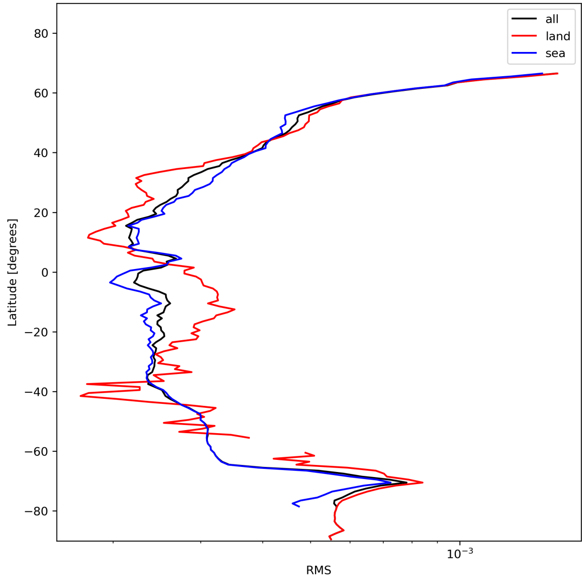
Figure 26: Zonal average of “RMS” for 2024-01-10 to 2024-01-11.
