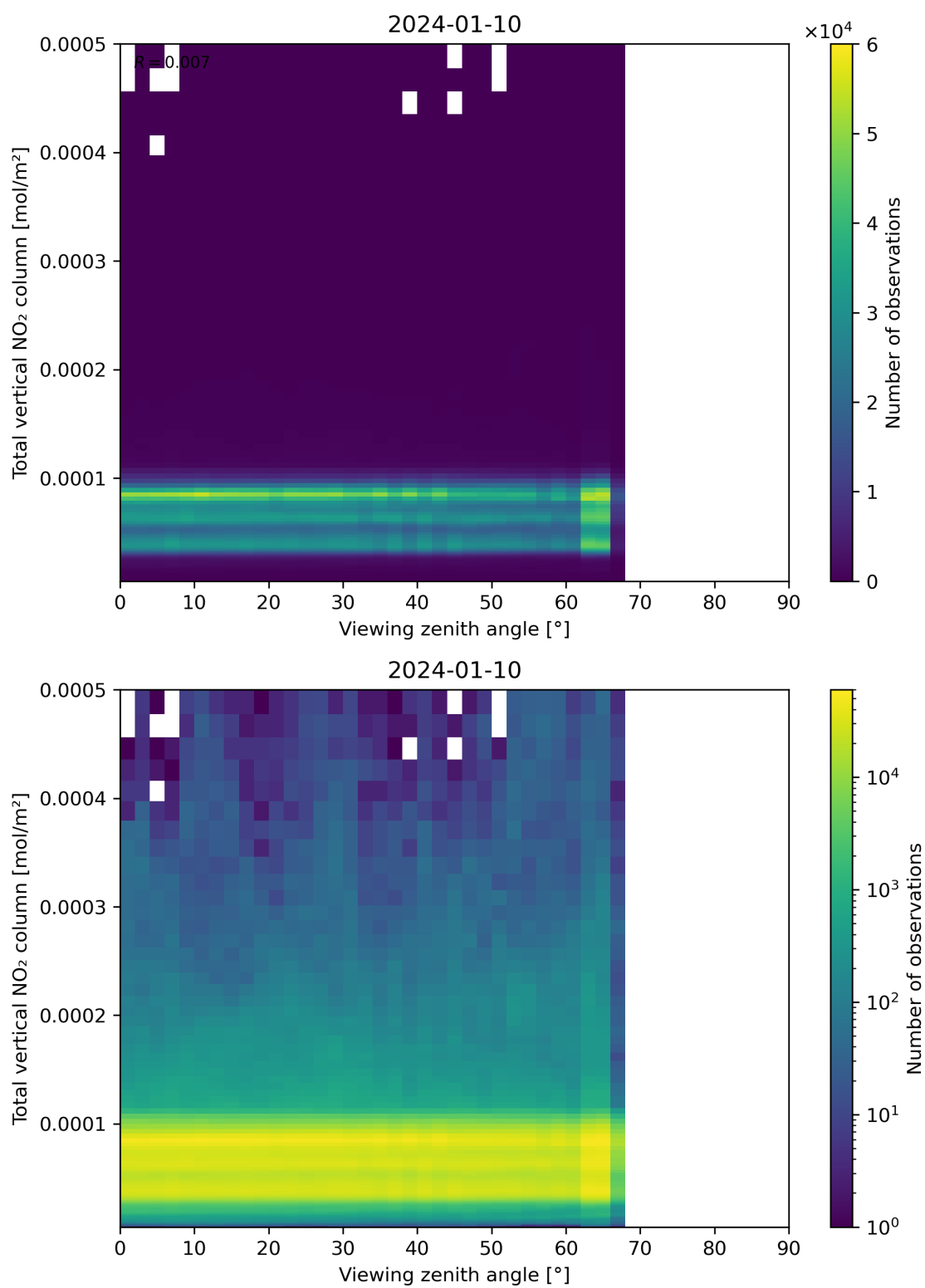
Figure 167: Scatter density plot of “Viewing zenith angle” against “Total vertical NO 2 column” for 2024-01-10 to 2024-01-11.
