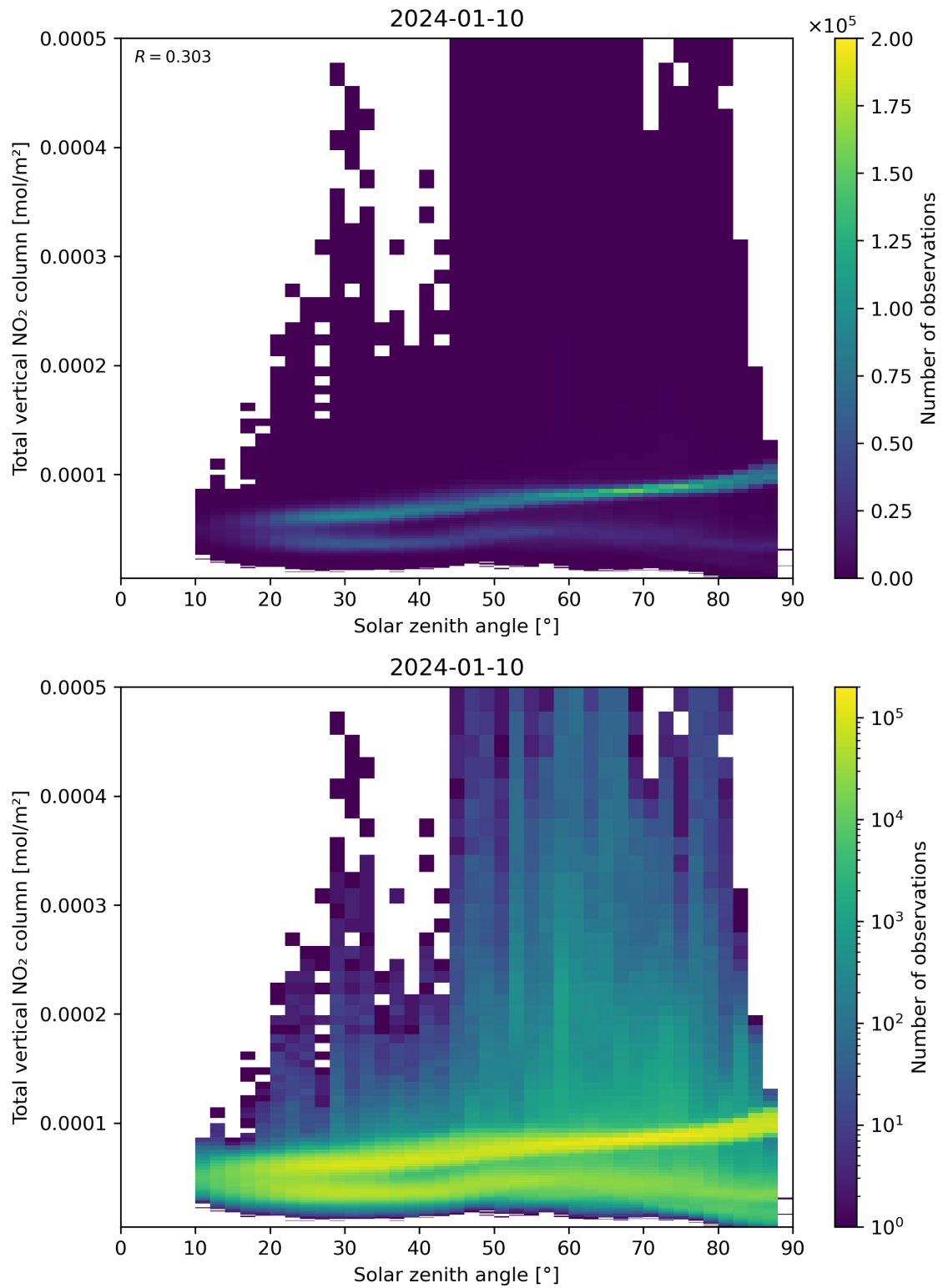
Figure 153: Scatter density plot of “Solar zenith angle” against “Total vertical NO 2 column” for 2024-01-10 to 2024-01-11.
