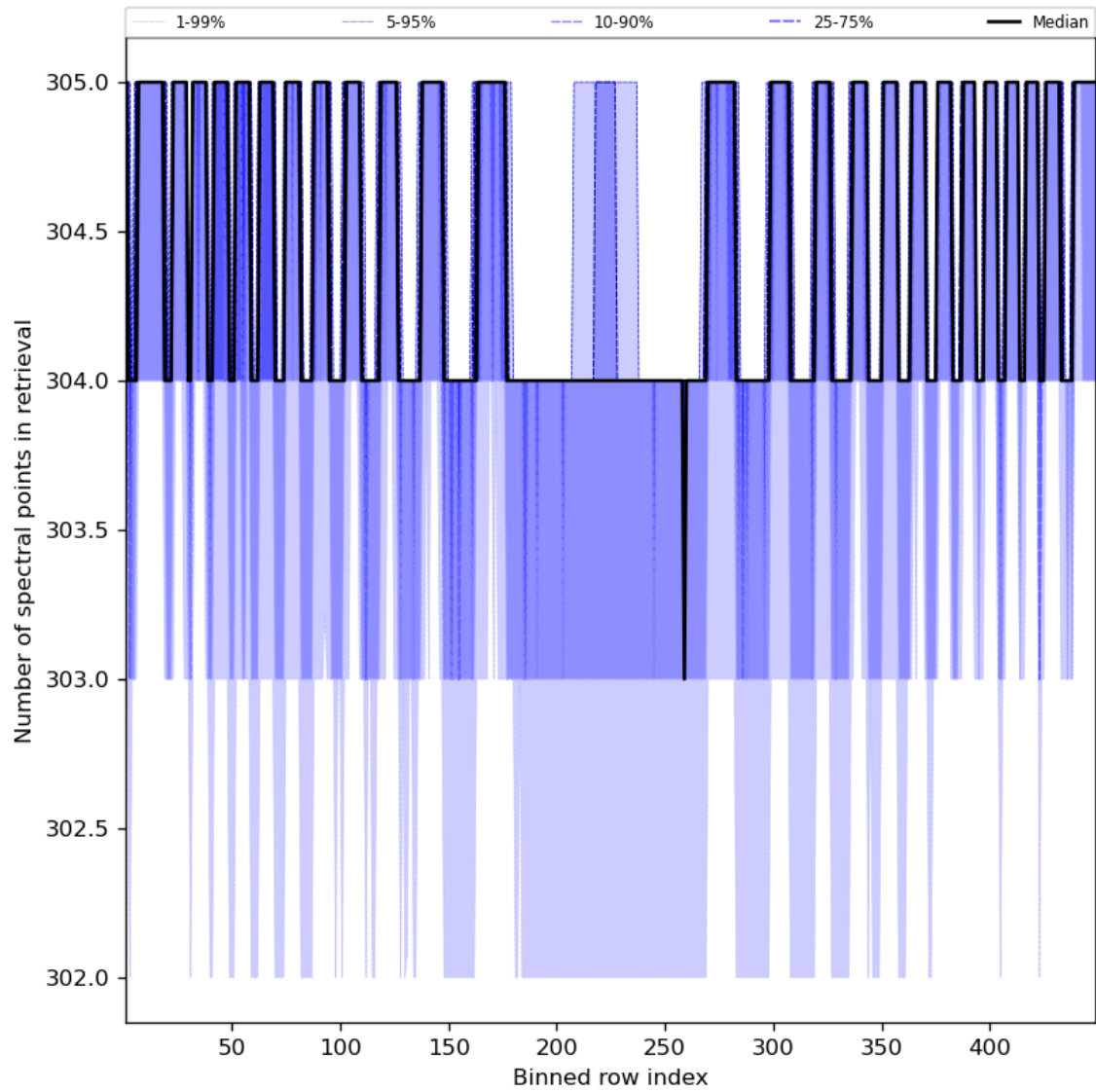
Figure 50: Along track statistics of “Number of spectral points in retrieval” for 2024-01-10 to 2024-01-11
