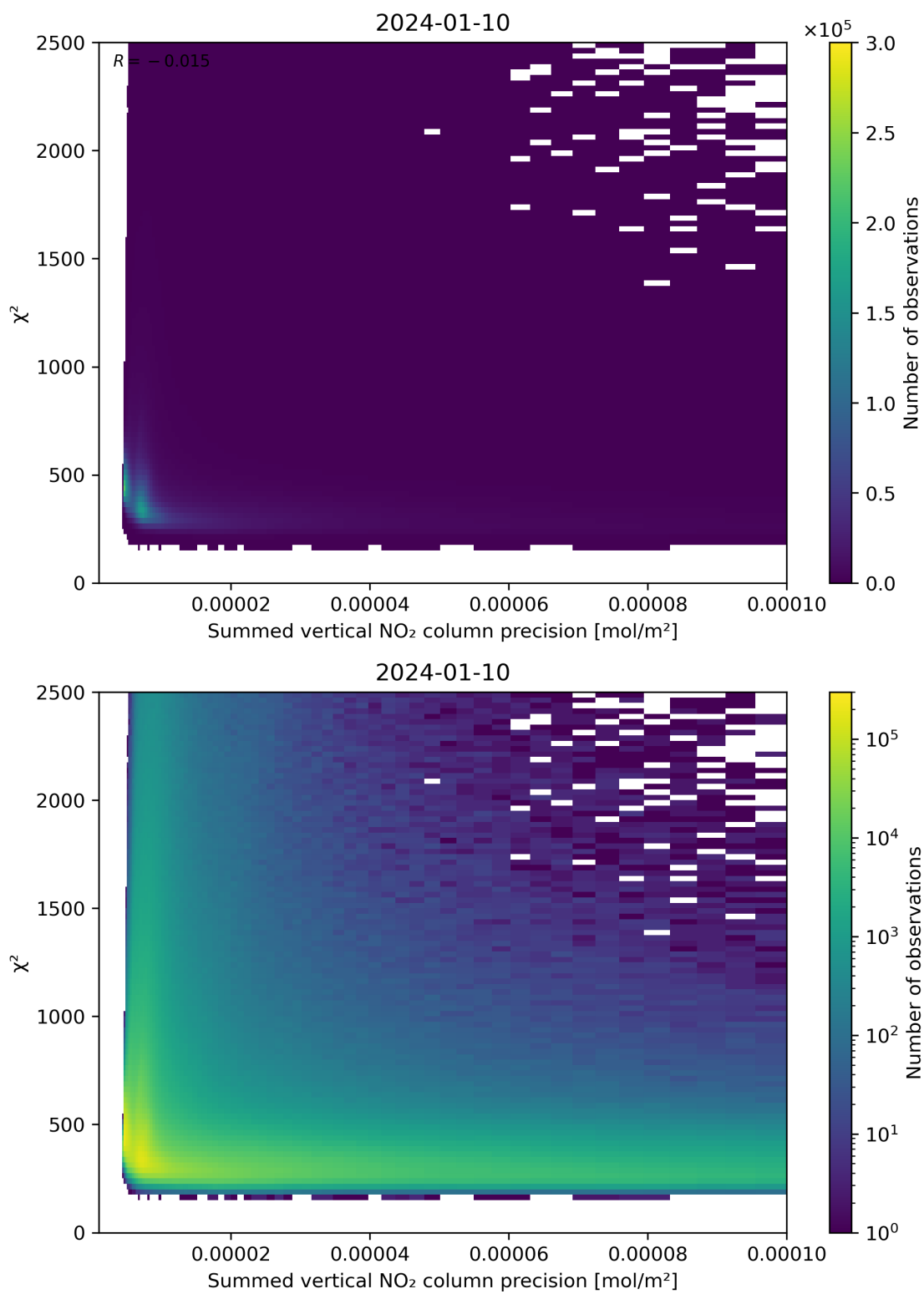
Figure 107: Scatter density plot of “Summed vertical NO 2 column precision” against “ \chi^2 ” for 2024-01-10 to 2024-01-11.
