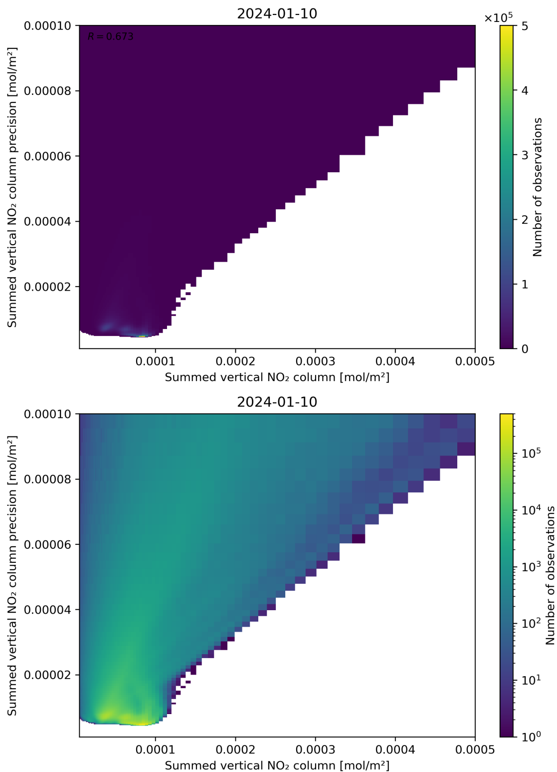
Figure 105: Scatter density plot of “Summed vertical NO 2 column” against “Summed vertical NO 2 column precision” for 2024-01-10 to 2024-01-11.
