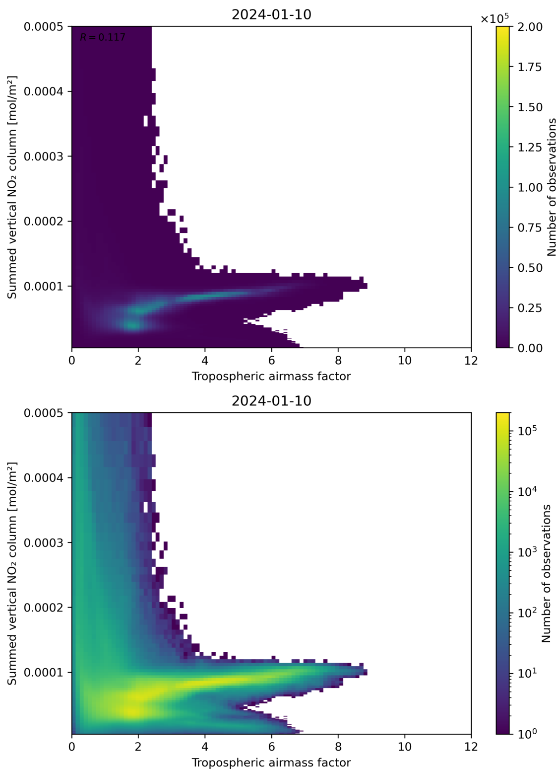
Figure 75: Scatter density plot of “Tropospheric air mass factor” against “Summed vertical NO 2 column” for 2024-01-10 to 2024-01-11.
