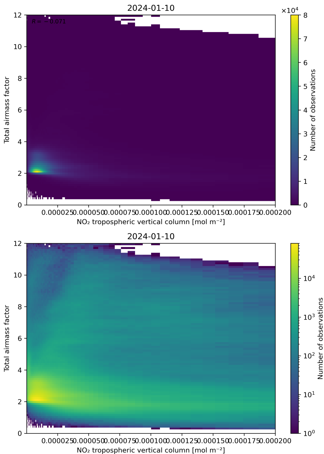
Figure 122: Scatter density plot of “NO 2 tropospheric vertical column” against “Total air mass factor” for 2024-01-10 to 2024-01-11.
