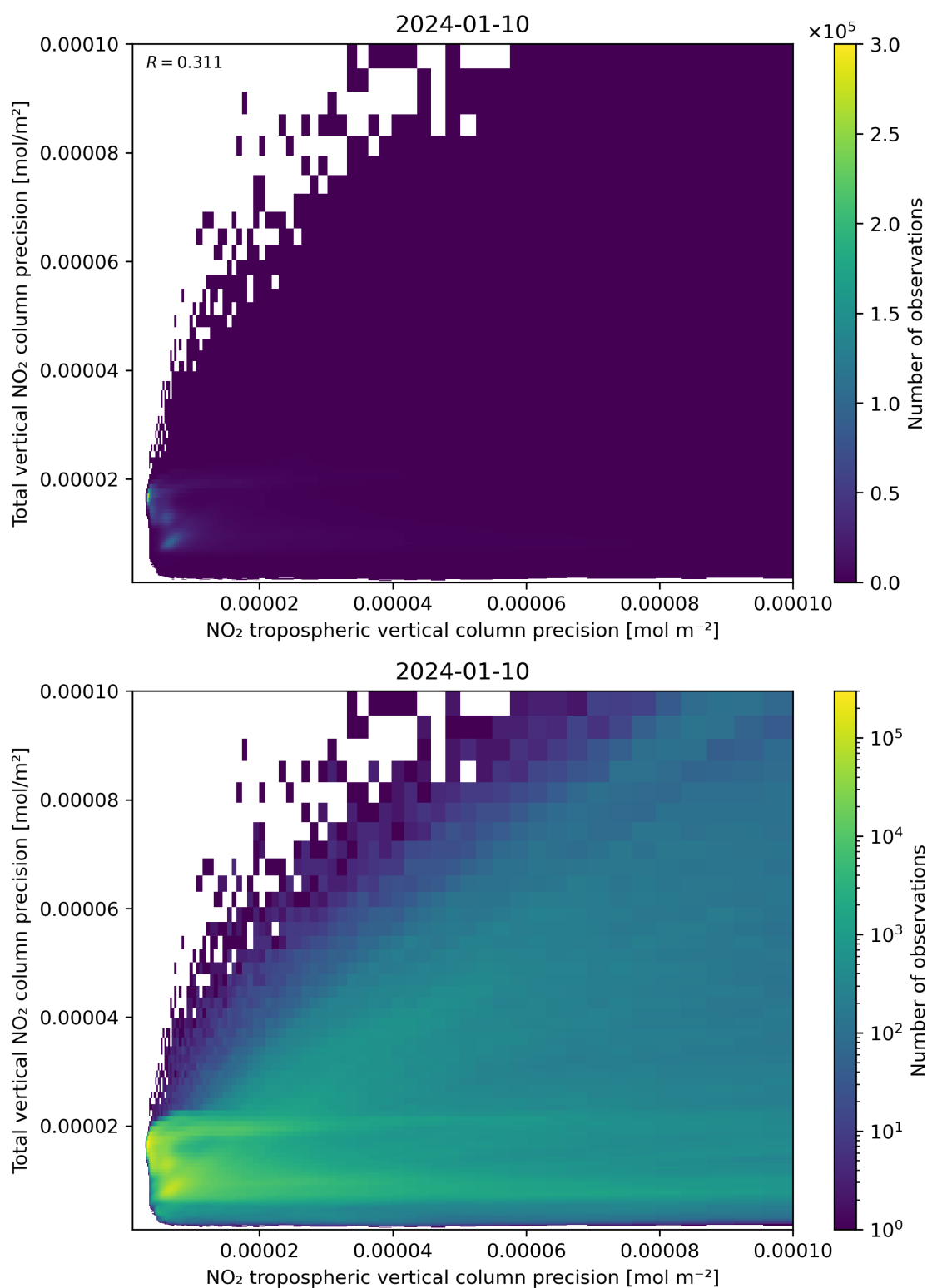
Figure 139: Scatter density plot of “NO 2 tropospheric vertical column precision” against “Total vertical NO 2 column precision” for 2024-01-10 to 2024-01-11.
