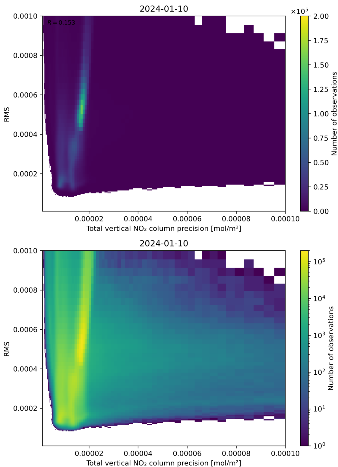
Figure 119: Scatter density plot of “Total vertical NO 2 column precision” against “RMS” for 2024-01-10 to 2024-01-11.
