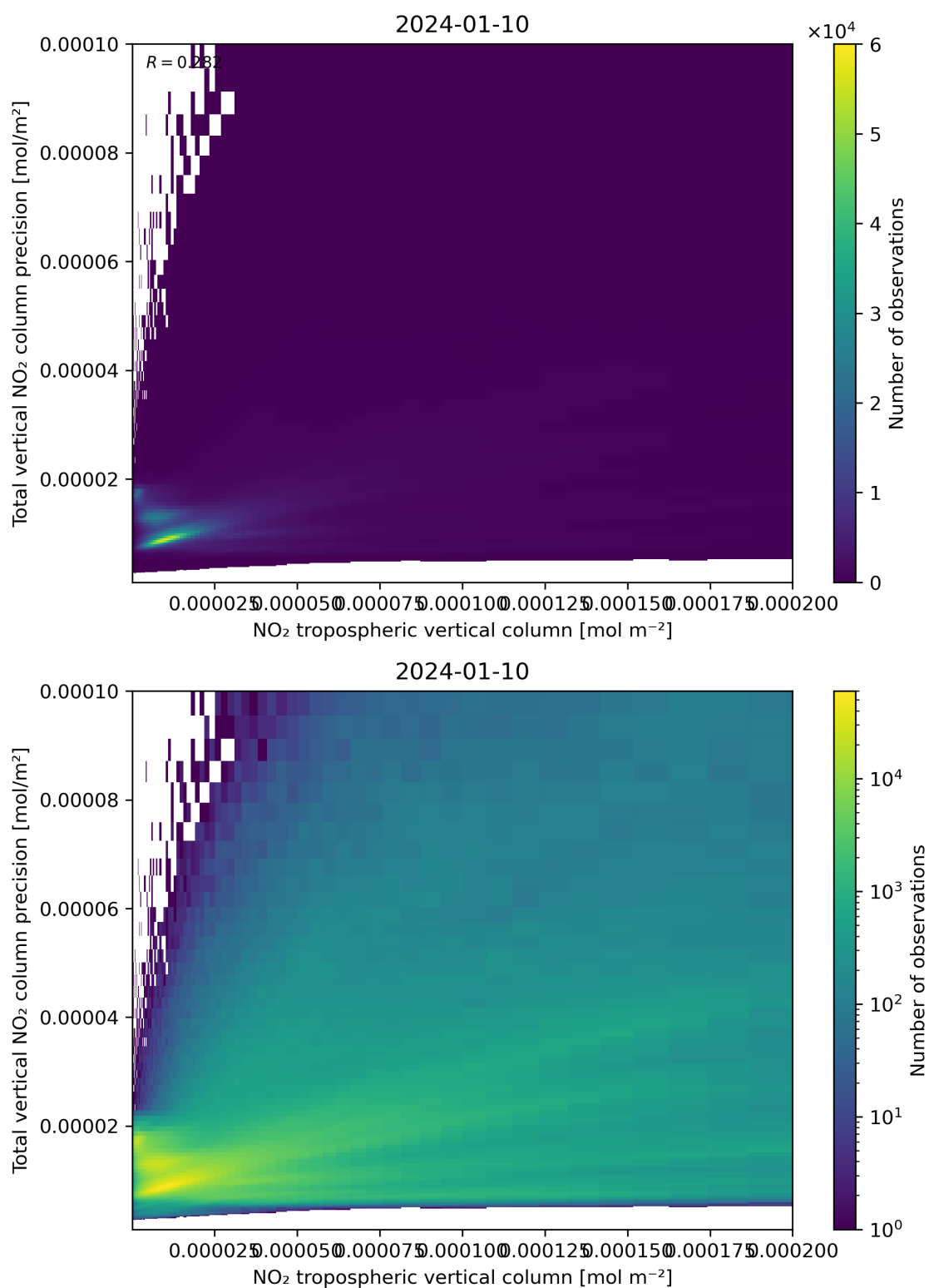
Figure 129: Scatter density plot of “NO 2 tropospheric vertical column” against “Total vertical NO 2 column precision” for 2024-01-10 to 2024-01-11.
