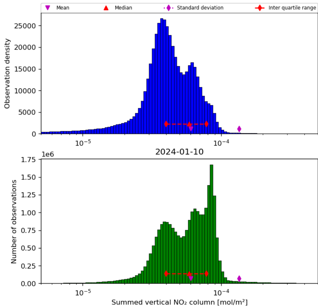
Figure 40: Histogram of “Summed vertical NO 2 column” for 2024-01-10 to 2024-01-11
