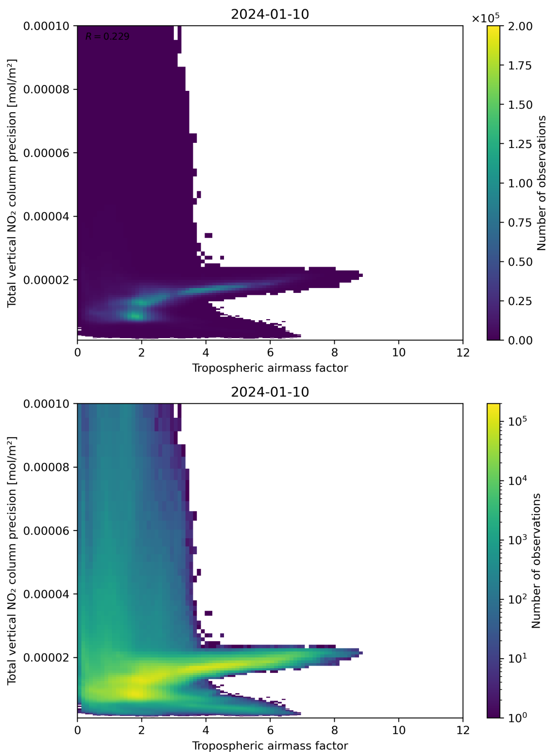
Figure 78: Scatter density plot of “Tropospheric air mass factor” against “Total vertical NO 2 column precision” for 2024-01-10 to 2024-01-11.
