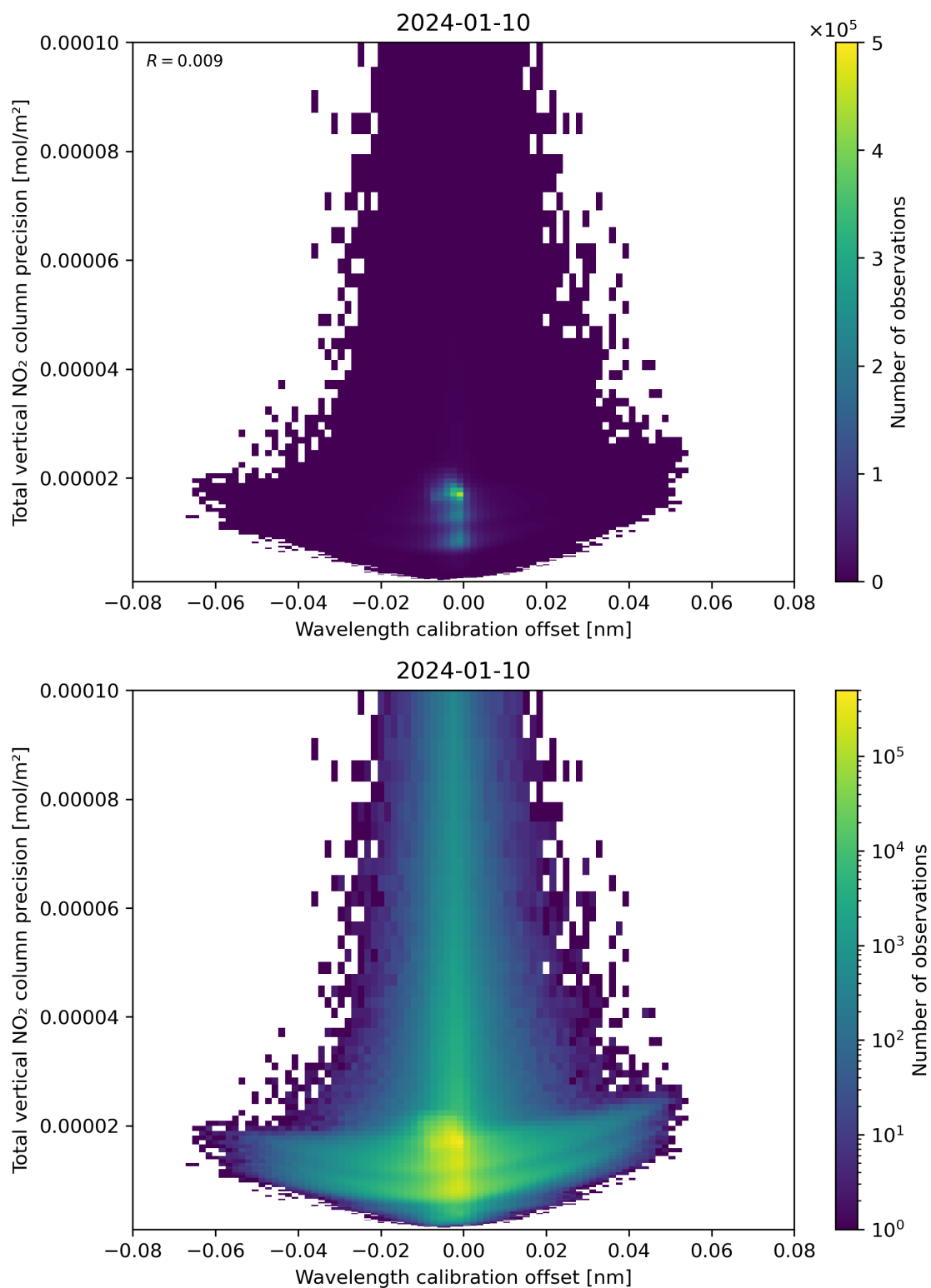
Figure 180: Scatter density plot of “Wavelength calibration offset” against “Total vertical NO 2 column precision” for 2024-01-10 to 2024-01-11.
