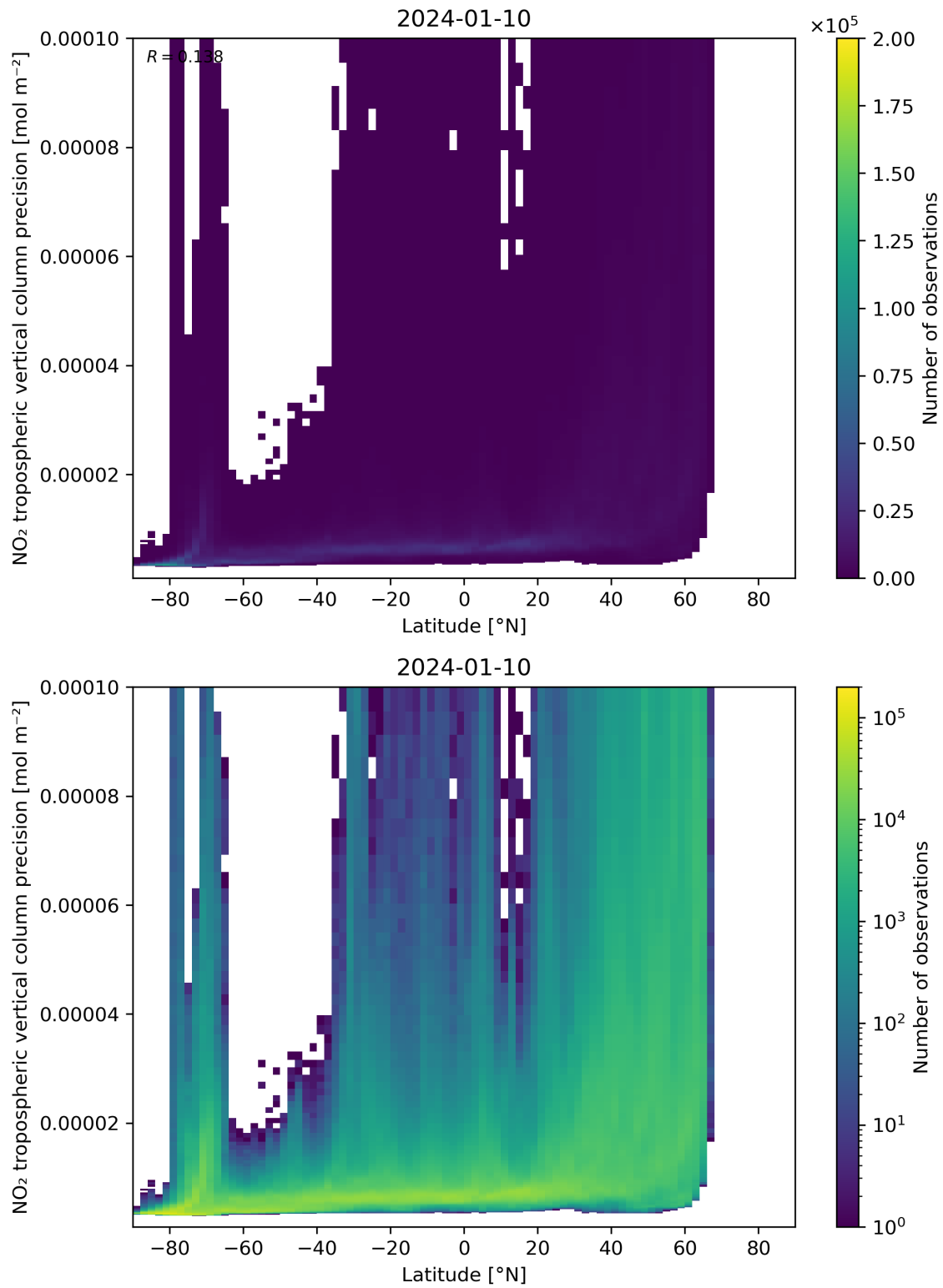
Figure 93: Scatter density plot of “Latitude” against “NO 2 tropospheric vertical column precision” for 2024-01-10 to 2024-01-11.
