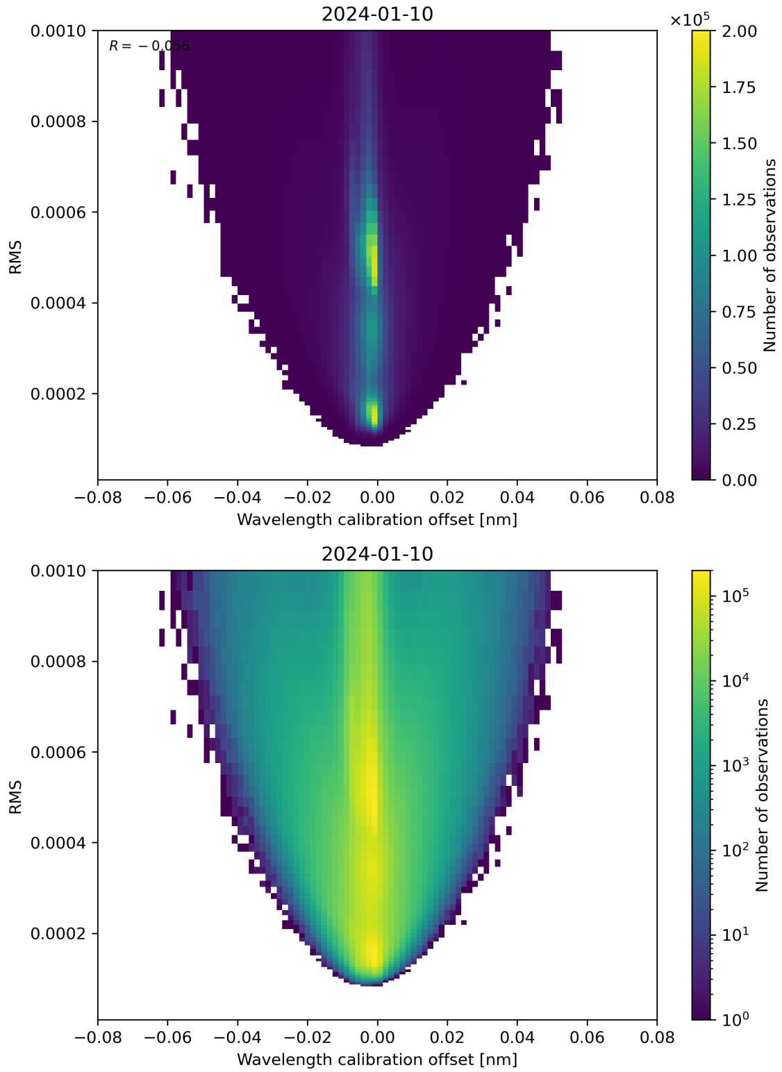
Figure 181: Scatter density plot of “Wavelength calibration offset” against “RMS” for 2024-01-10 to 2024-01-11.
