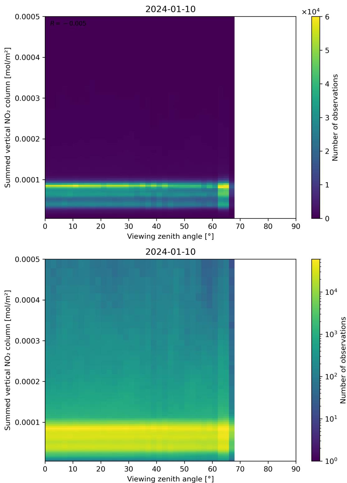
Figure 165: Scatter density plot of “Viewing zenith angle” against “Summed vertical NO 2 column” for 2024-01-10 to 2024-01-11.
