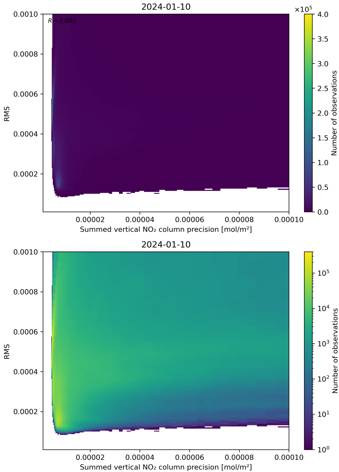
Figure 108: Scatter density plot of “Summed vertical NO 2 column precision” against “RMS” for 2024-01-10 to 2024-01-11.
