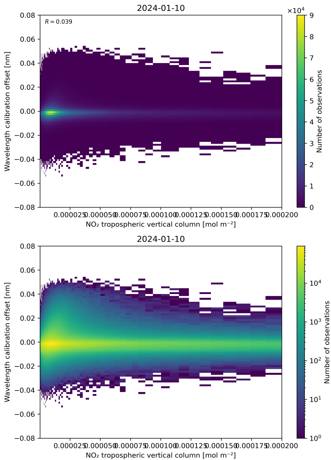
Figure 143: Scatter density plot of “NO 2 tropospheric vertical column” against “Wavelength calibration offset” for 2024-01-10 to 2024-01-11.
