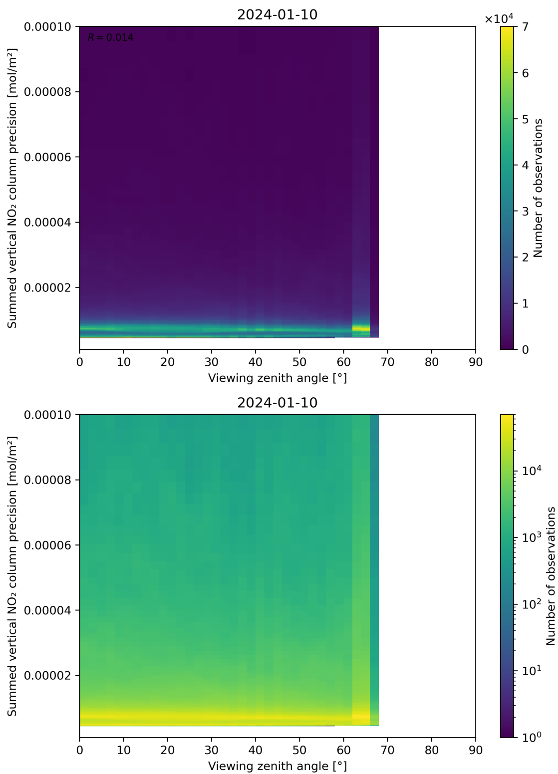
Figure 166: Scatter density plot of “Viewing zenith angle” against “Summed vertical NO 2 column precision” for 2024-01-10 to 2024-01-11.
