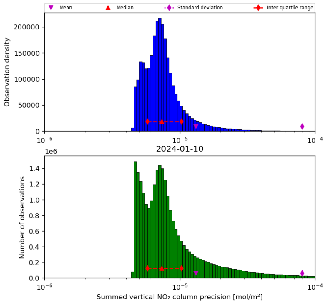
Figure 41: Histogram of “Summed vertical NO 2 column precision” for 2024-01-10 to 2024-01-11
