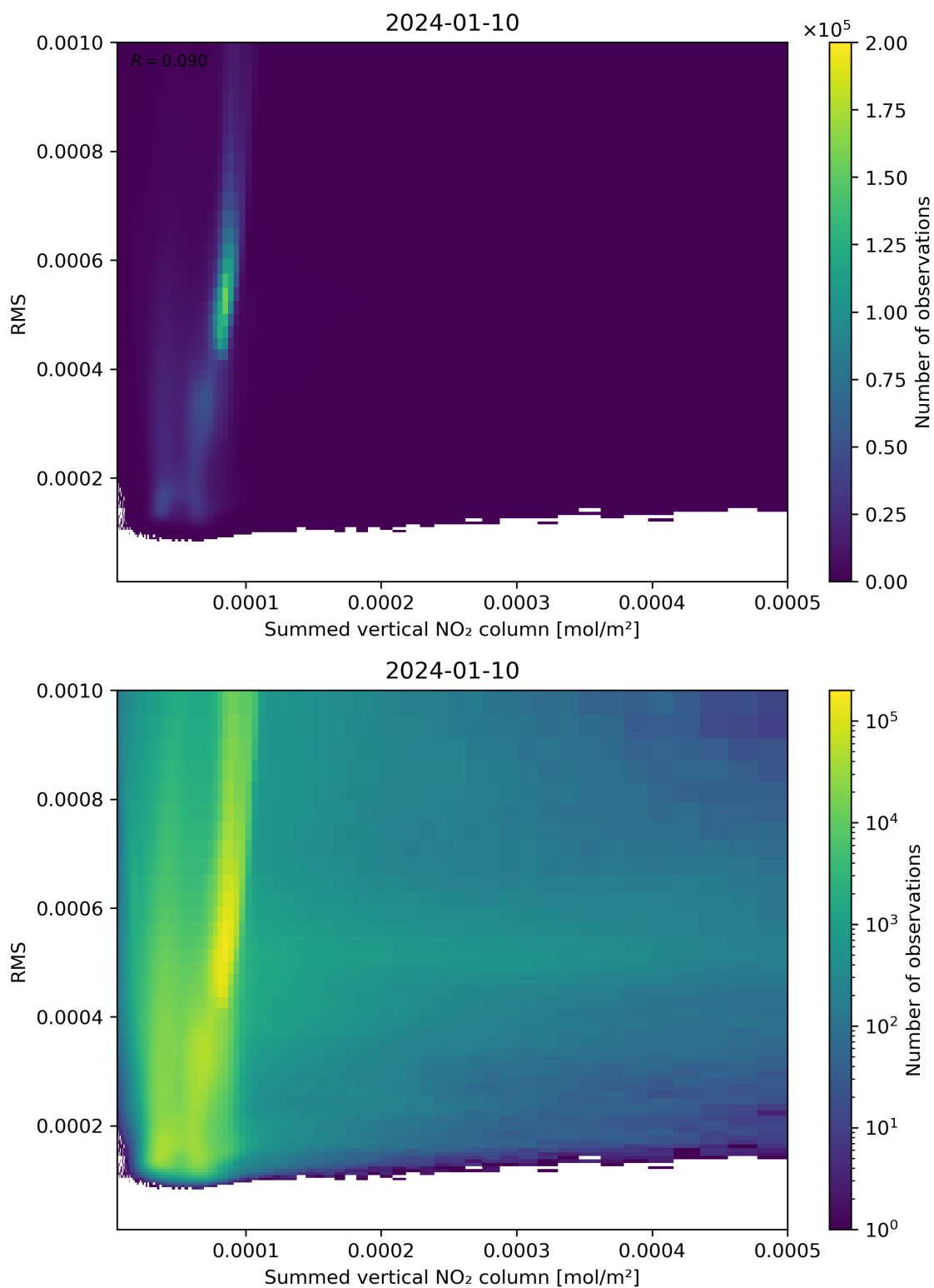
Figure 109: Scatter density plot of “Summed vertical NO 2 column” against “RMS” for 2024-01-10 to 2024-01-11.
