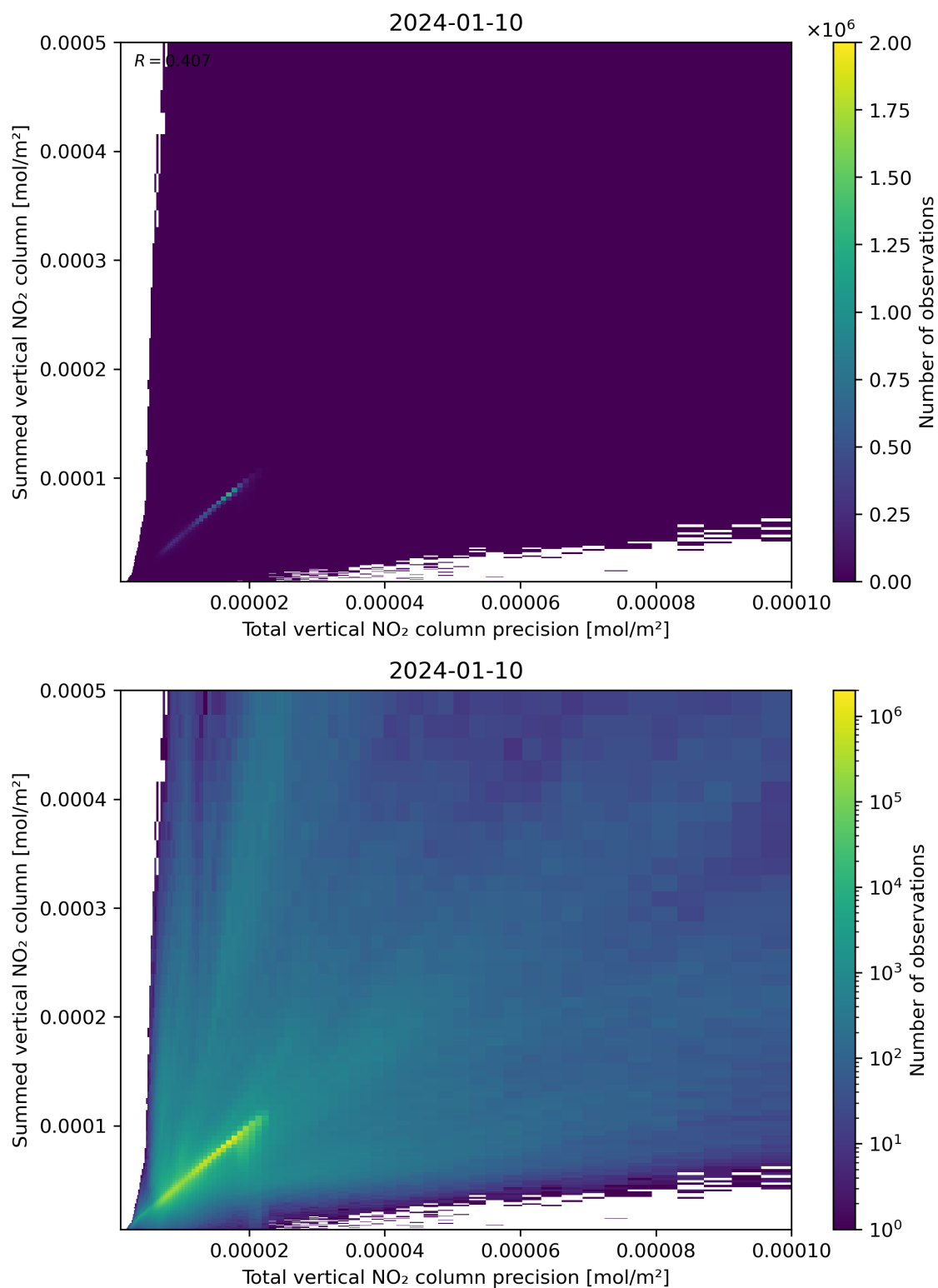
Figure 117: Scatter density plot of “Total vertical NO 2 column precision” against “Summed vertical NO 2 column” for 2024-01-10 to 2024-01-11.
