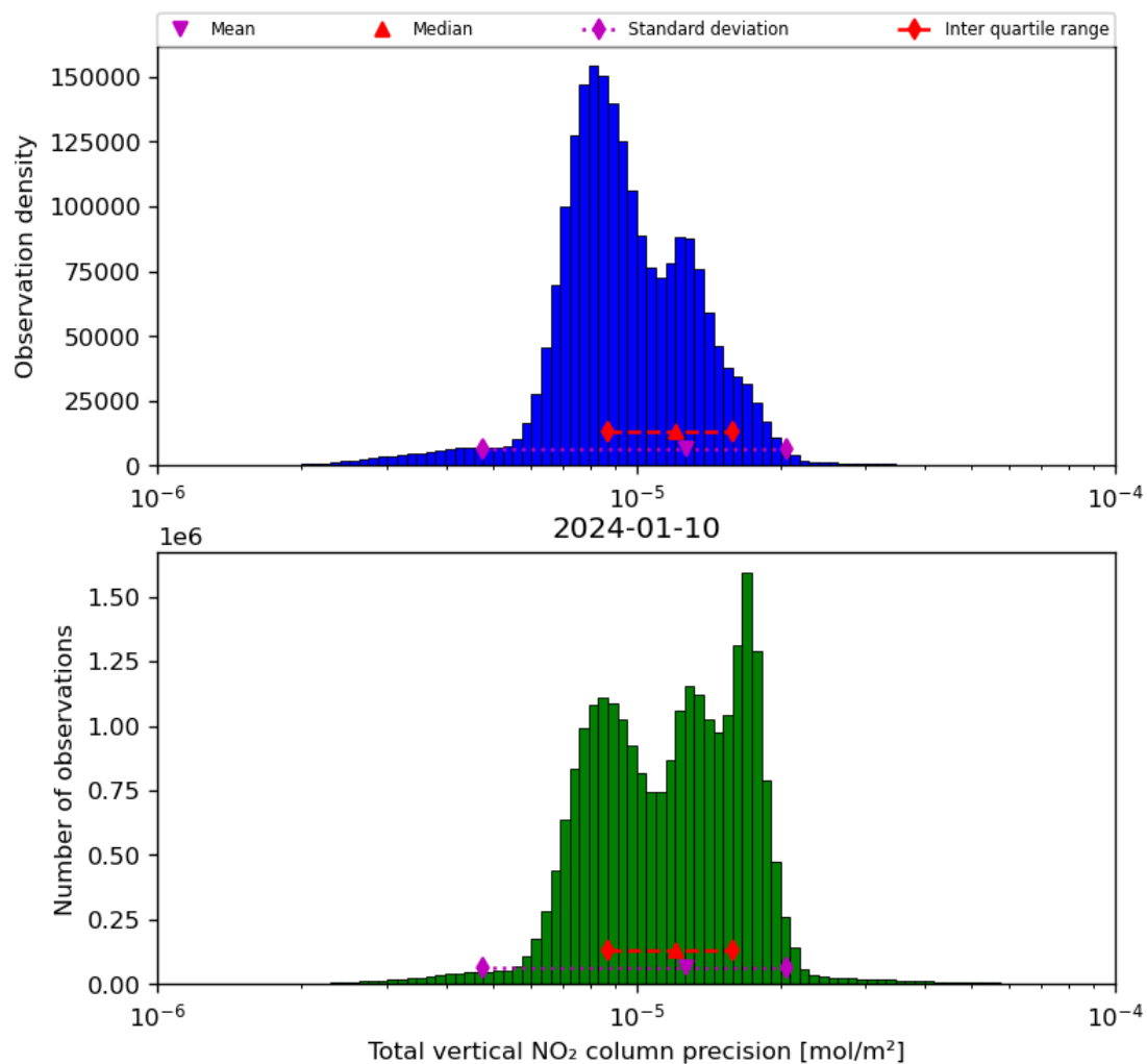
Figure 39: Histogram of “Total vertical NO 2 column precision” for 2024-01-10 to 2024-01-11
