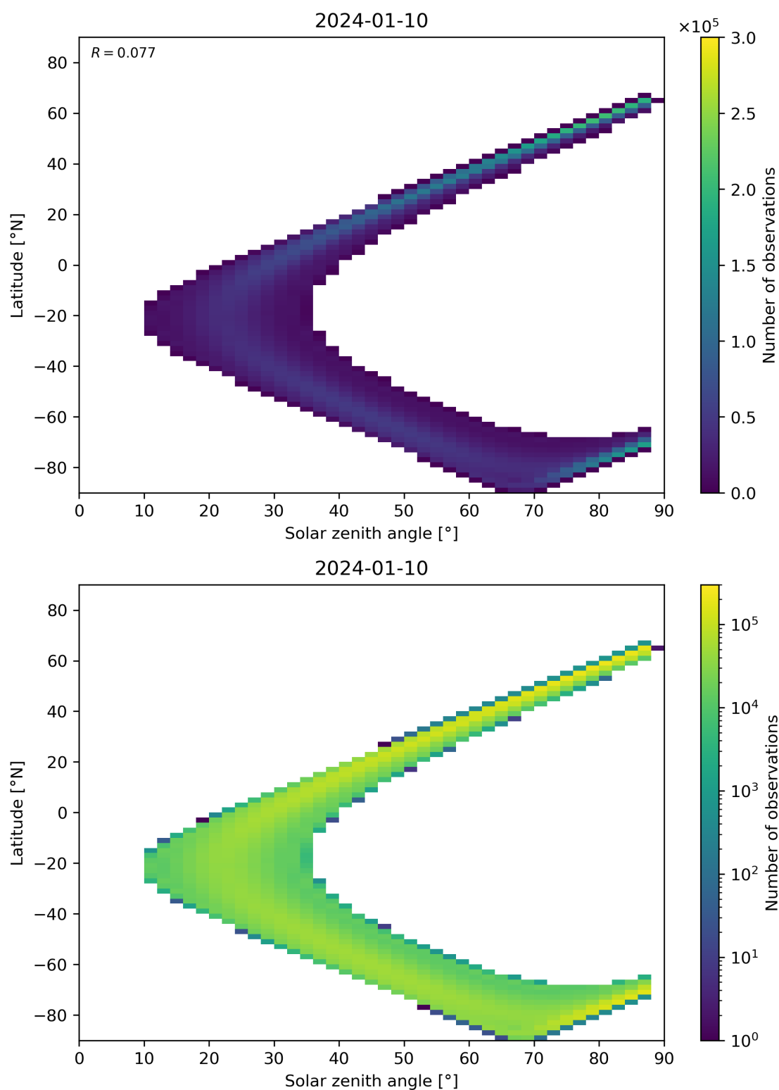
Figure 149: Scatter density plot of “Solar zenith angle” against “Latitude” for 2024-01-10 to 2024-01-11.
