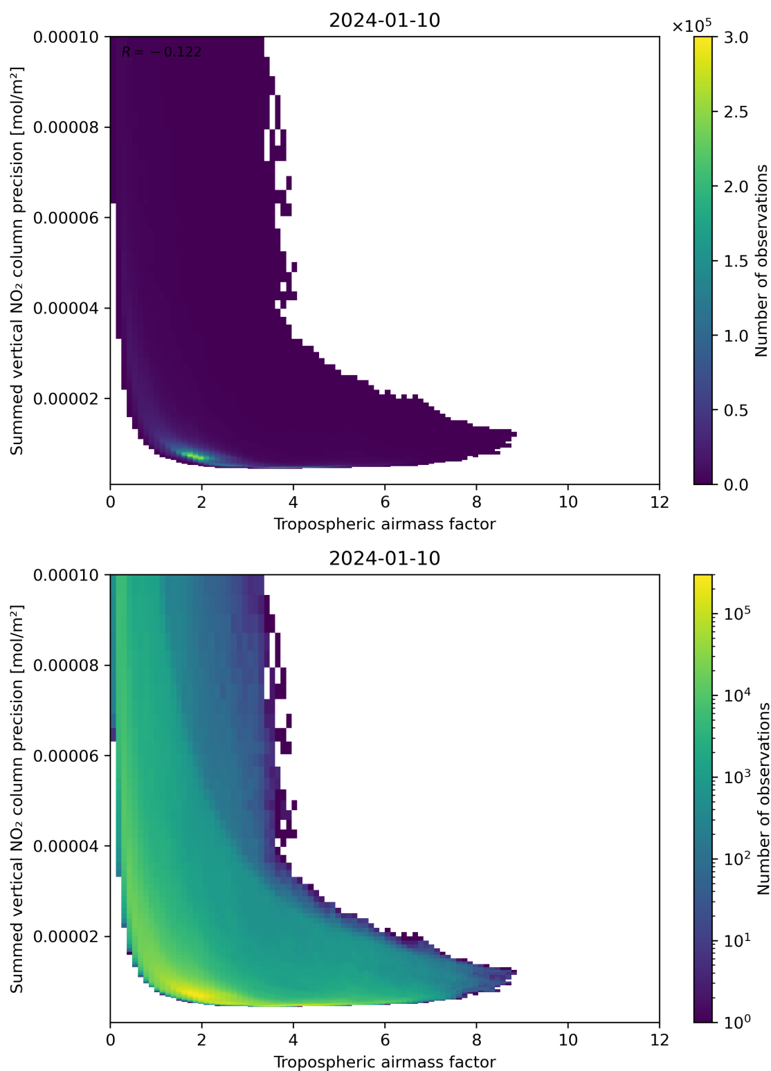
Figure 76: Scatter density plot of “Tropospheric air mass factor” against “Summed vertical NO 2 column precision” for 2024-01-10 to 2024-01-11.
