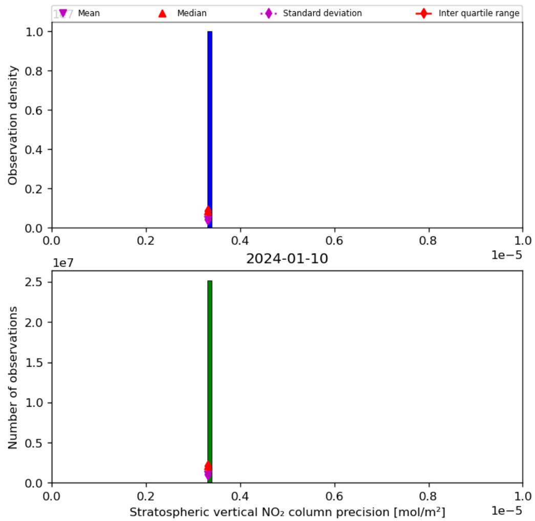
Figure 37: Histogram of “Stratospheric vertical NO 2 column precision” for 2024-01-10 to 2024-01-11
