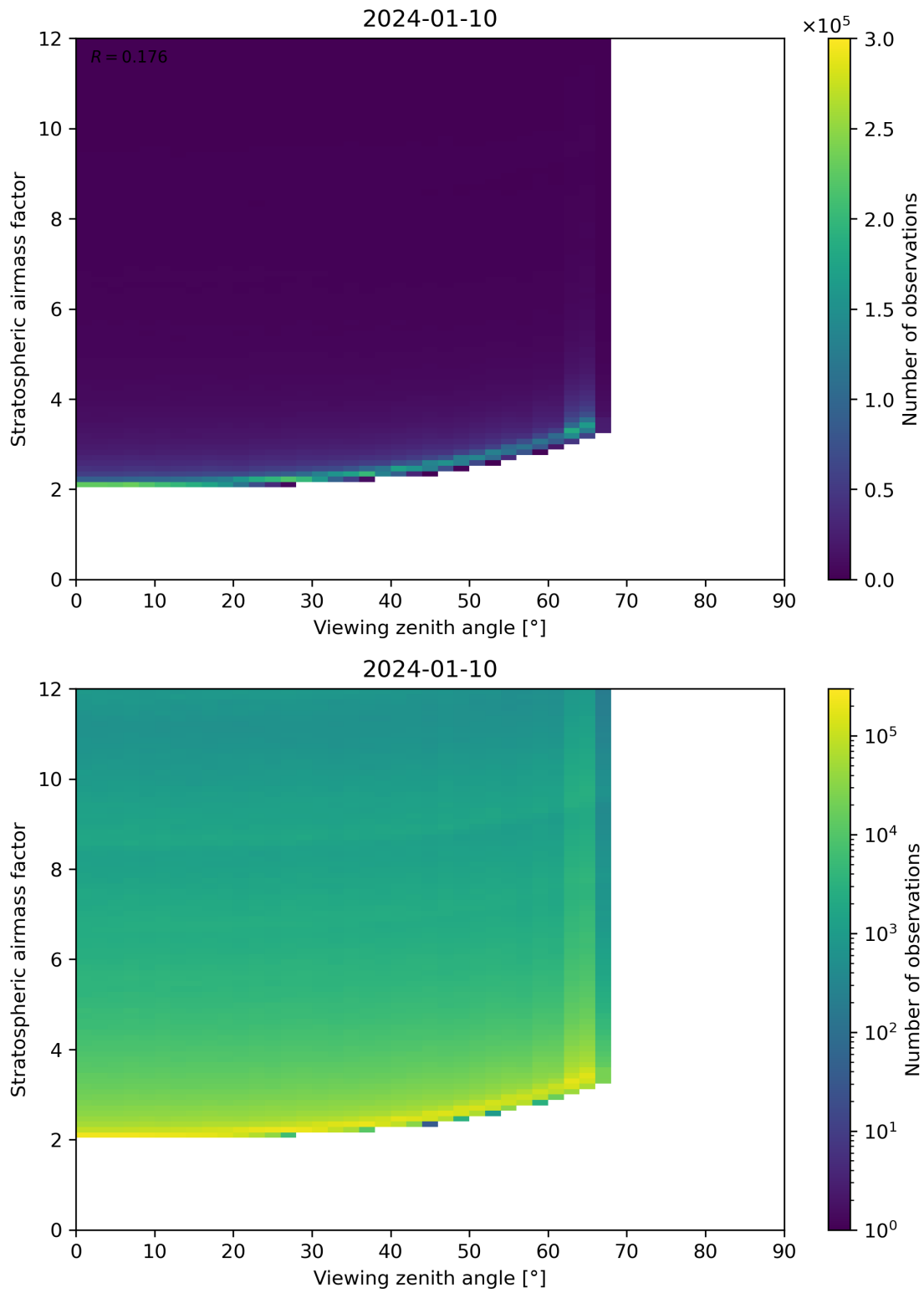
Figure 159: Scatter density plot of “Viewing zenith angle” against “Stratospheric airmass factor” for 2024-01-10 to 2024-01-11.
