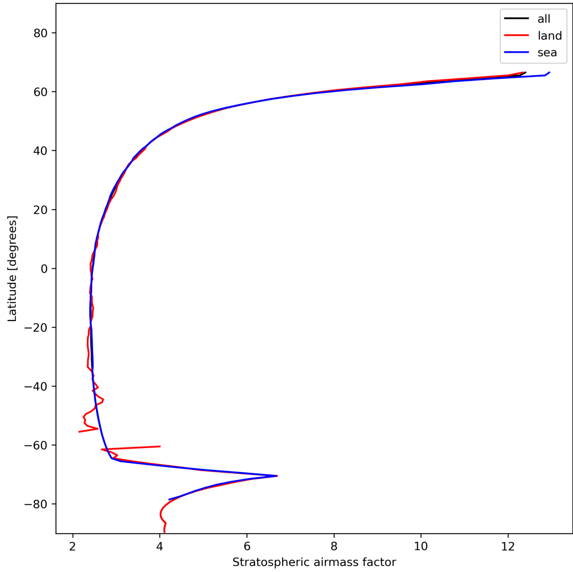
Figure 27: Zonal average of “Stratospheric air mass factor” for 2024-01-10 to 2024-01-11.
