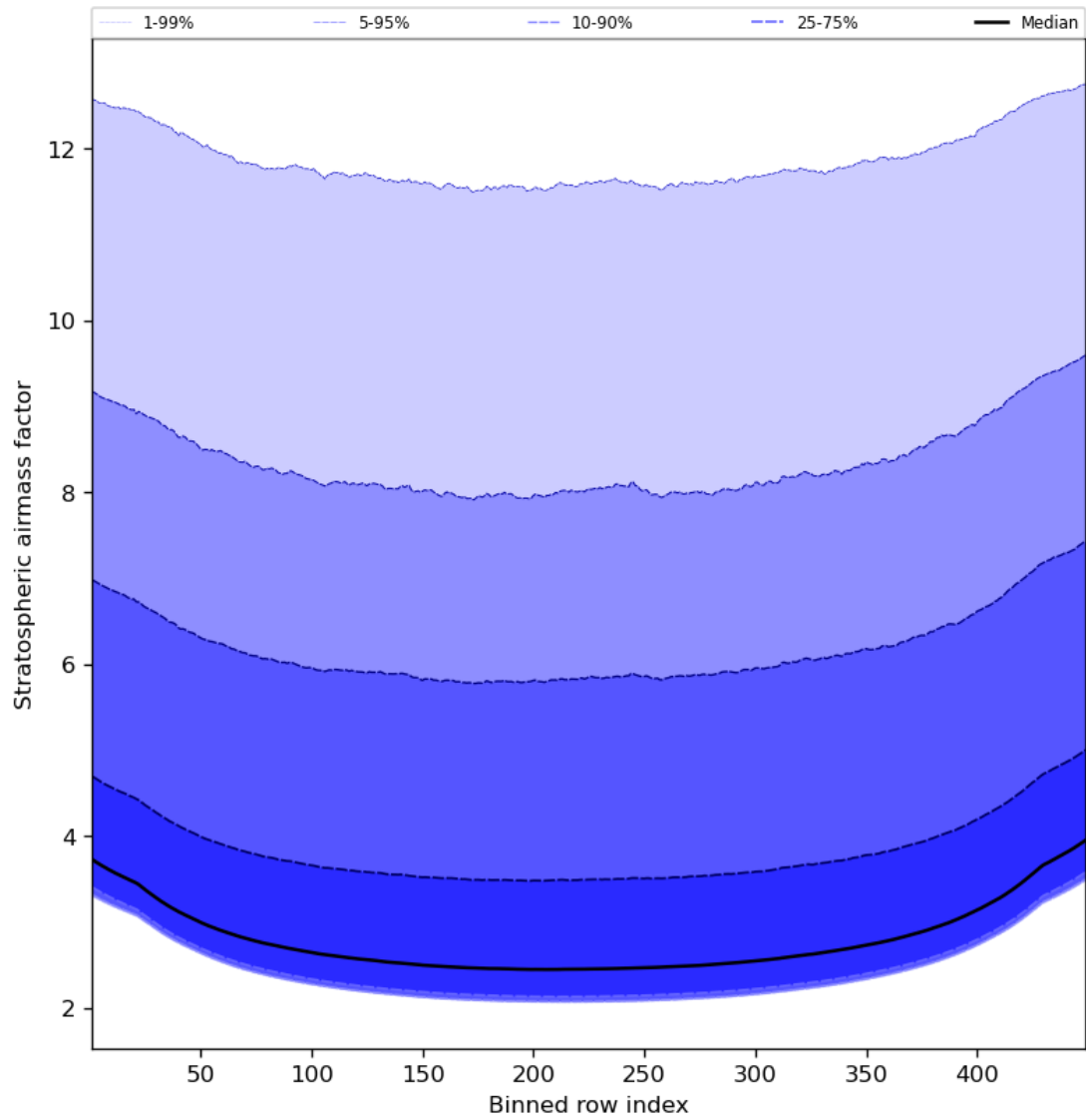
Figure 61: Along track statistics of “Stratospheric airmass factor” for 2024-01-10 to 2024-01-11
