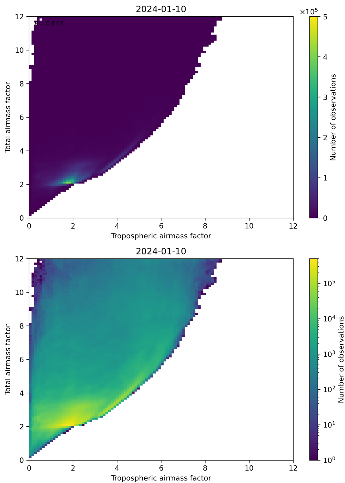
Figure 72: Scatter density plot of “Tropospheric airmass factor” against “Total airmass factor” for 2024-01-10 to 2024-01-11.
