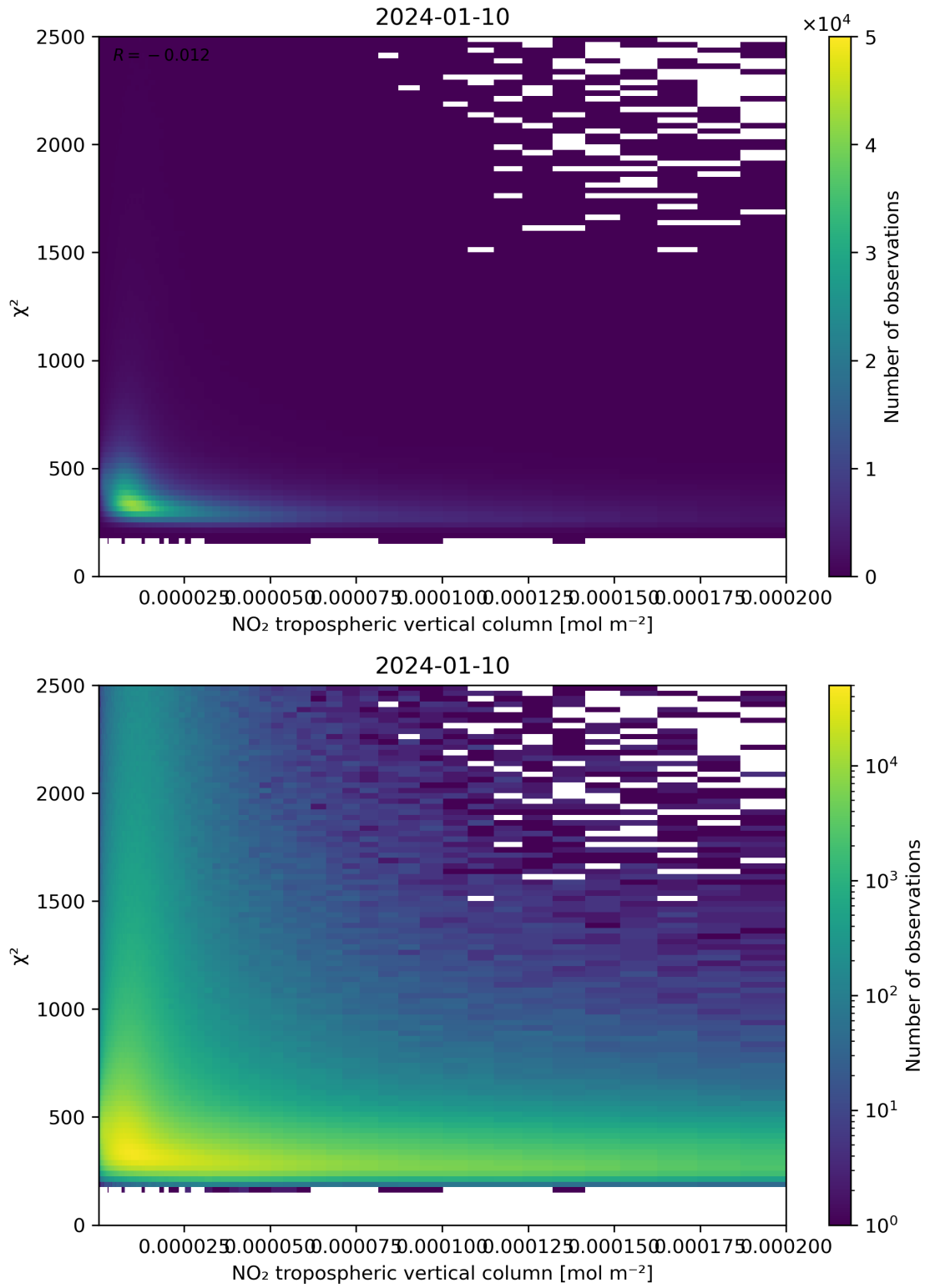
Figure 124: Scatter density plot of “NO 2 tropospheric vertical column” against “ \chi^2 ” for 2024-01-10 to 2024-01-11.
