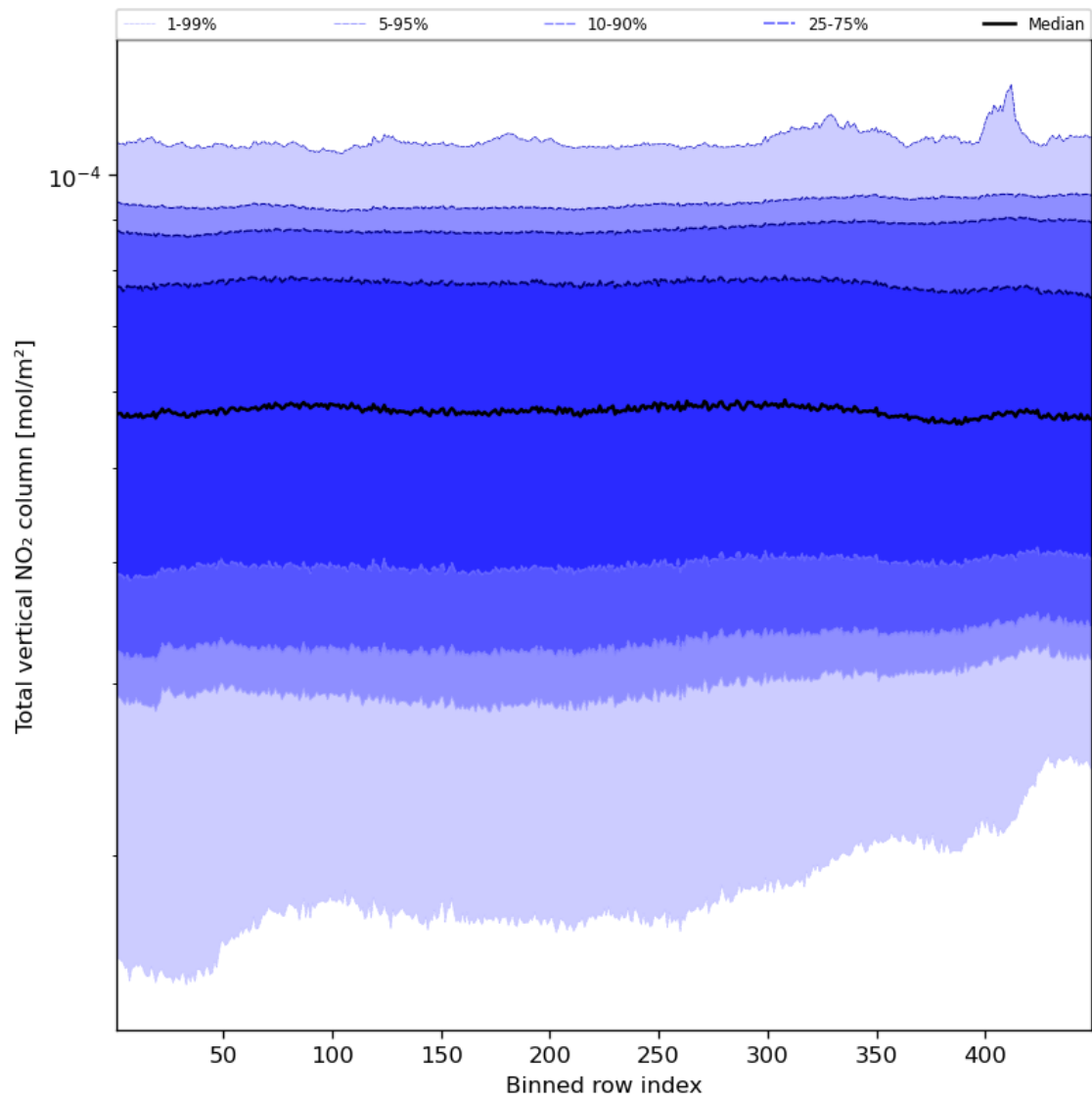
Figure 55: Along track statistics of “Total vertical NO 2 column” for 2024-01-10 to 2024-01-11
