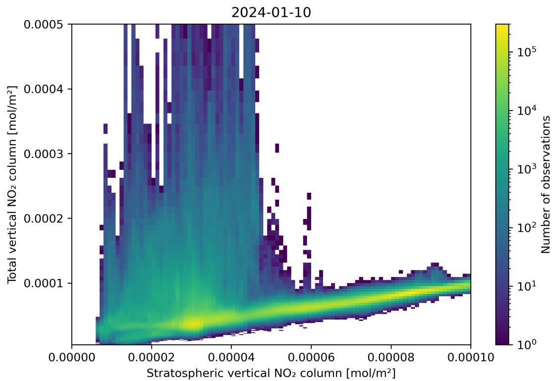
Figure 100: Scatter density plot of “Stratospheric vertical NO 2 column” against “Total vertical NO 2 column” for 2024-01-10 to 2024-01-11.
