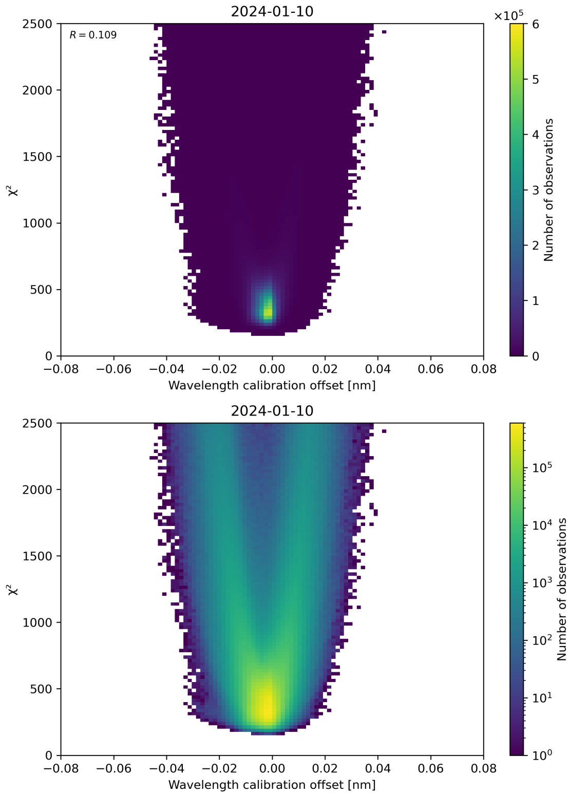
Figure 175: Scatter density plot of “Wavelength calibration offset” against “ \chi^2 ” for 2024-01-10 to 2024-01-11.
