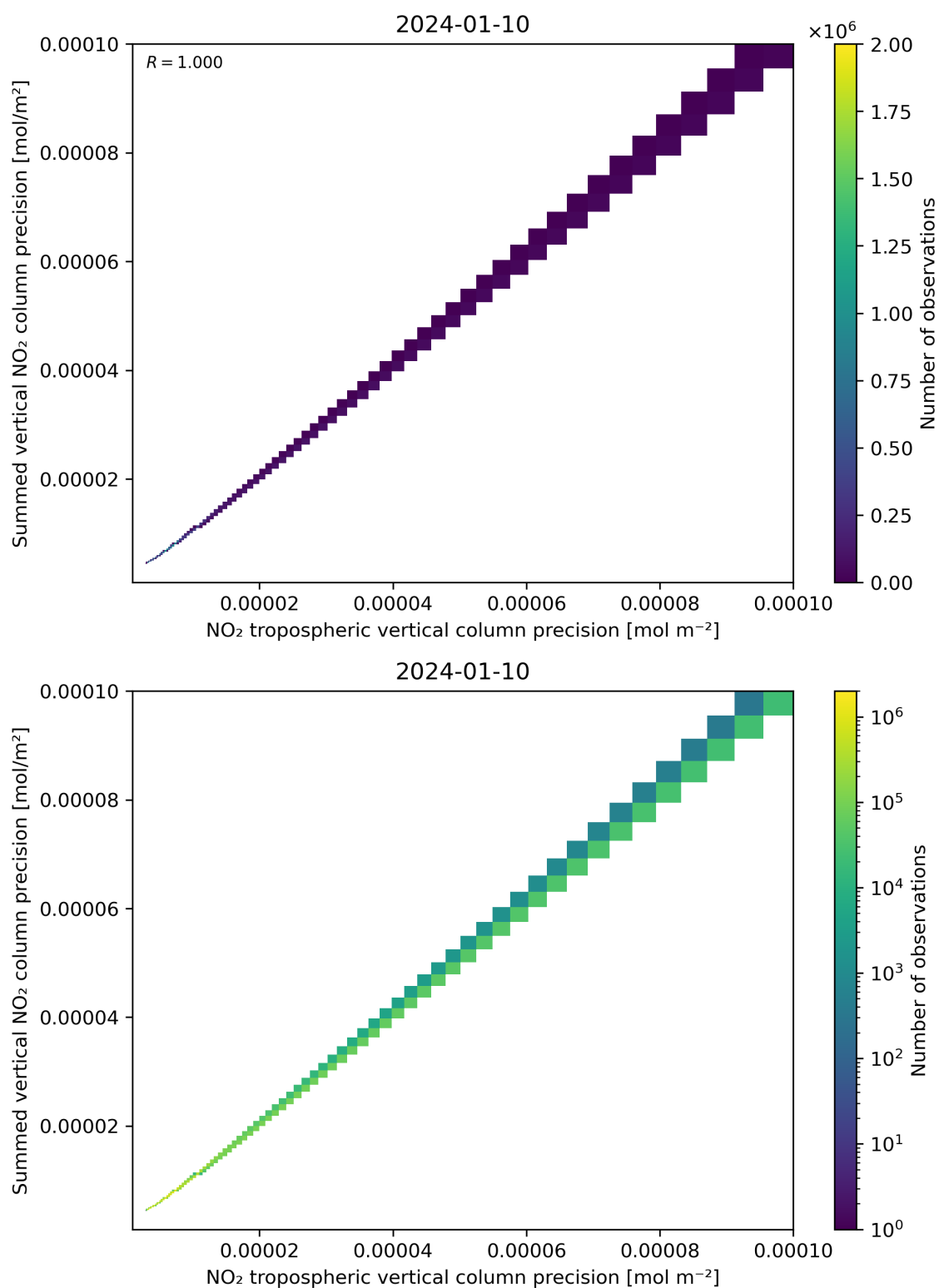
Figure 137: Scatter density plot of “NO 2 tropospheric vertical column precision” against “Summed vertical NO 2 column precision” for 2024-01-10 to 2024-01-11.
