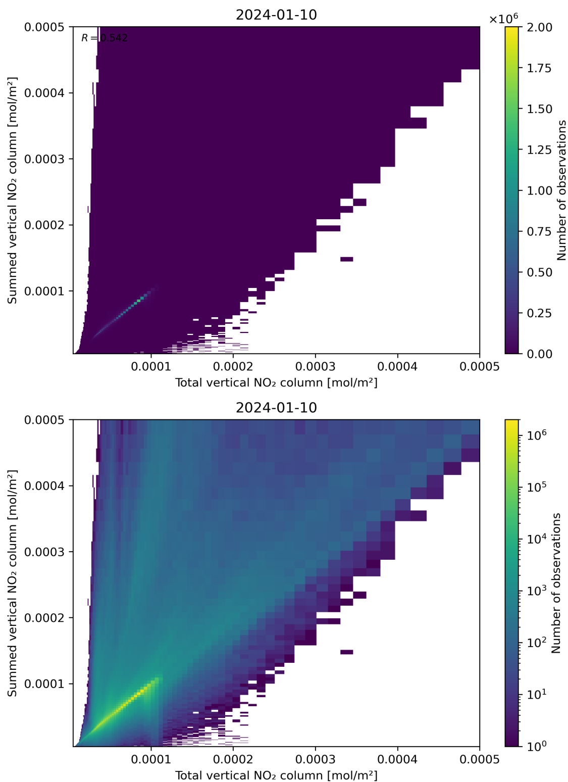
Figure 112: Scatter density plot of “Total vertical NO 2 column” against “Summed vertical NO 2 column” for 2024-01-10 to 2024-01-11.
