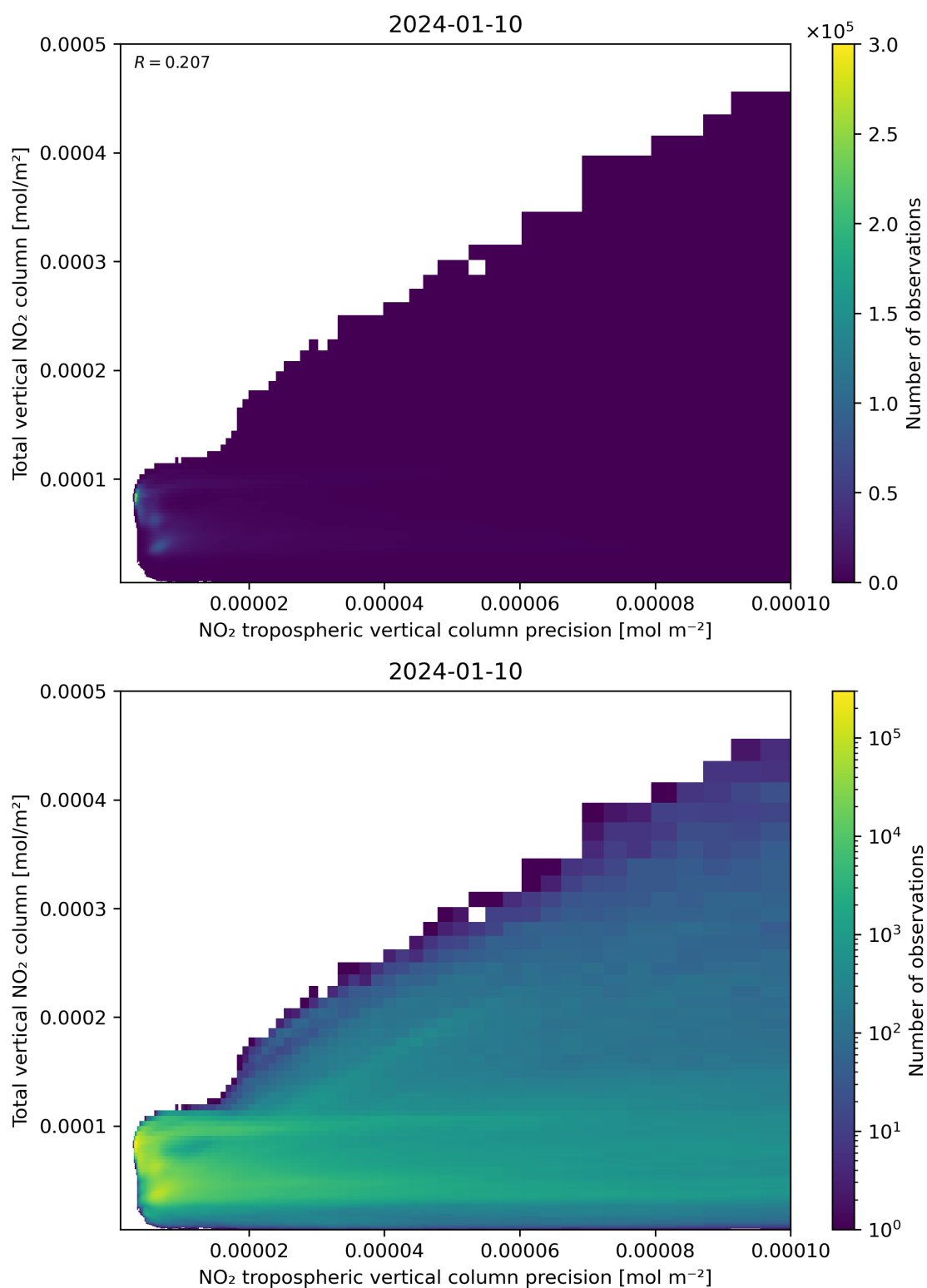
Figure 138: Scatter density plot of “NO 2 tropospheric vertical column precision” against “Total vertical NO 2 column” for 2024-01-10 to 2024-01-11.
