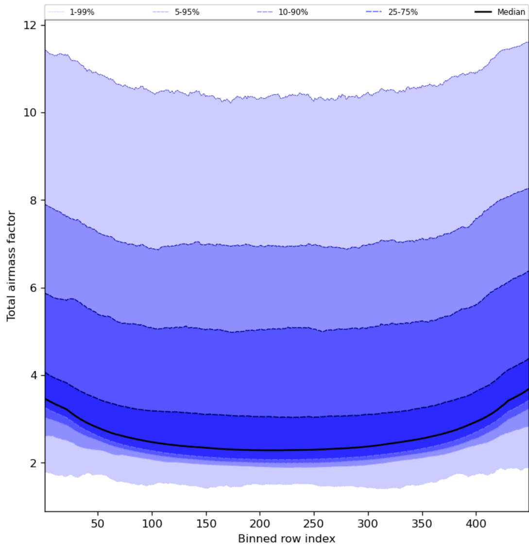
Figure 49: Along track statistics of “Total airmass factor” for 2024-01-10 to 2024-01-11
