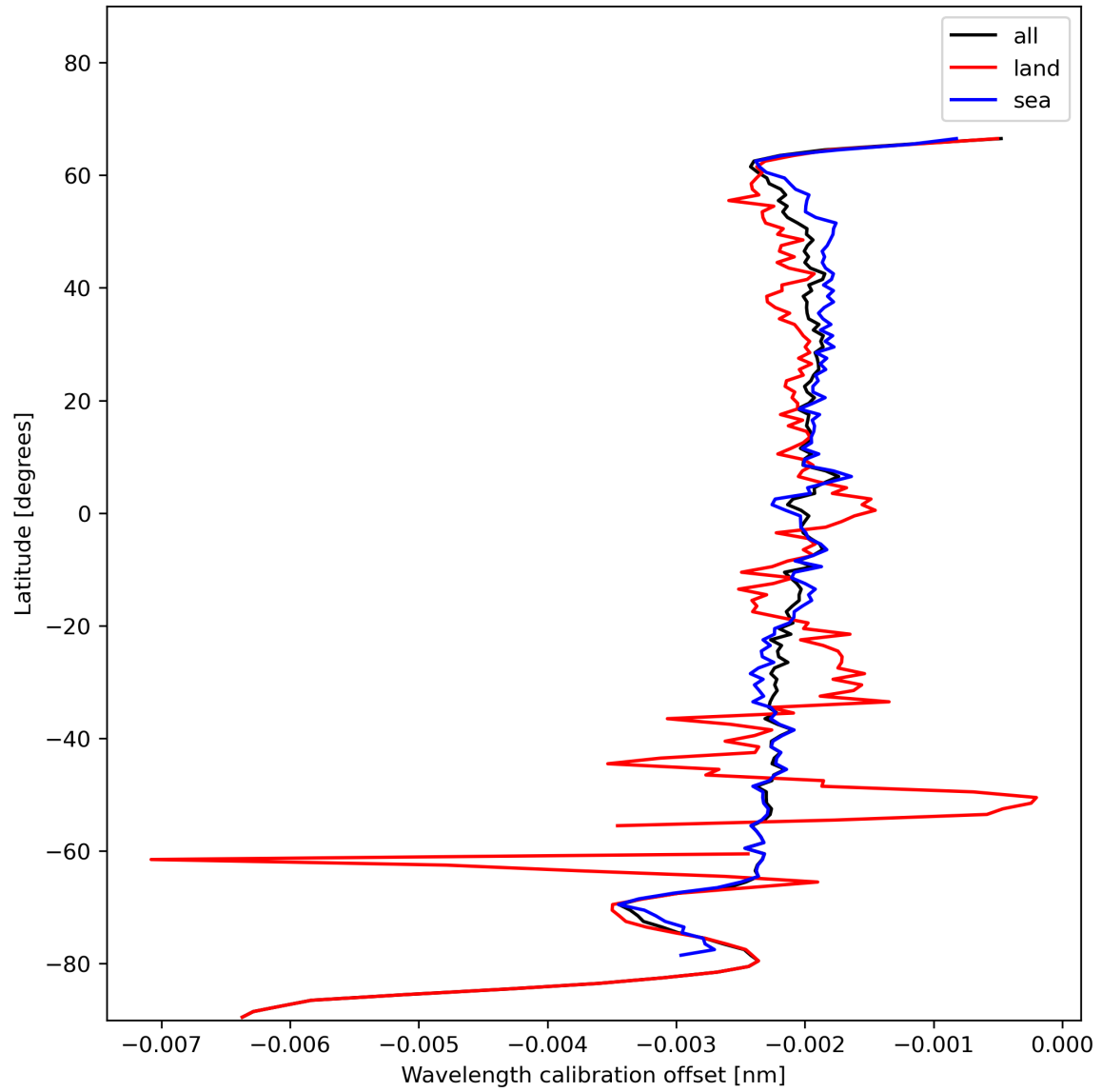
Figure 18: Zonal average of “Wavelength calibration offset” for 2024-01-10 to 2024-01-11.
