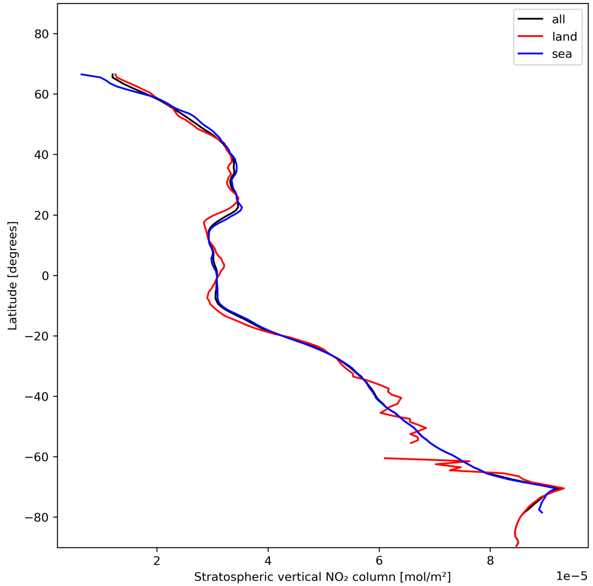
Figure 19: Zonal average of “Stratospheric vertical NO 2 column” for 2024-01-10 to 2024-01-11.
