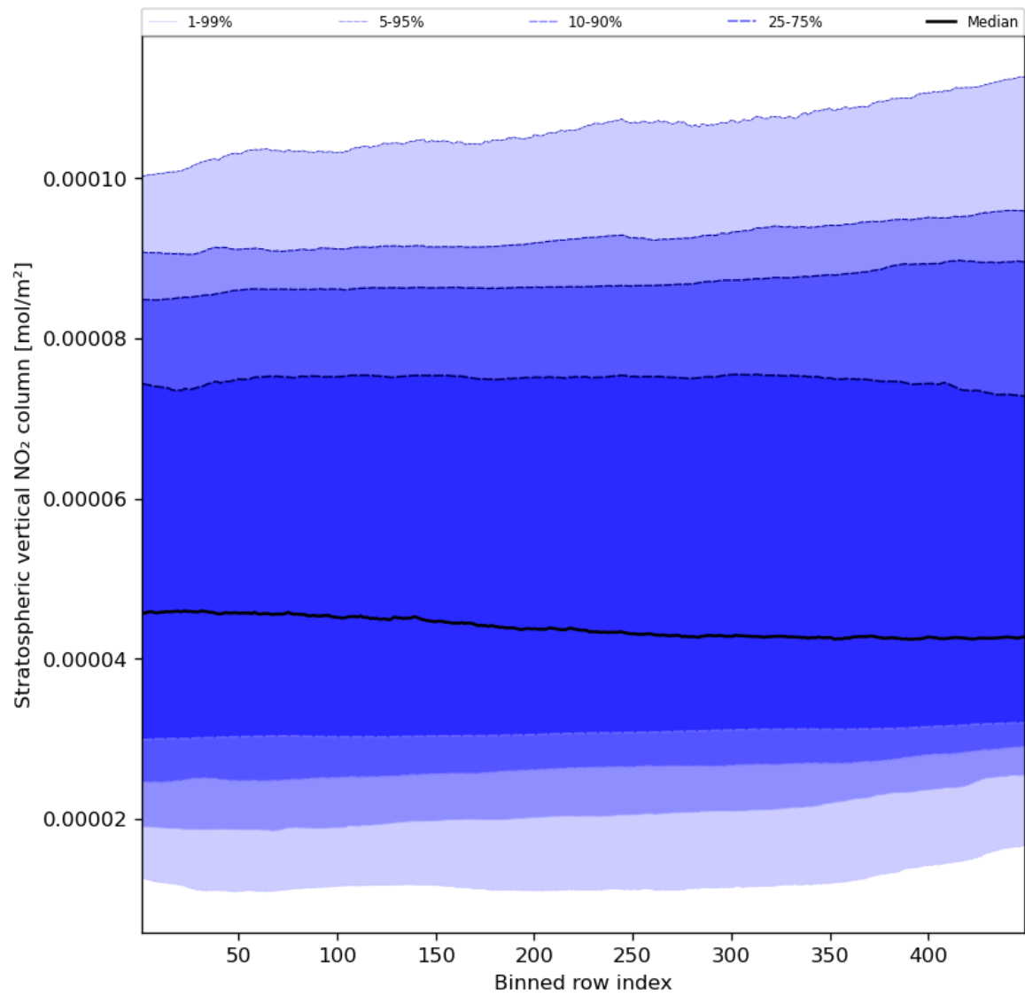
Figure 53: Along track statistics of “Stratospheric vertical NO 2 column” for 2024-01-10 to 2024-01-11
