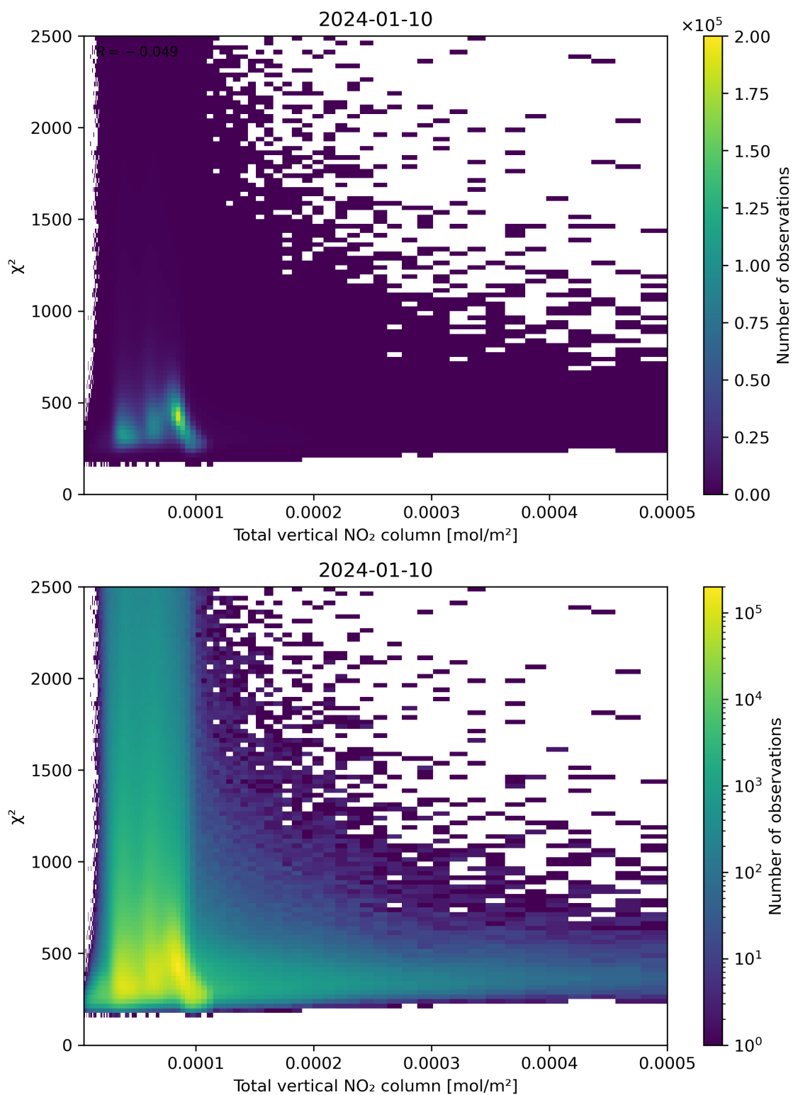
Figure 111: Scatter density plot of “Total vertical NO 2 column” against “ \chi^2 ” for 2024-01-10 to 2024-01-11.
