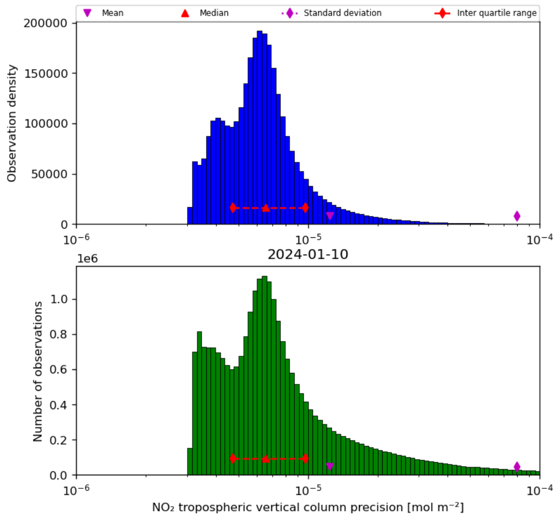
Figure 30: Histogram of “NO 2 tropospheric vertical column precision” for 2024-01-10 to 2024-01-11
