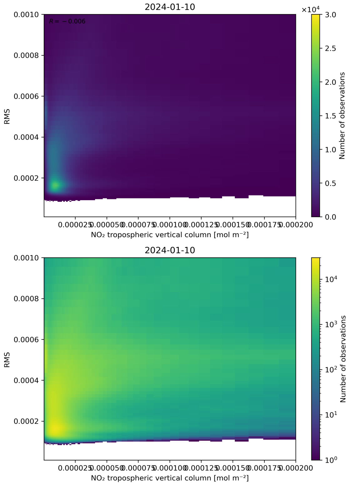
Figure 142: Scatter density plot of “NO 2 tropospheric vertical column” against “RMS” for 2024-01-10 to 2024-01-11.
