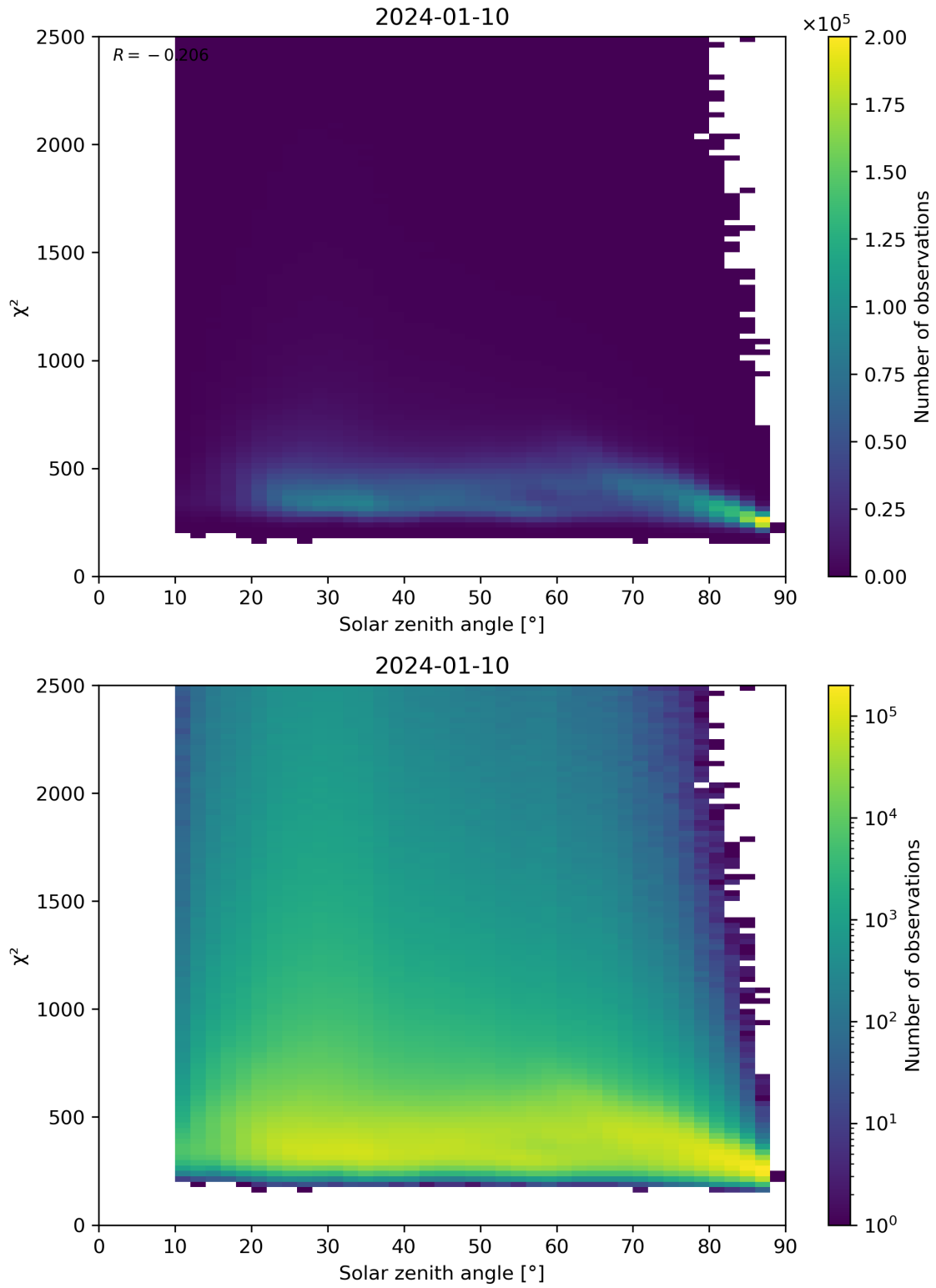
Figure 148: Scatter density plot of “Solar zenith angle” against “ \chi^2 ” for 2024-01-10 to 2024-01-11.
