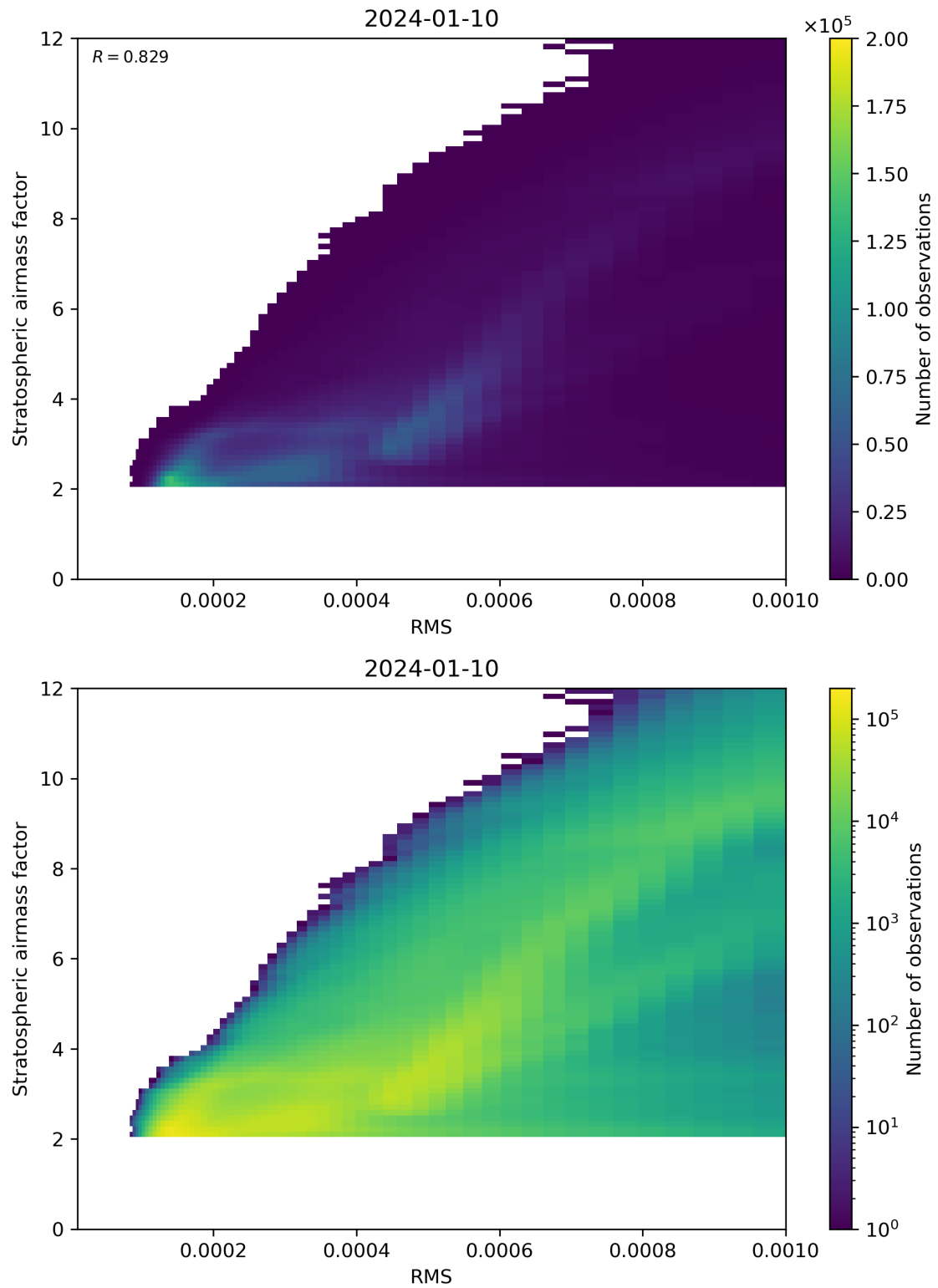
Figure 144: Scatter density plot of “RMS” against “Stratospheric airmass factor” for 2024-01-10 to 2024-01-11.
