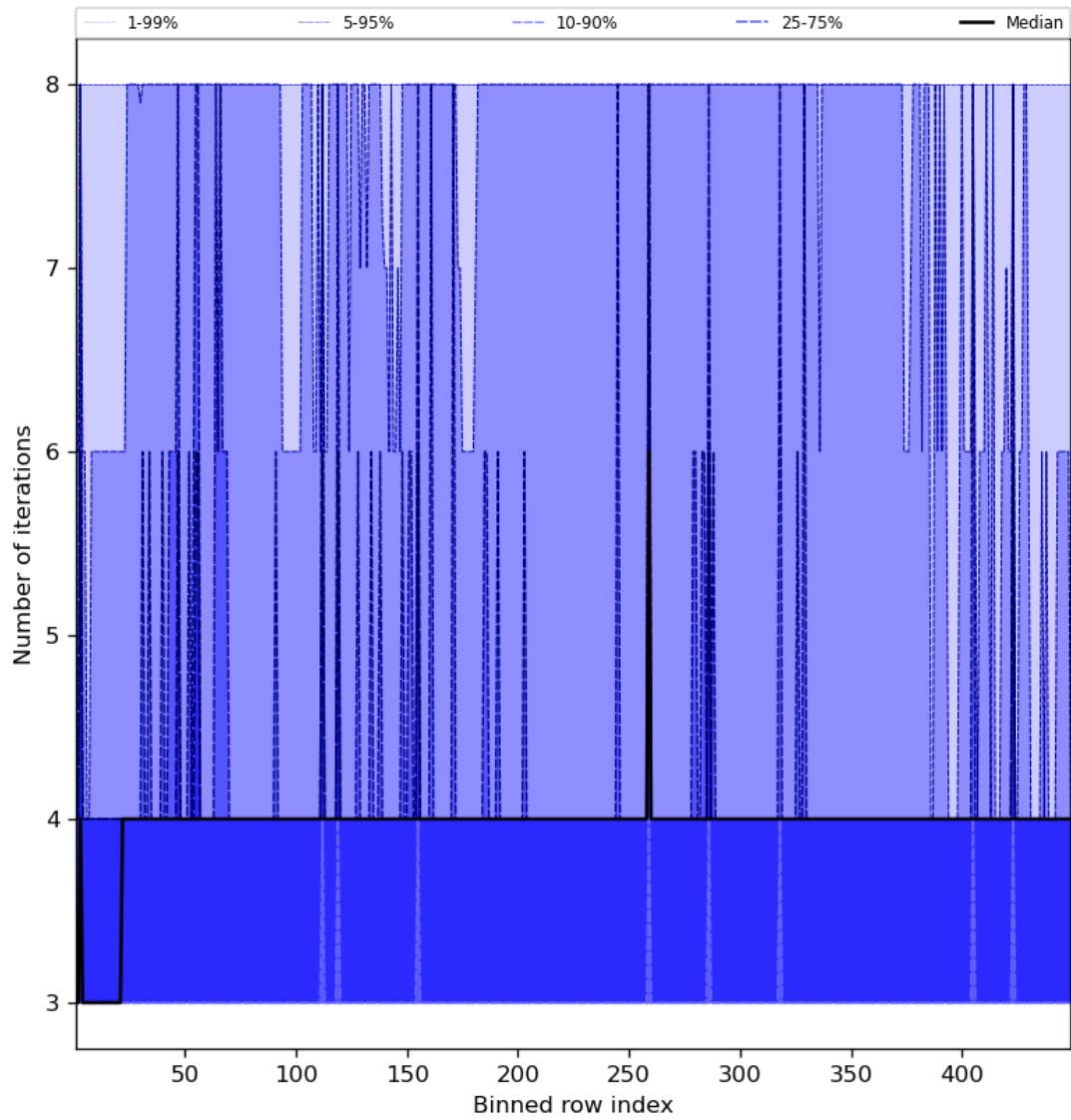
Figure 51: Along track statistics of “Number of iterations” for 2024-01-10 to 2024-01-11
