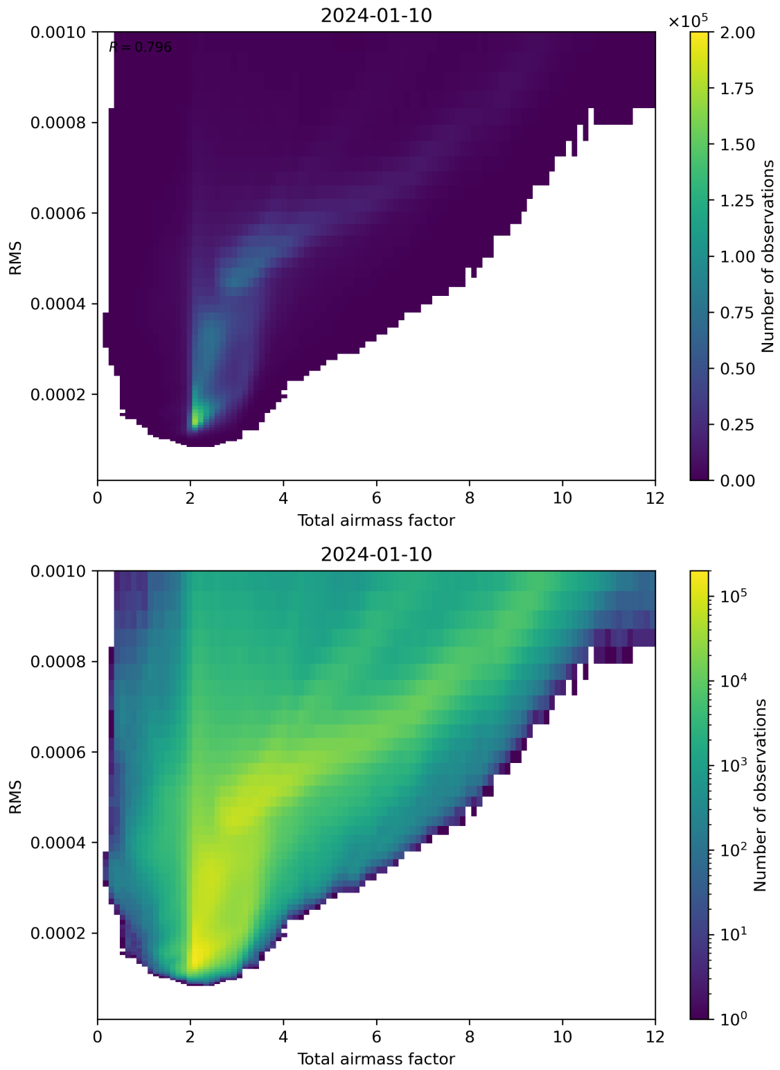
Figure 69: Scatter density plot of “Total airmass factor” against “RMS” for 2024-01-10 to 2024-01-11.
