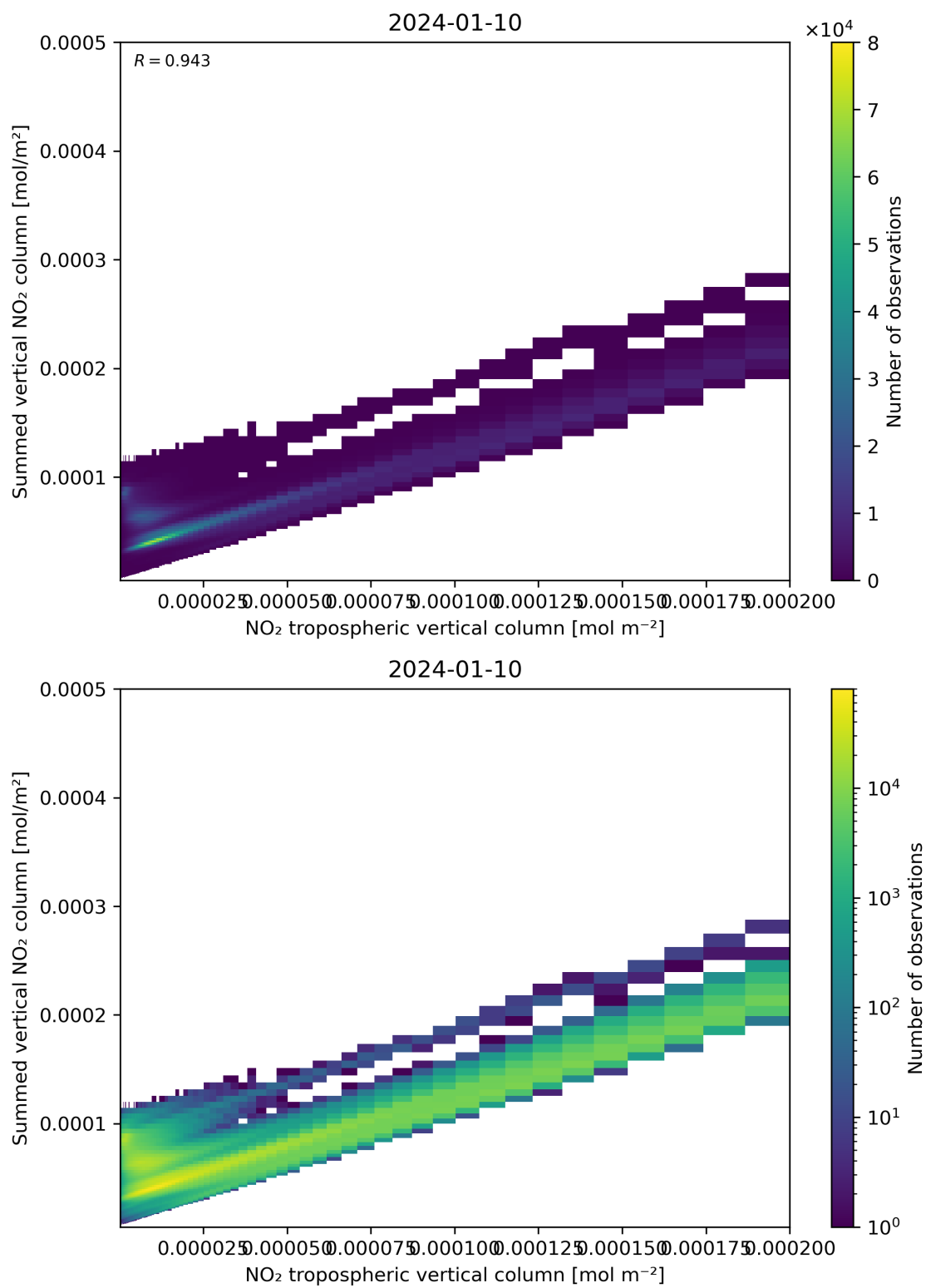
Figure 126: Scatter density plot of “NO 2 tropospheric vertical column” against “Summed vertical NO 2 column” for 2024-01-10 to 2024-01-11.
