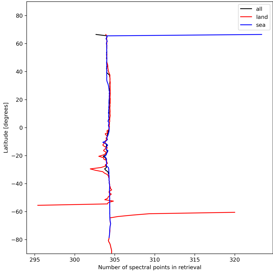
Figure 16: Zonal average of “Number of spectral points in retrieval” for 2024-01-10 to 2024-01-11.
