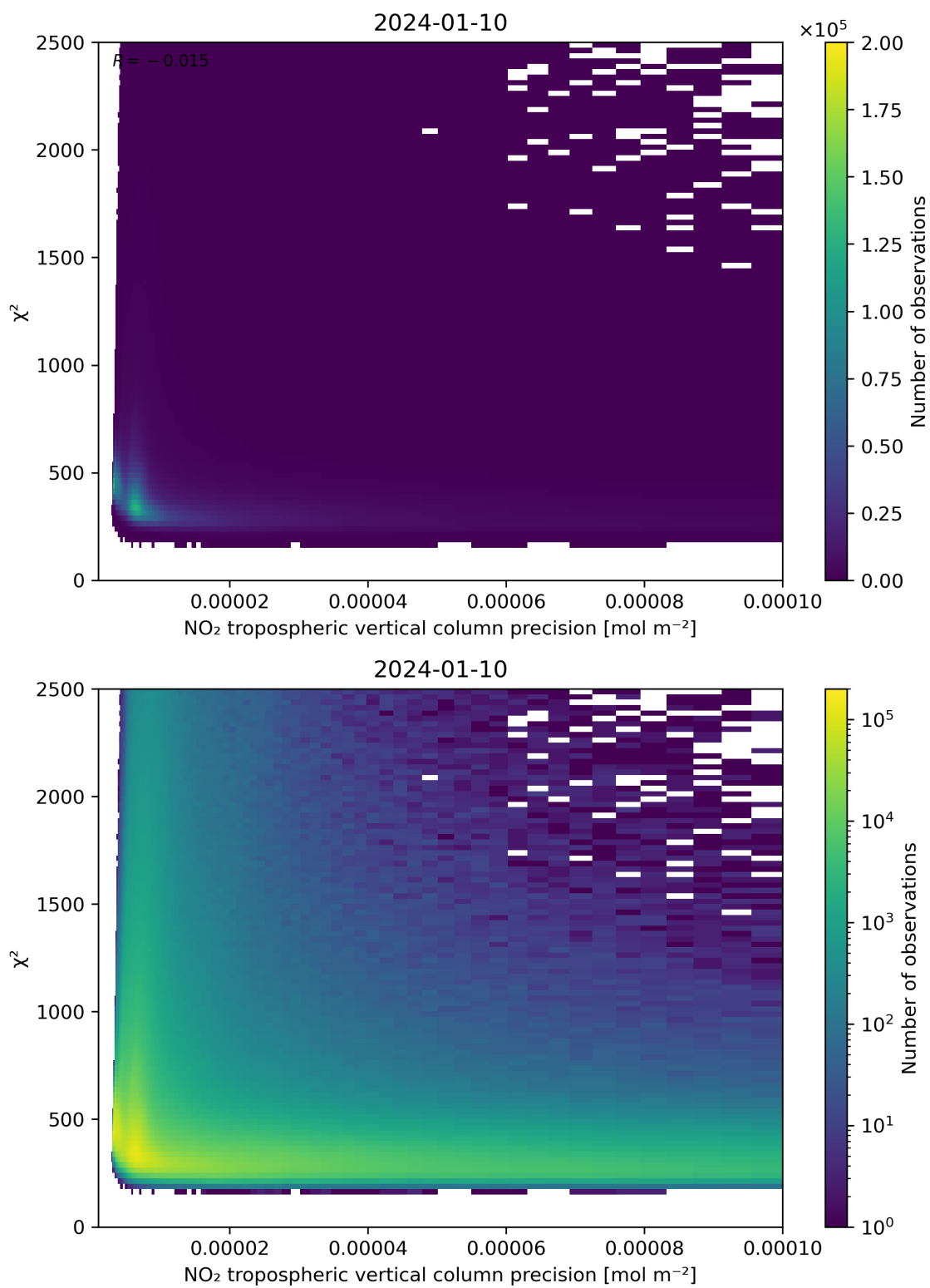
Figure 134: Scatter density plot of “NO 2 tropospheric vertical column precision” against “ \chi^2 ” for 2024-01-10 to 2024-01-11.
