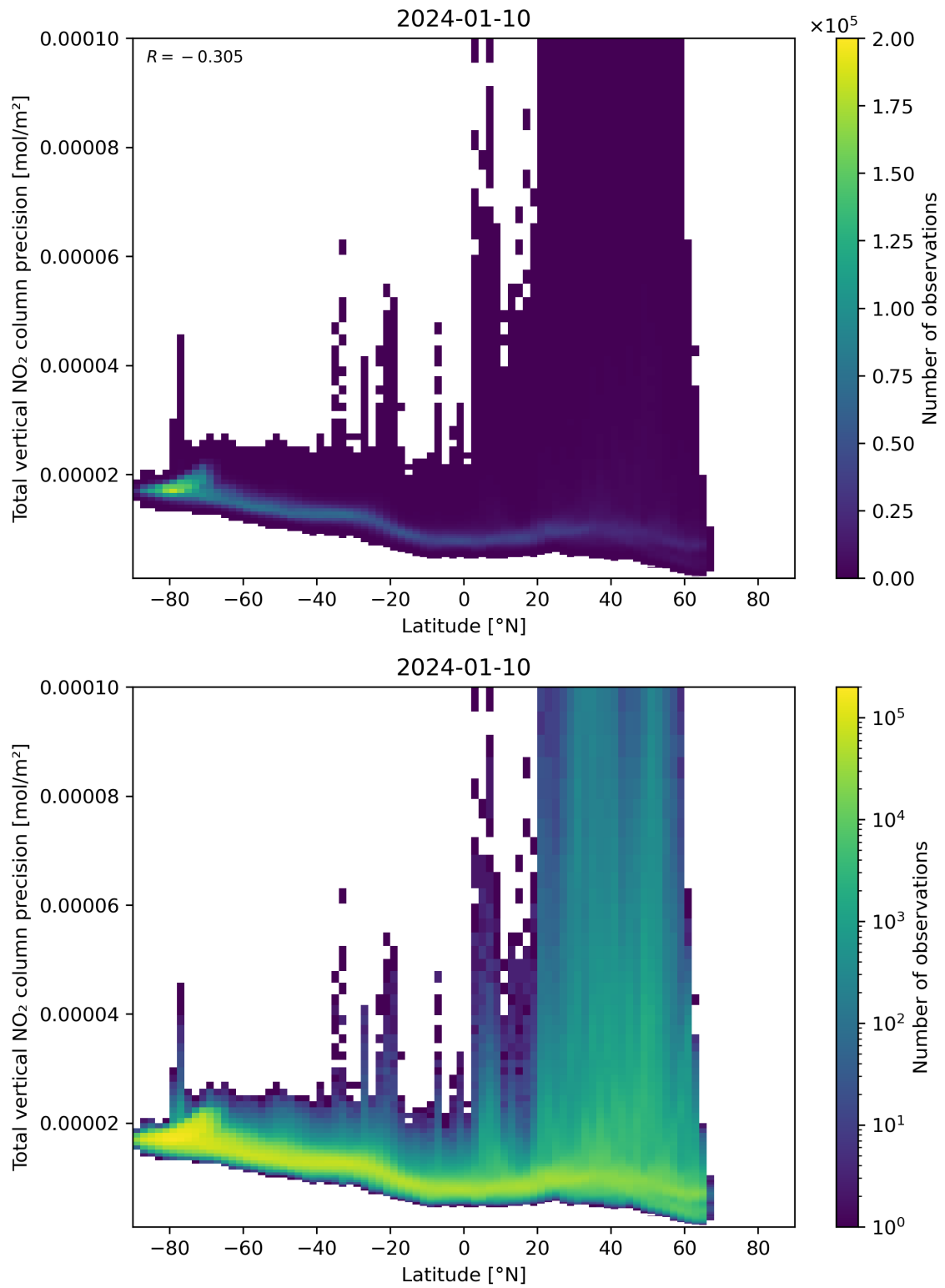
Figure 91: Scatter density plot of “Latitude” against “Total vertical NO 2 column precision” for 2024-01-10 to 2024-01-11.
