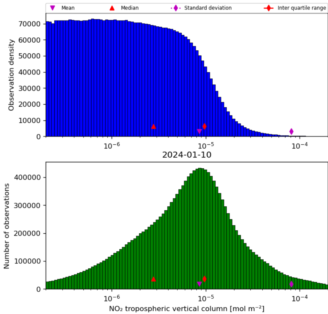
Figure 29: Histogram of “NO 2 tropospheric vertical column” for 2024-01-10 to 2024-01-11
