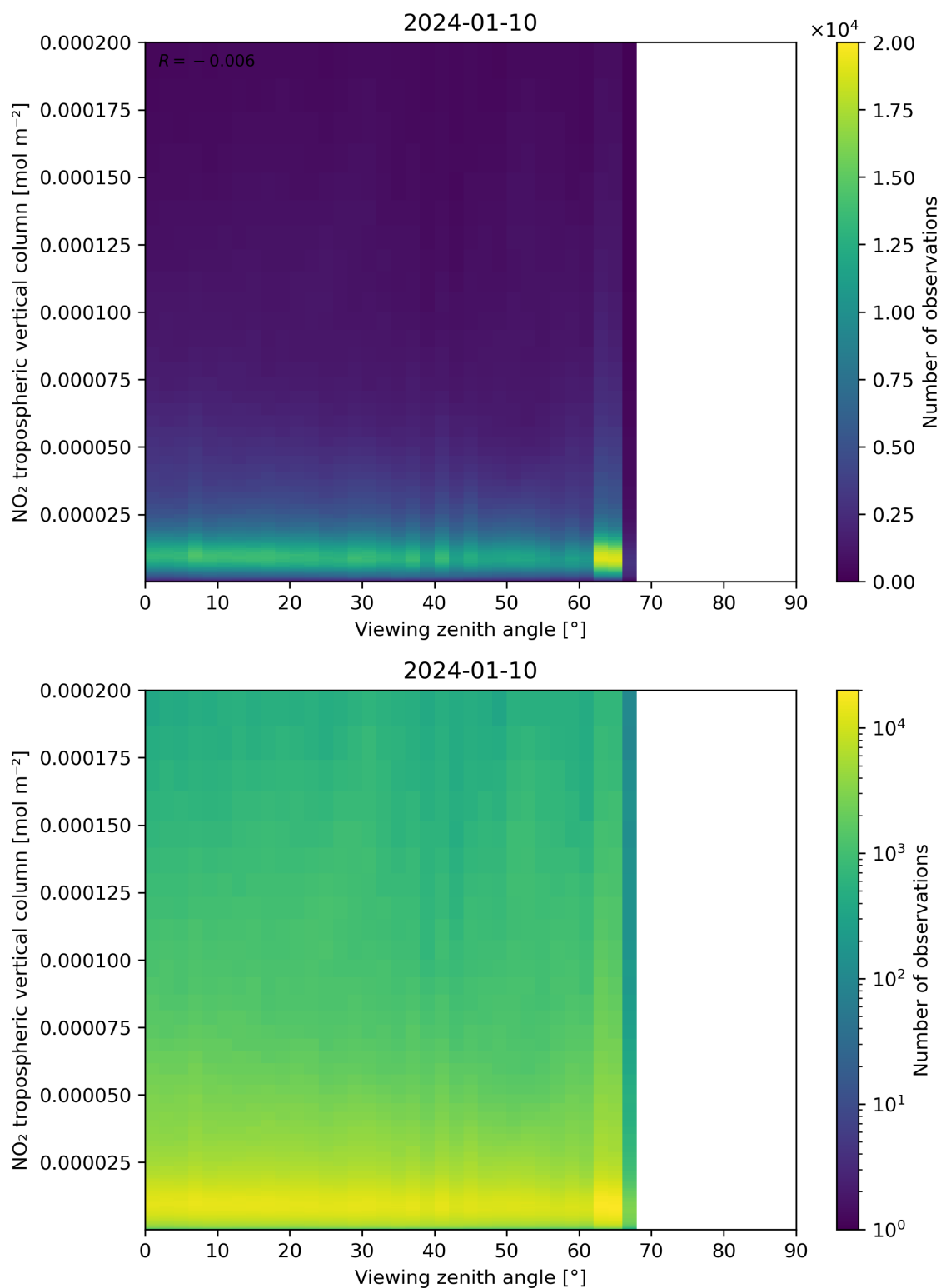
Figure 169: Scatter density plot of “Viewing zenith angle” against “NO 2 tropospheric vertical column” for 2024-01-10 to 2024-01-11.
