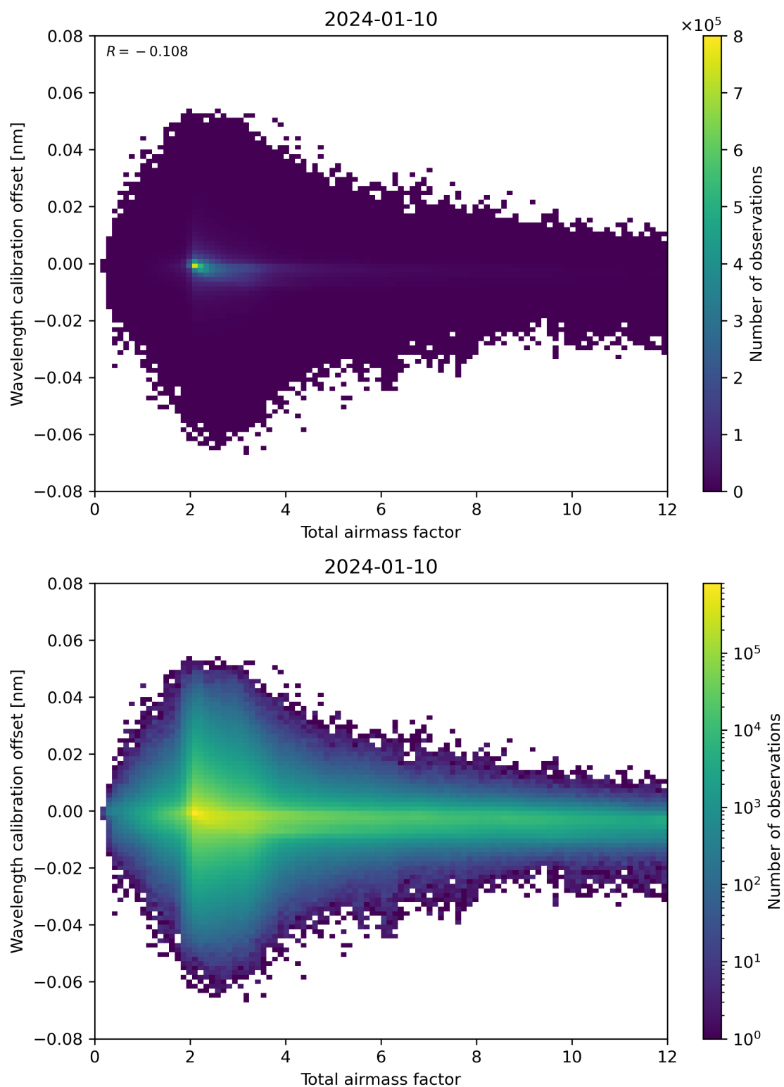
Figure 70: Scatter density plot of “Total airmass factor” against “Wavelength calibration offset” for 2024-01-10 to 2024-01-11.
