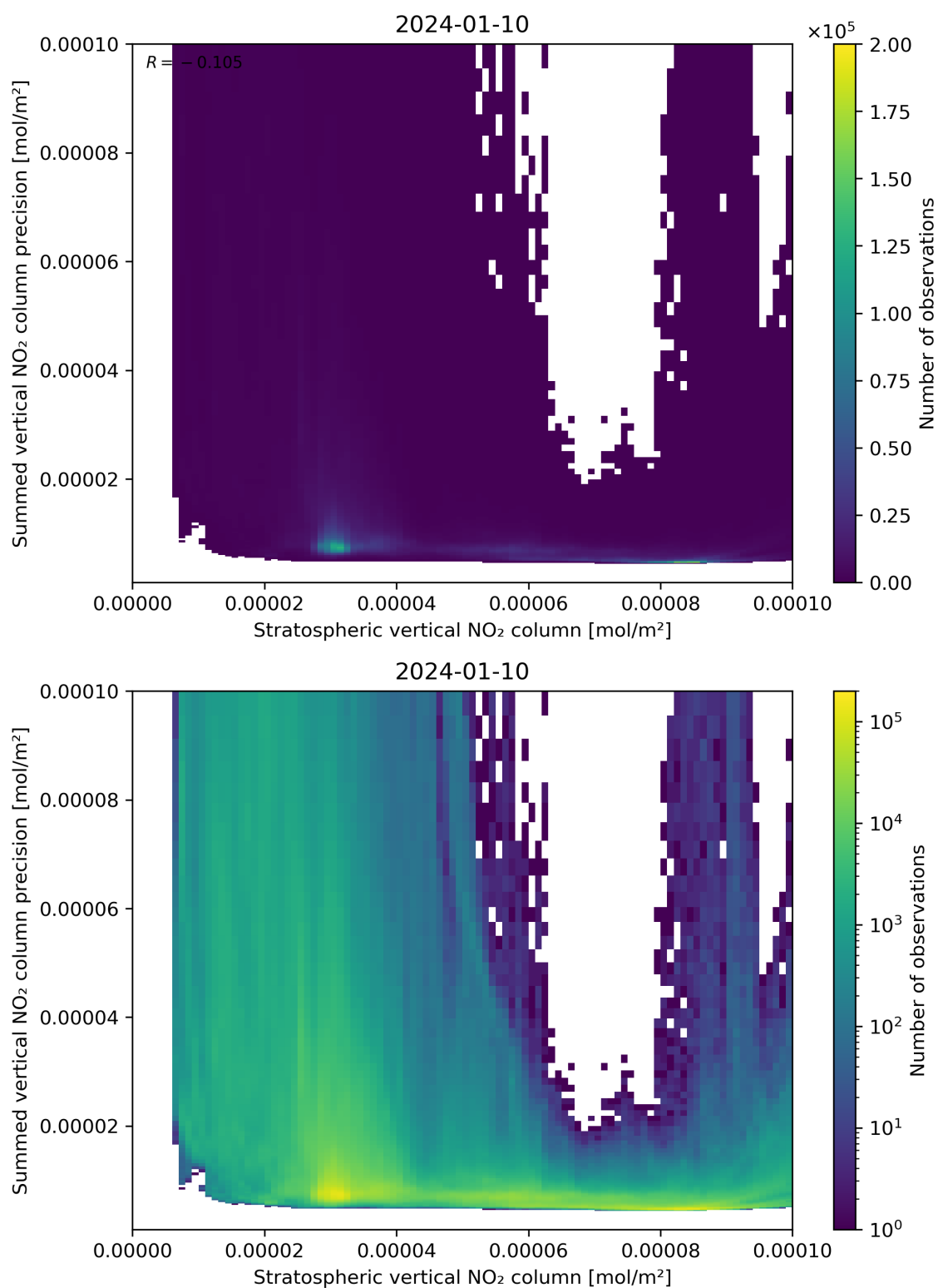
Figure 99: Scatter density plot of “Stratospheric vertical NO 2 column” against “Summed vertical NO 2 column precision” for 2024-01-10 to 2024-01-11.
