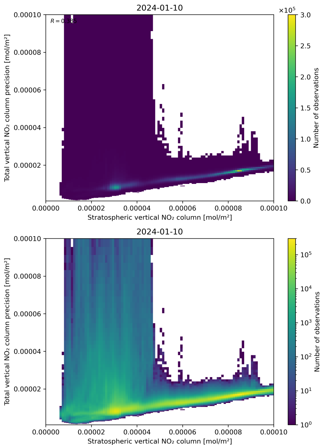
Figure 101: Scatter density plot of “Stratospheric vertical NO 2 column” against “Total vertical NO 2 column precision” for 2024-01-10 to 2024-01-11.
