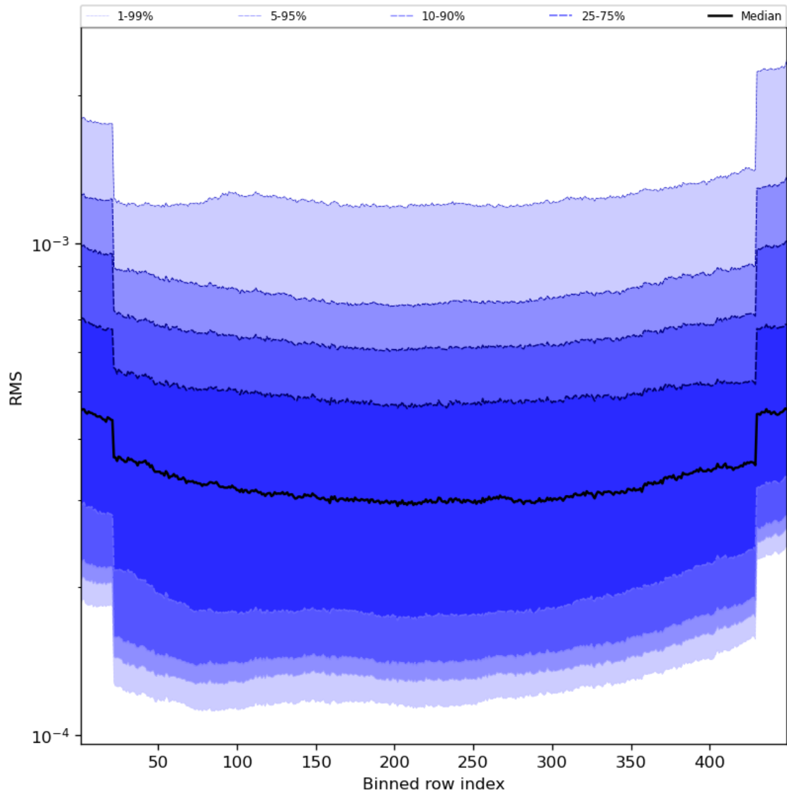
Figure 60: Along track statistics of “RMS” for 2024-01-10 to 2024-01-11
