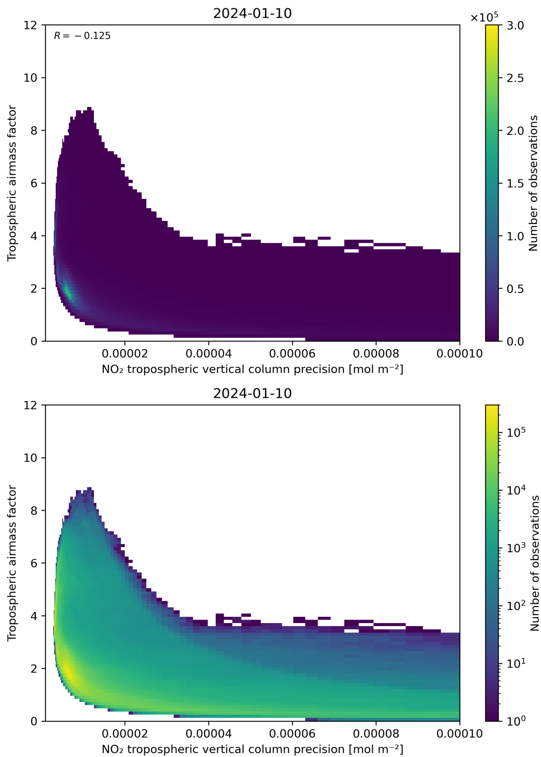
Figure 133: Scatter density plot of “NO 2 tropospheric vertical column precision” against “Tropospheric airmass factor” for 2024-01-10 to 2024-01-11.
