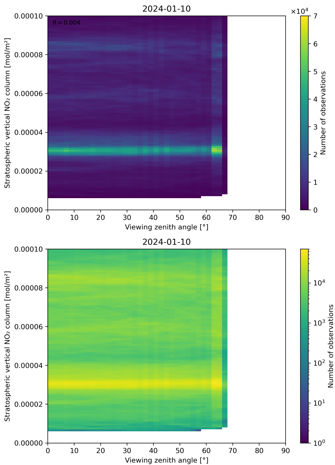
Figure 164: Scatter density plot of “Viewing zenith angle” against “Stratospheric vertical NO 2 column” for 2024-01-10 to 2024-01-11.
