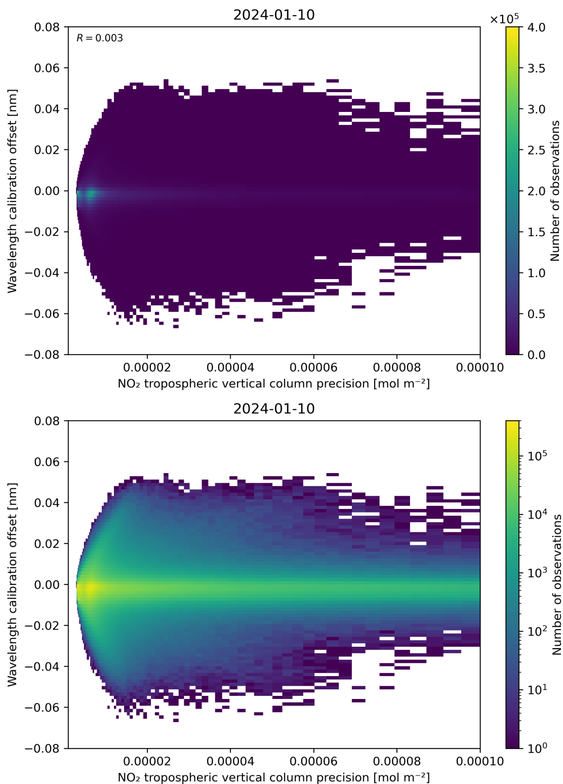
Figure 141: Scatter density plot of “NO 2 tropospheric vertical column precision” against “Wavelength calibration offset” for 2024-01-10 to 2024-01-11.
