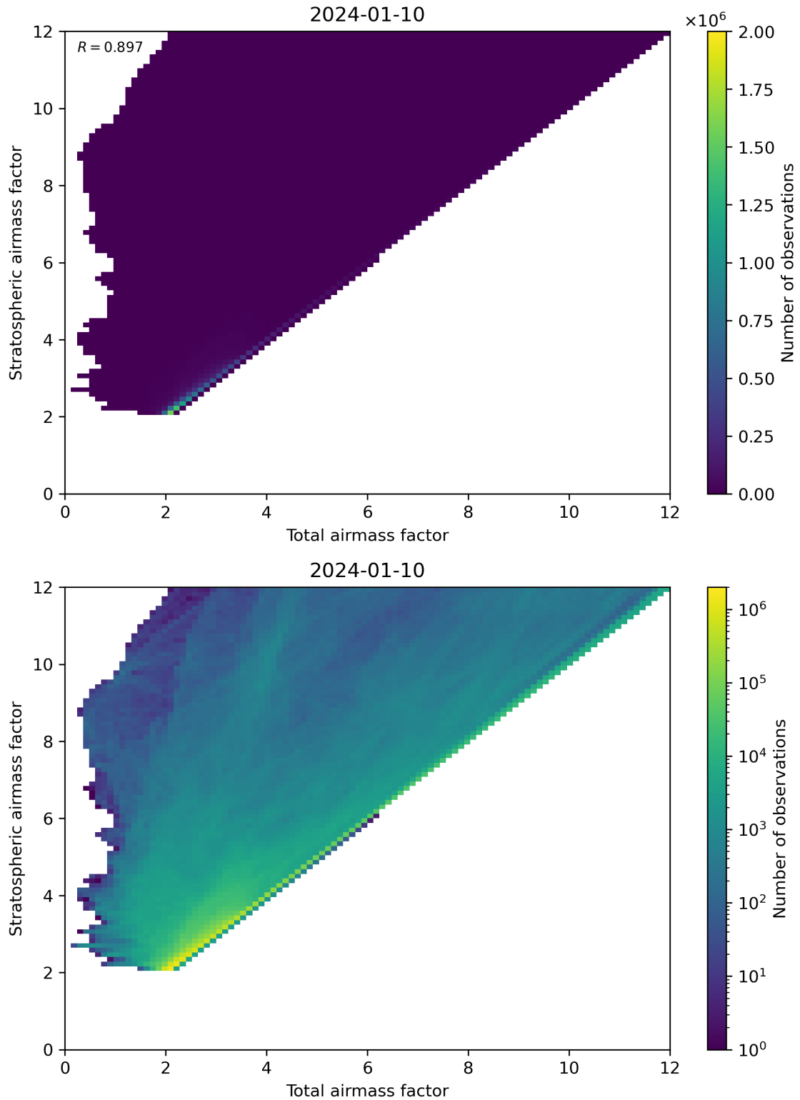
Figure 62: Scatter density plot of “Total airmass factor” against “Stratospheric airmass factor” for 2024-01-10 to 2024-01-11.
