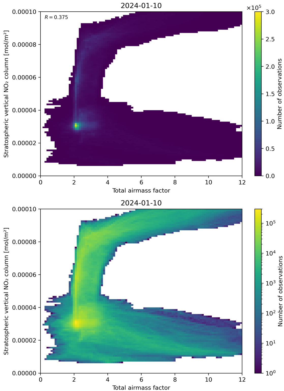
Figure 64: Scatter density plot of “Total airmass factor” against “Stratospheric vertical \text{NO}_2 column” for 2024-01-10 to 2024-01-11.
