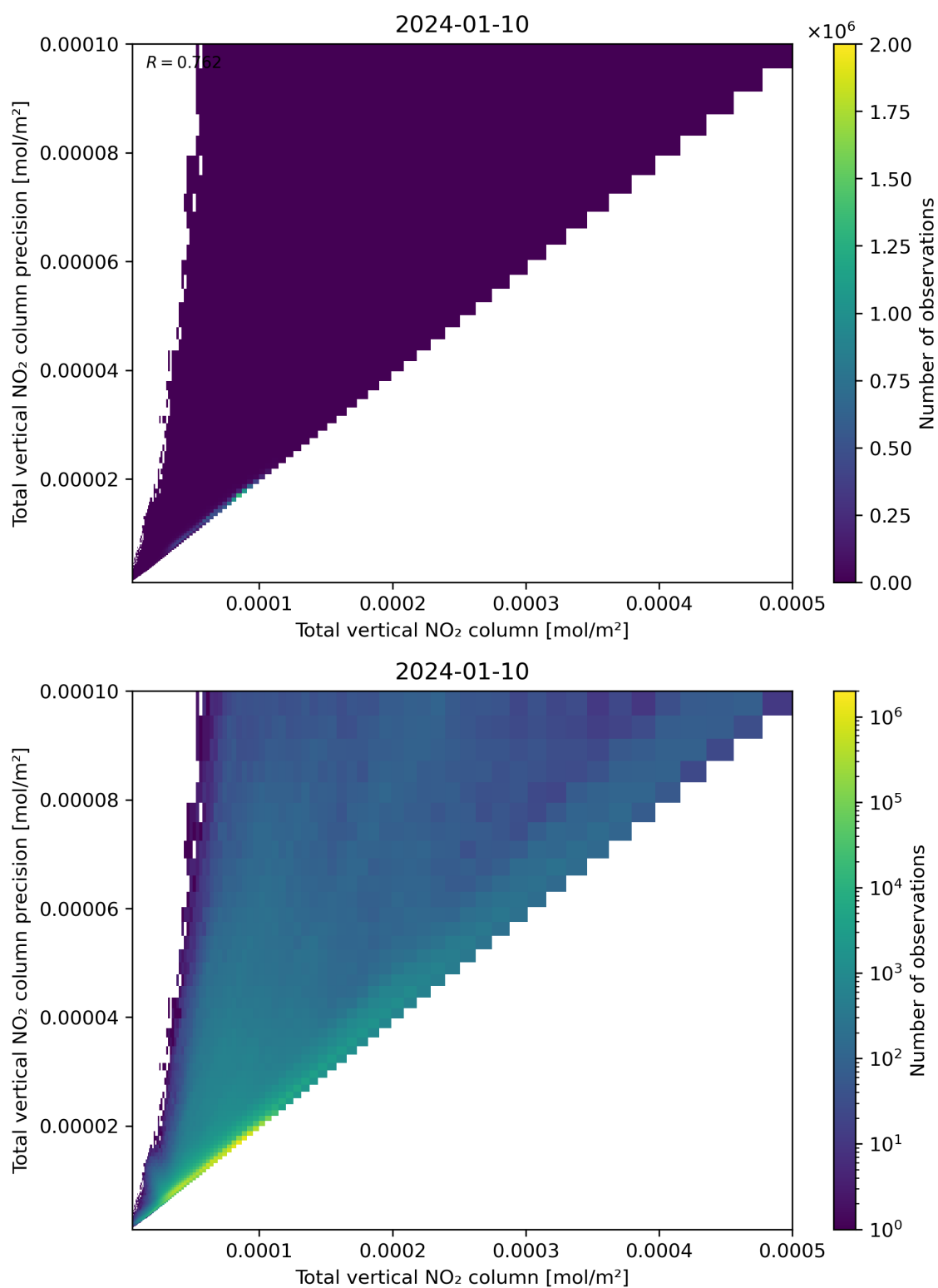
Figure 114: Scatter density plot of “Total vertical NO 2 column” against “Total vertical NO 2 column precision” for 2024-01-10 to 2024-01-11.
