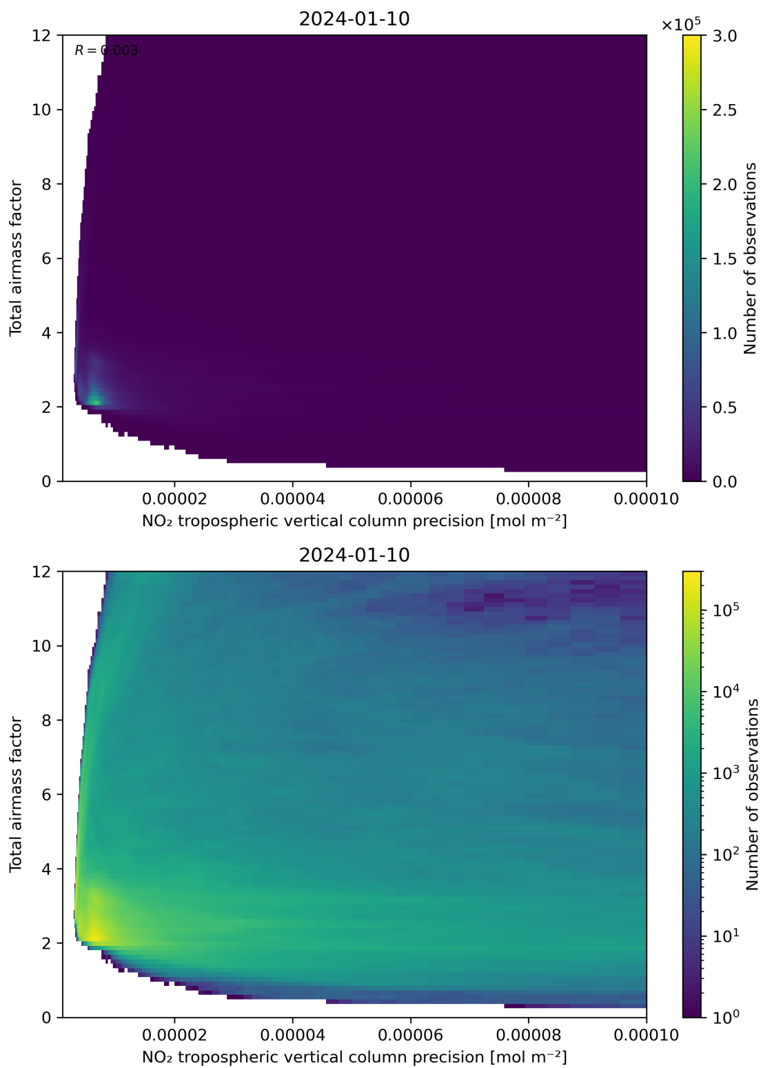
Figure 132: Scatter density plot of “NO 2 tropospheric vertical column precision” against “Total air mass factor” for 2024-01-10 to 2024-01-11.
