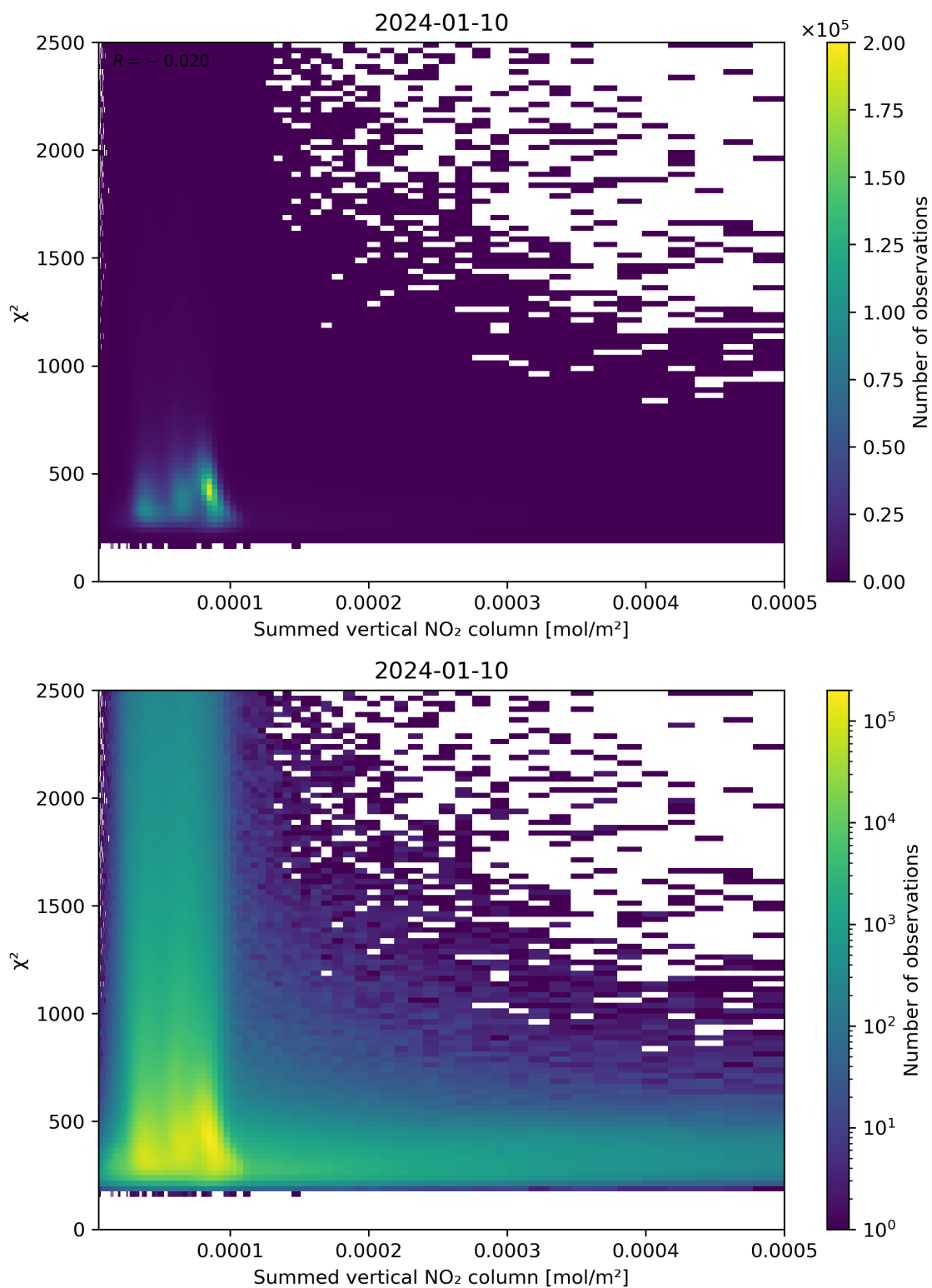
Figure 104: Scatter density plot of “Summed vertical NO 2 column” against “ \chi^2 ” for 2024-01-10 to 2024-01-11.
