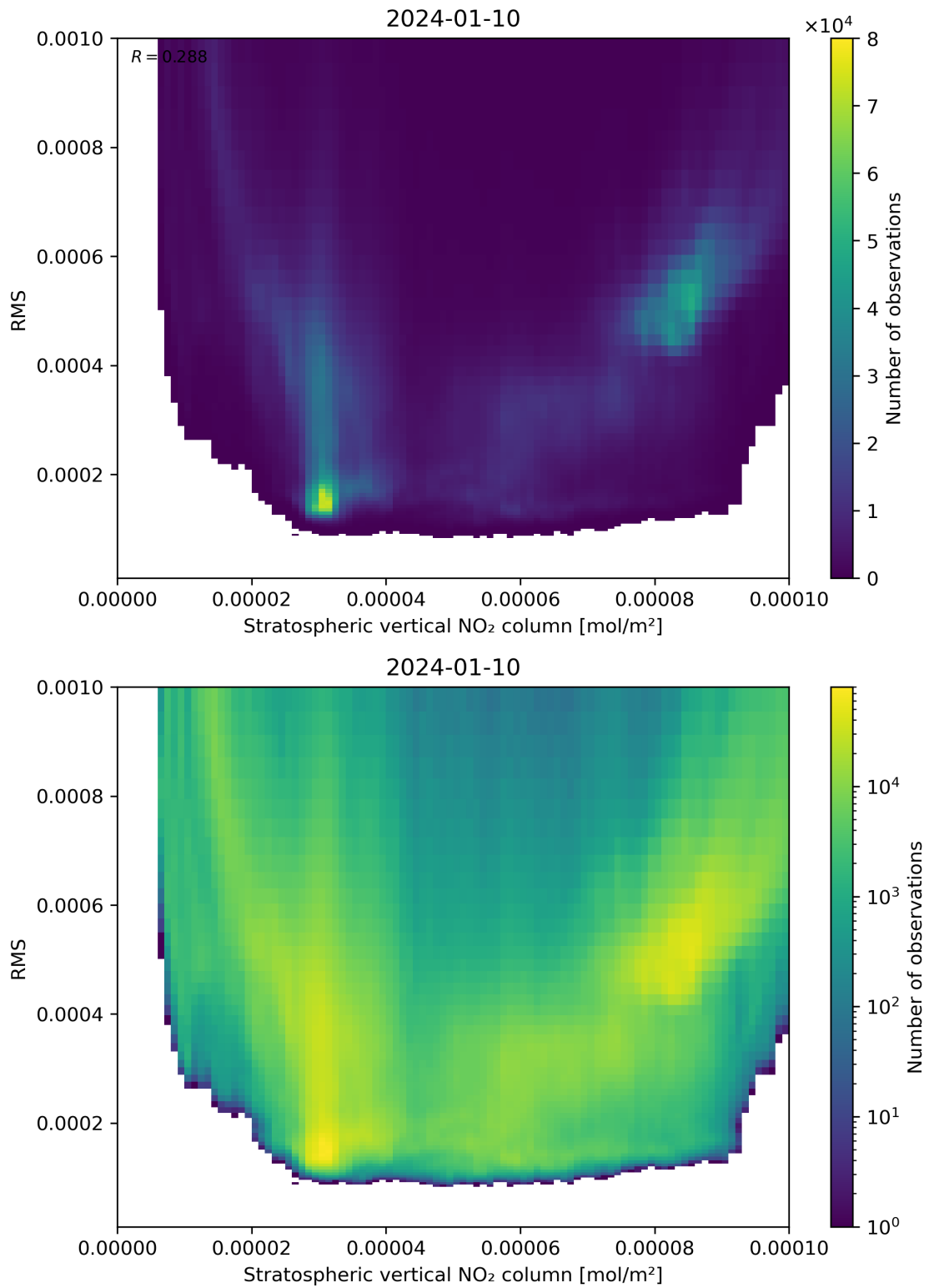
Figure 102: Scatter density plot of “Stratospheric vertical NO 2 column” against “RMS” for 2024-01-10 to 2024-01-11.
