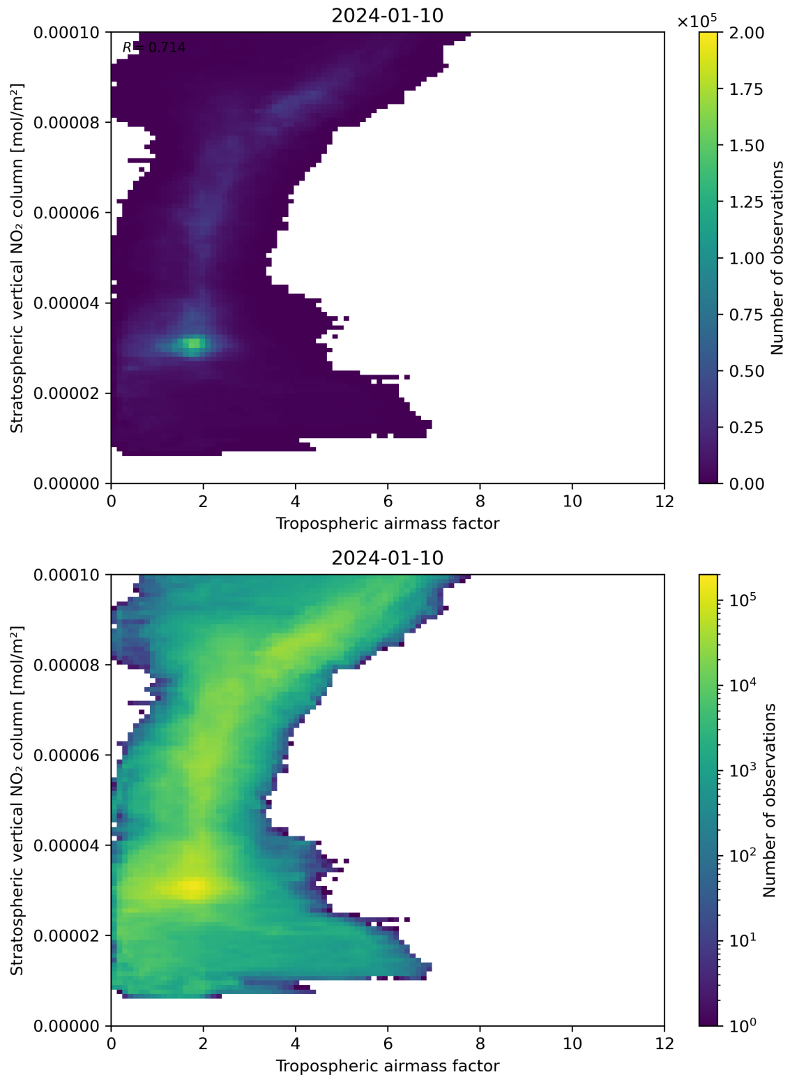
Figure 74: Scatter density plot of “Tropospheric air mass factor” against “Stratospheric vertical NO 2 column” for 2024-01-10 to 2024-01-11.
