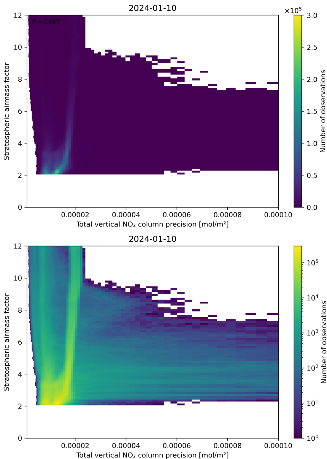
Figure 115: Scatter density plot of “Total vertical NO 2 column precision” against “Stratospheric air mass factor” for 2024-01-10 to 2024-01-11.
