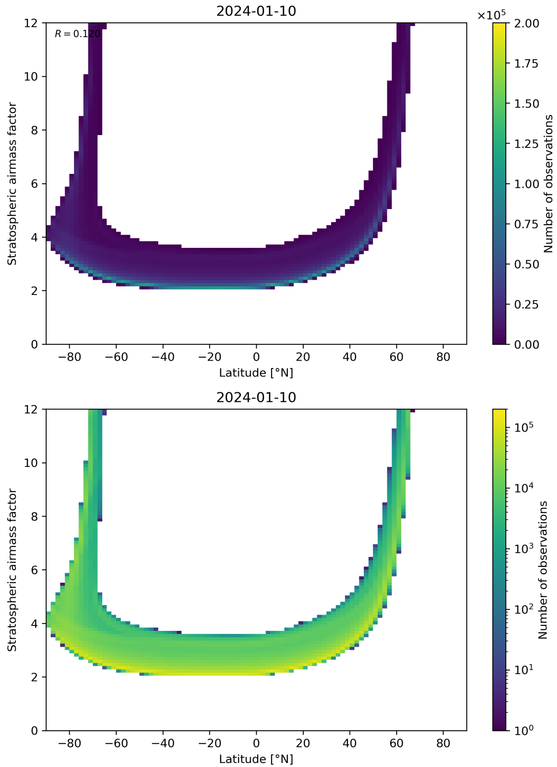
Figure 83: Scatter density plot of “Latitude” against “Stratospheric airmass factor” for 2024-01-10 to 2024-01-11.
