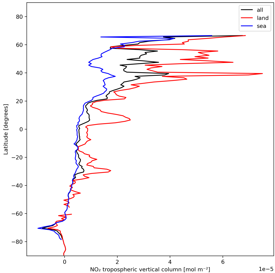
Figure 12: Zonal average of “NO 2 tropospheric vertical column” for 2024-01-10 to 2024-01-11.
