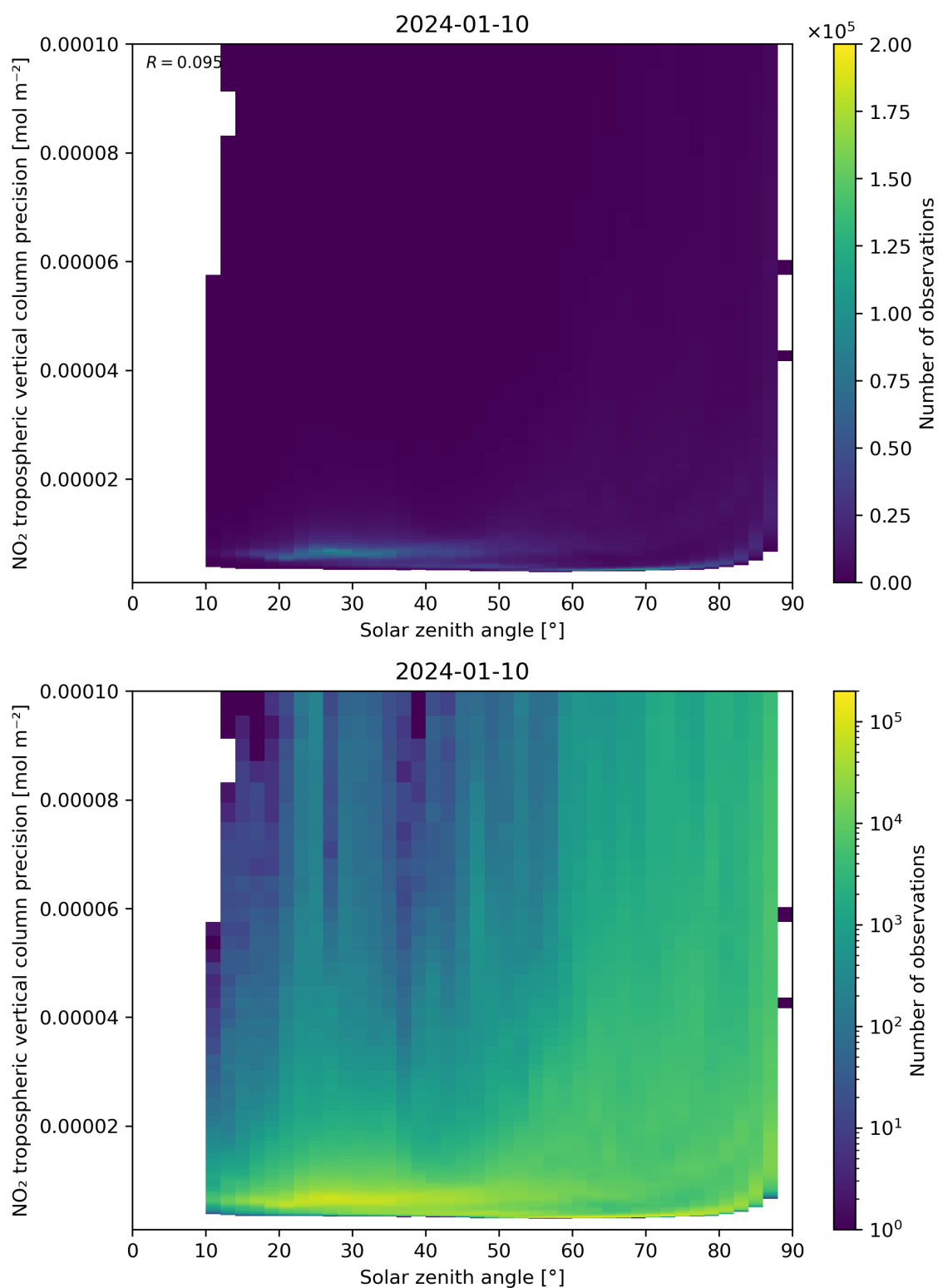
Figure 156: Scatter density plot of “Solar zenith angle” against “NO 2 tropospheric vertical column precision” for 2024-01-10 to 2024-01-11.
