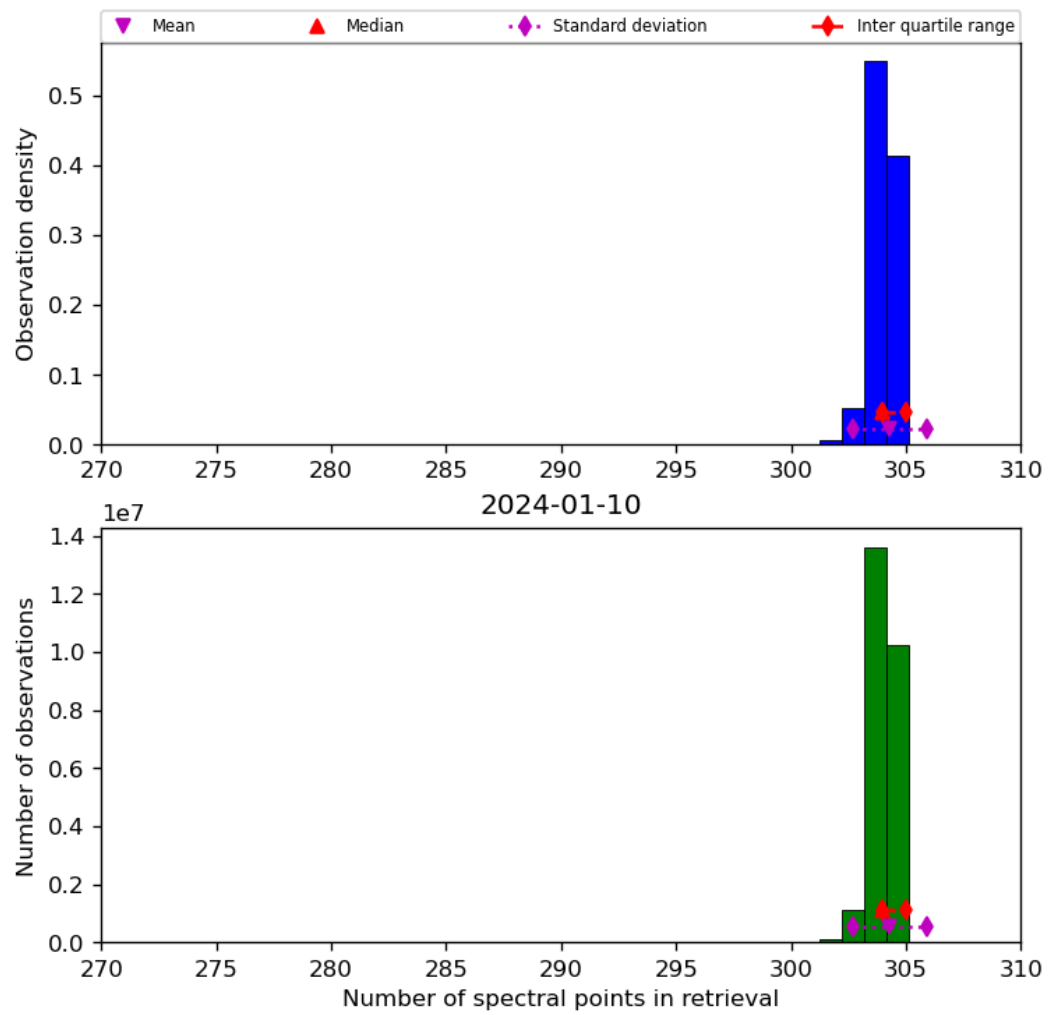
Figure 33: Histogram of “Number of spectral points in retrieval” for 2024-01-10 to 2024-01-11
