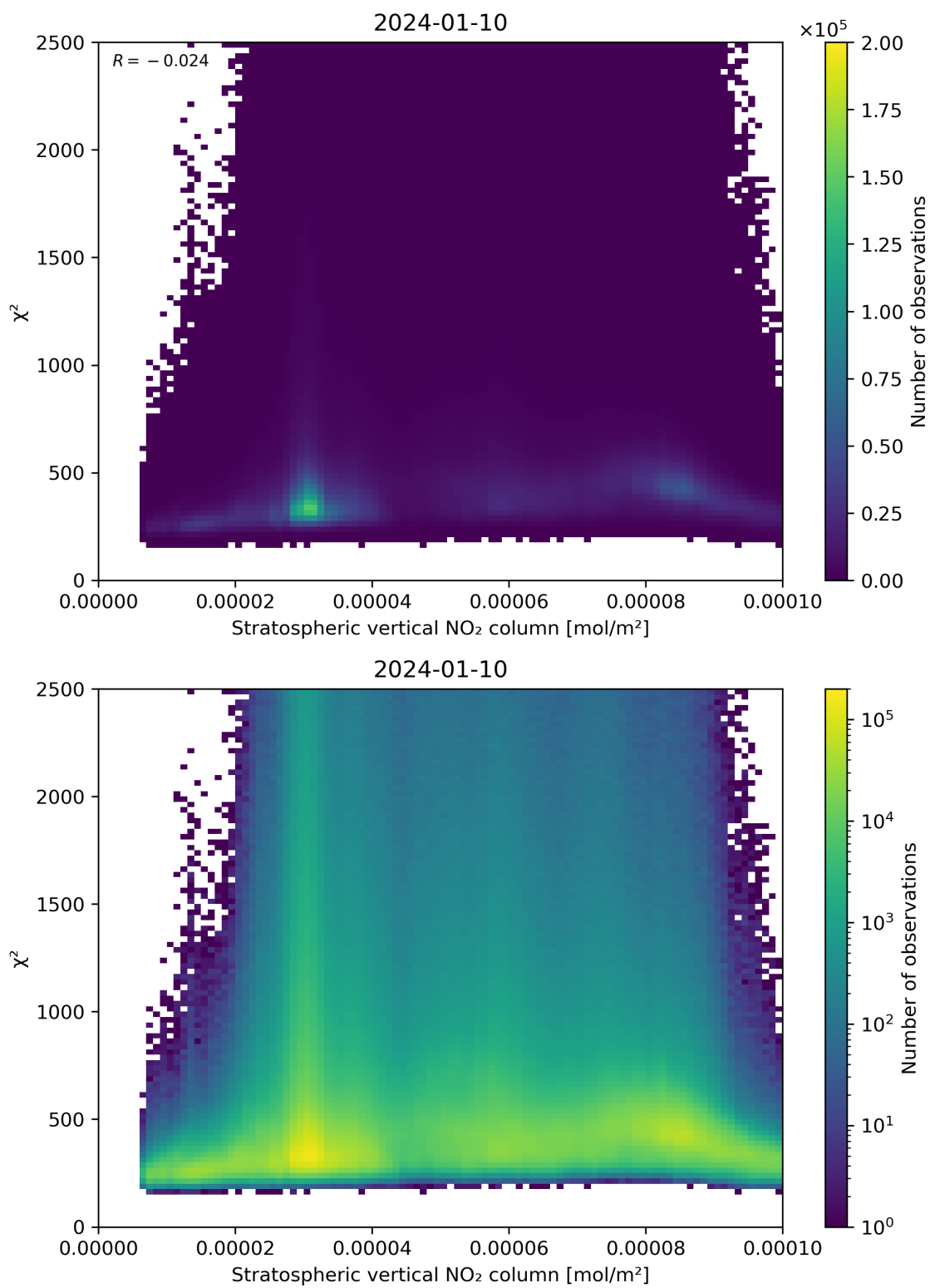
Figure 97: Scatter density plot of “Stratospheric vertical NO 2 column” against “ \chi^2 ” for 2024-01-10 to 2024-01-11.
