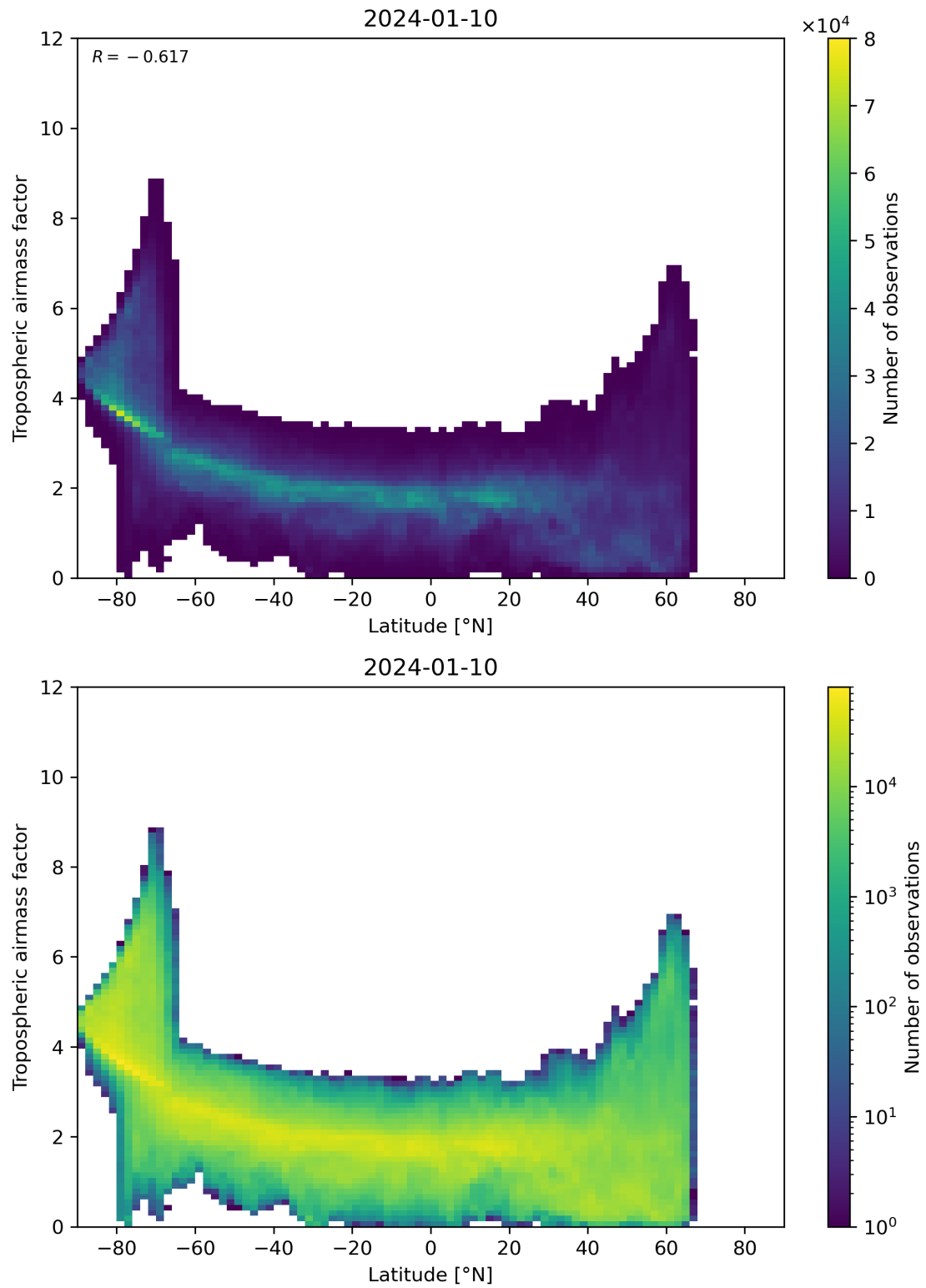
Figure 85: Scatter density plot of “Latitude” against “Tropospheric air mass factor” for 2024-01-10 to 2024-01-11.
