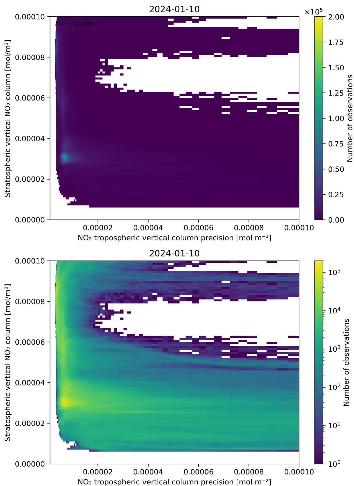
Figure 135: Scatter density plot of “NO 2 tropospheric vertical column precision” against “Stratospheric vertical NO 2 column” for 2024-01-10 to 2024-01-11.
