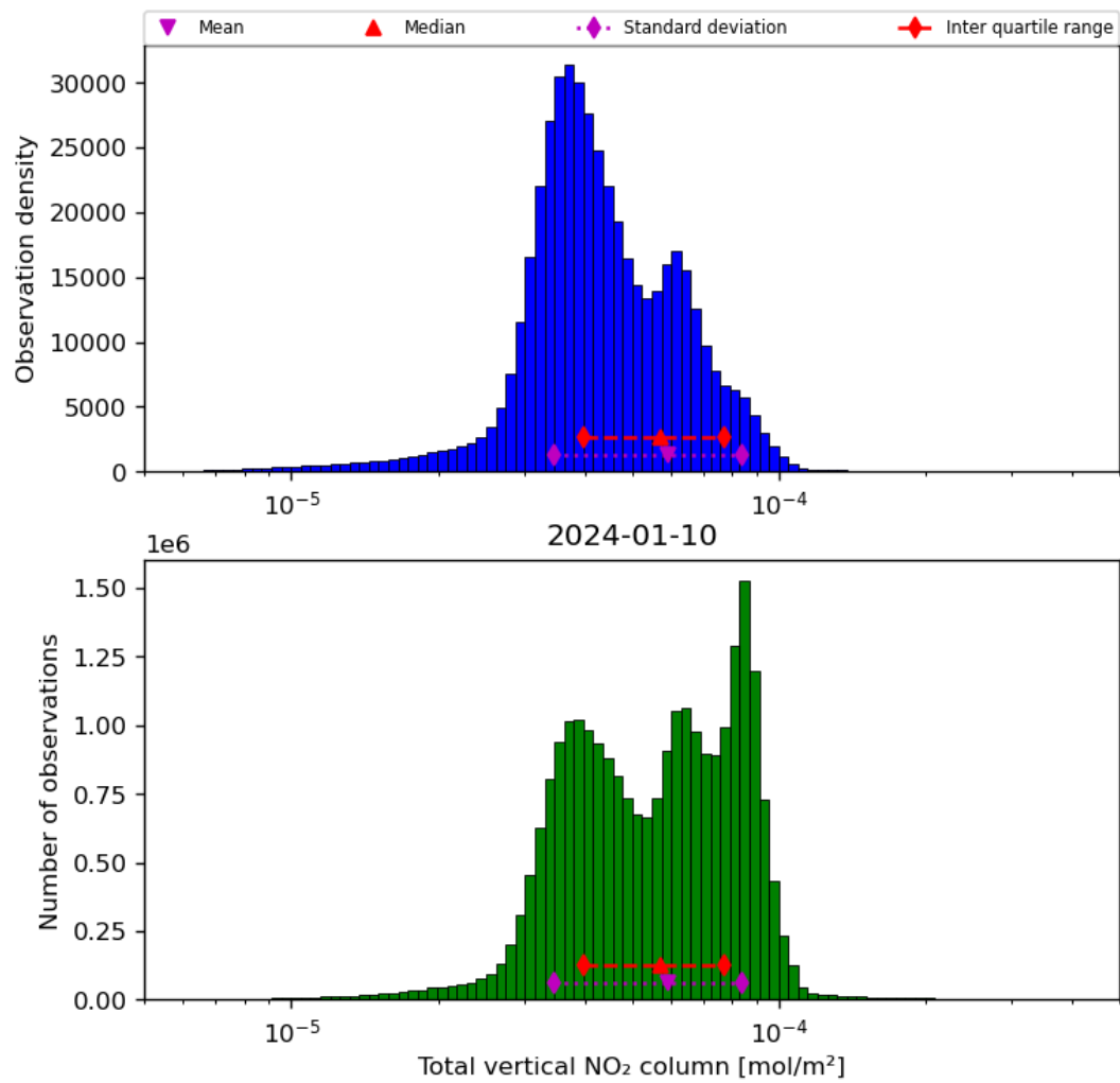
Figure 38: Histogram of “Total vertical NO 2 column” for 2024-01-10 to 2024-01-11
