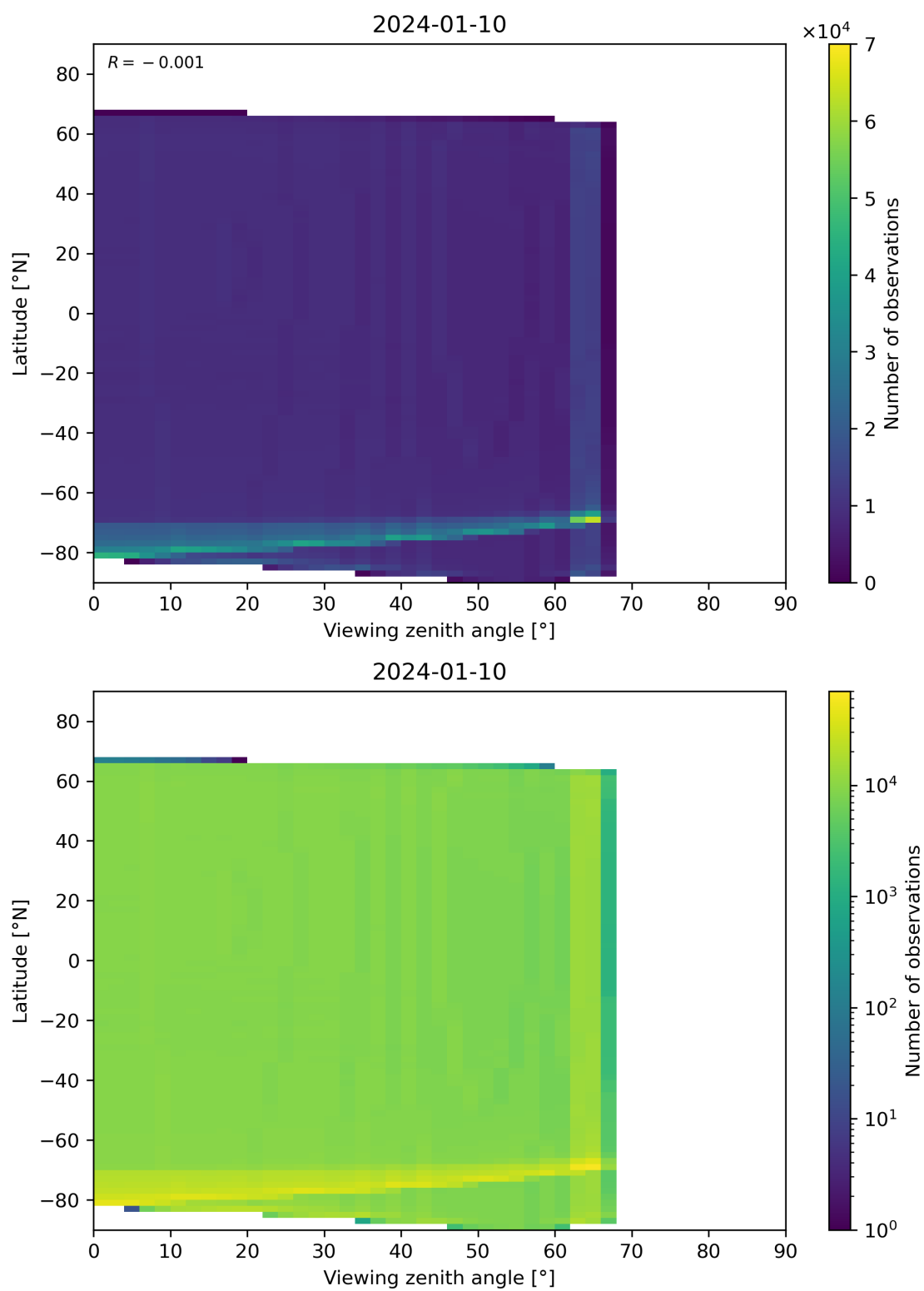
Figure 163: Scatter density plot of “Viewing zenith angle” against “Latitude” for 2024-01-10 to 2024-01-11.
