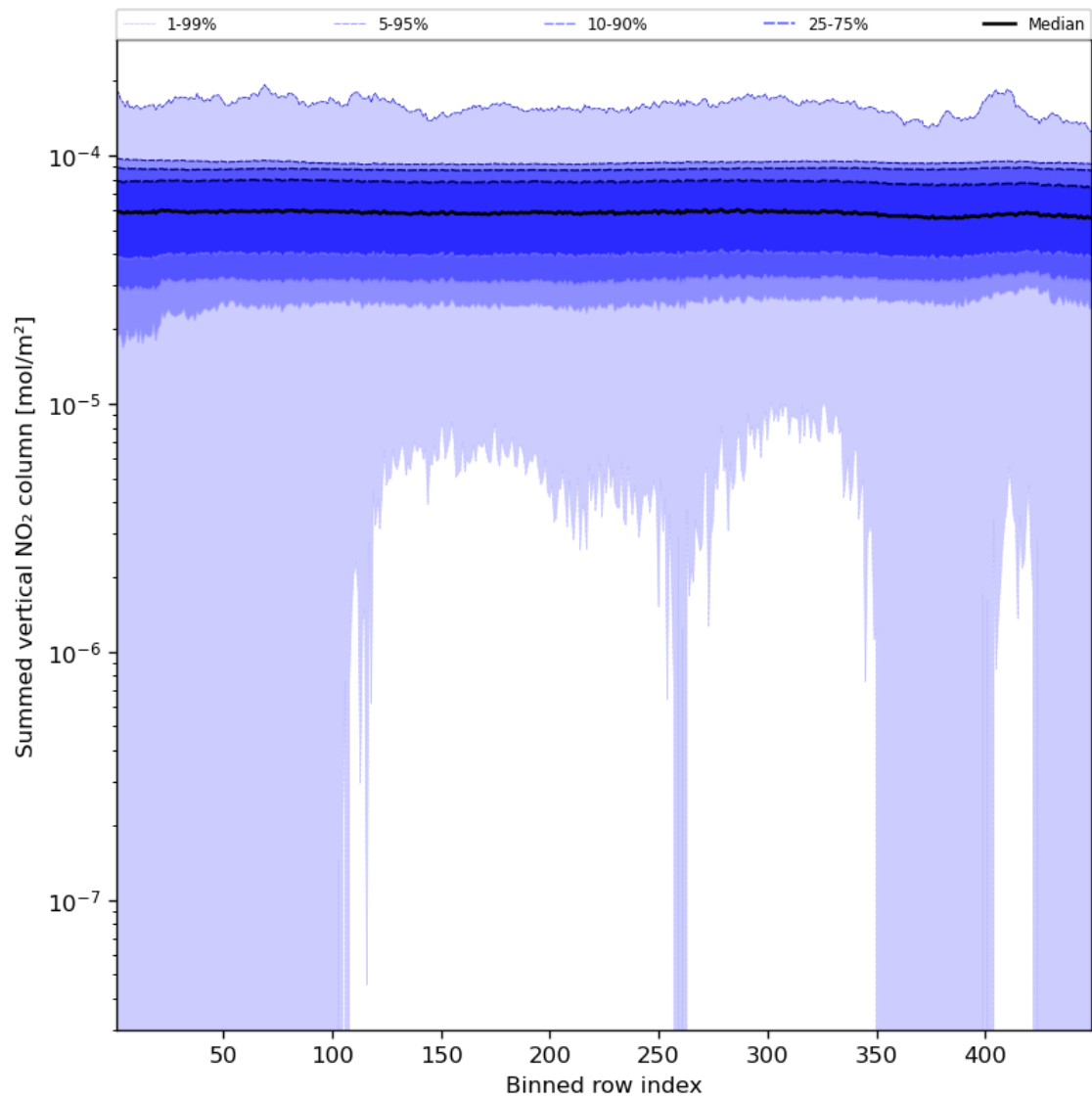
Figure 57: Along track statistics of “Summed vertical NO 2 column” for 2024-01-10 to 2024-01-11
