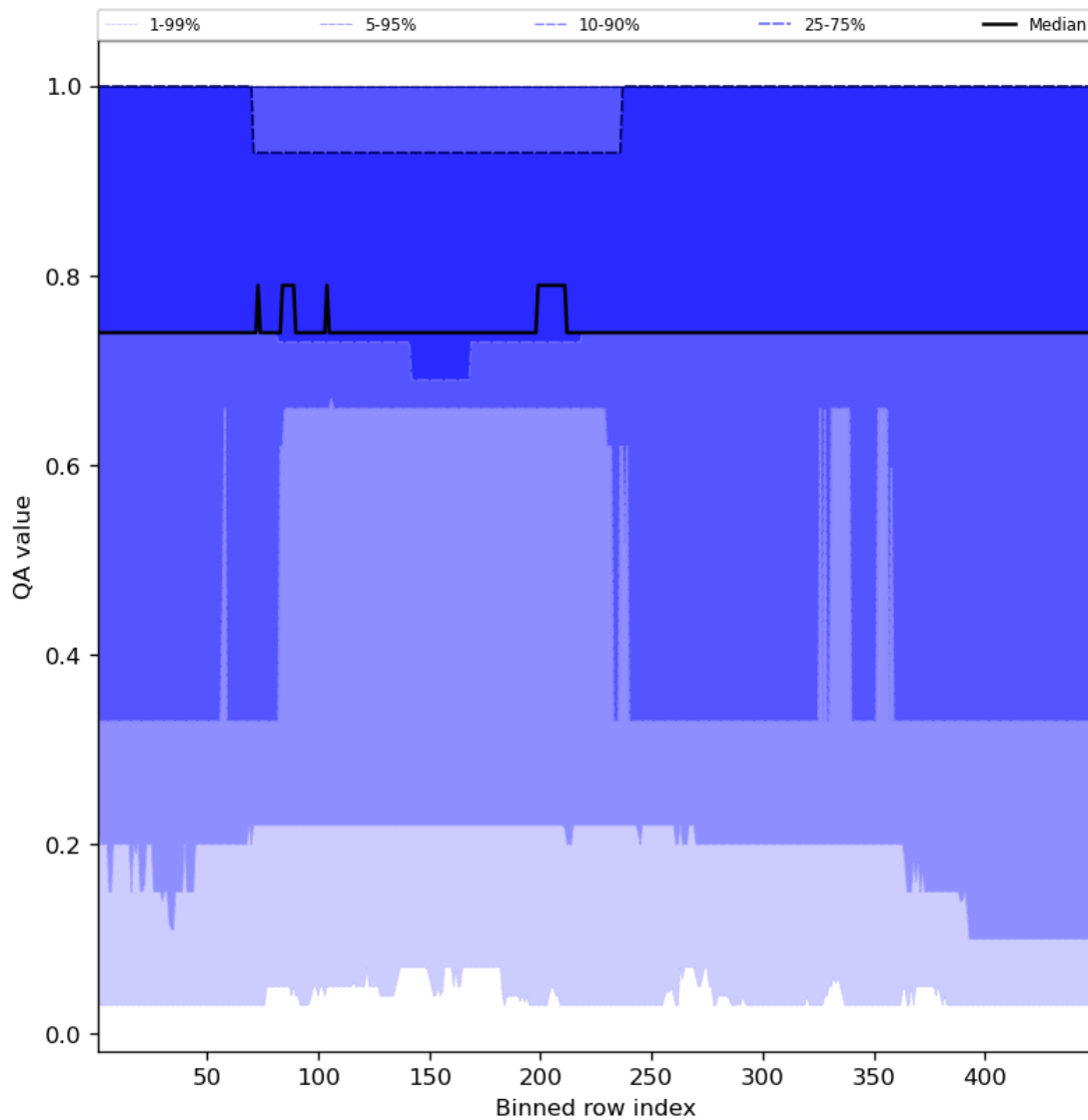
Figure 45: Along track statistics of “QA value” for 2024-01-10 to 2024-01-11
