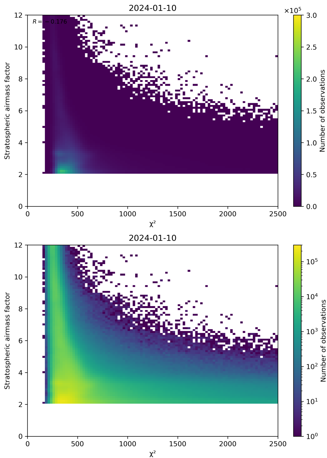
Figure 81: Scatter density plot of “ \chi^2 ” against “Stratospheric airmass factor” for 2024-01-10 to 2024-01-11.
