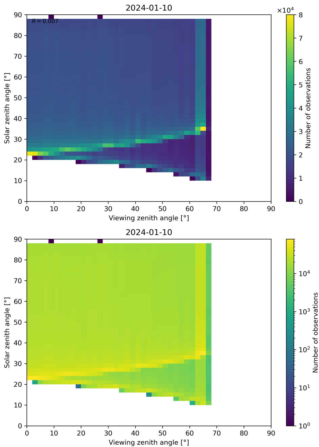
Figure 172: Scatter density plot of “Viewing zenith angle” against “Solar zenith angle” for 2024-01-10 to 2024-01-11.
