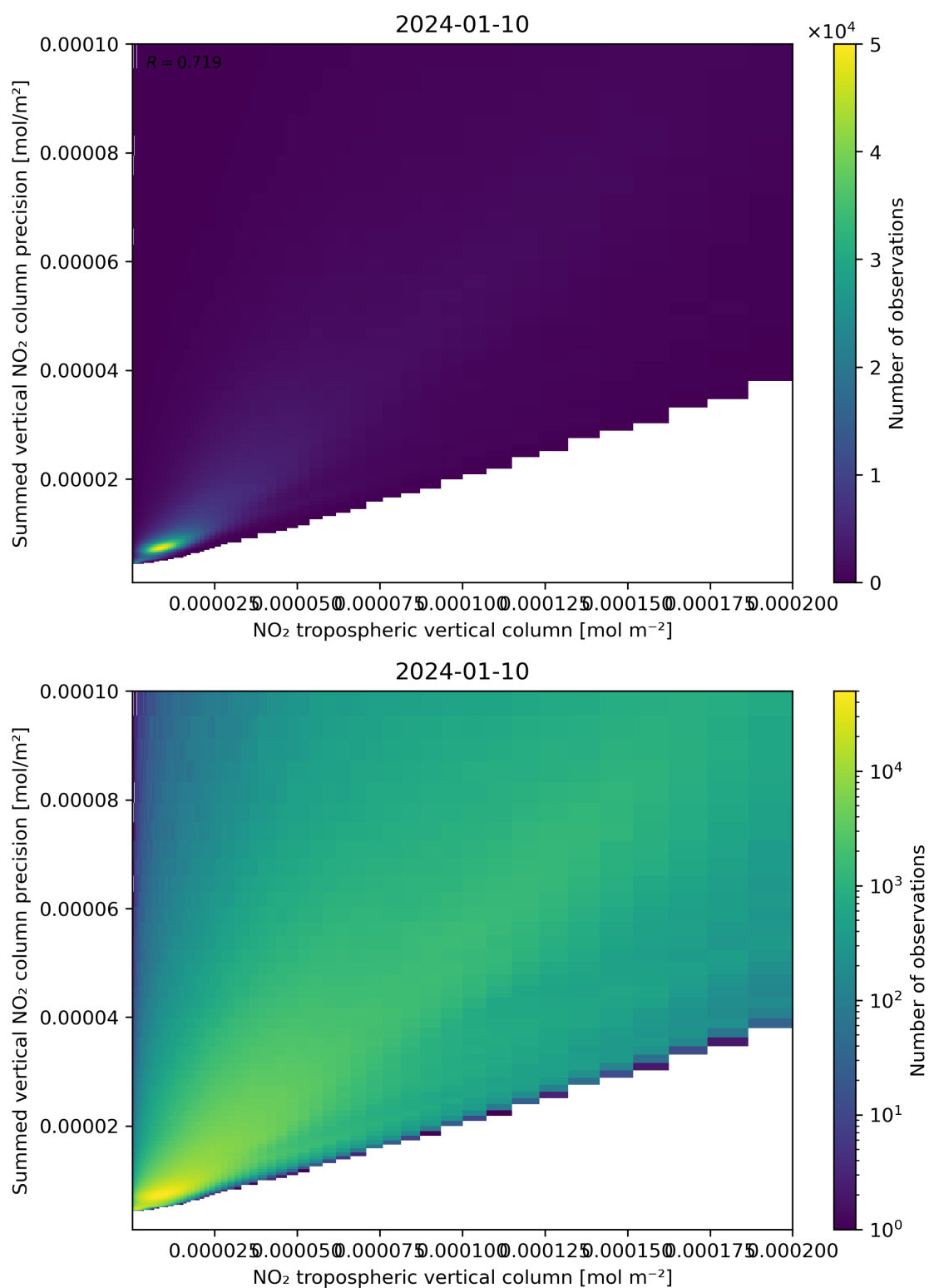
Figure 127: Scatter density plot of “NO 2 tropospheric vertical column” against “Summed vertical NO 2 column precision” for 2024-01-10 to 2024-01-11.
