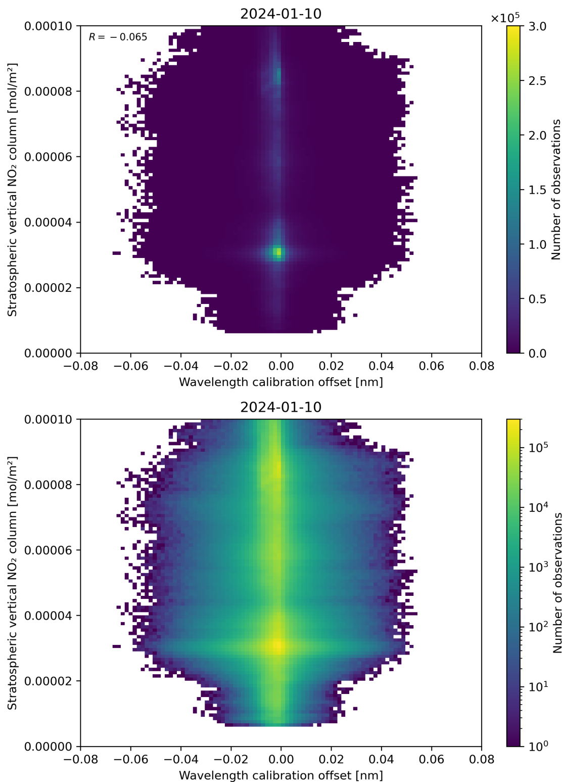
Figure 176: Scatter density plot of “Wavelength calibration offset” against “Stratospheric vertical NO 2 column” for 2024-01-10 to 2024-01-11.
