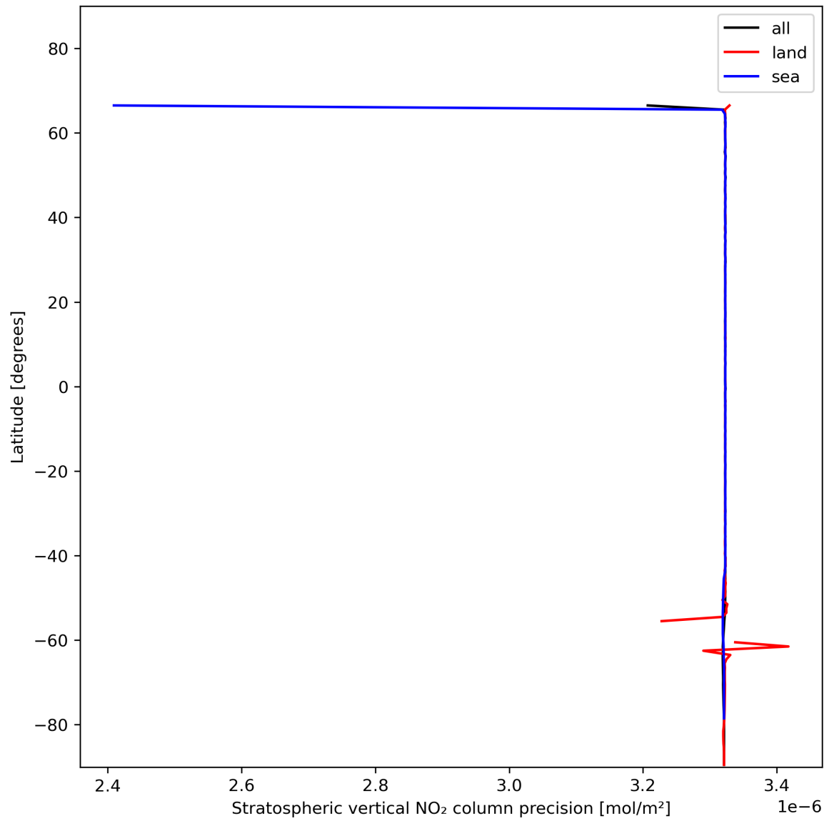
Figure 20: Zonal average of “Stratospheric vertical NO 2 column precision” for 2024-01-10 to 2024-01-11.
