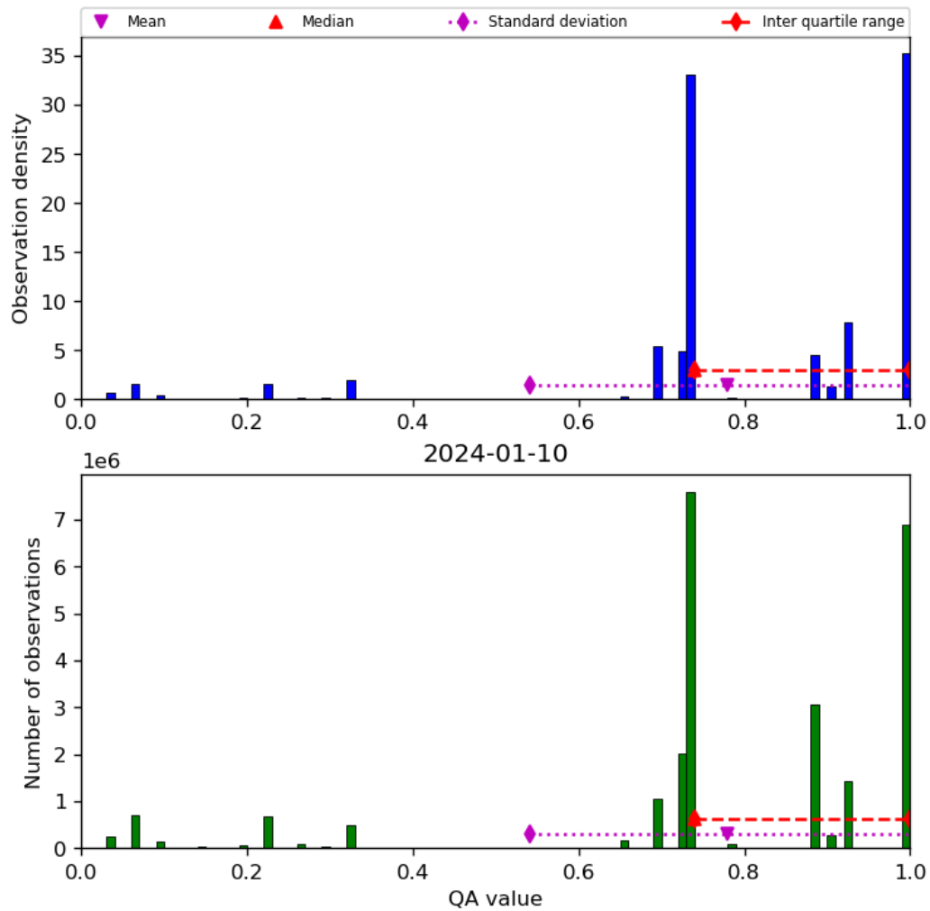
Figure 28: Histogram of “QA value” for 2024-01-10 to 2024-01-11
