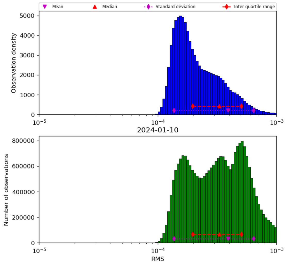
Figure 43: Histogram of “RMS” for 2024-01-10 to 2024-01-11
