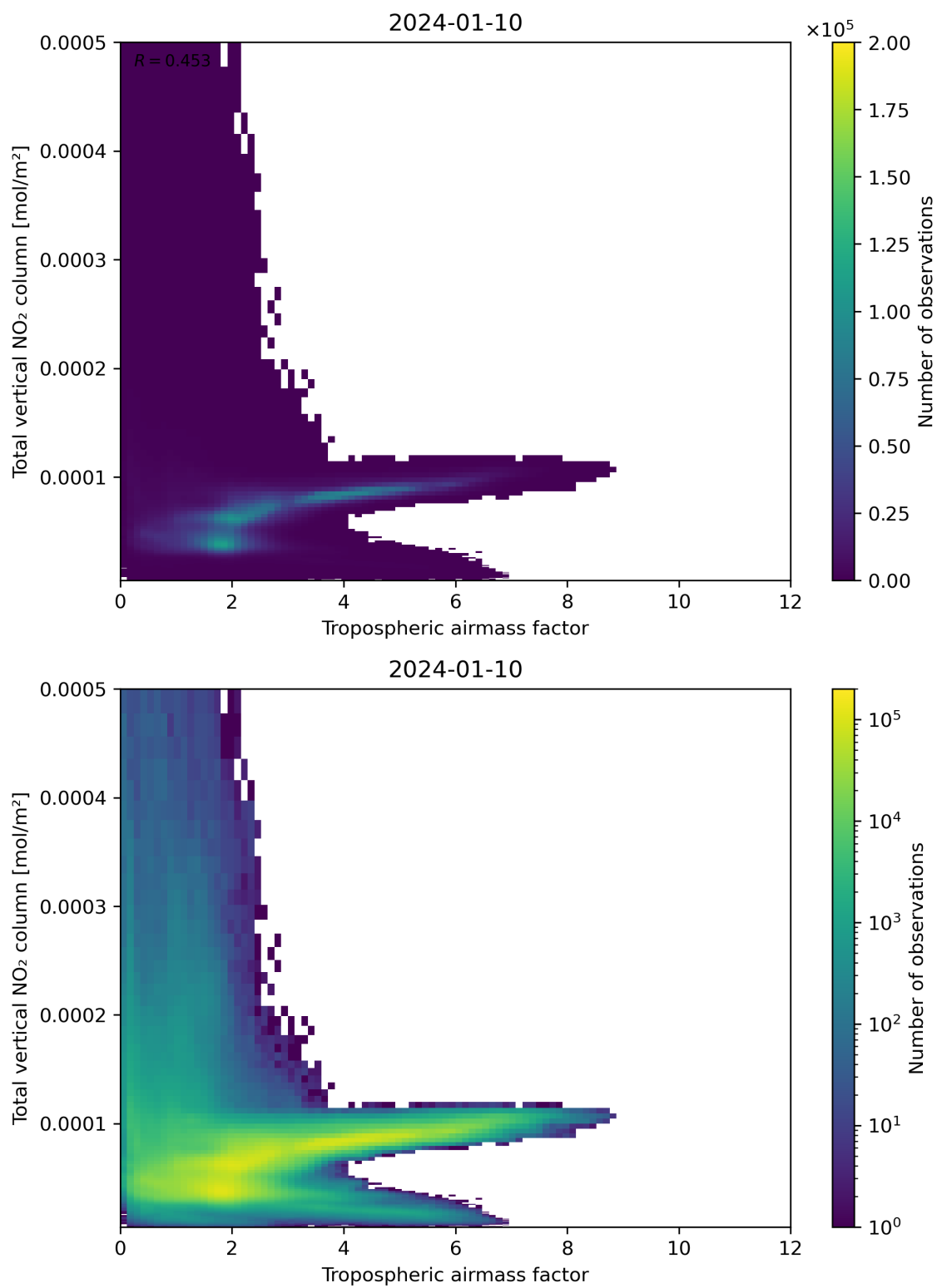
Figure 77: Scatter density plot of “Tropospheric airmass factor” against “Total vertical NO 2 column” for 2024-01-10 to 2024-01-11.
