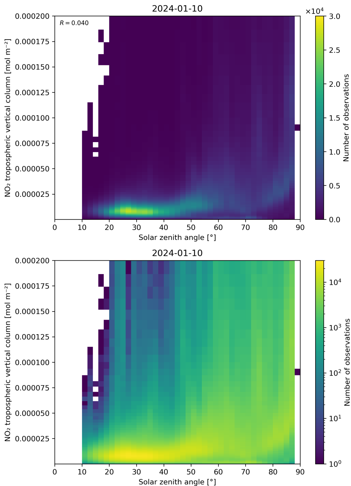
Figure 155: Scatter density plot of “Solar zenith angle” against “NO 2 tropospheric vertical column” for 2024-01-10 to 2024-01-11.
