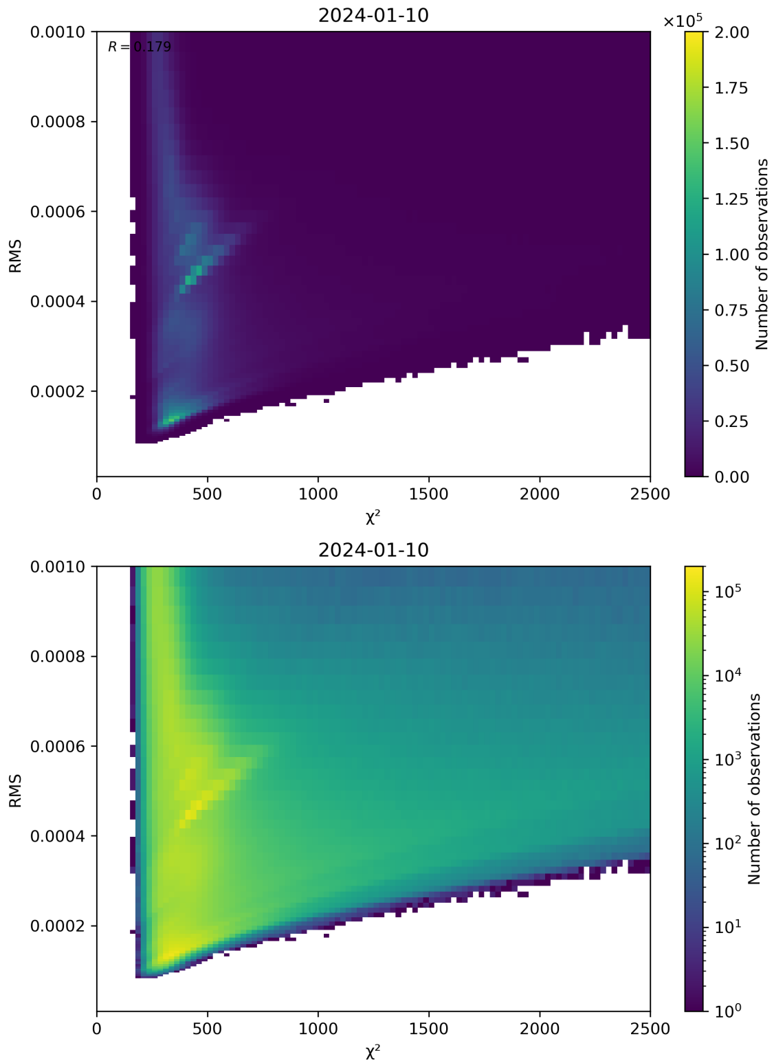
Figure 82: Scatter density plot of “ \chi^2 ” against “RMS” for 2024-01-10 to 2024-01-11.
