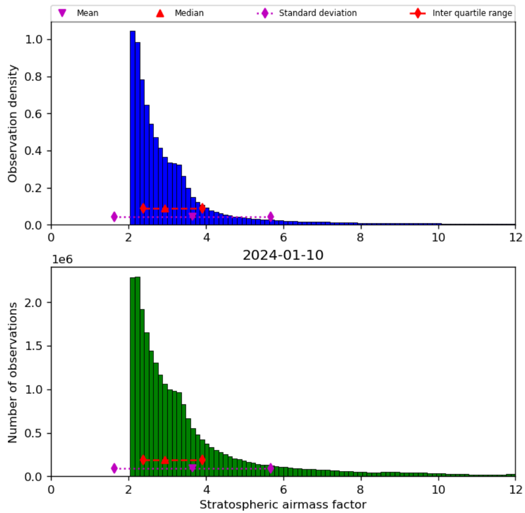
Figure 44: Histogram of “Stratospheric airmass factor” for 2024-01-10 to 2024-01-11
