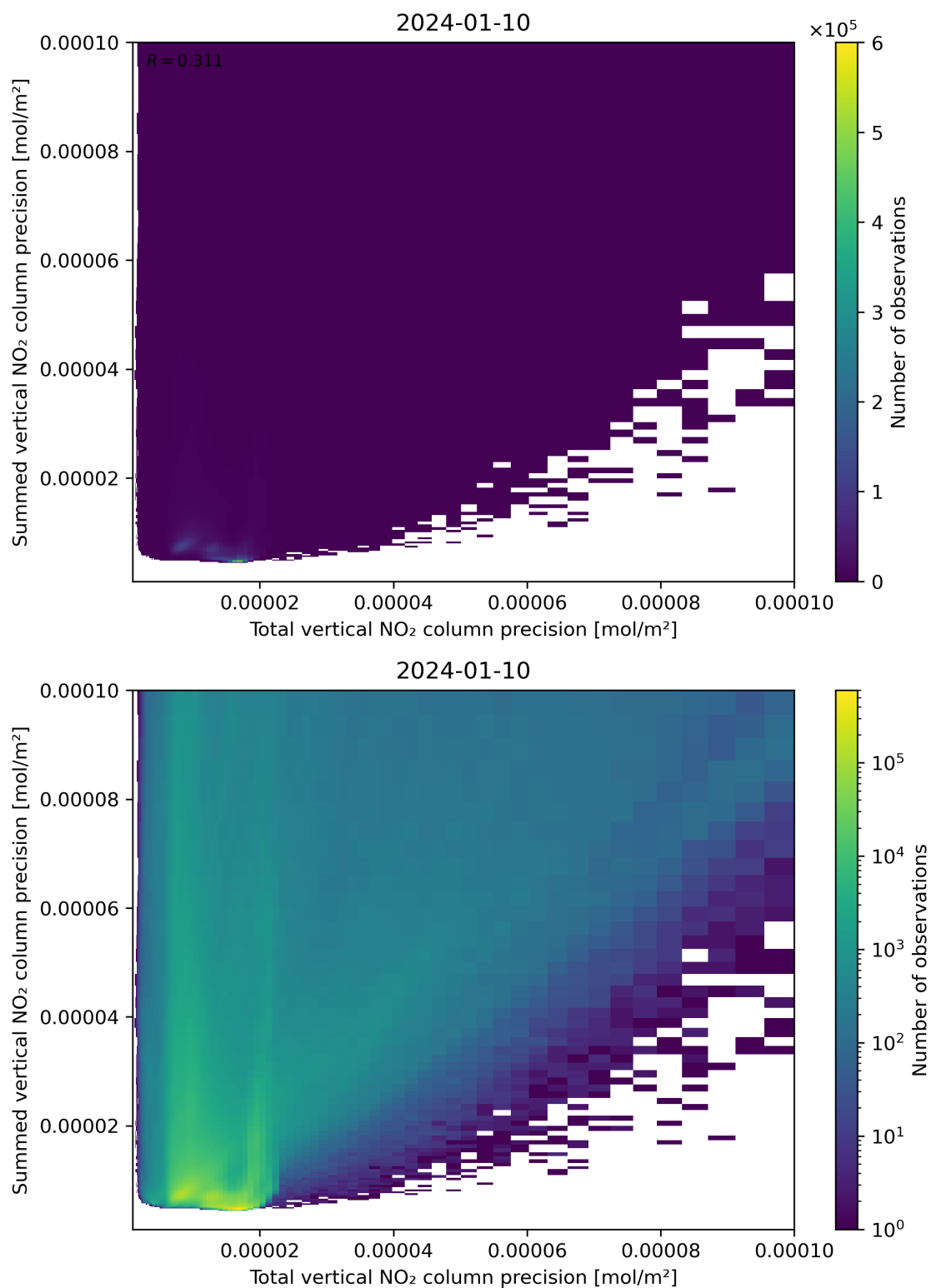
Figure 118: Scatter density plot of “Total vertical NO 2 column precision” against “Summed vertical NO 2 column precision” for 2024-01-10 to 2024-01-11.
