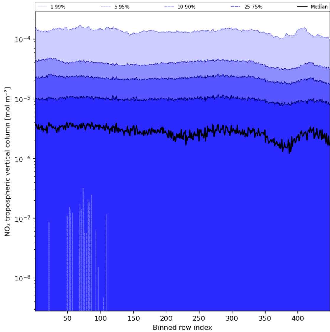
Figure 46: Along track statistics of “NO 2 tropospheric vertical column” for 2024-01-10 to 2024-01-11
