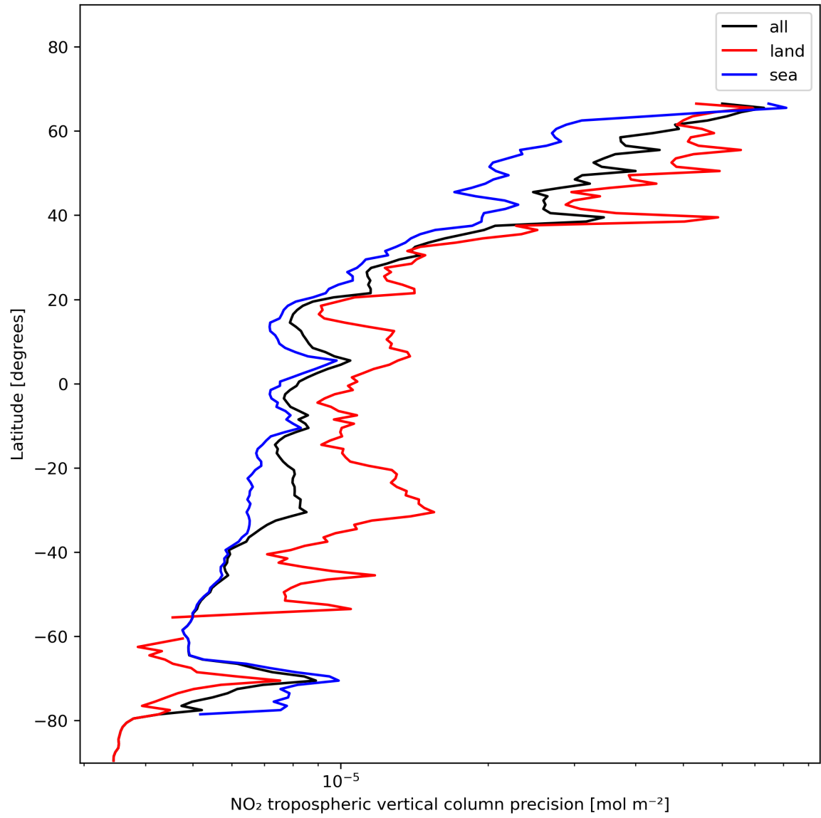
Figure 13: Zonal average of “NO 2 tropospheric vertical column precision” for 2024-01-10 to 2024-01-11.
