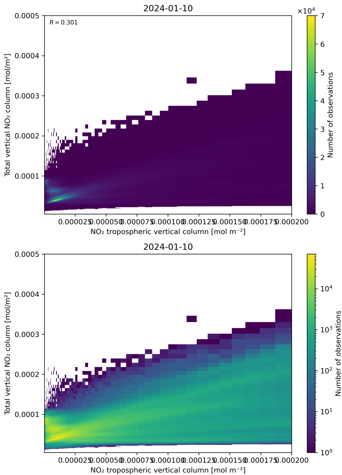
Figure 128: Scatter density plot of “NO 2 tropospheric vertical column” against “Total vertical NO 2 column” for 2024-01-10 to 2024-01-11.
