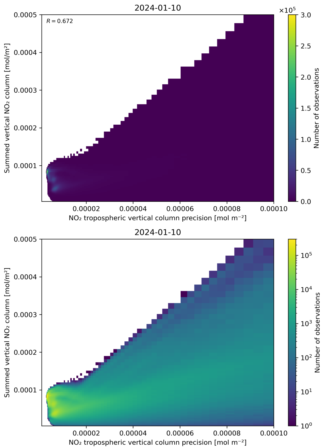
Figure 136: Scatter density plot of “NO 2 tropospheric vertical column precision” against “Summed vertical NO 2 column” for 2024-01-10 to 2024-01-11.
