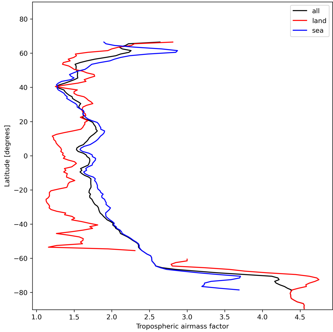
Figure 14: Zonal average of “Tropospheric airmass factor” for 2024-01-10 to 2024-01-11.
