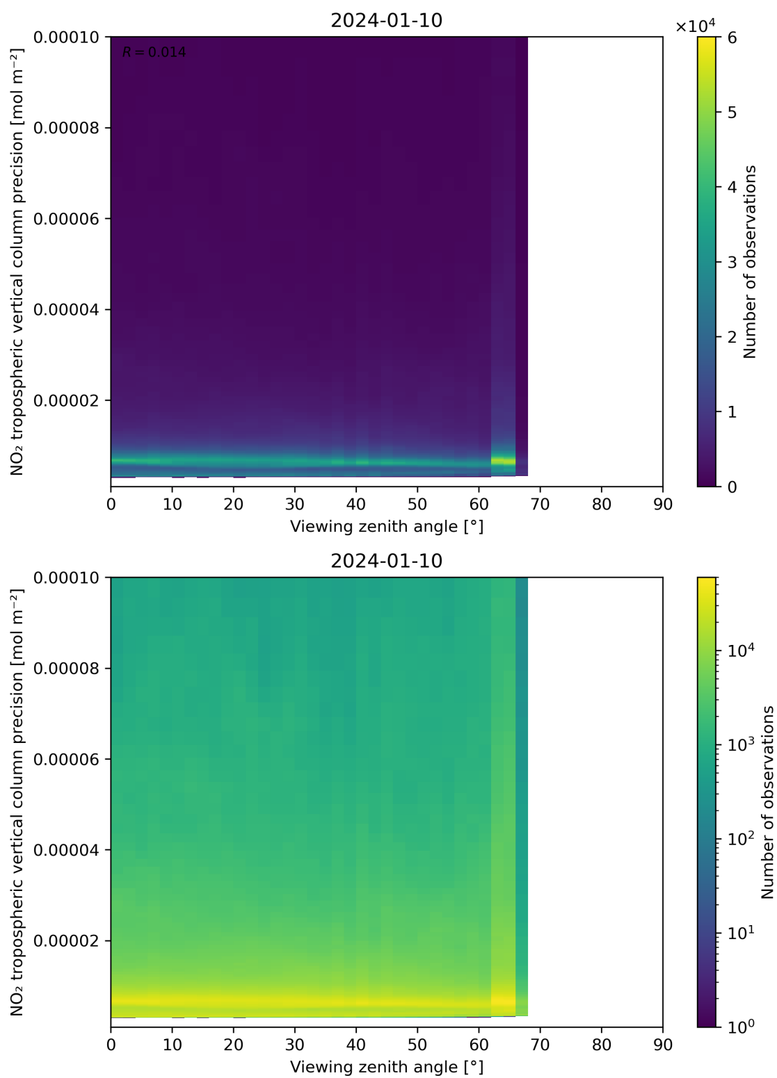
Figure 170: Scatter density plot of “Viewing zenith angle” against “NO 2 tropospheric vertical column precision” for 2024-01-10 to 2024-01-11.
