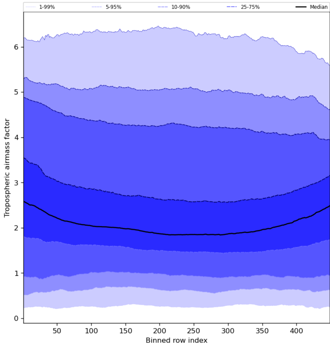
Figure 48: Along track statistics of “Tropospheric airmass factor” for 2024-01-10 to 2024-01-11
