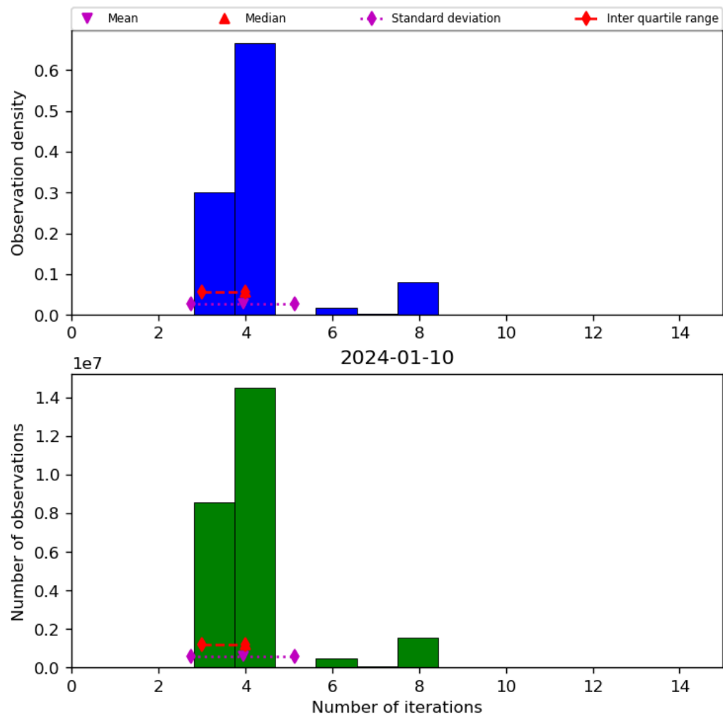
Figure 34: Histogram of “Number of iterations” for 2024-01-10 to 2024-01-11
