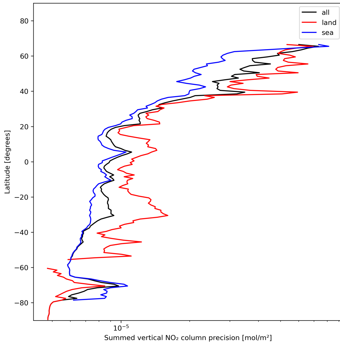
Figure 24: Zonal average of “Summed vertical NO 2 column precision” for 2024-01-10 to 2024-01-11.
