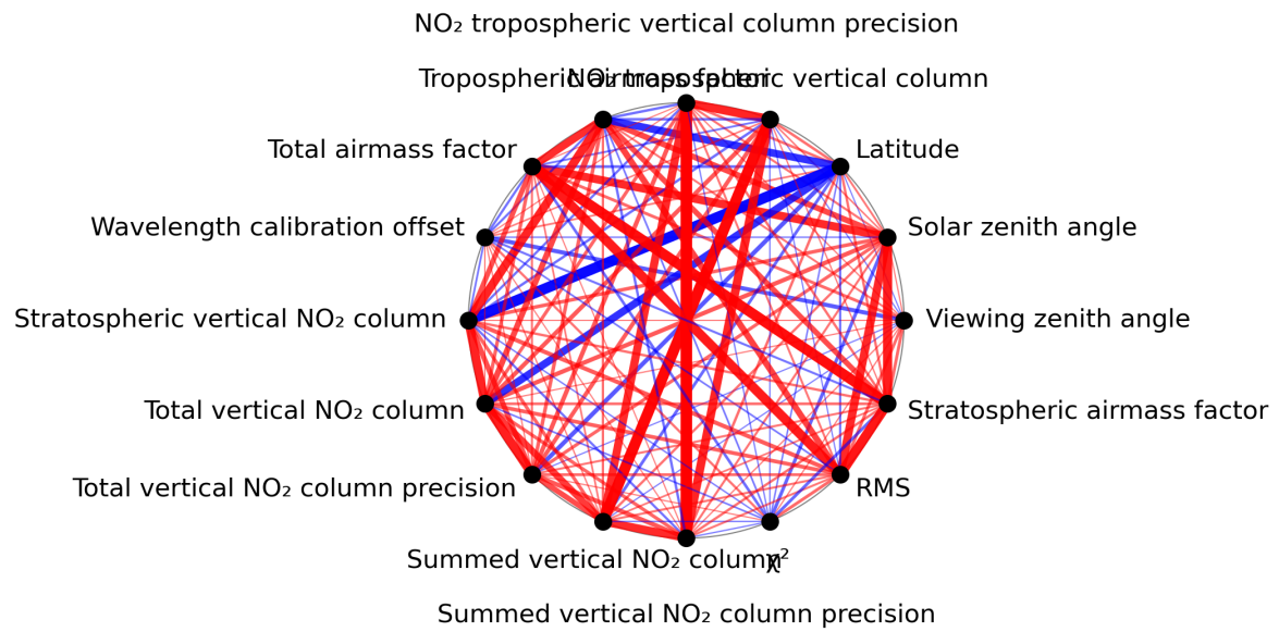
Figure 1: Map of correlation graph for 2024-01-10 to 2024-01-11.
