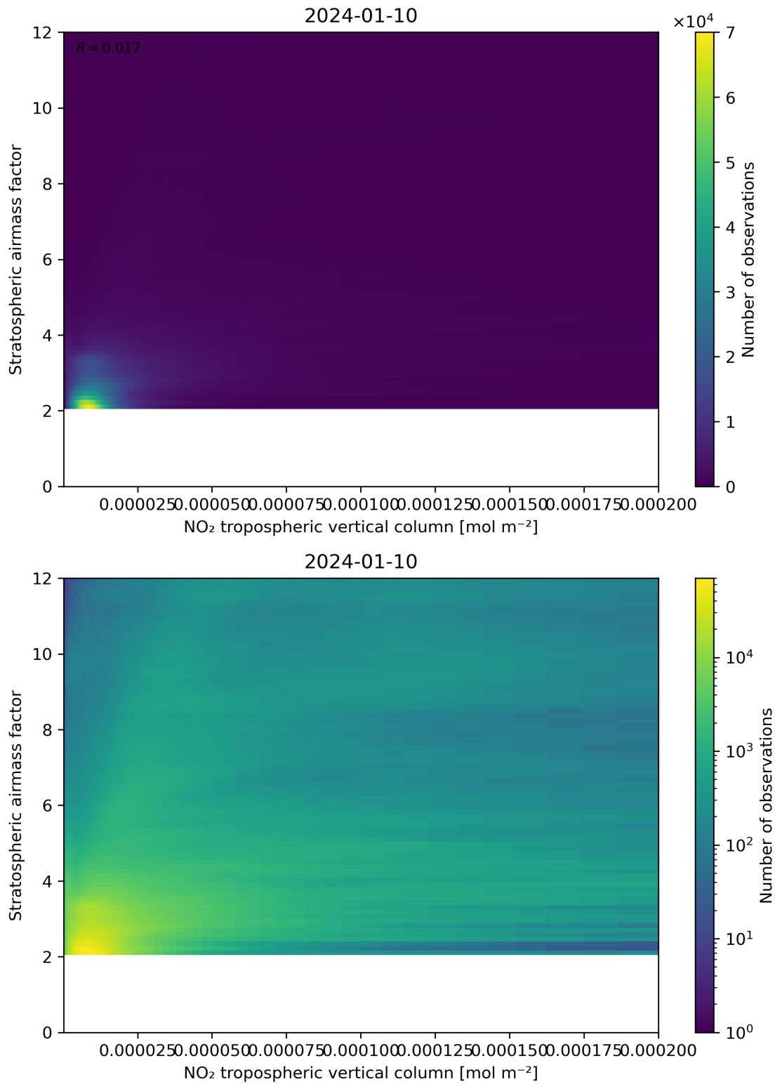
Figure 121: Scatter density plot of “NO 2 tropospheric vertical column” against “Stratospheric airmass factor” for 2024-01-10 to 2024-01-11.
