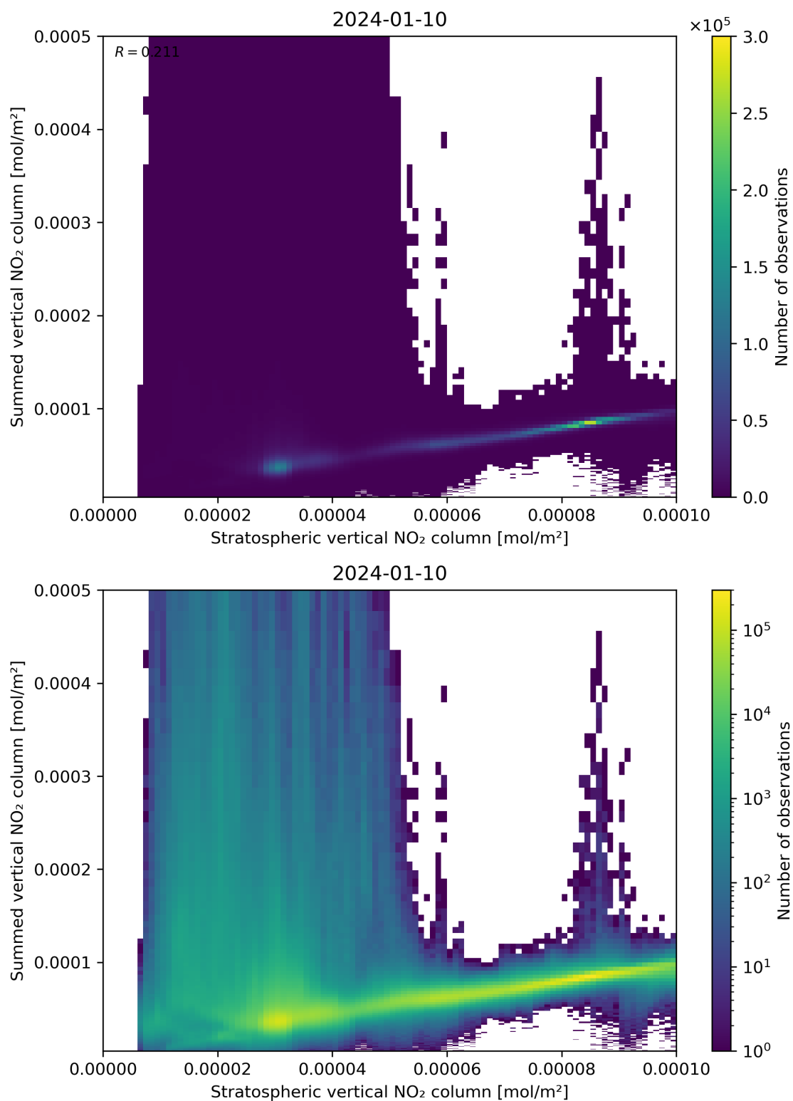
Figure 98: Scatter density plot of “Stratospheric vertical NO 2 column” against “Summed vertical NO 2 column” for 2024-01-10 to 2024-01-11.
