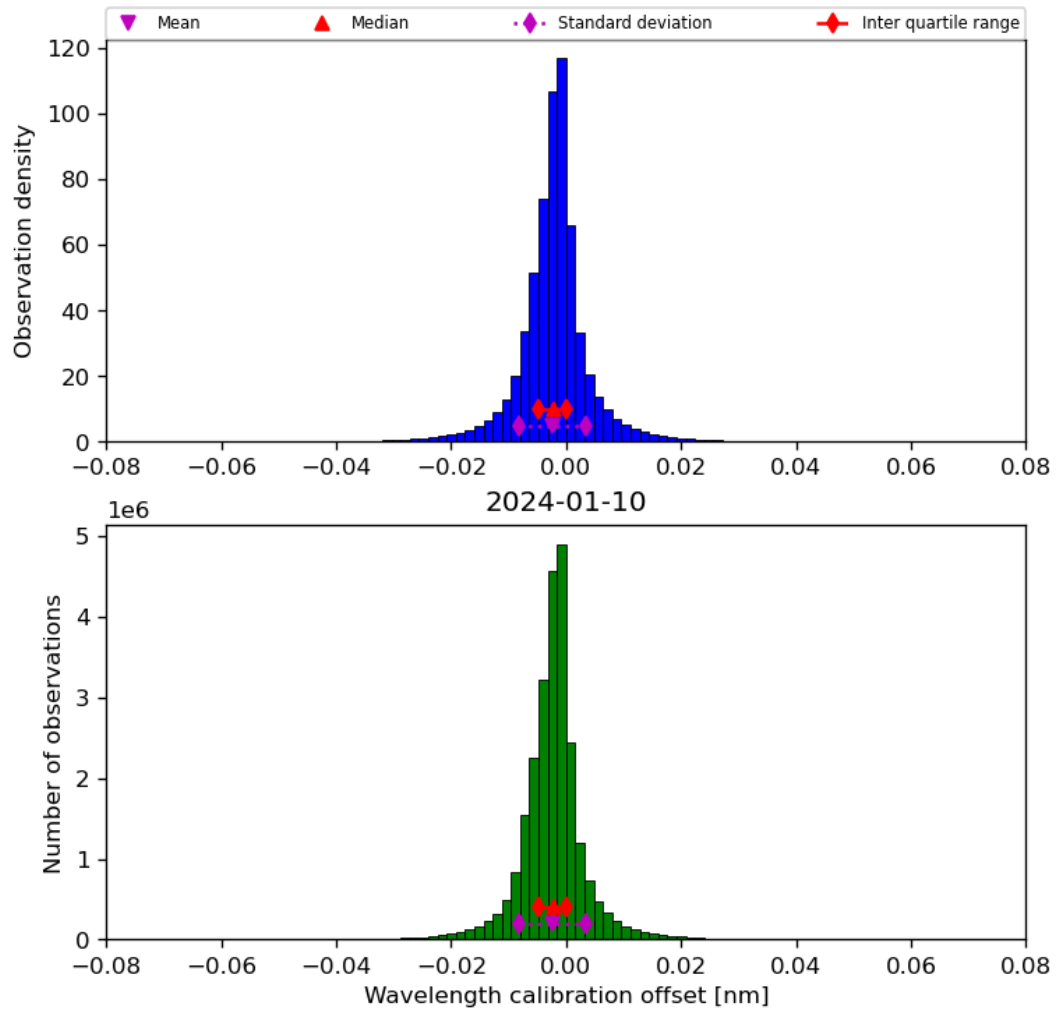
Figure 35: Histogram of “Wavelength calibration offset” for 2024-01-10 to 2024-01-11
