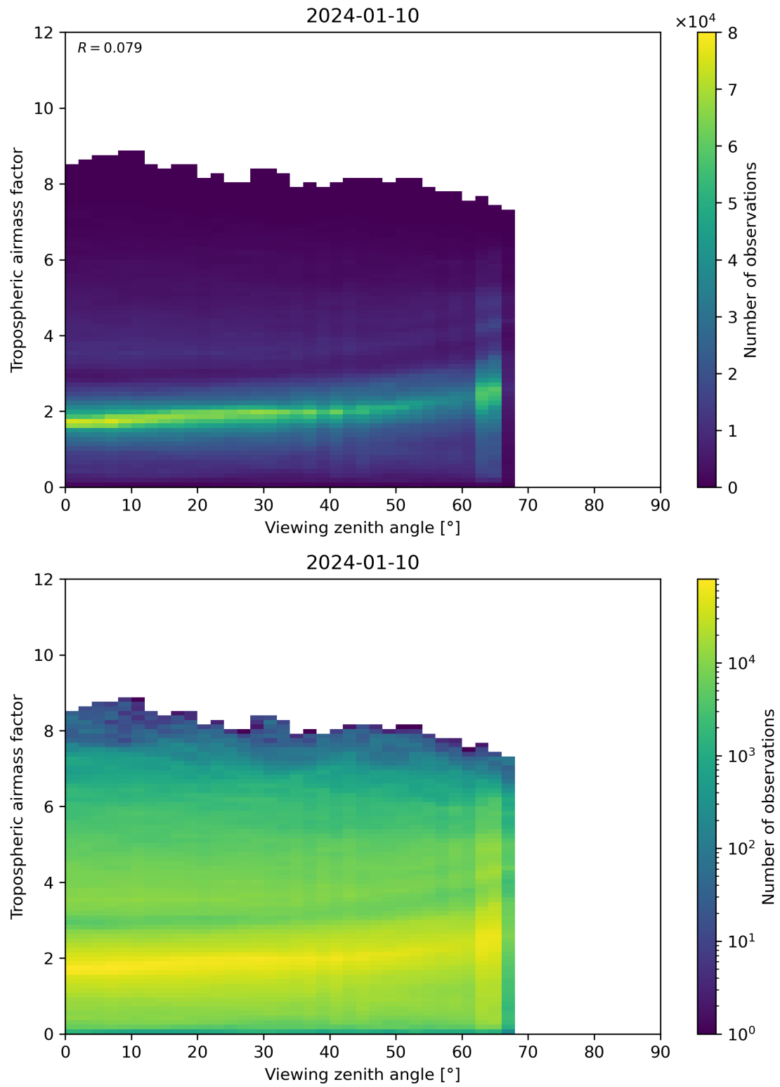
Figure 161: Scatter density plot of “Viewing zenith angle” against “Tropospheric airmass factor” for 2024-01-10 to 2024-01-11.
