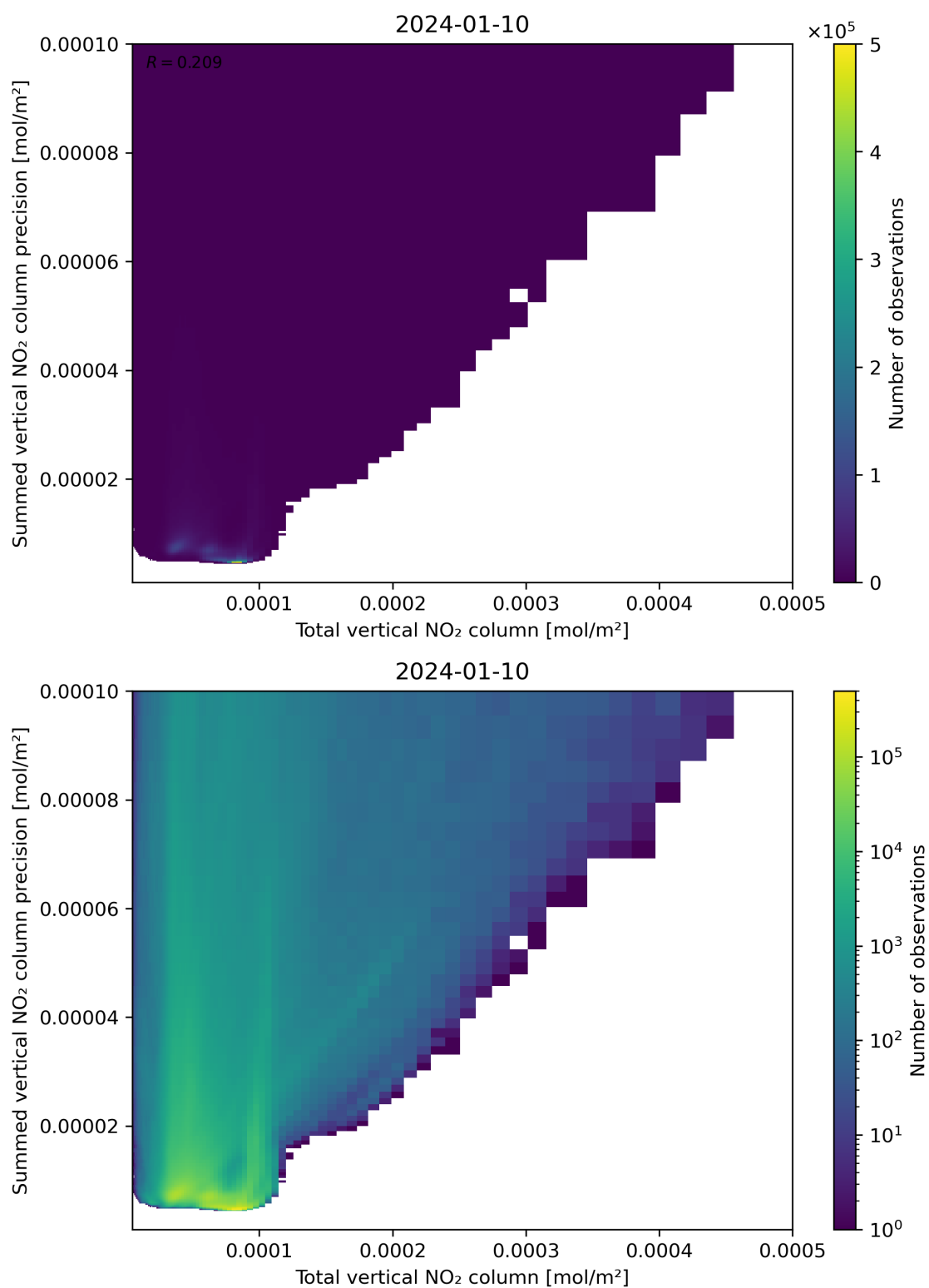
Figure 113: Scatter density plot of “Total vertical NO 2 column” against “Summed vertical NO 2 column precision” for 2024-01-10 to 2024-01-11.
