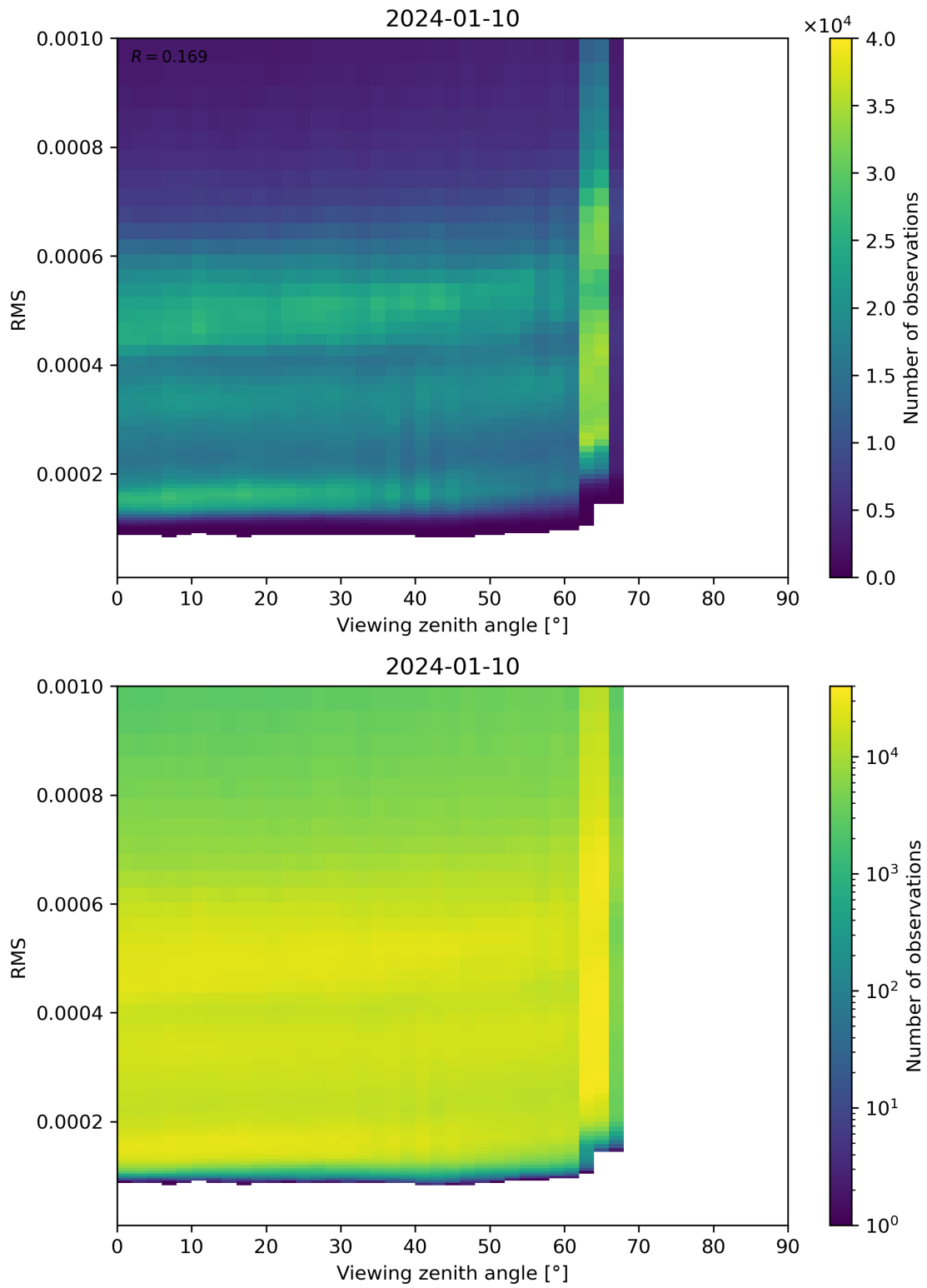
Figure 171: Scatter density plot of “Viewing zenith angle” against “RMS” for 2024-01-10 to 2024-01-11.
