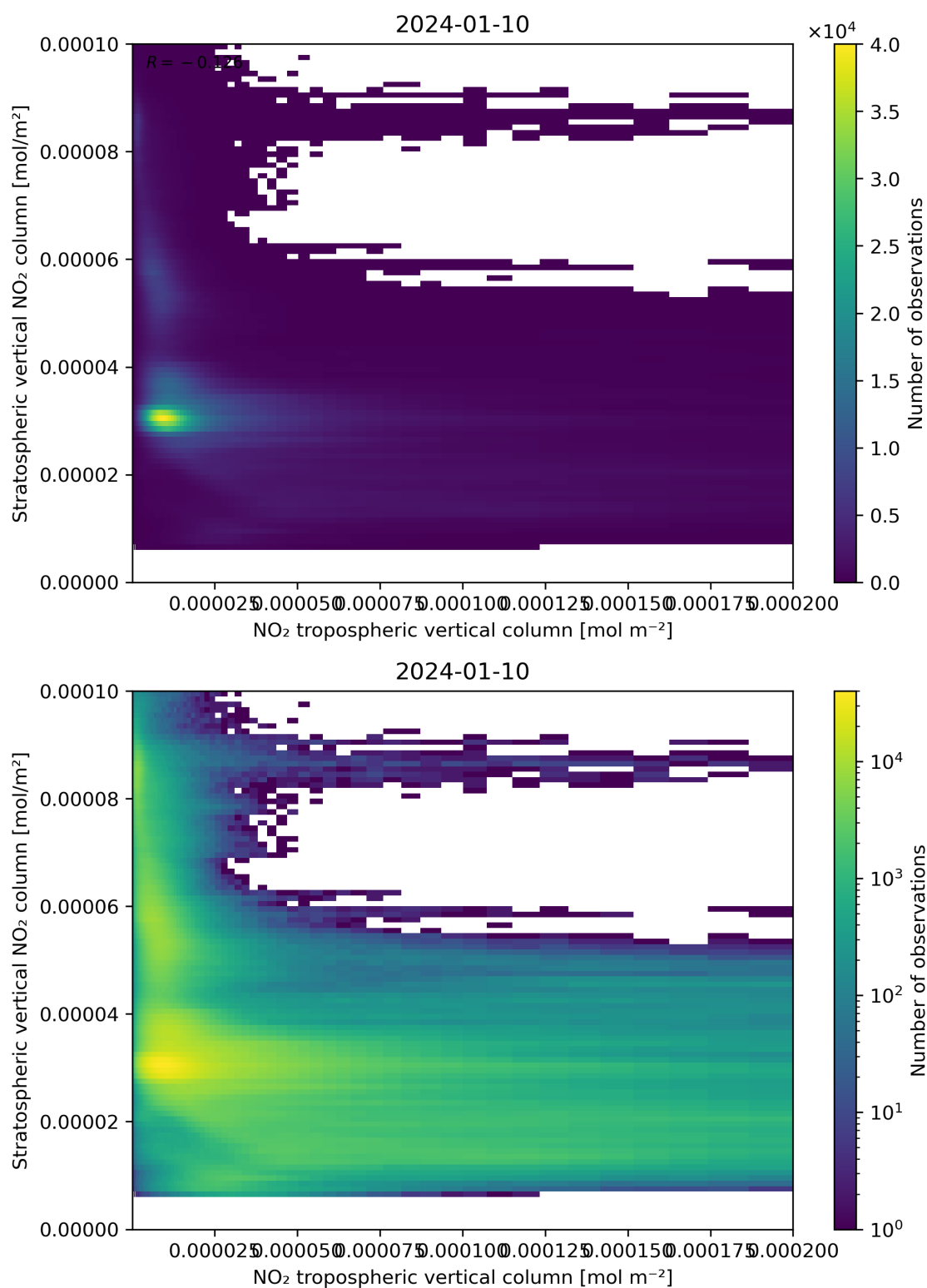
Figure 125: Scatter density plot of “NO 2 tropospheric vertical column” against “Stratospheric vertical NO 2 column” for 2024-01-10 to 2024-01-11.
