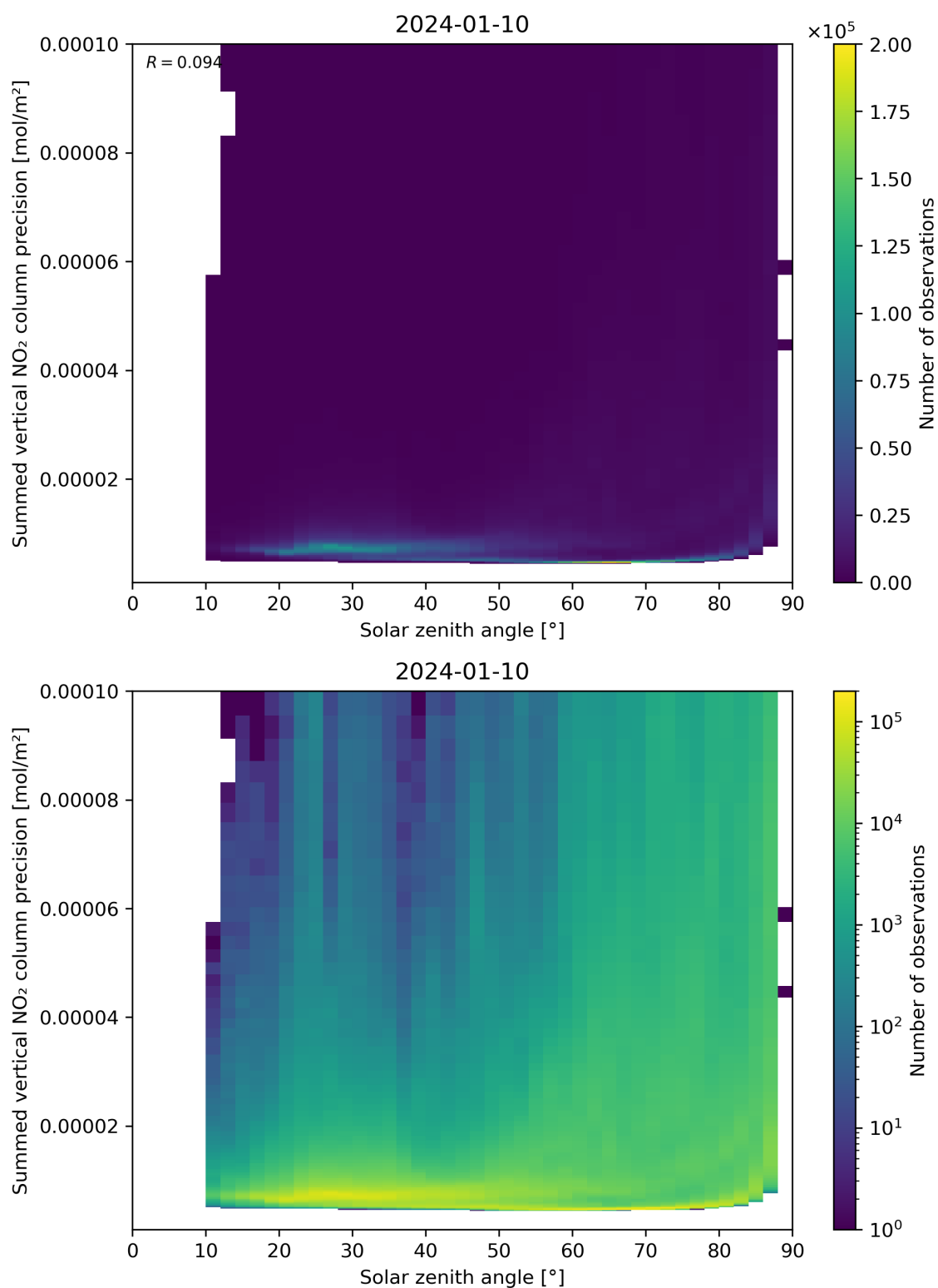
Figure 152: Scatter density plot of “Solar zenith angle” against “Summed vertical NO 2 column precision” for 2024-01-10 to 2024-01-11.
