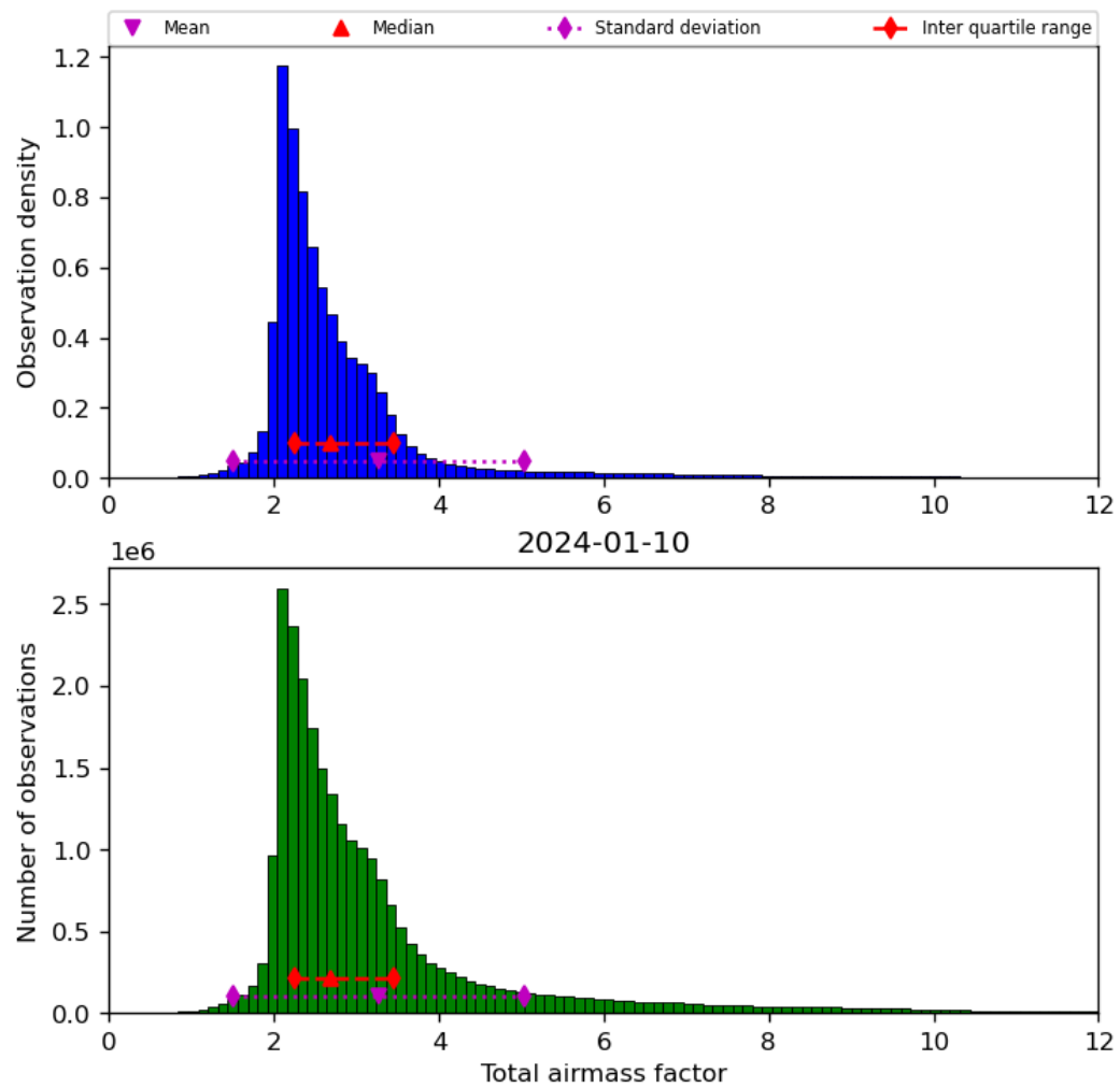
Figure 32: Histogram of “Total airmass factor” for 2024-01-10 to 2024-01-11
