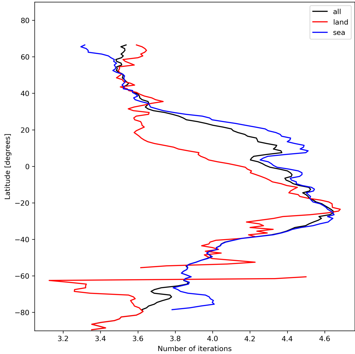
Figure 17: Zonal average of “Number of iterations” for 2024-01-10 to 2024-01-11.
