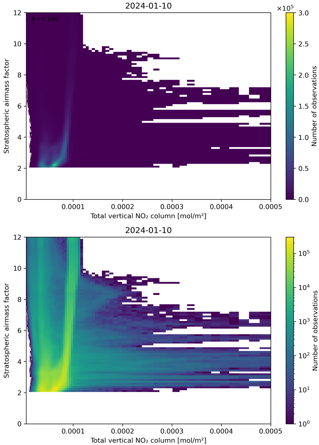
Figure 110: Scatter density plot of “Total vertical NO 2 column” against “Stratospheric airmass factor” for 2024-01-10 to 2024-01-11.
