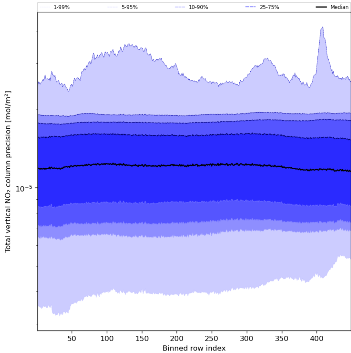
Figure 56: Along track statistics of “Total vertical NO 2 column precision” for 2024-01-10 to 2024-01-11
