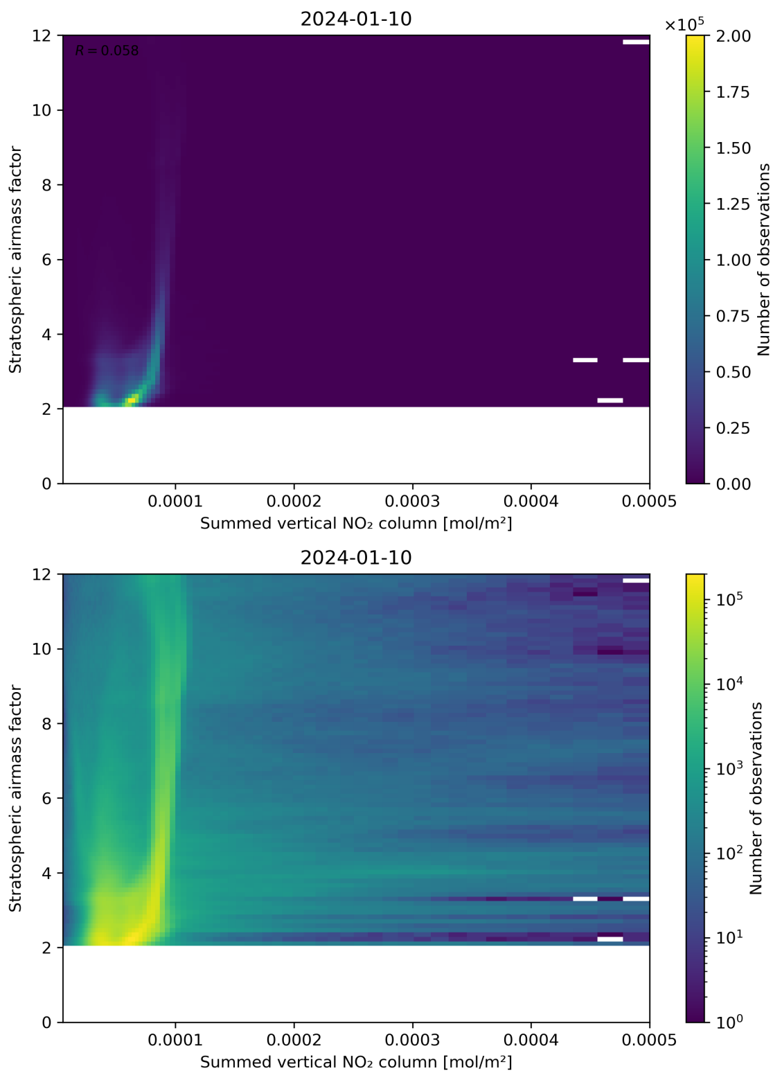
Figure 103: Scatter density plot of “Summed vertical NO 2 column” against “Stratospheric airmass factor” for 2024-01-10 to 2024-01-11.
