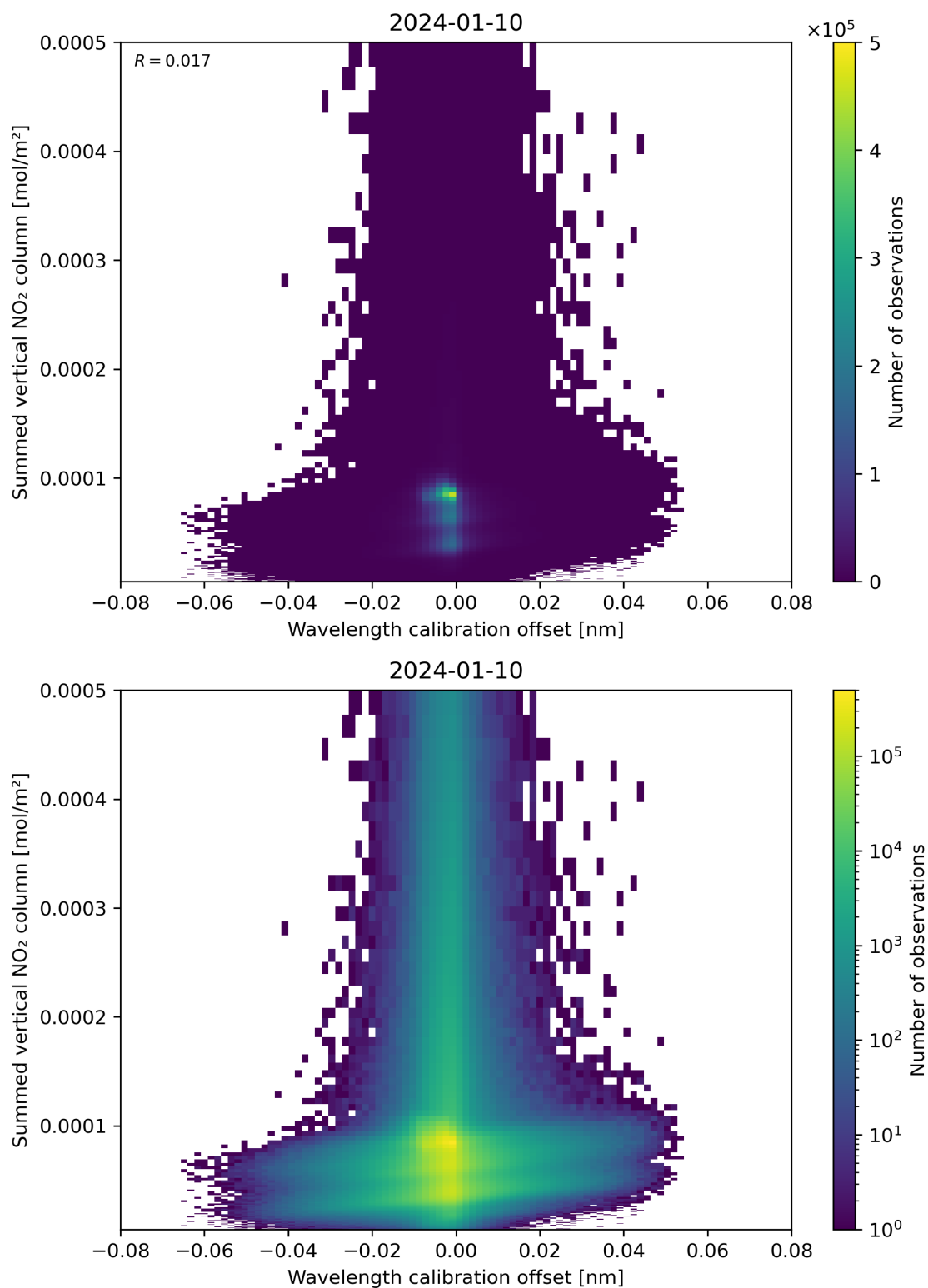
Figure 177: Scatter density plot of “Wavelength calibration offset” against “Summed vertical NO 2 column” for 2024-01-10 to 2024-01-11.
