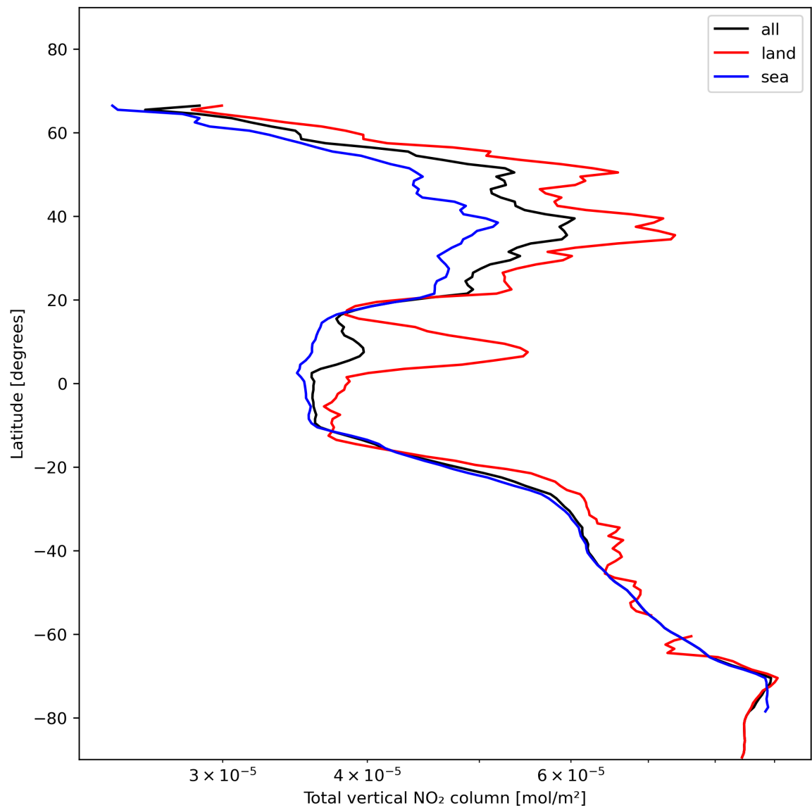
Figure 21: Zonal average of “Total vertical NO 2 column” for 2024-01-10 to 2024-01-11.
