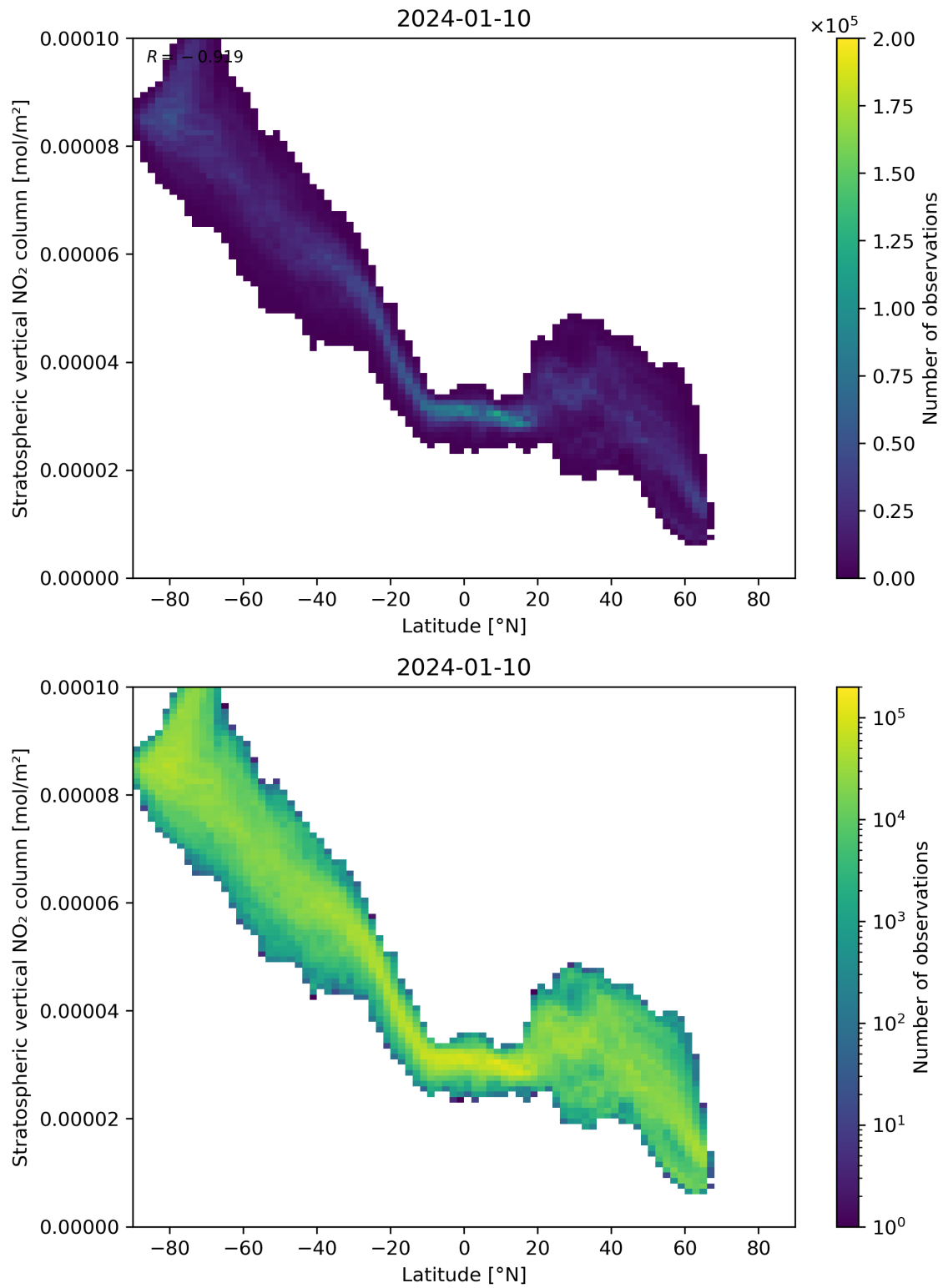
Figure 87: Scatter density plot of “Latitude” against “Stratospheric vertical NO 2 column” for 2024-01-10 to 2024-01-11.
