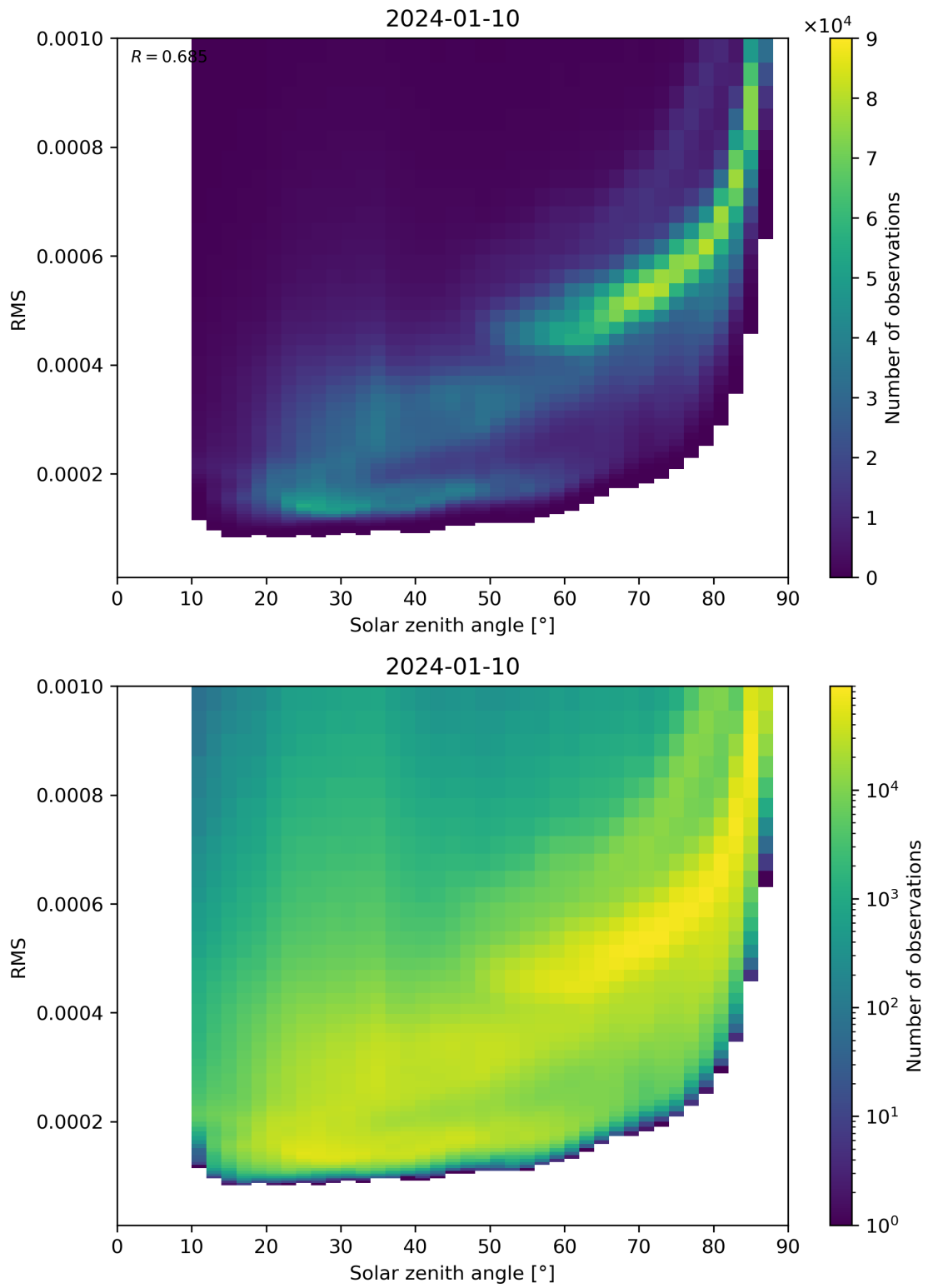
Figure 157: Scatter density plot of “Solar zenith angle” against “RMS” for 2024-01-10 to 2024-01-11.
