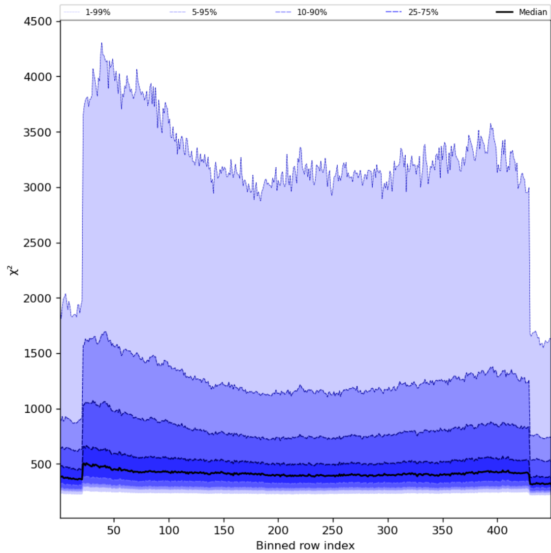
Figure 59: Along track statistics of “ \chi^2 ” for 2024-01-10 to 2024-01-11
