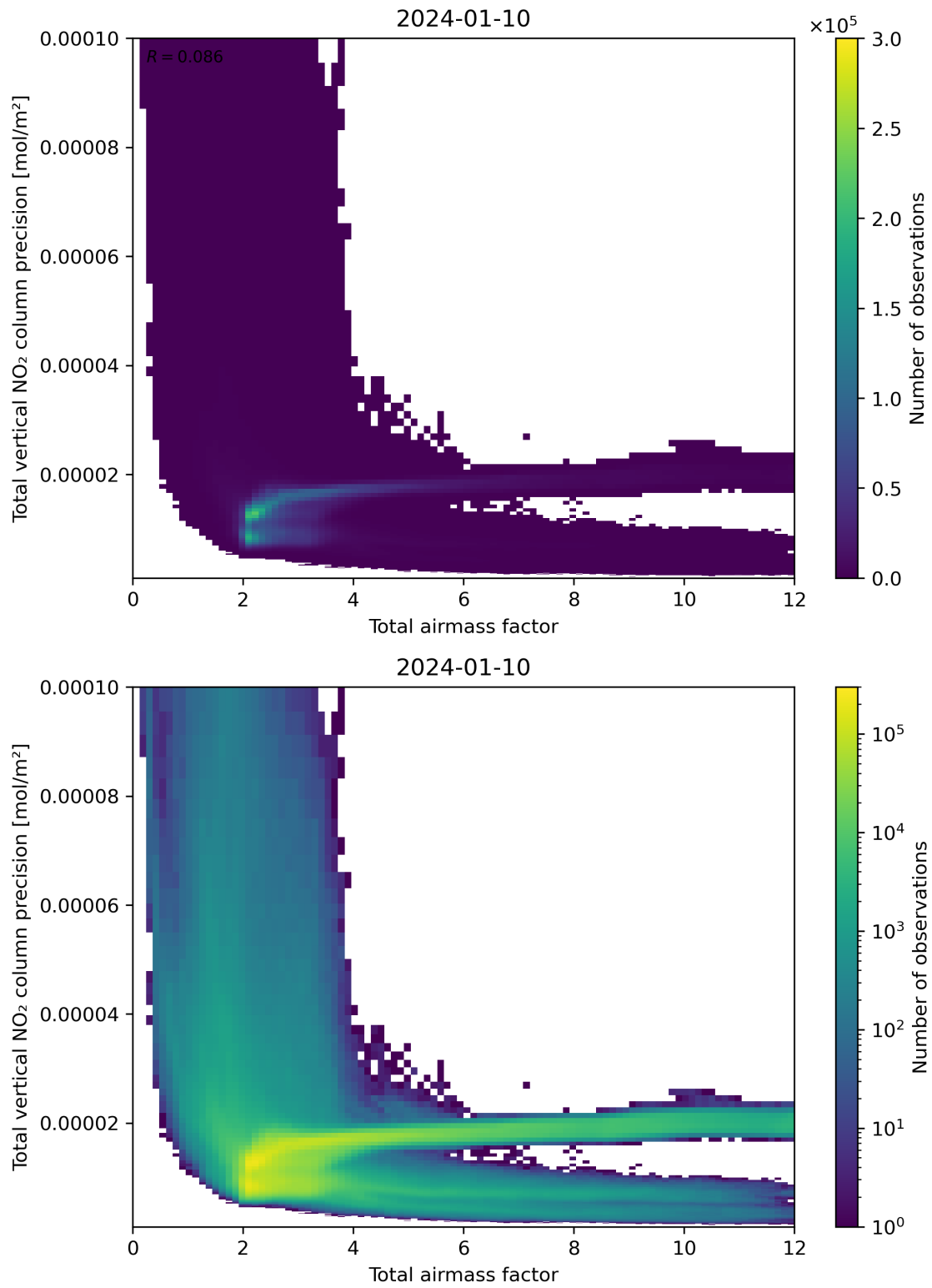
Figure 68: Scatter density plot of “Total airmass factor” against “Total vertical NO 2 column precision” for 2024-01-10 to 2024-01-11.
