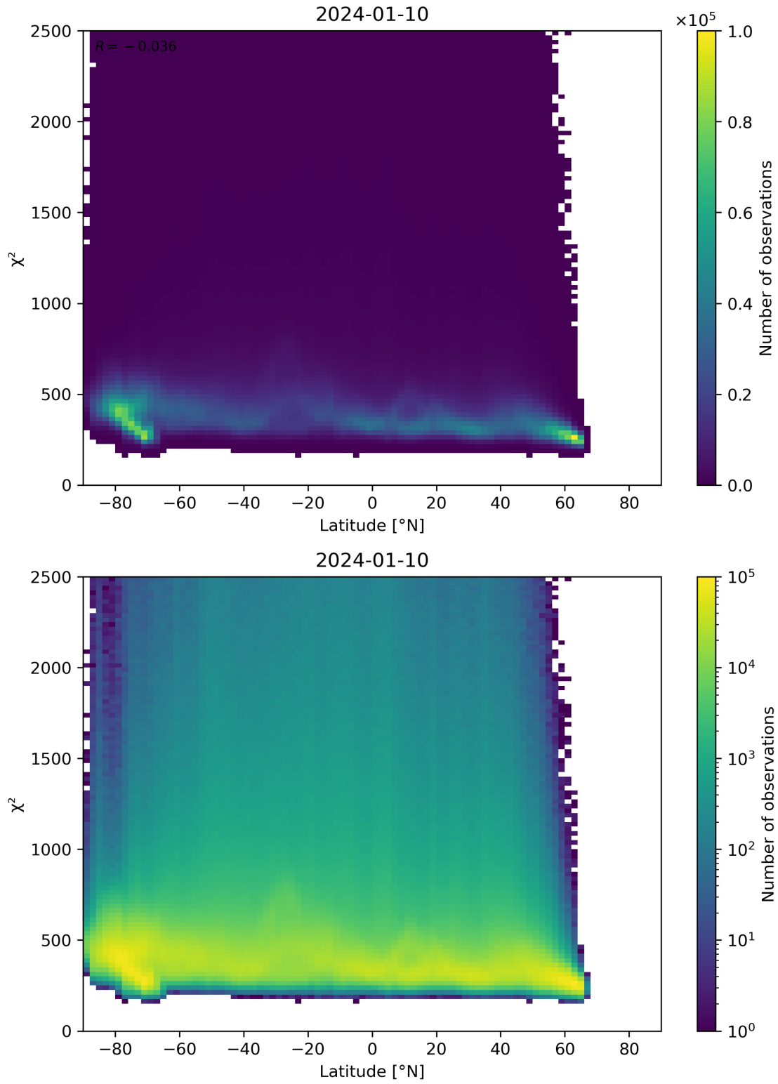
Figure 86: Scatter density plot of “Latitude” against “ \chi^2 ” for 2024-01-10 to 2024-01-11.
