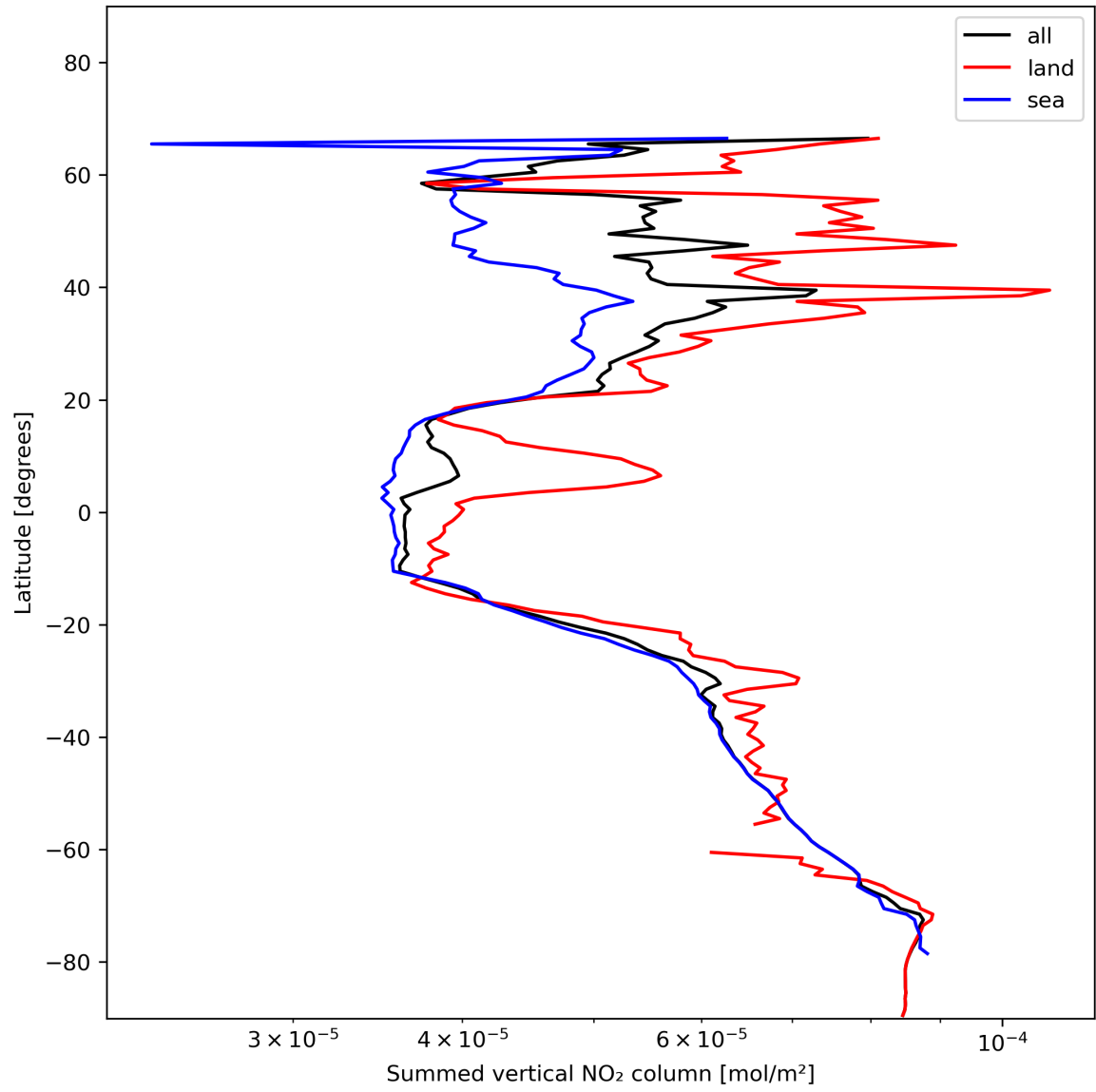
Figure 23: Zonal average of “Summed vertical NO 2 column” for 2024-01-10 to 2024-01-11.
