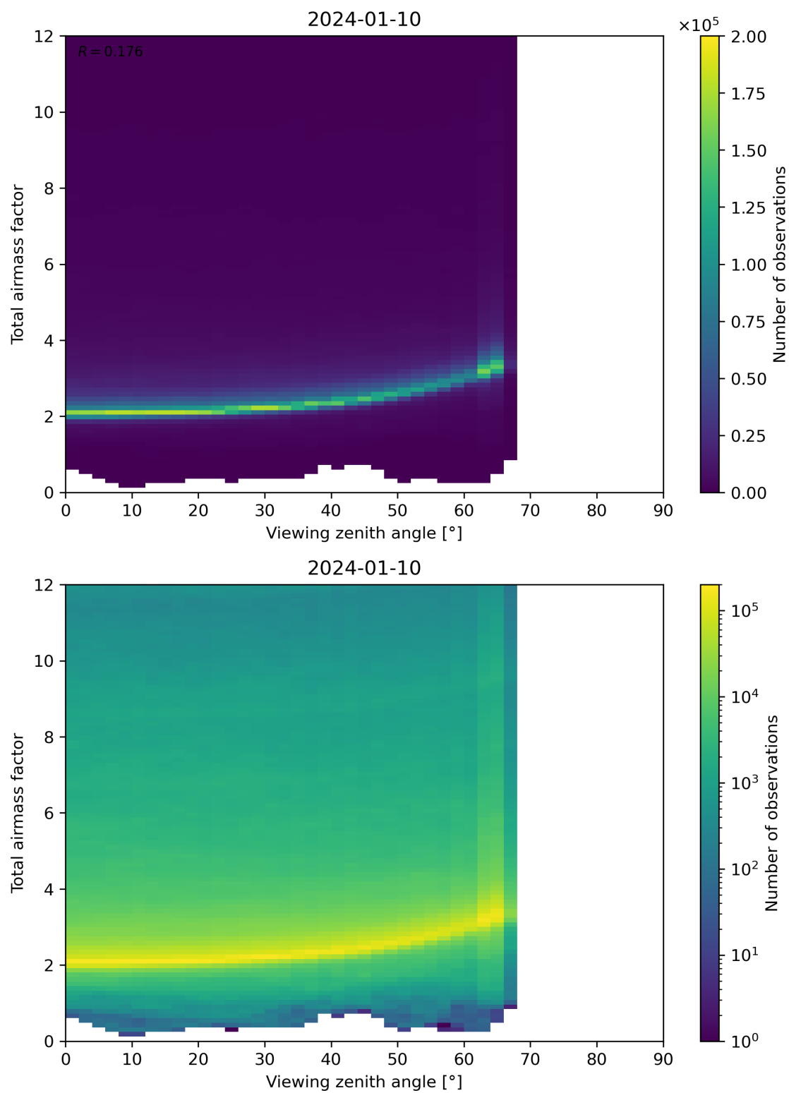
Figure 160: Scatter density plot of “Viewing zenith angle” against “Total airmass factor” for 2024-01-10 to 2024-01-11.
