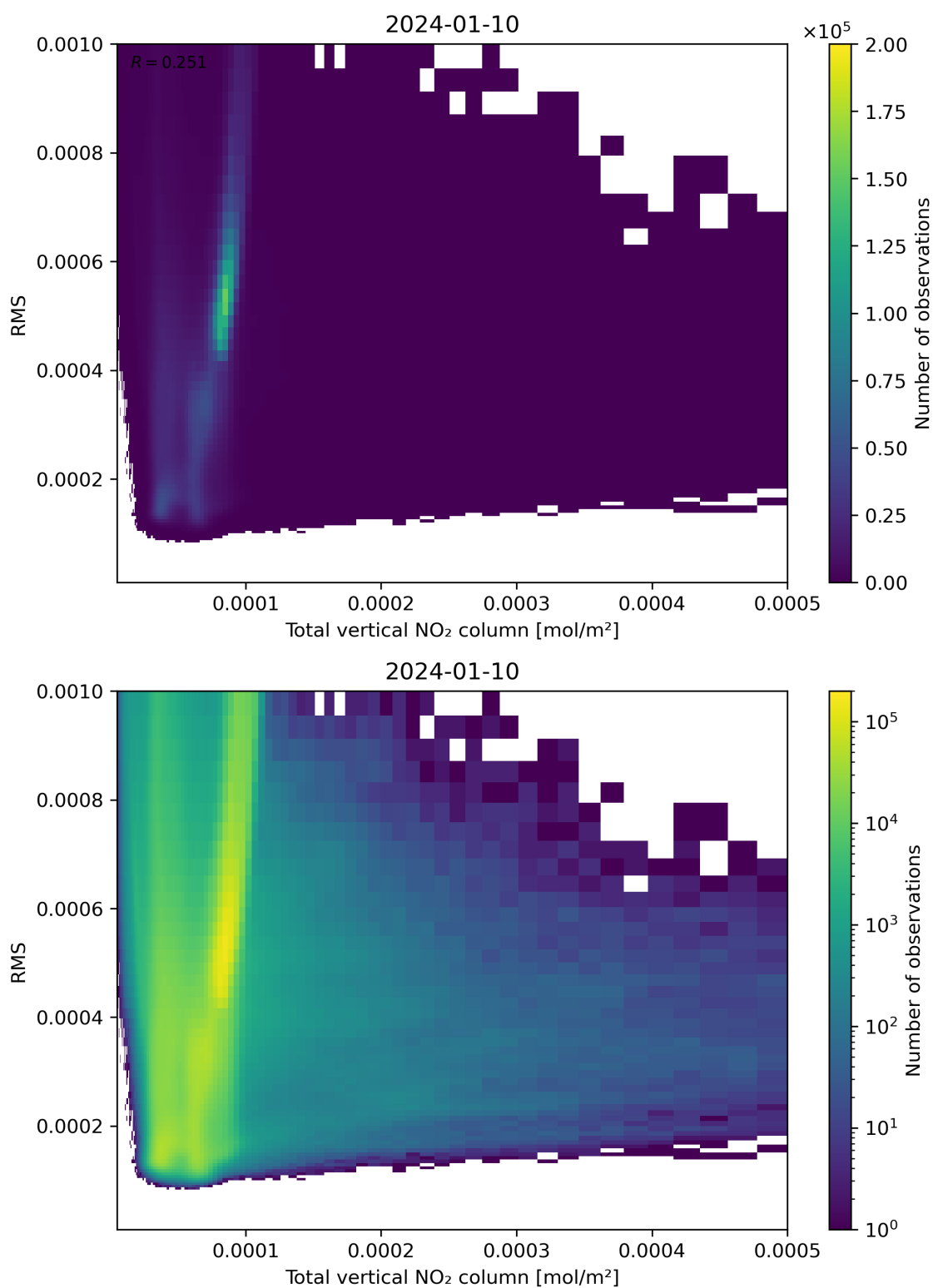
Figure 120: Scatter density plot of “Total vertical NO 2 column” against “RMS” for 2024-01-10 to 2024-01-11.
