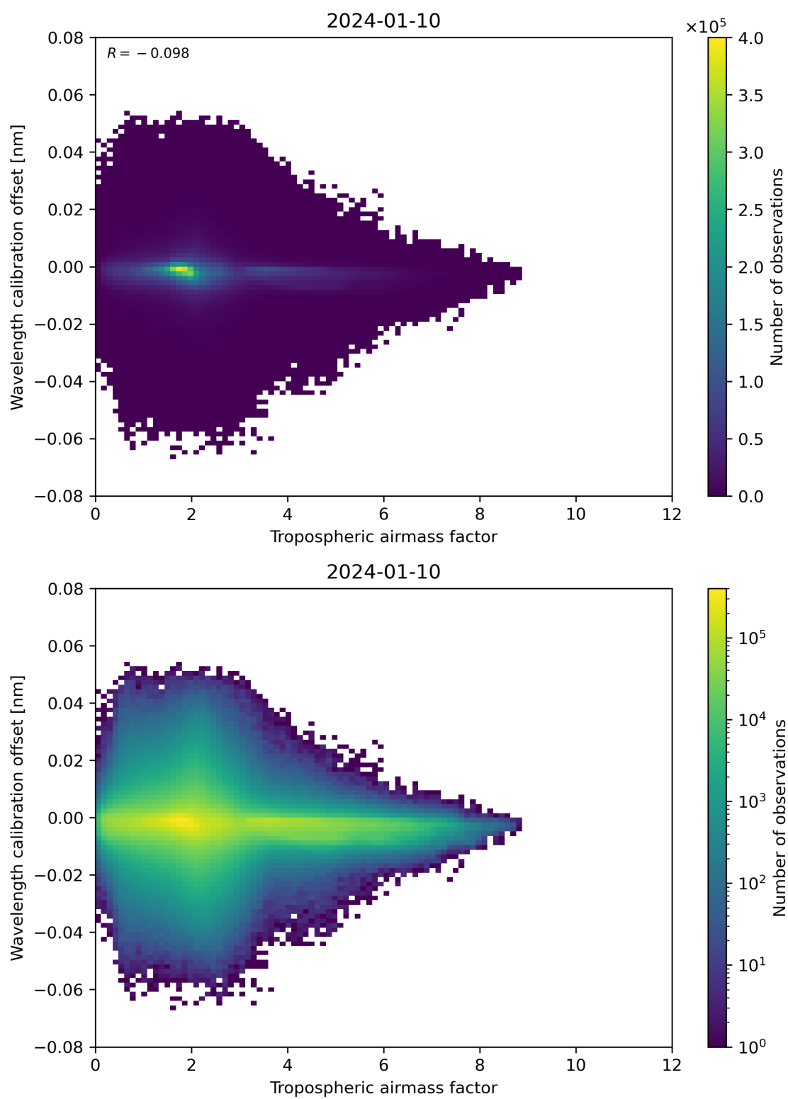
Figure 80: Scatter density plot of “Tropospheric air mass factor” against “Wavelength calibration offset” for 2024-01-10 to 2024-01-11.
