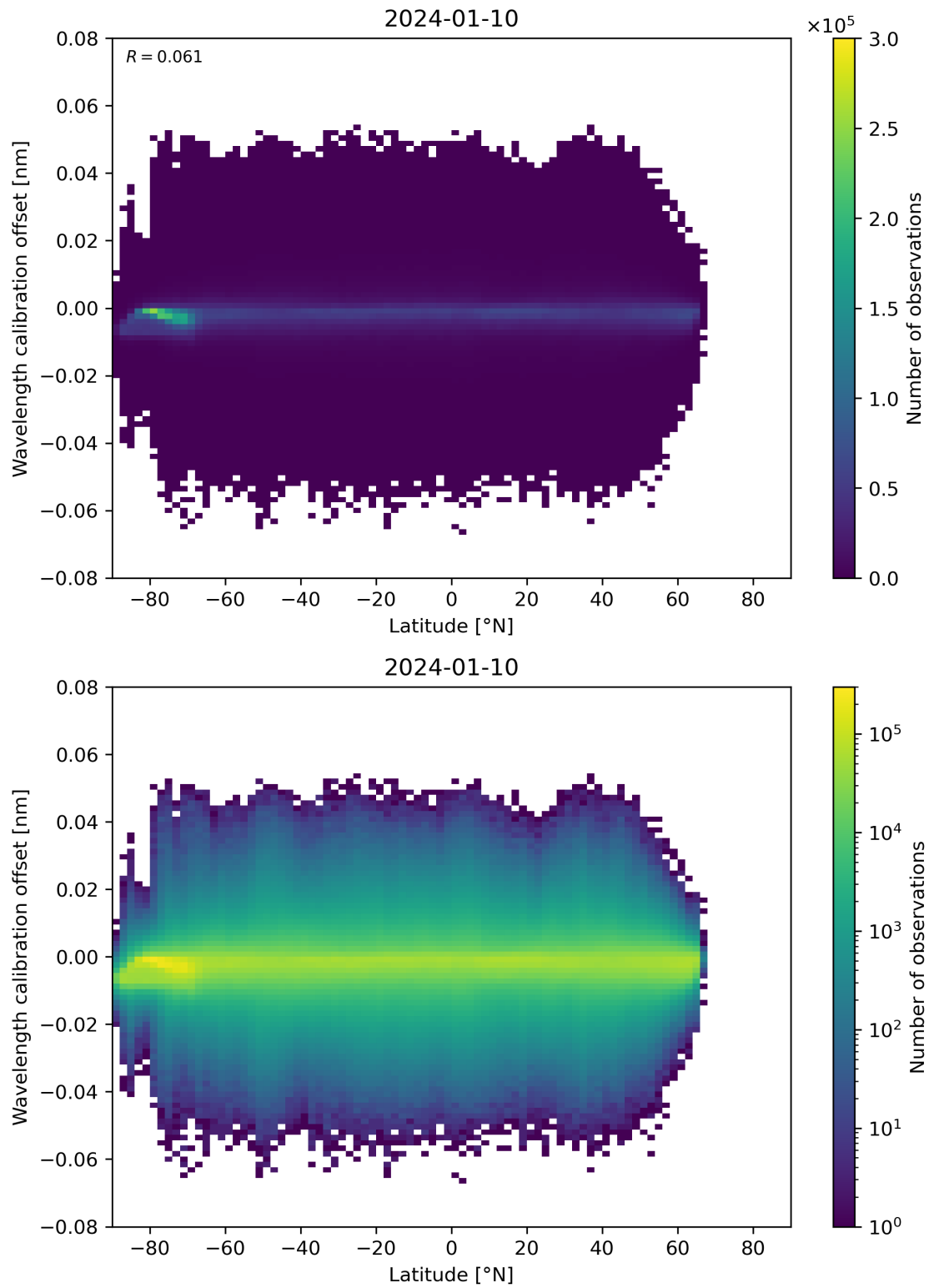
Figure 95: Scatter density plot of “Latitude” against “Wavelength calibration offset” for 2024-01-10 to 2024-01-11.
