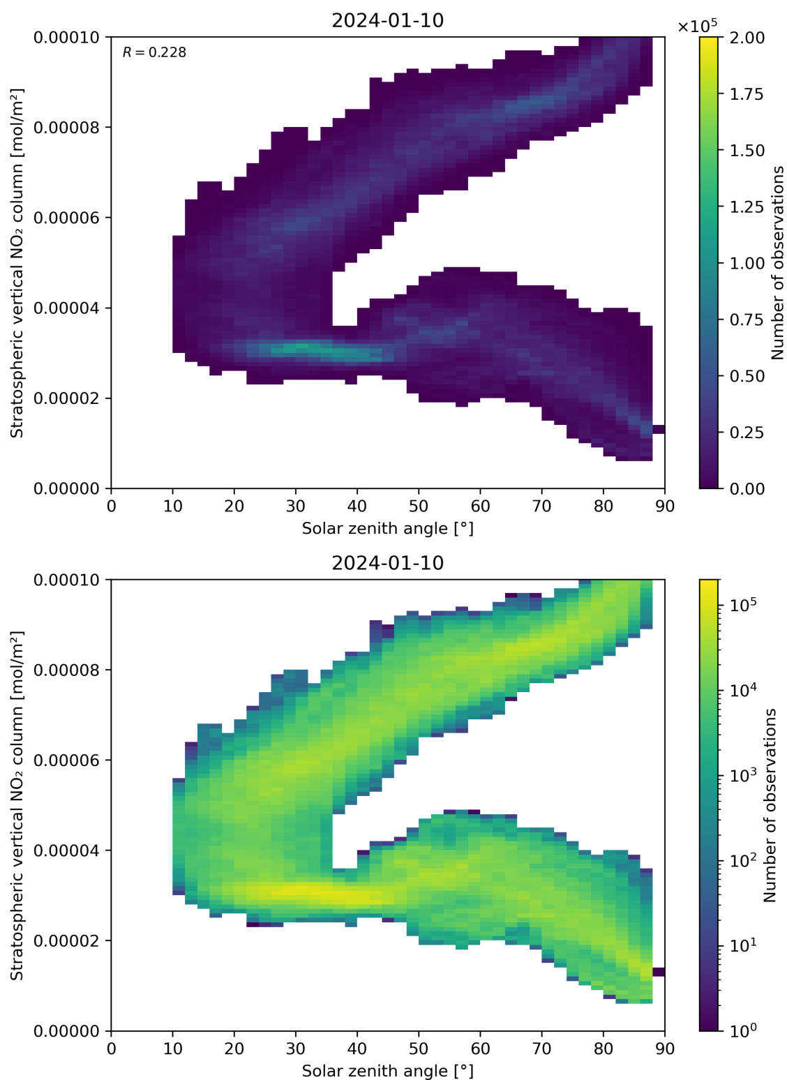
Figure 150: Scatter density plot of “Solar zenith angle” against “Stratospheric vertical NO 2 column” for 2024-01-10 to 2024-01-11.
