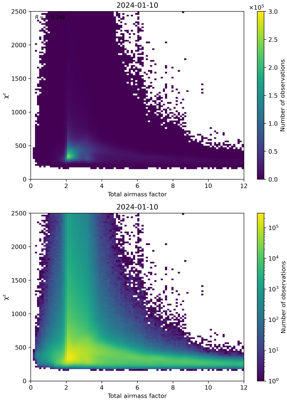
Figure 63: Scatter density plot of “Total airmass factor” against “ \chi^2 ” for 2024-01-10 to 2024-01-11.
