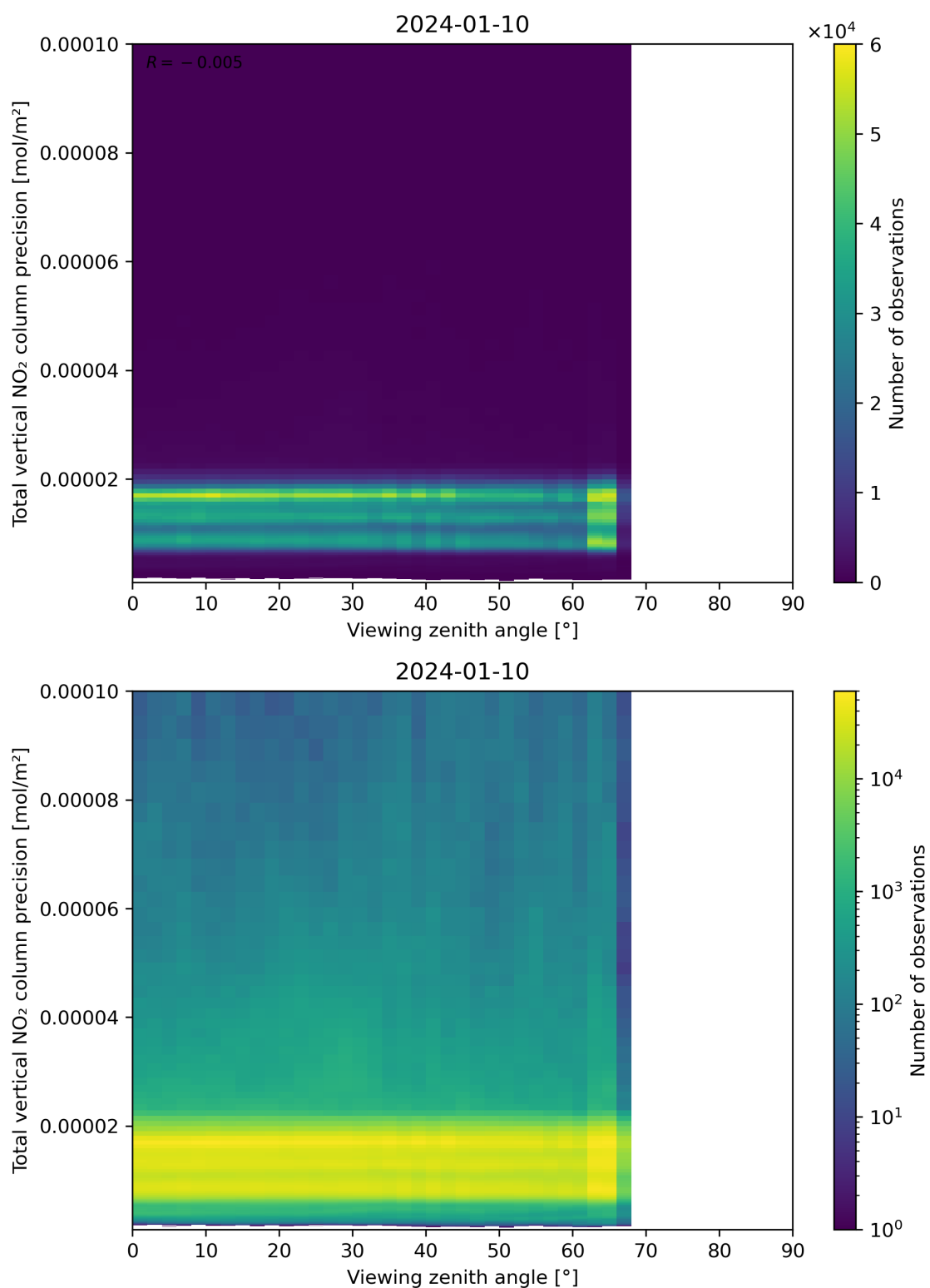
Figure 168: Scatter density plot of “Viewing zenith angle” against “Total vertical NO 2 column precision” for 2024-01-10 to 2024-01-11.
