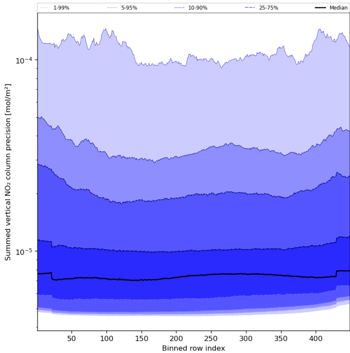
Figure 58: Along track statistics of “Summed vertical NO 2 column precision” for 2024-01-10 to 2024-01-11
