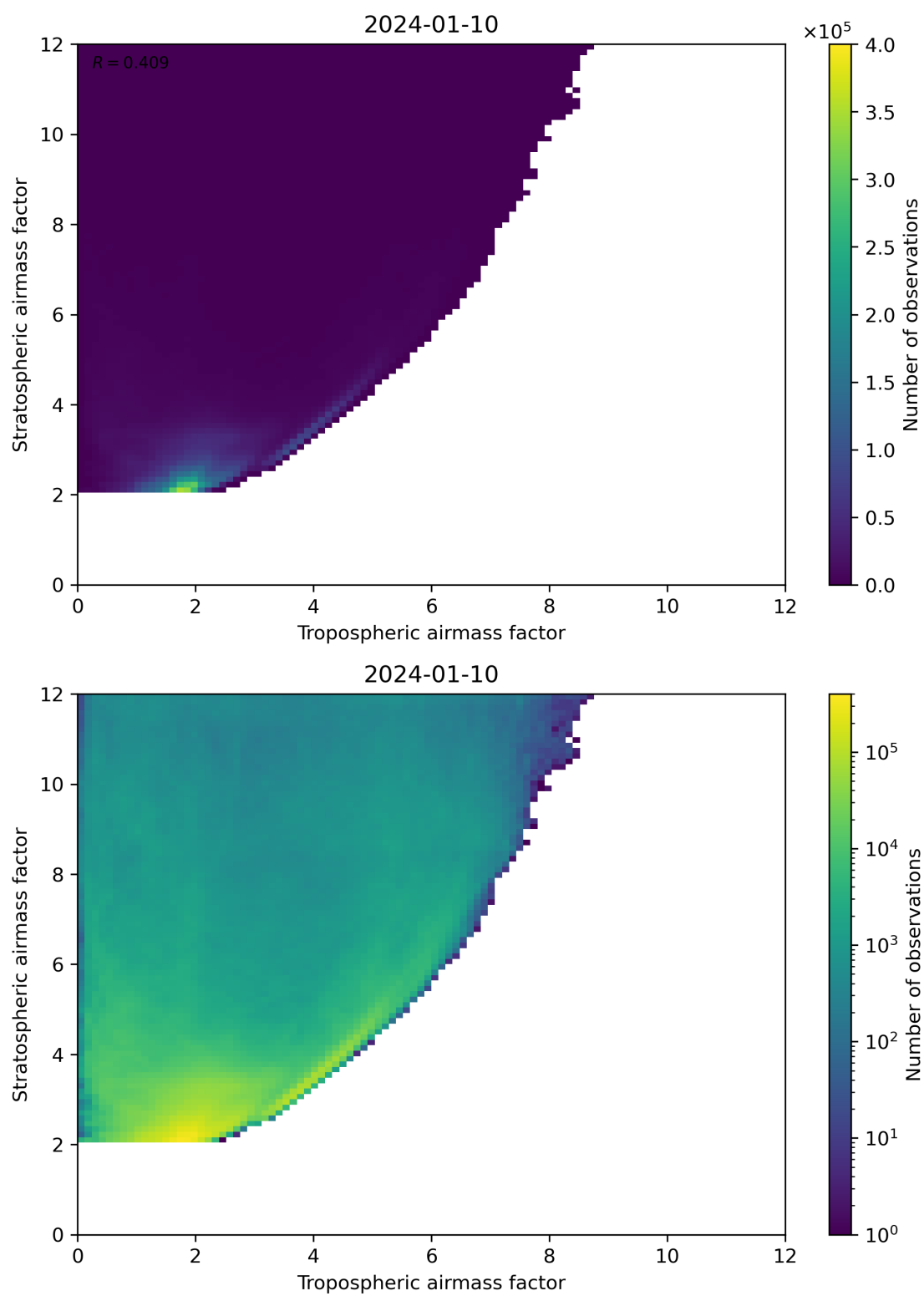
Figure 71: Scatter density plot of “Tropospheric airmass factor” against “Stratospheric airmass factor” for 2024-01-10 to 2024-01-11.
