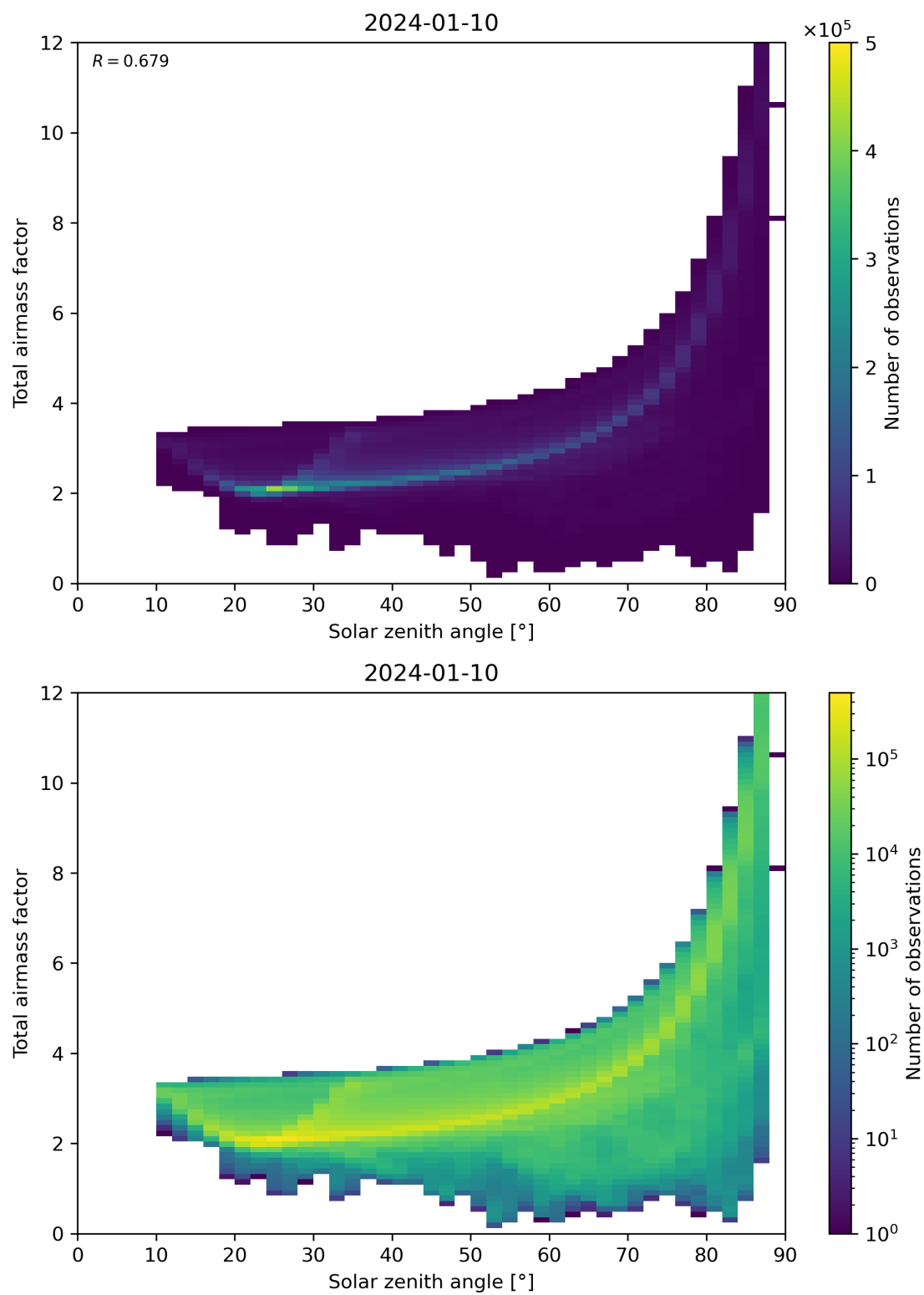
Figure 146: Scatter density plot of “Solar zenith angle” against “Total air mass factor” for 2024-01-10 to 2024-01-11.
