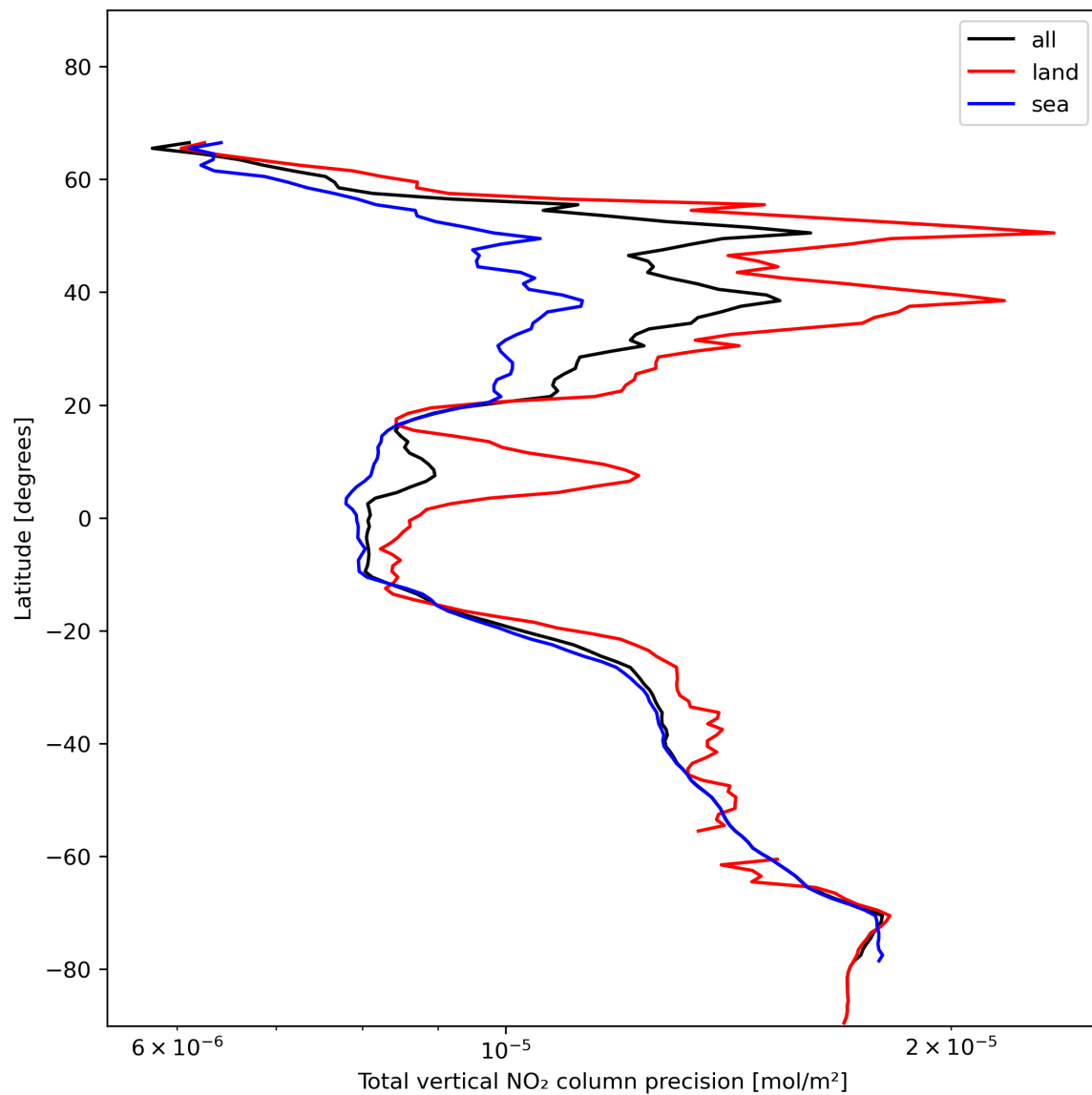
Figure 22: Zonal average of “Total vertical NO 2 column precision” for 2024-01-10 to 2024-01-11.
