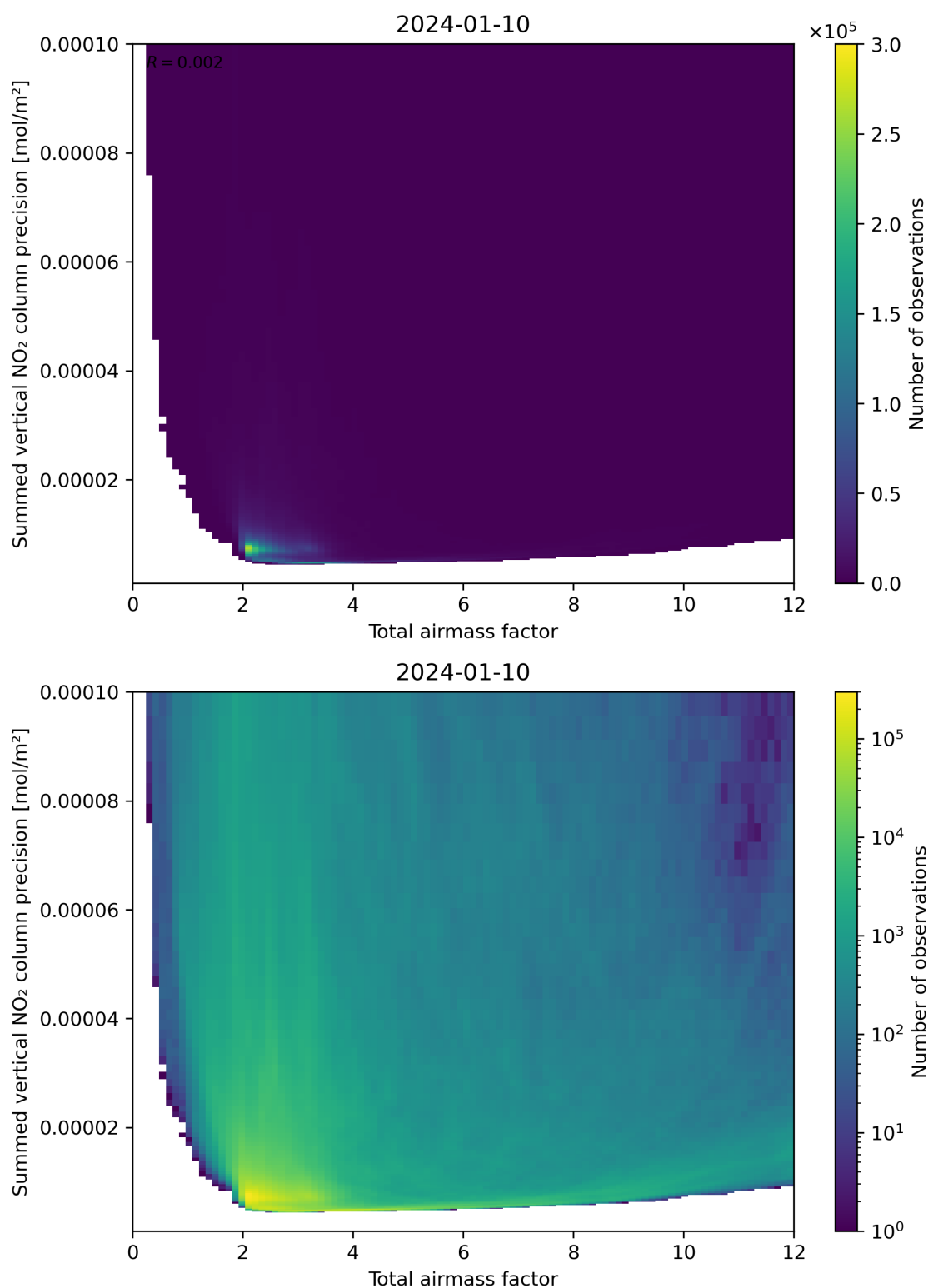
Figure 66: Scatter density plot of “Total airmass factor” against “Summed vertical NO 2 column precision” for 2024-01-10 to 2024-01-11.
