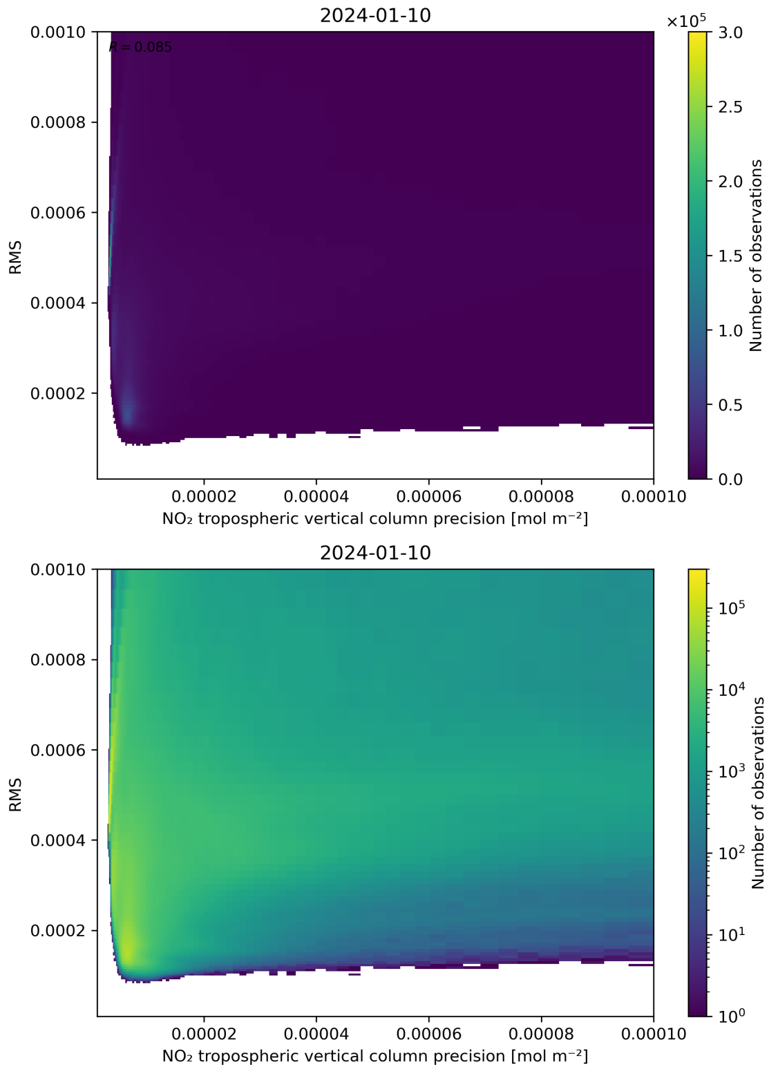
Figure 140: Scatter density plot of “NO 2 tropospheric vertical column precision” against “RMS” for 2024-01-10 to 2024-01-11.
