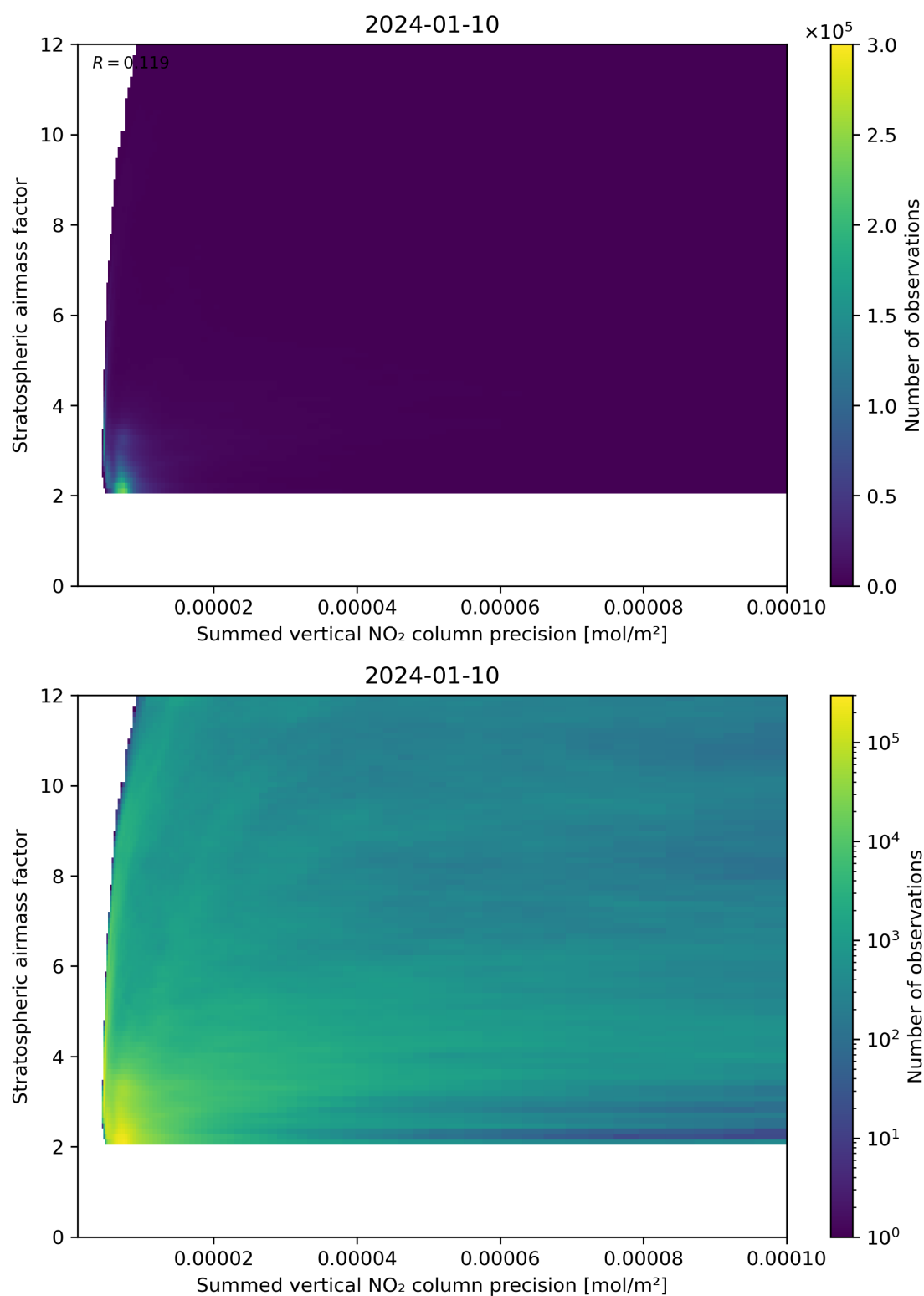
Figure 106: Scatter density plot of “Summed vertical NO 2 column precision” against “Stratospheric airmass factor” for 2024-01-10 to 2024-01-11.
