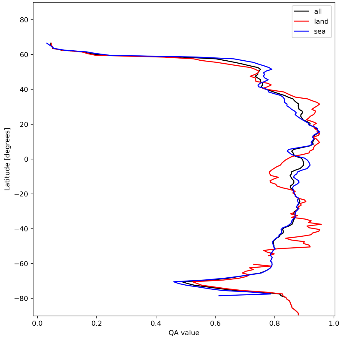
Figure 11: Zonal average of “QA value” for 2024-01-10 to 2024-01-11.
