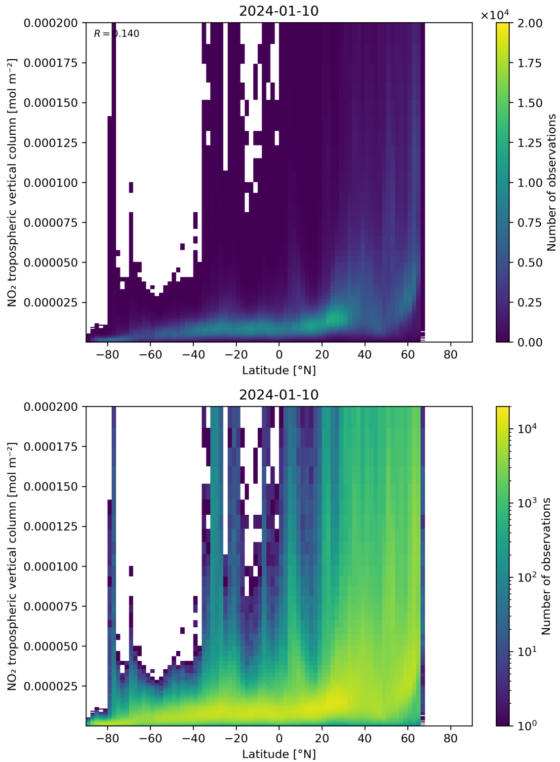
Figure 92: Scatter density plot of “Latitude” against “NO 2 tropospheric vertical column” for 2024-01-10 to 2024-01-11.
