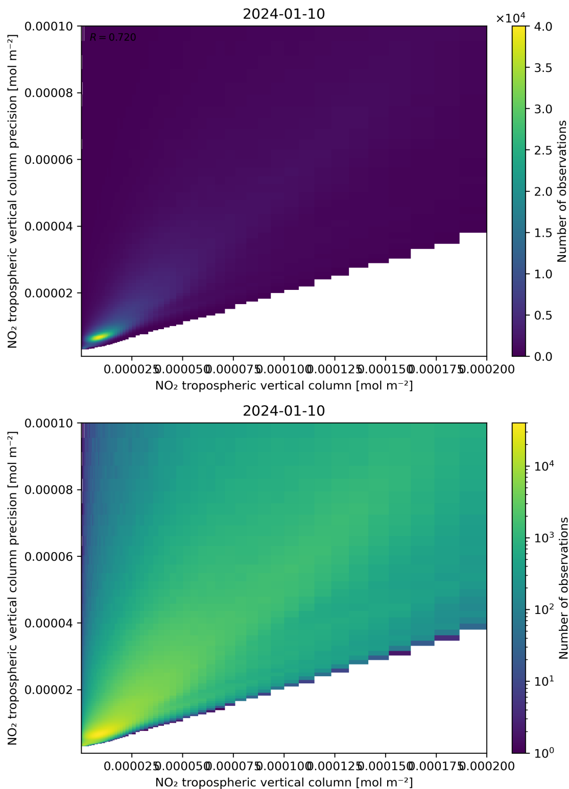
Figure 130: Scatter density plot of “NO 2 tropospheric vertical column” against “NO 2 tropospheric vertical column precision” for 2024-01-10 to 2024-01-11.
