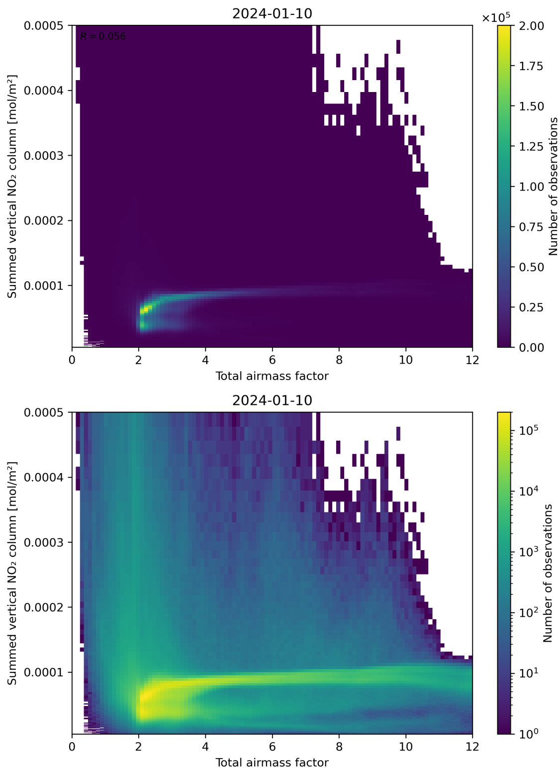
Figure 65: Scatter density plot of “Total airmass factor” against “Summed vertical NO 2 column” for 2024-01-10 to 2024-01-11.
