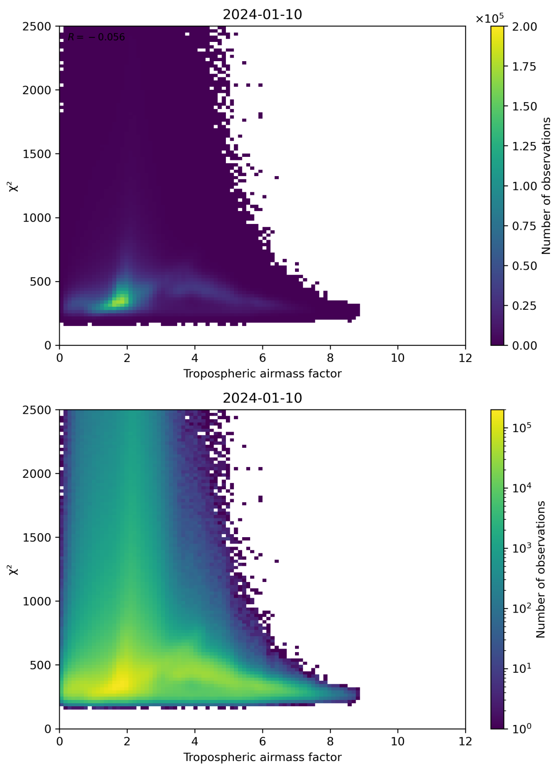
Figure 73: Scatter density plot of “Tropospheric airmass factor” against “ \chi^2 ” for 2024-01-10 to 2024-01-11.
