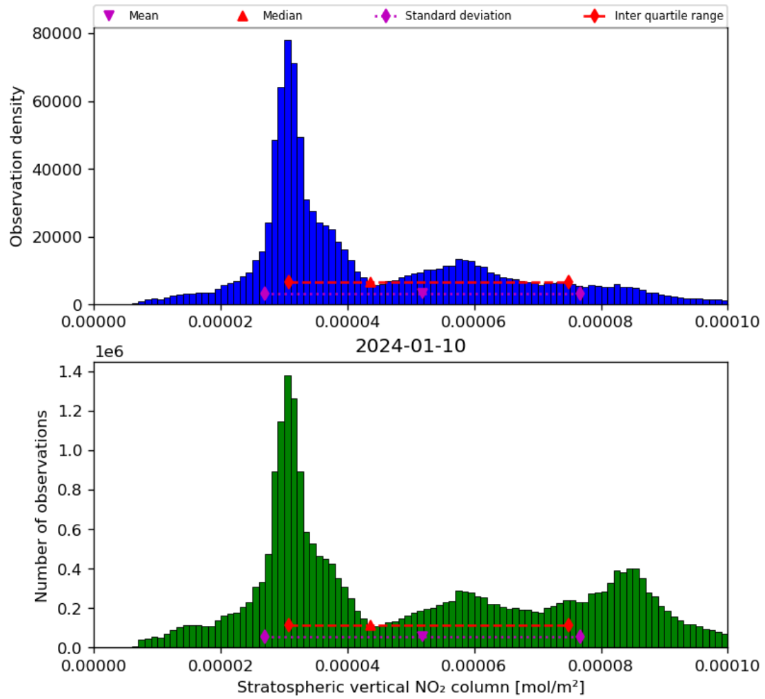
Figure 36: Histogram of “Stratospheric vertical NO 2 column” for 2024-01-10 to 2024-01-11
