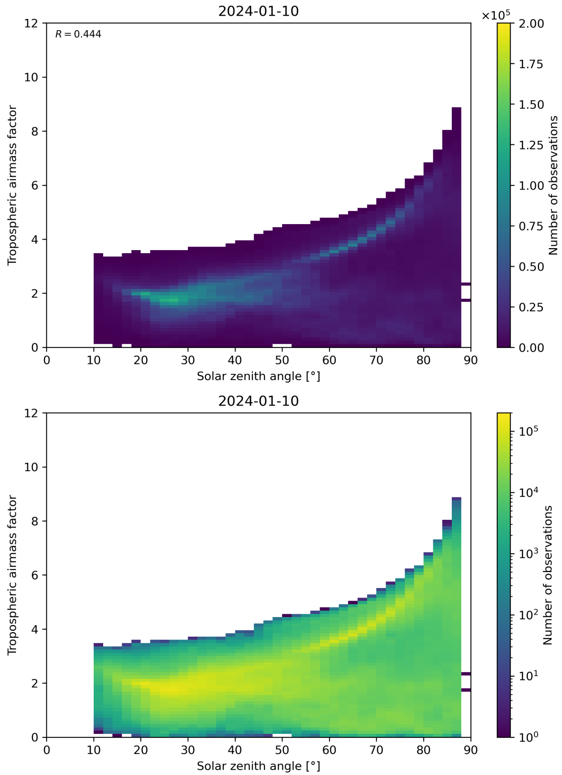
Figure 147: Scatter density plot of “Solar zenith angle” against “Tropospheric airmass factor” for 2024-01-10 to 2024-01-11.
