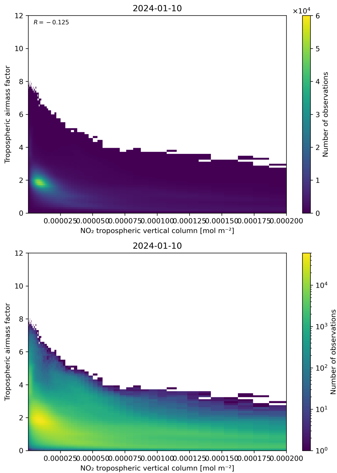
Figure 123: Scatter density plot of “NO 2 tropospheric vertical column” against “Tropospheric air mass factor” for 2024-01-10 to 2024-01-11.
