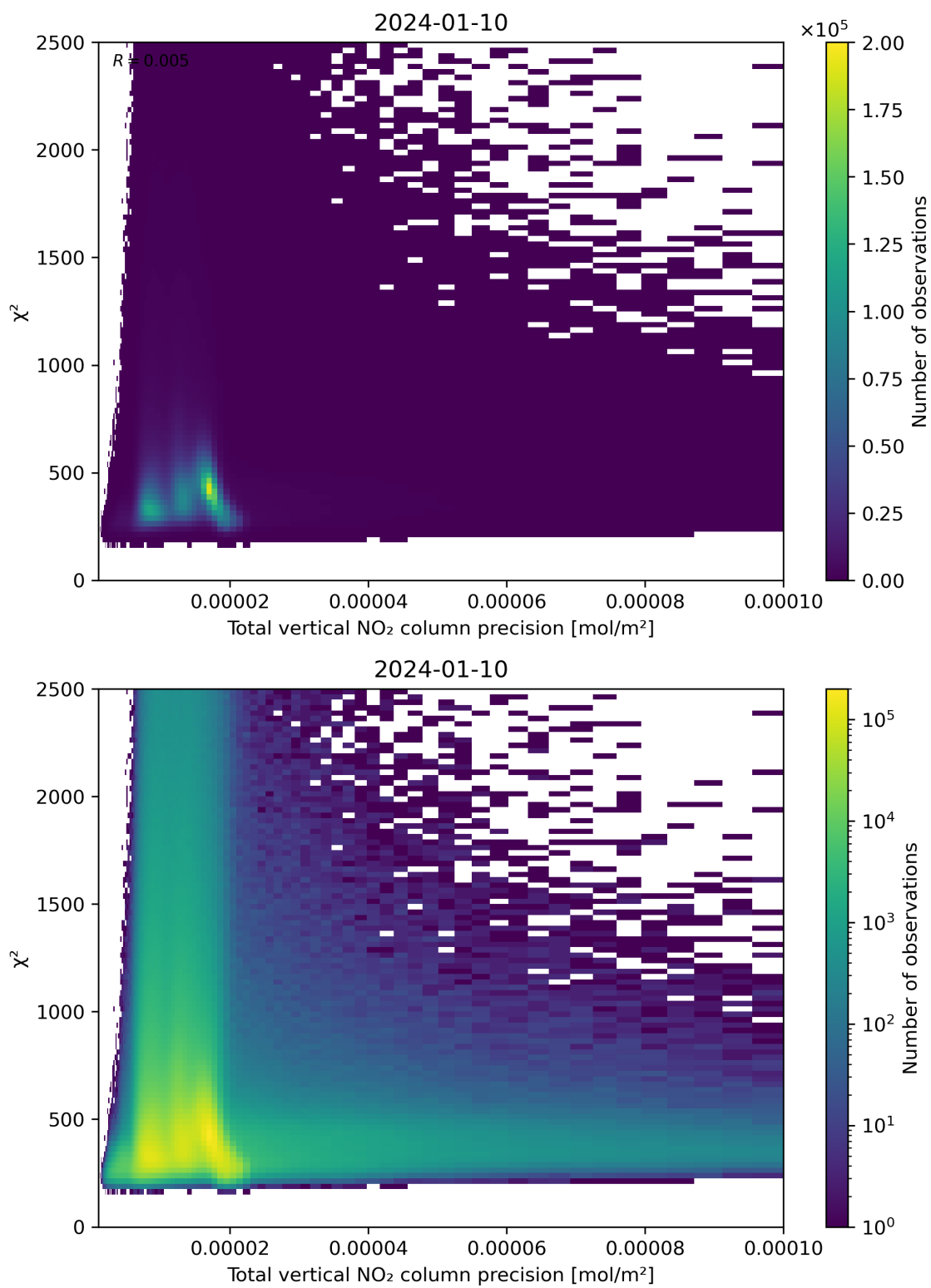
Figure 116: Scatter density plot of “Total vertical NO 2 column precision” against “ \chi^2 ” for 2024-01-10 to 2024-01-11.
