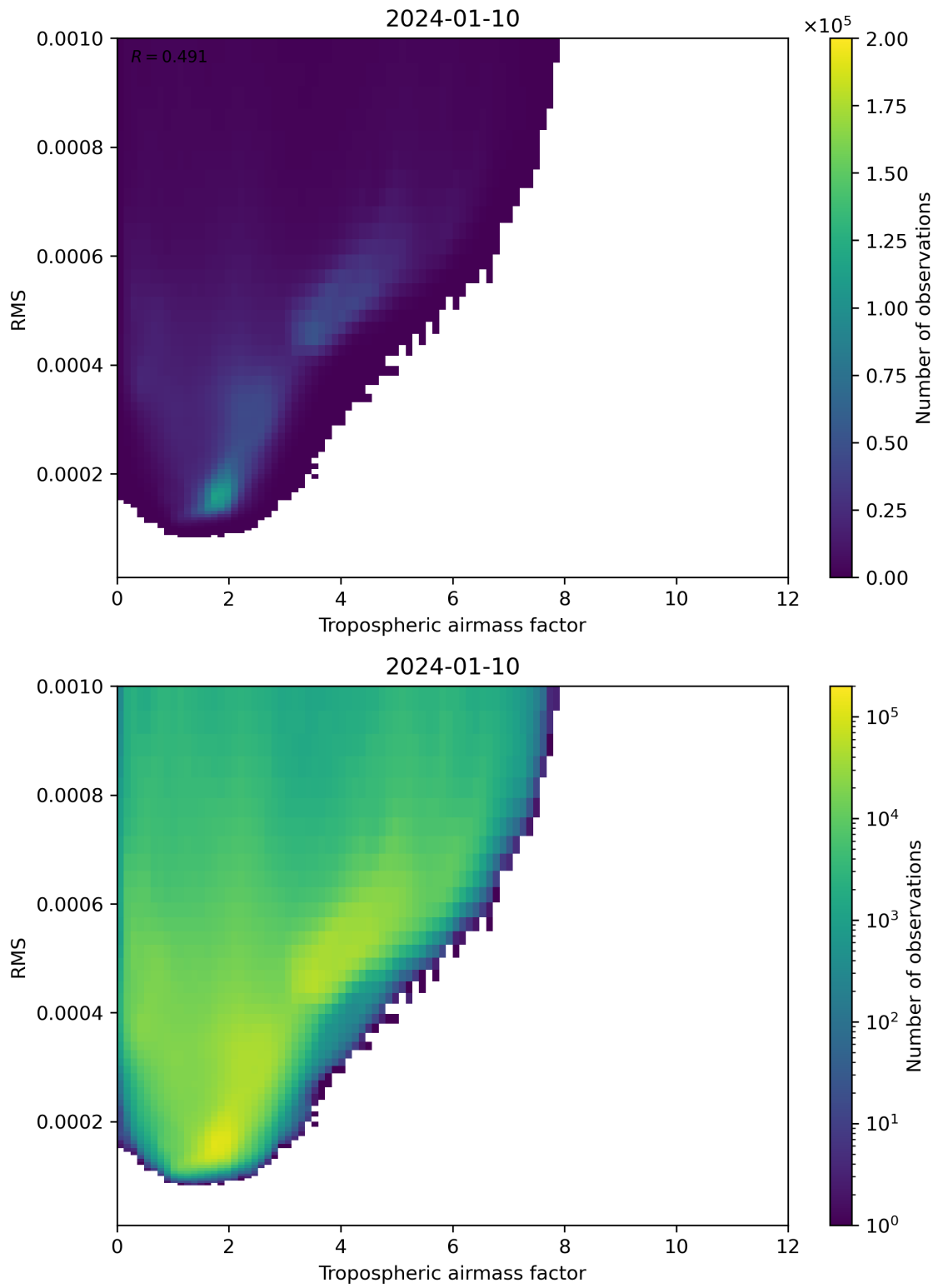
Figure 79: Scatter density plot of “Tropospheric airmass factor” against “RMS” for 2024-01-10 to 2024-01-11.
