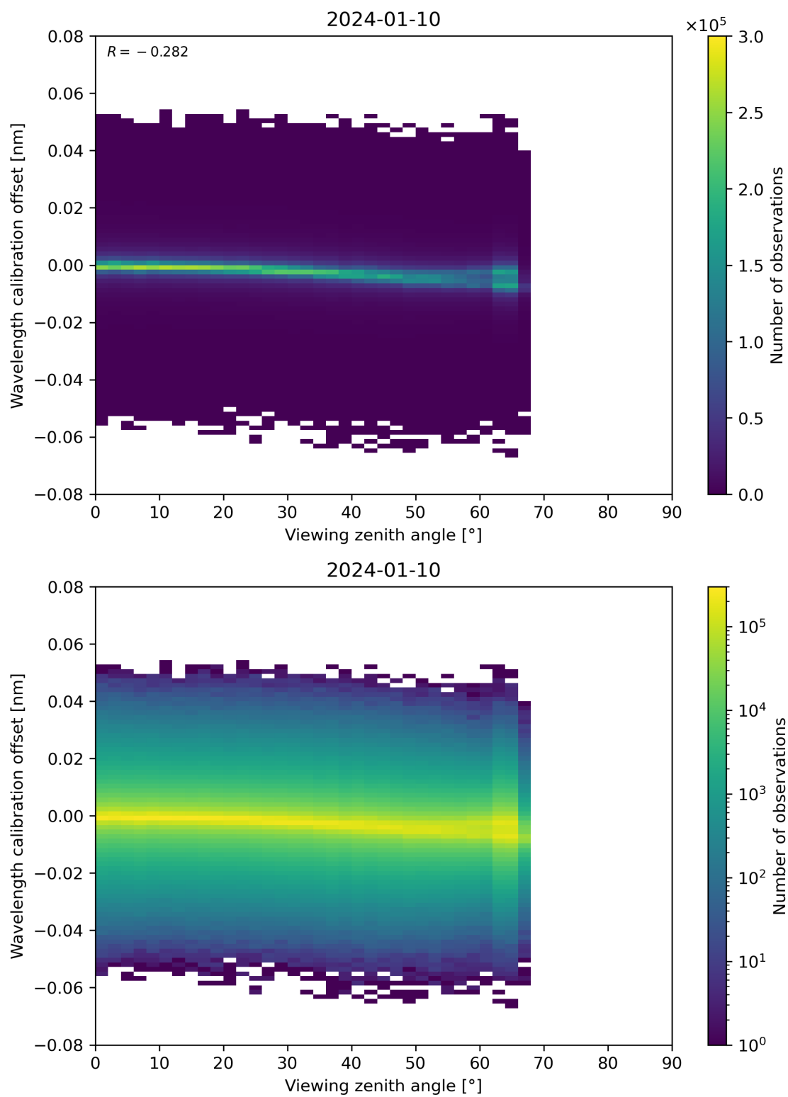
Figure 173: Scatter density plot of “Viewing zenith angle” against “Wavelength calibration offset” for 2024-01-10 to 2024-01-11.
