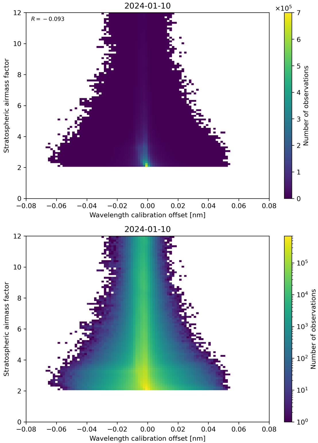
Figure 174: Scatter density plot of “Wavelength calibration offset” against “Stratospheric airmass factor” for 2024-01-10 to 2024-01-11.
