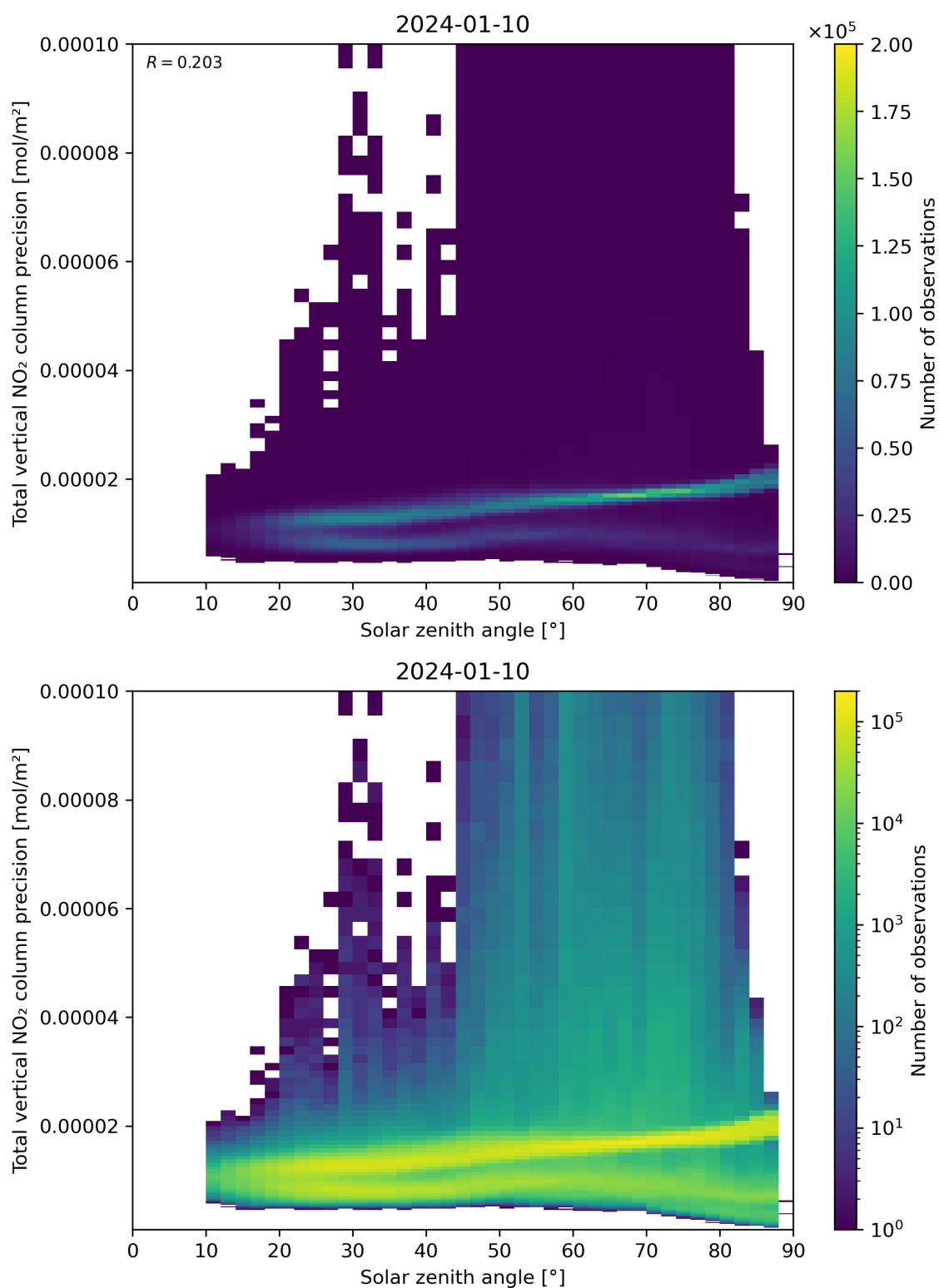
Figure 154: Scatter density plot of “Solar zenith angle” against “Total vertical NO 2 column precision” for 2024-01-10 to 2024-01-11.
