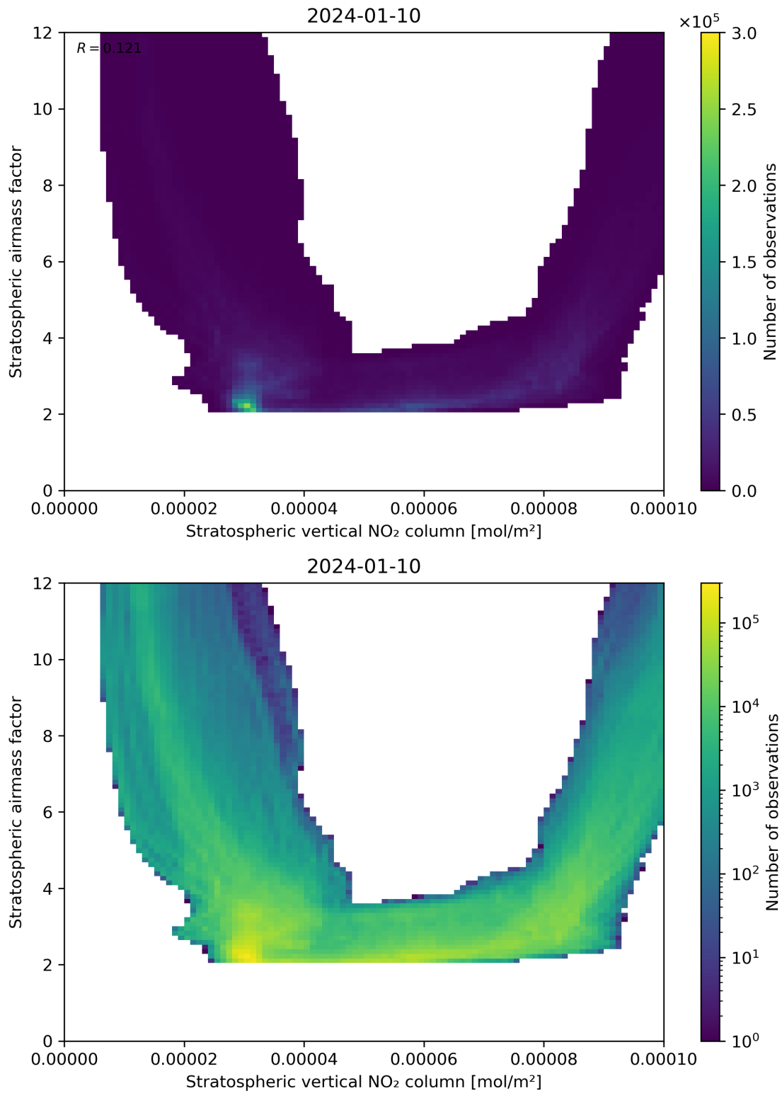
Figure 96: Scatter density plot of “Stratospheric vertical NO 2 column” against “Stratospheric airmass factor” for 2024-01-10 to 2024-01-11.
