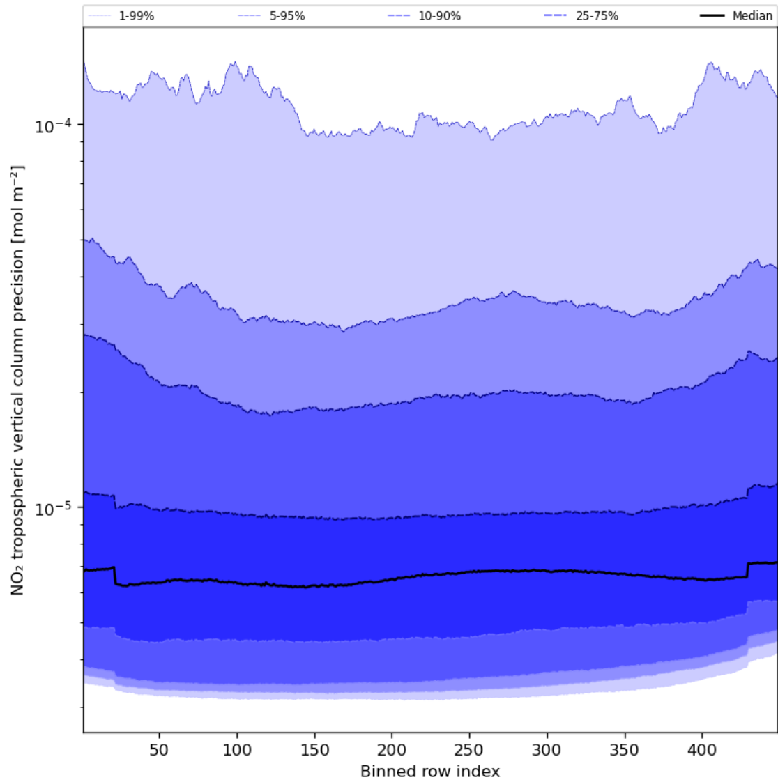
Figure 47: Along track statistics of “NO 2 tropospheric vertical column precision” for 2024-01-10 to 2024-01-11
