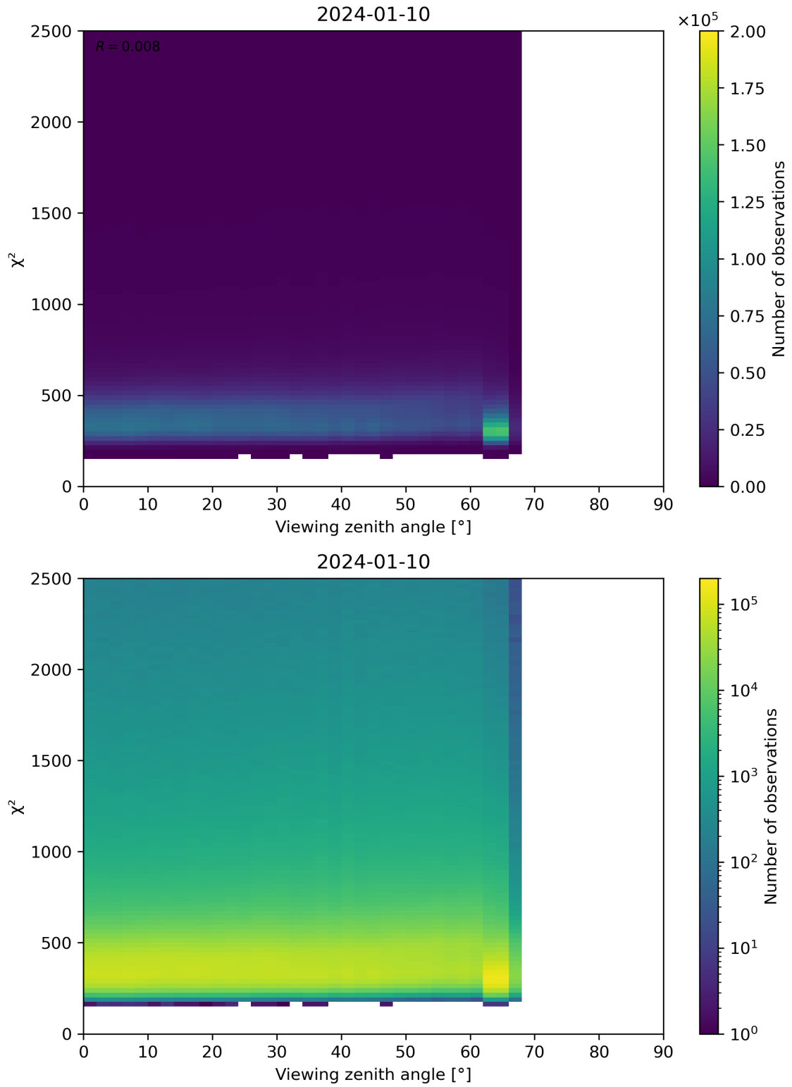
Figure 162: Scatter density plot of “Viewing zenith angle” against “ \chi^2 ” for 2024-01-10 to 2024-01-11.
