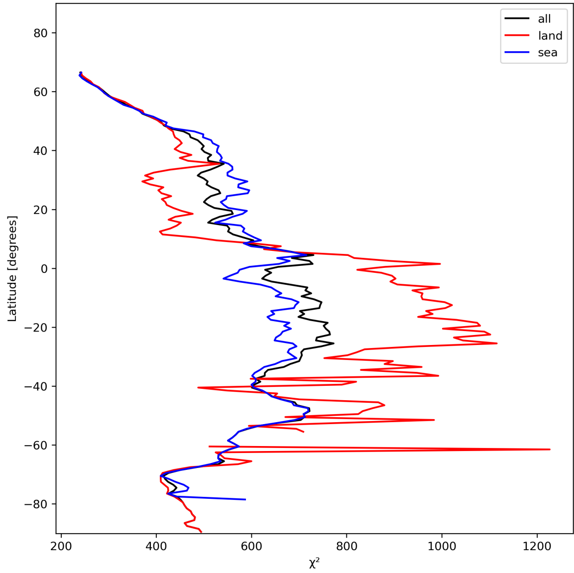
Figure 25: Zonal average of “ \chi^2 ” for 2024-01-10 to 2024-01-11.
