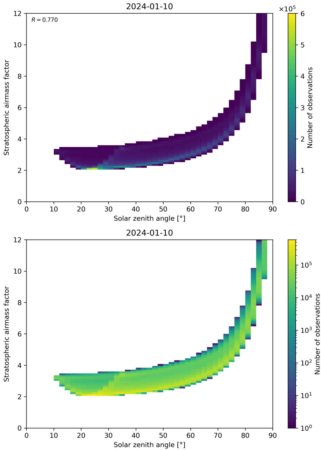
Figure 145: Scatter density plot of “Solar zenith angle” against “Stratospheric airmass factor” for 2024-01-10 to 2024-01-11.
