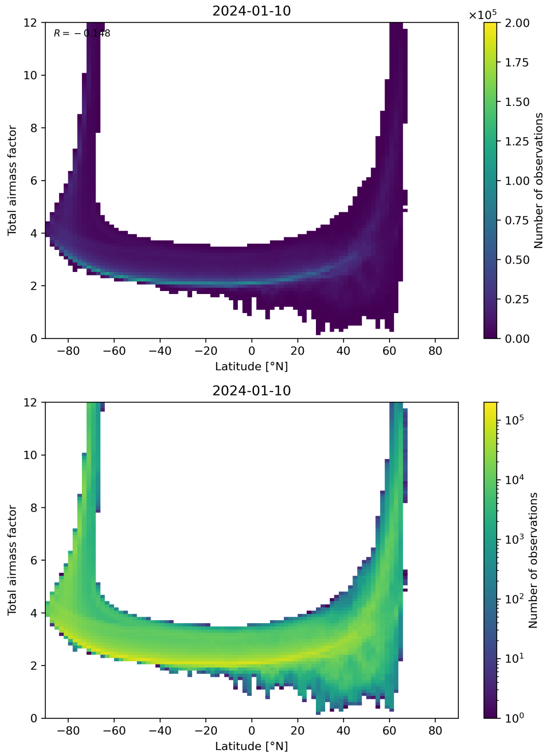
Figure 84: Scatter density plot of “Latitude” against “Total airmass factor” for 2024-01-10 to 2024-01-11.
