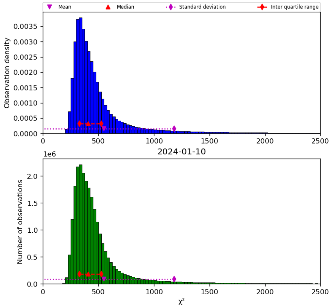
Figure 42: Histogram of “ \chi^2 ” for 2024-01-10 to 2024-01-11
