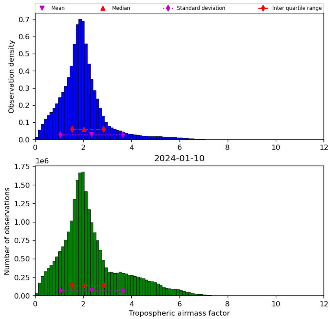
Figure 31: Histogram of “Tropospheric airmass factor” for 2024-01-10 to 2024-01-11
