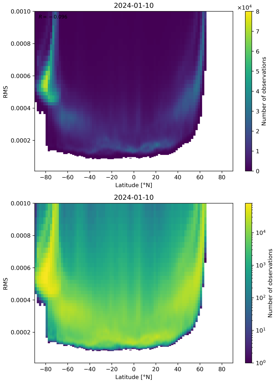
Figure 94: Scatter density plot of “Latitude” against “RMS” for 2024-01-10 to 2024-01-11.
