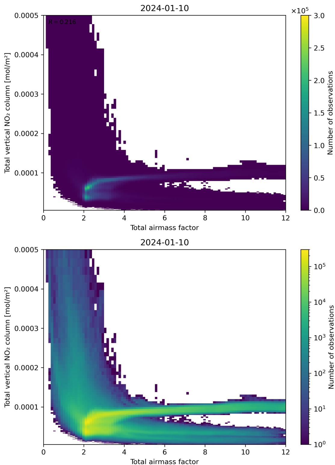
Figure 67: Scatter density plot of “Total airmass factor” against “Total vertical NO 2 column” for 2024-01-10 to 2024-01-11.
