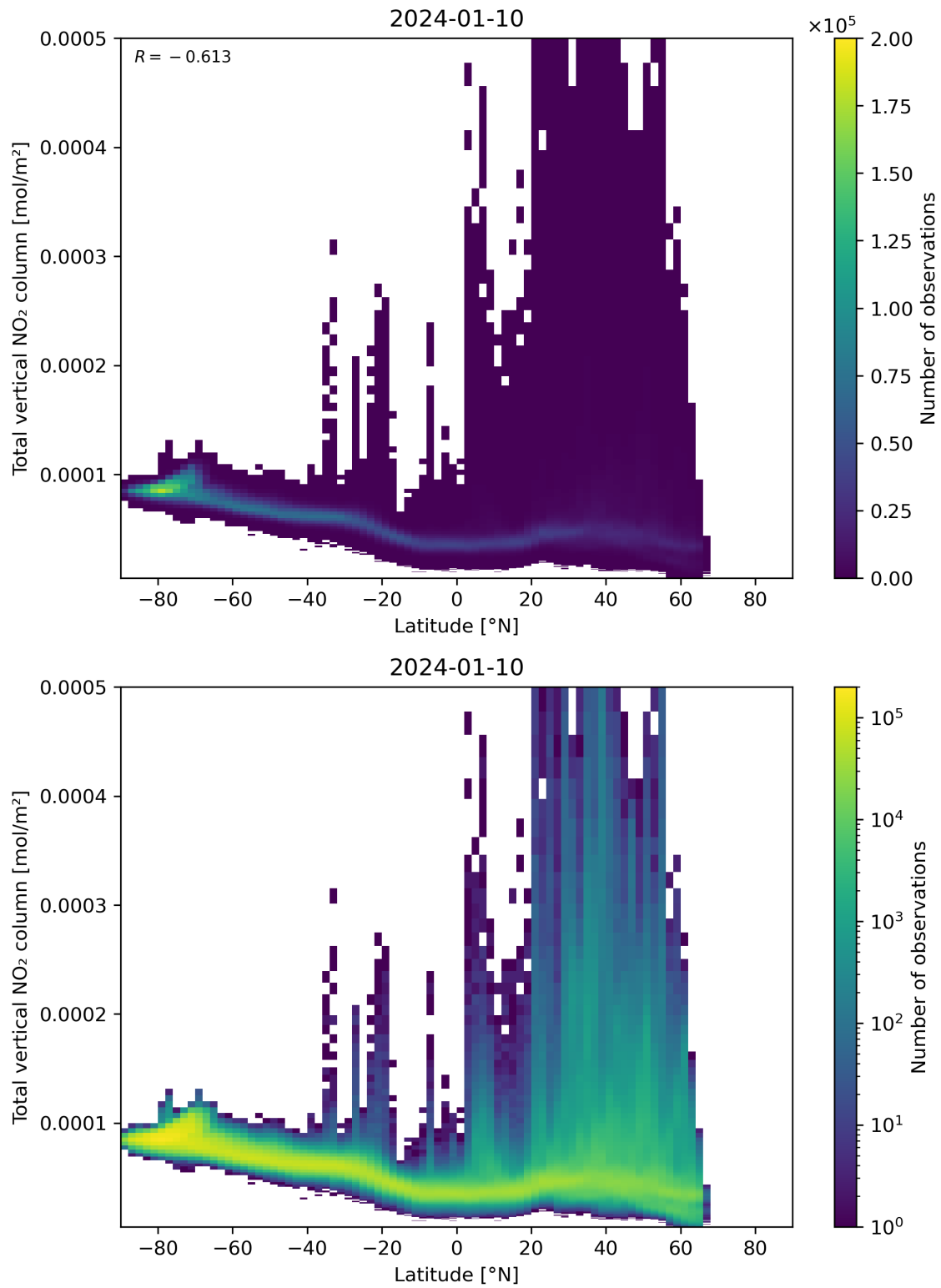
Figure 90: Scatter density plot of “Latitude” against “Total vertical NO 2 column” for 2024-01-10 to 2024-01-11.
