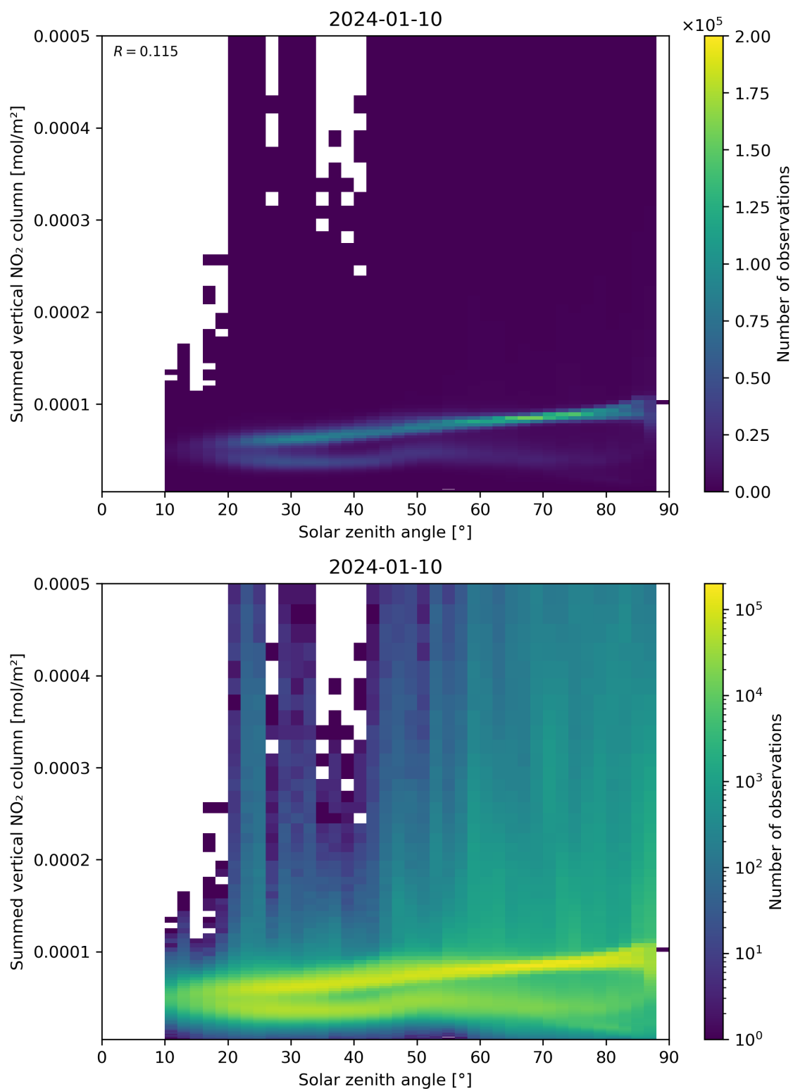
Figure 151: Scatter density plot of “Solar zenith angle” against “Summed vertical NO 2 column” for 2024-01-10 to 2024-01-11.
