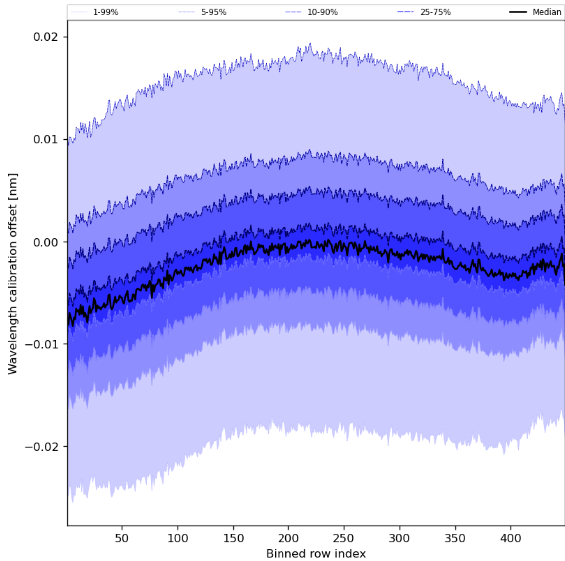
Figure 52: Along track statistics of “Wavelength calibration offset” for 2024-01-10 to 2024-01-11
