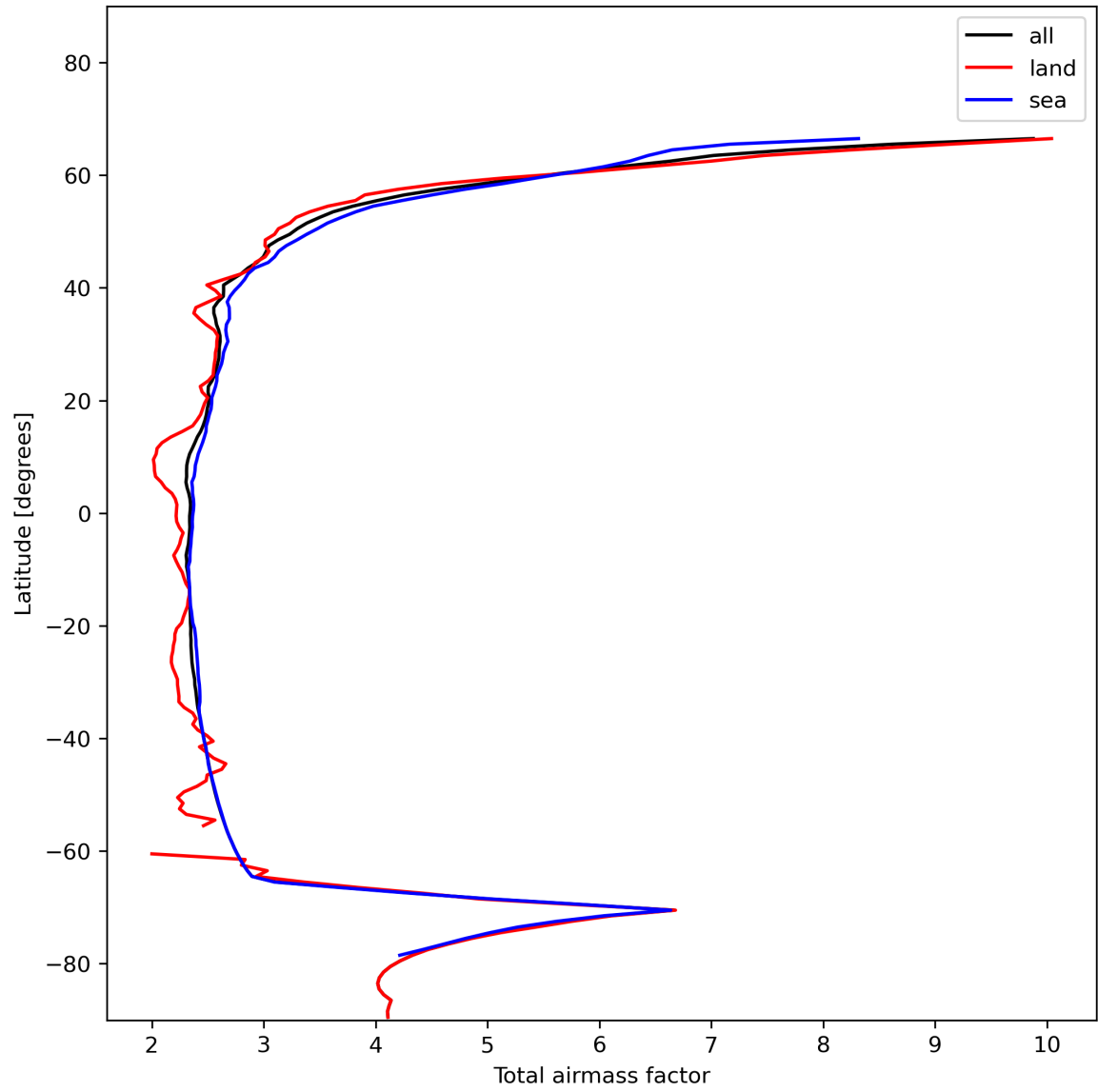
Figure 15: Zonal average of “Total airmass factor” for 2024-01-10 to 2024-01-11.
