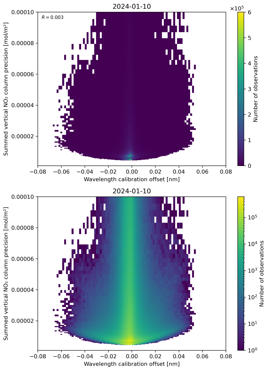
Figure 178: Scatter density plot of “Wavelength calibration offset” against “Summed vertical NO 2 column precision” for 2024-01-10 to 2024-01-11.
