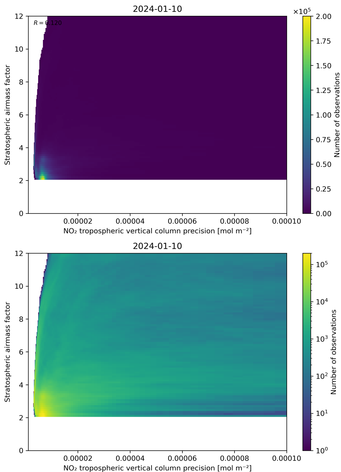
Figure 131: Scatter density plot of “NO 2 tropospheric vertical column precision” against “Stratospheric airmass factor” for 2024-01-10 to 2024-01-11.
