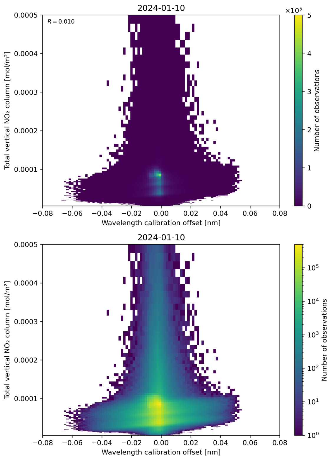
Figure 179: Scatter density plot of “Wavelength calibration offset” against “Total vertical NO 2 column” for 2024-01-10 to 2024-01-11.
