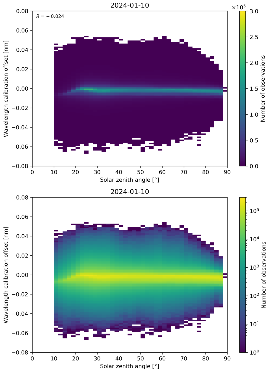
Figure 158: Scatter density plot of “Solar zenith angle” against “Wavelength calibration offset” for 2024-01-10 to 2024-01-11.
