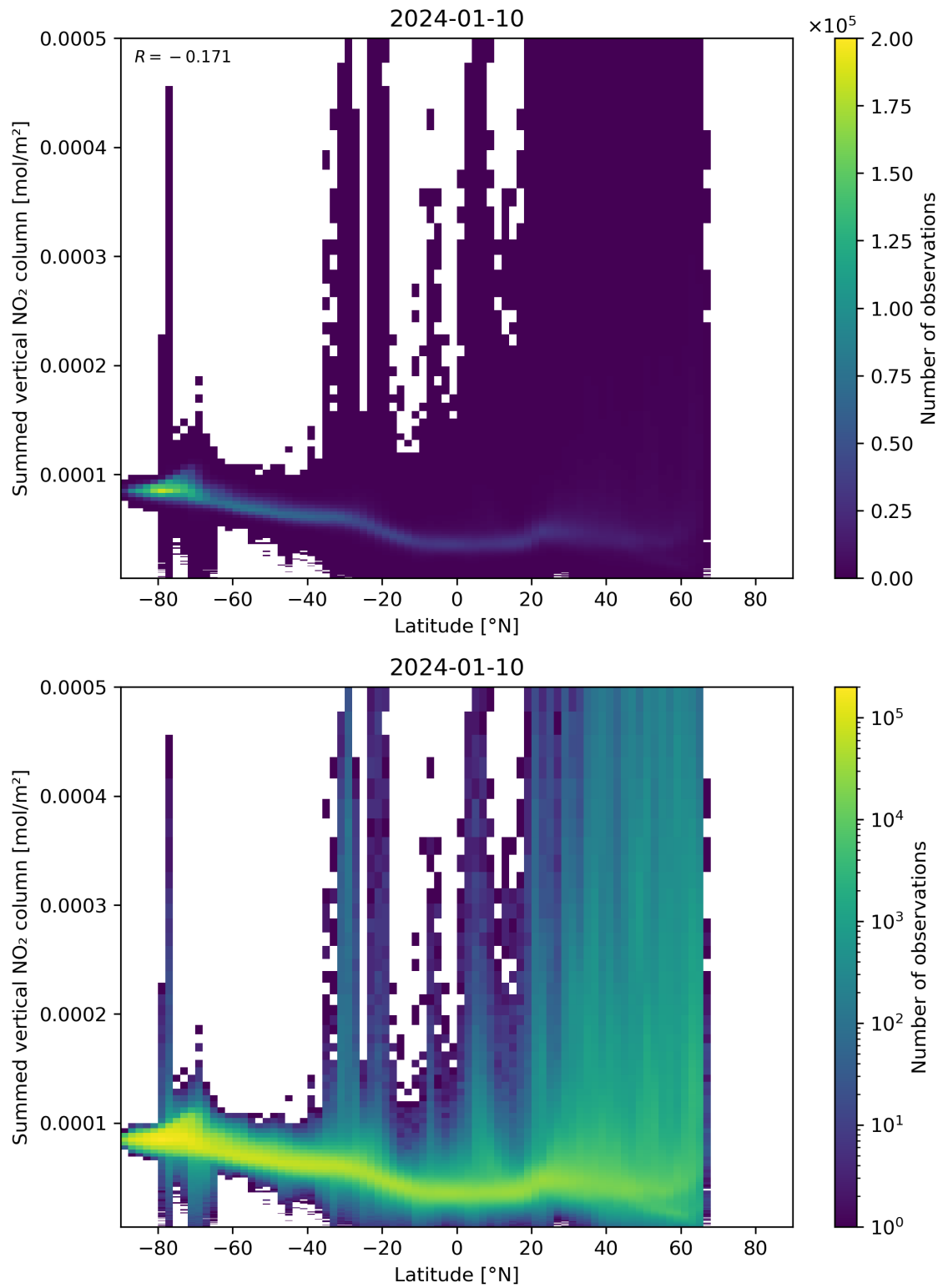
Figure 88: Scatter density plot of “Latitude” against “Summed vertical NO 2 column” for 2024-01-10 to 2024-01-11.
