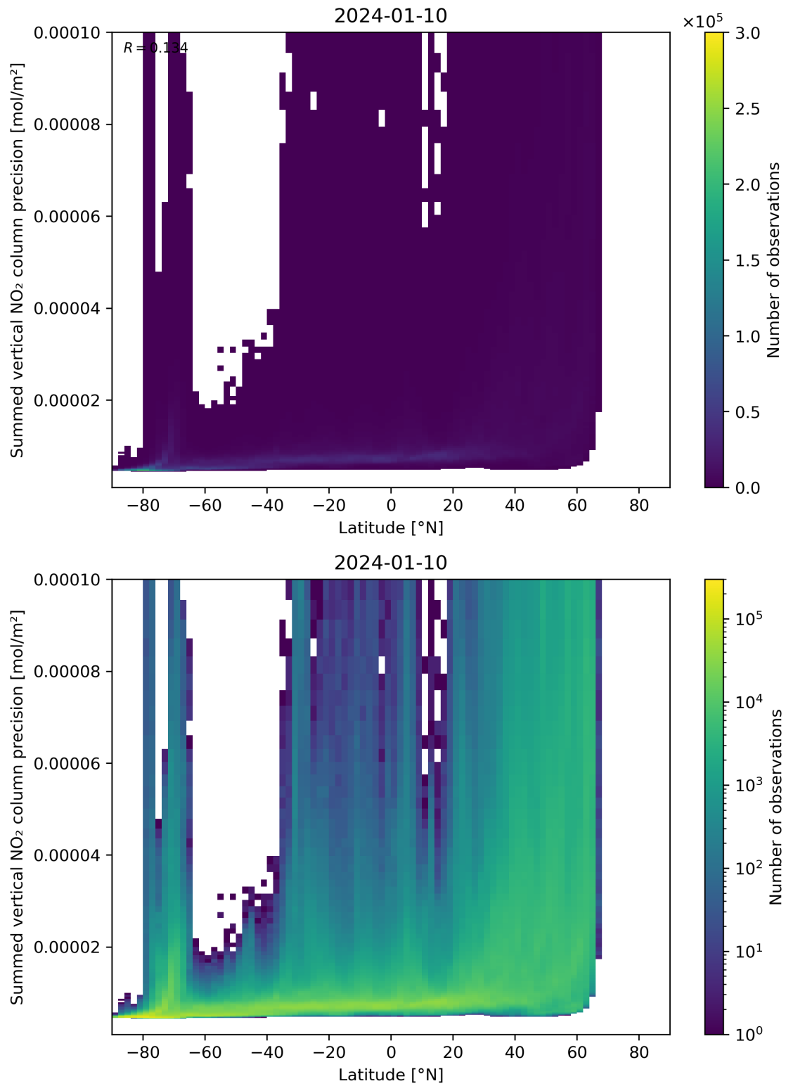
Figure 89: Scatter density plot of “Latitude” against “Summed vertical NO 2 column precision” for 2024-01-10 to 2024-01-11.
