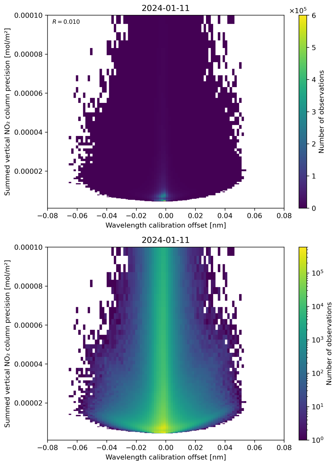
Figure 178: Scatter density plot of “Wavelength calibration offset” against “Summed vertical NO 2 column precision” for 2024-01-10 to 2024-01-12.
