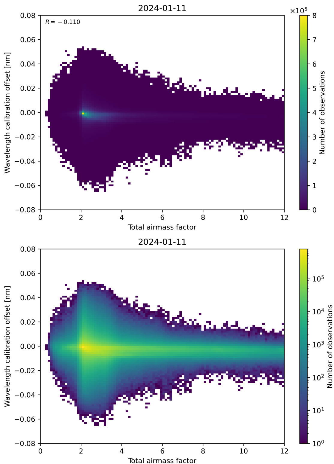
Figure 70: Scatter density plot of “Total airmass factor” against “Wavelength calibration offset” for 2024-01-10 to 2024-01-12.
