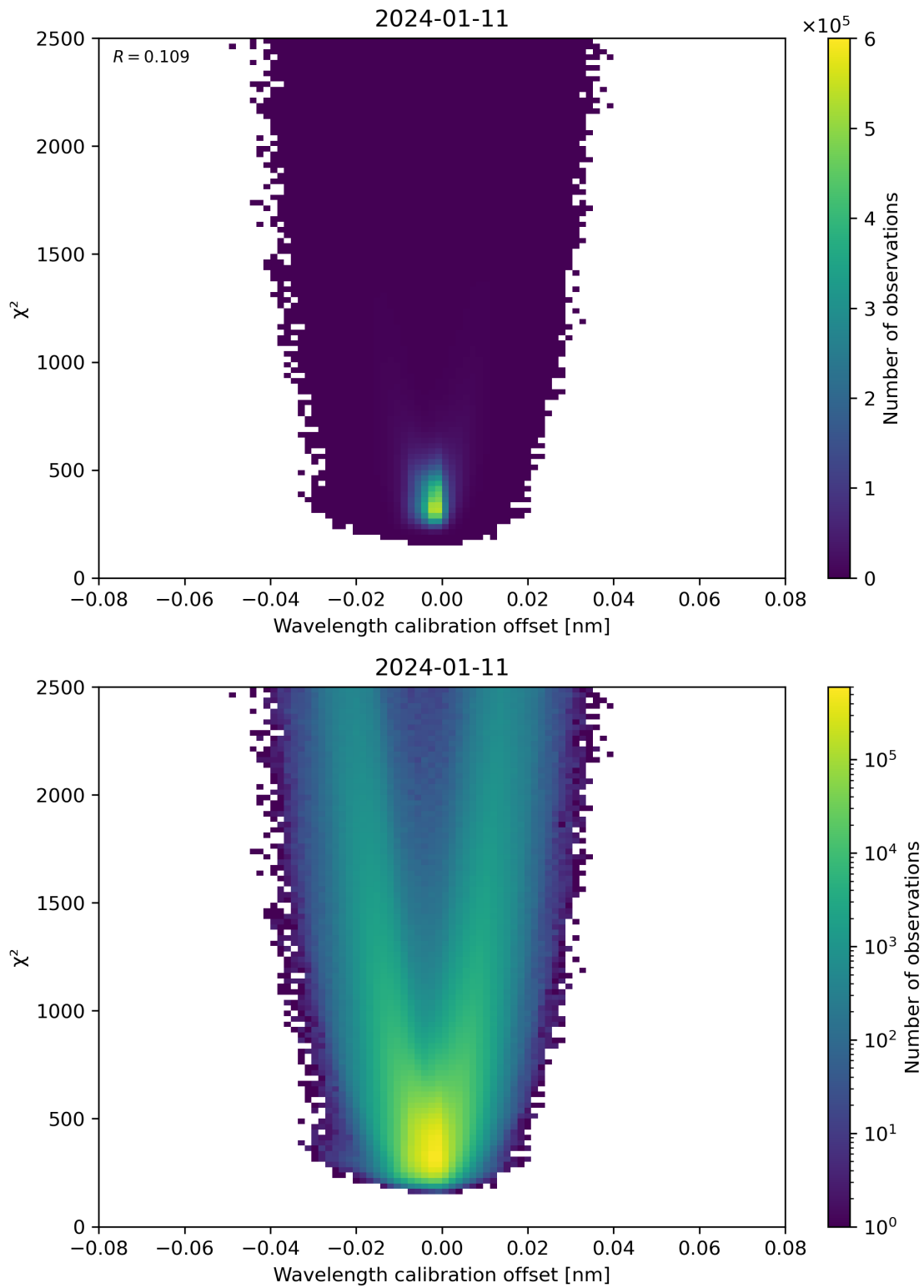
Figure 175: Scatter density plot of “Wavelength calibration offset” against “ \chi^2 ” for 2024-01-10 to 2024-01-12.
