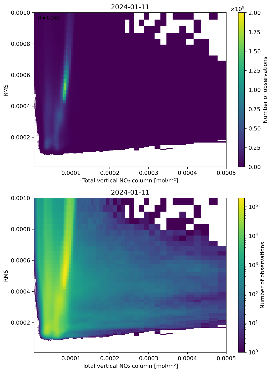
Figure 120: Scatter density plot of “Total vertical NO 2 column” against “RMS” for 2024-01-10 to 2024-01-12.
