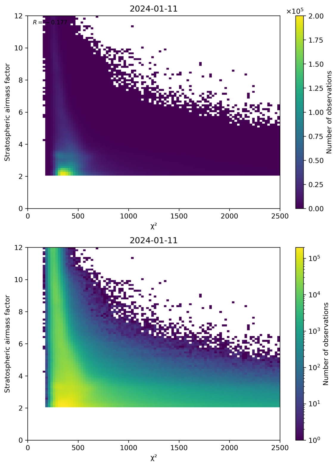
Figure 81: Scatter density plot of “ \chi^2 ” against “Stratospheric airmass factor” for 2024-01-10 to 2024-01-12.
