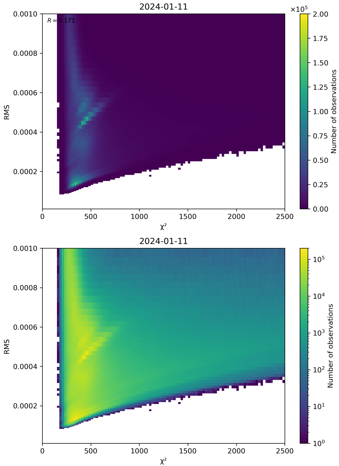
Figure 82: Scatter density plot of “ \chi^2 ” against “RMS” for 2024-01-10 to 2024-01-12.
