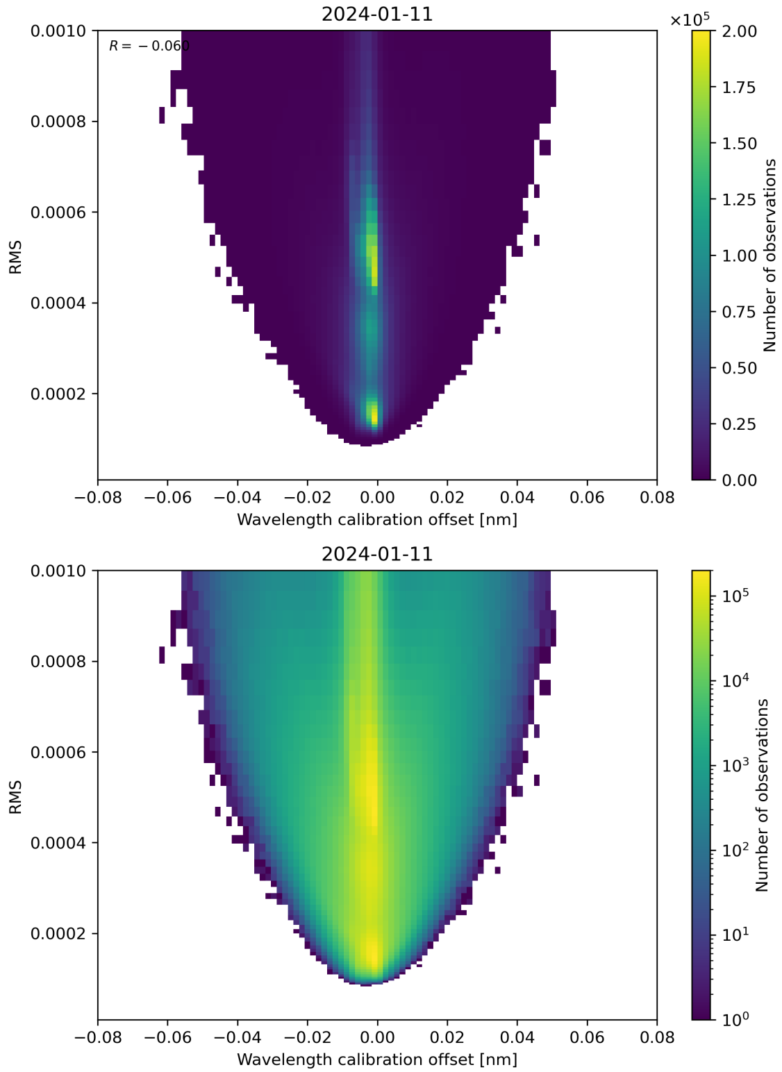
Figure 181: Scatter density plot of “Wavelength calibration offset” against “RMS” for 2024-01-10 to 2024-01-12.
