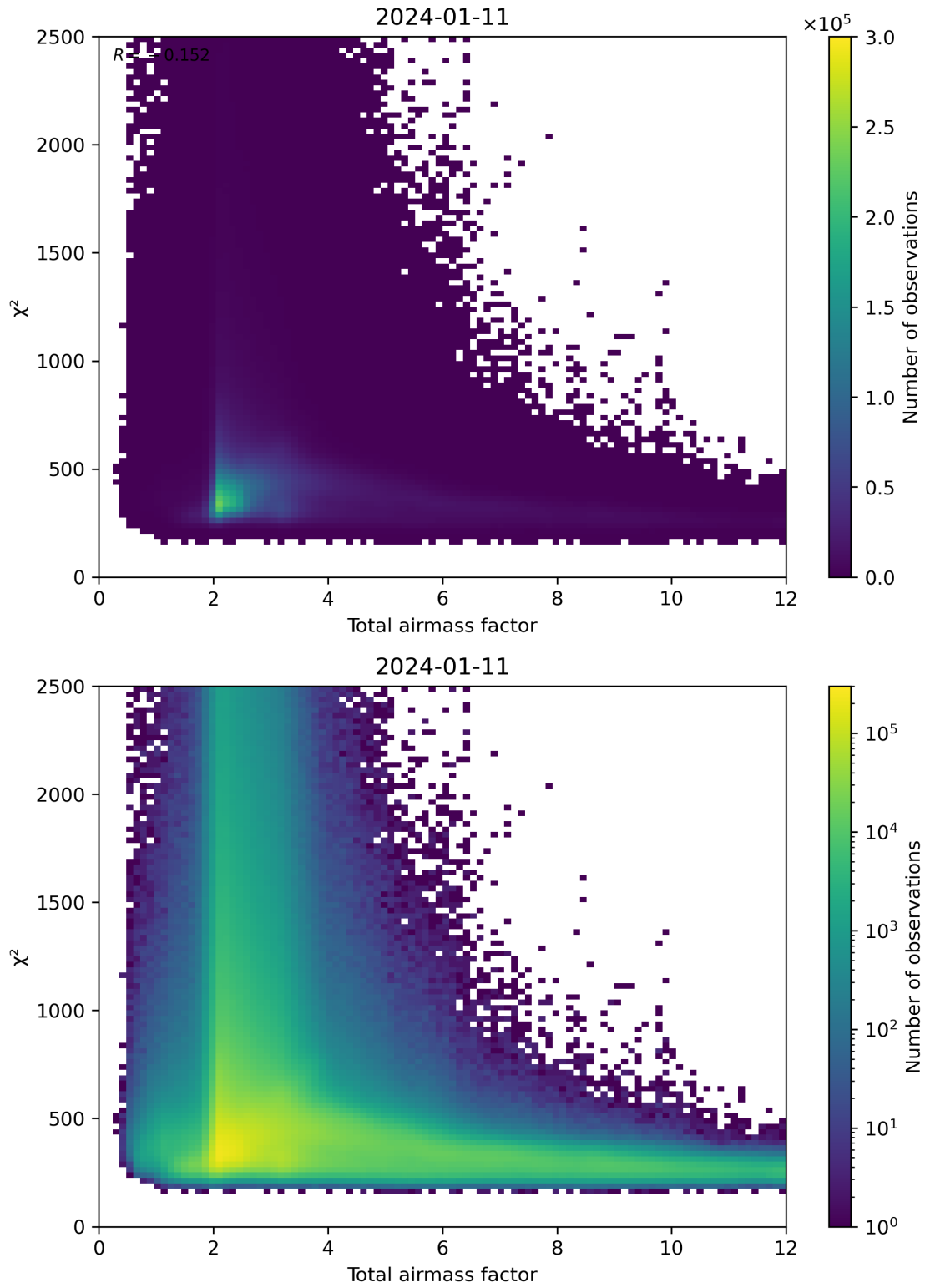
Figure 63: Scatter density plot of “Total airmass factor” against “ \chi^2 ” for 2024-01-10 to 2024-01-12.
