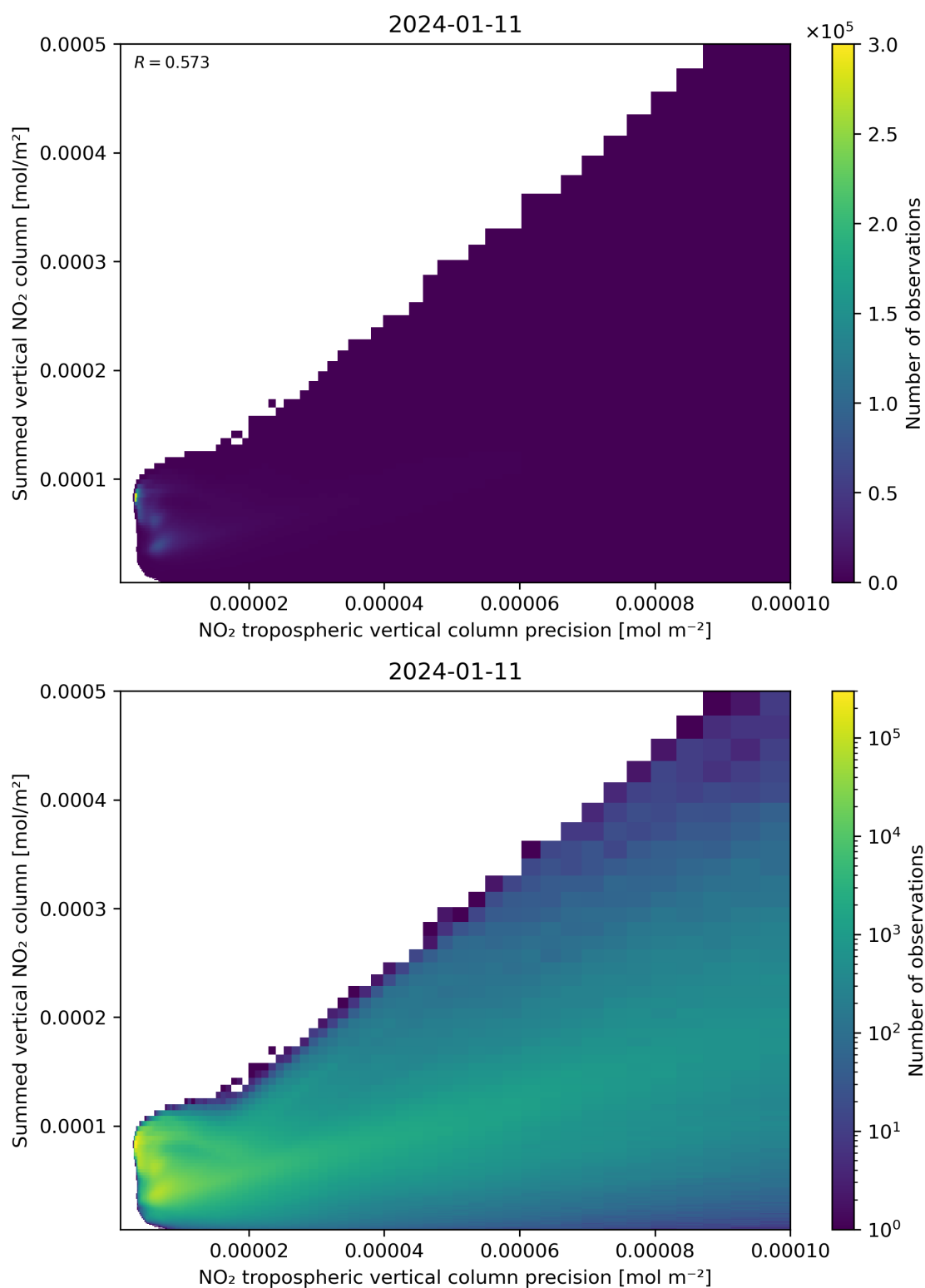
Figure 136: Scatter density plot of “NO 2 tropospheric vertical column precision” against “Summed vertical NO 2 column” for 2024-01-10 to 2024-01-12.
