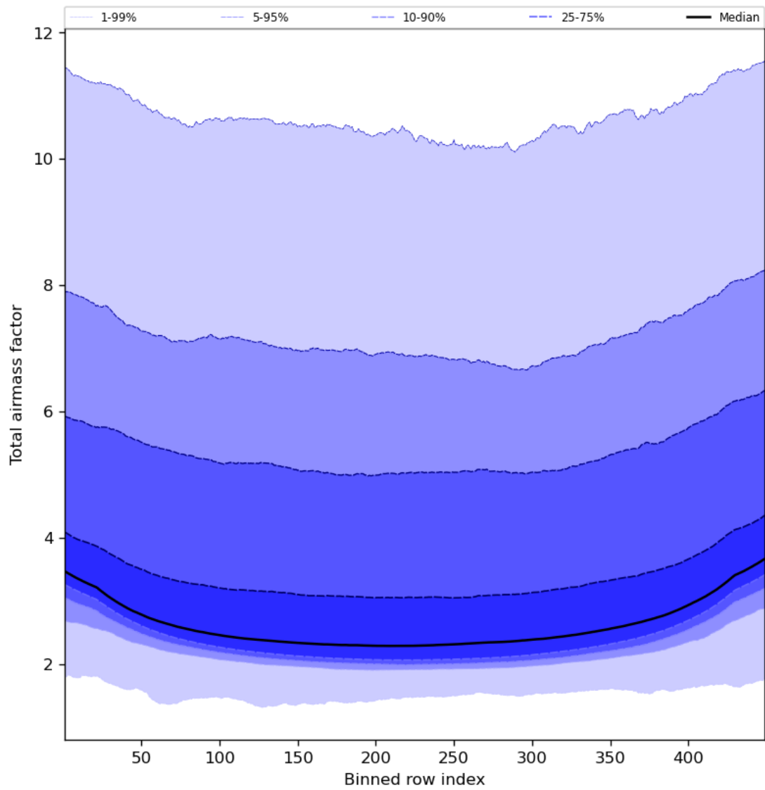
Figure 49: Along track statistics of “Total airmass factor” for 2024-01-10 to 2024-01-12
