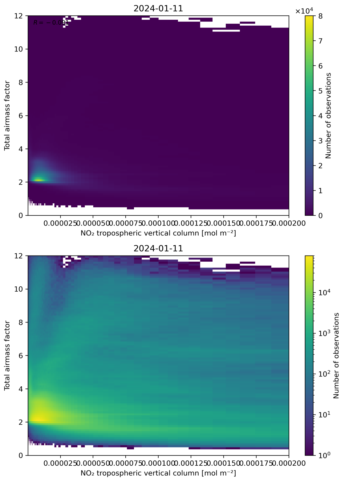
Figure 122: Scatter density plot of “NO 2 tropospheric vertical column” against “Total air mass factor” for 2024-01-10 to 2024-01-12.
