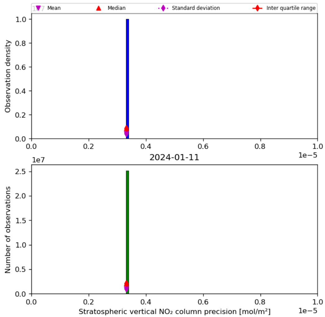
Figure 37: Histogram of “Stratospheric vertical NO 2 column precision” for 2024-01-10 to 2024-01-12
