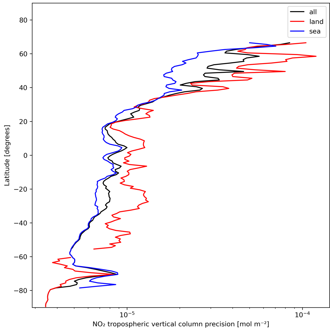
Figure 13: Zonal average of “NO 2 tropospheric vertical column precision” for 2024-01-10 to 2024-01-12.
