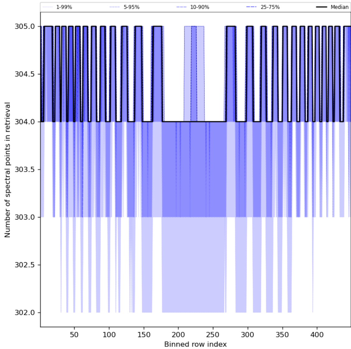
Figure 50: Along track statistics of “Number of spectral points in retrieval” for 2024-01-10 to 2024-01-12
