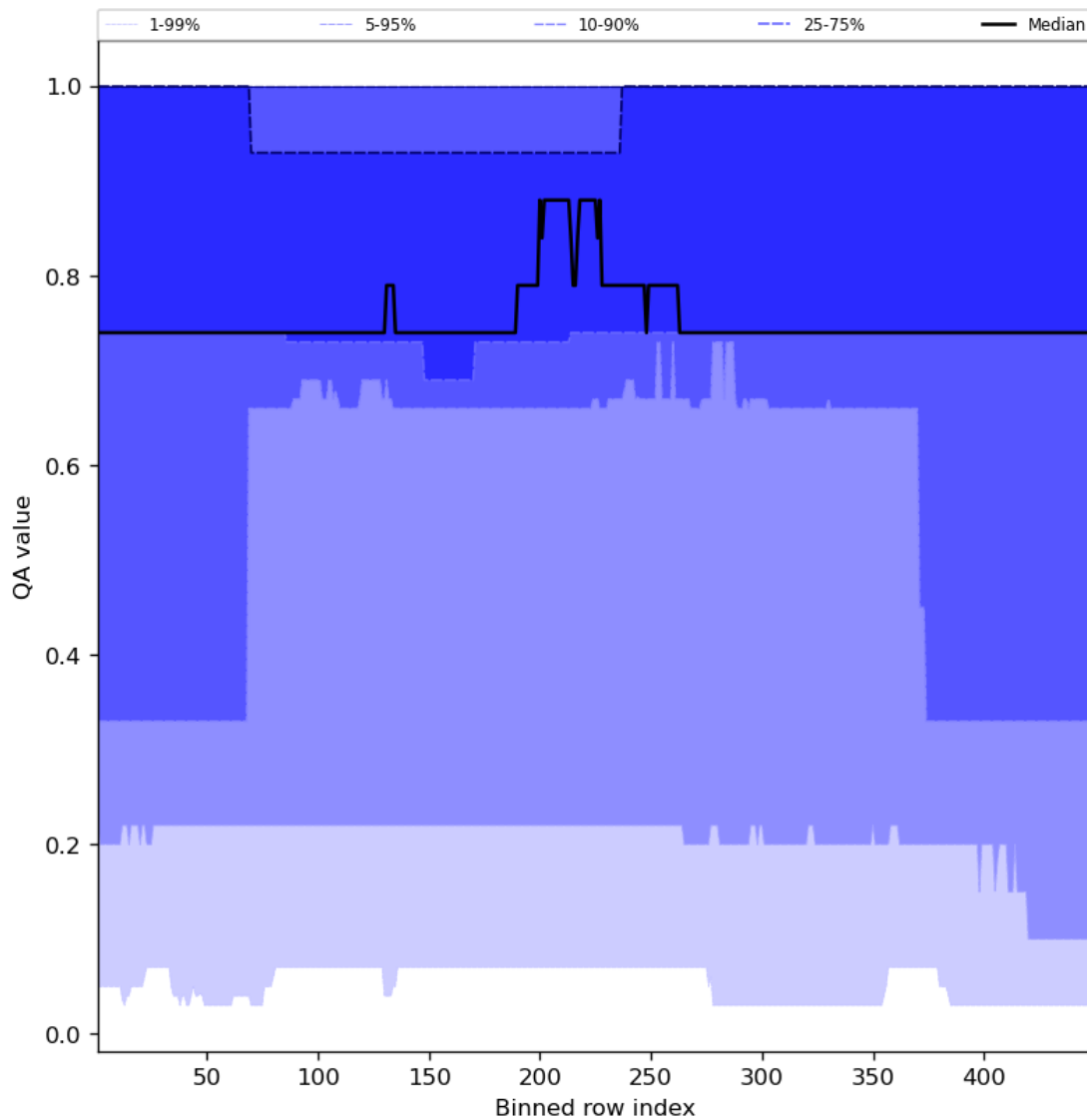
Figure 45: Along track statistics of “QA value” for 2024-01-10 to 2024-01-12
