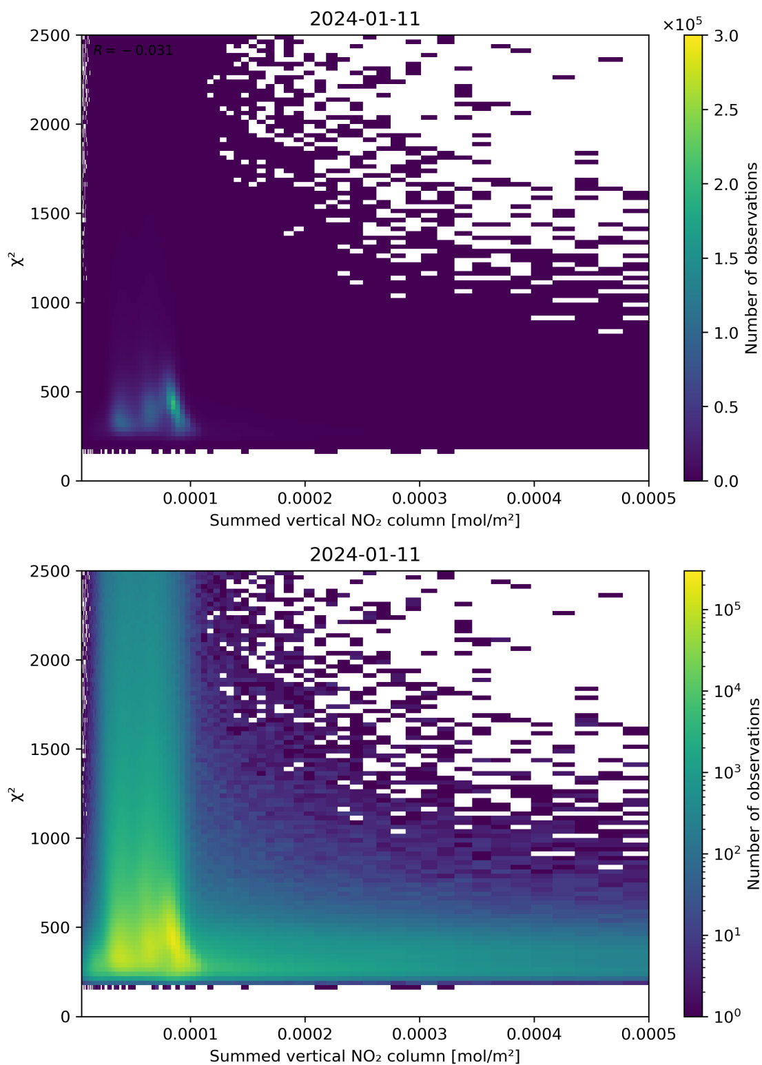
Figure 104: Scatter density plot of “Summed vertical NO 2 column” against “ \chi^2 ” for 2024-01-10 to 2024-01-12.
