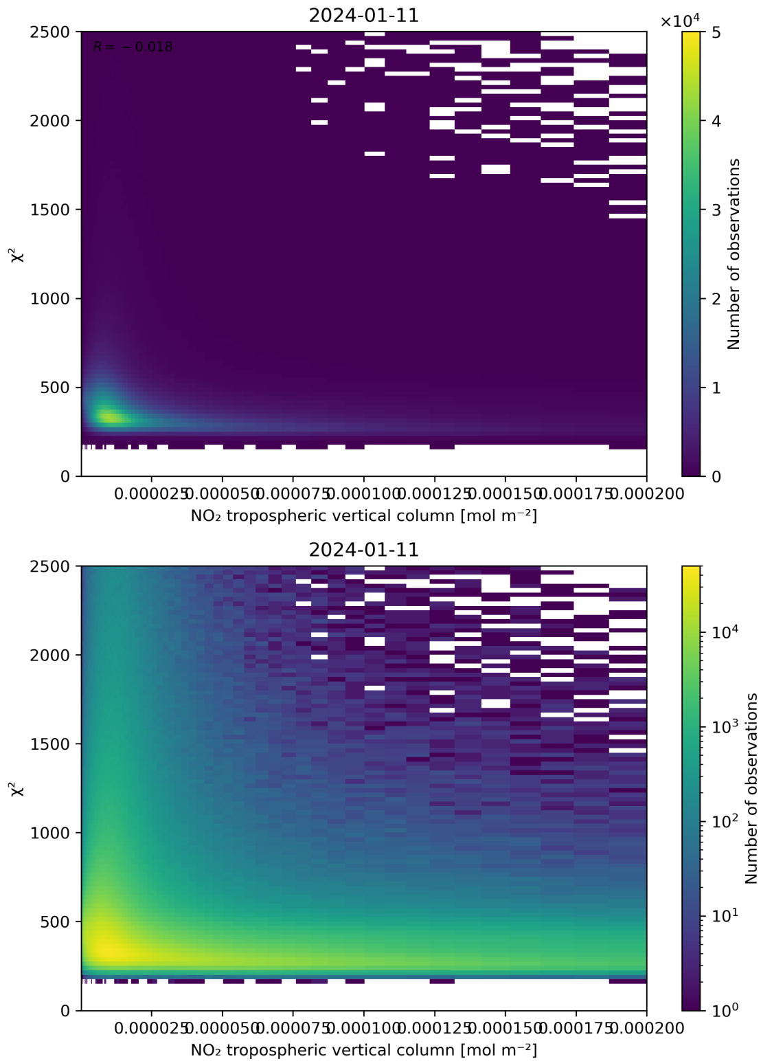
Figure 124: Scatter density plot of “NO 2 tropospheric vertical column” against “ \chi^2 ” for 2024-01-10 to 2024-01-12.
