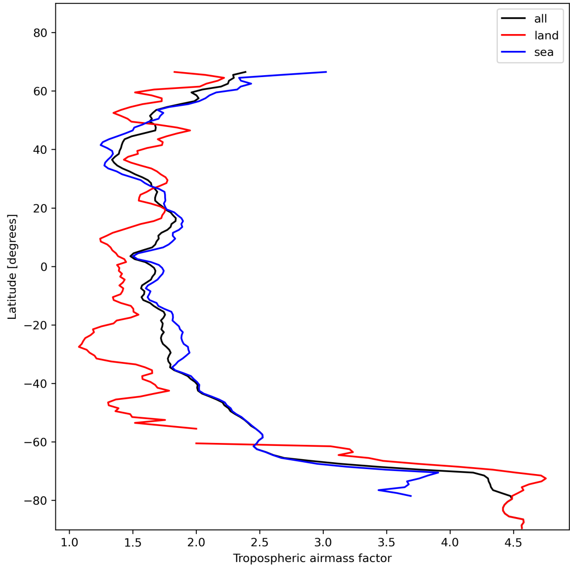
Figure 14: Zonal average of “Tropospheric airmass factor” for 2024-01-10 to 2024-01-12.
