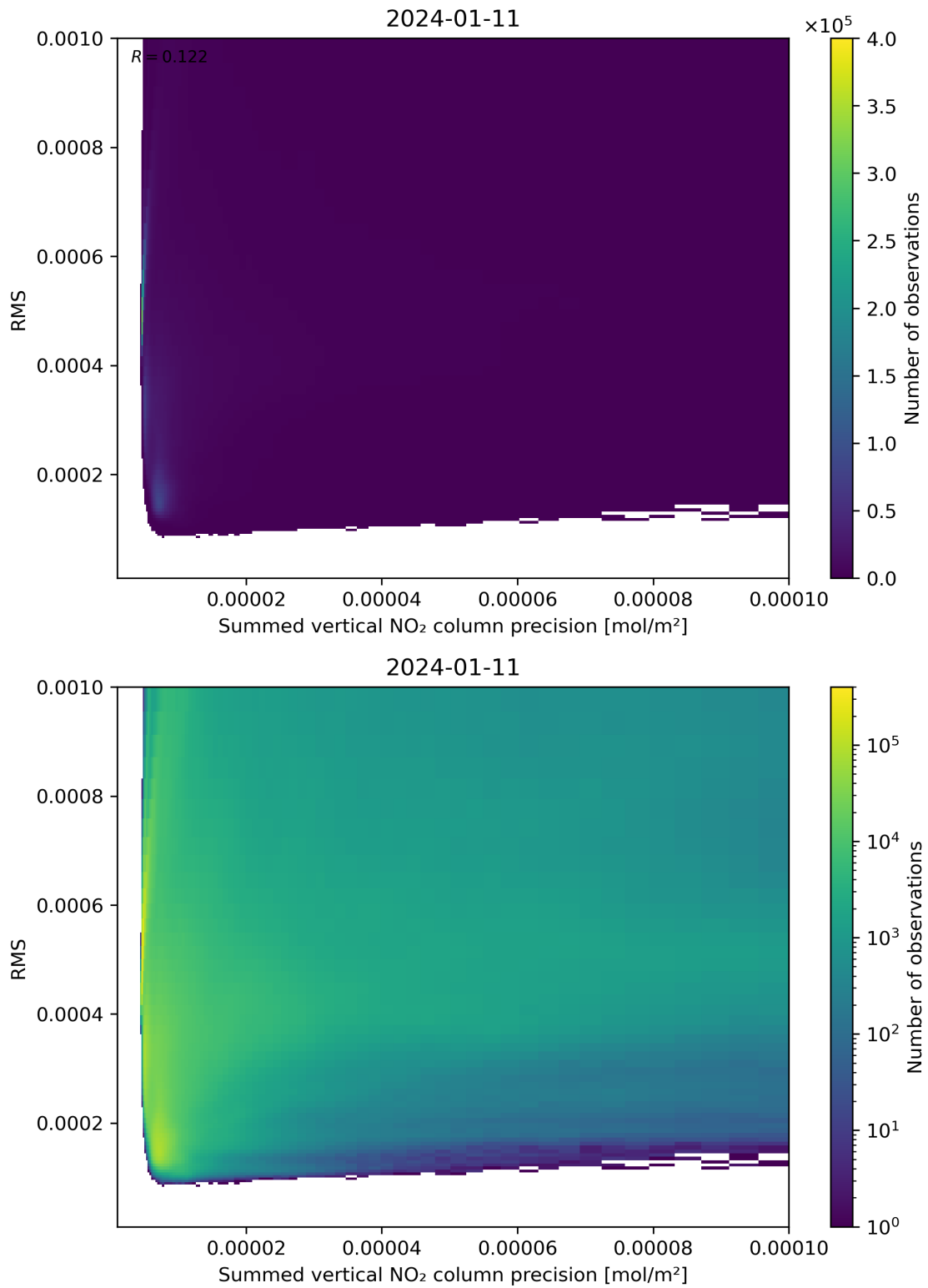
Figure 108: Scatter density plot of “Summed vertical NO 2 column precision” against “RMS” for 2024-01-10 to 2024-01-12.
