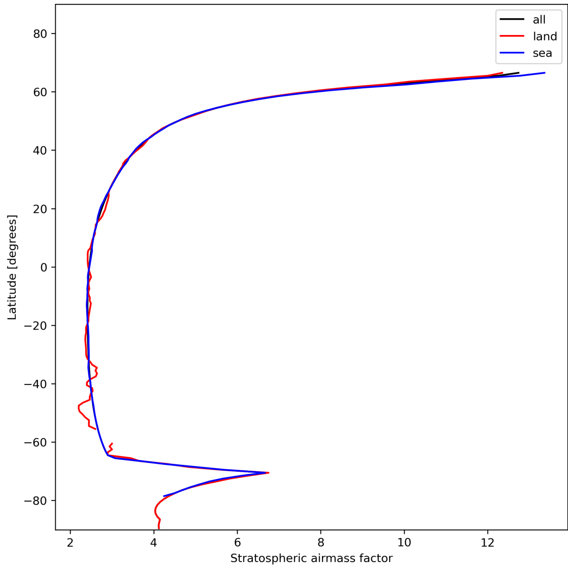
Figure 27: Zonal average of “Stratospheric air mass factor” for 2024-01-10 to 2024-01-12.
