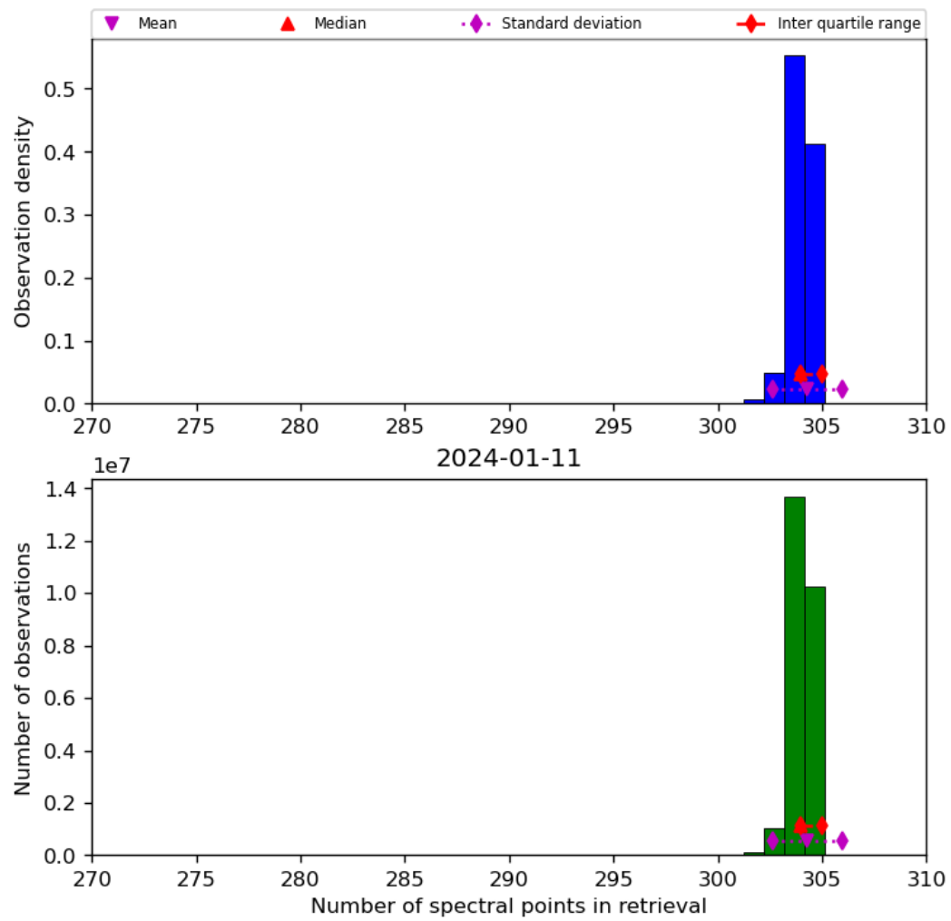
Figure 33: Histogram of “Number of spectral points in retrieval” for 2024-01-10 to 2024-01-12
