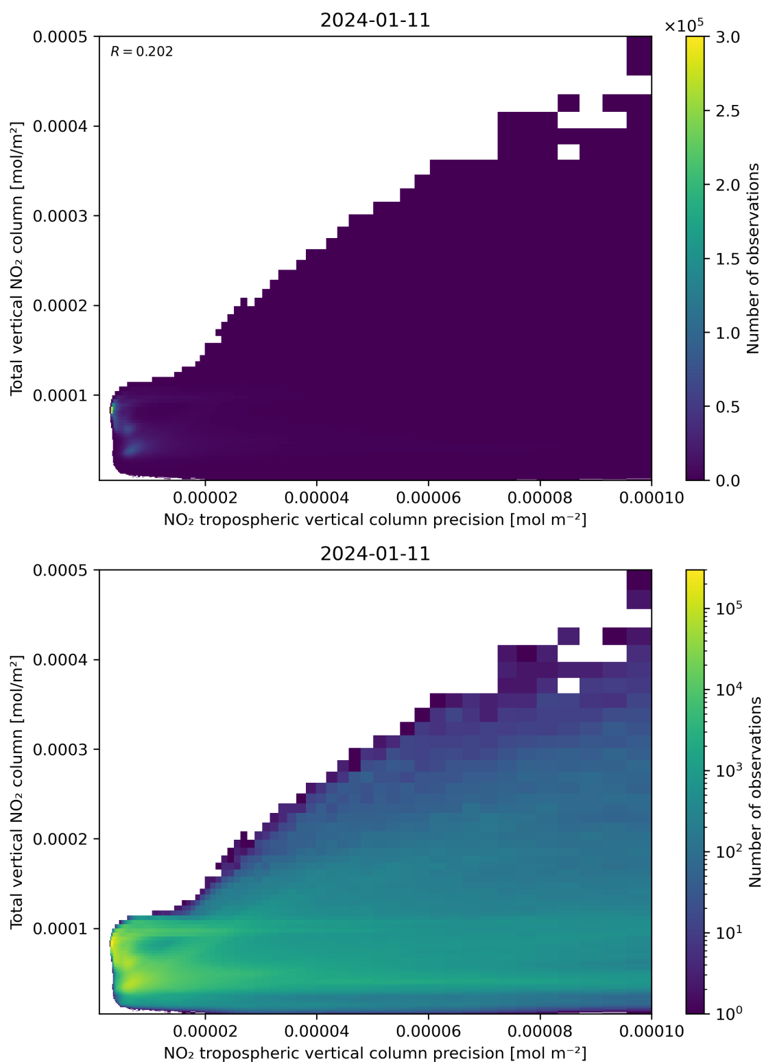
Figure 138: Scatter density plot of “NO 2 tropospheric vertical column precision” against “Total vertical NO 2 column” for 2024-01-10 to 2024-01-12.
