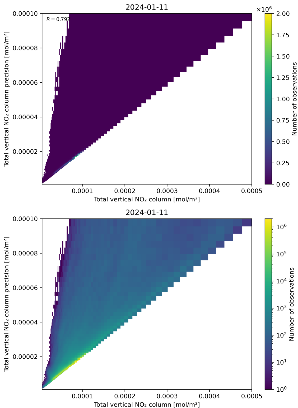
Figure 114: Scatter density plot of “Total vertical NO 2 column” against “Total vertical NO 2 column precision” for 2024-01-10 to 2024-01-12.
