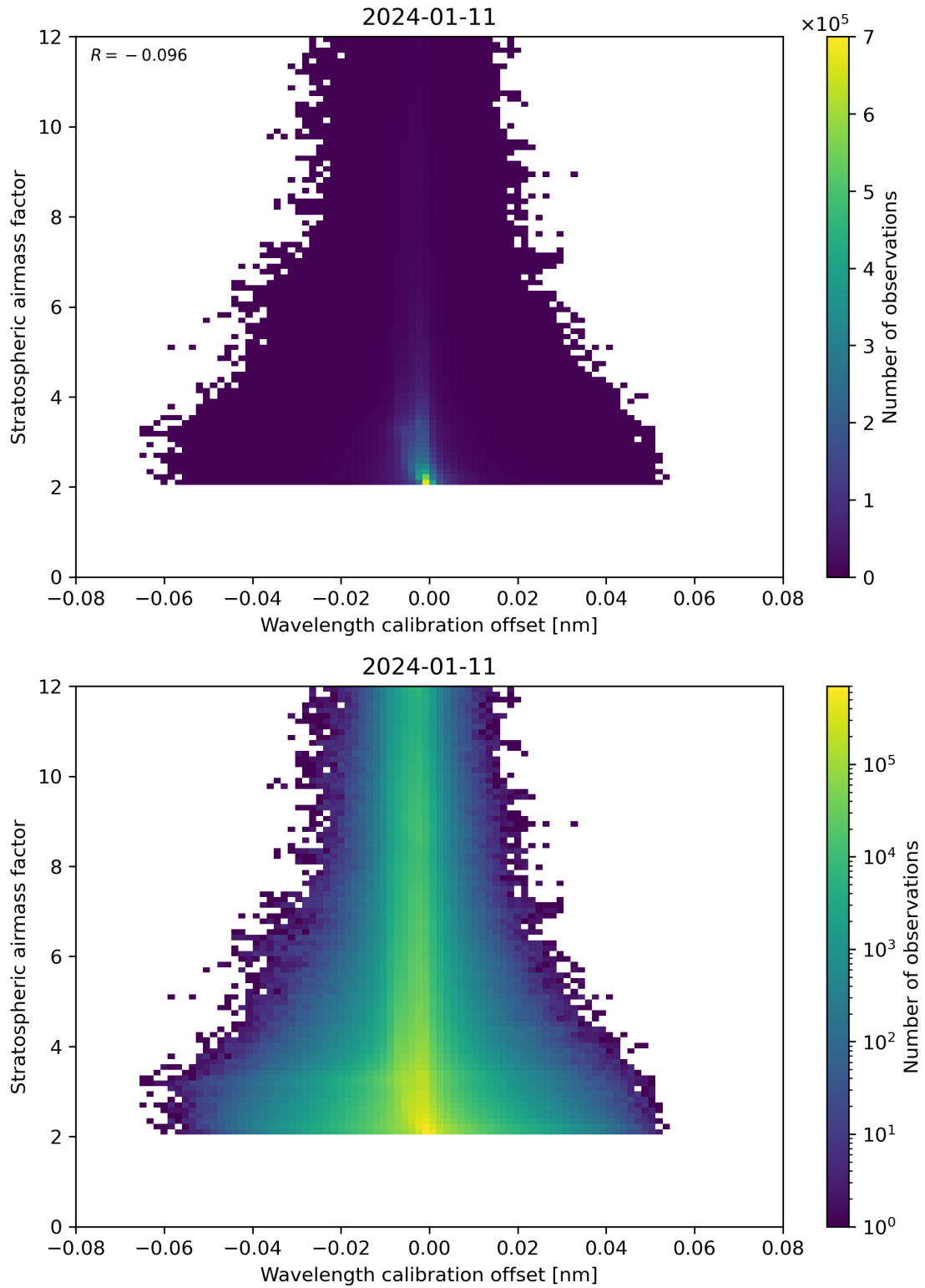
Figure 174: Scatter density plot of “Wavelength calibration offset” against “Stratospheric airmass factor” for 2024-01-10 to 2024-01-12.
