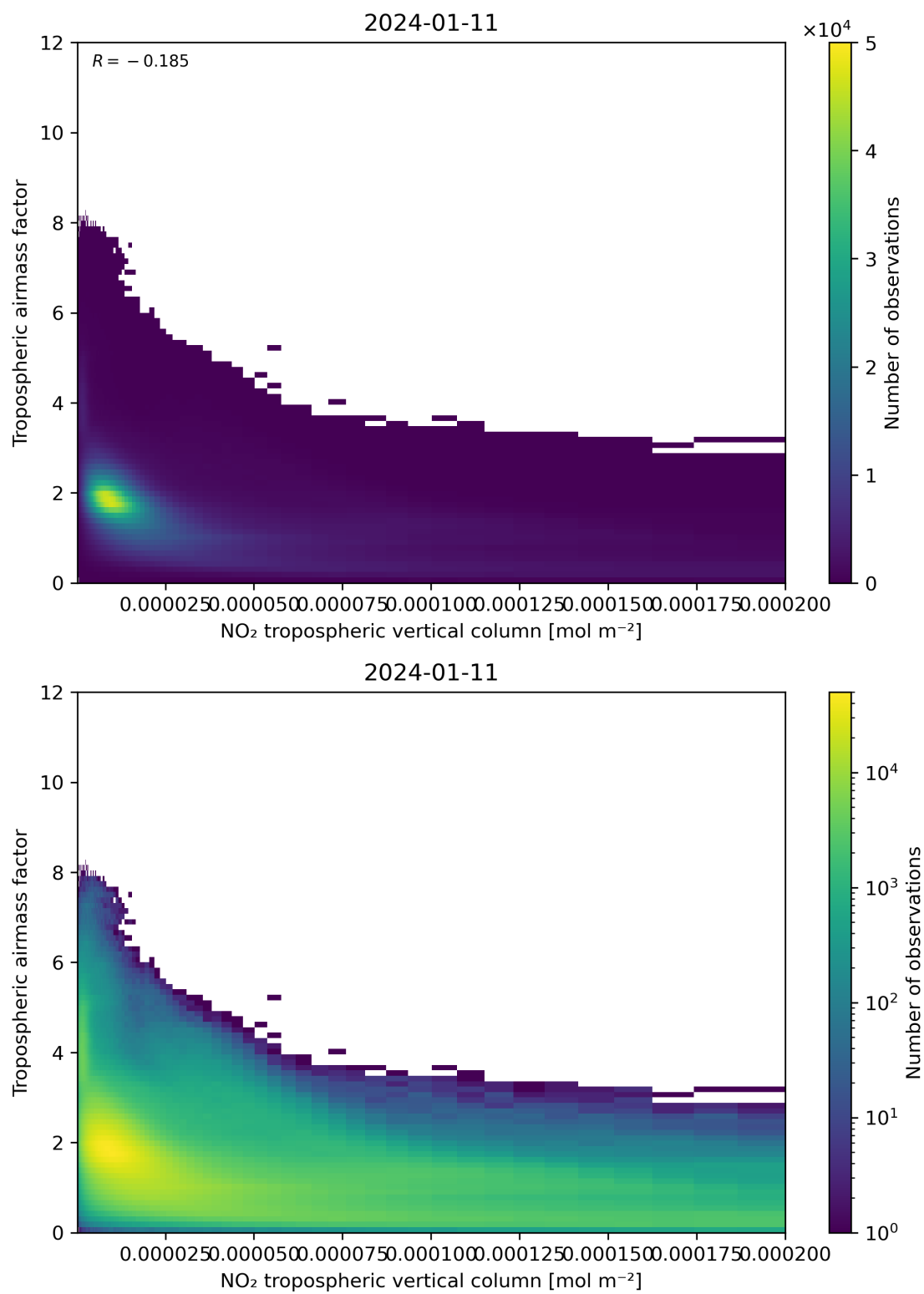
Figure 123: Scatter density plot of “NO 2 tropospheric vertical column” against “Tropospheric air mass factor” for 2024-01-10 to 2024-01-12.
