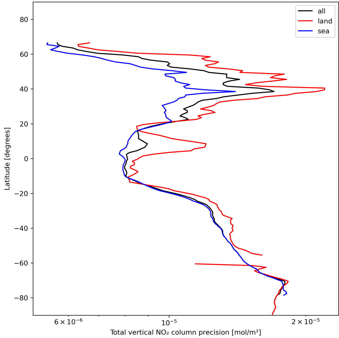
Figure 22: Zonal average of “Total vertical NO 2 column precision” for 2024-01-10 to 2024-01-12.
