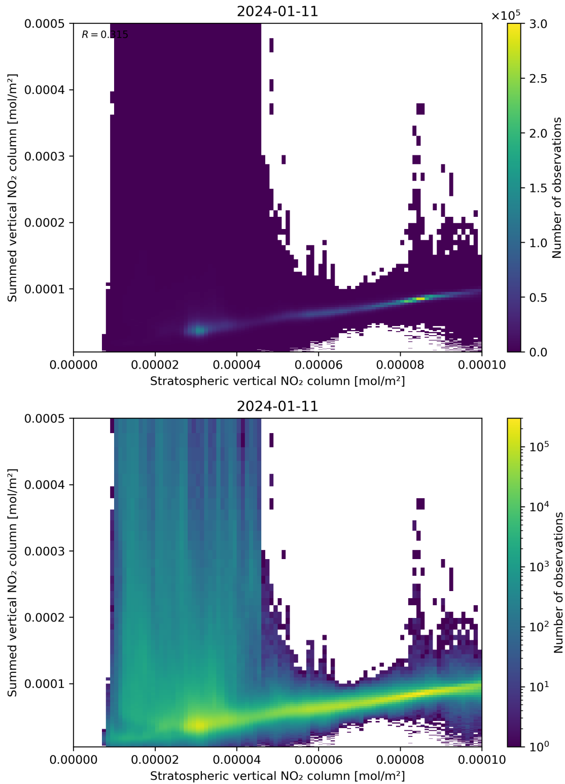
Figure 98: Scatter density plot of “Stratospheric vertical NO 2 column” against “Summed vertical NO 2 column” for 2024-01-10 to 2024-01-12.
