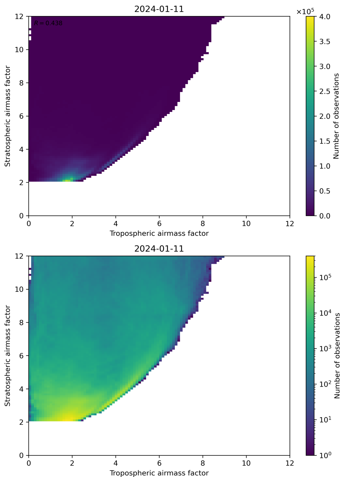
Figure 71: Scatter density plot of “Tropospheric airmass factor” against “Stratospheric airmass factor” for 2024-01-10 to 2024-01-12.
