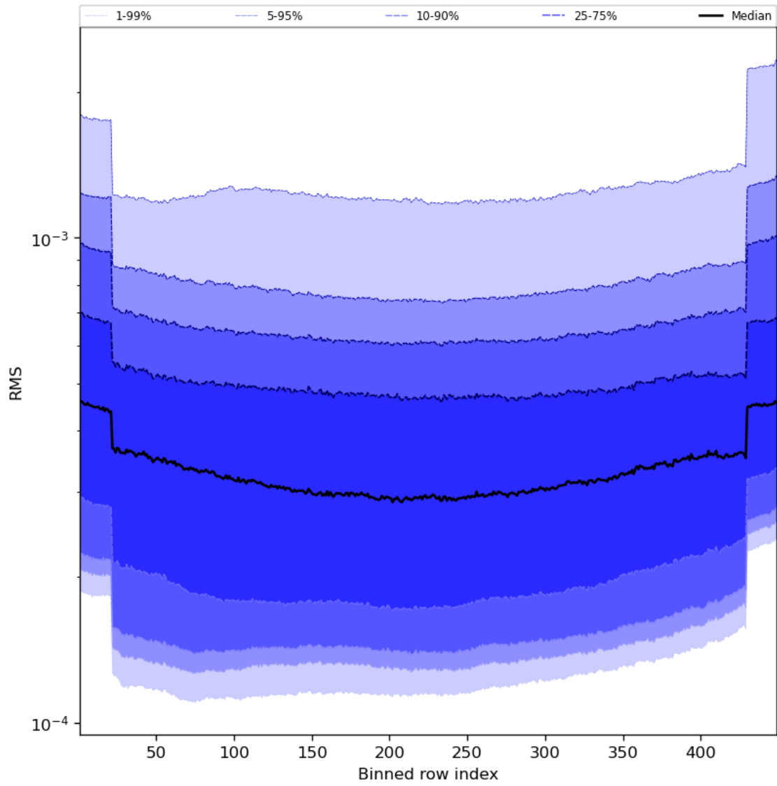
Figure 60: Along track statistics of “RMS” for 2024-01-10 to 2024-01-12
