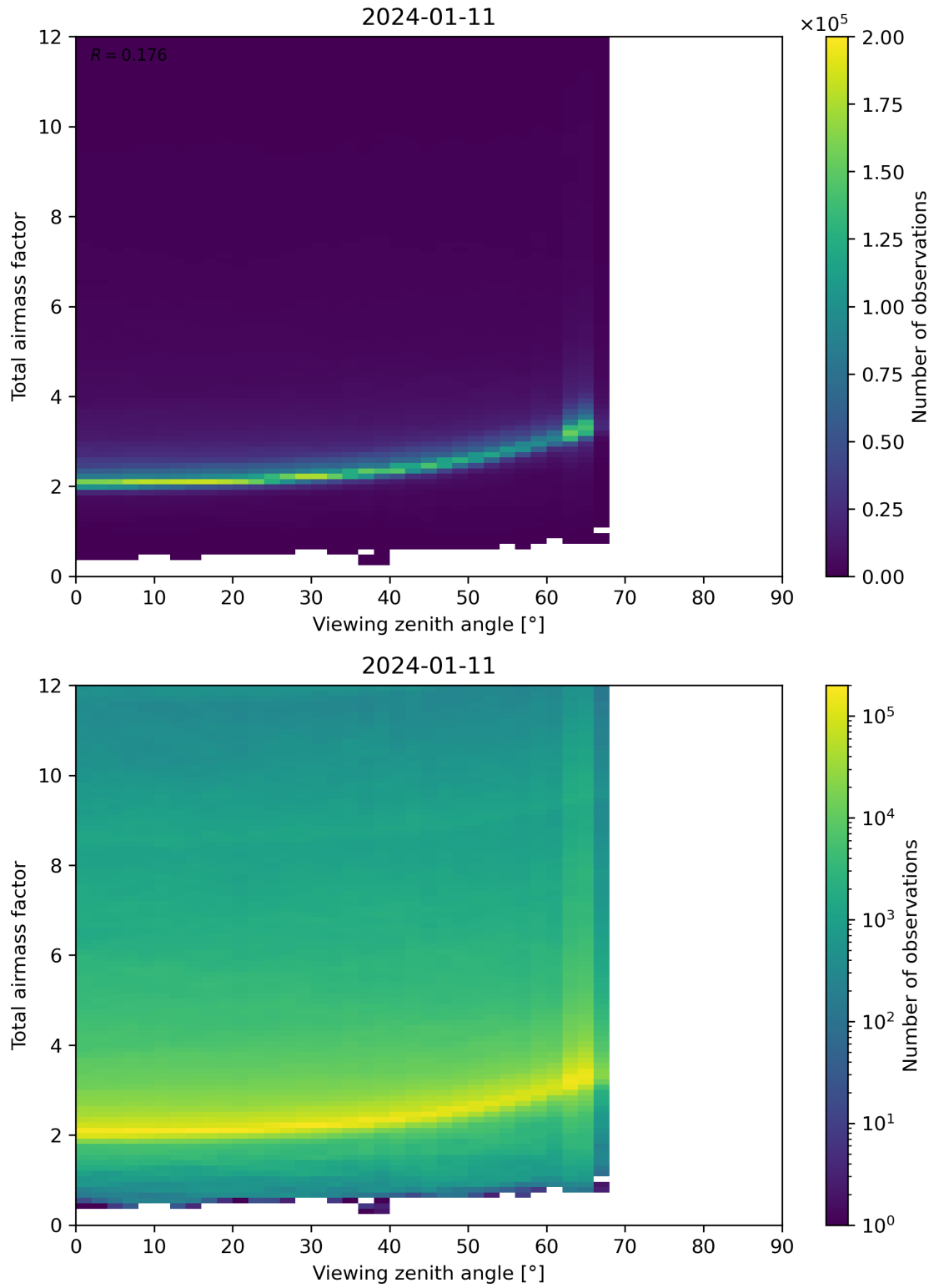
Figure 160: Scatter density plot of “Viewing zenith angle” against “Total airmass factor” for 2024-01-10 to 2024-01-12.
