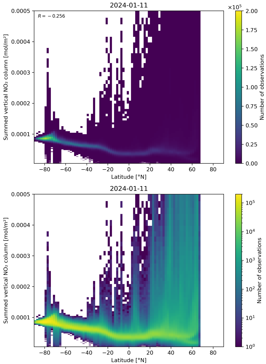
Figure 88: Scatter density plot of “Latitude” against “Summed vertical NO 2 column” for 2024-01-10 to 2024-01-12.
