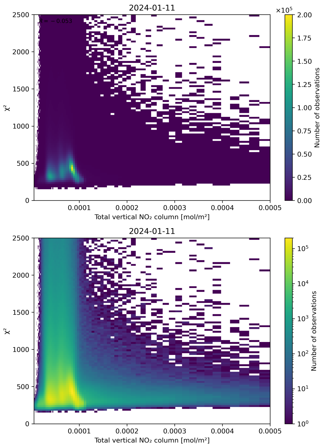
Figure 111: Scatter density plot of “Total vertical NO 2 column” against “ \chi^2 ” for 2024-01-10 to 2024-01-12.
