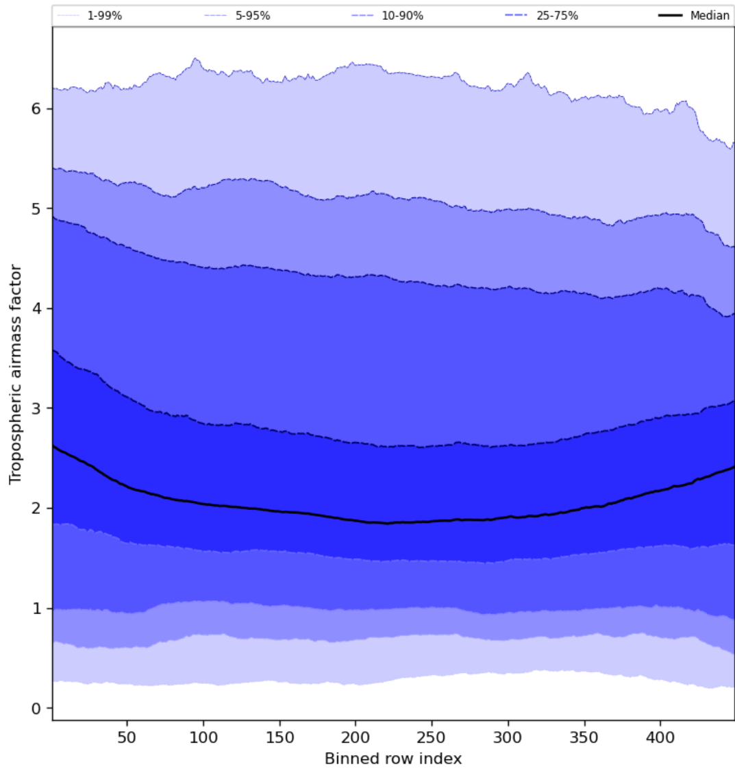
Figure 48: Along track statistics of “Tropospheric airmass factor” for 2024-01-10 to 2024-01-12
