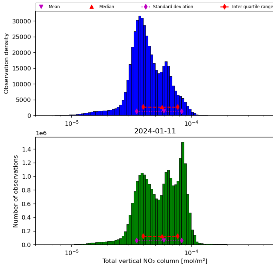
Figure 38: Histogram of “Total vertical NO 2 column” for 2024-01-10 to 2024-01-12
