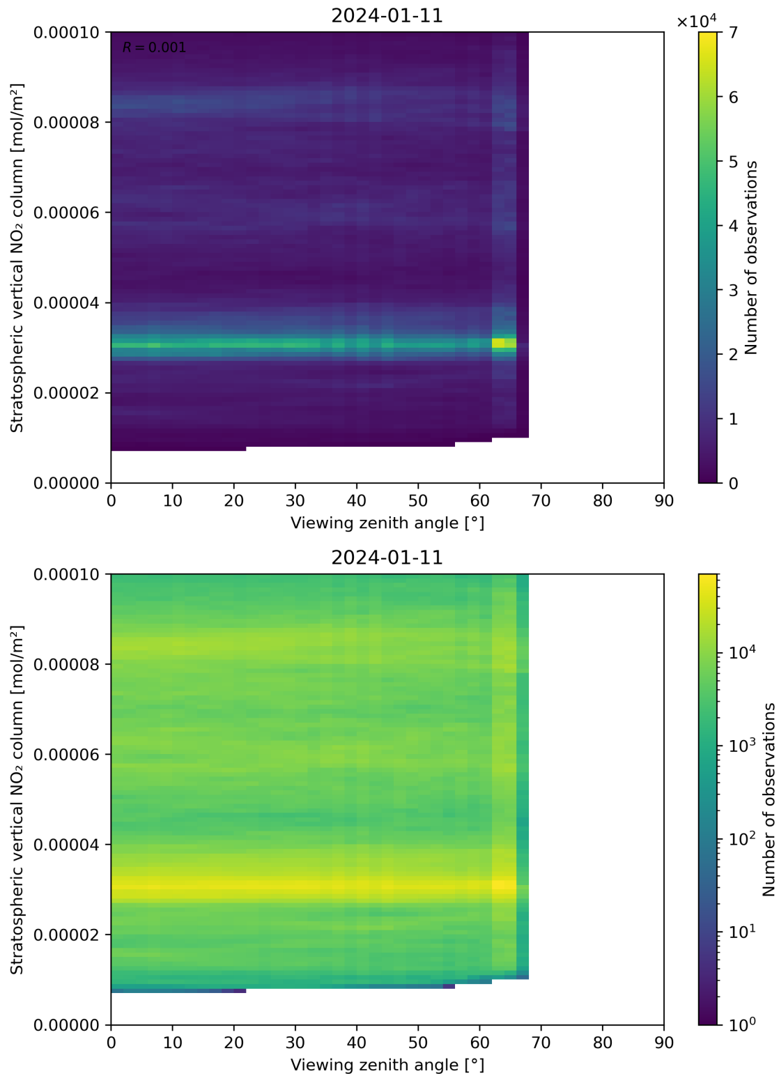
Figure 164: Scatter density plot of “Viewing zenith angle” against “Stratospheric vertical NO 2 column” for 2024-01-10 to 2024-01-12.
