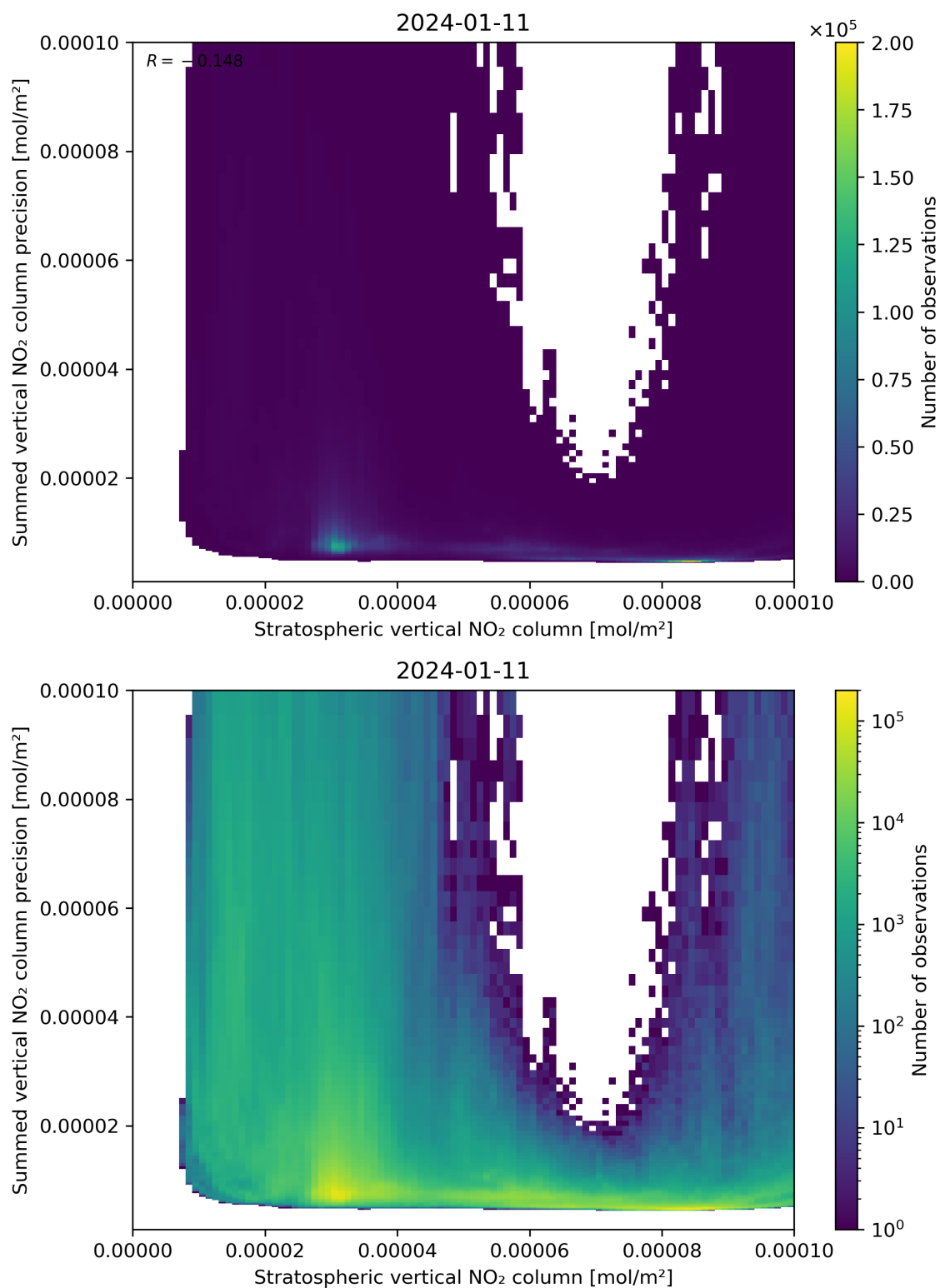
Figure 99: Scatter density plot of “Stratospheric vertical NO 2 column” against “Summed vertical NO 2 column precision” for 2024-01-10 to 2024-01-12.
