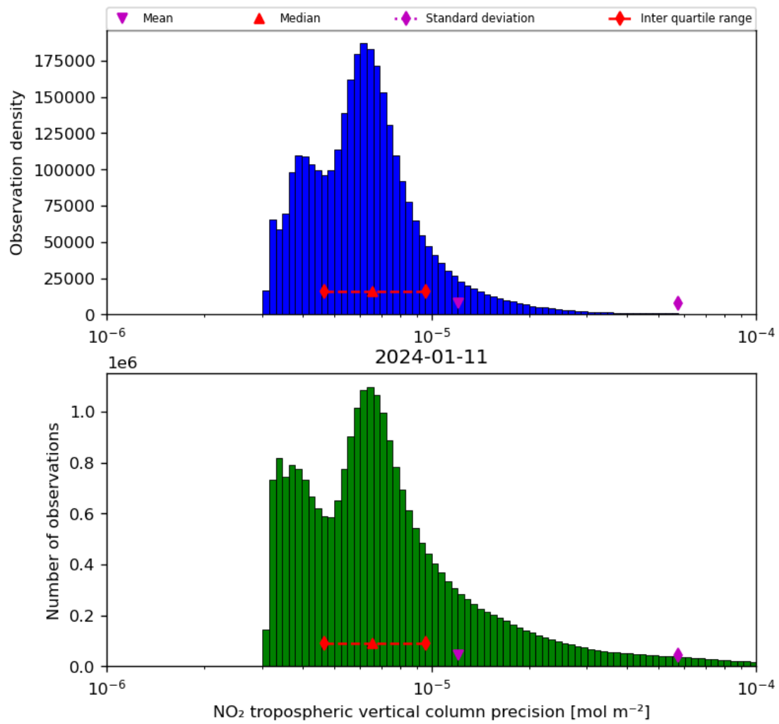
Figure 30: Histogram of “NO 2 tropospheric vertical column precision” for 2024-01-10 to 2024-01-12
