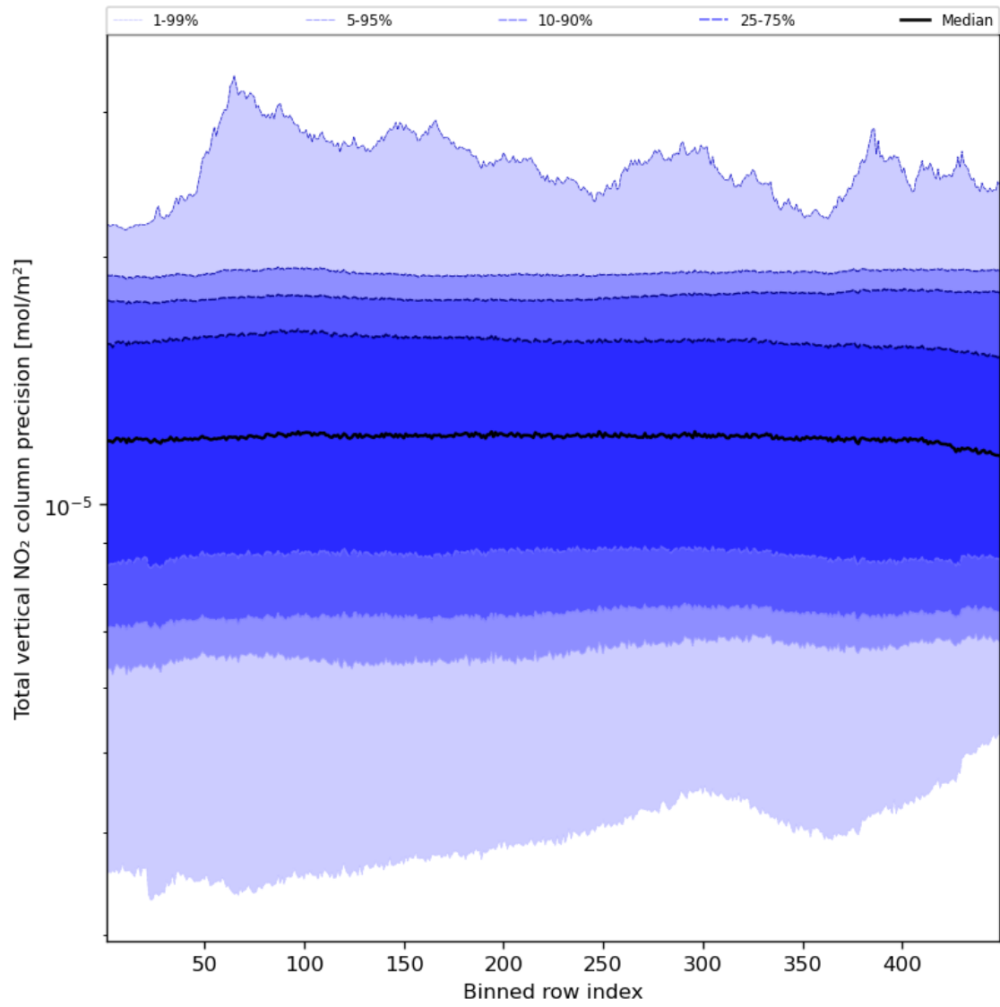
Figure 56: Along track statistics of “Total vertical NO 2 column precision” for 2024-01-10 to 2024-01-12
