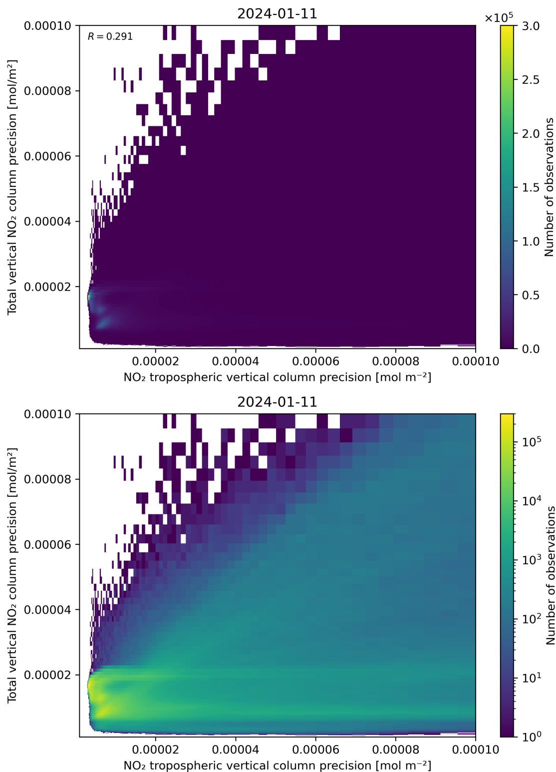
Figure 139: Scatter density plot of “NO 2 tropospheric vertical column precision” against “Total vertical NO 2 column precision” for 2024-01-10 to 2024-01-12.
