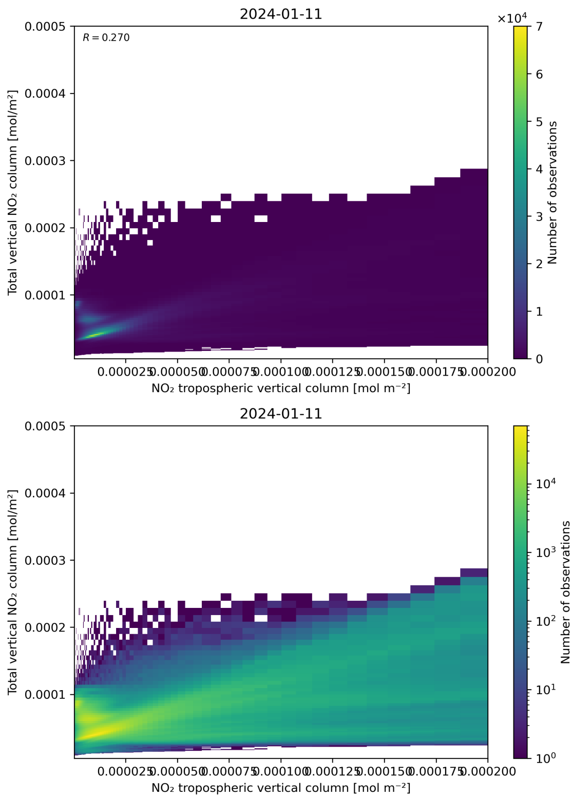
Figure 128: Scatter density plot of “NO 2 tropospheric vertical column” against “Total vertical NO 2 column” for 2024-01-10 to 2024-01-12.
