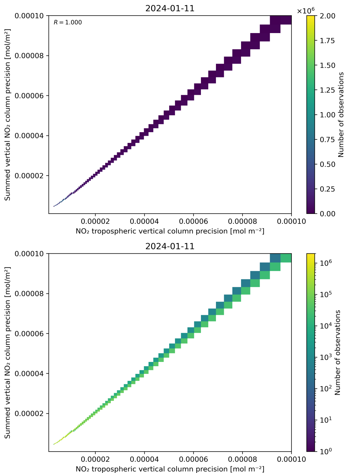
Figure 137: Scatter density plot of “NO 2 tropospheric vertical column precision” against “Summed vertical NO 2 column precision” for 2024-01-10 to 2024-01-12.
