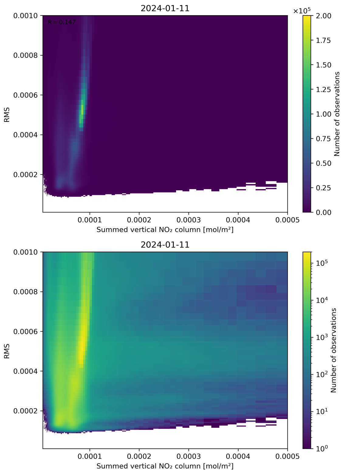
Figure 109: Scatter density plot of “Summed vertical NO 2 column” against “RMS” for 2024-01-10 to 2024-01-12.
