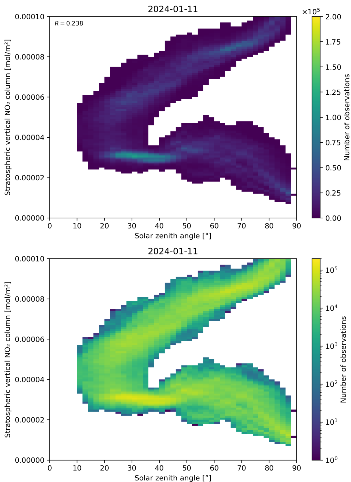
Figure 150: Scatter density plot of “Solar zenith angle” against “Stratospheric vertical NO 2 column” for 2024-01-10 to 2024-01-12.
