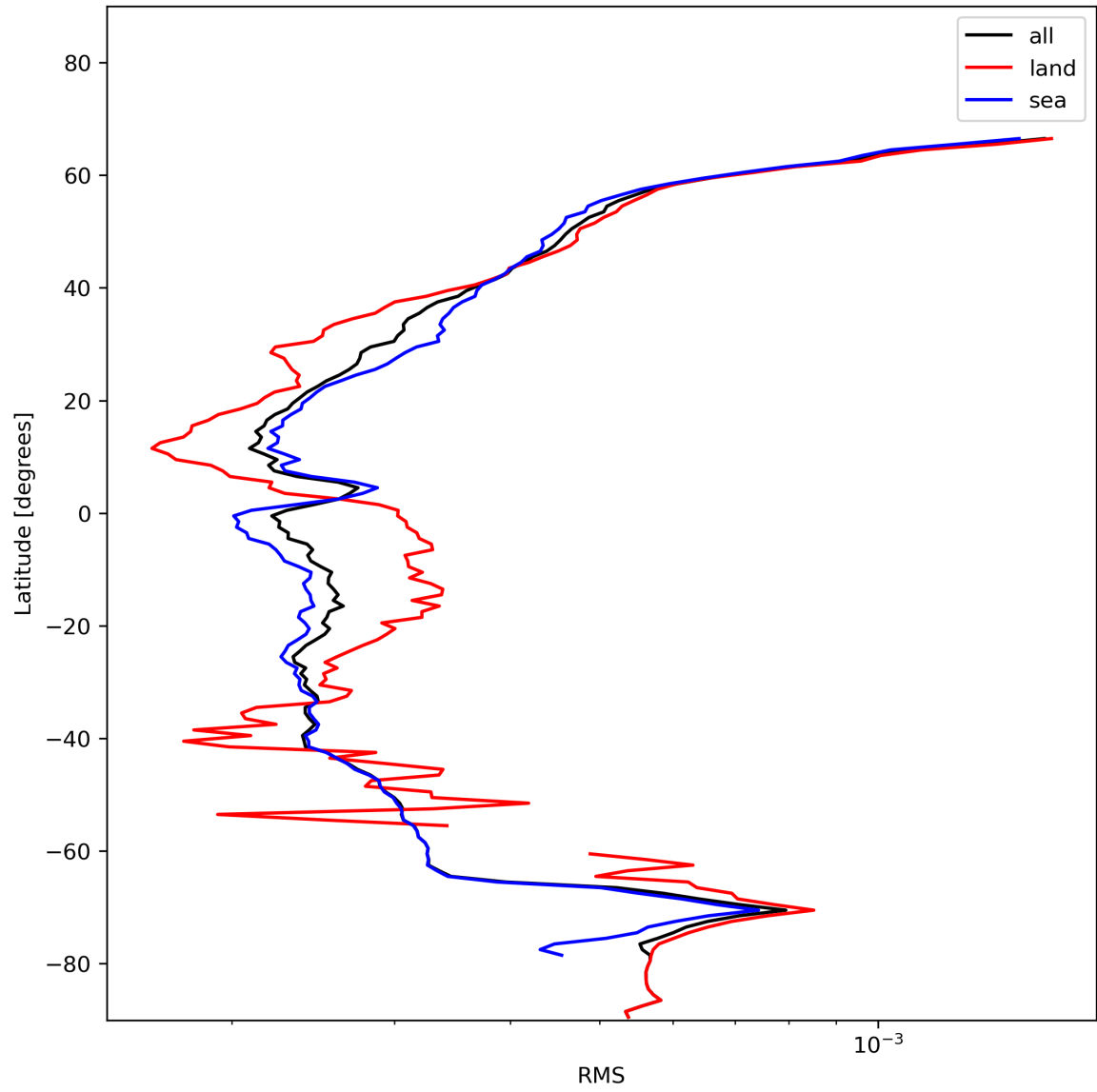
Figure 26: Zonal average of “RMS” for 2024-01-10 to 2024-01-12.
