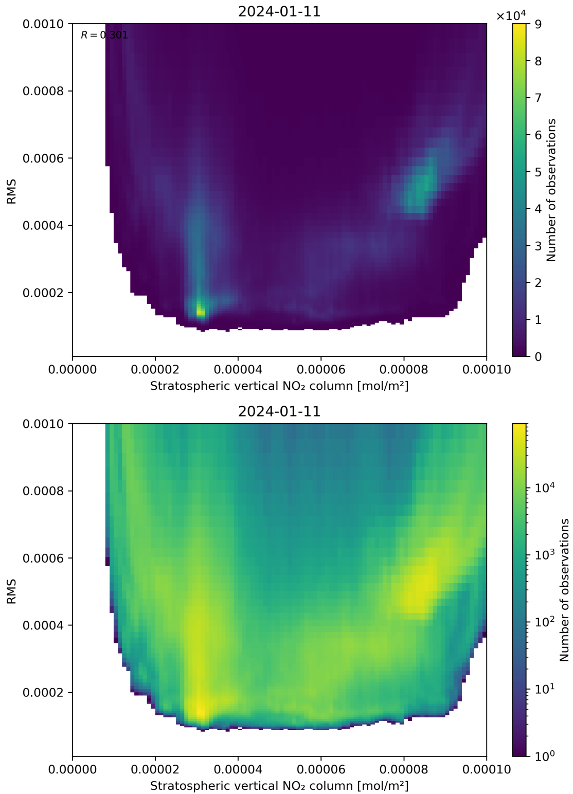
Figure 102: Scatter density plot of “Stratospheric vertical NO 2 column” against “RMS” for 2024-01-10 to 2024-01-12.
