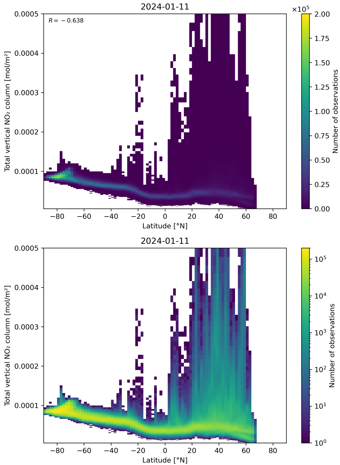
Figure 90: Scatter density plot of “Latitude” against “Total vertical NO 2 column” for 2024-01-10 to 2024-01-12.
