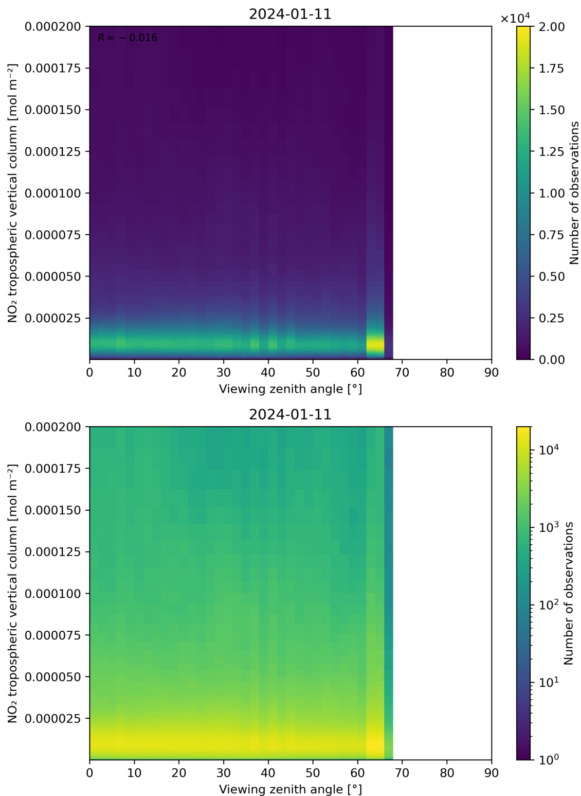
Figure 169: Scatter density plot of “Viewing zenith angle” against “NO 2 tropospheric vertical column” for 2024-01-10 to 2024-01-12.
