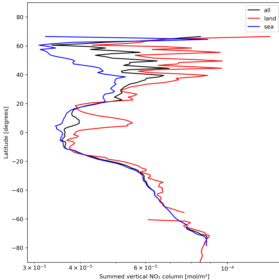
Figure 23: Zonal average of “Summed vertical NO 2 column” for 2024-01-10 to 2024-01-12.
