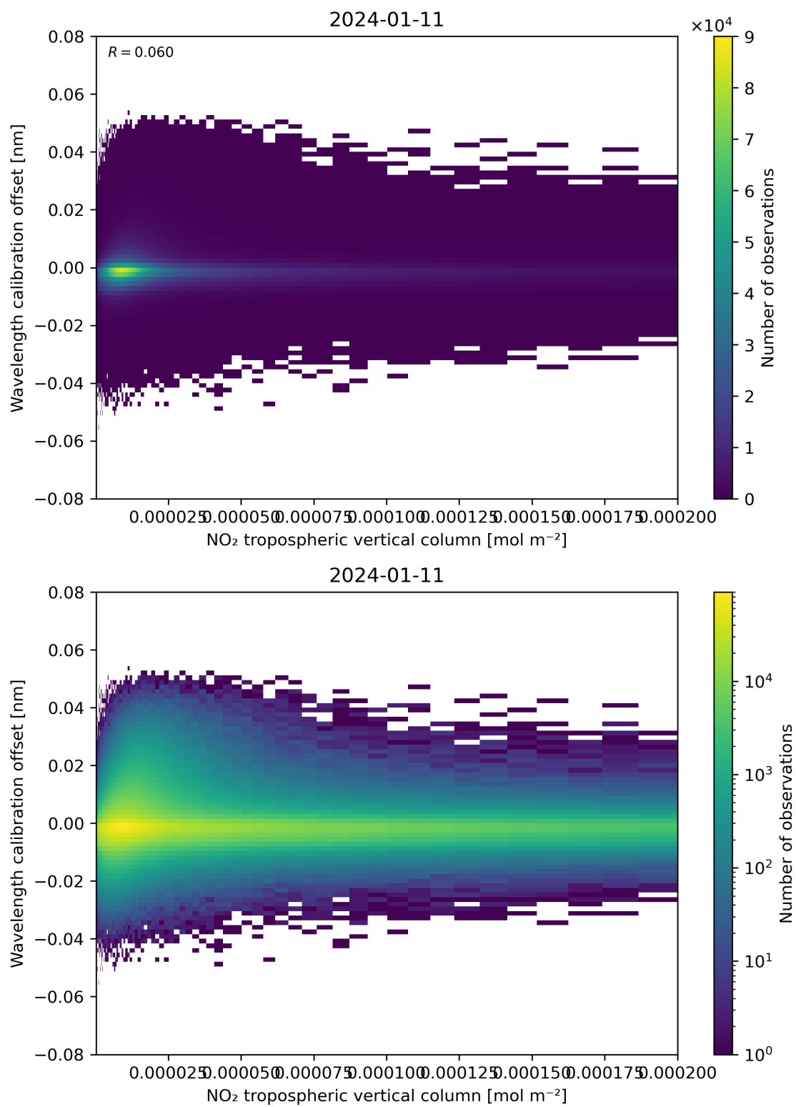
Figure 143: Scatter density plot of “NO 2 tropospheric vertical column” against “Wavelength calibration offset” for 2024-01-10 to 2024-01-12.
