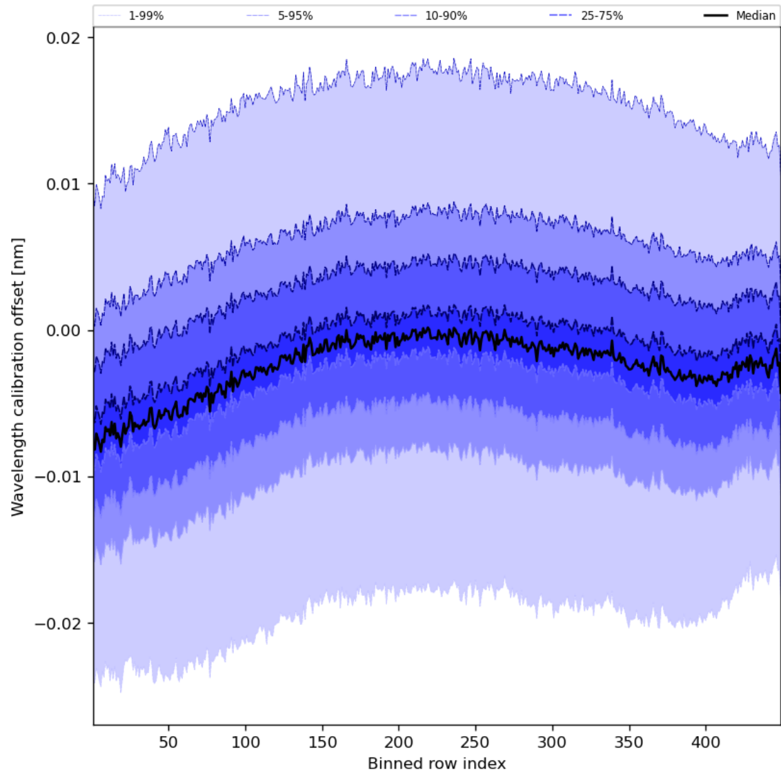
Figure 52: Along track statistics of “Wavelength calibration offset” for 2024-01-10 to 2024-01-12
