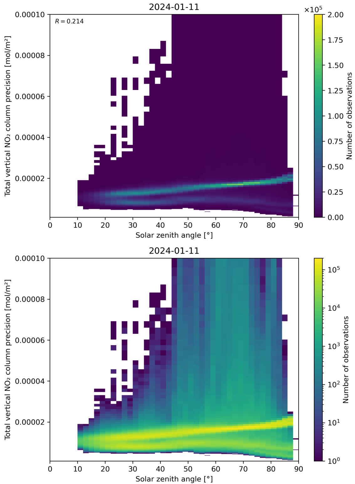
Figure 154: Scatter density plot of “Solar zenith angle” against “Total vertical NO 2 column precision” for 2024-01-10 to 2024-01-12.
