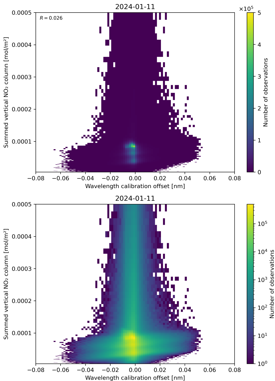
Figure 177: Scatter density plot of “Wavelength calibration offset” against “Summed vertical NO 2 column” for 2024-01-10 to 2024-01-12.
