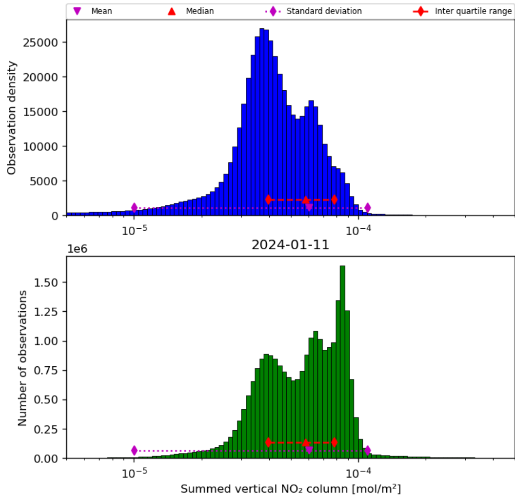
Figure 40: Histogram of “Summed vertical NO 2 column” for 2024-01-10 to 2024-01-12
