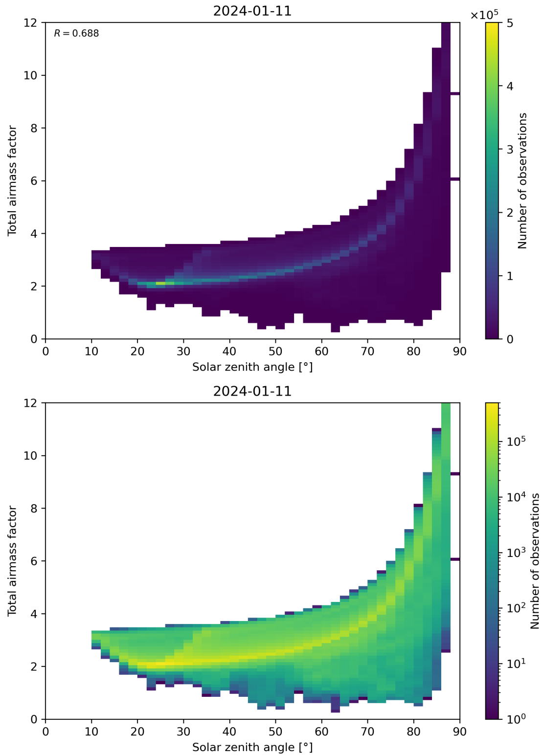
Figure 146: Scatter density plot of “Solar zenith angle” against “Total air mass factor” for 2024-01-10 to 2024-01-12.
