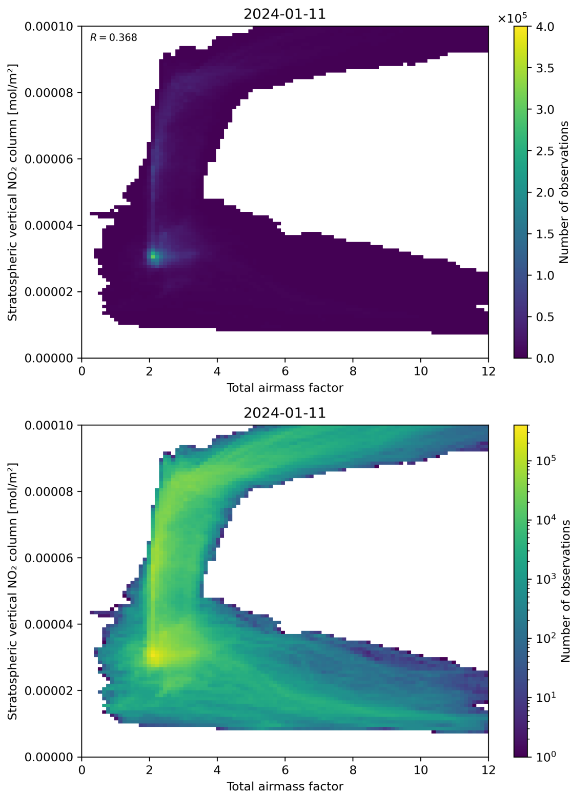
Figure 64: Scatter density plot of “Total airmass factor” against “Stratospheric vertical NO 2 column” for 2024-01-10 to 2024-01-12.
