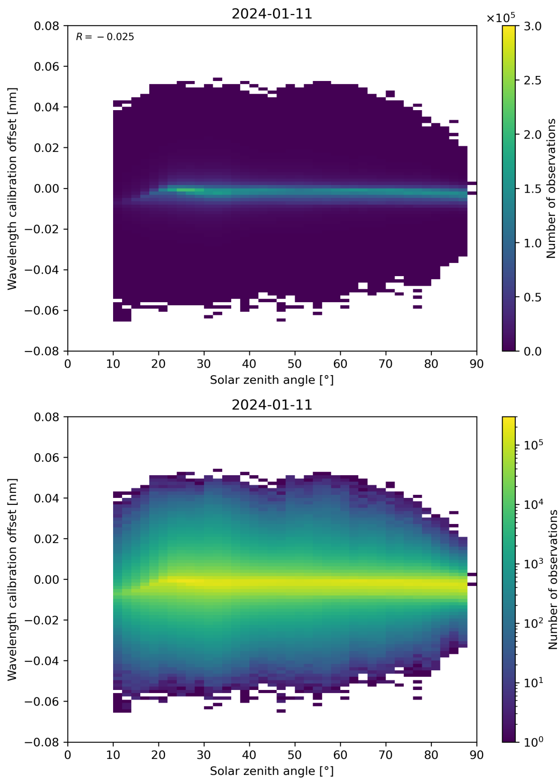
Figure 158: Scatter density plot of “Solar zenith angle” against “Wavelength calibration offset” for 2024-01-10 to 2024-01-12.
