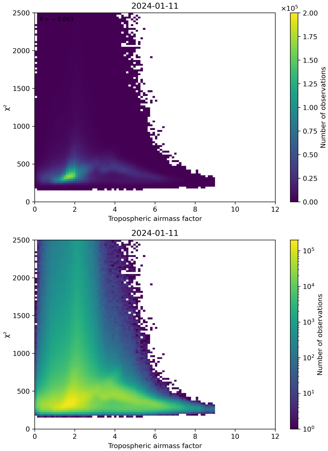
Figure 73: Scatter density plot of “Tropospheric airmass factor” against “ \chi^2 ” for 2024-01-10 to 2024-01-12.
