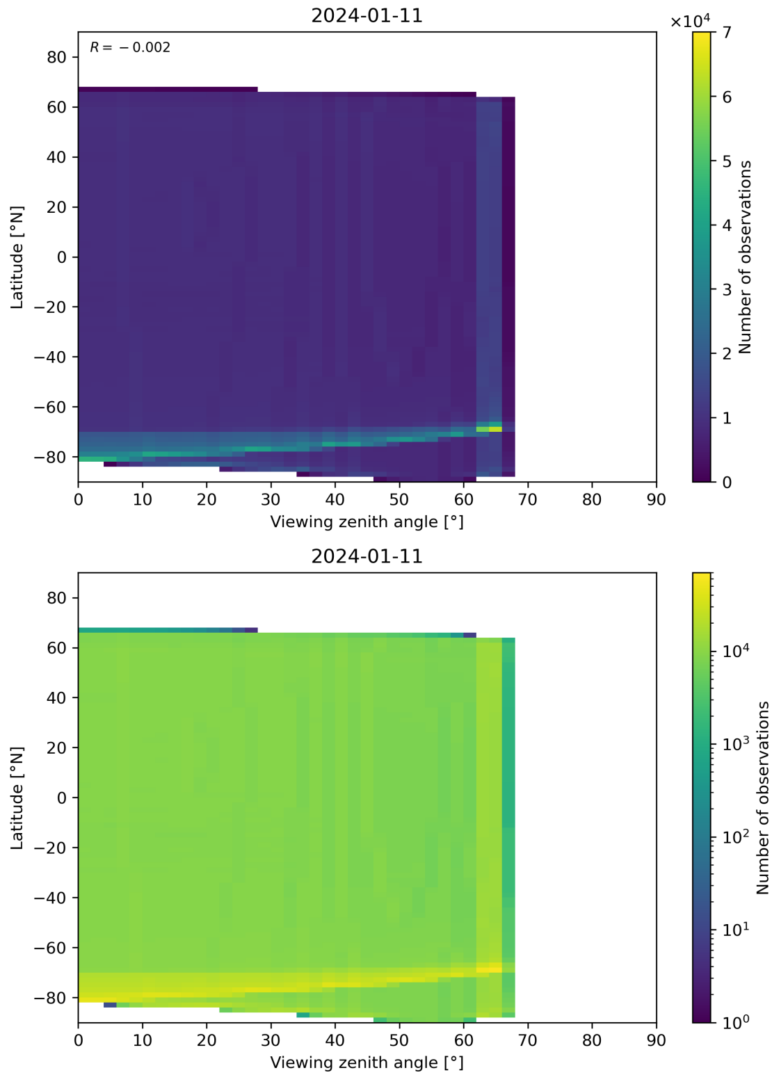
Figure 163: Scatter density plot of “Viewing zenith angle” against “Latitude” for 2024-01-10 to 2024-01-12.
