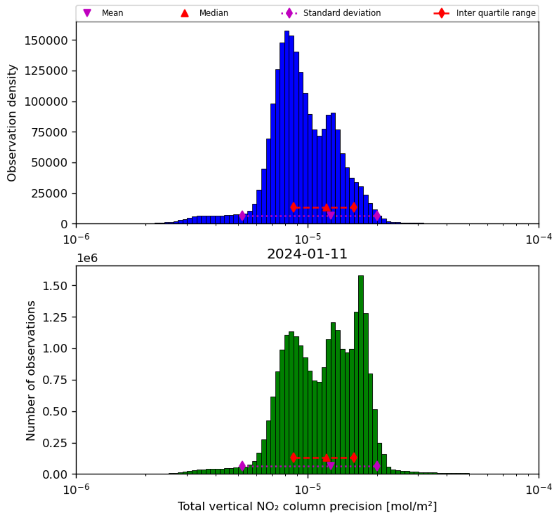
Figure 39: Histogram of “Total vertical NO 2 column precision” for 2024-01-10 to 2024-01-12
