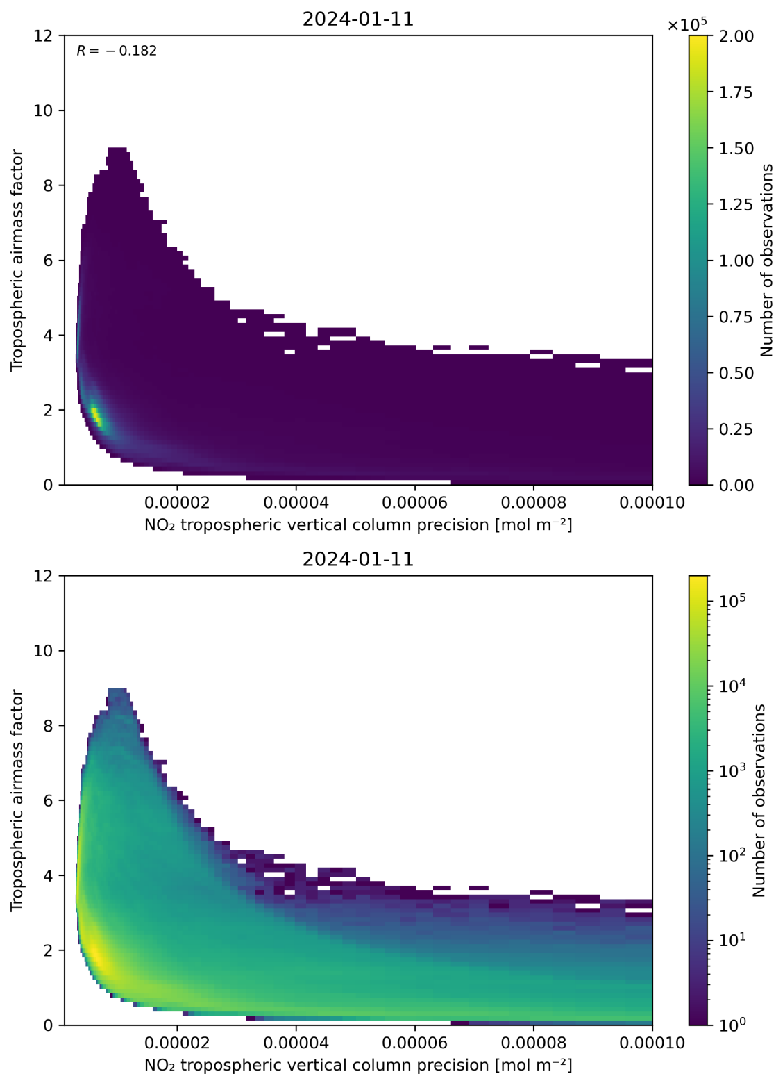
Figure 133: Scatter density plot of “NO 2 tropospheric vertical column precision” against “Tropospheric air mass factor” for 2024-01-10 to 2024-01-12.
