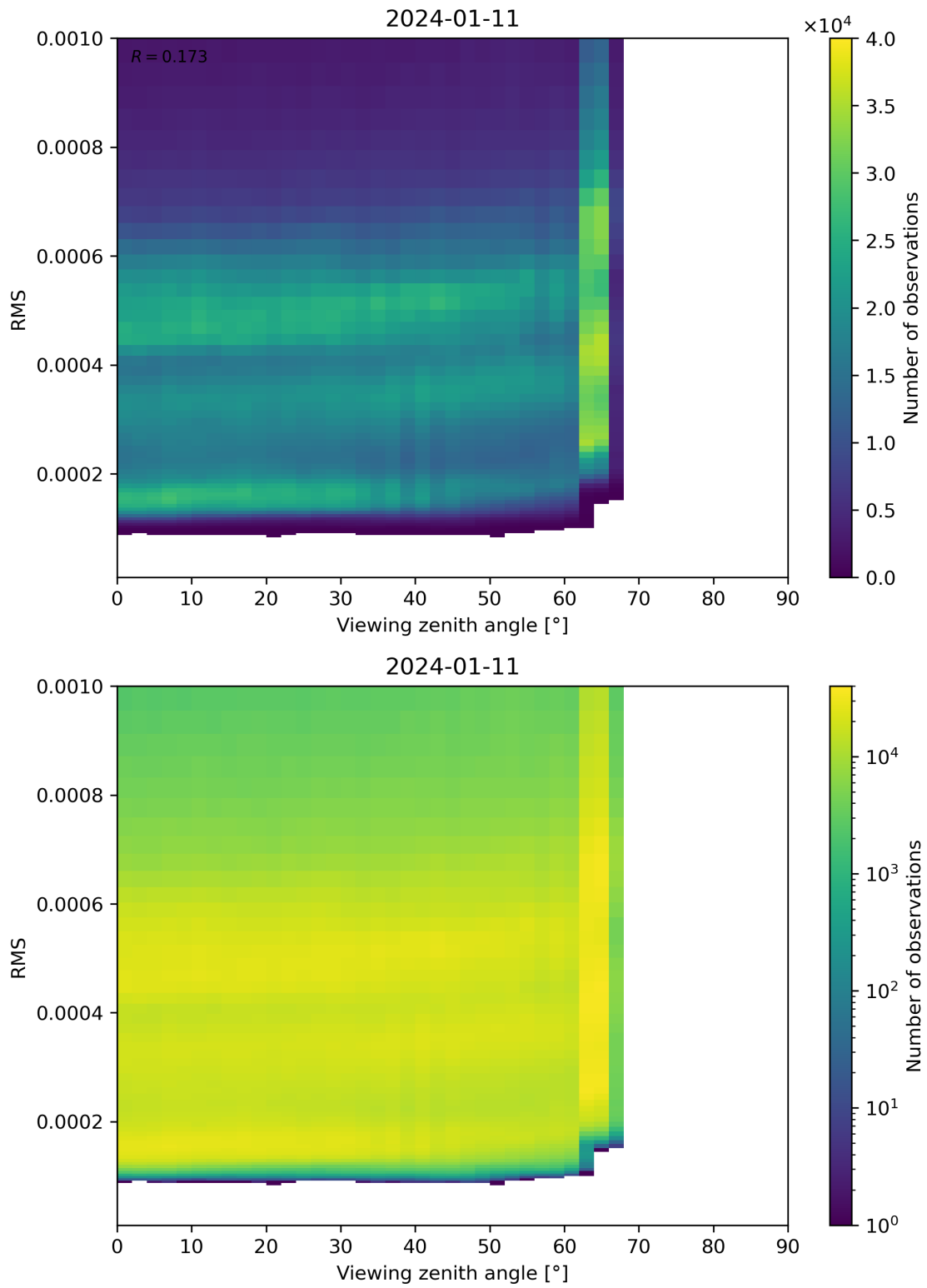
Figure 171: Scatter density plot of “Viewing zenith angle” against “RMS” for 2024-01-10 to 2024-01-12.
