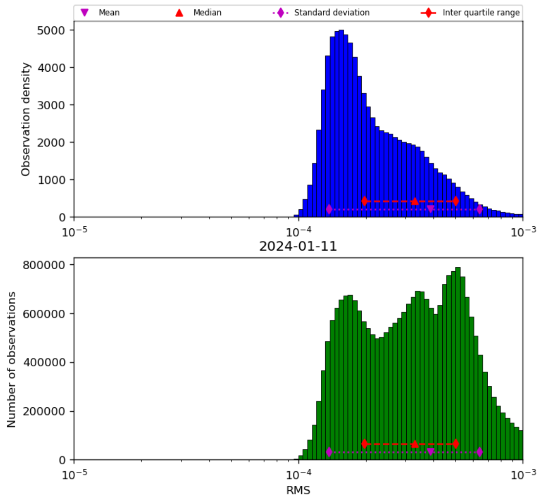
Figure 43: Histogram of “RMS” for 2024-01-10 to 2024-01-12
