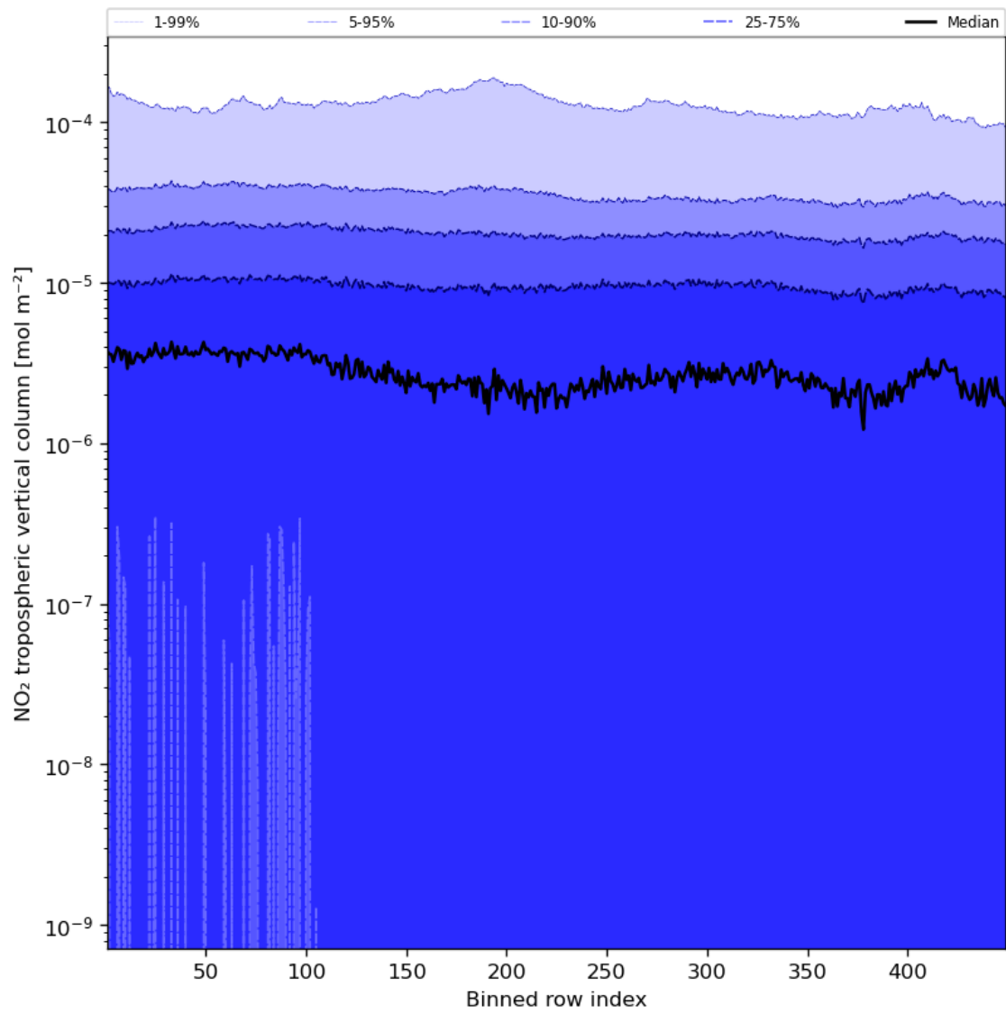
Figure 46: Along track statistics of “NO 2 tropospheric vertical column” for 2024-01-10 to 2024-01-12
