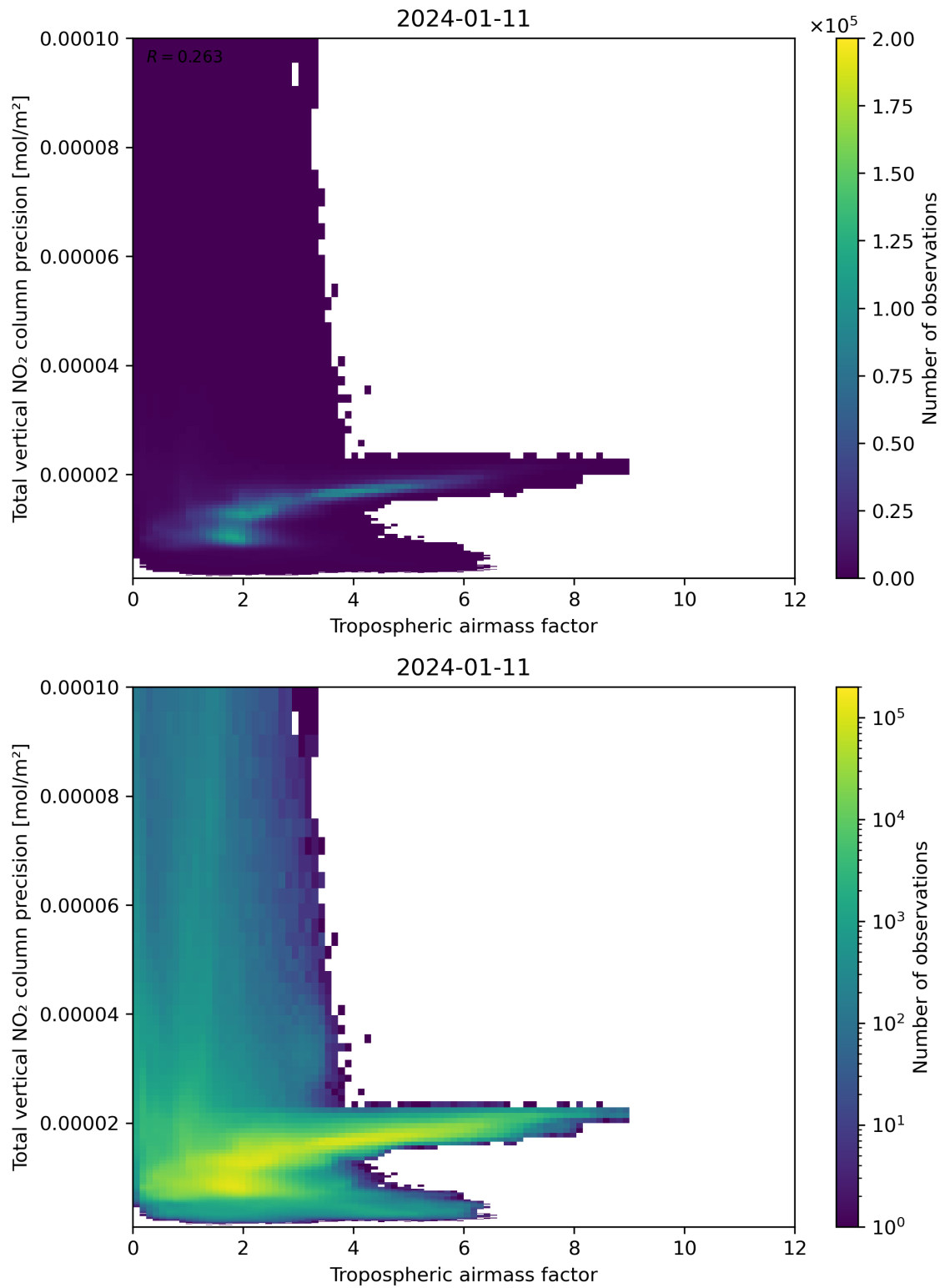
Figure 78: Scatter density plot of “Tropospheric air mass factor” against “Total vertical NO 2 column precision” for 2024-01-10 to 2024-01-12.
