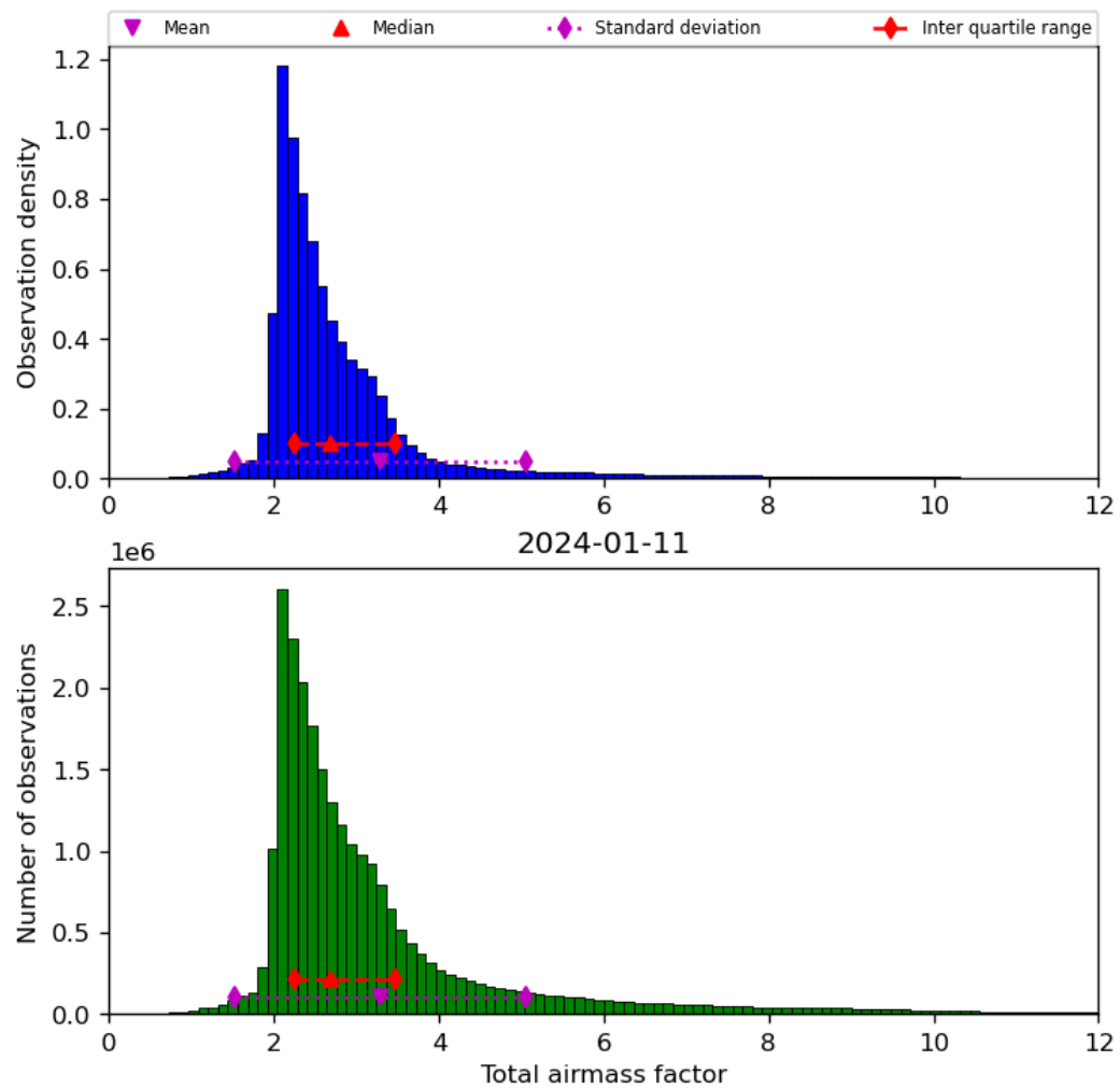
Figure 32: Histogram of “Total airmass factor” for 2024-01-10 to 2024-01-12
