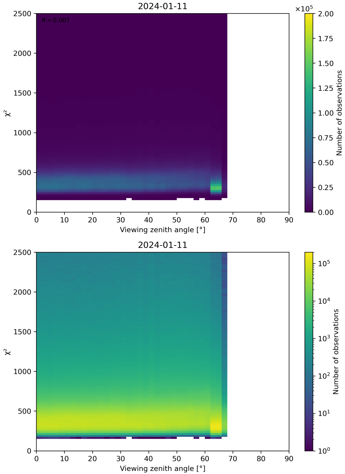
Figure 162: Scatter density plot of “Viewing zenith angle” against “ \chi^2 ” for 2024-01-10 to 2024-01-12.
