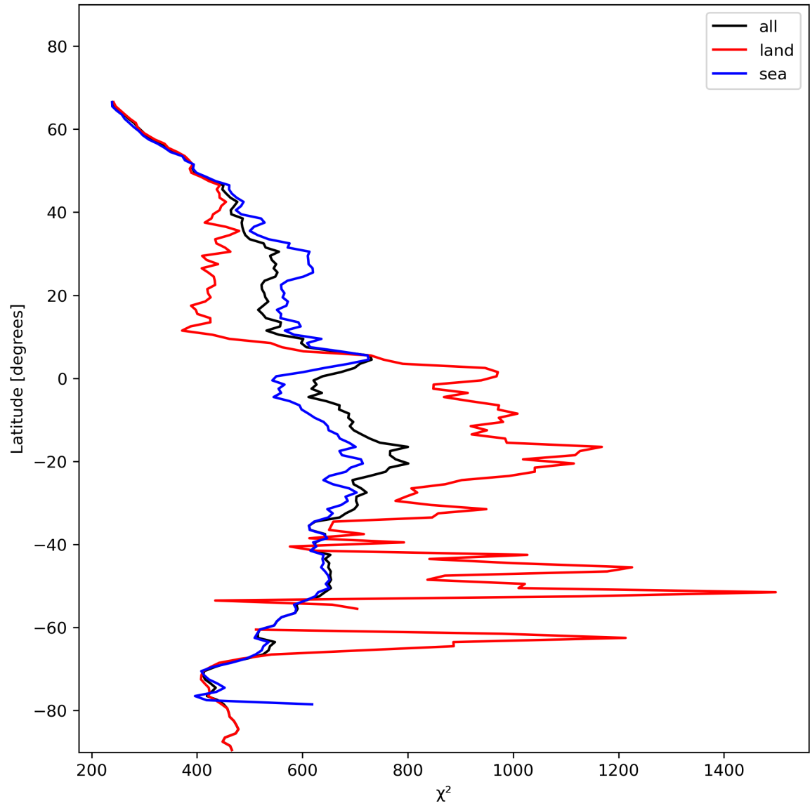
Figure 25: Zonal average of “ \chi^2 ” for 2024-01-10 to 2024-01-12.
