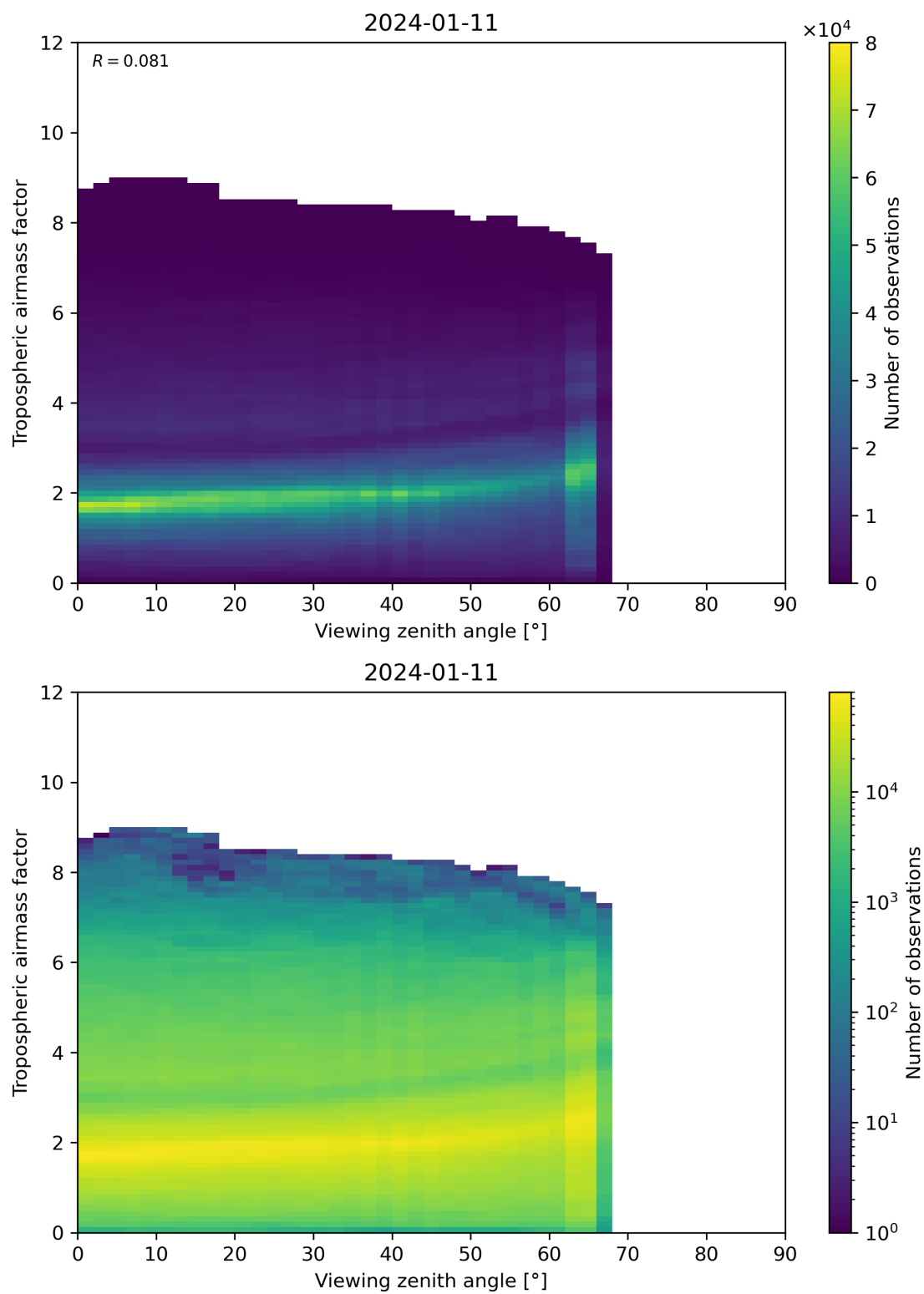
Figure 161: Scatter density plot of “Viewing zenith angle” against “Tropospheric airmass factor” for 2024-01-10 to 2024-01-12.
