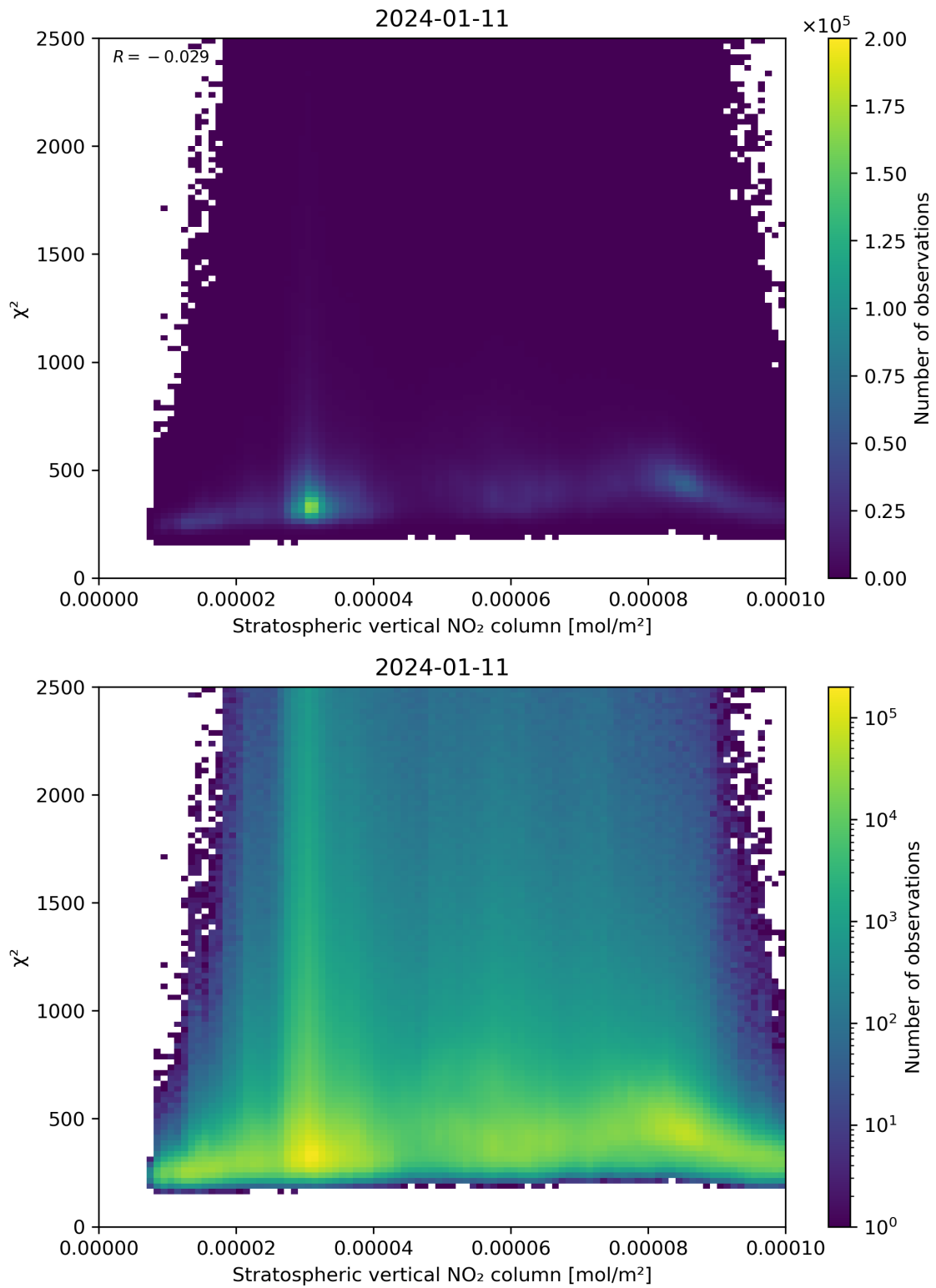
Figure 97: Scatter density plot of “Stratospheric vertical NO 2 column” against “ \chi^2 ” for 2024-01-10 to 2024-01-12.
