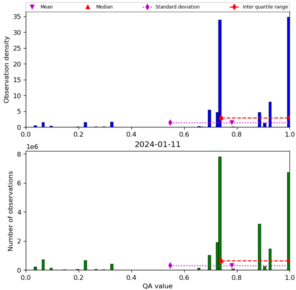
Figure 28: Histogram of “QA value” for 2024-01-10 to 2024-01-12
