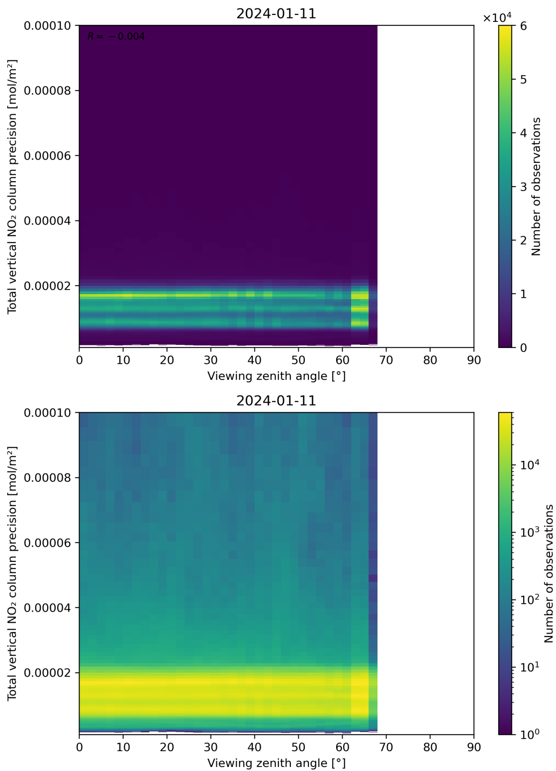
Figure 168: Scatter density plot of “Viewing zenith angle” against “Total vertical NO 2 column precision” for 2024-01-10 to 2024-01-12.
