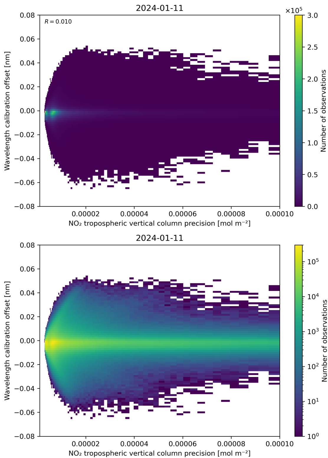
Figure 141: Scatter density plot of “NO 2 tropospheric vertical column precision” against “Wavelength calibration offset” for 2024-01-10 to 2024-01-12.
