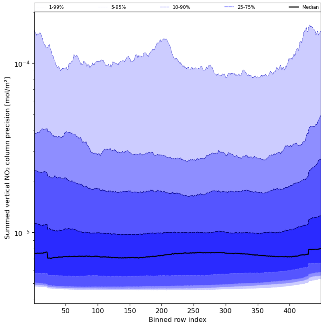
Figure 58: Along track statistics of “Summed vertical NO 2 column precision” for 2024-01-10 to 2024-01-12
