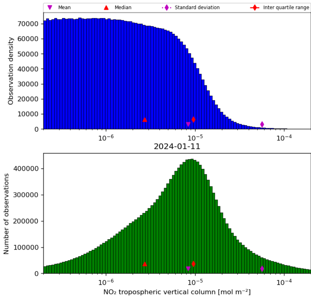
Figure 29: Histogram of “ \text{NO}_2 tropospheric vertical column” for 2024-01-10 to 2024-01-12
