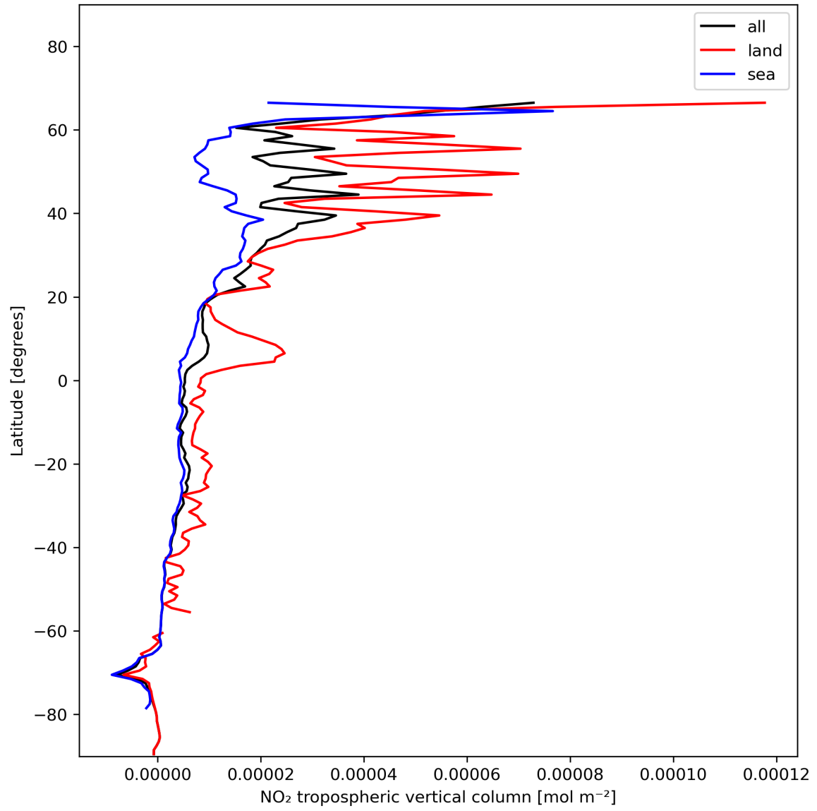
Figure 12: Zonal average of “NO 2 tropospheric vertical column” for 2024-01-10 to 2024-01-12.
