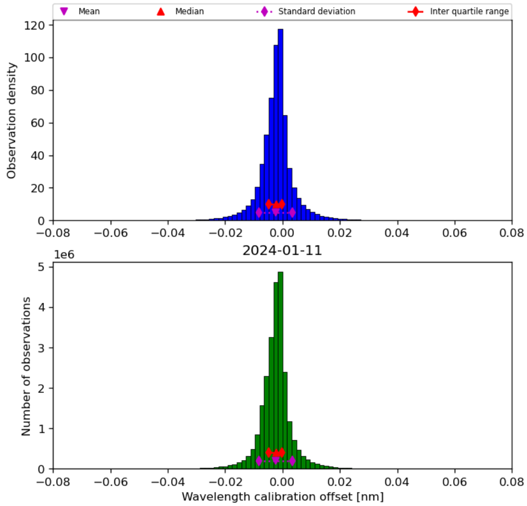
Figure 35: Histogram of “Wavelength calibration offset” for 2024-01-10 to 2024-01-12
