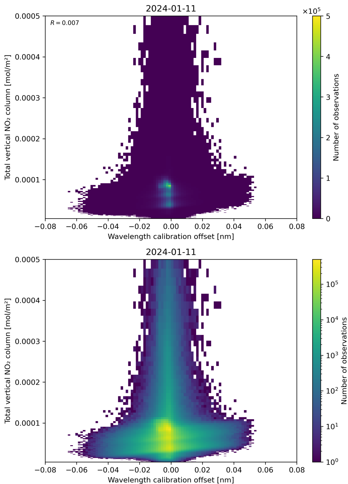
Figure 179: Scatter density plot of “Wavelength calibration offset” against “Total vertical NO 2 column” for 2024-01-10 to 2024-01-12.
