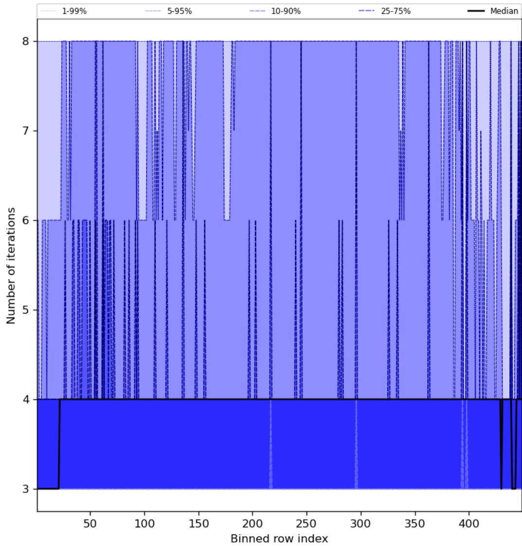
Figure 51: Along track statistics of “Number of iterations” for 2024-01-10 to 2024-01-12
