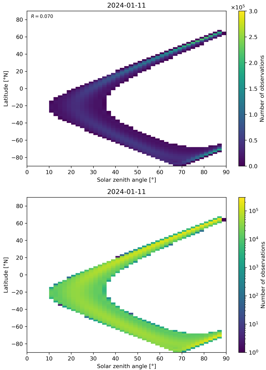
Figure 149: Scatter density plot of “Solar zenith angle” against “Latitude” for 2024-01-10 to 2024-01-12.
