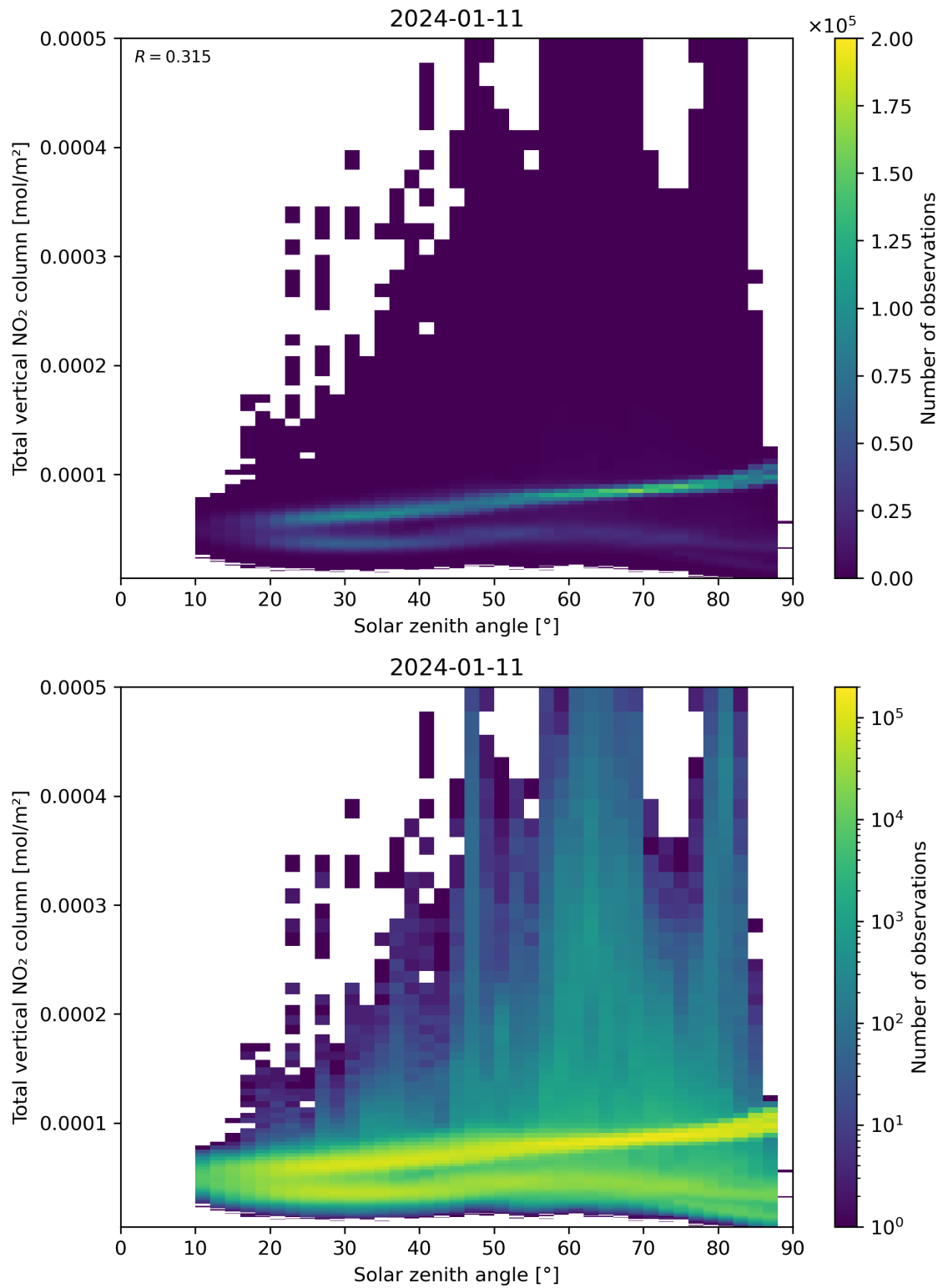
Figure 153: Scatter density plot of “Solar zenith angle” against “Total vertical NO 2 column” for 2024-01-10 to 2024-01-12.
