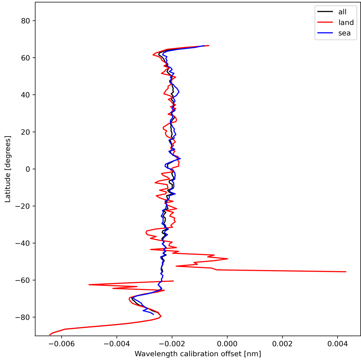
Figure 18: Zonal average of “Wavelength calibration offset” for 2024-01-10 to 2024-01-12.
