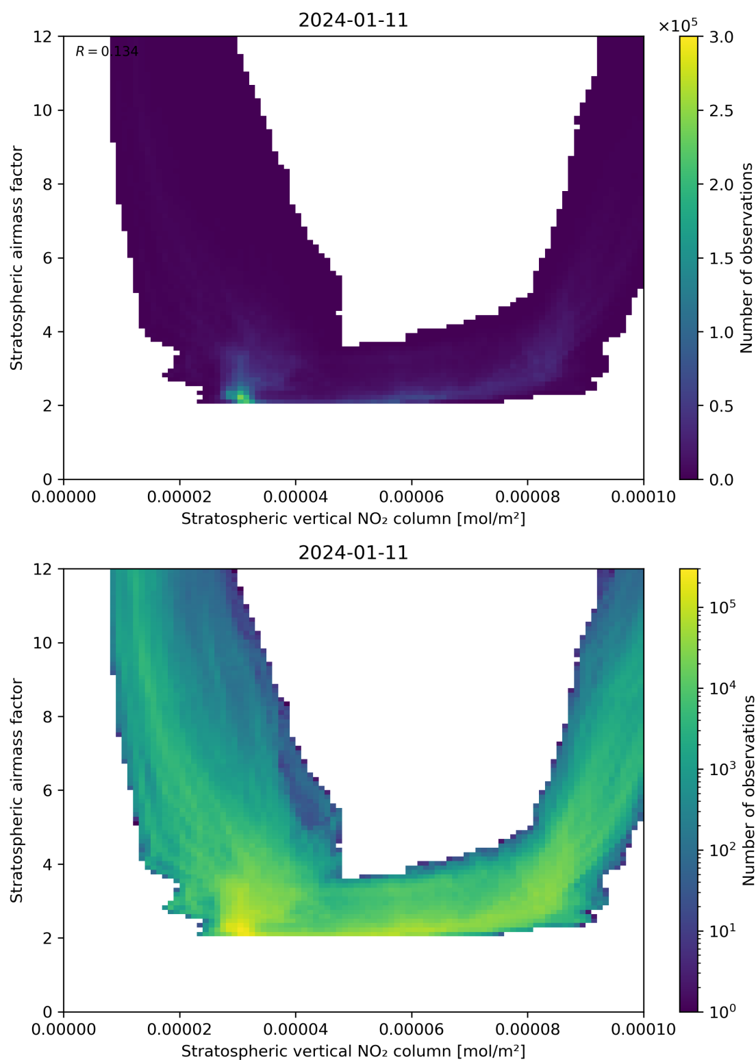
Figure 96: Scatter density plot of “Stratospheric vertical NO 2 column” against “Stratospheric airmass factor” for 2024-01-10 to 2024-01-12.
