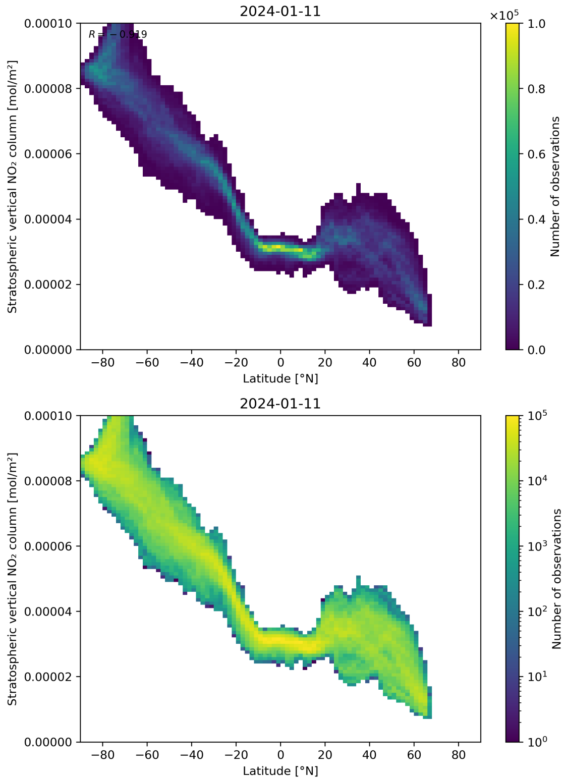
Figure 87: Scatter density plot of “Latitude” against “Stratospheric vertical NO 2 column” for 2024-01-10 to 2024-01-12.
