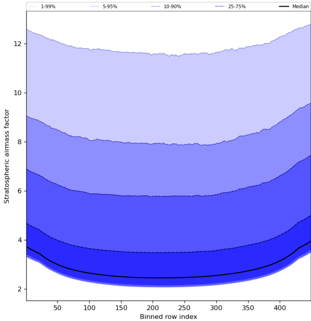
Figure 61: Along track statistics of “Stratospheric airmass factor” for 2024-01-10 to 2024-01-12
