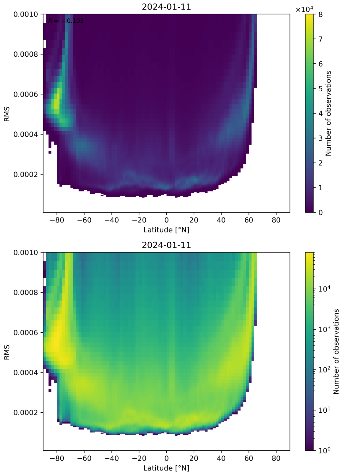
Figure 94: Scatter density plot of “Latitude” against “RMS” for 2024-01-10 to 2024-01-12.
