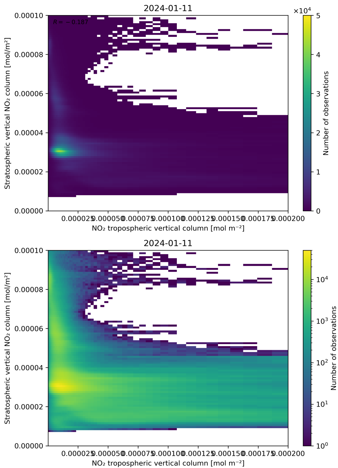
Figure 125: Scatter density plot of “NO 2 tropospheric vertical column” against “Stratospheric vertical NO 2 column” for 2024-01-10 to 2024-01-12.
