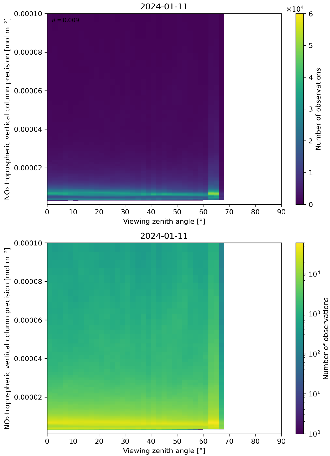
Figure 170: Scatter density plot of “Viewing zenith angle” against “NO 2 tropospheric vertical column precision” for 2024-01-10 to 2024-01-12.
