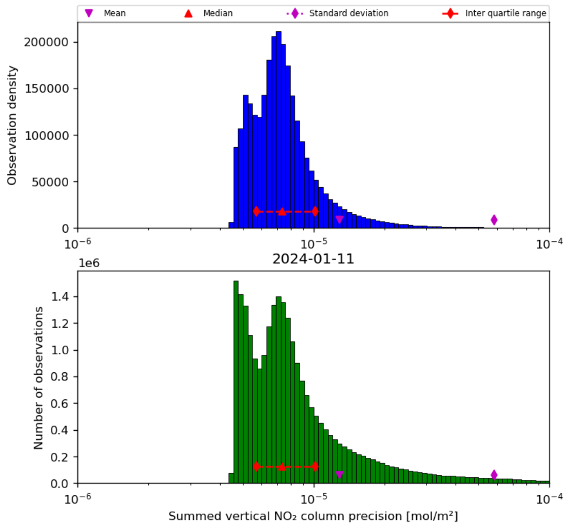
Figure 41: Histogram of “Summed vertical NO 2 column precision” for 2024-01-10 to 2024-01-12
