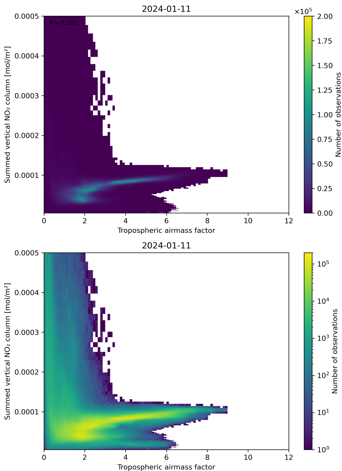
Figure 75: Scatter density plot of “Tropospheric airmass factor” against “Summed vertical NO 2 column” for 2024-01-10 to 2024-01-12.
