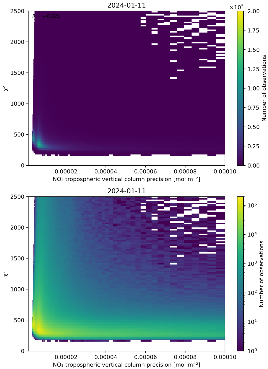
Figure 134: Scatter density plot of “NO 2 tropospheric vertical column precision” against “ \chi^2 ” for 2024-01-10 to 2024-01-12.
