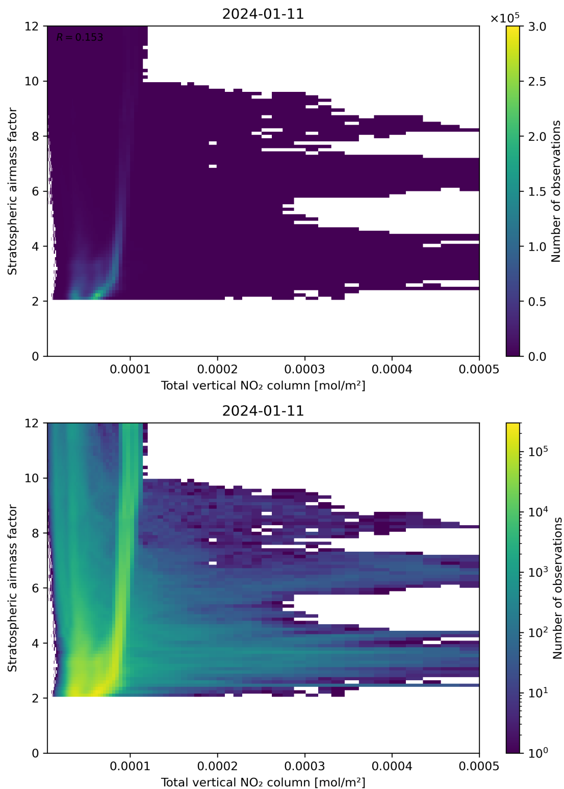
Figure 110: Scatter density plot of “Total vertical NO 2 column” against “Stratospheric air mass factor” for 2024-01-10 to 2024-01-12.
