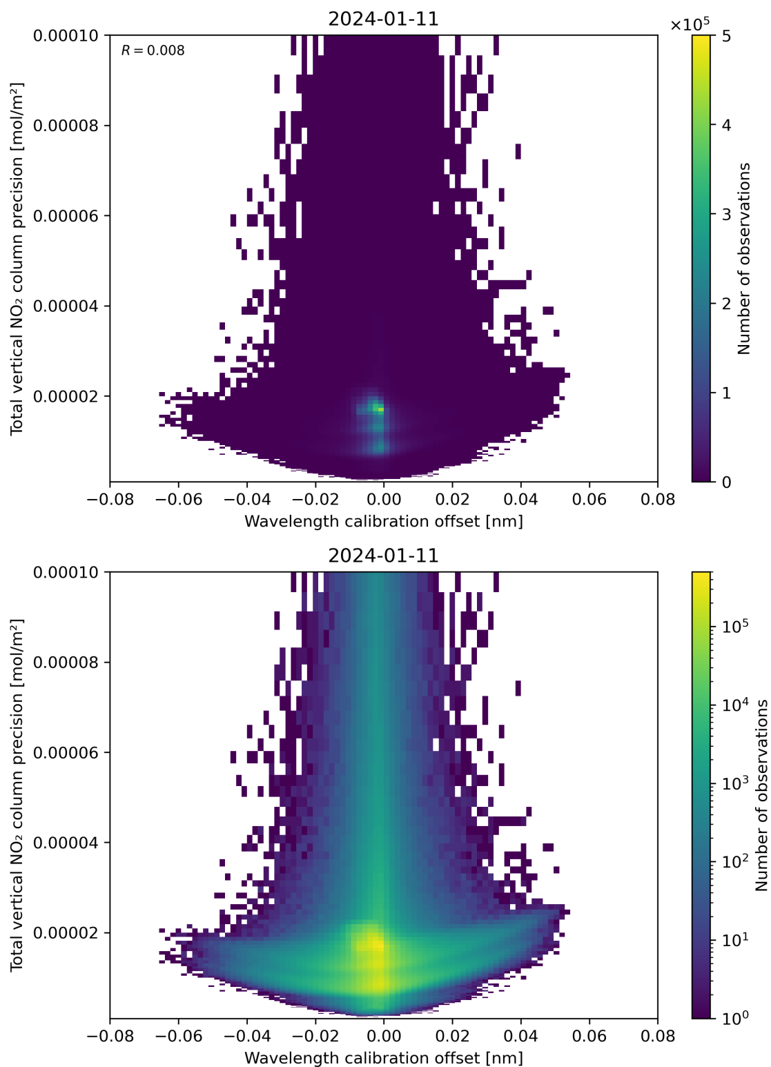
Figure 180: Scatter density plot of “Wavelength calibration offset” against “Total vertical NO 2 column precision” for 2024-01-10 to 2024-01-12.
