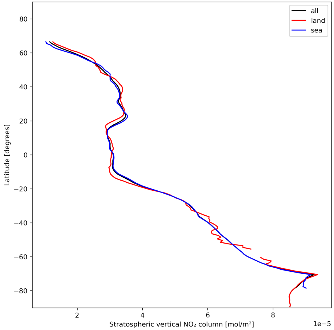
Figure 19: Zonal average of “Stratospheric vertical NO 2 column” for 2024-01-10 to 2024-01-12.
