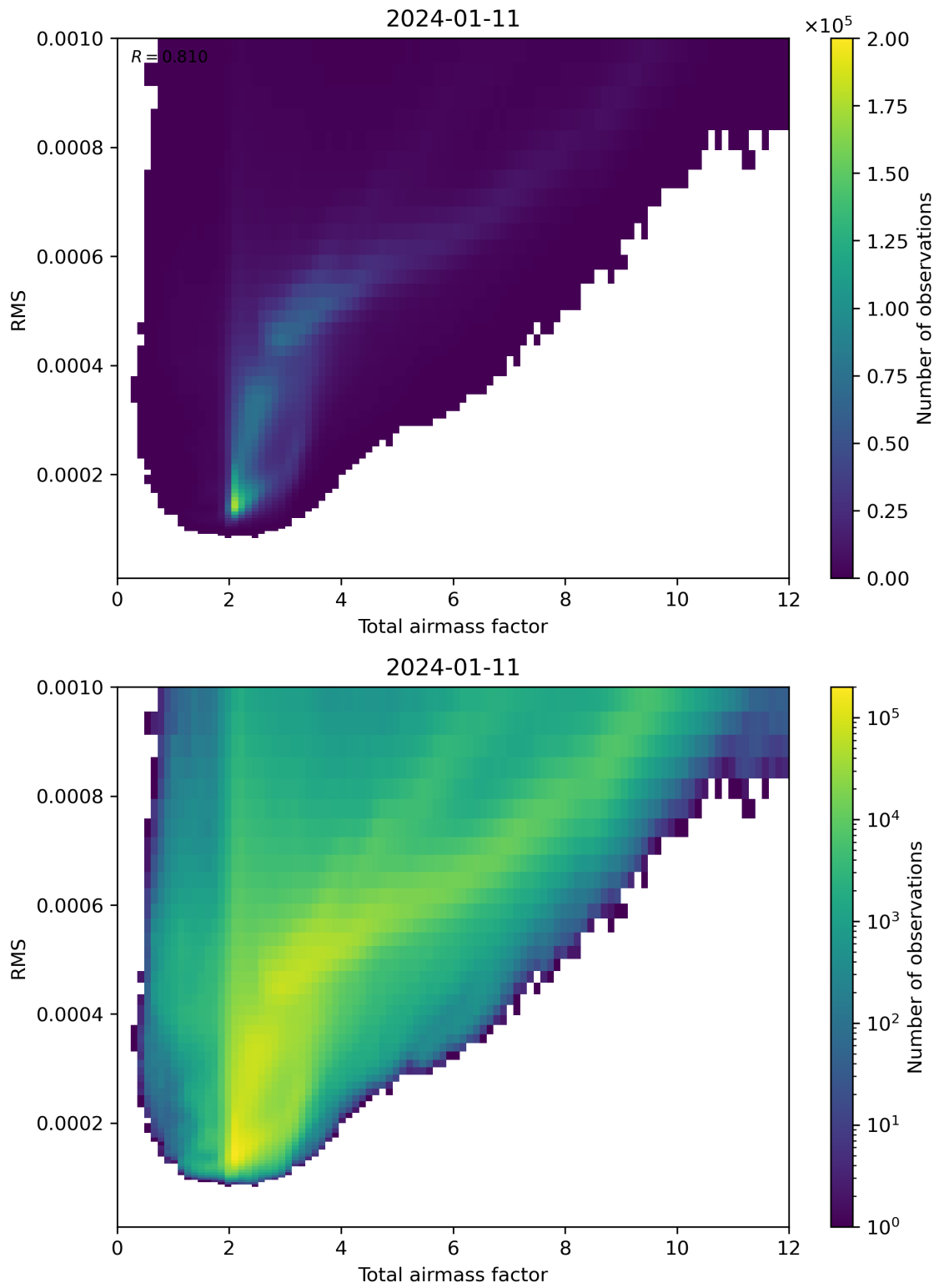
Figure 69: Scatter density plot of “Total airmass factor” against “RMS” for 2024-01-10 to 2024-01-12.
