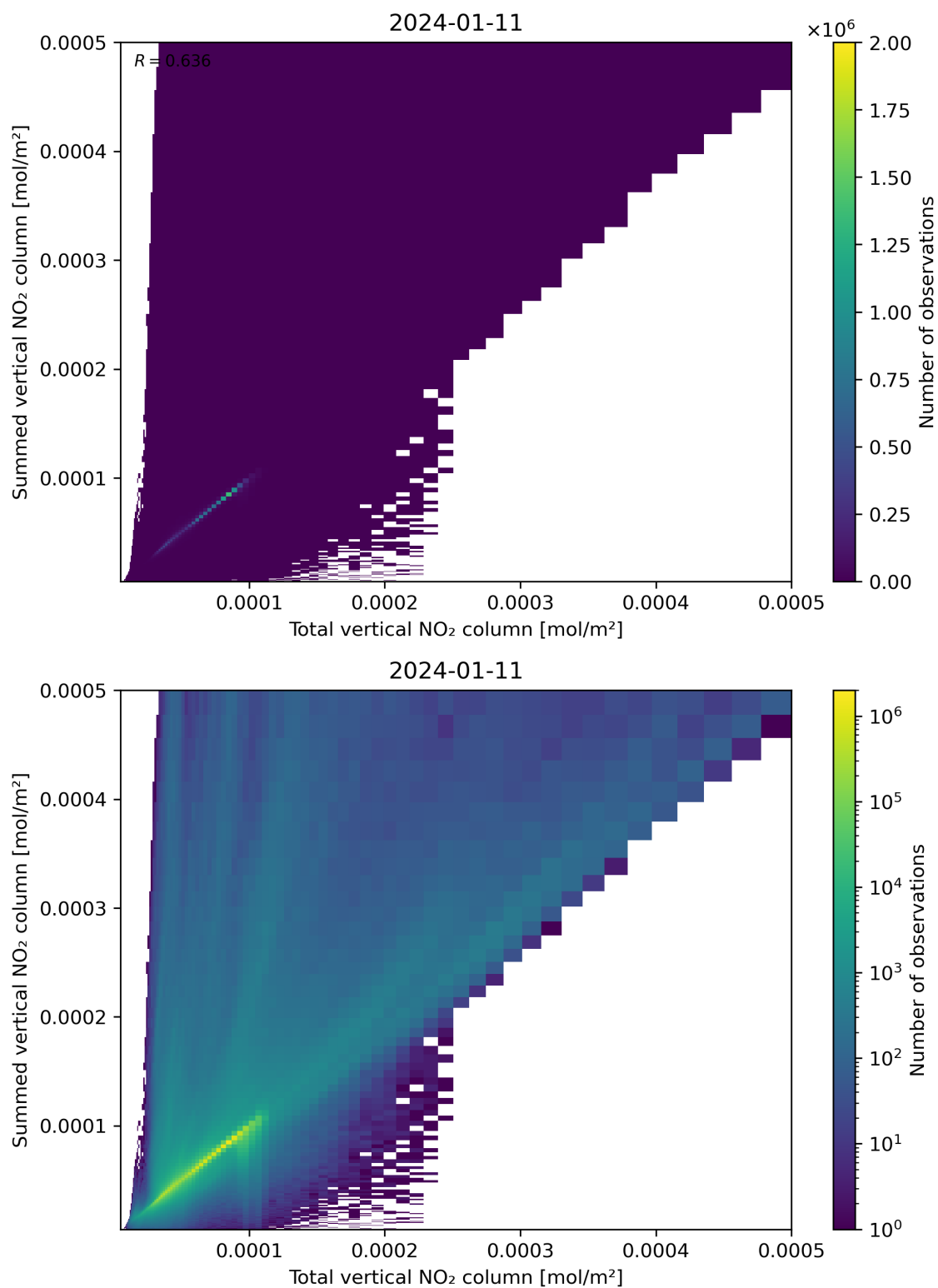
Figure 112: Scatter density plot of “Total vertical NO 2 column” against “Summed vertical NO 2 column” for 2024-01-10 to 2024-01-12.
