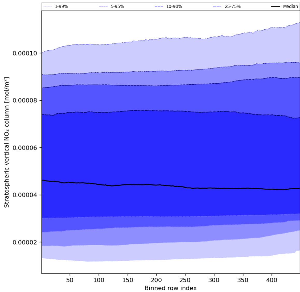
Figure 53: Along track statistics of “Stratospheric vertical NO 2 column” for 2024-01-10 to 2024-01-12
