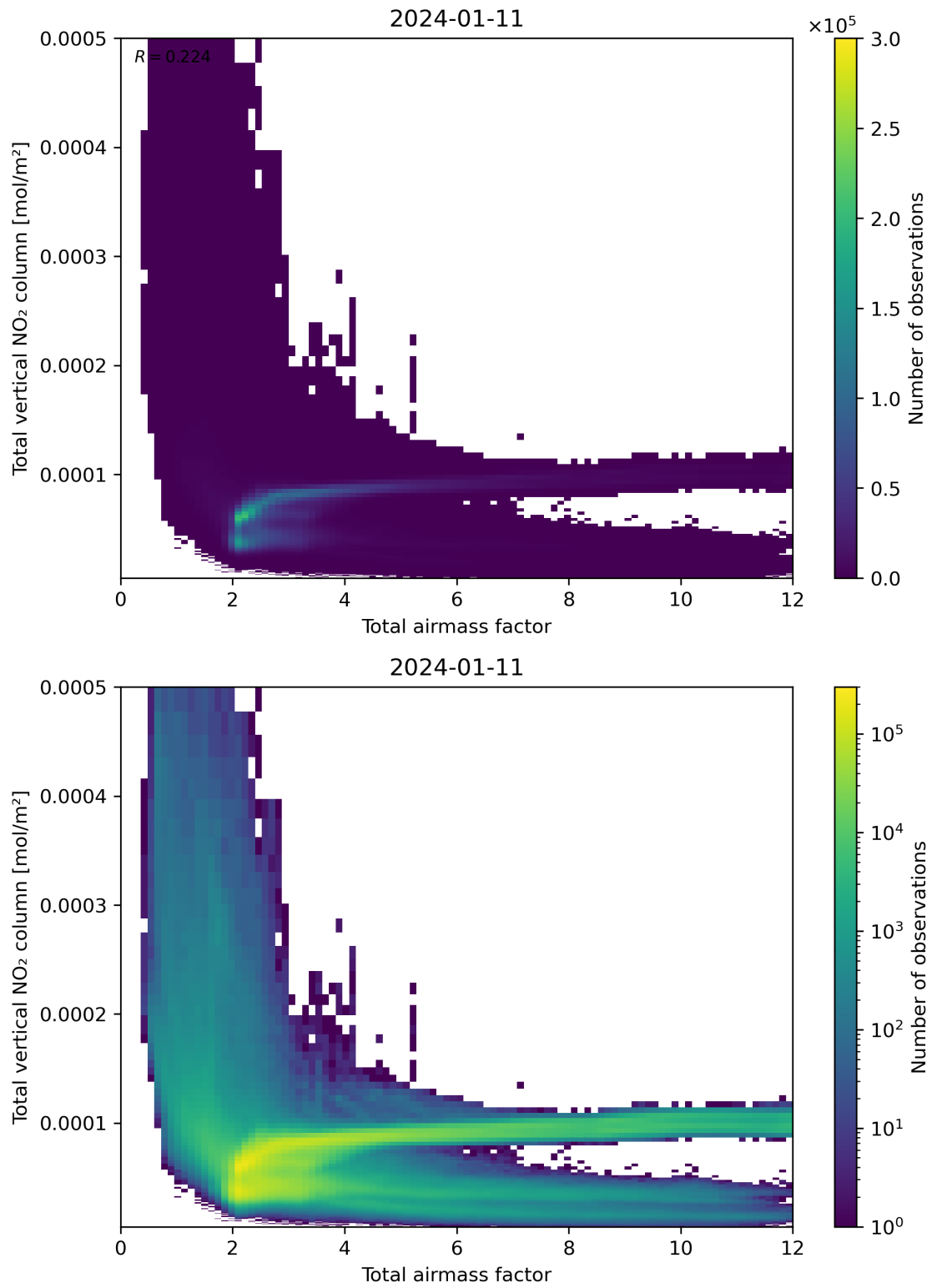
Figure 67: Scatter density plot of “Total airmass factor” against “Total vertical NO 2 column” for 2024-01-10 to 2024-01-12.
