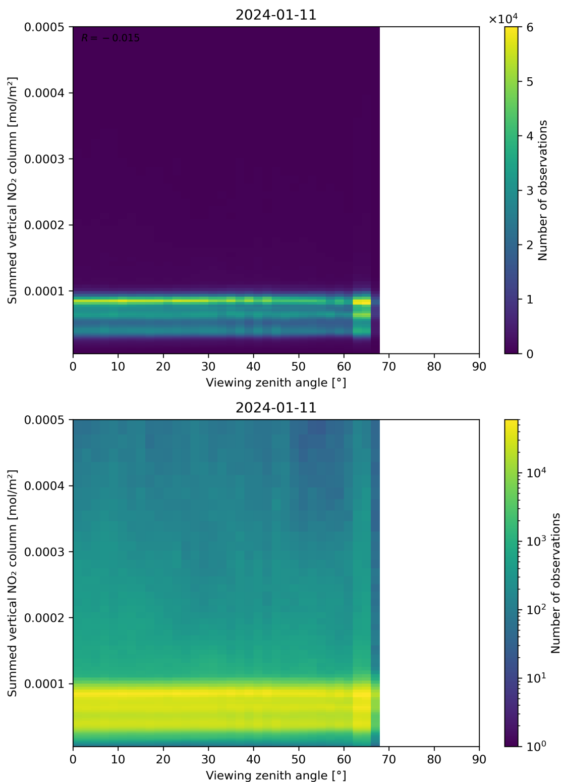
Figure 165: Scatter density plot of “Viewing zenith angle” against “Summed vertical NO 2 column” for 2024-01-10 to 2024-01-12.
