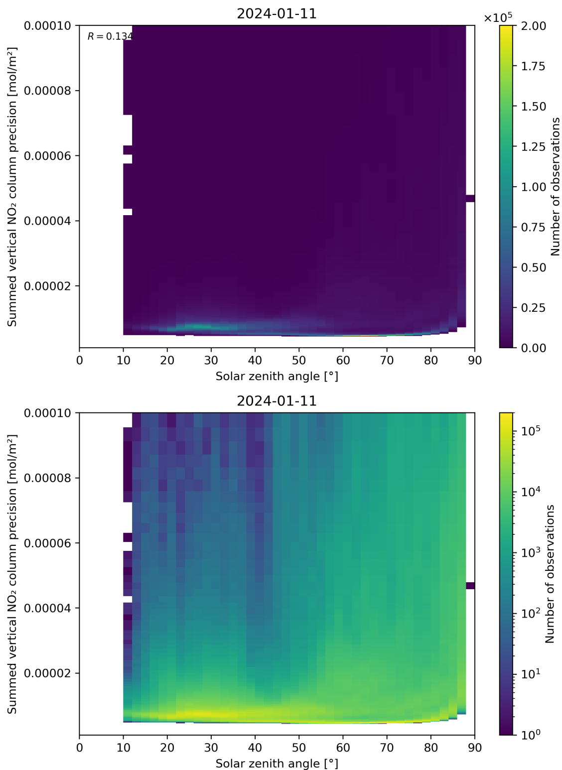
Figure 152: Scatter density plot of “Solar zenith angle” against “Summed vertical NO 2 column precision” for 2024-01-10 to 2024-01-12.
