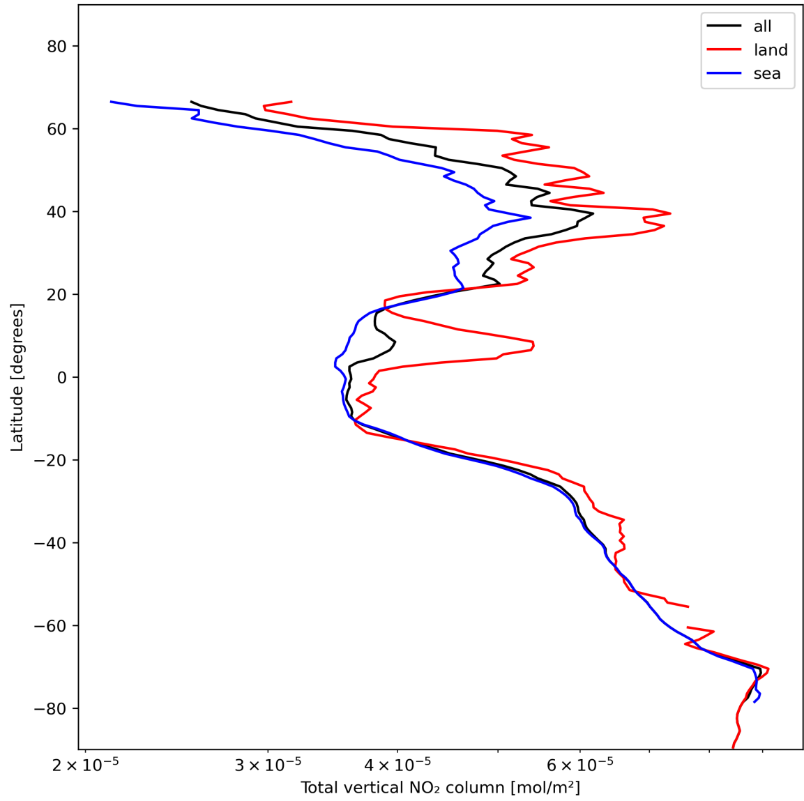
Figure 21: Zonal average of “Total vertical NO 2 column” for 2024-01-10 to 2024-01-12.
