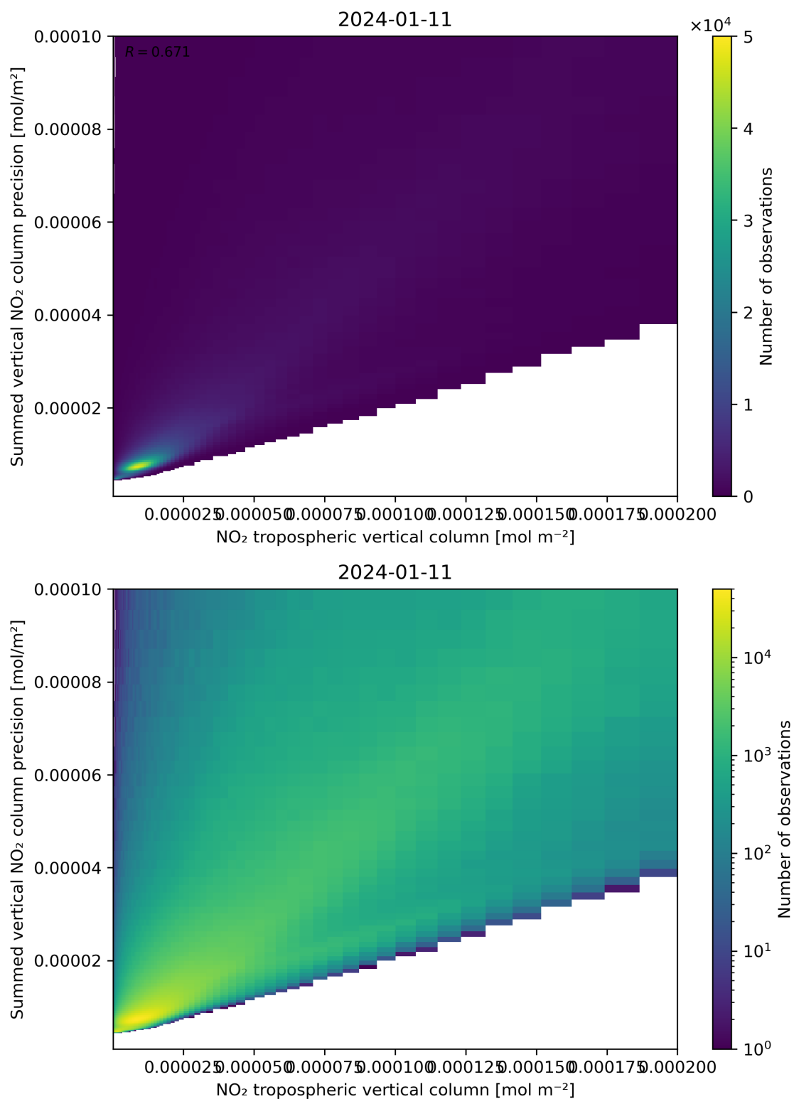
Figure 127: Scatter density plot of “NO 2 tropospheric vertical column” against “Summed vertical NO 2 column precision” for 2024-01-10 to 2024-01-12.
