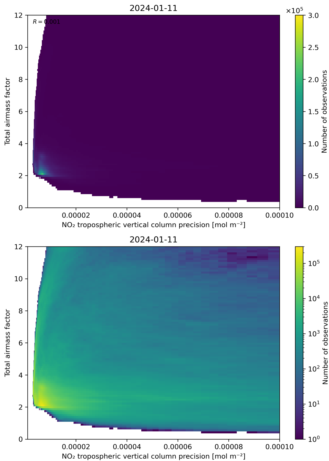
Figure 132: Scatter density plot of “NO 2 tropospheric vertical column precision” against “Total airmass factor” for 2024-01-10 to 2024-01-12.
