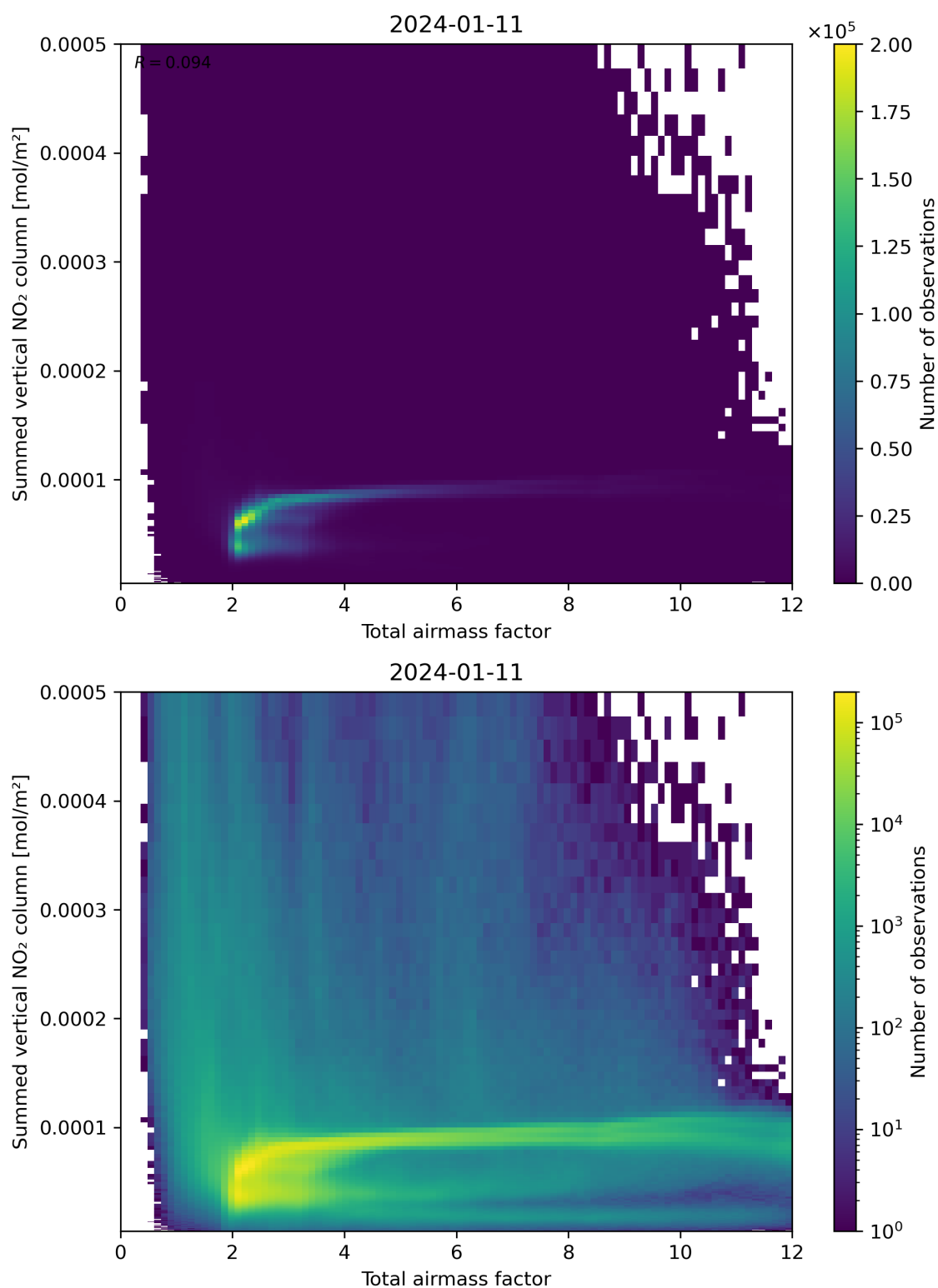
Figure 65: Scatter density plot of “Total airmass factor” against “Summed vertical NO 2 column” for 2024-01-10 to 2024-01-12.
