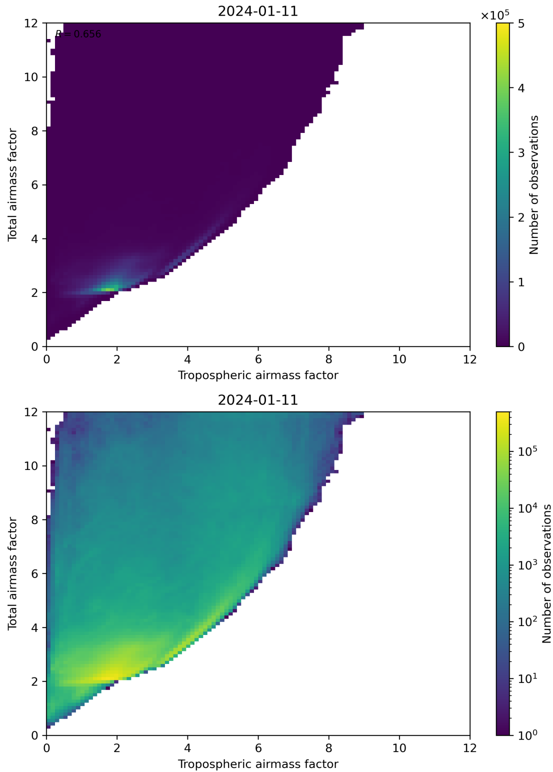
Figure 72: Scatter density plot of “Tropospheric airmass factor” against “Total airmass factor” for 2024-01-10 to 2024-01-12.
