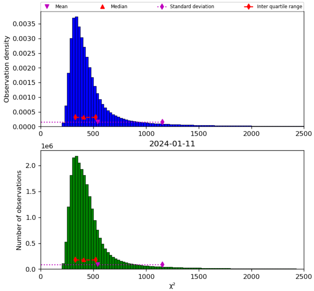
Figure 42: Histogram of “ \chi^2 ” for 2024-01-10 to 2024-01-12
