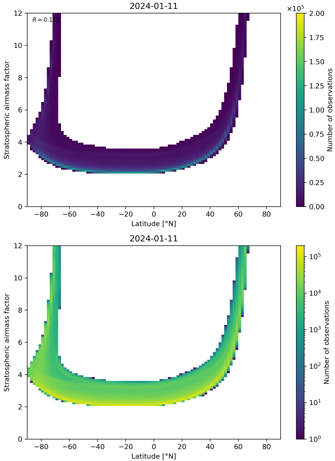
Figure 83: Scatter density plot of “Latitude” against “Stratospheric airmass factor” for 2024-01-10 to 2024-01-12.
