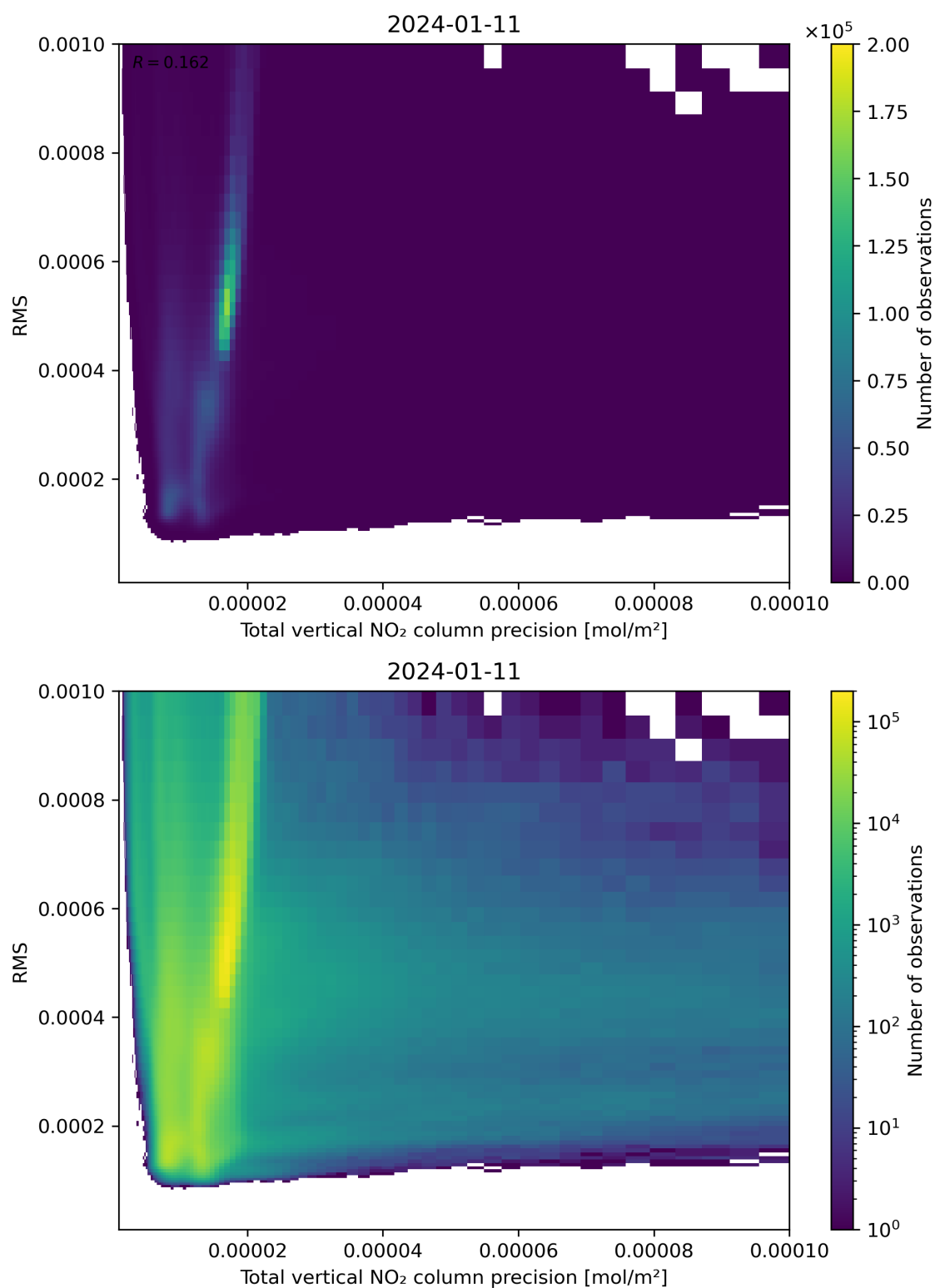
Figure 119: Scatter density plot of “Total vertical NO 2 column precision” against “RMS” for 2024-01-10 to 2024-01-12.
