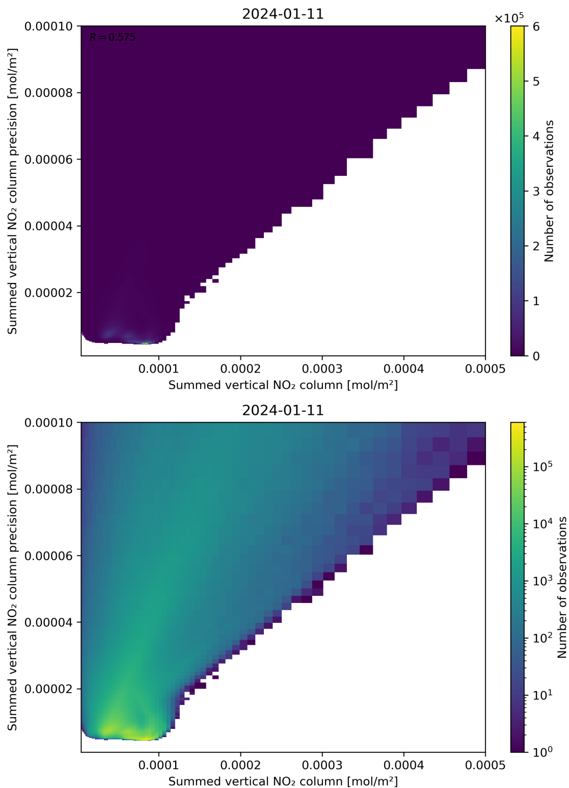
Figure 105: Scatter density plot of “Summed vertical NO 2 column” against “Summed vertical NO 2 column precision” for 2024-01-10 to 2024-01-12.
