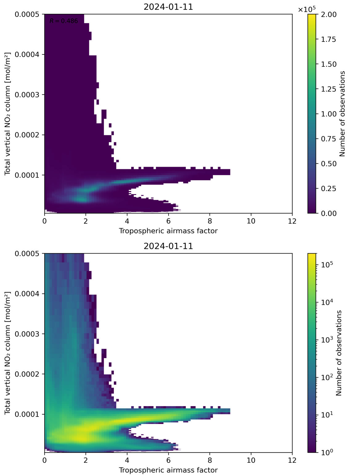
Figure 77: Scatter density plot of “Tropospheric airmass factor” against “Total vertical NO 2 column” for 2024-01-10 to 2024-01-12.
