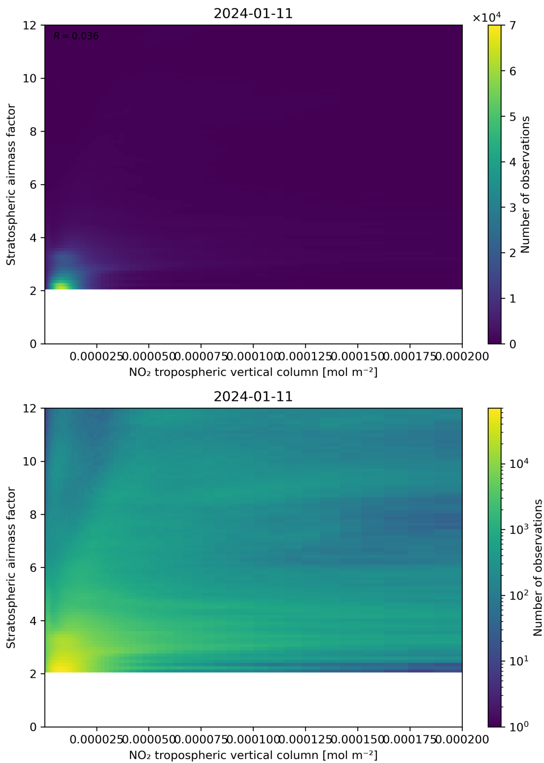
Figure 121: Scatter density plot of “NO 2 tropospheric vertical column” against “Stratospheric airmass factor” for 2024-01-10 to 2024-01-12.
