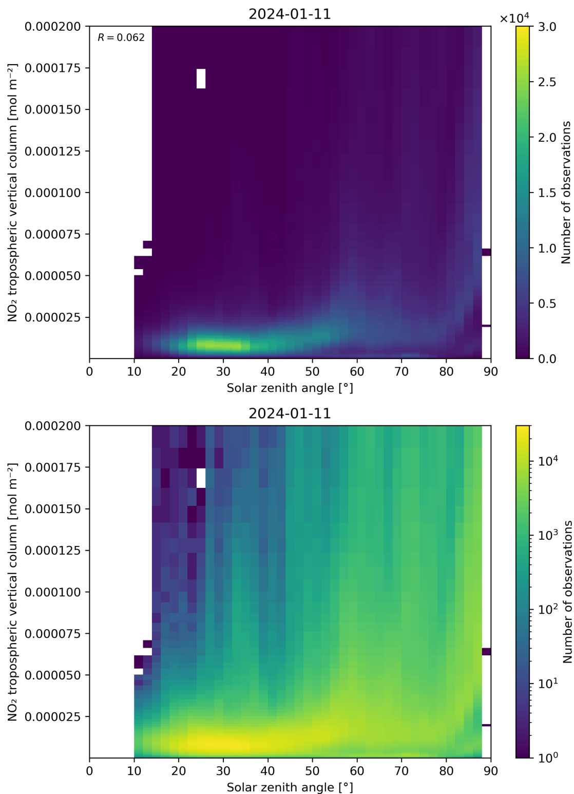
Figure 155: Scatter density plot of “Solar zenith angle” against “NO 2 tropospheric vertical column” for 2024-01-10 to 2024-01-12.
