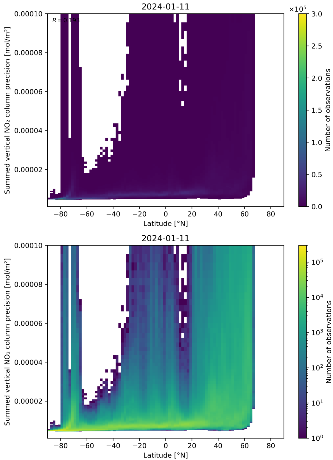
Figure 89: Scatter density plot of “Latitude” against “Summed vertical NO 2 column precision” for 2024-01-10 to 2024-01-12.
