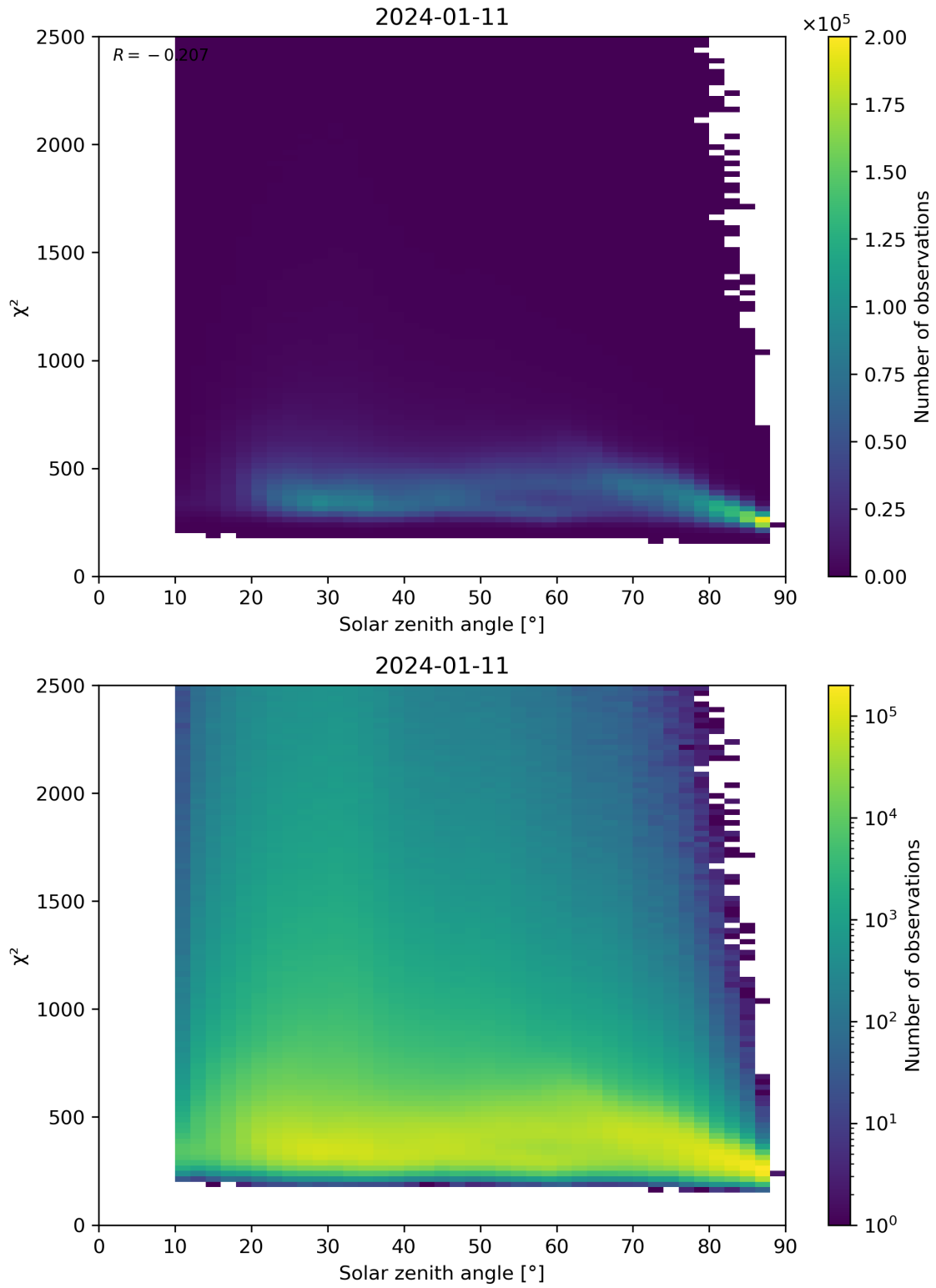
Figure 148: Scatter density plot of “Solar zenith angle” against “ \chi^2 ” for 2024-01-10 to 2024-01-12.
