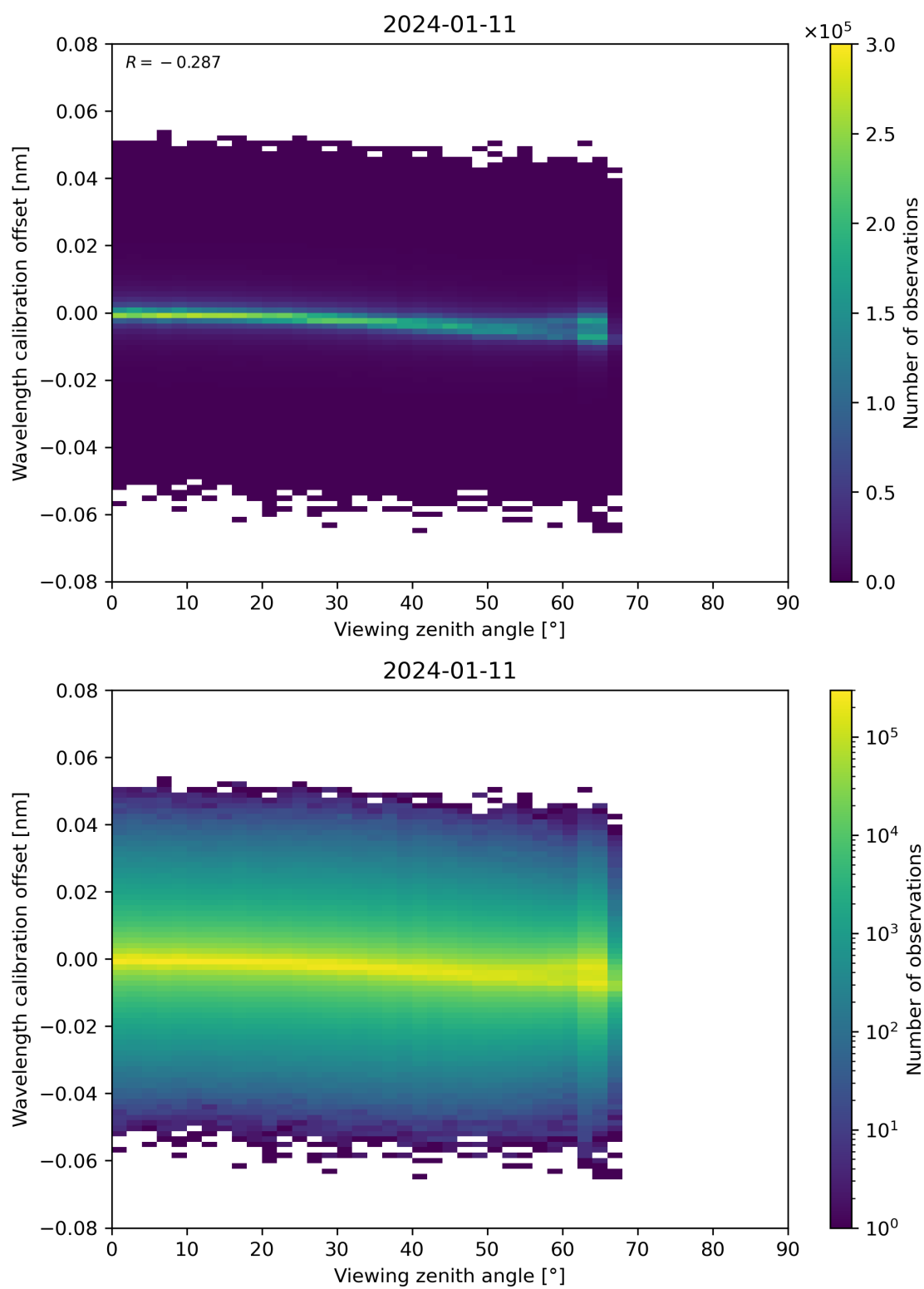
Figure 173: Scatter density plot of “Viewing zenith angle” against “Wavelength calibration offset” for 2024-01-10 to 2024-01-12.
