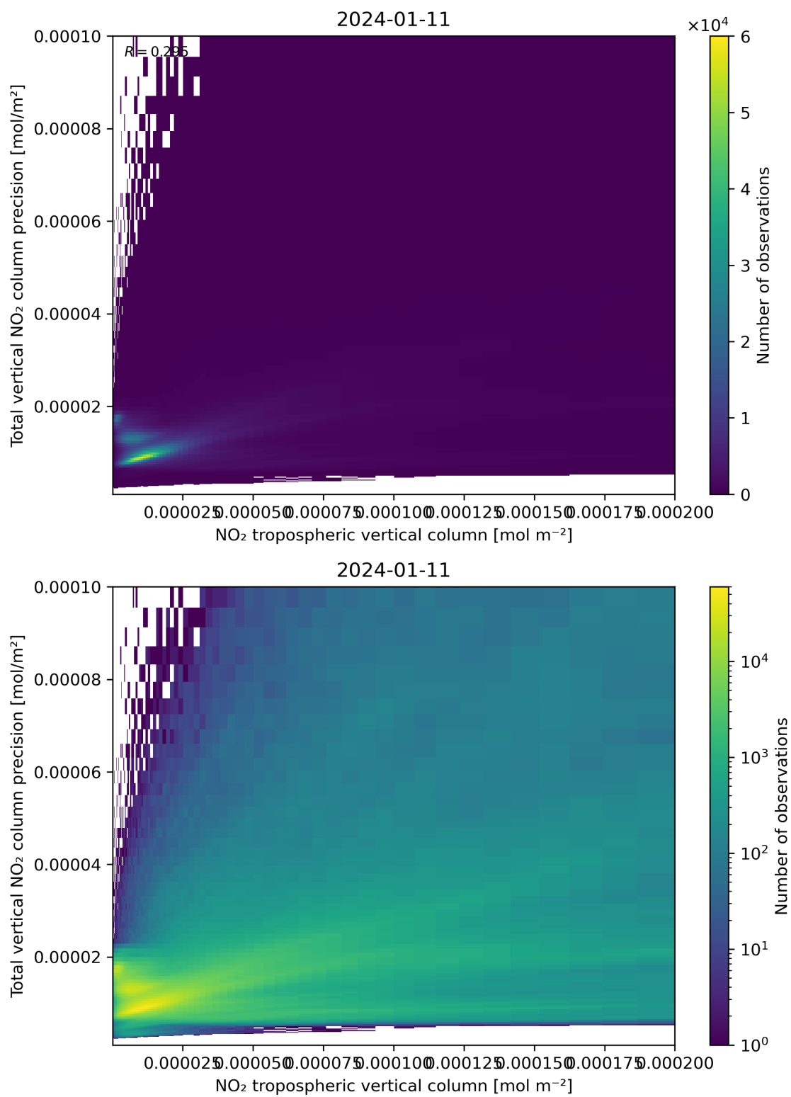
Figure 129: Scatter density plot of “NO 2 tropospheric vertical column” against “Total vertical NO 2 column precision” for 2024-01-10 to 2024-01-12.
