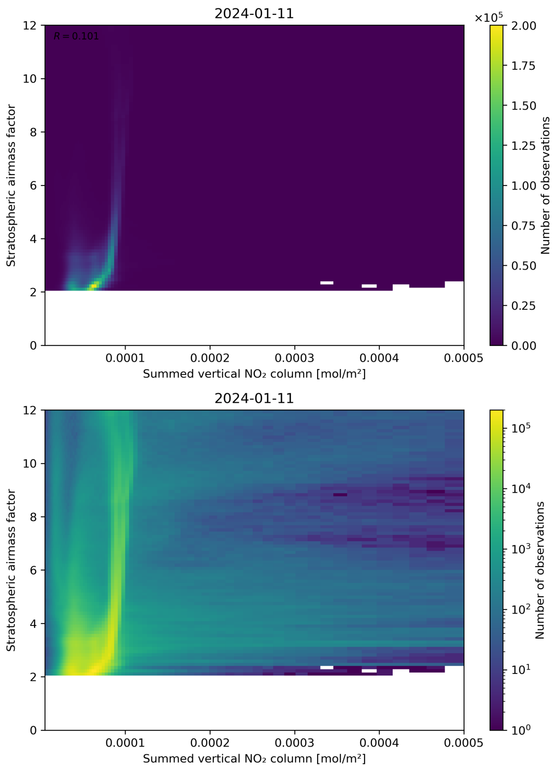
Figure 103: Scatter density plot of “Summed vertical NO 2 column” against “Stratospheric airmass factor” for 2024-01-10 to 2024-01-12.
