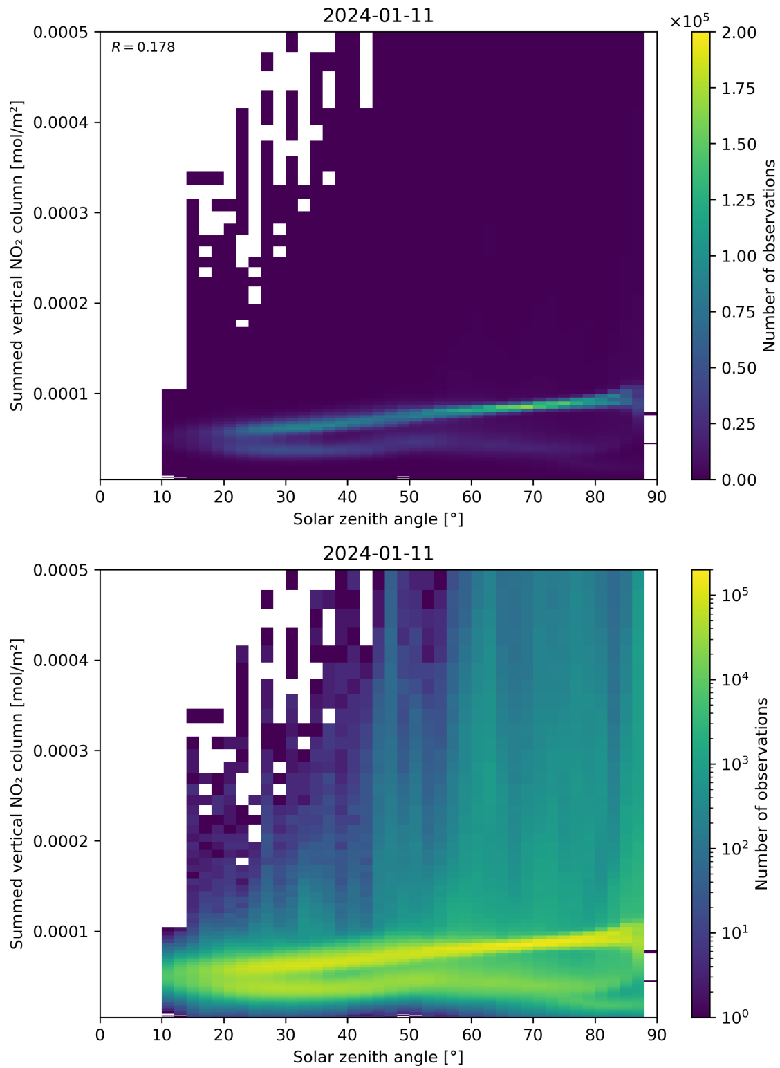
Figure 151: Scatter density plot of “Solar zenith angle” against “Summed vertical NO 2 column” for 2024-01-10 to 2024-01-12.
