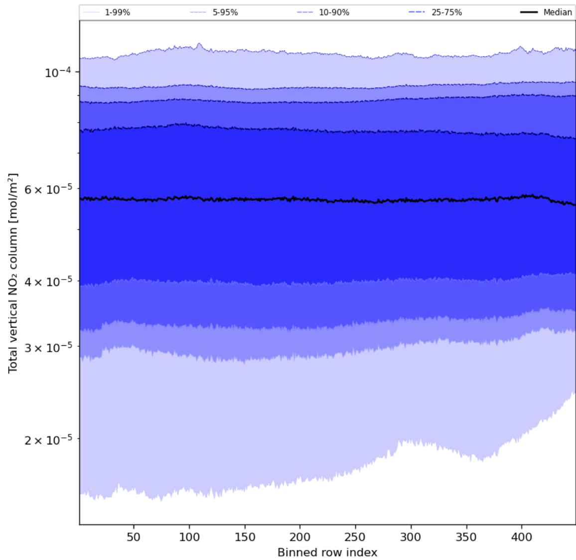
Figure 55: Along track statistics of “Total vertical NO 2 column” for 2024-01-10 to 2024-01-12
