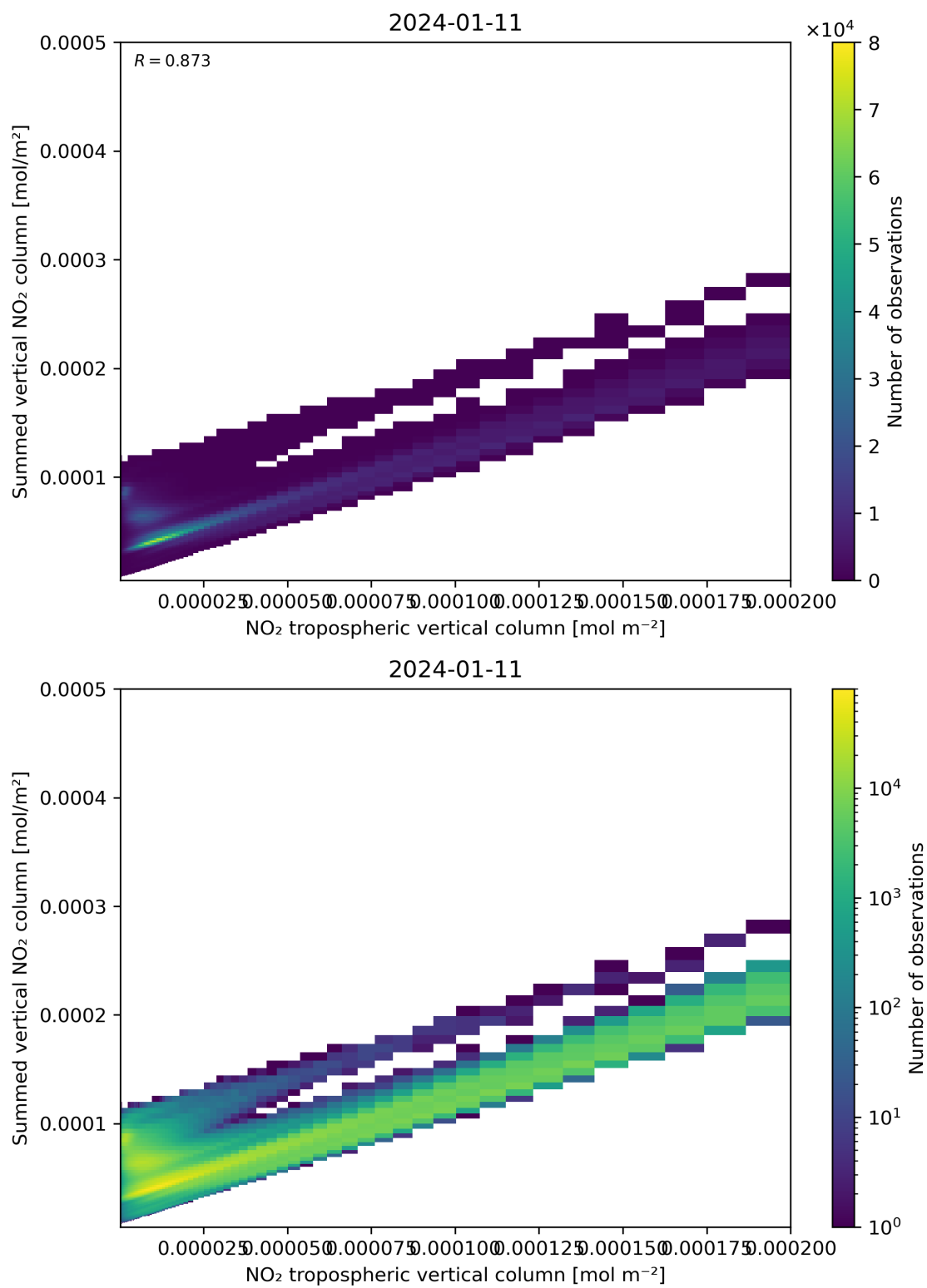
Figure 126: Scatter density plot of “NO 2 tropospheric vertical column” against “Summed vertical NO 2 column” for 2024-01-10 to 2024-01-12.
