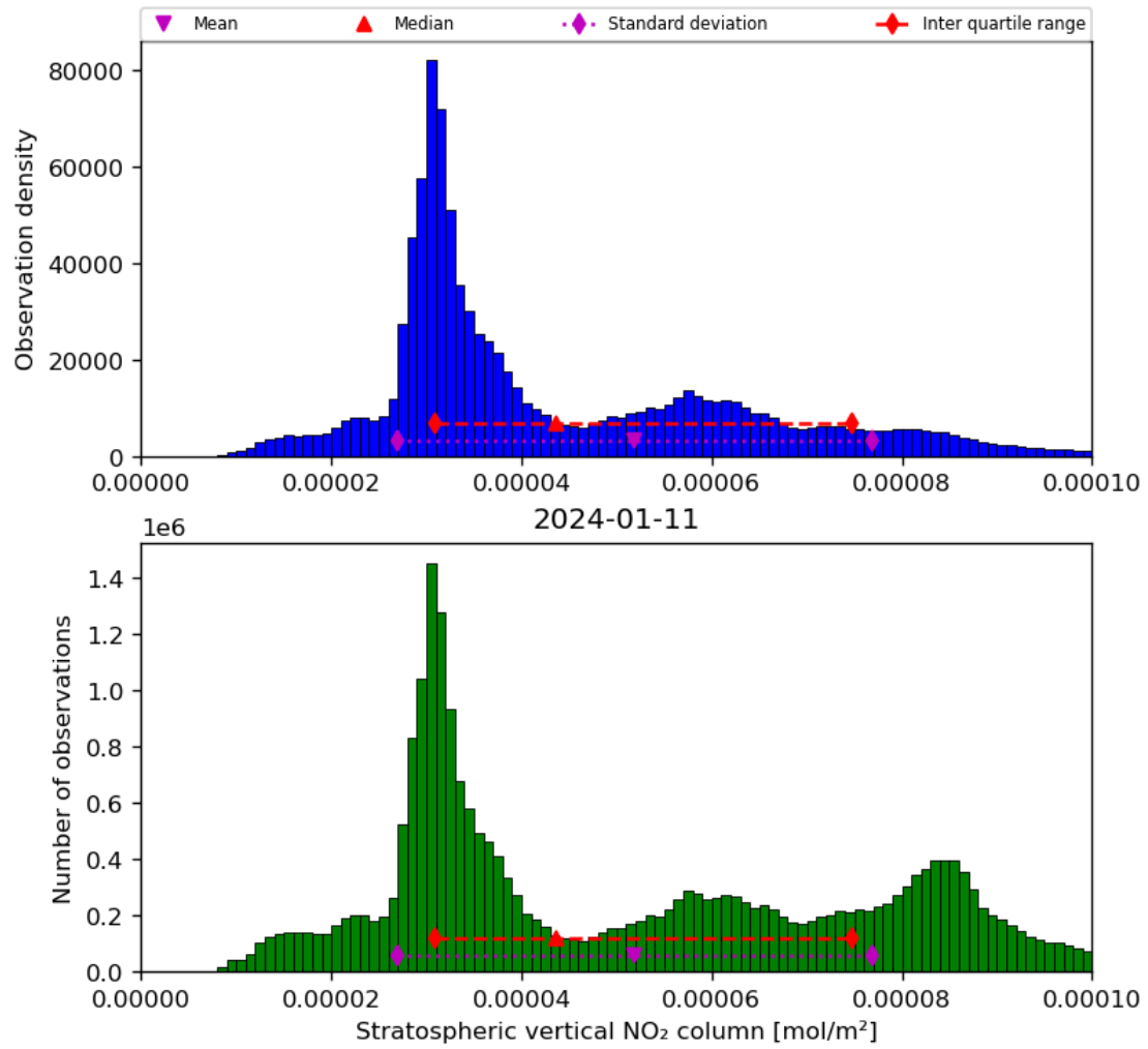
Figure 36: Histogram of “Stratospheric vertical NO 2 column” for 2024-01-10 to 2024-01-12
