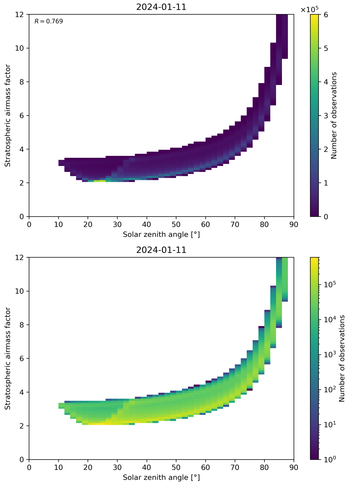
Figure 145: Scatter density plot of “Solar zenith angle” against “Stratospheric airmass factor” for 2024-01-10 to 2024-01-12.
