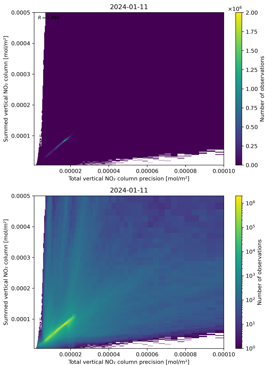
Figure 117: Scatter density plot of “Total vertical NO 2 column precision” against “Summed vertical NO 2 column” for 2024-01-10 to 2024-01-12.
