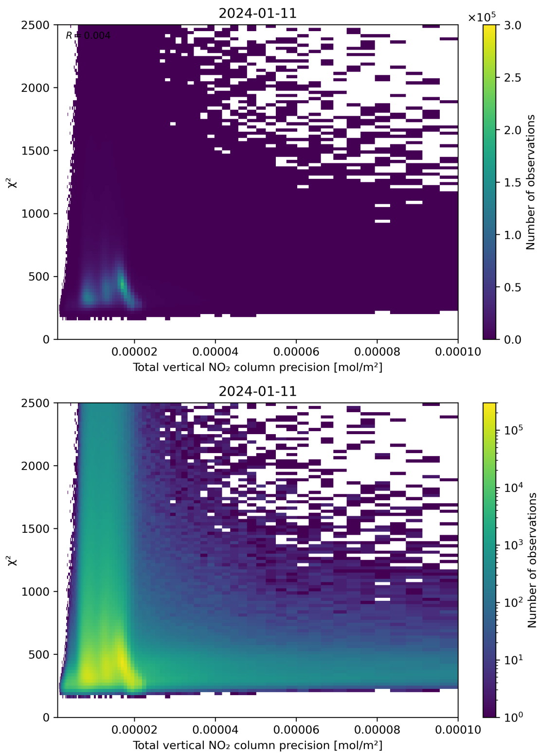
Figure 116: Scatter density plot of “Total vertical NO 2 column precision” against “ \chi^2 ” for 2024-01-10 to 2024-01-12.
