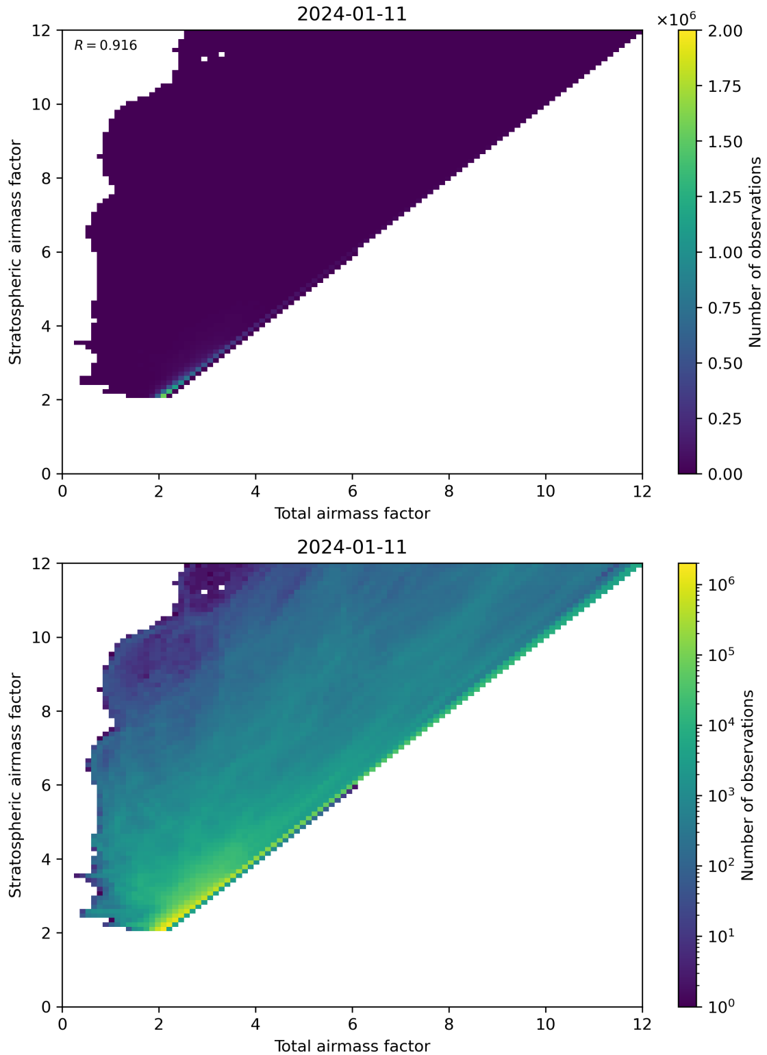
Figure 62: Scatter density plot of “Total airmass factor” against “Stratospheric airmass factor” for 2024-01-10 to 2024-01-12.
