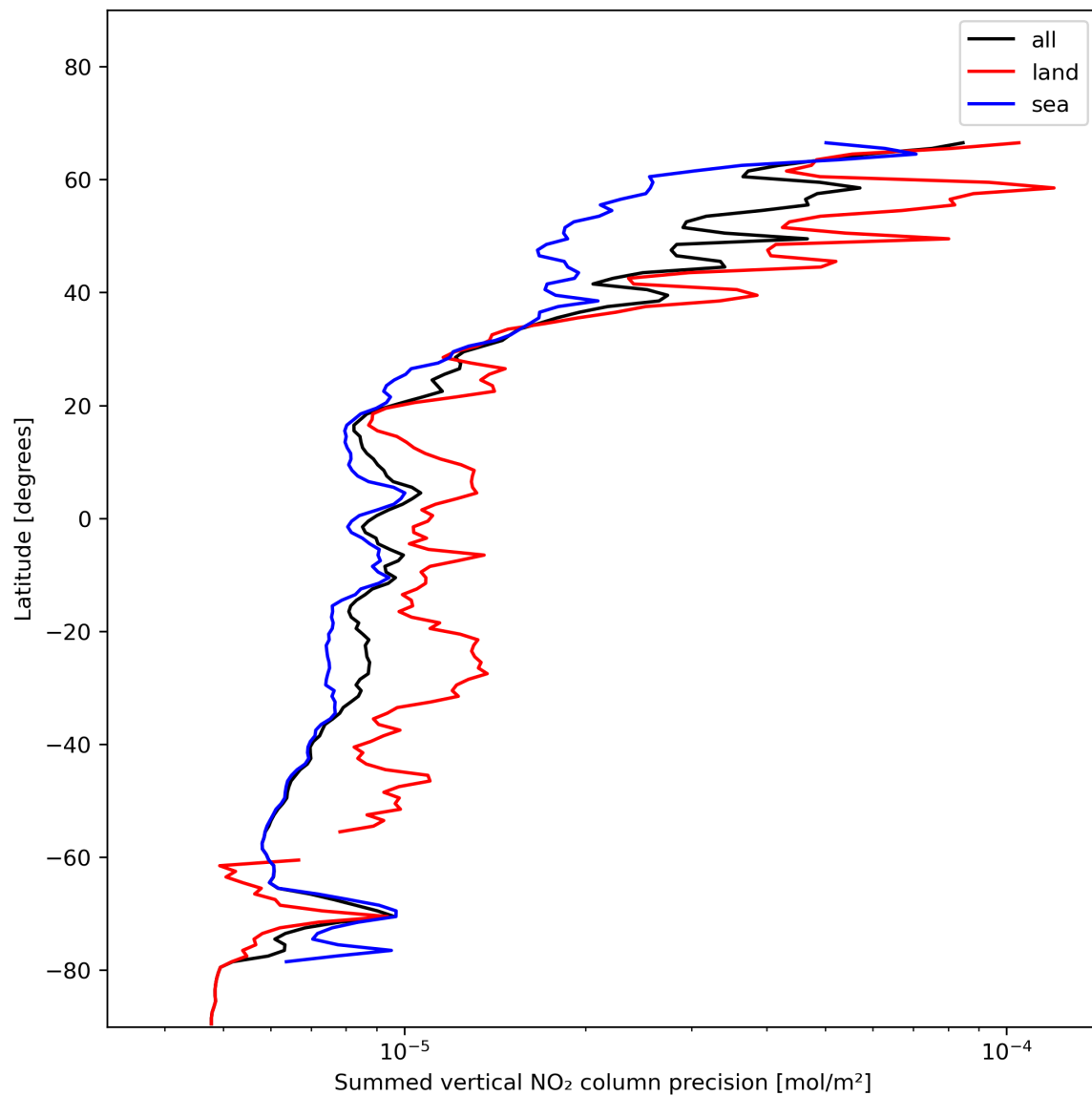
Figure 24: Zonal average of “Summed vertical NO 2 column precision” for 2024-01-10 to 2024-01-12.
