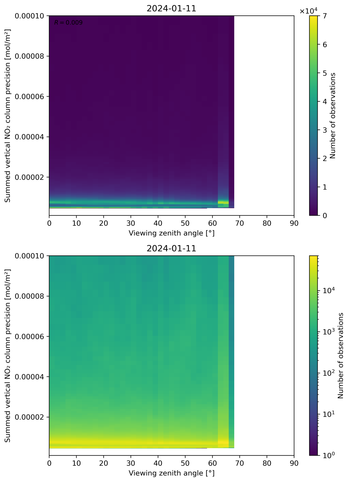
Figure 166: Scatter density plot of “Viewing zenith angle” against “Summed vertical NO 2 column precision” for 2024-01-10 to 2024-01-12.
