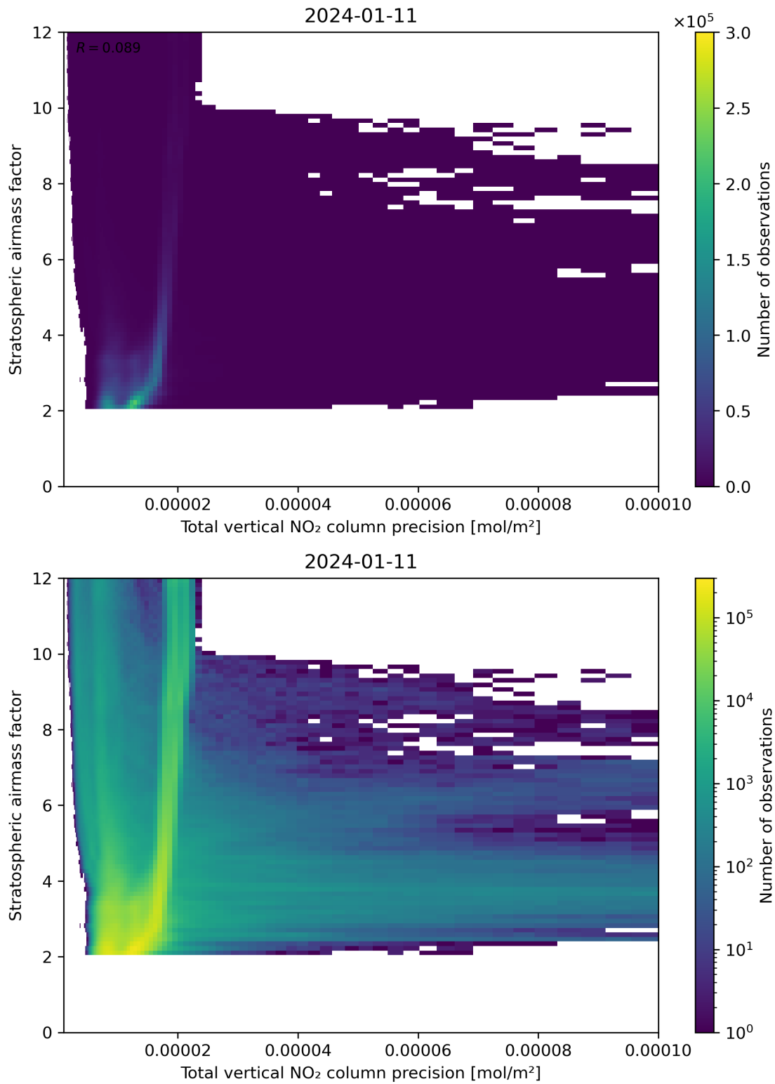
Figure 115: Scatter density plot of “Total vertical NO 2 column precision” against “Stratospheric air mass factor” for 2024-01-10 to 2024-01-12.
