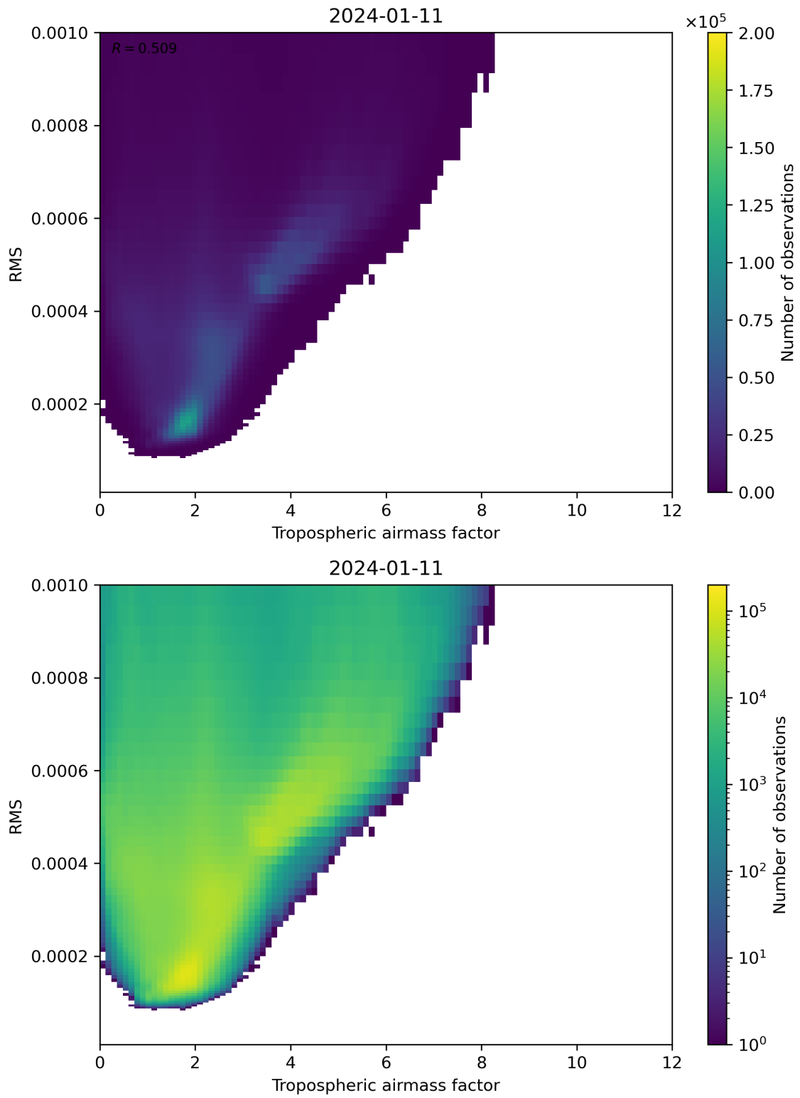
Figure 79: Scatter density plot of “Tropospheric airmass factor” against “RMS” for 2024-01-10 to 2024-01-12.
