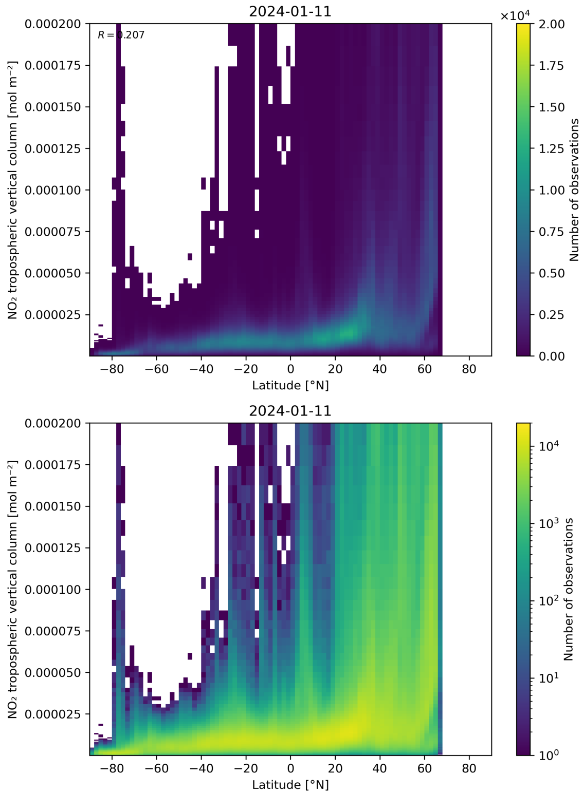
Figure 92: Scatter density plot of “Latitude” against “NO 2 tropospheric vertical column” for 2024-01-10 to 2024-01-12.
