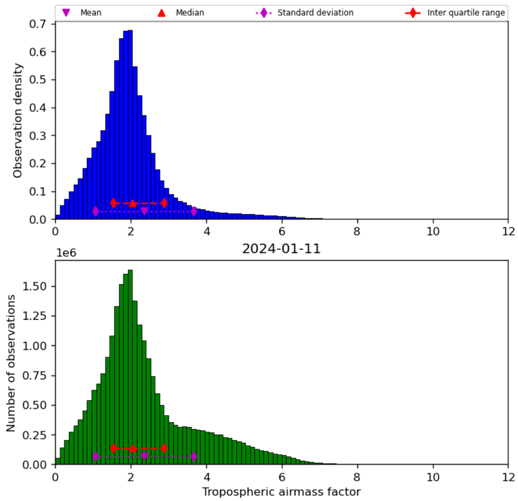
Figure 31: Histogram of “Tropospheric airmass factor” for 2024-01-10 to 2024-01-12
