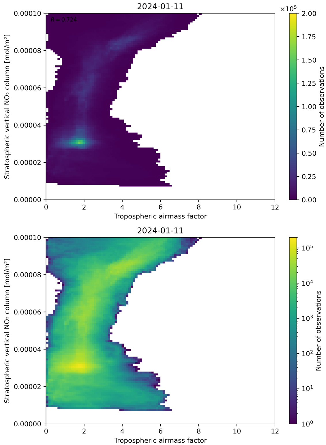
Figure 74: Scatter density plot of “Tropospheric air mass factor” against “Stratospheric vertical NO 2 column” for 2024-01-10 to 2024-01-12.
