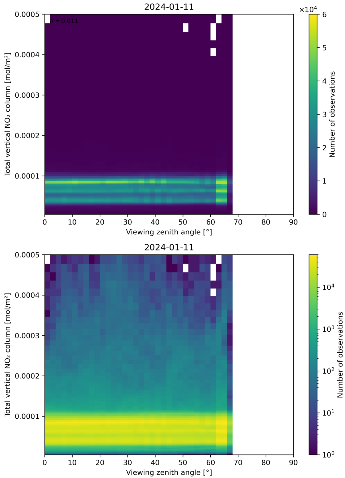
Figure 167: Scatter density plot of “Viewing zenith angle” against “Total vertical NO 2 column” for 2024-01-10 to 2024-01-12.
