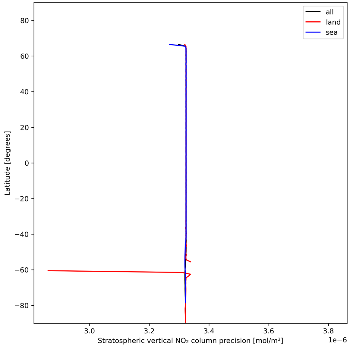
Figure 20: Zonal average of “Stratospheric vertical NO 2 column precision” for 2024-01-10 to 2024-01-12.
