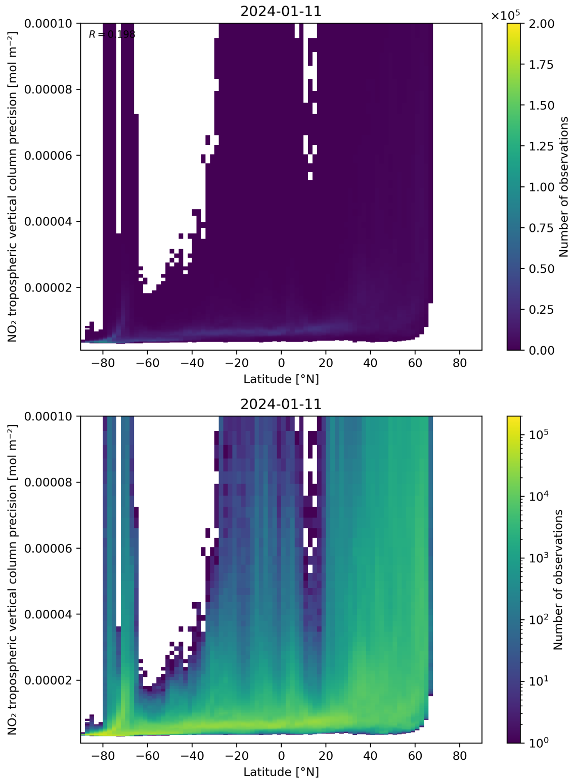
Figure 93: Scatter density plot of “Latitude” against “NO 2 tropospheric vertical column precision” for 2024-01-10 to 2024-01-12.
