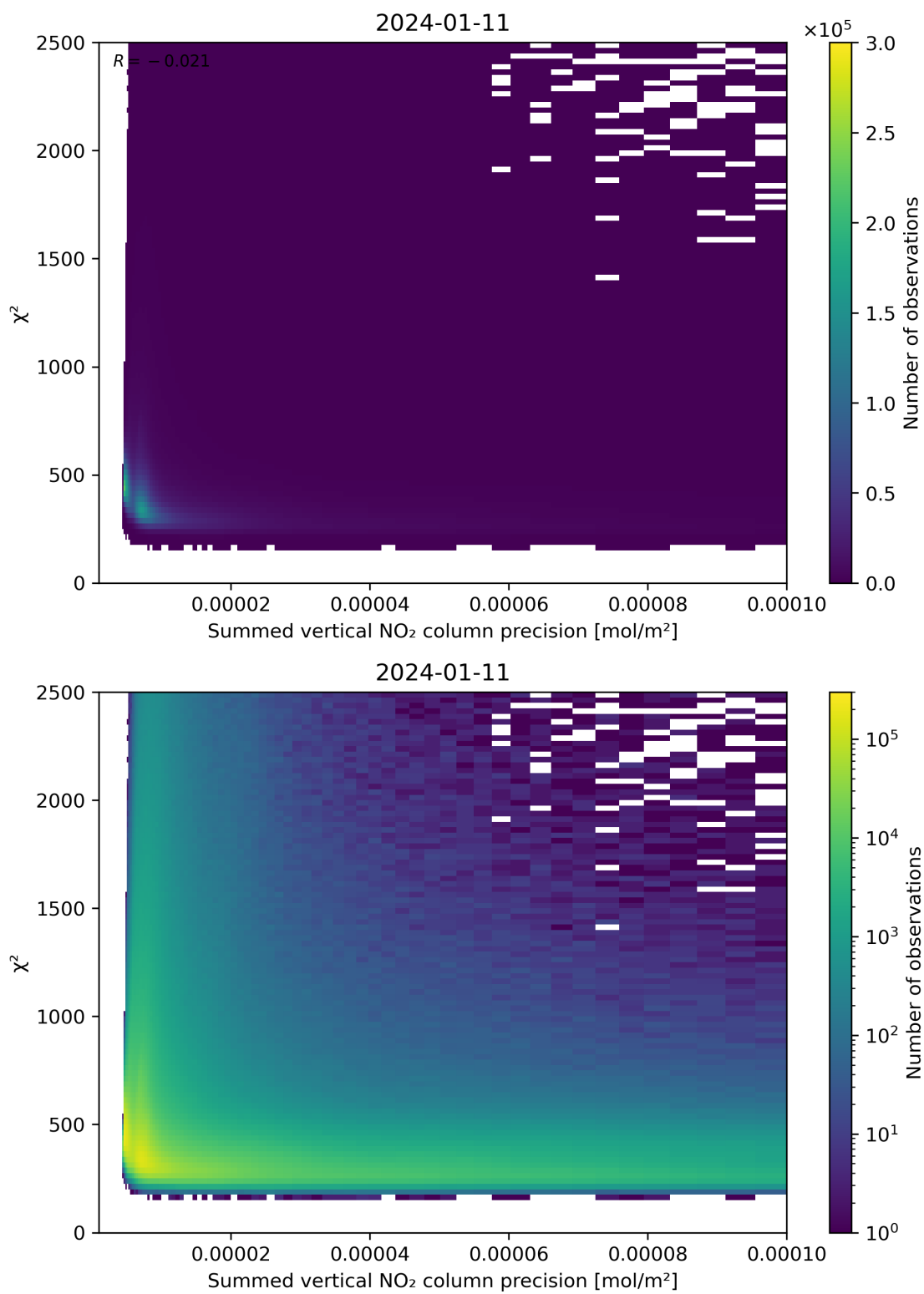
Figure 107: Scatter density plot of “Summed vertical NO 2 column precision” against “ \chi^2 ” for 2024-01-10 to 2024-01-12.
