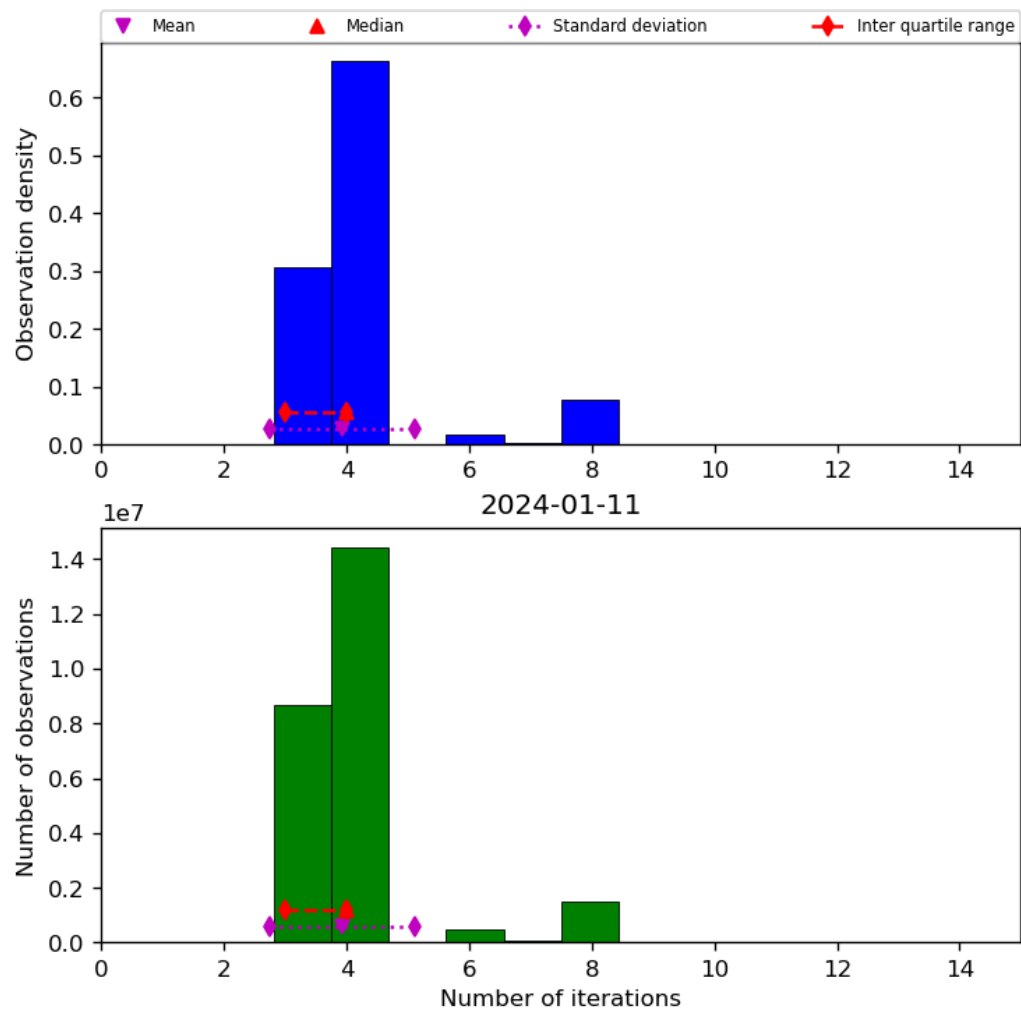
Figure 34: Histogram of “Number of iterations” for 2024-01-10 to 2024-01-12
