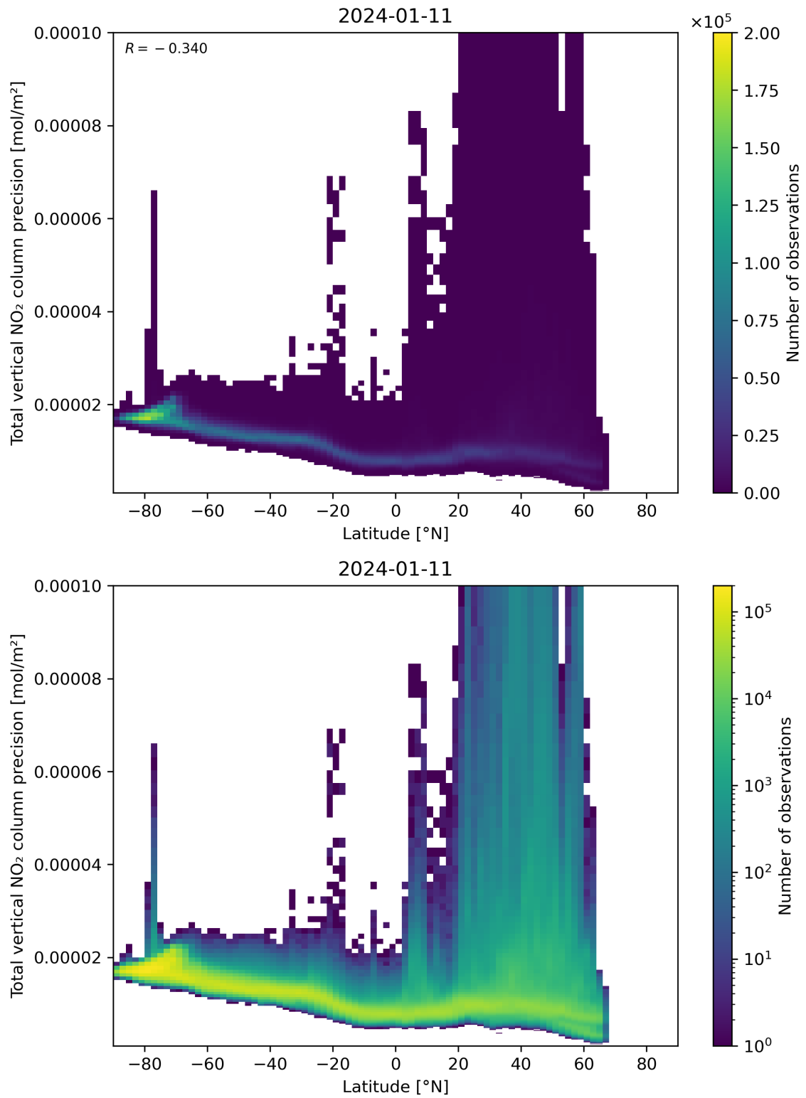
Figure 91: Scatter density plot of “Latitude” against “Total vertical NO 2 column precision” for 2024-01-10 to 2024-01-12.
