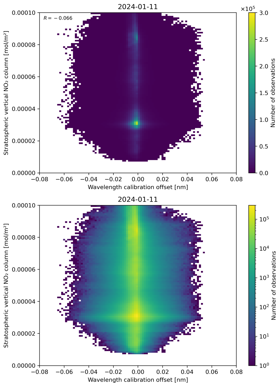
Figure 176: Scatter density plot of “Wavelength calibration offset” against “Stratospheric vertical NO 2 column” for 2024-01-10 to 2024-01-12.
