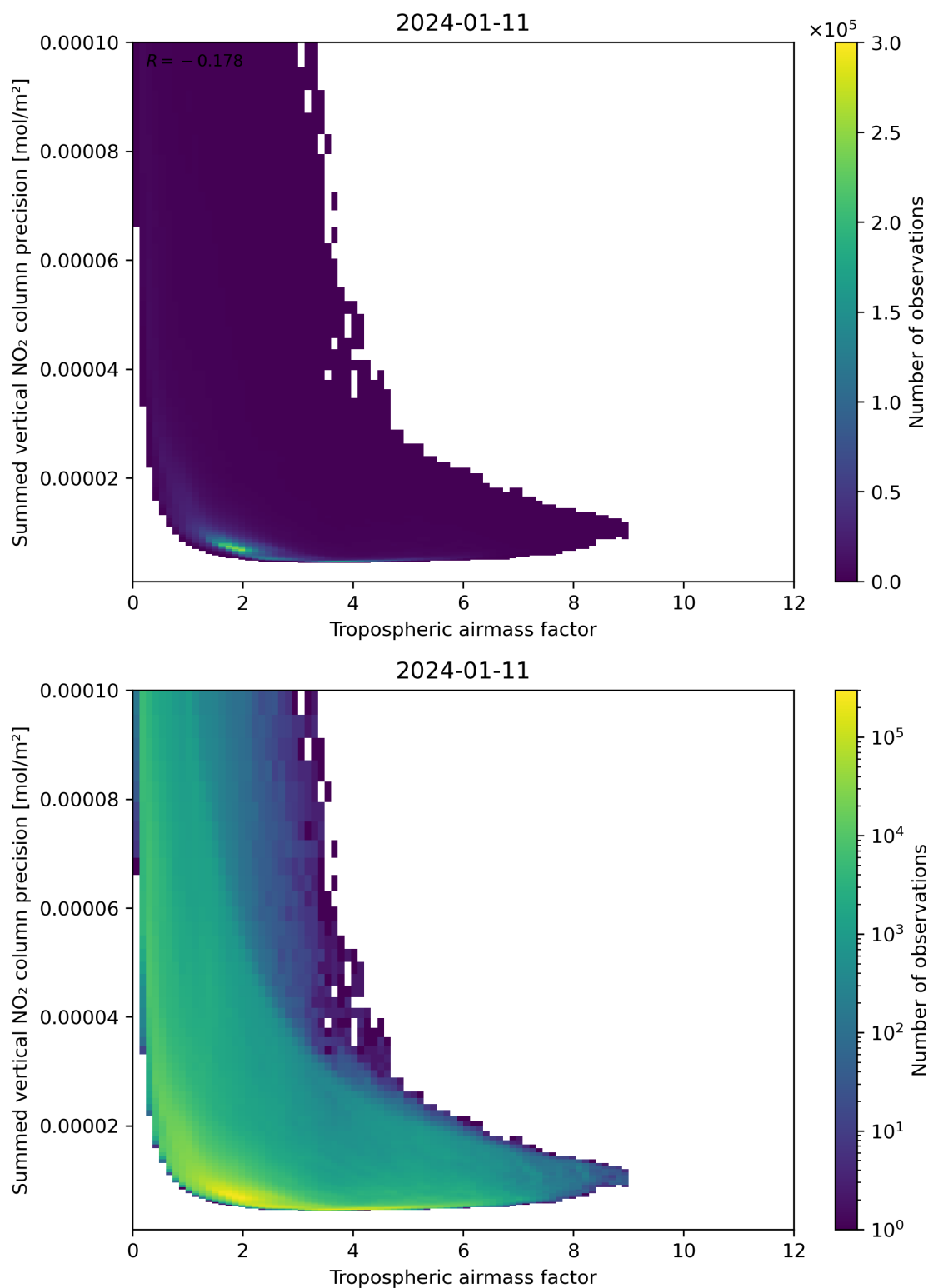
Figure 76: Scatter density plot of “Tropospheric air mass factor” against “Summed vertical NO 2 column precision” for 2024-01-10 to 2024-01-12.
