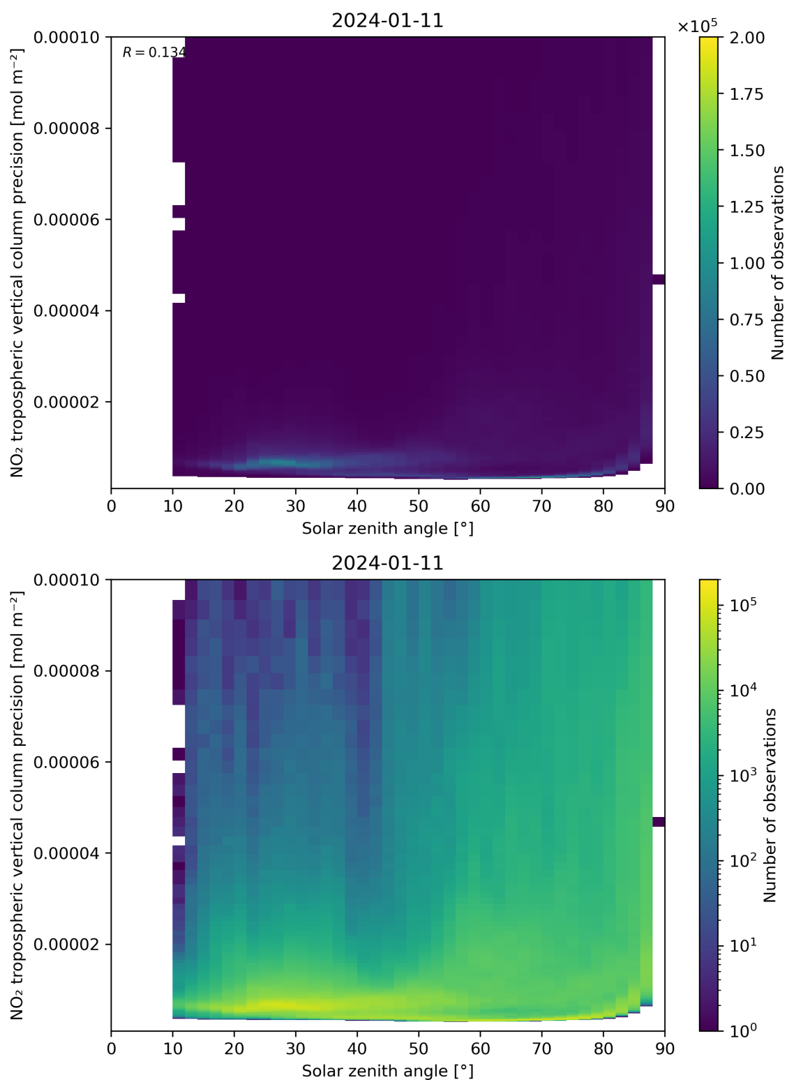
Figure 156: Scatter density plot of “Solar zenith angle” against “NO 2 tropospheric vertical column precision” for 2024-01-10 to 2024-01-12.
