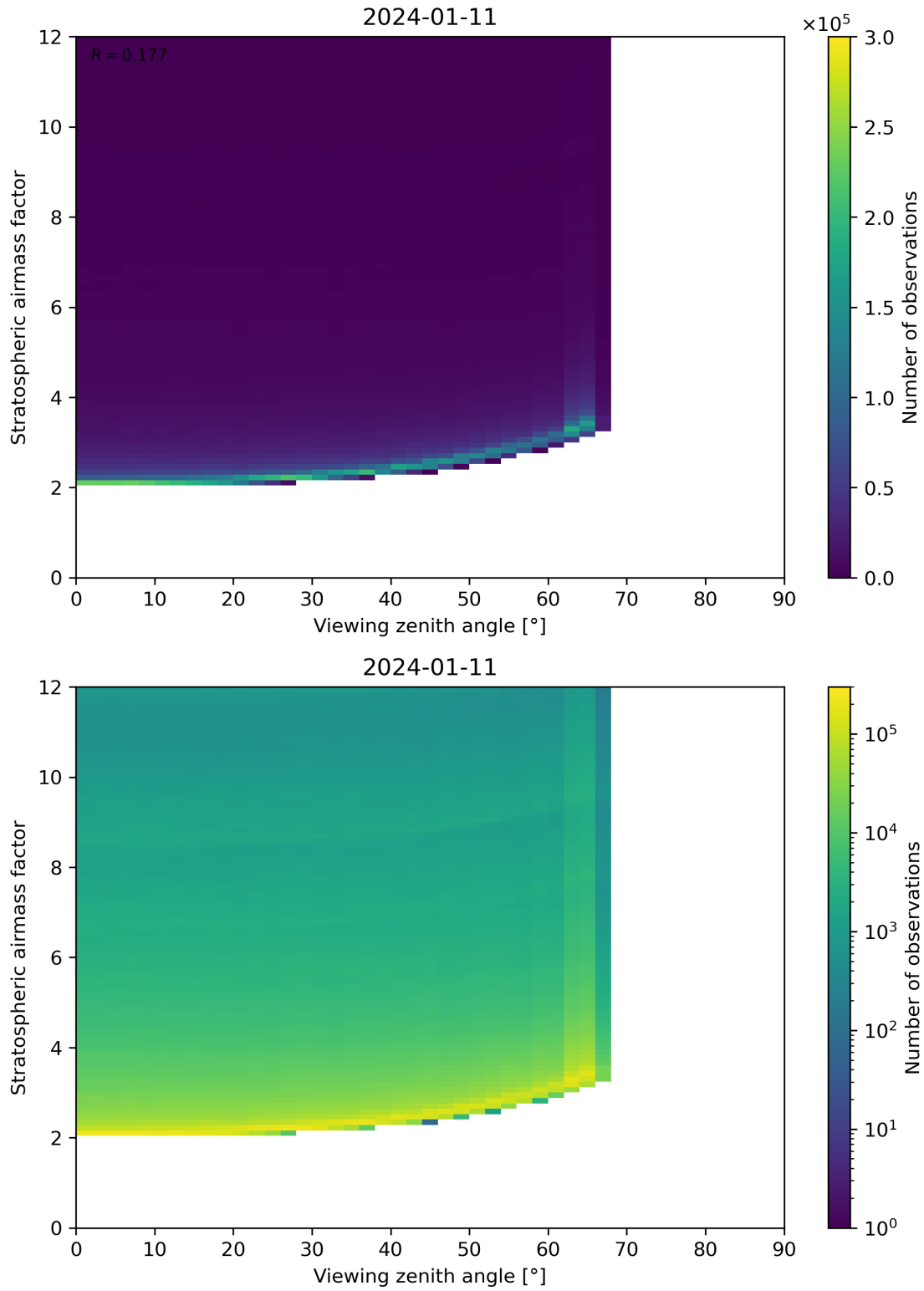
Figure 159: Scatter density plot of “Viewing zenith angle” against “Stratospheric airmass factor” for 2024-01-10 to 2024-01-12.
