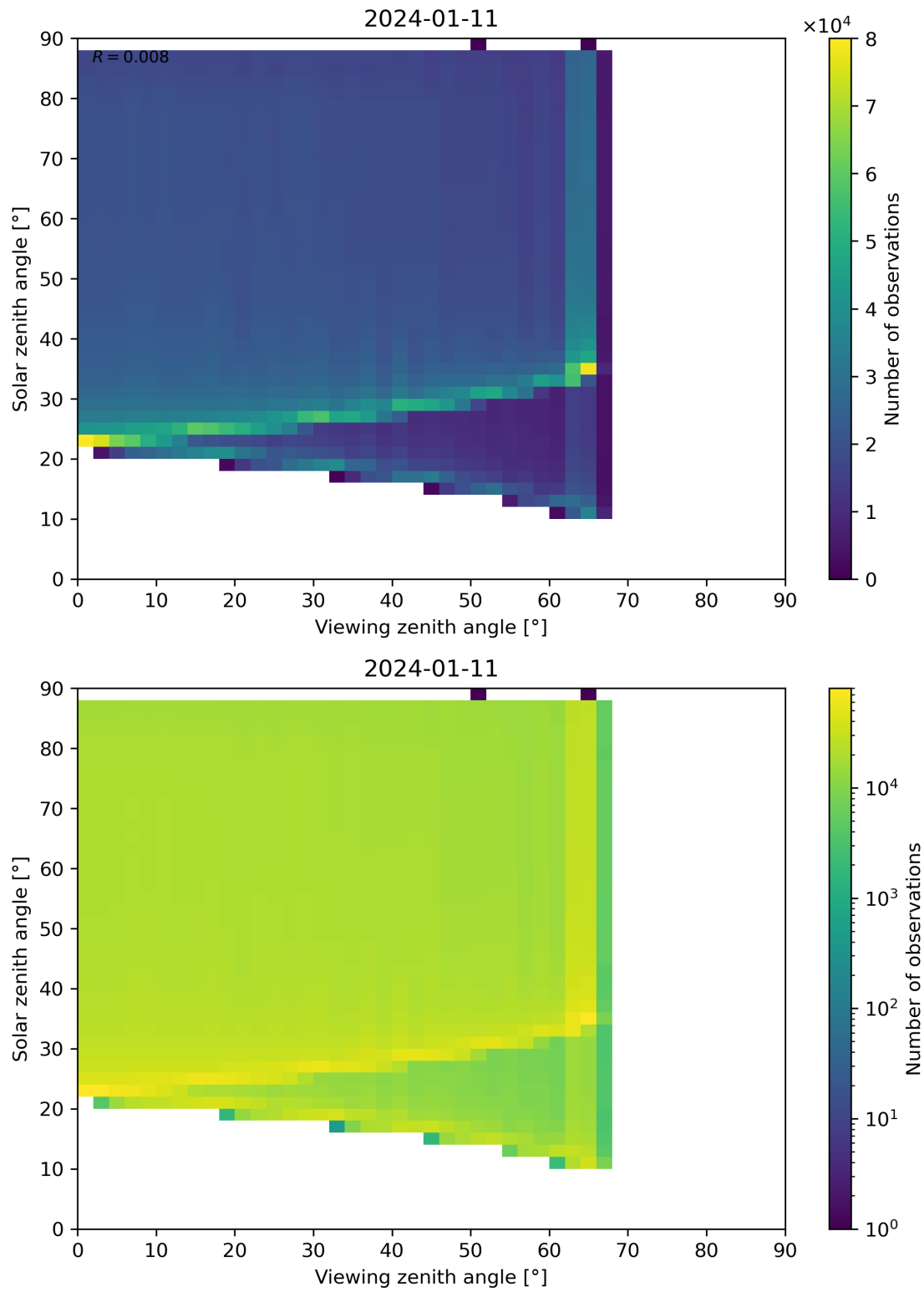
Figure 172: Scatter density plot of “Viewing zenith angle” against “Solar zenith angle” for 2024-01-10 to 2024-01-12.
