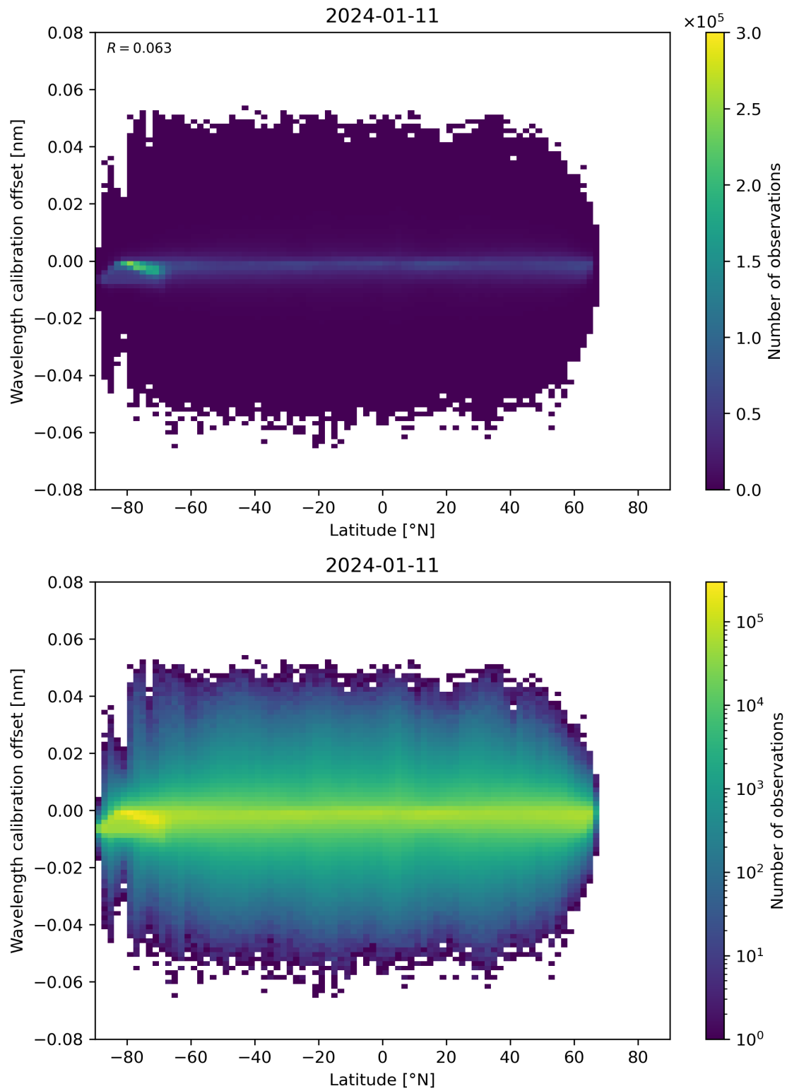
Figure 95: Scatter density plot of “Latitude” against “Wavelength calibration offset” for 2024-01-10 to 2024-01-12.
