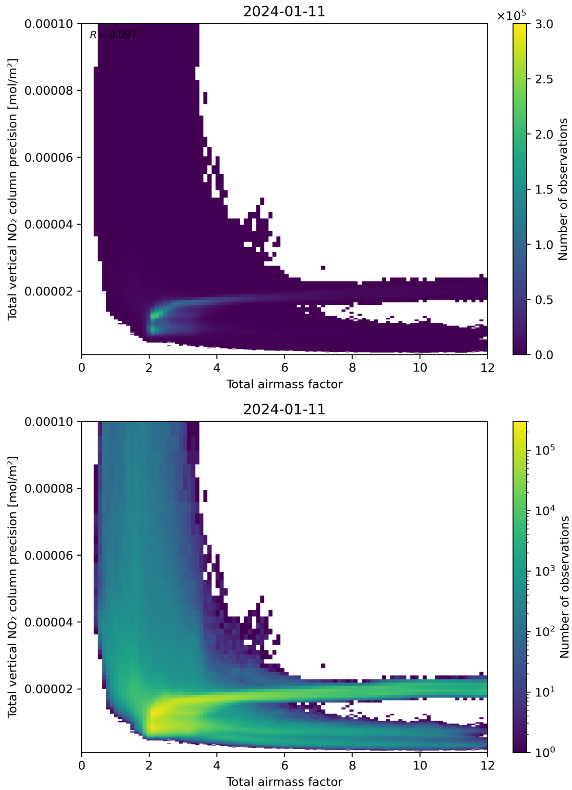
Figure 68: Scatter density plot of “Total airmass factor” against “Total vertical NO 2 column precision” for 2024-01-10 to 2024-01-12.
