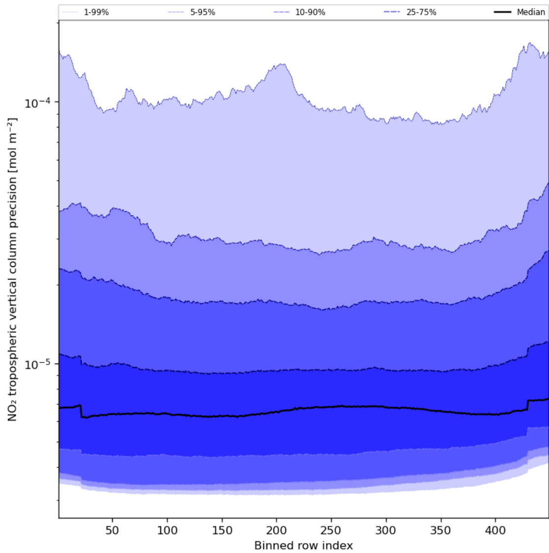
Figure 47: Along track statistics of “NO 2 tropospheric vertical column precision” for 2024-01-10 to 2024-01-12
