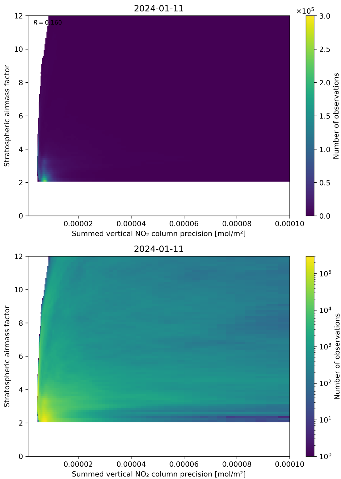
Figure 106: Scatter density plot of “Summed vertical NO 2 column precision” against “Stratospheric airmass factor” for 2024-01-10 to 2024-01-12.
