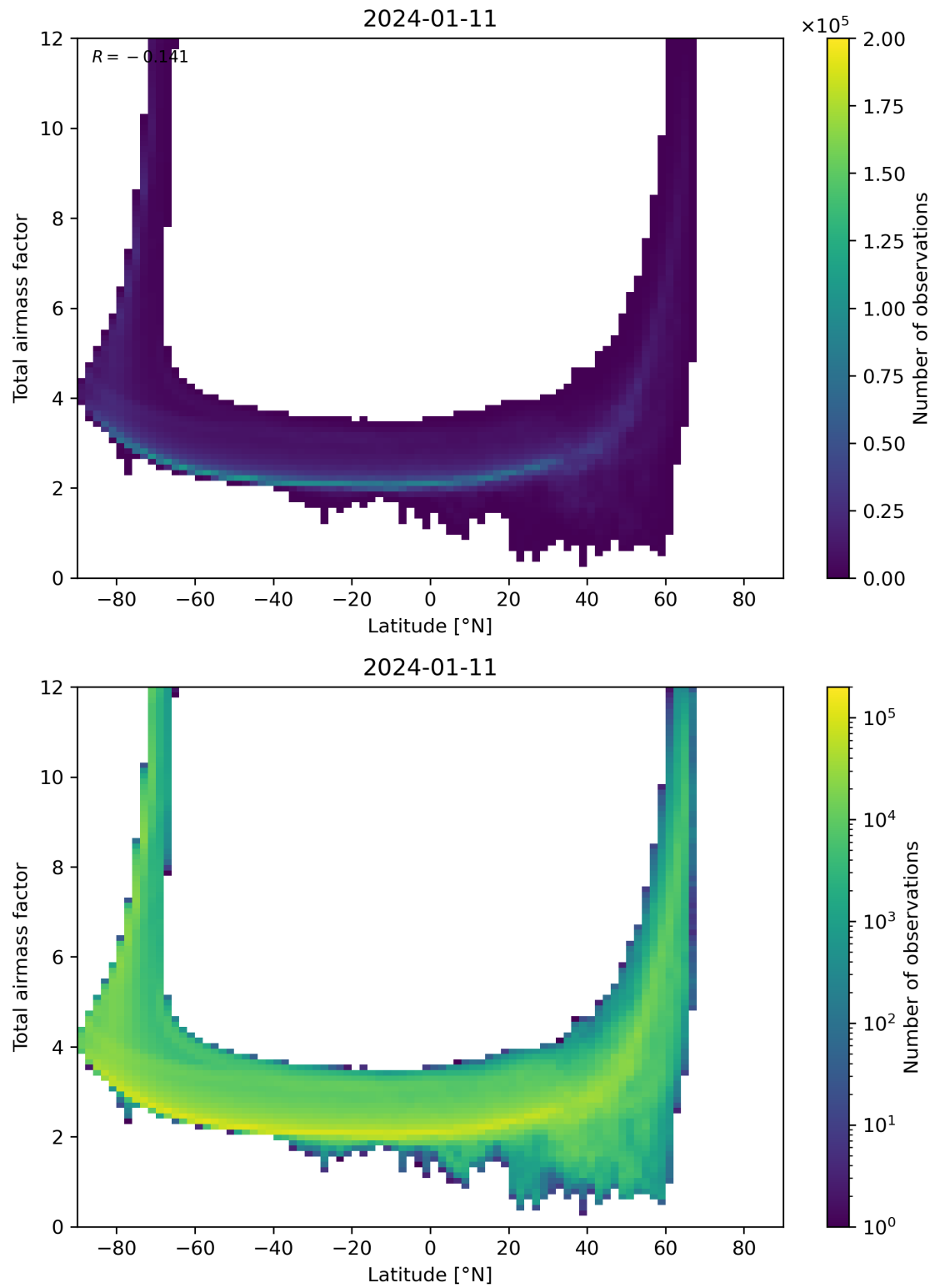
Figure 84: Scatter density plot of “Latitude” against “Total airmass factor” for 2024-01-10 to 2024-01-12.
