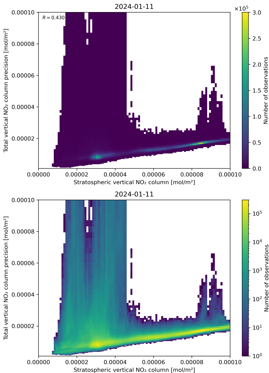
Figure 101: Scatter density plot of “Stratospheric vertical NO 2 column” against “Total vertical NO 2 column precision” for 2024-01-10 to 2024-01-12.
