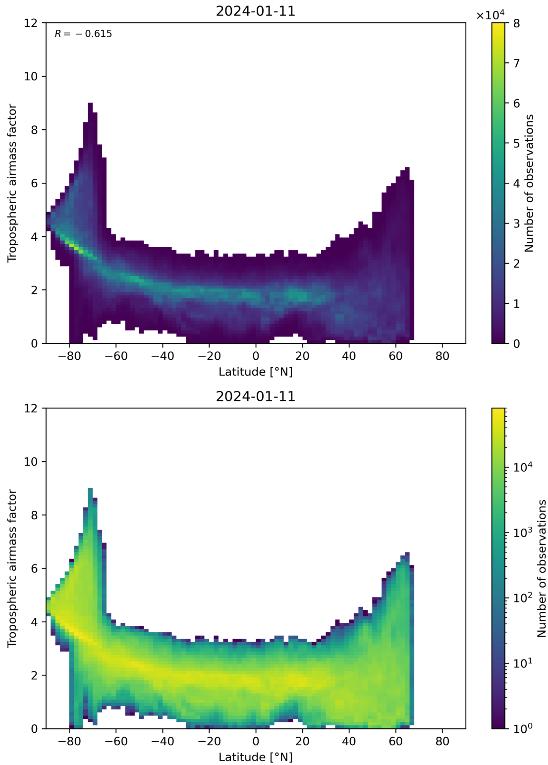
Figure 85: Scatter density plot of “Latitude” against “Tropospheric air mass factor” for 2024-01-10 to 2024-01-12.
