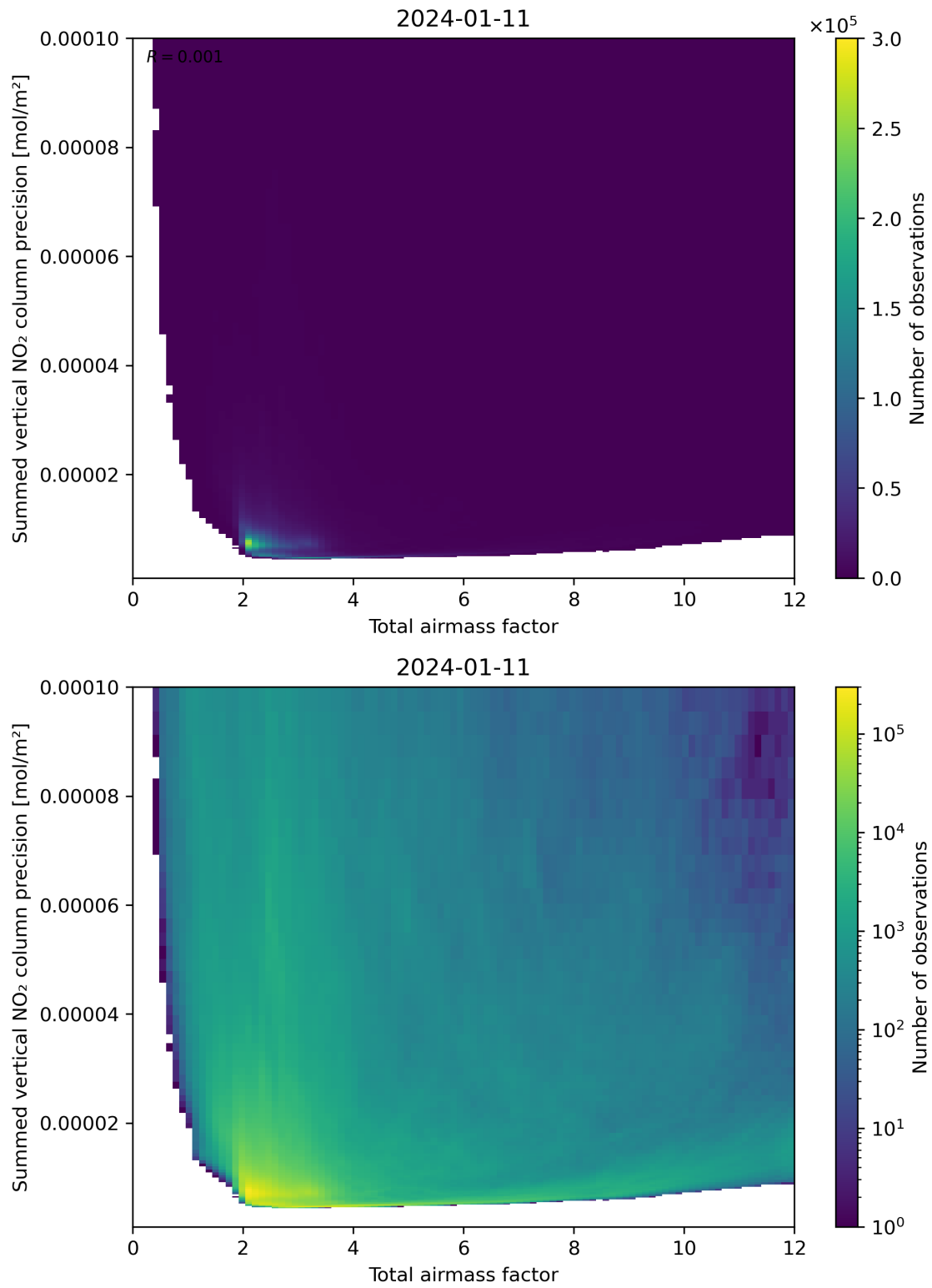
Figure 66: Scatter density plot of “Total airmass factor” against “Summed vertical NO 2 column precision” for 2024-01-10 to 2024-01-12.
