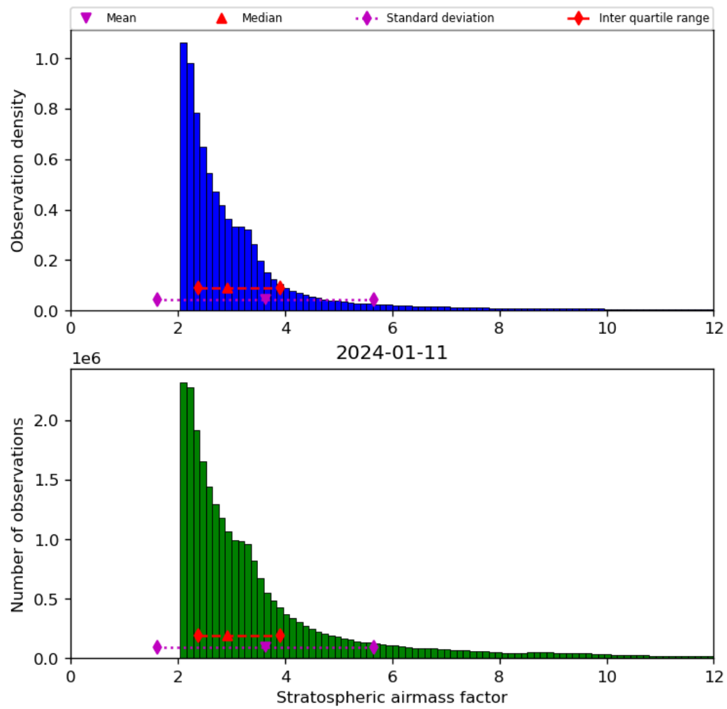
Figure 44: Histogram of “Stratospheric airmass factor” for 2024-01-10 to 2024-01-12
