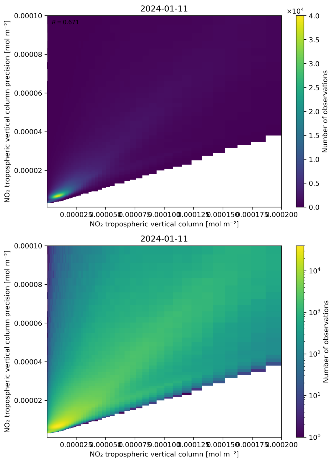
Figure 130: Scatter density plot of “NO 2 tropospheric vertical column” against “NO 2 tropospheric vertical column precision” for 2024-01-10 to 2024-01-12.
