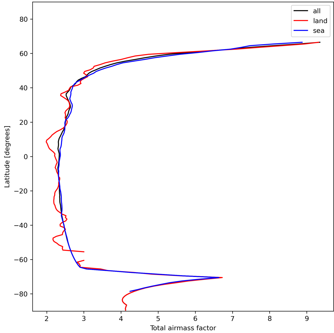
Figure 15: Zonal average of “Total airmass factor” for 2024-01-10 to 2024-01-12.
