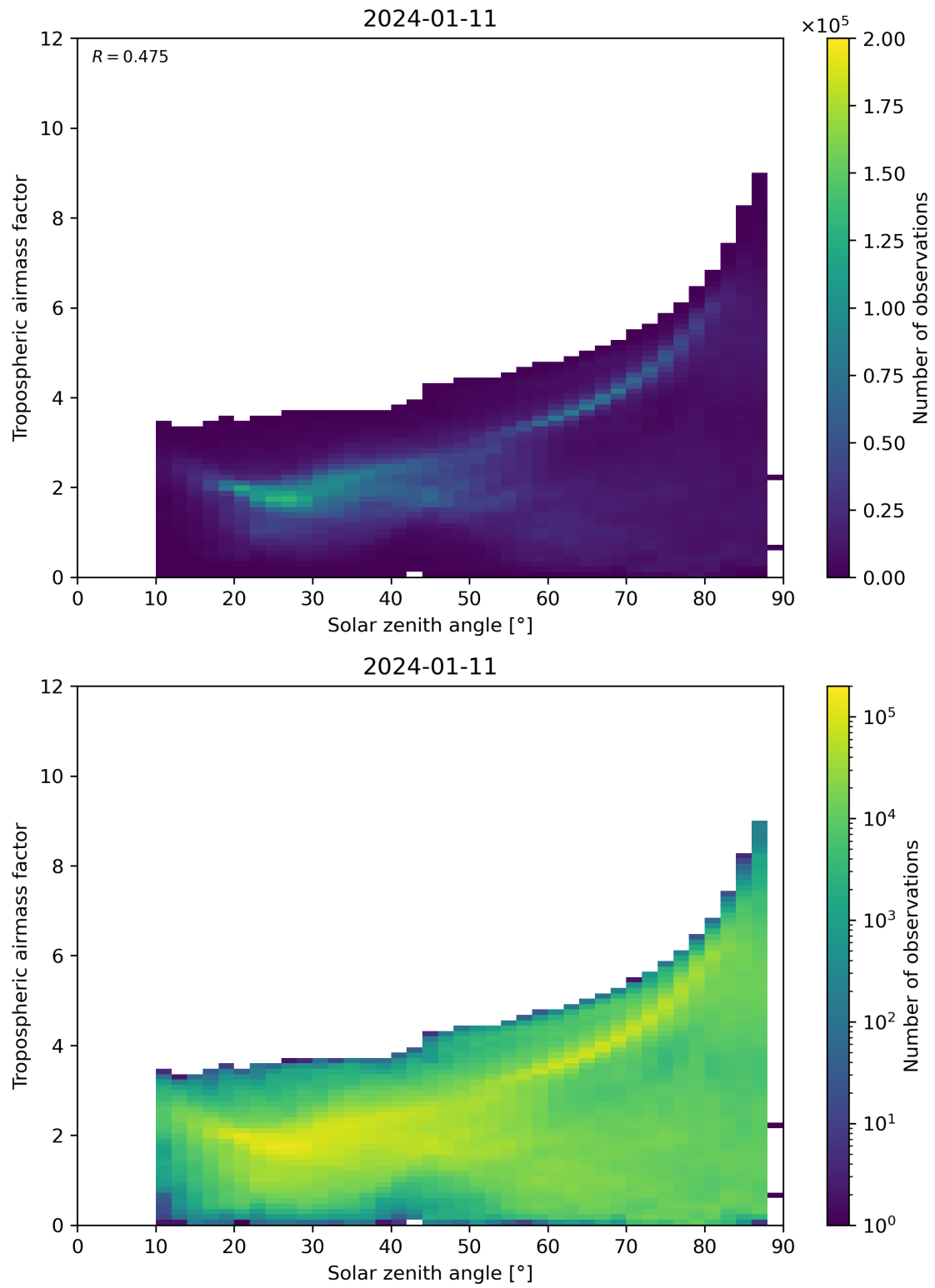
Figure 147: Scatter density plot of “Solar zenith angle” against “Tropospheric airmass factor” for 2024-01-10 to 2024-01-12.
