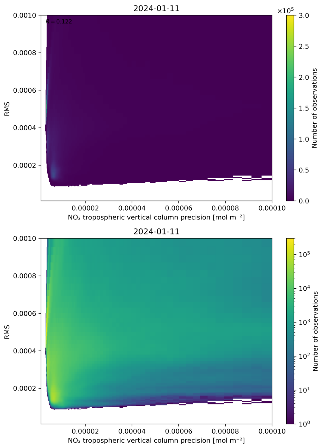
Figure 140: Scatter density plot of “NO 2 tropospheric vertical column precision” against “RMS” for 2024-01-10 to 2024-01-12.
