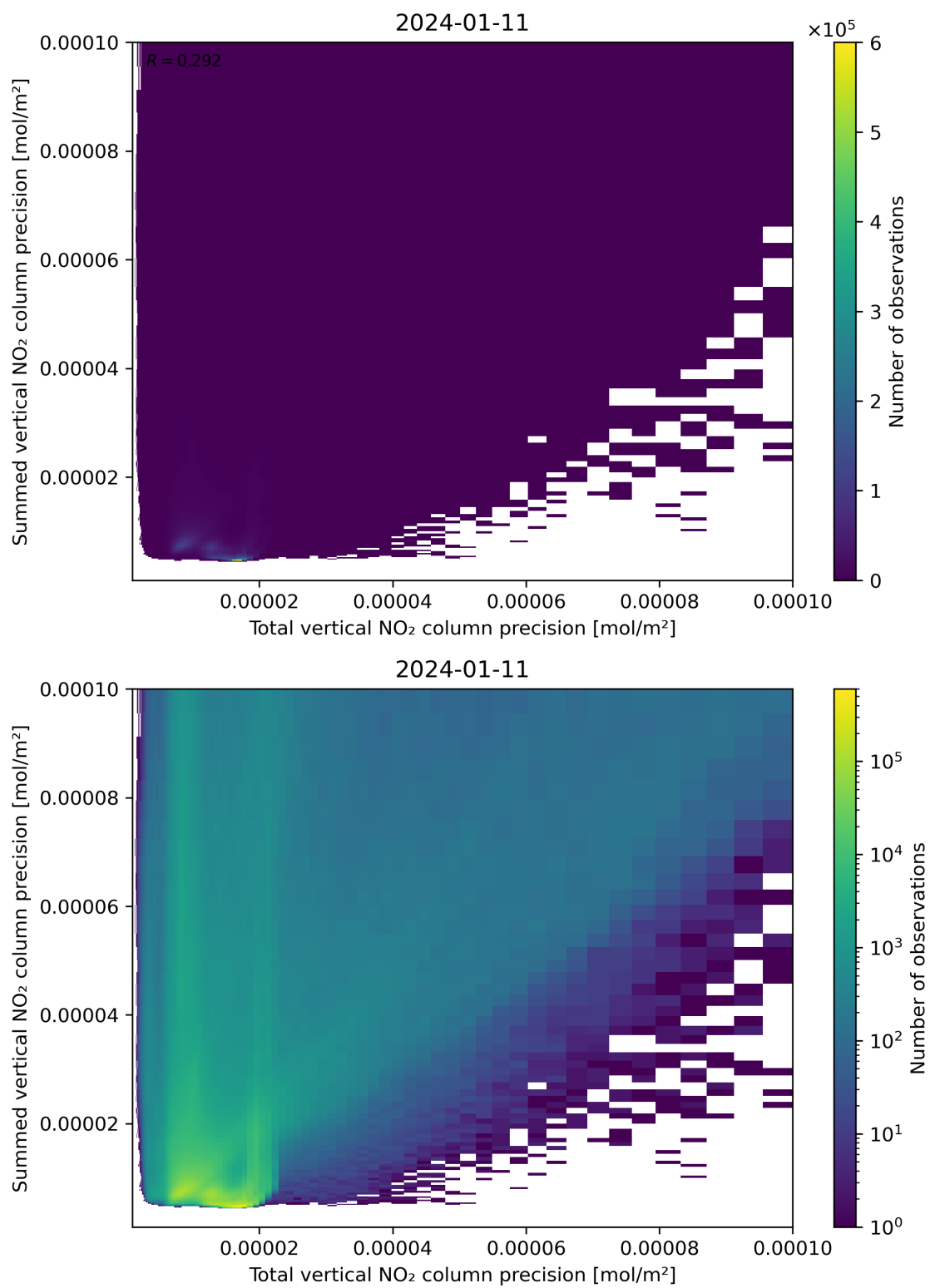
Figure 118: Scatter density plot of “Total vertical NO 2 column precision” against “Summed vertical NO 2 column precision” for 2024-01-10 to 2024-01-12.
