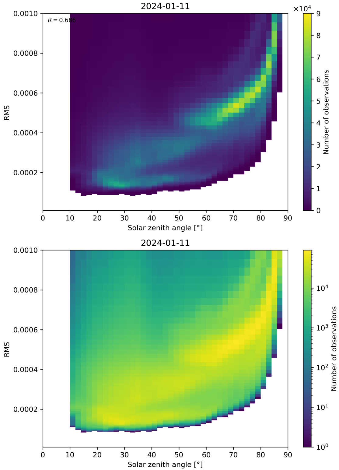
Figure 157: Scatter density plot of “Solar zenith angle” against “RMS” for 2024-01-10 to 2024-01-12.
