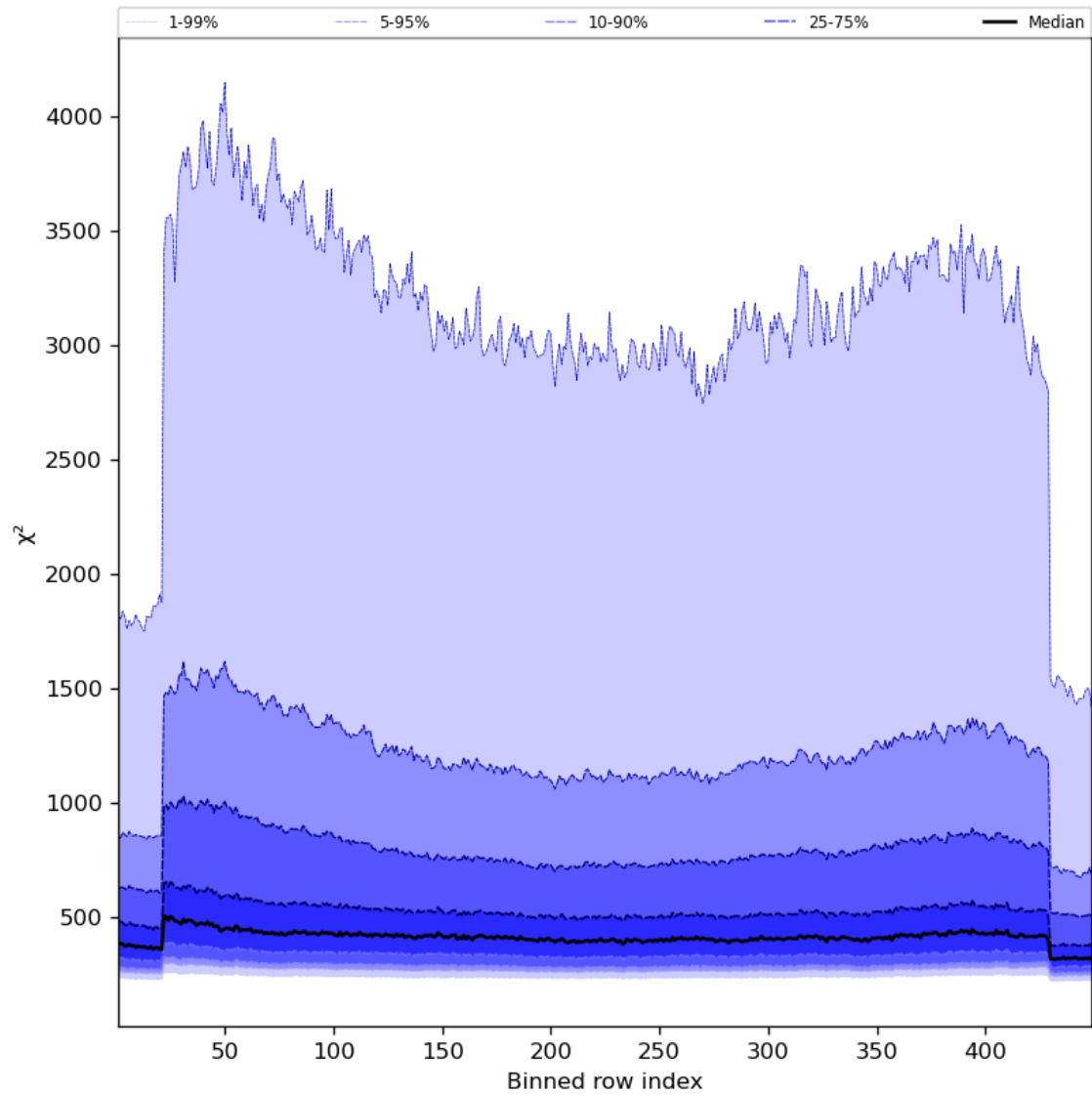
Figure 59: Along track statistics of “ \chi^2 ” for 2024-01-10 to 2024-01-12
