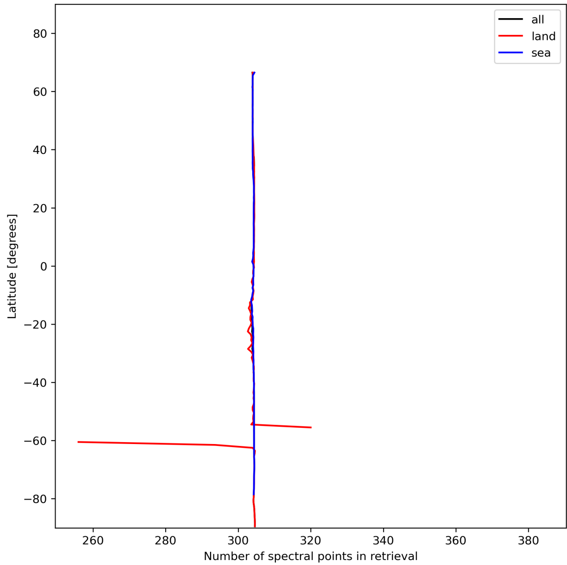
Figure 16: Zonal average of “Number of spectral points in retrieval” for 2024-01-10 to 2024-01-12.
