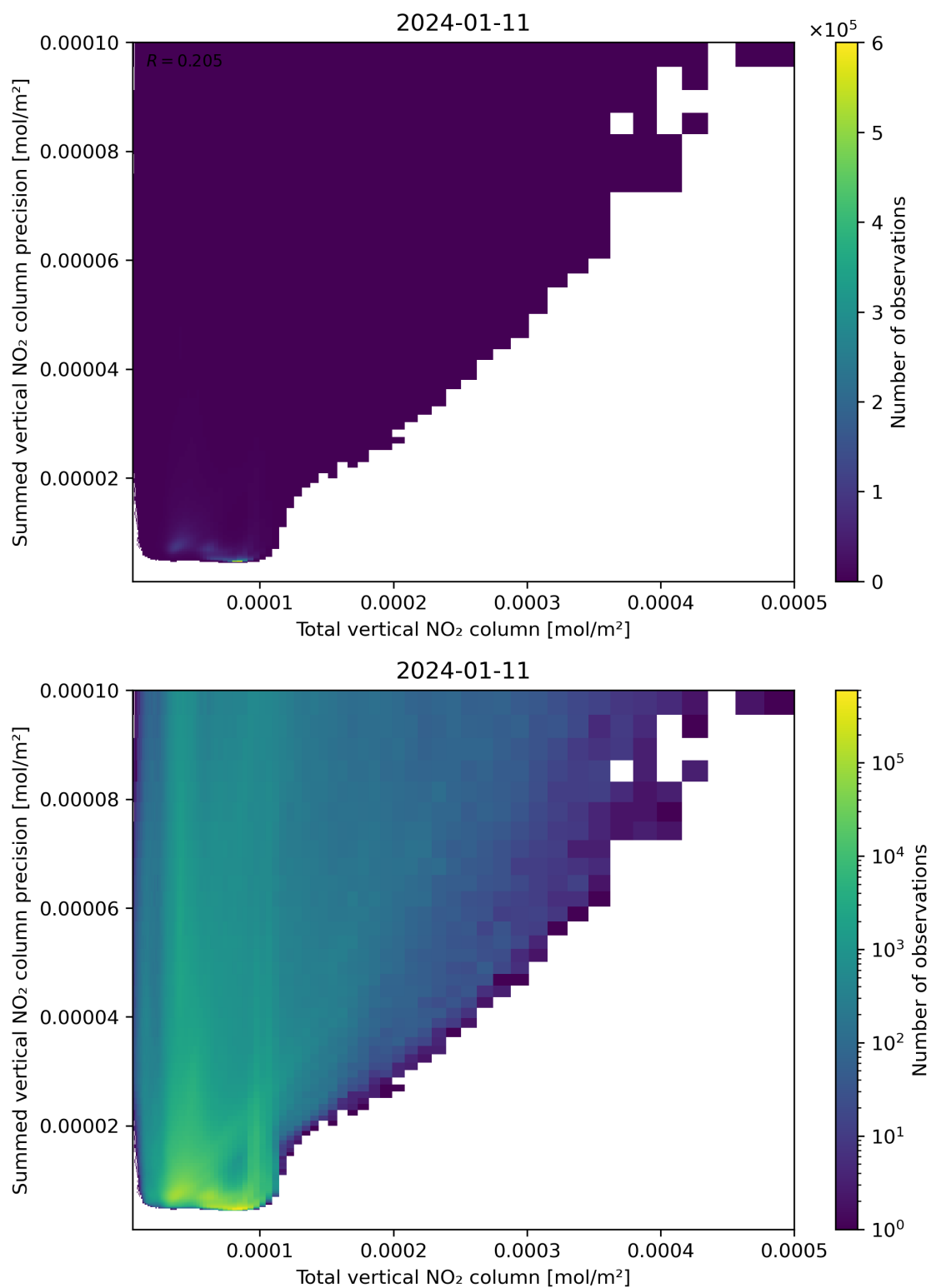
Figure 113: Scatter density plot of “Total vertical NO 2 column” against “Summed vertical NO 2 column precision” for 2024-01-10 to 2024-01-12.
