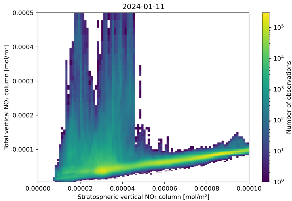
Figure 100: Scatter density plot of “Stratospheric vertical NO 2 column” against “Total vertical NO 2 column” for 2024-01-10 to 2024-01-12.
