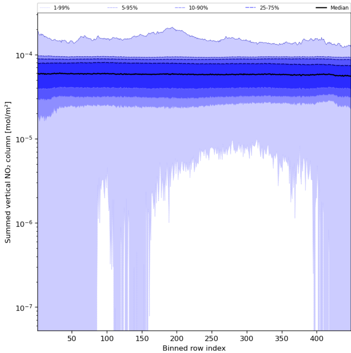
Figure 57: Along track statistics of “Summed vertical NO 2 column” for 2024-01-10 to 2024-01-12
