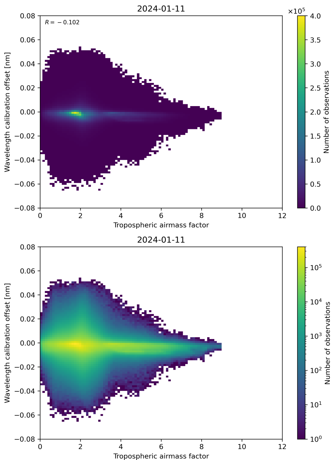
Figure 80: Scatter density plot of “Tropospheric airmass factor” against “Wavelength calibration offset” for 2024-01-10 to 2024-01-12.
