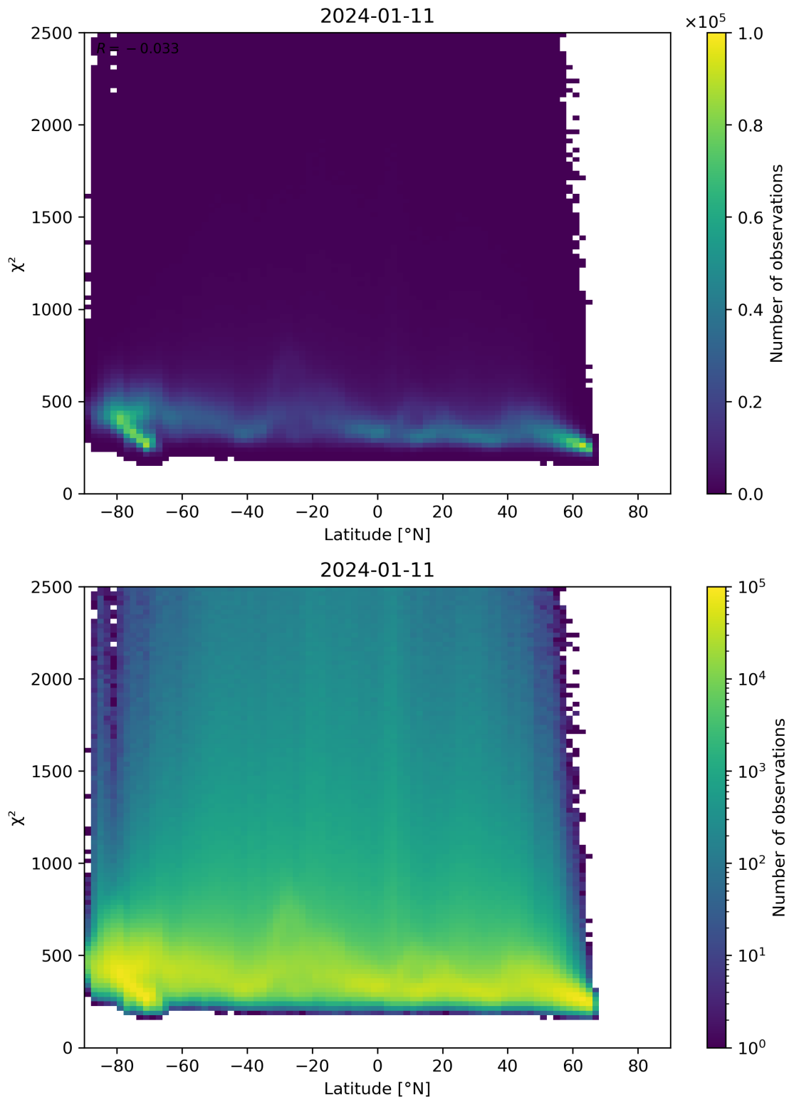
Figure 86: Scatter density plot of “Latitude” against “ \chi^2 ” for 2024-01-10 to 2024-01-12.
