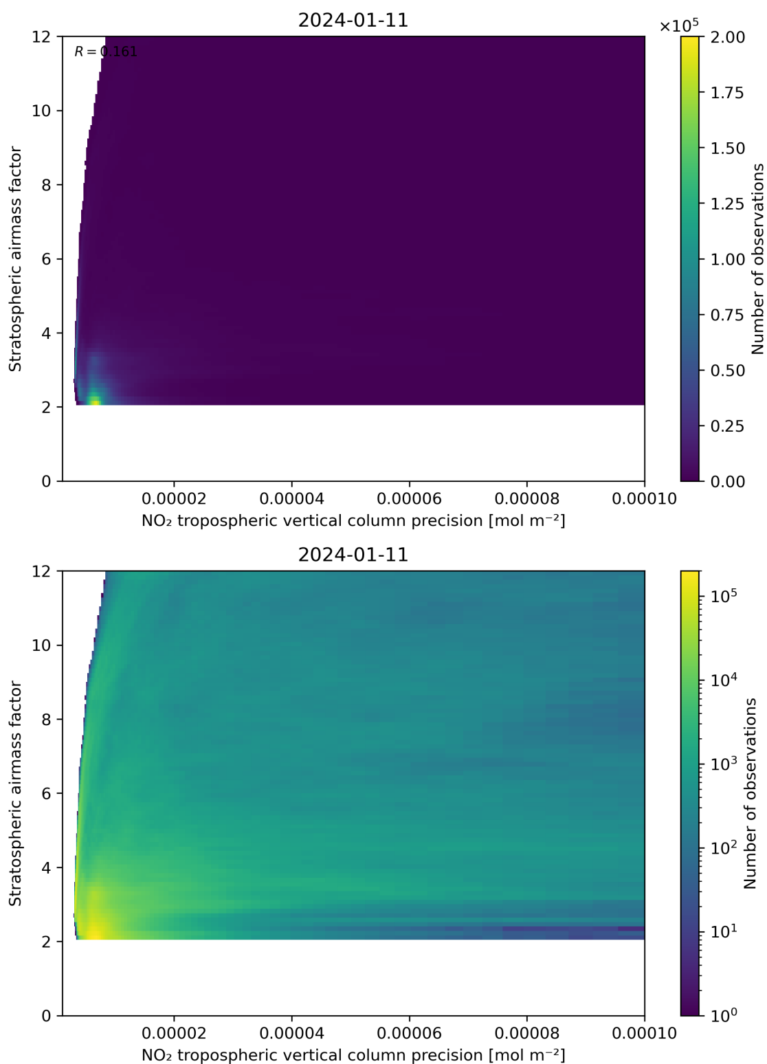
Figure 131: Scatter density plot of “NO 2 tropospheric vertical column precision” against “Stratospheric airmass factor” for 2024-01-10 to 2024-01-12.
