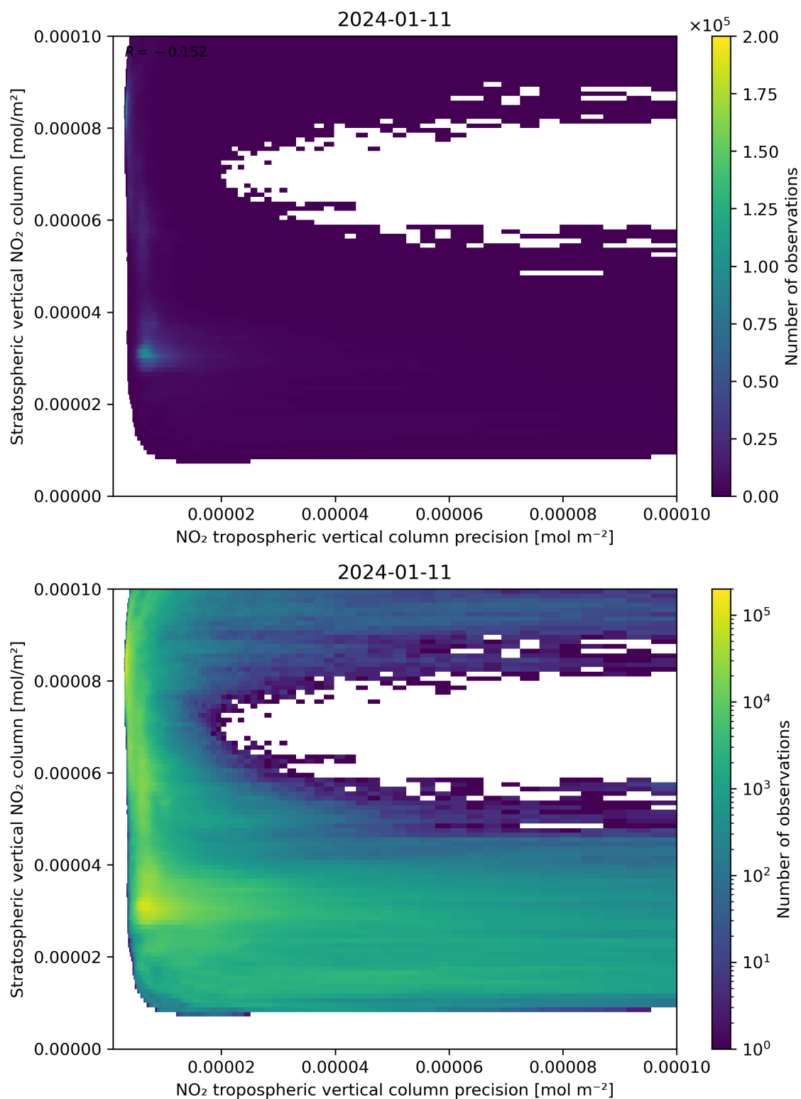
Figure 135: Scatter density plot of “NO 2 tropospheric vertical column precision” against “Stratospheric vertical NO 2 column” for 2024-01-10 to 2024-01-12.
