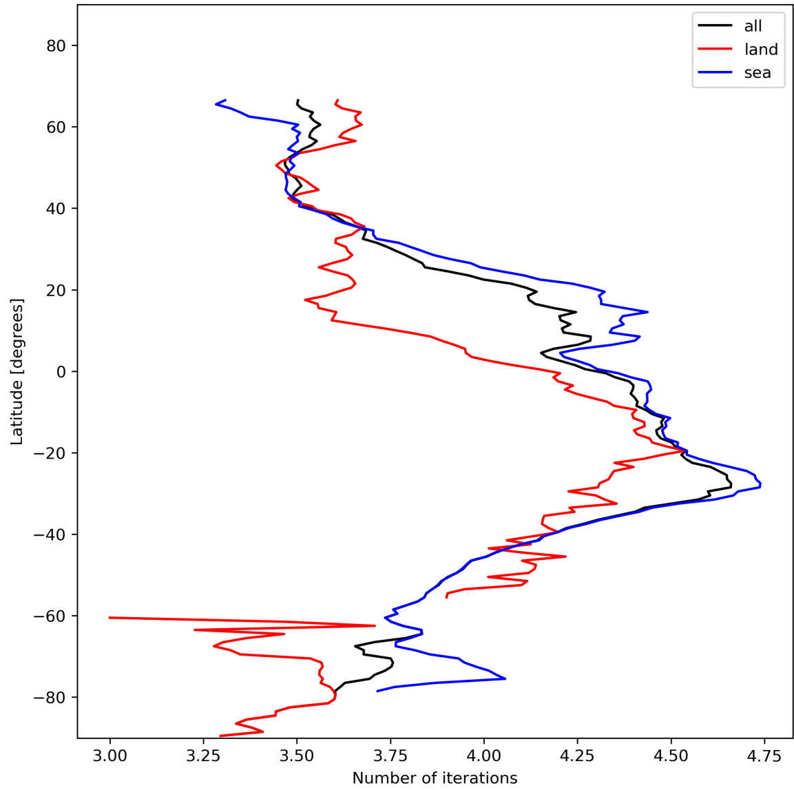
Figure 17: Zonal average of “Number of iterations” for 2024-01-10 to 2024-01-12.
