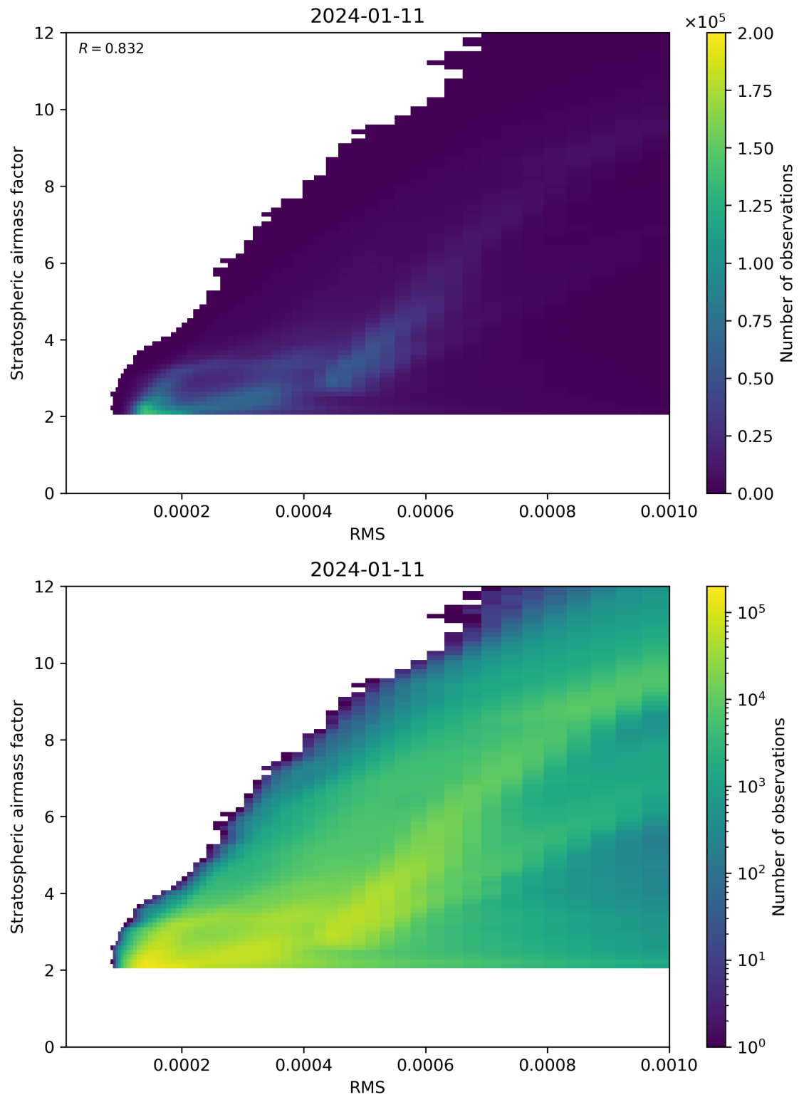
Figure 144: Scatter density plot of “RMS” against “Stratospheric airmass factor” for 2024-01-10 to 2024-01-12.
