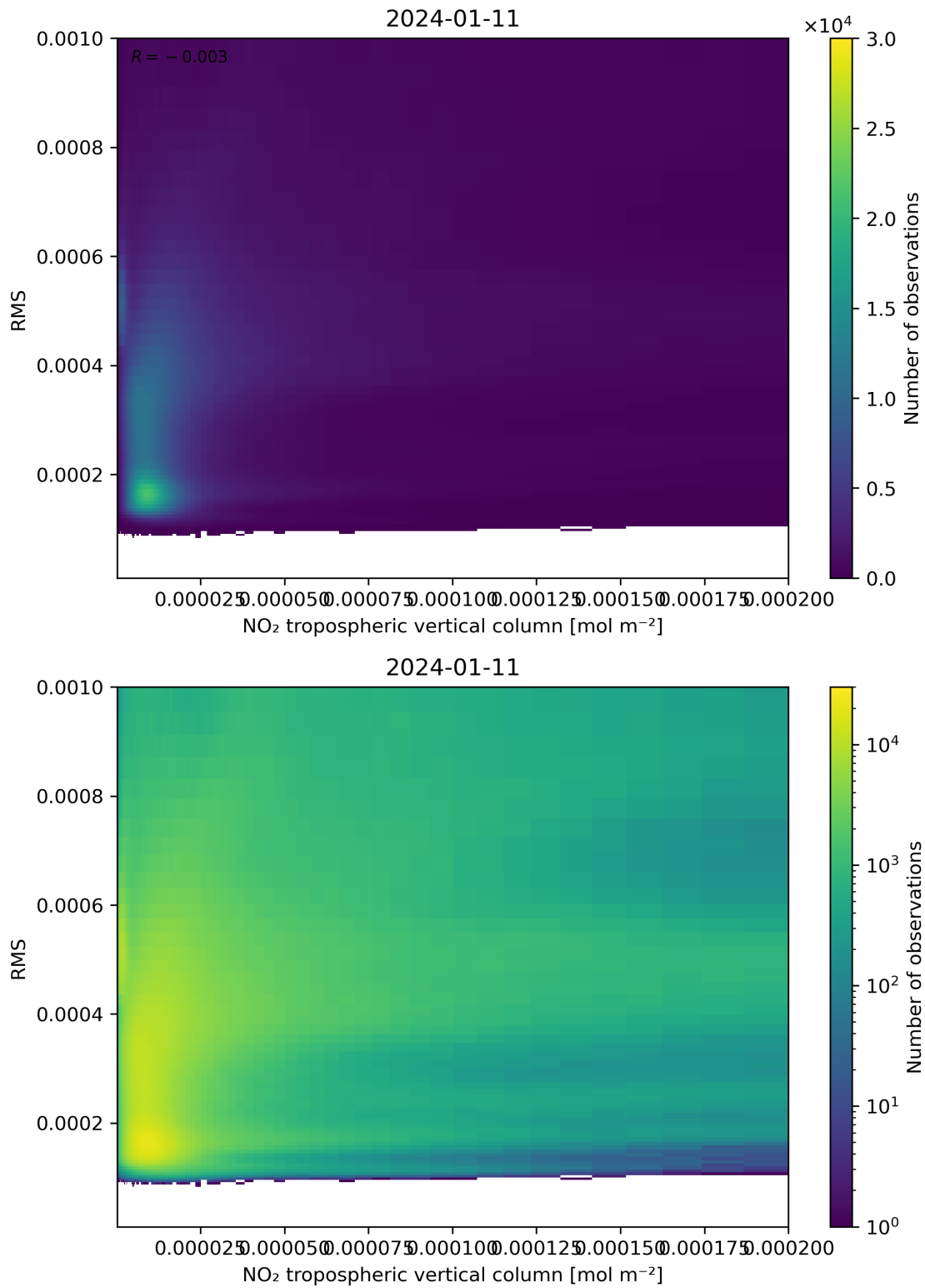
Figure 142: Scatter density plot of “NO 2 tropospheric vertical column” against “RMS” for 2024-01-10 to 2024-01-12.
