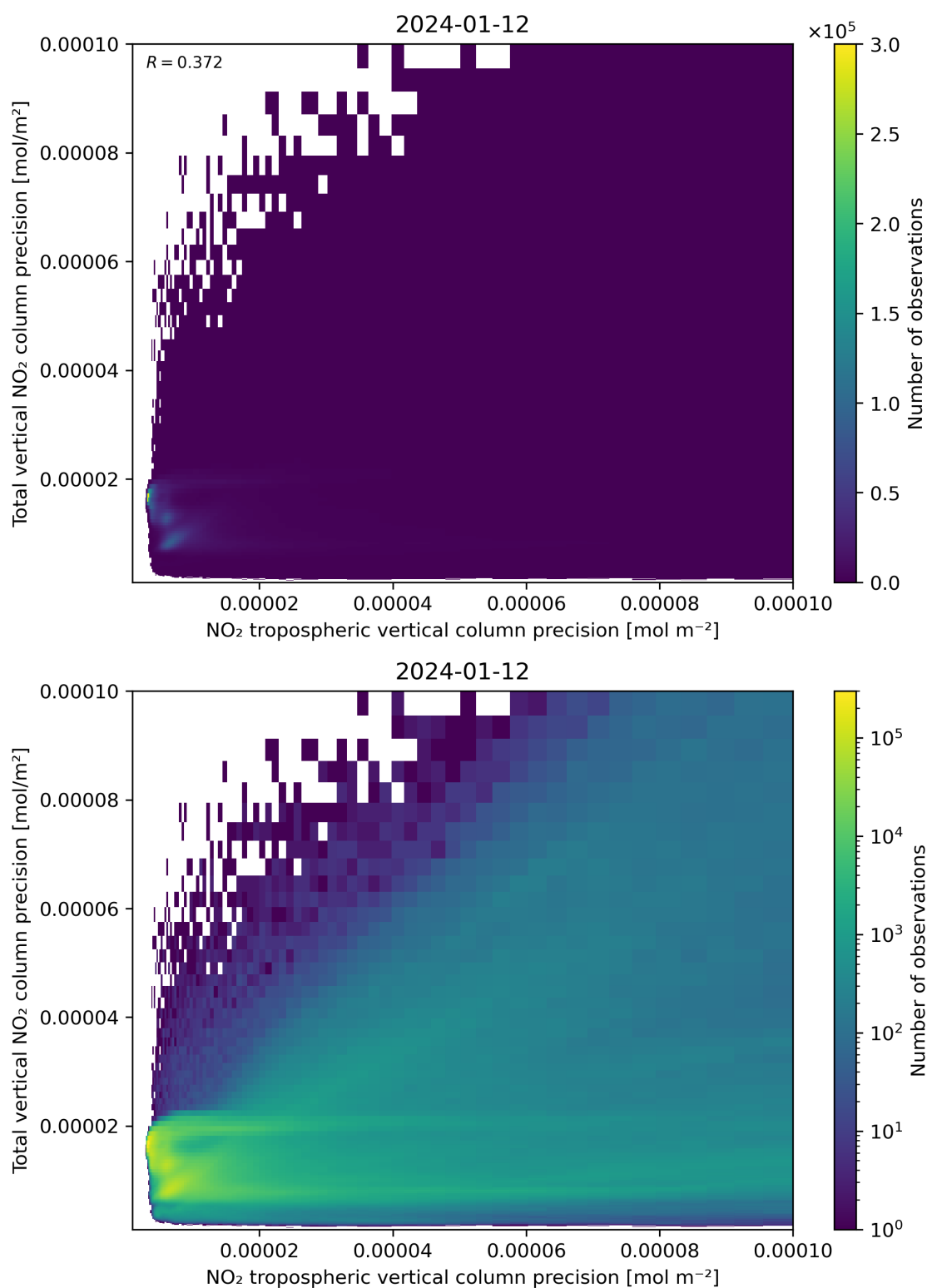
Figure 139: Scatter density plot of “NO 2 tropospheric vertical column precision” against “Total vertical NO 2 column precision” for 2024-01-11 to 2024-01-13.
