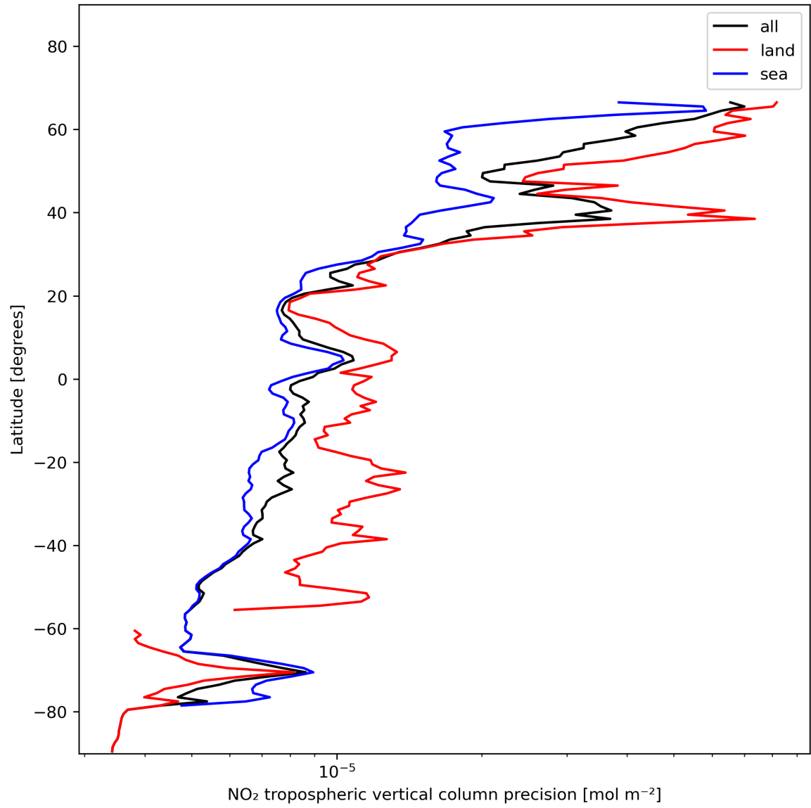
Figure 13: Zonal average of “NO 2 tropospheric vertical column precision” for 2024-01-11 to 2024-01-13.
