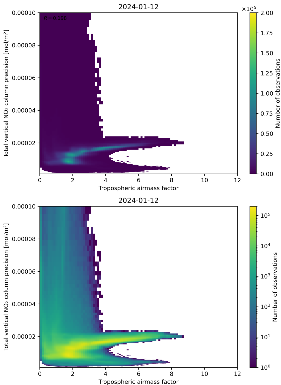
Figure 78: Scatter density plot of “Tropospheric air mass factor” against “Total vertical NO 2 column precision” for 2024-01-11 to 2024-01-13.
