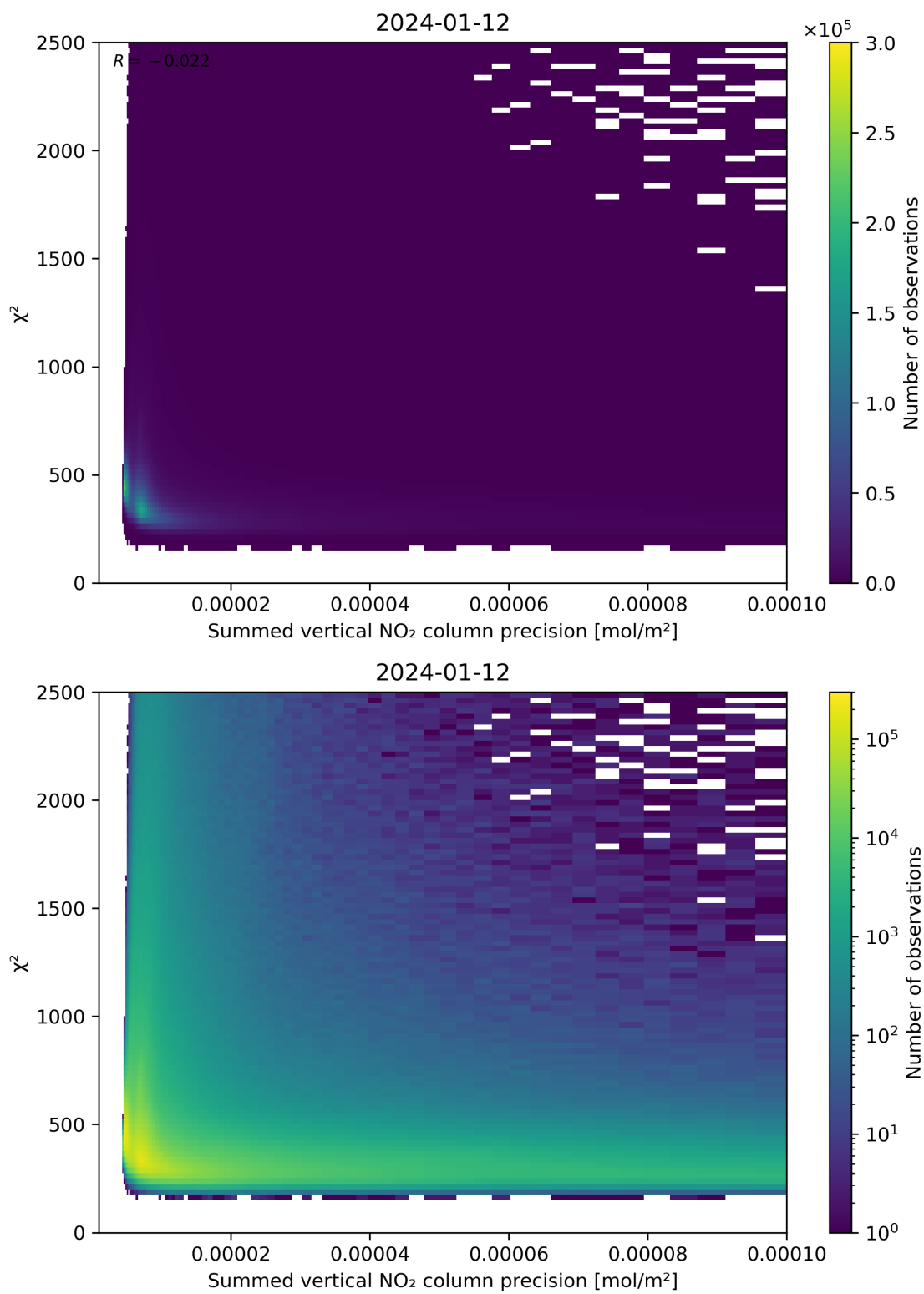
Figure 107: Scatter density plot of “Summed vertical NO 2 column precision” against “ \chi^2 ” for 2024-01-11 to 2024-01-13.
