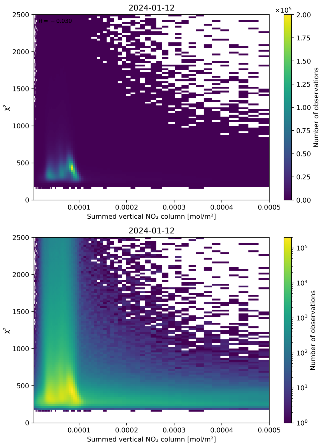
Figure 104: Scatter density plot of “Summed vertical NO 2 column” against “ \chi^2 ” for 2024-01-11 to 2024-01-13.
