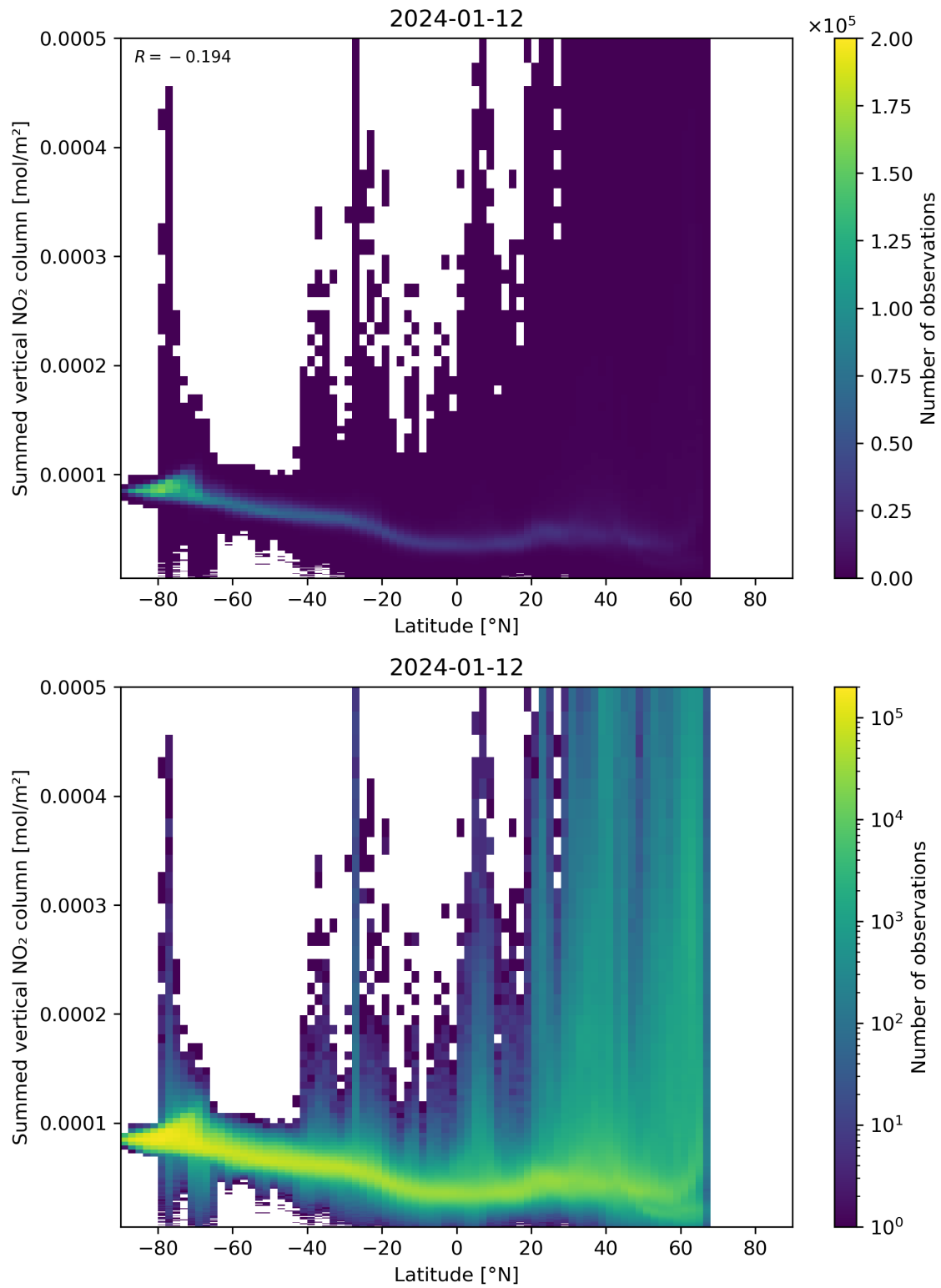
Figure 88: Scatter density plot of “Latitude” against “Summed vertical NO 2 column” for 2024-01-11 to 2024-01-13.
