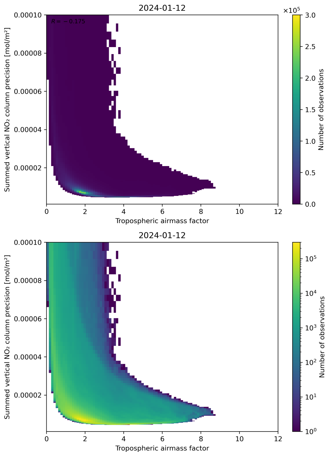
Figure 76: Scatter density plot of “Tropospheric air mass factor” against “Summed vertical NO 2 column precision” for 2024-01-11 to 2024-01-13.
