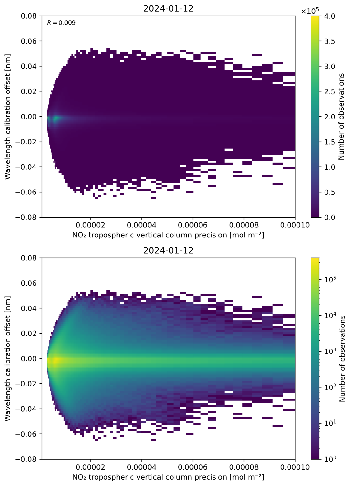
Figure 141: Scatter density plot of “NO 2 tropospheric vertical column precision” against “Wavelength calibration offset” for 2024-01-11 to 2024-01-13.
