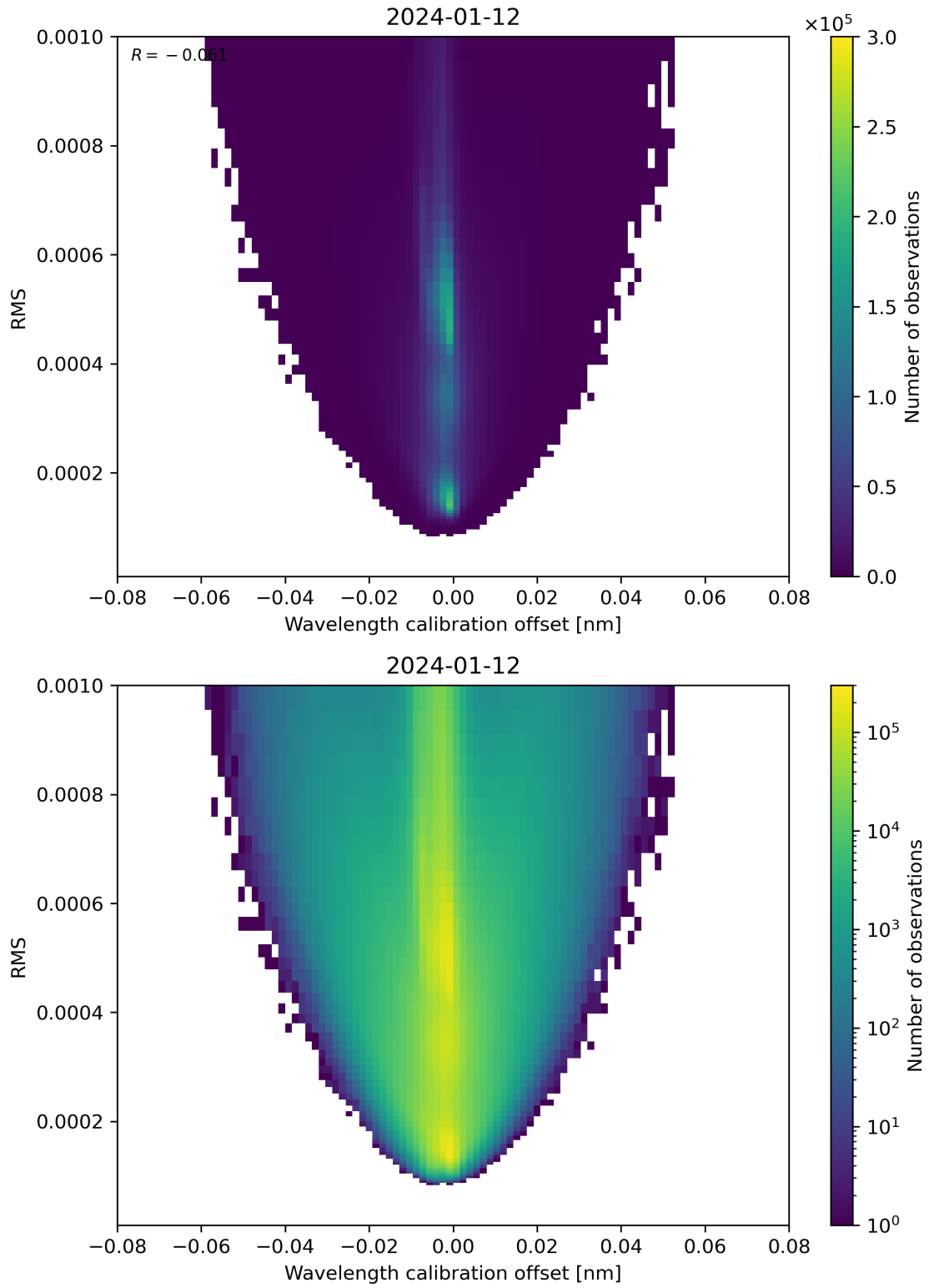
Figure 181: Scatter density plot of “Wavelength calibration offset” against “RMS” for 2024-01-11 to 2024-01-13.
