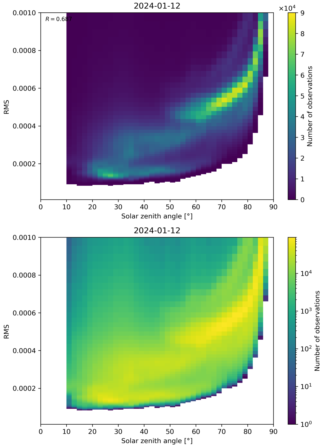
Figure 157: Scatter density plot of “Solar zenith angle” against “RMS” for 2024-01-11 to 2024-01-13.
