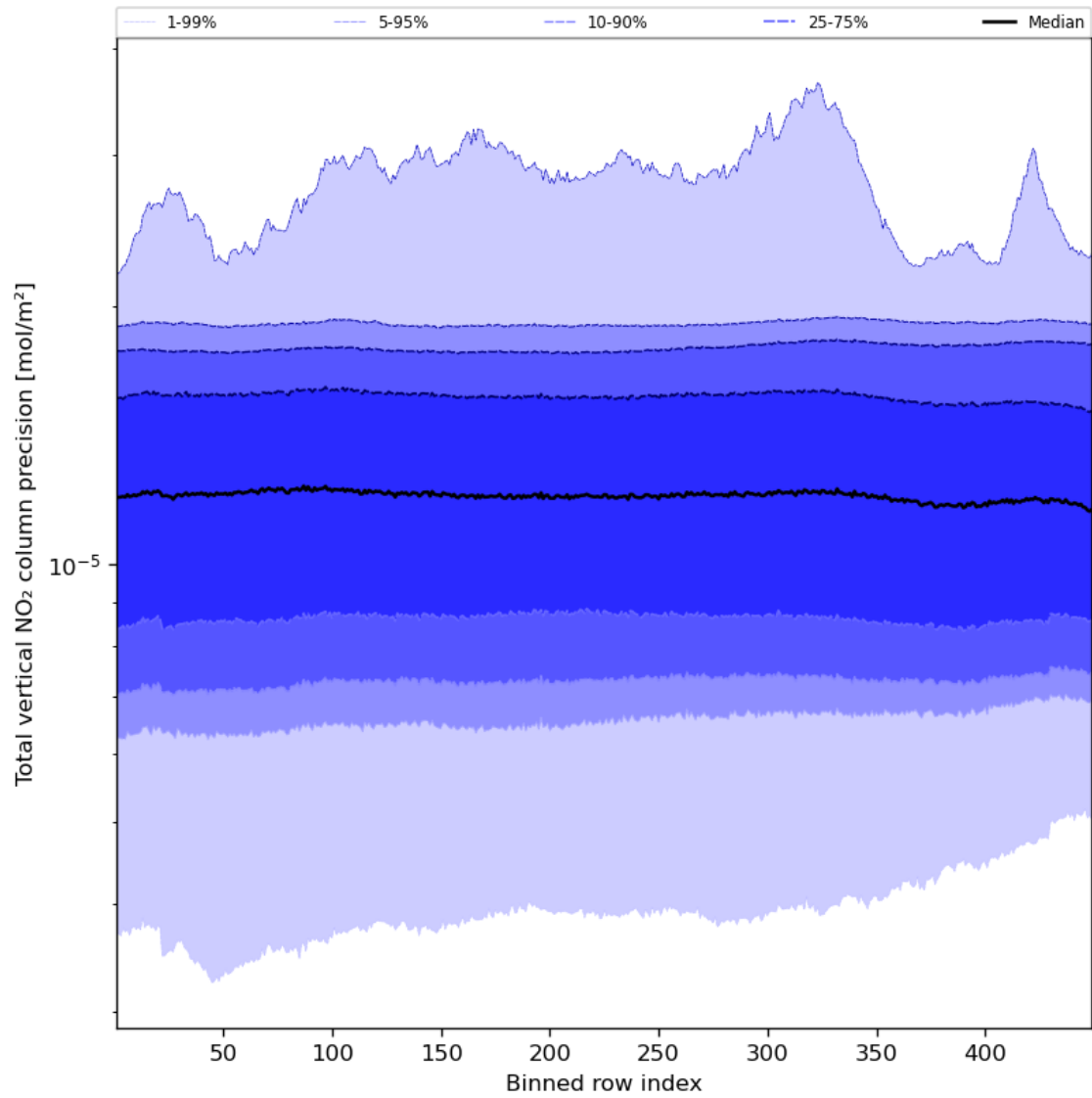
Figure 56: Along track statistics of “Total vertical NO 2 column precision” for 2024-01-11 to 2024-01-13
