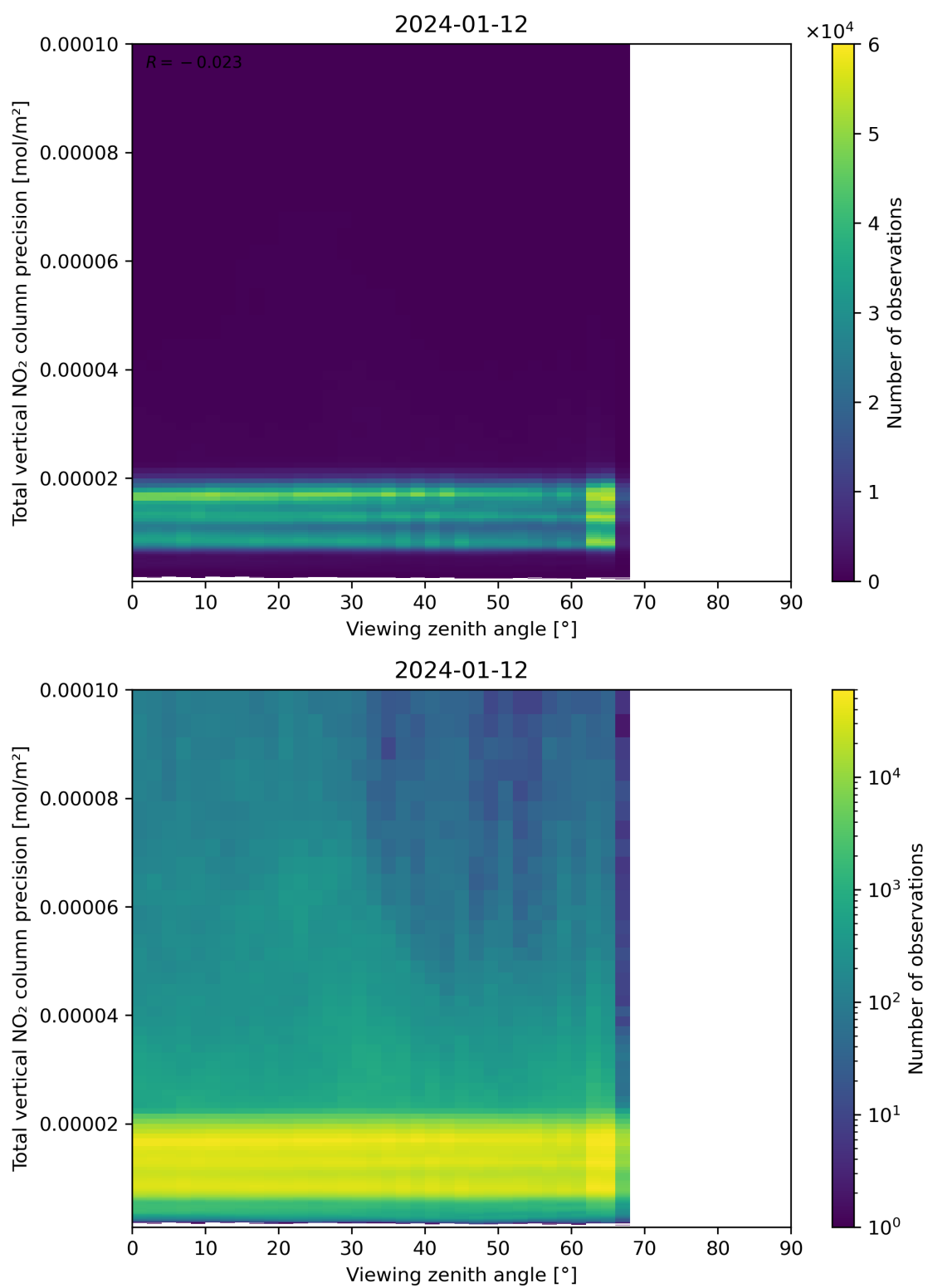
Figure 168: Scatter density plot of “Viewing zenith angle” against “Total vertical NO 2 column precision” for 2024-01-11 to 2024-01-13.
