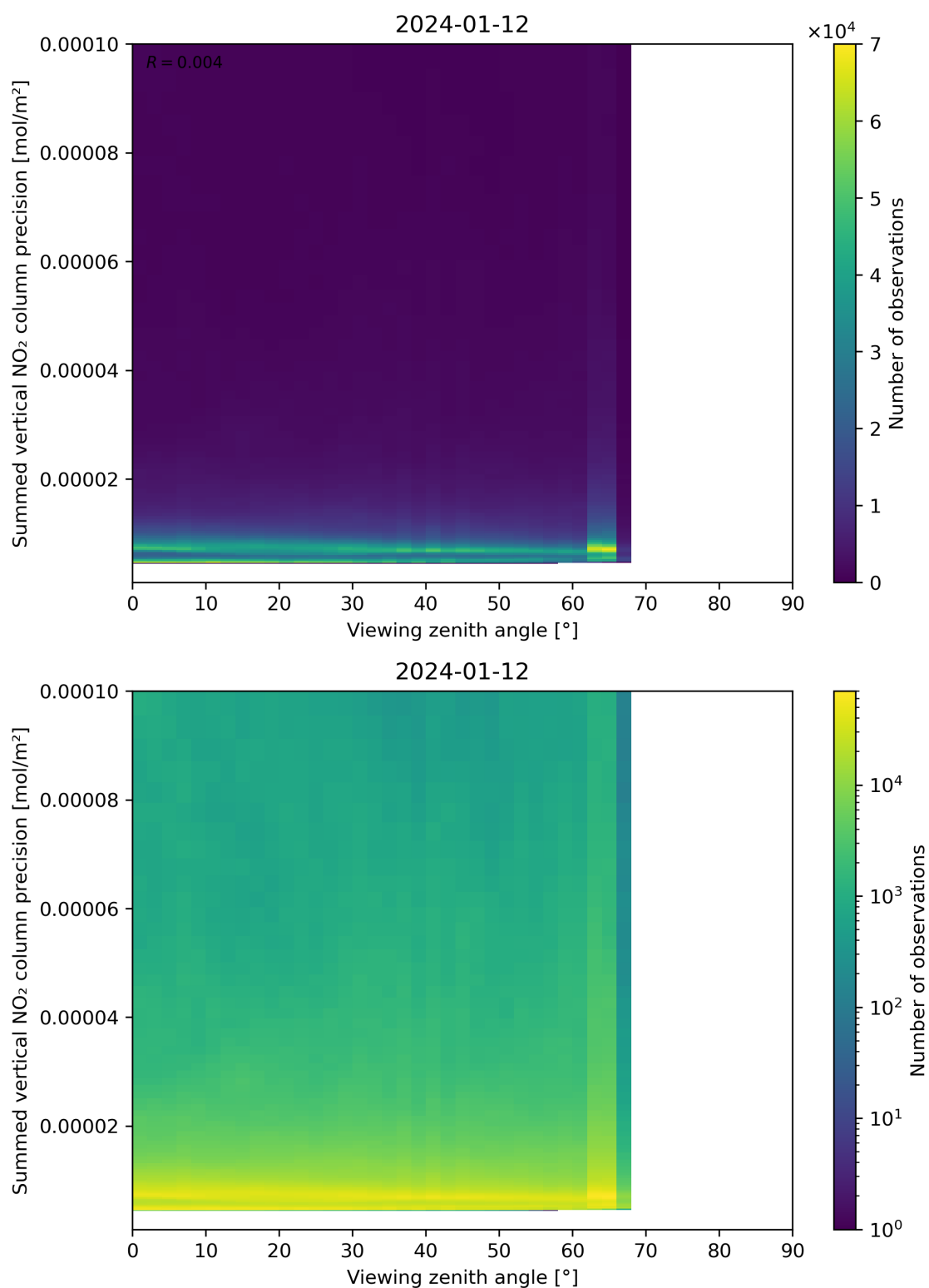
Figure 166: Scatter density plot of “Viewing zenith angle” against “Summed vertical NO 2 column precision” for 2024-01-11 to 2024-01-13.
