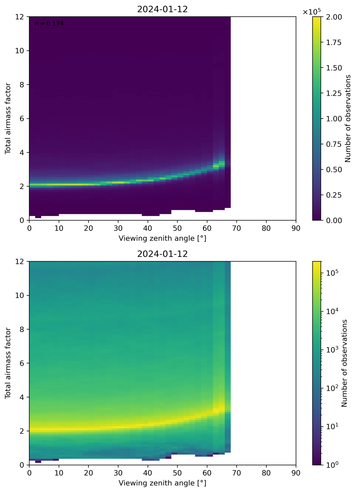
Figure 160: Scatter density plot of “Viewing zenith angle” against “Total airmass factor” for 2024-01-11 to 2024-01-13.
