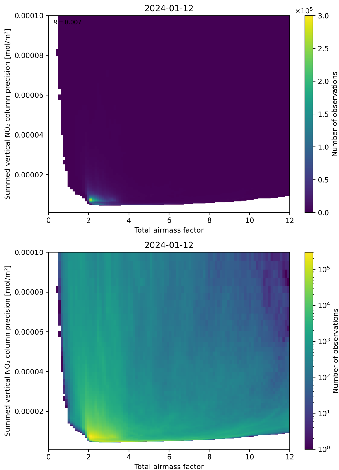
Figure 66: Scatter density plot of “Total airmass factor” against “Summed vertical NO 2 column precision” for 2024-01-11 to 2024-01-13.
