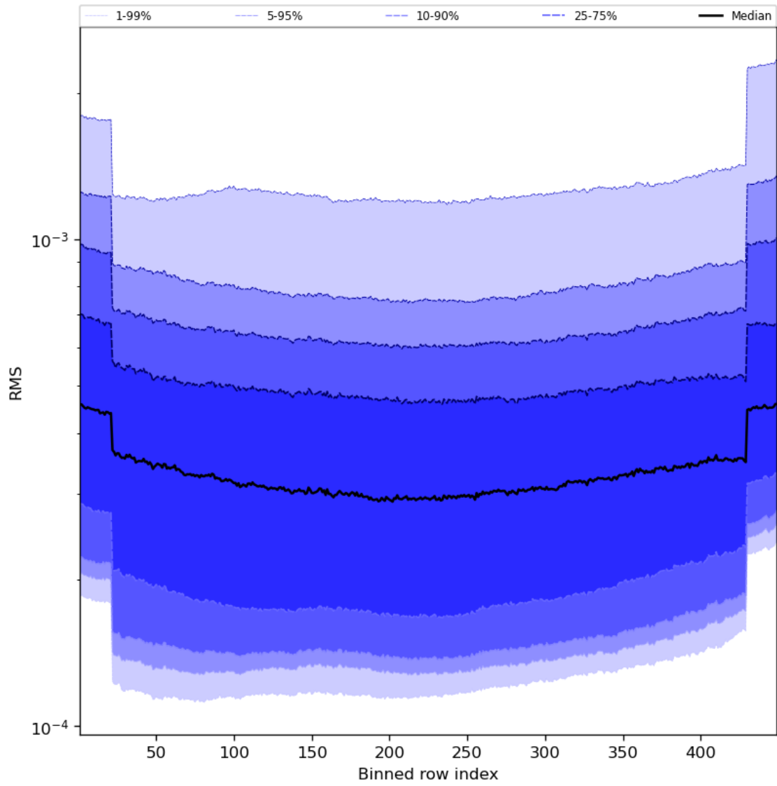
Figure 60: Along track statistics of “RMS” for 2024-01-11 to 2024-01-13
