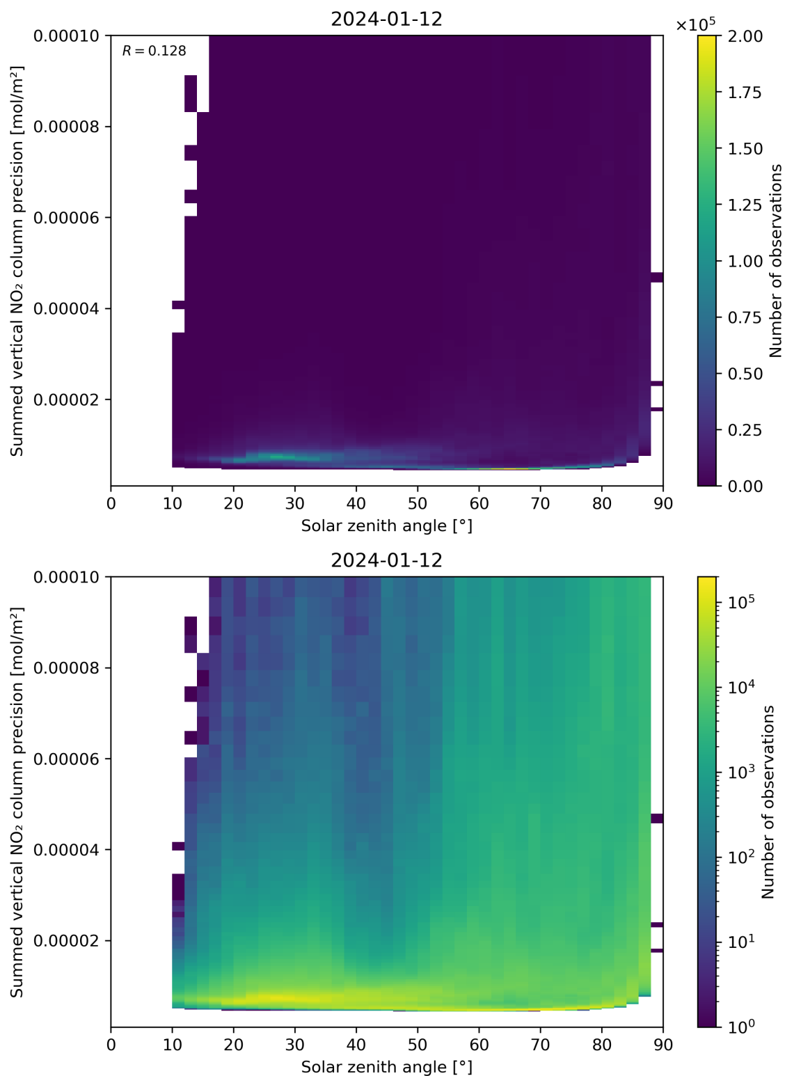
Figure 152: Scatter density plot of “Solar zenith angle” against “Summed vertical NO 2 column precision” for 2024-01-11 to 2024-01-13.
