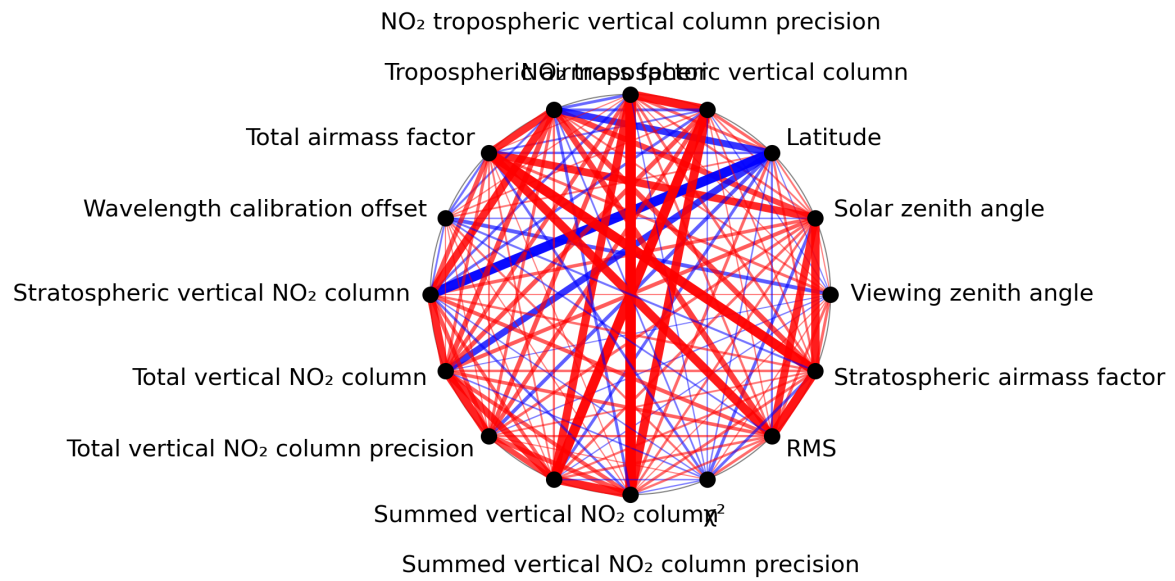
Figure 1: Map of correlation graph for 2024-01-11 to 2024-01-13.
