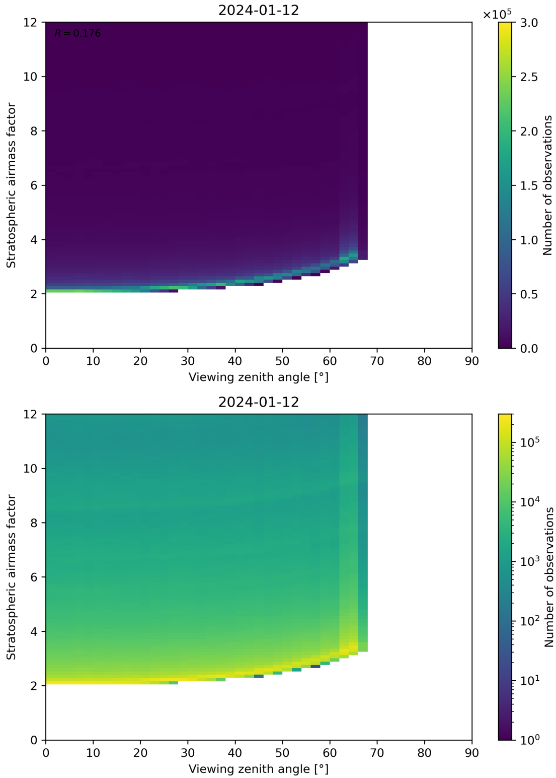
Figure 159: Scatter density plot of “Viewing zenith angle” against “Stratospheric airmass factor” for 2024-01-11 to 2024-01-13.
