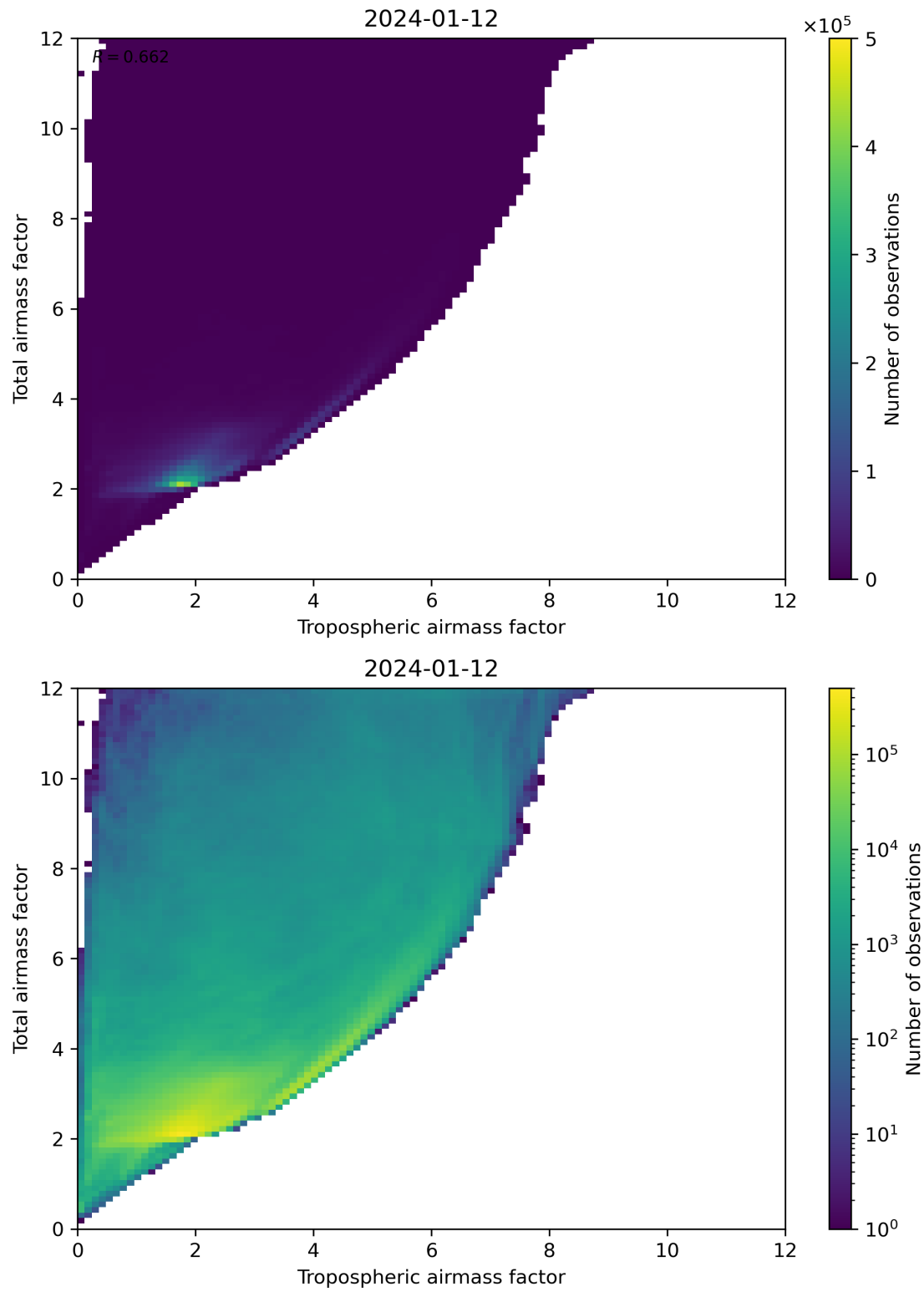
Figure 72: Scatter density plot of “Tropospheric airmass factor” against “Total airmass factor” for 2024-01-11 to 2024-01-13.
