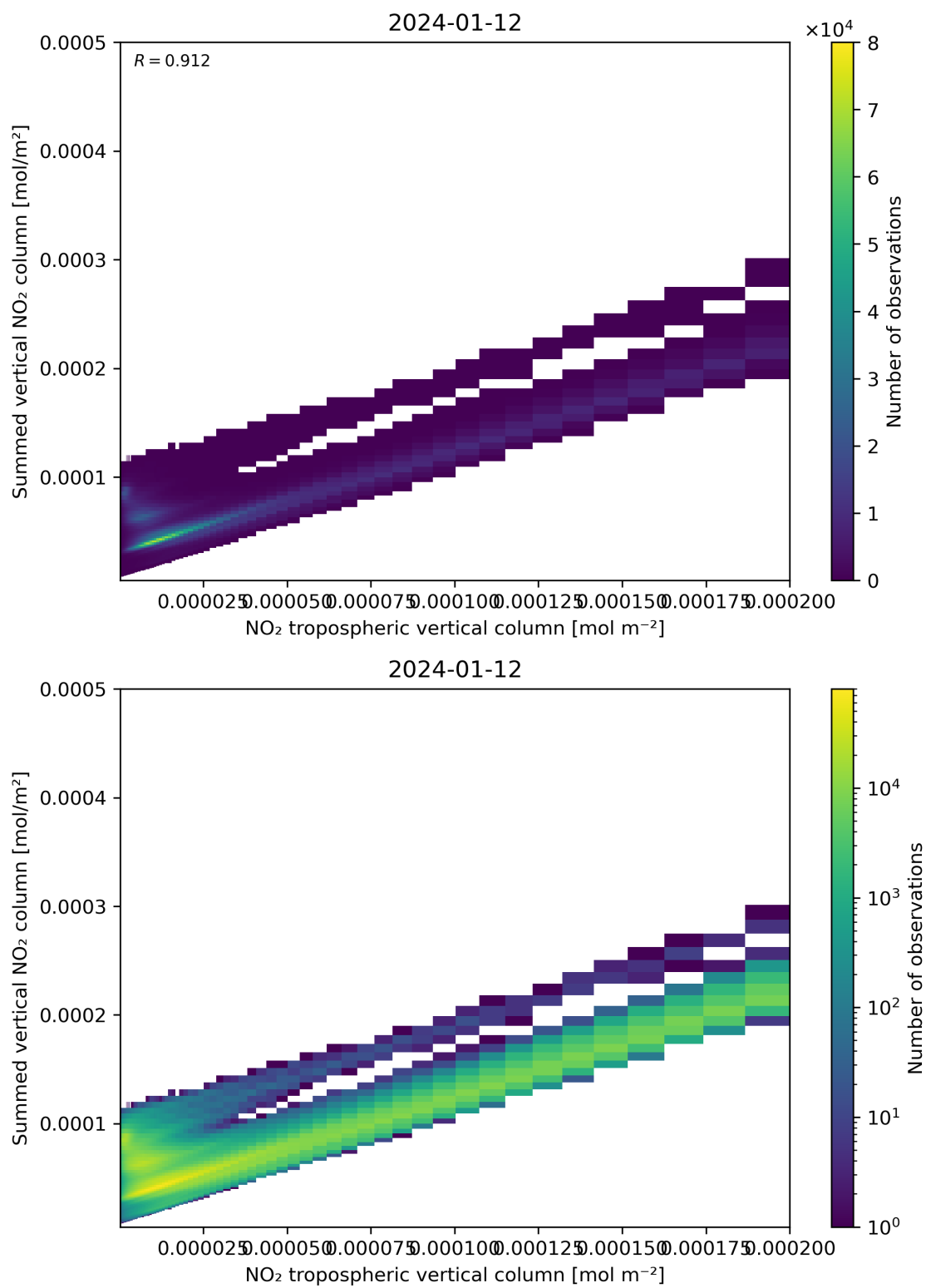
Figure 126: Scatter density plot of “NO 2 tropospheric vertical column” against “Summed vertical NO 2 column” for 2024-01-11 to 2024-01-13.
