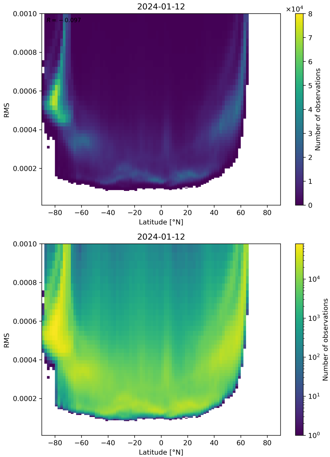
Figure 94: Scatter density plot of “Latitude” against “RMS” for 2024-01-11 to 2024-01-13.
