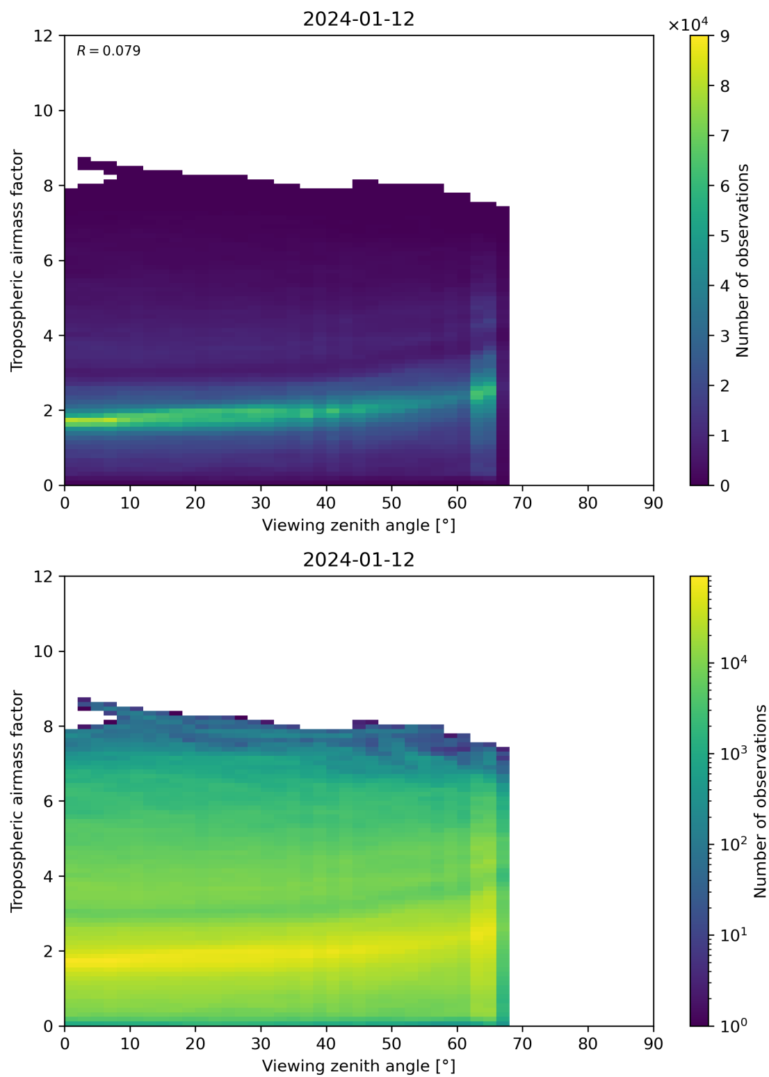
Figure 161: Scatter density plot of “Viewing zenith angle” against “Tropospheric airmass factor” for 2024-01-11 to 2024-01-13.
