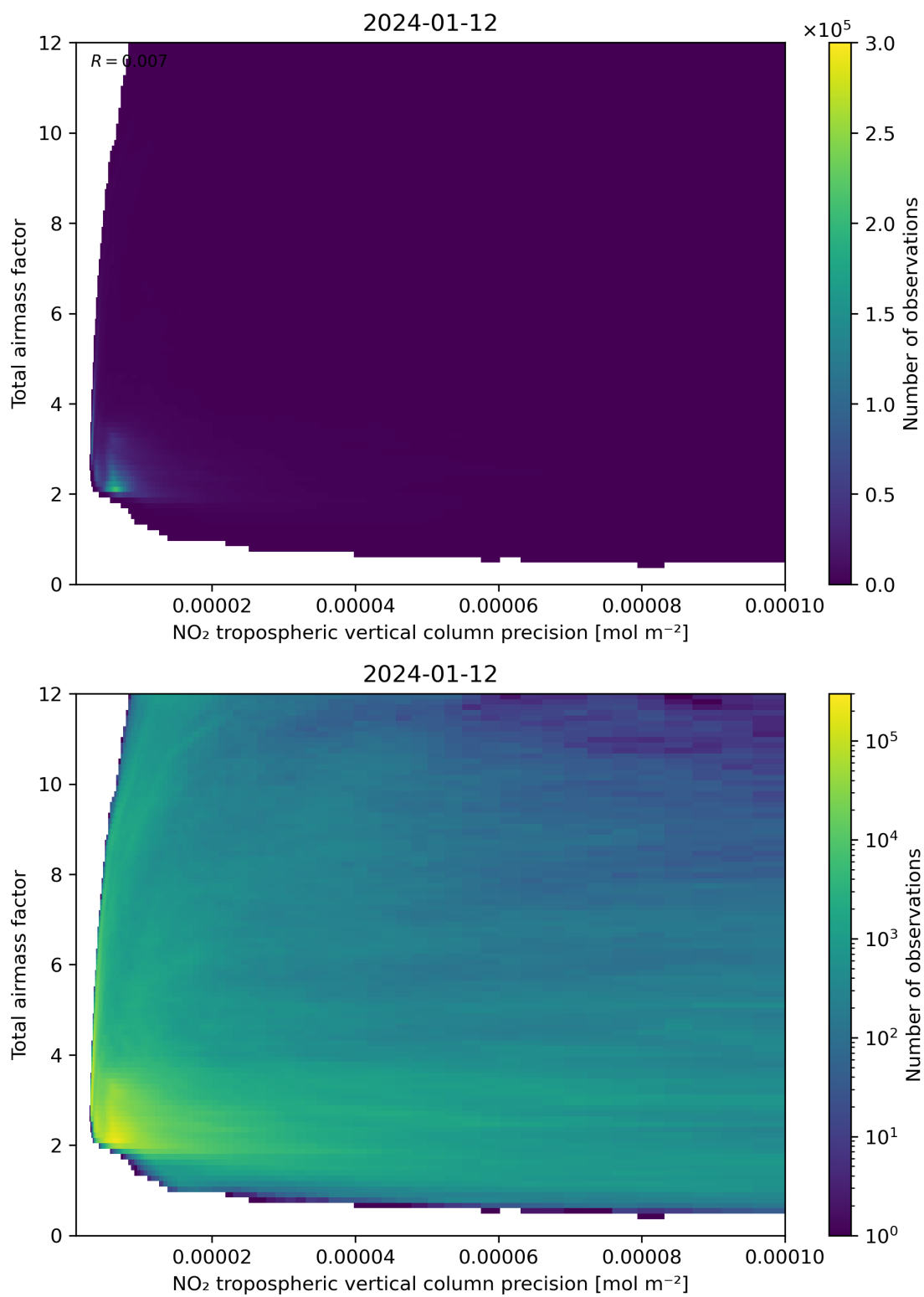
Figure 132: Scatter density plot of “NO 2 tropospheric vertical column precision” against “Total air mass factor” for 2024-01-11 to 2024-01-13.
