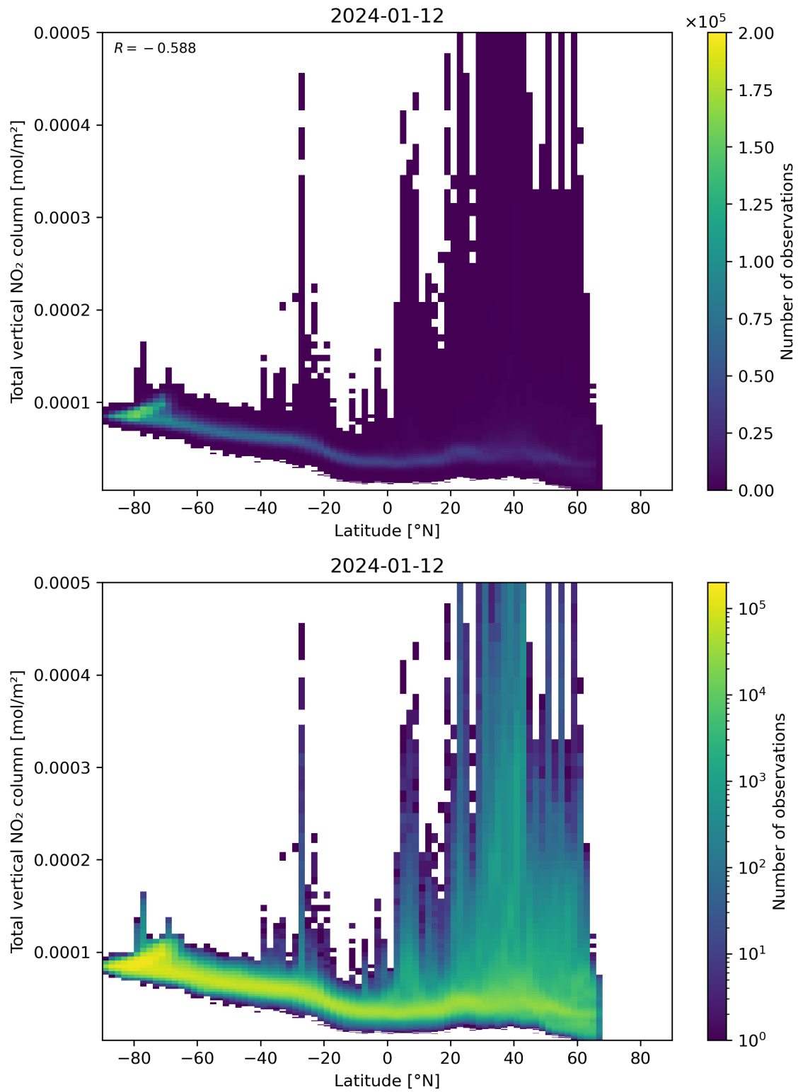
Figure 90: Scatter density plot of “Latitude” against “Total vertical NO 2 column” for 2024-01-11 to 2024-01-13.
