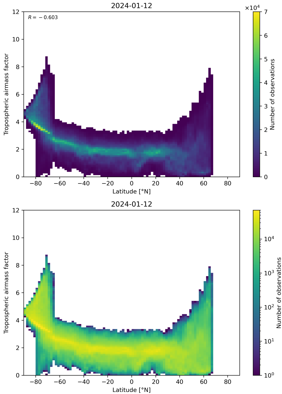
Figure 85: Scatter density plot of “Latitude” against “Tropospheric airmass factor” for 2024-01-11 to 2024-01-13.
