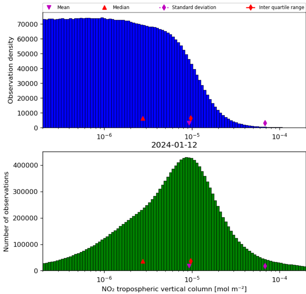
Figure 29: Histogram of “NO 2 tropospheric vertical column” for 2024-01-11 to 2024-01-13
