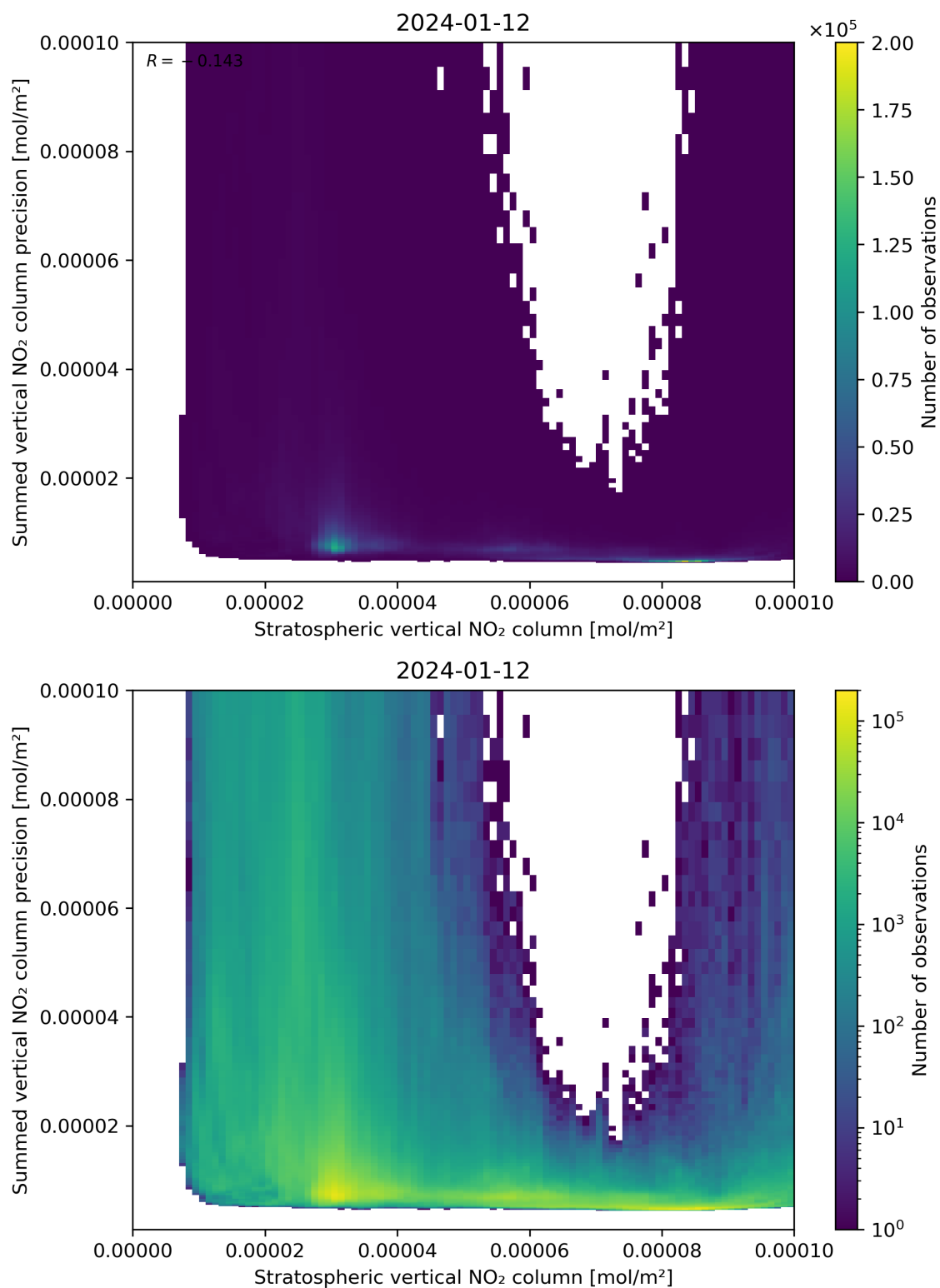
Figure 99: Scatter density plot of “Stratospheric vertical NO 2 column” against “Summed vertical NO 2 column precision” for 2024-01-11 to 2024-01-13.
