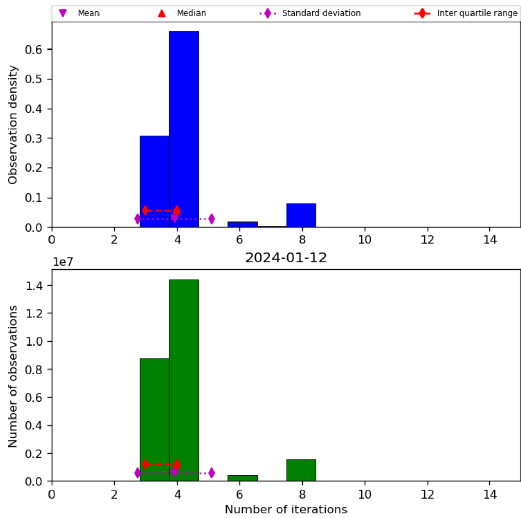
Figure 34: Histogram of “Number of iterations” for 2024-01-11 to 2024-01-13
