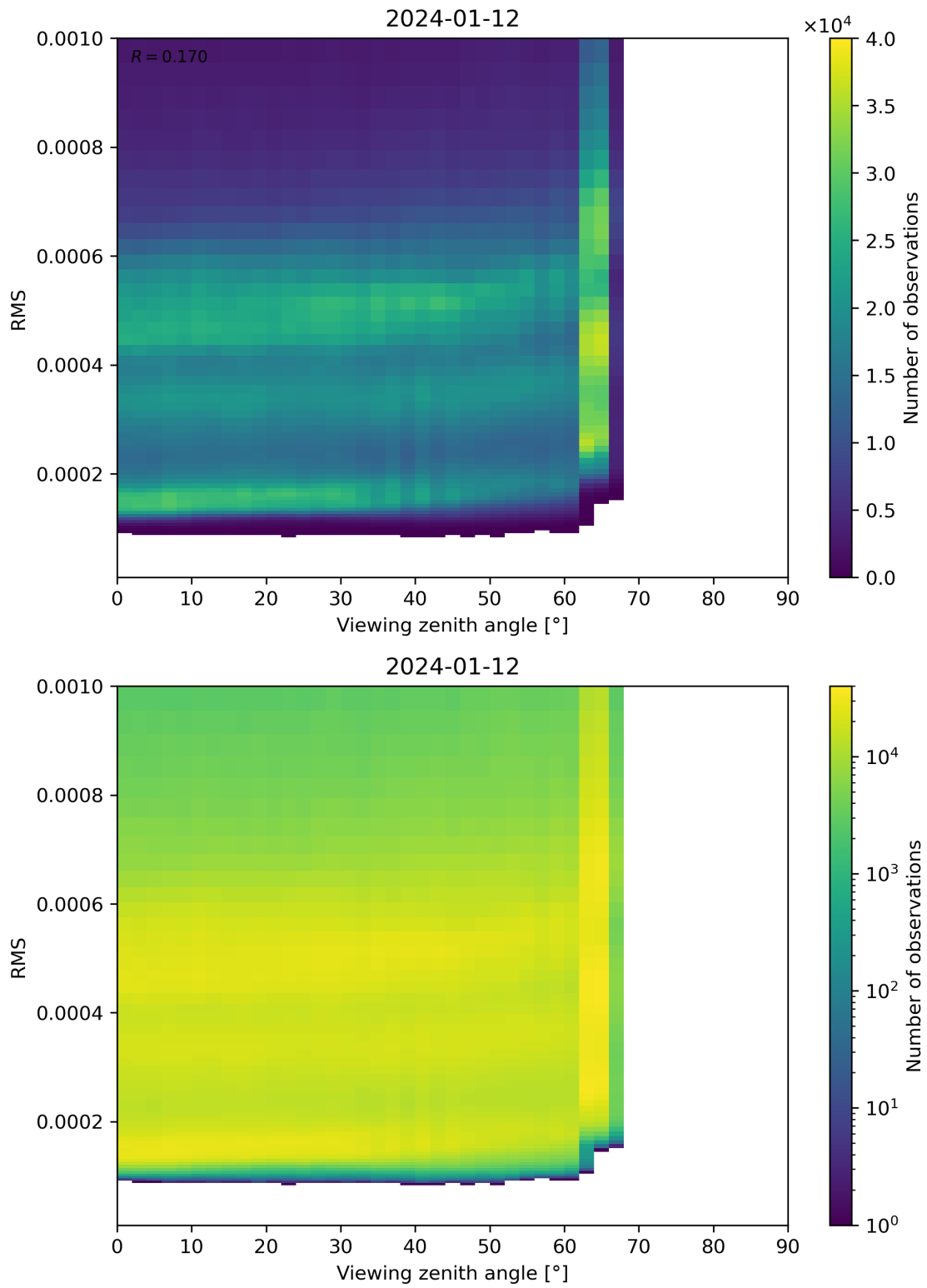
Figure 171: Scatter density plot of “Viewing zenith angle” against “RMS” for 2024-01-11 to 2024-01-13.
