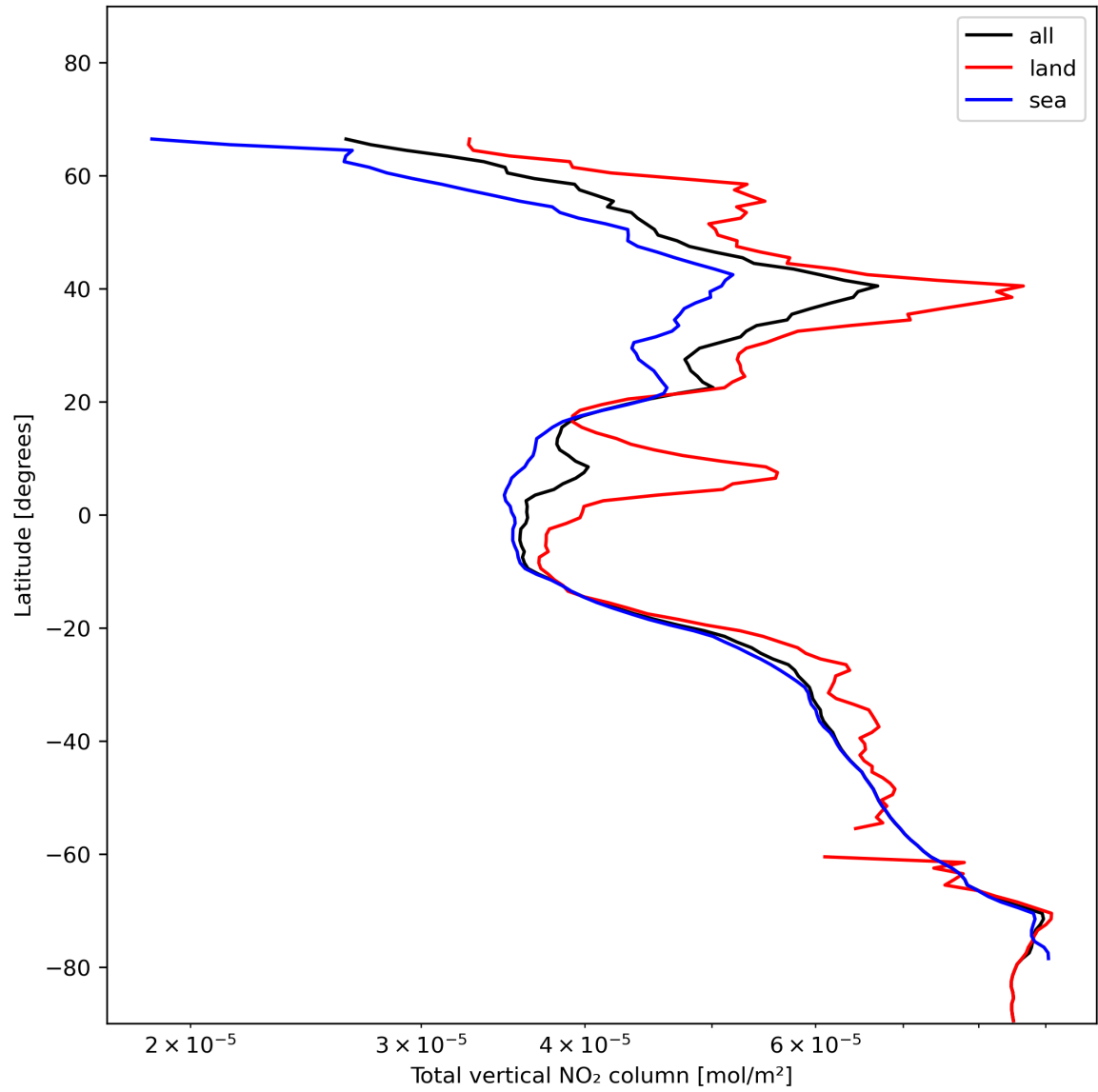
Figure 21: Zonal average of “Total vertical NO 2 column” for 2024-01-11 to 2024-01-13.
