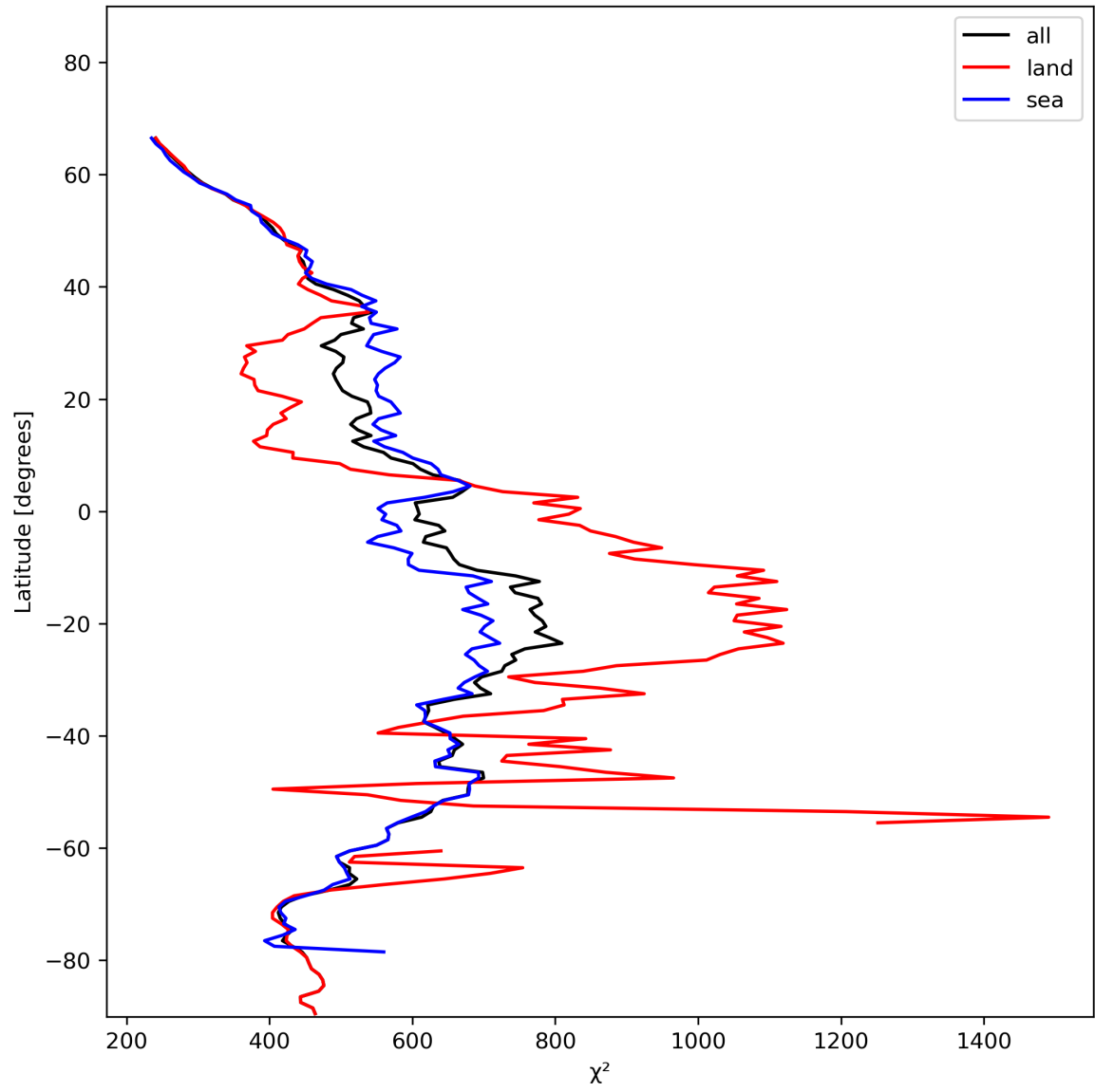
Figure 25: Zonal average of “ \chi^2 ” for 2024-01-11 to 2024-01-13.
