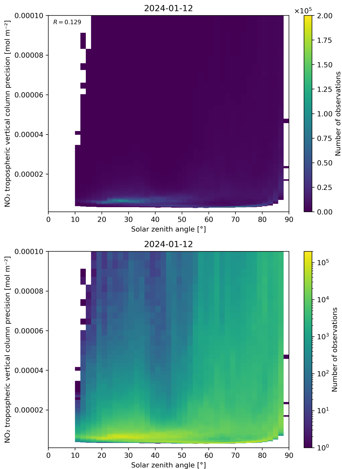
Figure 156: Scatter density plot of “Solar zenith angle” against “NO 2 tropospheric vertical column precision” for 2024-01-11 to 2024-01-13.
