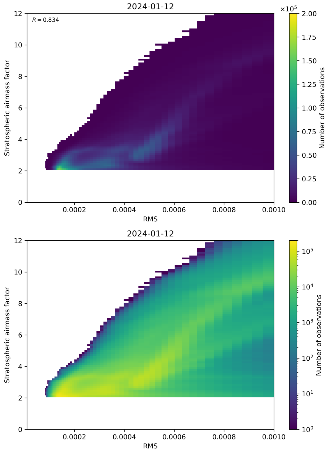
Figure 144: Scatter density plot of “RMS” against “Stratospheric airmass factor” for 2024-01-11 to 2024-01-13.
