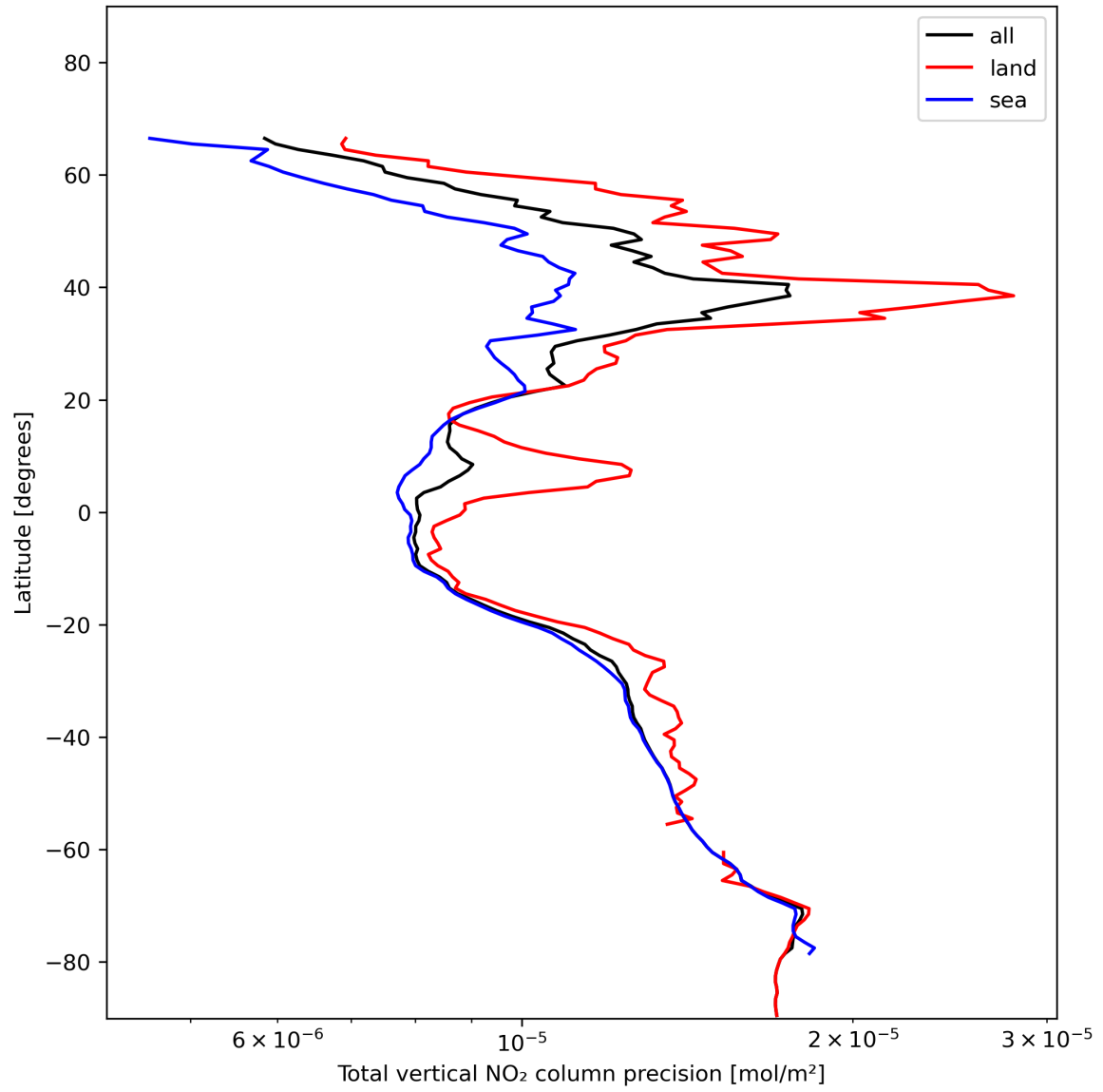
Figure 22: Zonal average of “Total vertical NO 2 column precision” for 2024-01-11 to 2024-01-13.
