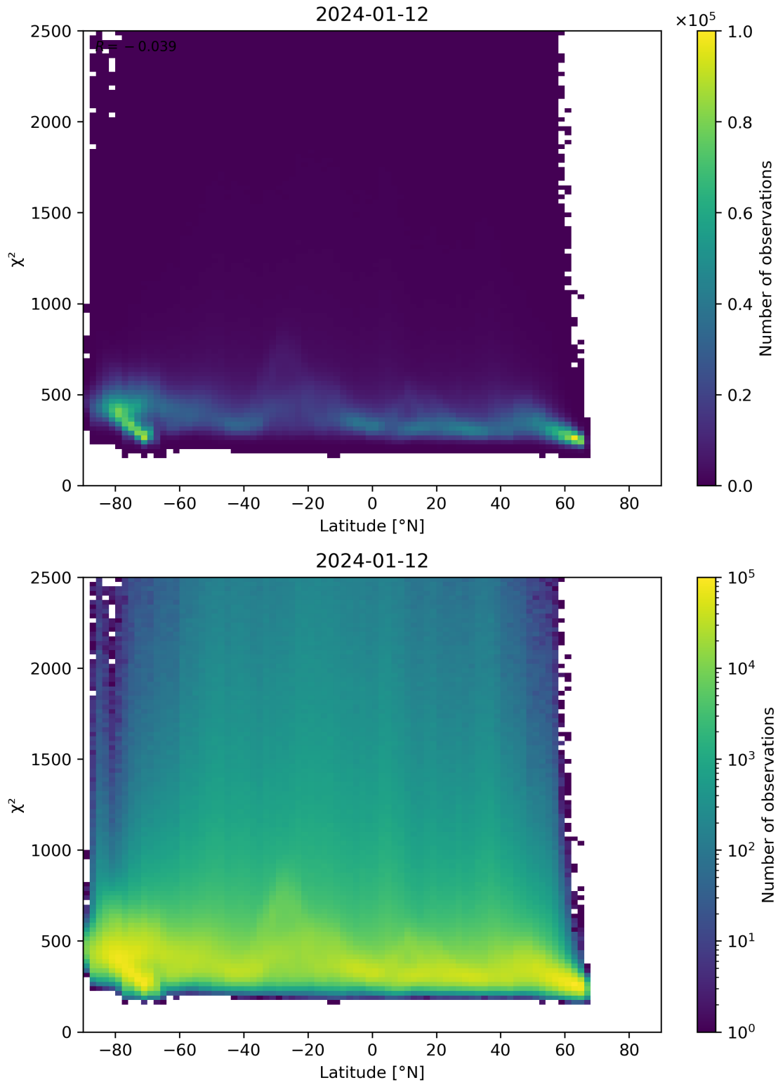
Figure 86: Scatter density plot of “Latitude” against “ \chi^2 ” for 2024-01-11 to 2024-01-13.
