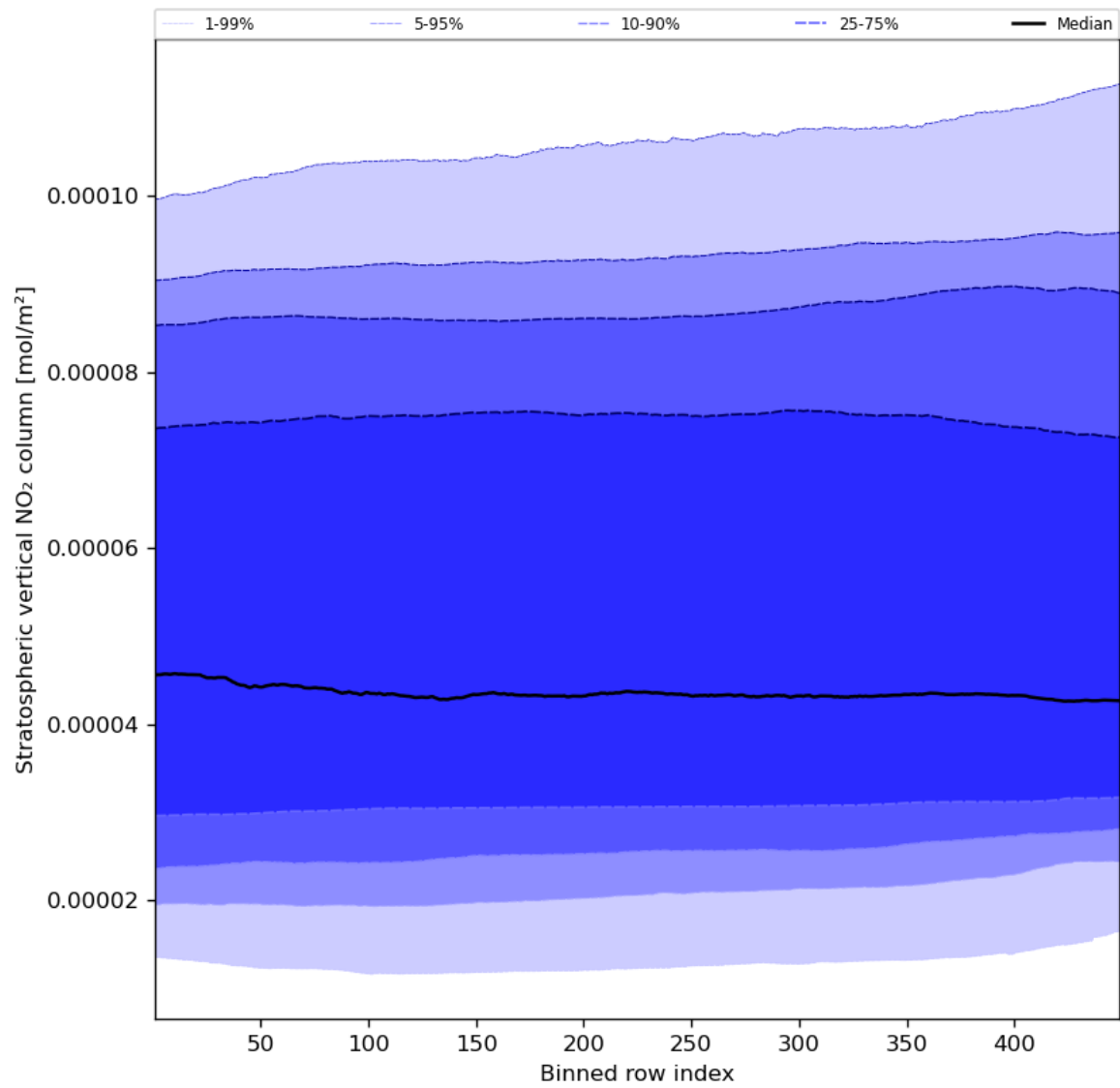
Figure 53: Along track statistics of “Stratospheric vertical NO 2 column” for 2024-01-11 to 2024-01-13
