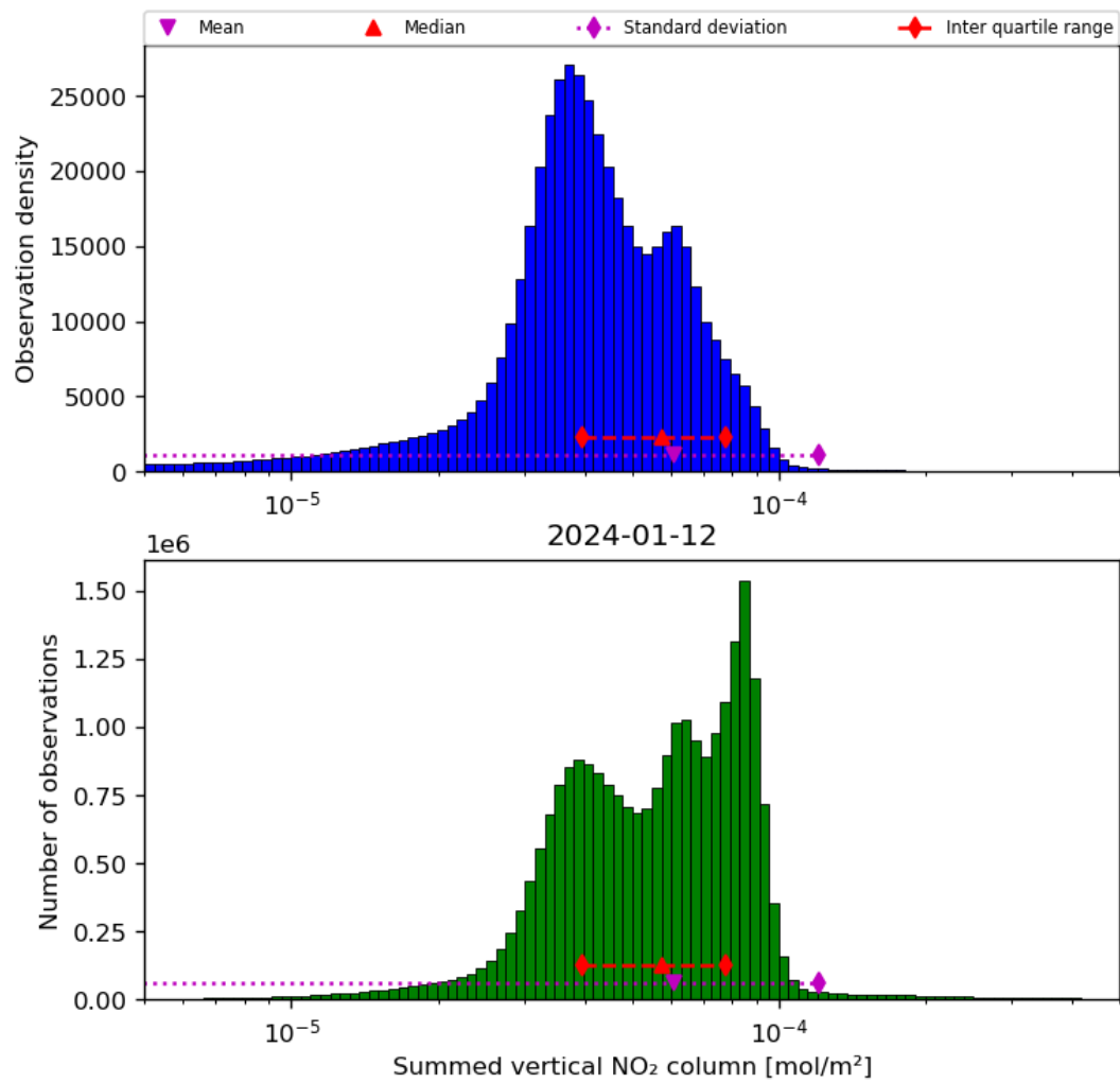
Figure 40: Histogram of “Summed vertical NO 2 column” for 2024-01-11 to 2024-01-13
