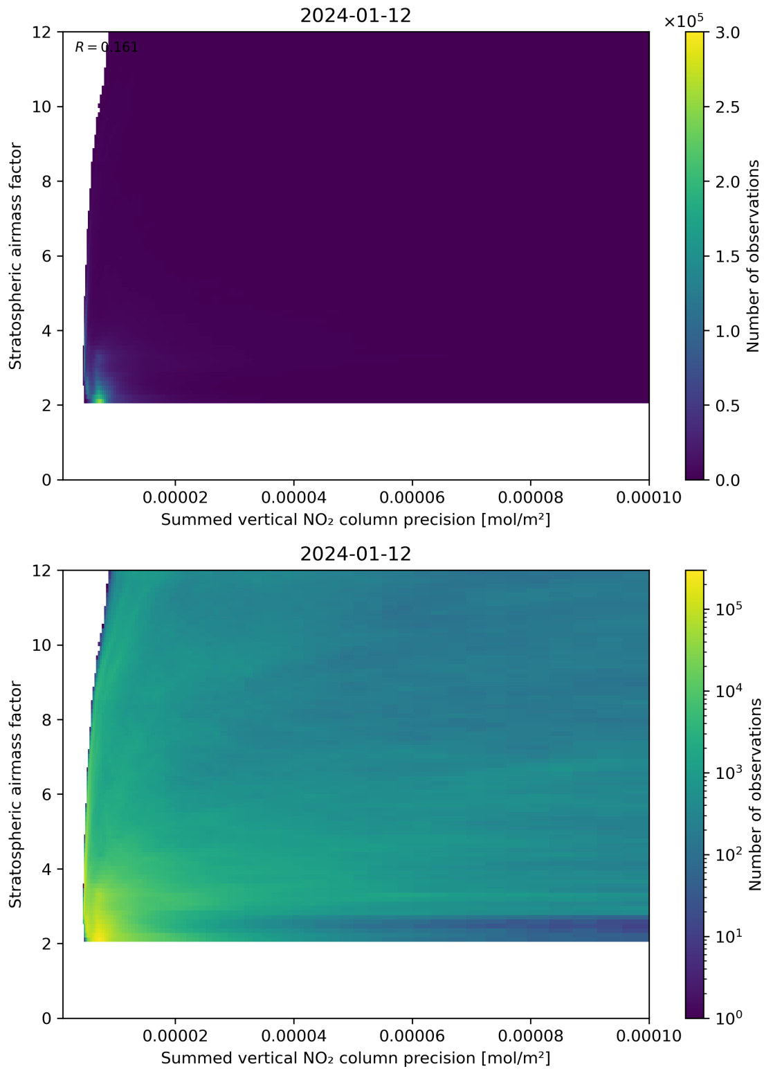
Figure 106: Scatter density plot of “Summed vertical NO 2 column precision” against “Stratospheric airmass factor” for 2024-01-11 to 2024-01-13.
