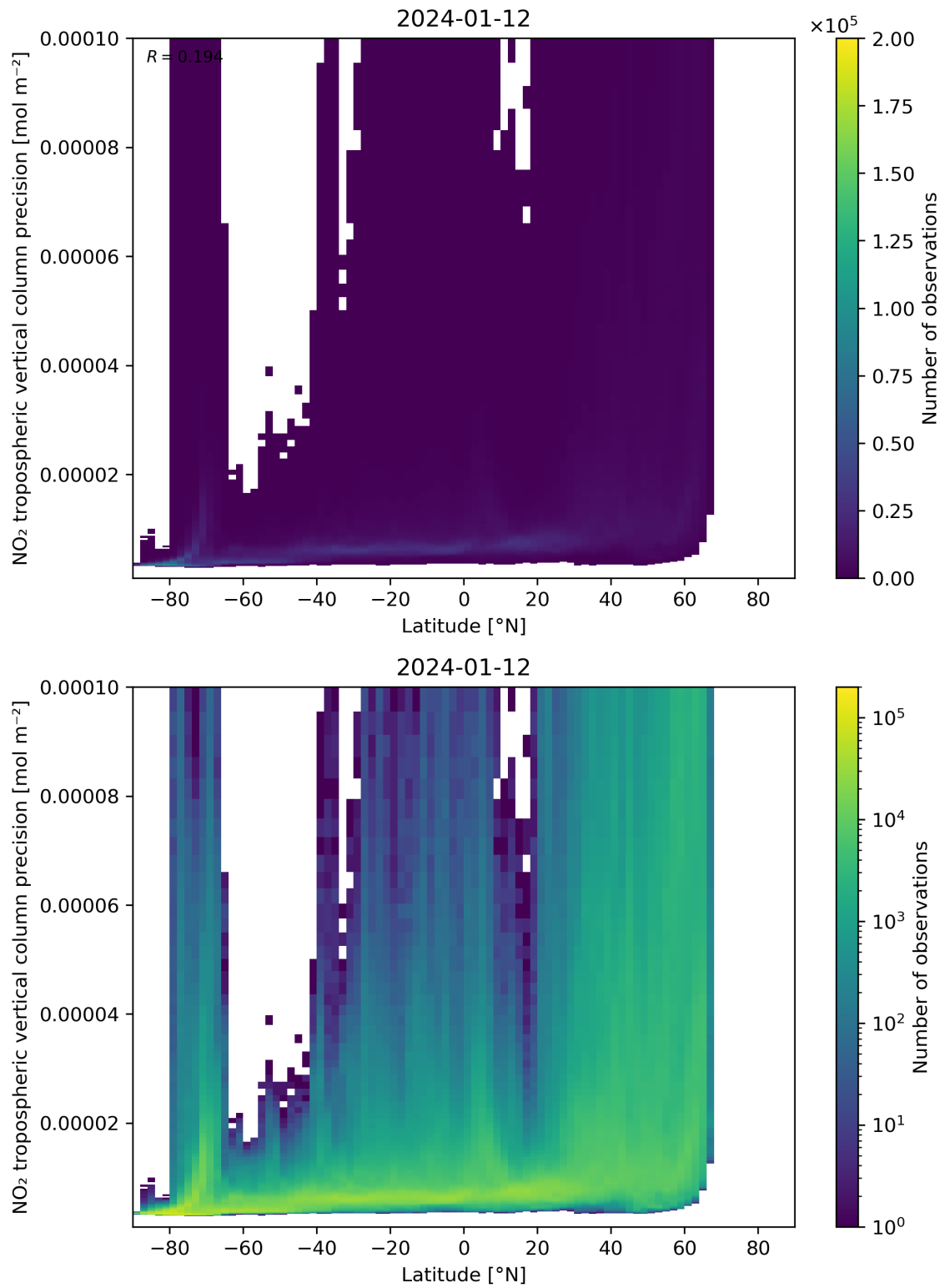
Figure 93: Scatter density plot of “Latitude” against “NO 2 tropospheric vertical column precision” for 2024-01-11 to 2024-01-13.
