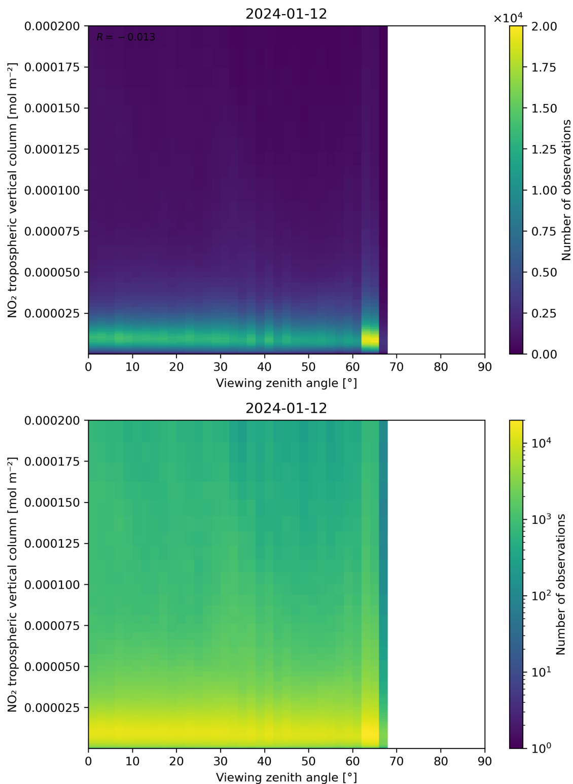
Figure 169: Scatter density plot of “Viewing zenith angle” against “NO 2 tropospheric vertical column” for 2024-01-11 to 2024-01-13.
