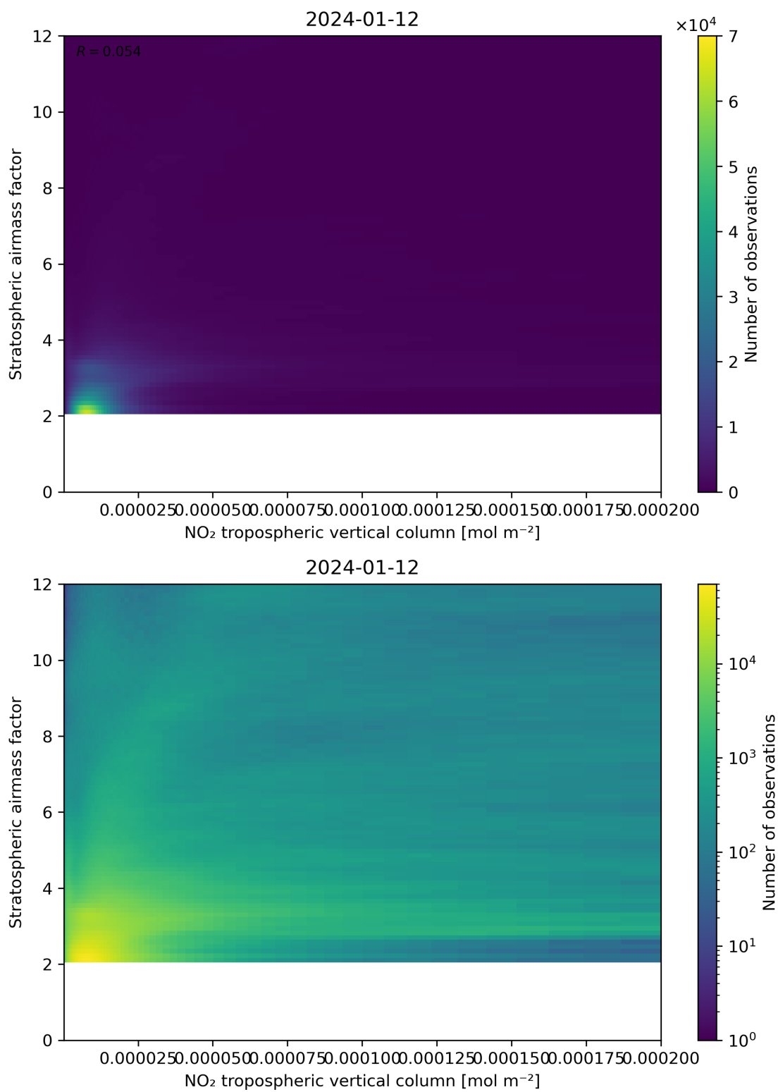
Figure 121: Scatter density plot of “NO 2 tropospheric vertical column” against “Stratospheric airmass factor” for 2024-01-11 to 2024-01-13.
