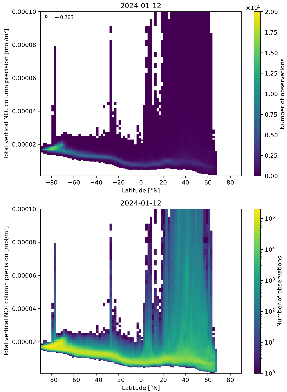
Figure 91: Scatter density plot of “Latitude” against “Total vertical NO 2 column precision” for 2024-01-11 to 2024-01-13.
