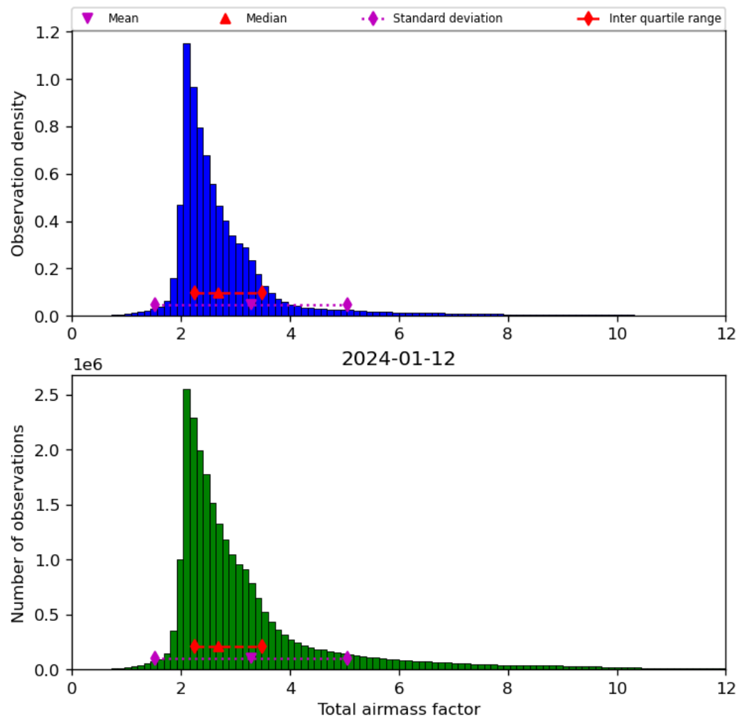
Figure 32: Histogram of “Total airmass factor” for 2024-01-11 to 2024-01-13
