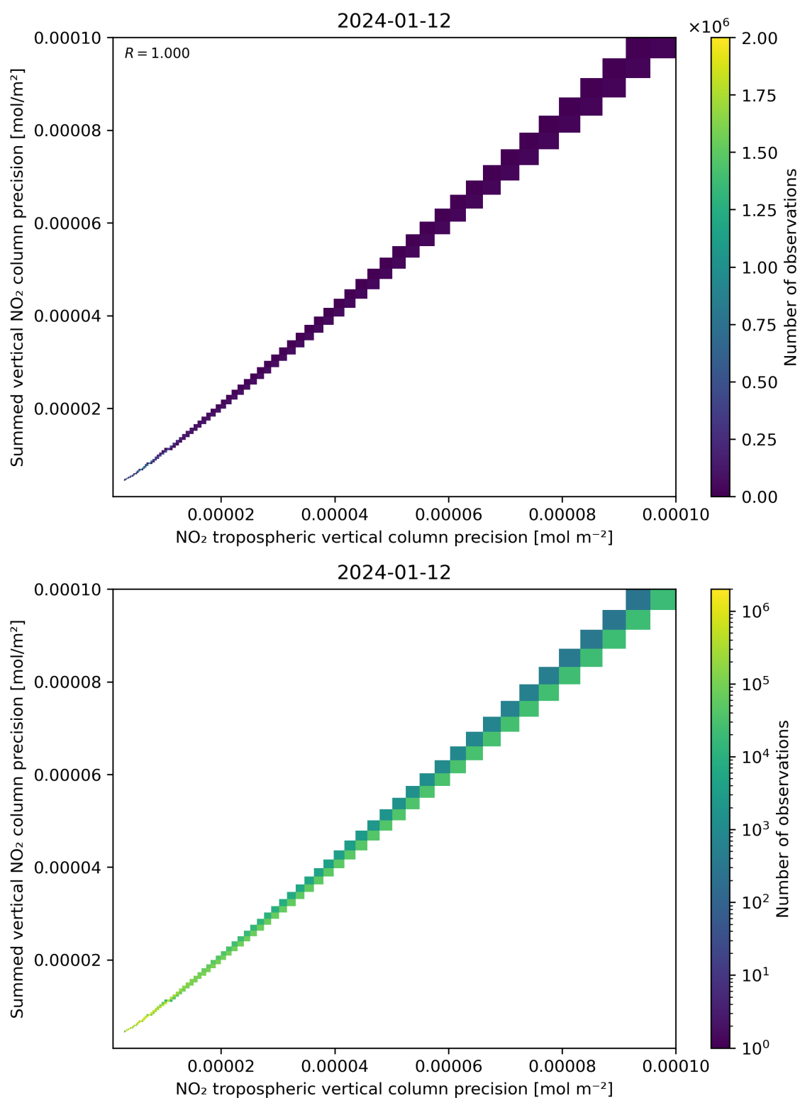
Figure 137: Scatter density plot of “NO 2 tropospheric vertical column precision” against “Summed vertical NO 2 column precision” for 2024-01-11 to 2024-01-13.
