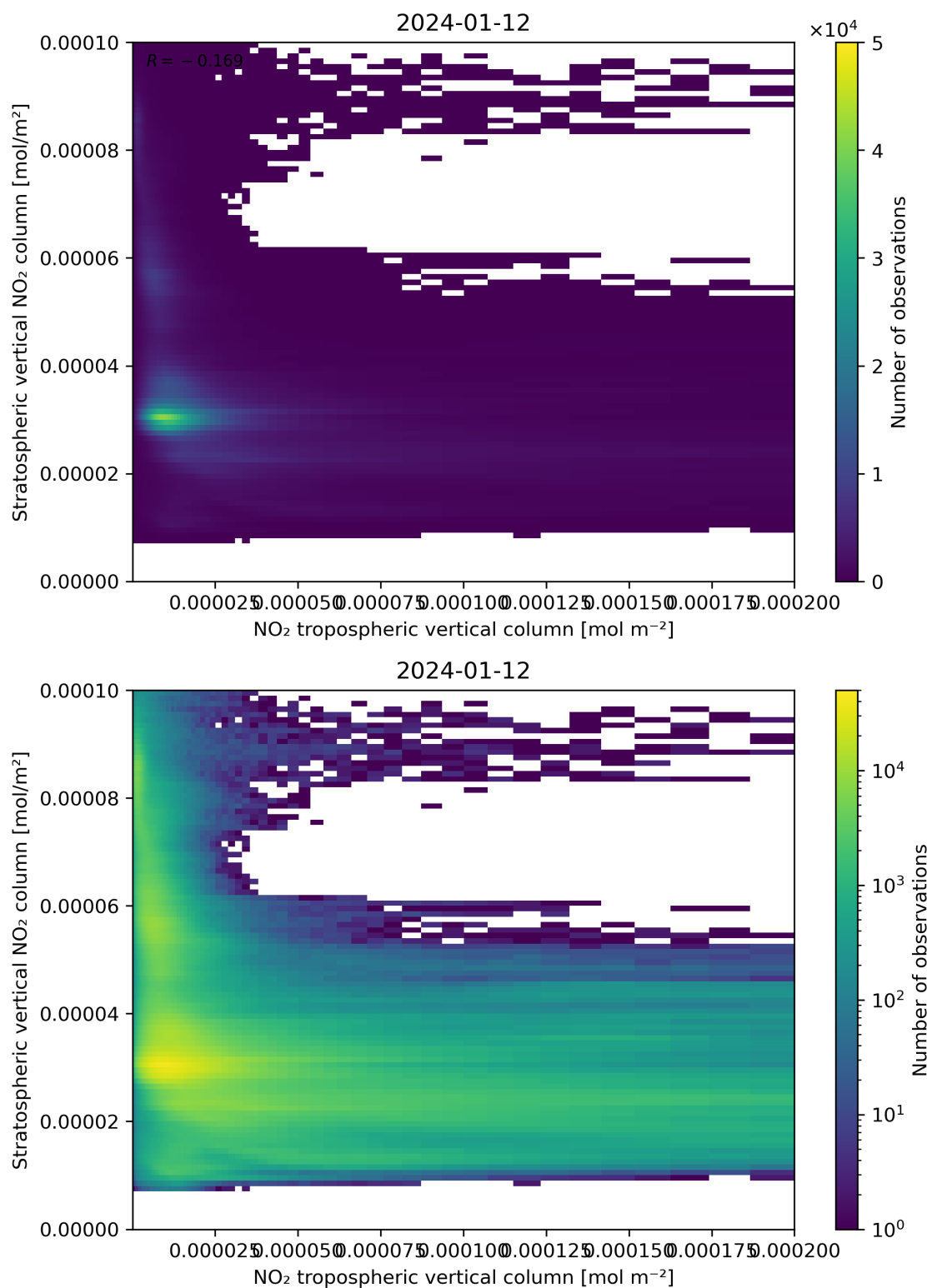
Figure 125: Scatter density plot of “NO 2 tropospheric vertical column” against “Stratospheric vertical NO 2 column” for 2024-01-11 to 2024-01-13.
