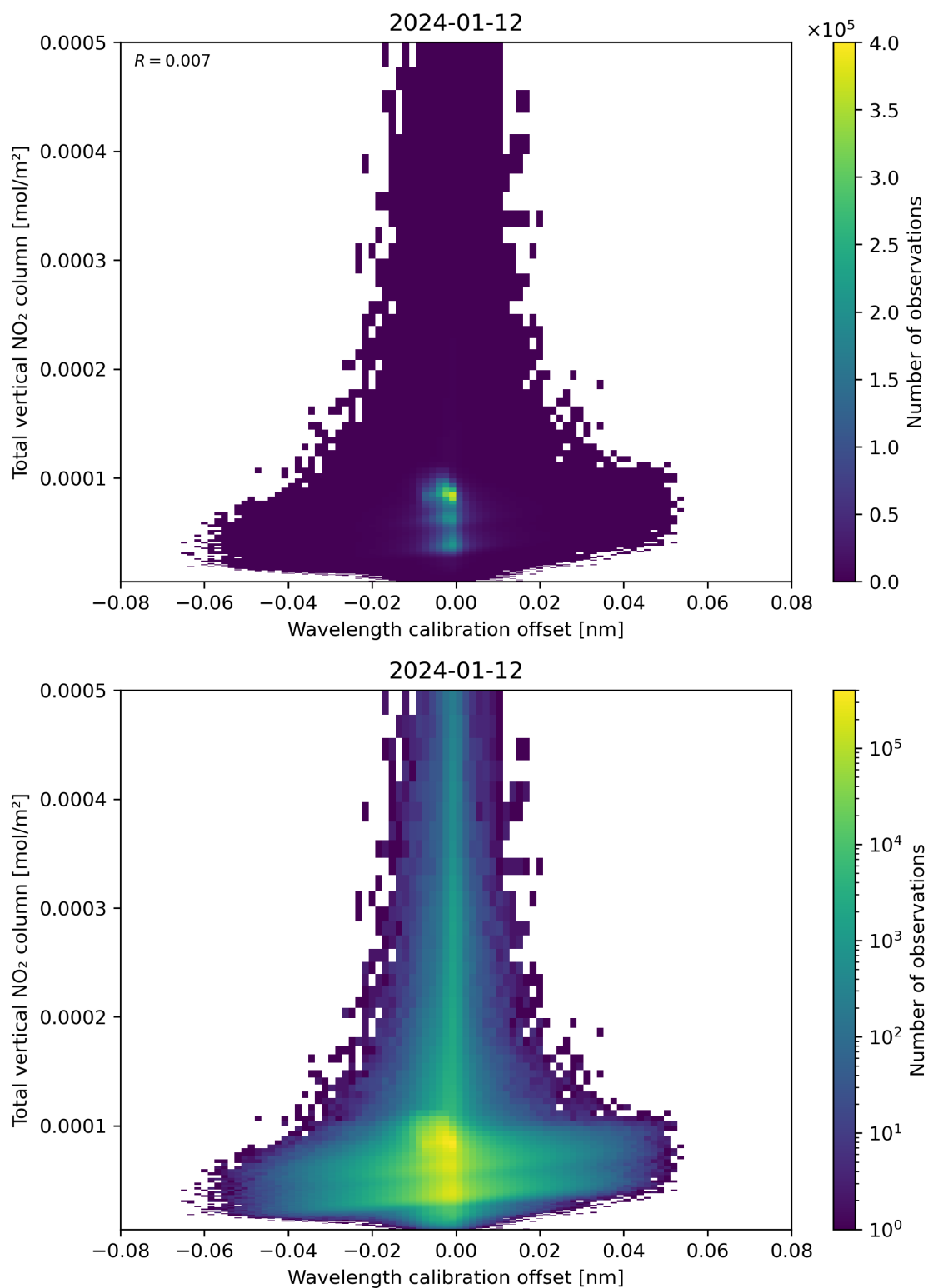
Figure 179: Scatter density plot of “Wavelength calibration offset” against “Total vertical NO 2 column” for 2024-01-11 to 2024-01-13.
