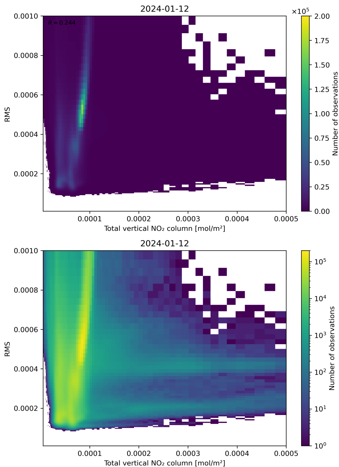
Figure 120: Scatter density plot of “Total vertical NO 2 column” against “RMS” for 2024-01-11 to 2024-01-13.
