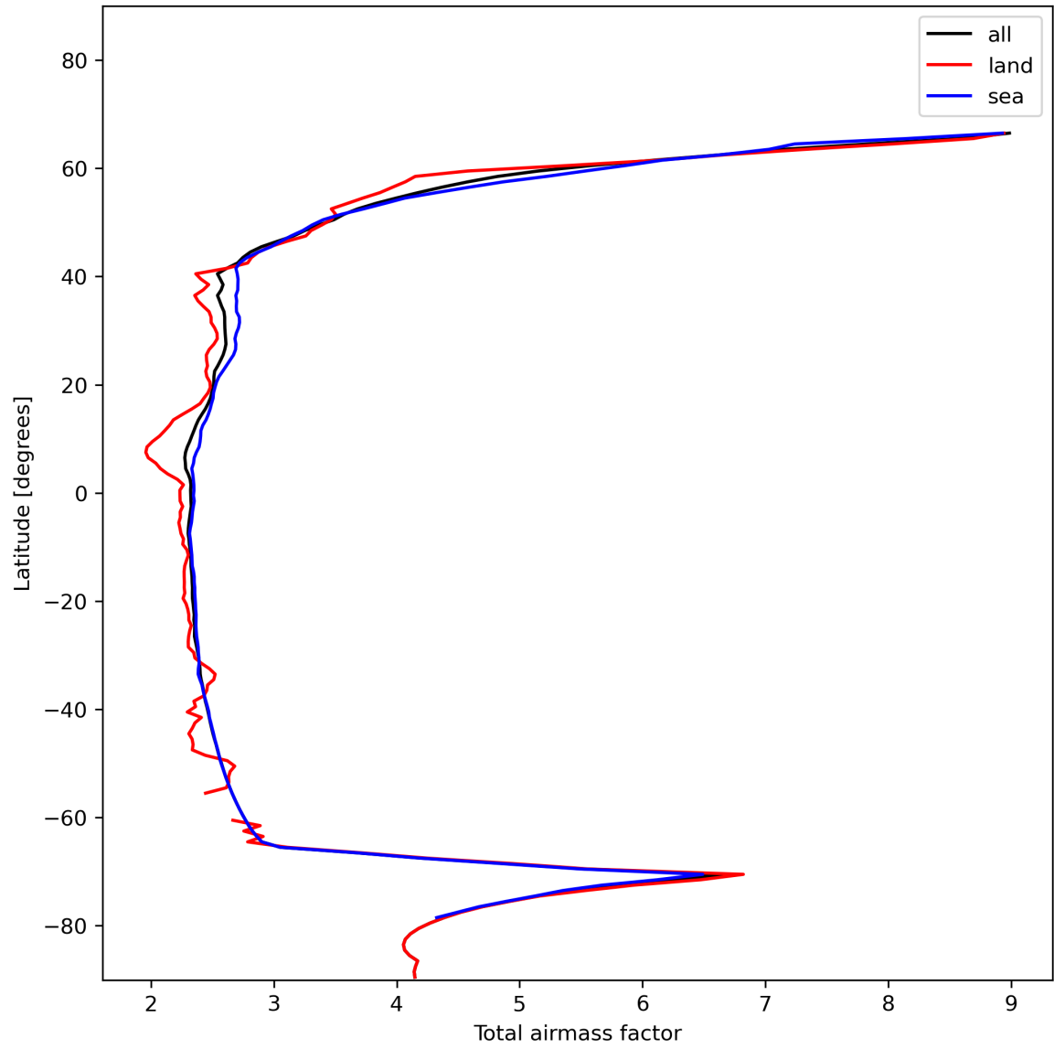
Figure 15: Zonal average of “Total airmass factor” for 2024-01-11 to 2024-01-13.
