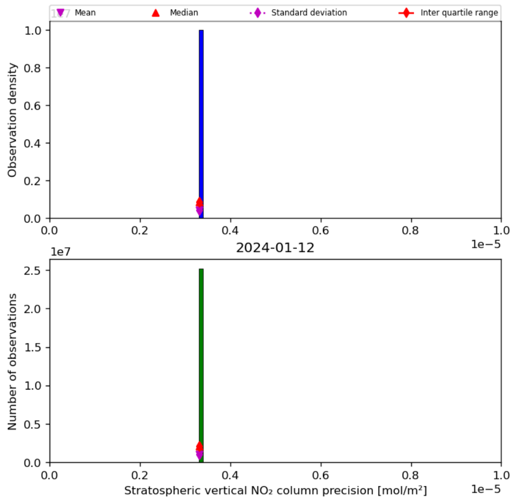
Figure 37: Histogram of “Stratospheric vertical NO 2 column precision” for 2024-01-11 to 2024-01-13
