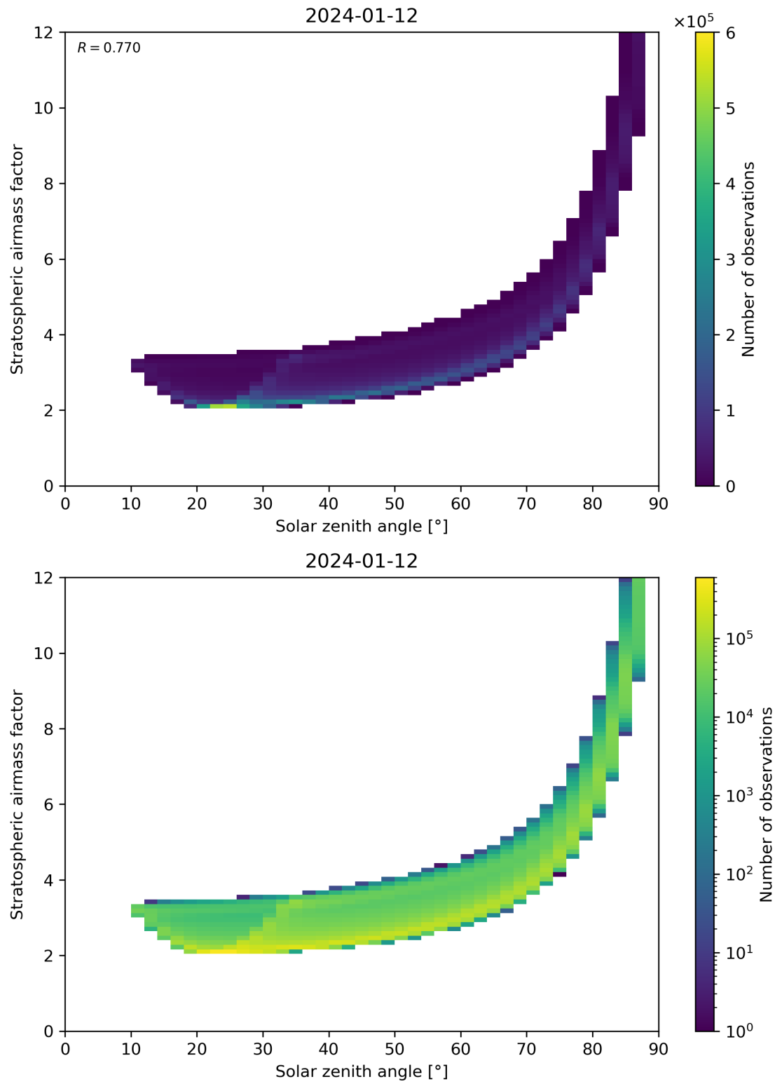
Figure 145: Scatter density plot of “Solar zenith angle” against “Stratospheric airmass factor” for 2024-01-11 to 2024-01-13.
