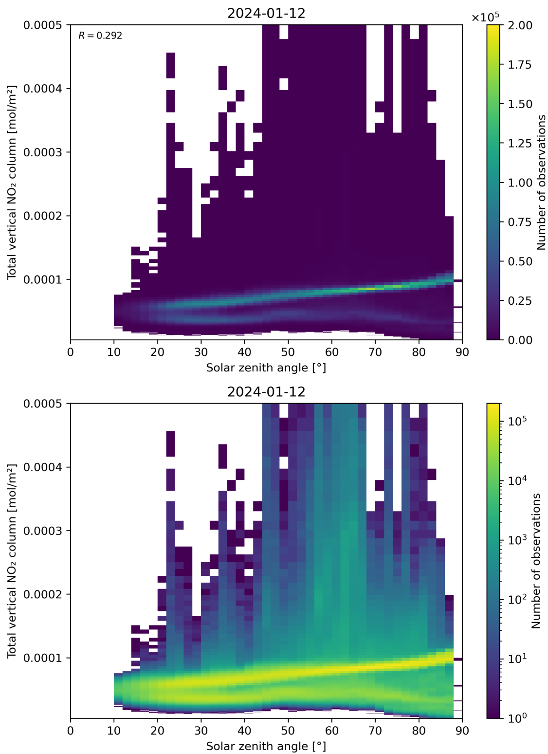
Figure 153: Scatter density plot of “Solar zenith angle” against “Total vertical NO 2 column” for 2024-01-11 to 2024-01-13.
