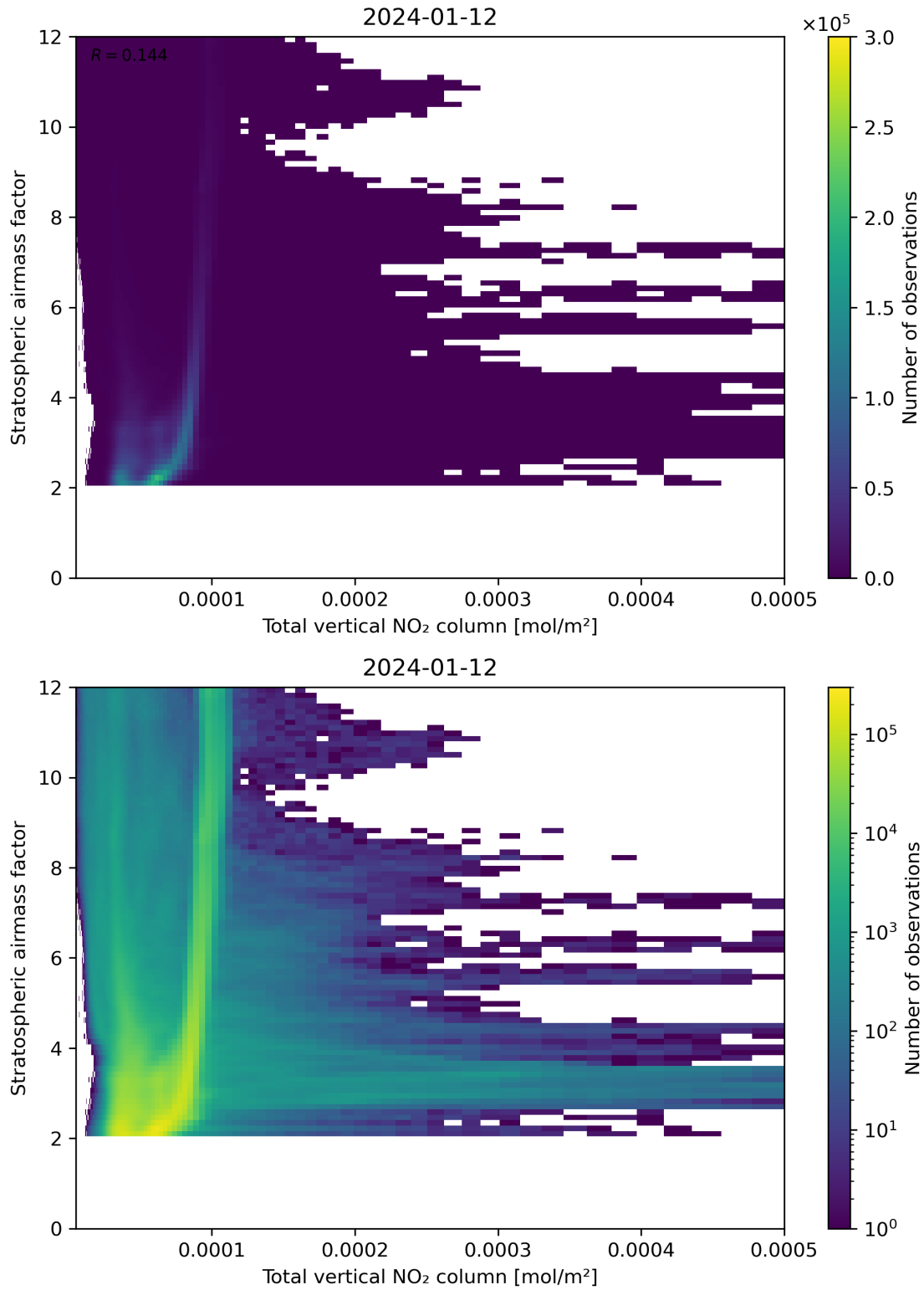
Figure 110: Scatter density plot of “Total vertical NO 2 column” against “Stratospheric airmass factor” for 2024-01-11 to 2024-01-13.
