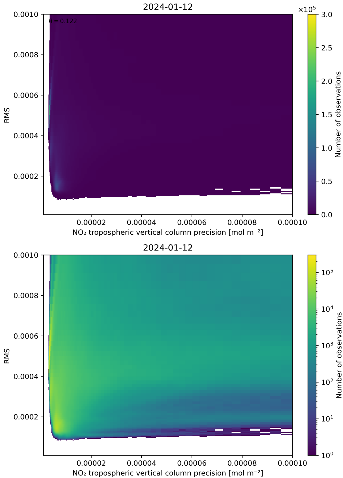
Figure 140: Scatter density plot of “NO 2 tropospheric vertical column precision” against “RMS” for 2024-01-11 to 2024-01-13.
