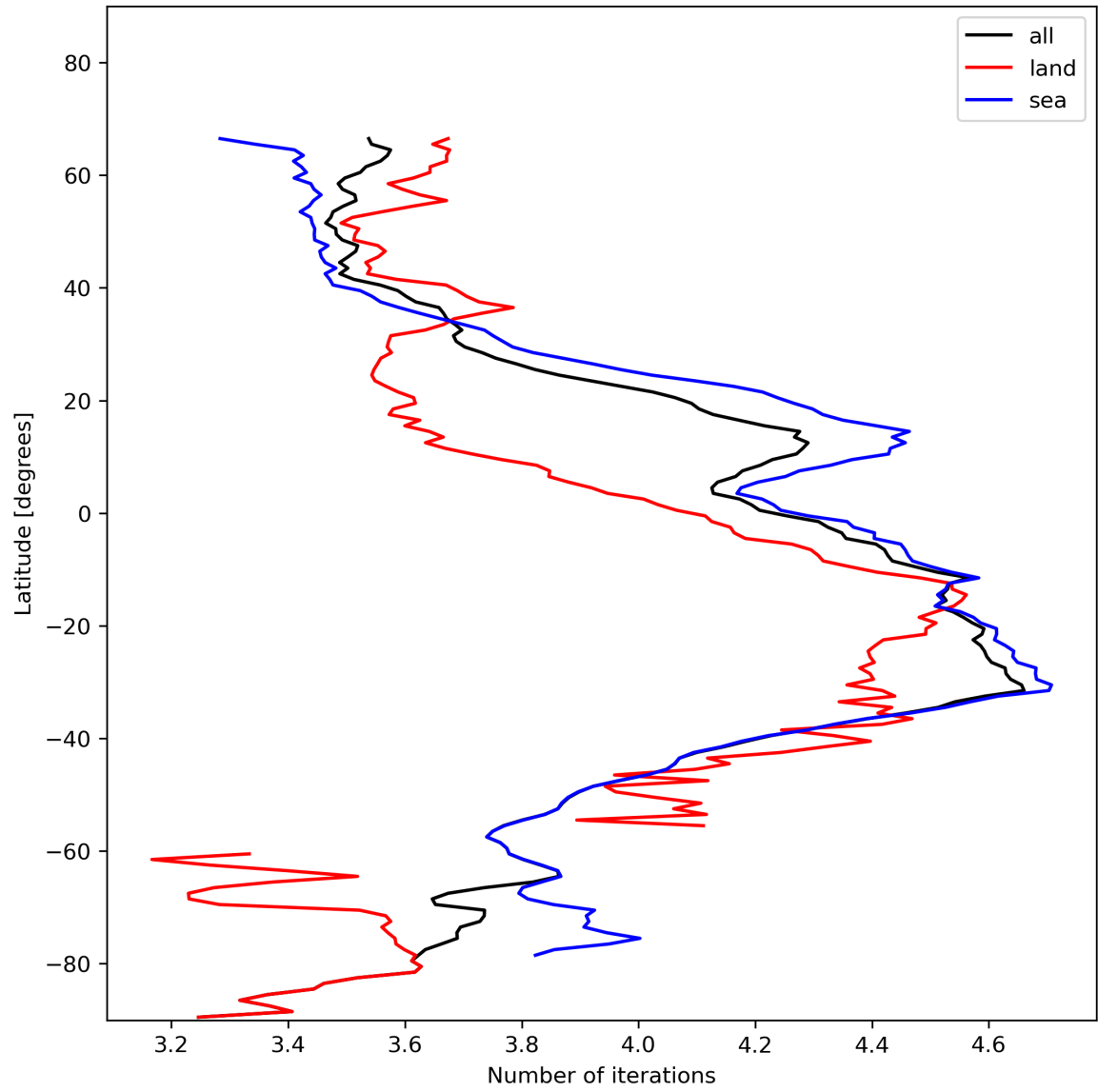
Figure 17: Zonal average of “Number of iterations” for 2024-01-11 to 2024-01-13.
