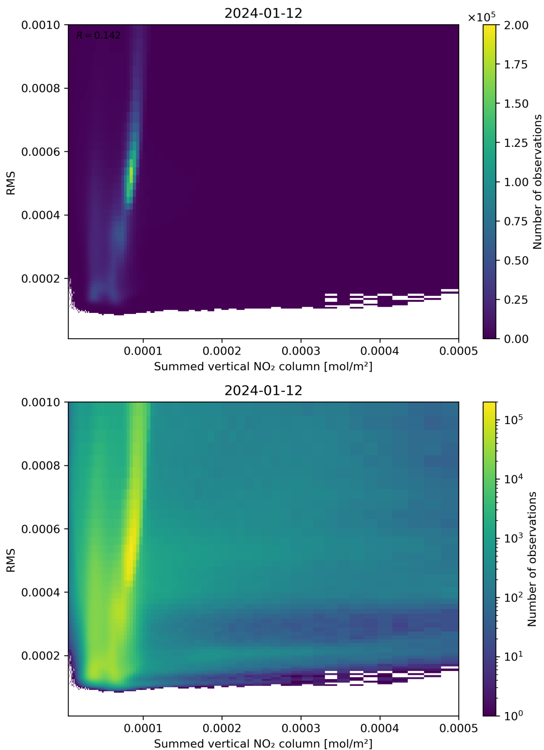
Figure 109: Scatter density plot of “Summed vertical NO 2 column” against “RMS” for 2024-01-11 to 2024-01-13.
