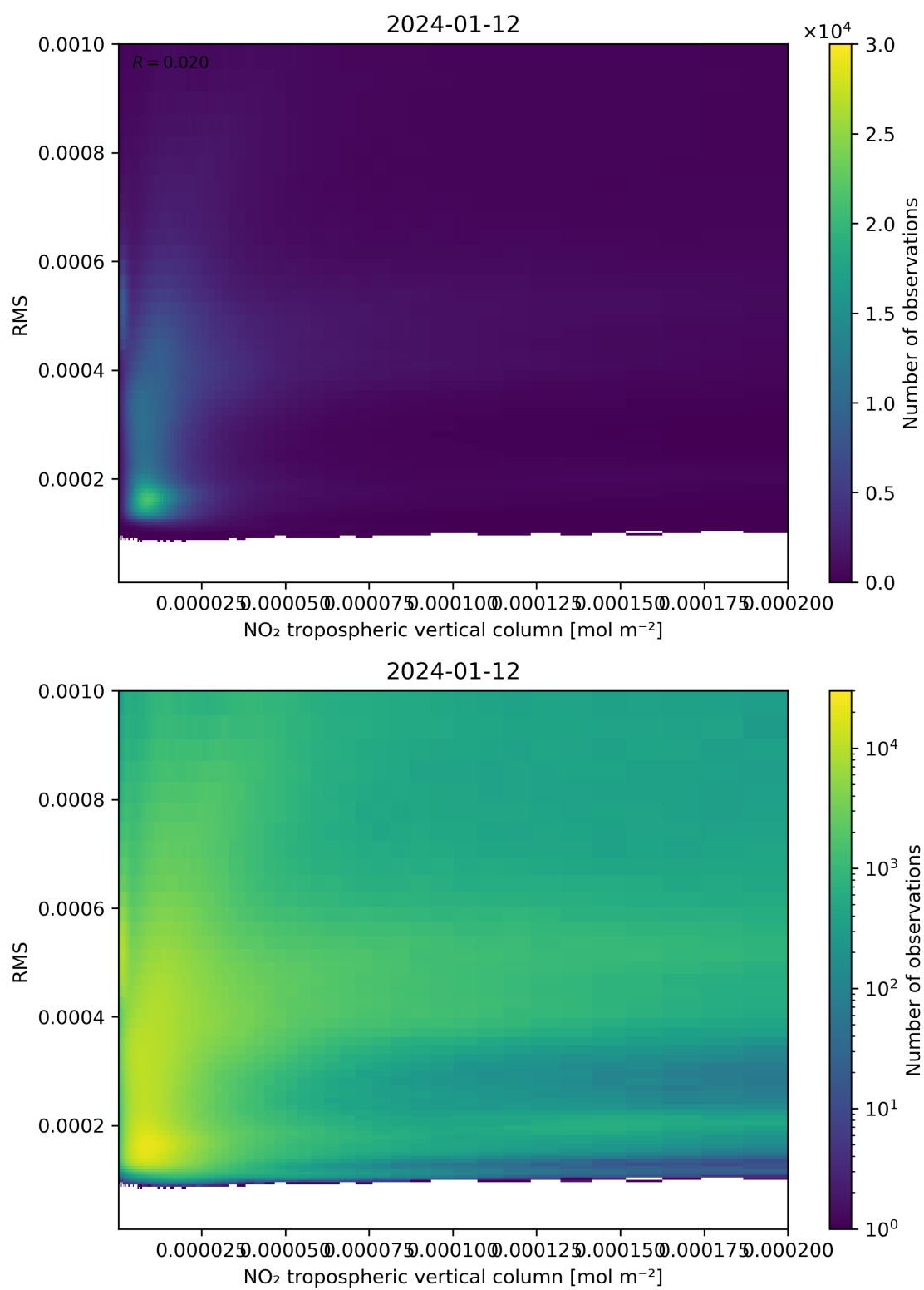
Figure 142: Scatter density plot of “NO 2 tropospheric vertical column” against “RMS” for 2024-01-11 to 2024-01-13.
