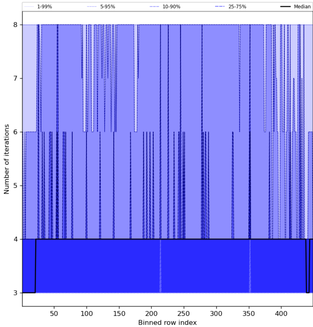
Figure 51: Along track statistics of “Number of iterations” for 2024-01-11 to 2024-01-13
