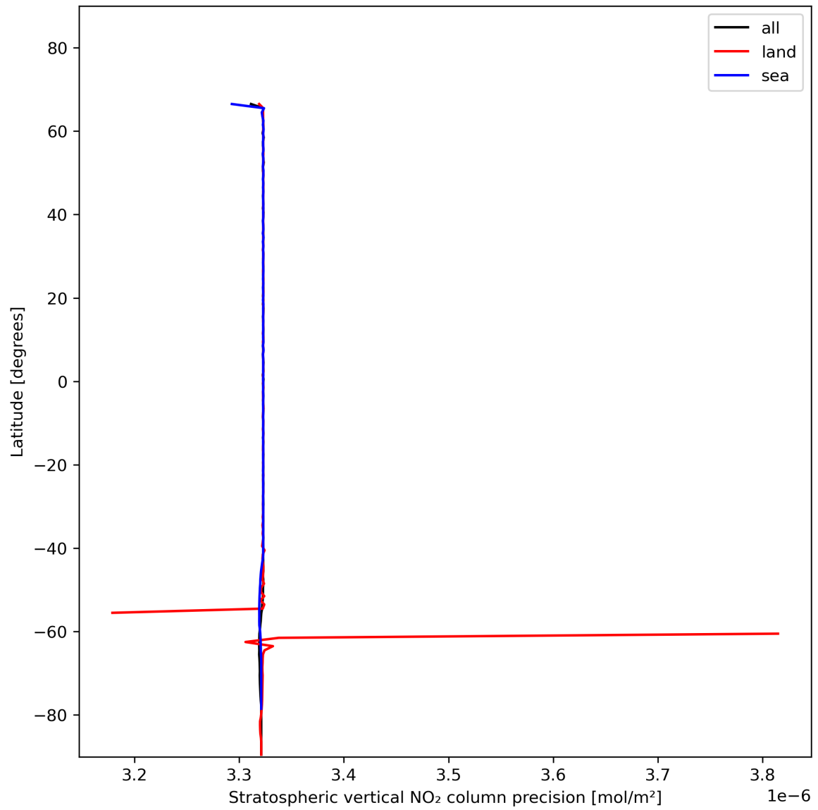
Figure 20: Zonal average of “Stratospheric vertical NO 2 column precision” for 2024-01-11 to 2024-01-13.
