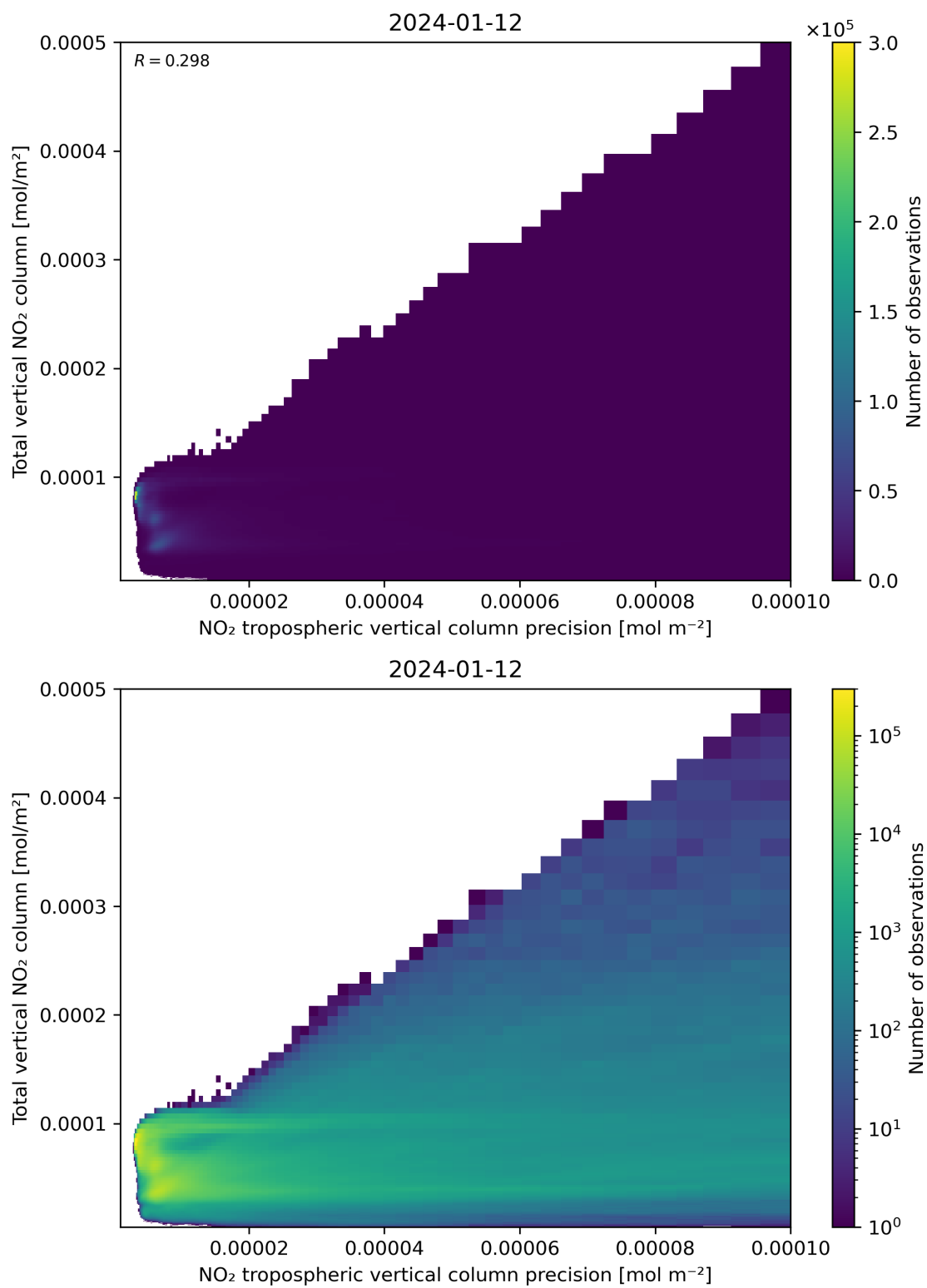
Figure 138: Scatter density plot of “NO 2 tropospheric vertical column precision” against “Total vertical NO 2 column” for 2024-01-11 to 2024-01-13.
