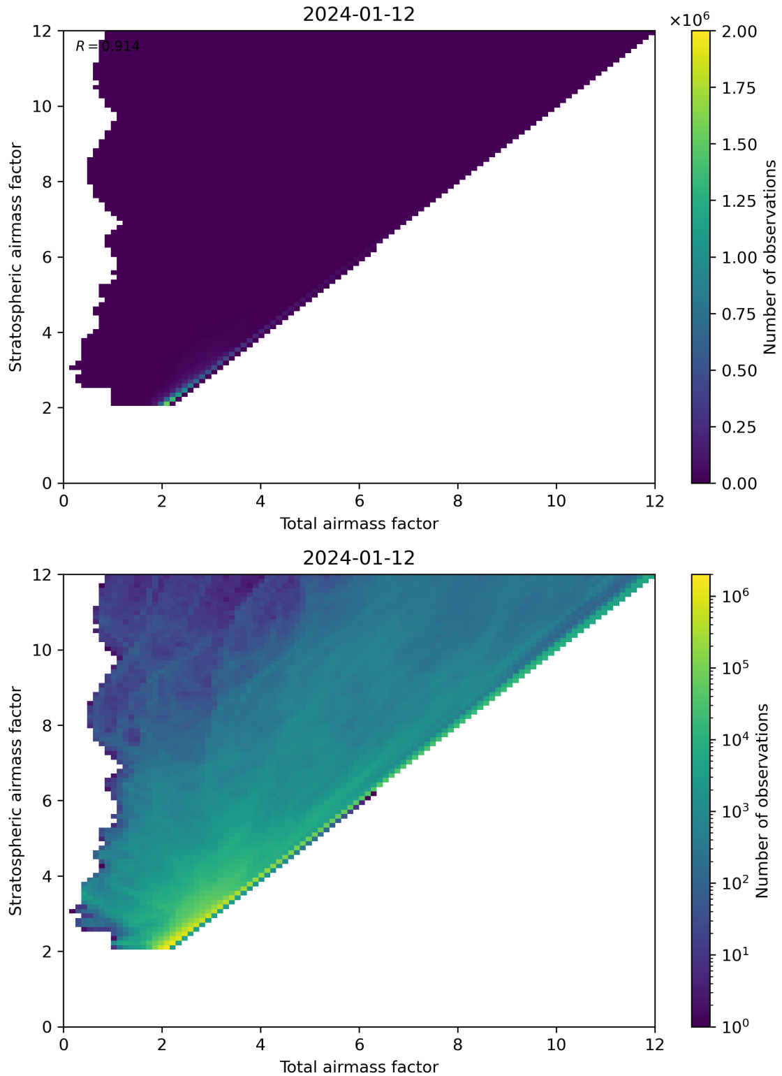
Figure 62: Scatter density plot of “Total airmass factor” against “Stratospheric airmass factor” for 2024-01-11 to 2024-01-13.
