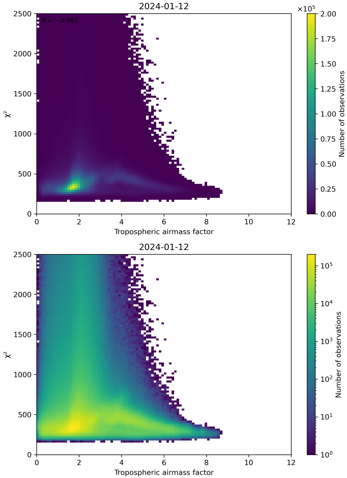
Figure 73: Scatter density plot of “Tropospheric airmass factor” against “ \chi^2 ” for 2024-01-11 to 2024-01-13.
