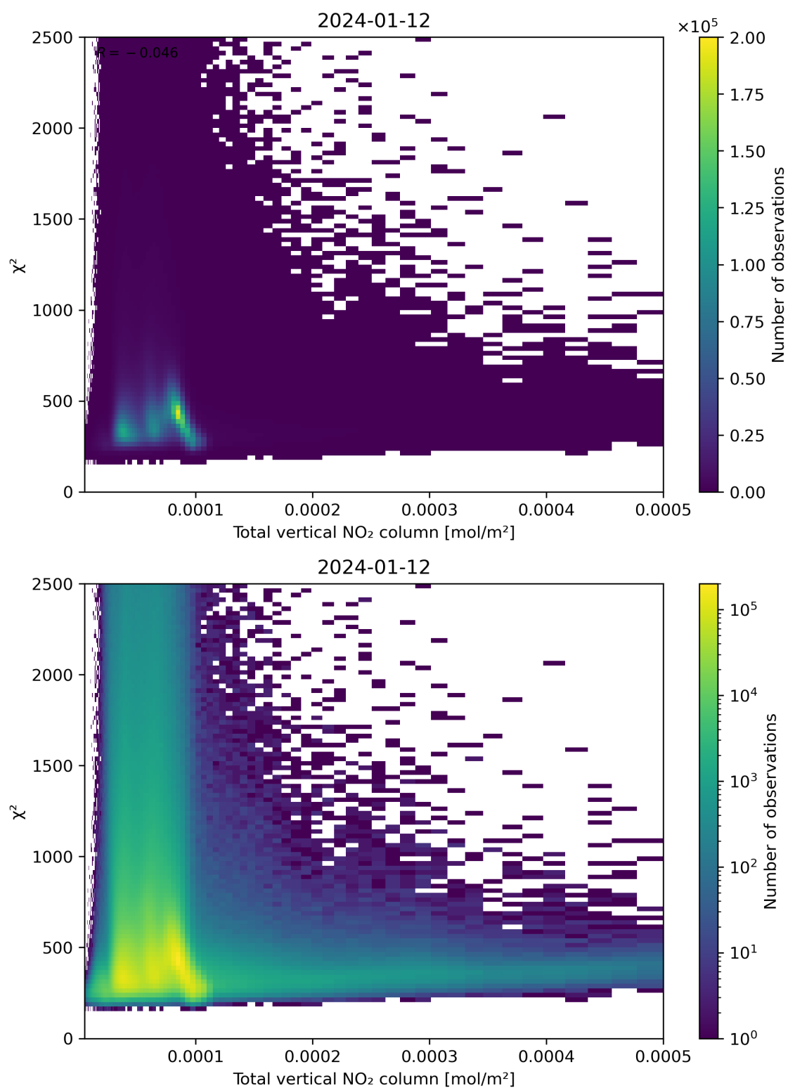
Figure 111: Scatter density plot of “Total vertical NO 2 column” against “ \chi^2 ” for 2024-01-11 to 2024-01-13.
