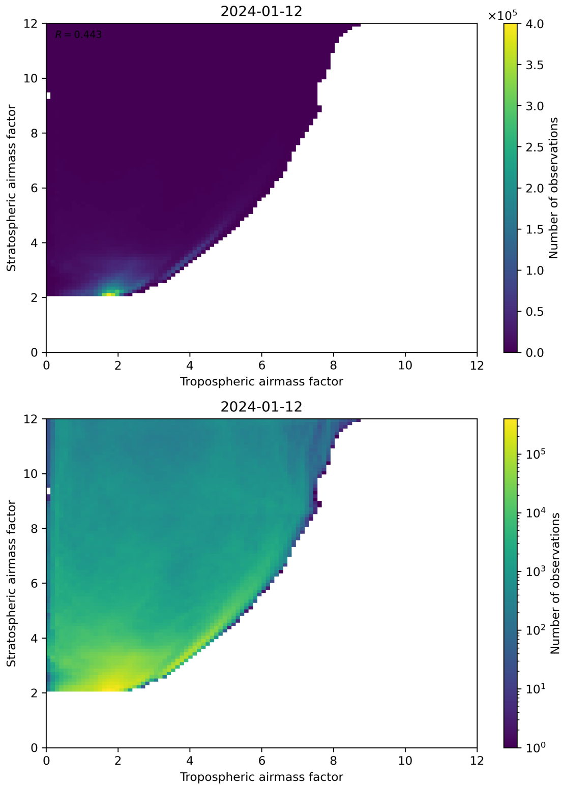
Figure 71: Scatter density plot of “Tropospheric airmass factor” against “Stratospheric airmass factor” for 2024-01-11 to 2024-01-13.
