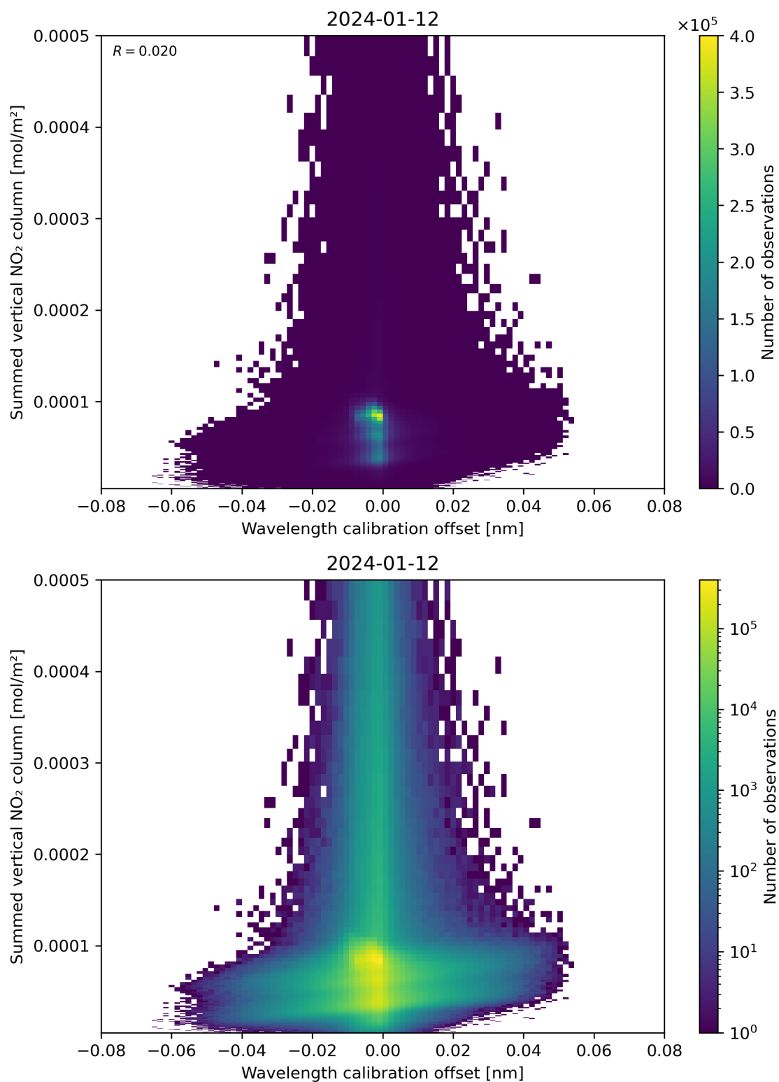
Figure 177: Scatter density plot of “Wavelength calibration offset” against “Summed vertical NO 2 column” for 2024-01-11 to 2024-01-13.
