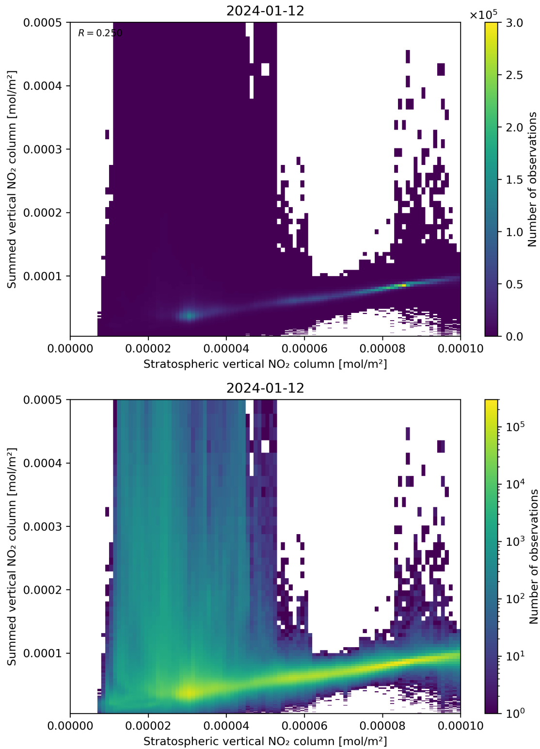
Figure 98: Scatter density plot of “Stratospheric vertical NO 2 column” against “Summed vertical NO 2 column” for 2024-01-11 to 2024-01-13.
