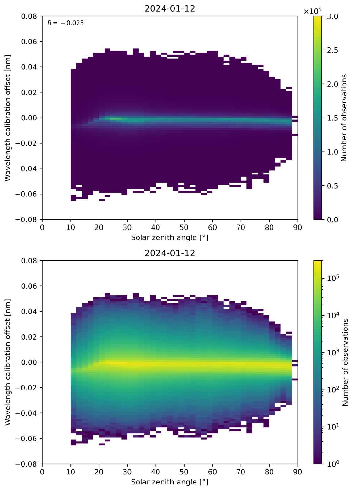
Figure 158: Scatter density plot of “Solar zenith angle” against “Wavelength calibration offset” for 2024-01-11 to 2024-01-13.
