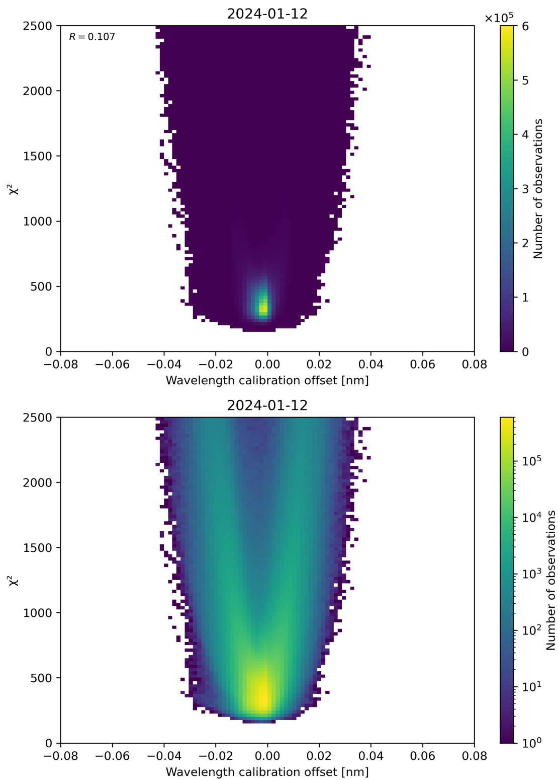
Figure 175: Scatter density plot of “Wavelength calibration offset” against “ \chi^2 ” for 2024-01-11 to 2024-01-13.
