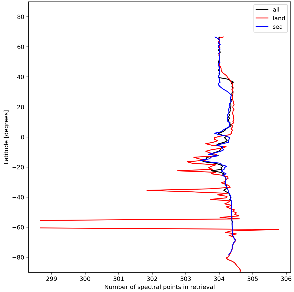
Figure 16: Zonal average of “Number of spectral points in retrieval” for 2024-01-11 to 2024-01-13.
