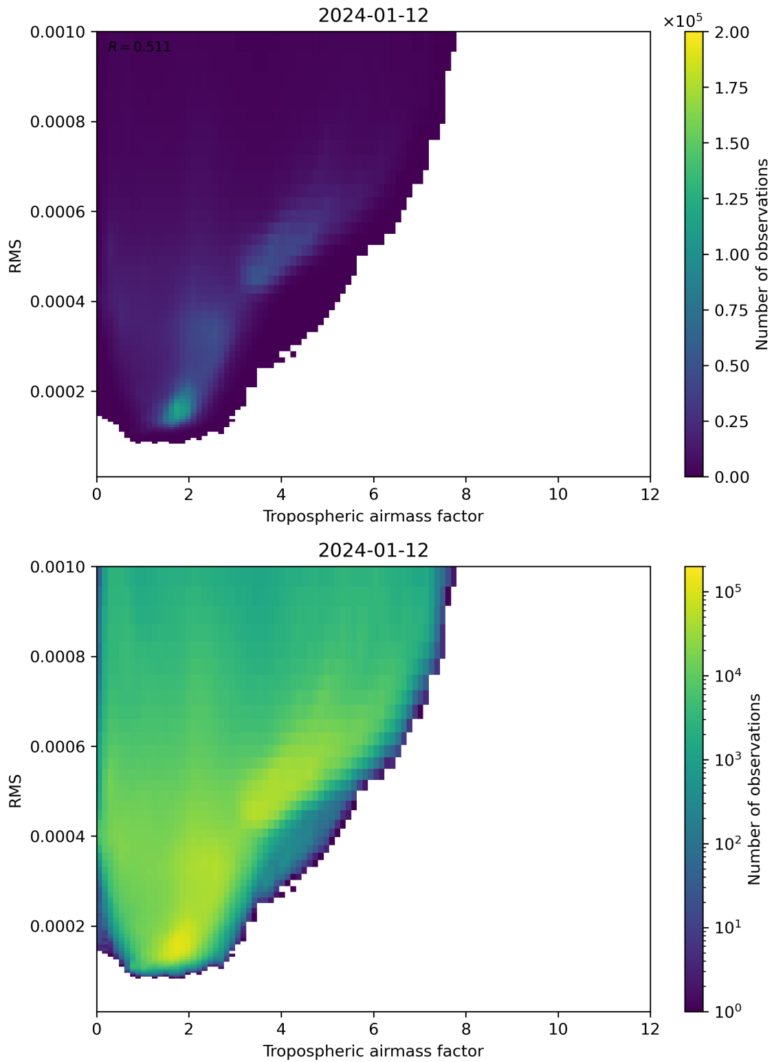
Figure 79: Scatter density plot of “Tropospheric airmass factor” against “RMS” for 2024-01-11 to 2024-01-13.
