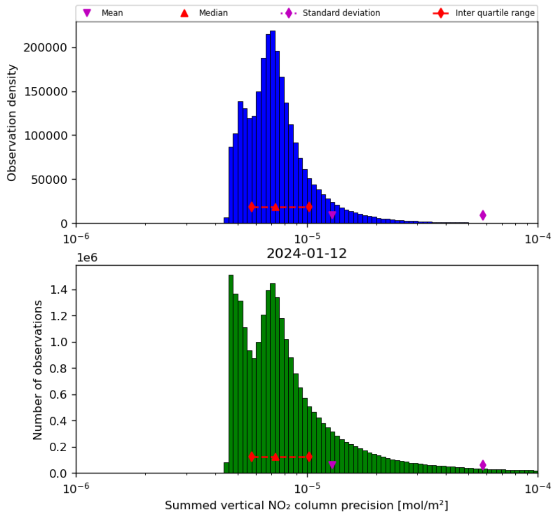
Figure 41: Histogram of “Summed vertical NO 2 column precision” for 2024-01-11 to 2024-01-13
