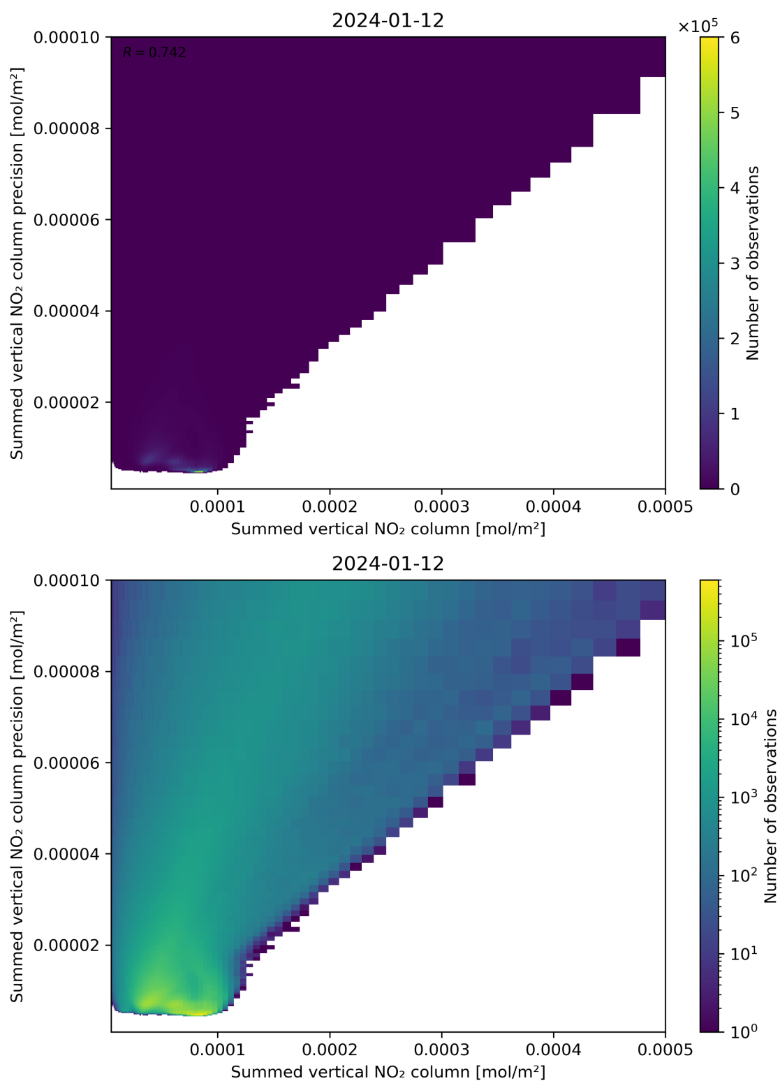
Figure 105: Scatter density plot of “Summed vertical NO 2 column” against “Summed vertical NO 2 column precision” for 2024-01-11 to 2024-01-13.
