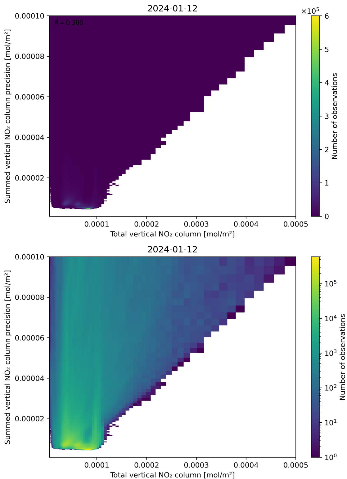
Figure 113: Scatter density plot of “Total vertical NO 2 column” against “Summed vertical NO 2 column precision” for 2024-01-11 to 2024-01-13.
