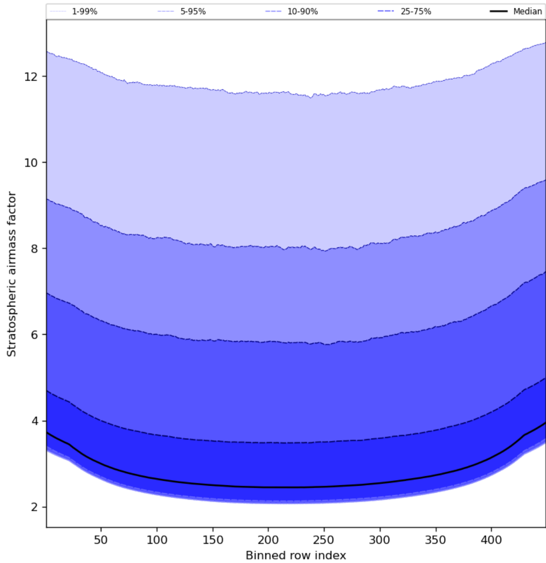
Figure 61: Along track statistics of “Stratospheric airmass factor” for 2024-01-11 to 2024-01-13
