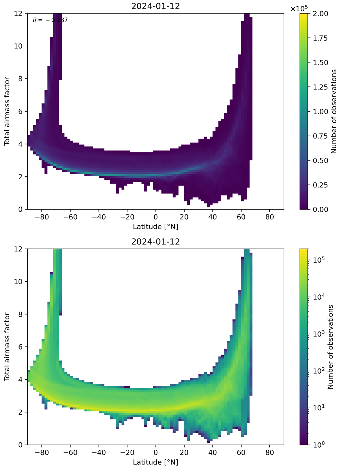
Figure 84: Scatter density plot of “Latitude” against “Total airmass factor” for 2024-01-11 to 2024-01-13.
