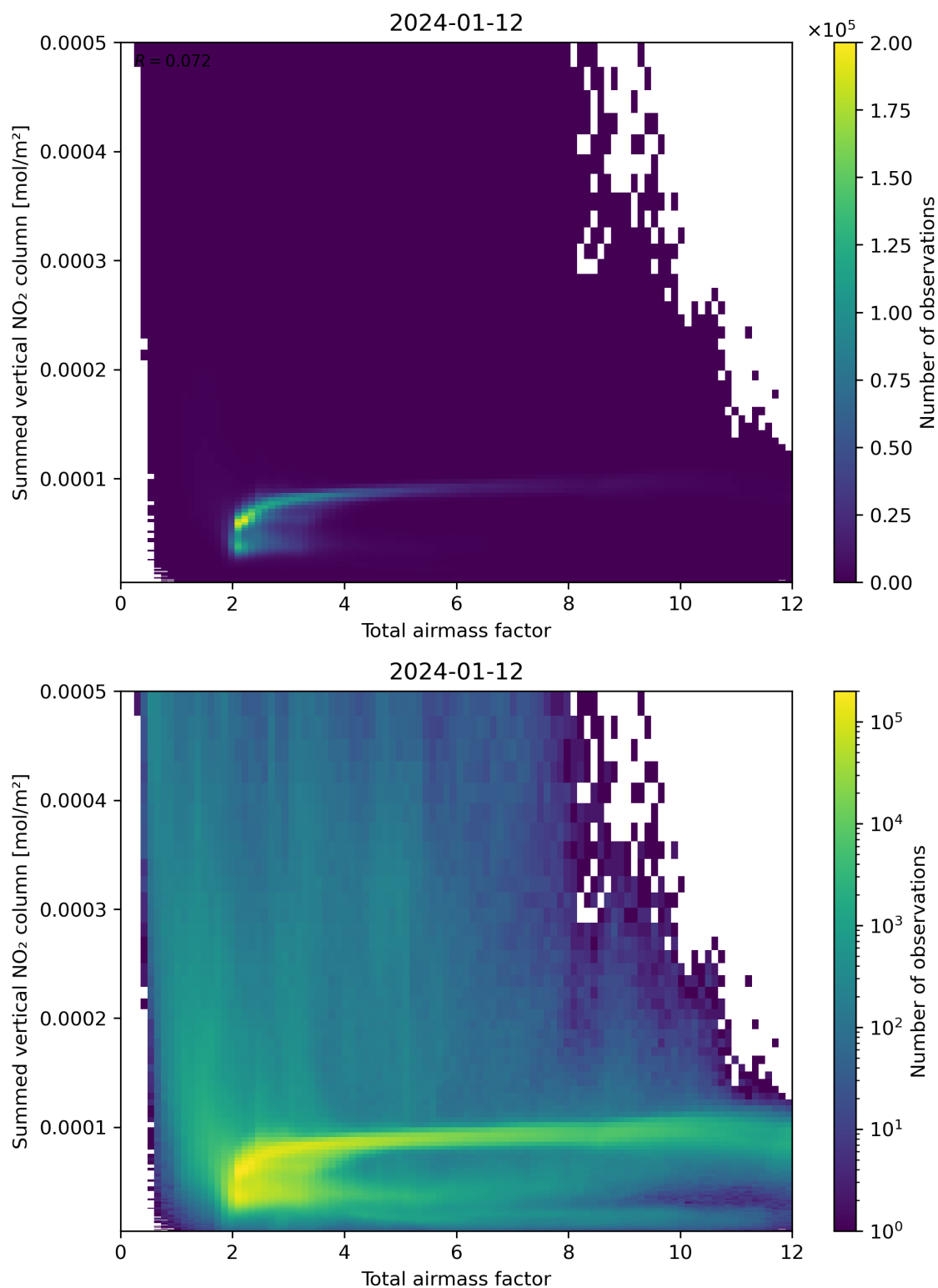
Figure 65: Scatter density plot of “Total airmass factor” against “Summed vertical NO 2 column” for 2024-01-11 to 2024-01-13.
