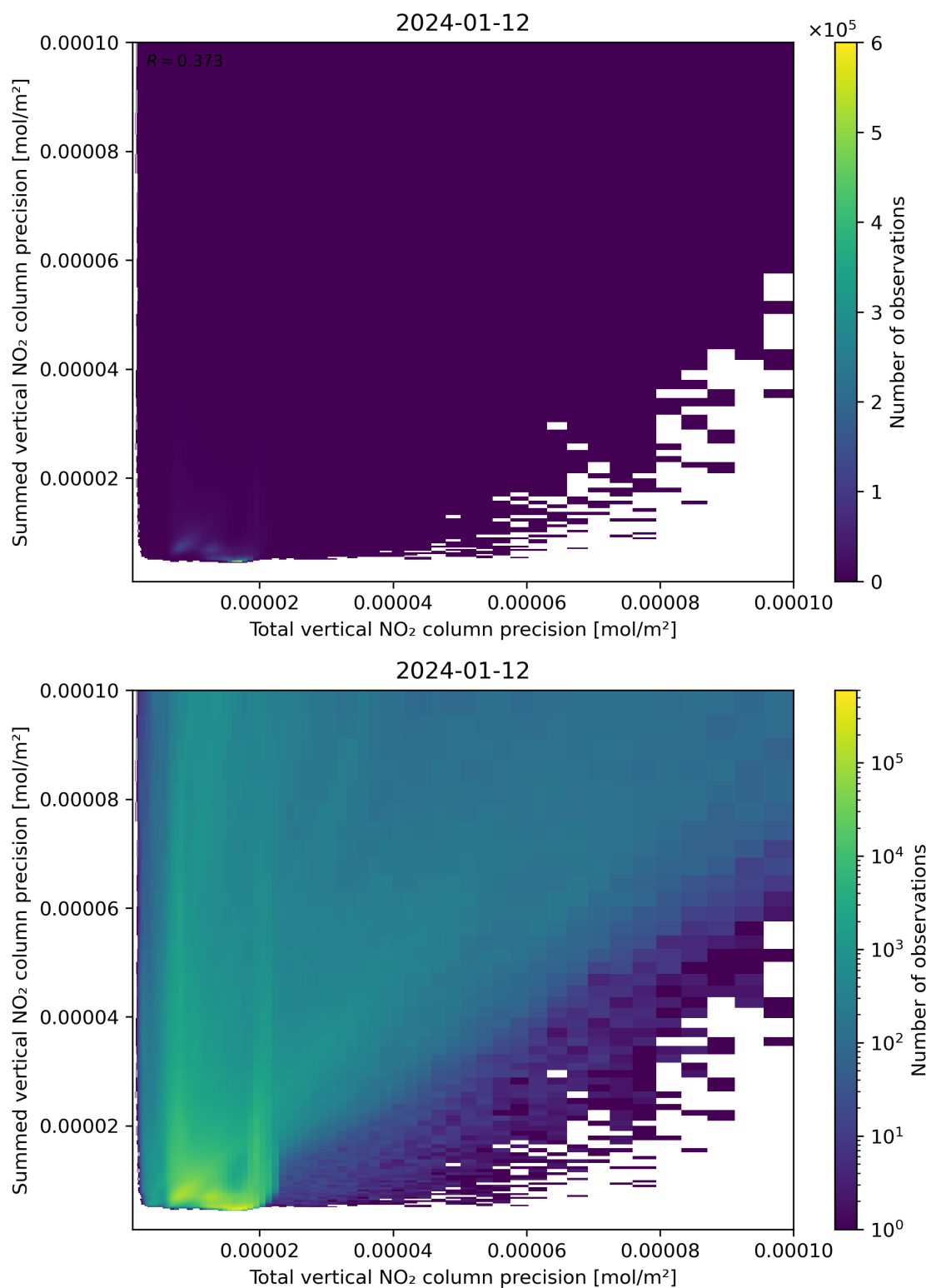
Figure 118: Scatter density plot of “Total vertical NO 2 column precision” against “Summed vertical NO 2 column precision” for 2024-01-11 to 2024-01-13.
