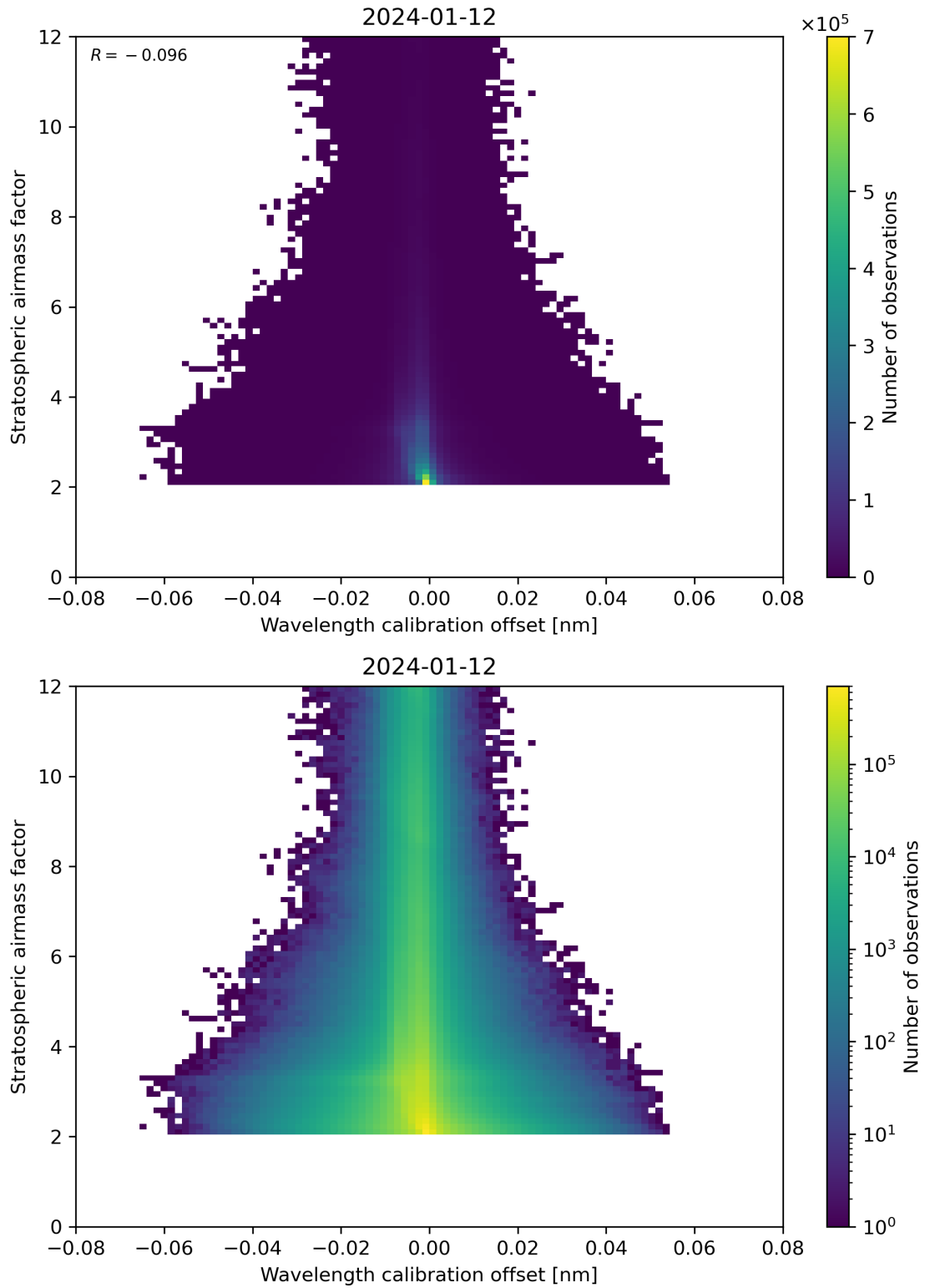
Figure 174: Scatter density plot of “Wavelength calibration offset” against “Stratospheric air mass factor” for 2024-01-11 to 2024-01-13.
