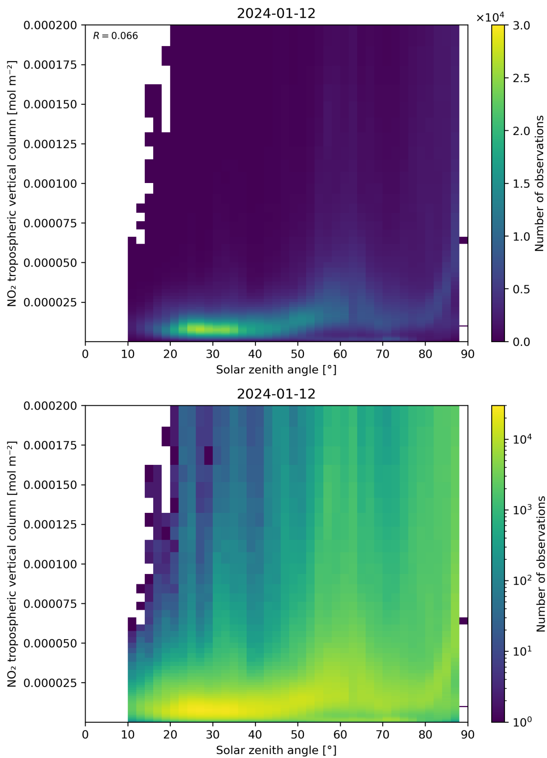
Figure 155: Scatter density plot of “Solar zenith angle” against “NO 2 tropospheric vertical column” for 2024-01-11 to 2024-01-13.
