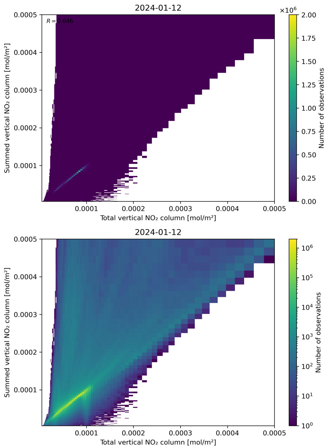
Figure 112: Scatter density plot of “Total vertical NO 2 column” against “Summed vertical NO 2 column” for 2024-01-11 to 2024-01-13.
