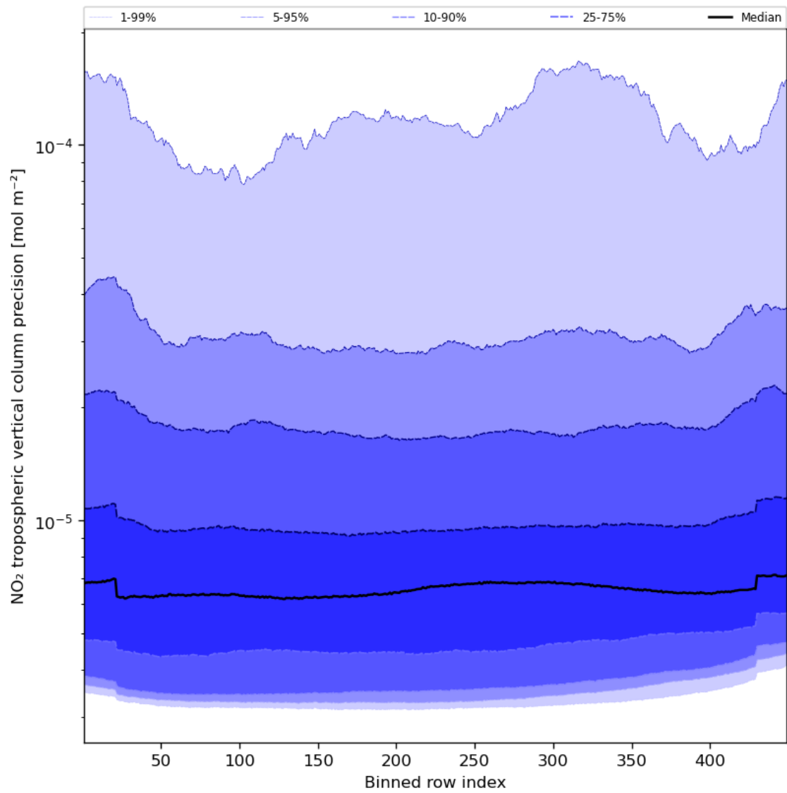
Figure 47: Along track statistics of “NO 2 tropospheric vertical column precision” for 2024-01-11 to 2024-01-13
