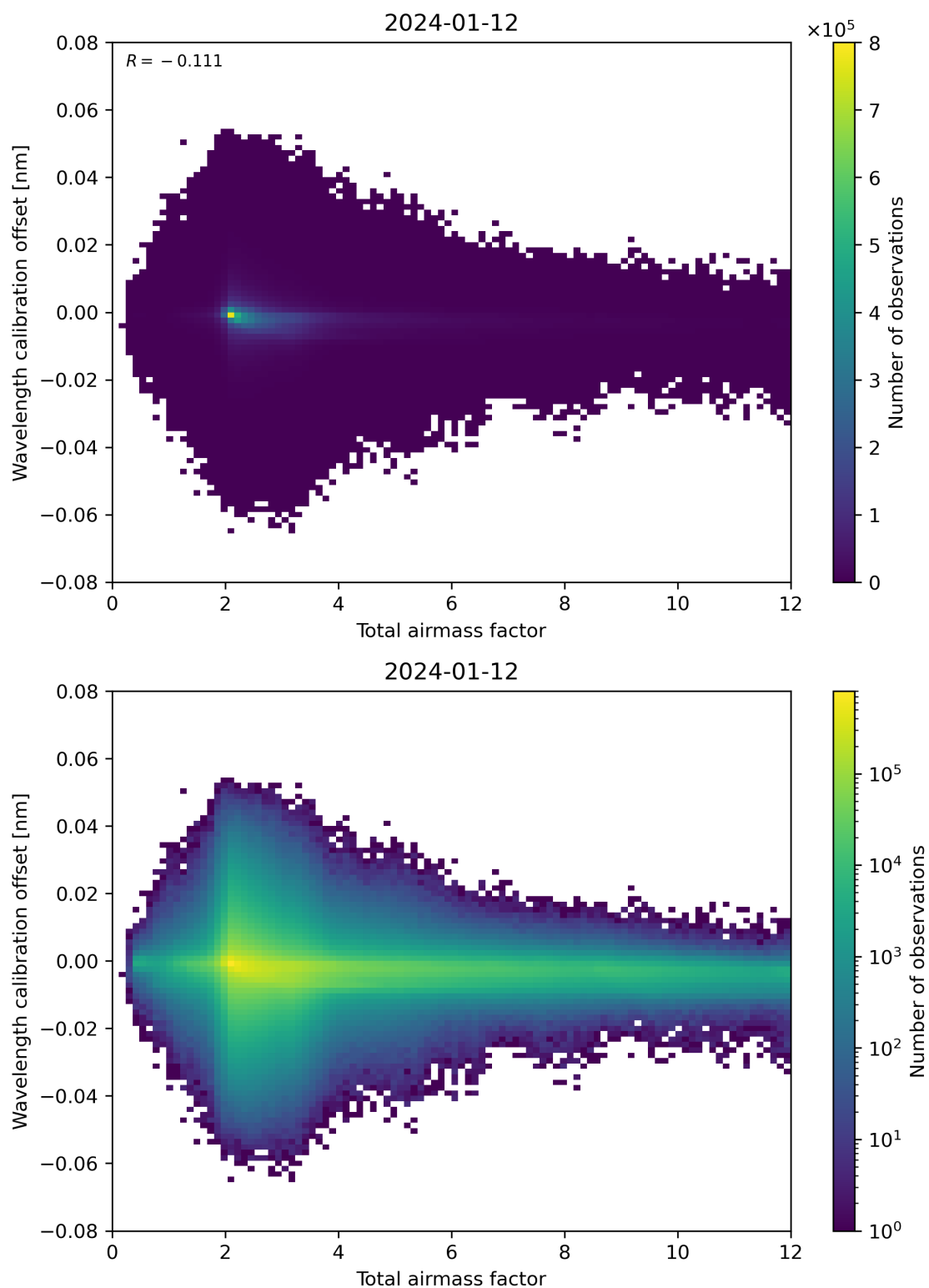
Figure 70: Scatter density plot of “Total airmass factor” against “Wavelength calibration offset” for 2024-01-11 to 2024-01-13.
