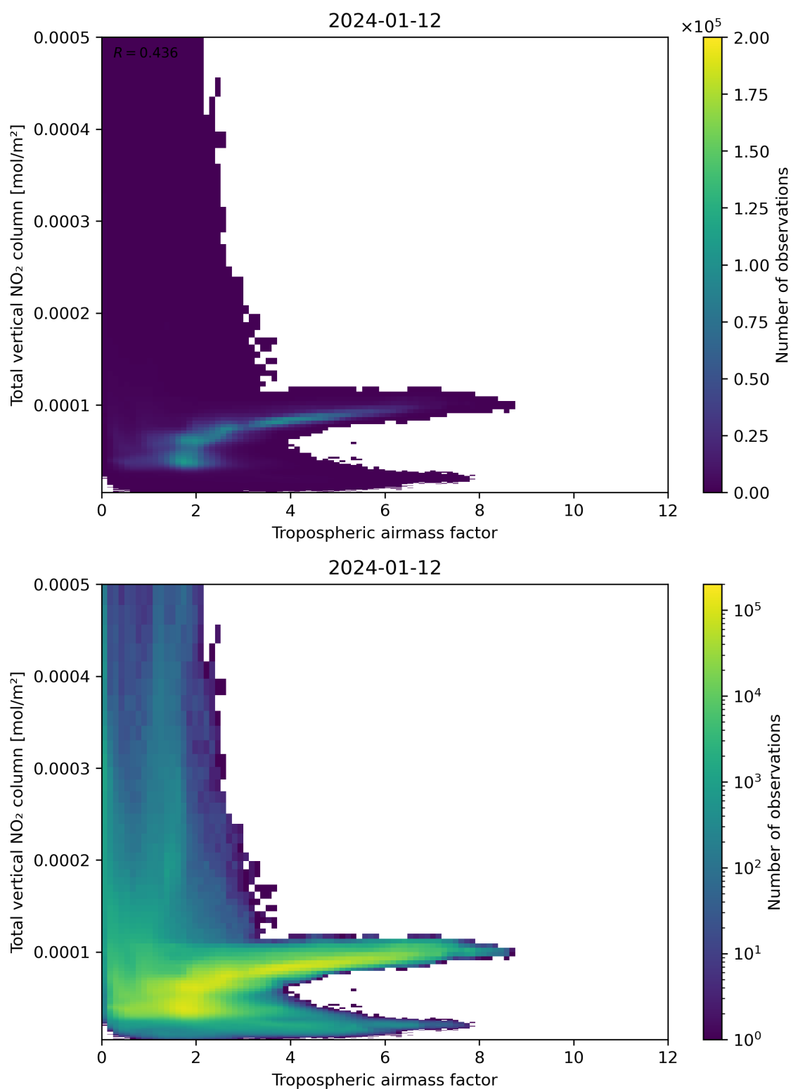
Figure 77: Scatter density plot of “Tropospheric airmass factor” against “Total vertical NO 2 column” for 2024-01-11 to 2024-01-13.
