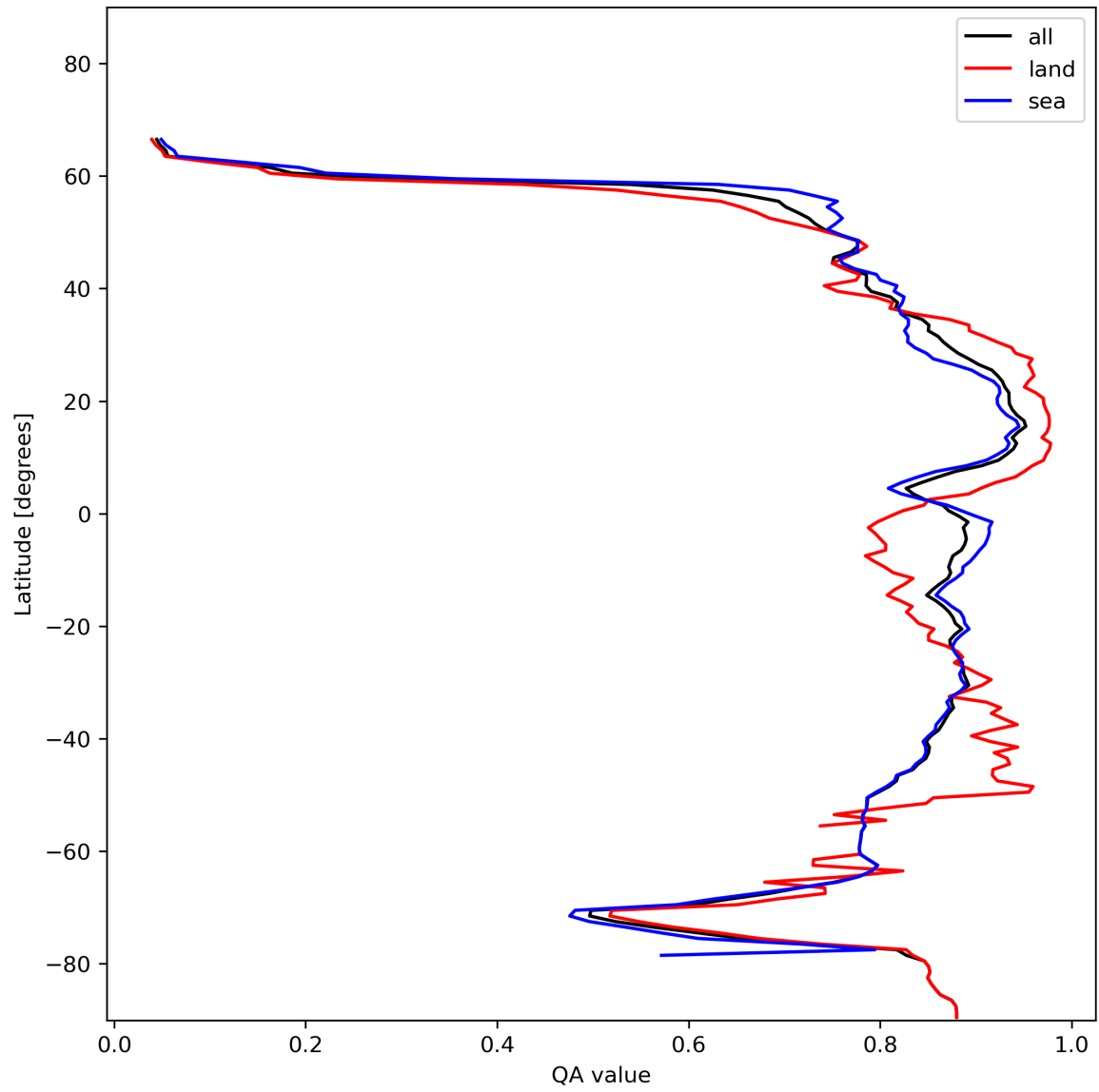
Figure 11: Zonal average of “QA value” for 2024-01-11 to 2024-01-13.
