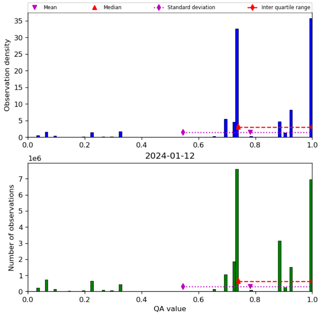
Figure 28: Histogram of “QA value” for 2024-01-11 to 2024-01-13
