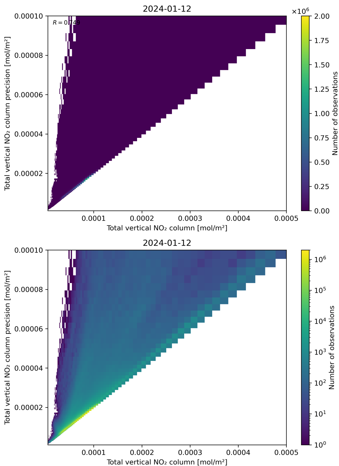
Figure 114: Scatter density plot of “Total vertical NO 2 column” against “Total vertical NO 2 column precision” for 2024-01-11 to 2024-01-13.
