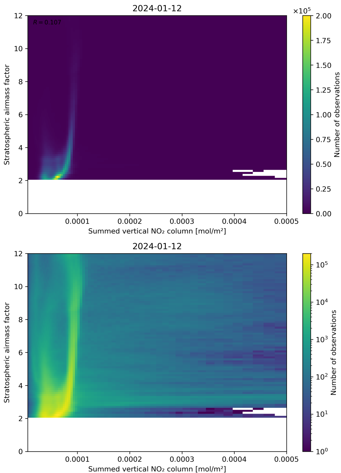
Figure 103: Scatter density plot of “Summed vertical NO 2 column” against “Stratospheric airmass factor” for 2024-01-11 to 2024-01-13.
