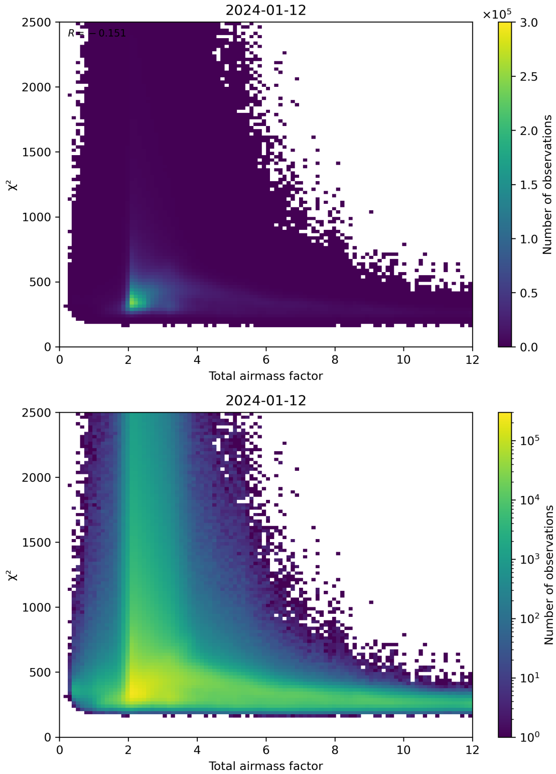
Figure 63: Scatter density plot of “Total airmass factor” against “ \chi^2 ” for 2024-01-11 to 2024-01-13.
