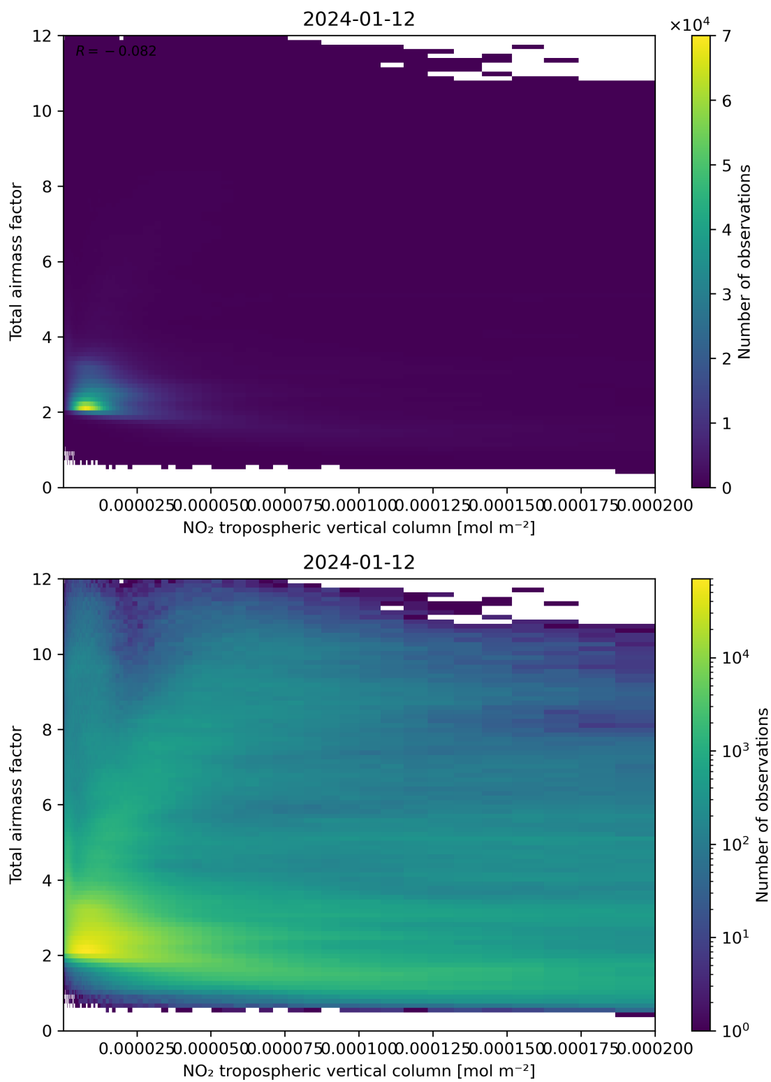
Figure 122: Scatter density plot of “NO 2 tropospheric vertical column” against “Total air mass factor” for 2024-01-11 to 2024-01-13.
