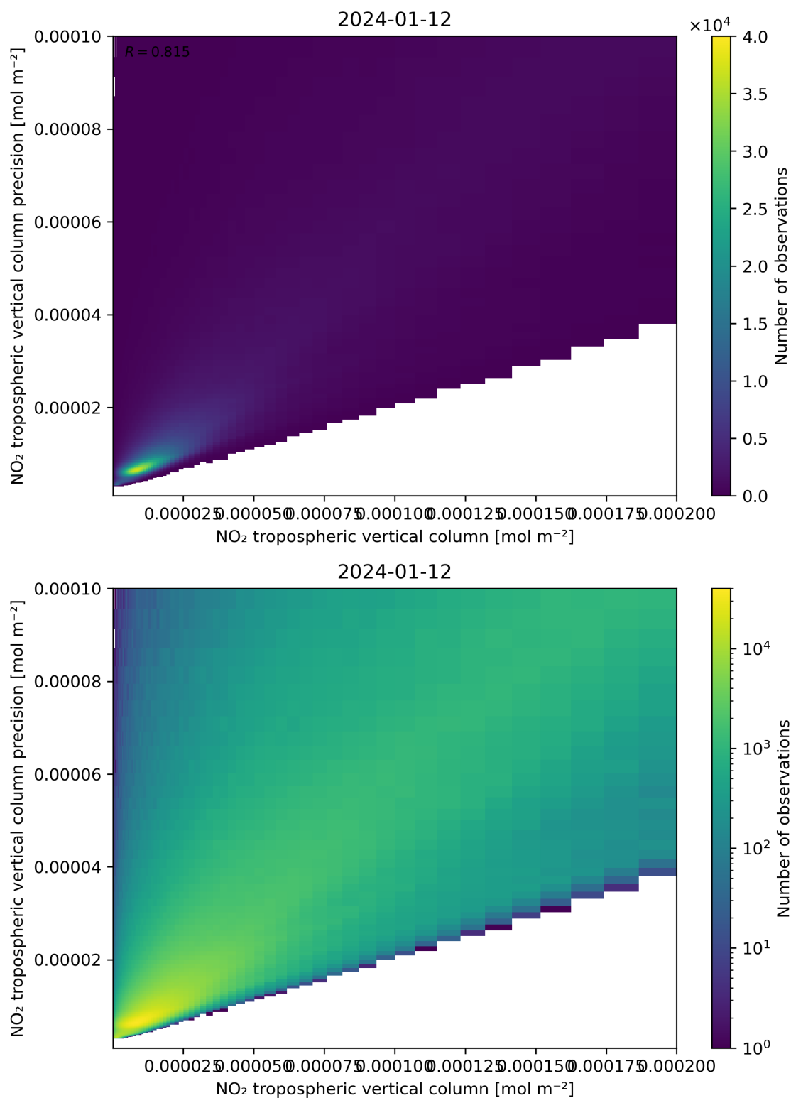
Figure 130: Scatter density plot of “NO 2 tropospheric vertical column” against “NO 2 tropospheric vertical column precision” for 2024-01-11 to 2024-01-13.
