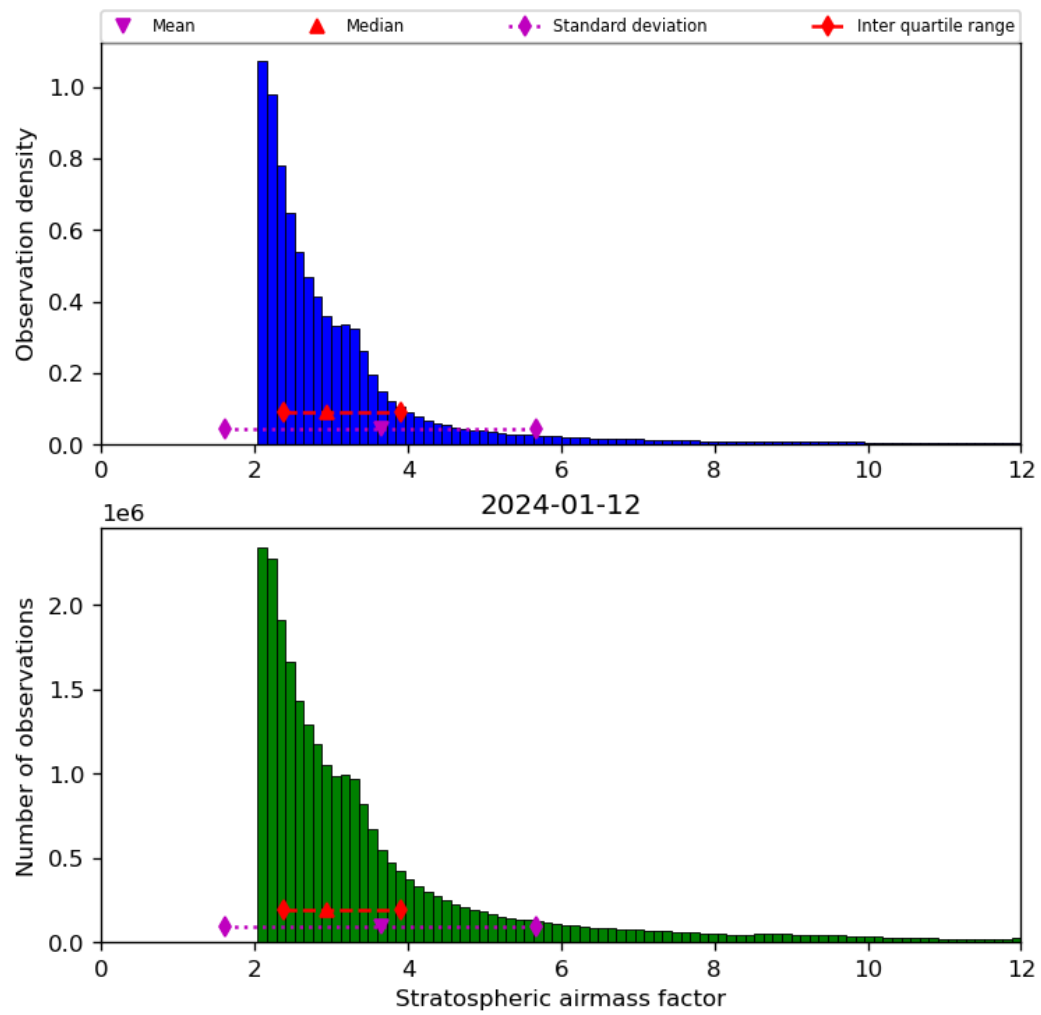
Figure 44: Histogram of “Stratospheric airmass factor” for 2024-01-11 to 2024-01-13
