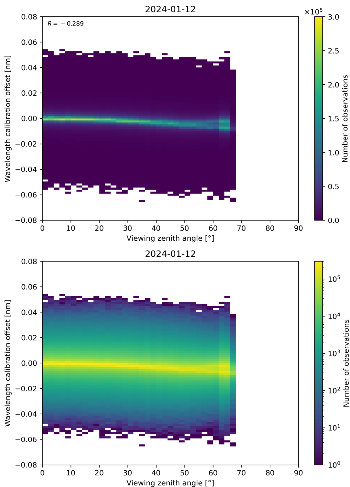
Figure 173: Scatter density plot of “Viewing zenith angle” against “Wavelength calibration offset” for 2024-01-11 to 2024-01-13.
