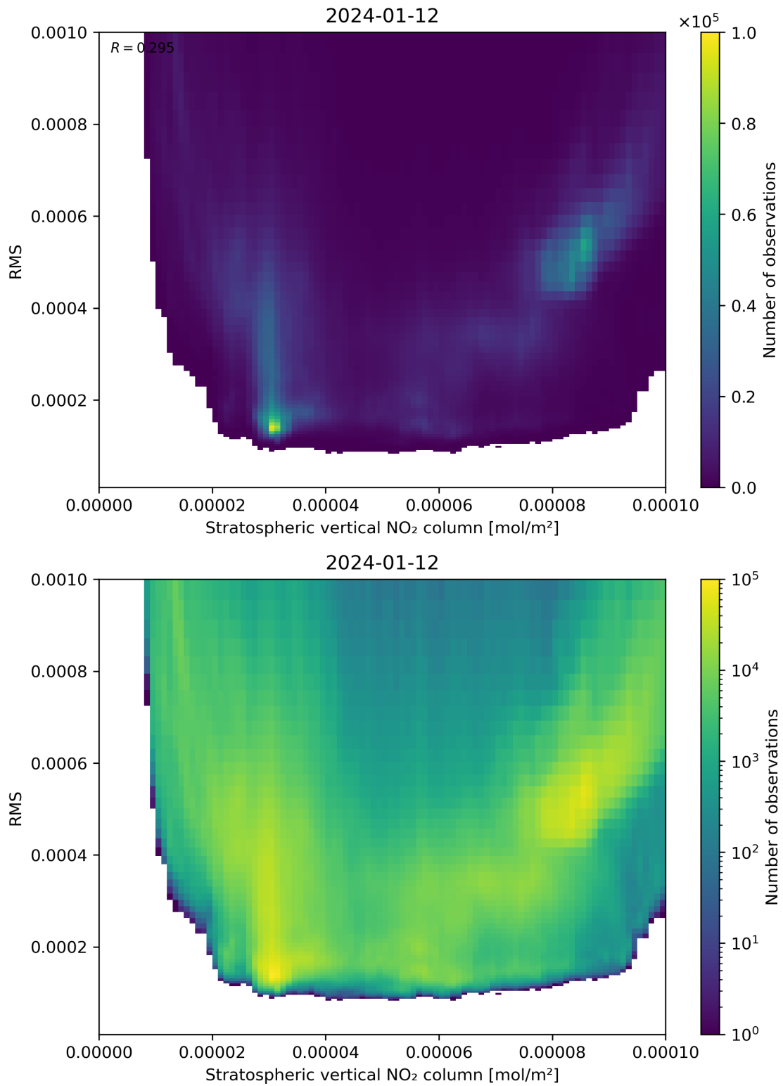
Figure 102: Scatter density plot of “Stratospheric vertical NO 2 column” against “RMS” for 2024-01-11 to 2024-01-13.
