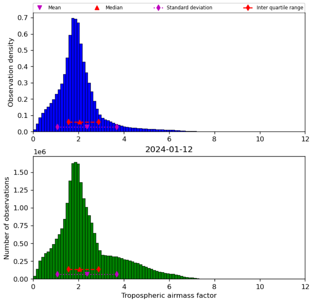
Figure 31: Histogram of “Tropospheric airmass factor” for 2024-01-11 to 2024-01-13
