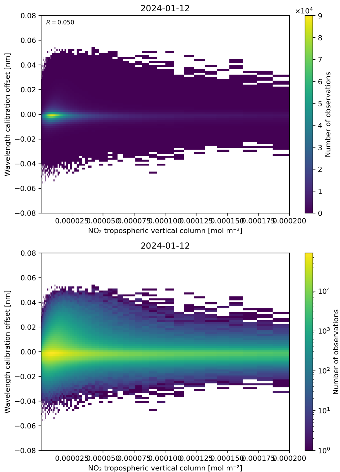
Figure 143: Scatter density plot of “NO 2 tropospheric vertical column” against “Wavelength calibration offset” for 2024-01-11 to 2024-01-13.
