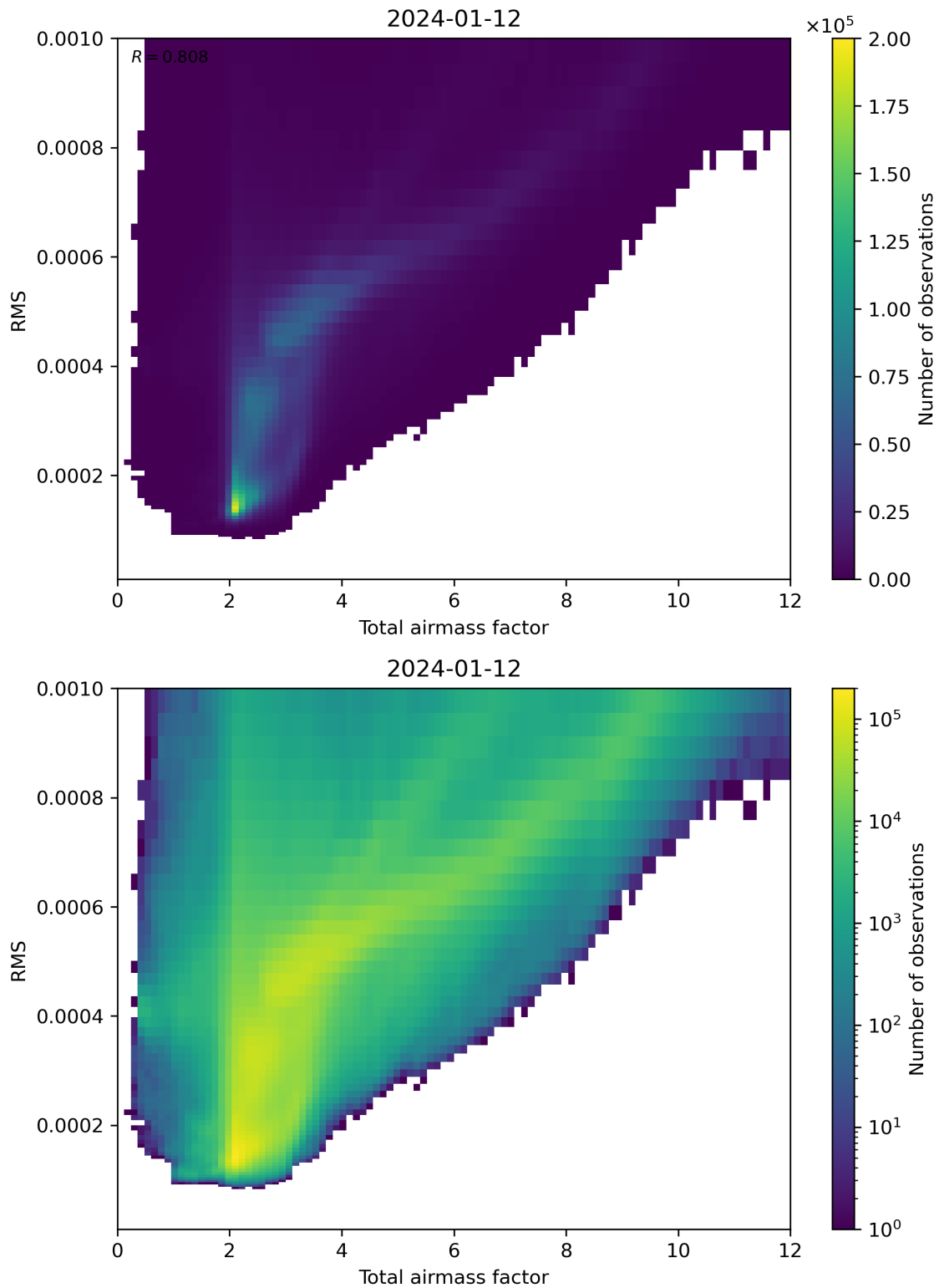
Figure 69: Scatter density plot of “Total airmass factor” against “RMS” for 2024-01-11 to 2024-01-13.
