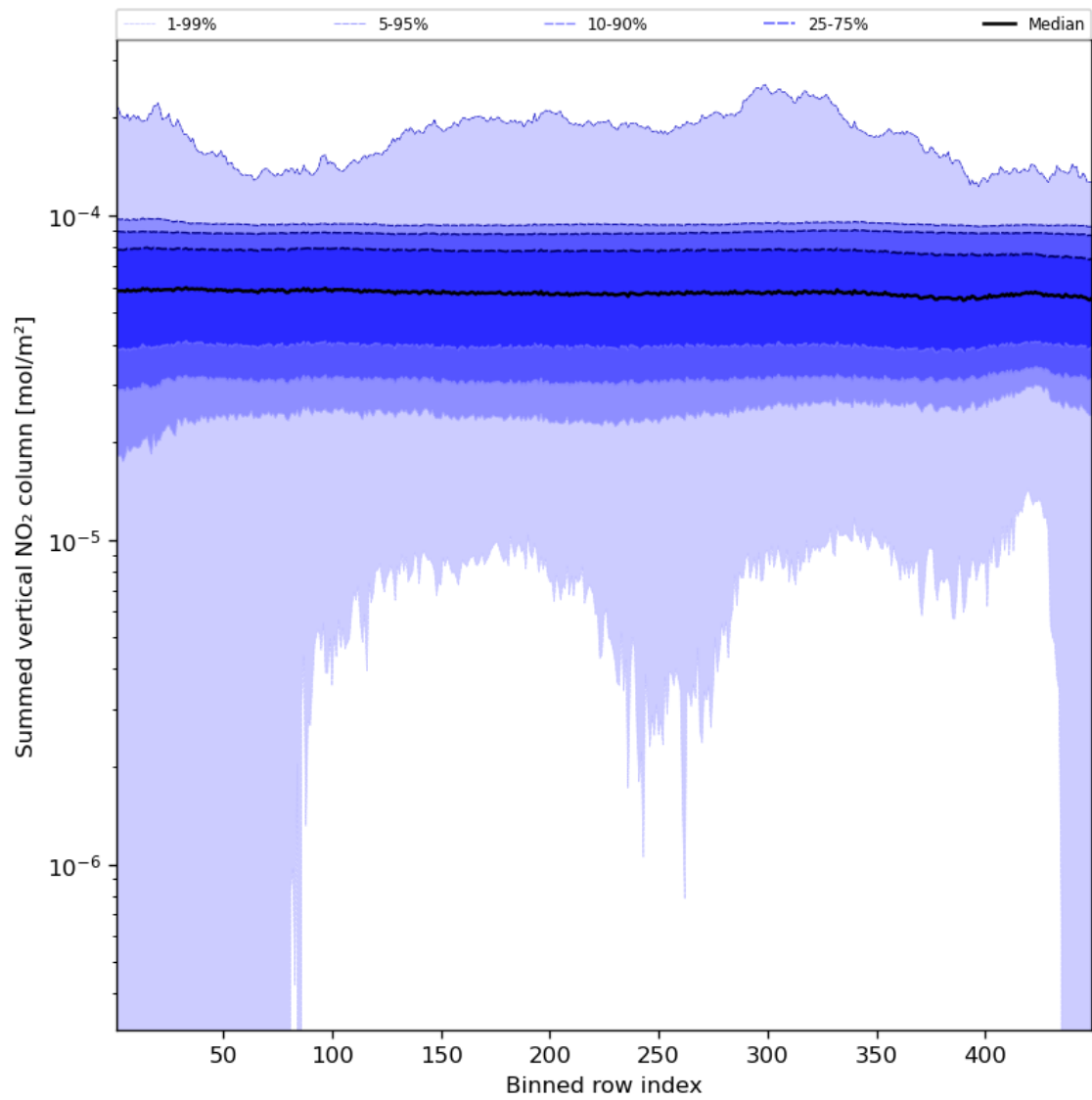
Figure 57: Along track statistics of “Summed vertical NO 2 column” for 2024-01-11 to 2024-01-13
