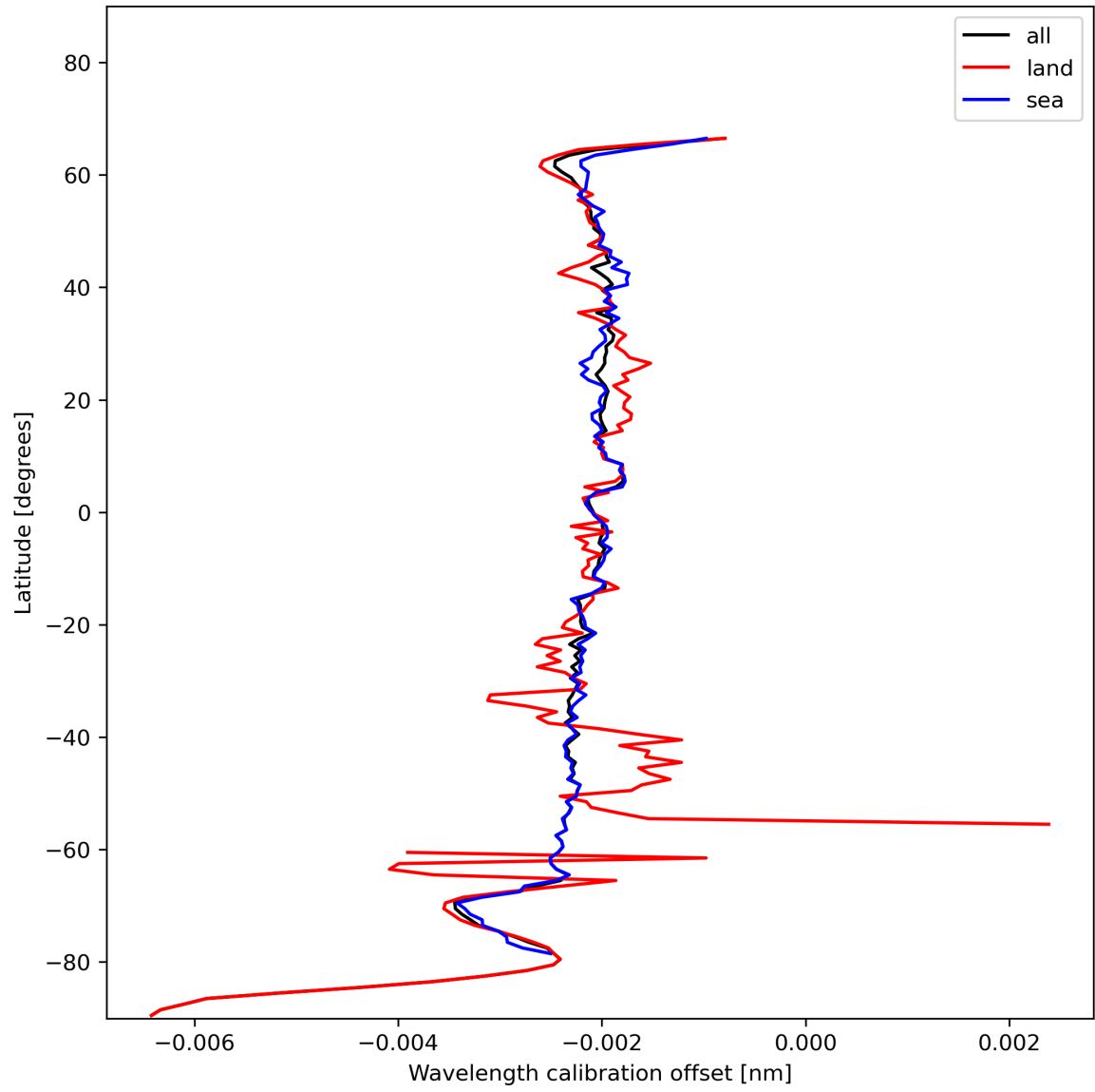
Figure 18: Zonal average of “Wavelength calibration offset” for 2024-01-11 to 2024-01-13.
