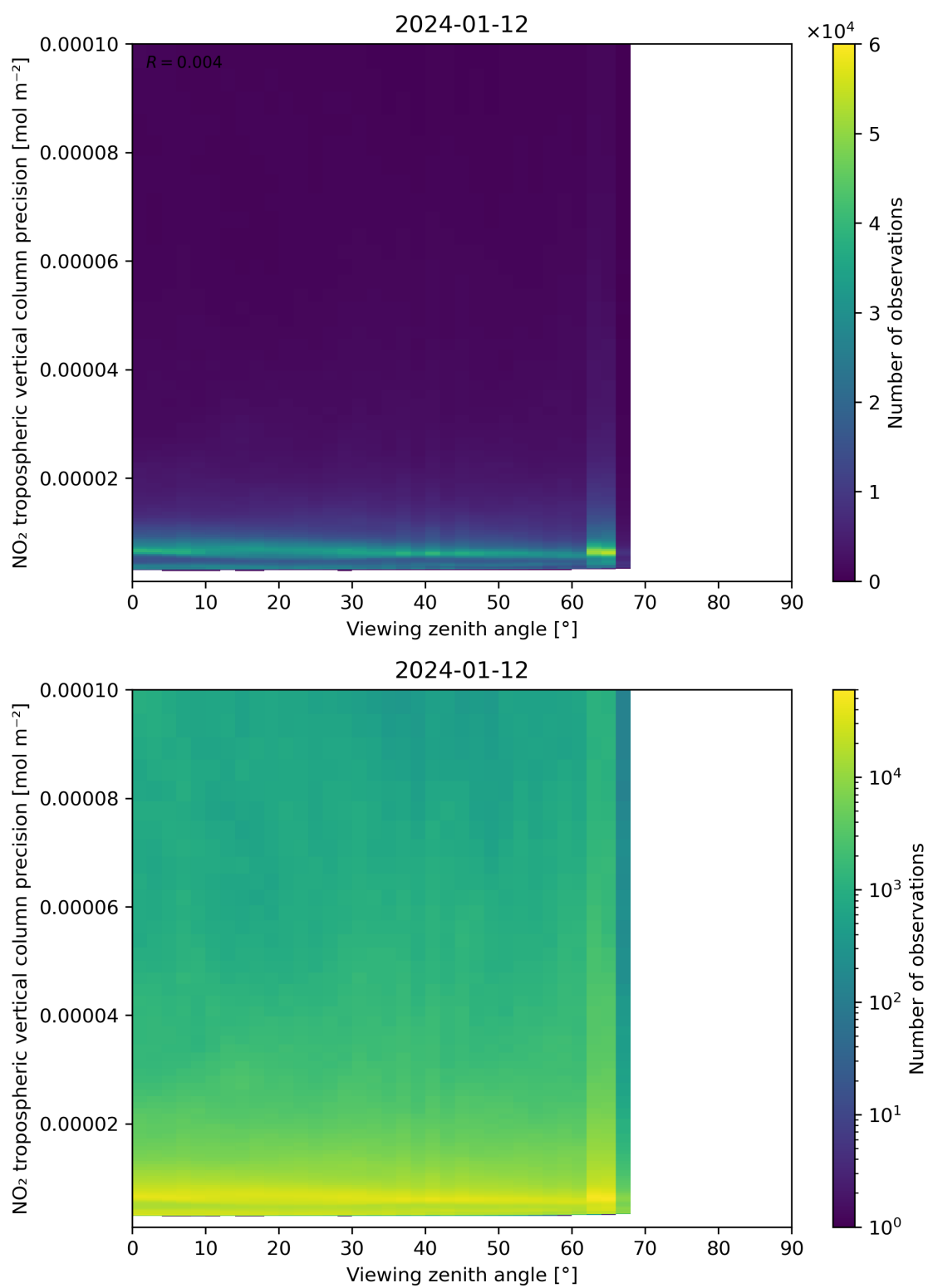
Figure 170: Scatter density plot of “Viewing zenith angle” against “NO 2 tropospheric vertical column precision” for 2024-01-11 to 2024-01-13.
