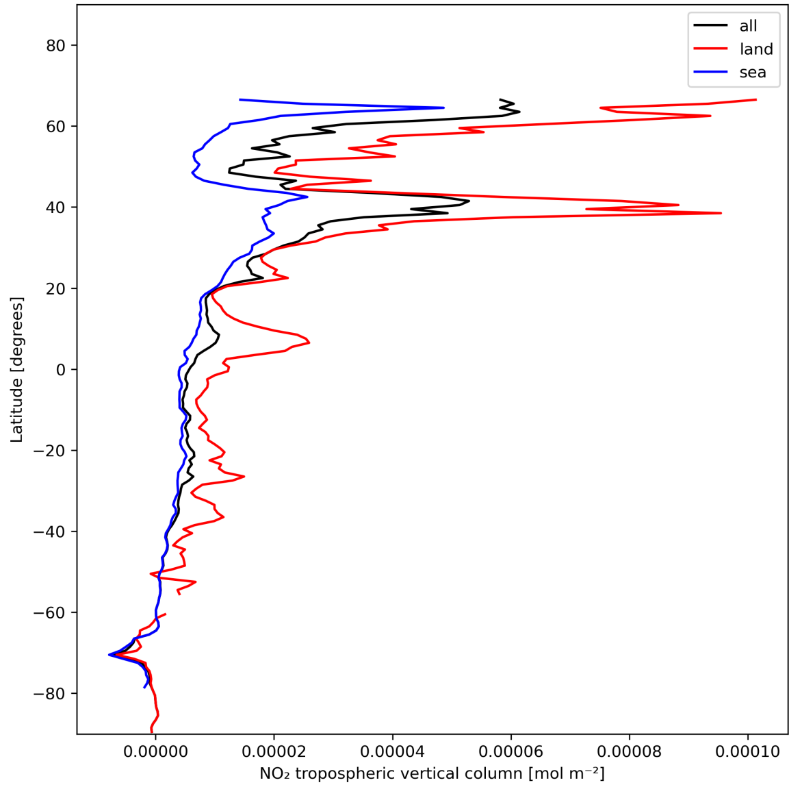
Figure 12: Zonal average of “NO 2 tropospheric vertical column” for 2024-01-11 to 2024-01-13.
