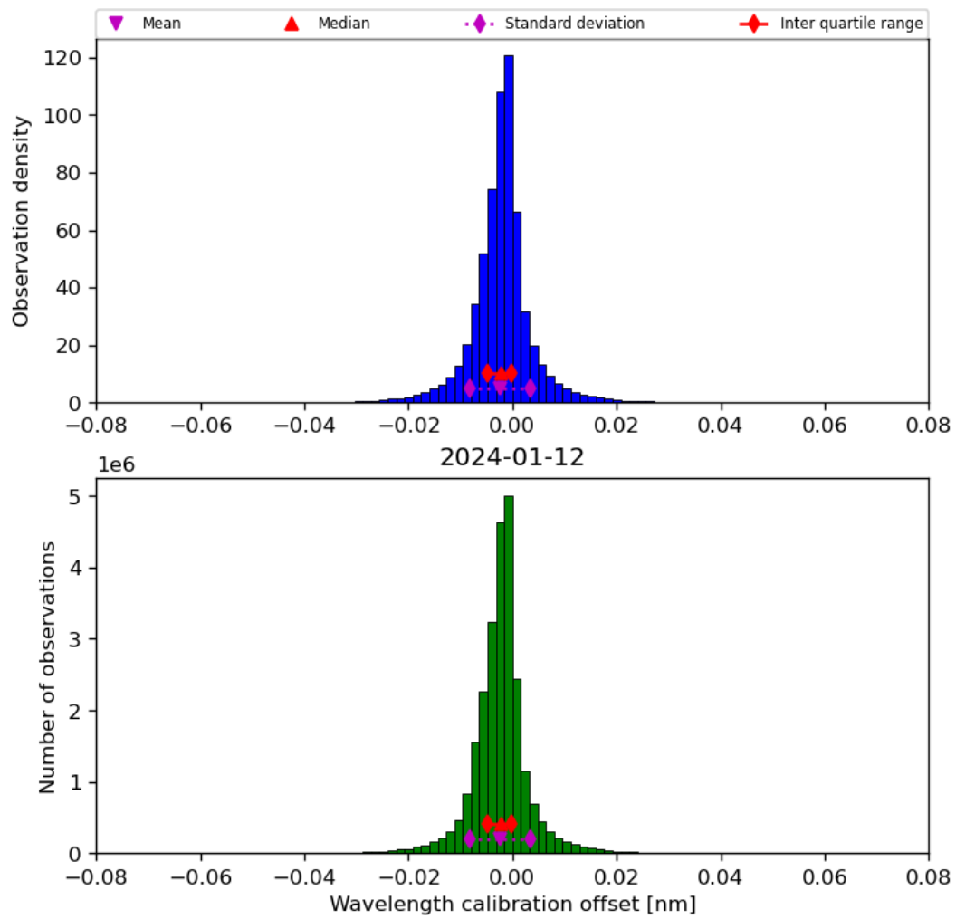
Figure 35: Histogram of “Wavelength calibration offset” for 2024-01-11 to 2024-01-13
