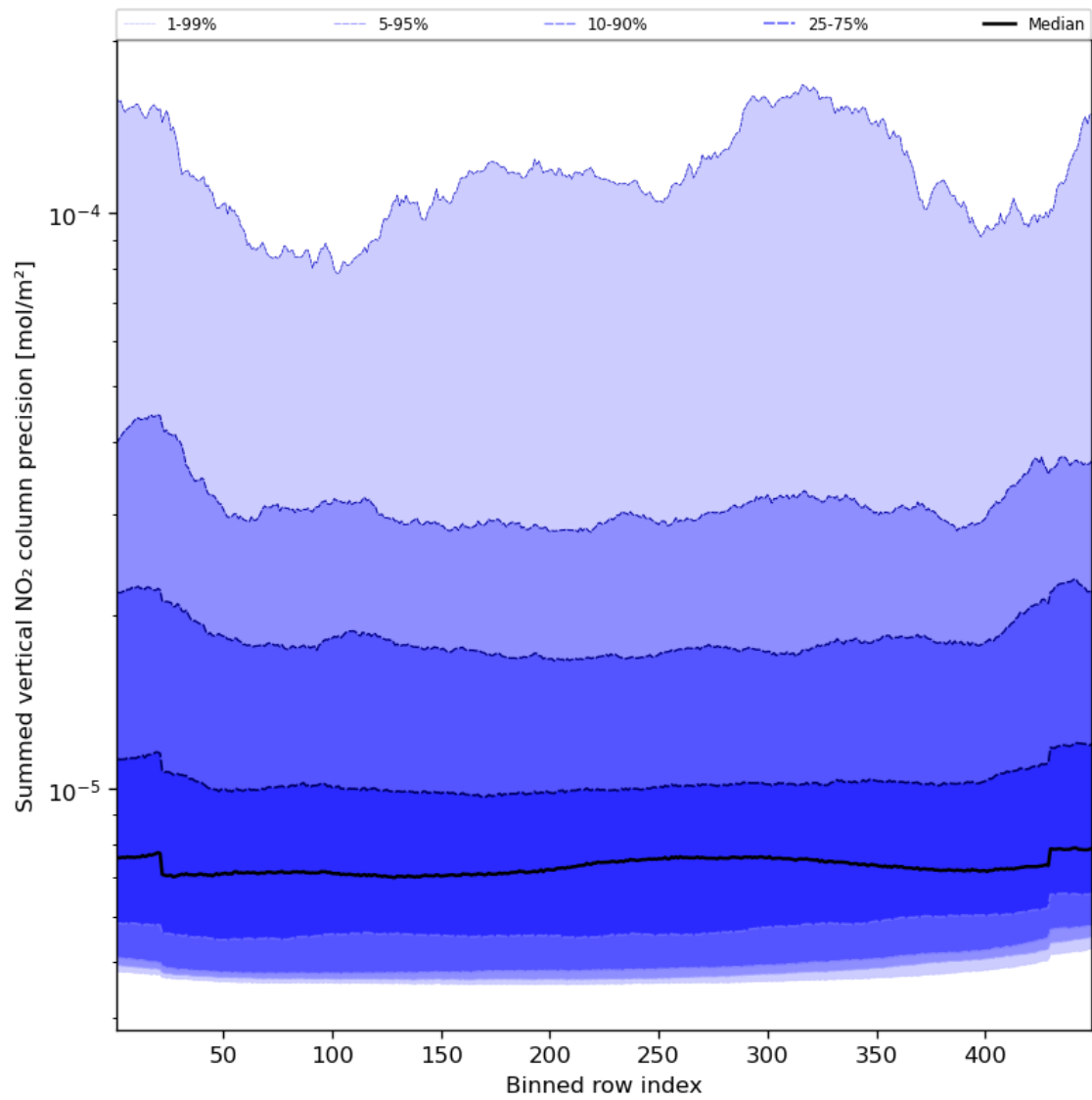
Figure 58: Along track statistics of “Summed vertical NO 2 column precision” for 2024-01-11 to 2024-01-13
