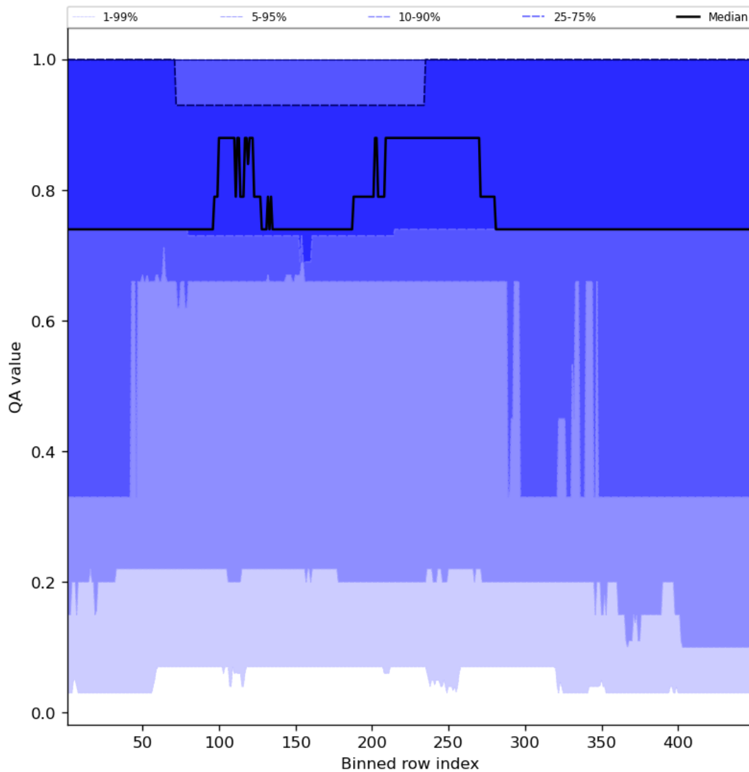
Figure 45: Along track statistics of “QA value” for 2024-01-11 to 2024-01-13
