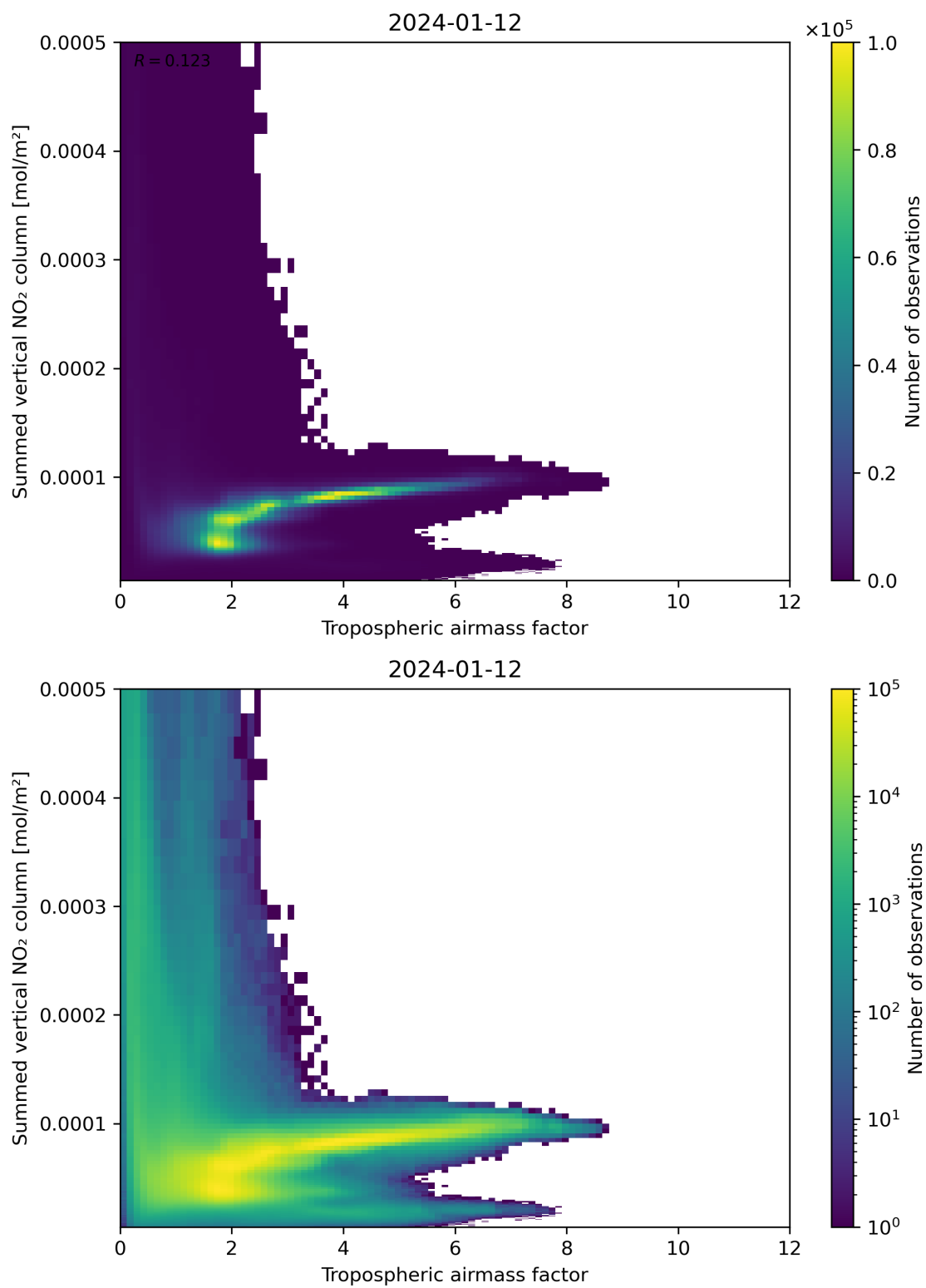
Figure 75: Scatter density plot of “Tropospheric airmass factor” against “Summed vertical NO 2 column” for 2024-01-11 to 2024-01-13.
