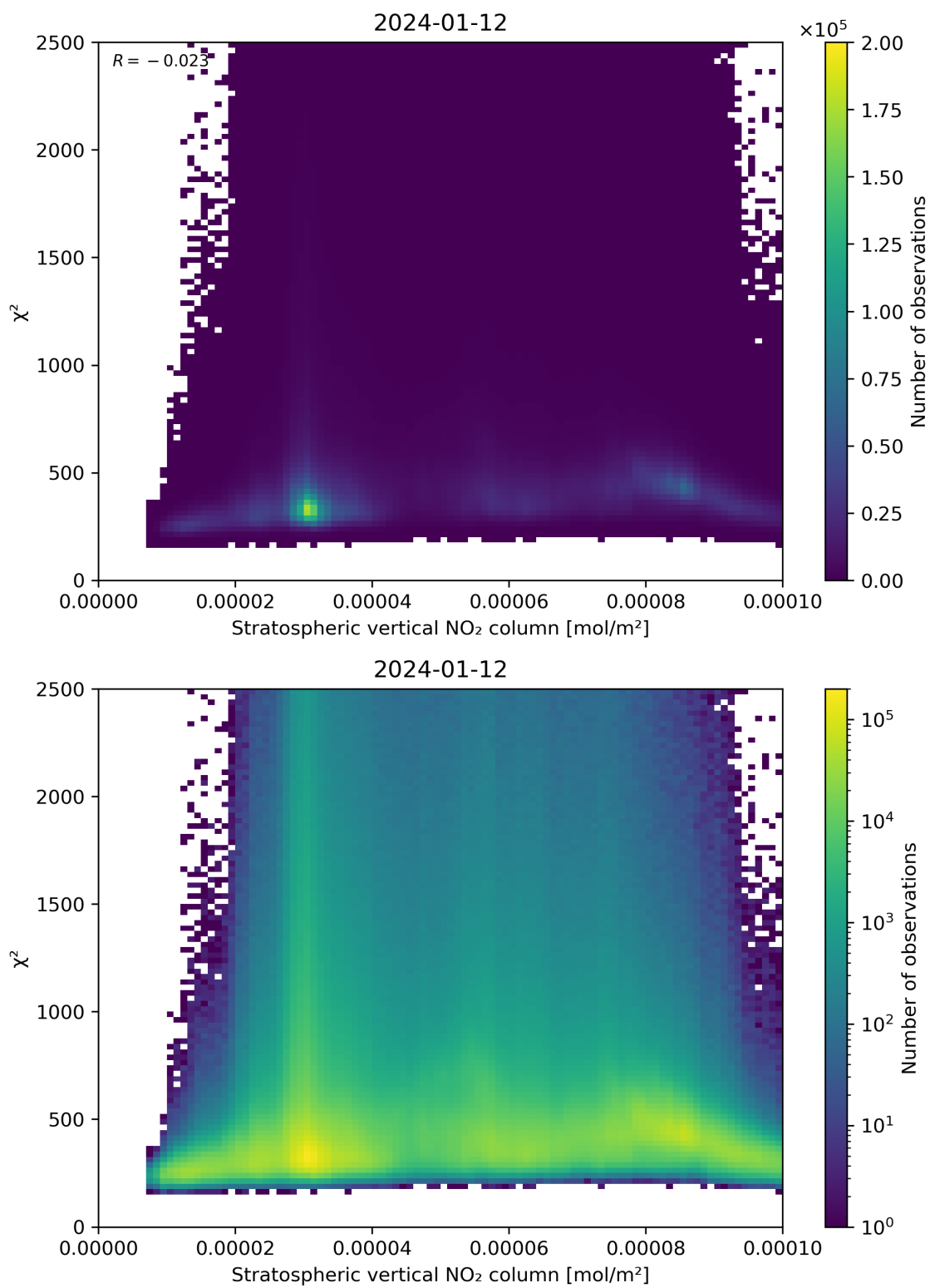
Figure 97: Scatter density plot of “Stratospheric vertical NO 2 column” against “ \chi^2 ” for 2024-01-11 to 2024-01-13.
