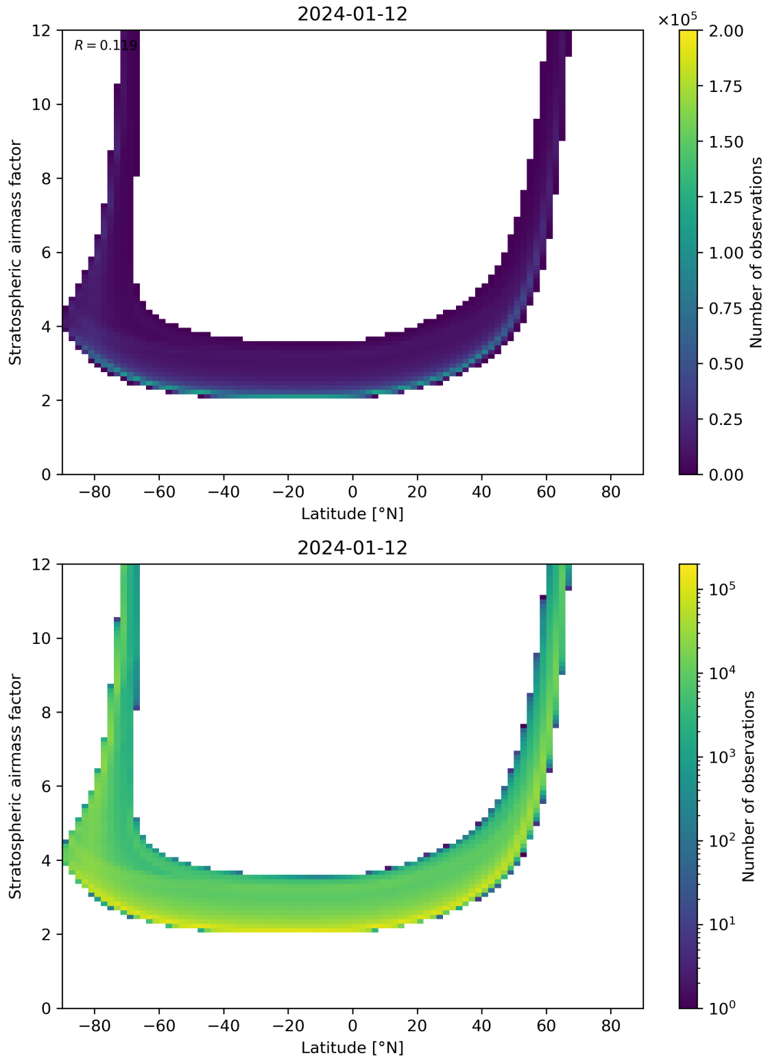
Figure 83: Scatter density plot of “Latitude” against “Stratospheric air mass factor” for 2024-01-11 to 2024-01-13.
