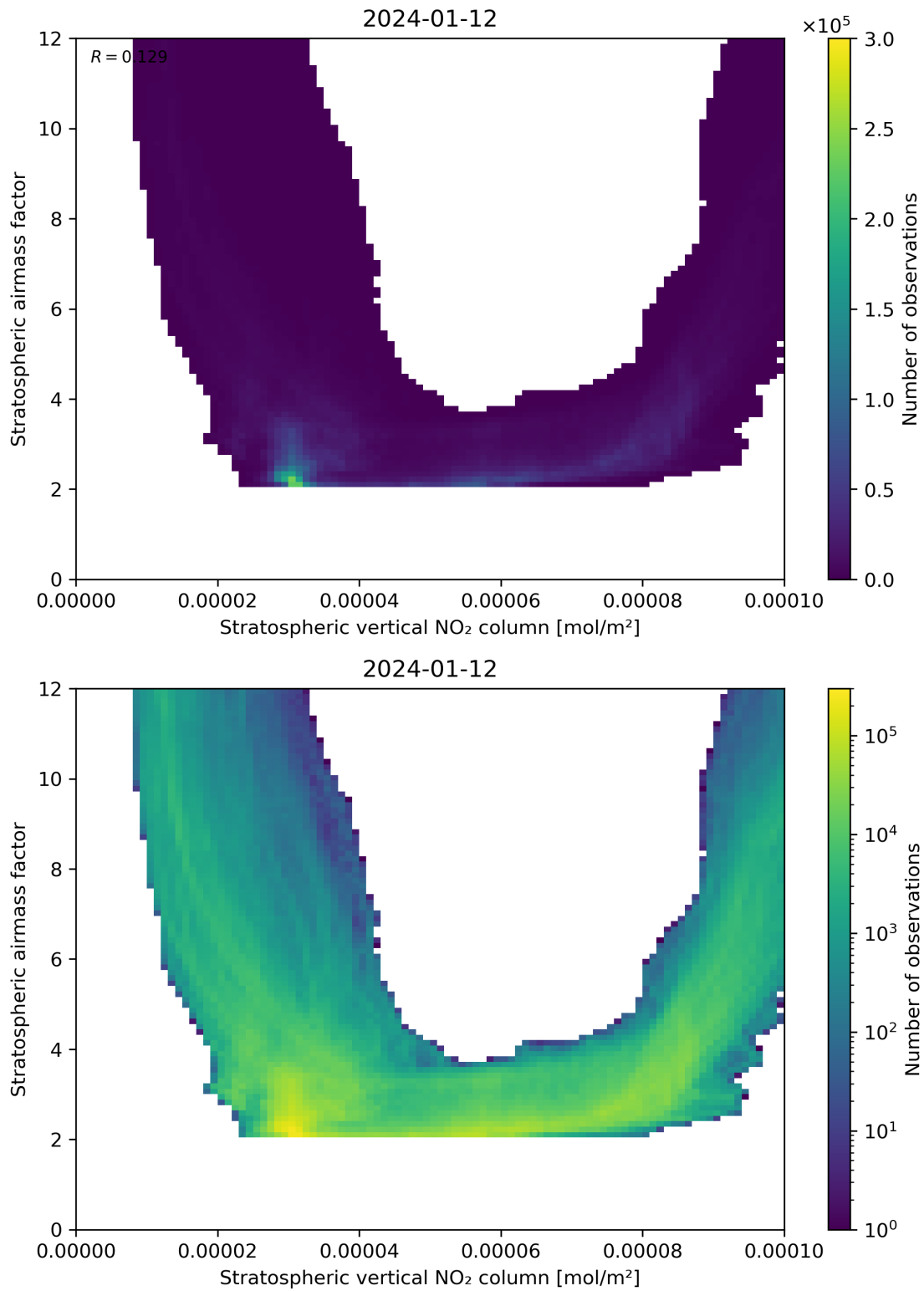
Figure 96: Scatter density plot of “Stratospheric vertical NO 2 column” against “Stratospheric airmass factor” for 2024-01-11 to 2024-01-13.
