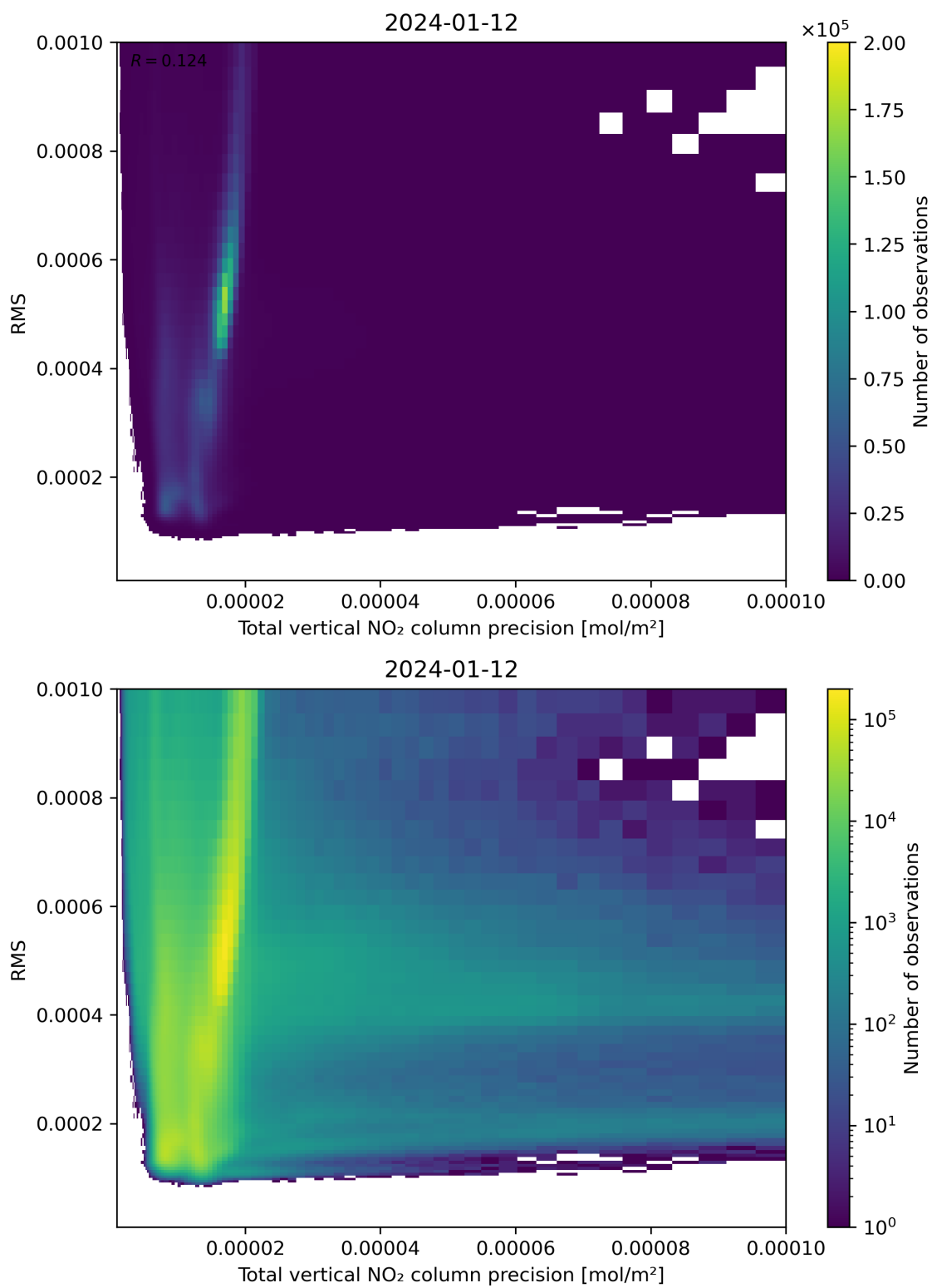
Figure 119: Scatter density plot of “Total vertical NO 2 column precision” against “RMS” for 2024-01-11 to 2024-01-13.
