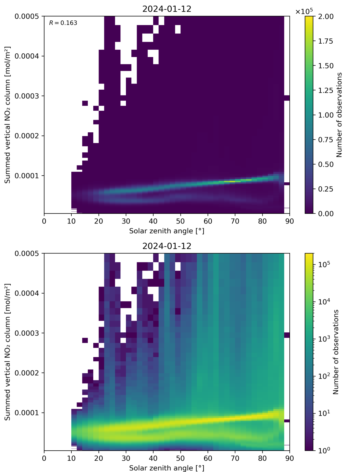
Figure 151: Scatter density plot of “Solar zenith angle” against “Summed vertical NO 2 column” for 2024-01-11 to 2024-01-13.
