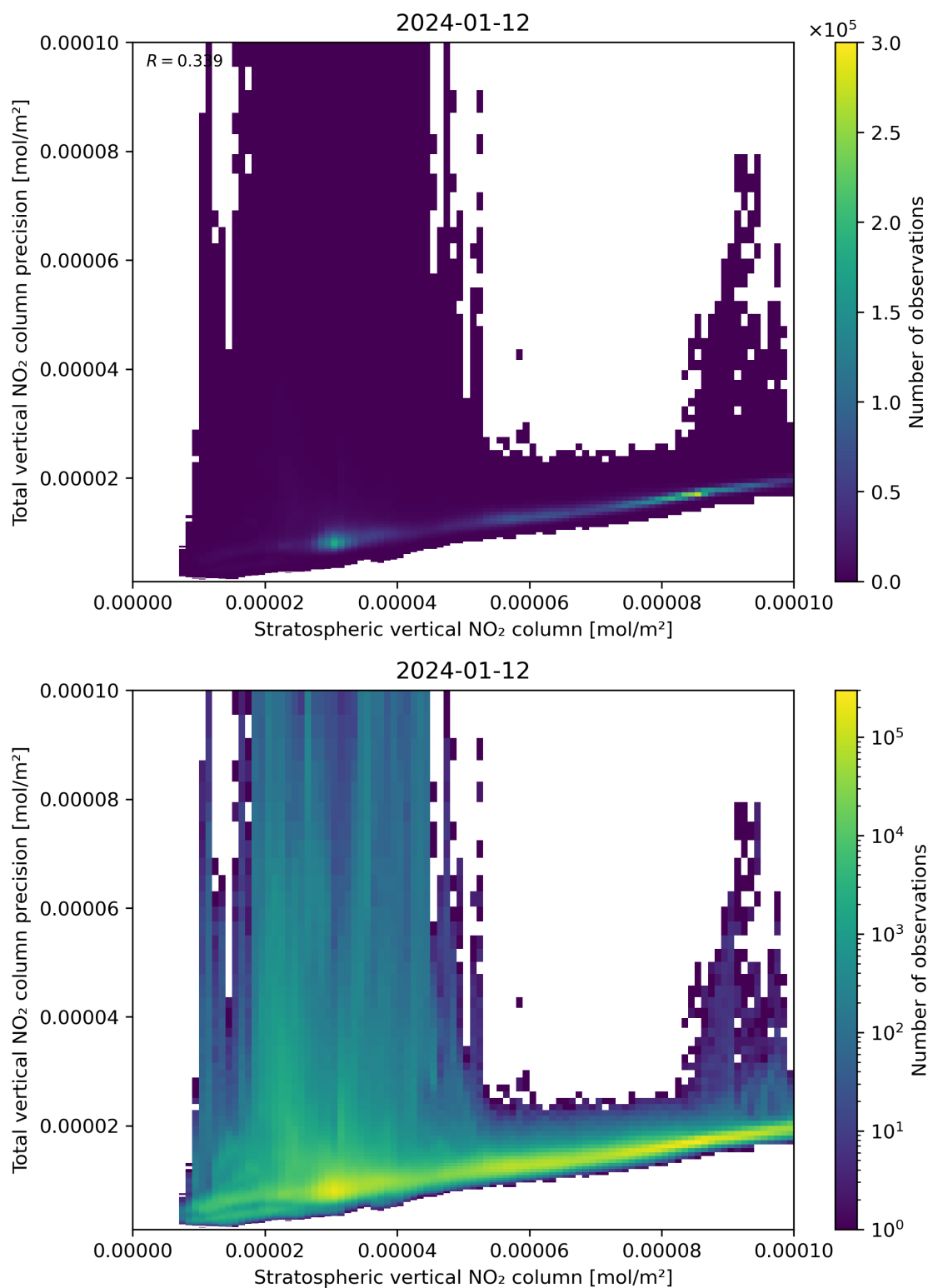
Figure 101: Scatter density plot of “Stratospheric vertical NO 2 column” against “Total vertical NO 2 column precision” for 2024-01-11 to 2024-01-13.
