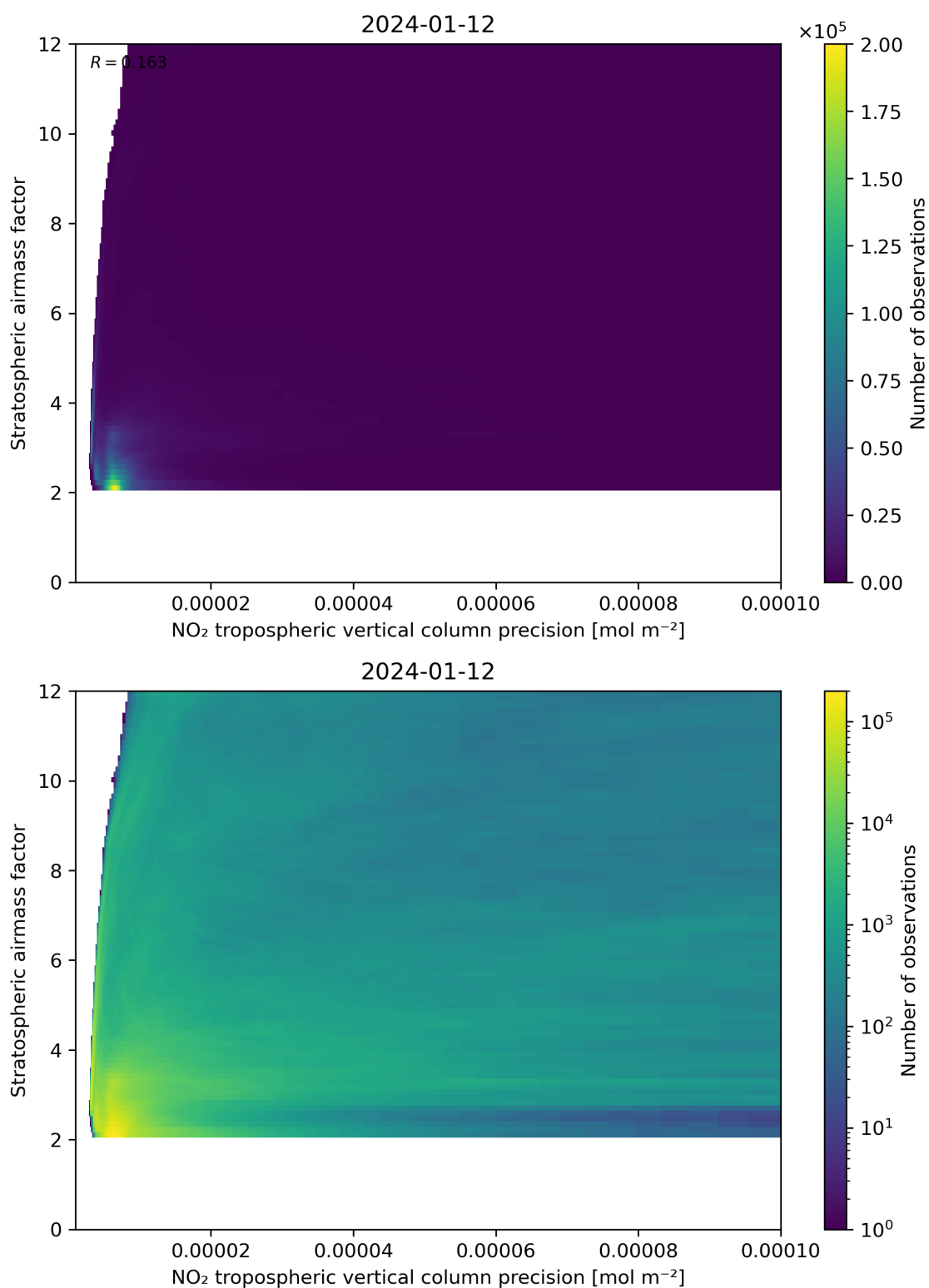
Figure 131: Scatter density plot of “NO 2 tropospheric vertical column precision” against “Stratospheric airmass factor” for 2024-01-11 to 2024-01-13.
