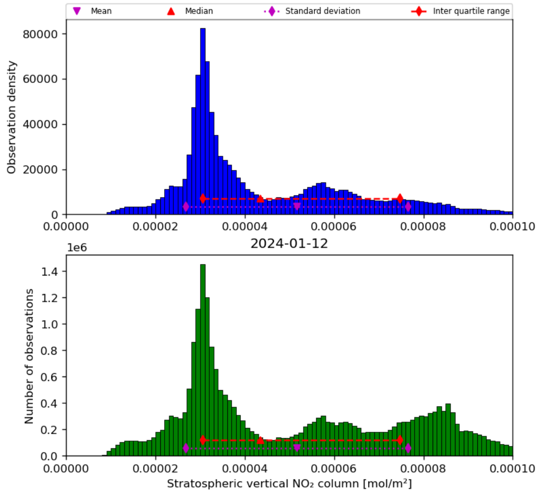
Figure 36: Histogram of “Stratospheric vertical NO 2 column” for 2024-01-11 to 2024-01-13
