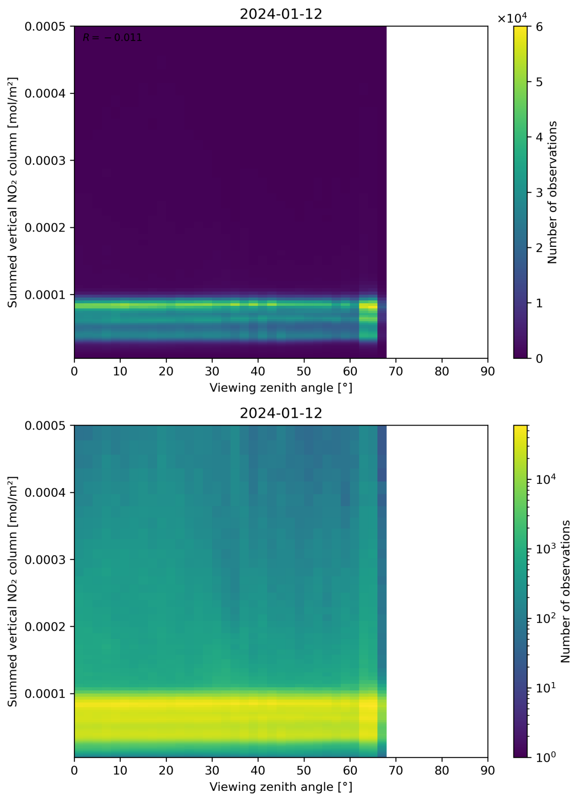
Figure 165: Scatter density plot of “Viewing zenith angle” against “Summed vertical NO 2 column” for 2024-01-11 to 2024-01-13.
