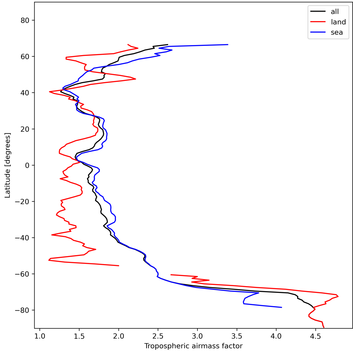
Figure 14: Zonal average of “Tropospheric airmass factor” for 2024-01-11 to 2024-01-13.
