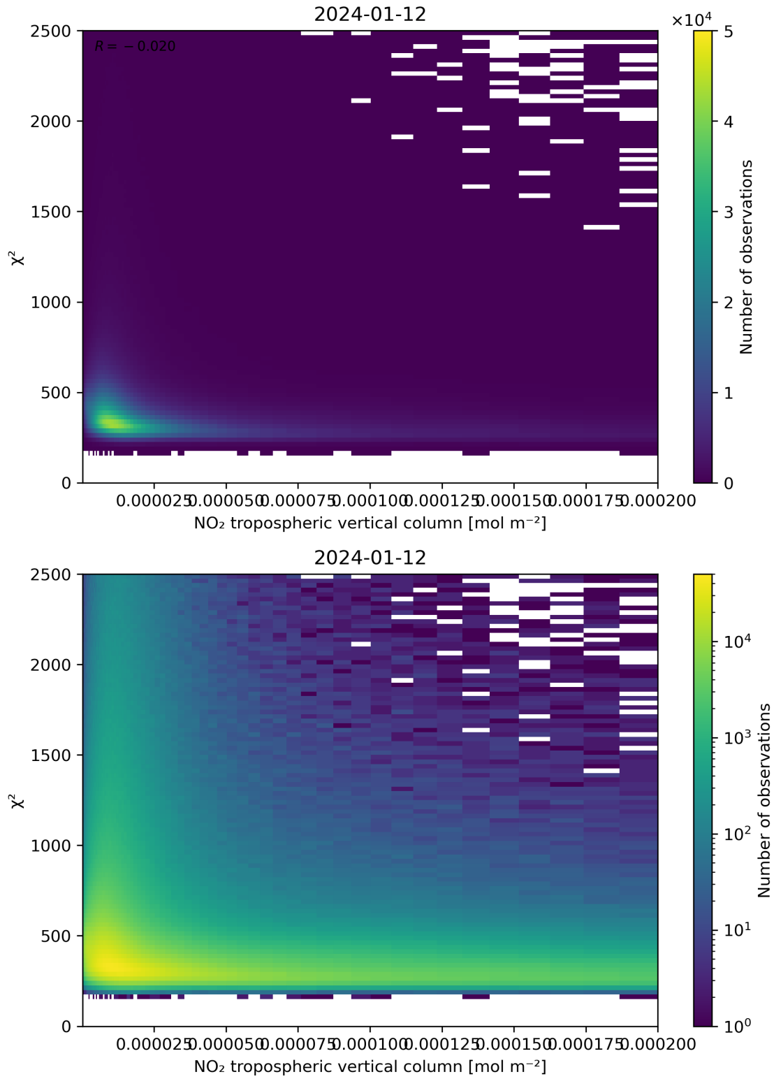
Figure 124: Scatter density plot of “NO 2 tropospheric vertical column” against “ \chi^2 ” for 2024-01-11 to 2024-01-13.
