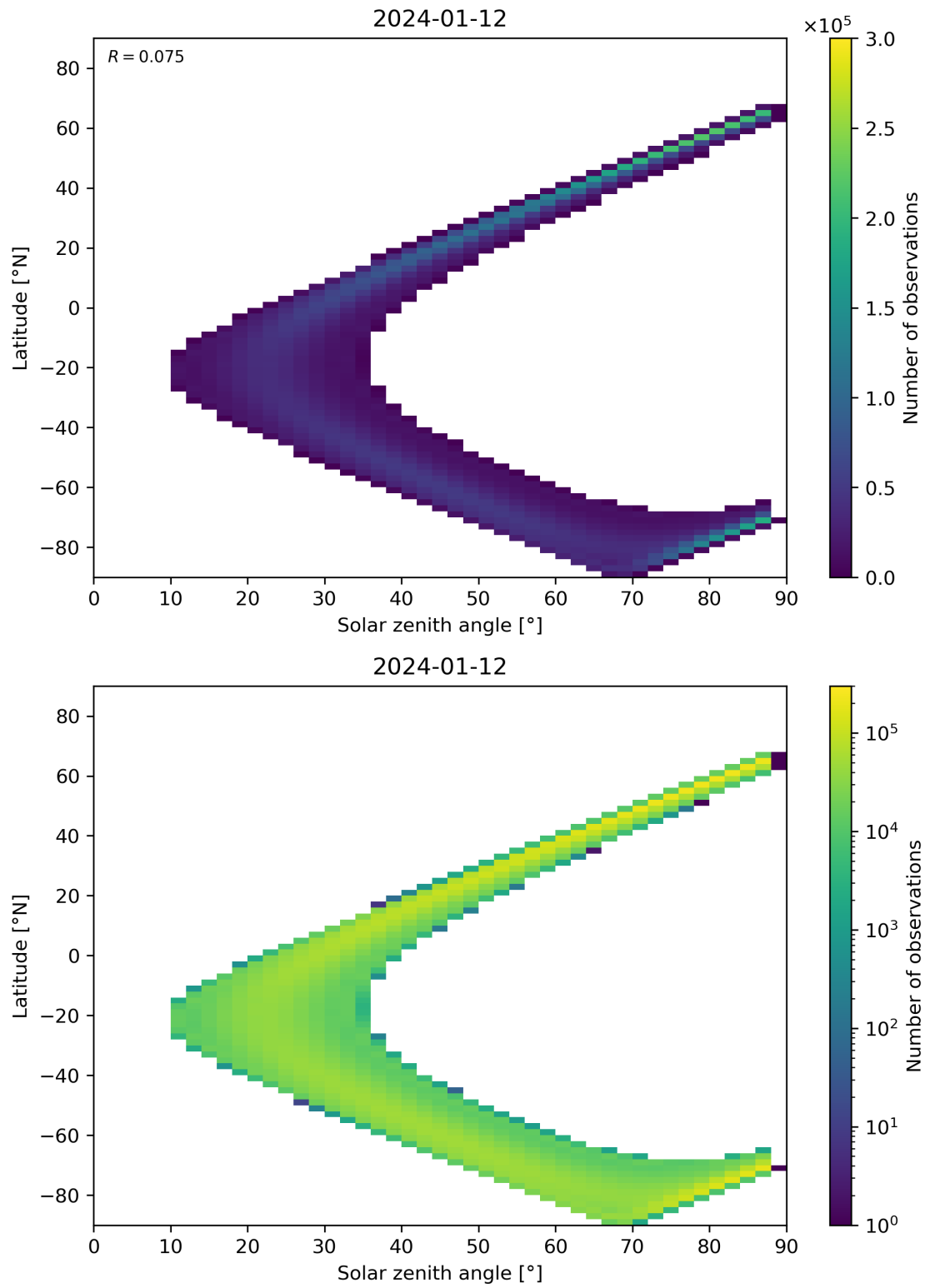
Figure 149: Scatter density plot of “Solar zenith angle” against “Latitude” for 2024-01-11 to 2024-01-13.
