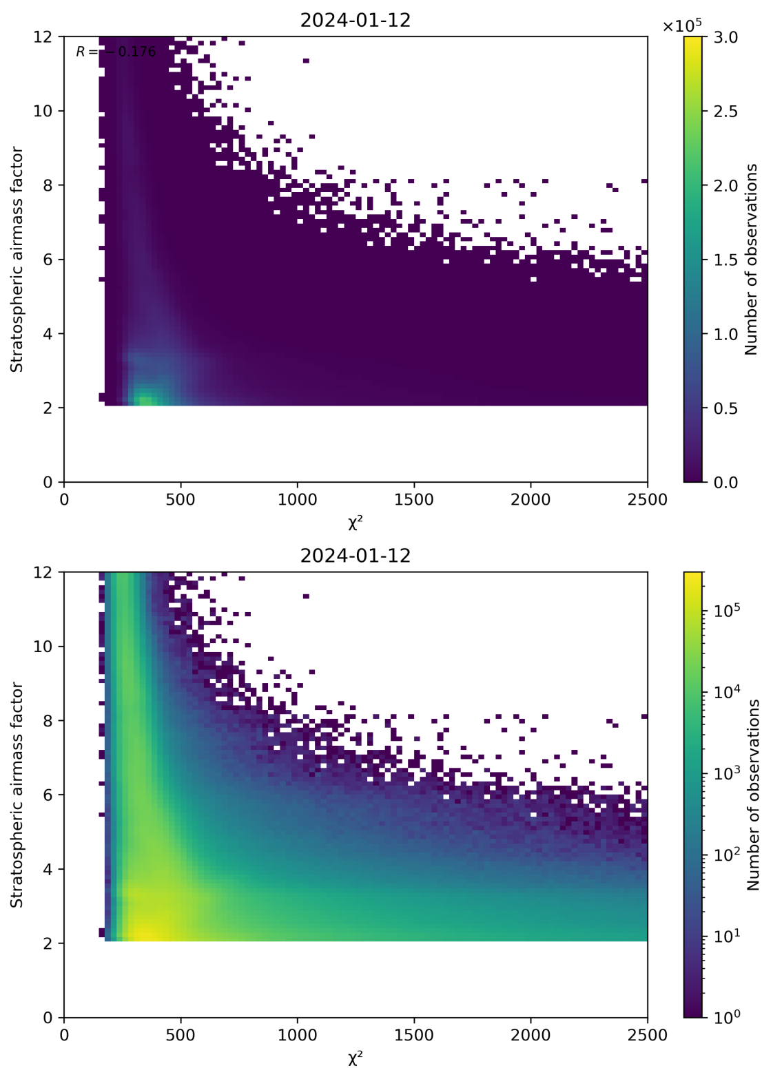
Figure 81: Scatter density plot of “ \chi^2 ” against “Stratospheric airmass factor” for 2024-01-11 to 2024-01-13.
