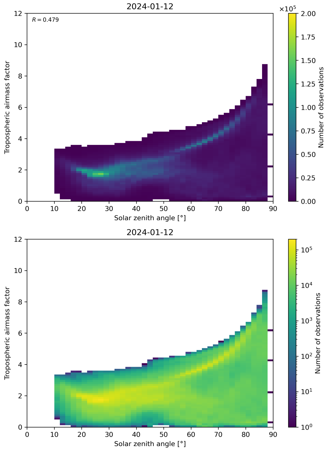
Figure 147: Scatter density plot of “Solar zenith angle” against “Tropospheric airmass factor” for 2024-01-11 to 2024-01-13.
