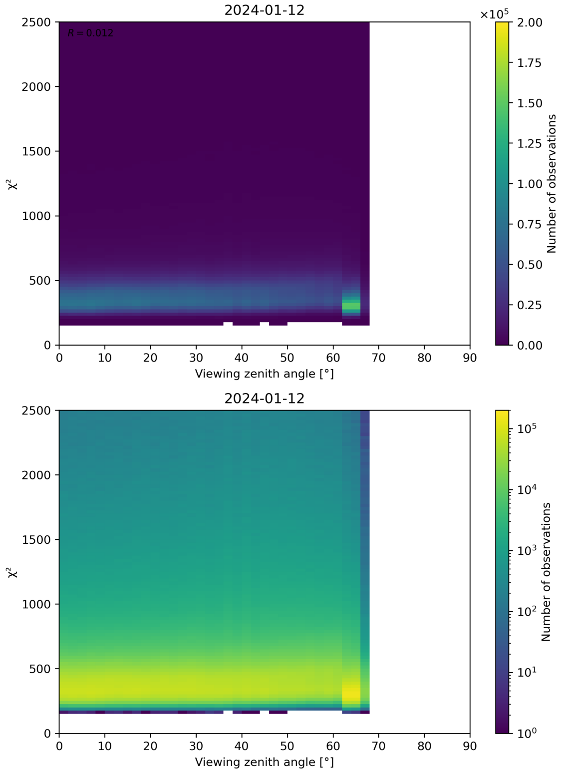
Figure 162: Scatter density plot of “Viewing zenith angle” against “ \chi^2 ” for 2024-01-11 to 2024-01-13.
