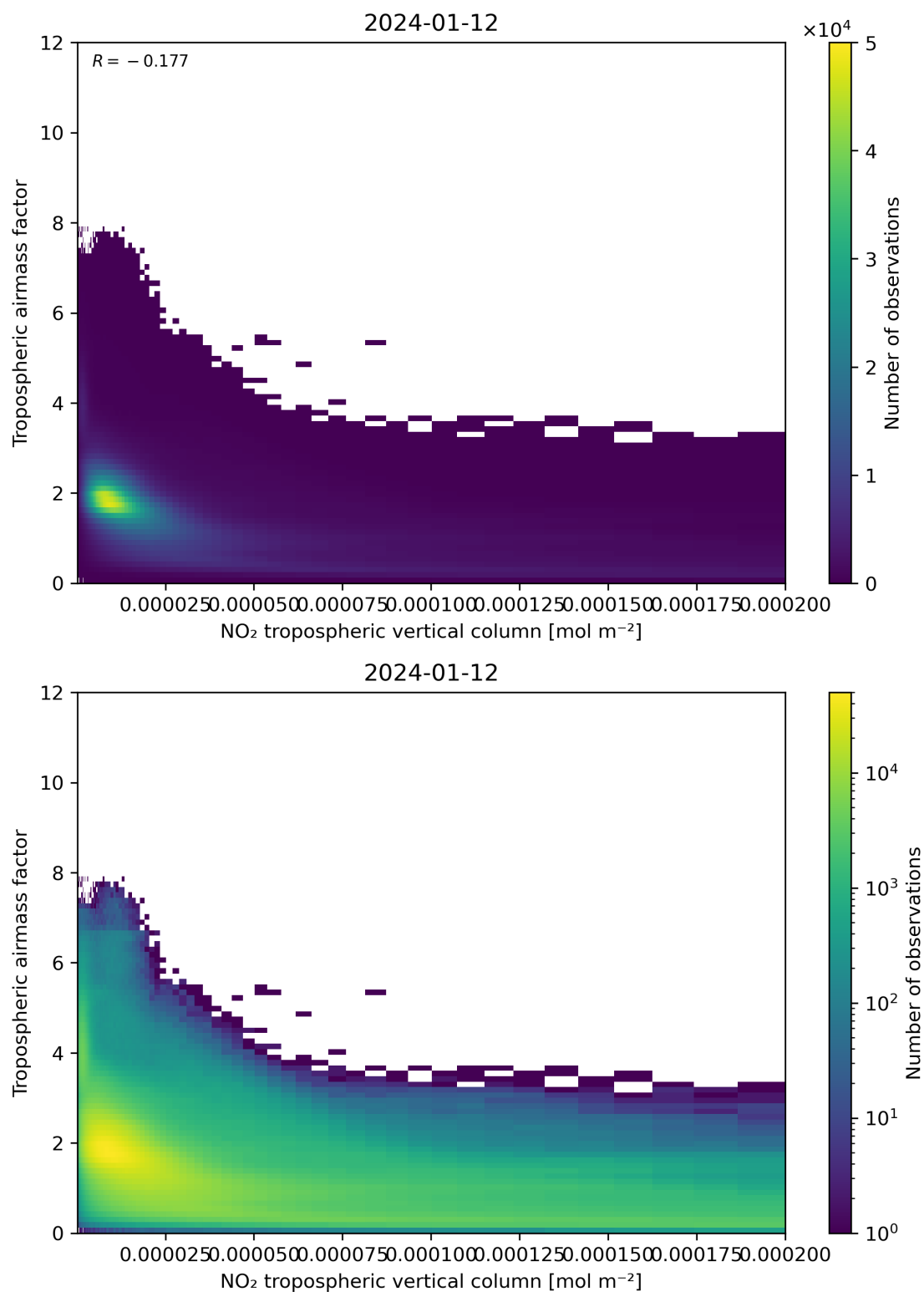
Figure 123: Scatter density plot of “NO 2 tropospheric vertical column” against “Tropospheric air mass factor” for 2024-01-11 to 2024-01-13.
