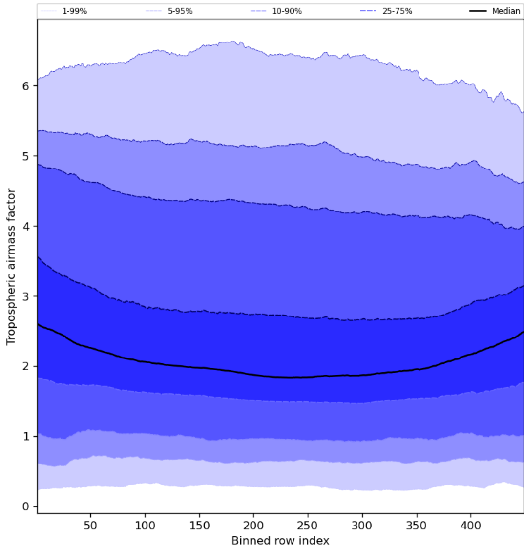
Figure 48: Along track statistics of “Tropospheric air mass factor” for 2024-01-11 to 2024-01-13
