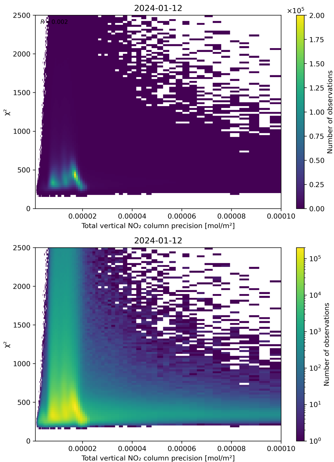
Figure 116: Scatter density plot of “Total vertical NO 2 column precision” against “ \chi^2 ” for 2024-01-11 to 2024-01-13.
