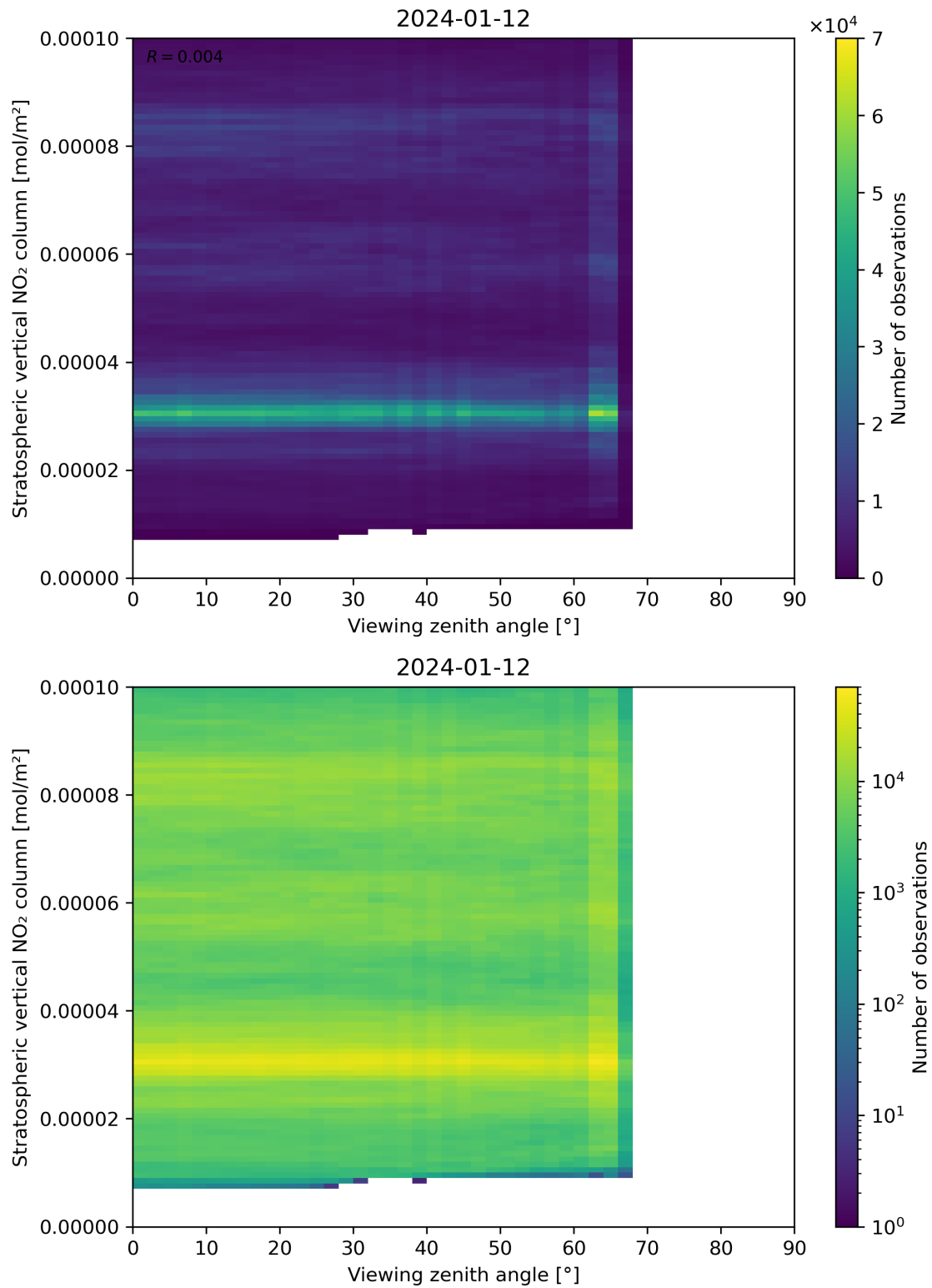
Figure 164: Scatter density plot of “Viewing zenith angle” against “Stratospheric vertical NO 2 column” for 2024-01-11 to 2024-01-13.
