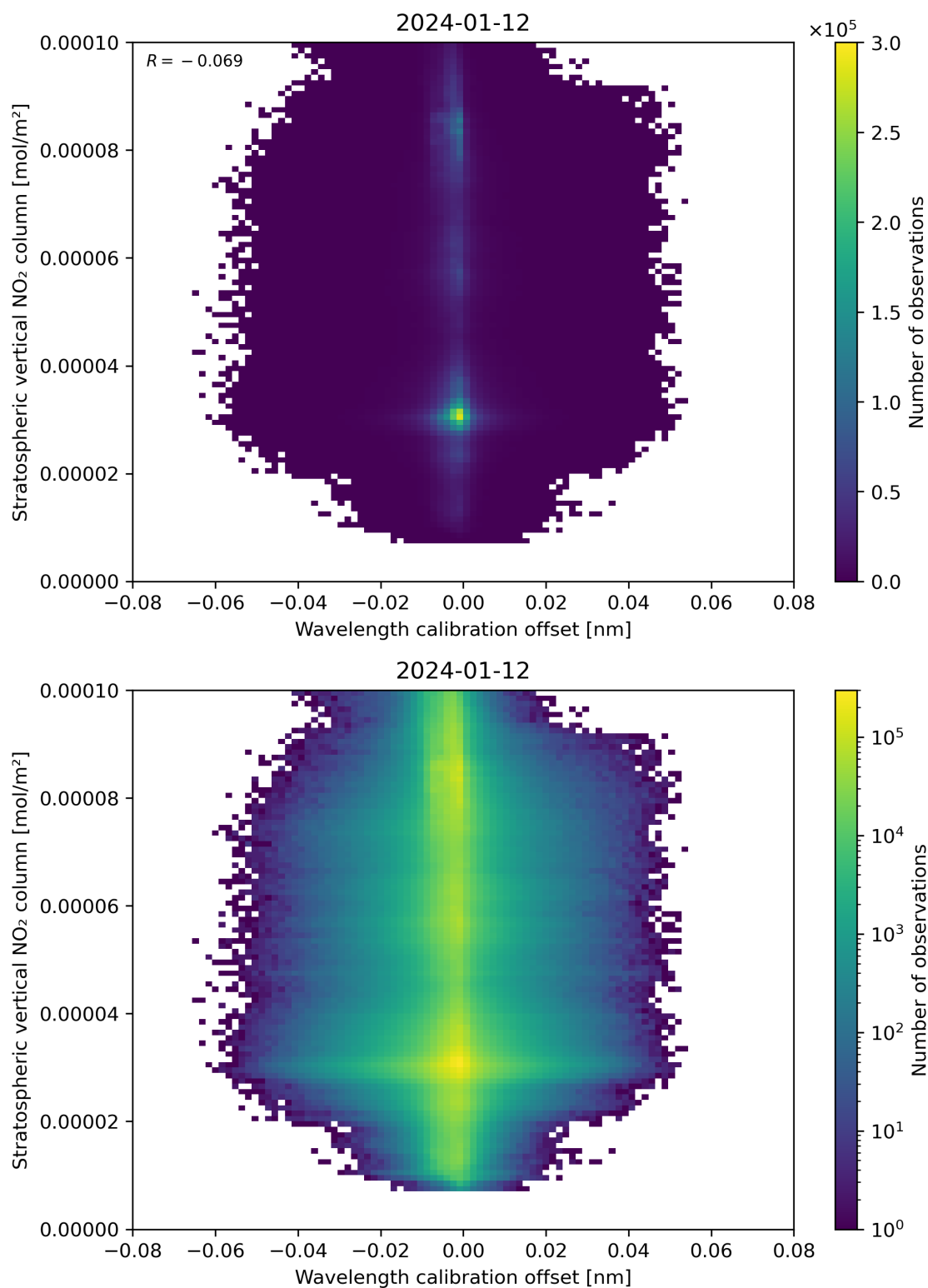
Figure 176: Scatter density plot of “Wavelength calibration offset” against “Stratospheric vertical NO 2 column” for 2024-01-11 to 2024-01-13.
