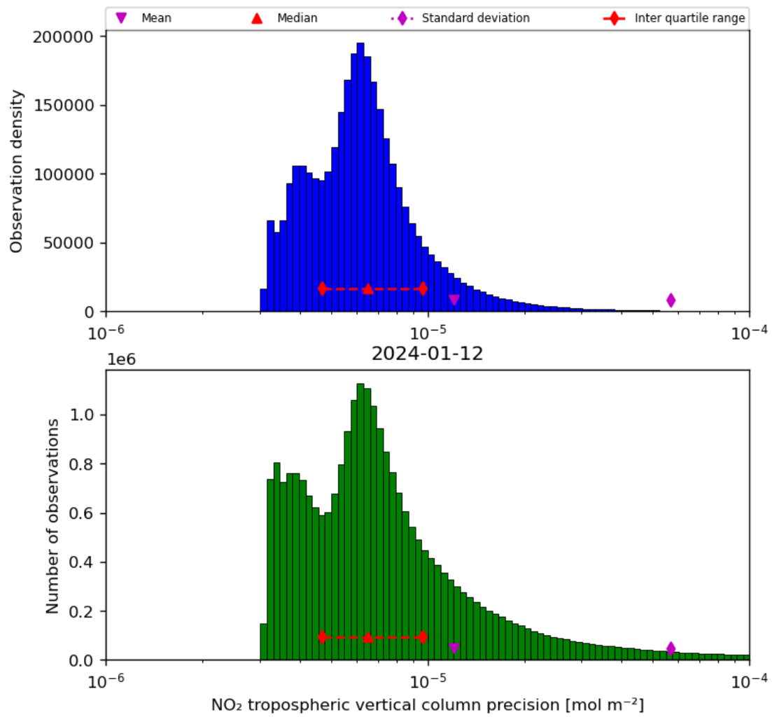
Figure 30: Histogram of “NO 2 tropospheric vertical column precision” for 2024-01-11 to 2024-01-13
