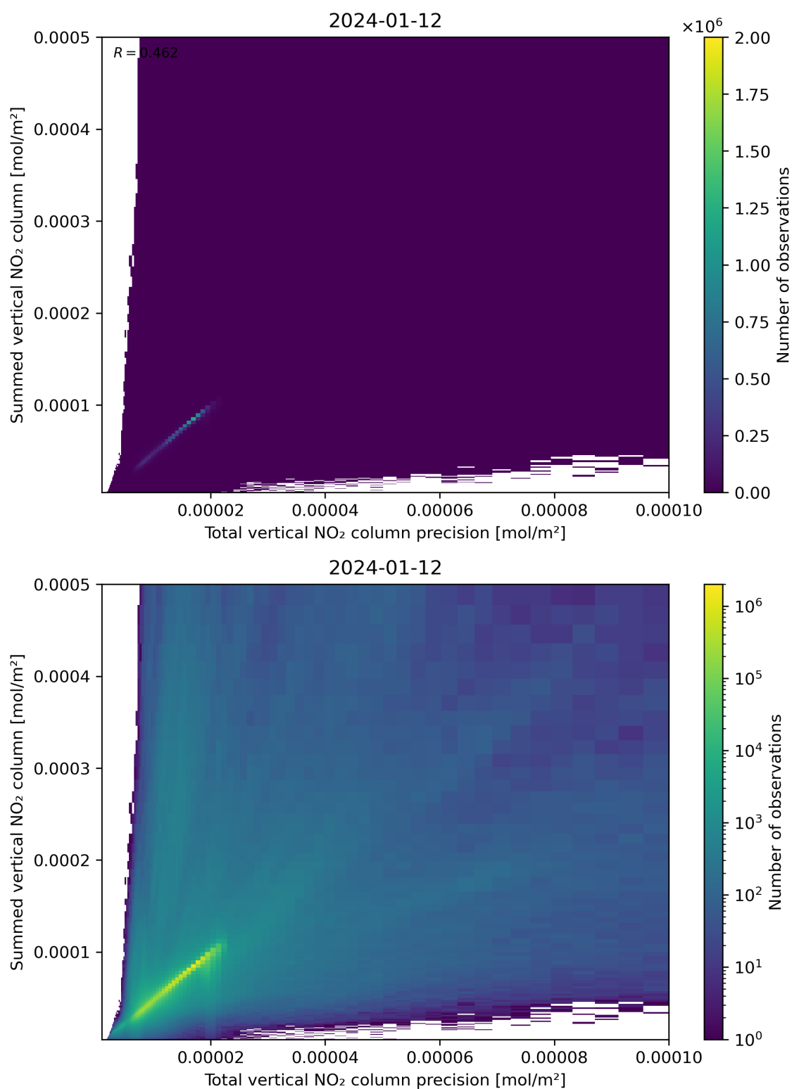
Figure 117: Scatter density plot of “Total vertical NO 2 column precision” against “Summed vertical NO 2 column” for 2024-01-11 to 2024-01-13.
