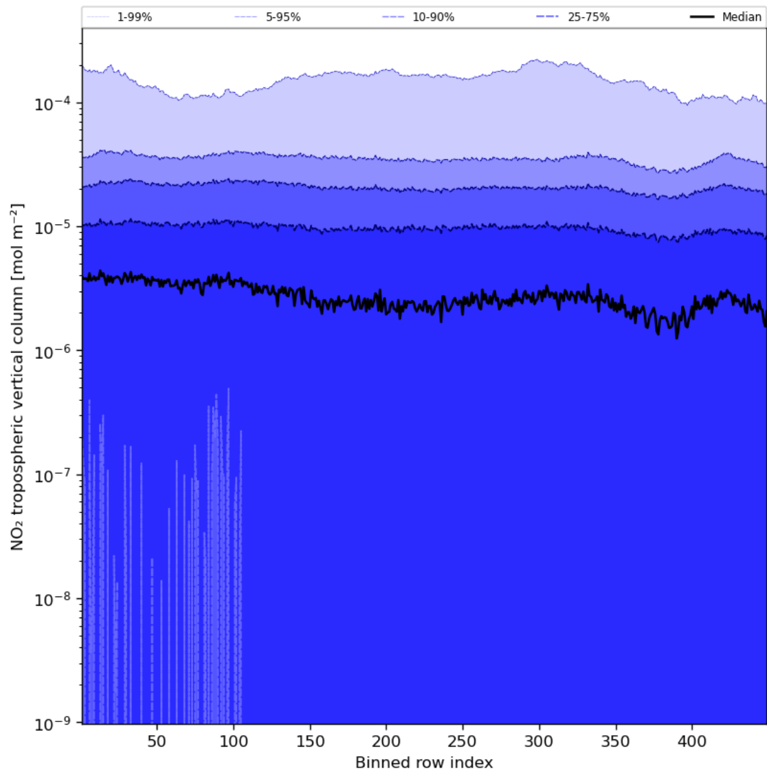
Figure 46: Along track statistics of “NO 2 tropospheric vertical column” for 2024-01-11 to 2024-01-13
