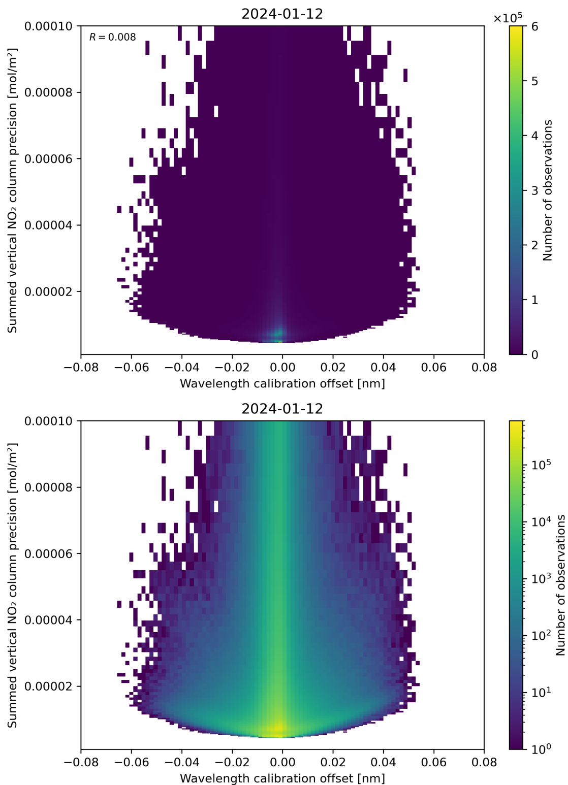
Figure 178: Scatter density plot of “Wavelength calibration offset” against “Summed vertical NO 2 column precision” for 2024-01-11 to 2024-01-13.
