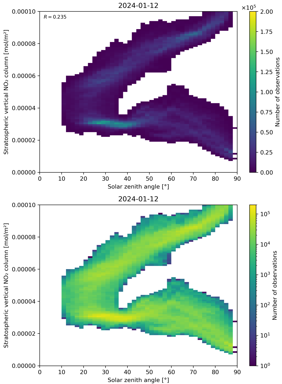
Figure 150: Scatter density plot of “Solar zenith angle” against “Stratospheric vertical NO 2 column” for 2024-01-11 to 2024-01-13.
