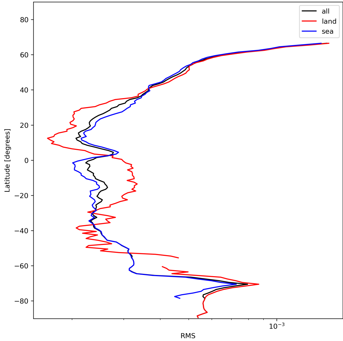
Figure 26: Zonal average of “RMS” for 2024-01-11 to 2024-01-13.
