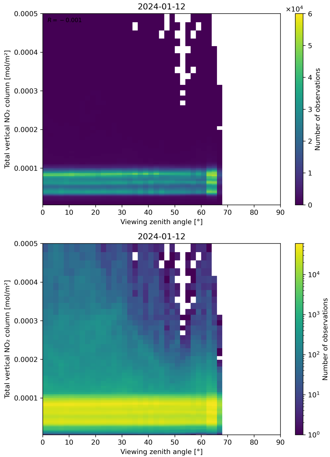
Figure 167: Scatter density plot of “Viewing zenith angle” against “Total vertical NO 2 column” for 2024-01-11 to 2024-01-13.
