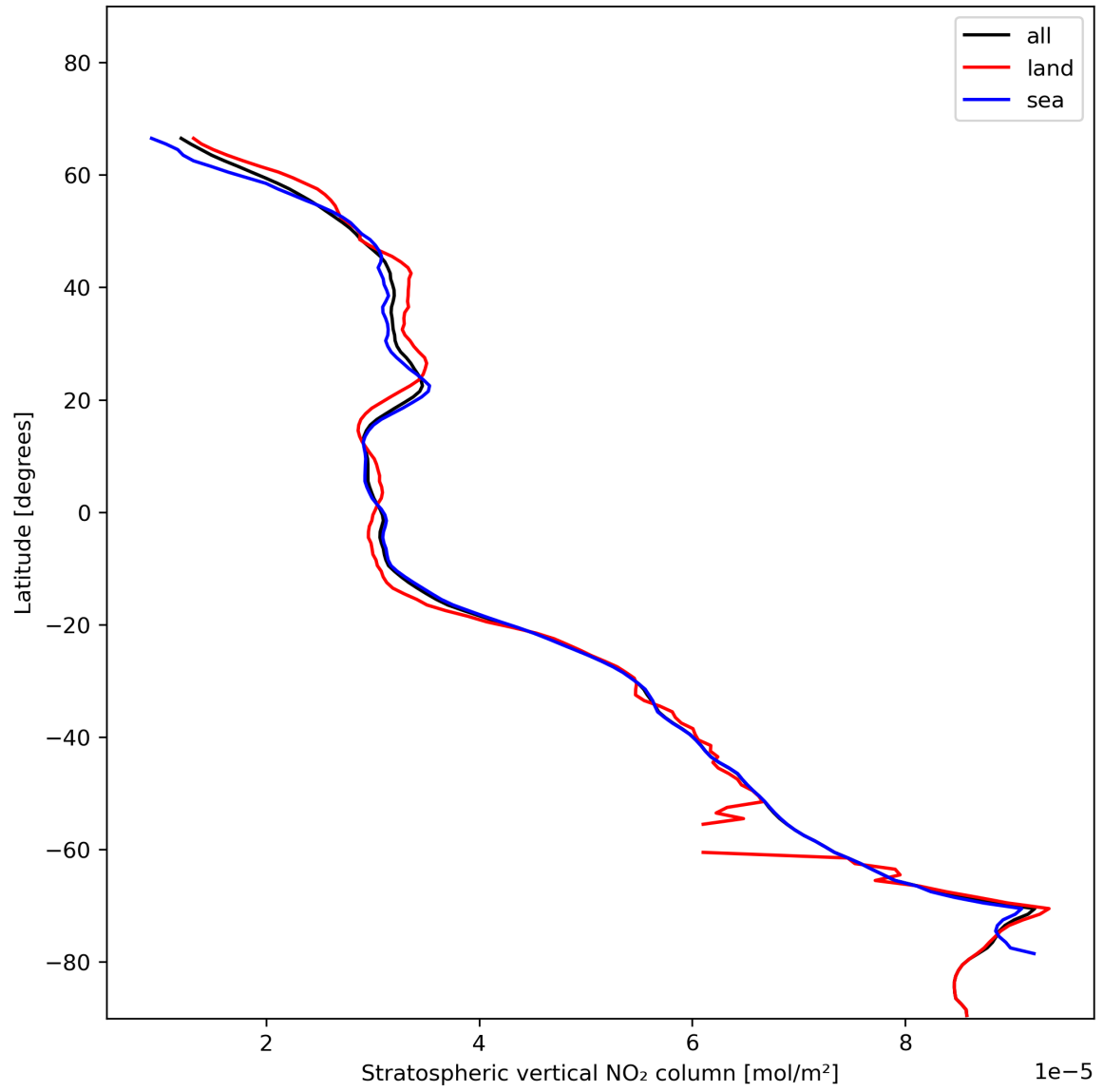
Figure 19: Zonal average of “Stratospheric vertical NO 2 column” for 2024-01-11 to 2024-01-13.
