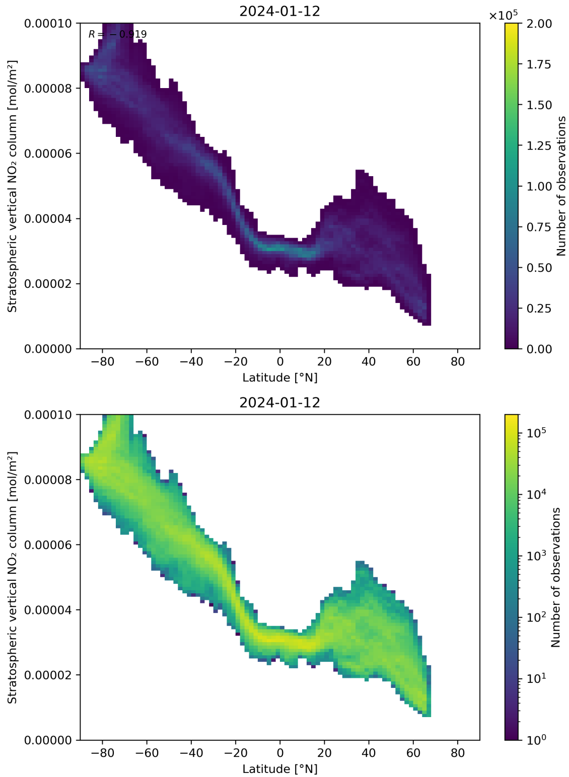
Figure 87: Scatter density plot of “Latitude” against “Stratospheric vertical NO 2 column” for 2024-01-11 to 2024-01-13.
