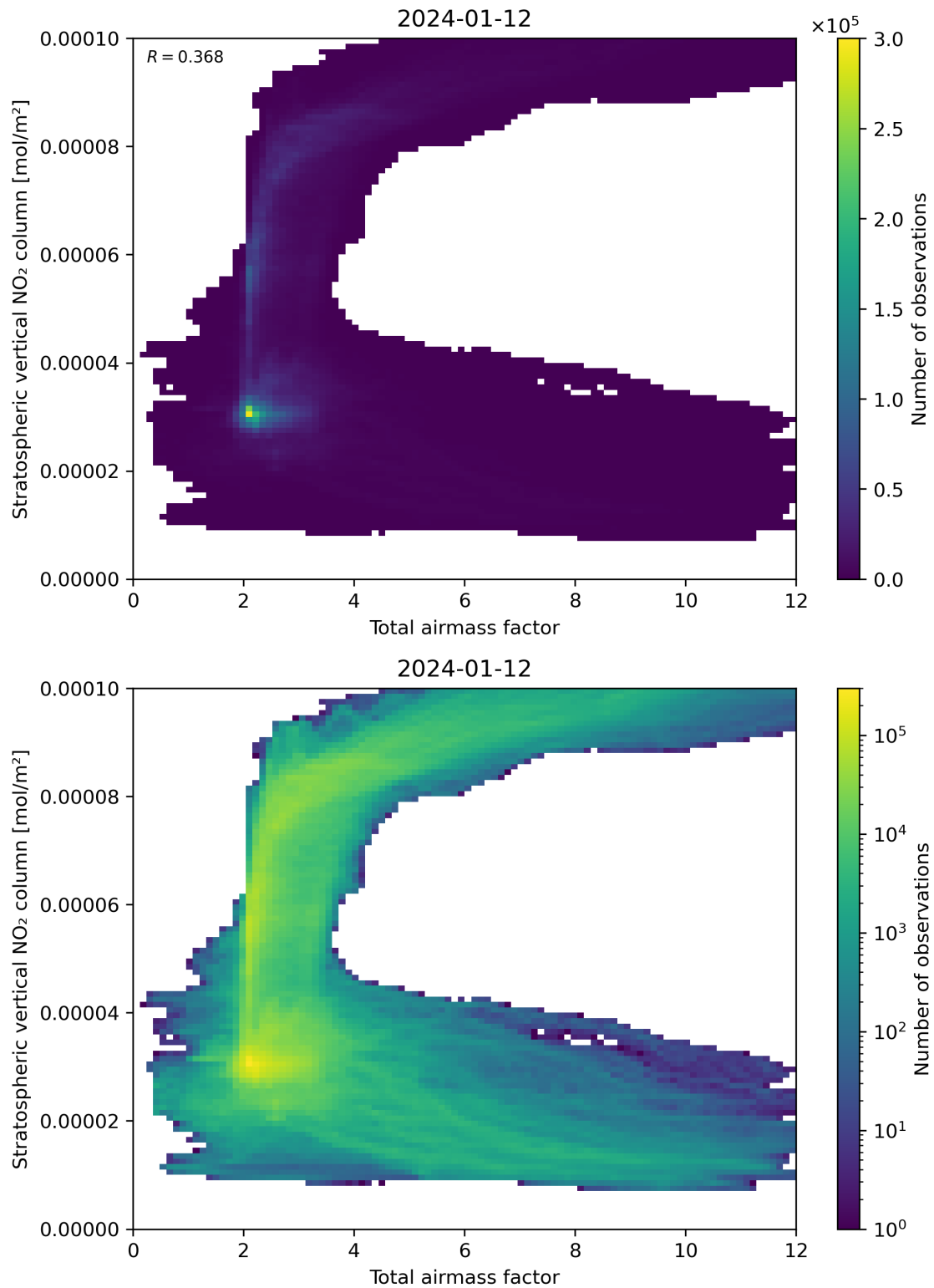
Figure 64: Scatter density plot of “Total airmass factor” against “Stratospheric vertical NO 2 column” for 2024-01-11 to 2024-01-13.
