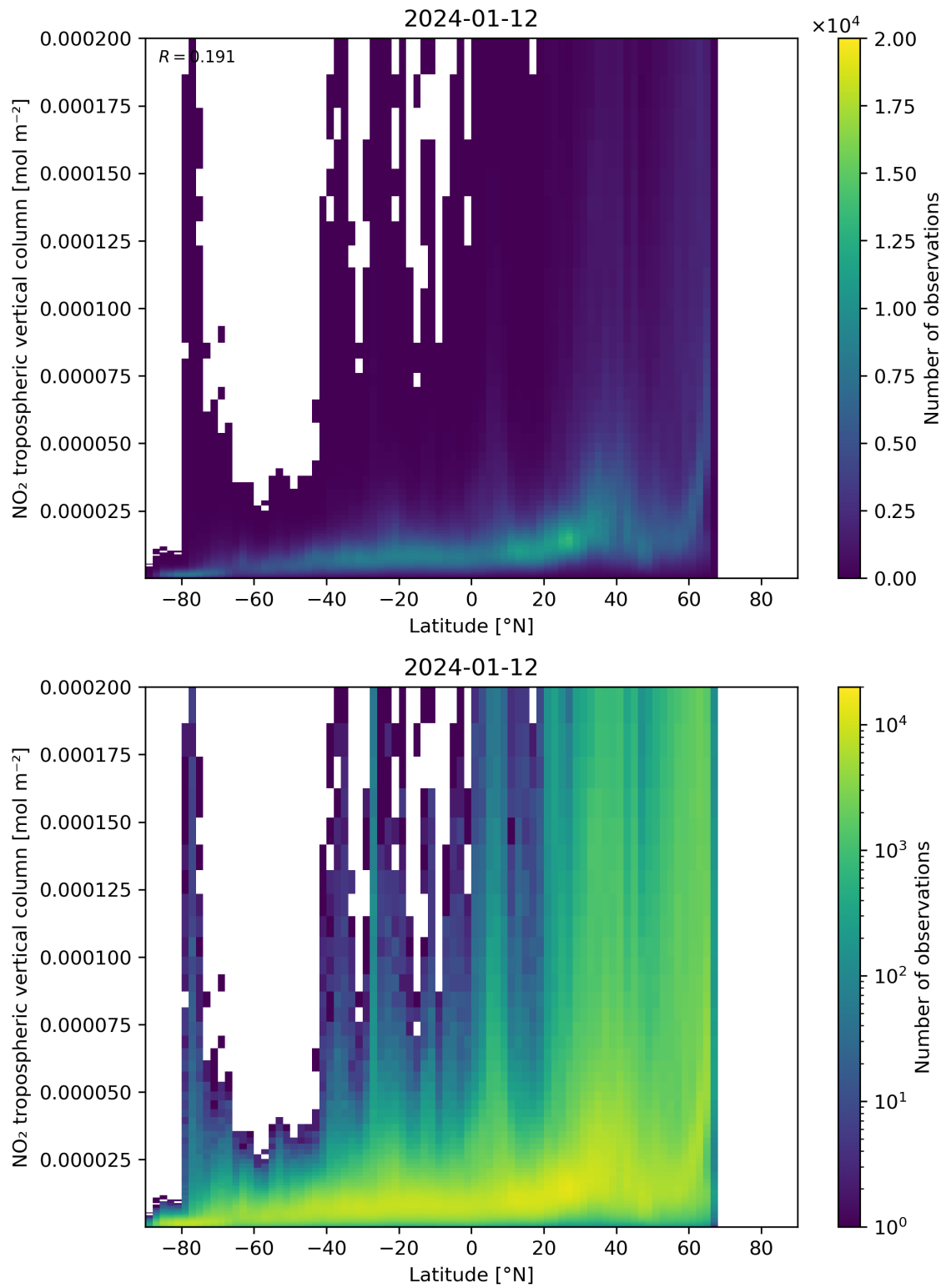
Figure 92: Scatter density plot of “Latitude” against “NO 2 tropospheric vertical column” for 2024-01-11 to 2024-01-13.
