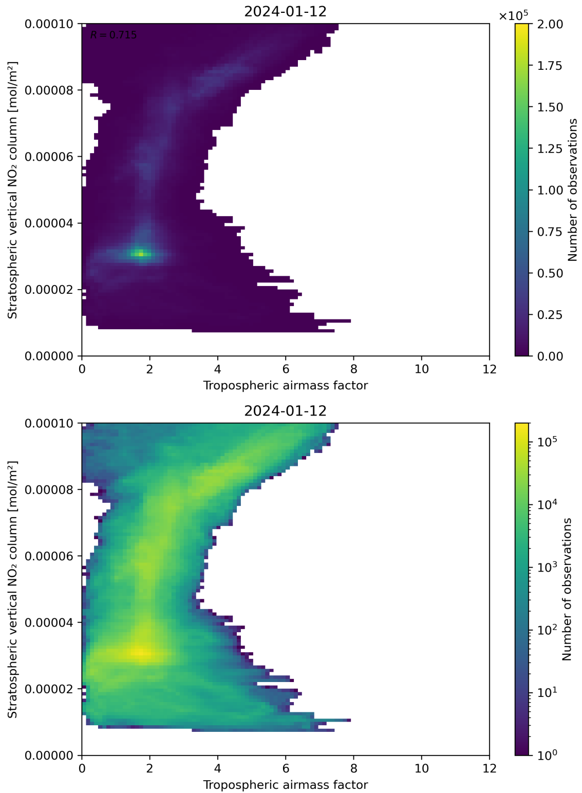
Figure 74: Scatter density plot of “Tropospheric air mass factor” against “Stratospheric vertical NO 2 column” for 2024-01-11 to 2024-01-13.
