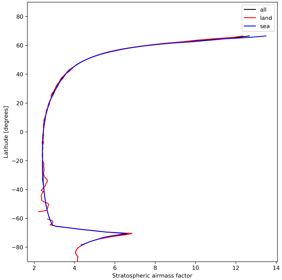
Figure 27: Zonal average of “Stratospheric airmass factor” for 2024-01-11 to 2024-01-13.
