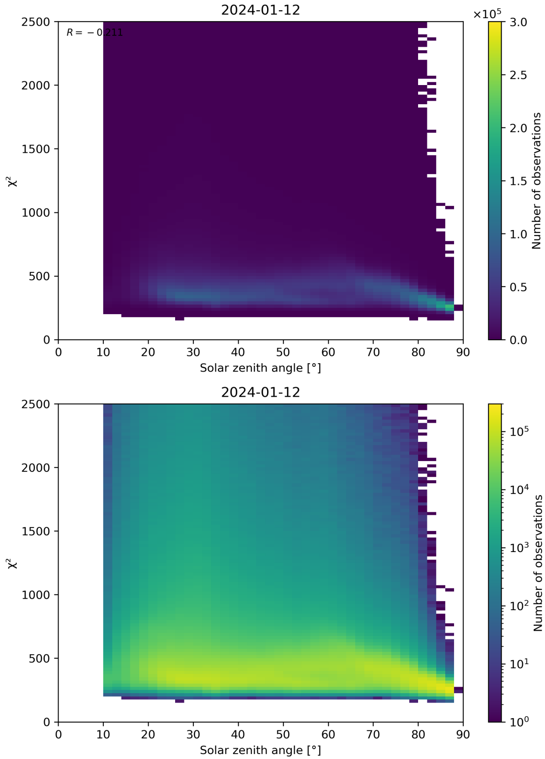
Figure 148: Scatter density plot of “Solar zenith angle” against “ \chi^2 ” for 2024-01-11 to 2024-01-13.
