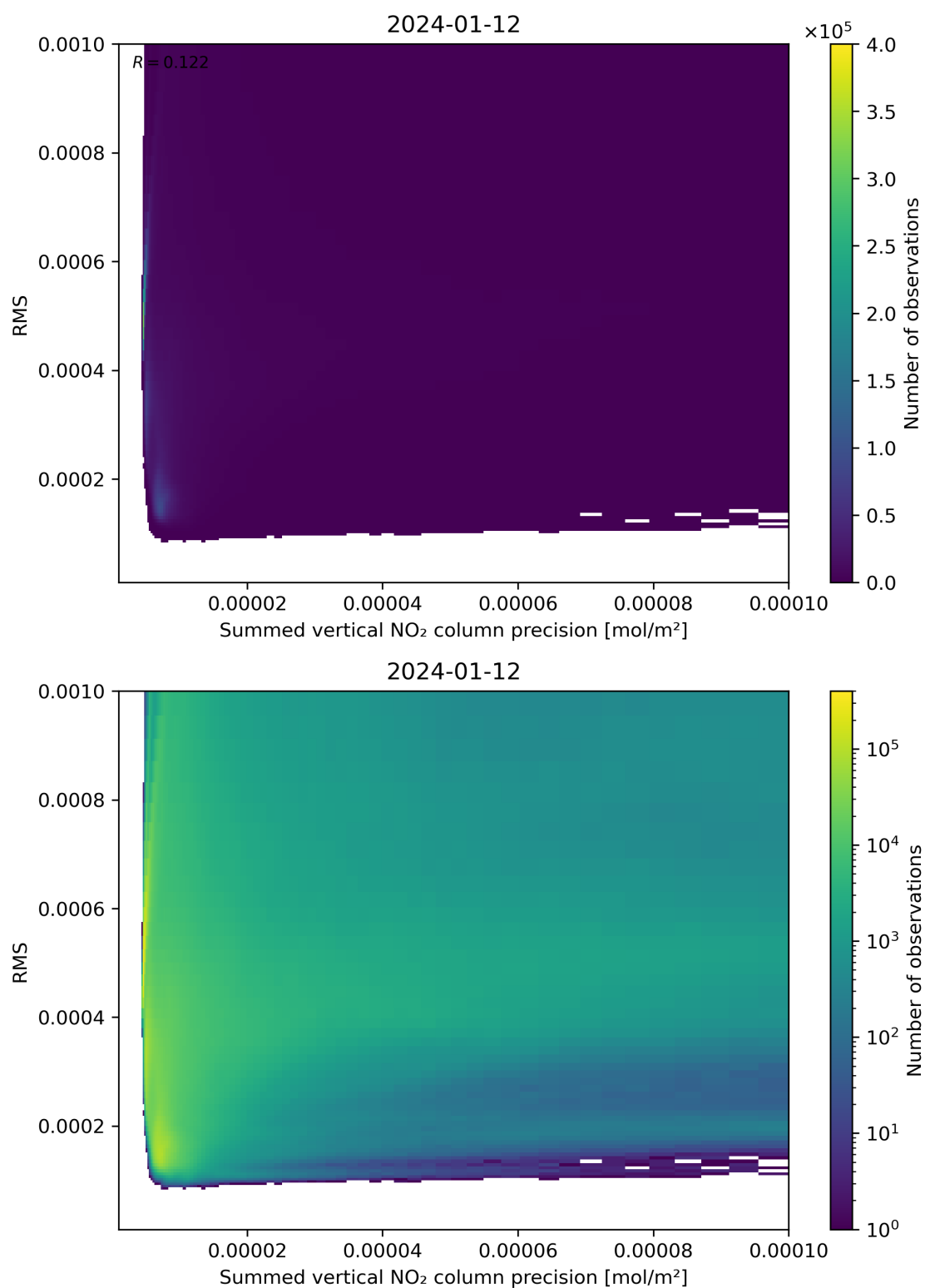
Figure 108: Scatter density plot of “Summed vertical NO 2 column precision” against “RMS” for 2024-01-11 to 2024-01-13.
