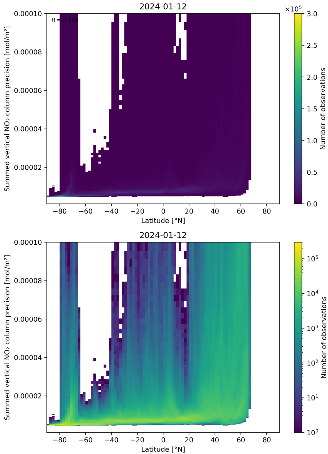
Figure 89: Scatter density plot of “Latitude” against “Summed vertical NO 2 column precision” for 2024-01-11 to 2024-01-13.
