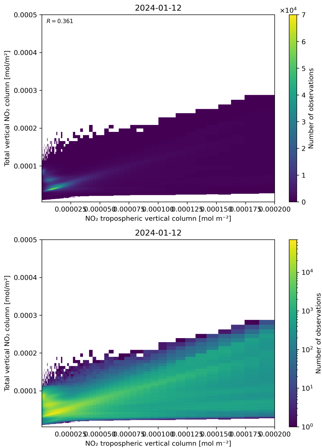
Figure 128: Scatter density plot of “NO 2 tropospheric vertical column” against “Total vertical NO 2 column” for 2024-01-11 to 2024-01-13.
