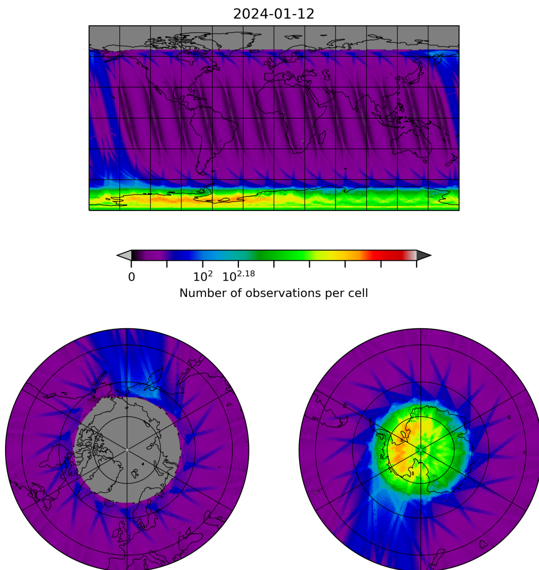
Figure 10: Map of the number of observations for 2024-01-11 to 2024-01-13
