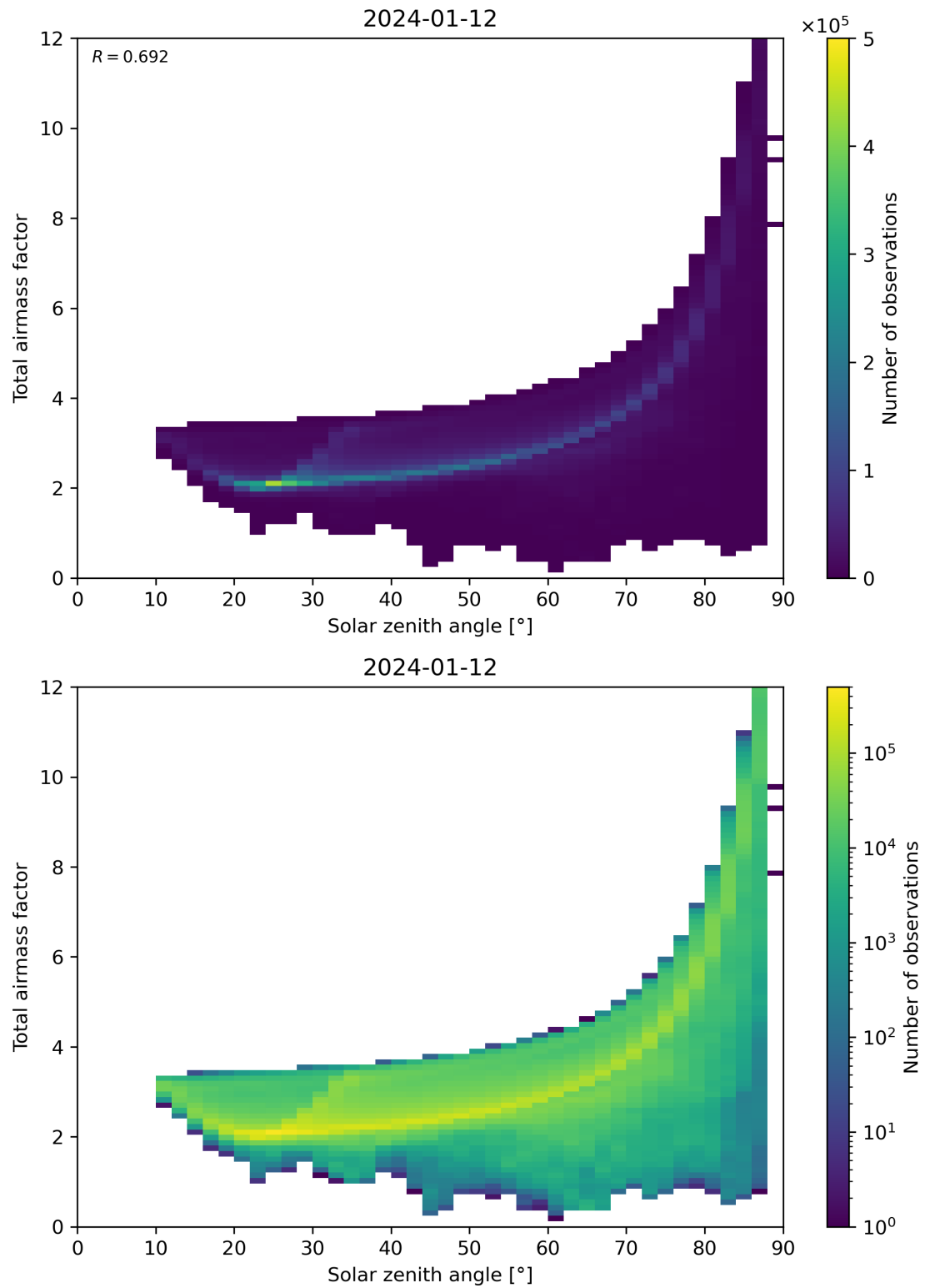
Figure 146: Scatter density plot of “Solar zenith angle” against “Total air mass factor” for 2024-01-11 to 2024-01-13.
