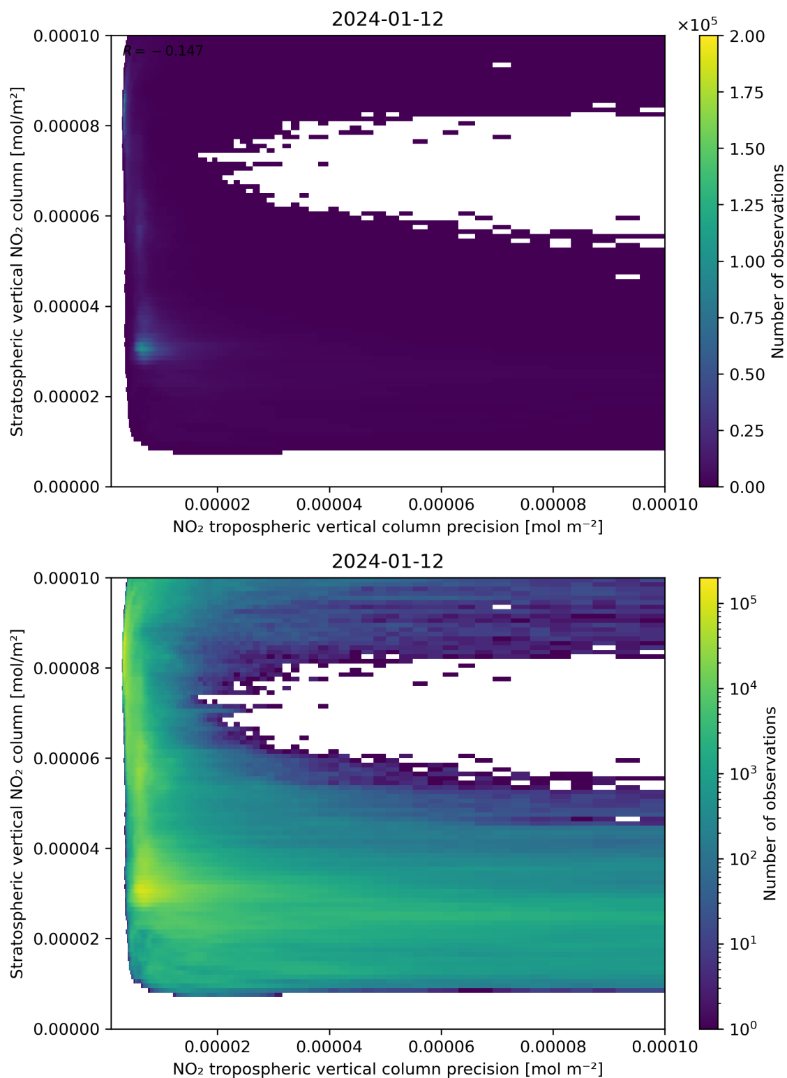
Figure 135: Scatter density plot of “NO 2 tropospheric vertical column precision” against “Stratospheric vertical NO 2 column” for 2024-01-11 to 2024-01-13.
