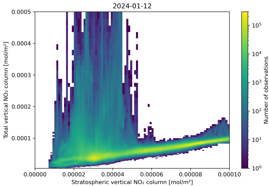
Figure 100: Scatter density plot of “Stratospheric vertical NO 2 column” against “Total vertical NO 2 column” for 2024-01-11 to 2024-01-13.
