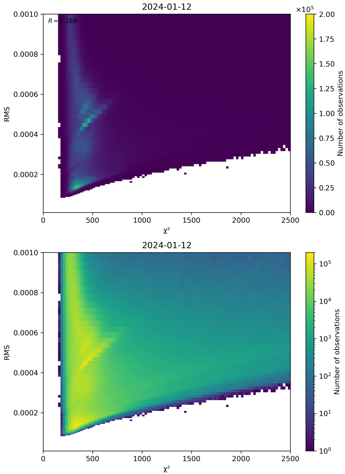
Figure 82: Scatter density plot of “ \chi^2 ” against “RMS” for 2024-01-11 to 2024-01-13.
