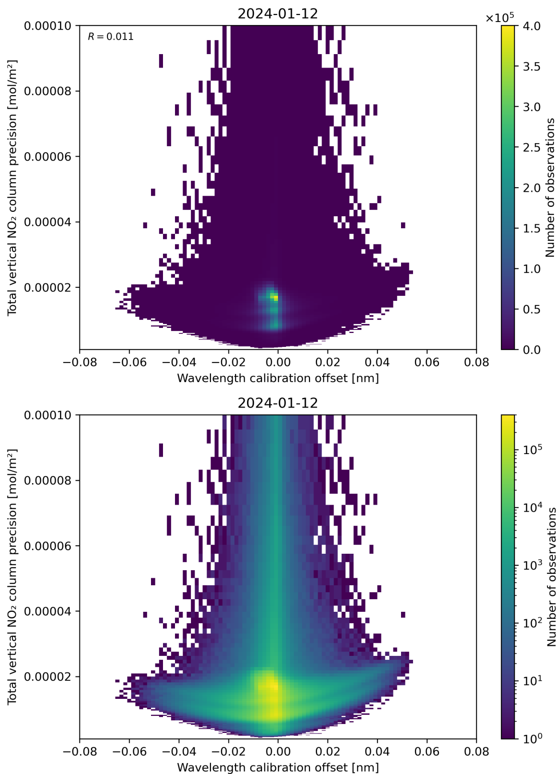
Figure 180: Scatter density plot of “Wavelength calibration offset” against “Total vertical NO 2 column precision” for 2024-01-11 to 2024-01-13.
