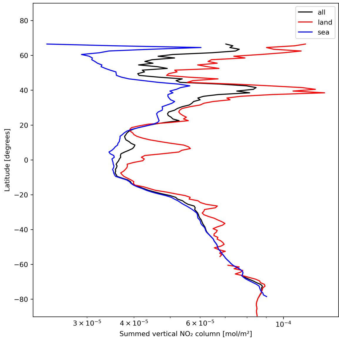
Figure 23: Zonal average of “Summed vertical NO 2 column” for 2024-01-11 to 2024-01-13.
