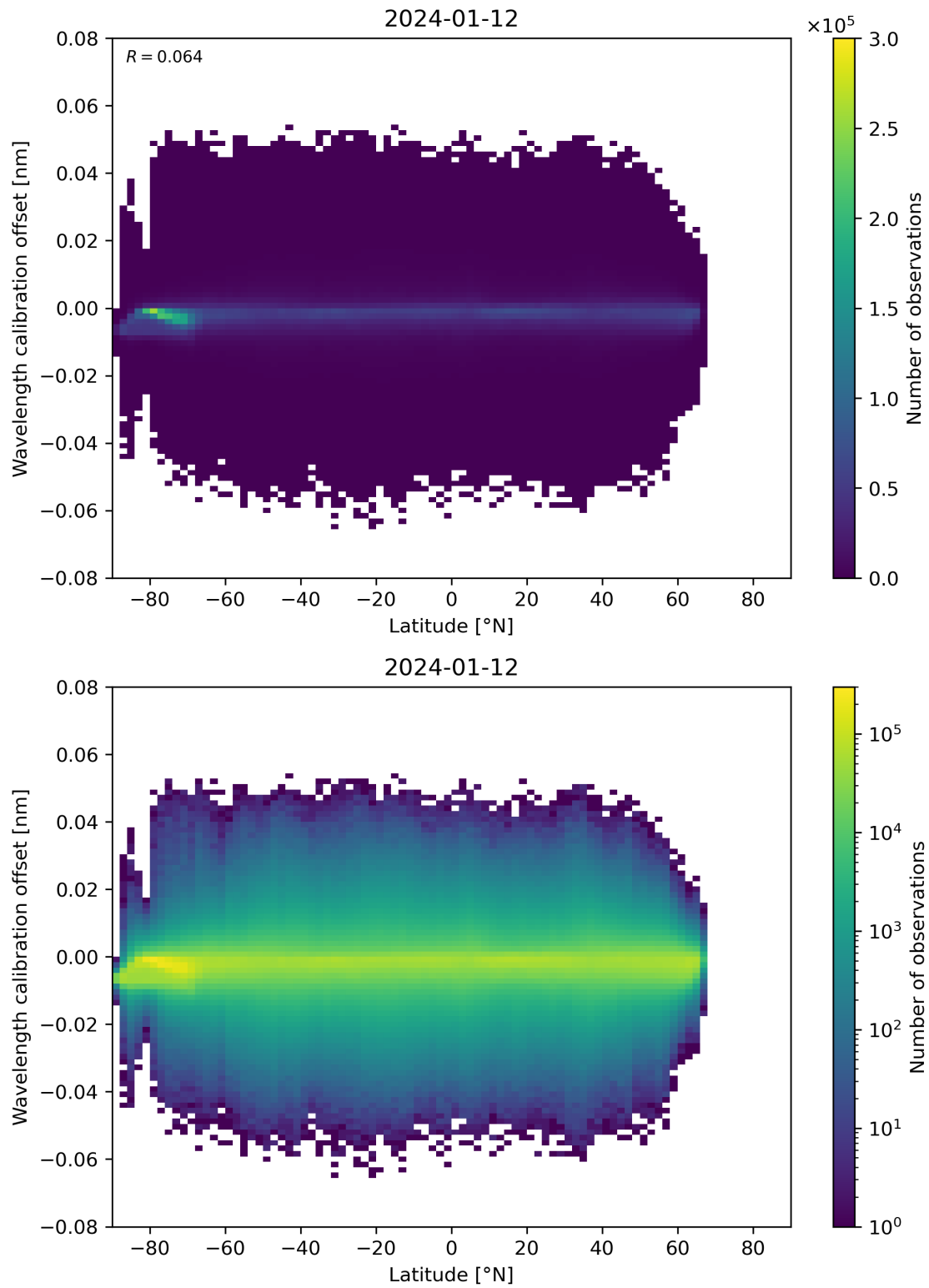
Figure 95: Scatter density plot of “Latitude” against “Wavelength calibration offset” for 2024-01-11 to 2024-01-13.
