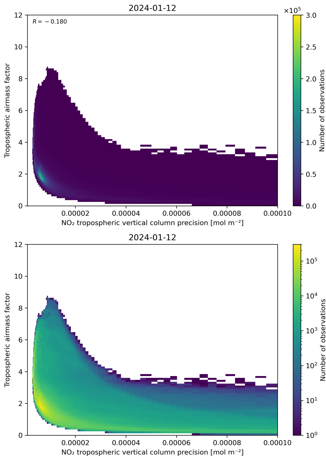
Figure 133: Scatter density plot of “NO 2 tropospheric vertical column precision” against “Tropospheric airmass factor” for 2024-01-11 to 2024-01-13.
