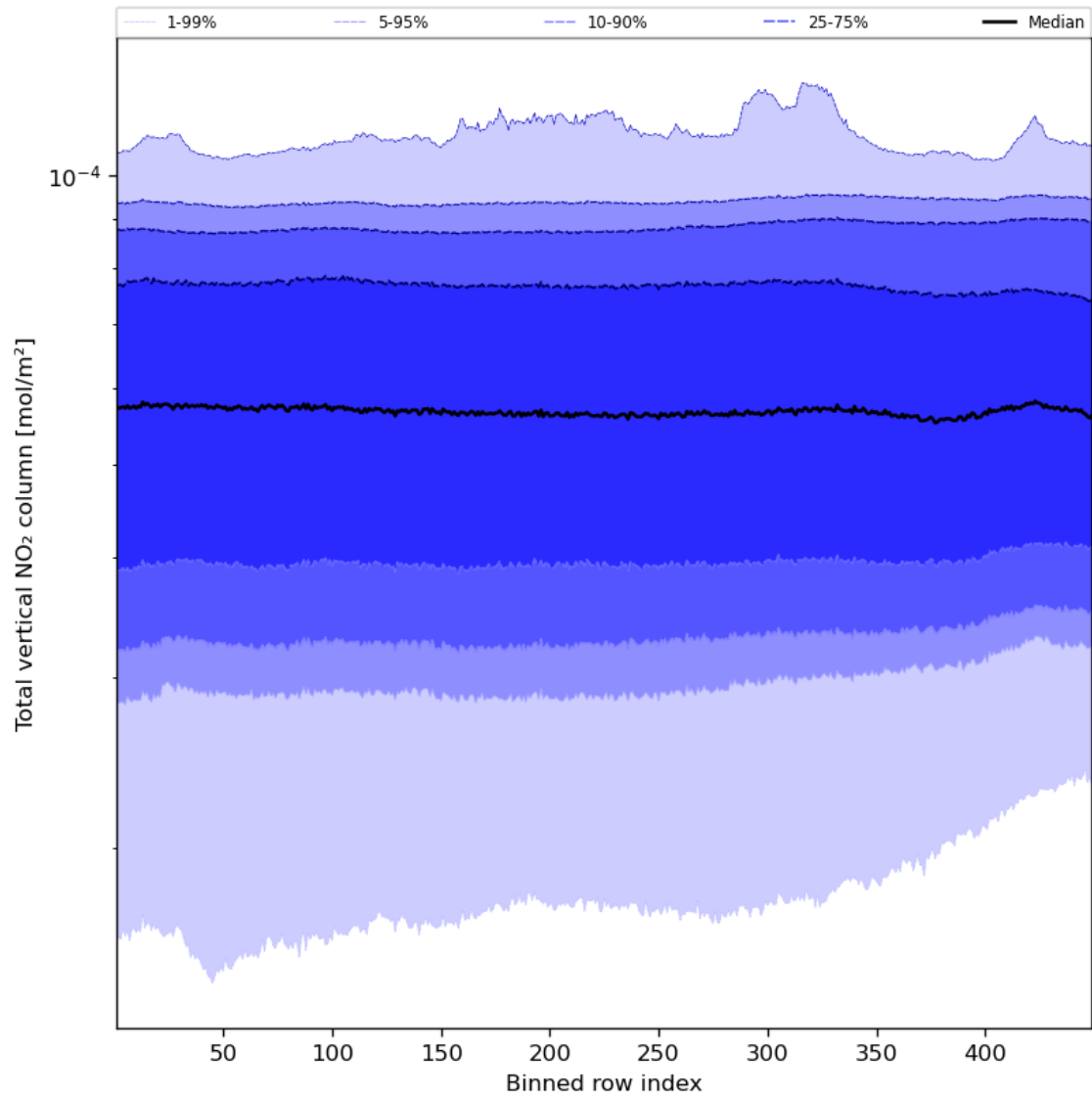
Figure 55: Along track statistics of “Total vertical NO 2 column” for 2024-01-11 to 2024-01-13
