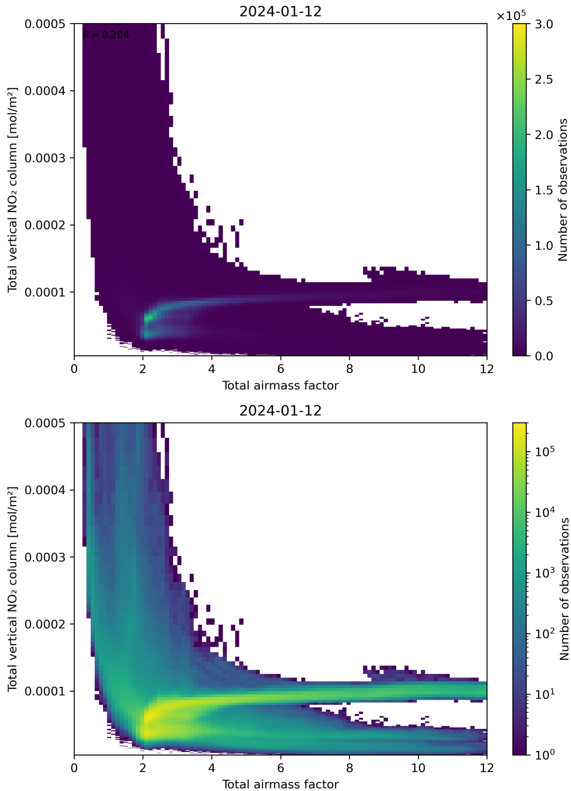
Figure 67: Scatter density plot of “Total airmass factor” against “Total vertical NO 2 column” for 2024-01-11 to 2024-01-13.
