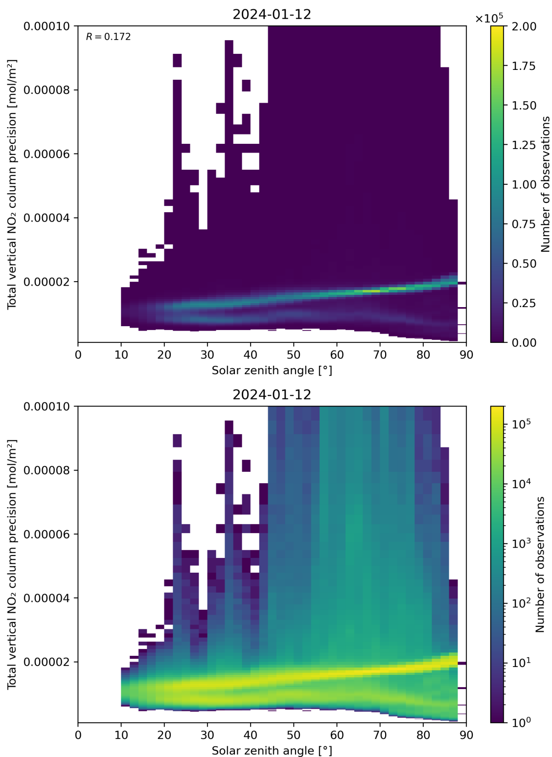
Figure 154: Scatter density plot of “Solar zenith angle” against “Total vertical NO 2 column precision” for 2024-01-11 to 2024-01-13.
