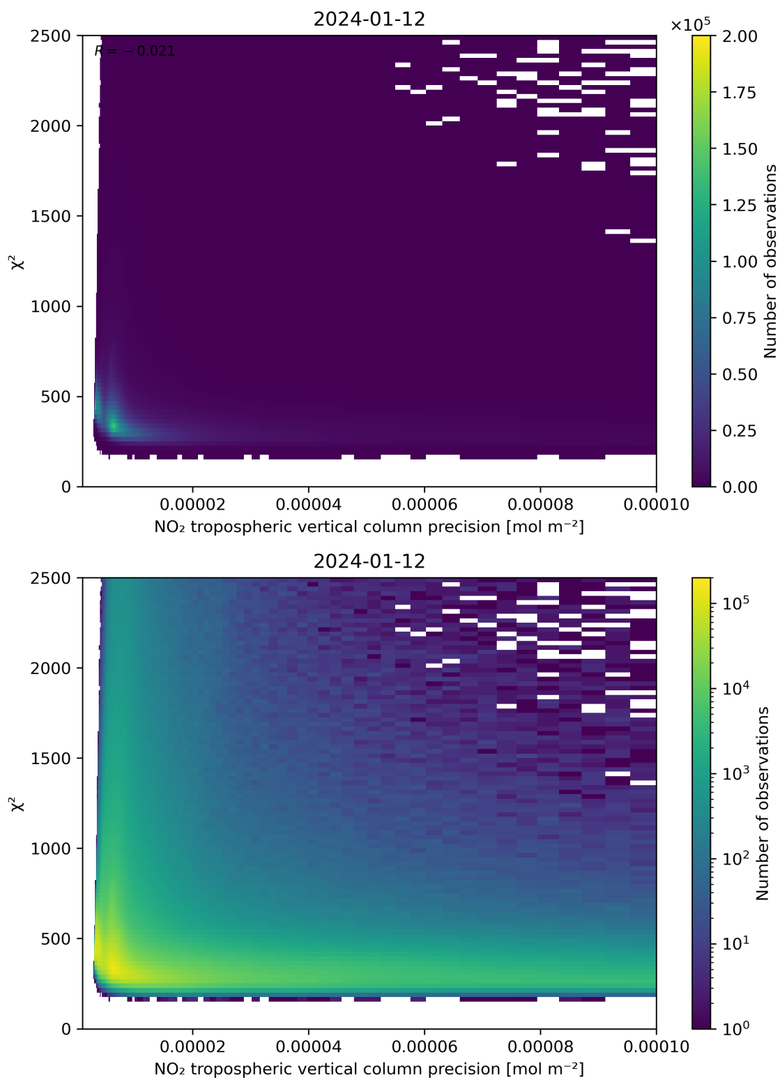
Figure 134: Scatter density plot of “NO 2 tropospheric vertical column precision” against “ \chi^2 ” for 2024-01-11 to 2024-01-13.
