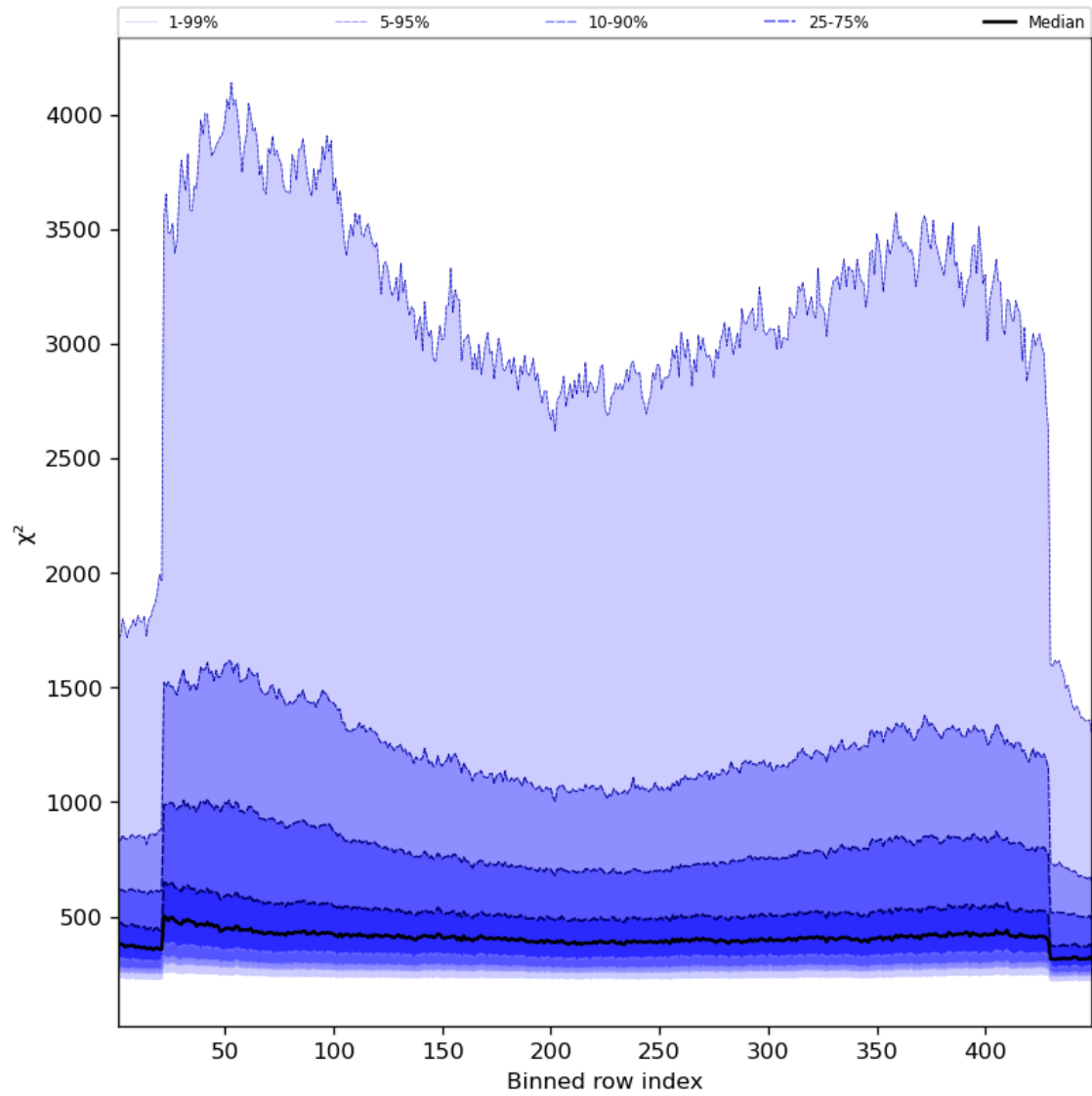
Figure 59: Along track statistics of “ \chi^2 ” for 2024-01-11 to 2024-01-13
