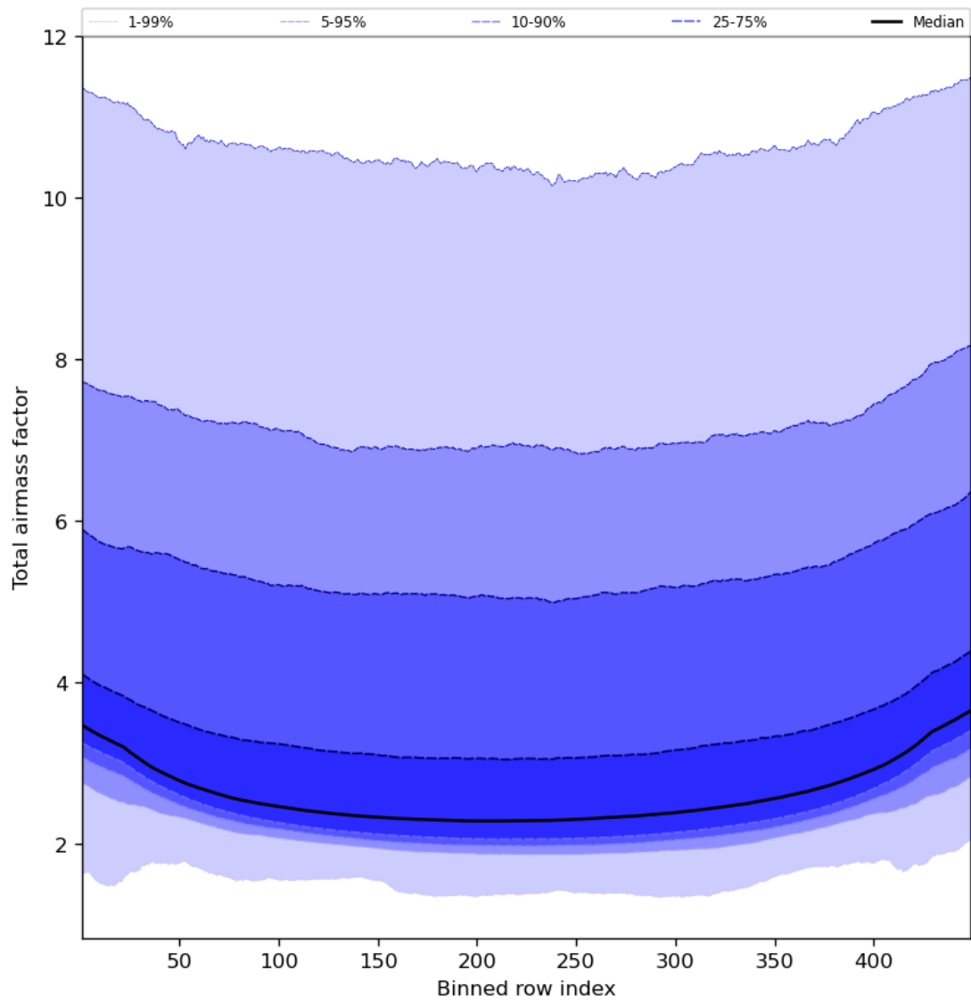
Figure 49: Along track statistics of “Total airmass factor” for 2024-01-11 to 2024-01-13
