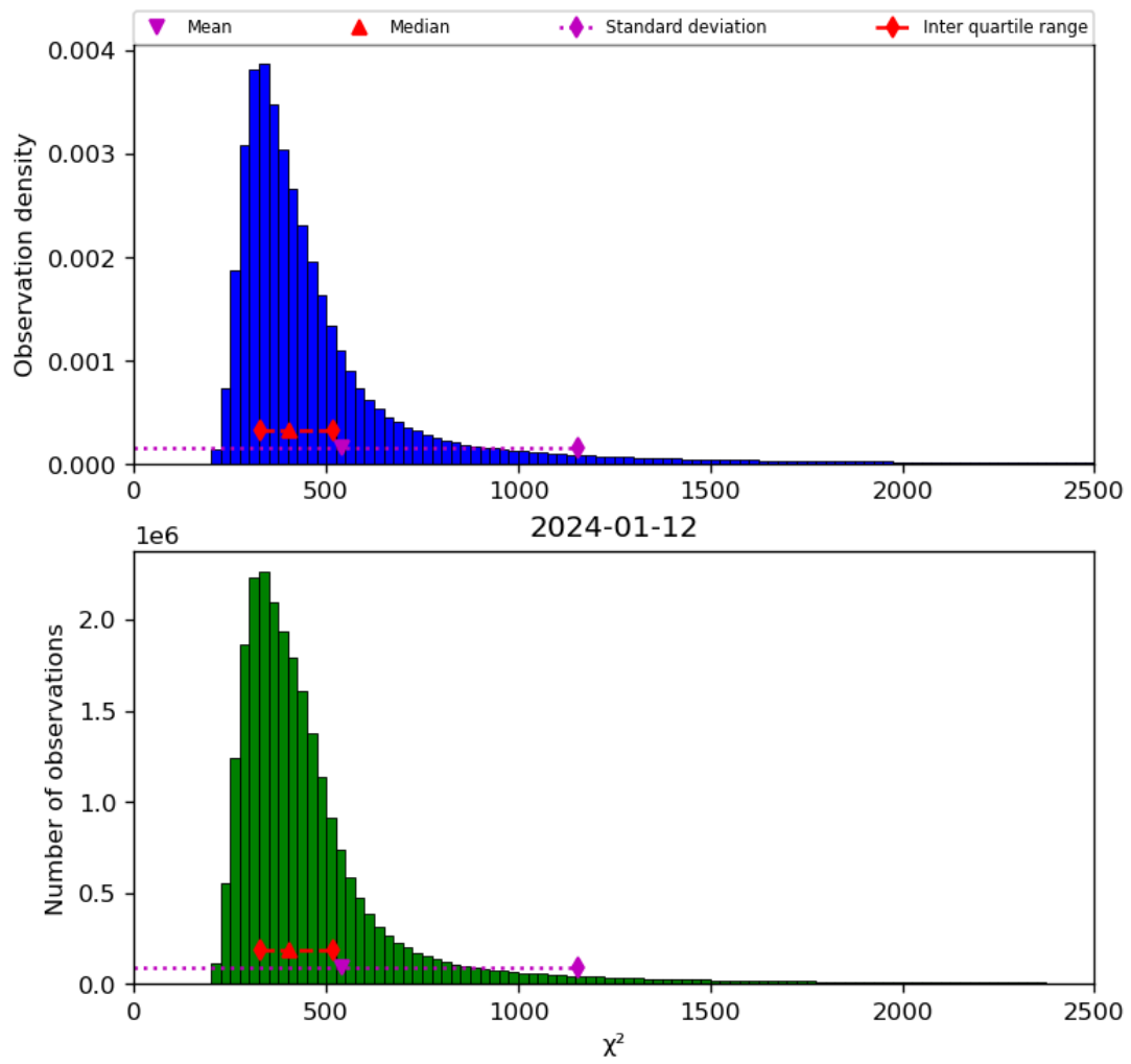
Figure 42: Histogram of “ \chi^2 ” for 2024-01-11 to 2024-01-13
