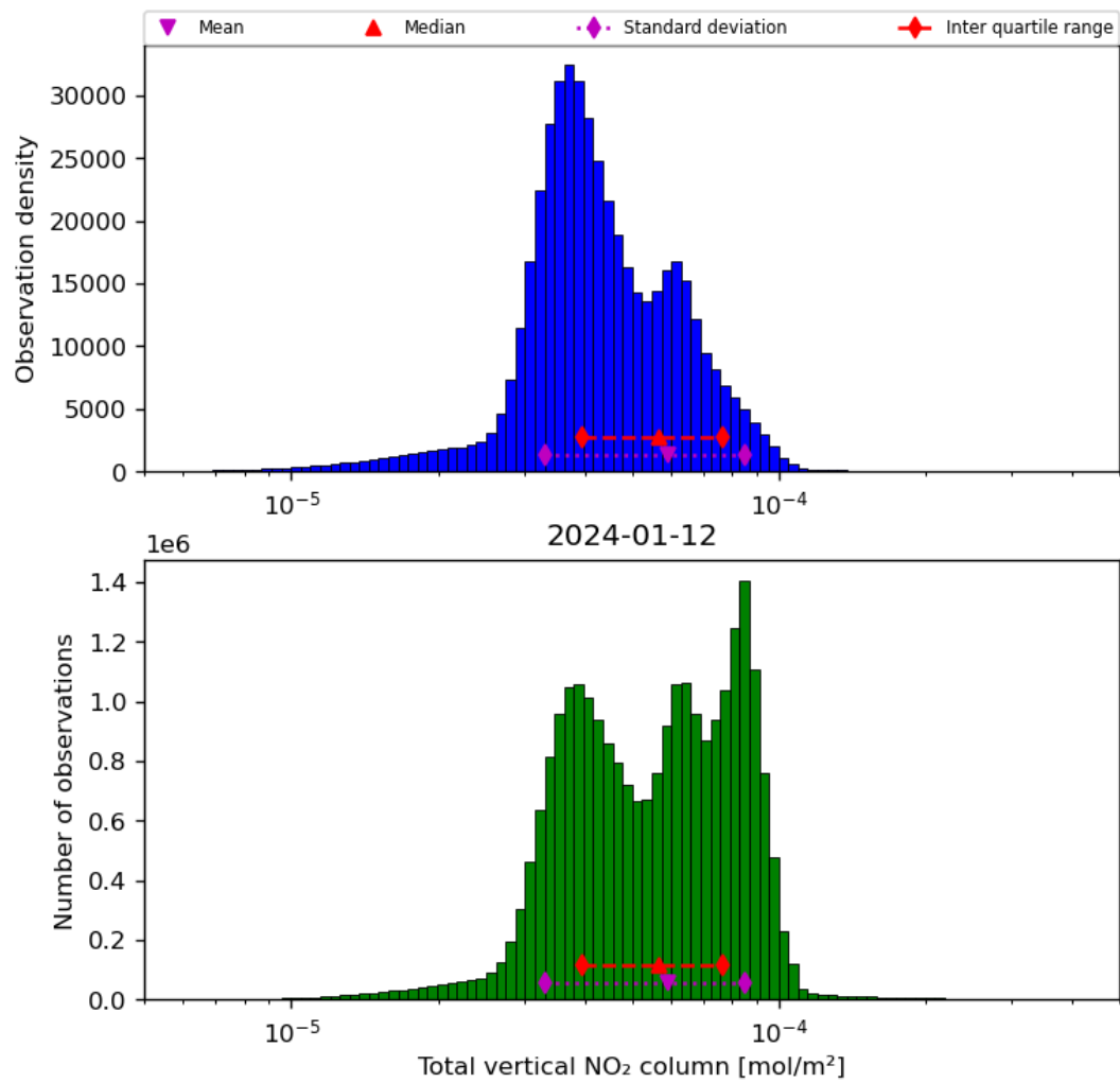
Figure 38: Histogram of “Total vertical NO 2 column” for 2024-01-11 to 2024-01-13
