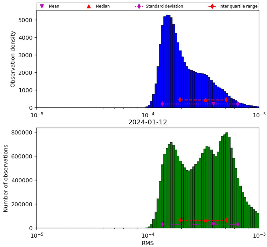
Figure 43: Histogram of “RMS” for 2024-01-11 to 2024-01-13
