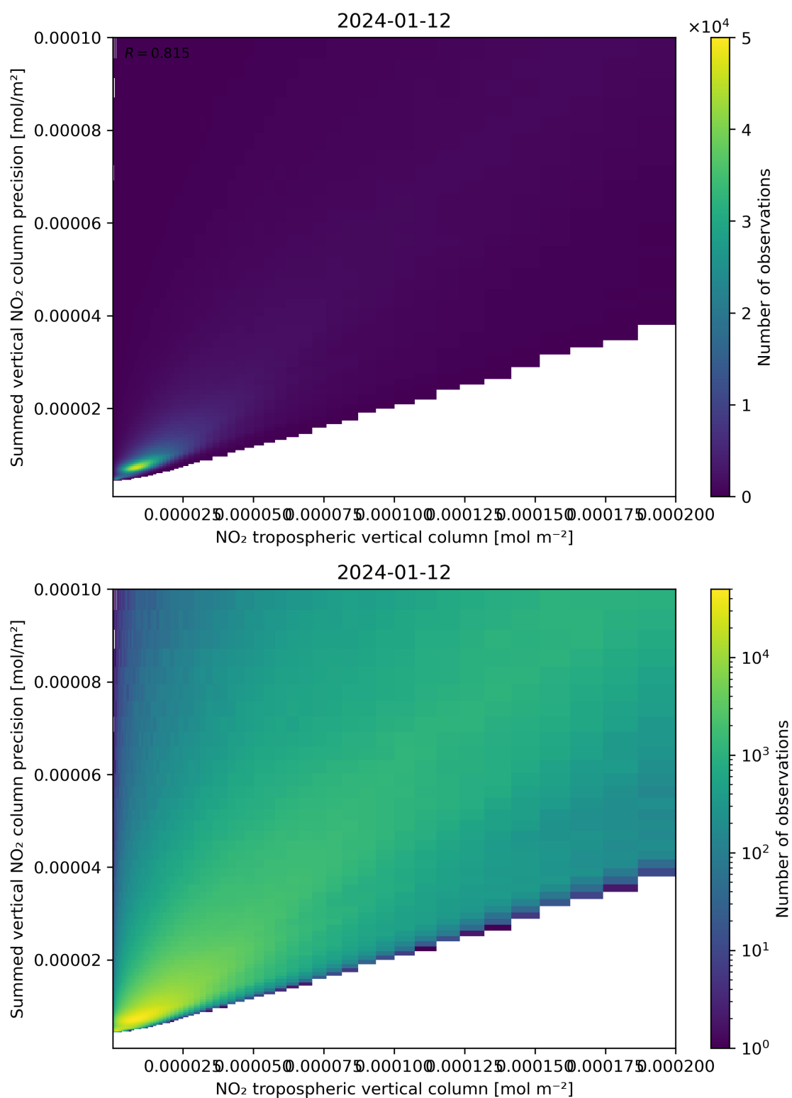
Figure 127: Scatter density plot of “NO 2 tropospheric vertical column” against “Summed vertical NO 2 column precision” for 2024-01-11 to 2024-01-13.
