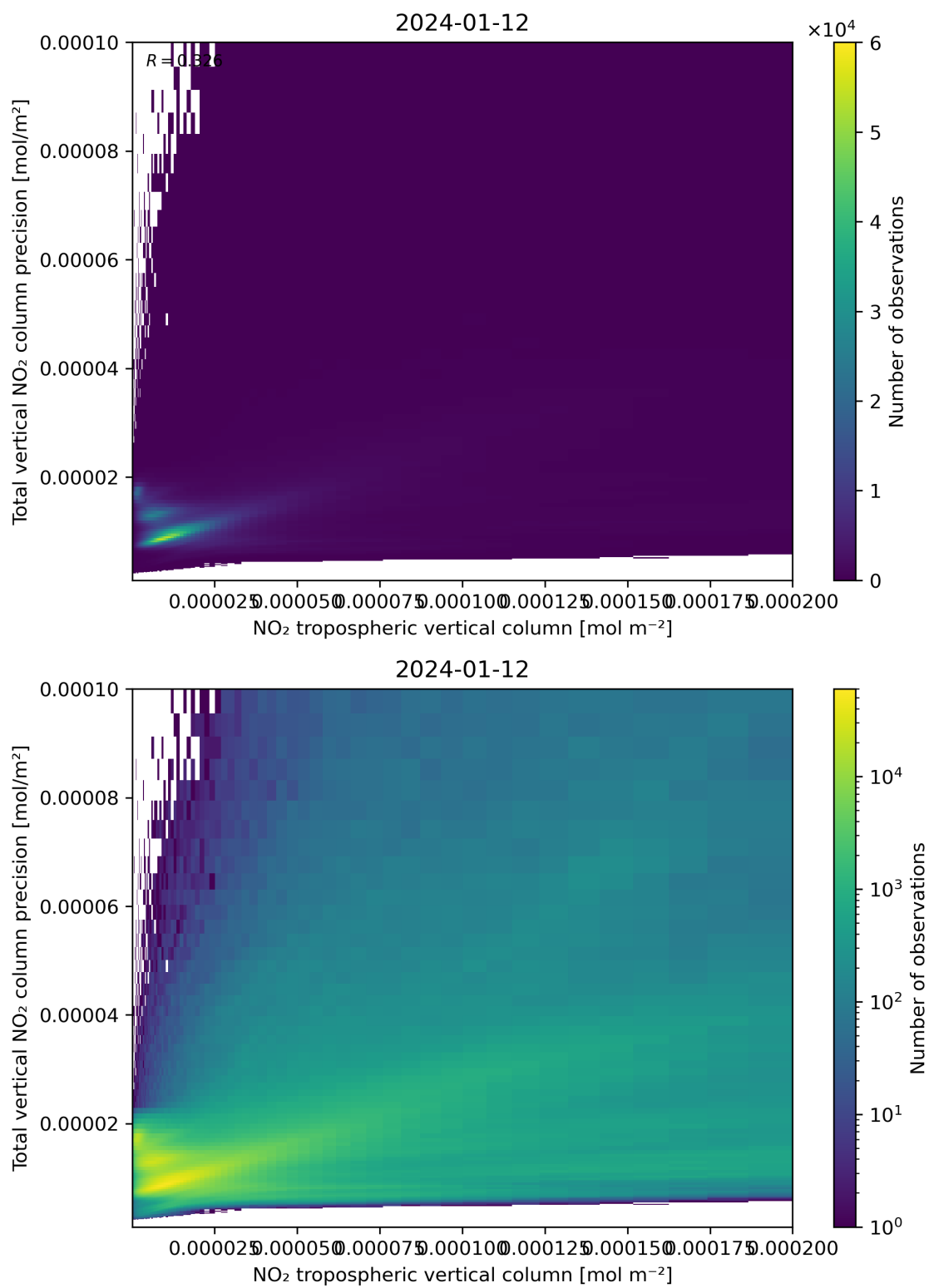
Figure 129: Scatter density plot of “NO 2 tropospheric vertical column” against “Total vertical NO 2 column precision” for 2024-01-11 to 2024-01-13.
