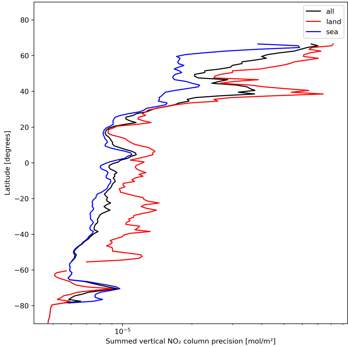
Figure 24: Zonal average of “Summed vertical NO 2 column precision” for 2024-01-11 to 2024-01-13.
