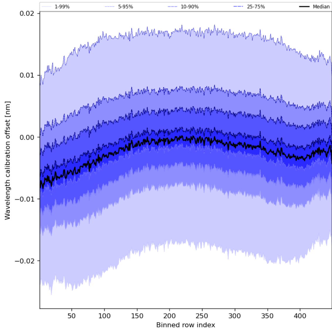
Figure 52: Along track statistics of “Wavelength calibration offset” for 2024-01-11 to 2024-01-13
