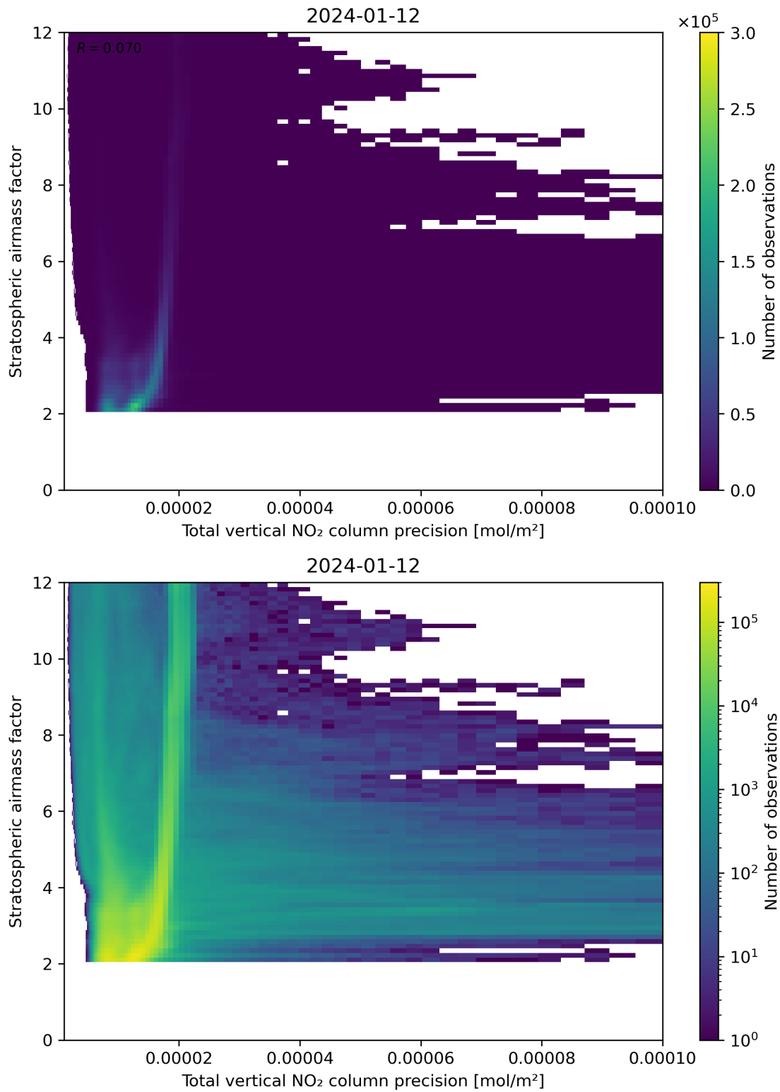
Figure 115: Scatter density plot of “Total vertical NO 2 column precision” against “Stratospheric air mass factor” for 2024-01-11 to 2024-01-13.
