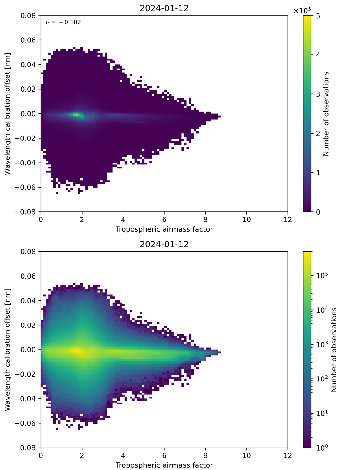
Figure 80: Scatter density plot of “Tropospheric air mass factor” against “Wavelength calibration offset” for 2024-01-11 to 2024-01-13.
