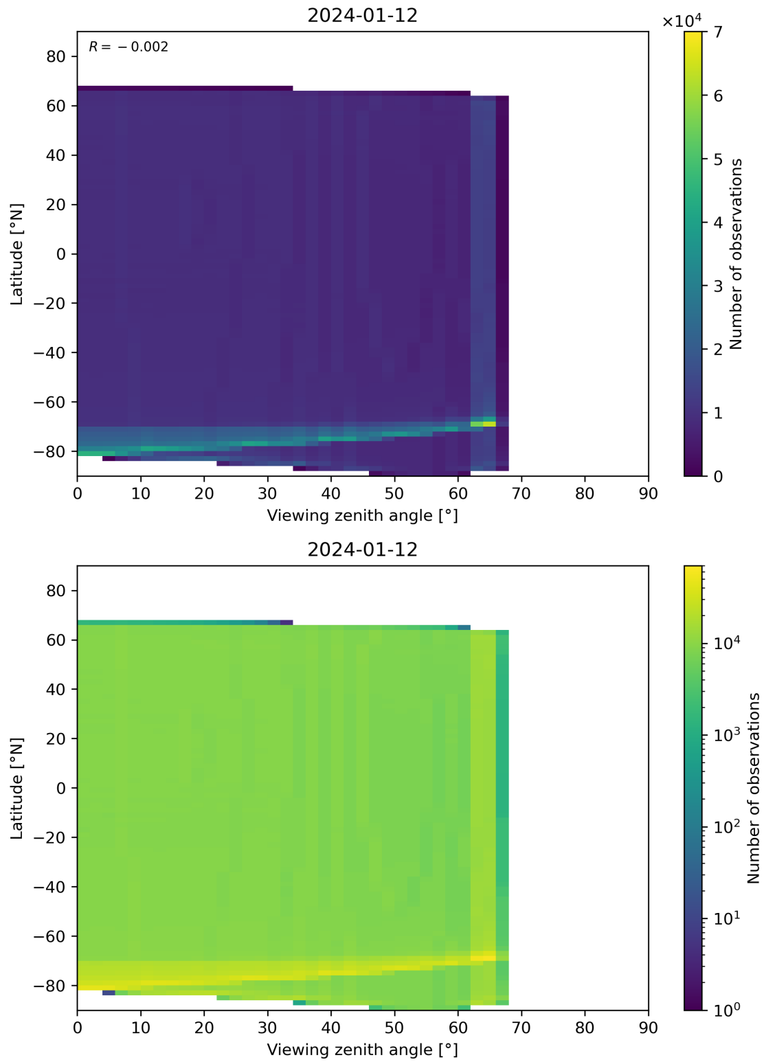
Figure 163: Scatter density plot of “Viewing zenith angle” against “Latitude” for 2024-01-11 to 2024-01-13.
