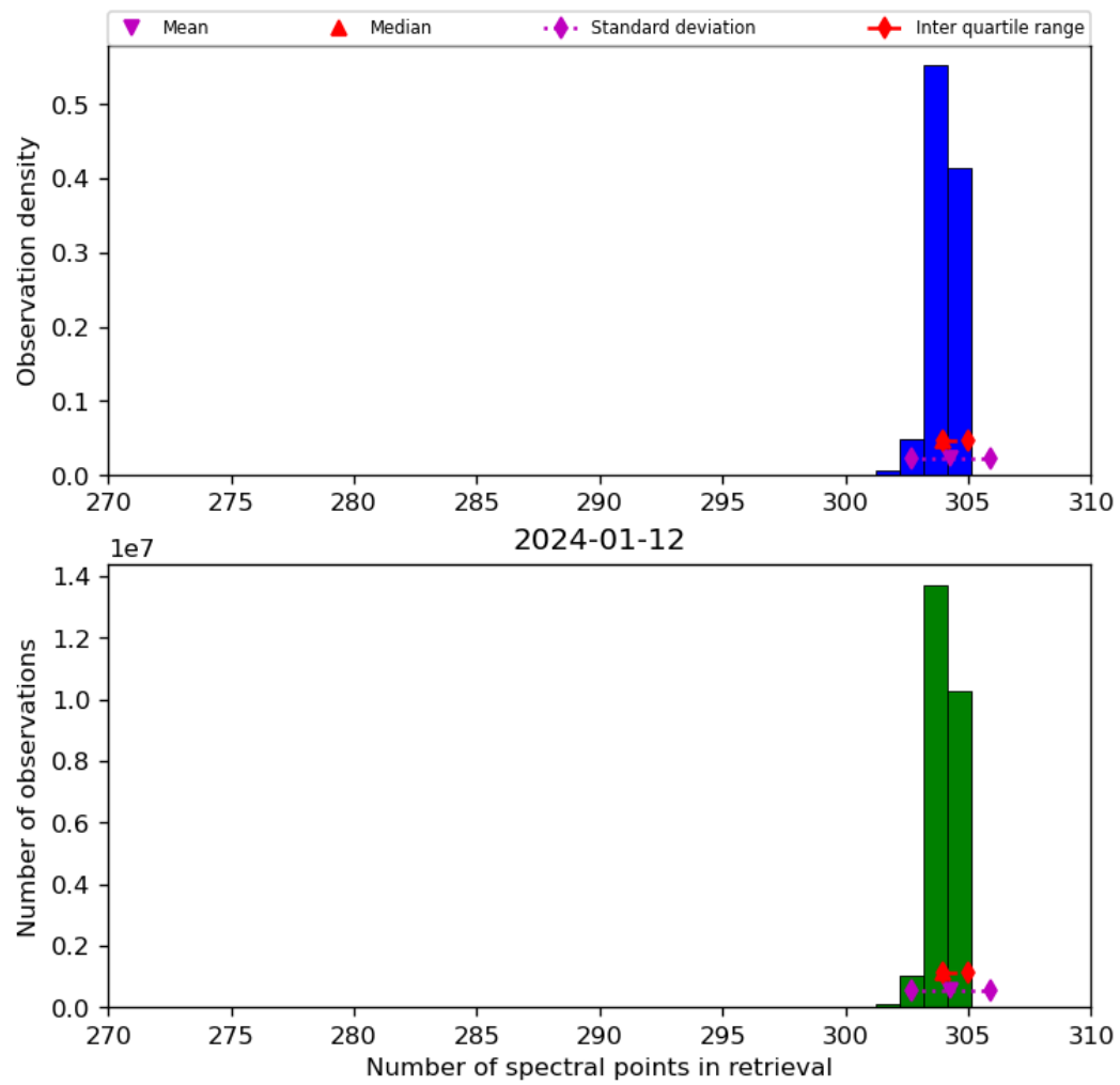
Figure 33: Histogram of “Number of spectral points in retrieval” for 2024-01-11 to 2024-01-13
