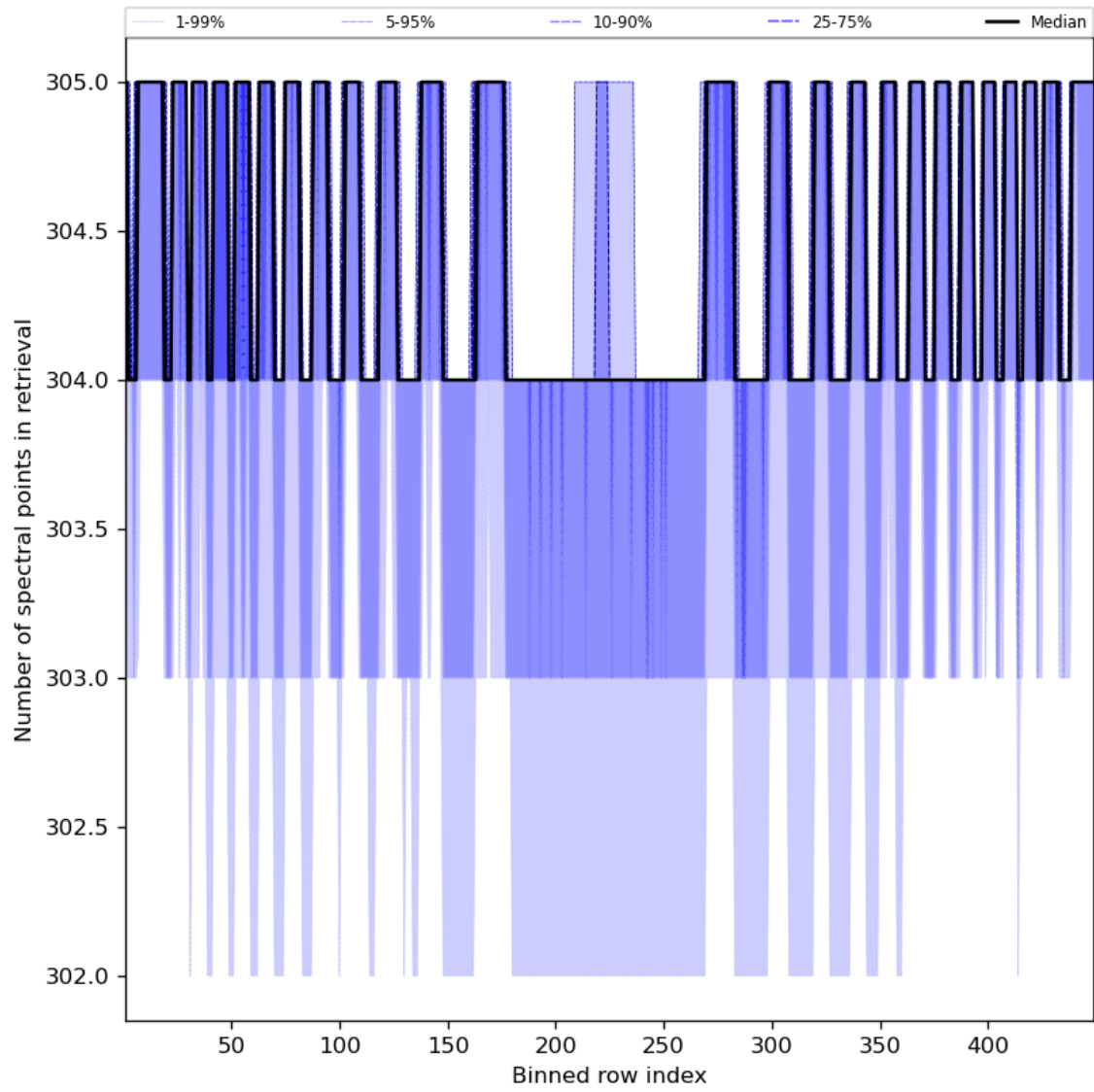
Figure 50: Along track statistics of “Number of spectral points in retrieval” for 2024-01-11 to 2024-01-13
