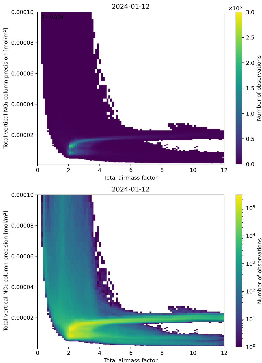
Figure 68: Scatter density plot of “Total airmass factor” against “Total vertical NO 2 column precision” for 2024-01-11 to 2024-01-13.
