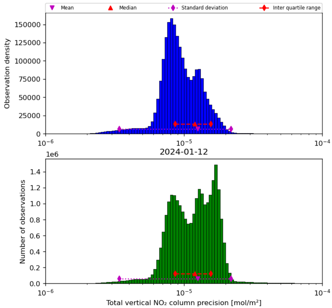
Figure 39: Histogram of “Total vertical NO 2 column precision” for 2024-01-11 to 2024-01-13
