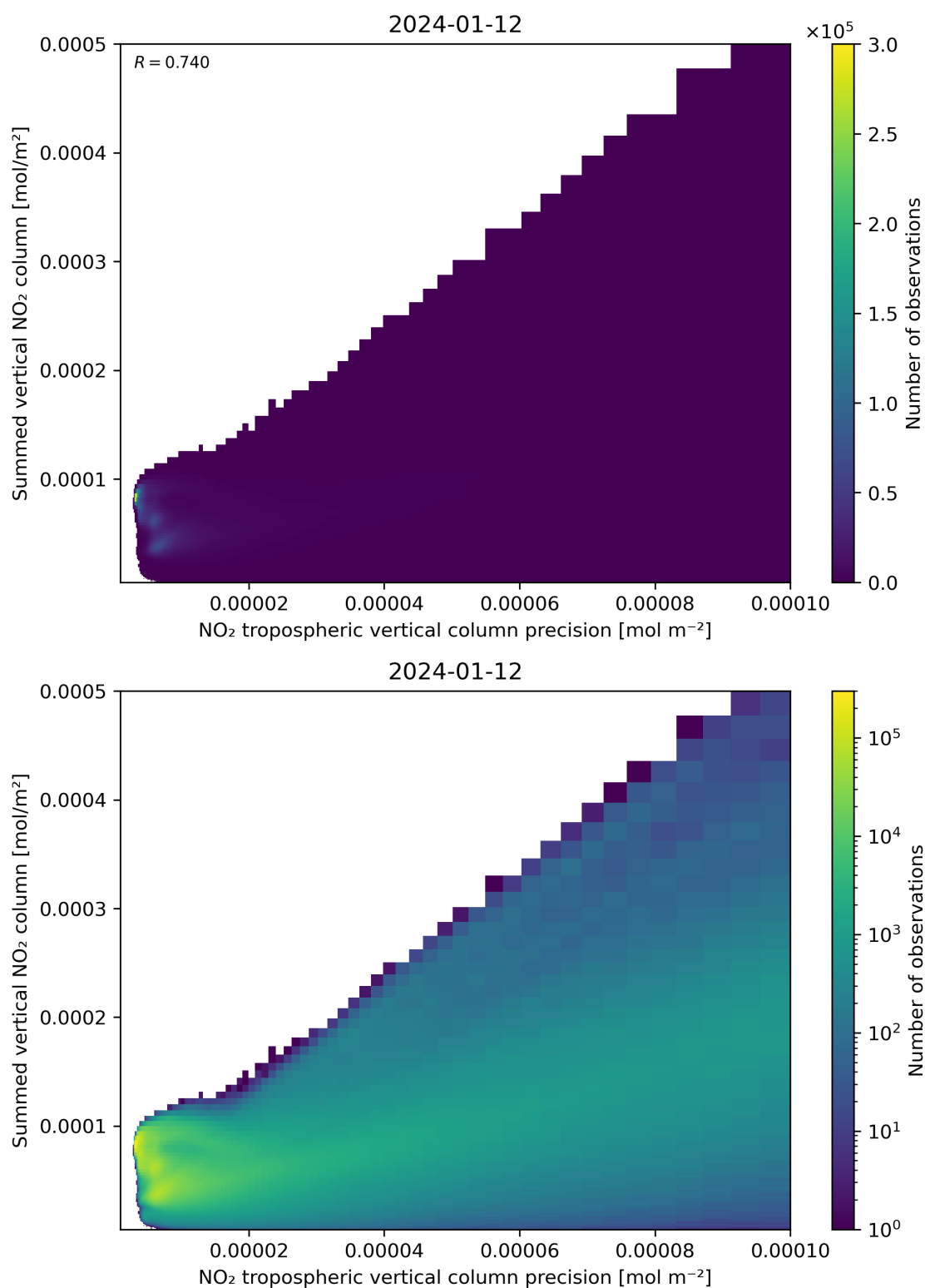
Figure 136: Scatter density plot of “NO 2 tropospheric vertical column precision” against “Summed vertical NO 2 column” for 2024-01-11 to 2024-01-13.
