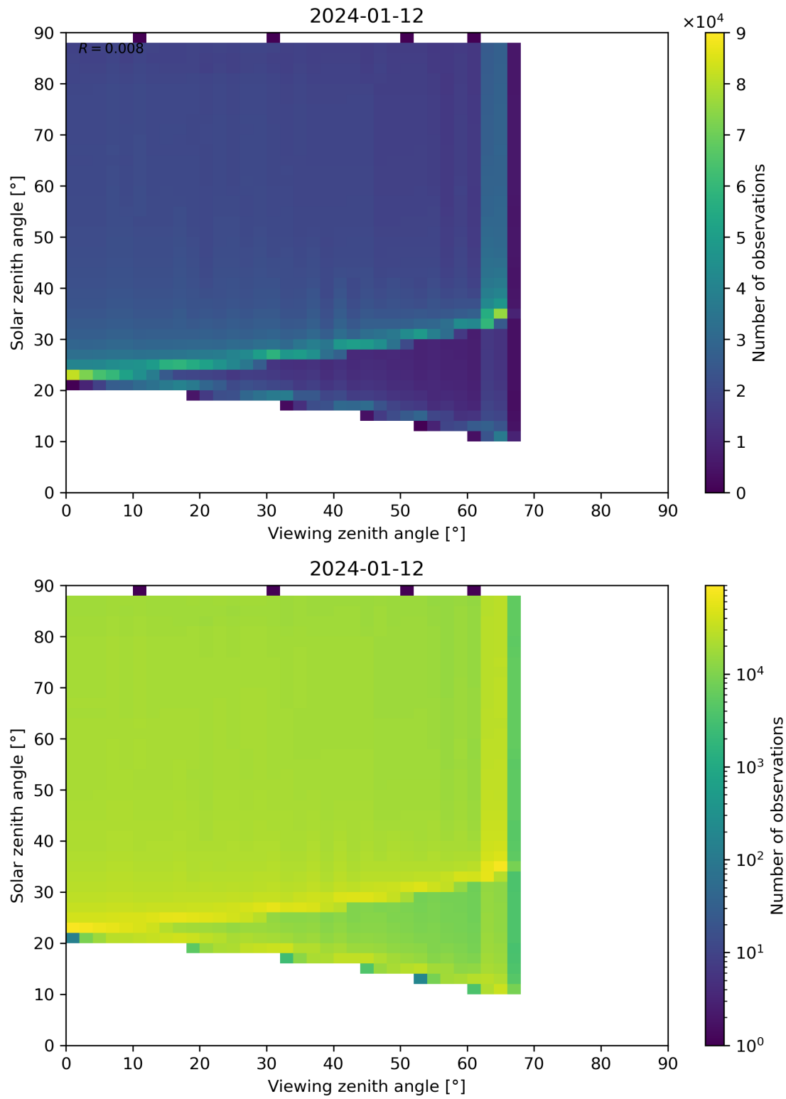
Figure 172: Scatter density plot of “Viewing zenith angle” against “Solar zenith angle” for 2024-01-11 to 2024-01-13.
