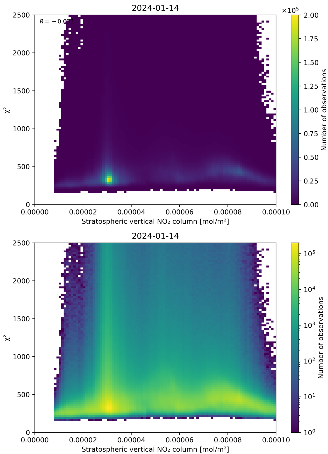
Figure 97: Scatter density plot of “Stratospheric vertical NO 2 column” against “ \chi^2 ” for 2024-01-13 to 2024-01-15.
