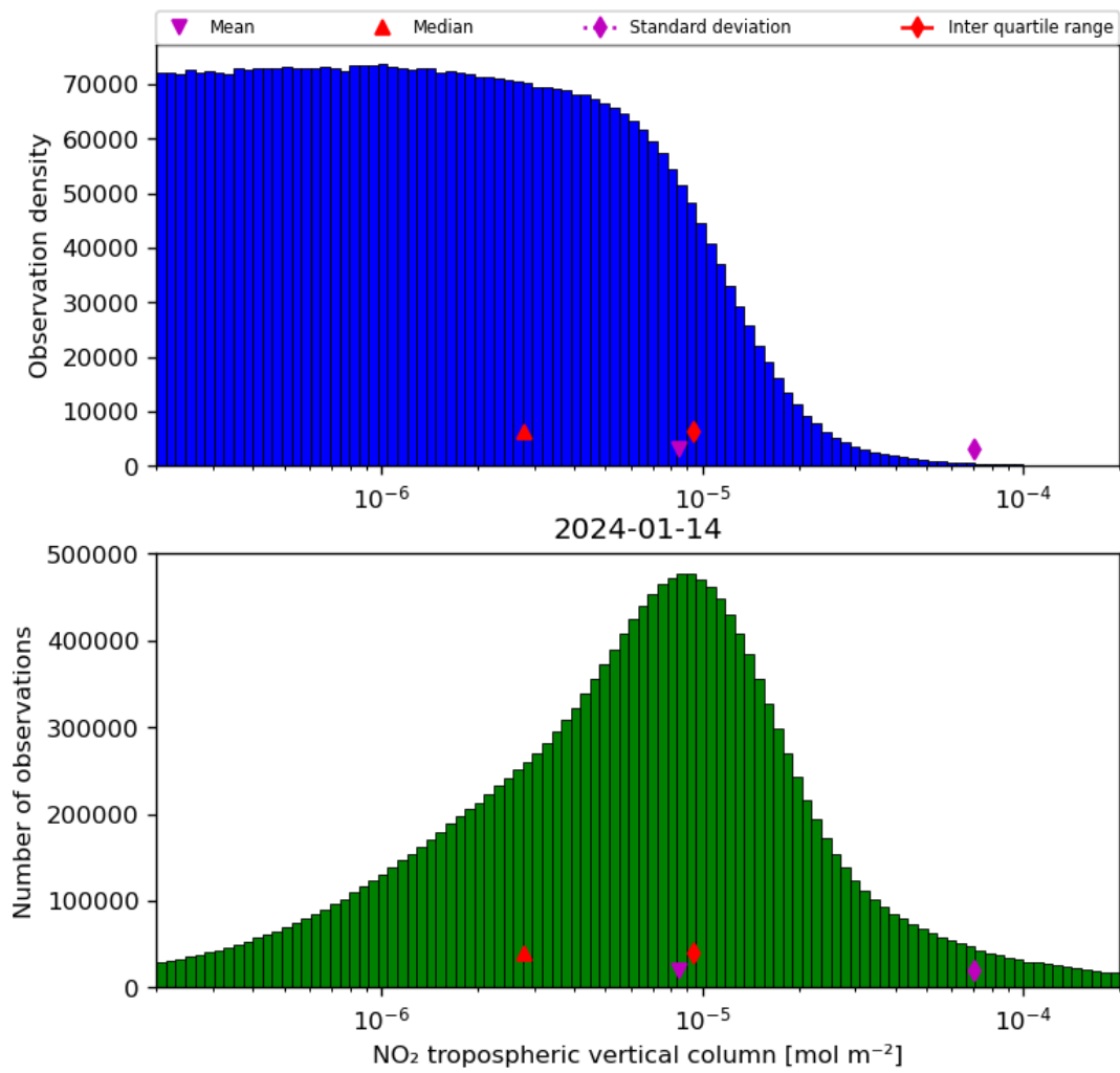
Figure 29: Histogram of “NO 2 tropospheric vertical column” for 2024-01-13 to 2024-01-15
