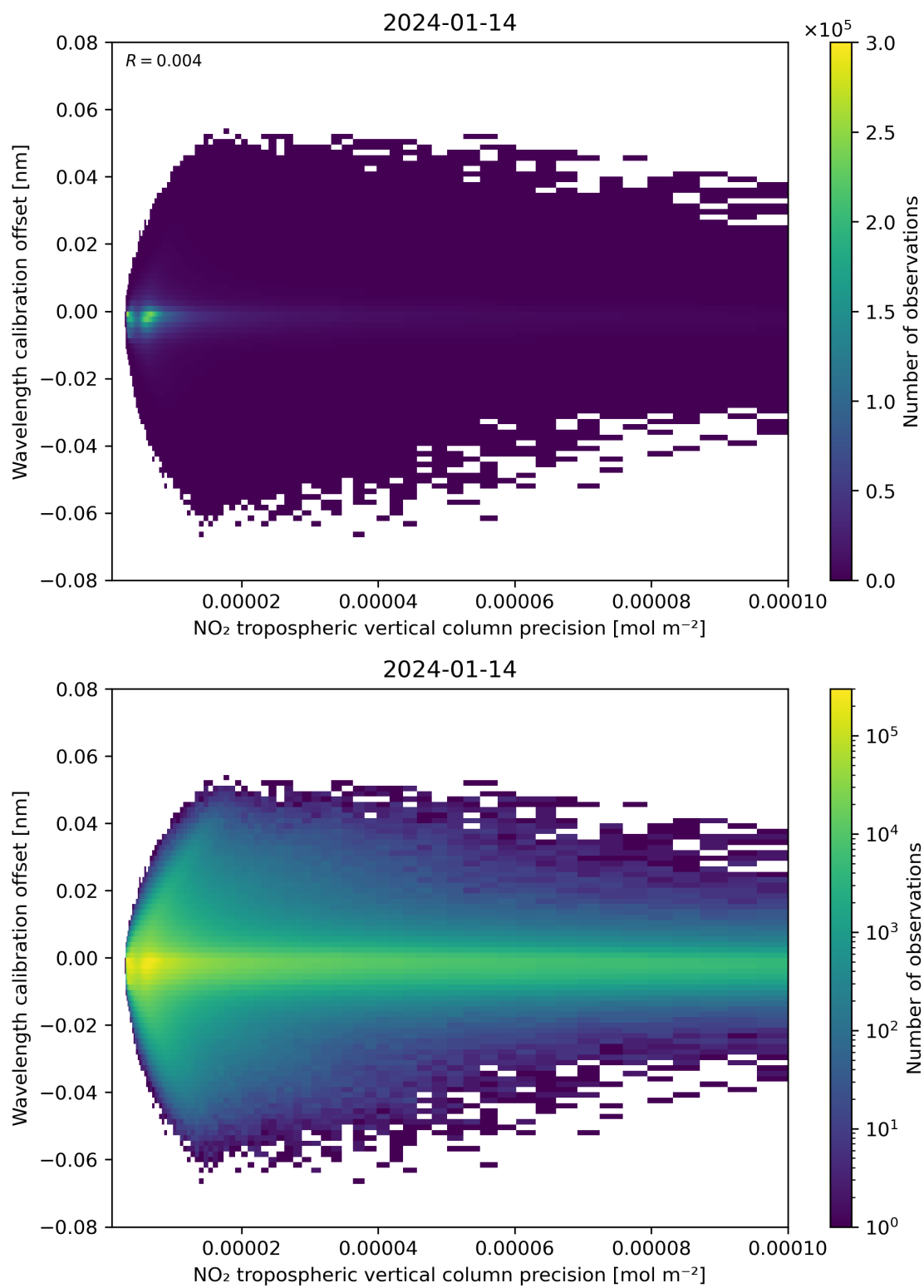
Figure 141: Scatter density plot of “NO 2 tropospheric vertical column precision” against “Wavelength calibration offset” for 2024-01-13 to 2024-01-15.
