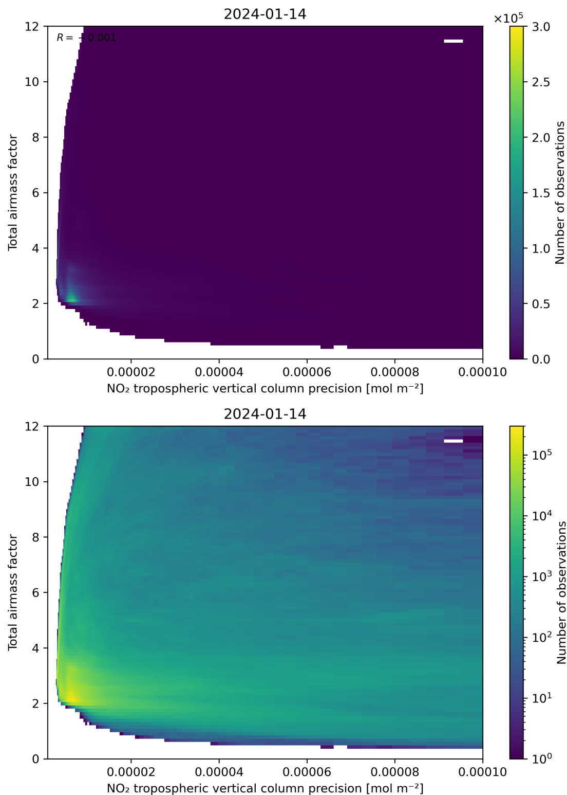
Figure 132: Scatter density plot of “NO 2 tropospheric vertical column precision” against “Total air mass factor” for 2024-01-13 to 2024-01-15.
