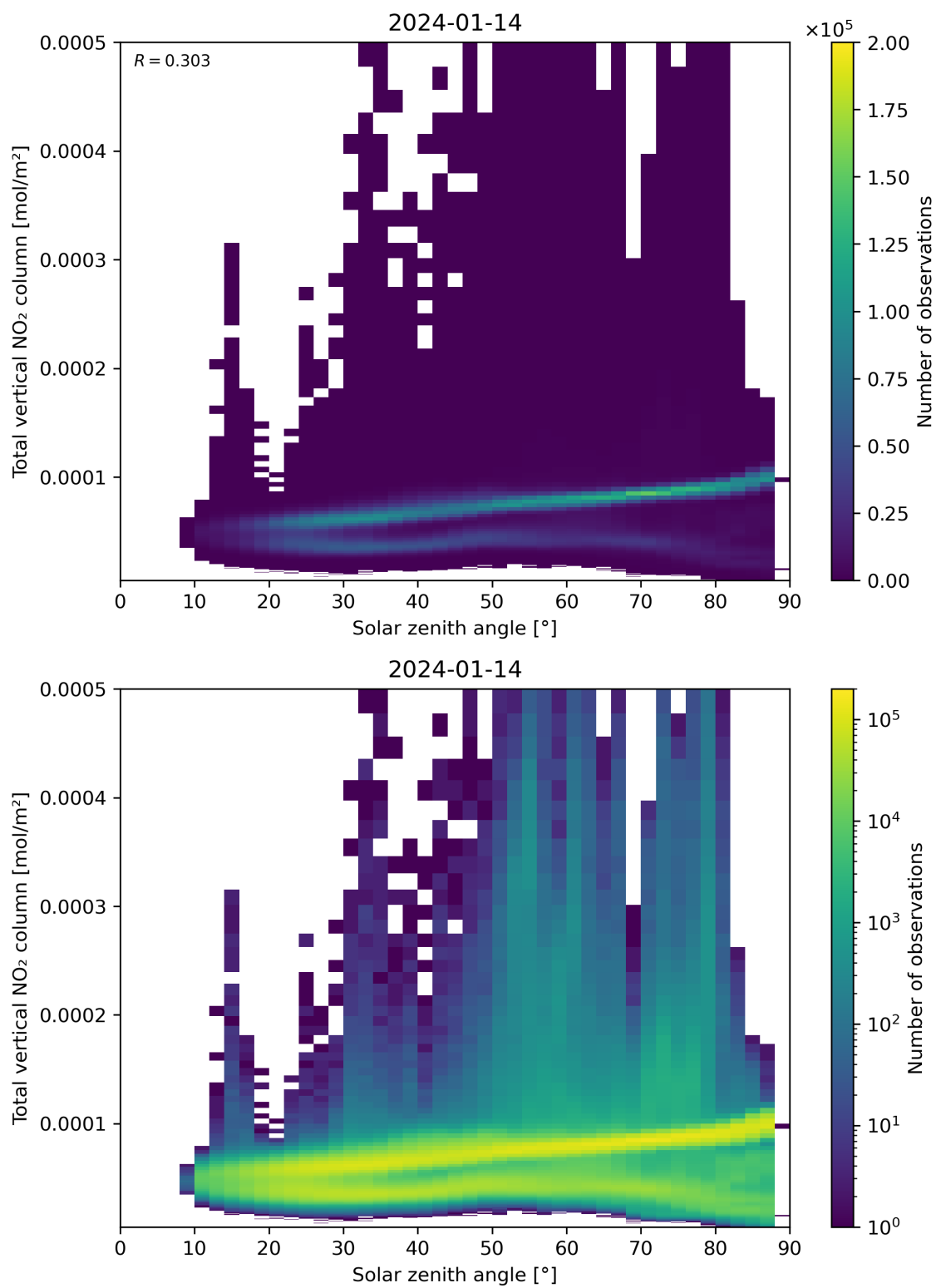
Figure 153: Scatter density plot of “Solar zenith angle” against “Total vertical NO 2 column” for 2024-01-13 to 2024-01-15.
