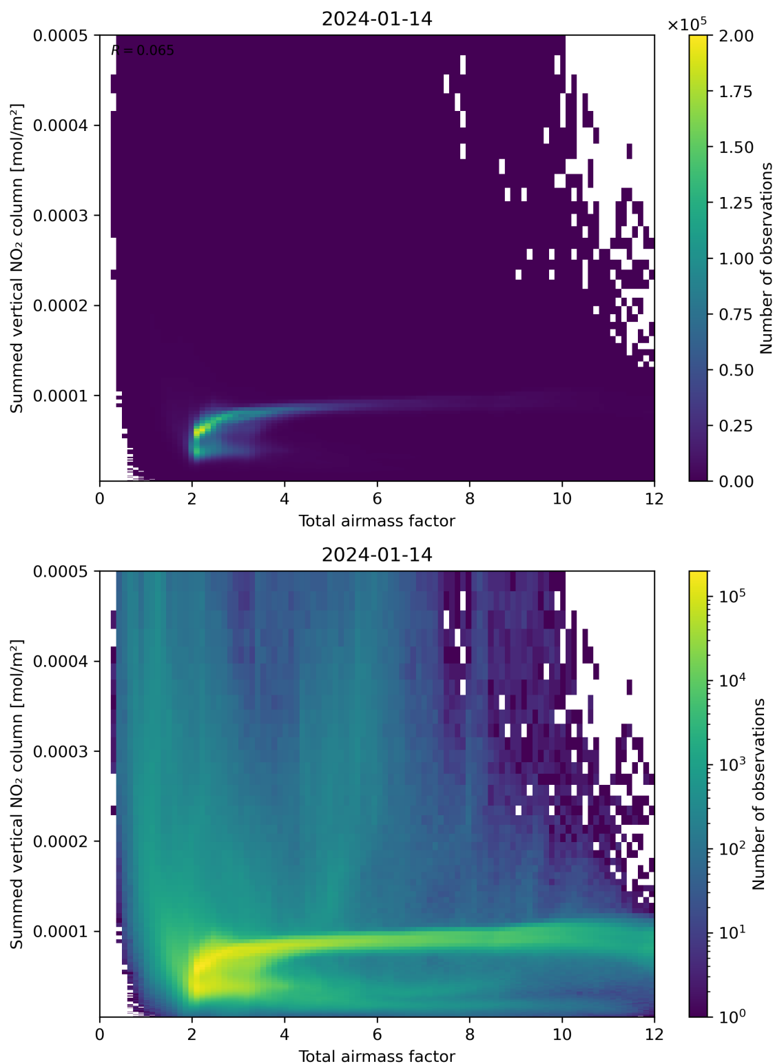
Figure 65: Scatter density plot of “Total airmass factor” against “Summed vertical NO 2 column” for 2024-01-13 to 2024-01-15.
