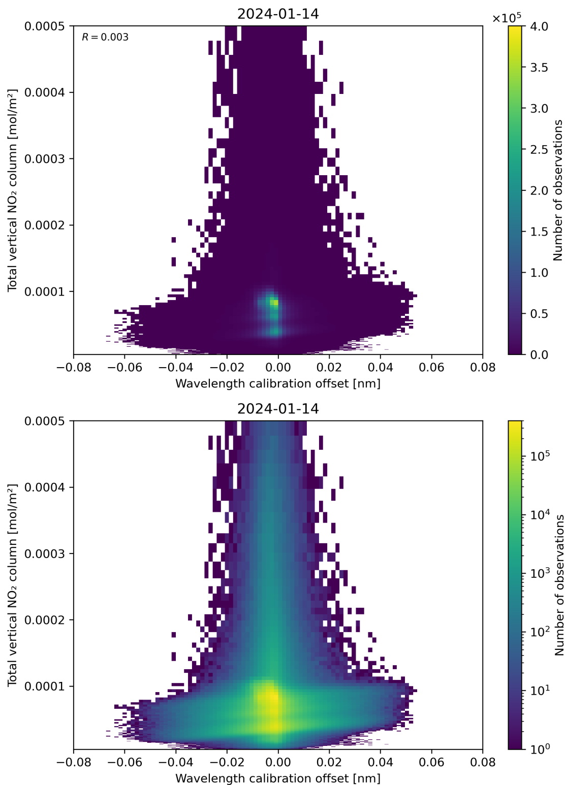
Figure 179: Scatter density plot of “Wavelength calibration offset” against “Total vertical NO 2 column” for 2024-01-13 to 2024-01-15.
