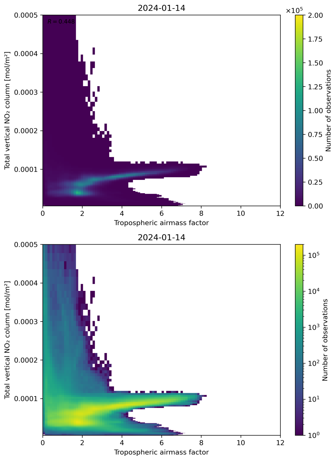
Figure 77: Scatter density plot of “Tropospheric airmass factor” against “Total vertical NO 2 column” for 2024-01-13 to 2024-01-15.
