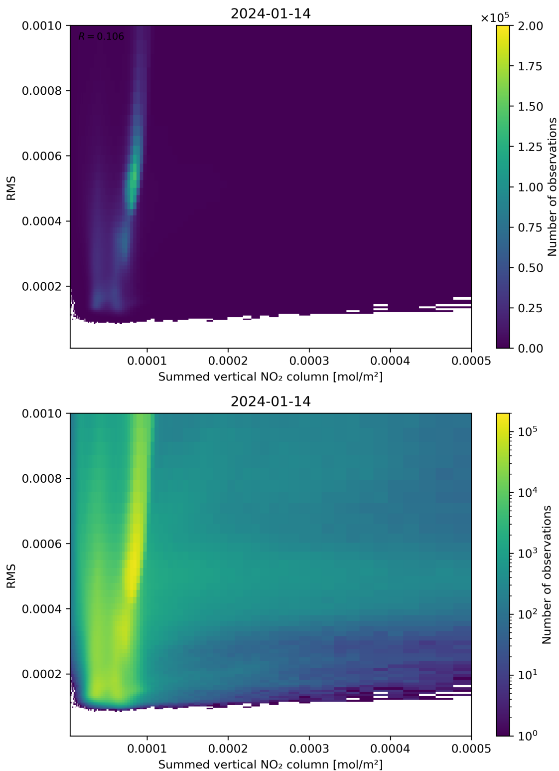
Figure 109: Scatter density plot of “Summed vertical NO 2 column” against “RMS” for 2024-01-13 to 2024-01-15.
