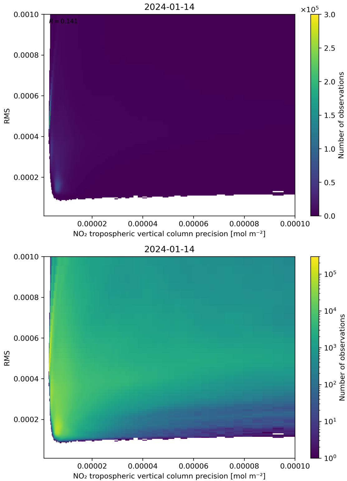
Figure 140: Scatter density plot of “NO 2 tropospheric vertical column precision” against “RMS” for 2024-01-13 to 2024-01-15.
