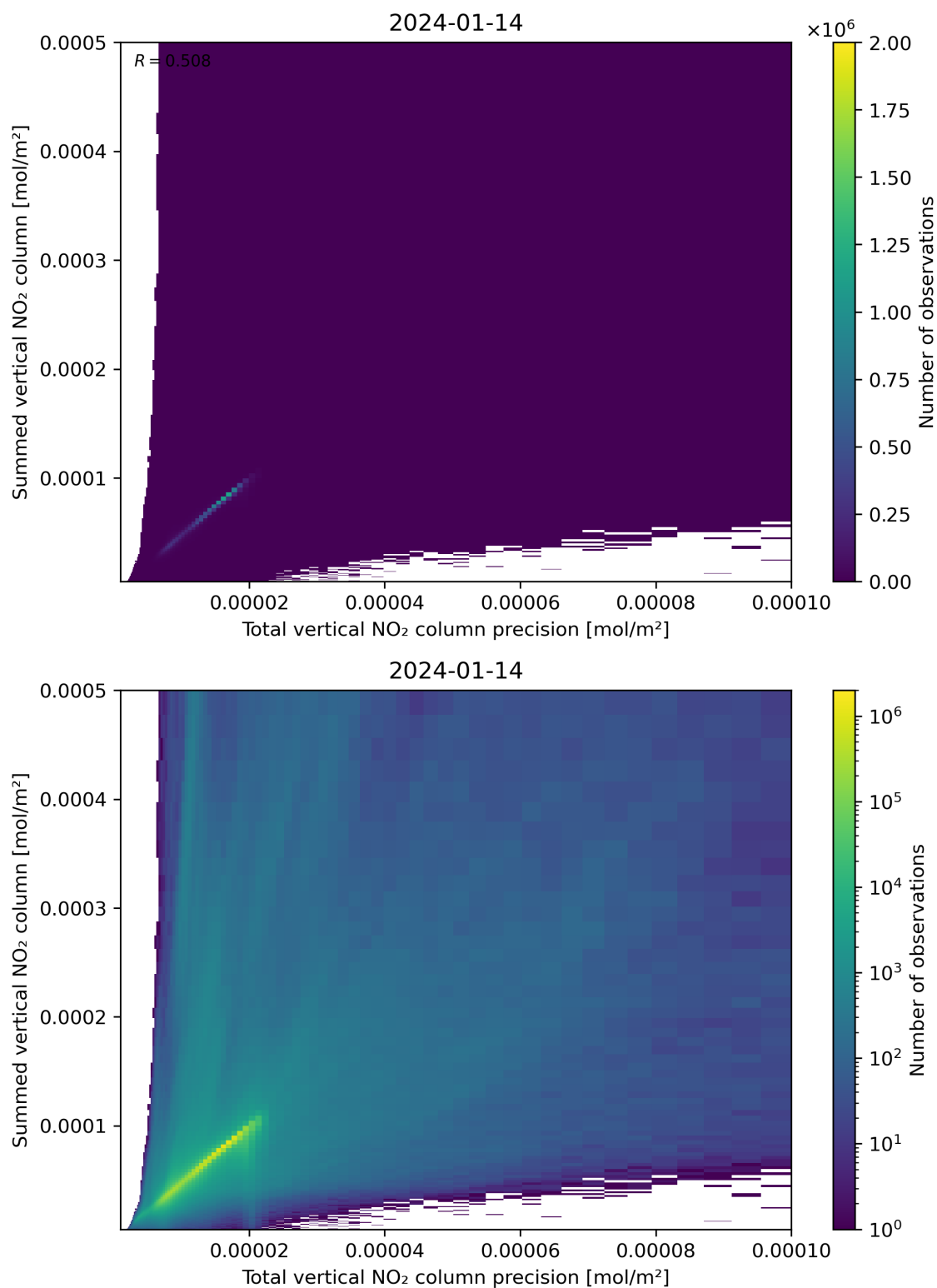
Figure 117: Scatter density plot of “Total vertical NO 2 column precision” against “Summed vertical NO 2 column” for 2024-01-13 to 2024-01-15.
