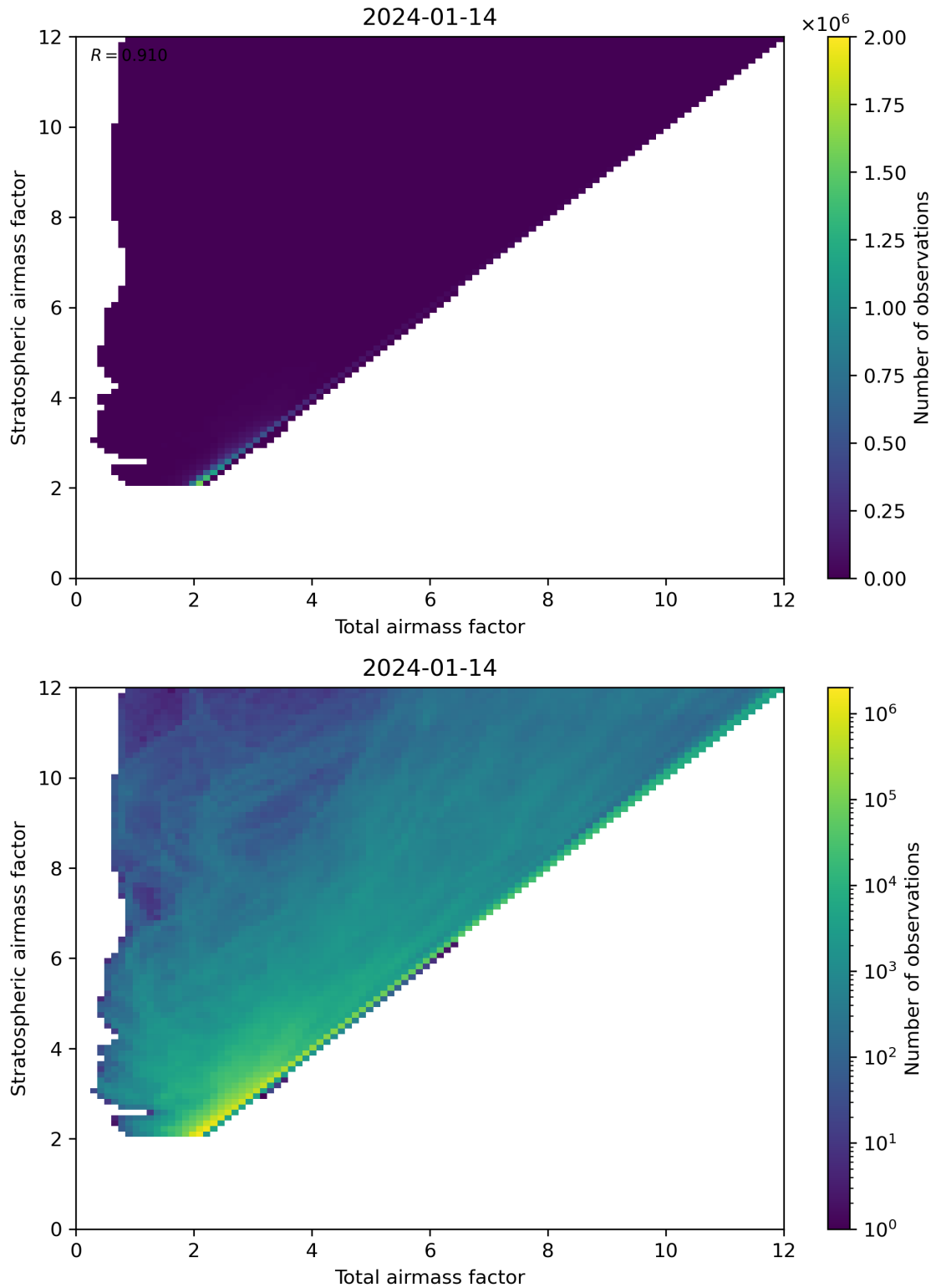
Figure 62: Scatter density plot of “Total air mass factor” against “Stratospheric air mass factor” for 2024-01-13 to 2024-01-15.
