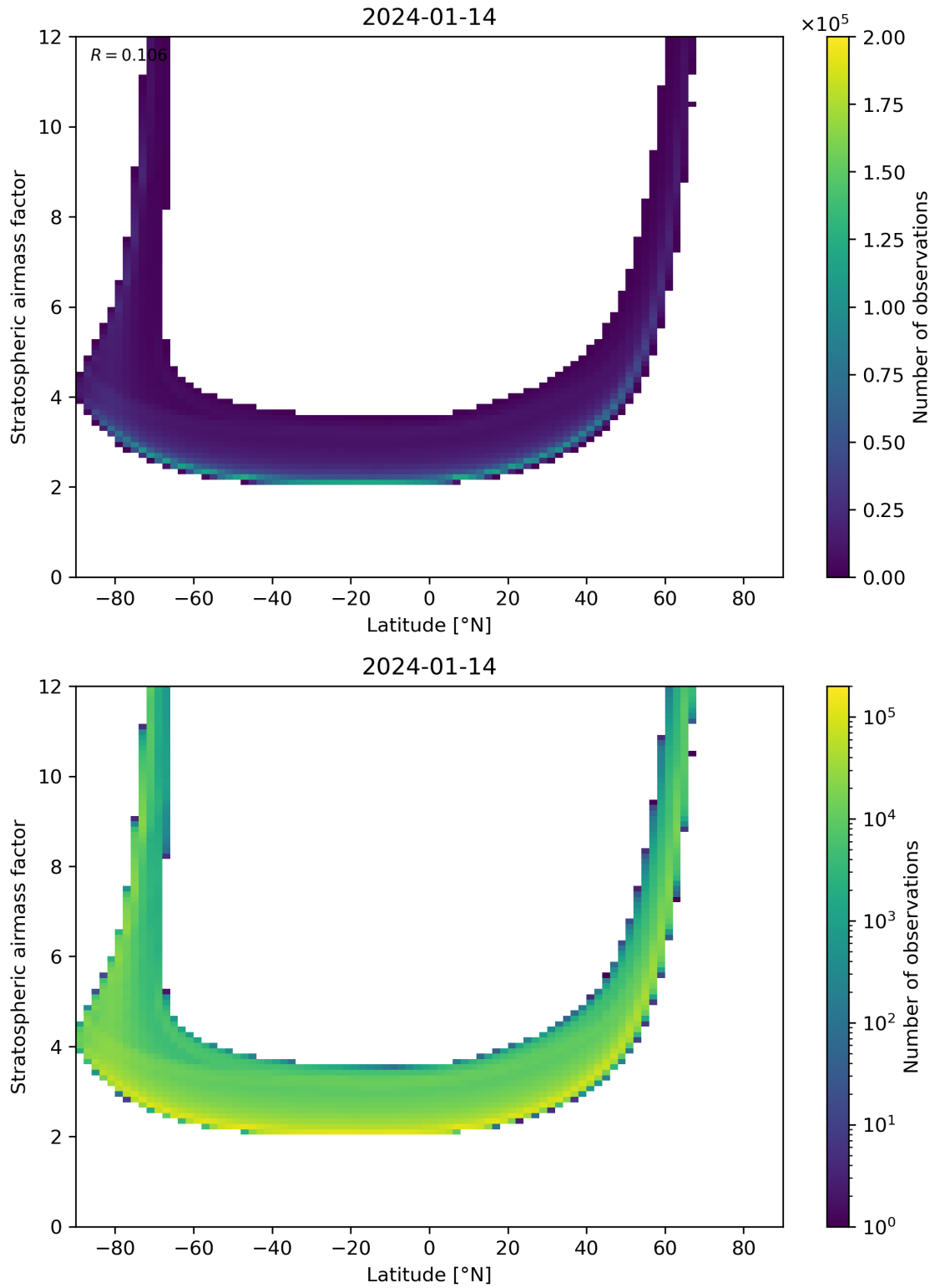
Figure 83: Scatter density plot of “Latitude” against “Stratospheric airmass factor” for 2024-01-13 to 2024-01-15.
