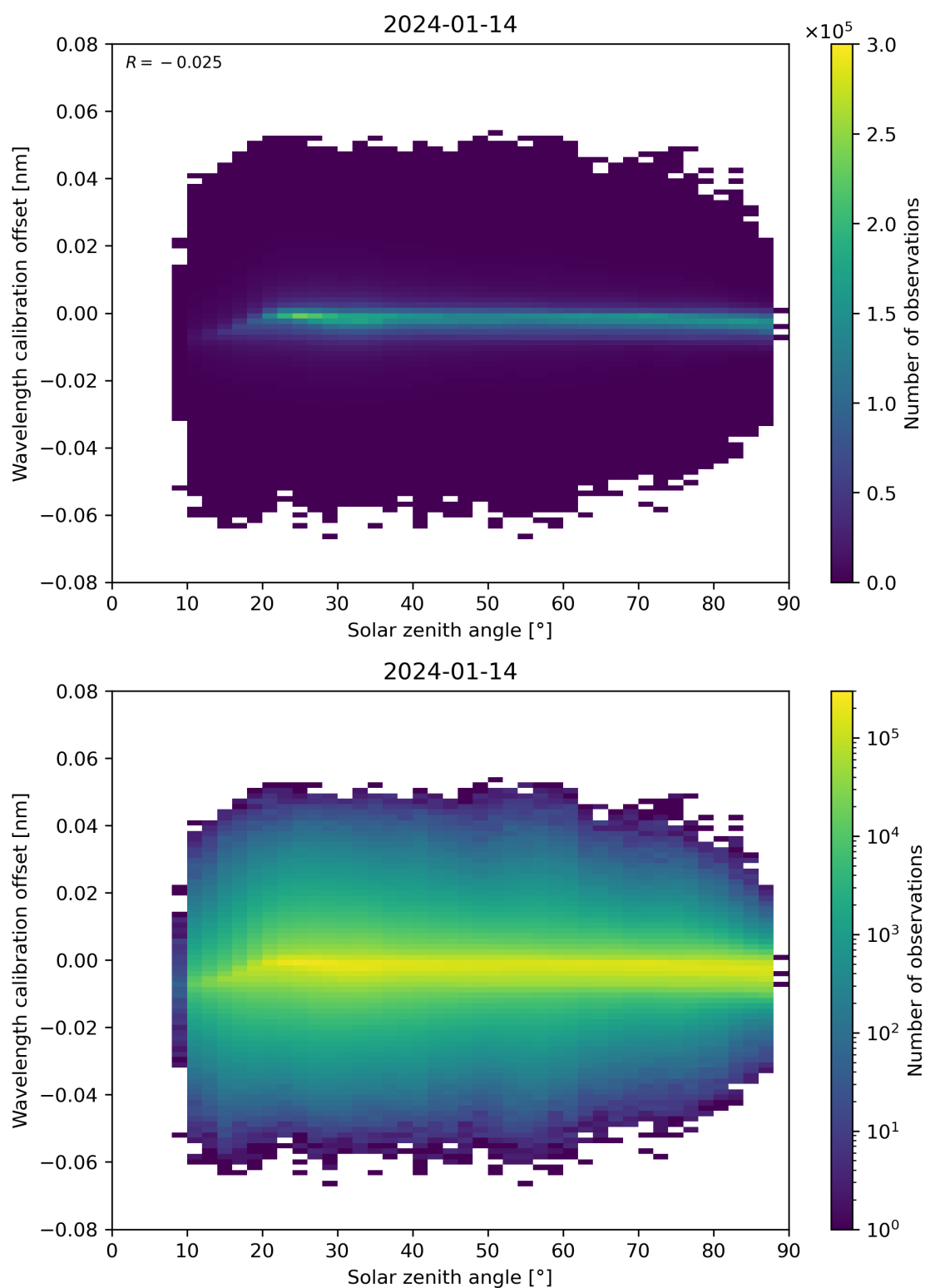
Figure 158: Scatter density plot of “Solar zenith angle” against “Wavelength calibration offset” for 2024-01-13 to 2024-01-15.
