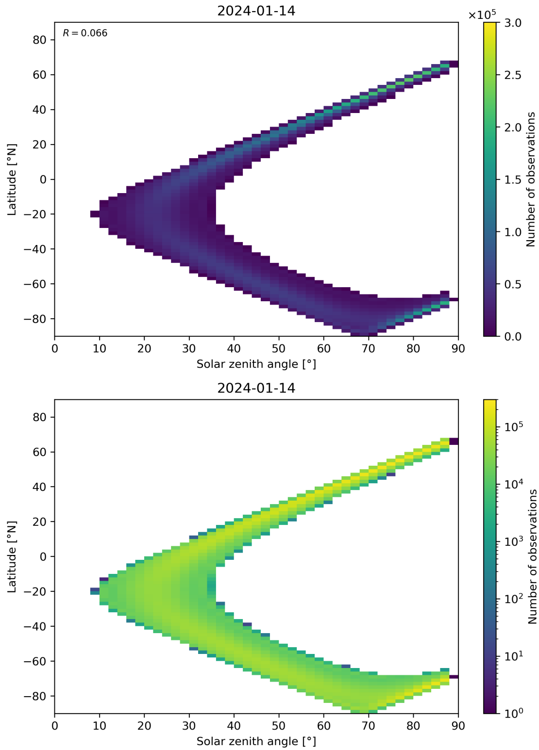
Figure 149: Scatter density plot of “Solar zenith angle” against “Latitude” for 2024-01-13 to 2024-01-15.
