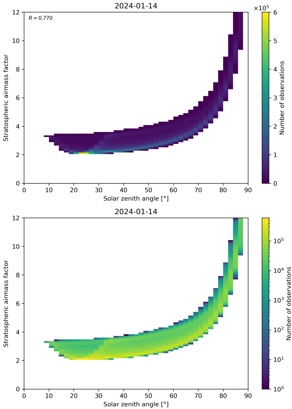
Figure 145: Scatter density plot of “Solar zenith angle” against “Stratospheric airmass factor” for 2024-01-13 to 2024-01-15.
