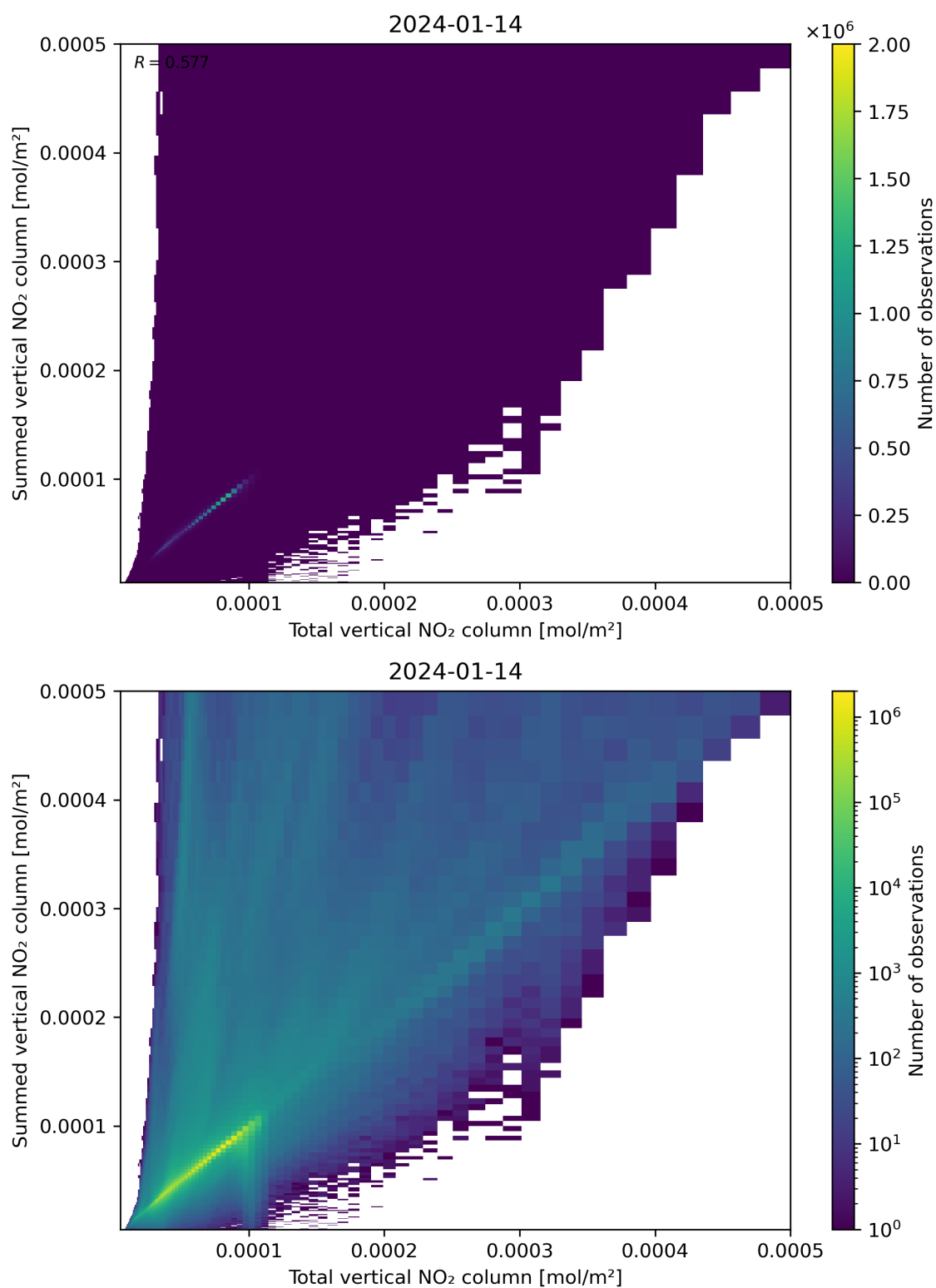
Figure 112: Scatter density plot of “Total vertical NO 2 column” against “Summed vertical NO 2 column” for 2024-01-13 to 2024-01-15.
