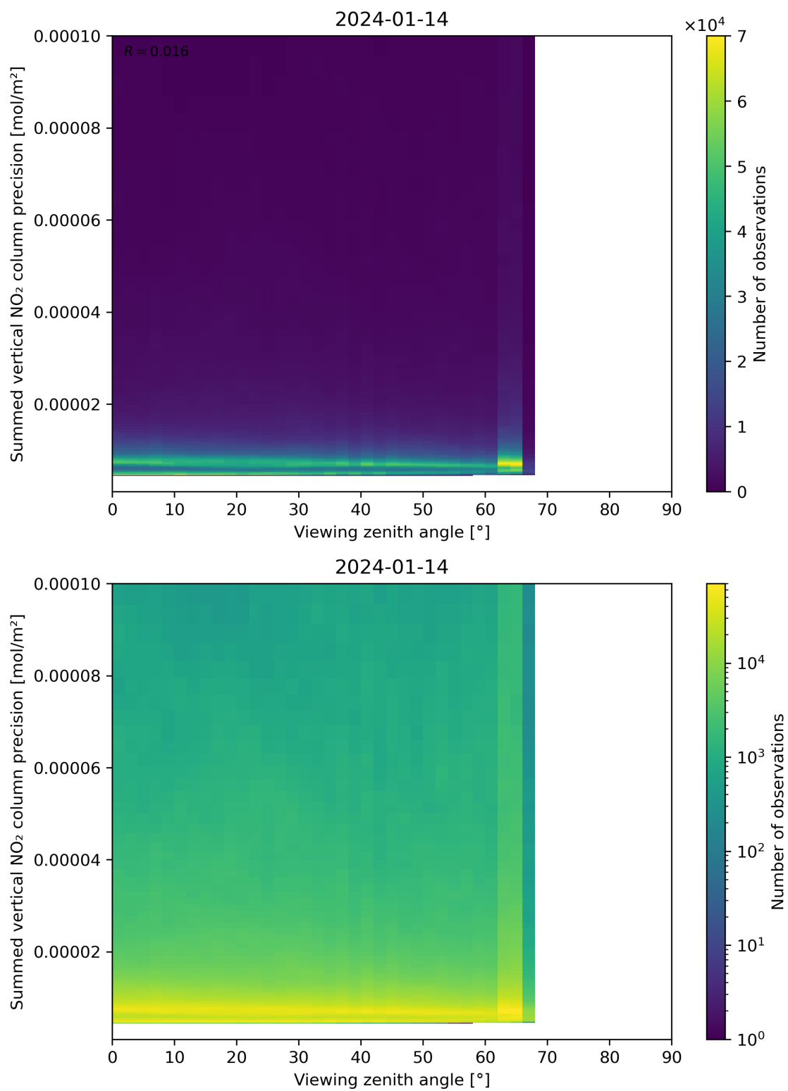
Figure 166: Scatter density plot of “Viewing zenith angle” against “Summed vertical NO 2 column precision” for 2024-01-13 to 2024-01-15.
