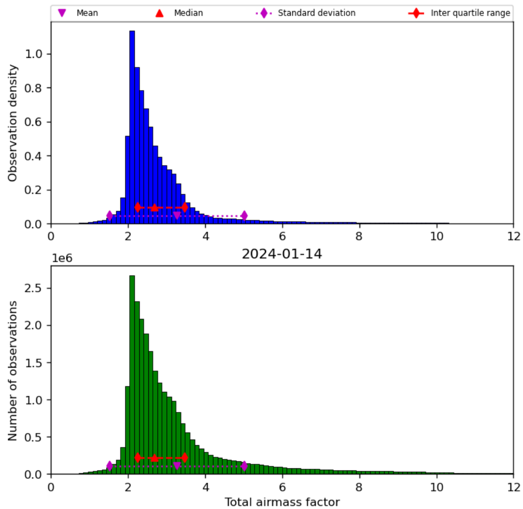
Figure 32: Histogram of “Total airmass factor” for 2024-01-13 to 2024-01-15
