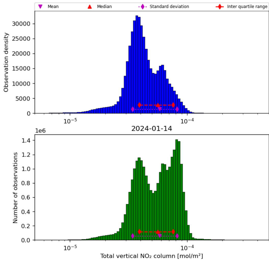
Figure 38: Histogram of “Total vertical NO 2 column” for 2024-01-13 to 2024-01-15
