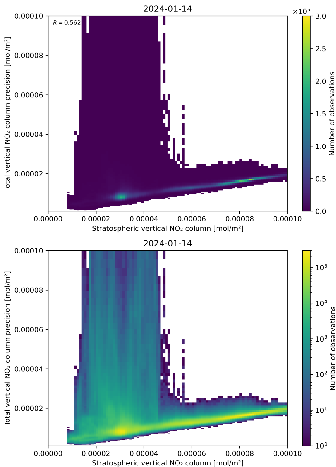
Figure 101: Scatter density plot of “Stratospheric vertical NO 2 column” against “Total vertical NO 2 column precision” for 2024-01-13 to 2024-01-15.
