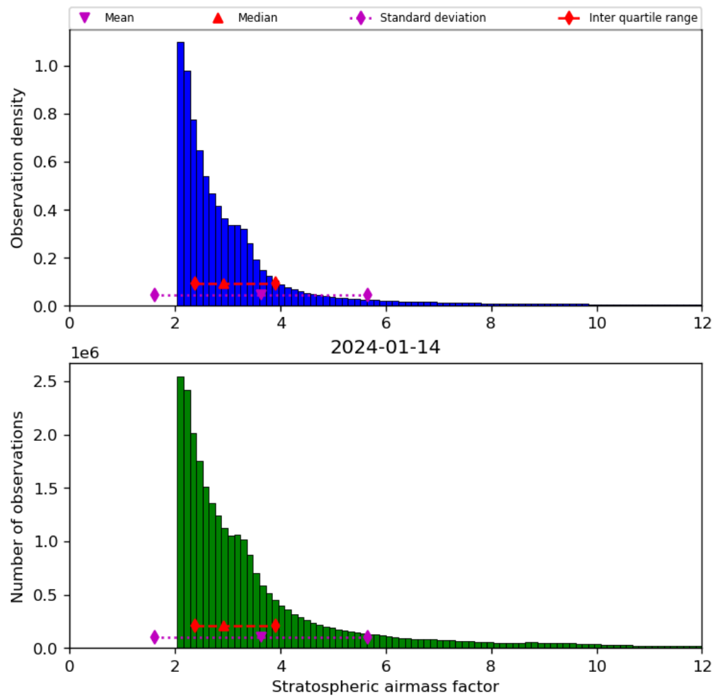
Figure 44: Histogram of “Stratospheric airmass factor” for 2024-01-13 to 2024-01-15
