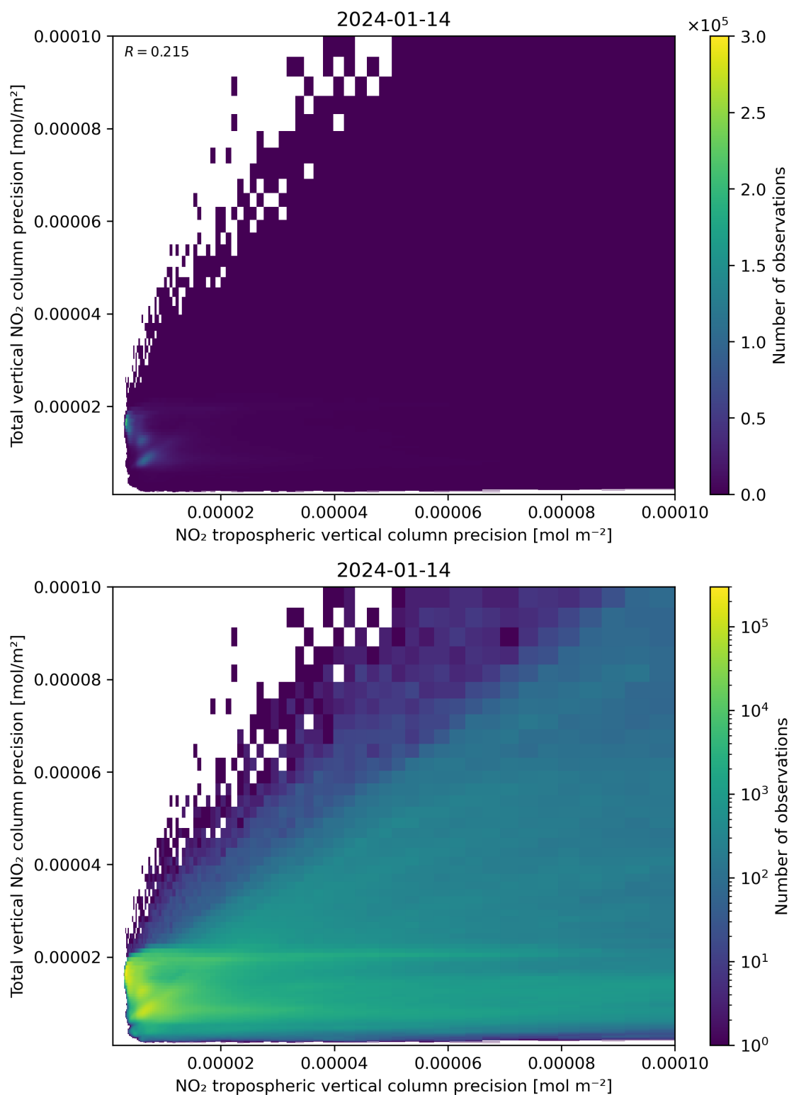
Figure 139: Scatter density plot of “NO 2 tropospheric vertical column precision” against “Total vertical NO 2 column precision” for 2024-01-13 to 2024-01-15.
