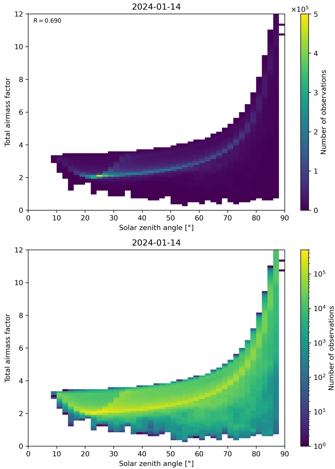
Figure 146: Scatter density plot of “Solar zenith angle” against “Total air mass factor” for 2024-01-13 to 2024-01-15.
