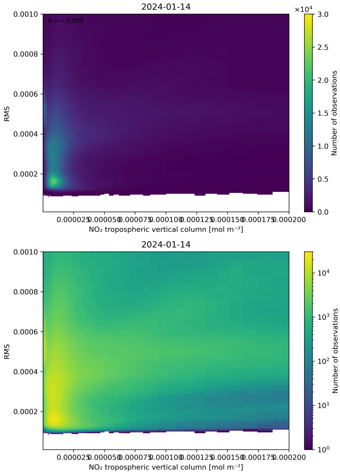
Figure 142: Scatter density plot of “NO 2 tropospheric vertical column” against “RMS” for 2024-01-13 to 2024-01-15.
