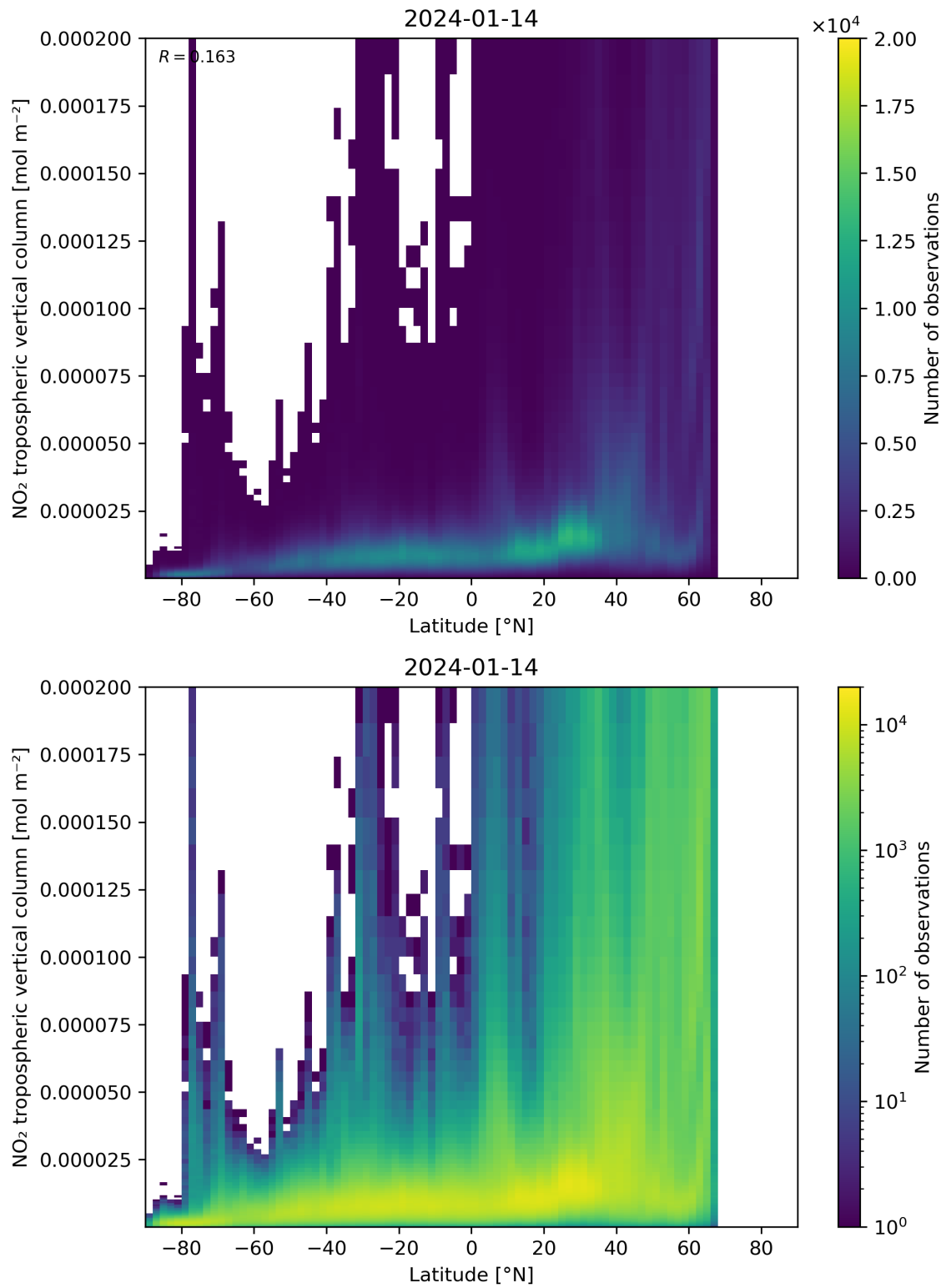
Figure 92: Scatter density plot of “Latitude” against “NO 2 tropospheric vertical column” for 2024-01-13 to 2024-01-15.
