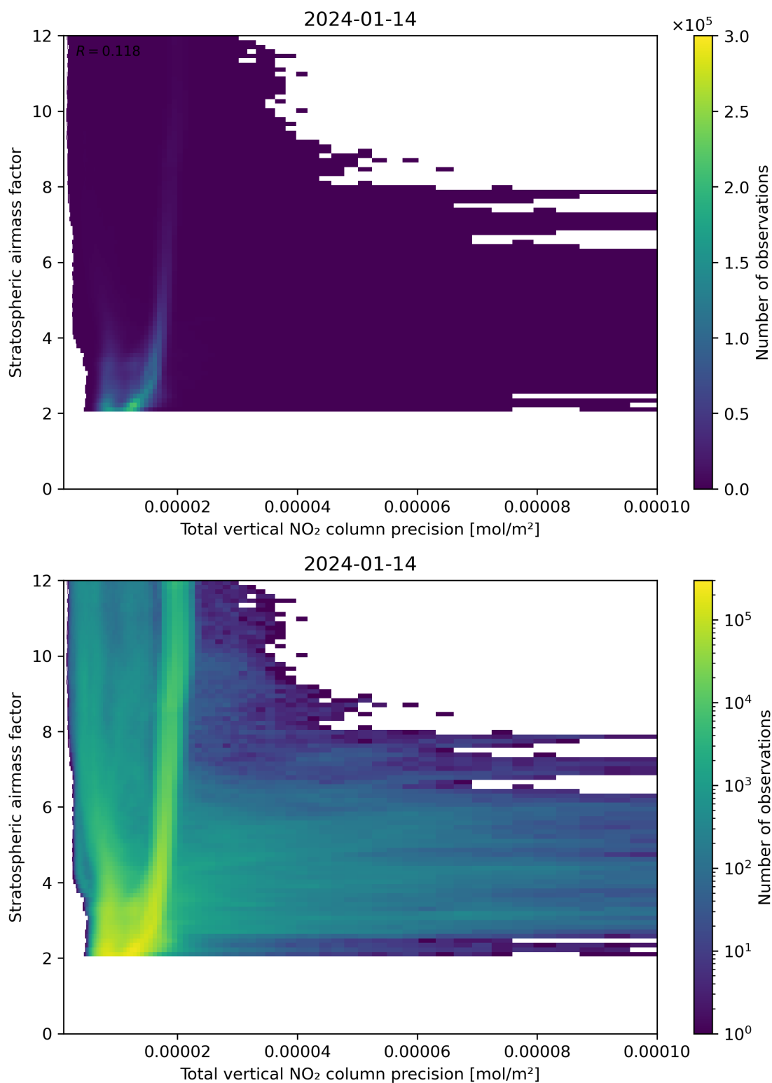
Figure 115: Scatter density plot of “Total vertical NO 2 column precision” against “Stratospheric air mass factor” for 2024-01-13 to 2024-01-15.
