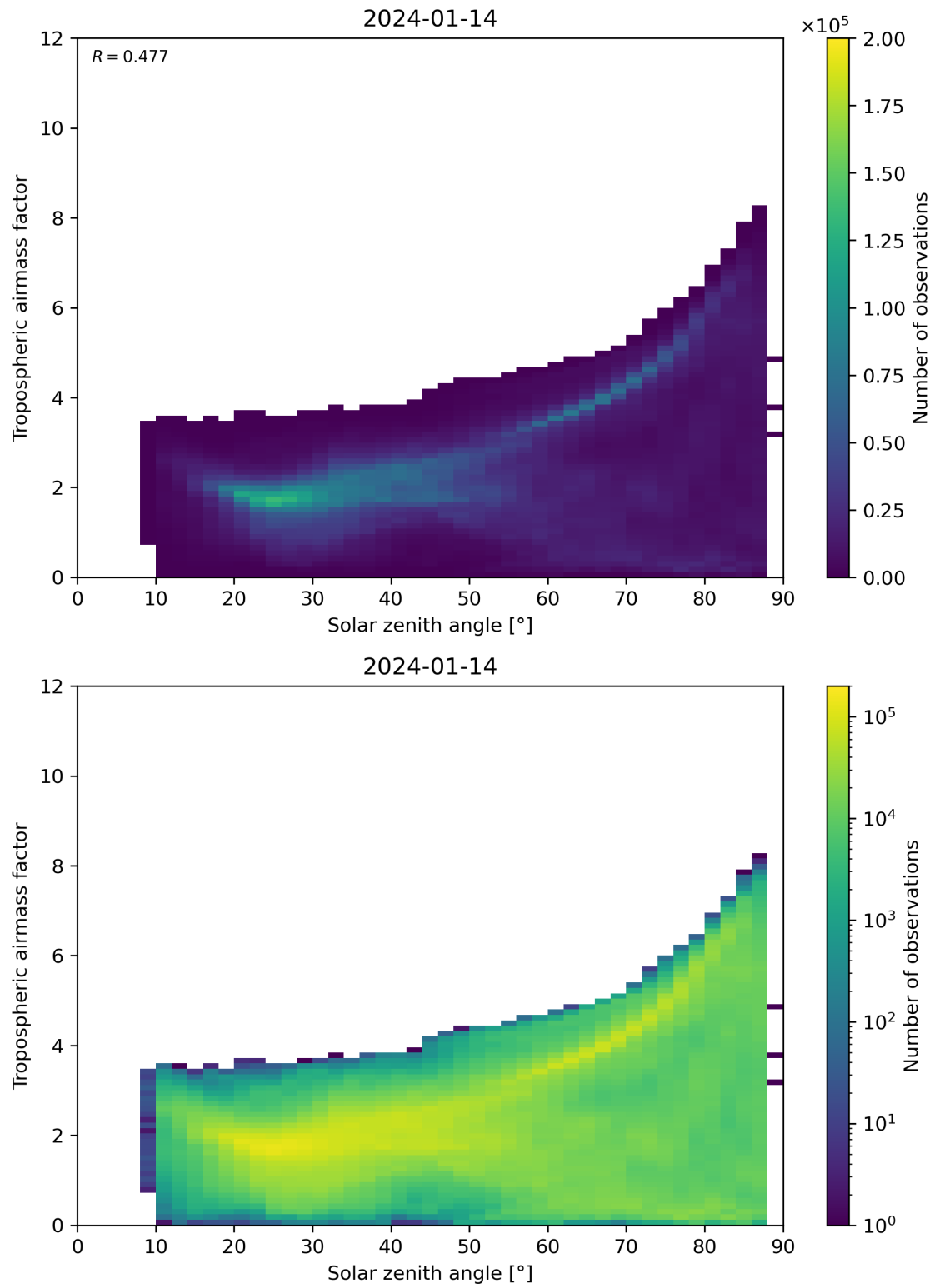
Figure 147: Scatter density plot of “Solar zenith angle” against “Tropospheric airmass factor” for 2024-01-13 to 2024-01-15.
