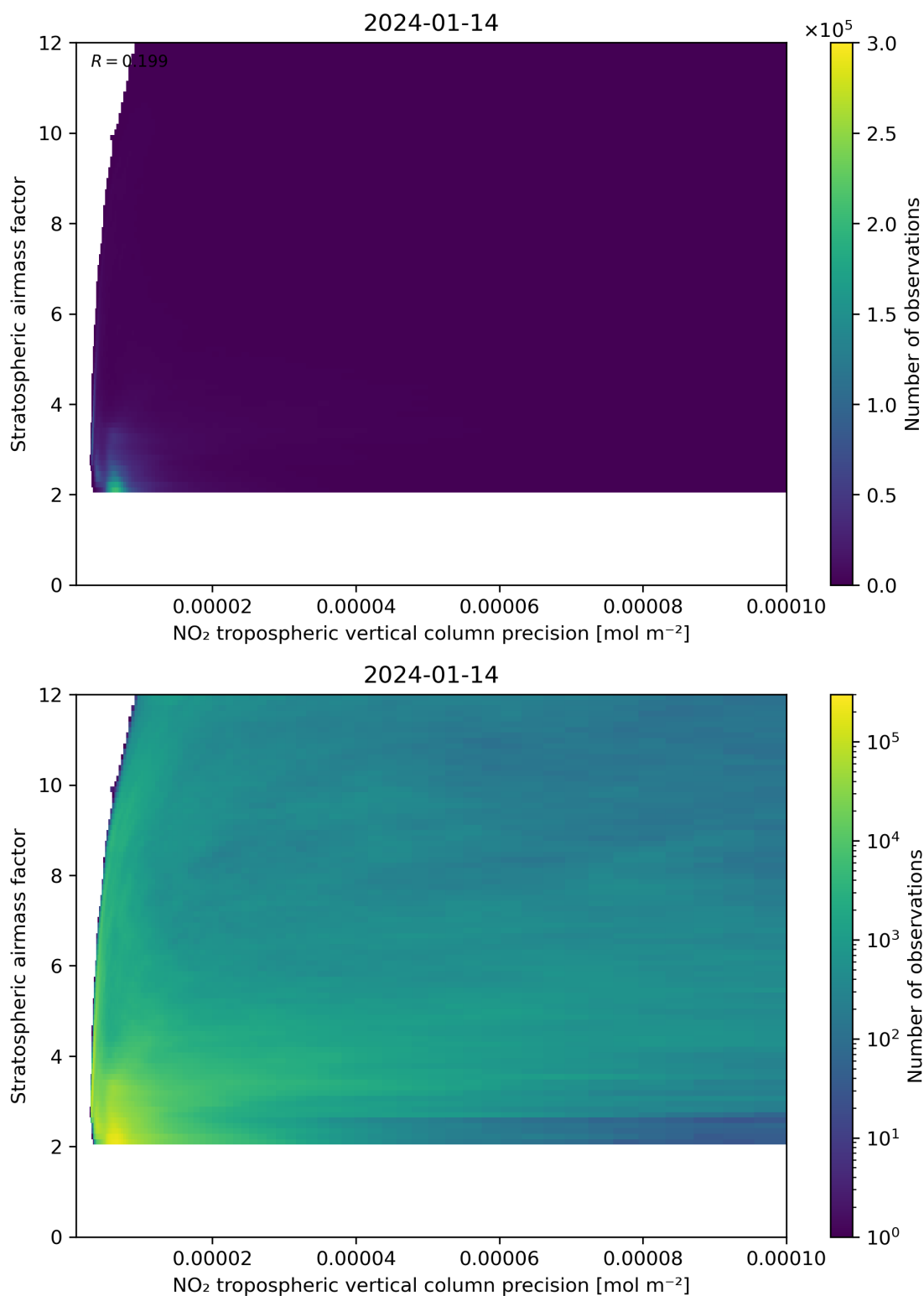
Figure 131: Scatter density plot of “NO 2 tropospheric vertical column precision” against “Stratospheric airmass factor” for 2024-01-13 to 2024-01-15.
