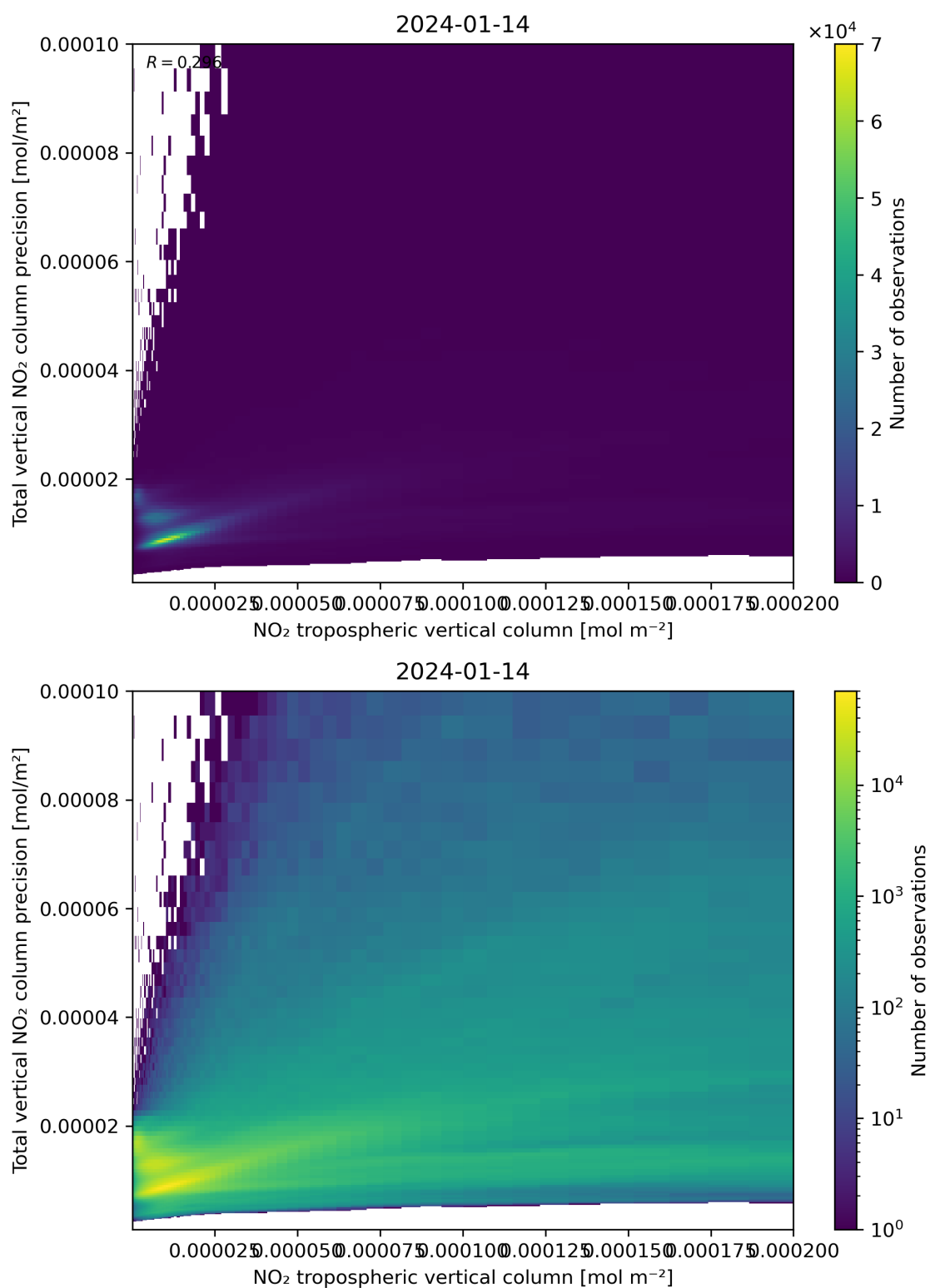
Figure 129: Scatter density plot of “NO 2 tropospheric vertical column” against “Total vertical NO 2 column precision” for 2024-01-13 to 2024-01-15.
