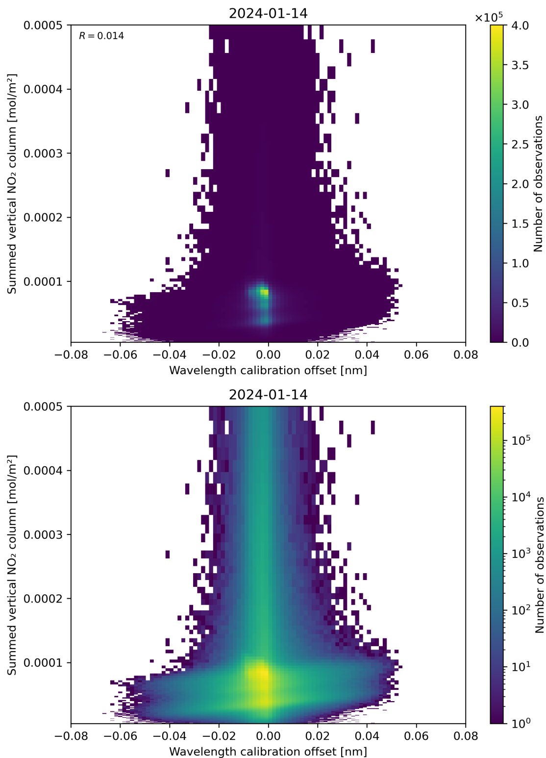
Figure 177: Scatter density plot of “Wavelength calibration offset” against “Summed vertical NO 2 column” for 2024-01-13 to 2024-01-15.
