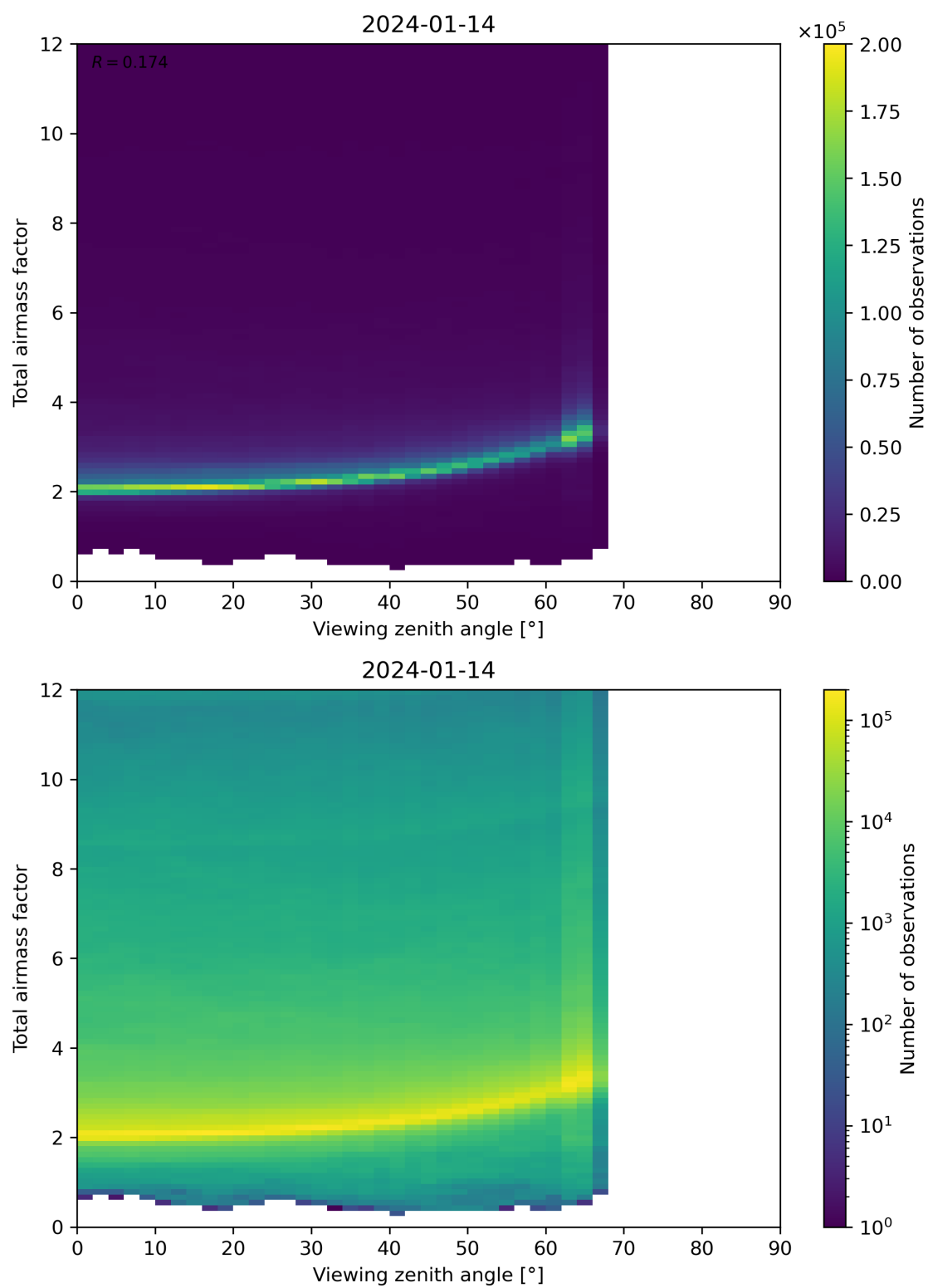
Figure 160: Scatter density plot of “Viewing zenith angle” against “Total airmass factor” for 2024-01-13 to 2024-01-15.
