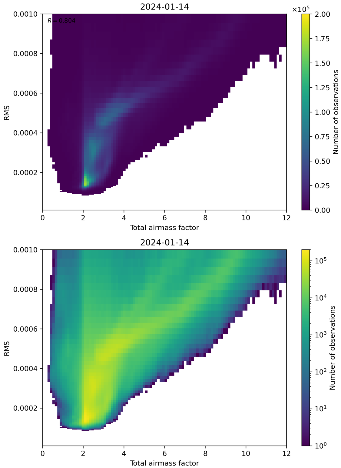
Figure 69: Scatter density plot of “Total airmass factor” against “RMS” for 2024-01-13 to 2024-01-15.
