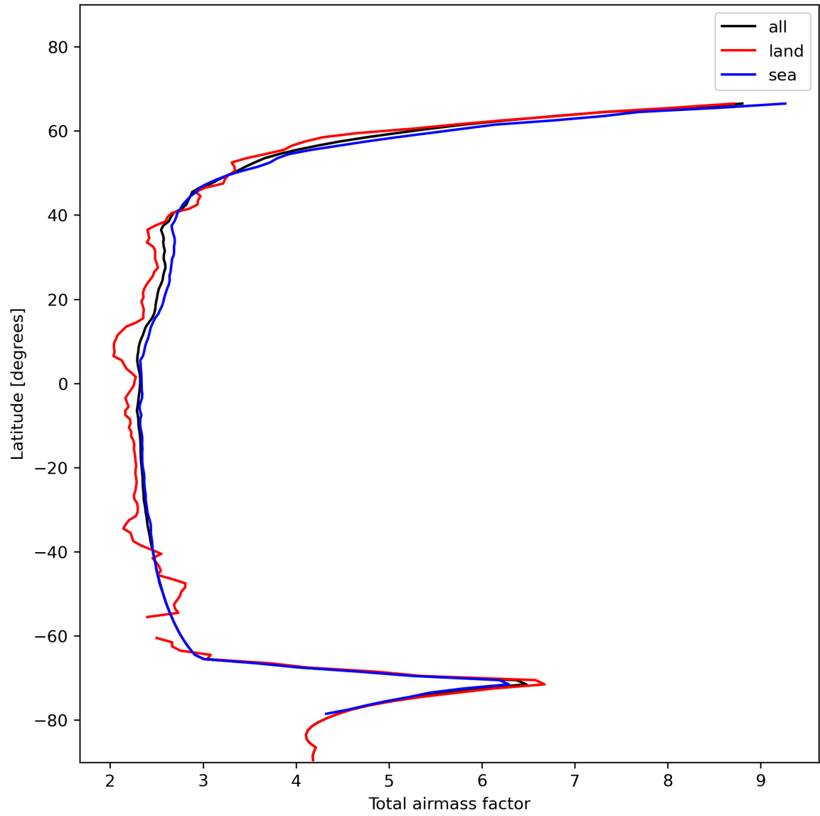
Figure 15: Zonal average of “Total airmass factor” for 2024-01-13 to 2024-01-15.
