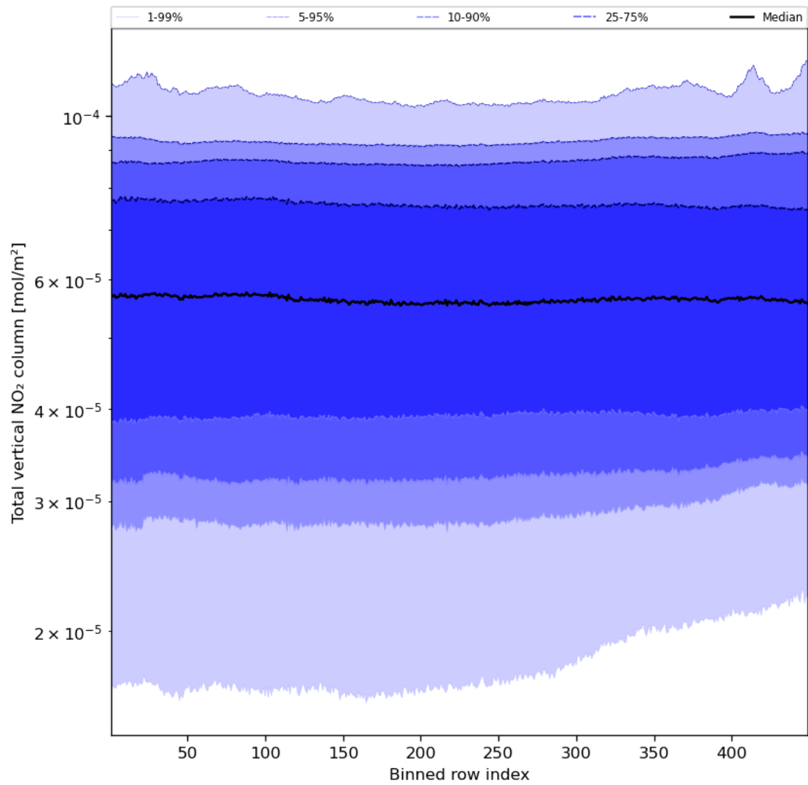
Figure 55: Along track statistics of “Total vertical NO 2 column” for 2024-01-13 to 2024-01-15
