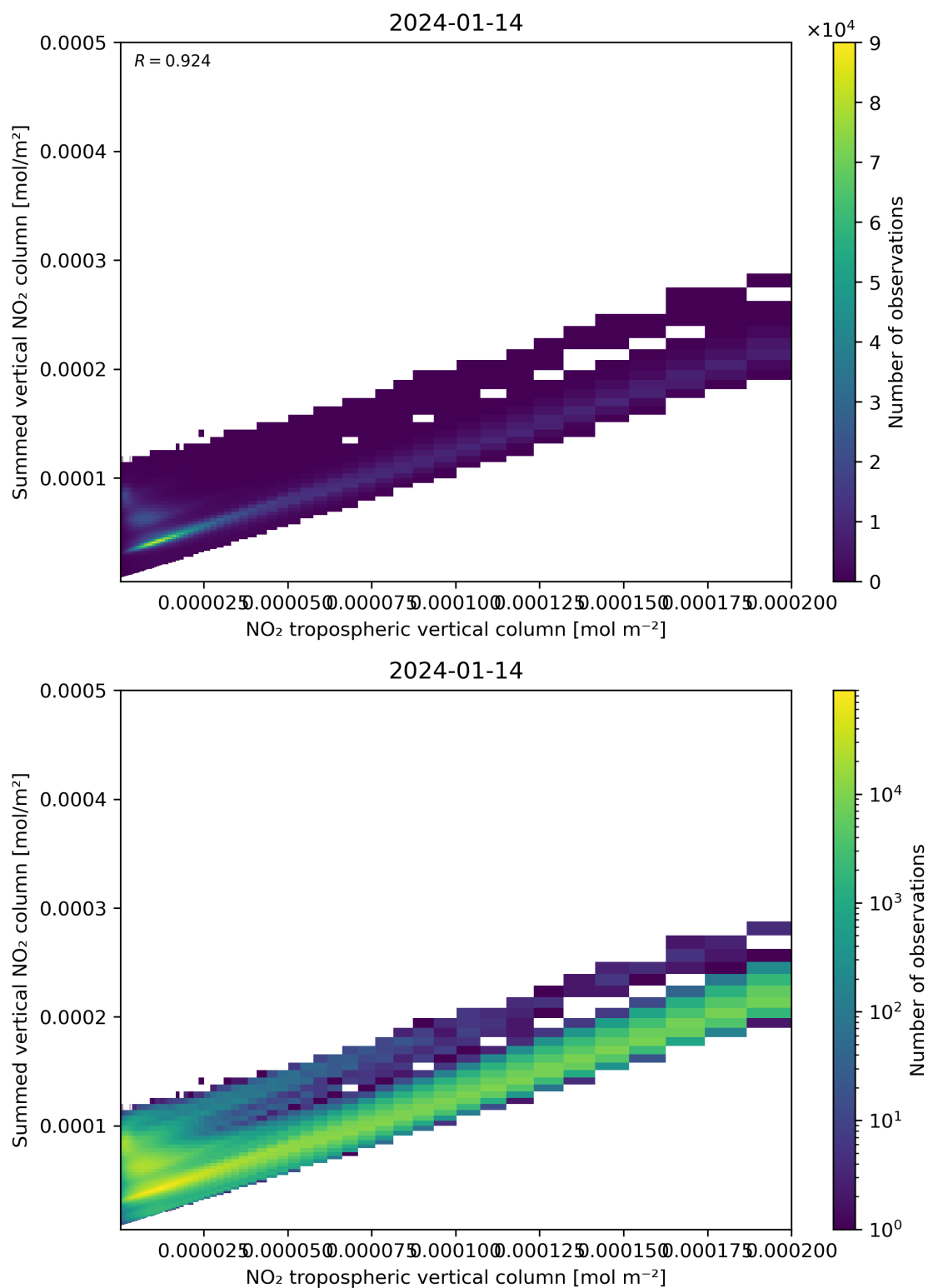
Figure 126: Scatter density plot of “NO 2 tropospheric vertical column” against “Summed vertical NO 2 column” for 2024-01-13 to 2024-01-15.
