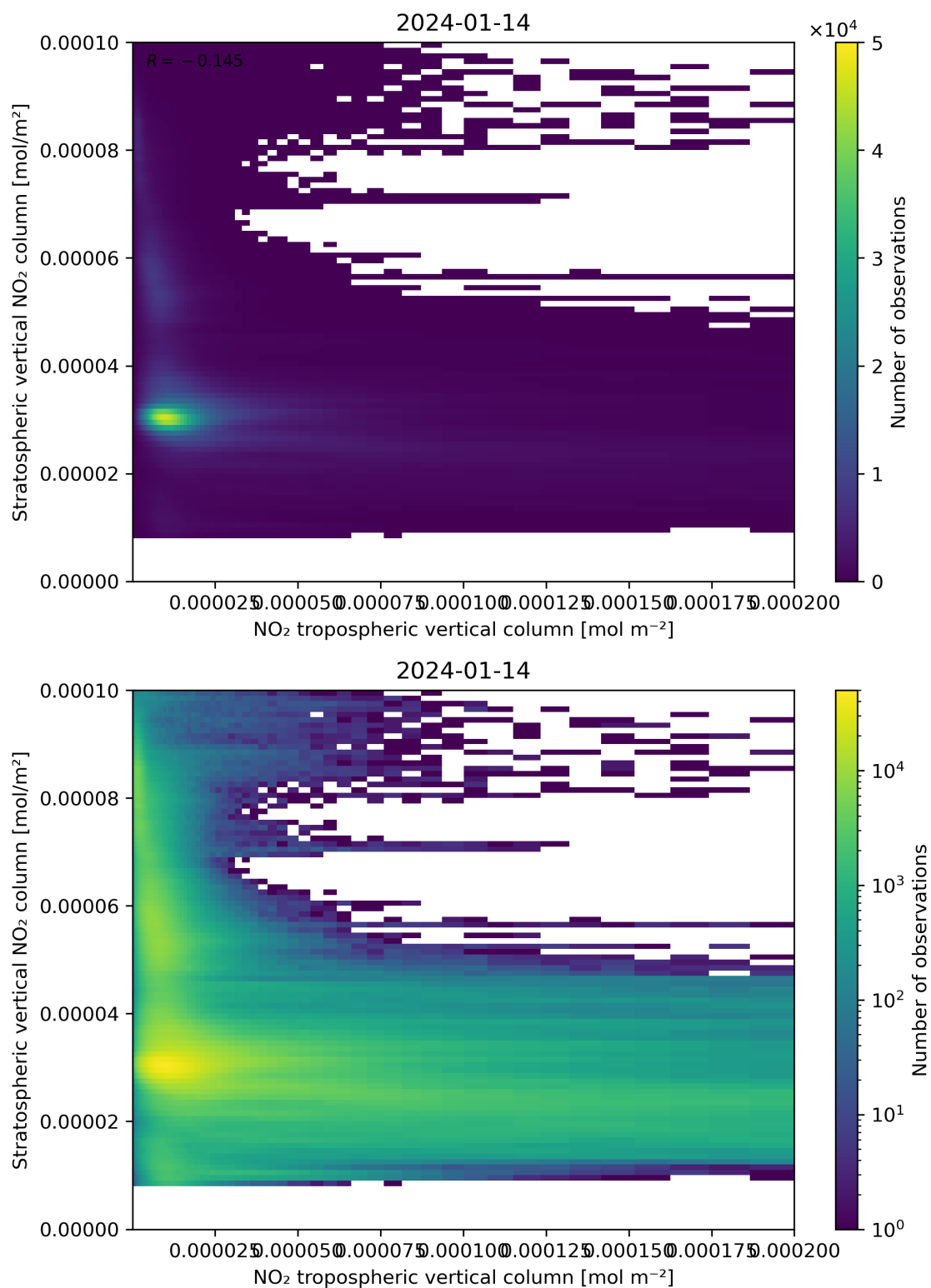
Figure 125: Scatter density plot of “NO 2 tropospheric vertical column” against “Stratospheric vertical NO 2 column” for 2024-01-13 to 2024-01-15.
