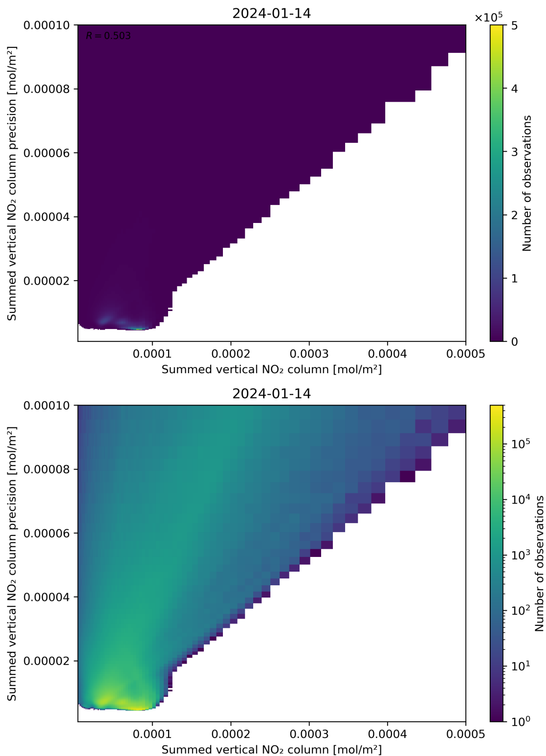
Figure 105: Scatter density plot of “Summed vertical NO 2 column” against “Summed vertical NO 2 column precision” for 2024-01-13 to 2024-01-15.
