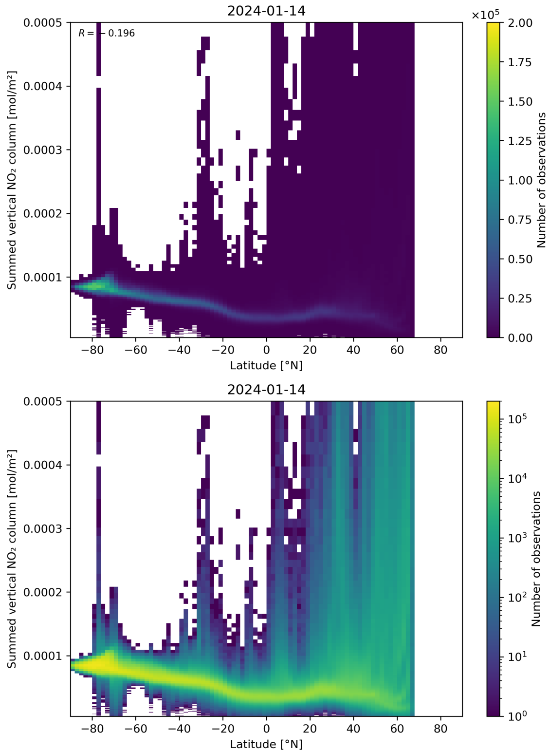
Figure 88: Scatter density plot of “Latitude” against “Summed vertical NO 2 column” for 2024-01-13 to 2024-01-15.
