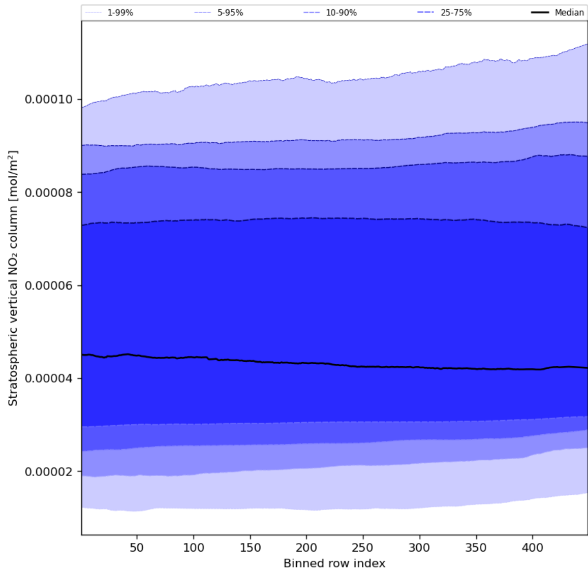
Figure 53: Along track statistics of “Stratospheric vertical NO 2 column” for 2024-01-13 to 2024-01-15
