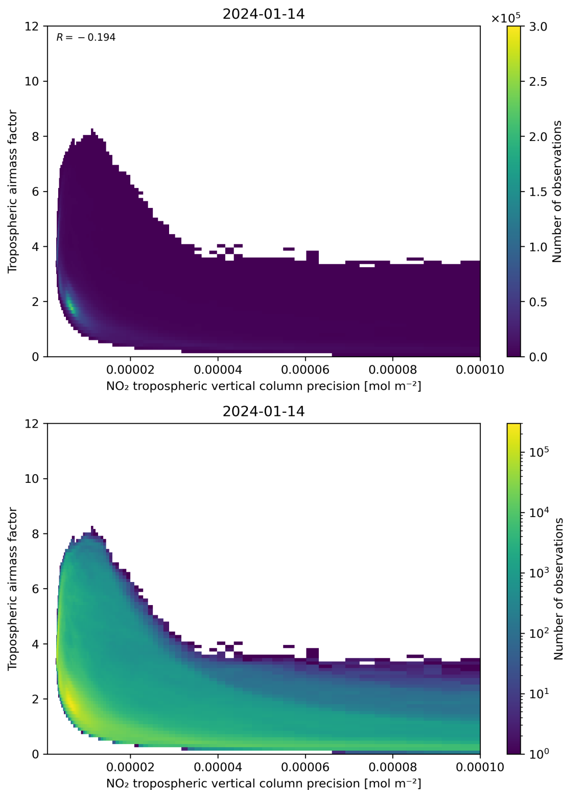
Figure 133: Scatter density plot of “NO 2 tropospheric vertical column precision” against “Tropospheric airmass factor” for 2024-01-13 to 2024-01-15.
