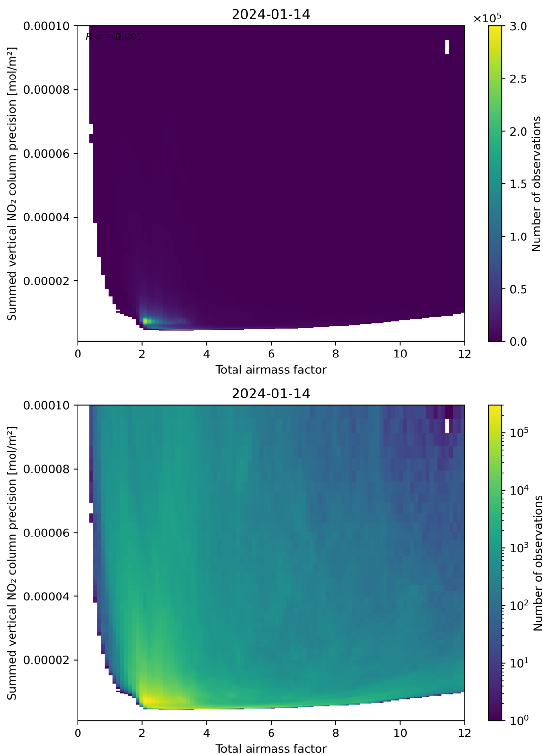
Figure 66: Scatter density plot of “Total airmass factor” against “Summed vertical NO 2 column precision” for 2024-01-13 to 2024-01-15.
