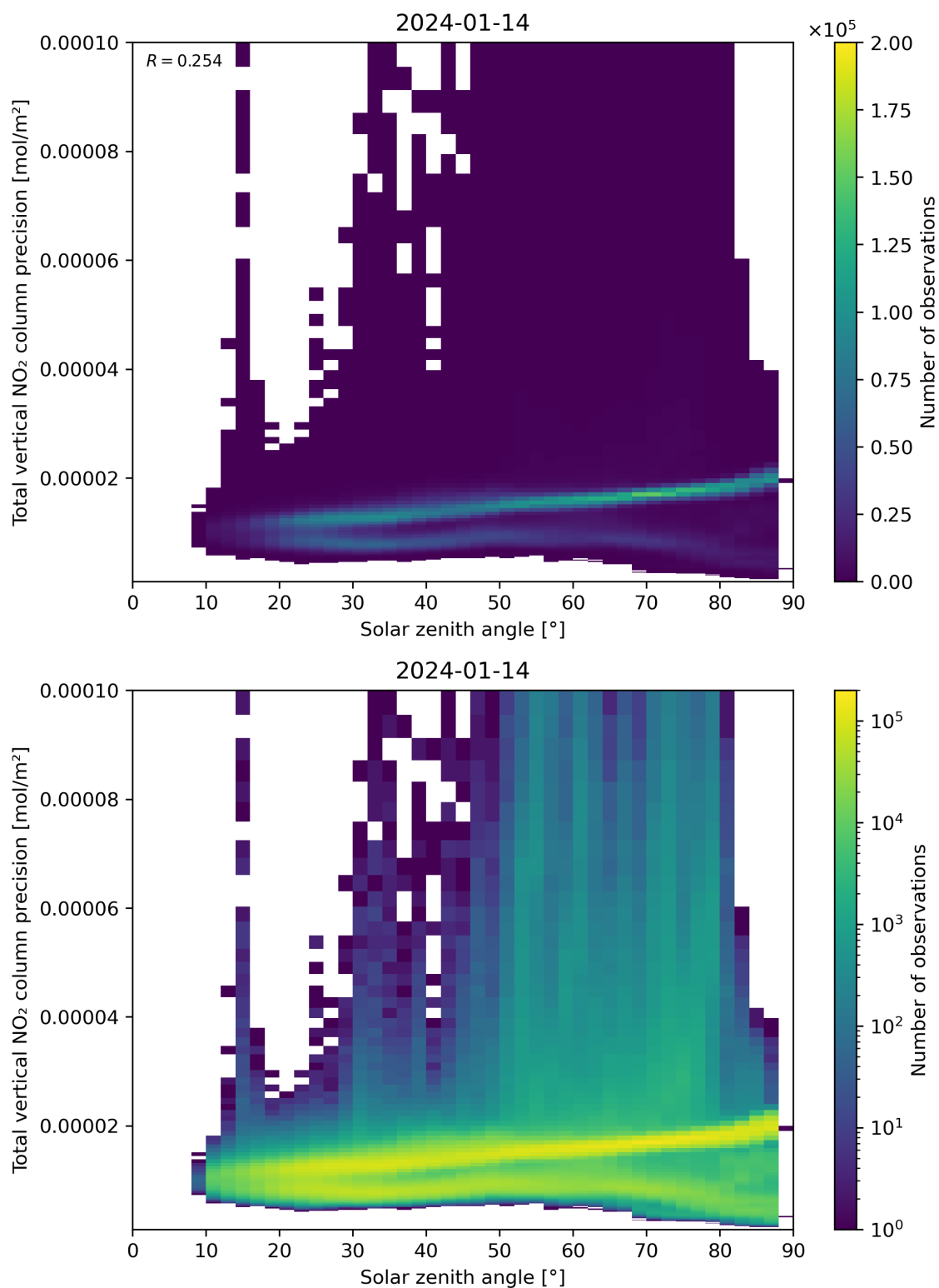
Figure 154: Scatter density plot of “Solar zenith angle” against “Total vertical NO 2 column precision” for 2024-01-13 to 2024-01-15.
