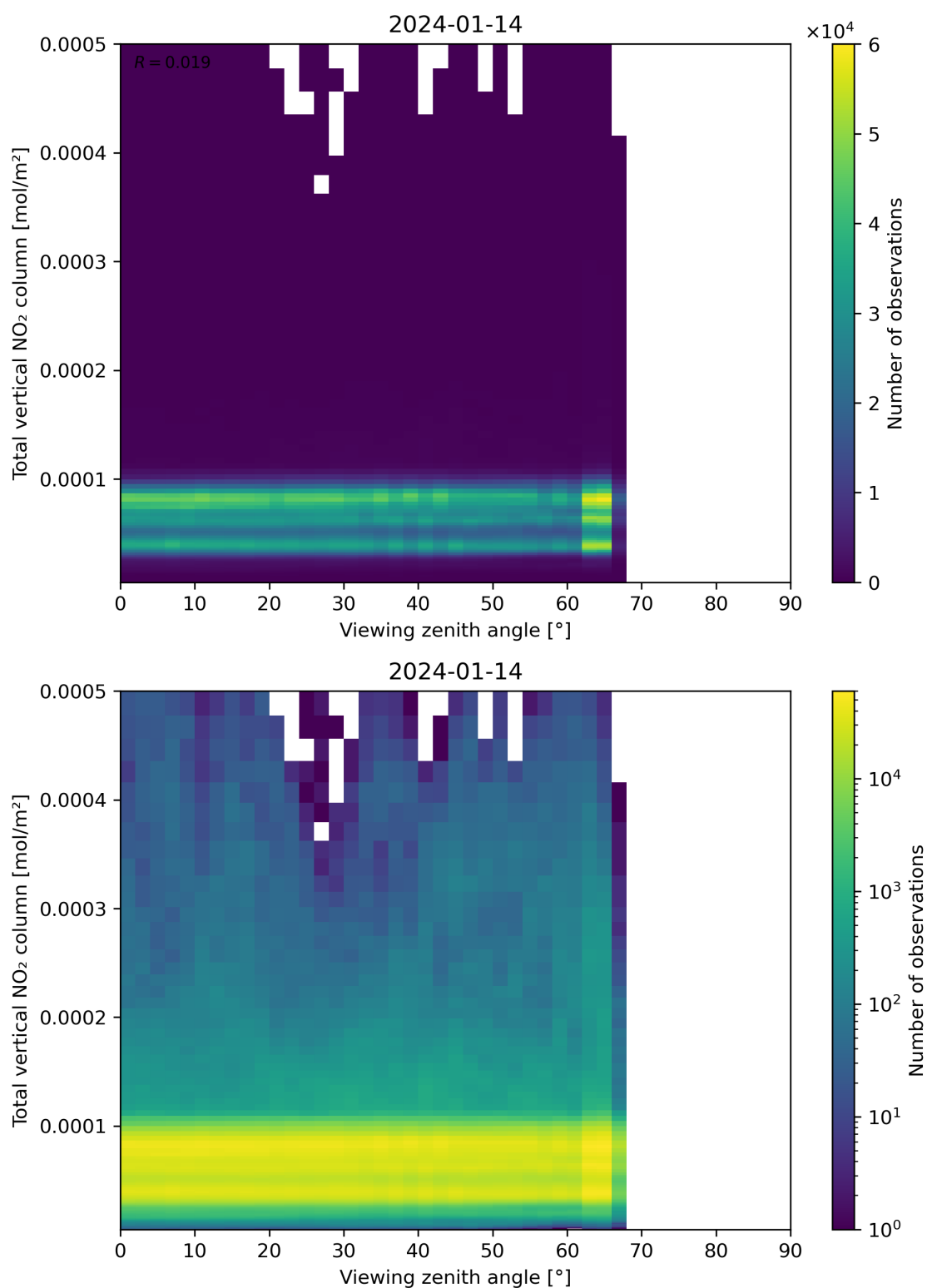
Figure 167: Scatter density plot of “Viewing zenith angle” against “Total vertical NO 2 column” for 2024-01-13 to 2024-01-15.
