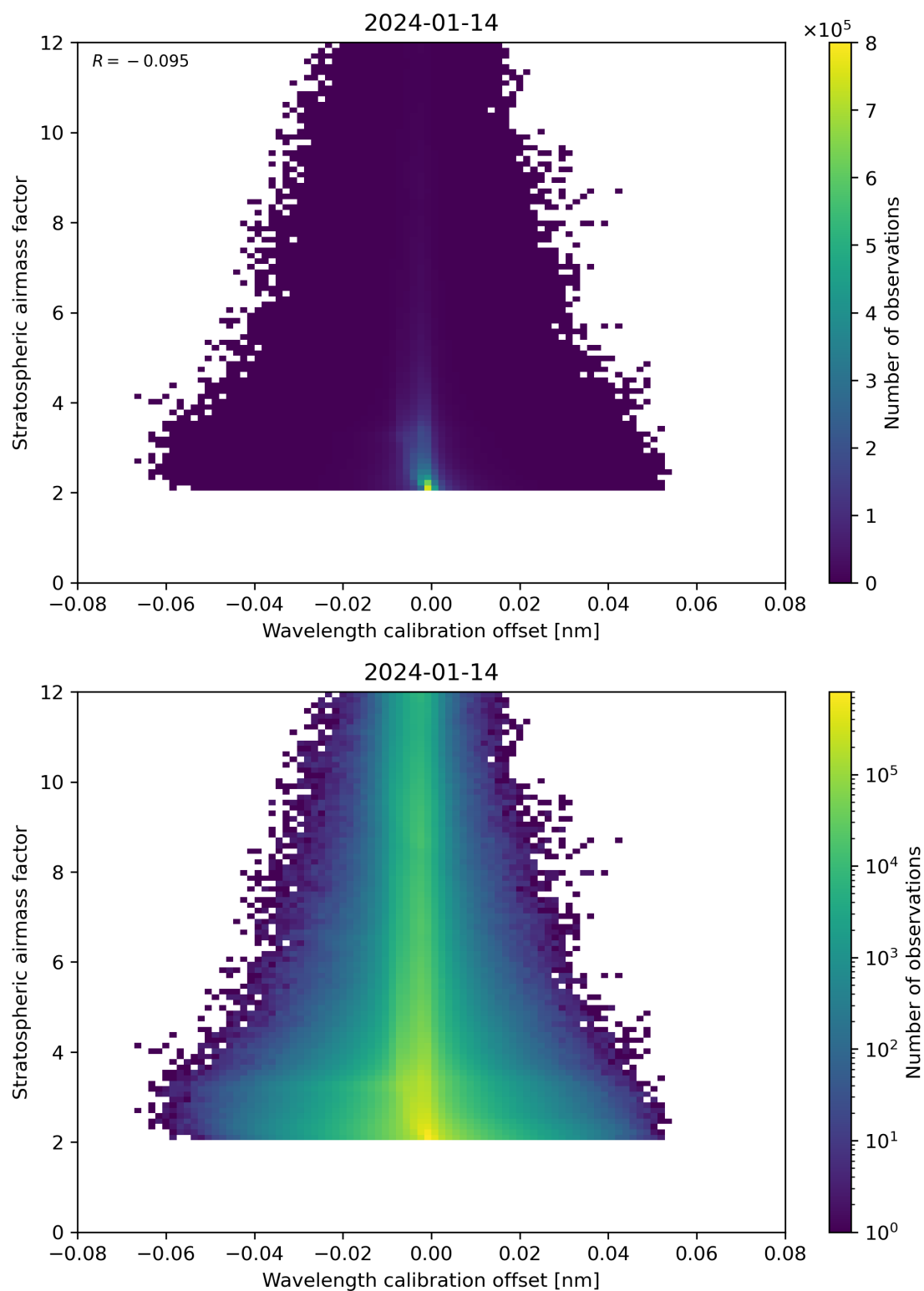
Figure 174: Scatter density plot of “Wavelength calibration offset” against “Stratospheric airmass factor” for 2024-01-13 to 2024-01-15.
