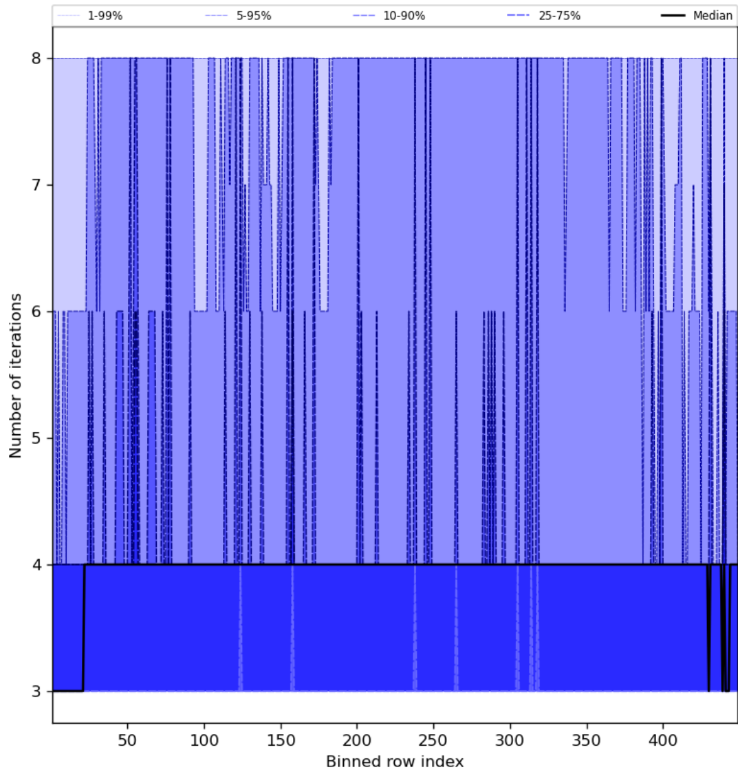
Figure 51: Along track statistics of “Number of iterations” for 2024-01-13 to 2024-01-15
