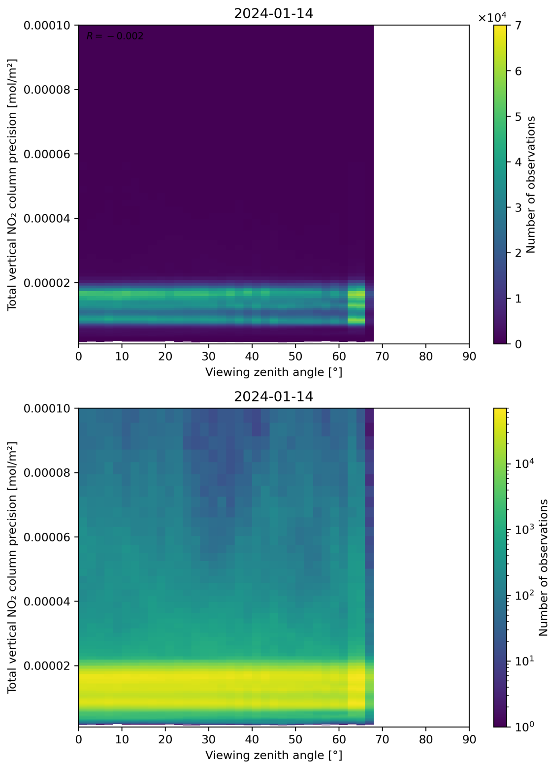
Figure 168: Scatter density plot of “Viewing zenith angle” against “Total vertical NO 2 column precision” for 2024-01-13 to 2024-01-15.
