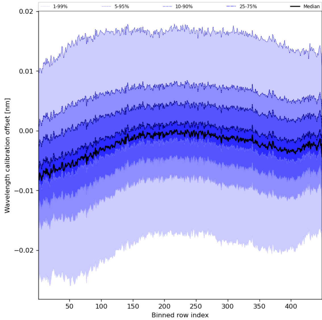
Figure 52: Along track statistics of “Wavelength calibration offset” for 2024-01-13 to 2024-01-15
