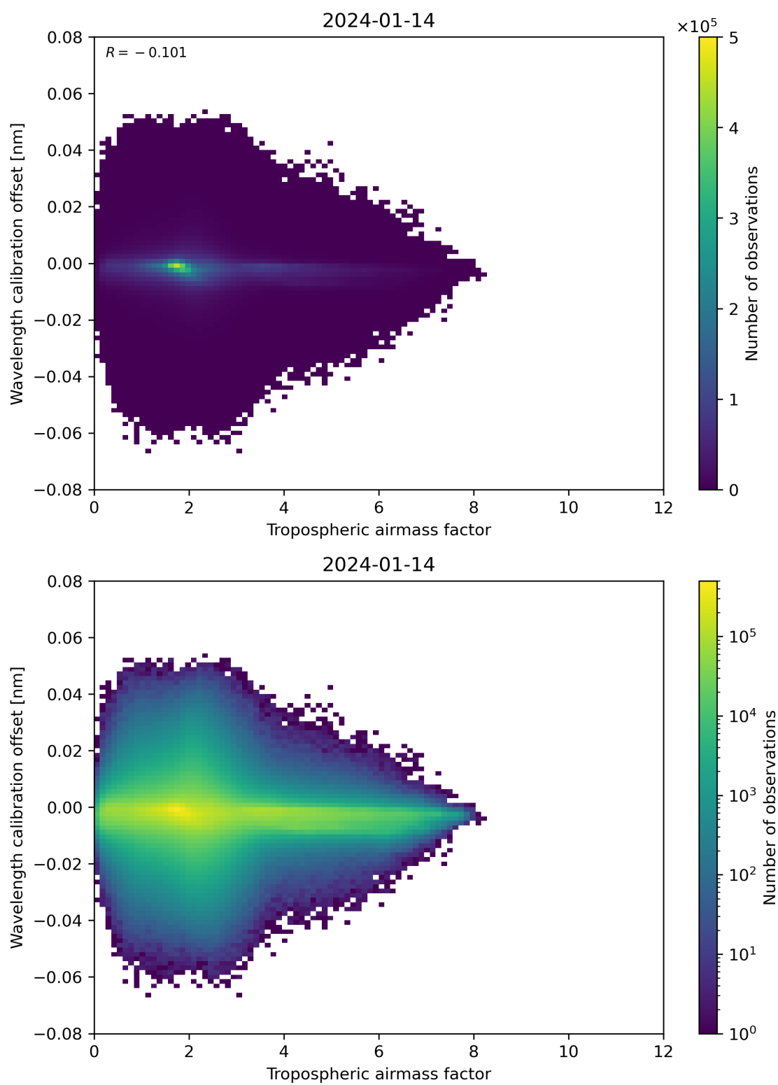
Figure 80: Scatter density plot of “Tropospheric airmass factor” against “Wavelength calibration offset” for 2024-01-13 to 2024-01-15.
