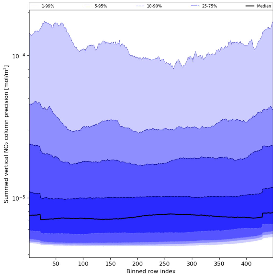
Figure 58: Along track statistics of “Summed vertical NO 2 column precision” for 2024-01-13 to 2024-01-15
