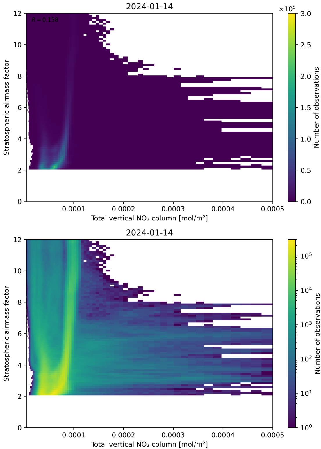
Figure 110: Scatter density plot of “Total vertical NO 2 column” against “Stratospheric air mass factor” for 2024-01-13 to 2024-01-15.
