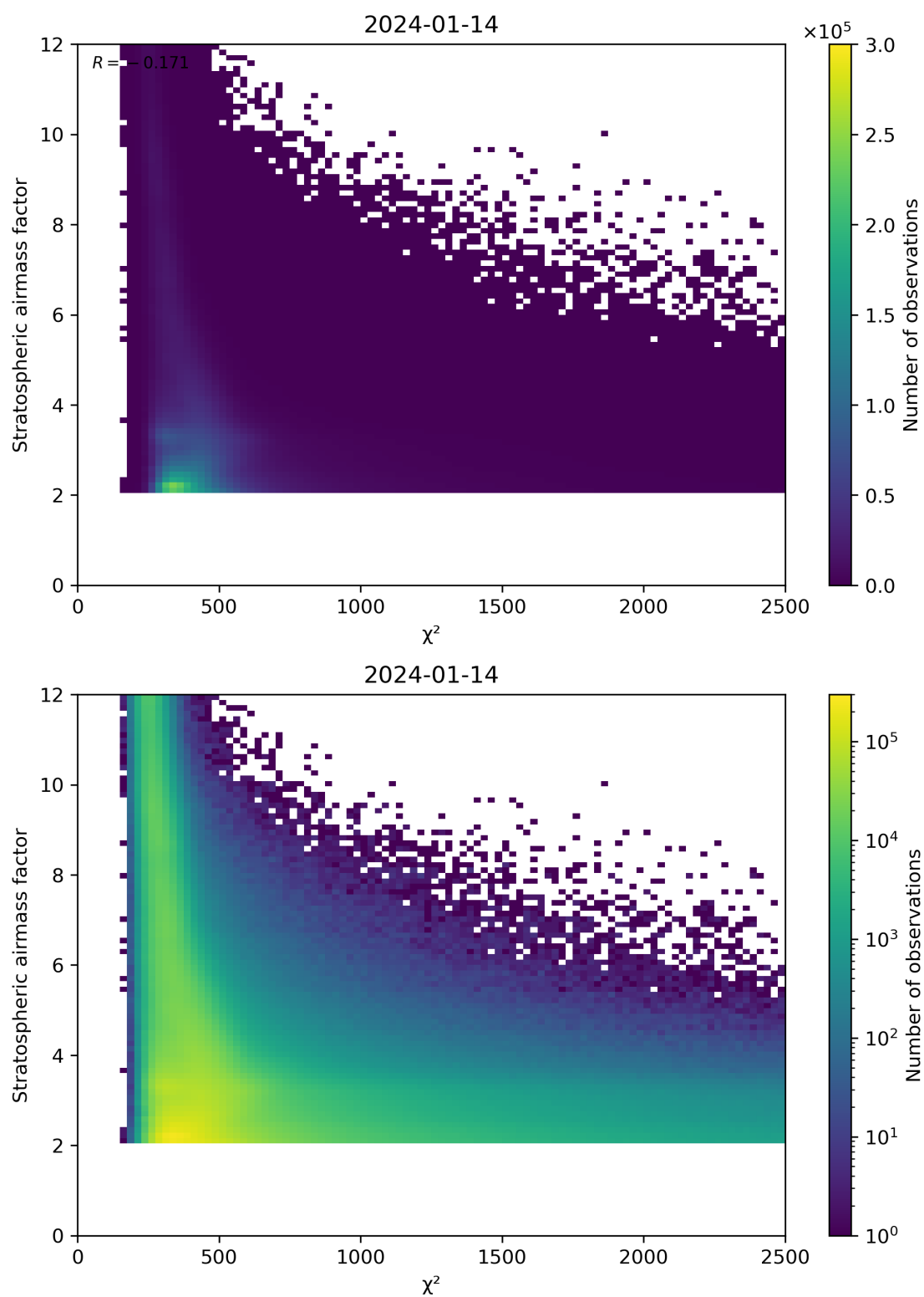
Figure 81: Scatter density plot of “ \chi^2 ” against “Stratospheric airmass factor” for 2024-01-13 to 2024-01-15.
