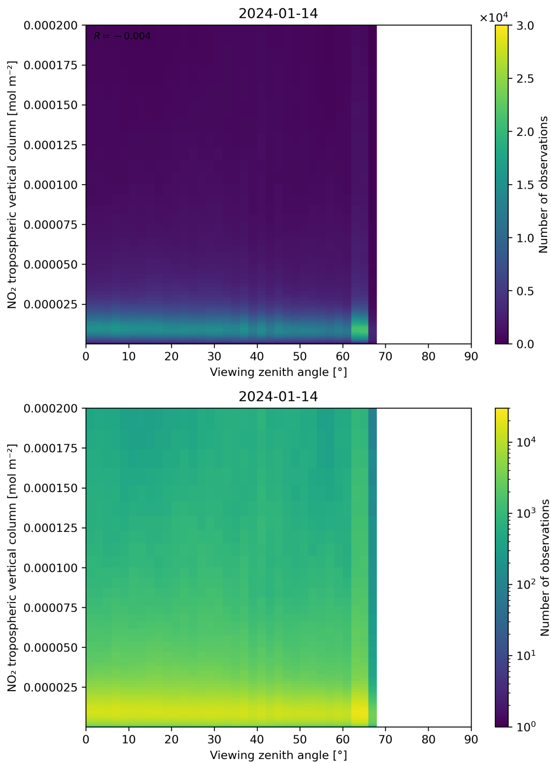
Figure 169: Scatter density plot of “Viewing zenith angle” against “NO 2 tropospheric vertical column” for 2024-01-13 to 2024-01-15.
