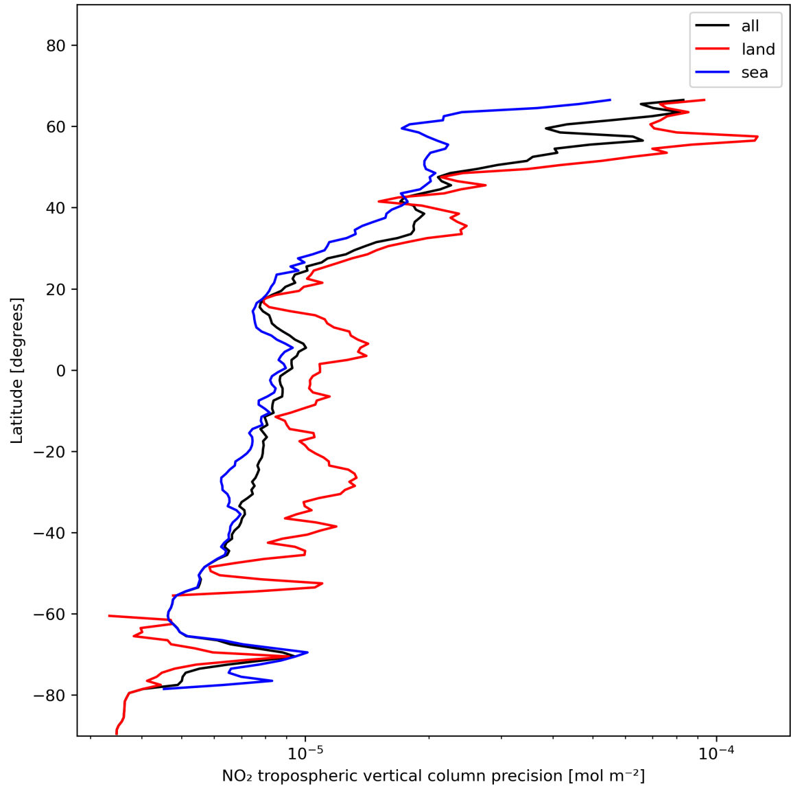
Figure 13: Zonal average of “NO 2 tropospheric vertical column precision” for 2024-01-13 to 2024-01-15.
