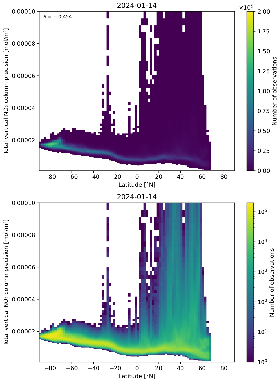
Figure 91: Scatter density plot of “Latitude” against “Total vertical NO 2 column precision” for 2024-01-13 to 2024-01-15.
