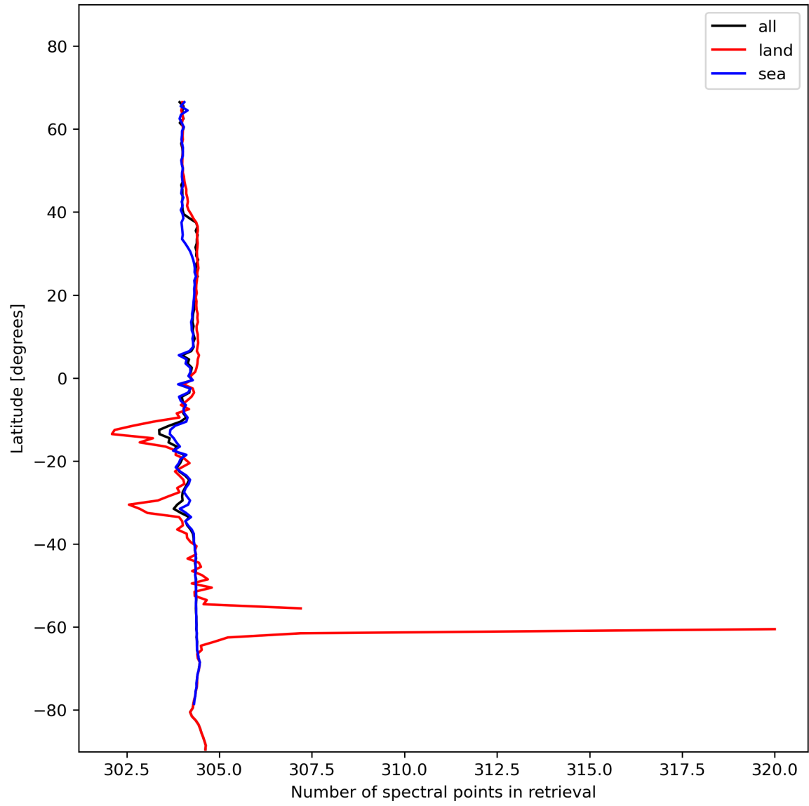
Figure 16: Zonal average of “Number of spectral points in retrieval” for 2024-01-13 to 2024-01-15.
