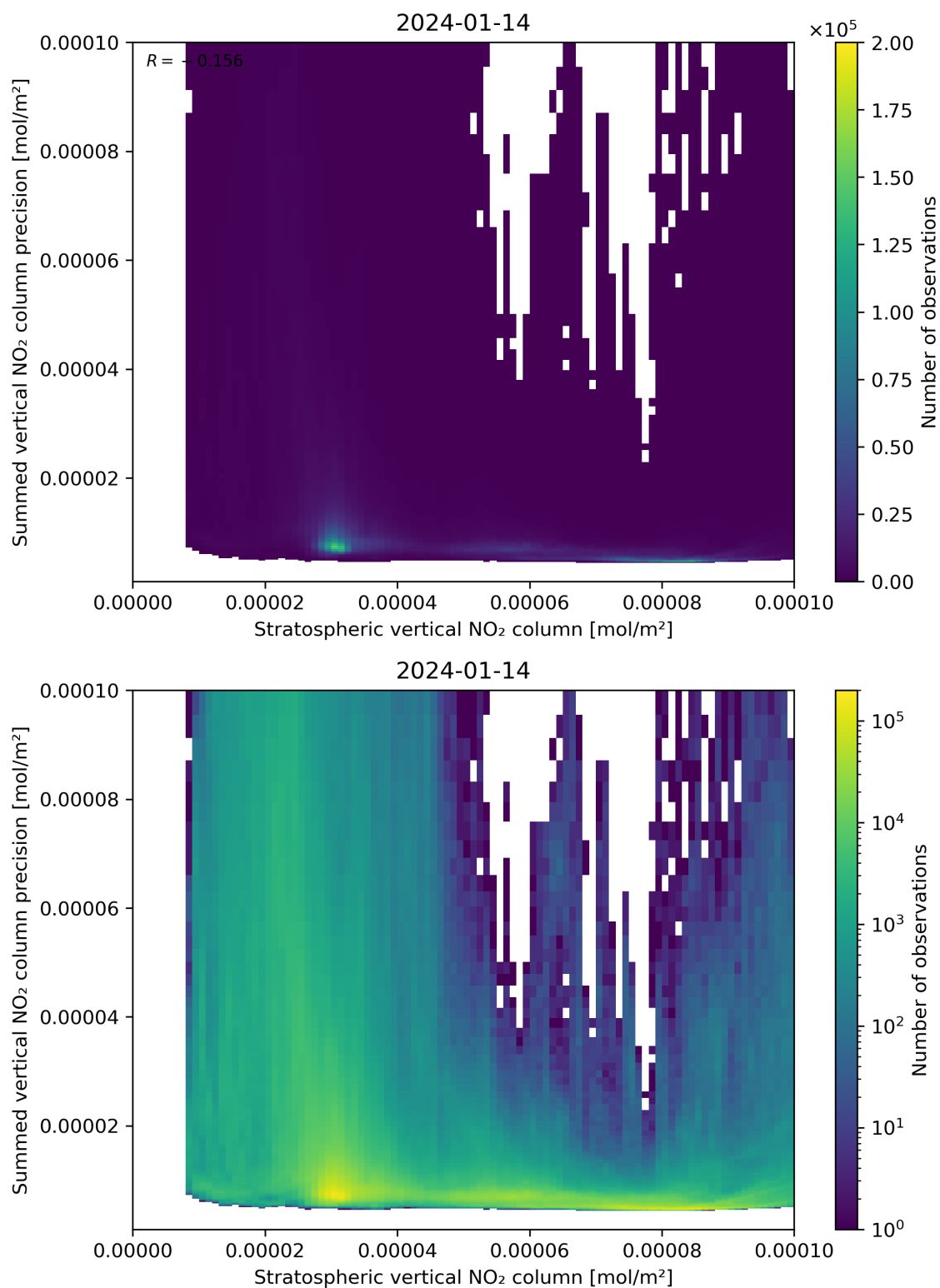
Figure 99: Scatter density plot of “Stratospheric vertical NO 2 column” against “Summed vertical NO 2 column precision” for 2024-01-13 to 2024-01-15.
