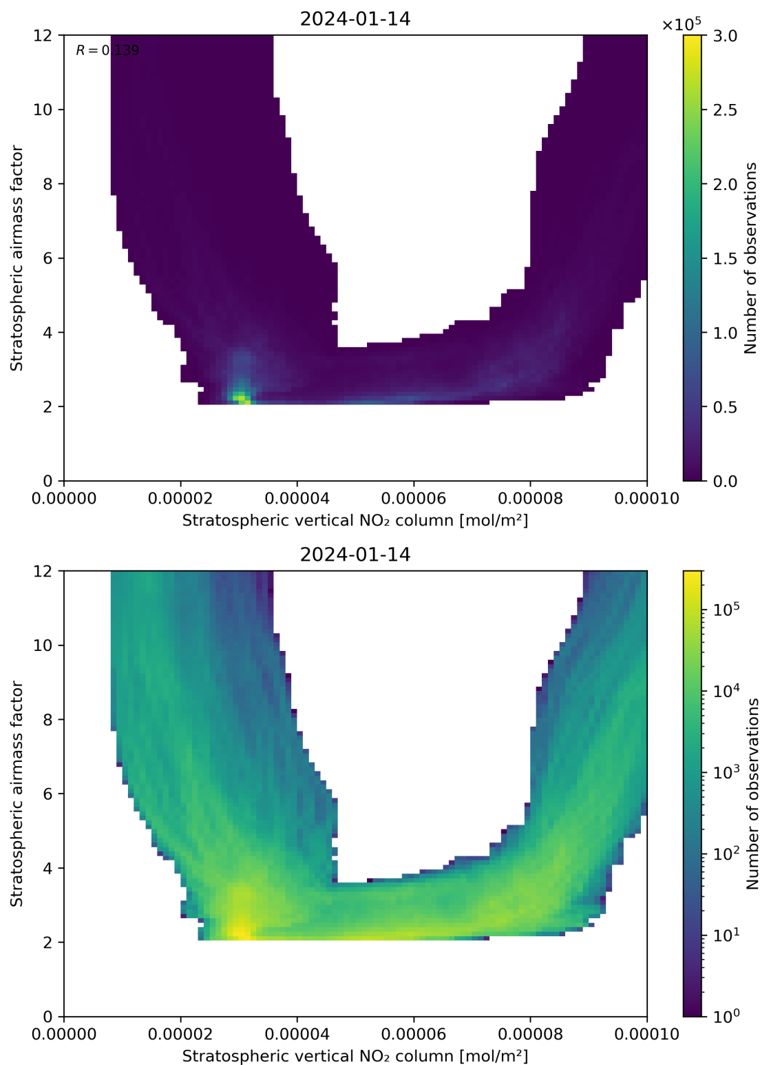
Figure 96: Scatter density plot of “Stratospheric vertical NO 2 column” against “Stratospheric airmass factor” for 2024-01-13 to 2024-01-15.
