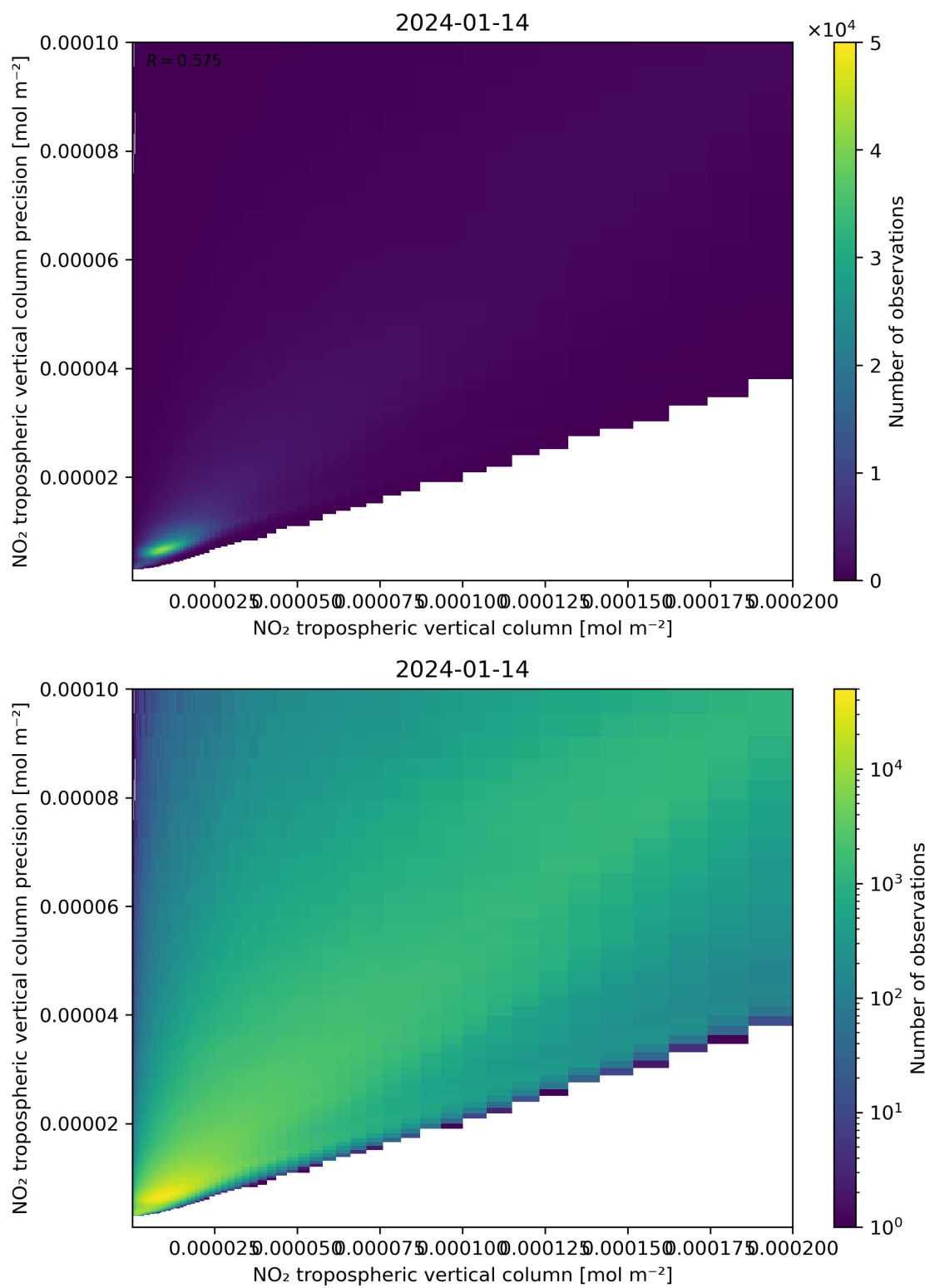
Figure 130: Scatter density plot of “NO 2 tropospheric vertical column” against “NO 2 tropospheric vertical column precision” for 2024-01-13 to 2024-01-15.
