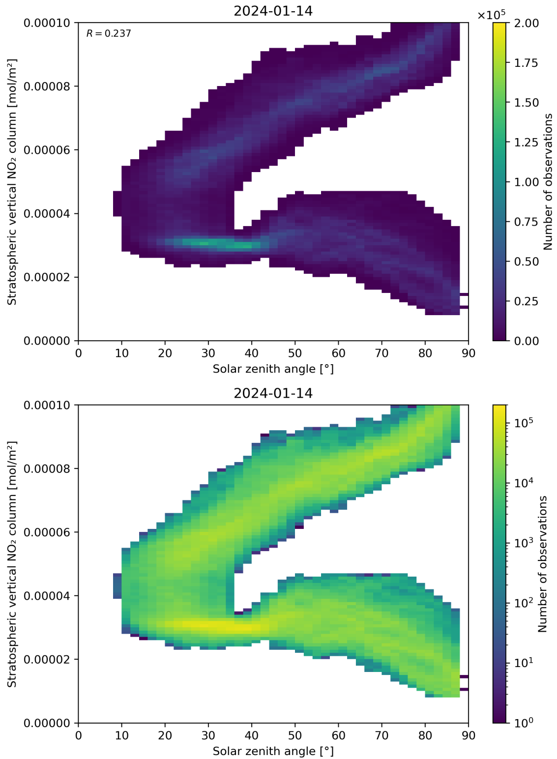
Figure 150: Scatter density plot of “Solar zenith angle” against “Stratospheric vertical NO 2 column” for 2024-01-13 to 2024-01-15.
