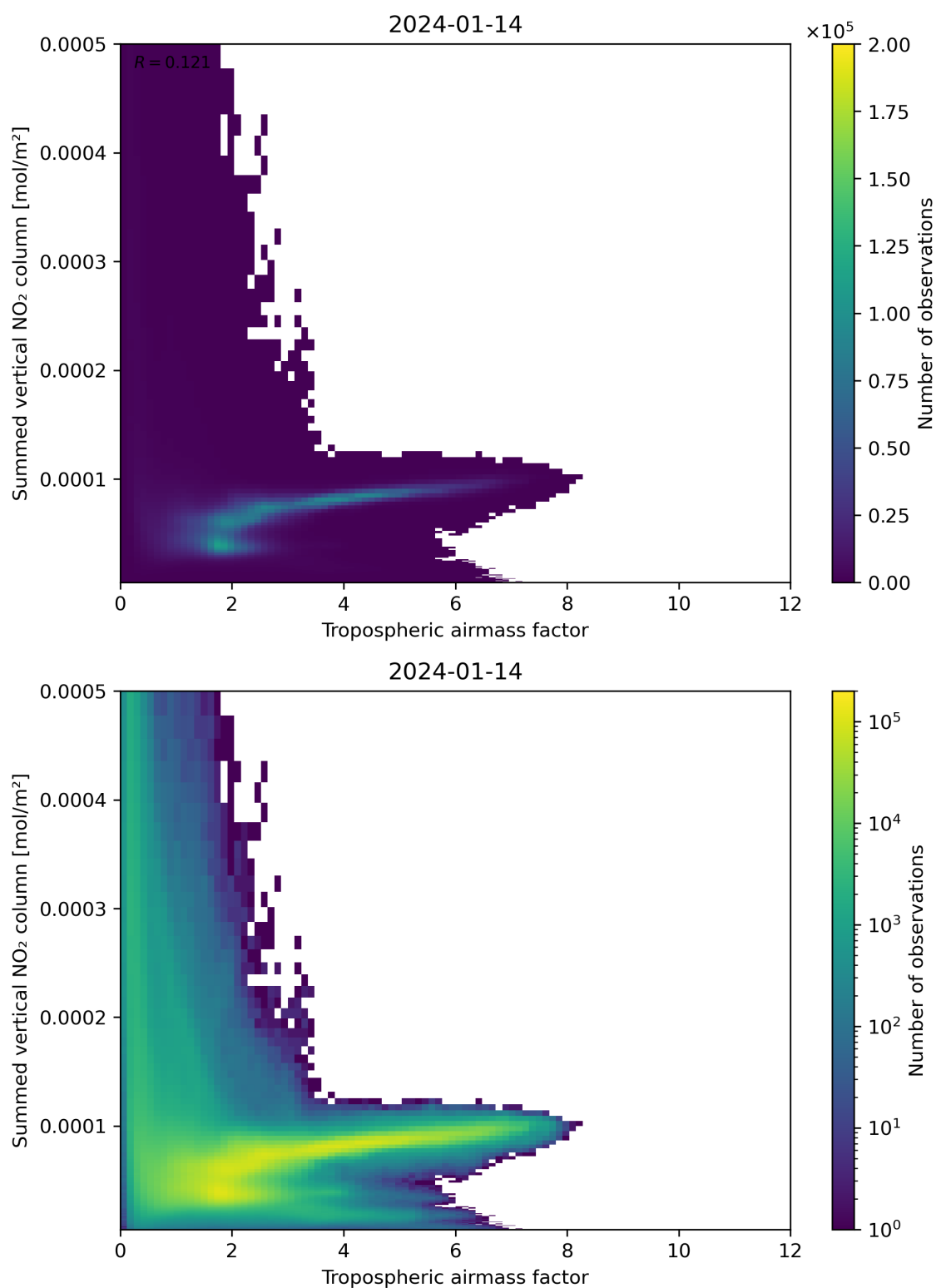
Figure 75: Scatter density plot of “Tropospheric airmass factor” against “Summed vertical NO 2 column” for 2024-01-13 to 2024-01-15.
