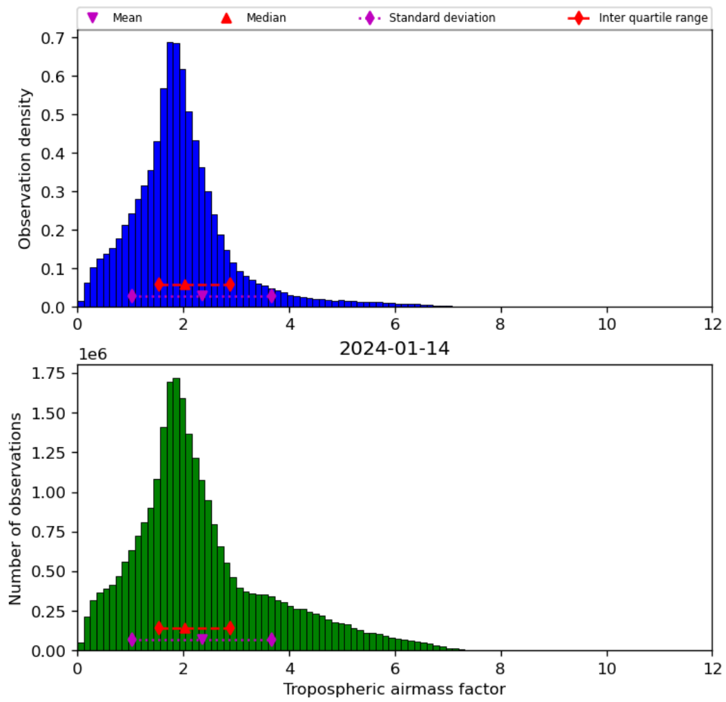
Figure 31: Histogram of “Tropospheric airmass factor” for 2024-01-13 to 2024-01-15
