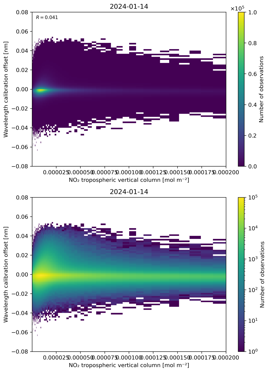
Figure 143: Scatter density plot of “NO 2 tropospheric vertical column” against “Wavelength calibration offset” for 2024-01-13 to 2024-01-15.
