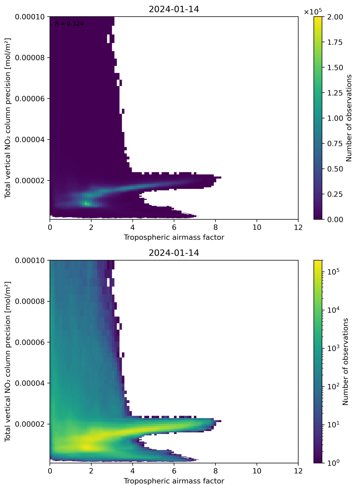
Figure 78: Scatter density plot of “Tropospheric air mass factor” against “Total vertical NO 2 column precision” for 2024-01-13 to 2024-01-15.
