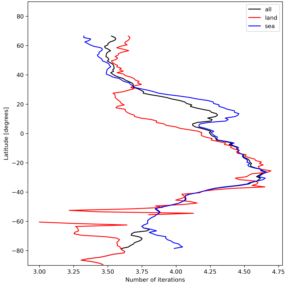
Figure 17: Zonal average of “Number of iterations” for 2024-01-13 to 2024-01-15.
