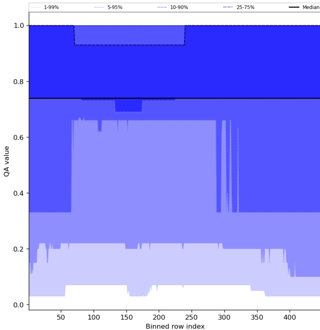
Figure 45: Along track statistics of “QA value” for 2024-01-13 to 2024-01-15
