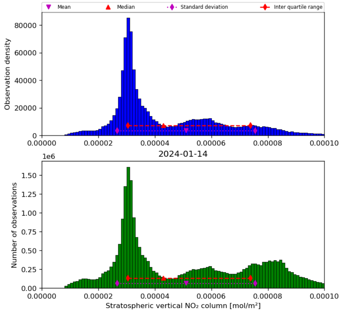
Figure 36: Histogram of “Stratospheric vertical NO 2 column” for 2024-01-13 to 2024-01-15
