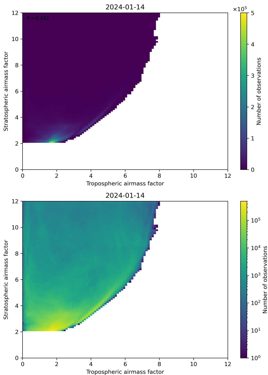
Figure 71: Scatter density plot of “Tropospheric airmass factor” against “Stratospheric airmass factor” for 2024-01-13 to 2024-01-15.
