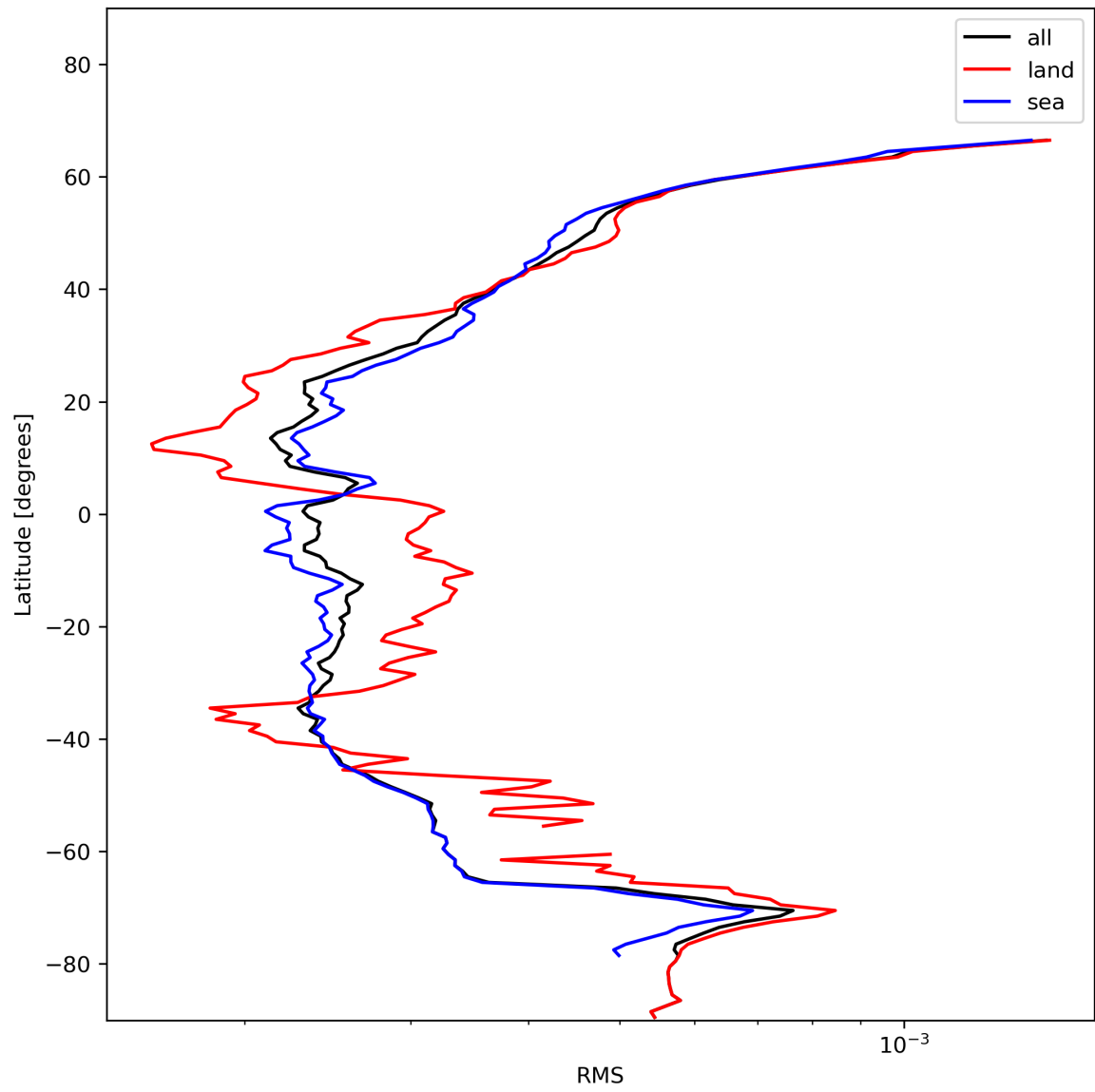
Figure 26: Zonal average of “RMS” for 2024-01-13 to 2024-01-15.
