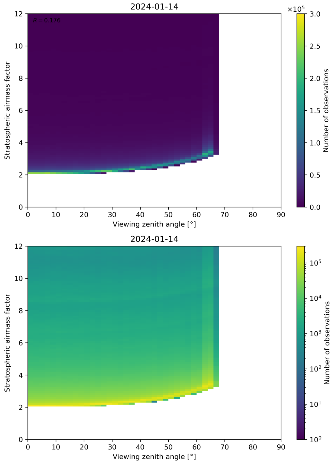
Figure 159: Scatter density plot of “Viewing zenith angle” against “Stratospheric airmass factor” for 2024-01-13 to 2024-01-15.
