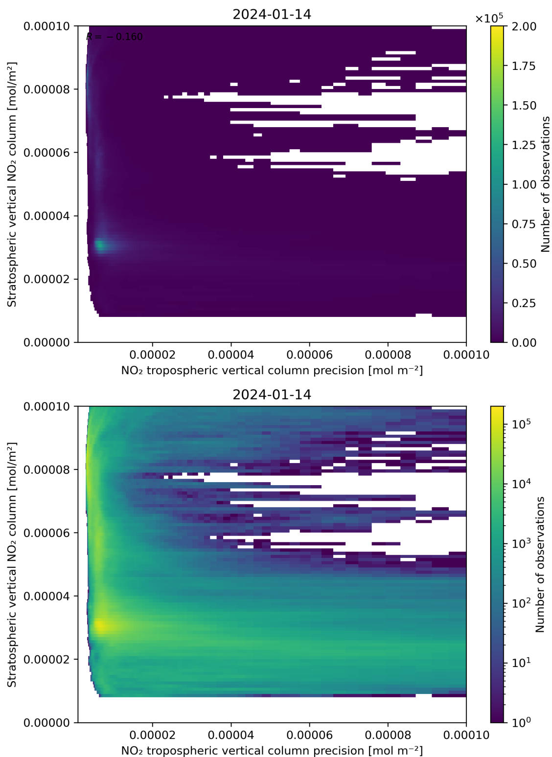
Figure 135: Scatter density plot of “NO 2 tropospheric vertical column precision” against “Stratospheric vertical NO 2 column” for 2024-01-13 to 2024-01-15.
