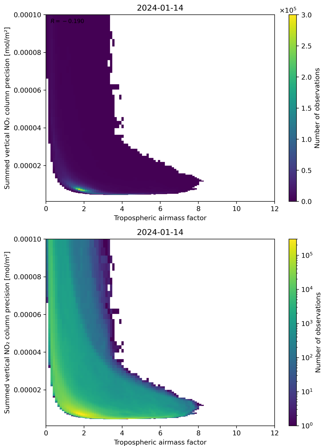
Figure 76: Scatter density plot of “Tropospheric air mass factor” against “Summed vertical NO 2 column precision” for 2024-01-13 to 2024-01-15.
