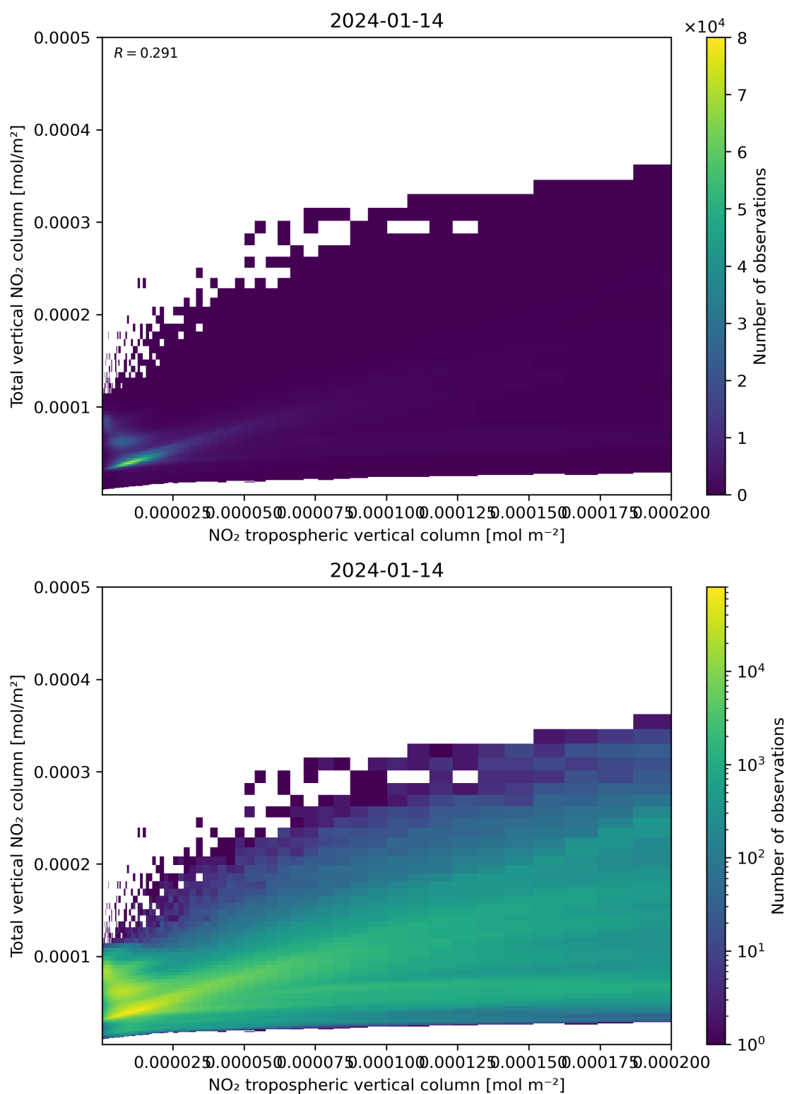
Figure 128: Scatter density plot of “NO 2 tropospheric vertical column” against “Total vertical NO 2 column” for 2024-01-13 to 2024-01-15.
