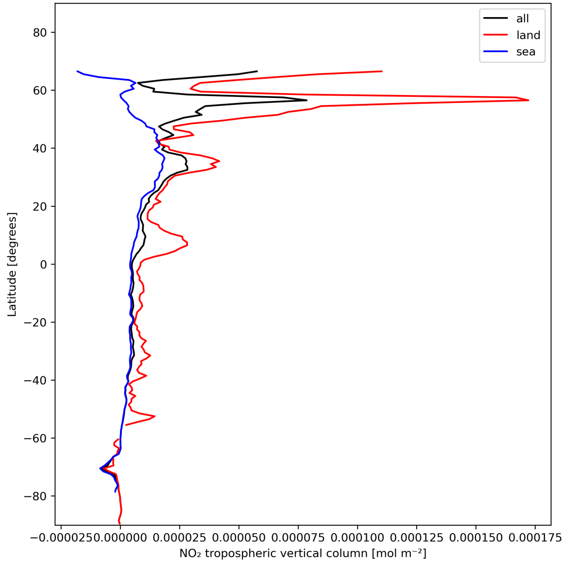
Figure 12: Zonal average of “NO 2 tropospheric vertical column” for 2024-01-13 to 2024-01-15.
