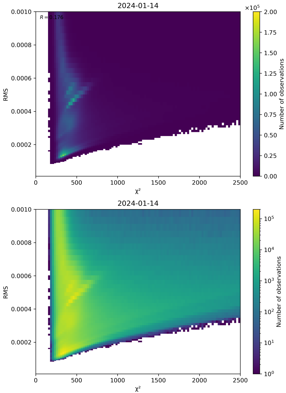
Figure 82: Scatter density plot of “ \chi^2 ” against “RMS” for 2024-01-13 to 2024-01-15.
