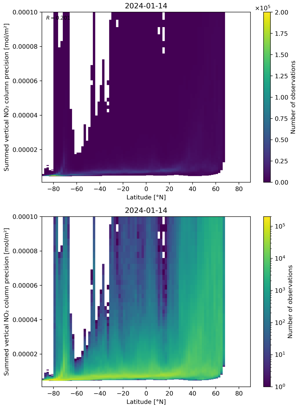
Figure 89: Scatter density plot of “Latitude” against “Summed vertical NO 2 column precision” for 2024-01-13 to 2024-01-15.
