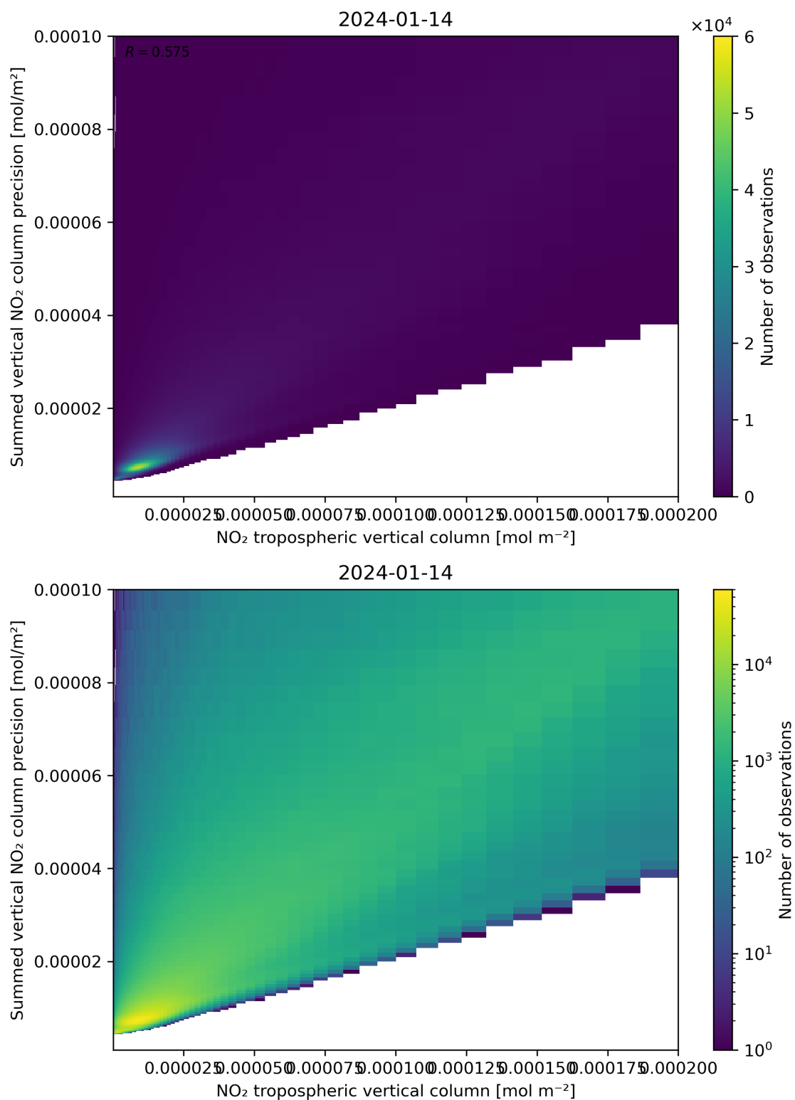
Figure 127: Scatter density plot of “NO 2 tropospheric vertical column” against “Summed vertical NO 2 column precision” for 2024-01-13 to 2024-01-15.
