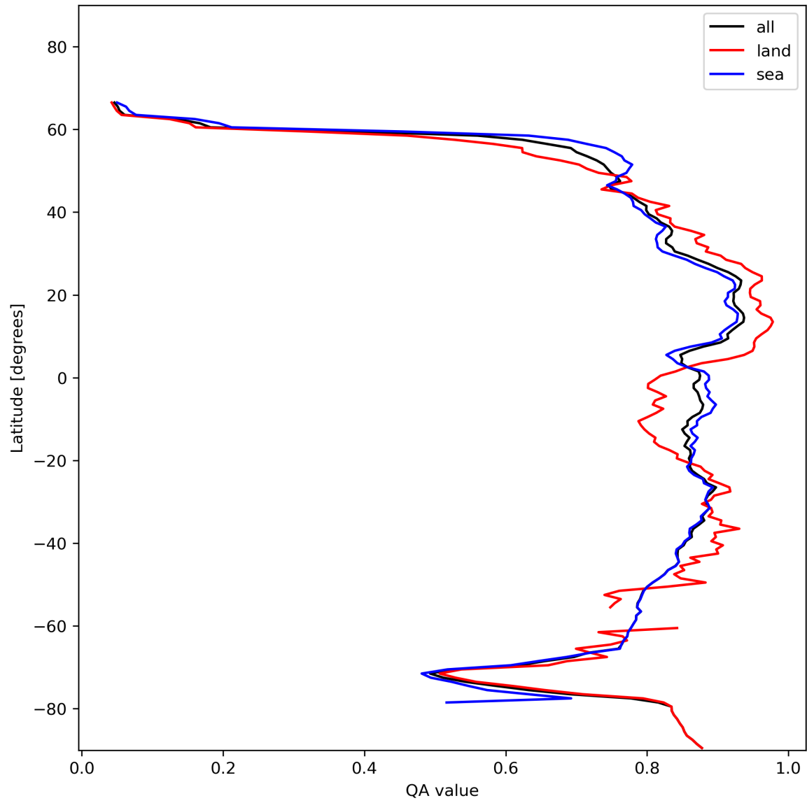
Figure 11: Zonal average of “QA value” for 2024-01-13 to 2024-01-15.
