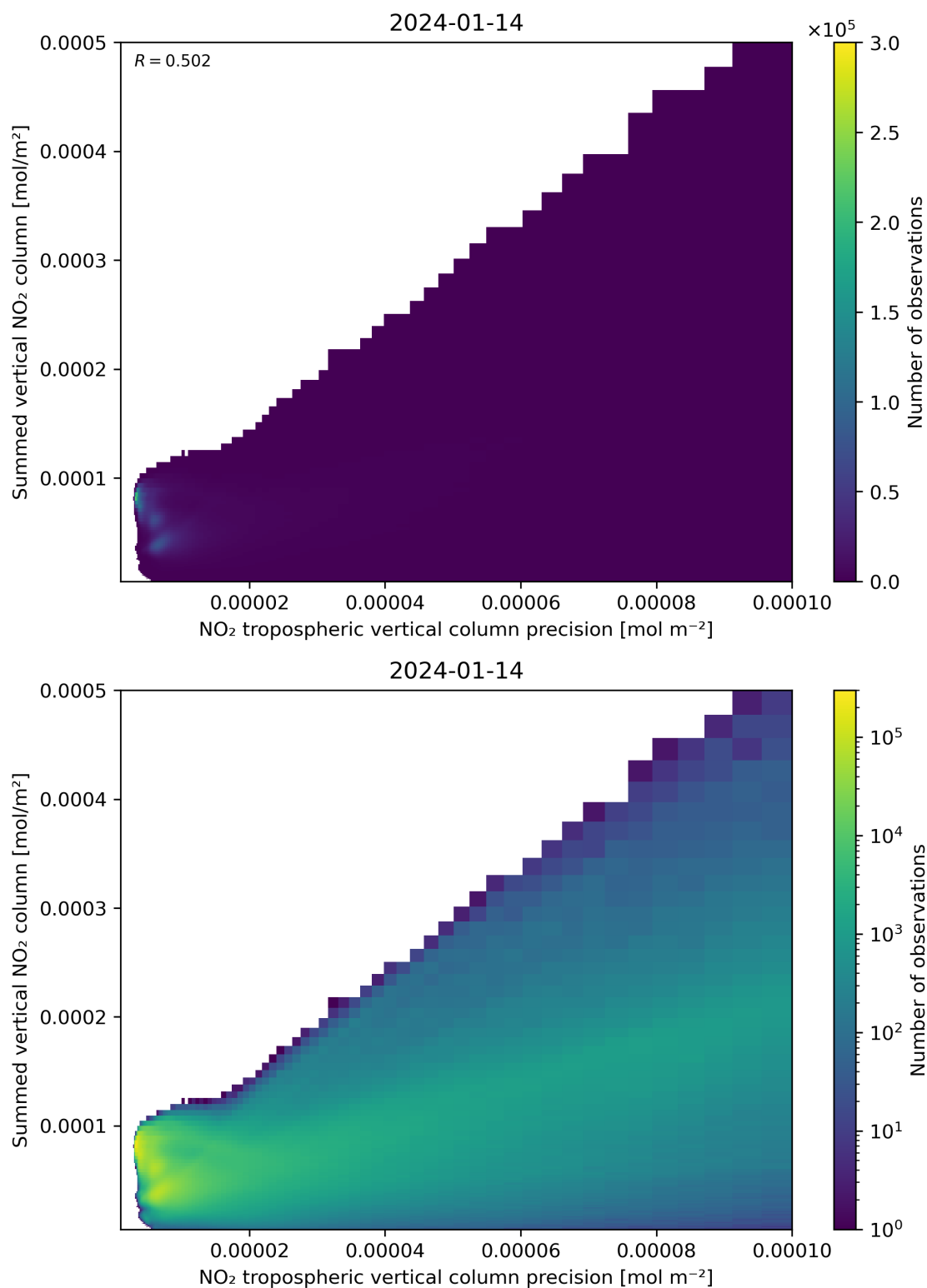
Figure 136: Scatter density plot of “NO 2 tropospheric vertical column precision” against “Summed vertical NO 2 column” for 2024-01-13 to 2024-01-15.
