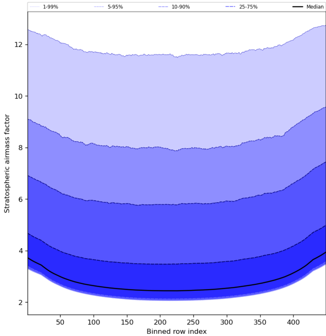
Figure 61: Along track statistics of “Stratospheric airmass factor” for 2024-01-13 to 2024-01-15
