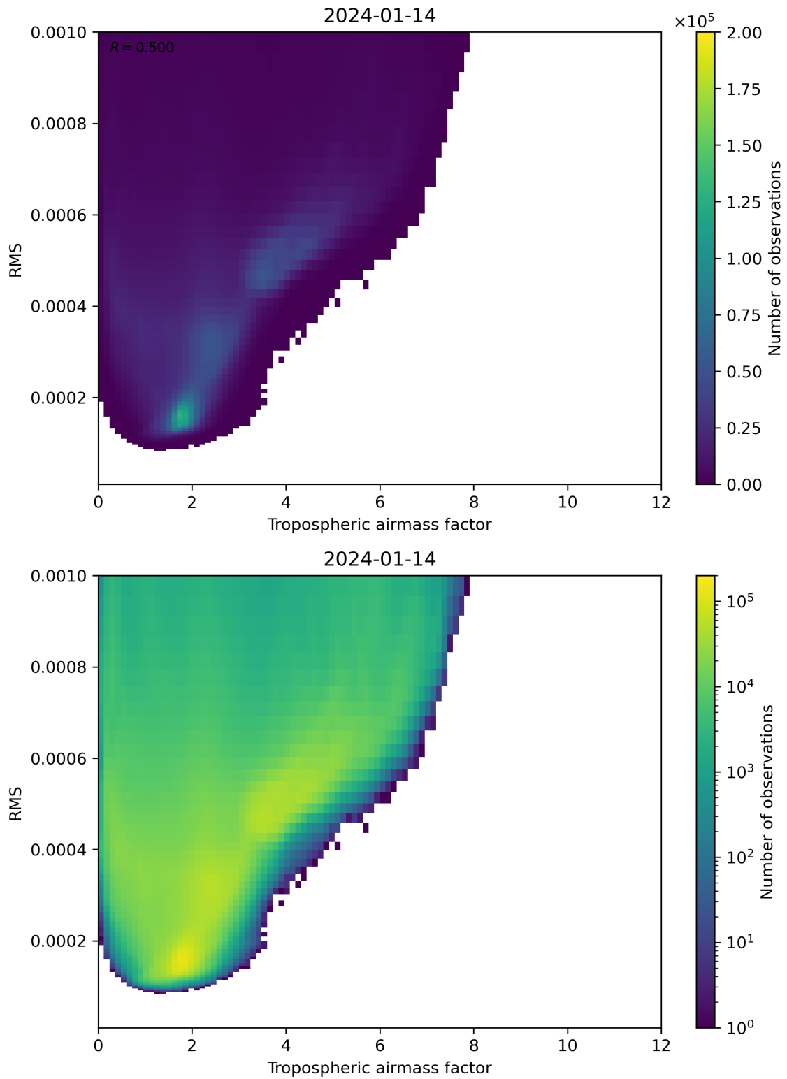
Figure 79: Scatter density plot of “Tropospheric airmass factor” against “RMS” for 2024-01-13 to 2024-01-15.
