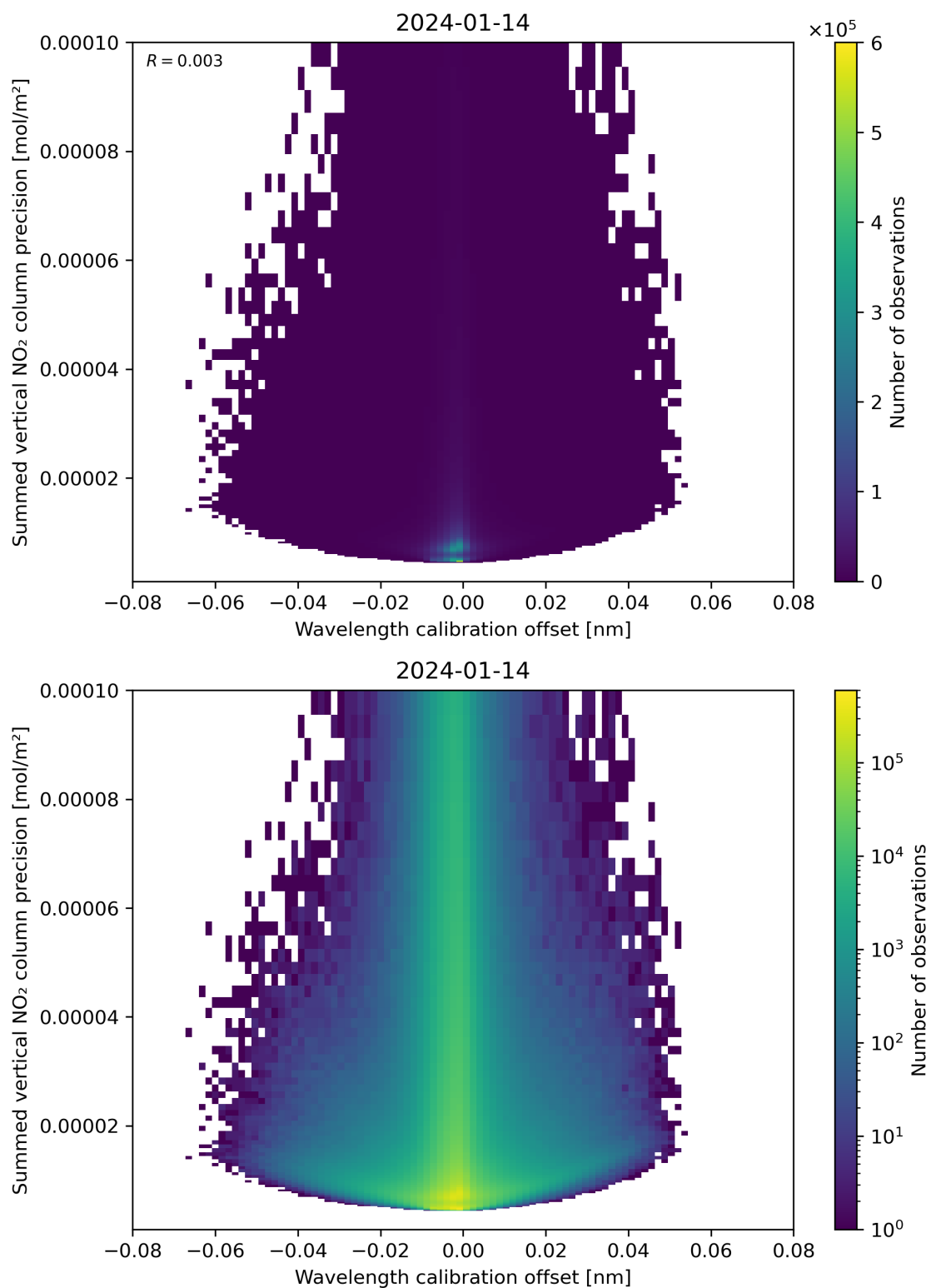
Figure 178: Scatter density plot of “Wavelength calibration offset” against “Summed vertical NO 2 column precision” for 2024-01-13 to 2024-01-15.
