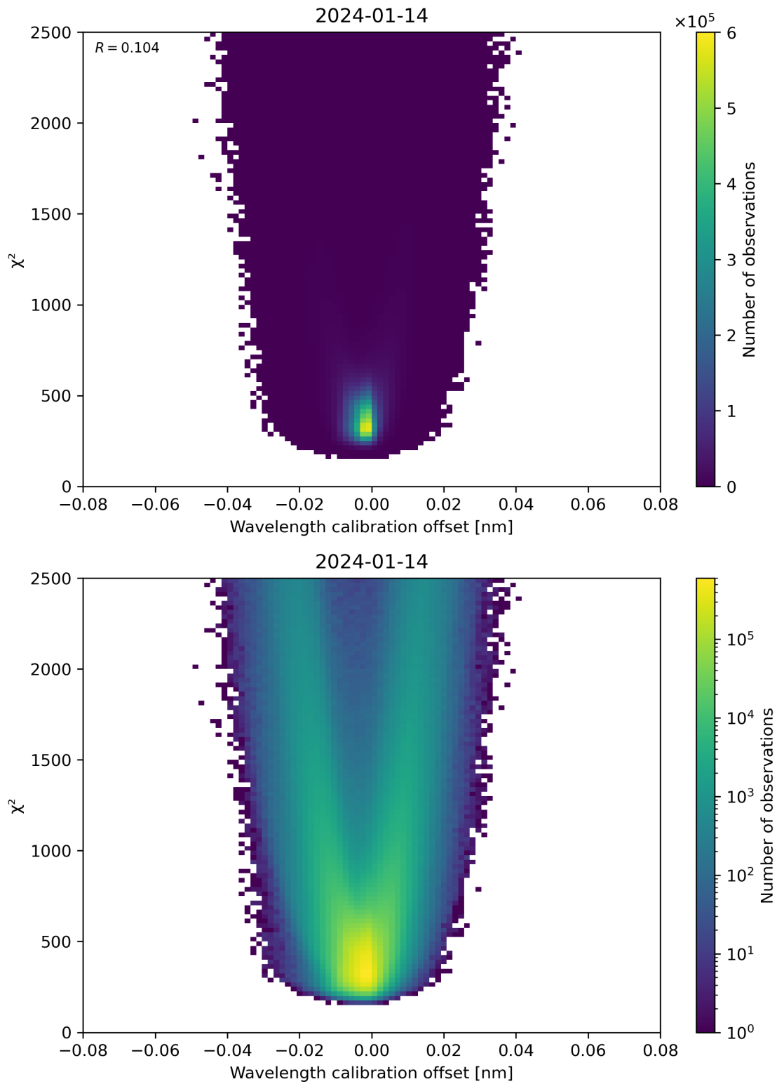
Figure 175: Scatter density plot of “Wavelength calibration offset” against “ \chi^2 ” for 2024-01-13 to 2024-01-15.
