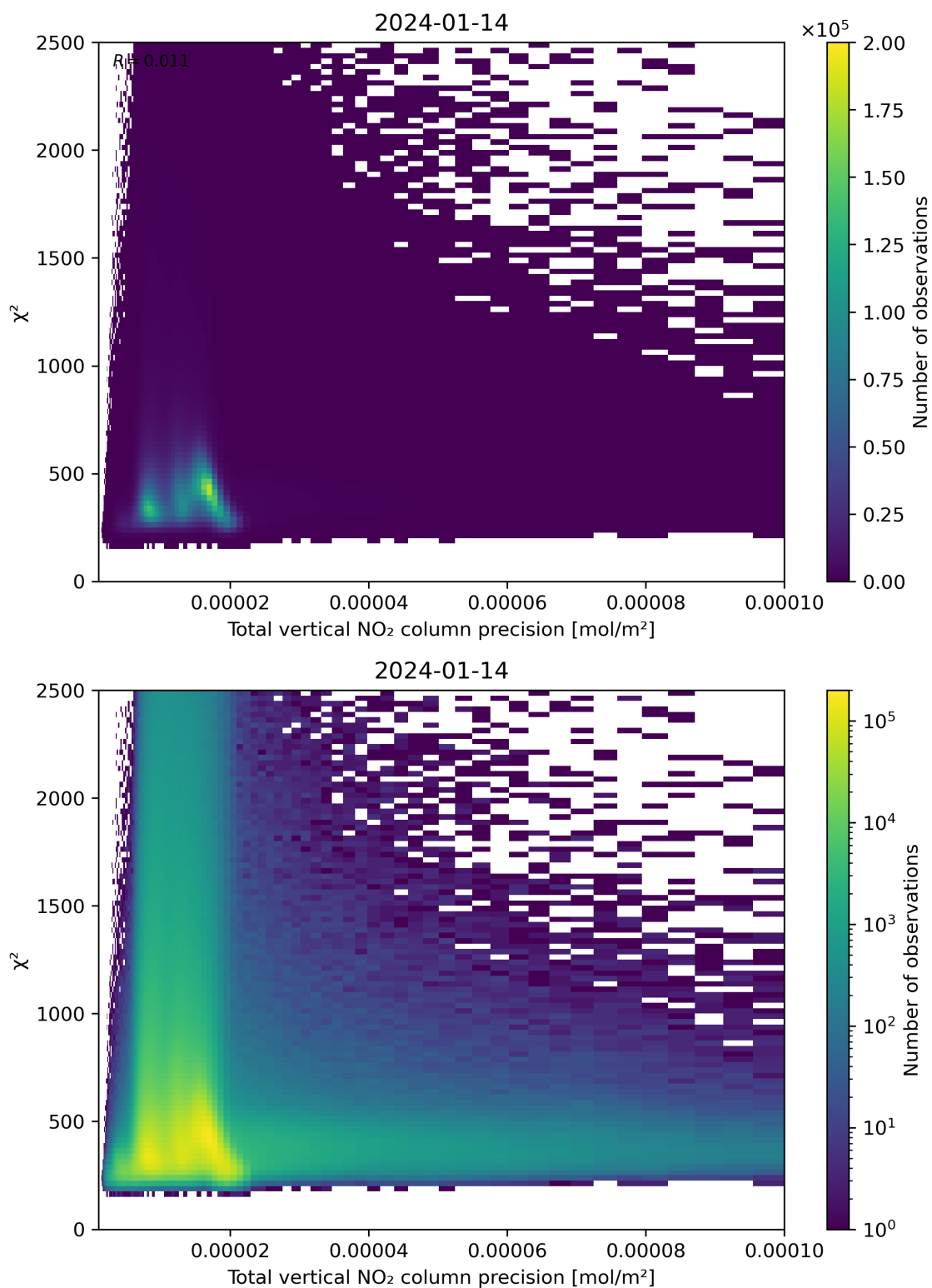
Figure 116: Scatter density plot of “Total vertical NO 2 column precision” against “ \chi^2 ” for 2024-01-13 to 2024-01-15.
