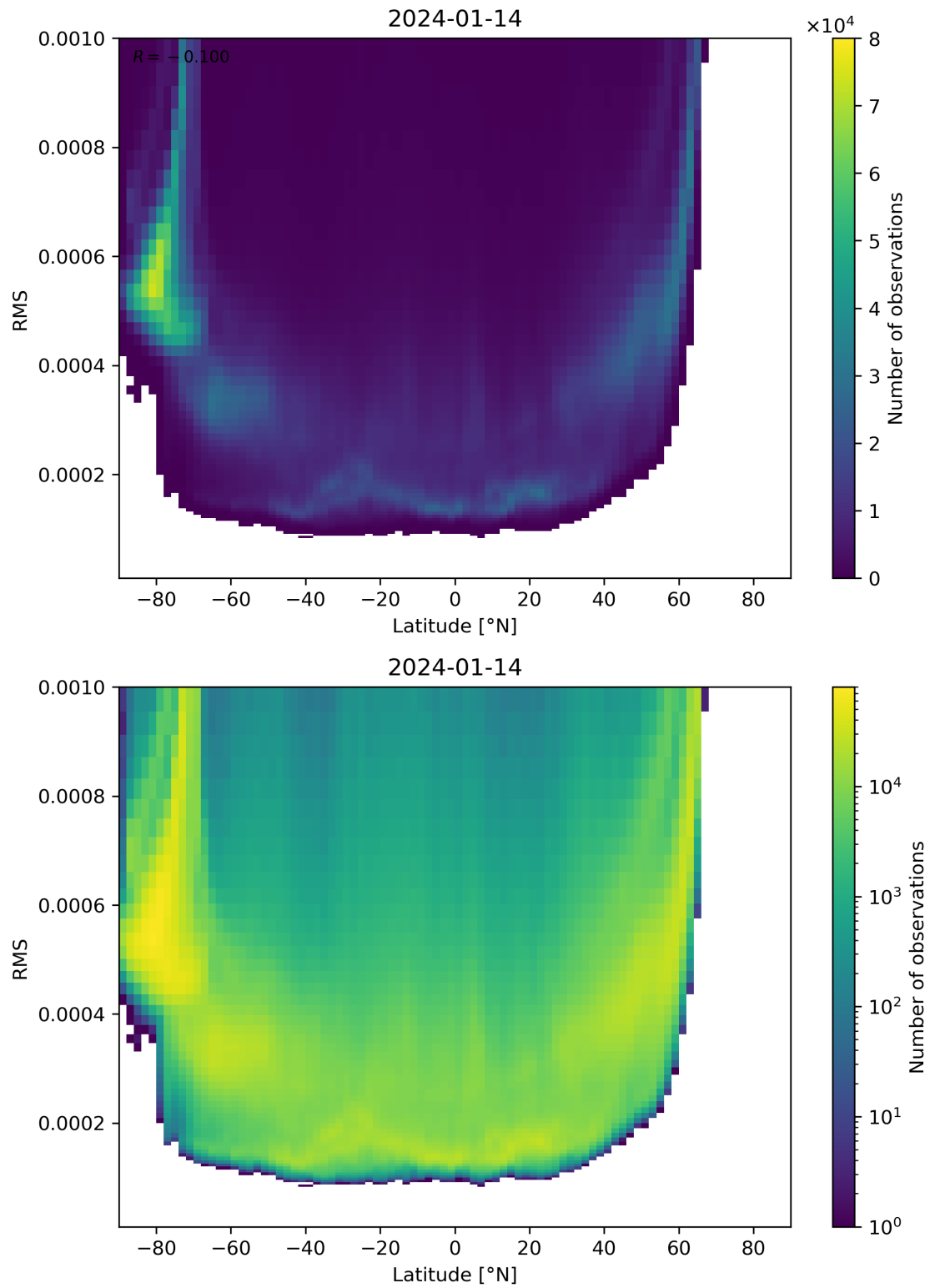
Figure 94: Scatter density plot of “Latitude” against “RMS” for 2024-01-13 to 2024-01-15.
