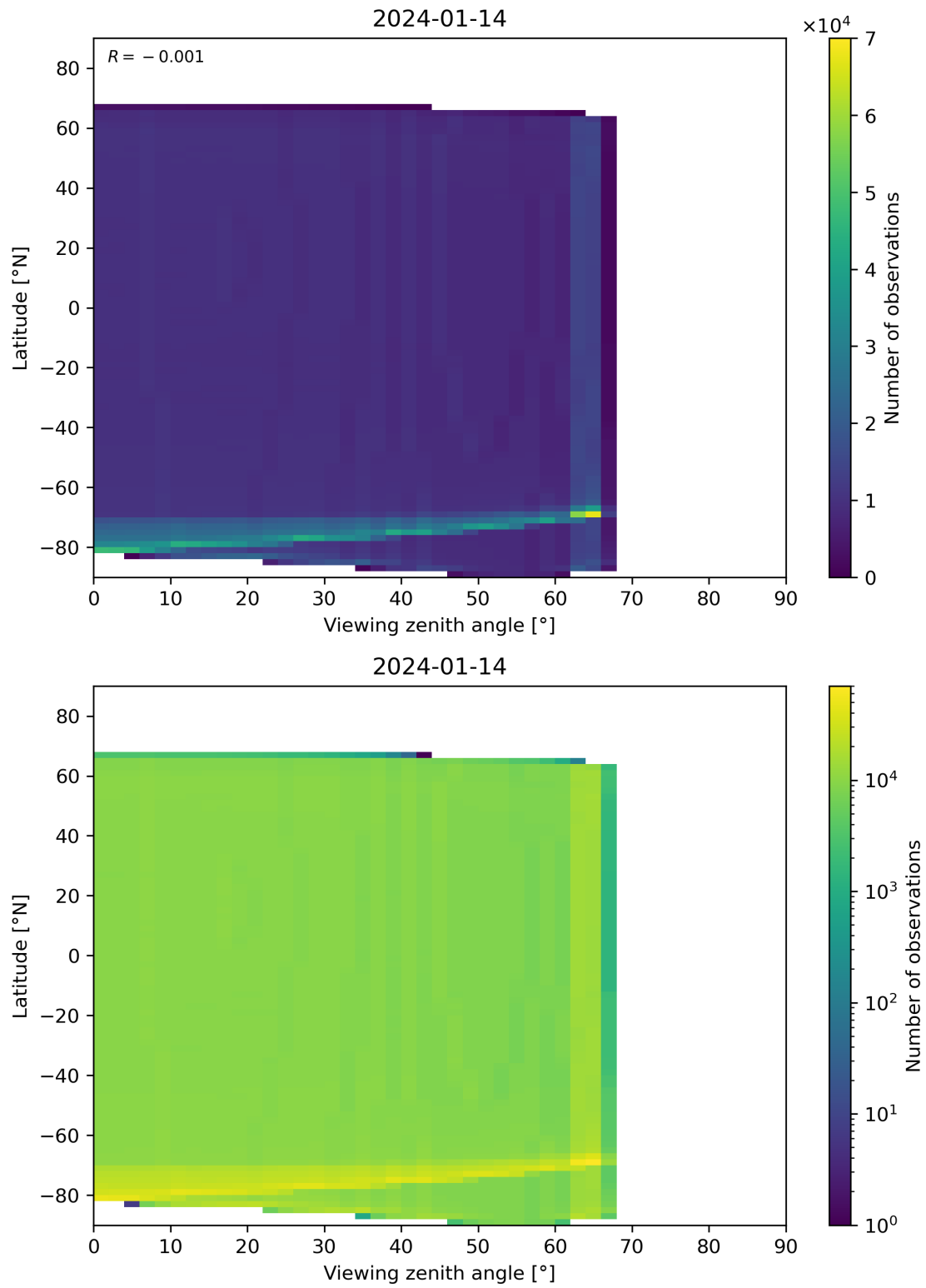
Figure 163: Scatter density plot of “Viewing zenith angle” against “Latitude” for 2024-01-13 to 2024-01-15.
