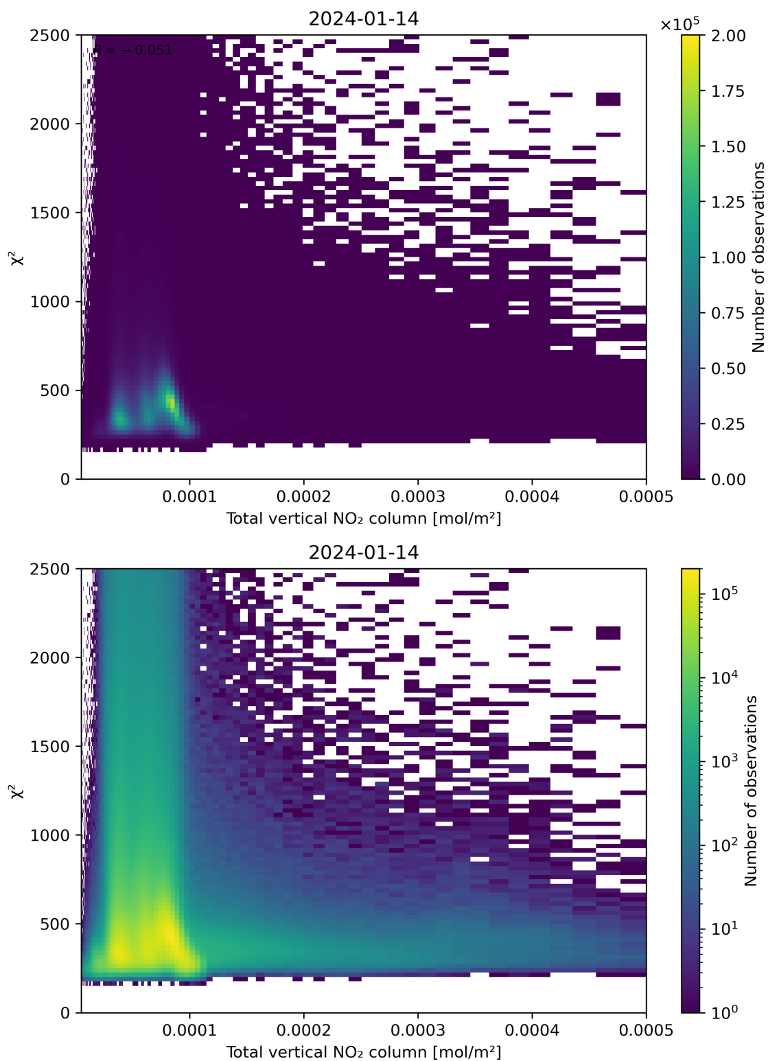
Figure 111: Scatter density plot of “Total vertical NO 2 column” against “ \chi^2 ” for 2024-01-13 to 2024-01-15.
