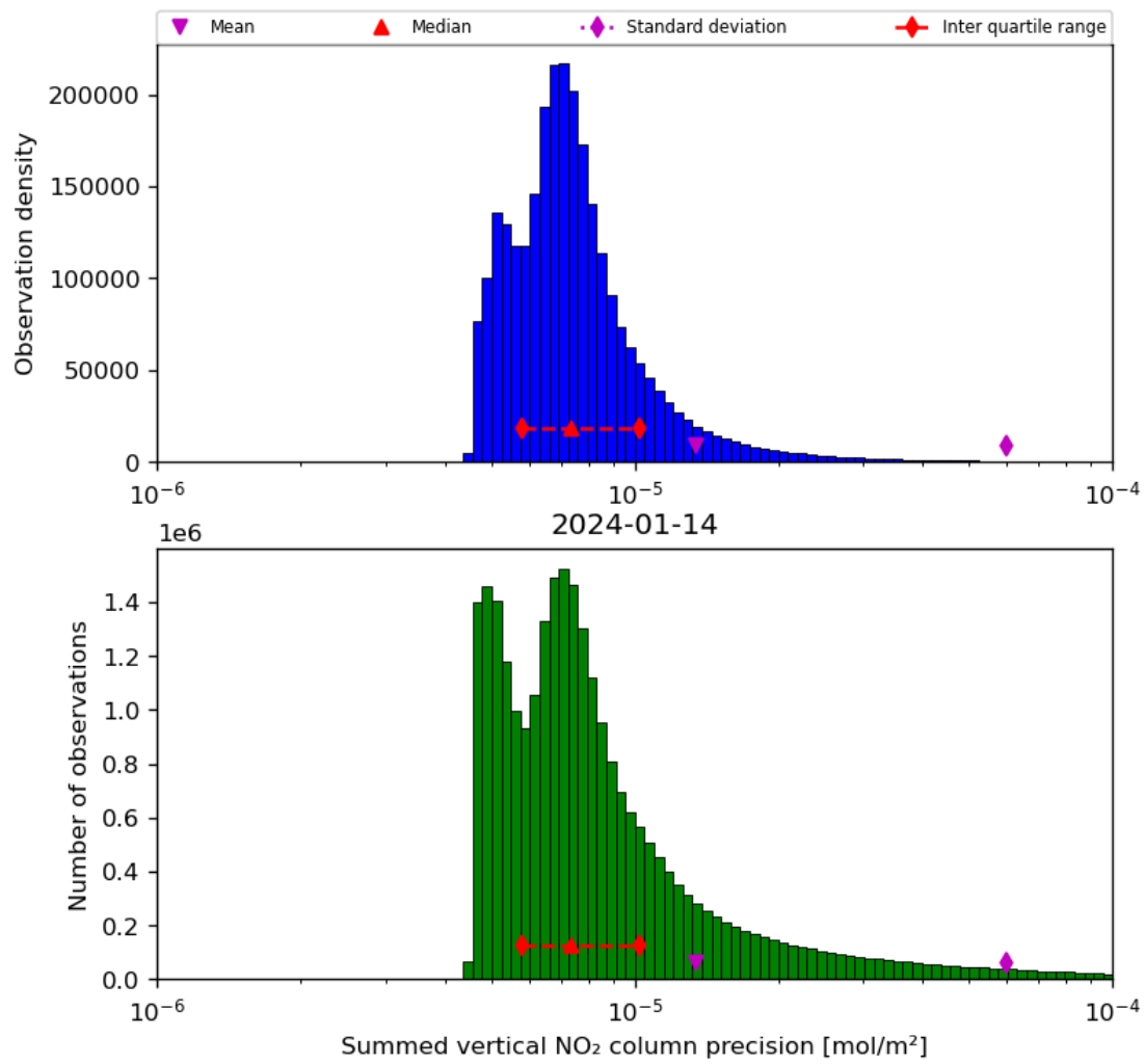
Figure 41: Histogram of “Summed vertical NO 2 column precision” for 2024-01-13 to 2024-01-15
