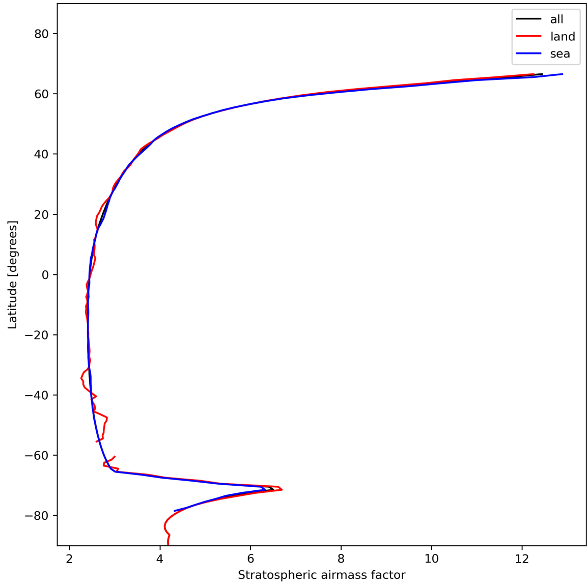
Figure 27: Zonal average of “Stratospheric airmass factor” for 2024-01-13 to 2024-01-15.
