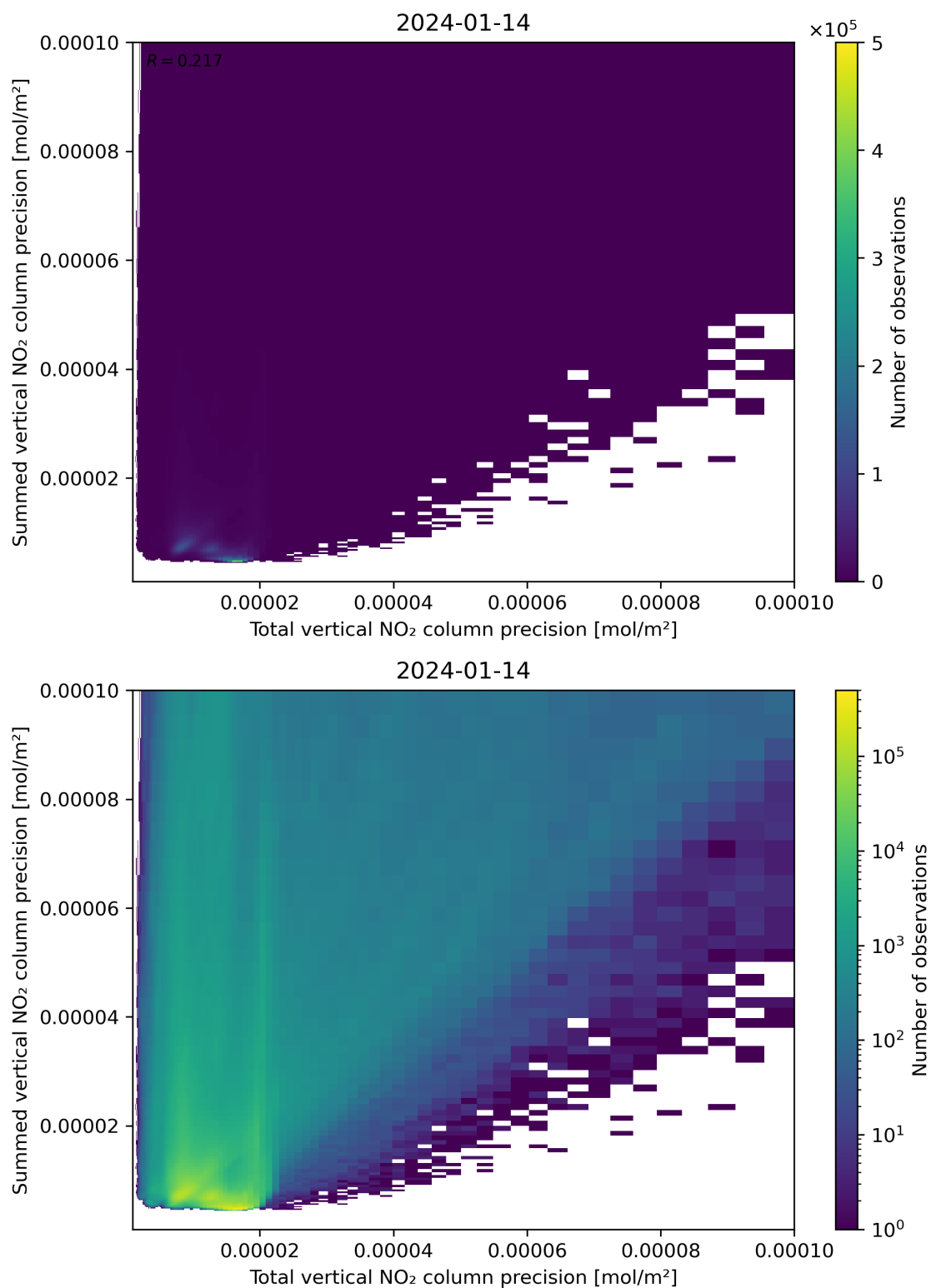
Figure 118: Scatter density plot of “Total vertical NO 2 column precision” against “Summed vertical NO 2 column precision” for 2024-01-13 to 2024-01-15.
