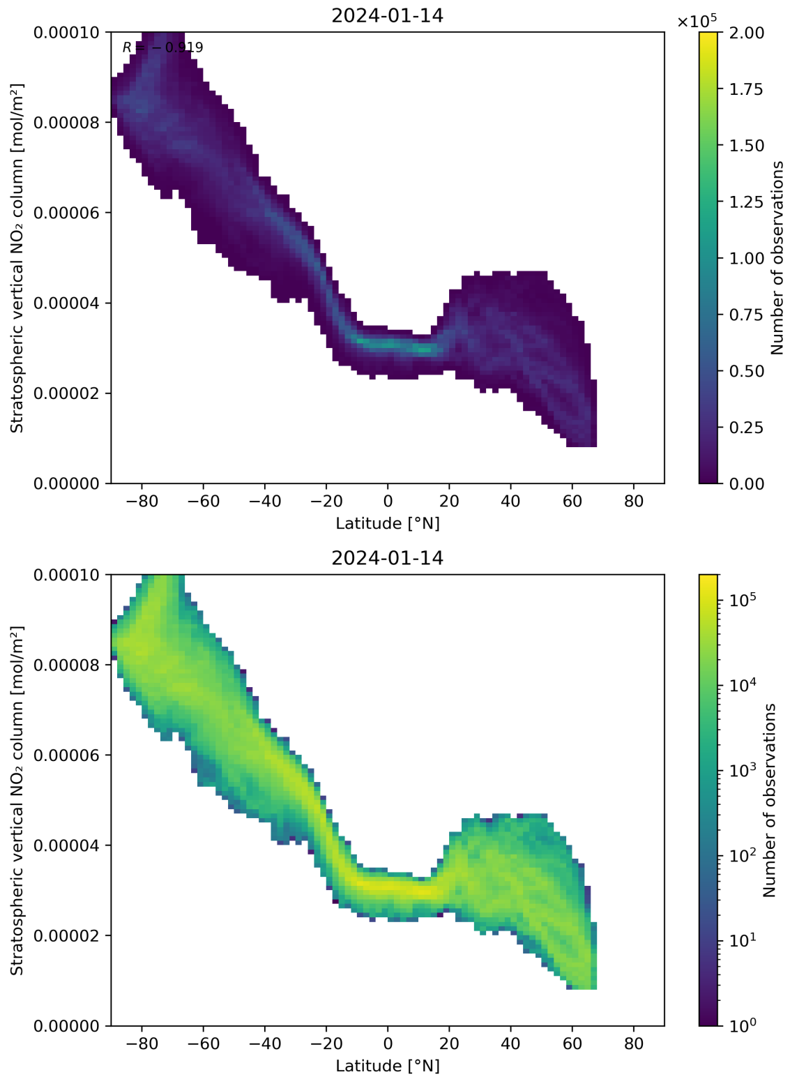
Figure 87: Scatter density plot of “Latitude” against “Stratospheric vertical NO 2 column” for 2024-01-13 to 2024-01-15.
