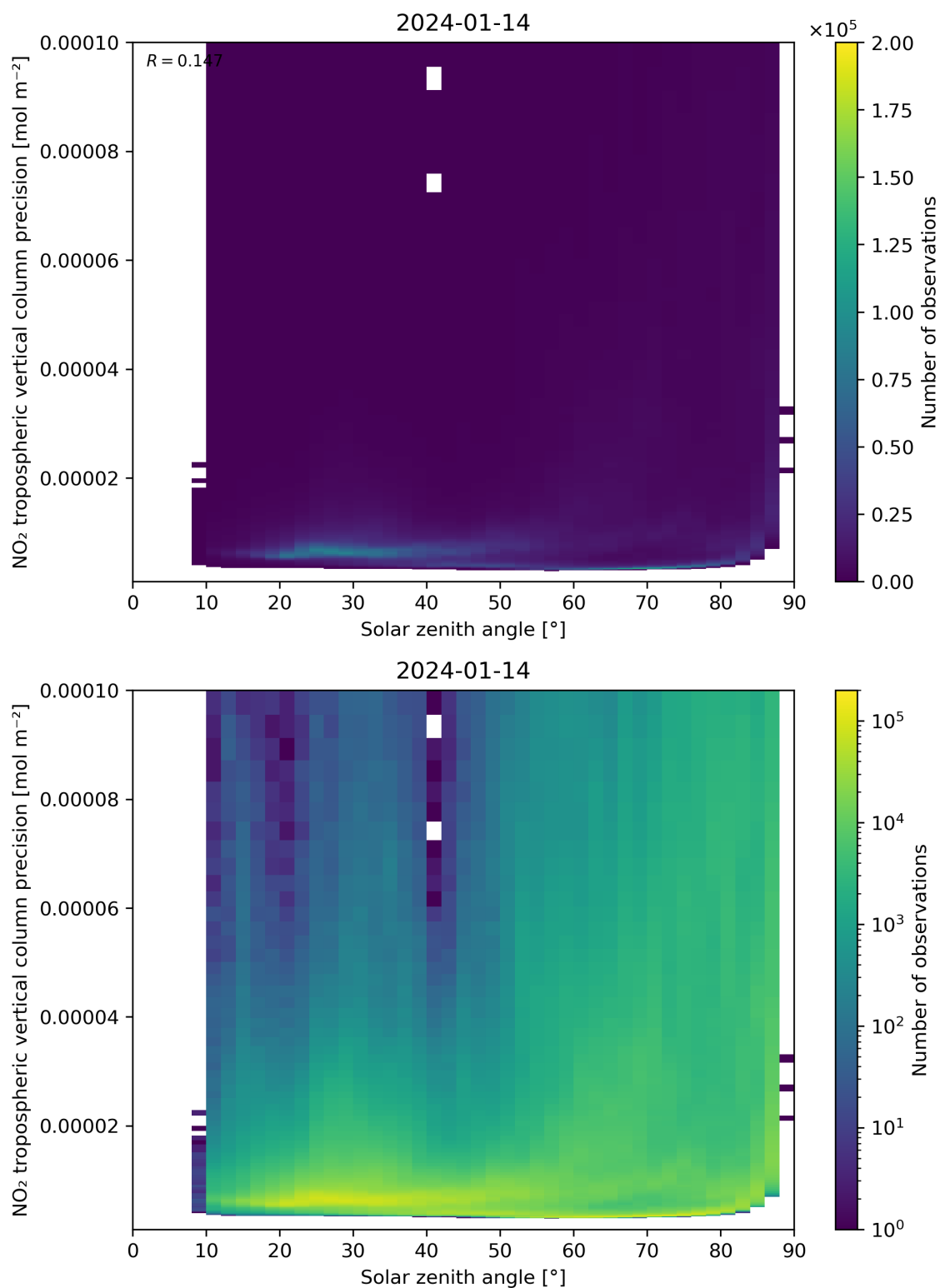
Figure 156: Scatter density plot of “Solar zenith angle” against “NO 2 tropospheric vertical column precision” for 2024-01-13 to 2024-01-15.
