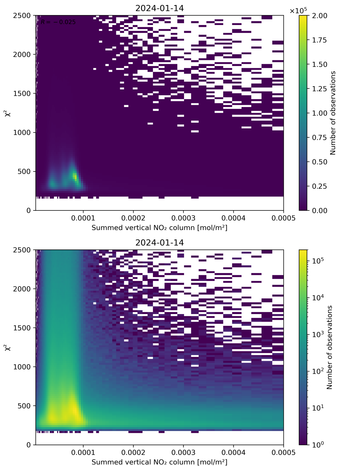
Figure 104: Scatter density plot of “Summed vertical NO 2 column” against “ \chi^2 ” for 2024-01-13 to 2024-01-15.
