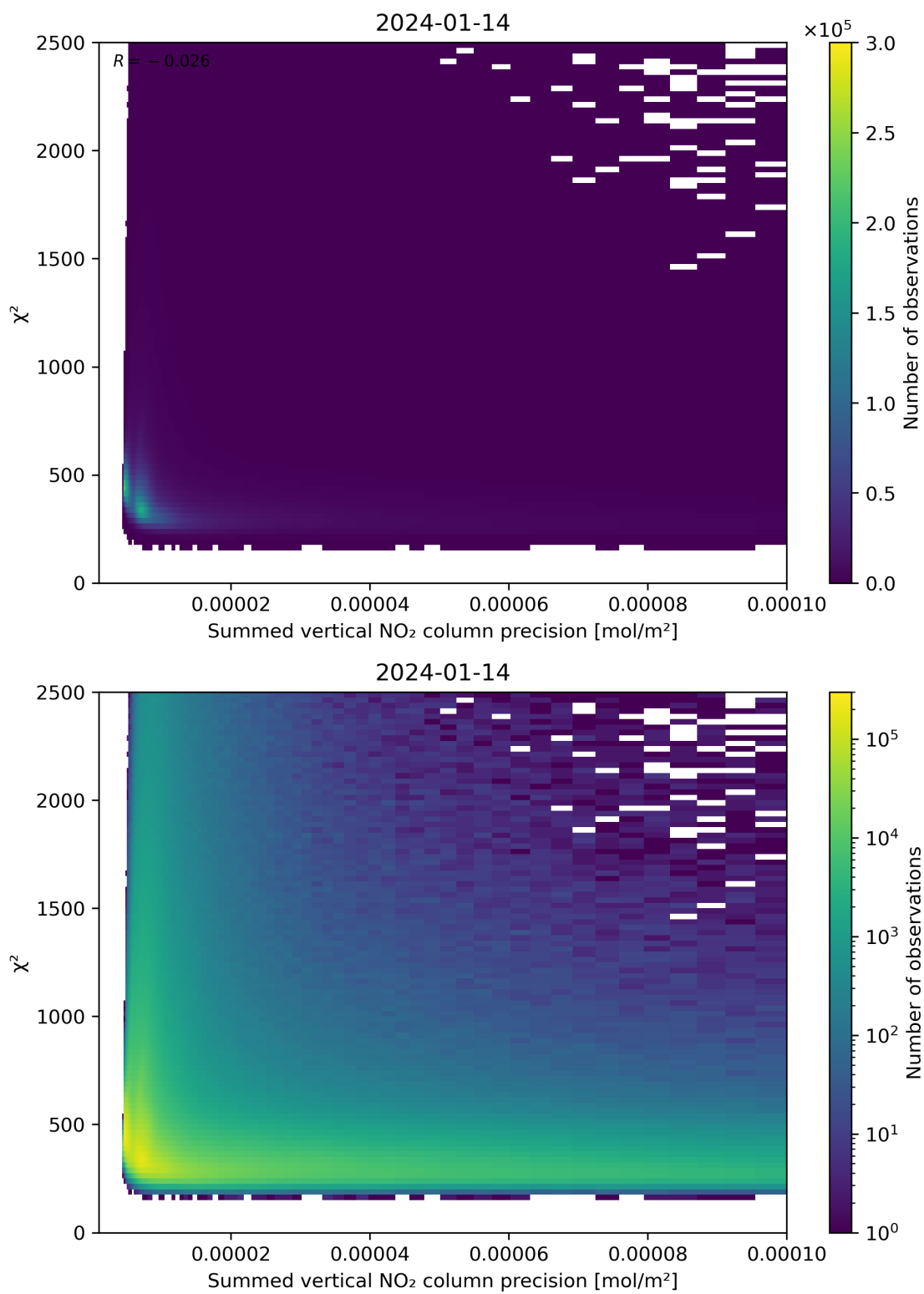
Figure 107: Scatter density plot of “Summed vertical NO 2 column precision” against “ \chi^2 ” for 2024-01-13 to 2024-01-15.
