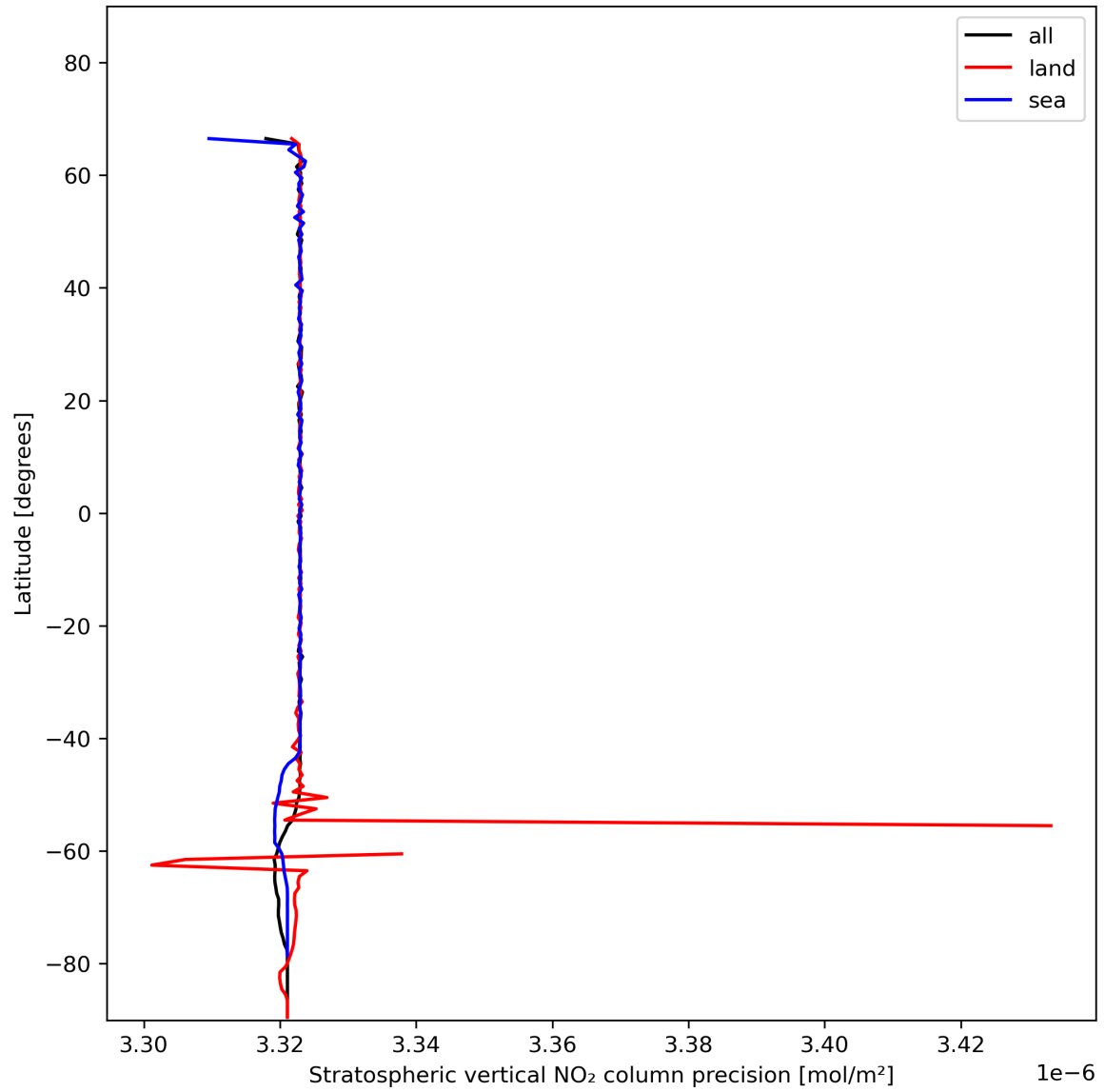
Figure 20: Zonal average of “Stratospheric vertical NO 2 column precision” for 2024-01-13 to 2024-01-15.
