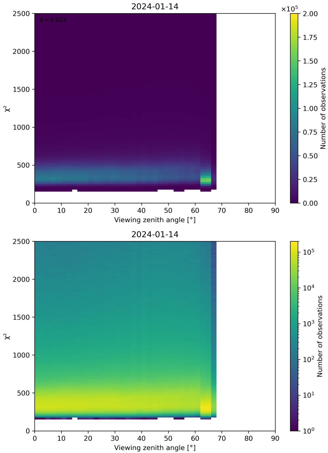
Figure 162: Scatter density plot of “Viewing zenith angle” against “ \chi^2 ” for 2024-01-13 to 2024-01-15.
