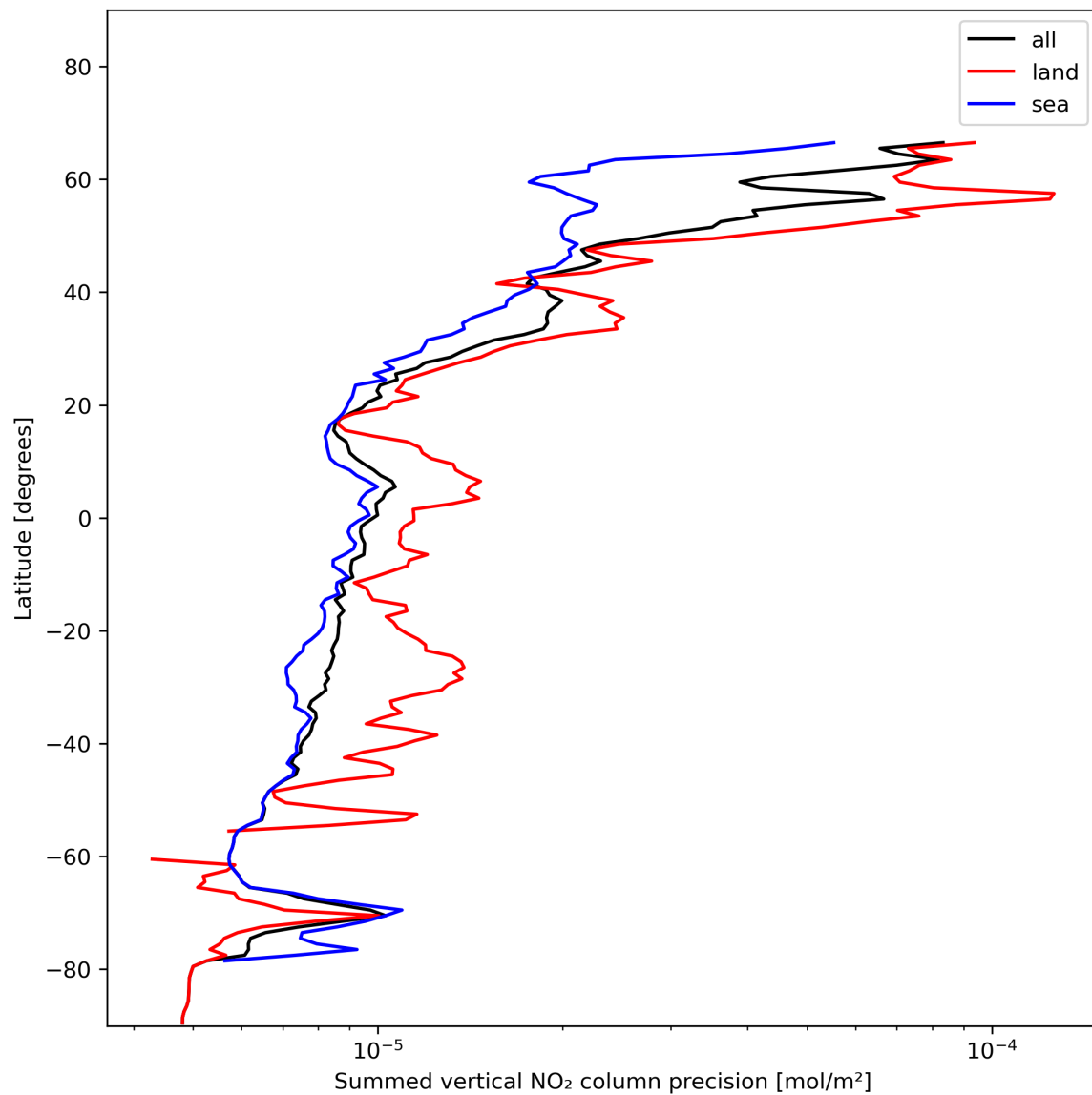
Figure 24: Zonal average of “Summed vertical NO 2 column precision” for 2024-01-13 to 2024-01-15.
