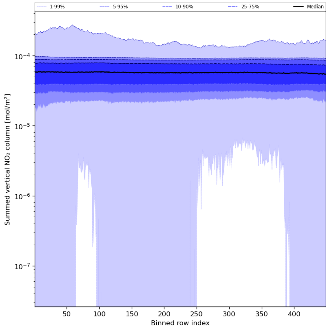
Figure 57: Along track statistics of “Summed vertical NO 2 column” for 2024-01-13 to 2024-01-15
