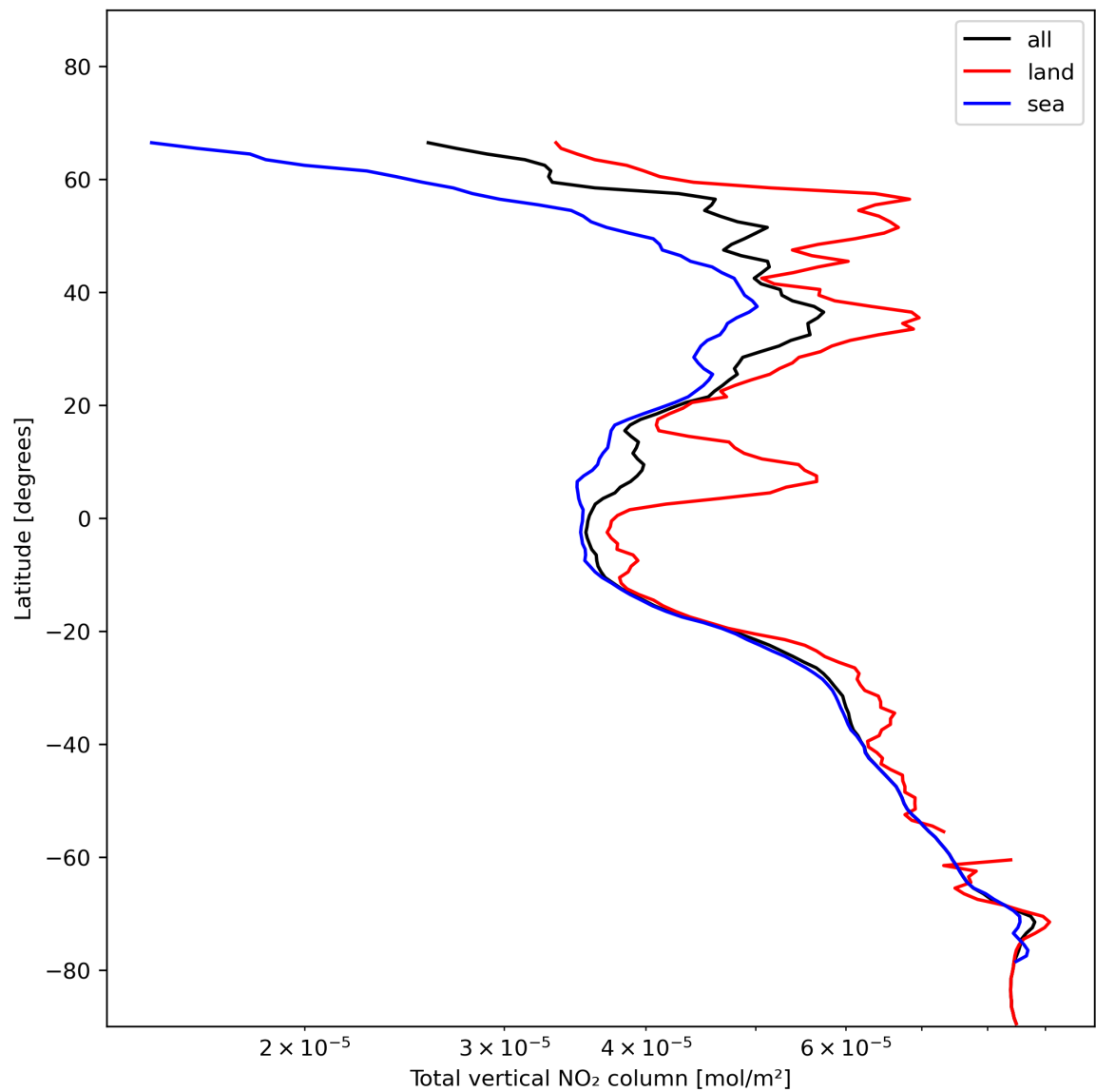
Figure 21: Zonal average of “Total vertical NO 2 column” for 2024-01-13 to 2024-01-15.
