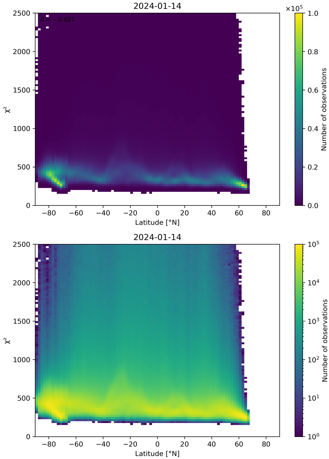
Figure 86: Scatter density plot of “Latitude” against “ \chi^2 ” for 2024-01-13 to 2024-01-15.
