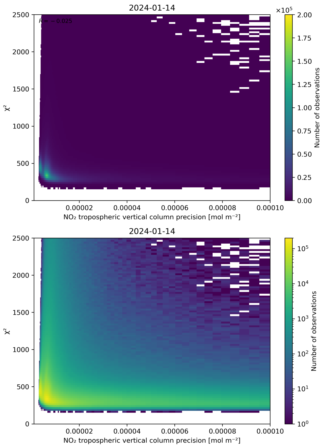
Figure 134: Scatter density plot of “NO 2 tropospheric vertical column precision” against “ \chi^2 ” for 2024-01-13 to 2024-01-15.
