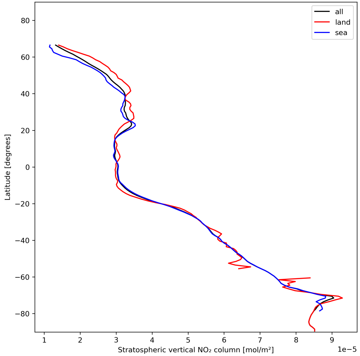
Figure 19: Zonal average of “Stratospheric vertical NO 2 column” for 2024-01-13 to 2024-01-15.
