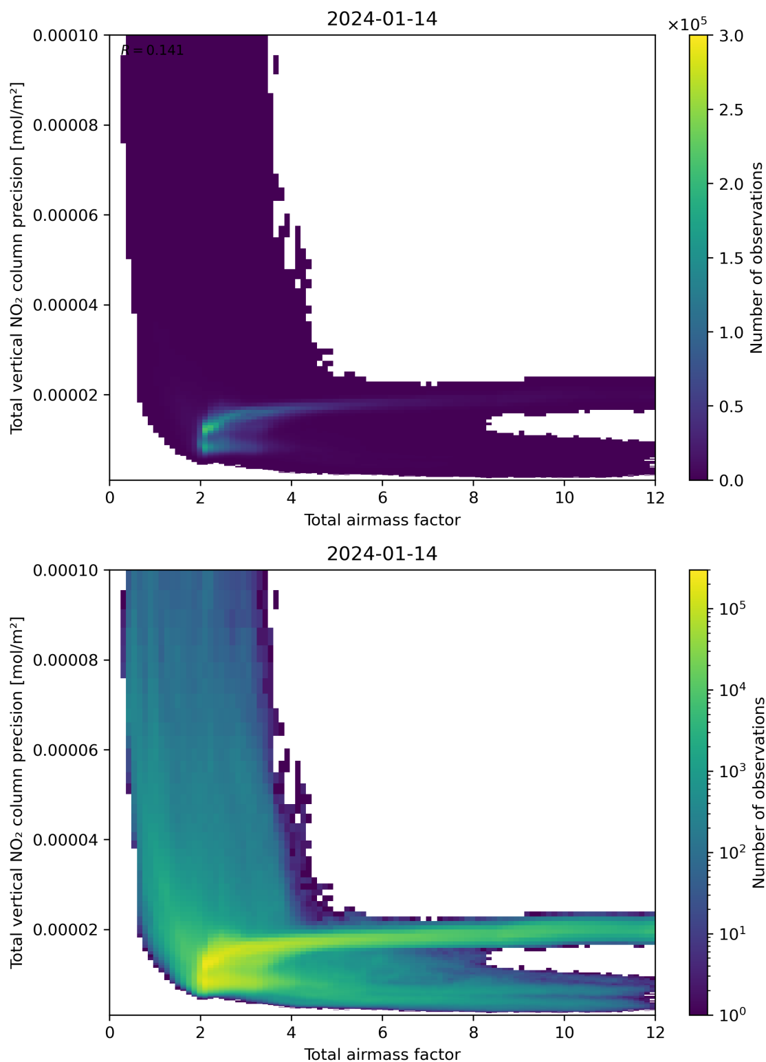
Figure 68: Scatter density plot of “Total airmass factor” against “Total vertical NO 2 column precision” for 2024-01-13 to 2024-01-15.
