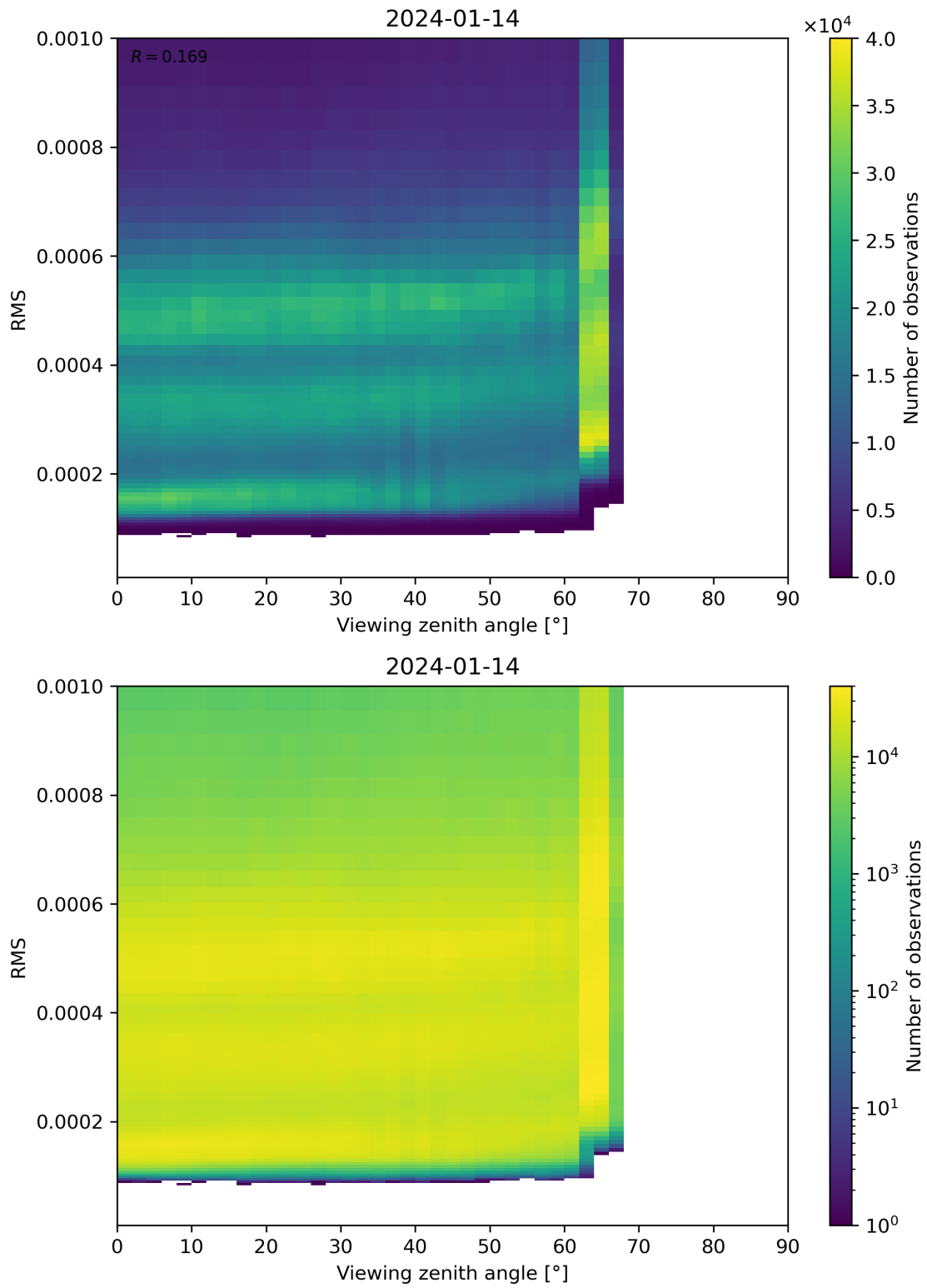
Figure 171: Scatter density plot of “Viewing zenith angle” against “RMS” for 2024-01-13 to 2024-01-15.
