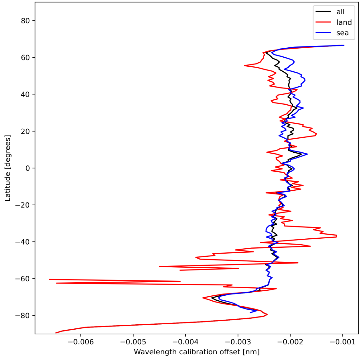
Figure 18: Zonal average of “Wavelength calibration offset” for 2024-01-13 to 2024-01-15.
