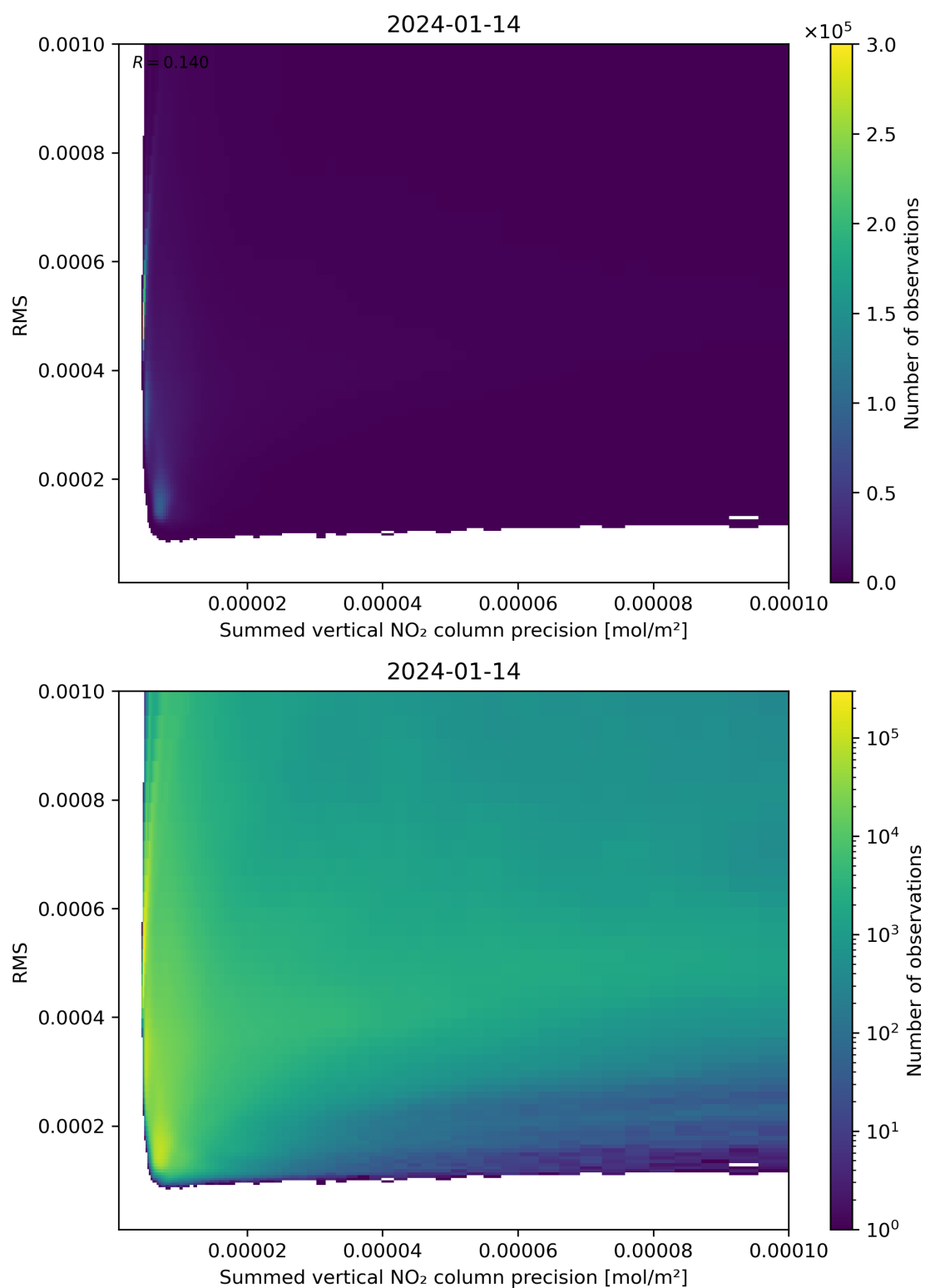
Figure 108: Scatter density plot of “Summed vertical NO 2 column precision” against “RMS” for 2024-01-13 to 2024-01-15.
