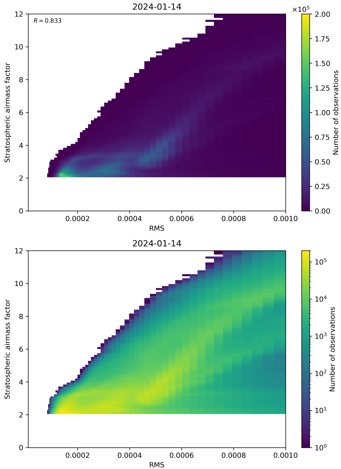
Figure 144: Scatter density plot of “RMS” against “Stratospheric airmass factor” for 2024-01-13 to 2024-01-15.
