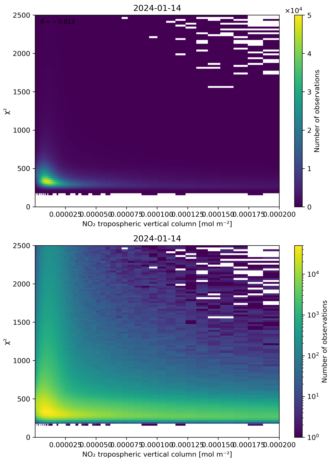
Figure 124: Scatter density plot of “NO 2 tropospheric vertical column” against “ \chi^2 ” for 2024-01-13 to 2024-01-15.
