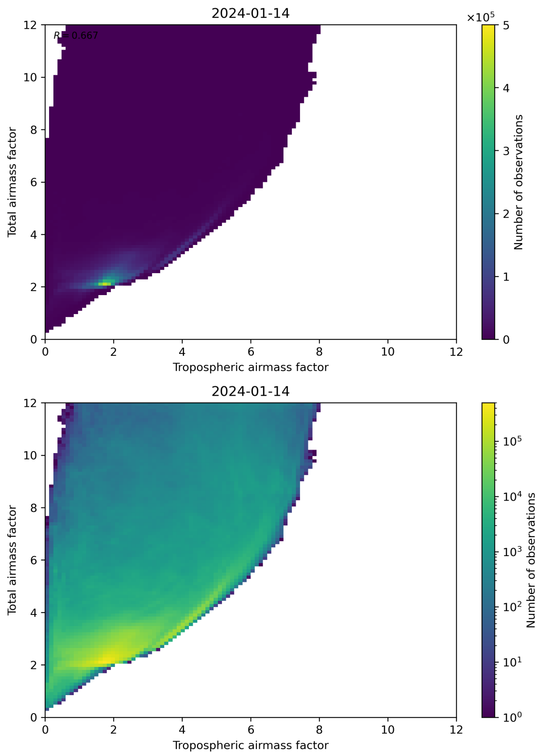
Figure 72: Scatter density plot of “Tropospheric airmass factor” against “Total airmass factor” for 2024-01-13 to 2024-01-15.
