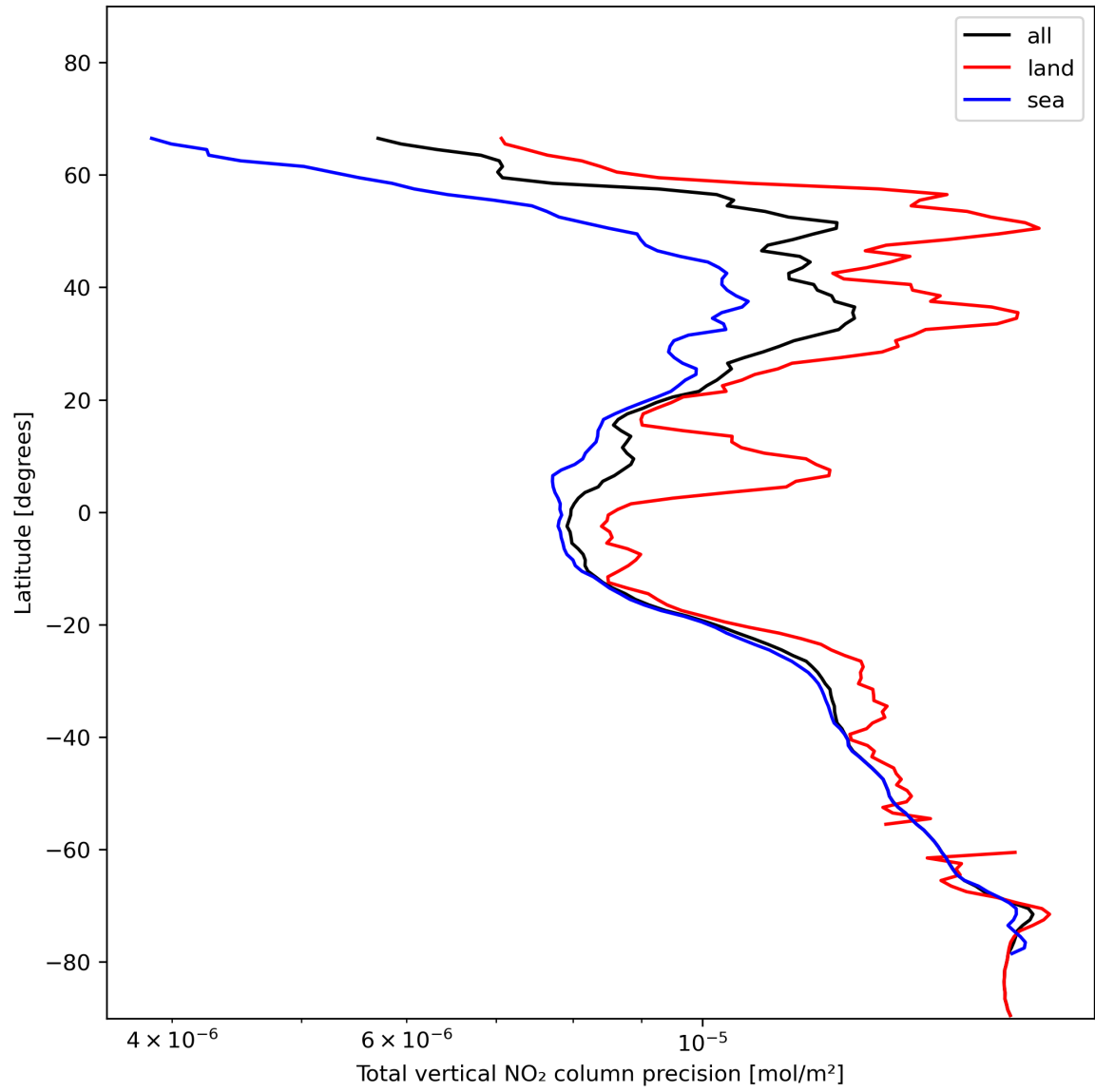
Figure 22: Zonal average of “Total vertical NO 2 column precision” for 2024-01-13 to 2024-01-15.
