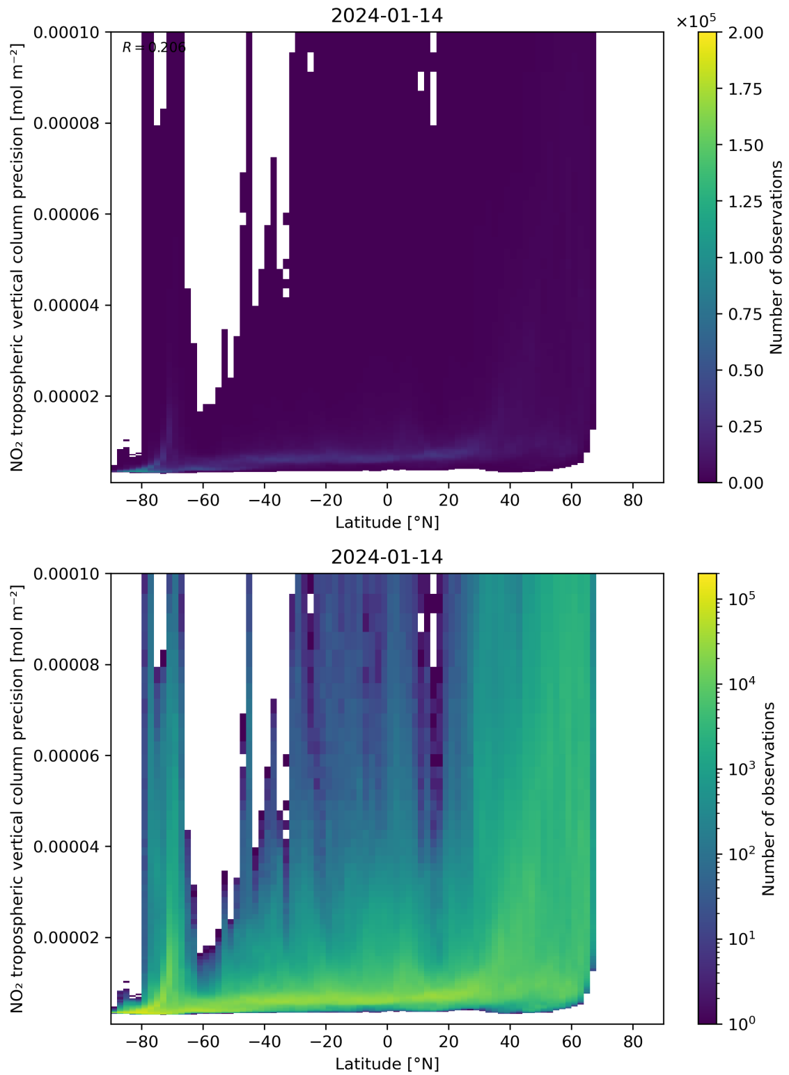
Figure 93: Scatter density plot of “Latitude” against “NO 2 tropospheric vertical column precision” for 2024-01-13 to 2024-01-15.
