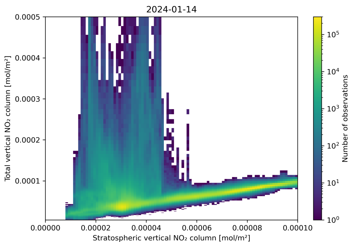
Figure 100: Scatter density plot of “Stratospheric vertical NO 2 column” against “Total vertical NO 2 column” for 2024-01-13 to 2024-01-15.
