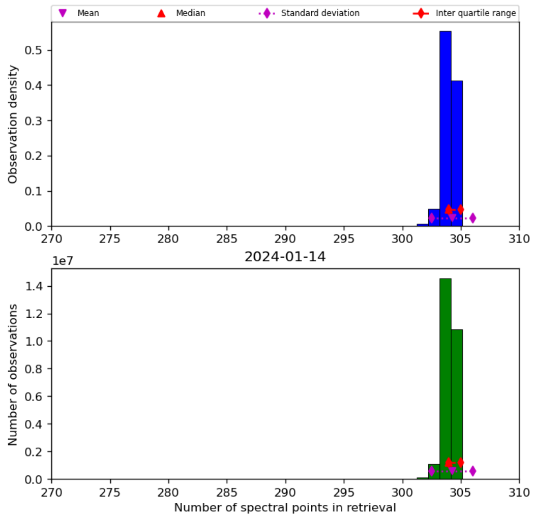
Figure 33: Histogram of “Number of spectral points in retrieval” for 2024-01-13 to 2024-01-15
