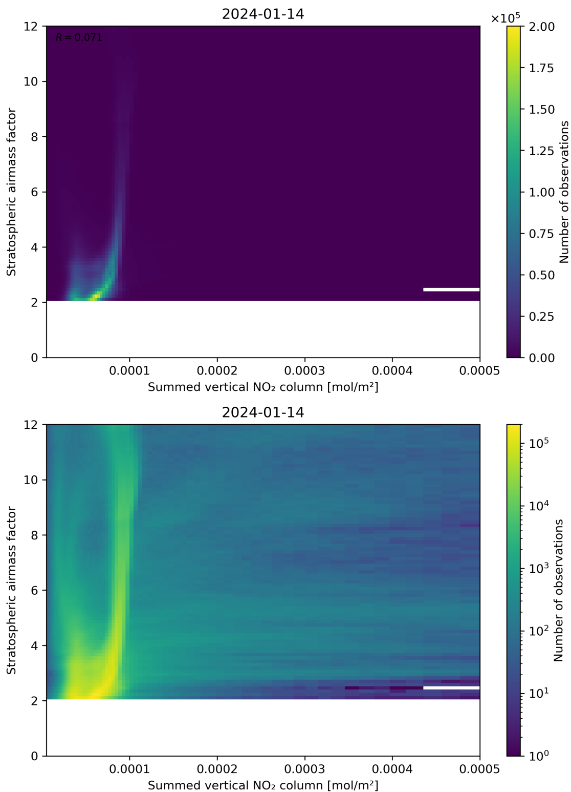
Figure 103: Scatter density plot of “Summed vertical NO 2 column” against “Stratospheric airmass factor” for 2024-01-13 to 2024-01-15.
