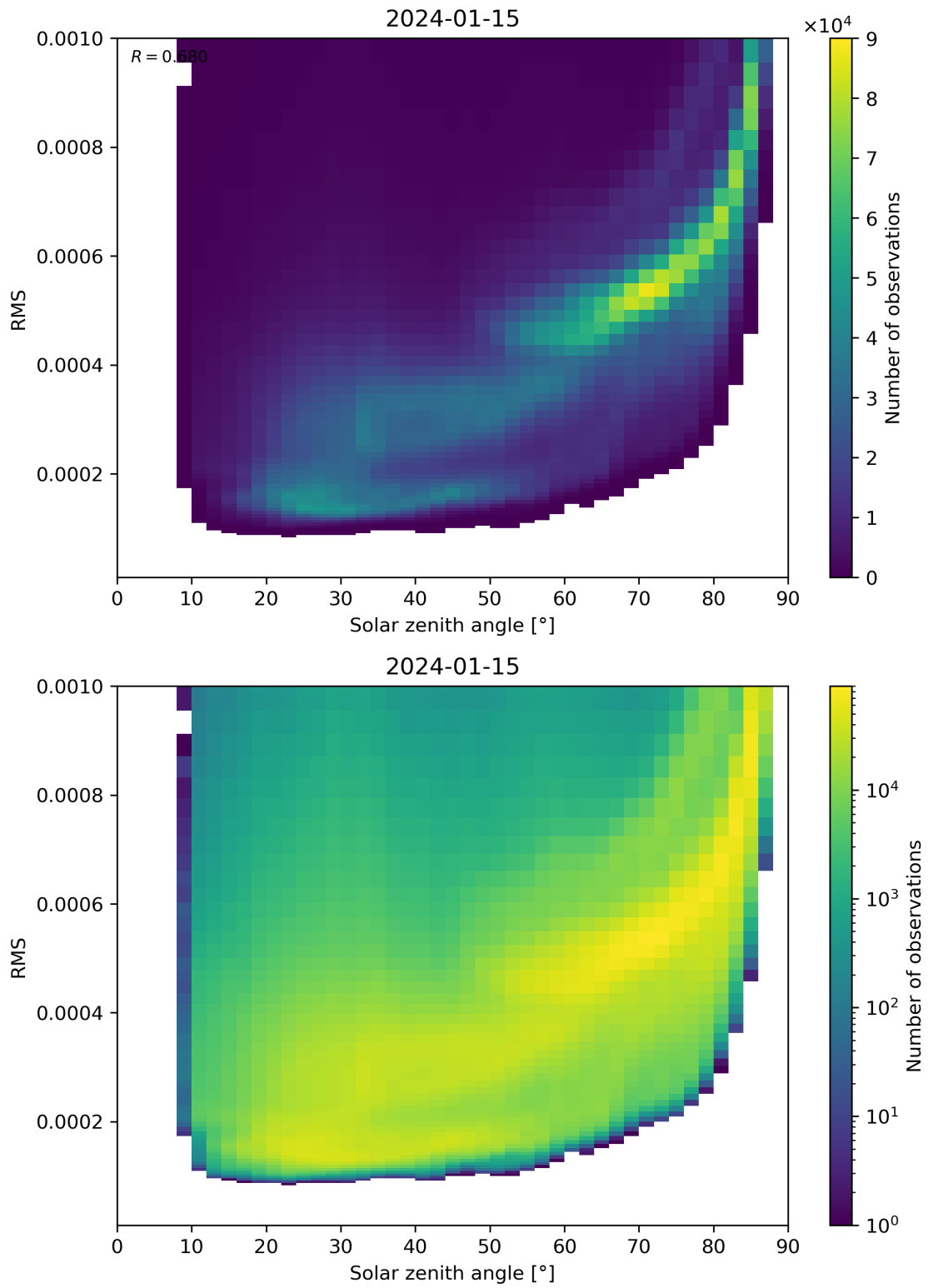
Figure 157: Scatter density plot of “Solar zenith angle” against “RMS” for 2024-01-15 to 2024-01-16.
