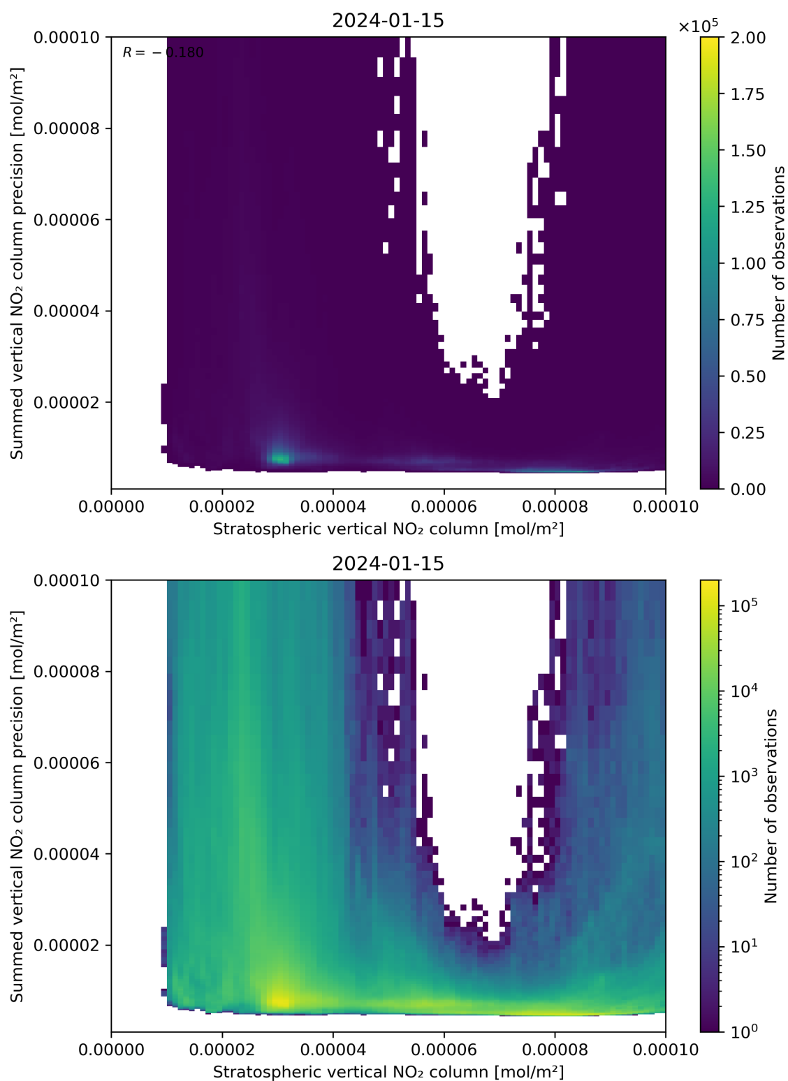
Figure 99: Scatter density plot of “Stratospheric vertical NO 2 column” against “Summed vertical NO 2 column precision” for 2024-01-15 to 2024-01-16.
