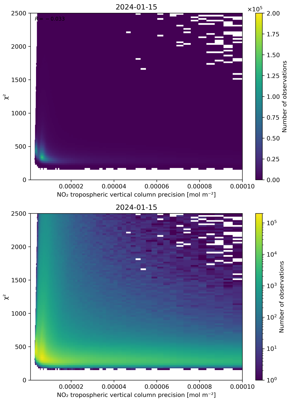
Figure 134: Scatter density plot of “NO 2 tropospheric vertical column precision” against “ \chi^2 ” for 2024-01-15 to 2024-01-16.
