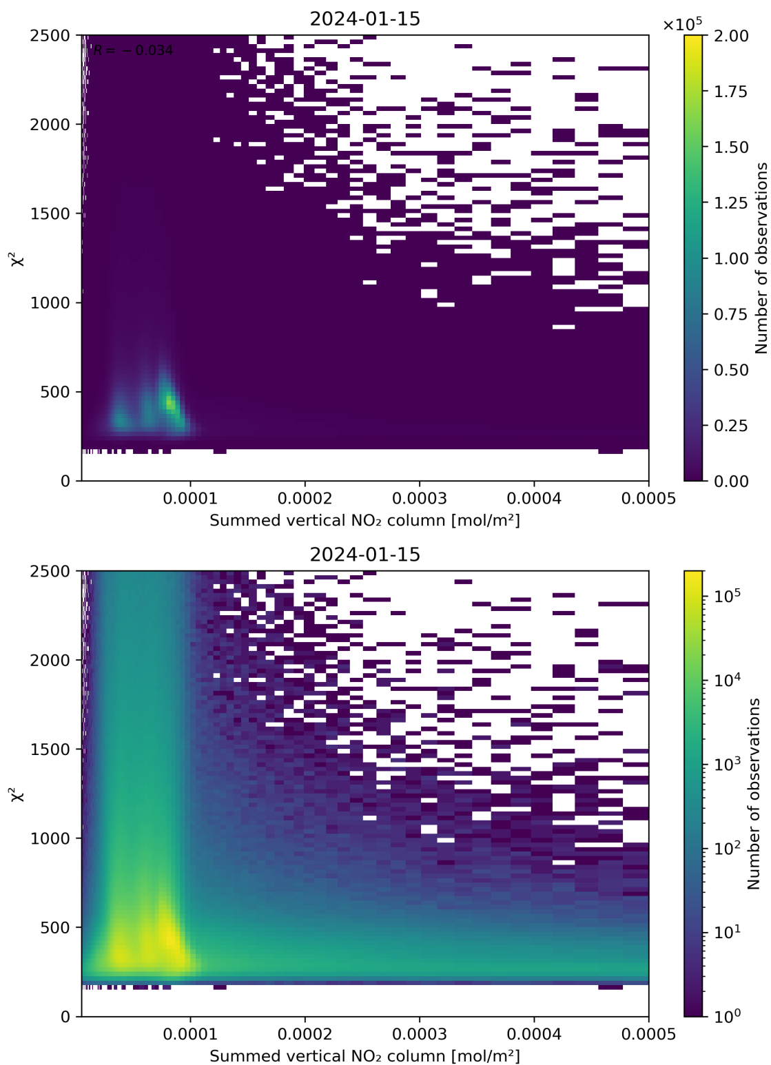
Figure 104: Scatter density plot of “Summed vertical NO 2 column” against “ \chi^2 ” for 2024-01-15 to 2024-01-16.
