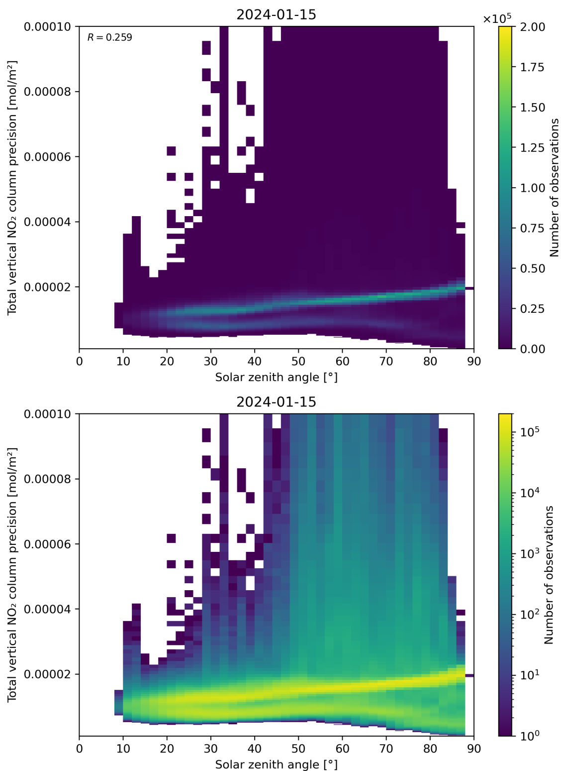
Figure 154: Scatter density plot of “Solar zenith angle” against “Total vertical NO 2 column precision” for 2024-01-15 to 2024-01-16.
