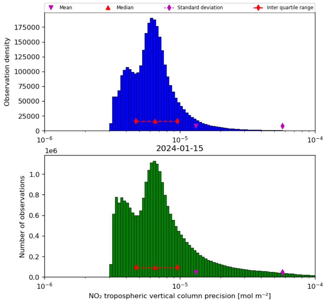
Figure 30: Histogram of “NO 2 tropospheric vertical column precision” for 2024-01-15 to 2024-01-16
