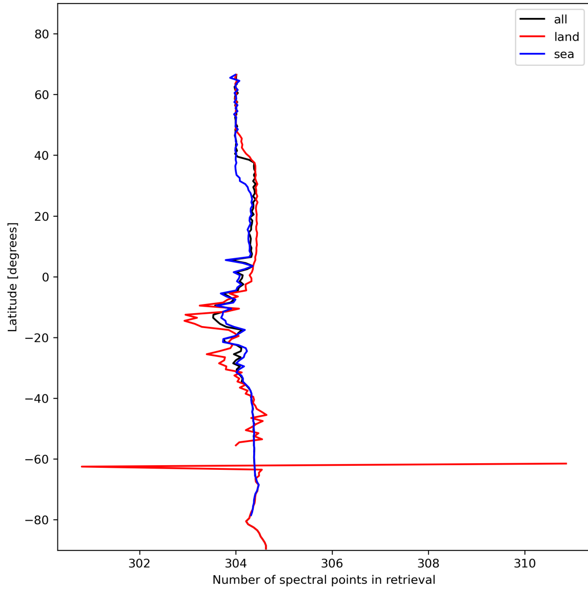
Figure 16: Zonal average of “Number of spectral points in retrieval” for 2024-01-15 to 2024-01-16.
