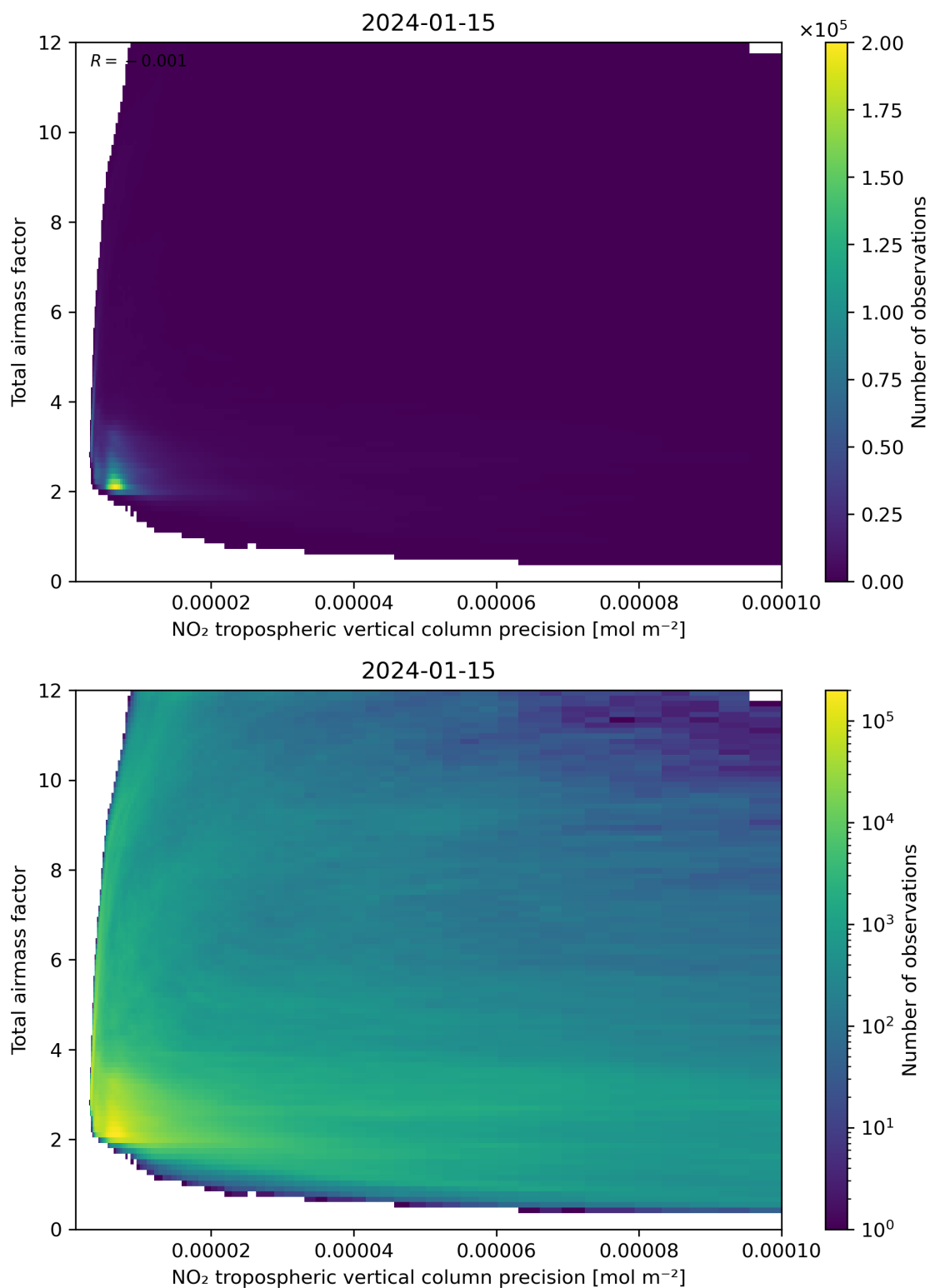
Figure 132: Scatter density plot of “NO 2 tropospheric vertical column precision” against “Total airmass factor” for 2024-01-15 to 2024-01-16.
