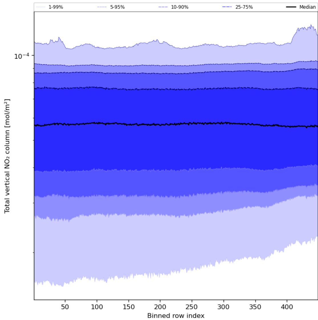
Figure 55: Along track statistics of “Total vertical NO 2 column” for 2024-01-15 to 2024-01-16
