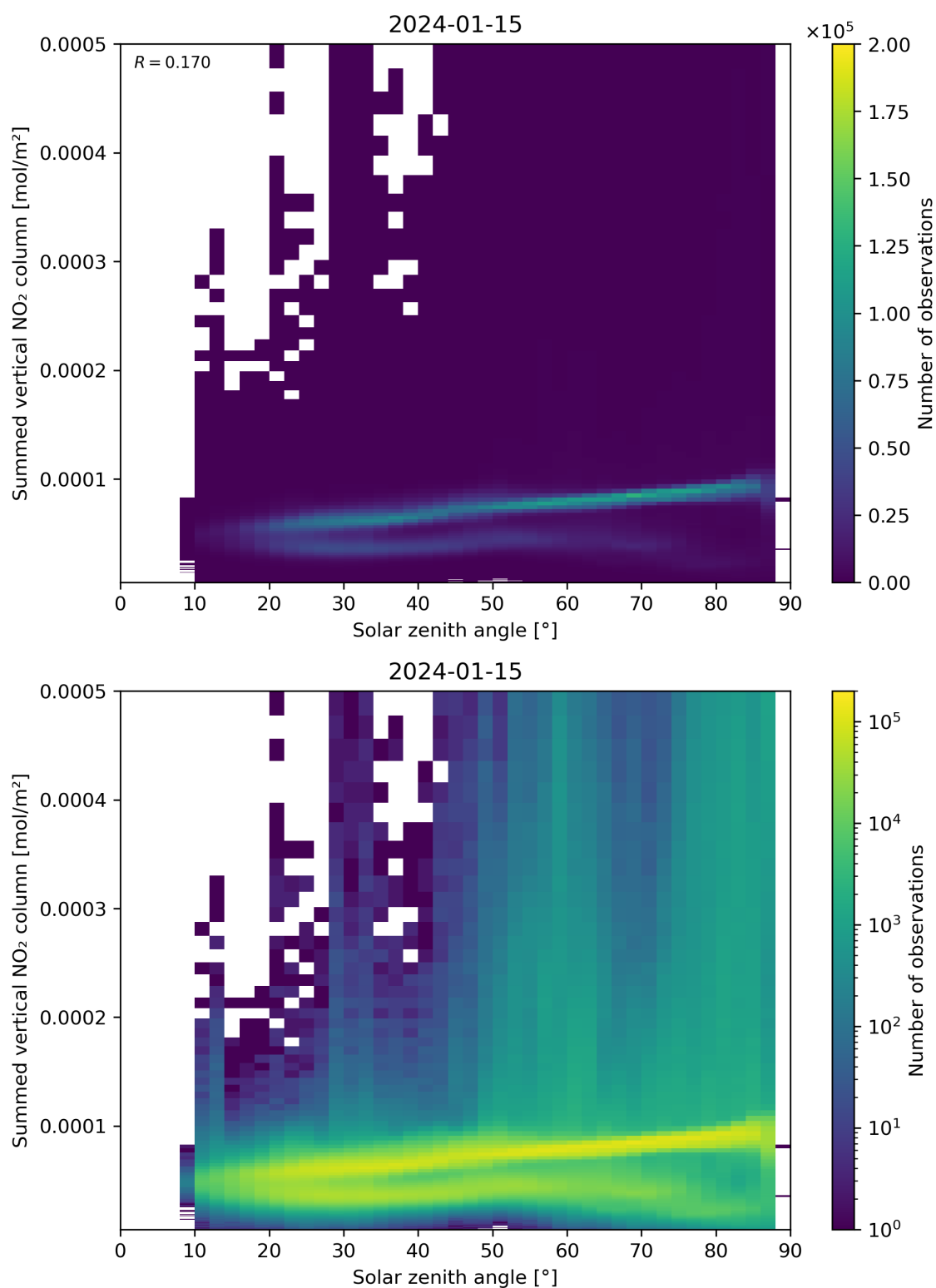
Figure 151: Scatter density plot of “Solar zenith angle” against “Summed vertical NO 2 column” for 2024-01-15 to 2024-01-16.
