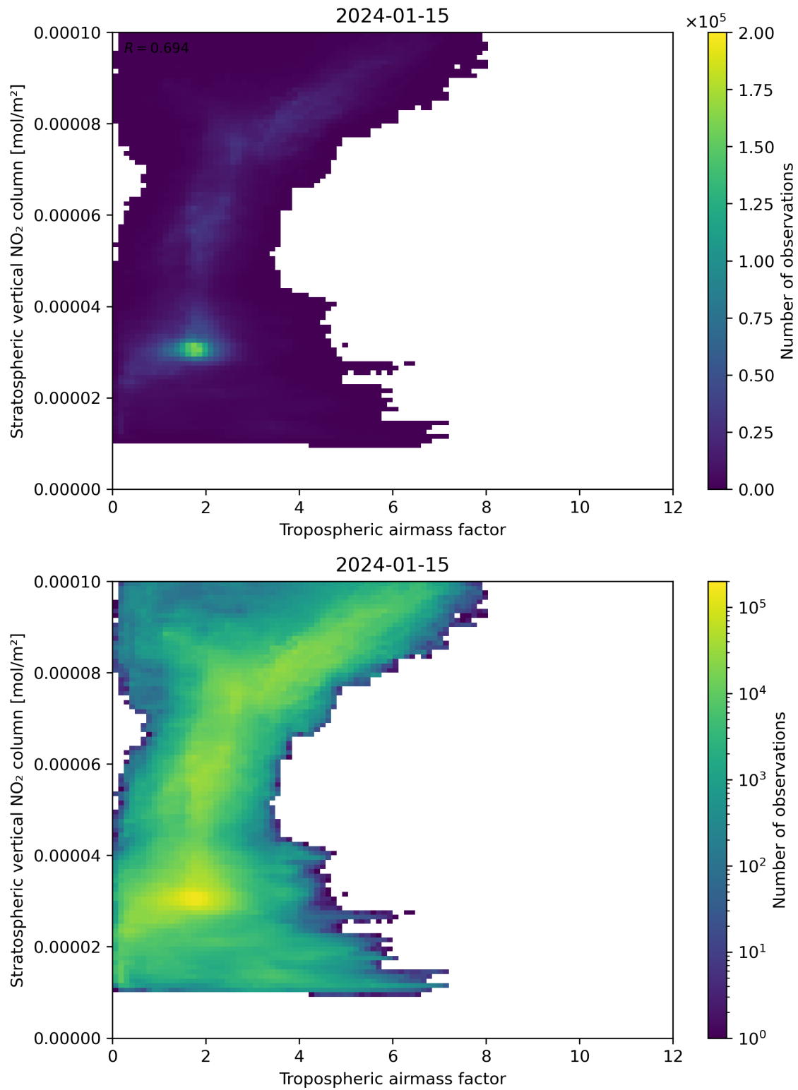
Figure 74: Scatter density plot of “Tropospheric air mass factor” against “Stratospheric vertical NO 2 column” for 2024-01-15 to 2024-01-16.
