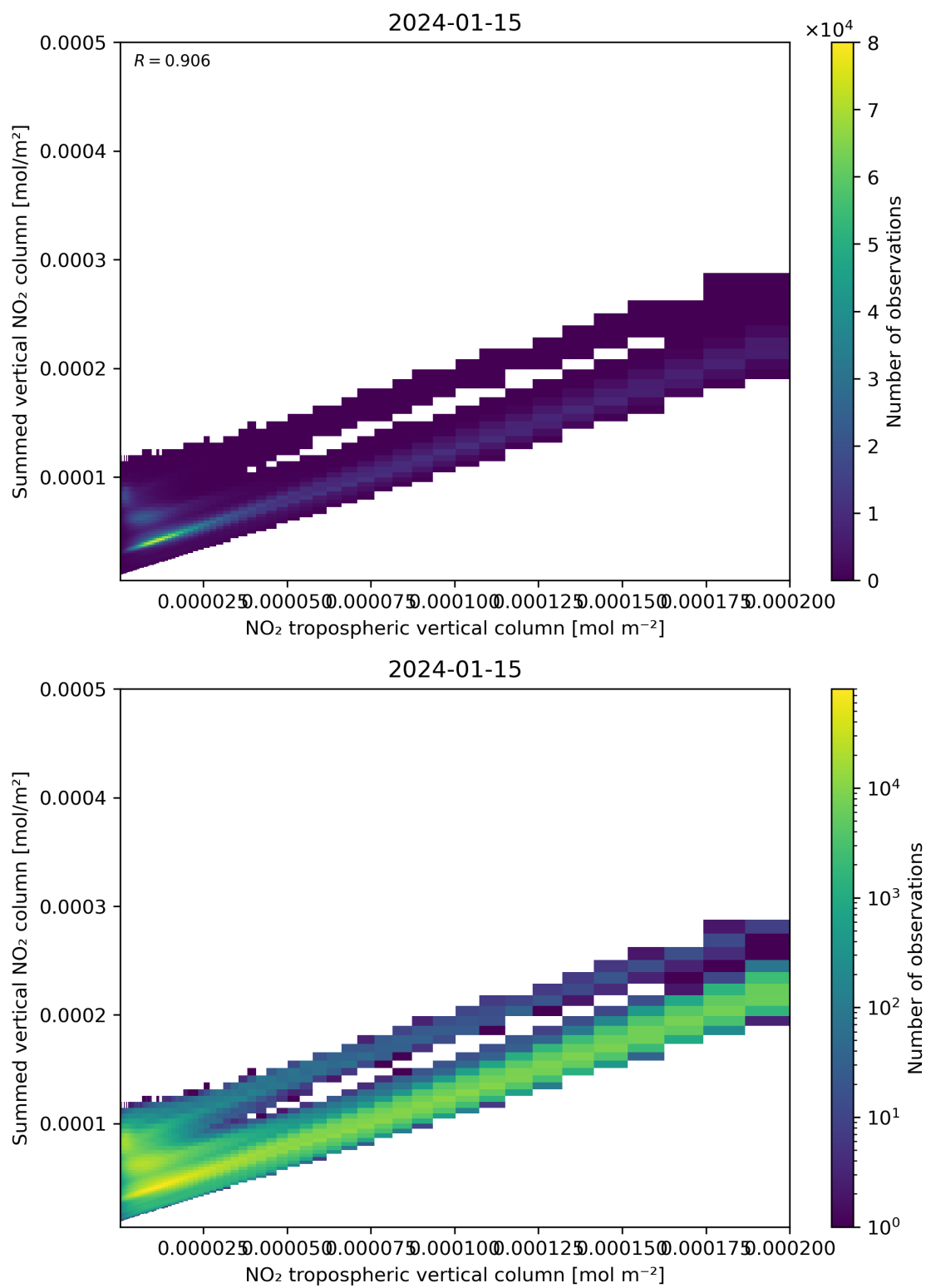
Figure 126: Scatter density plot of “NO 2 tropospheric vertical column” against “Summed vertical NO 2 column” for 2024-01-15 to 2024-01-16.
