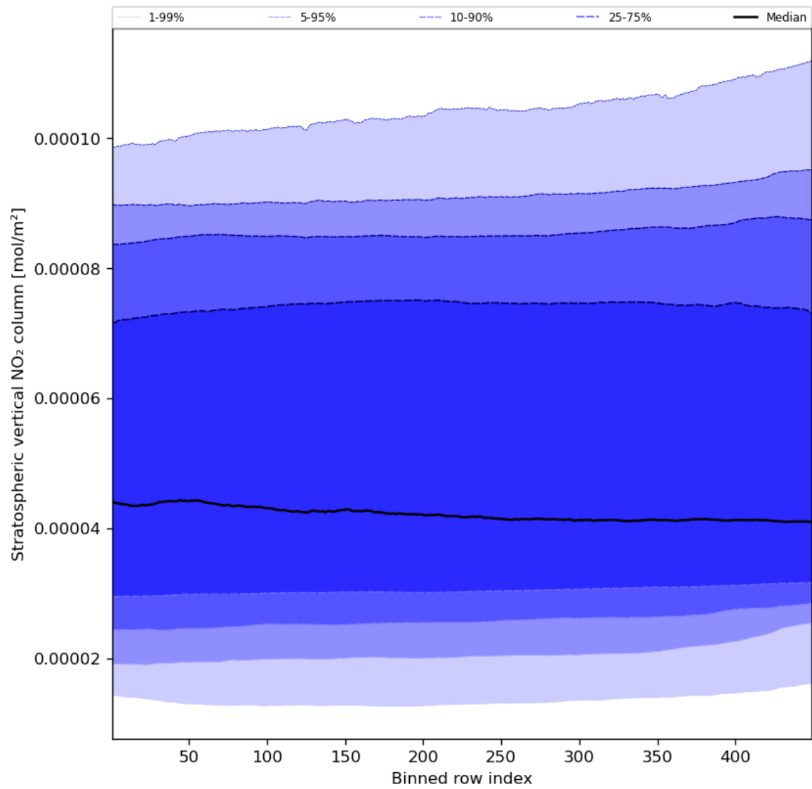
Figure 53: Along track statistics of “Stratospheric vertical NO 2 column” for 2024-01-15 to 2024-01-16
