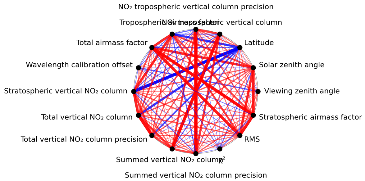
Figure 1: Map of correlation graph for 2024-01-15 to 2024-01-16.
