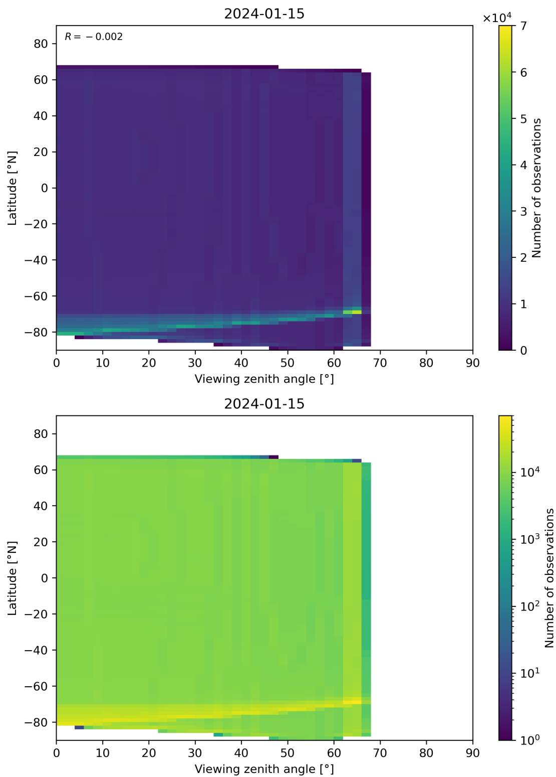
Figure 163: Scatter density plot of “Viewing zenith angle” against “Latitude” for 2024-01-15 to 2024-01-16.
