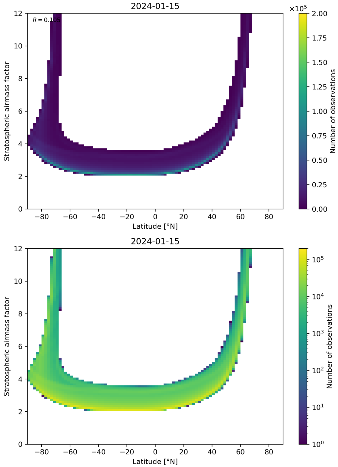
Figure 83: Scatter density plot of “Latitude” against “Stratospheric air mass factor” for 2024-01-15 to 2024-01-16.
