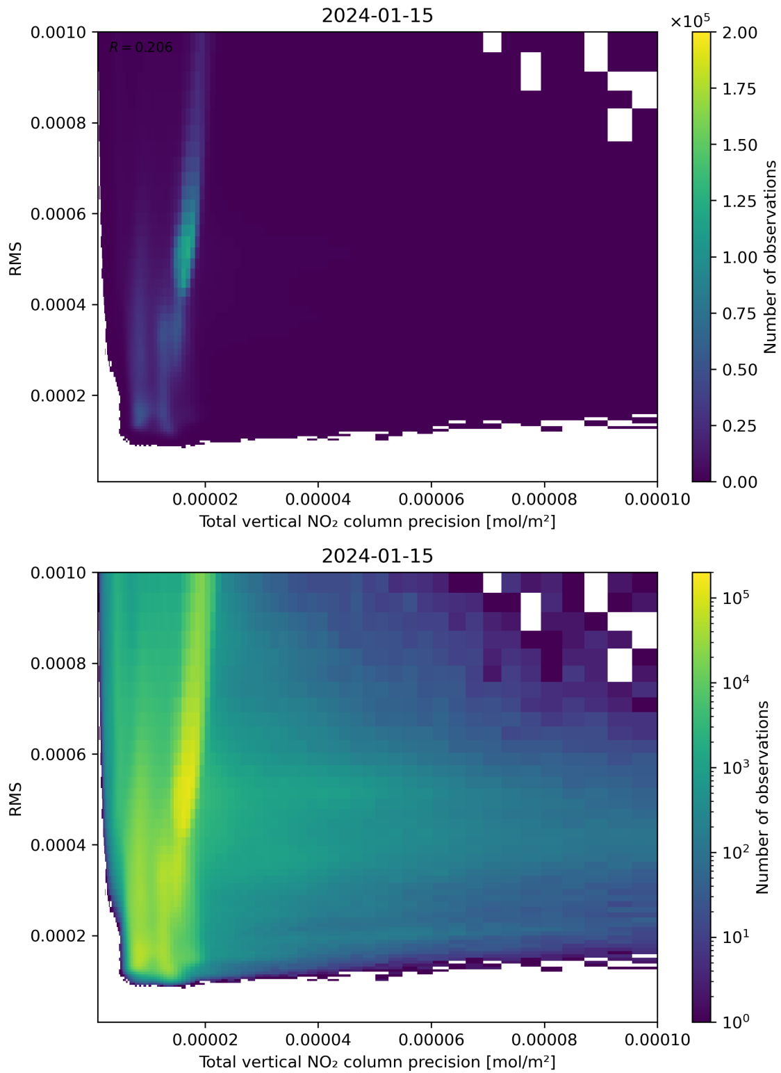
Figure 119: Scatter density plot of “Total vertical NO 2 column precision” against “RMS” for 2024-01-15 to 2024-01-16.
