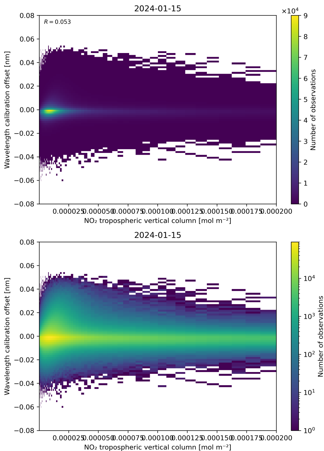
Figure 143: Scatter density plot of “NO 2 tropospheric vertical column” against “Wavelength calibration offset” for 2024-01-15 to 2024-01-16.
