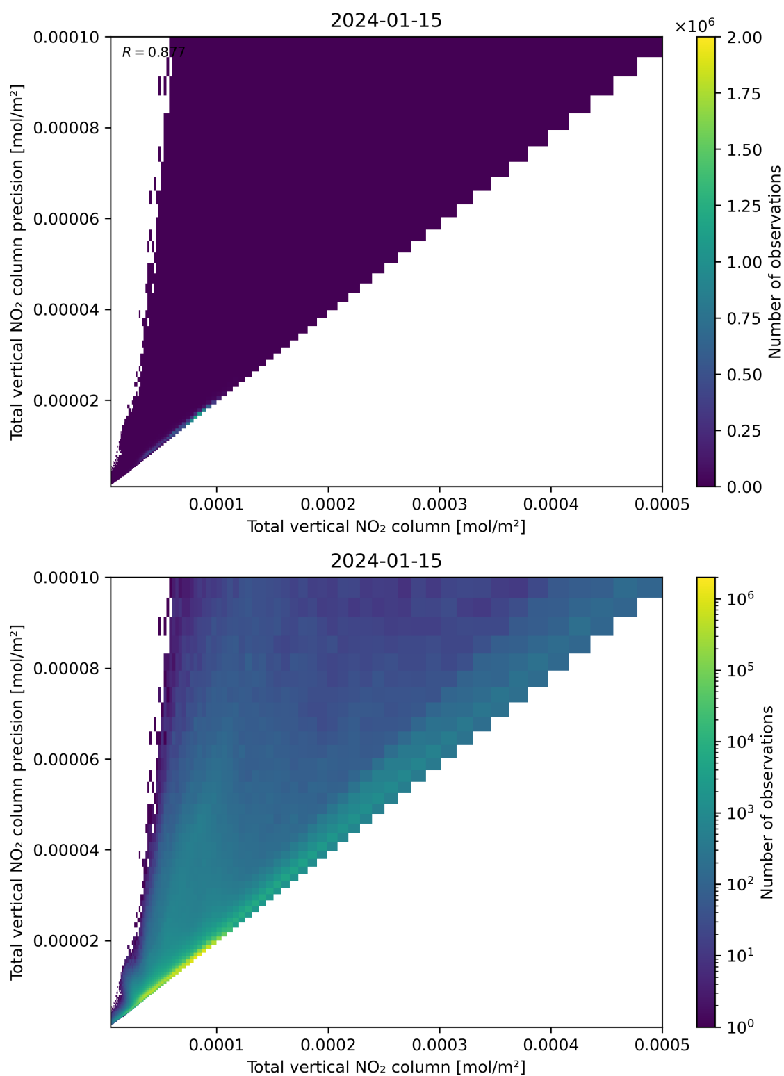
Figure 114: Scatter density plot of “Total vertical NO 2 column” against “Total vertical NO 2 column precision” for 2024-01-15 to 2024-01-16.
