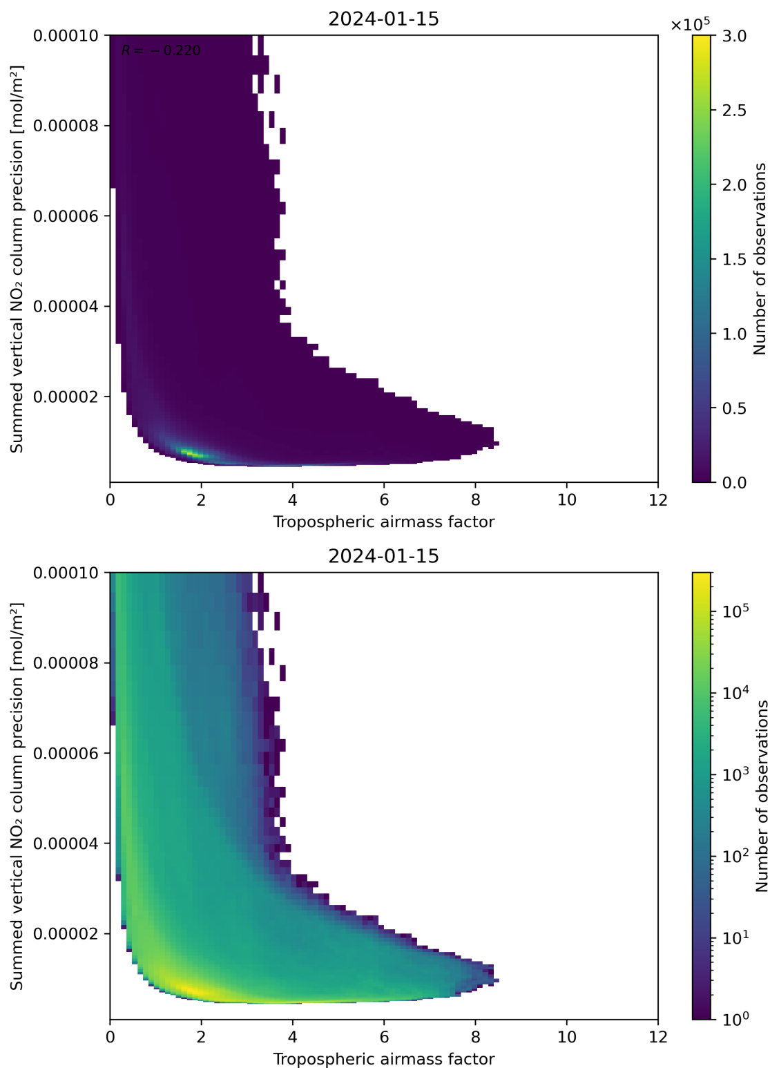
Figure 76: Scatter density plot of “Tropospheric air mass factor” against “Summed vertical NO 2 column precision” for 2024-01-15 to 2024-01-16.
