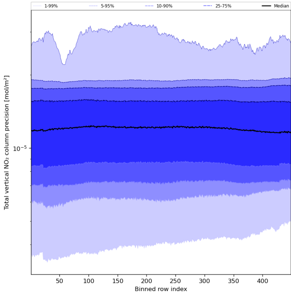
Figure 56: Along track statistics of “Total vertical NO 2 column precision” for 2024-01-15 to 2024-01-16
