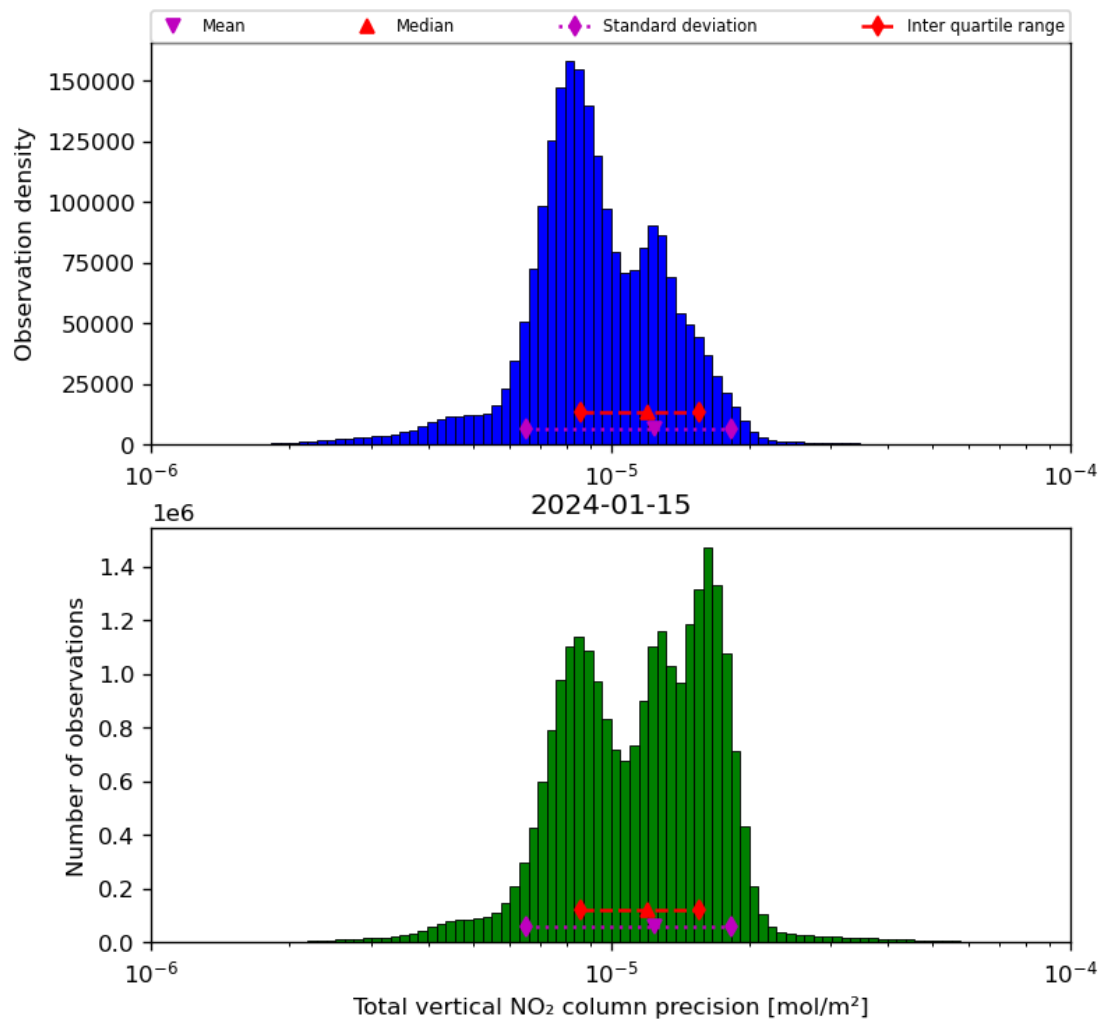
Figure 39: Histogram of “Total vertical NO 2 column precision” for 2024-01-15 to 2024-01-16
