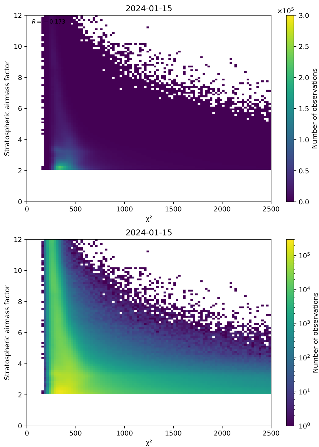
Figure 81: Scatter density plot of “ \chi^2 ” against “Stratospheric airmass factor” for 2024-01-15 to 2024-01-16.
