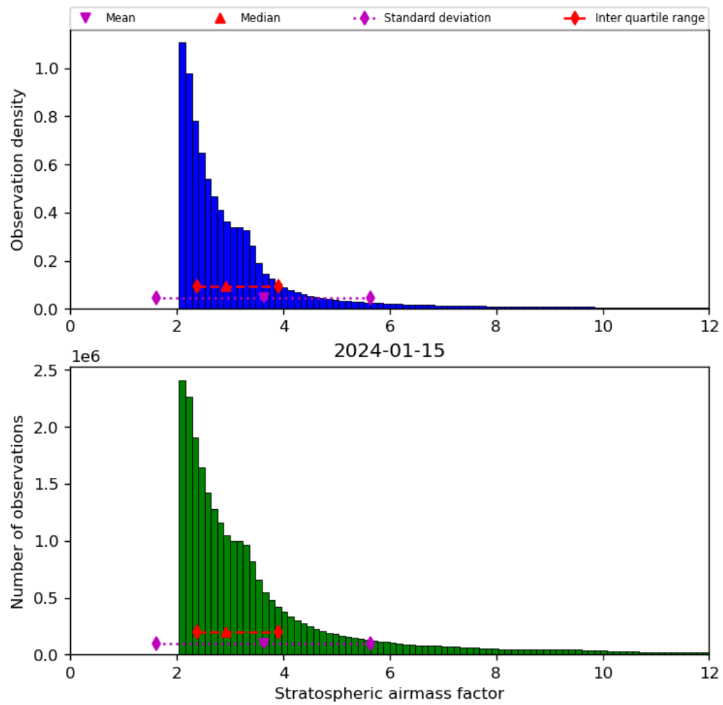
Figure 44: Histogram of “Stratospheric airmass factor” for 2024-01-15 to 2024-01-16
