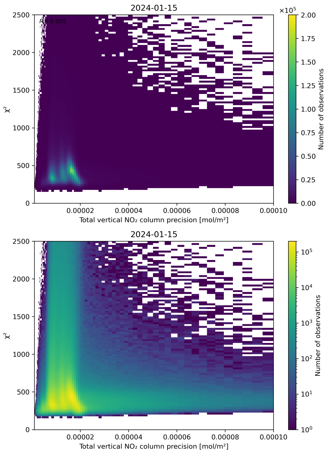
Figure 116: Scatter density plot of “Total vertical NO 2 column precision” against “ \chi^2 ” for 2024-01-15 to 2024-01-16.
