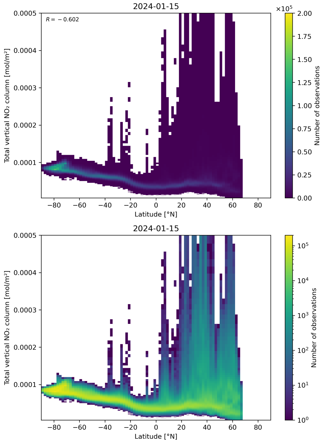
Figure 90: Scatter density plot of “Latitude” against “Total vertical NO 2 column” for 2024-01-15 to 2024-01-16.
