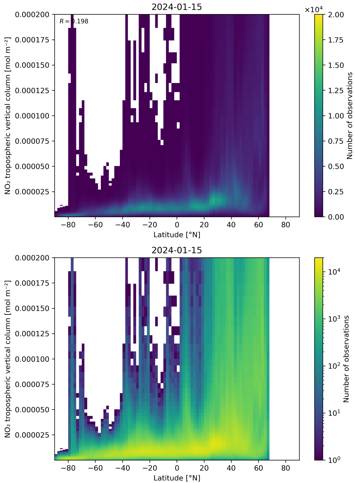
Figure 92: Scatter density plot of “Latitude” against “NO 2 tropospheric vertical column” for 2024-01-15 to 2024-01-16.
