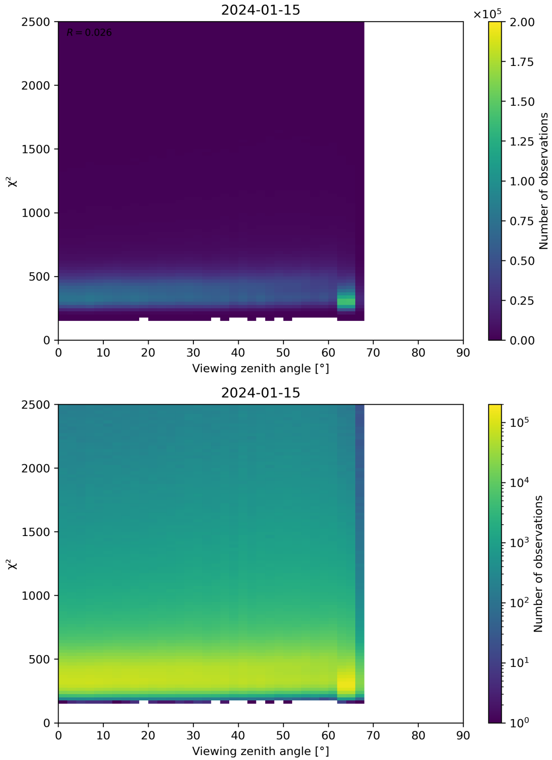
Figure 162: Scatter density plot of “Viewing zenith angle” against “ \chi^2 ” for 2024-01-15 to 2024-01-16.
