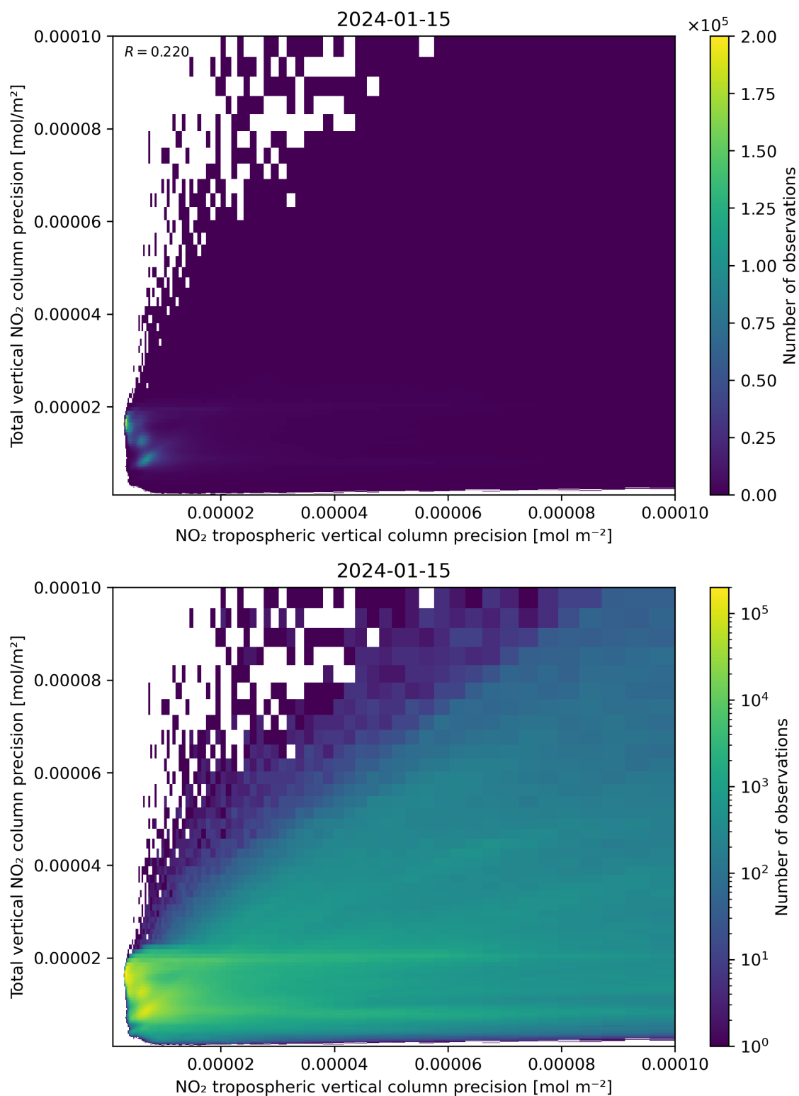
Figure 139: Scatter density plot of “NO 2 tropospheric vertical column precision” against “Total vertical NO 2 column precision” for 2024-01-15 to 2024-01-16.
