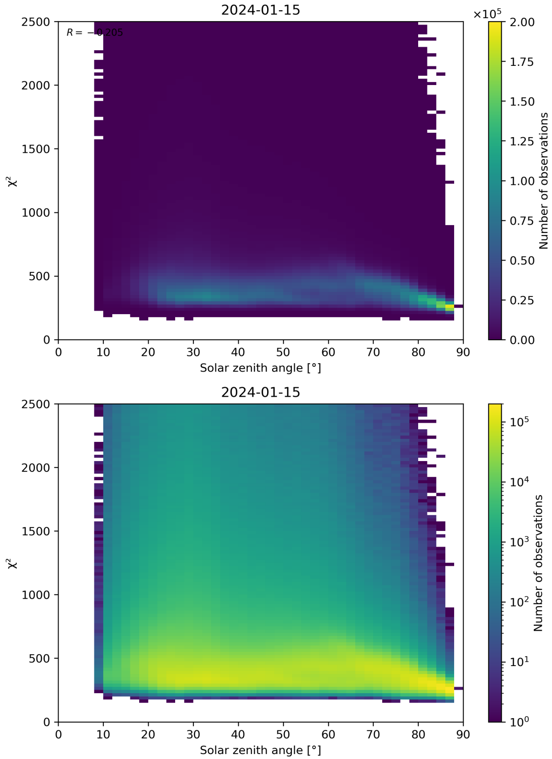
Figure 148: Scatter density plot of “Solar zenith angle” against “ \chi^2 ” for 2024-01-15 to 2024-01-16.
