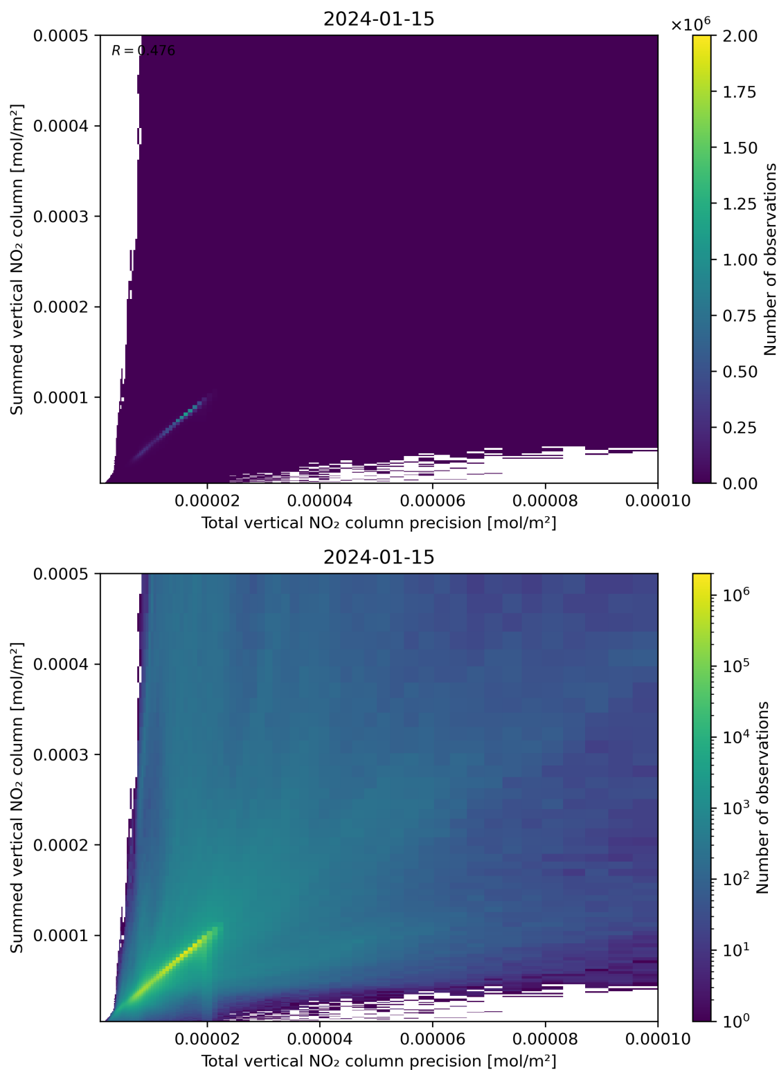
Figure 117: Scatter density plot of “Total vertical NO 2 column precision” against “Summed vertical NO 2 column” for 2024-01-15 to 2024-01-16.
