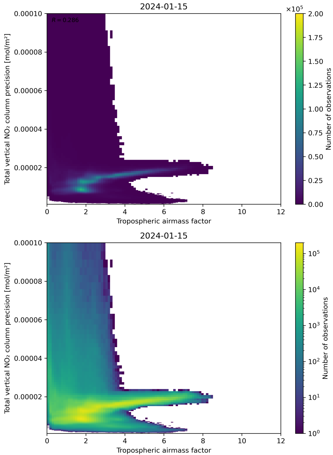
Figure 78: Scatter density plot of “Tropospheric air mass factor” against “Total vertical NO 2 column precision” for 2024-01-15 to 2024-01-16.
