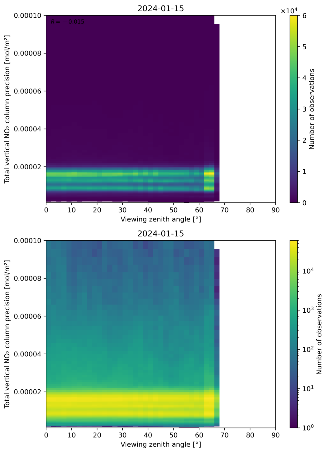
Figure 168: Scatter density plot of “Viewing zenith angle” against “Total vertical NO 2 column precision” for 2024-01-15 to 2024-01-16.
