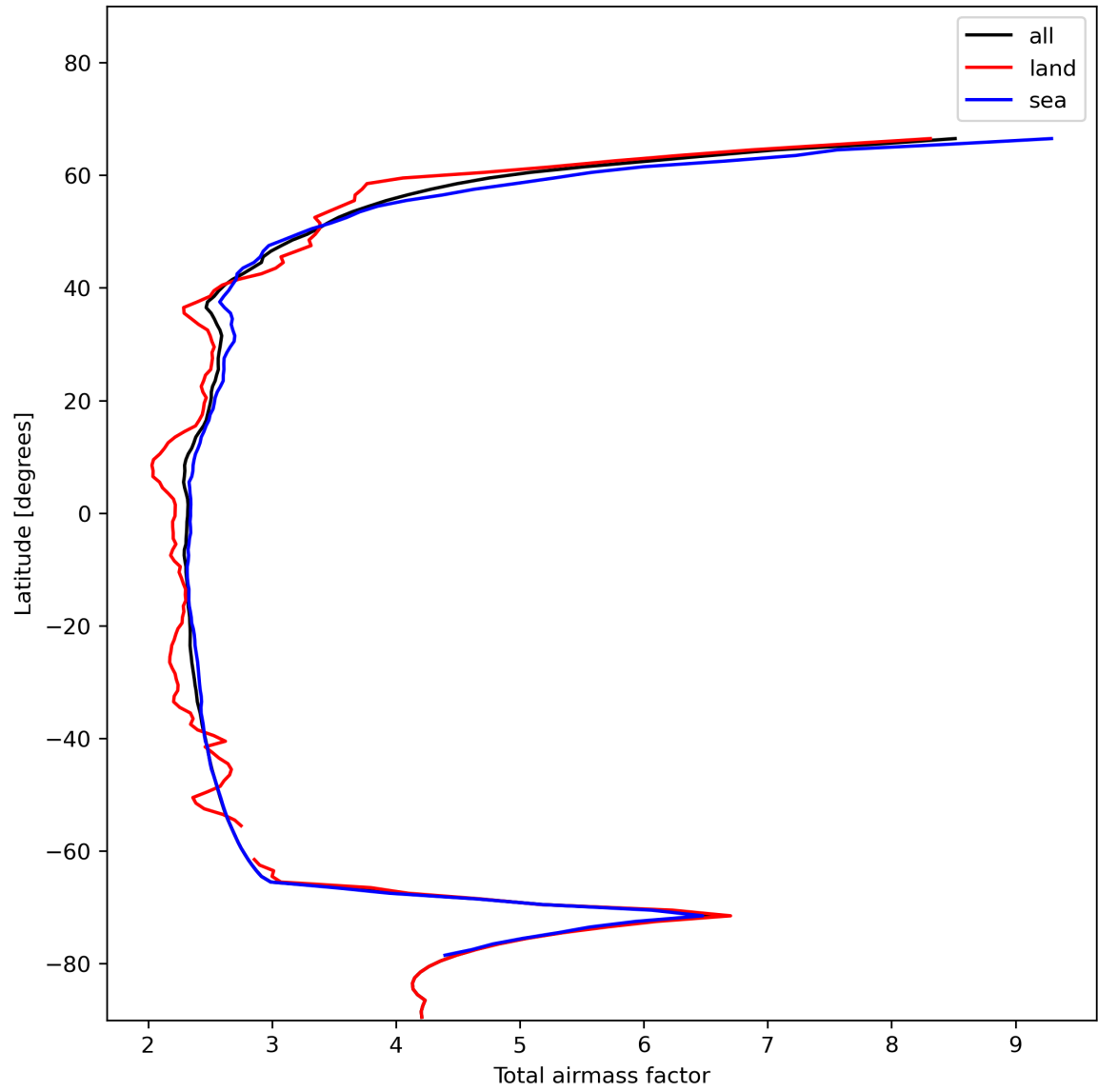
Figure 15: Zonal average of “Total airmass factor” for 2024-01-15 to 2024-01-16.
