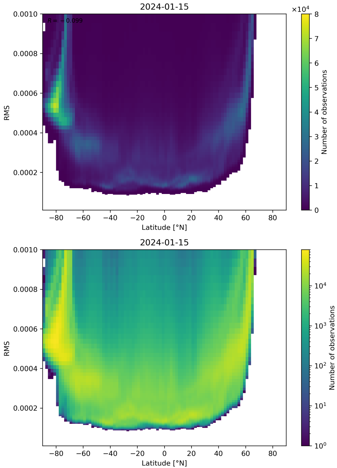
Figure 94: Scatter density plot of “Latitude” against “RMS” for 2024-01-15 to 2024-01-16.
