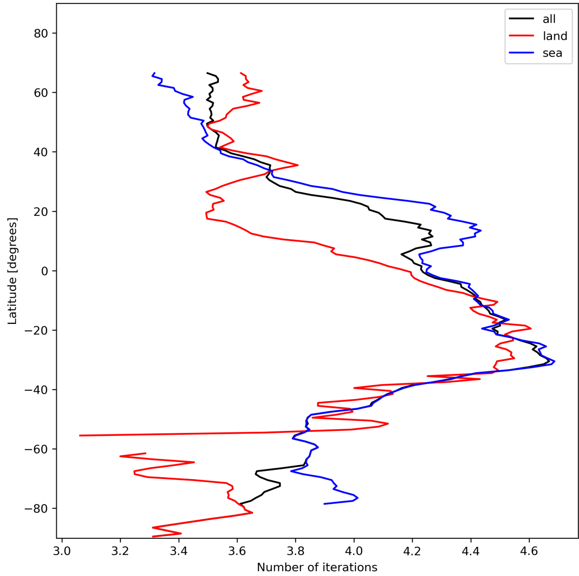
Figure 17: Zonal average of “Number of iterations” for 2024-01-15 to 2024-01-16.
