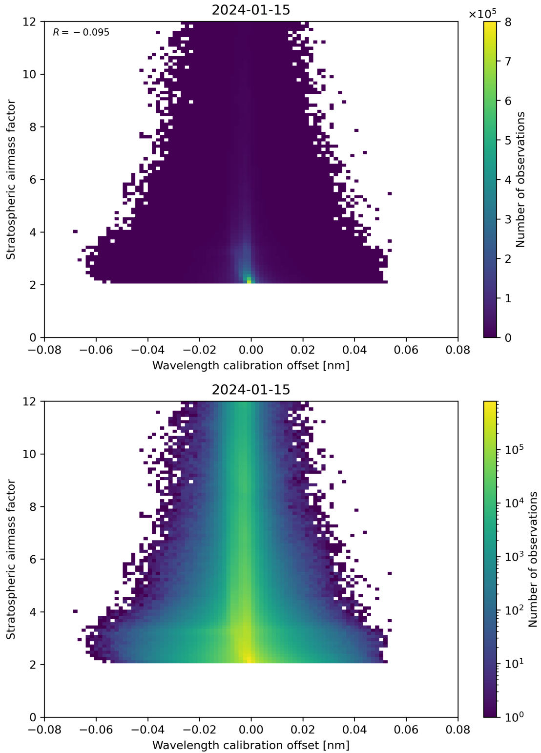
Figure 174: Scatter density plot of “Wavelength calibration offset” against “Stratospheric air mass factor” for 2024-01-15 to 2024-01-16.
