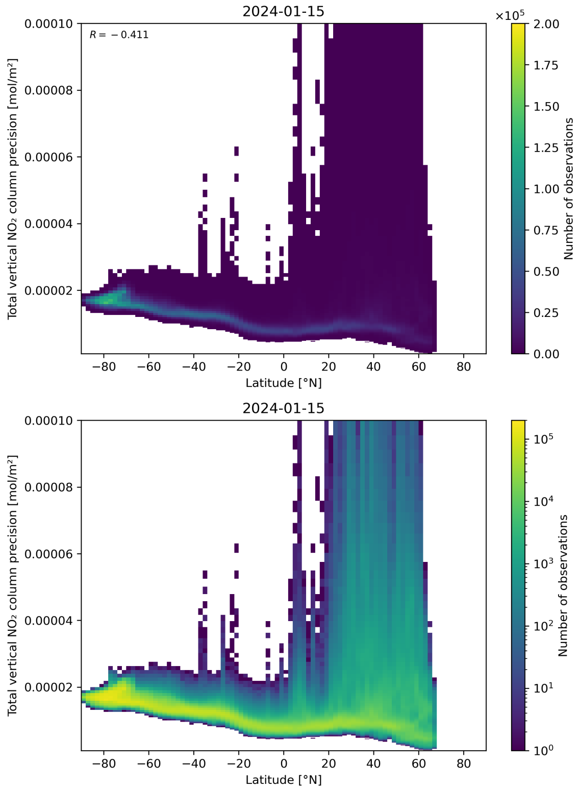
Figure 91: Scatter density plot of “Latitude” against “Total vertical NO 2 column precision” for 2024-01-15 to 2024-01-16.
