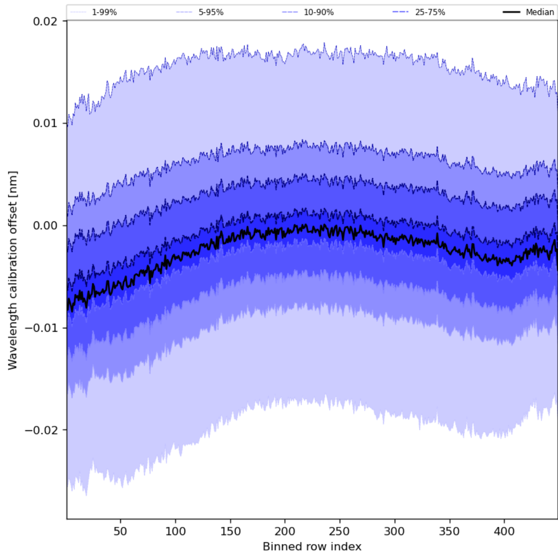
Figure 52: Along track statistics of “Wavelength calibration offset” for 2024-01-15 to 2024-01-16
