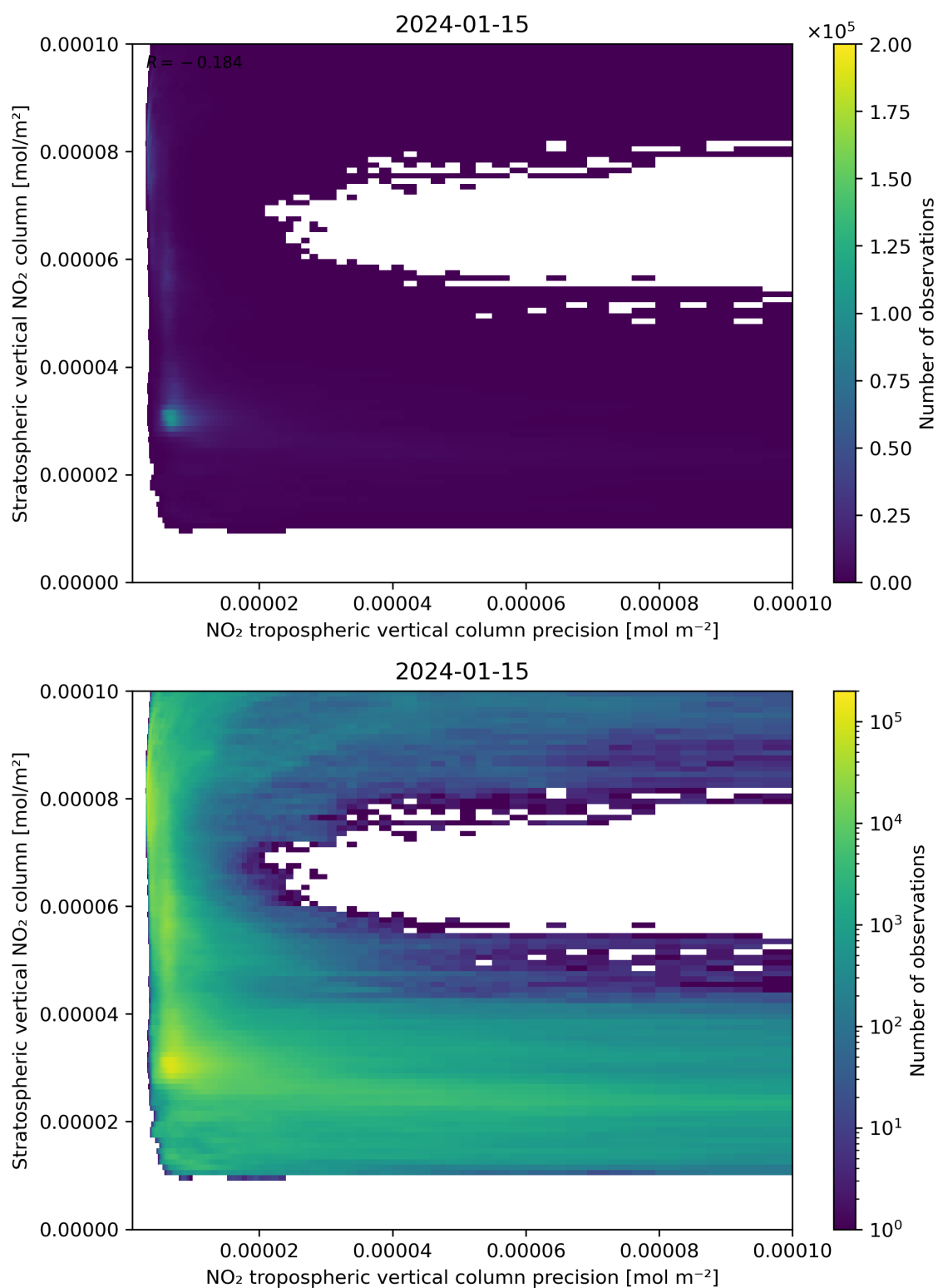
Figure 135: Scatter density plot of “NO 2 tropospheric vertical column precision” against “Stratospheric vertical NO 2 column” for 2024-01-15 to 2024-01-16.
