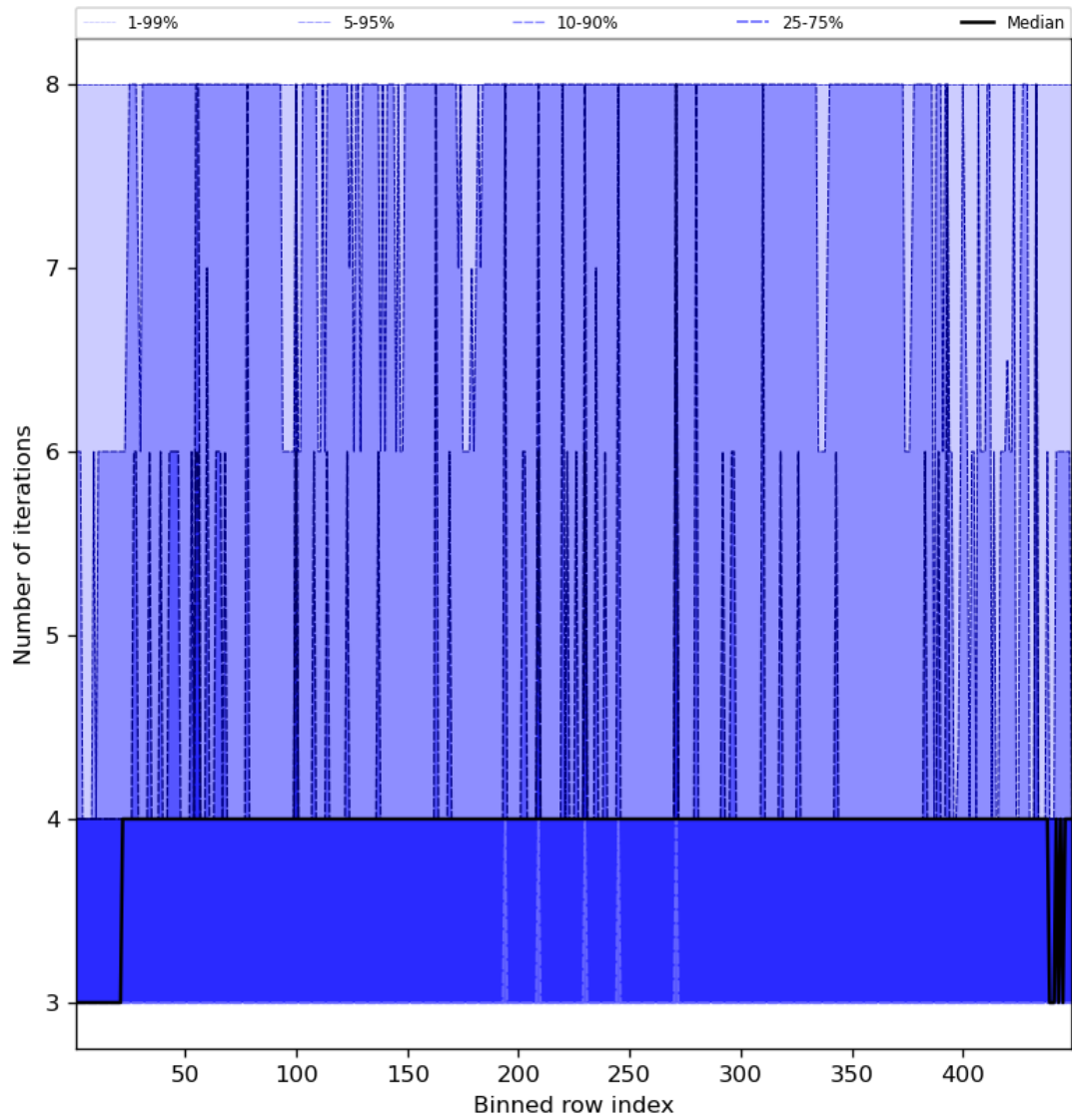
Figure 51: Along track statistics of “Number of iterations” for 2024-01-15 to 2024-01-16
