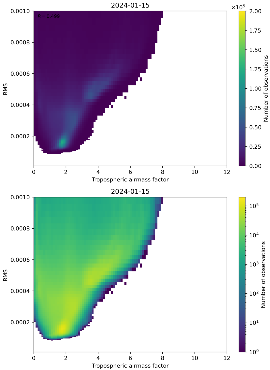
Figure 79: Scatter density plot of “Tropospheric airmass factor” against “RMS” for 2024-01-15 to 2024-01-16.
