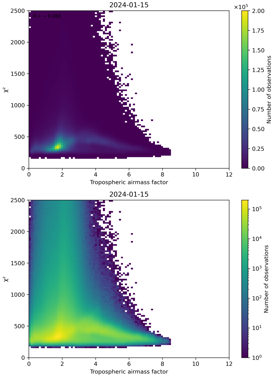
Figure 73: Scatter density plot of “Tropospheric airmass factor” against “ \chi^2 ” for 2024-01-15 to 2024-01-16.
