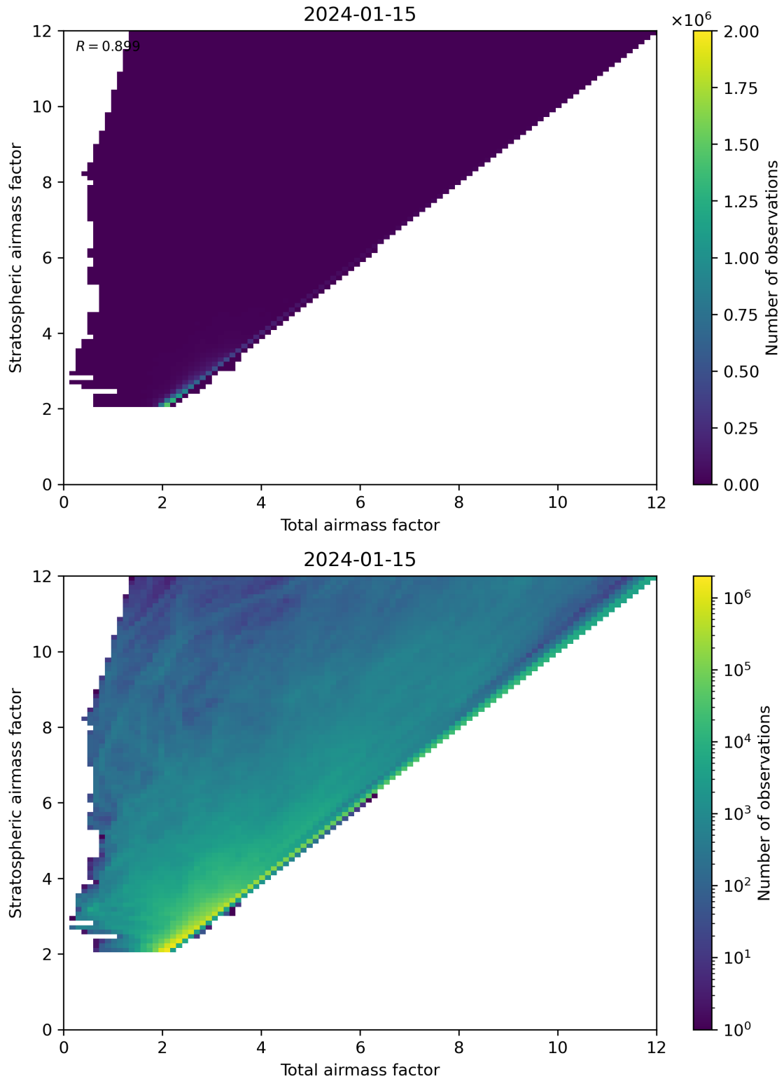
Figure 62: Scatter density plot of “Total airmass factor” against “Stratospheric airmass factor” for 2024-01-15 to 2024-01-16.
