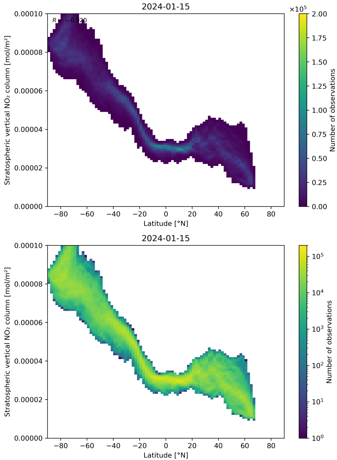
Figure 87: Scatter density plot of “Latitude” against “Stratospheric vertical NO 2 column” for 2024-01-15 to 2024-01-16.
