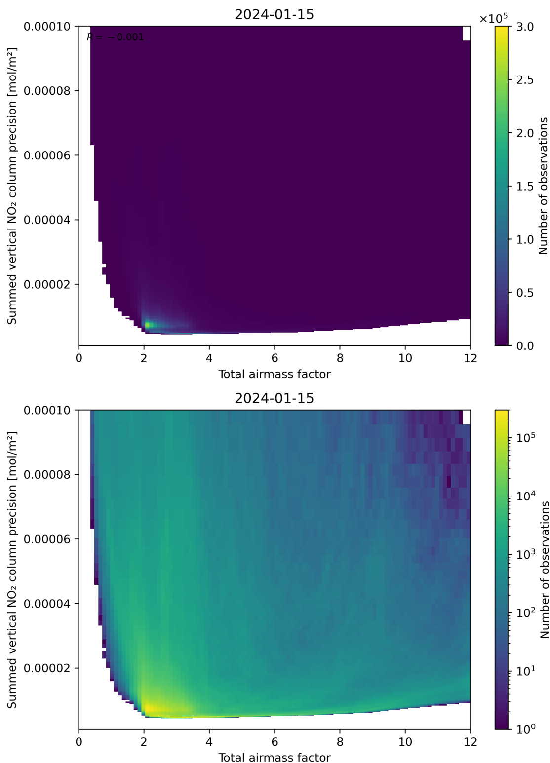
Figure 66: Scatter density plot of “Total airmass factor” against “Summed vertical NO 2 column precision” for 2024-01-15 to 2024-01-16.
