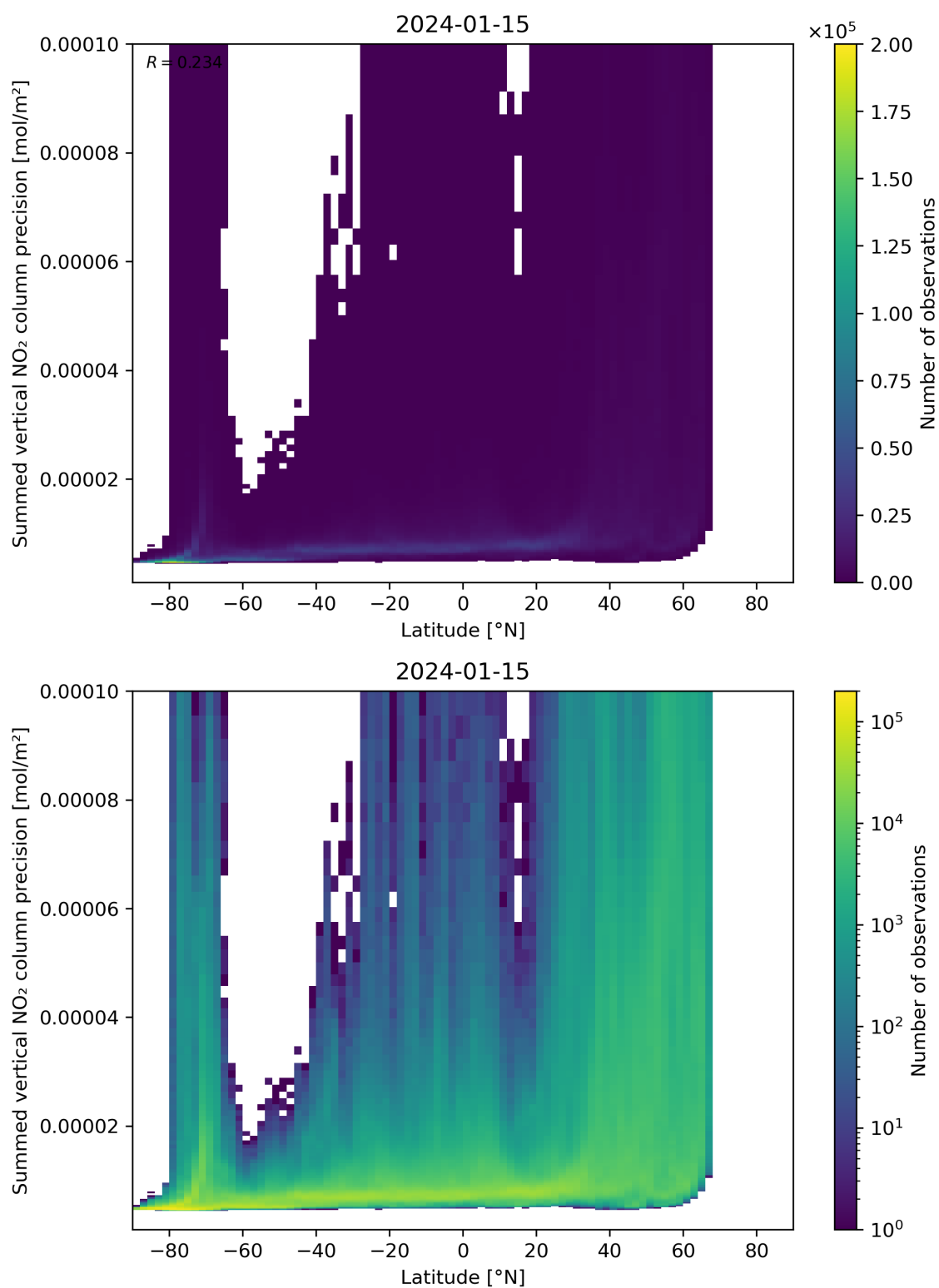
Figure 89: Scatter density plot of “Latitude” against “Summed vertical NO 2 column precision” for 2024-01-15 to 2024-01-16.
