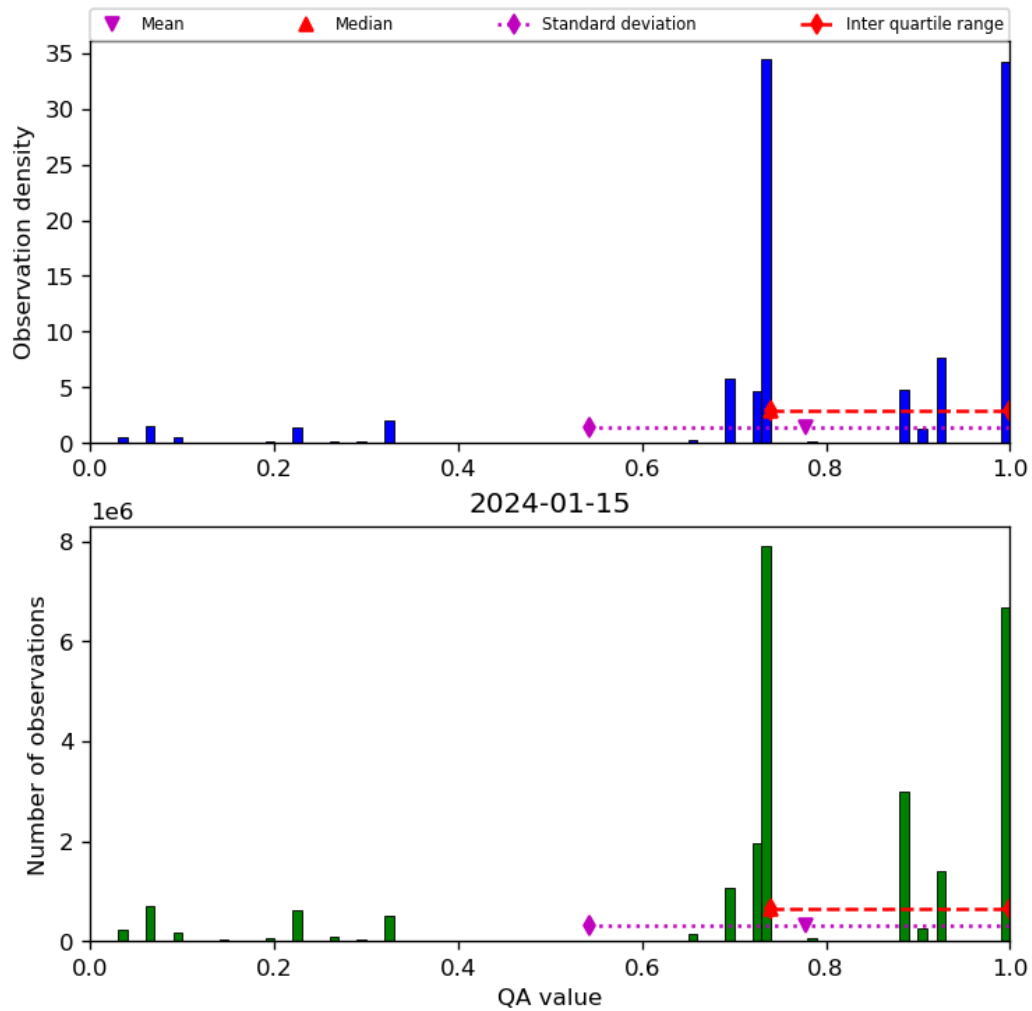
Figure 28: Histogram of “QA value” for 2024-01-15 to 2024-01-16
