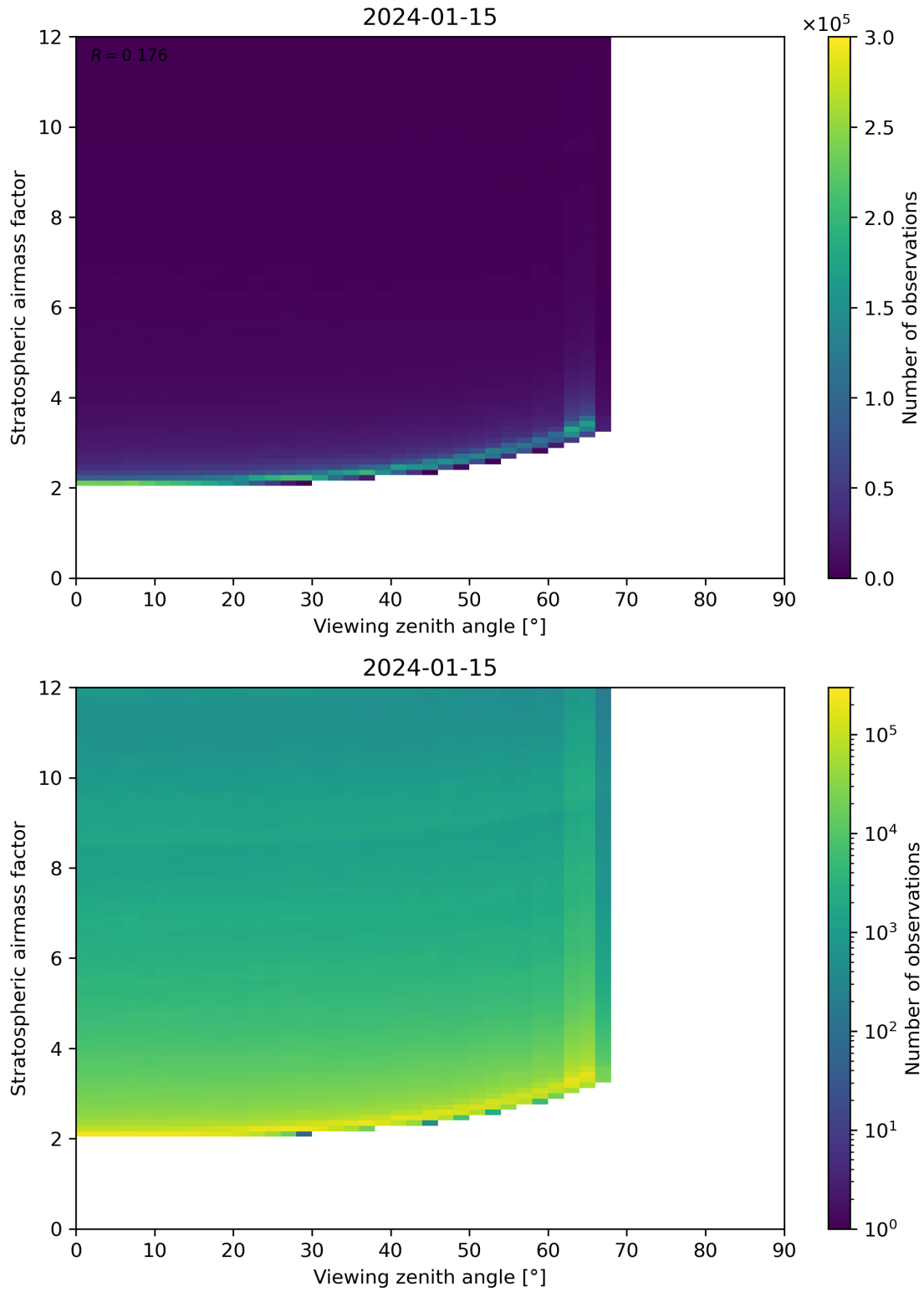
Figure 159: Scatter density plot of “Viewing zenith angle” against “Stratospheric airmass factor” for 2024-01-15 to 2024-01-16.
