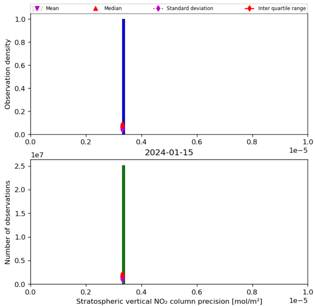
Figure 37: Histogram of “Stratospheric vertical NO 2 column precision” for 2024-01-15 to 2024-01-16
