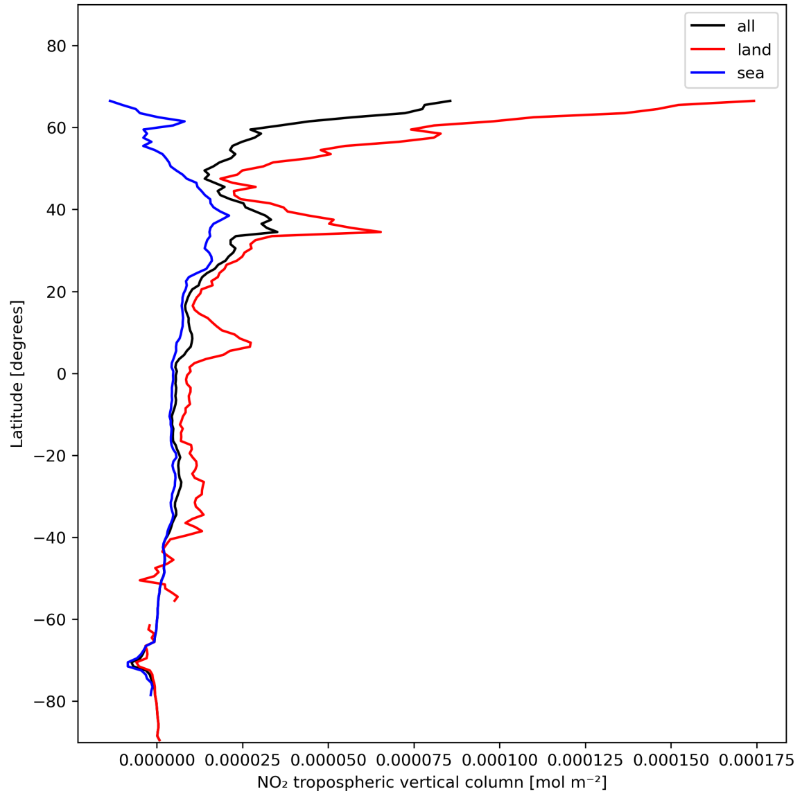
Figure 12: Zonal average of “NO 2 tropospheric vertical column” for 2024-01-15 to 2024-01-16.
