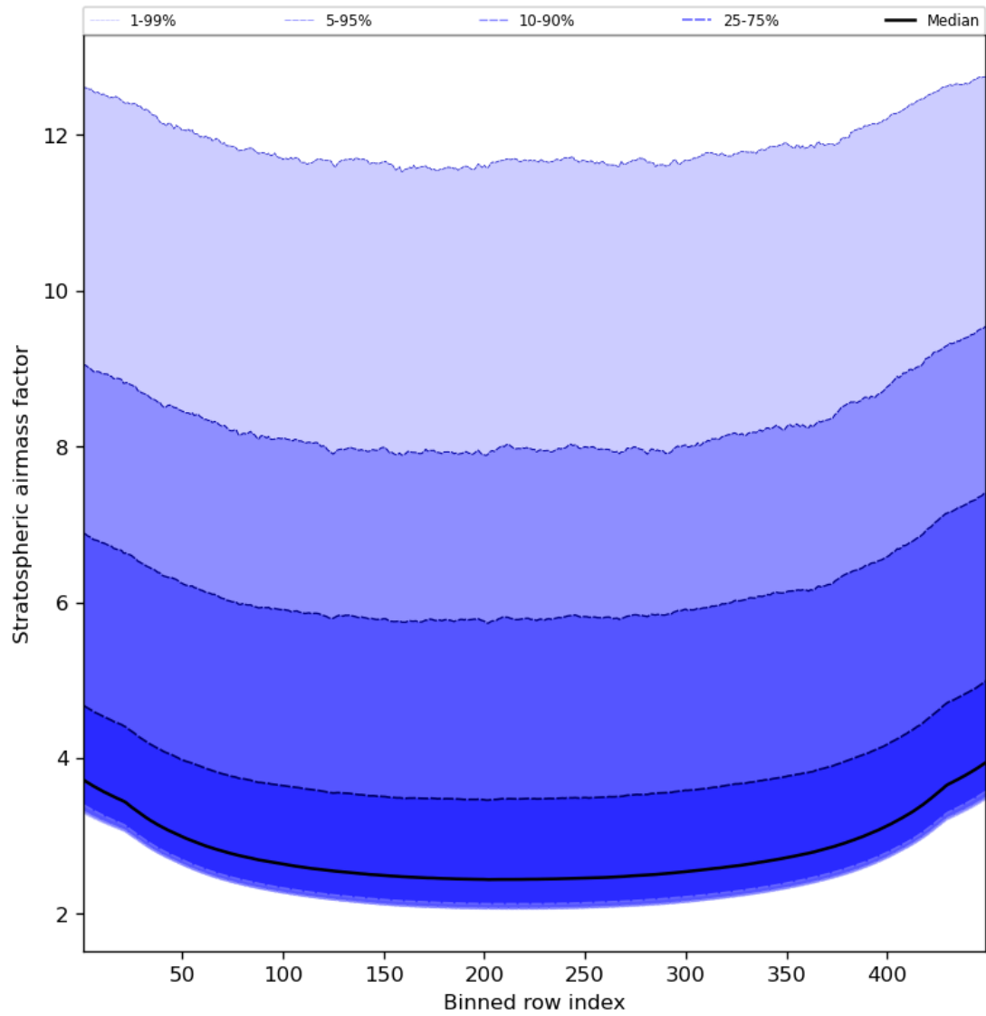
Figure 61: Along track statistics of “Stratospheric airmass factor” for 2024-01-15 to 2024-01-16
