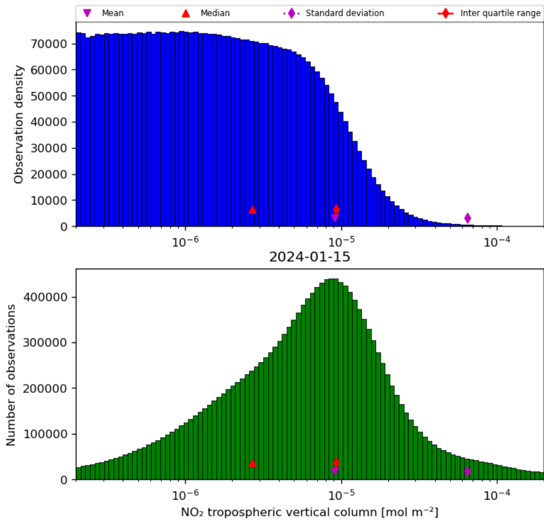
Figure 29: Histogram of “NO 2 tropospheric vertical column” for 2024-01-15 to 2024-01-16
