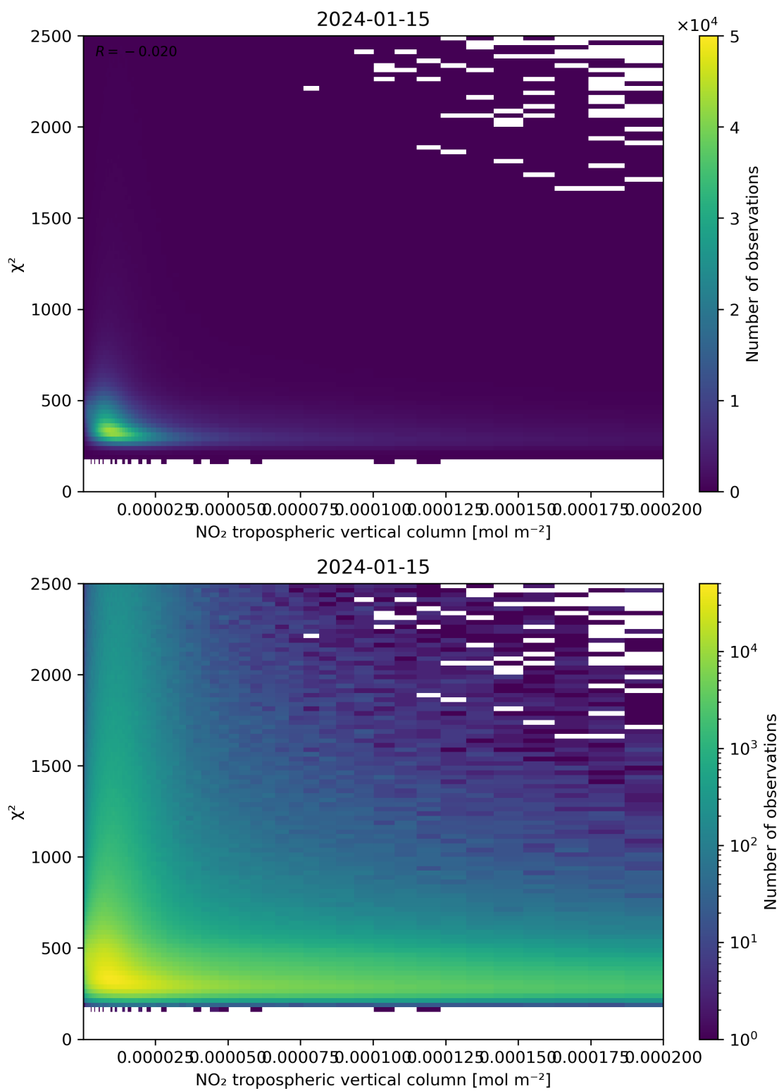
Figure 124: Scatter density plot of “NO 2 tropospheric vertical column” against “ \chi^2 ” for 2024-01-15 to 2024-01-16.
