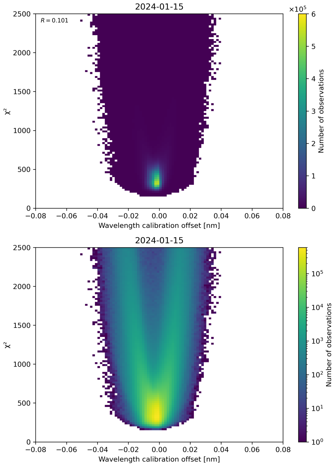
Figure 175: Scatter density plot of “Wavelength calibration offset” against “ \chi^2 ” for 2024-01-15 to 2024-01-16.
