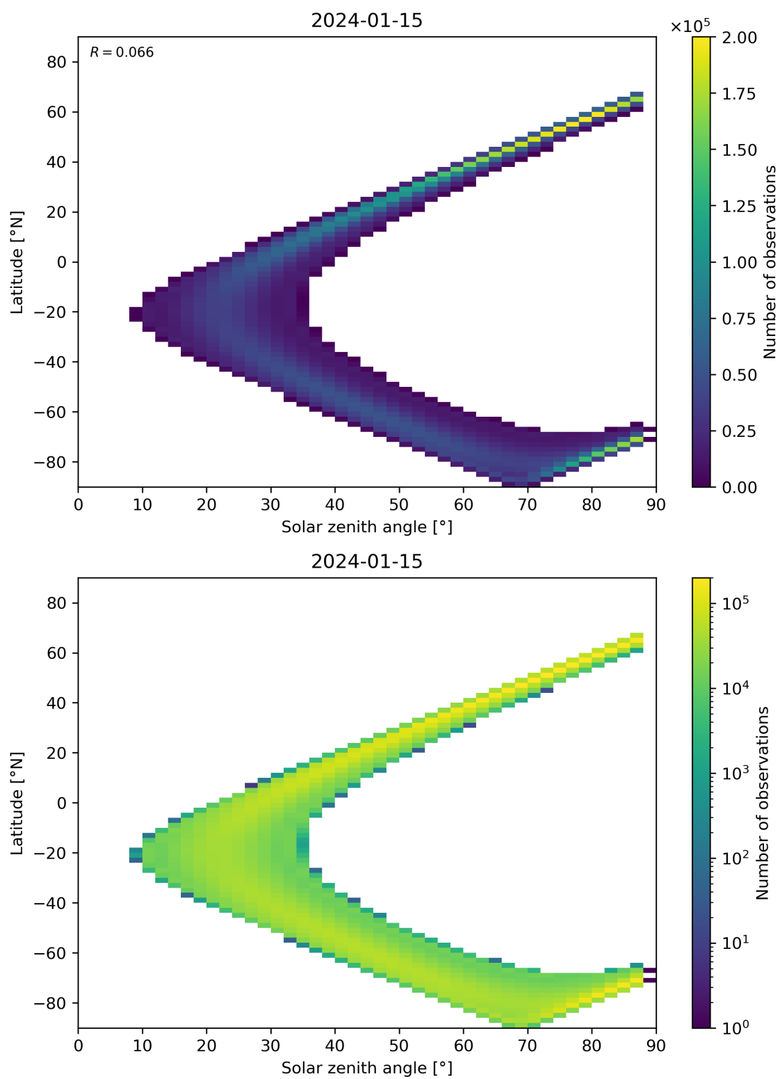
Figure 149: Scatter density plot of “Solar zenith angle” against “Latitude” for 2024-01-15 to 2024-01-16.
