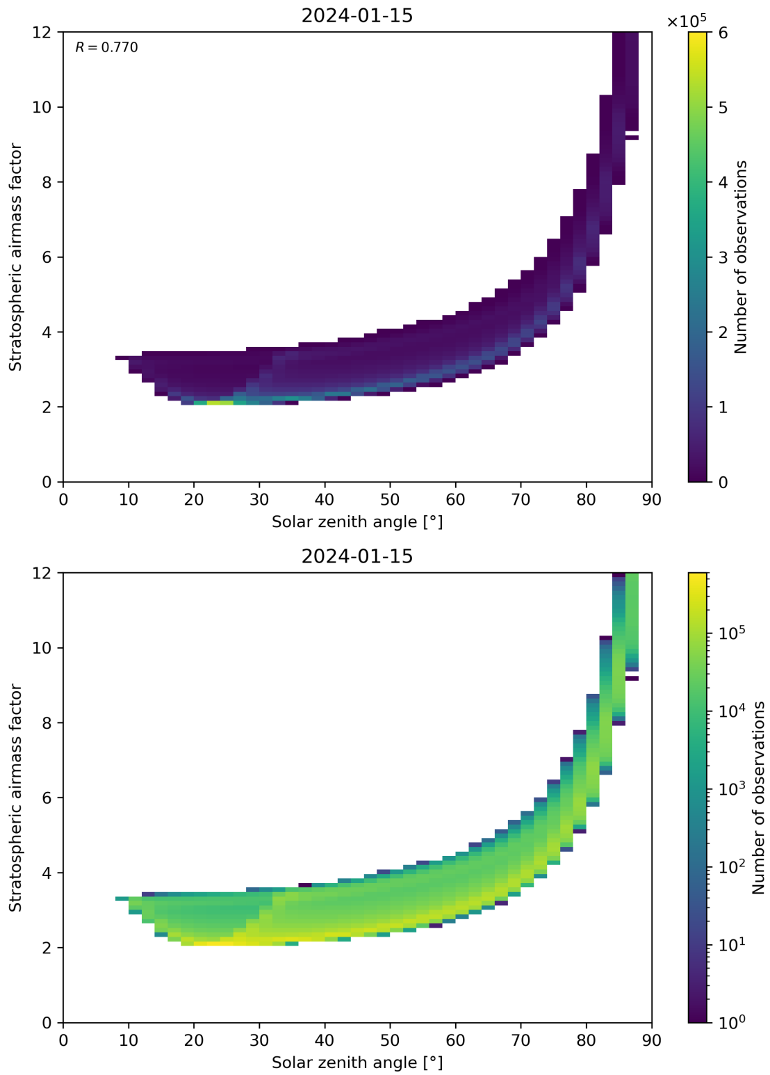
Figure 145: Scatter density plot of “Solar zenith angle” against “Stratospheric airmass factor” for 2024-01-15 to 2024-01-16.
