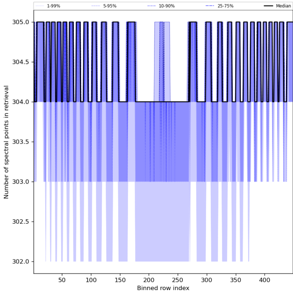
Figure 50: Along track statistics of “Number of spectral points in retrieval” for 2024-01-15 to 2024-01-16
