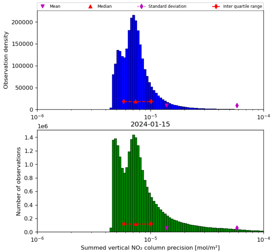
Figure 41: Histogram of "Summed vertical NO 2 column precision" for 2024-01-15 to 2024-01-16
