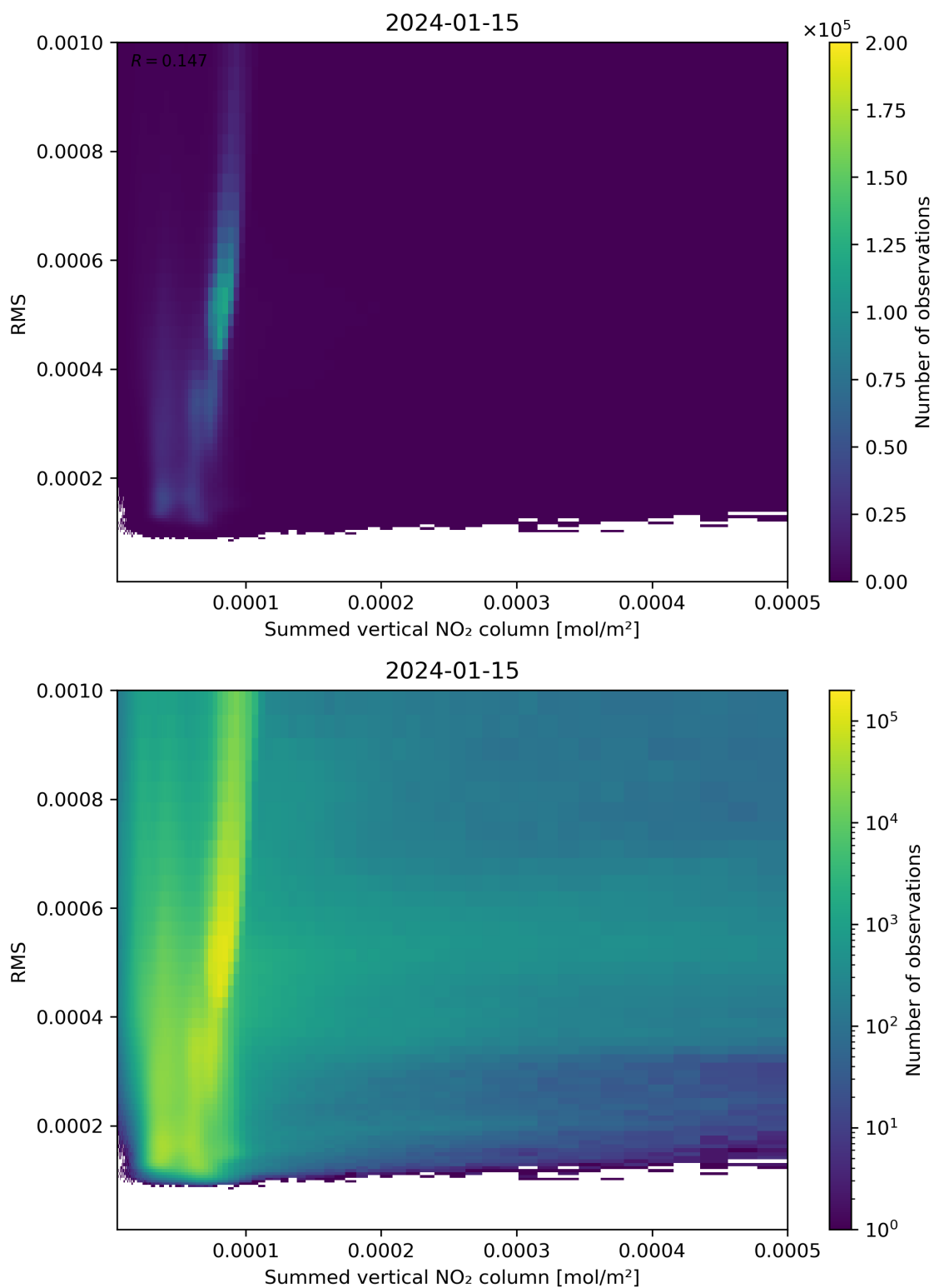
Figure 109: Scatter density plot of “Summed vertical NO 2 column” against “RMS” for 2024-01-15 to 2024-01-16.
