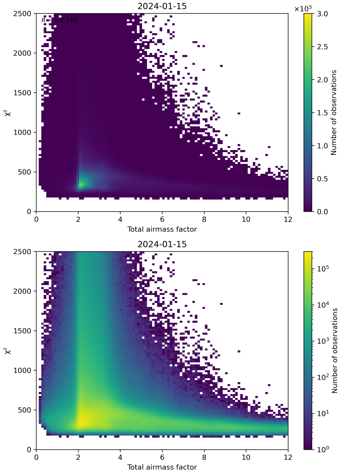
Figure 63: Scatter density plot of “Total airmass factor” against “ \chi^2 ” for 2024-01-15 to 2024-01-16.
