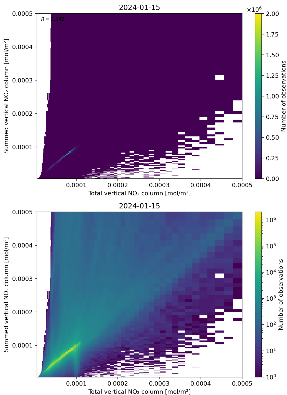
Figure 112: Scatter density plot of “Total vertical NO 2 column” against “Summed vertical NO 2 column” for 2024-01-15 to 2024-01-16.
