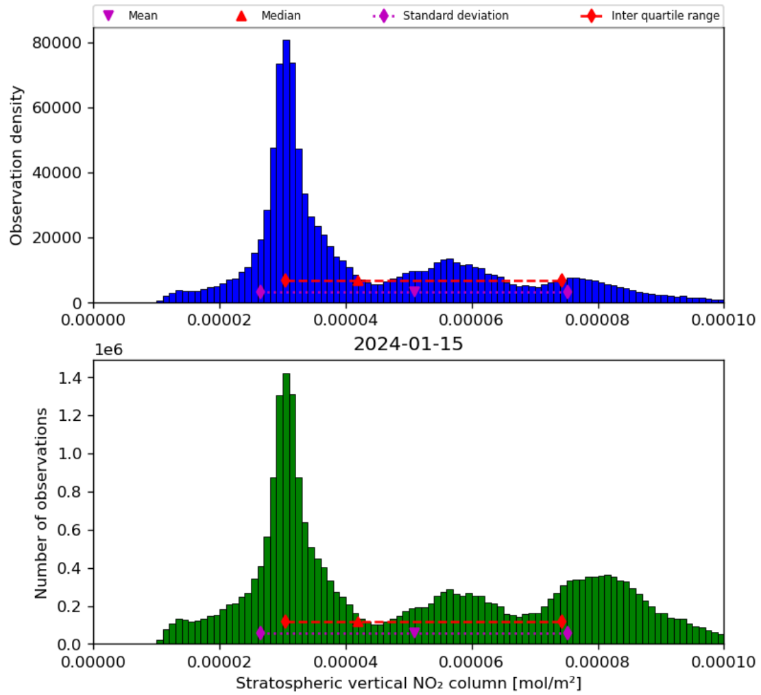
Figure 36: Histogram of “Stratospheric vertical NO 2 column” for 2024-01-15 to 2024-01-16
