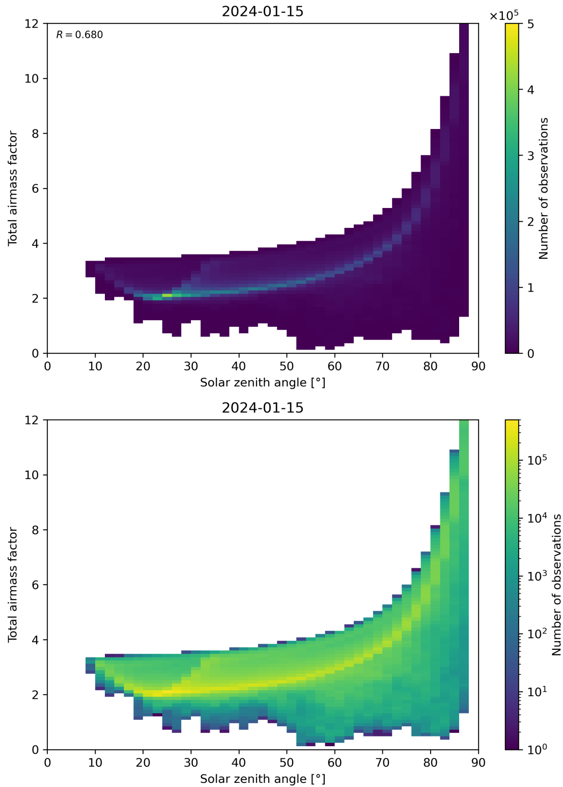
Figure 146: Scatter density plot of “Solar zenith angle” against “Total air mass factor” for 2024-01-15 to 2024-01-16.
