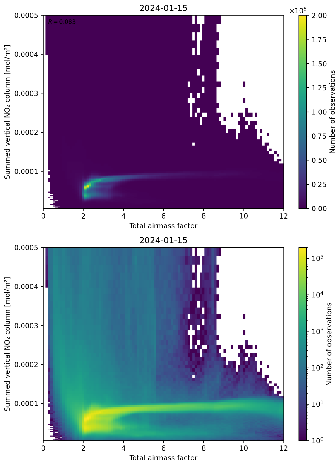
Figure 65: Scatter density plot of “Total airmass factor” against “Summed vertical NO 2 column” for 2024-01-15 to 2024-01-16.
