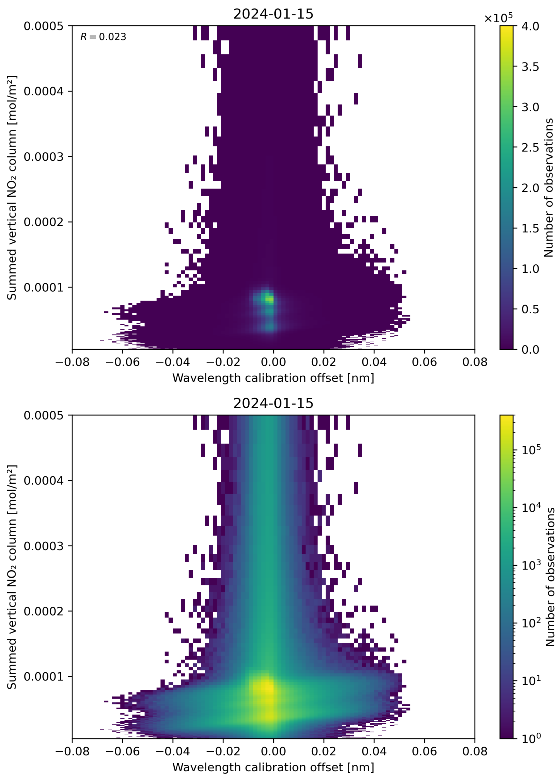
Figure 177: Scatter density plot of “Wavelength calibration offset” against “Summed vertical NO 2 column” for 2024-01-15 to 2024-01-16.
