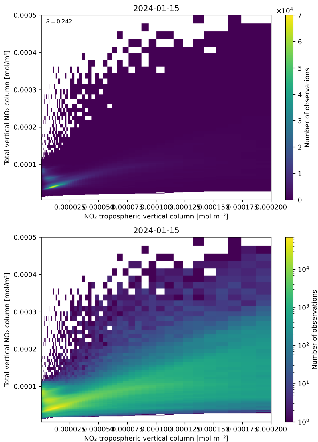
Figure 128: Scatter density plot of “NO 2 tropospheric vertical column” against “Total vertical NO 2 column” for 2024-01-15 to 2024-01-16.
