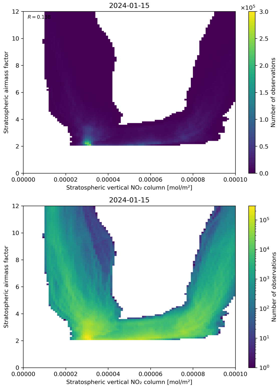
Figure 96: Scatter density plot of “Stratospheric vertical NO 2 column” against “Stratospheric airmass factor” for 2024-01-15 to 2024-01-16.
