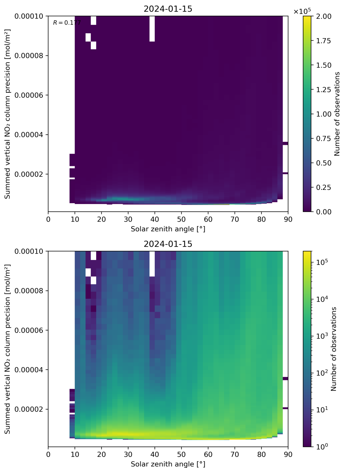
Figure 152: Scatter density plot of “Solar zenith angle” against “Summed vertical NO 2 column precision” for 2024-01-15 to 2024-01-16.
