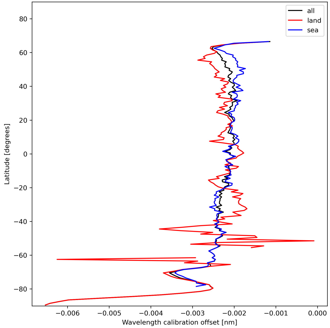
Figure 18: Zonal average of “Wavelength calibration offset” for 2024-01-15 to 2024-01-16.
