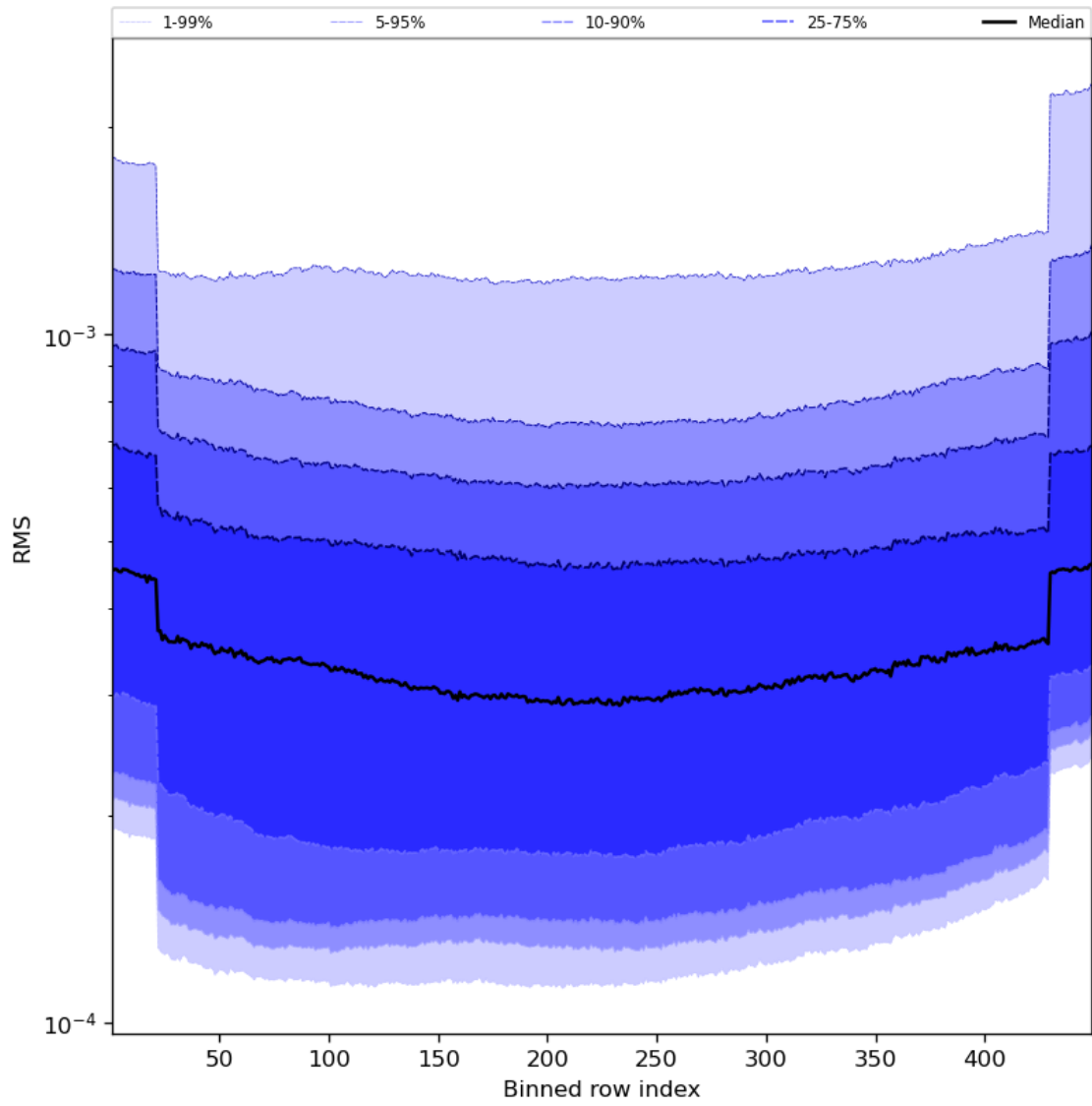
Figure 60: Along track statistics of “RMS” for 2024-01-15 to 2024-01-16
