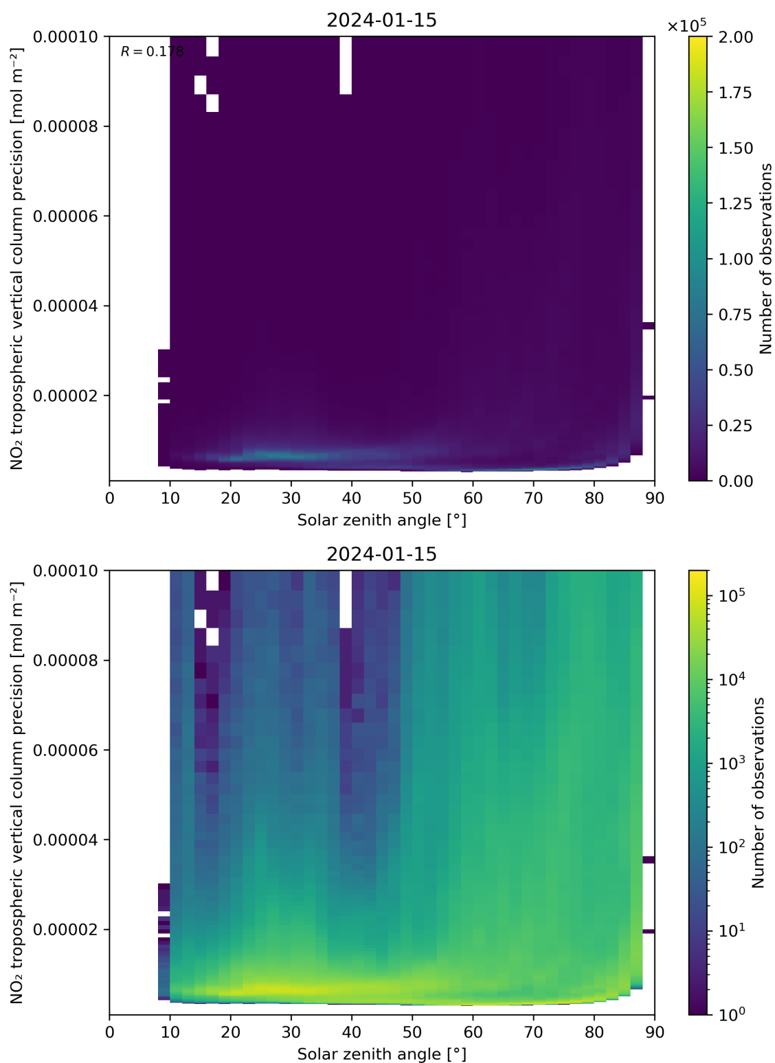
Figure 156: Scatter density plot of “Solar zenith angle” against “NO 2 tropospheric vertical column precision” for 2024-01-15 to 2024-01-16.
