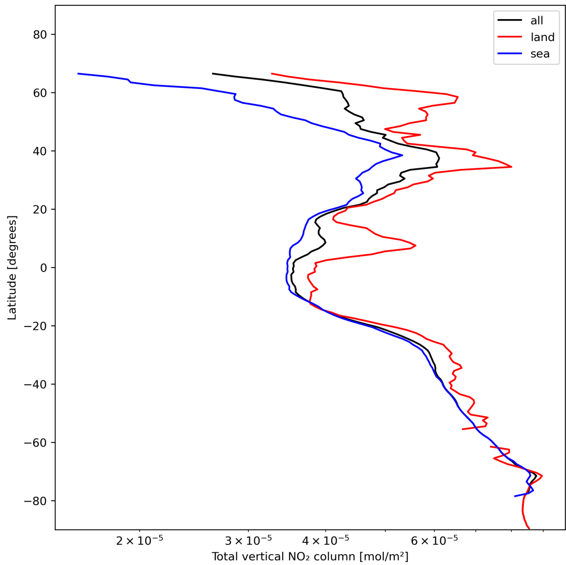
Figure 21: Zonal average of “Total vertical NO 2 column” for 2024-01-15 to 2024-01-16.
