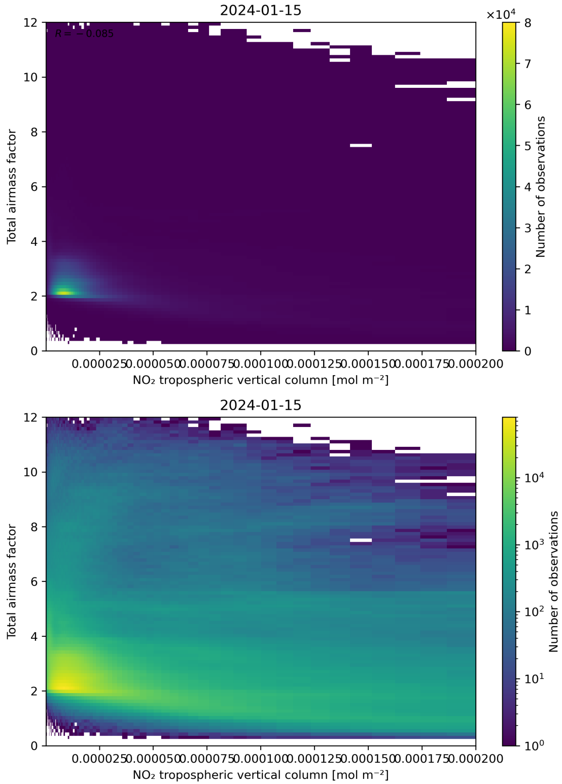
Figure 122: Scatter density plot of “NO 2 tropospheric vertical column” against “Total air mass factor” for 2024-01-15 to 2024-01-16.
