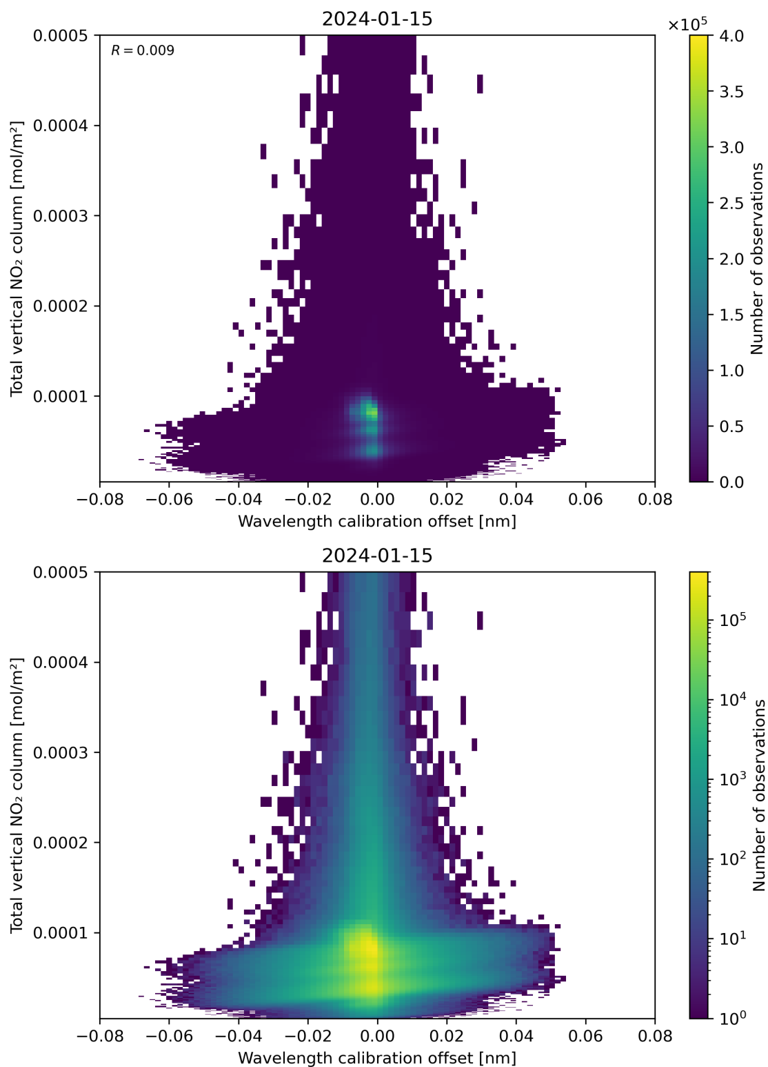
Figure 179: Scatter density plot of “Wavelength calibration offset” against “Total vertical NO 2 column” for 2024-01-15 to 2024-01-16.
