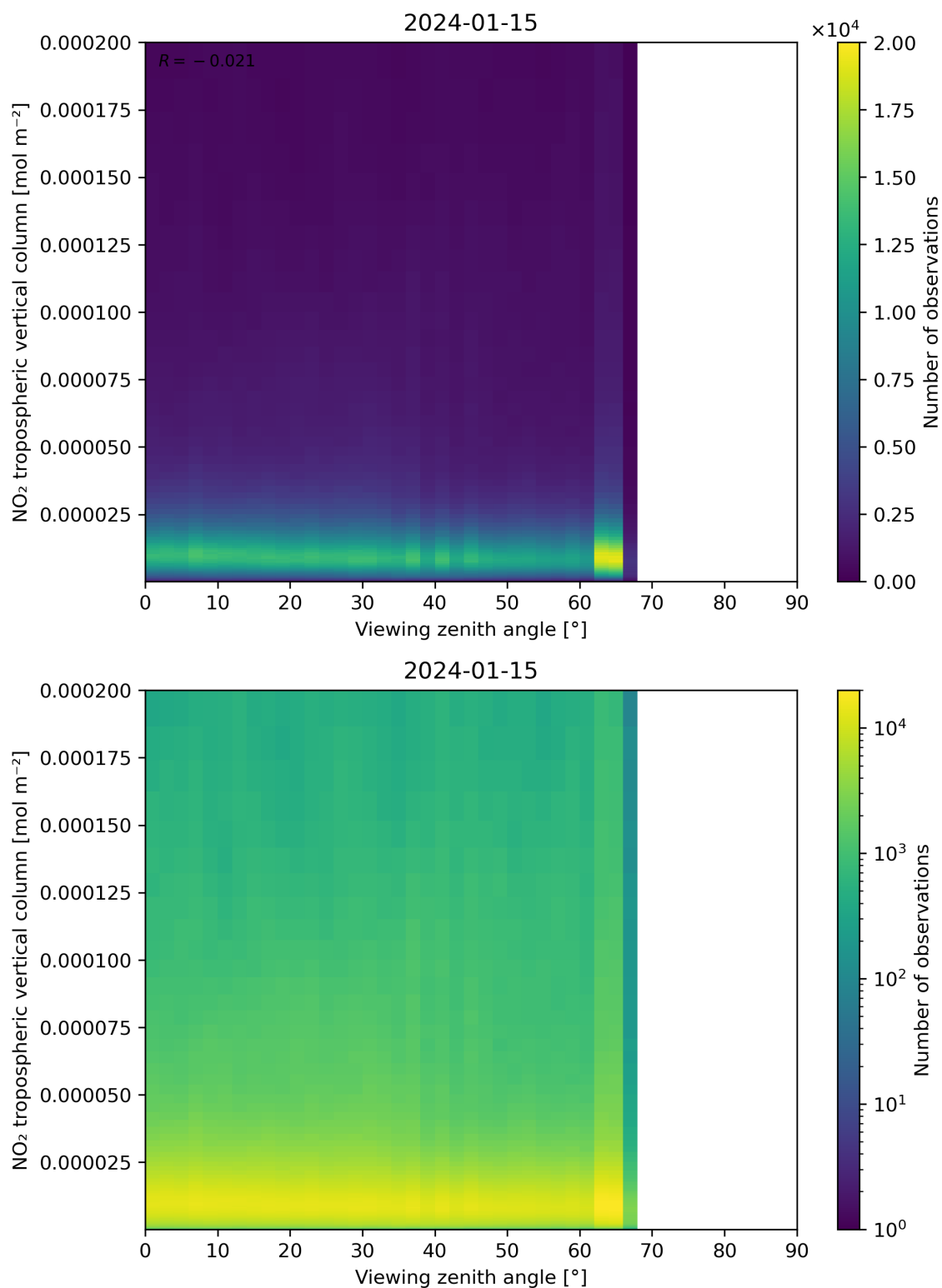
Figure 169: Scatter density plot of “Viewing zenith angle” against “NO 2 tropospheric vertical column” for 2024-01-15 to 2024-01-16.
