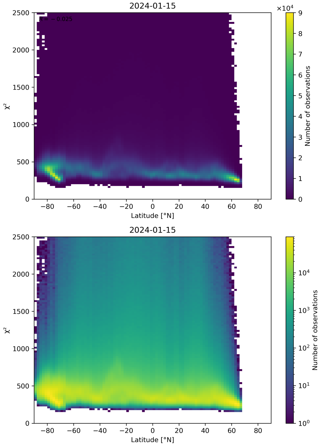
Figure 86: Scatter density plot of “Latitude” against “ \chi^2 ” for 2024-01-15 to 2024-01-16.
