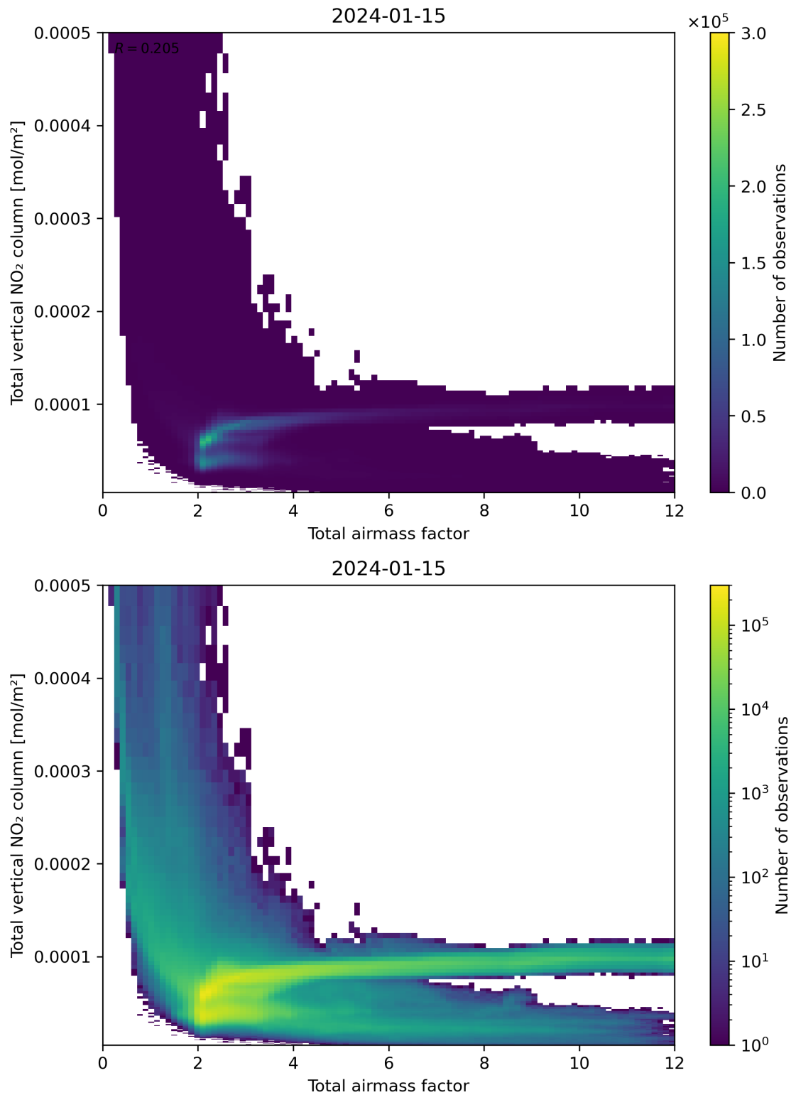
Figure 67: Scatter density plot of “Total airmass factor” against “Total vertical NO 2 column” for 2024-01-15 to 2024-01-16.
