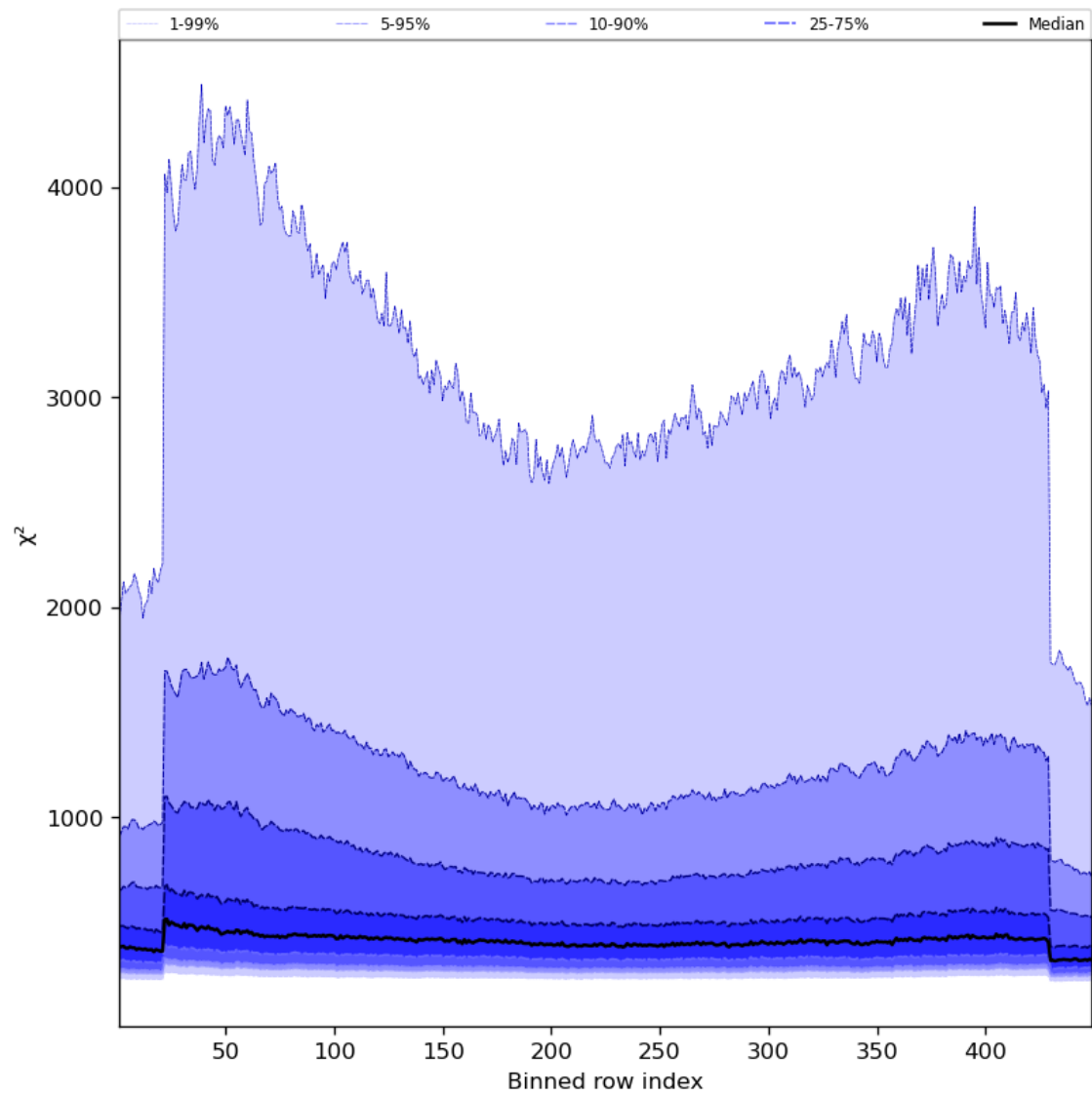
Figure 59: Along track statistics of “ \chi^2 ” for 2024-01-15 to 2024-01-16
