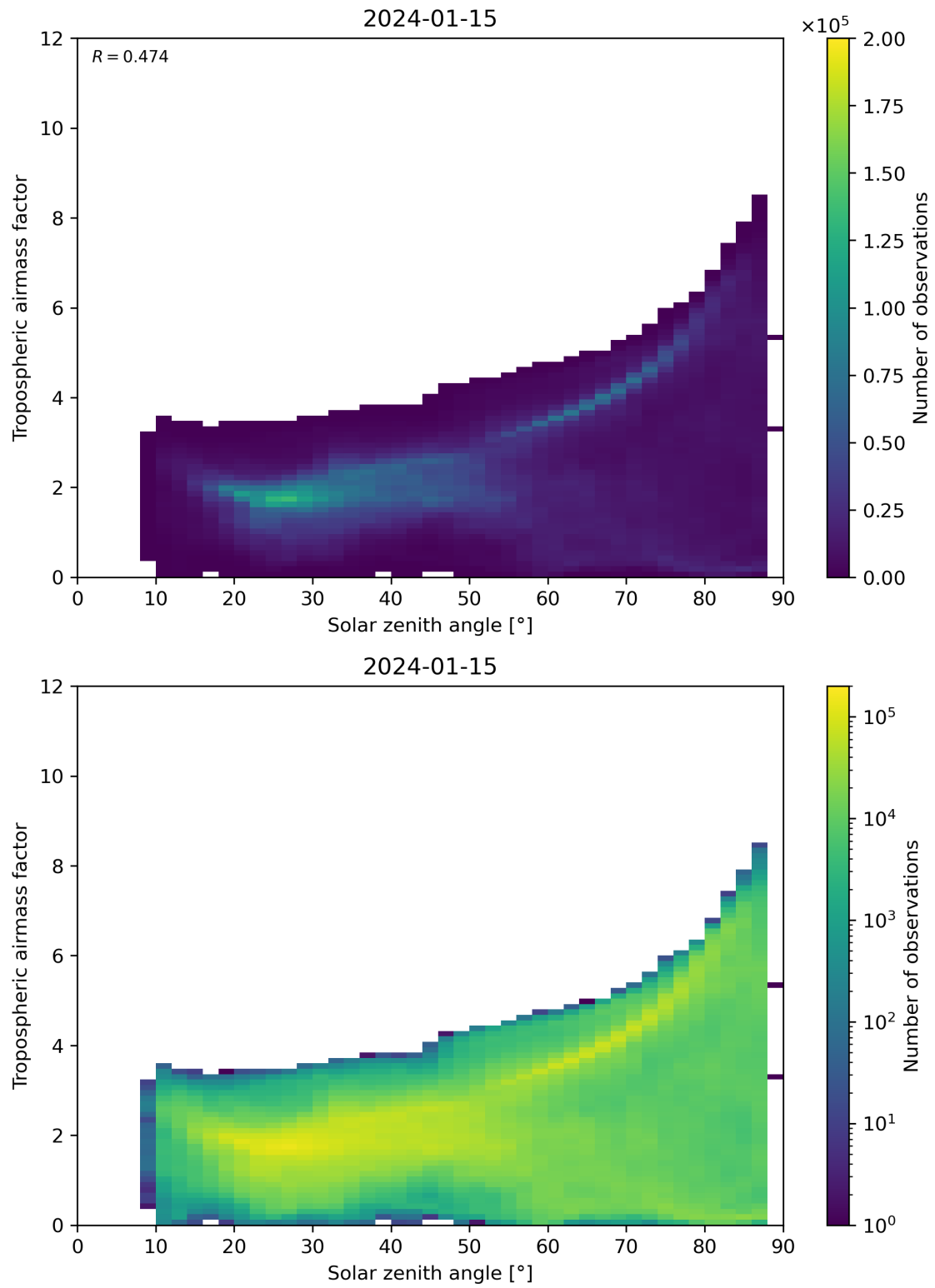
Figure 147: Scatter density plot of “Solar zenith angle” against “Tropospheric airmass factor” for 2024-01-15 to 2024-01-16.
