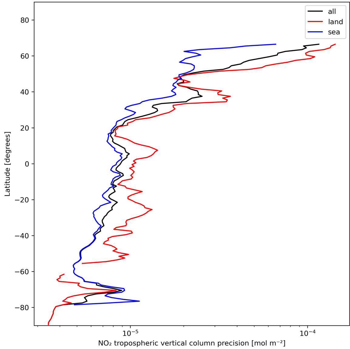
Figure 13: Zonal average of “NO 2 tropospheric vertical column precision” for 2024-01-15 to 2024-01-16.
