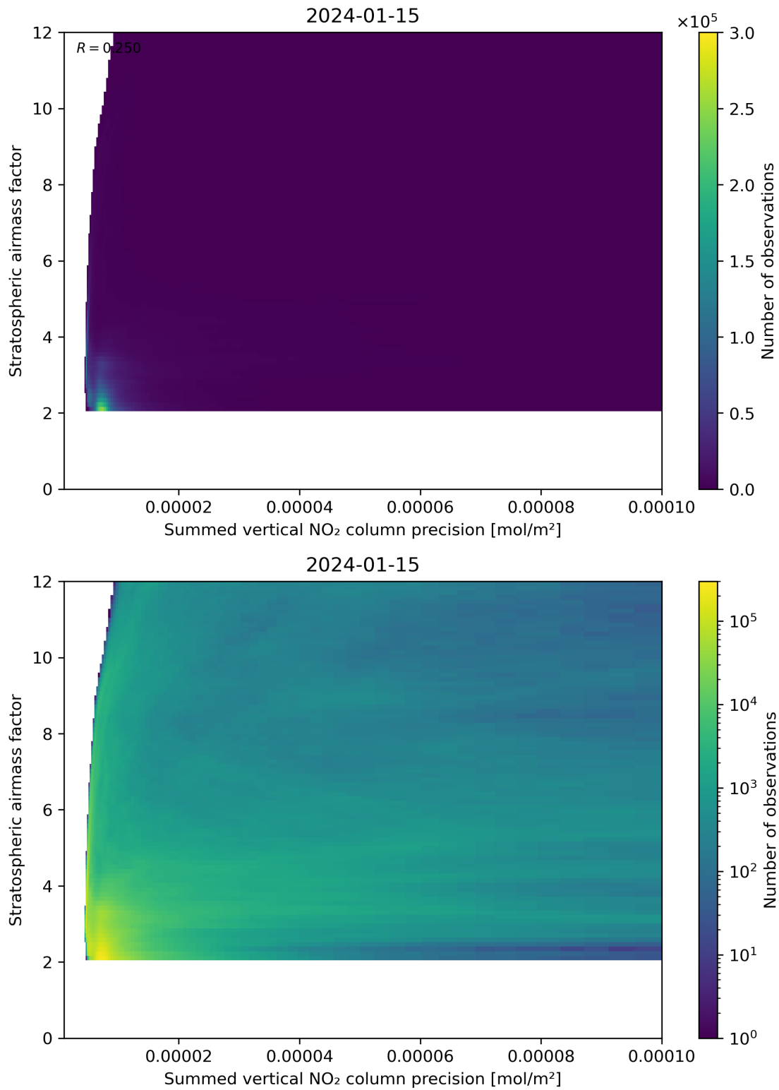
Figure 106: Scatter density plot of “Summed vertical NO 2 column precision” against “Stratospheric airmass factor” for 2024-01-15 to 2024-01-16.
