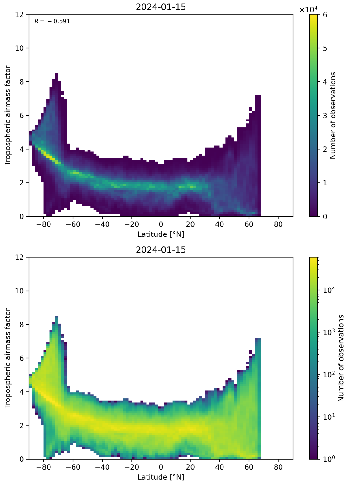
Figure 85: Scatter density plot of “Latitude” against “Tropospheric air mass factor” for 2024-01-15 to 2024-01-16.
