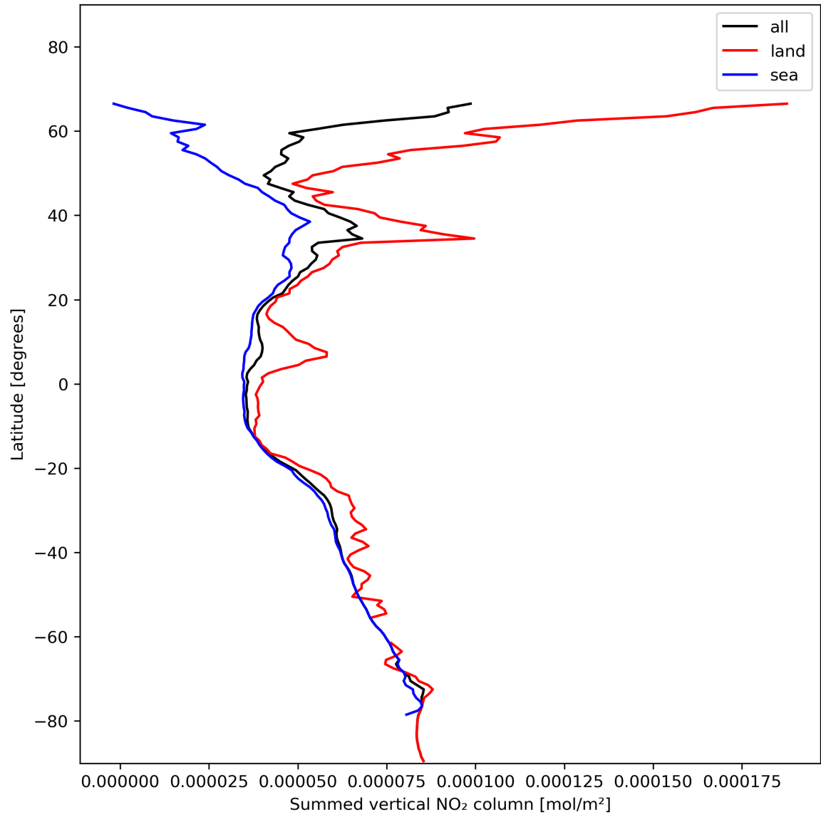
Figure 23: Zonal average of “Summed vertical NO 2 column” for 2024-01-15 to 2024-01-16.
