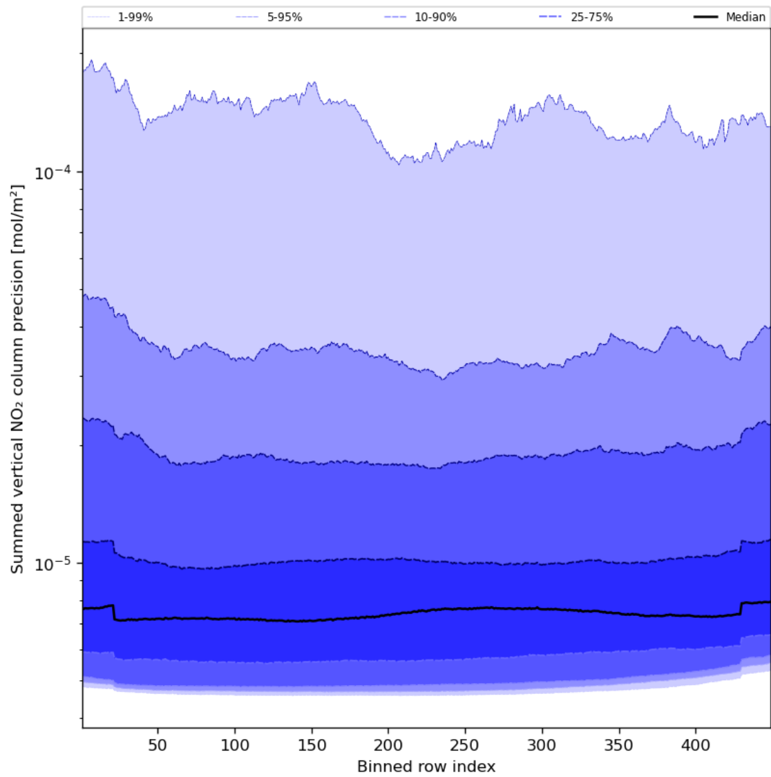
Figure 58: Along track statistics of “Summed vertical NO 2 column precision” for 2024-01-15 to 2024-01-16
