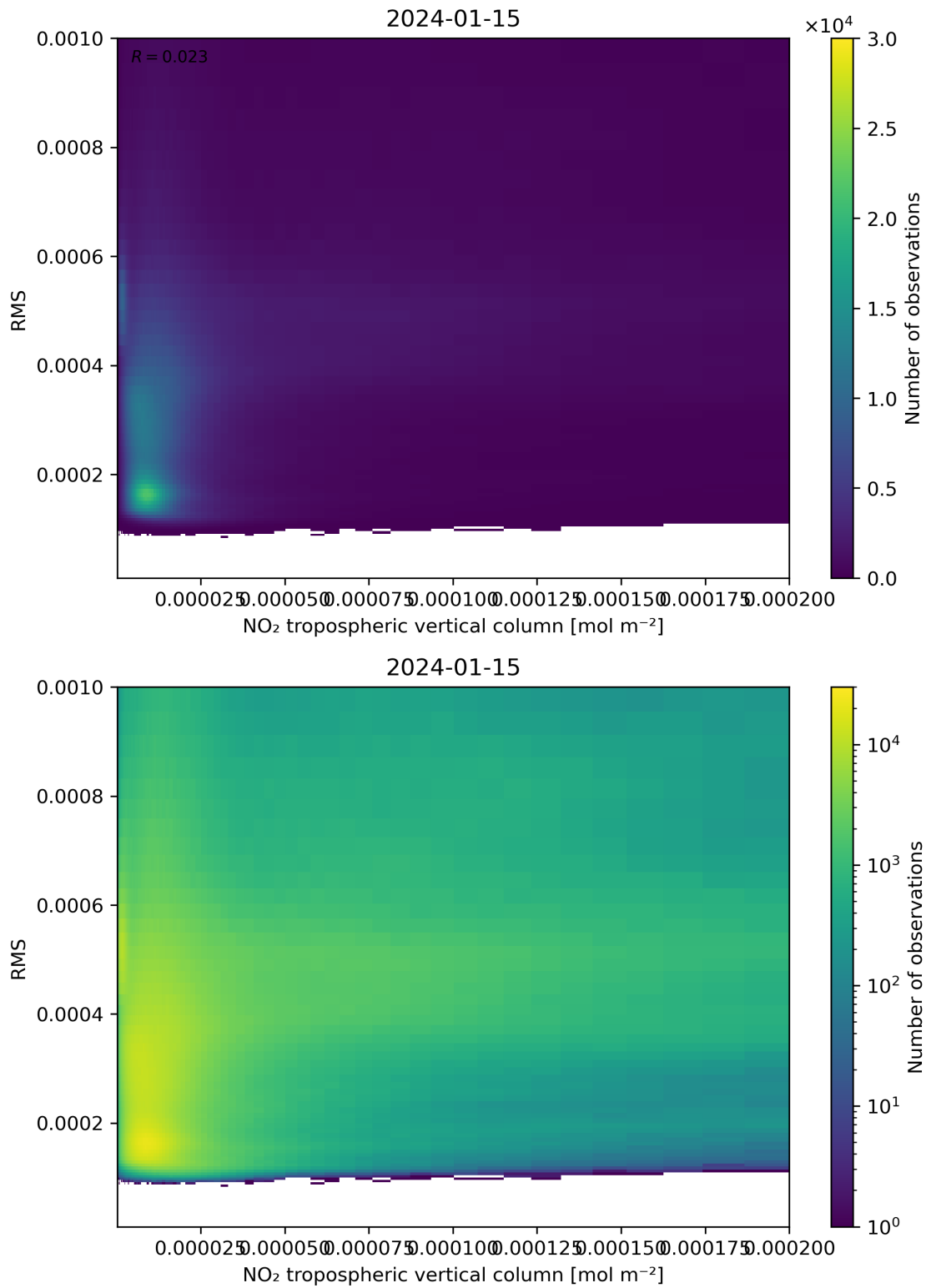
Figure 142: Scatter density plot of “NO 2 tropospheric vertical column” against “RMS” for 2024-01-15 to 2024-01-16.
