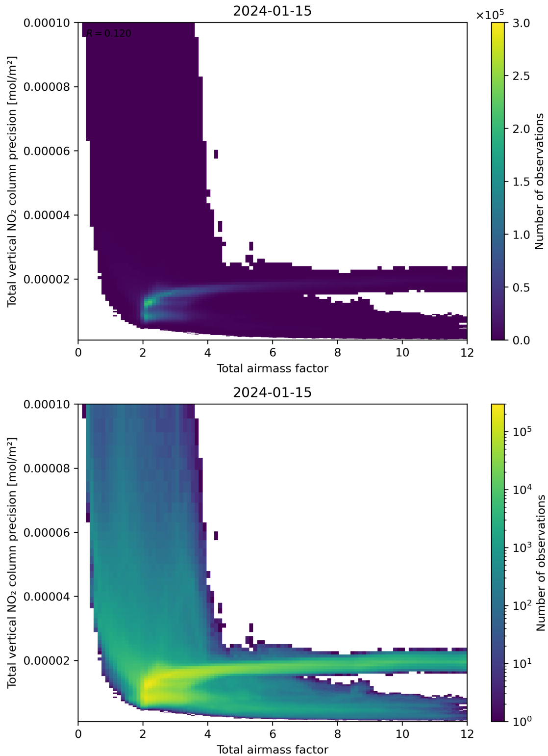
Figure 68: Scatter density plot of “Total airmass factor” against “Total vertical NO 2 column precision” for 2024-01-15 to 2024-01-16.
