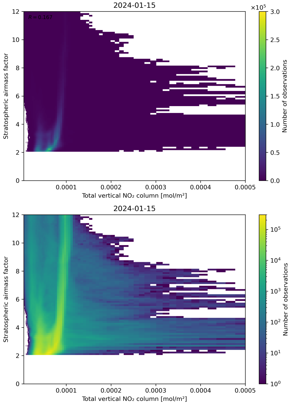
Figure 110: Scatter density plot of “Total vertical NO 2 column” against “Stratospheric airmass factor” for 2024-01-15 to 2024-01-16.
