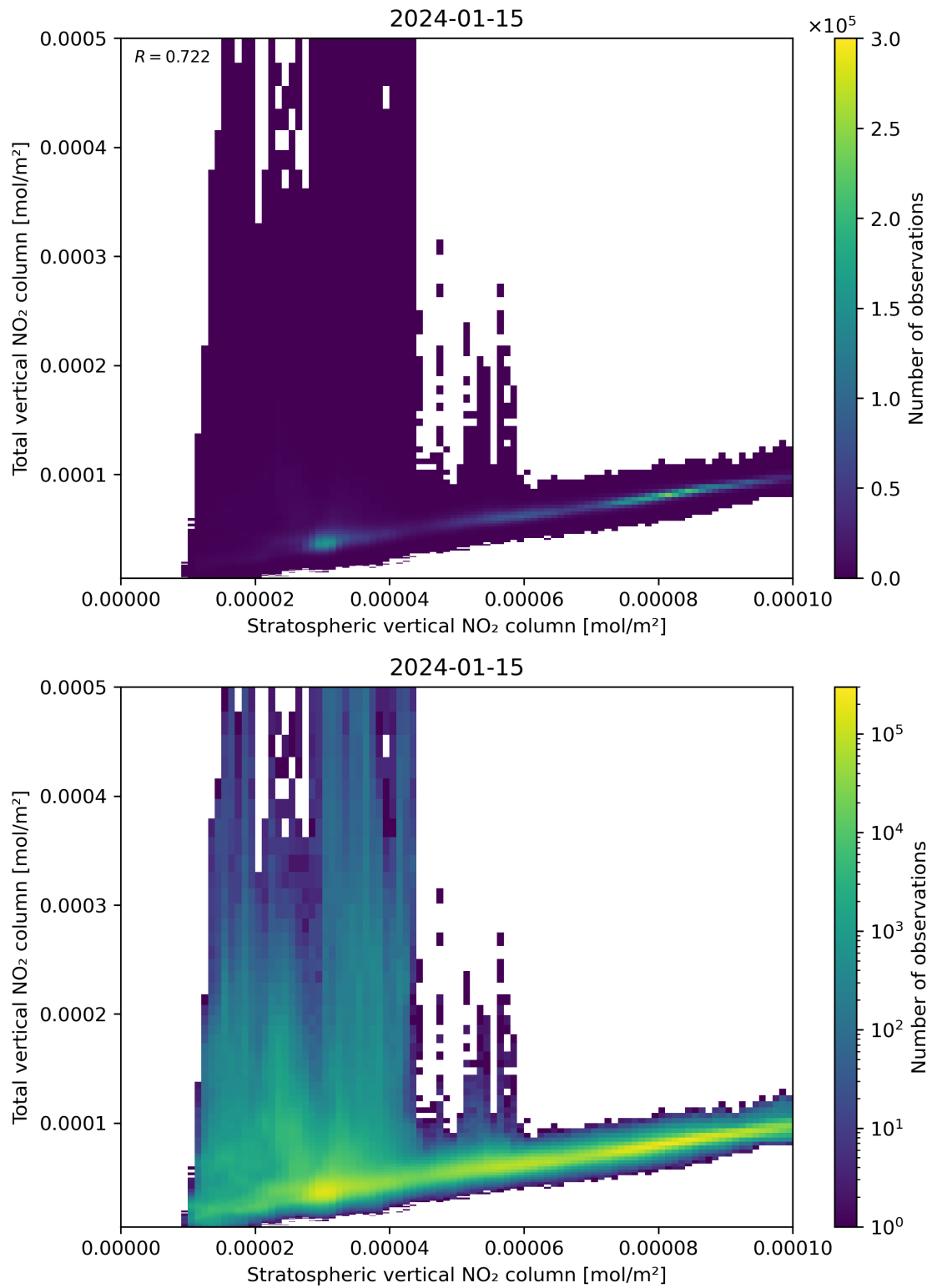
Figure 100: Scatter density plot of “Stratospheric vertical NO 2 column” against “Total vertical NO 2 column” for 2024-01-15 to 2024-01-16.
