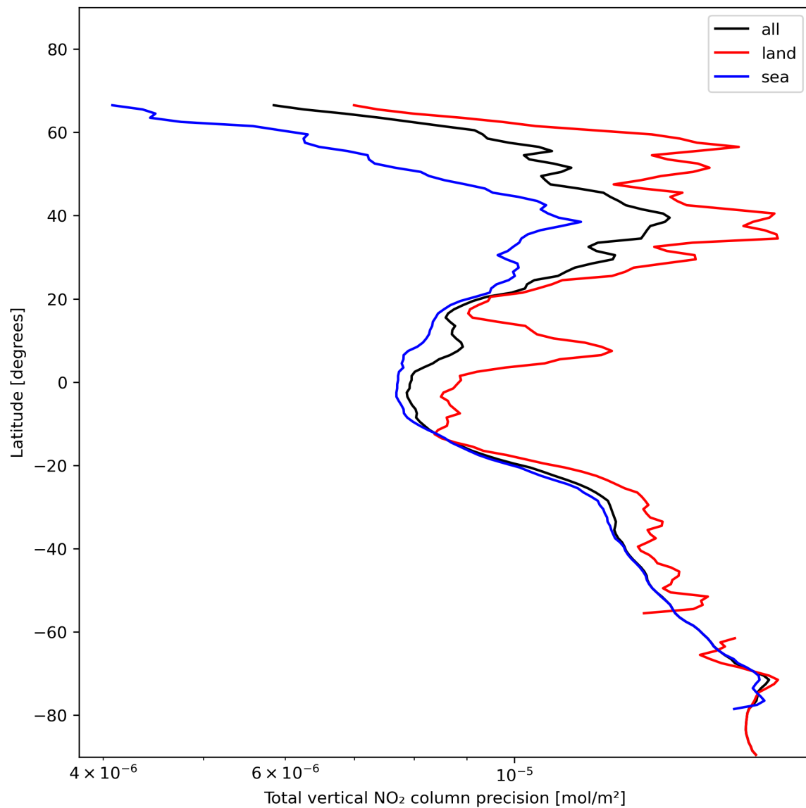
Figure 22: Zonal average of “Total vertical NO 2 column precision” for 2024-01-15 to 2024-01-16.
