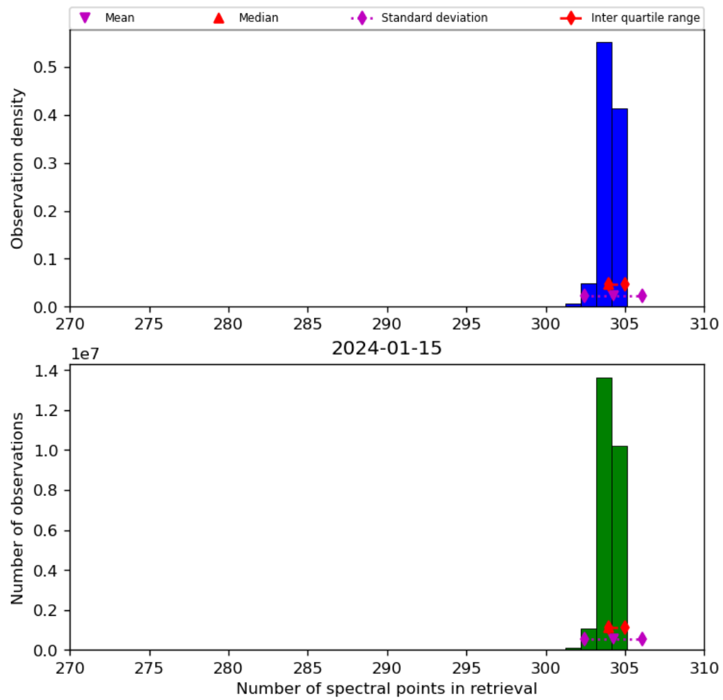
Figure 33: Histogram of “Number of spectral points in retrieval” for 2024-01-15 to 2024-01-16
