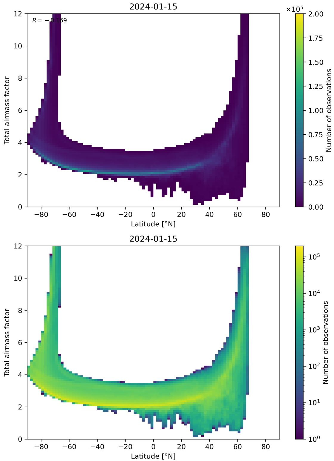
Figure 84: Scatter density plot of “Latitude” against “Total airmass factor” for 2024-01-15 to 2024-01-16.
