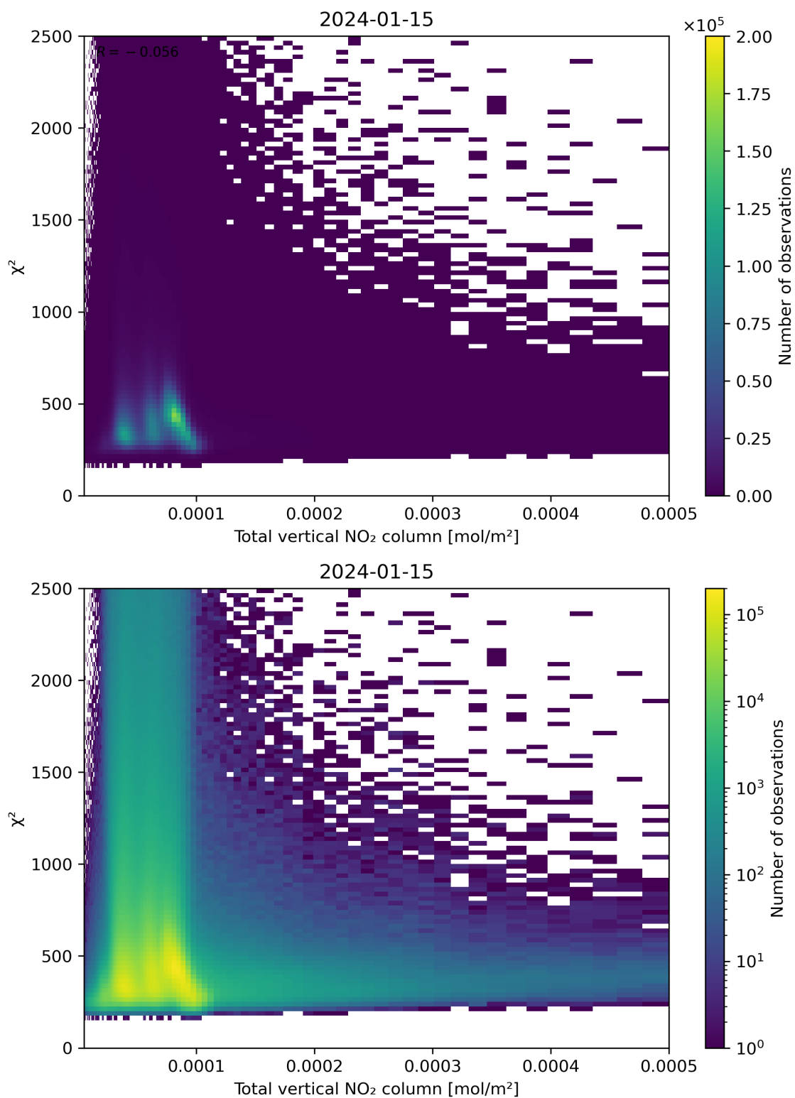
Figure 111: Scatter density plot of “Total vertical NO 2 column” against “ \chi^2 ” for 2024-01-15 to 2024-01-16.
