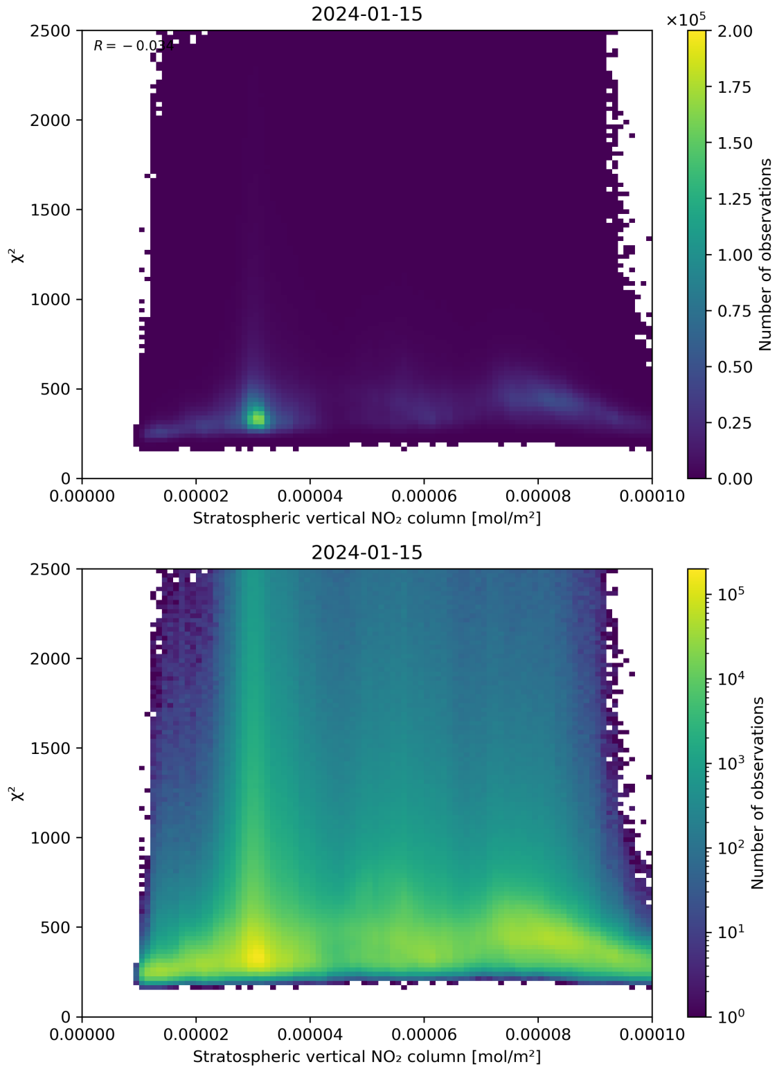
Figure 97: Scatter density plot of “Stratospheric vertical NO 2 column” against “ \chi^2 ” for 2024-01-15 to 2024-01-16.
