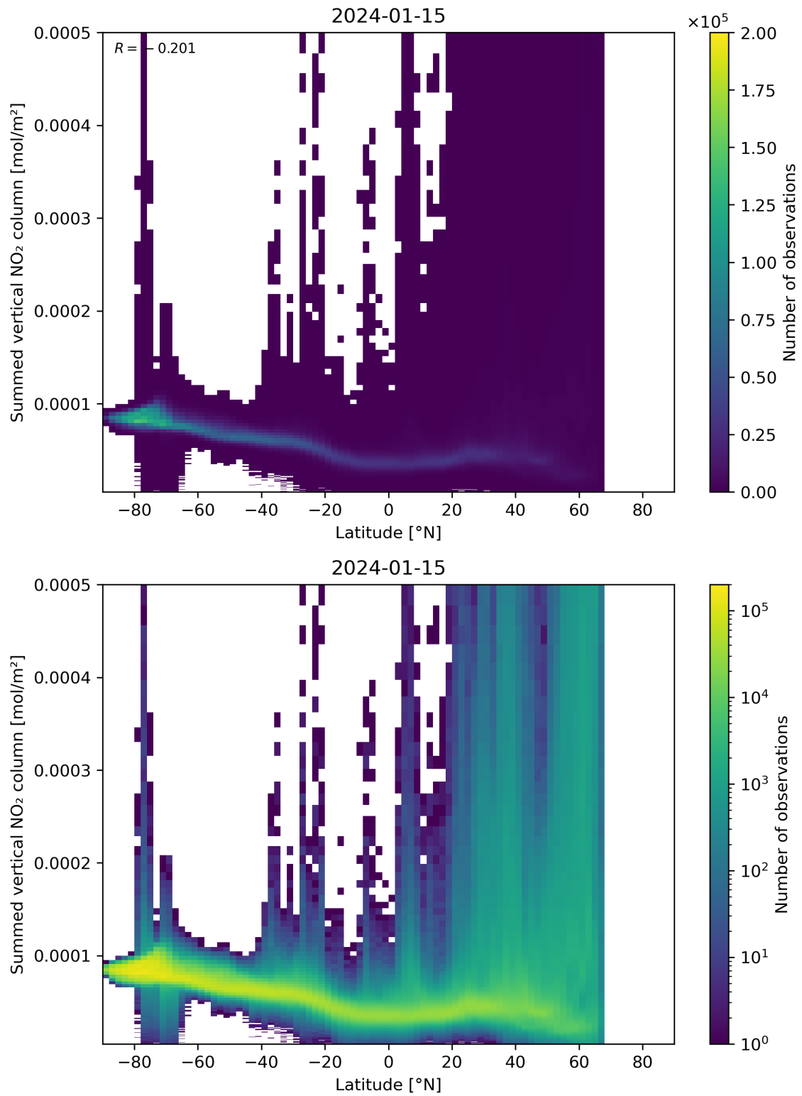
Figure 88: Scatter density plot of “Latitude” against “Summed vertical NO 2 column” for 2024-01-15 to 2024-01-16.
