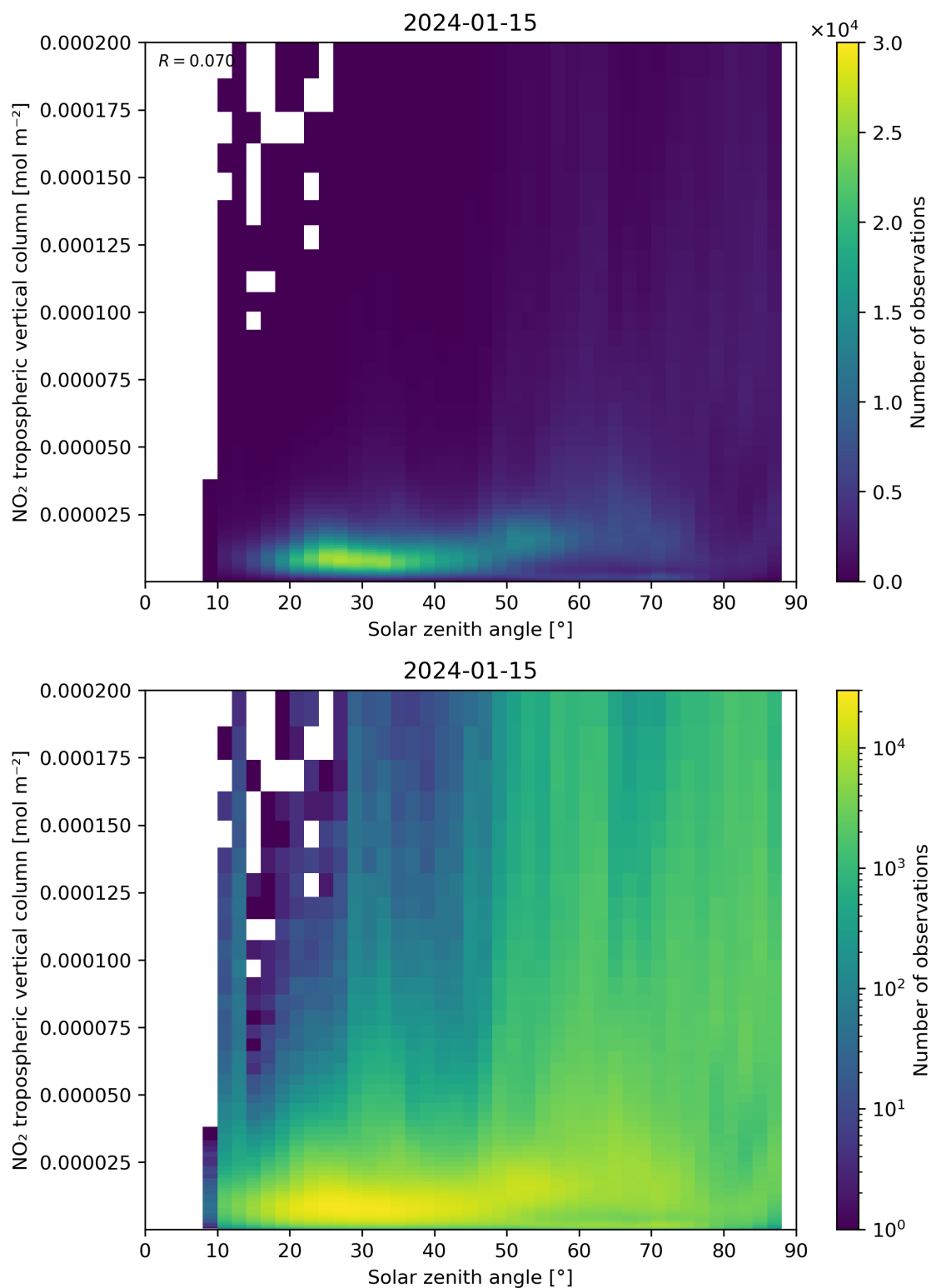
Figure 155: Scatter density plot of “Solar zenith angle” against “NO 2 tropospheric vertical column” for 2024-01-15 to 2024-01-16.
