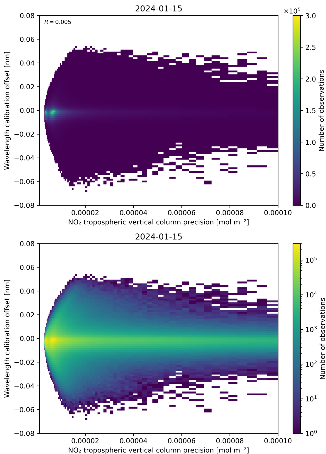
Figure 141: Scatter density plot of “NO 2 tropospheric vertical column precision” against “Wavelength calibration offset” for 2024-01-15 to 2024-01-16.
