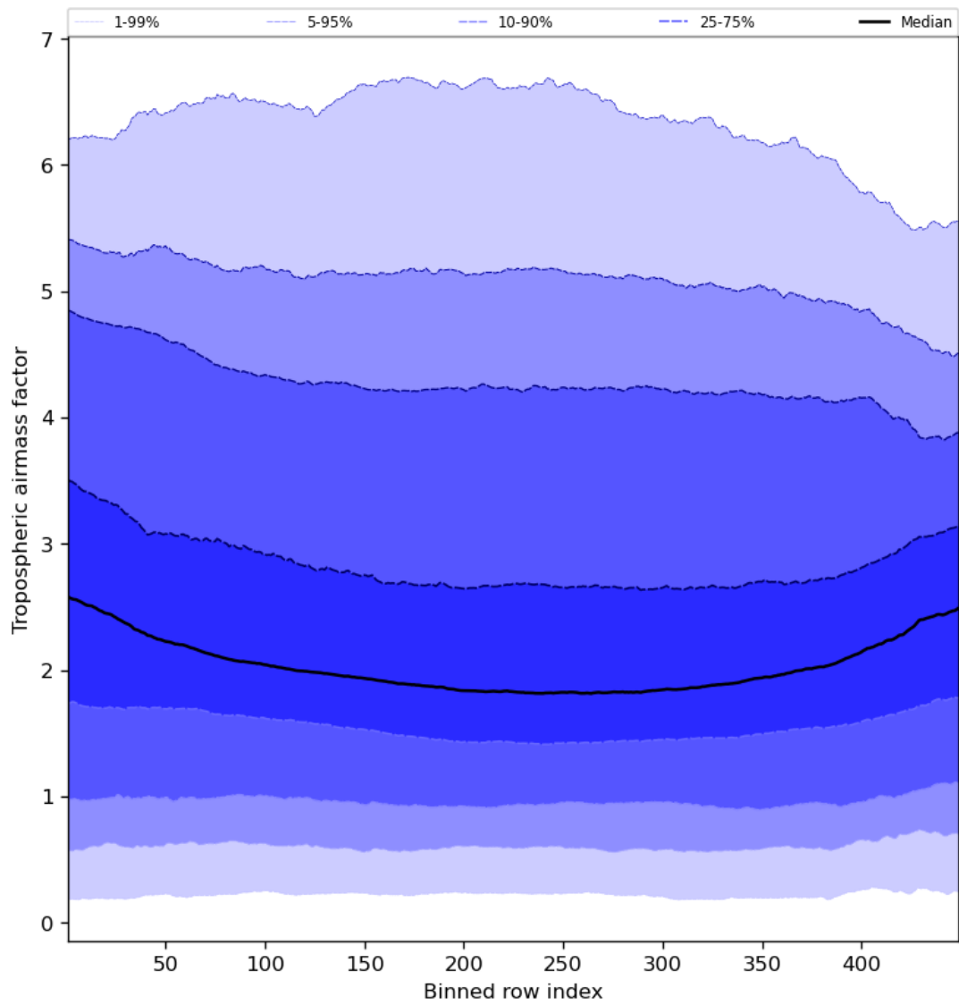
Figure 48: Along track statistics of “Tropospheric airmass factor” for 2024-01-15 to 2024-01-16
