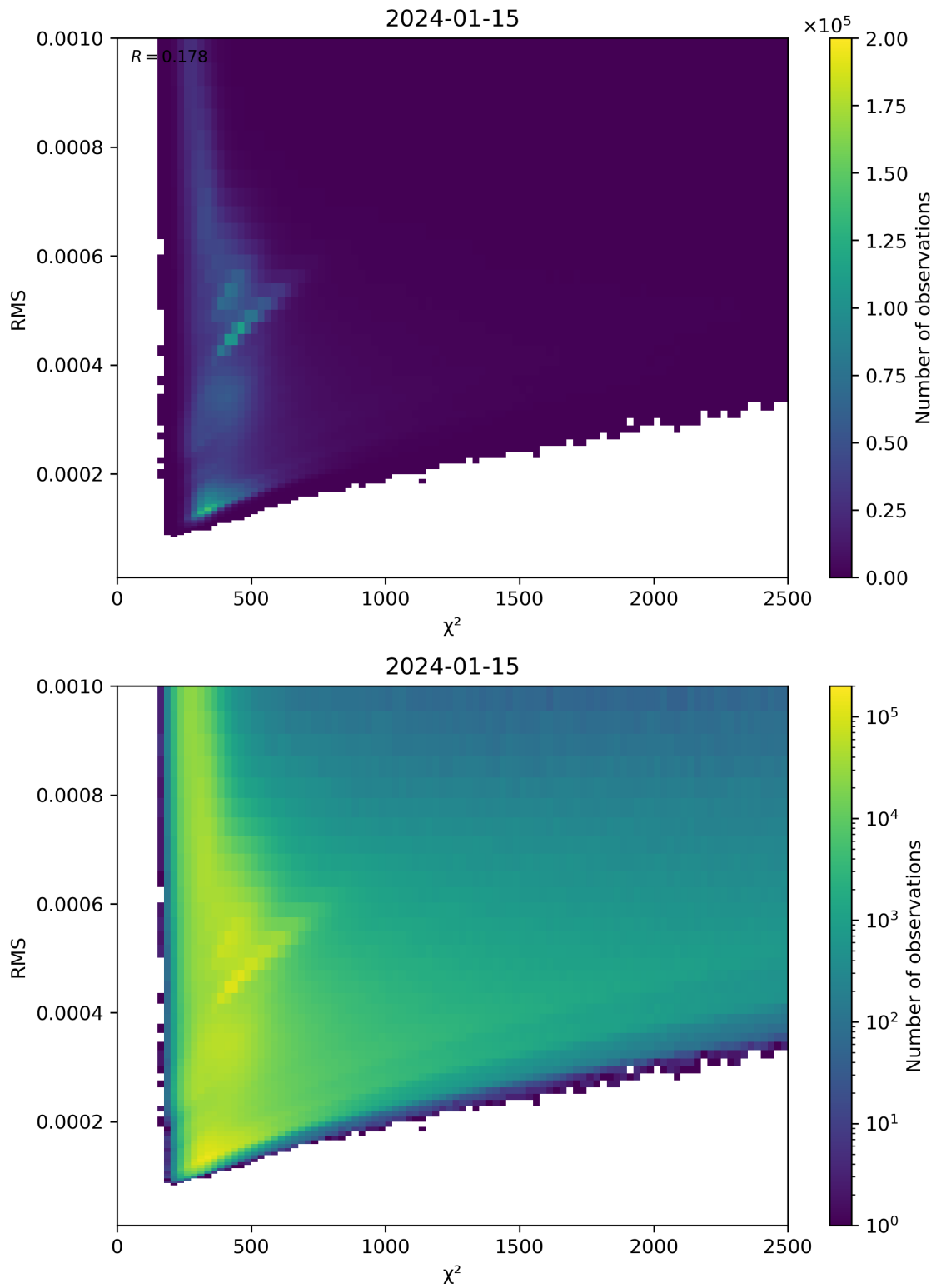
Figure 82: Scatter density plot of “ \chi^2 ” against “RMS” for 2024-01-15 to 2024-01-16.
