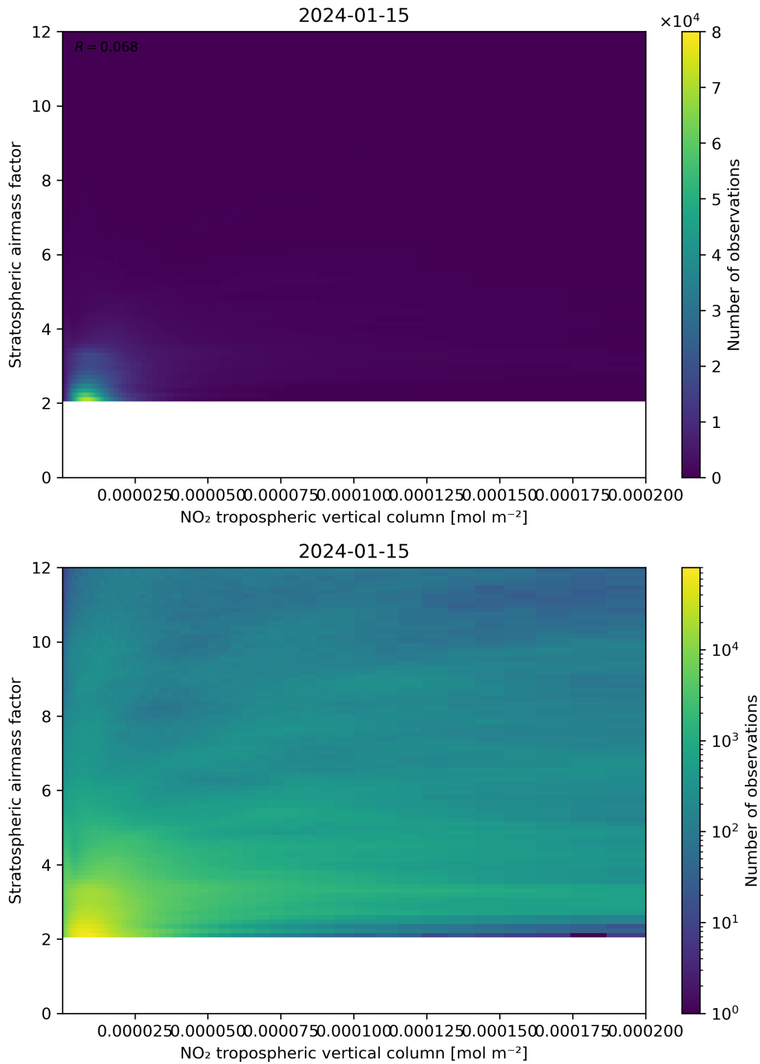
Figure 121: Scatter density plot of “NO 2 tropospheric vertical column” against “Stratospheric air mass factor” for 2024-01-15 to 2024-01-16.
