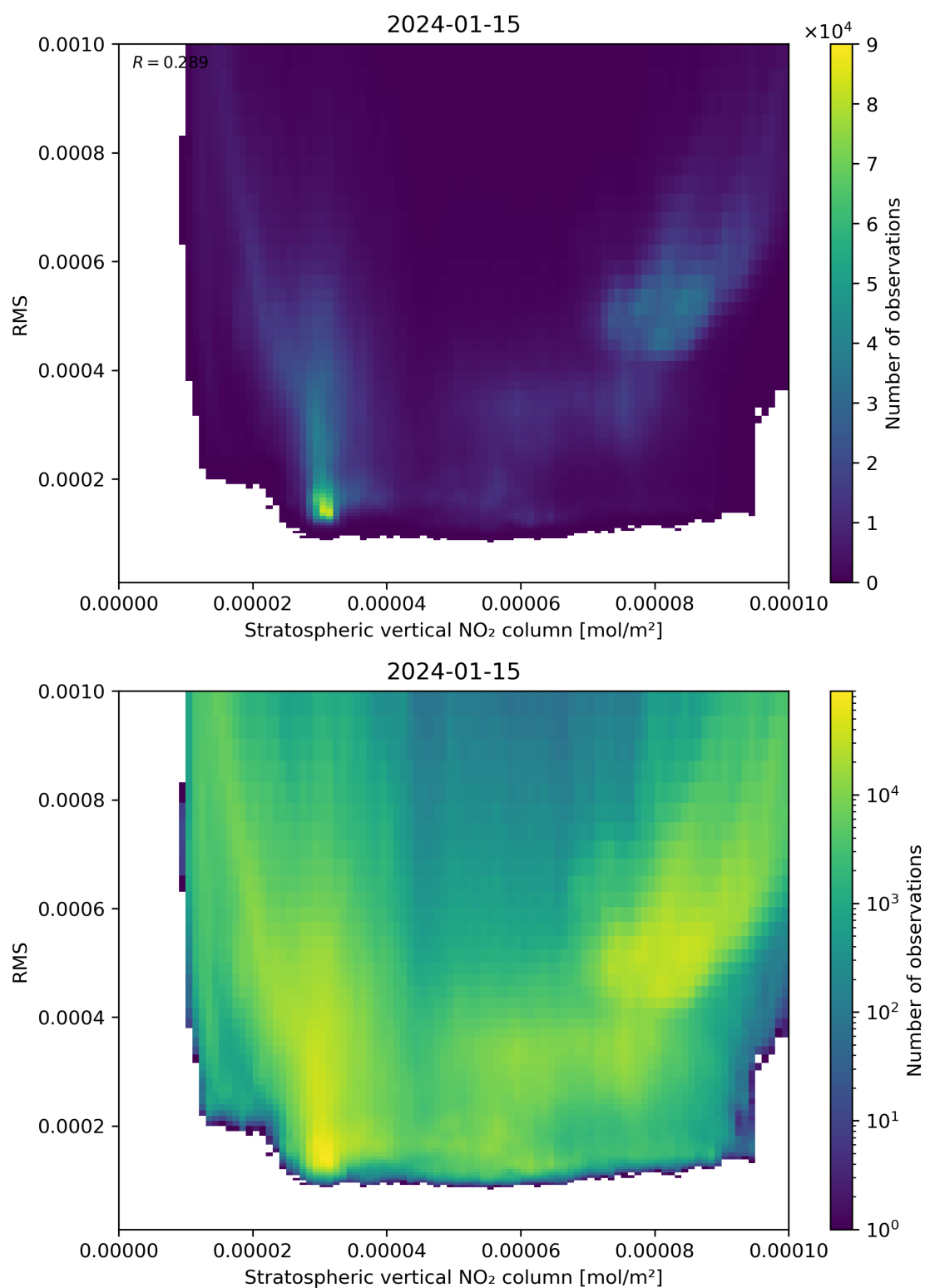
Figure 102: Scatter density plot of “Stratospheric vertical NO 2 column” against “RMS” for 2024-01-15 to 2024-01-16.
