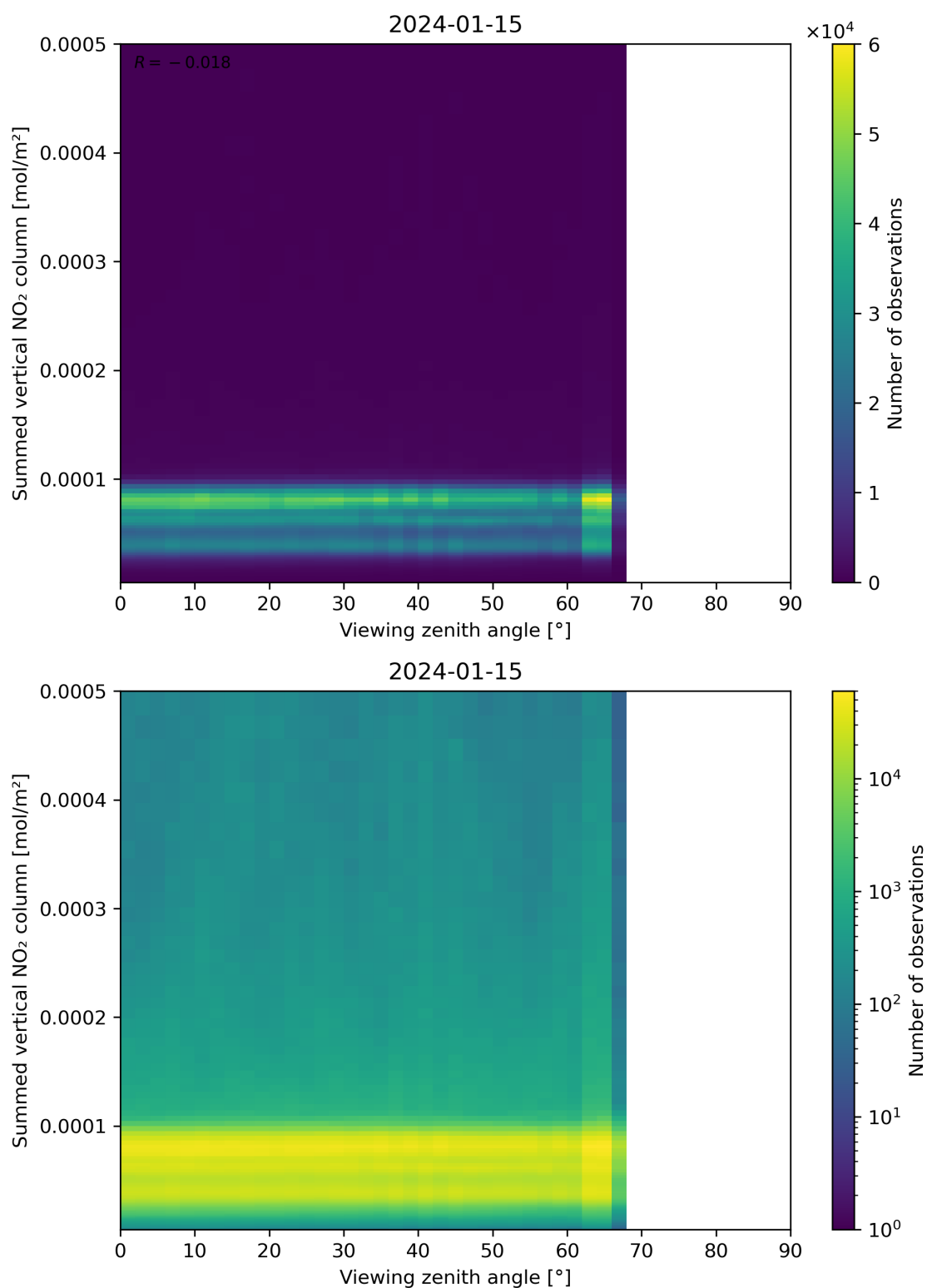
Figure 165: Scatter density plot of “Viewing zenith angle” against “Summed vertical NO 2 column” for 2024-01-15 to 2024-01-16.
