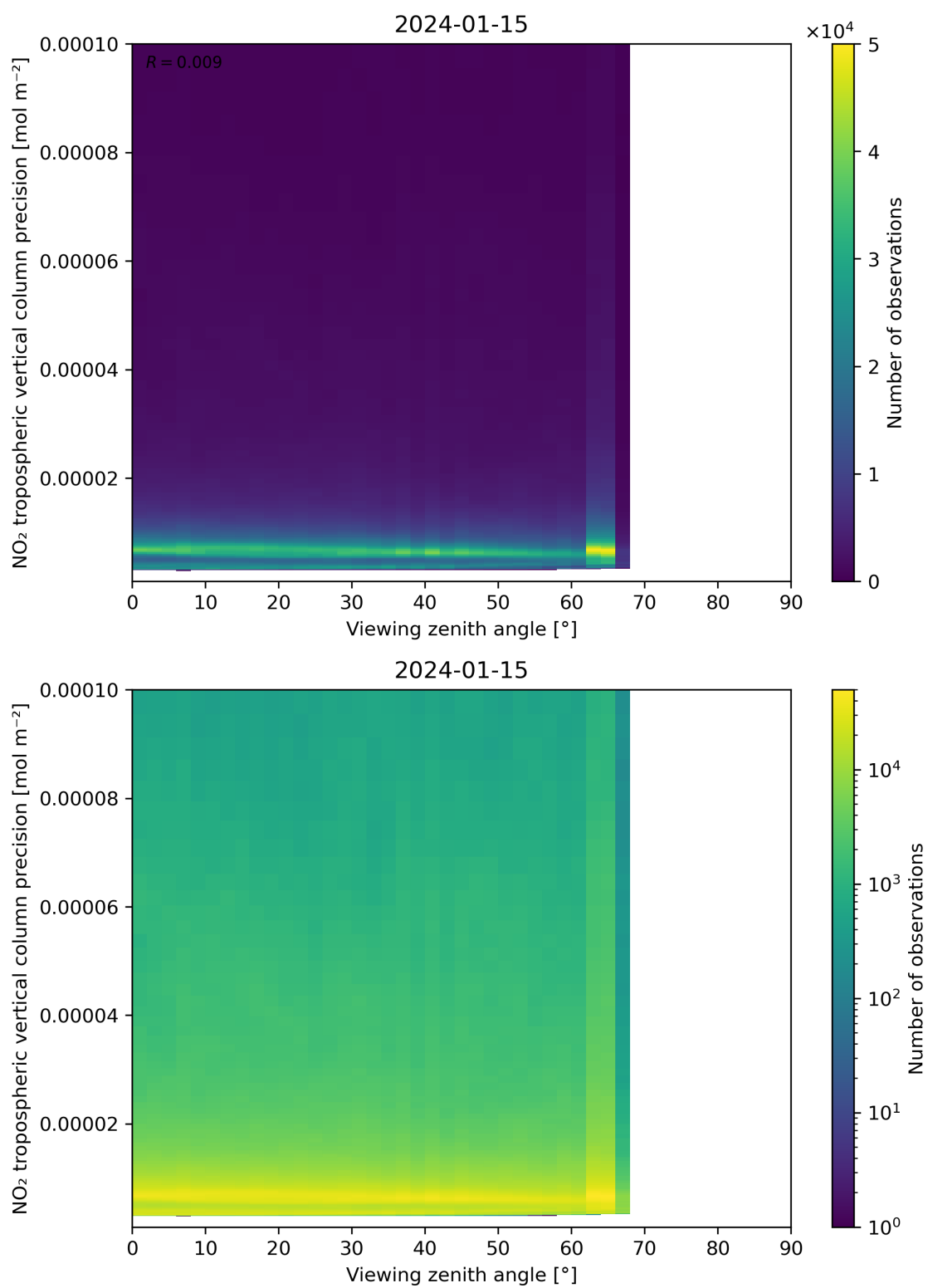
Figure 170: Scatter density plot of “Viewing zenith angle” against “NO 2 tropospheric vertical column precision” for 2024-01-15 to 2024-01-16.
