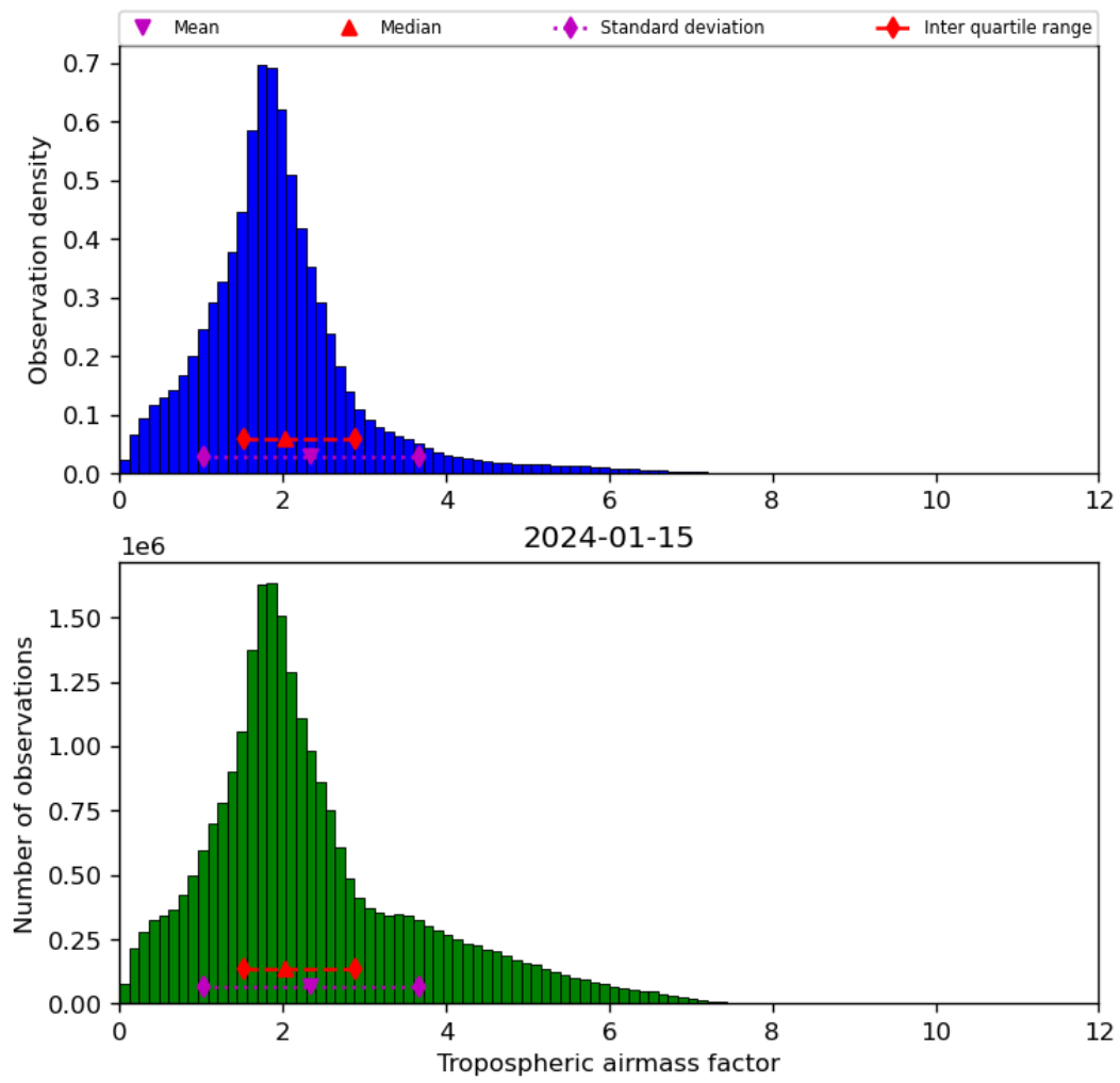
Figure 31: Histogram of “Tropospheric airmass factor” for 2024-01-15 to 2024-01-16
