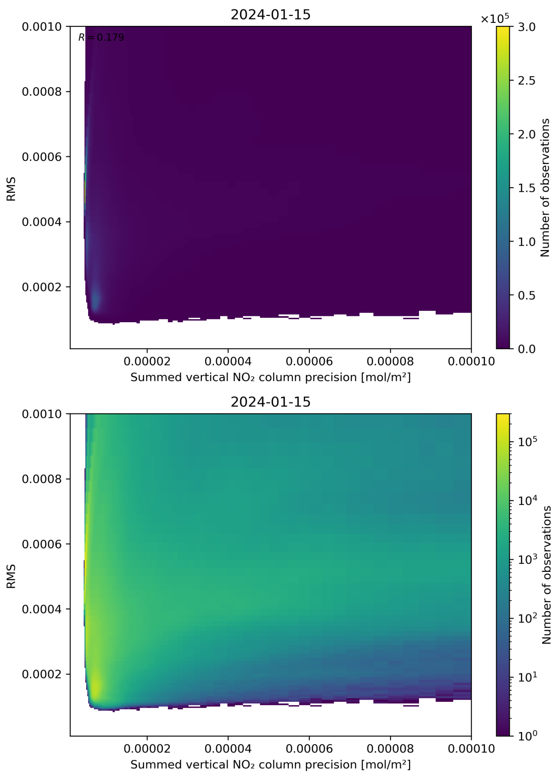
Figure 108: Scatter density plot of “Summed vertical NO 2 column precision” against “RMS” for 2024-01-15 to 2024-01-16.
