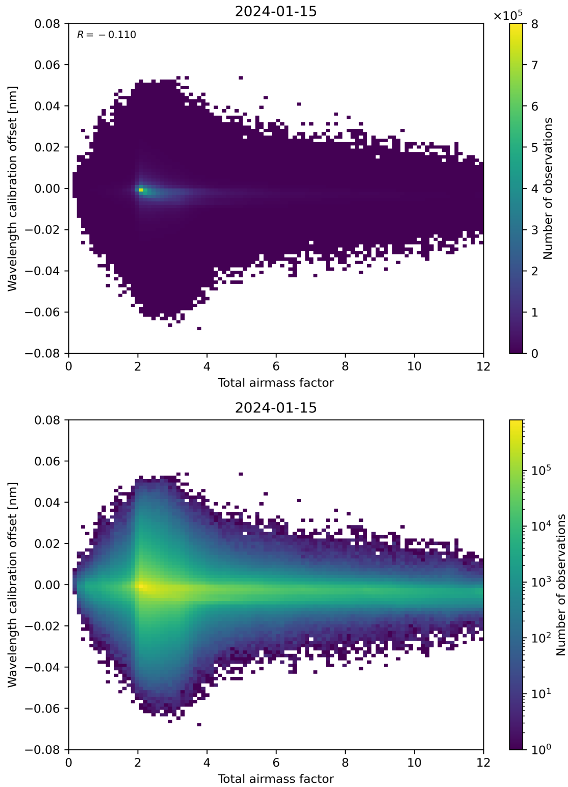
Figure 70: Scatter density plot of “Total airmass factor” against “Wavelength calibration offset” for 2024-01-15 to 2024-01-16.
