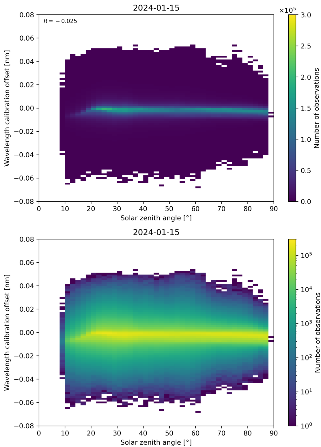
Figure 158: Scatter density plot of “Solar zenith angle” against “Wavelength calibration offset” for 2024-01-15 to 2024-01-16.
