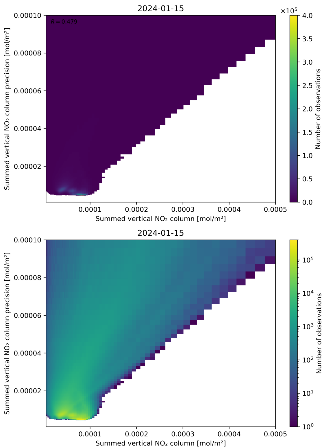
Figure 105: Scatter density plot of “Summed vertical NO 2 column” against “Summed vertical NO 2 column precision” for 2024-01-15 to 2024-01-16.
