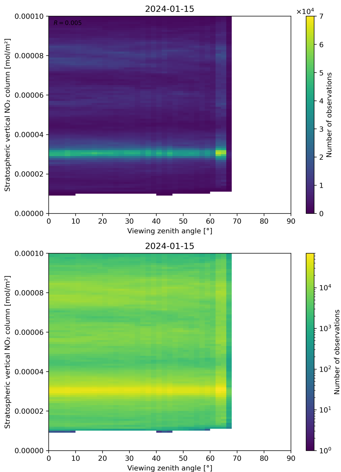
Figure 164: Scatter density plot of “Viewing zenith angle” against “Stratospheric vertical NO 2 column” for 2024-01-15 to 2024-01-16.
