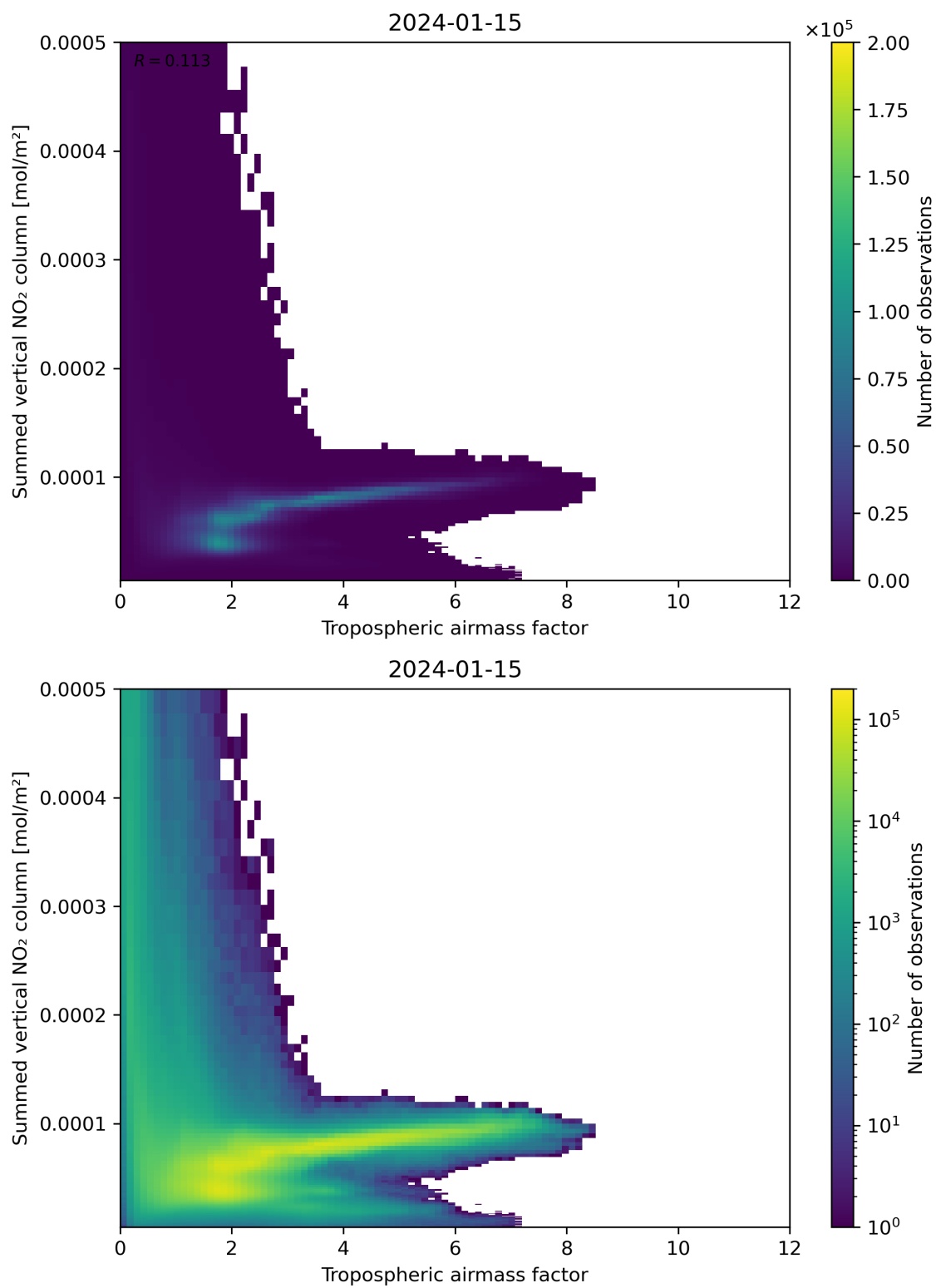
Figure 75: Scatter density plot of “Tropospheric airmass factor” against “Summed vertical NO 2 column” for 2024-01-15 to 2024-01-16.
