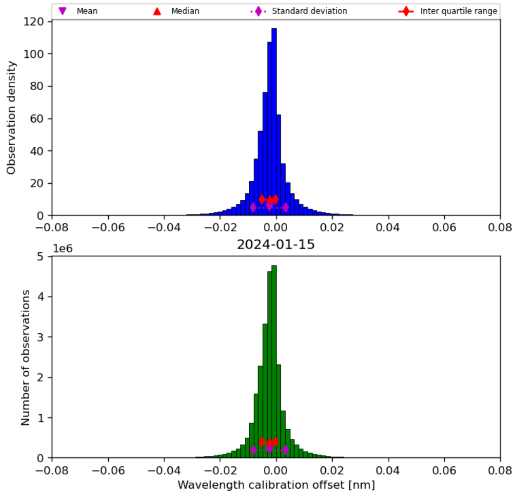
Figure 35: Histogram of “Wavelength calibration offset” for 2024-01-15 to 2024-01-16
