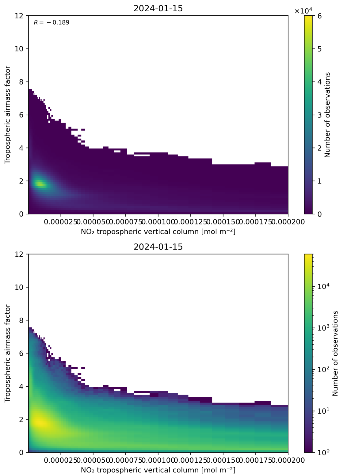
Figure 123: Scatter density plot of “NO 2 tropospheric vertical column” against “Tropospheric air mass factor” for 2024-01-15 to 2024-01-16.
