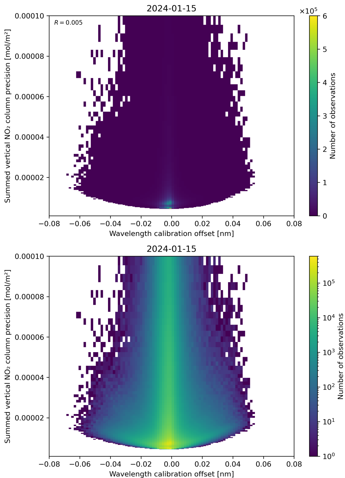
Figure 178: Scatter density plot of “Wavelength calibration offset” against “Summed vertical NO 2 column precision” for 2024-01-15 to 2024-01-16.
