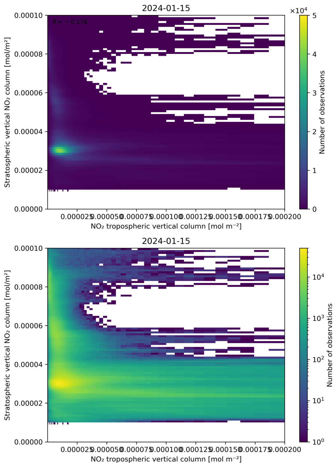
Figure 125: Scatter density plot of “NO 2 tropospheric vertical column” against “Stratospheric vertical NO 2 column” for 2024-01-15 to 2024-01-16.
