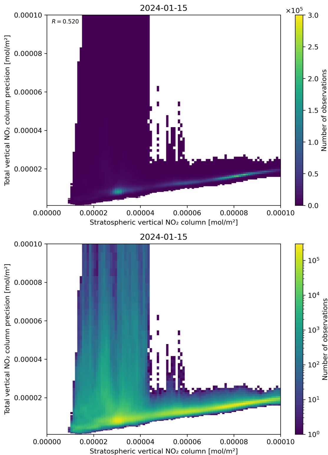
Figure 101: Scatter density plot of “Stratospheric vertical NO 2 column” against “Total vertical NO 2 column precision” for 2024-01-15 to 2024-01-16.
