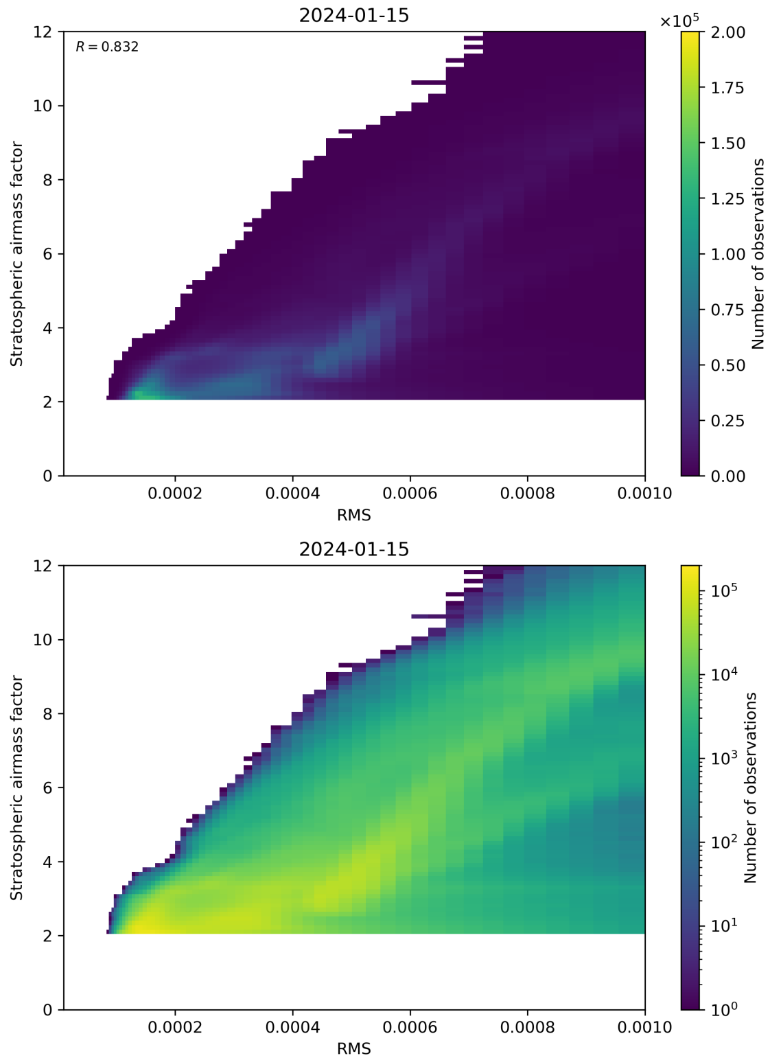
Figure 144: Scatter density plot of “RMS” against “Stratospheric airmass factor” for 2024-01-15 to 2024-01-16.
