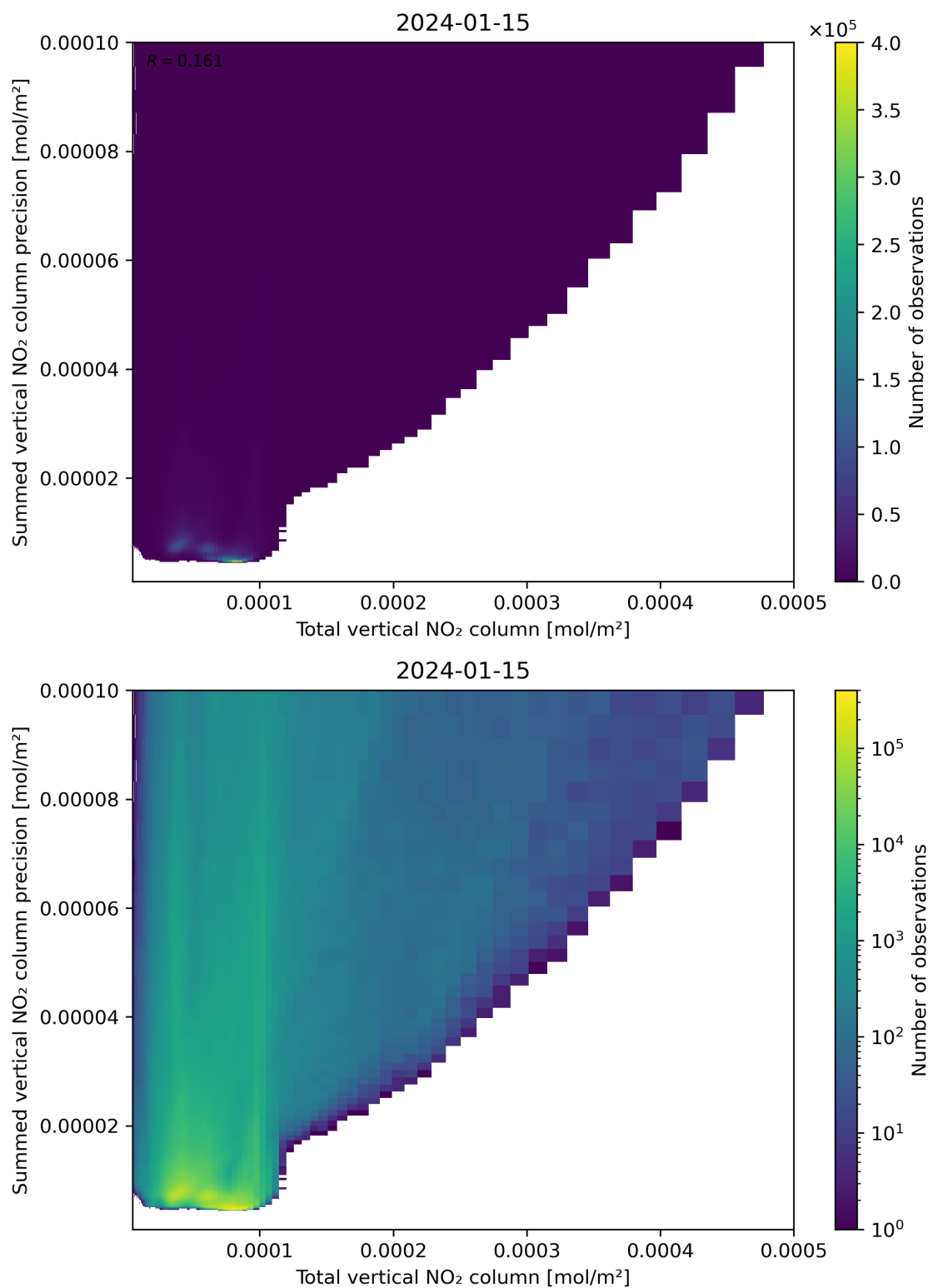
Figure 113: Scatter density plot of “Total vertical NO 2 column” against “Summed vertical NO 2 column precision” for 2024-01-15 to 2024-01-16.
