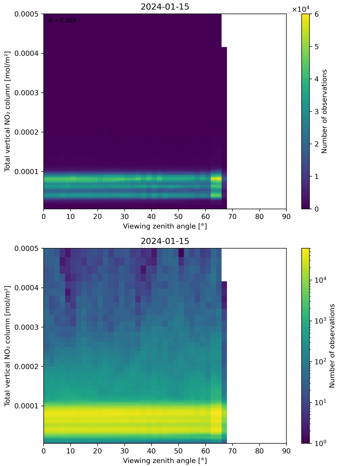
Figure 167: Scatter density plot of “Viewing zenith angle” against “Total vertical NO 2 column” for 2024-01-15 to 2024-01-16.
