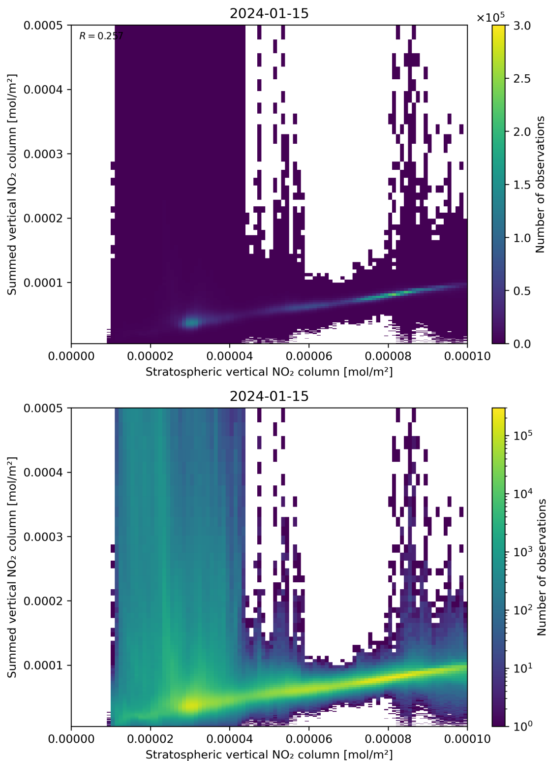
Figure 98: Scatter density plot of “Stratospheric vertical NO 2 column” against “Summed vertical NO 2 column” for 2024-01-15 to 2024-01-16.
