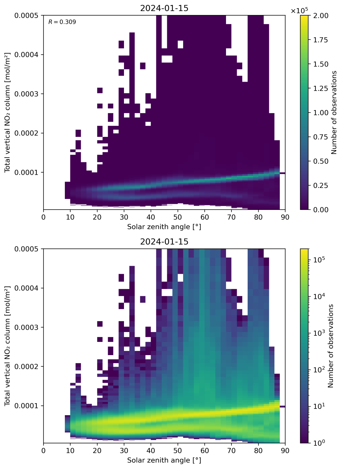
Figure 153: Scatter density plot of “Solar zenith angle” against “Total vertical NO 2 column” for 2024-01-15 to 2024-01-16.
