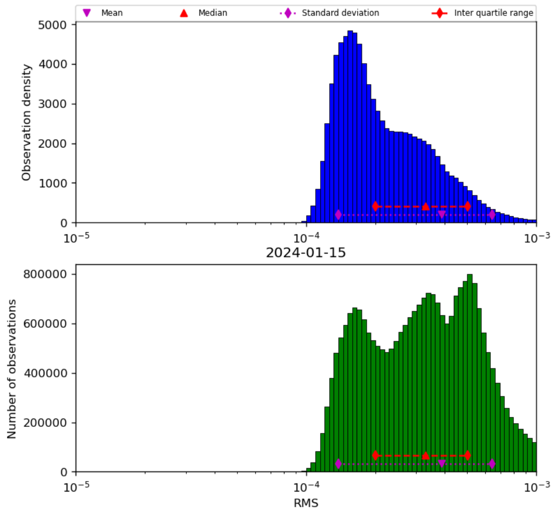
Figure 43: Histogram of “RMS” for 2024-01-15 to 2024-01-16
