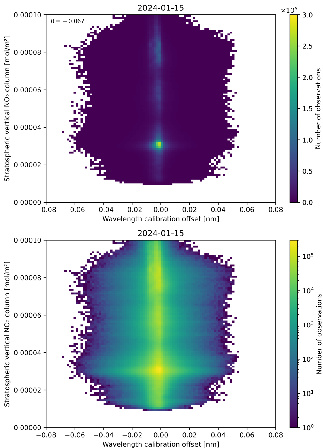
Figure 176: Scatter density plot of “Wavelength calibration offset” against “Stratospheric vertical NO 2 column” for 2024-01-15 to 2024-01-16.
