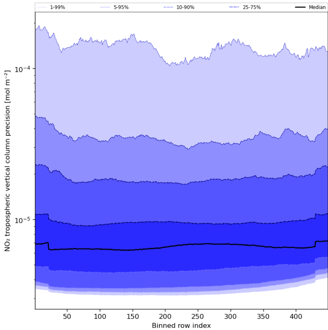
Figure 47: Along track statistics of “NO 2 tropospheric vertical column precision” for 2024-01-15 to 2024-01-16
