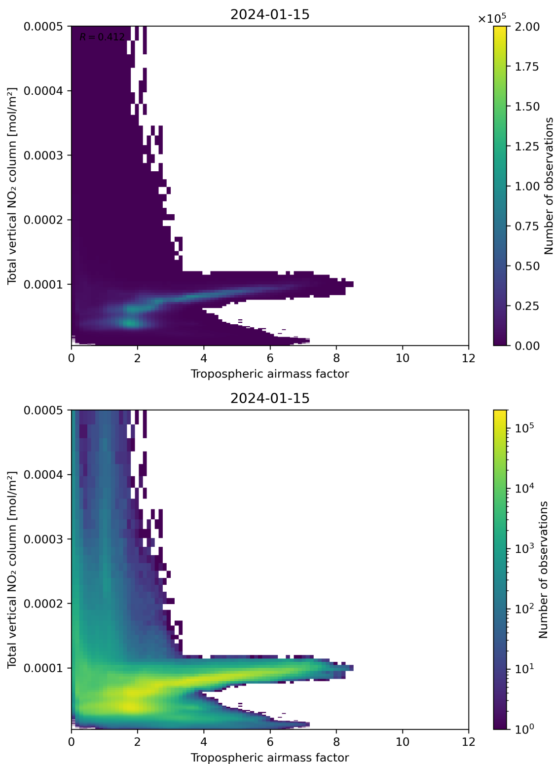
Figure 77: Scatter density plot of “Tropospheric airmass factor” against “Total vertical NO 2 column” for 2024-01-15 to 2024-01-16.
