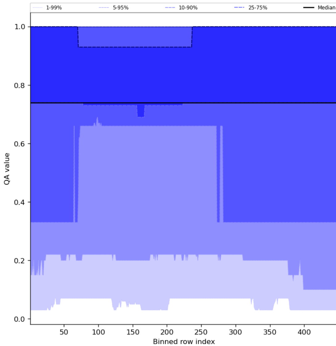
Figure 45: Along track statistics of “QA value” for 2024-01-15 to 2024-01-16
