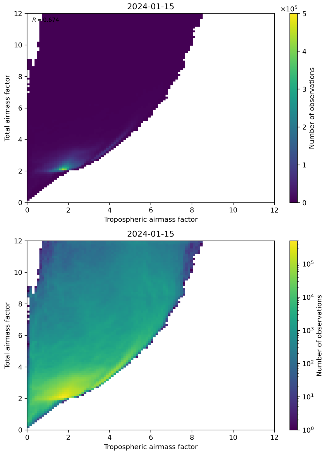
Figure 72: Scatter density plot of “Tropospheric airmass factor” against “Total airmass factor” for 2024-01-15 to 2024-01-16.
