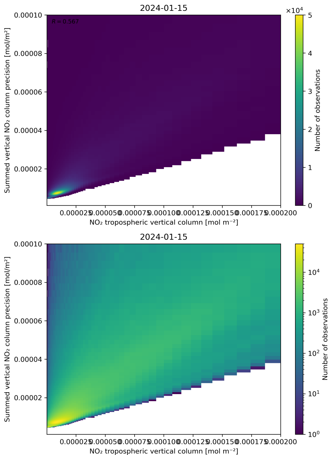
Figure 127: Scatter density plot of “NO 2 tropospheric vertical column” against “Summed vertical NO 2 column precision” for 2024-01-15 to 2024-01-16.
