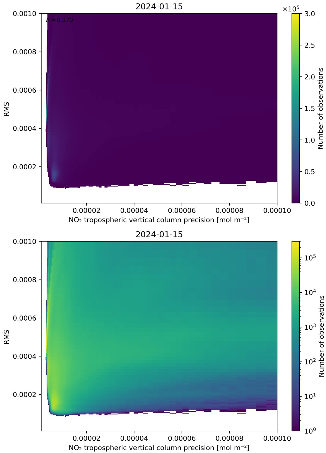
Figure 140: Scatter density plot of “NO 2 tropospheric vertical column precision” against “RMS” for 2024-01-15 to 2024-01-16.
