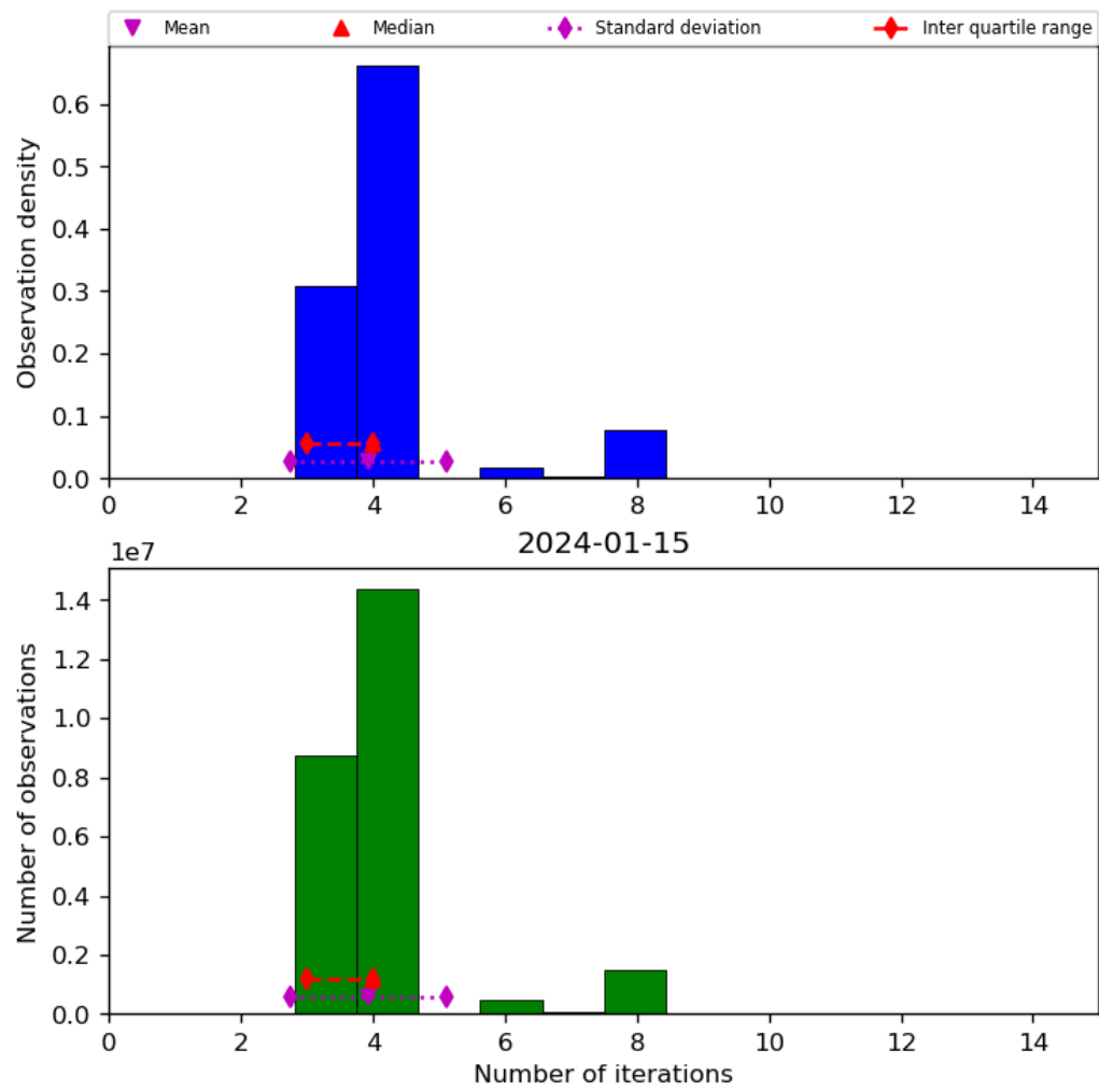
Figure 34: Histogram of “Number of iterations” for 2024-01-15 to 2024-01-16
