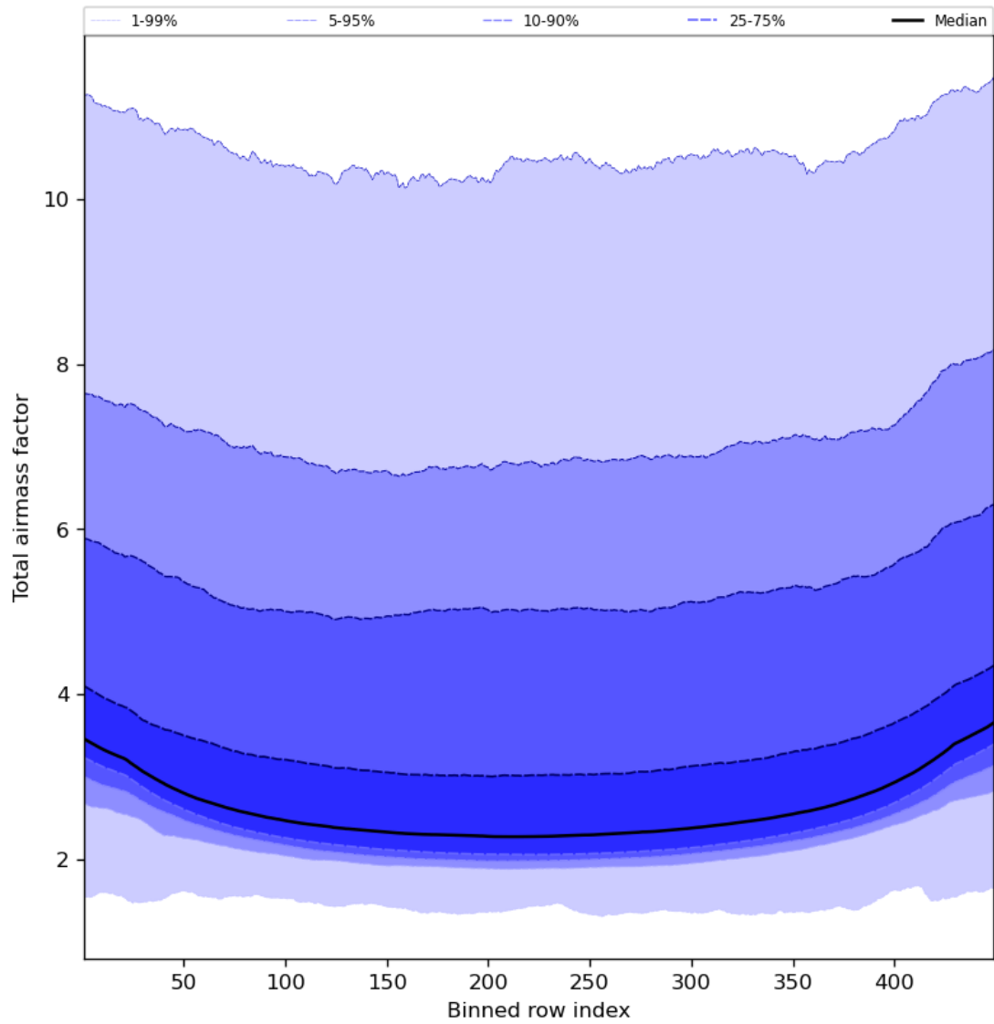
Figure 49: Along track statistics of “Total airmass factor” for 2024-01-15 to 2024-01-16
