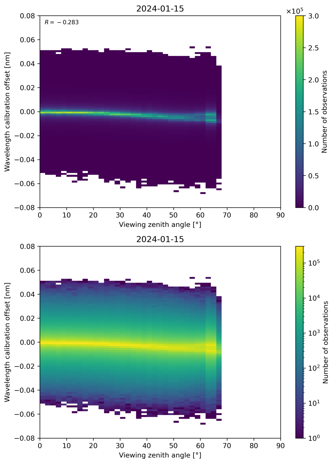
Figure 173: Scatter density plot of “Viewing zenith angle” against “Wavelength calibration offset” for 2024-01-15 to 2024-01-16.
