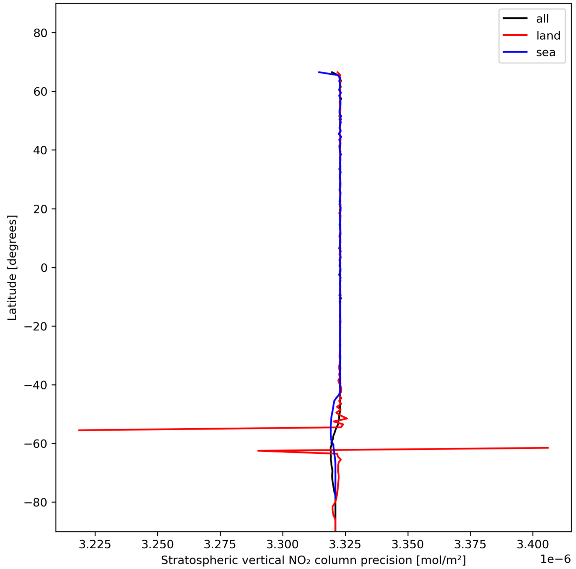
Figure 20: Zonal average of "Stratospheric vertical NO 2 column precision" for 2024-01-15 to 2024-01-16.
