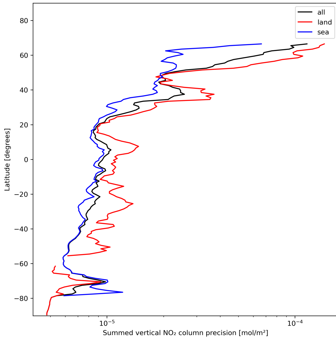
Figure 24: Zonal average of “Summed vertical NO 2 column precision” for 2024-01-15 to 2024-01-16.
