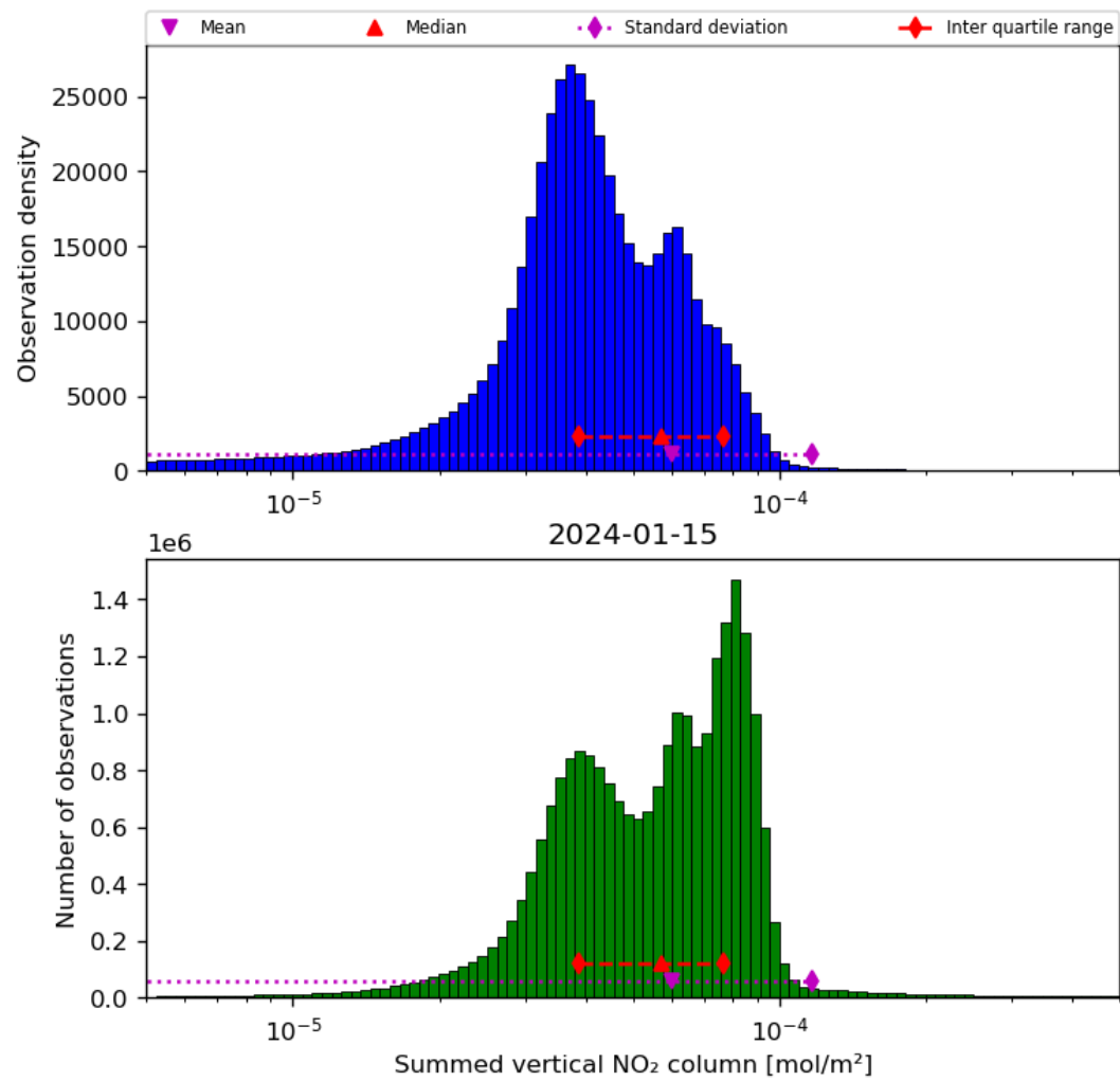
Figure 40: Histogram of “Summed vertical NO 2 column” for 2024-01-15 to 2024-01-16
