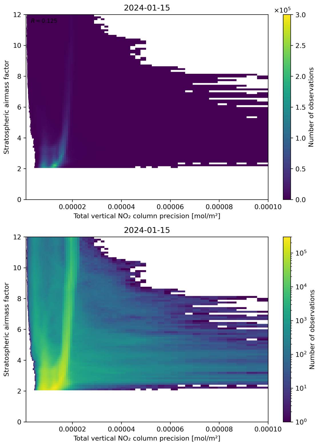
Figure 115: Scatter density plot of “Total vertical NO 2 column precision” against “Stratospheric air mass factor” for 2024-01-15 to 2024-01-16.
