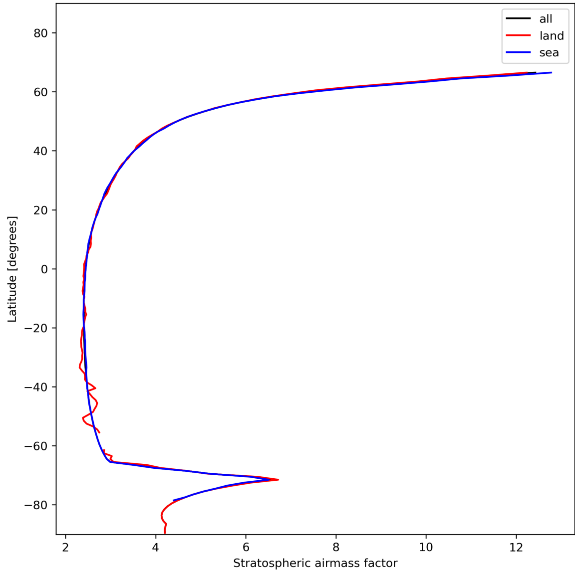
Figure 27: Zonal average of “Stratospheric airmass factor” for 2024-01-15 to 2024-01-16.
