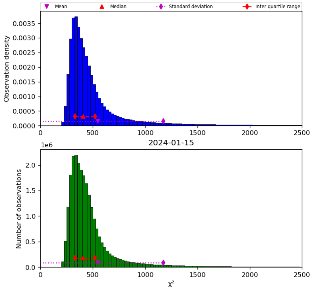
Figure 42: Histogram of “ \chi^2 ” for 2024-01-15 to 2024-01-16
