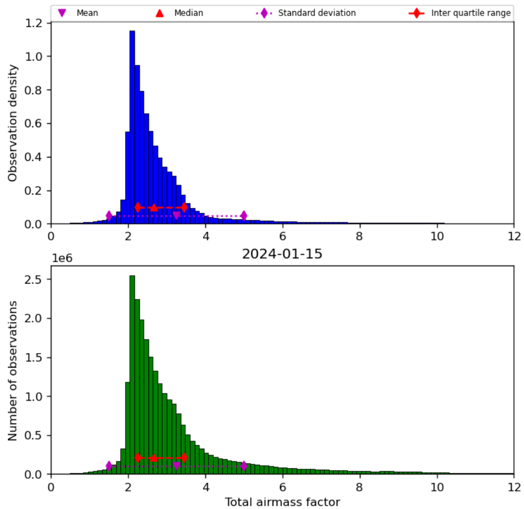
Figure 32: Histogram of “Total airmass factor” for 2024-01-15 to 2024-01-16
