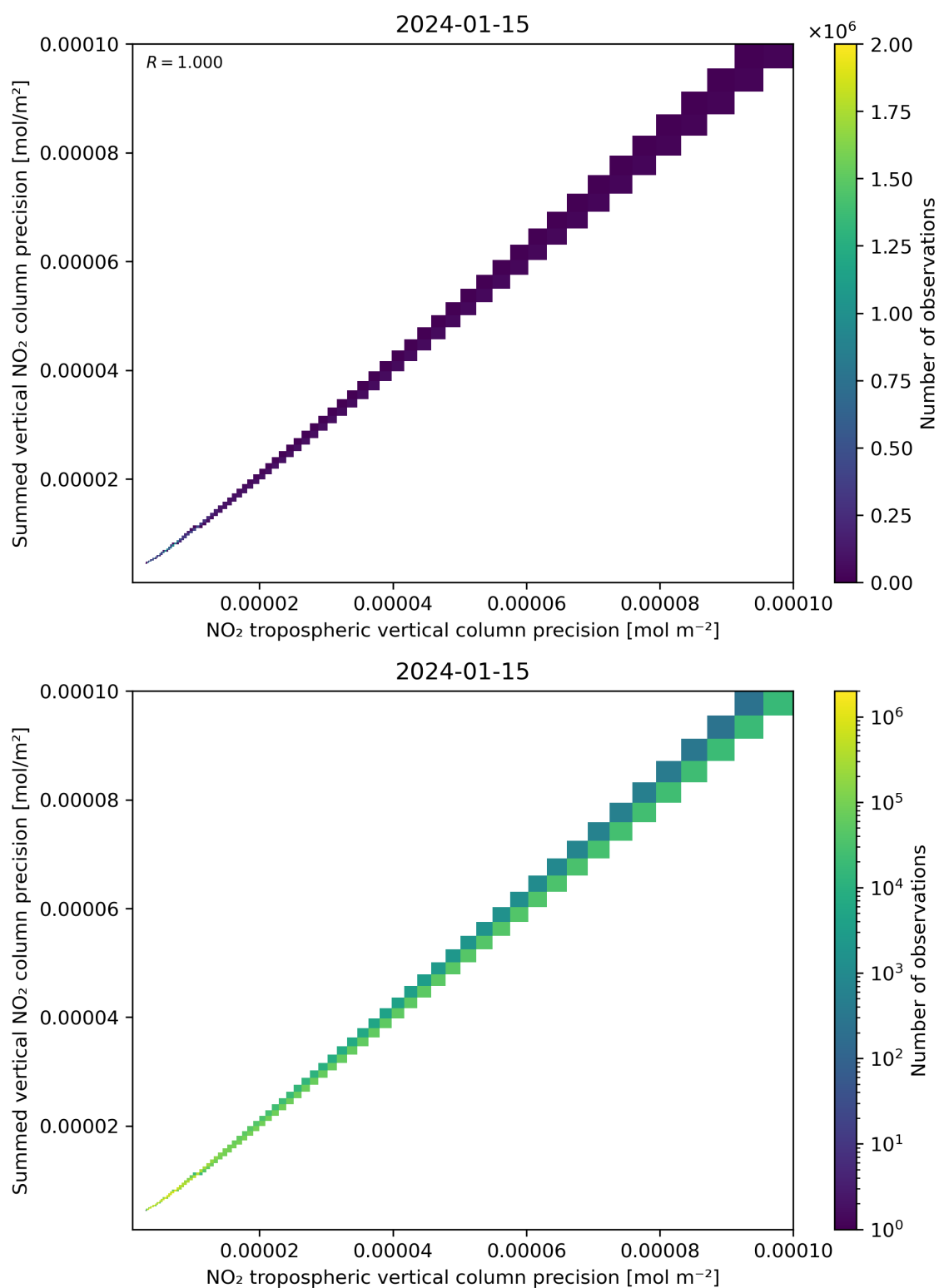
Figure 137: Scatter density plot of “NO 2 tropospheric vertical column precision” against “Summed vertical NO 2 column precision” for 2024-01-15 to 2024-01-16.
