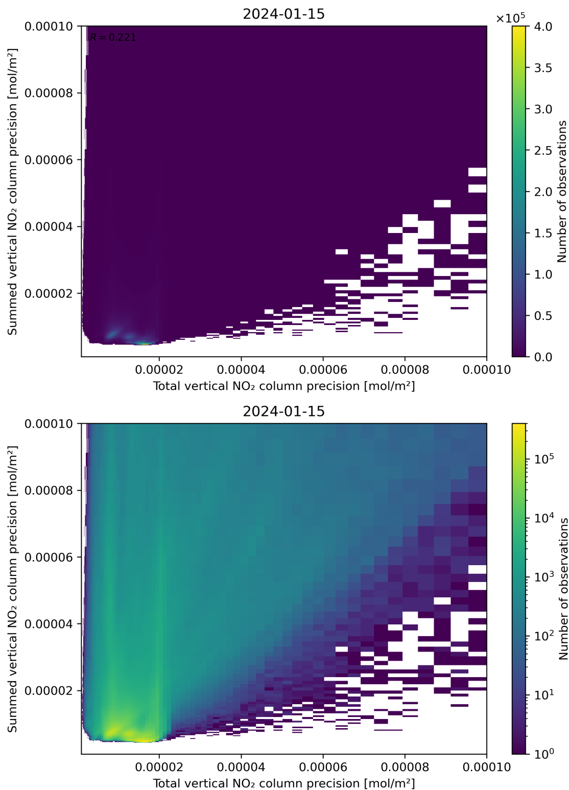
Figure 118: Scatter density plot of “Total vertical NO 2 column precision” against “Summed vertical NO 2 column precision” for 2024-01-15 to 2024-01-16.
