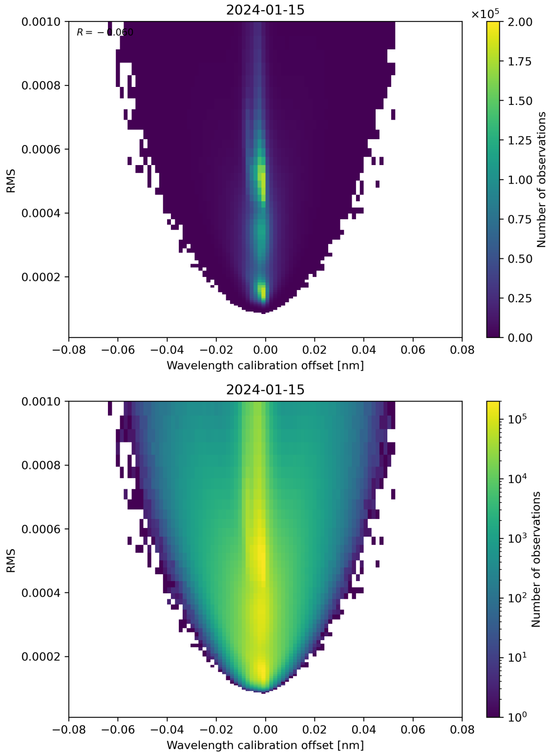
Figure 181: Scatter density plot of “Wavelength calibration offset” against “RMS” for 2024-01-15 to 2024-01-16.
