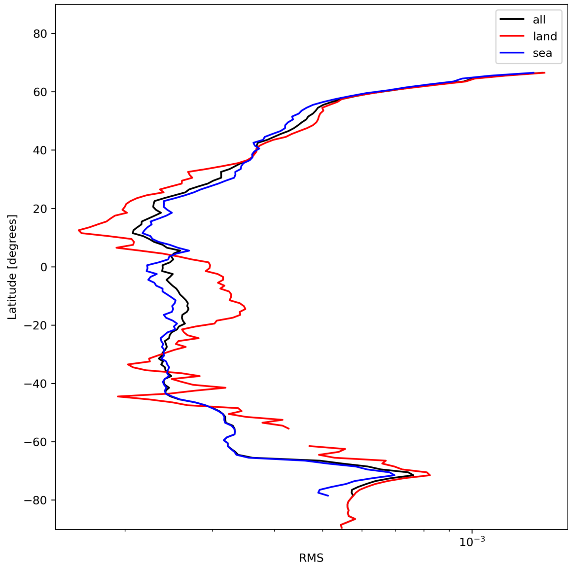
Figure 26: Zonal average of “RMS” for 2024-01-15 to 2024-01-16.
