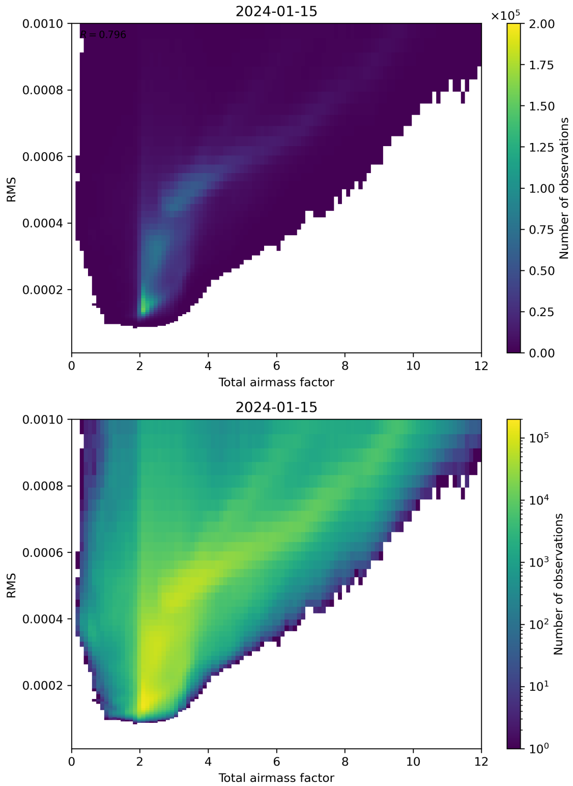
Figure 69: Scatter density plot of “Total airmass factor” against “RMS” for 2024-01-15 to 2024-01-16.
