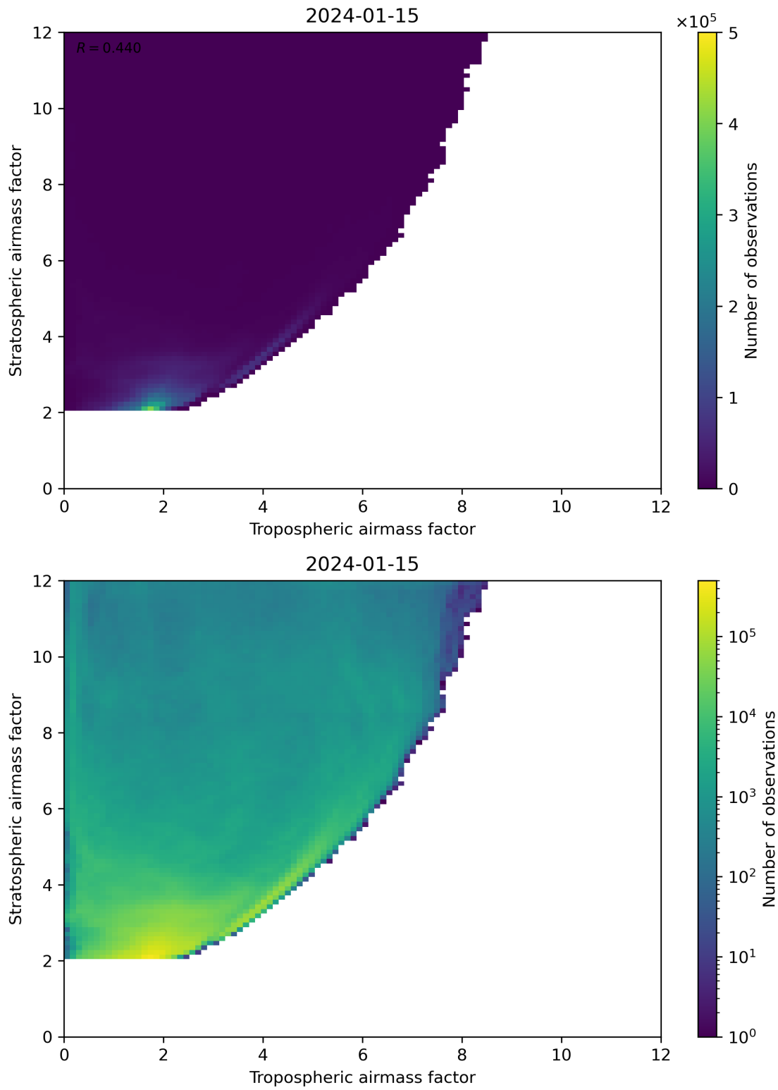
Figure 71: Scatter density plot of “Tropospheric airmass factor” against “Stratospheric airmass factor” for 2024-01-15 to 2024-01-16.
