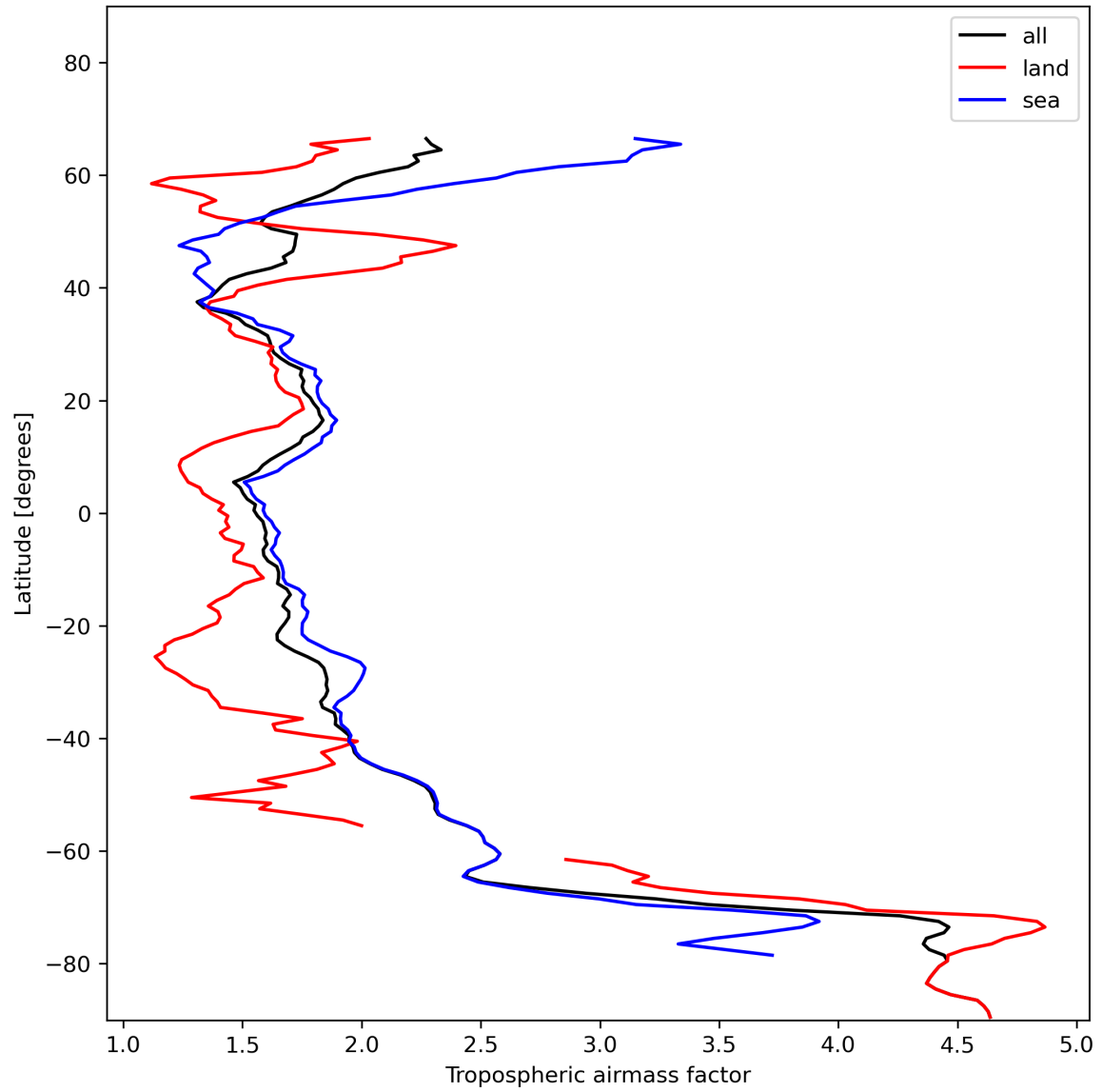
Figure 14: Zonal average of “Tropospheric airmass factor” for 2024-01-15 to 2024-01-16.
