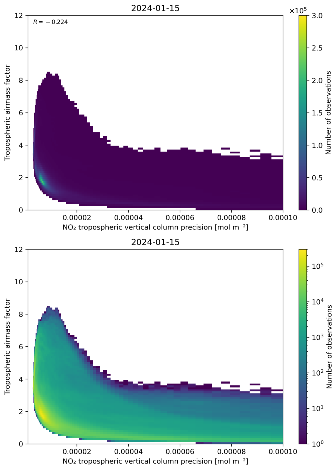
Figure 133: Scatter density plot of “NO 2 tropospheric vertical column precision” against “Tropospheric airmass factor” for 2024-01-15 to 2024-01-16.
