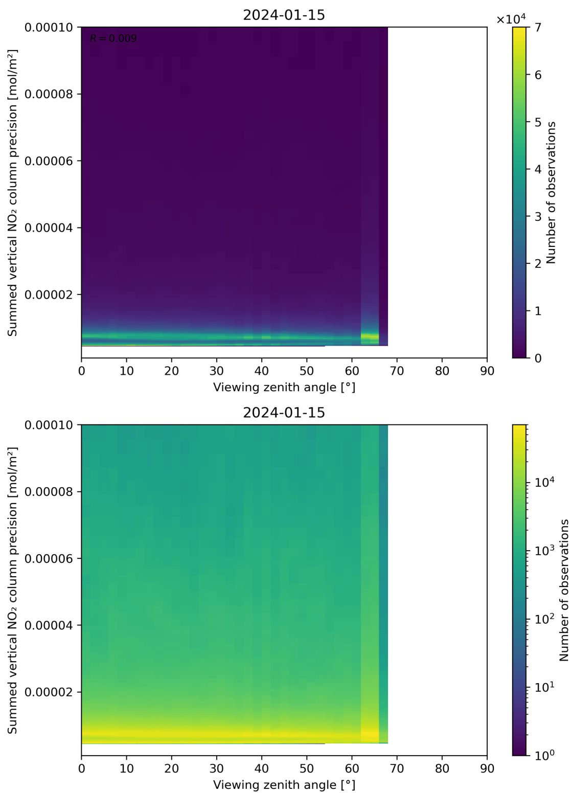
Figure 166: Scatter density plot of “Viewing zenith angle” against “Summed vertical NO 2 column precision” for 2024-01-15 to 2024-01-16.
