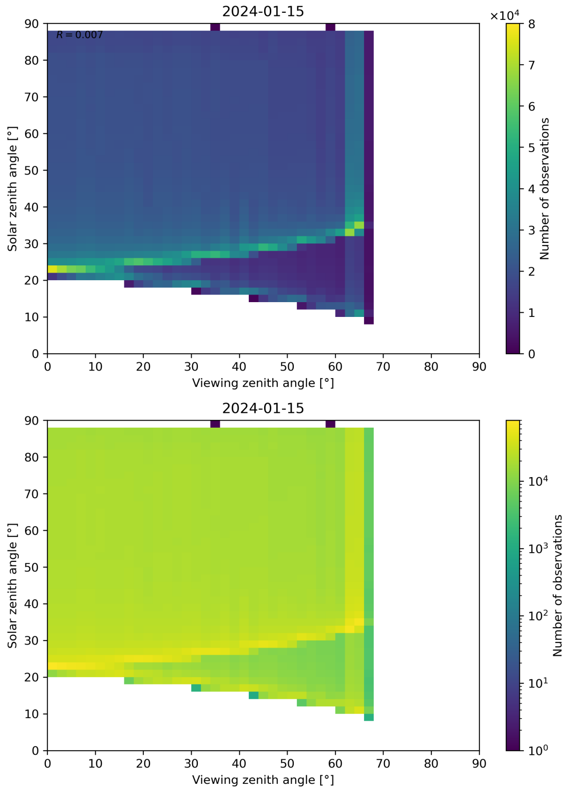
Figure 172: Scatter density plot of “Viewing zenith angle” against “Solar zenith angle” for 2024-01-15 to 2024-01-16.
