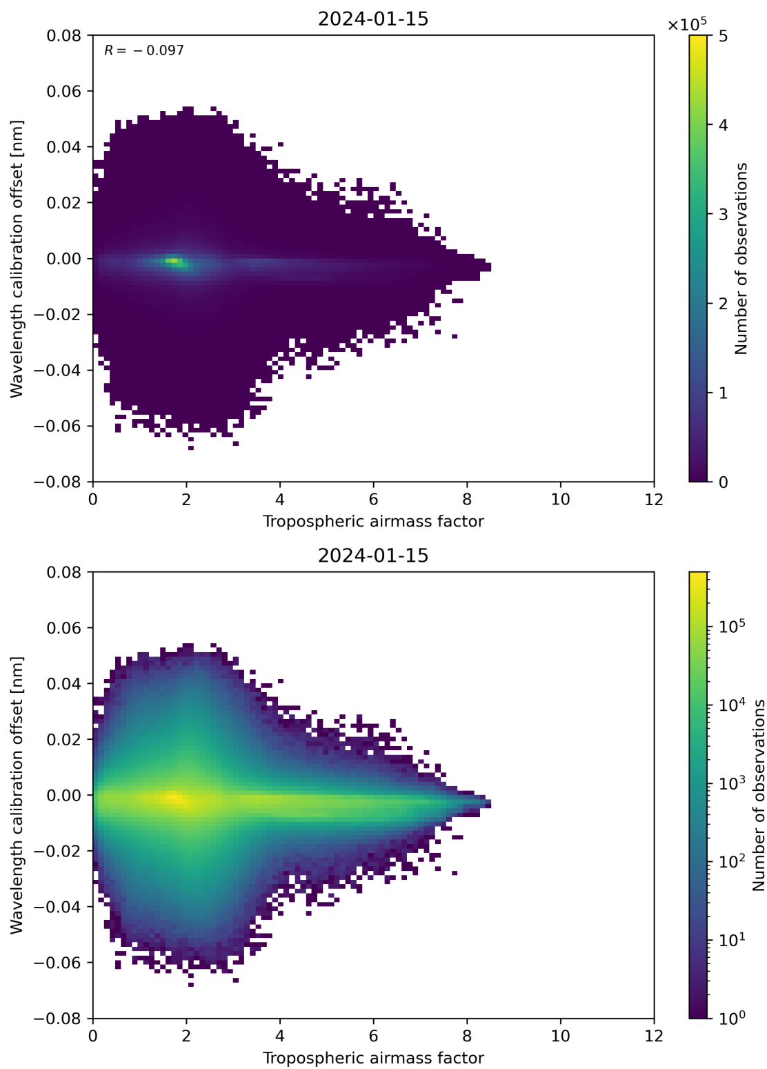
Figure 80: Scatter density plot of “Tropospheric air mass factor” against “Wavelength calibration offset” for 2024-01-15 to 2024-01-16.
