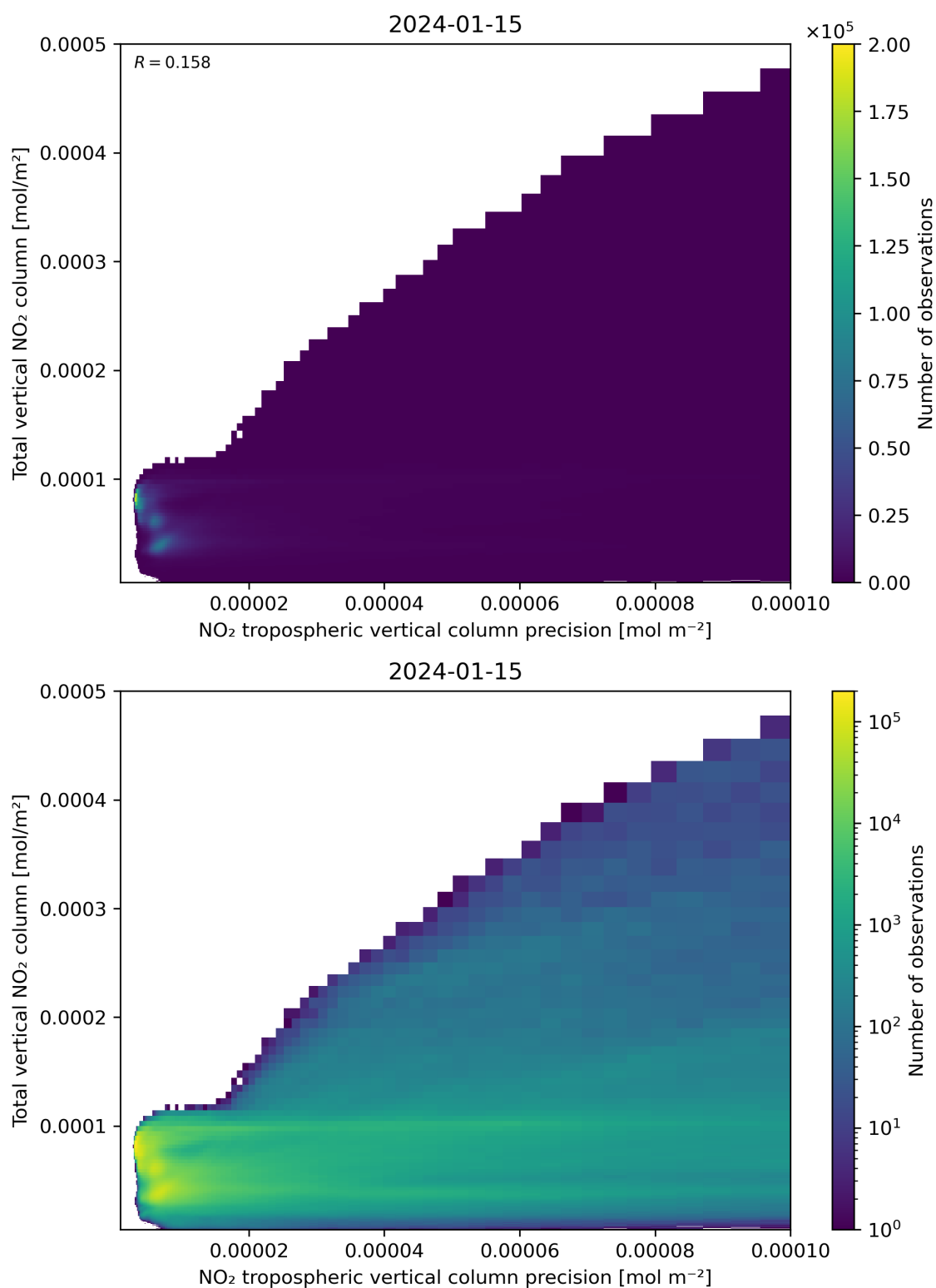
Figure 138: Scatter density plot of “NO 2 tropospheric vertical column precision” against “Total vertical NO 2 column” for 2024-01-15 to 2024-01-16.
