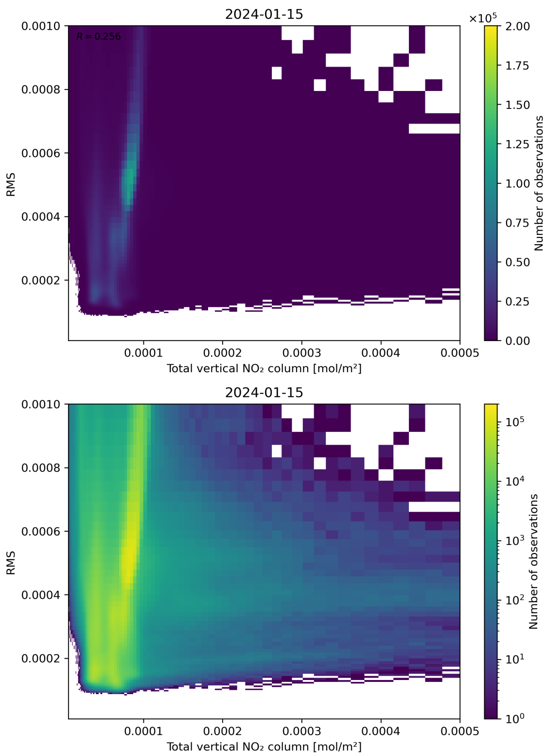
Figure 120: Scatter density plot of “Total vertical NO 2 column” against “RMS” for 2024-01-15 to 2024-01-16.
