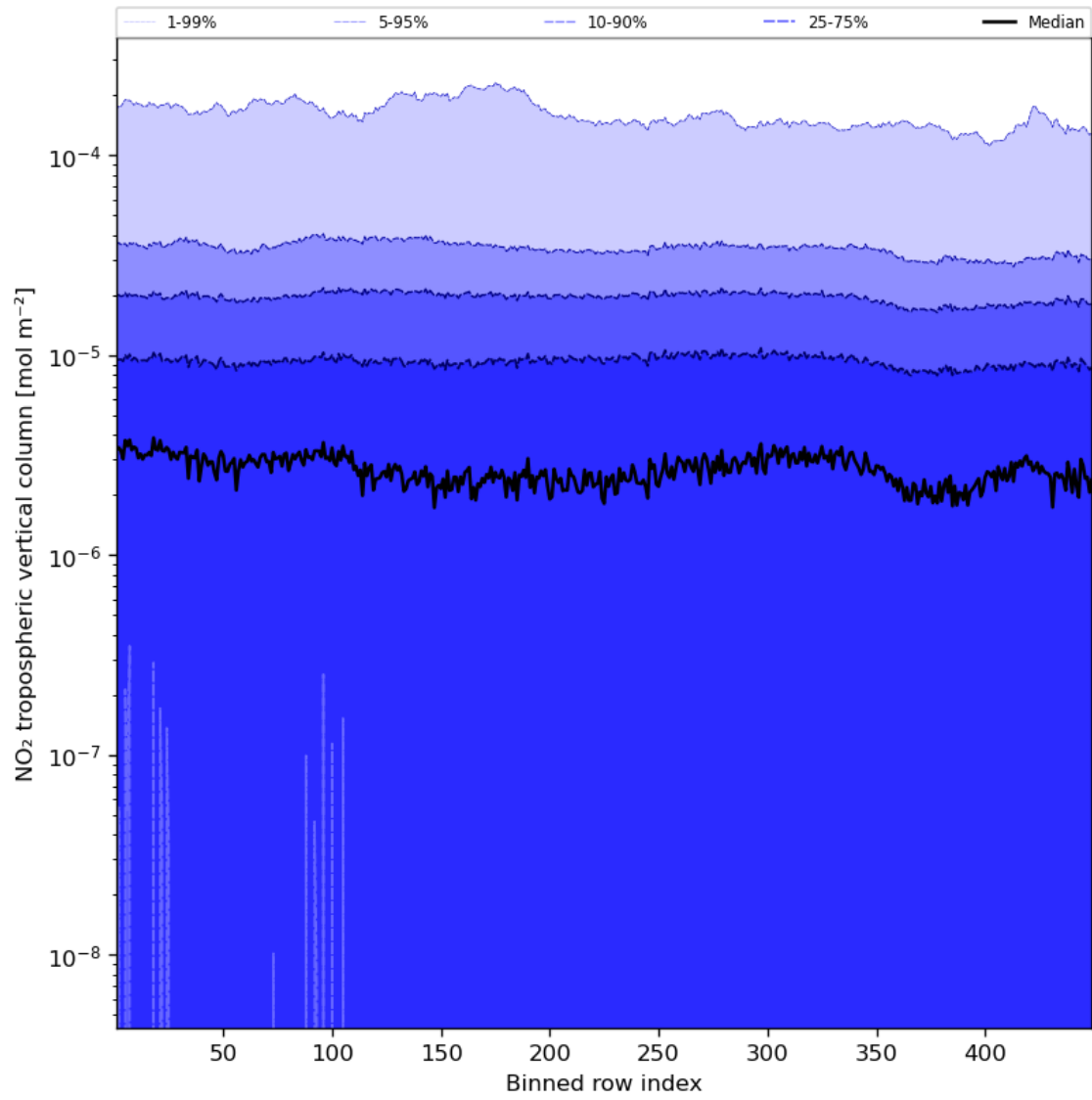
Figure 46: Along track statistics of “NO 2 tropospheric vertical column” for 2024-01-15 to 2024-01-16
