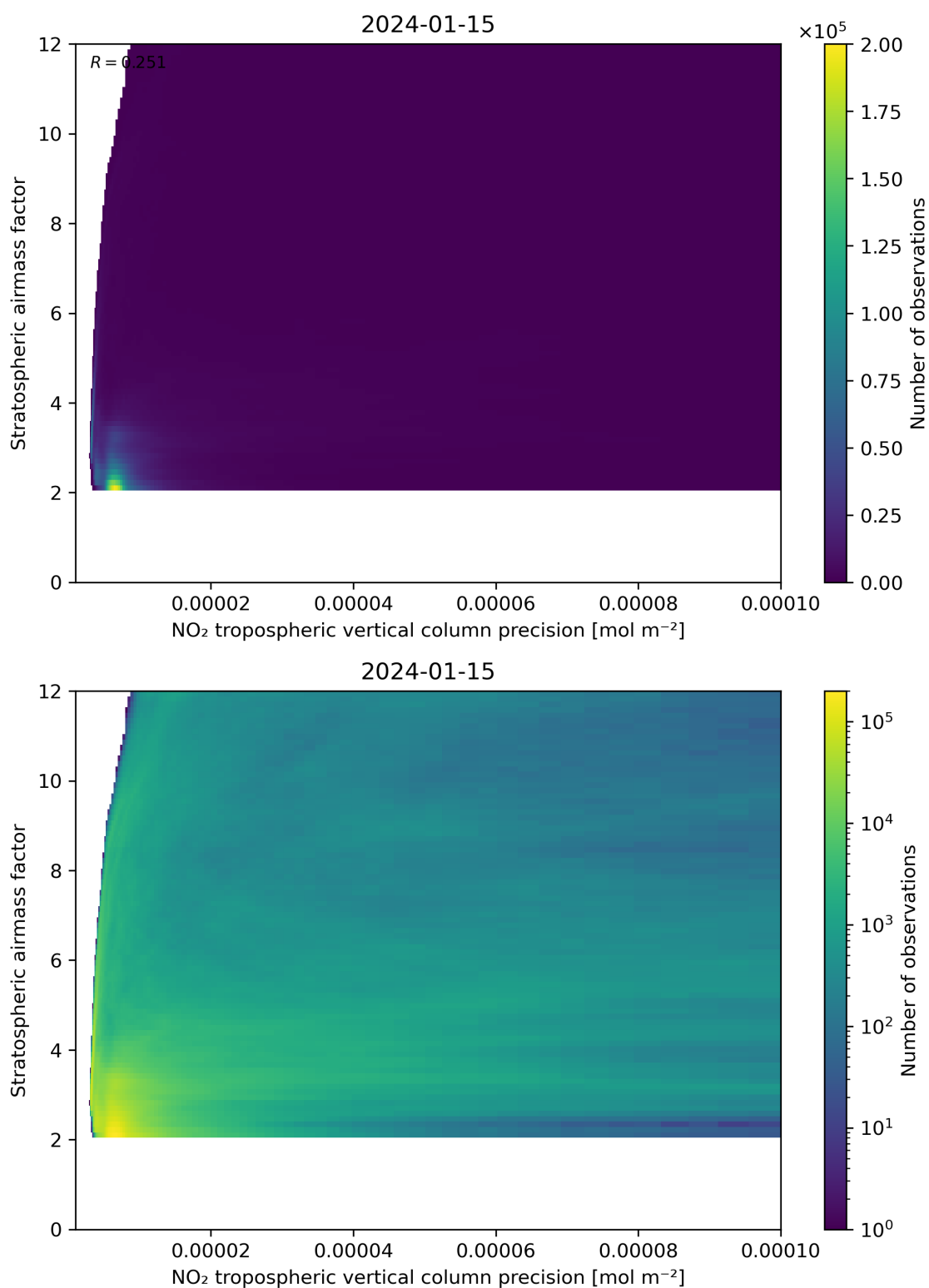
Figure 131: Scatter density plot of “NO 2 tropospheric vertical column precision” against “Stratospheric airmass factor” for 2024-01-15 to 2024-01-16.
