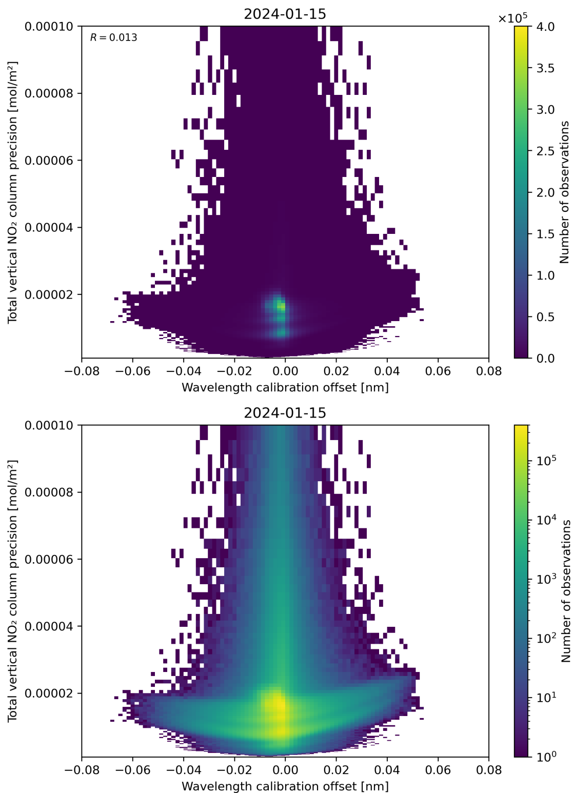
Figure 180: Scatter density plot of “Wavelength calibration offset” against “Total vertical NO 2 column precision” for 2024-01-15 to 2024-01-16.
