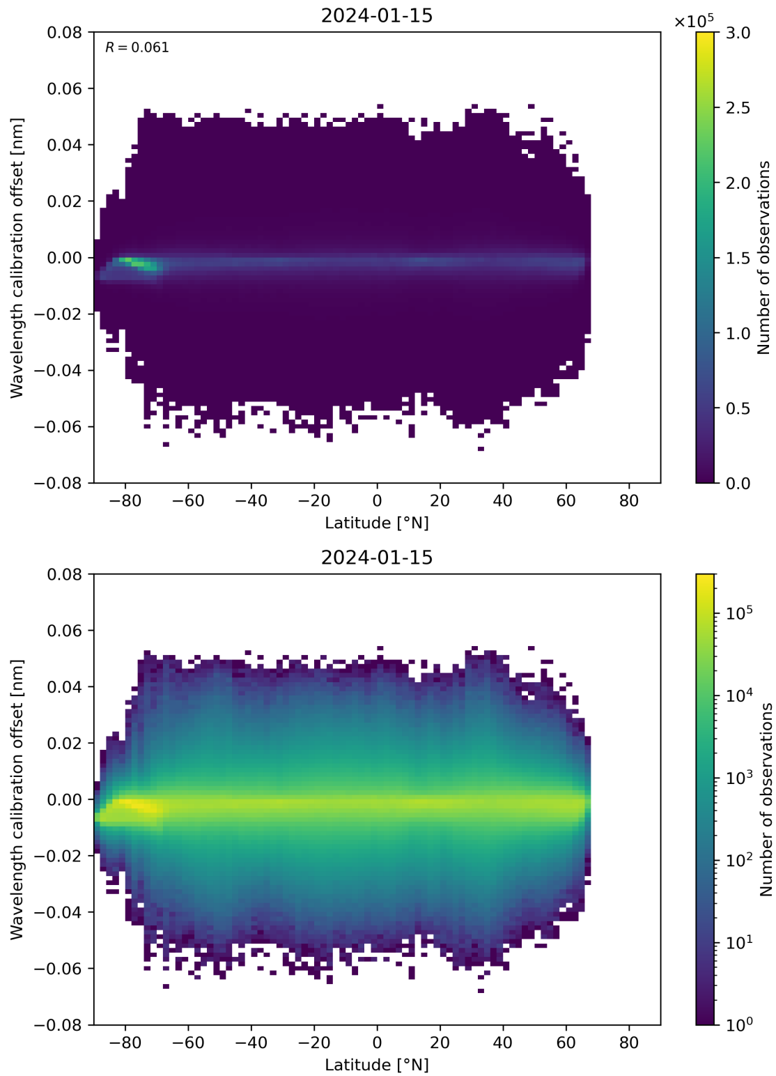
Figure 95: Scatter density plot of “Latitude” against “Wavelength calibration offset” for 2024-01-15 to 2024-01-16.
