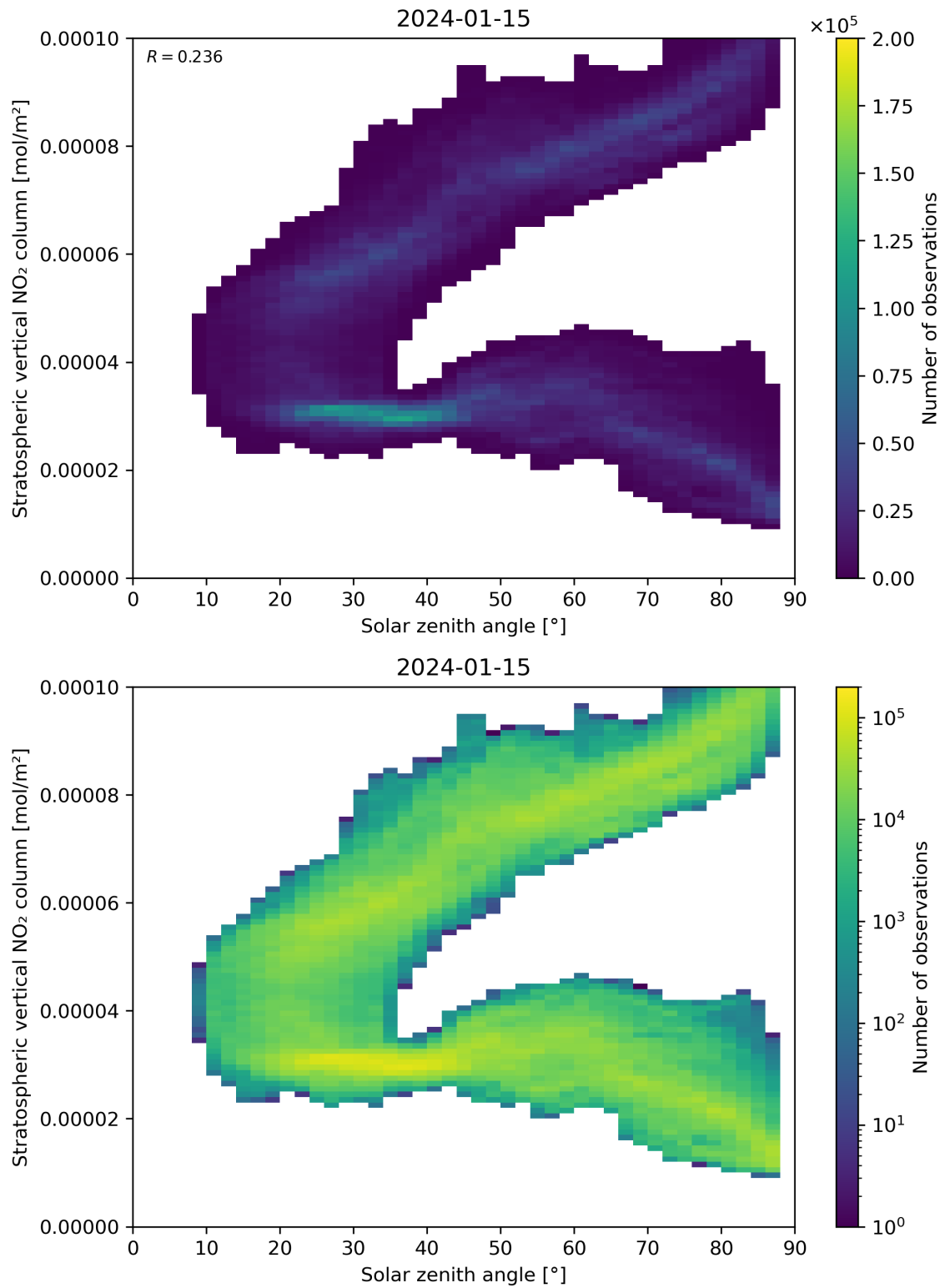
Figure 150: Scatter density plot of “Solar zenith angle” against “Stratospheric vertical NO 2 column” for 2024-01-15 to 2024-01-16.
