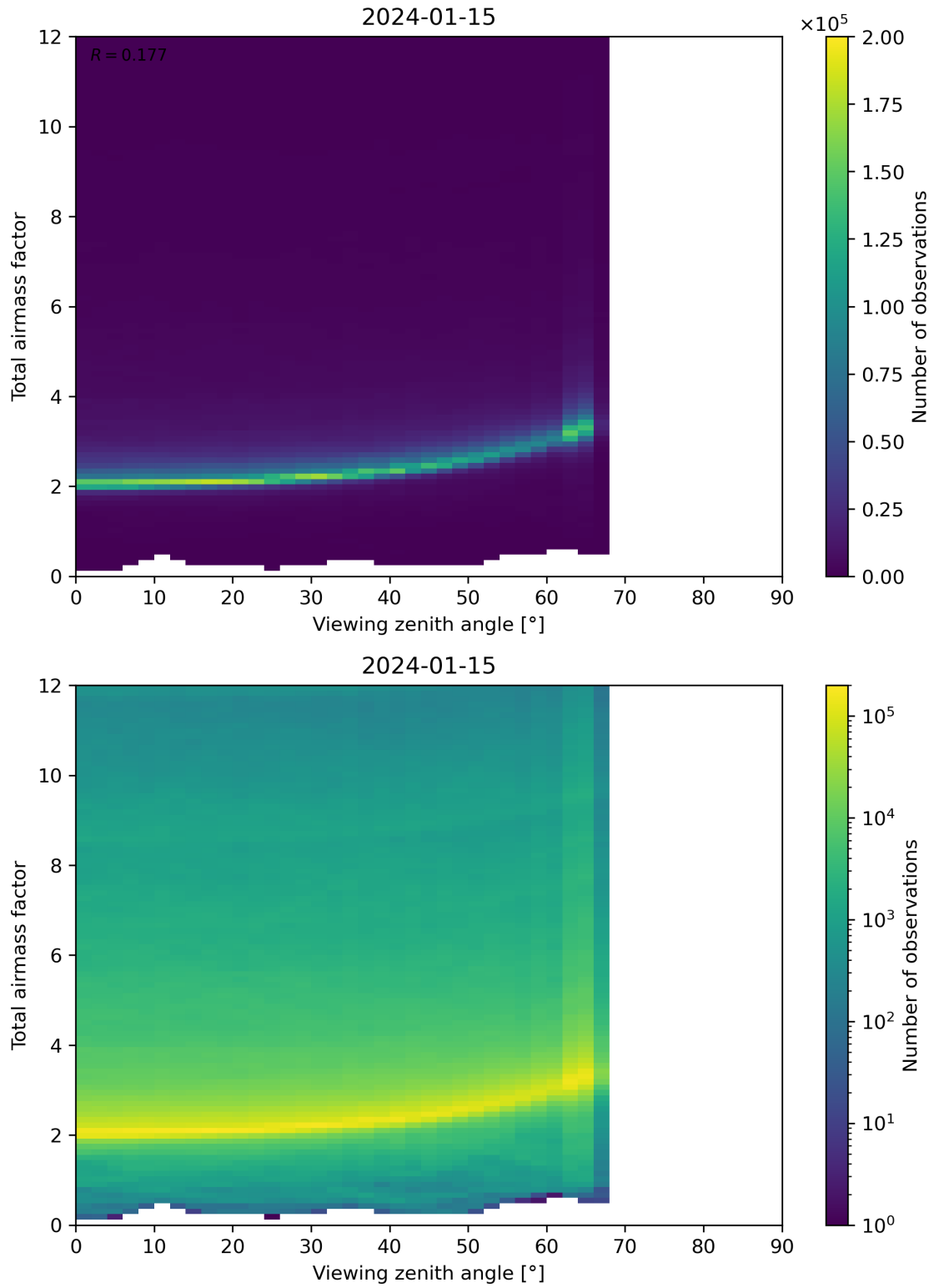
Figure 160: Scatter density plot of “Viewing zenith angle” against “Total airmass factor” for 2024-01-15 to 2024-01-16.
