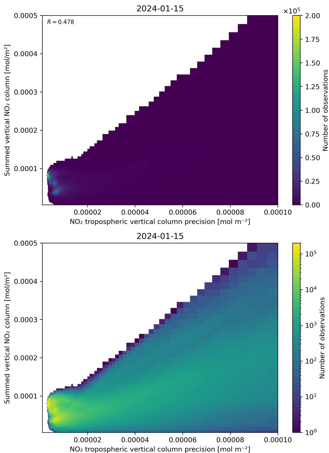
Figure 136: Scatter density plot of “NO 2 tropospheric vertical column precision” against “Summed vertical NO 2 column” for 2024-01-15 to 2024-01-16.
