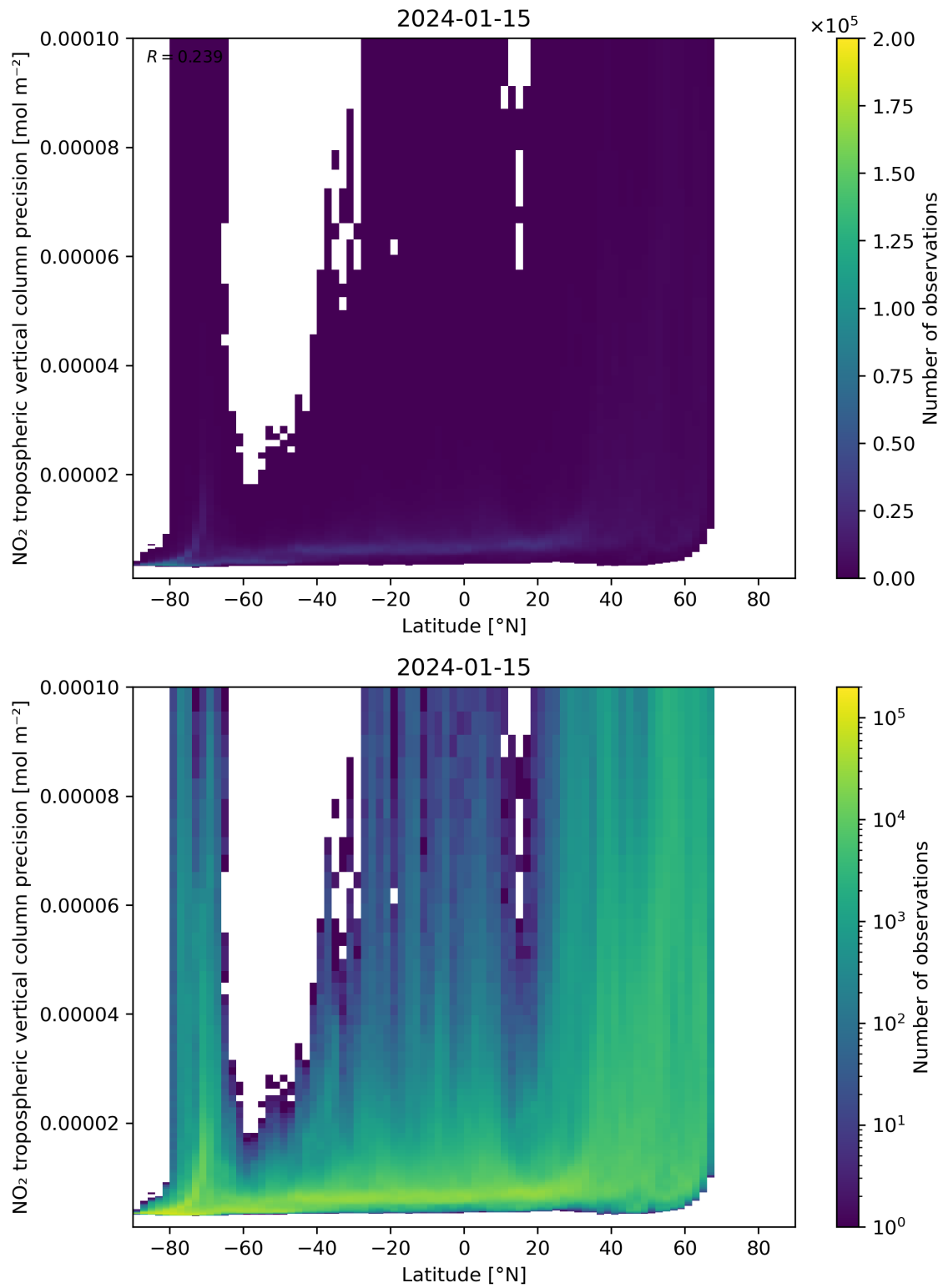
Figure 93: Scatter density plot of “Latitude” against “NO 2 tropospheric vertical column precision” for 2024-01-15 to 2024-01-16.
