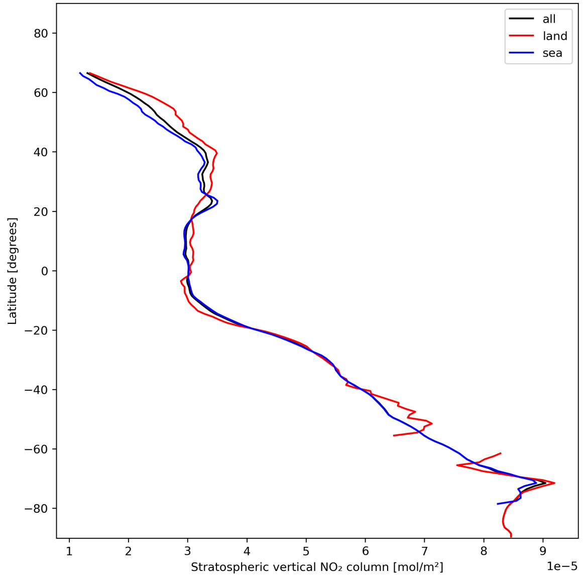
Figure 19: Zonal average of “Stratospheric vertical NO 2 column” for 2024-01-15 to 2024-01-16.
