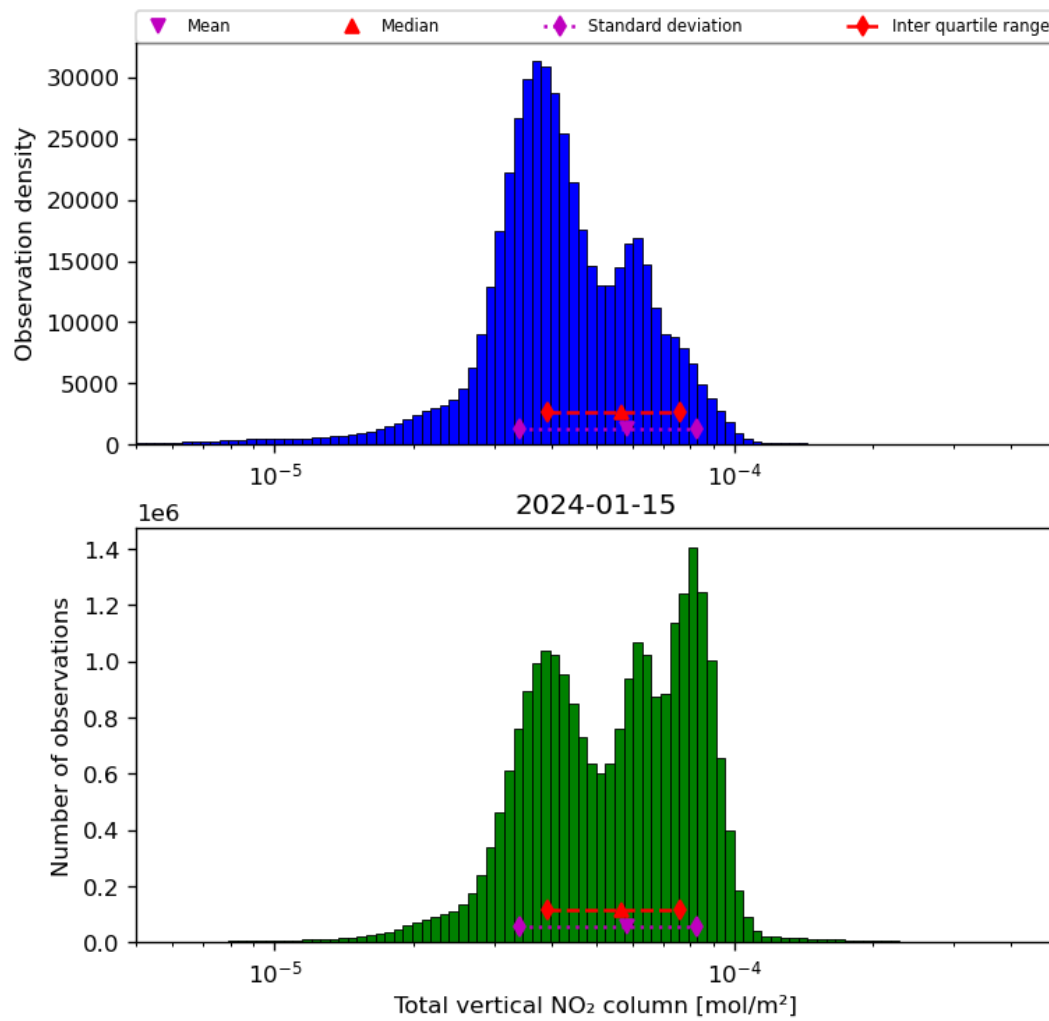
Figure 38: Histogram of “Total vertical NO 2 column” for 2024-01-15 to 2024-01-16
