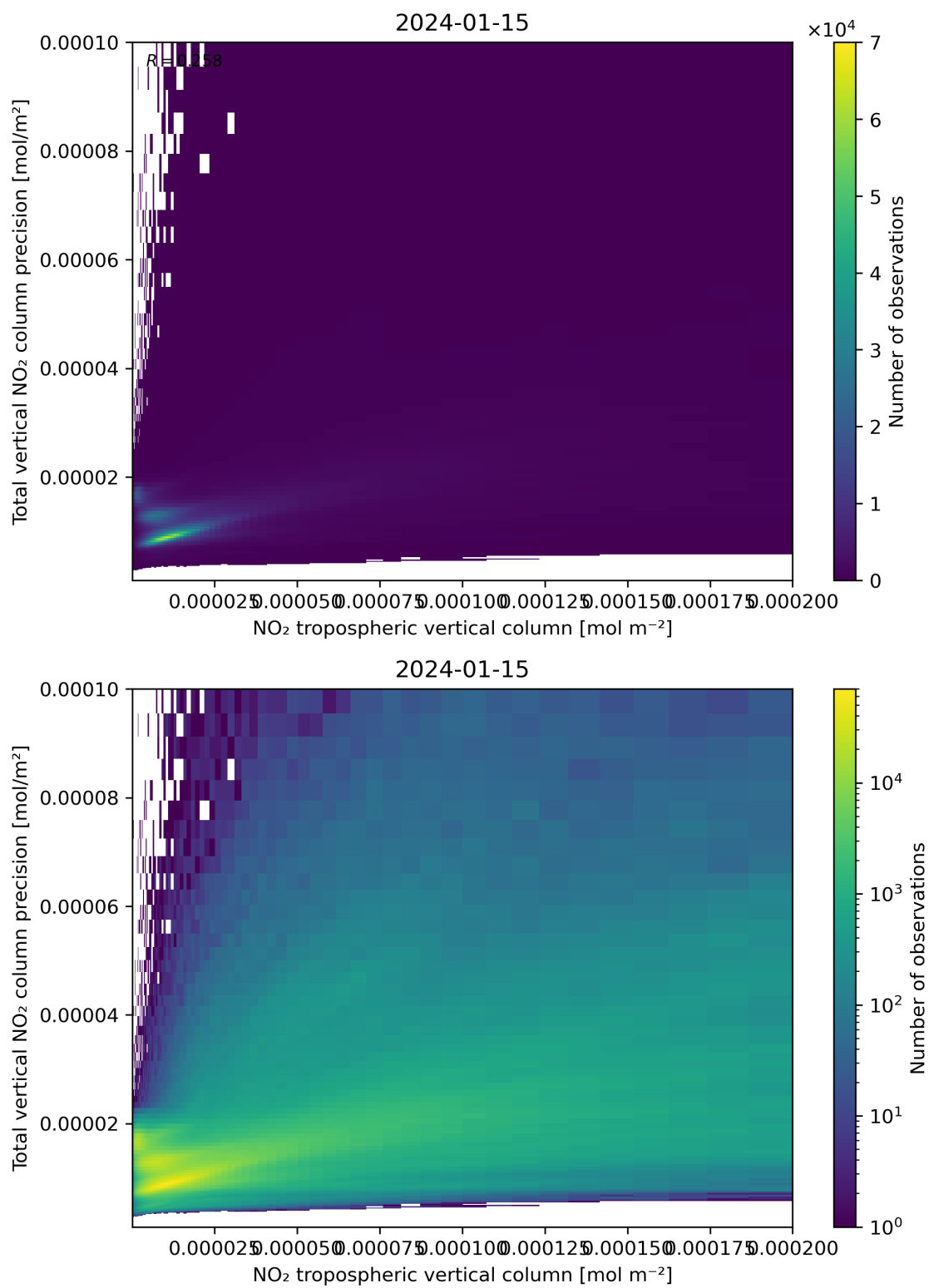
Figure 129: Scatter density plot of “NO 2 tropospheric vertical column” against “Total vertical NO 2 column precision” for 2024-01-15 to 2024-01-16.
