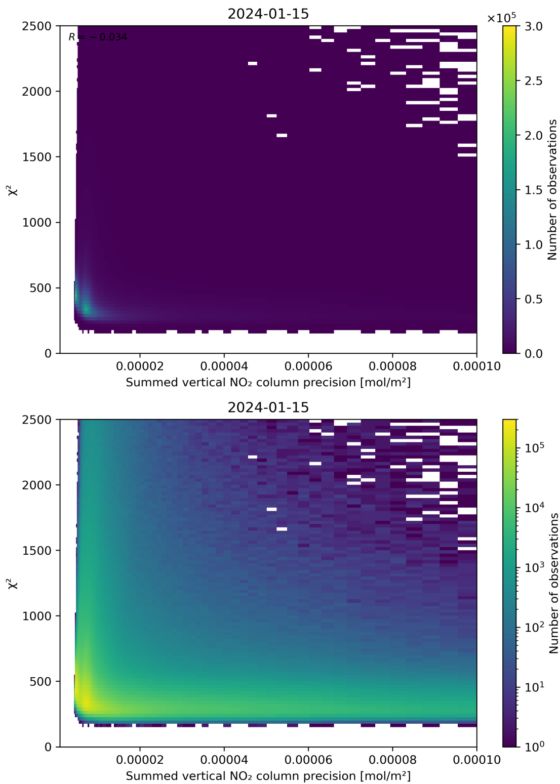
Figure 107: Scatter density plot of “Summed vertical NO 2 column precision” against “ \chi^2 ” for 2024-01-15 to 2024-01-16.
