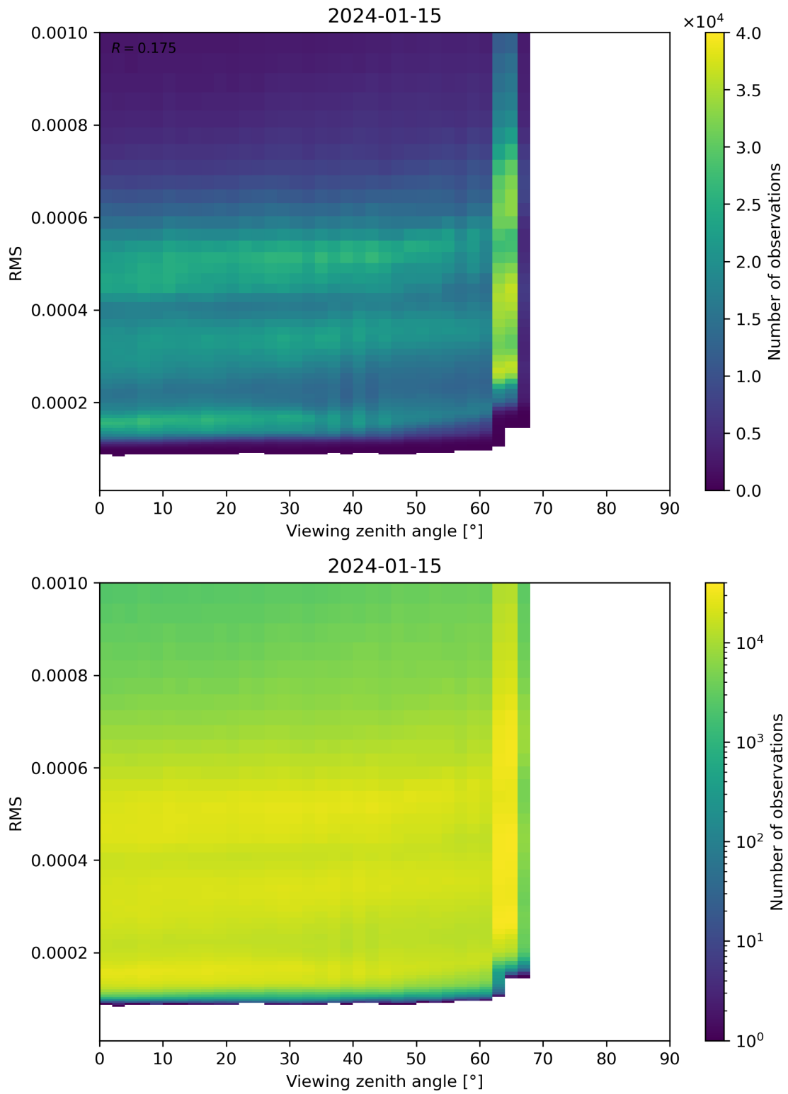
Figure 171: Scatter density plot of “Viewing zenith angle” against “RMS” for 2024-01-15 to 2024-01-16.
