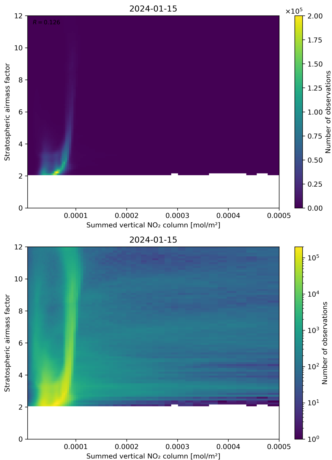
Figure 103: Scatter density plot of “Summed vertical NO 2 column” against “Stratospheric airmass factor” for 2024-01-15 to 2024-01-16.
