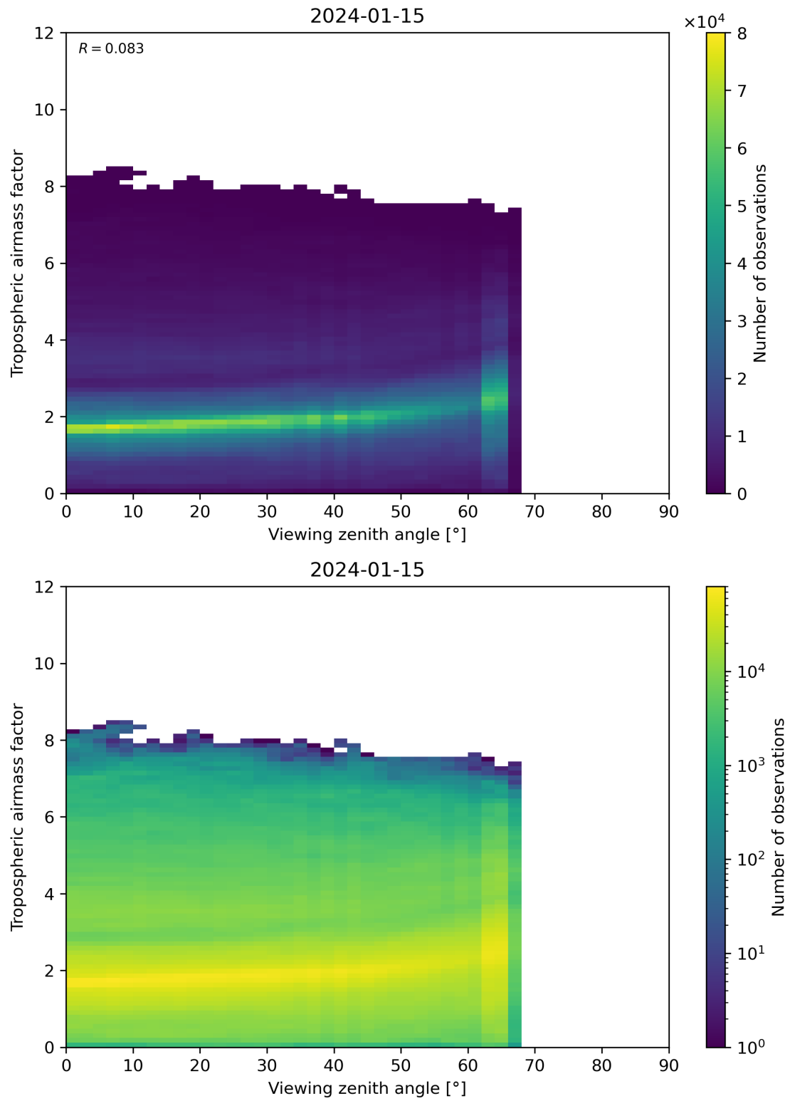
Figure 161: Scatter density plot of “Viewing zenith angle” against “Tropospheric airmass factor” for 2024-01-15 to 2024-01-16.
