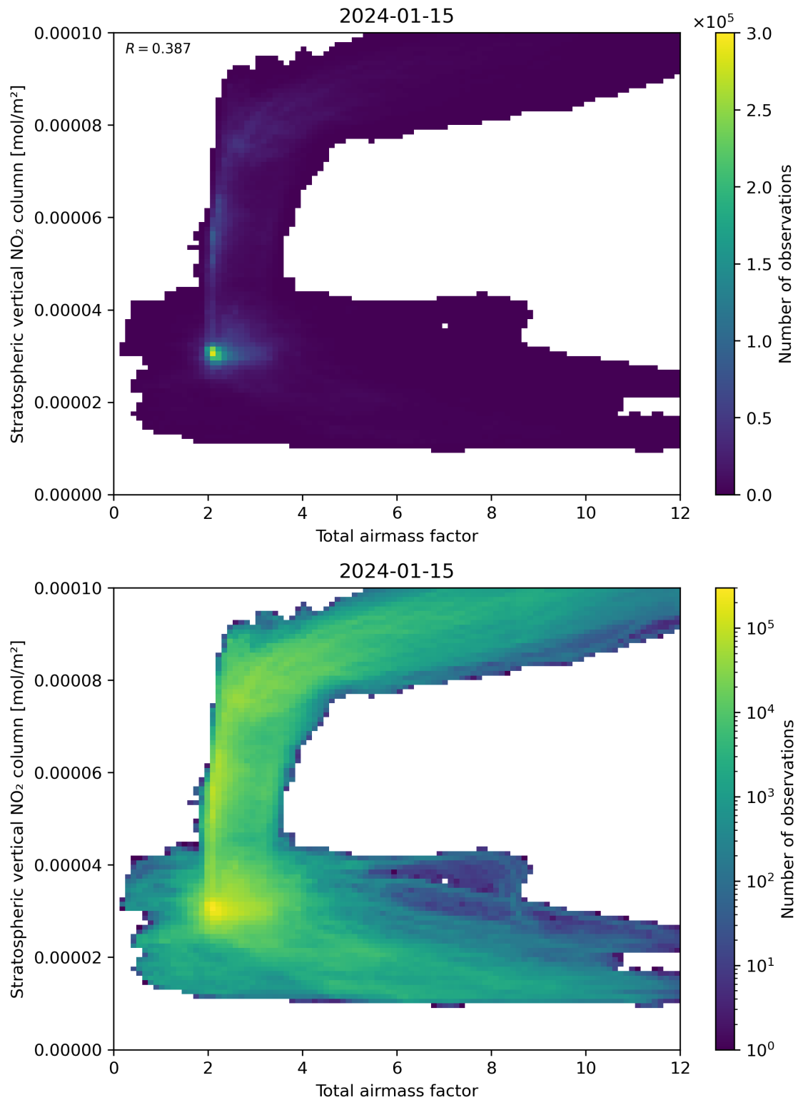
Figure 64: Scatter density plot of “Total airmass factor” against “Stratospheric vertical NO 2 column” for 2024-01-15 to 2024-01-16.
