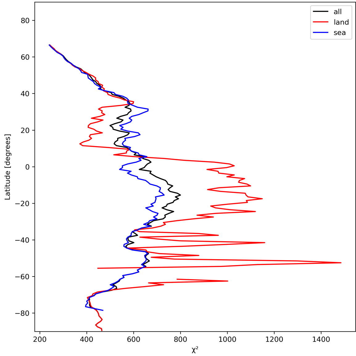
Figure 25: Zonal average of “ \chi^2 ” for 2024-01-15 to 2024-01-16.
