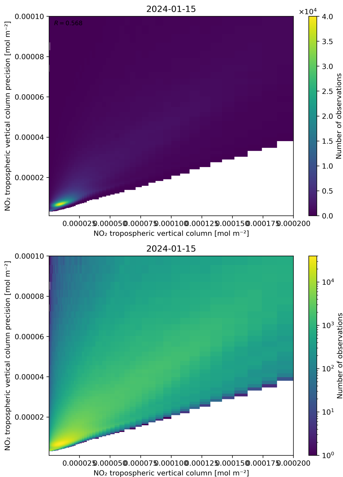
Figure 130: Scatter density plot of “NO 2 tropospheric vertical column” against “NO 2 tropospheric vertical column precision” for 2024-01-15 to 2024-01-16.
