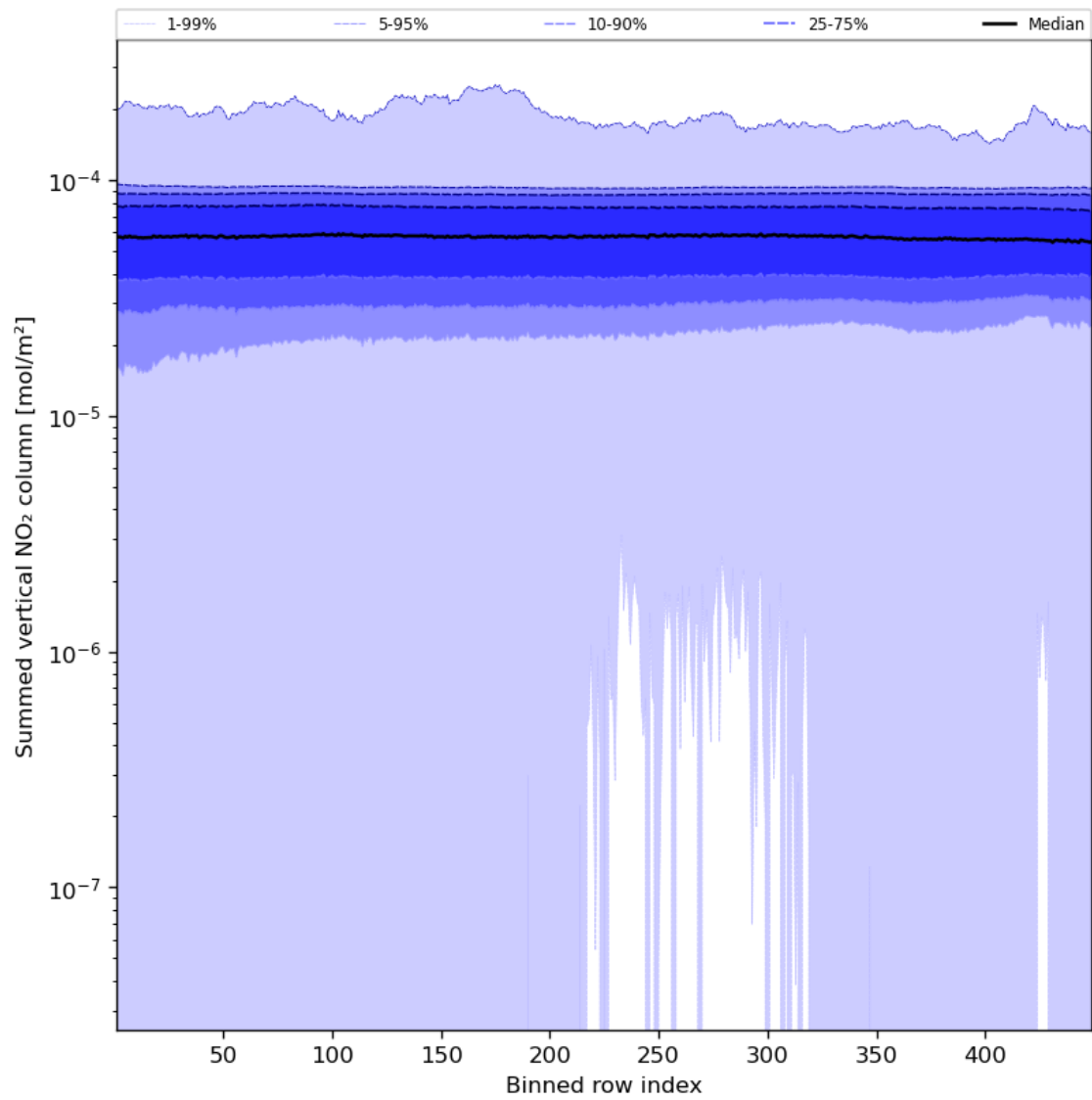
Figure 57: Along track statistics of “Summed vertical NO 2 column” for 2024-01-15 to 2024-01-16
