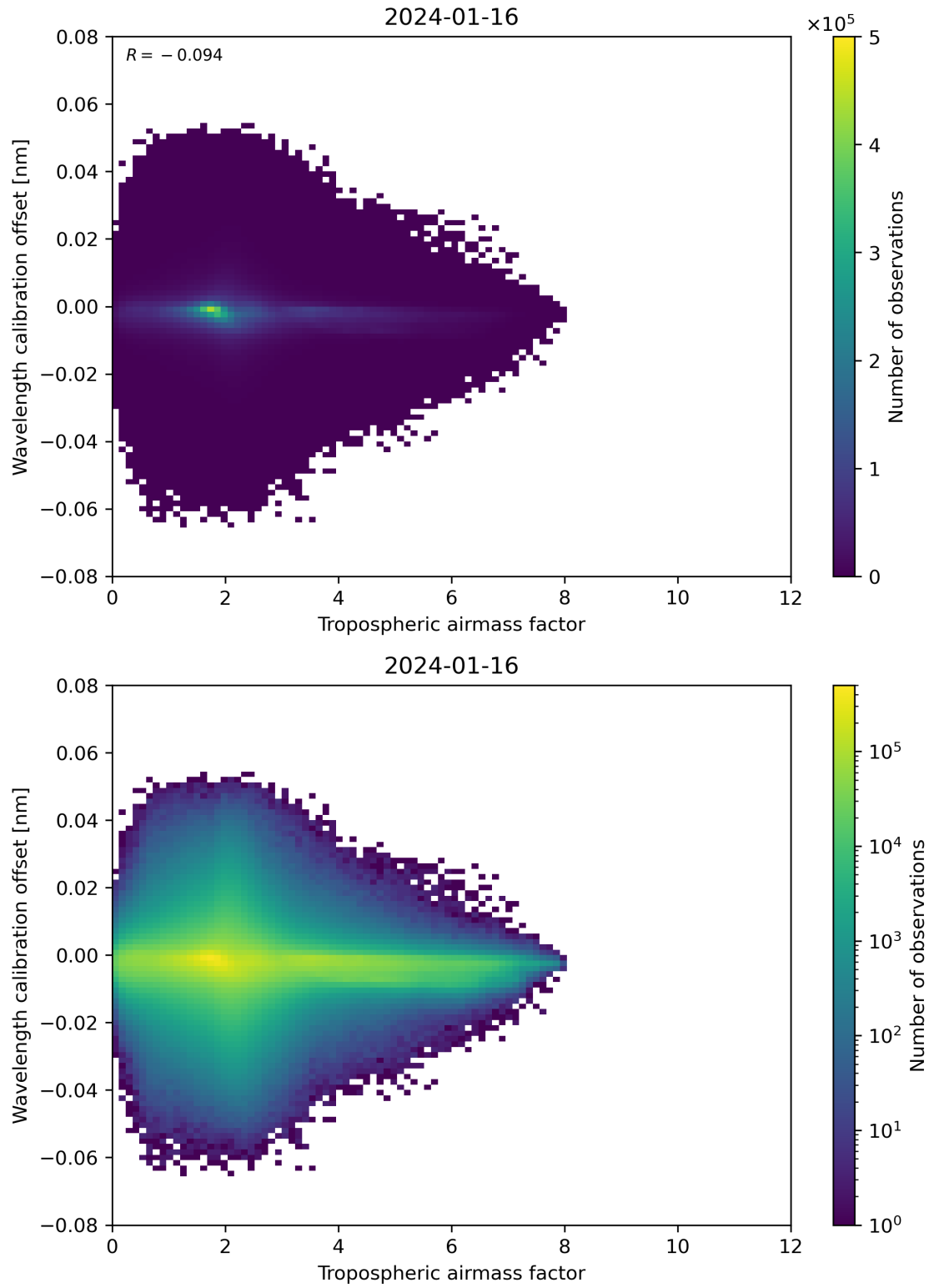
Figure 80: Scatter density plot of “Tropospheric airmass factor” against “Wavelength calibration offset” for 2024-01-15 to 2024-01-17.
