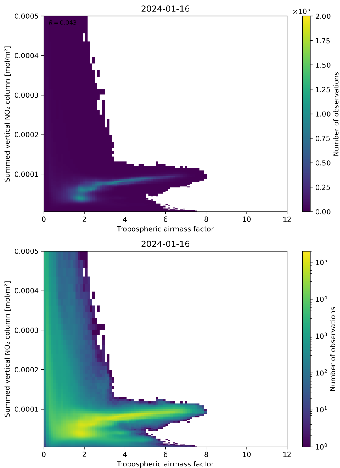
Figure 75: Scatter density plot of “Tropospheric airmass factor” against “Summed vertical NO 2 column” for 2024-01-15 to 2024-01-17.
