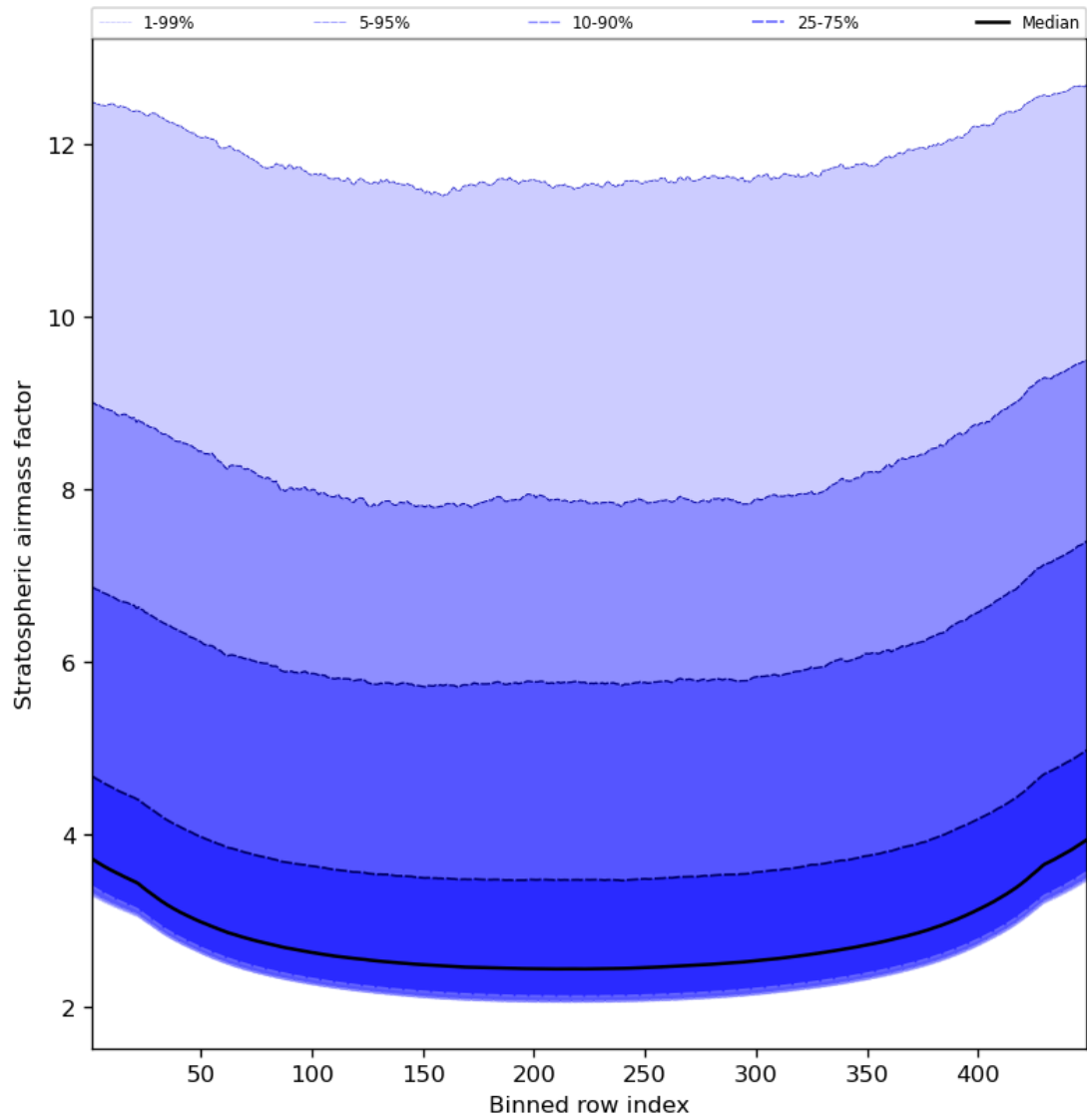
Figure 61: Along track statistics of “Stratospheric airmass factor” for 2024-01-15 to 2024-01-17
