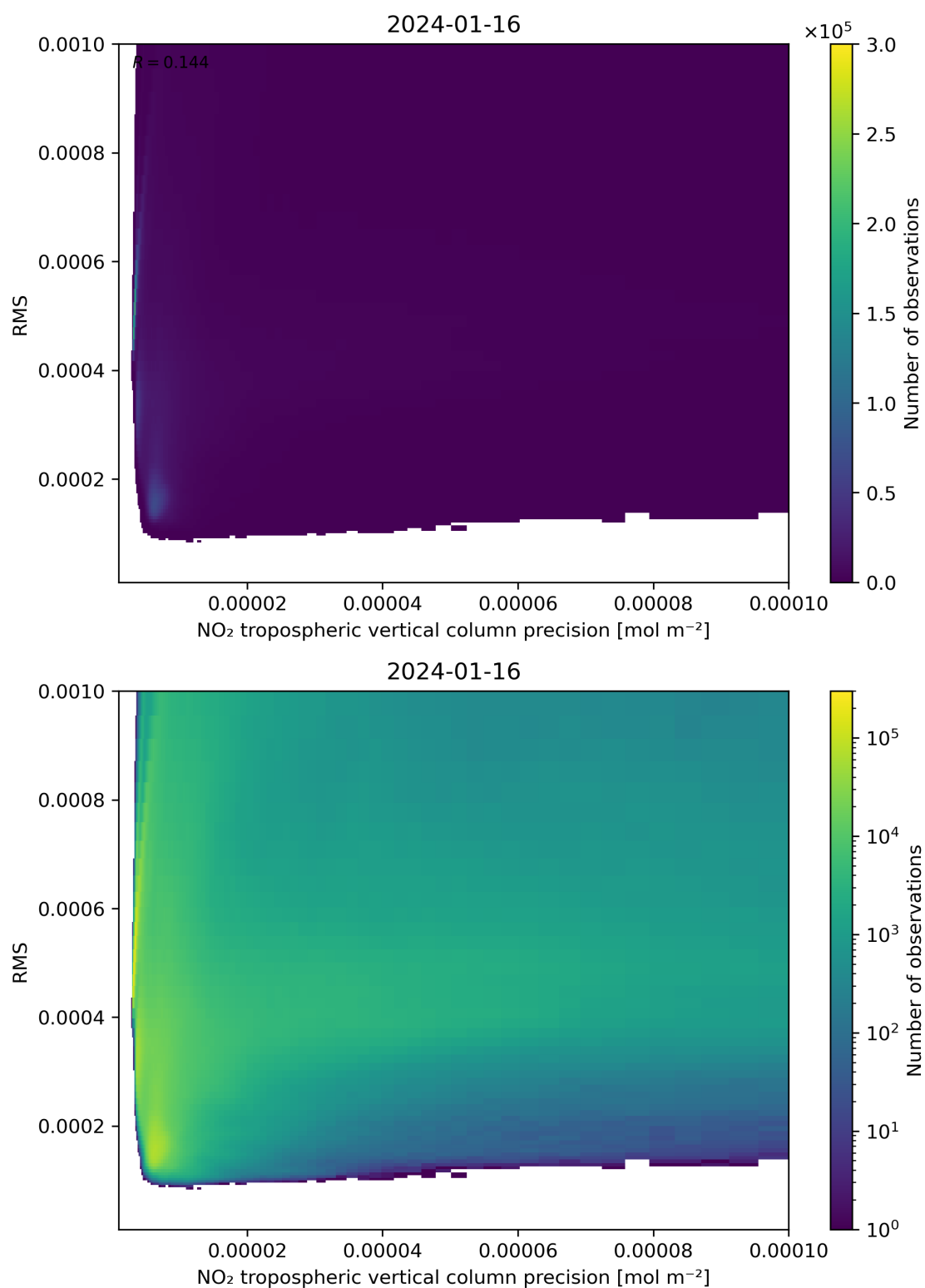
Figure 140: Scatter density plot of “NO 2 tropospheric vertical column precision” against “RMS” for 2024-01-15 to 2024-01-17.
