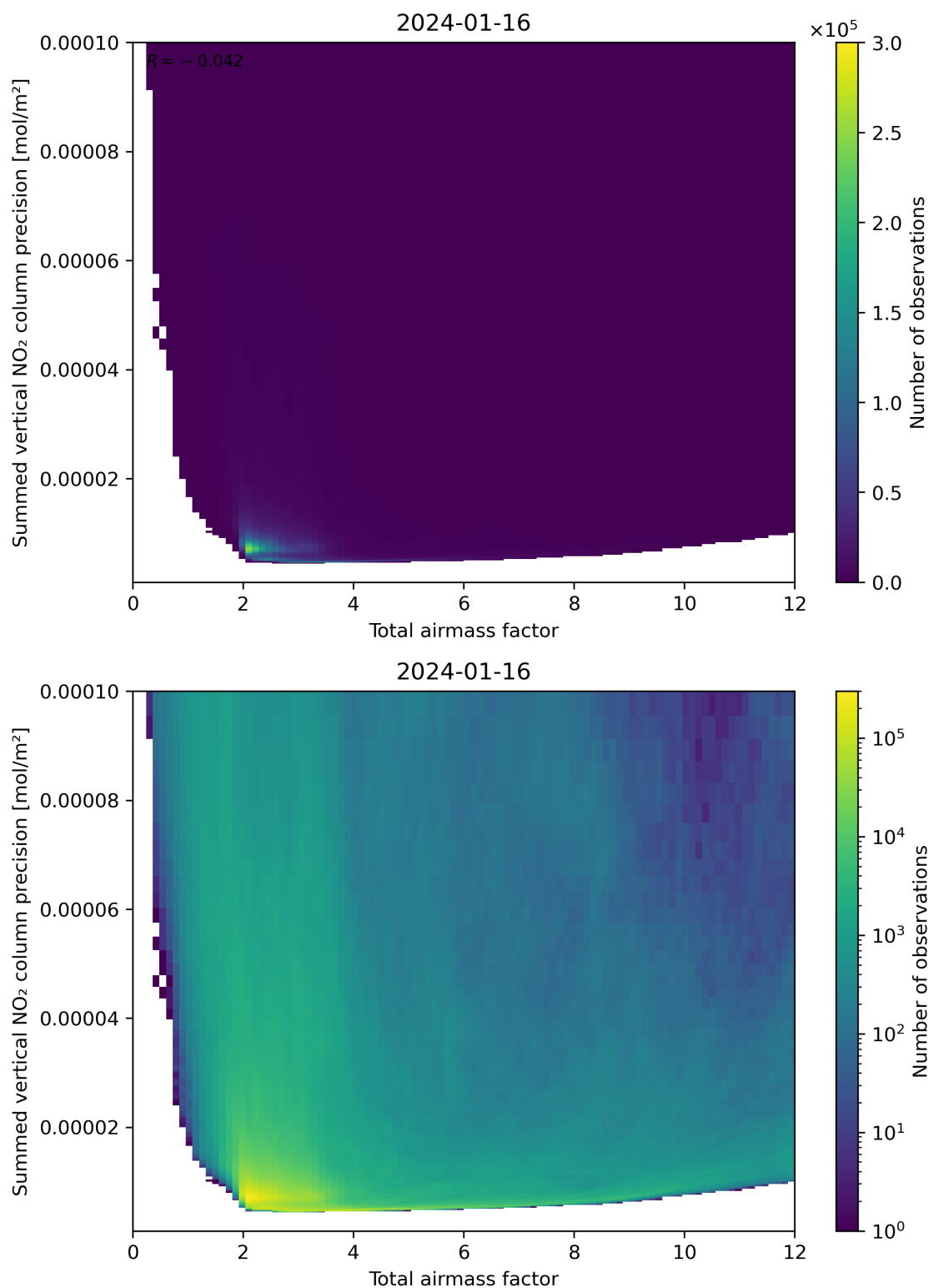
Figure 66: Scatter density plot of “Total airmass factor” against “Summed vertical NO 2 column precision” for 2024-01-15 to 2024-01-17.
