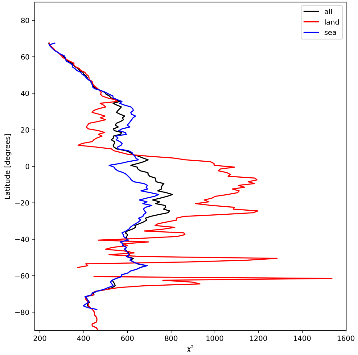
Figure 25: Zonal average of “ \chi^2 ” for 2024-01-15 to 2024-01-17.
