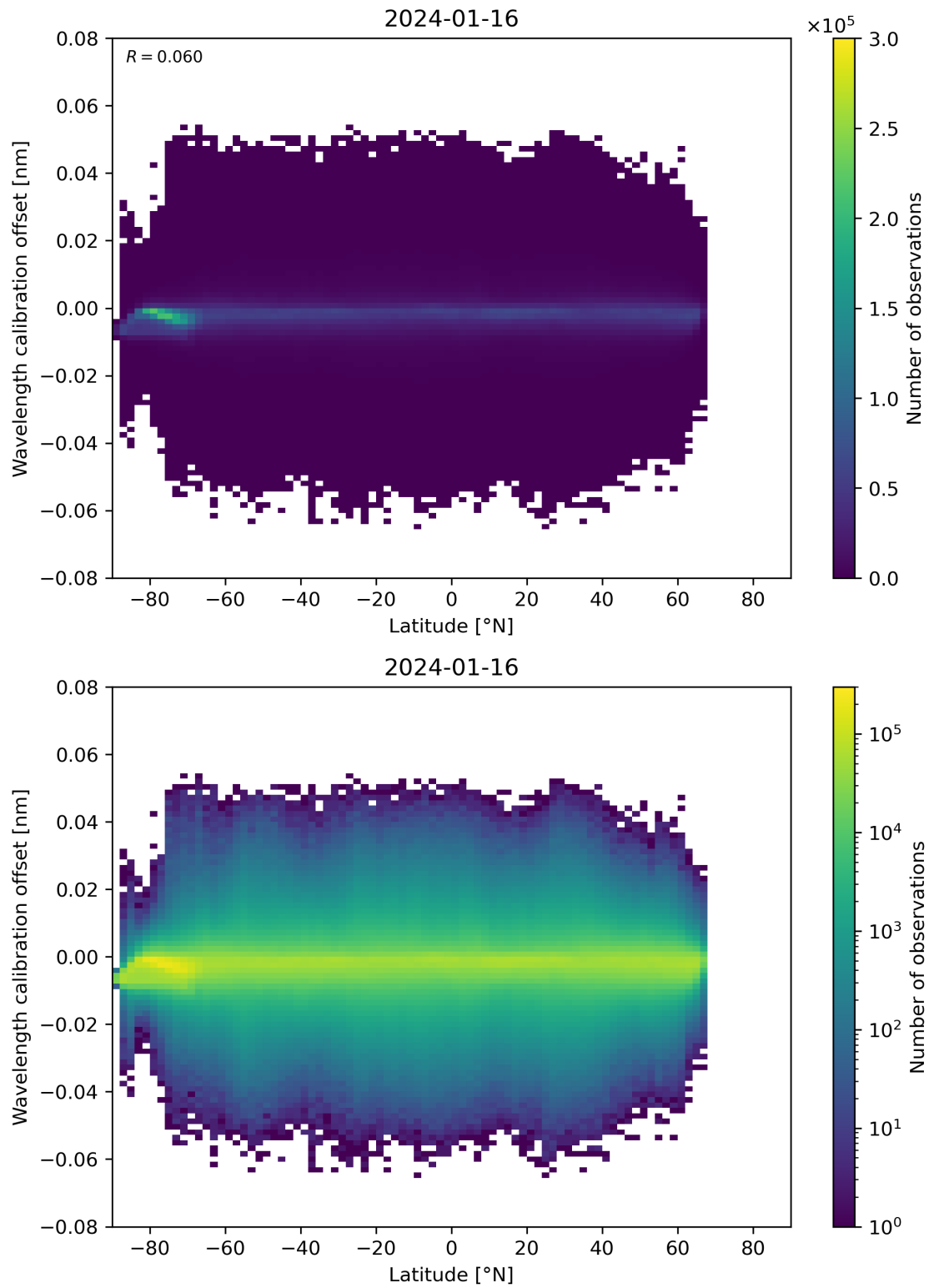
Figure 95: Scatter density plot of “Latitude” against “Wavelength calibration offset” for 2024-01-15 to 2024-01-17.
