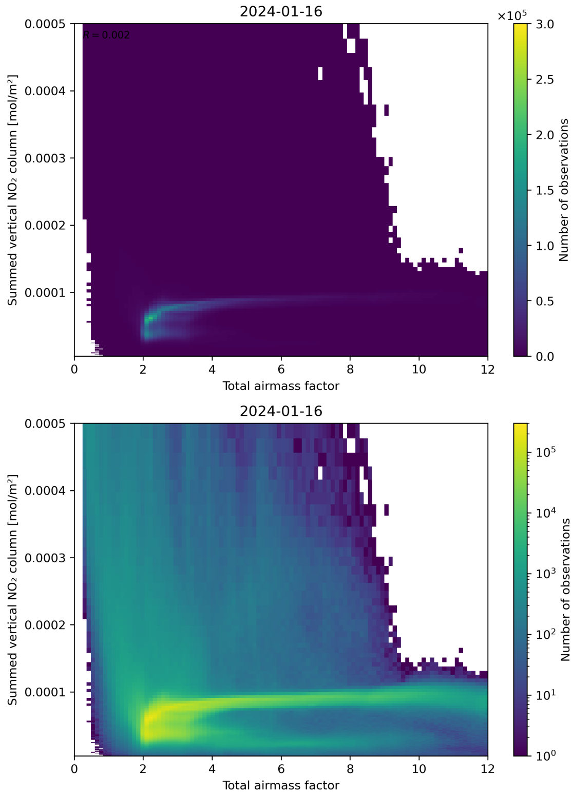
Figure 65: Scatter density plot of “Total airmass factor” against “Summed vertical NO 2 column” for 2024-01-15 to 2024-01-17.
