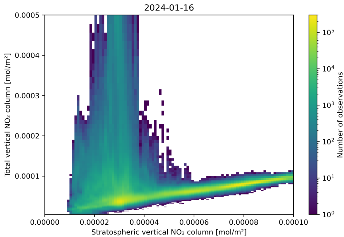
Figure 100: Scatter density plot of “Stratospheric vertical NO 2 column” against “Total vertical NO 2 column” for 2024-01-15 to 2024-01-17.
