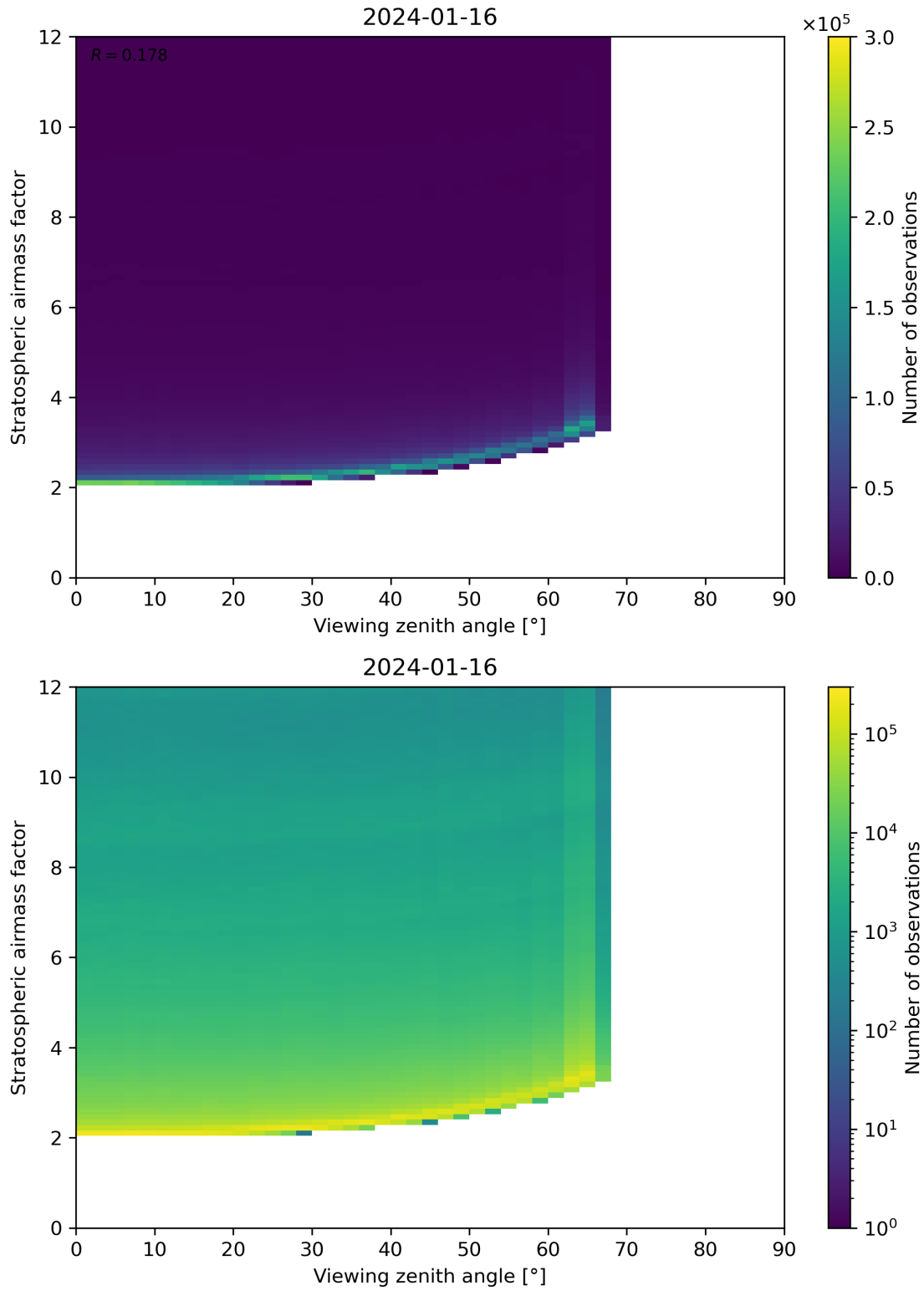
Figure 159: Scatter density plot of “Viewing zenith angle” against “Stratospheric airmass factor” for 2024-01-15 to 2024-01-17.
