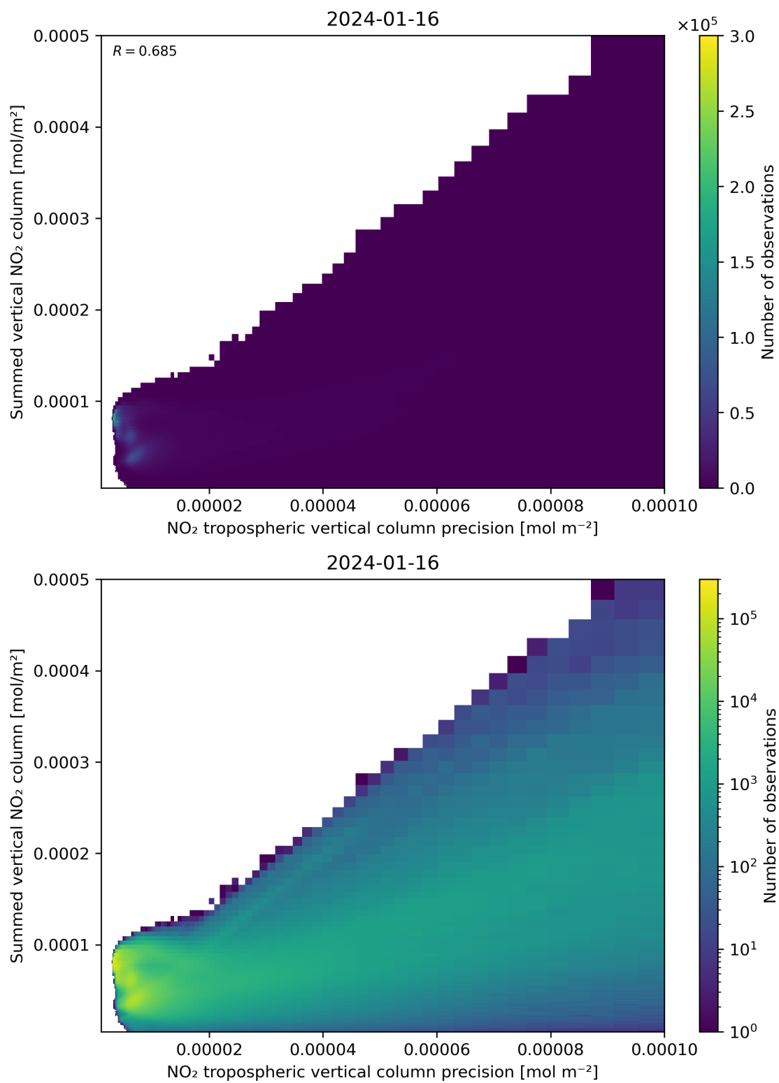
Figure 136: Scatter density plot of “NO 2 tropospheric vertical column precision” against “Summed vertical NO 2 column” for 2024-01-15 to 2024-01-17.
