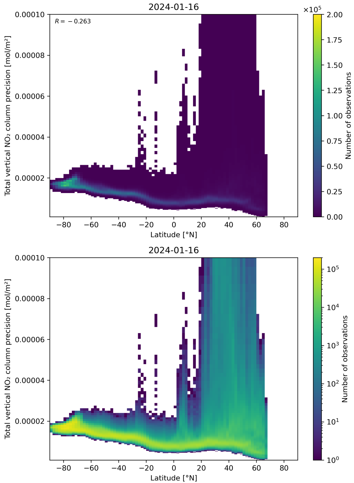
Figure 91: Scatter density plot of “Latitude” against “Total vertical NO 2 column precision” for 2024-01-15 to 2024-01-17.
