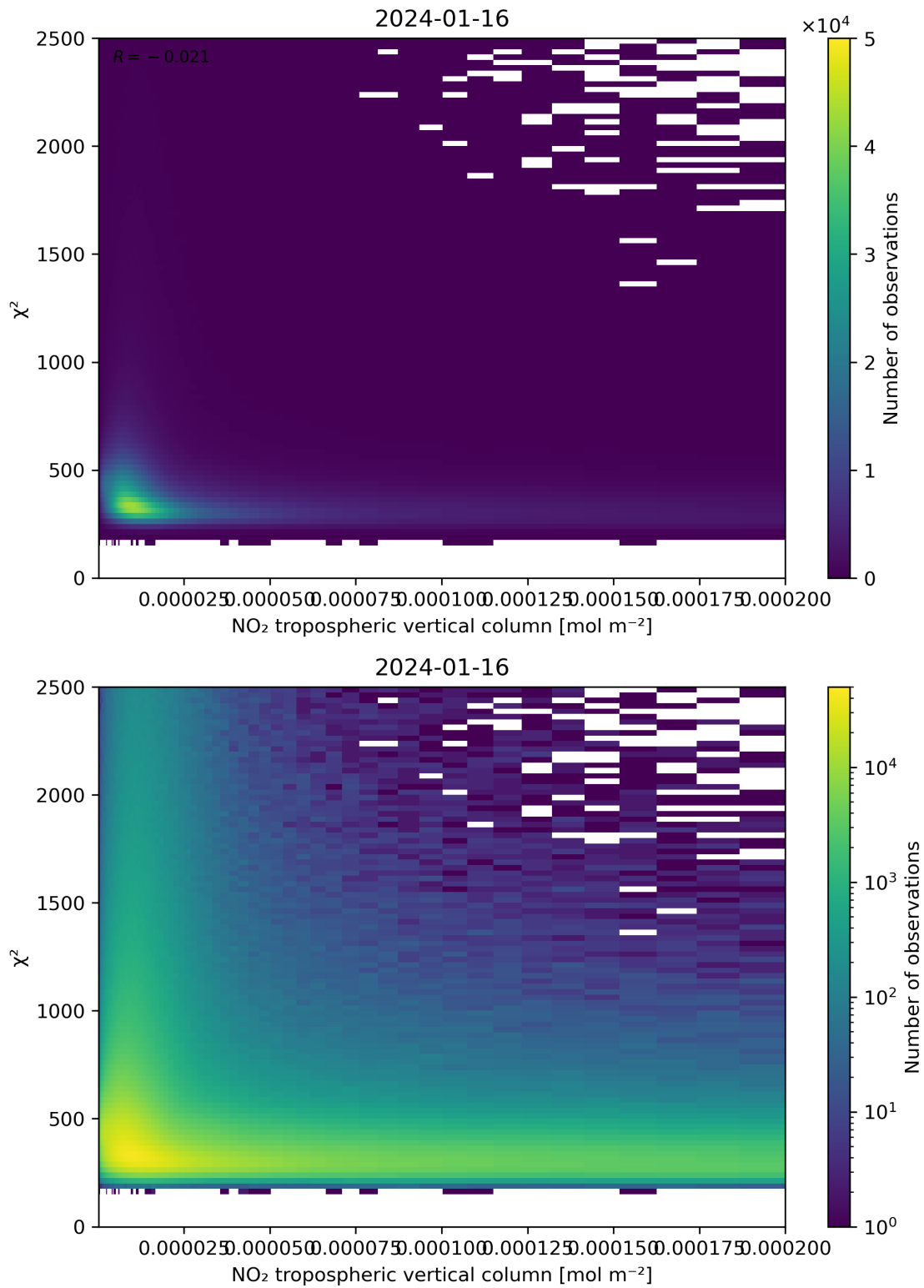
Figure 124: Scatter density plot of “NO 2 tropospheric vertical column” against “ \chi^2 ” for 2024-01-15 to 2024-01-17.
