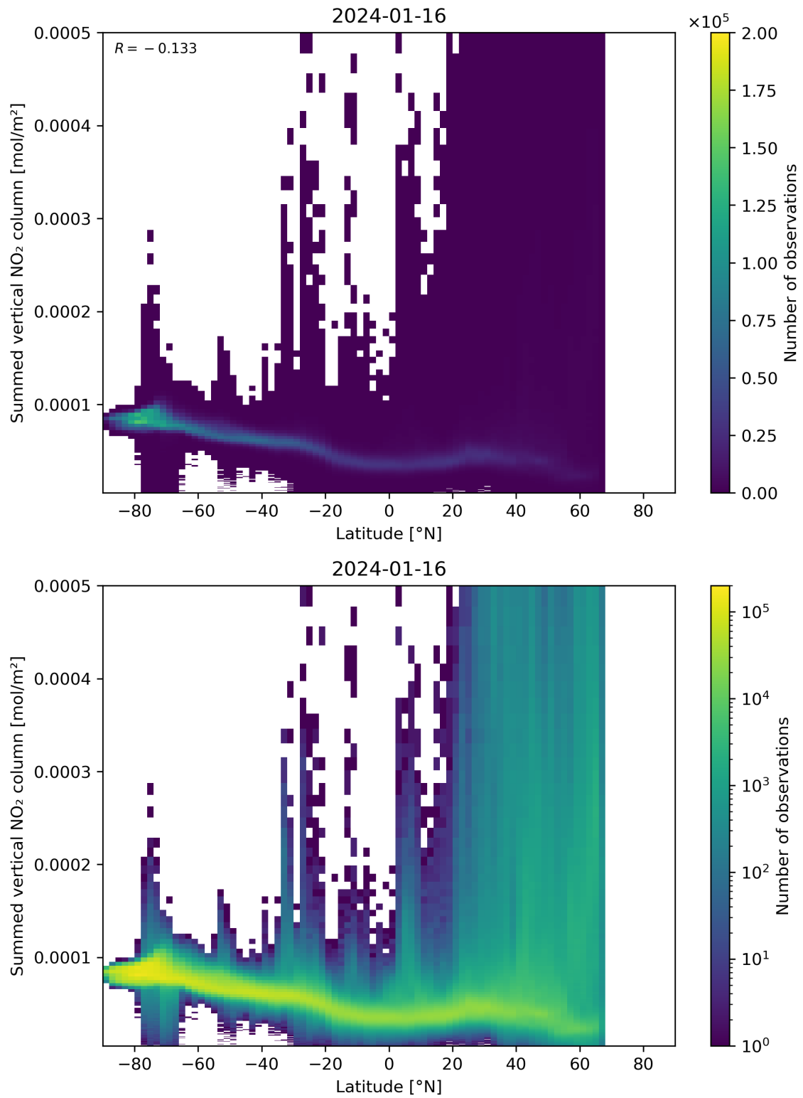
Figure 88: Scatter density plot of “Latitude” against “Summed vertical NO 2 column” for 2024-01-15 to 2024-01-17.
