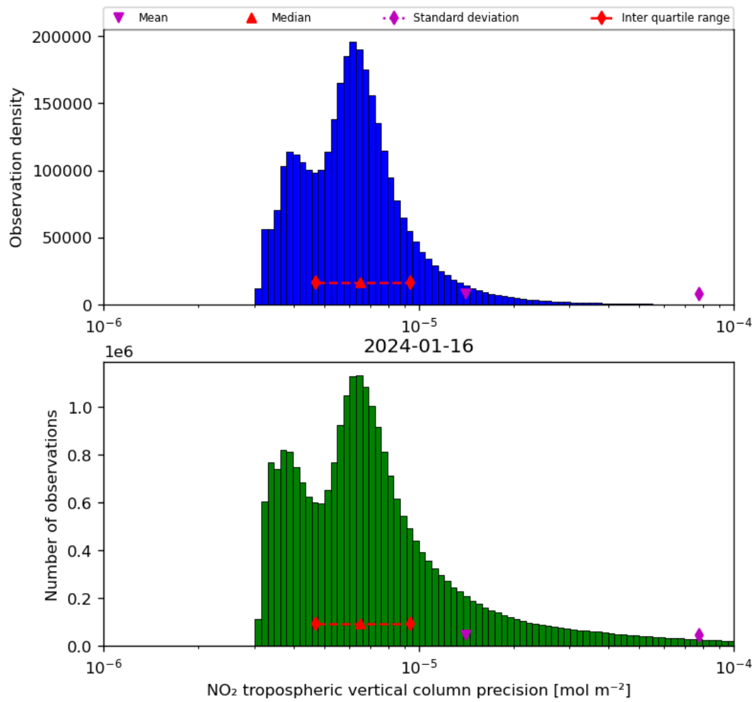
Figure 30: Histogram of “NO 2 tropospheric vertical column precision” for 2024-01-15 to 2024-01-17
