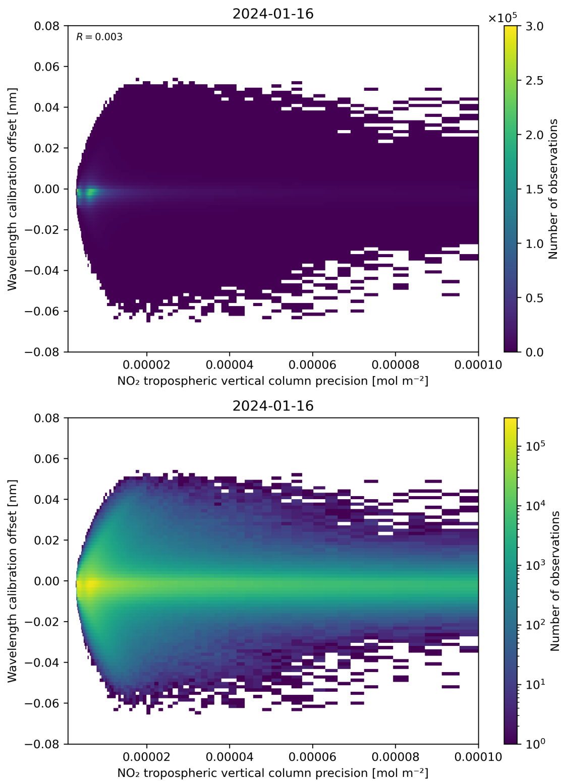
Figure 141: Scatter density plot of “NO 2 tropospheric vertical column precision” against “Wavelength calibration offset” for 2024-01-15 to 2024-01-17.
