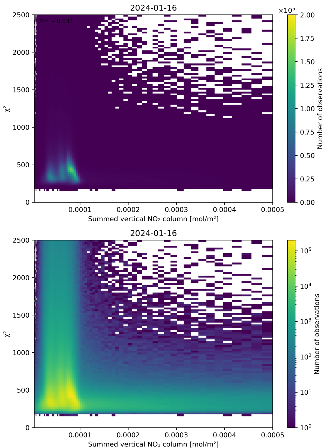
Figure 104: Scatter density plot of “Summed vertical NO 2 column” against “ \chi^2 ” for 2024-01-15 to 2024-01-17.
