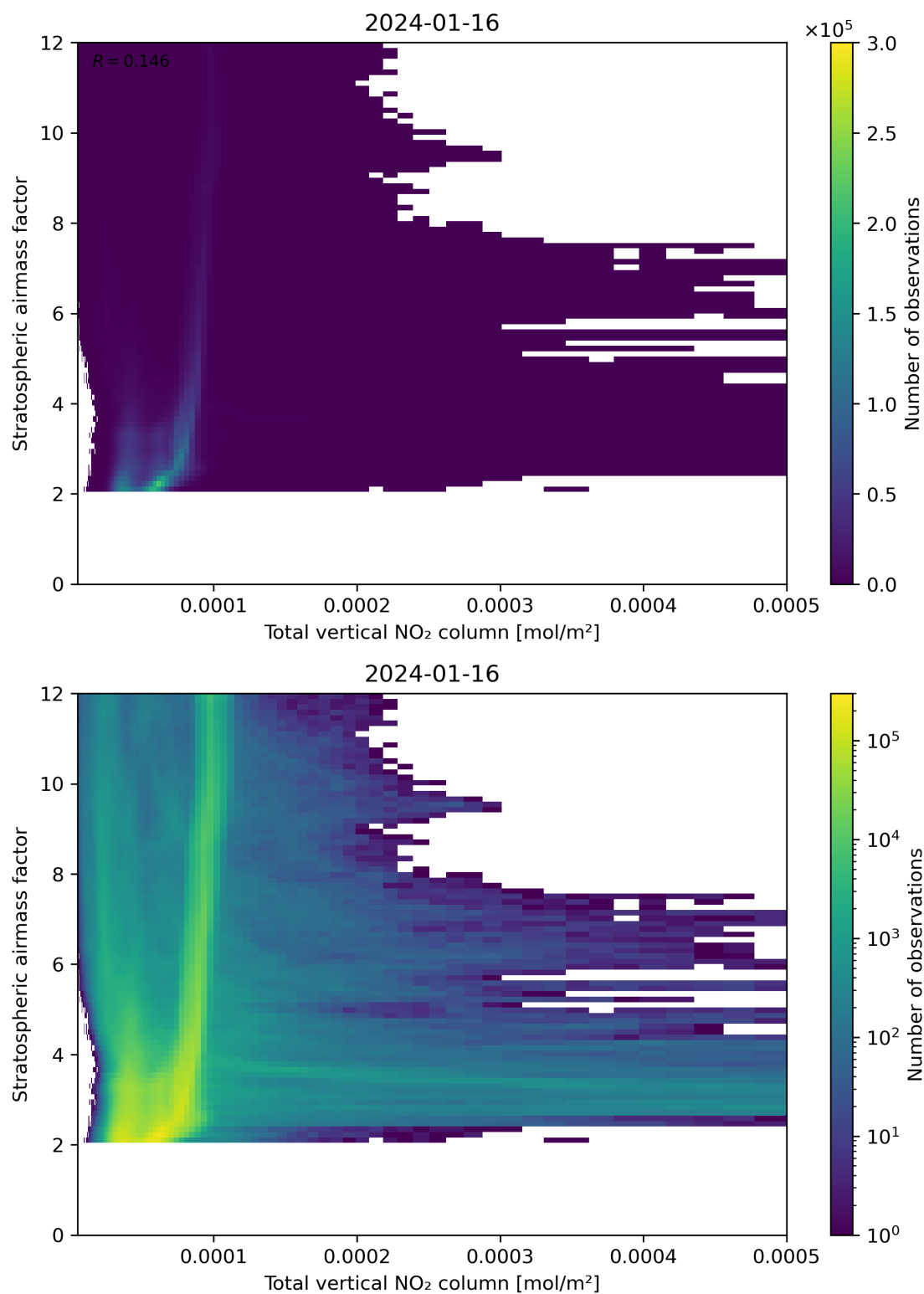
Figure 110: Scatter density plot of “Total vertical NO 2 column” against “Stratospheric airmass factor” for 2024-01-15 to 2024-01-17.
