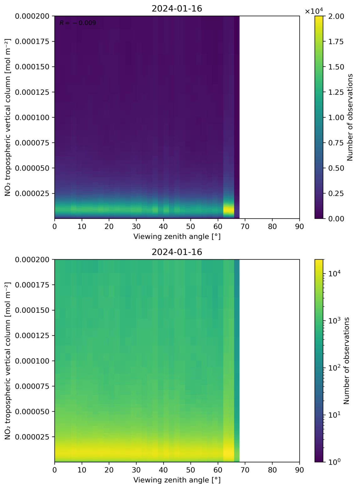
Figure 169: Scatter density plot of “Viewing zenith angle” against “NO 2 tropospheric vertical column” for 2024-01-15 to 2024-01-17.
