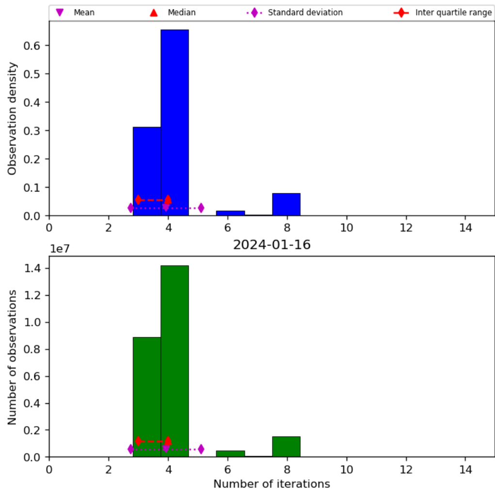
Figure 34: Histogram of “Number of iterations” for 2024-01-15 to 2024-01-17
