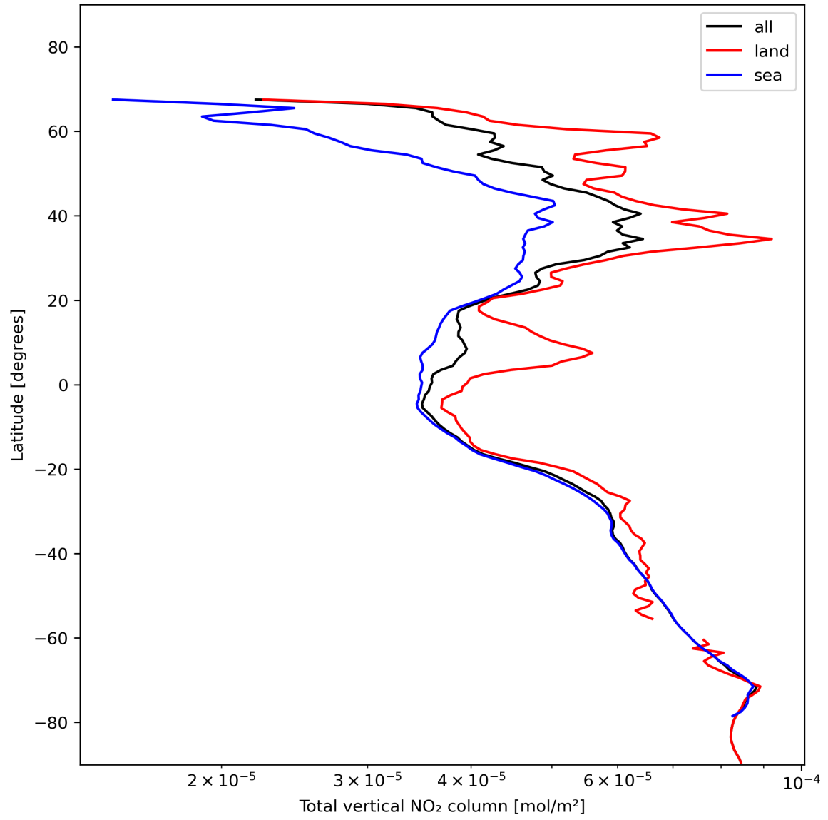
Figure 21: Zonal average of “Total vertical NO 2 column” for 2024-01-15 to 2024-01-17.
