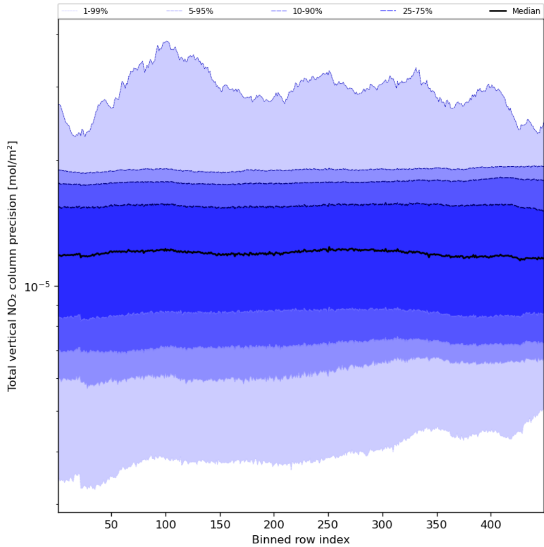
Figure 56: Along track statistics of “Total vertical NO 2 column precision” for 2024-01-15 to 2024-01-17
