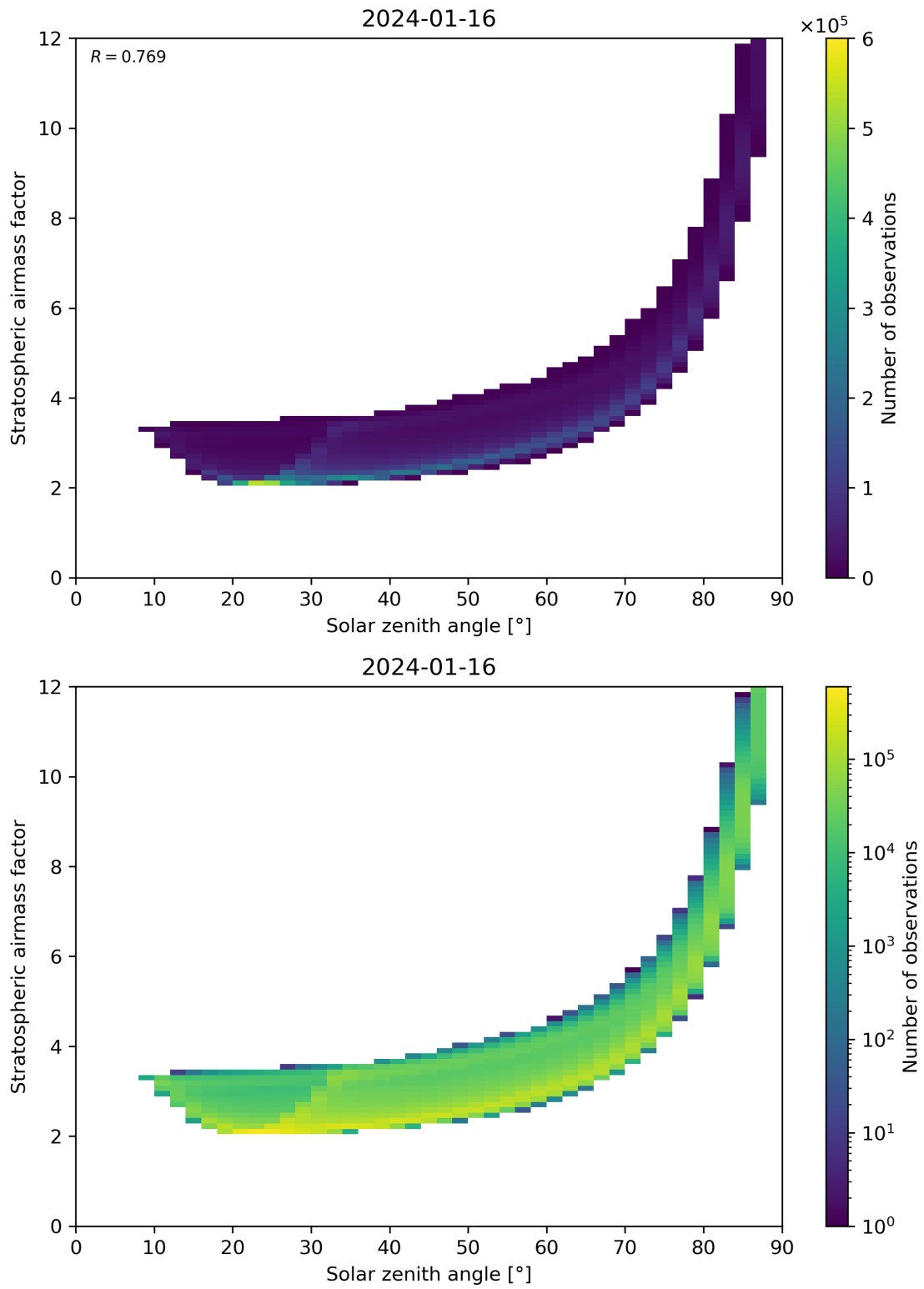
Figure 145: Scatter density plot of “Solar zenith angle” against “Stratospheric airmass factor” for 2024-01-15 to 2024-01-17.
