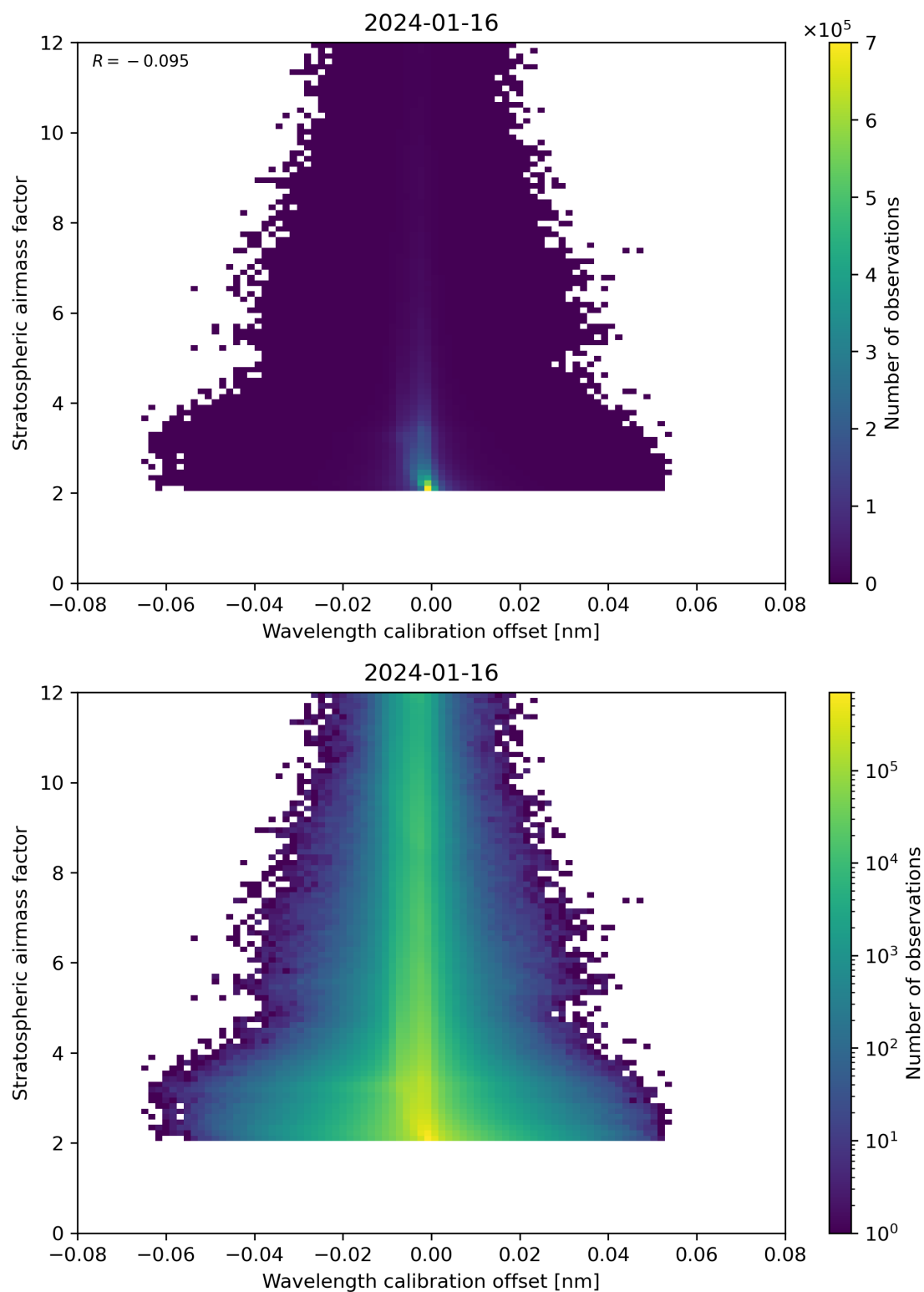
Figure 174: Scatter density plot of “Wavelength calibration offset” against “Stratospheric air mass factor” for 2024-01-15 to 2024-01-17.
