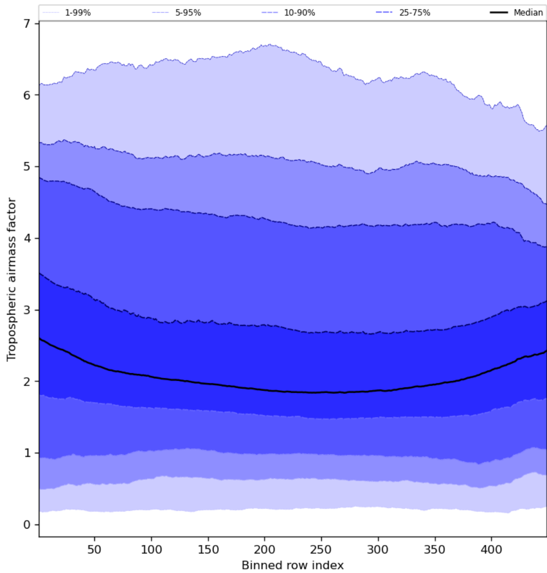
Figure 48: Along track statistics of “Tropospheric air mass factor” for 2024-01-15 to 2024-01-17
