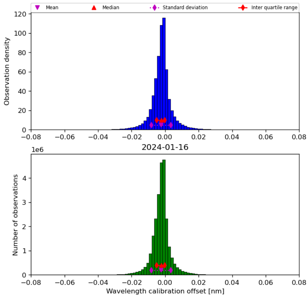
Figure 35: Histogram of “Wavelength calibration offset” for 2024-01-15 to 2024-01-17
