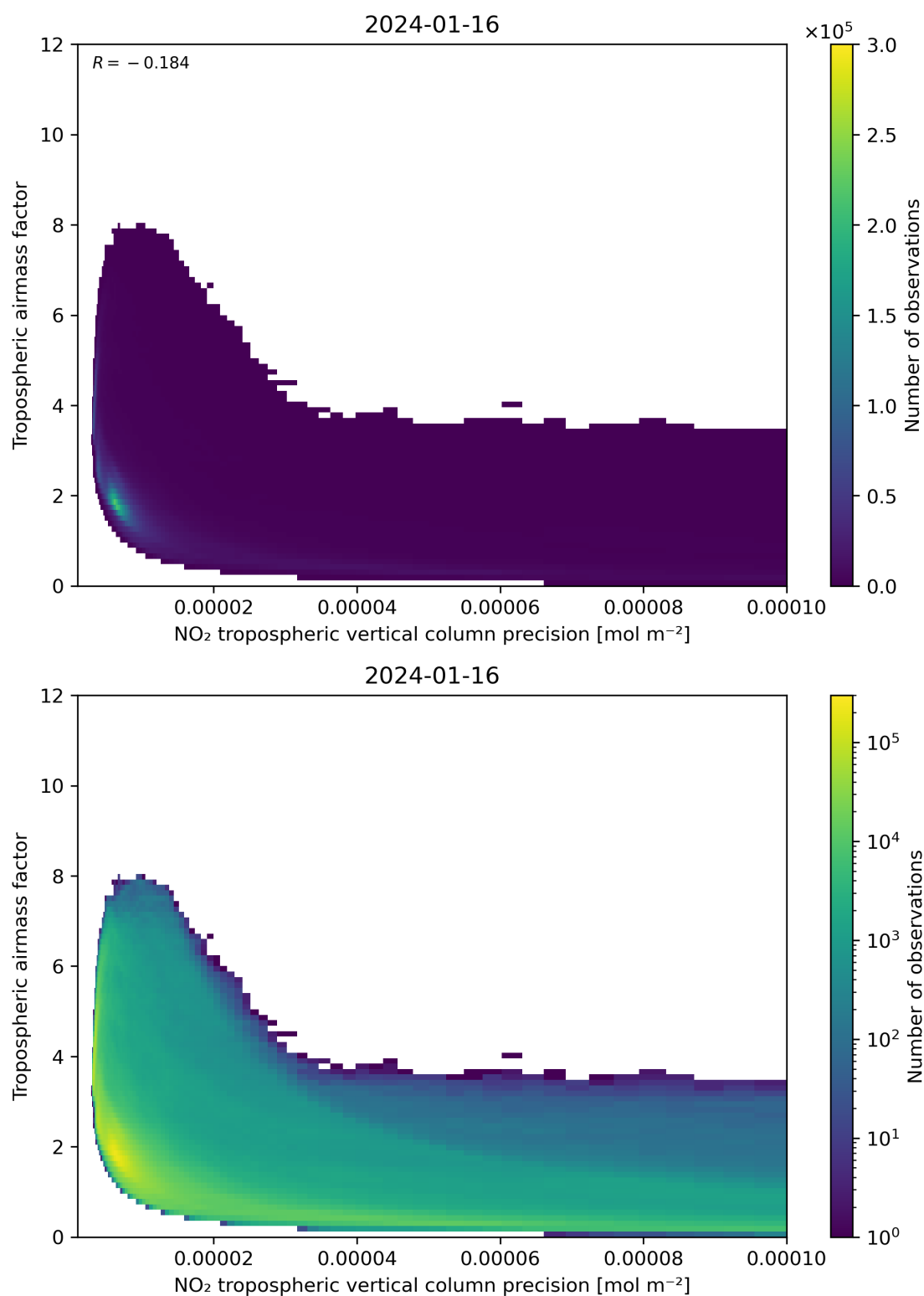
Figure 133: Scatter density plot of “NO 2 tropospheric vertical column precision” against “Tropospheric airmass factor” for 2024-01-15 to 2024-01-17.
