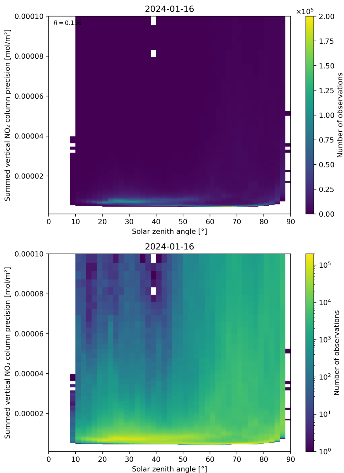
Figure 152: Scatter density plot of “Solar zenith angle” against “Summed vertical NO 2 column precision” for 2024-01-15 to 2024-01-17.
