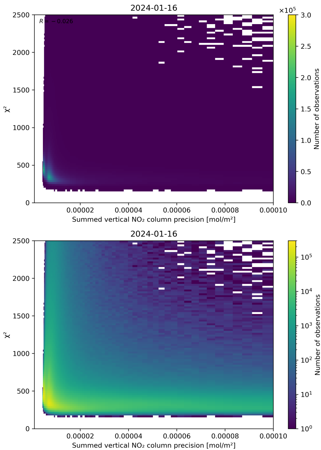
Figure 107: Scatter density plot of “Summed vertical NO 2 column precision” against “ \chi^2 ” for 2024-01-15 to 2024-01-17.
