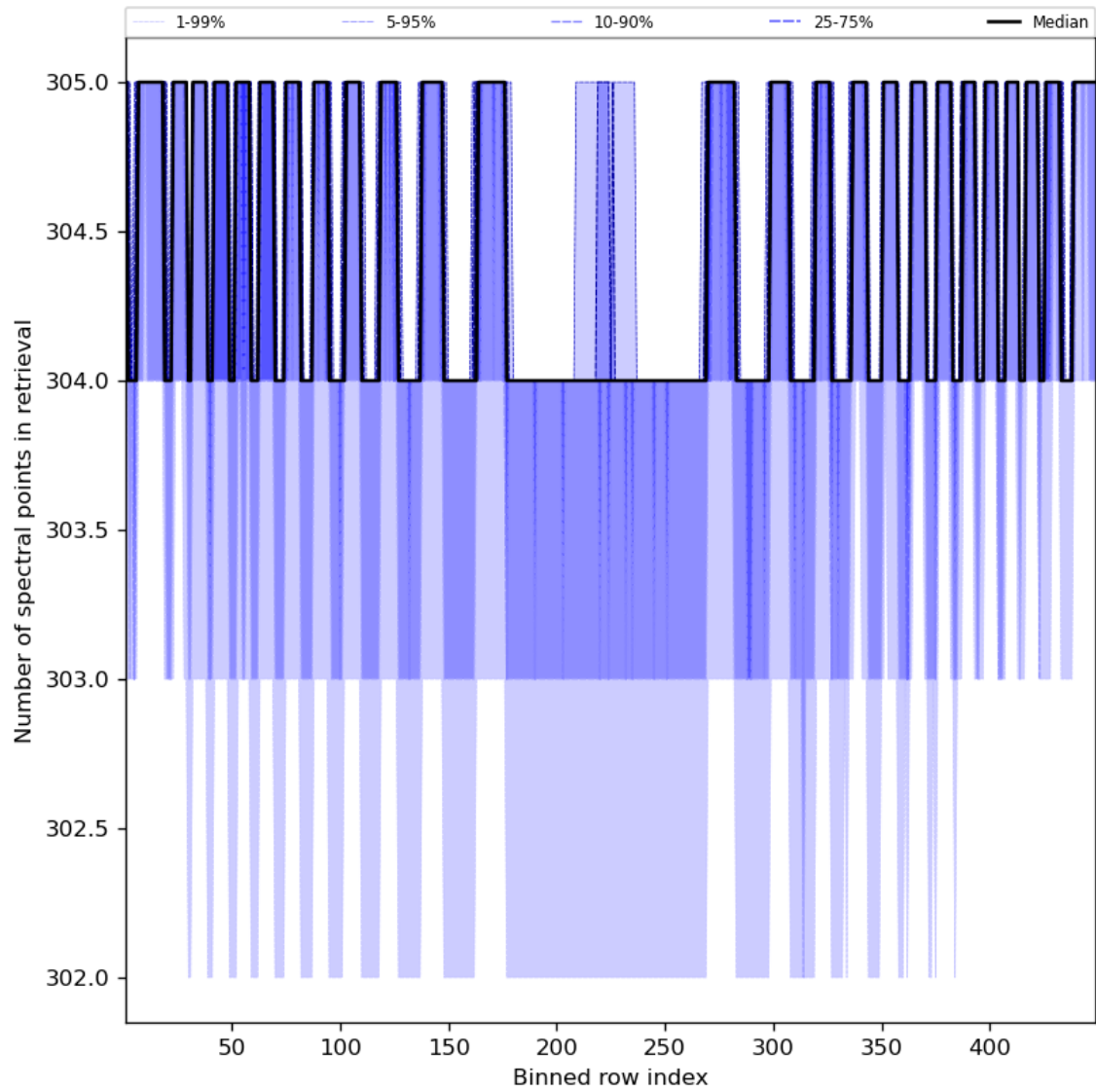
Figure 50: Along track statistics of “Number of spectral points in retrieval” for 2024-01-15 to 2024-01-17
