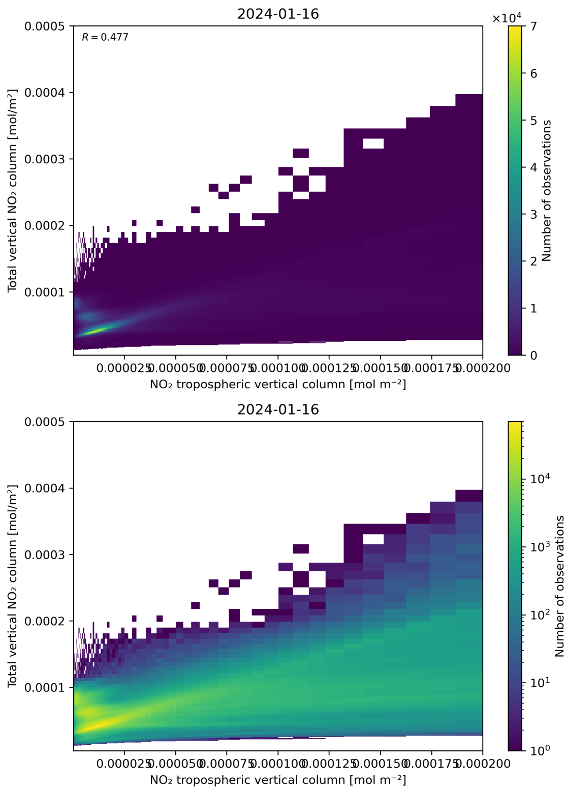
Figure 128: Scatter density plot of “NO 2 tropospheric vertical column” against “Total vertical NO 2 column” for 2024-01-15 to 2024-01-17.
