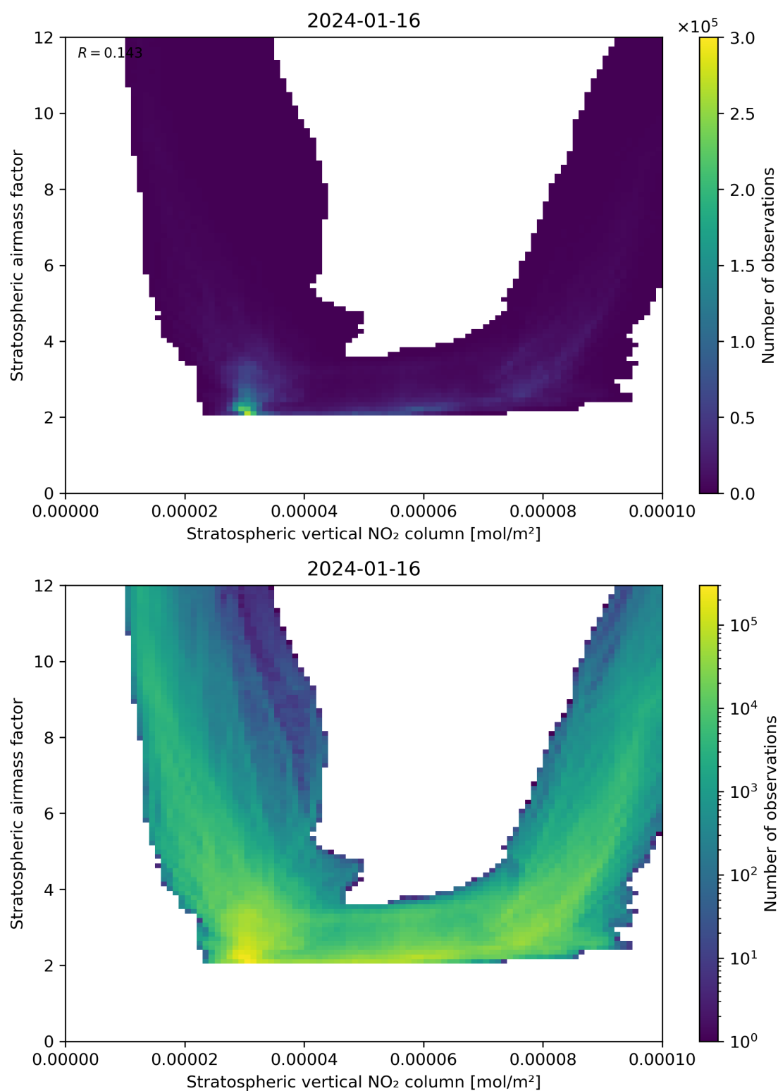
Figure 96: Scatter density plot of “Stratospheric vertical NO 2 column” against “Stratospheric airmass factor” for 2024-01-15 to 2024-01-17.
