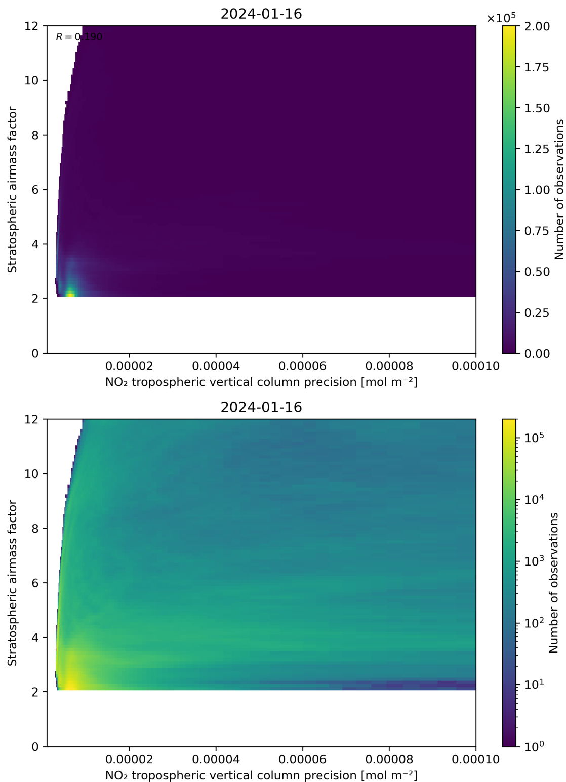
Figure 131: Scatter density plot of “NO 2 tropospheric vertical column precision” against “Stratospheric airmass factor” for 2024-01-15 to 2024-01-17.
