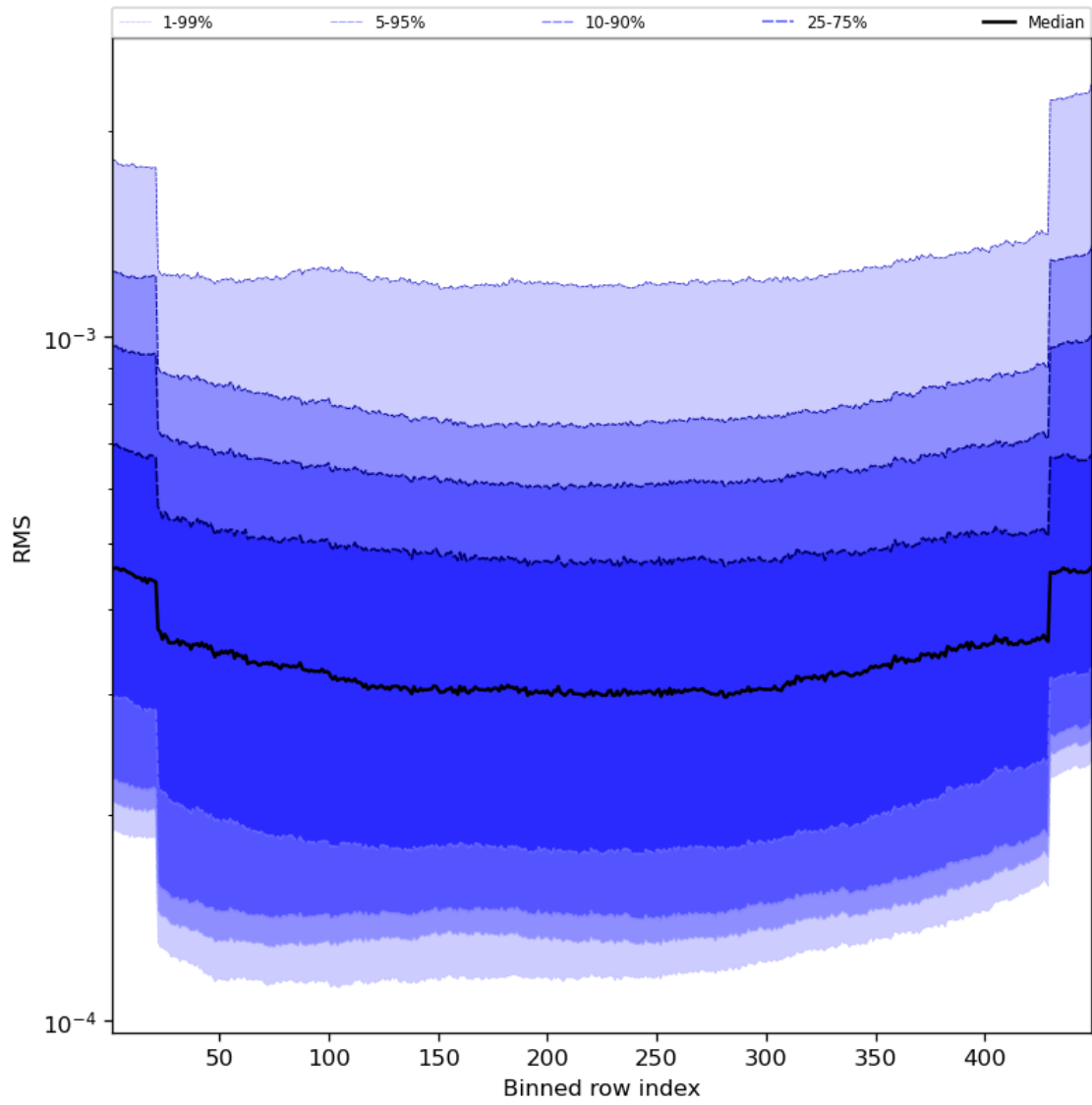
Figure 60: Along track statistics of “RMS” for 2024-01-15 to 2024-01-17
