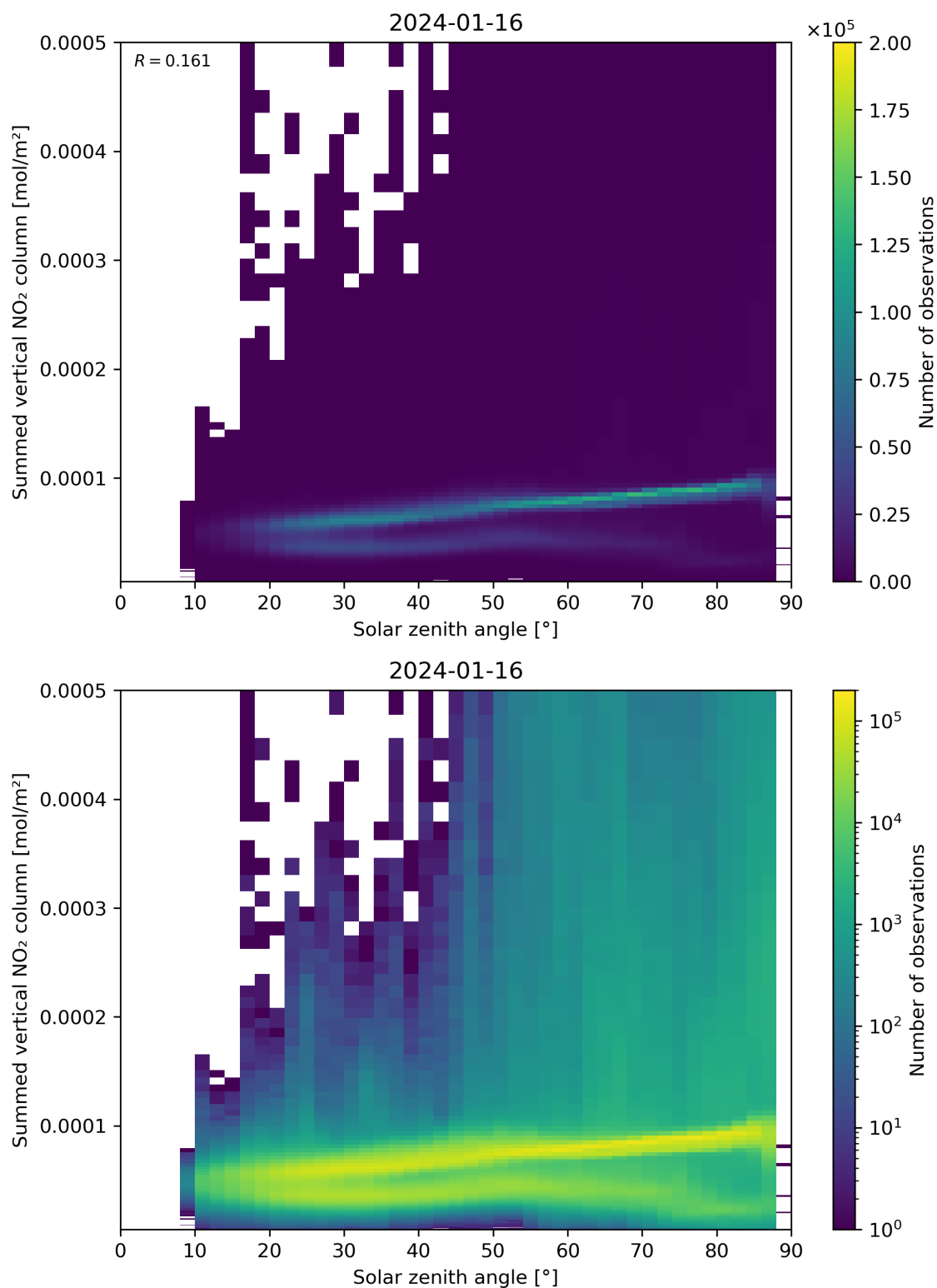
Figure 151: Scatter density plot of “Solar zenith angle” against “Summed vertical NO 2 column” for 2024-01-15 to 2024-01-17.
