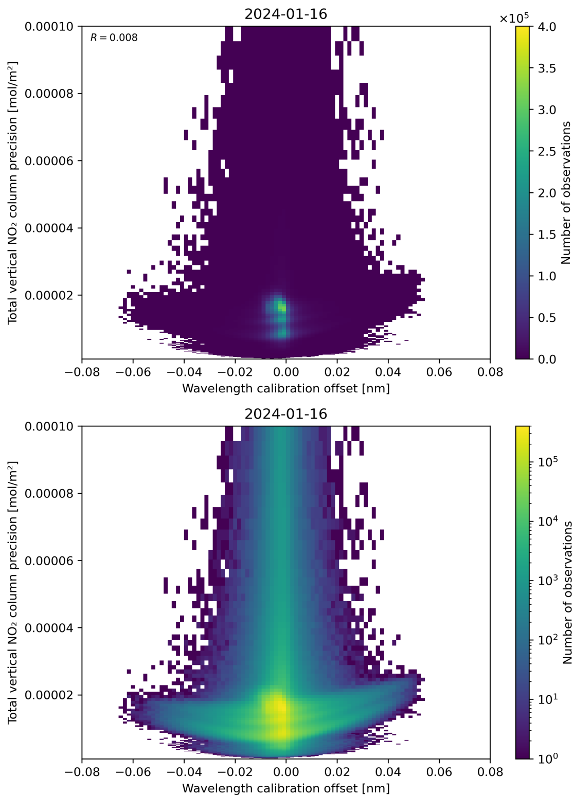
Figure 180: Scatter density plot of “Wavelength calibration offset” against “Total vertical NO 2 column precision” for 2024-01-15 to 2024-01-17.
