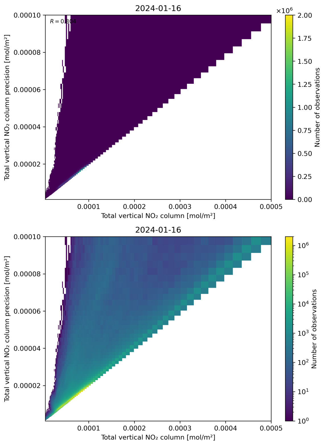
Figure 114: Scatter density plot of “Total vertical NO 2 column” against “Total vertical NO 2 column precision” for 2024-01-15 to 2024-01-17.
