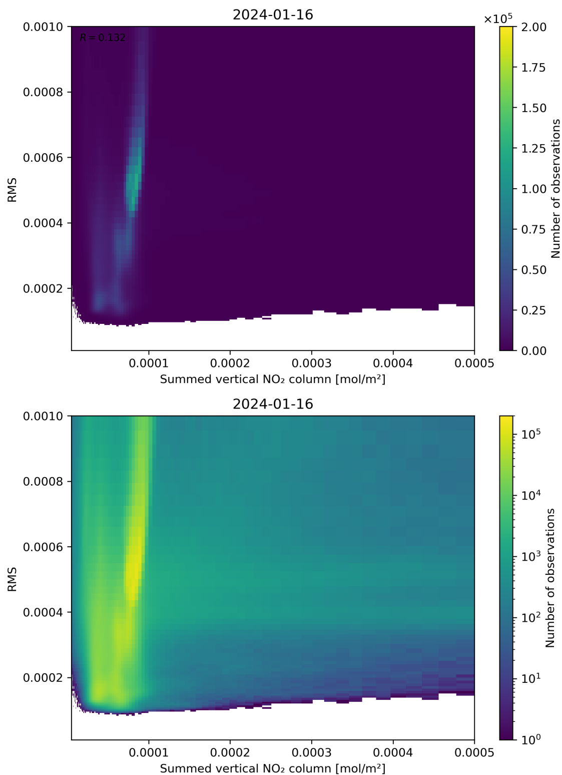
Figure 109: Scatter density plot of “Summed vertical NO 2 column” against “RMS” for 2024-01-15 to 2024-01-17.
