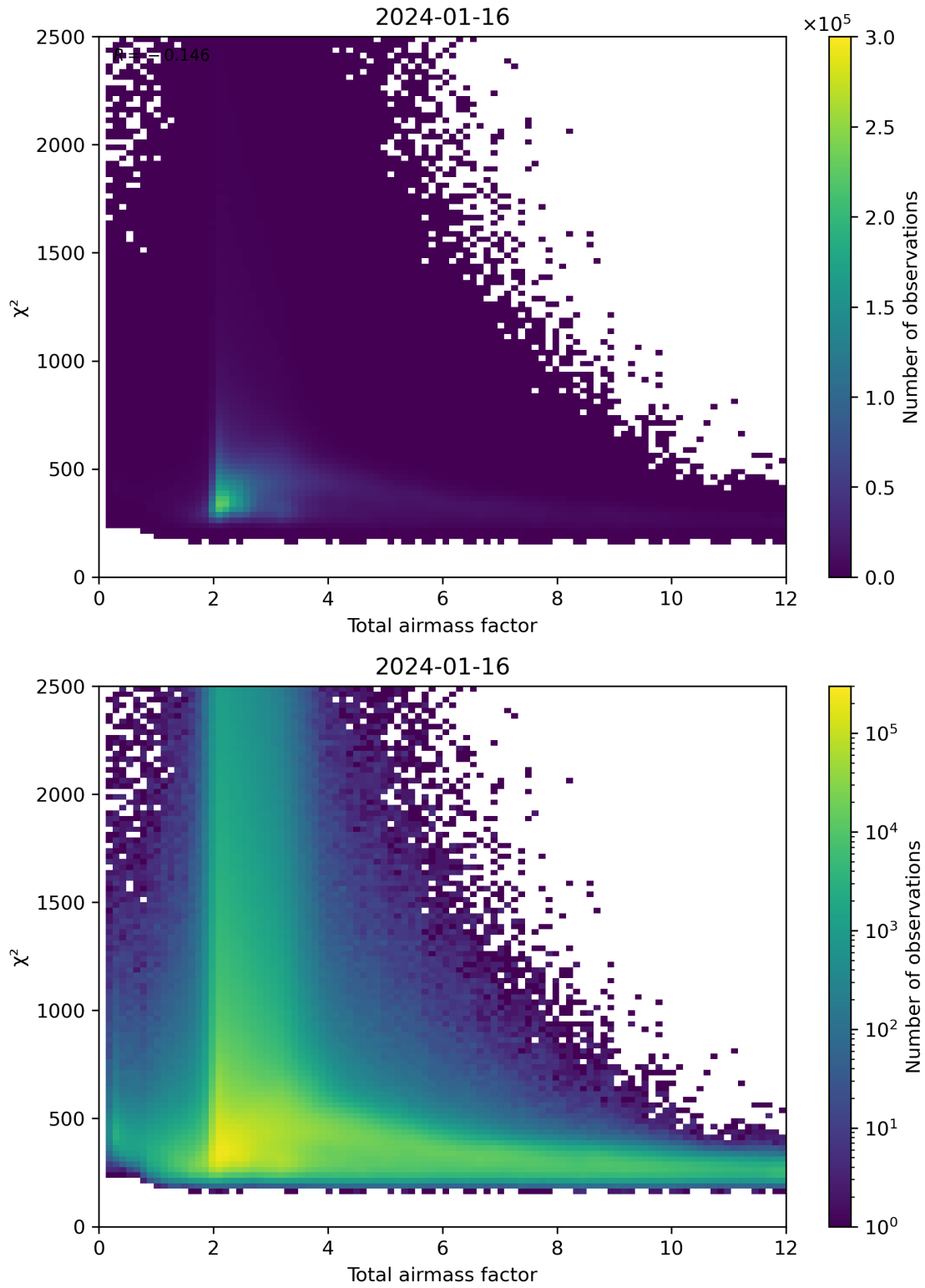
Figure 63: Scatter density plot of “Total airmass factor” against “ \chi^2 ” for 2024-01-15 to 2024-01-17.
