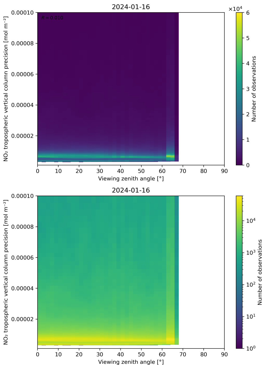
Figure 170: Scatter density plot of “Viewing zenith angle” against “NO 2 tropospheric vertical column precision” for 2024-01-15 to 2024-01-17.
