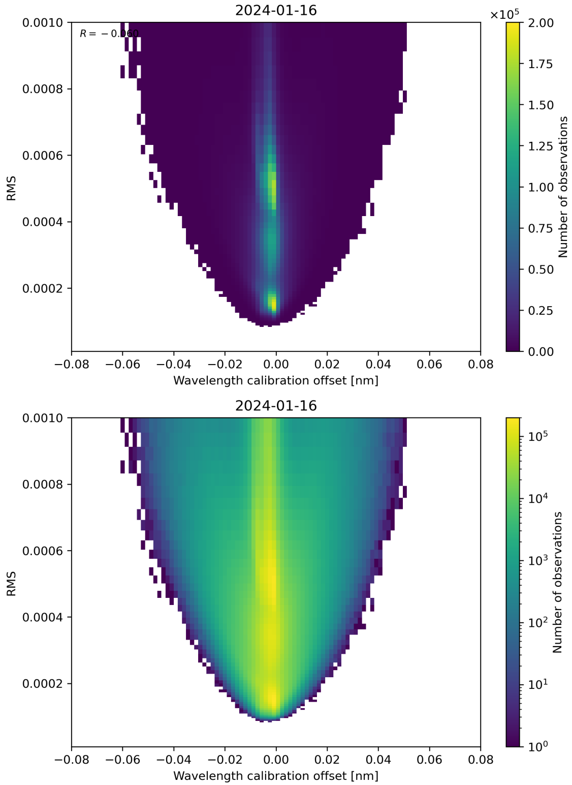
Figure 181: Scatter density plot of “Wavelength calibration offset” against “RMS” for 2024-01-15 to 2024-01-17.
