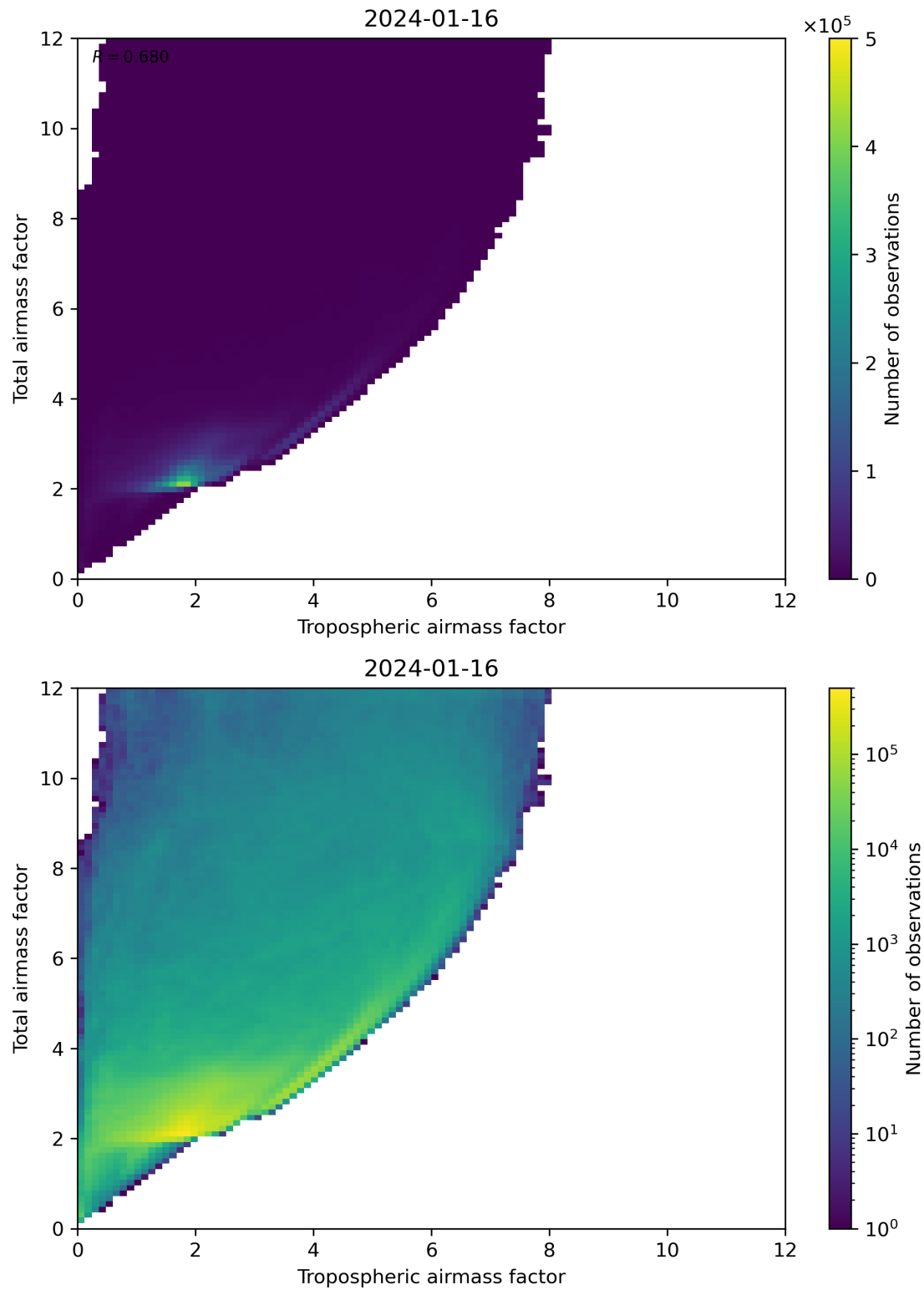
Figure 72: Scatter density plot of “Tropospheric airmass factor” against “Total airmass factor” for 2024-01-15 to 2024-01-17.
