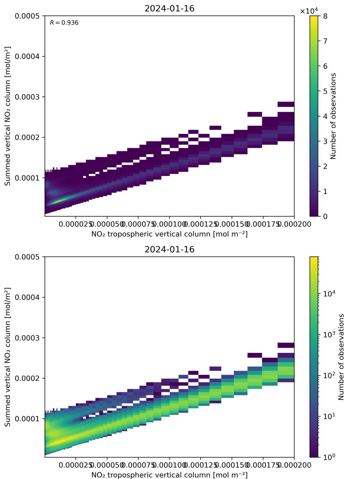
Figure 126: Scatter density plot of “NO 2 tropospheric vertical column” against “Summed vertical NO 2 column” for 2024-01-15 to 2024-01-17.
