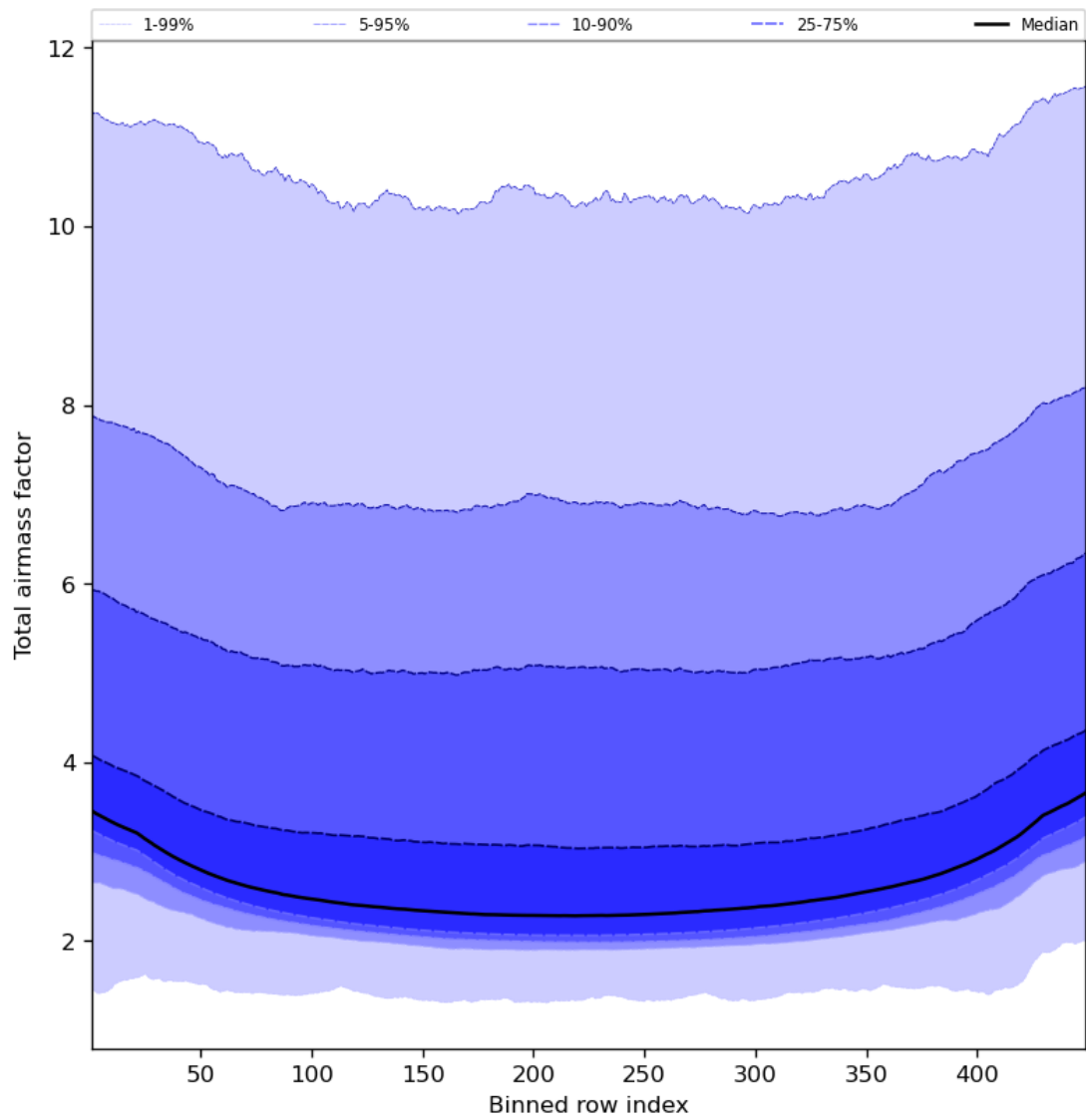
Figure 49: Along track statistics of “Total airmass factor” for 2024-01-15 to 2024-01-17
