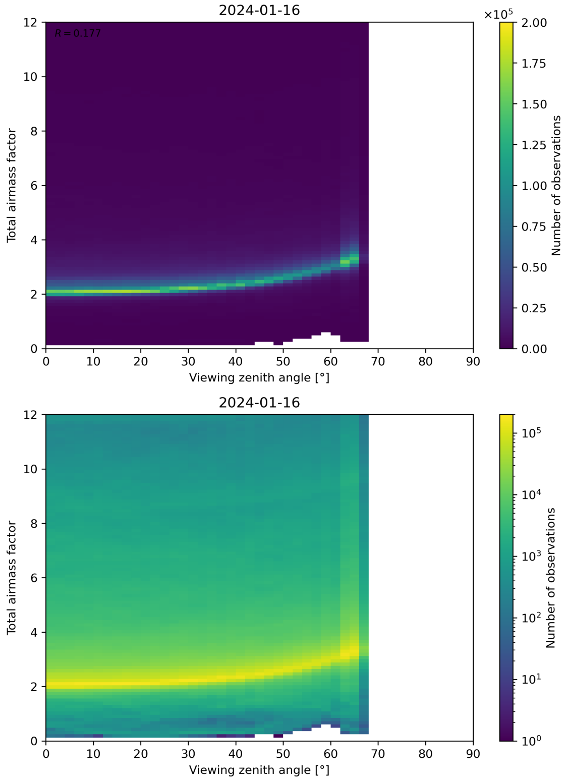
Figure 160: Scatter density plot of “Viewing zenith angle” against “Total airmass factor” for 2024-01-15 to 2024-01-17.
