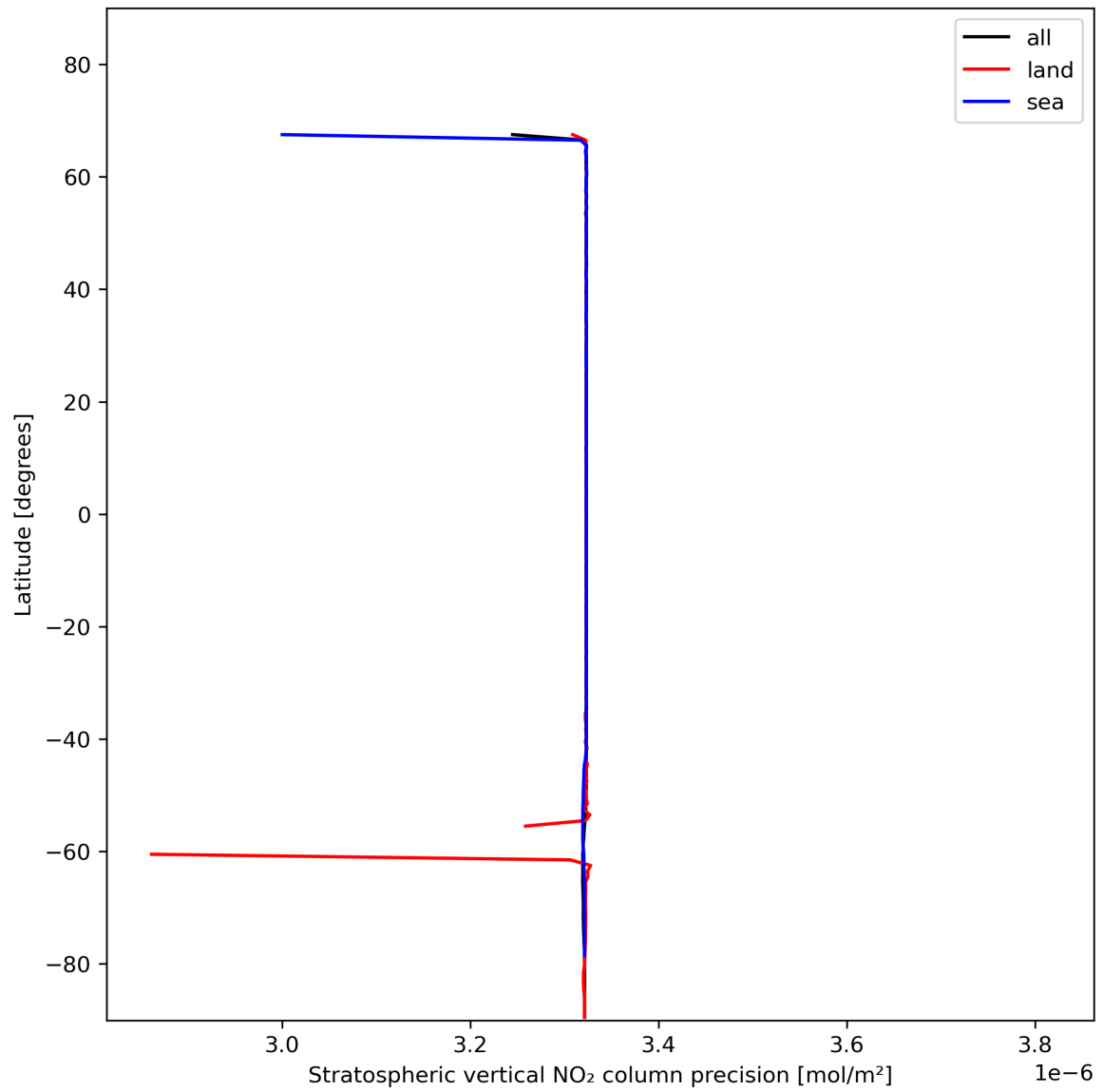
Figure 20: Zonal average of “Stratospheric vertical NO 2 column precision” for 2024-01-15 to 2024-01-17.
