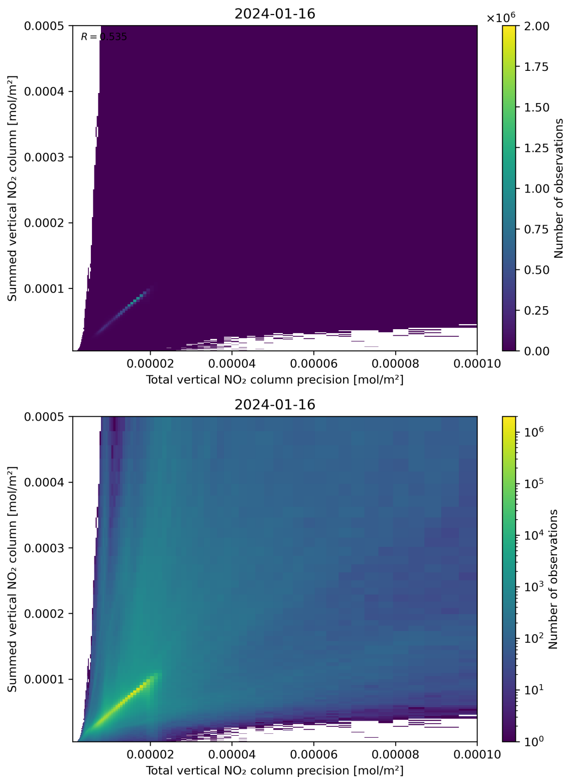
Figure 117: Scatter density plot of “Total vertical NO 2 column precision” against “Summed vertical NO 2 column” for 2024-01-15 to 2024-01-17.
