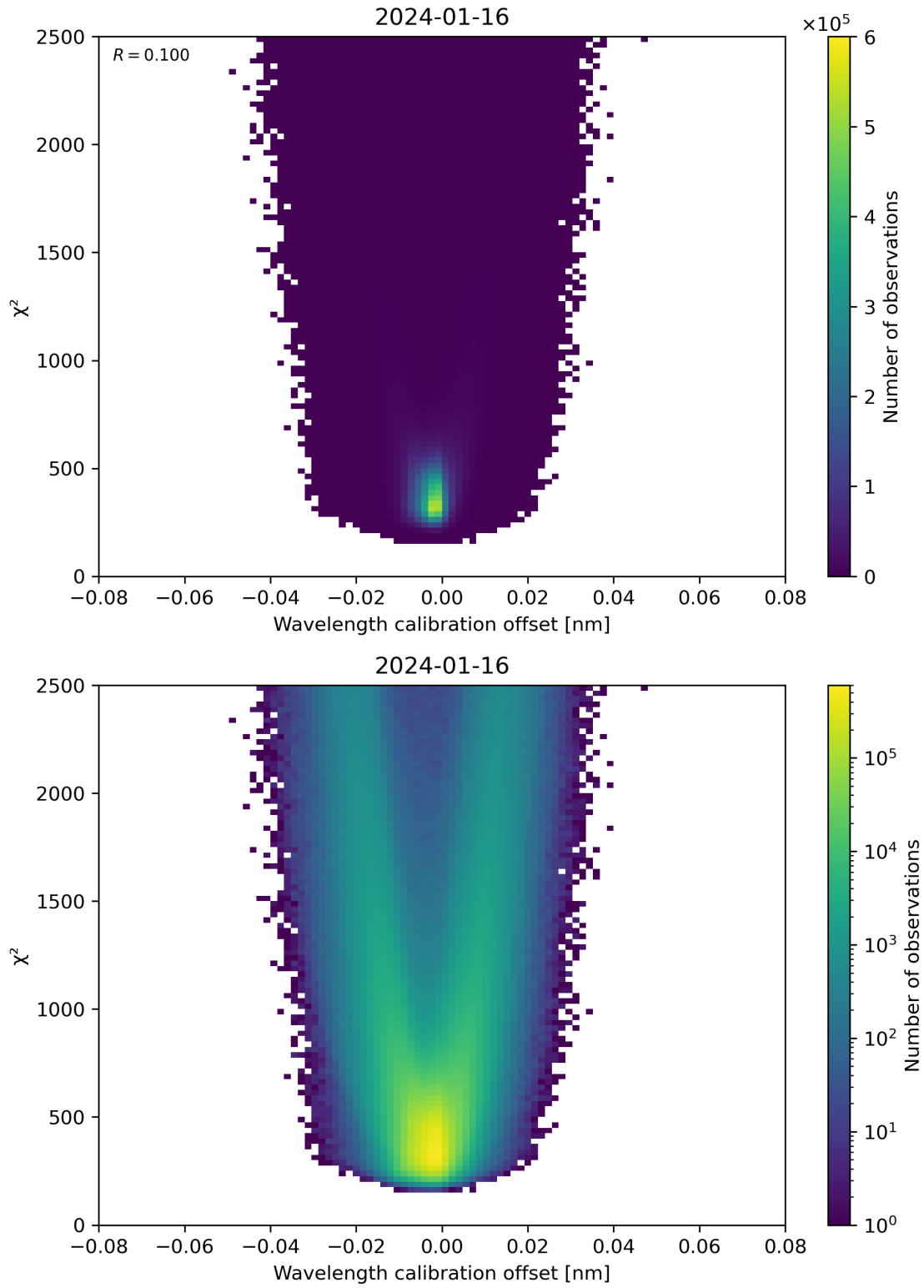
Figure 175: Scatter density plot of “Wavelength calibration offset” against “ \chi^2 ” for 2024-01-15 to 2024-01-17.
