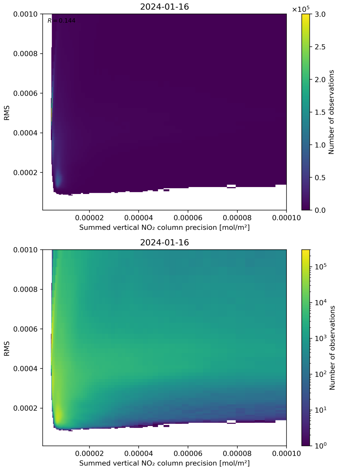
Figure 108: Scatter density plot of “Summed vertical NO 2 column precision” against “RMS” for 2024-01-15 to 2024-01-17.
