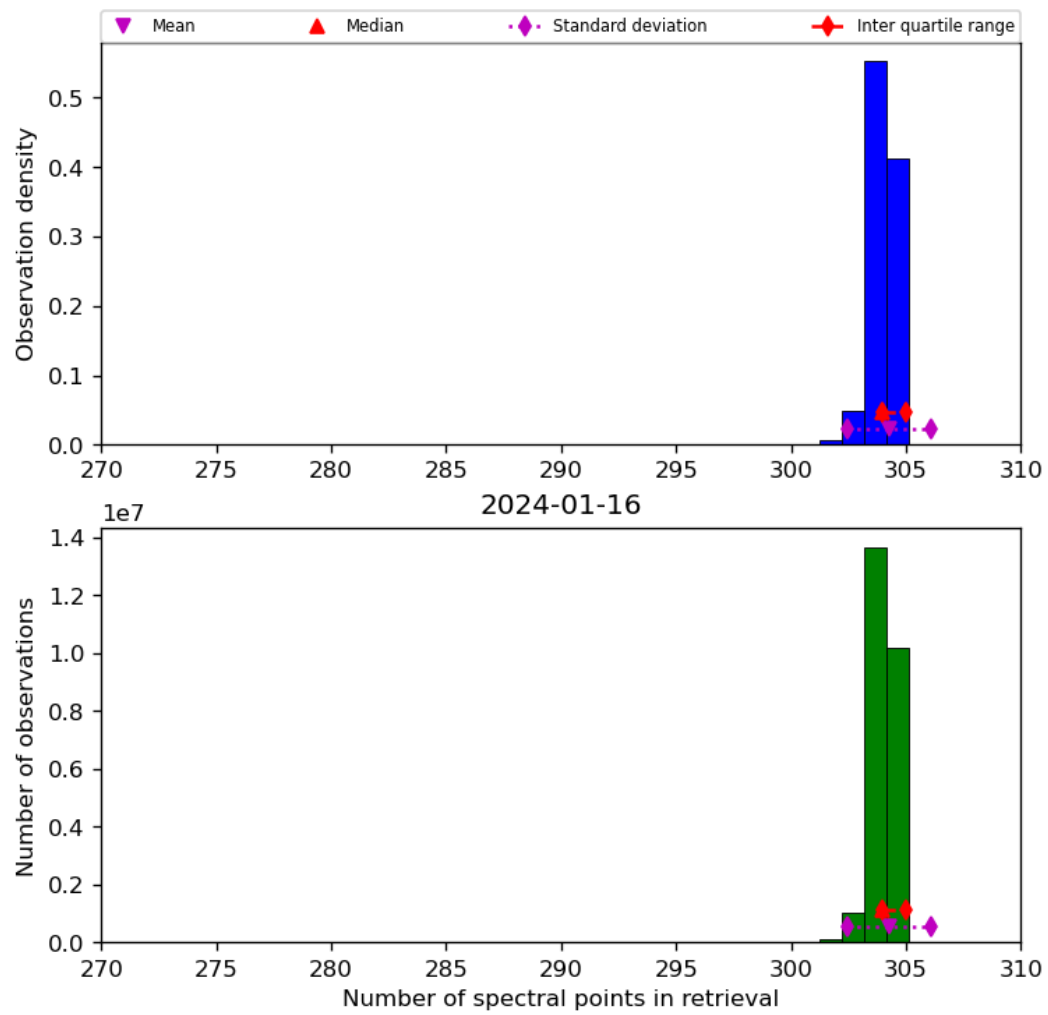
Figure 33: Histogram of “Number of spectral points in retrieval” for 2024-01-15 to 2024-01-17
