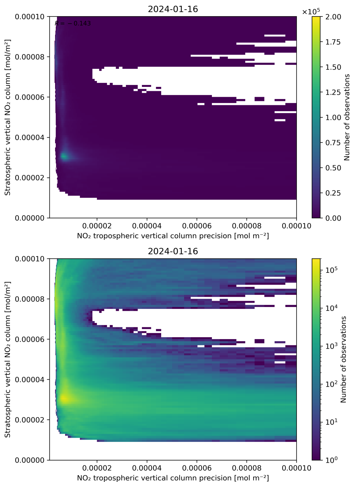
Figure 135: Scatter density plot of “NO 2 tropospheric vertical column precision” against “Stratospheric vertical NO 2 column” for 2024-01-15 to 2024-01-17.
