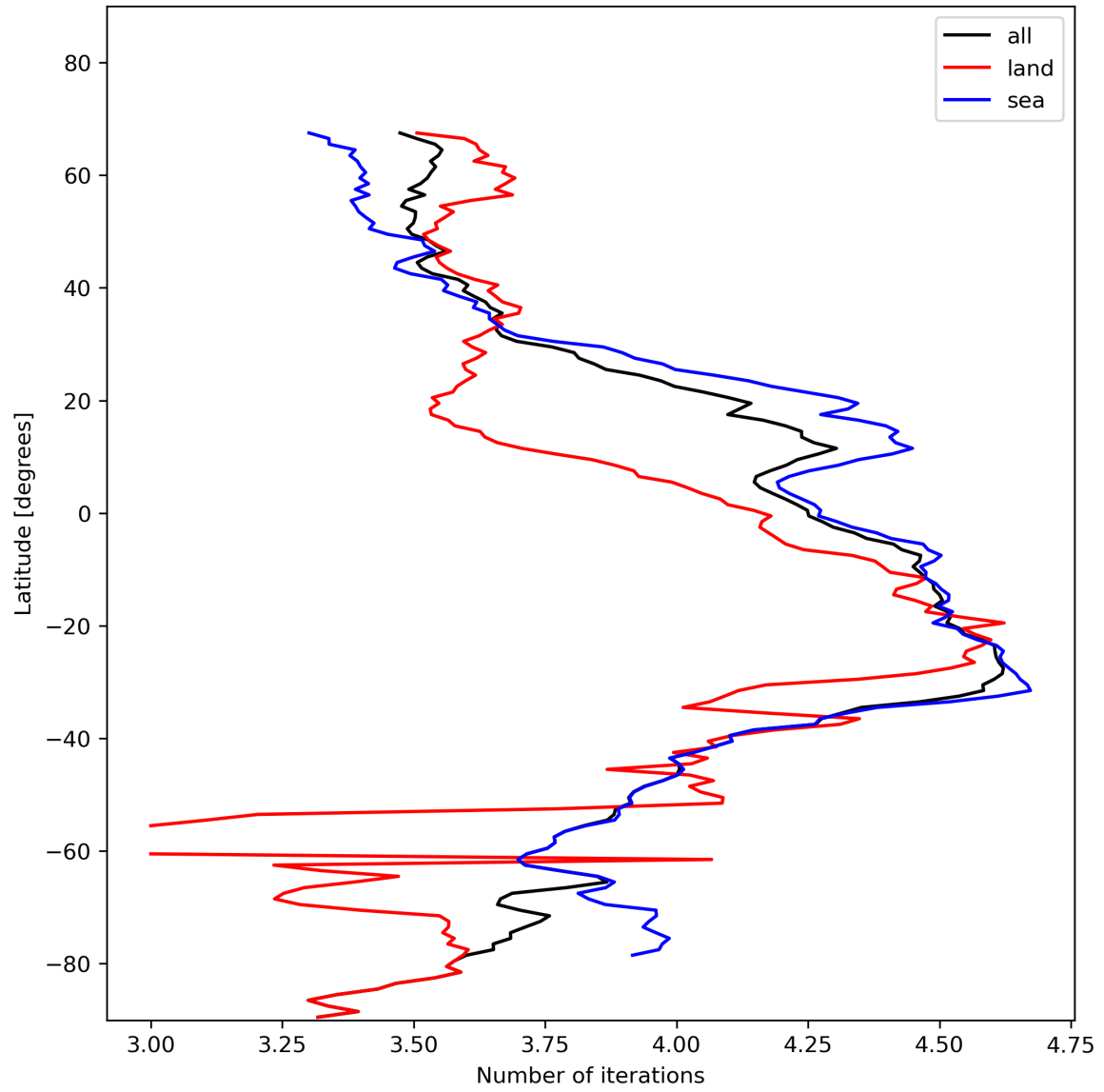
Figure 17: Zonal average of “Number of iterations” for 2024-01-15 to 2024-01-17.
