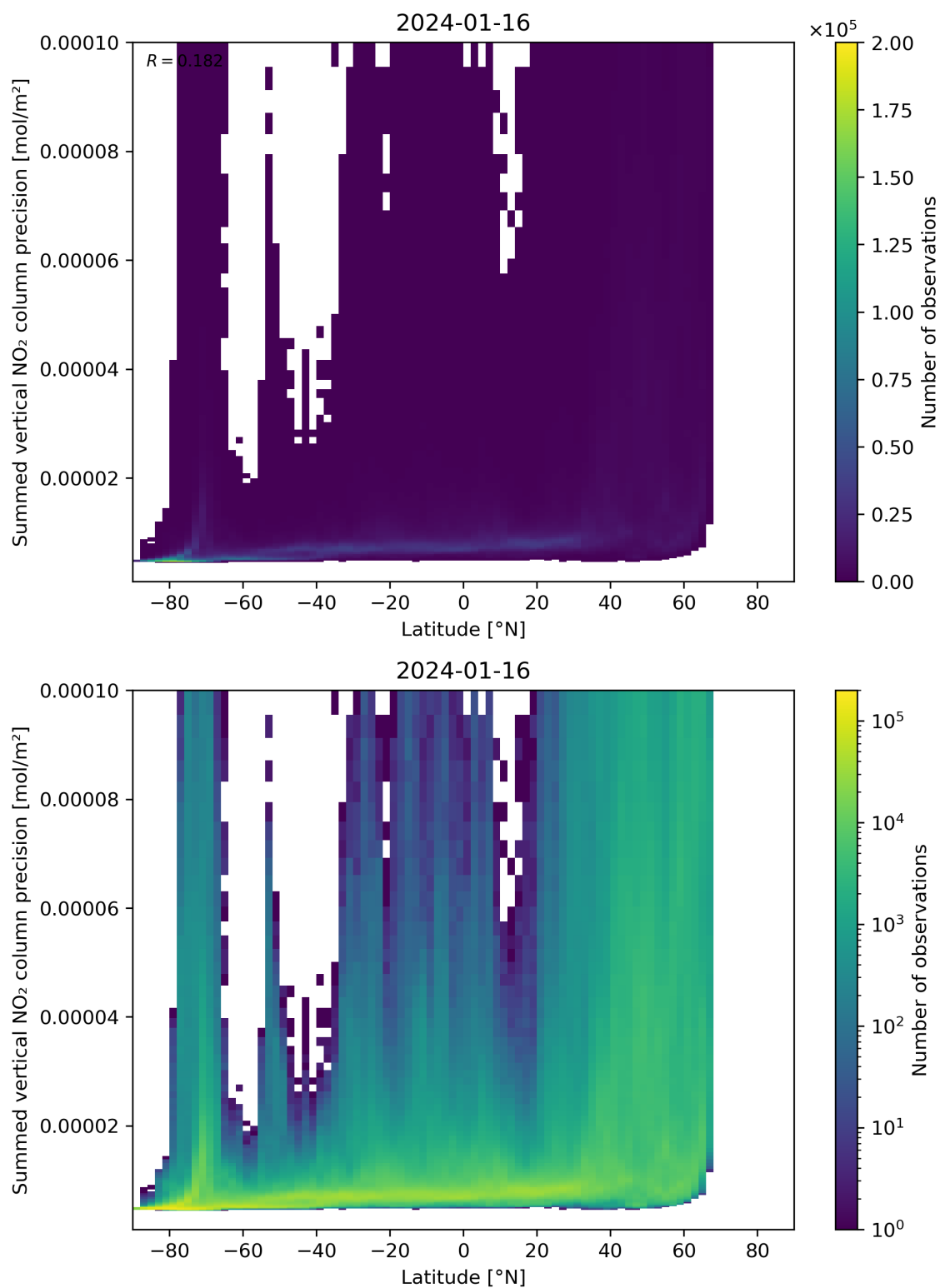
Figure 89: Scatter density plot of “Latitude” against “Summed vertical NO 2 column precision” for 2024-01-15 to 2024-01-17.
