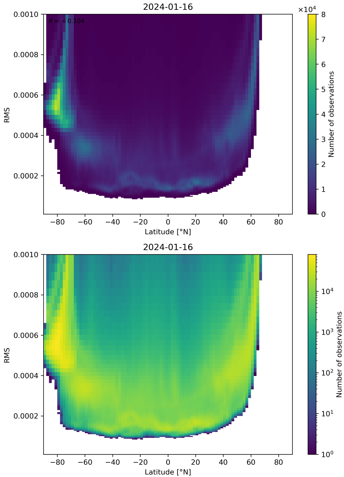
Figure 94: Scatter density plot of “Latitude” against “RMS” for 2024-01-15 to 2024-01-17.
