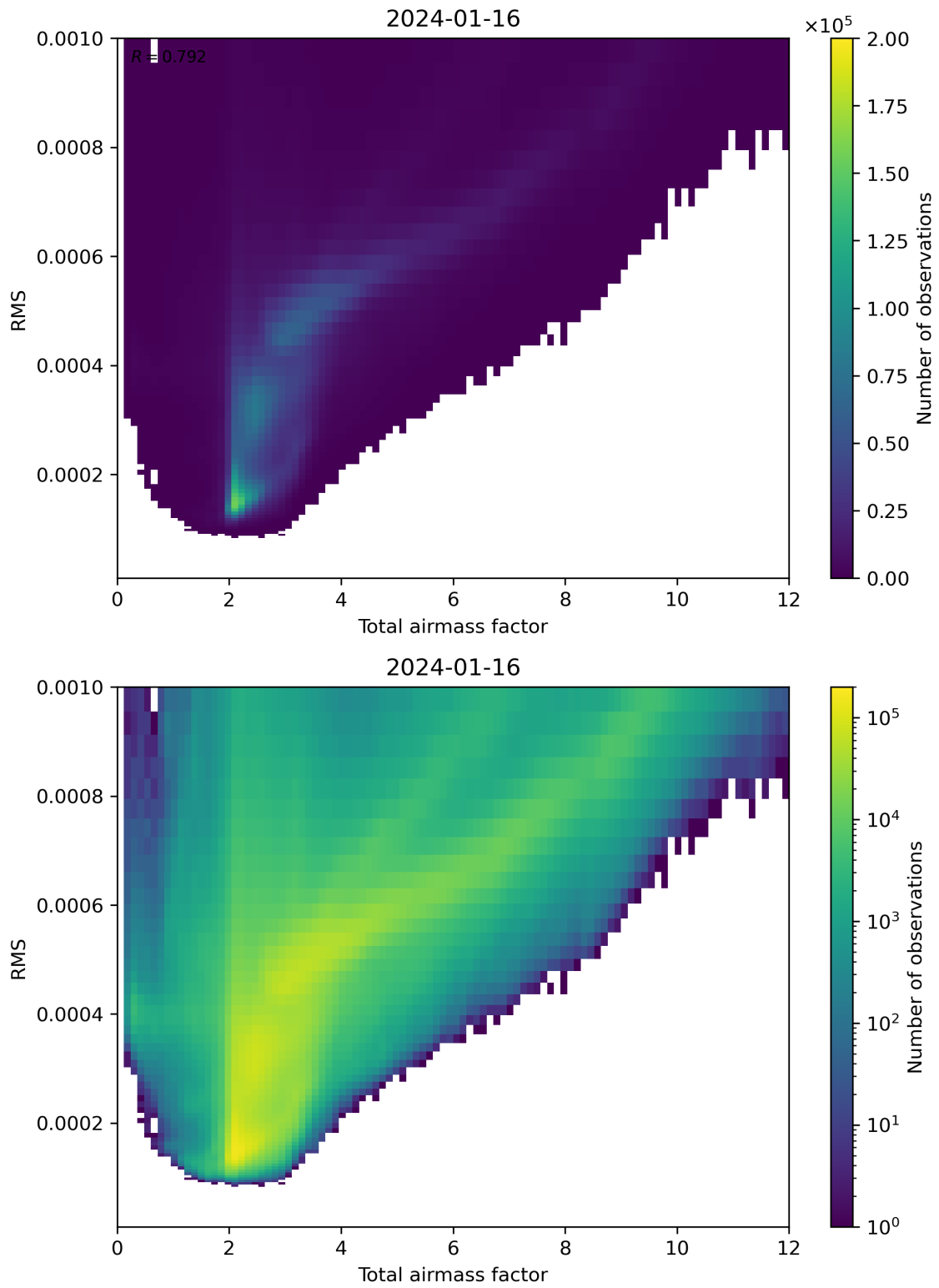
Figure 69: Scatter density plot of “Total airmass factor” against “RMS” for 2024-01-15 to 2024-01-17.
