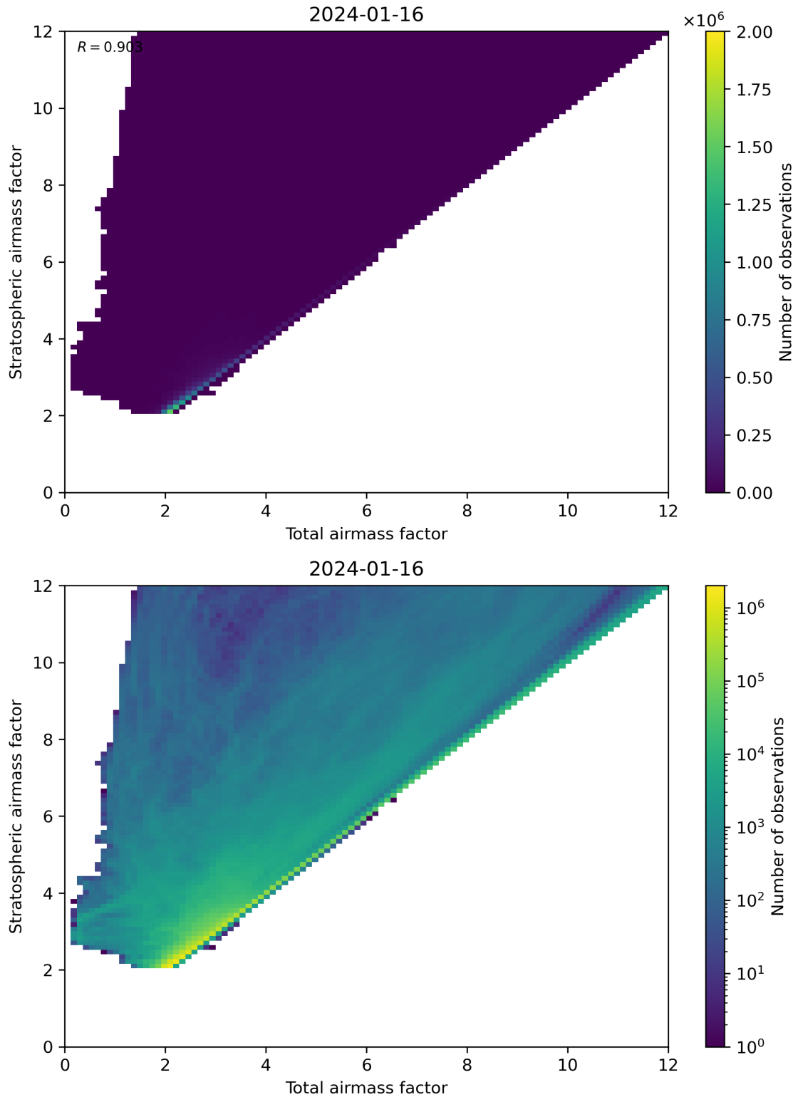
Figure 62: Scatter density plot of “Total airmass factor” against “Stratospheric airmass factor” for 2024-01-15 to 2024-01-17.
