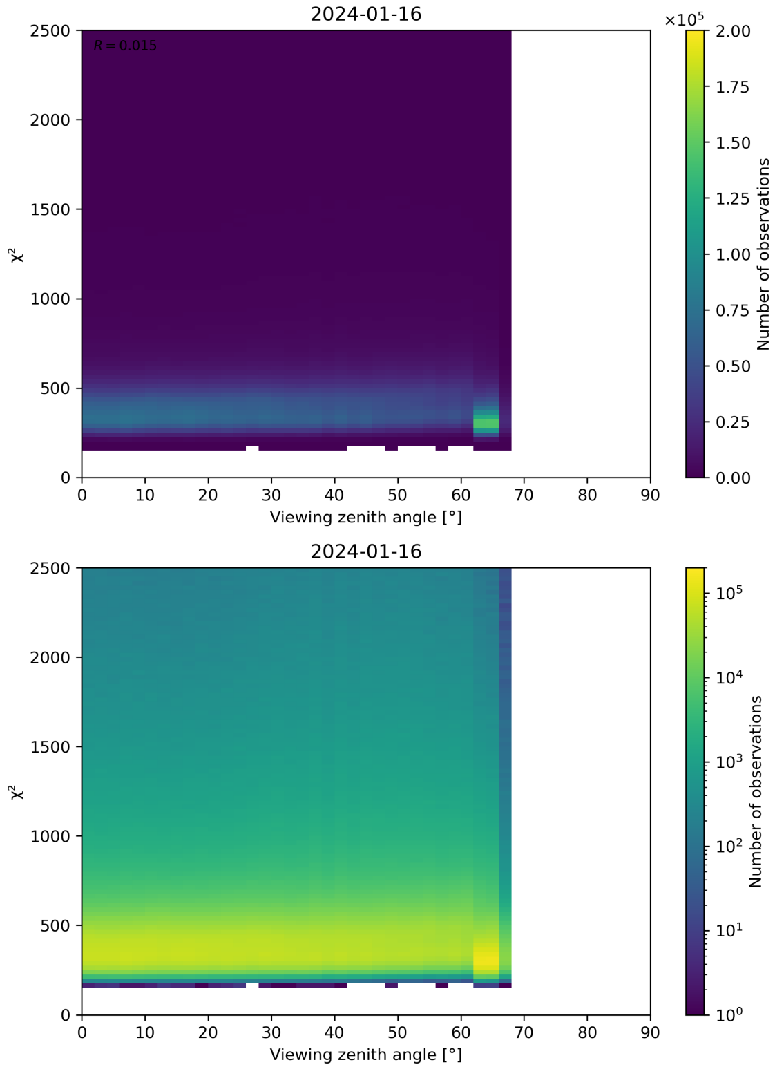
Figure 162: Scatter density plot of “Viewing zenith angle” against “ \chi^2 ” for 2024-01-15 to 2024-01-17.
