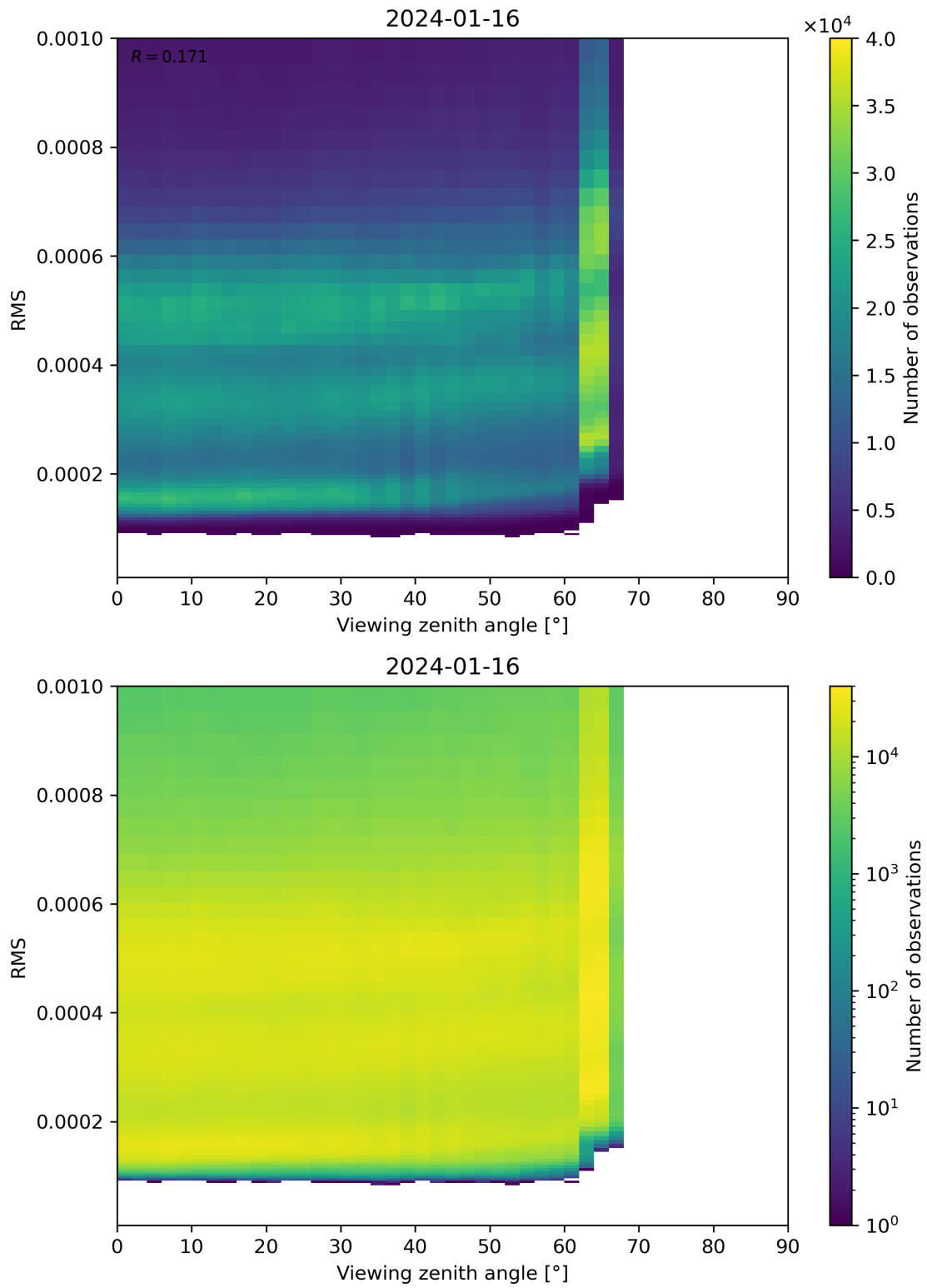
Figure 171: Scatter density plot of “Viewing zenith angle” against “RMS” for 2024-01-15 to 2024-01-17.
