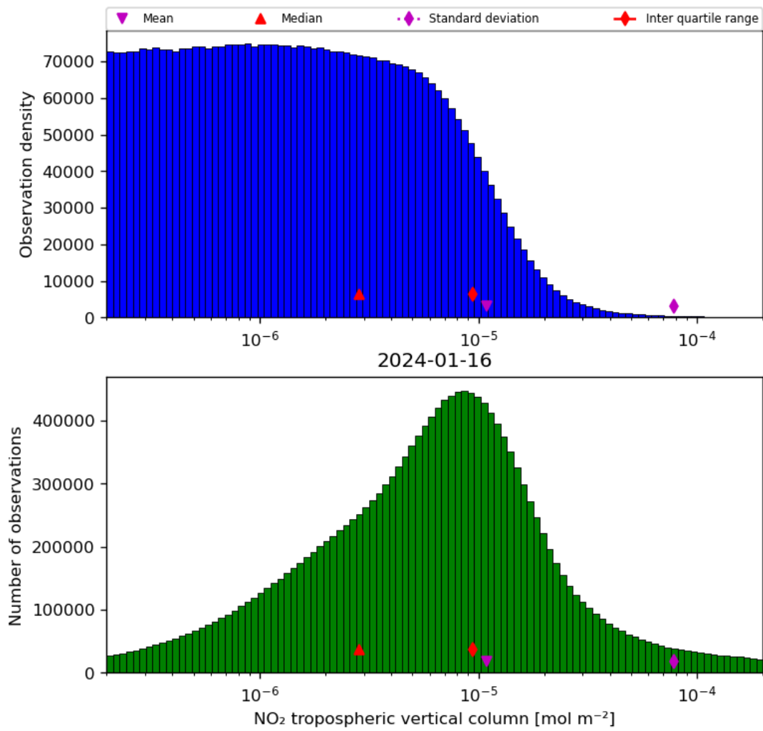
Figure 29: Histogram of “NO 2 tropospheric vertical column” for 2024-01-15 to 2024-01-17
