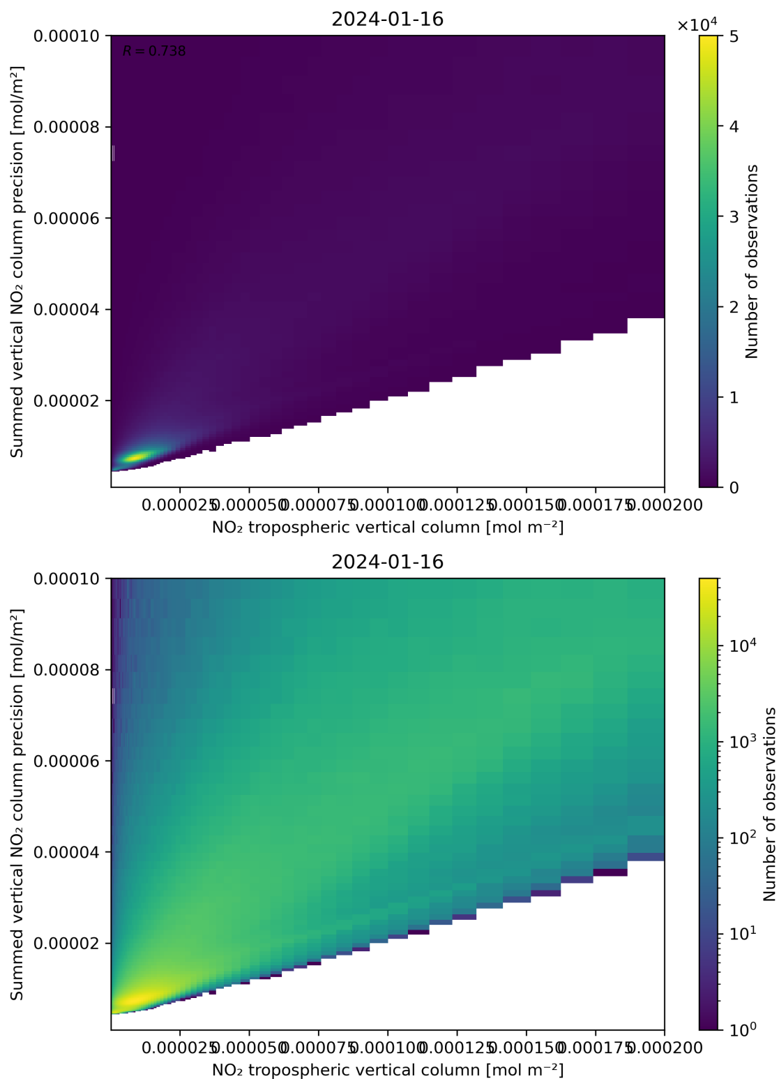
Figure 127: Scatter density plot of “NO 2 tropospheric vertical column” against “Summed vertical NO 2 column precision” for 2024-01-15 to 2024-01-17.
