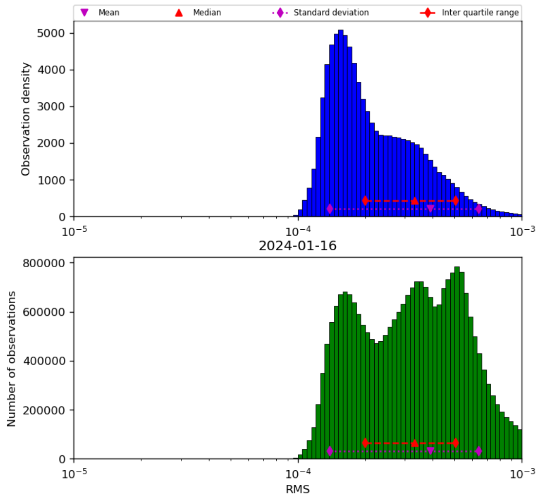
Figure 43: Histogram of “RMS” for 2024-01-15 to 2024-01-17
