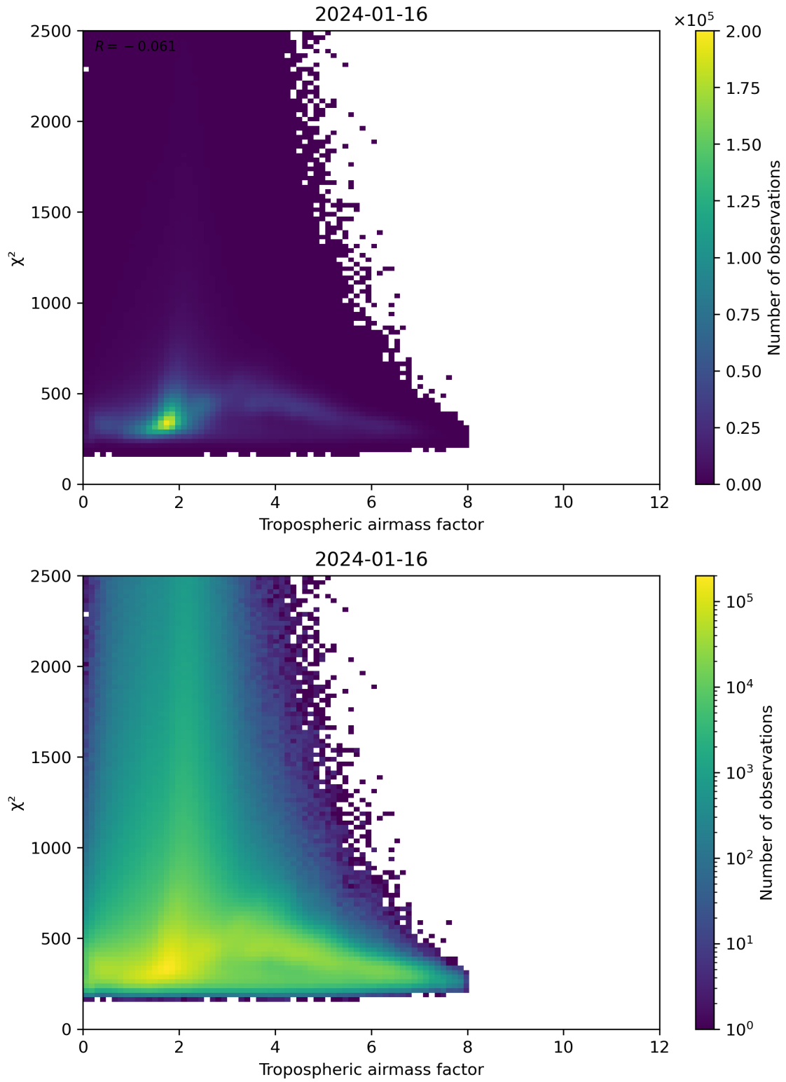
Figure 73: Scatter density plot of “Tropospheric airmass factor” against “ \chi^2 ” for 2024-01-15 to 2024-01-17.
