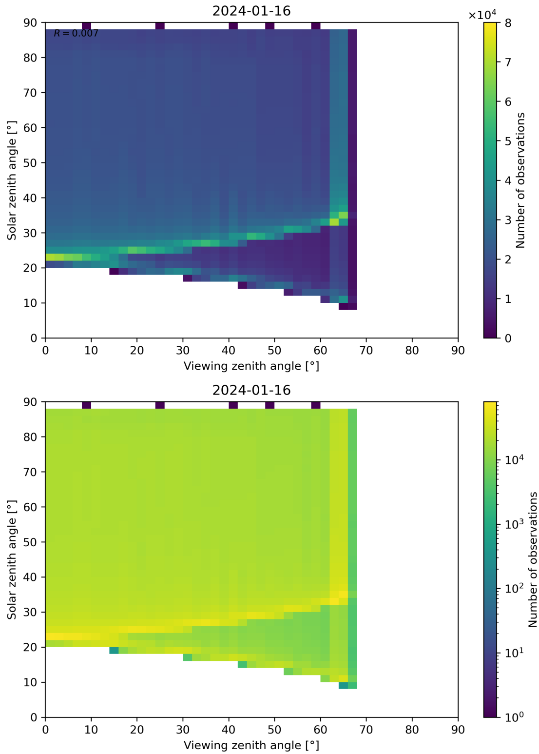
Figure 172: Scatter density plot of “Viewing zenith angle” against “Solar zenith angle” for 2024-01-15 to 2024-01-17.
