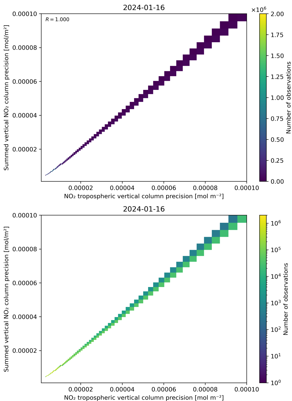
Figure 137: Scatter density plot of “NO 2 tropospheric vertical column precision” against “Summed vertical NO 2 column precision” for 2024-01-15 to 2024-01-17.
