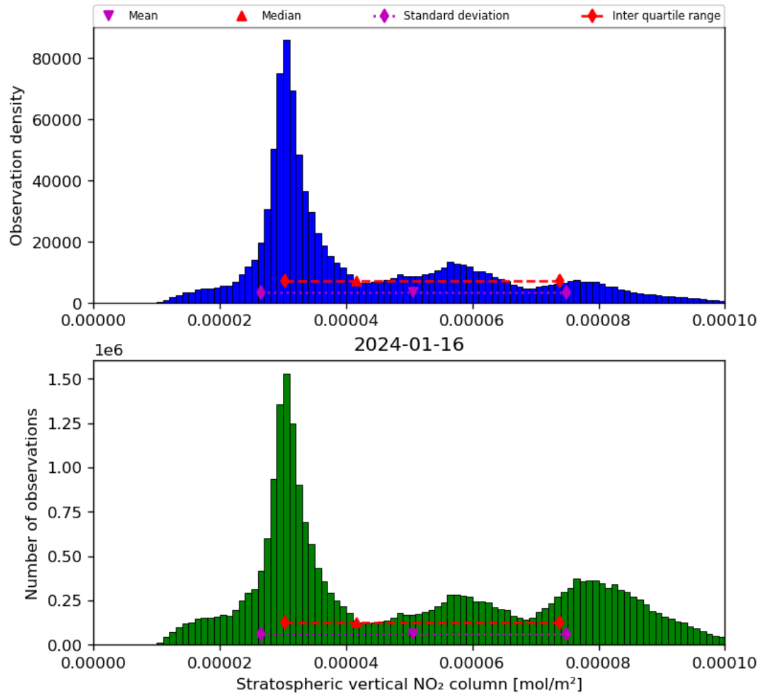
Figure 36: Histogram of “Stratospheric vertical NO 2 column” for 2024-01-15 to 2024-01-17
