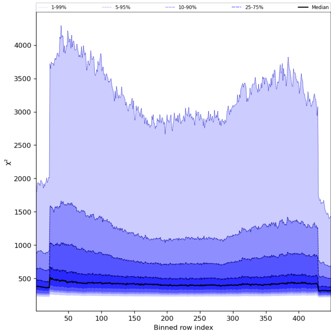
Figure 59: Along track statistics of “ \chi^2 ” for 2024-01-15 to 2024-01-17
