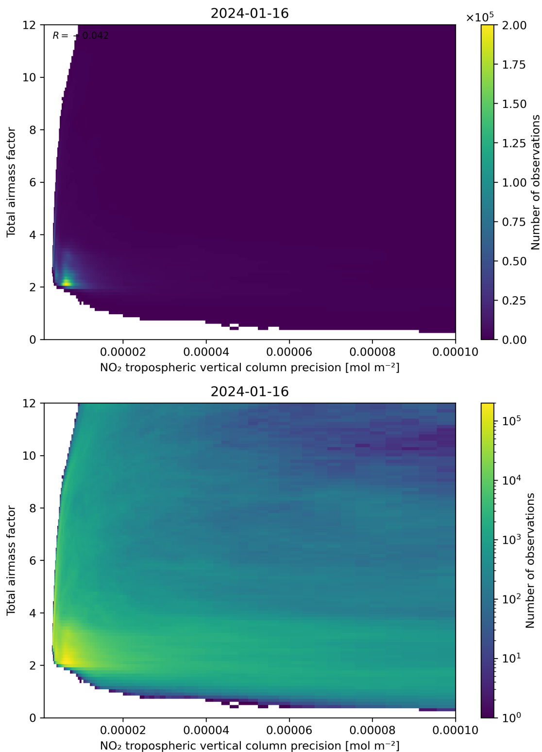
Figure 132: Scatter density plot of “NO 2 tropospheric vertical column precision” against “Total air mass factor” for 2024-01-15 to 2024-01-17.
