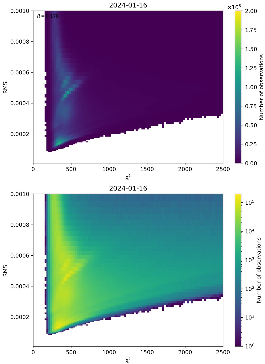
Figure 82: Scatter density plot of “ \chi^2 ” against “RMS” for 2024-01-15 to 2024-01-17.
