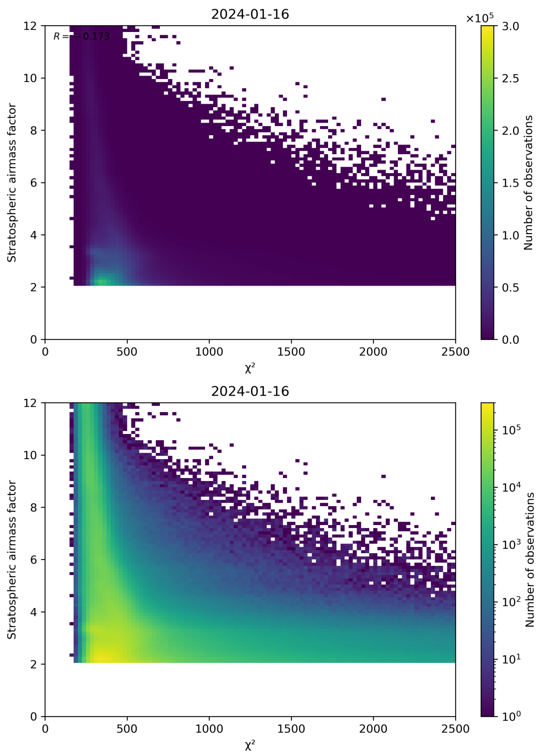
Figure 81: Scatter density plot of “ \chi^2 ” against “Stratospheric airmass factor” for 2024-01-15 to 2024-01-17.
