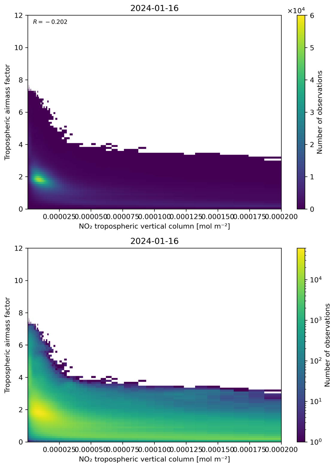
Figure 123: Scatter density plot of “NO 2 tropospheric vertical column” against “Tropospheric air mass factor” for 2024-01-15 to 2024-01-17.
