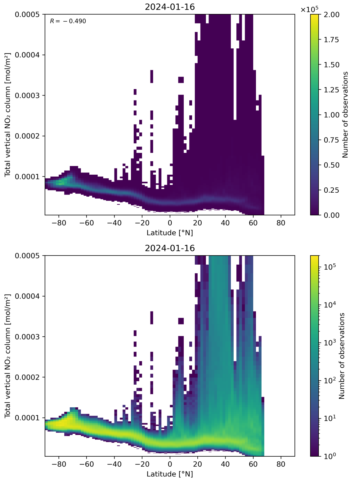
Figure 90: Scatter density plot of “Latitude” against “Total vertical NO 2 column” for 2024-01-15 to 2024-01-17.
