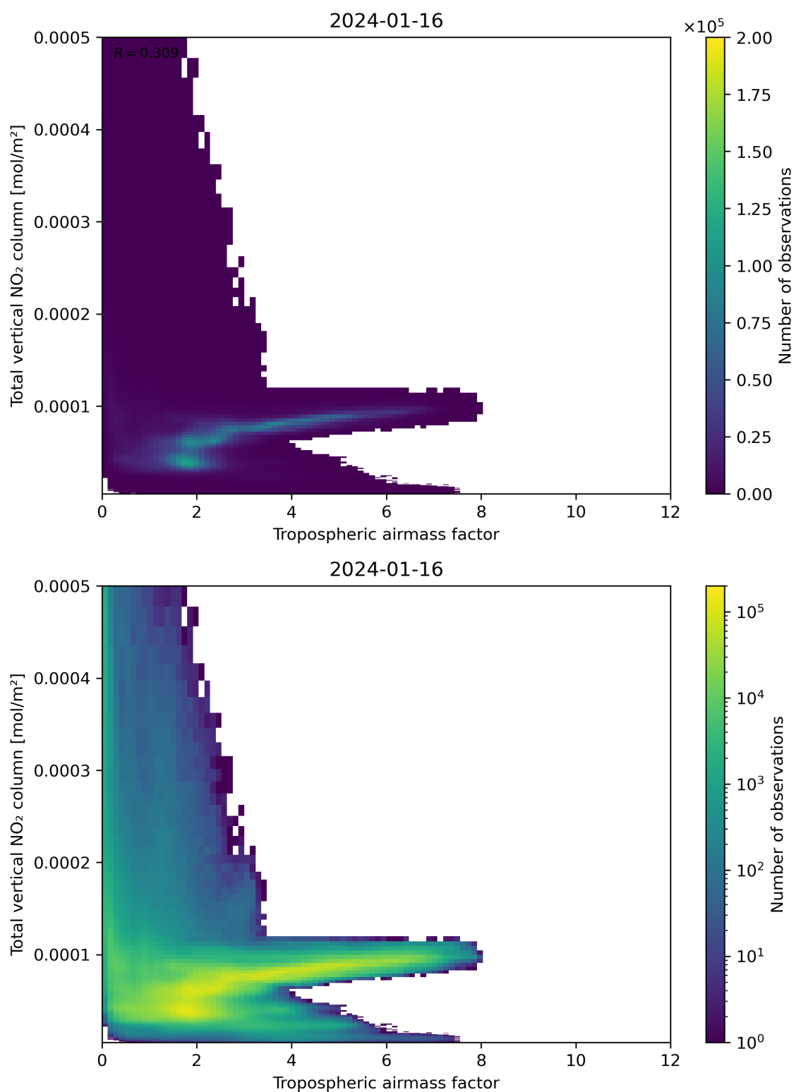
Figure 77: Scatter density plot of “Tropospheric airmass factor” against “Total vertical NO 2 column” for 2024-01-15 to 2024-01-17.
