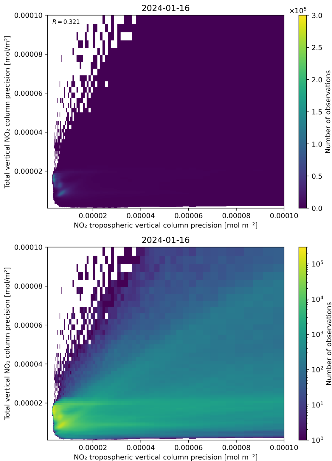
Figure 139: Scatter density plot of “NO 2 tropospheric vertical column precision” against “Total vertical NO 2 column precision” for 2024-01-15 to 2024-01-17.
