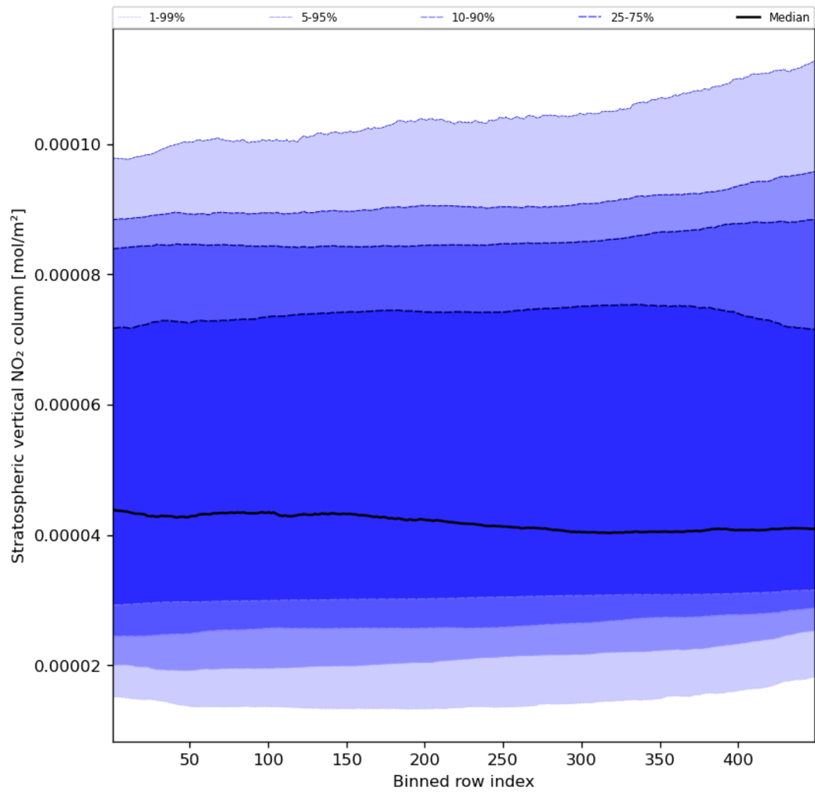
Figure 53: Along track statistics of “Stratospheric vertical NO 2 column” for 2024-01-15 to 2024-01-17
