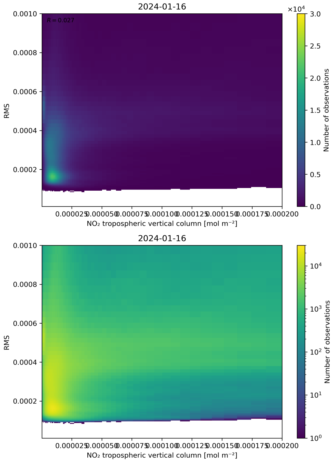
Figure 142: Scatter density plot of “NO 2 tropospheric vertical column” against “RMS” for 2024-01-15 to 2024-01-17.
