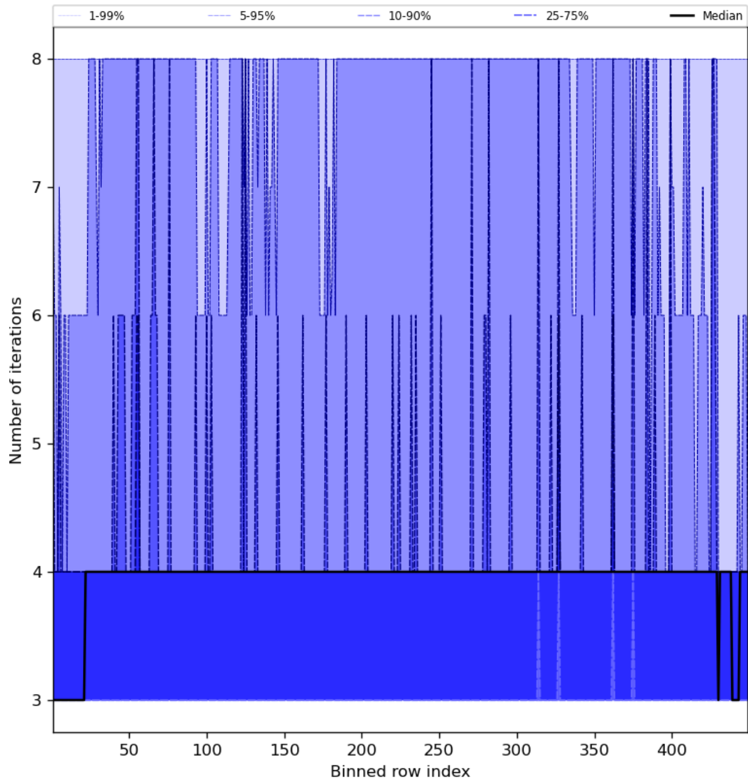
Figure 51: Along track statistics of “Number of iterations” for 2024-01-15 to 2024-01-17
