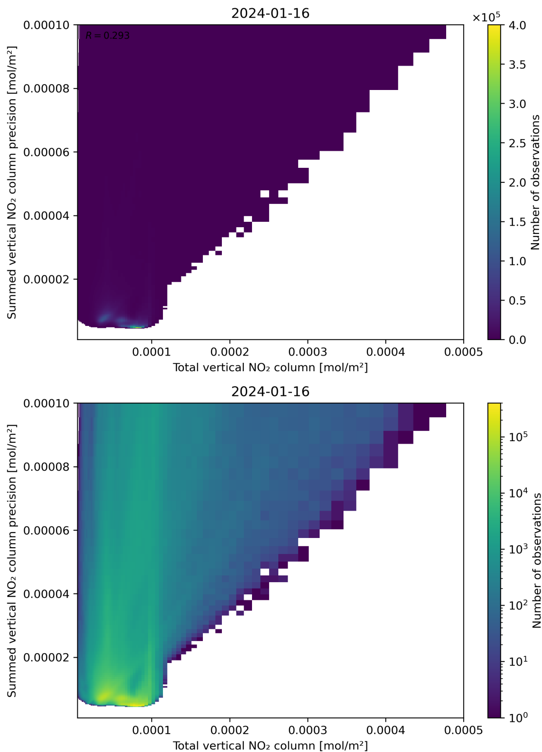
Figure 113: Scatter density plot of “Total vertical NO 2 column” against “Summed vertical NO 2 column precision” for 2024-01-15 to 2024-01-17.
