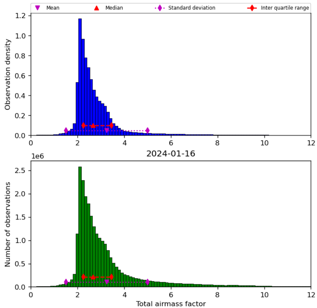
Figure 32: Histogram of “Total airmass factor” for 2024-01-15 to 2024-01-17
