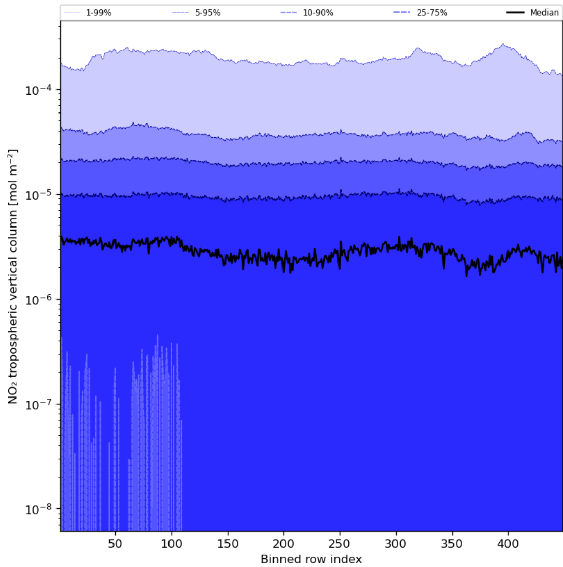
Figure 46: Along track statistics of "NO 2 tropospheric vertical column" for 2024-01-15 to 2024-01-17
