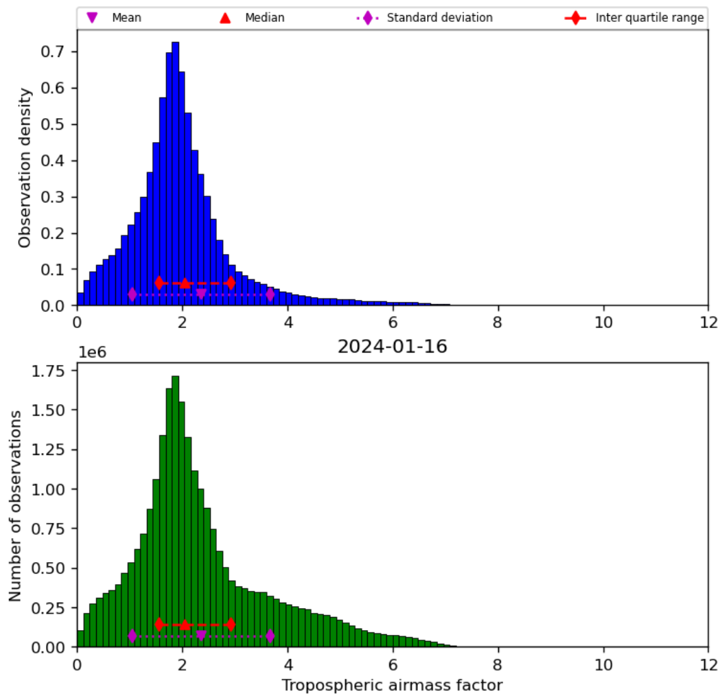
Figure 31: Histogram of “Tropospheric airmass factor” for 2024-01-15 to 2024-01-17
