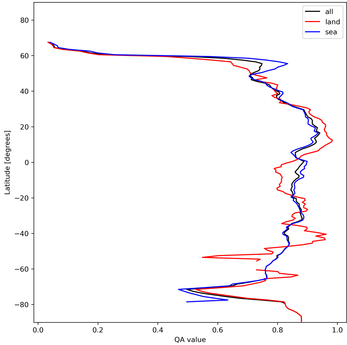
Figure 11: Zonal average of “QA value” for 2024-01-15 to 2024-01-17.
