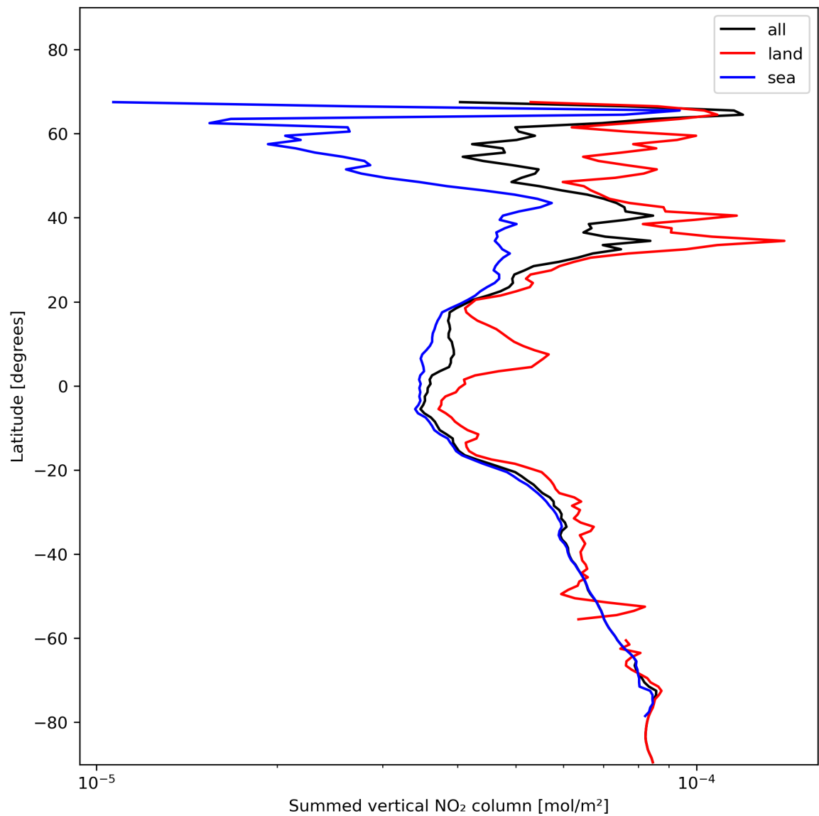
Figure 23: Zonal average of “Summed vertical NO 2 column” for 2024-01-15 to 2024-01-17.
