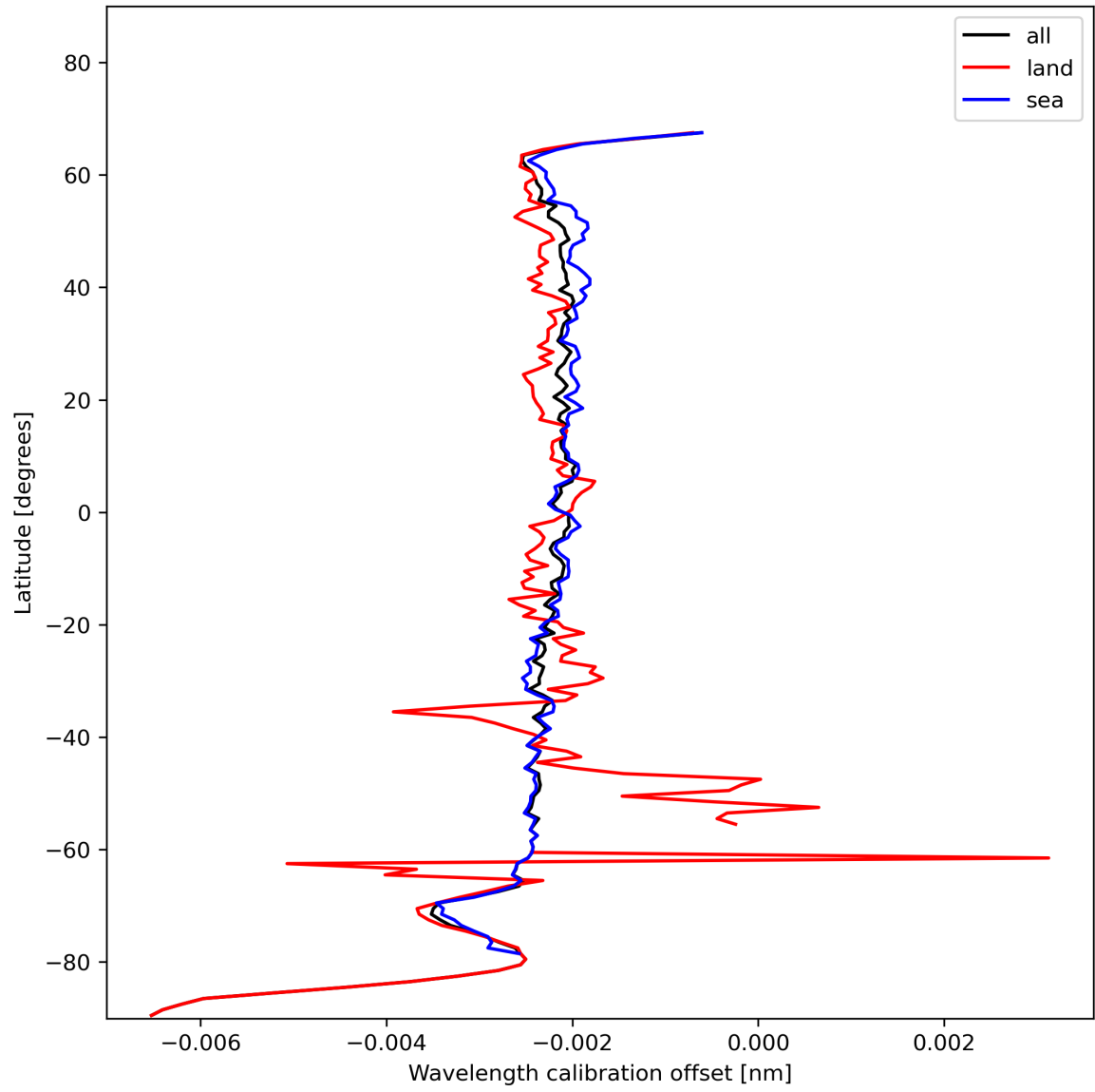
Figure 18: Zonal average of “Wavelength calibration offset” for 2024-01-15 to 2024-01-17.
