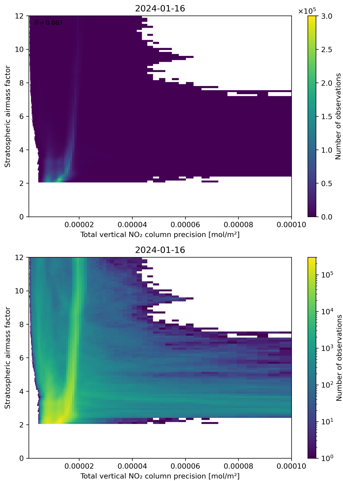
Figure 115: Scatter density plot of “Total vertical NO 2 column precision” against “Stratospheric airmass factor” for 2024-01-15 to 2024-01-17.
