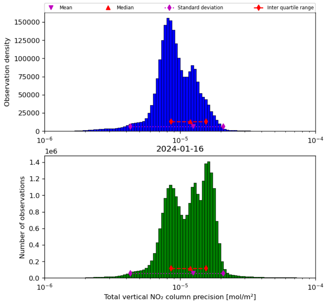
Figure 39: Histogram of “Total vertical NO 2 column precision” for 2024-01-15 to 2024-01-17
