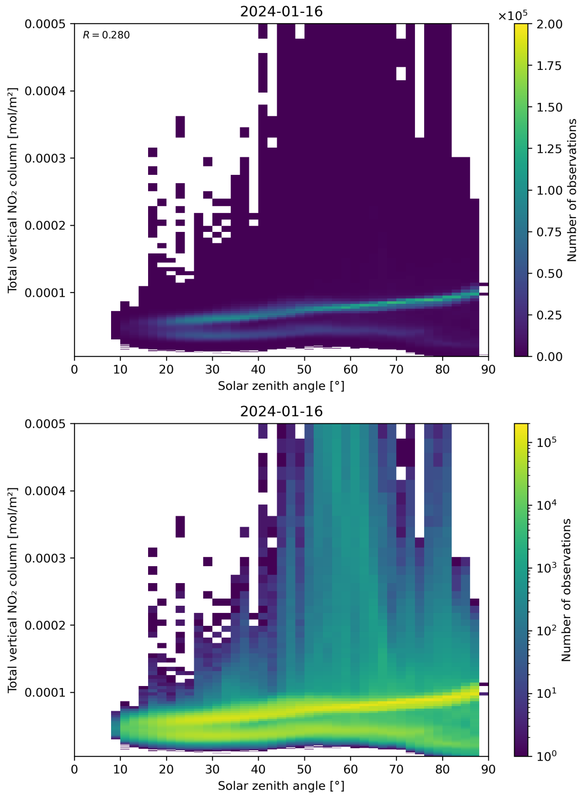
Figure 153: Scatter density plot of “Solar zenith angle” against “Total vertical NO 2 column” for 2024-01-15 to 2024-01-17.
