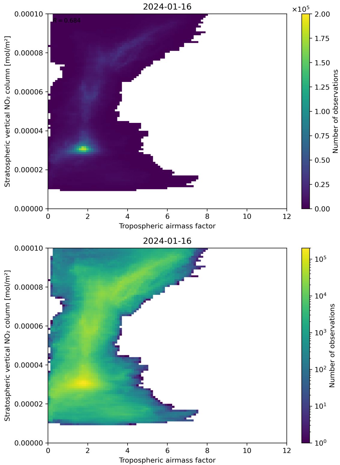
Figure 74: Scatter density plot of “Tropospheric air mass factor” against “Stratospheric vertical NO 2 column” for 2024-01-15 to 2024-01-17.
