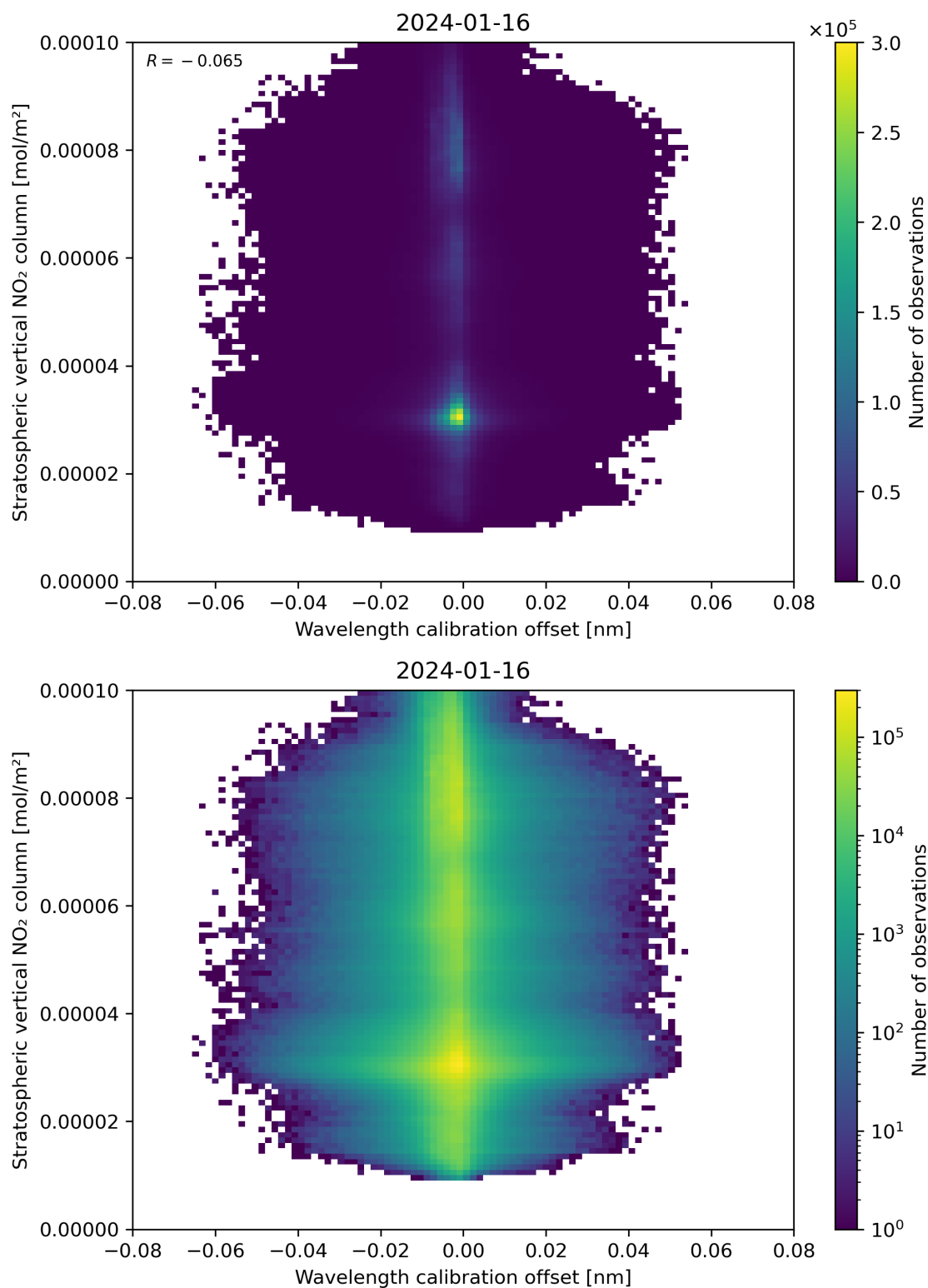
Figure 176: Scatter density plot of “Wavelength calibration offset” against “Stratospheric vertical NO 2 column” for 2024-01-15 to 2024-01-17.
