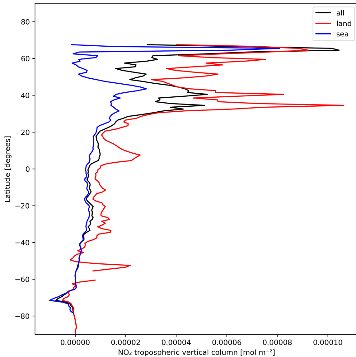
Figure 12: Zonal average of “NO 2 tropospheric vertical column” for 2024-01-15 to 2024-01-17.
