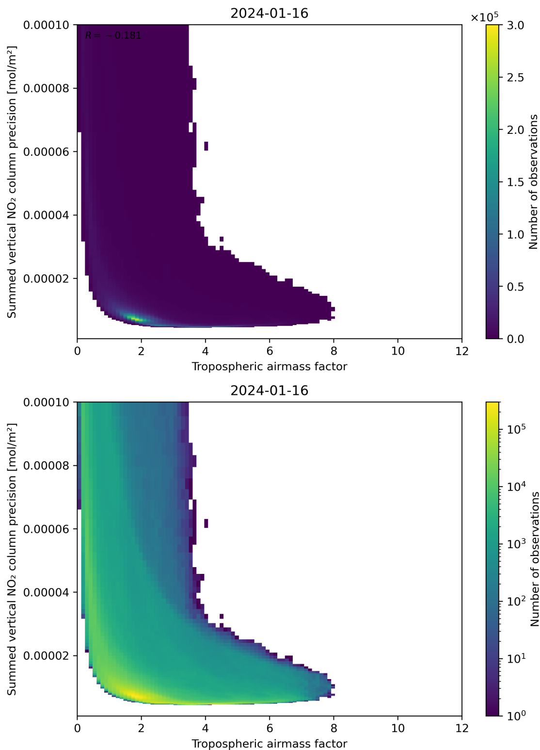
Figure 76: Scatter density plot of “Tropospheric air mass factor” against “Summed vertical NO 2 column precision” for 2024-01-15 to 2024-01-17.
