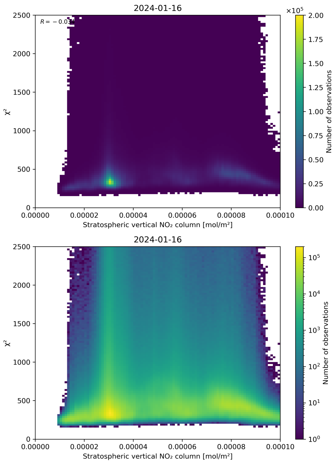
Figure 97: Scatter density plot of “Stratospheric vertical NO 2 column” against “ \chi^2 ” for 2024-01-15 to 2024-01-17.
