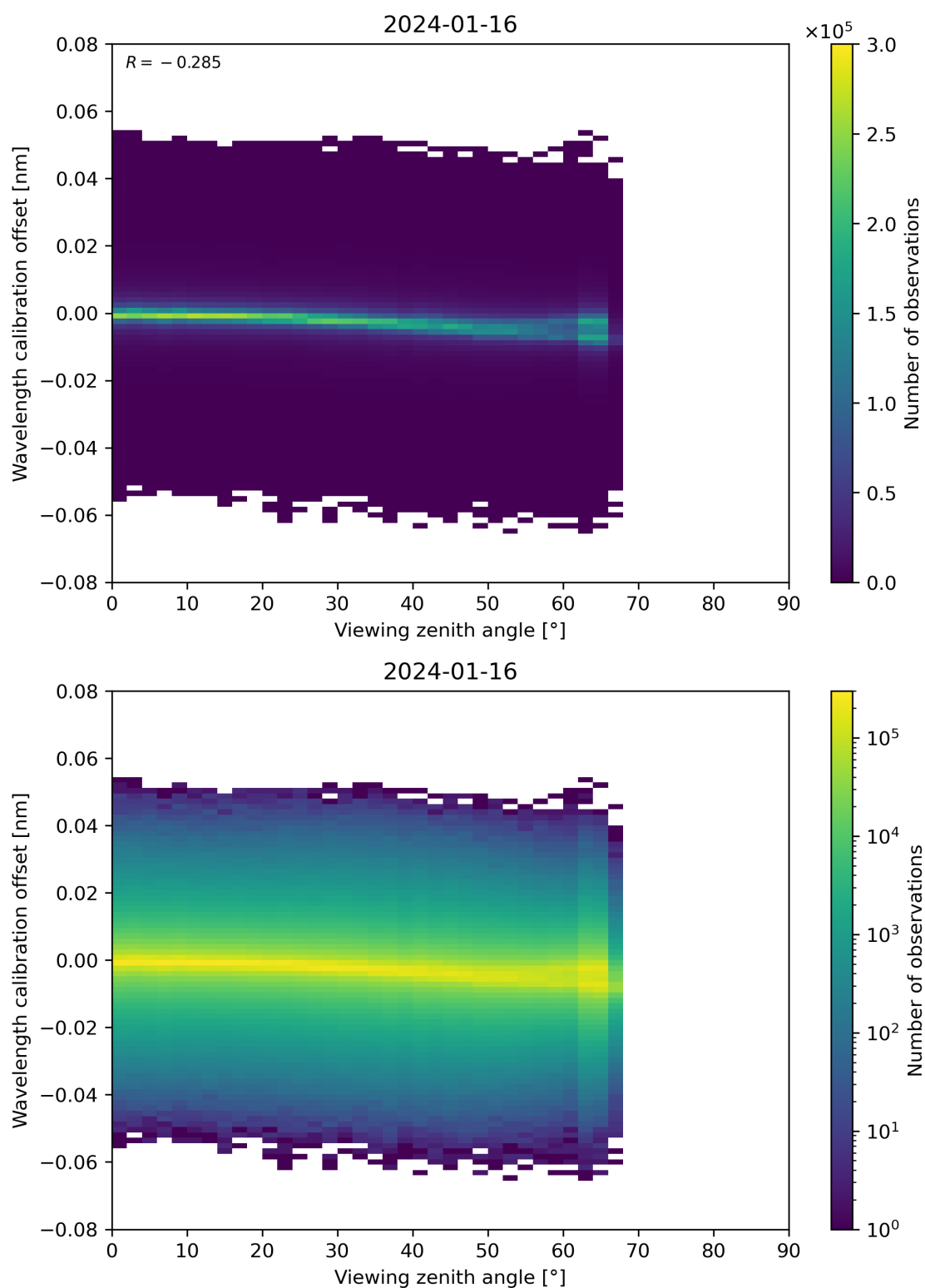
Figure 173: Scatter density plot of “Viewing zenith angle” against “Wavelength calibration offset” for 2024-01-15 to 2024-01-17.
