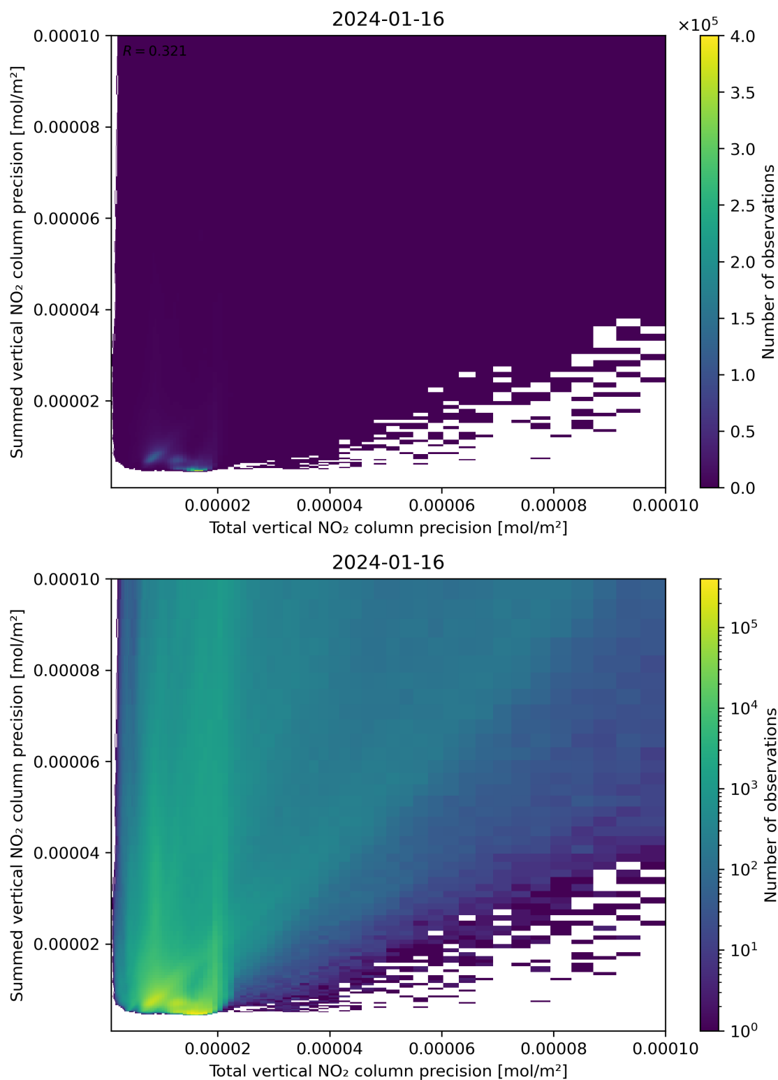
Figure 118: Scatter density plot of “Total vertical NO 2 column precision” against “Summed vertical NO 2 column precision” for 2024-01-15 to 2024-01-17.
