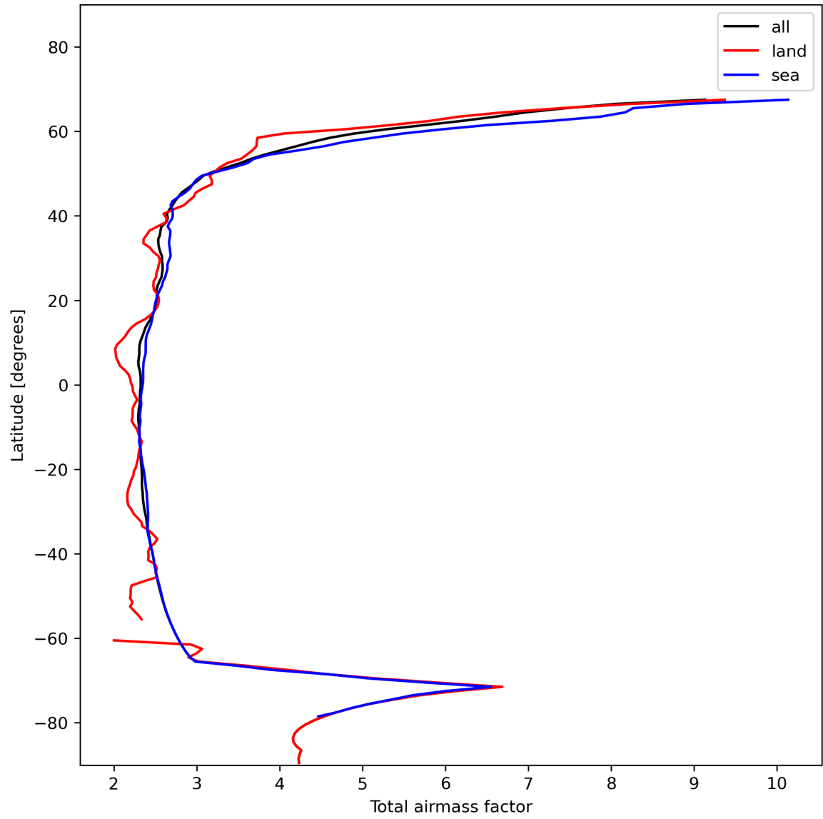
Figure 15: Zonal average of “Total airmass factor” for 2024-01-15 to 2024-01-17.
