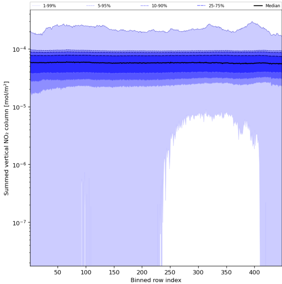
Figure 57: Along track statistics of “Summed vertical NO 2 column” for 2024-01-15 to 2024-01-17
