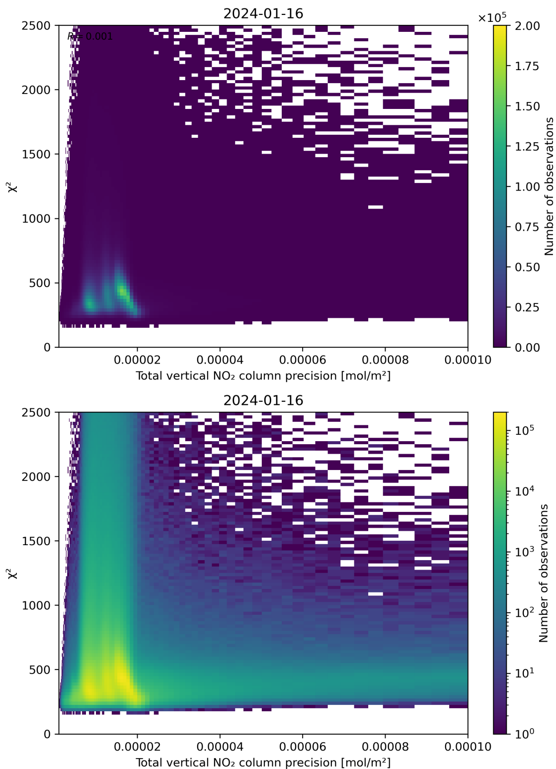
Figure 116: Scatter density plot of “Total vertical NO 2 column precision” against “ \chi^2 ” for 2024-01-15 to 2024-01-17.
