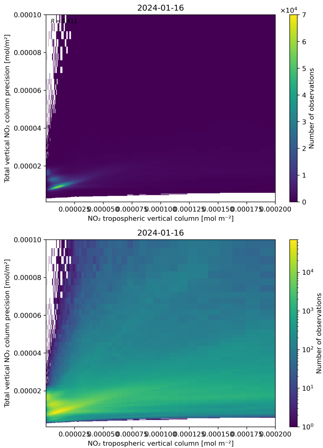
Figure 129: Scatter density plot of “NO 2 tropospheric vertical column” against “Total vertical NO 2 column precision” for 2024-01-15 to 2024-01-17.
