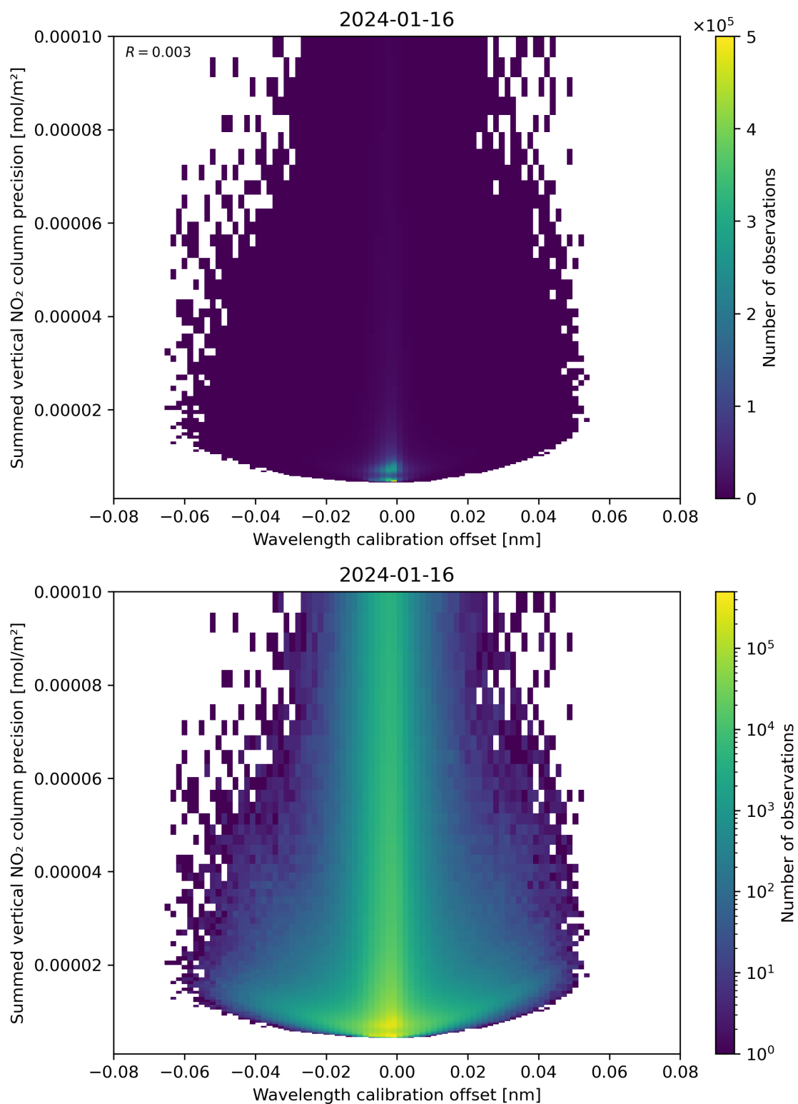
Figure 178: Scatter density plot of “Wavelength calibration offset” against “Summed vertical NO 2 column precision” for 2024-01-15 to 2024-01-17.
