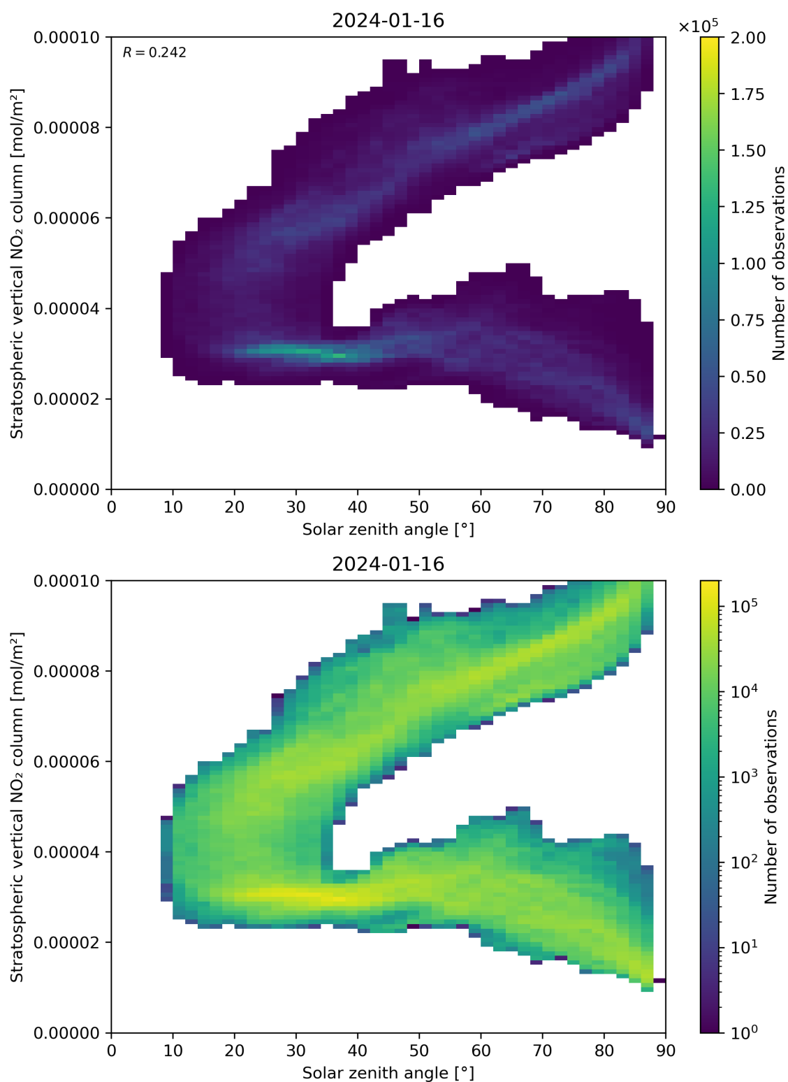
Figure 150: Scatter density plot of “Solar zenith angle” against “Stratospheric vertical NO 2 column” for 2024-01-15 to 2024-01-17.
