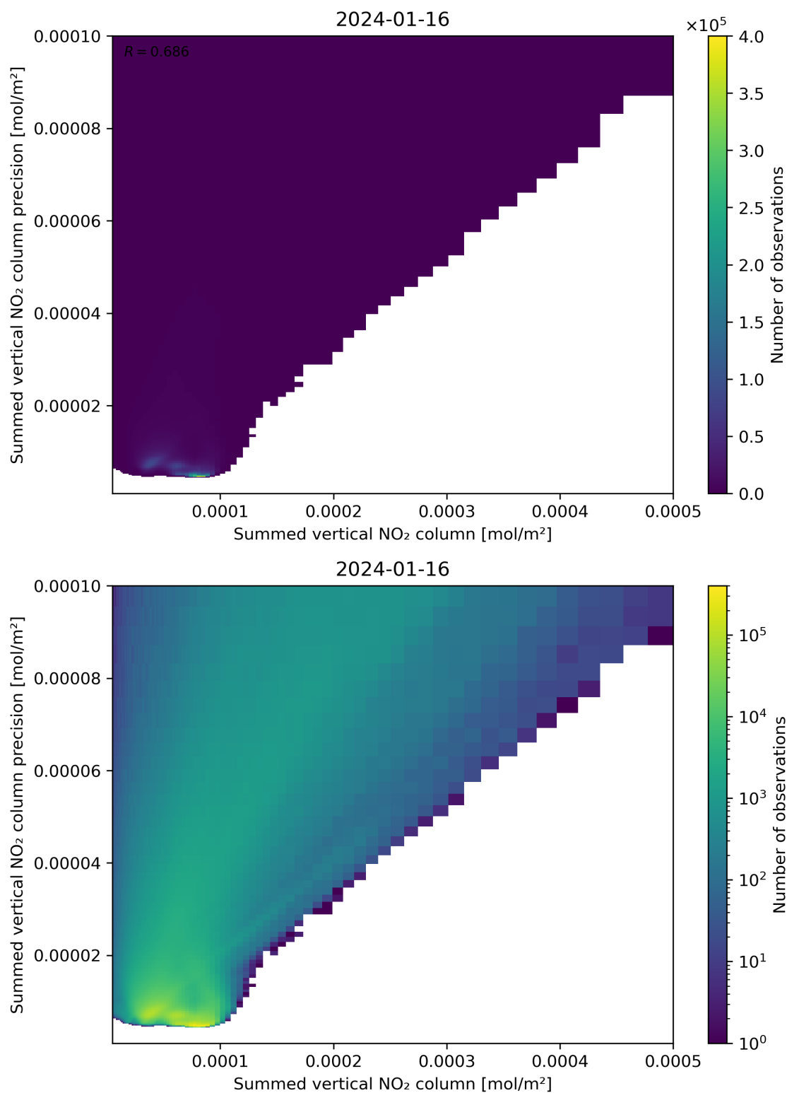
Figure 105: Scatter density plot of “Summed vertical NO 2 column” against “Summed vertical NO 2 column precision” for 2024-01-15 to 2024-01-17.
