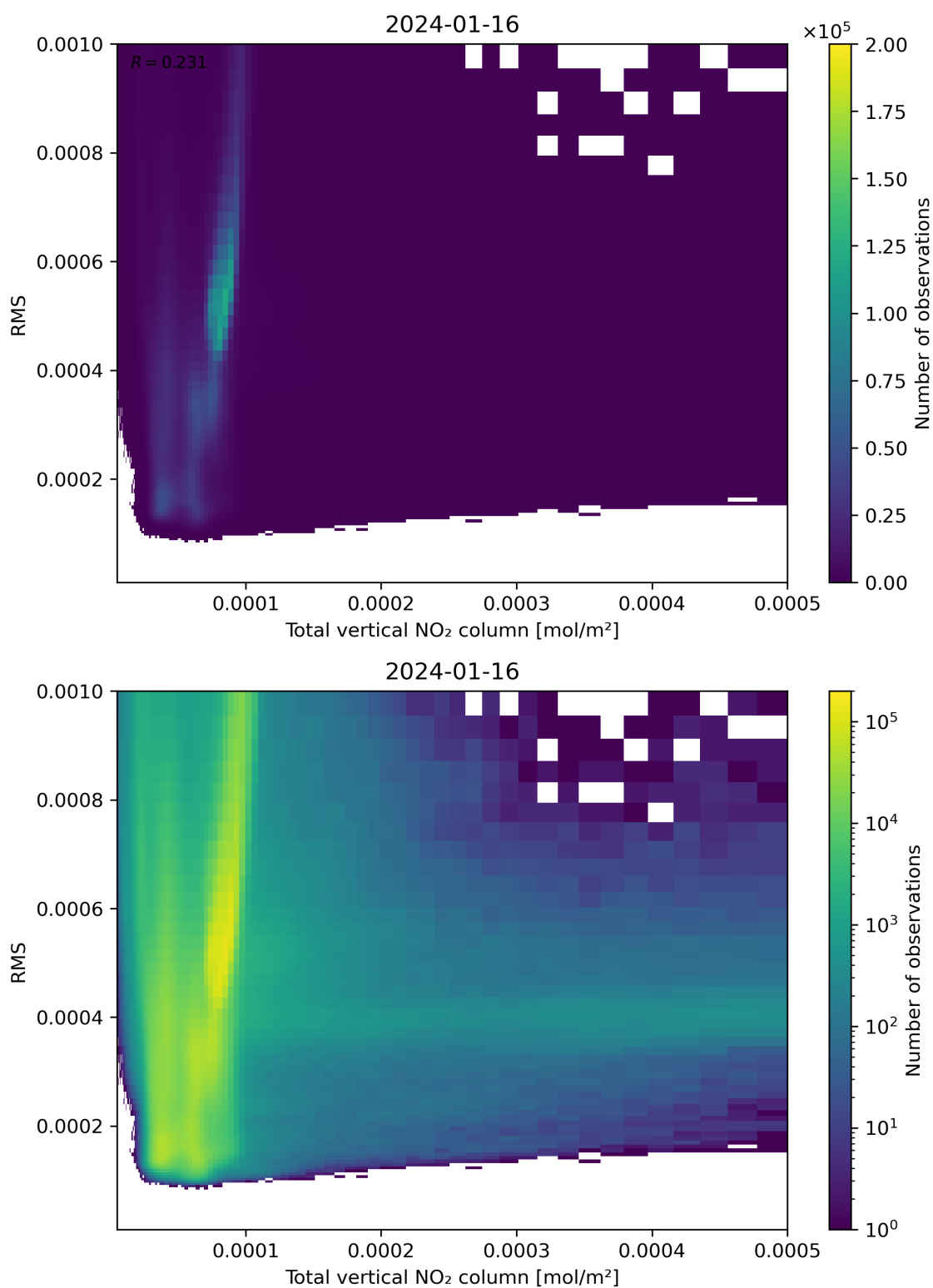
Figure 120: Scatter density plot of “Total vertical NO 2 column” against “RMS” for 2024-01-15 to 2024-01-17.
