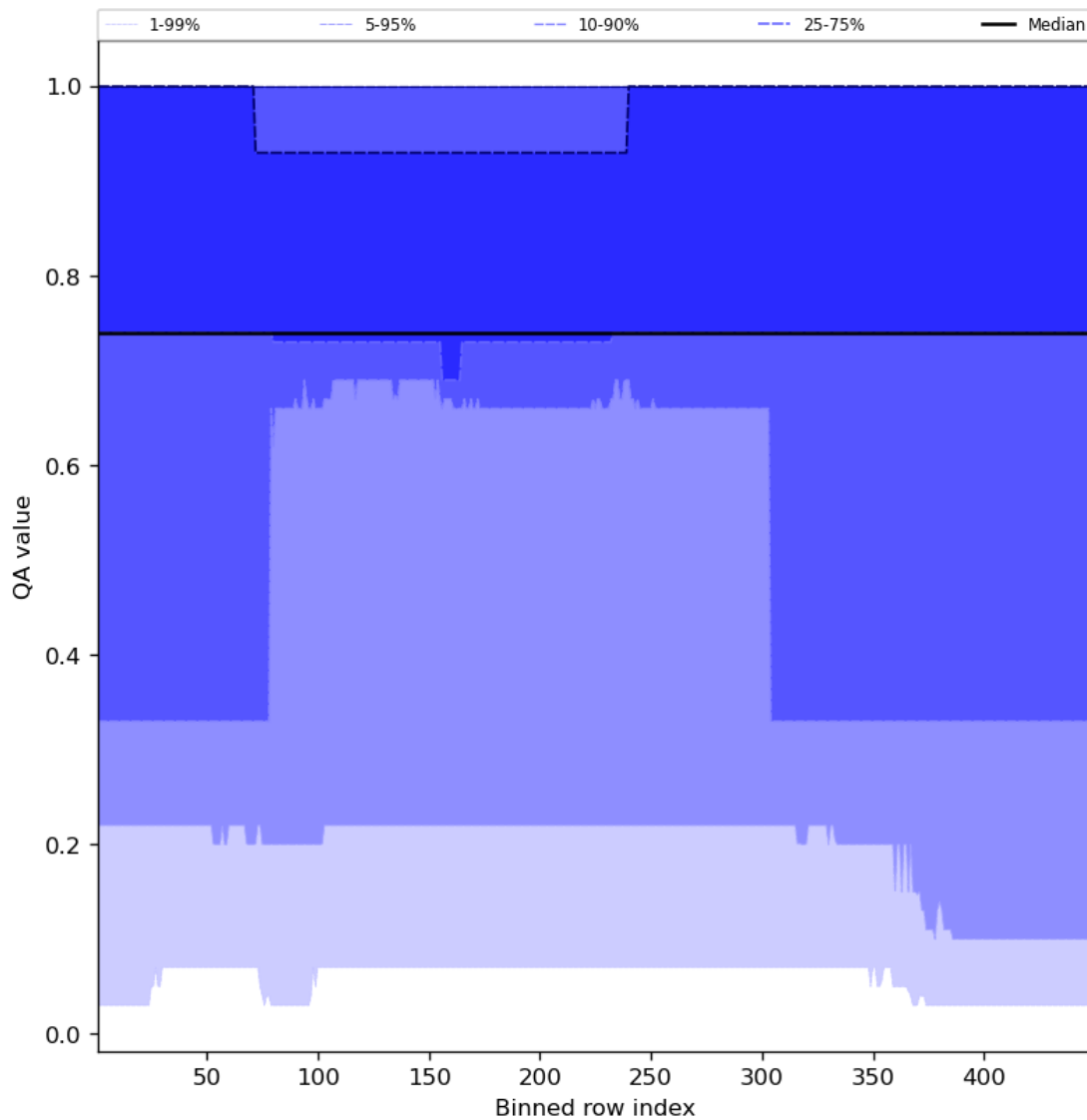
Figure 45: Along track statistics of “QA value” for 2024-01-15 to 2024-01-17
