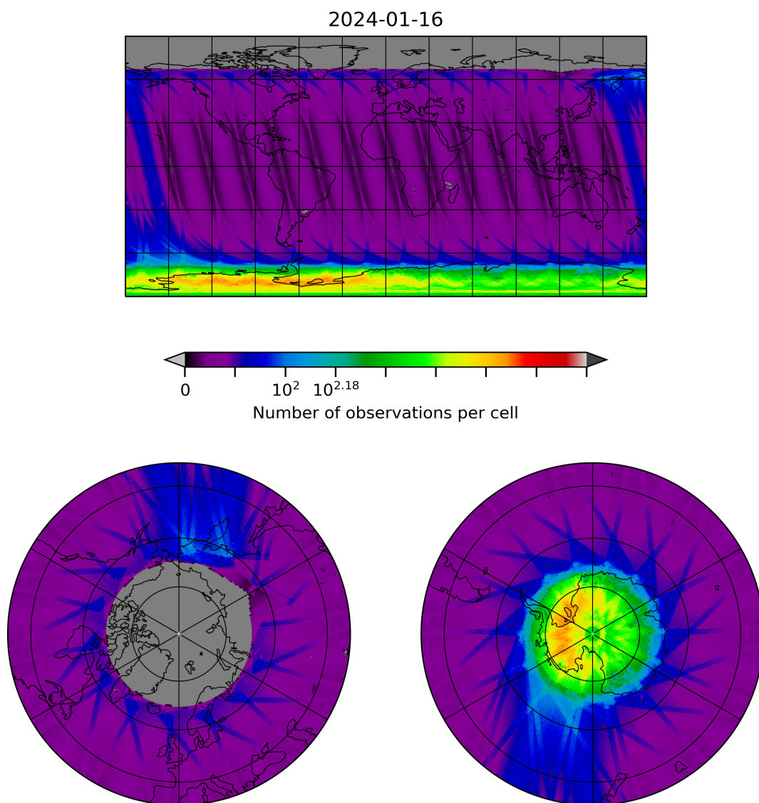
Figure 10: Map of the number of observations for 2024-01-15 to 2024-01-17
