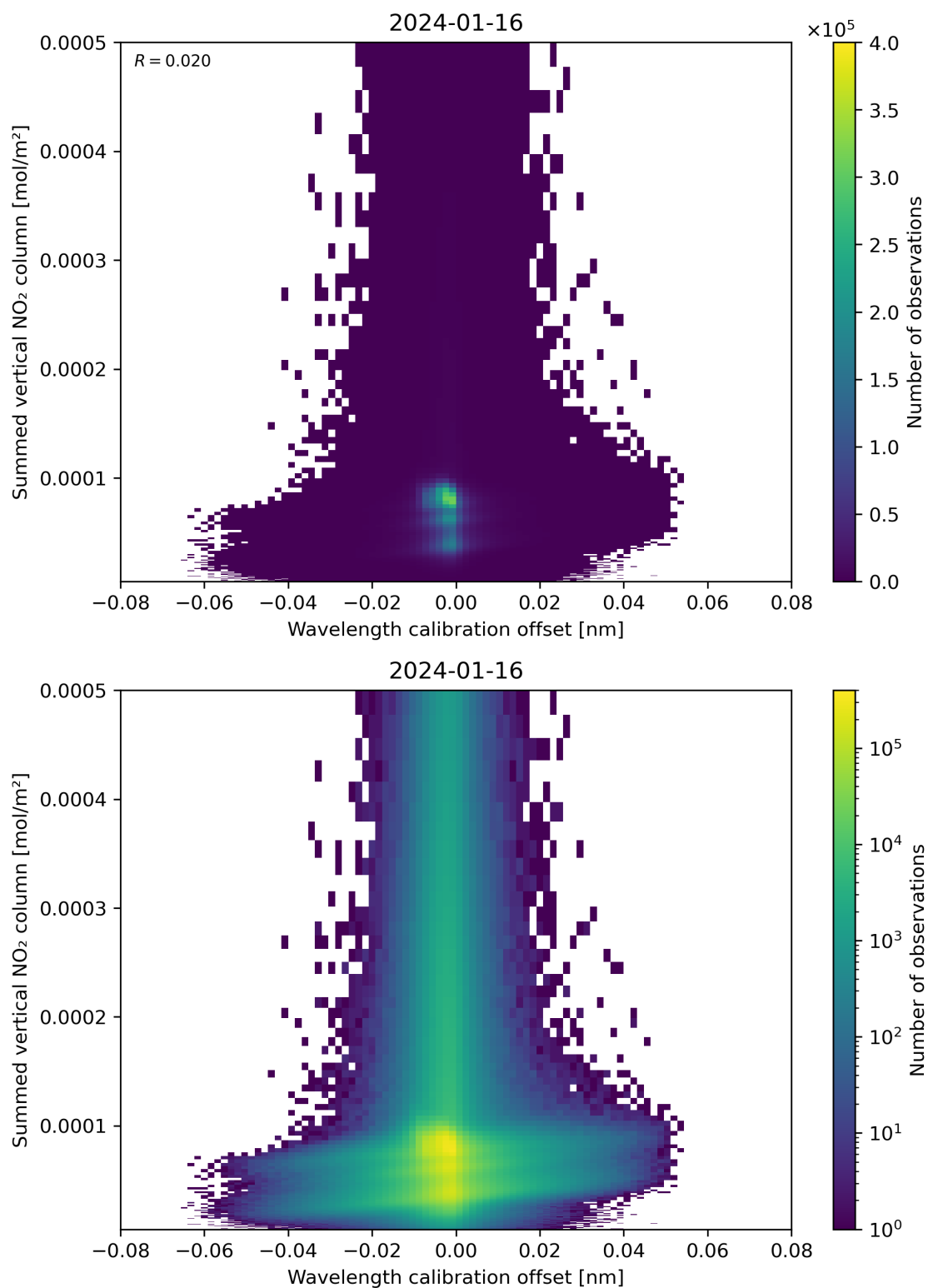
Figure 177: Scatter density plot of “Wavelength calibration offset” against “Summed vertical NO 2 column” for 2024-01-15 to 2024-01-17.
