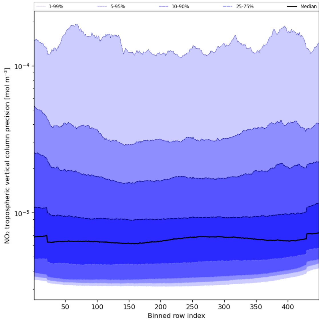
Figure 47: Along track statistics of “NO 2 tropospheric vertical column precision” for 2024-01-15 to 2024-01-17
