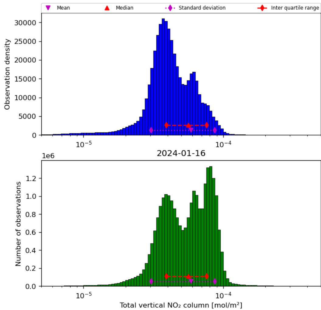
Figure 38: Histogram of "Total vertical NO 2 column" for 2024-01-15 to 2024-01-17
