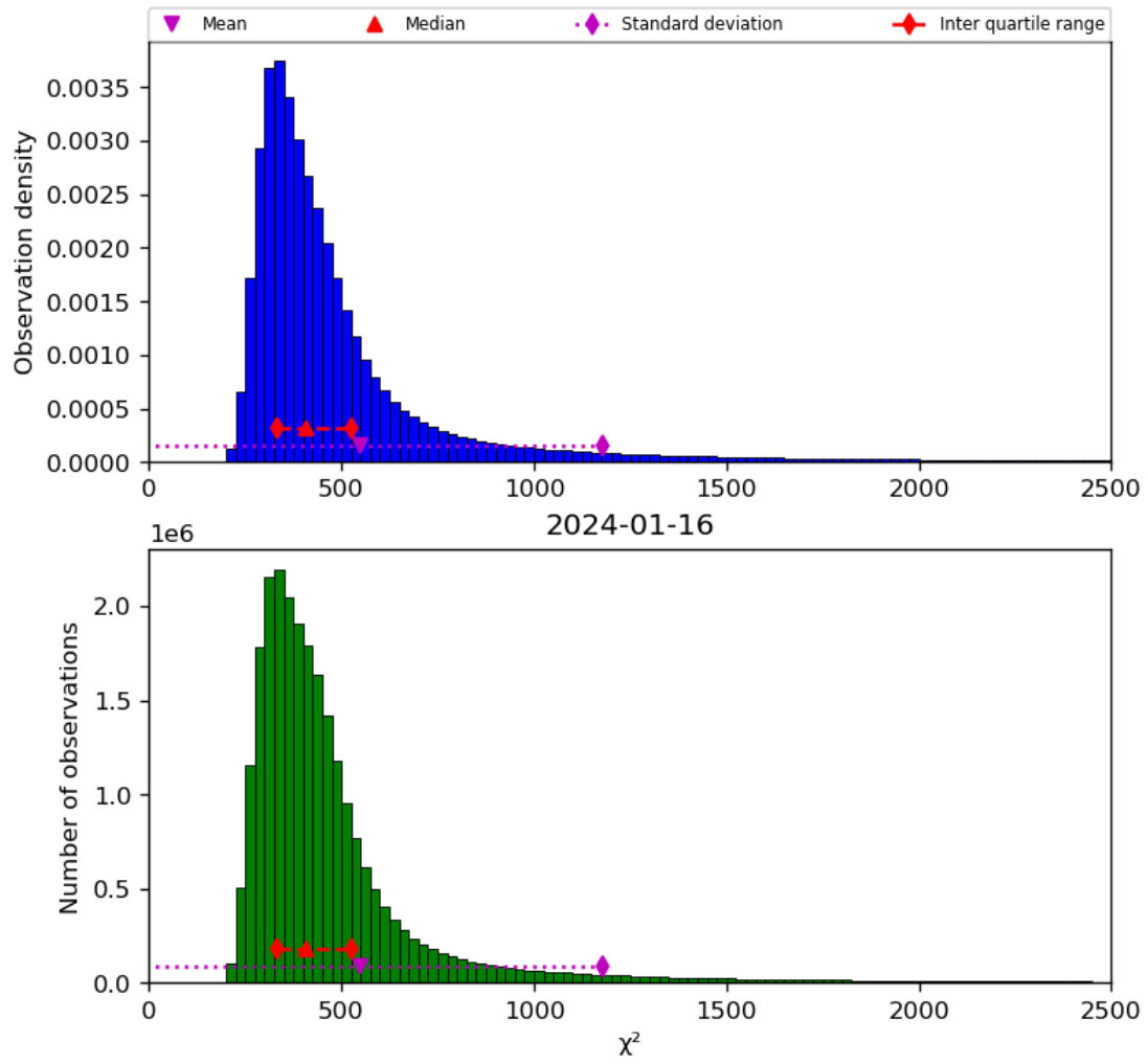
Figure 42: Histogram of " \chi^2 " for 2024-01-15 to 2024-01-17
