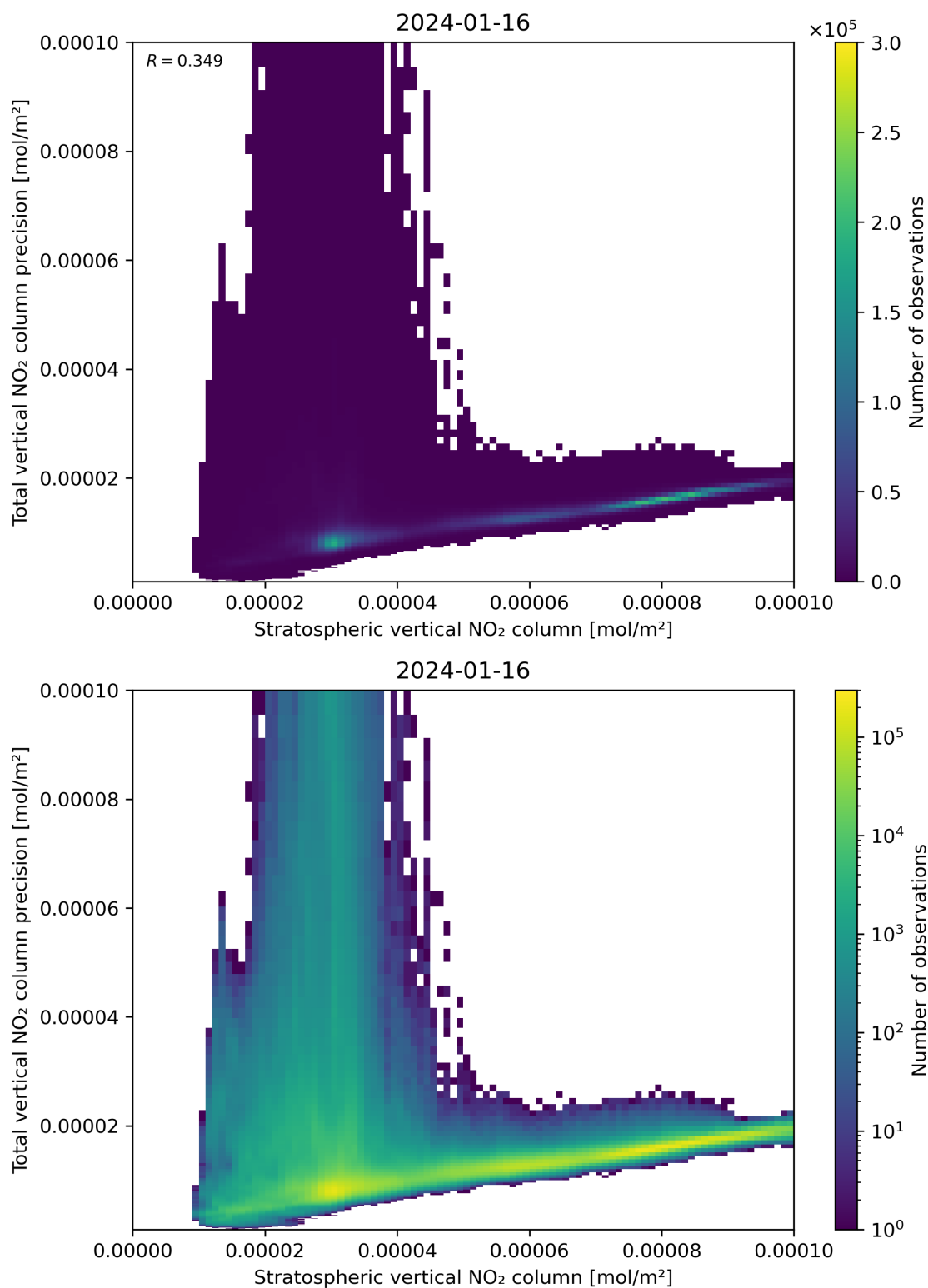
Figure 101: Scatter density plot of “Stratospheric vertical NO 2 column” against “Total vertical NO 2 column precision” for 2024-01-15 to 2024-01-17.
