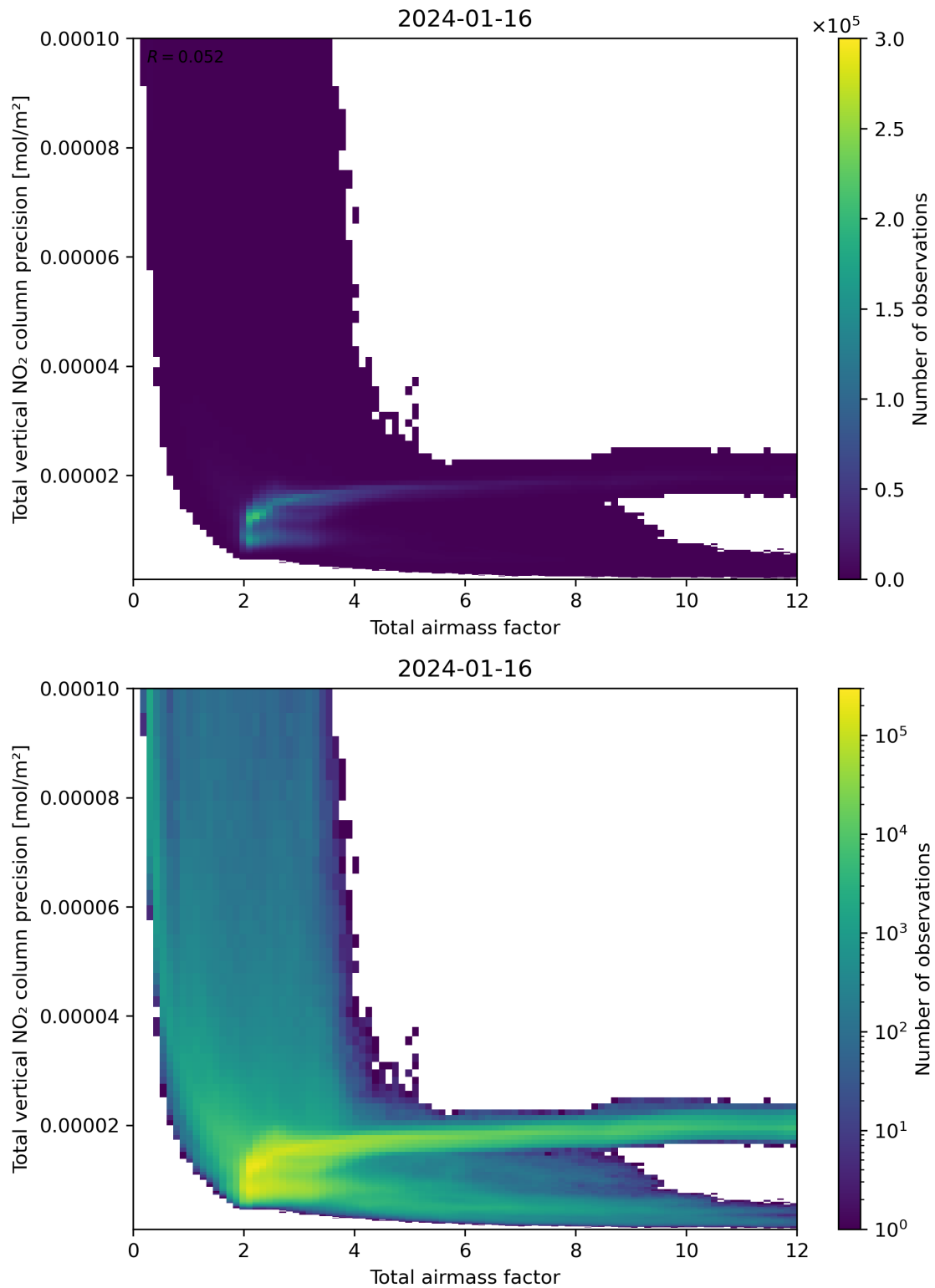
Figure 68: Scatter density plot of “Total airmass factor” against “Total vertical NO 2 column precision” for 2024-01-15 to 2024-01-17.
