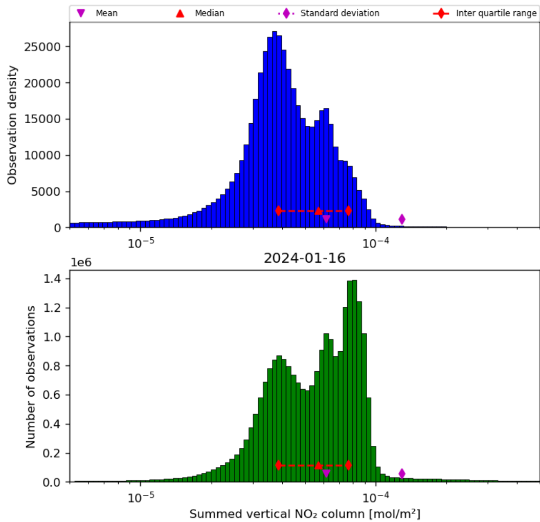
Figure 40: Histogram of “Summed vertical NO 2 column” for 2024-01-15 to 2024-01-17
