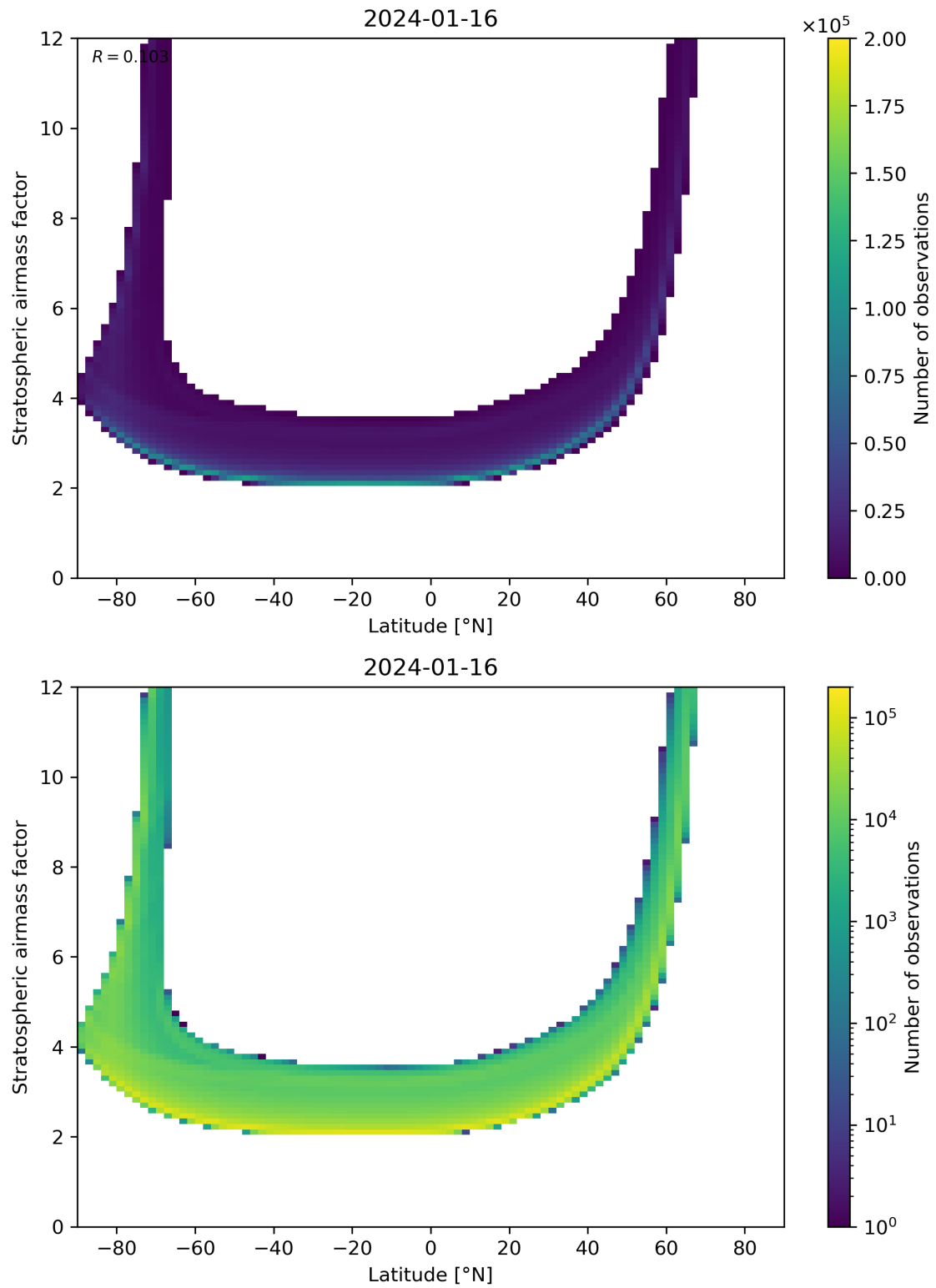
Figure 83: Scatter density plot of “Latitude” against “Stratospheric air mass factor” for 2024-01-15 to 2024-01-17.
