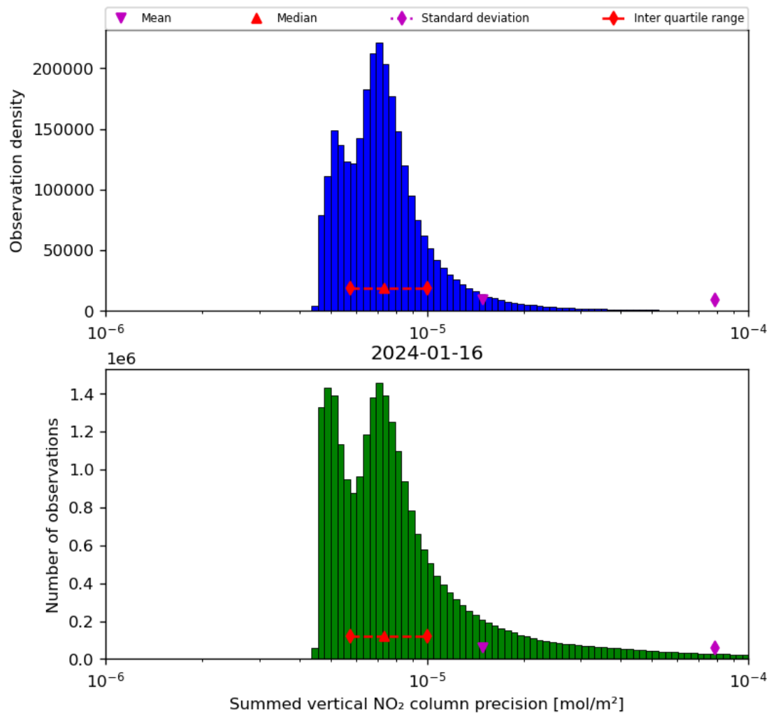
Figure 41: Histogram of “Summed vertical NO 2 column precision” for 2024-01-15 to 2024-01-17
