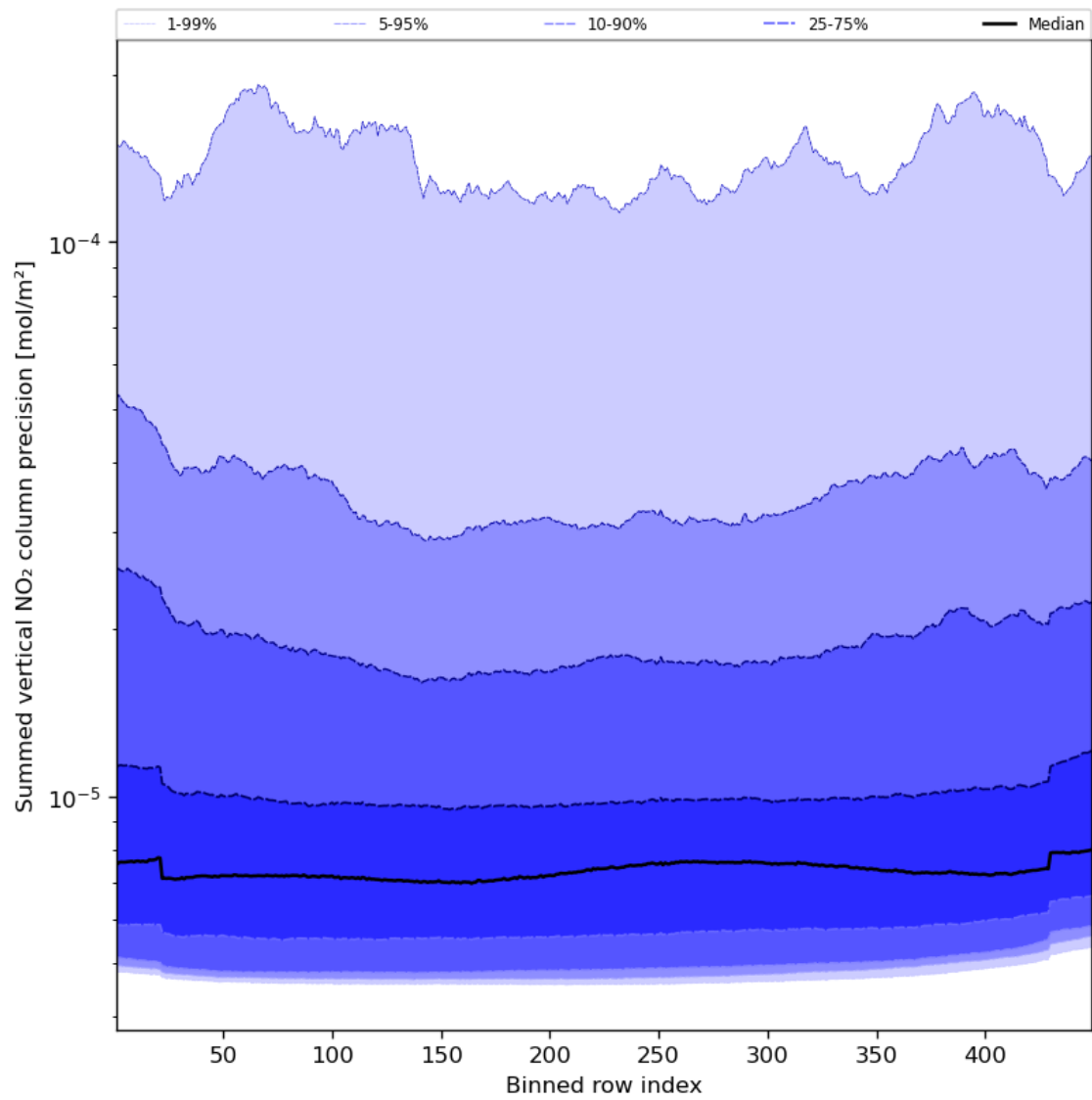
Figure 58: Along track statistics of “Summed vertical NO 2 column precision” for 2024-01-15 to 2024-01-17
