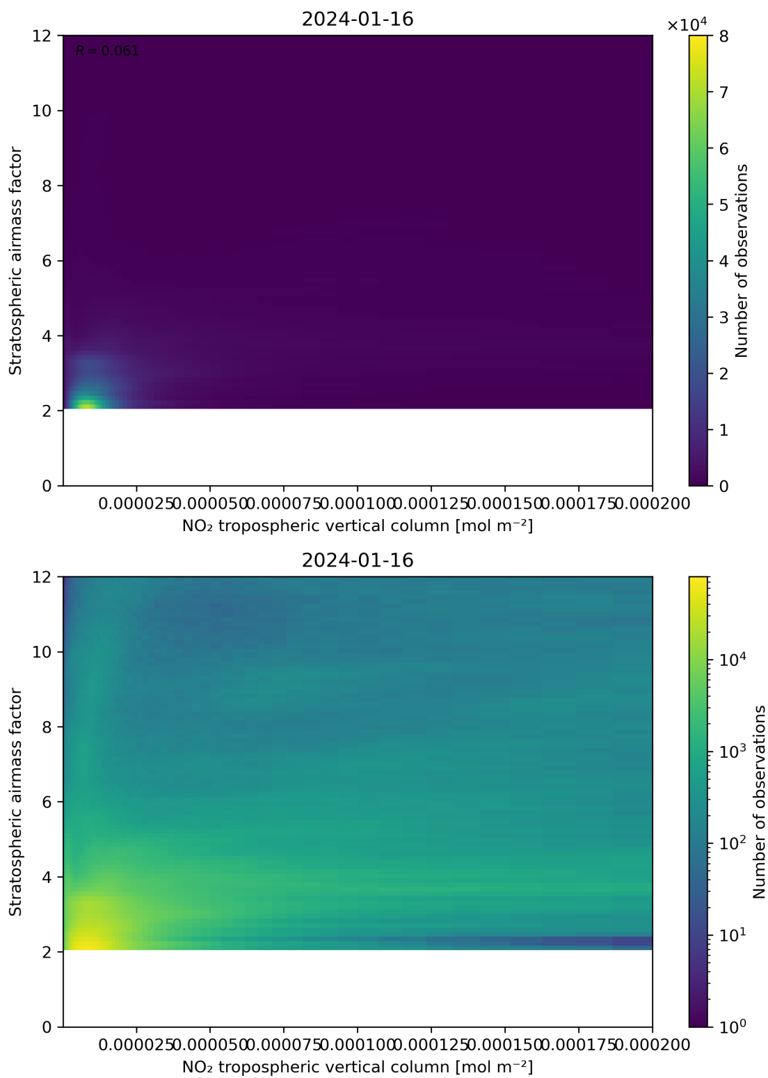
Figure 121: Scatter density plot of “NO 2 tropospheric vertical column” against “Stratospheric airmass factor” for 2024-01-15 to 2024-01-17.
