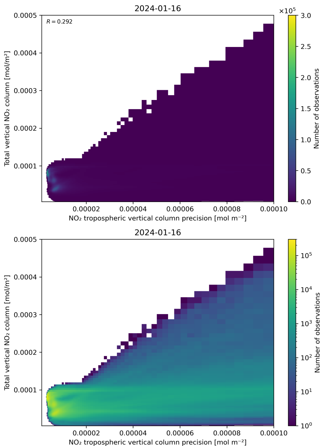
Figure 138: Scatter density plot of “NO 2 tropospheric vertical column precision” against “Total vertical NO 2 column” for 2024-01-15 to 2024-01-17.
