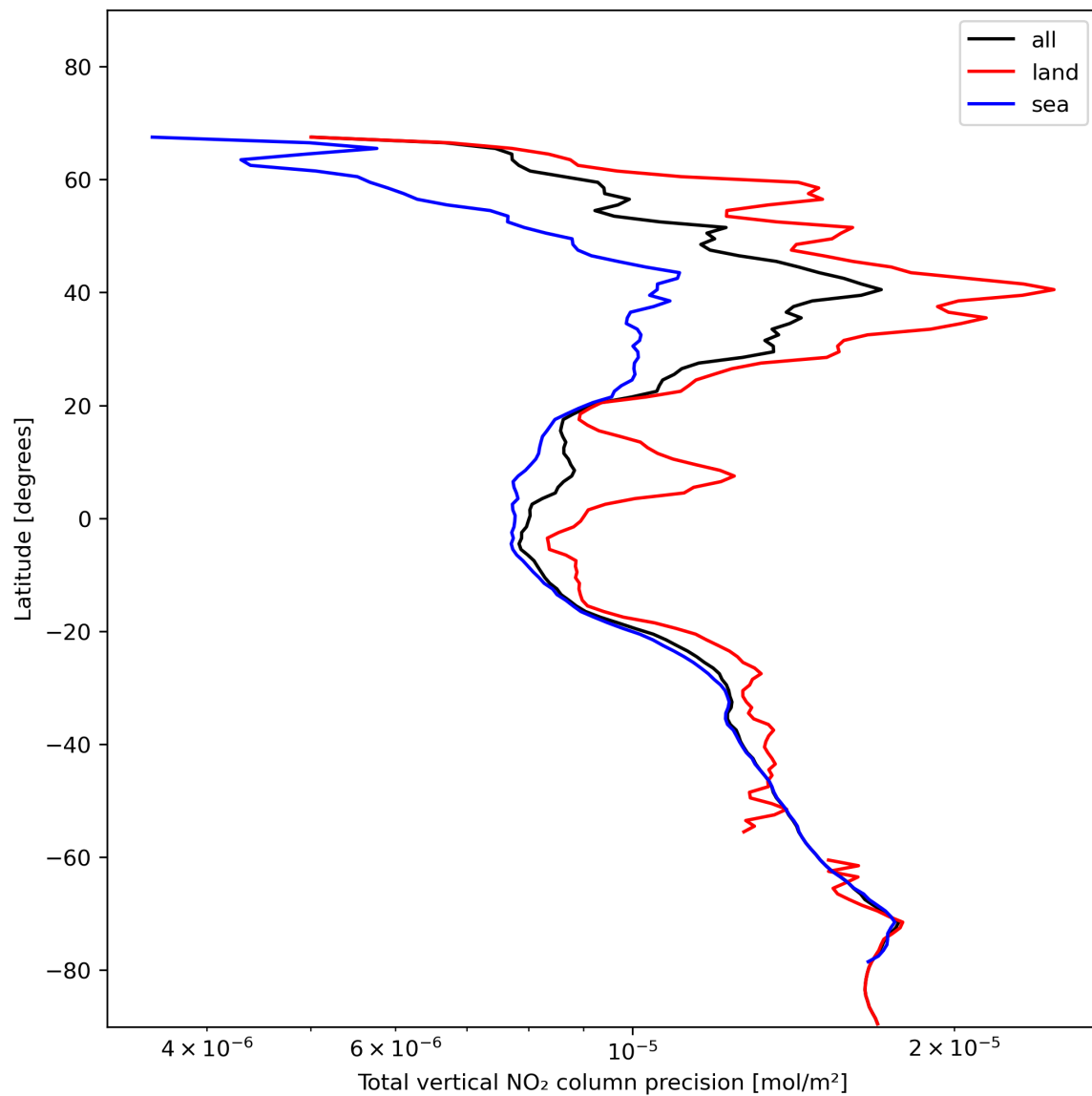
Figure 22: Zonal average of “Total vertical NO 2 column precision” for 2024-01-15 to 2024-01-17.
