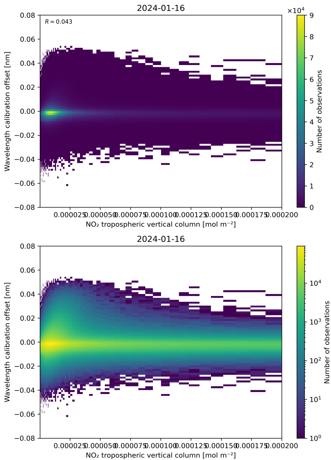
Figure 143: Scatter density plot of “NO 2 tropospheric vertical column” against “Wavelength calibration offset” for 2024-01-15 to 2024-01-17.
