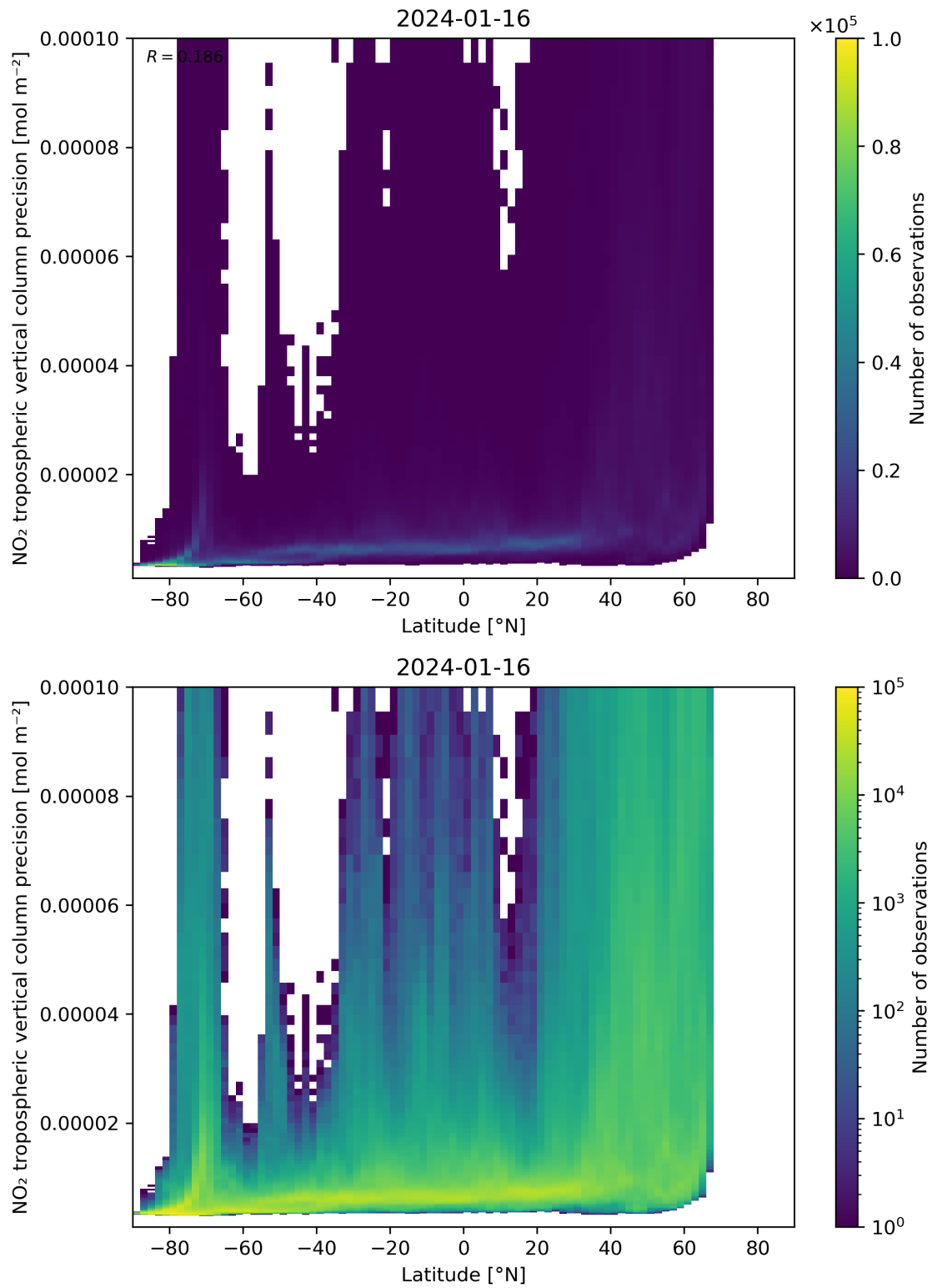
Figure 93: Scatter density plot of “Latitude” against “NO 2 tropospheric vertical column precision” for 2024-01-15 to 2024-01-17.
