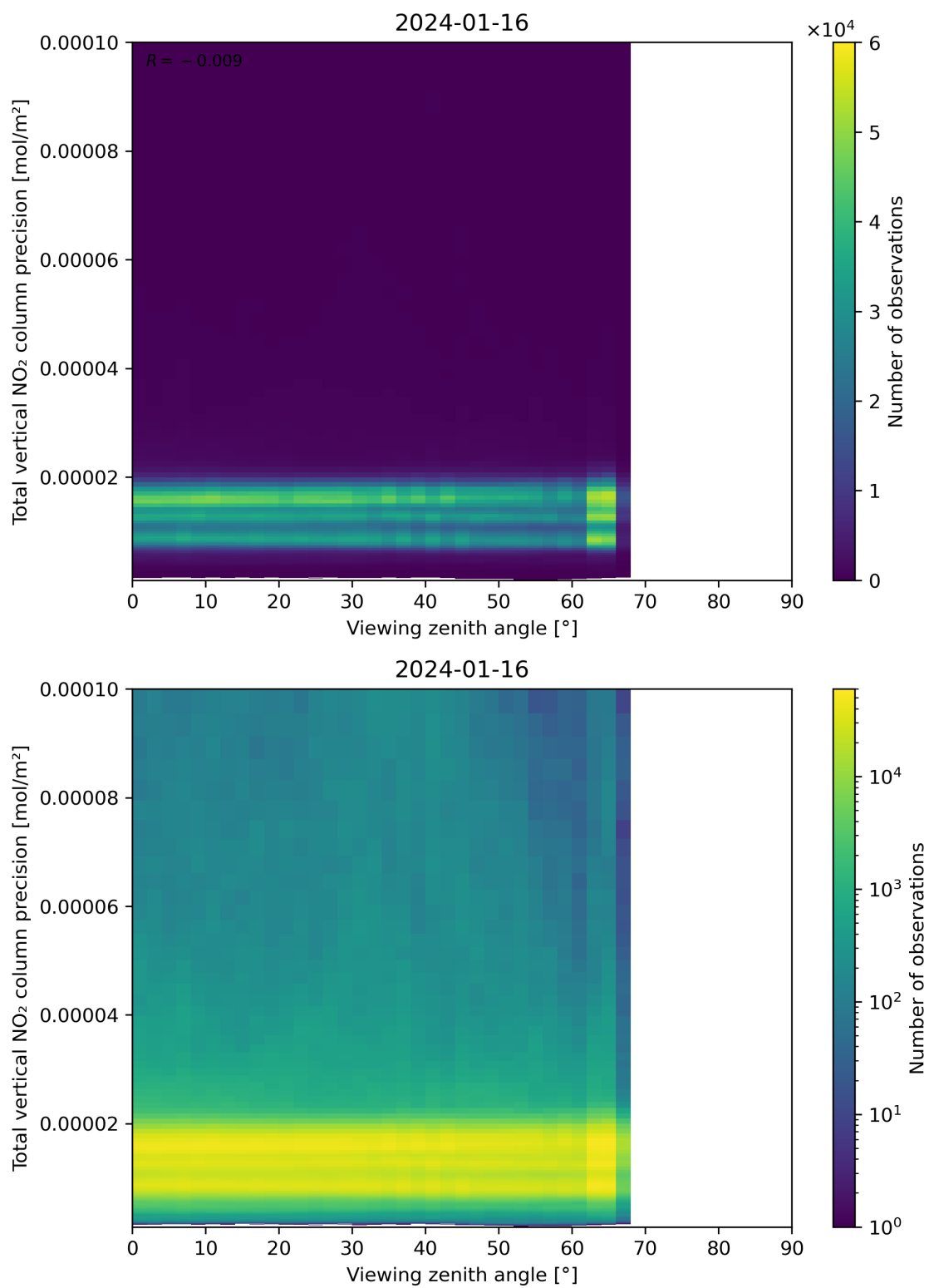
Figure 168: Scatter density plot of “Viewing zenith angle” against “Total vertical NO 2 column precision” for 2024-01-15 to 2024-01-17.
