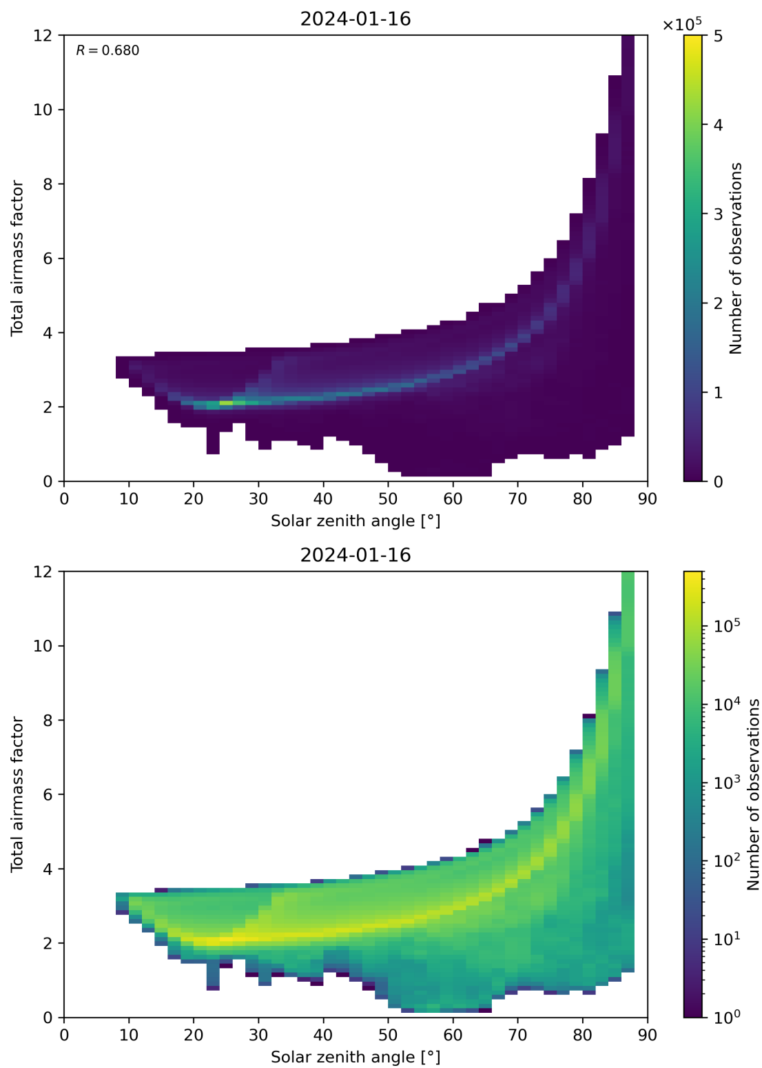
Figure 146: Scatter density plot of “Solar zenith angle” against “Total air mass factor” for 2024-01-15 to 2024-01-17.
