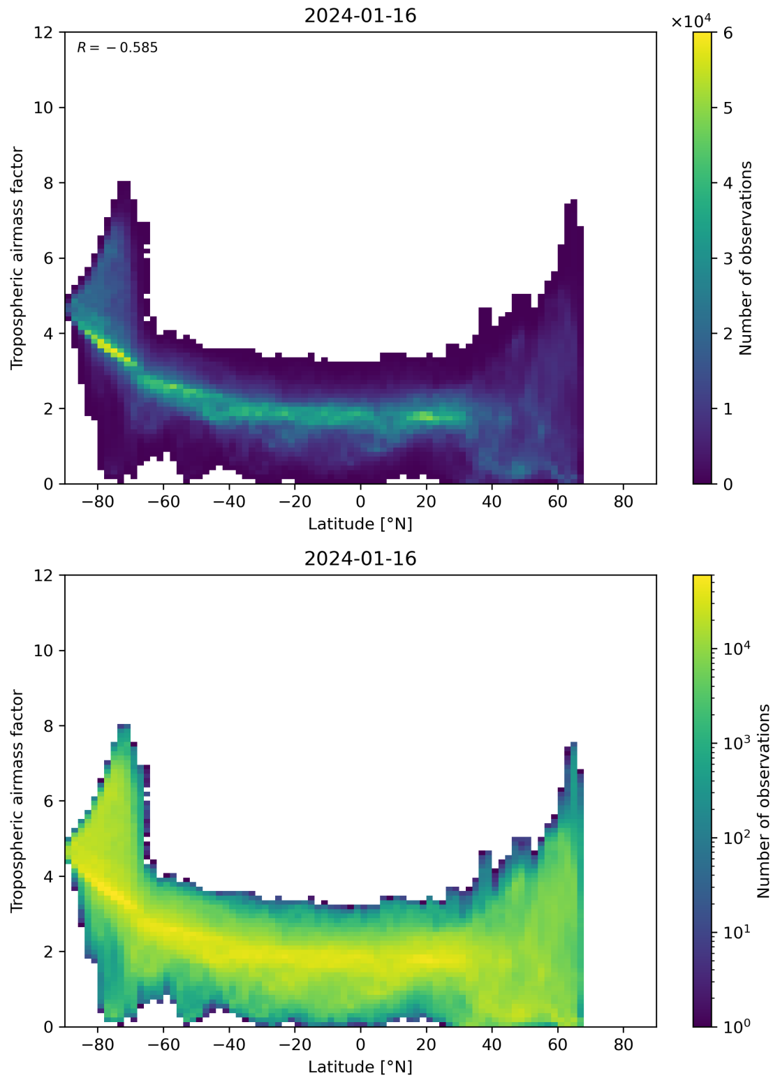
Figure 85: Scatter density plot of “Latitude” against “Tropospheric airmass factor” for 2024-01-15 to 2024-01-17.
