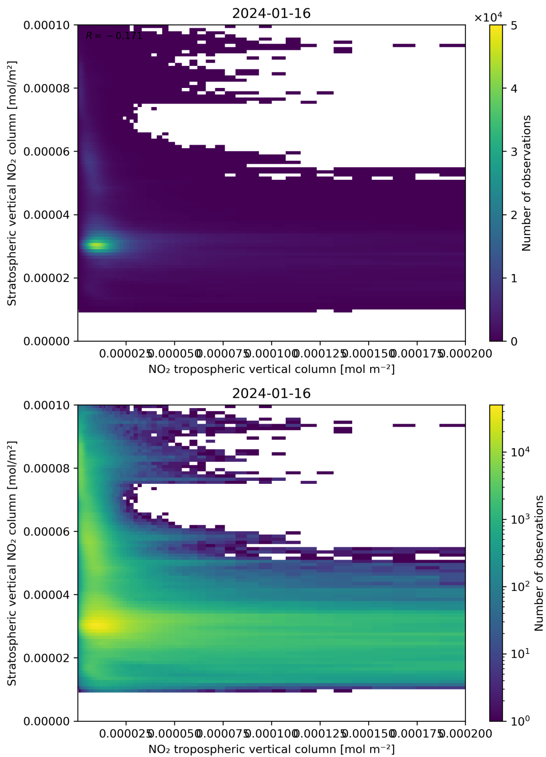
Figure 125: Scatter density plot of “NO 2 tropospheric vertical column” against “Stratospheric vertical NO 2 column” for 2024-01-15 to 2024-01-17.
