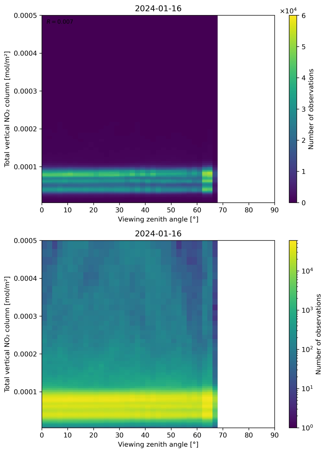
Figure 167: Scatter density plot of “Viewing zenith angle” against “Total vertical NO 2 column” for 2024-01-15 to 2024-01-17.
