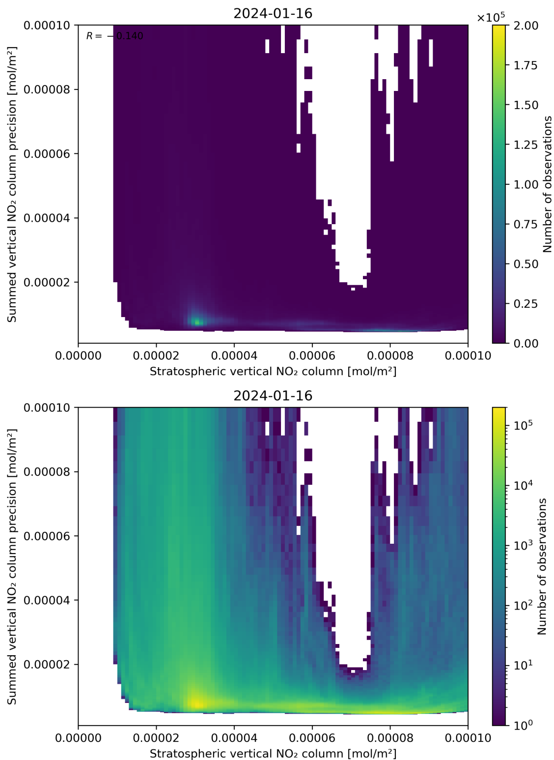
Figure 99: Scatter density plot of “Stratospheric vertical NO 2 column” against “Summed vertical NO 2 column precision” for 2024-01-15 to 2024-01-17.
