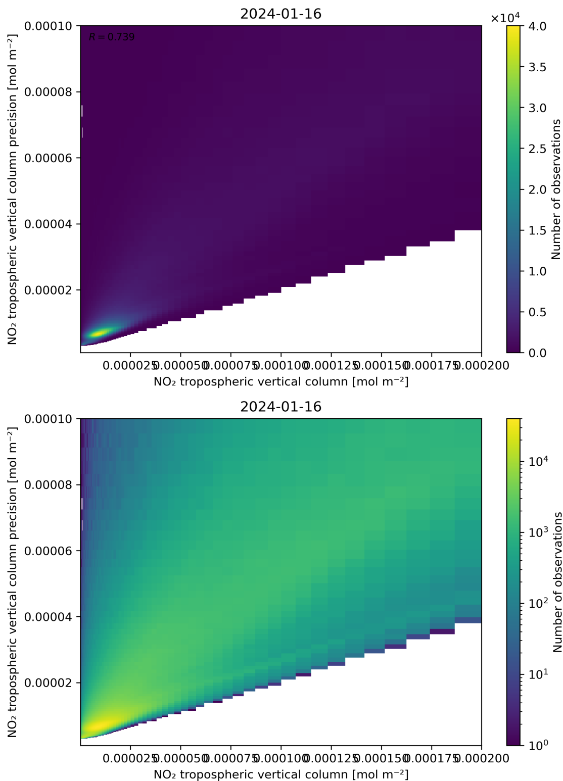
Figure 130: Scatter density plot of “NO 2 tropospheric vertical column” against “NO 2 tropospheric vertical column precision” for 2024-01-15 to 2024-01-17.
