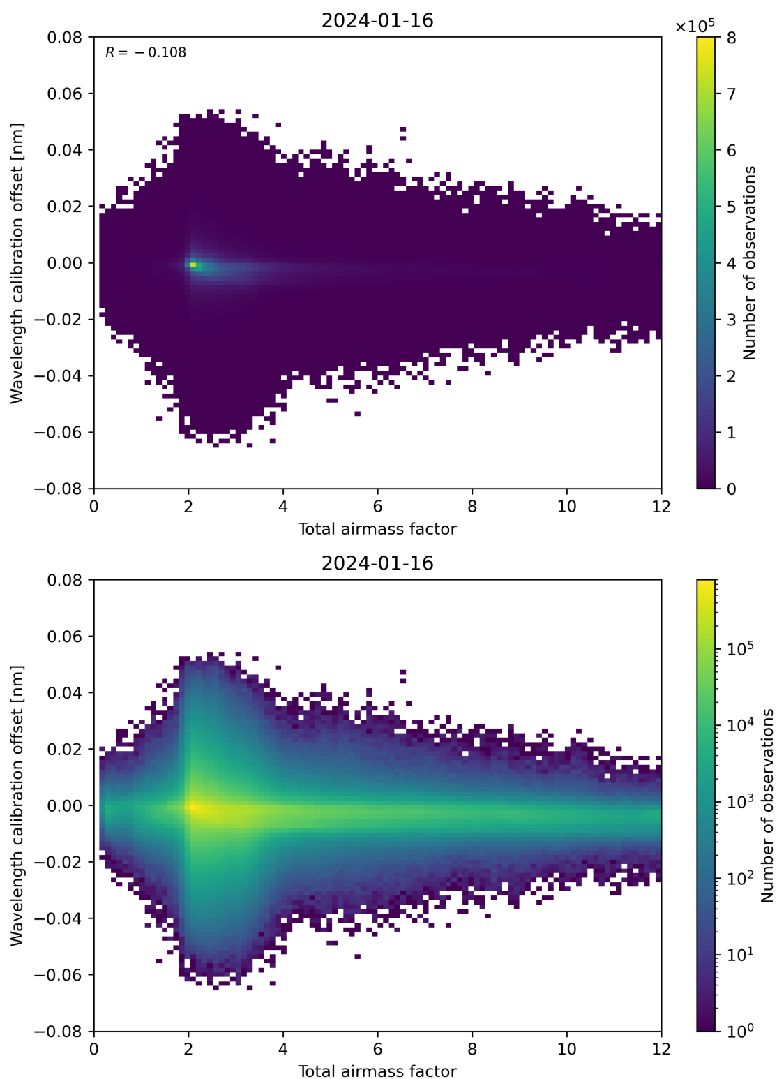
Figure 70: Scatter density plot of “Total airmass factor” against “Wavelength calibration offset” for 2024-01-15 to 2024-01-17.
