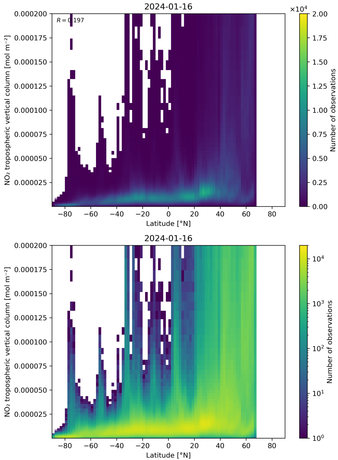
Figure 92: Scatter density plot of “Latitude” against “NO 2 tropospheric vertical column” for 2024-01-15 to 2024-01-17.
