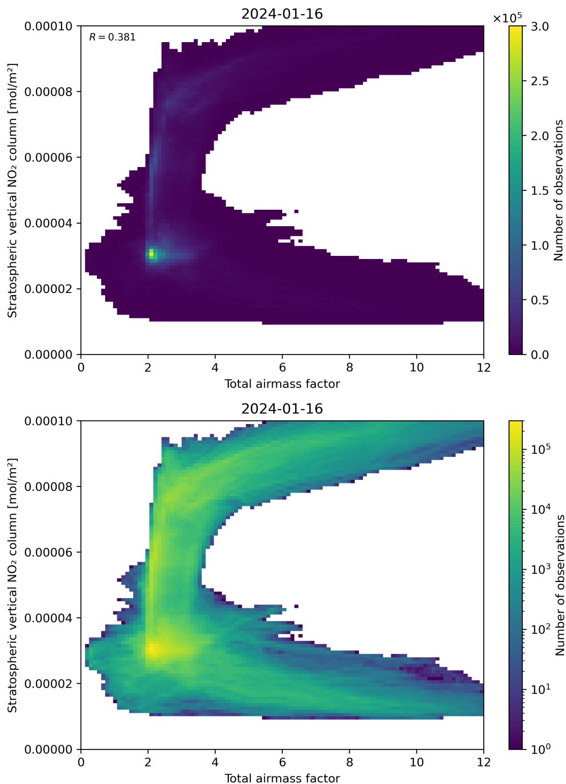
Figure 64: Scatter density plot of “Total airmass factor” against “Stratospheric vertical \text{NO}_2 column” for 2024-01-15 to 2024-01-17.
