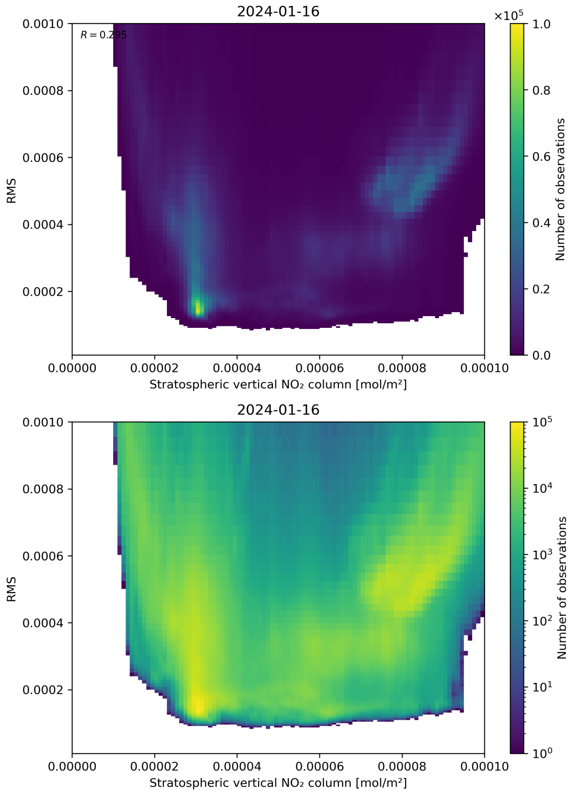
Figure 102: Scatter density plot of “Stratospheric vertical NO 2 column” against “RMS” for 2024-01-15 to 2024-01-17.
