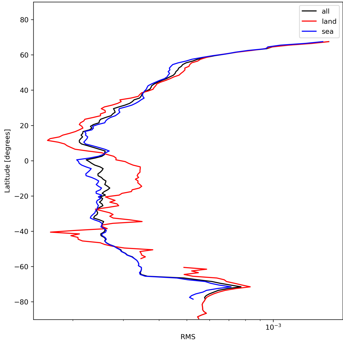
Figure 26: Zonal average of “RMS” for 2024-01-15 to 2024-01-17.
