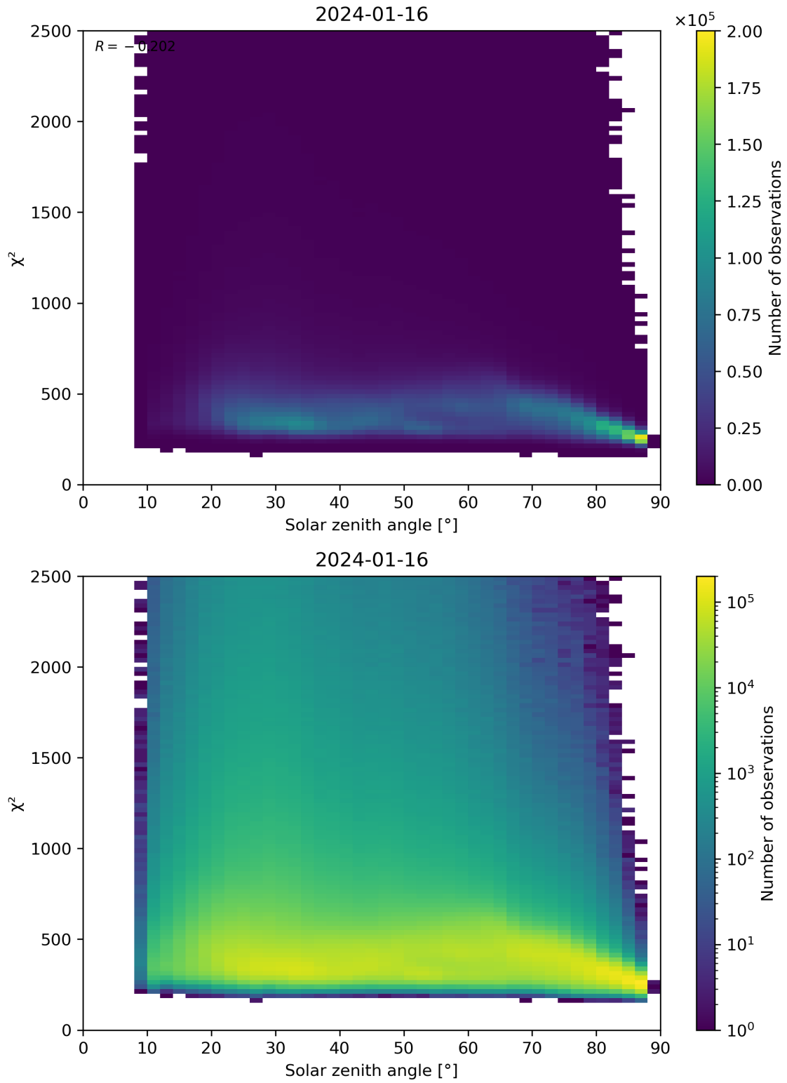
Figure 148: Scatter density plot of “Solar zenith angle” against “ \chi^2 ” for 2024-01-15 to 2024-01-17.
