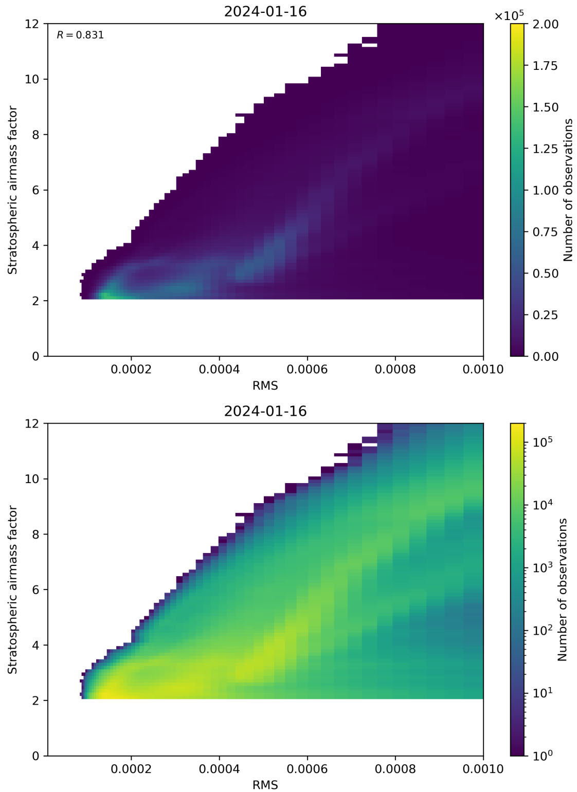
Figure 144: Scatter density plot of “RMS” against “Stratospheric airmass factor” for 2024-01-15 to 2024-01-17.
