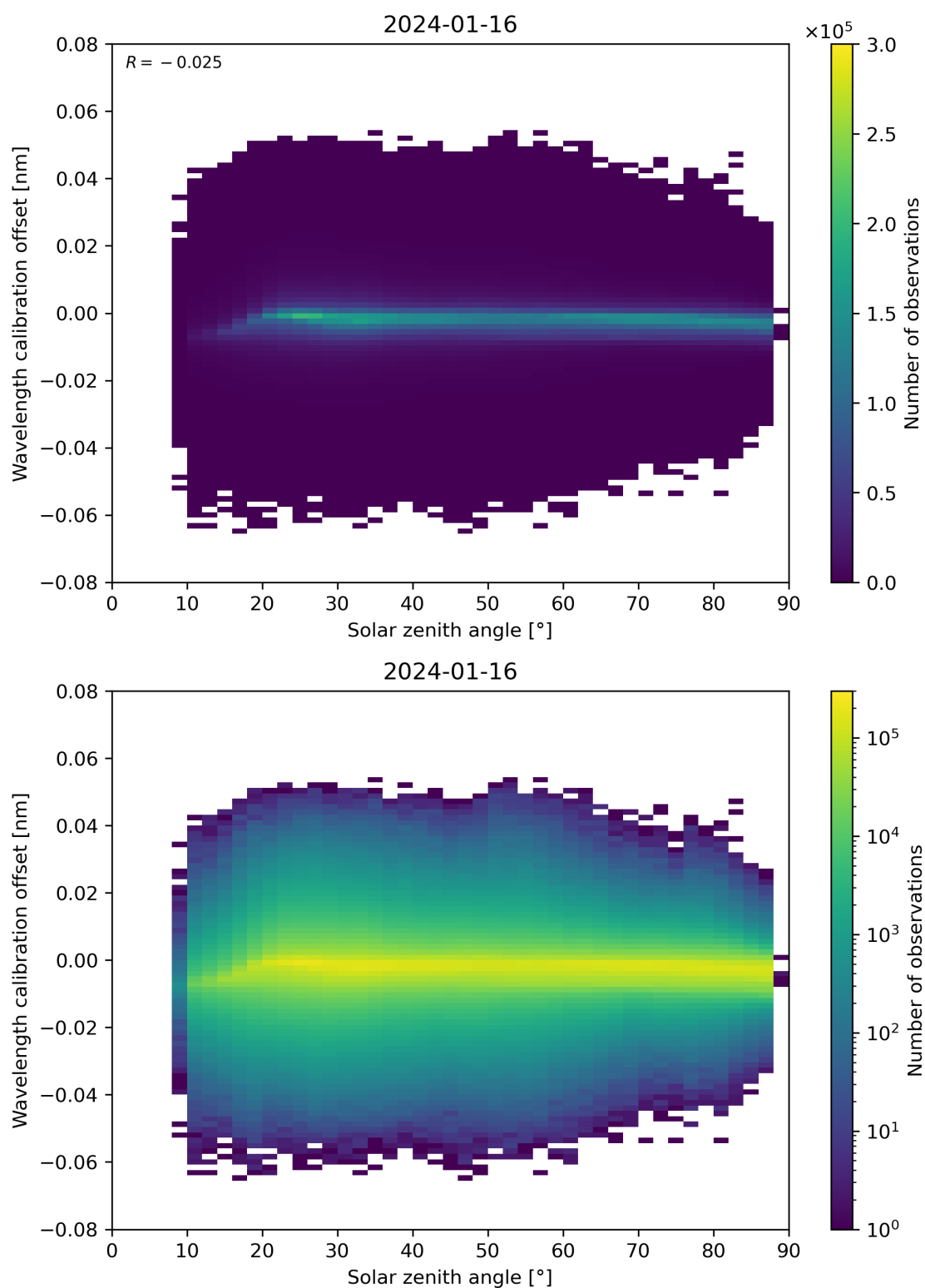
Figure 158: Scatter density plot of “Solar zenith angle” against “Wavelength calibration offset” for 2024-01-15 to 2024-01-17.
