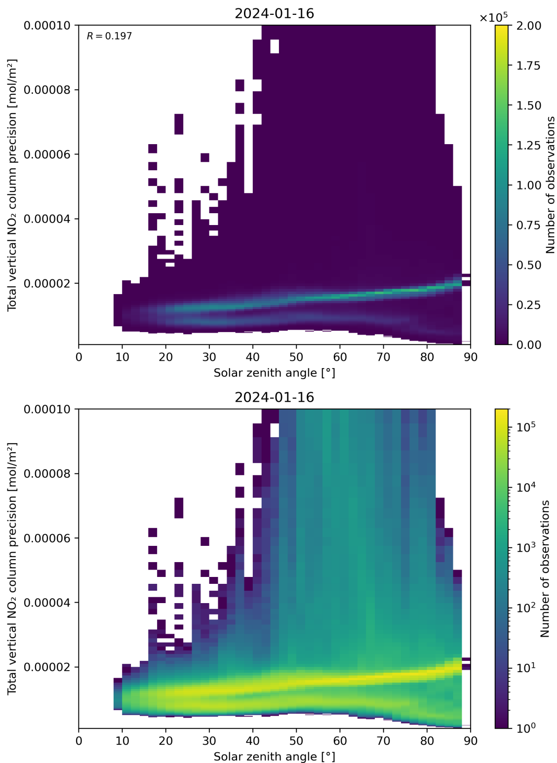
Figure 154: Scatter density plot of “Solar zenith angle” against “Total vertical NO 2 column precision” for 2024-01-15 to 2024-01-17.
