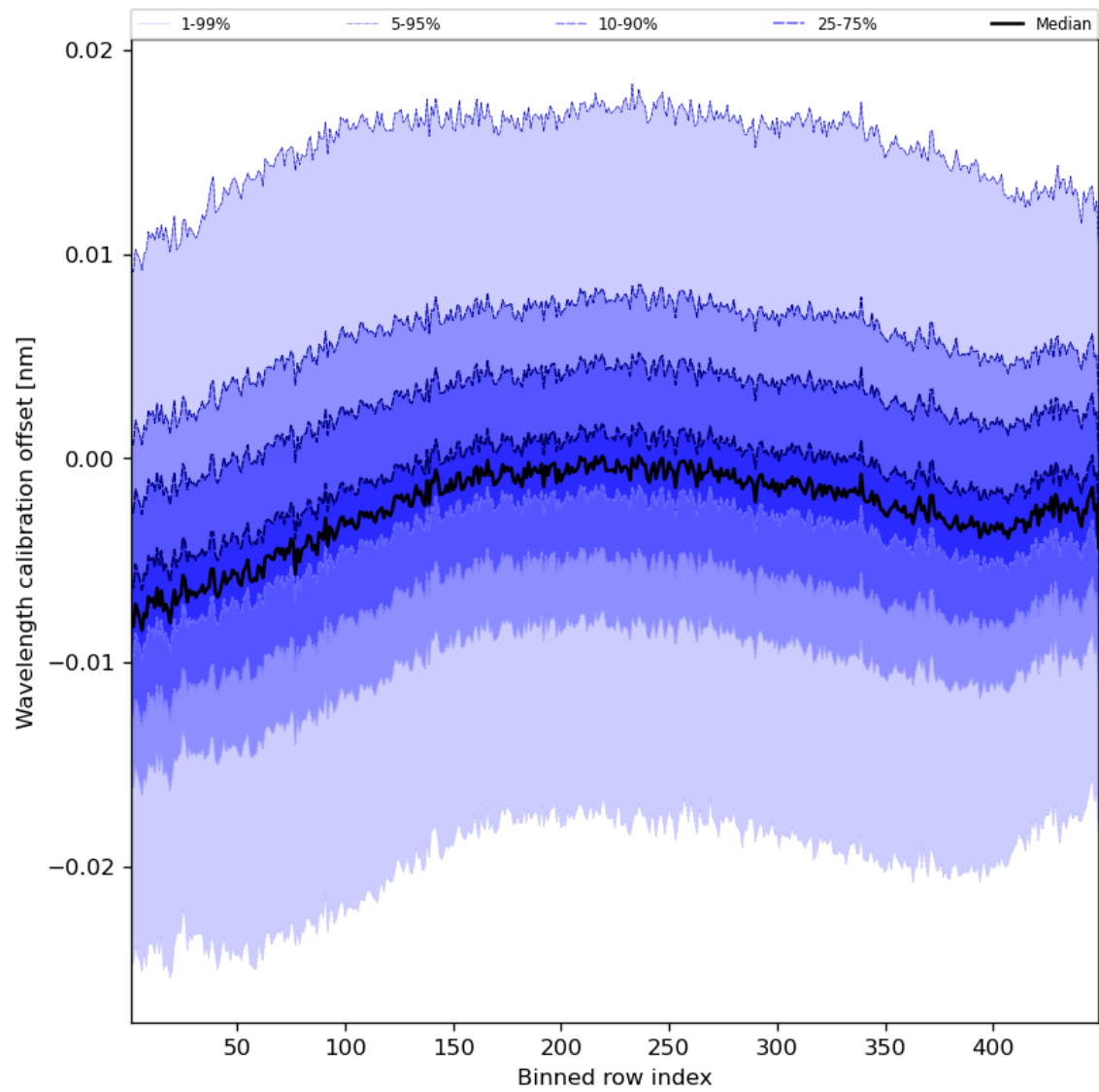
Figure 52: Along track statistics of “Wavelength calibration offset” for 2024-01-15 to 2024-01-17
