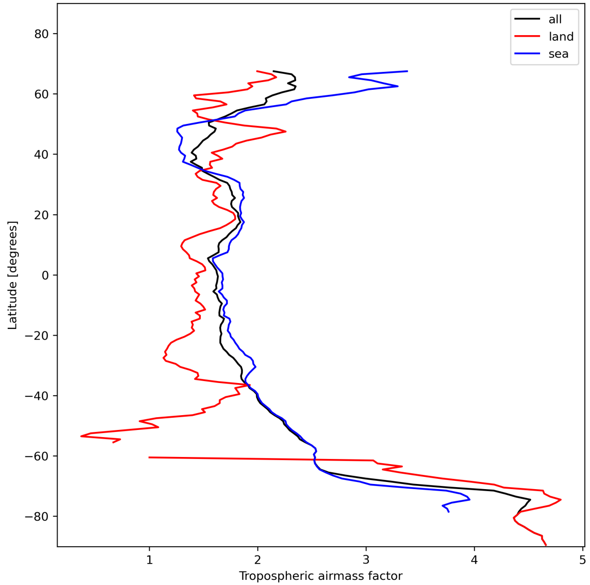
Figure 14: Zonal average of “Tropospheric airmass factor” for 2024-01-15 to 2024-01-17.
