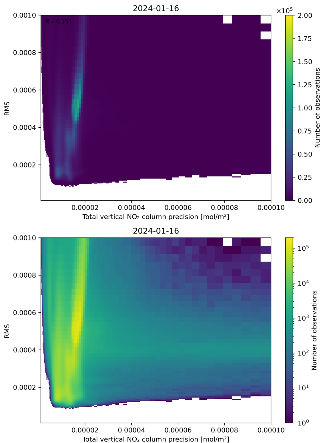
Figure 119: Scatter density plot of “Total vertical NO 2 column precision” against “RMS” for 2024-01-15 to 2024-01-17.
