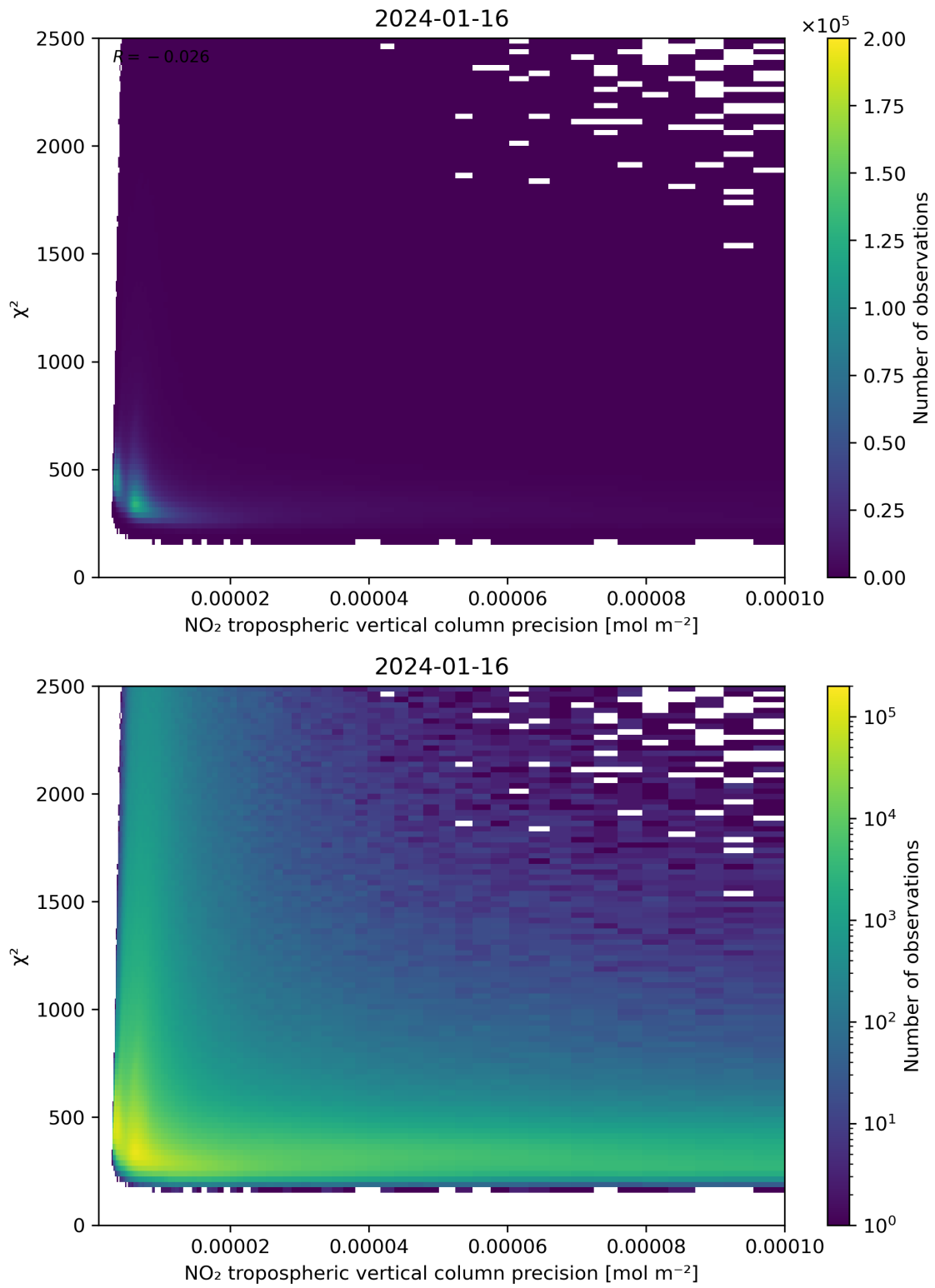
Figure 134: Scatter density plot of “NO 2 tropospheric vertical column precision” against “ \chi^2 ” for 2024-01-15 to 2024-01-17.
