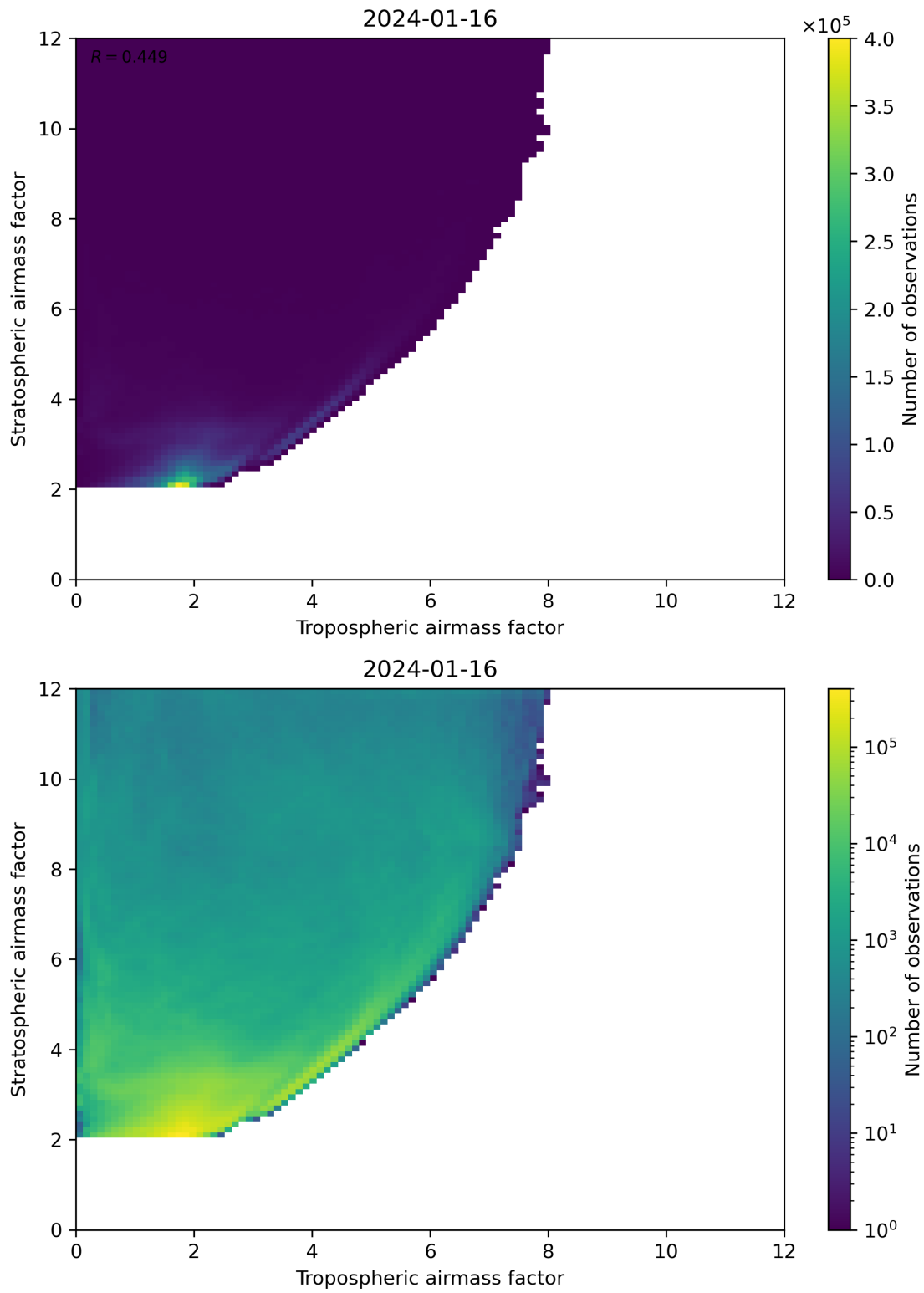
Figure 71: Scatter density plot of “Tropospheric airmass factor” against “Stratospheric airmass factor” for 2024-01-15 to 2024-01-17.
