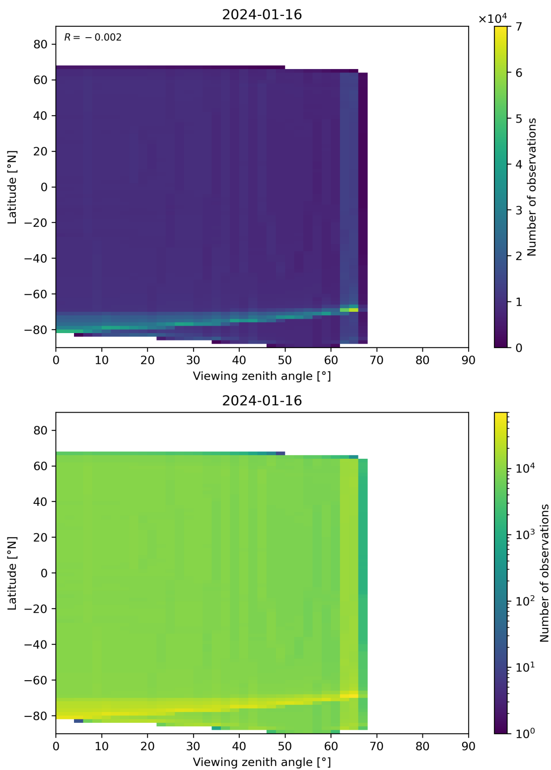
Figure 163: Scatter density plot of “Viewing zenith angle” against “Latitude” for 2024-01-15 to 2024-01-17.
