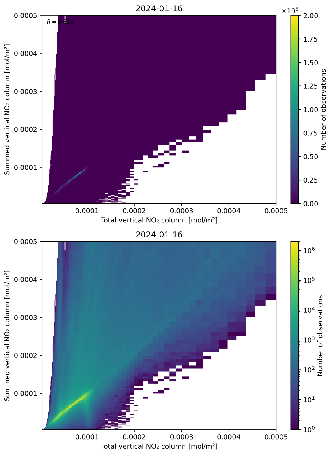
Figure 112: Scatter density plot of “Total vertical NO 2 column” against “Summed vertical NO 2 column” for 2024-01-15 to 2024-01-17.
