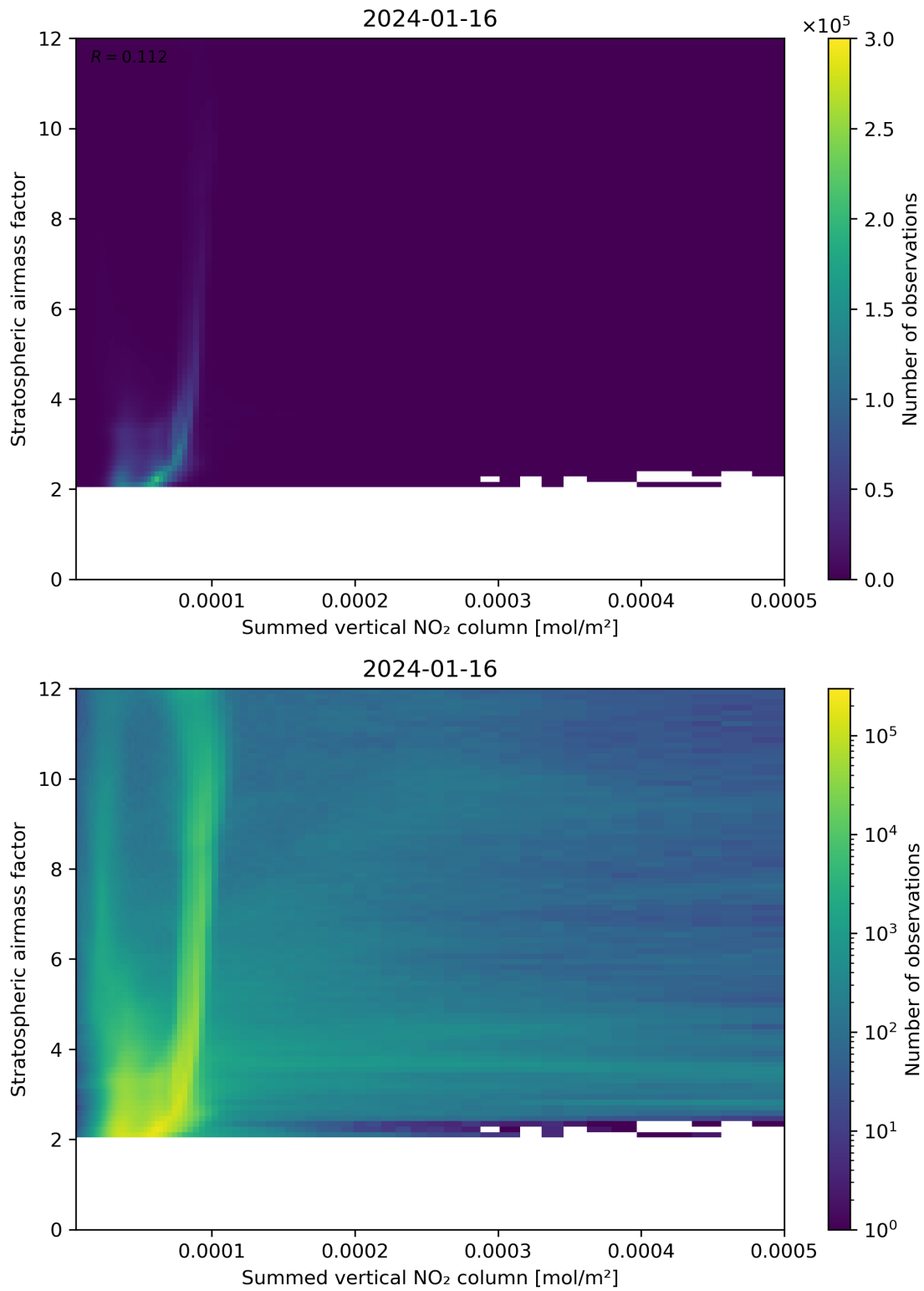
Figure 103: Scatter density plot of “Summed vertical NO 2 column” against “Stratospheric air mass factor” for 2024-01-15 to 2024-01-17.
