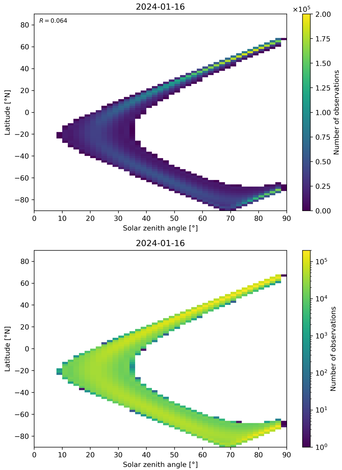
Figure 149: Scatter density plot of “Solar zenith angle” against “Latitude” for 2024-01-15 to 2024-01-17.
