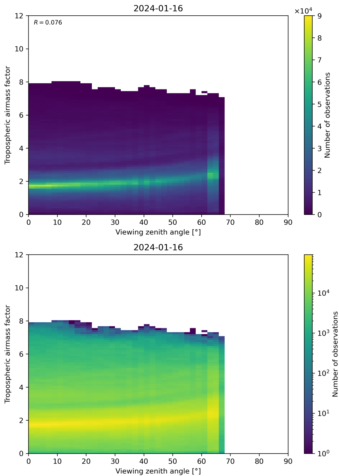
Figure 161: Scatter density plot of “Viewing zenith angle” against “Tropospheric airmass factor” for 2024-01-15 to 2024-01-17.
