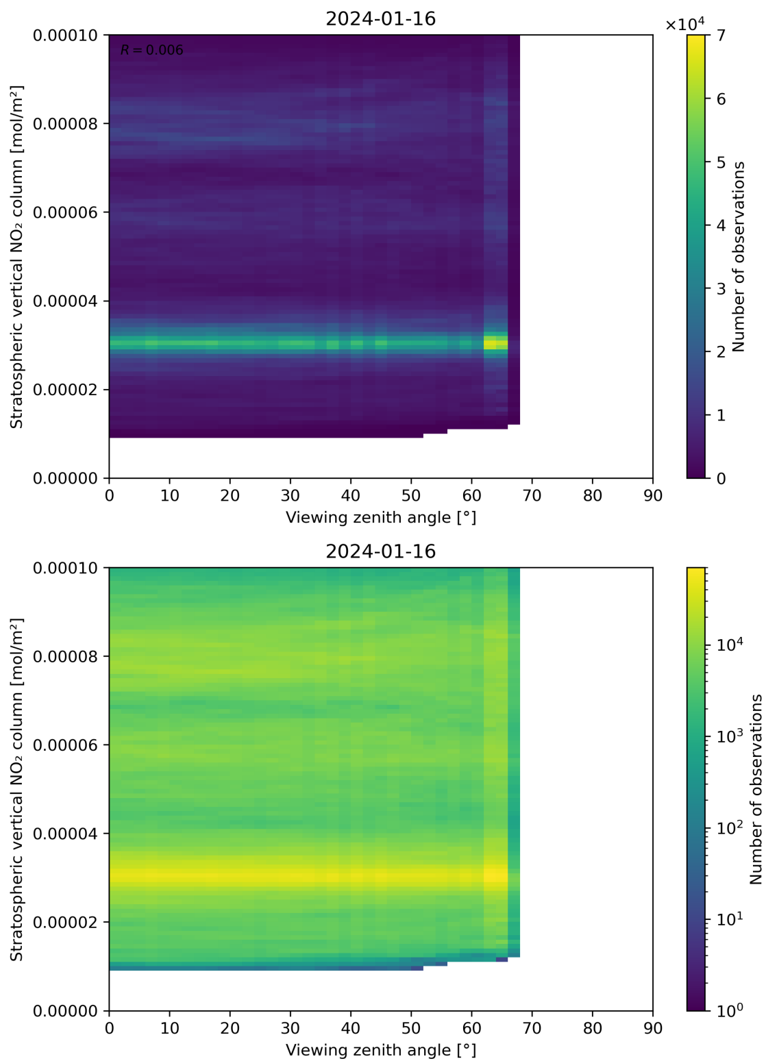
Figure 164: Scatter density plot of “Viewing zenith angle” against “Stratospheric vertical NO 2 column” for 2024-01-15 to 2024-01-17.
