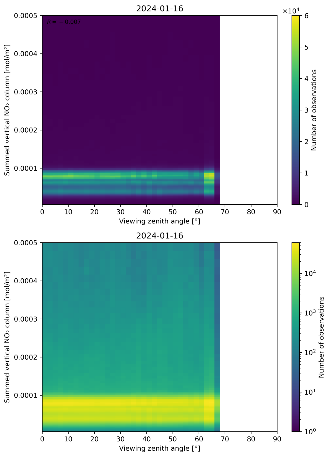
Figure 165: Scatter density plot of “Viewing zenith angle” against “Summed vertical NO 2 column” for 2024-01-15 to 2024-01-17.
