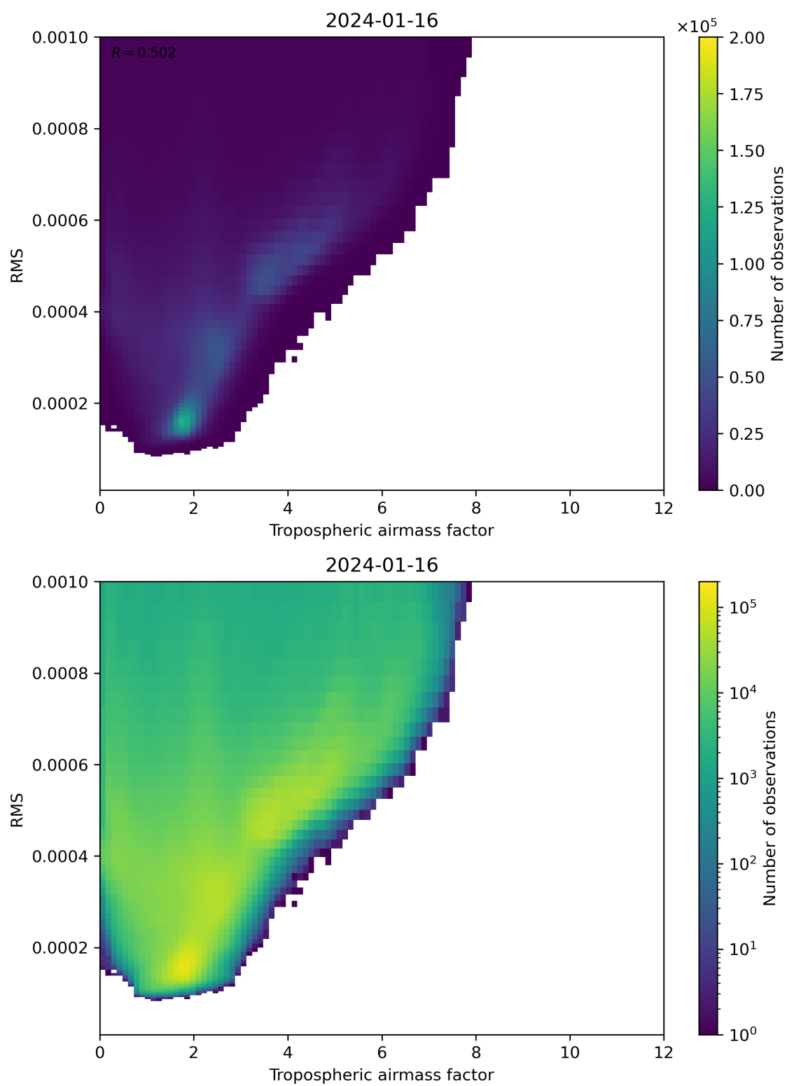
Figure 79: Scatter density plot of “Tropospheric airmass factor” against “RMS” for 2024-01-15 to 2024-01-17.
