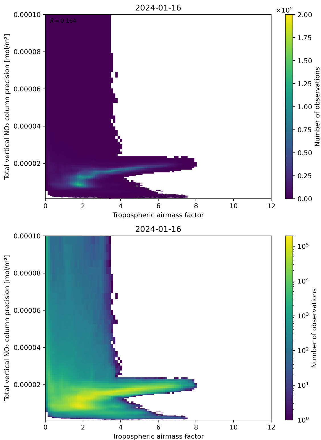
Figure 78: Scatter density plot of “Tropospheric air mass factor” against “Total vertical NO 2 column precision” for 2024-01-15 to 2024-01-17.
