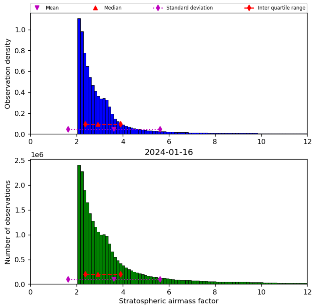
Figure 44: Histogram of “Stratospheric airmass factor” for 2024-01-15 to 2024-01-17
