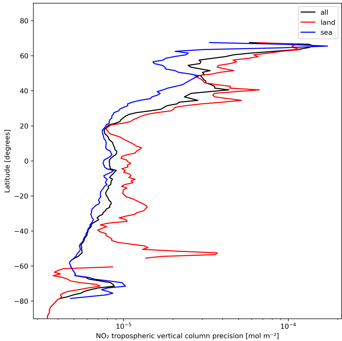
Figure 13: Zonal average of “NO 2 tropospheric vertical column precision” for 2024-01-15 to 2024-01-17.
