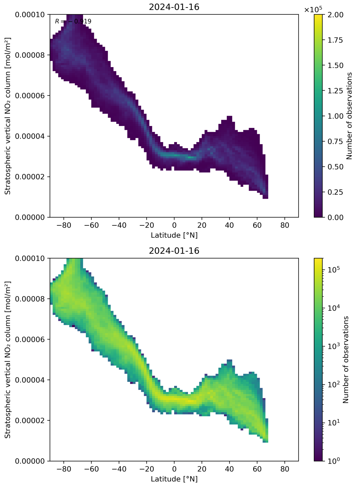
Figure 87: Scatter density plot of “Latitude” against “Stratospheric vertical NO 2 column” for 2024-01-15 to 2024-01-17.
