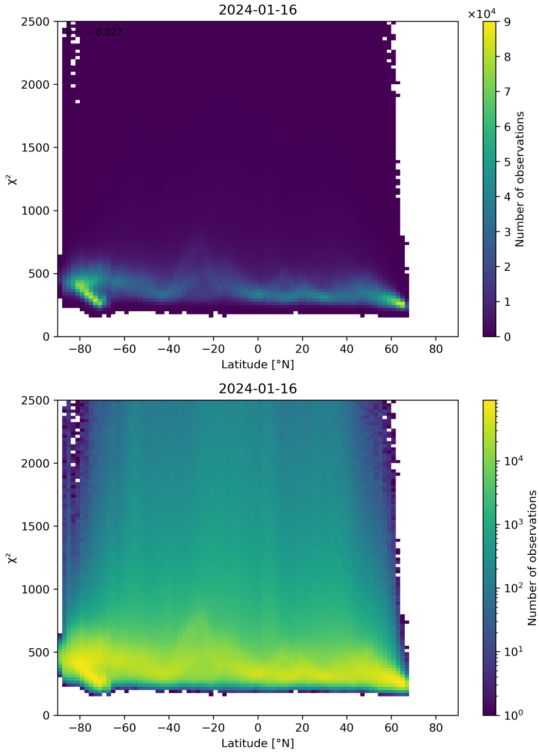
Figure 86: Scatter density plot of “Latitude” against “ \chi^2 ” for 2024-01-15 to 2024-01-17.
