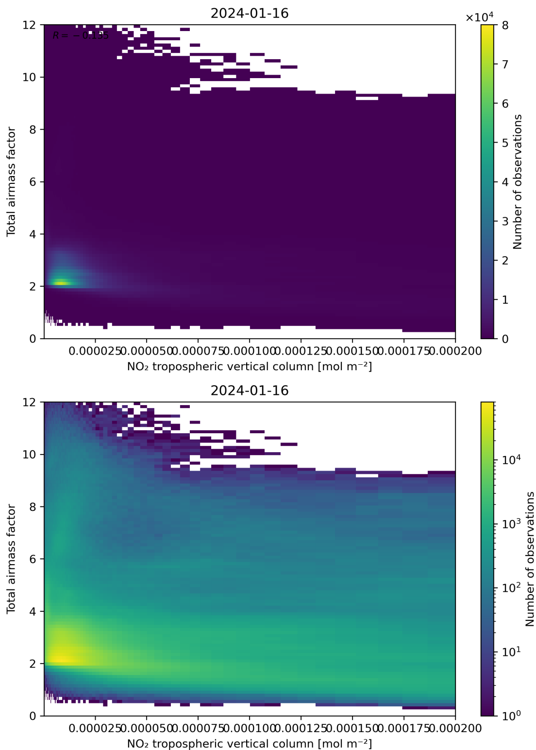
Figure 122: Scatter density plot of “NO 2 tropospheric vertical column” against “Total air mass factor” for 2024-01-15 to 2024-01-17.
