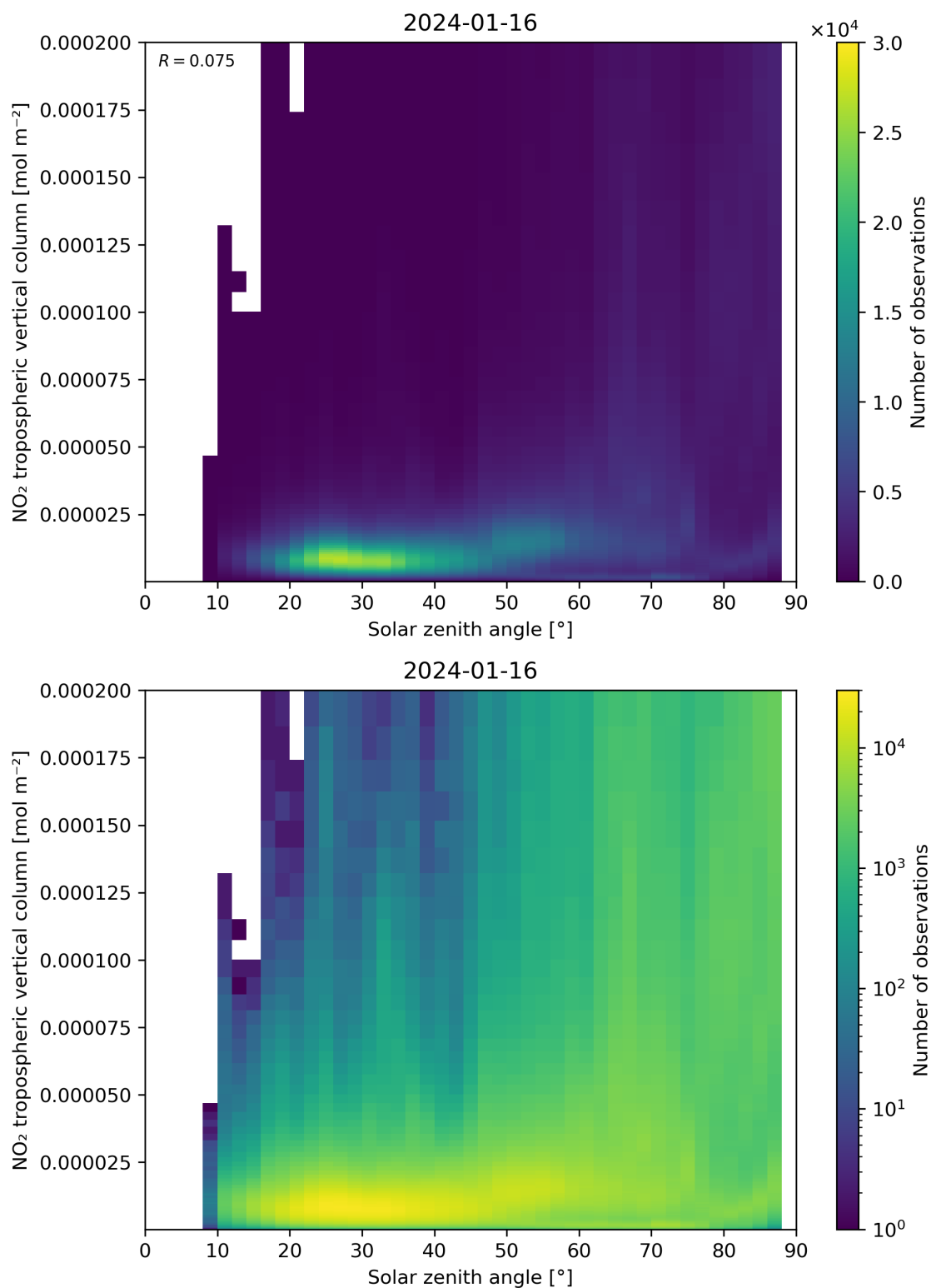
Figure 155: Scatter density plot of “Solar zenith angle” against “NO 2 tropospheric vertical column” for 2024-01-15 to 2024-01-17.
