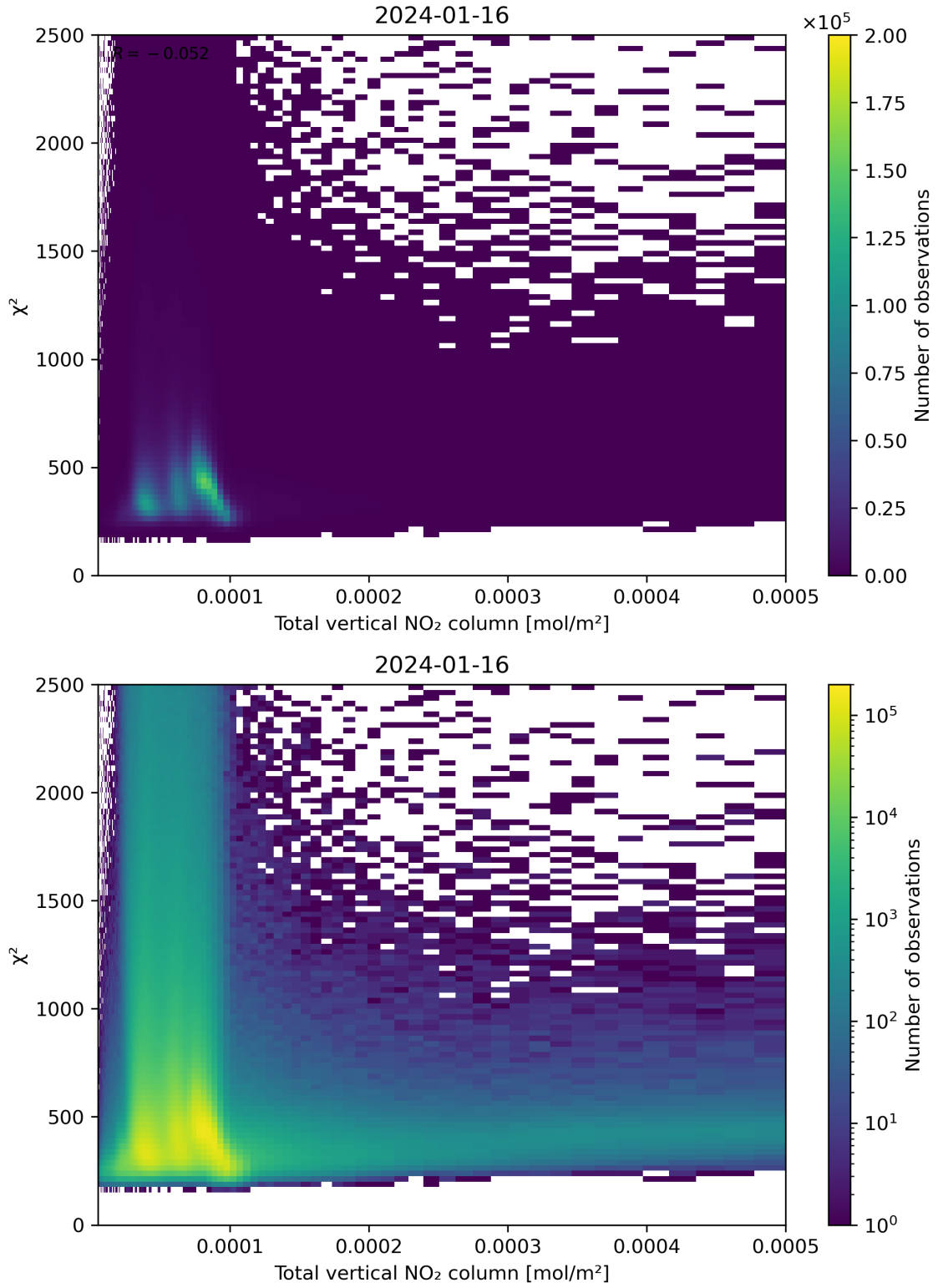
Figure 111: Scatter density plot of “Total vertical NO 2 column” against “ \chi^2 ” for 2024-01-15 to 2024-01-17.
