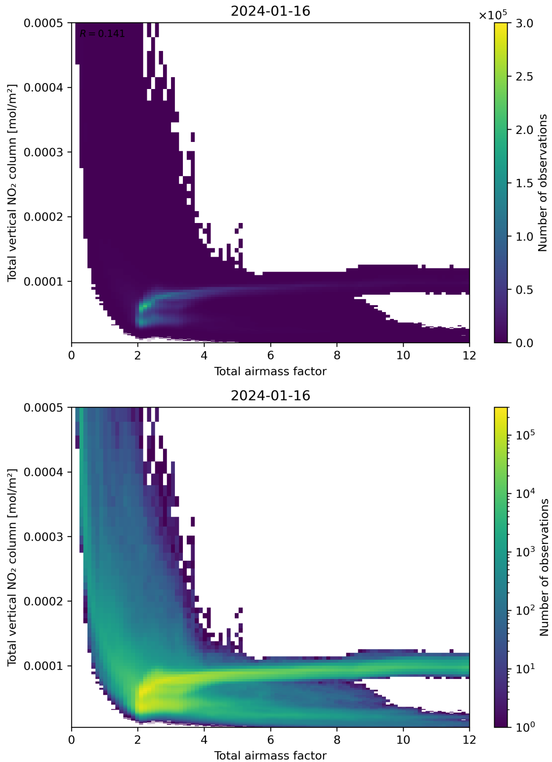
Figure 67: Scatter density plot of “Total airmass factor” against “Total vertical NO 2 column” for 2024-01-15 to 2024-01-17.
