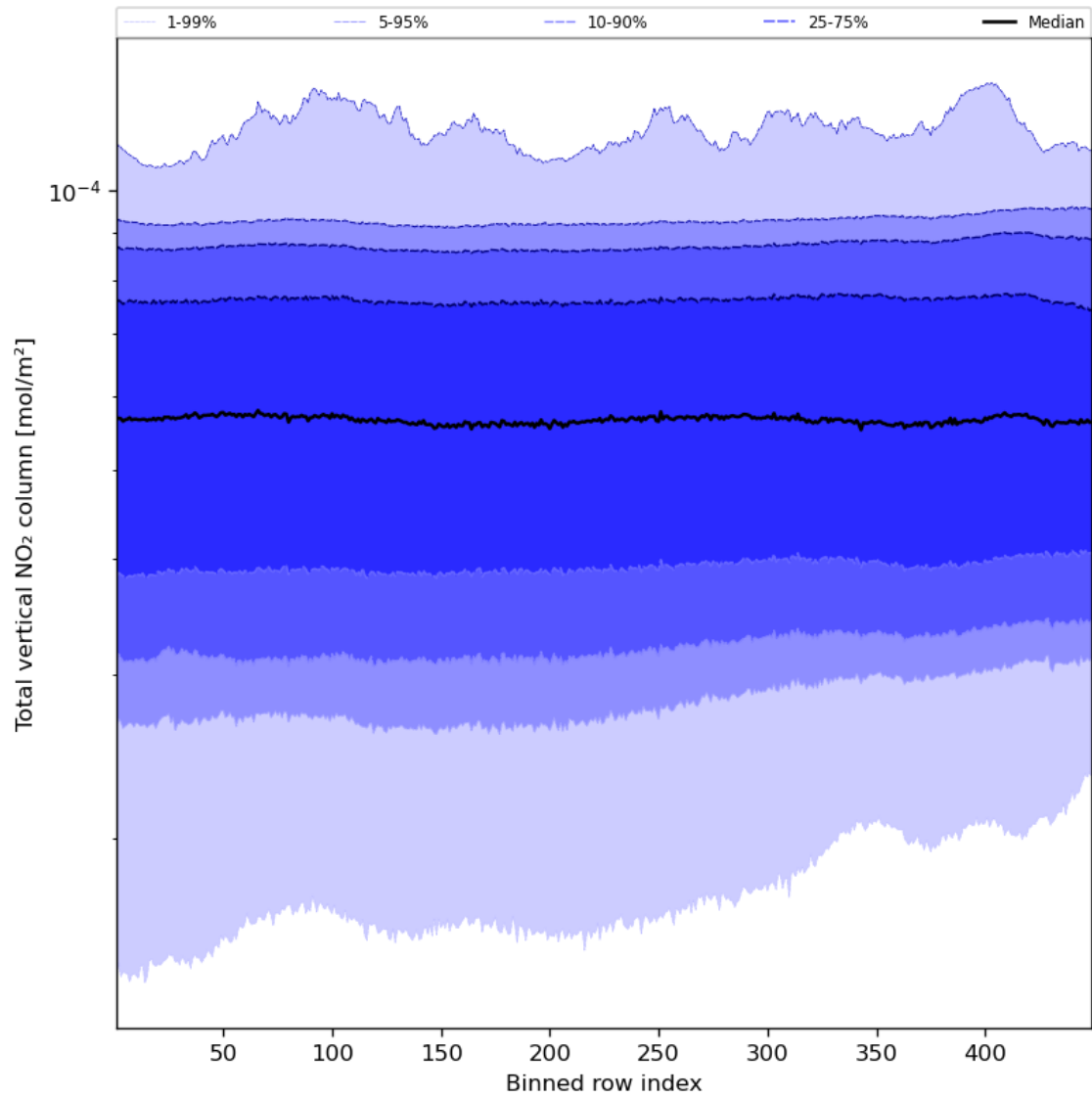
Figure 55: Along track statistics of “Total vertical NO 2 column” for 2024-01-15 to 2024-01-17
