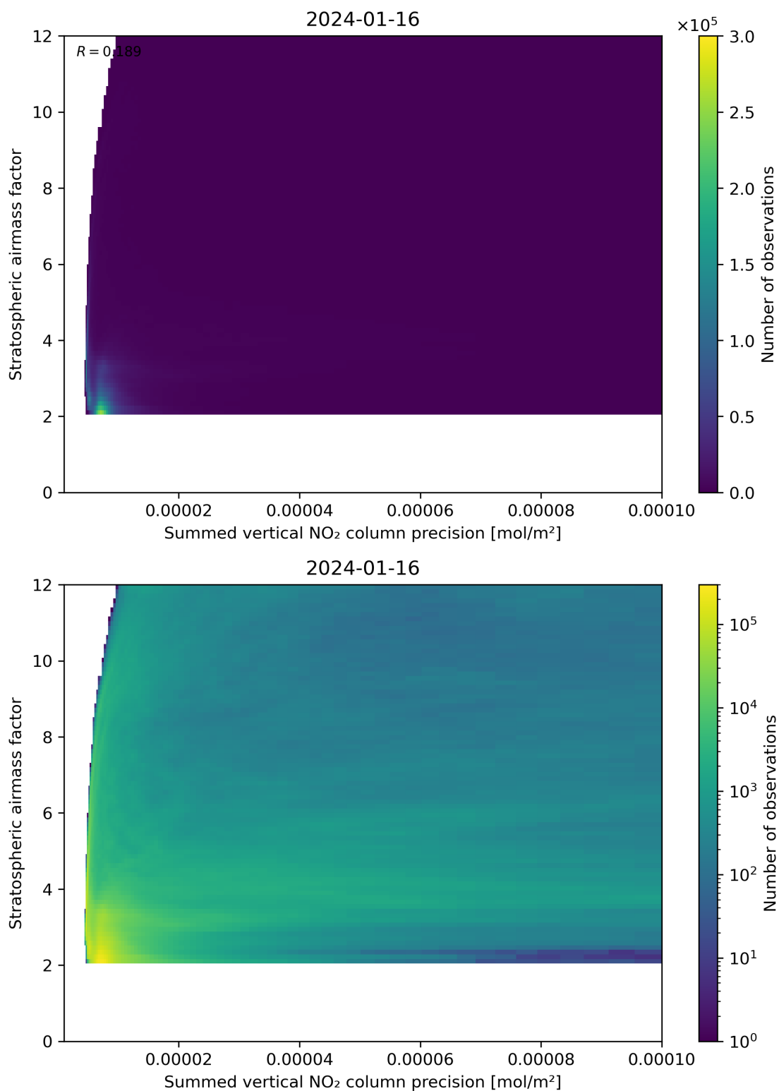
Figure 106: Scatter density plot of “Summed vertical NO 2 column precision” against “Stratospheric airmass factor” for 2024-01-15 to 2024-01-17.
