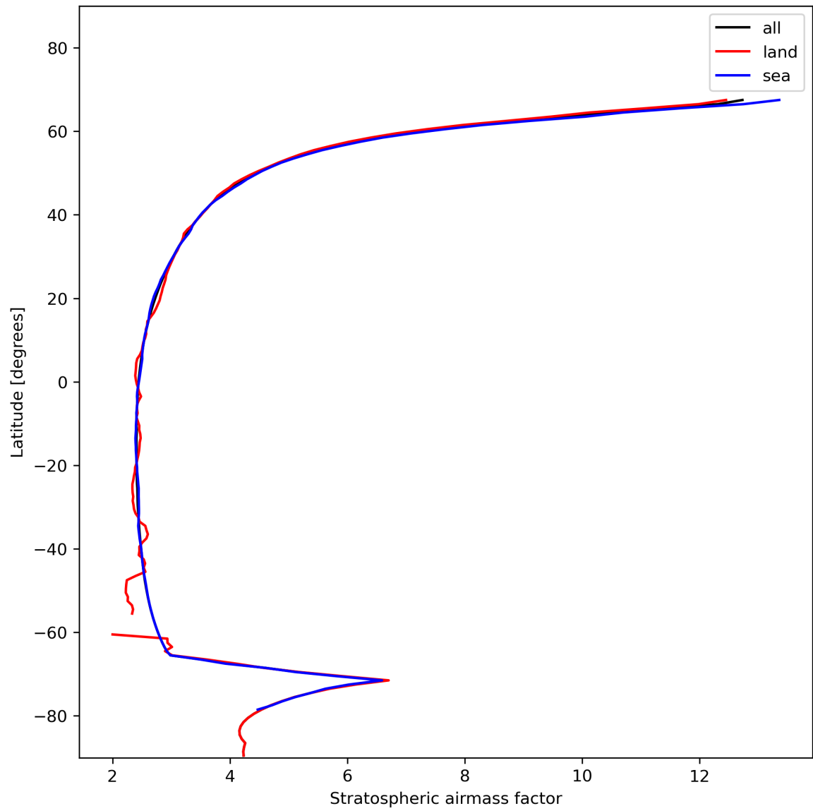
Figure 27: Zonal average of “Stratospheric airmass factor” for 2024-01-15 to 2024-01-17.
