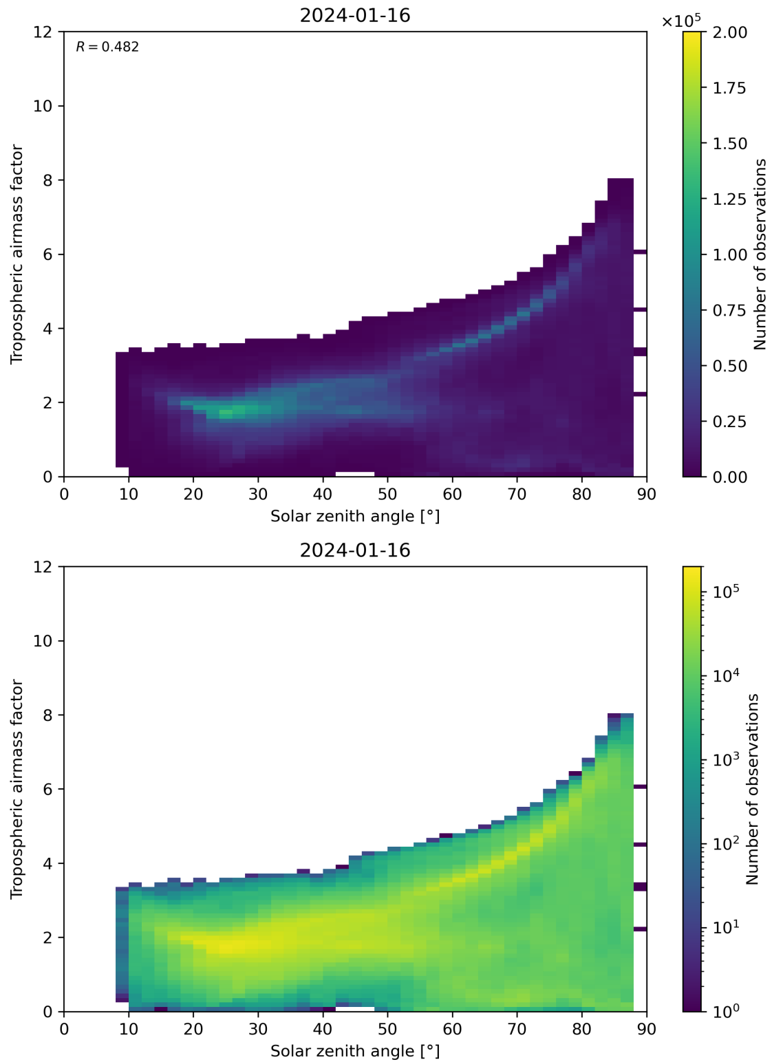
Figure 147: Scatter density plot of “Solar zenith angle” against “Tropospheric airmass factor” for 2024-01-15 to 2024-01-17.
