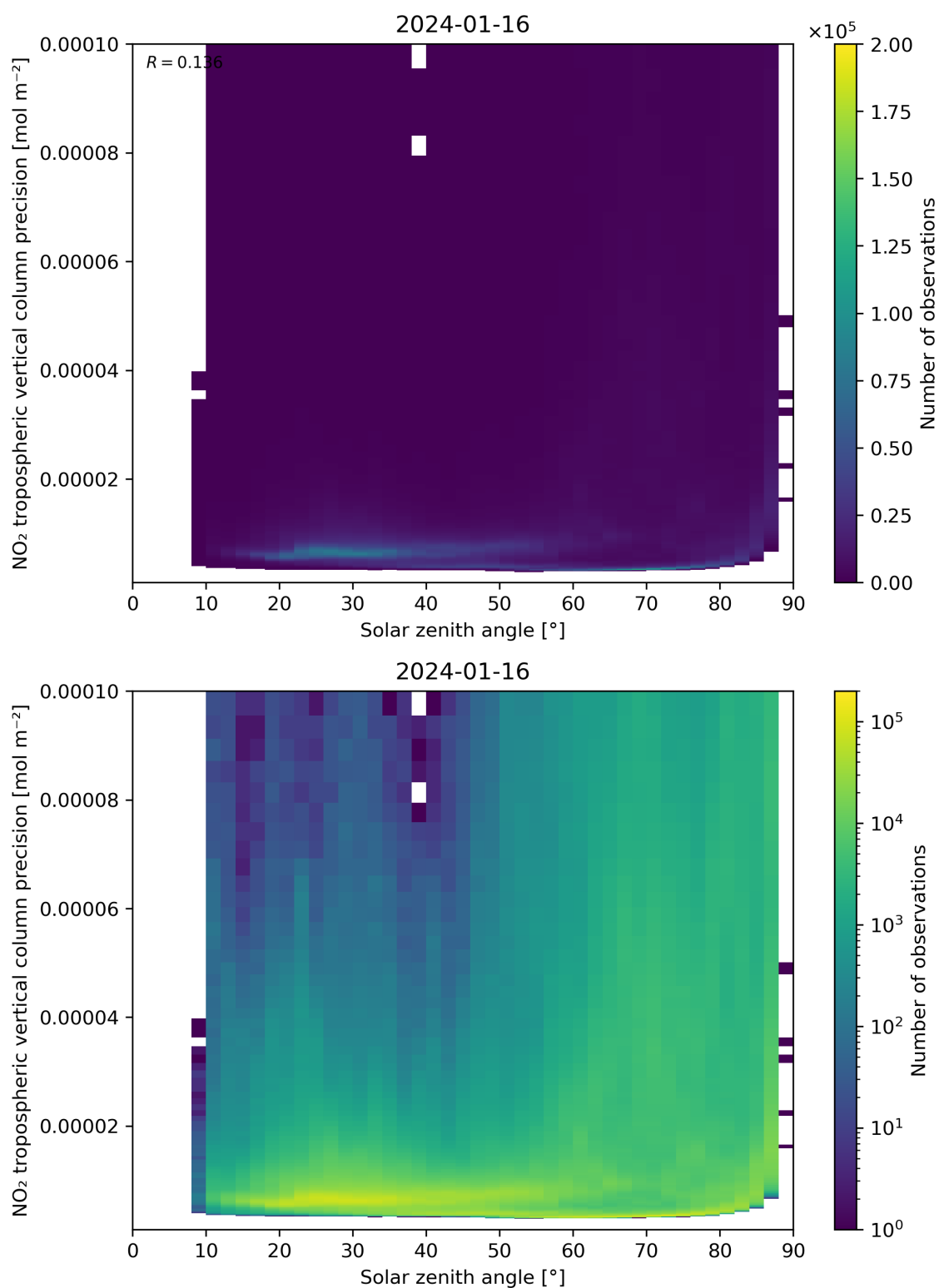
Figure 156: Scatter density plot of “Solar zenith angle” against “NO 2 tropospheric vertical column precision” for 2024-01-15 to 2024-01-17.
