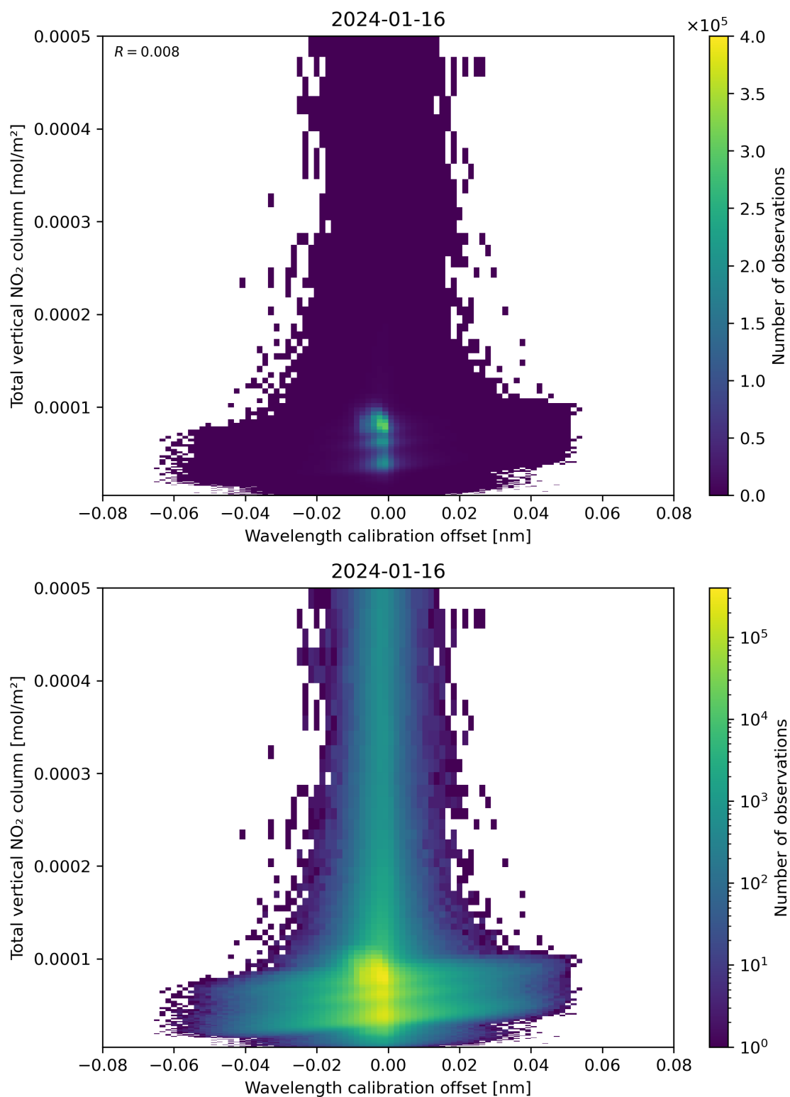
Figure 179: Scatter density plot of “Wavelength calibration offset” against “Total vertical NO 2 column” for 2024-01-15 to 2024-01-17.
