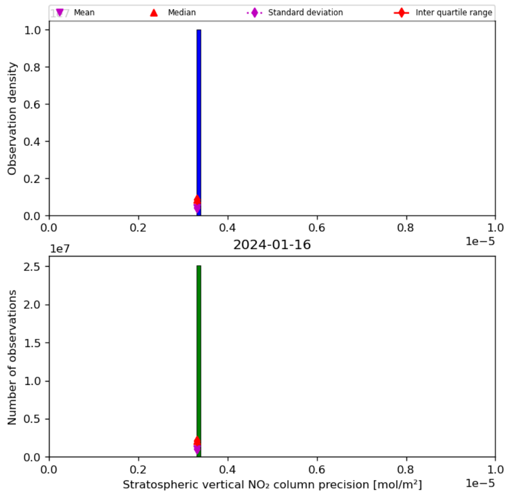
Figure 37: Histogram of “Stratospheric vertical NO 2 column precision” for 2024-01-15 to 2024-01-17
