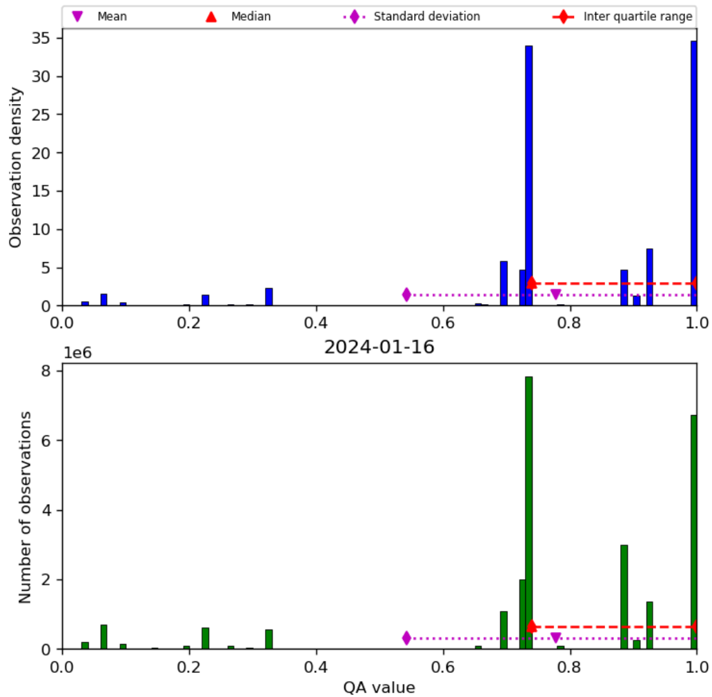
Figure 28: Histogram of “QA value” for 2024-01-15 to 2024-01-17
