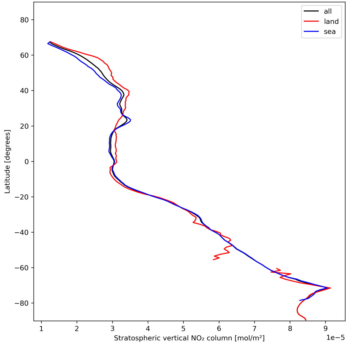
Figure 19: Zonal average of “Stratospheric vertical NO 2 column” for 2024-01-15 to 2024-01-17.
