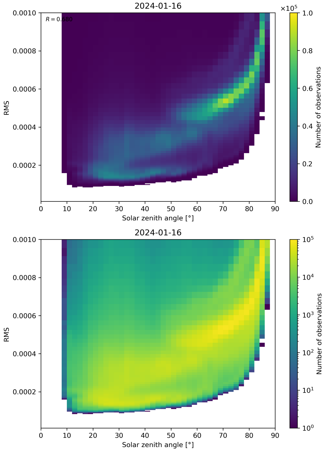
Figure 157: Scatter density plot of “Solar zenith angle” against “RMS” for 2024-01-15 to 2024-01-17.
