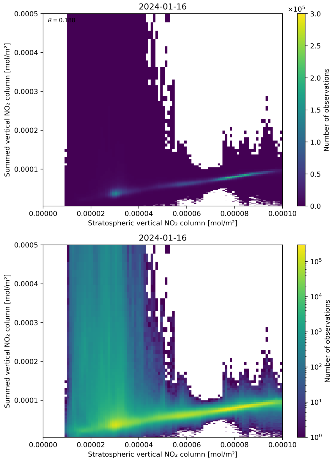
Figure 98: Scatter density plot of “Stratospheric vertical NO 2 column” against “Summed vertical NO 2 column” for 2024-01-15 to 2024-01-17.
