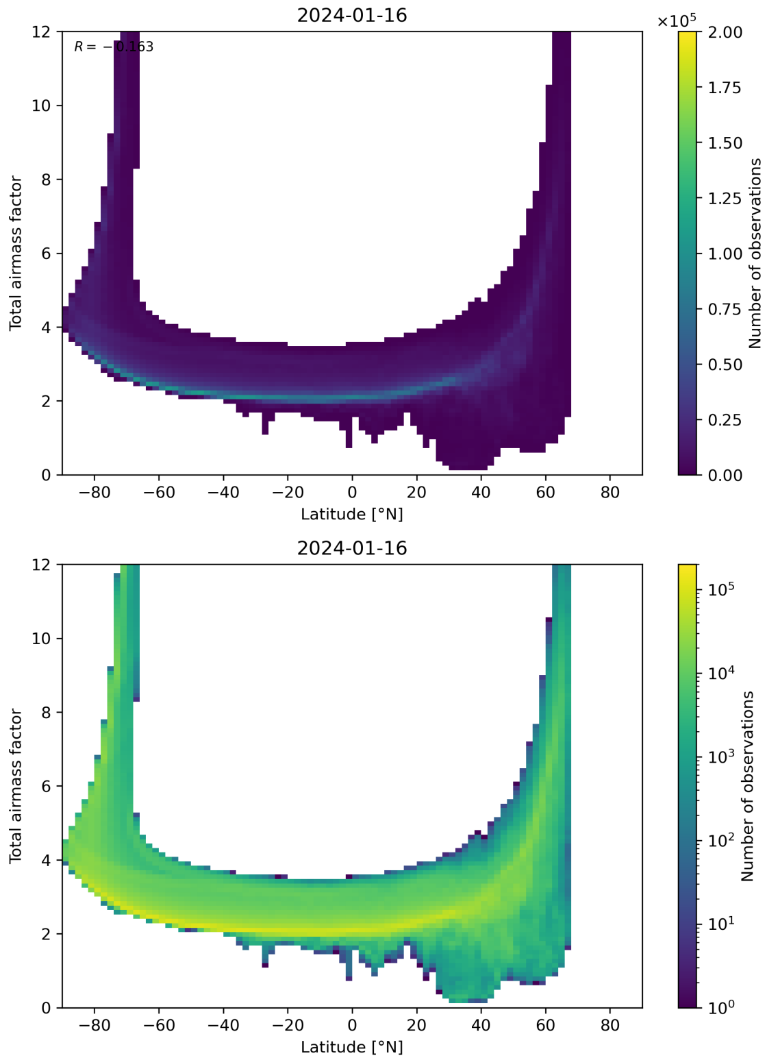
Figure 84: Scatter density plot of “Latitude” against “Total airmass factor” for 2024-01-15 to 2024-01-17.
