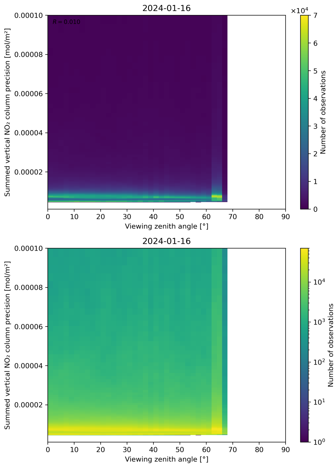
Figure 166: Scatter density plot of “Viewing zenith angle” against “Summed vertical NO 2 column precision” for 2024-01-15 to 2024-01-17.
