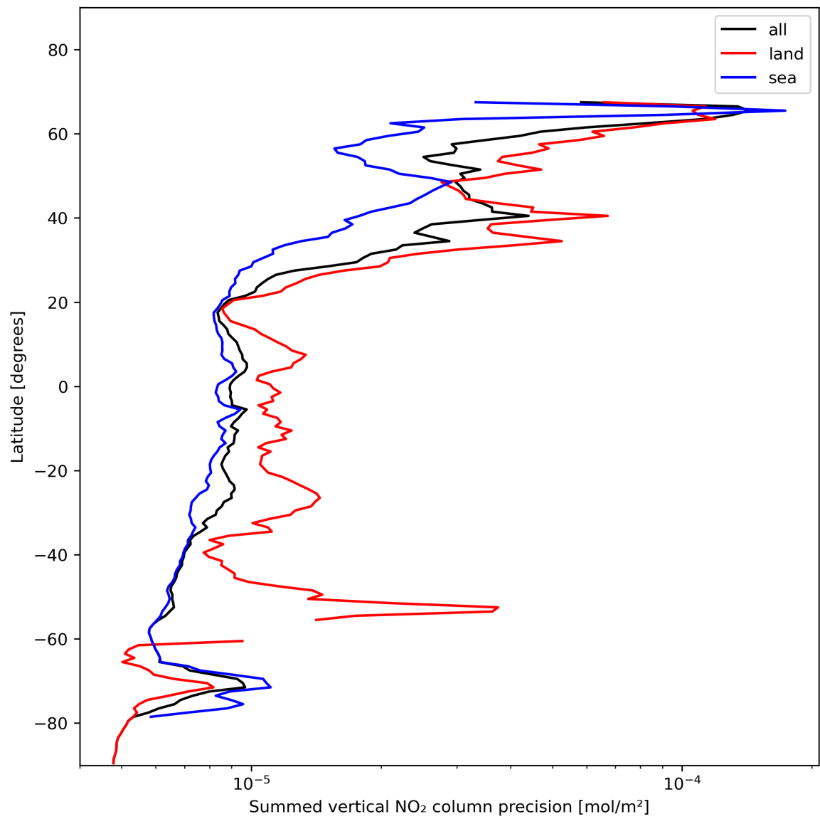
Figure 24: Zonal average of “Summed vertical NO 2 column precision” for 2024-01-15 to 2024-01-17.
