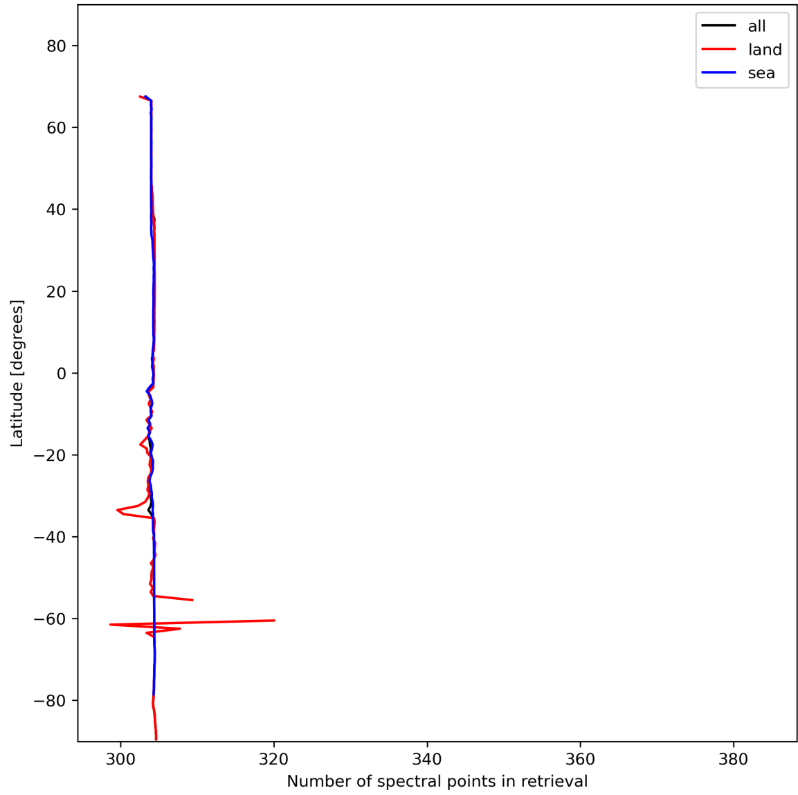
Figure 16: Zonal average of “Number of spectral points in retrieval” for 2024-01-15 to 2024-01-17.
