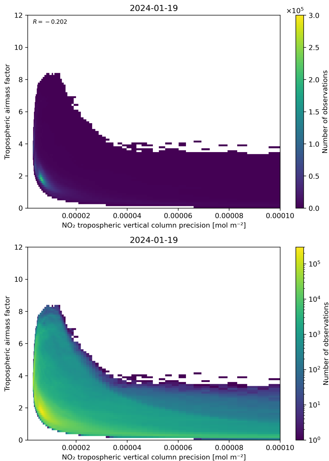
Figure 133: Scatter density plot of “NO 2 tropospheric vertical column precision” against “Tropospheric airmass factor” for 2024-01-18 to 2024-01-20.
