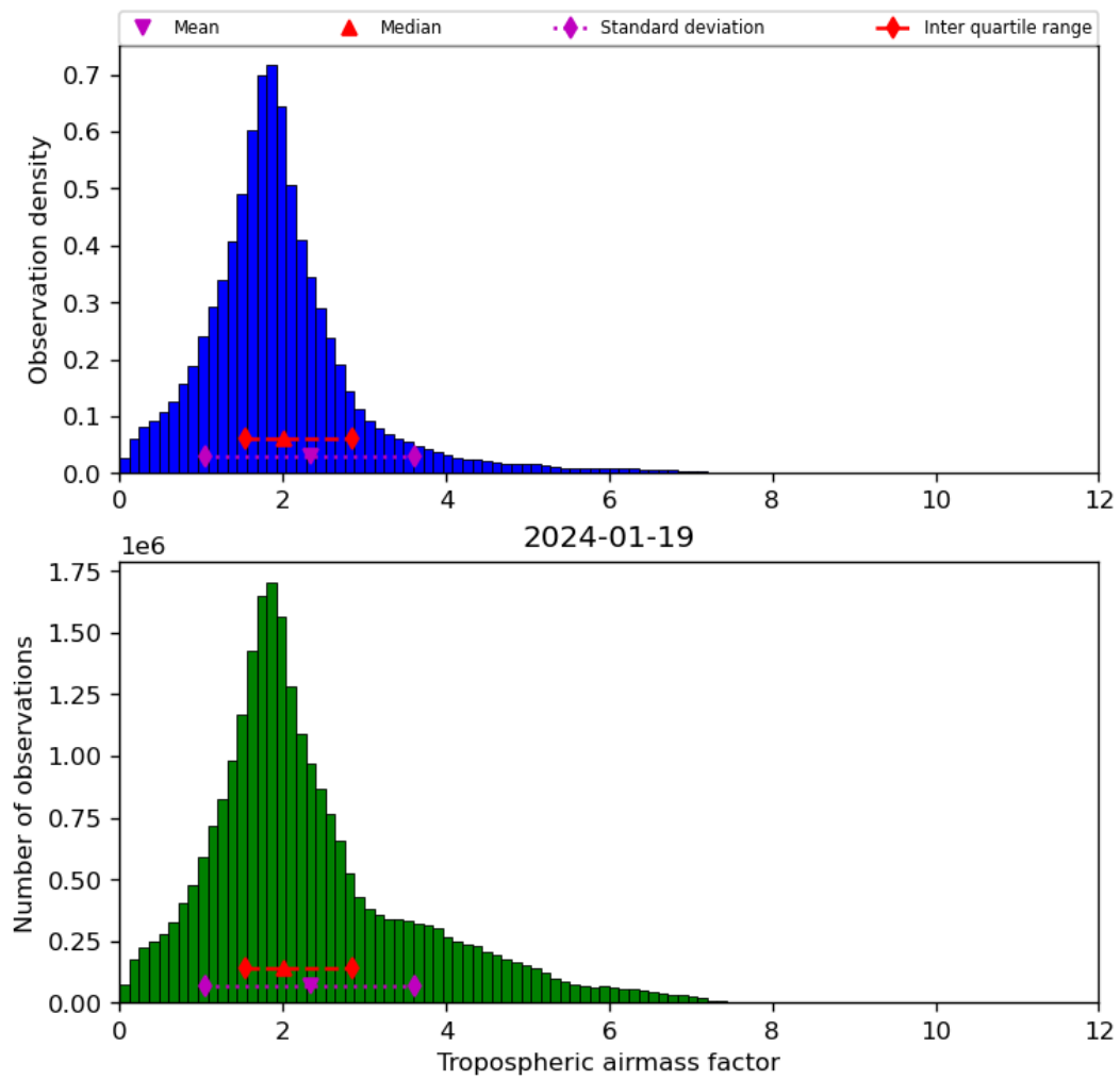
Figure 31: Histogram of “Tropospheric airmass factor” for 2024-01-18 to 2024-01-20
