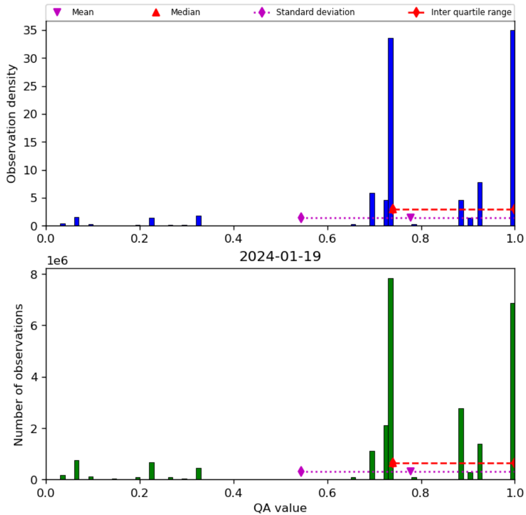
Figure 28: Histogram of “QA value” for 2024-01-18 to 2024-01-20
