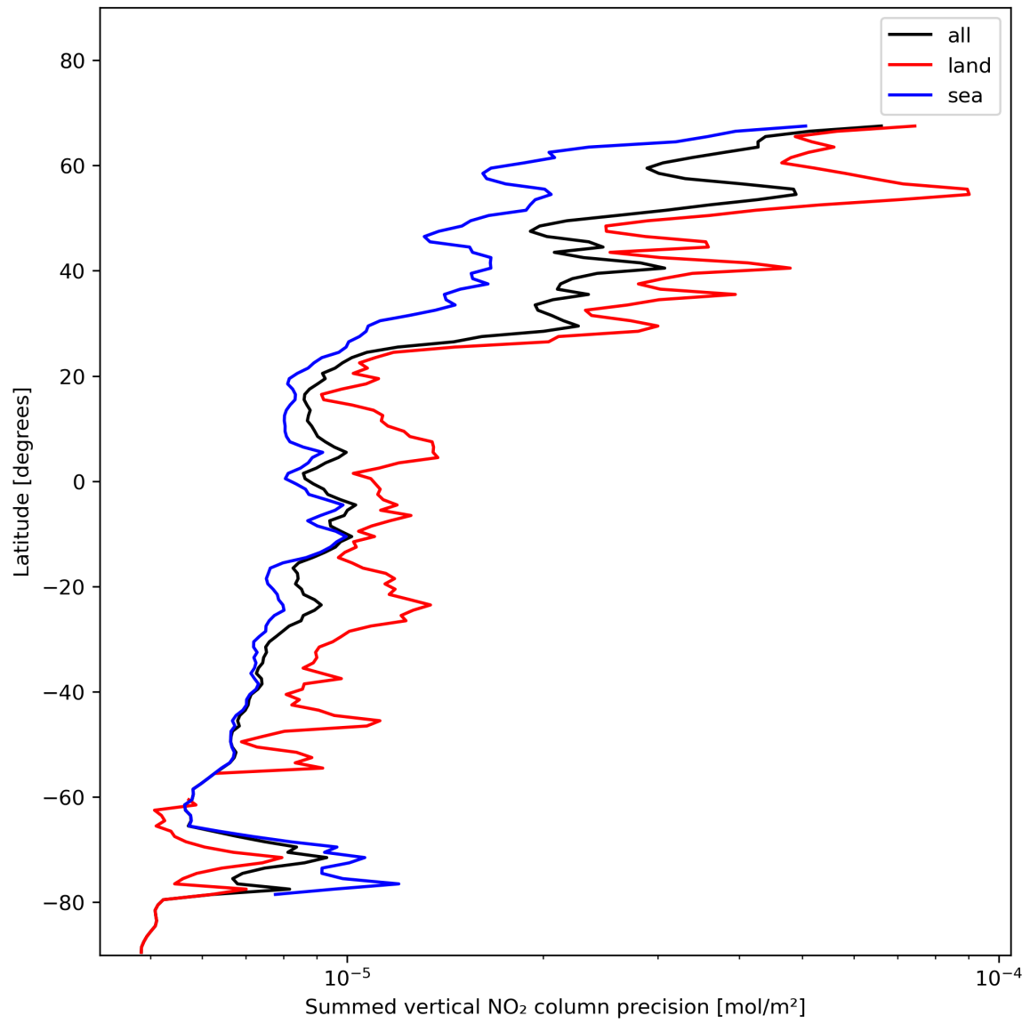
Figure 24: Zonal average of “Summed vertical NO 2 column precision” for 2024-01-18 to 2024-01-20.
