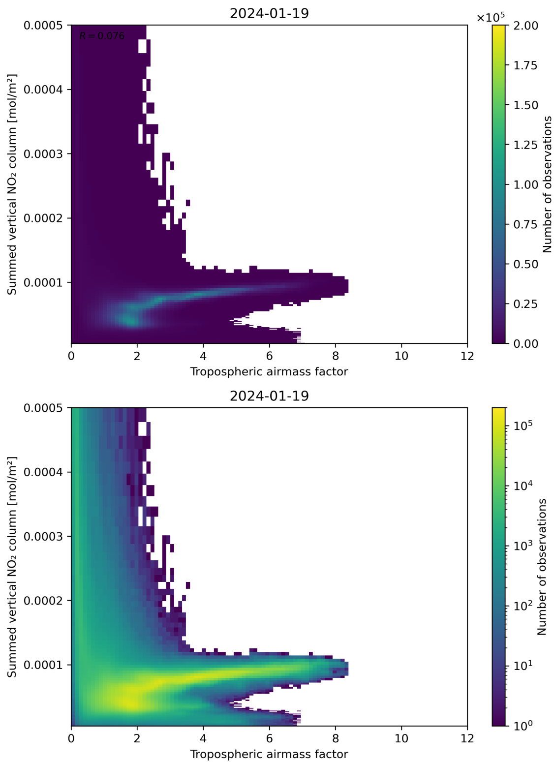
Figure 75: Scatter density plot of “Tropospheric air mass factor” against “Summed vertical NO 2 column” for 2024-01-18 to 2024-01-20.
