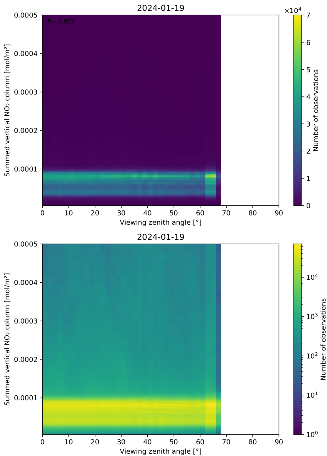
Figure 165: Scatter density plot of “Viewing zenith angle” against “Summed vertical NO 2 column” for 2024-01-18 to 2024-01-20.
