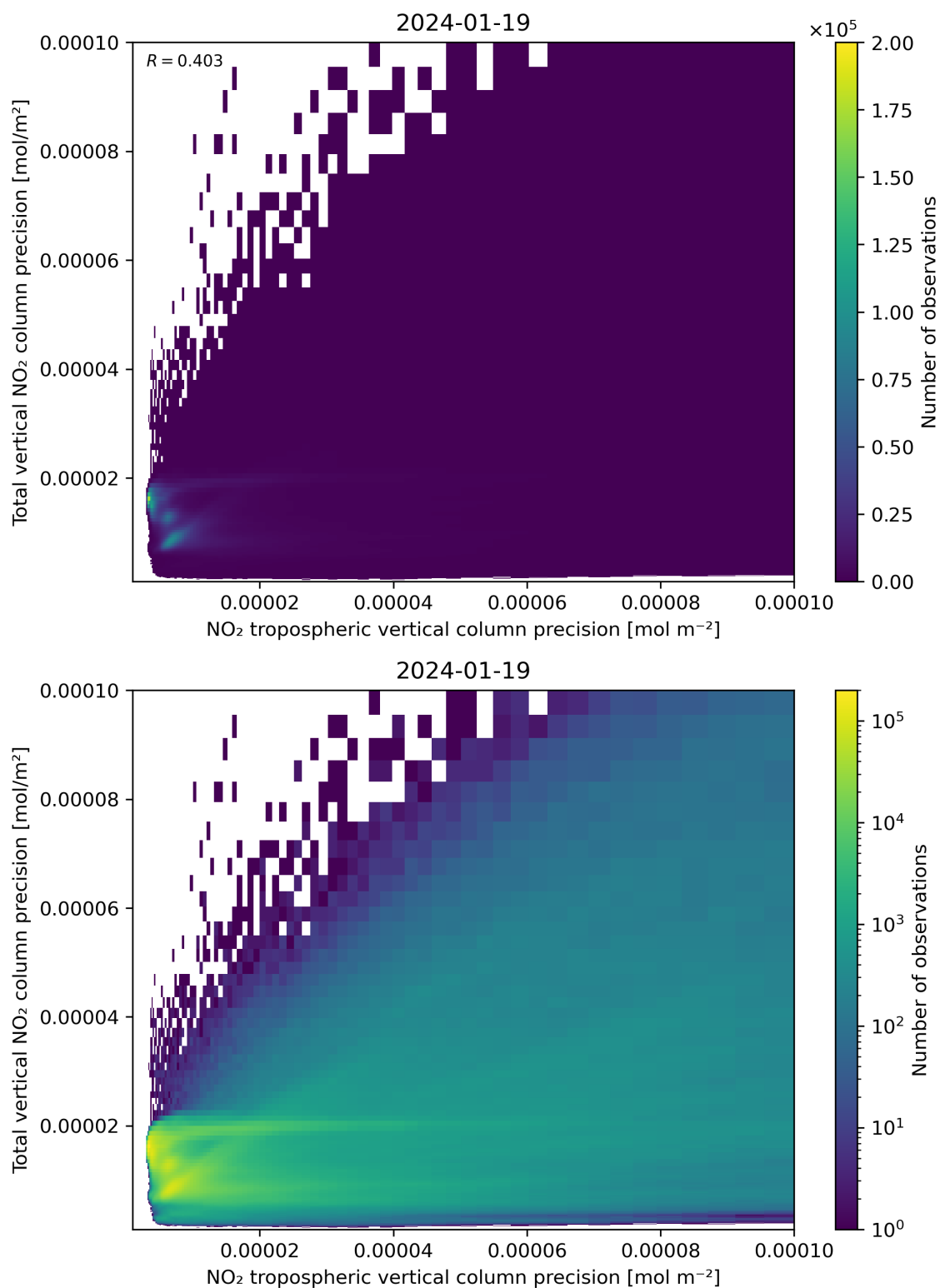
Figure 139: Scatter density plot of “NO 2 tropospheric vertical column precision” against “Total vertical NO 2 column precision” for 2024-01-18 to 2024-01-20.
