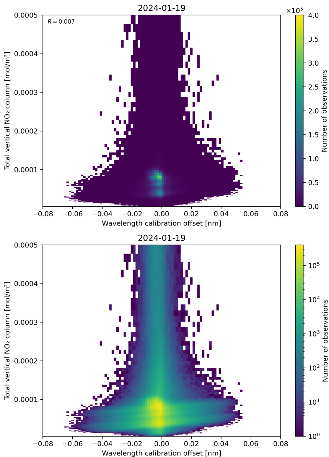
Figure 179: Scatter density plot of “Wavelength calibration offset” against “Total vertical NO 2 column” for 2024-01-18 to 2024-01-20.
