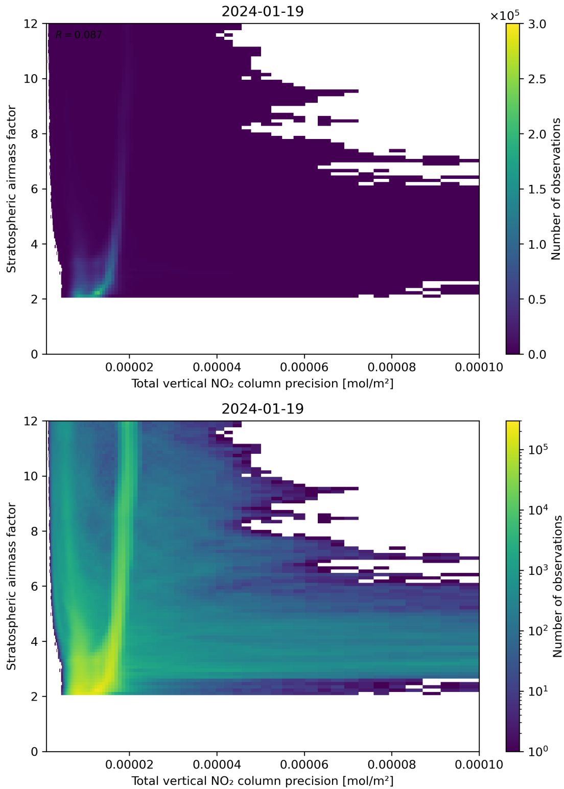
Figure 115: Scatter density plot of “Total vertical NO 2 column precision” against “Stratospheric air mass factor” for 2024-01-18 to 2024-01-20.
