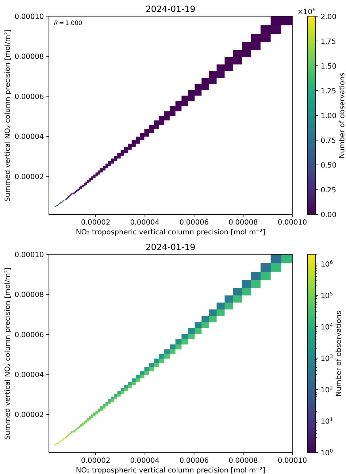
Figure 137: Scatter density plot of “NO 2 tropospheric vertical column precision” against “Summed vertical NO 2 column precision” for 2024-01-18 to 2024-01-20.
