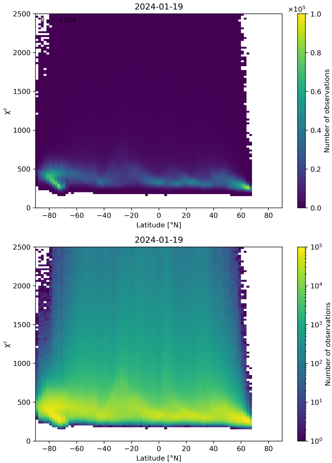
Figure 86: Scatter density plot of “Latitude” against “ \chi^2 ” for 2024-01-18 to 2024-01-20.
