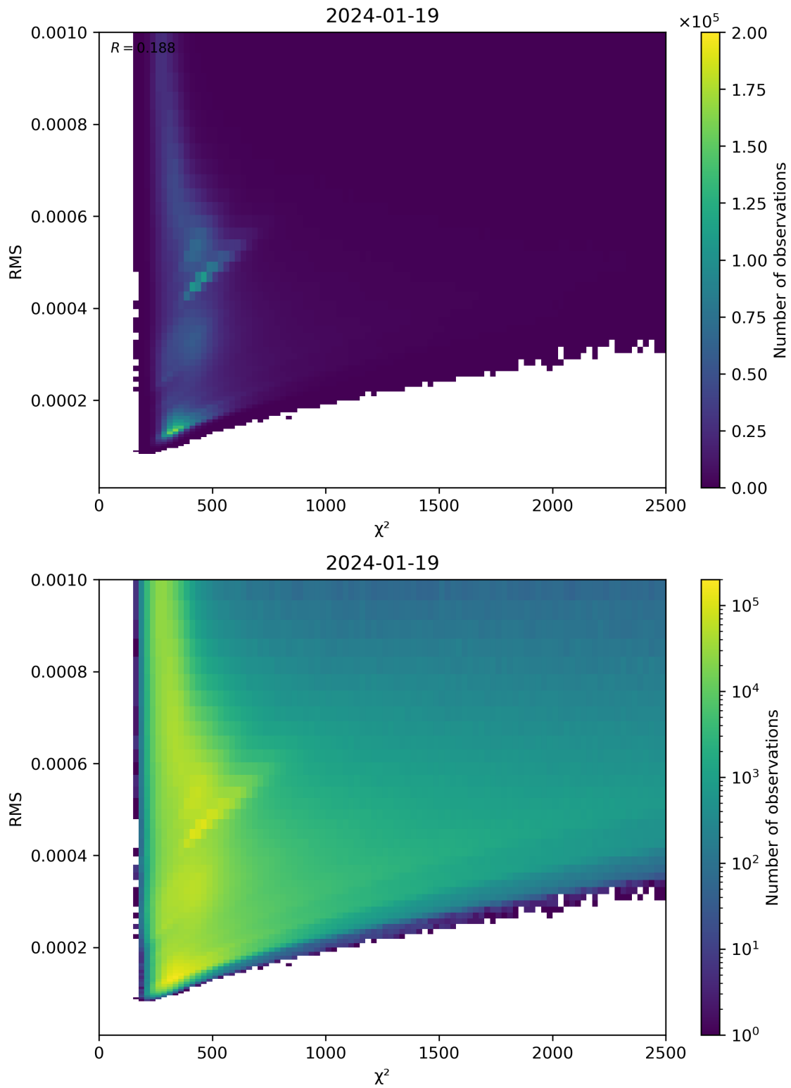
Figure 82: Scatter density plot of “ \chi^2 ” against “RMS” for 2024-01-18 to 2024-01-20.
