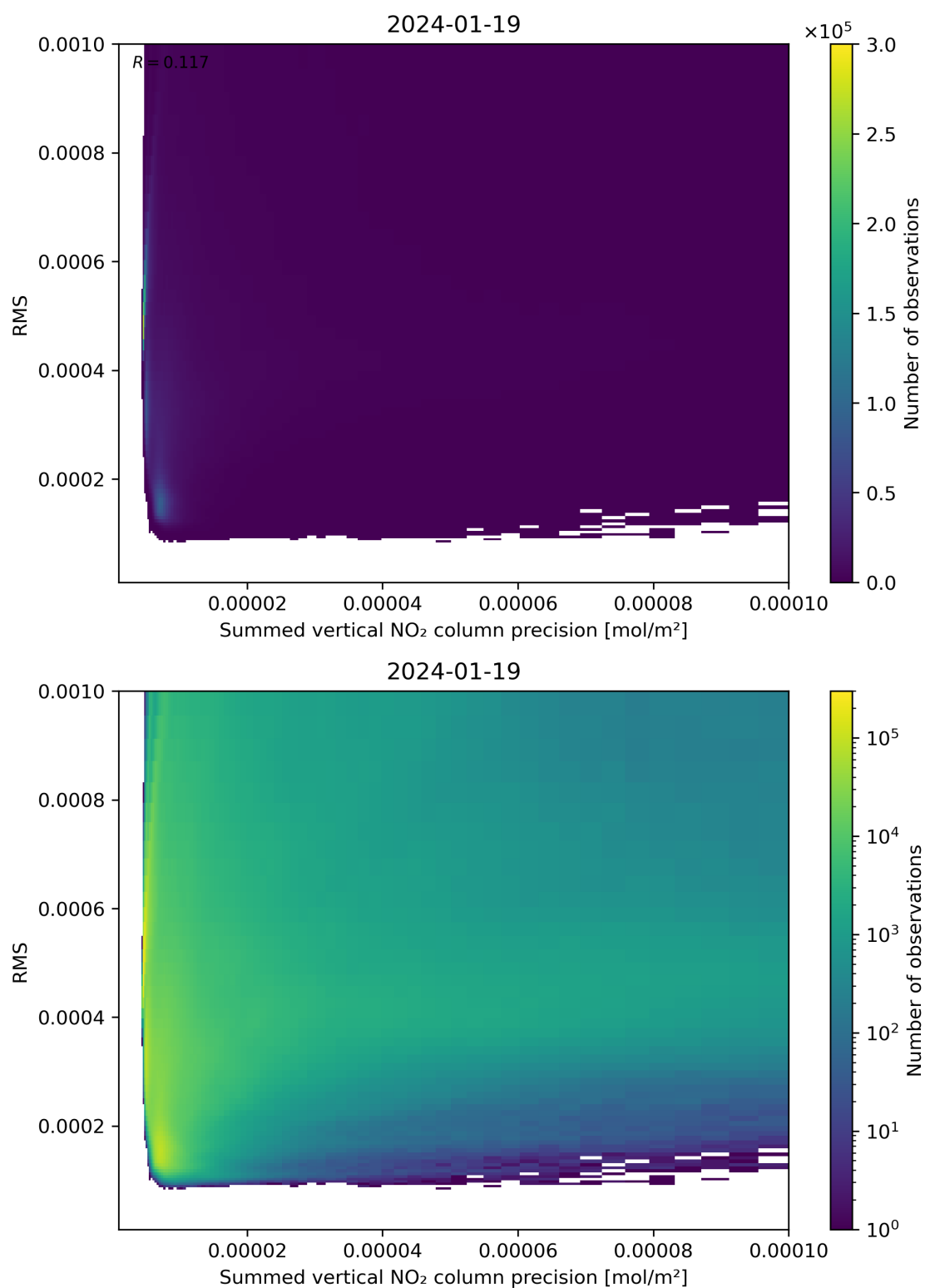
Figure 108: Scatter density plot of “Summed vertical NO 2 column precision” against “RMS” for 2024-01-18 to 2024-01-20.
