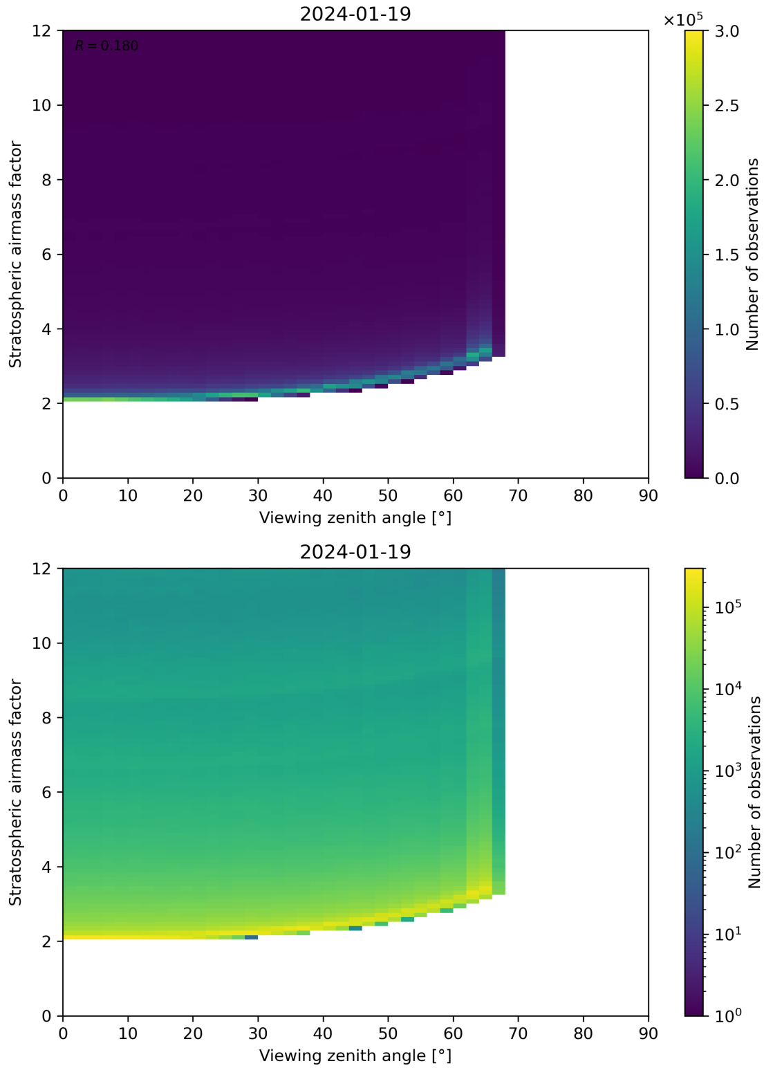
Figure 159: Scatter density plot of “Viewing zenith angle” against “Stratospheric airmass factor” for 2024-01-18 to 2024-01-20.
