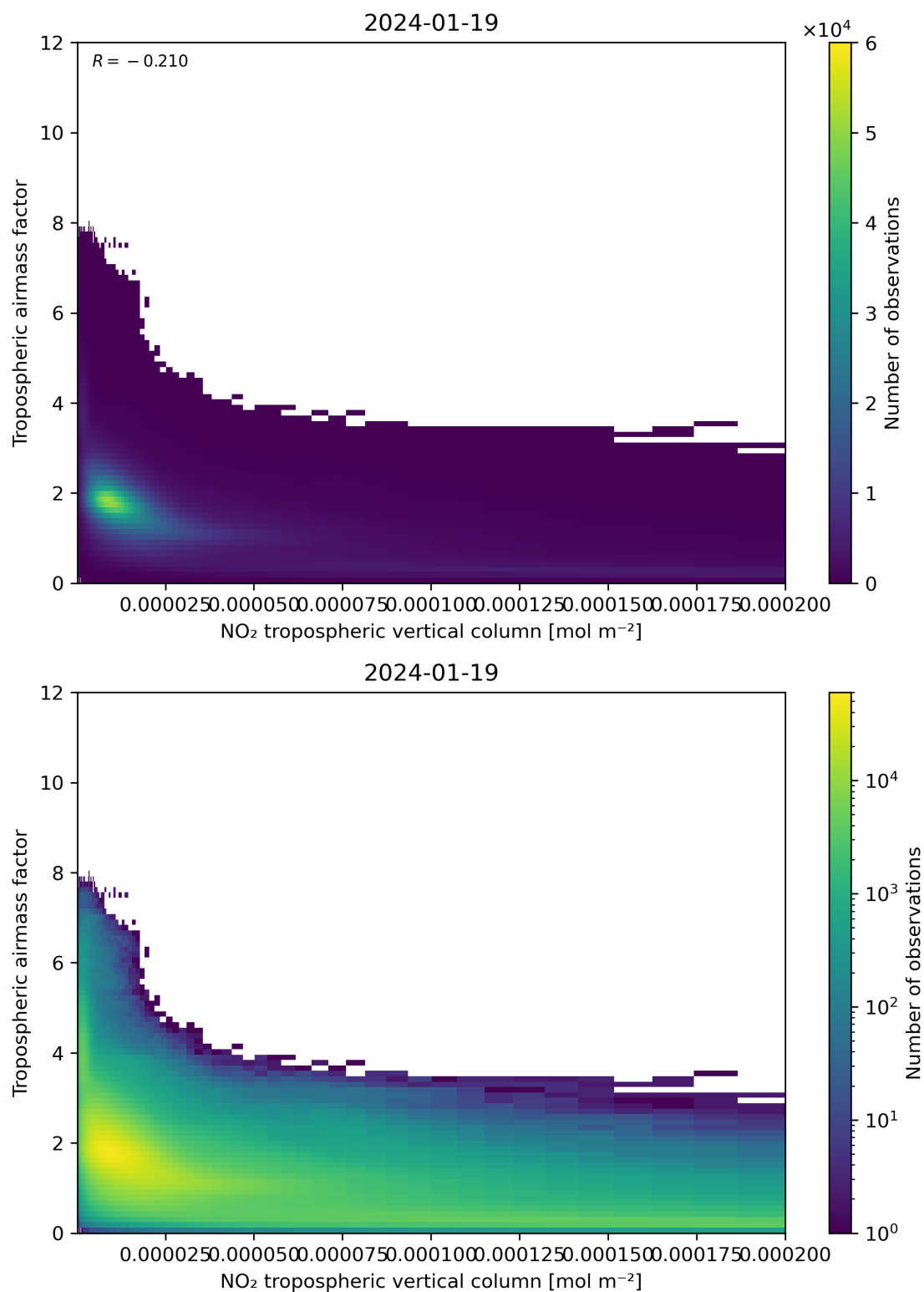
Figure 123: Scatter density plot of “NO 2 tropospheric vertical column” against “Tropospheric airmass factor” for 2024-01-18 to 2024-01-20.
