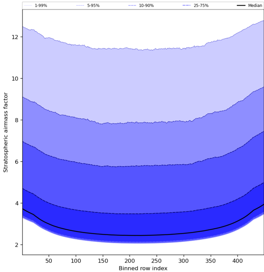
Figure 61: Along track statistics of “Stratospheric airmass factor” for 2024-01-18 to 2024-01-20
