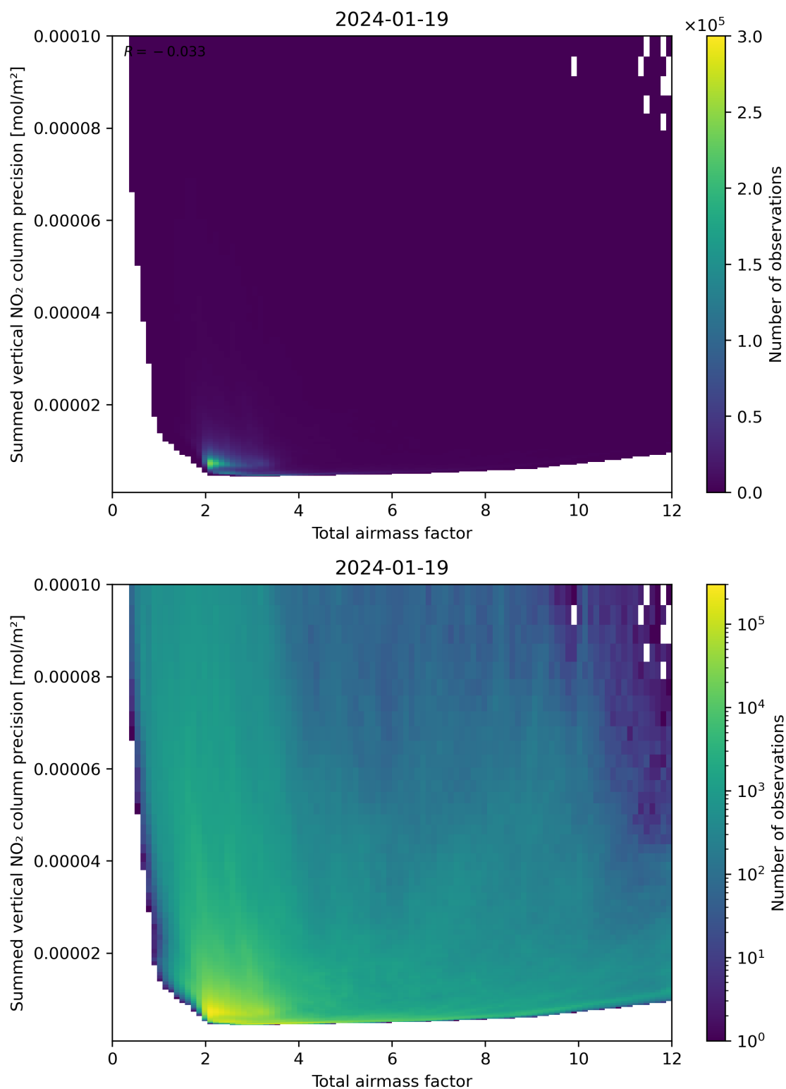
Figure 66: Scatter density plot of “Total airmass factor” against “Summed vertical NO 2 column precision” for 2024-01-18 to 2024-01-20.
