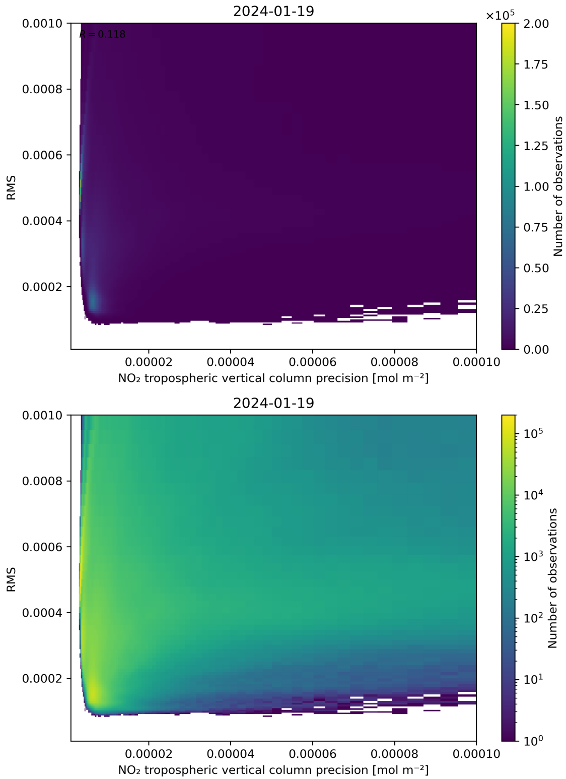
Figure 140: Scatter density plot of “NO 2 tropospheric vertical column precision” against “RMS” for 2024-01-18 to 2024-01-20.
