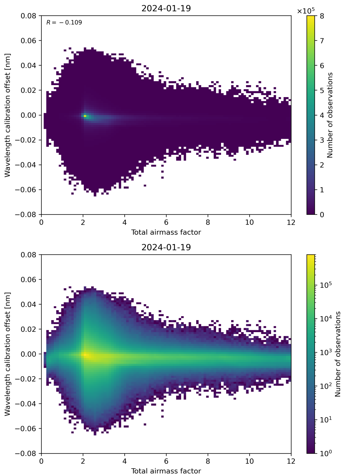
Figure 70: Scatter density plot of “Total airmass factor” against “Wavelength calibration offset” for 2024-01-18 to 2024-01-20.
