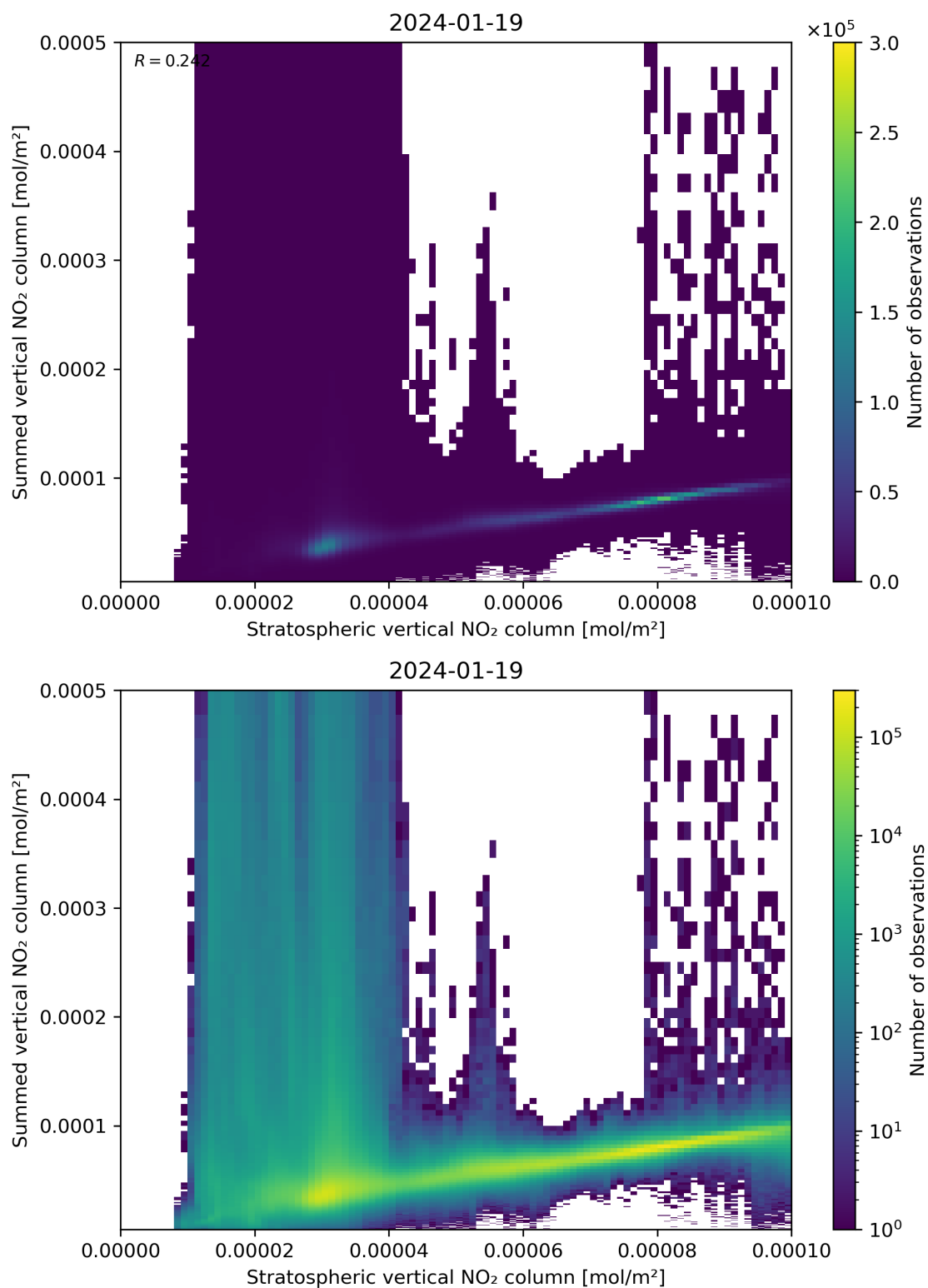
Figure 98: Scatter density plot of “Stratospheric vertical NO 2 column” against “Summed vertical NO 2 column” for 2024-01-18 to 2024-01-20.
