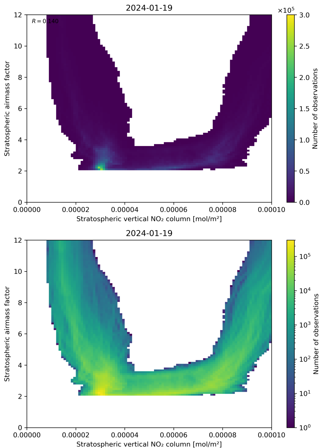
Figure 96: Scatter density plot of “Stratospheric vertical NO 2 column” against “Stratospheric airmass factor” for 2024-01-18 to 2024-01-20.
