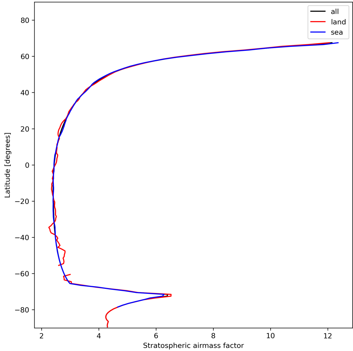
Figure 27: Zonal average of “Stratospheric airmass factor” for 2024-01-18 to 2024-01-20.
