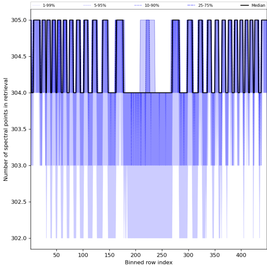
Figure 50: Along track statistics of “Number of spectral points in retrieval” for 2024-01-18 to 2024-01-20
