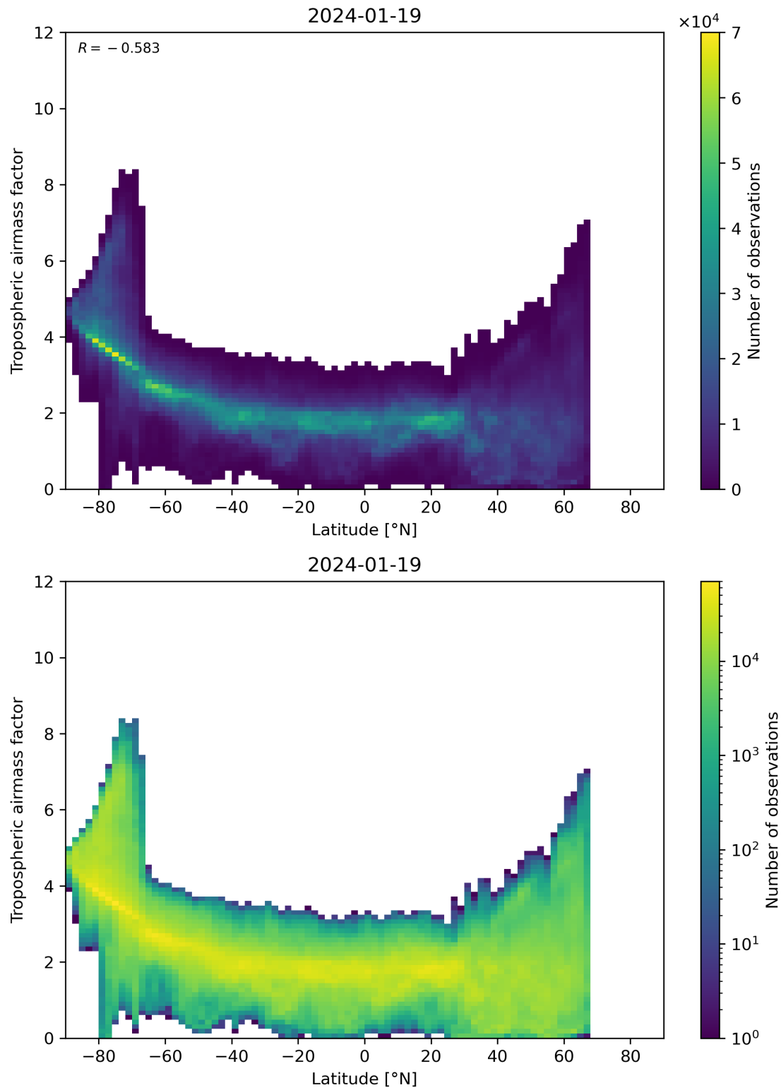
Figure 85: Scatter density plot of “Latitude” against “Tropospheric air mass factor” for 2024-01-18 to 2024-01-20.
