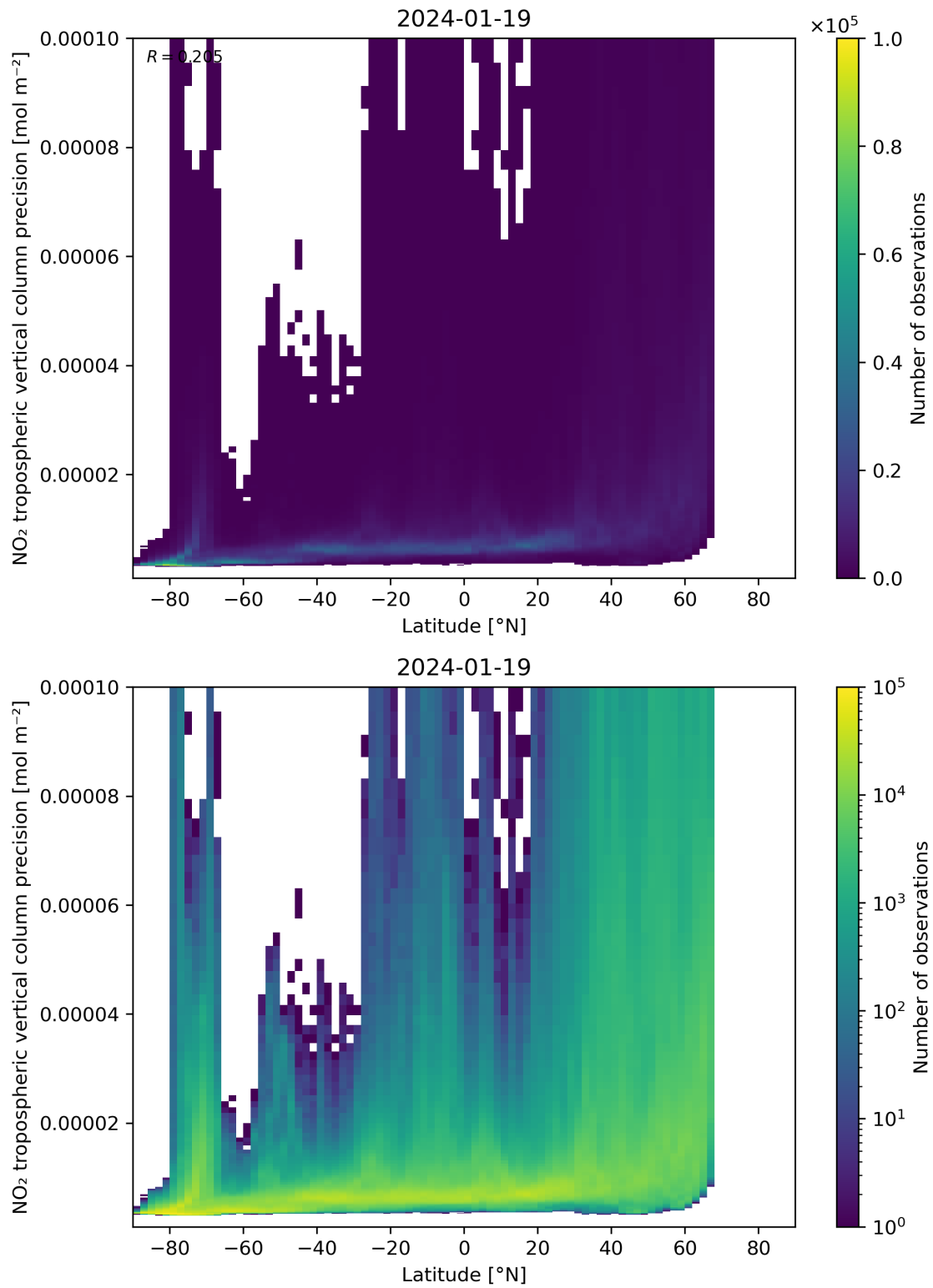
Figure 93: Scatter density plot of “Latitude” against “NO 2 tropospheric vertical column precision” for 2024-01-18 to 2024-01-20.
