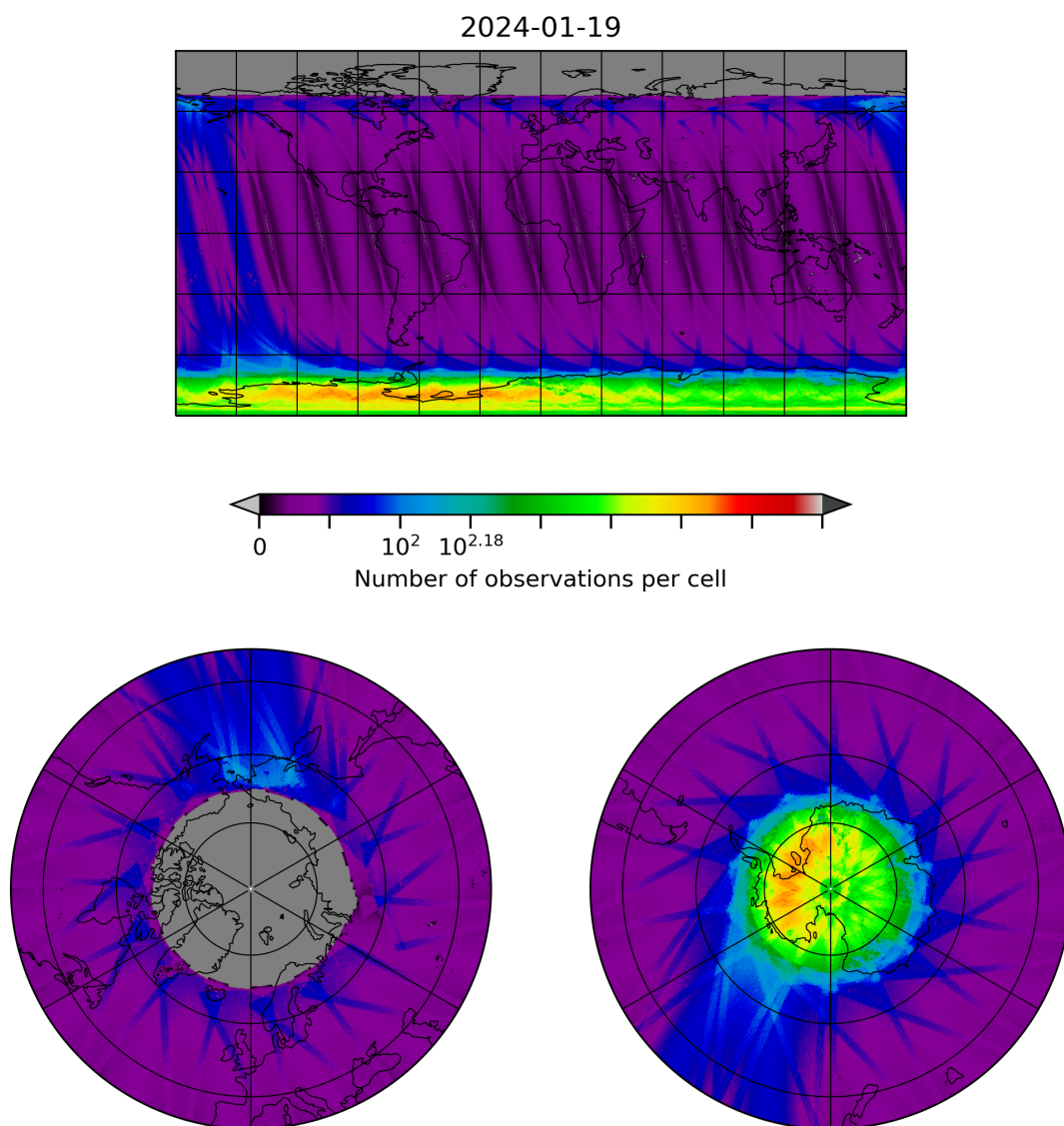
Figure 10: Map of the number of observations for 2024-01-18 to 2024-01-20
