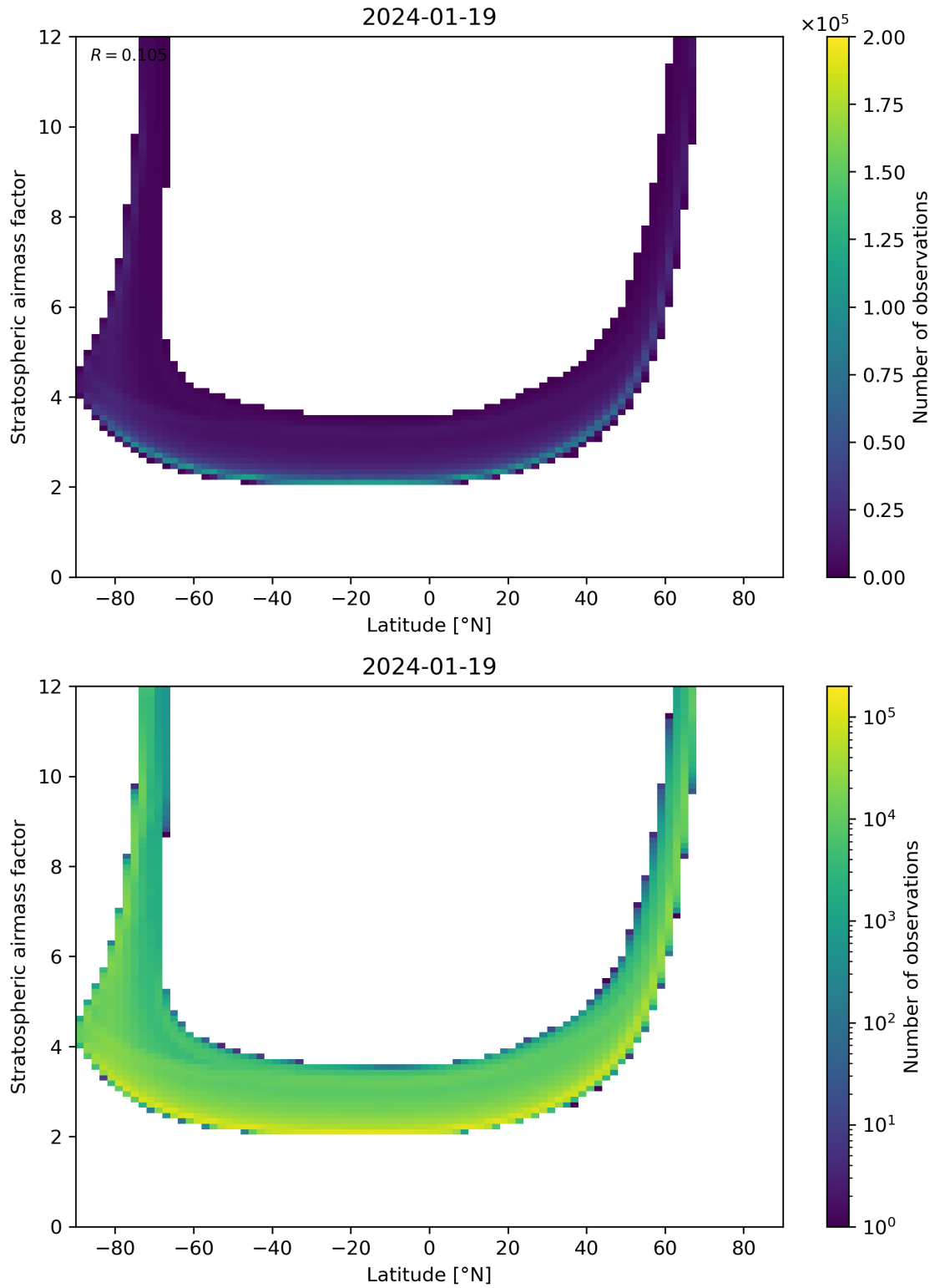
Figure 83: Scatter density plot of “Latitude” against “Stratospheric airmass factor” for 2024-01-18 to 2024-01-20.
