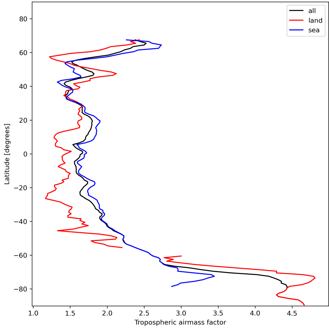
Figure 14: Zonal average of “Tropospheric airmass factor” for 2024-01-18 to 2024-01-20.
