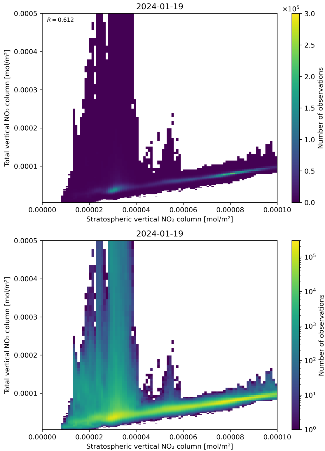
Figure 100: Scatter density plot of “Stratospheric vertical NO 2 column” against “Total vertical NO 2 column” for 2024-01-18 to 2024-01-20.
