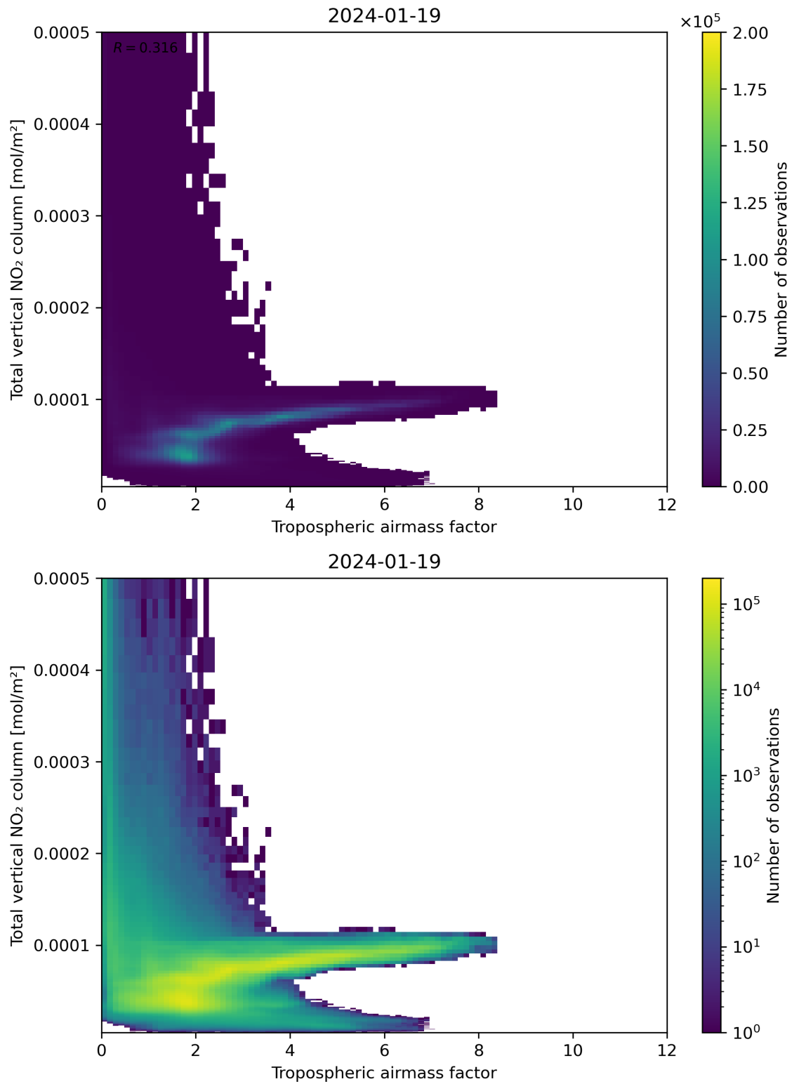
Figure 77: Scatter density plot of “Tropospheric airmass factor” against “Total vertical NO 2 column” for 2024-01-18 to 2024-01-20.
