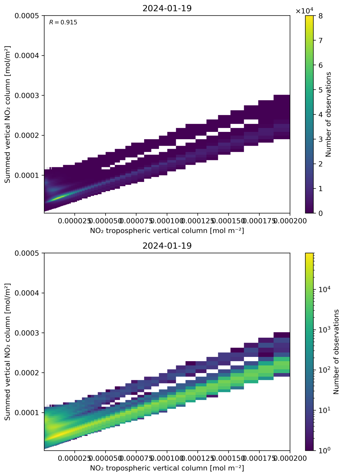
Figure 126: Scatter density plot of “NO 2 tropospheric vertical column” against “Summed vertical NO 2 column” for 2024-01-18 to 2024-01-20.
