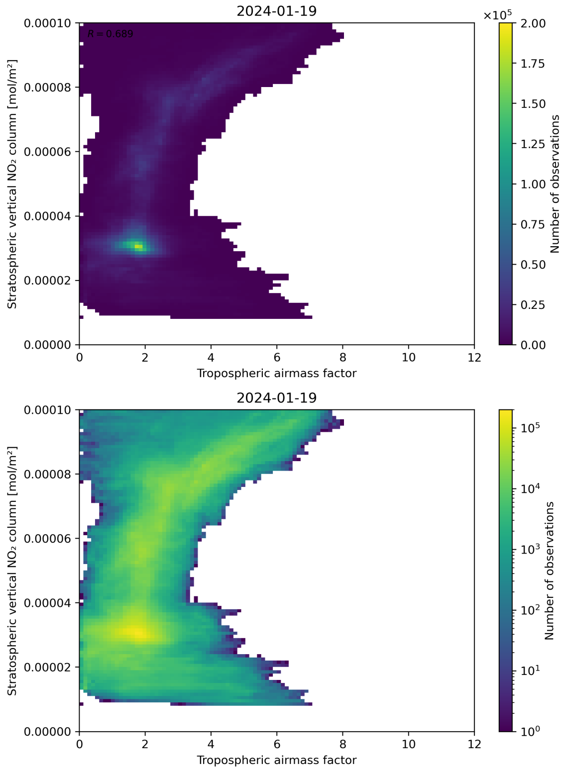
Figure 74: Scatter density plot of “Tropospheric air mass factor” against “Stratospheric vertical NO 2 column” for 2024-01-18 to 2024-01-20.
