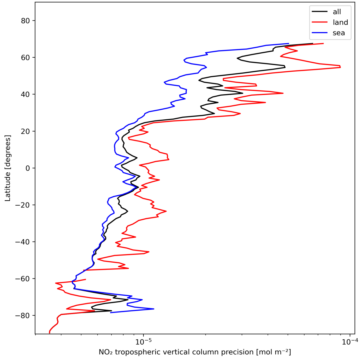
Figure 13: Zonal average of “NO 2 tropospheric vertical column precision” for 2024-01-18 to 2024-01-20.
