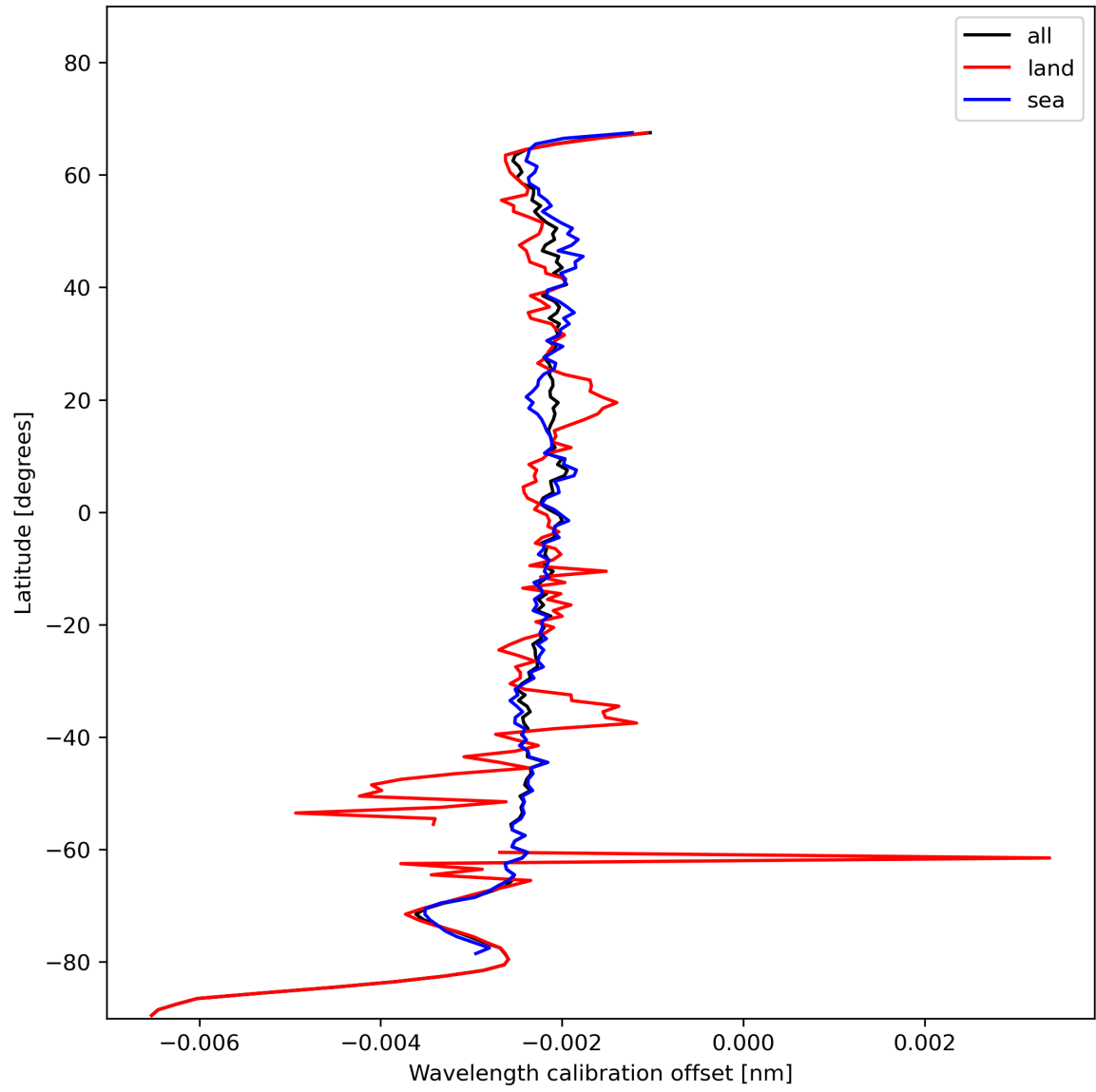
Figure 18: Zonal average of “Wavelength calibration offset” for 2024-01-18 to 2024-01-20.
