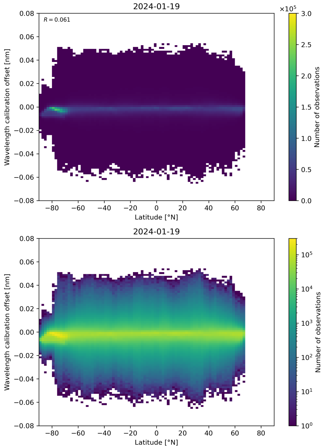
Figure 95: Scatter density plot of “Latitude” against “Wavelength calibration offset” for 2024-01-18 to 2024-01-20.
