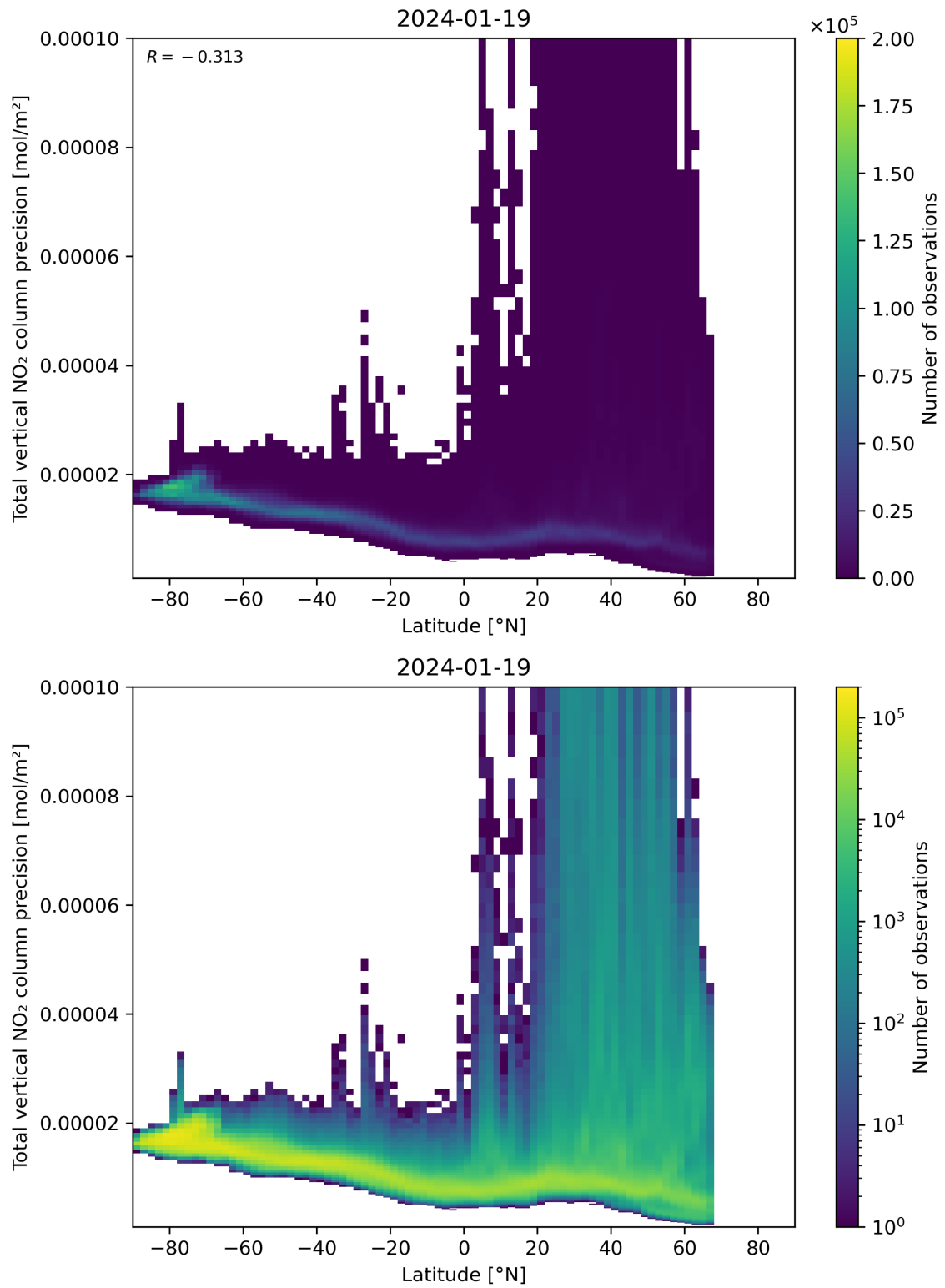
Figure 91: Scatter density plot of “Latitude” against “Total vertical NO 2 column precision” for 2024-01-18 to 2024-01-20.
