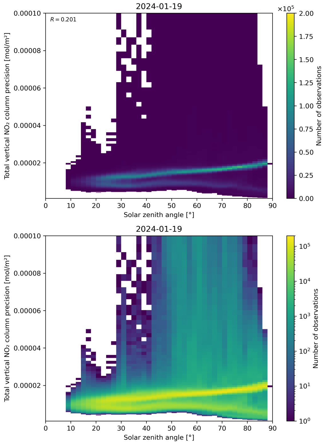
Figure 154: Scatter density plot of “Solar zenith angle” against “Total vertical NO 2 column precision” for 2024-01-18 to 2024-01-20.
