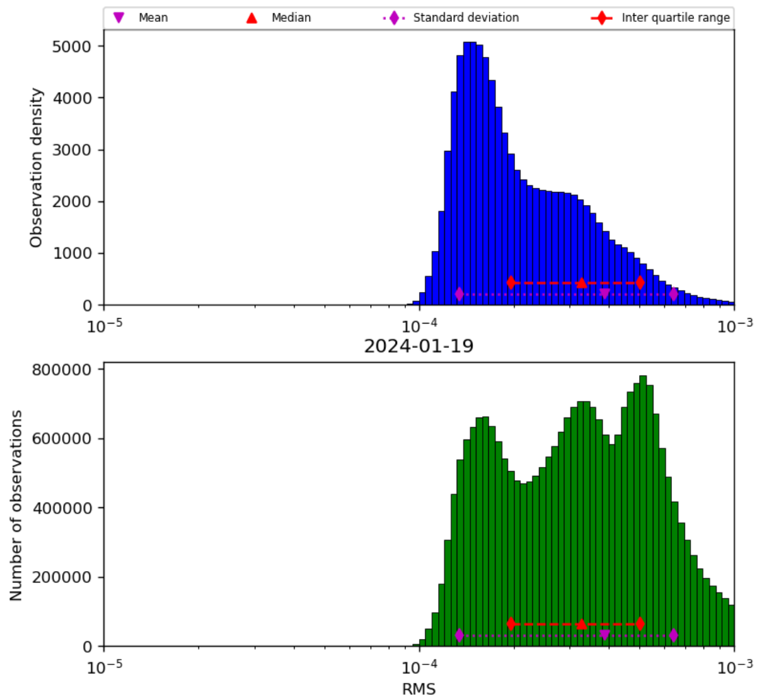
Figure 43: Histogram of “RMS” for 2024-01-18 to 2024-01-20
