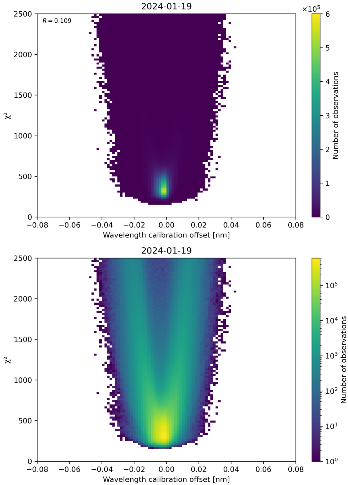
Figure 175: Scatter density plot of “Wavelength calibration offset” against “ \chi^2 ” for 2024-01-18 to 2024-01-20.
