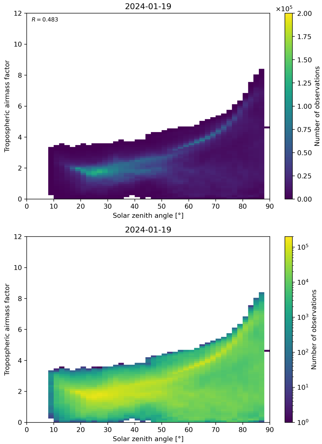
Figure 147: Scatter density plot of “Solar zenith angle” against “Tropospheric airmass factor” for 2024-01-18 to 2024-01-20.
