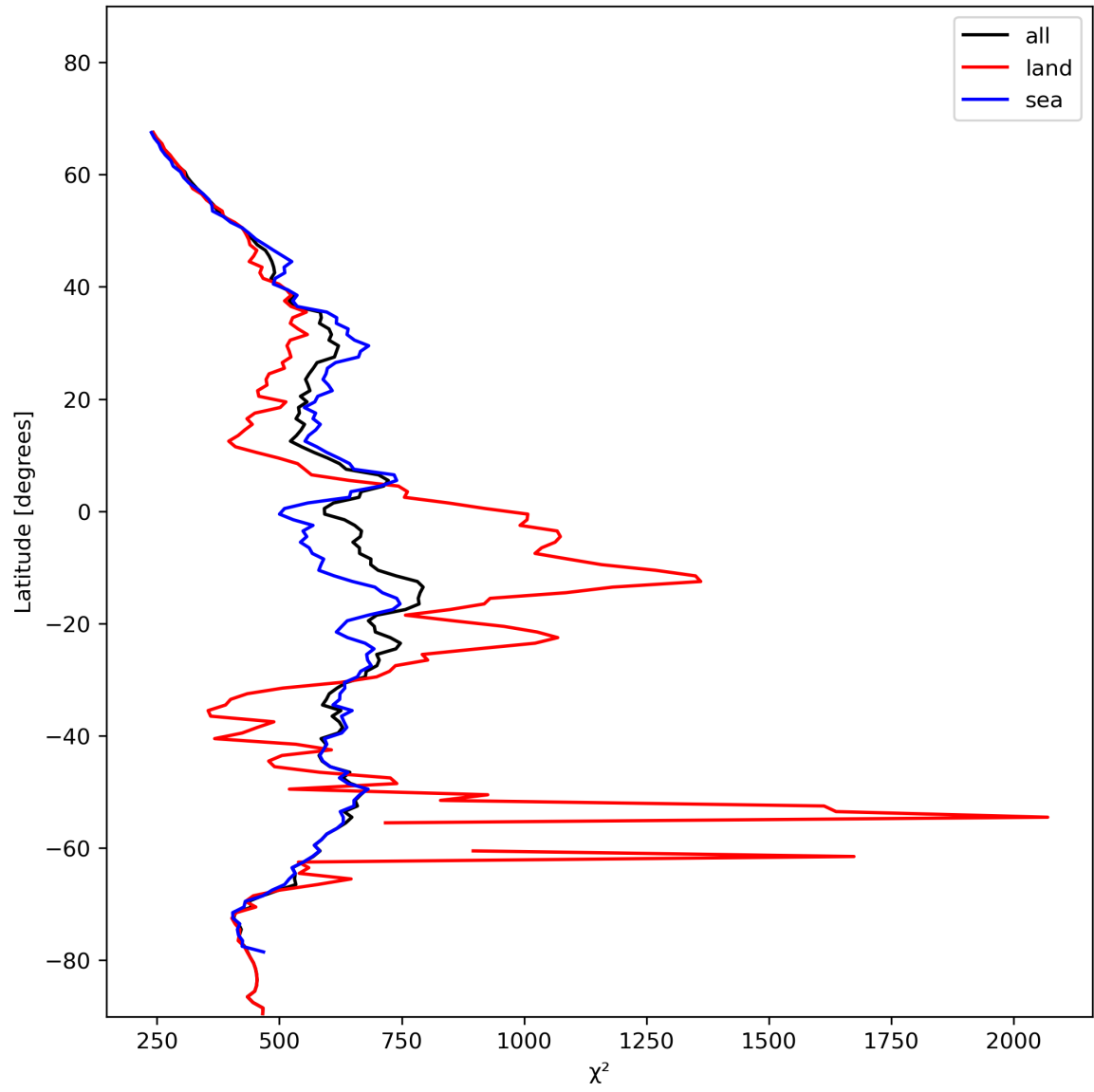
Figure 25: Zonal average of “ \chi^2 ” for 2024-01-18 to 2024-01-20.
