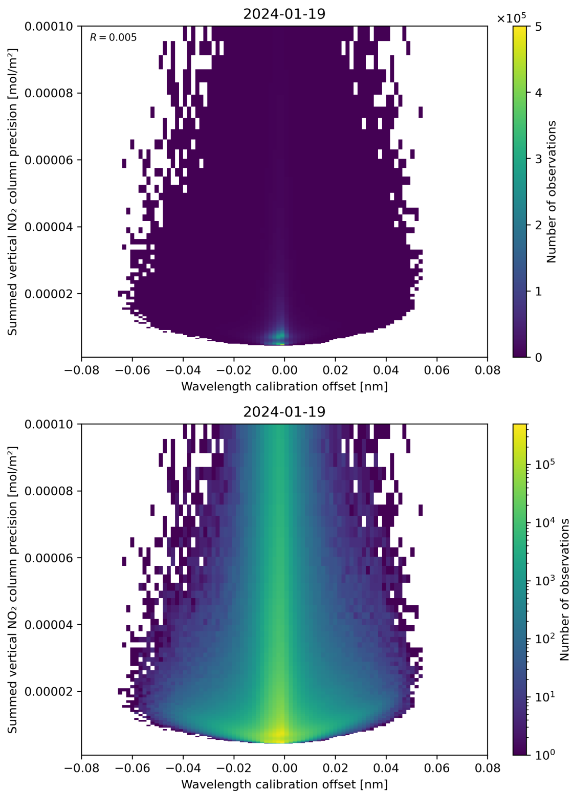
Figure 178: Scatter density plot of “Wavelength calibration offset” against “Summed vertical NO 2 column precision” for 2024-01-18 to 2024-01-20.
