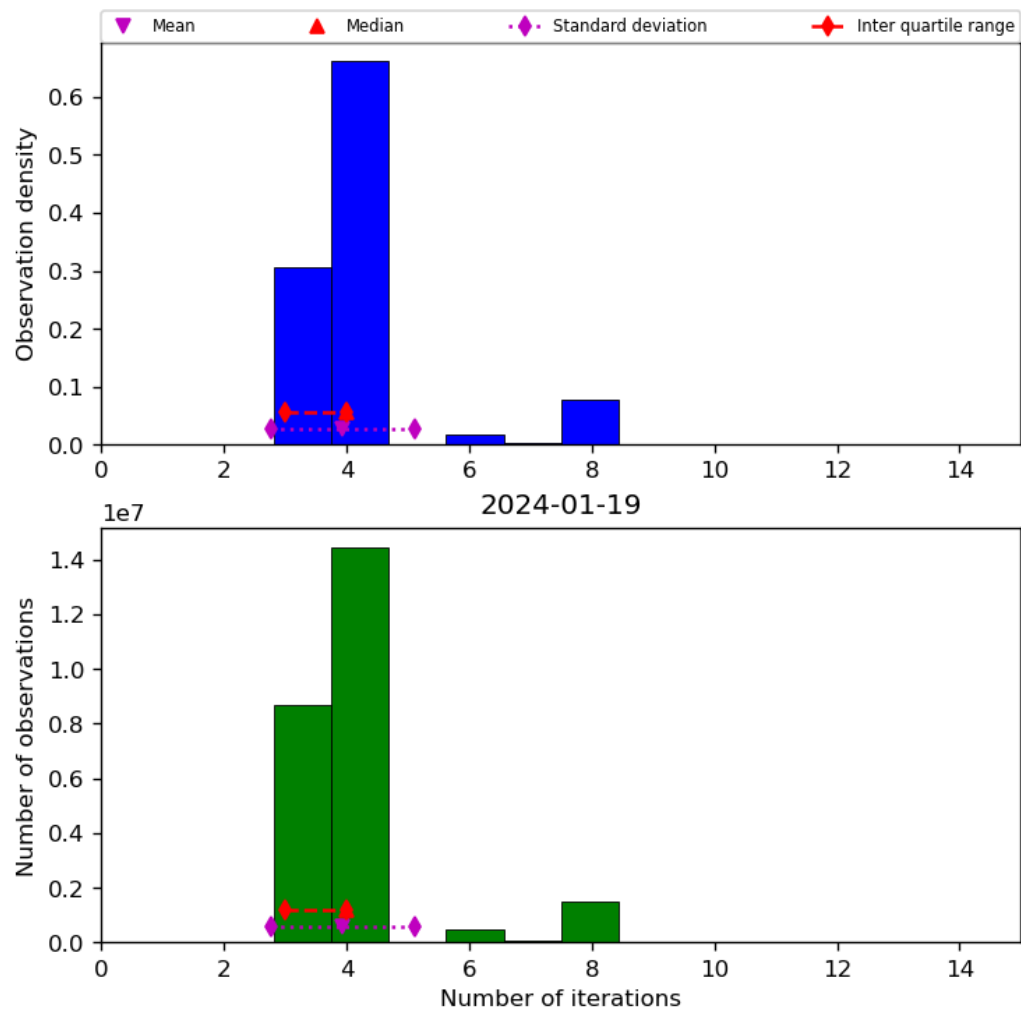
Figure 34: Histogram of “Number of iterations” for 2024-01-18 to 2024-01-20
