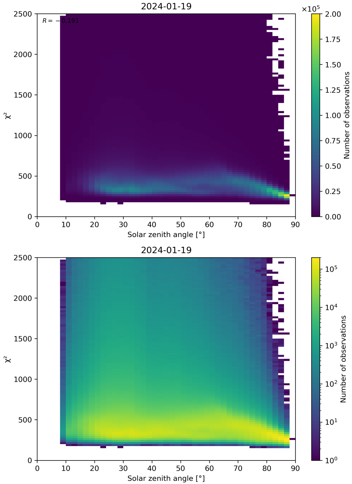
Figure 148: Scatter density plot of “Solar zenith angle” against “ \chi^2 ” for 2024-01-18 to 2024-01-20.
