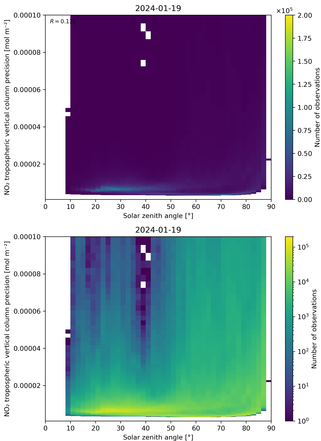
Figure 156: Scatter density plot of “Solar zenith angle” against “NO 2 tropospheric vertical column precision” for 2024-01-18 to 2024-01-20.
