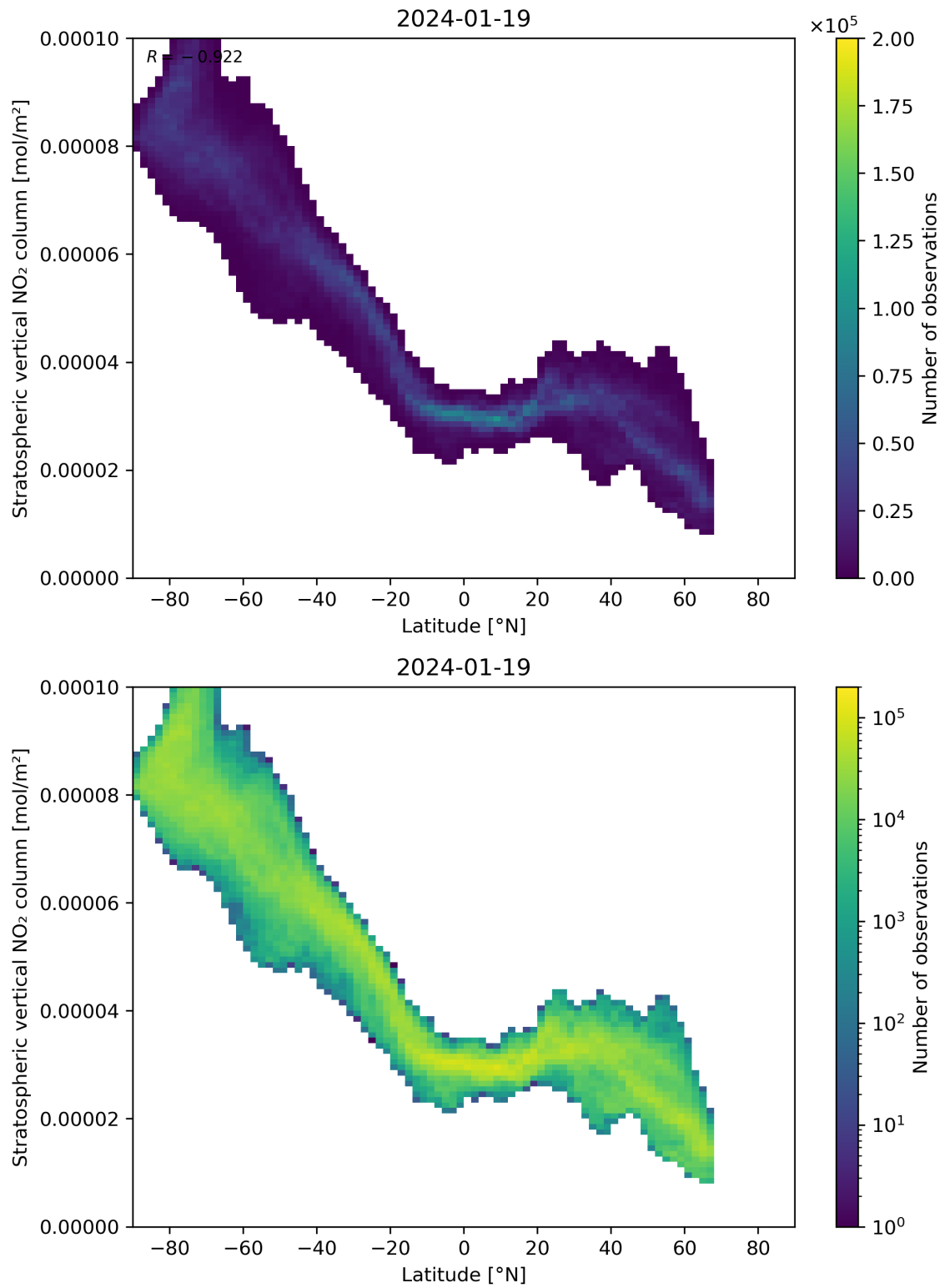
Figure 87: Scatter density plot of “Latitude” against “Stratospheric vertical NO 2 column” for 2024-01-18 to 2024-01-20.
