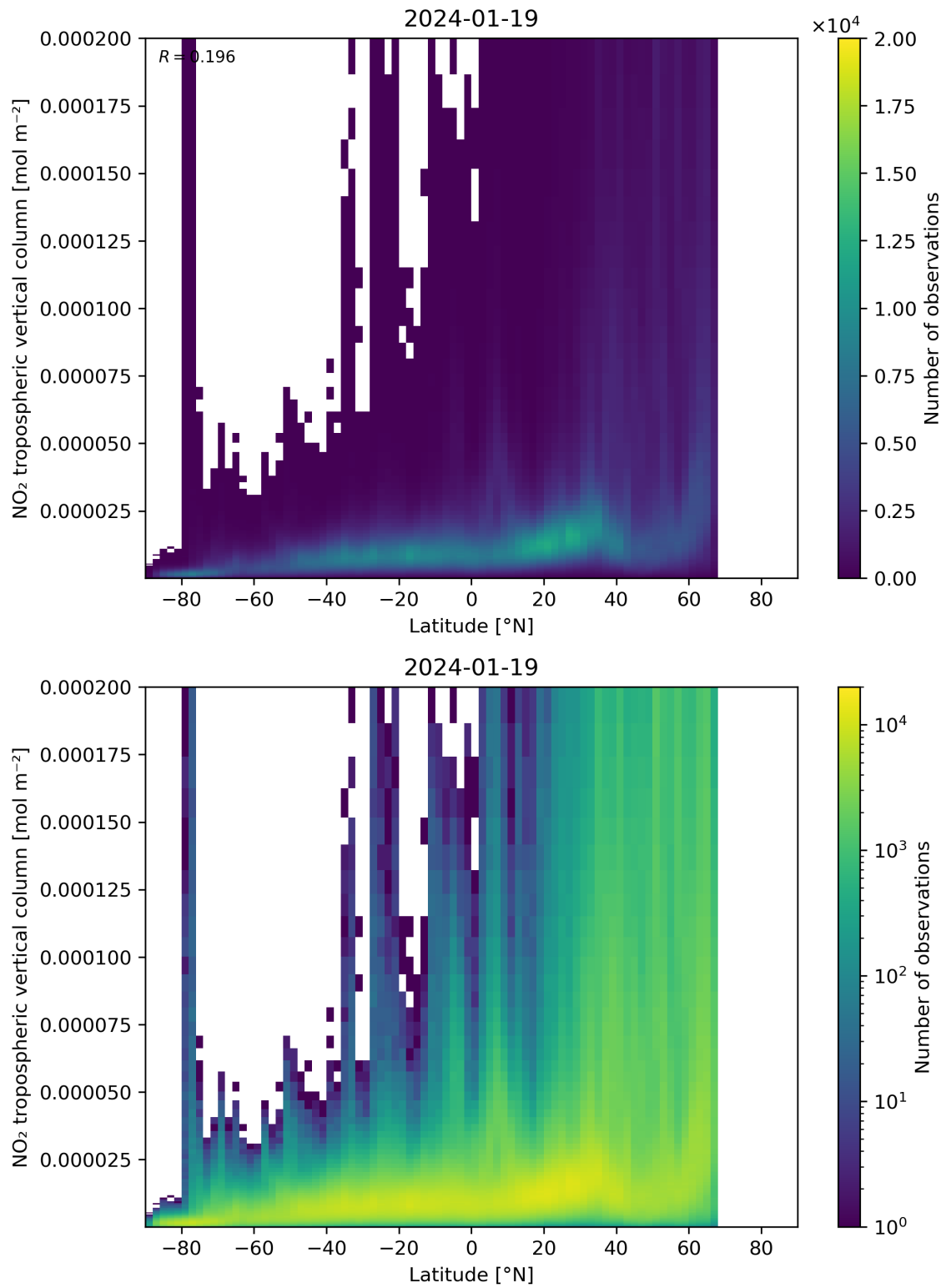
Figure 92: Scatter density plot of “Latitude” against “NO 2 tropospheric vertical column” for 2024-01-18 to 2024-01-20.
