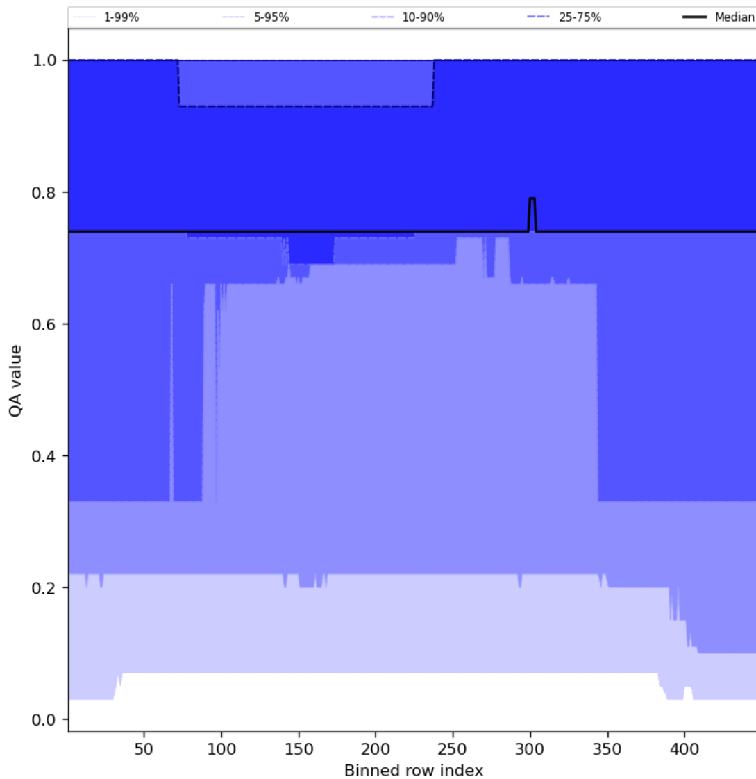
Figure 45: Along track statistics of “QA value” for 2024-01-18 to 2024-01-20
