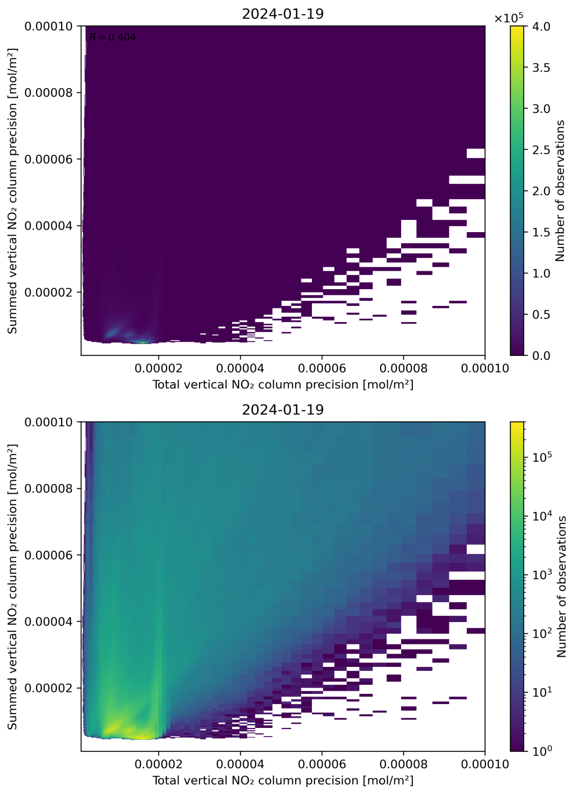
Figure 118: Scatter density plot of “Total vertical NO 2 column precision” against “Summed vertical NO 2 column precision” for 2024-01-18 to 2024-01-20.
