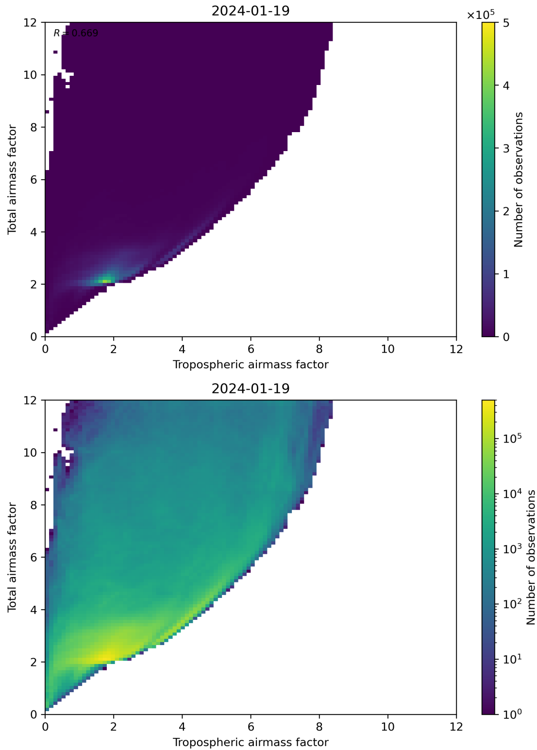
Figure 72: Scatter density plot of “Tropospheric airmass factor” against “Total airmass factor” for 2024-01-18 to 2024-01-20.
