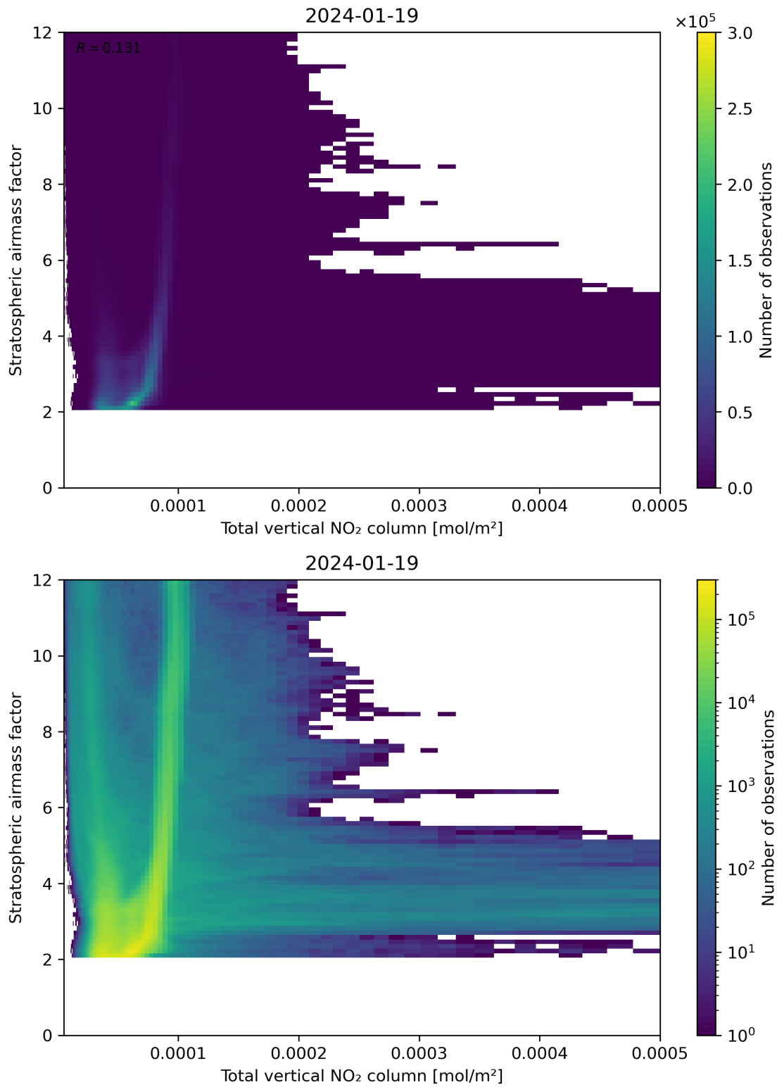
Figure 110: Scatter density plot of “Total vertical NO 2 column” against “Stratospheric airmass factor” for 2024-01-18 to 2024-01-20.
