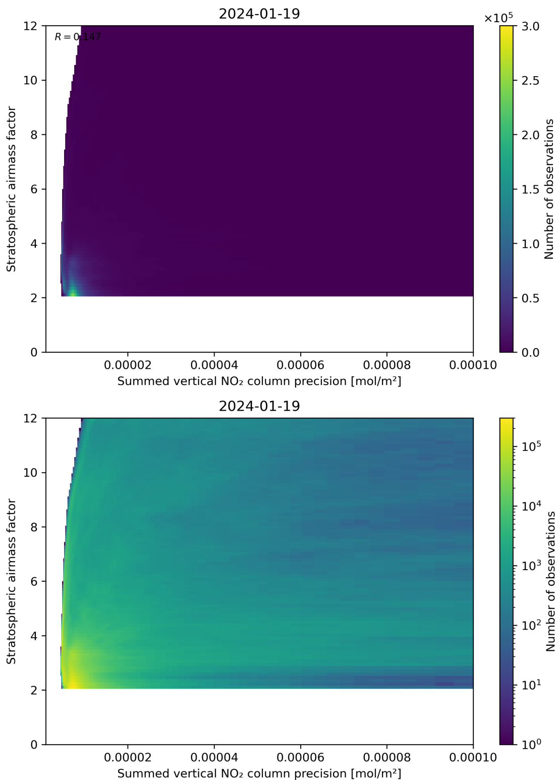
Figure 106: Scatter density plot of “Summed vertical NO 2 column precision” against “Stratospheric airmass factor” for 2024-01-18 to 2024-01-20.
