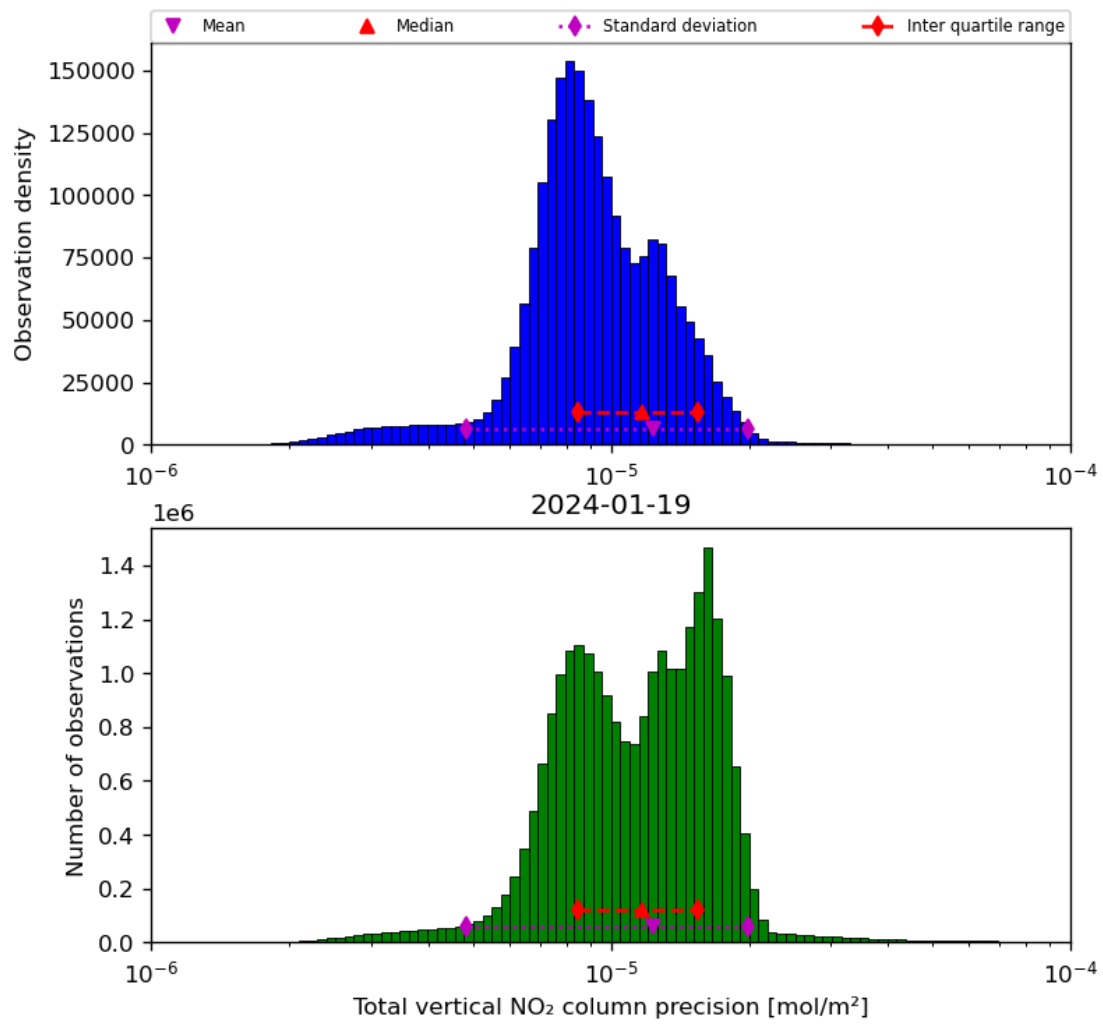
Figure 39: Histogram of “Total vertical NO 2 column precision” for 2024-01-18 to 2024-01-20
