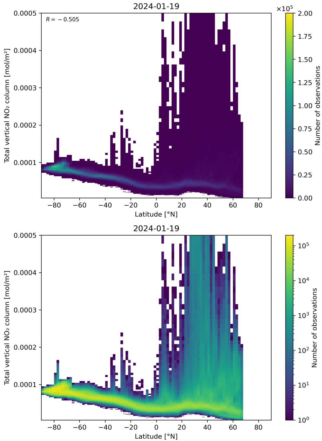
Figure 90: Scatter density plot of “Latitude” against “Total vertical NO 2 column” for 2024-01-18 to 2024-01-20.
