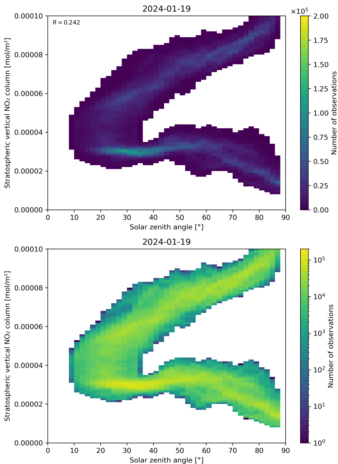
Figure 150: Scatter density plot of “Solar zenith angle” against “Stratospheric vertical NO 2 column” for 2024-01-18 to 2024-01-20.
