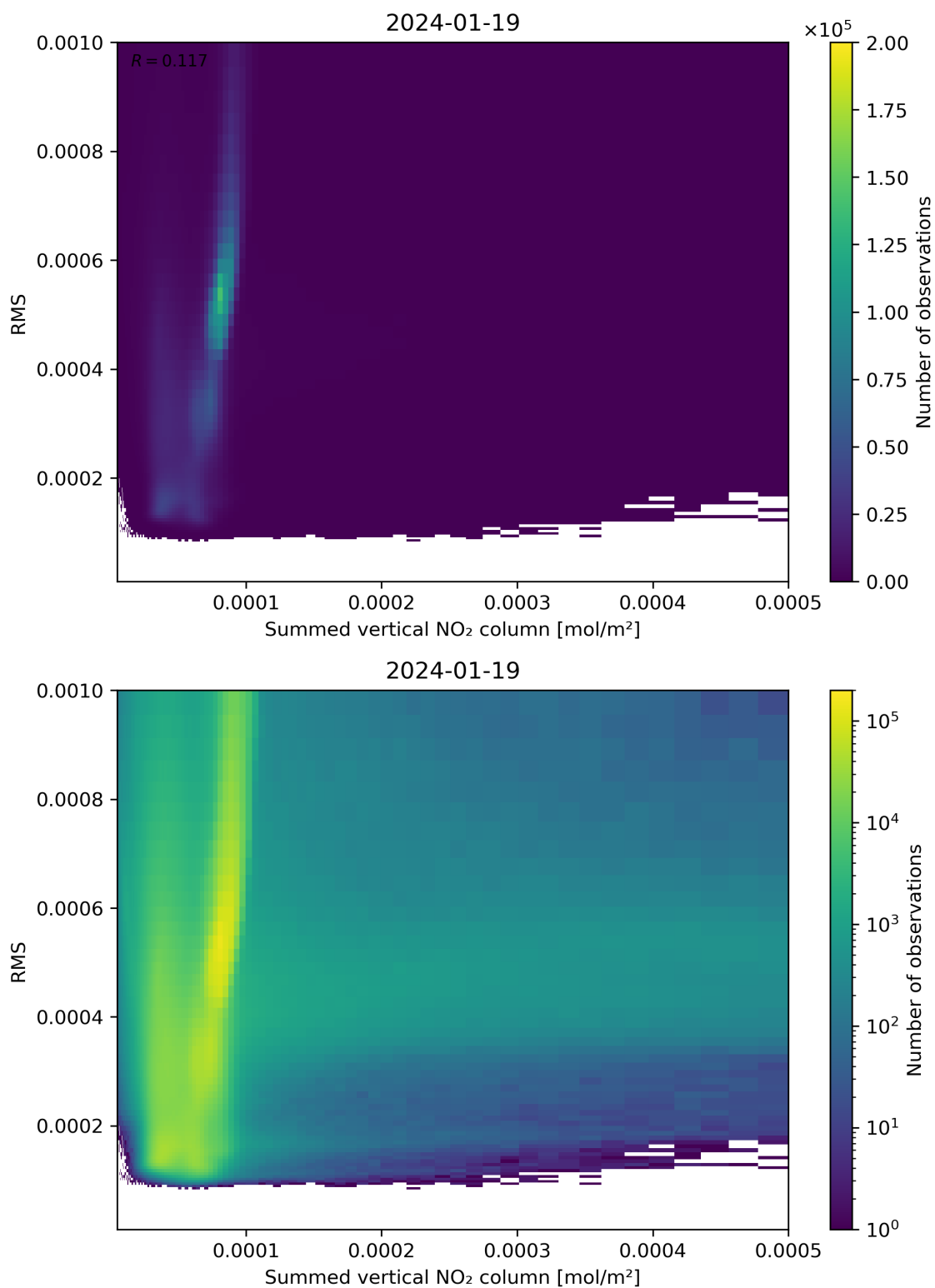
Figure 109: Scatter density plot of “Summed vertical NO 2 column” against “RMS” for 2024-01-18 to 2024-01-20.
