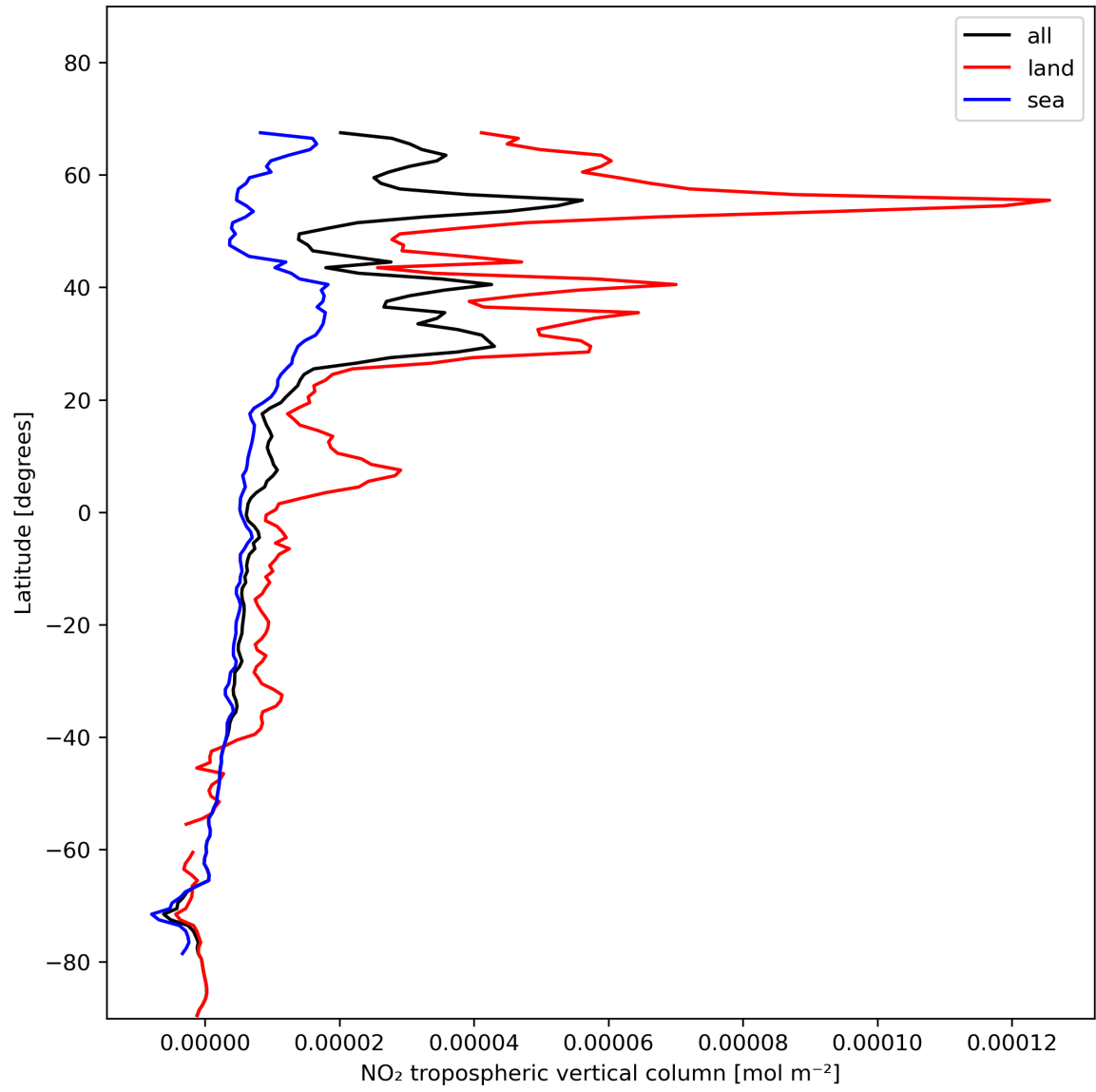
Figure 12: Zonal average of “NO 2 tropospheric vertical column” for 2024-01-18 to 2024-01-20.
