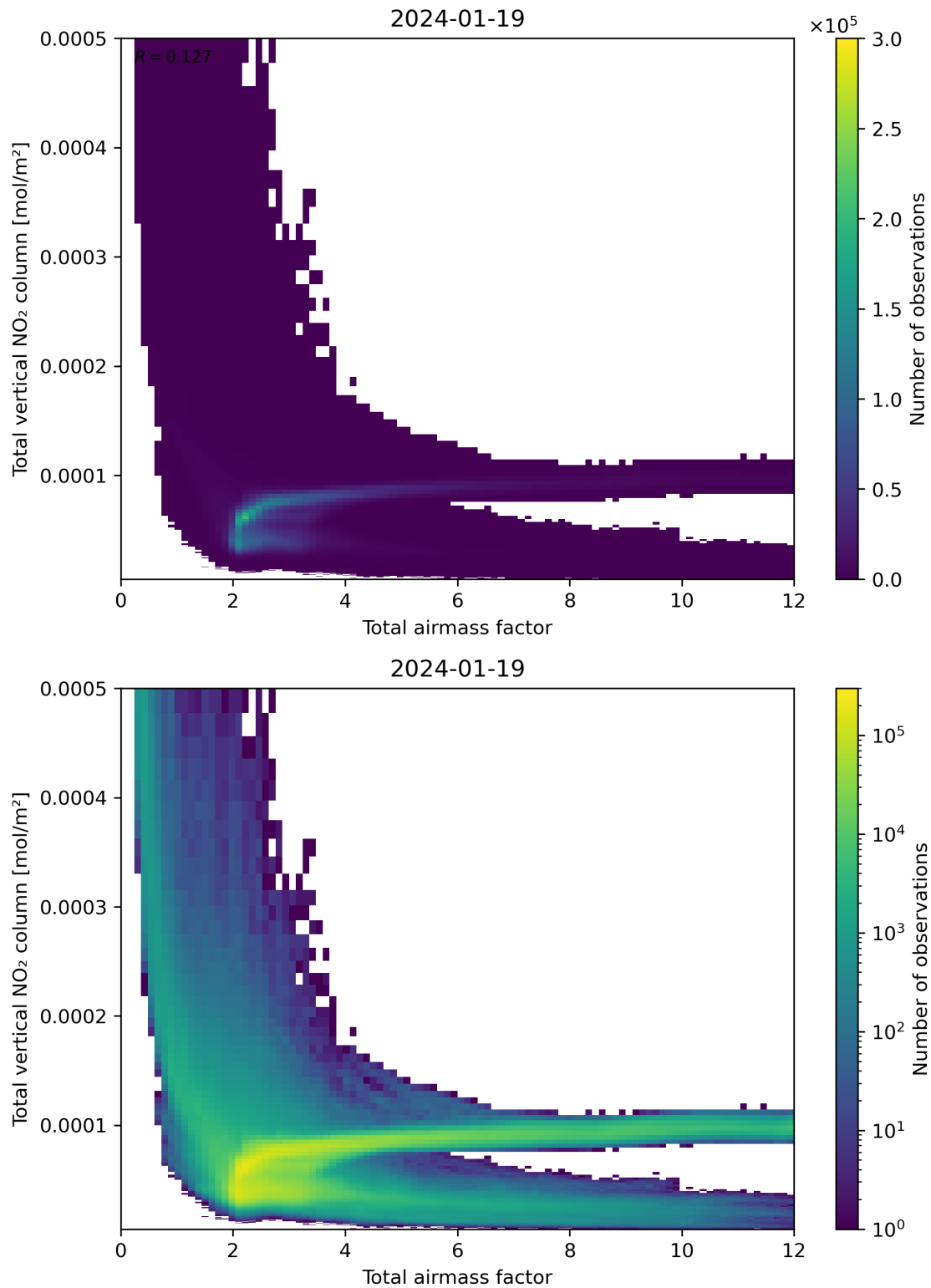
Figure 67: Scatter density plot of “Total airmass factor” against “Total vertical NO 2 column” for 2024-01-18 to 2024-01-20.
