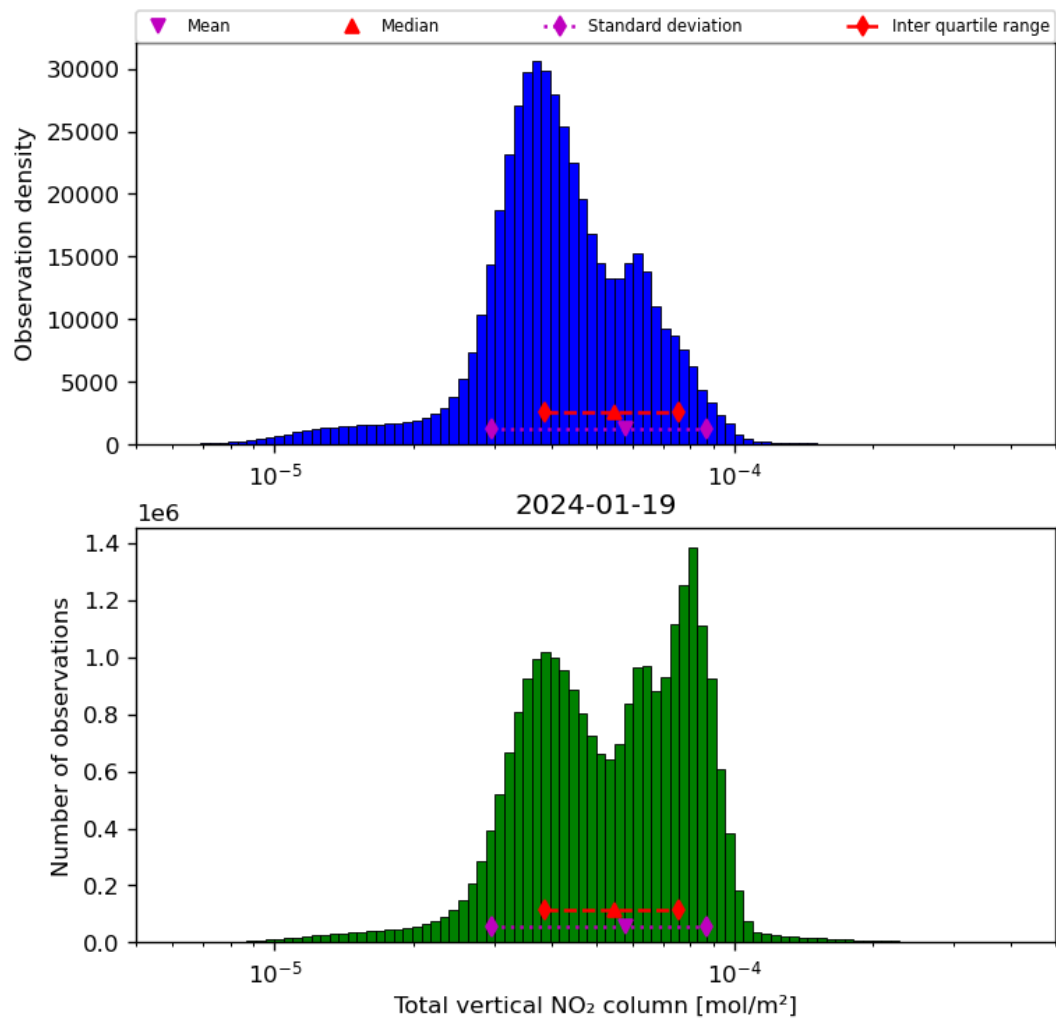
Figure 38: Histogram of “Total vertical NO 2 column” for 2024-01-18 to 2024-01-20
