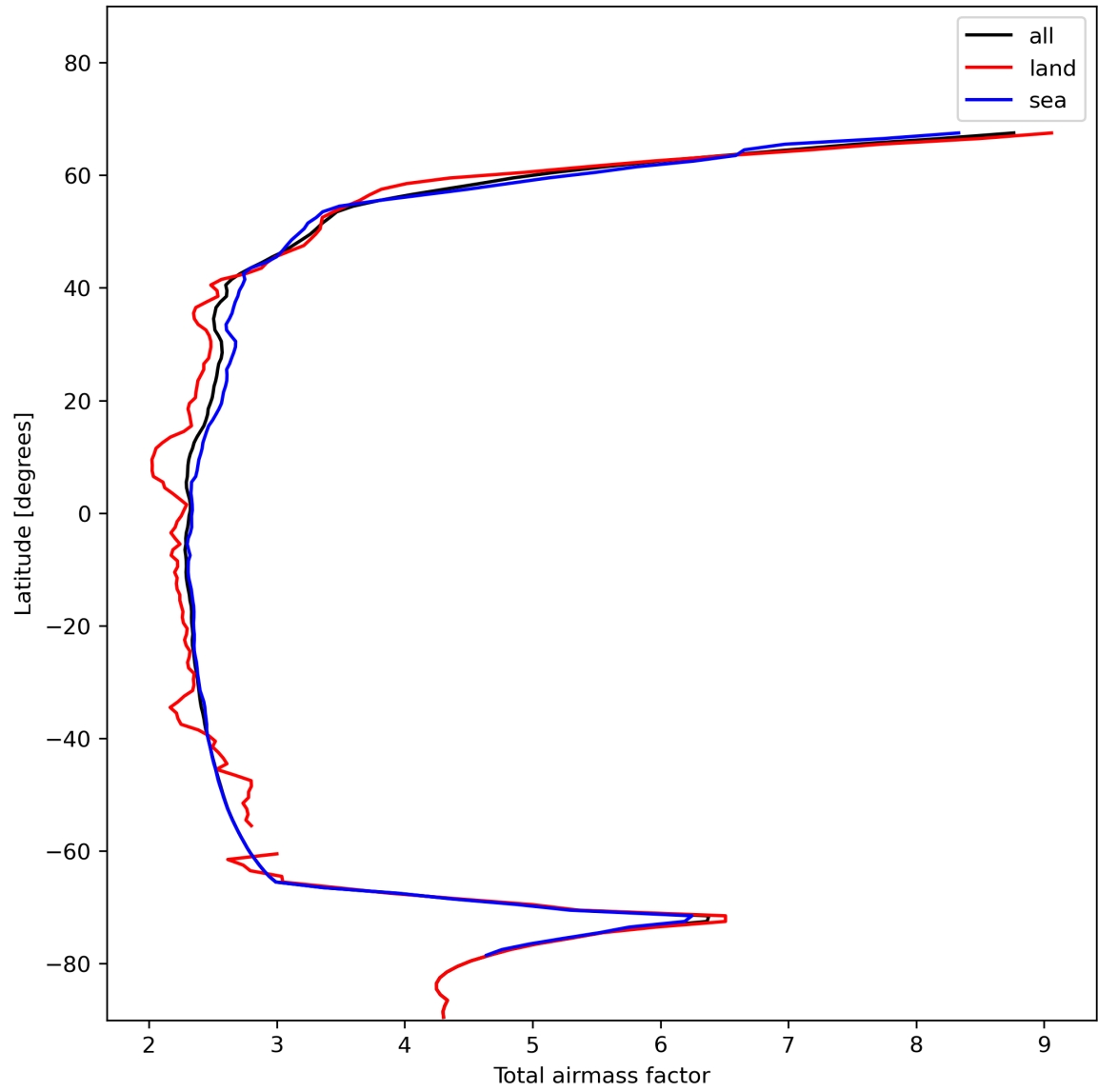
Figure 15: Zonal average of “Total airmass factor” for 2024-01-18 to 2024-01-20.
