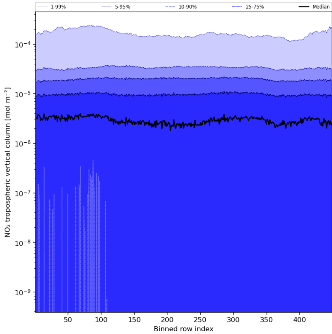
Figure 46: Along track statistics of “ \text{NO}_2 tropospheric vertical column” for 2024-01-18 to 2024-01-20
