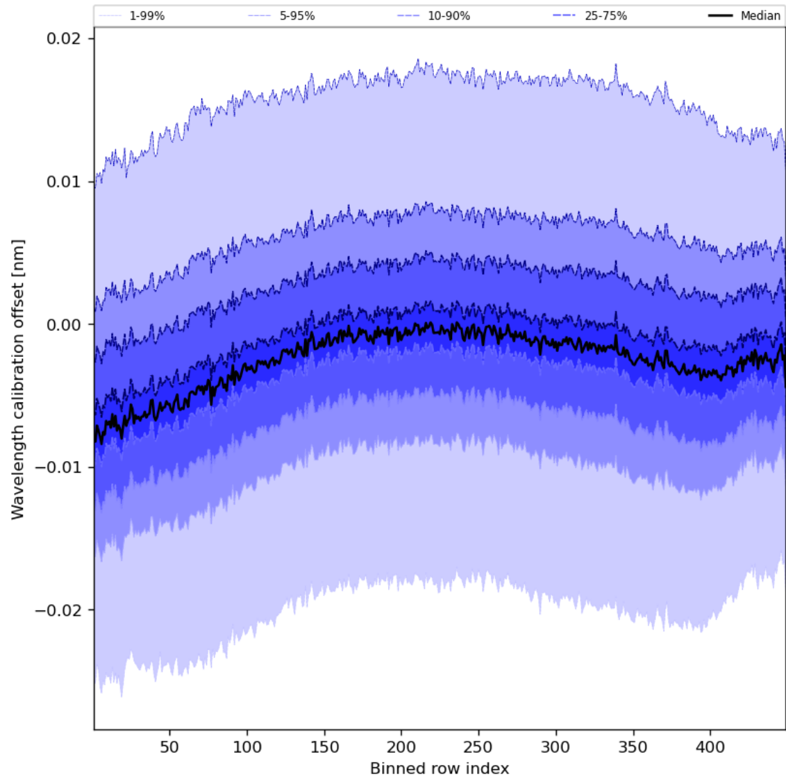
Figure 52: Along track statistics of “Wavelength calibration offset” for 2024-01-18 to 2024-01-20
