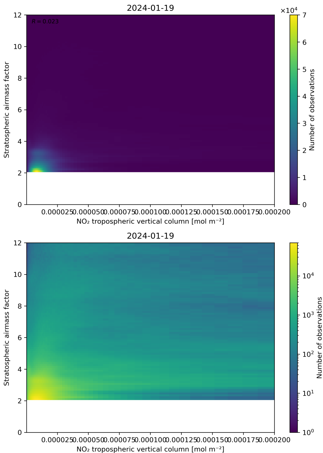
Figure 121: Scatter density plot of “NO 2 tropospheric vertical column” against “Stratospheric airmass factor” for 2024-01-18 to 2024-01-20.
