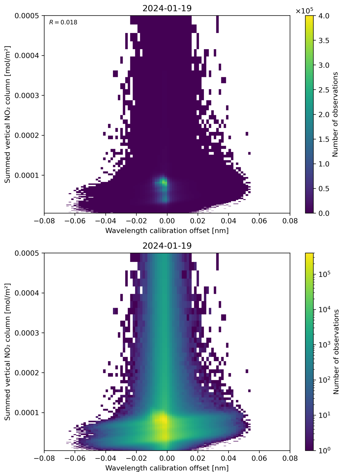
Figure 177: Scatter density plot of “Wavelength calibration offset” against “Summed vertical NO 2 column” for 2024-01-18 to 2024-01-20.
