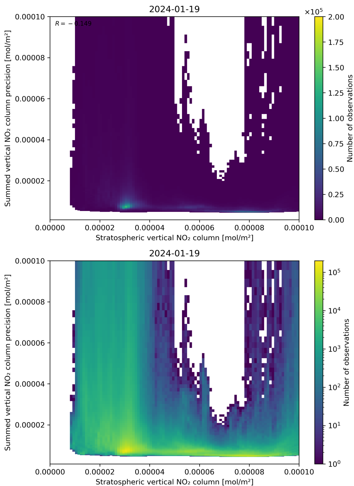
Figure 99: Scatter density plot of “Stratospheric vertical NO 2 column” against “Summed vertical NO 2 column precision” for 2024-01-18 to 2024-01-20.
