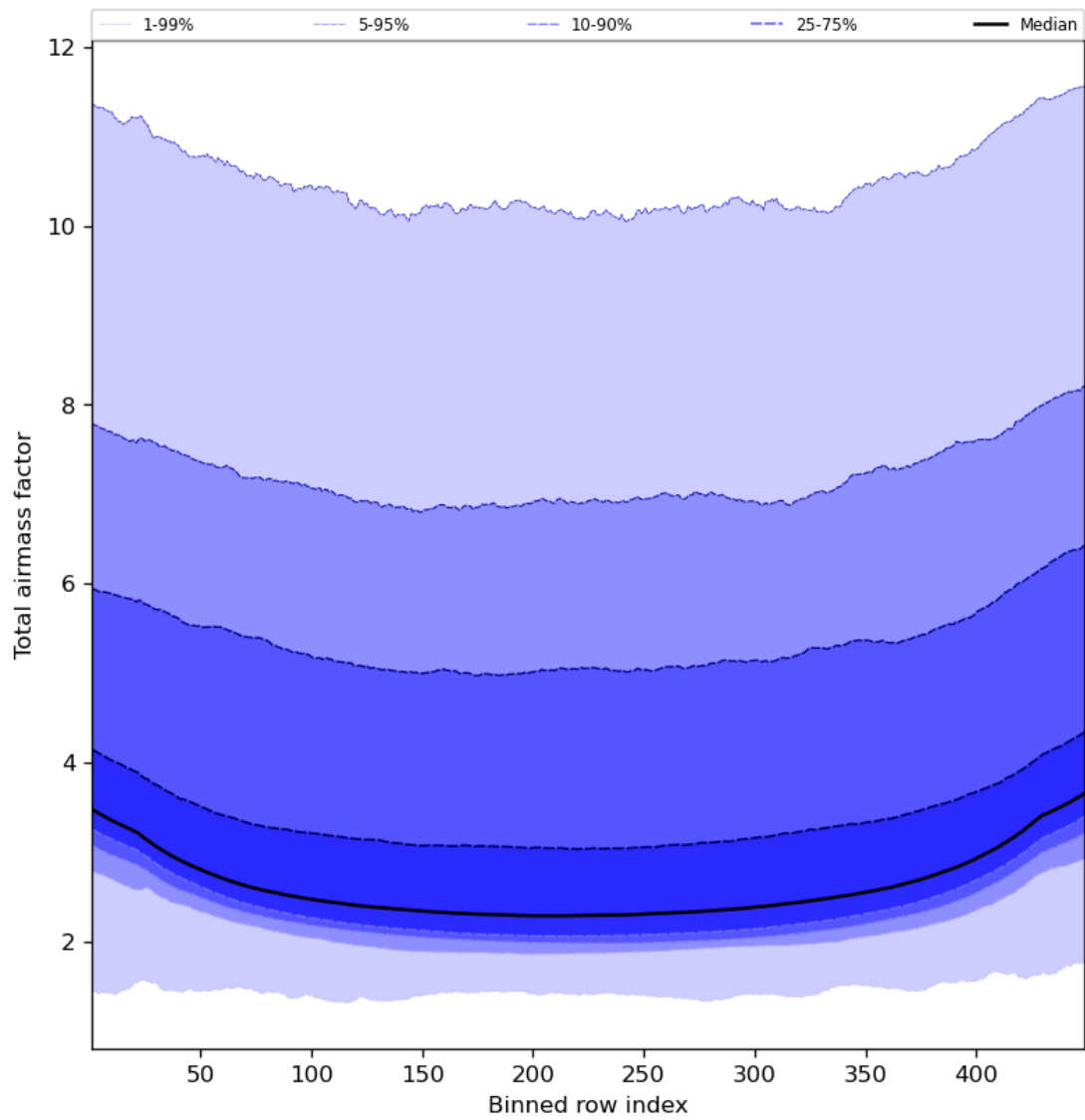
Figure 49: Along track statistics of “Total airmass factor” for 2024-01-18 to 2024-01-20
