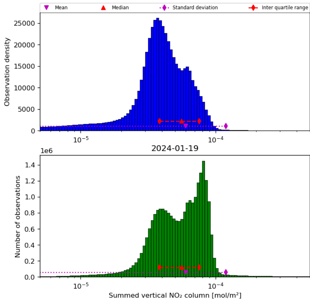
Figure 40: Histogram of “Summed vertical NO 2 column” for 2024-01-18 to 2024-01-20
