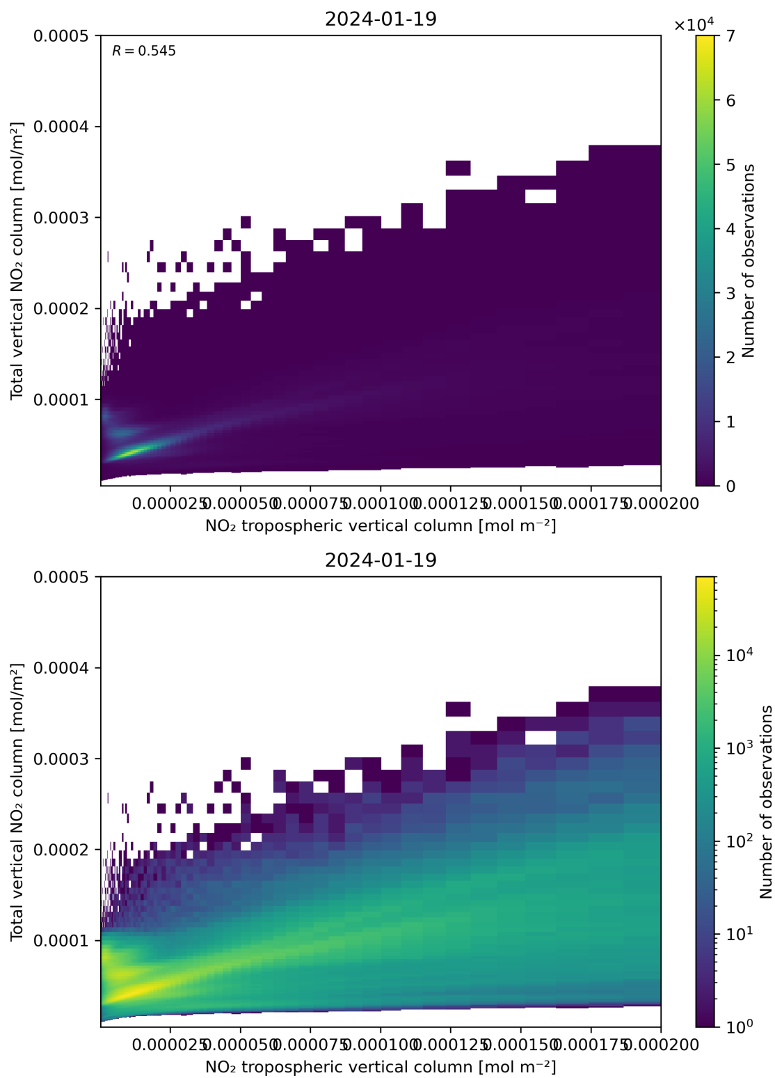
Figure 128: Scatter density plot of “NO 2 tropospheric vertical column” against “Total vertical NO 2 column” for 2024-01-18 to 2024-01-20.
