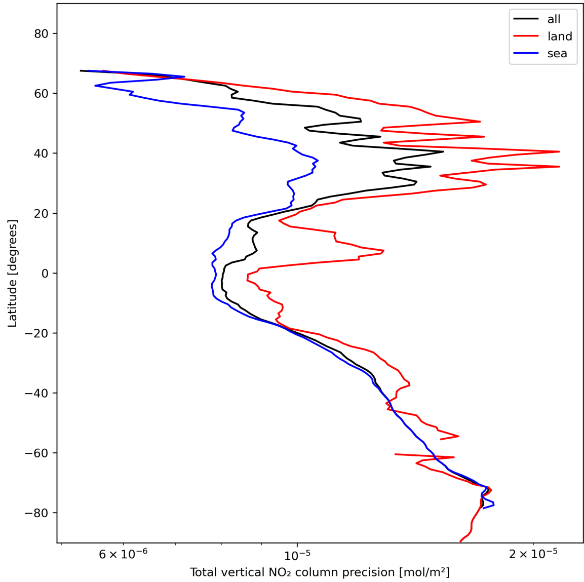
Figure 22: Zonal average of “Total vertical NO 2 column precision” for 2024-01-18 to 2024-01-20.
