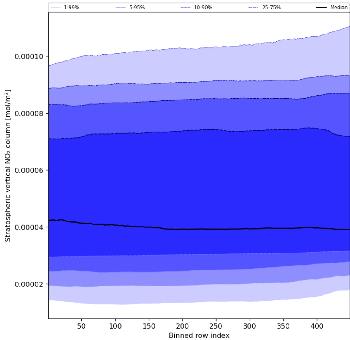
Figure 53: Along track statistics of “Stratospheric vertical NO 2 column” for 2024-01-18 to 2024-01-20
