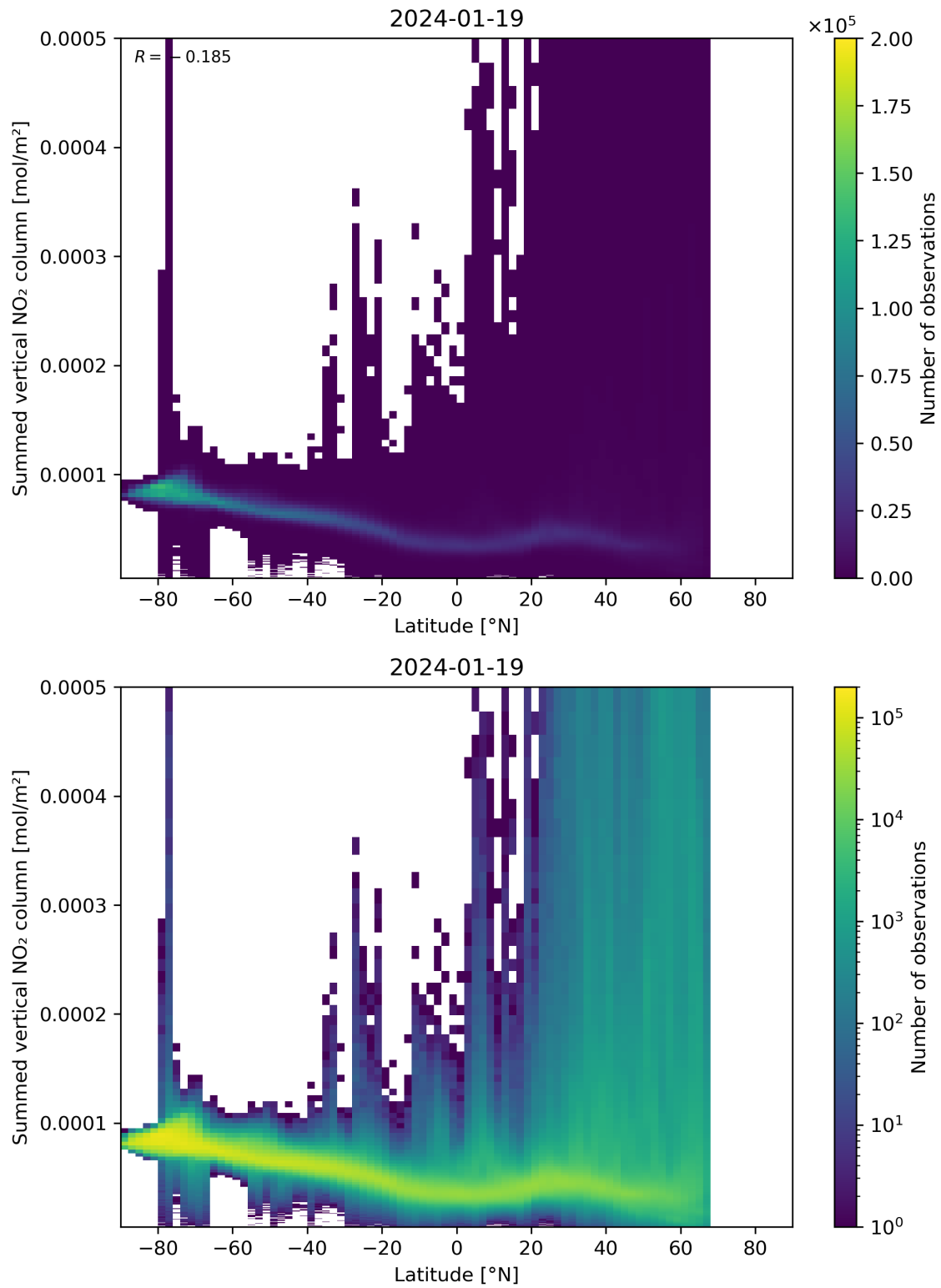
Figure 88: Scatter density plot of “Latitude” against “Summed vertical NO 2 column” for 2024-01-18 to 2024-01-20.
