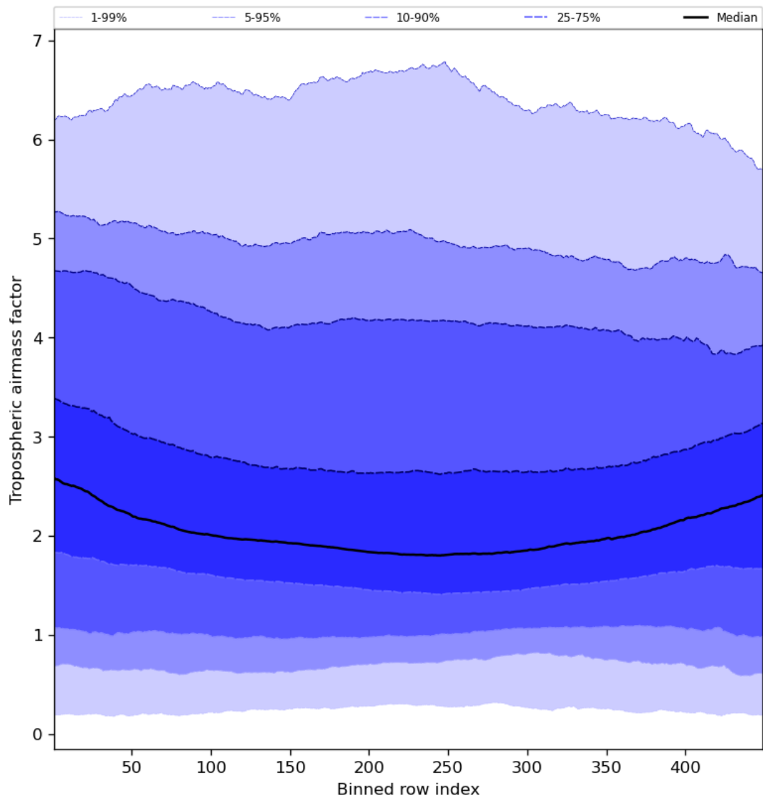
Figure 48: Along track statistics of “Tropospheric airmass factor” for 2024-01-18 to 2024-01-20
