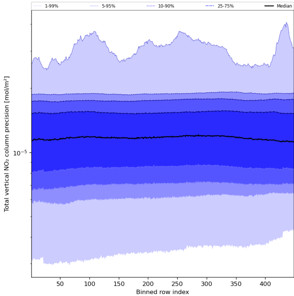
Figure 56: Along track statistics of “Total vertical NO 2 column precision” for 2024-01-18 to 2024-01-20
