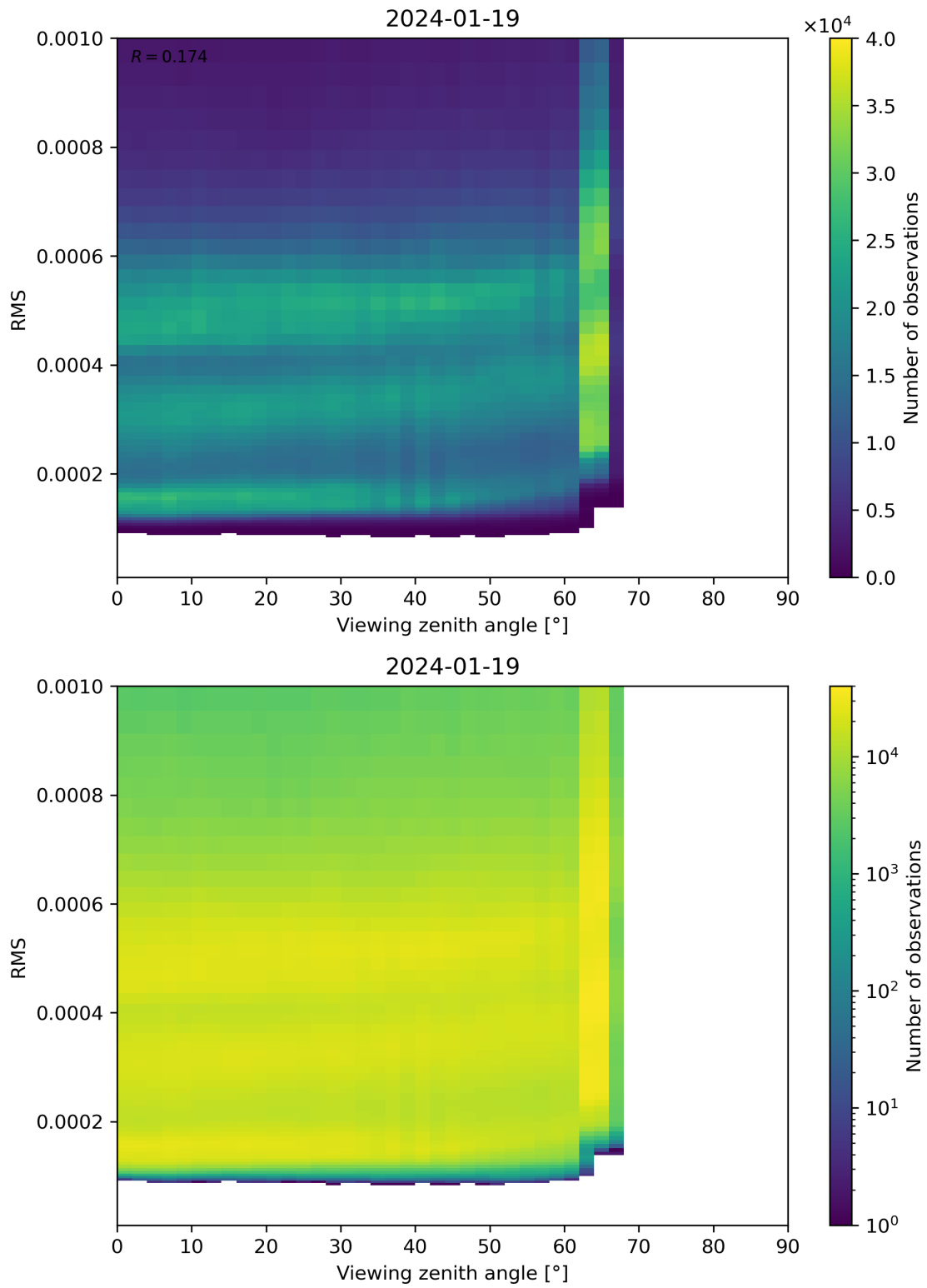
Figure 171: Scatter density plot of “Viewing zenith angle” against “RMS” for 2024-01-18 to 2024-01-20.
