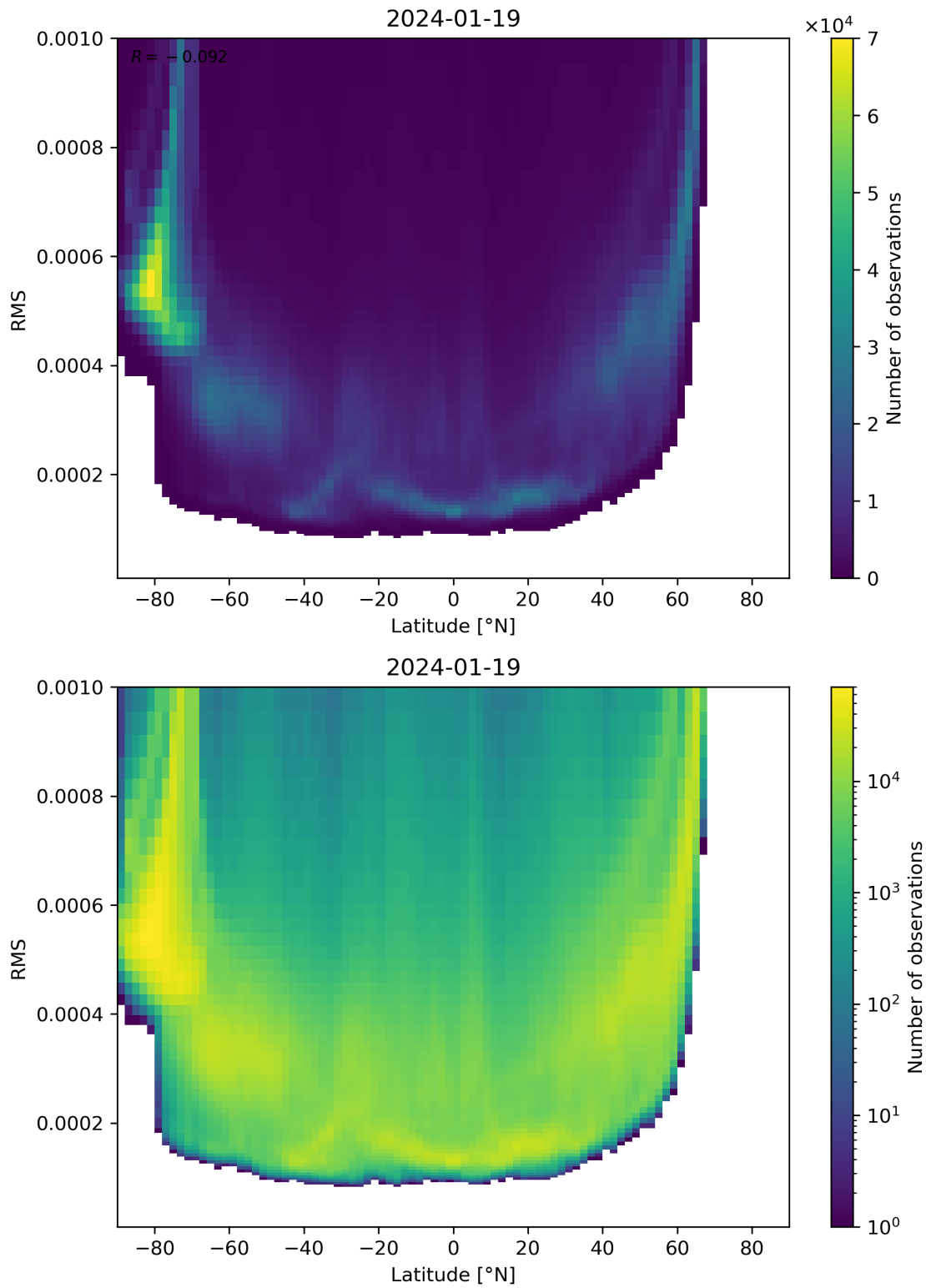
Figure 94: Scatter density plot of “Latitude” against “RMS” for 2024-01-18 to 2024-01-20.
