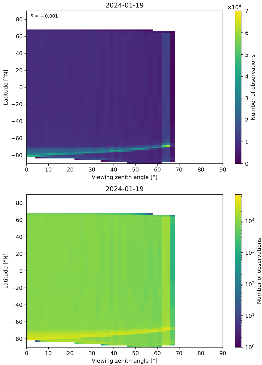
Figure 163: Scatter density plot of “Viewing zenith angle” against “Latitude” for 2024-01-18 to 2024-01-20.
