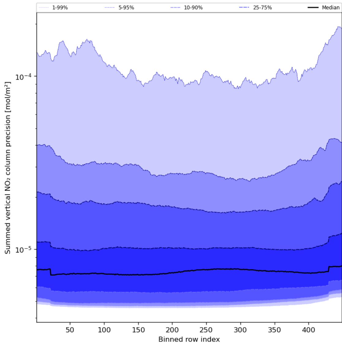
Figure 58: Along track statistics of “Summed vertical NO 2 column precision” for 2024-01-18 to 2024-01-20
