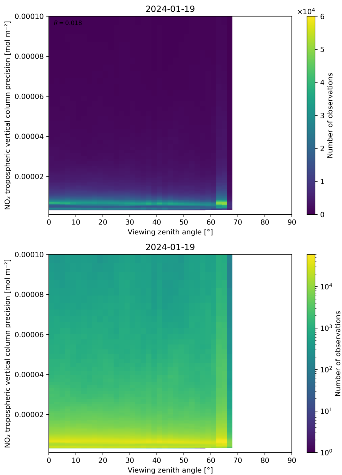
Figure 170: Scatter density plot of “Viewing zenith angle” against “NO 2 tropospheric vertical column precision” for 2024-01-18 to 2024-01-20.
