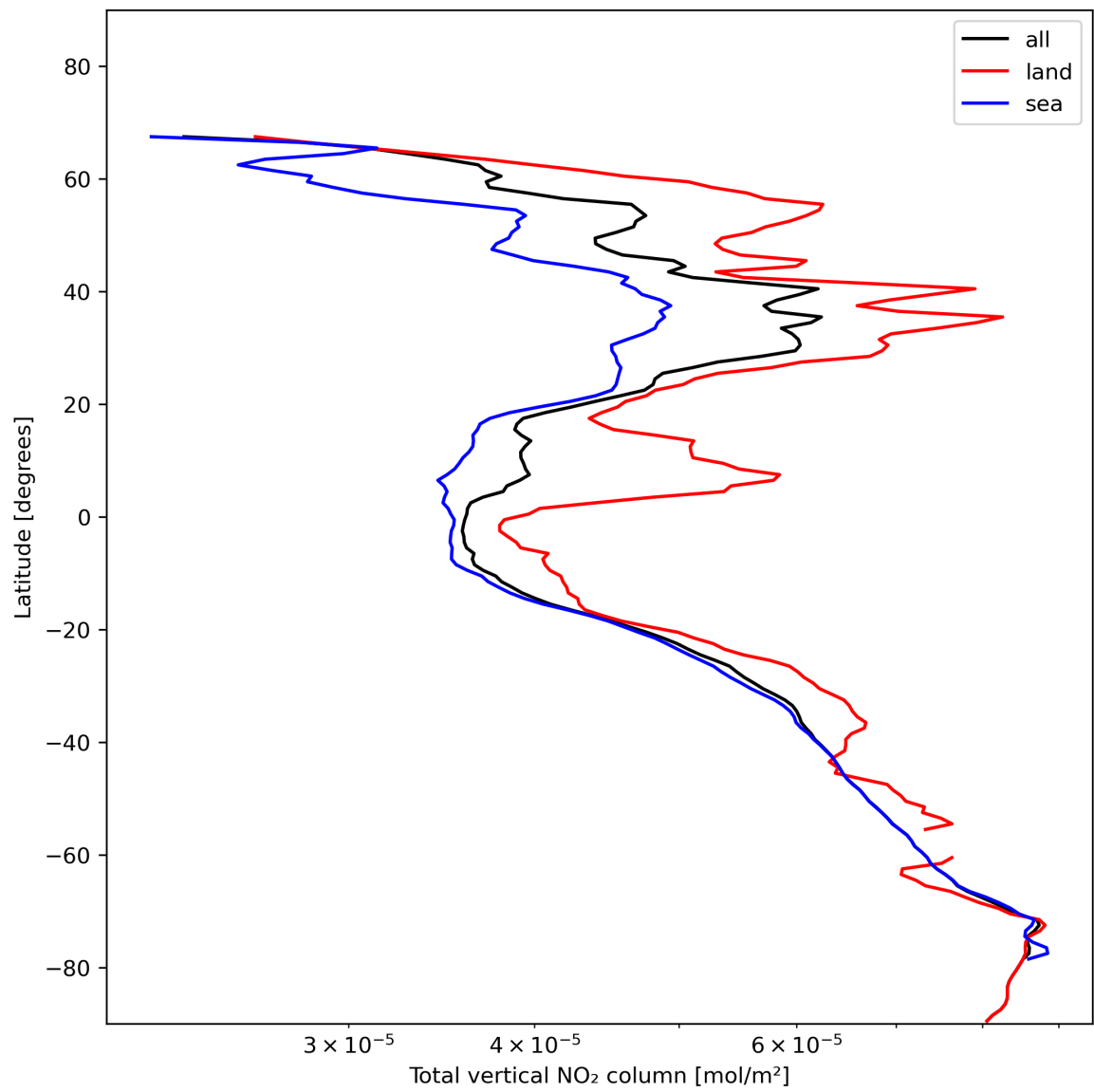
Figure 21: Zonal average of “Total vertical NO 2 column” for 2024-01-18 to 2024-01-20.
