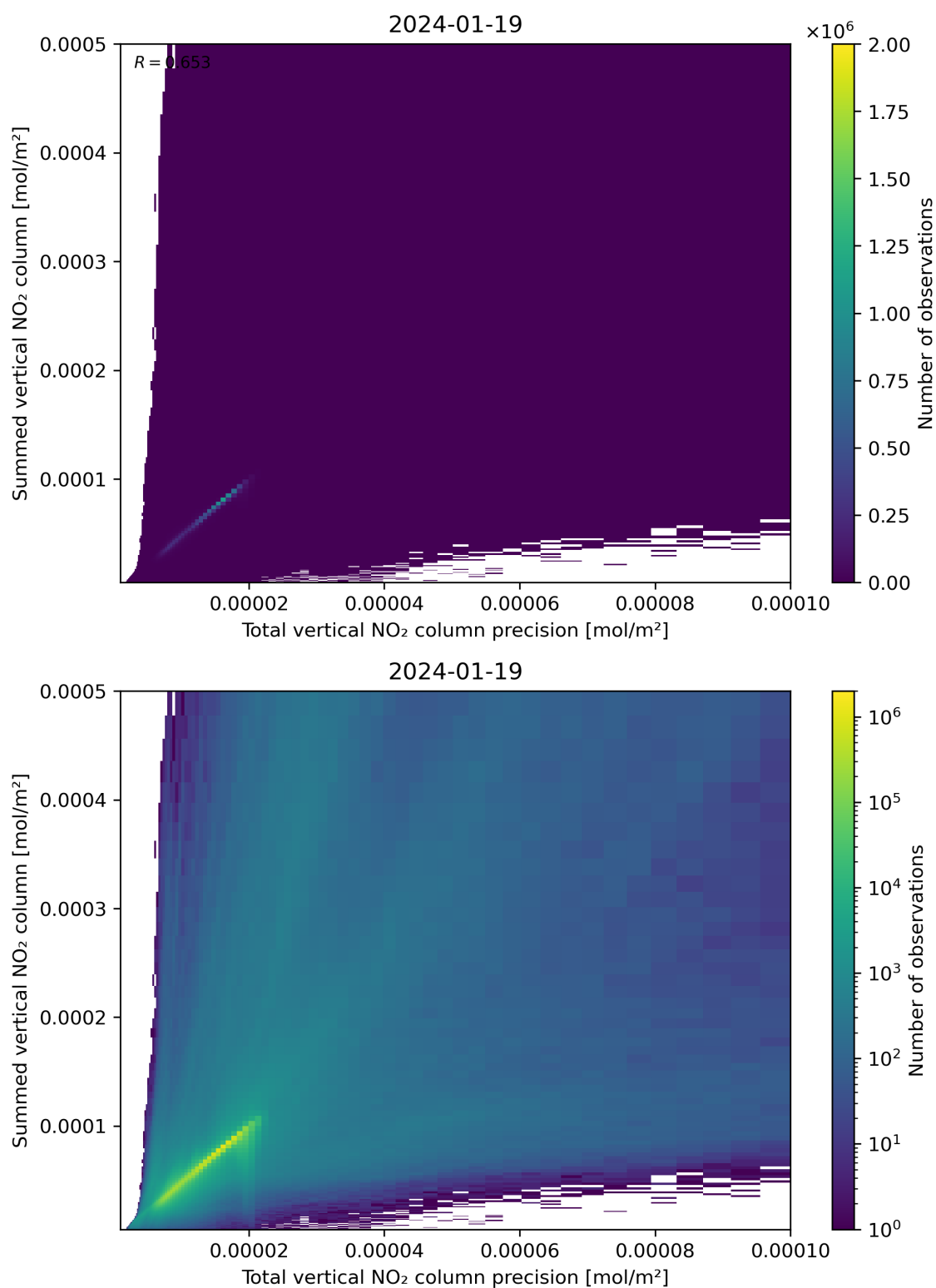
Figure 117: Scatter density plot of “Total vertical NO 2 column precision” against “Summed vertical NO 2 column” for 2024-01-18 to 2024-01-20.
