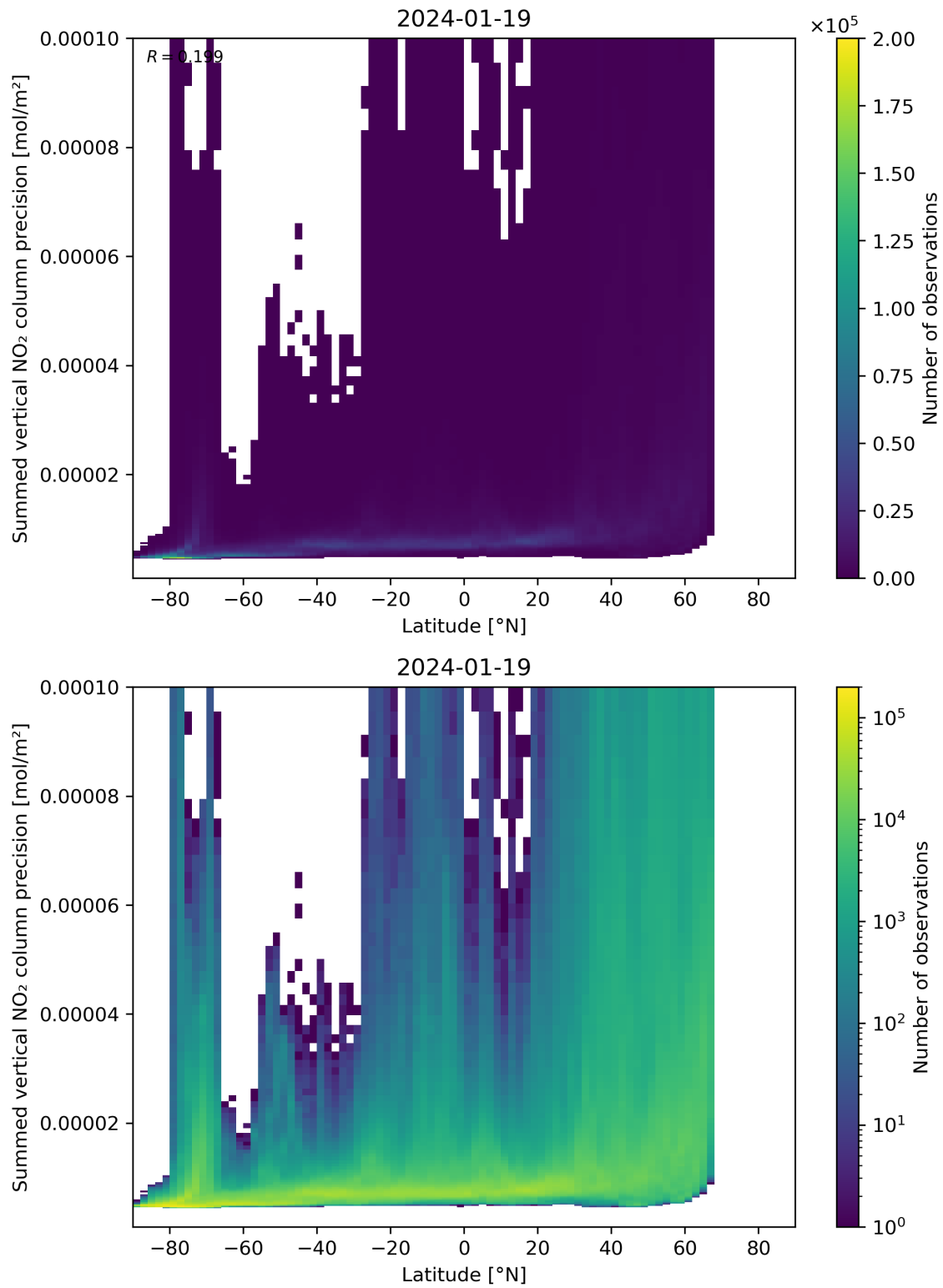
Figure 89: Scatter density plot of “Latitude” against “Summed vertical NO 2 column precision” for 2024-01-18 to 2024-01-20.
