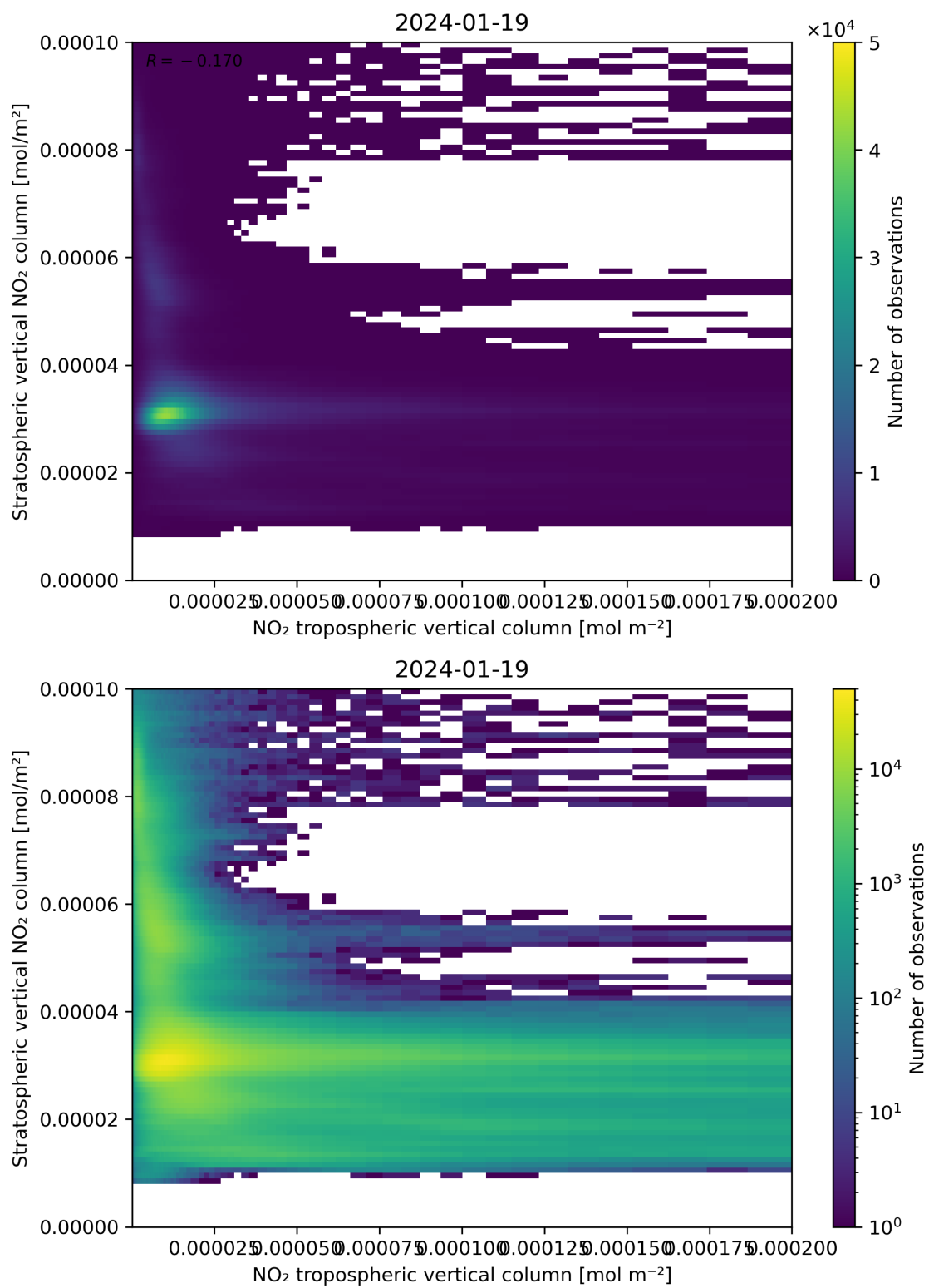
Figure 125: Scatter density plot of “NO 2 tropospheric vertical column” against “Stratospheric vertical NO 2 column” for 2024-01-18 to 2024-01-20.
