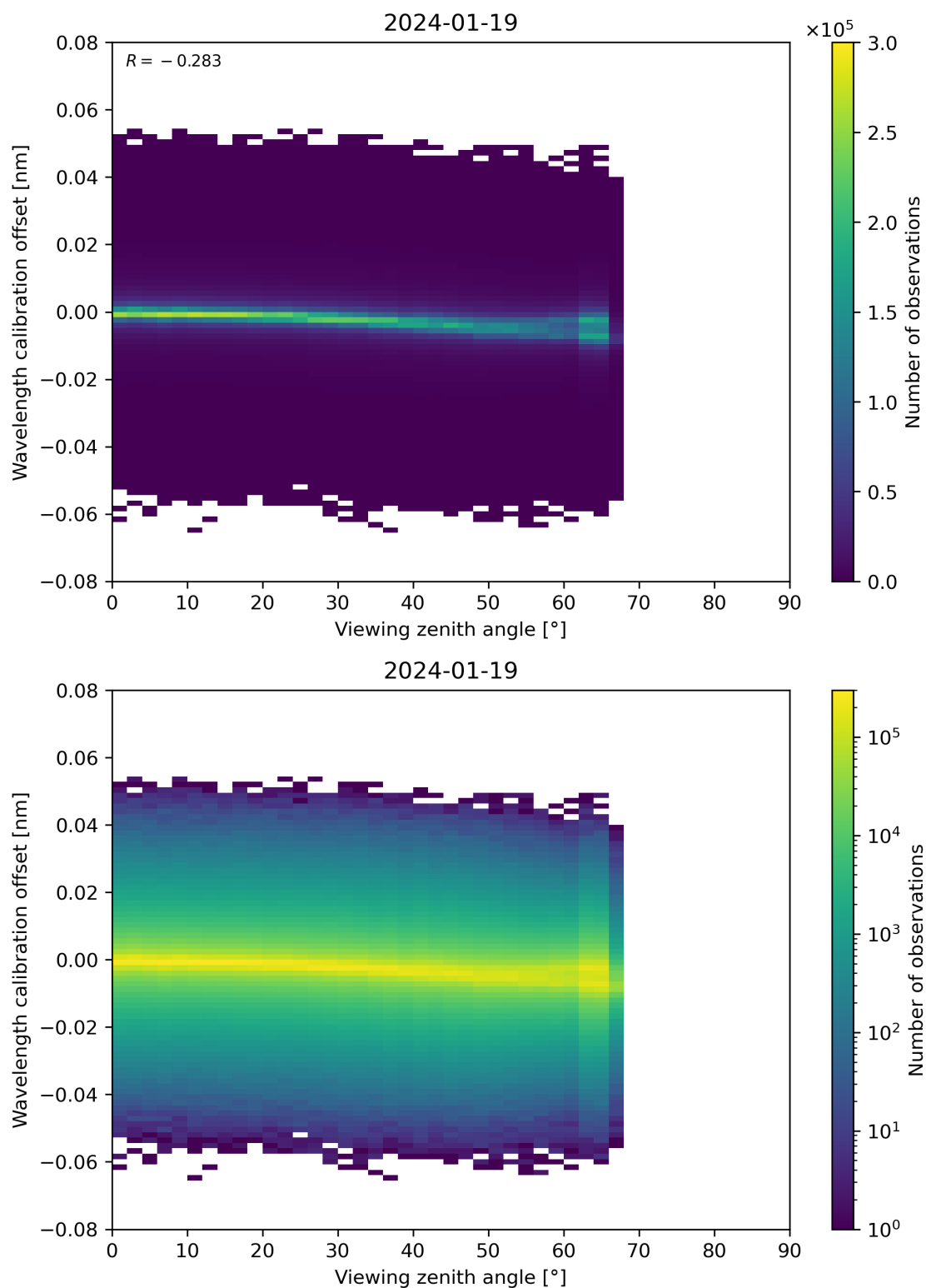
Figure 173: Scatter density plot of “Viewing zenith angle” against “Wavelength calibration offset” for 2024-01-18 to 2024-01-20.
