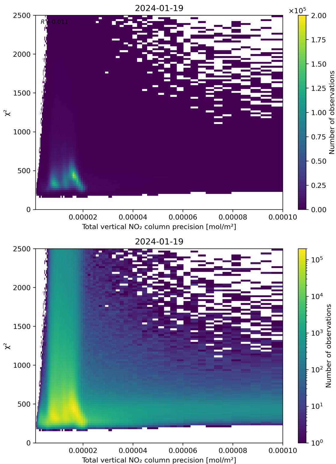
Figure 116: Scatter density plot of “Total vertical NO 2 column precision” against “ \chi^2 ” for 2024-01-18 to 2024-01-20.
