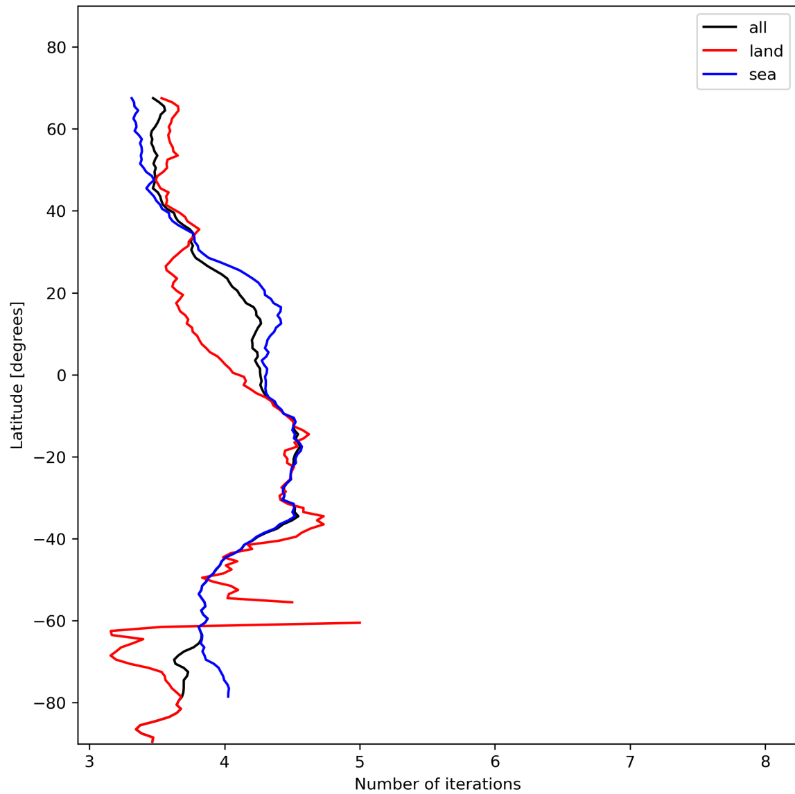
Figure 17: Zonal average of “Number of iterations” for 2024-01-18 to 2024-01-20.
