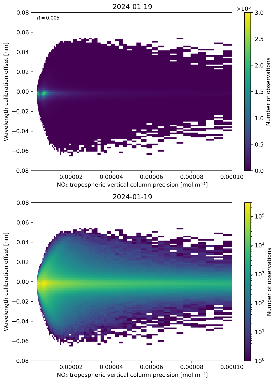
Figure 141: Scatter density plot of “NO 2 tropospheric vertical column precision” against “Wavelength calibration offset” for 2024-01-18 to 2024-01-20.
