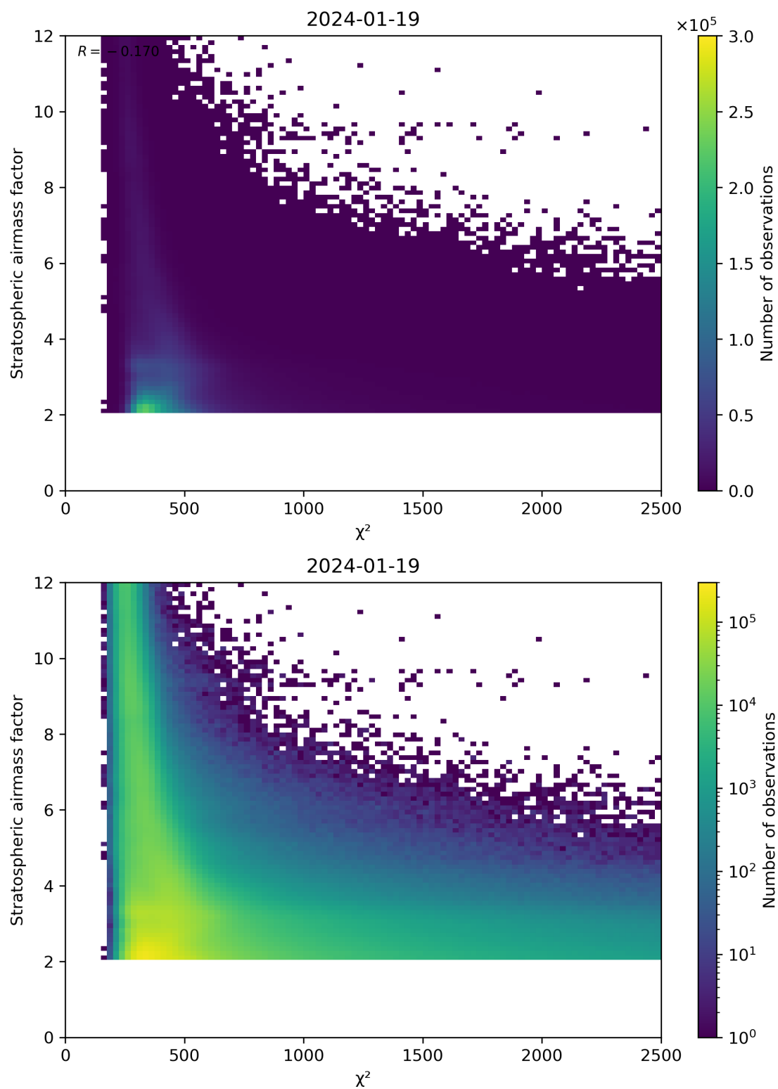
Figure 81: Scatter density plot of “ \chi^2 ” against “Stratospheric airmass factor” for 2024-01-18 to 2024-01-20.
