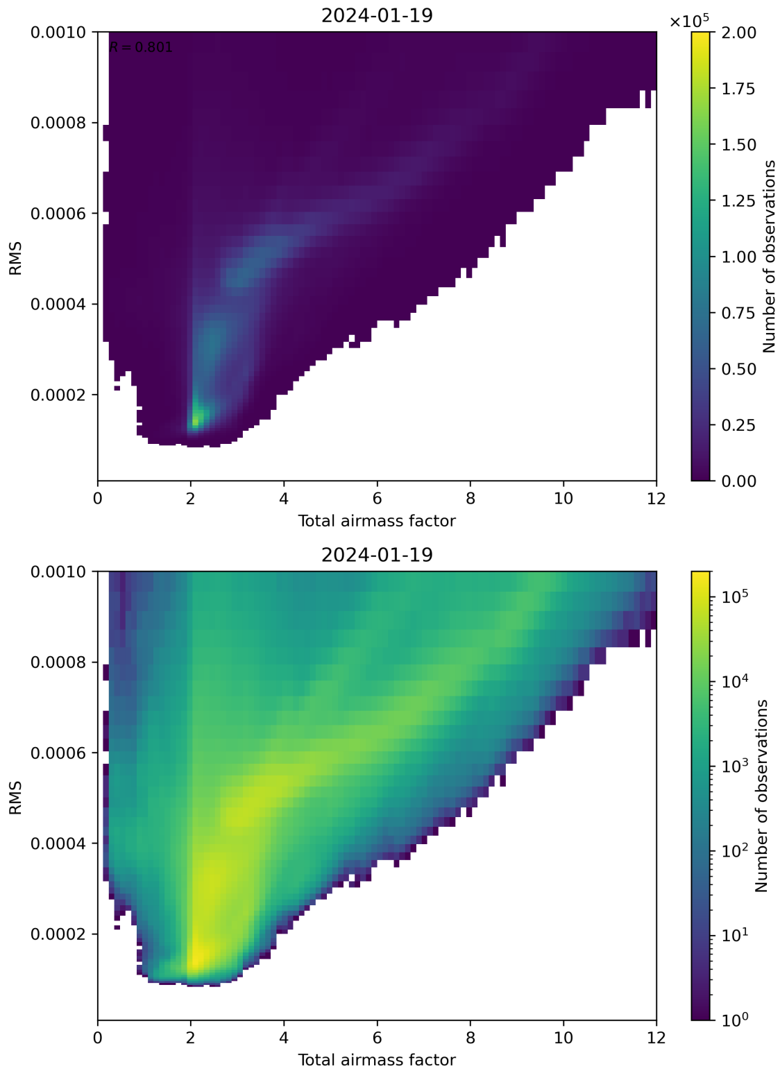
Figure 69: Scatter density plot of “Total airmass factor” against “RMS” for 2024-01-18 to 2024-01-20.
