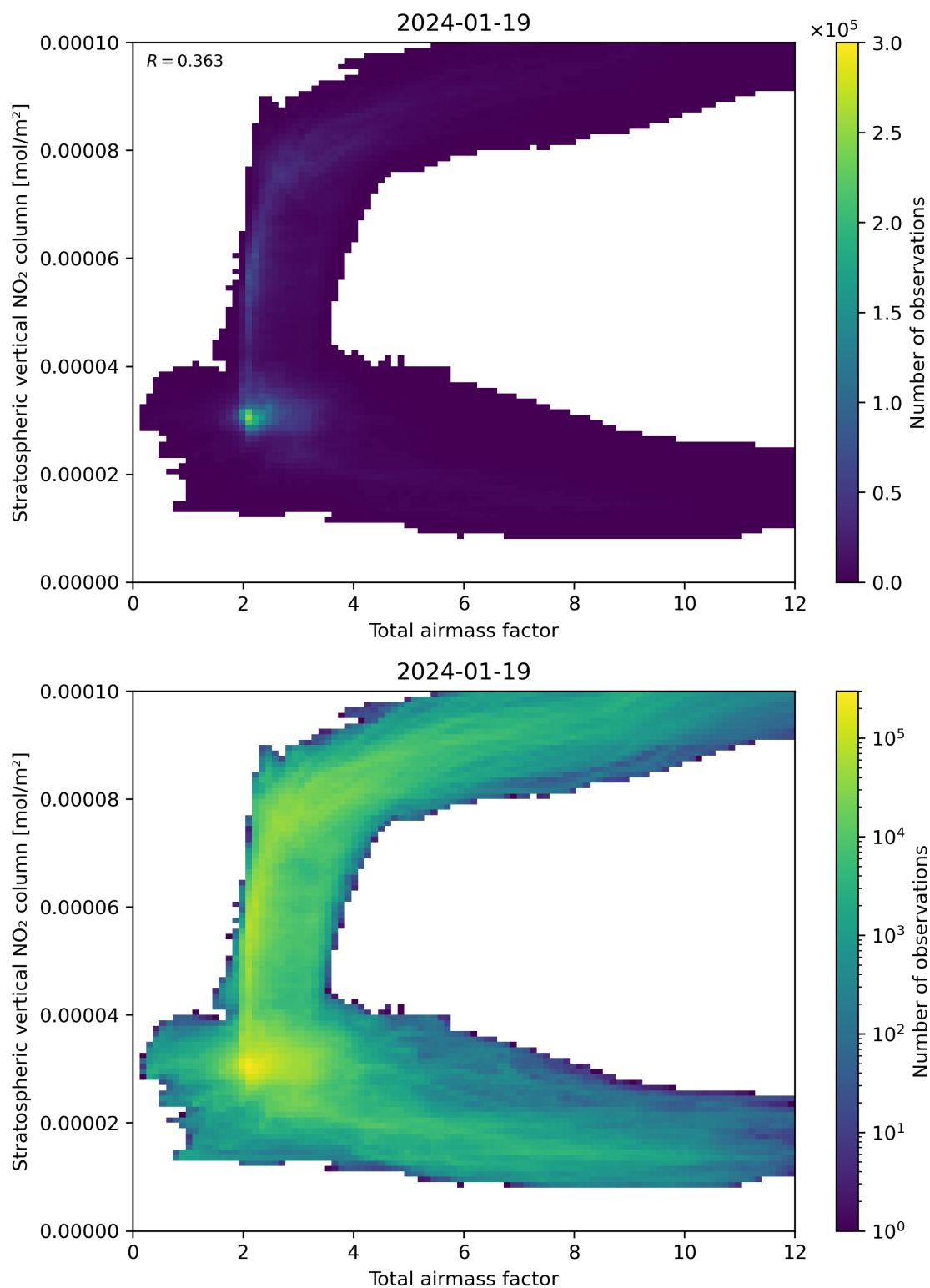
Figure 64: Scatter density plot of “Total airmass factor” against “Stratospheric vertical NO 2 column” for 2024-01-18 to 2024-01-20.
