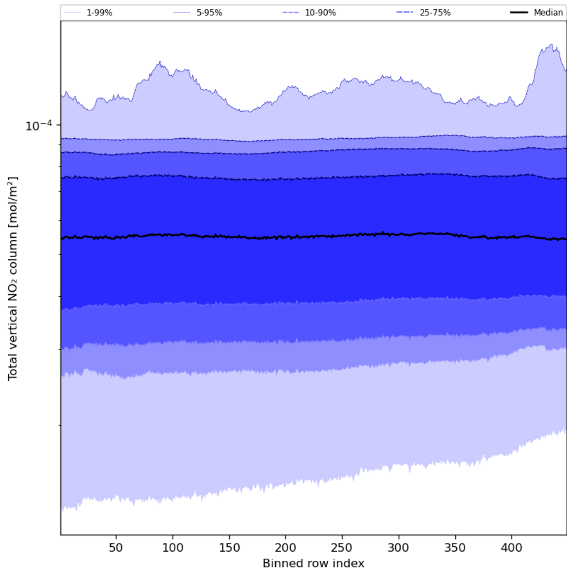
Figure 55: Along track statistics of “Total vertical NO 2 column” for 2024-01-18 to 2024-01-20
