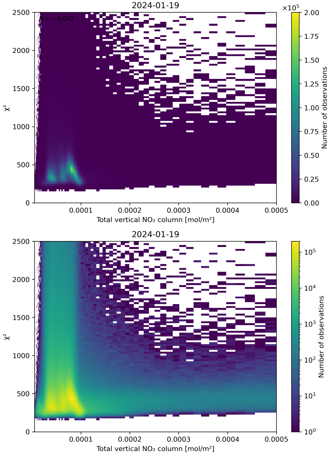
Figure 111: Scatter density plot of “Total vertical NO 2 column” against “ \chi^2 ” for 2024-01-18 to 2024-01-20.
