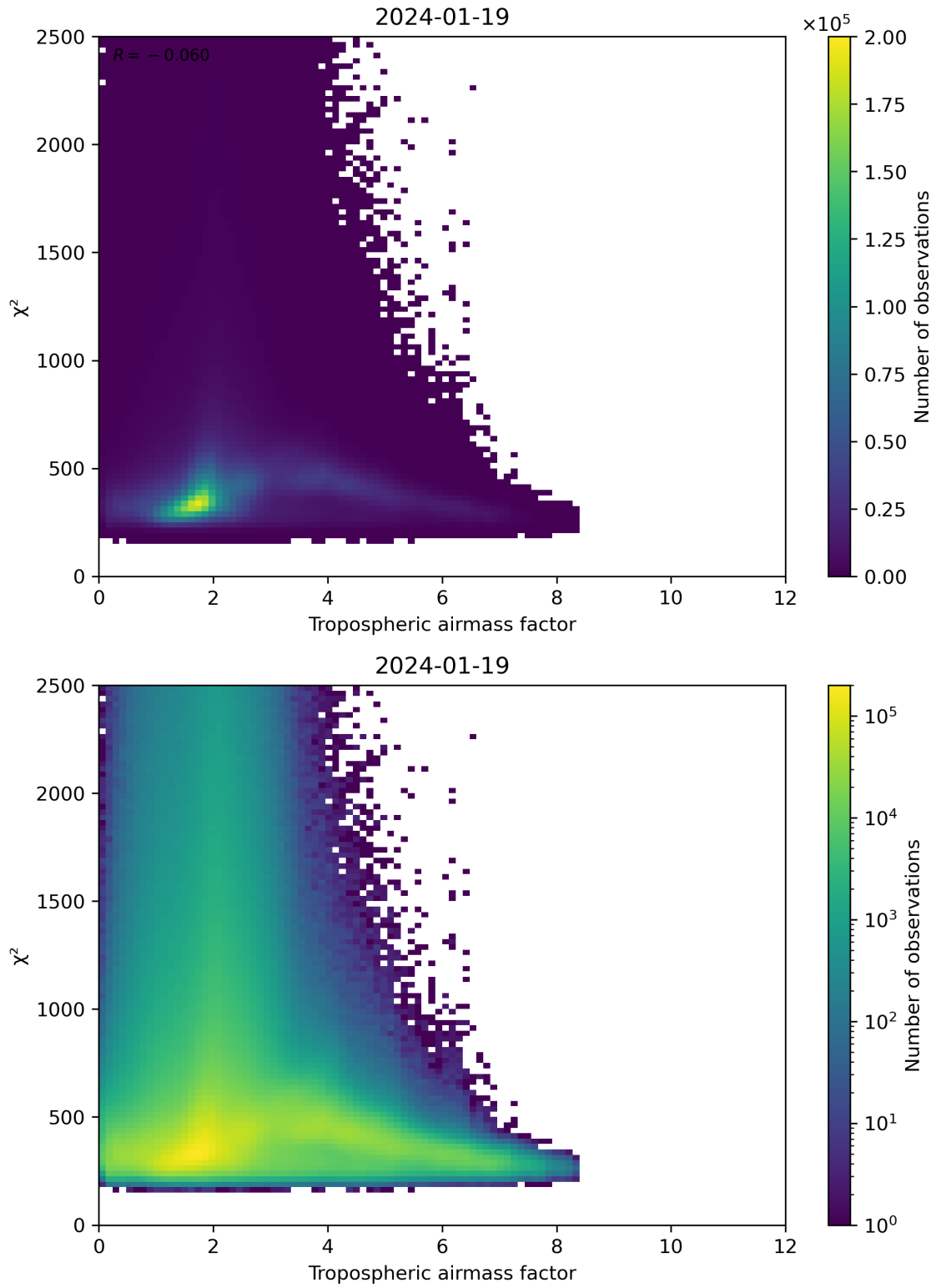
Figure 73: Scatter density plot of “Tropospheric airmass factor” against “ \chi^2 ” for 2024-01-18 to 2024-01-20.
