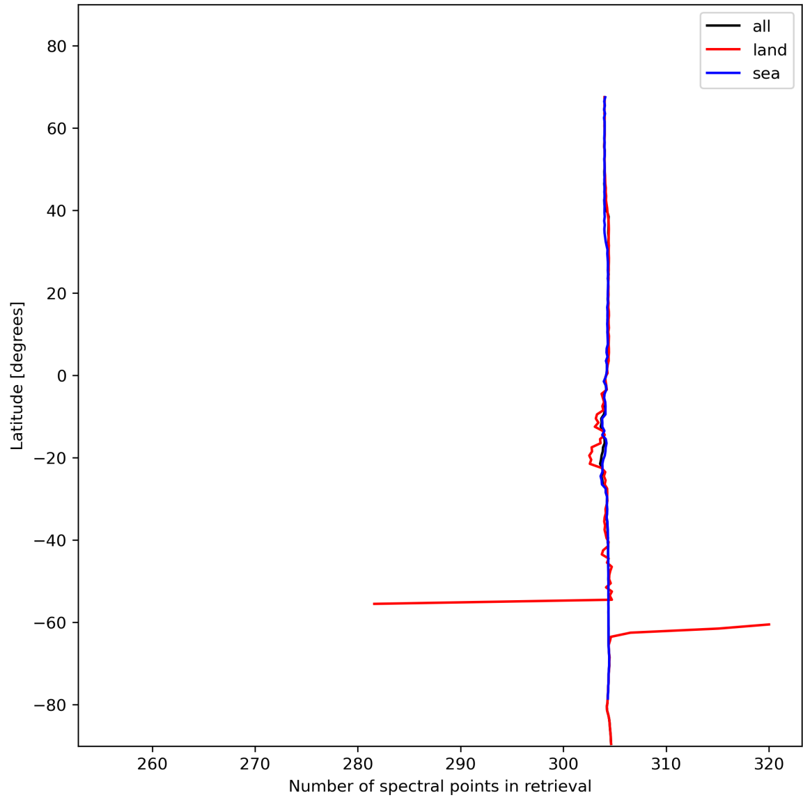
Figure 16: Zonal average of “Number of spectral points in retrieval” for 2024-01-18 to 2024-01-20.
