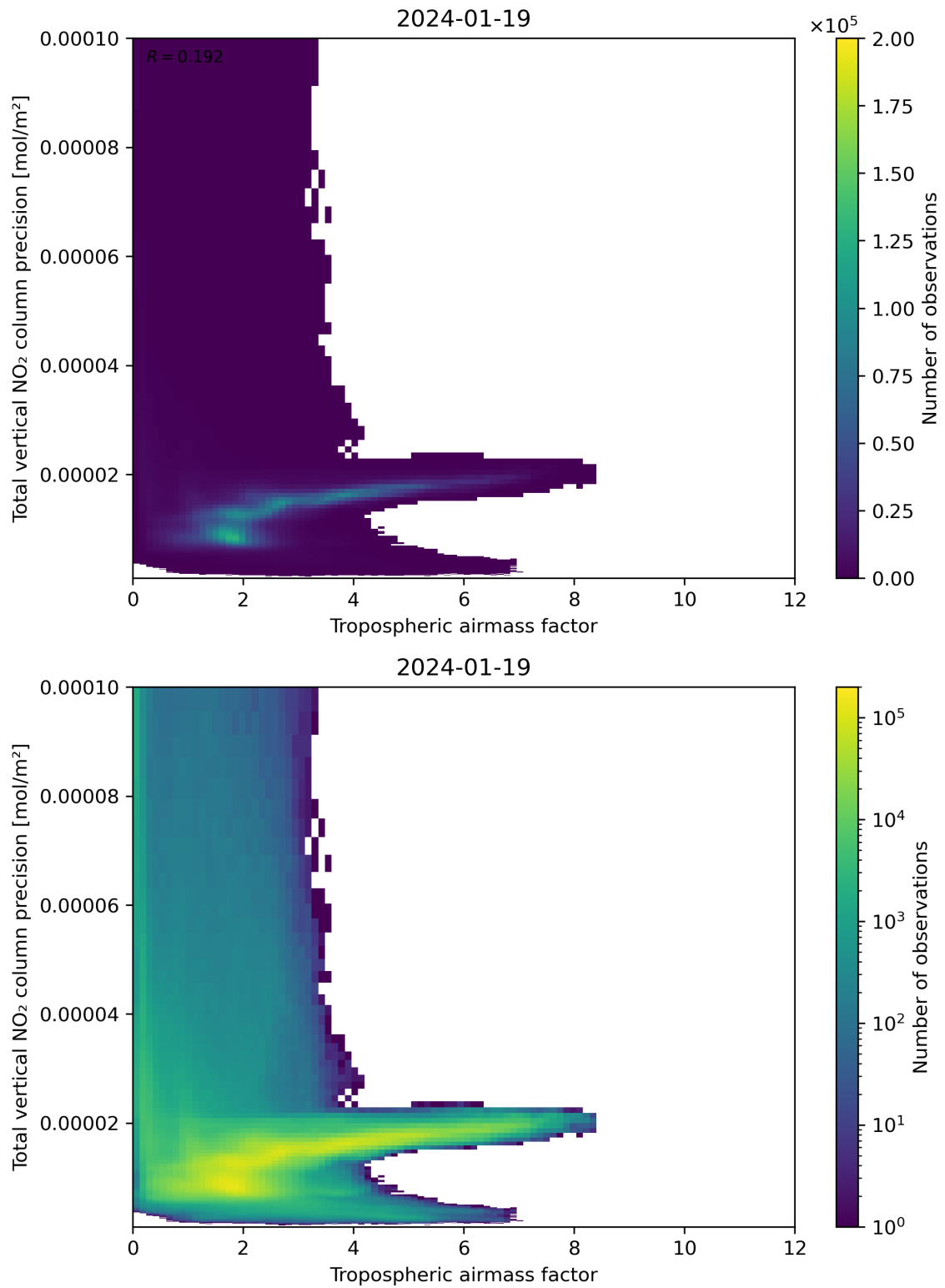
Figure 78: Scatter density plot of “Tropospheric air mass factor” against “Total vertical NO 2 column precision” for 2024-01-18 to 2024-01-20.
