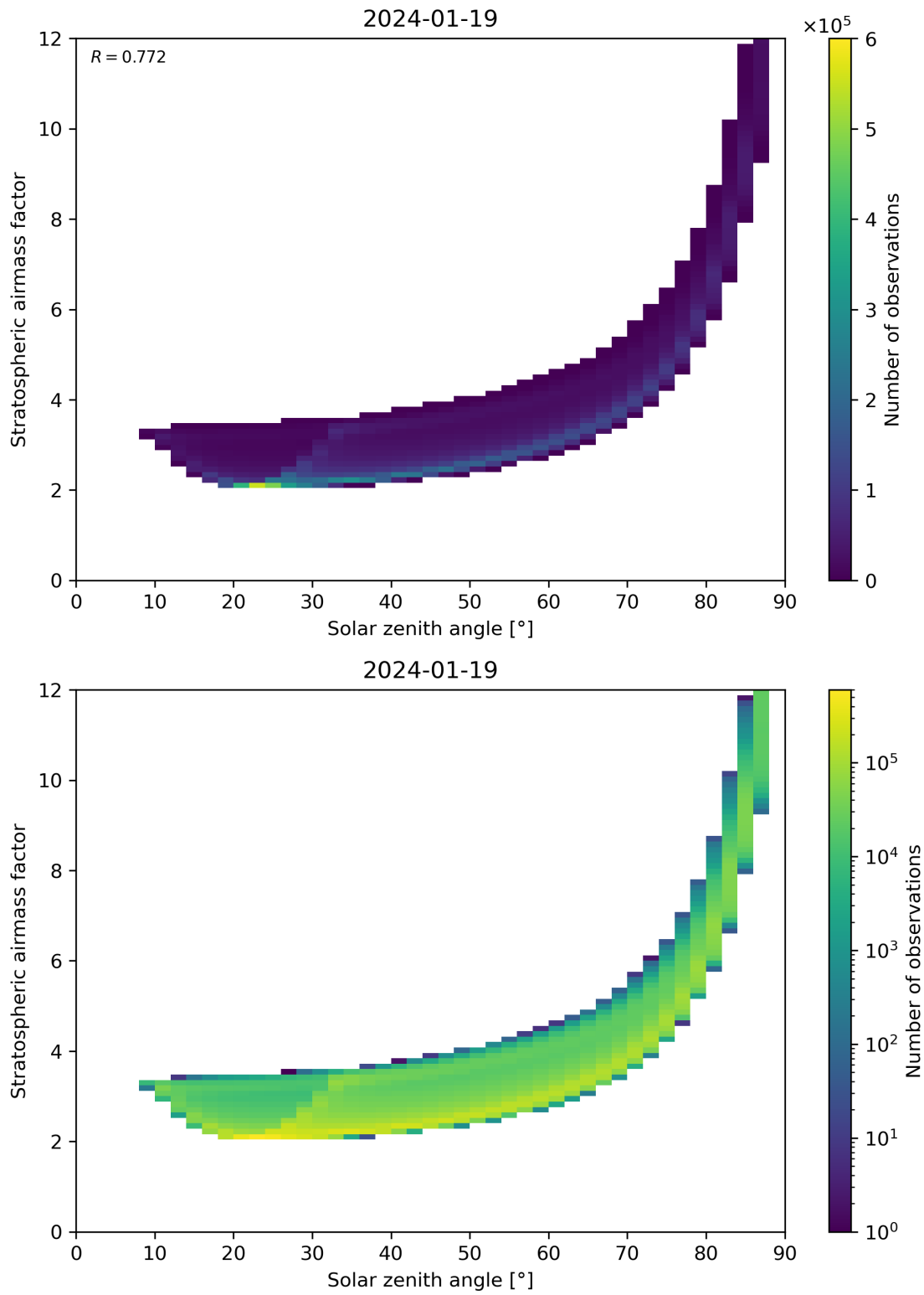
Figure 145: Scatter density plot of “Solar zenith angle” against “Stratospheric airmass factor” for 2024-01-18 to 2024-01-20.
