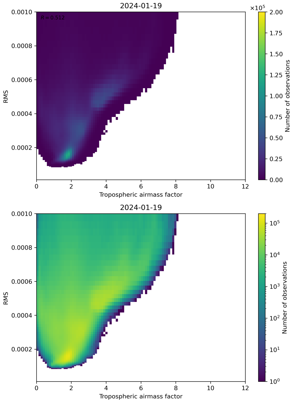
Figure 79: Scatter density plot of “Tropospheric airmass factor” against “RMS” for 2024-01-18 to 2024-01-20.
