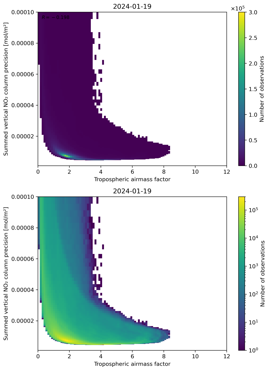
Figure 76: Scatter density plot of “Tropospheric air mass factor” against “Summed vertical NO 2 column precision” for 2024-01-18 to 2024-01-20.
