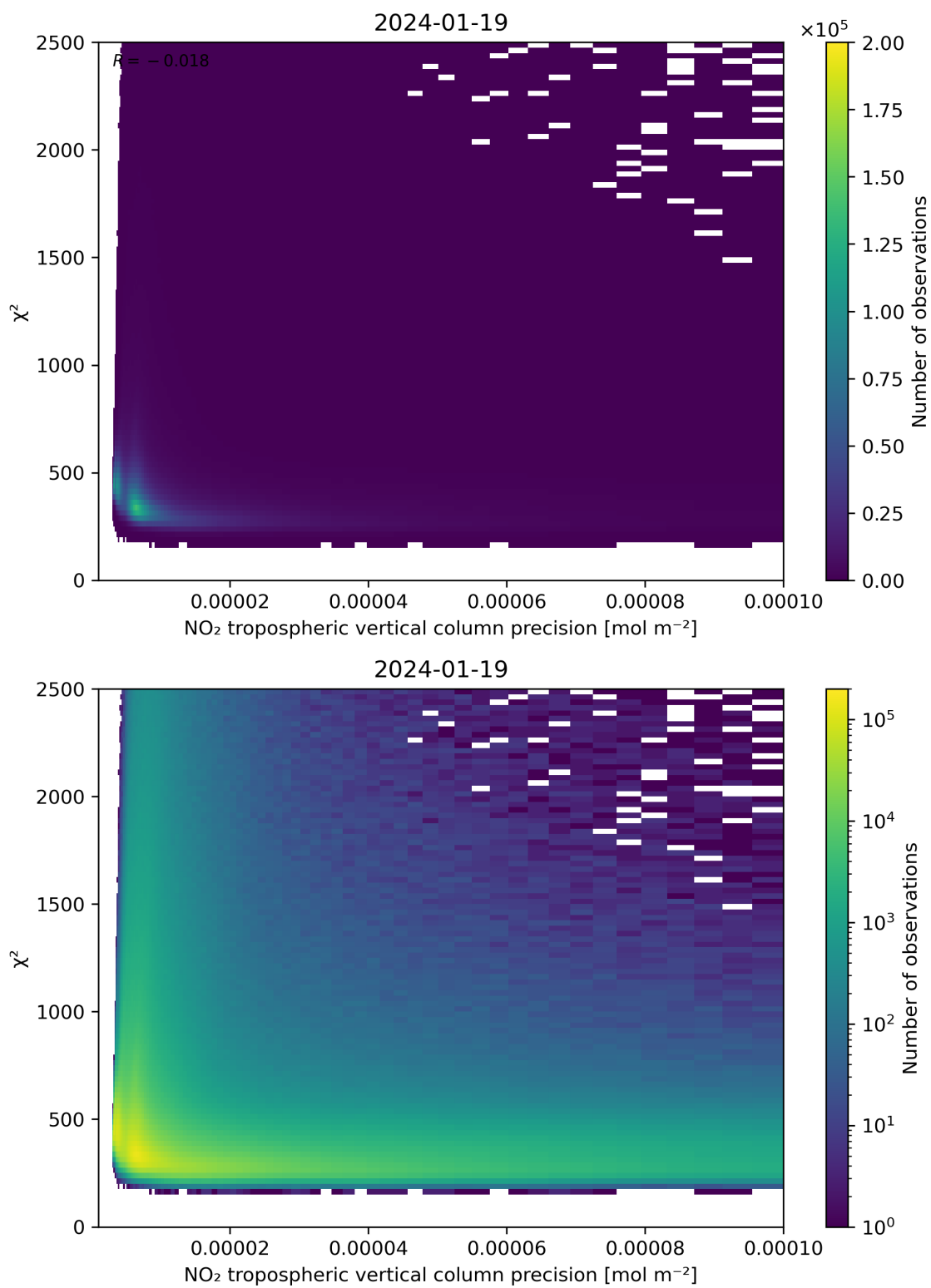
Figure 134: Scatter density plot of “NO 2 tropospheric vertical column precision” against “ \chi^2 ” for 2024-01-18 to 2024-01-20.
