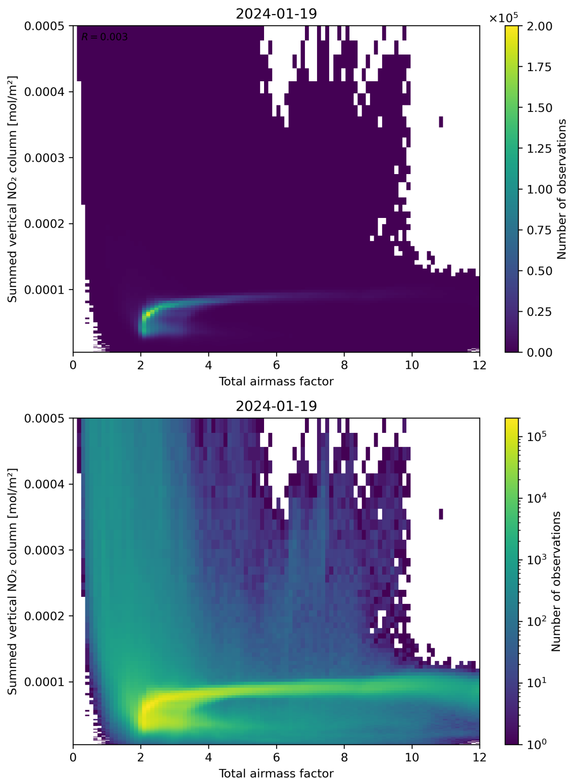
Figure 65: Scatter density plot of “Total airmass factor” against “Summed vertical NO 2 column” for 2024-01-18 to 2024-01-20.
