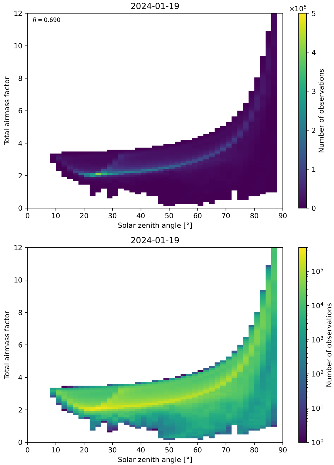
Figure 146: Scatter density plot of “Solar zenith angle” against “Total air mass factor” for 2024-01-18 to 2024-01-20.
