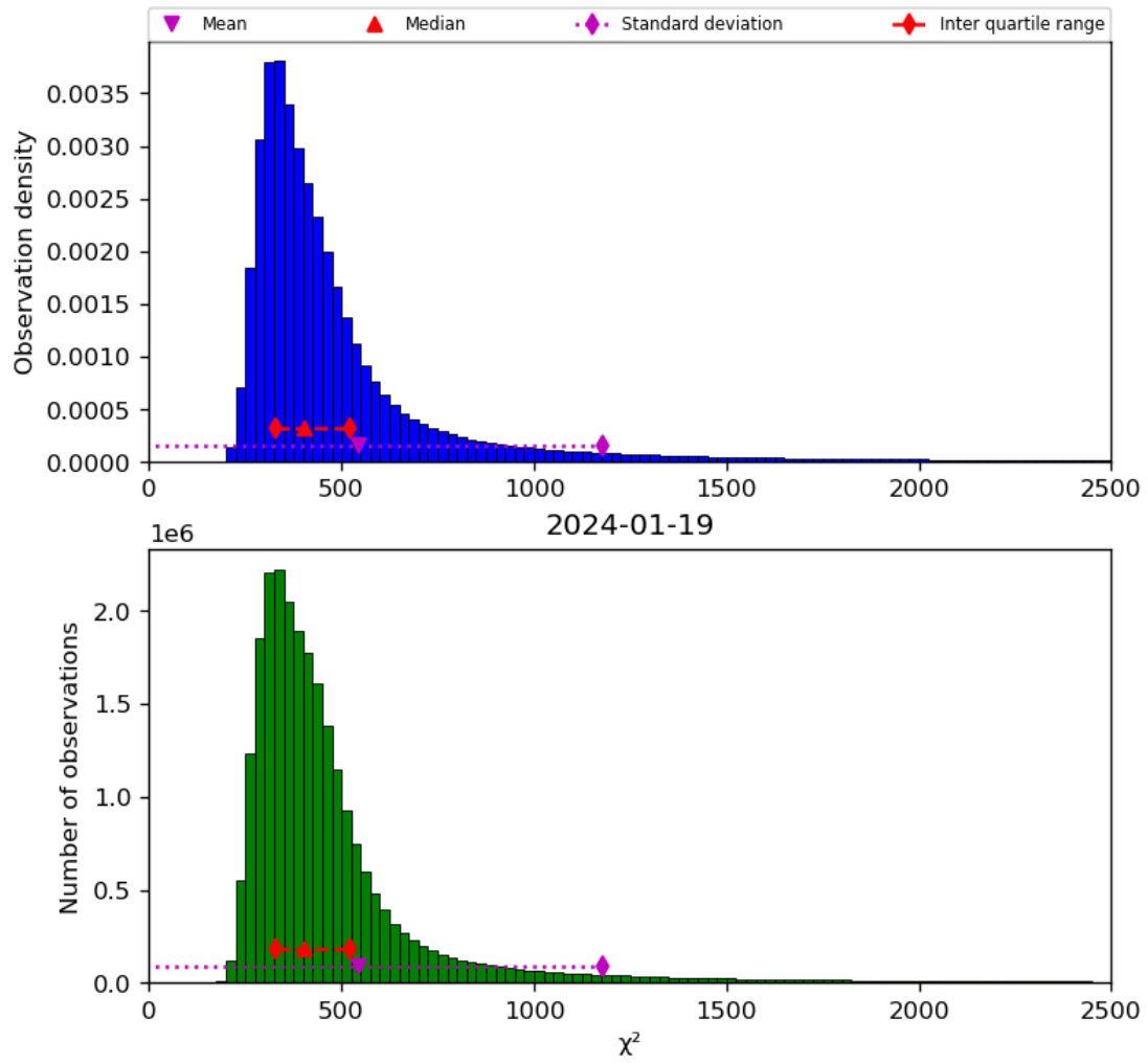
Figure 42: Histogram of “ \chi^2 ” for 2024-01-18 to 2024-01-20
