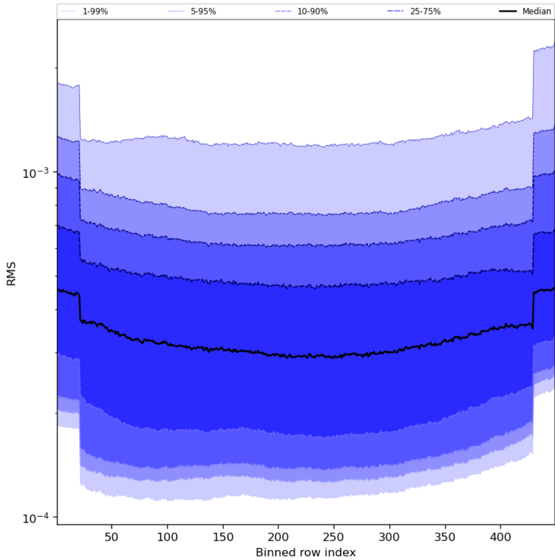
Figure 60: Along track statistics of “RMS” for 2024-01-18 to 2024-01-20
