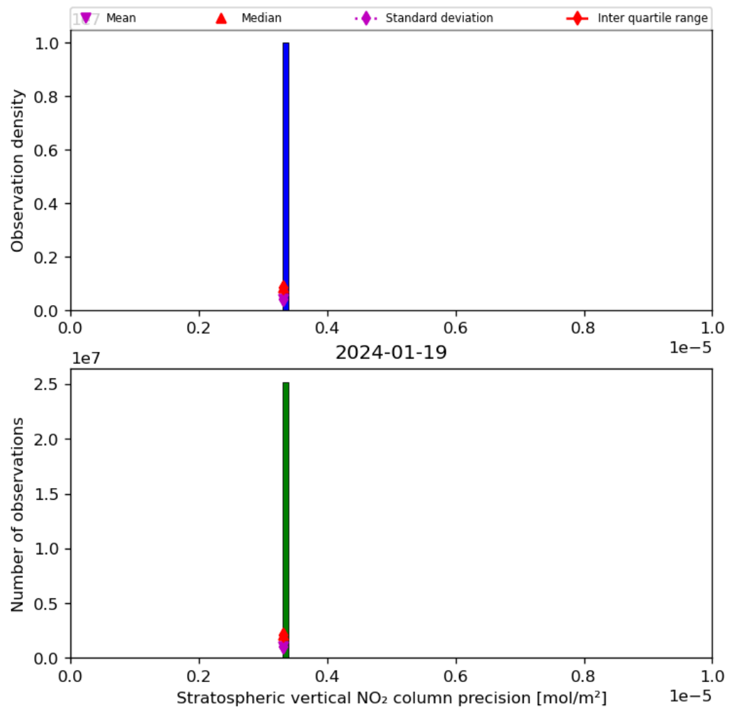
Figure 37: Histogram of “Stratospheric vertical NO 2 column precision” for 2024-01-18 to 2024-01-20
