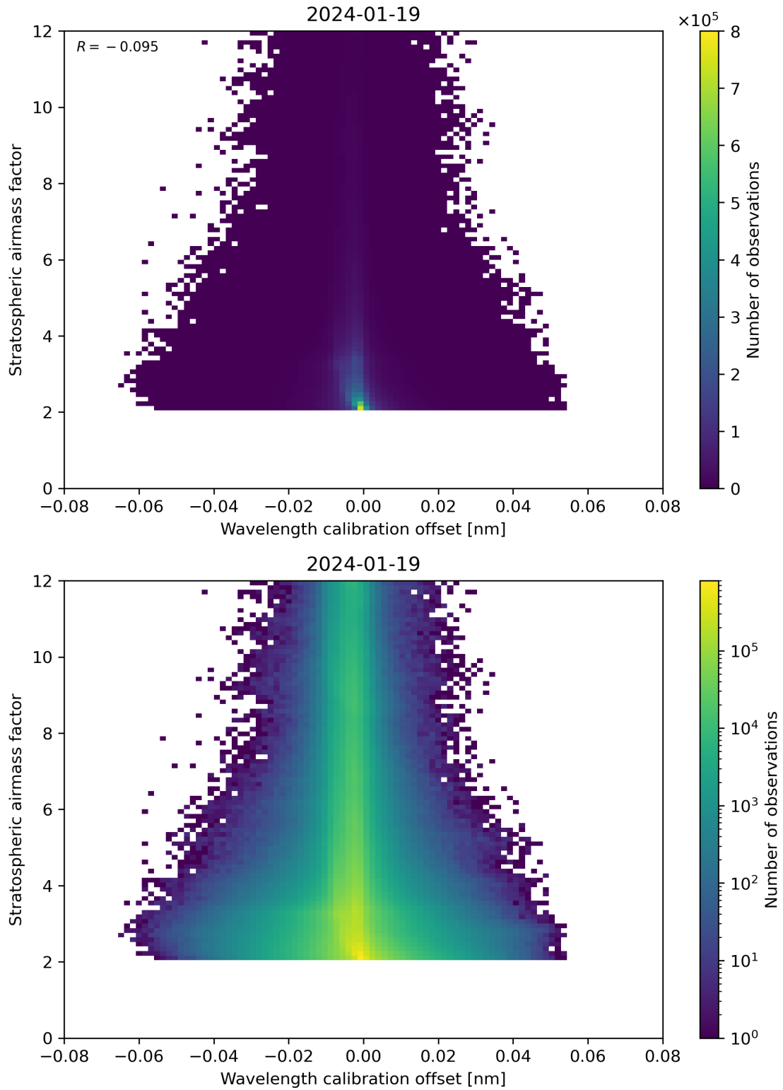
Figure 174: Scatter density plot of “Wavelength calibration offset” against “Stratospheric airmass factor” for 2024-01-18 to 2024-01-20.
