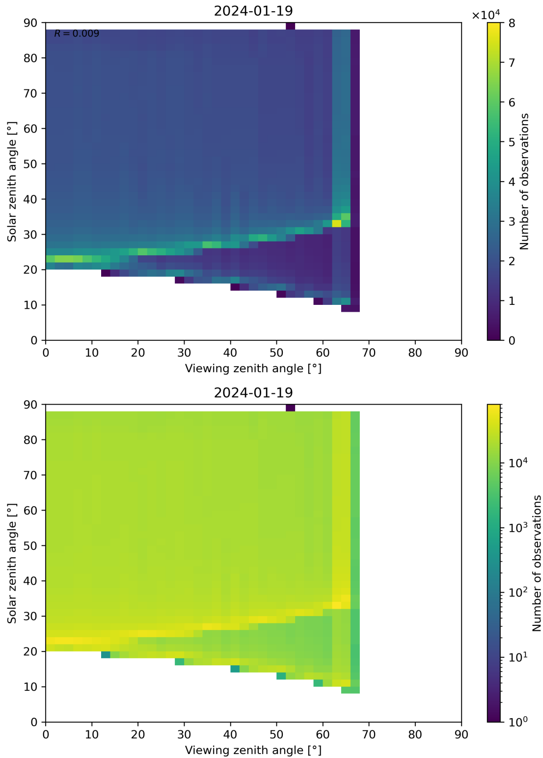
Figure 172: Scatter density plot of “Viewing zenith angle” against “Solar zenith angle” for 2024-01-18 to 2024-01-20.
