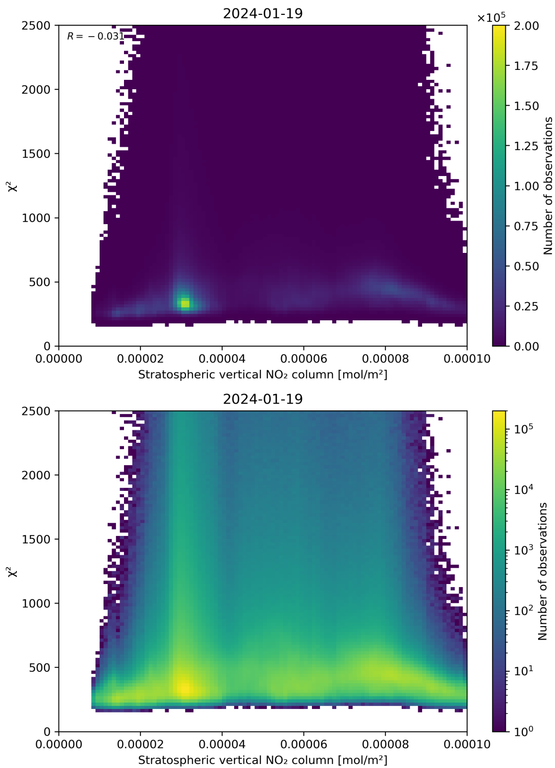
Figure 97: Scatter density plot of “Stratospheric vertical NO 2 column” against “ \chi^2 ” for 2024-01-18 to 2024-01-20.
