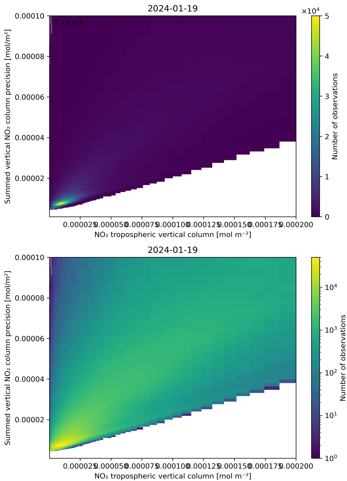
Figure 127: Scatter density plot of “NO 2 tropospheric vertical column” against “Summed vertical NO 2 column precision” for 2024-01-18 to 2024-01-20.
