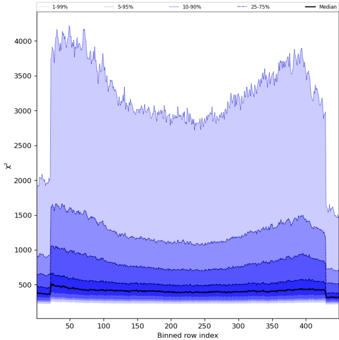
Figure 59: Along track statistics of “ \chi^2 ” for 2024-01-18 to 2024-01-20
