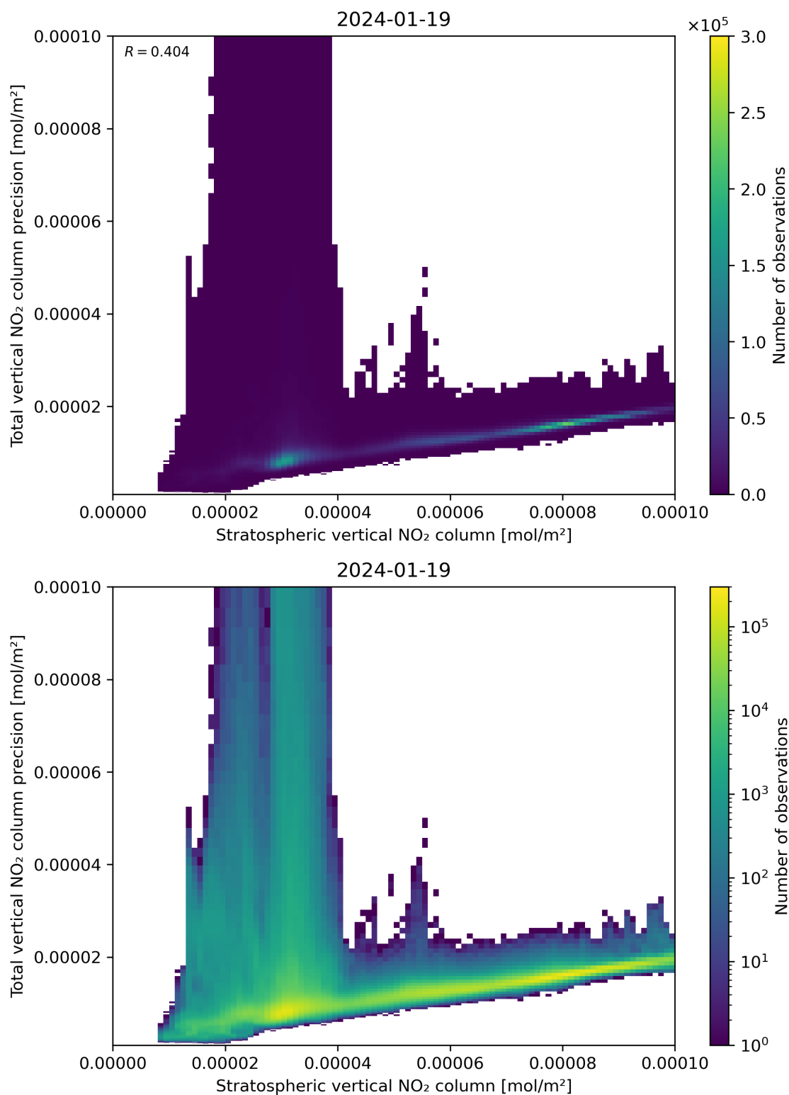
Figure 101: Scatter density plot of “Stratospheric vertical NO 2 column” against “Total vertical NO 2 column precision” for 2024-01-18 to 2024-01-20.
