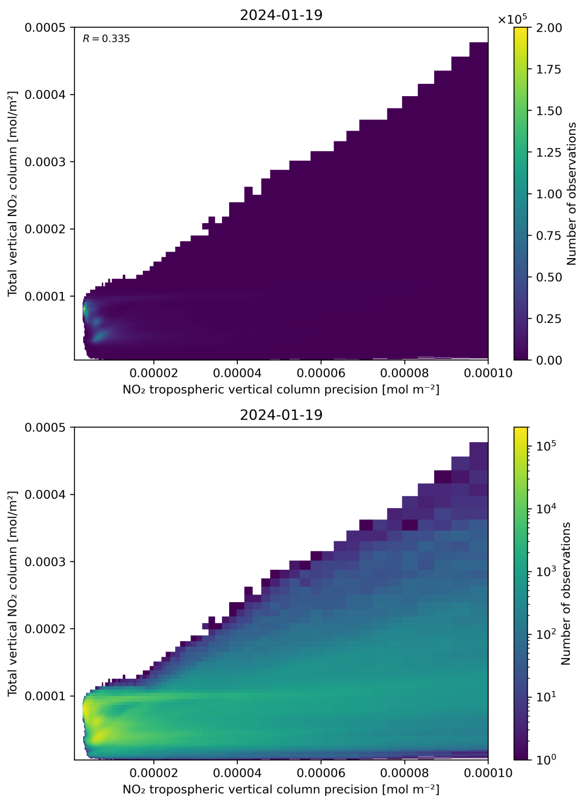
Figure 138: Scatter density plot of “NO 2 tropospheric vertical column precision” against “Total vertical NO 2 column” for 2024-01-18 to 2024-01-20.
