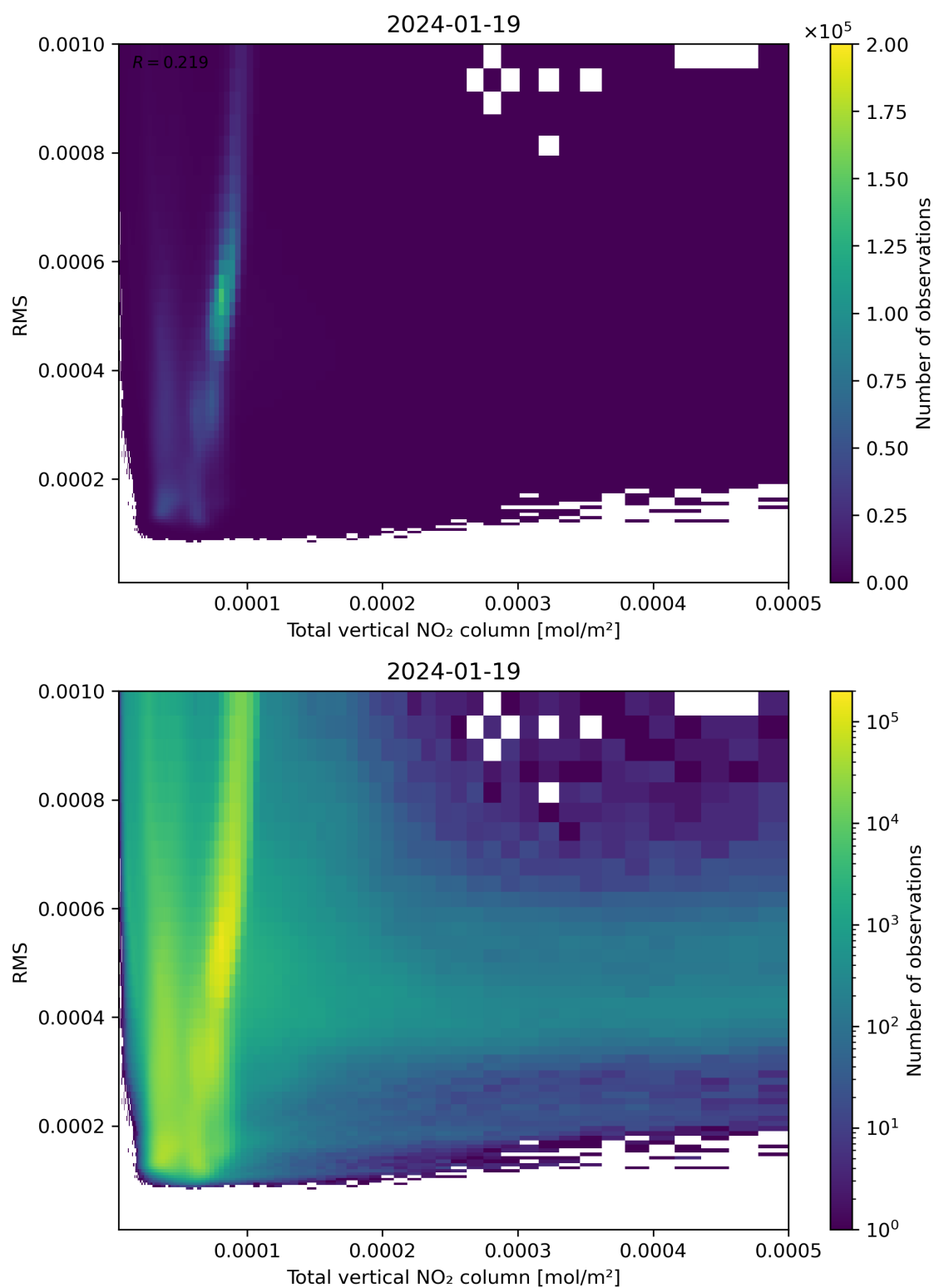
Figure 120: Scatter density plot of “Total vertical NO 2 column” against “RMS” for 2024-01-18 to 2024-01-20.
