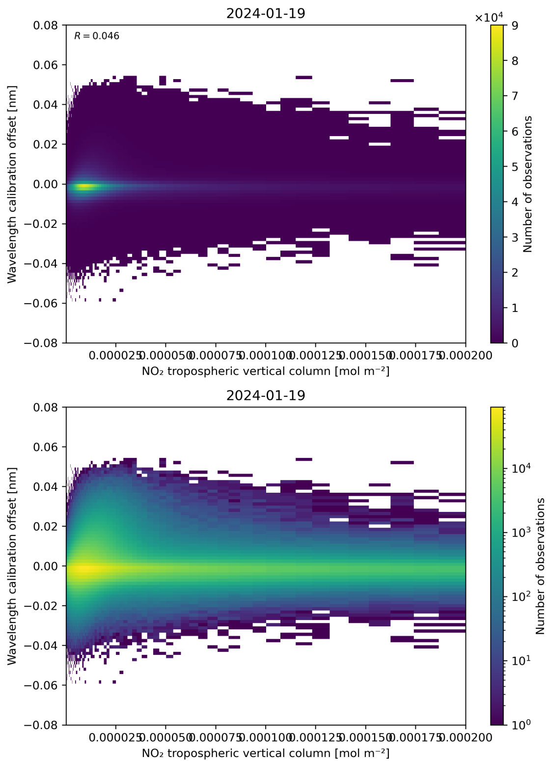
Figure 143: Scatter density plot of “NO 2 tropospheric vertical column” against “Wavelength calibration offset” for 2024-01-18 to 2024-01-20.
