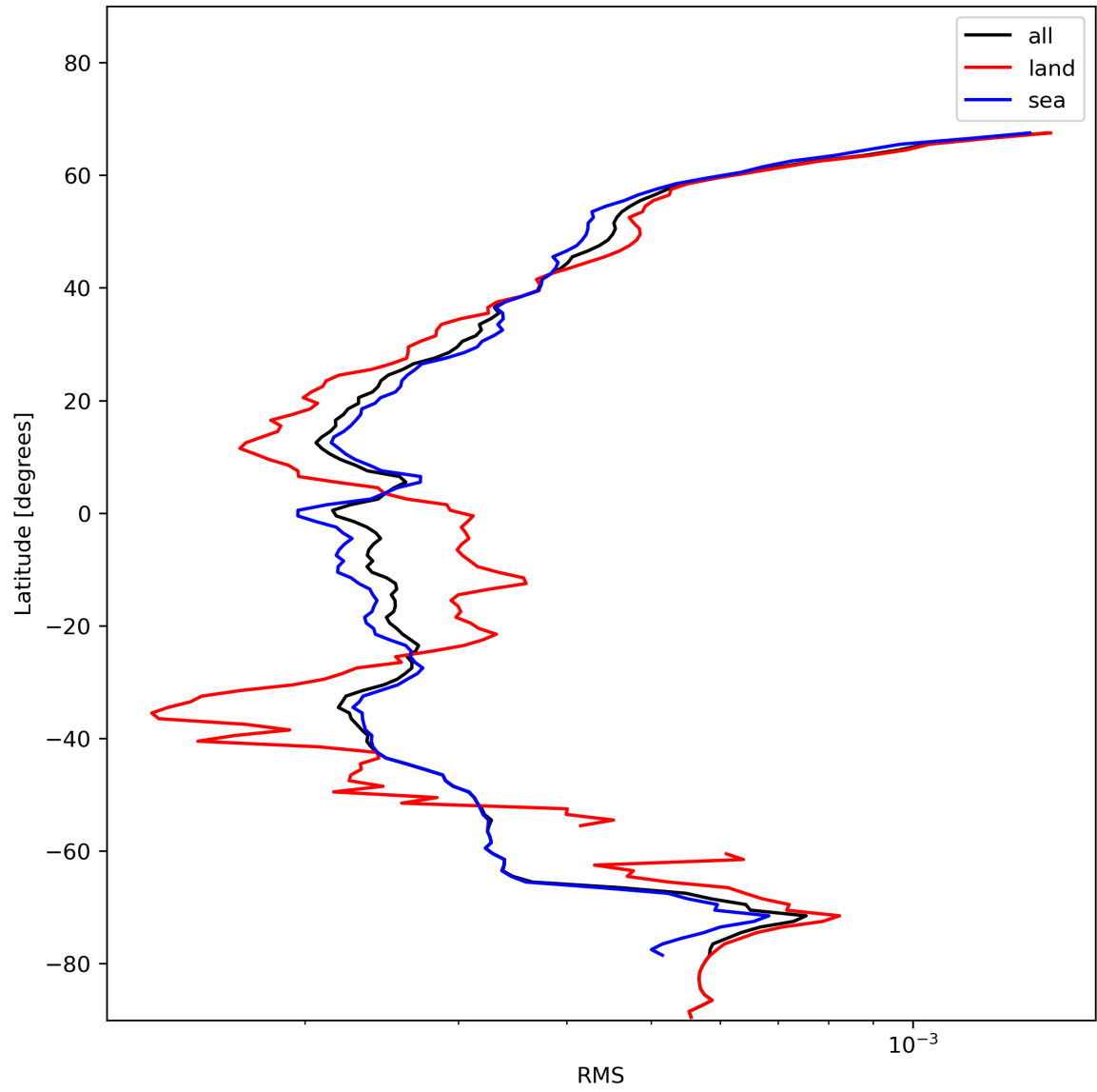
Figure 26: Zonal average of “RMS” for 2024-01-18 to 2024-01-20.
