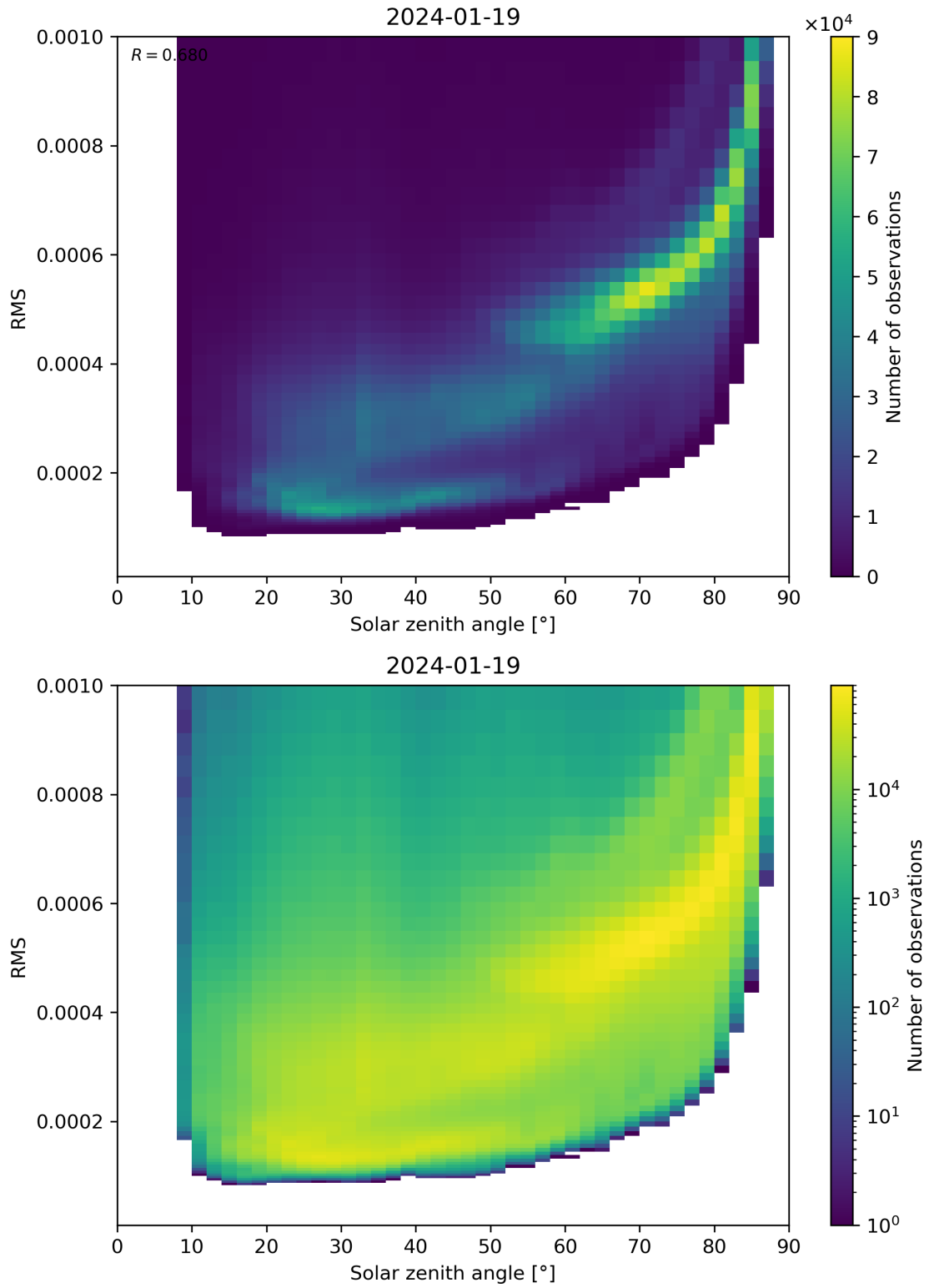
Figure 157: Scatter density plot of “Solar zenith angle” against “RMS” for 2024-01-18 to 2024-01-20.
