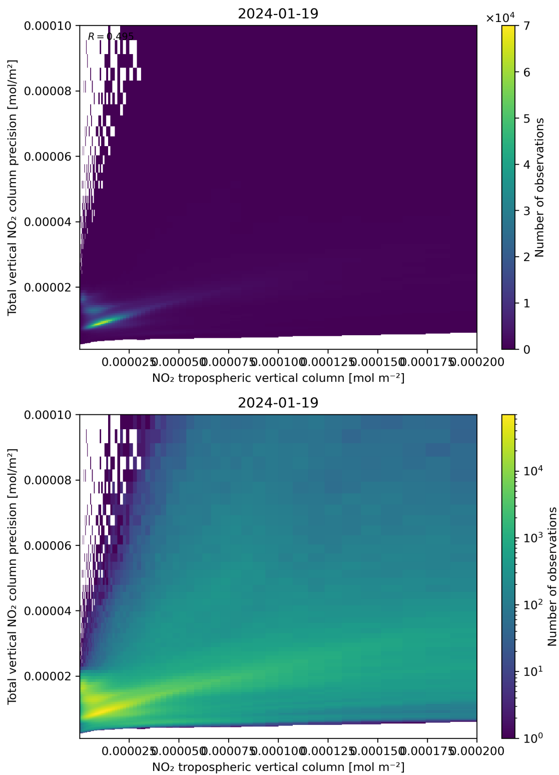
Figure 129: Scatter density plot of “NO 2 tropospheric vertical column” against “Total vertical NO 2 column precision” for 2024-01-18 to 2024-01-20.
