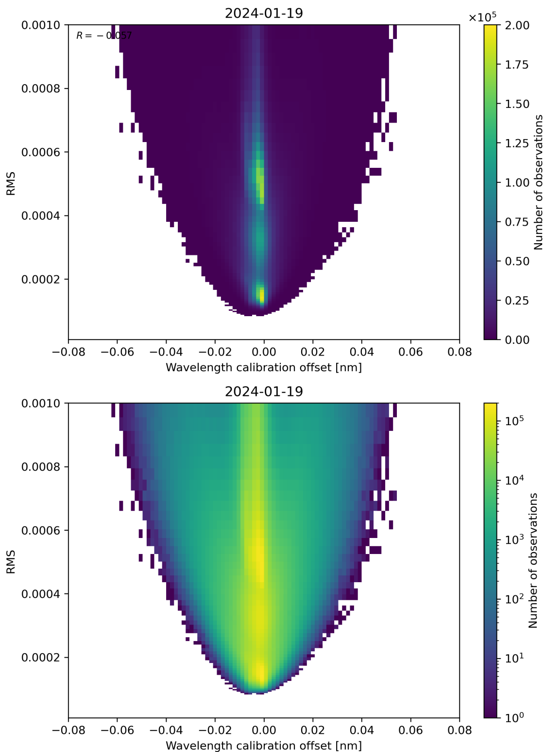
Figure 181: Scatter density plot of “Wavelength calibration offset” against “RMS” for 2024-01-18 to 2024-01-20.
