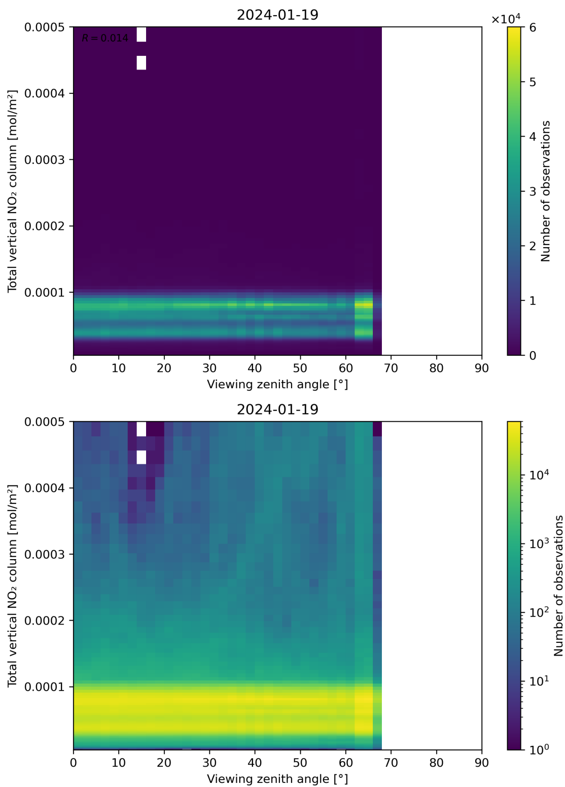
Figure 167: Scatter density plot of “Viewing zenith angle” against “Total vertical NO 2 column” for 2024-01-18 to 2024-01-20.
