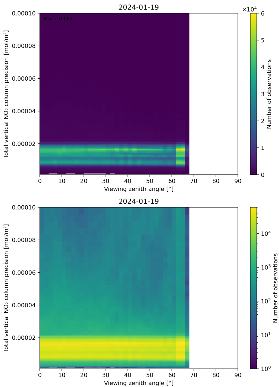
Figure 168: Scatter density plot of “Viewing zenith angle” against “Total vertical NO 2 column precision” for 2024-01-18 to 2024-01-20.
