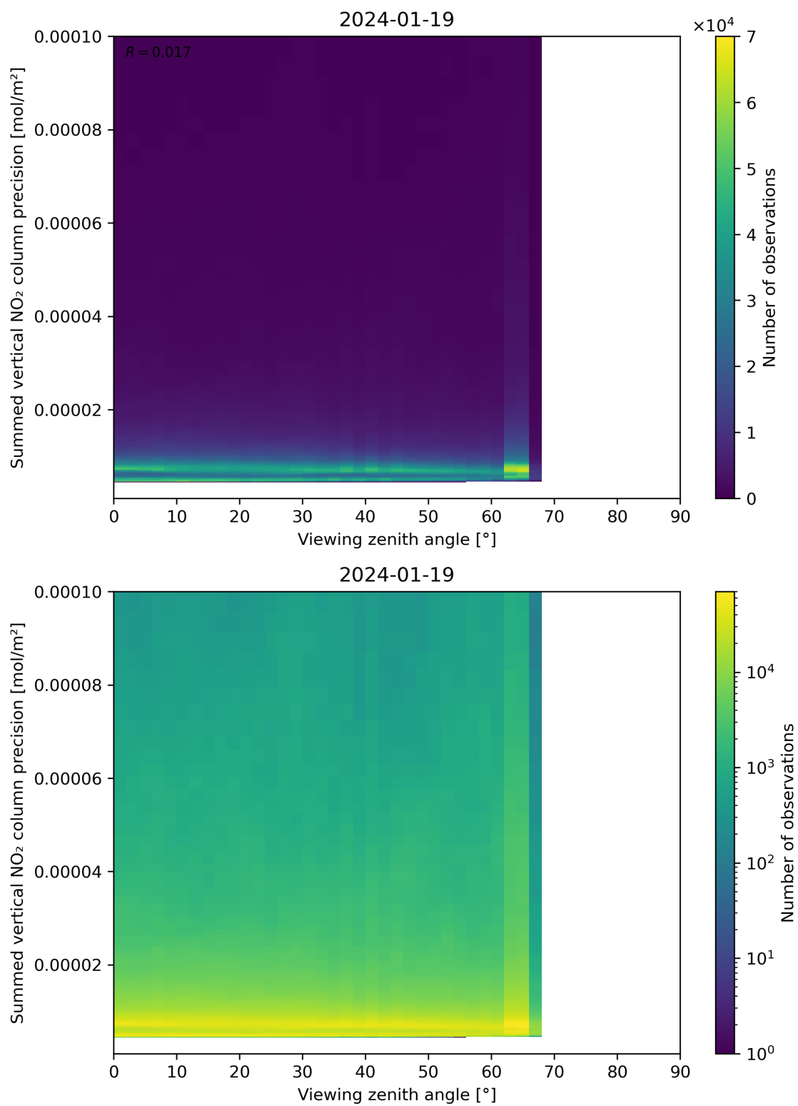
Figure 166: Scatter density plot of “Viewing zenith angle” against “Summed vertical NO 2 column precision” for 2024-01-18 to 2024-01-20.
