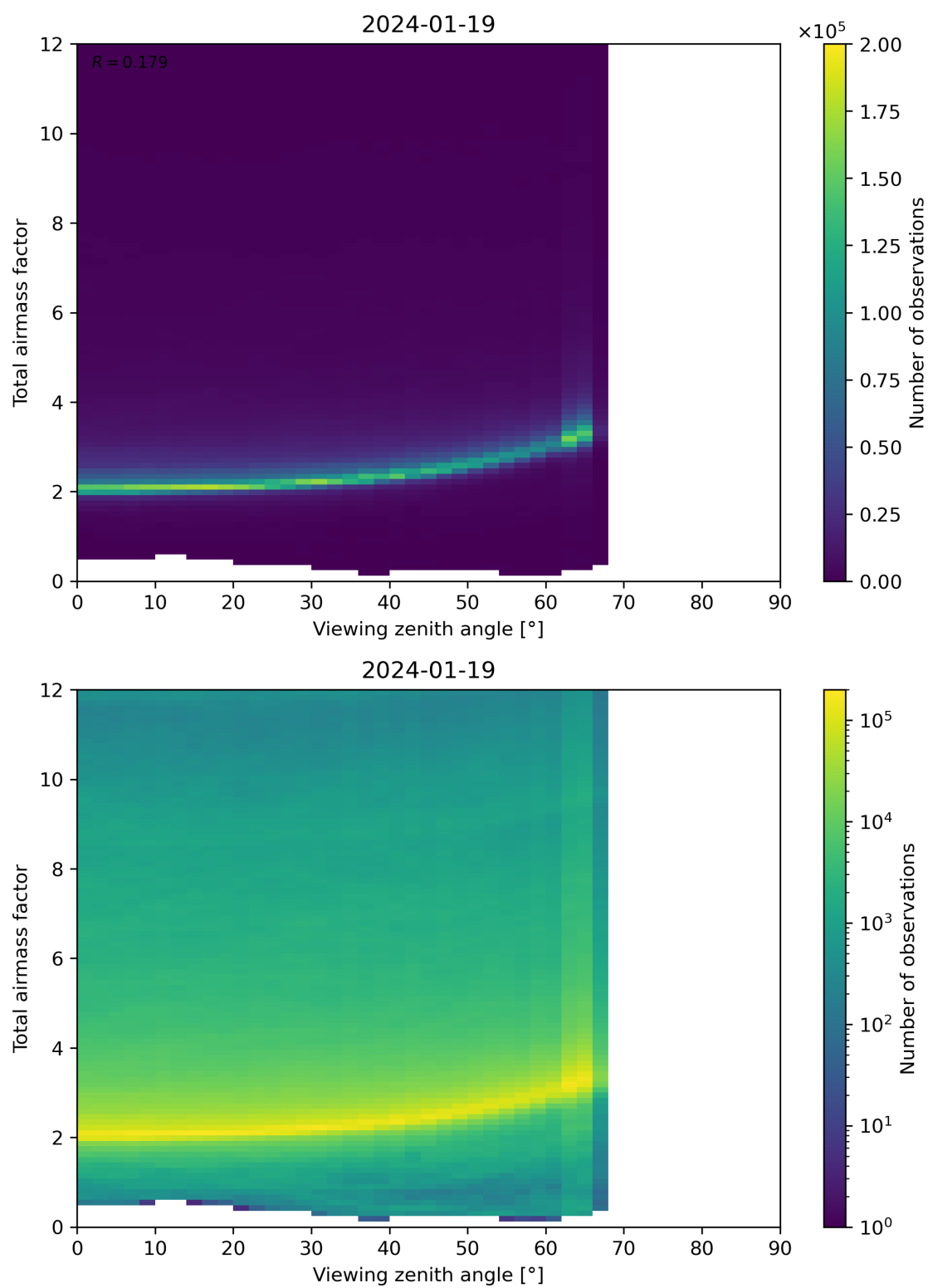
Figure 160: Scatter density plot of “Viewing zenith angle” against “Total airmass factor” for 2024-01-18 to 2024-01-20.
