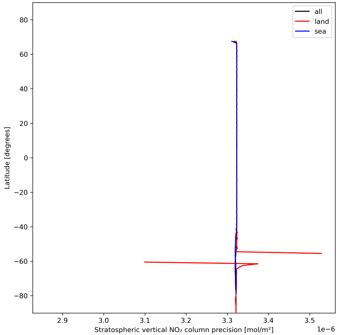
Figure 20: Zonal average of “Stratospheric vertical NO 2 column precision” for 2024-01-18 to 2024-01-20.
