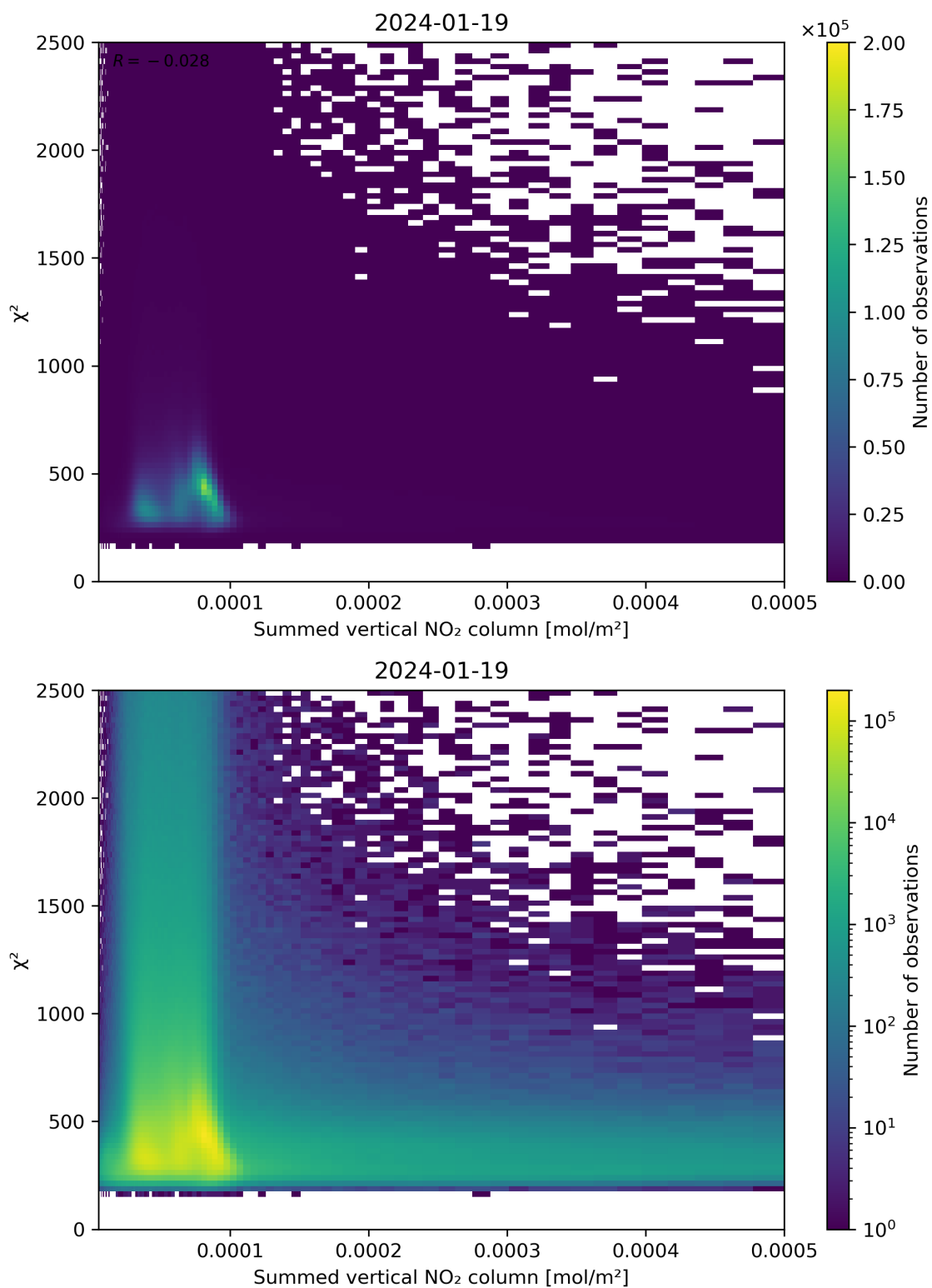
Figure 104: Scatter density plot of “Summed vertical NO 2 column” against “ \chi^2 ” for 2024-01-18 to 2024-01-20.
