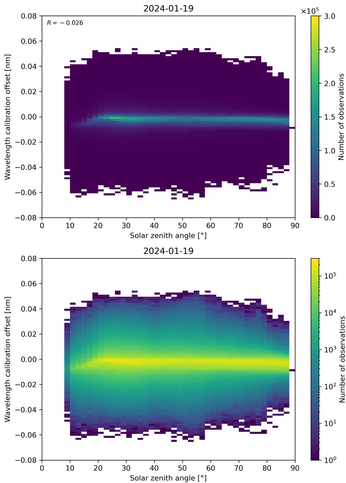
Figure 158: Scatter density plot of “Solar zenith angle” against “Wavelength calibration offset” for 2024-01-18 to 2024-01-20.
