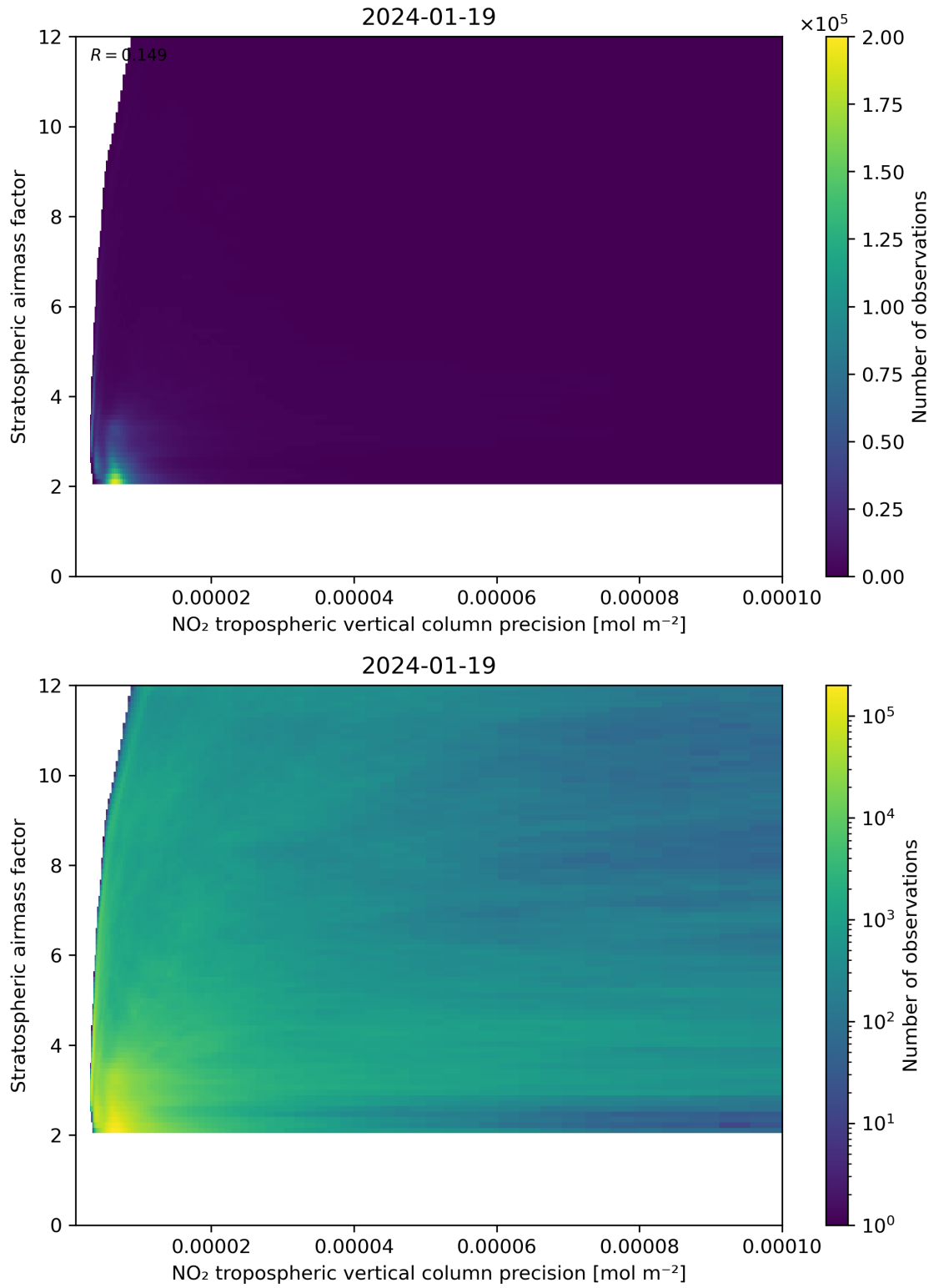
Figure 131: Scatter density plot of “NO 2 tropospheric vertical column precision” against “Stratospheric airmass factor” for 2024-01-18 to 2024-01-20.
