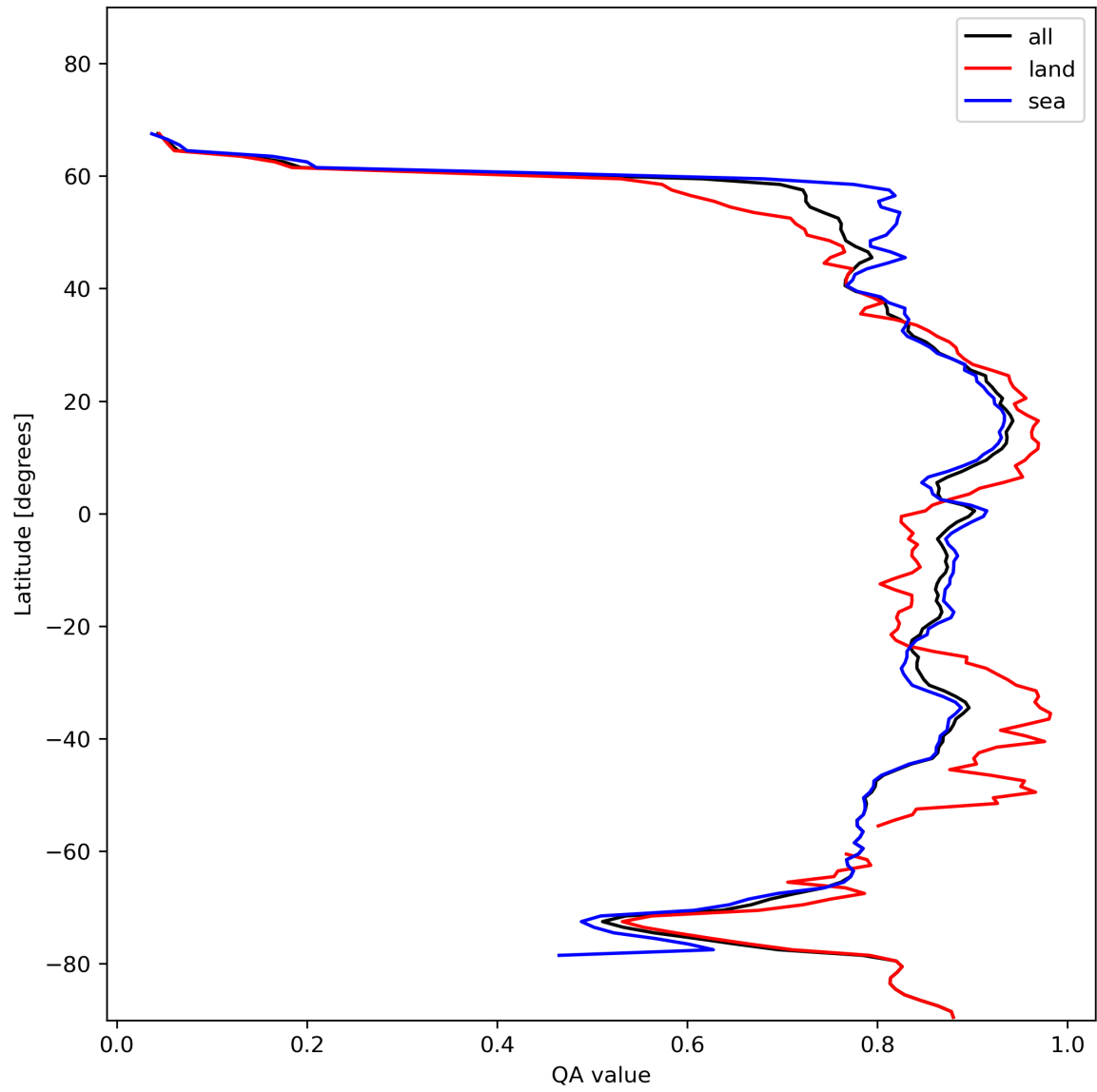
Figure 11: Zonal average of “QA value” for 2024-01-18 to 2024-01-20.
