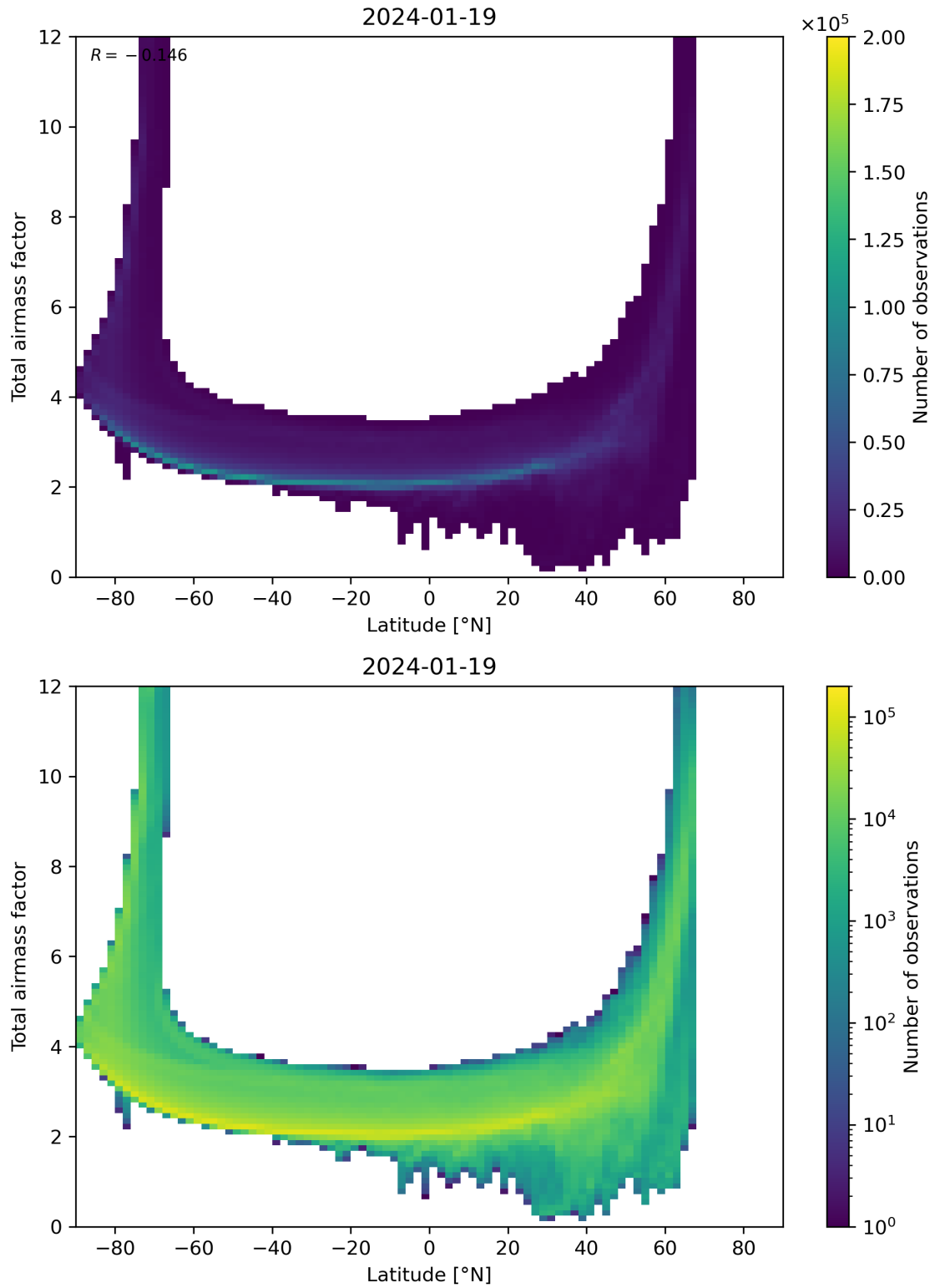
Figure 84: Scatter density plot of “Latitude” against “Total airmass factor” for 2024-01-18 to 2024-01-20.
