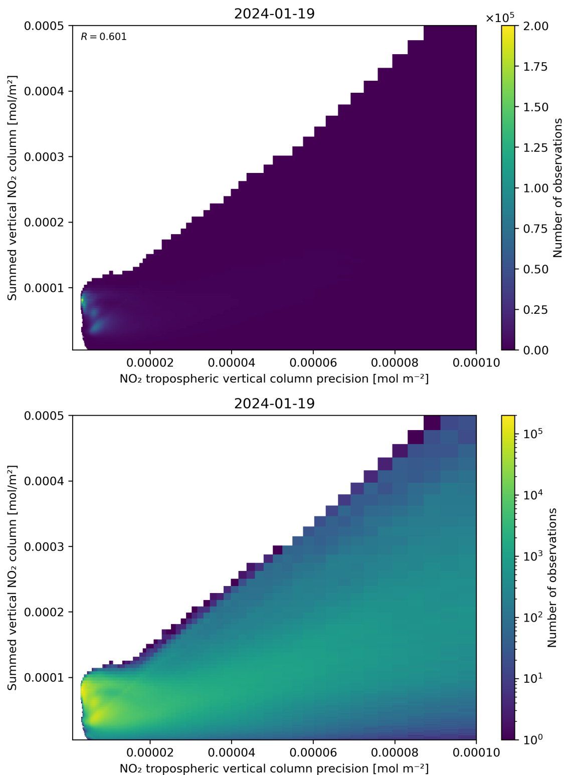
Figure 136: Scatter density plot of “NO 2 tropospheric vertical column precision” against “Summed vertical NO 2 column” for 2024-01-18 to 2024-01-20.
