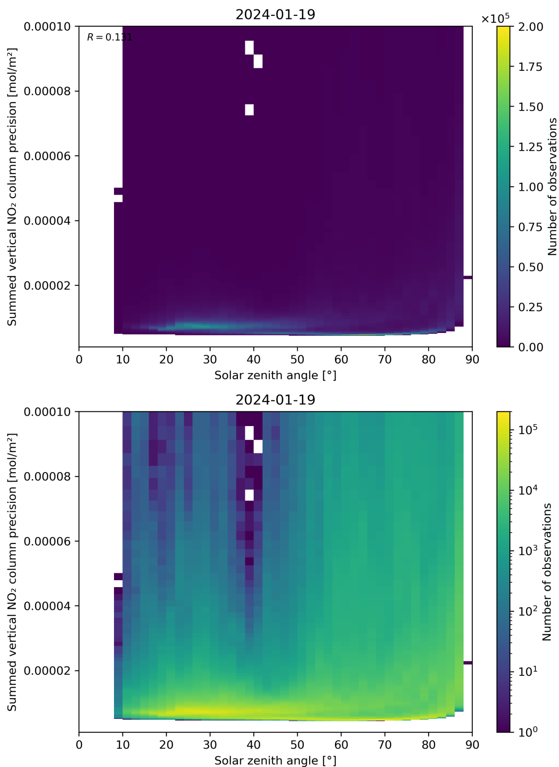
Figure 152: Scatter density plot of “Solar zenith angle” against “Summed vertical NO 2 column precision” for 2024-01-18 to 2024-01-20.
