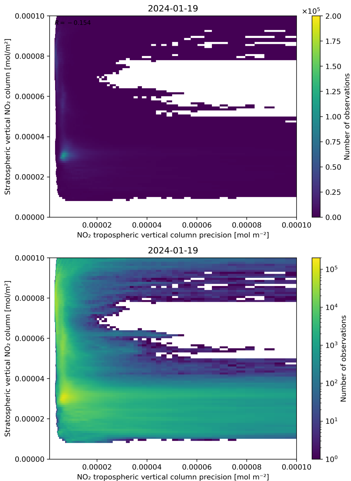
Figure 135: Scatter density plot of “NO 2 tropospheric vertical column precision” against “Stratospheric vertical NO 2 column” for 2024-01-18 to 2024-01-20.
