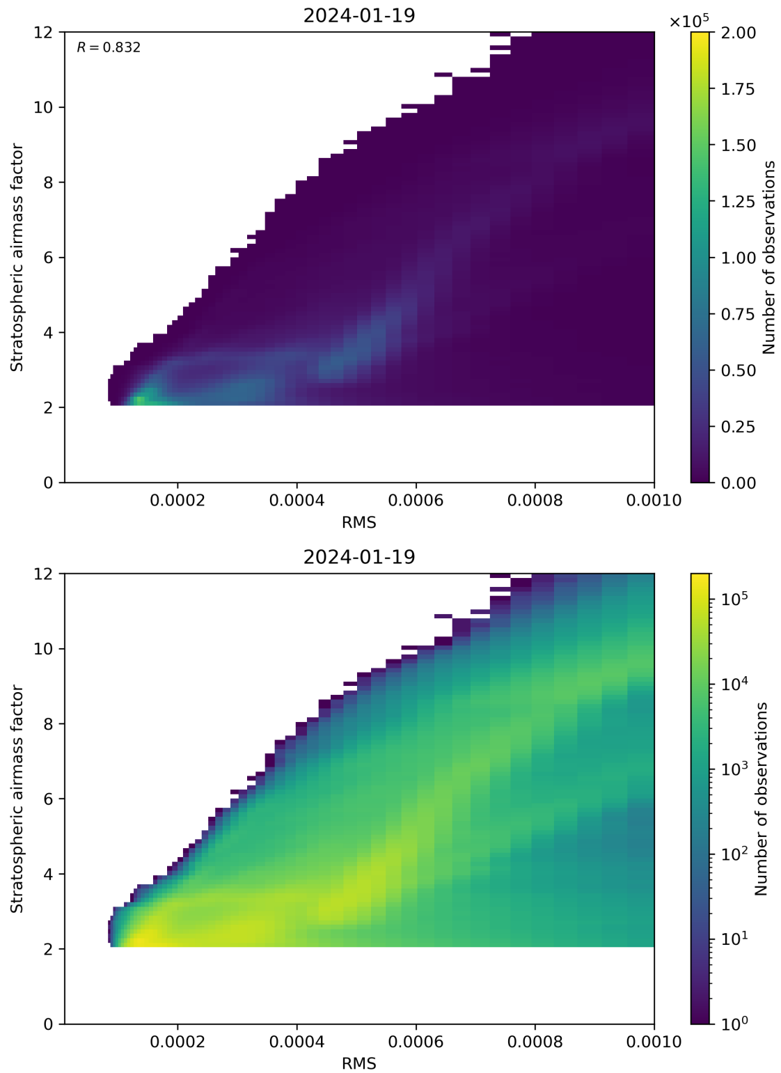
Figure 144: Scatter density plot of “RMS” against “Stratospheric airmass factor” for 2024-01-18 to 2024-01-20.
