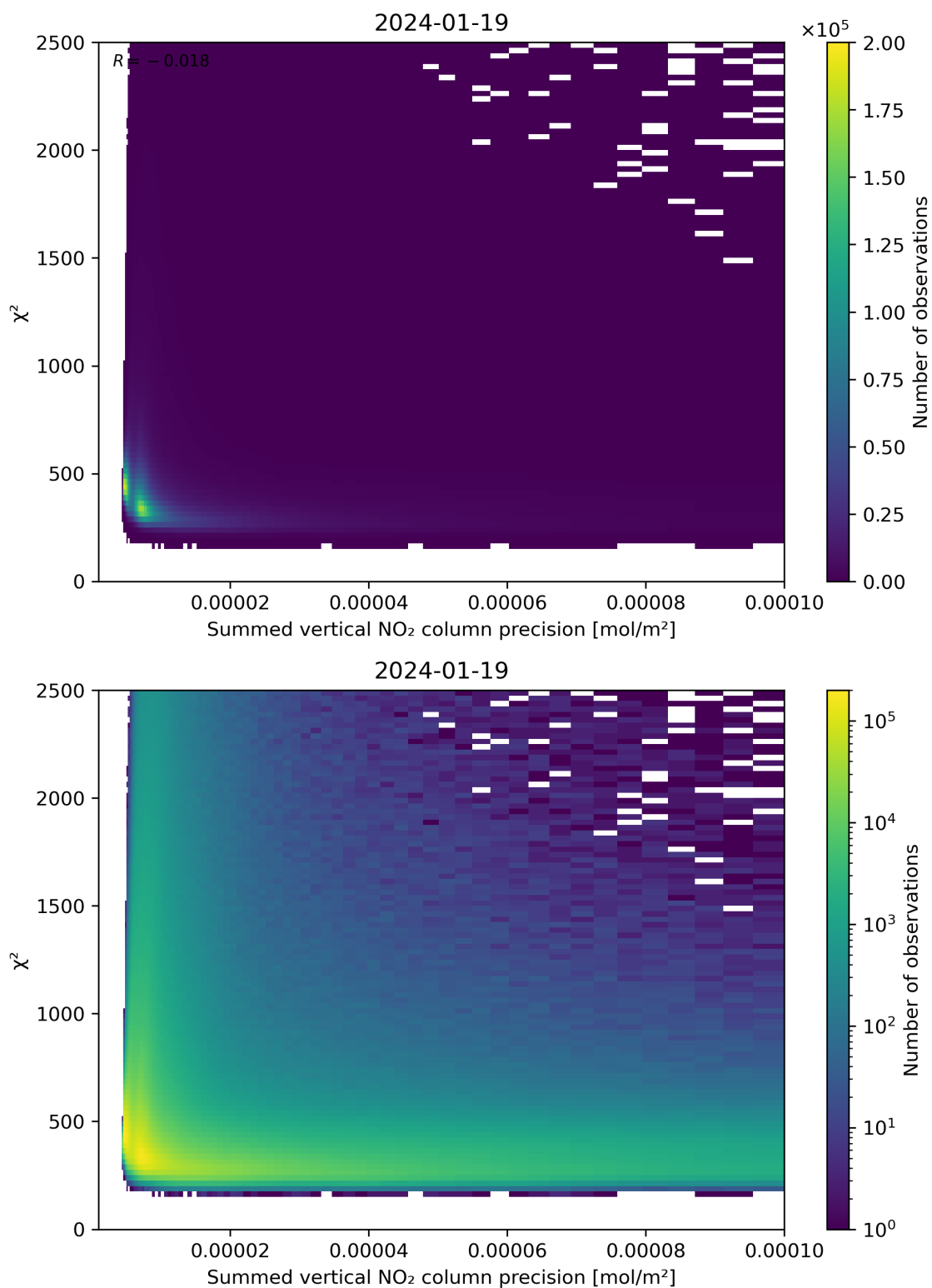
Figure 107: Scatter density plot of “Summed vertical NO 2 column precision” against “ \chi^2 ” for 2024-01-18 to 2024-01-20.
