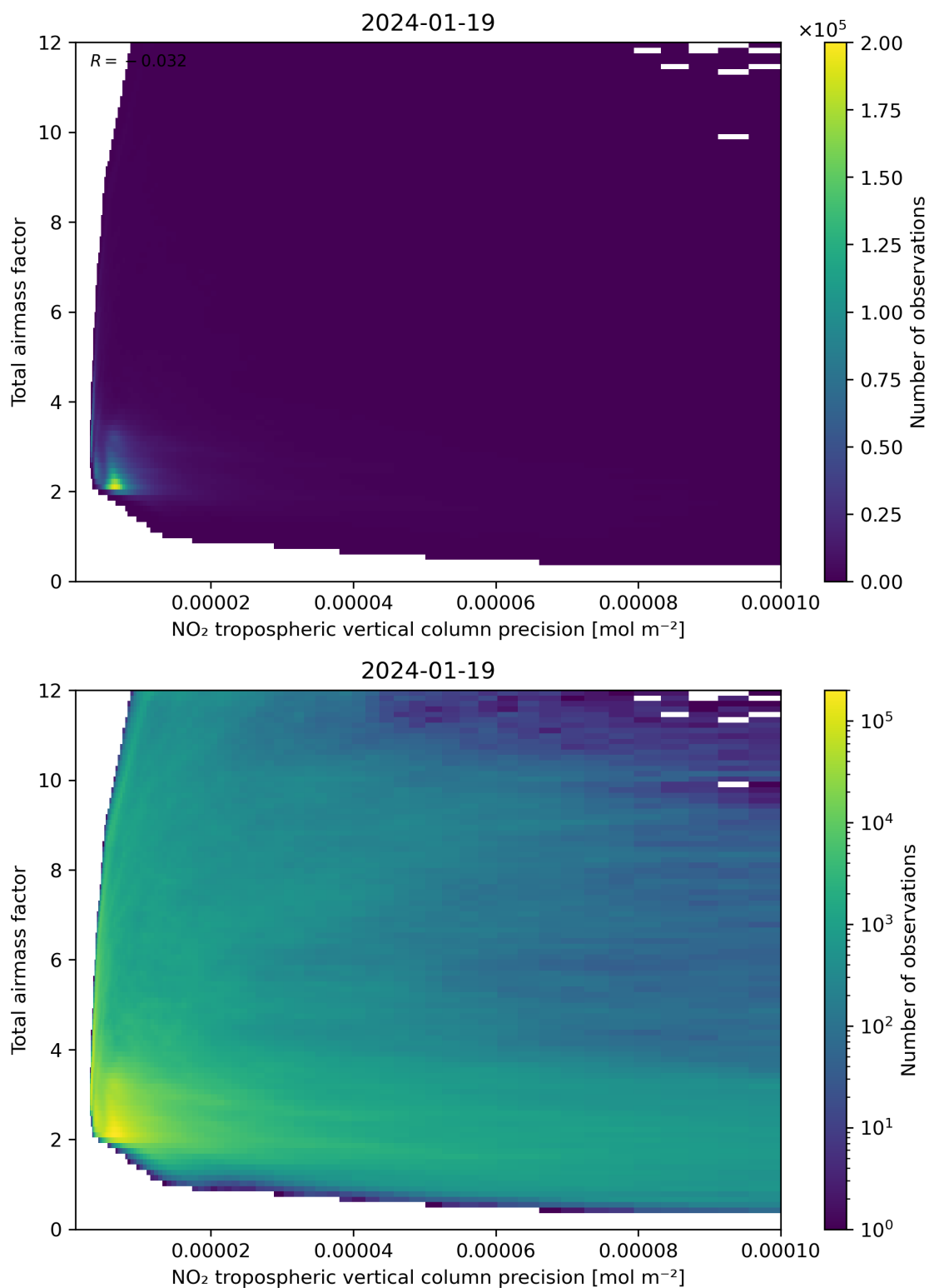
Figure 132: Scatter density plot of “NO 2 tropospheric vertical column precision” against “Total air mass factor” for 2024-01-18 to 2024-01-20.
