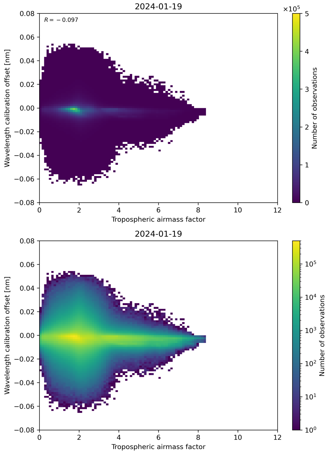
Figure 80: Scatter density plot of “Tropospheric airmass factor” against “Wavelength calibration offset” for 2024-01-18 to 2024-01-20.
