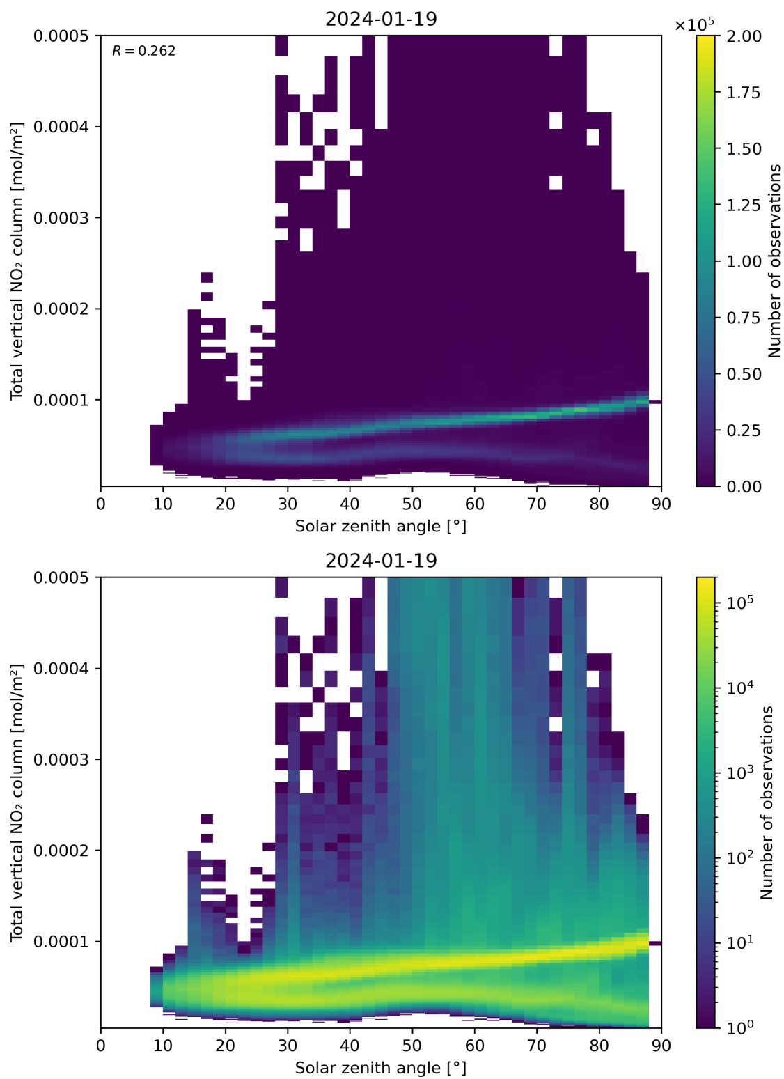
Figure 153: Scatter density plot of “Solar zenith angle” against “Total vertical NO 2 column” for 2024-01-18 to 2024-01-20.
