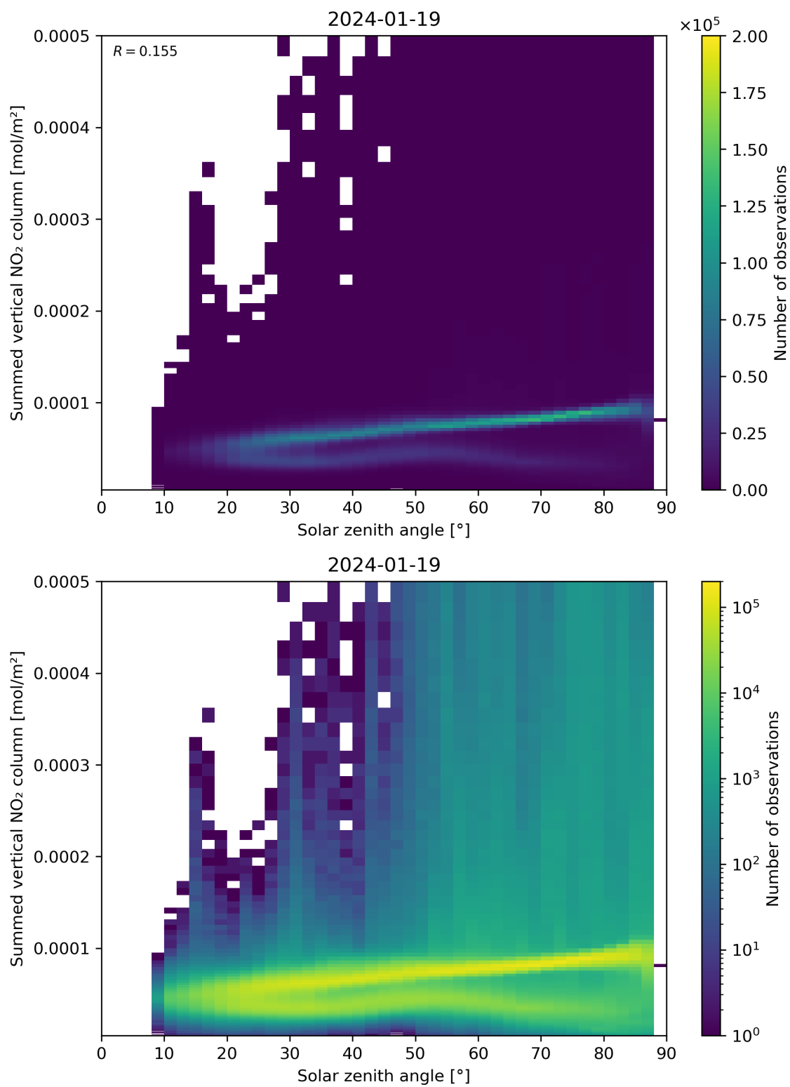
Figure 151: Scatter density plot of “Solar zenith angle” against “Summed vertical NO 2 column” for 2024-01-18 to 2024-01-20.
