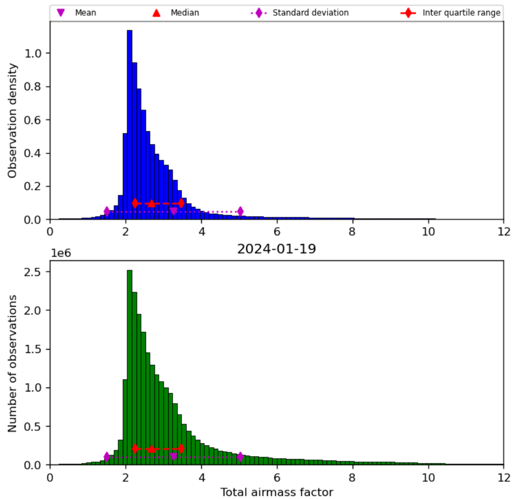
Figure 32: Histogram of “Total airmass factor” for 2024-01-18 to 2024-01-20
