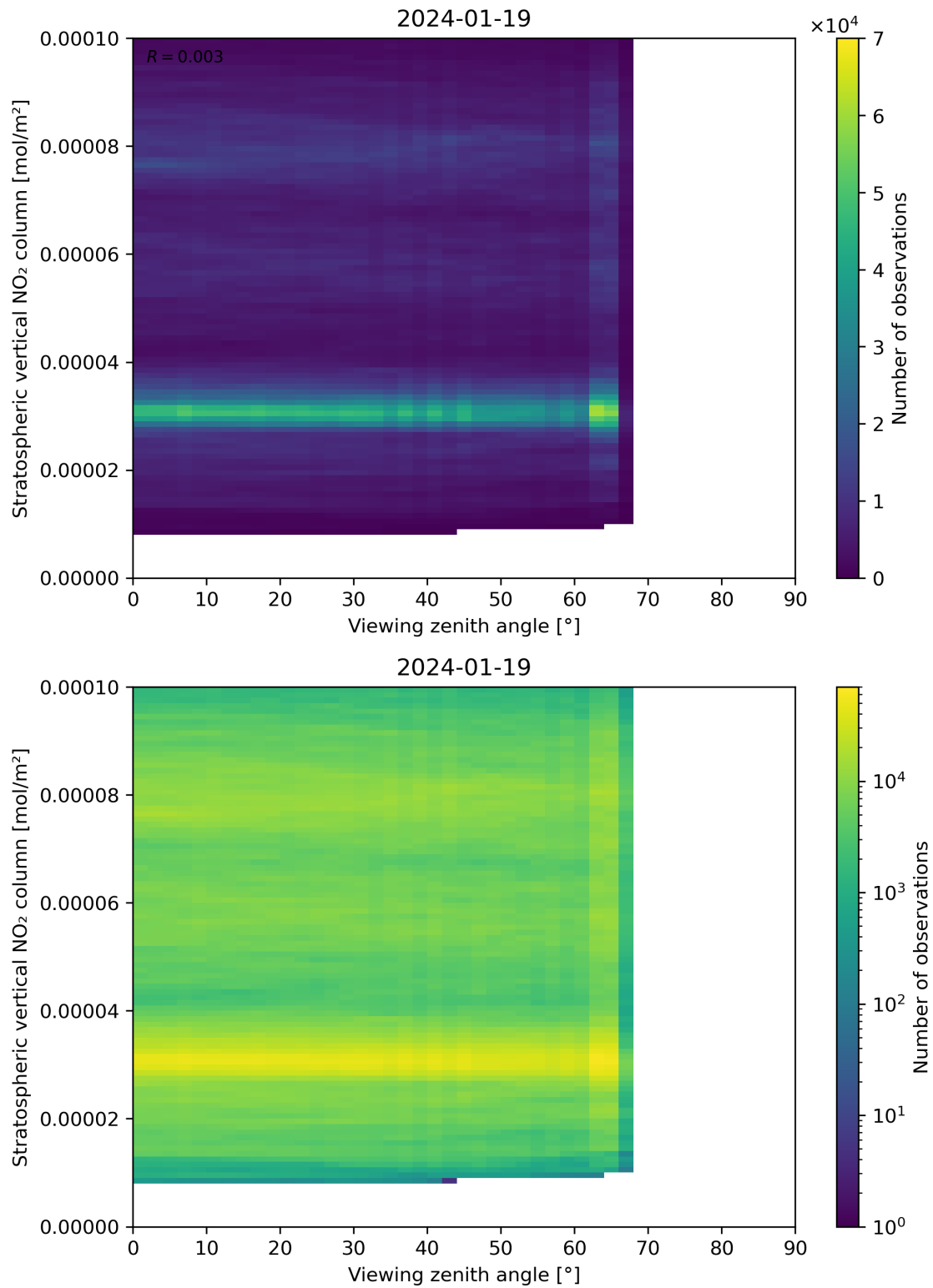
Figure 164: Scatter density plot of “Viewing zenith angle” against “Stratospheric vertical NO 2 column” for 2024-01-18 to 2024-01-20.
