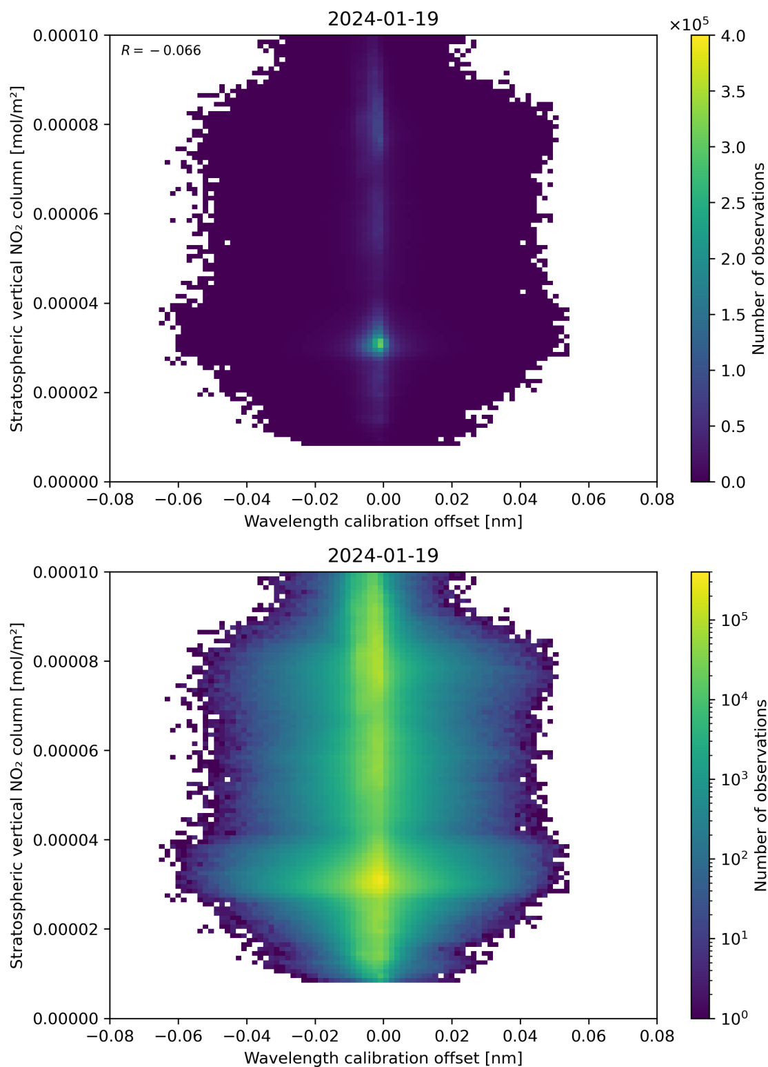
Figure 176: Scatter density plot of “Wavelength calibration offset” against “Stratospheric vertical NO 2 column” for 2024-01-18 to 2024-01-20.
