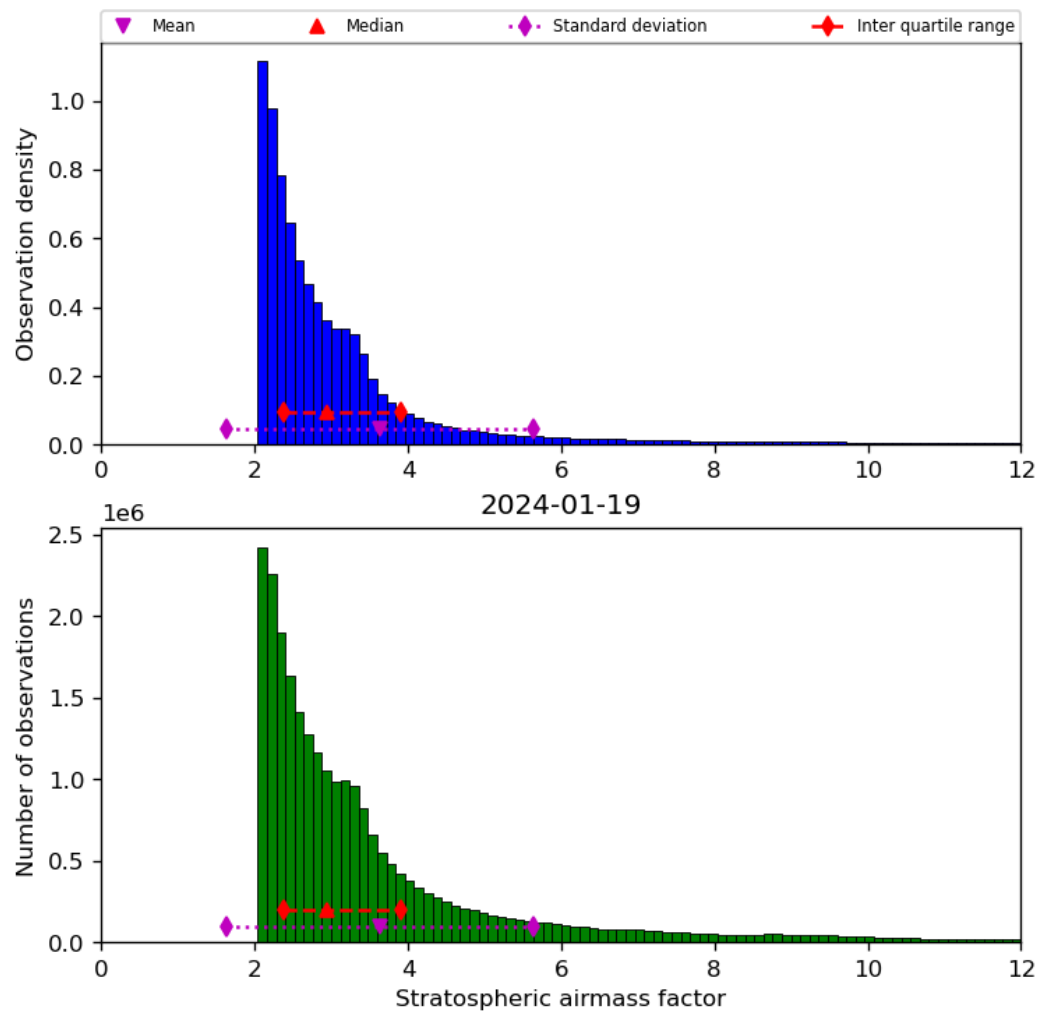
Figure 44: Histogram of “Stratospheric airmass factor” for 2024-01-18 to 2024-01-20
