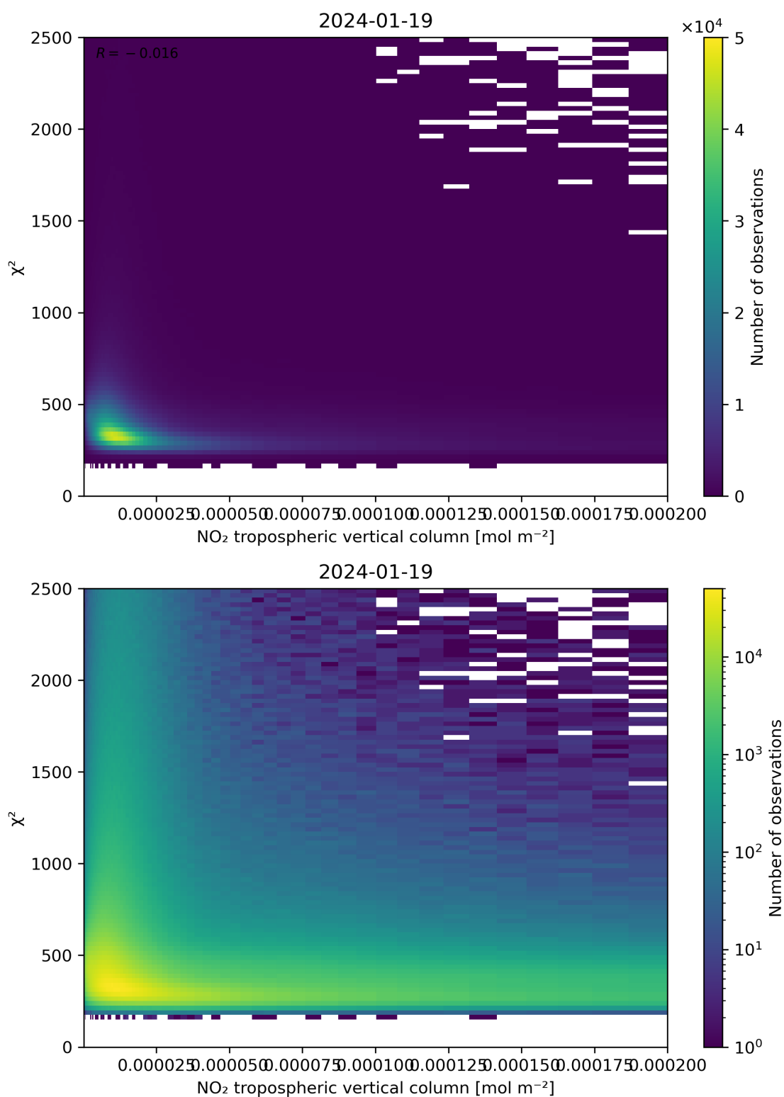
Figure 124: Scatter density plot of “NO 2 tropospheric vertical column” against “ \chi^2 ” for 2024-01-18 to 2024-01-20.
