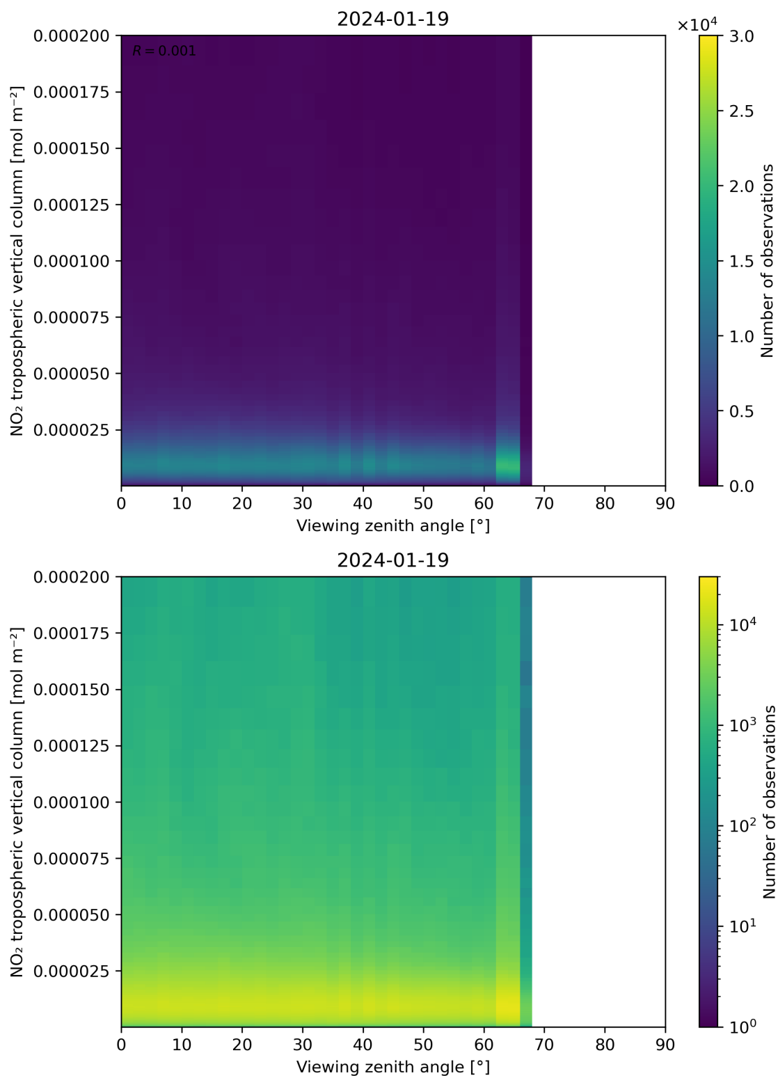
Figure 169: Scatter density plot of “Viewing zenith angle” against “NO 2 tropospheric vertical column” for 2024-01-18 to 2024-01-20.
