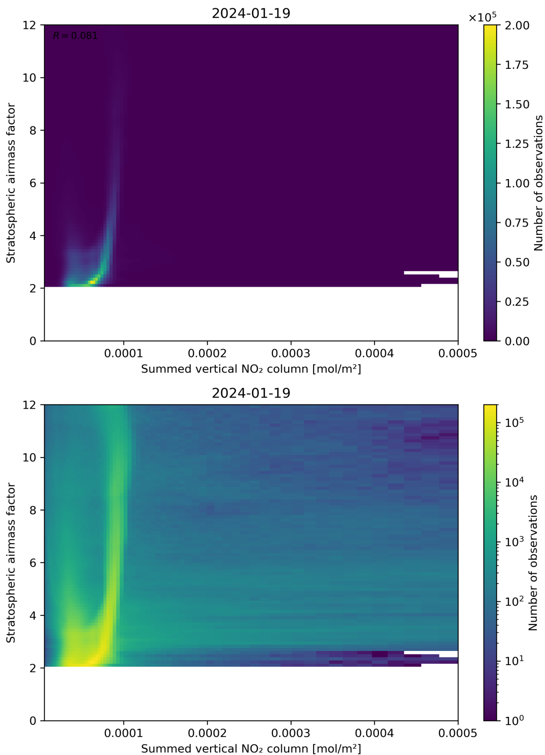
Figure 103: Scatter density plot of “Summed vertical NO 2 column” against “Stratospheric airmass factor” for 2024-01-18 to 2024-01-20.
