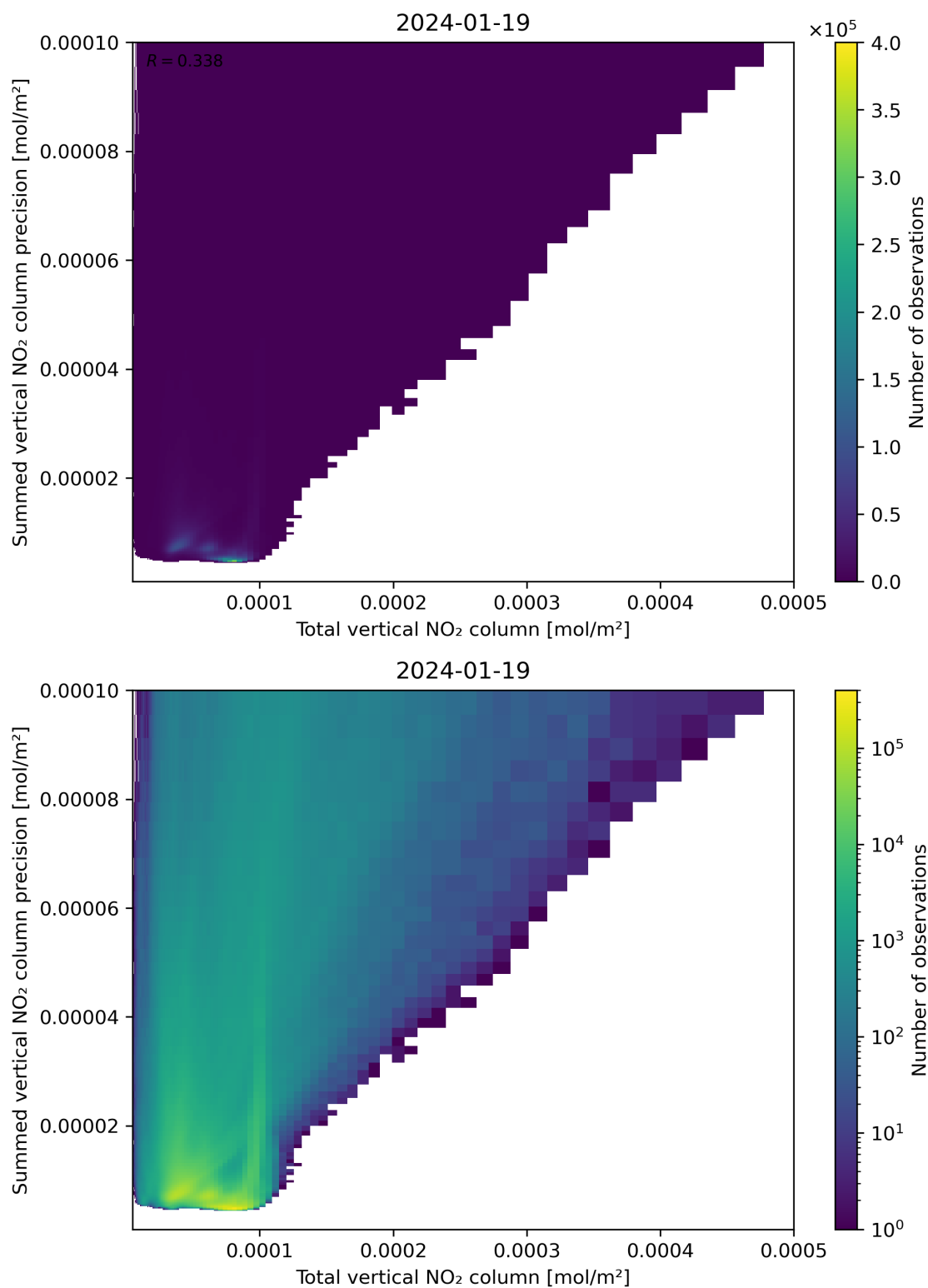
Figure 113: Scatter density plot of “Total vertical NO 2 column” against “Summed vertical NO 2 column precision” for 2024-01-18 to 2024-01-20.
