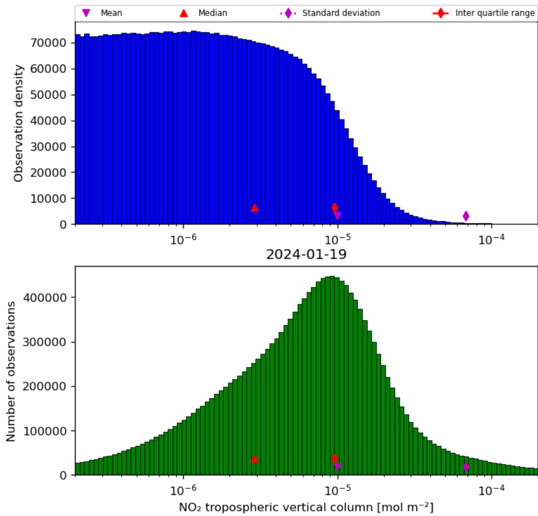
Figure 29: Histogram of “NO 2 tropospheric vertical column” for 2024-01-18 to 2024-01-20
