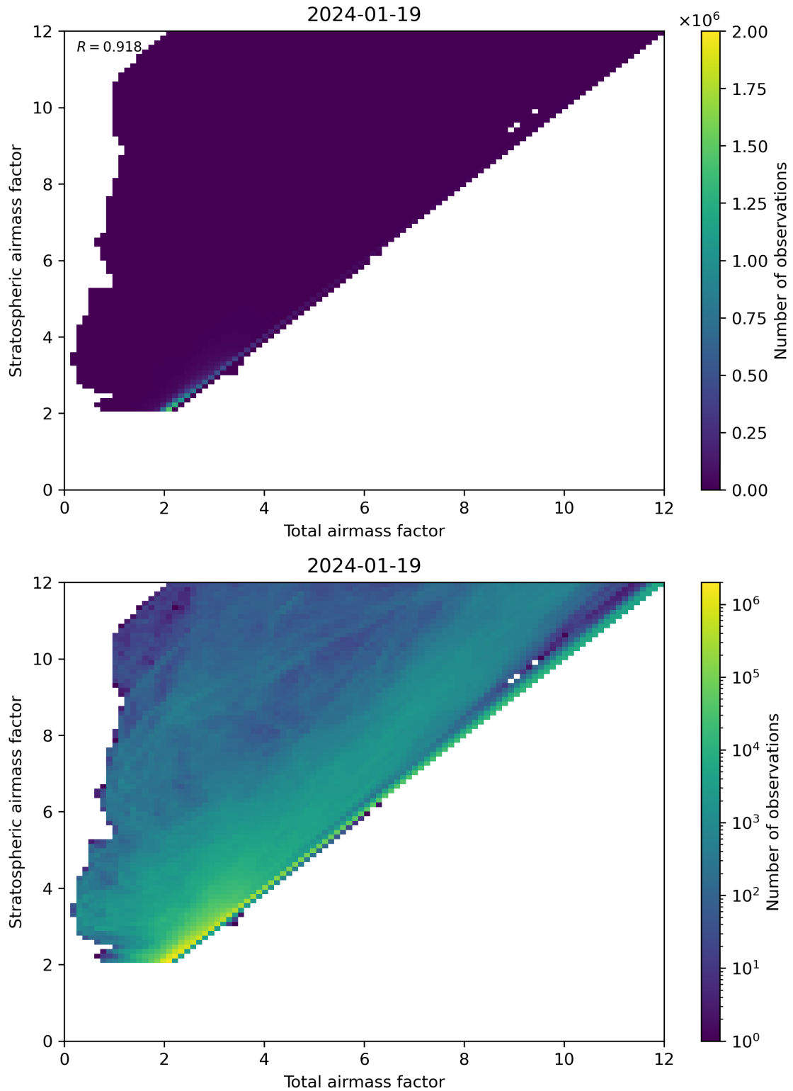
Figure 62: Scatter density plot of “Total airmass factor” against “Stratospheric airmass factor” for 2024-01-18 to 2024-01-20.
