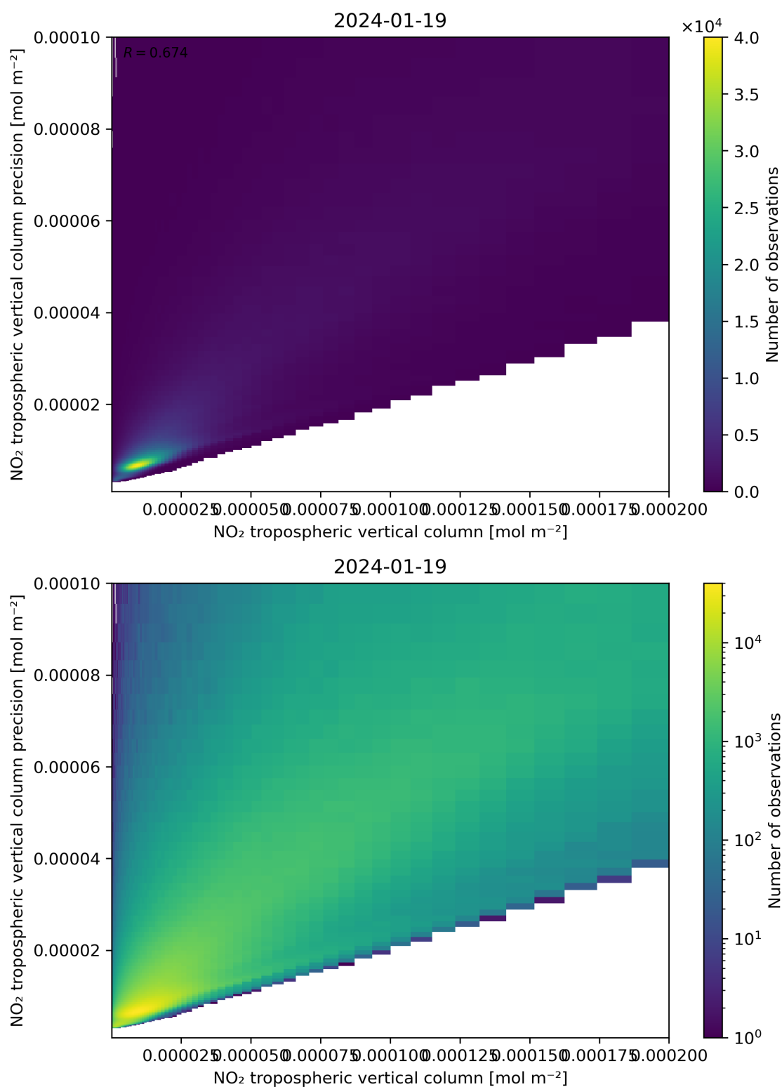
Figure 130: Scatter density plot of “NO 2 tropospheric vertical column” against “NO 2 tropospheric vertical column precision” for 2024-01-18 to 2024-01-20.
