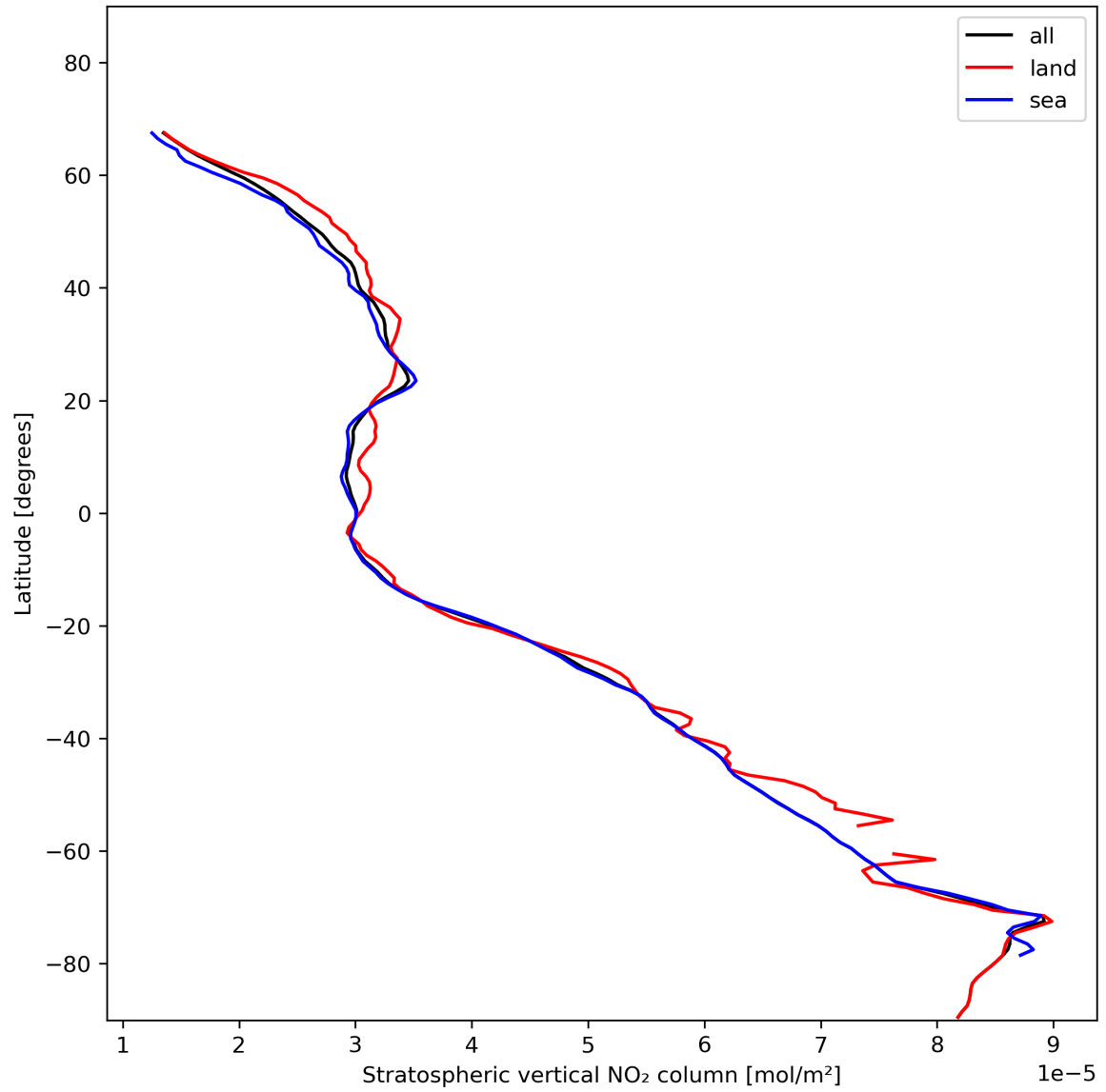
Figure 19: Zonal average of “Stratospheric vertical NO 2 column” for 2024-01-18 to 2024-01-20.
