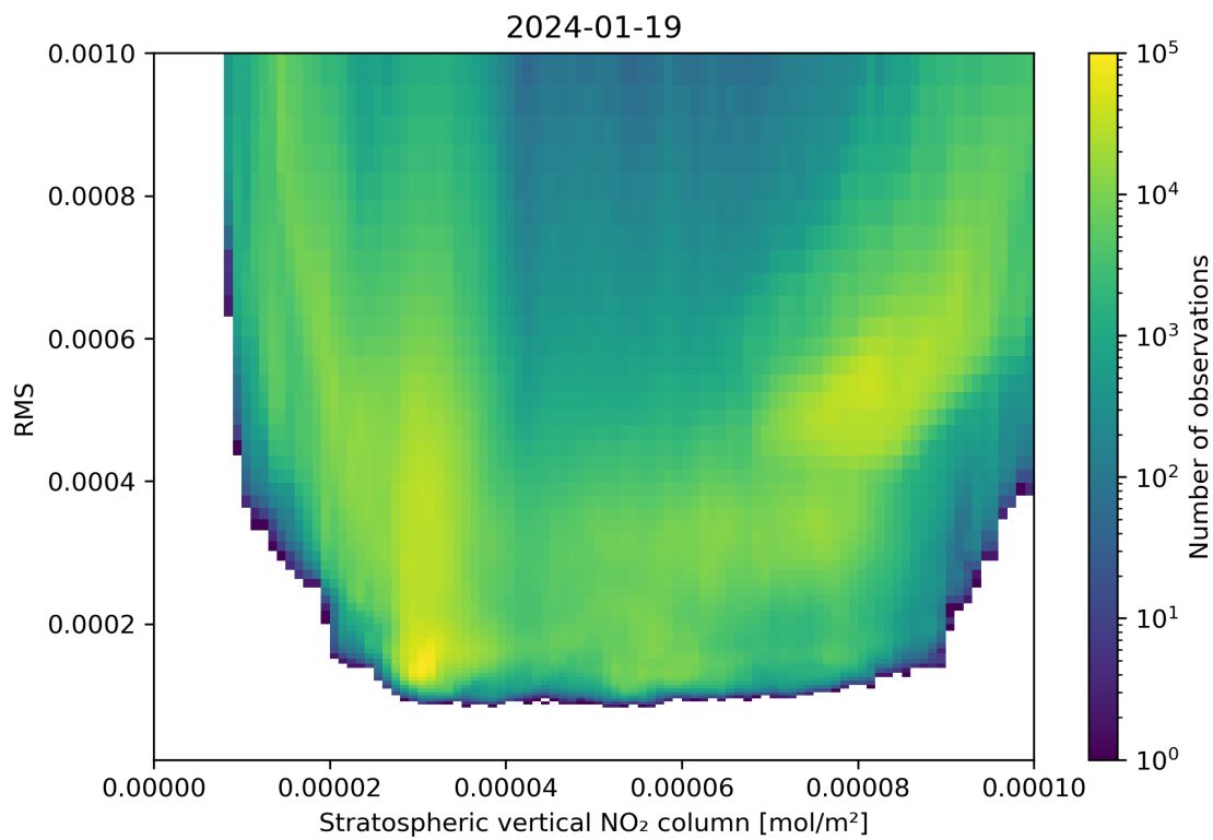
Figure 102: Scatter density plot of “Stratospheric vertical NO 2 column” against “RMS” for 2024-01-18 to 2024-01-20.
