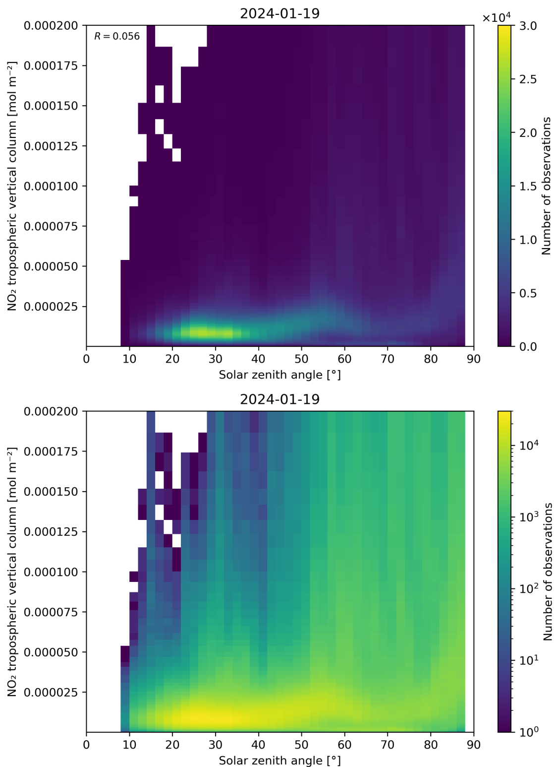
Figure 155: Scatter density plot of “Solar zenith angle” against “NO 2 tropospheric vertical column” for 2024-01-18 to 2024-01-20.
