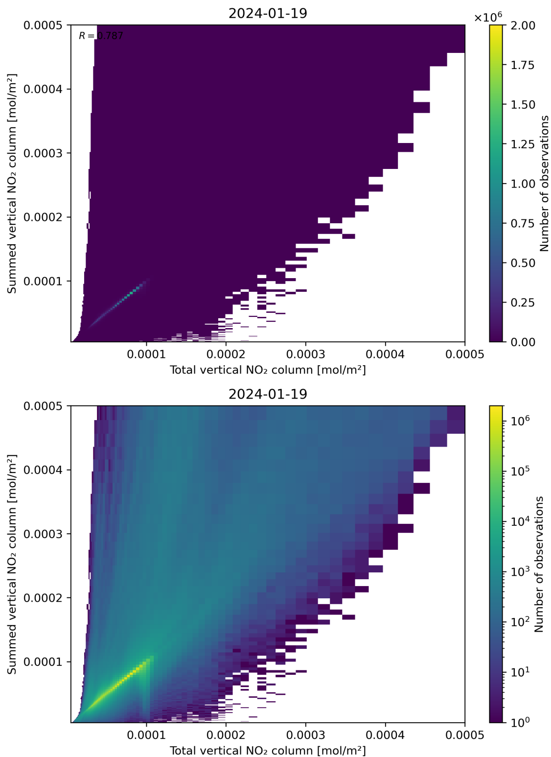
Figure 112: Scatter density plot of “Total vertical NO 2 column” against “Summed vertical NO 2 column” for 2024-01-18 to 2024-01-20.
