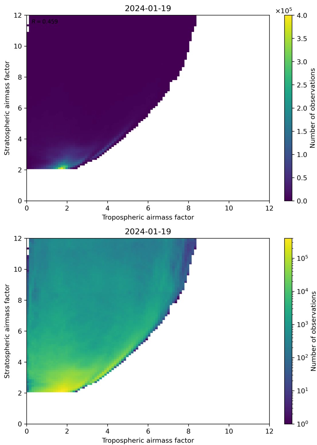
Figure 71: Scatter density plot of “Tropospheric airmass factor” against “Stratospheric airmass factor” for 2024-01-18 to 2024-01-20.
