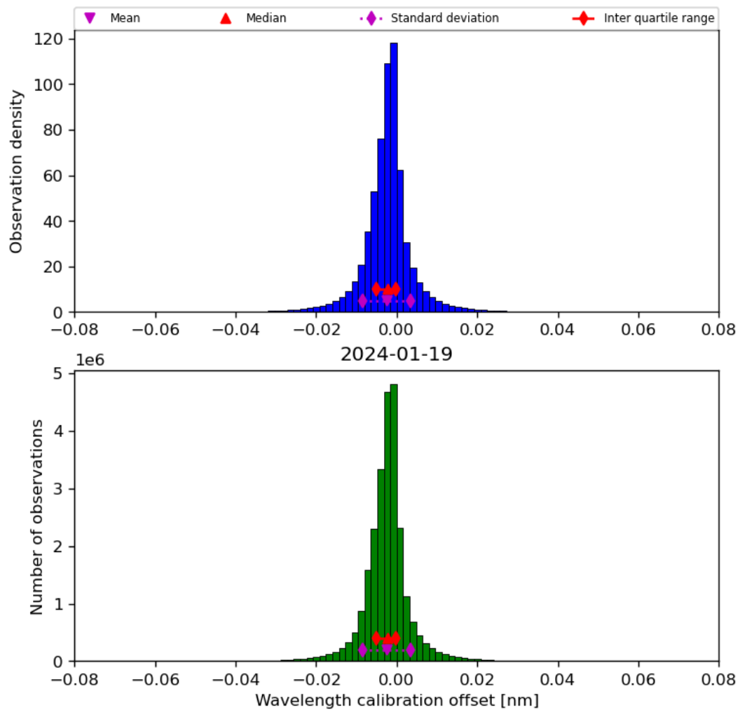
Figure 35: Histogram of “Wavelength calibration offset” for 2024-01-18 to 2024-01-20
