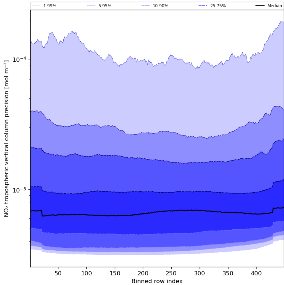
Figure 47: Along track statistics of “NO 2 tropospheric vertical column precision” for 2024-01-18 to 2024-01-20
