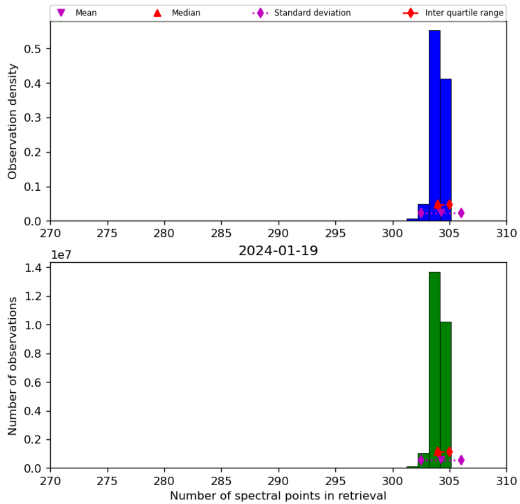
Figure 33: Histogram of “Number of spectral points in retrieval” for 2024-01-18 to 2024-01-20
