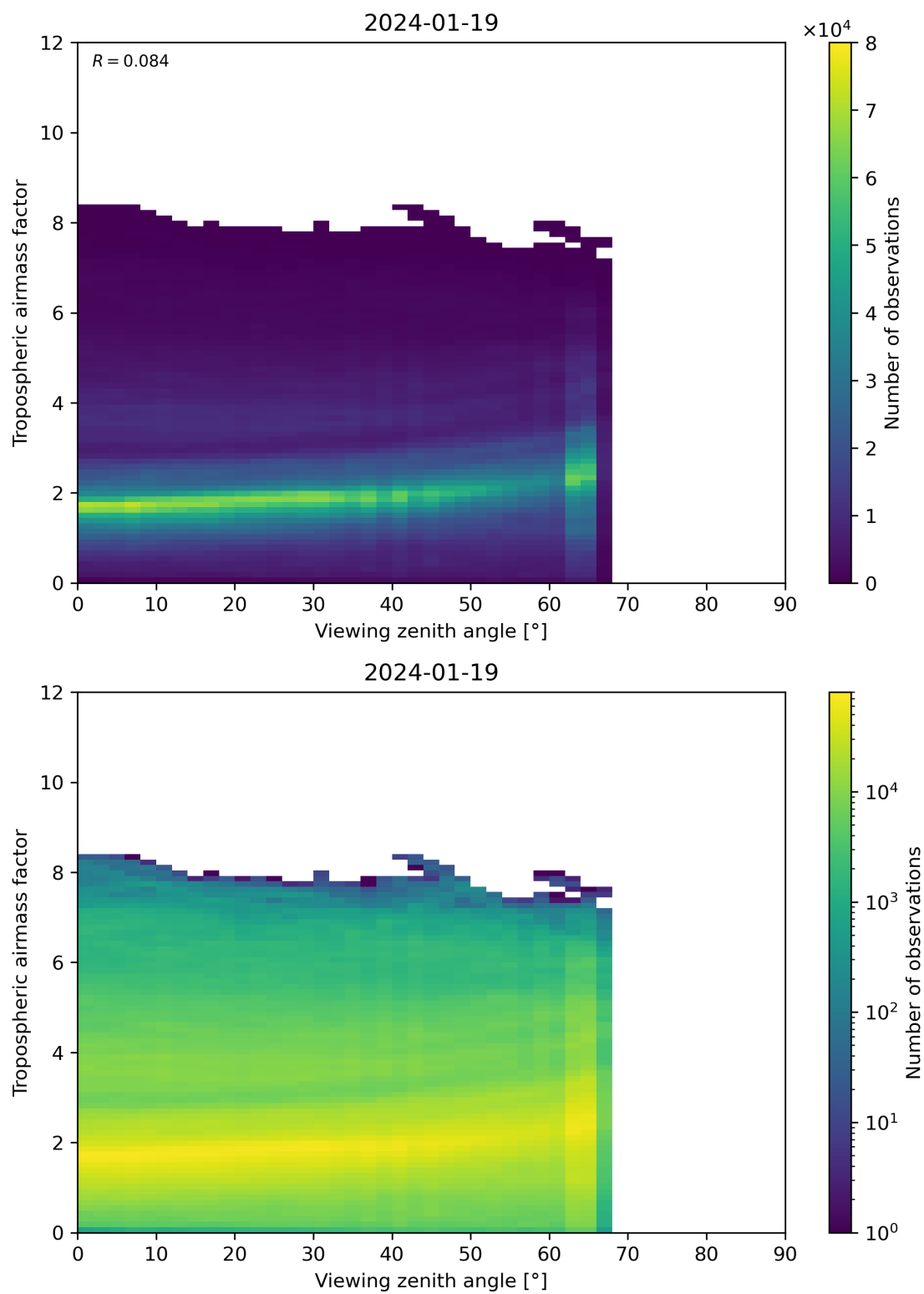
Figure 161: Scatter density plot of “Viewing zenith angle” against “Tropospheric airmass factor” for 2024-01-18 to 2024-01-20.
