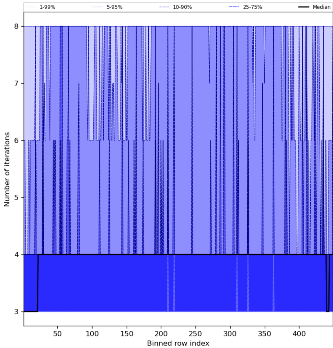
Figure 51: Along track statistics of “Number of iterations” for 2024-01-18 to 2024-01-20
