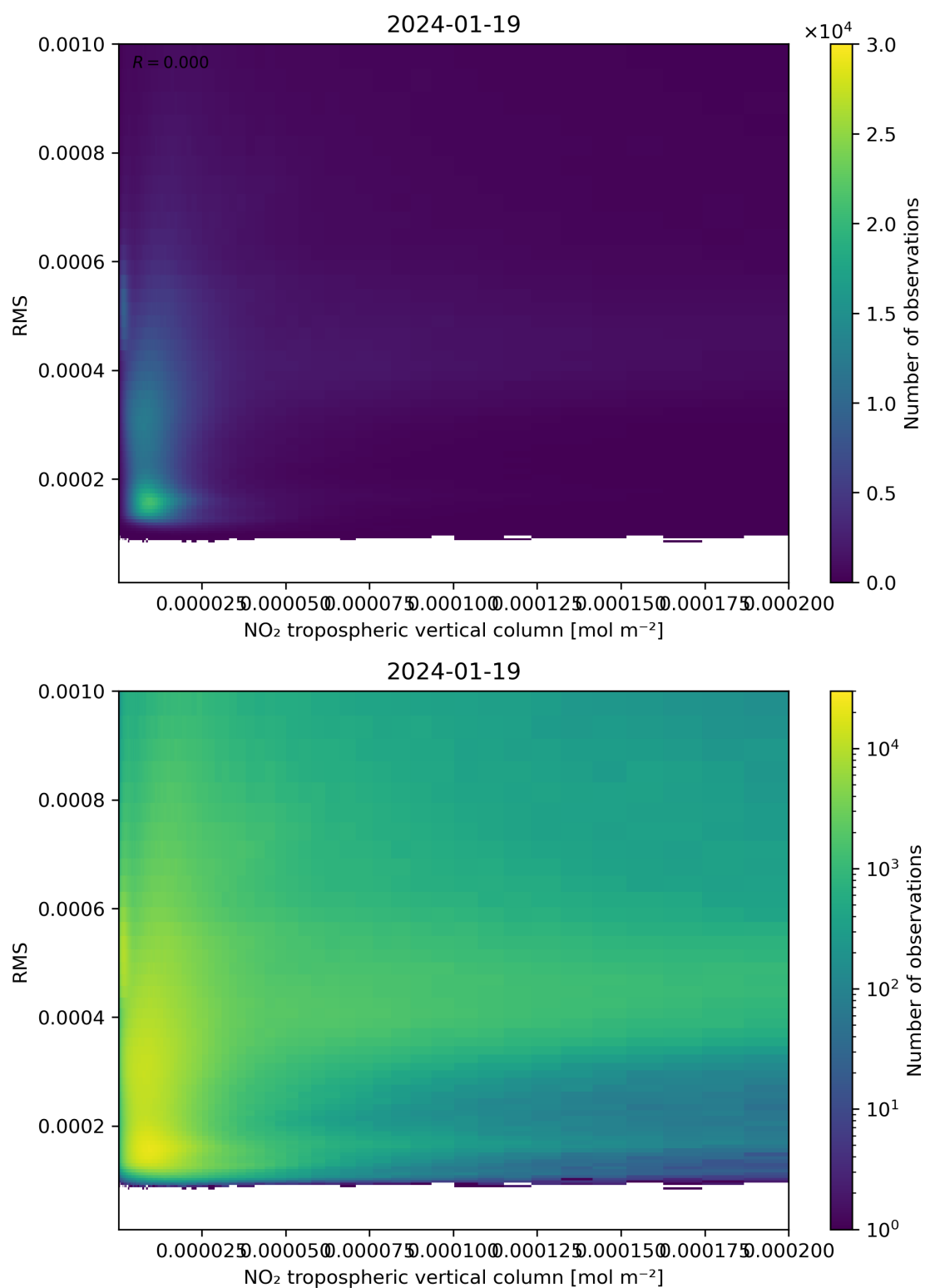
Figure 142: Scatter density plot of “NO 2 tropospheric vertical column” against “RMS” for 2024-01-18 to 2024-01-20.
