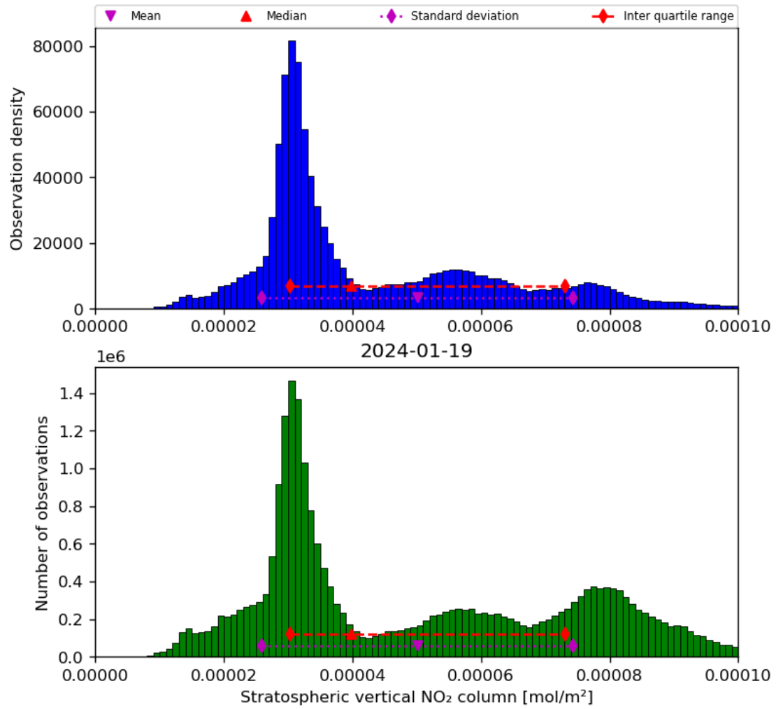
Figure 36: Histogram of “Stratospheric vertical NO 2 column” for 2024-01-18 to 2024-01-20
