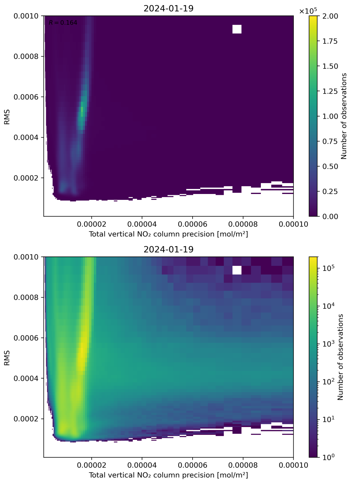
Figure 119: Scatter density plot of “Total vertical NO 2 column precision” against “RMS” for 2024-01-18 to 2024-01-20.
