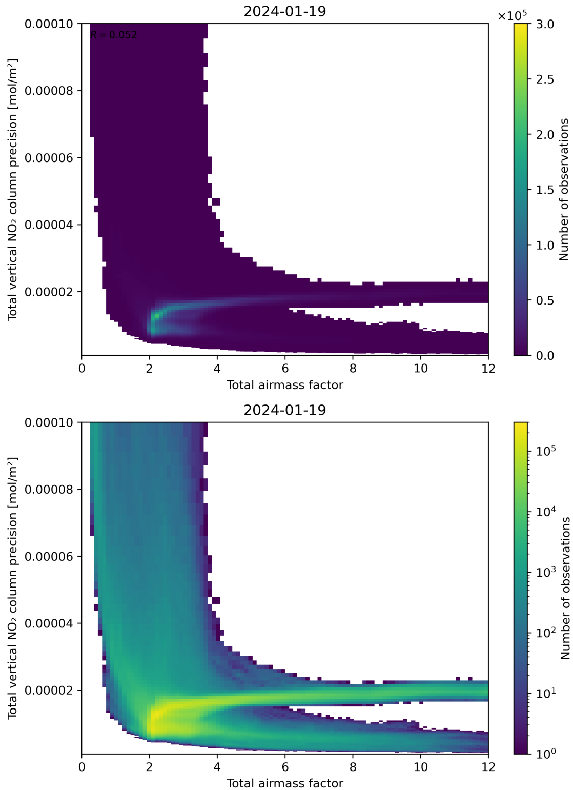
Figure 68: Scatter density plot of “Total airmass factor” against “Total vertical NO 2 column precision” for 2024-01-18 to 2024-01-20.
