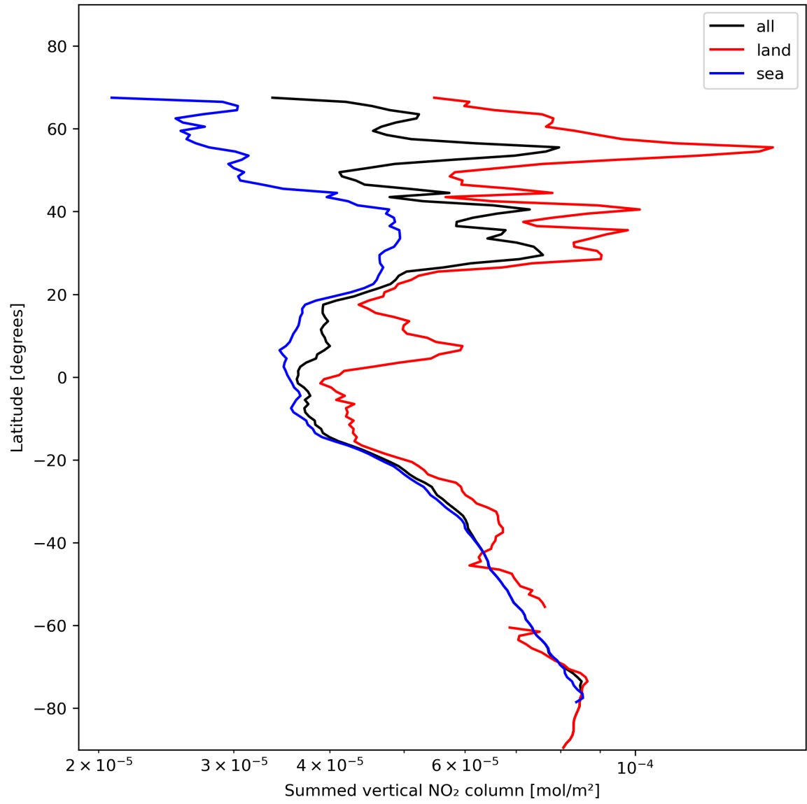
Figure 23: Zonal average of “Summed vertical NO 2 column” for 2024-01-18 to 2024-01-20.
