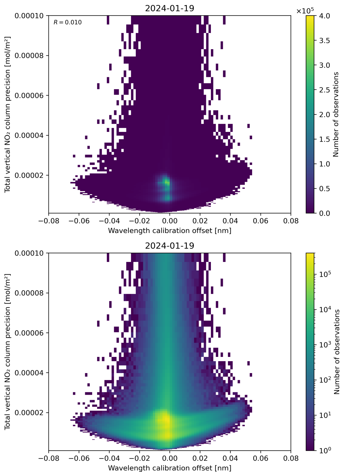
Figure 180: Scatter density plot of “Wavelength calibration offset” against “Total vertical NO 2 column precision” for 2024-01-18 to 2024-01-20.
