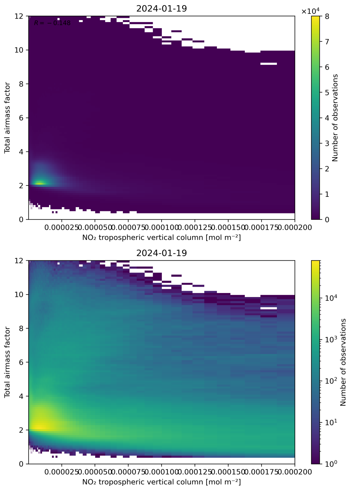
Figure 122: Scatter density plot of “NO 2 tropospheric vertical column” against “Total air mass factor” for 2024-01-18 to 2024-01-20.
