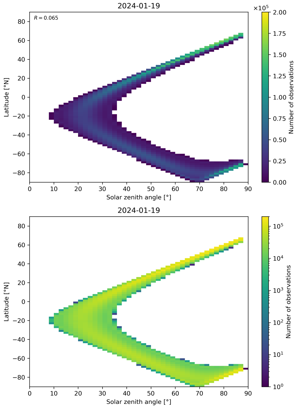
Figure 149: Scatter density plot of “Solar zenith angle” against “Latitude” for 2024-01-18 to 2024-01-20.
