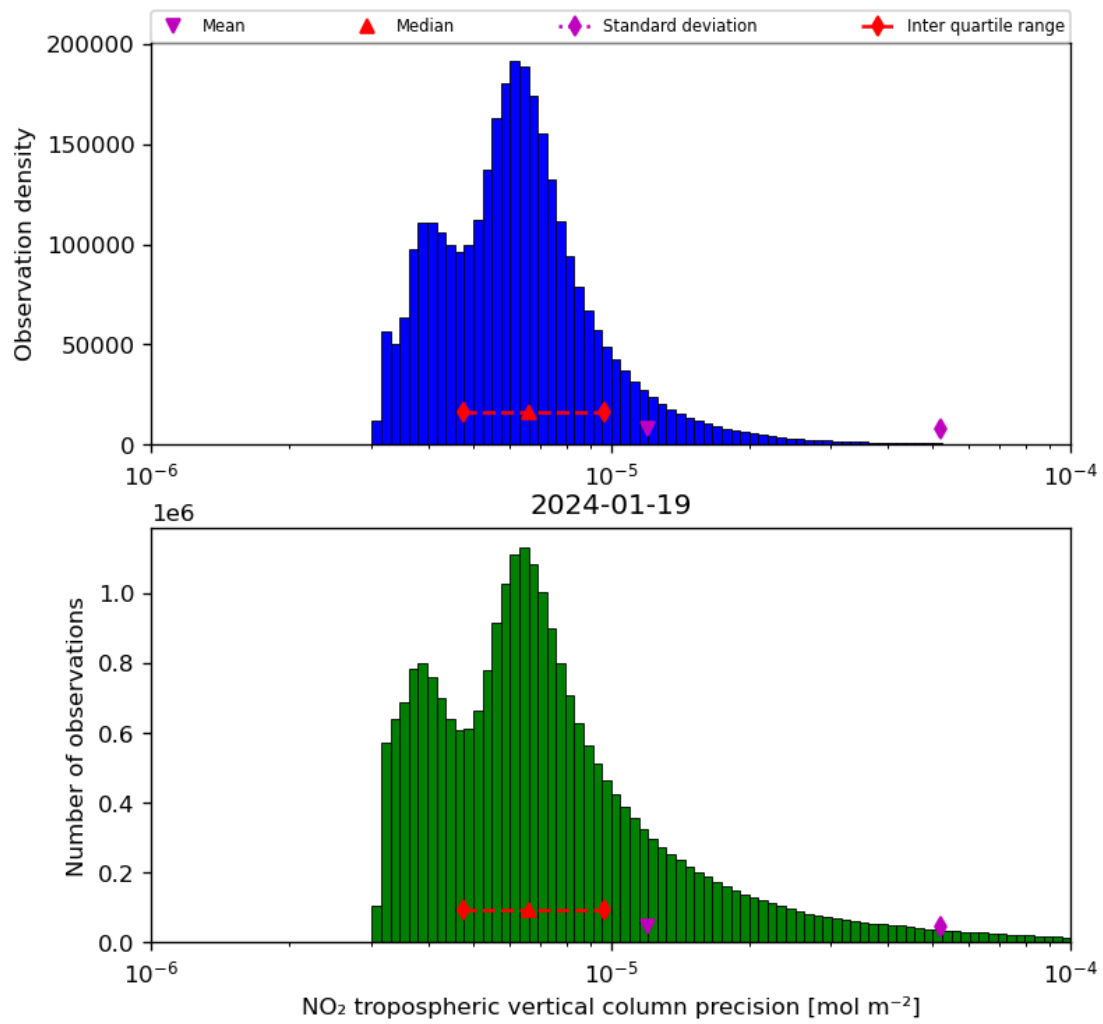
Figure 30: Histogram of “NO 2 tropospheric vertical column precision” for 2024-01-18 to 2024-01-20
