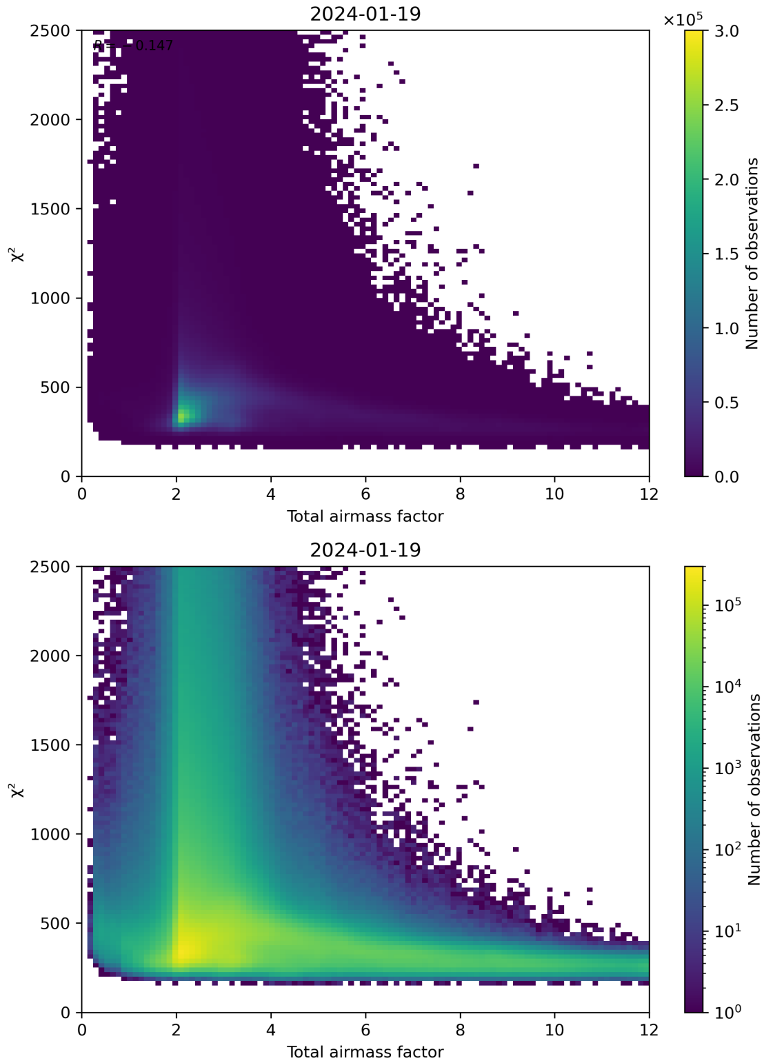
Figure 63: Scatter density plot of “Total airmass factor” against “ \chi^2 ” for 2024-01-18 to 2024-01-20.
