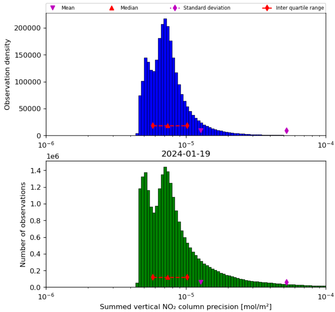
Figure 41: Histogram of “Summed vertical NO 2 column precision” for 2024-01-18 to 2024-01-20
