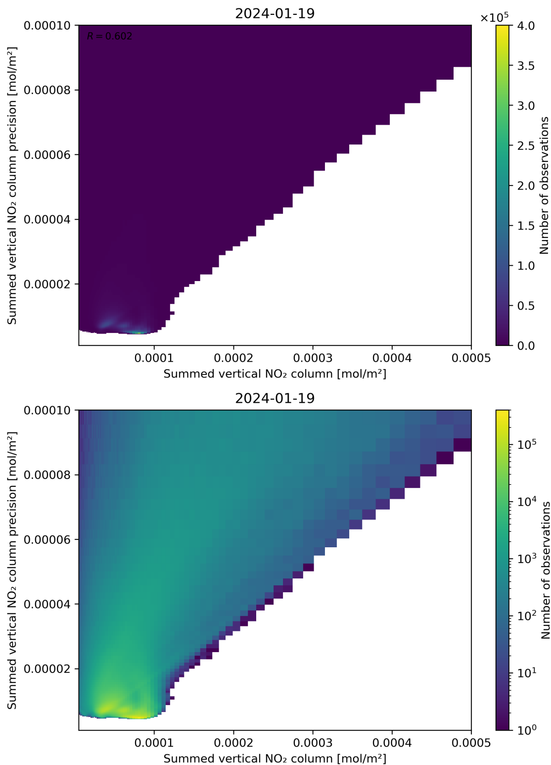
Figure 105: Scatter density plot of “Summed vertical NO 2 column” against “Summed vertical NO 2 column precision” for 2024-01-18 to 2024-01-20.
