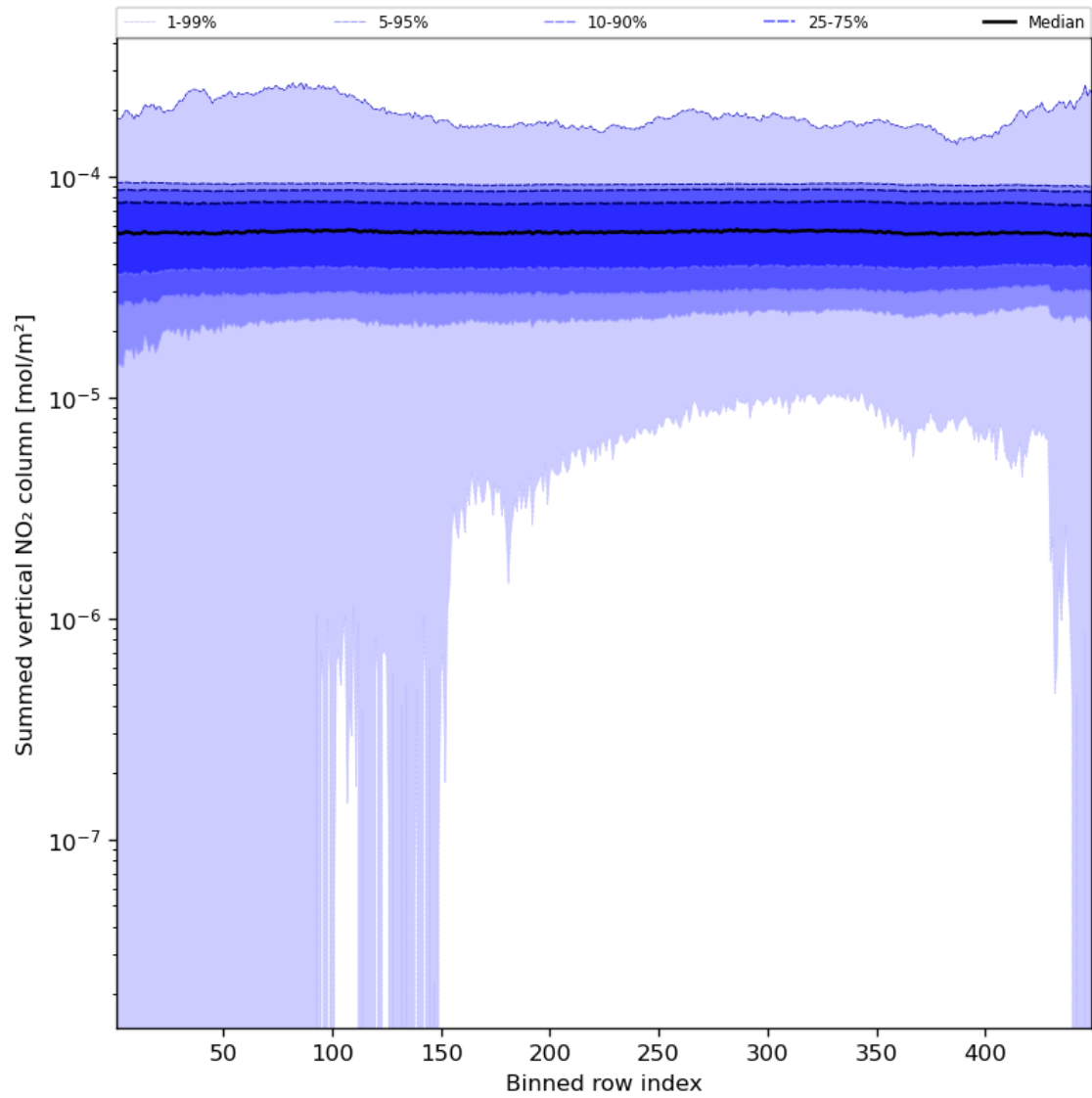
Figure 57: Along track statistics of “Summed vertical NO 2 column” for 2024-01-18 to 2024-01-20
