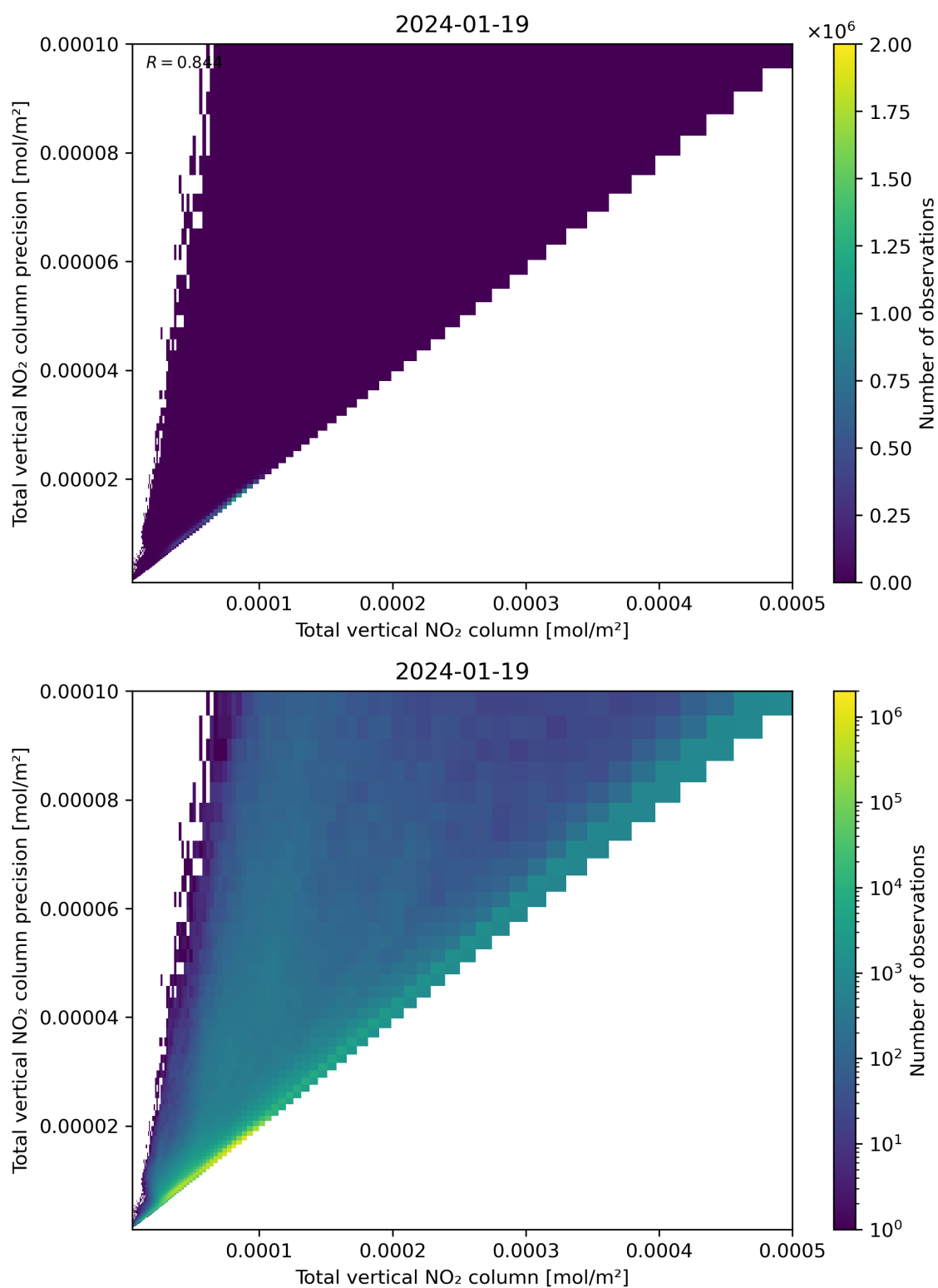
Figure 114: Scatter density plot of “Total vertical NO 2 column” against “Total vertical NO 2 column precision” for 2024-01-18 to 2024-01-20.
