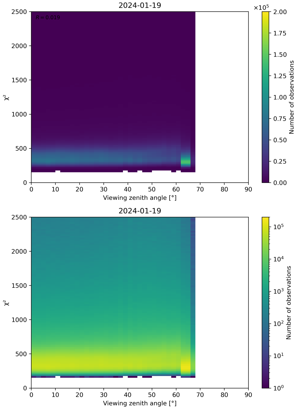
Figure 162: Scatter density plot of “Viewing zenith angle” against “ \chi^2 ” for 2024-01-18 to 2024-01-20.
