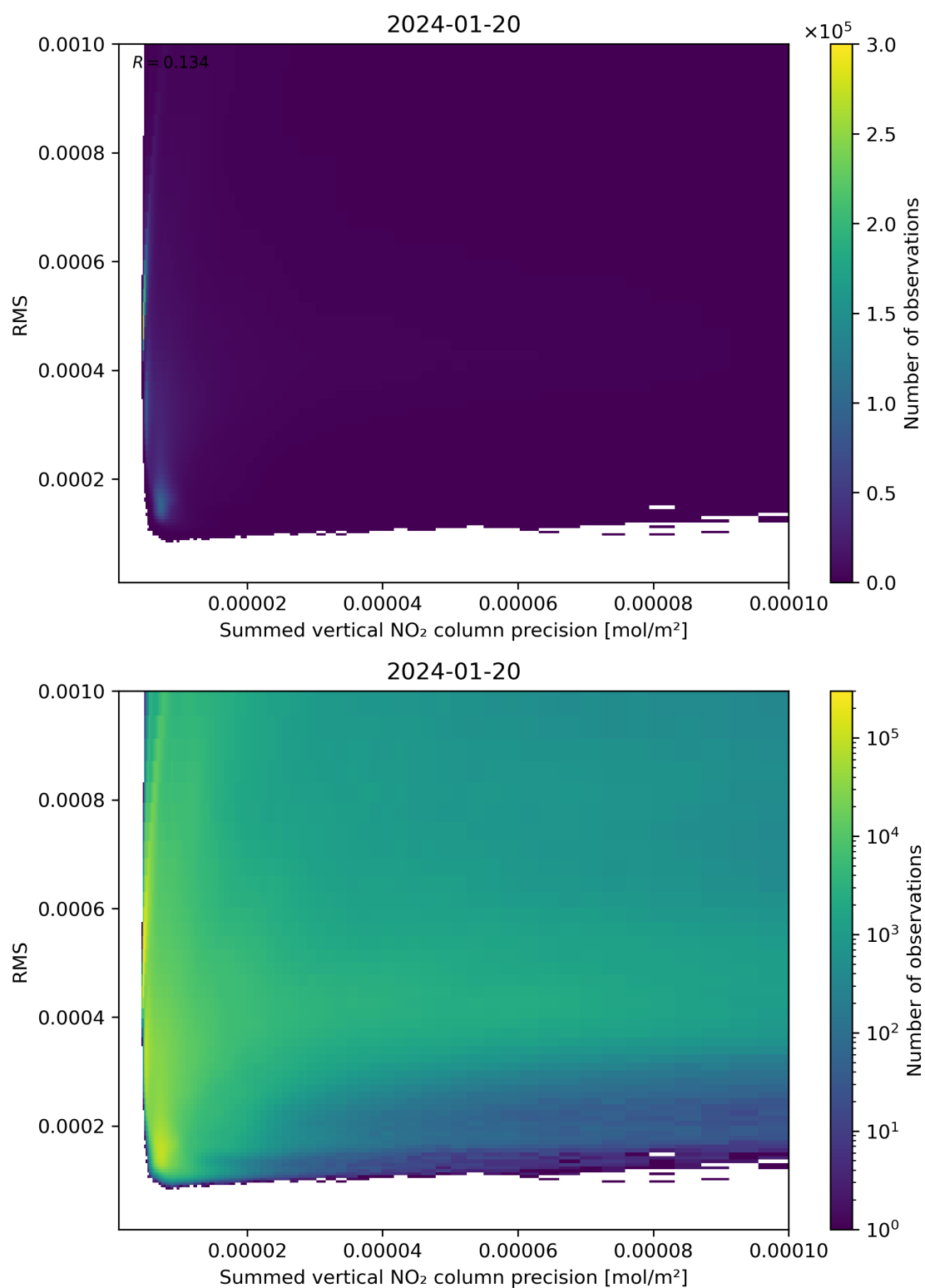
Figure 108: Scatter density plot of “Summed vertical NO 2 column precision” against “RMS” for 2024-01-19 to 2024-01-21.
