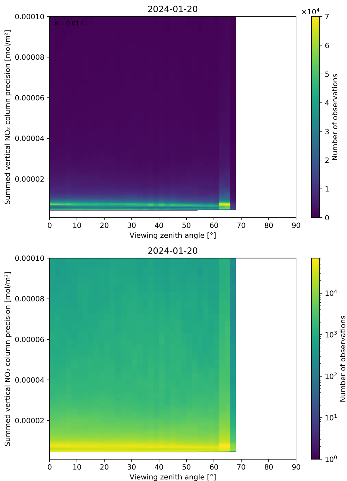
Figure 166: Scatter density plot of “Viewing zenith angle” against “Summed vertical NO 2 column precision” for 2024-01-19 to 2024-01-21.
