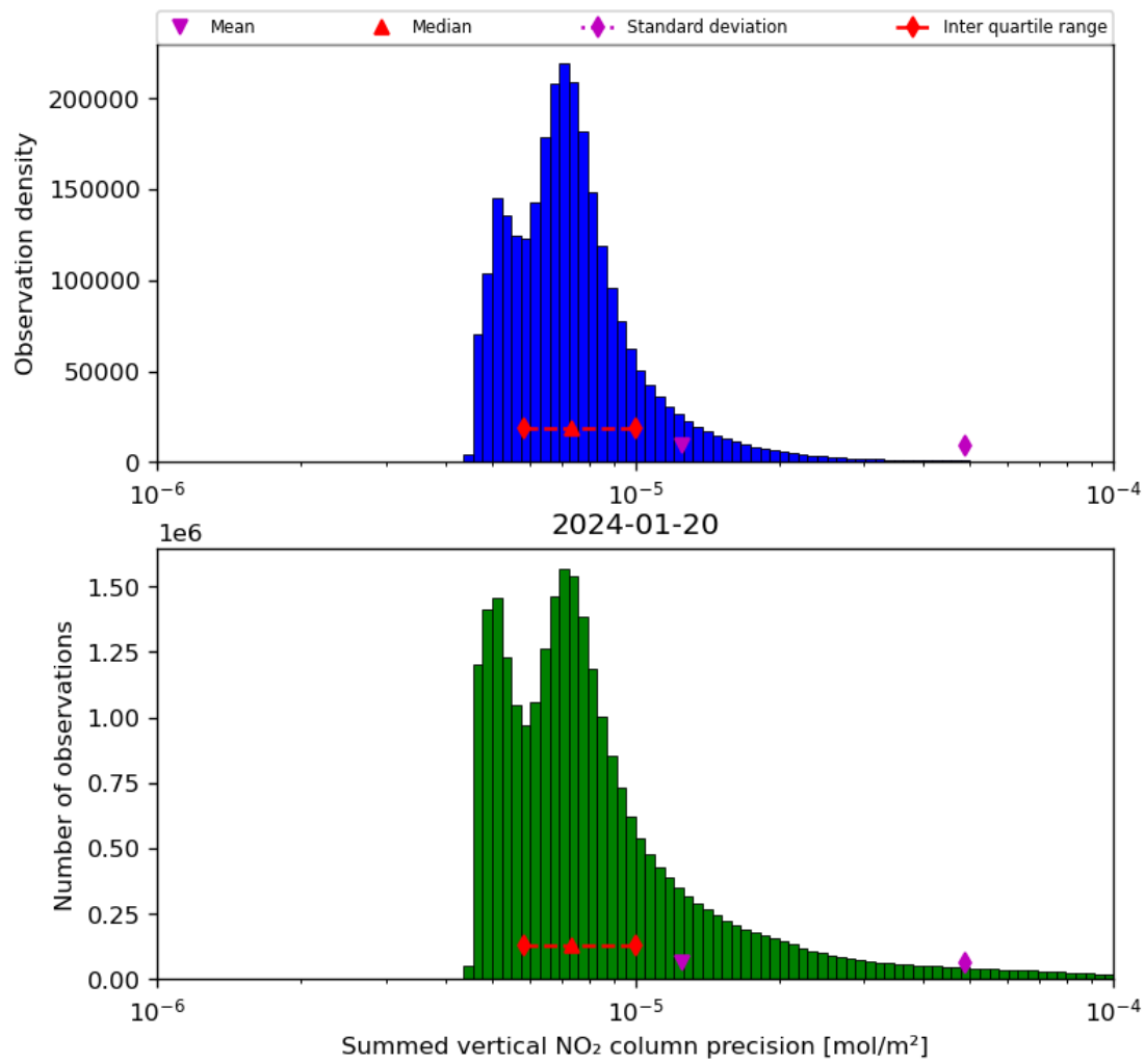
Figure 41: Histogram of “Summed vertical NO 2 column precision” for 2024-01-19 to 2024-01-21
