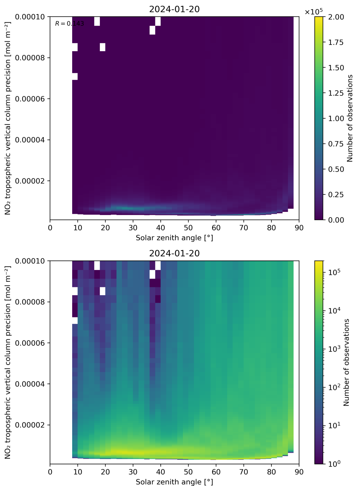
Figure 156: Scatter density plot of “Solar zenith angle” against “NO 2 tropospheric vertical column precision” for 2024-01-19 to 2024-01-21.
