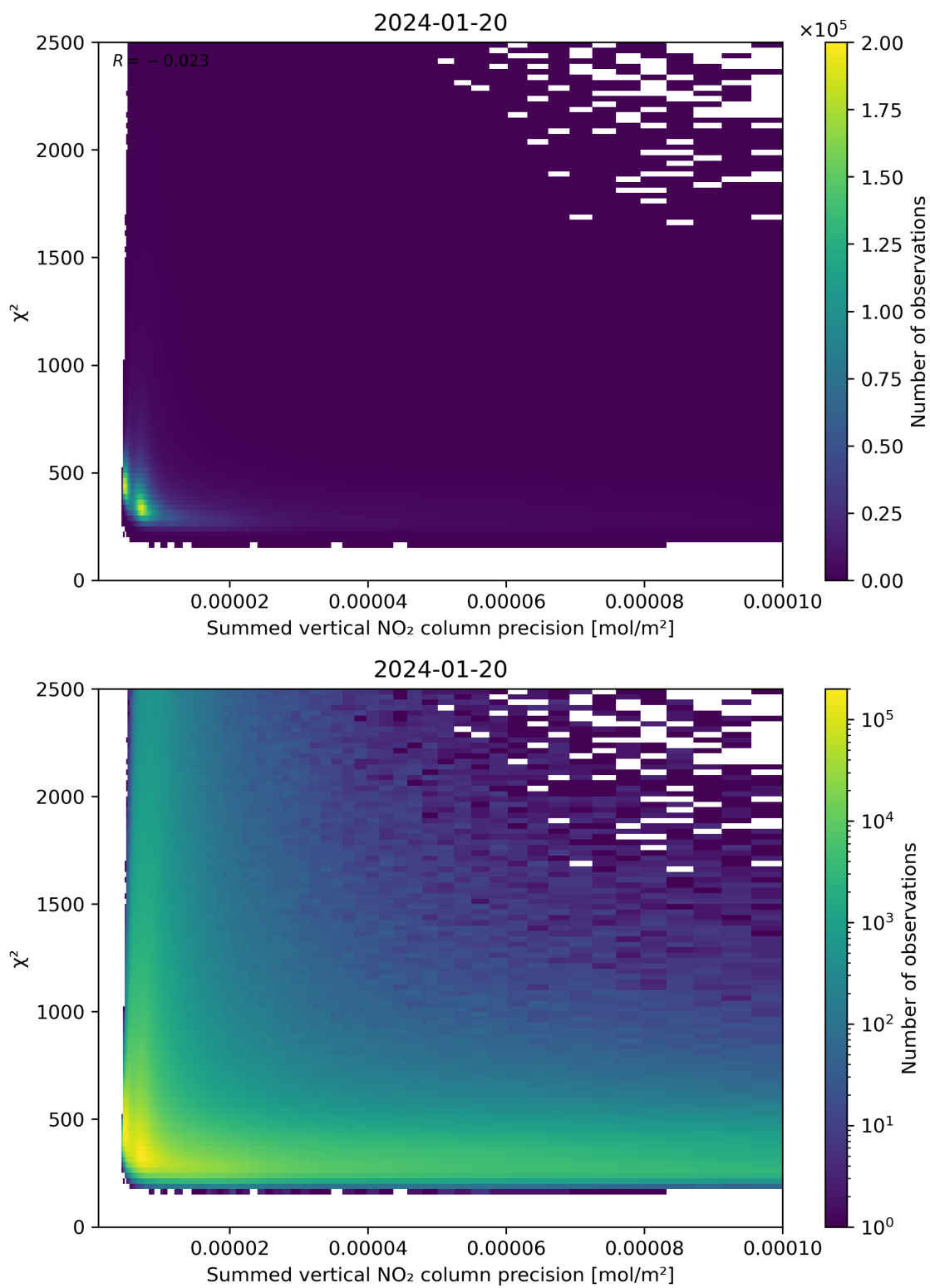
Figure 107: Scatter density plot of “Summed vertical NO 2 column precision” against “ \chi^2 ” for 2024-01-19 to 2024-01-21.
