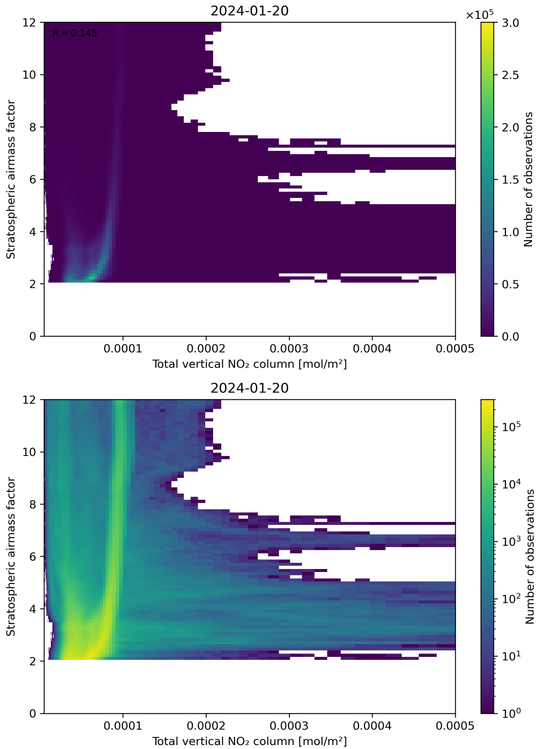
Figure 110: Scatter density plot of “Total vertical NO 2 column” against “Stratospheric air mass factor” for 2024-01-19 to 2024-01-21.
