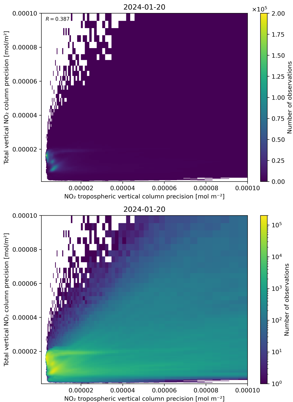
Figure 139: Scatter density plot of “NO 2 tropospheric vertical column precision” against “Total vertical NO 2 column precision” for 2024-01-19 to 2024-01-21.
