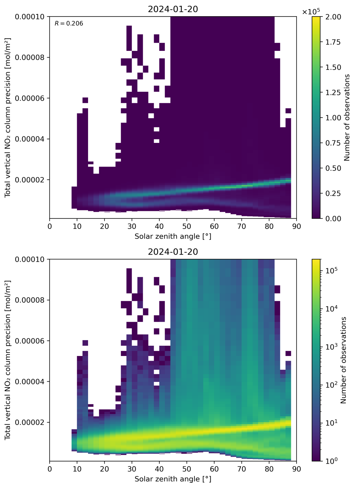
Figure 154: Scatter density plot of “Solar zenith angle” against “Total vertical NO 2 column precision” for 2024-01-19 to 2024-01-21.
