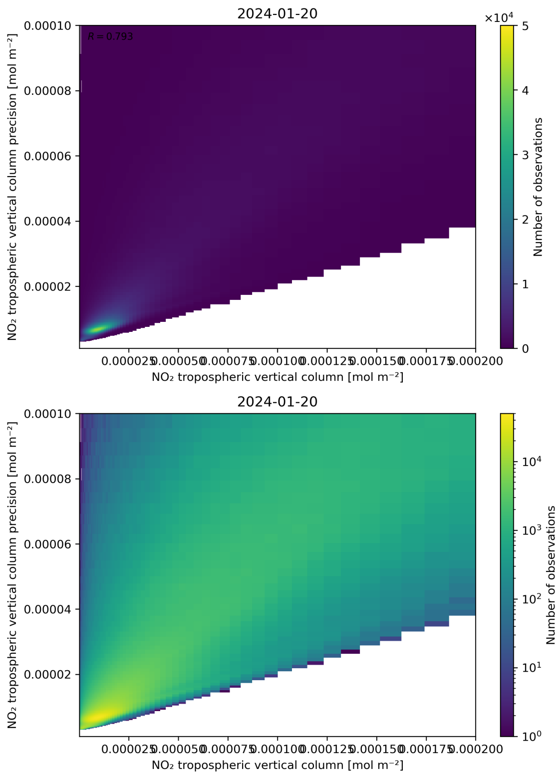
Figure 130: Scatter density plot of “NO 2 tropospheric vertical column” against “NO 2 tropospheric vertical column precision” for 2024-01-19 to 2024-01-21.
