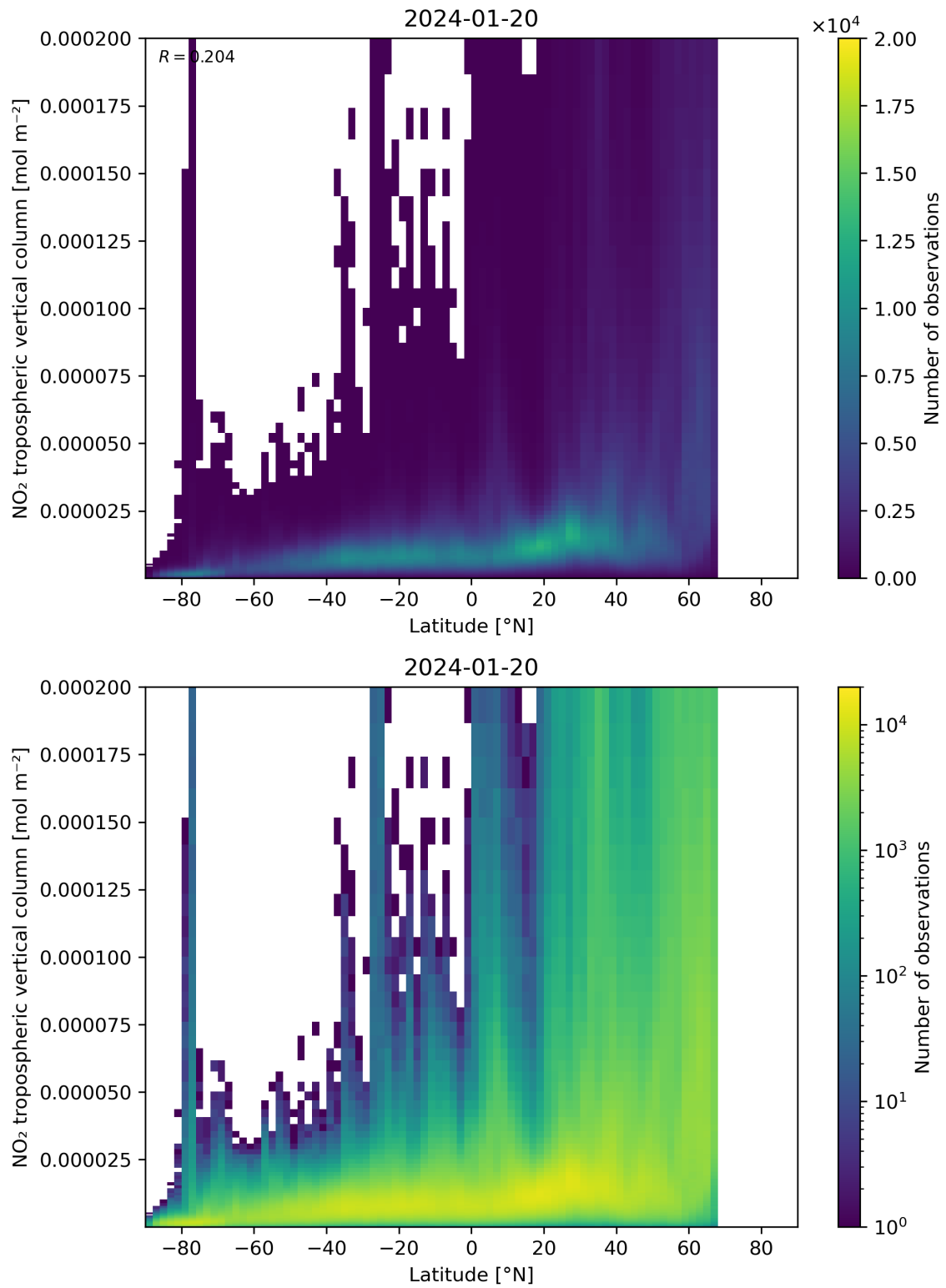
Figure 92: Scatter density plot of “Latitude” against “NO 2 tropospheric vertical column” for 2024-01-19 to 2024-01-21.
