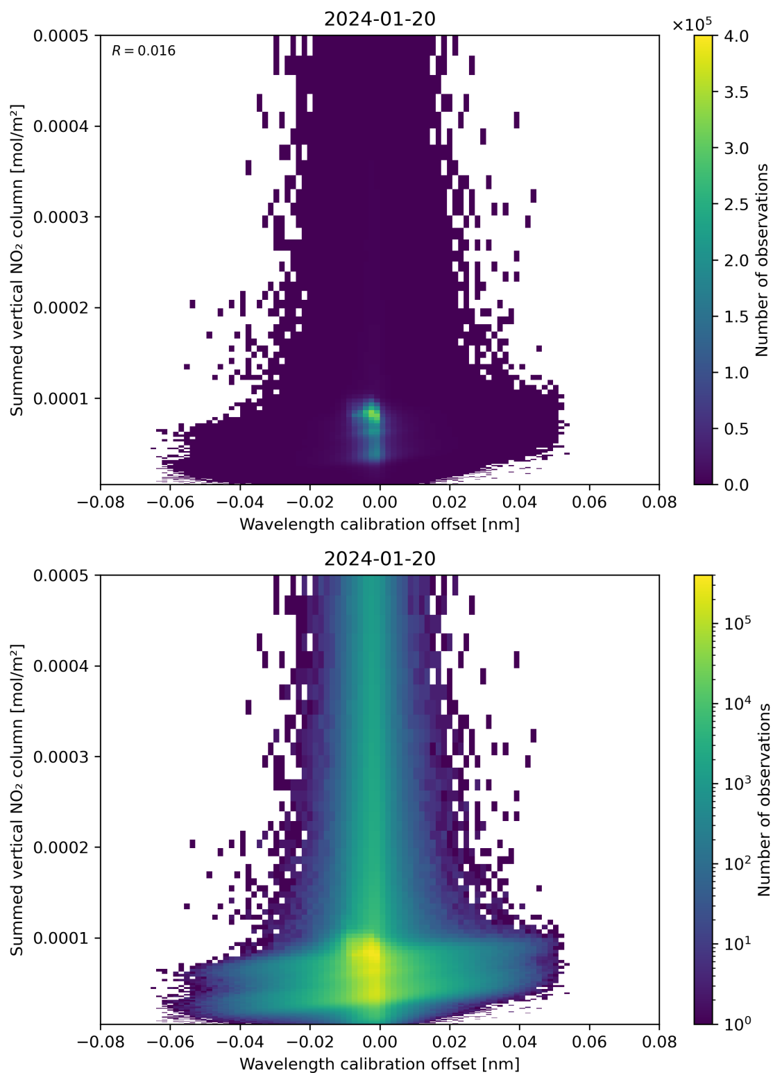
Figure 177: Scatter density plot of “Wavelength calibration offset” against “Summed vertical NO 2 column” for 2024-01-19 to 2024-01-21.
