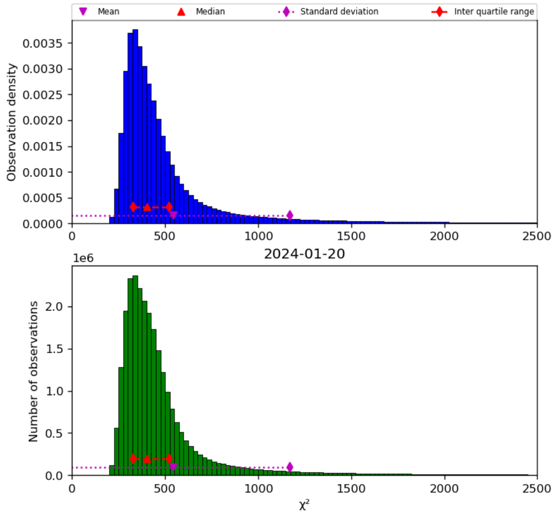
Figure 42: Histogram of “ \chi^2 ” for 2024-01-19 to 2024-01-21
