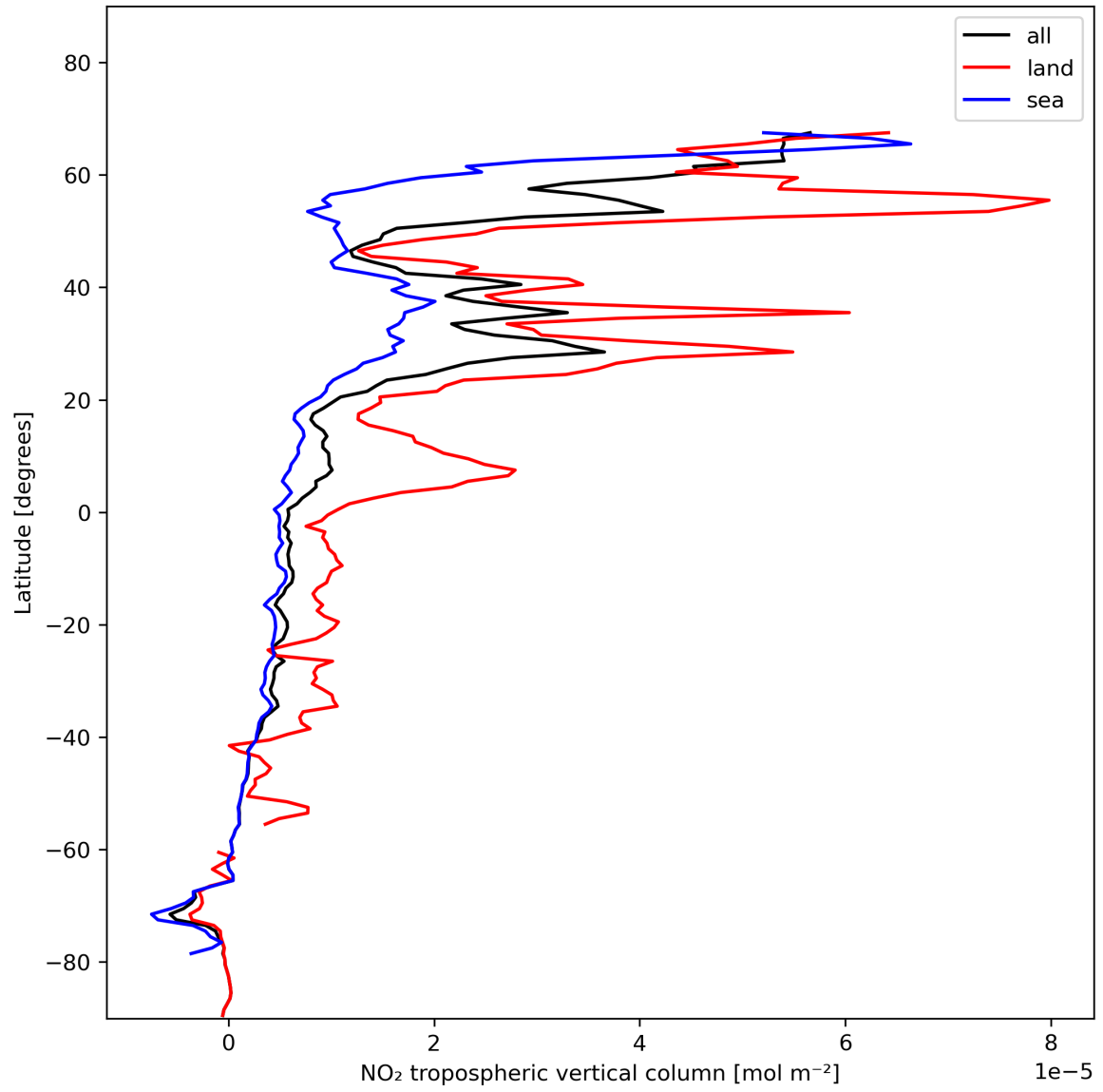
Figure 12: Zonal average of “NO 2 tropospheric vertical column” for 2024-01-19 to 2024-01-21.
