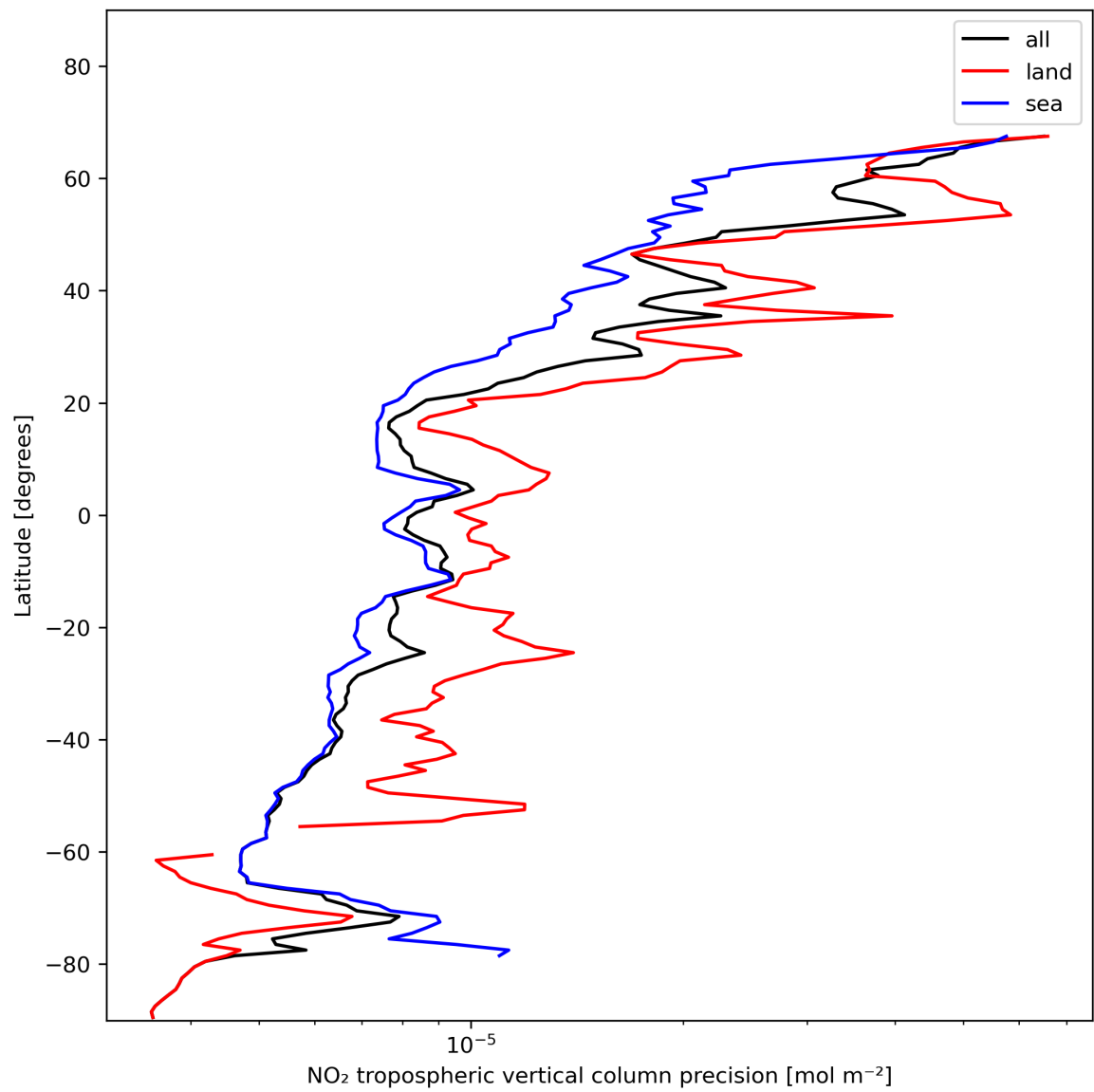
Figure 13: Zonal average of “NO 2 tropospheric vertical column precision” for 2024-01-19 to 2024-01-21.
