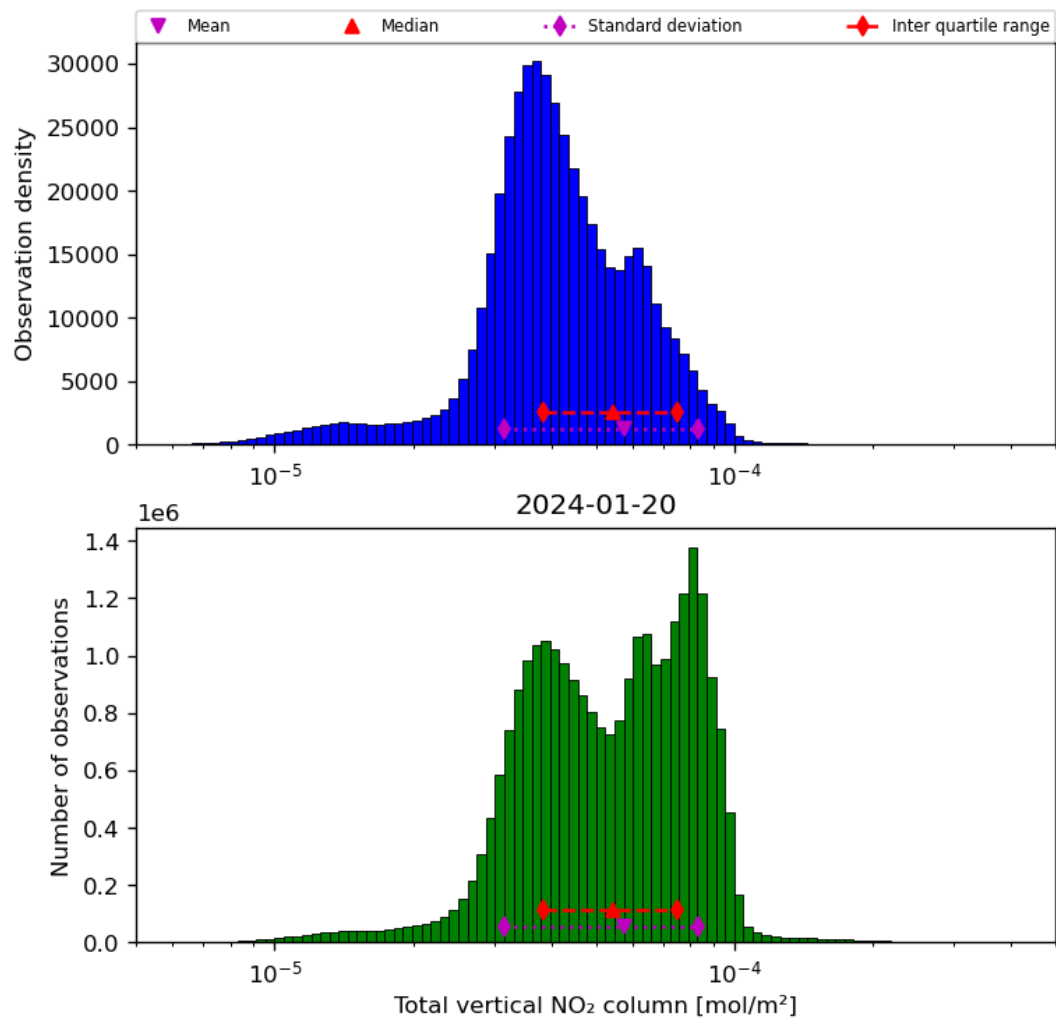
Figure 38: Histogram of “Total vertical NO 2 column” for 2024-01-19 to 2024-01-21
