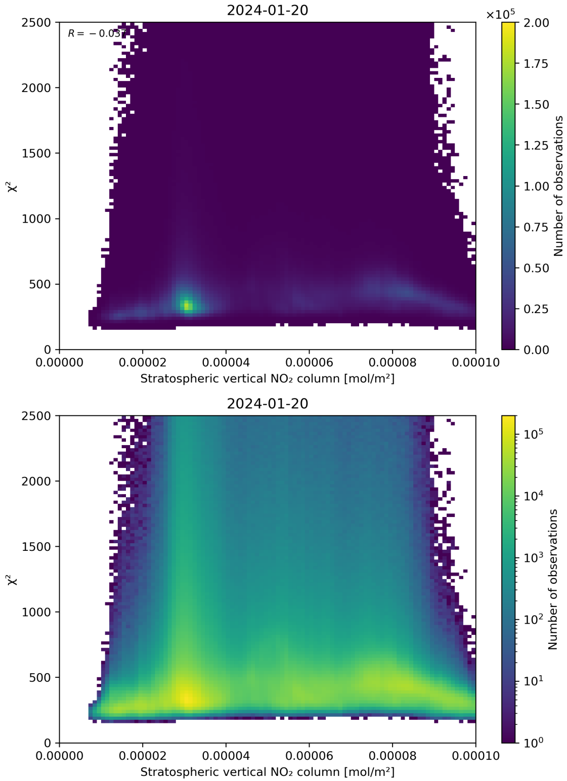
Figure 97: Scatter density plot of “Stratospheric vertical NO 2 column” against “ \chi^2 ” for 2024-01-19 to 2024-01-21.
