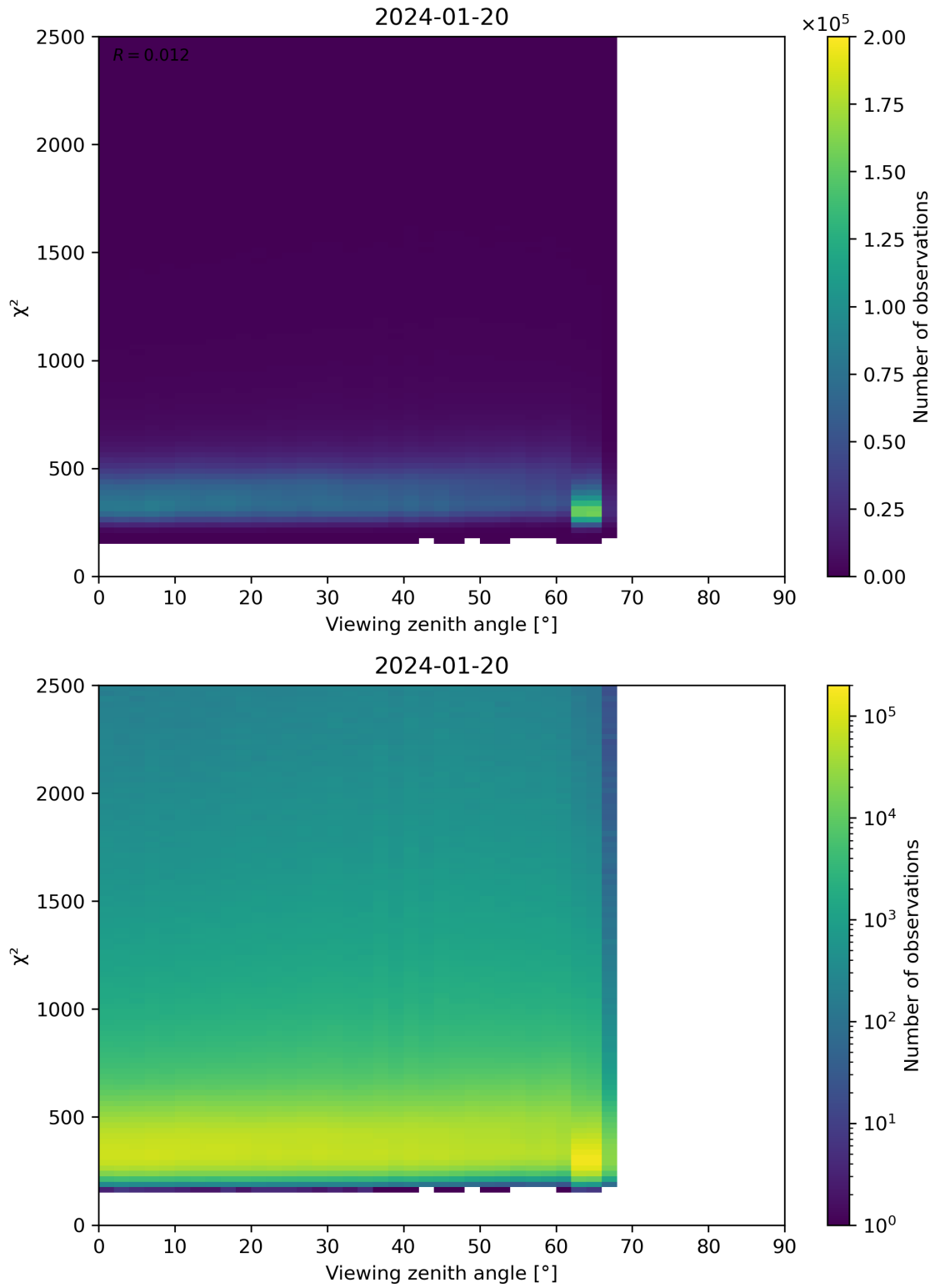
Figure 162: Scatter density plot of “Viewing zenith angle” against “ \chi^2 ” for 2024-01-19 to 2024-01-21.
