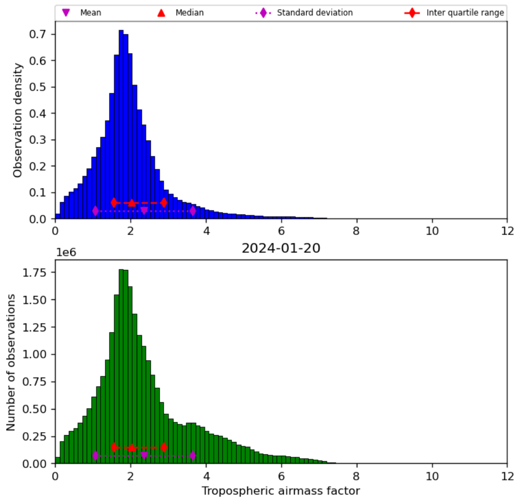
Figure 31: Histogram of “Tropospheric airmass factor” for 2024-01-19 to 2024-01-21
