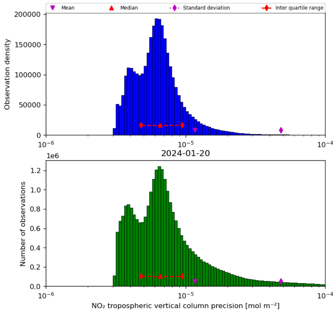
Figure 30: Histogram of “NO 2 tropospheric vertical column precision” for 2024-01-19 to 2024-01-21
