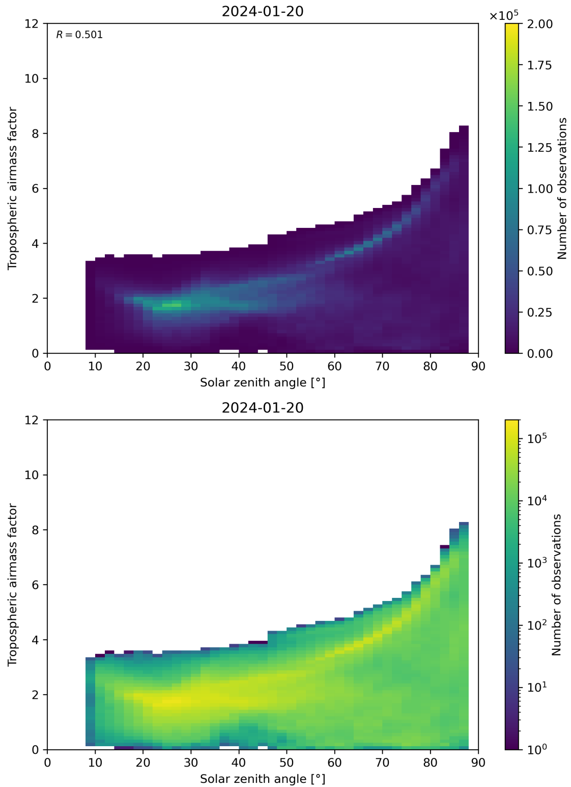
Figure 147: Scatter density plot of “Solar zenith angle” against “Tropospheric airmass factor” for 2024-01-19 to 2024-01-21.
