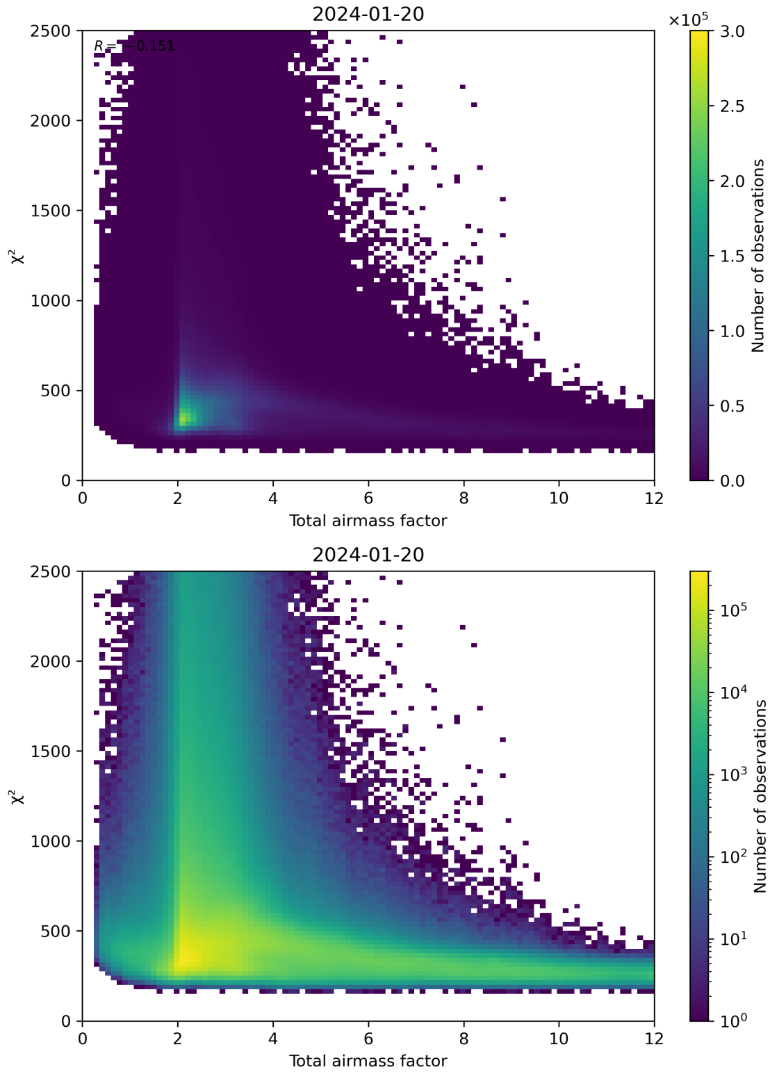
Figure 63: Scatter density plot of “Total airmass factor” against “ \chi^2 ” for 2024-01-19 to 2024-01-21.
