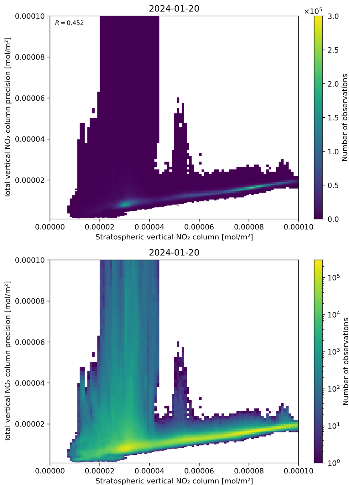
Figure 101: Scatter density plot of “Stratospheric vertical NO 2 column” against “Total vertical NO 2 column precision” for 2024-01-19 to 2024-01-21.
