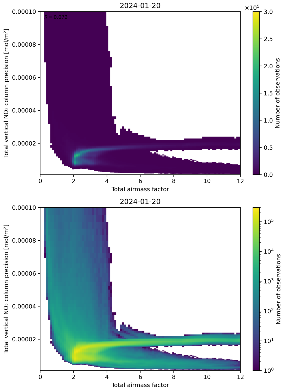
Figure 68: Scatter density plot of “Total airmass factor” against “Total vertical NO 2 column precision” for 2024-01-19 to 2024-01-21.
