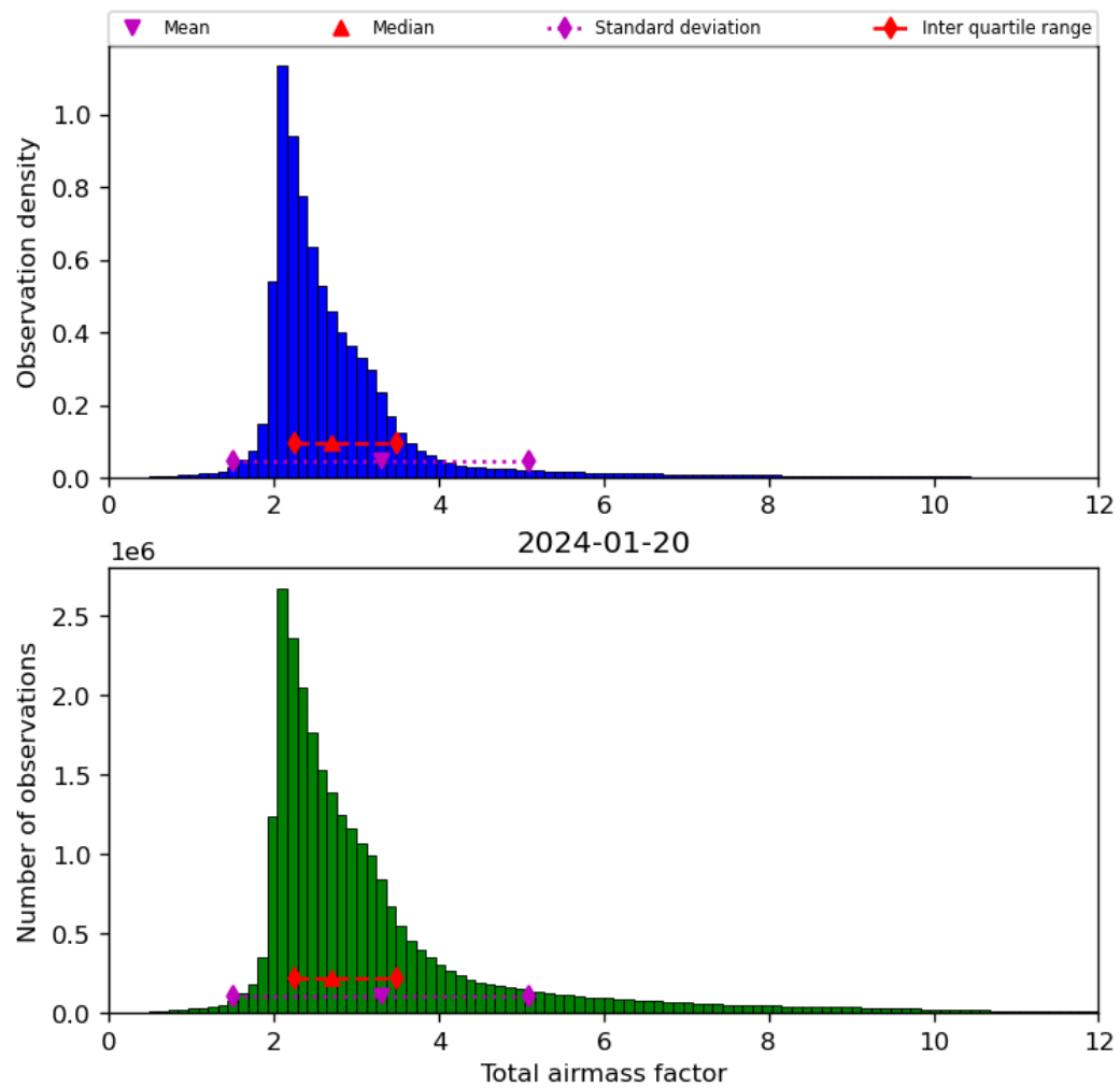
Figure 32: Histogram of “Total airmass factor” for 2024-01-19 to 2024-01-21
