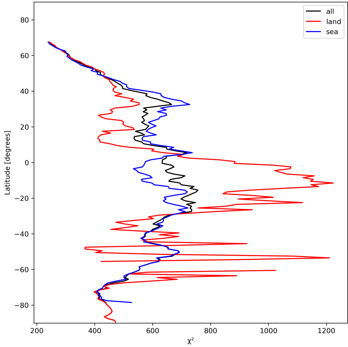
Figure 25: Zonal average of “ \chi^2 ” for 2024-01-19 to 2024-01-21.
