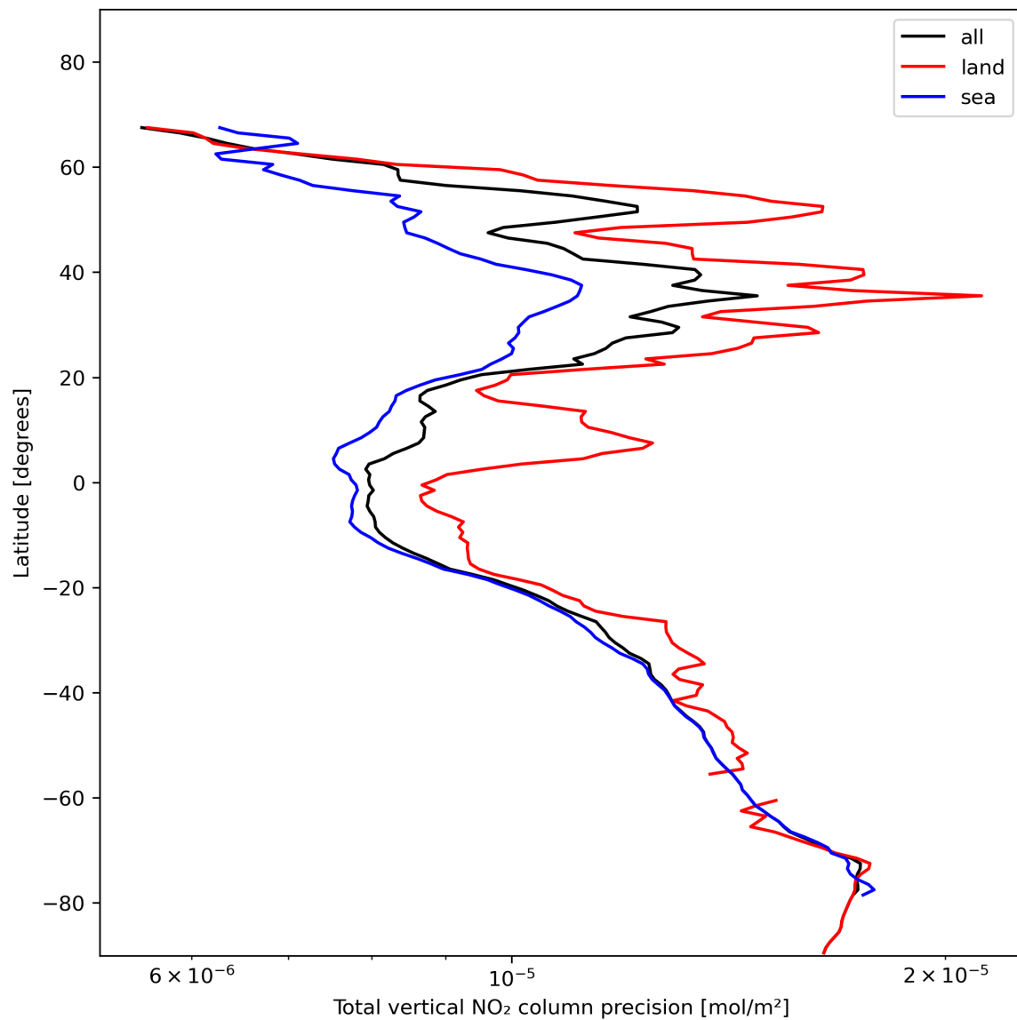
Figure 22: Zonal average of “Total vertical NO 2 column precision” for 2024-01-19 to 2024-01-21.
