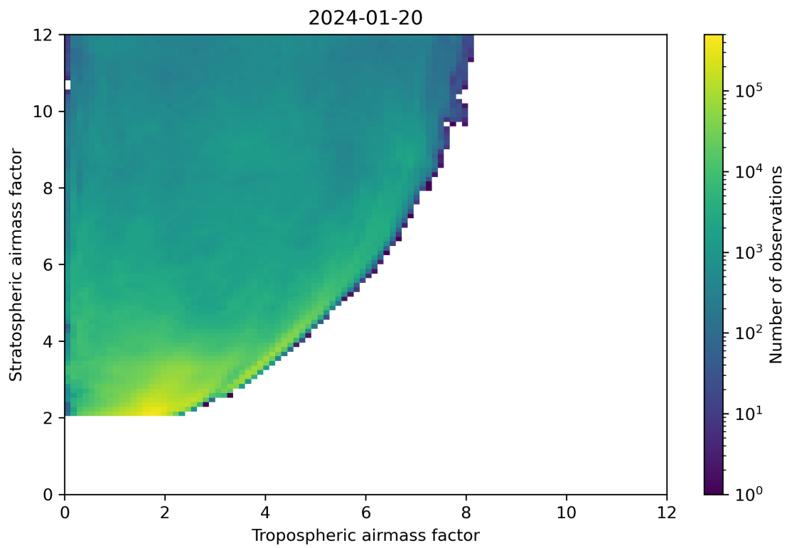
Figure 71: Scatter density plot of “Tropospheric airmass factor” against “Stratospheric airmass factor” for 2024-01-19 to 2024-01-21.
