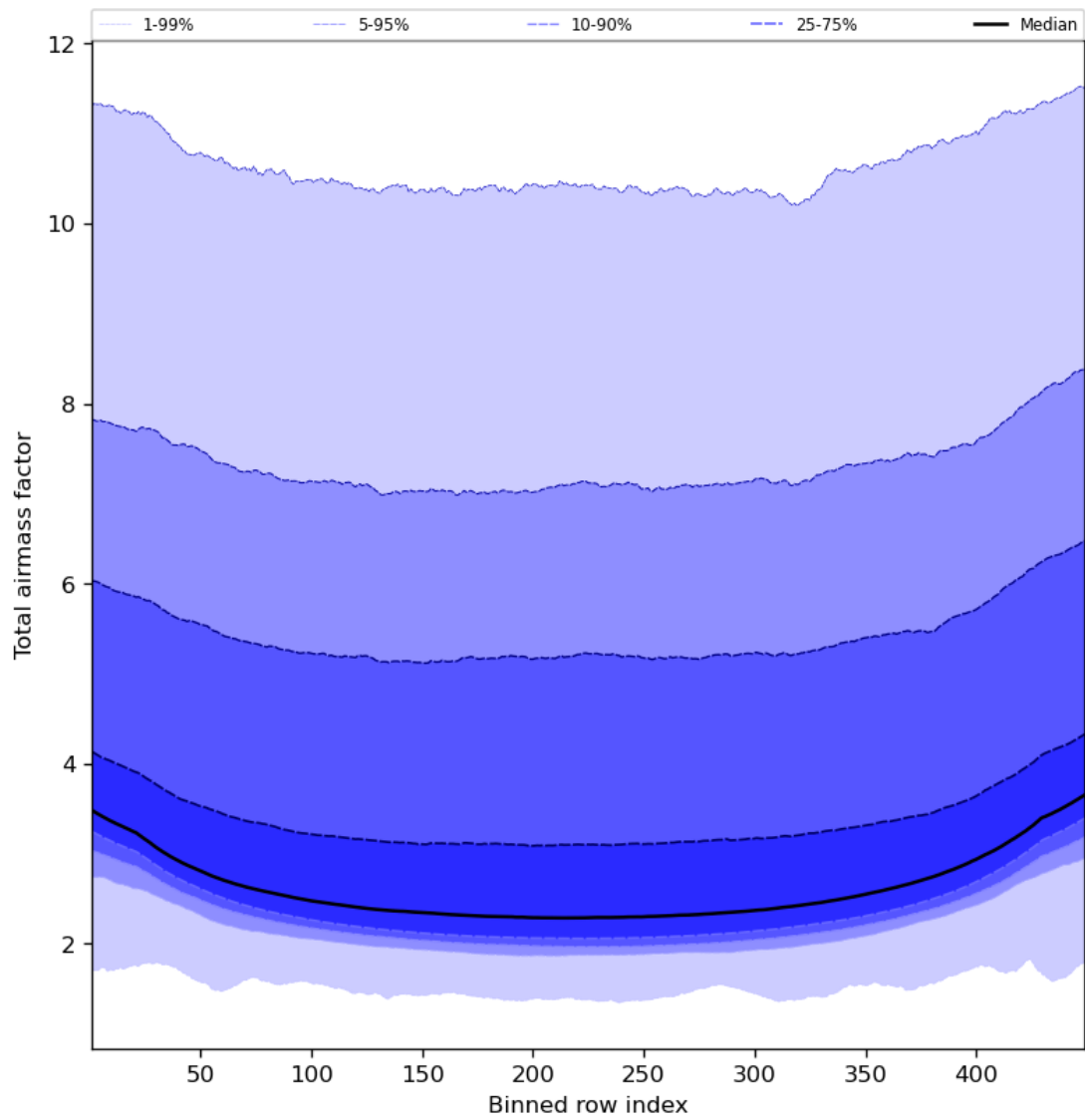
Figure 49: Along track statistics of “Total airmass factor” for 2024-01-19 to 2024-01-21
