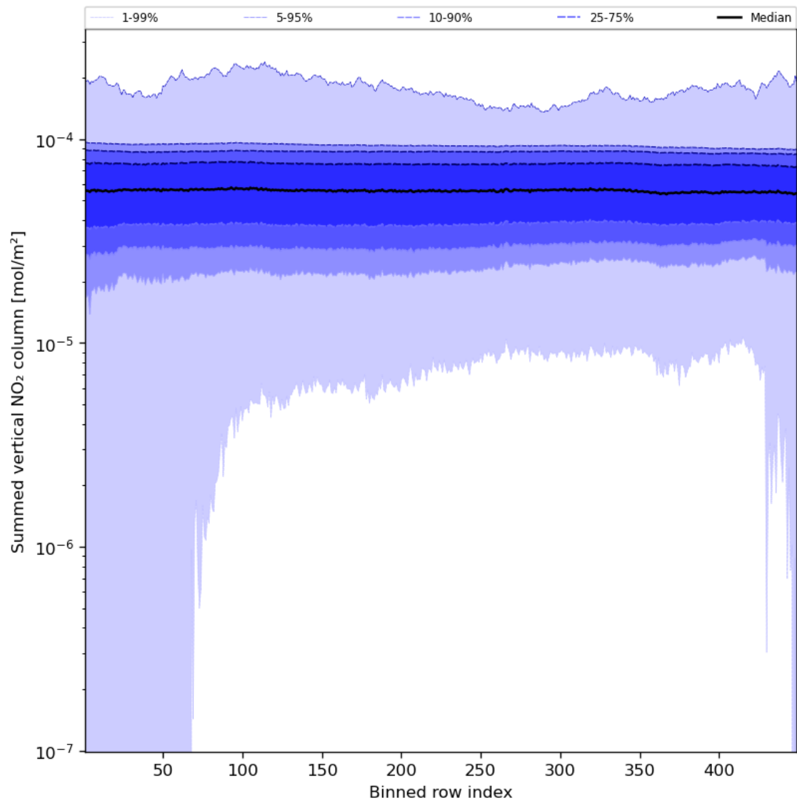
Figure 57: Along track statistics of “Summed vertical NO 2 column” for 2024-01-19 to 2024-01-21
