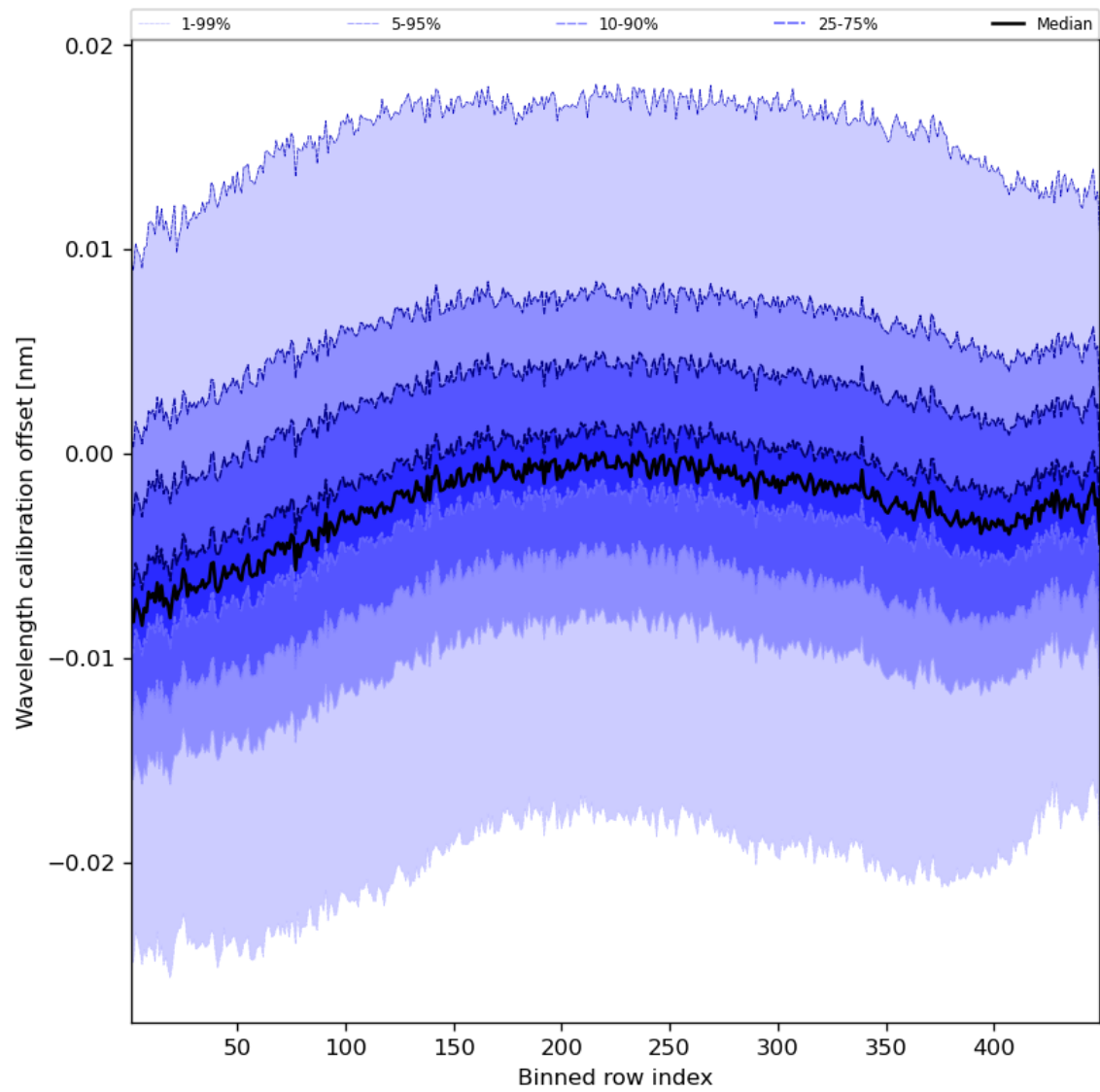
Figure 52: Along track statistics of “Wavelength calibration offset” for 2024-01-19 to 2024-01-21
