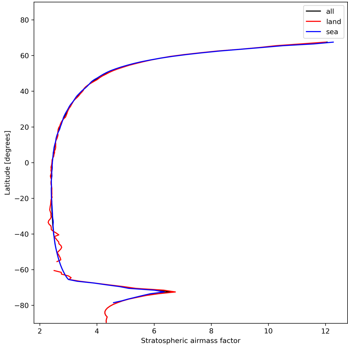
Figure 27: Zonal average of “Stratospheric airmass factor” for 2024-01-19 to 2024-01-21.
