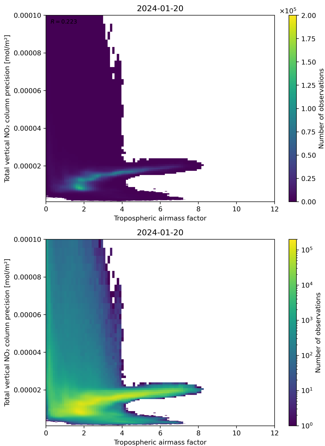
Figure 78: Scatter density plot of “Tropospheric air mass factor” against “Total vertical NO 2 column precision” for 2024-01-19 to 2024-01-21.
