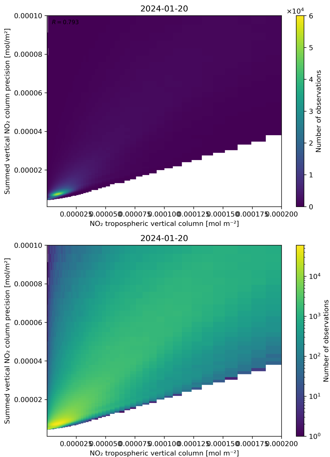
Figure 127: Scatter density plot of “NO 2 tropospheric vertical column” against “Summed vertical NO 2 column precision” for 2024-01-19 to 2024-01-21.
