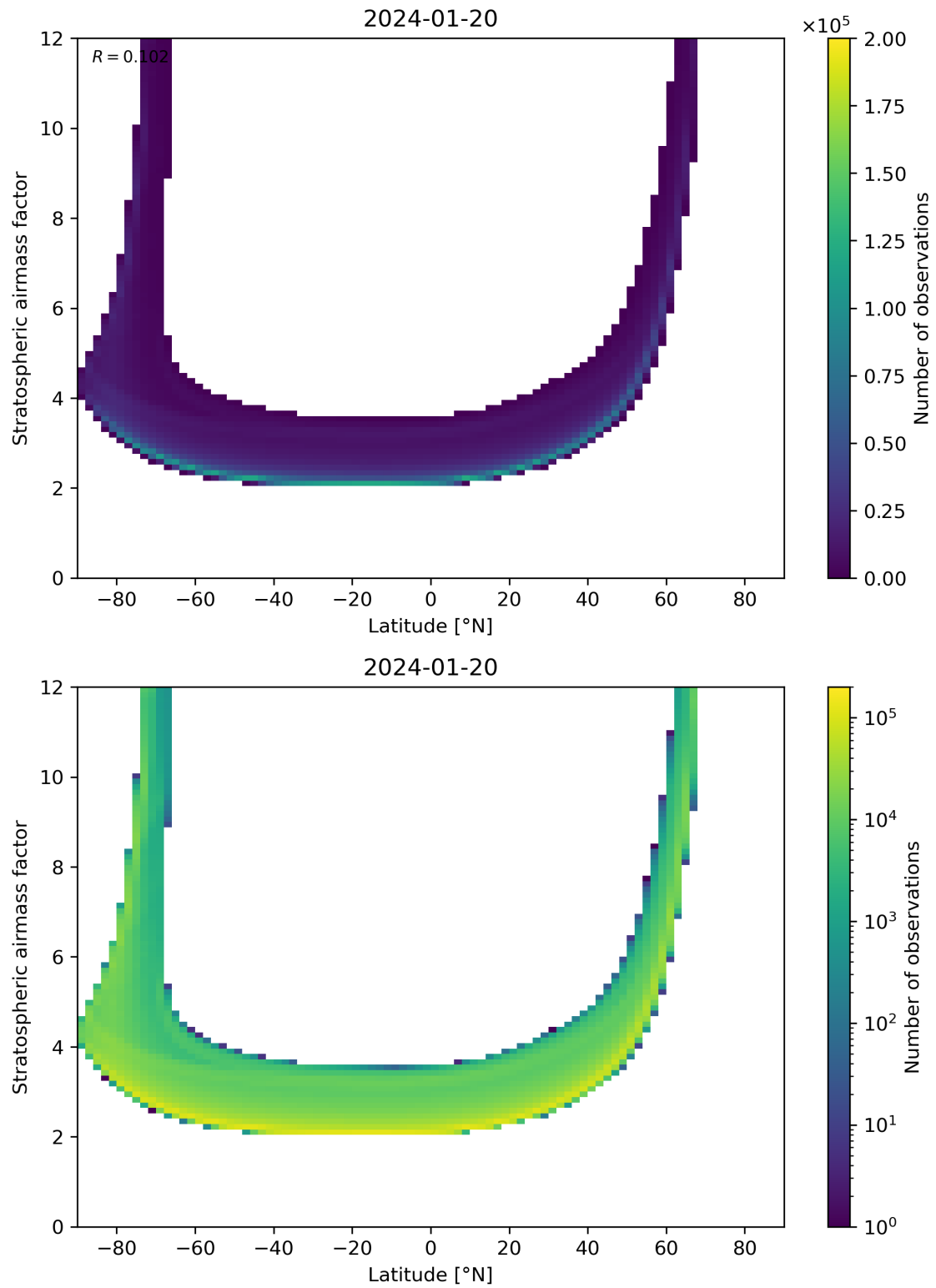
Figure 83: Scatter density plot of “Latitude” against “Stratospheric airmass factor” for 2024-01-19 to 2024-01-21.
