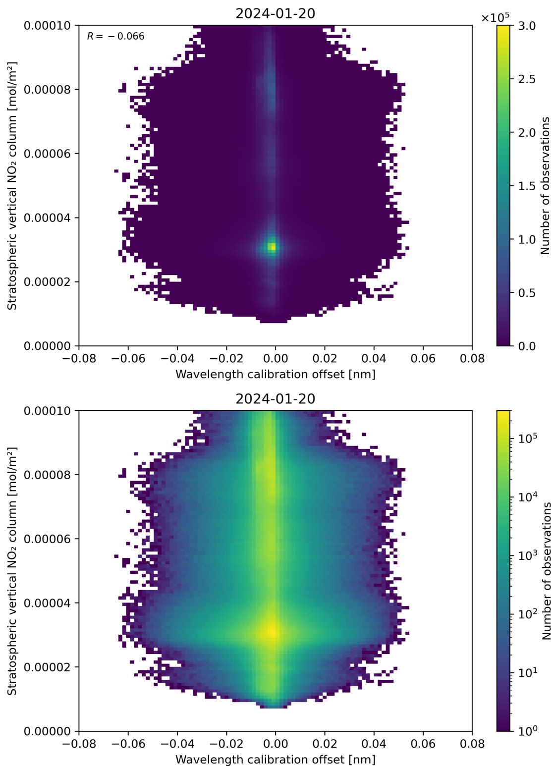
Figure 176: Scatter density plot of “Wavelength calibration offset” against “Stratospheric vertical NO 2 column” for 2024-01-19 to 2024-01-21.
