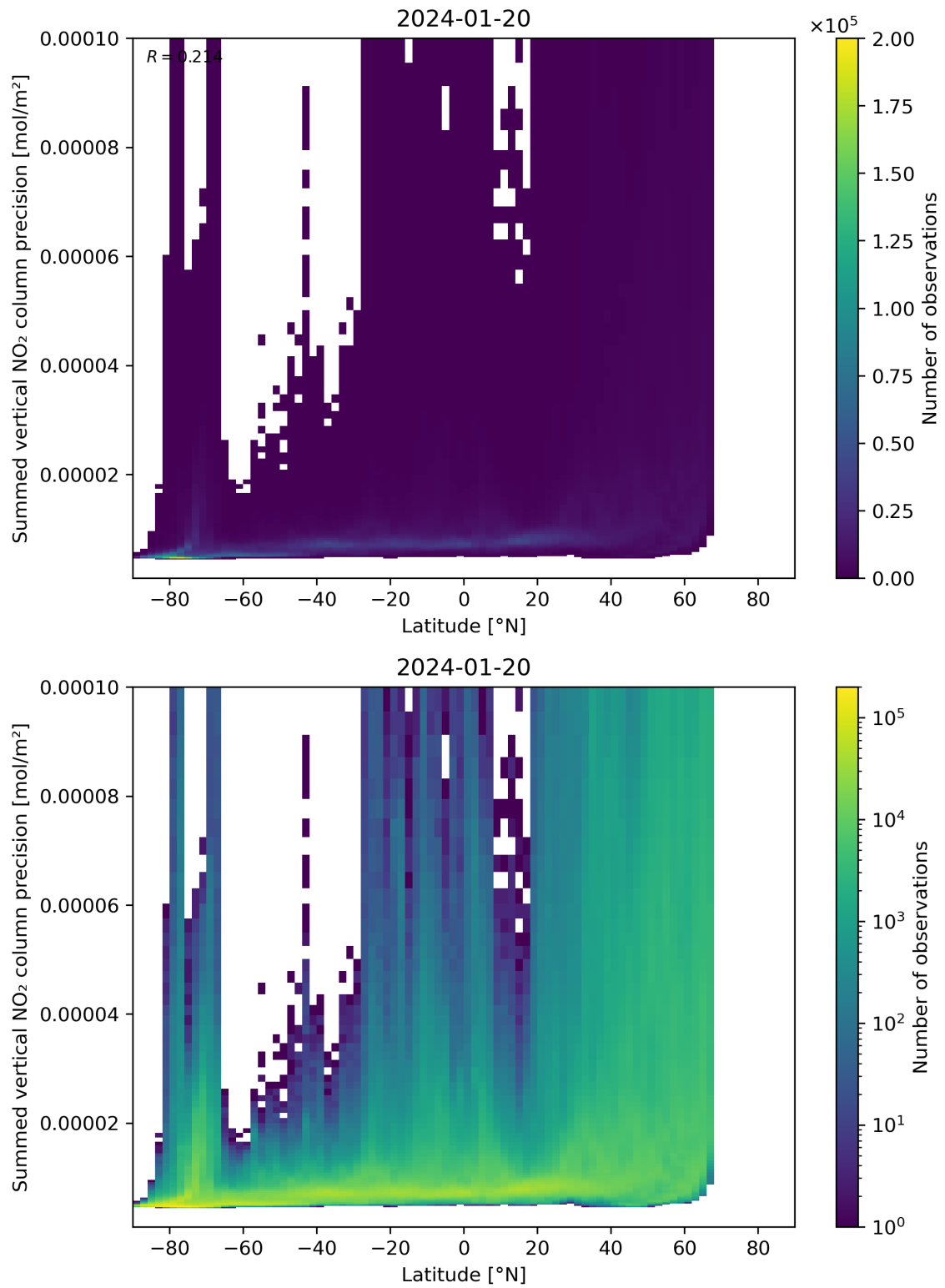
Figure 89: Scatter density plot of “Latitude” against “Summed vertical NO 2 column precision” for 2024-01-19 to 2024-01-21.
