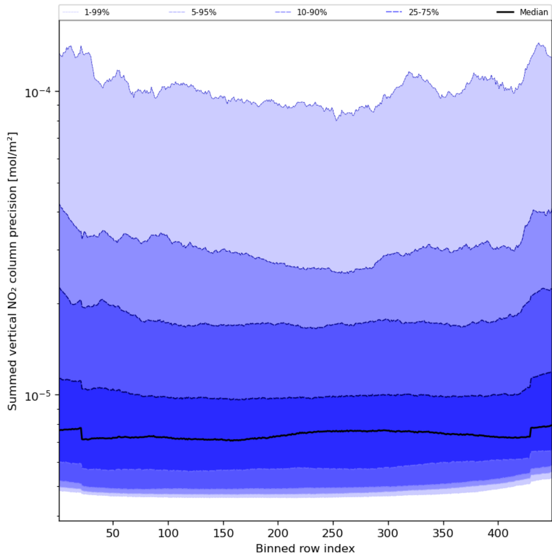
Figure 58: Along track statistics of “Summed vertical NO 2 column precision” for 2024-01-19 to 2024-01-21
