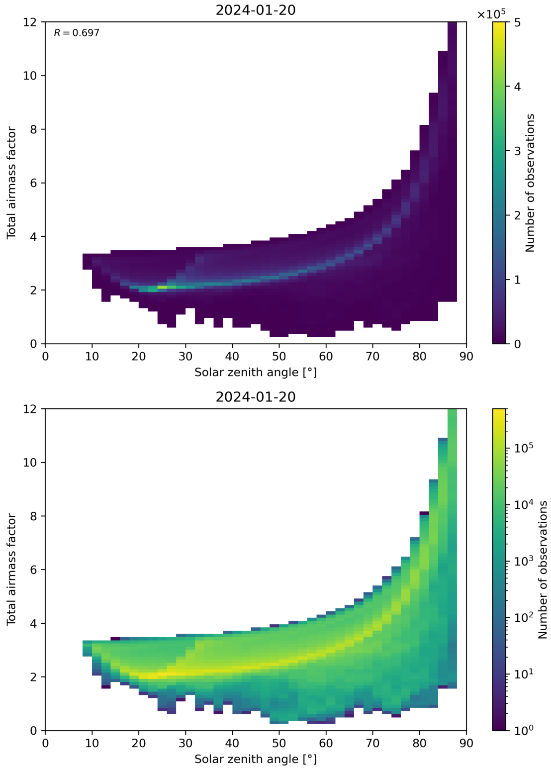
Figure 146: Scatter density plot of “Solar zenith angle” against “Total air mass factor” for 2024-01-19 to 2024-01-21.
