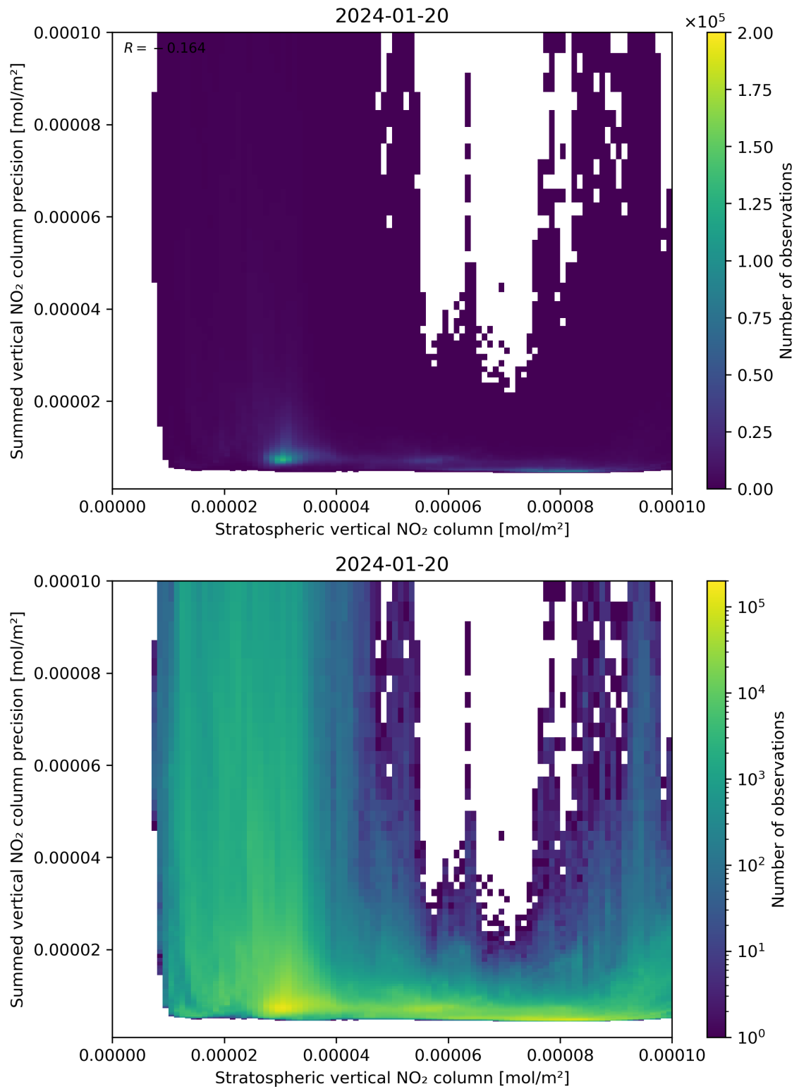
Figure 99: Scatter density plot of “Stratospheric vertical NO 2 column” against “Summed vertical NO 2 column precision” for 2024-01-19 to 2024-01-21.
