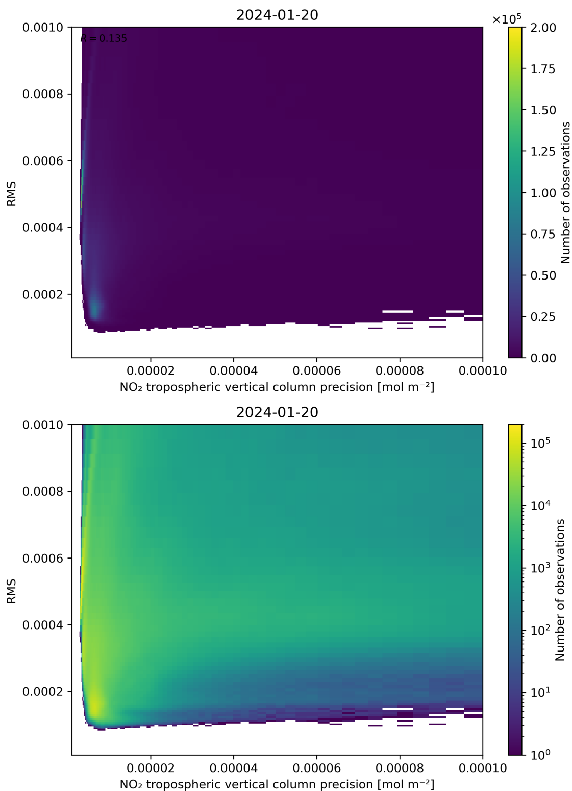
Figure 140: Scatter density plot of “NO 2 tropospheric vertical column precision” against “RMS” for 2024-01-19 to 2024-01-21.
