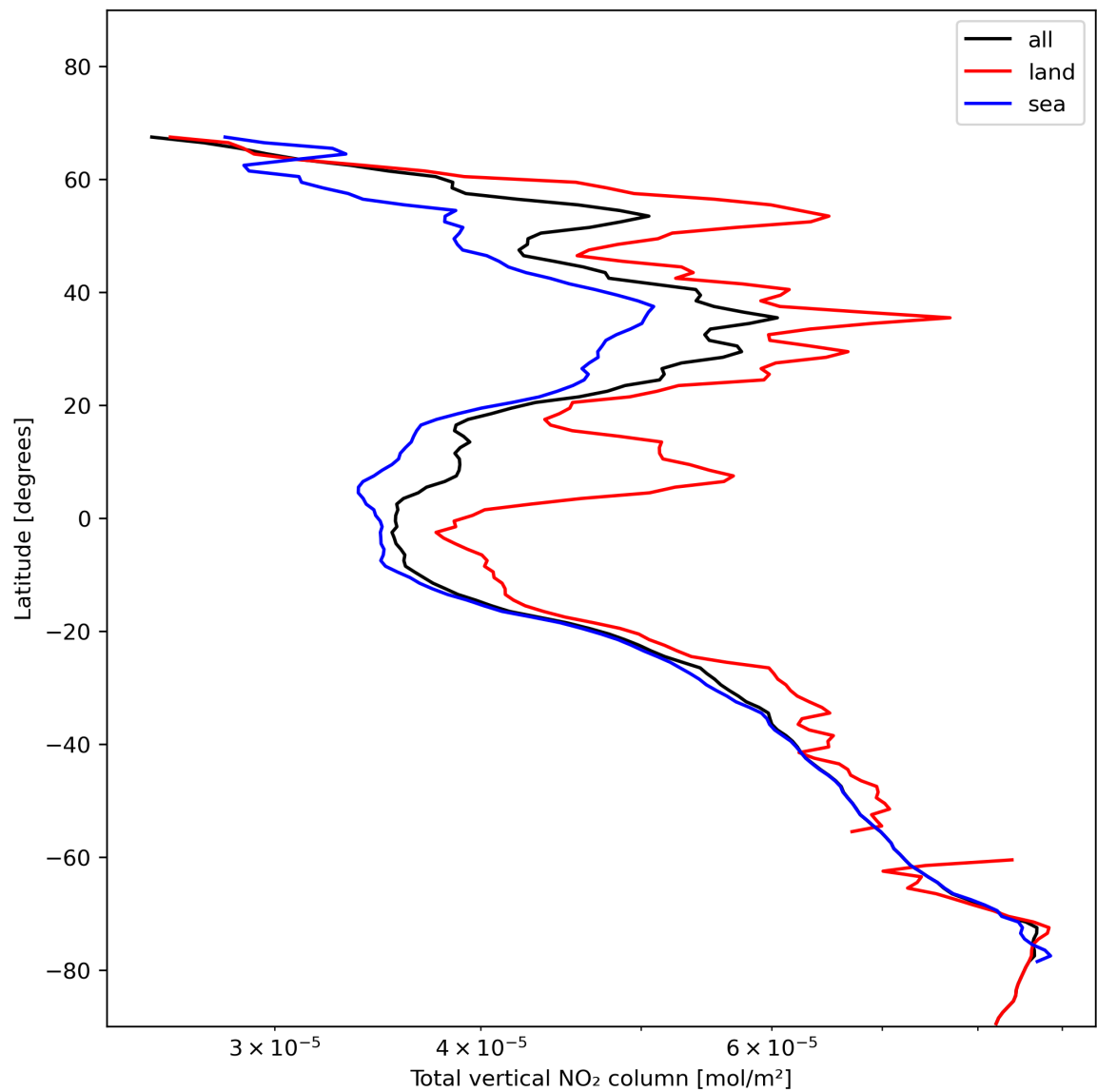
Figure 21: Zonal average of “Total vertical NO 2 column” for 2024-01-19 to 2024-01-21.
