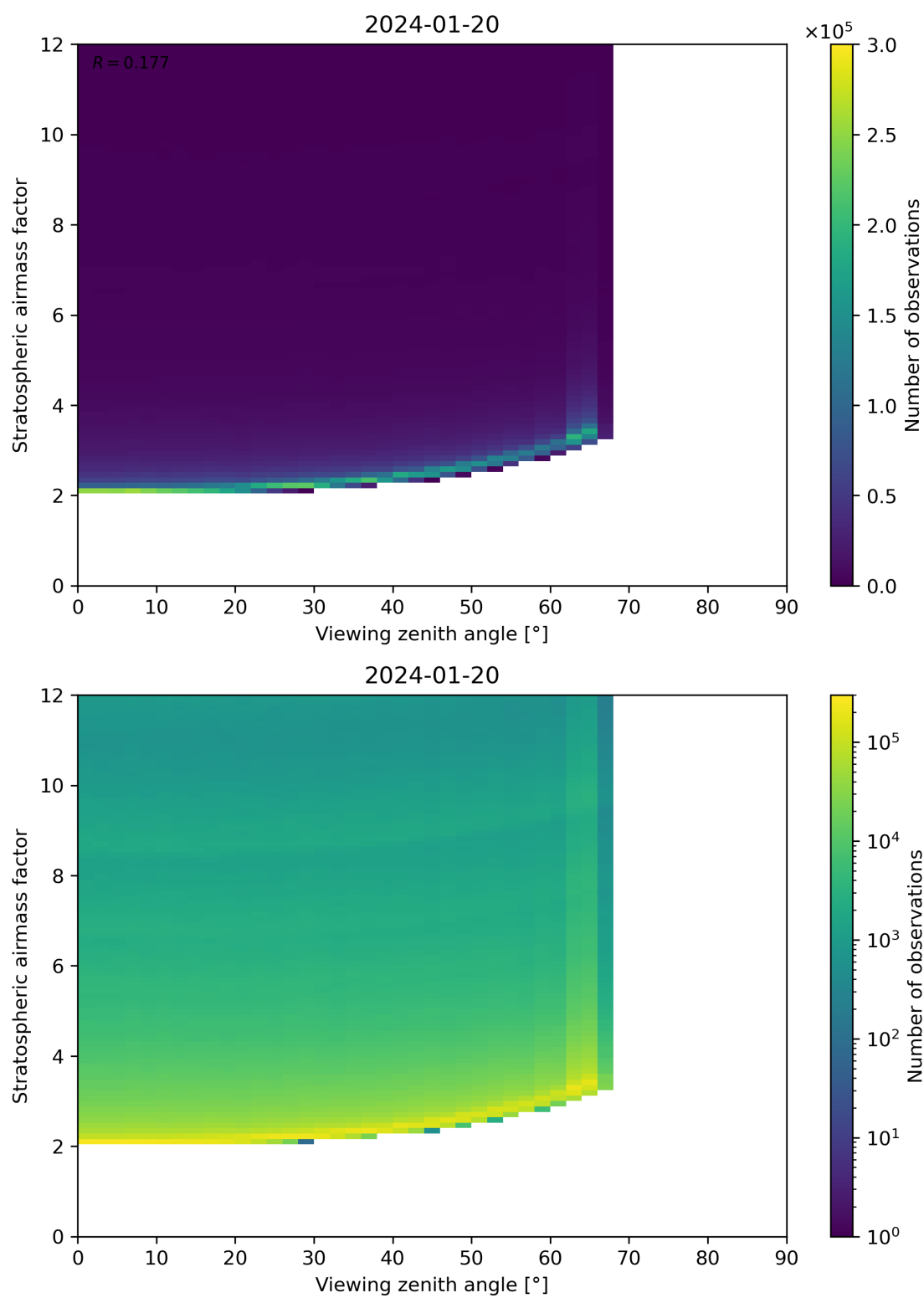
Figure 159: Scatter density plot of “Viewing zenith angle” against “Stratospheric airmass factor” for 2024-01-19 to 2024-01-21.
