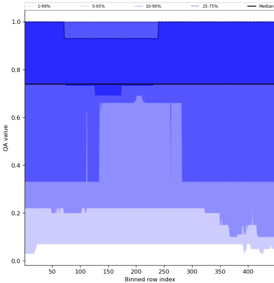
Figure 45: Along track statistics of “QA value” for 2024-01-19 to 2024-01-21
