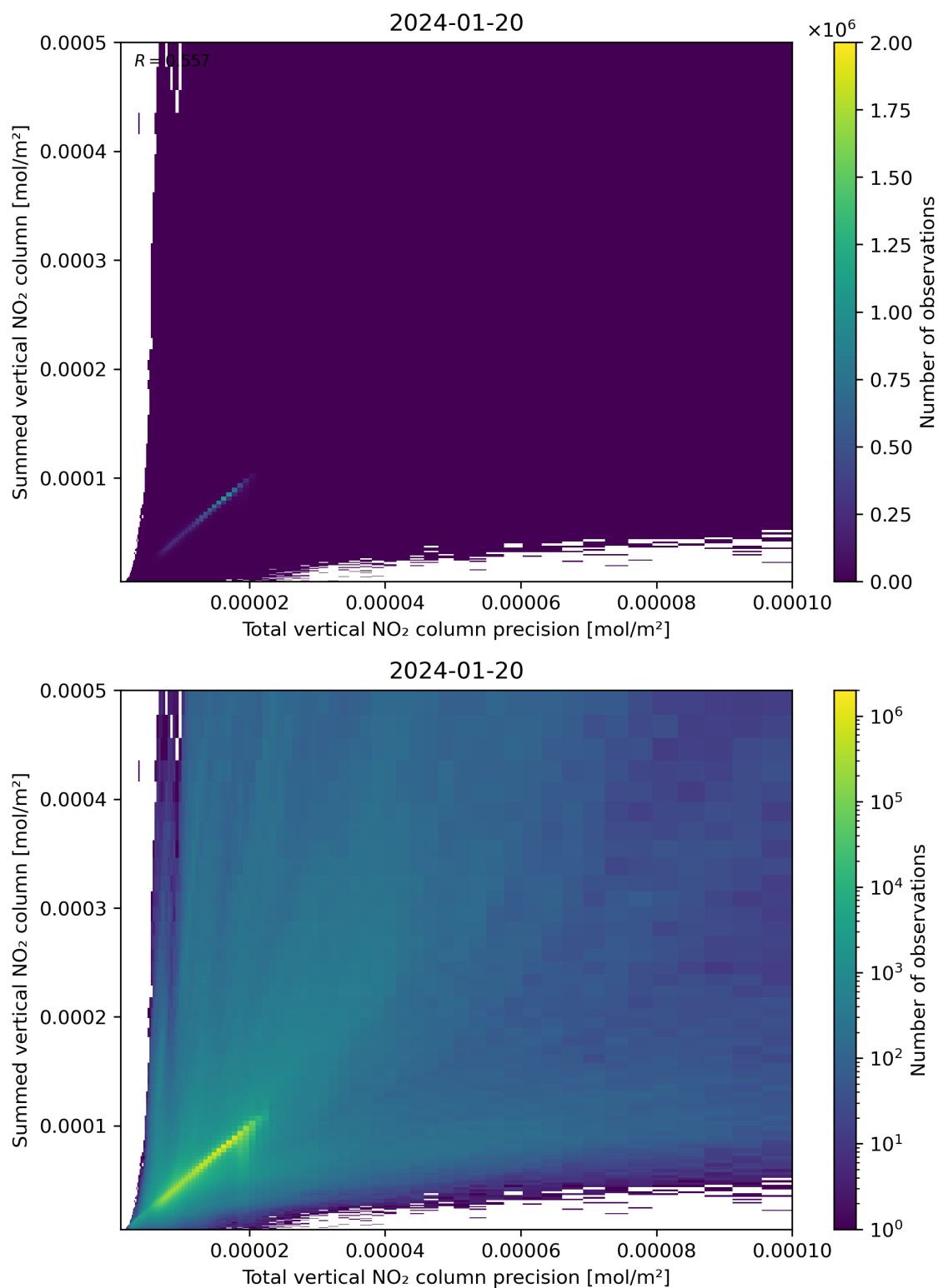
Figure 117: Scatter density plot of “Total vertical NO 2 column precision” against “Summed vertical NO 2 column” for 2024-01-19 to 2024-01-21.
