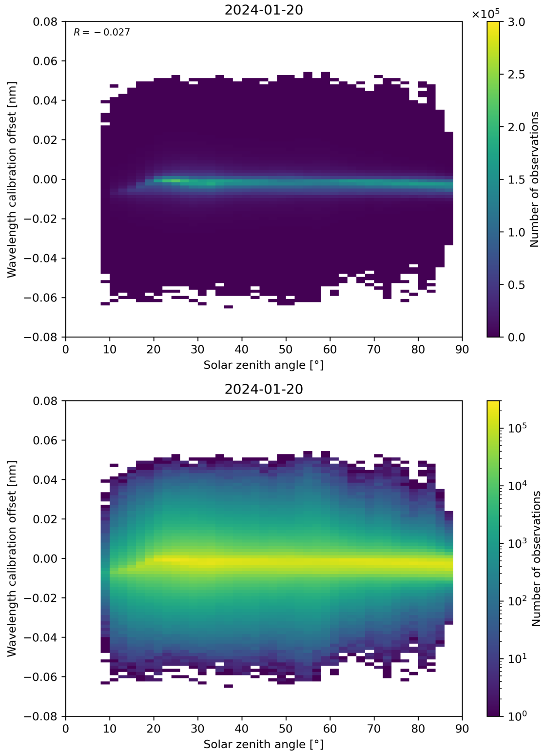
Figure 158: Scatter density plot of “Solar zenith angle” against “Wavelength calibration offset” for 2024-01-19 to 2024-01-21.
