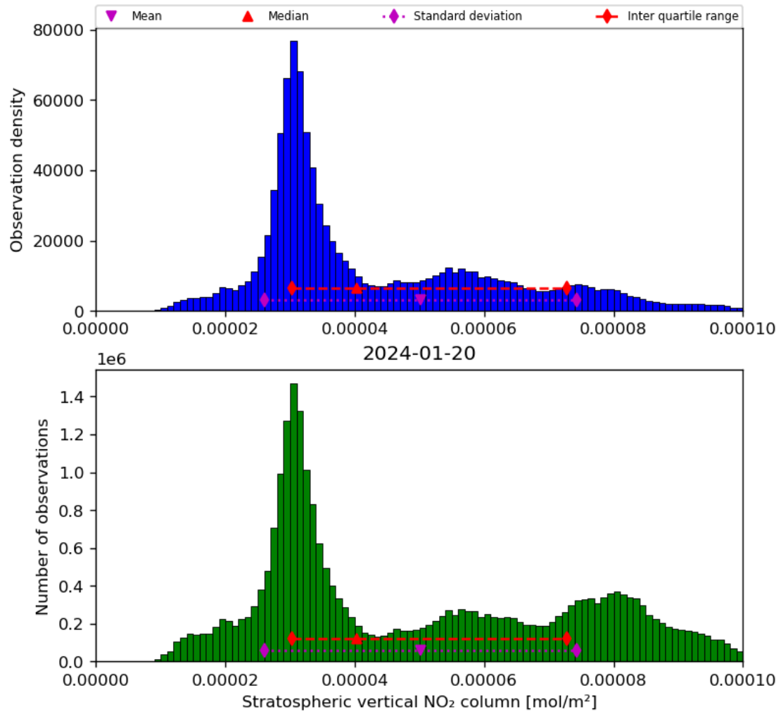
Figure 36: Histogram of “Stratospheric vertical NO 2 column” for 2024-01-19 to 2024-01-21
