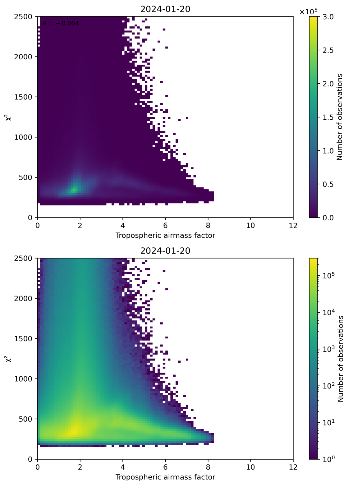
Figure 73: Scatter density plot of “Tropospheric airmass factor” against “ \chi^2 ” for 2024-01-19 to 2024-01-21.
