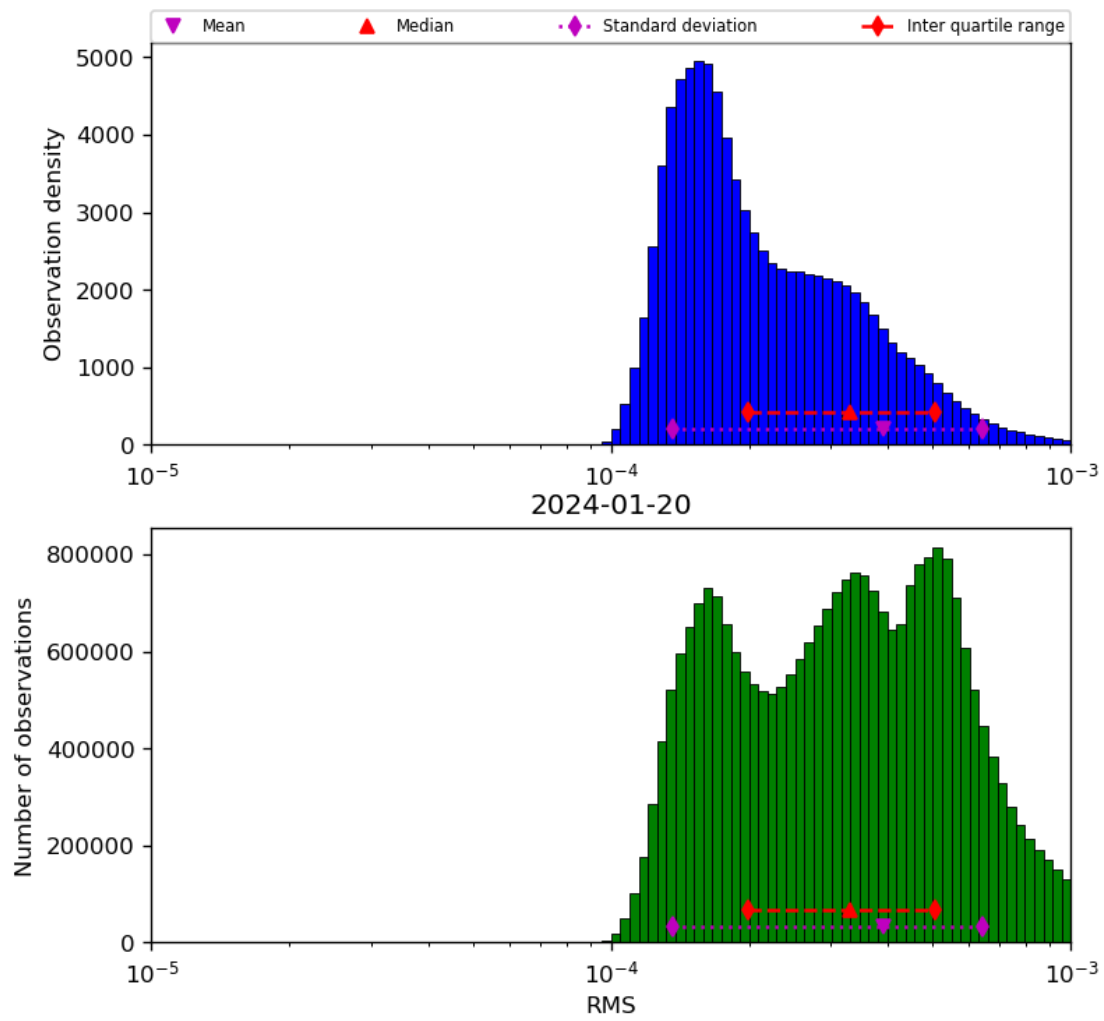
Figure 43: Histogram of “RMS” for 2024-01-19 to 2024-01-21
