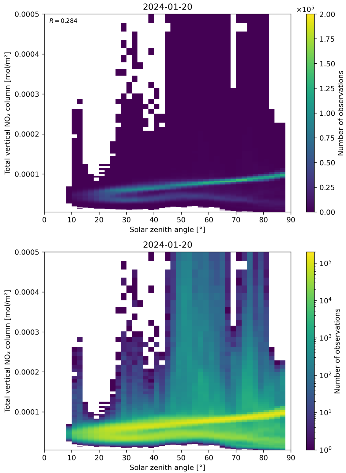
Figure 153: Scatter density plot of “Solar zenith angle” against “Total vertical NO 2 column” for 2024-01-19 to 2024-01-21.
