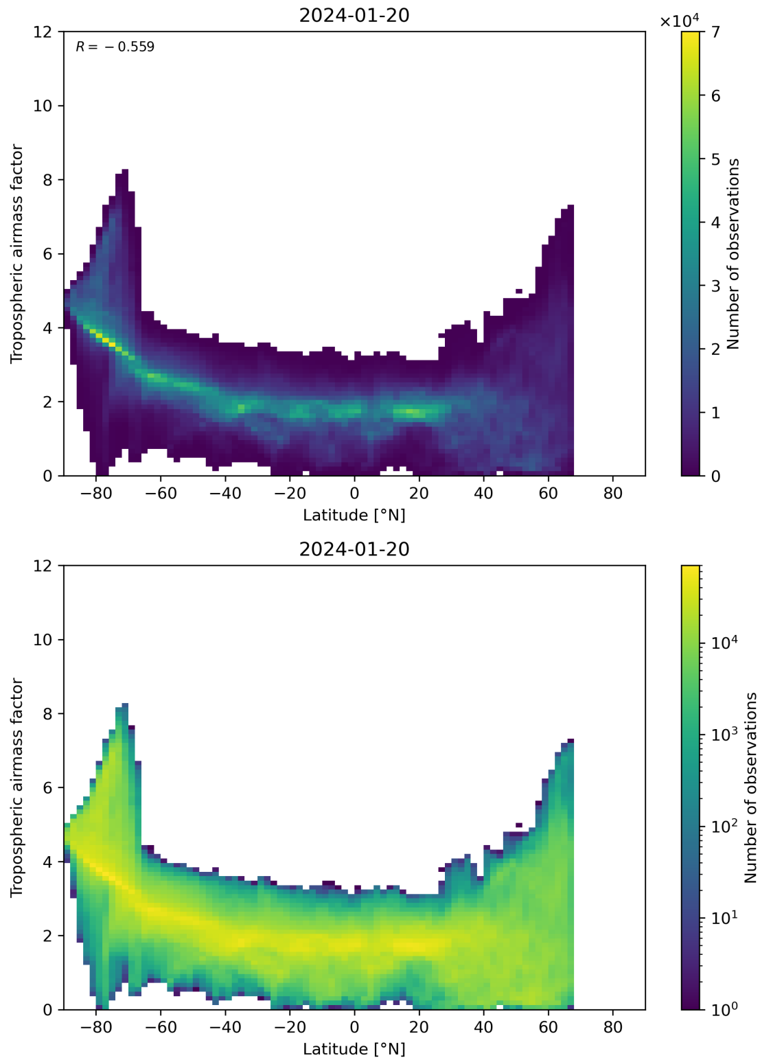
Figure 85: Scatter density plot of “Latitude” against “Tropospheric airmass factor” for 2024-01-19 to 2024-01-21.
