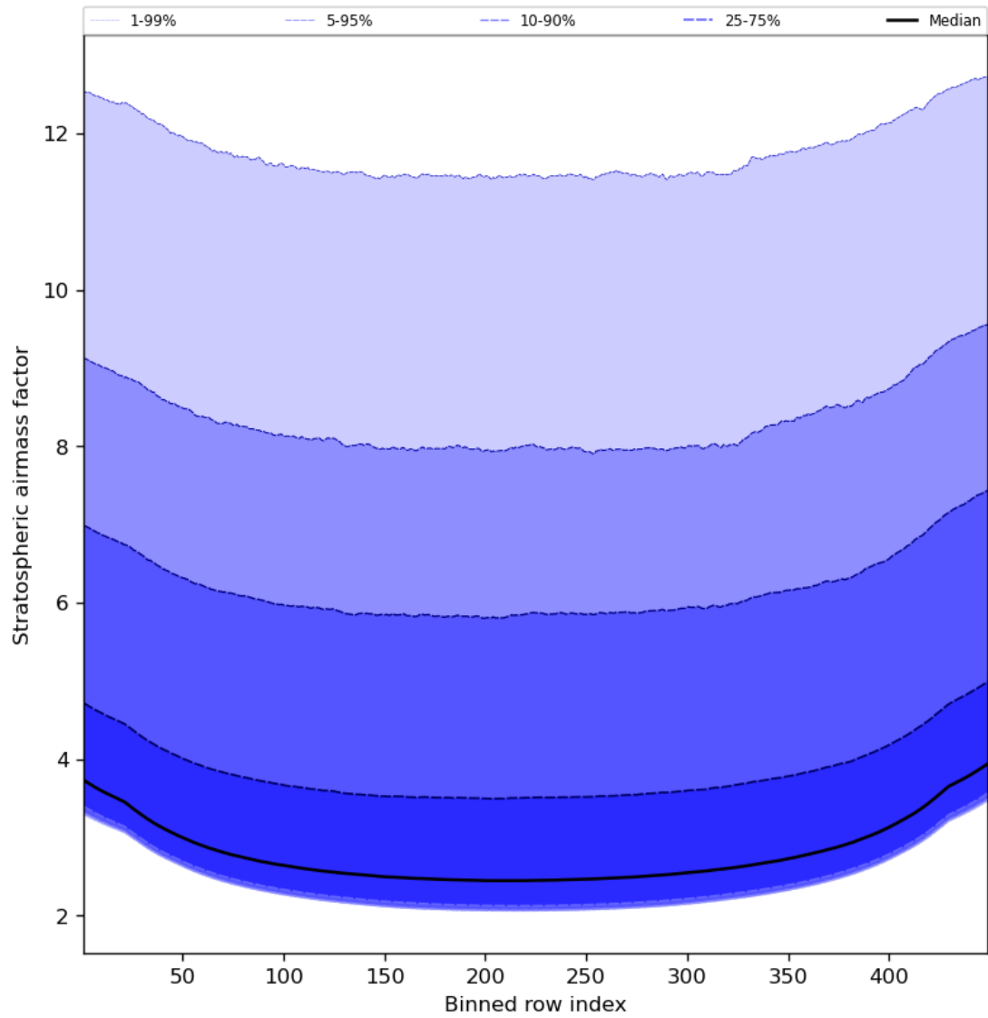
Figure 61: Along track statistics of “Stratospheric airmass factor” for 2024-01-19 to 2024-01-21
