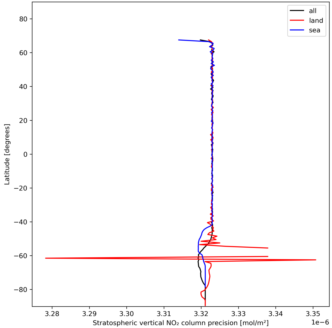
Figure 20: Zonal average of “Stratospheric vertical NO 2 column precision” for 2024-01-19 to 2024-01-21.
