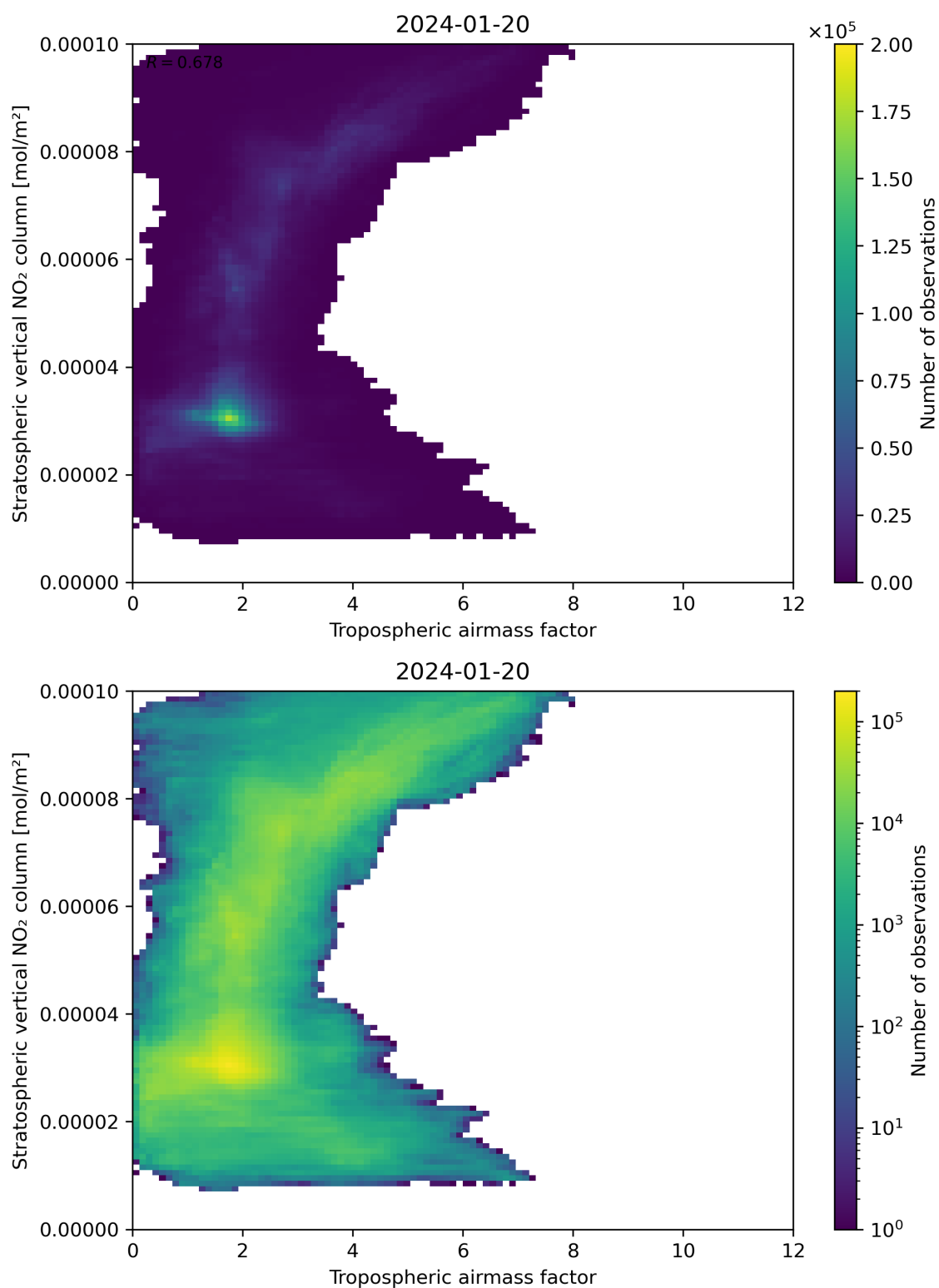
Figure 74: Scatter density plot of “Tropospheric air mass factor” against “Stratospheric vertical NO 2 column” for 2024-01-19 to 2024-01-21.
