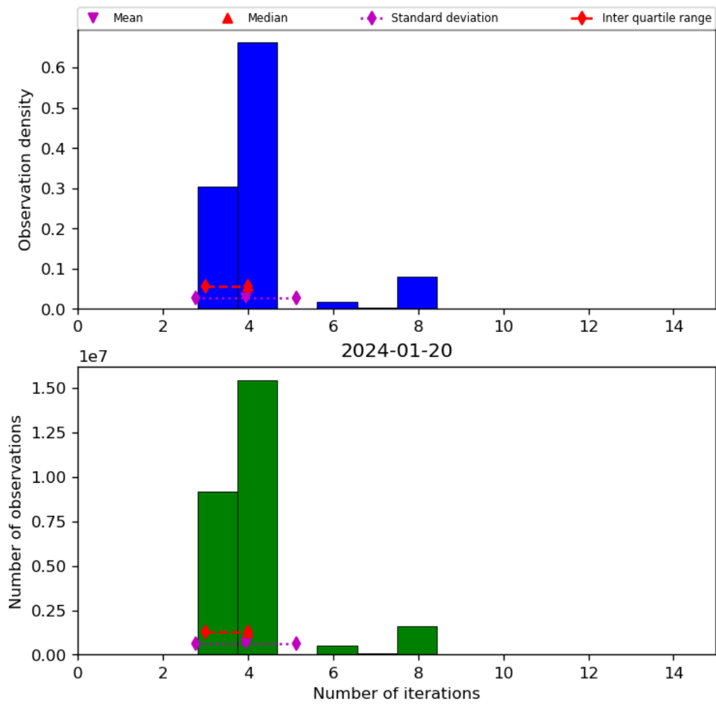
Figure 34: Histogram of “Number of iterations” for 2024-01-19 to 2024-01-21
