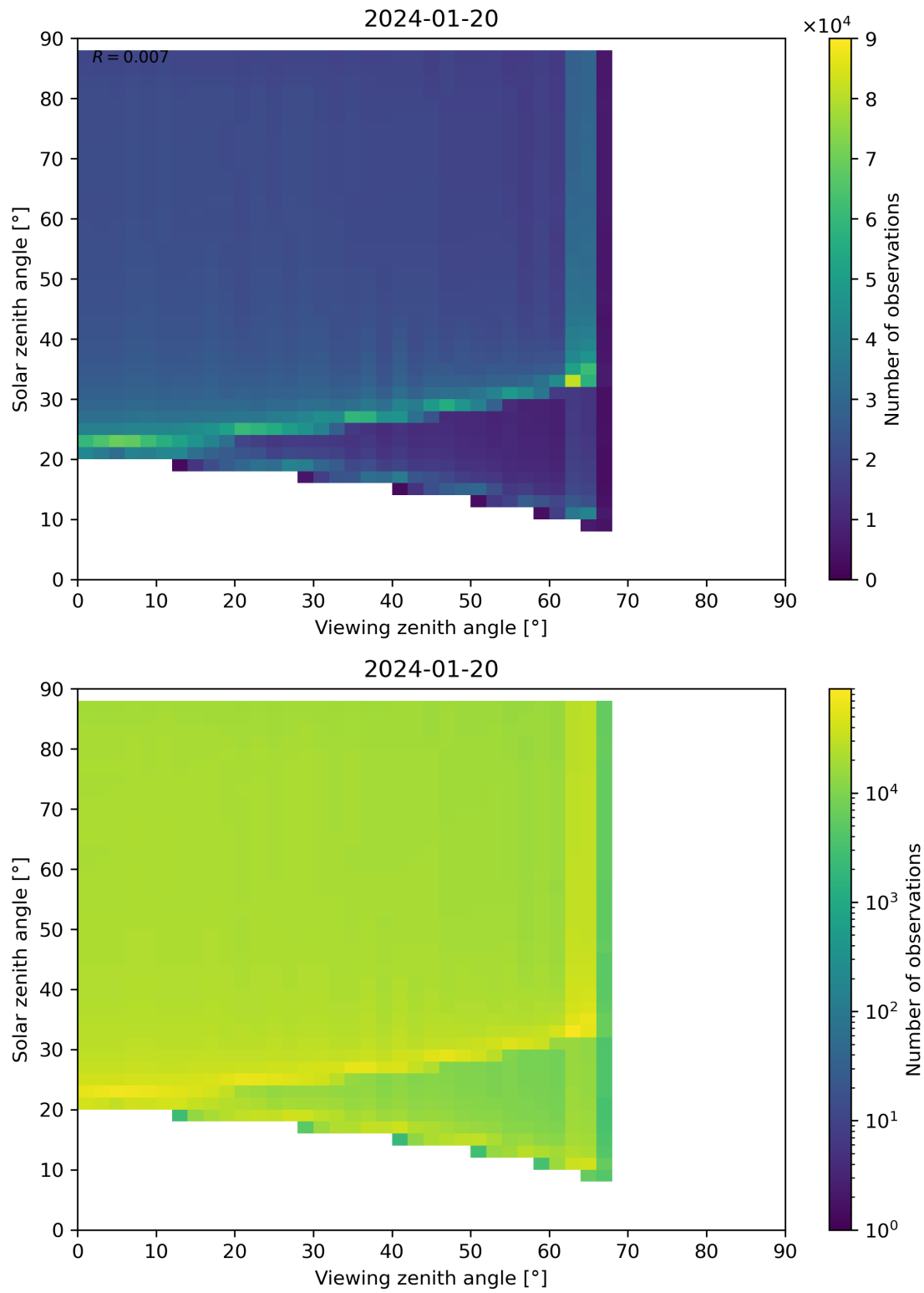
Figure 172: Scatter density plot of “Viewing zenith angle” against “Solar zenith angle” for 2024-01-19 to 2024-01-21.
