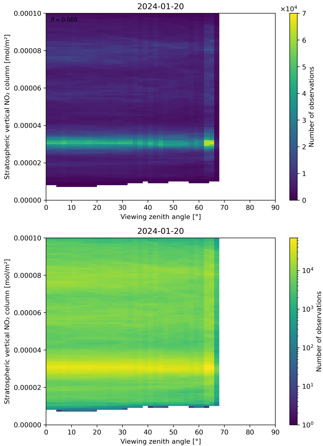
Figure 164: Scatter density plot of “Viewing zenith angle” against “Stratospheric vertical NO 2 column” for 2024-01-19 to 2024-01-21.
