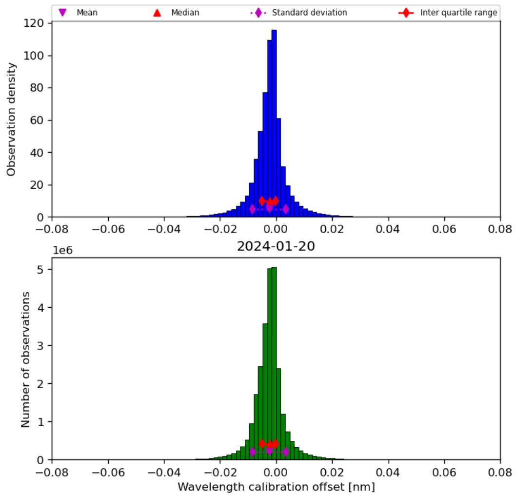
Figure 35: Histogram of “Wavelength calibration offset” for 2024-01-19 to 2024-01-21
