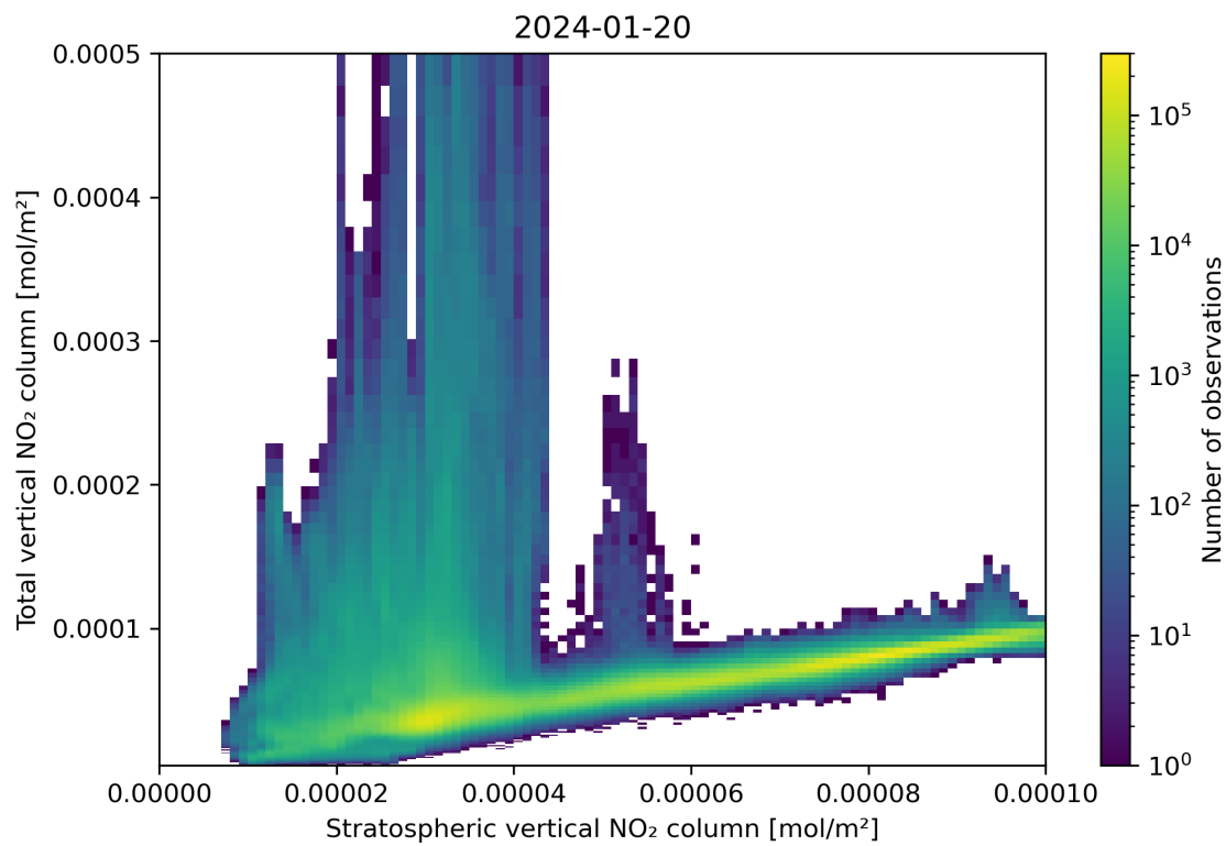
Figure 100: Scatter density plot of “Stratospheric vertical NO 2 column” against “Total vertical NO 2 column” for 2024-01-19 to 2024-01-21.
