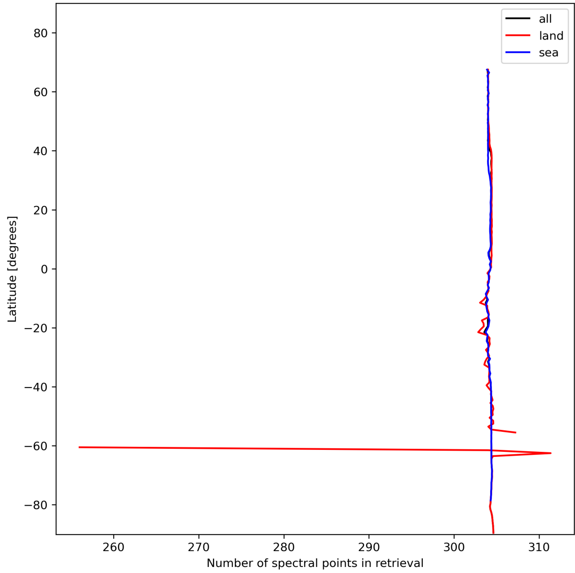
Figure 16: Zonal average of “Number of spectral points in retrieval” for 2024-01-19 to 2024-01-21.
