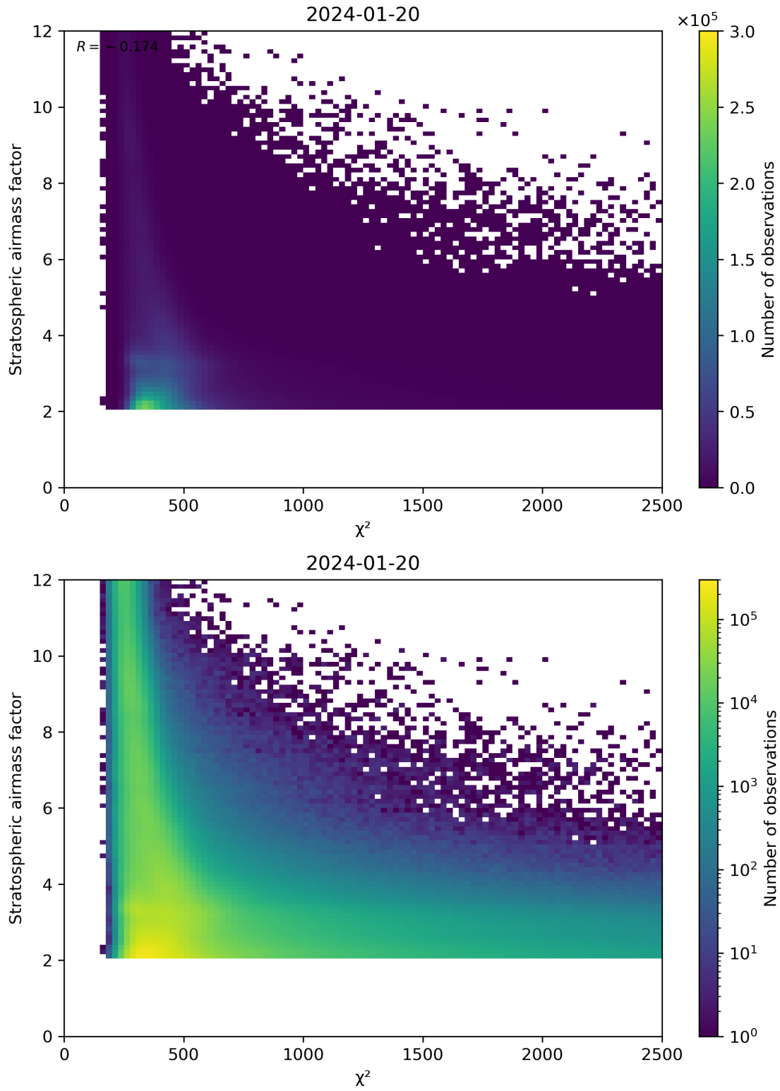
Figure 81: Scatter density plot of “ \chi^2 ” against “Stratospheric airmass factor” for 2024-01-19 to 2024-01-21.
