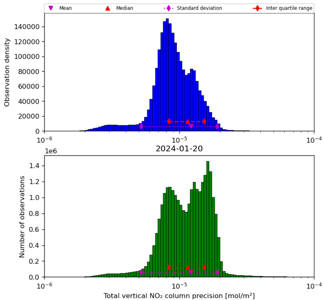
Figure 39: Histogram of “Total vertical NO 2 column precision” for 2024-01-19 to 2024-01-21
