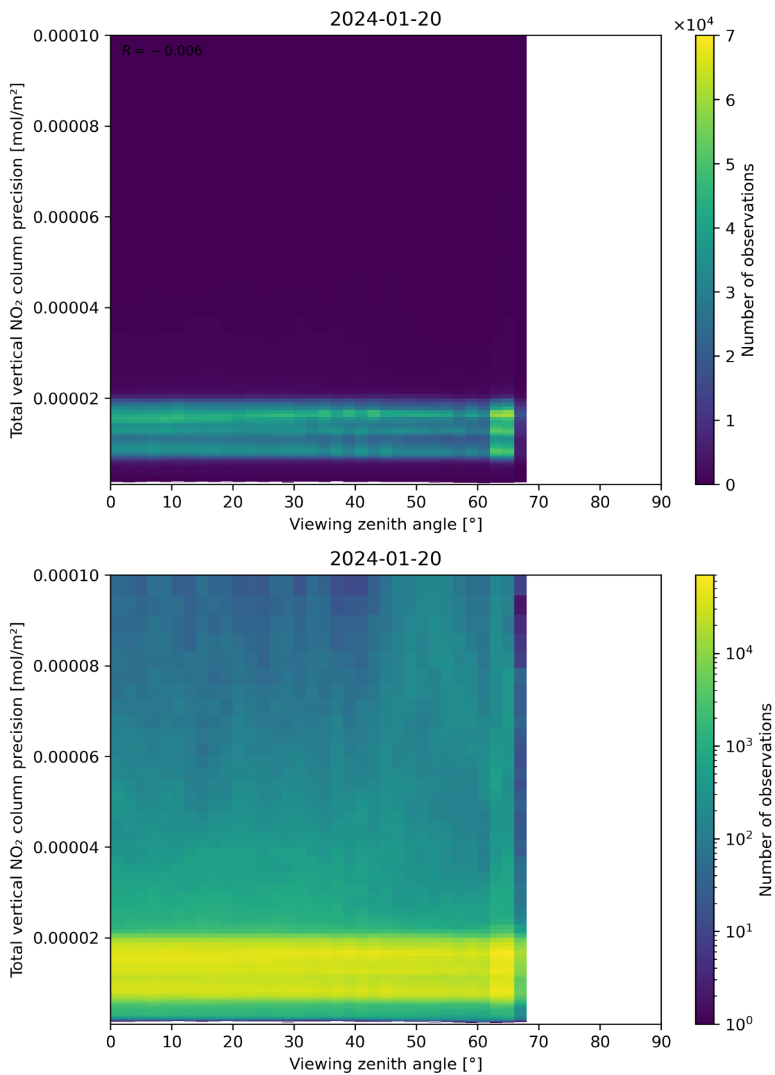
Figure 168: Scatter density plot of “Viewing zenith angle” against “Total vertical NO 2 column precision” for 2024-01-19 to 2024-01-21.
