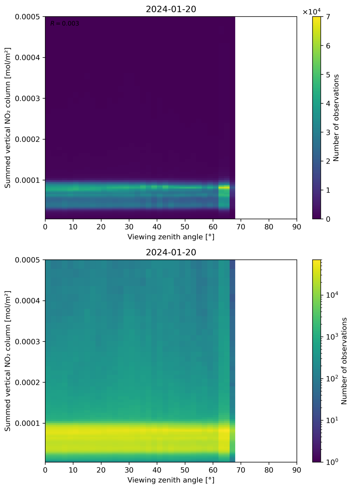
Figure 165: Scatter density plot of “Viewing zenith angle” against “Summed vertical NO 2 column” for 2024-01-19 to 2024-01-21.
