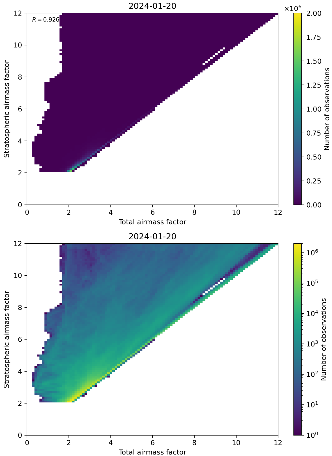
Figure 62: Scatter density plot of “Total airmass factor” against “Stratospheric airmass factor” for 2024-01-19 to 2024-01-21.
