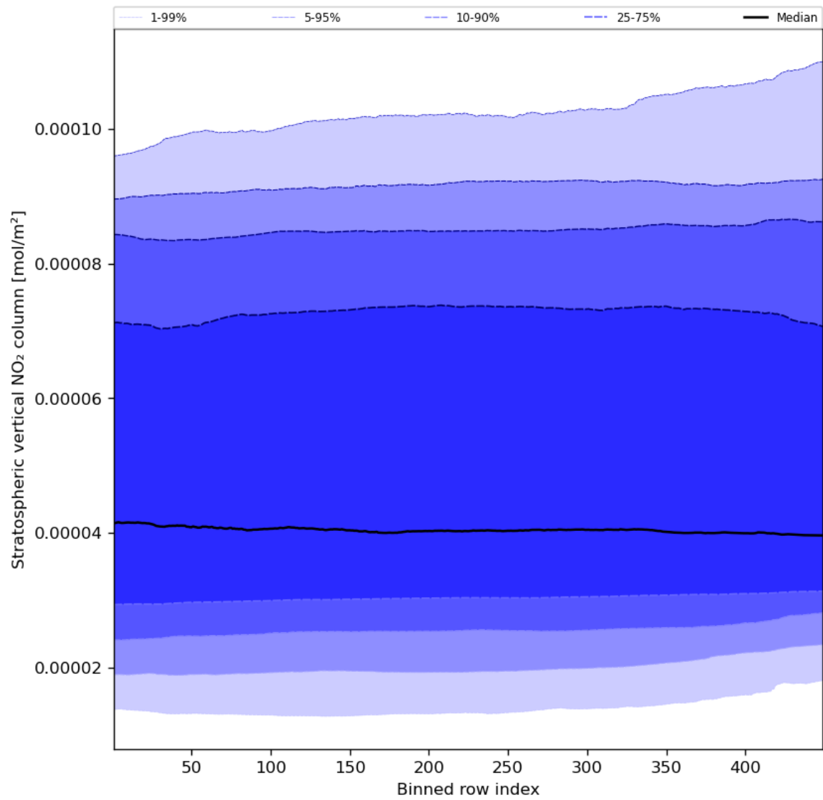
Figure 53: Along track statistics of “Stratospheric vertical NO 2 column” for 2024-01-19 to 2024-01-21
