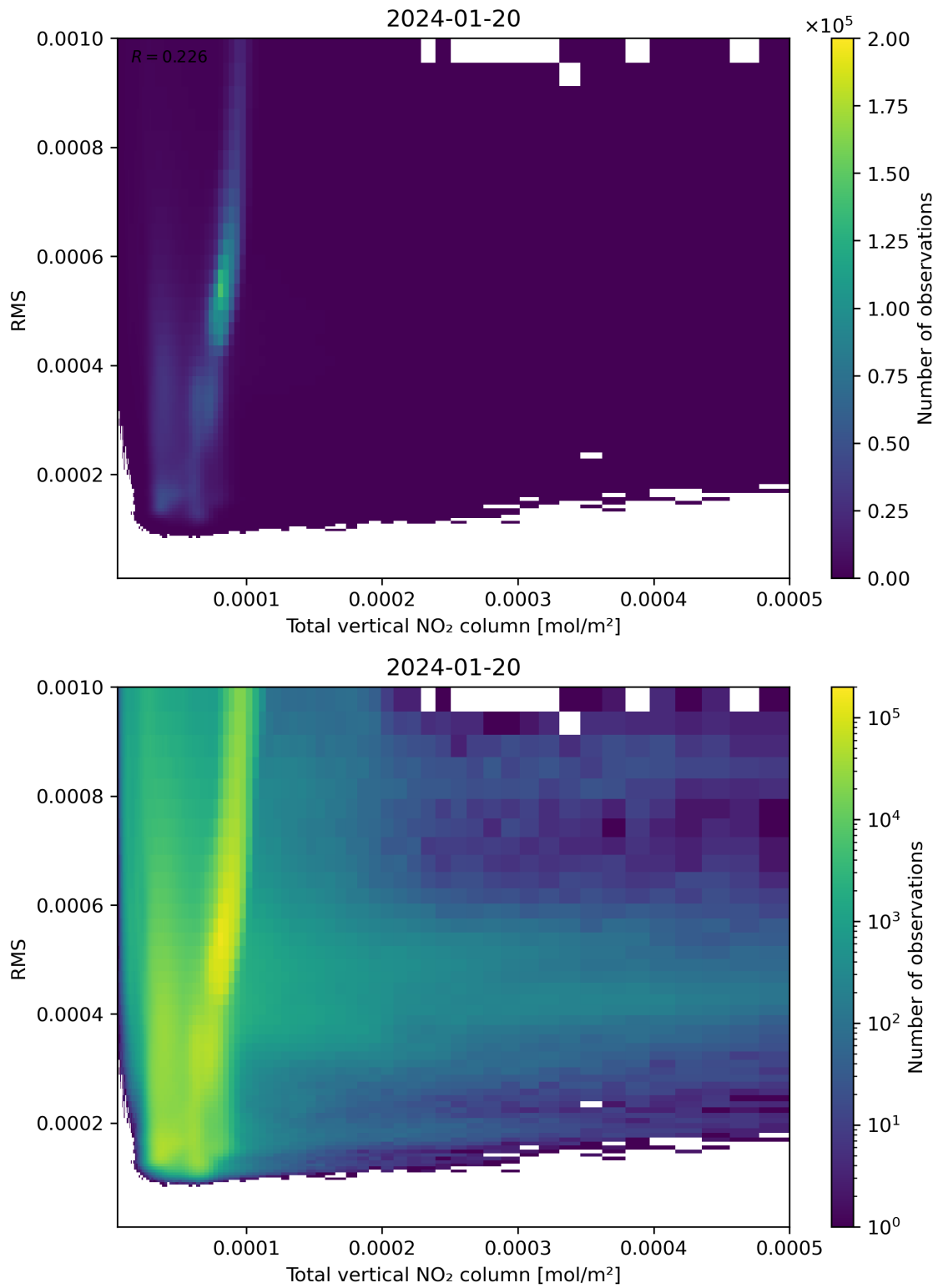
Figure 120: Scatter density plot of “Total vertical NO 2 column” against “RMS” for 2024-01-19 to 2024-01-21.
