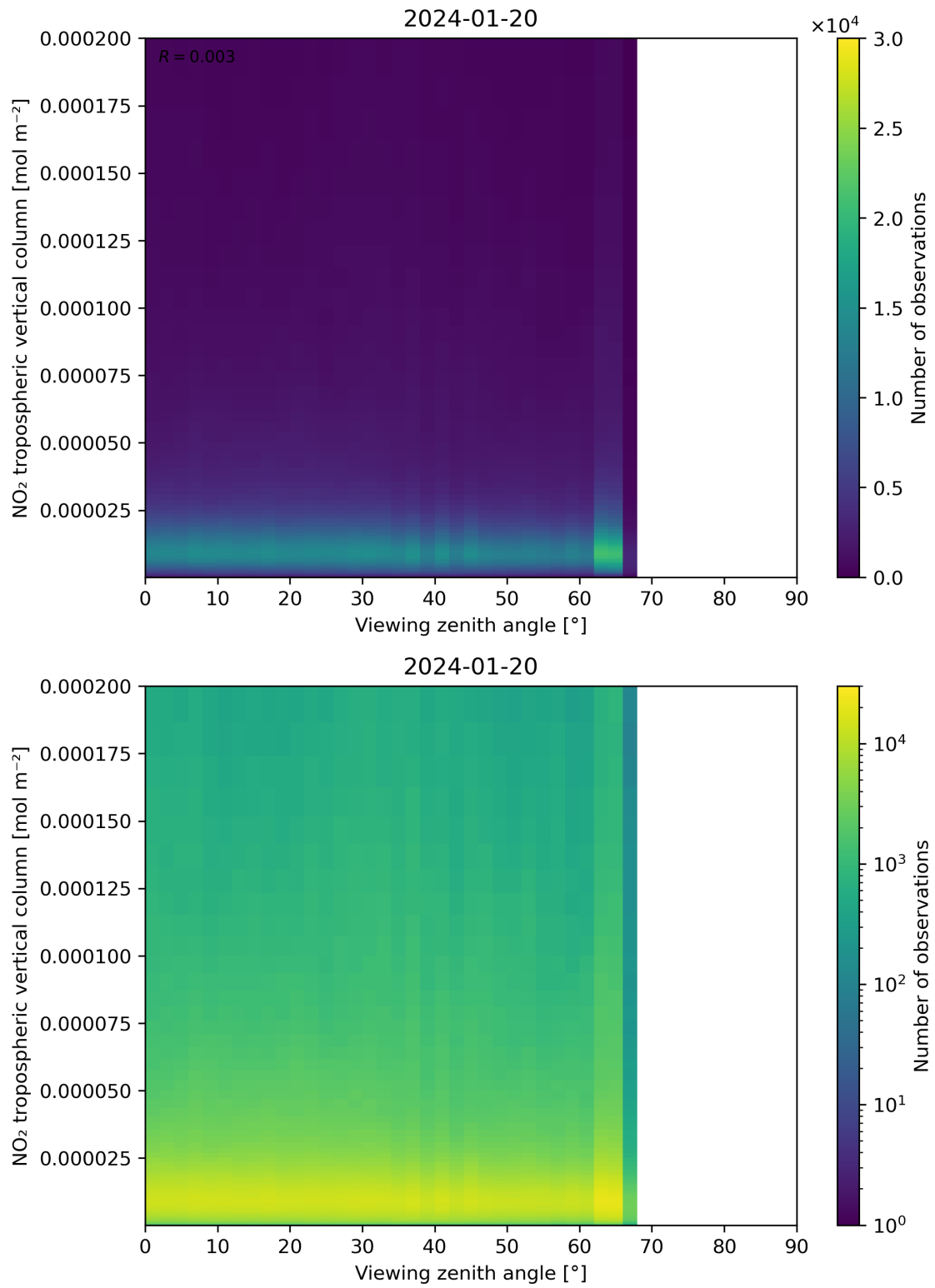
Figure 169: Scatter density plot of “Viewing zenith angle” against “NO 2 tropospheric vertical column” for 2024-01-19 to 2024-01-21.
