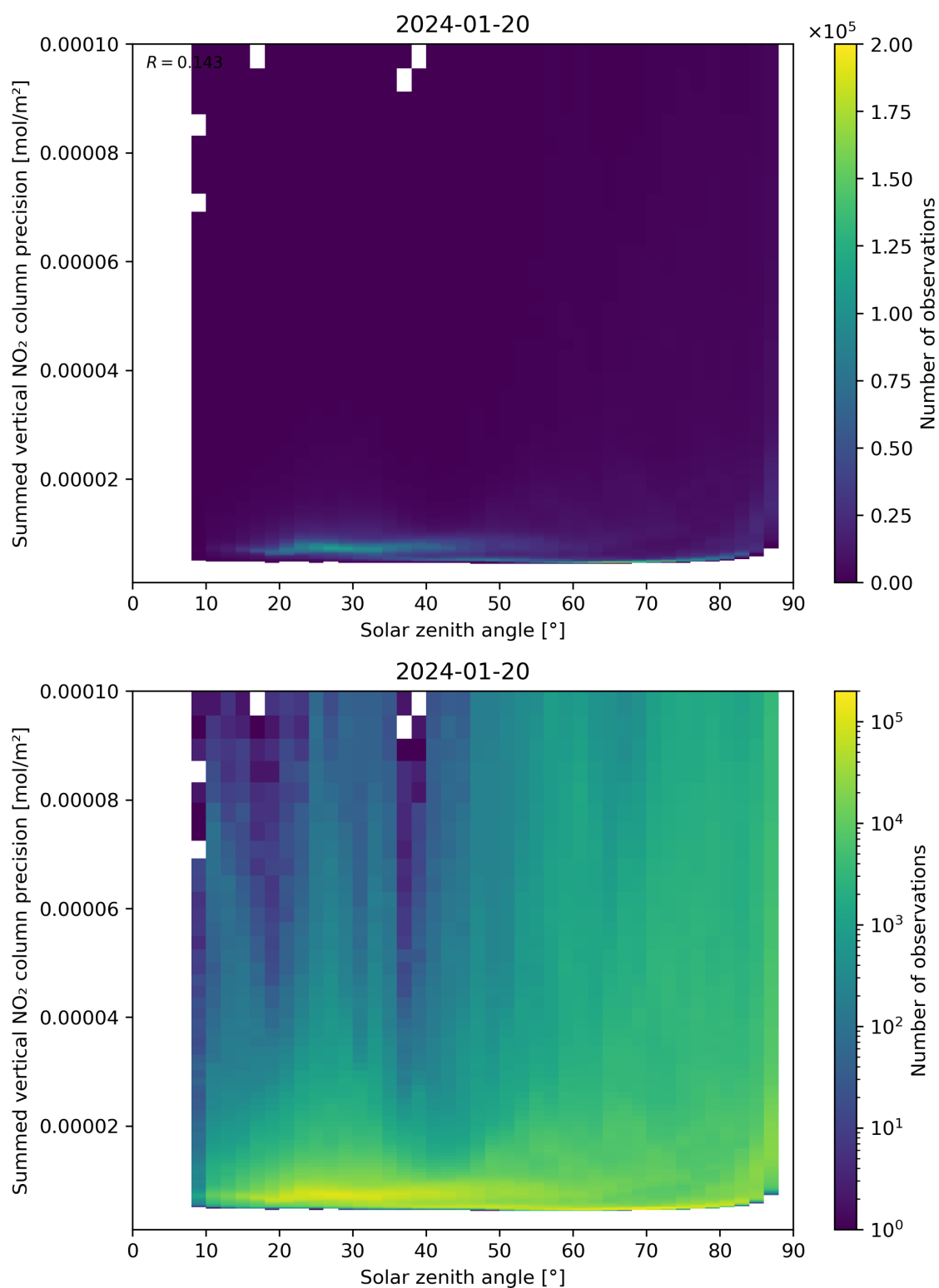
Figure 152: Scatter density plot of “Solar zenith angle” against “Summed vertical NO 2 column precision” for 2024-01-19 to 2024-01-21.
