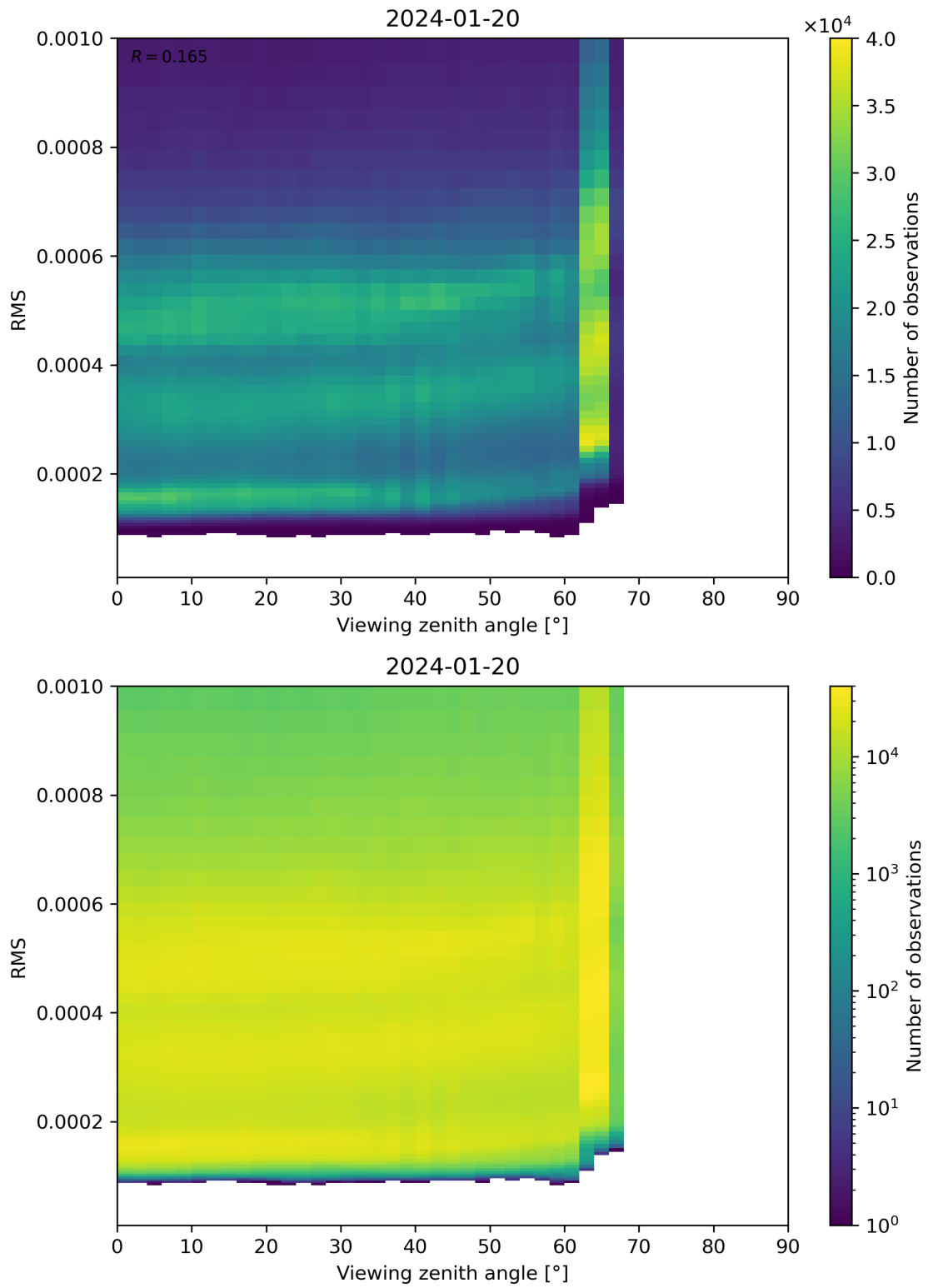
Figure 171: Scatter density plot of “Viewing zenith angle” against “RMS” for 2024-01-19 to 2024-01-21.
