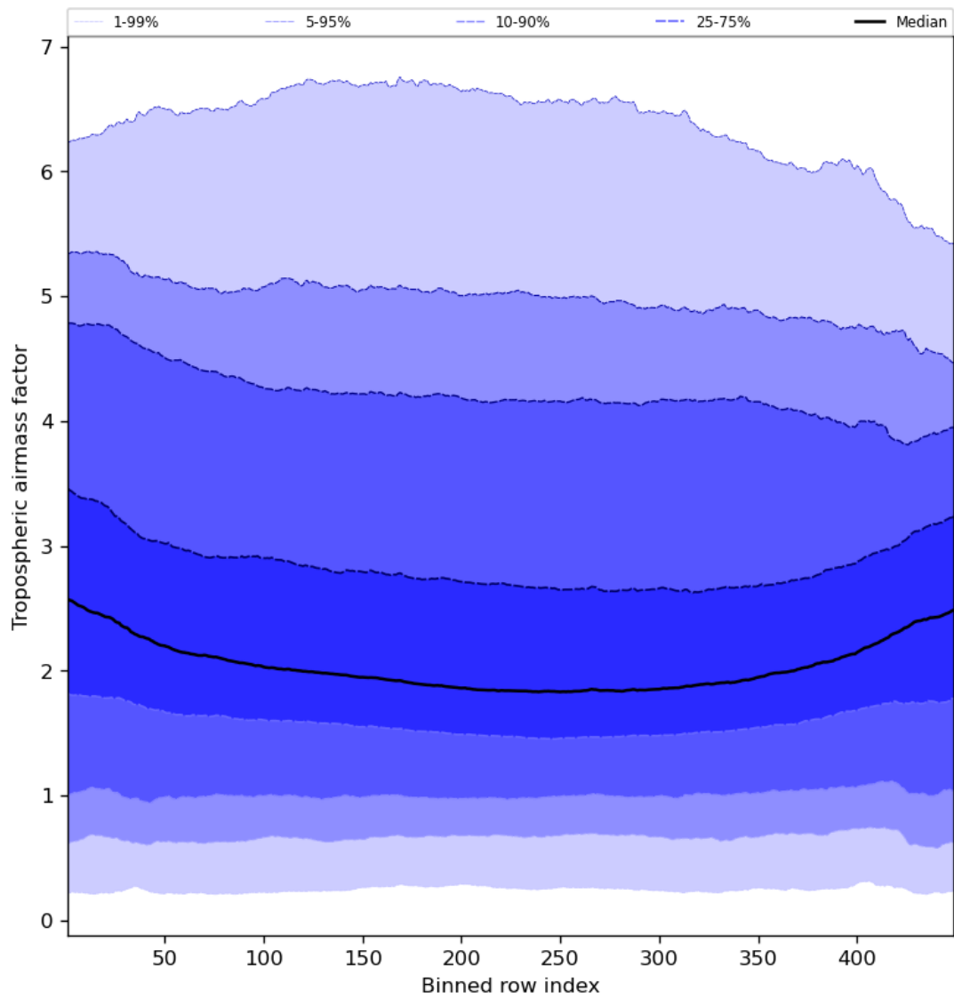
Figure 48: Along track statistics of “Tropospheric air mass factor” for 2024-01-19 to 2024-01-21
