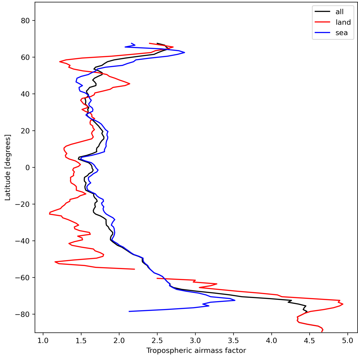
Figure 14: Zonal average of “Tropospheric airmass factor” for 2024-01-19 to 2024-01-21.
