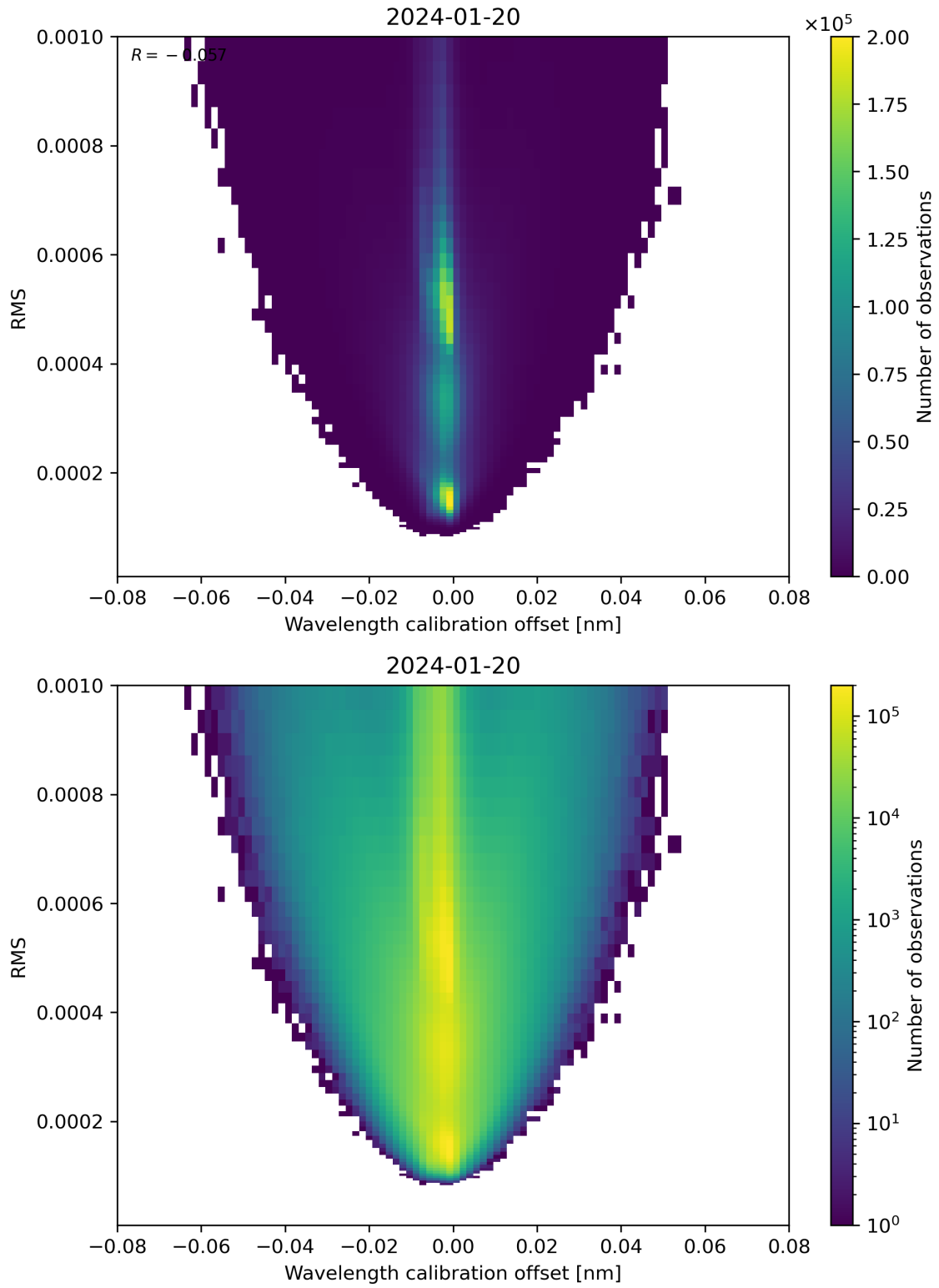
Figure 181: Scatter density plot of “Wavelength calibration offset” against “RMS” for 2024-01-19 to 2024-01-21.
