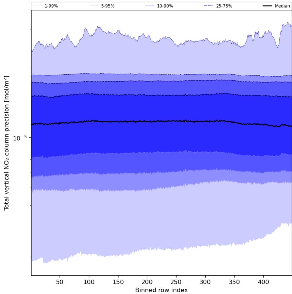
Figure 56: Along track statistics of "Total vertical NO 2 column precision" for 2024-01-19 to 2024-01-21
