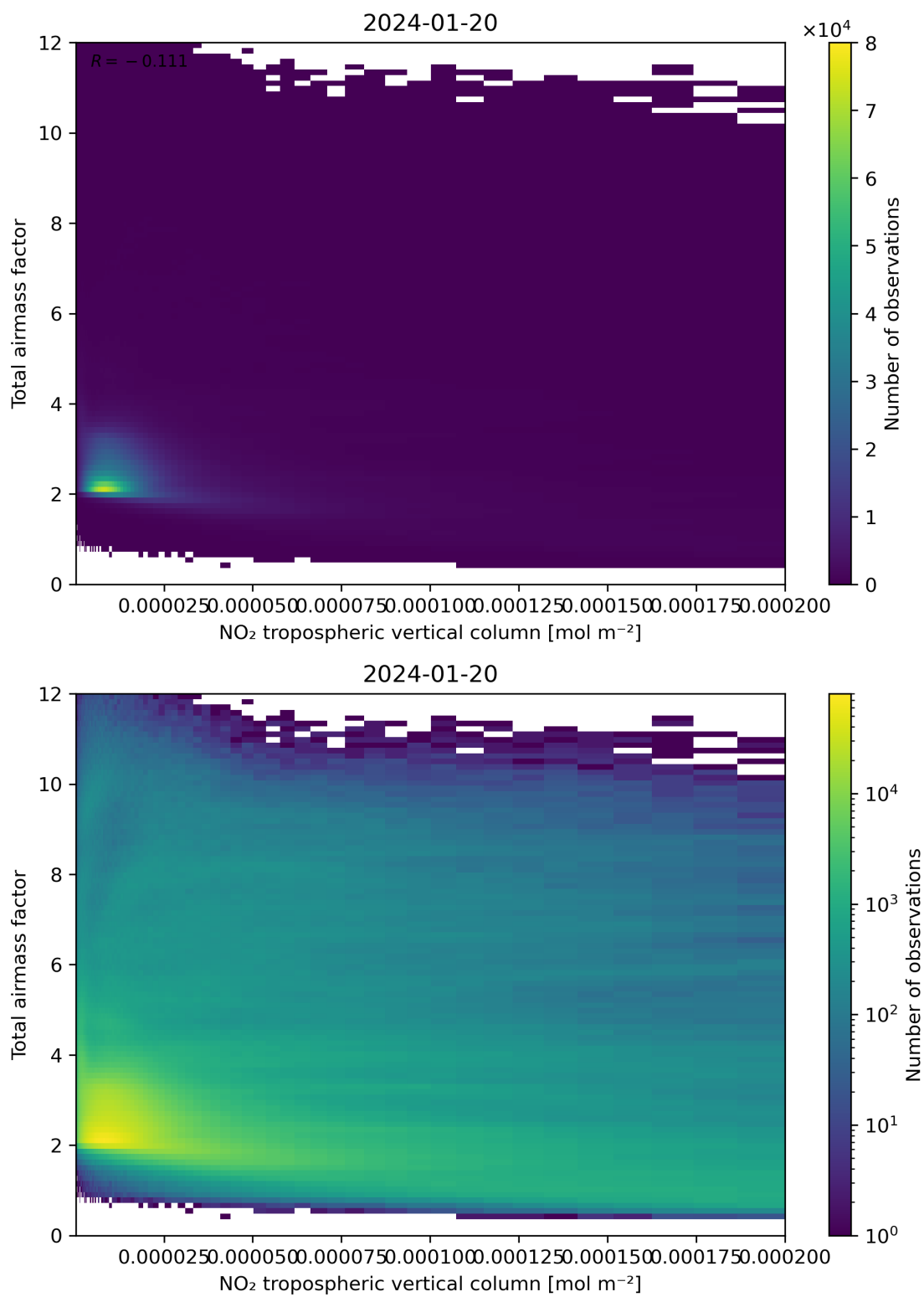
Figure 122: Scatter density plot of “NO 2 tropospheric vertical column” against “Total air mass factor” for 2024-01-19 to 2024-01-21.
