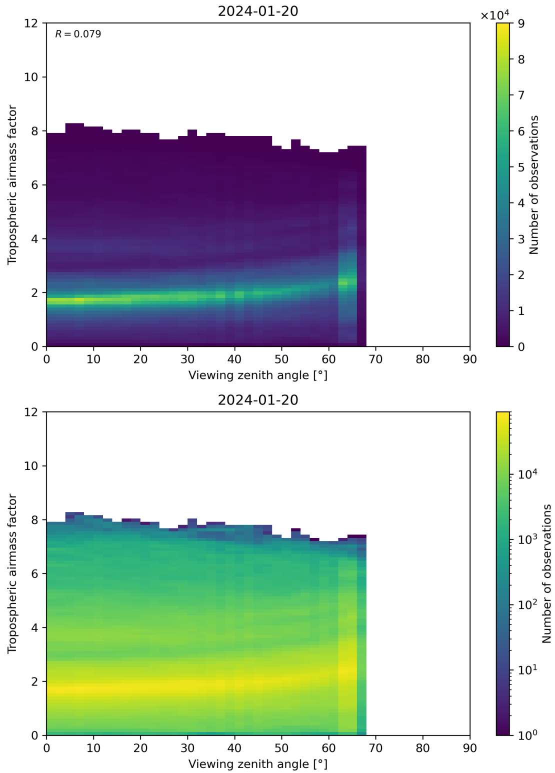
Figure 161: Scatter density plot of “Viewing zenith angle” against “Tropospheric airmass factor” for 2024-01-19 to 2024-01-21.
