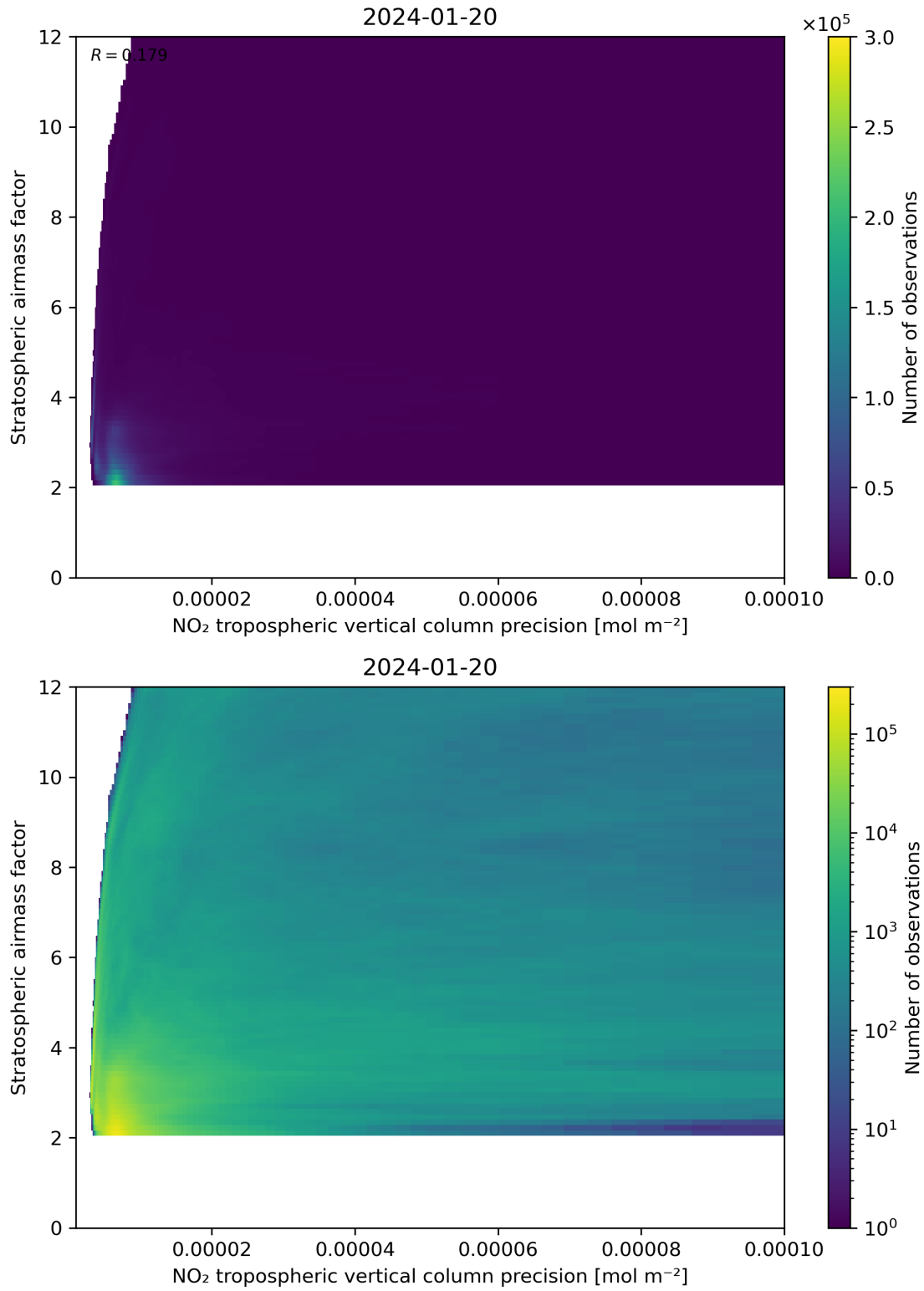
Figure 131: Scatter density plot of “NO 2 tropospheric vertical column precision” against “Stratospheric airmass factor” for 2024-01-19 to 2024-01-21.
