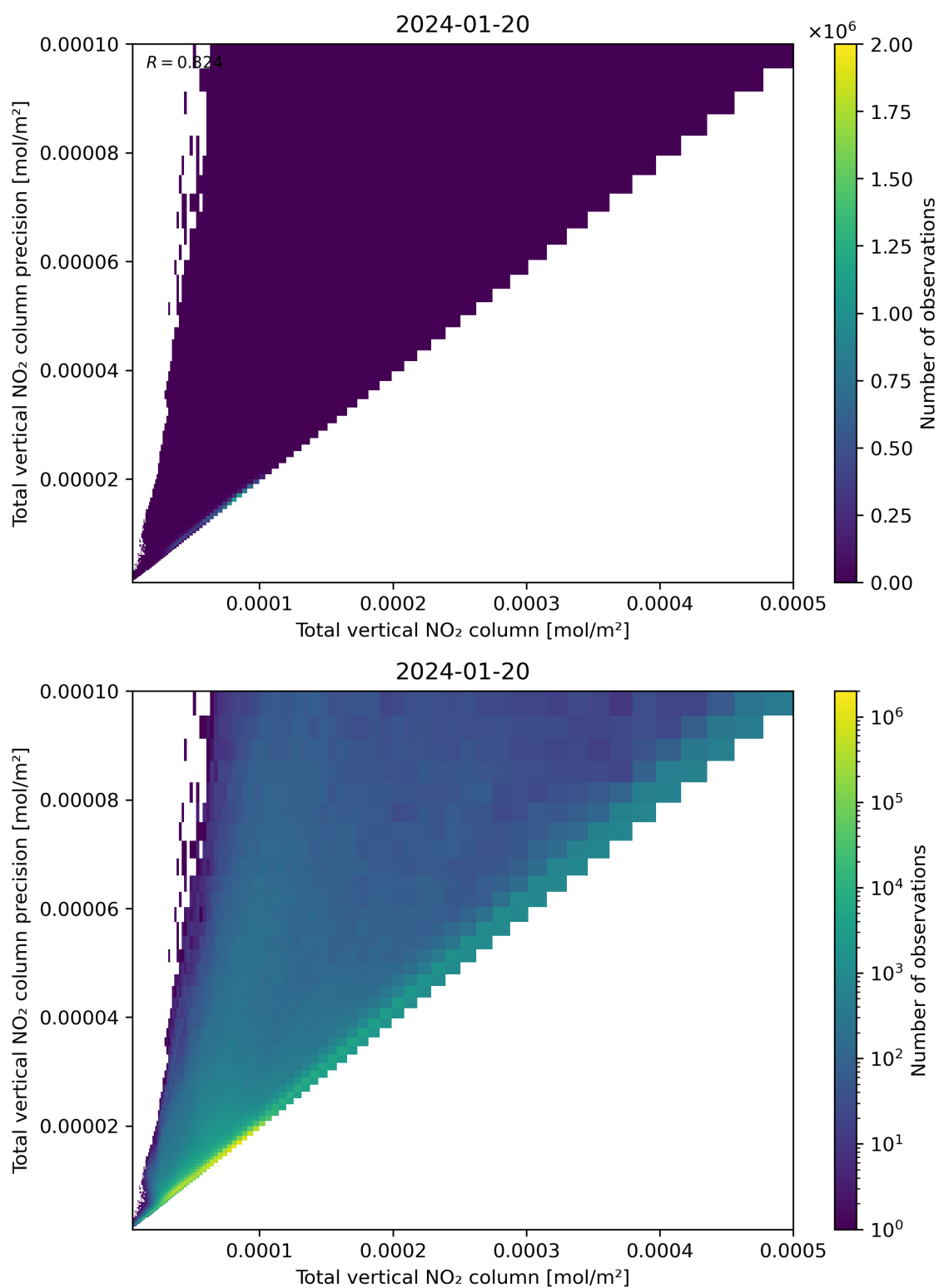
Figure 114: Scatter density plot of “Total vertical NO 2 column” against “Total vertical NO 2 column precision” for 2024-01-19 to 2024-01-21.
