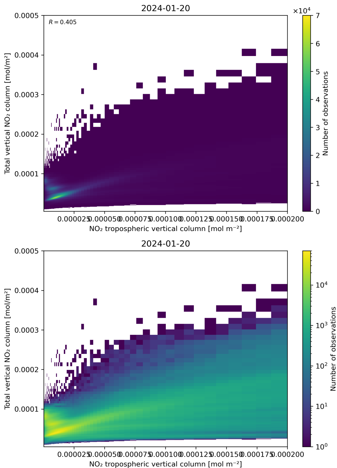
Figure 128: Scatter density plot of “NO 2 tropospheric vertical column” against “Total vertical NO 2 column” for 2024-01-19 to 2024-01-21.
