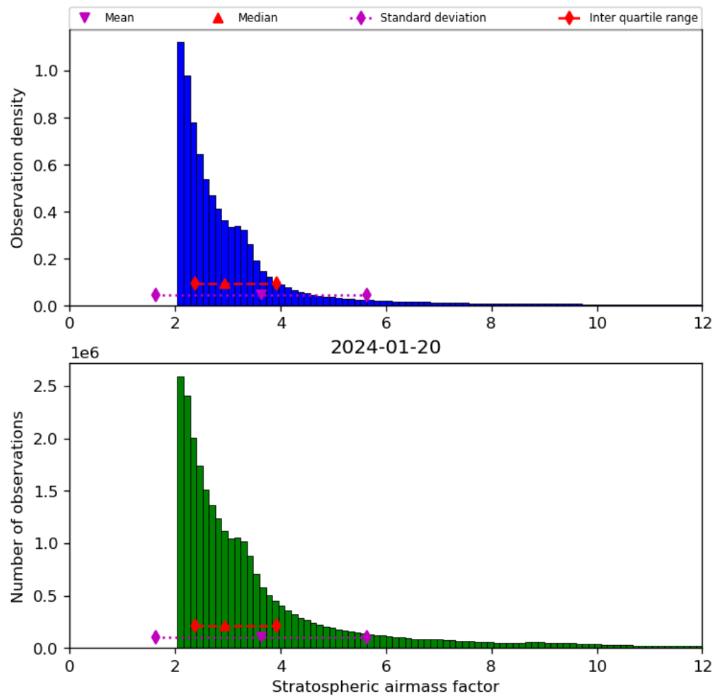
Figure 44: Histogram of “Stratospheric airmass factor” for 2024-01-19 to 2024-01-21
