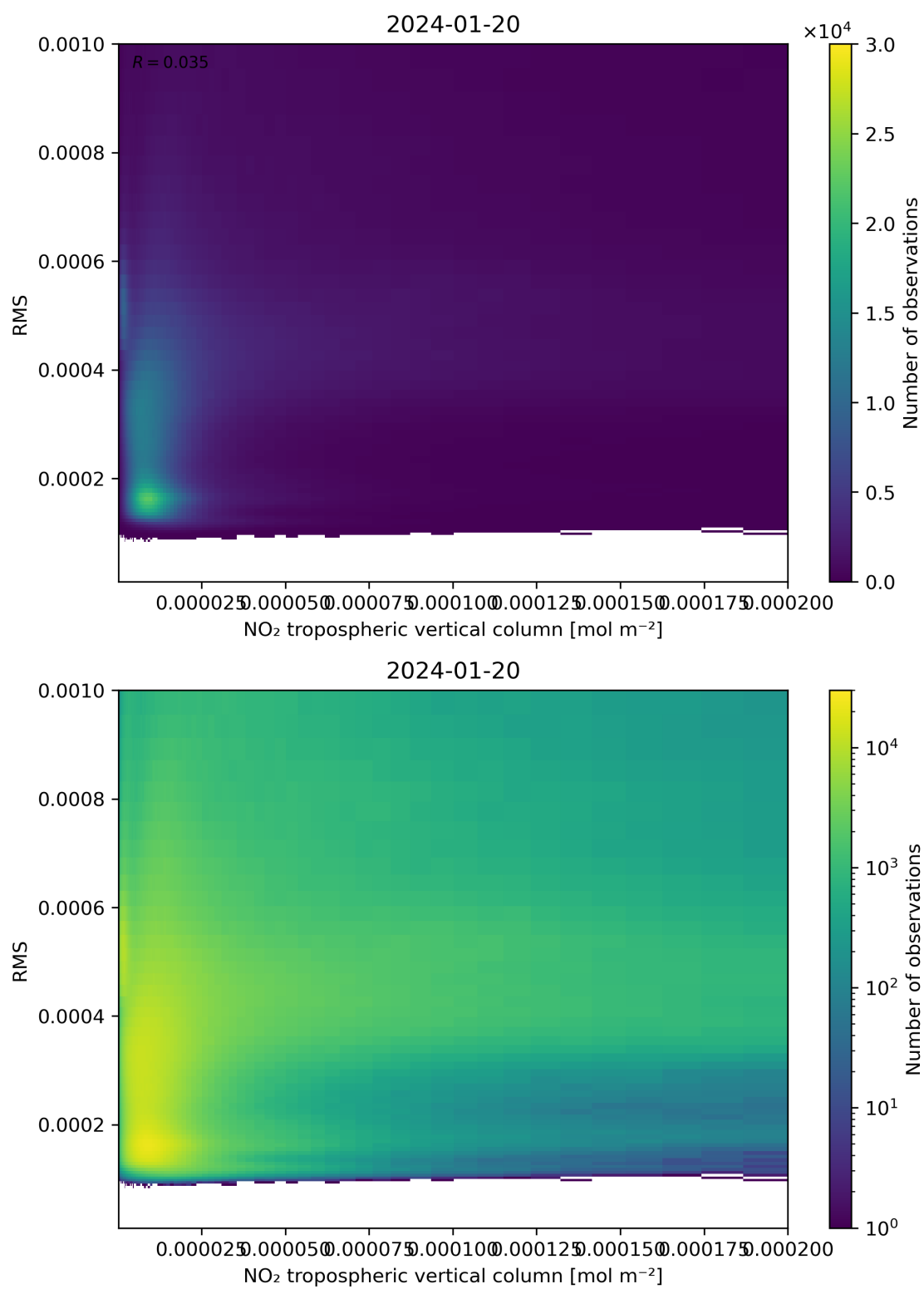
Figure 142: Scatter density plot of “NO 2 tropospheric vertical column” against “RMS” for 2024-01-19 to 2024-01-21.
