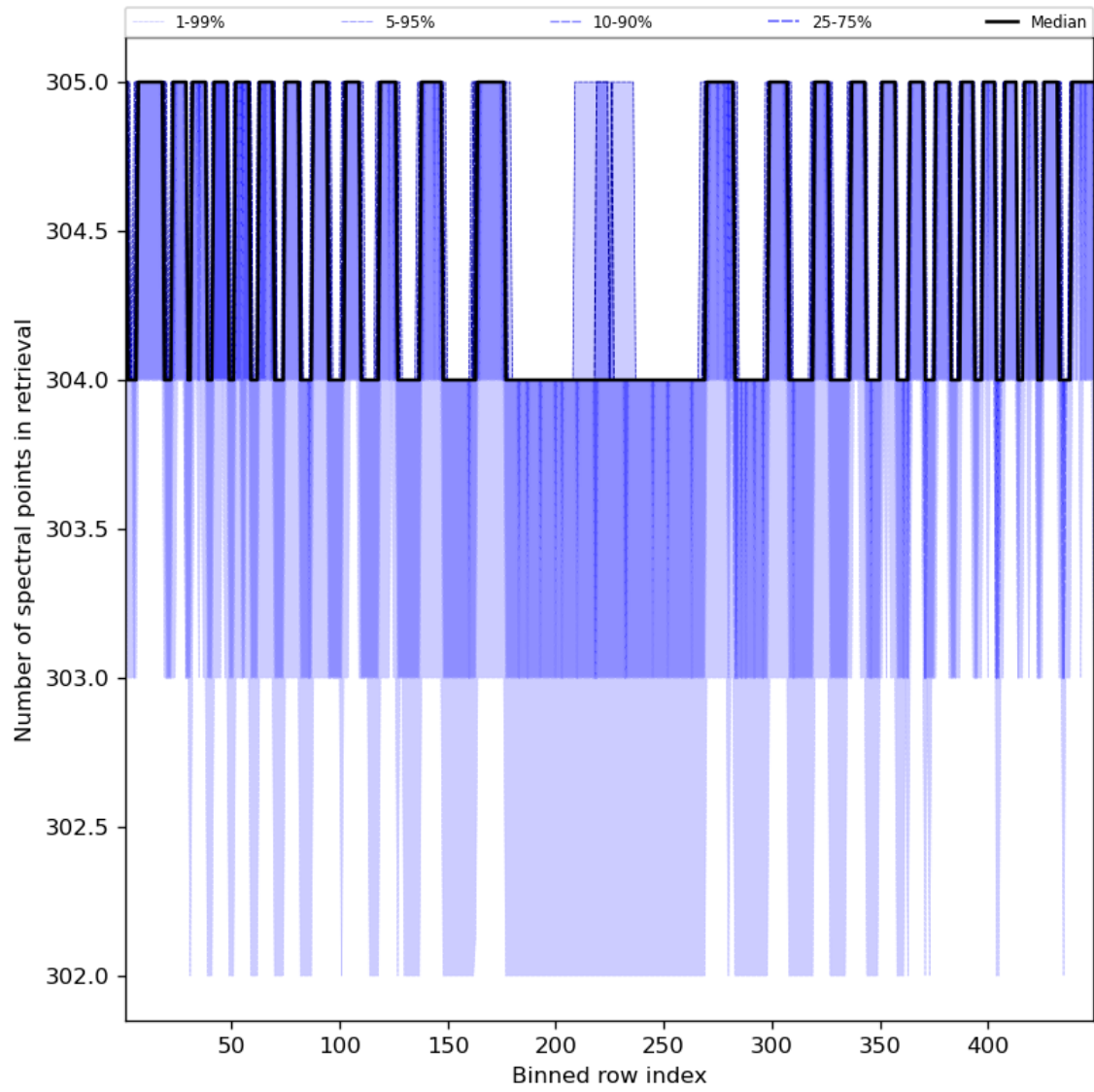
Figure 50: Along track statistics of “Number of spectral points in retrieval” for 2024-01-19 to 2024-01-21
