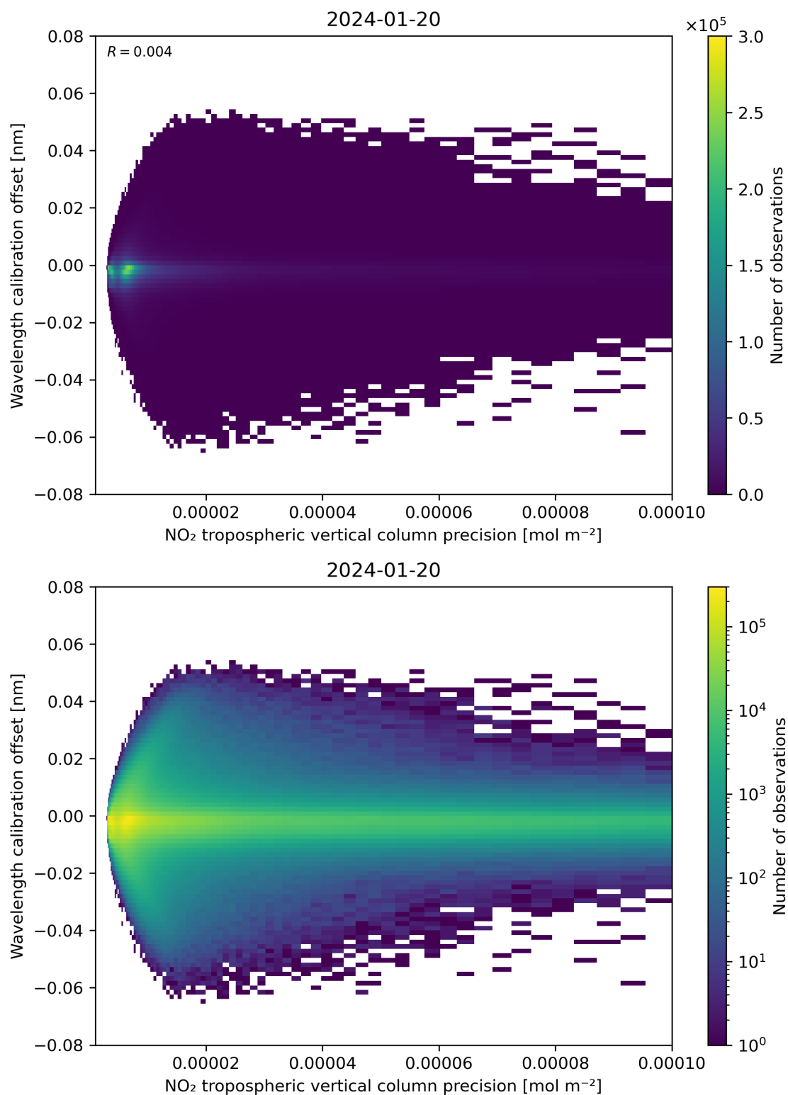
Figure 141: Scatter density plot of “NO 2 tropospheric vertical column precision” against “Wavelength calibration offset” for 2024-01-19 to 2024-01-21.
