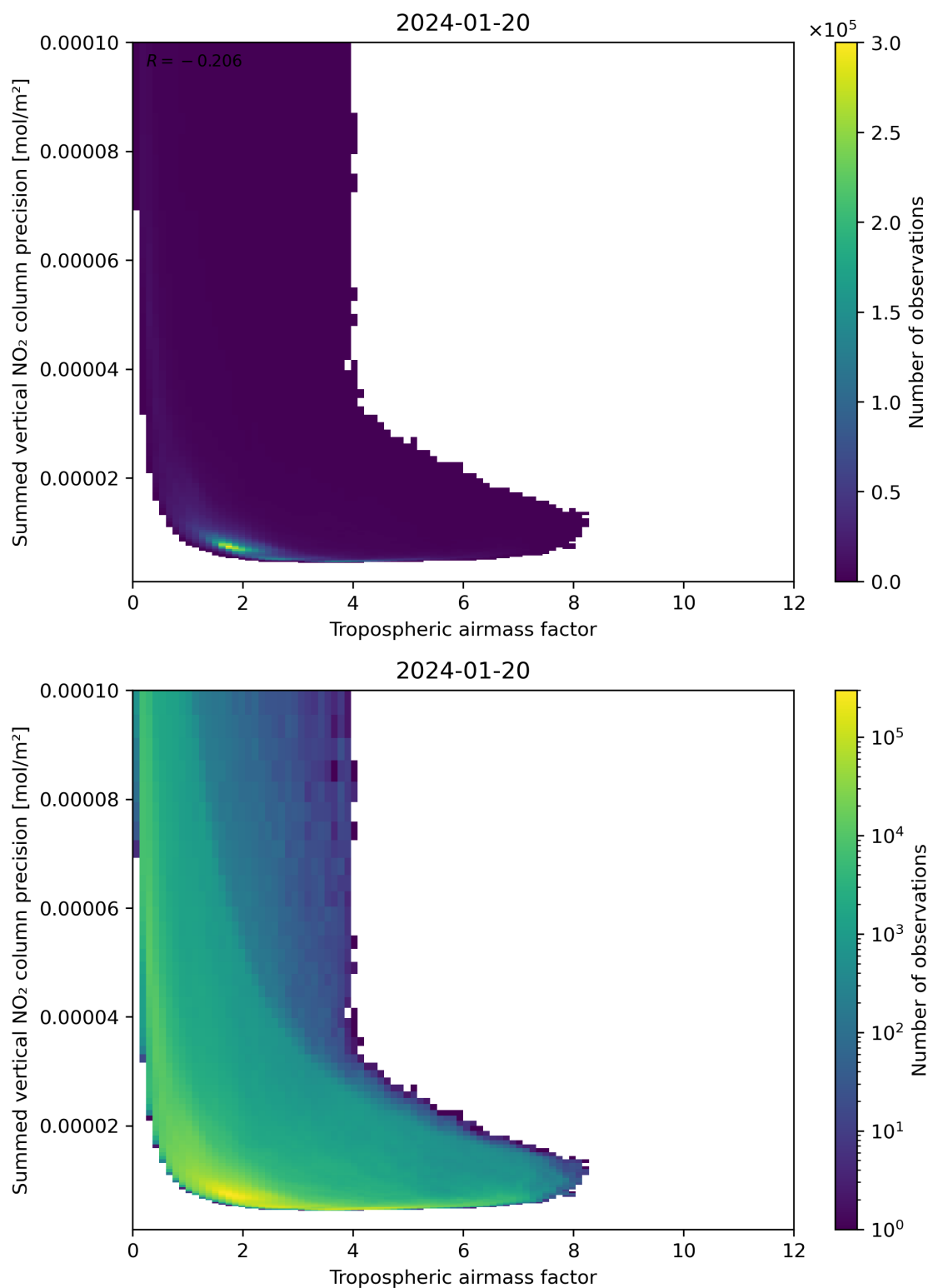
Figure 76: Scatter density plot of “Tropospheric airmass factor” against “Summed vertical NO 2 column precision” for 2024-01-19 to 2024-01-21.
