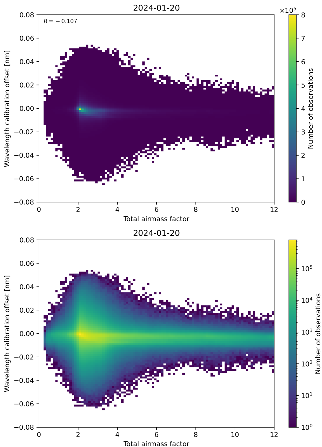
Figure 70: Scatter density plot of “Total airmass factor” against “Wavelength calibration offset” for 2024-01-19 to 2024-01-21.
