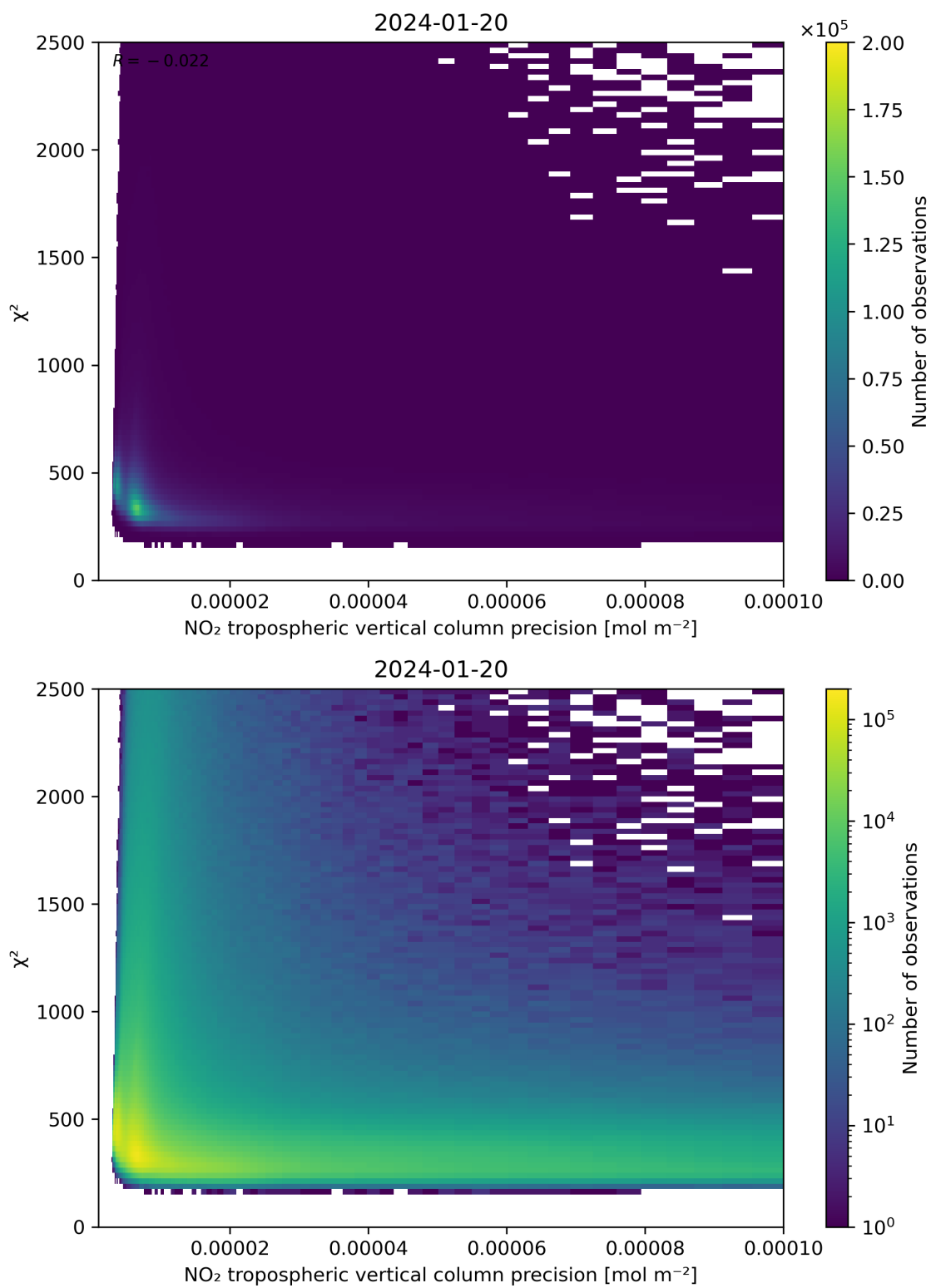
Figure 134: Scatter density plot of “NO 2 tropospheric vertical column precision” against “ \chi^2 ” for 2024-01-19 to 2024-01-21.
