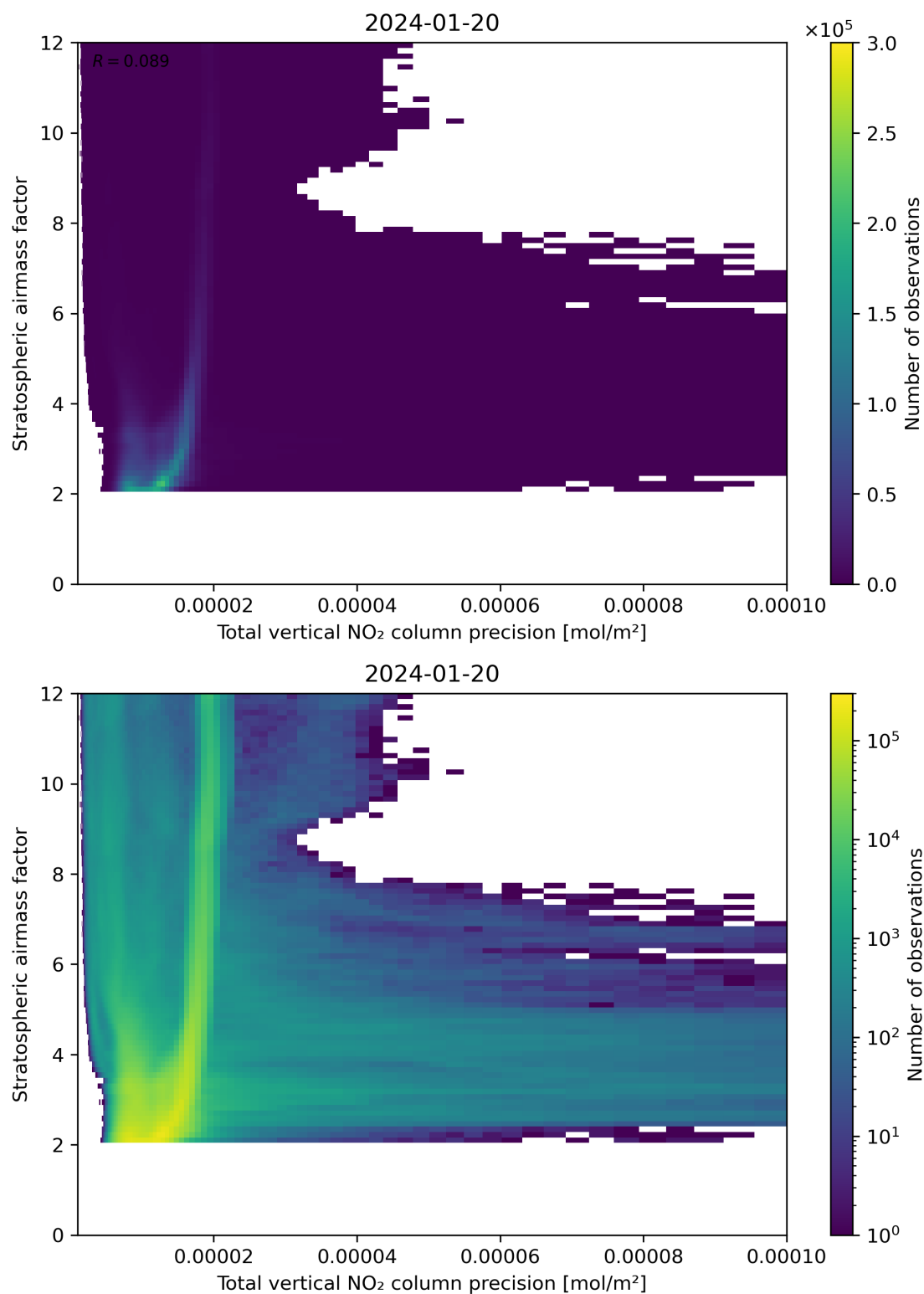
Figure 115: Scatter density plot of “Total vertical NO 2 column precision” against “Stratospheric air mass factor” for 2024-01-19 to 2024-01-21.
