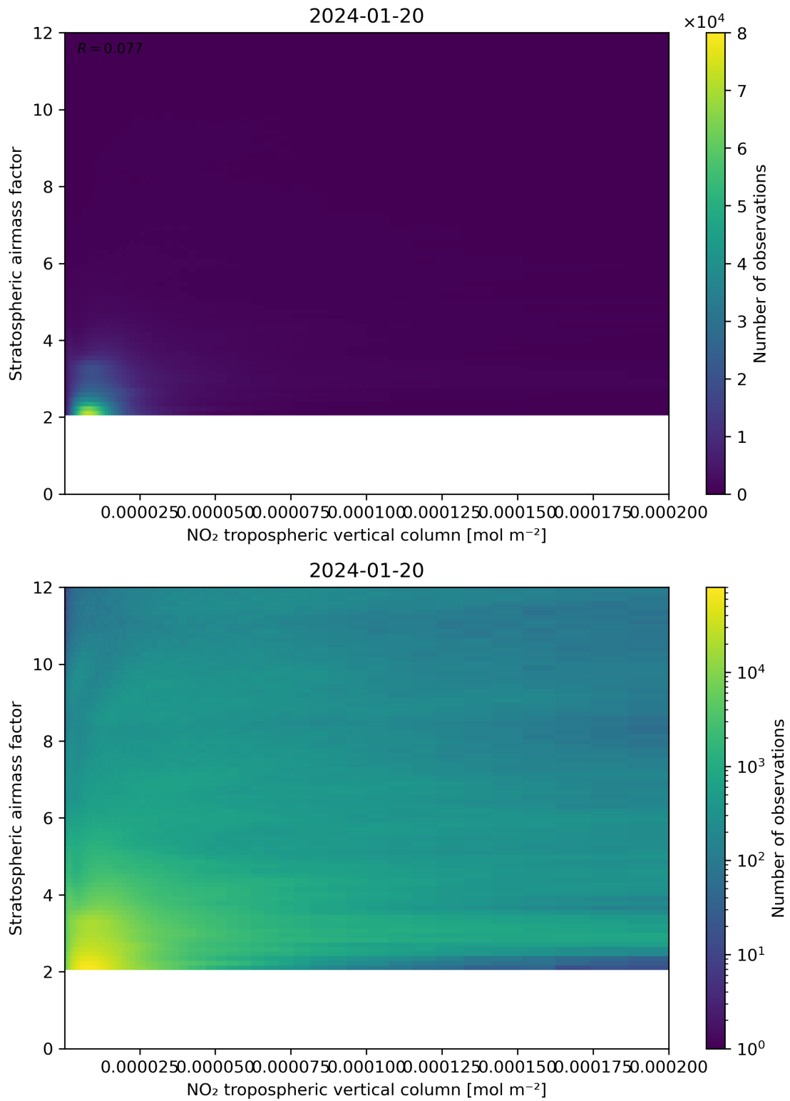
Figure 121: Scatter density plot of “NO 2 tropospheric vertical column” against “Stratospheric airmass factor” for 2024-01-19 to 2024-01-21.
