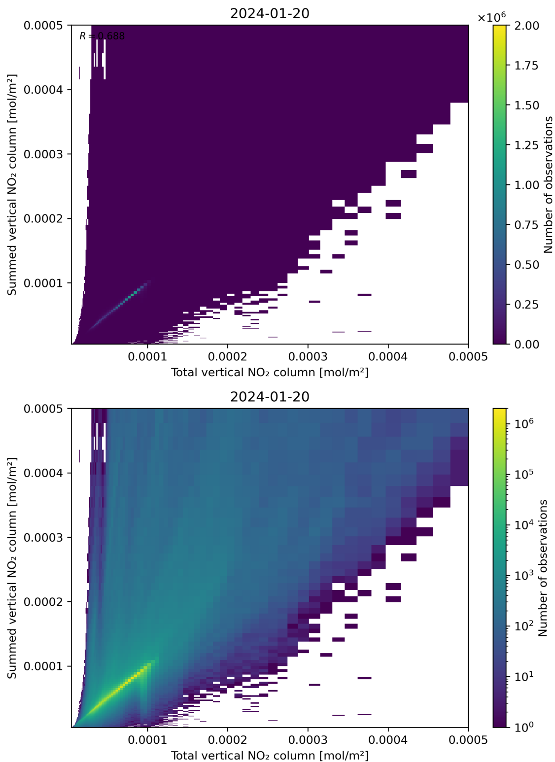
Figure 112: Scatter density plot of “Total vertical NO 2 column” against “Summed vertical NO 2 column” for 2024-01-19 to 2024-01-21.
