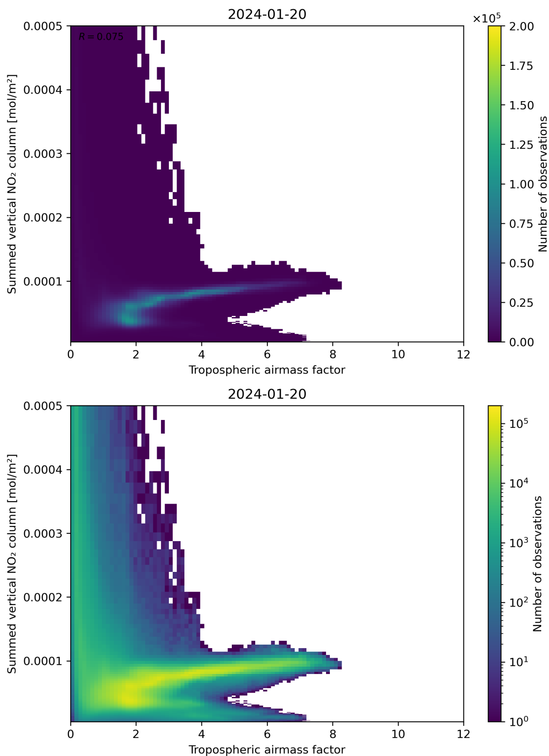
Figure 75: Scatter density plot of “Tropospheric air mass factor” against “Summed vertical NO 2 column” for 2024-01-19 to 2024-01-21.
