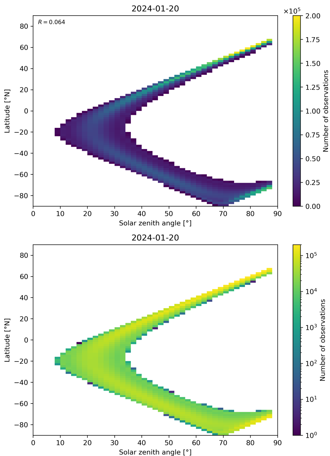
Figure 149: Scatter density plot of “Solar zenith angle” against “Latitude” for 2024-01-19 to 2024-01-21.
