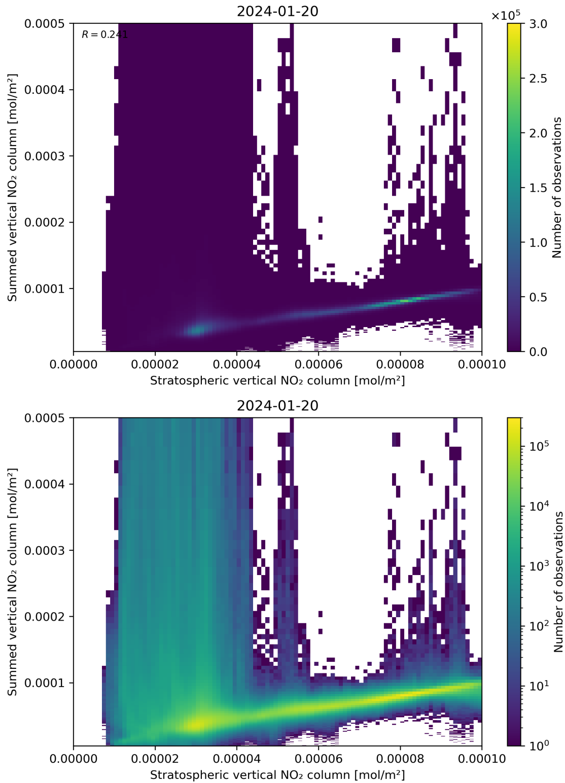
Figure 98: Scatter density plot of “Stratospheric vertical NO 2 column” against “Summed vertical NO 2 column” for 2024-01-19 to 2024-01-21.
