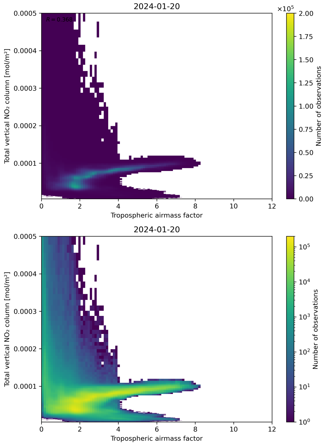
Figure 77: Scatter density plot of “Tropospheric airmass factor” against “Total vertical NO 2 column” for 2024-01-19 to 2024-01-21.
