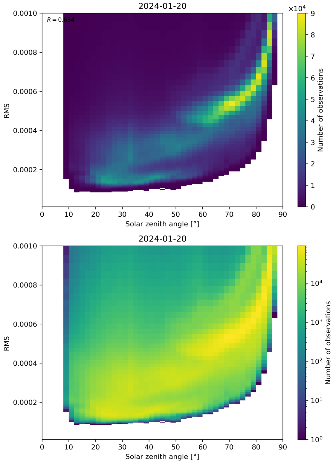
Figure 157: Scatter density plot of “Solar zenith angle” against “RMS” for 2024-01-19 to 2024-01-21.
