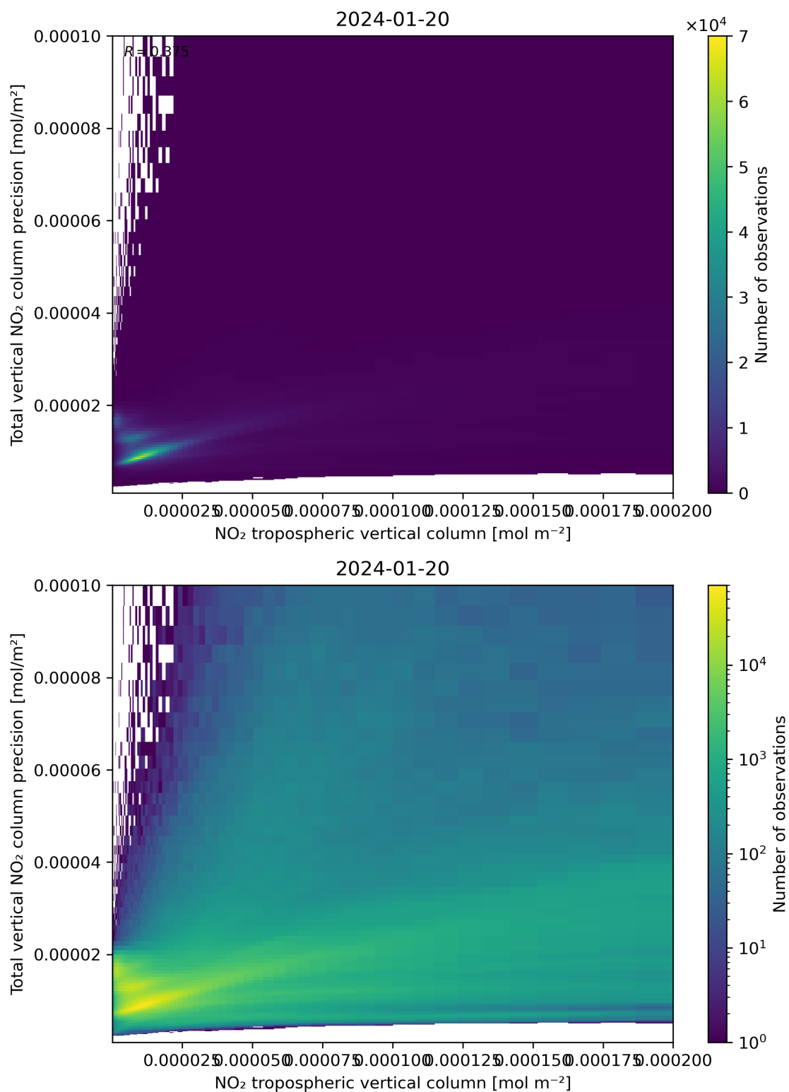
Figure 129: Scatter density plot of “NO 2 tropospheric vertical column” against “Total vertical NO 2 column precision” for 2024-01-19 to 2024-01-21.
