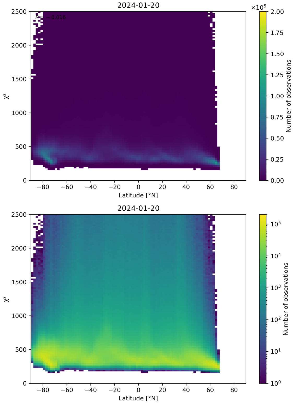
Figure 86: Scatter density plot of “Latitude” against “ \chi^2 ” for 2024-01-19 to 2024-01-21.
