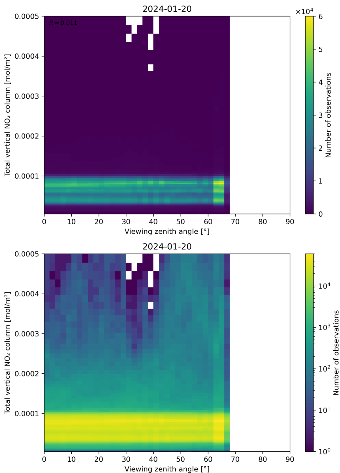
Figure 167: Scatter density plot of “Viewing zenith angle” against “Total vertical NO 2 column” for 2024-01-19 to 2024-01-21.
