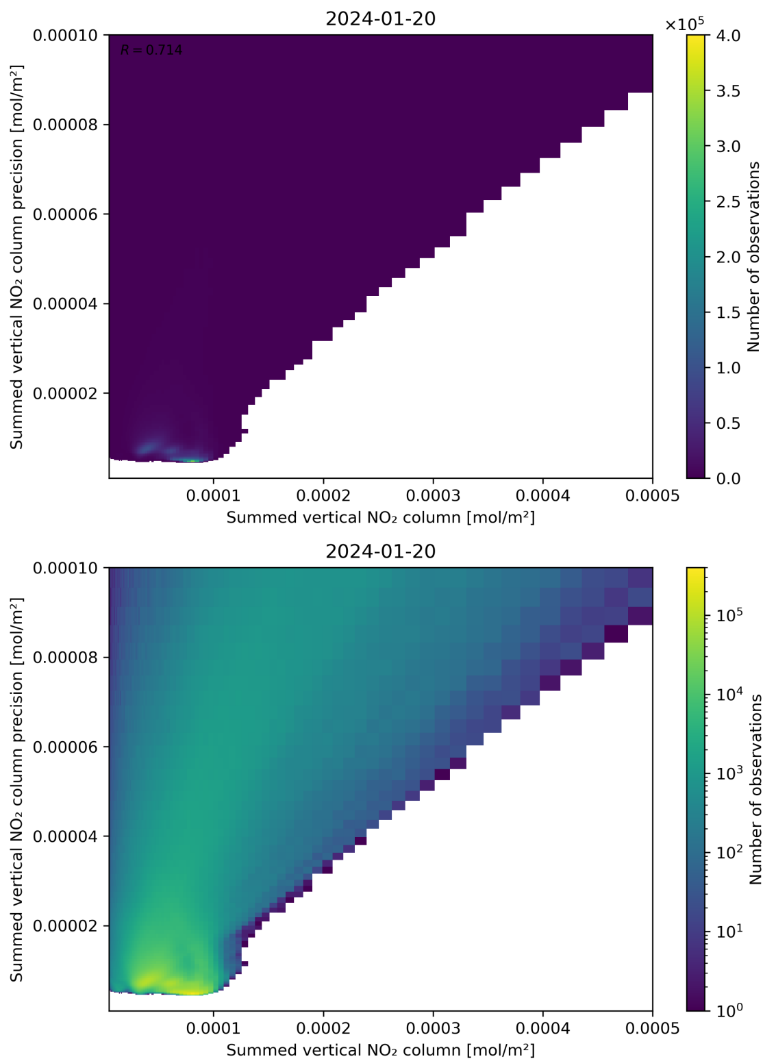
Figure 105: Scatter density plot of “Summed vertical NO 2 column” against “Summed vertical NO 2 column precision” for 2024-01-19 to 2024-01-21.
