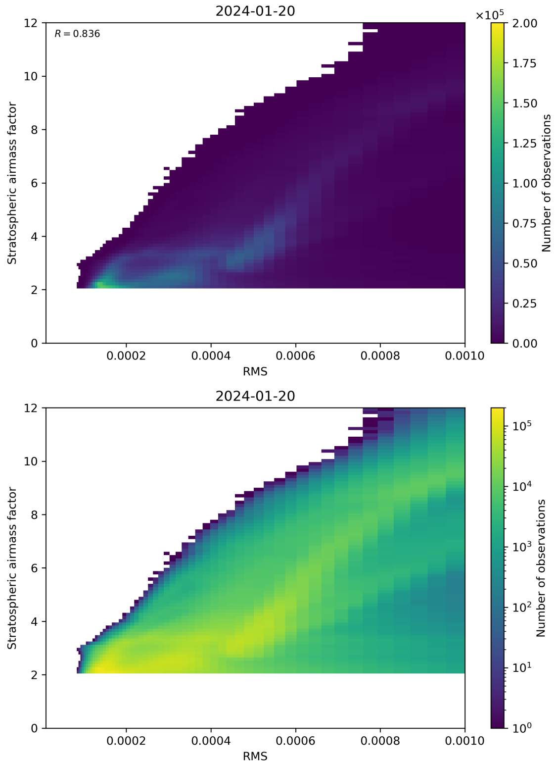
Figure 144: Scatter density plot of “RMS” against “Stratospheric airmass factor” for 2024-01-19 to 2024-01-21.
