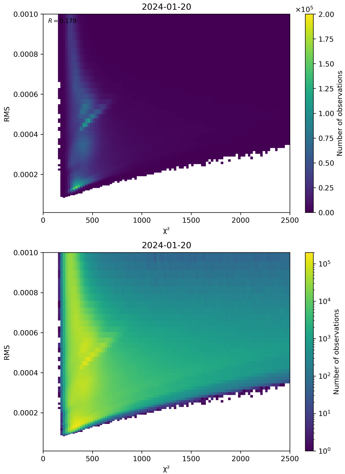
Figure 82: Scatter density plot of “ \chi^2 ” against “RMS” for 2024-01-19 to 2024-01-21.
