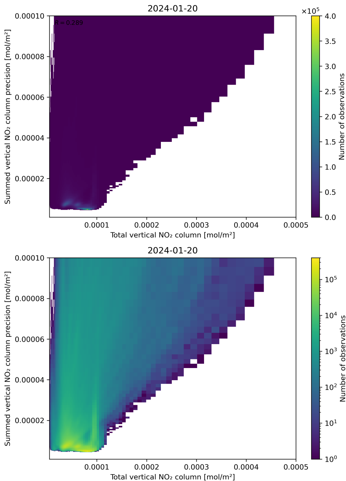
Figure 113: Scatter density plot of “Total vertical NO 2 column” against “Summed vertical NO 2 column precision” for 2024-01-19 to 2024-01-21.
