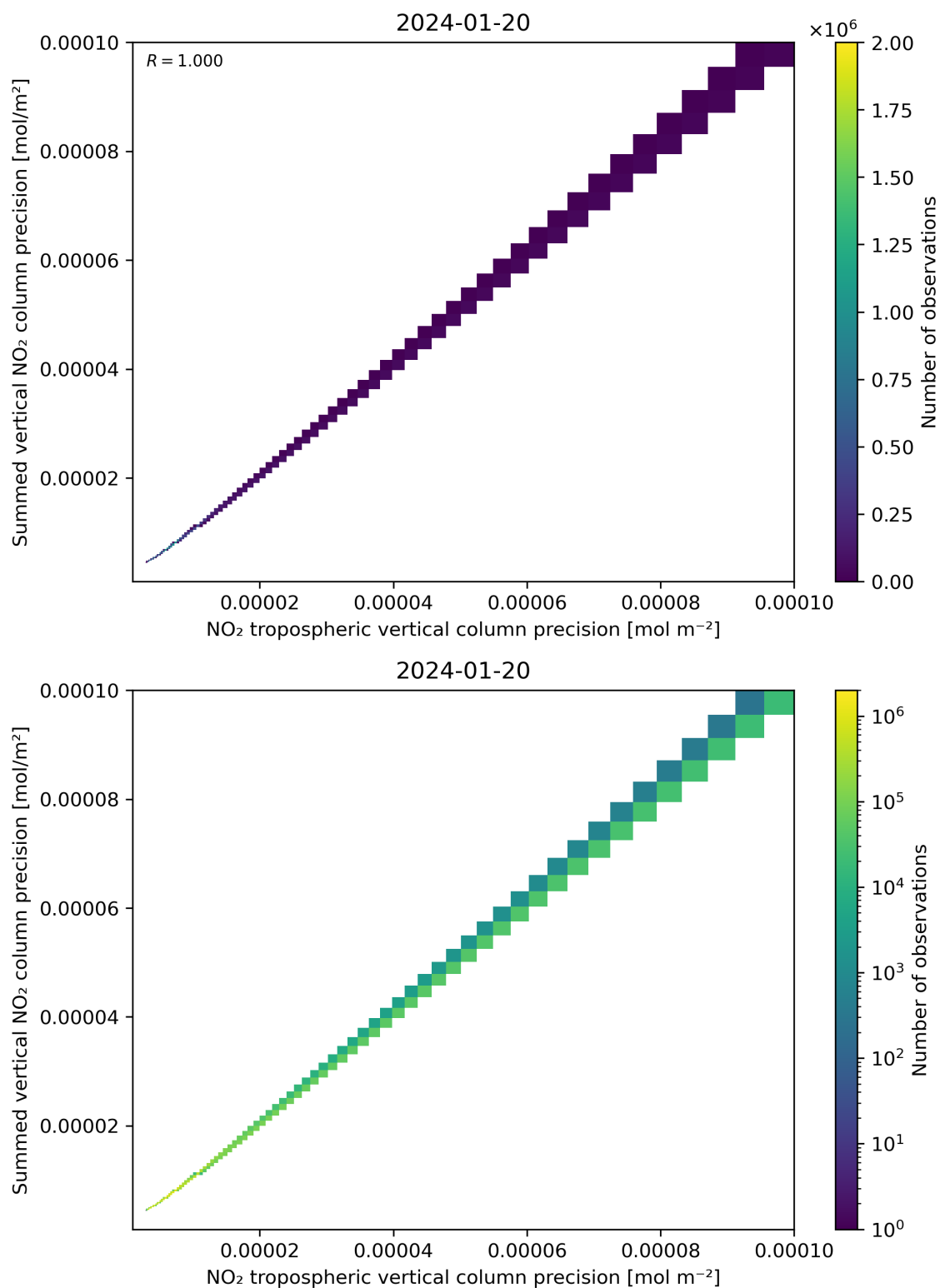
Figure 137: Scatter density plot of “NO 2 tropospheric vertical column precision” against “Summed vertical NO 2 column precision” for 2024-01-19 to 2024-01-21.
