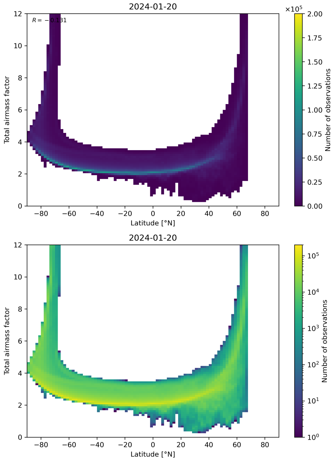
Figure 84: Scatter density plot of “Latitude” against “Total airmass factor” for 2024-01-19 to 2024-01-21.
