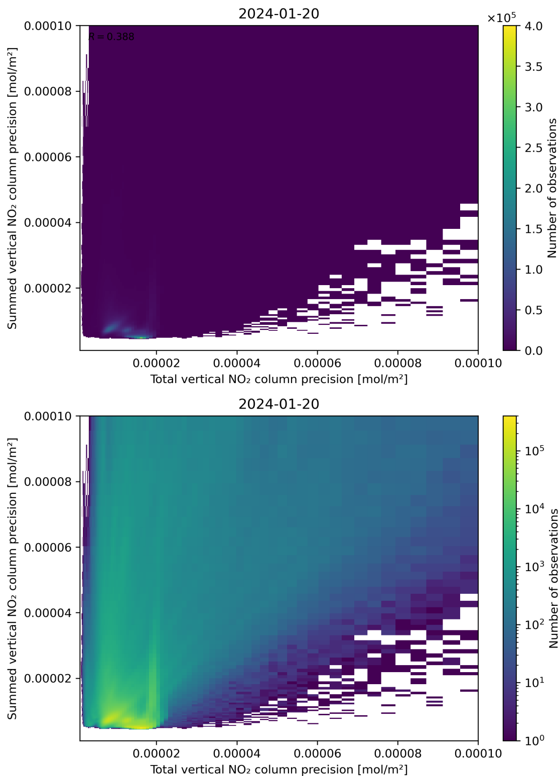
Figure 118: Scatter density plot of “Total vertical NO 2 column precision” against “Summed vertical NO 2 column precision” for 2024-01-19 to 2024-01-21.
