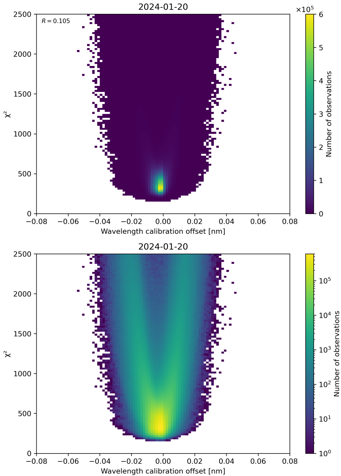
Figure 175: Scatter density plot of “Wavelength calibration offset” against “ \chi^2 ” for 2024-01-19 to 2024-01-21.
