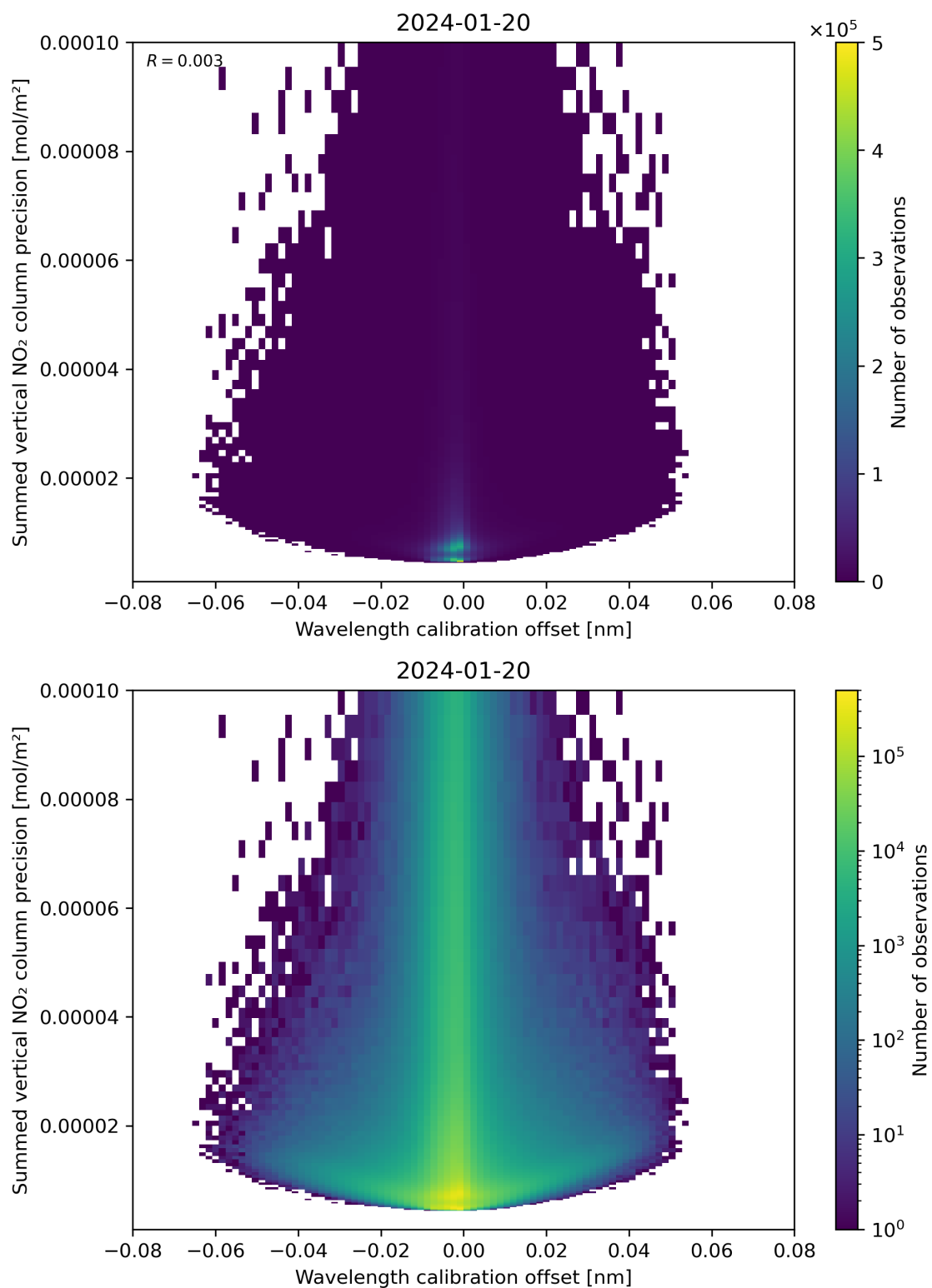
Figure 178: Scatter density plot of “Wavelength calibration offset” against “Summed vertical NO 2 column precision” for 2024-01-19 to 2024-01-21.
