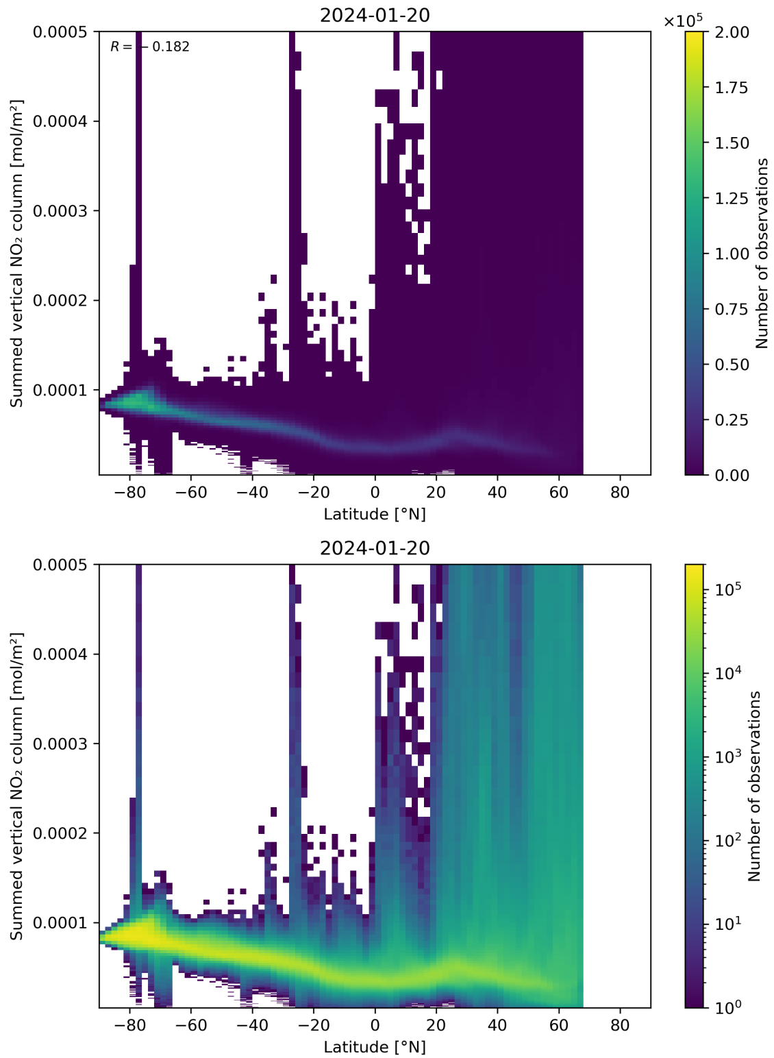
Figure 88: Scatter density plot of “Latitude” against “Summed vertical NO 2 column” for 2024-01-19 to 2024-01-21.
