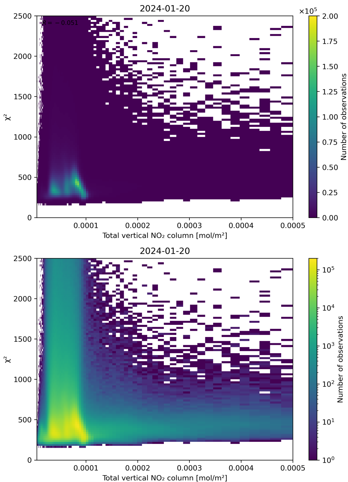
Figure 111: Scatter density plot of “Total vertical NO 2 column” against “ \chi^2 ” for 2024-01-19 to 2024-01-21.
