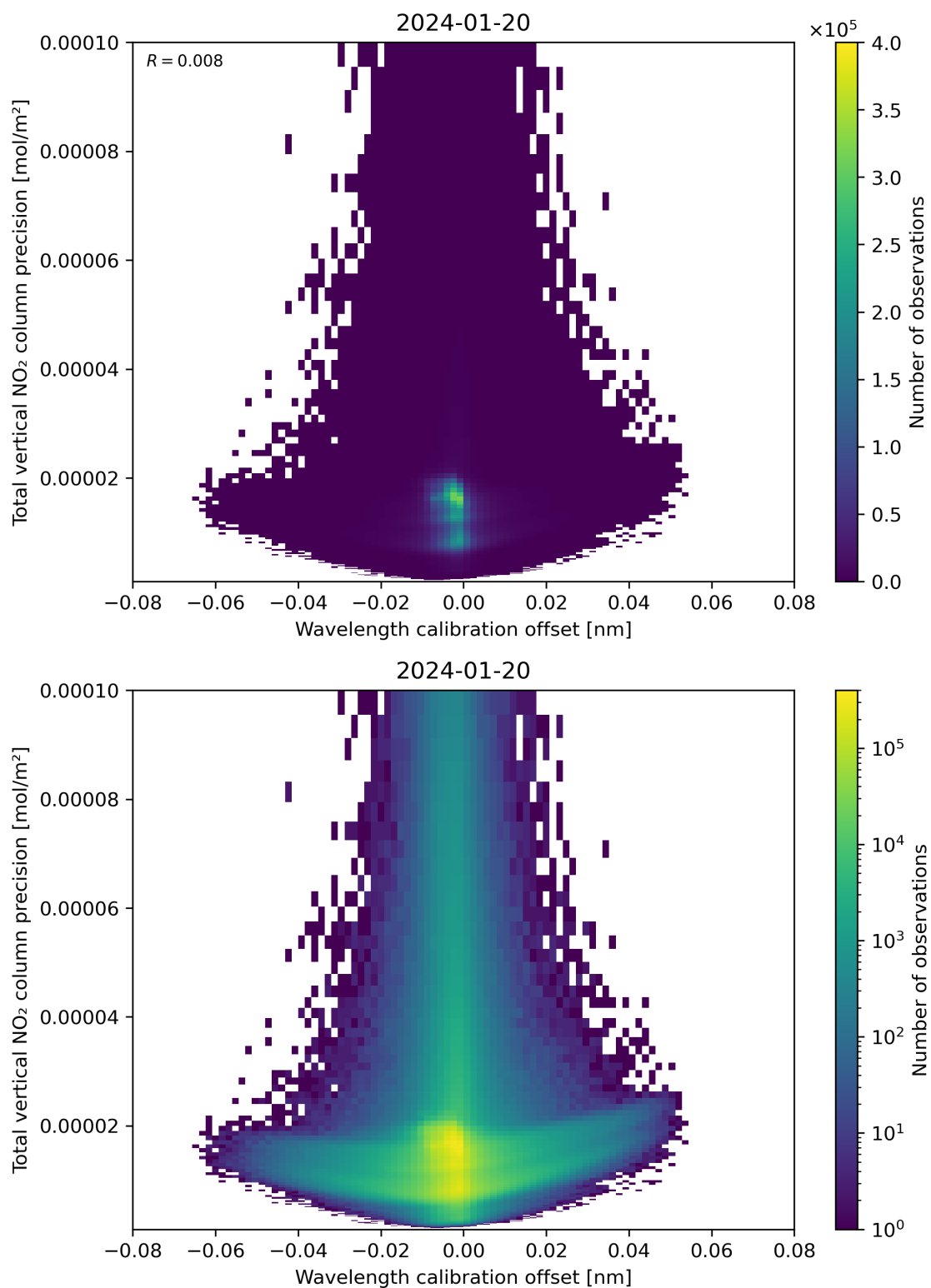
Figure 180: Scatter density plot of “Wavelength calibration offset” against “Total vertical NO 2 column precision” for 2024-01-19 to 2024-01-21.
