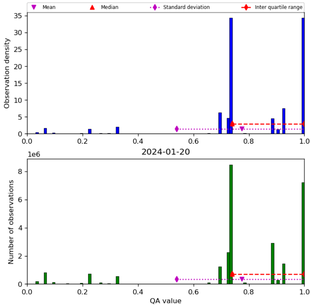
Figure 28: Histogram of “QA value” for 2024-01-19 to 2024-01-21
