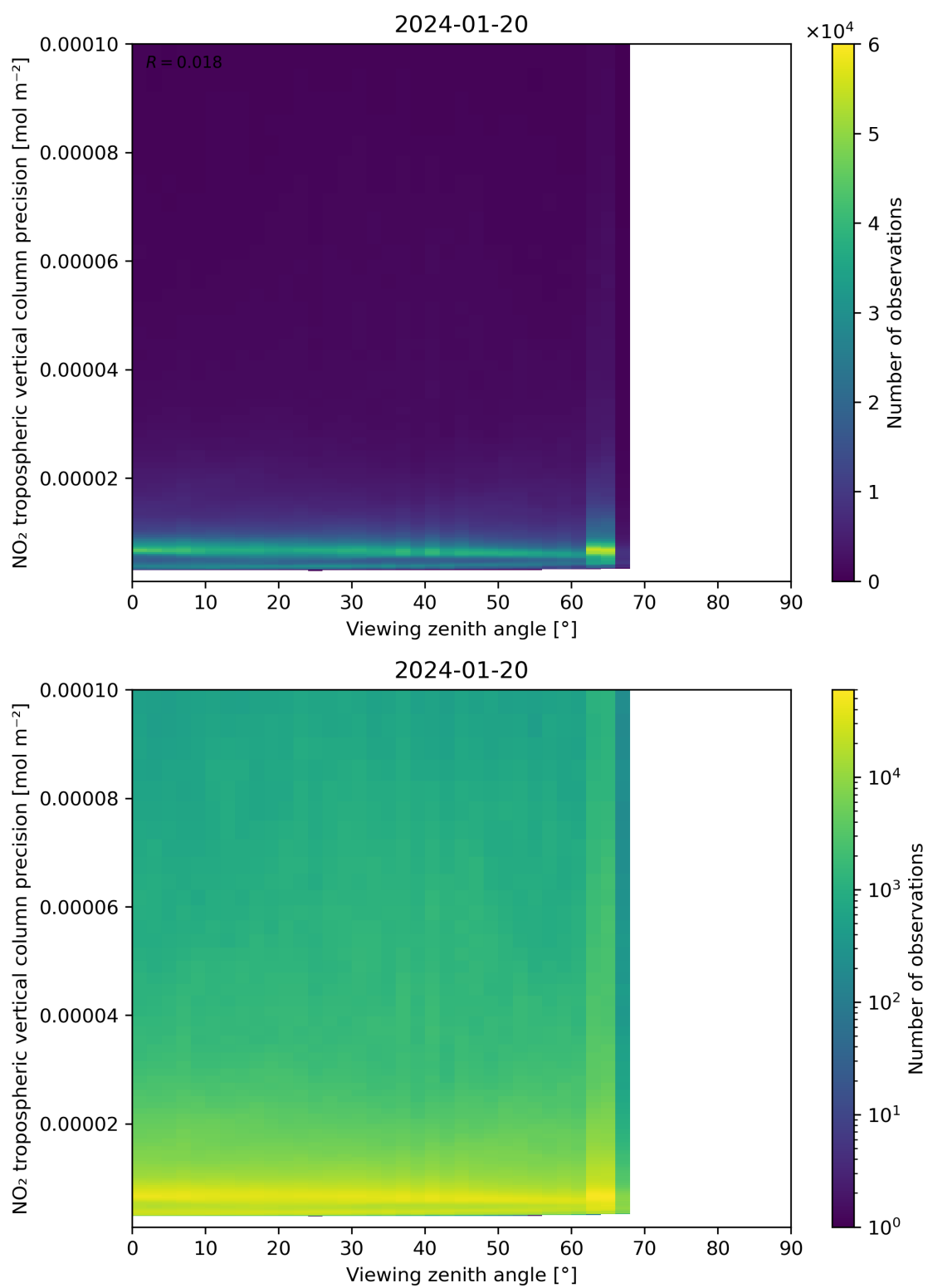
Figure 170: Scatter density plot of “Viewing zenith angle” against “NO 2 tropospheric vertical column precision” for 2024-01-19 to 2024-01-21.
