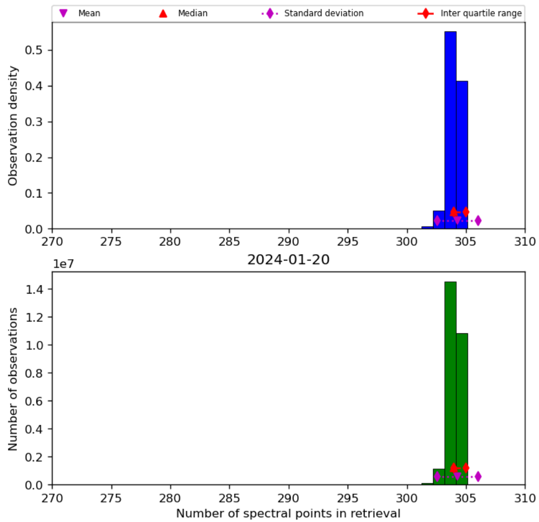
Figure 33: Histogram of “Number of spectral points in retrieval” for 2024-01-19 to 2024-01-21
