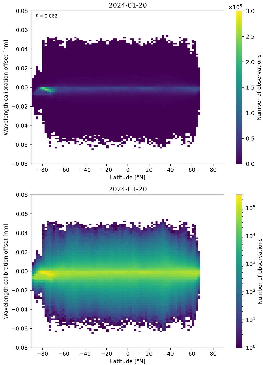
Figure 95: Scatter density plot of “Latitude” against “Wavelength calibration offset” for 2024-01-19 to 2024-01-21.
