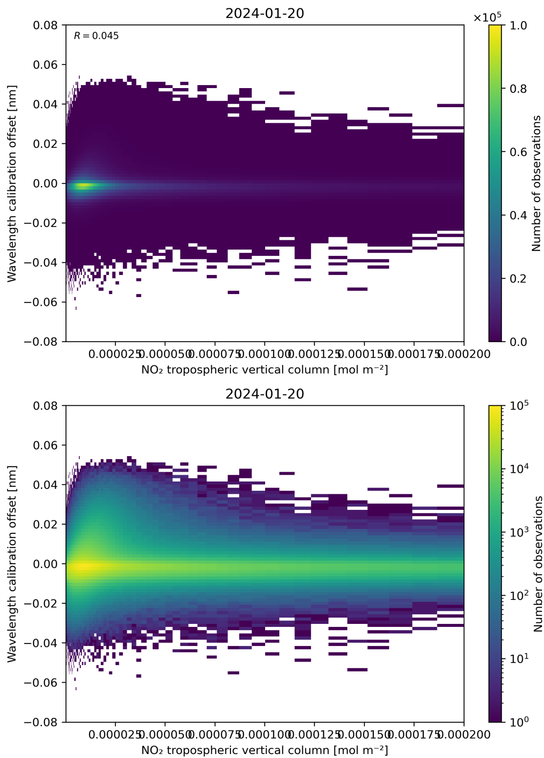
Figure 143: Scatter density plot of “NO 2 tropospheric vertical column” against “Wavelength calibration offset” for 2024-01-19 to 2024-01-21.
