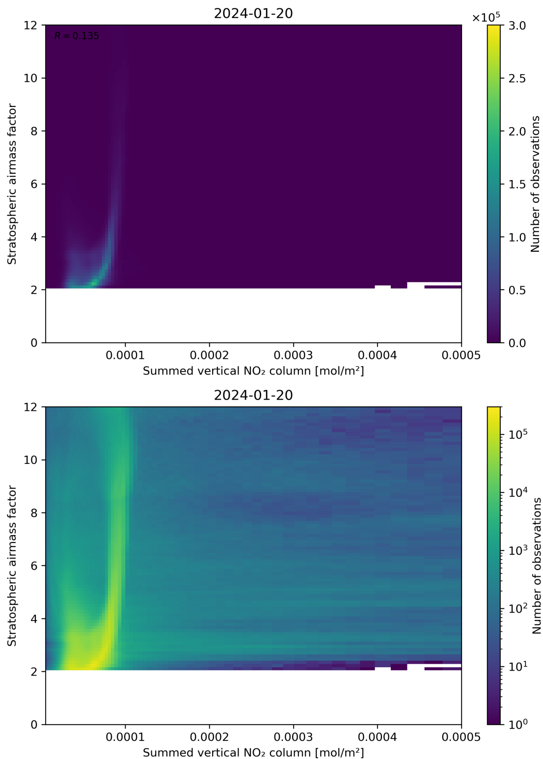
Figure 103: Scatter density plot of “Summed vertical NO 2 column” against “Stratospheric airmass factor” for 2024-01-19 to 2024-01-21.
