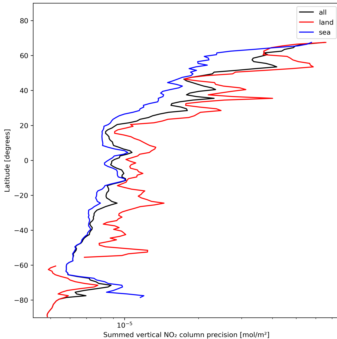
Figure 24: Zonal average of “Summed vertical NO 2 column precision” for 2024-01-19 to 2024-01-21.
