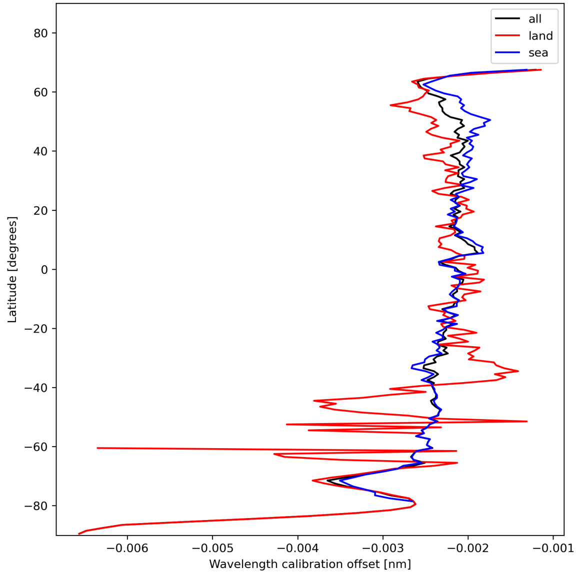
Figure 18: Zonal average of “Wavelength calibration offset” for 2024-01-19 to 2024-01-21.
