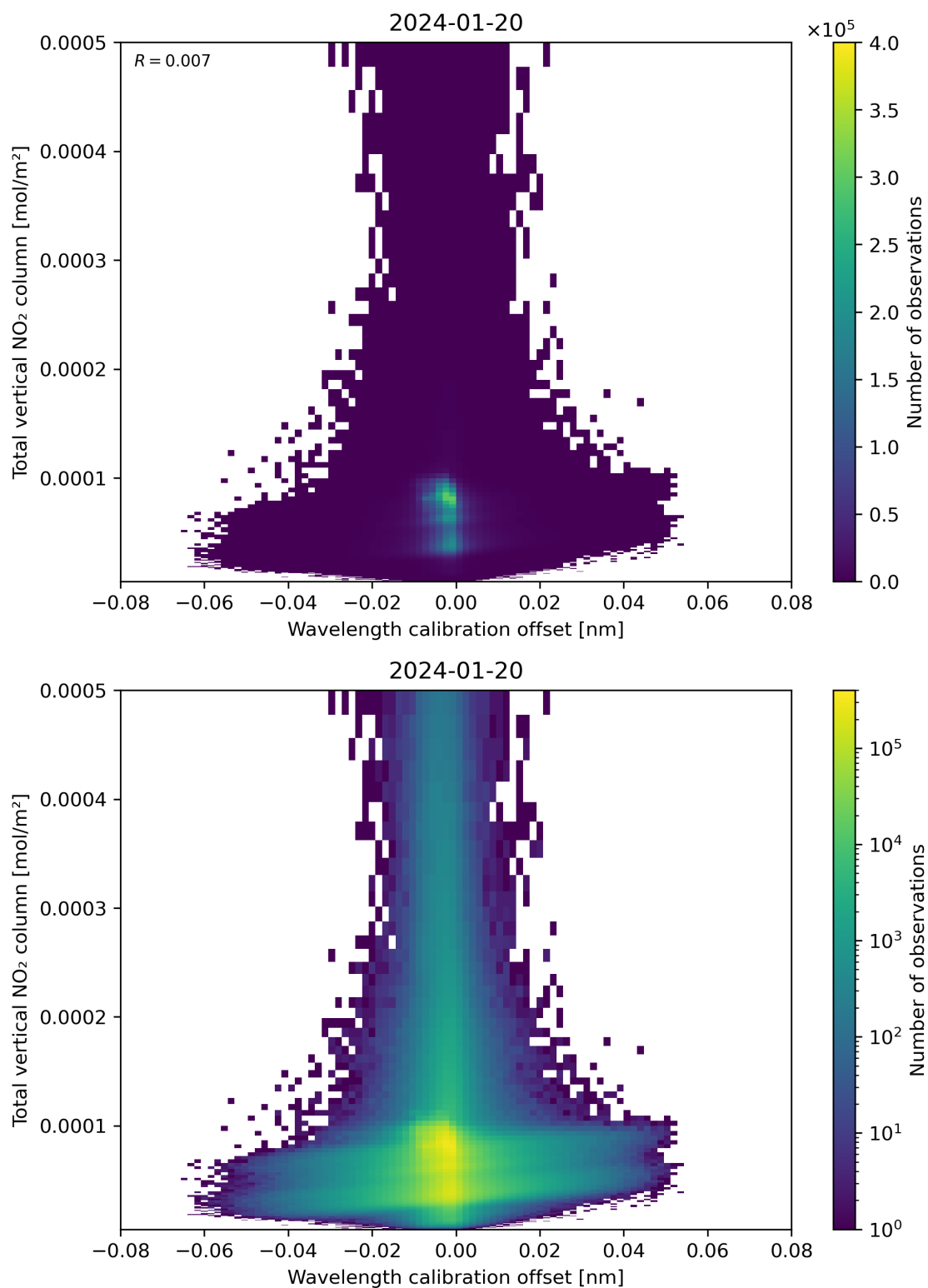
Figure 179: Scatter density plot of “Wavelength calibration offset” against “Total vertical NO 2 column” for 2024-01-19 to 2024-01-21.
