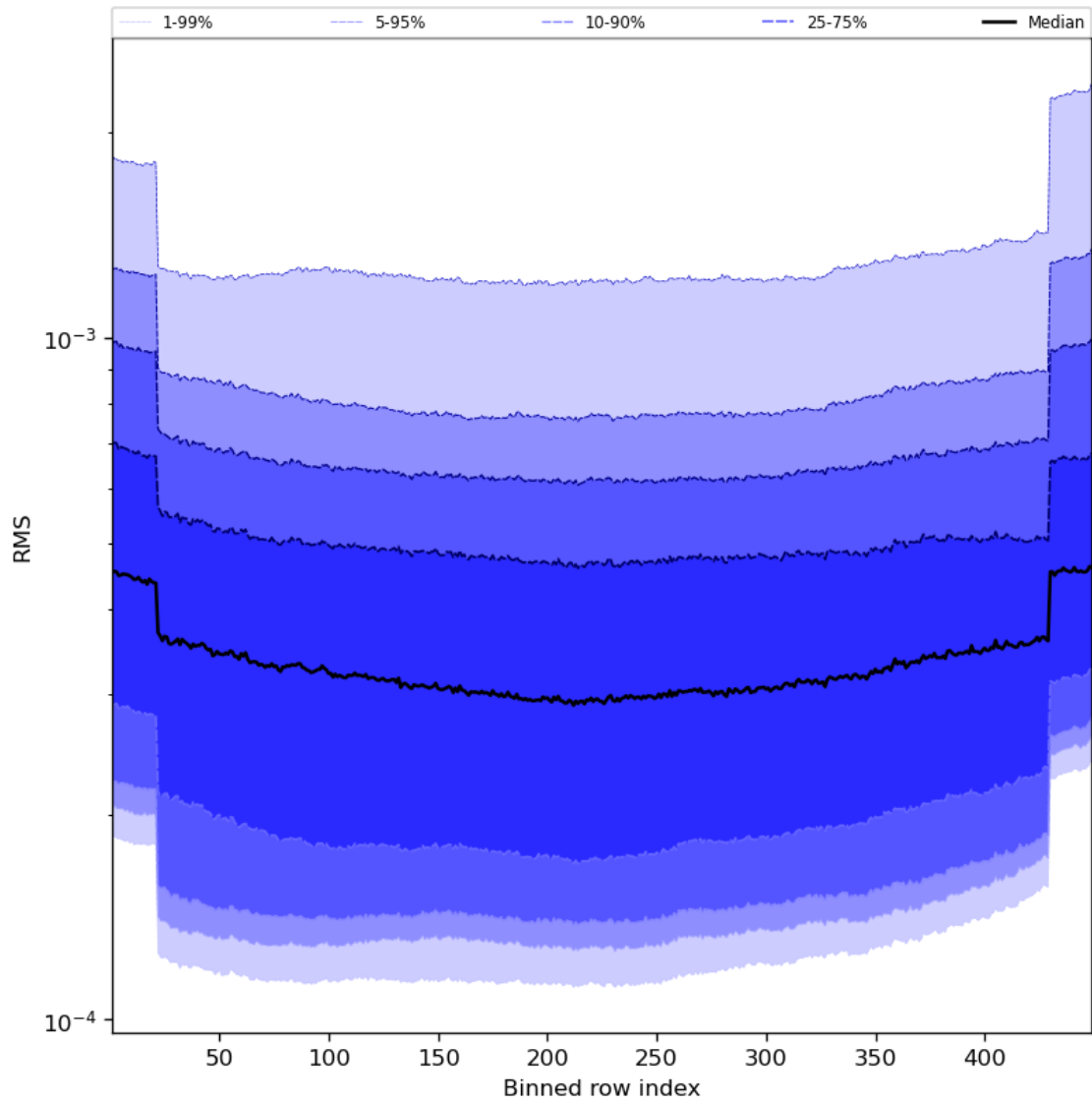
Figure 60: Along track statistics of “RMS” for 2024-01-19 to 2024-01-21
