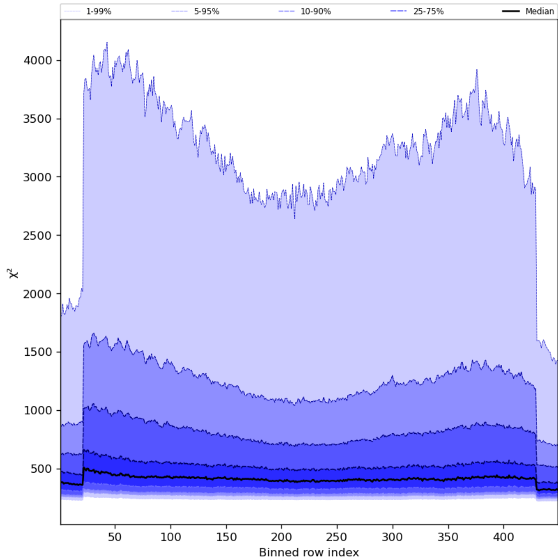
Figure 59: Along track statistics of “ \chi^2 ” for 2024-01-19 to 2024-01-21
