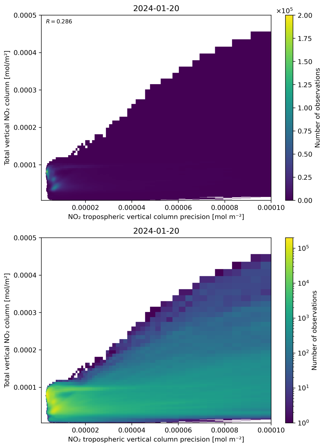
Figure 138: Scatter density plot of “NO 2 tropospheric vertical column precision” against “Total vertical NO 2 column” for 2024-01-19 to 2024-01-21.
