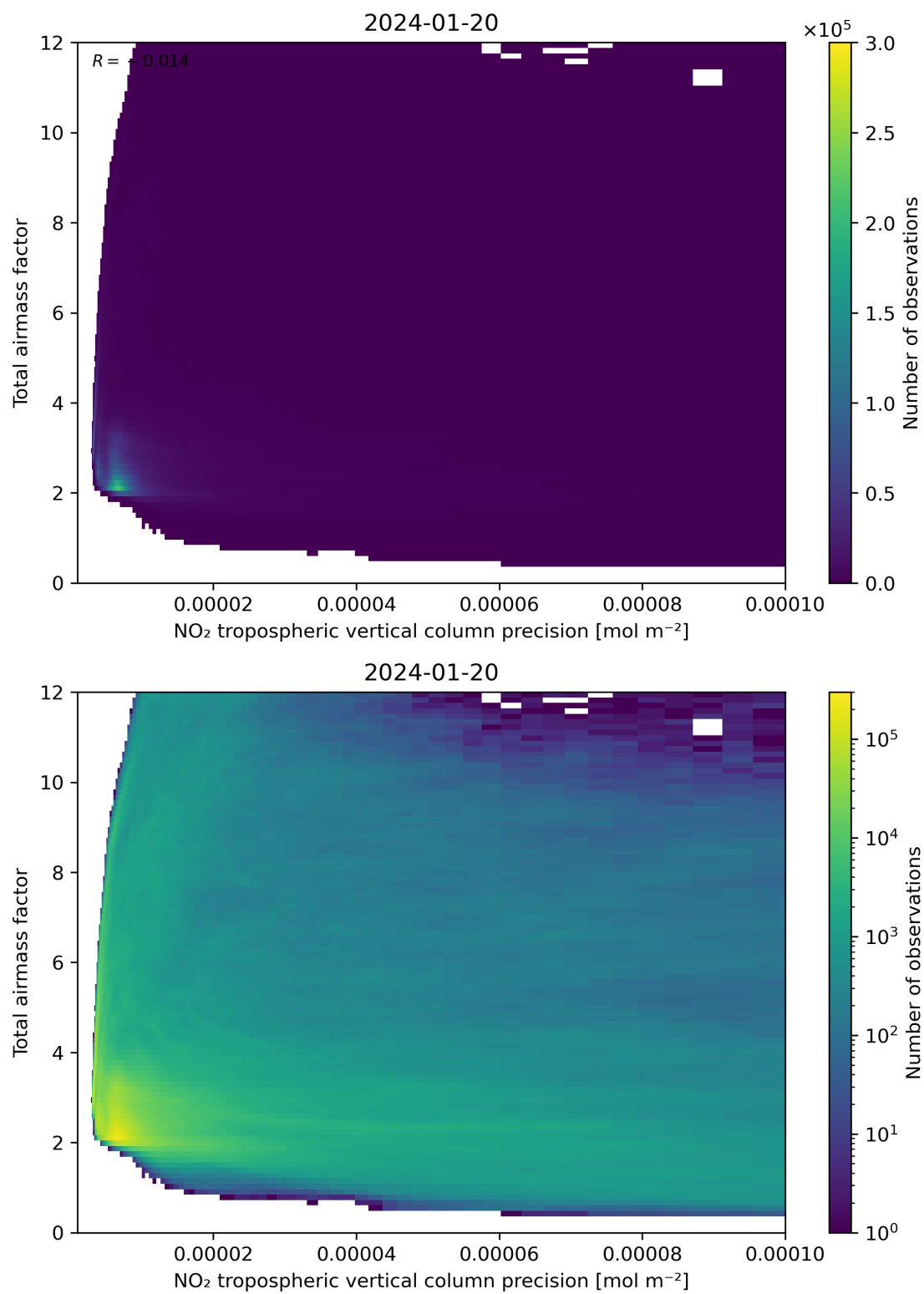
Figure 132: Scatter density plot of “NO 2 tropospheric vertical column precision” against “Total air mass factor” for 2024-01-19 to 2024-01-21.
