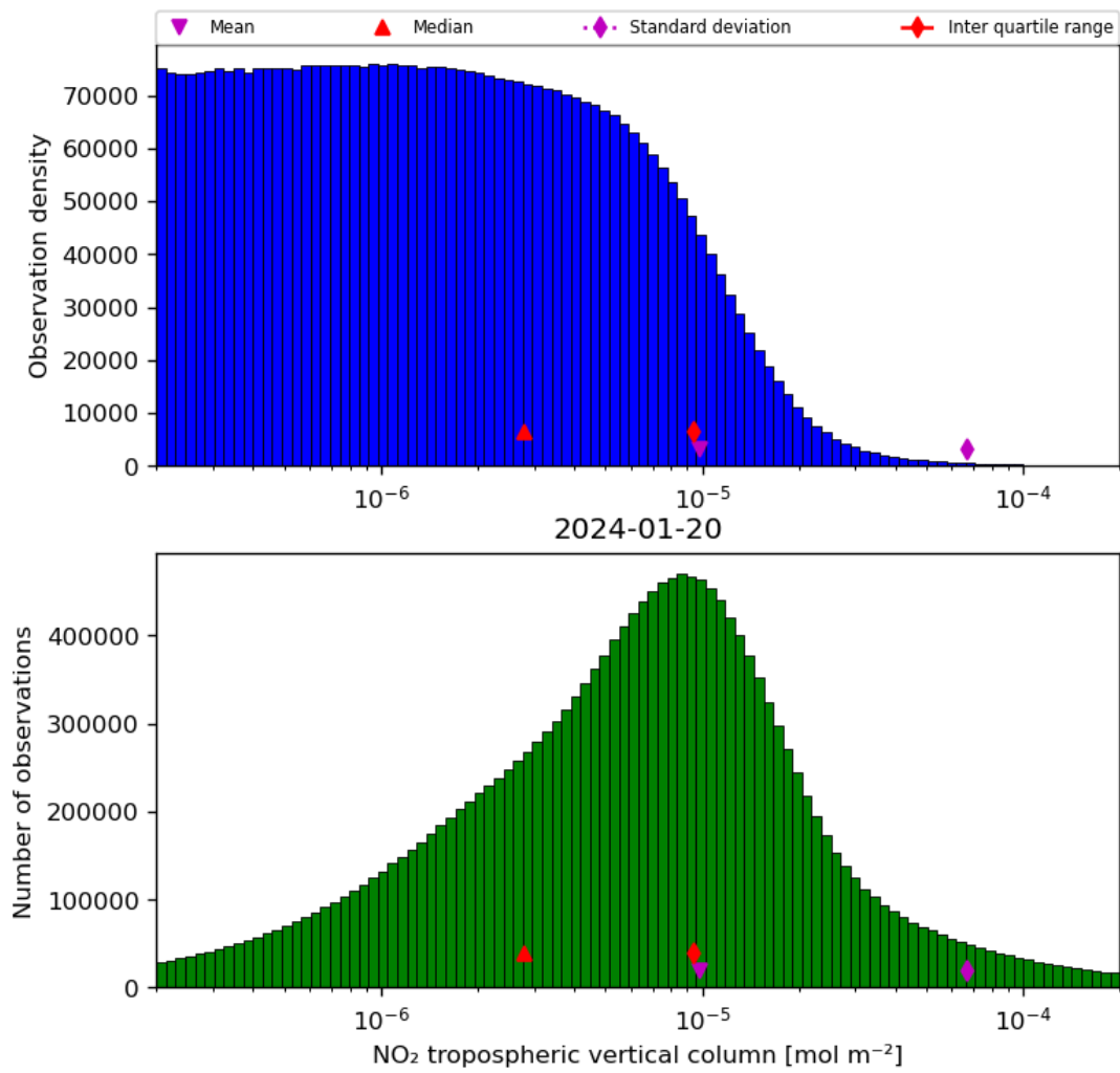
Figure 29: Histogram of “NO 2 tropospheric vertical column” for 2024-01-19 to 2024-01-21
