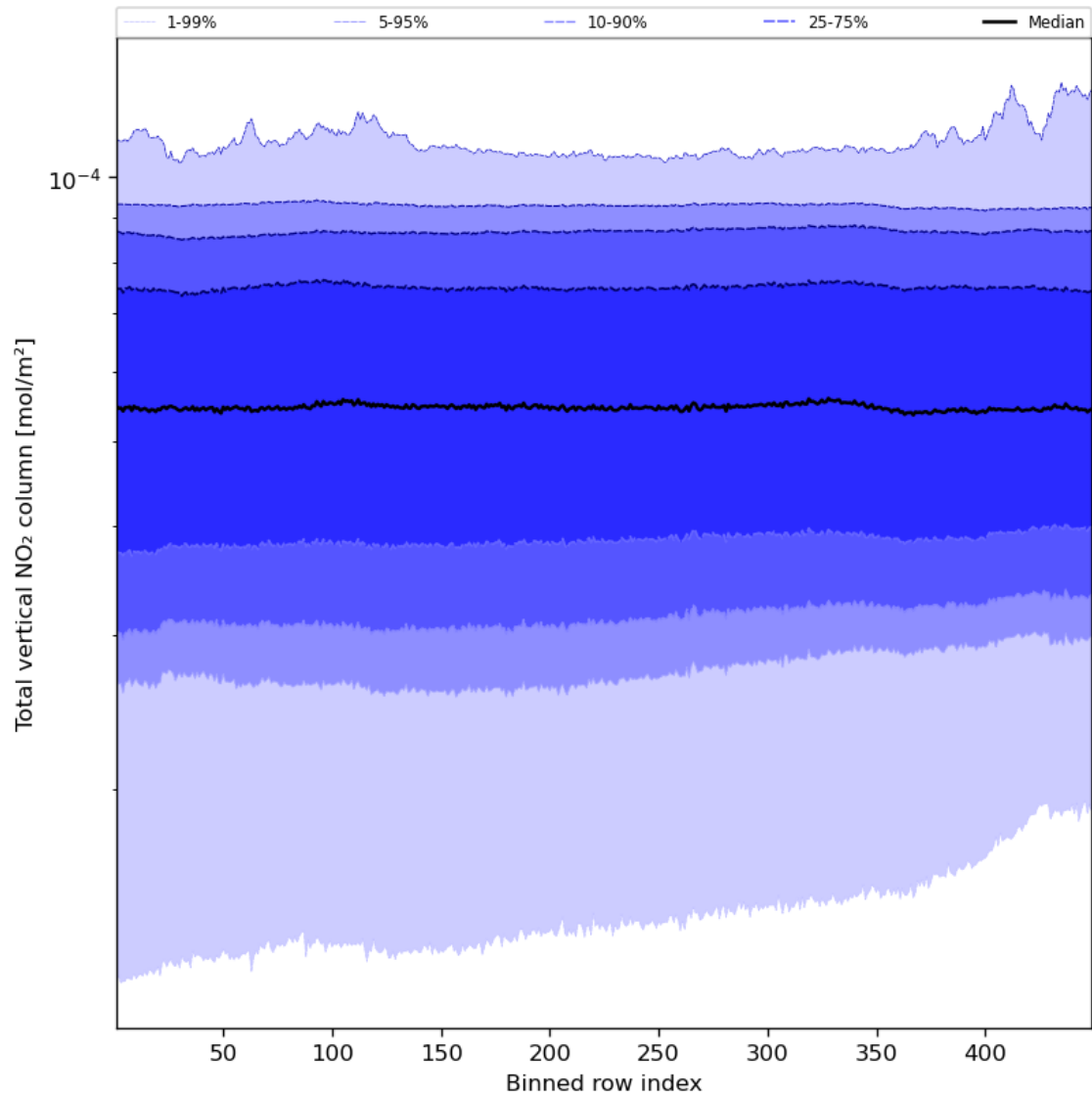
Figure 55: Along track statistics of “Total vertical NO 2 column” for 2024-01-19 to 2024-01-21
