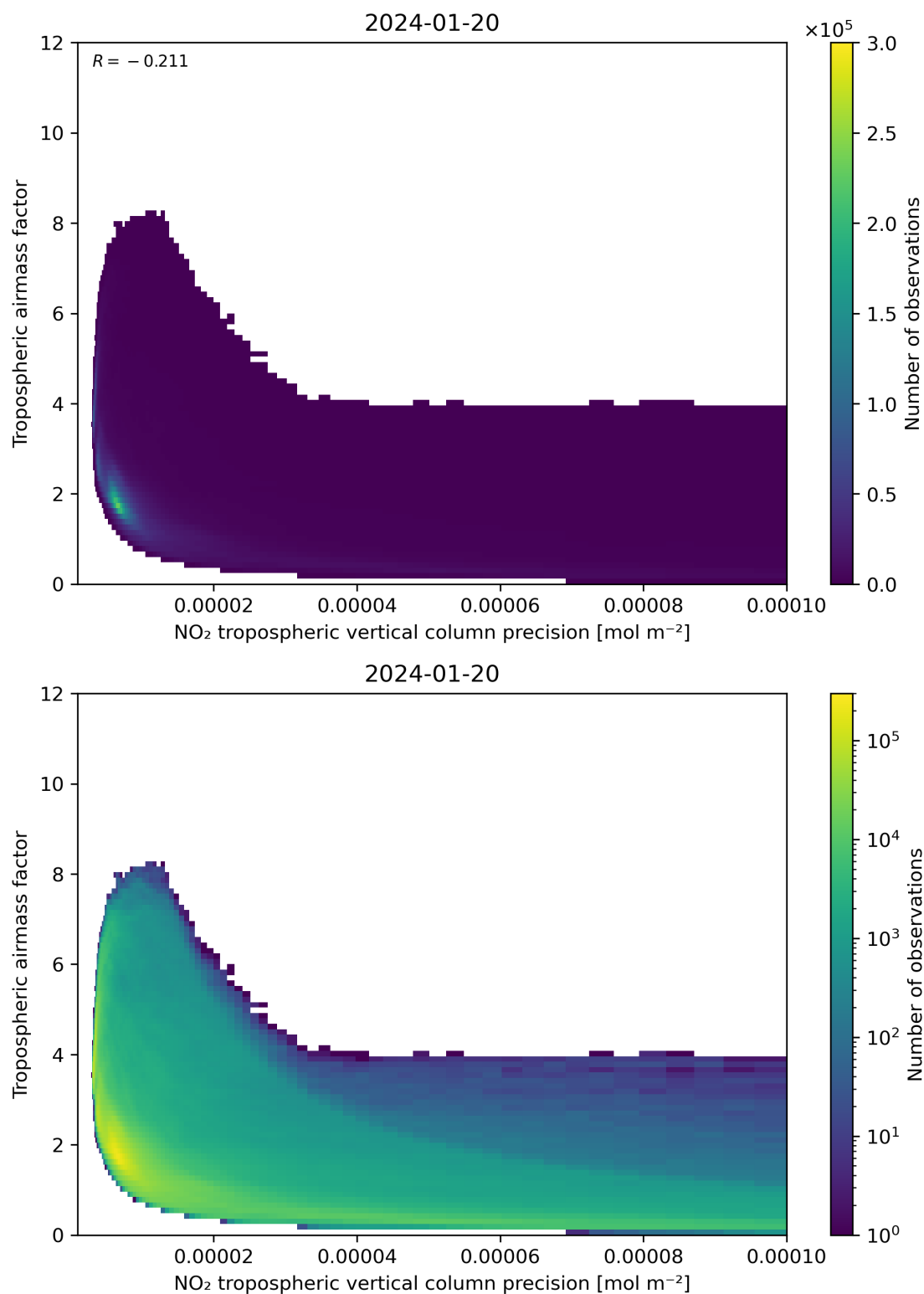
Figure 133: Scatter density plot of “NO 2 tropospheric vertical column precision” against “Tropospheric airmass factor” for 2024-01-19 to 2024-01-21.
