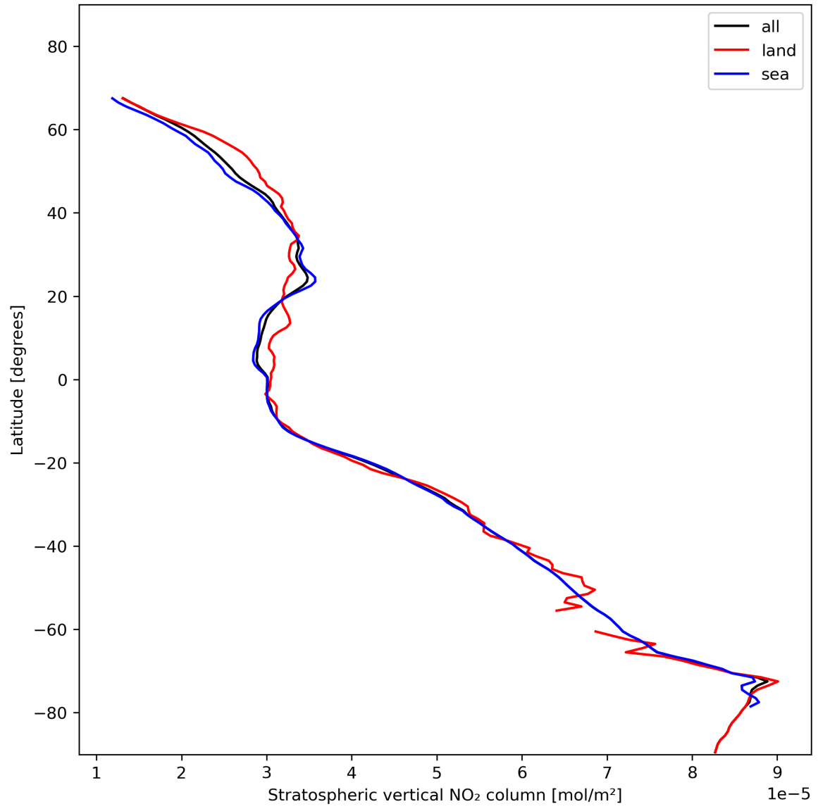
Figure 19: Zonal average of “Stratospheric vertical NO 2 column” for 2024-01-19 to 2024-01-21.
