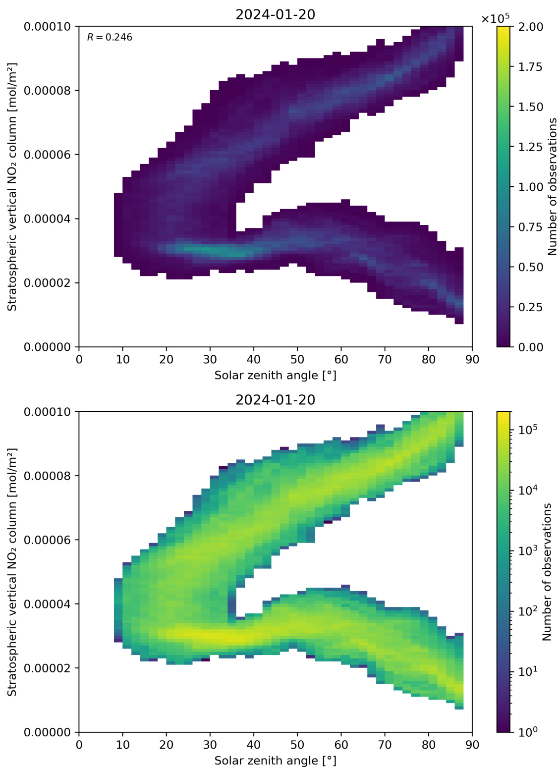
Figure 150: Scatter density plot of “Solar zenith angle” against “Stratospheric vertical NO 2 column” for 2024-01-19 to 2024-01-21.
