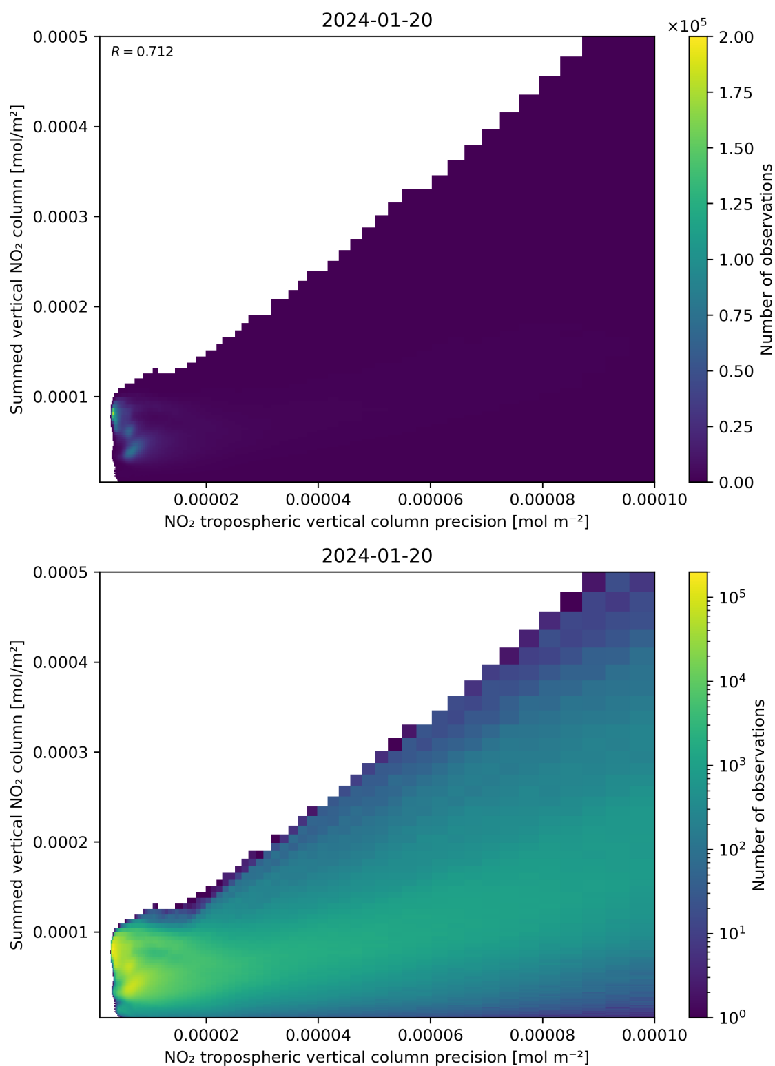
Figure 136: Scatter density plot of “NO 2 tropospheric vertical column precision” against “Summed vertical NO 2 column” for 2024-01-19 to 2024-01-21.
