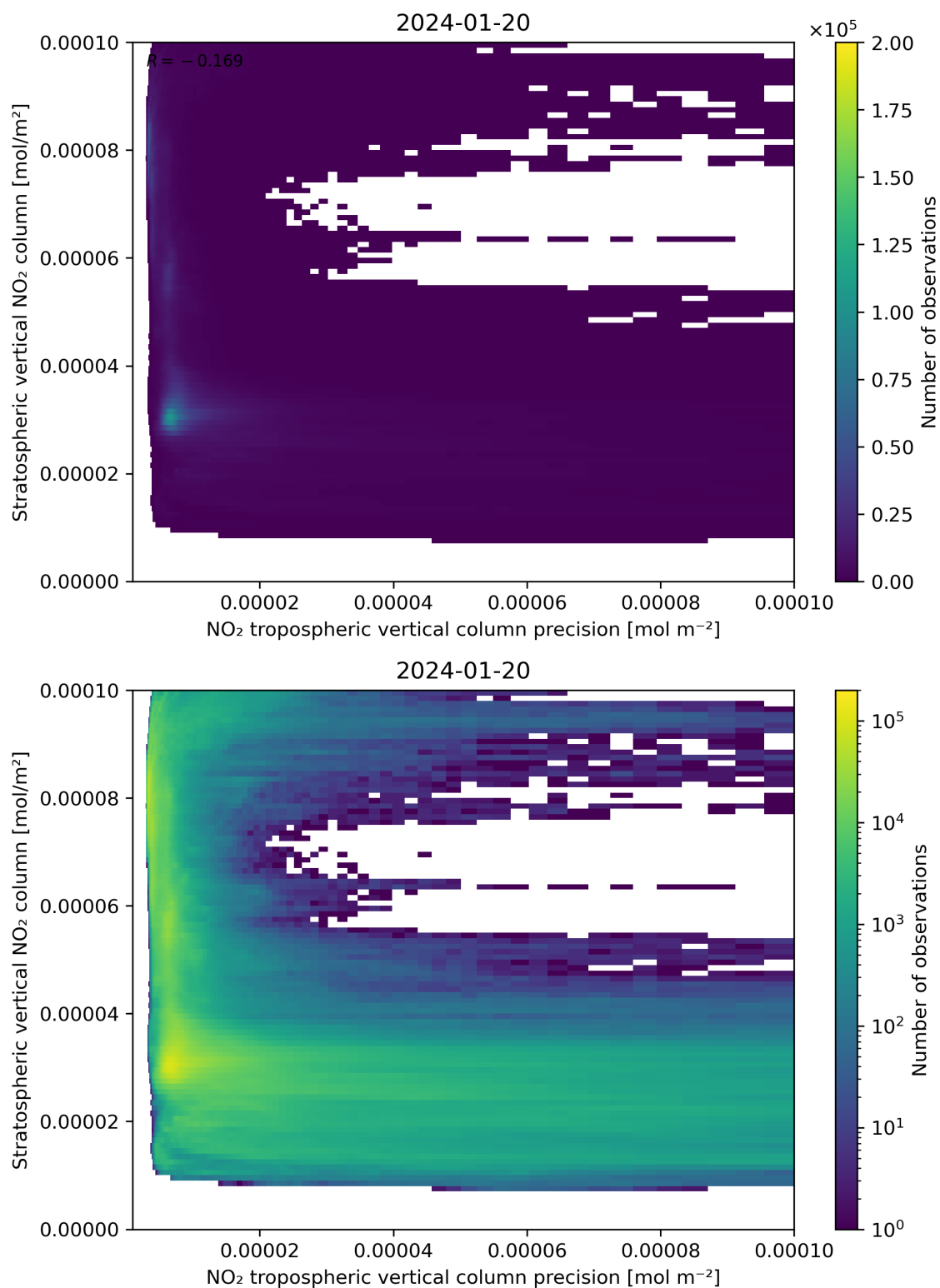
Figure 135: Scatter density plot of “NO 2 tropospheric vertical column precision” against “Stratospheric vertical NO 2 column” for 2024-01-19 to 2024-01-21.
