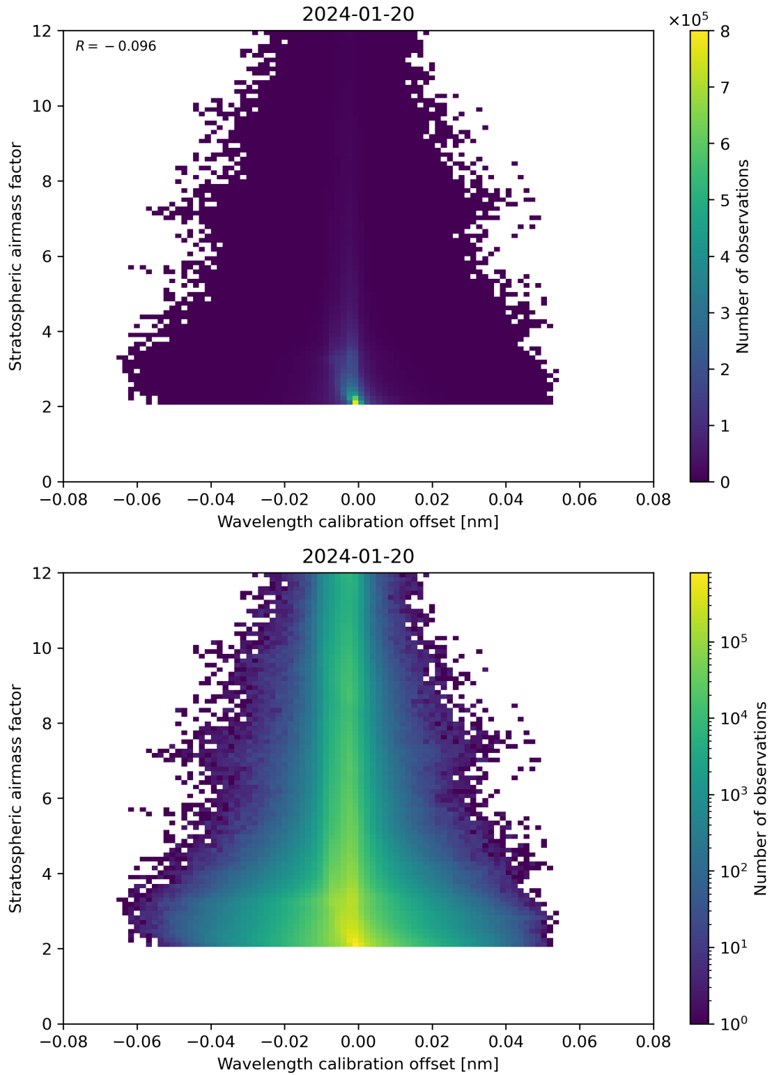
Figure 174: Scatter density plot of “Wavelength calibration offset” against “Stratospheric airmass factor” for 2024-01-19 to 2024-01-21.
