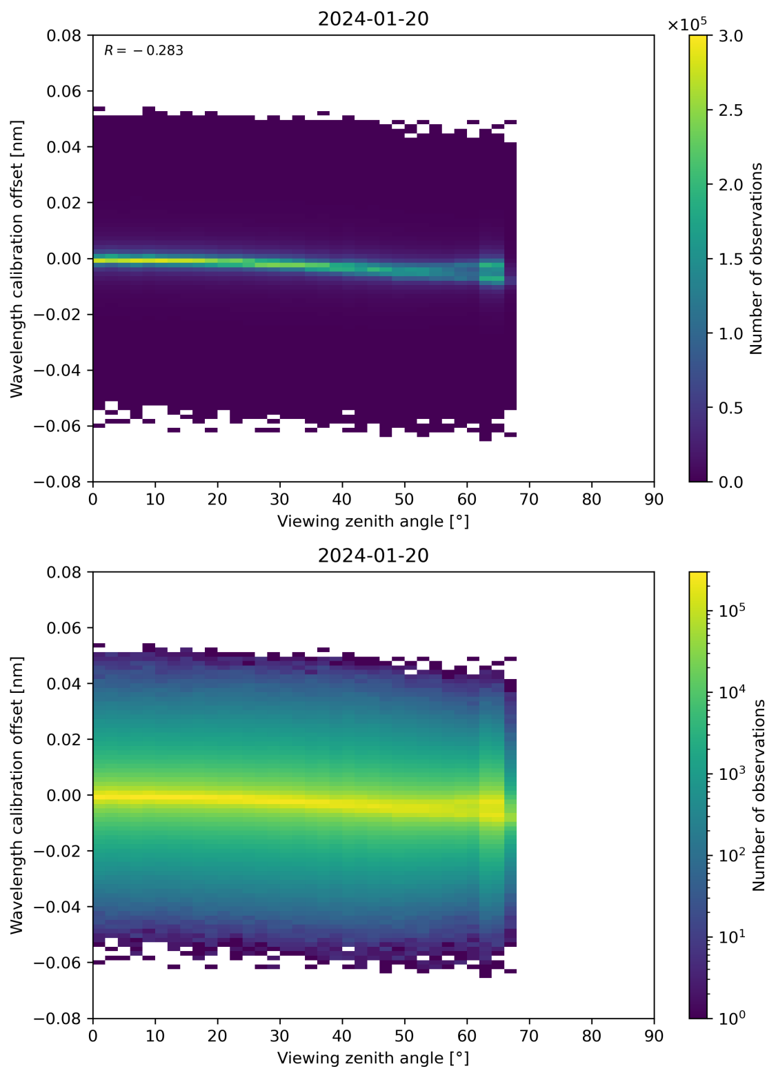
Figure 173: Scatter density plot of “Viewing zenith angle” against “Wavelength calibration offset” for 2024-01-19 to 2024-01-21.
