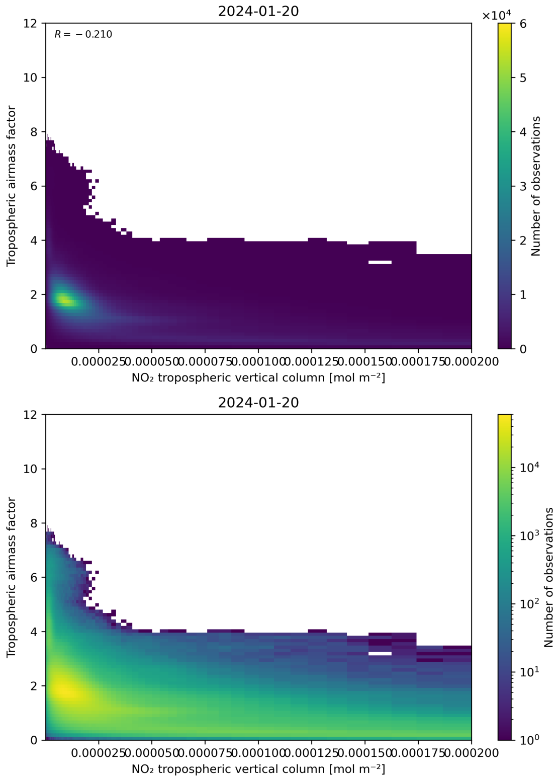
Figure 123: Scatter density plot of “NO 2 tropospheric vertical column” against “Tropospheric air mass factor” for 2024-01-19 to 2024-01-21.
