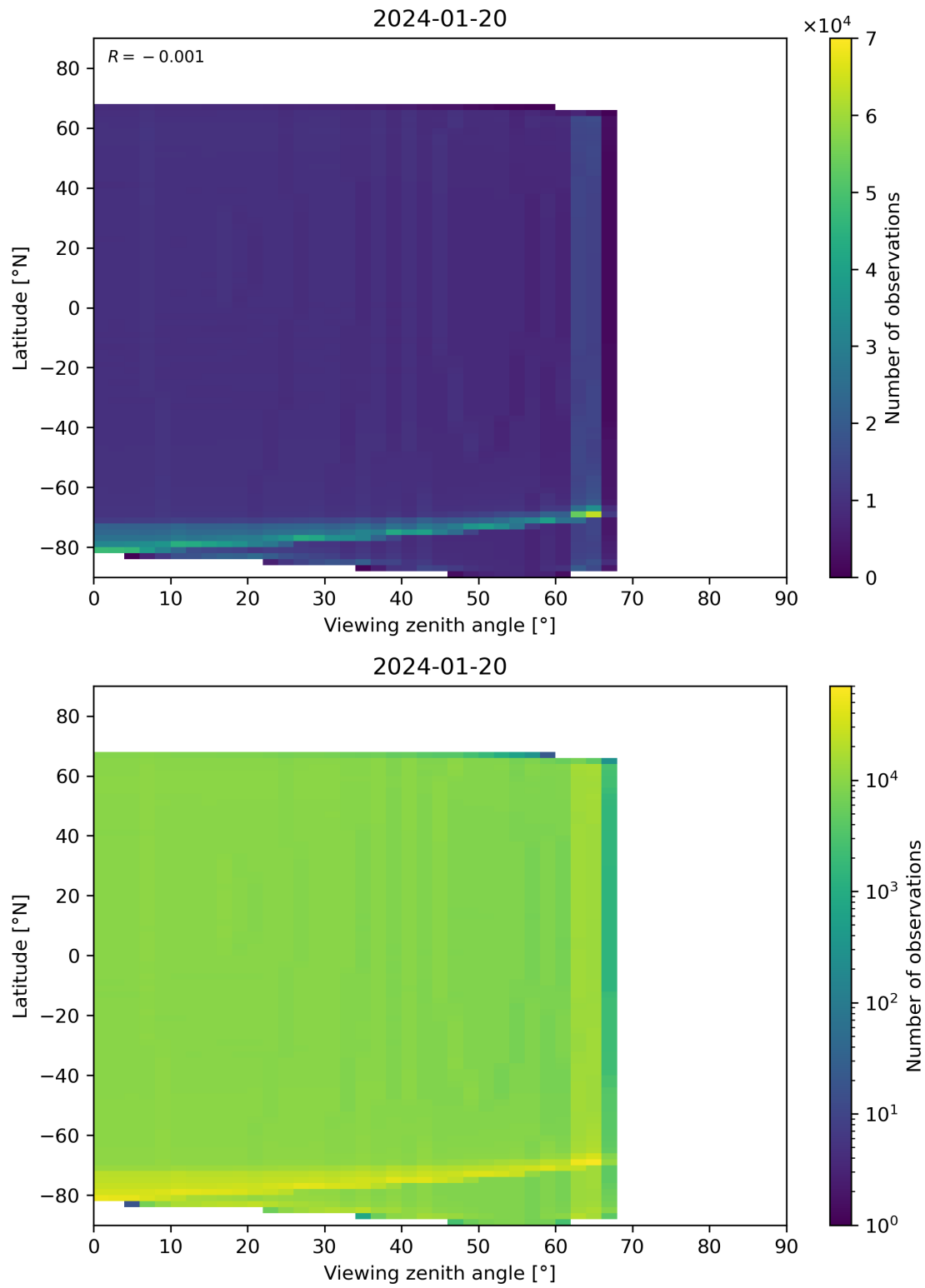
Figure 163: Scatter density plot of “Viewing zenith angle” against “Latitude” for 2024-01-19 to 2024-01-21.
