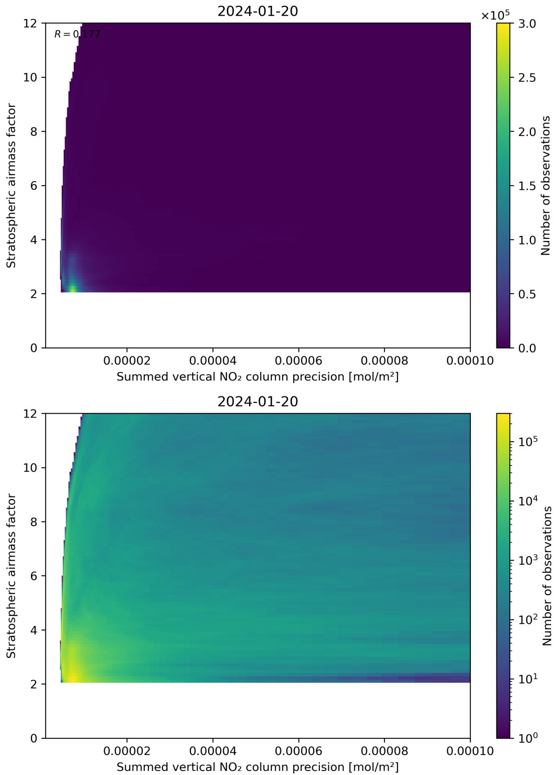
Figure 106: Scatter density plot of “Summed vertical NO 2 column precision” against “Stratospheric airmass factor” for 2024-01-19 to 2024-01-21.
