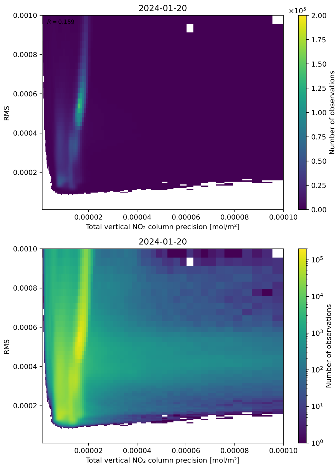
Figure 119: Scatter density plot of “Total vertical NO 2 column precision” against “RMS” for 2024-01-19 to 2024-01-21.
