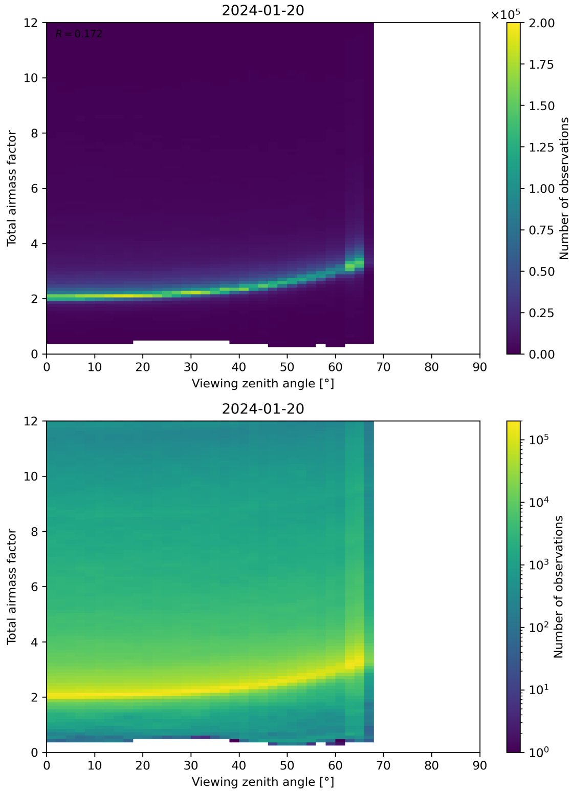
Figure 160: Scatter density plot of “Viewing zenith angle” against “Total airmass factor” for 2024-01-19 to 2024-01-21.
