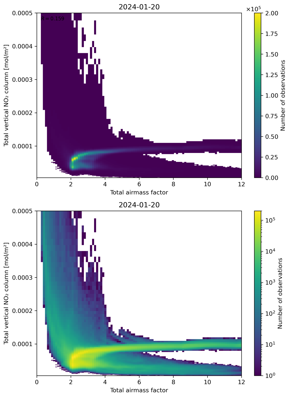
Figure 67: Scatter density plot of “Total airmass factor” against “Total vertical NO 2 column” for 2024-01-19 to 2024-01-21.
