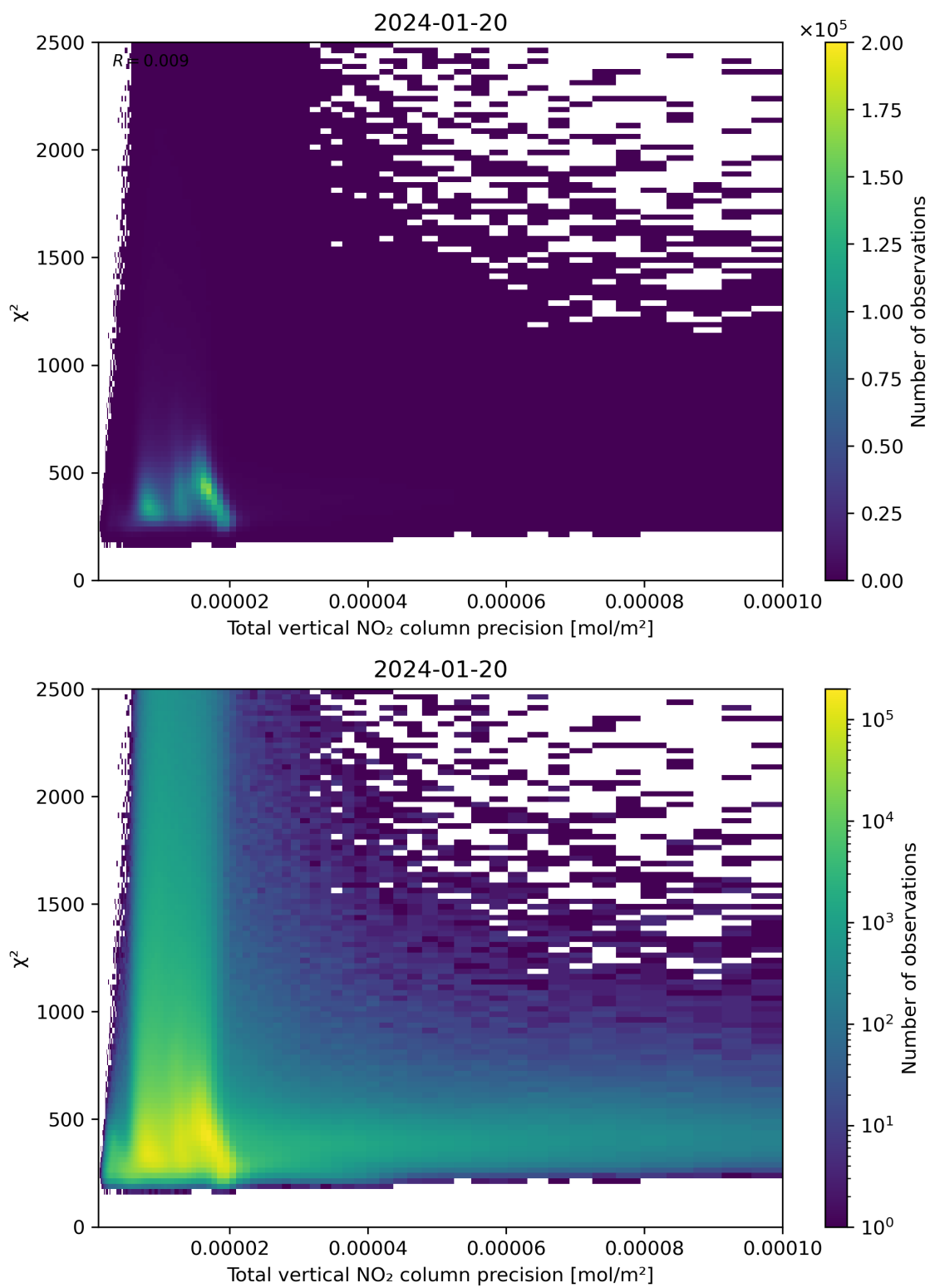
Figure 116: Scatter density plot of “Total vertical NO 2 column precision” against “ \chi^2 ” for 2024-01-19 to 2024-01-21.
