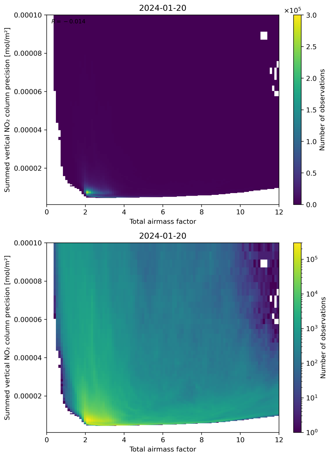
Figure 66: Scatter density plot of “Total airmass factor” against “Summed vertical NO 2 column precision” for 2024-01-19 to 2024-01-21.
