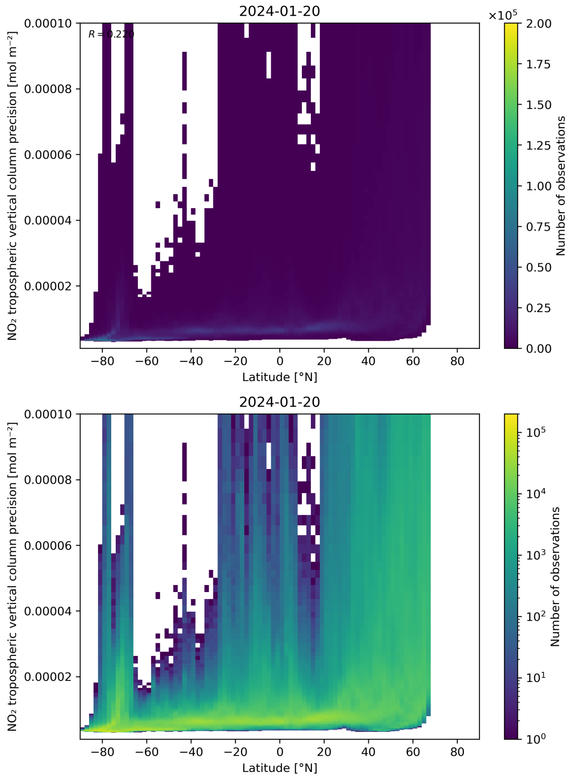
Figure 93: Scatter density plot of “Latitude” against “NO 2 tropospheric vertical column precision” for 2024-01-19 to 2024-01-21.
