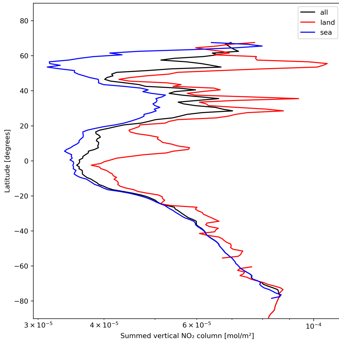
Figure 23: Zonal average of “Summed vertical NO 2 column” for 2024-01-19 to 2024-01-21.
