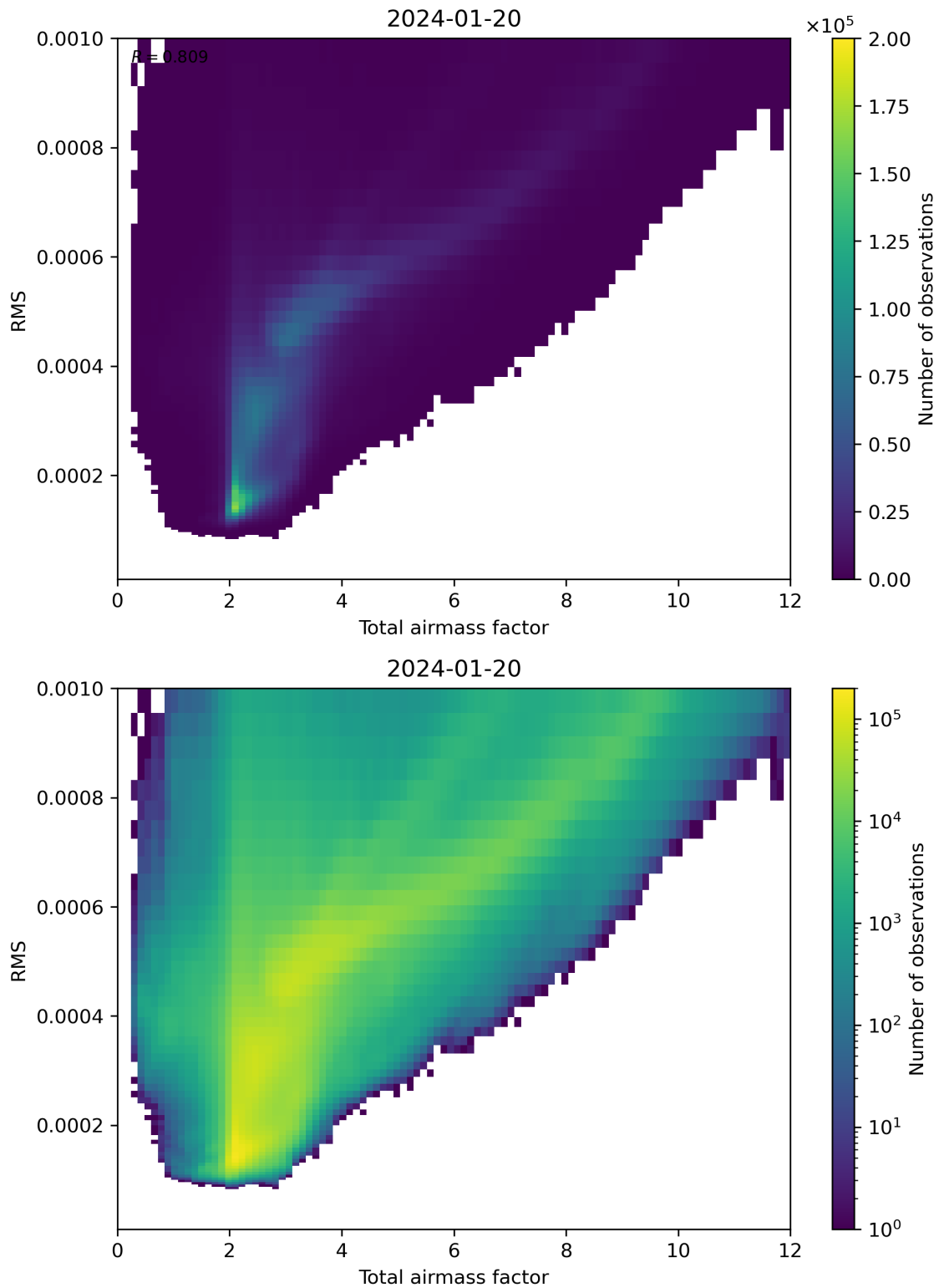
Figure 69: Scatter density plot of “Total airmass factor” against “RMS” for 2024-01-19 to 2024-01-21.
