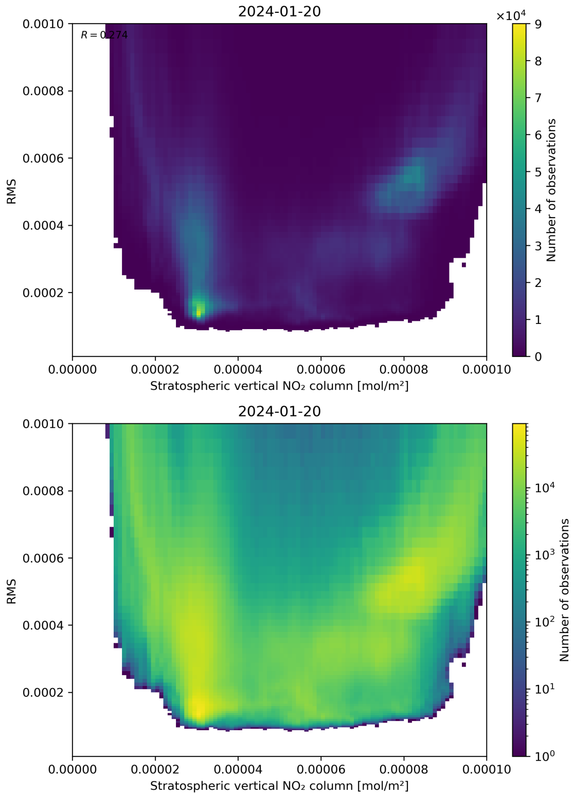
Figure 102: Scatter density plot of “Stratospheric vertical NO 2 column” against “RMS” for 2024-01-19 to 2024-01-21.
