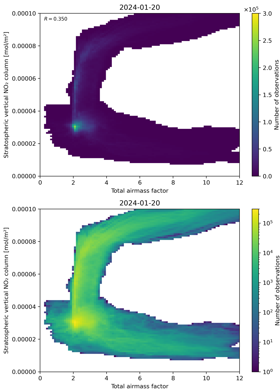
Figure 64: Scatter density plot of “Total airmass factor” against “Stratospheric vertical \text{NO}_2 column” for 2024-01-19 to 2024-01-21.
