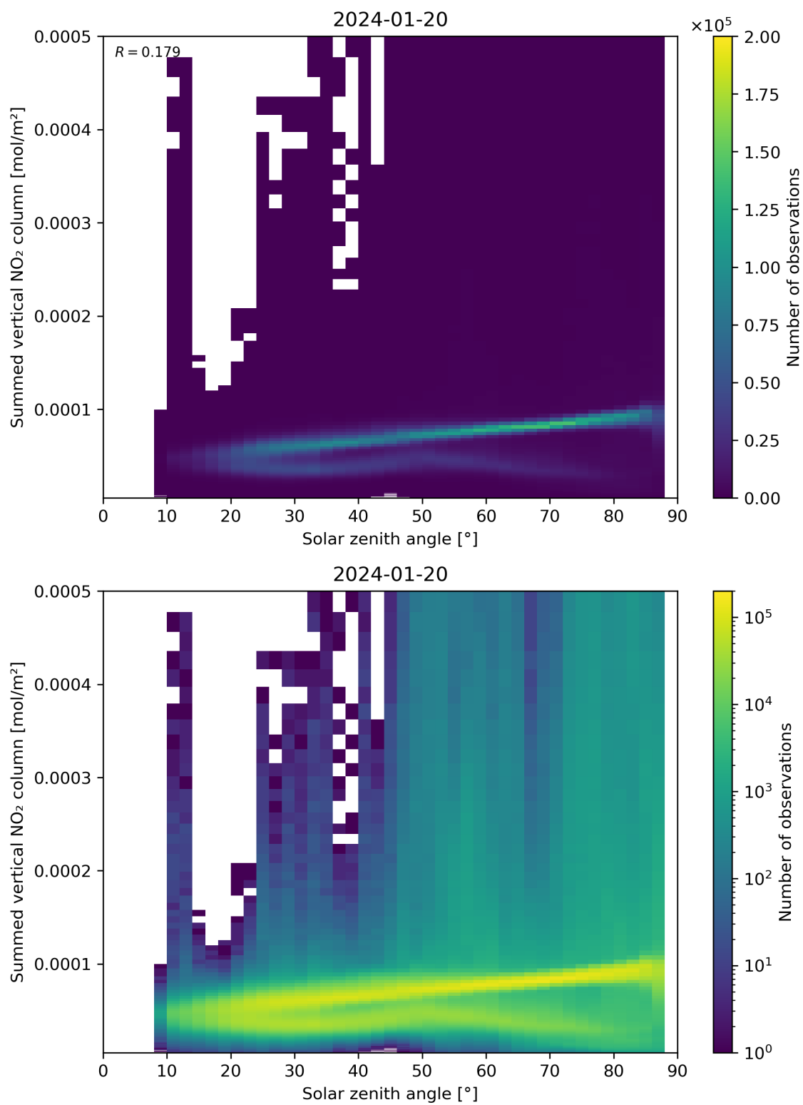
Figure 151: Scatter density plot of “Solar zenith angle” against “Summed vertical NO 2 column” for 2024-01-19 to 2024-01-21.
