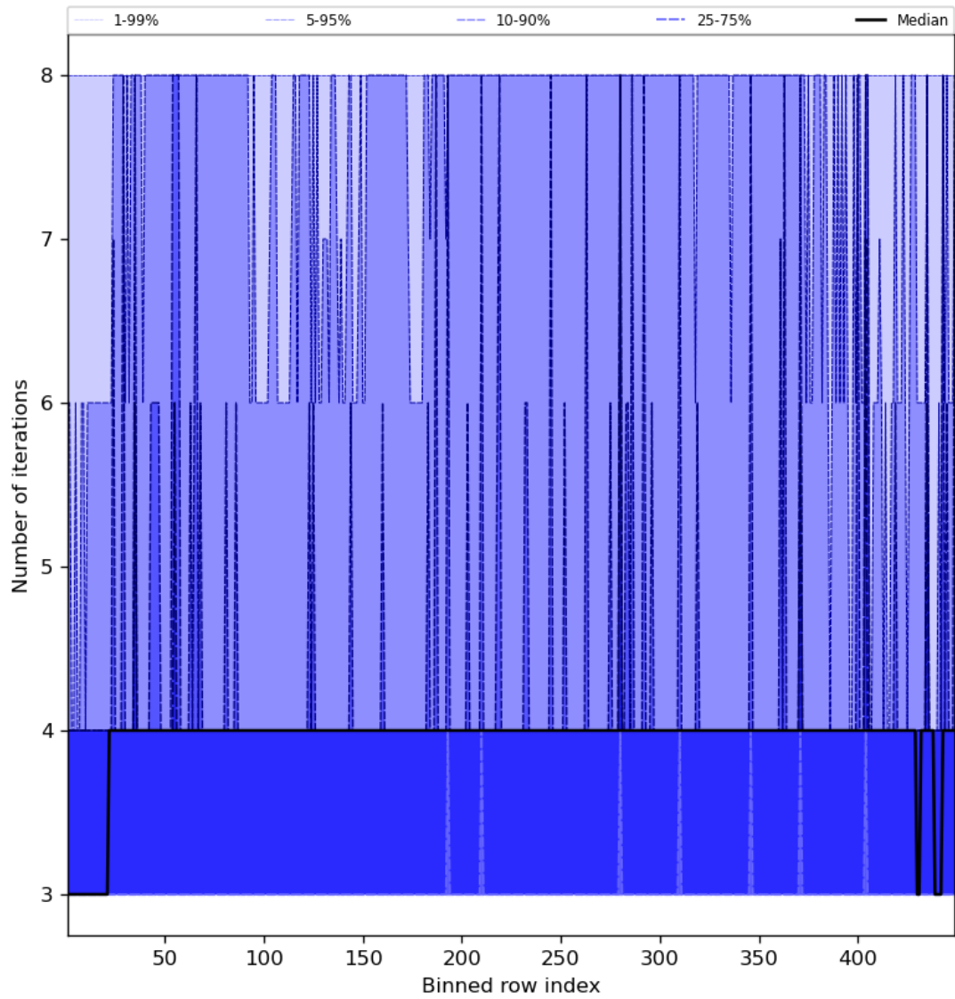
Figure 51: Along track statistics of “Number of iterations” for 2024-01-19 to 2024-01-21
