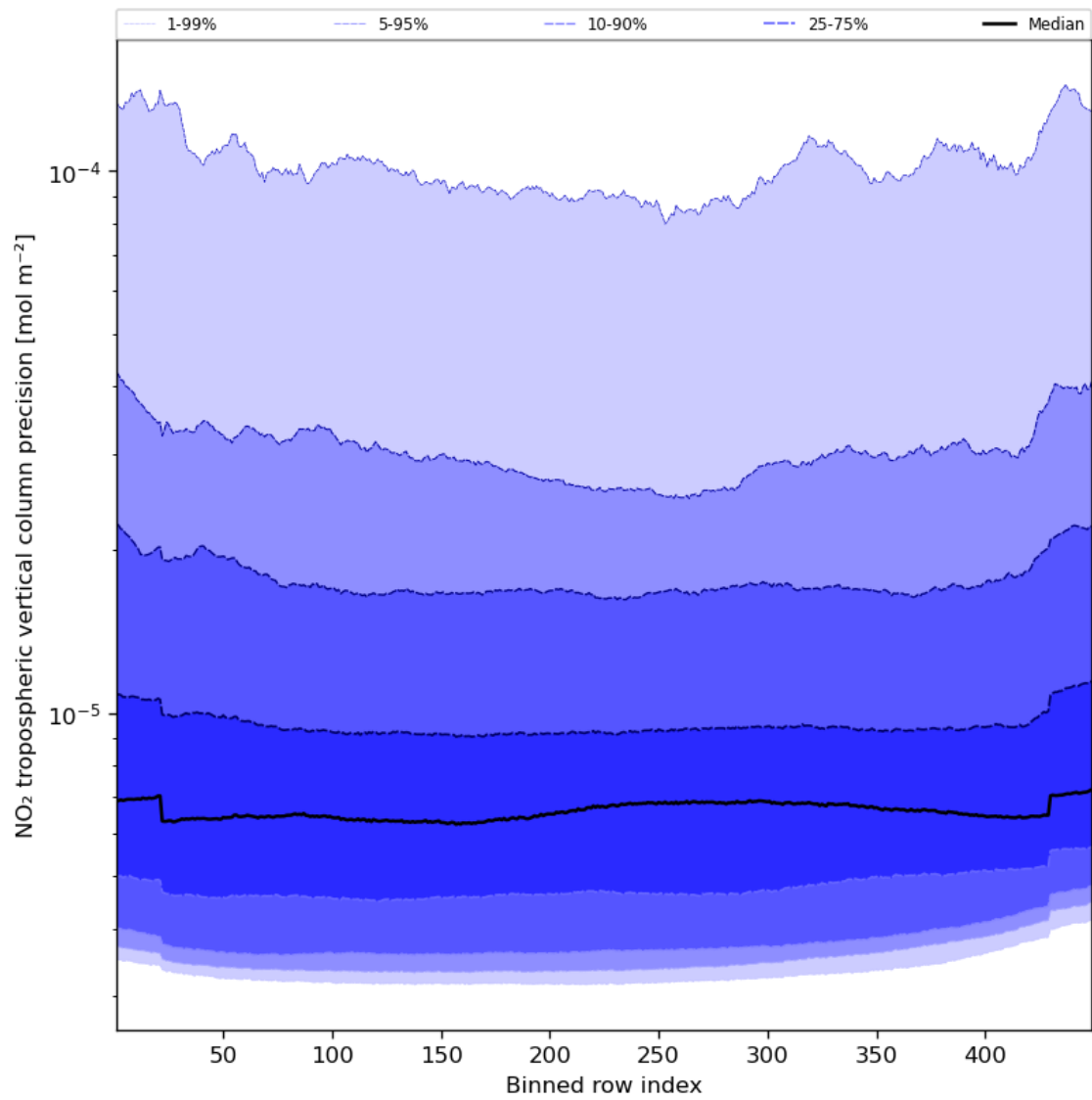
Figure 47: Along track statistics of “NO 2 tropospheric vertical column precision” for 2024-01-19 to 2024-01-21
