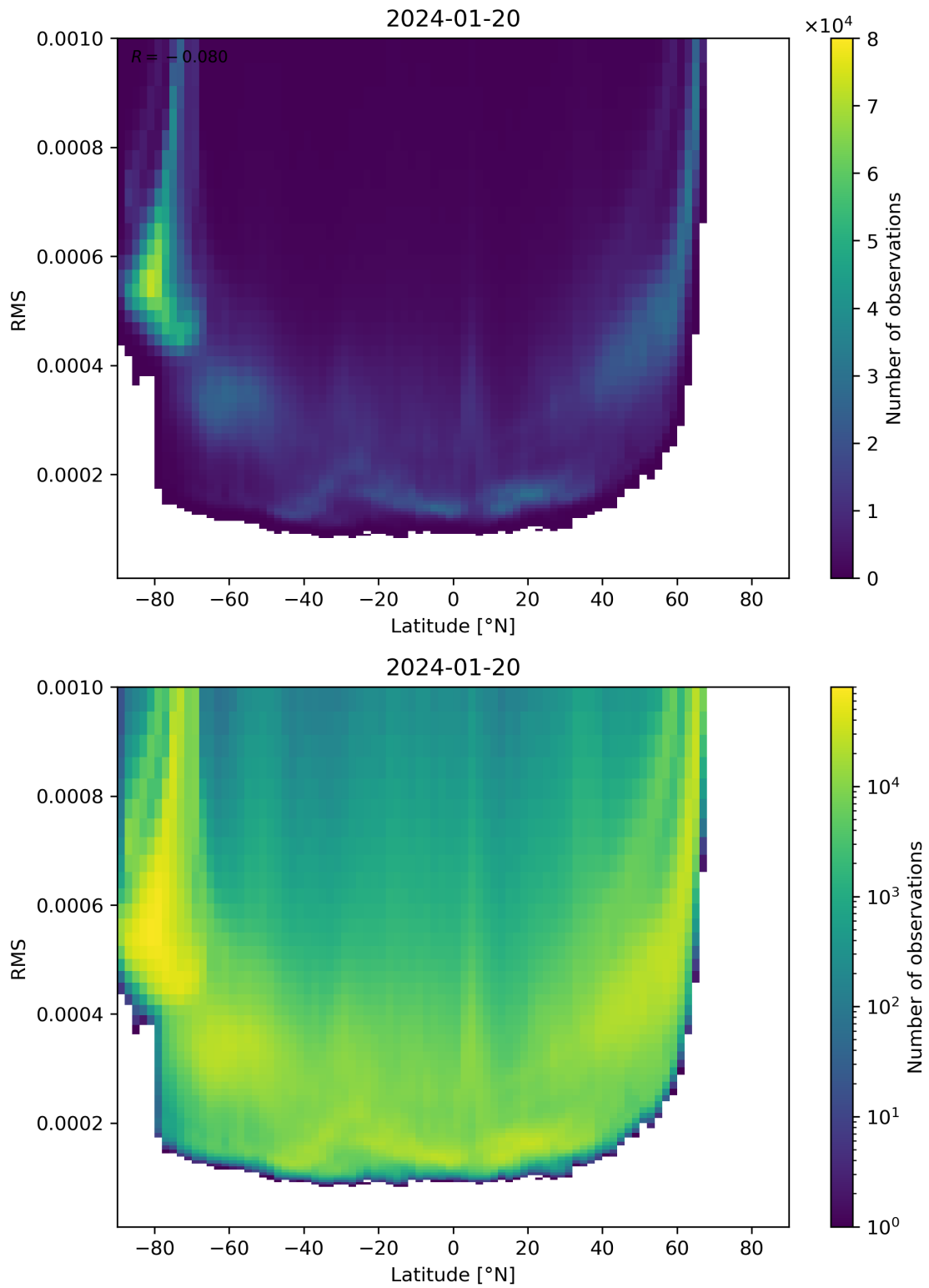
Figure 94: Scatter density plot of “Latitude” against “RMS” for 2024-01-19 to 2024-01-21.
