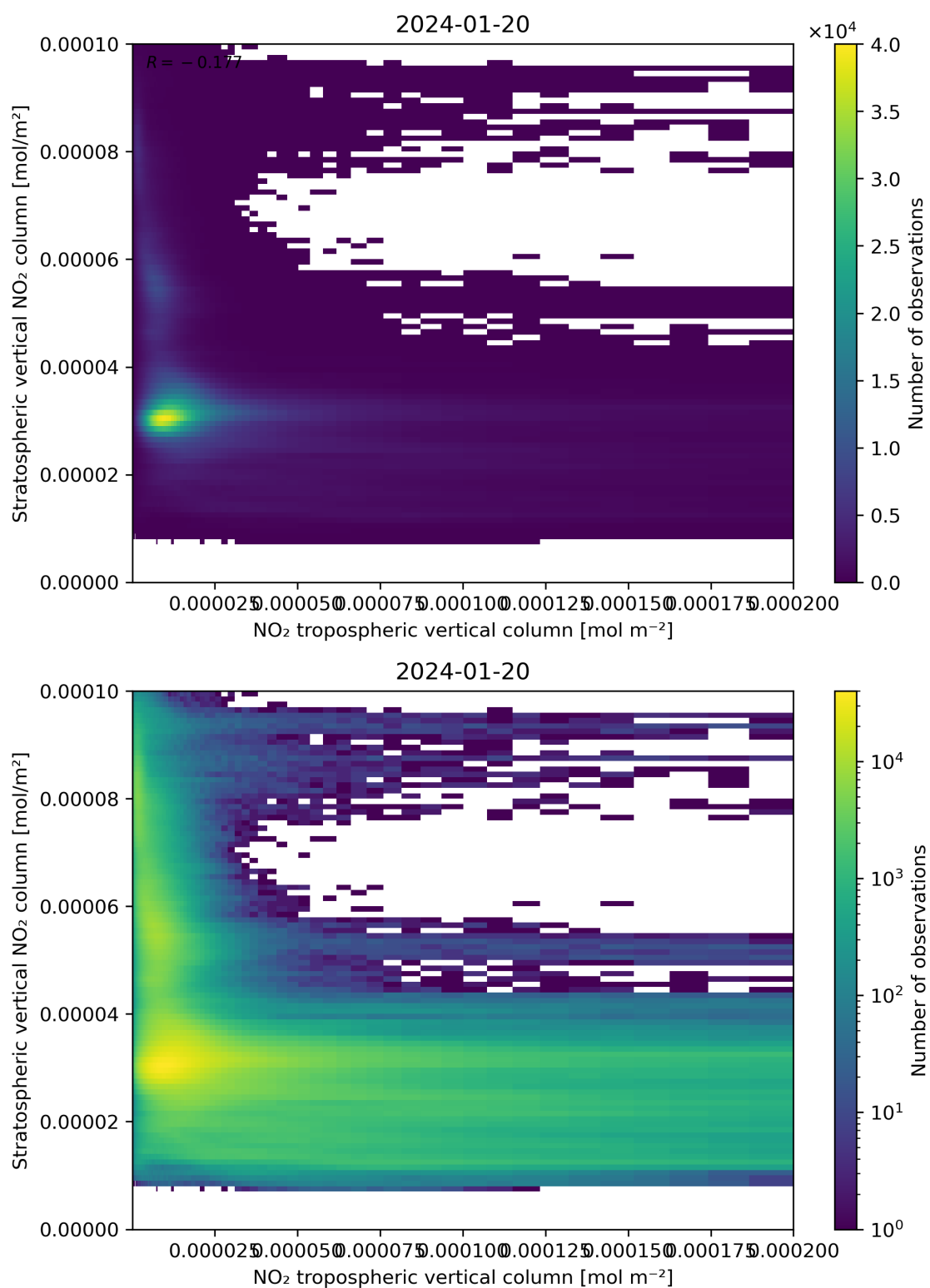
Figure 125: Scatter density plot of “NO 2 tropospheric vertical column” against “Stratospheric vertical NO 2 column” for 2024-01-19 to 2024-01-21.
