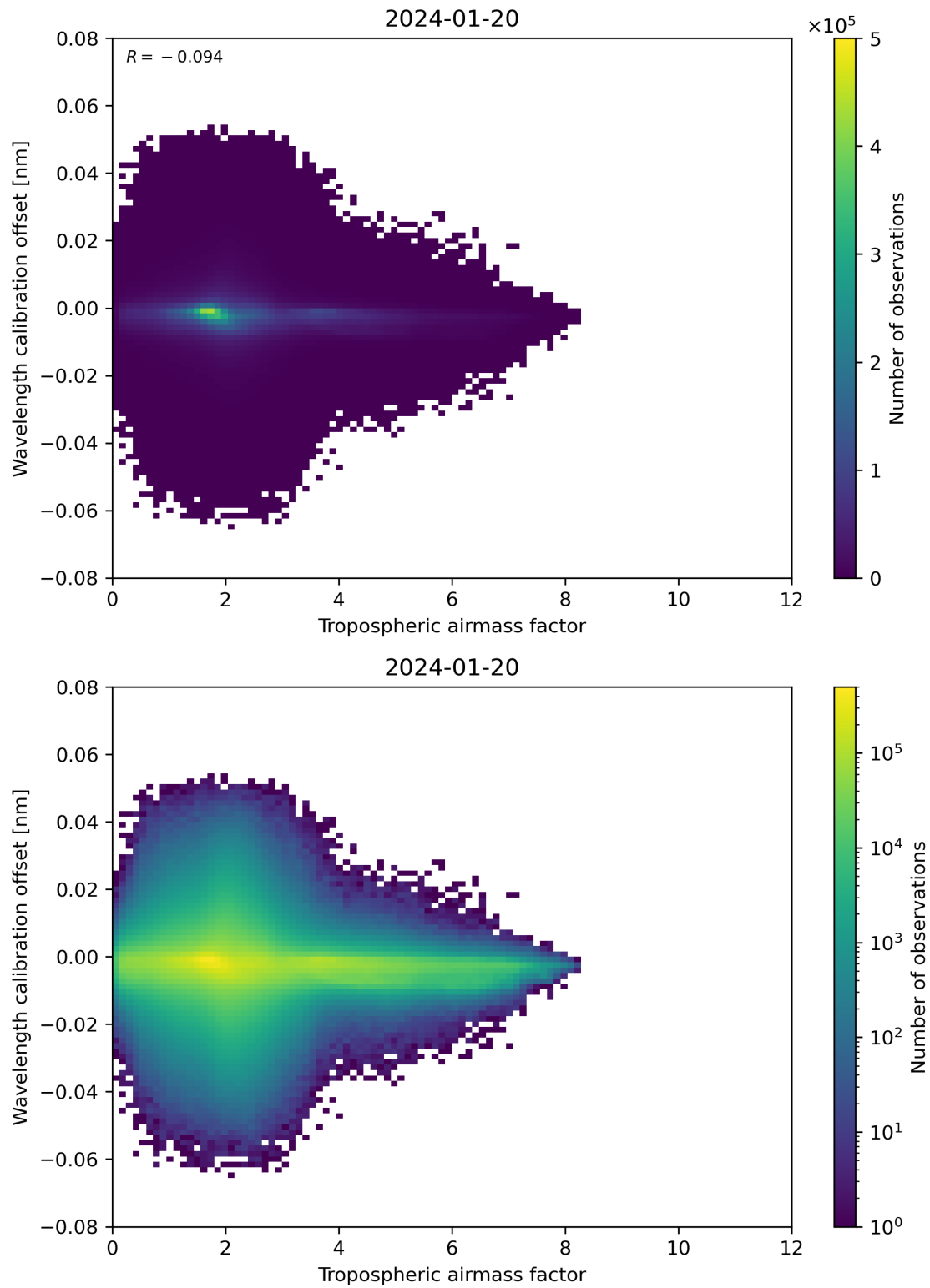
Figure 80: Scatter density plot of “Tropospheric airmass factor” against “Wavelength calibration offset” for 2024-01-19 to 2024-01-21.
