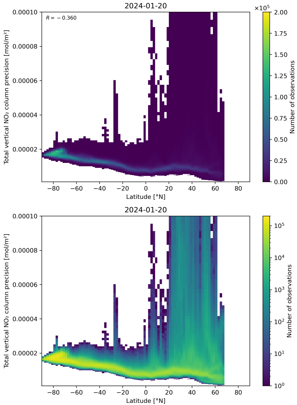
Figure 91: Scatter density plot of “Latitude” against “Total vertical NO 2 column precision” for 2024-01-19 to 2024-01-21.
