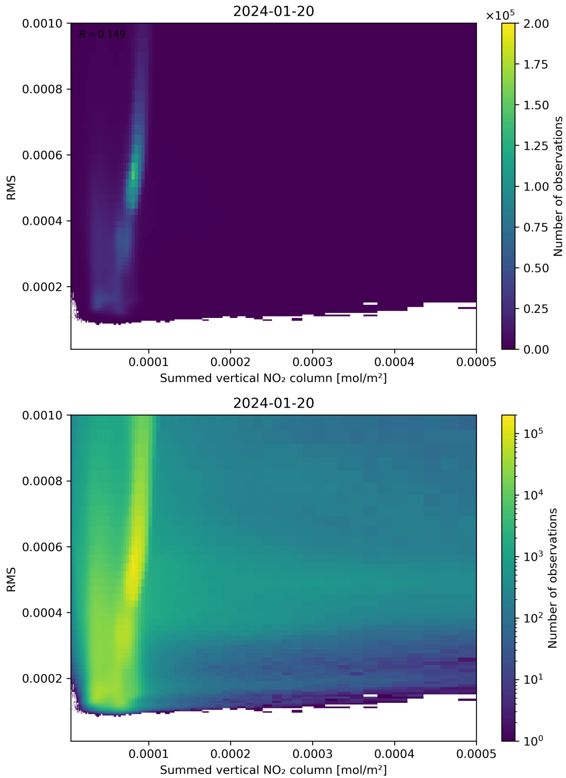
Figure 109: Scatter density plot of “Summed vertical NO 2 column” against “RMS” for 2024-01-19 to 2024-01-21.
