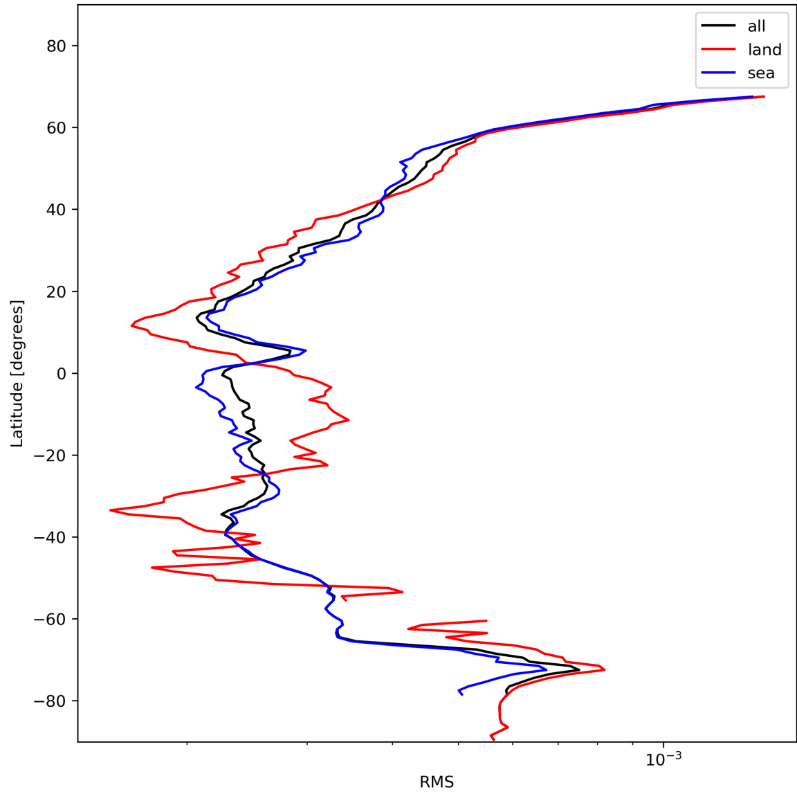
Figure 26: Zonal average of “RMS” for 2024-01-19 to 2024-01-21.
