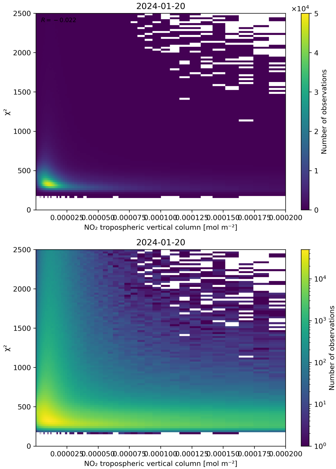
Figure 124: Scatter density plot of “NO 2 tropospheric vertical column” against “ \chi^2 ” for 2024-01-19 to 2024-01-21.
