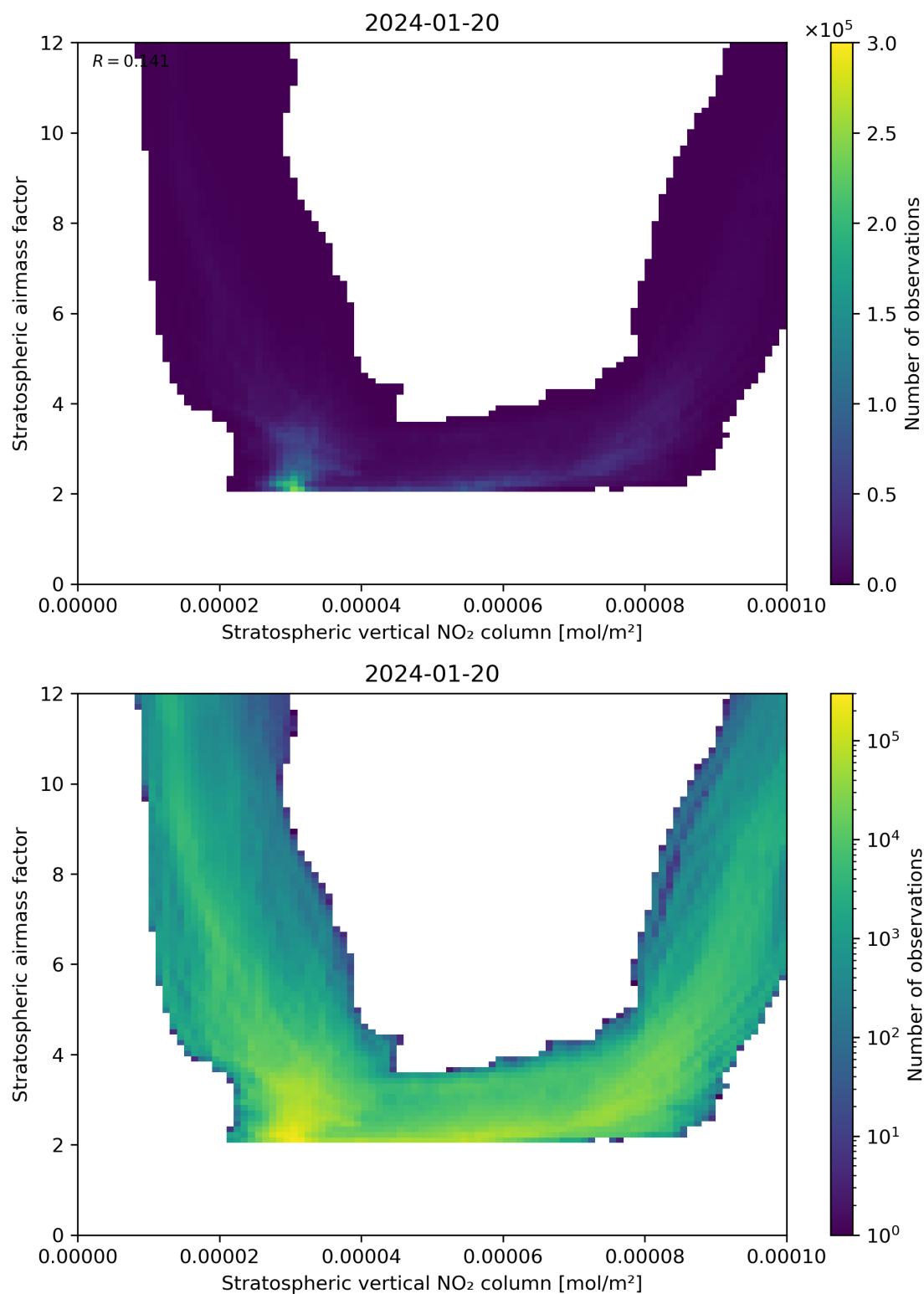
Figure 96: Scatter density plot of “Stratospheric vertical NO 2 column” against “Stratospheric airmass factor” for 2024-01-19 to 2024-01-21.
