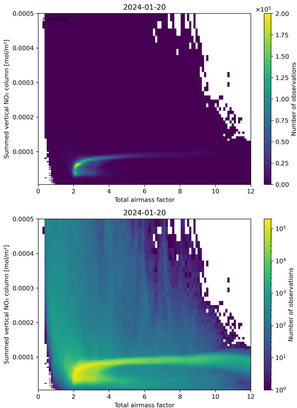
Figure 65: Scatter density plot of “Total airmass factor” against “Summed vertical NO 2 column” for 2024-01-19 to 2024-01-21.
