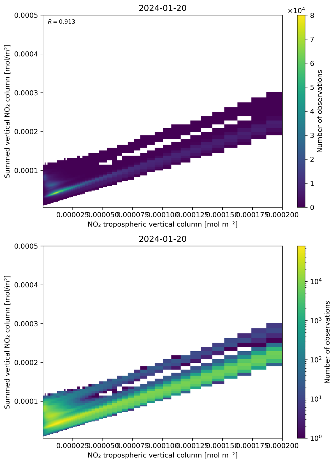
Figure 126: Scatter density plot of “NO 2 tropospheric vertical column” against “Summed vertical NO 2 column” for 2024-01-19 to 2024-01-21.
