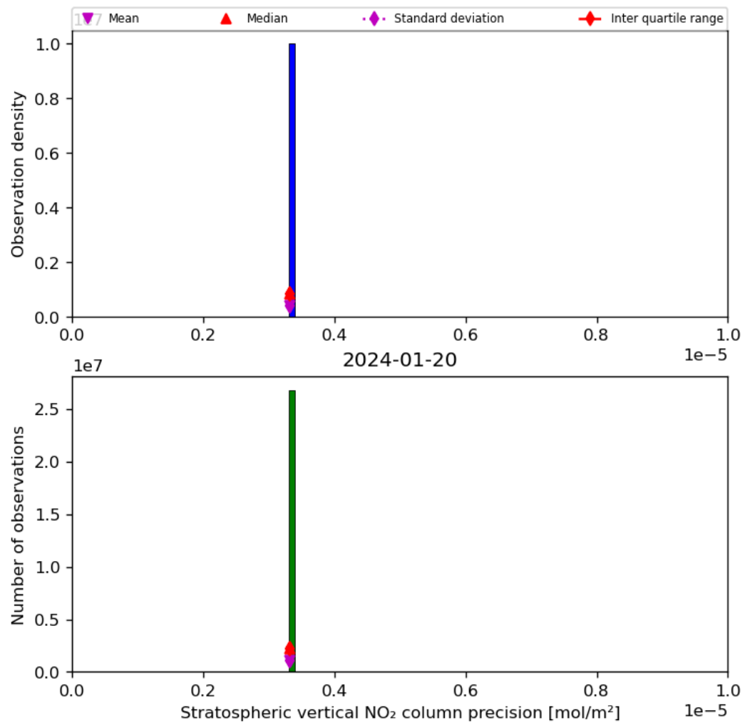
Figure 37: Histogram of “Stratospheric vertical NO 2 column precision” for 2024-01-19 to 2024-01-21
