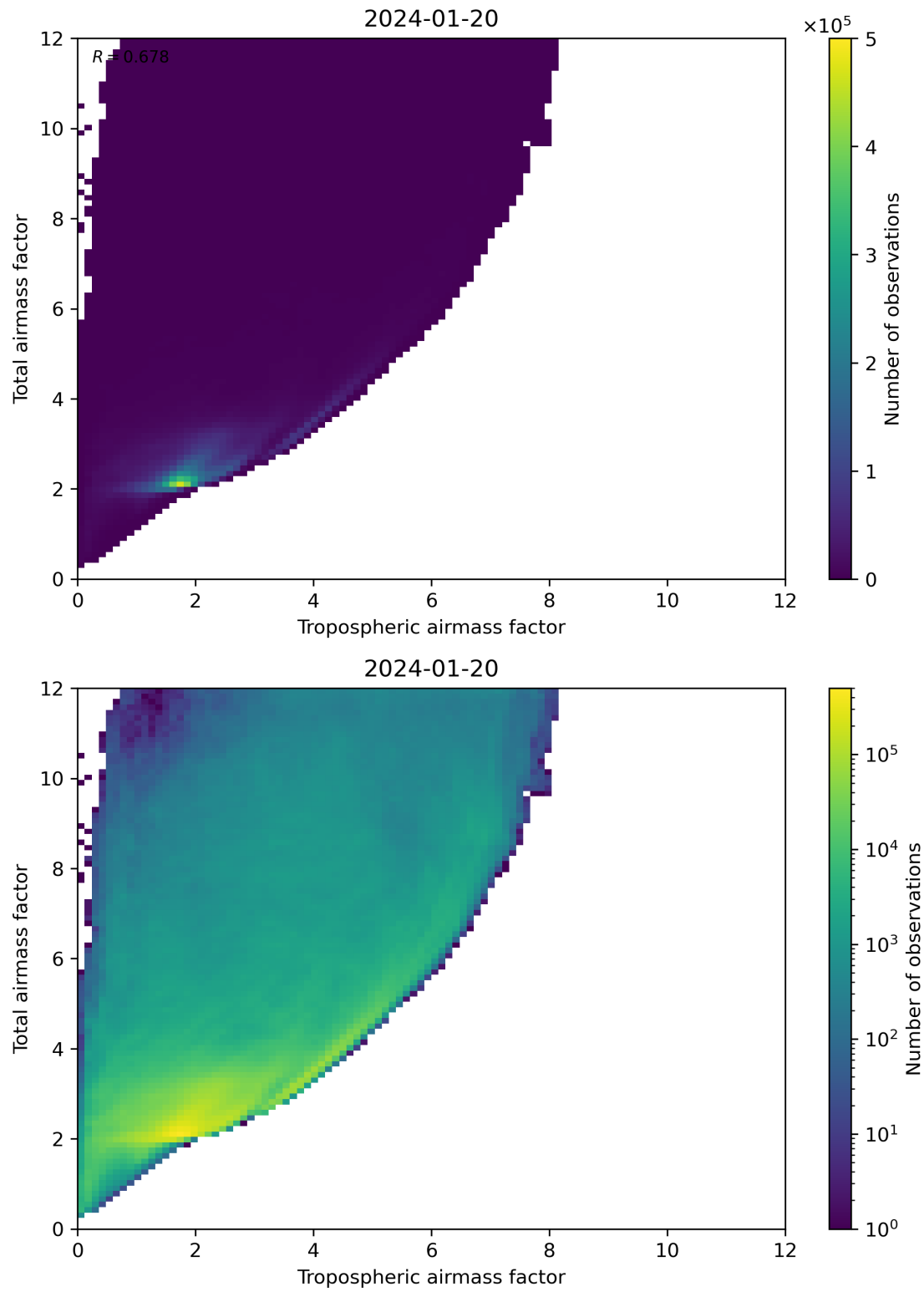
Figure 72: Scatter density plot of “Tropospheric airmass factor” against “Total airmass factor” for 2024-01-19 to 2024-01-21.
