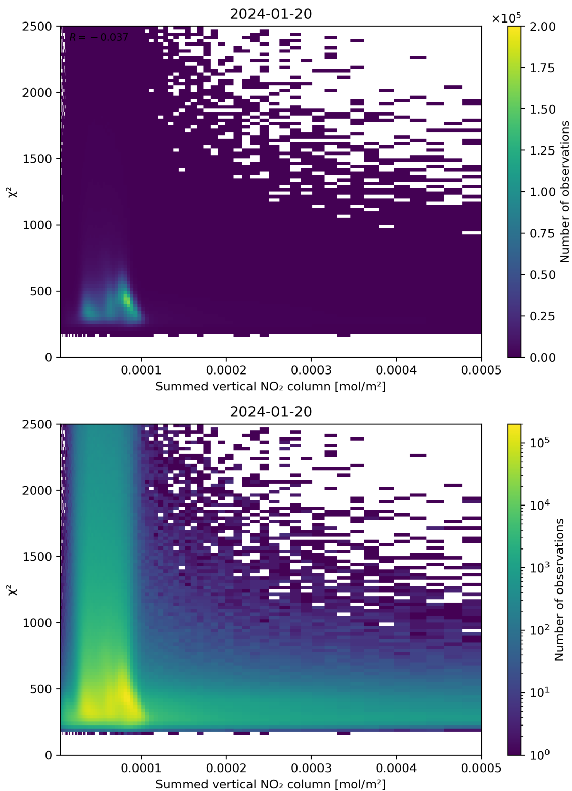
Figure 104: Scatter density plot of “Summed vertical NO 2 column” against “ \chi^2 ” for 2024-01-19 to 2024-01-21.
