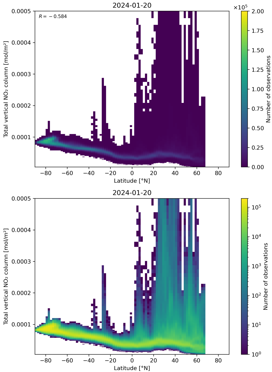
Figure 90: Scatter density plot of “Latitude” against “Total vertical NO 2 column” for 2024-01-19 to 2024-01-21.
