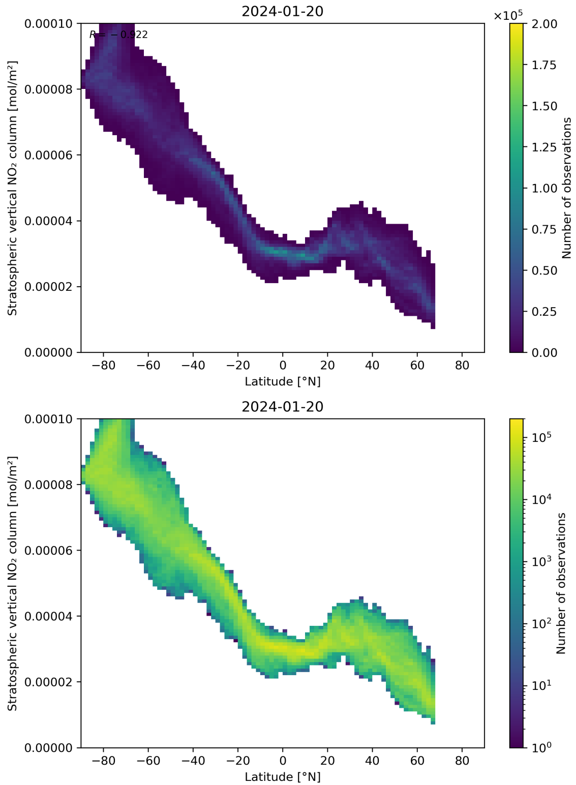
Figure 87: Scatter density plot of “Latitude” against “Stratospheric vertical NO 2 column” for 2024-01-19 to 2024-01-21.
