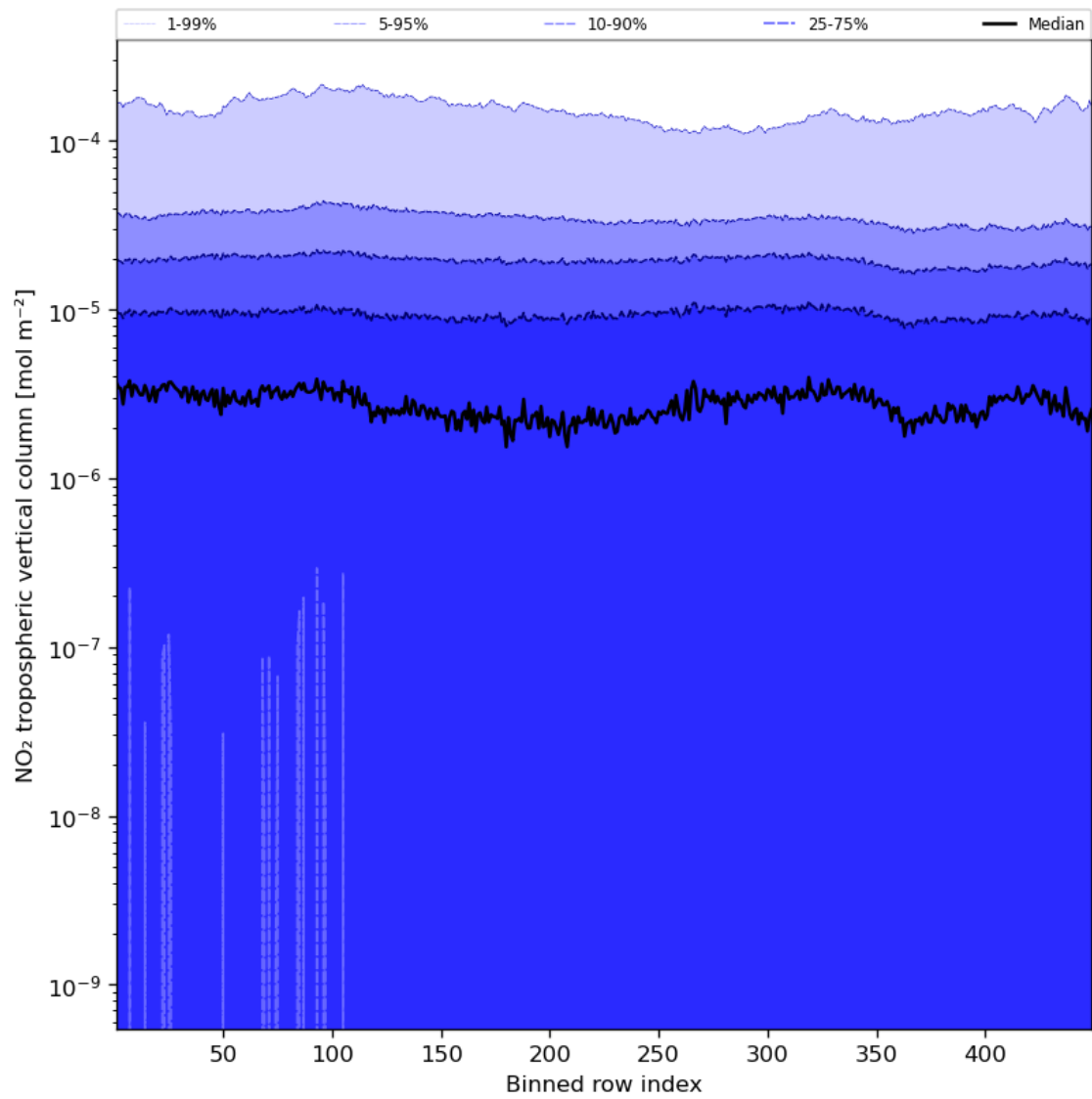
Figure 46: Along track statistics of “NO 2 tropospheric vertical column” for 2024-01-19 to 2024-01-21
