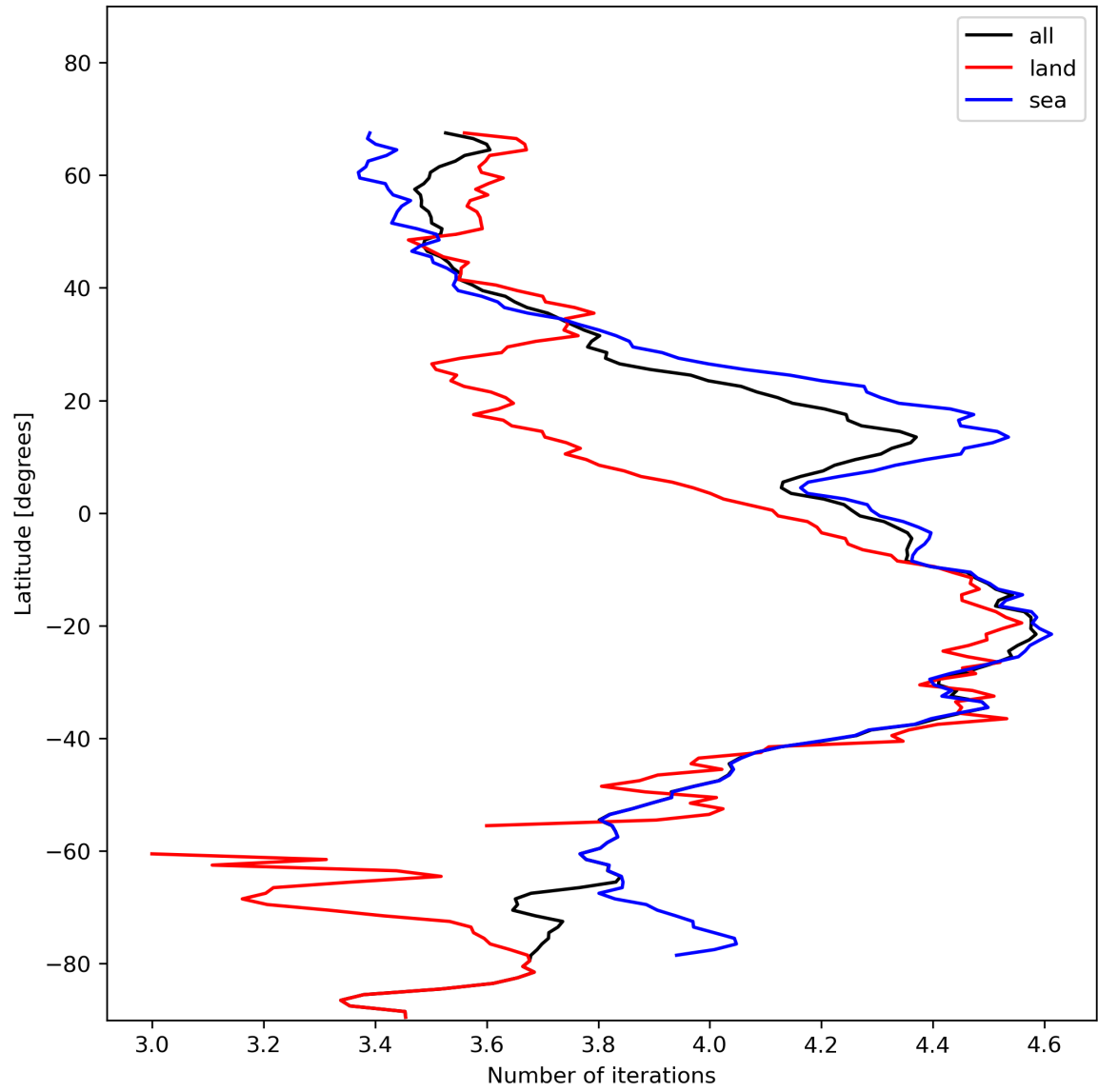
Figure 17: Zonal average of “Number of iterations” for 2024-01-19 to 2024-01-21.
