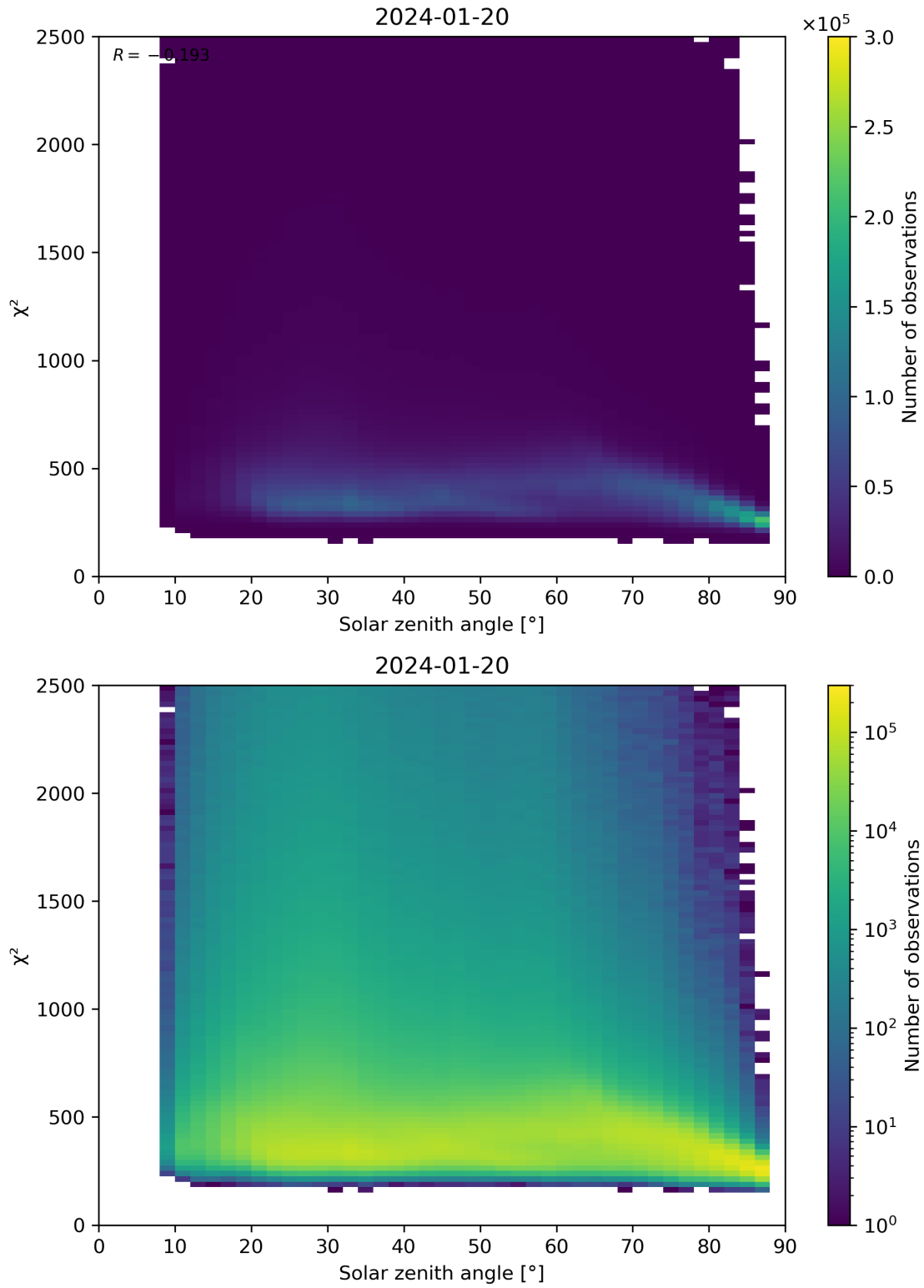
Figure 148: Scatter density plot of “Solar zenith angle” against “ \chi^2 ” for 2024-01-19 to 2024-01-21.
