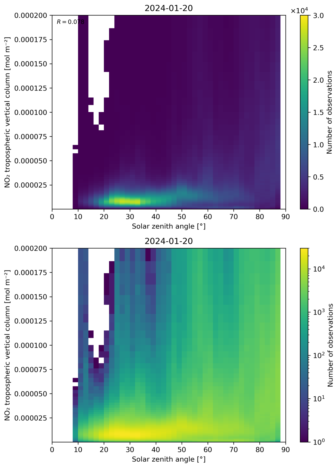
Figure 155: Scatter density plot of “Solar zenith angle” against “NO 2 tropospheric vertical column” for 2024-01-19 to 2024-01-21.
