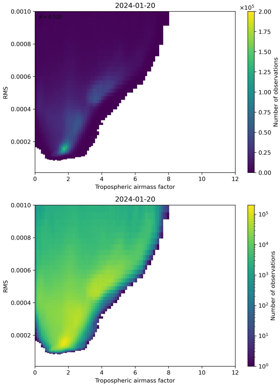
Figure 79: Scatter density plot of “Tropospheric airmass factor” against “RMS” for 2024-01-19 to 2024-01-21.
