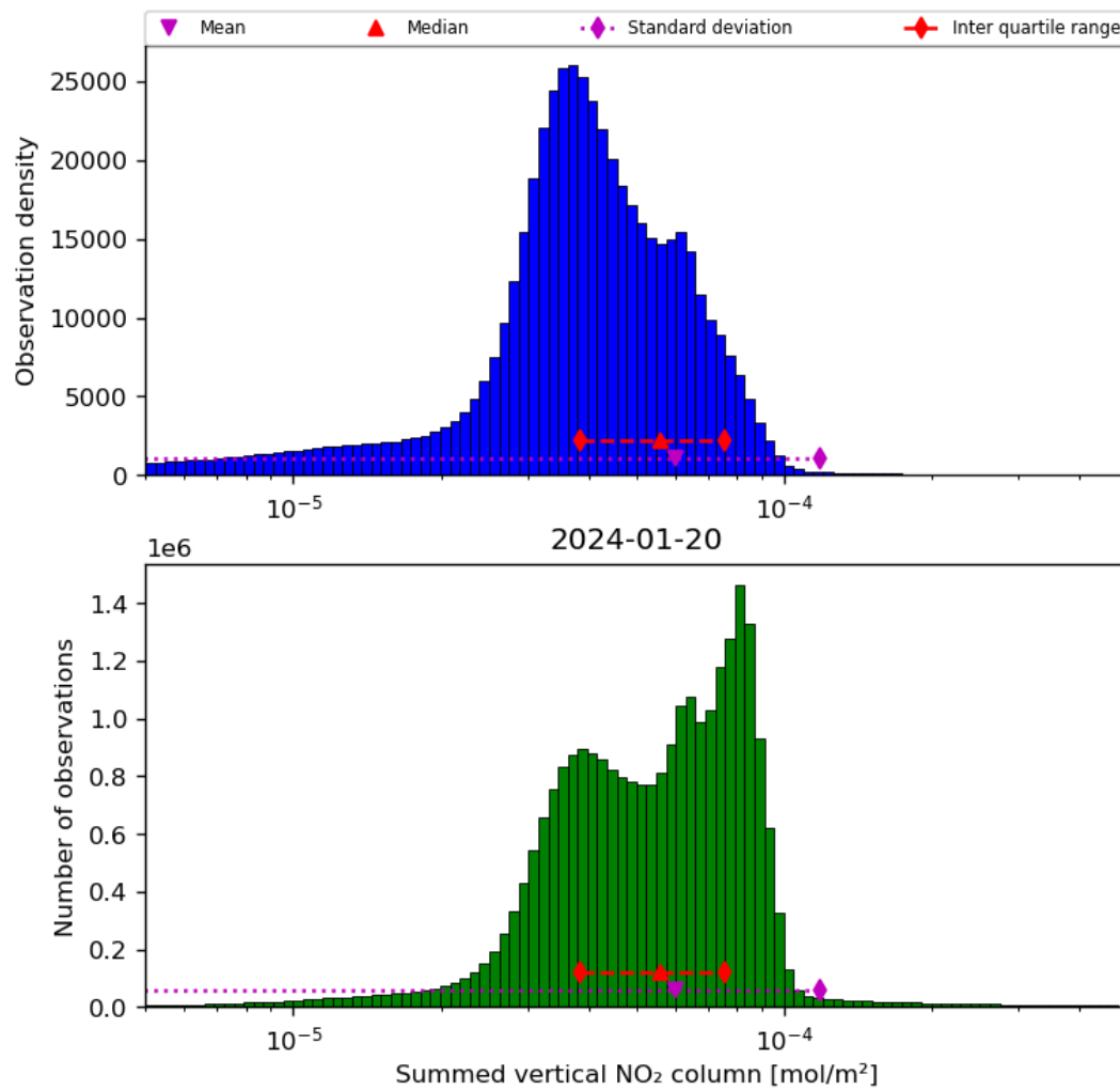
Figure 40: Histogram of "Summed vertical NO 2 column" for 2024-01-19 to 2024-01-21
