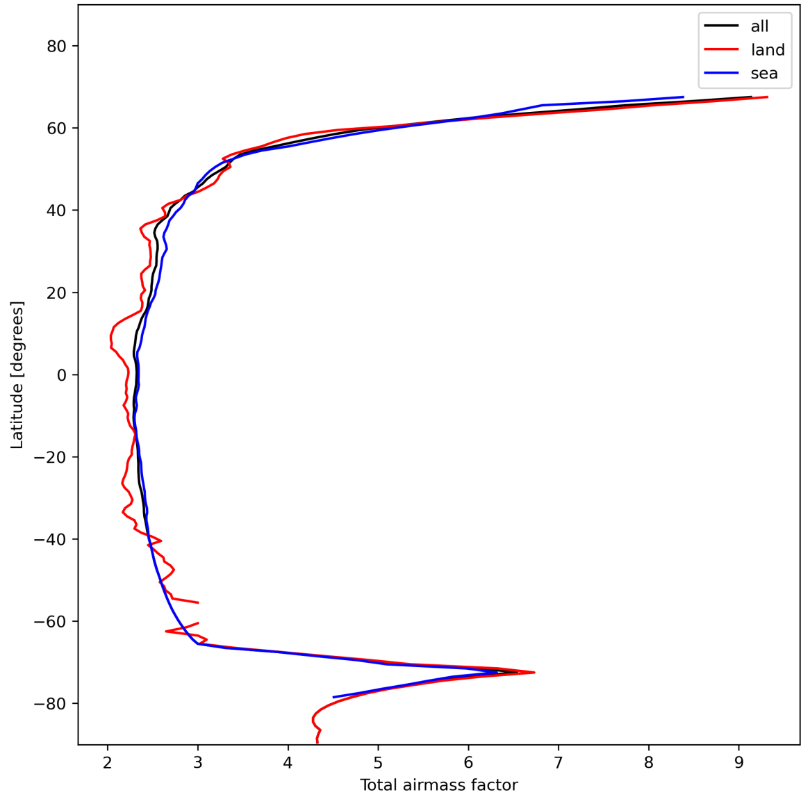
Figure 15: Zonal average of “Total airmass factor” for 2024-01-19 to 2024-01-21.
