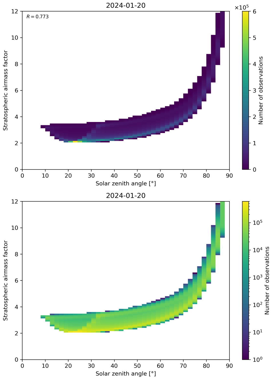
Figure 145: Scatter density plot of “Solar zenith angle” against “Stratospheric airmass factor” for 2024-01-19 to 2024-01-21.
