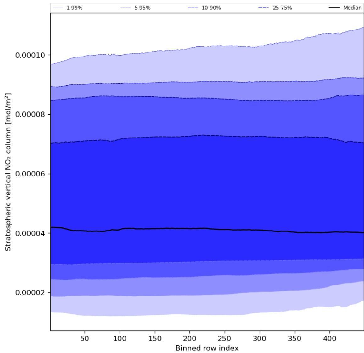
Figure 53: Along track statistics of “Stratospheric vertical NO 2 column” for 2024-01-21 to 2024-01-22
