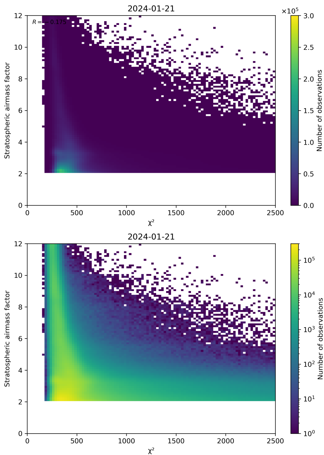
Figure 81: Scatter density plot of " \chi^2 " against "Stratospheric airmass factor" for 2024-01-21 to 2024-01-22.
