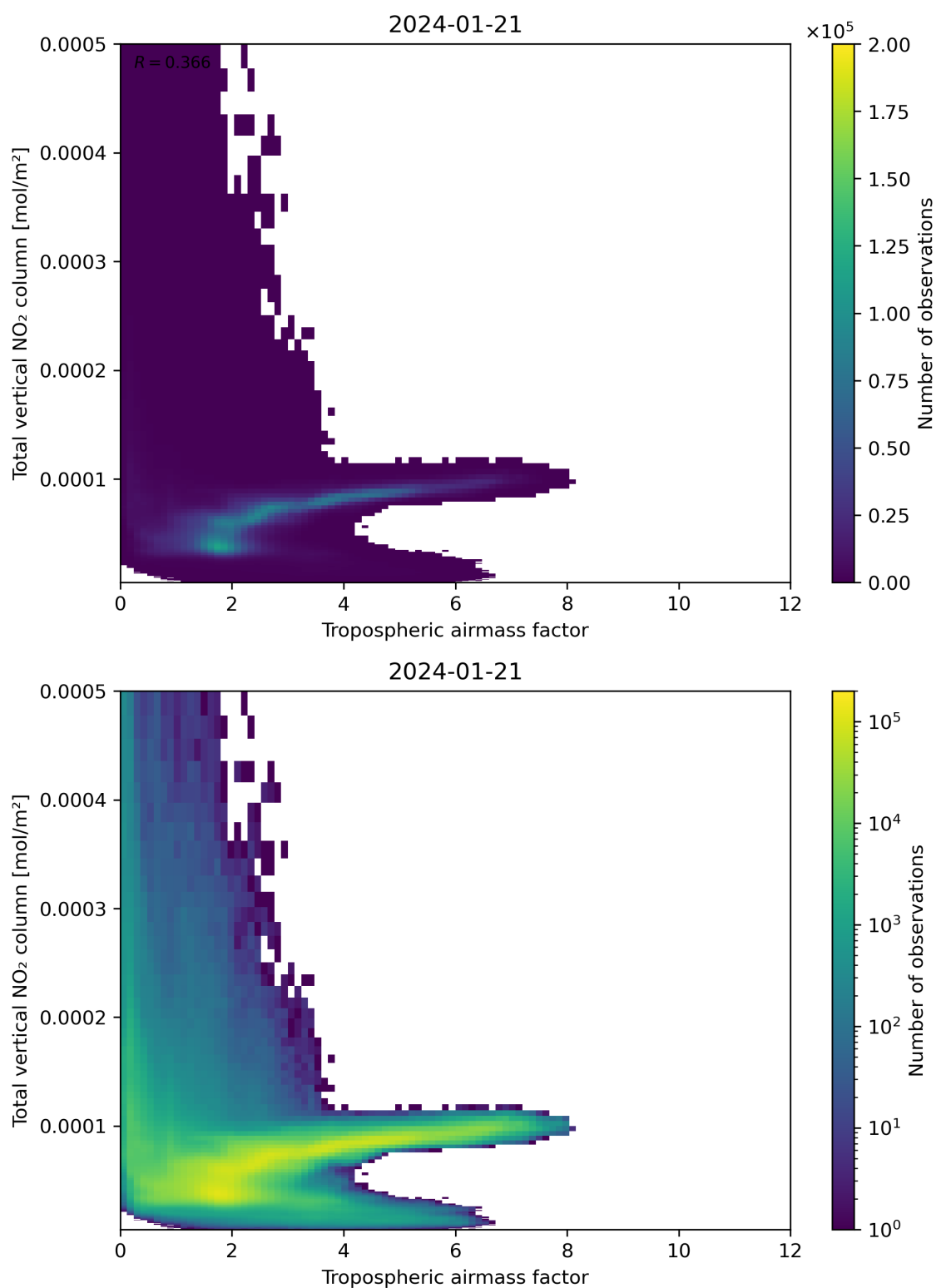
Figure 77: Scatter density plot of “Tropospheric airmass factor” against “Total vertical NO 2 column” for 2024-01-21 to 2024-01-22.
