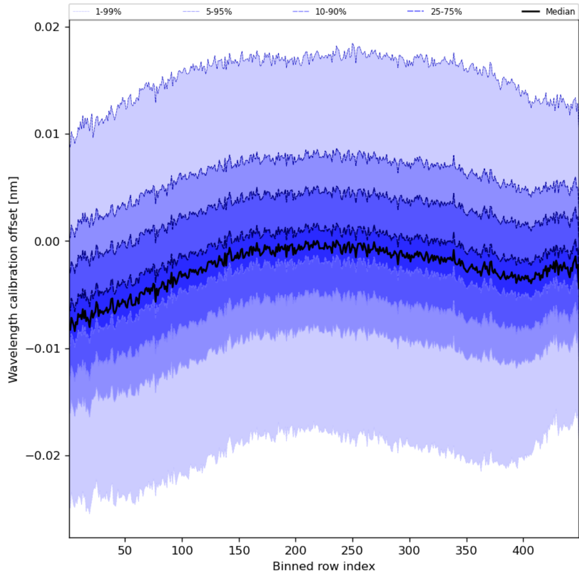
Figure 52: Along track statistics of “Wavelength calibration offset” for 2024-01-21 to 2024-01-22
