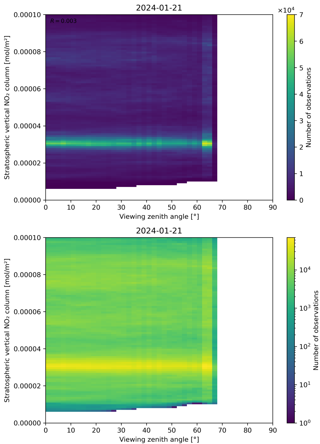
Figure 164: Scatter density plot of “Viewing zenith angle” against “Stratospheric vertical NO 2 column” for 2024-01-21 to 2024-01-22.
