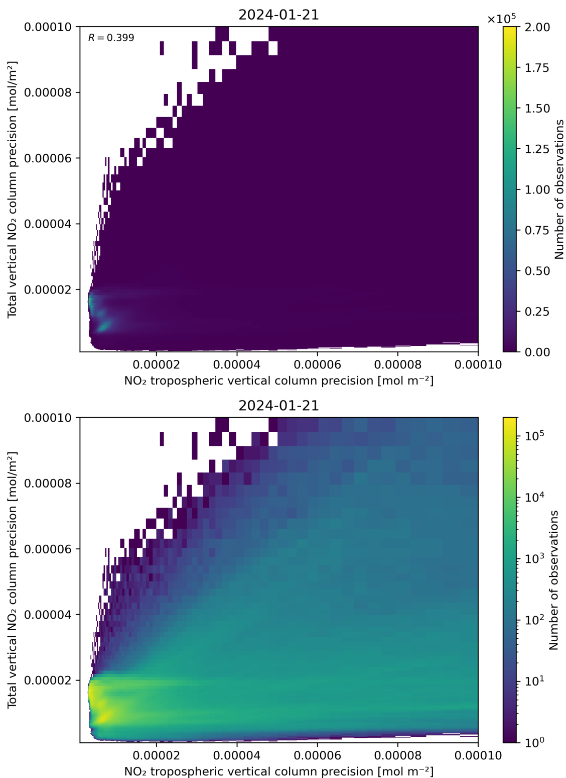
Figure 139: Scatter density plot of “NO 2 tropospheric vertical column precision” against “Total vertical NO 2 column precision” for 2024-01-21 to 2024-01-22.
