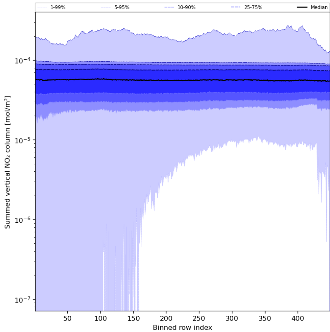
Figure 57: Along track statistics of “Summed vertical NO 2 column” for 2024-01-21 to 2024-01-22
