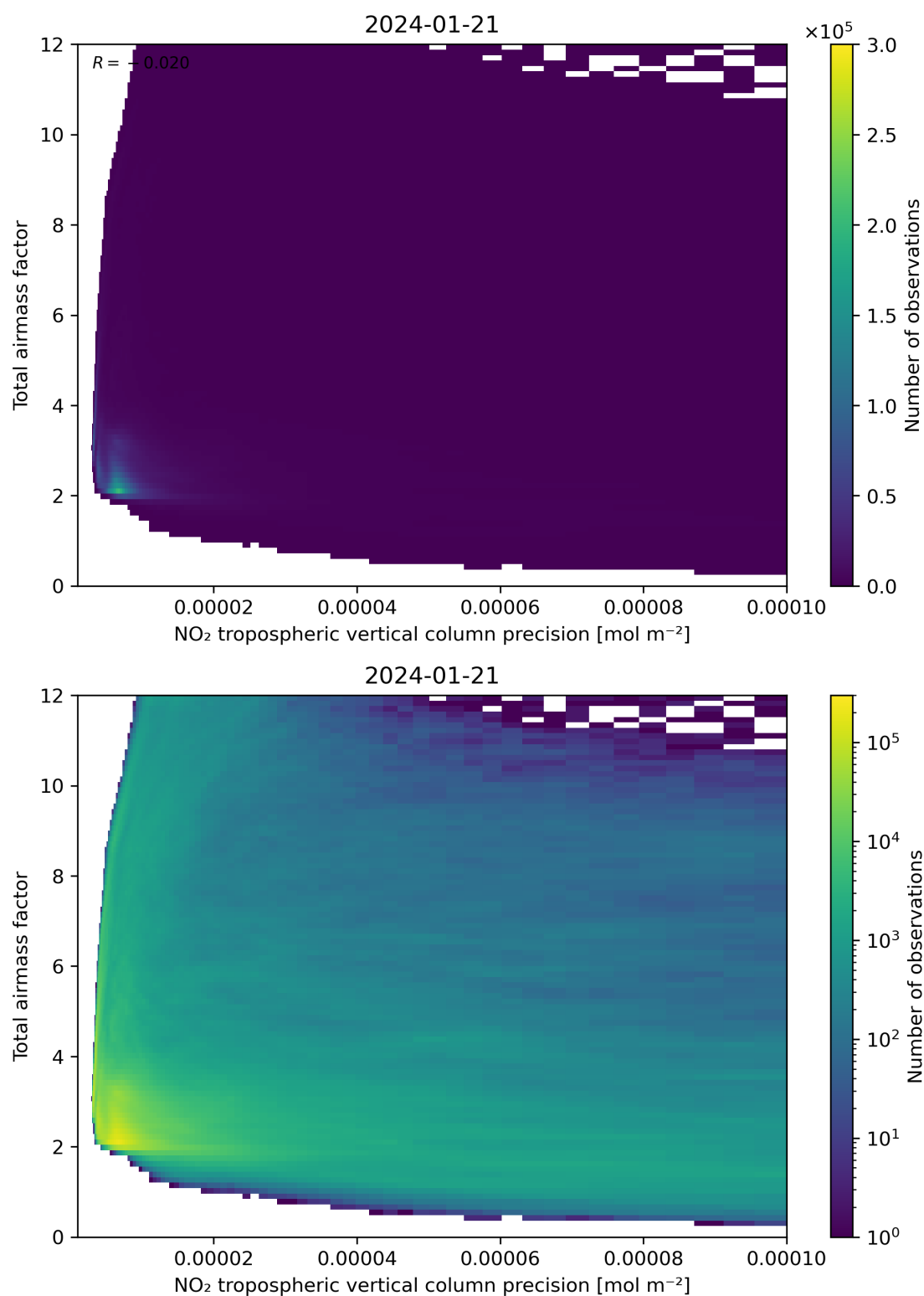
Figure 132: Scatter density plot of “NO 2 tropospheric vertical column precision” against “Total air mass factor” for 2024-01-21 to 2024-01-22.
