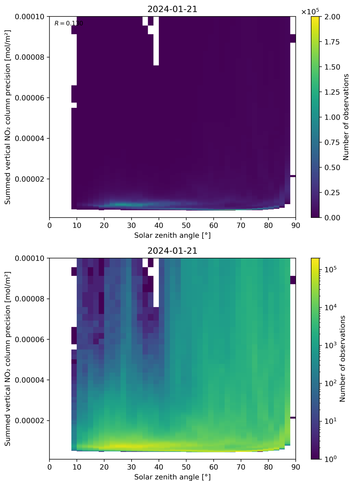
Figure 152: Scatter density plot of “Solar zenith angle” against “Summed vertical NO 2 column precision” for 2024-01-21 to 2024-01-22.
