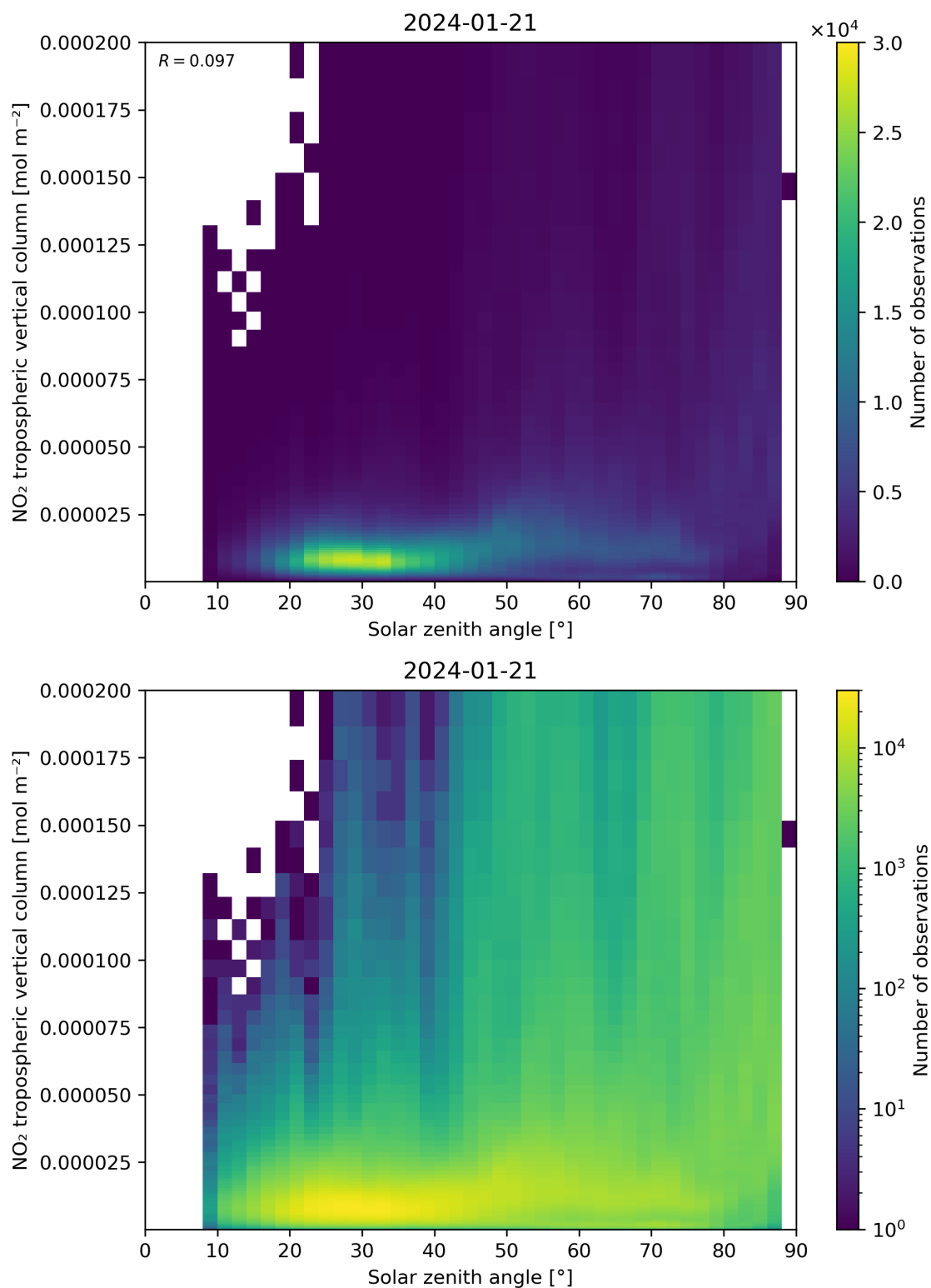
Figure 155: Scatter density plot of “Solar zenith angle” against “NO 2 tropospheric vertical column” for 2024-01-21 to 2024-01-22.
