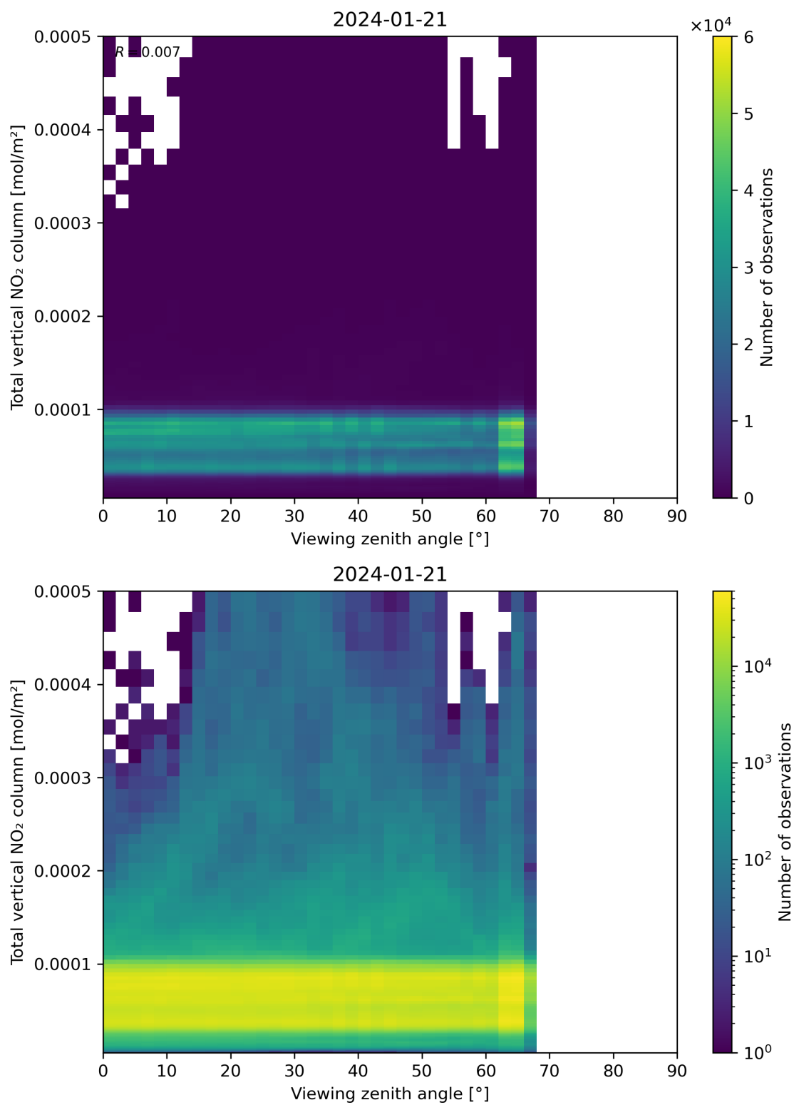
Figure 167: Scatter density plot of “Viewing zenith angle” against “Total vertical NO 2 column” for 2024-01-21 to 2024-01-22.
