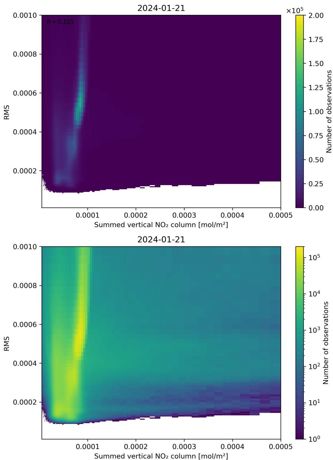
Figure 109: Scatter density plot of “Summed vertical NO 2 column” against “RMS” for 2024-01-21 to 2024-01-22.
