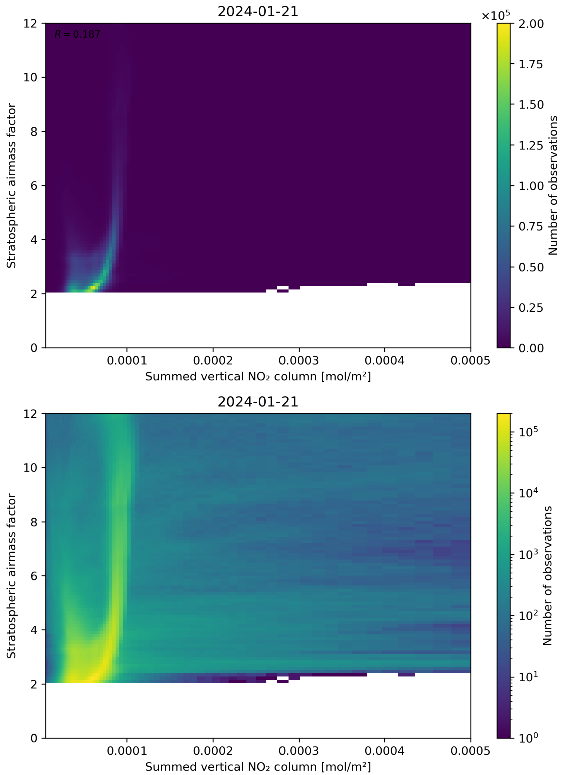
Figure 103: Scatter density plot of “Summed vertical NO 2 column” against “Stratospheric airmass factor” for 2024-01-21 to 2024-01-22.
