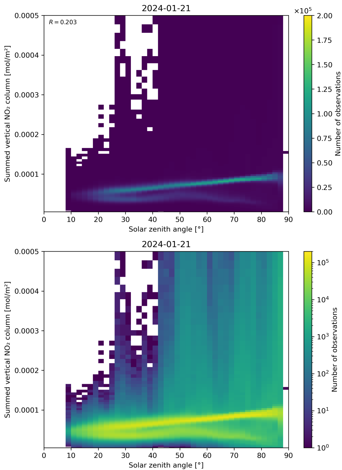
Figure 151: Scatter density plot of “Solar zenith angle” against “Summed vertical NO 2 column” for 2024-01-21 to 2024-01-22.
