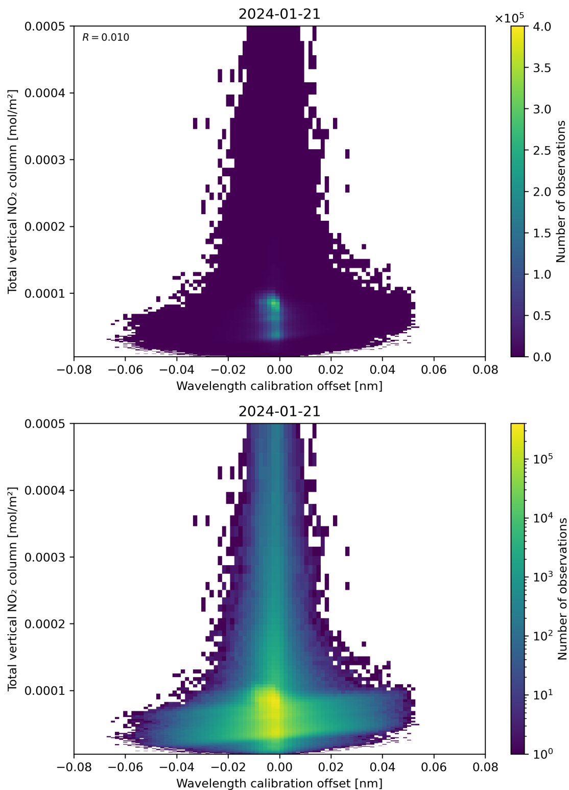
Figure 179: Scatter density plot of “Wavelength calibration offset” against “Total vertical NO 2 column” for 2024-01-21 to 2024-01-22.
