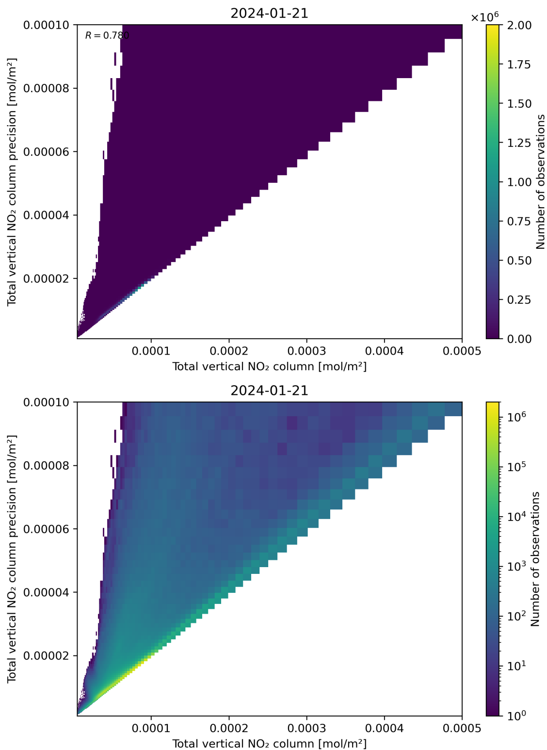
Figure 114: Scatter density plot of “Total vertical NO 2 column” against “Total vertical NO 2 column precision” for 2024-01-21 to 2024-01-22.
