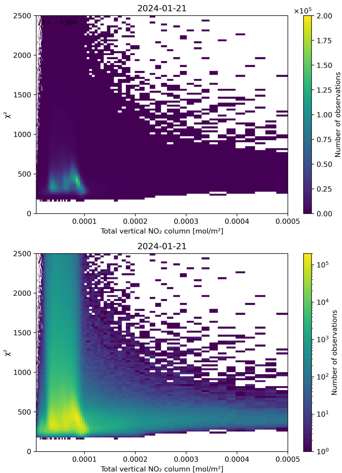
Figure 111: Scatter density plot of “Total vertical NO 2 column” against “ \chi^2 ” for 2024-01-21 to 2024-01-22.
