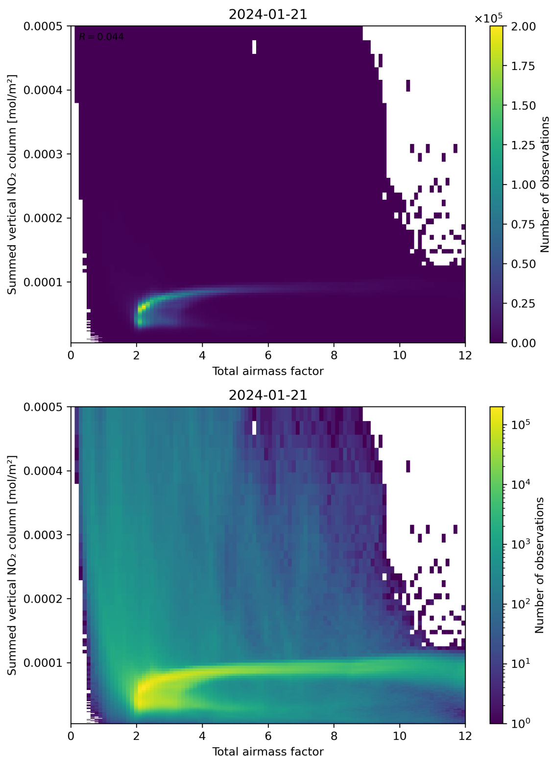
Figure 65: Scatter density plot of “Total airmass factor” against “Summed vertical NO 2 column” for 2024-01-21 to 2024-01-22.
