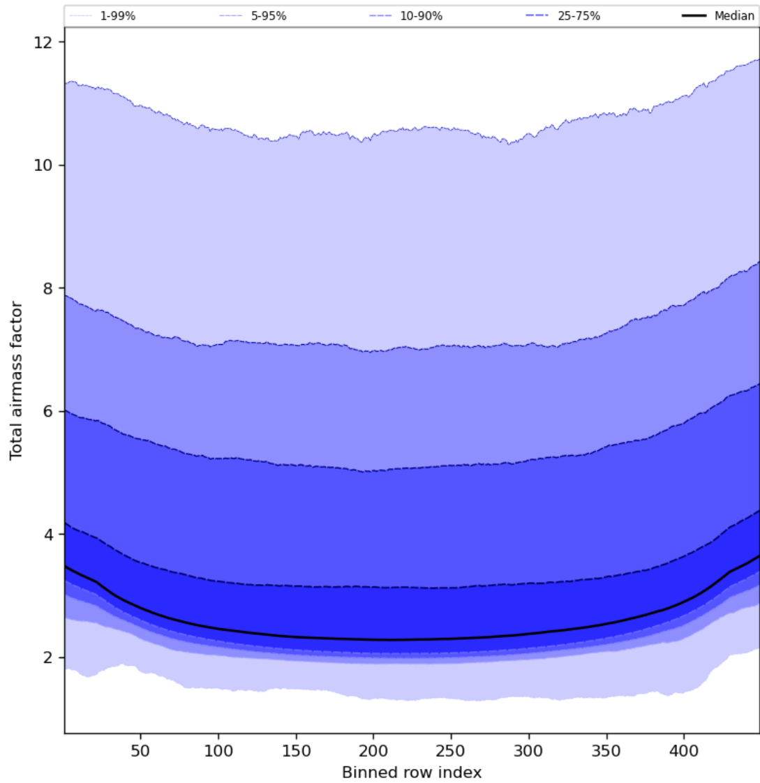
Figure 49: Along track statistics of “Total airmass factor” for 2024-01-21 to 2024-01-22
