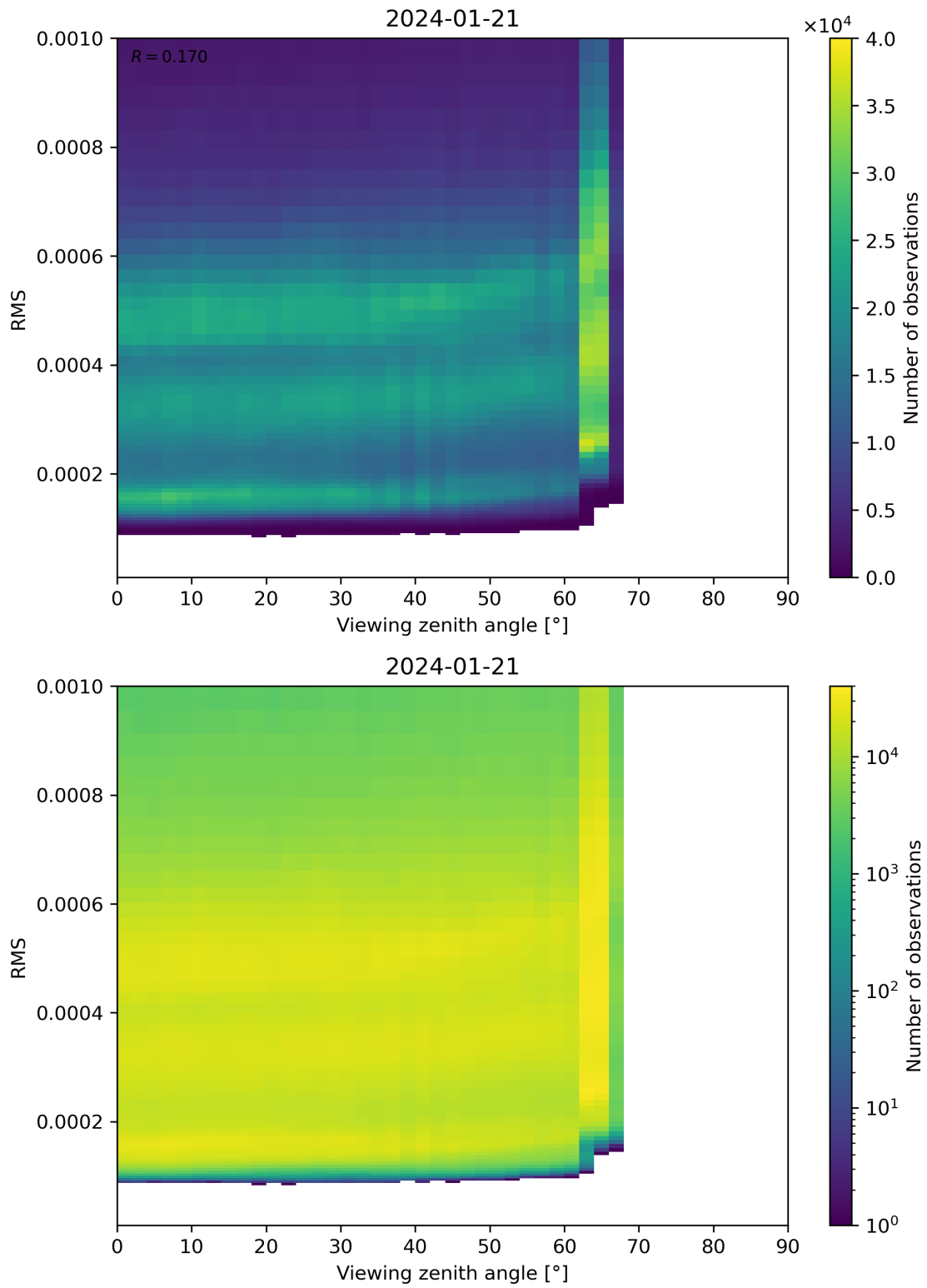
Figure 171: Scatter density plot of “Viewing zenith angle” against “RMS” for 2024-01-21 to 2024-01-22.
