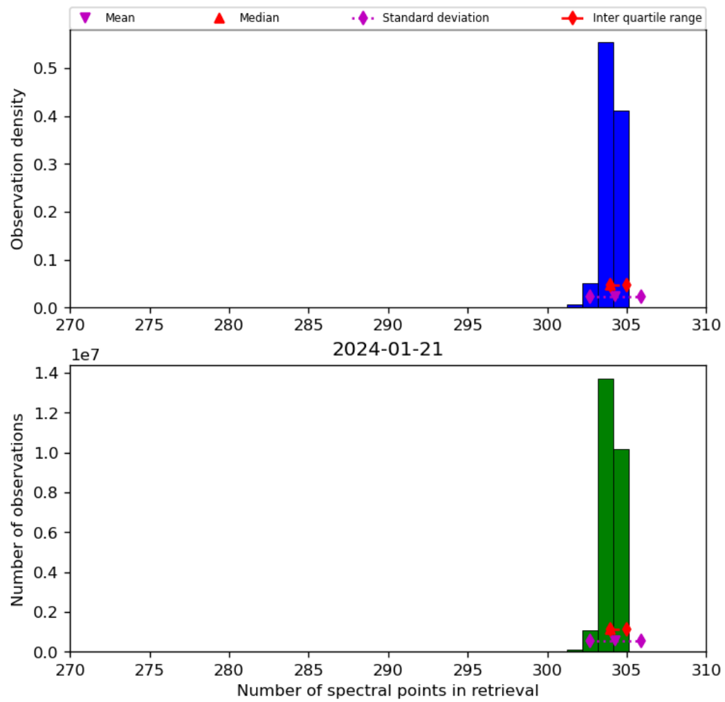
Figure 33: Histogram of “Number of spectral points in retrieval” for 2024-01-21 to 2024-01-22
