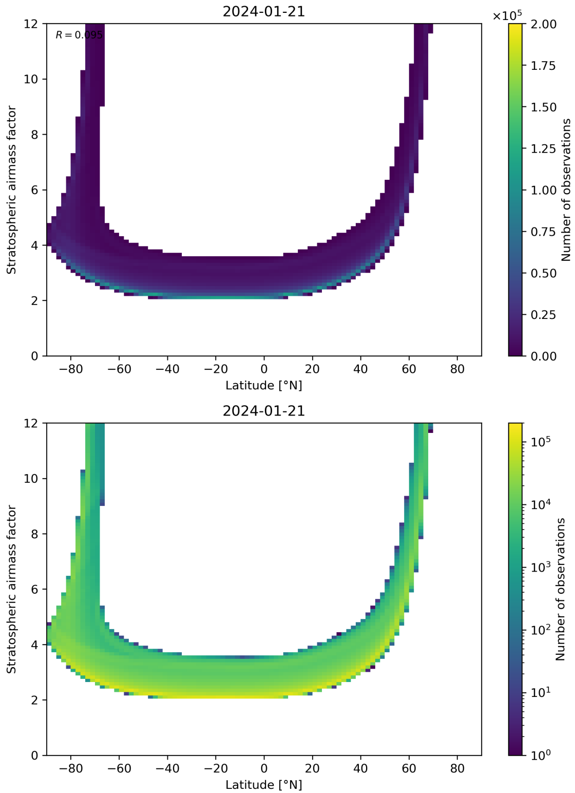
Figure 83: Scatter density plot of “Latitude” against “Stratospheric airmass factor” for 2024-01-21 to 2024-01-22.
