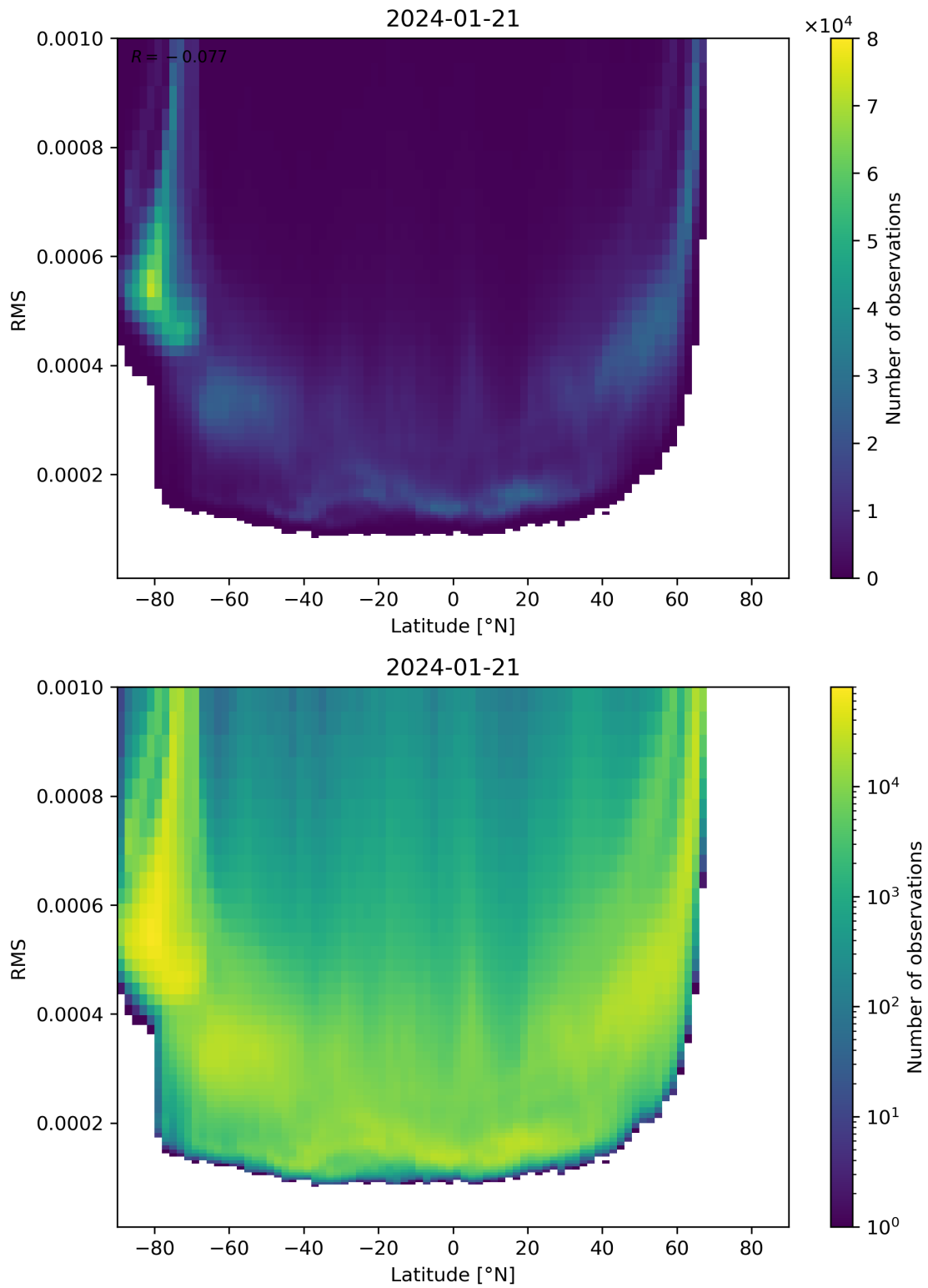
Figure 94: Scatter density plot of “Latitude” against “RMS” for 2024-01-21 to 2024-01-22.
