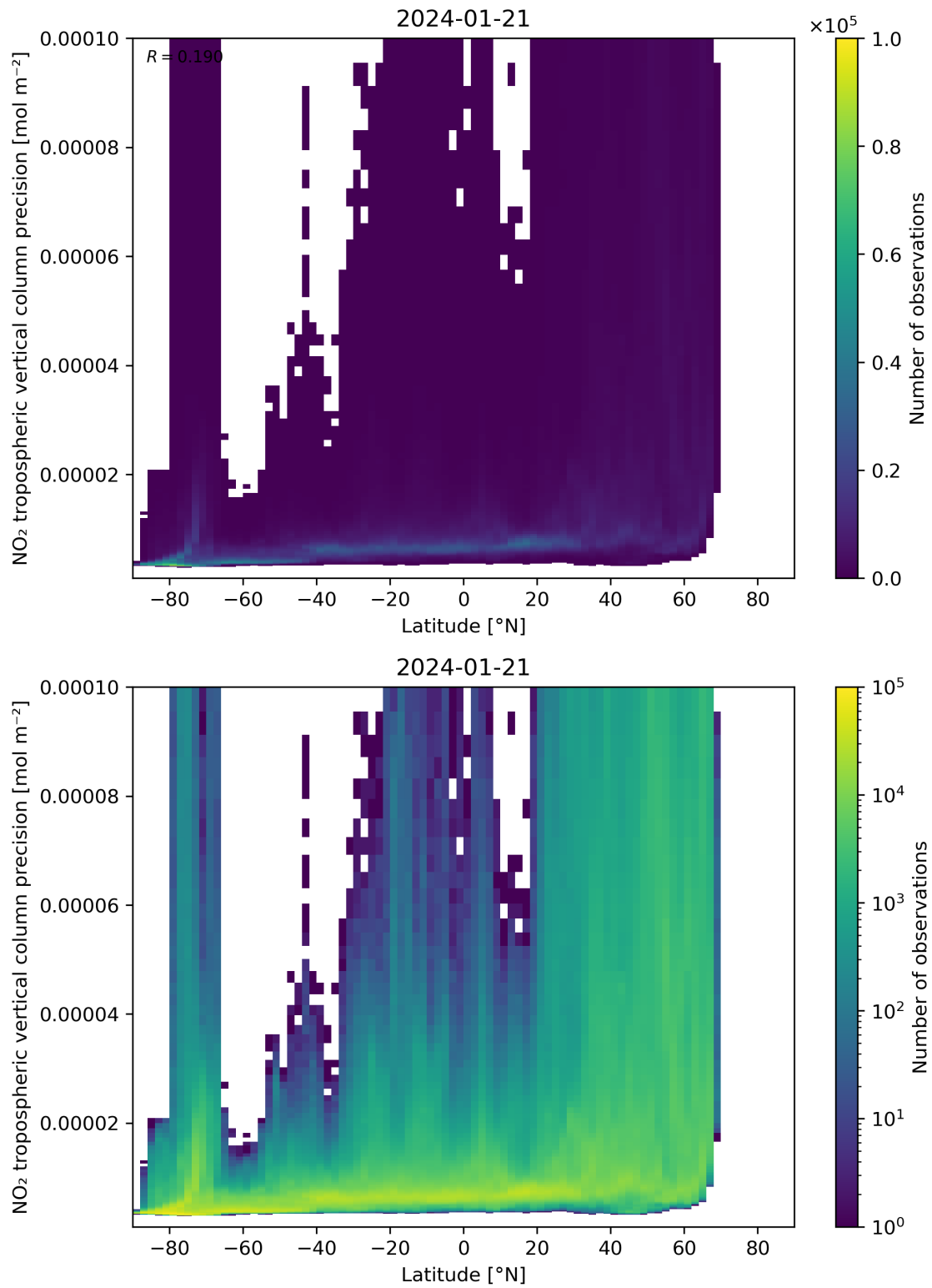
Figure 93: Scatter density plot of “Latitude” against “NO 2 tropospheric vertical column precision” for 2024-01-21 to 2024-01-22.
