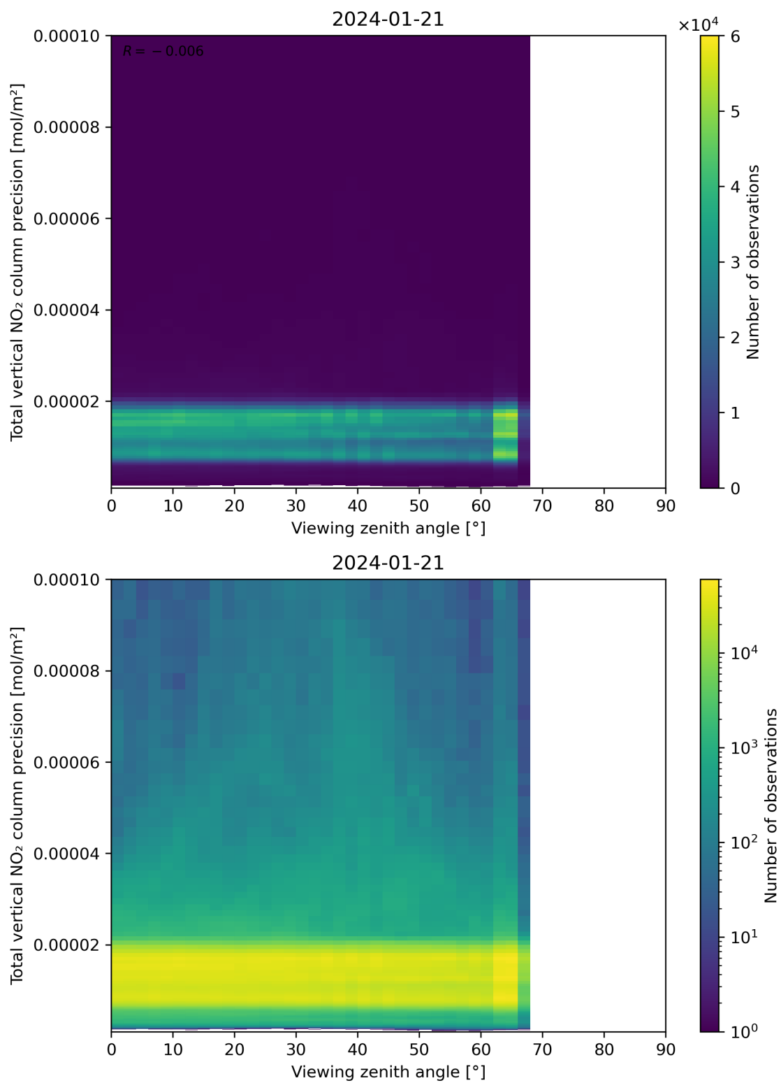
Figure 168: Scatter density plot of “Viewing zenith angle” against “Total vertical NO 2 column precision” for 2024-01-21 to 2024-01-22.
