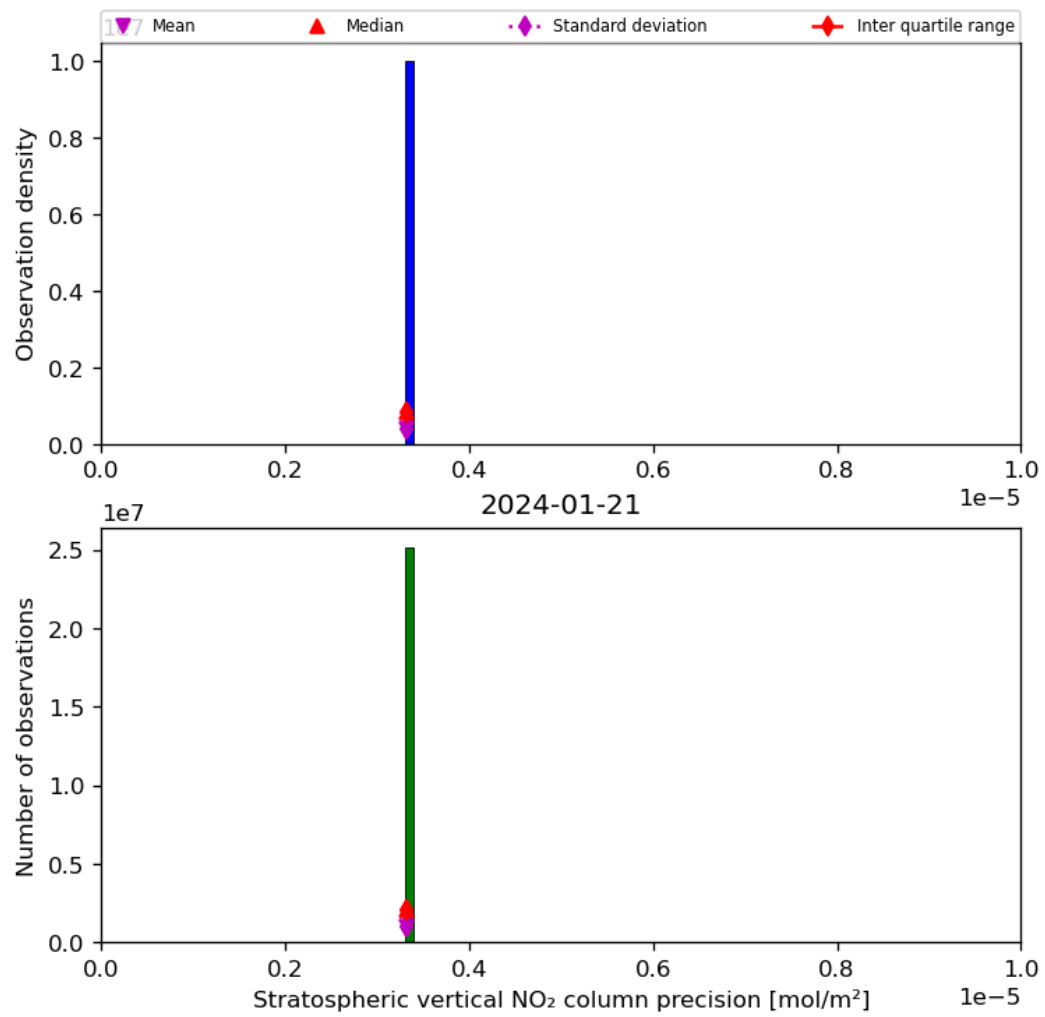
Figure 37: Histogram of “Stratospheric vertical NO 2 column precision” for 2024-01-21 to 2024-01-22
