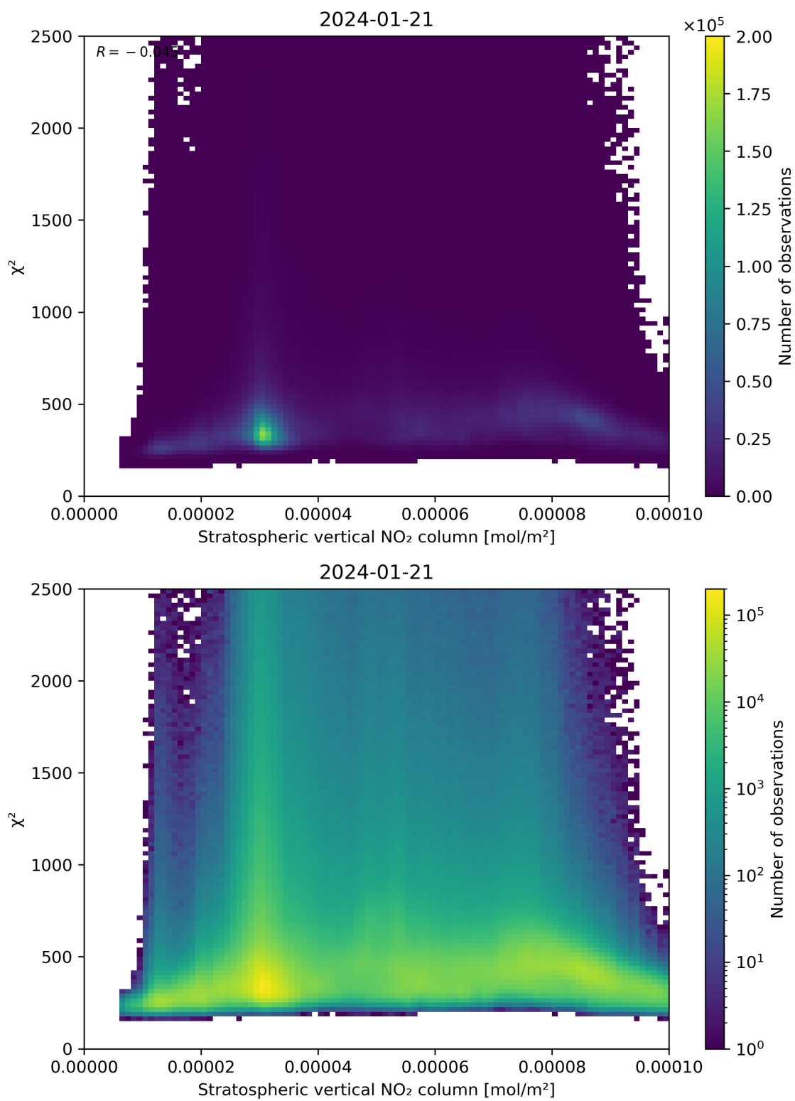
Figure 97: Scatter density plot of “Stratospheric vertical NO 2 column” against “ \chi^2 ” for 2024-01-21 to 2024-01-22.
