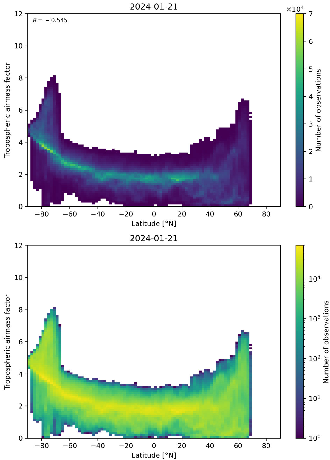
Figure 85: Scatter density plot of “Latitude” against “Tropospheric airmass factor” for 2024-01-21 to 2024-01-22.
