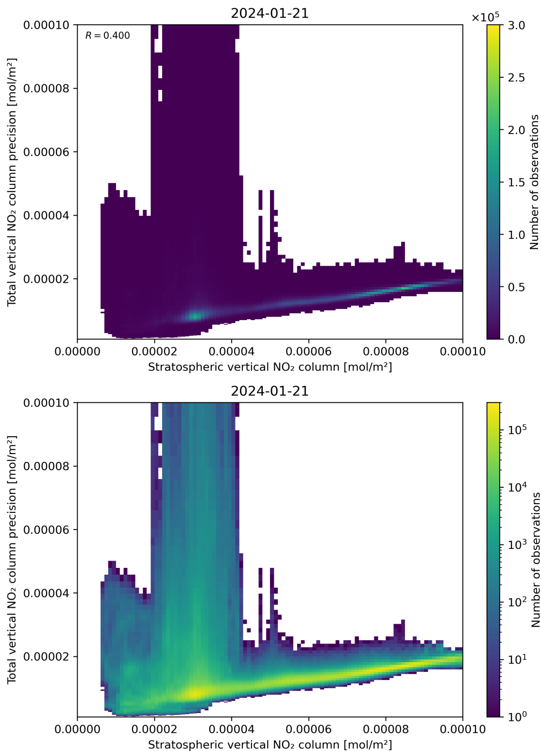
Figure 101: Scatter density plot of “Stratospheric vertical NO 2 column” against “Total vertical NO 2 column precision” for 2024-01-21 to 2024-01-22.
