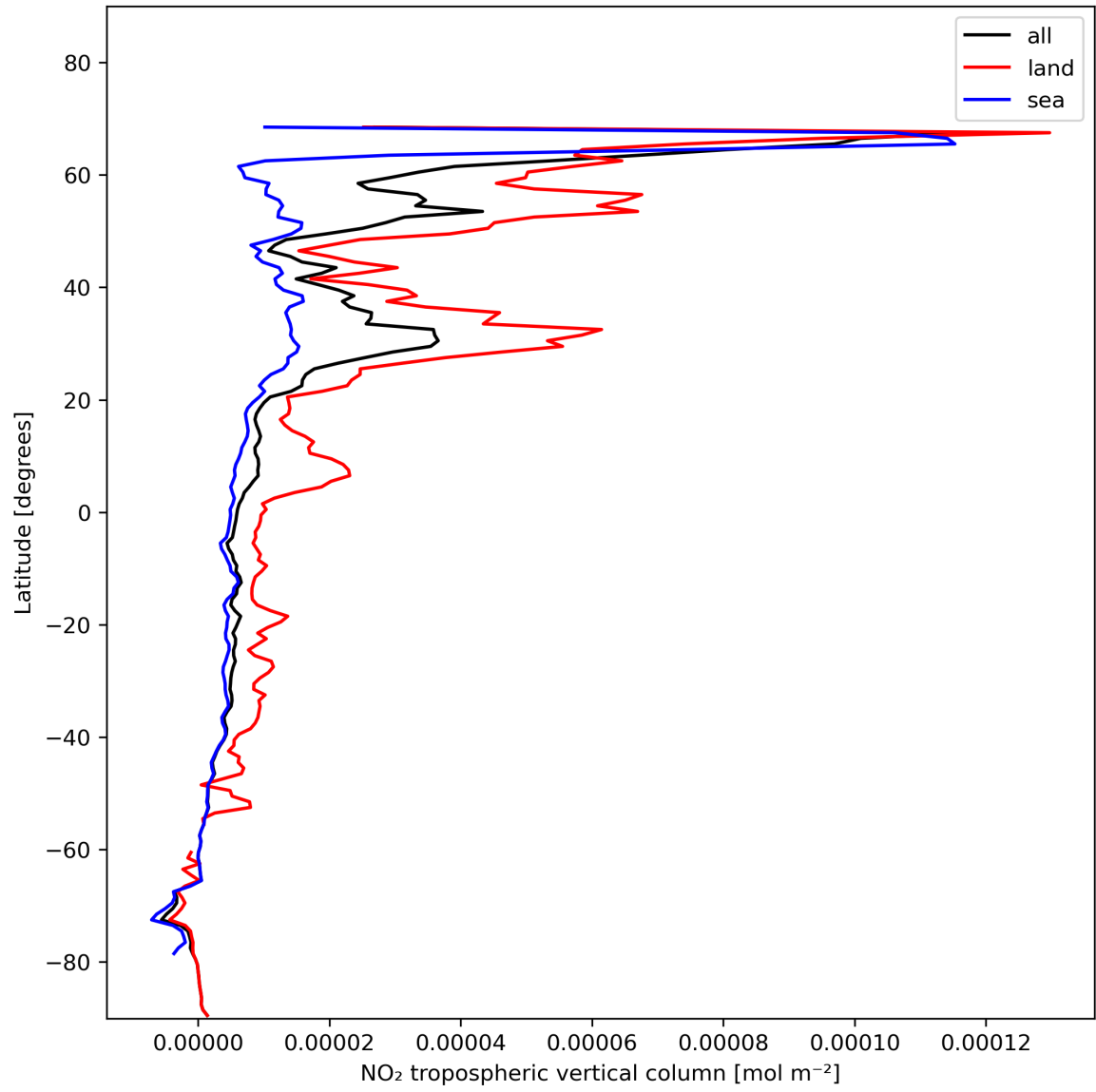
Figure 12: Zonal average of “NO 2 tropospheric vertical column” for 2024-01-21 to 2024-01-22.
