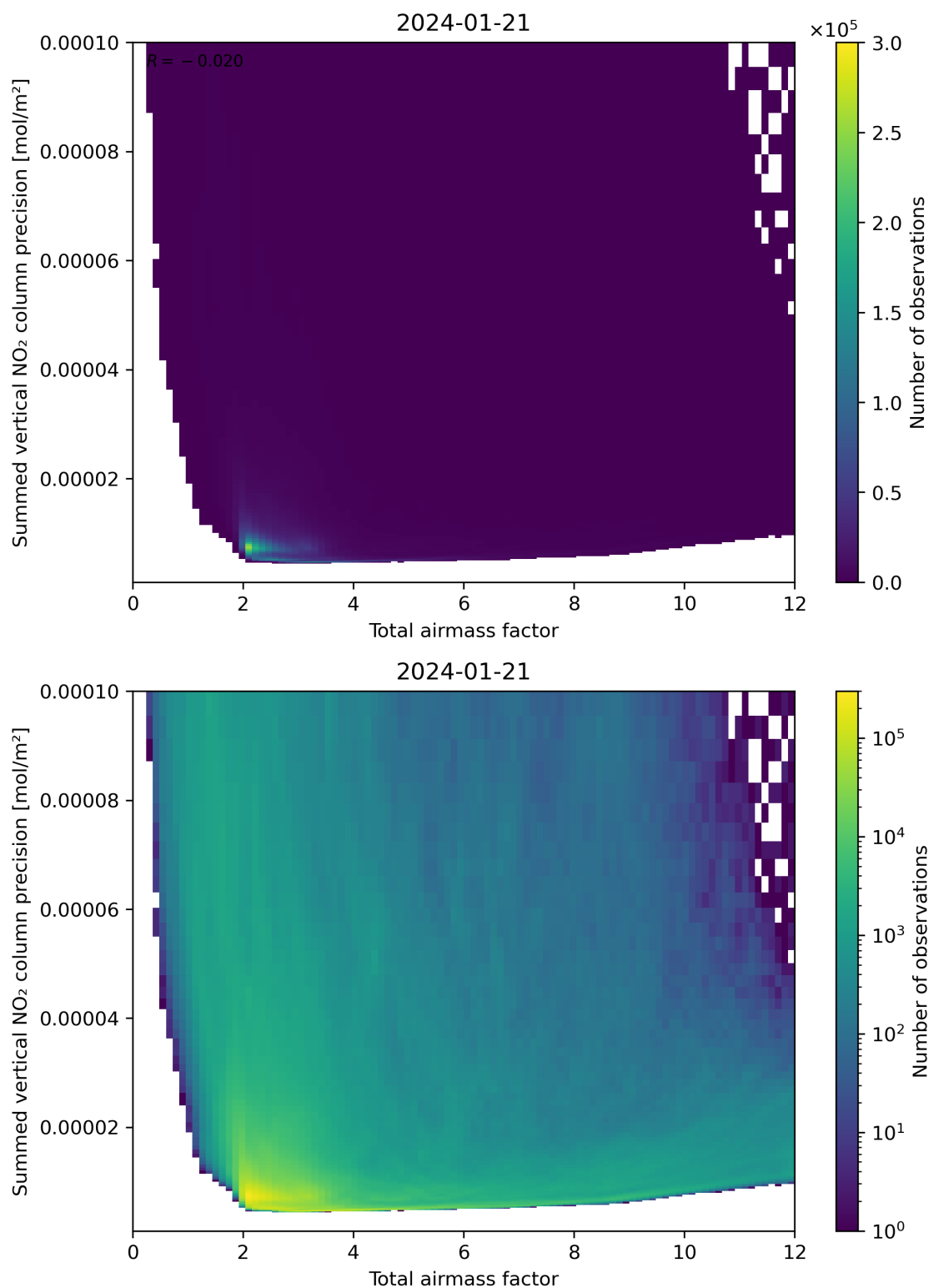
Figure 66: Scatter density plot of “Total airmass factor” against “Summed vertical NO 2 column precision” for 2024-01-21 to 2024-01-22.
