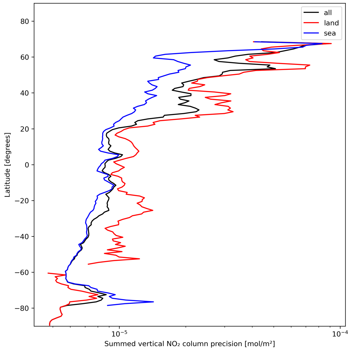
Figure 24: Zonal average of “Summed vertical NO 2 column precision” for 2024-01-21 to 2024-01-22.
