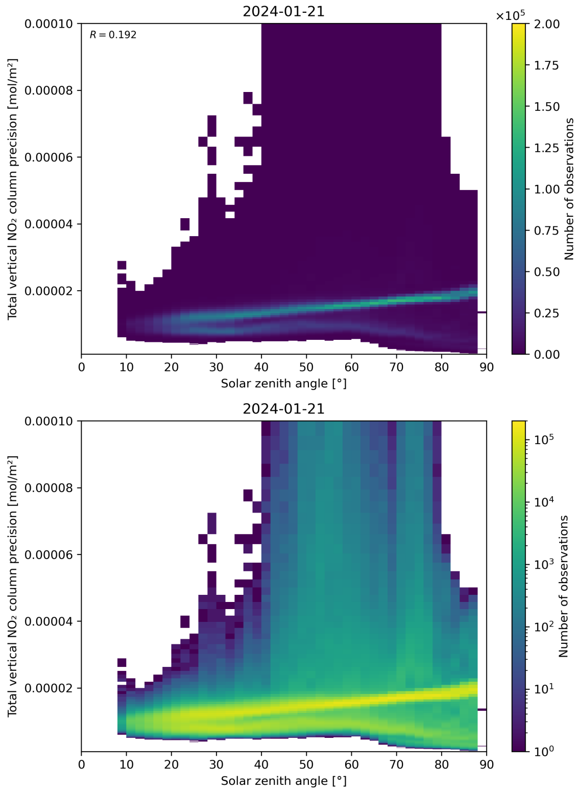
Figure 154: Scatter density plot of “Solar zenith angle” against “Total vertical NO 2 column precision” for 2024-01-21 to 2024-01-22.
