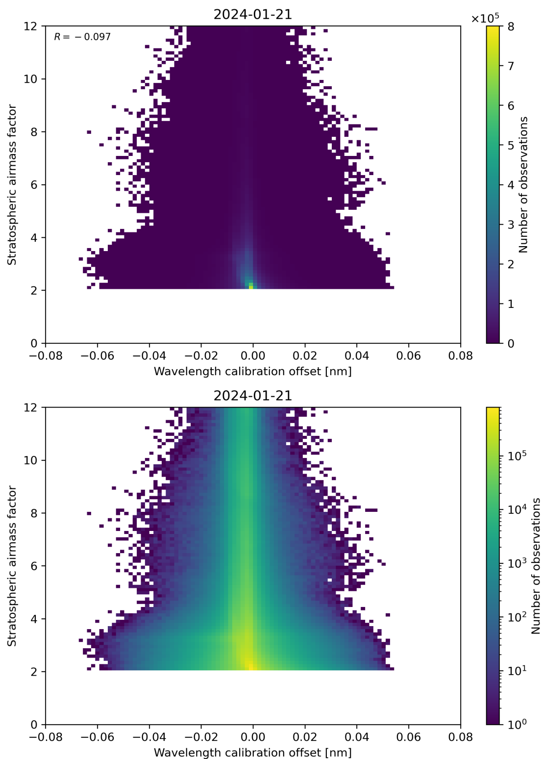
Figure 174: Scatter density plot of “Wavelength calibration offset” against “Stratospheric airmass factor” for 2024-01-21 to 2024-01-22.
