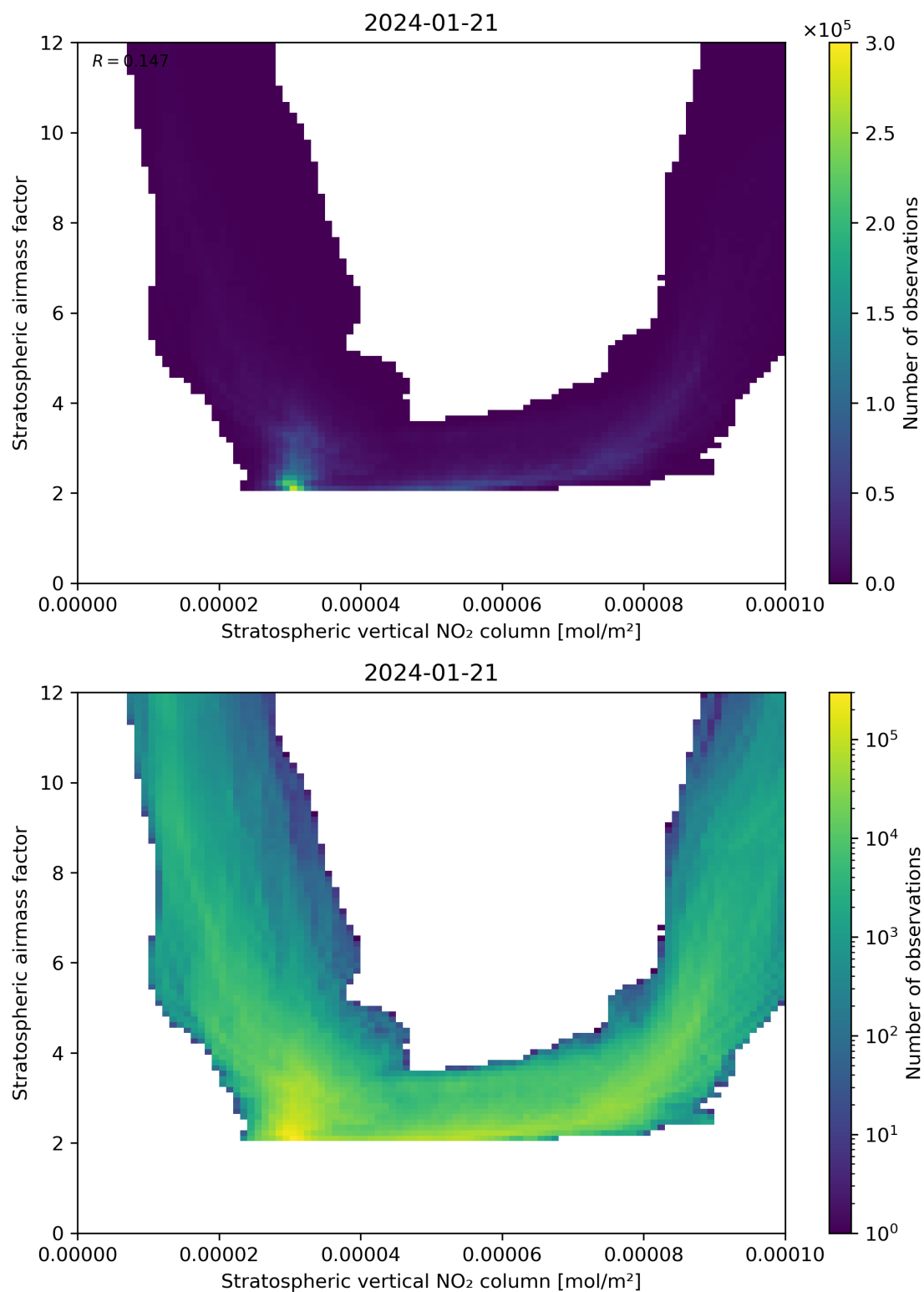
Figure 96: Scatter density plot of “Stratospheric vertical NO 2 column” against “Stratospheric airmass factor” for 2024-01-21 to 2024-01-22.
