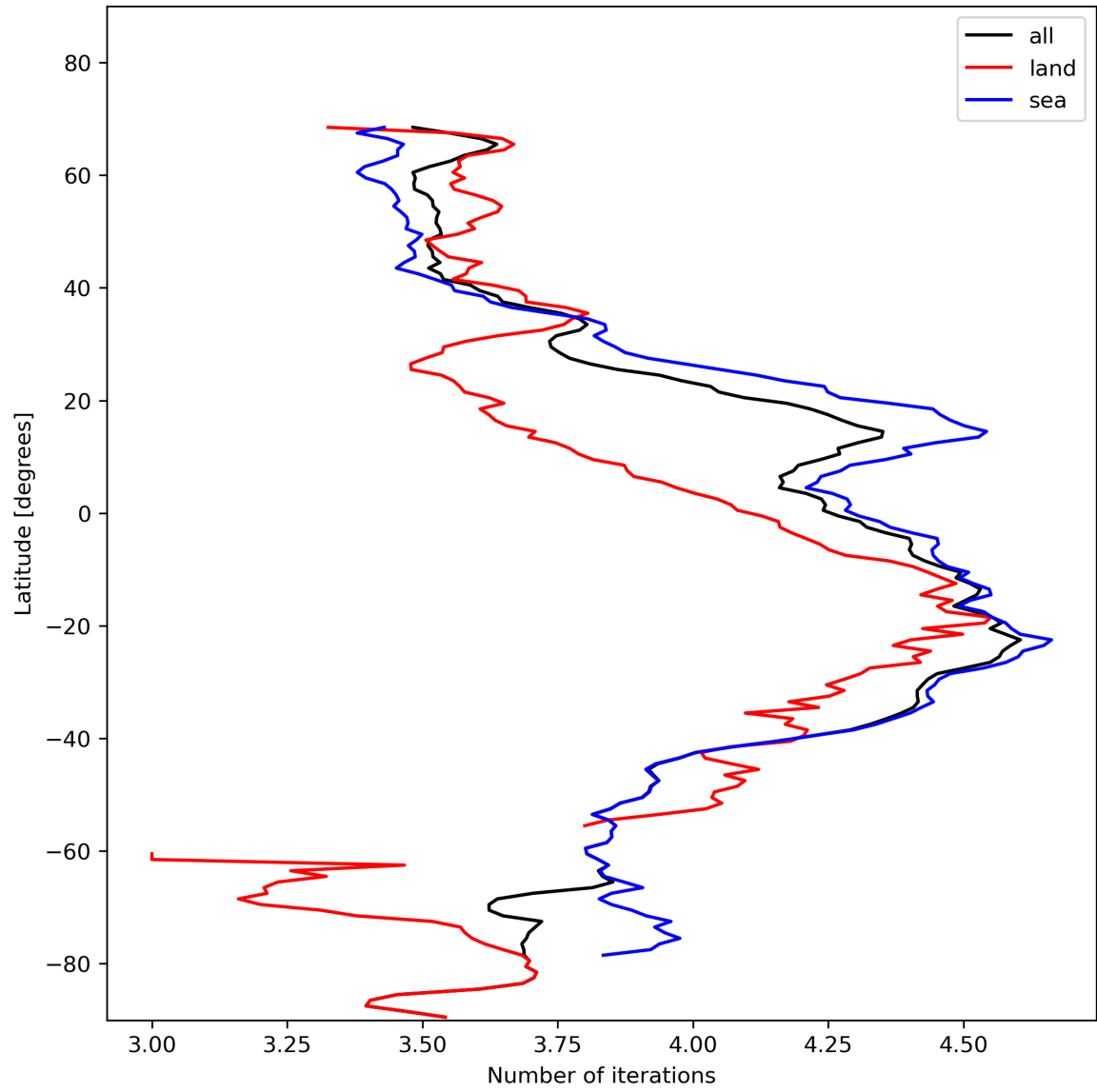
Figure 17: Zonal average of “Number of iterations” for 2024-01-21 to 2024-01-22.
