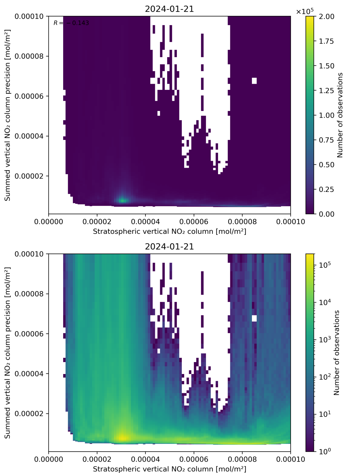
Figure 99: Scatter density plot of “Stratospheric vertical NO 2 column” against “Summed vertical NO 2 column precision” for 2024-01-21 to 2024-01-22.
