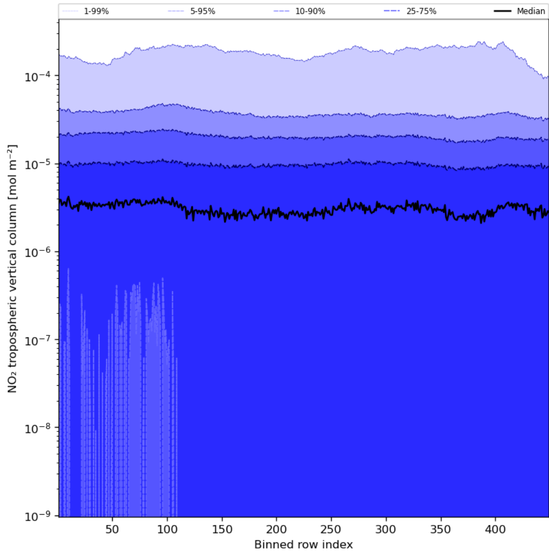
Figure 46: Along track statistics of “ \text{NO}_2 tropospheric vertical column” for 2024-01-21 to 2024-01-22
