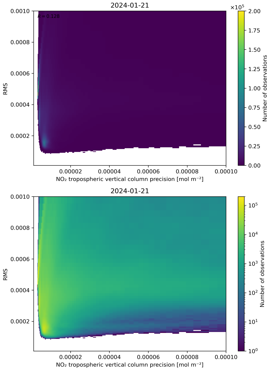
Figure 140: Scatter density plot of “NO 2 tropospheric vertical column precision” against “RMS” for 2024-01-21 to 2024-01-22.
