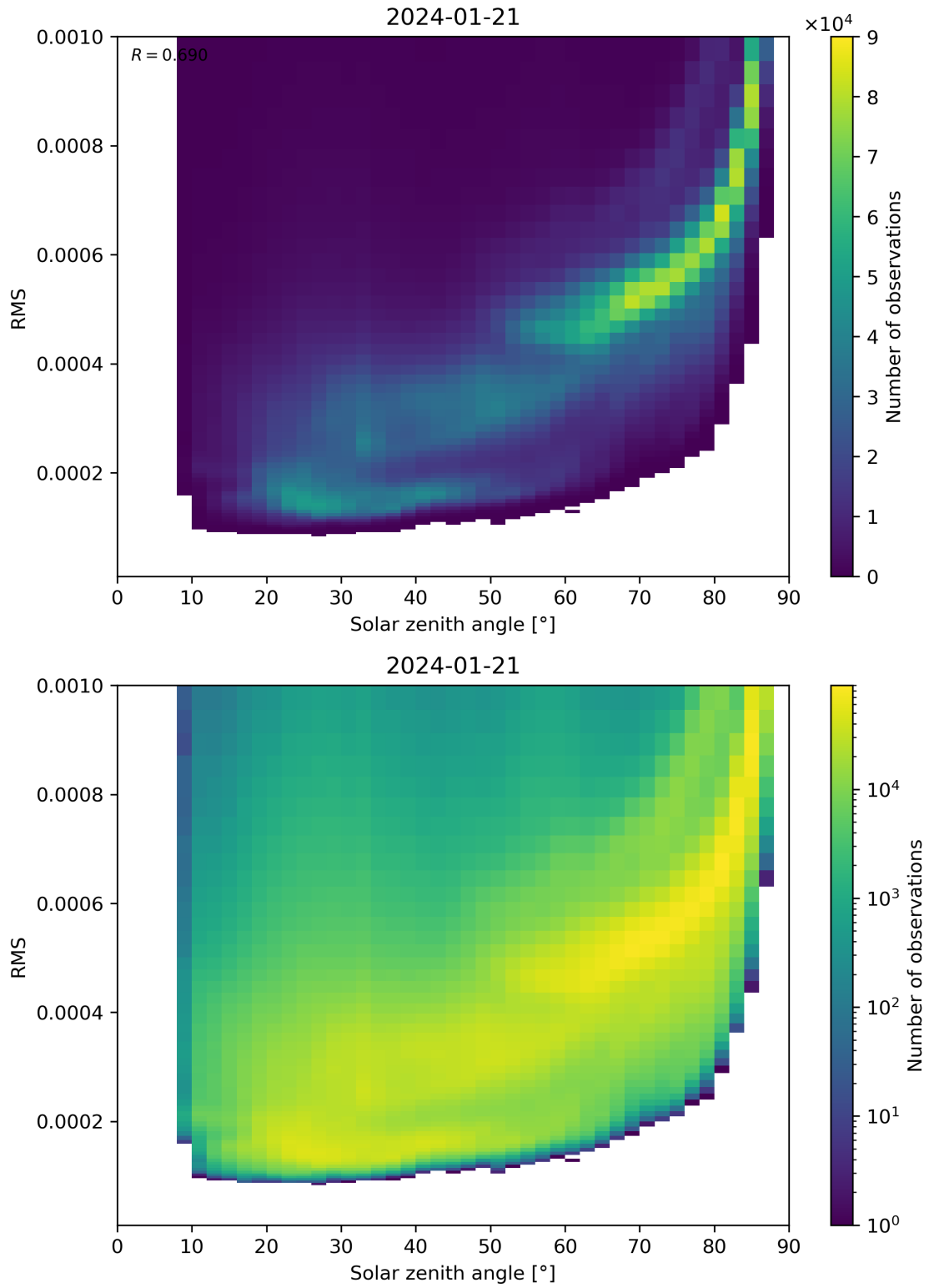
Figure 157: Scatter density plot of “Solar zenith angle” against “RMS” for 2024-01-21 to 2024-01-22.
