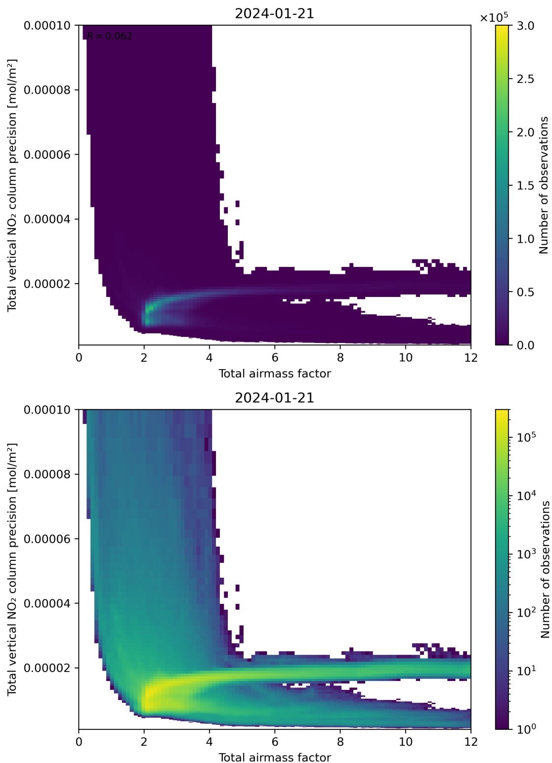
Figure 68: Scatter density plot of “Total airmass factor” against “Total vertical NO 2 column precision” for 2024-01-21 to 2024-01-22.
