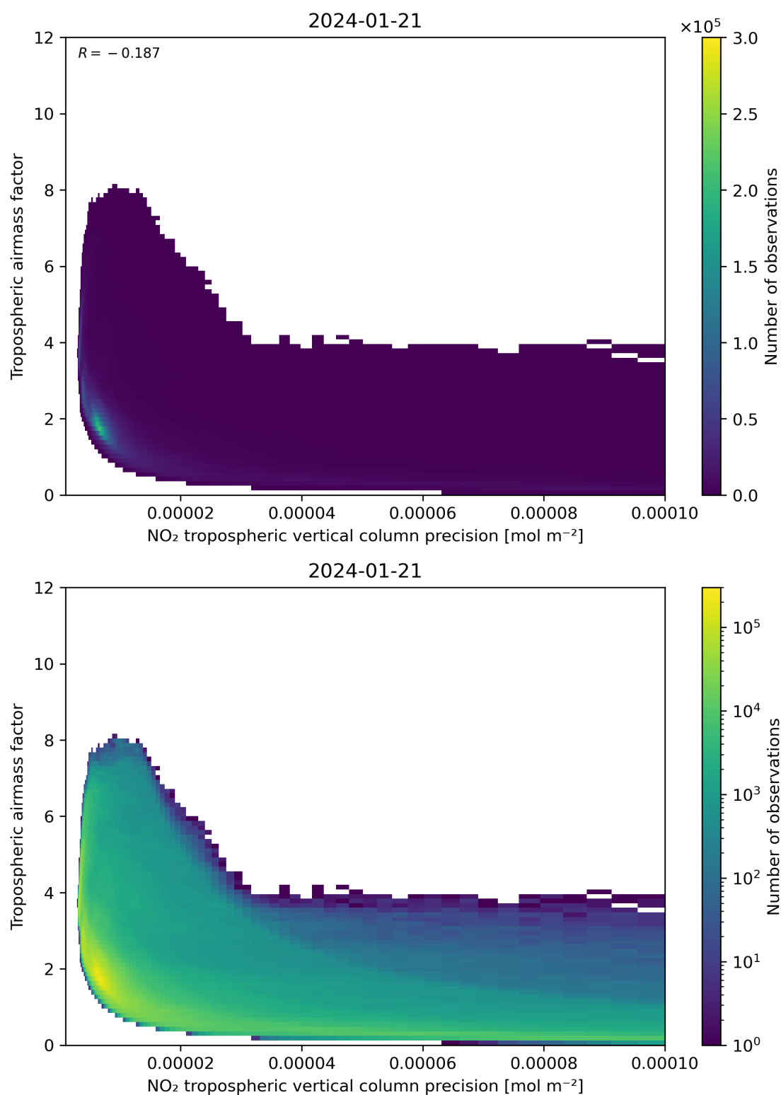
Figure 133: Scatter density plot of “NO 2 tropospheric vertical column precision” against “Tropospheric air mass factor” for 2024-01-21 to 2024-01-22.
