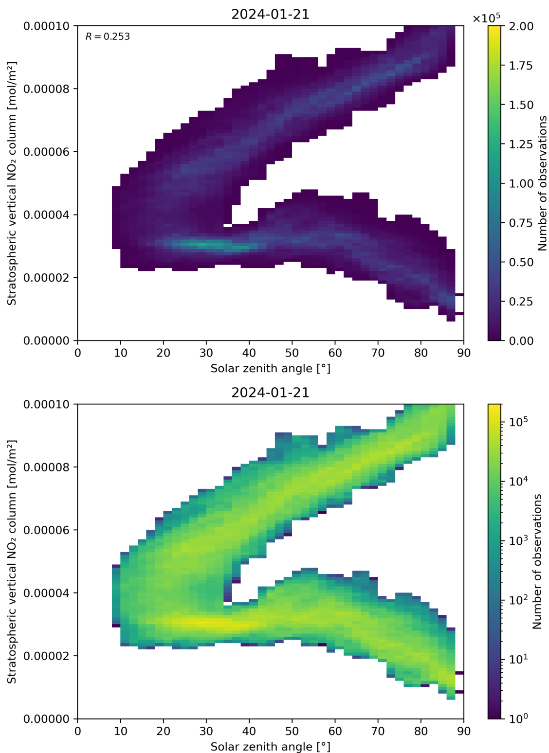
Figure 150: Scatter density plot of “Solar zenith angle” against “Stratospheric vertical NO 2 column” for 2024-01-21 to 2024-01-22.
