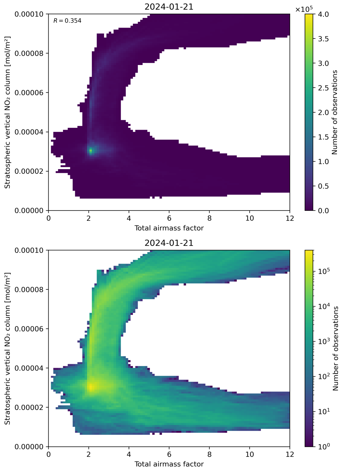
Figure 64: Scatter density plot of “Total airmass factor” against “Stratospheric vertical NO 2 column” for 2024-01-21 to 2024-01-22.
