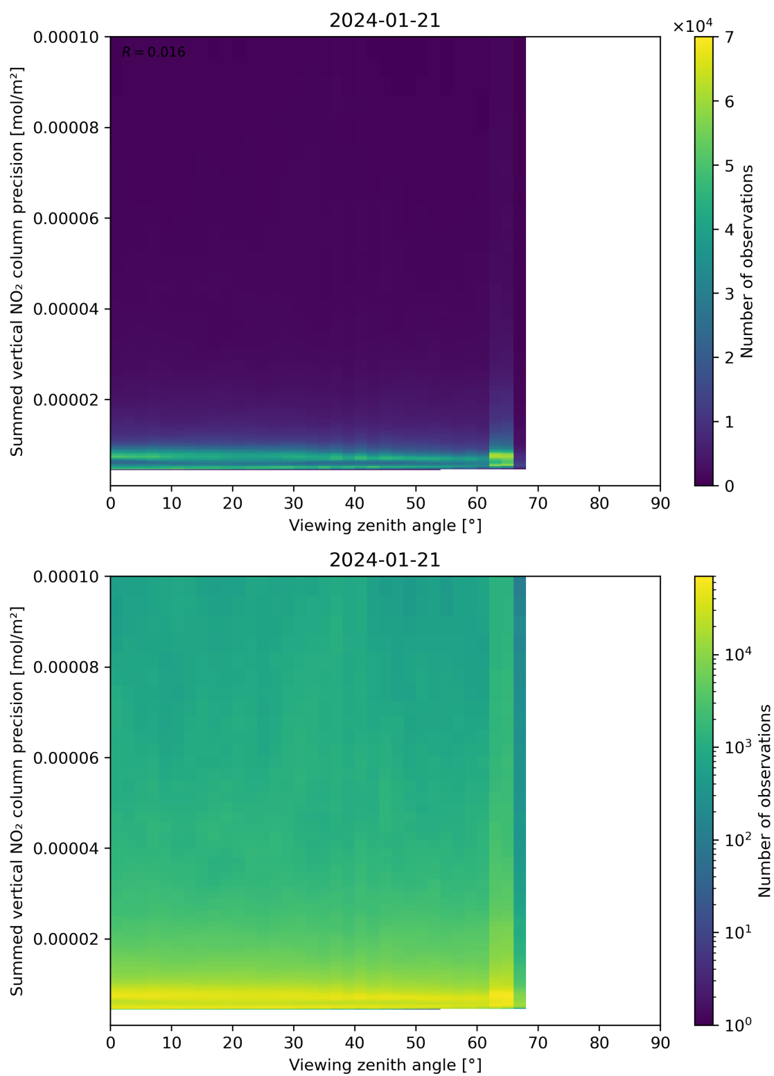
Figure 166: Scatter density plot of “Viewing zenith angle” against “Summed vertical NO 2 column precision” for 2024-01-21 to 2024-01-22.
