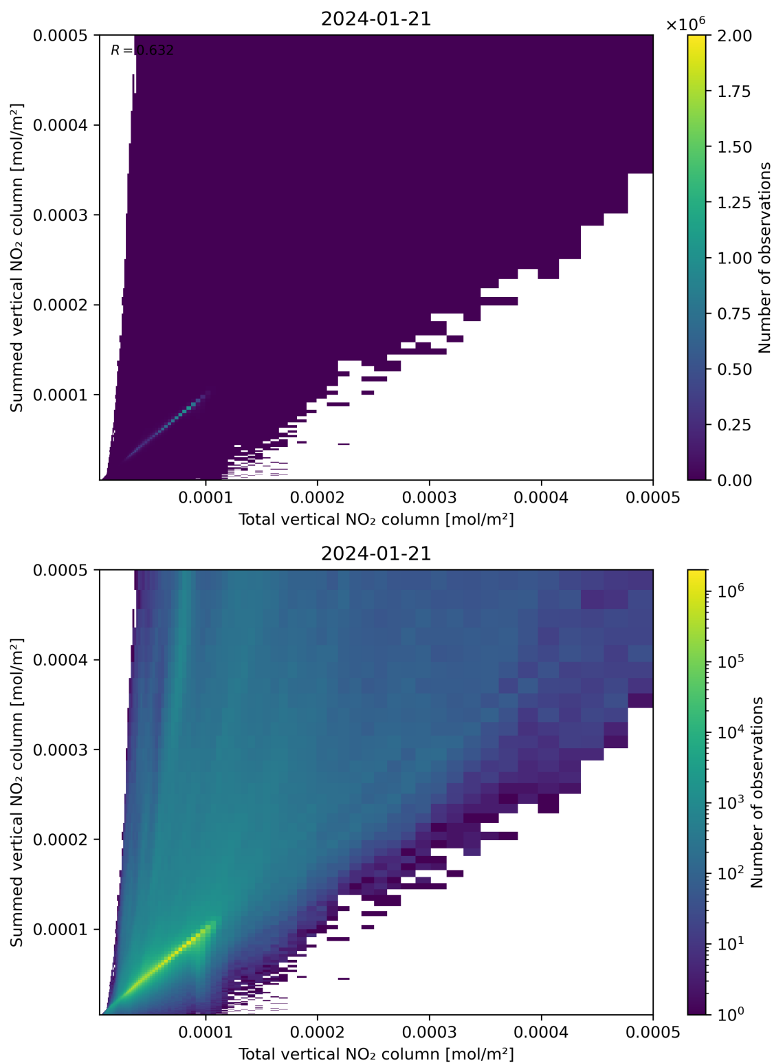
Figure 112: Scatter density plot of “Total vertical NO 2 column” against “Summed vertical NO 2 column” for 2024-01-21 to 2024-01-22.
