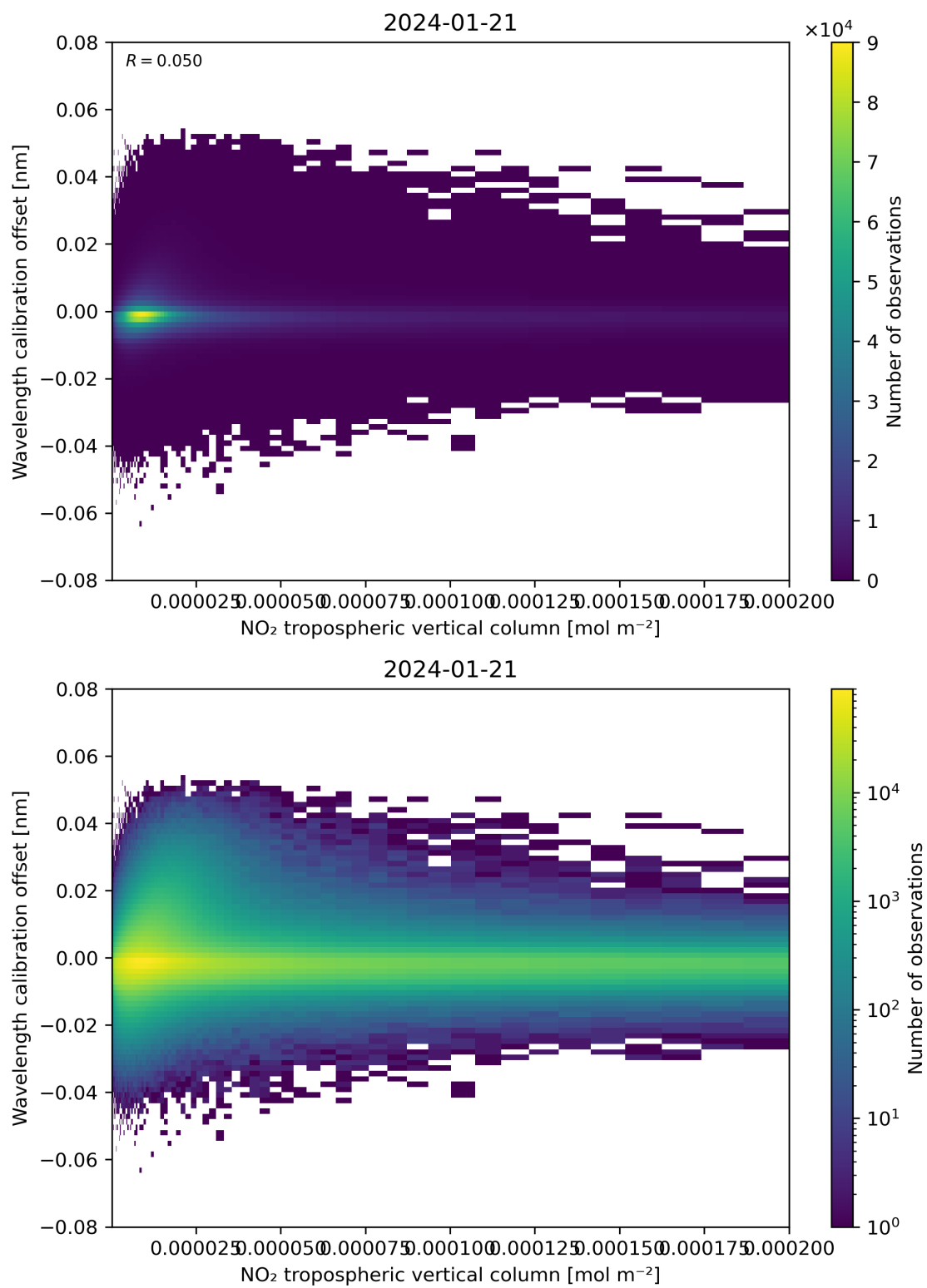
Figure 143: Scatter density plot of “NO 2 tropospheric vertical column” against “Wavelength calibration offset” for 2024-01-21 to 2024-01-22.
