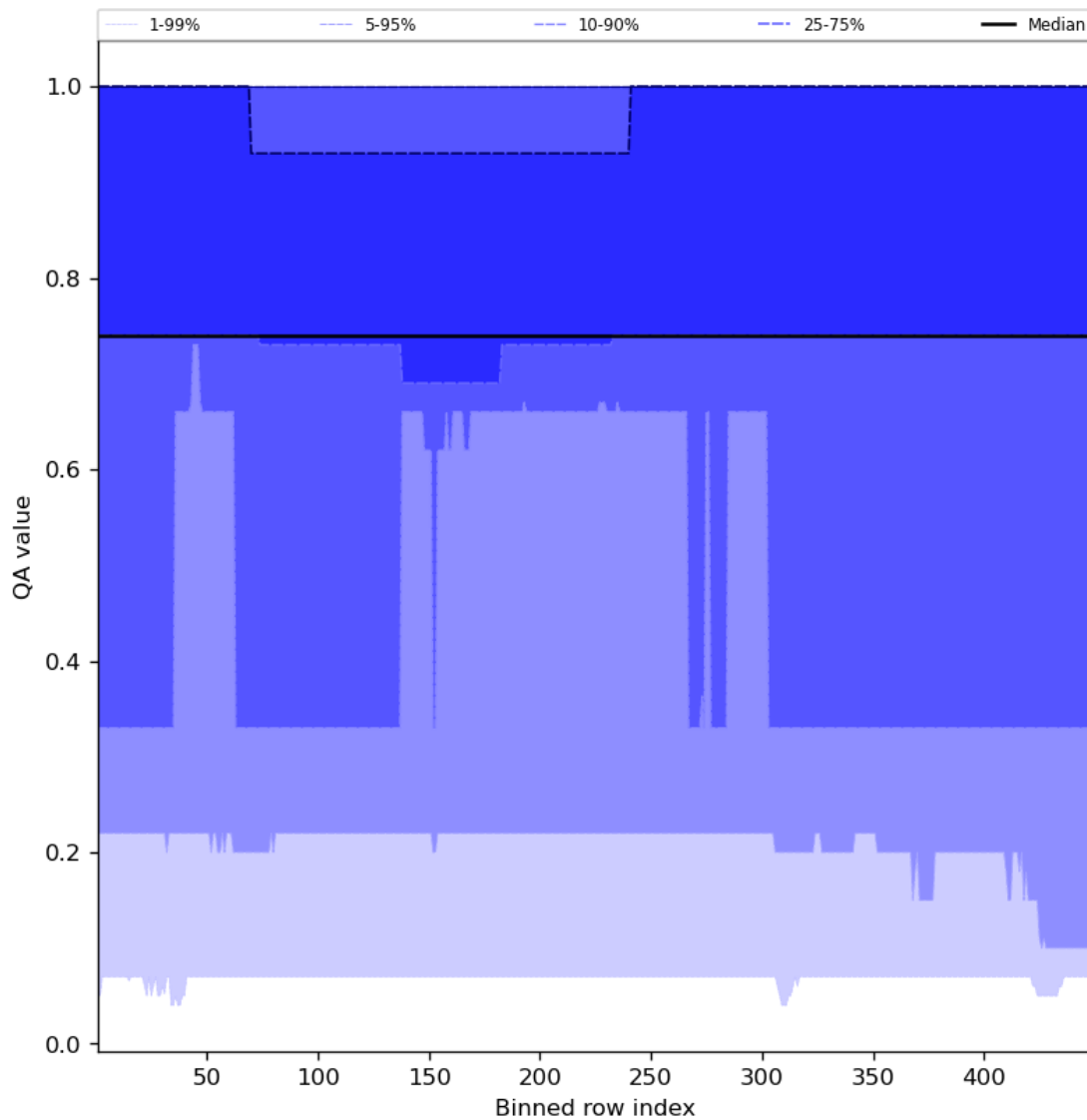
Figure 45: Along track statistics of “QA value” for 2024-01-21 to 2024-01-22
