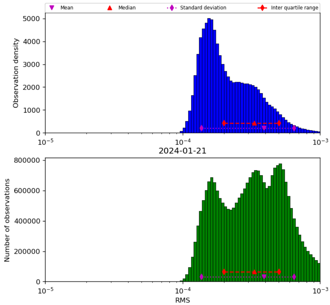
Figure 43: Histogram of “RMS” for 2024-01-21 to 2024-01-22
