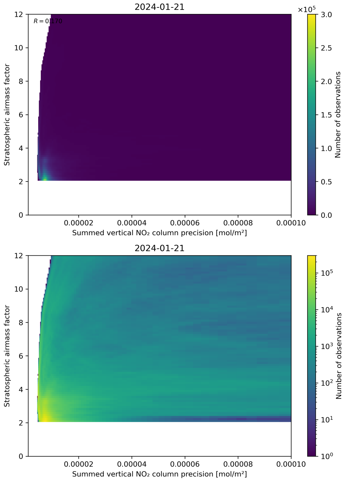
Figure 106: Scatter density plot of “Summed vertical NO 2 column precision” against “Stratospheric airmass factor” for 2024-01-21 to 2024-01-22.
