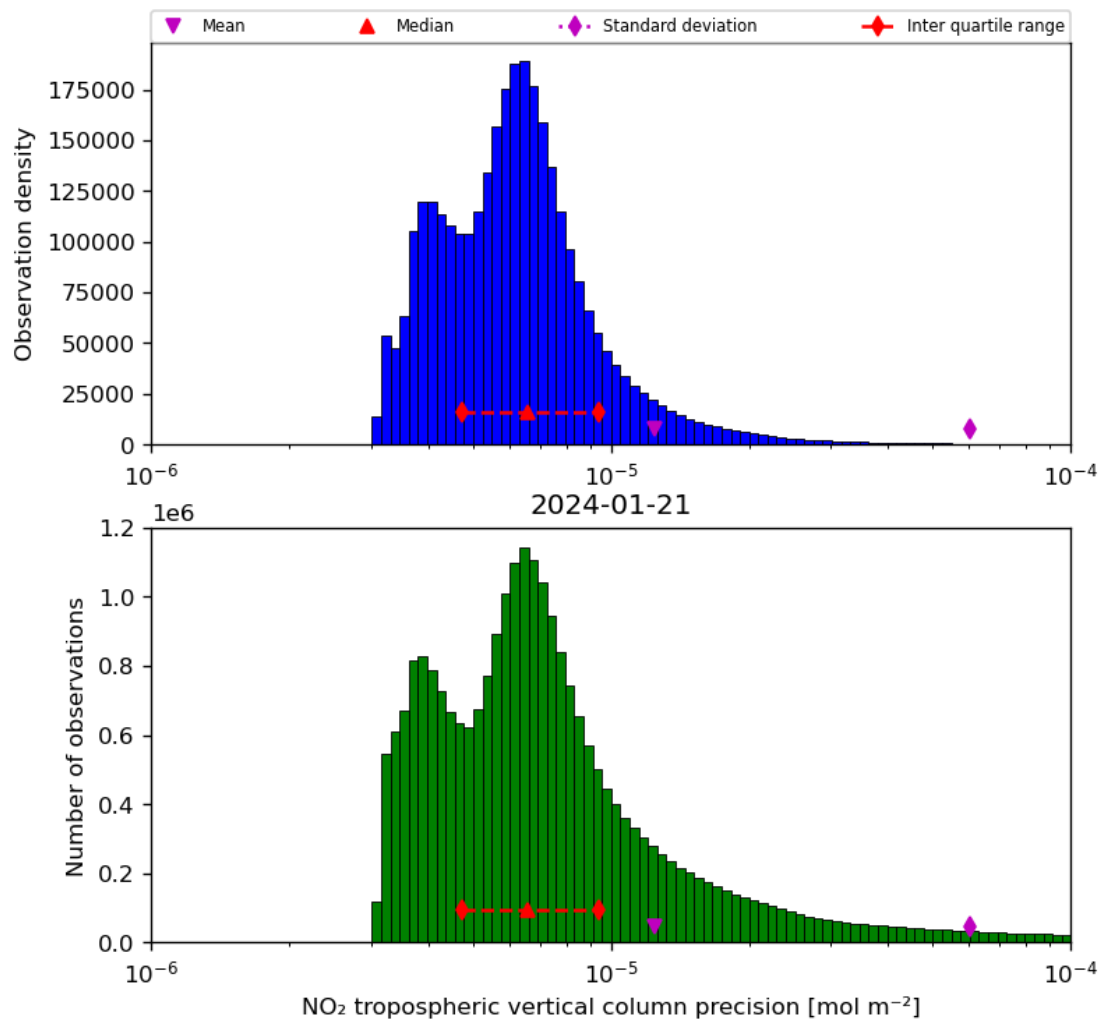
Figure 30: Histogram of “NO 2 tropospheric vertical column precision” for 2024-01-21 to 2024-01-22
