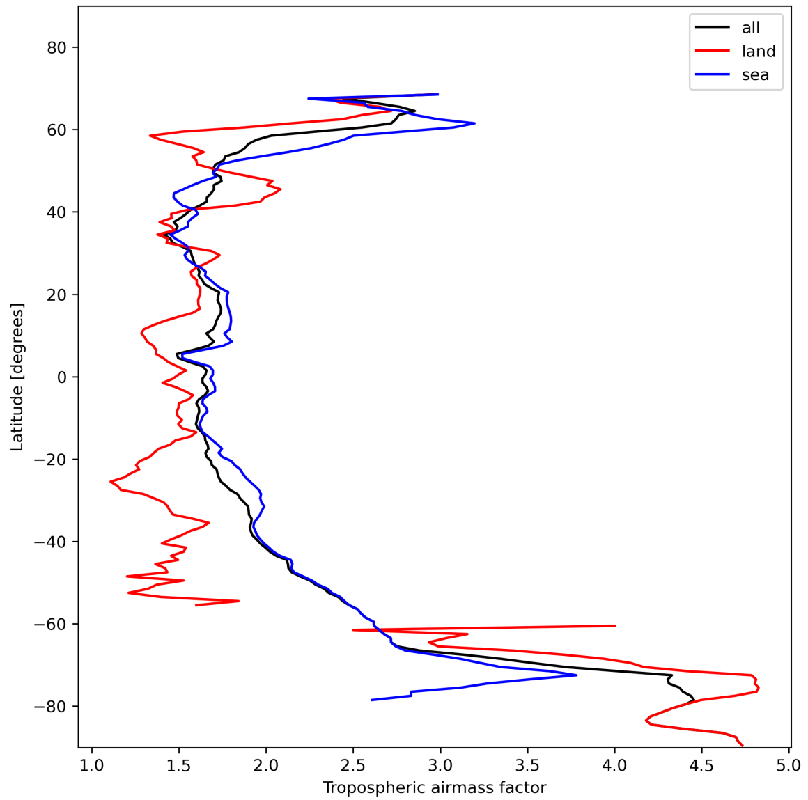
Figure 14: Zonal average of “Tropospheric airmass factor” for 2024-01-21 to 2024-01-22.
