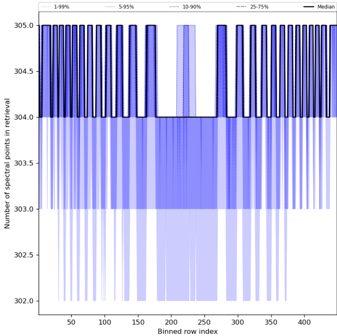
Figure 50: Along track statistics of “Number of spectral points in retrieval” for 2024-01-21 to 2024-01-22
