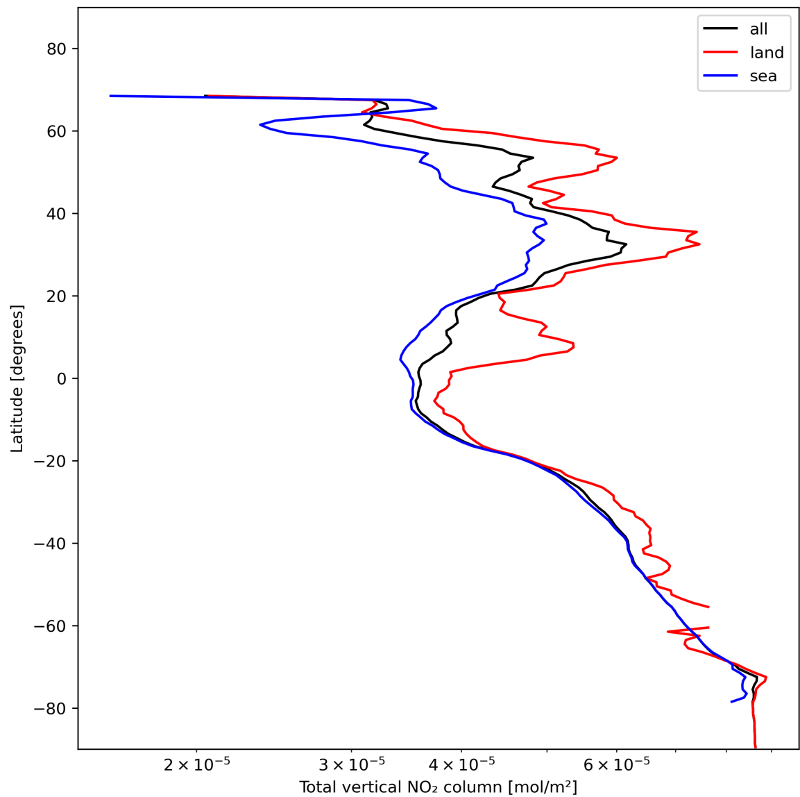
Figure 21: Zonal average of “Total vertical NO 2 column” for 2024-01-21 to 2024-01-22.
