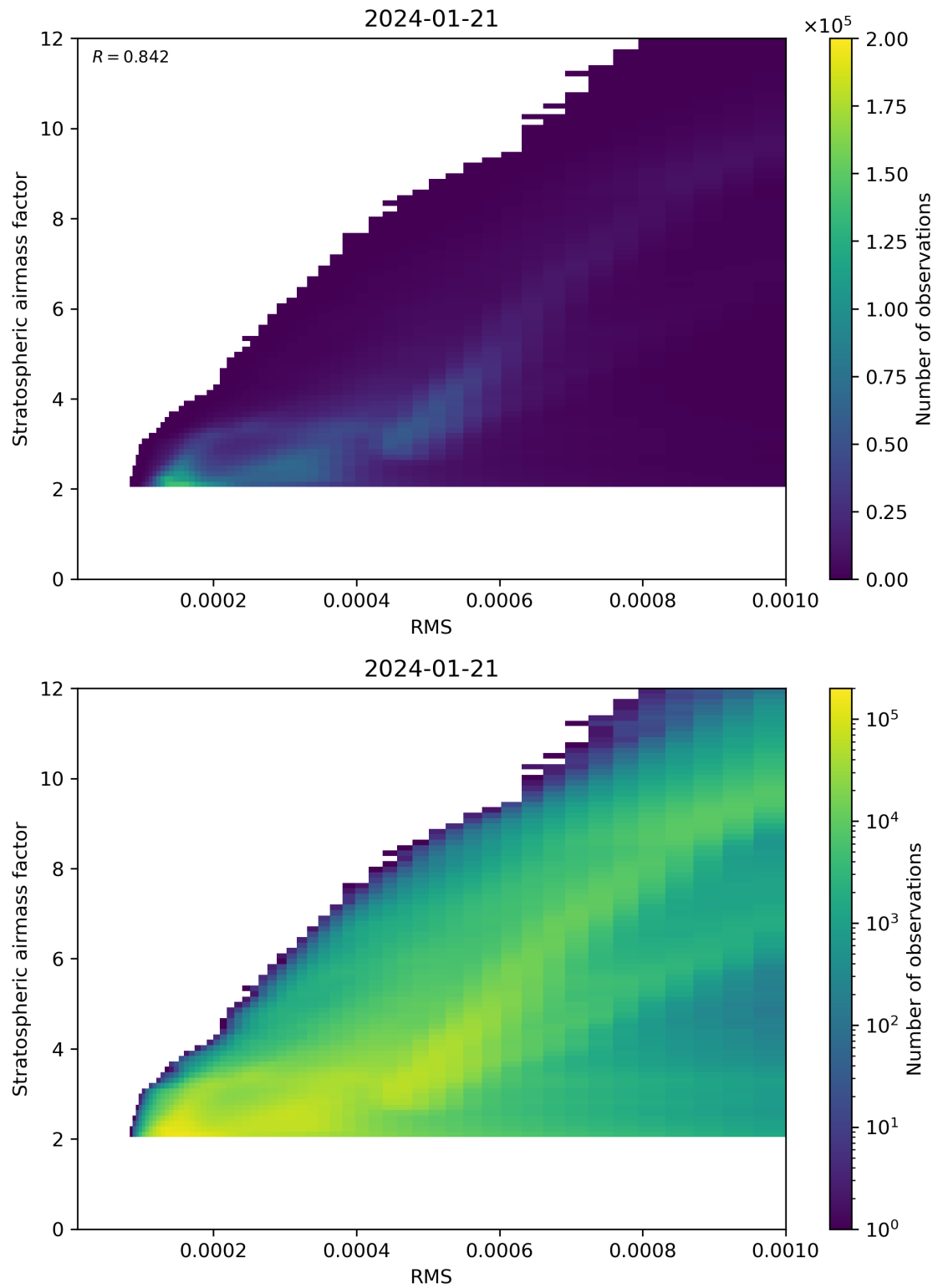
Figure 144: Scatter density plot of “RMS” against “Stratospheric airmass factor” for 2024-01-21 to 2024-01-22.
