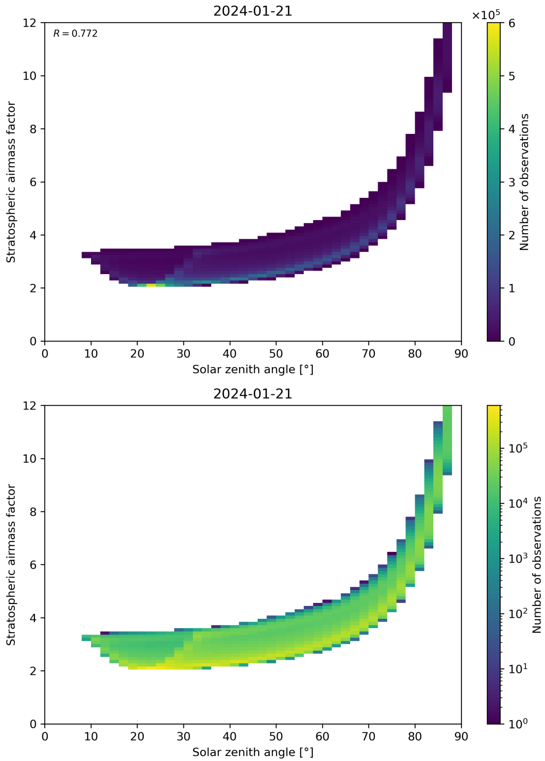
Figure 145: Scatter density plot of “Solar zenith angle” against “Stratospheric airmass factor” for 2024-01-21 to 2024-01-22.
