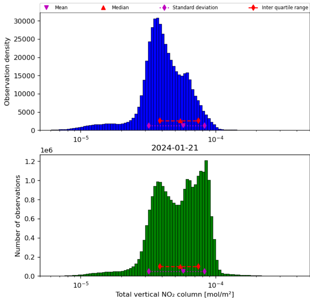
Figure 38: Histogram of "Total vertical NO 2 column" for 2024-01-21 to 2024-01-22
