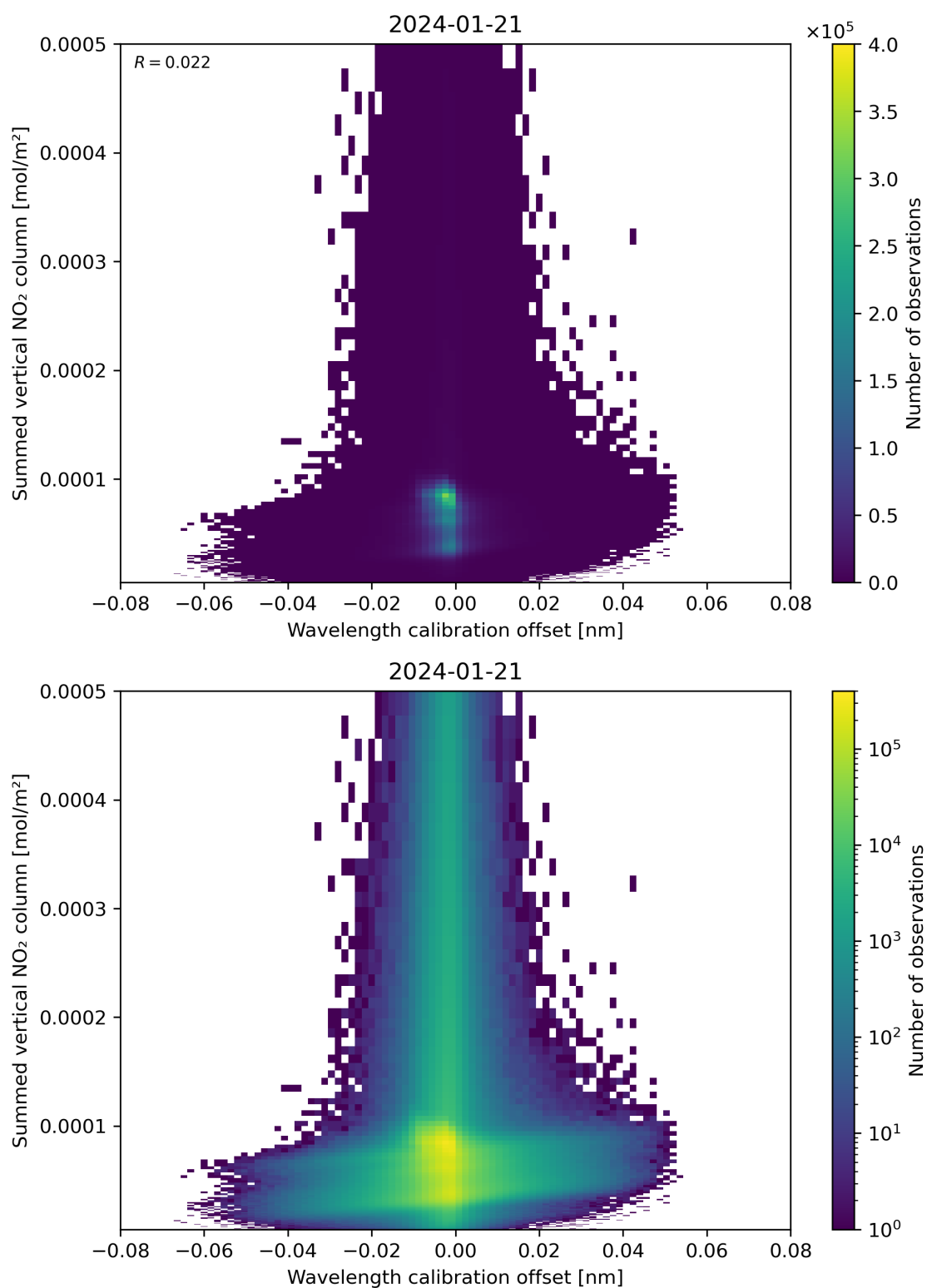
Figure 177: Scatter density plot of “Wavelength calibration offset” against “Summed vertical NO 2 column” for 2024-01-21 to 2024-01-22.
