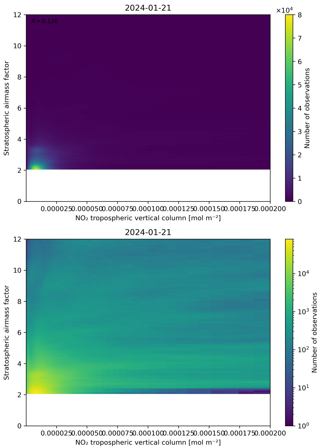
Figure 121: Scatter density plot of “NO 2 tropospheric vertical column” against “Stratospheric airmass factor” for 2024-01-21 to 2024-01-22.
