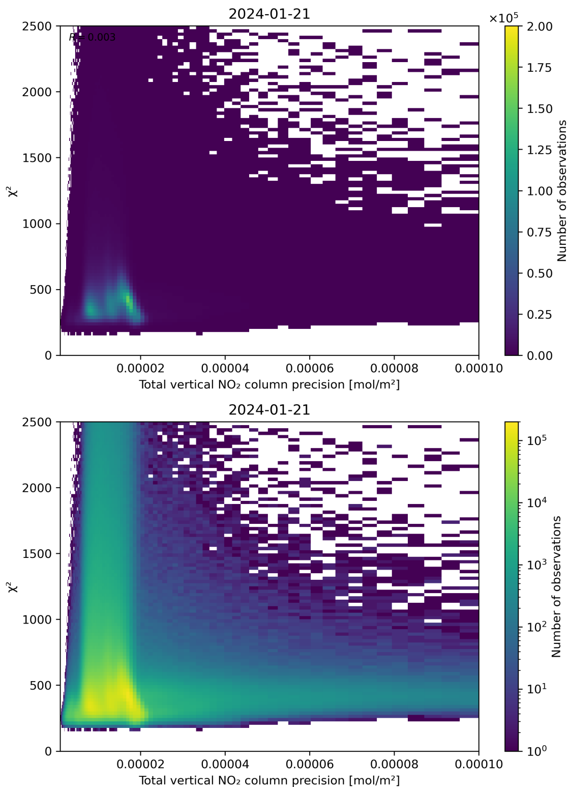
Figure 116: Scatter density plot of “Total vertical NO 2 column precision” against “ \chi^2 ” for 2024-01-21 to 2024-01-22.
