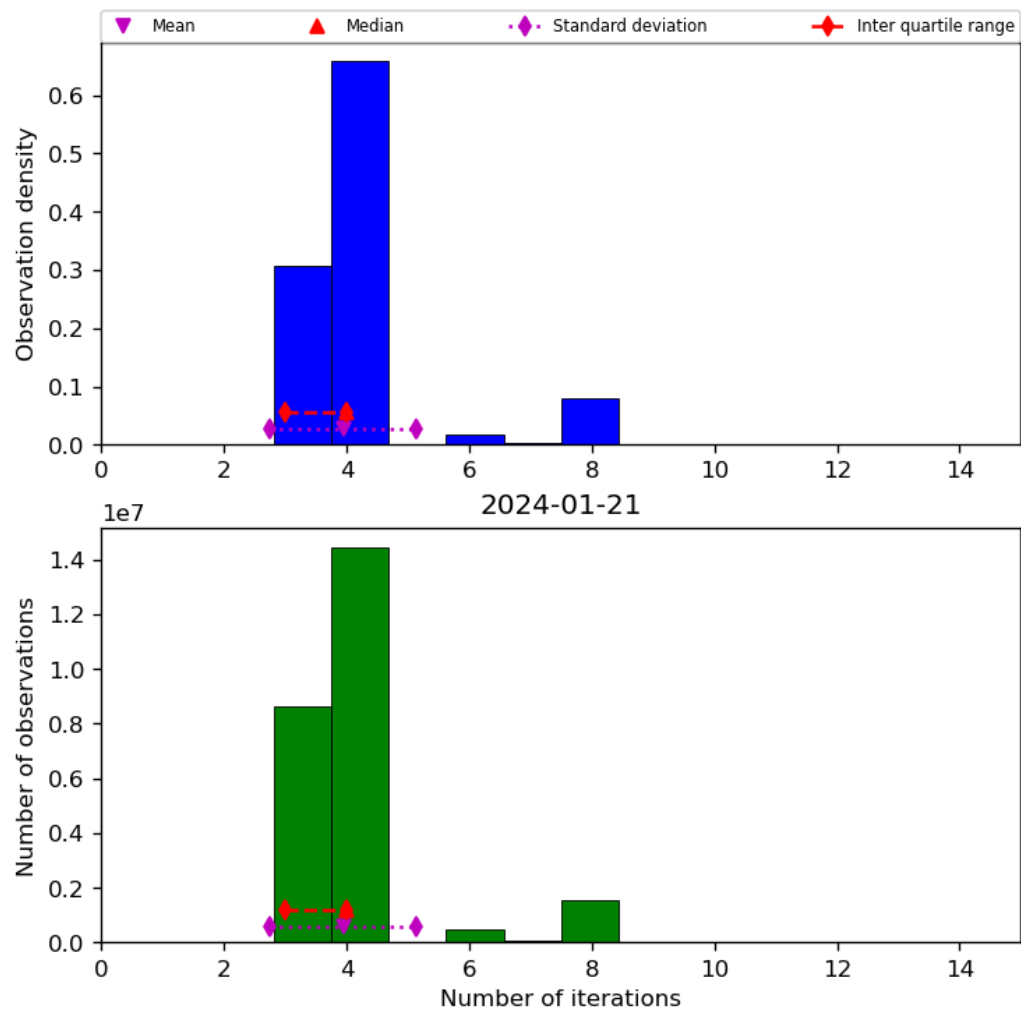
Figure 34: Histogram of “Number of iterations” for 2024-01-21 to 2024-01-22
