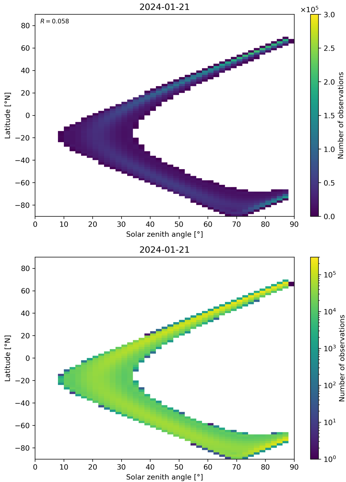
Figure 149: Scatter density plot of “Solar zenith angle” against “Latitude” for 2024-01-21 to 2024-01-22.
