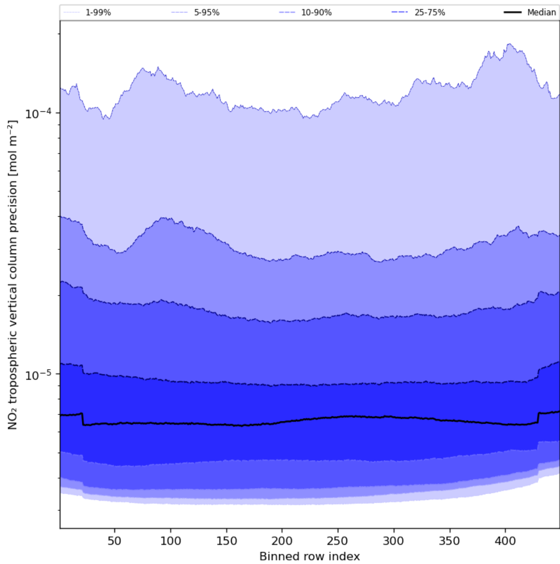
Figure 47: Along track statistics of “NO 2 tropospheric vertical column precision” for 2024-01-21 to 2024-01-22
