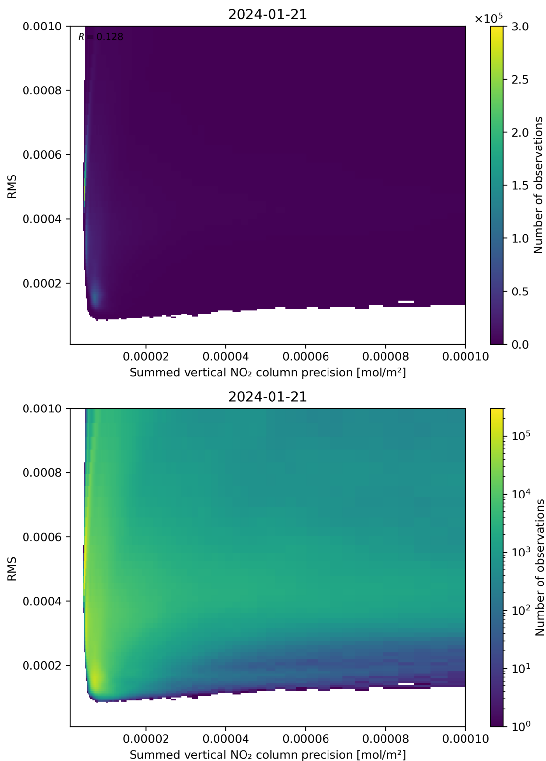
Figure 108: Scatter density plot of “Summed vertical NO 2 column precision” against “RMS” for 2024-01-21 to 2024-01-22.
