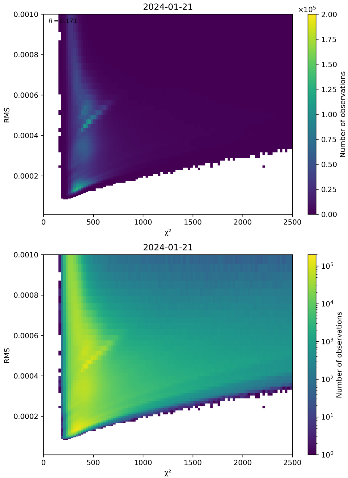
Figure 82: Scatter density plot of “ \chi^2 ” against “RMS” for 2024-01-21 to 2024-01-22.
