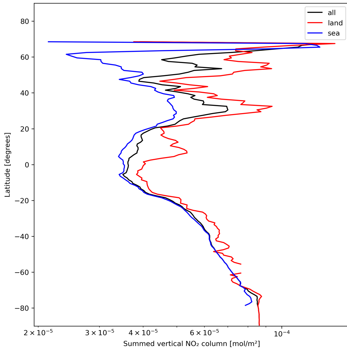
Figure 23: Zonal average of “Summed vertical NO 2 column” for 2024-01-21 to 2024-01-22.
