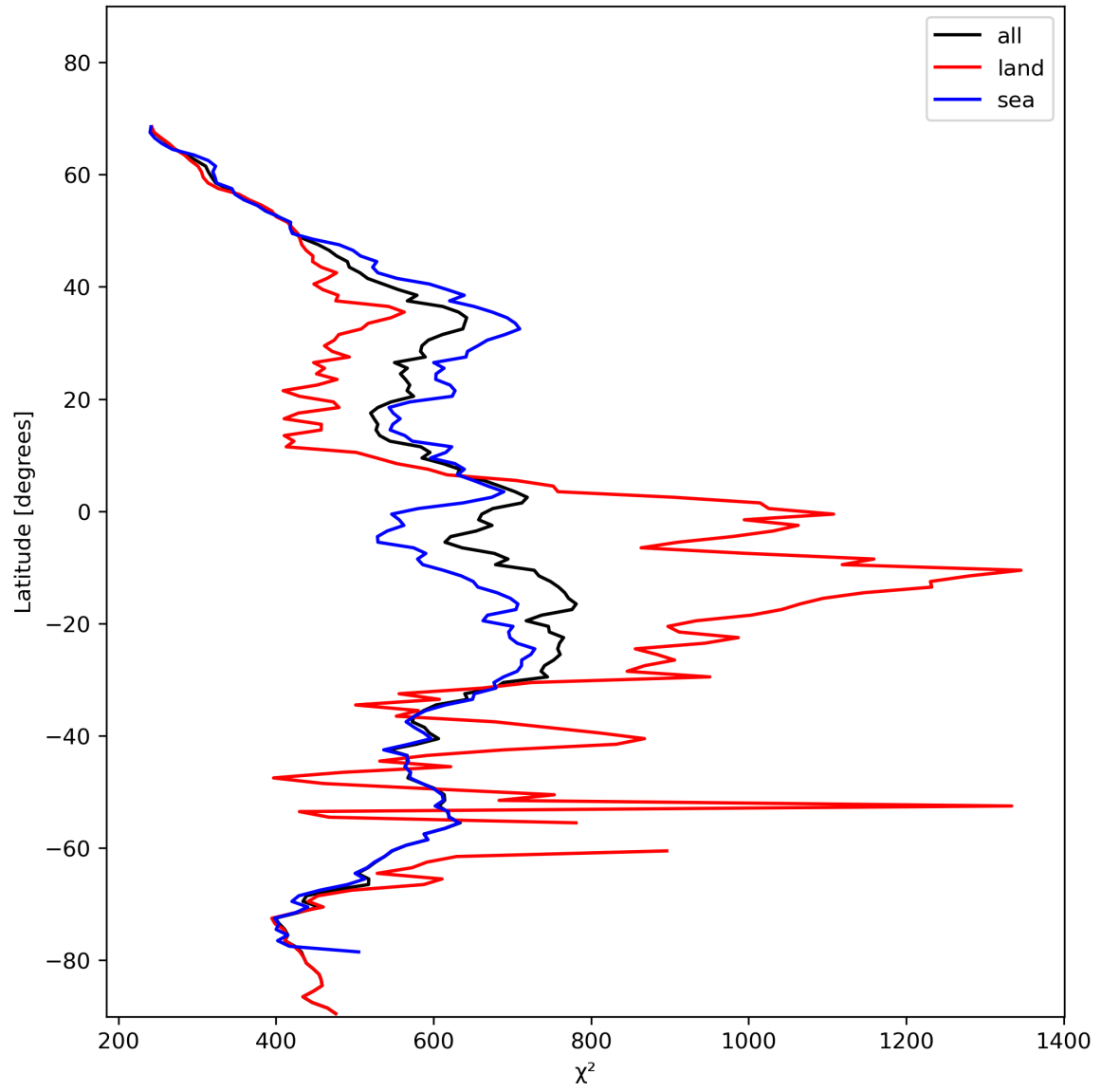
Figure 25: Zonal average of “ \chi^2 ” for 2024-01-21 to 2024-01-22.
