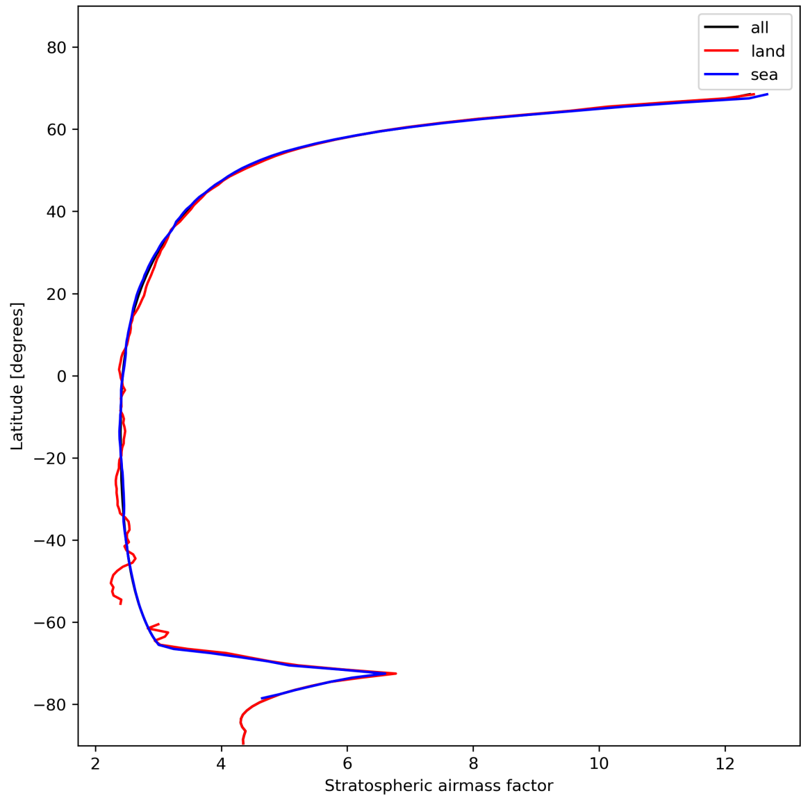
Figure 27: Zonal average of “Stratospheric airmass factor” for 2024-01-21 to 2024-01-22.
