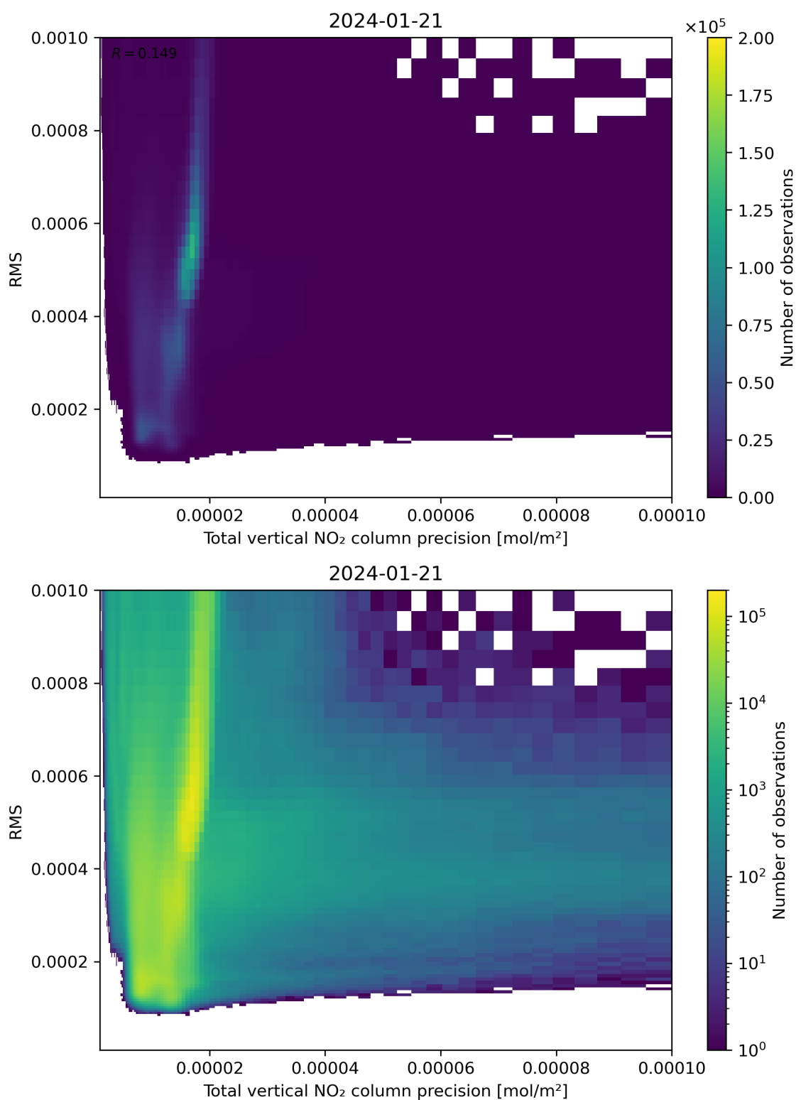
Figure 119: Scatter density plot of “Total vertical NO 2 column precision” against “RMS” for 2024-01-21 to 2024-01-22.
