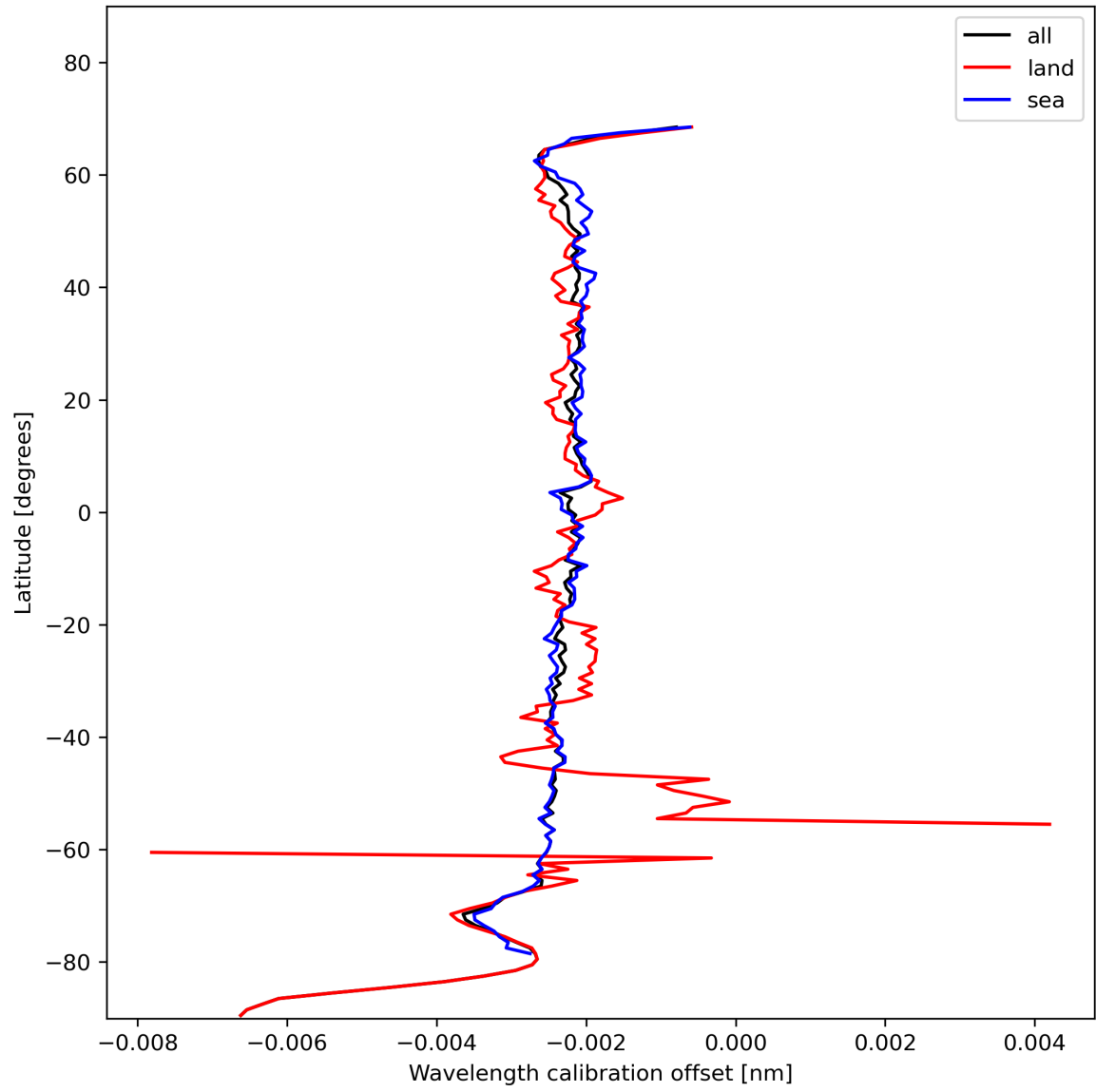
Figure 18: Zonal average of “Wavelength calibration offset” for 2024-01-21 to 2024-01-22.
