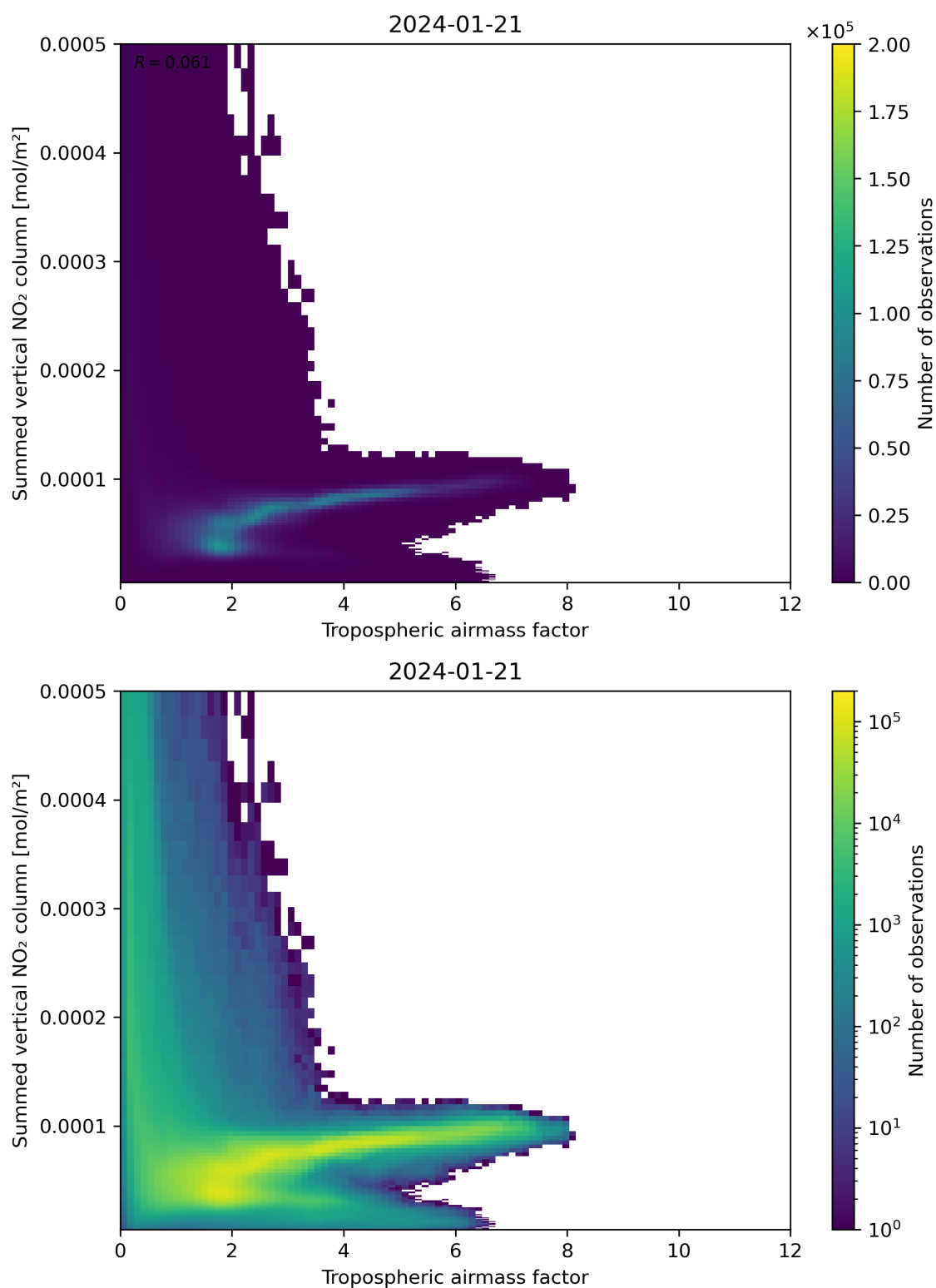
Figure 75: Scatter density plot of “Tropospheric airmass factor” against “Summed vertical NO 2 column” for 2024-01-21 to 2024-01-22.
