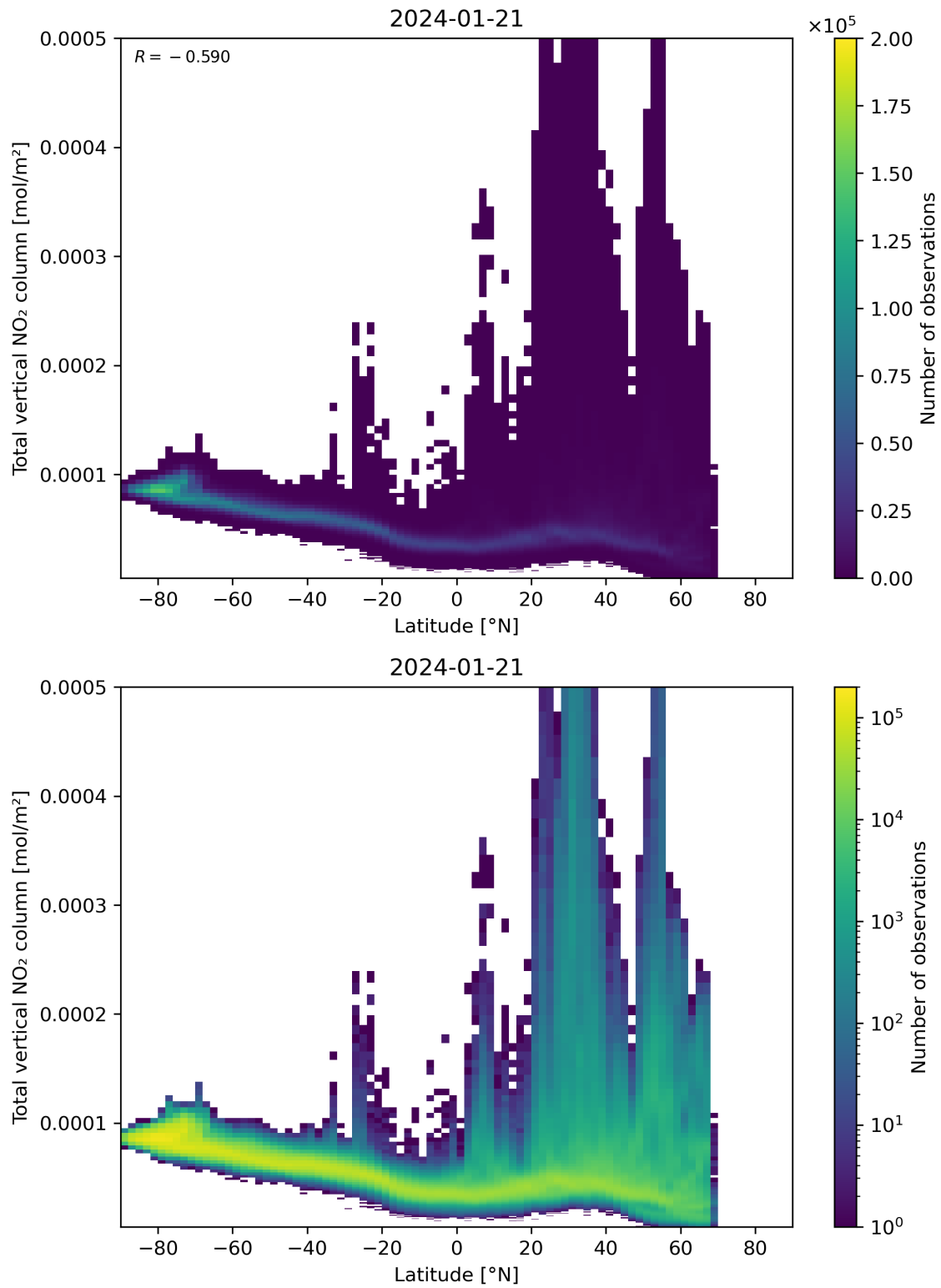
Figure 90: Scatter density plot of “Latitude” against “Total vertical NO 2 column” for 2024-01-21 to 2024-01-22.
