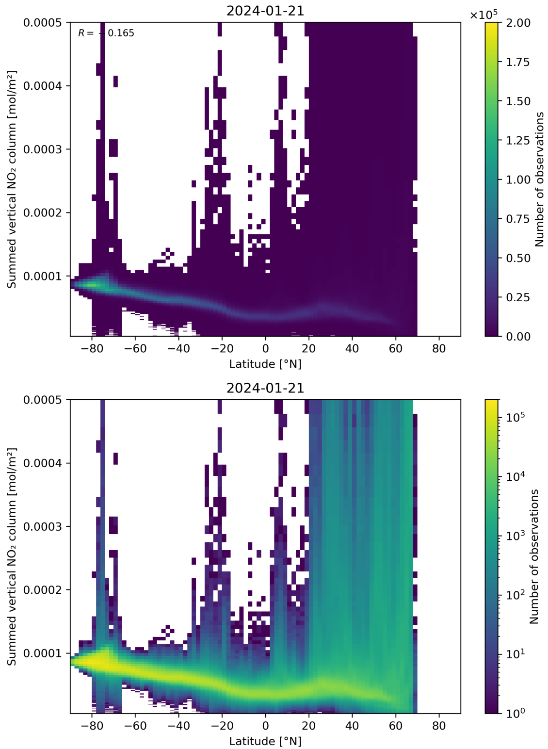
Figure 88: Scatter density plot of “Latitude” against “Summed vertical NO 2 column” for 2024-01-21 to 2024-01-22.
