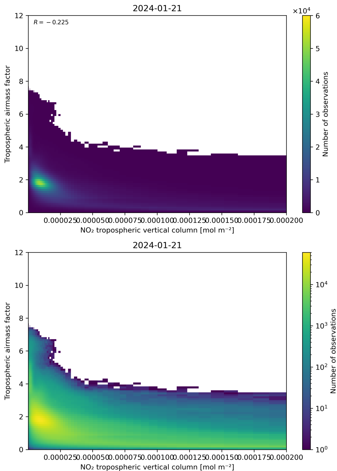
Figure 123: Scatter density plot of “NO 2 tropospheric vertical column” against “Tropospheric air mass factor” for 2024-01-21 to 2024-01-22.
