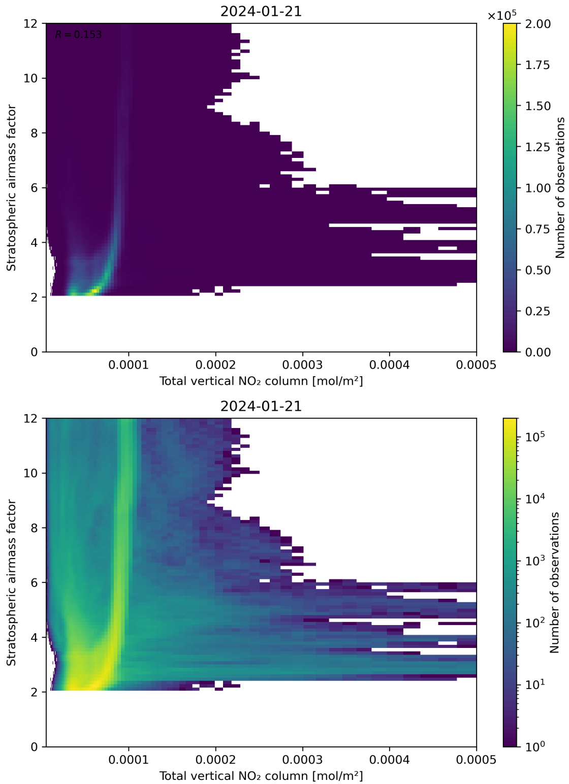
Figure 110: Scatter density plot of “Total vertical NO 2 column” against “Stratospheric airmass factor” for 2024-01-21 to 2024-01-22.
