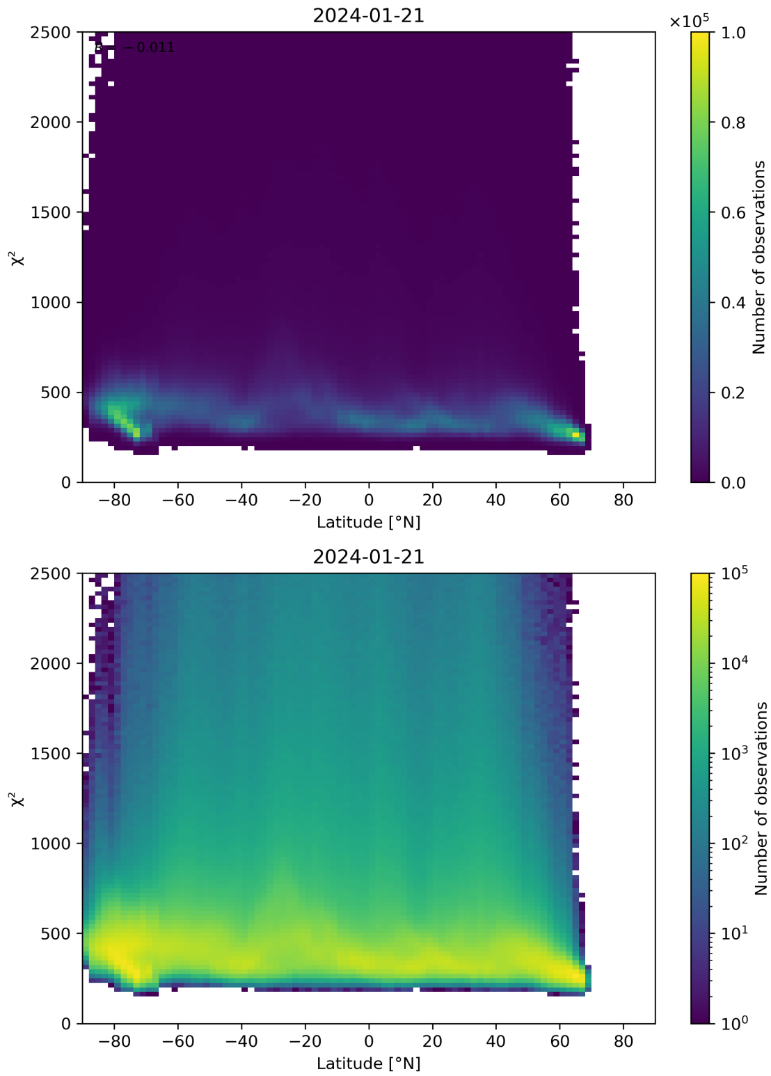
Figure 86: Scatter density plot of “Latitude” against “ \chi^2 ” for 2024-01-21 to 2024-01-22.
