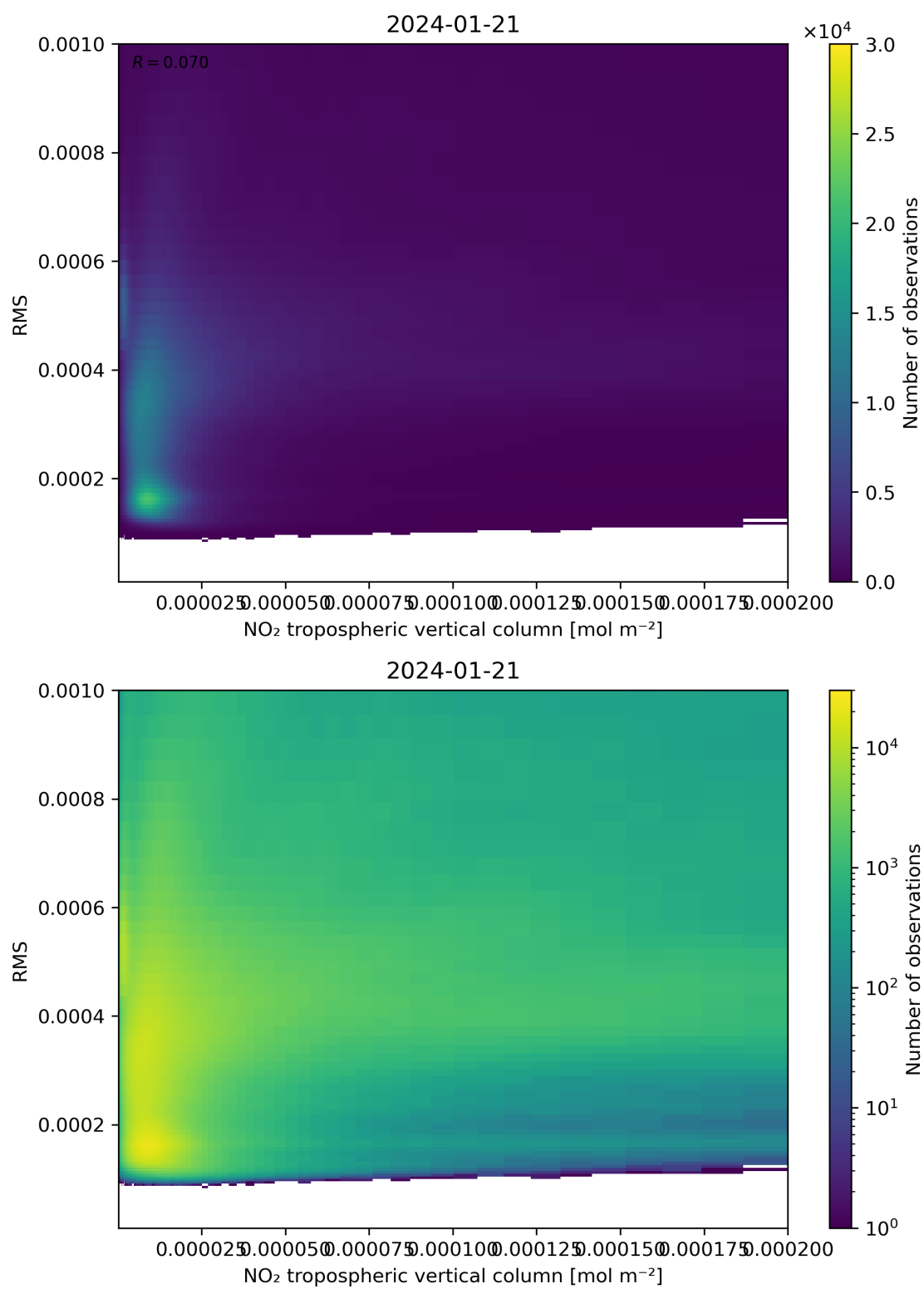
Figure 142: Scatter density plot of “NO 2 tropospheric vertical column” against “RMS” for 2024-01-21 to 2024-01-22.
