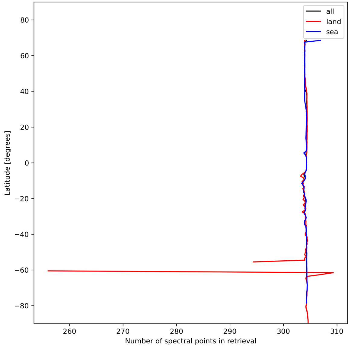
Figure 16: Zonal average of “Number of spectral points in retrieval” for 2024-01-21 to 2024-01-22.
