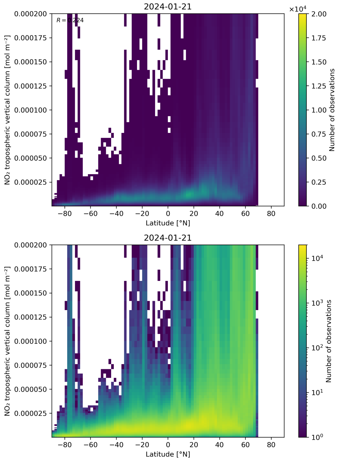
Figure 92: Scatter density plot of “Latitude” against “NO 2 tropospheric vertical column” for 2024-01-21 to 2024-01-22.
