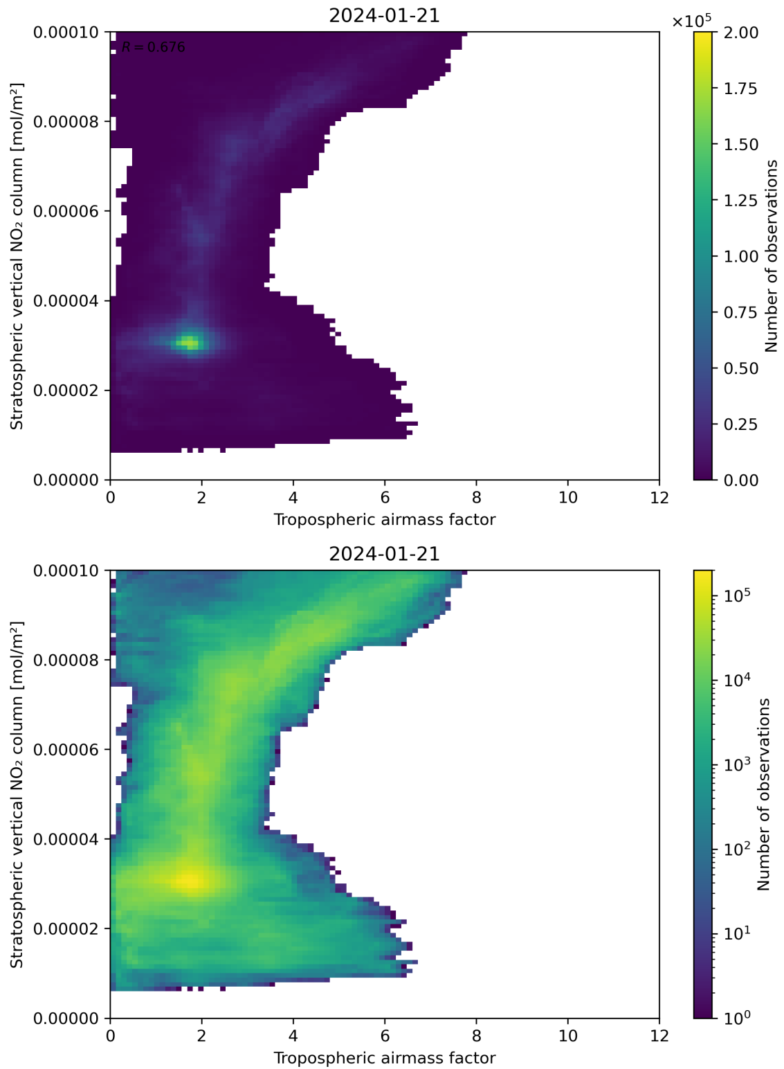
Figure 74: Scatter density plot of “Tropospheric air mass factor” against “Stratospheric vertical NO 2 column” for 2024-01-21 to 2024-01-22.
