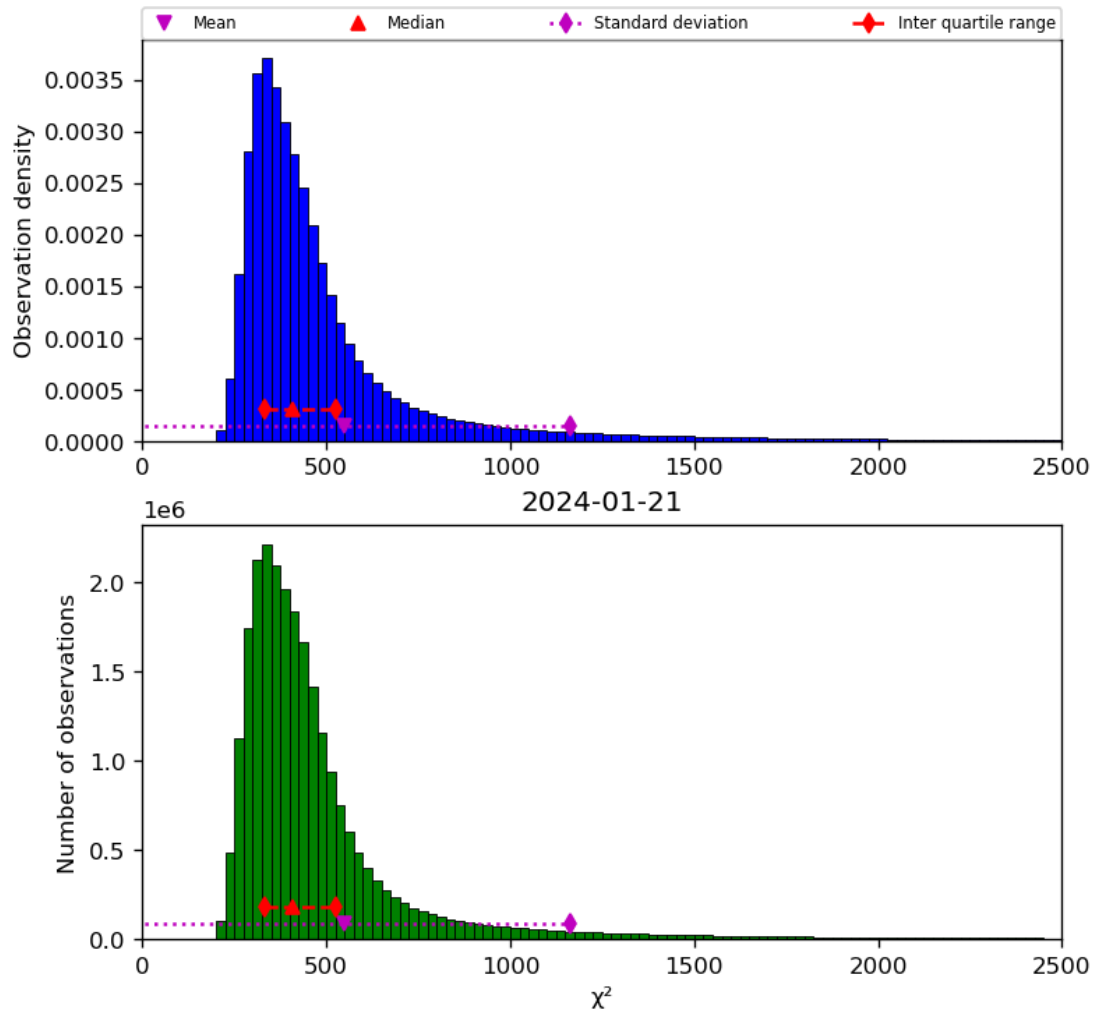
Figure 42: Histogram of “ \chi^2 ” for 2024-01-21 to 2024-01-22
