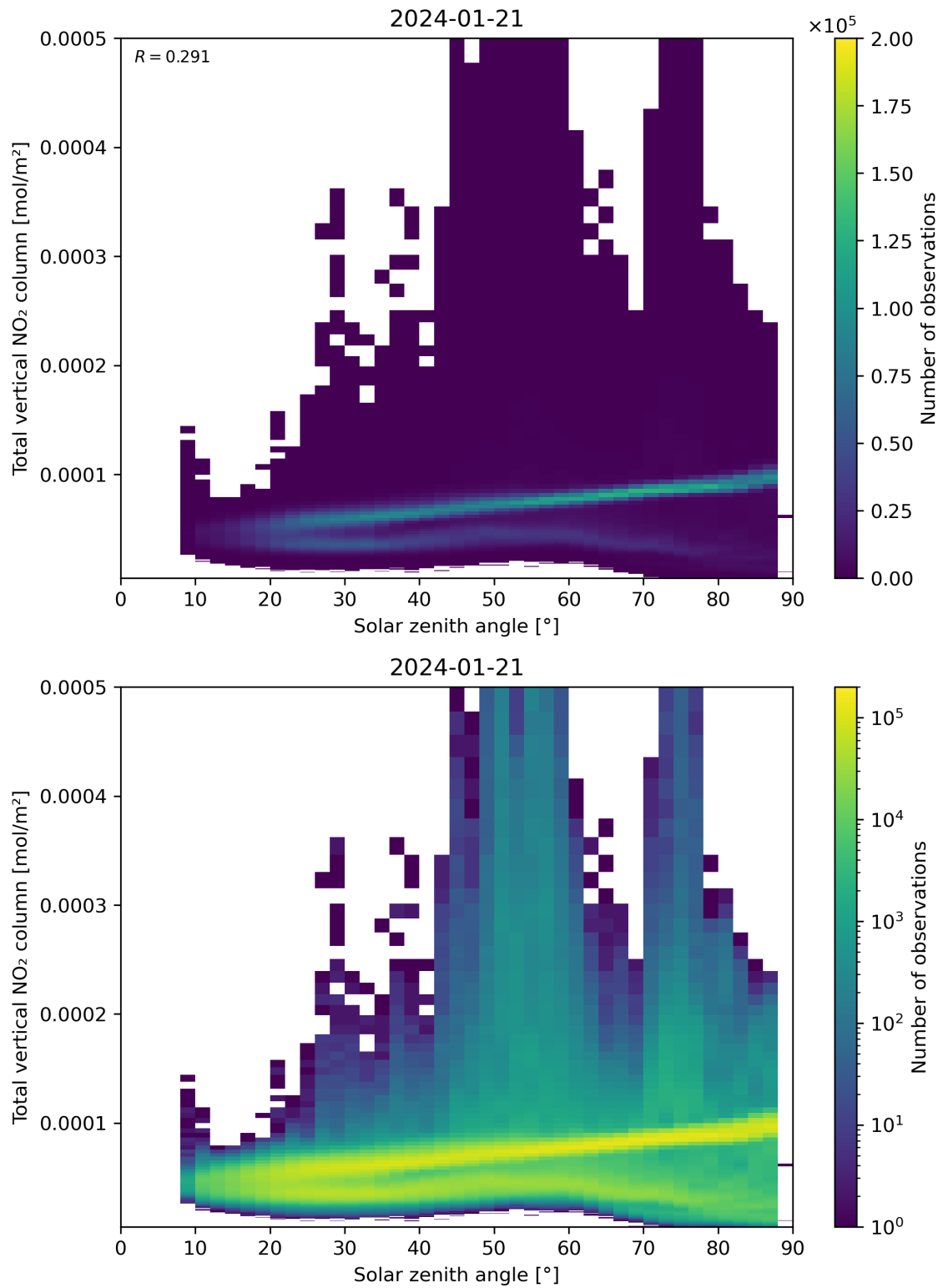
Figure 153: Scatter density plot of “Solar zenith angle” against “Total vertical NO 2 column” for 2024-01-21 to 2024-01-22.
