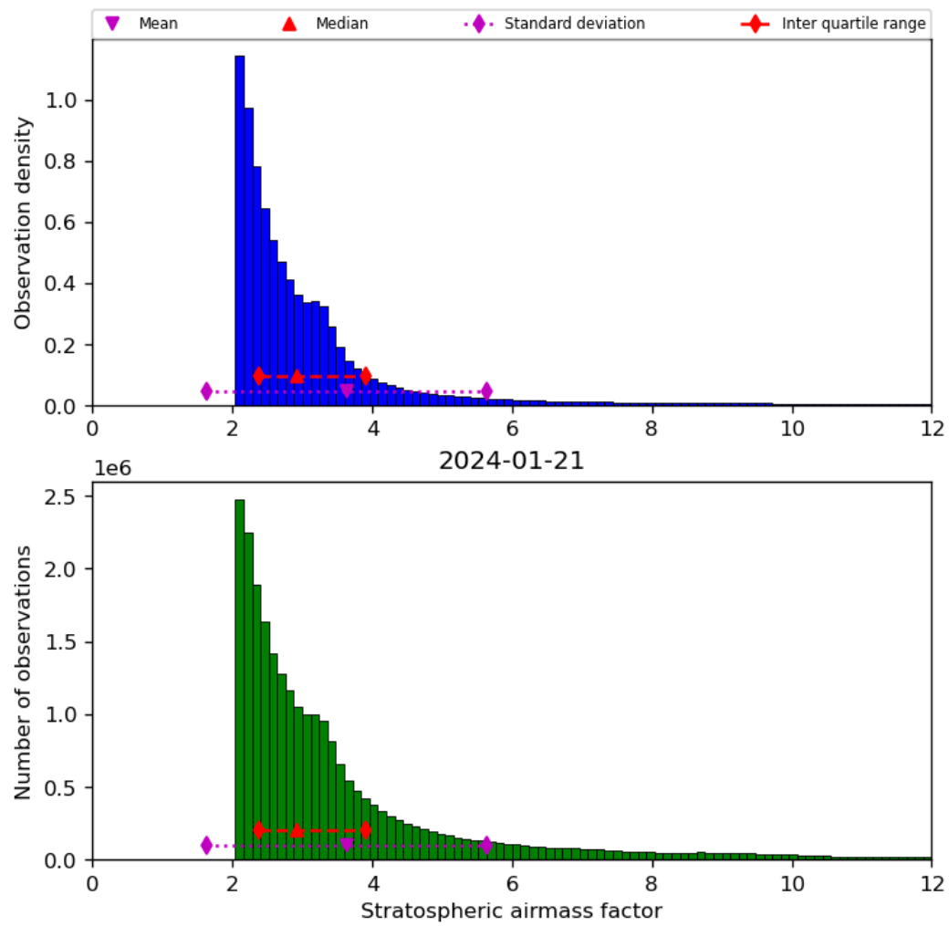
Figure 44: Histogram of “Stratospheric airmass factor” for 2024-01-21 to 2024-01-22
