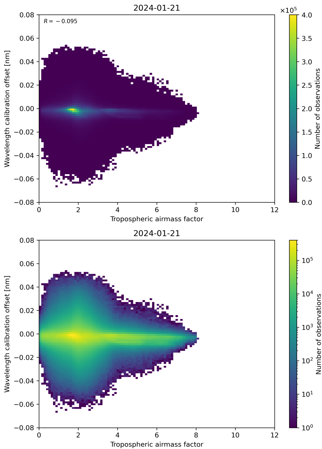
Figure 80: Scatter density plot of “Tropospheric airmass factor” against “Wavelength calibration offset” for 2024-01-21 to 2024-01-22.
