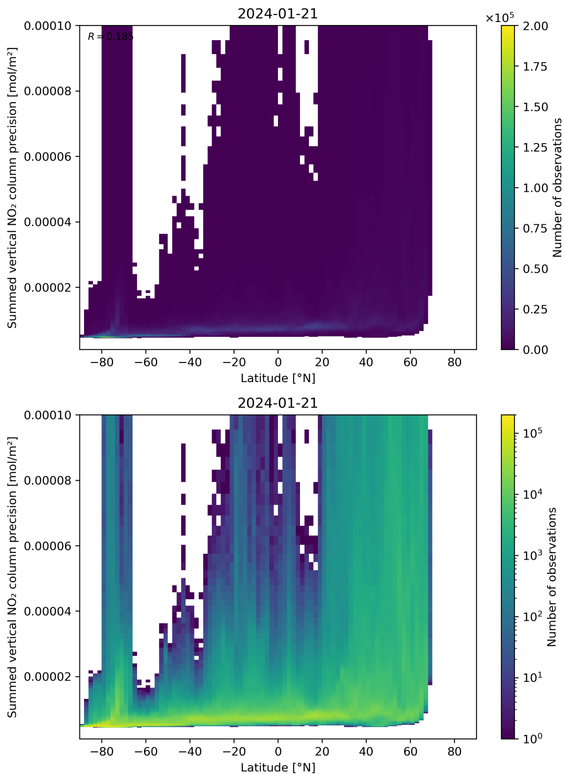
Figure 89: Scatter density plot of “Latitude” against “Summed vertical NO 2 column precision” for 2024-01-21 to 2024-01-22.
