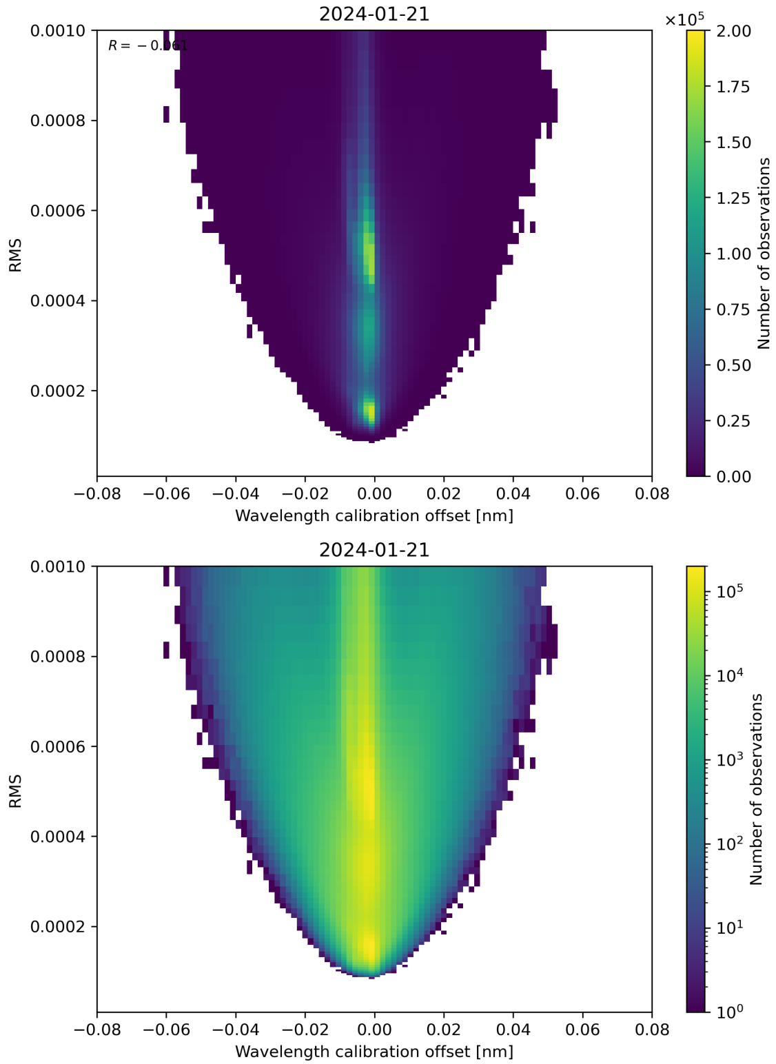
Figure 181: Scatter density plot of “Wavelength calibration offset” against “RMS” for 2024-01-21 to 2024-01-22.
