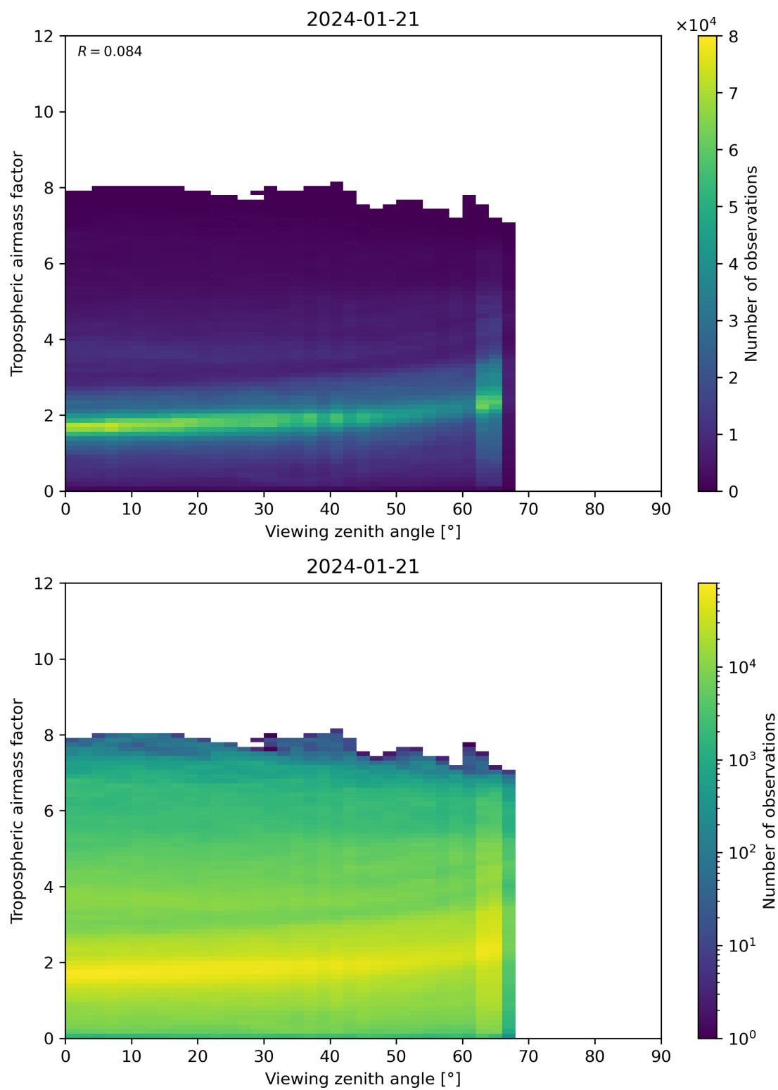
Figure 161: Scatter density plot of “Viewing zenith angle” against “Tropospheric airmass factor” for 2024-01-21 to 2024-01-22.
