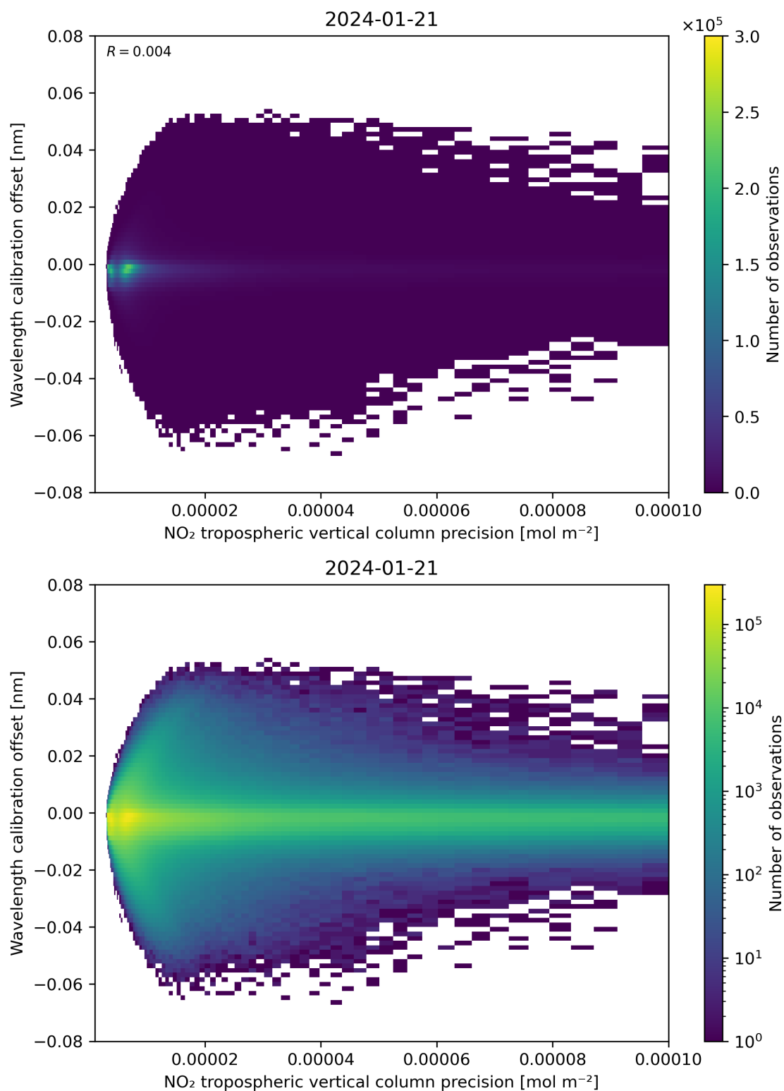
Figure 141: Scatter density plot of “NO 2 tropospheric vertical column precision” against “Wavelength calibration offset” for 2024-01-21 to 2024-01-22.
