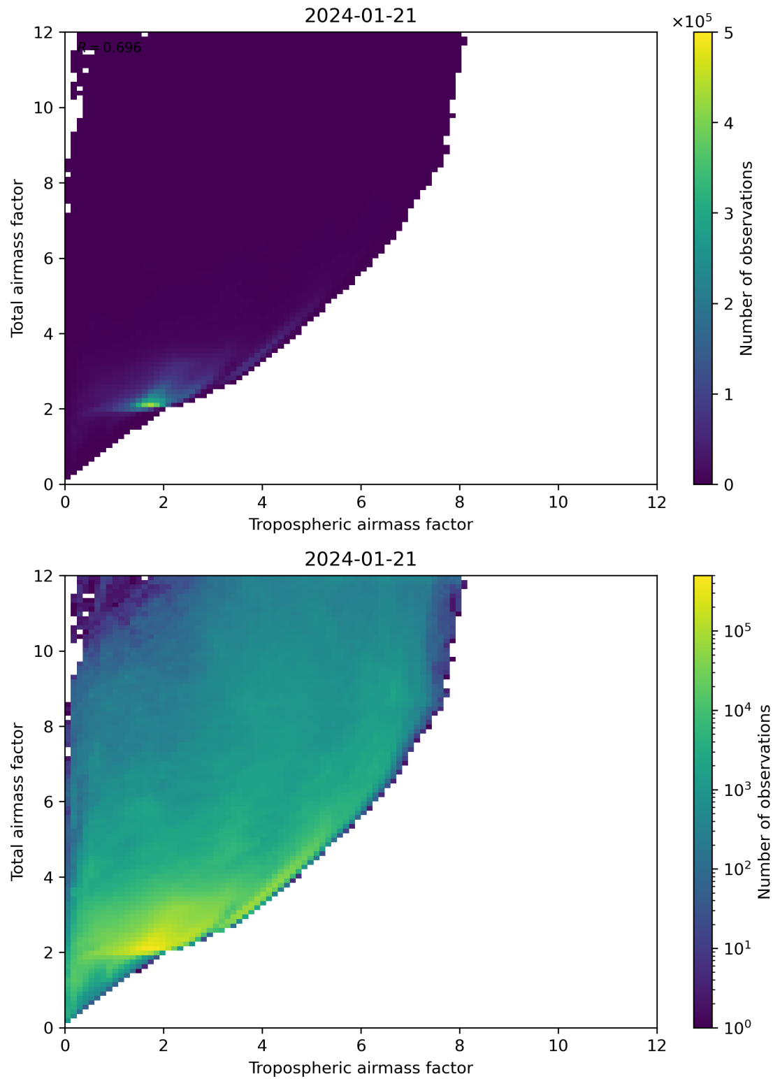
Figure 72: Scatter density plot of “Tropospheric airmass factor” against “Total airmass factor” for 2024-01-21 to 2024-01-22.
