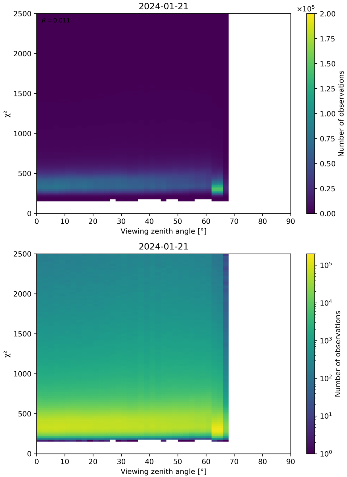
Figure 162: Scatter density plot of “Viewing zenith angle” against “ \chi^2 ” for 2024-01-21 to 2024-01-22.
