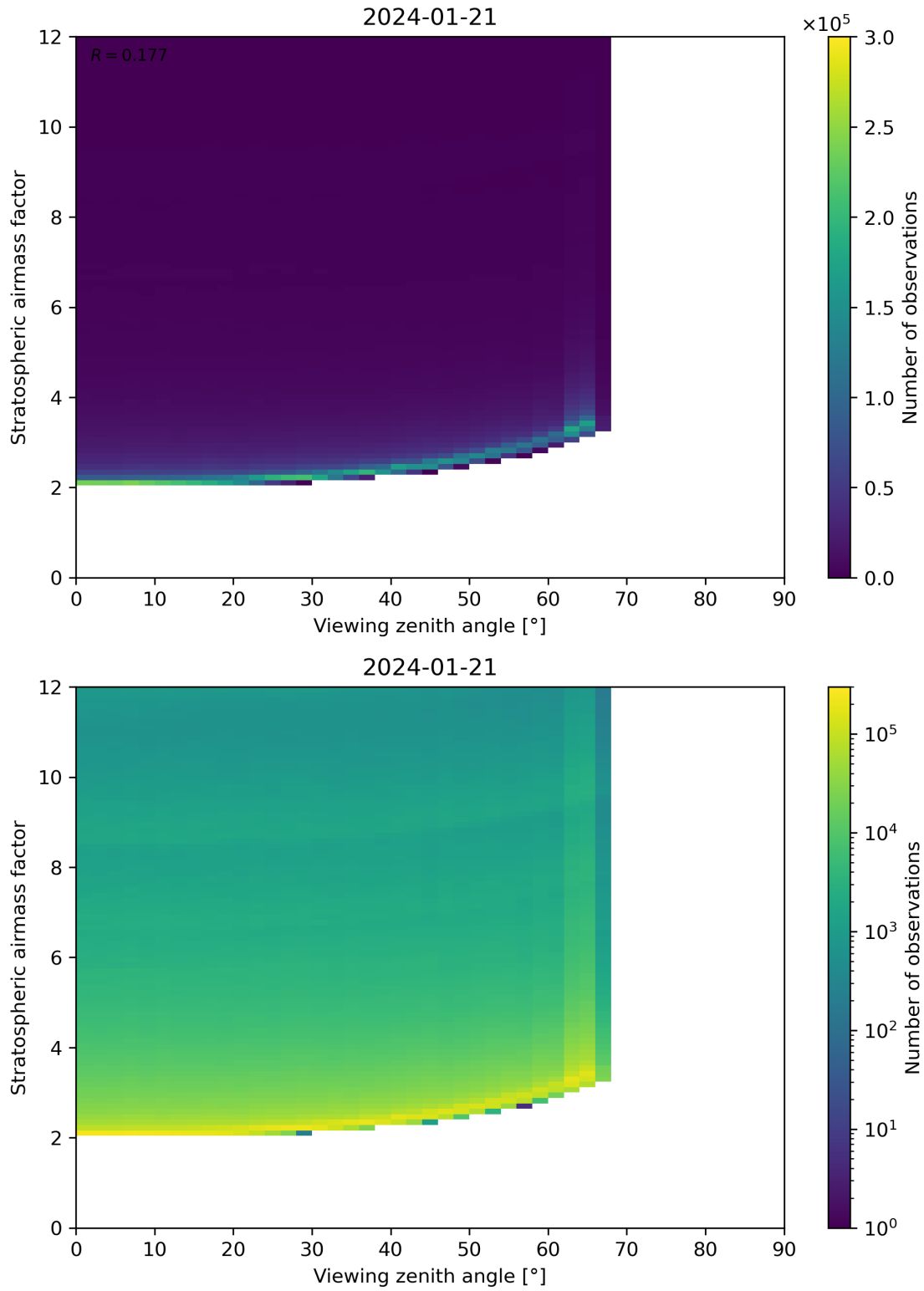
Figure 159: Scatter density plot of “Viewing zenith angle” against “Stratospheric airmass factor” for 2024-01-21 to 2024-01-22.
