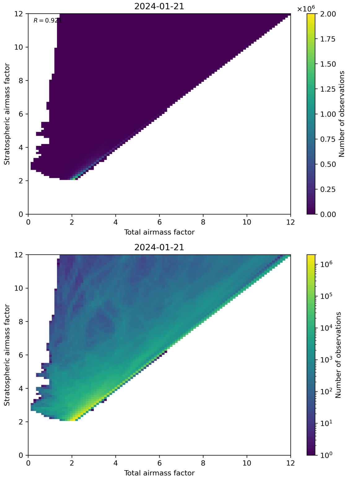
Figure 62: Scatter density plot of “Total airmass factor” against “Stratospheric airmass factor” for 2024-01-21 to 2024-01-22.
