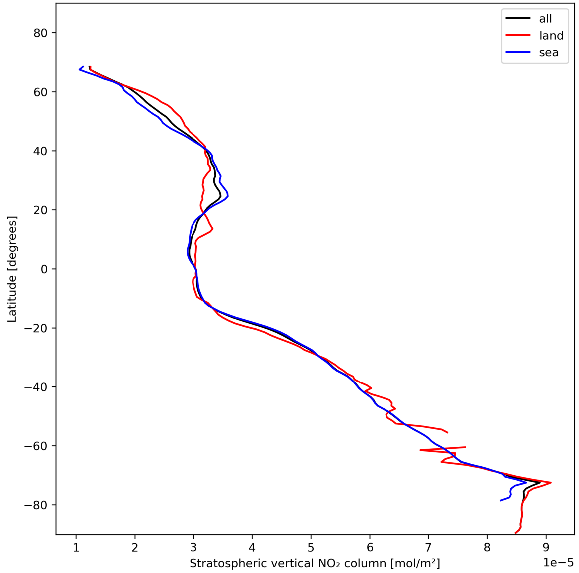
Figure 19: Zonal average of “Stratospheric vertical NO 2 column” for 2024-01-21 to 2024-01-22.
