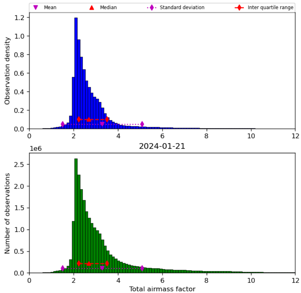
Figure 32: Histogram of “Total airmass factor” for 2024-01-21 to 2024-01-22
