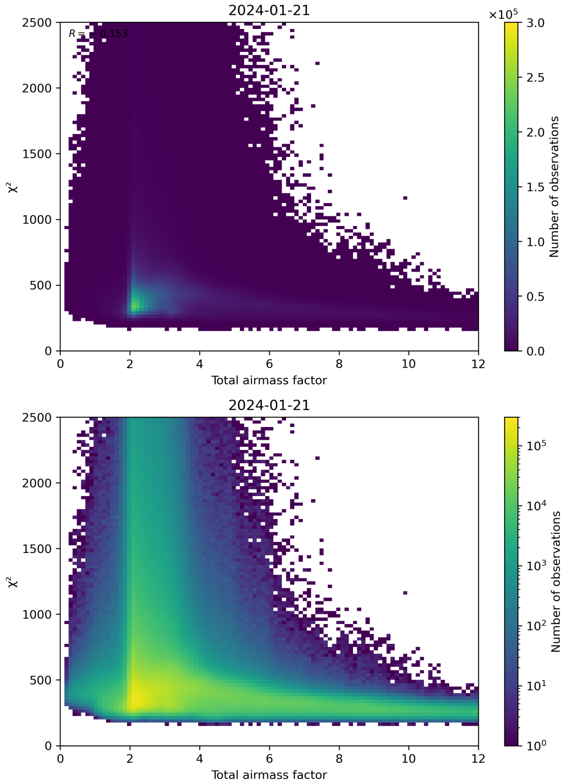
Figure 63: Scatter density plot of “Total airmass factor” against “ \chi^2 ” for 2024-01-21 to 2024-01-22.
