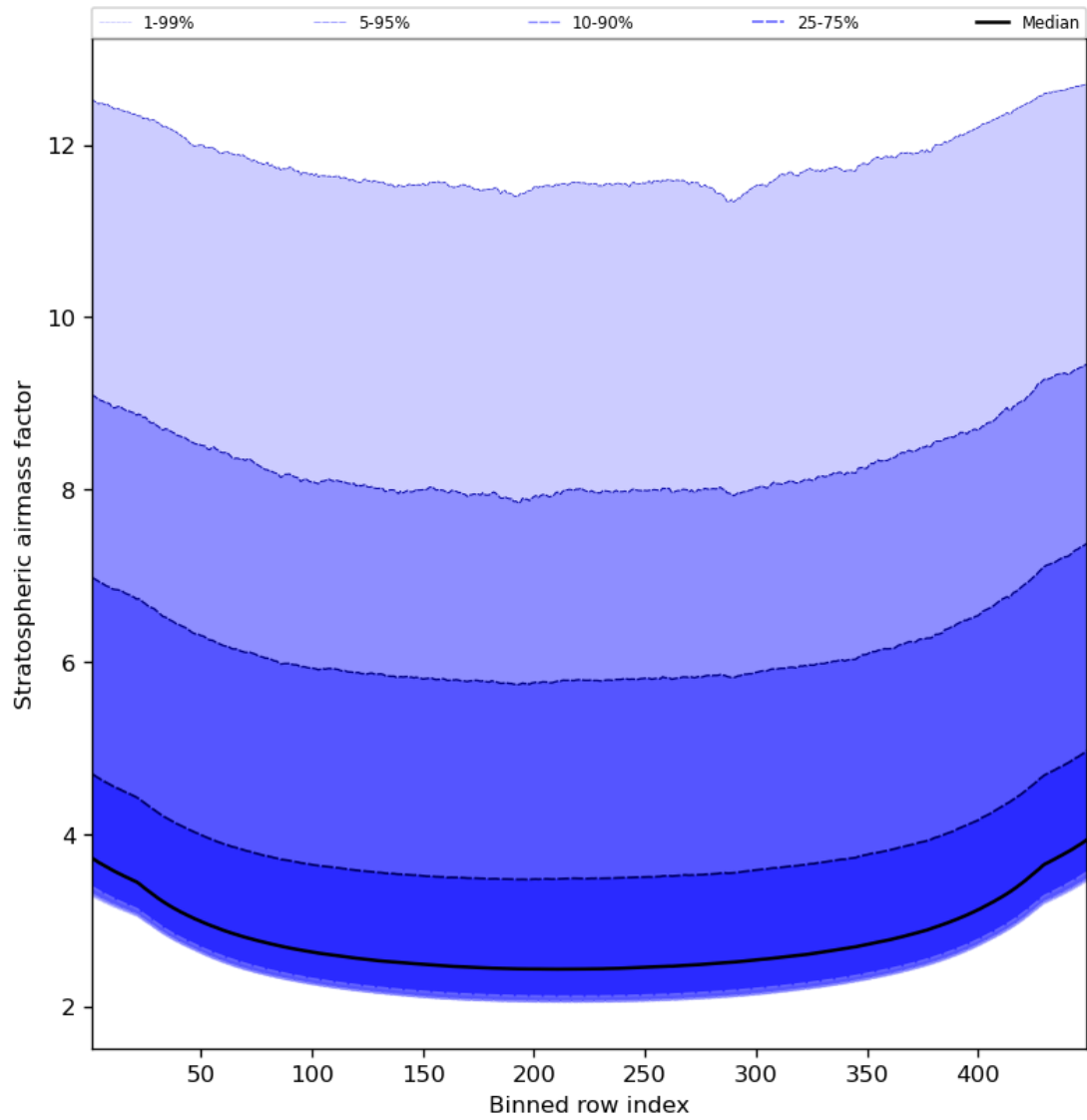
Figure 61: Along track statistics of “Stratospheric airmass factor” for 2024-01-21 to 2024-01-22
