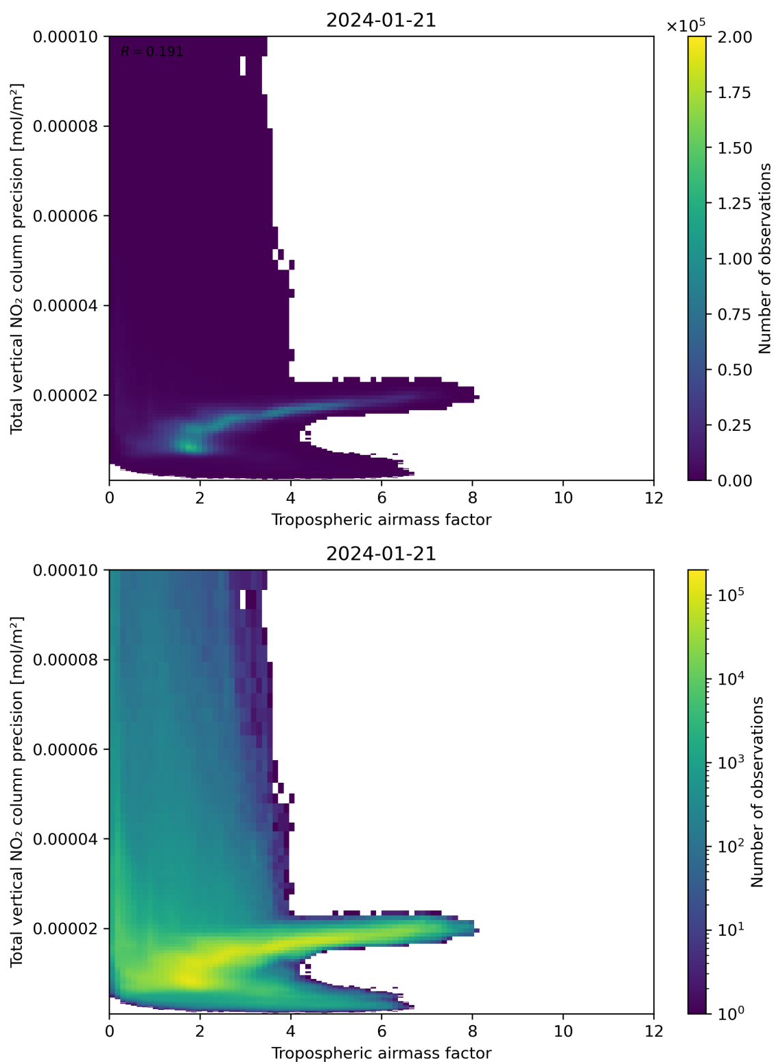
Figure 78: Scatter density plot of “Tropospheric air mass factor” against “Total vertical NO 2 column precision” for 2024-01-21 to 2024-01-22.
