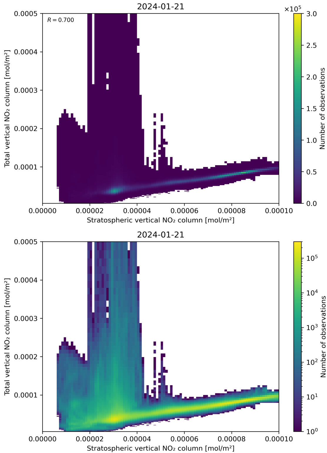
Figure 100: Scatter density plot of “Stratospheric vertical NO 2 column” against “Total vertical NO 2 column” for 2024-01-21 to 2024-01-22.
