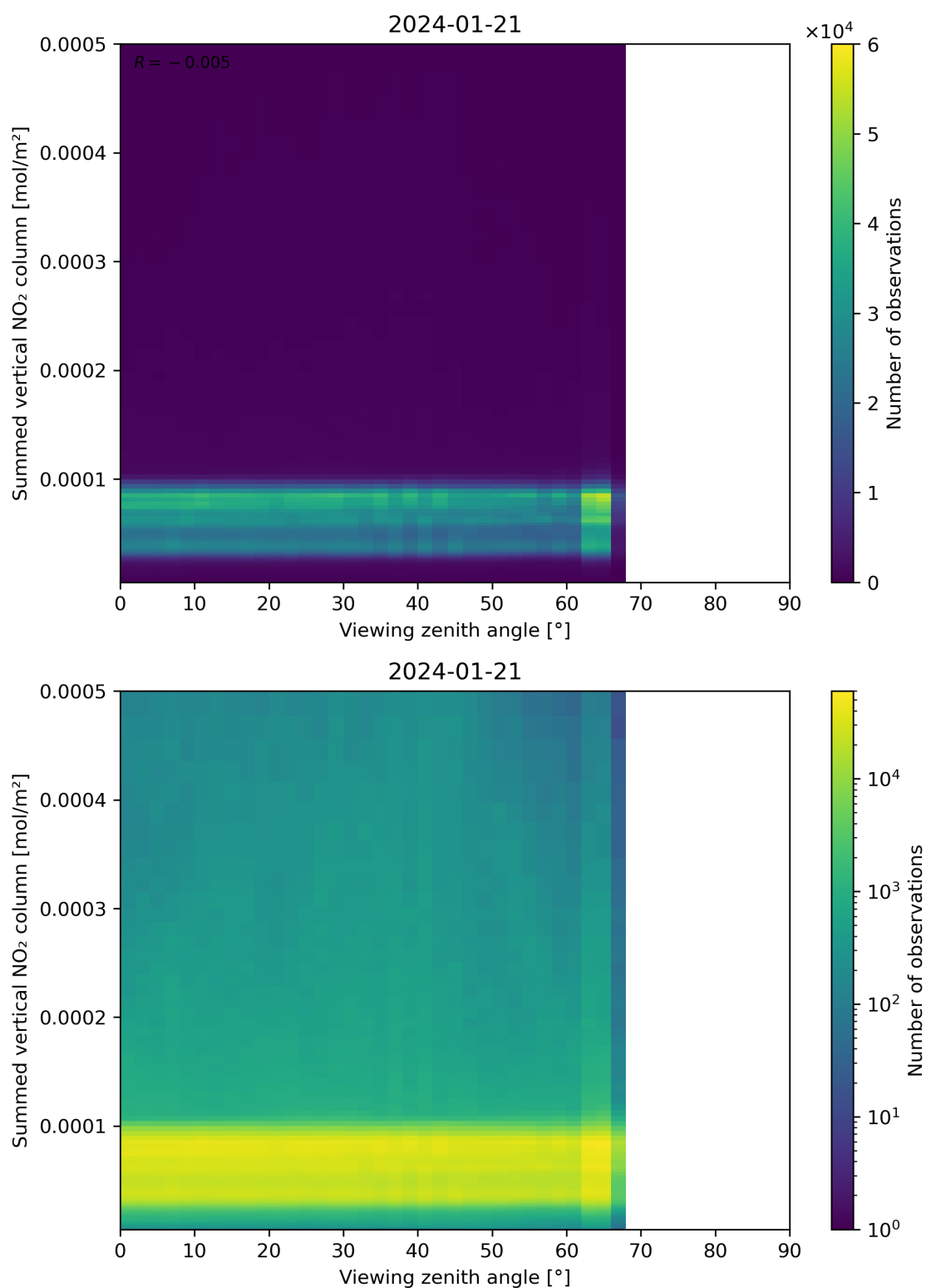
Figure 165: Scatter density plot of “Viewing zenith angle” against “Summed vertical NO 2 column” for 2024-01-21 to 2024-01-22.
