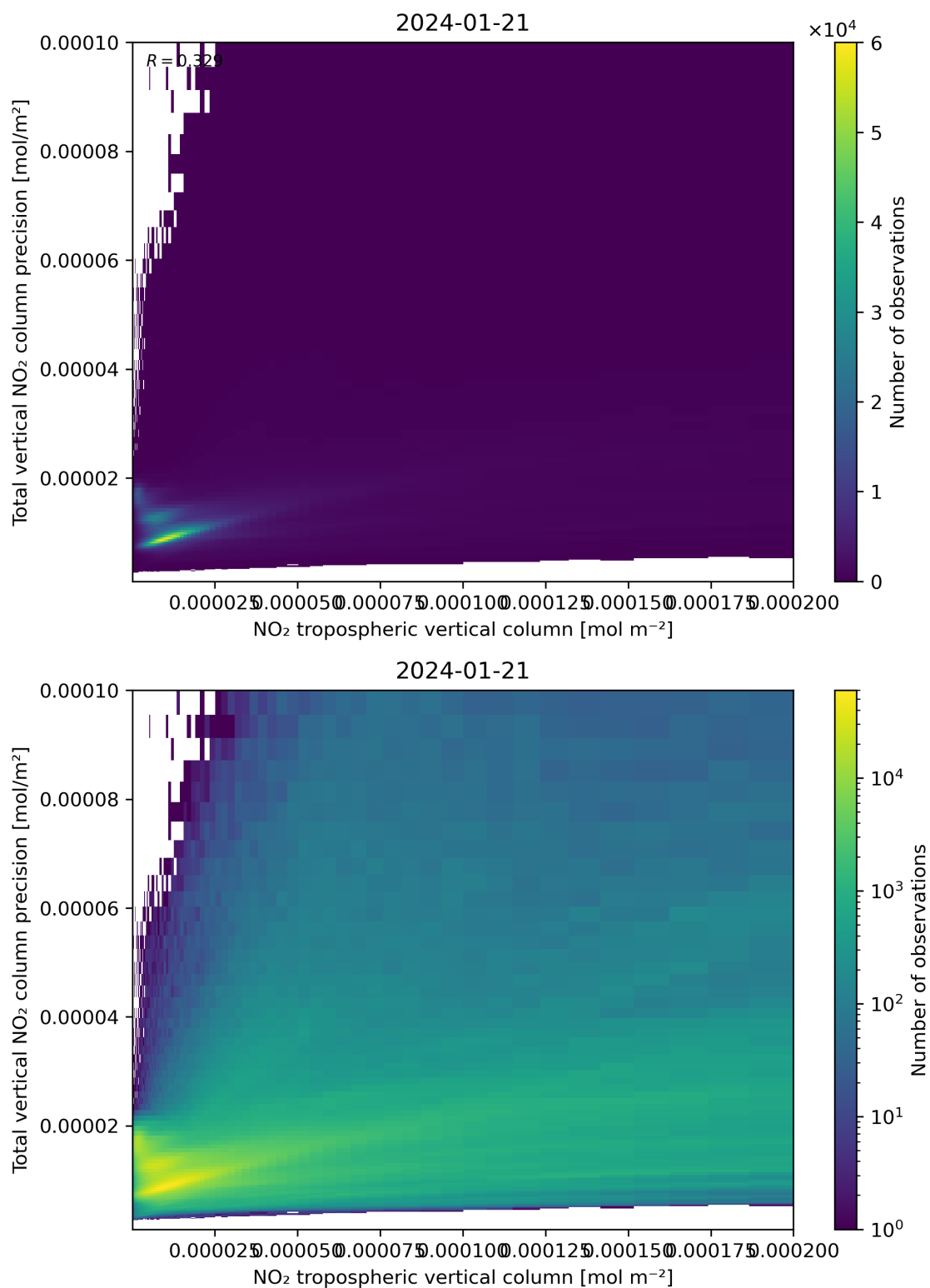
Figure 129: Scatter density plot of “NO 2 tropospheric vertical column” against “Total vertical NO 2 column precision” for 2024-01-21 to 2024-01-22.
