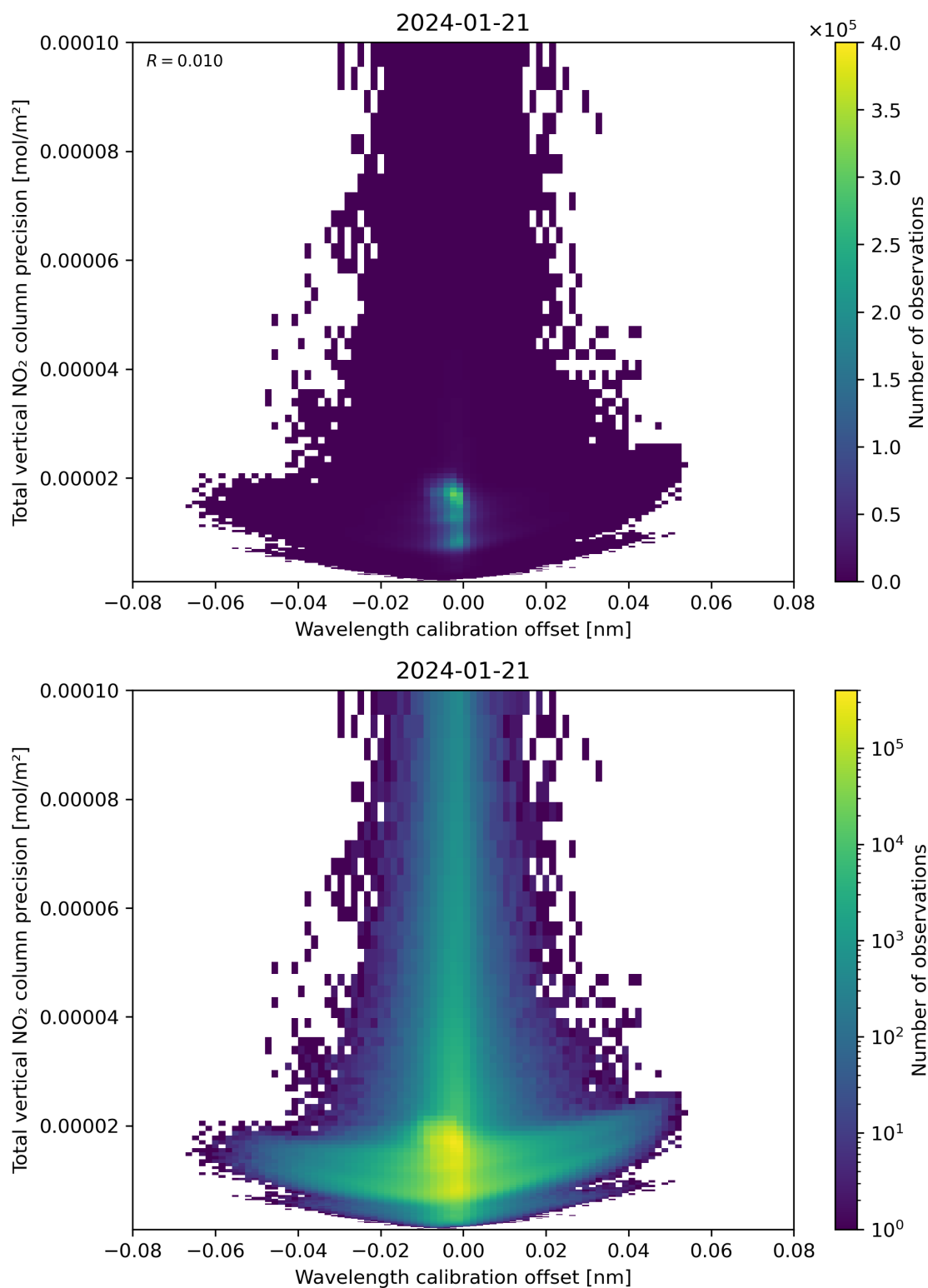
Figure 180: Scatter density plot of “Wavelength calibration offset” against “Total vertical NO 2 column precision” for 2024-01-21 to 2024-01-22.
