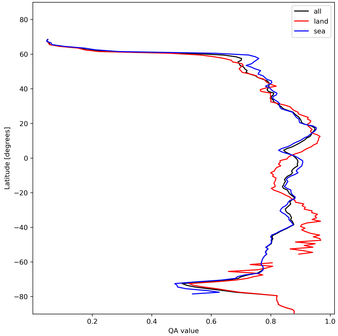
Figure 11: Zonal average of “QA value” for 2024-01-21 to 2024-01-22.
