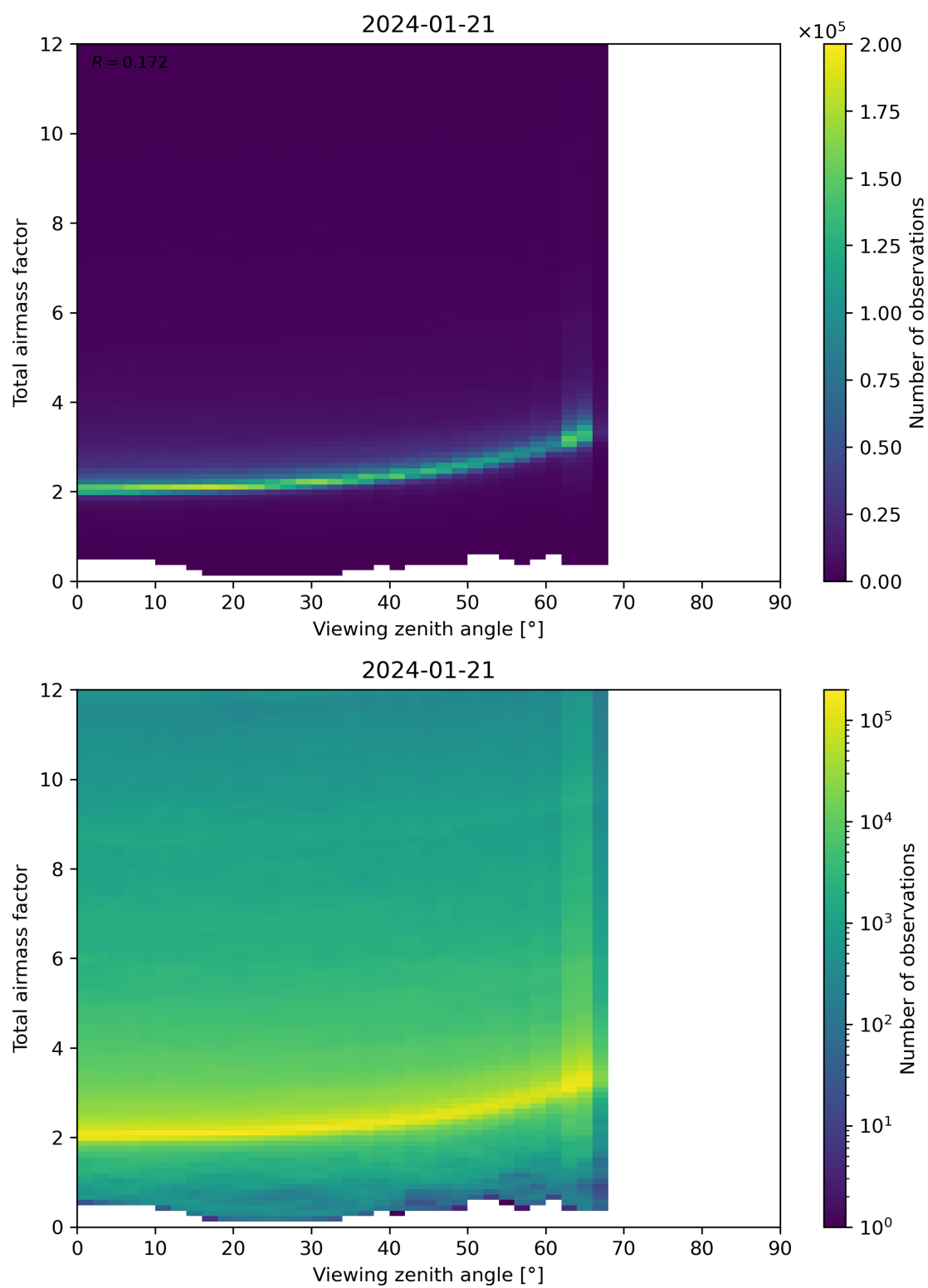
Figure 160: Scatter density plot of “Viewing zenith angle” against “Total airmass factor” for 2024-01-21 to 2024-01-22.
