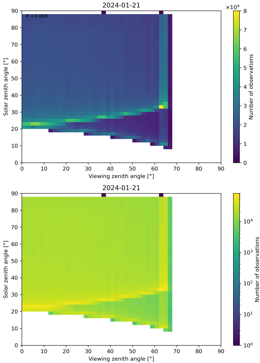
Figure 172: Scatter density plot of “Viewing zenith angle” against “Solar zenith angle” for 2024-01-21 to 2024-01-22.
