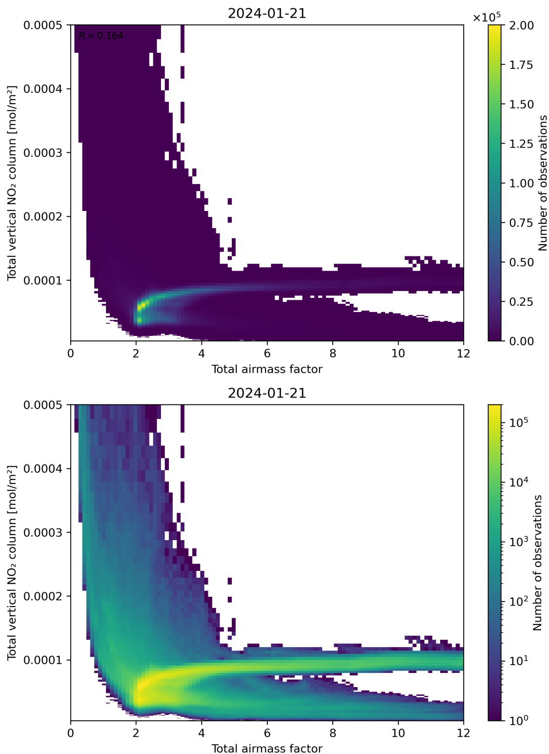
Figure 67: Scatter density plot of “Total airmass factor” against “Total vertical NO 2 column” for 2024-01-21 to 2024-01-22.
