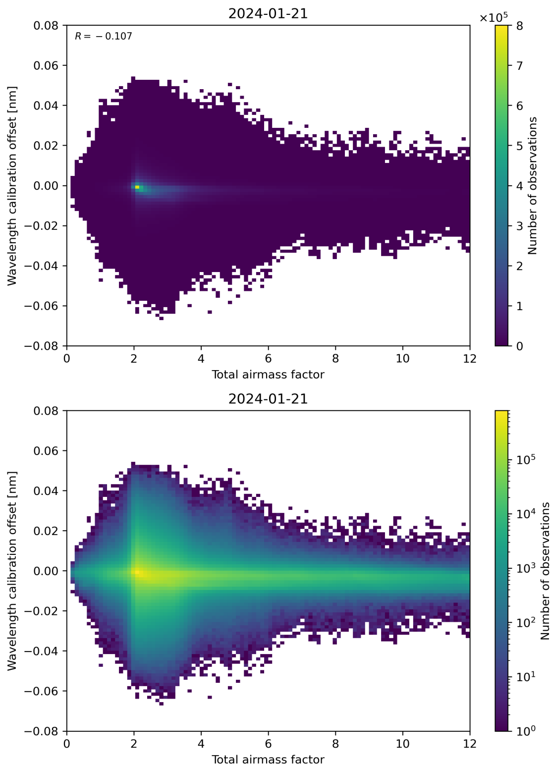
Figure 70: Scatter density plot of “Total airmass factor” against “Wavelength calibration offset” for 2024-01-21 to 2024-01-22.
