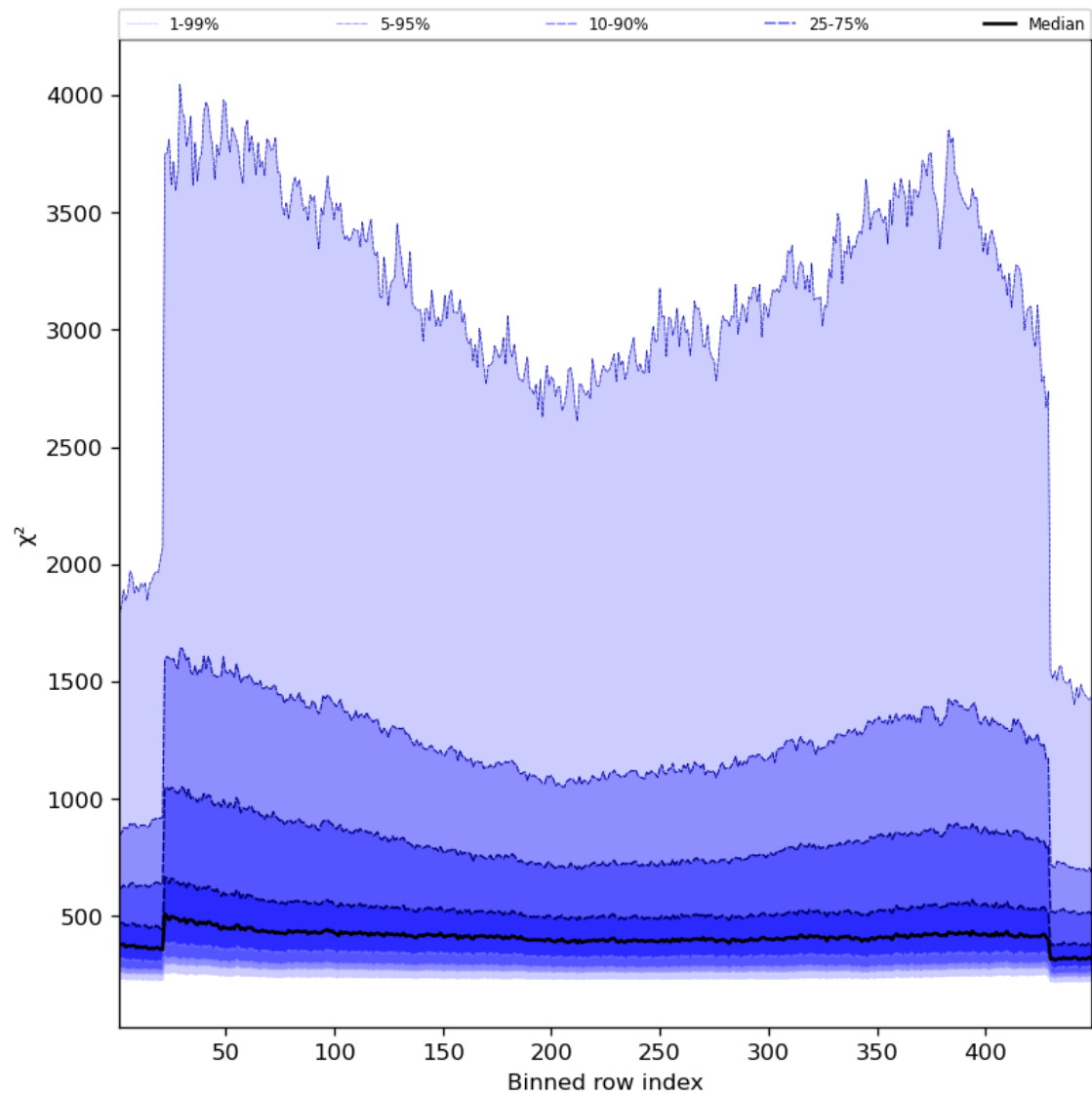
Figure 59: Along track statistics of “ \chi^2 ” for 2024-01-21 to 2024-01-22
