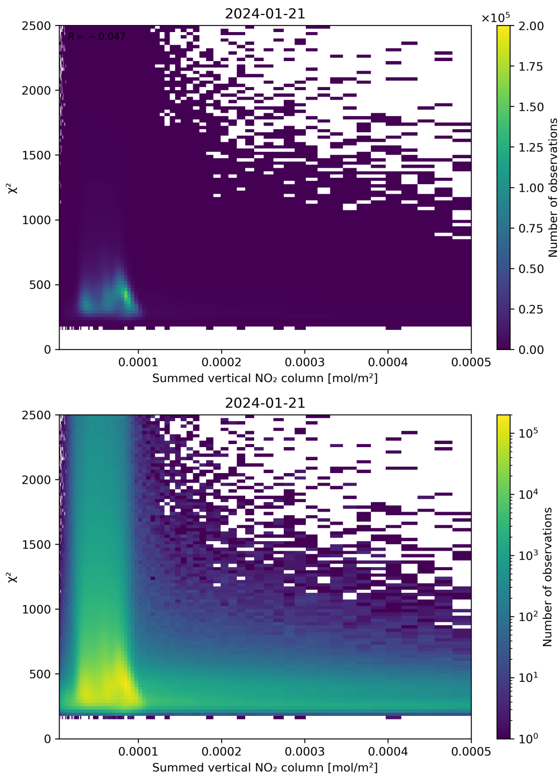
Figure 104: Scatter density plot of “Summed vertical NO 2 column” against “ \chi^2 ” for 2024-01-21 to 2024-01-22.
