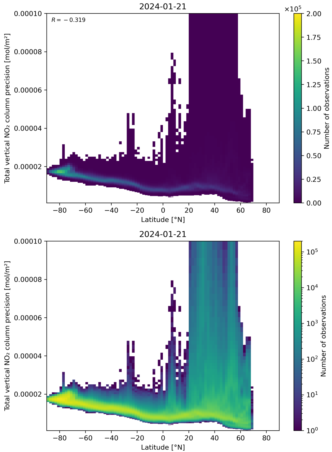
Figure 91: Scatter density plot of “Latitude” against “Total vertical NO 2 column precision” for 2024-01-21 to 2024-01-22.
