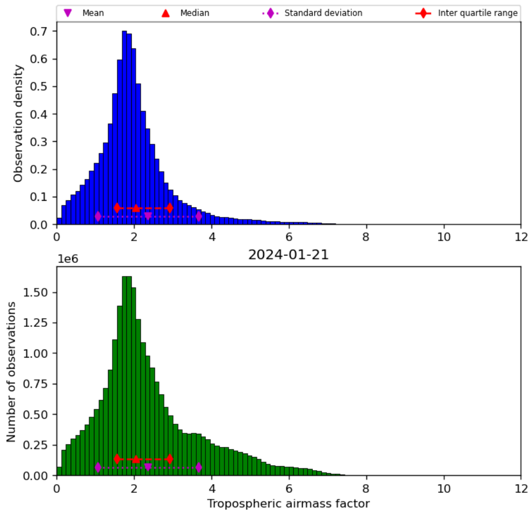
Figure 31: Histogram of “Tropospheric airmass factor” for 2024-01-21 to 2024-01-22
