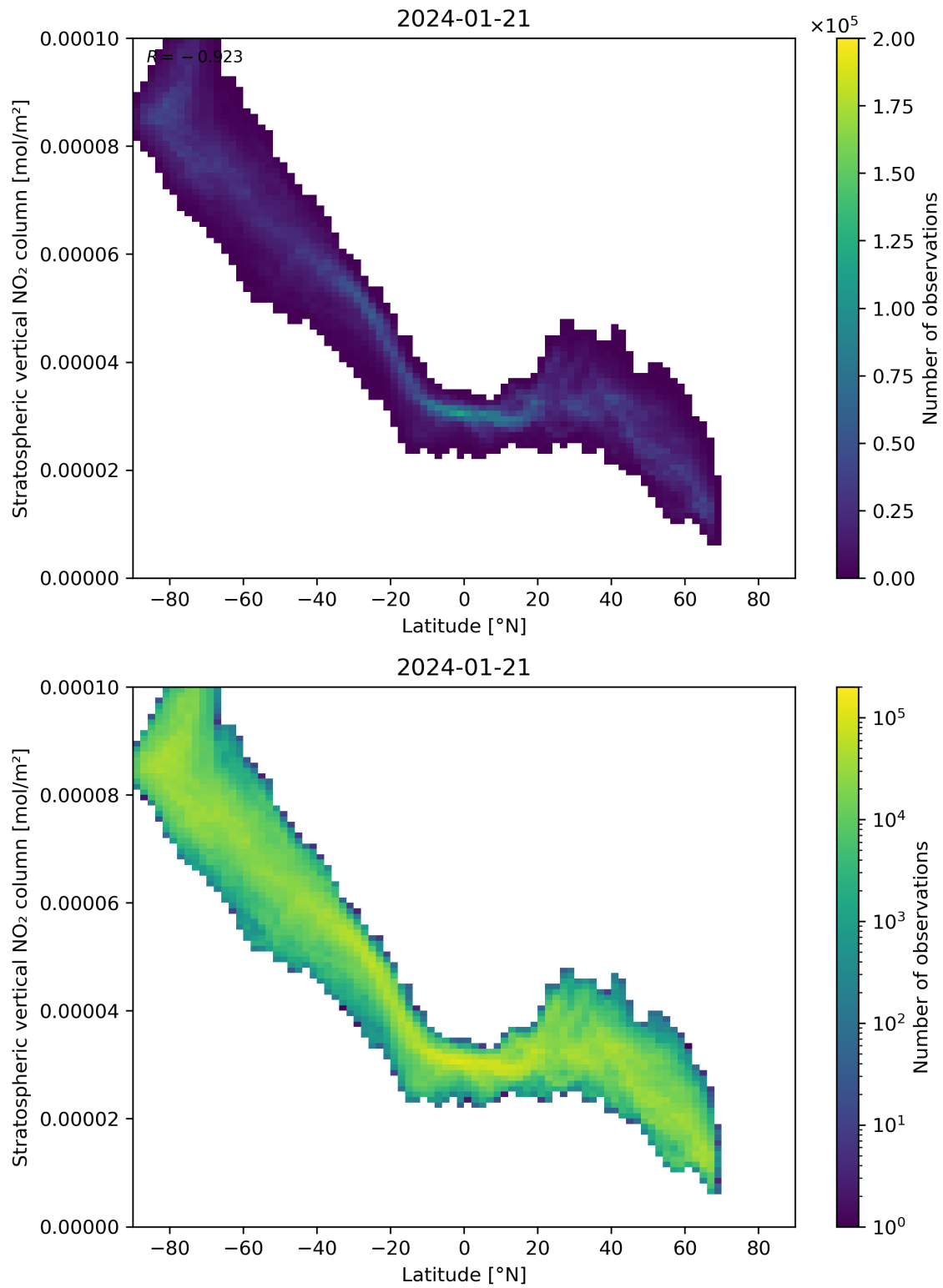
Figure 87: Scatter density plot of “Latitude” against “Stratospheric vertical NO 2 column” for 2024-01-21 to 2024-01-22.
