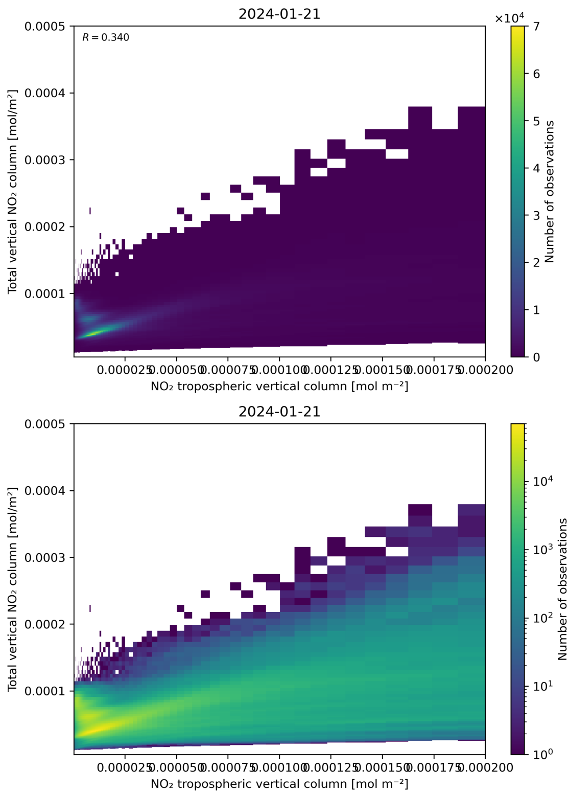
Figure 128: Scatter density plot of “NO 2 tropospheric vertical column” against “Total vertical NO 2 column” for 2024-01-21 to 2024-01-22.
