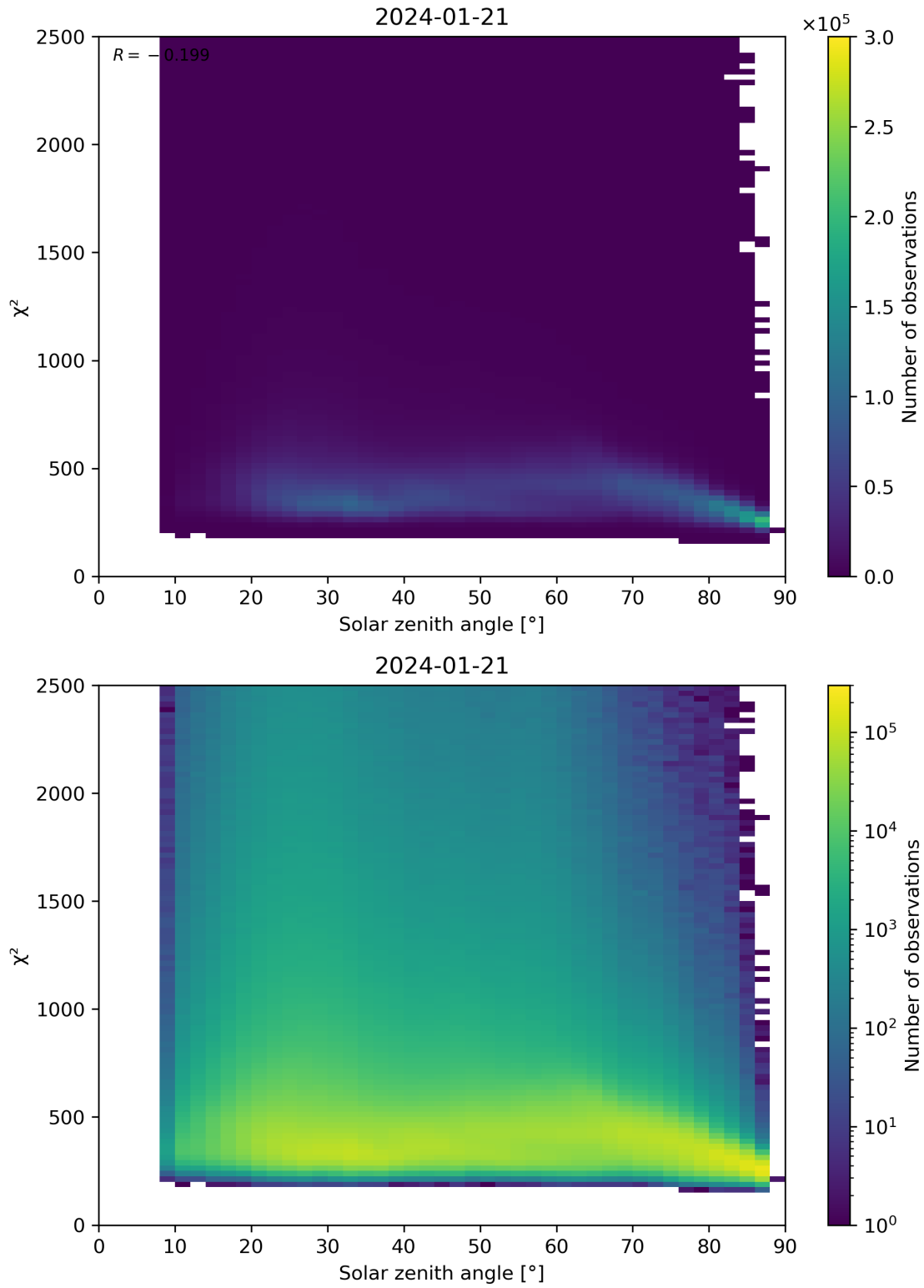
Figure 148: Scatter density plot of “Solar zenith angle” against “ \chi^2 ” for 2024-01-21 to 2024-01-22.
