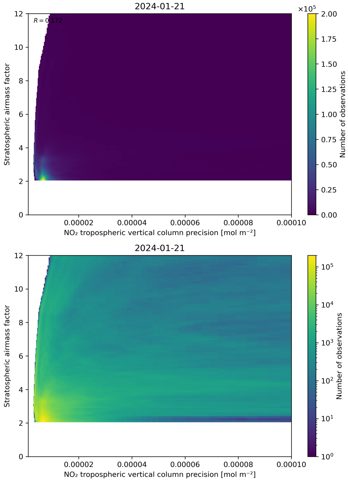
Figure 131: Scatter density plot of “NO 2 tropospheric vertical column precision” against “Stratospheric airmass factor” for 2024-01-21 to 2024-01-22.
