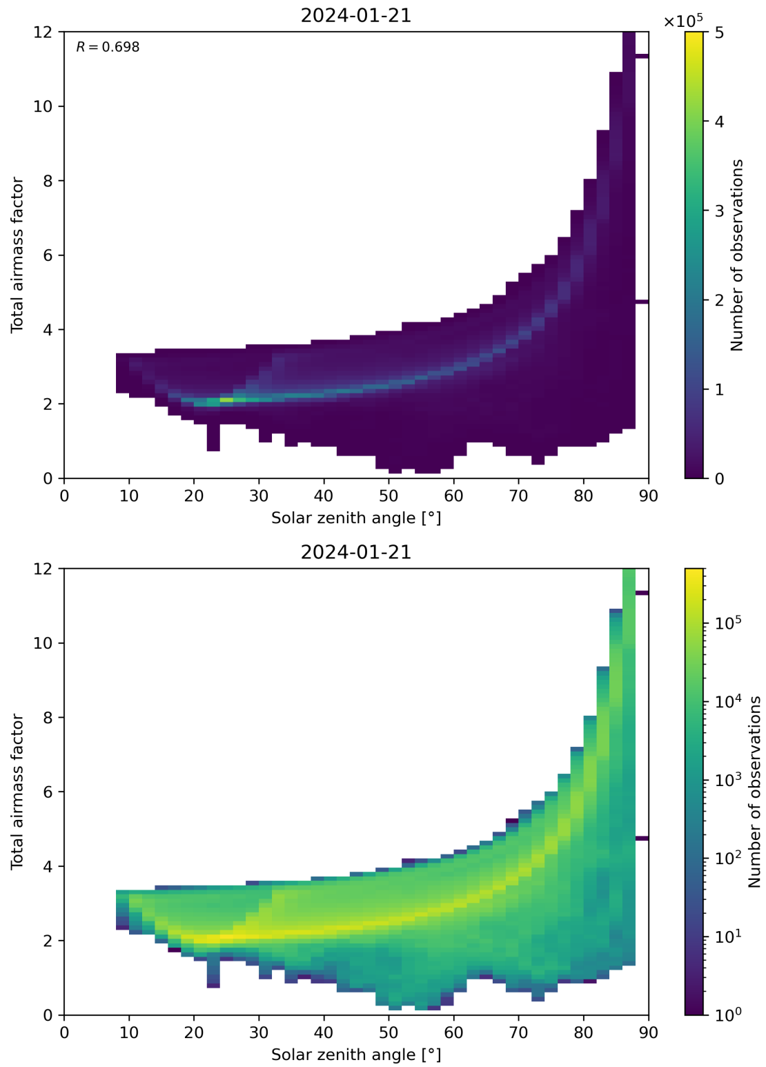
Figure 146: Scatter density plot of “Solar zenith angle” against “Total air mass factor” for 2024-01-21 to 2024-01-22.
