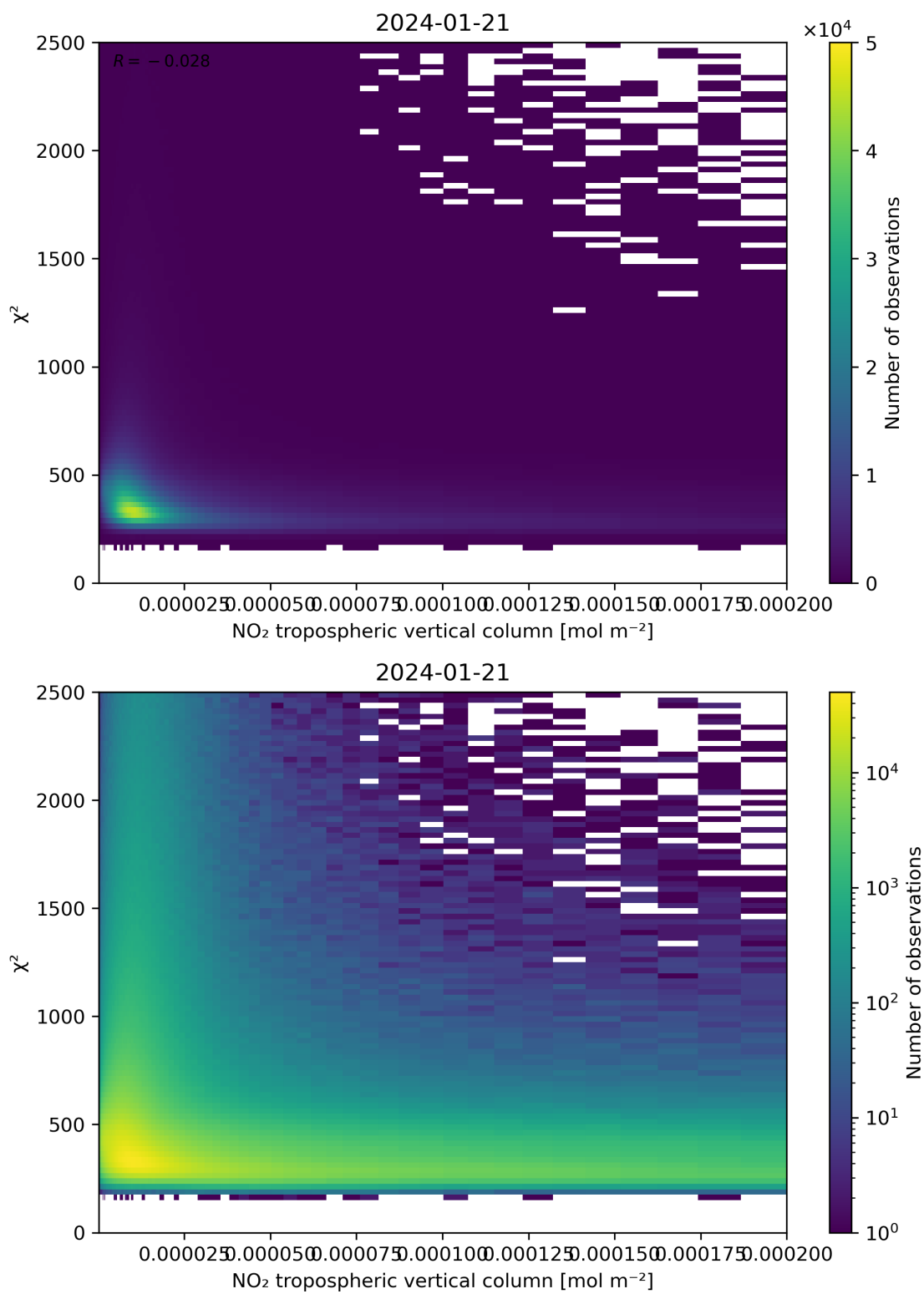
Figure 124: Scatter density plot of “NO 2 tropospheric vertical column” against “ \chi^2 ” for 2024-01-21 to 2024-01-22.
