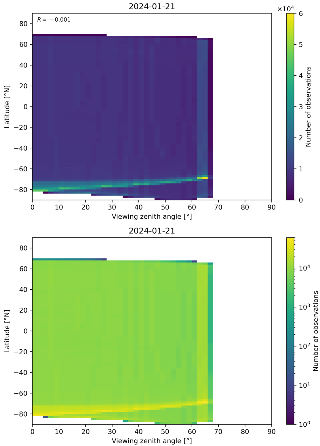
Figure 163: Scatter density plot of “Viewing zenith angle” against “Latitude” for 2024-01-21 to 2024-01-22.
