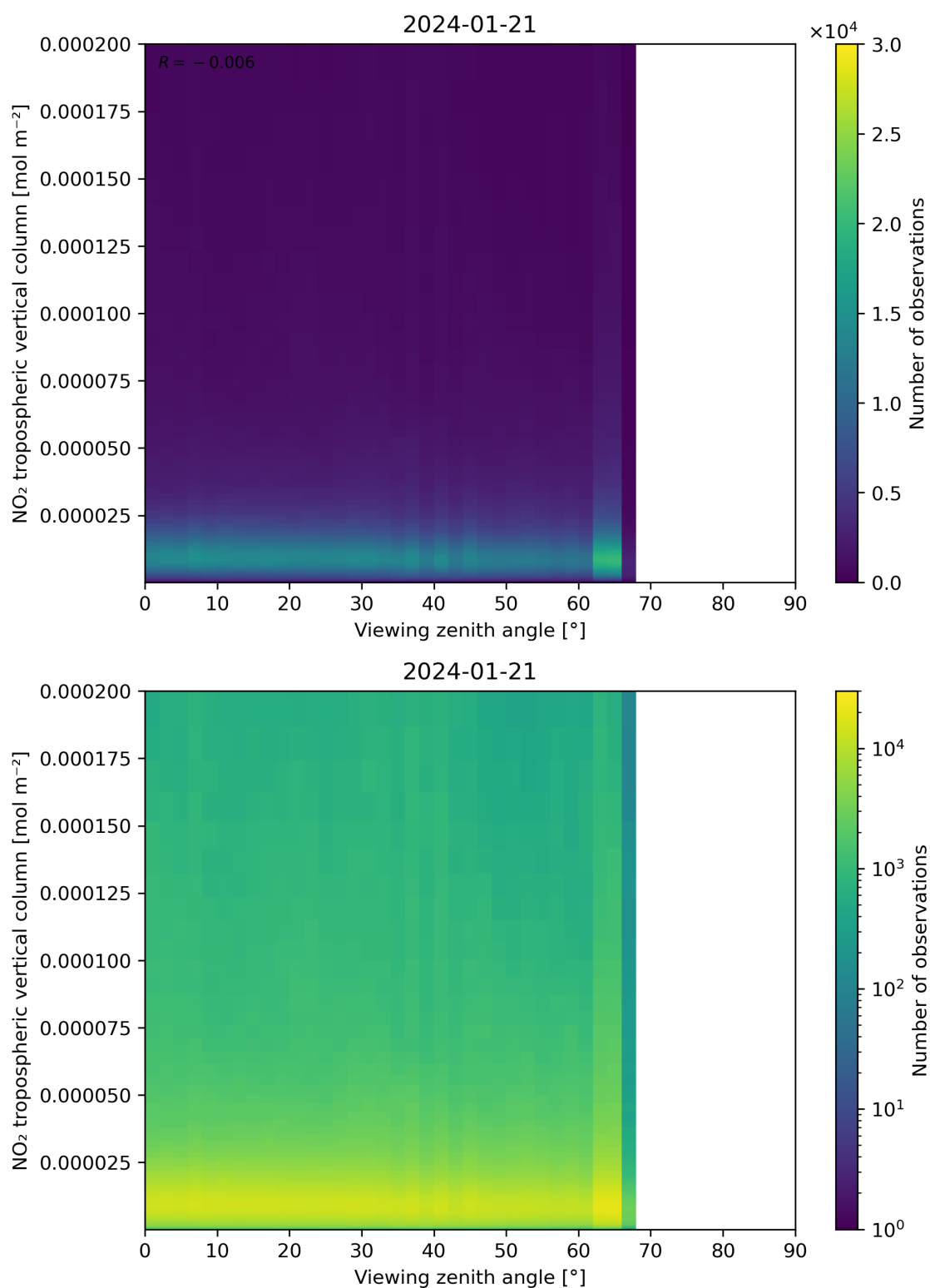
Figure 169: Scatter density plot of “Viewing zenith angle” against “NO 2 tropospheric vertical column” for 2024-01-21 to 2024-01-22.
