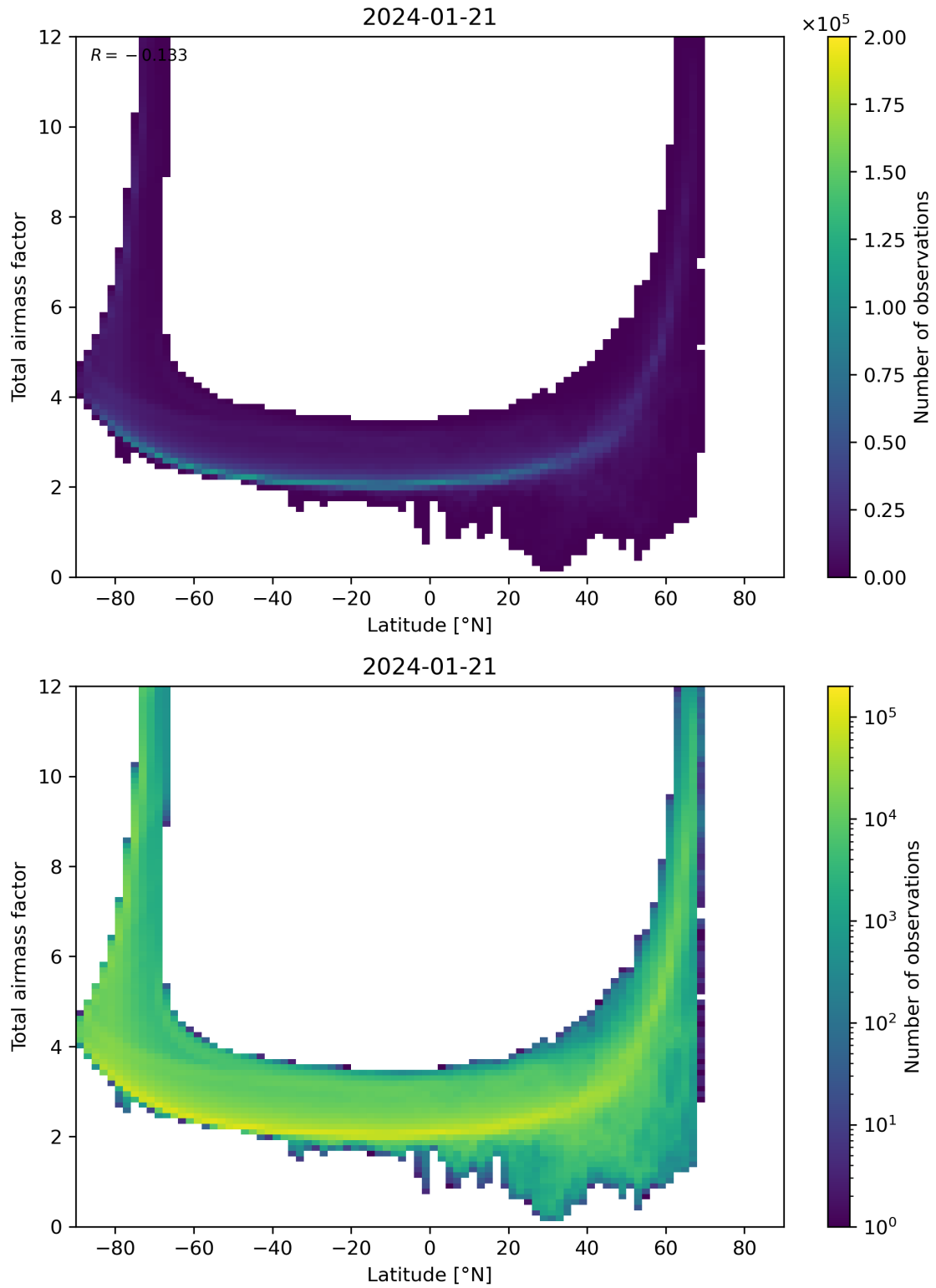
Figure 84: Scatter density plot of “Latitude” against “Total airmass factor” for 2024-01-21 to 2024-01-22.
