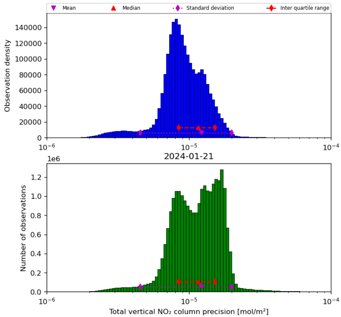
Figure 39: Histogram of “Total vertical NO 2 column precision” for 2024-01-21 to 2024-01-22
