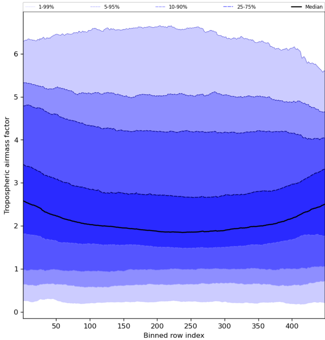
Figure 48: Along track statistics of “Tropospheric airmass factor” for 2024-01-21 to 2024-01-22
