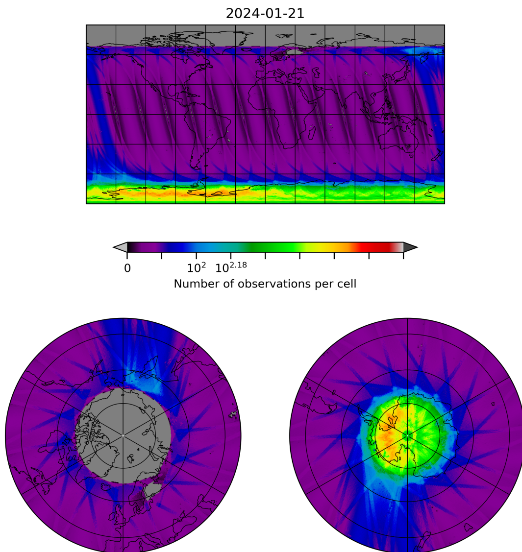
Figure 10: Map of the number of observations for 2024-01-21 to 2024-01-22
