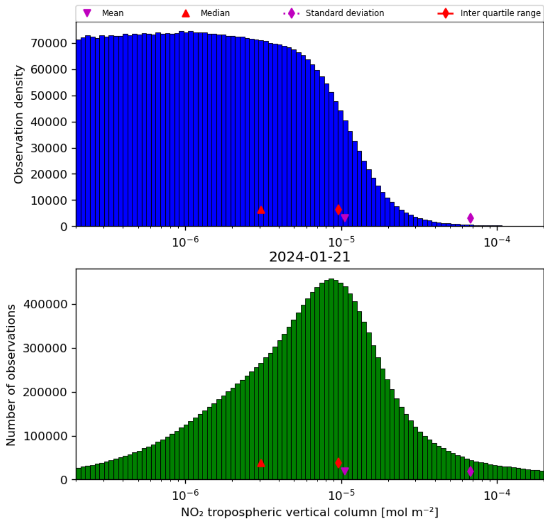
Figure 29: Histogram of “NO 2 tropospheric vertical column” for 2024-01-21 to 2024-01-22
