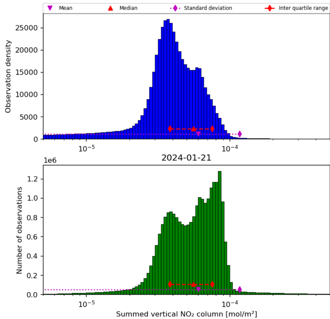
Figure 40: Histogram of “Summed vertical NO 2 column” for 2024-01-21 to 2024-01-22
