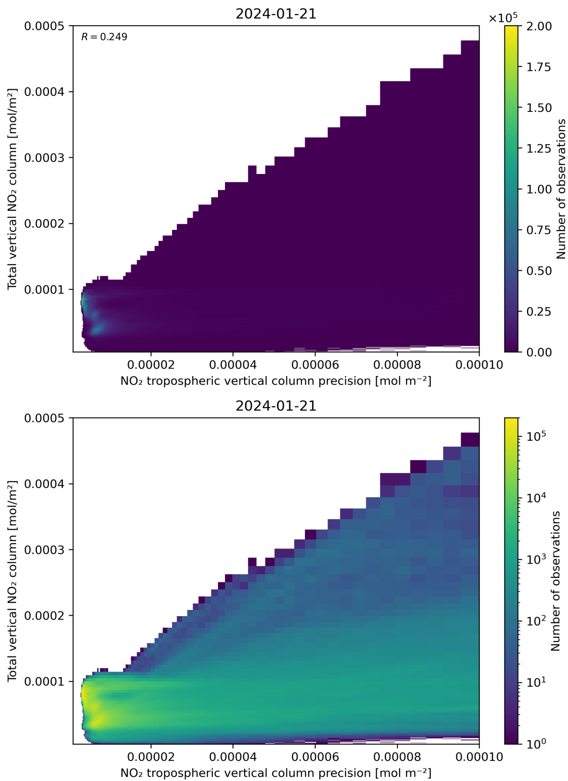
Figure 138: Scatter density plot of “NO 2 tropospheric vertical column precision” against “Total vertical NO 2 column” for 2024-01-21 to 2024-01-22.
