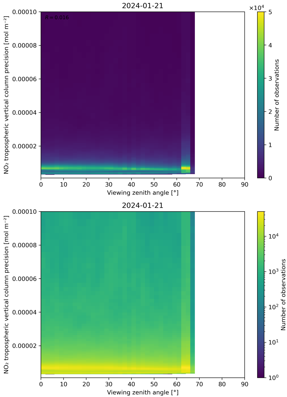
Figure 170: Scatter density plot of “Viewing zenith angle” against “NO 2 tropospheric vertical column precision” for 2024-01-21 to 2024-01-22.
