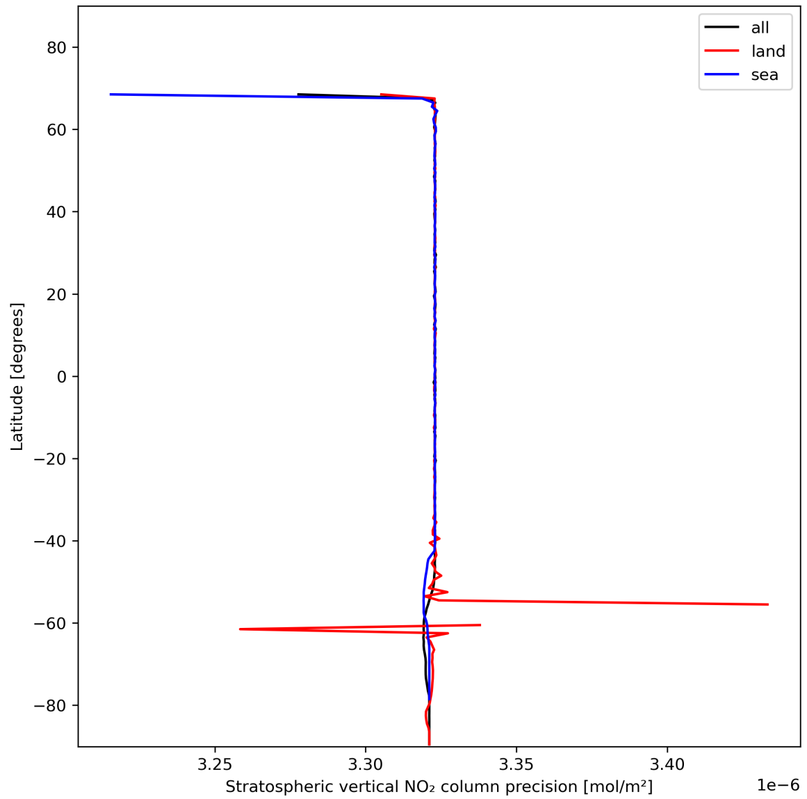
Figure 20: Zonal average of “Stratospheric vertical NO 2 column precision” for 2024-01-21 to 2024-01-22.
