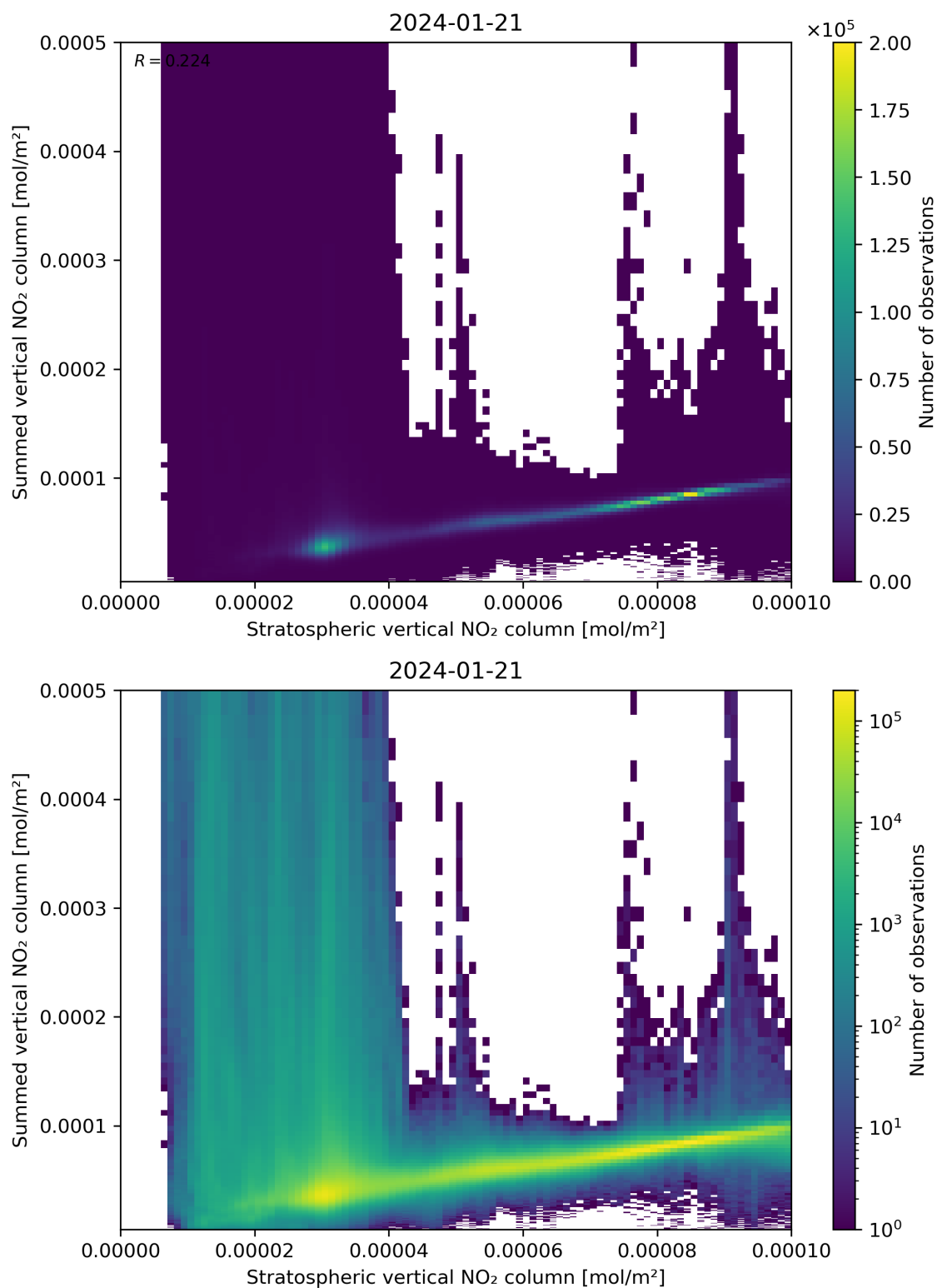
Figure 98: Scatter density plot of “Stratospheric vertical NO 2 column” against “Summed vertical NO 2 column” for 2024-01-21 to 2024-01-22.
