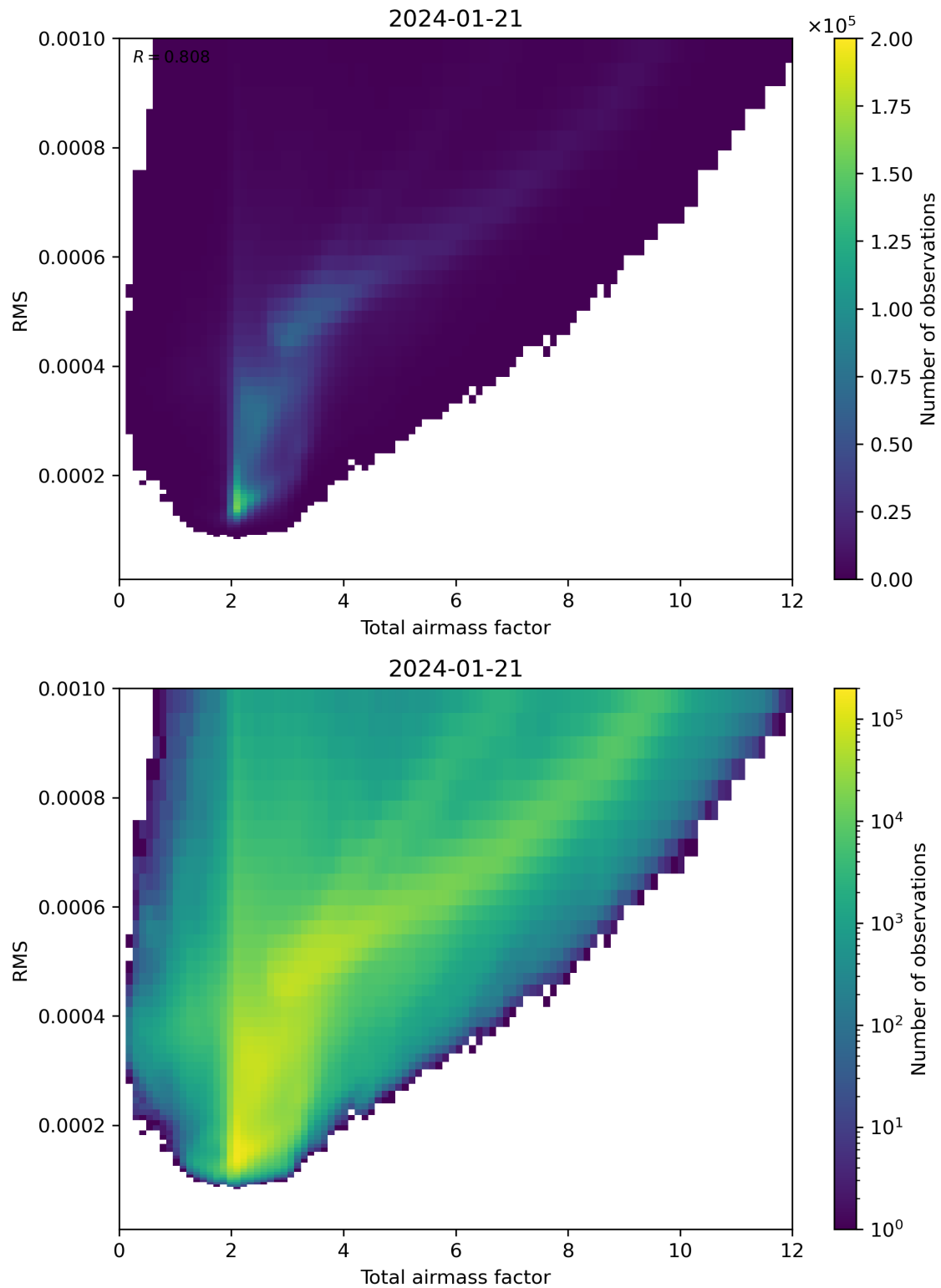
Figure 69: Scatter density plot of “Total airmass factor” against “RMS” for 2024-01-21 to 2024-01-22.
