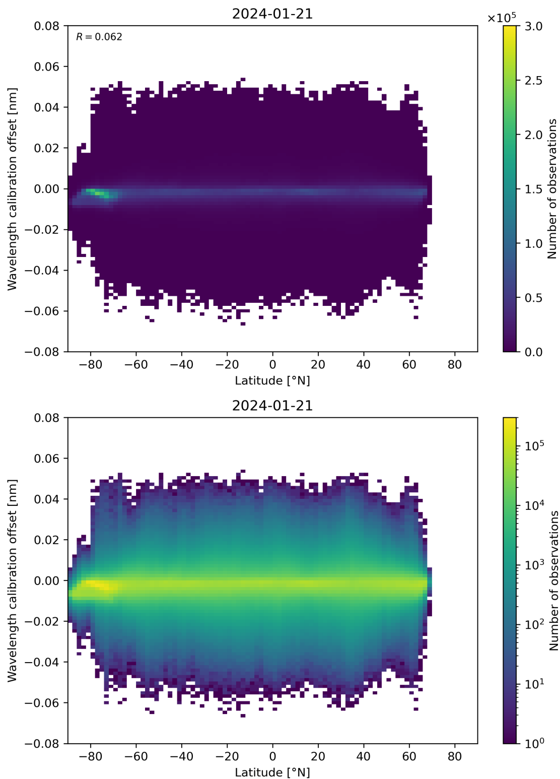
Figure 95: Scatter density plot of “Latitude” against “Wavelength calibration offset” for 2024-01-21 to 2024-01-22.
