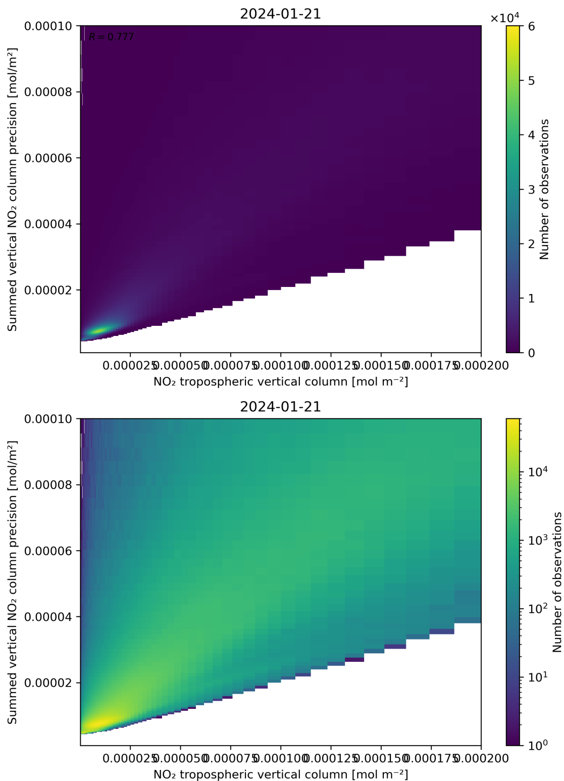
Figure 127: Scatter density plot of “NO 2 tropospheric vertical column” against “Summed vertical NO 2 column precision” for 2024-01-21 to 2024-01-22.
