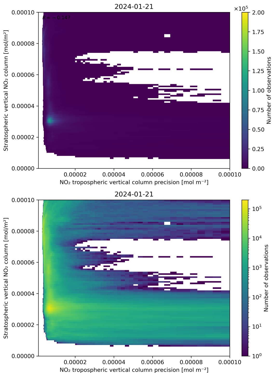
Figure 135: Scatter density plot of “NO 2 tropospheric vertical column precision” against “Stratospheric vertical NO 2 column” for 2024-01-21 to 2024-01-22.
