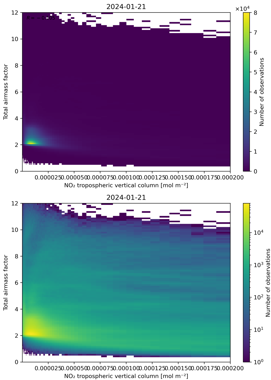
Figure 122: Scatter density plot of “NO 2 tropospheric vertical column” against “Total air mass factor” for 2024-01-21 to 2024-01-22.
