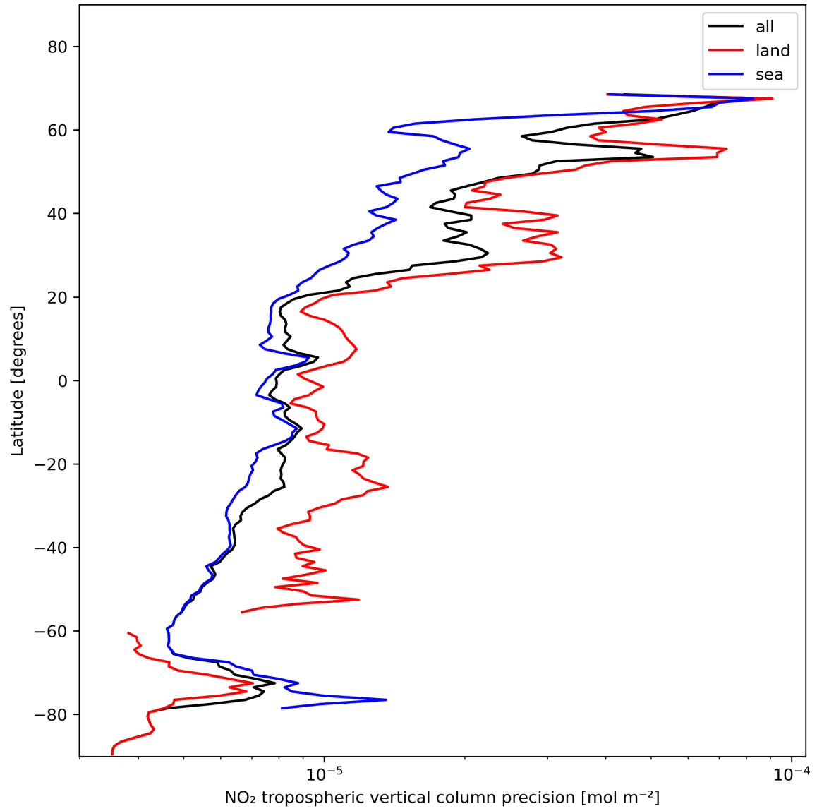
Figure 13: Zonal average of “NO 2 tropospheric vertical column precision” for 2024-01-21 to 2024-01-22.
