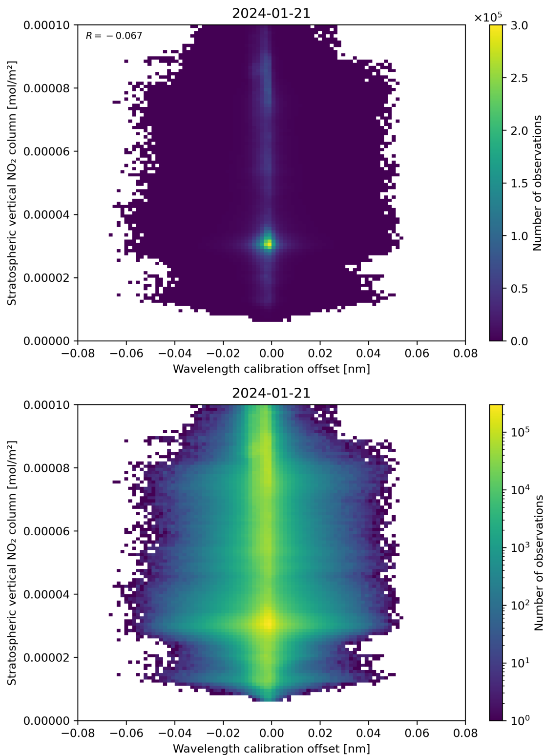
Figure 176: Scatter density plot of “Wavelength calibration offset” against “Stratospheric vertical NO 2 column” for 2024-01-21 to 2024-01-22.
