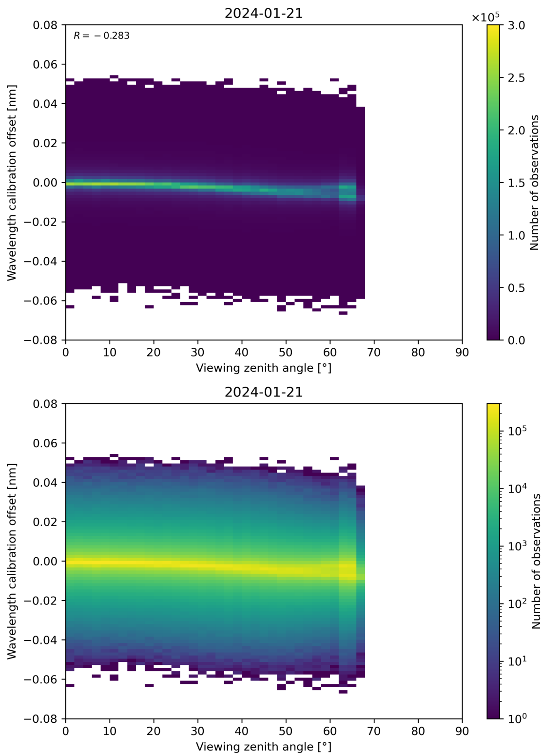
Figure 173: Scatter density plot of “Viewing zenith angle” against “Wavelength calibration offset” for 2024-01-21 to 2024-01-22.
