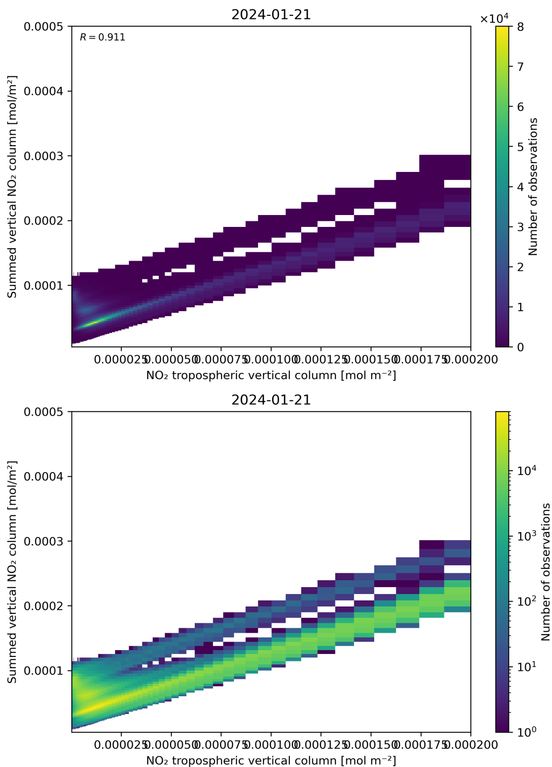
Figure 126: Scatter density plot of “NO 2 tropospheric vertical column” against “Summed vertical NO 2 column” for 2024-01-21 to 2024-01-22.
