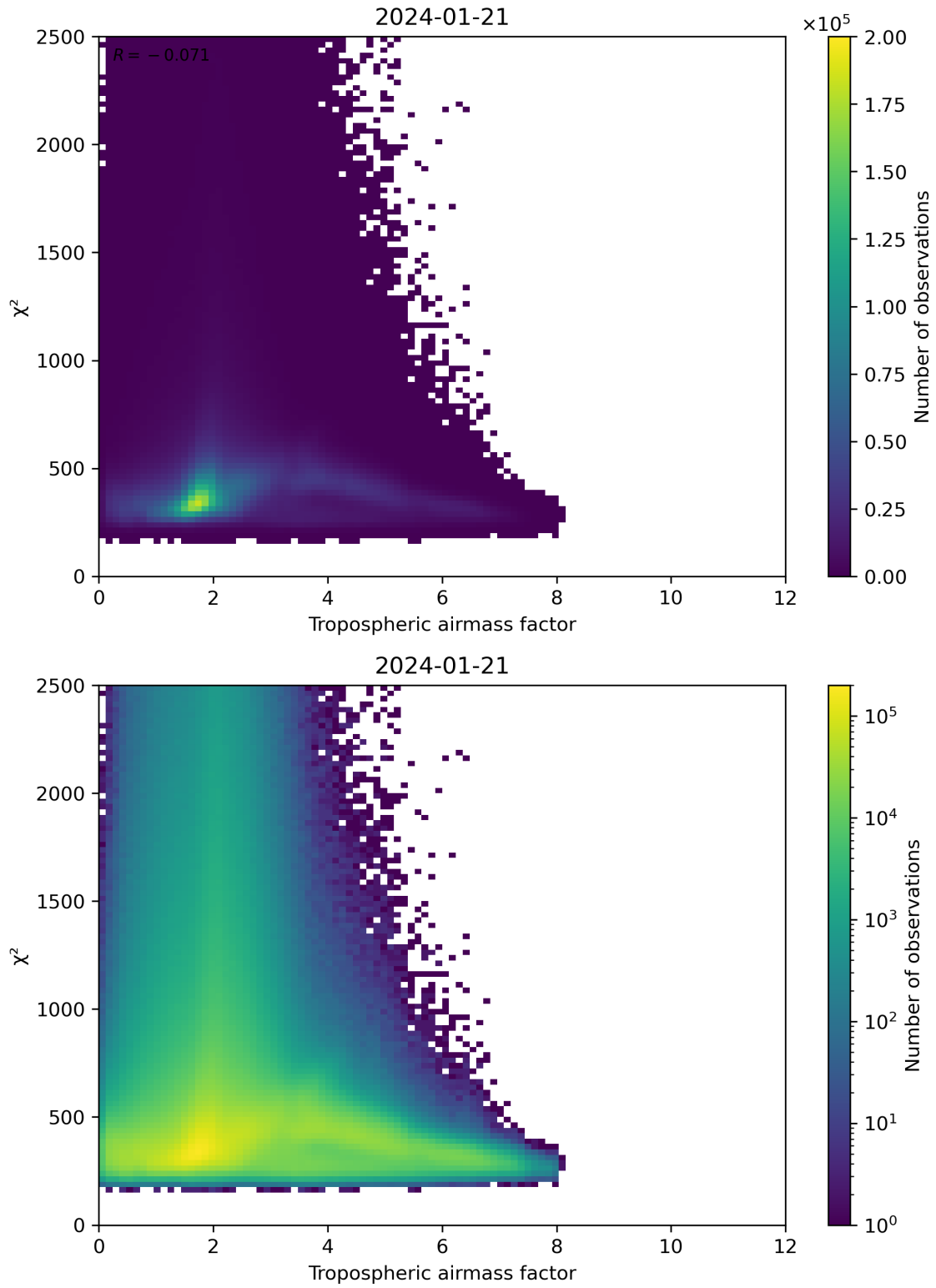
Figure 73: Scatter density plot of “Tropospheric airmass factor” against “ \chi^2 ” for 2024-01-21 to 2024-01-22.
