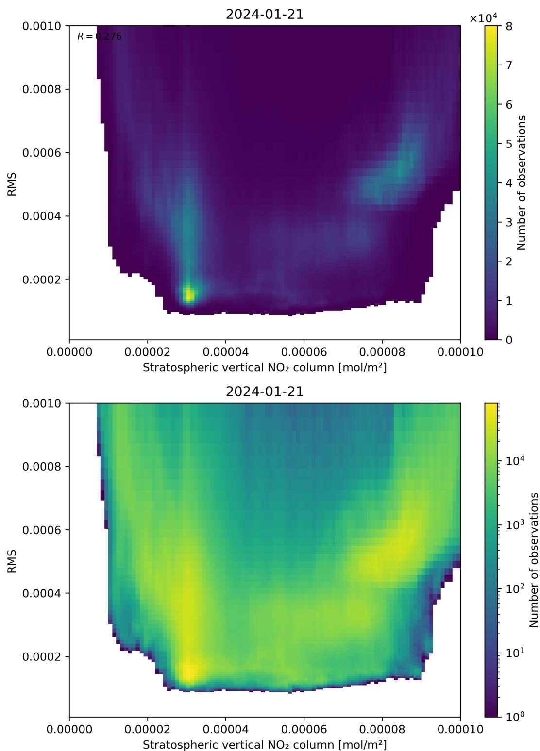
Figure 102: Scatter density plot of “Stratospheric vertical NO 2 column” against “RMS” for 2024-01-21 to 2024-01-22.
