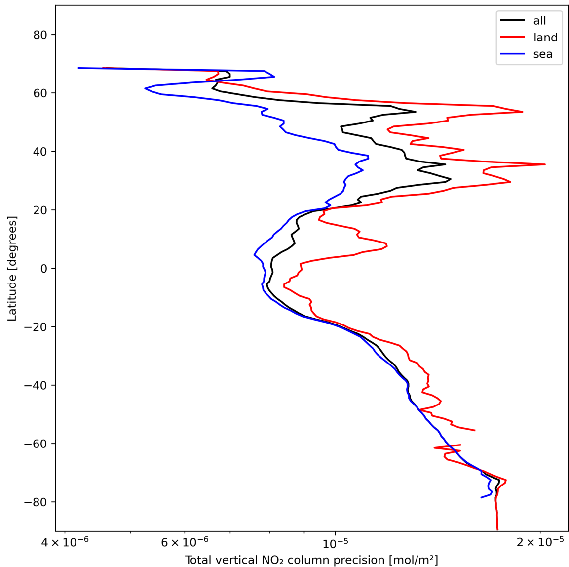
Figure 22: Zonal average of “Total vertical NO 2 column precision” for 2024-01-21 to 2024-01-22.
