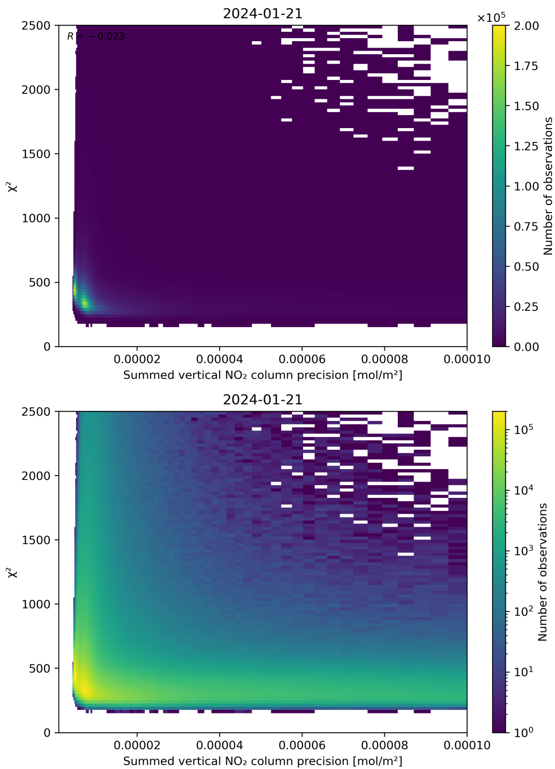
Figure 107: Scatter density plot of “Summed vertical NO 2 column precision” against “ \chi^2 ” for 2024-01-21 to 2024-01-22.
