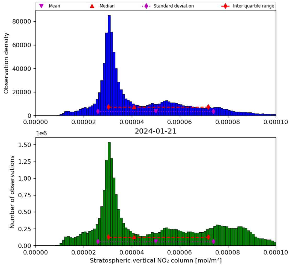
Figure 36: Histogram of “Stratospheric vertical NO 2 column” for 2024-01-21 to 2024-01-22
