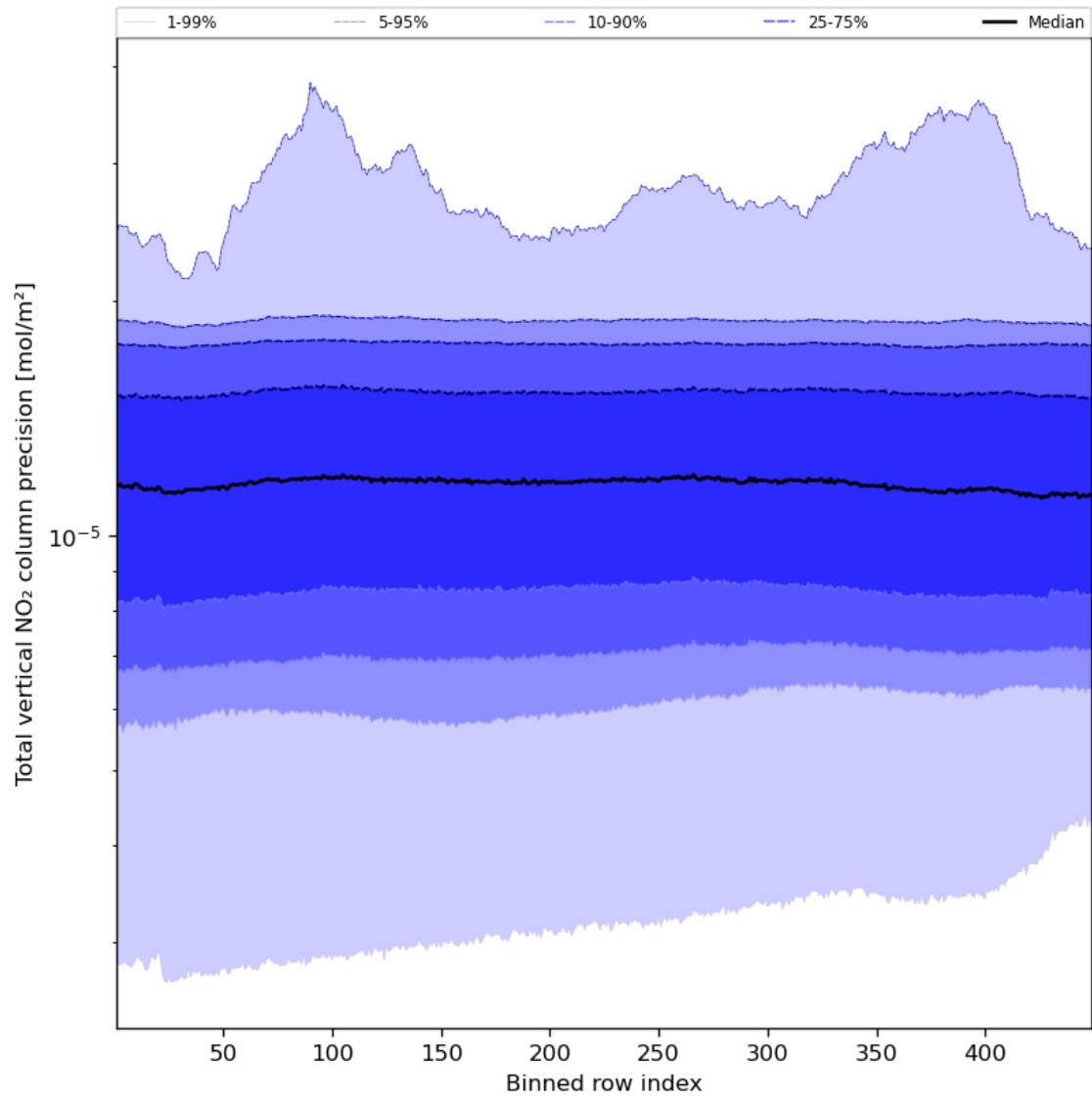
Figure 56: Along track statistics of “Total vertical NO 2 column precision” for 2024-01-21 to 2024-01-22
