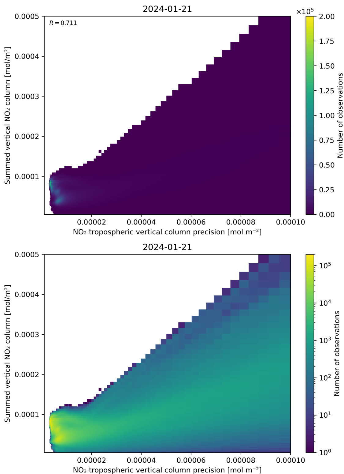
Figure 136: Scatter density plot of “NO 2 tropospheric vertical column precision” against “Summed vertical NO 2 column” for 2024-01-21 to 2024-01-22.
