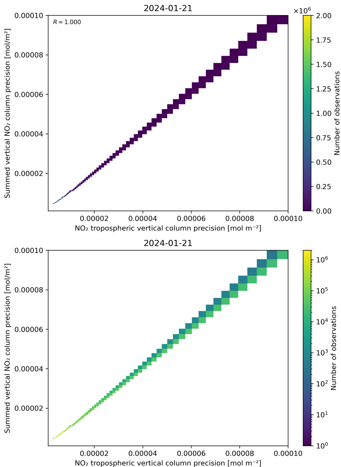
Figure 137: Scatter density plot of “NO 2 tropospheric vertical column precision” against “Summed vertical NO 2 column precision” for 2024-01-21 to 2024-01-22.
