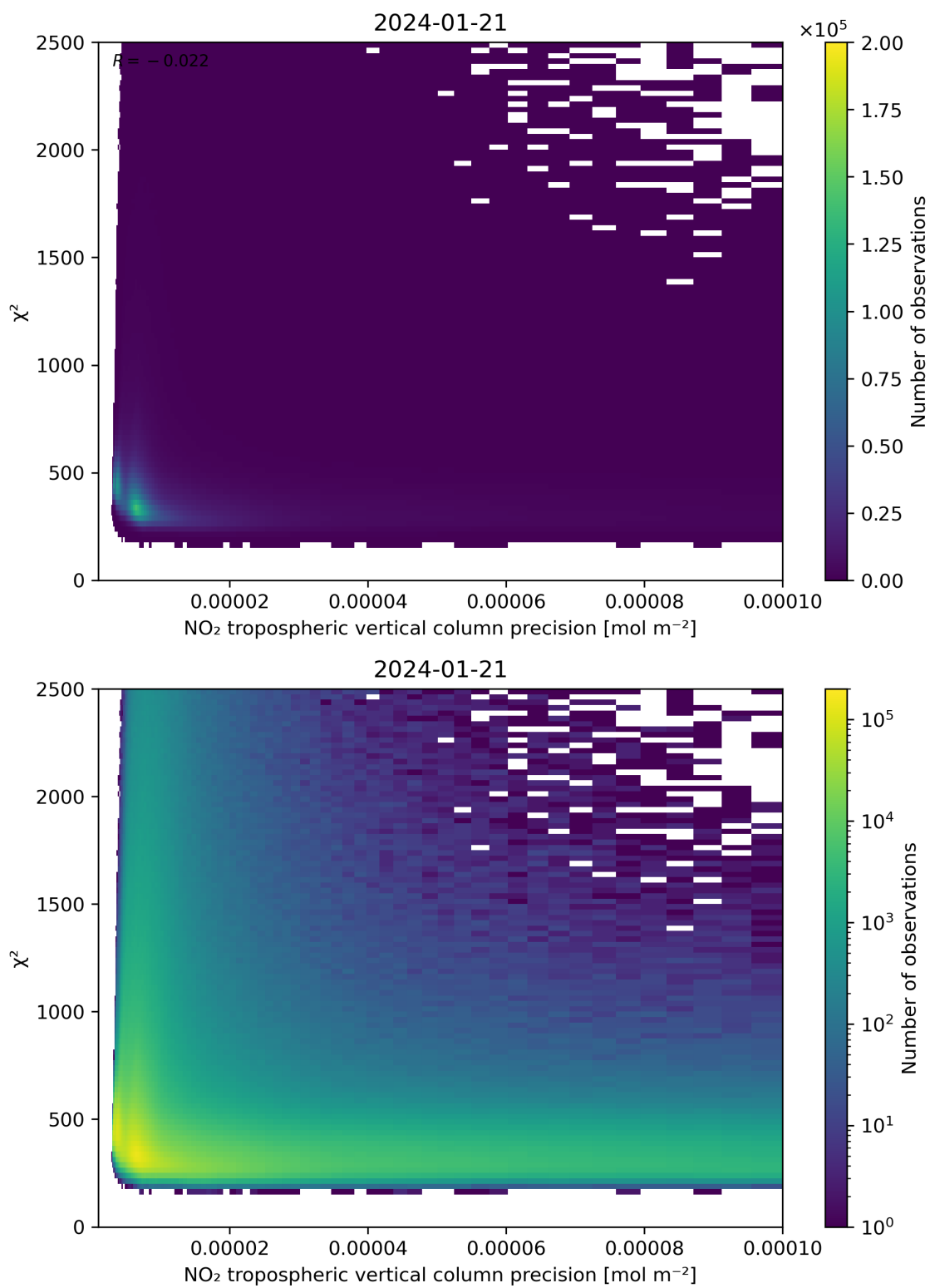
Figure 134: Scatter density plot of “NO 2 tropospheric vertical column precision” against “ \chi^2 ” for 2024-01-21 to 2024-01-22.
