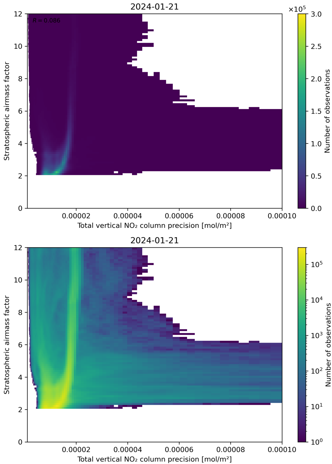
Figure 115: Scatter density plot of “Total vertical NO 2 column precision” against “Stratospheric airmass factor” for 2024-01-21 to 2024-01-22.
