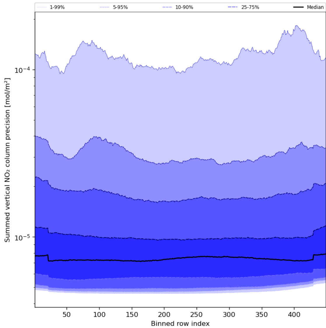
Figure 58: Along track statistics of “Summed vertical NO 2 column precision” for 2024-01-21 to 2024-01-22
