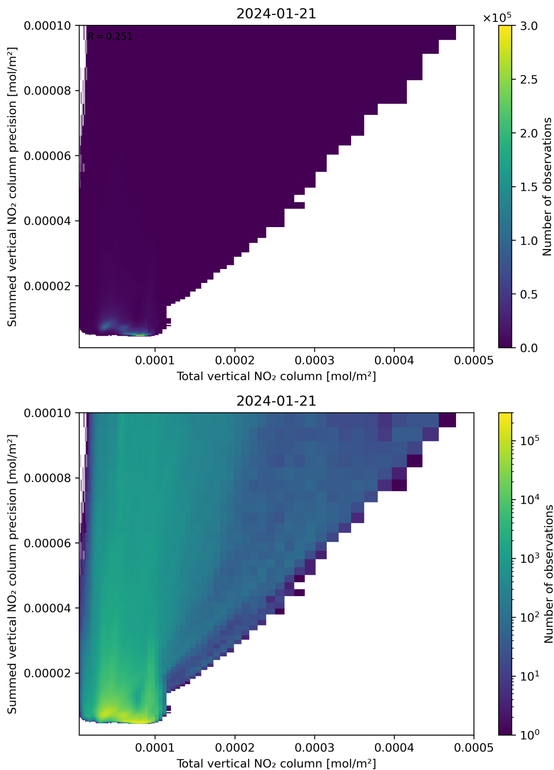
Figure 113: Scatter density plot of “Total vertical NO 2 column” against “Summed vertical NO 2 column precision” for 2024-01-21 to 2024-01-22.
