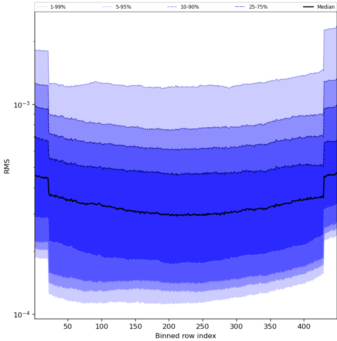
Figure 60: Along track statistics of “RMS” for 2024-01-21 to 2024-01-22
