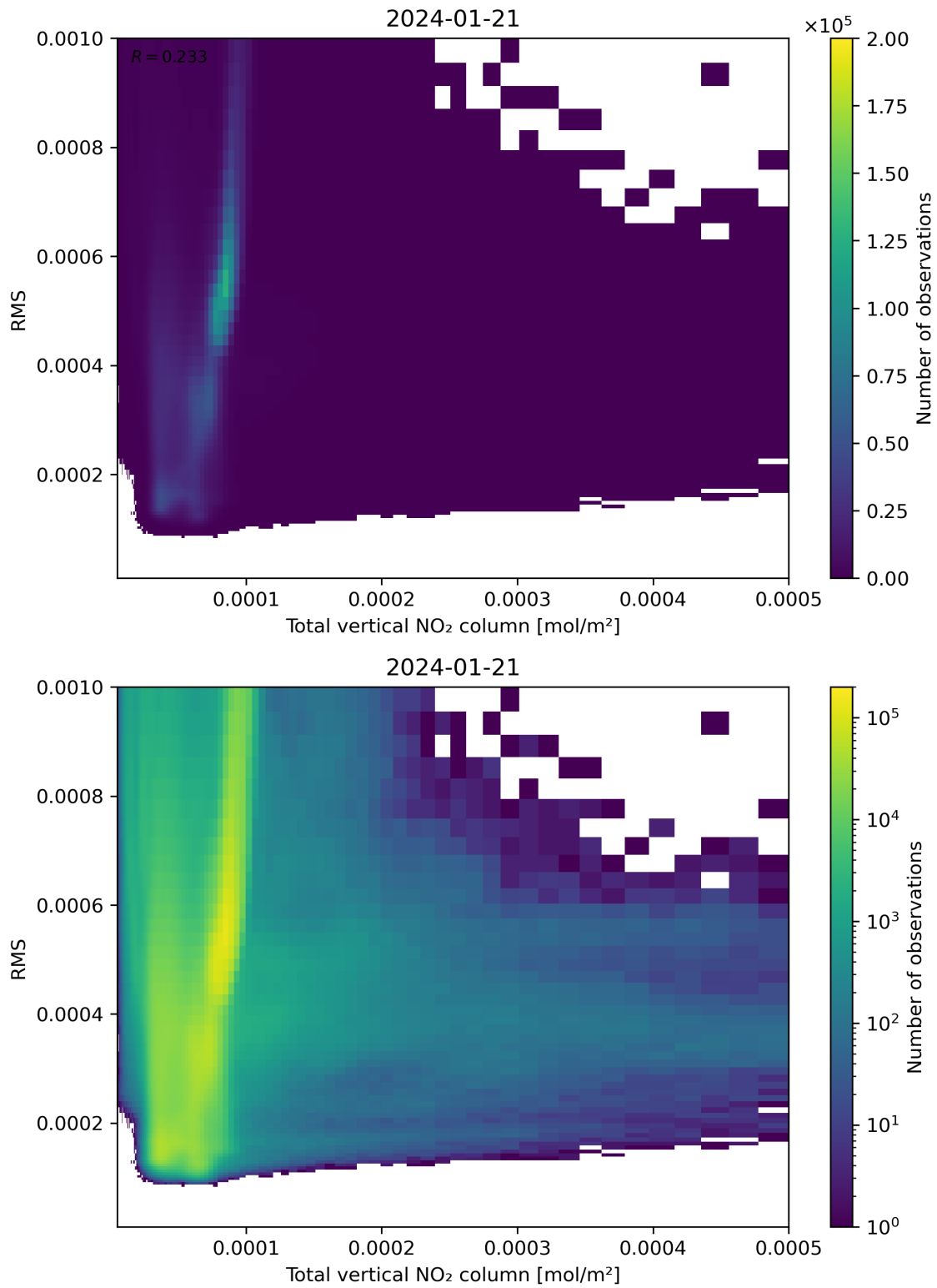
Figure 120: Scatter density plot of “Total vertical NO 2 column” against “RMS” for 2024-01-21 to 2024-01-22.
