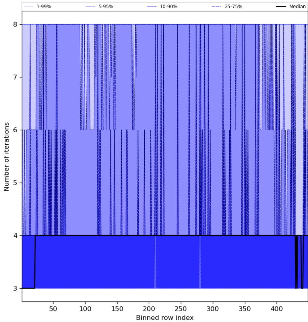
Figure 51: Along track statistics of “Number of iterations” for 2024-01-21 to 2024-01-22
