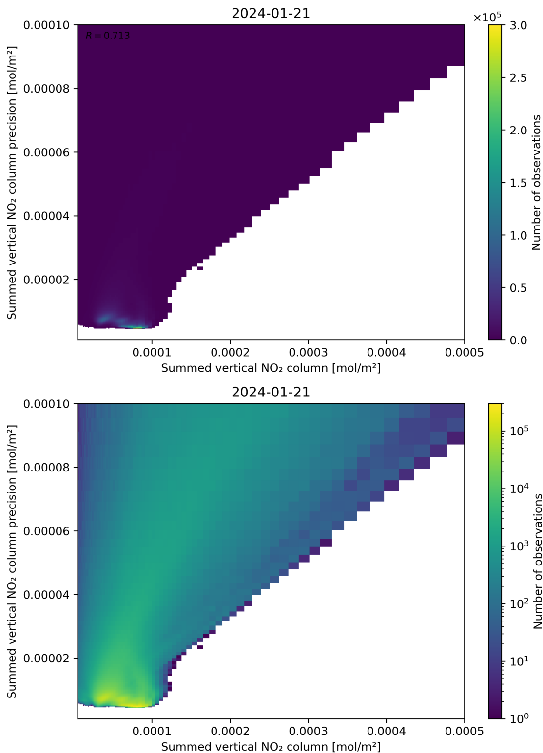
Figure 105: Scatter density plot of “Summed vertical NO 2 column” against “Summed vertical NO 2 column precision” for 2024-01-21 to 2024-01-22.
