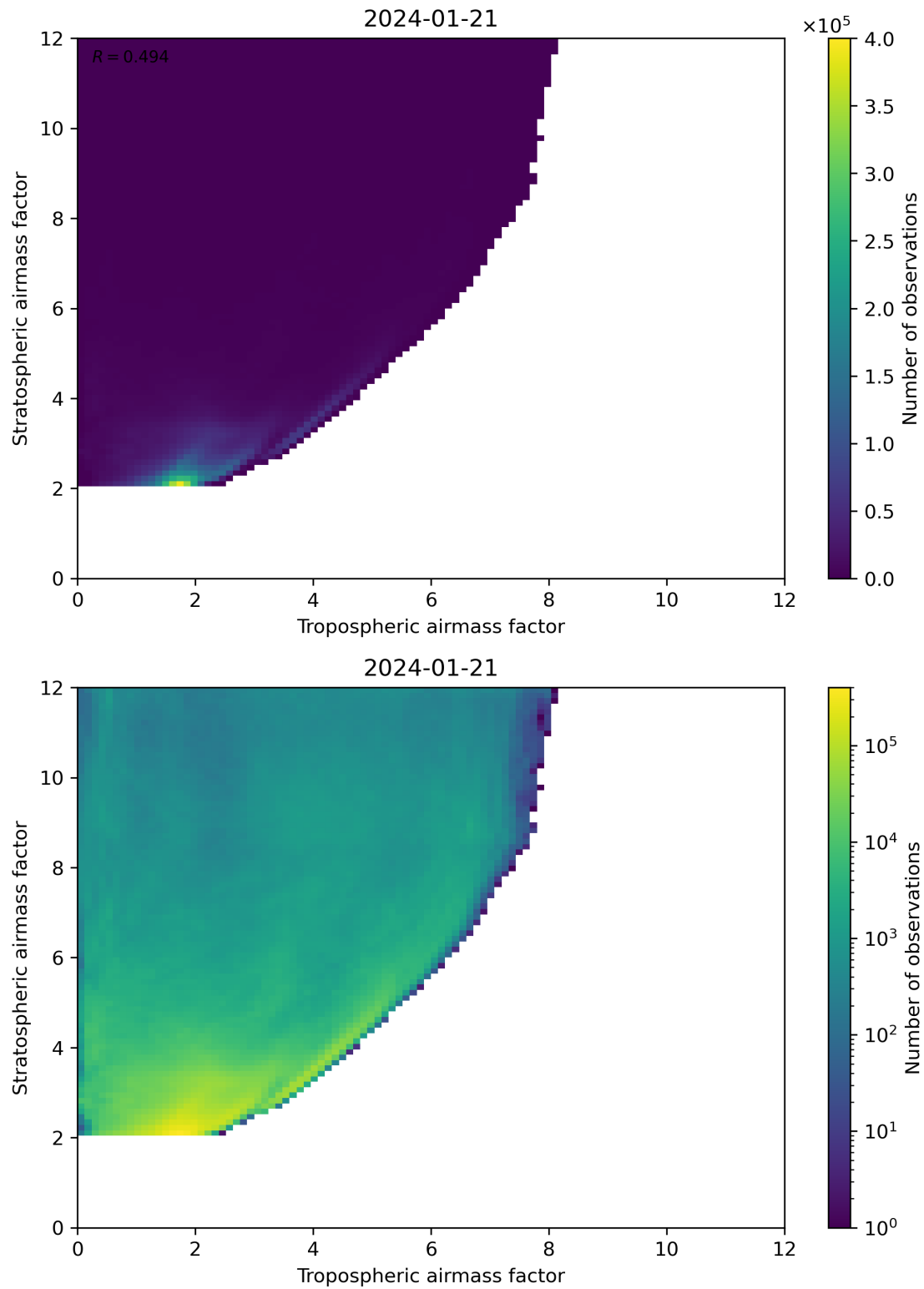
Figure 71: Scatter density plot of “Tropospheric airmass factor” against “Stratospheric airmass factor” for 2024-01-21 to 2024-01-22.
