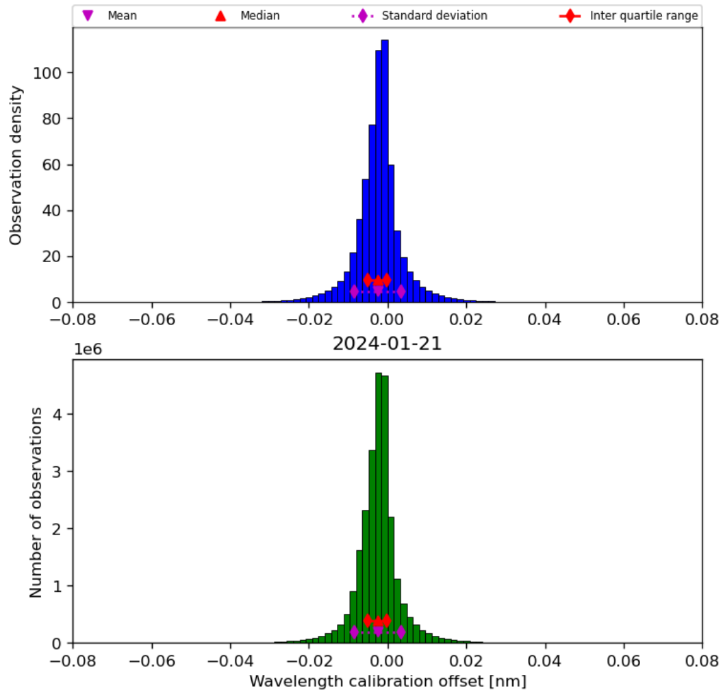
Figure 35: Histogram of “Wavelength calibration offset” for 2024-01-21 to 2024-01-22
