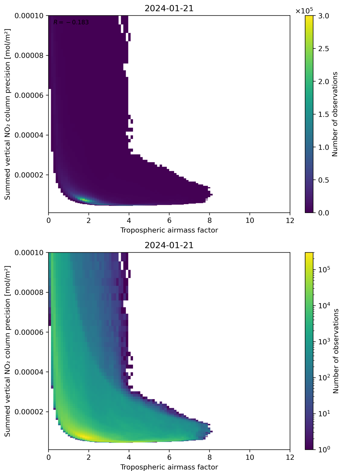
Figure 76: Scatter density plot of “Tropospheric air mass factor” against “Summed vertical NO 2 column precision” for 2024-01-21 to 2024-01-22.
