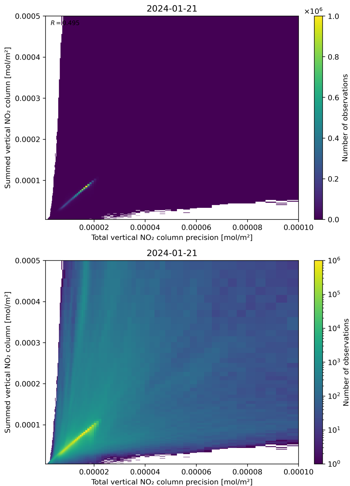
Figure 117: Scatter density plot of “Total vertical NO 2 column precision” against “Summed vertical NO 2 column” for 2024-01-21 to 2024-01-22.
