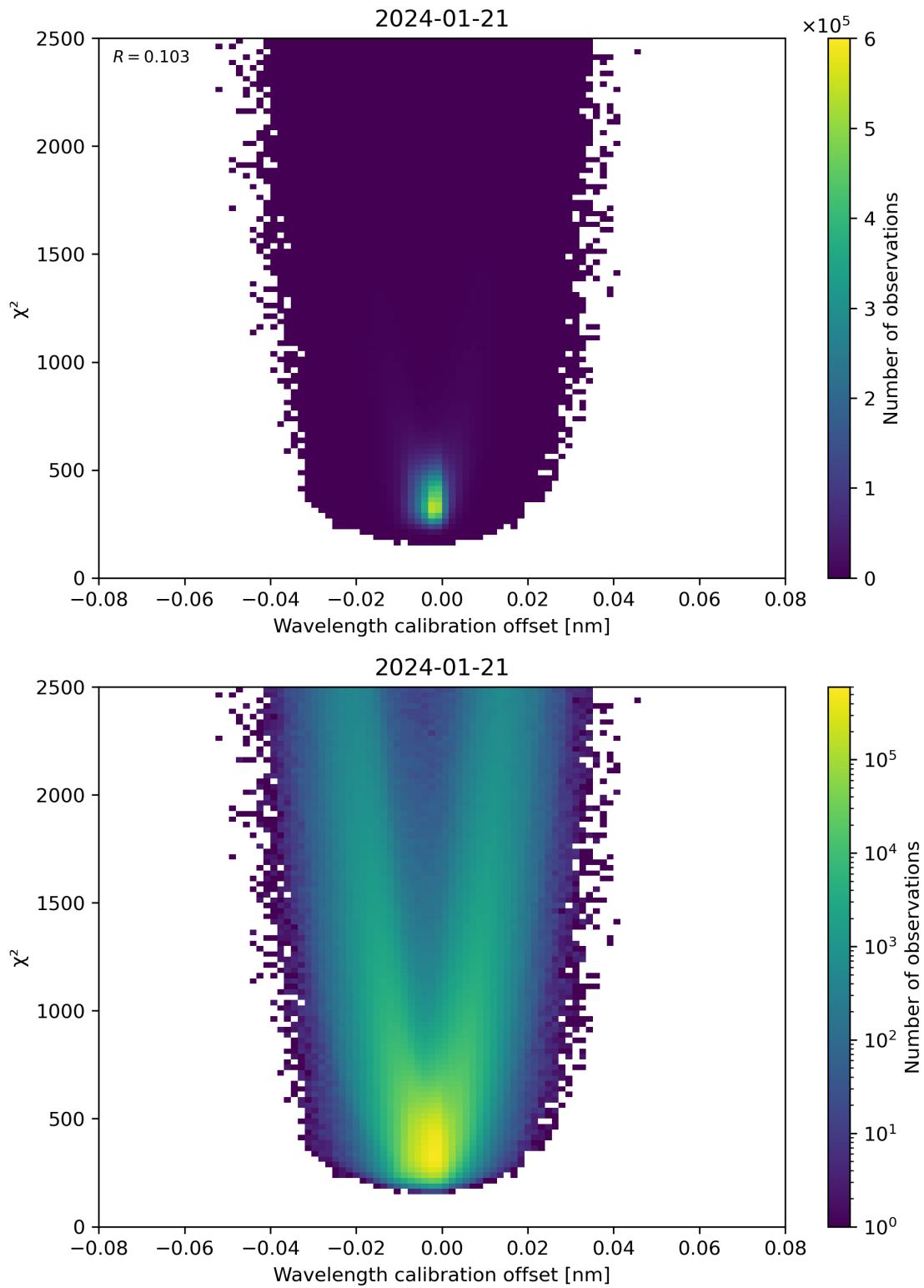
Figure 175: Scatter density plot of “Wavelength calibration offset” against “ \chi^2 ” for 2024-01-21 to 2024-01-22.
