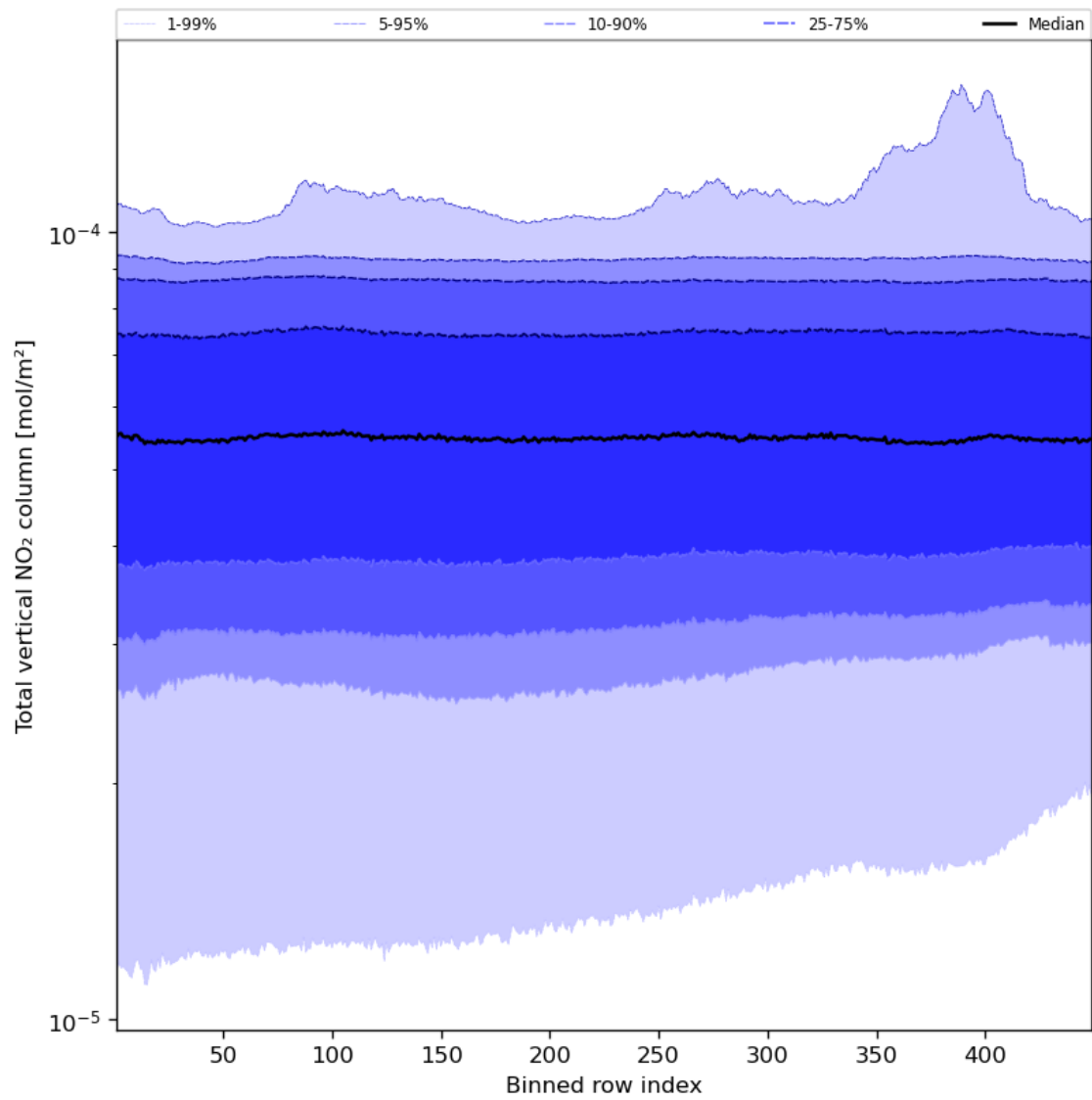
Figure 55: Along track statistics of “Total vertical NO 2 column” for 2024-01-21 to 2024-01-22
