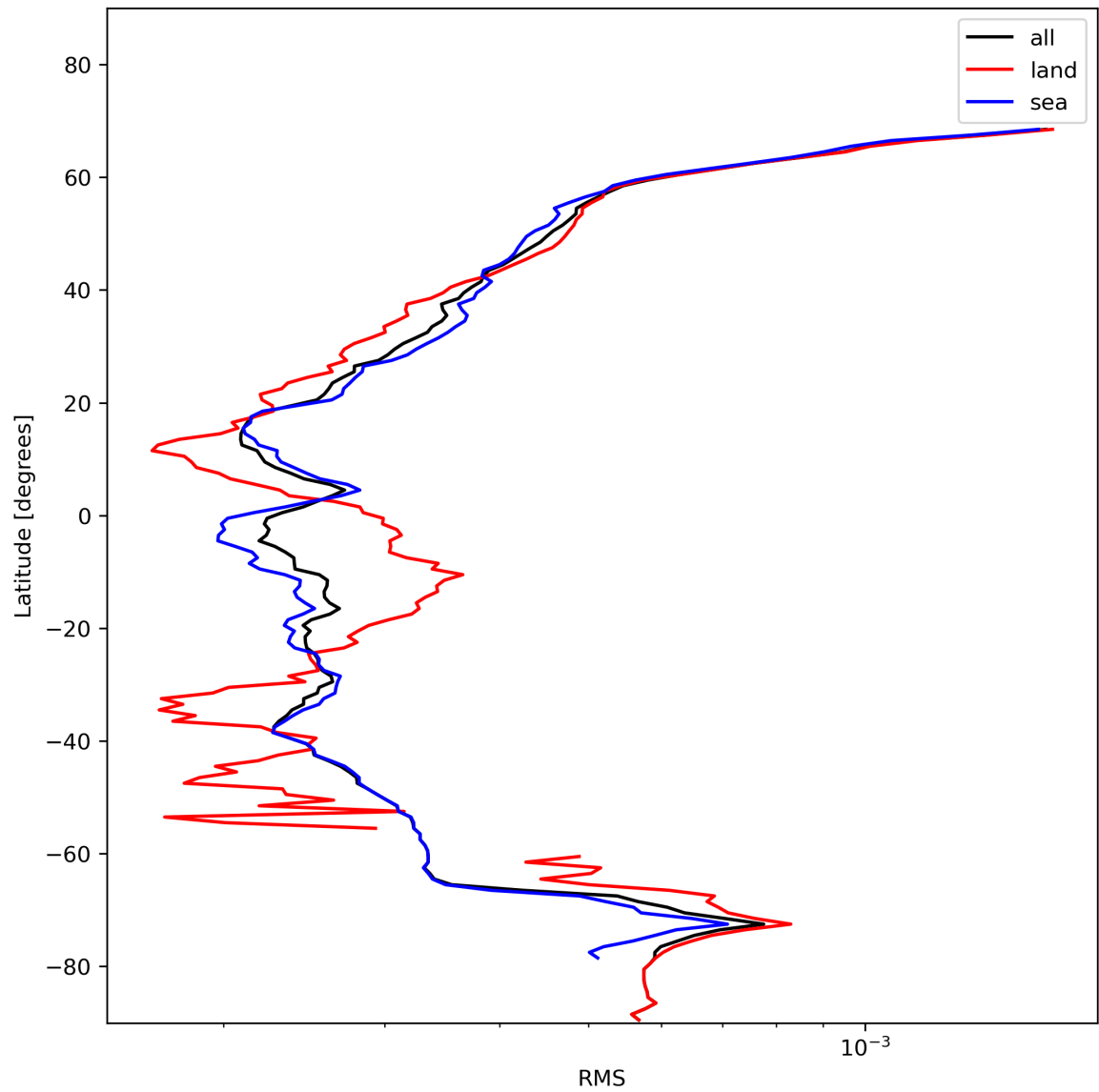
Figure 26: Zonal average of “RMS” for 2024-01-21 to 2024-01-22.
