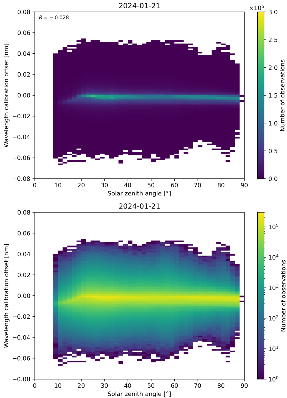
Figure 158: Scatter density plot of “Solar zenith angle” against “Wavelength calibration offset” for 2024-01-21 to 2024-01-22.
