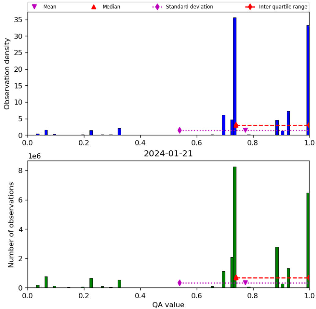
Figure 28: Histogram of “QA value” for 2024-01-21 to 2024-01-22
