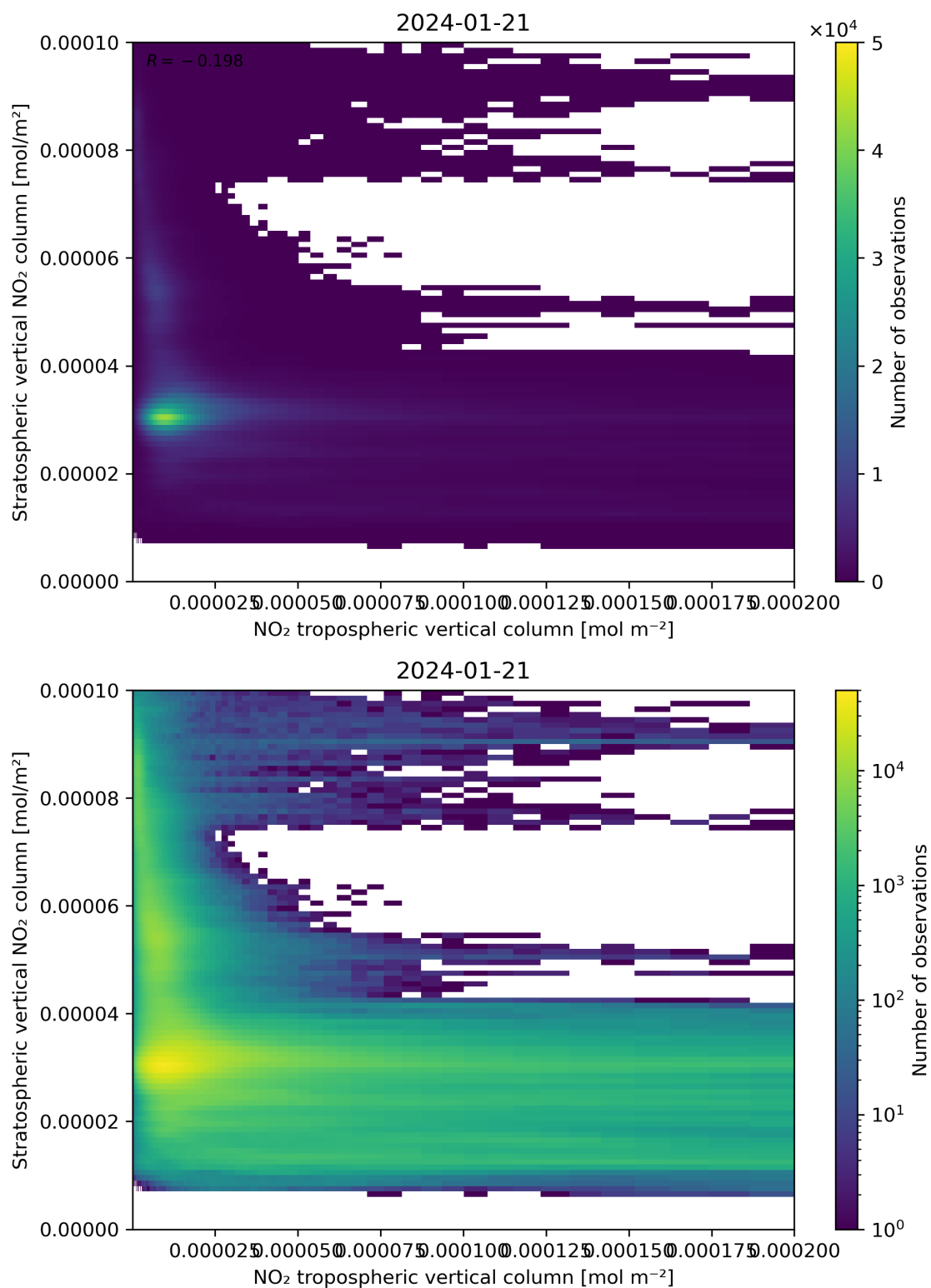
Figure 125: Scatter density plot of “NO 2 tropospheric vertical column” against “Stratospheric vertical NO 2 column” for 2024-01-21 to 2024-01-22.
