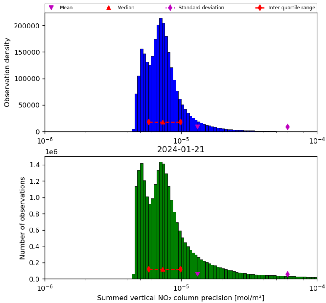
Figure 41: Histogram of "Summed vertical NO 2 column precision" for 2024-01-21 to 2024-01-22
