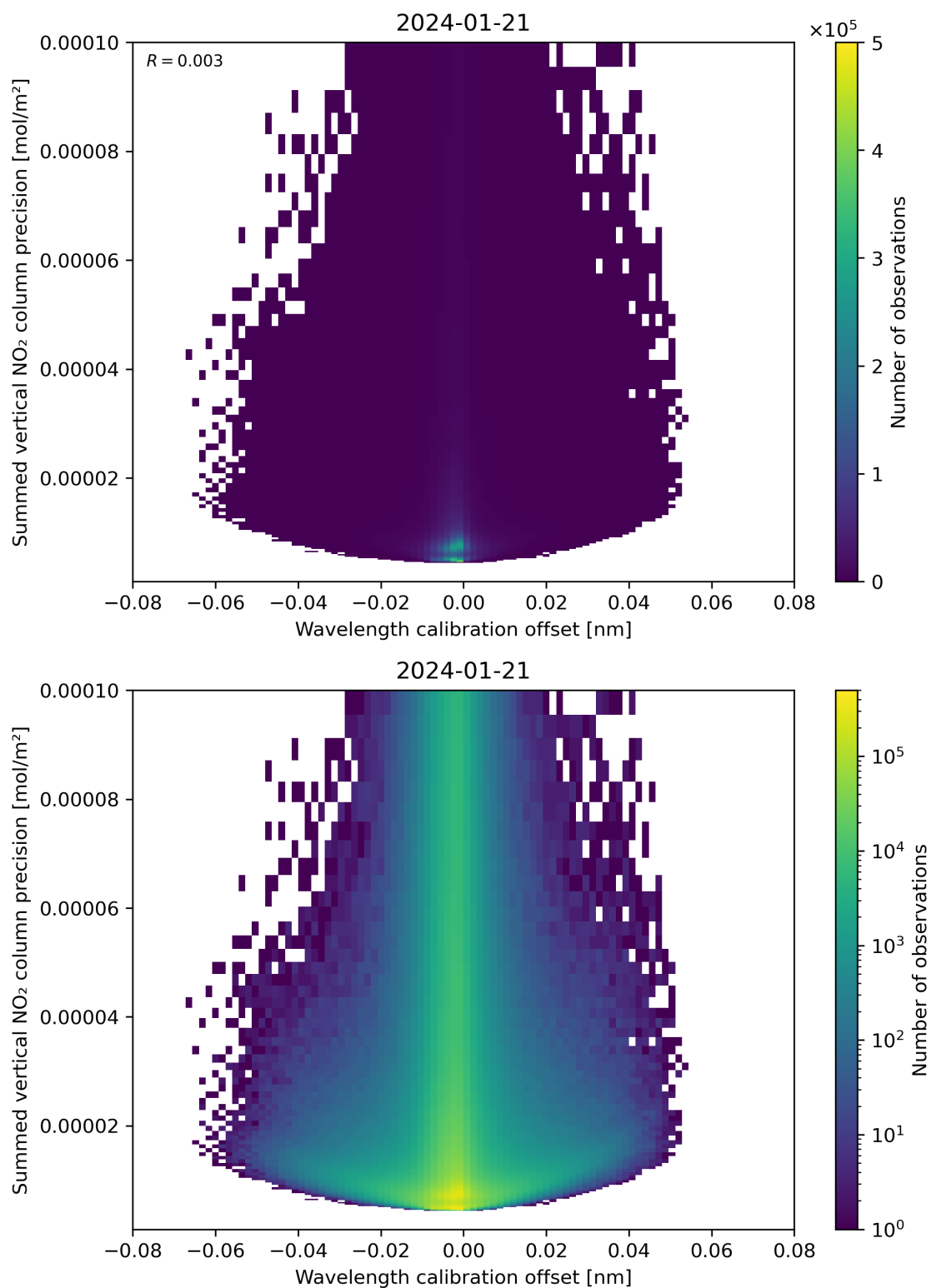
Figure 178: Scatter density plot of “Wavelength calibration offset” against “Summed vertical NO 2 column precision” for 2024-01-21 to 2024-01-22.
