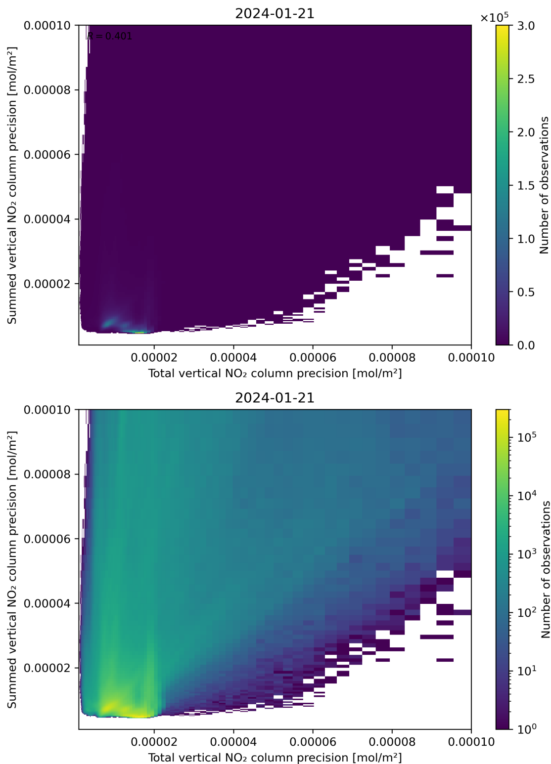
Figure 118: Scatter density plot of “Total vertical NO 2 column precision” against “Summed vertical NO 2 column precision” for 2024-01-21 to 2024-01-22.
