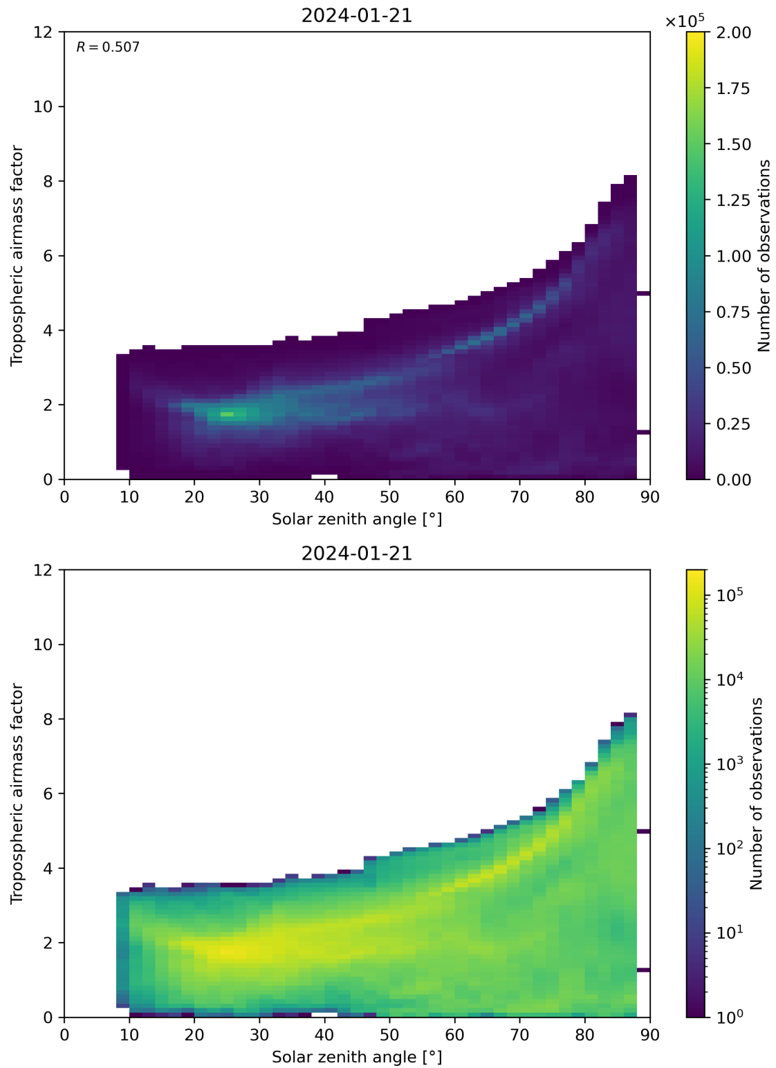
Figure 147: Scatter density plot of “Solar zenith angle” against “Tropospheric airmass factor” for 2024-01-21 to 2024-01-22.
