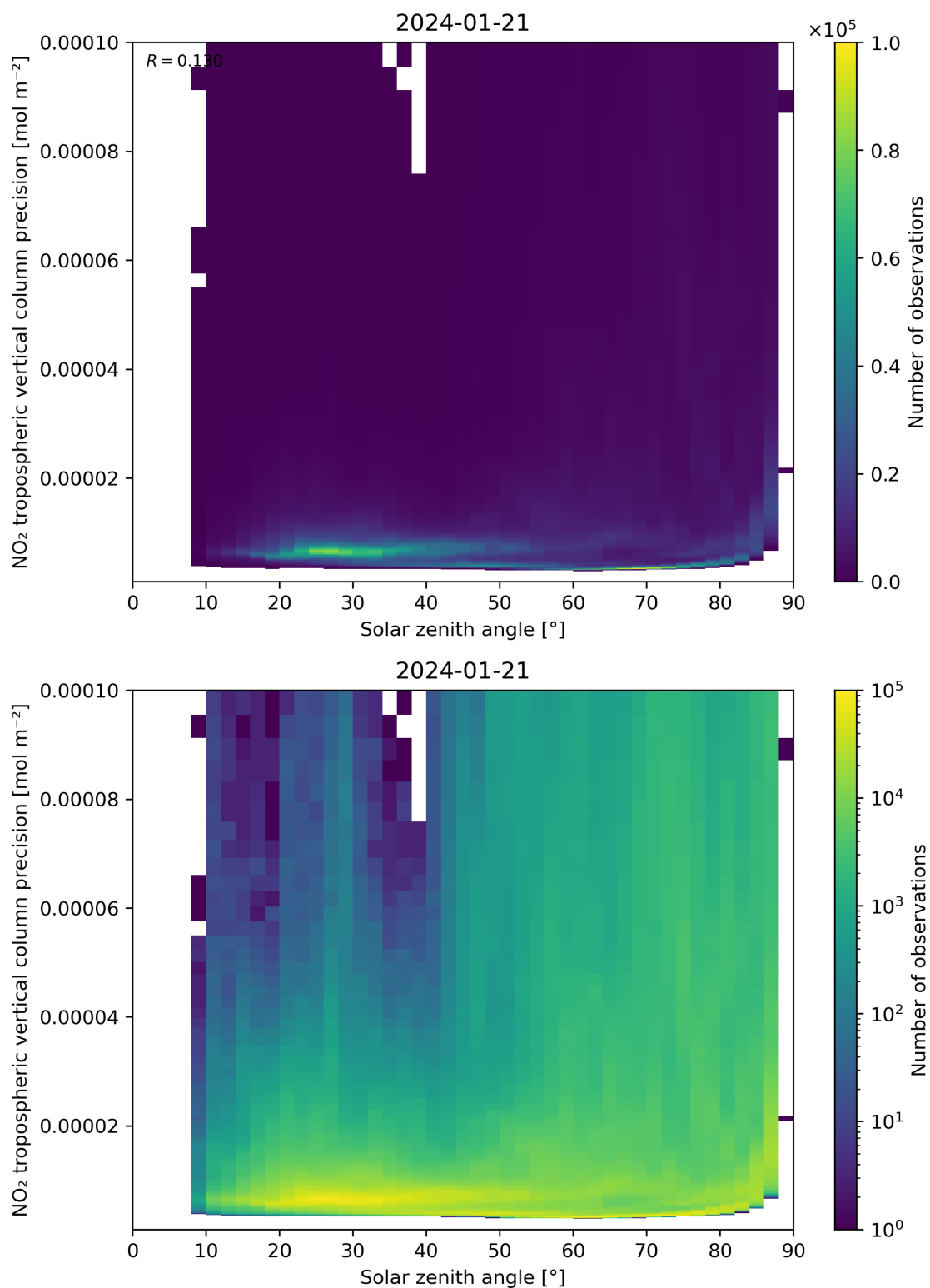
Figure 156: Scatter density plot of “Solar zenith angle” against “NO 2 tropospheric vertical column precision” for 2024-01-21 to 2024-01-22.
