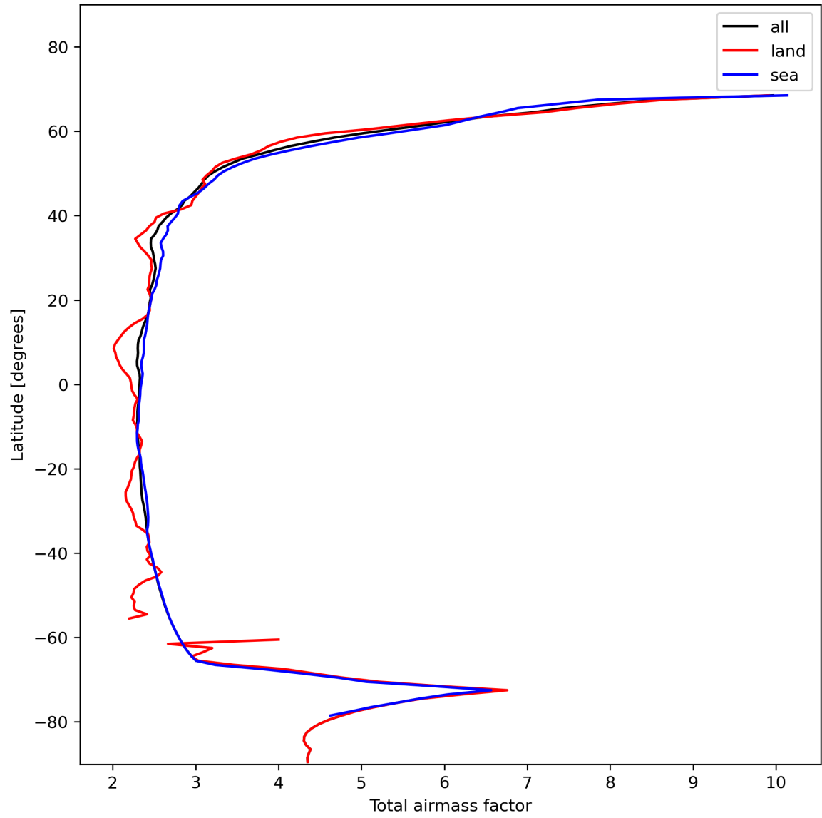
Figure 15: Zonal average of “Total airmass factor” for 2024-01-21 to 2024-01-22.
