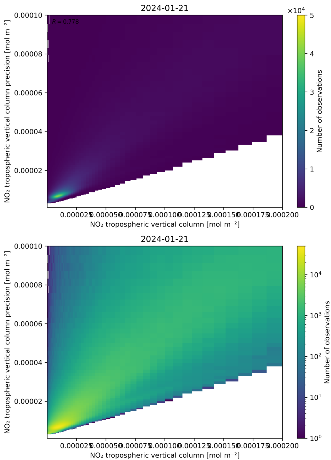
Figure 130: Scatter density plot of “NO 2 tropospheric vertical column” against “NO 2 tropospheric vertical column precision” for 2024-01-21 to 2024-01-22.
