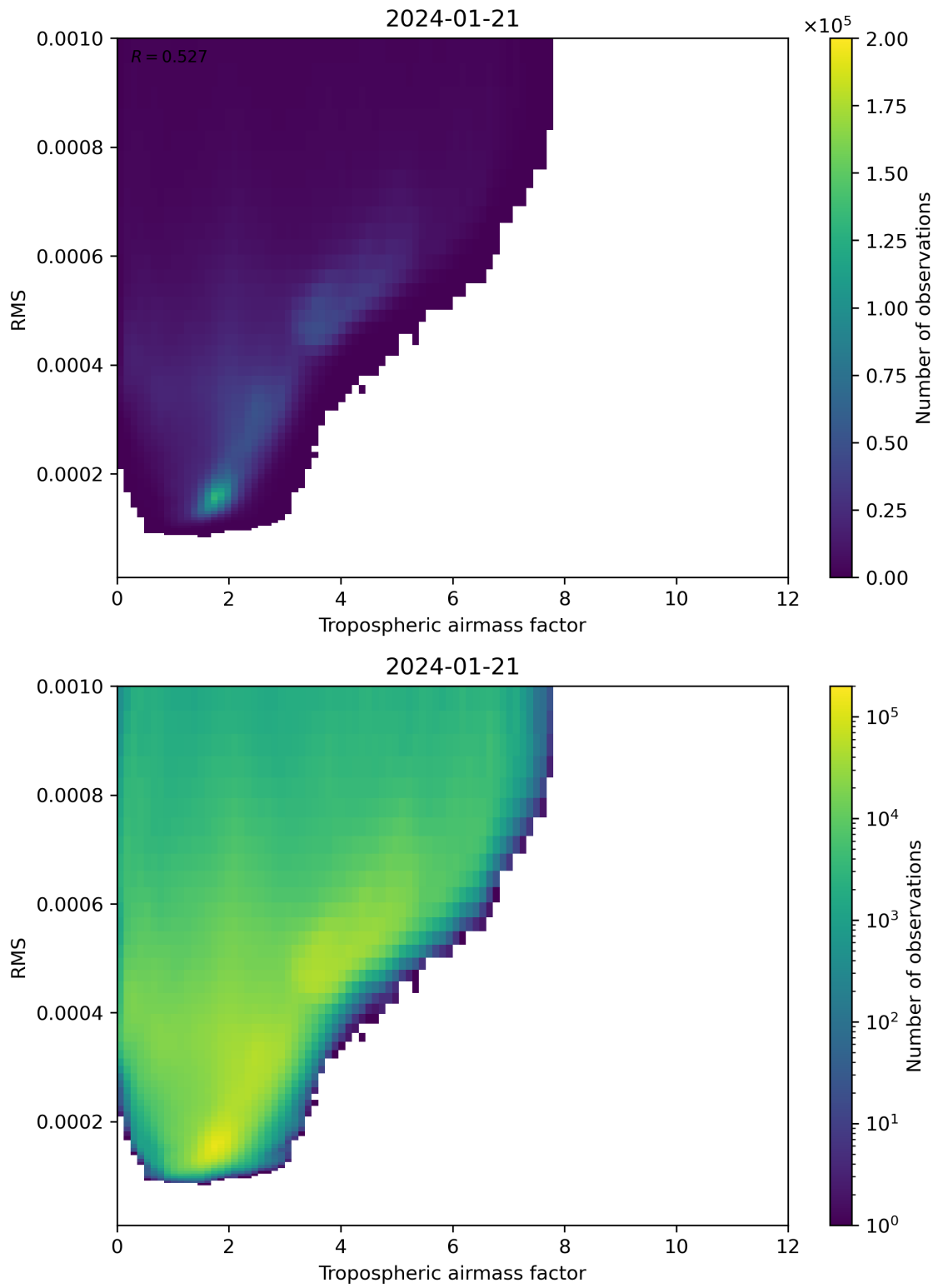
Figure 79: Scatter density plot of “Tropospheric airmass factor” against “RMS” for 2024-01-21 to 2024-01-22.
