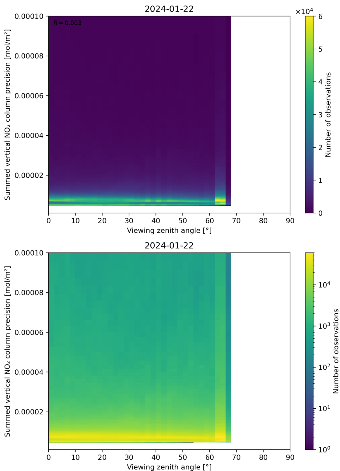
Figure 166: Scatter density plot of “Viewing zenith angle” against “Summed vertical NO 2 column precision” for 2024-01-21 to 2024-01-23.
