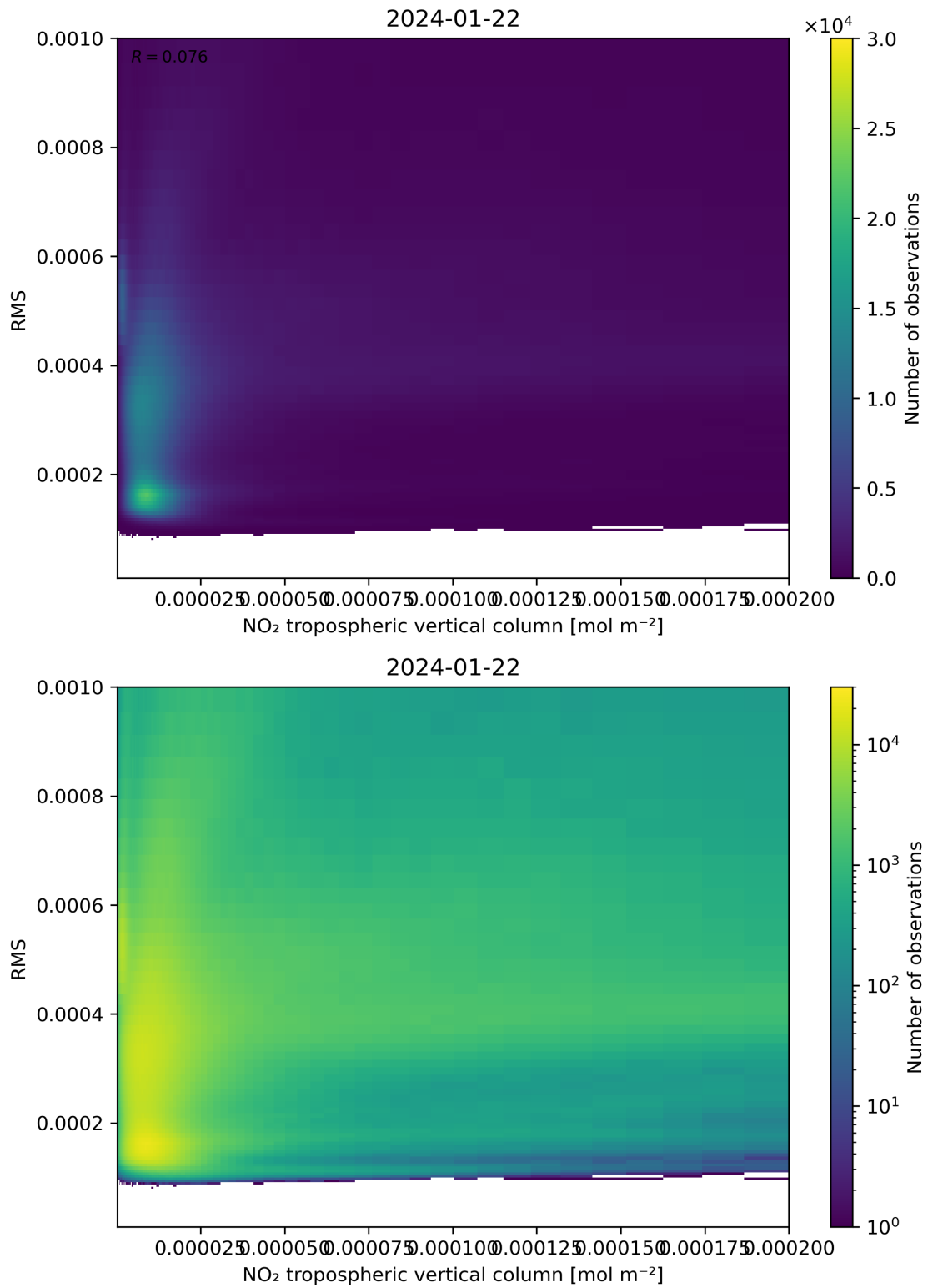
Figure 142: Scatter density plot of “NO 2 tropospheric vertical column” against “RMS” for 2024-01-21 to 2024-01-23.
