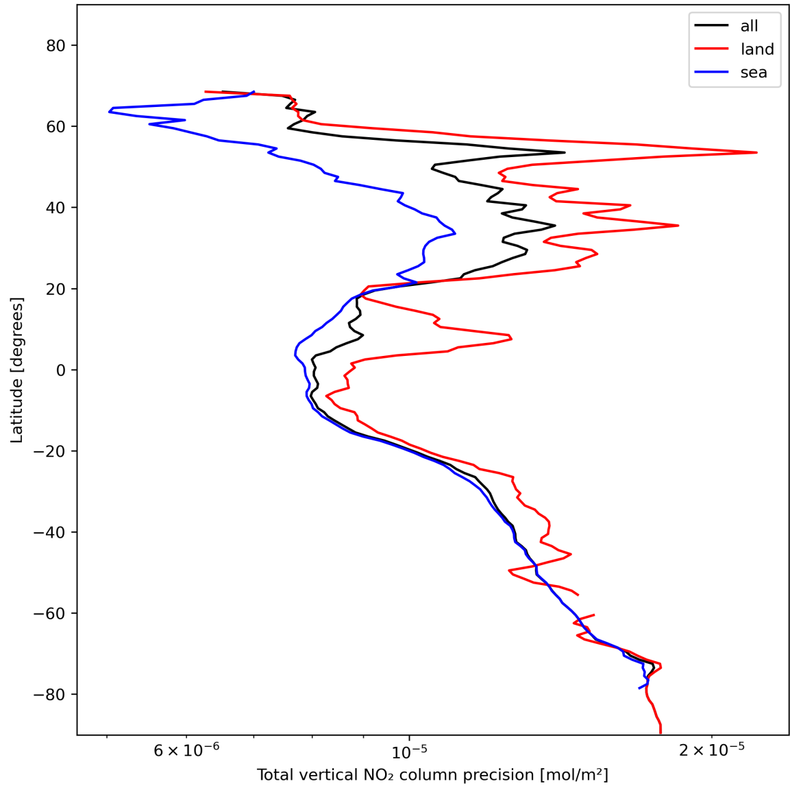
Figure 22: Zonal average of “Total vertical NO 2 column precision” for 2024-01-21 to 2024-01-23.
