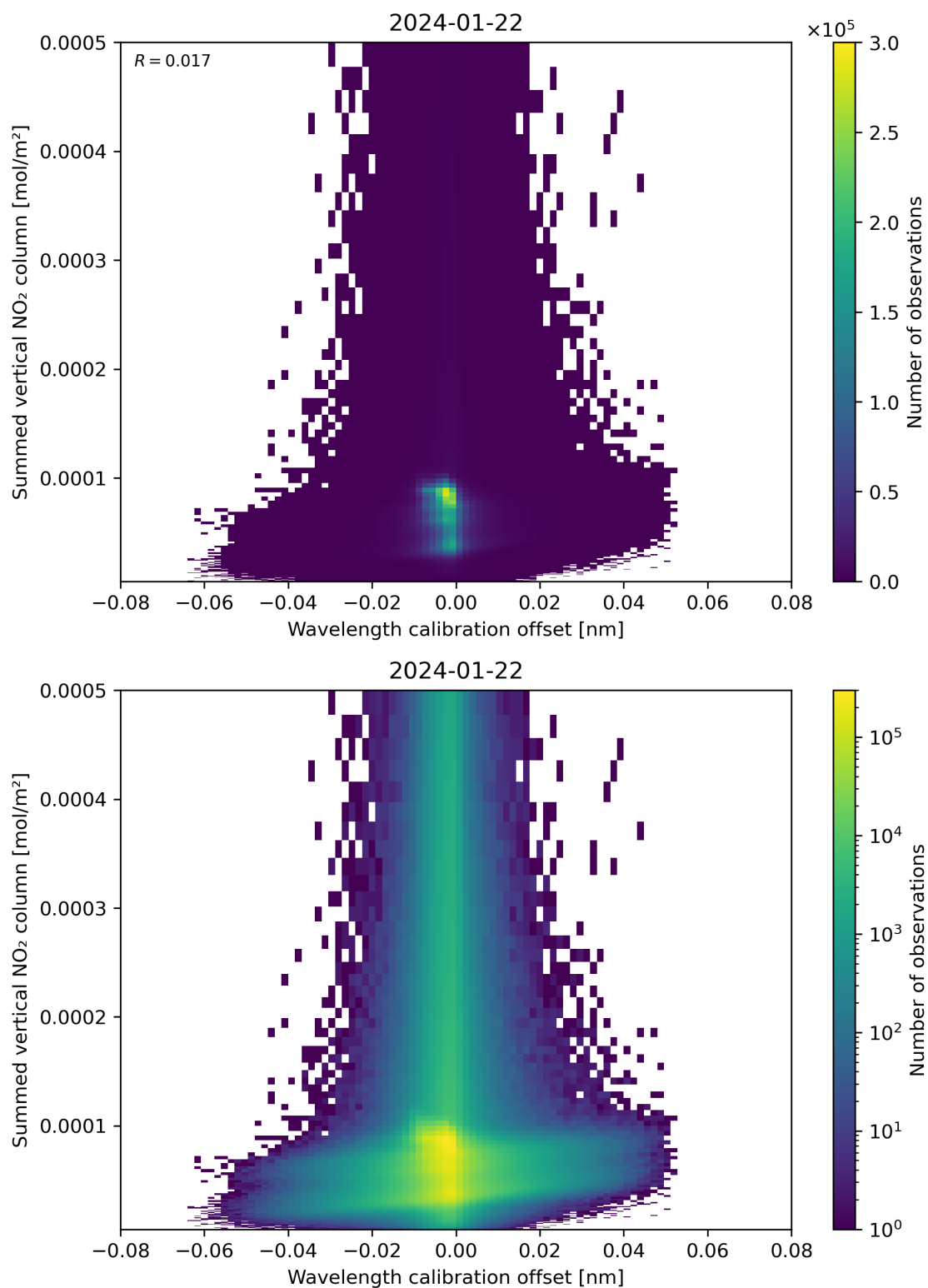
Figure 177: Scatter density plot of “Wavelength calibration offset” against “Summed vertical NO 2 column” for 2024-01-21 to 2024-01-23.
