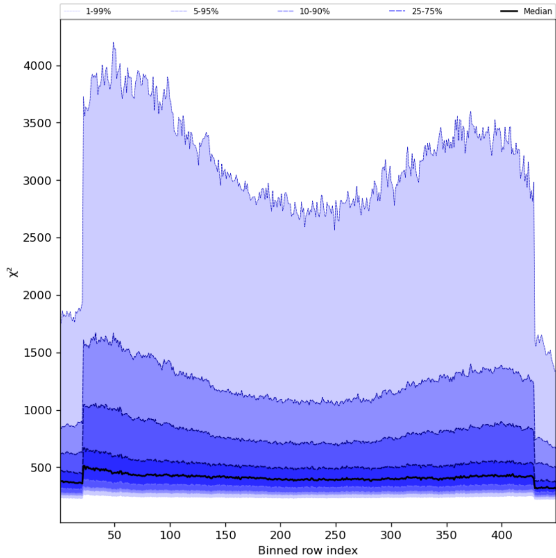
Figure 59: Along track statistics of “ \chi^2 ” for 2024-01-21 to 2024-01-23
