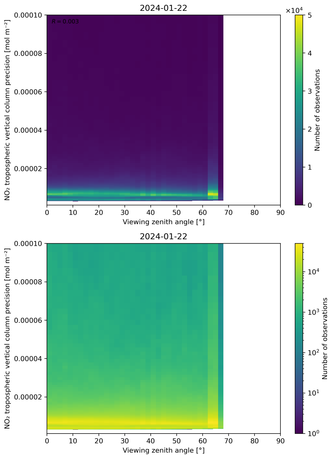
Figure 170: Scatter density plot of “Viewing zenith angle” against “NO 2 tropospheric vertical column precision” for 2024-01-21 to 2024-01-23.
