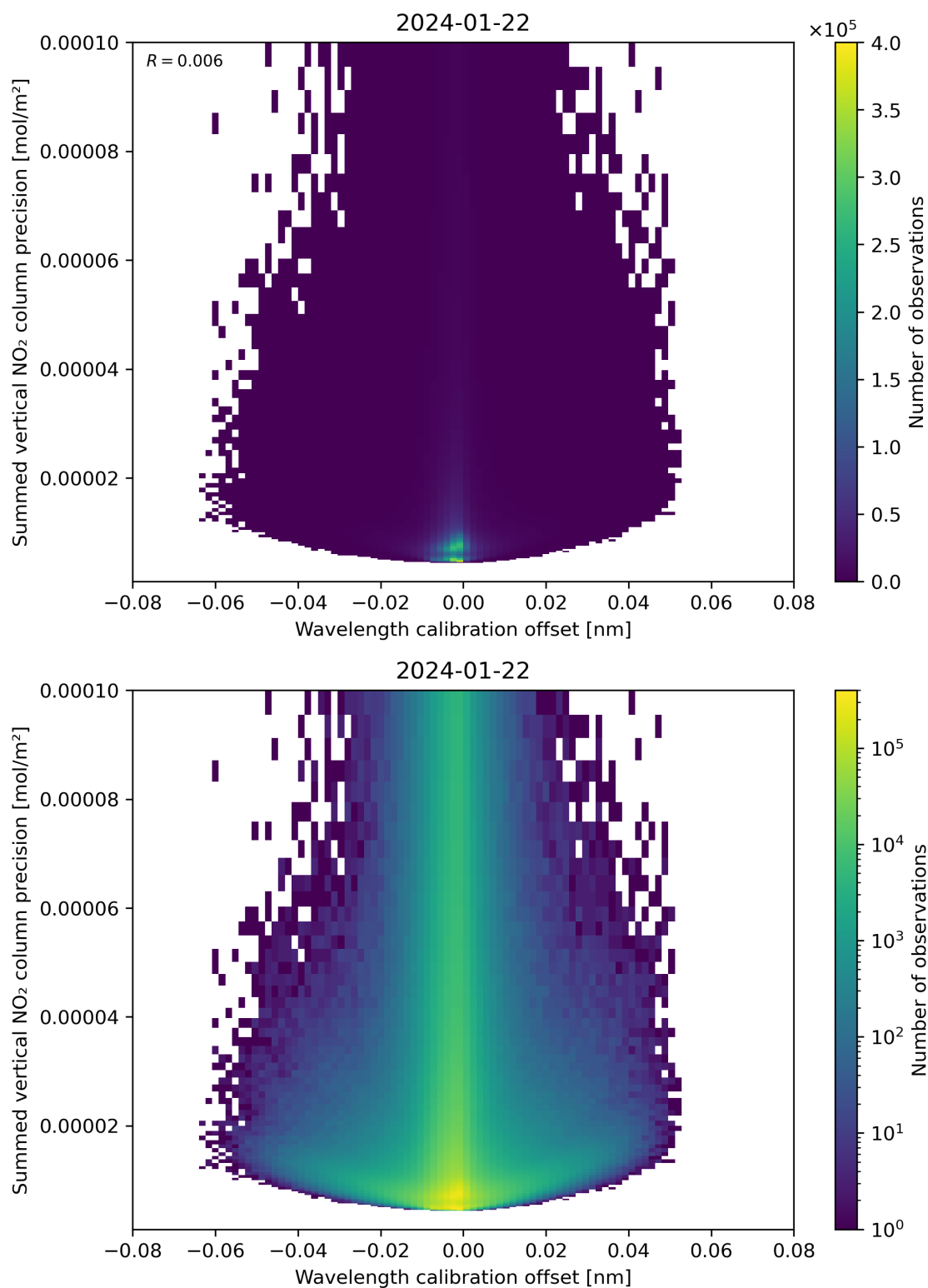
Figure 178: Scatter density plot of “Wavelength calibration offset” against “Summed vertical NO 2 column precision” for 2024-01-21 to 2024-01-23.
