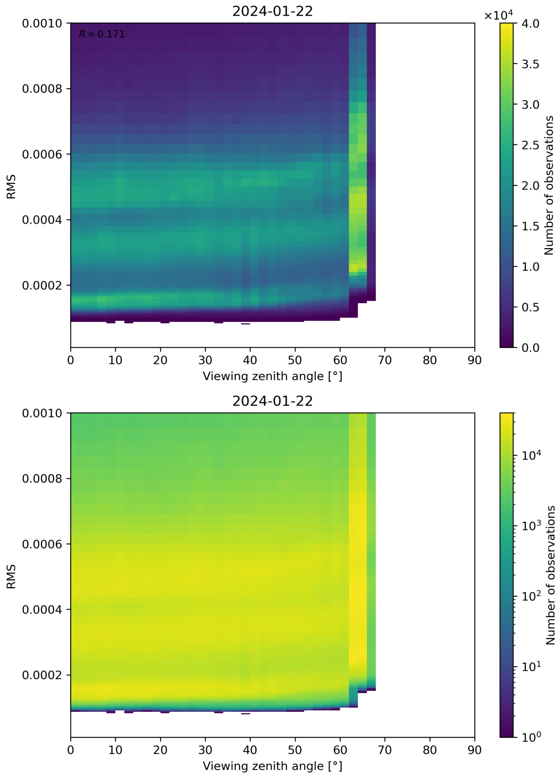
Figure 171: Scatter density plot of “Viewing zenith angle” against “RMS” for 2024-01-21 to 2024-01-23.
