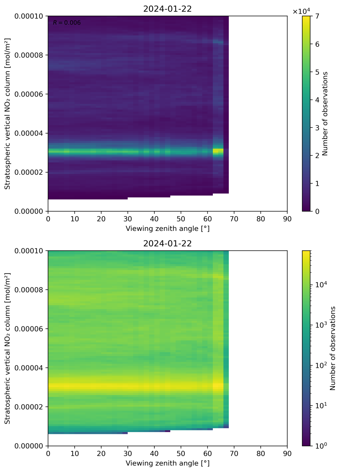
Figure 164: Scatter density plot of “Viewing zenith angle” against “Stratospheric vertical NO 2 column” for 2024-01-21 to 2024-01-23.
