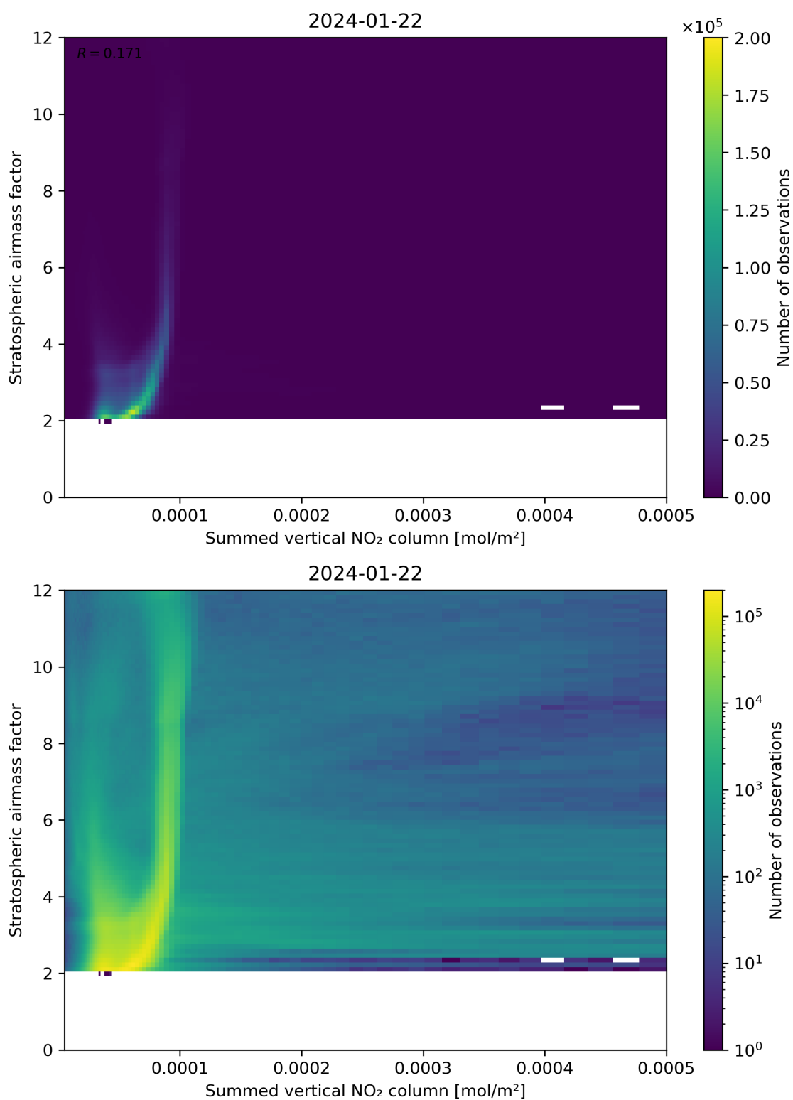
Figure 103: Scatter density plot of “Summed vertical NO 2 column” against “Stratospheric airmass factor” for 2024-01-21 to 2024-01-23.
