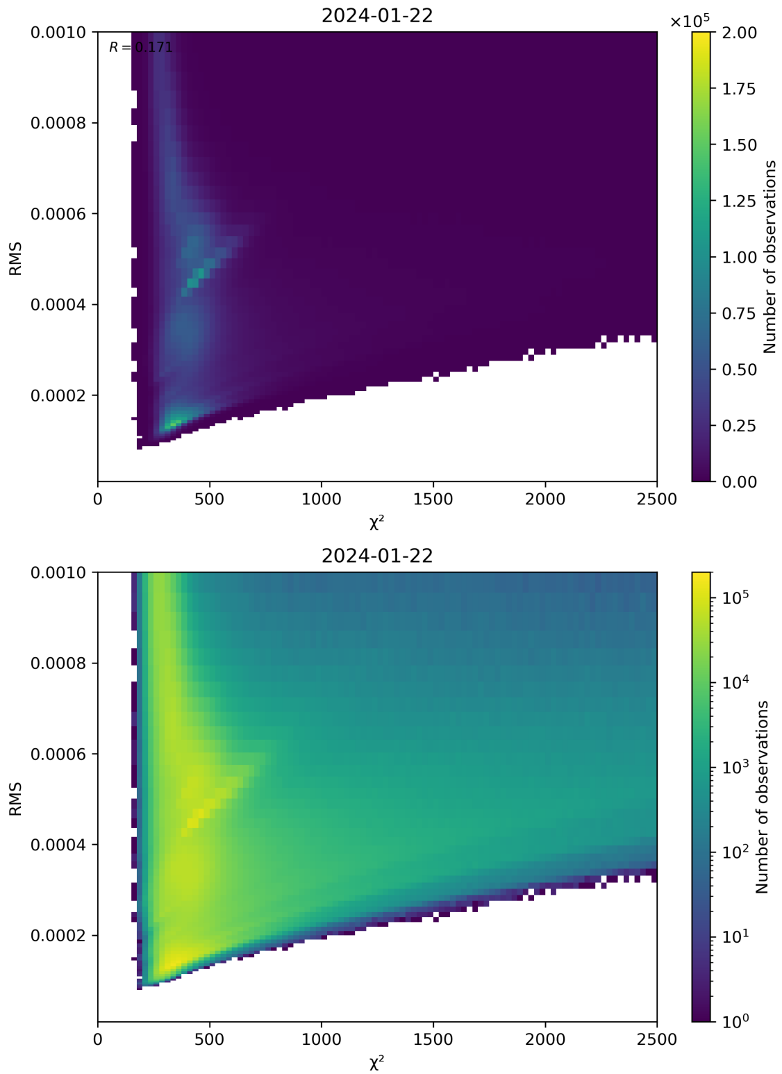
Figure 82: Scatter density plot of “ \chi^2 ” against “RMS” for 2024-01-21 to 2024-01-23.
