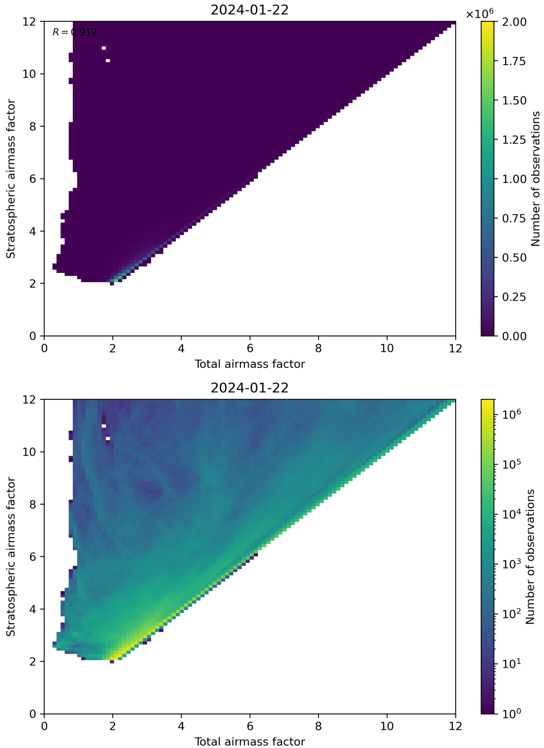
Figure 62: Scatter density plot of “Total airmass factor” against “Stratospheric airmass factor” for 2024-01-21 to 2024-01-23.
