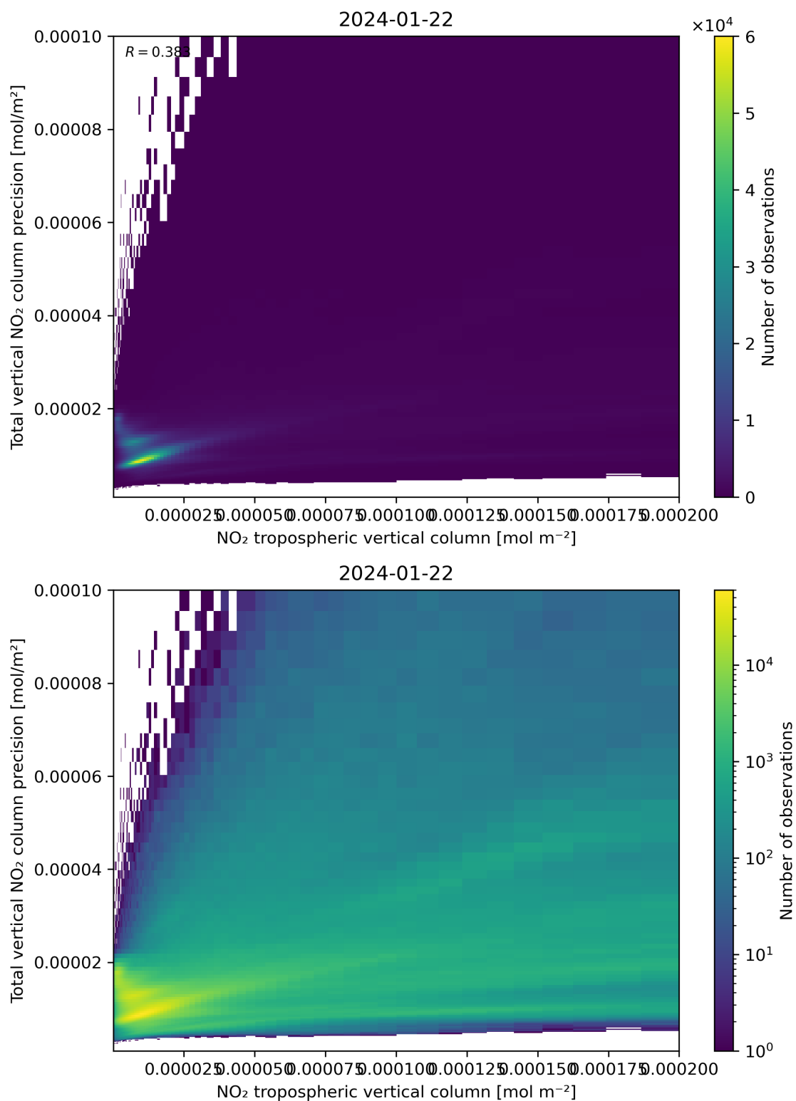
Figure 129: Scatter density plot of “NO 2 tropospheric vertical column” against “Total vertical NO 2 column precision” for 2024-01-21 to 2024-01-23.
