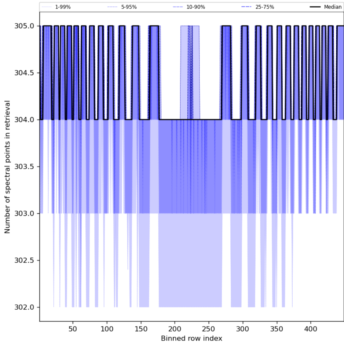
Figure 50: Along track statistics of “Number of spectral points in retrieval” for 2024-01-21 to 2024-01-23
