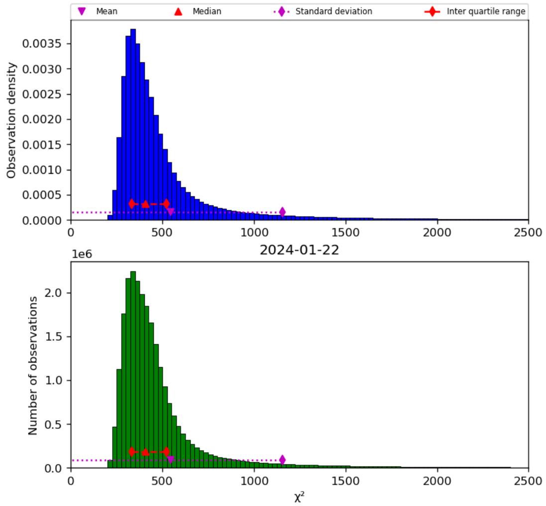
Figure 42: Histogram of “ \chi^2 ” for 2024-01-21 to 2024-01-23
