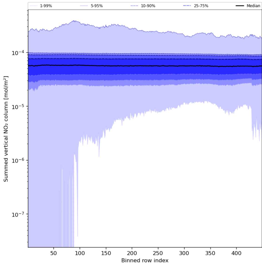
Figure 57: Along track statistics of “Summed vertical NO 2 column” for 2024-01-21 to 2024-01-23
