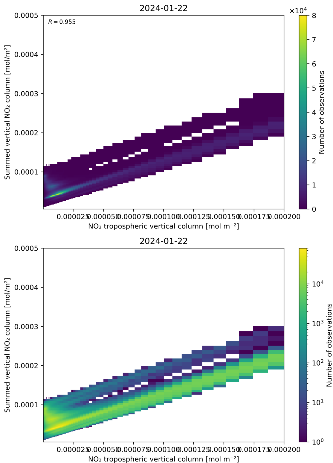
Figure 126: Scatter density plot of “NO 2 tropospheric vertical column” against “Summed vertical NO 2 column” for 2024-01-21 to 2024-01-23.
