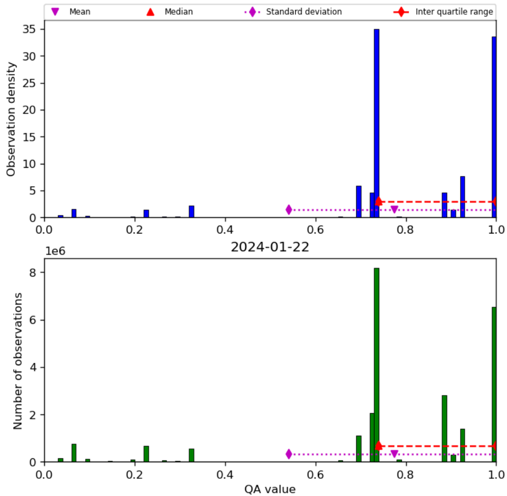
Figure 28: Histogram of “QA value” for 2024-01-21 to 2024-01-23
