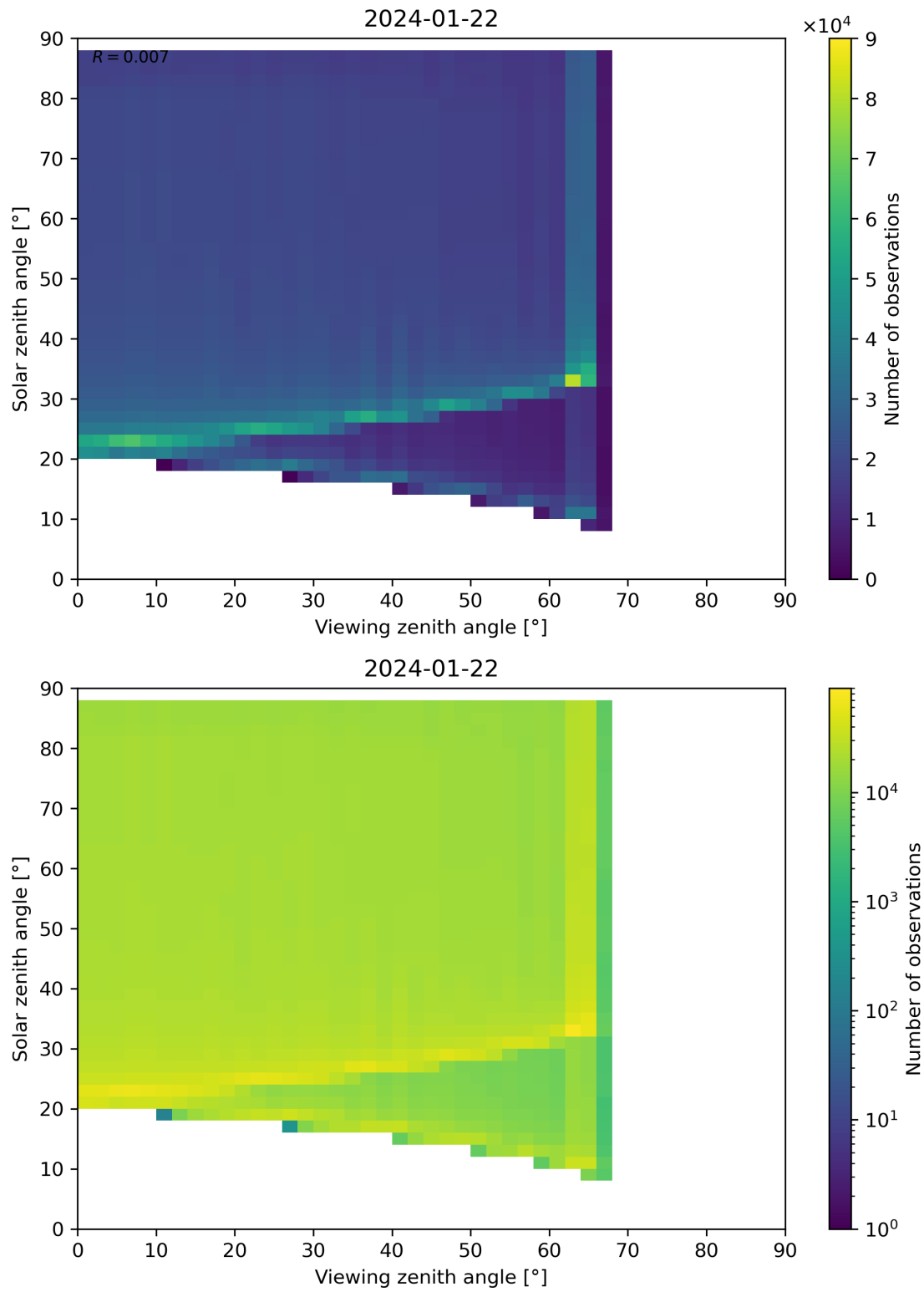
Figure 172: Scatter density plot of “Viewing zenith angle” against “Solar zenith angle” for 2024-01-21 to 2024-01-23.
