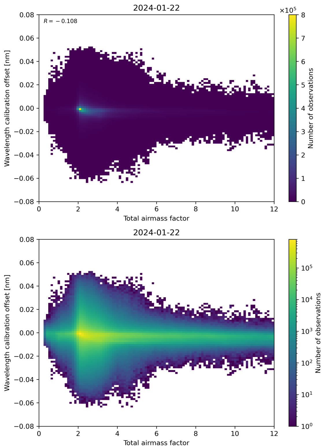
Figure 70: Scatter density plot of “Total airmass factor” against “Wavelength calibration offset” for 2024-01-21 to 2024-01-23.
