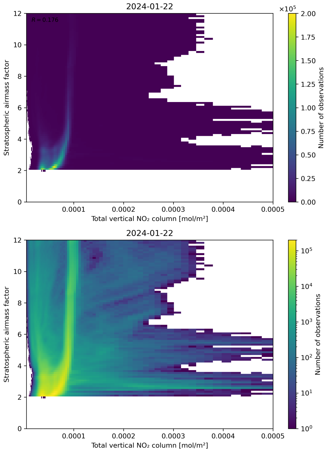
Figure 110: Scatter density plot of “Total vertical NO 2 column” against “Stratospheric airmass factor” for 2024-01-21 to 2024-01-23.
