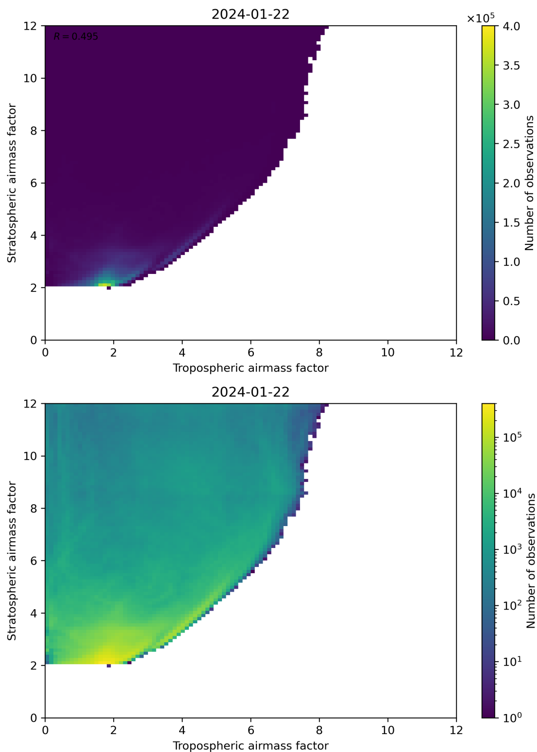
Figure 71: Scatter density plot of “Tropospheric airmass factor” against “Stratospheric airmass factor” for 2024-01-21 to 2024-01-23.
