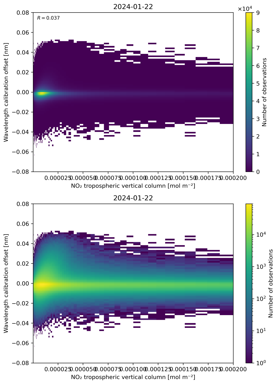
Figure 143: Scatter density plot of “NO 2 tropospheric vertical column” against “Wavelength calibration offset” for 2024-01-21 to 2024-01-23.
