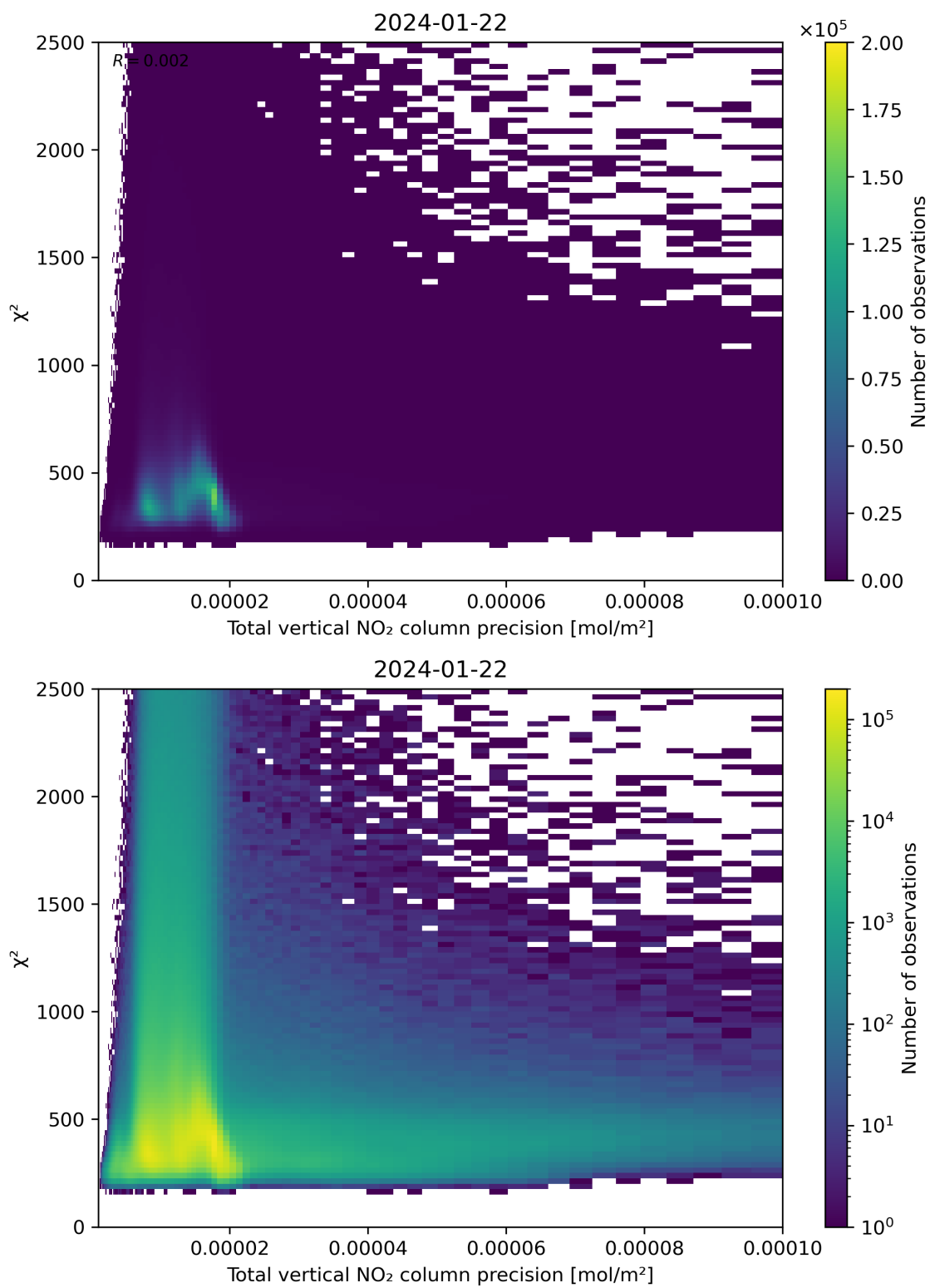
Figure 116: Scatter density plot of “Total vertical NO 2 column precision” against “ \chi^2 ” for 2024-01-21 to 2024-01-23.
