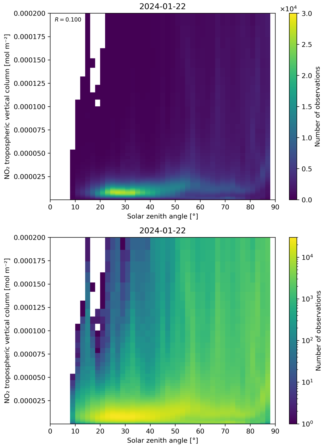
Figure 155: Scatter density plot of “Solar zenith angle” against “NO 2 tropospheric vertical column” for 2024-01-21 to 2024-01-23.
