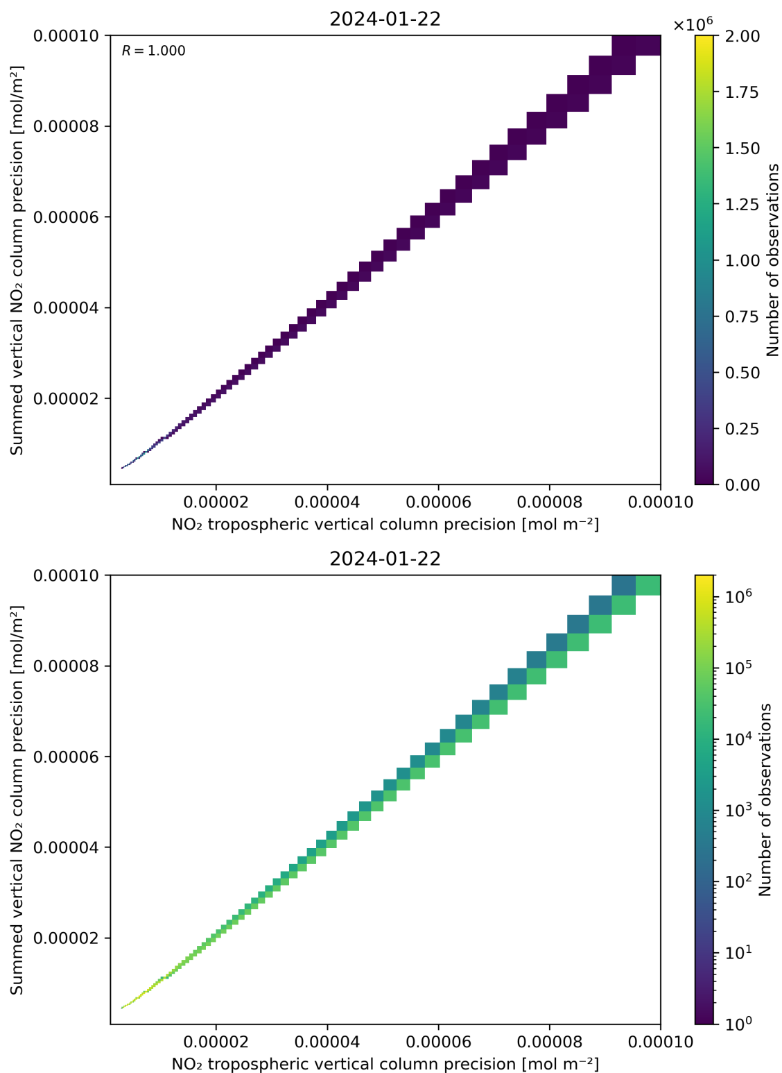
Figure 137: Scatter density plot of “NO 2 tropospheric vertical column precision” against “Summed vertical NO 2 column precision” for 2024-01-21 to 2024-01-23.
