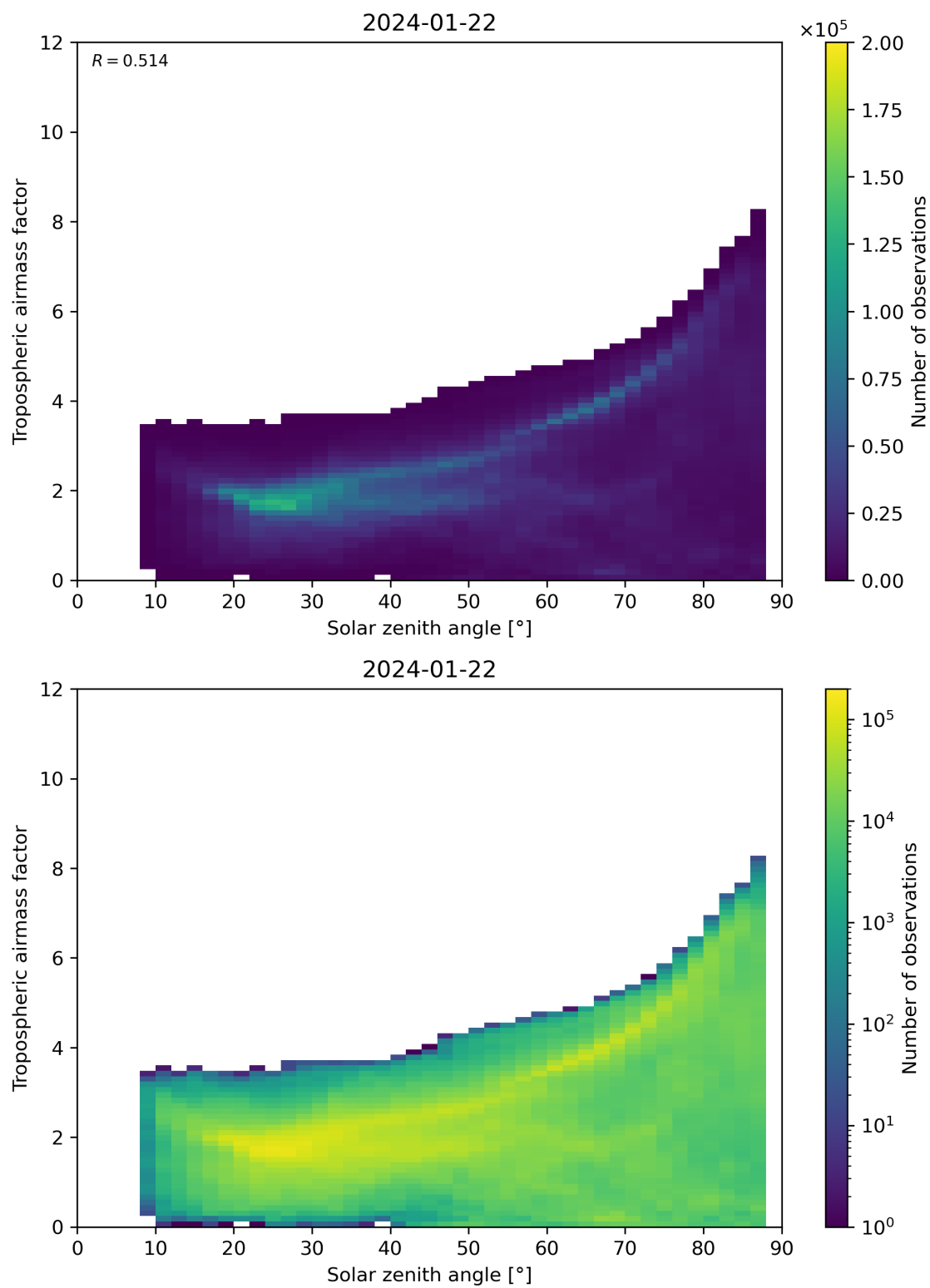
Figure 147: Scatter density plot of “Solar zenith angle” against “Tropospheric airmass factor” for 2024-01-21 to 2024-01-23.
