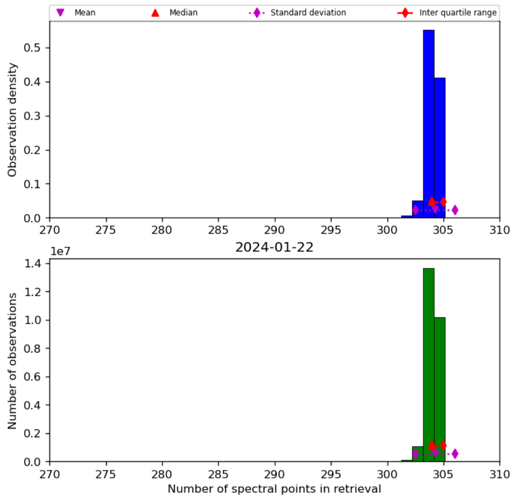
Figure 33: Histogram of “Number of spectral points in retrieval” for 2024-01-21 to 2024-01-23
