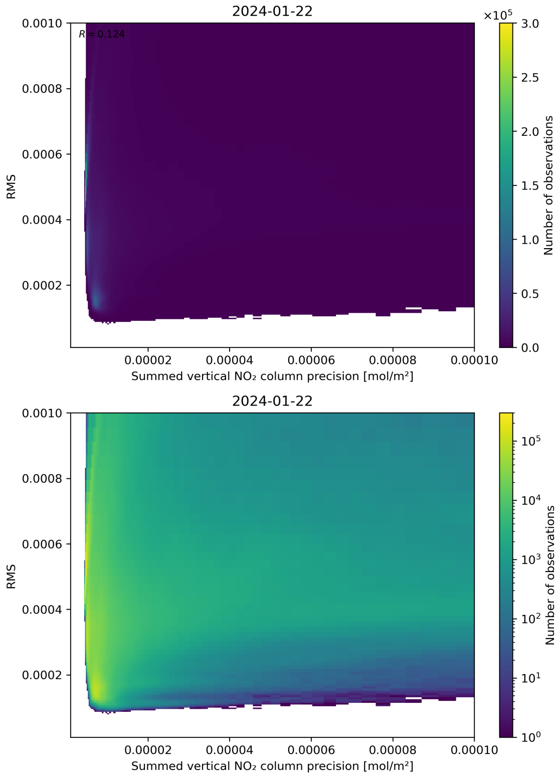
Figure 108: Scatter density plot of “Summed vertical NO 2 column precision” against “RMS” for 2024-01-21 to 2024-01-23.
