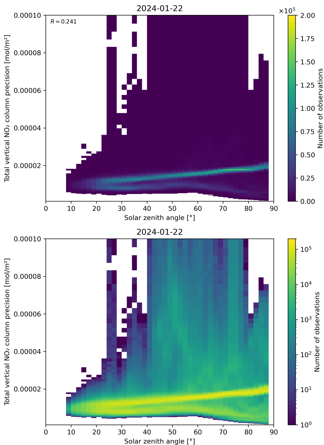
Figure 154: Scatter density plot of “Solar zenith angle” against “Total vertical NO 2 column precision” for 2024-01-21 to 2024-01-23.
