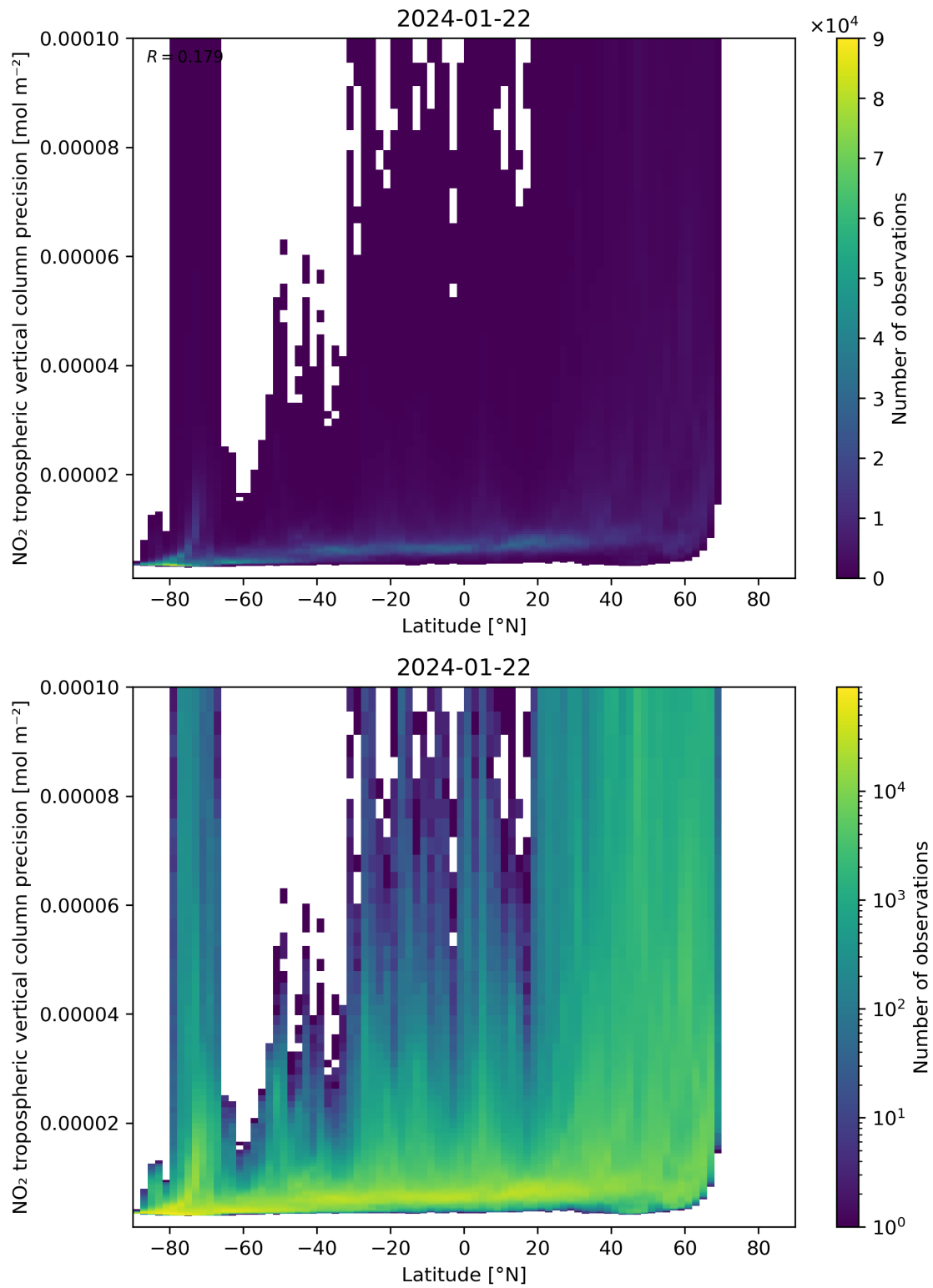
Figure 93: Scatter density plot of “Latitude” against “NO 2 tropospheric vertical column precision” for 2024-01-21 to 2024-01-23.
