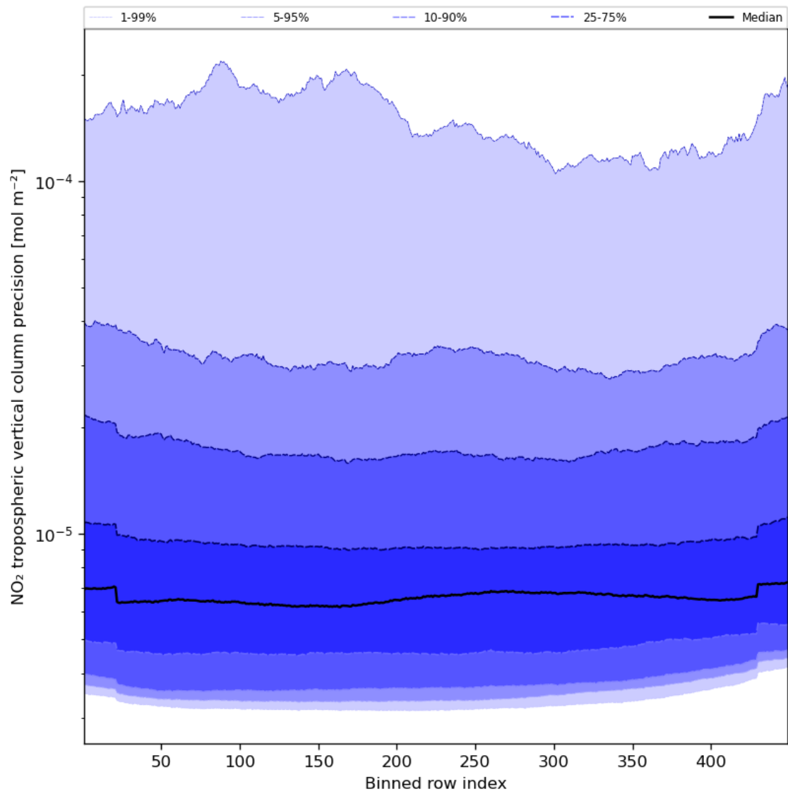
Figure 47: Along track statistics of “NO 2 tropospheric vertical column precision” for 2024-01-21 to 2024-01-23
