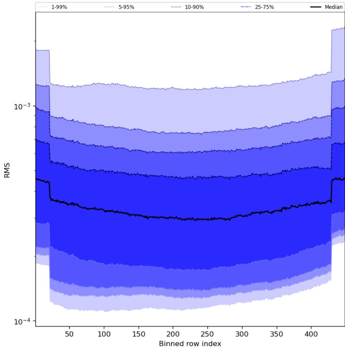
Figure 60: Along track statistics of “RMS” for 2024-01-21 to 2024-01-23
