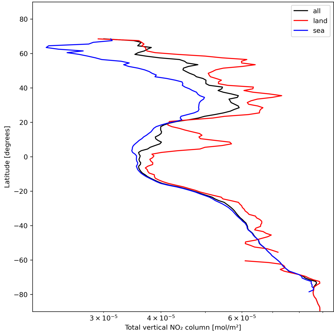
Figure 21: Zonal average of “Total vertical NO 2 column” for 2024-01-21 to 2024-01-23.
