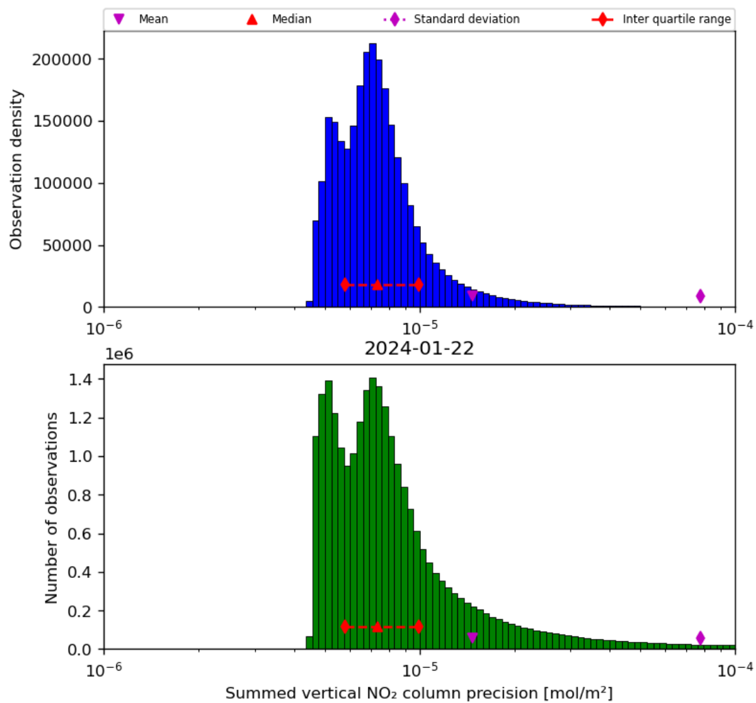
Figure 41: Histogram of “Summed vertical NO 2 column precision” for 2024-01-21 to 2024-01-23
