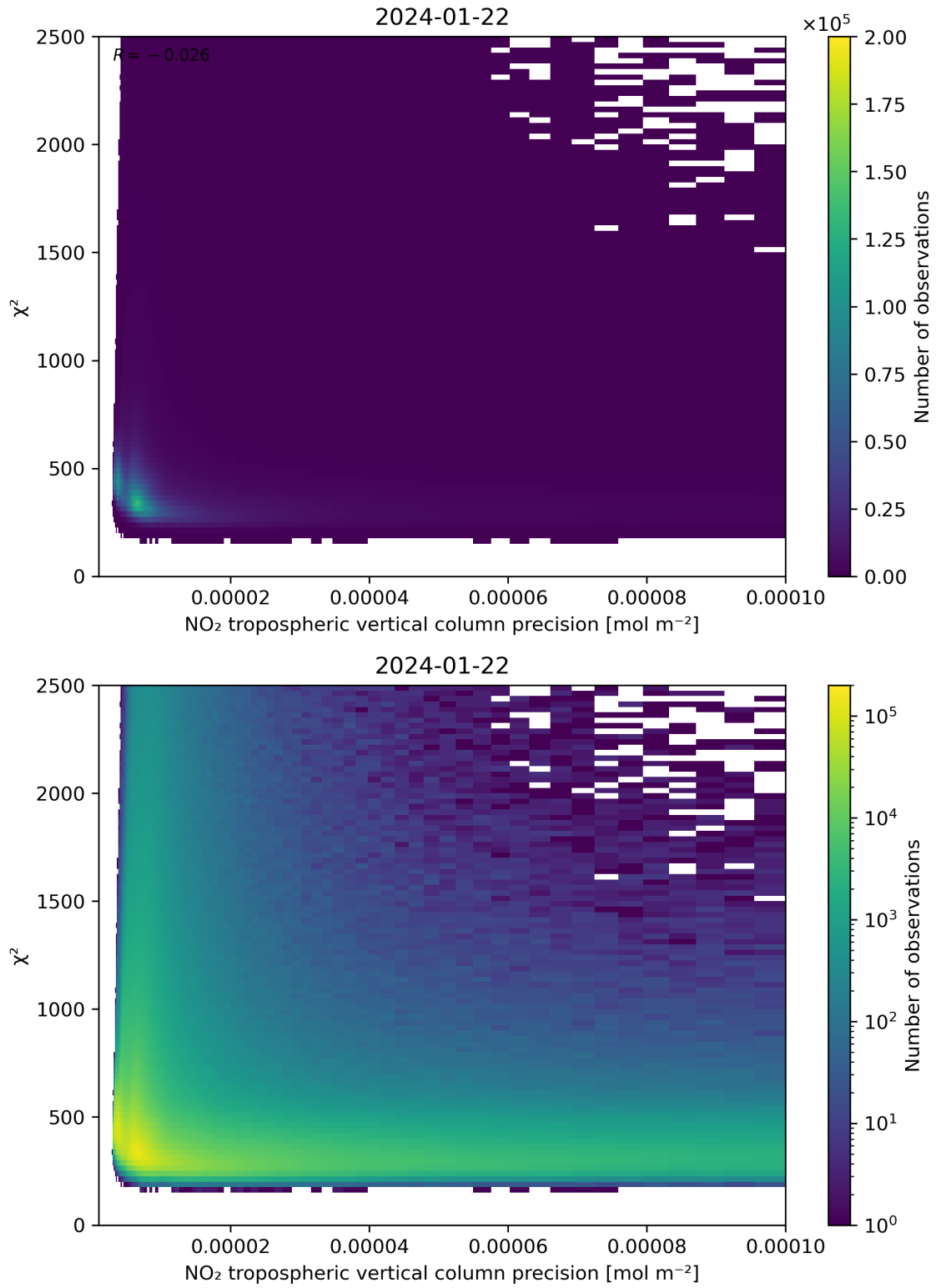
Figure 134: Scatter density plot of “NO 2 tropospheric vertical column precision” against “ \chi^2 ” for 2024-01-21 to 2024-01-23.
