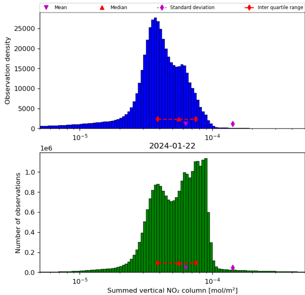
Figure 40: Histogram of “Summed vertical NO 2 column” for 2024-01-21 to 2024-01-23
