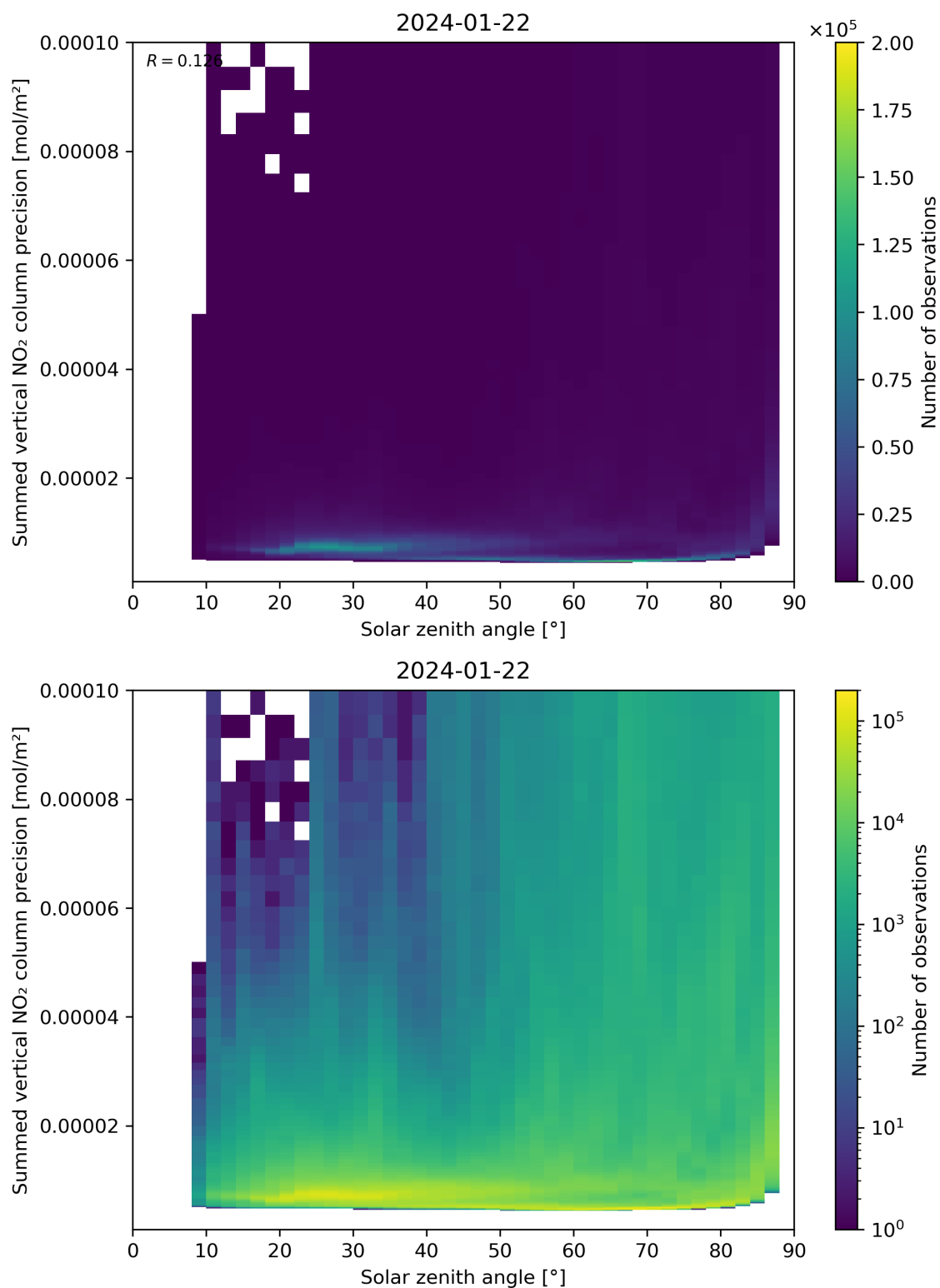
Figure 152: Scatter density plot of “Solar zenith angle” against “Summed vertical NO 2 column precision” for 2024-01-21 to 2024-01-23.
