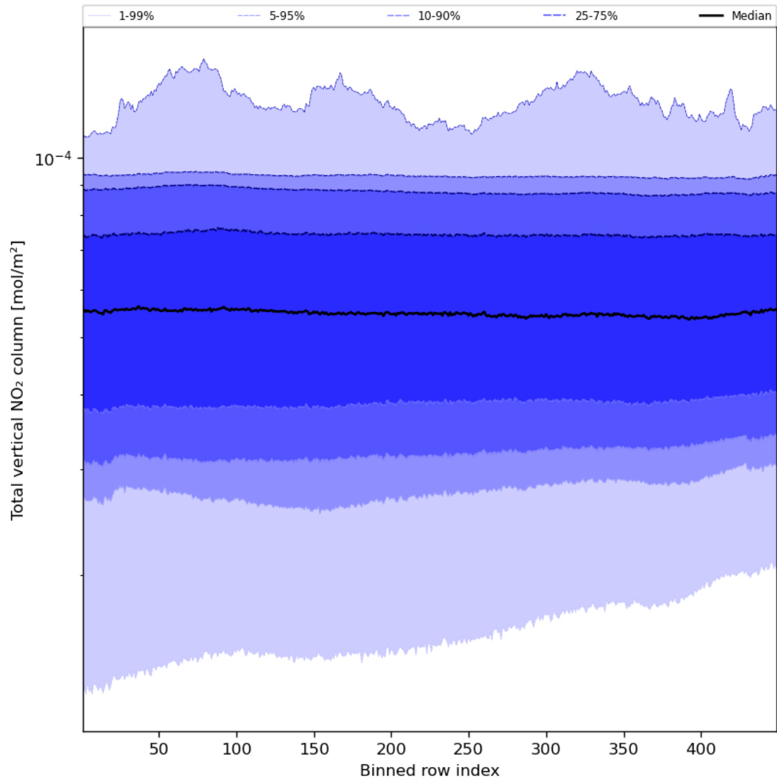
Figure 55: Along track statistics of “Total vertical NO 2 column” for 2024-01-21 to 2024-01-23
