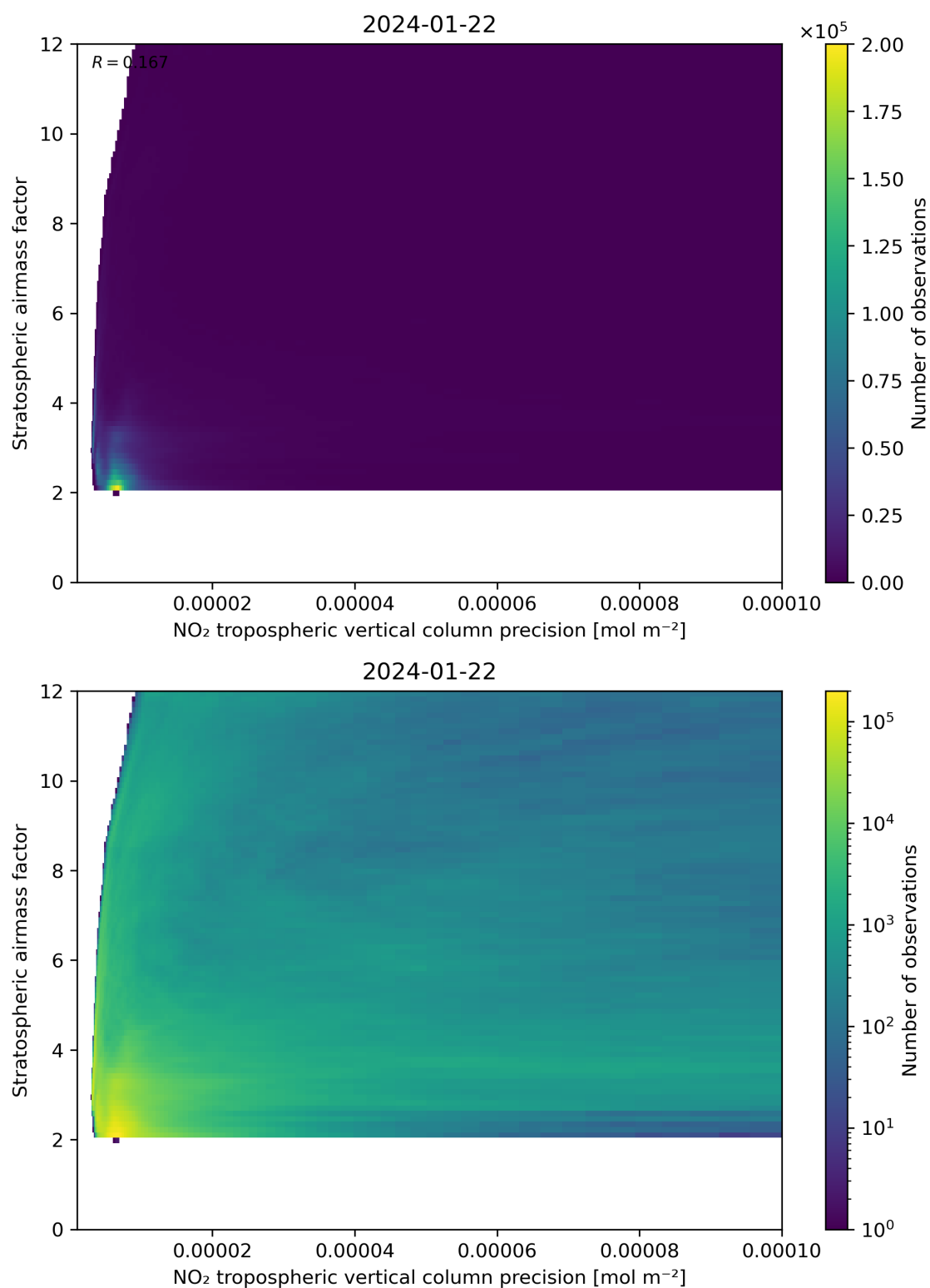
Figure 131: Scatter density plot of “NO 2 tropospheric vertical column precision” against “Stratospheric airmass factor” for 2024-01-21 to 2024-01-23.
