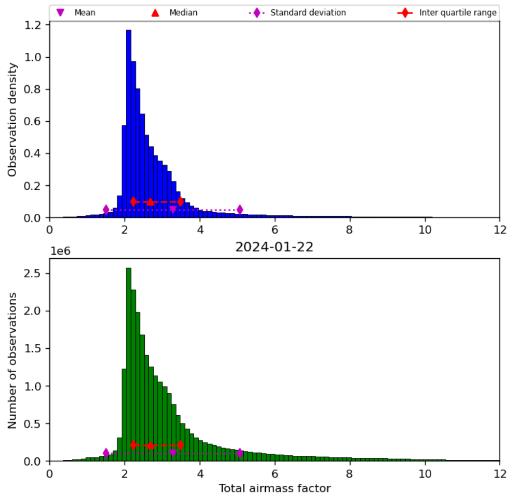
Figure 32: Histogram of “Total airmass factor” for 2024-01-21 to 2024-01-23
