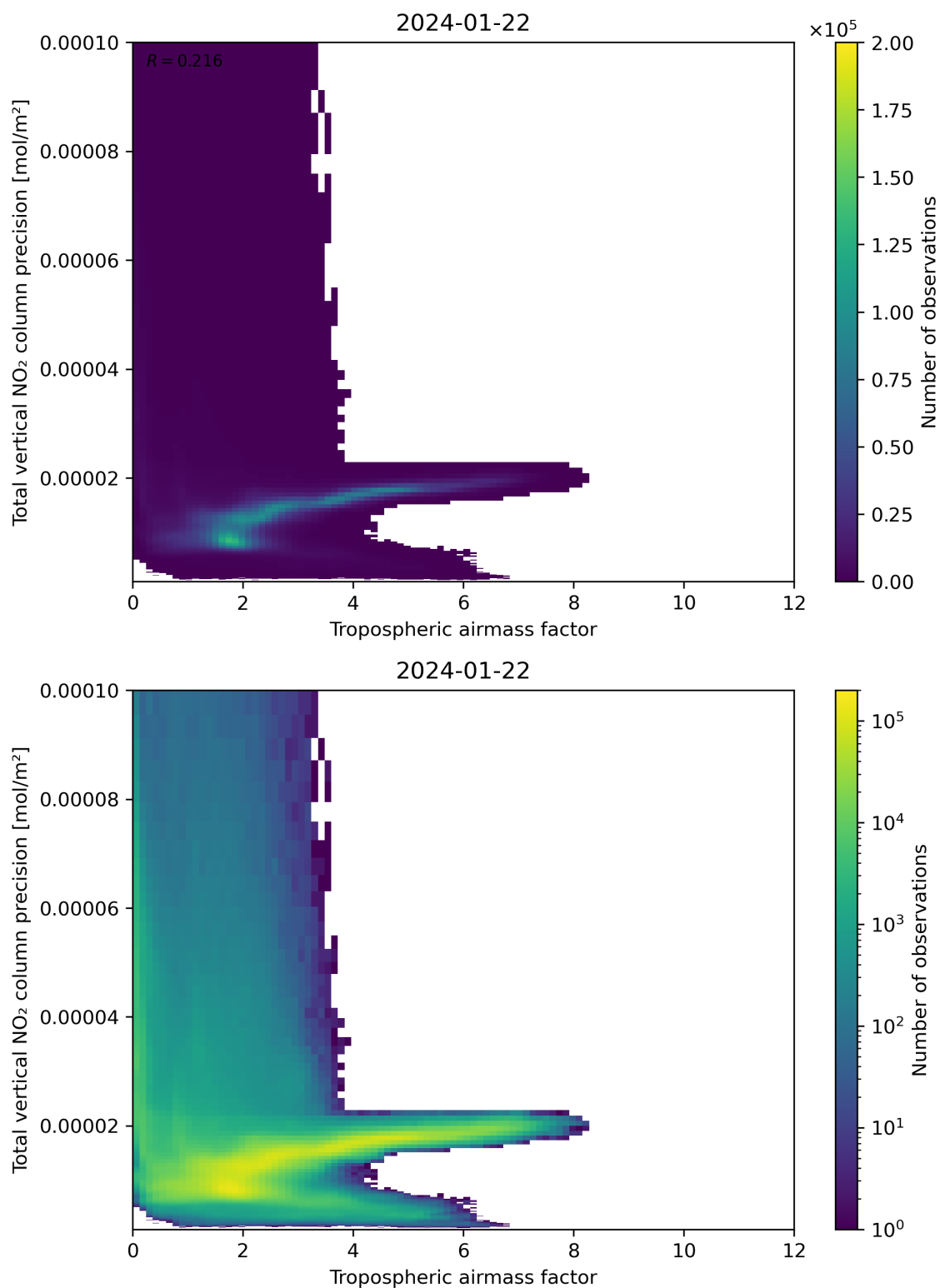
Figure 78: Scatter density plot of “Tropospheric air mass factor” against “Total vertical NO 2 column precision” for 2024-01-21 to 2024-01-23.
