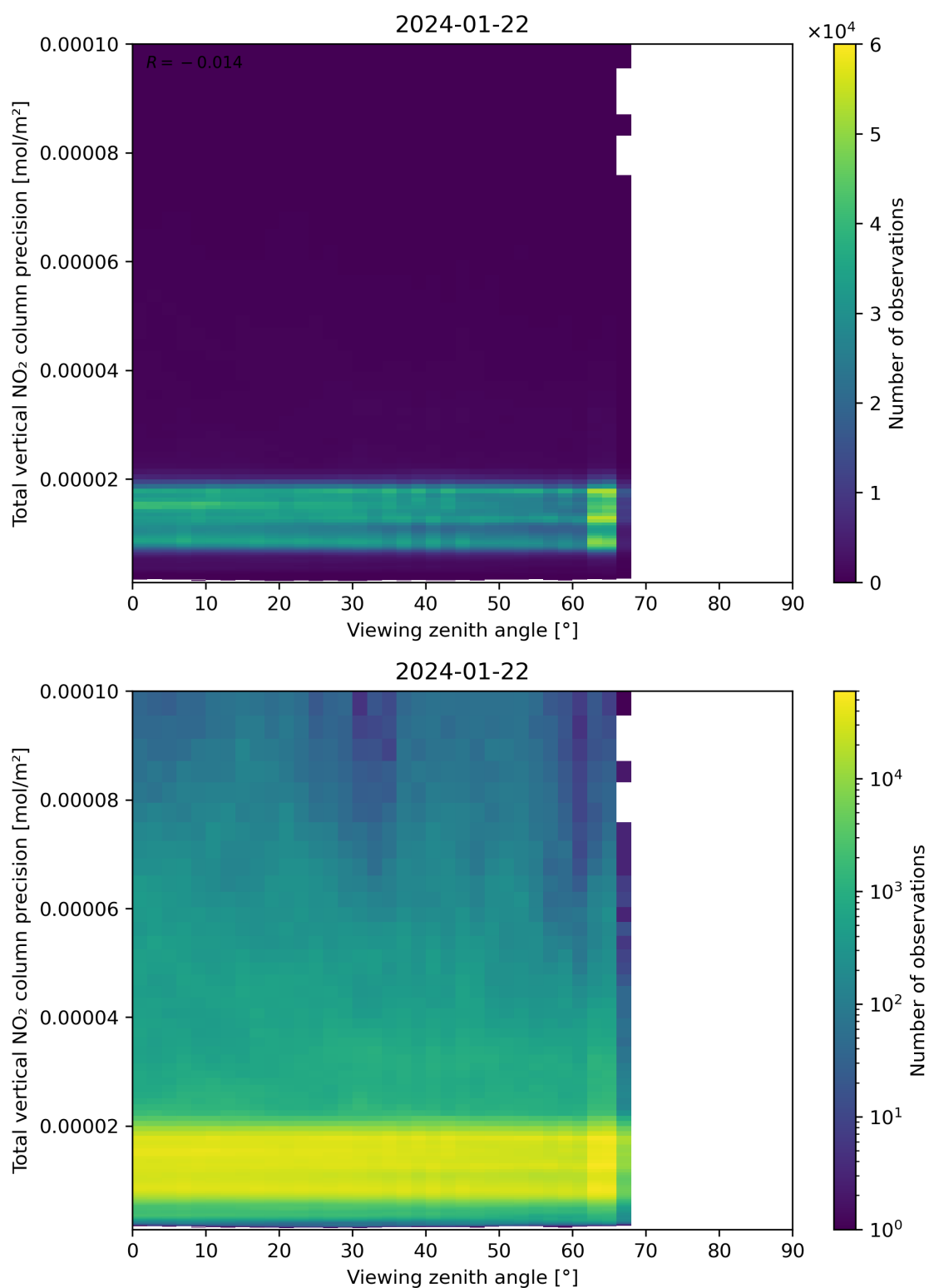
Figure 168: Scatter density plot of “Viewing zenith angle” against “Total vertical NO 2 column precision” for 2024-01-21 to 2024-01-23.
