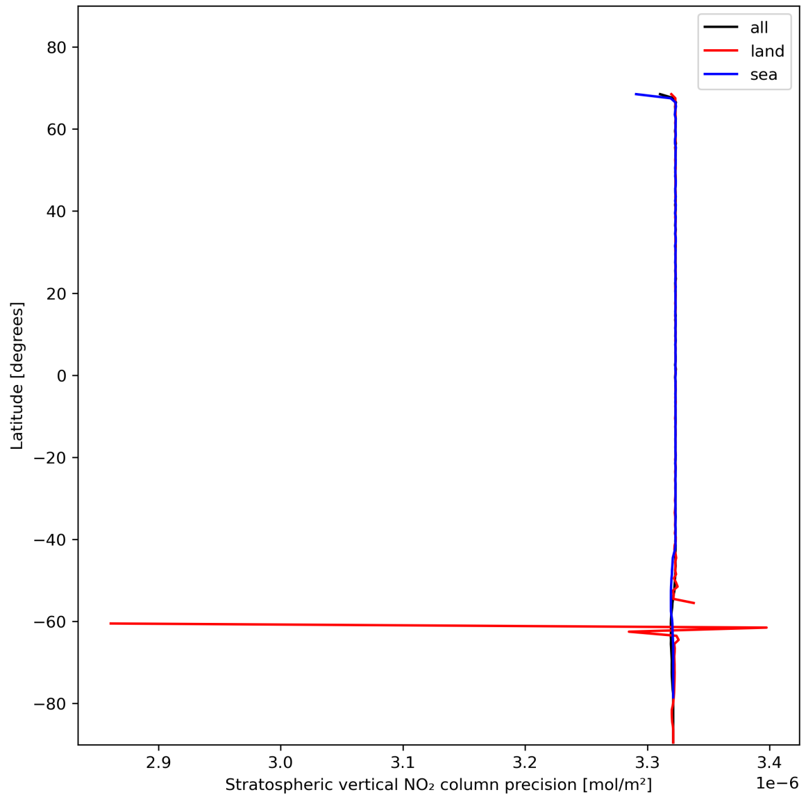
Figure 20: Zonal average of “Stratospheric vertical NO 2 column precision” for 2024-01-21 to 2024-01-23.
