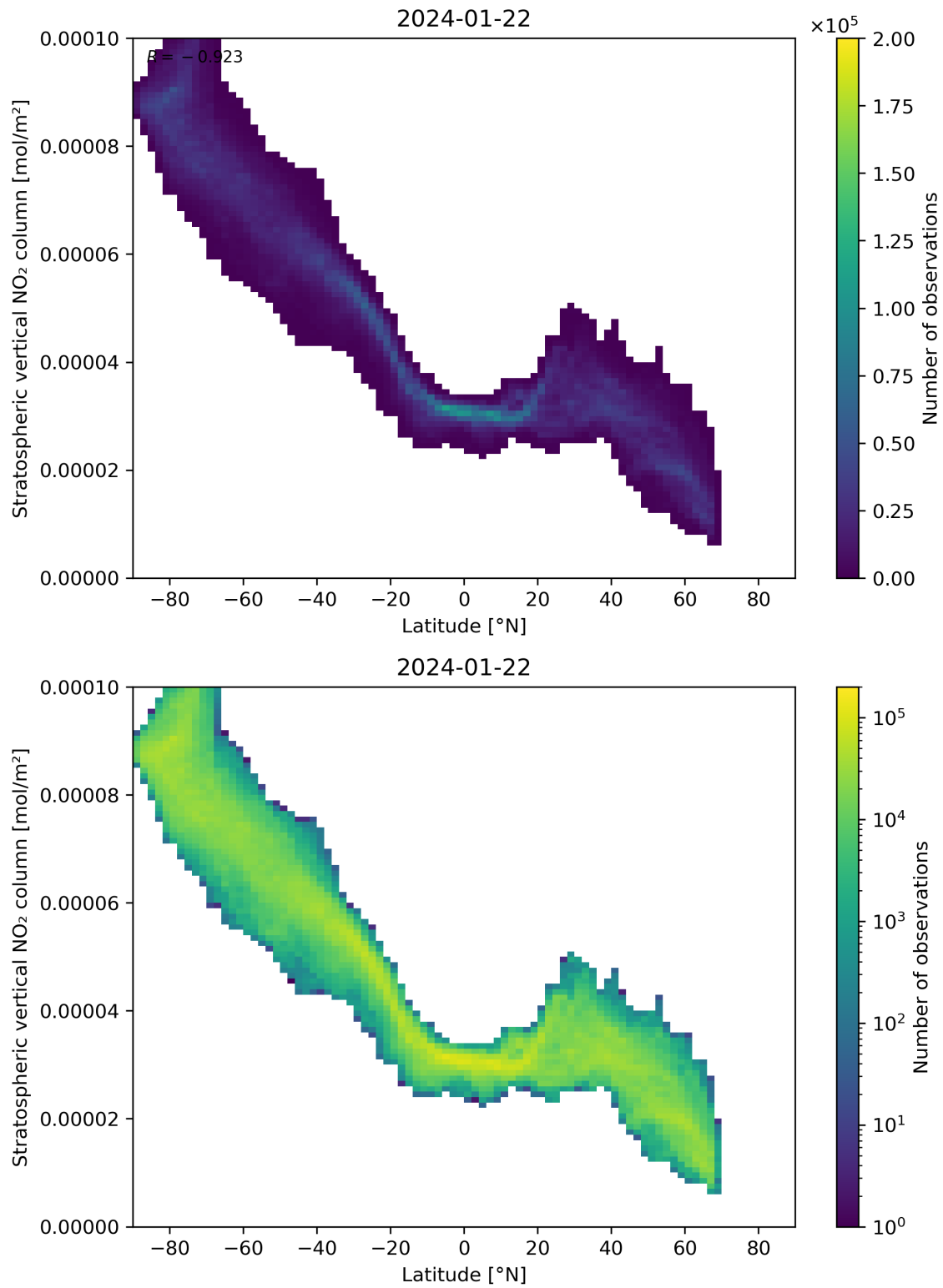
Figure 87: Scatter density plot of “Latitude” against “Stratospheric vertical NO 2 column” for 2024-01-21 to 2024-01-23.
