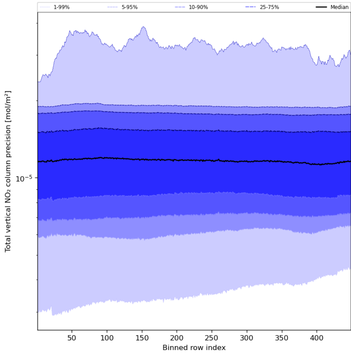
Figure 56: Along track statistics of “Total vertical NO 2 column precision” for 2024-01-21 to 2024-01-23
