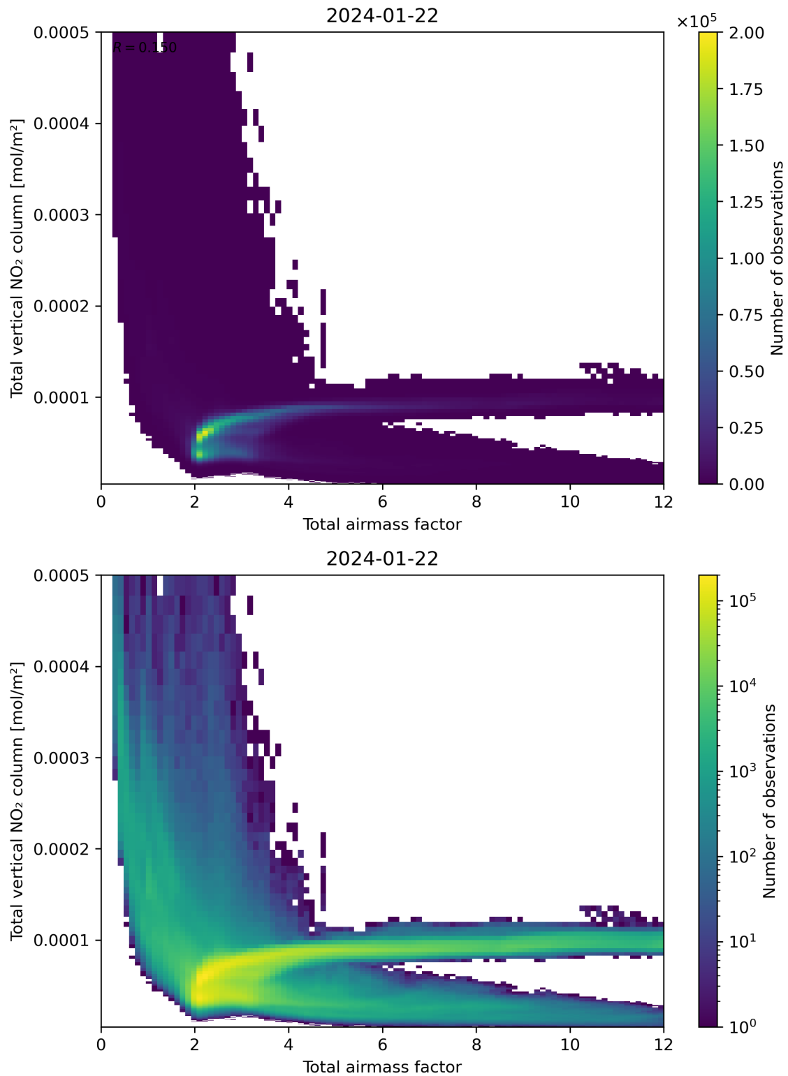
Figure 67: Scatter density plot of “Total airmass factor” against “Total vertical NO 2 column” for 2024-01-21 to 2024-01-23.
