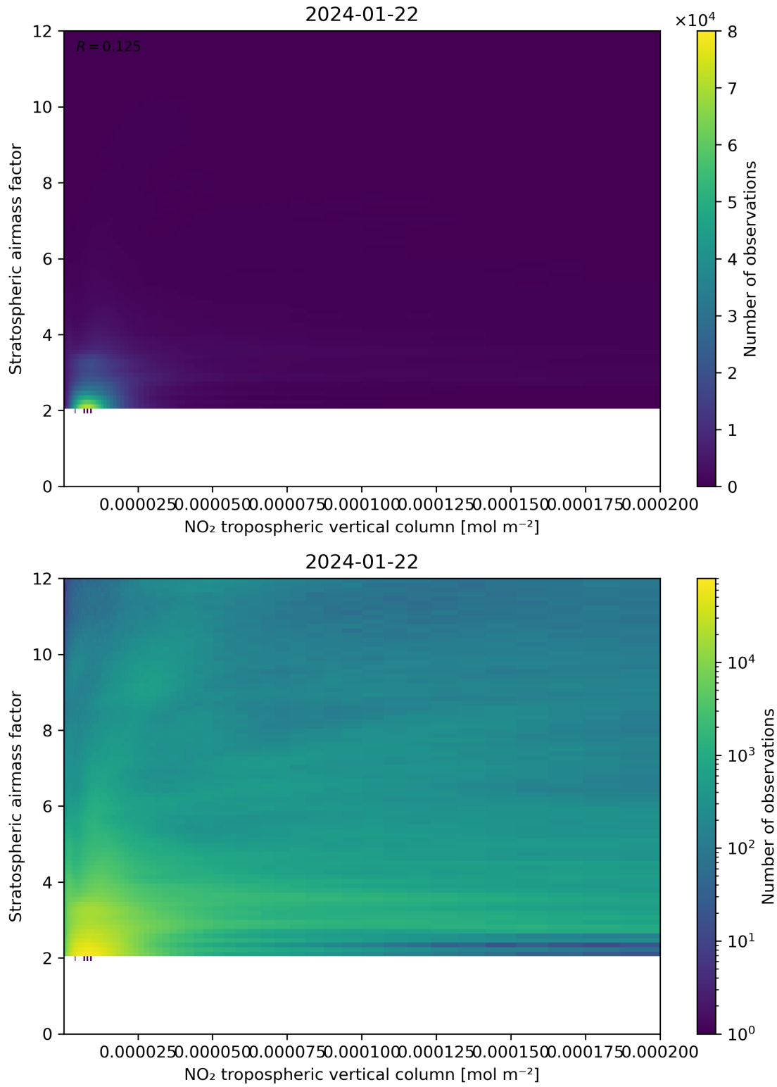
Figure 121: Scatter density plot of “NO 2 tropospheric vertical column” against “Stratospheric airmass factor” for 2024-01-21 to 2024-01-23.
