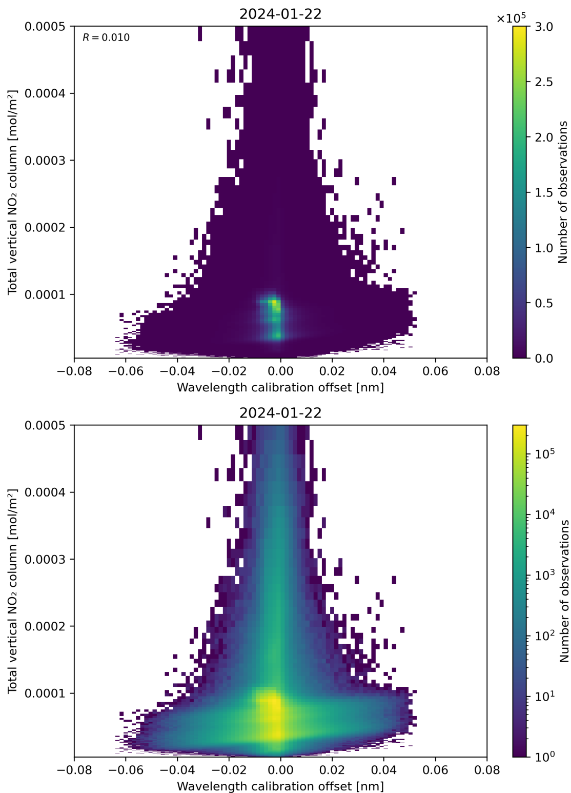
Figure 179: Scatter density plot of “Wavelength calibration offset” against “Total vertical NO 2 column” for 2024-01-21 to 2024-01-23.
