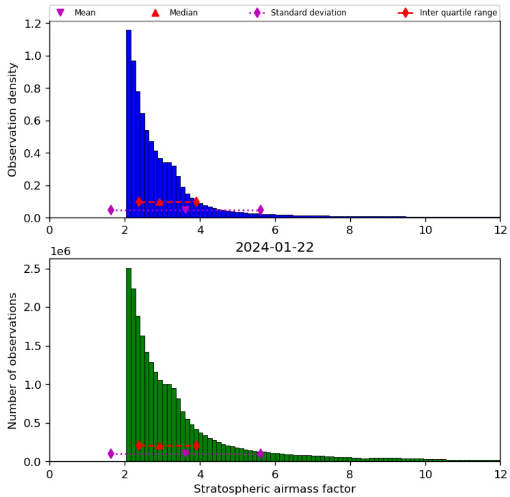
Figure 44: Histogram of “Stratospheric airmass factor” for 2024-01-21 to 2024-01-23
