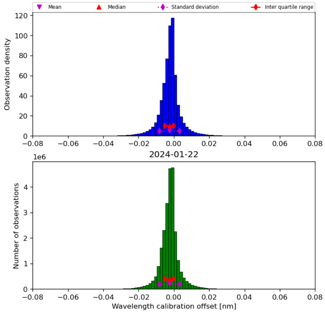
Figure 35: Histogram of “Wavelength calibration offset” for 2024-01-21 to 2024-01-23
