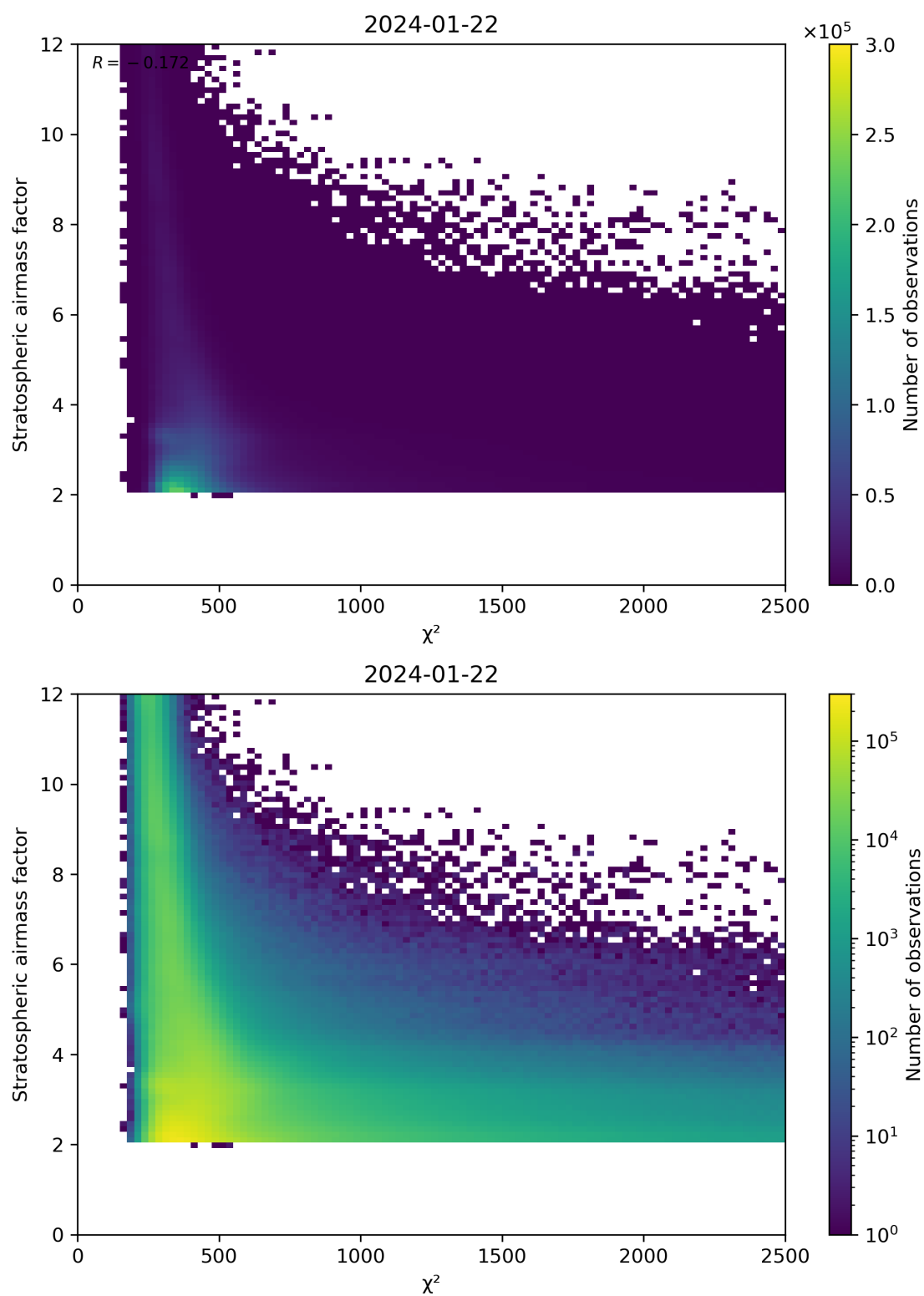
Figure 81: Scatter density plot of “ \chi^2 ” against “Stratospheric airmass factor” for 2024-01-21 to 2024-01-23.
