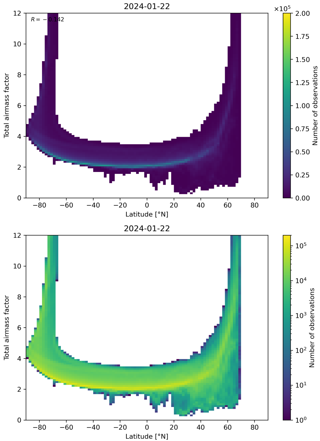
Figure 84: Scatter density plot of “Latitude” against “Total airmass factor” for 2024-01-21 to 2024-01-23.
