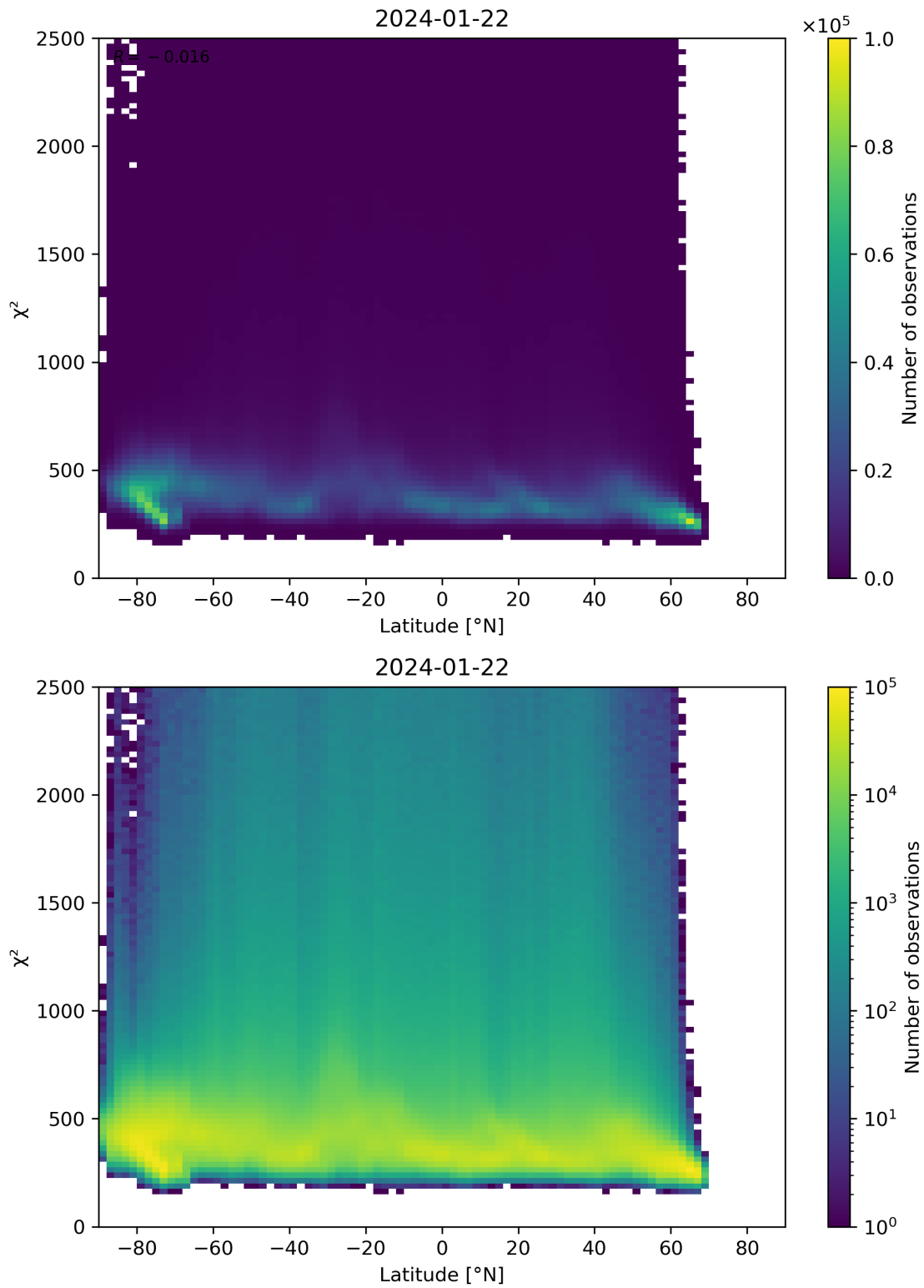
Figure 86: Scatter density plot of “Latitude” against “ \chi^2 ” for 2024-01-21 to 2024-01-23.
