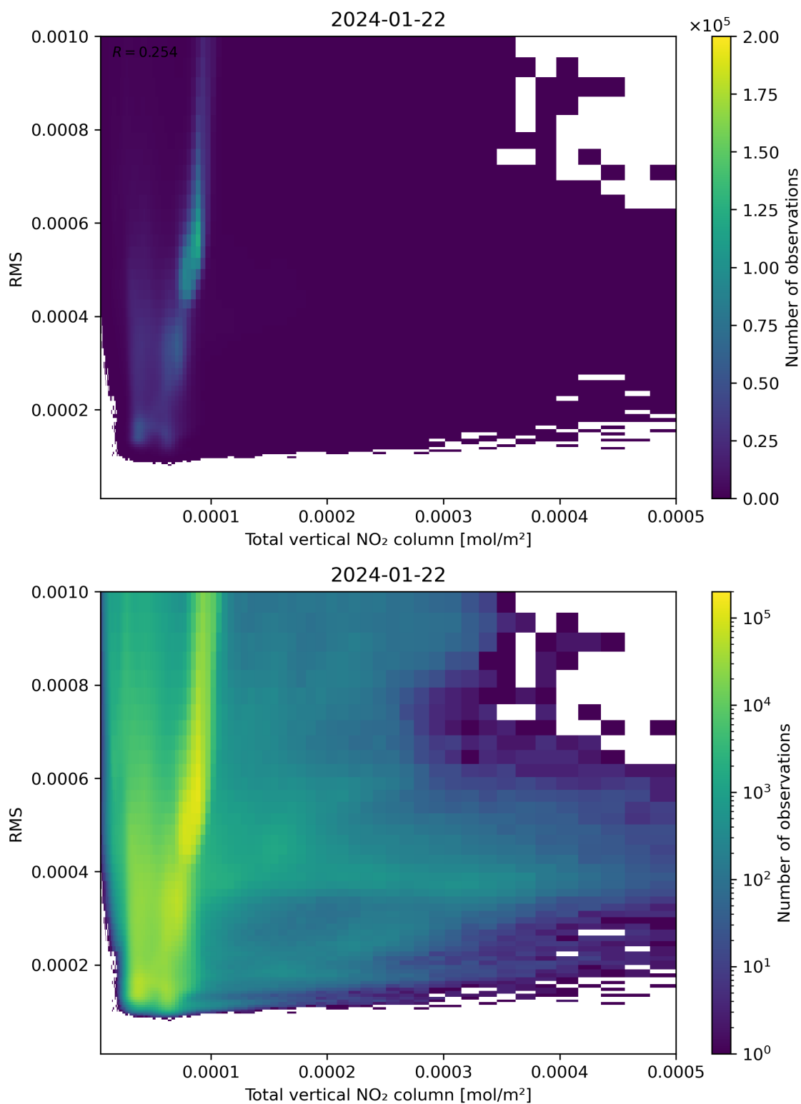
Figure 120: Scatter density plot of “Total vertical NO 2 column” against “RMS” for 2024-01-21 to 2024-01-23.
