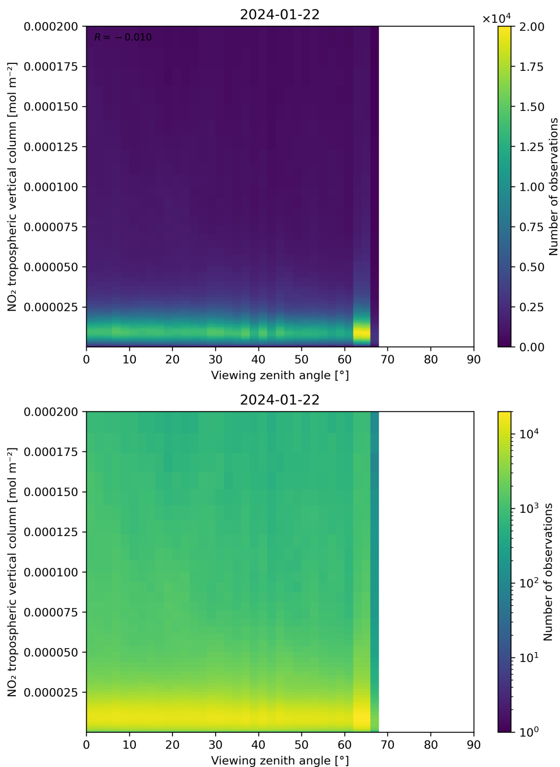
Figure 169: Scatter density plot of “Viewing zenith angle” against “NO 2 tropospheric vertical column” for 2024-01-21 to 2024-01-23.
