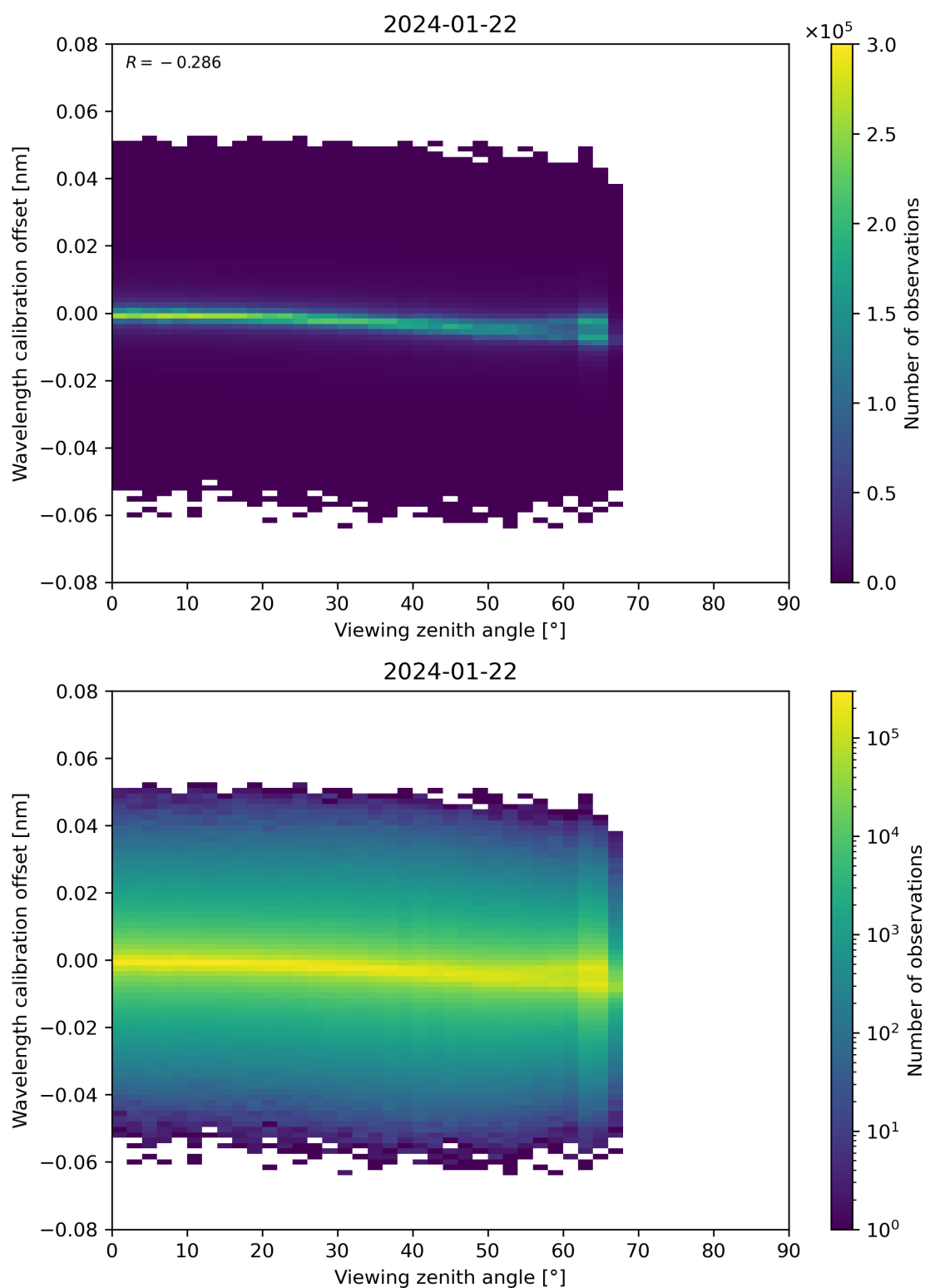
Figure 173: Scatter density plot of “Viewing zenith angle” against “Wavelength calibration offset” for 2024-01-21 to 2024-01-23.
