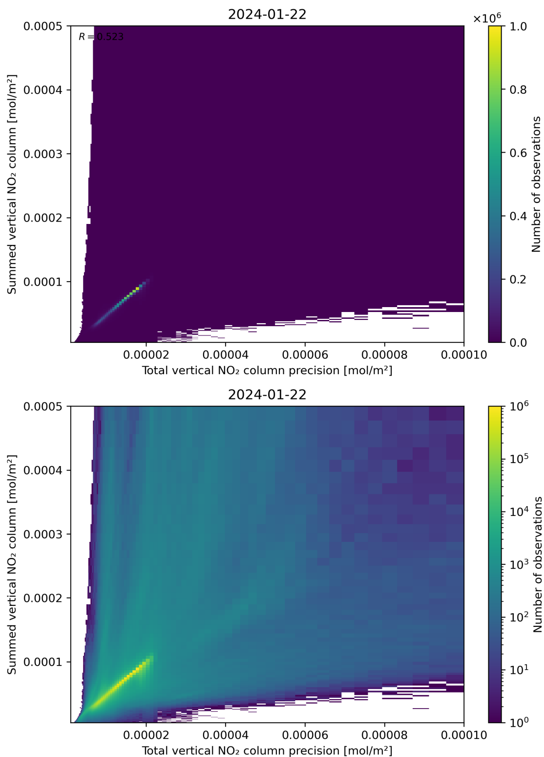
Figure 117: Scatter density plot of “Total vertical NO 2 column precision” against “Summed vertical NO 2 column” for 2024-01-21 to 2024-01-23.
