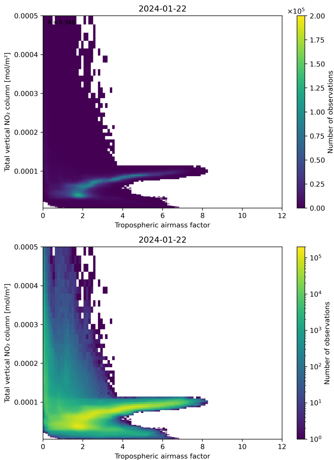
Figure 77: Scatter density plot of “Tropospheric airmass factor” against “Total vertical \text{NO}_2 column” for 2024-01-21 to 2024-01-23.
