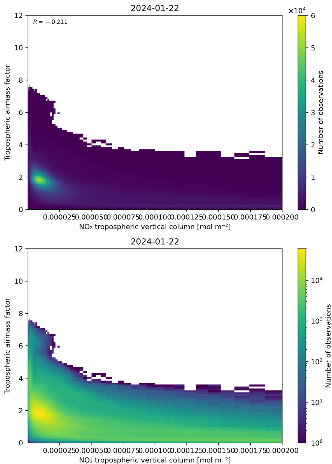
Figure 123: Scatter density plot of “NO 2 tropospheric vertical column” against “Tropospheric airmass factor” for 2024-01-21 to 2024-01-23.
