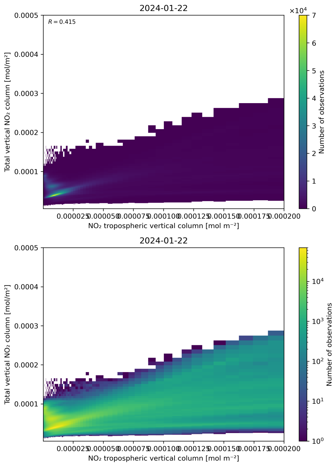
Figure 128: Scatter density plot of “NO 2 tropospheric vertical column” against “Total vertical NO 2 column” for 2024-01-21 to 2024-01-23.
