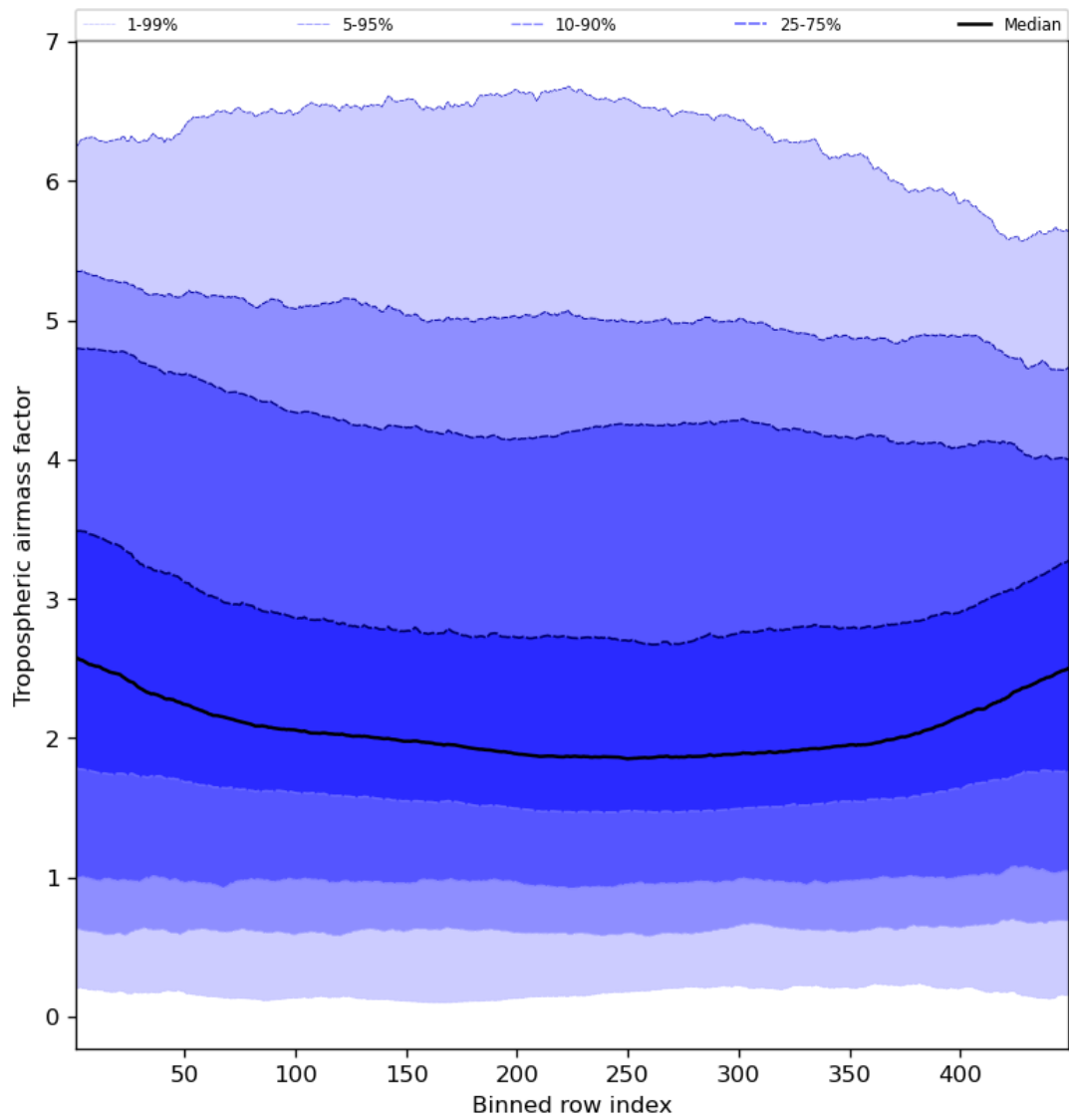
Figure 48: Along track statistics of “Tropospheric airmass factor” for 2024-01-21 to 2024-01-23
