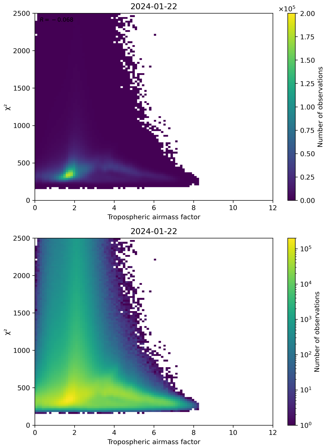
Figure 73: Scatter density plot of “Tropospheric airmass factor” against “ \chi^2 ” for 2024-01-21 to 2024-01-23.
