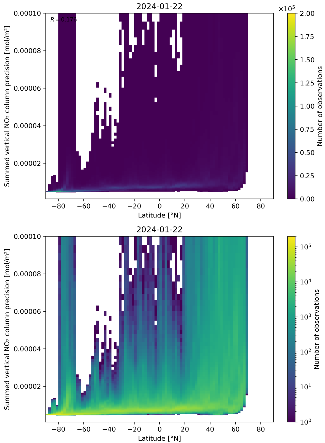
Figure 89: Scatter density plot of “Latitude” against “Summed vertical NO 2 column precision” for 2024-01-21 to 2024-01-23.
