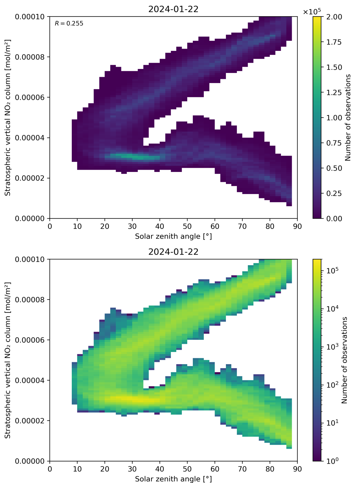
Figure 150: Scatter density plot of “Solar zenith angle” against “Stratospheric vertical NO 2 column” for 2024-01-21 to 2024-01-23.
