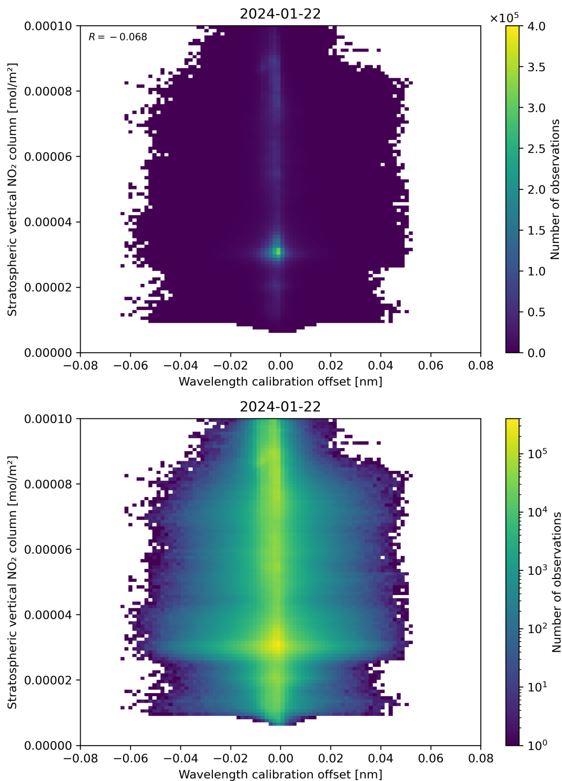
Figure 176: Scatter density plot of “Wavelength calibration offset” against “Stratospheric vertical NO 2 column” for 2024-01-21 to 2024-01-23.
