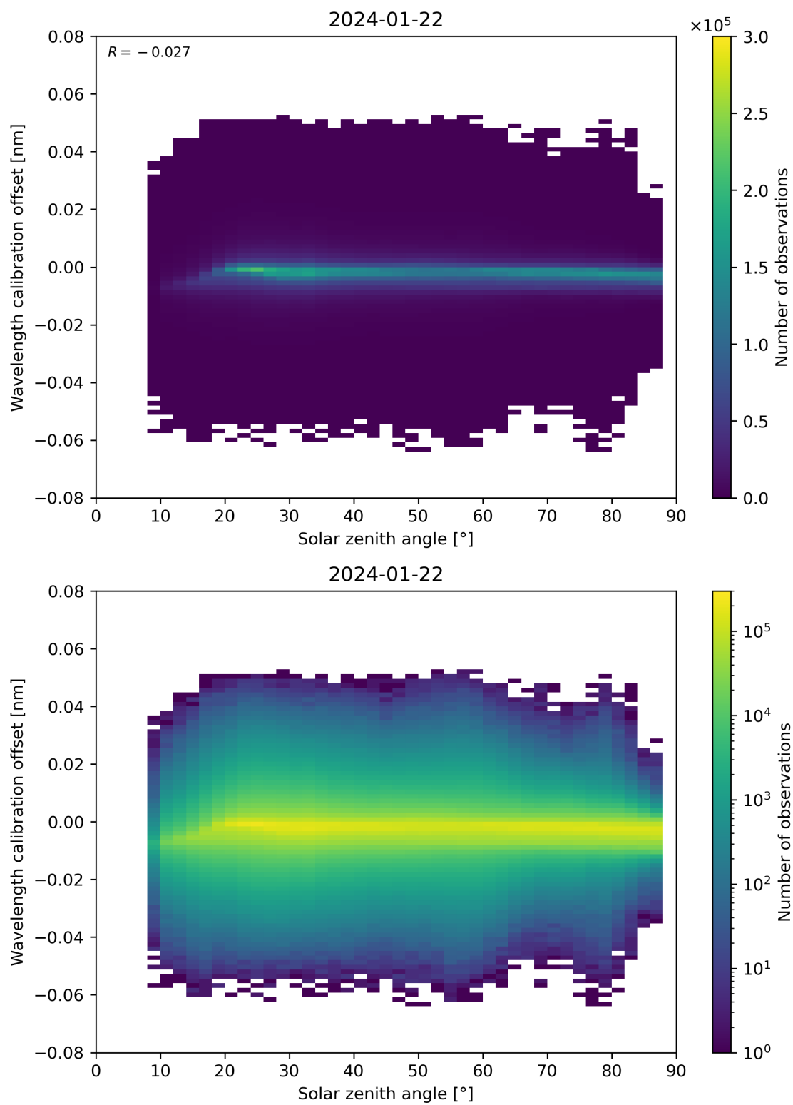
Figure 158: Scatter density plot of “Solar zenith angle” against “Wavelength calibration offset” for 2024-01-21 to 2024-01-23.
