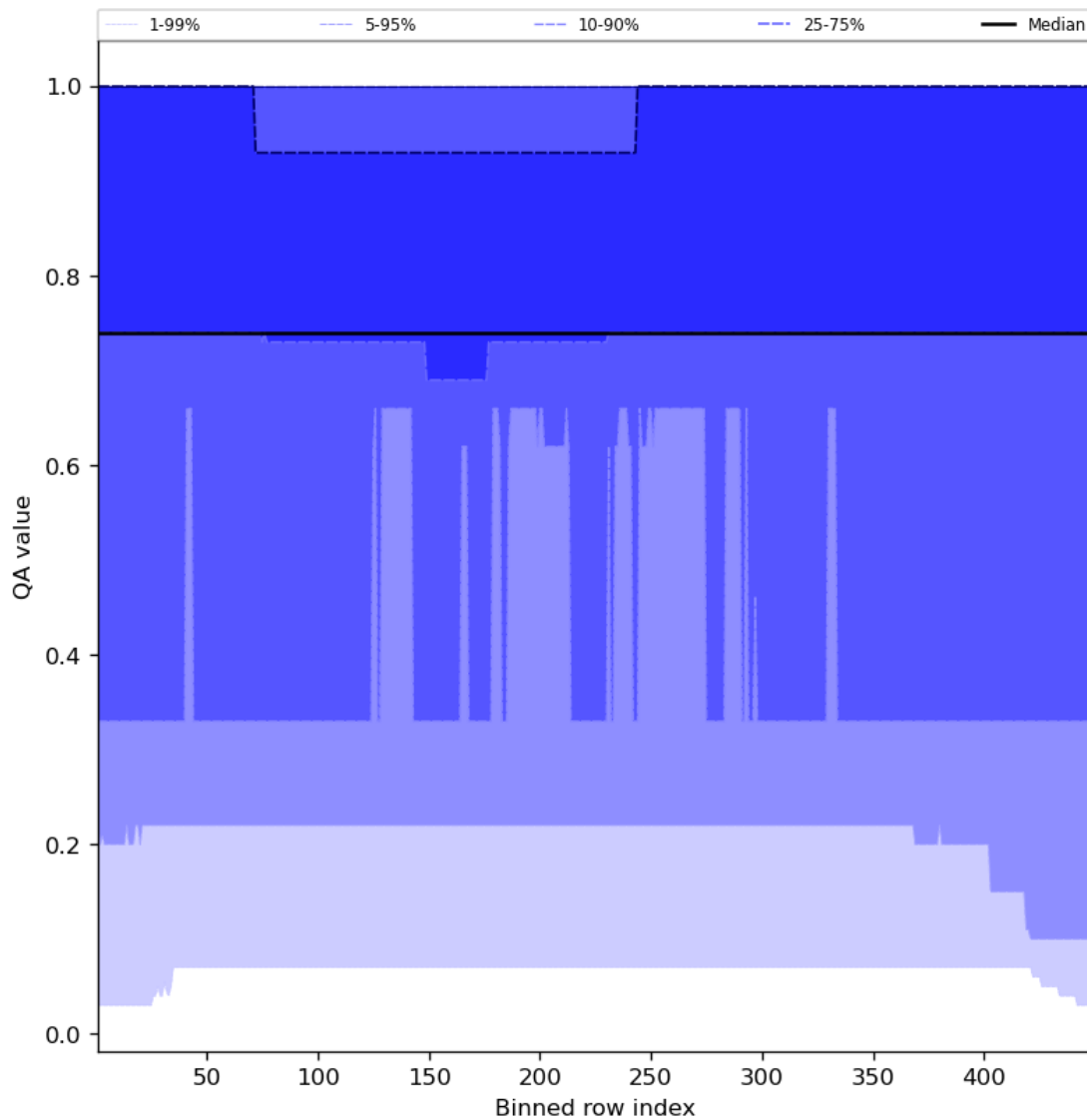
Figure 45: Along track statistics of “QA value” for 2024-01-21 to 2024-01-23
