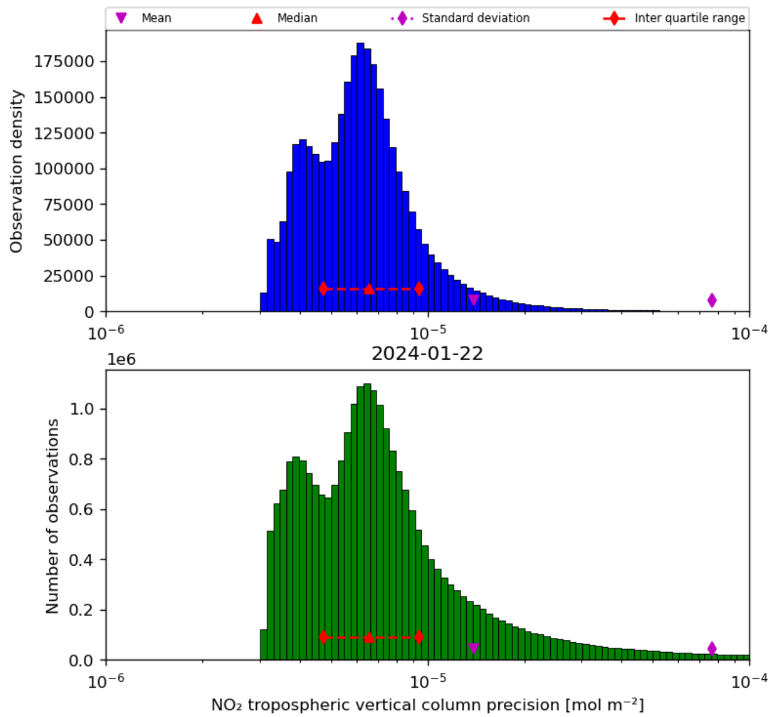
Figure 30: Histogram of “NO 2 tropospheric vertical column precision” for 2024-01-21 to 2024-01-23
