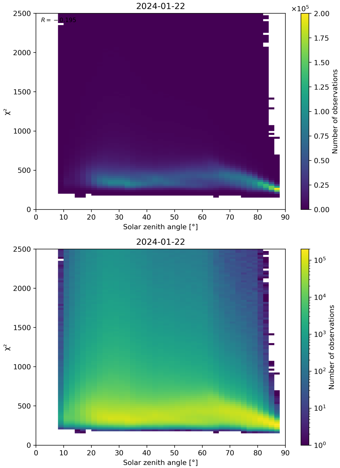
Figure 148: Scatter density plot of “Solar zenith angle” against “ \chi^2 ” for 2024-01-21 to 2024-01-23.
