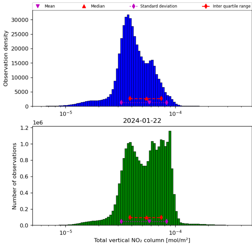
Figure 38: Histogram of “Total vertical NO 2 column” for 2024-01-21 to 2024-01-23
