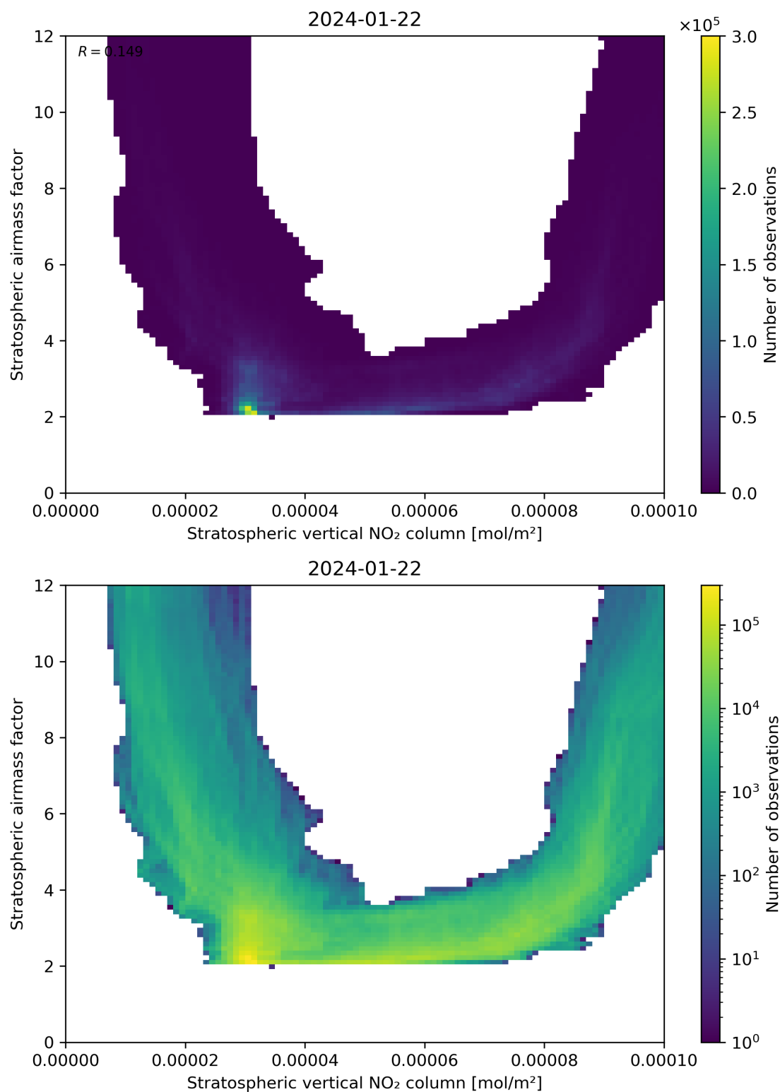
Figure 96: Scatter density plot of “Stratospheric vertical NO 2 column” against “Stratospheric airmass factor” for 2024-01-21 to 2024-01-23.
