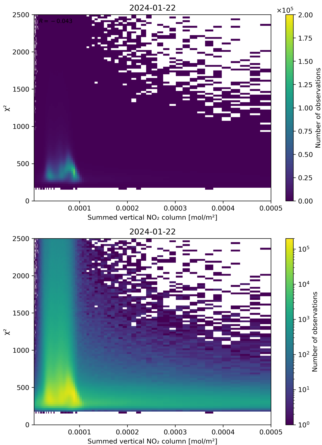
Figure 104: Scatter density plot of “Summed vertical NO 2 column” against “ \chi^2 ” for 2024-01-21 to 2024-01-23.
