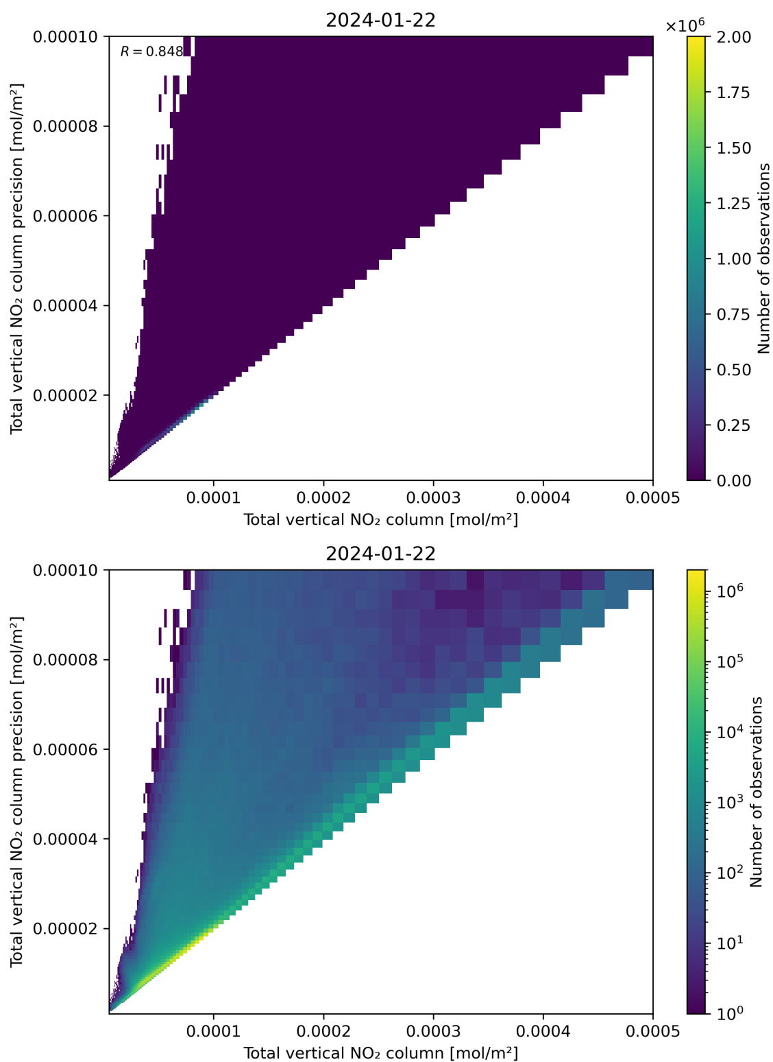
Figure 114: Scatter density plot of “Total vertical NO 2 column” against “Total vertical NO 2 column precision” for 2024-01-21 to 2024-01-23.
