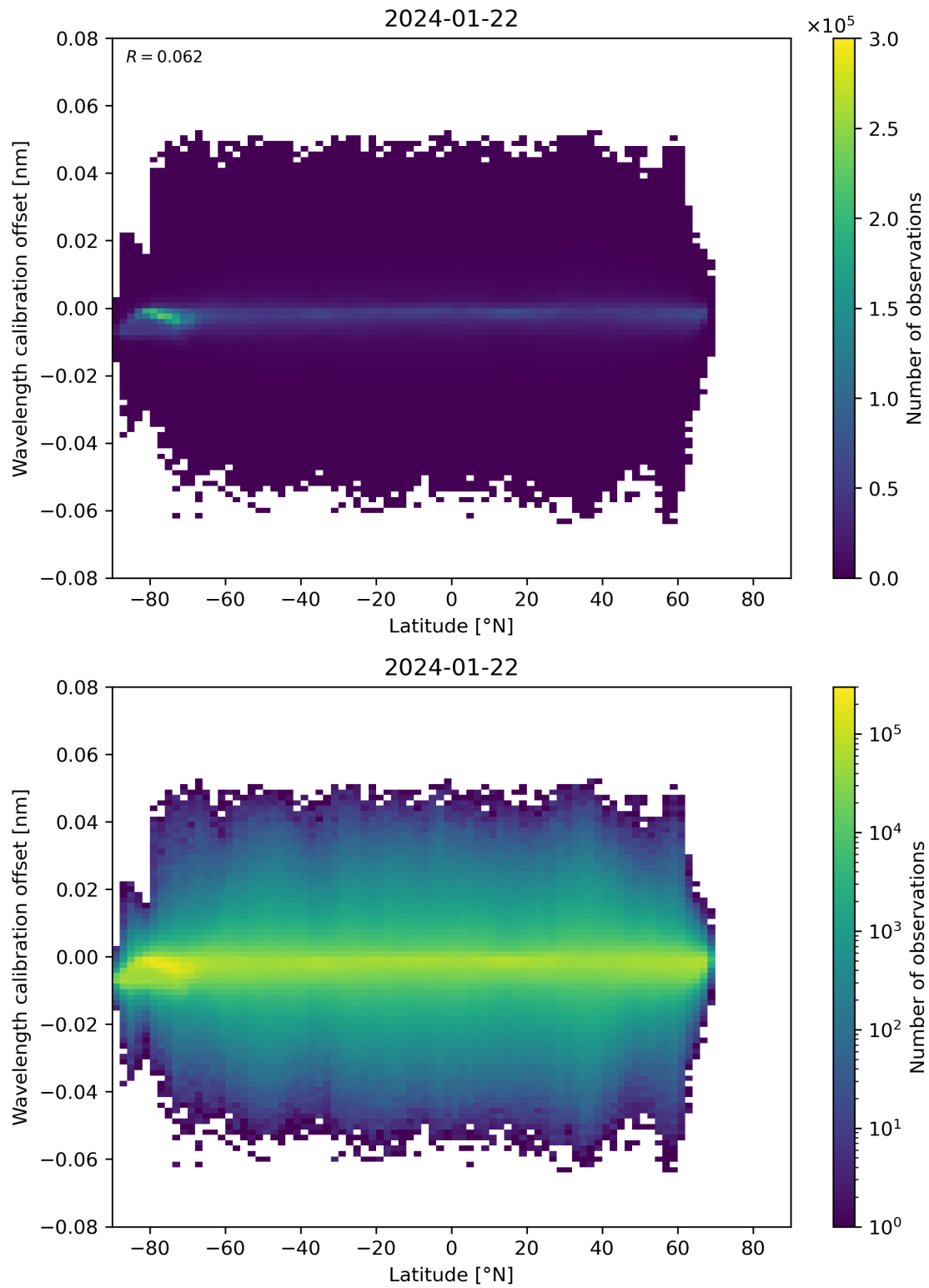
Figure 95: Scatter density plot of “Latitude” against “Wavelength calibration offset” for 2024-01-21 to 2024-01-23.
