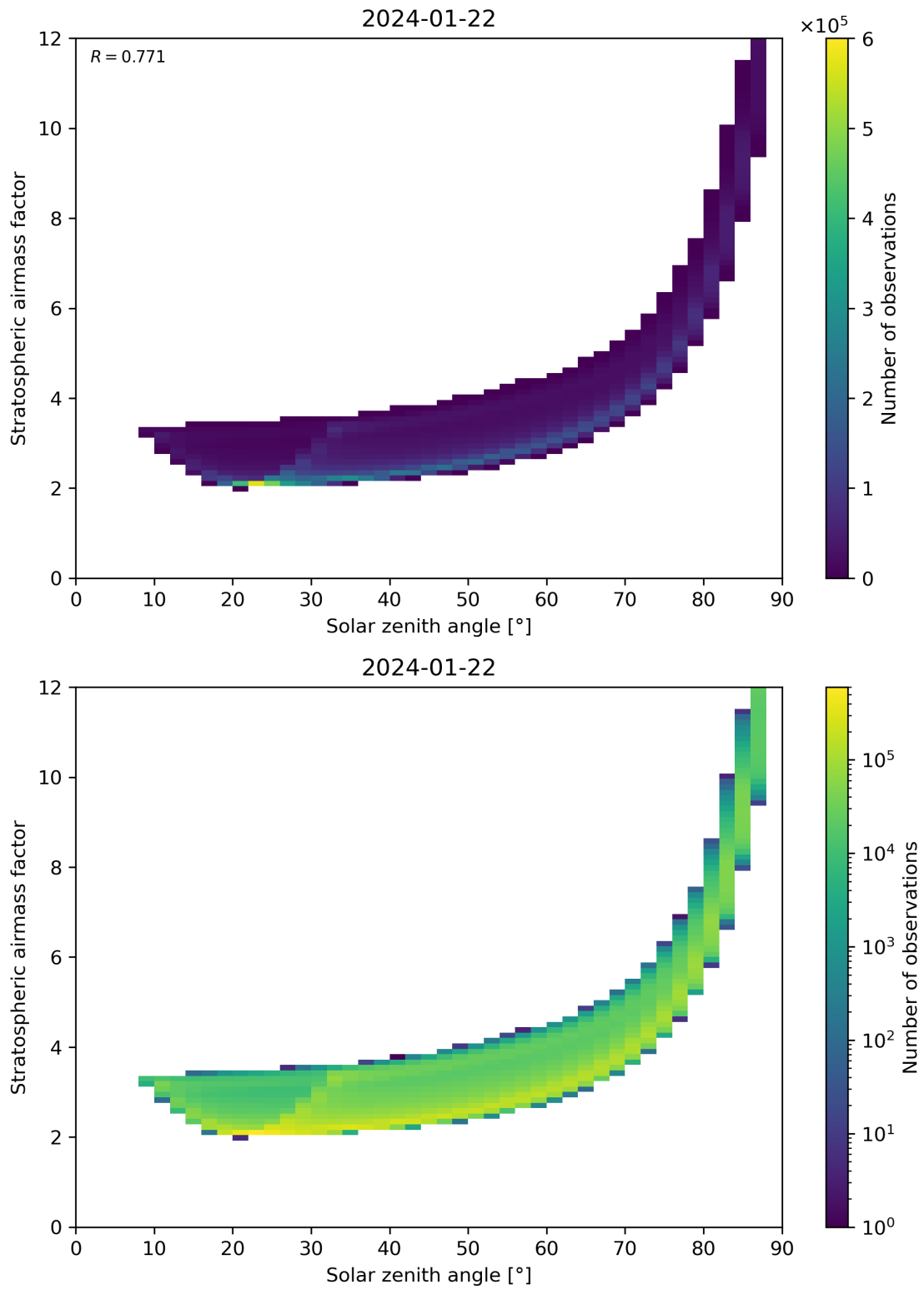
Figure 145: Scatter density plot of “Solar zenith angle” against “Stratospheric airmass factor” for 2024-01-21 to 2024-01-23.
