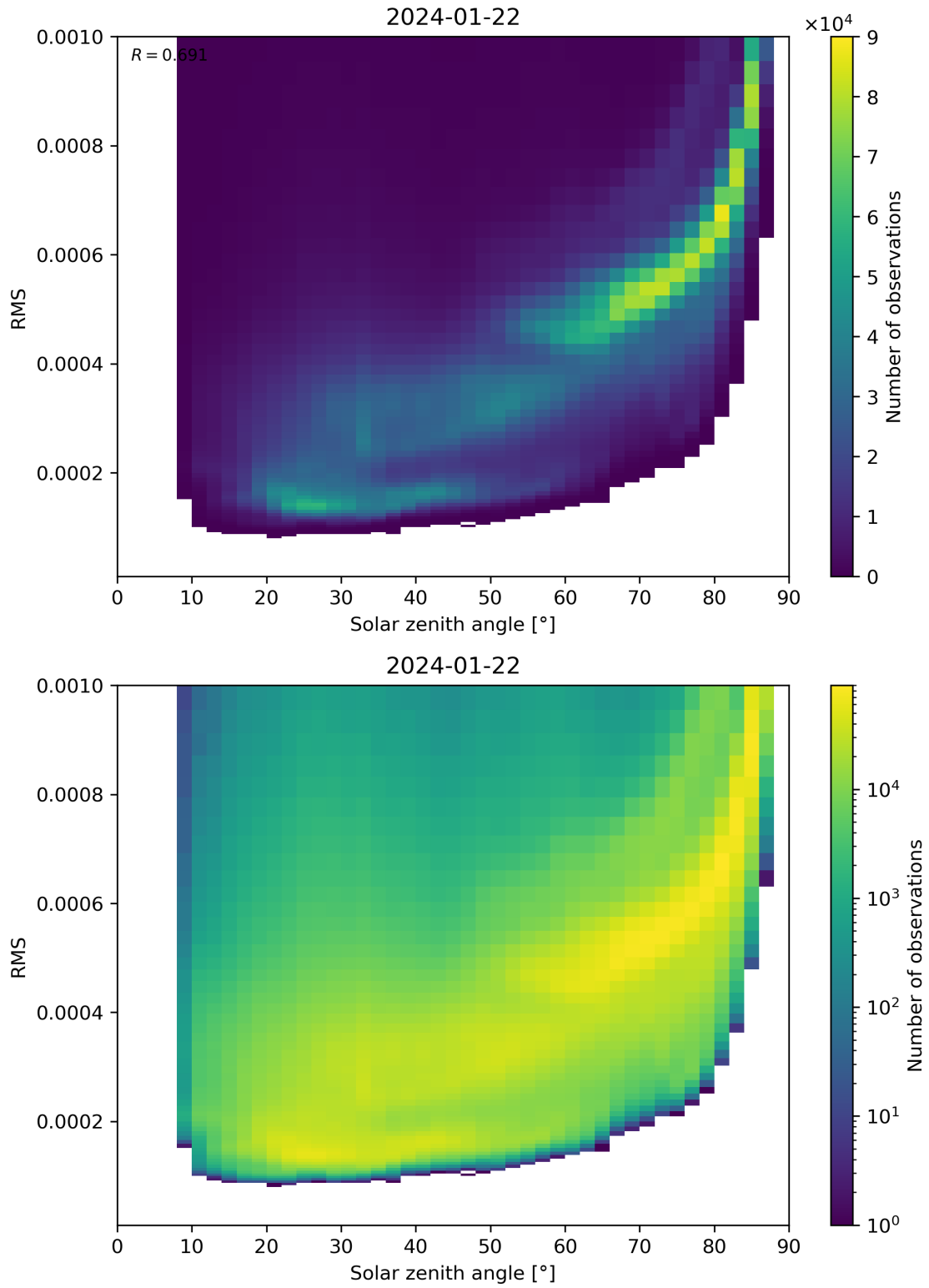
Figure 157: Scatter density plot of “Solar zenith angle” against “RMS” for 2024-01-21 to 2024-01-23.
