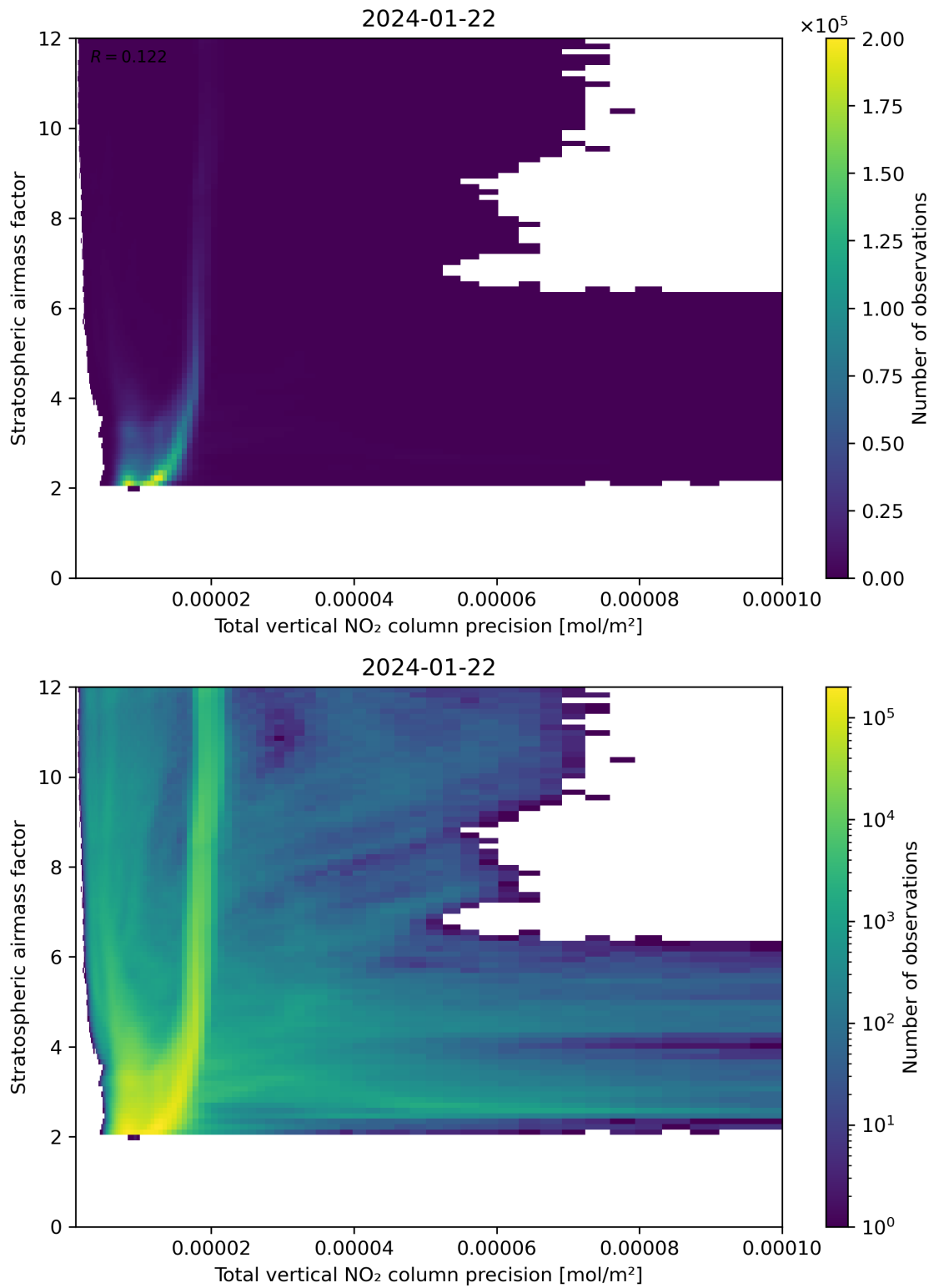
Figure 115: Scatter density plot of “Total vertical NO 2 column precision” against “Stratospheric air mass factor” for 2024-01-21 to 2024-01-23.
