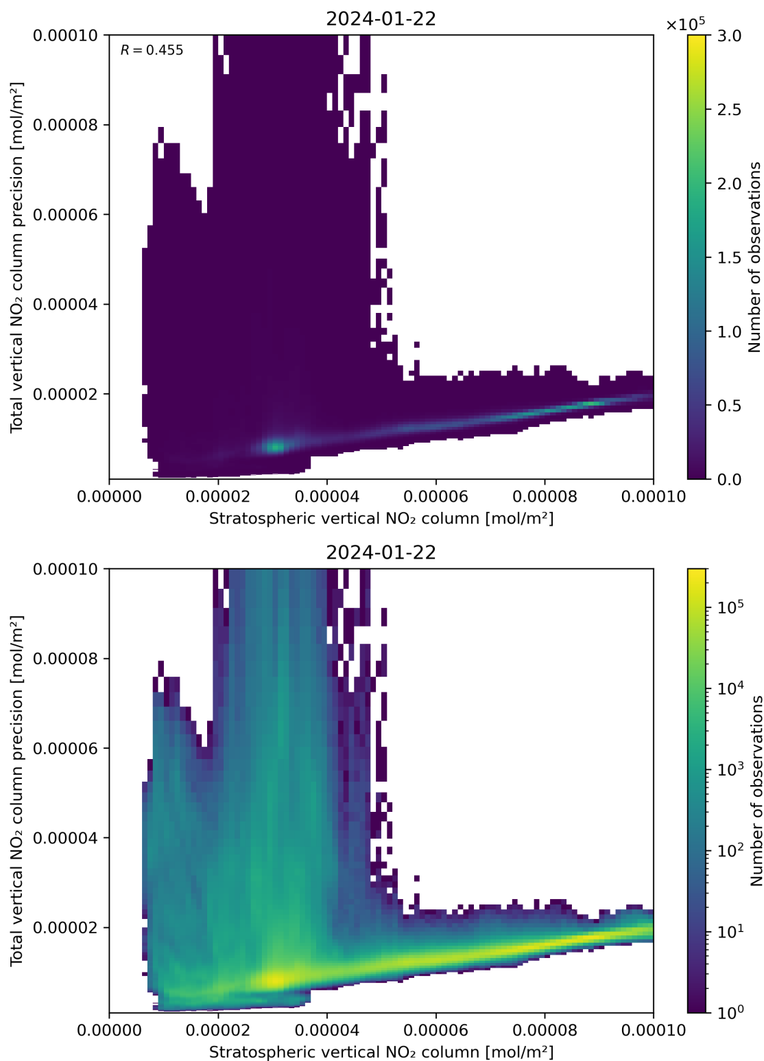
Figure 101: Scatter density plot of “Stratospheric vertical NO 2 column” against “Total vertical NO 2 column precision” for 2024-01-21 to 2024-01-23.
