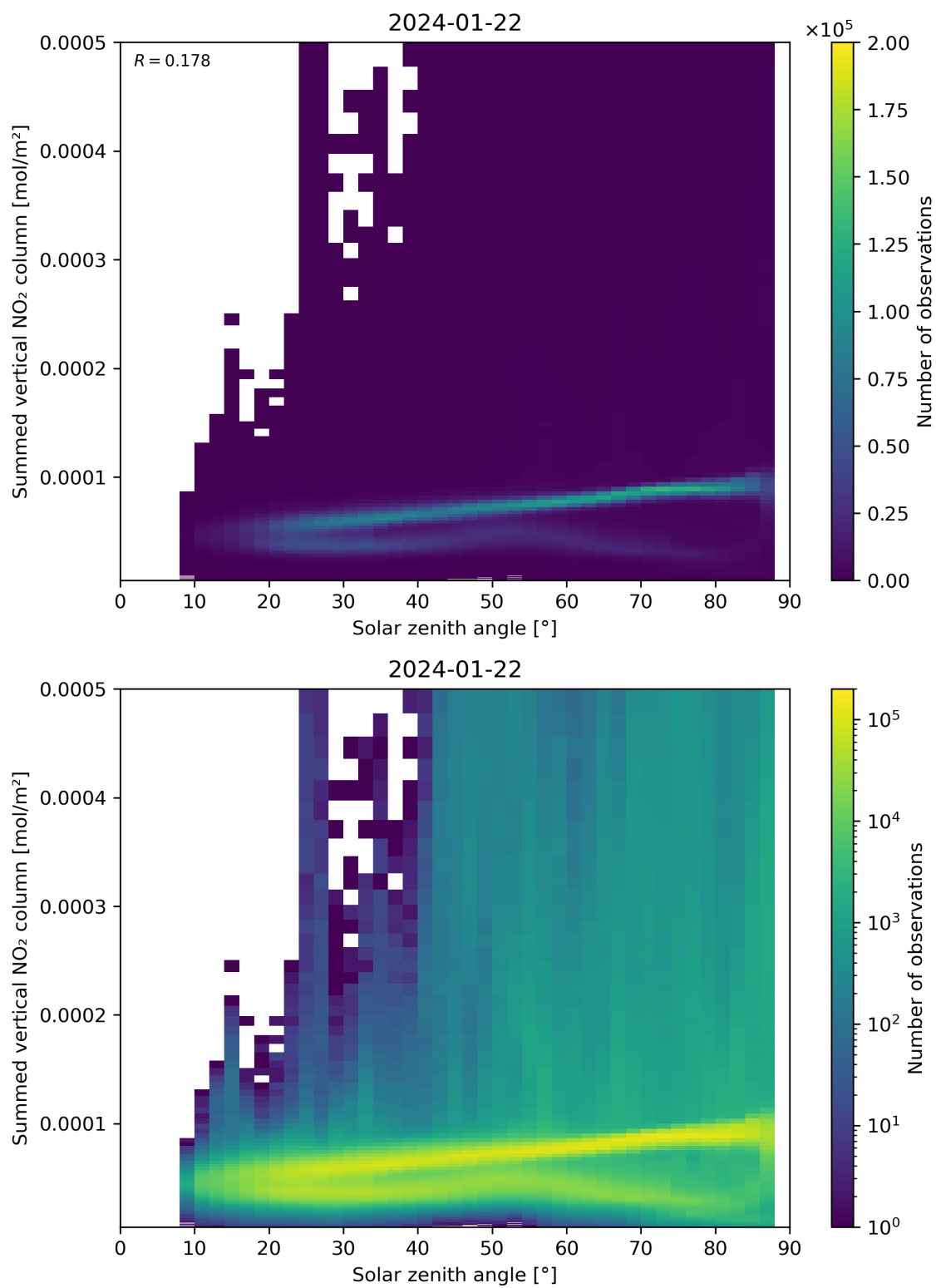
Figure 151: Scatter density plot of “Solar zenith angle” against “Summed vertical NO 2 column” for 2024-01-21 to 2024-01-23.
