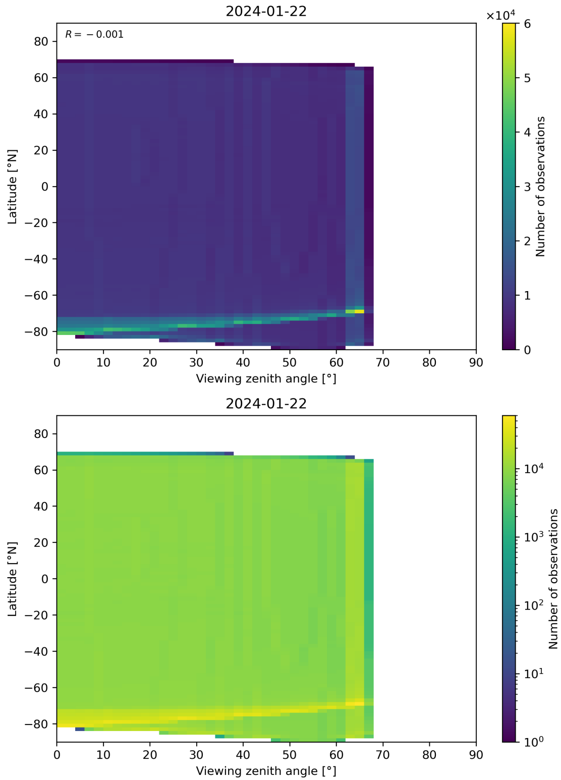
Figure 163: Scatter density plot of “Viewing zenith angle” against “Latitude” for 2024-01-21 to 2024-01-23.
