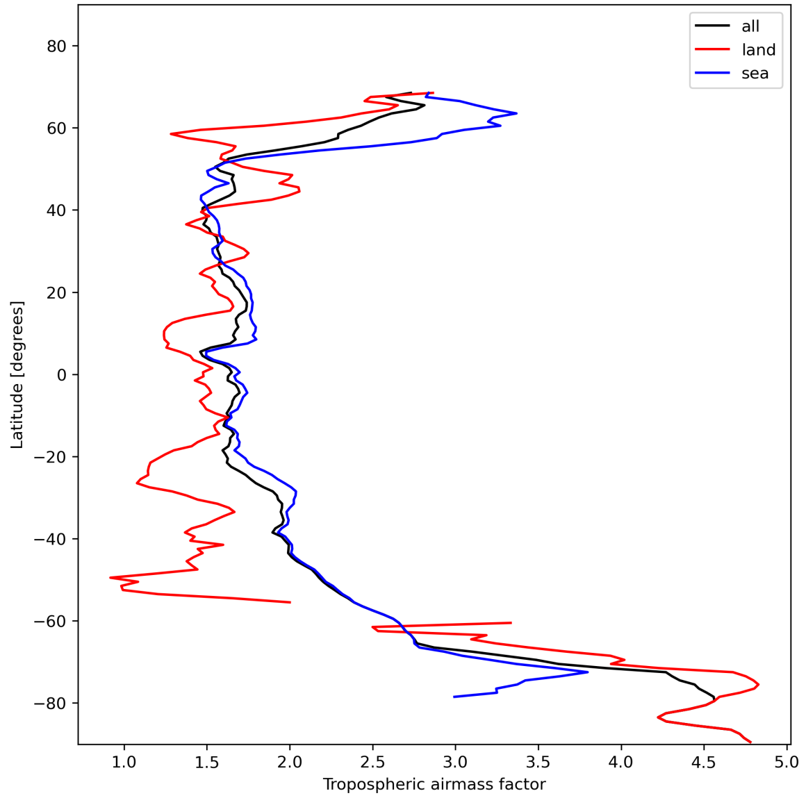
Figure 14: Zonal average of “Tropospheric airmass factor” for 2024-01-21 to 2024-01-23.
