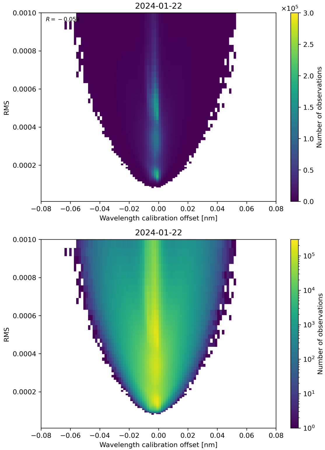
Figure 181: Scatter density plot of “Wavelength calibration offset” against “RMS” for 2024-01-21 to 2024-01-23.
