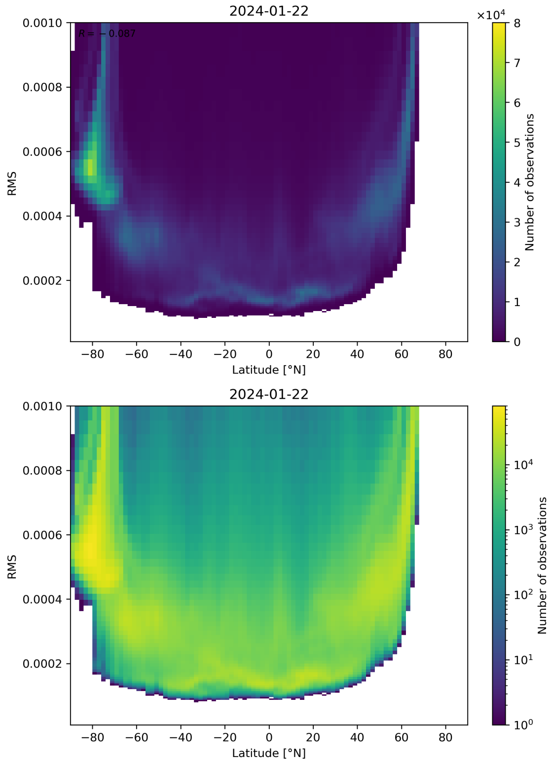
Figure 94: Scatter density plot of “Latitude” against “RMS” for 2024-01-21 to 2024-01-23.
