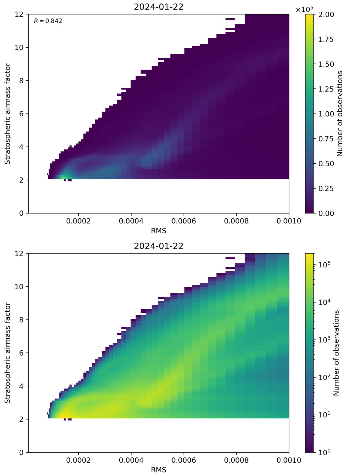
Figure 144: Scatter density plot of “RMS” against “Stratospheric airmass factor” for 2024-01-21 to 2024-01-23.
