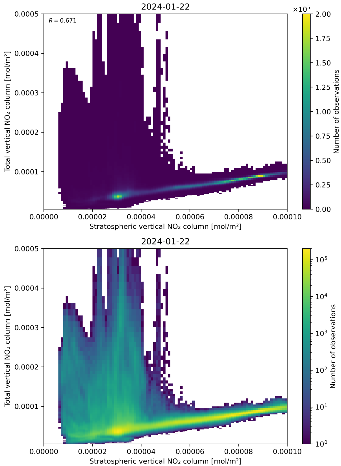
Figure 100: Scatter density plot of “Stratospheric vertical NO 2 column” against “Total vertical NO 2 column” for 2024-01-21 to 2024-01-23.
