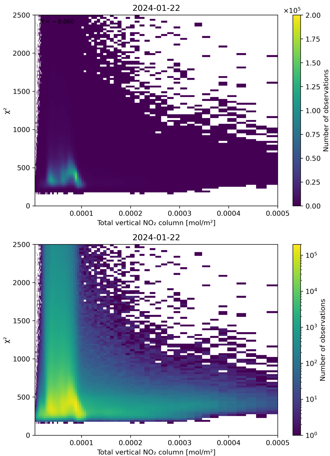
Figure 111: Scatter density plot of “Total vertical NO 2 column” against “ \chi^2 ” for 2024-01-21 to 2024-01-23.
