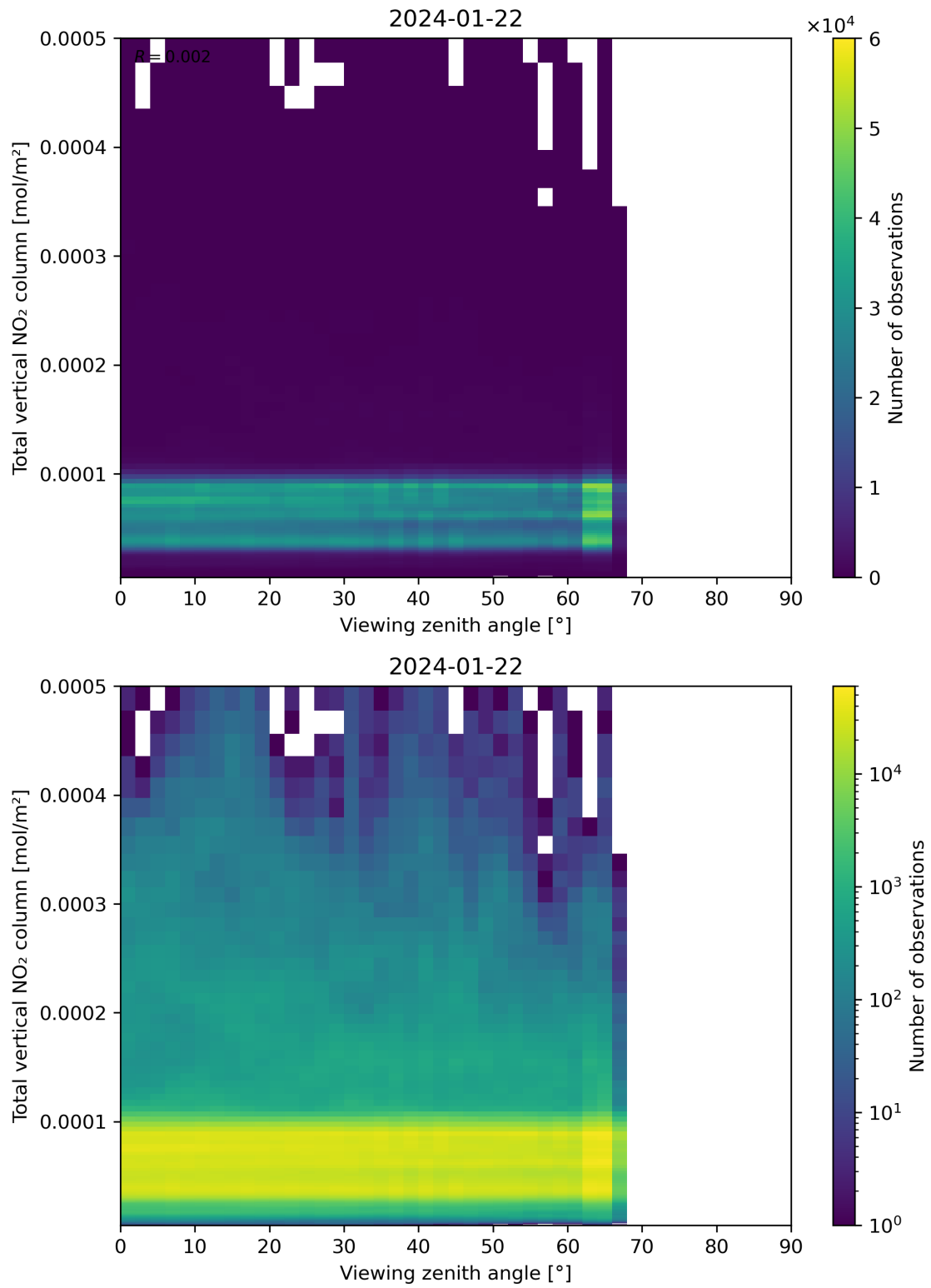
Figure 167: Scatter density plot of “Viewing zenith angle” against “Total vertical NO 2 column” for 2024-01-21 to 2024-01-23.
