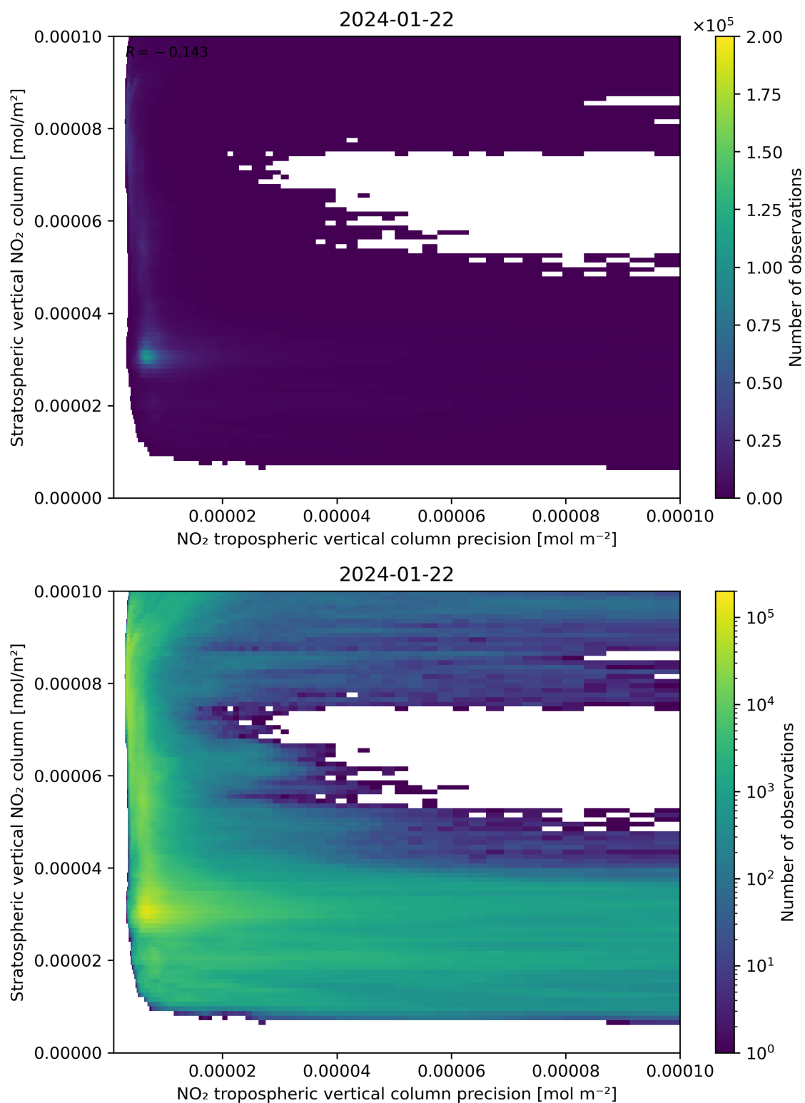
Figure 135: Scatter density plot of “NO 2 tropospheric vertical column precision” against “Stratospheric vertical NO 2 column” for 2024-01-21 to 2024-01-23.
