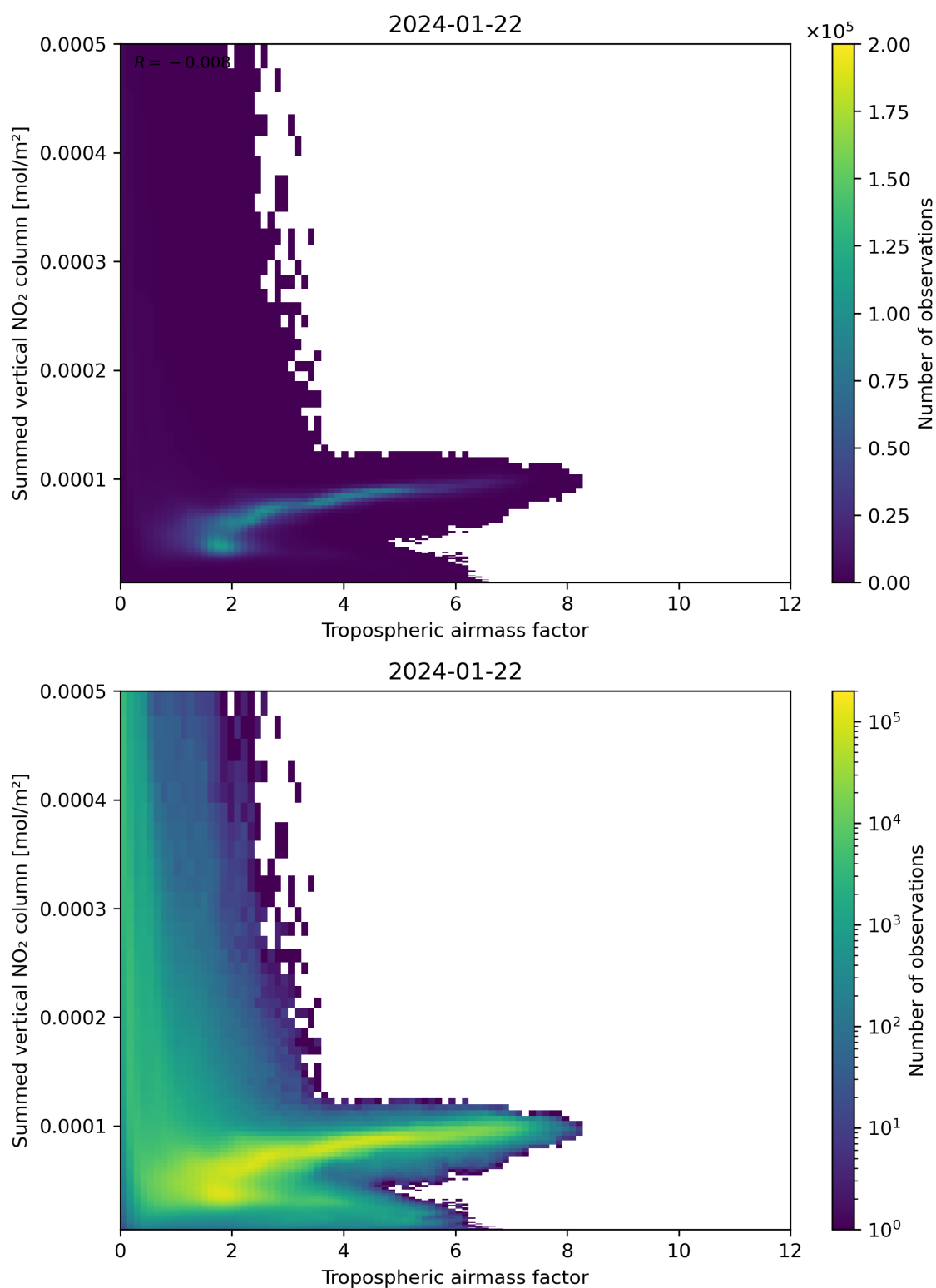
Figure 75: Scatter density plot of “Tropospheric airmass factor” against “Summed vertical NO 2 column” for 2024-01-21 to 2024-01-23.
