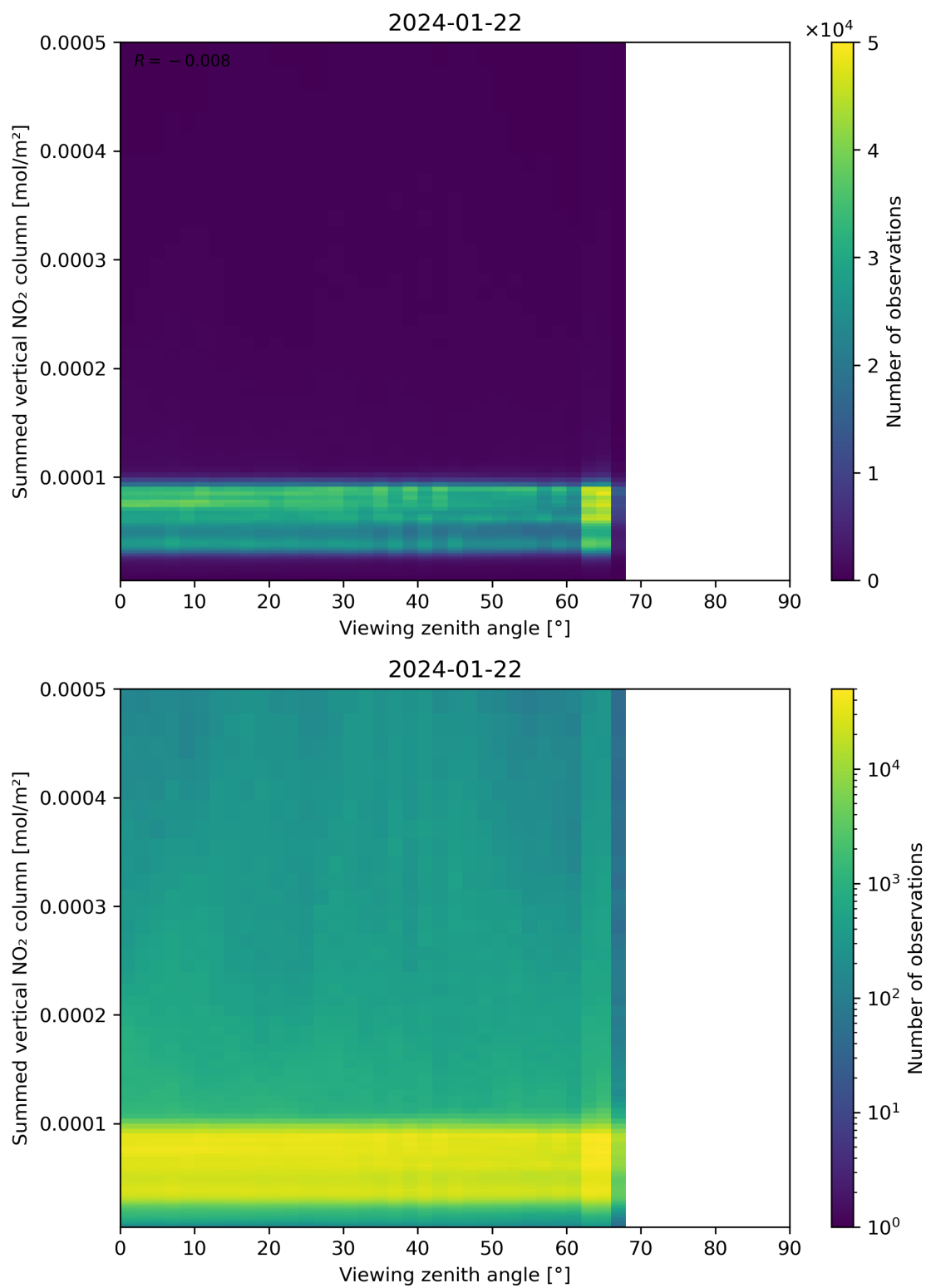
Figure 165: Scatter density plot of “Viewing zenith angle” against “Summed vertical NO 2 column” for 2024-01-21 to 2024-01-23.
