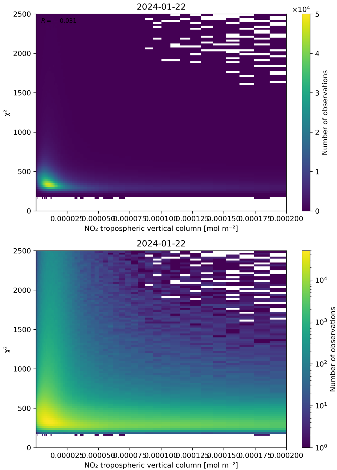
Figure 124: Scatter density plot of “NO 2 tropospheric vertical column” against “ \chi^2 ” for 2024-01-21 to 2024-01-23.
