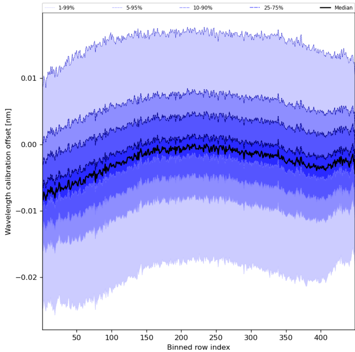
Figure 52: Along track statistics of “Wavelength calibration offset” for 2024-01-21 to 2024-01-23
