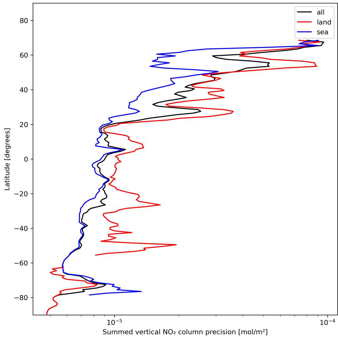
Figure 24: Zonal average of “Summed vertical NO 2 column precision” for 2024-01-21 to 2024-01-23.
