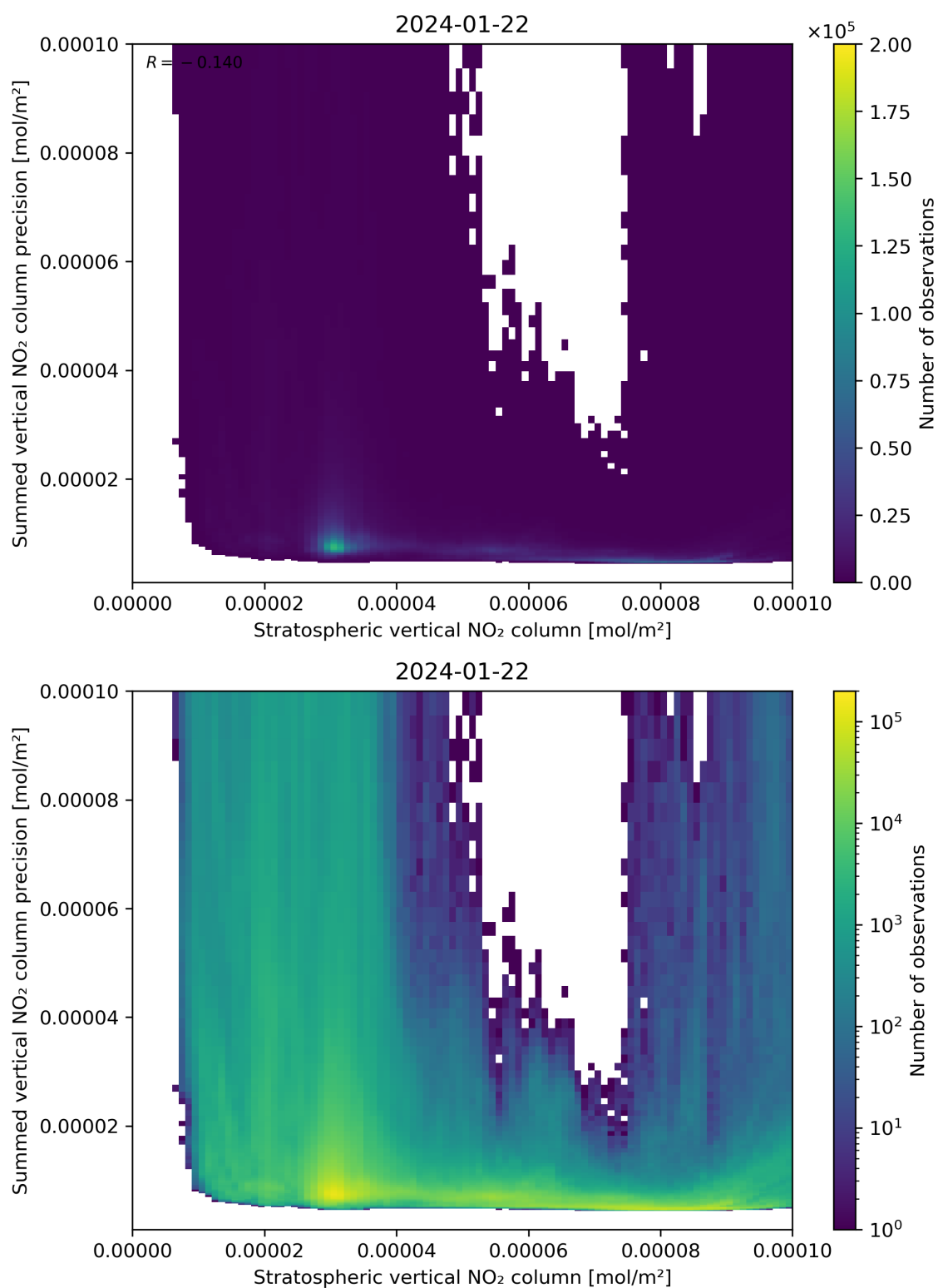
Figure 99: Scatter density plot of “Stratospheric vertical NO 2 column” against “Summed vertical NO 2 column precision” for 2024-01-21 to 2024-01-23.
