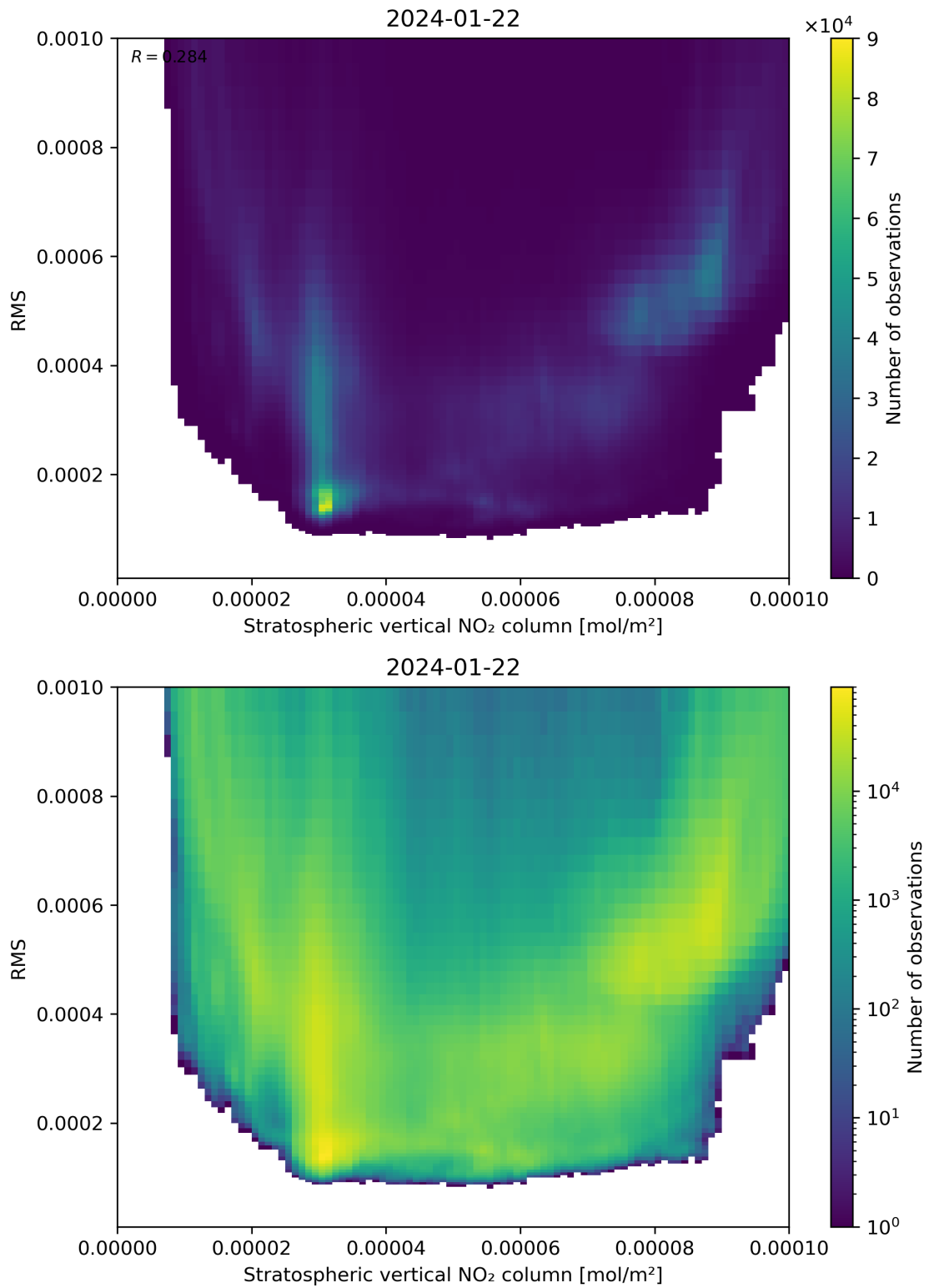
Figure 102: Scatter density plot of “Stratospheric vertical NO 2 column” against “RMS” for 2024-01-21 to 2024-01-23.
