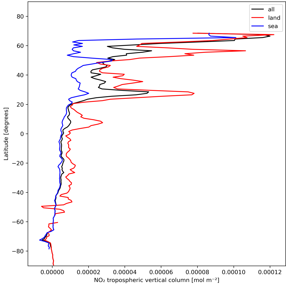
Figure 12: Zonal average of “NO 2 tropospheric vertical column” for 2024-01-21 to 2024-01-23.
