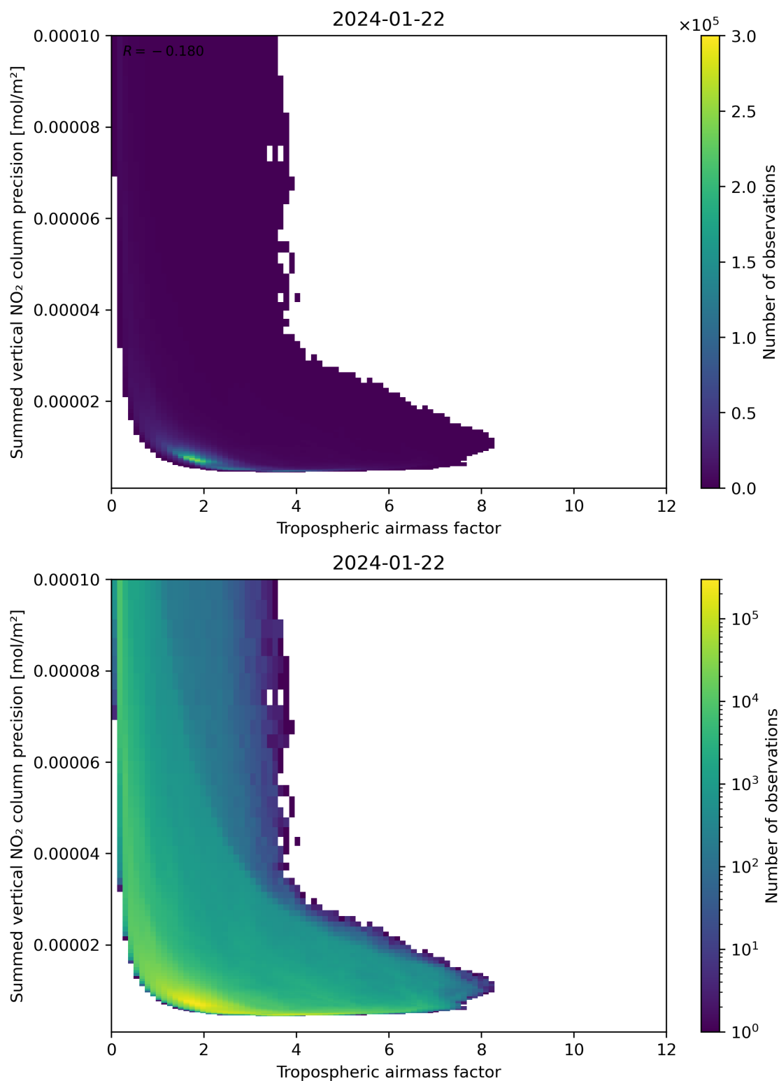
Figure 76: Scatter density plot of “Tropospheric air mass factor” against “Summed vertical NO 2 column precision” for 2024-01-21 to 2024-01-23.
