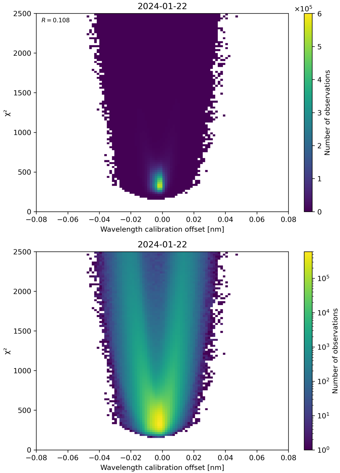
Figure 175: Scatter density plot of “Wavelength calibration offset” against “ \chi^2 ” for 2024-01-21 to 2024-01-23.
