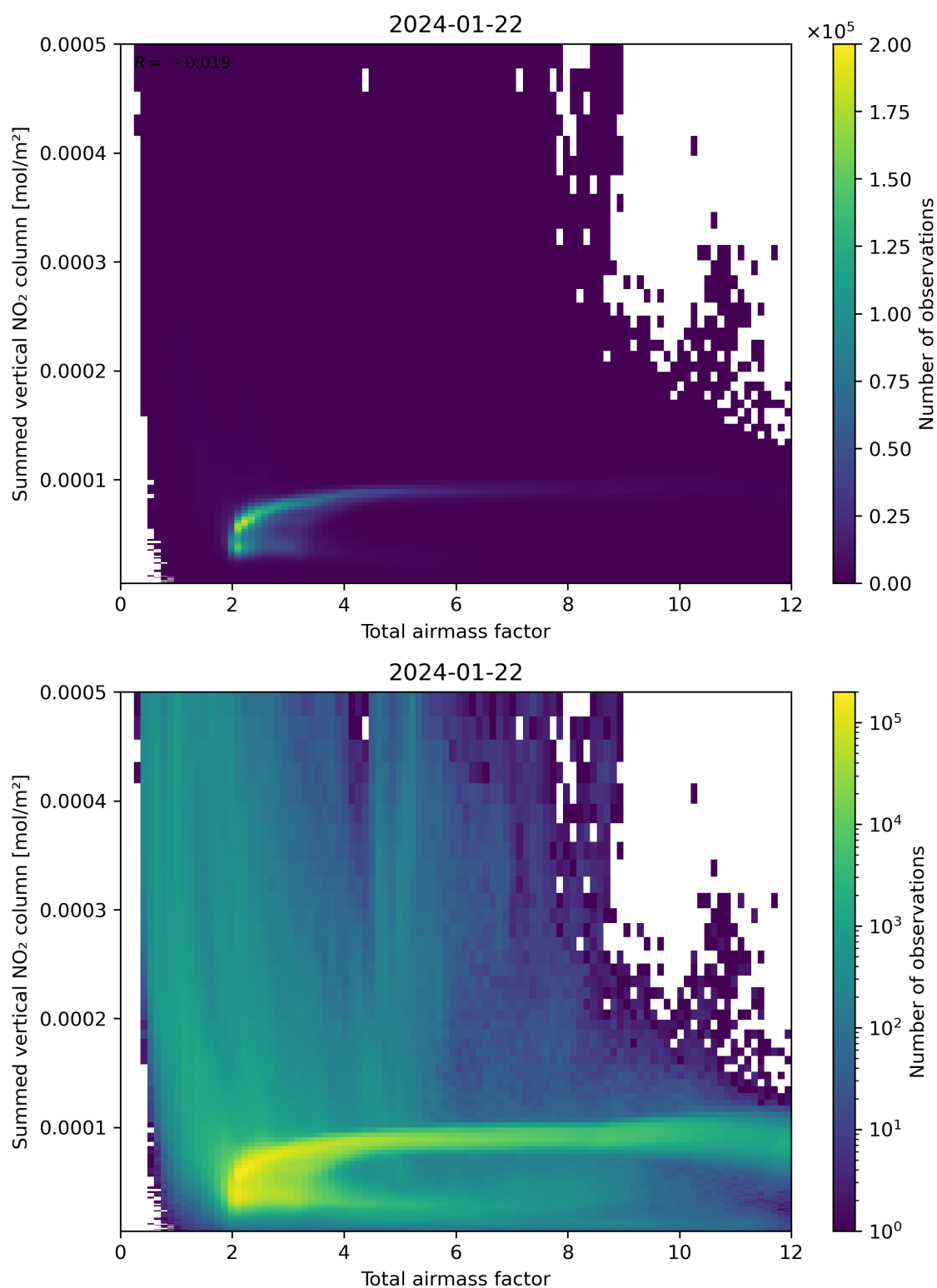
Figure 65: Scatter density plot of “Total airmass factor” against “Summed vertical NO 2 column” for 2024-01-21 to 2024-01-23.
