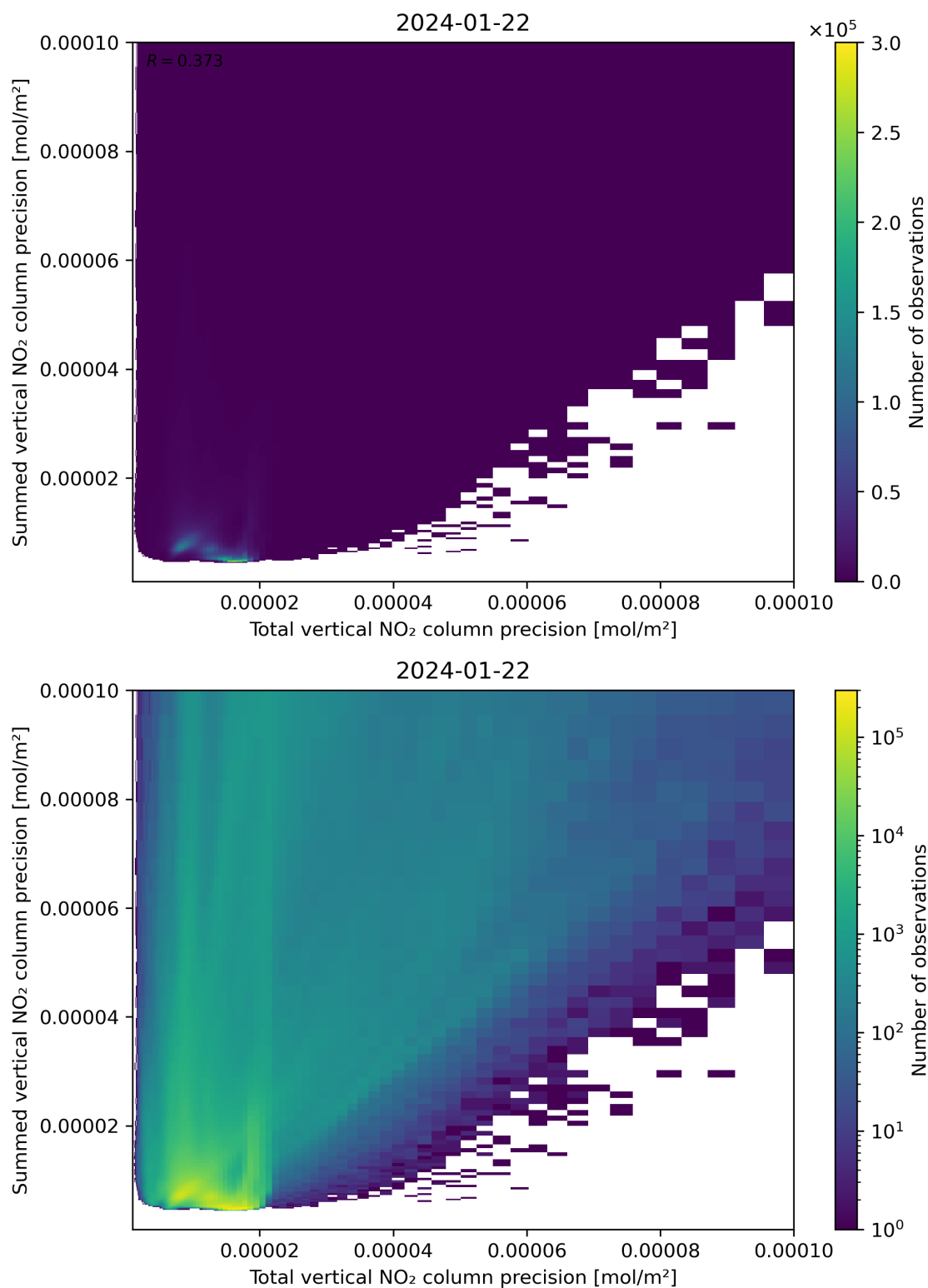
Figure 118: Scatter density plot of “Total vertical NO 2 column precision” against “Summed vertical NO 2 column precision” for 2024-01-21 to 2024-01-23.
