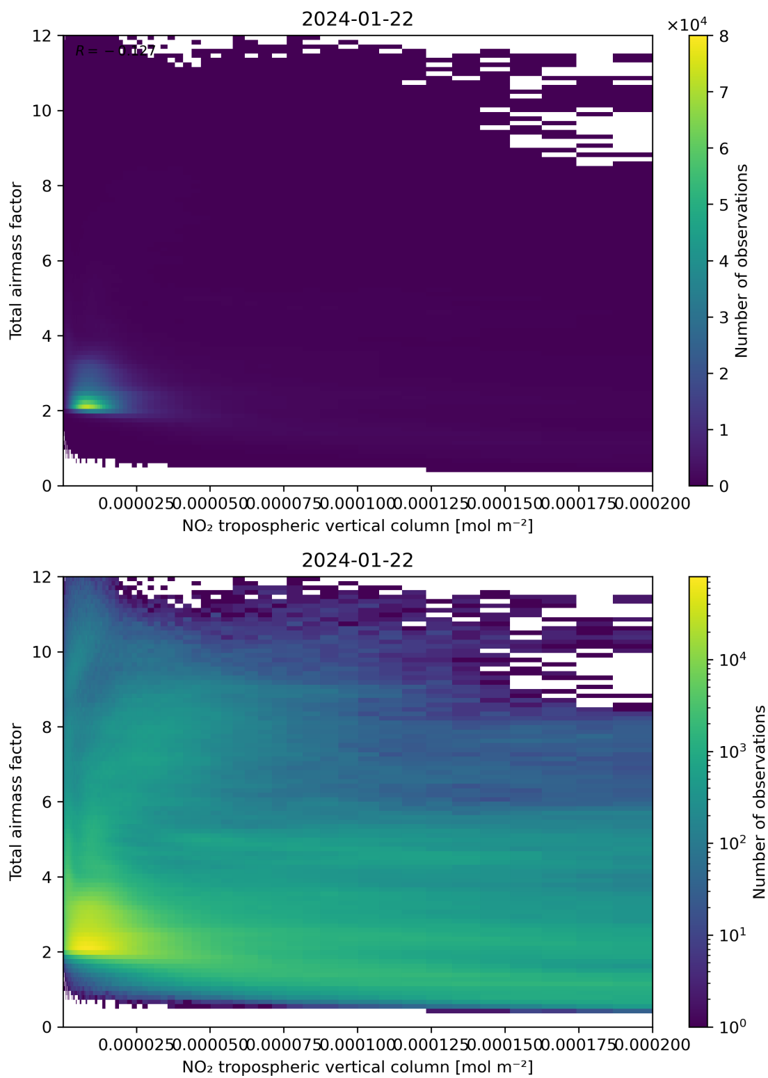
Figure 122: Scatter density plot of “NO 2 tropospheric vertical column” against “Total air mass factor” for 2024-01-21 to 2024-01-23.
