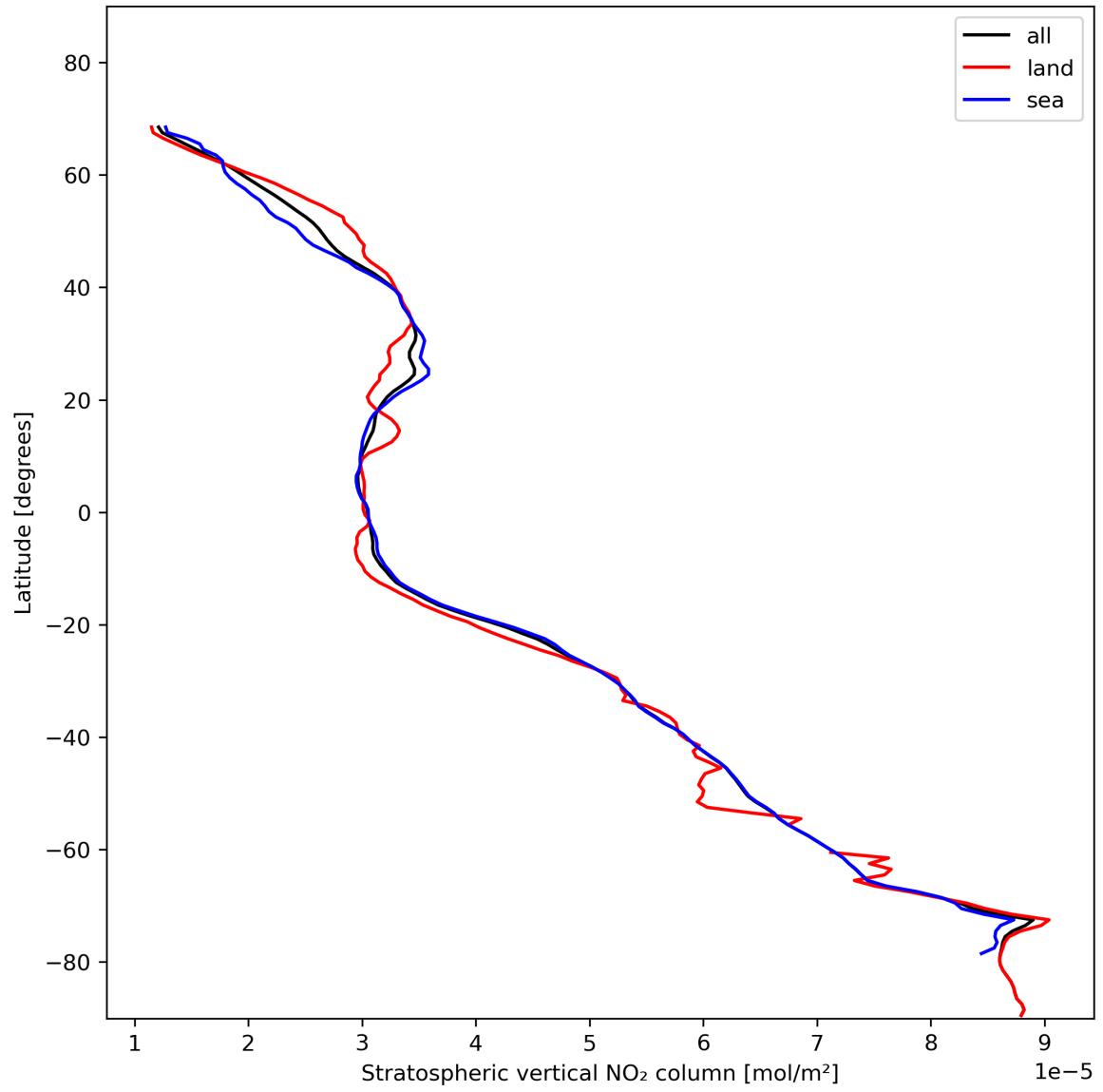
Figure 19: Zonal average of “Stratospheric vertical NO 2 column” for 2024-01-21 to 2024-01-23.
