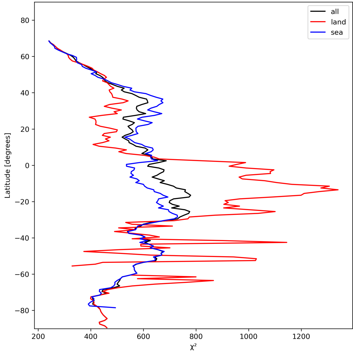
Figure 25: Zonal average of “ \chi^2 ” for 2024-01-21 to 2024-01-23.
