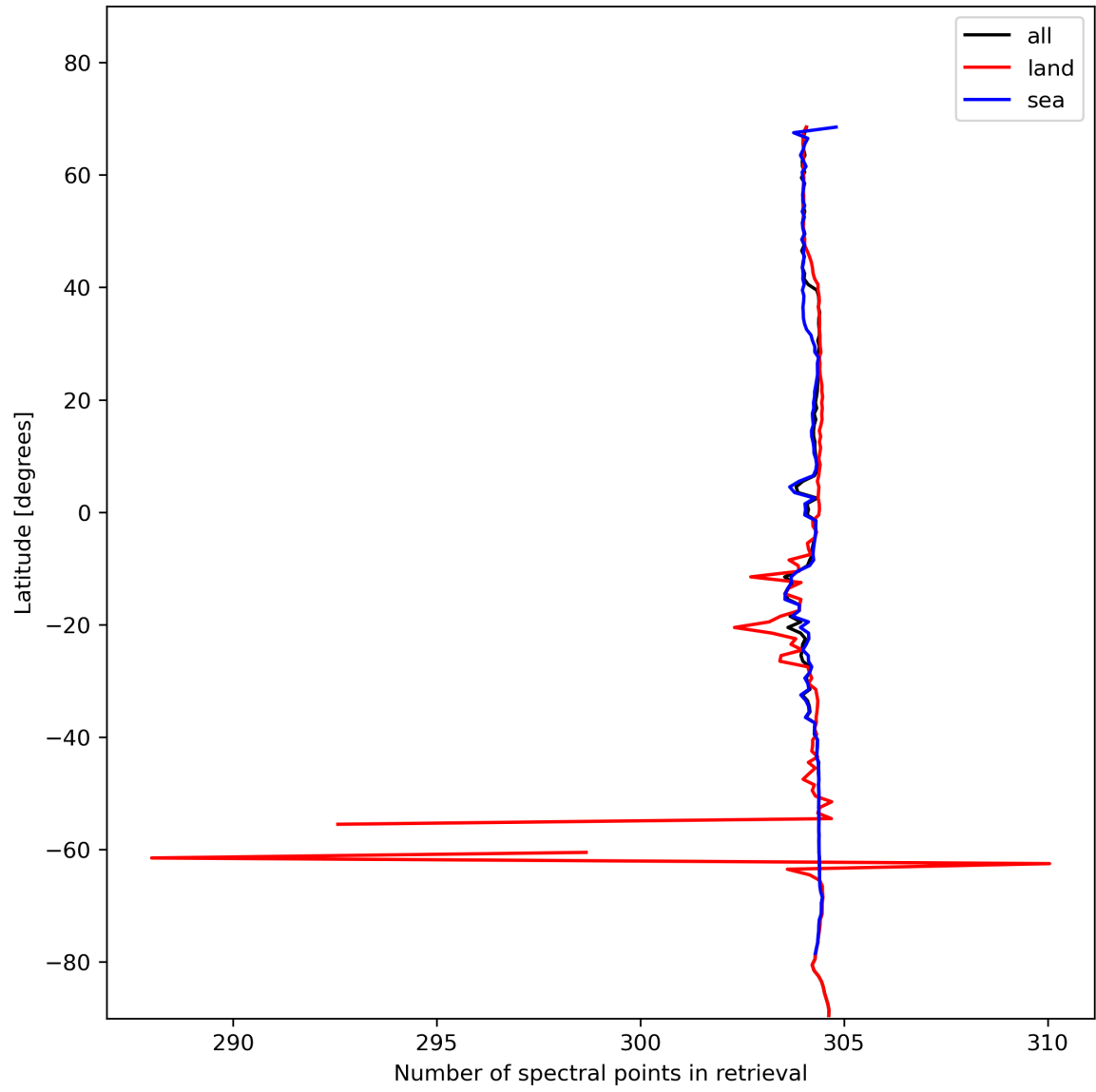
Figure 16: Zonal average of “Number of spectral points in retrieval” for 2024-01-21 to 2024-01-23.
