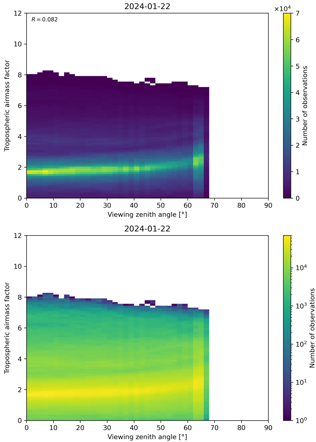
Figure 161: Scatter density plot of “Viewing zenith angle” against “Tropospheric airmass factor” for 2024-01-21 to 2024-01-23.
