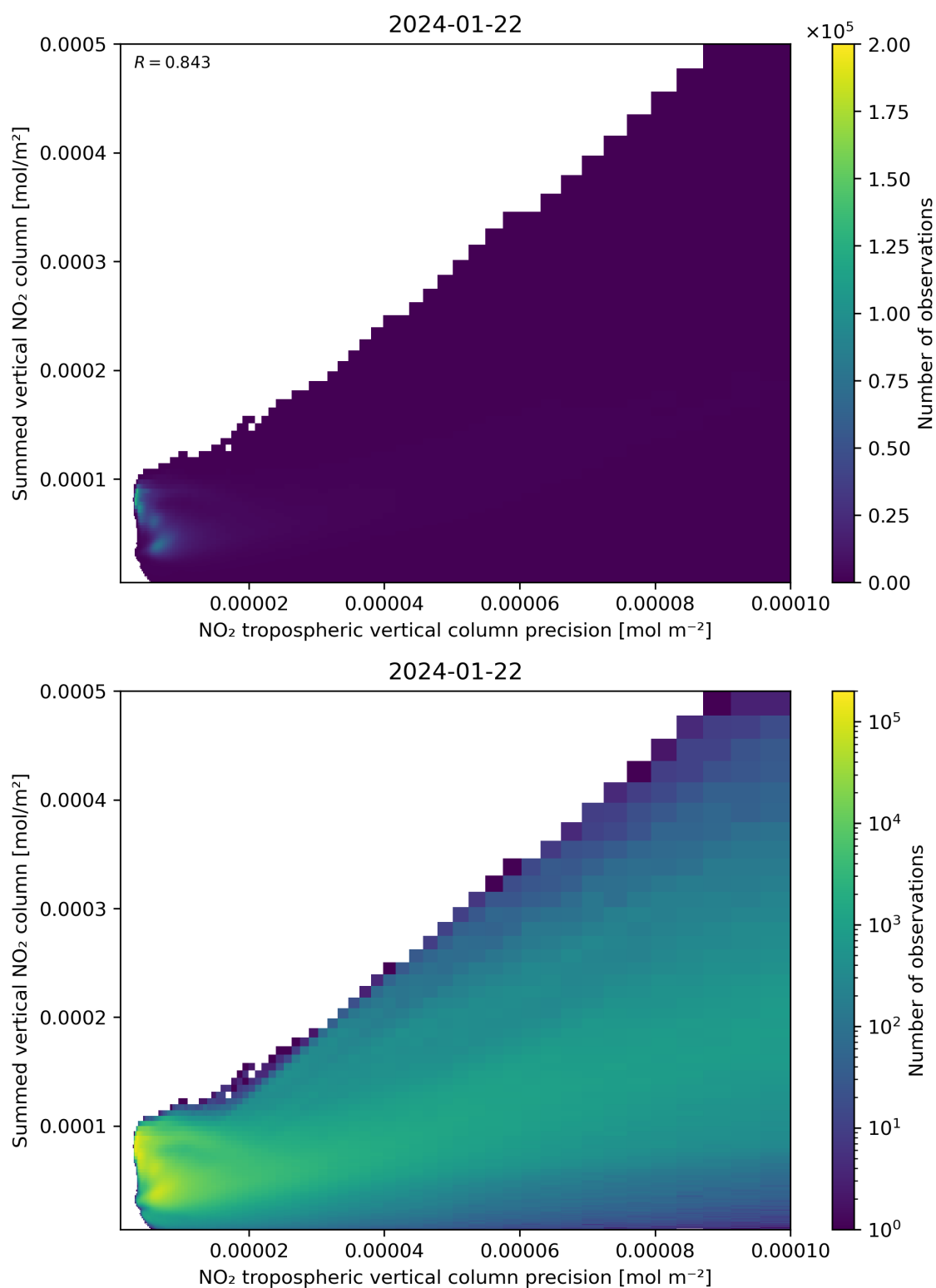
Figure 136: Scatter density plot of “NO 2 tropospheric vertical column precision” against “Summed vertical NO 2 column” for 2024-01-21 to 2024-01-23.
