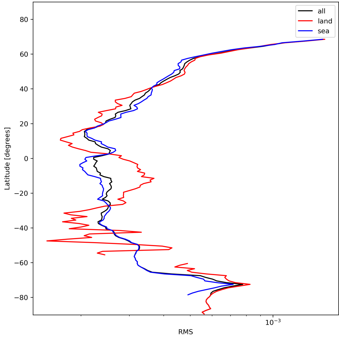
Figure 26: Zonal average of “RMS” for 2024-01-21 to 2024-01-23.
