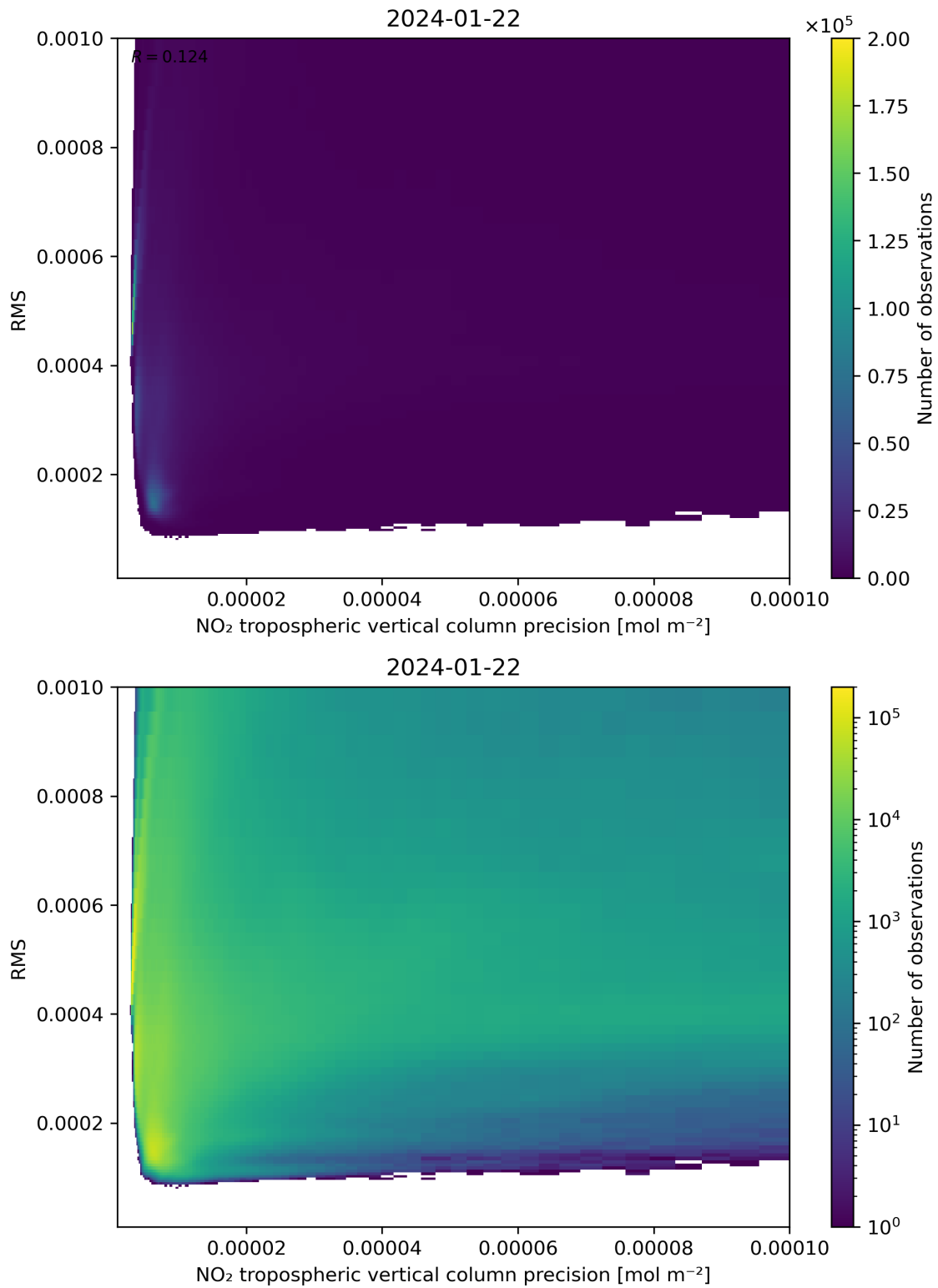
Figure 140: Scatter density plot of “NO 2 tropospheric vertical column precision” against “RMS” for 2024-01-21 to 2024-01-23.
