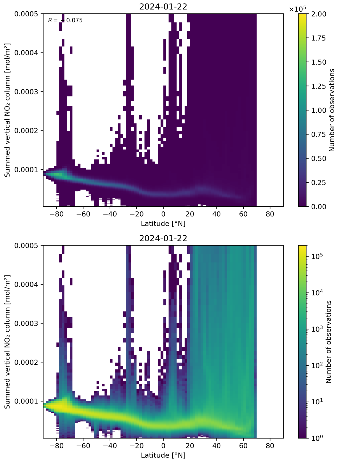
Figure 88: Scatter density plot of “Latitude” against “Summed vertical NO 2 column” for 2024-01-21 to 2024-01-23.
