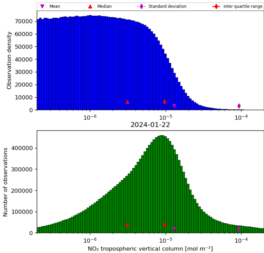
Figure 29: Histogram of “NO 2 tropospheric vertical column” for 2024-01-21 to 2024-01-23
