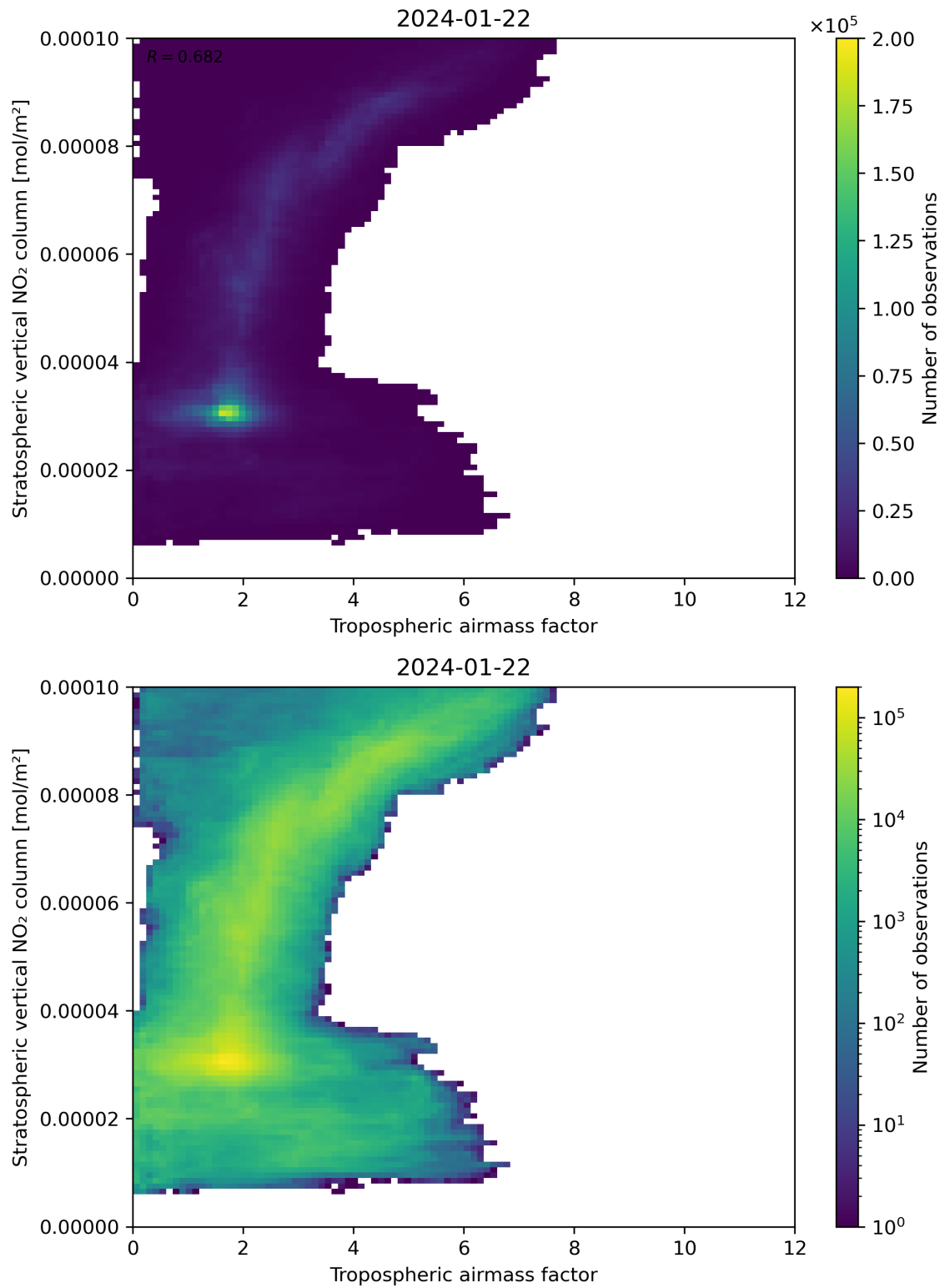
Figure 74: Scatter density plot of “Tropospheric air mass factor” against “Stratospheric vertical NO 2 column” for 2024-01-21 to 2024-01-23.
