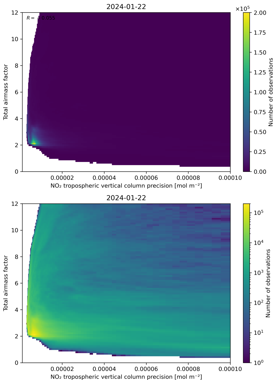
Figure 132: Scatter density plot of “NO 2 tropospheric vertical column precision” against “Total air mass factor” for 2024-01-21 to 2024-01-23.
