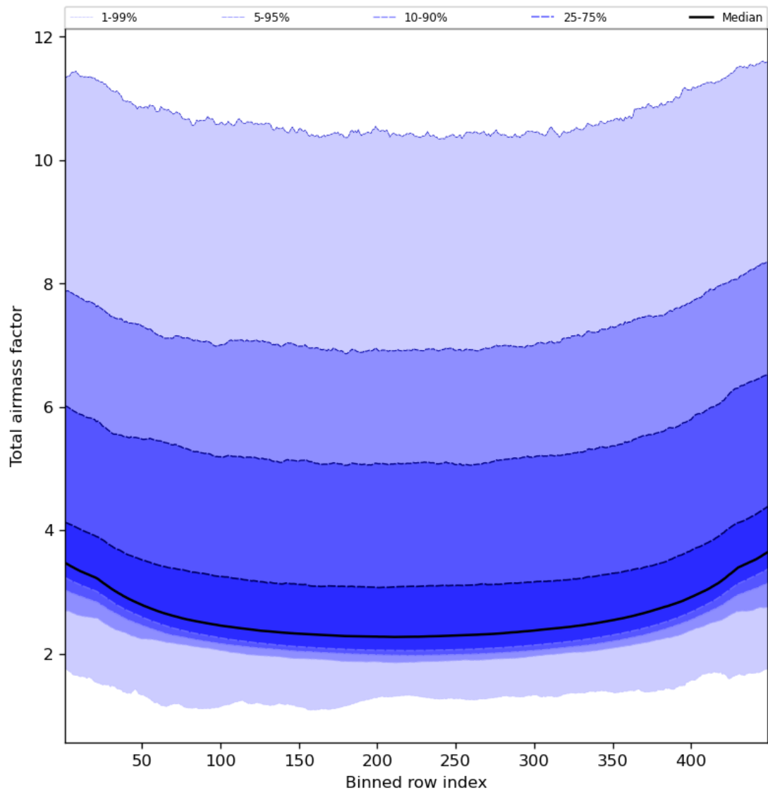
Figure 49: Along track statistics of “Total airmass factor” for 2024-01-21 to 2024-01-23
