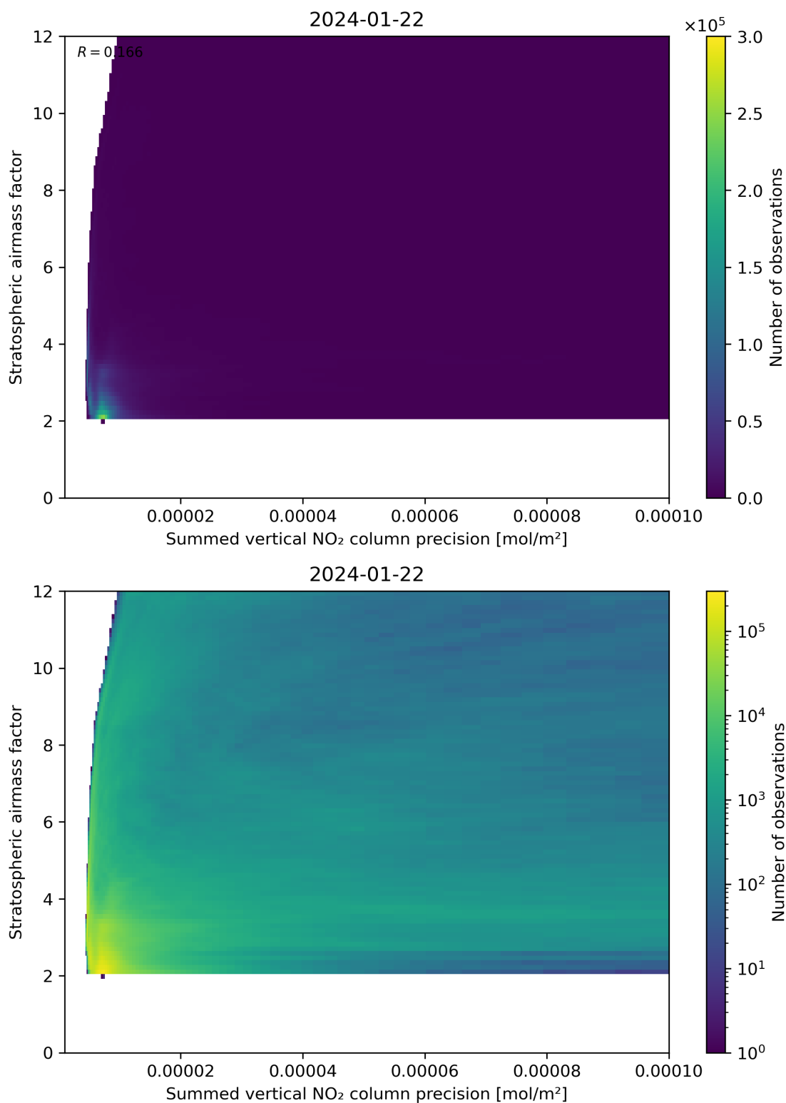
Figure 106: Scatter density plot of “Summed vertical NO 2 column precision” against “Stratospheric airmass factor” for 2024-01-21 to 2024-01-23.
