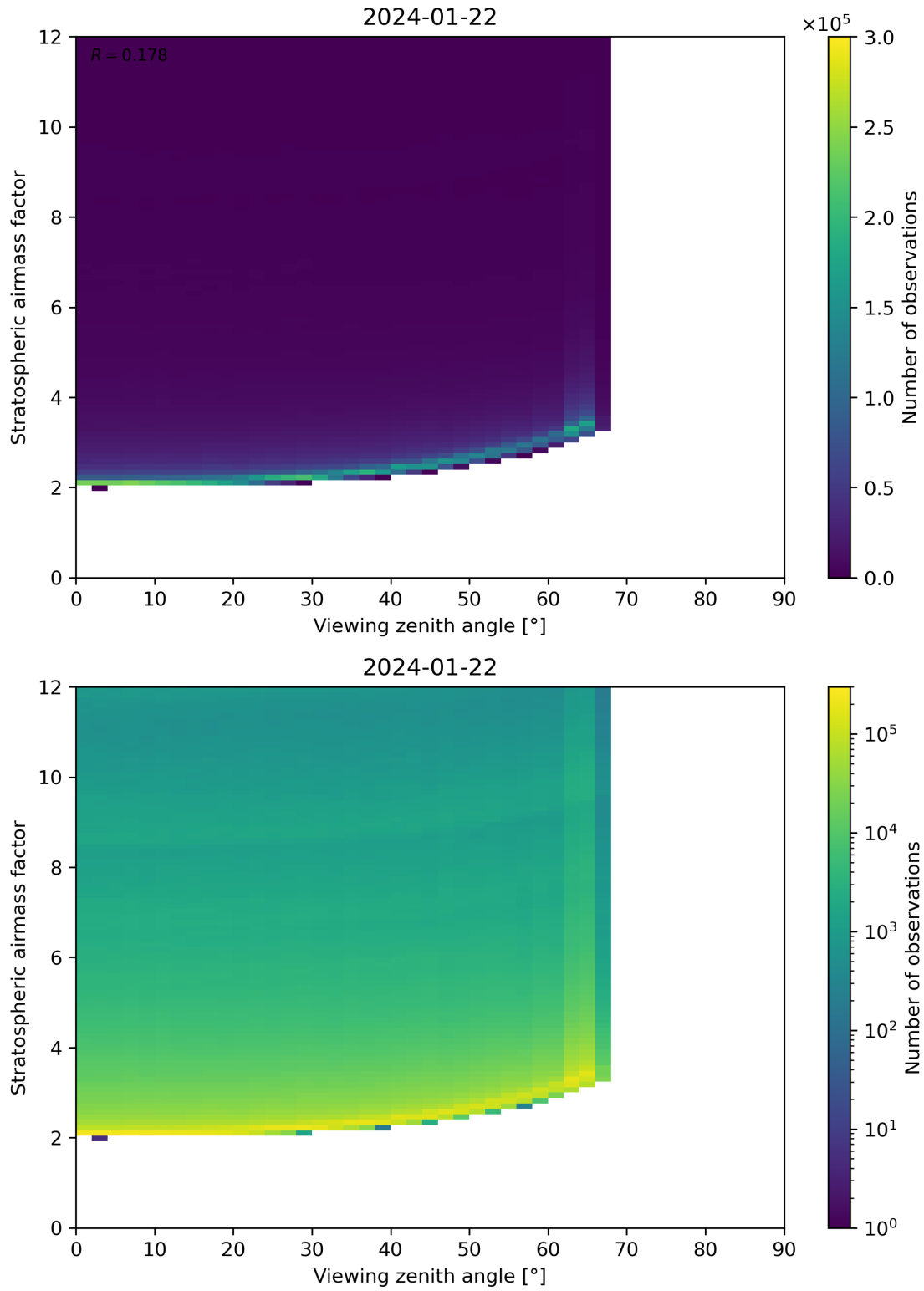
Figure 159: Scatter density plot of “Viewing zenith angle” against “Stratospheric airmass factor” for 2024-01-21 to 2024-01-23.
