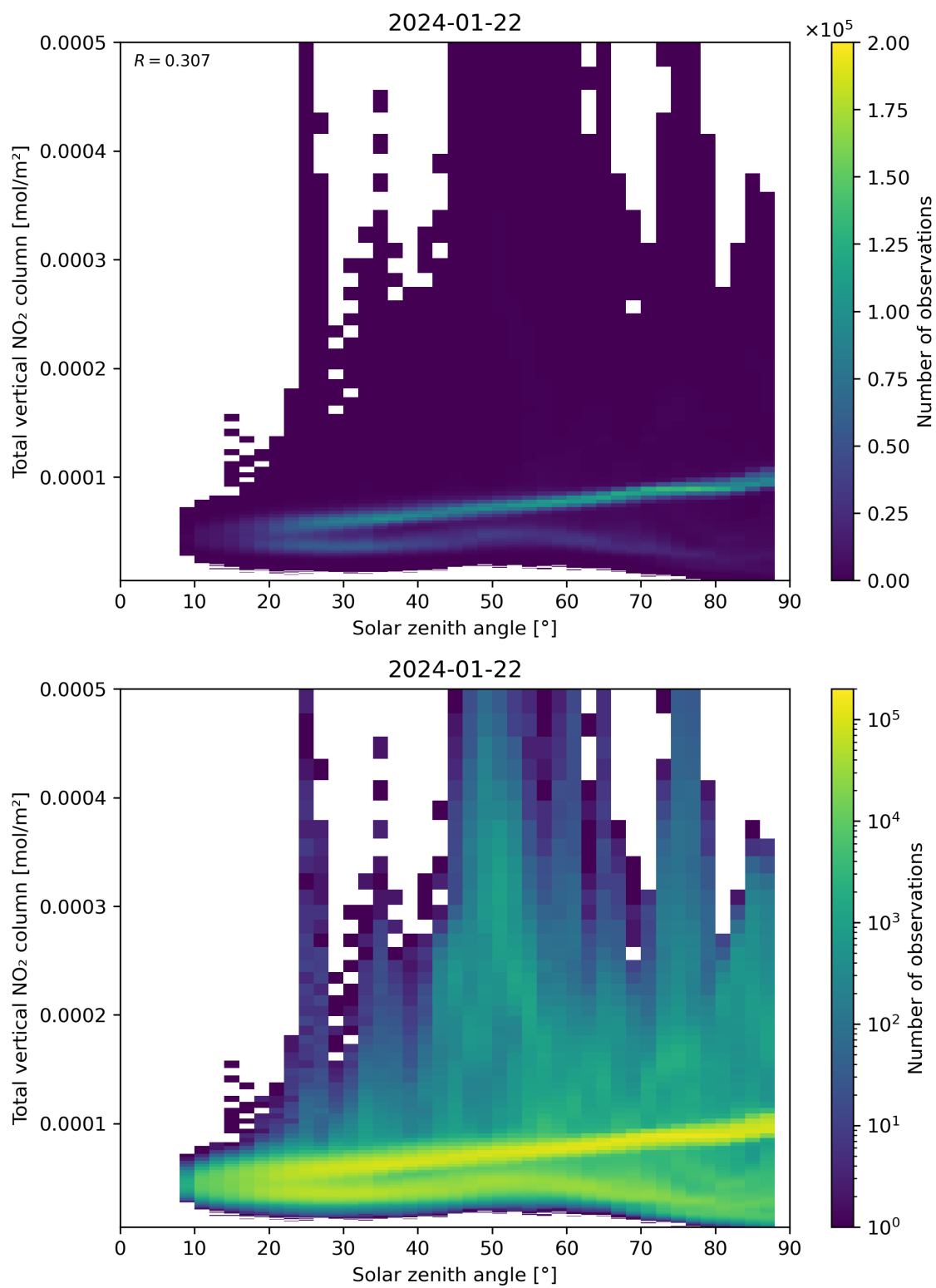
Figure 153: Scatter density plot of “Solar zenith angle” against “Total vertical NO 2 column” for 2024-01-21 to 2024-01-23.
