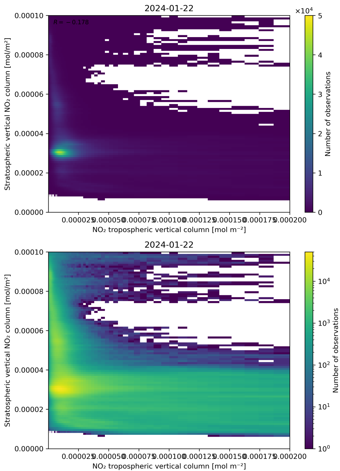
Figure 125: Scatter density plot of “NO 2 tropospheric vertical column” against “Stratospheric vertical NO 2 column” for 2024-01-21 to 2024-01-23.
