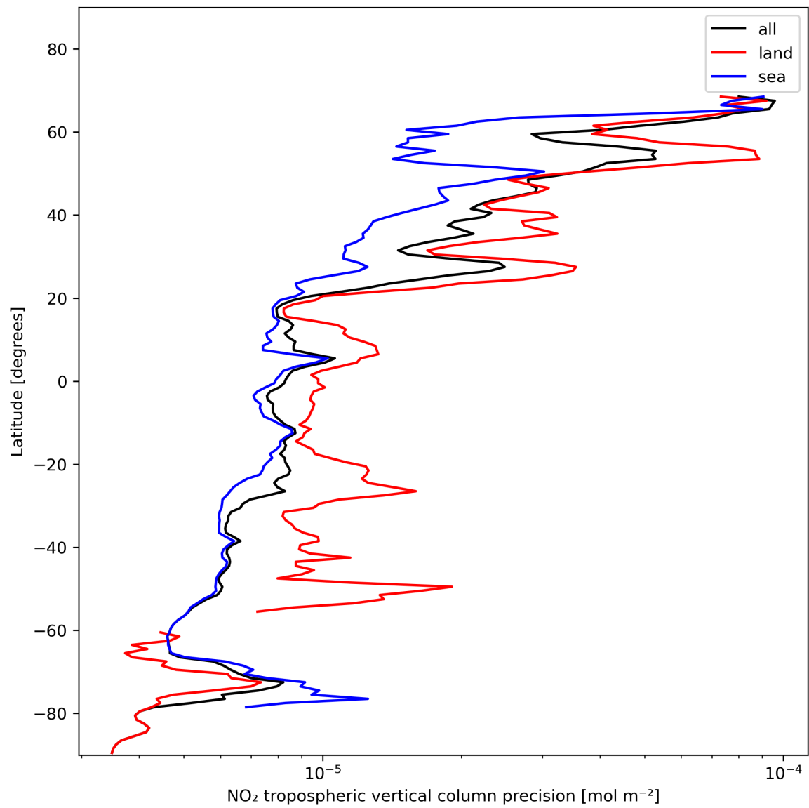
Figure 13: Zonal average of “NO 2 tropospheric vertical column precision” for 2024-01-21 to 2024-01-23.
