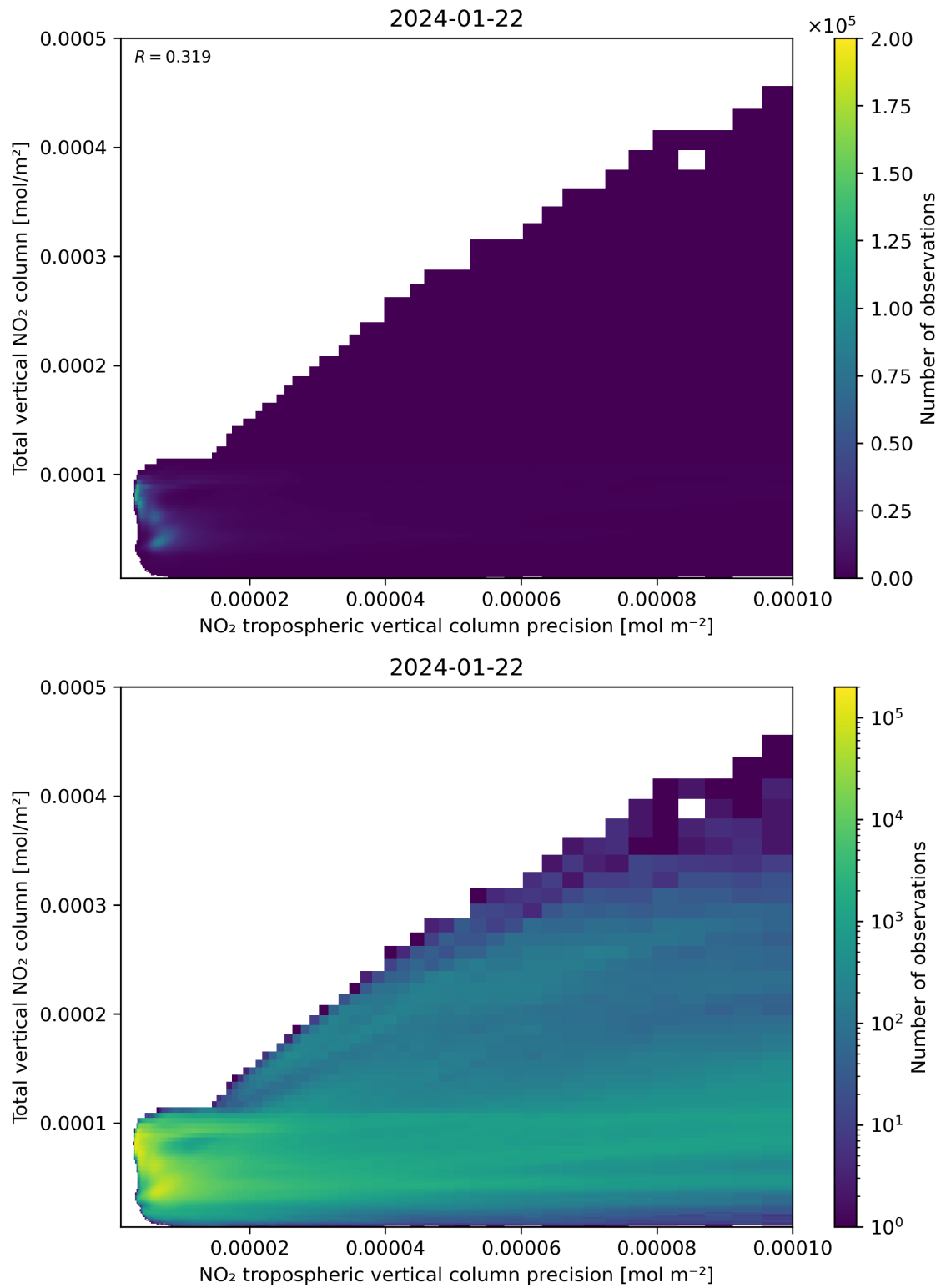
Figure 138: Scatter density plot of “NO 2 tropospheric vertical column precision” against “Total vertical NO 2 column” for 2024-01-21 to 2024-01-23.
