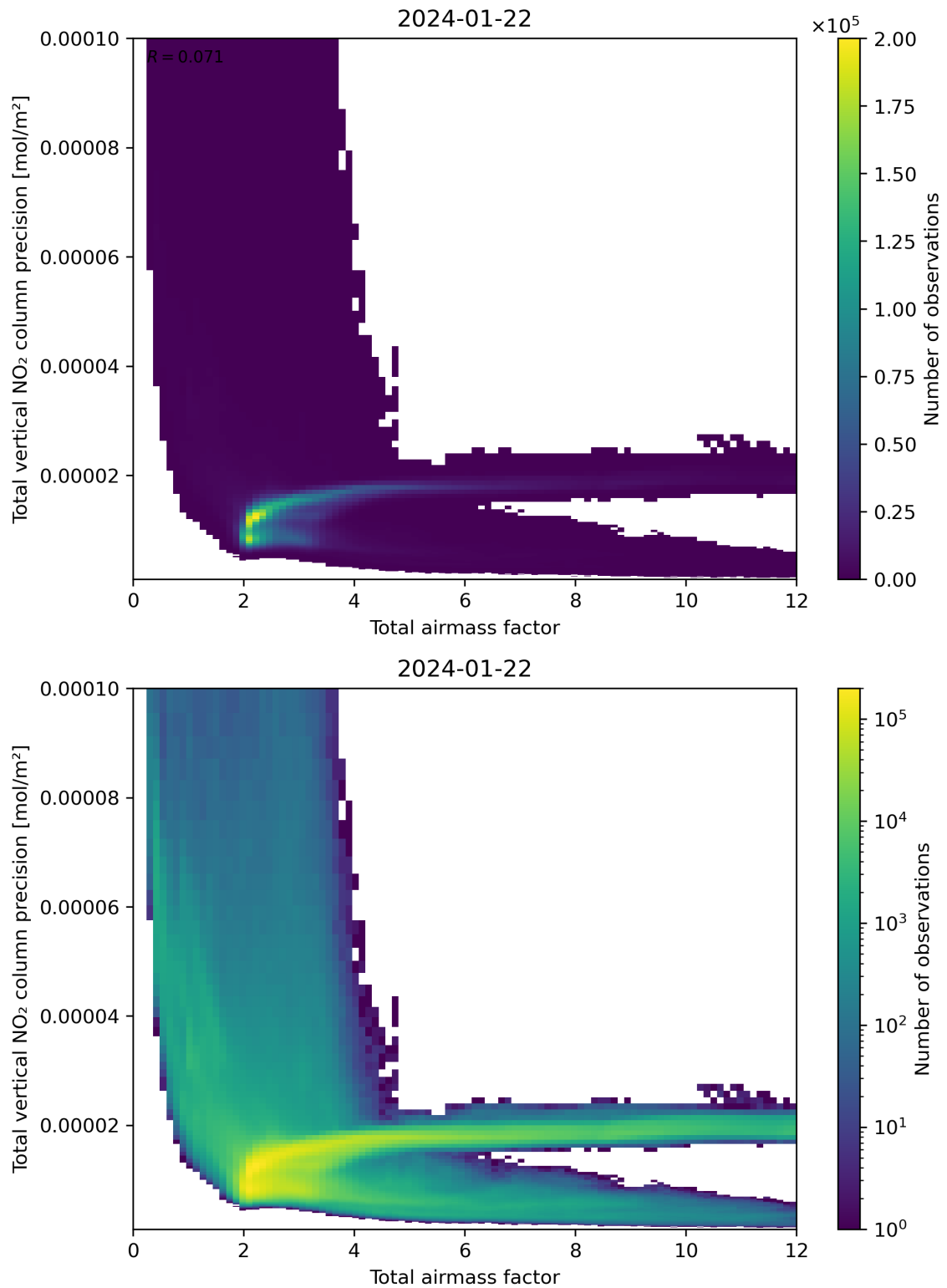
Figure 68: Scatter density plot of “Total airmass factor” against “Total vertical NO 2 column precision” for 2024-01-21 to 2024-01-23.
