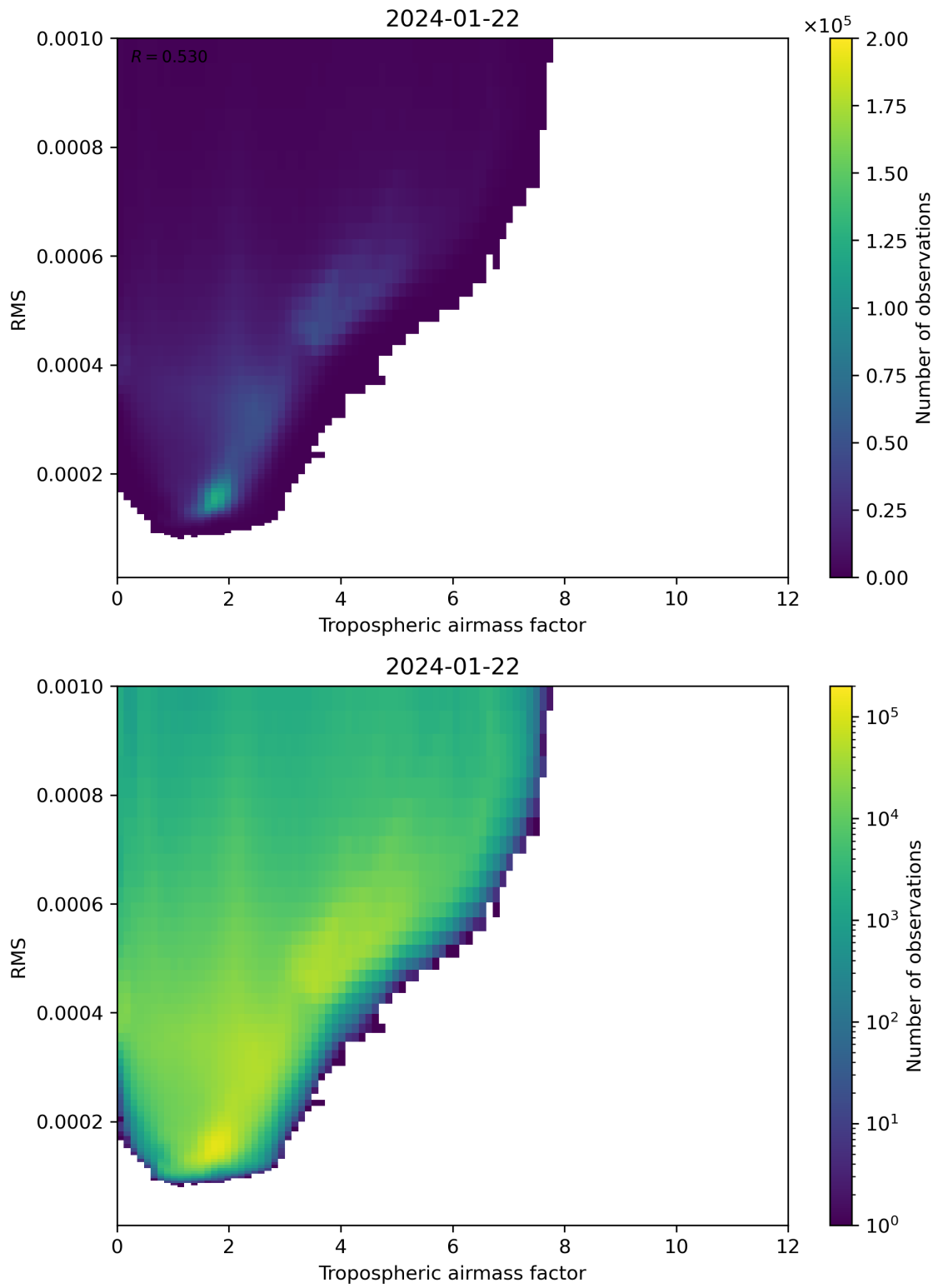
Figure 79: Scatter density plot of “Tropospheric airmass factor” against “RMS” for 2024-01-21 to 2024-01-23.
