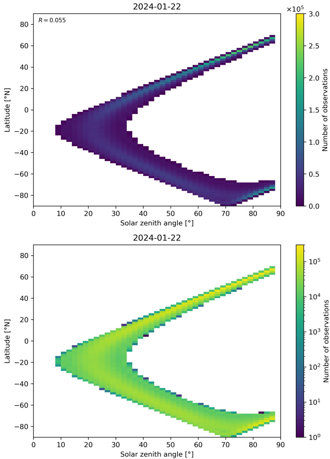
Figure 149: Scatter density plot of “Solar zenith angle” against “Latitude” for 2024-01-21 to 2024-01-23.
