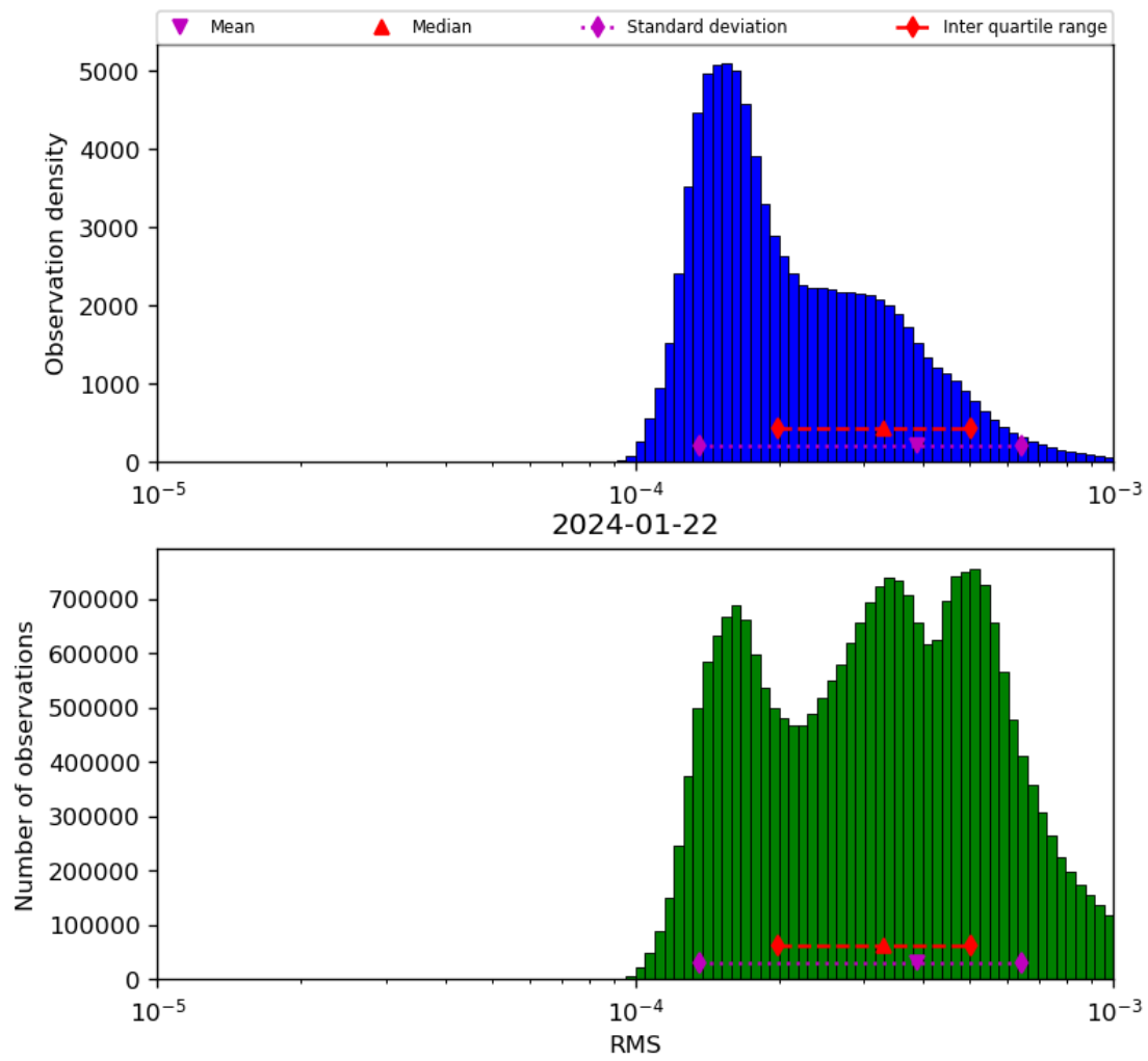
Figure 43: Histogram of “RMS” for 2024-01-21 to 2024-01-23
