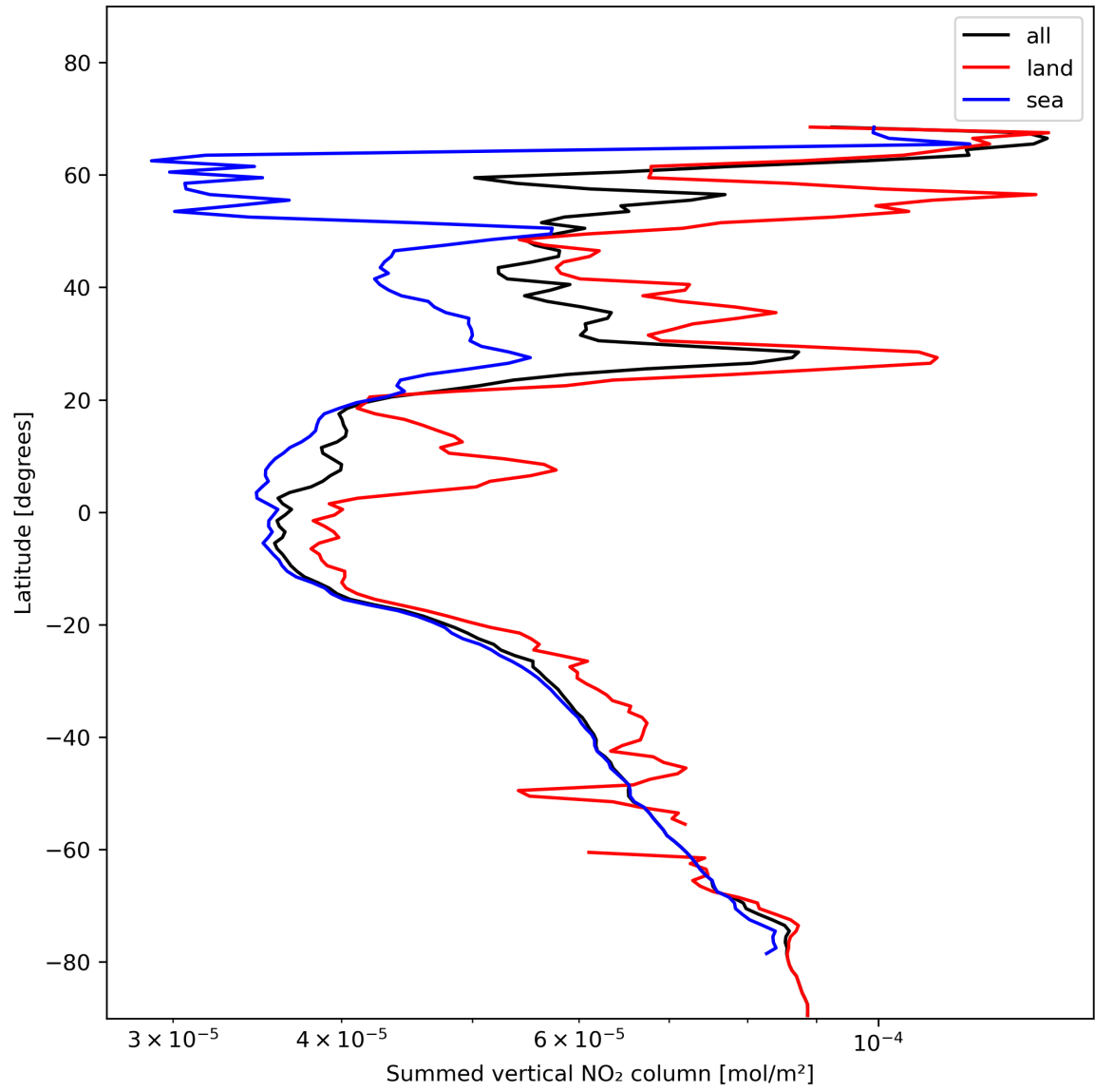
Figure 23: Zonal average of “Summed vertical NO 2 column” for 2024-01-21 to 2024-01-23.
