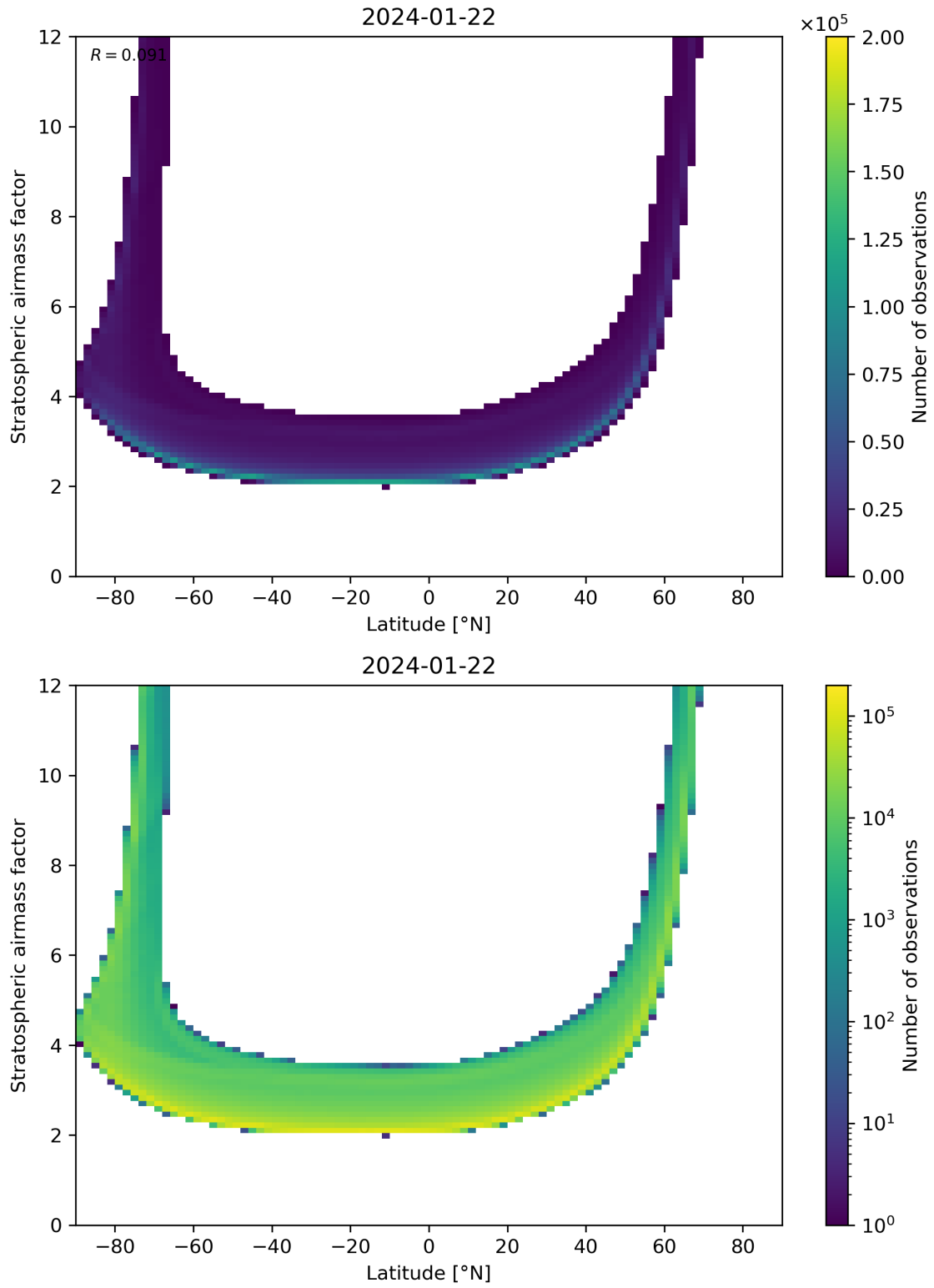
Figure 83: Scatter density plot of “Latitude” against “Stratospheric airmass factor” for 2024-01-21 to 2024-01-23.
