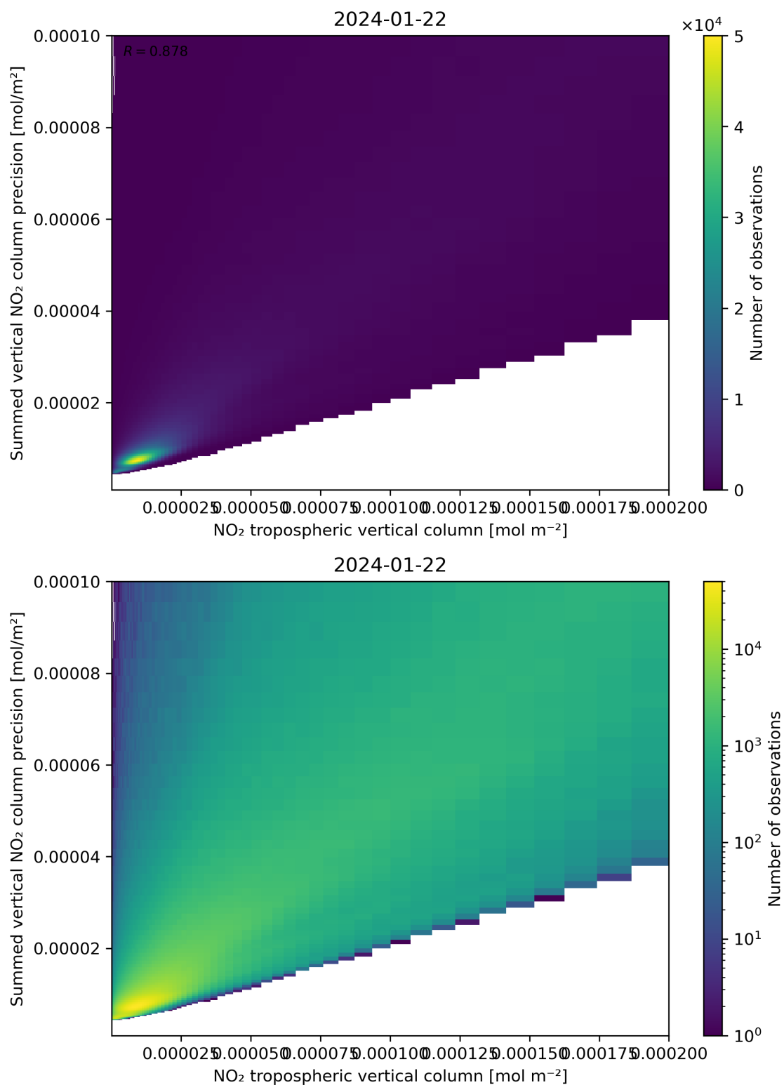
Figure 127: Scatter density plot of “NO 2 tropospheric vertical column” against “Summed vertical NO 2 column precision” for 2024-01-21 to 2024-01-23.
