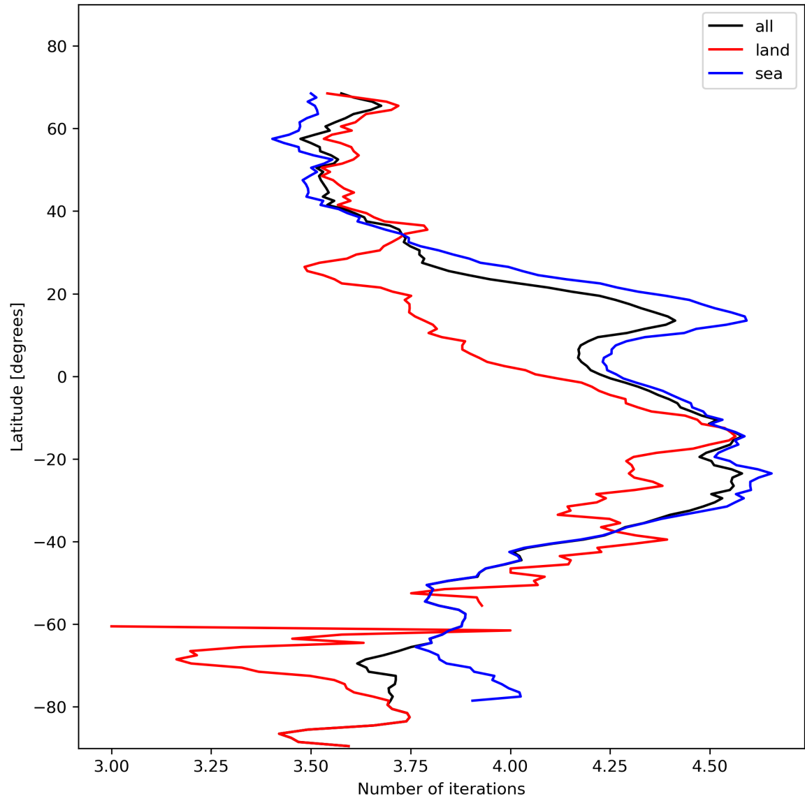
Figure 17: Zonal average of “Number of iterations” for 2024-01-21 to 2024-01-23.
