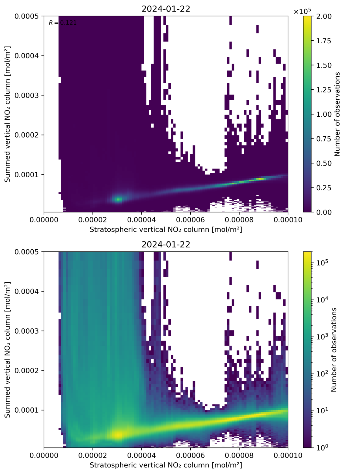
Figure 98: Scatter density plot of “Stratospheric vertical NO 2 column” against “Summed vertical NO 2 column” for 2024-01-21 to 2024-01-23.
