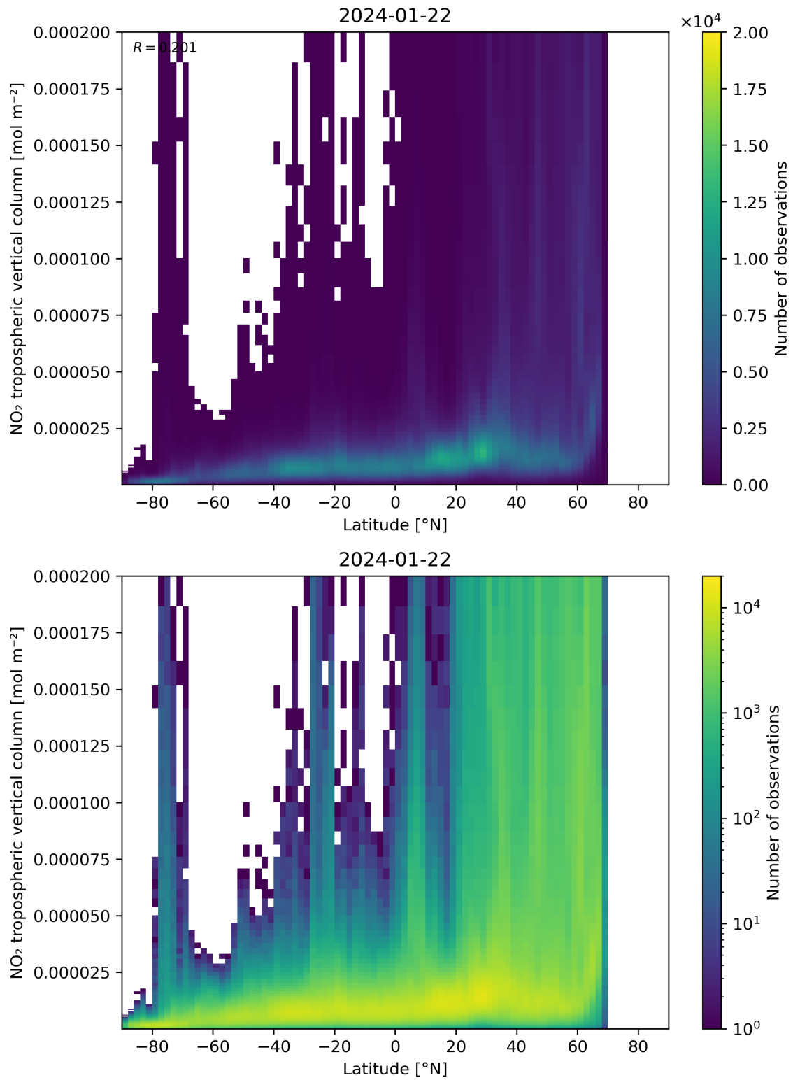
Figure 92: Scatter density plot of “Latitude” against “NO 2 tropospheric vertical column” for 2024-01-21 to 2024-01-23.
