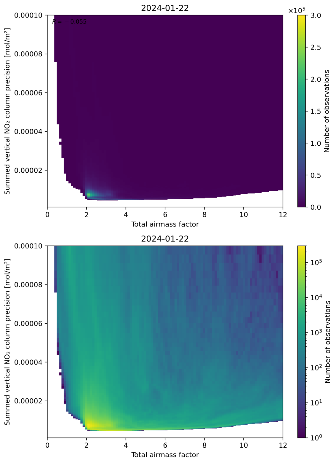
Figure 66: Scatter density plot of “Total airmass factor” against “Summed vertical NO 2 column precision” for 2024-01-21 to 2024-01-23.
