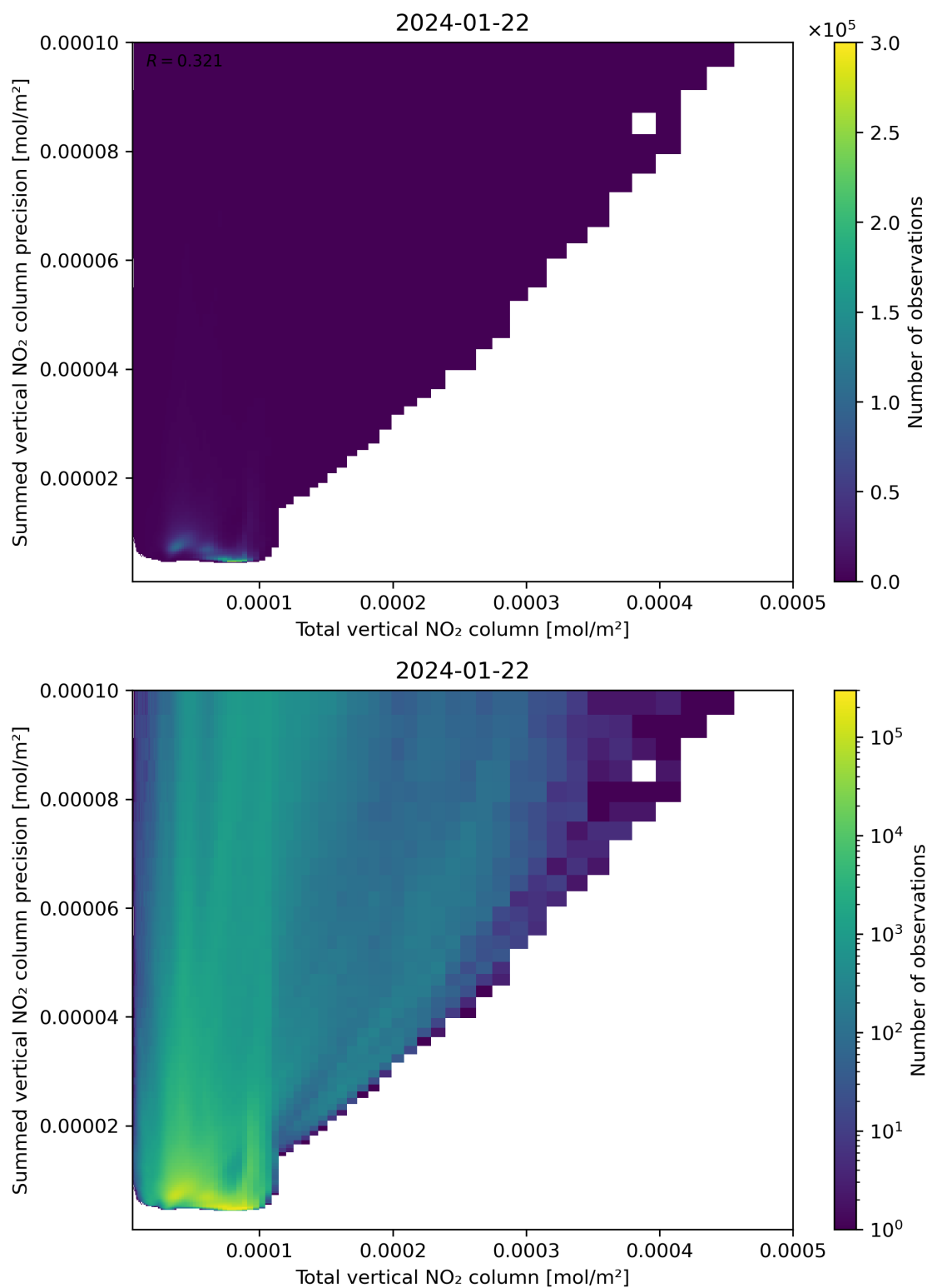
Figure 113: Scatter density plot of “Total vertical NO 2 column” against “Summed vertical NO 2 column precision” for 2024-01-21 to 2024-01-23.
