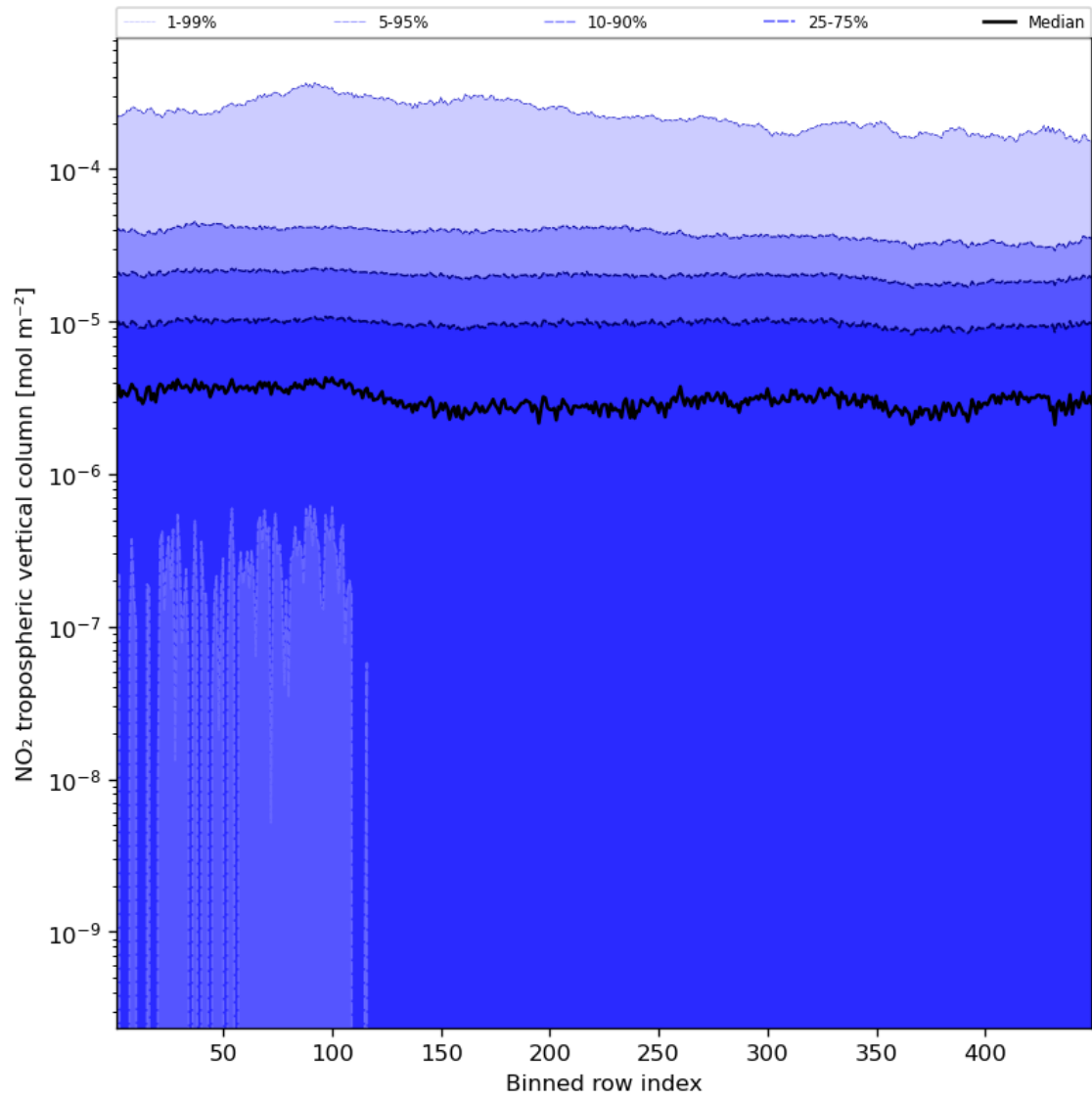
Figure 46: Along track statistics of “NO 2 tropospheric vertical column” for 2024-01-21 to 2024-01-23
