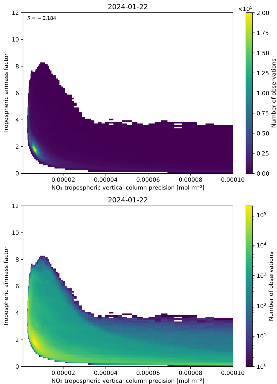
Figure 133: Scatter density plot of “NO 2 tropospheric vertical column precision” against “Tropospheric airmass factor” for 2024-01-21 to 2024-01-23.
