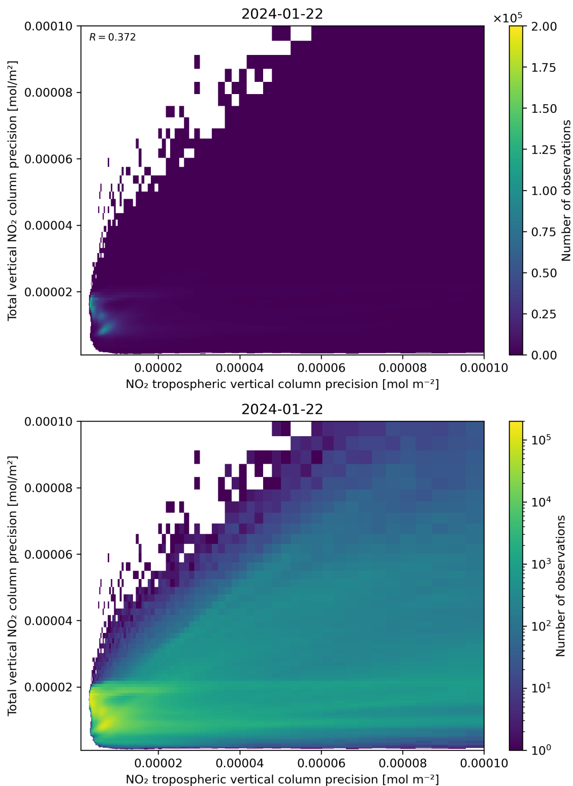
Figure 139: Scatter density plot of “NO 2 tropospheric vertical column precision” against “Total vertical NO 2 column precision” for 2024-01-21 to 2024-01-23.
