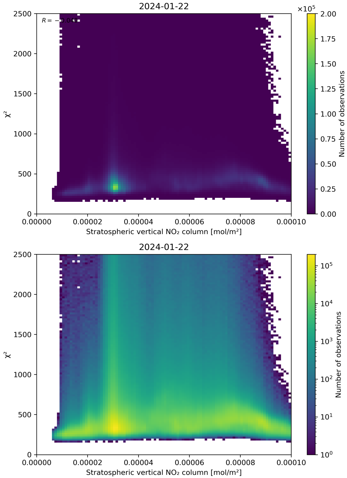
Figure 97: Scatter density plot of “Stratospheric vertical NO 2 column” against “ \chi^2 ” for 2024-01-21 to 2024-01-23.
