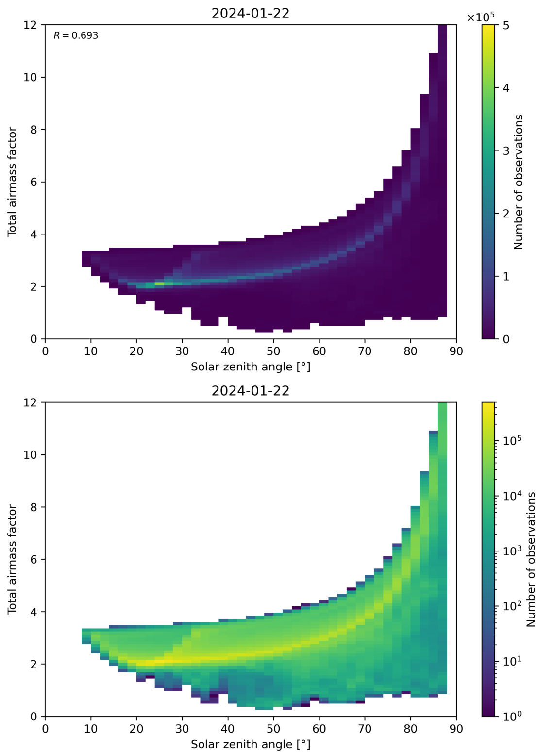
Figure 146: Scatter density plot of “Solar zenith angle” against “Total air mass factor” for 2024-01-21 to 2024-01-23.
