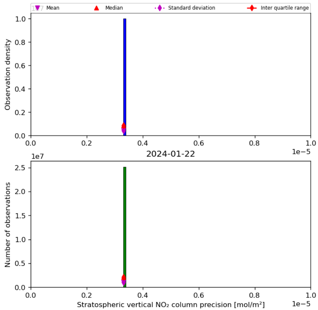
Figure 37: Histogram of “Stratospheric vertical NO 2 column precision” for 2024-01-21 to 2024-01-23
