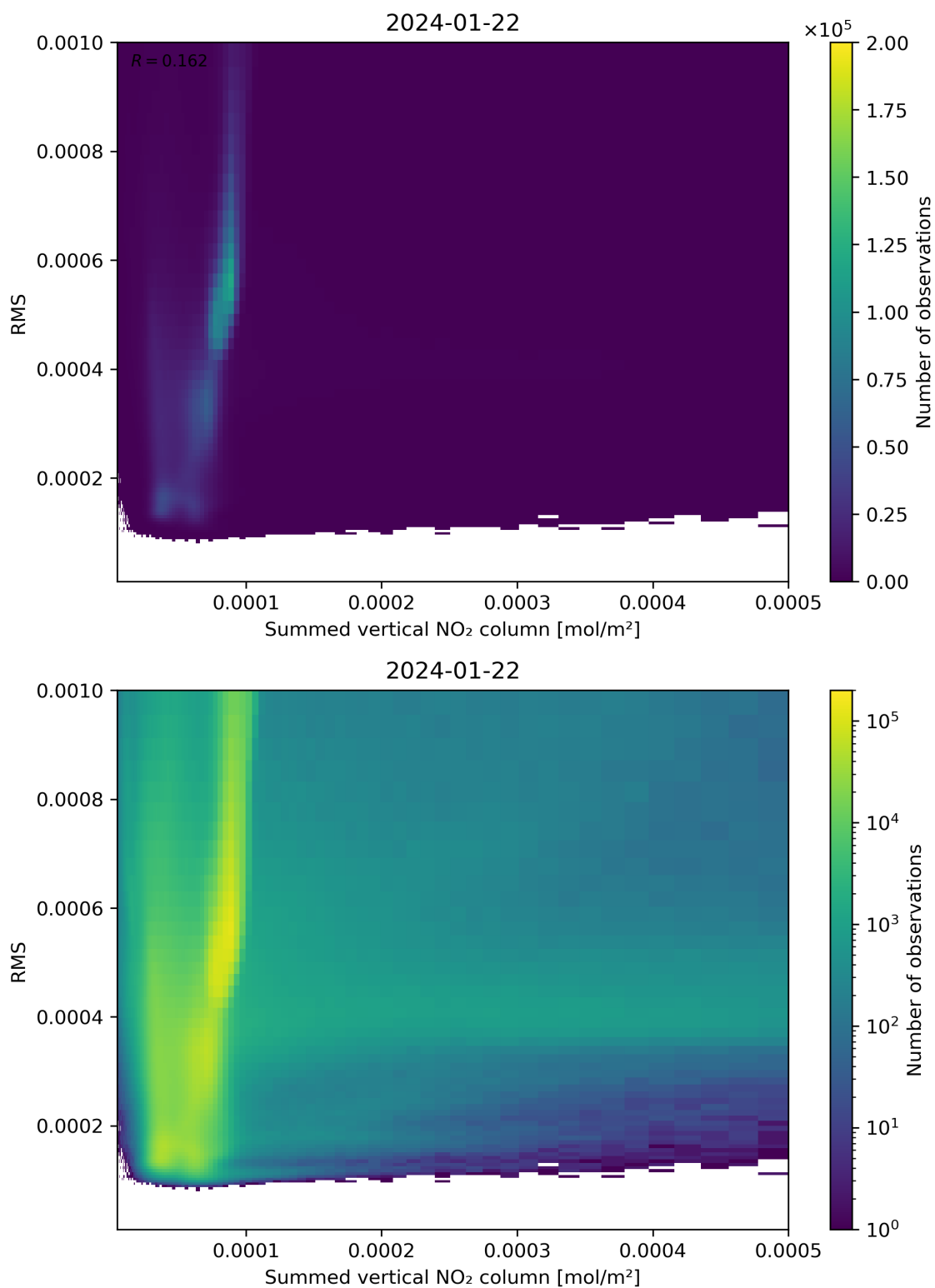
Figure 109: Scatter density plot of “Summed vertical NO 2 column” against “RMS” for 2024-01-21 to 2024-01-23.
