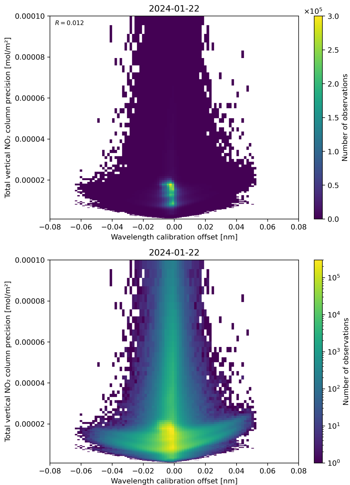
Figure 180: Scatter density plot of “Wavelength calibration offset” against “Total vertical NO 2 column precision” for 2024-01-21 to 2024-01-23.
