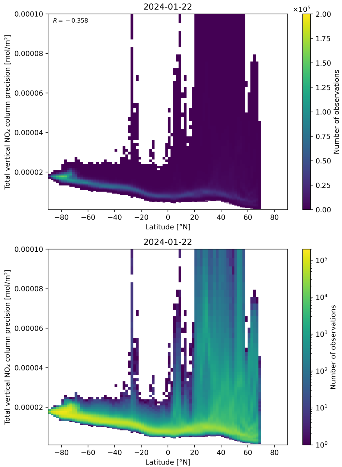
Figure 91: Scatter density plot of “Latitude” against “Total vertical NO 2 column precision” for 2024-01-21 to 2024-01-23.
