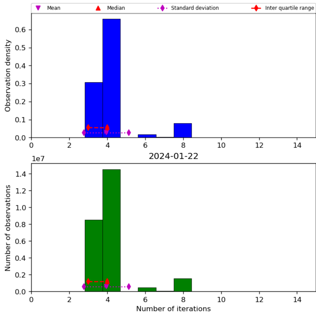
Figure 34: Histogram of “Number of iterations” for 2024-01-21 to 2024-01-23
