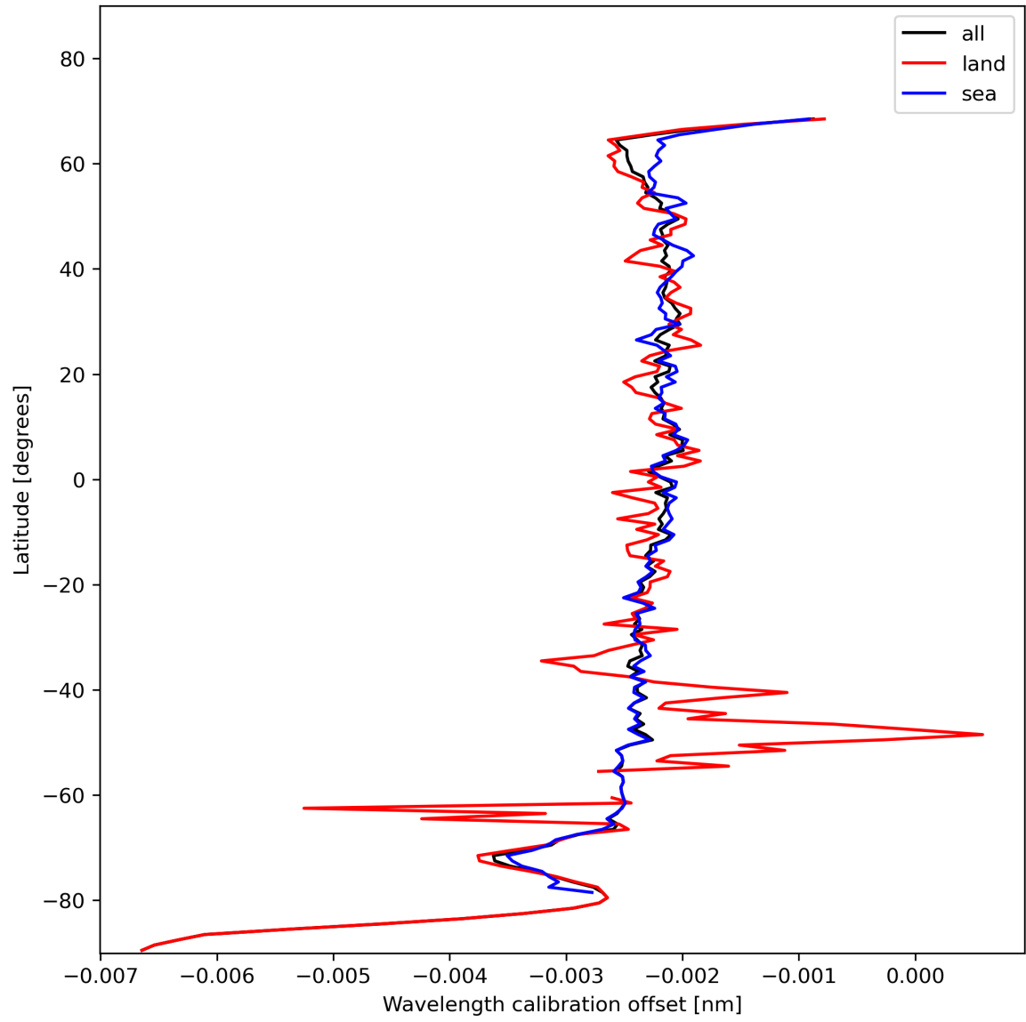
Figure 18: Zonal average of “Wavelength calibration offset” for 2024-01-21 to 2024-01-23.
