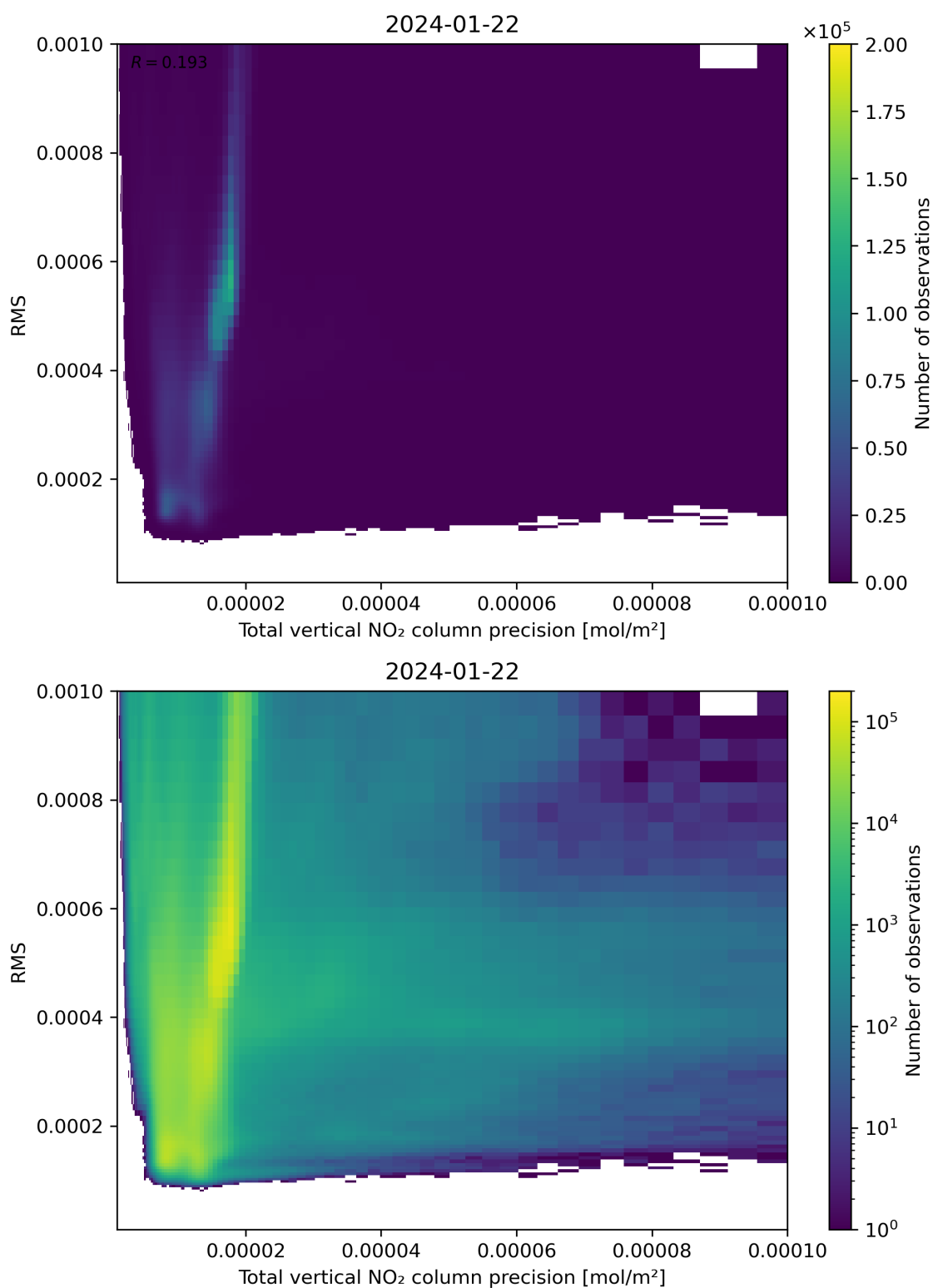
Figure 119: Scatter density plot of “Total vertical NO 2 column precision” against “RMS” for 2024-01-21 to 2024-01-23.
