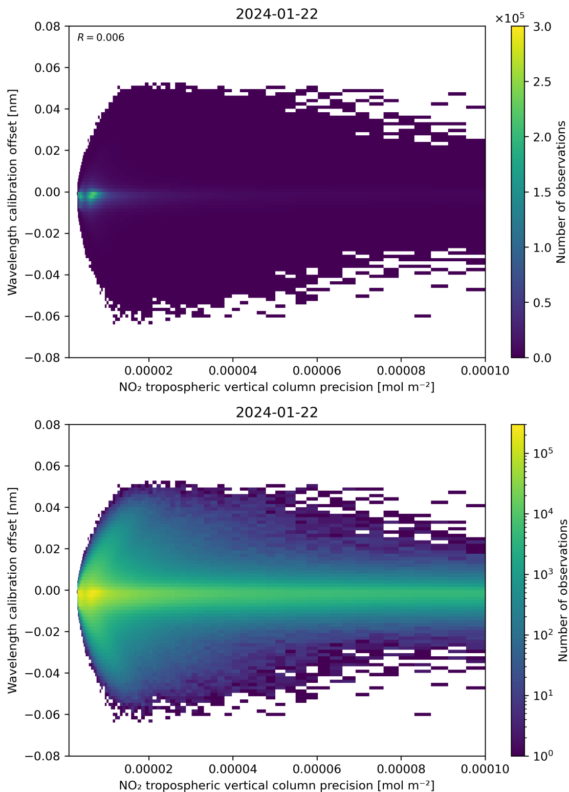
Figure 141: Scatter density plot of “NO 2 tropospheric vertical column precision” against “Wavelength calibration offset” for 2024-01-21 to 2024-01-23.
