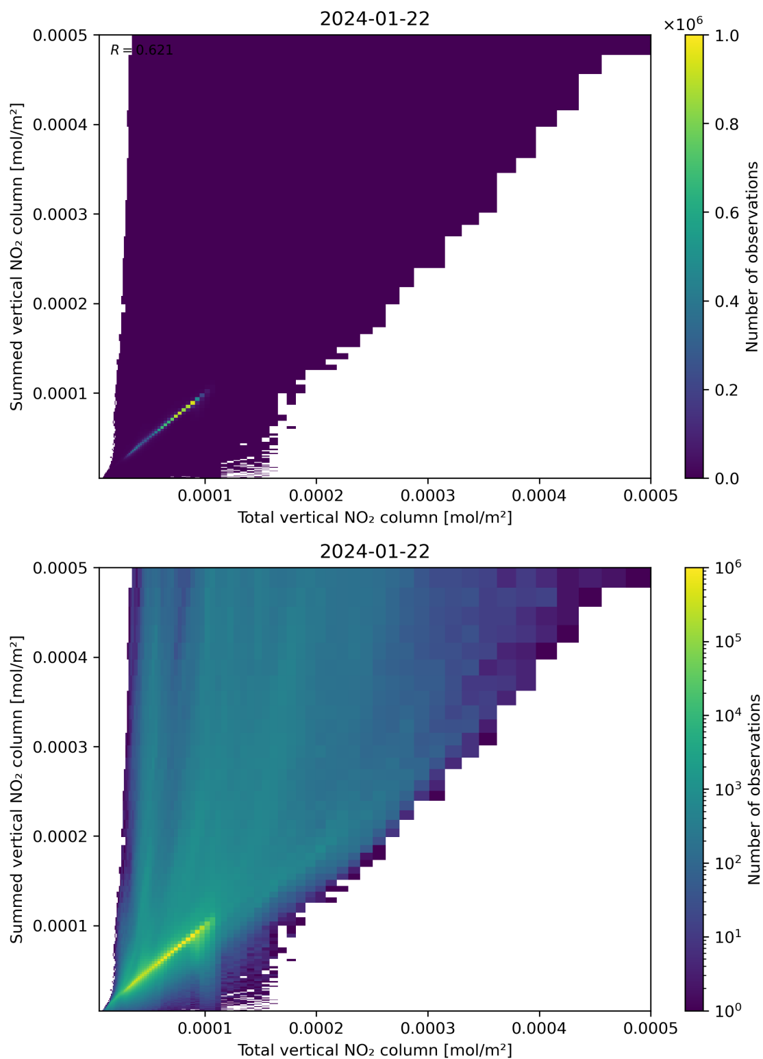
Figure 112: Scatter density plot of “Total vertical NO 2 column” against “Summed vertical NO 2 column” for 2024-01-21 to 2024-01-23.
