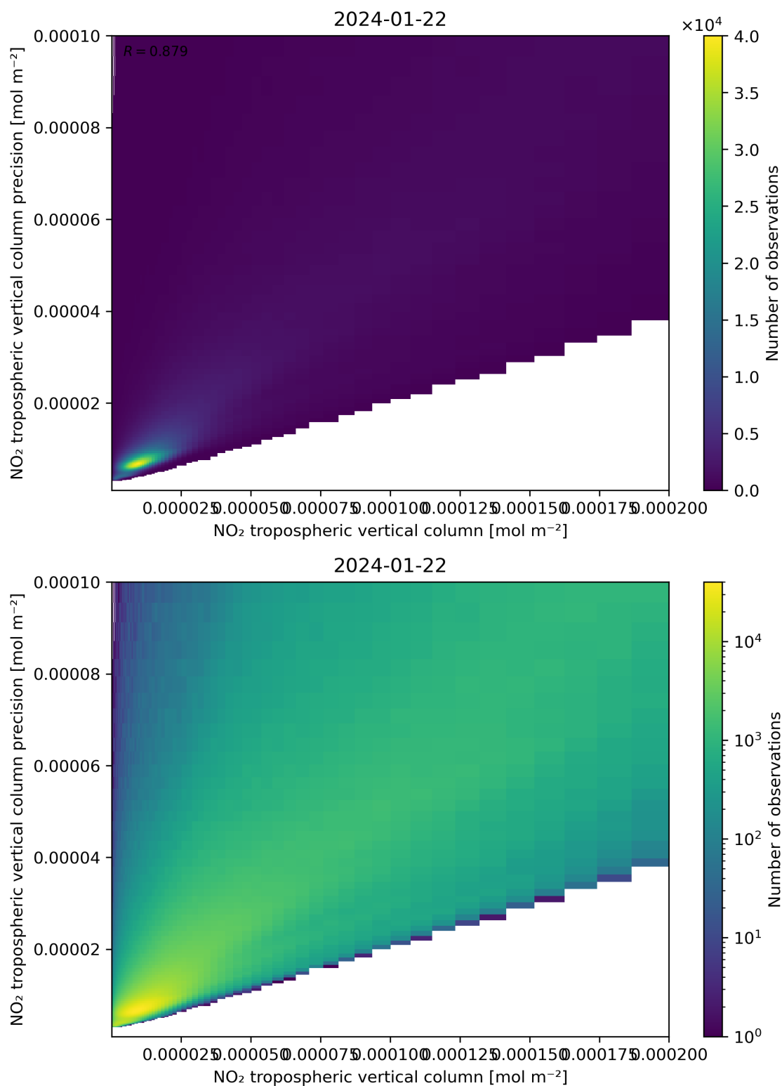
Figure 130: Scatter density plot of “NO 2 tropospheric vertical column” against “NO 2 tropospheric vertical column precision” for 2024-01-21 to 2024-01-23.
