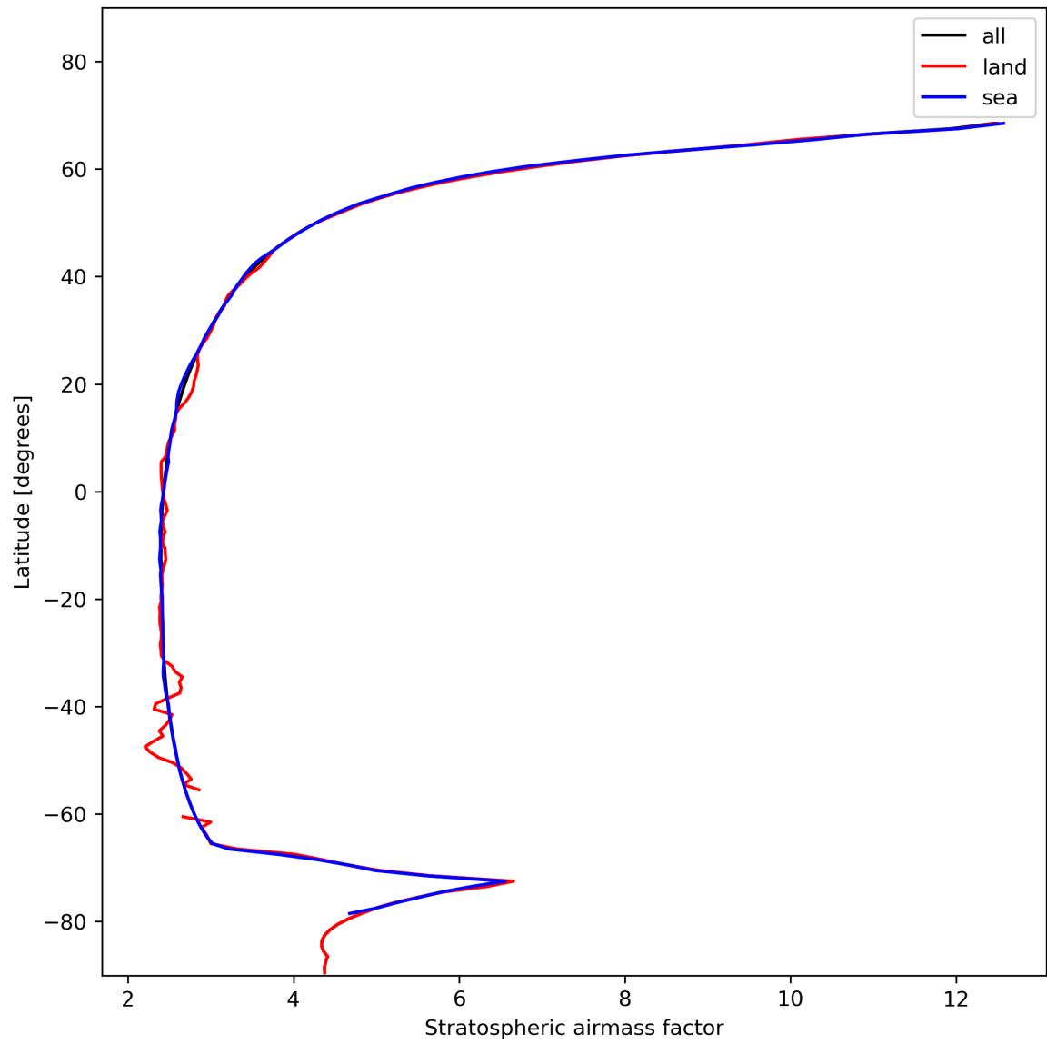
Figure 27: Zonal average of “Stratospheric airmass factor” for 2024-01-21 to 2024-01-23.
