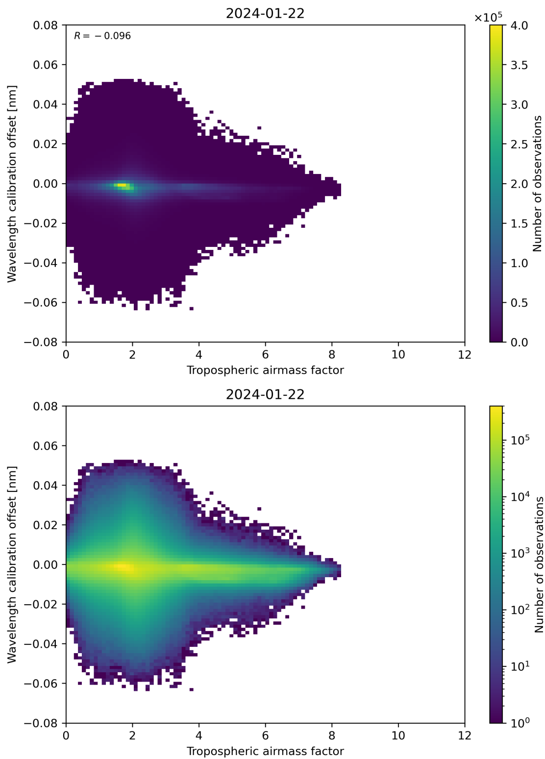
Figure 80: Scatter density plot of “Tropospheric airmass factor” against “Wavelength calibration offset” for 2024-01-21 to 2024-01-23.
