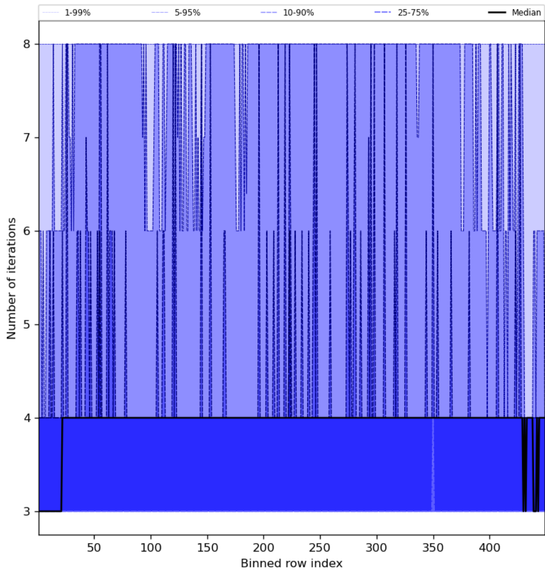
Figure 51: Along track statistics of “Number of iterations” for 2024-01-21 to 2024-01-23
