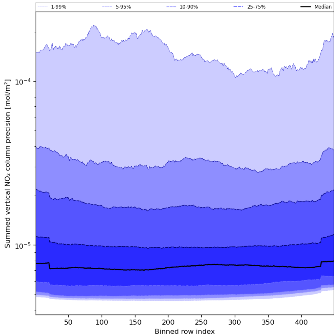
Figure 58: Along track statistics of “Summed vertical NO 2 column precision” for 2024-01-21 to 2024-01-23
