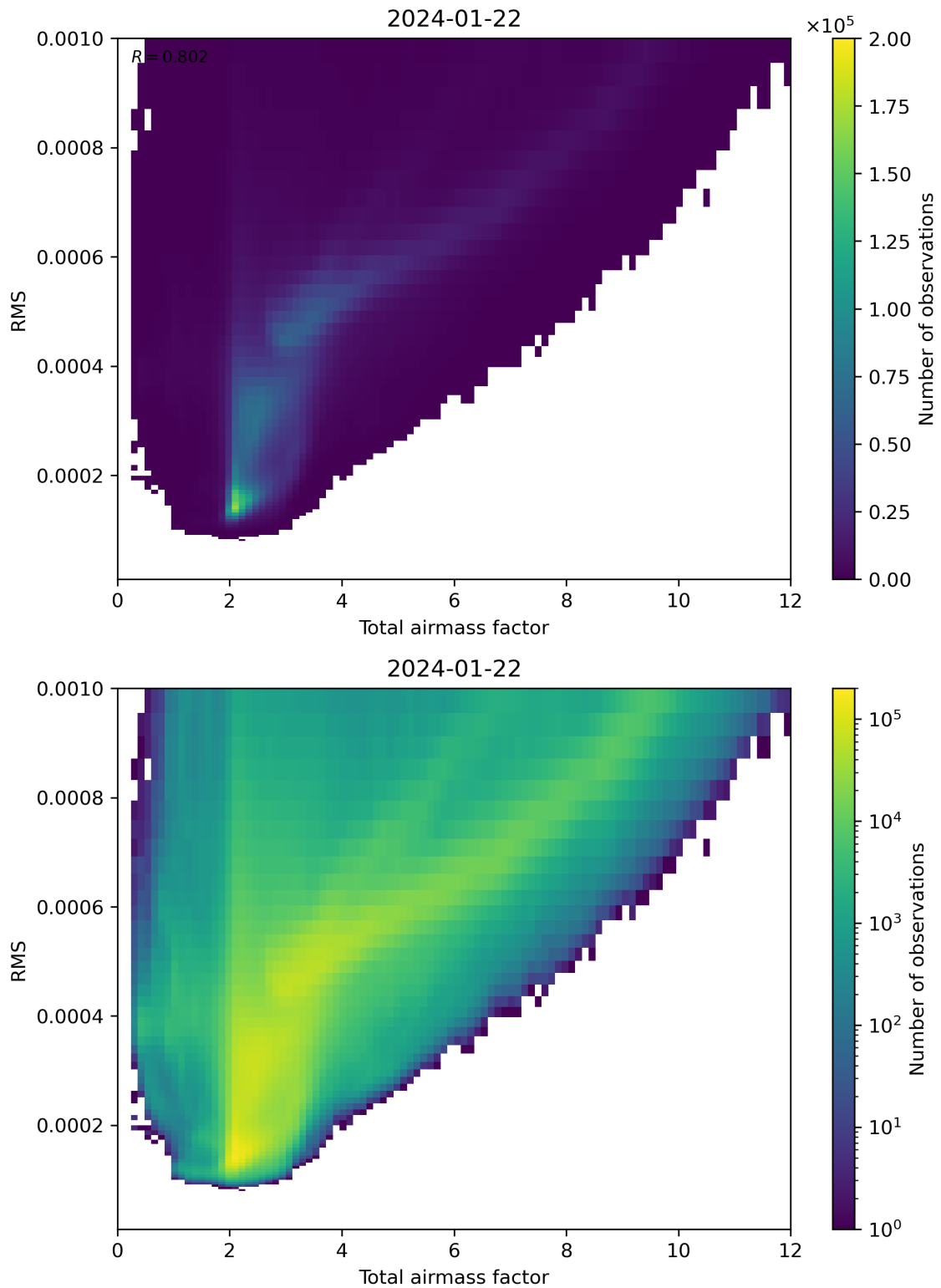
Figure 69: Scatter density plot of “Total airmass factor” against “RMS” for 2024-01-21 to 2024-01-23.
