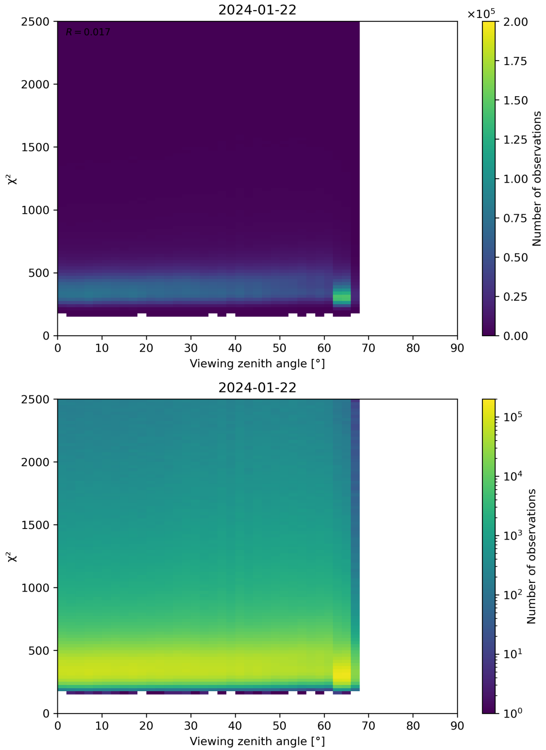
Figure 162: Scatter density plot of “Viewing zenith angle” against “ \chi^2 ” for 2024-01-21 to 2024-01-23.
