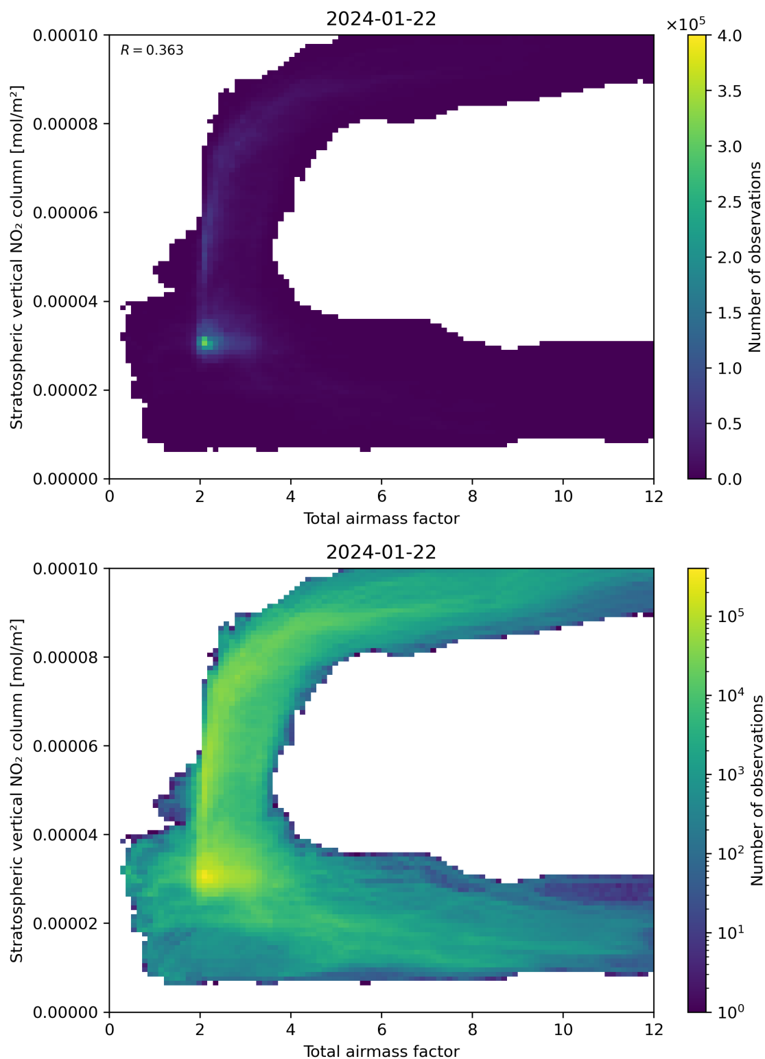
Figure 64: Scatter density plot of “Total airmass factor” against “Stratospheric vertical \text{NO}_2 column” for 2024-01-21 to 2024-01-23.
