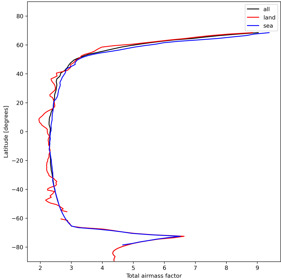
Figure 15: Zonal average of “Total airmass factor” for 2024-01-21 to 2024-01-23.
