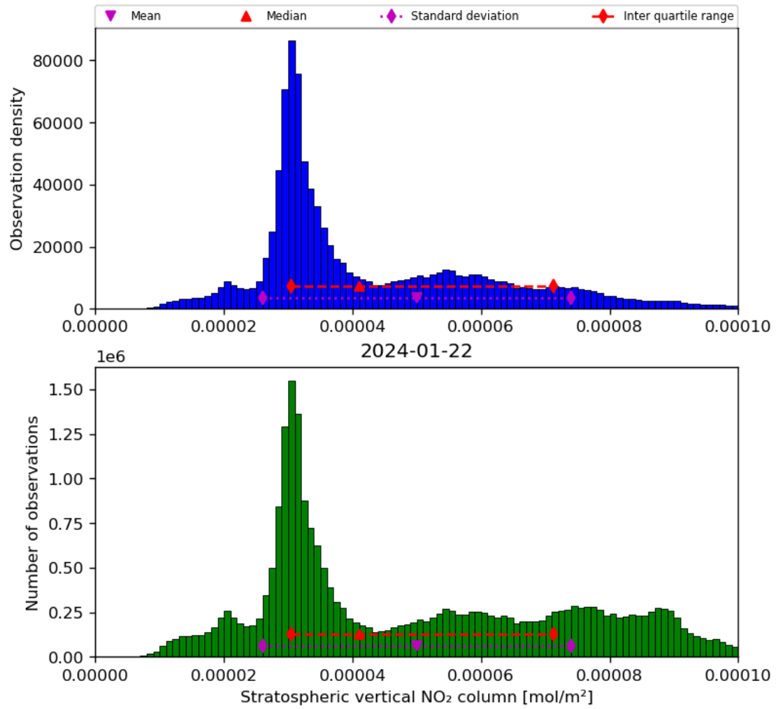
Figure 36: Histogram of “Stratospheric vertical NO 2 column” for 2024-01-21 to 2024-01-23
