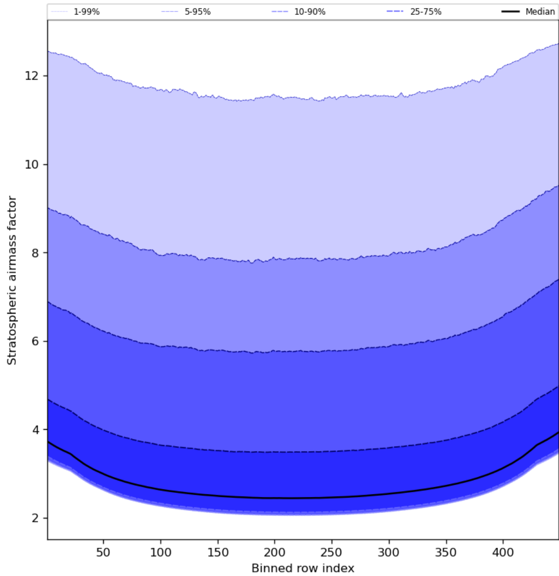
Figure 61: Along track statistics of “Stratospheric airmass factor” for 2024-01-21 to 2024-01-23
