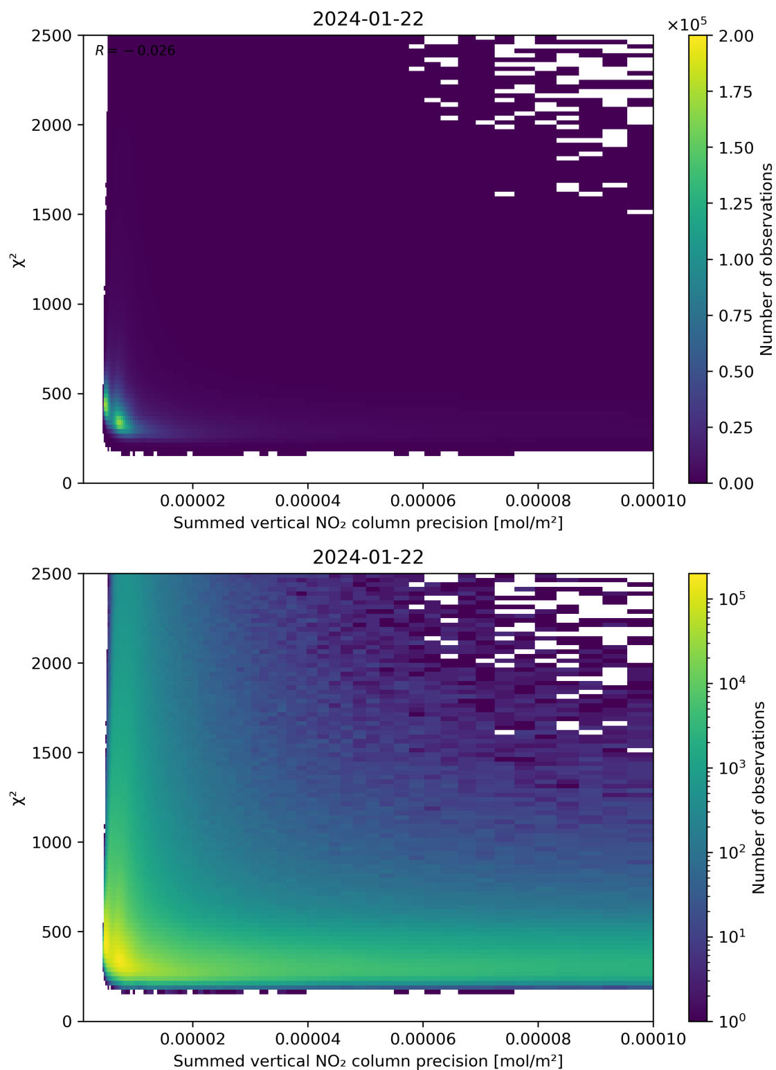
Figure 107: Scatter density plot of “Summed vertical NO 2 column precision” against “ \chi^2 ” for 2024-01-21 to 2024-01-23.
