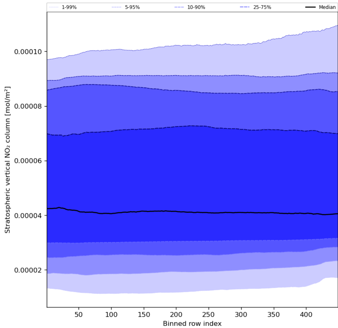
Figure 53: Along track statistics of “Stratospheric vertical NO 2 column” for 2024-01-21 to 2024-01-23
