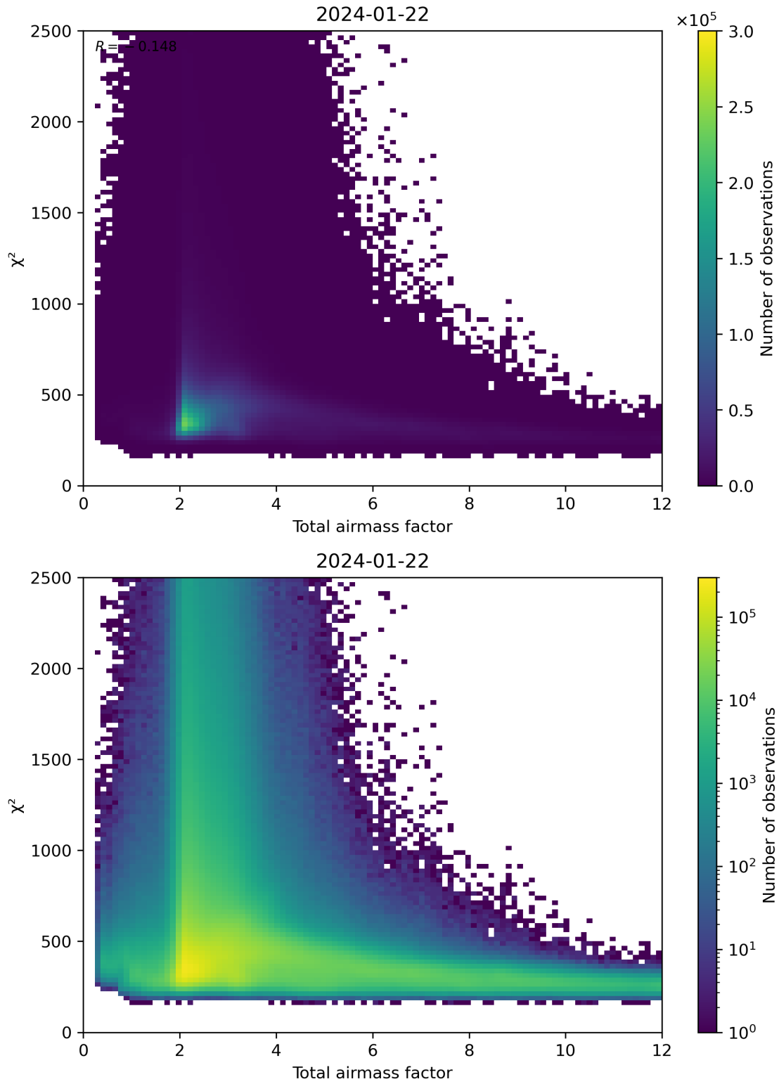
Figure 63: Scatter density plot of “Total airmass factor” against “ \chi^2 ” for 2024-01-21 to 2024-01-23.
