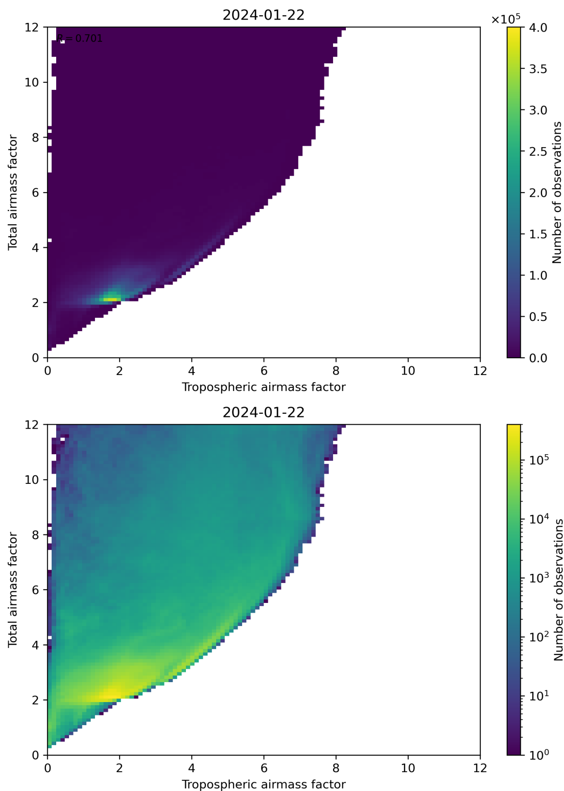
Figure 72: Scatter density plot of “Tropospheric airmass factor” against “Total airmass factor” for 2024-01-21 to 2024-01-23.
