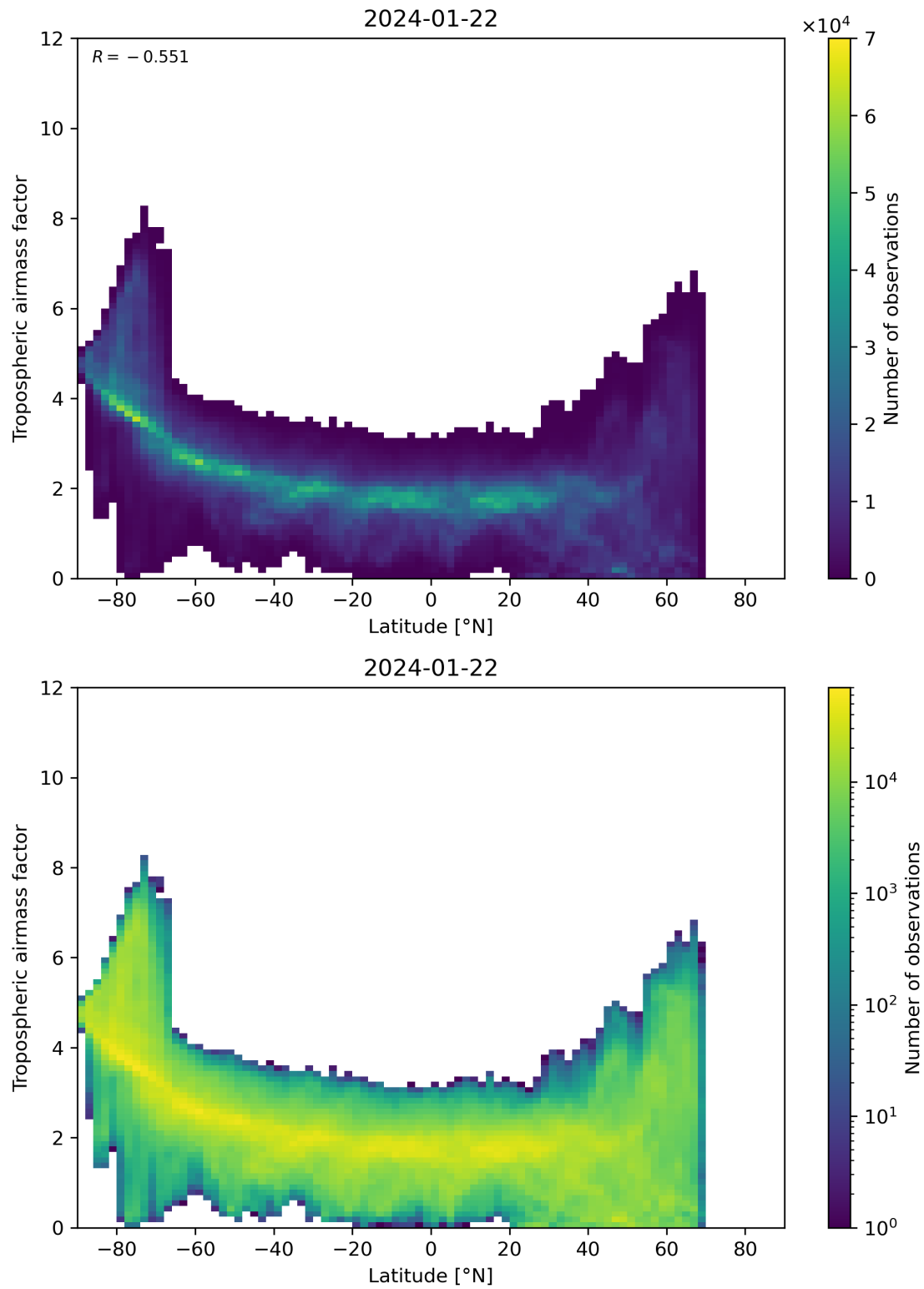
Figure 85: Scatter density plot of “Latitude” against “Tropospheric airmass factor” for 2024-01-21 to 2024-01-23.
