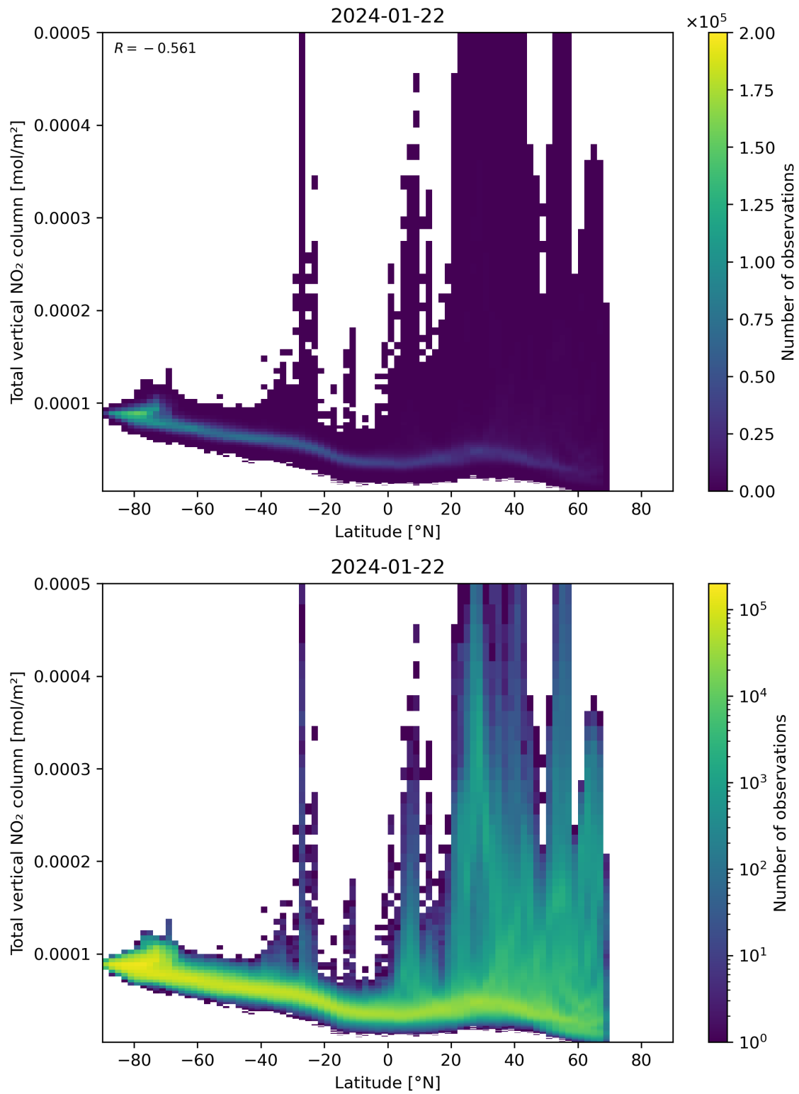
Figure 90: Scatter density plot of “Latitude” against “Total vertical NO 2 column” for 2024-01-21 to 2024-01-23.
