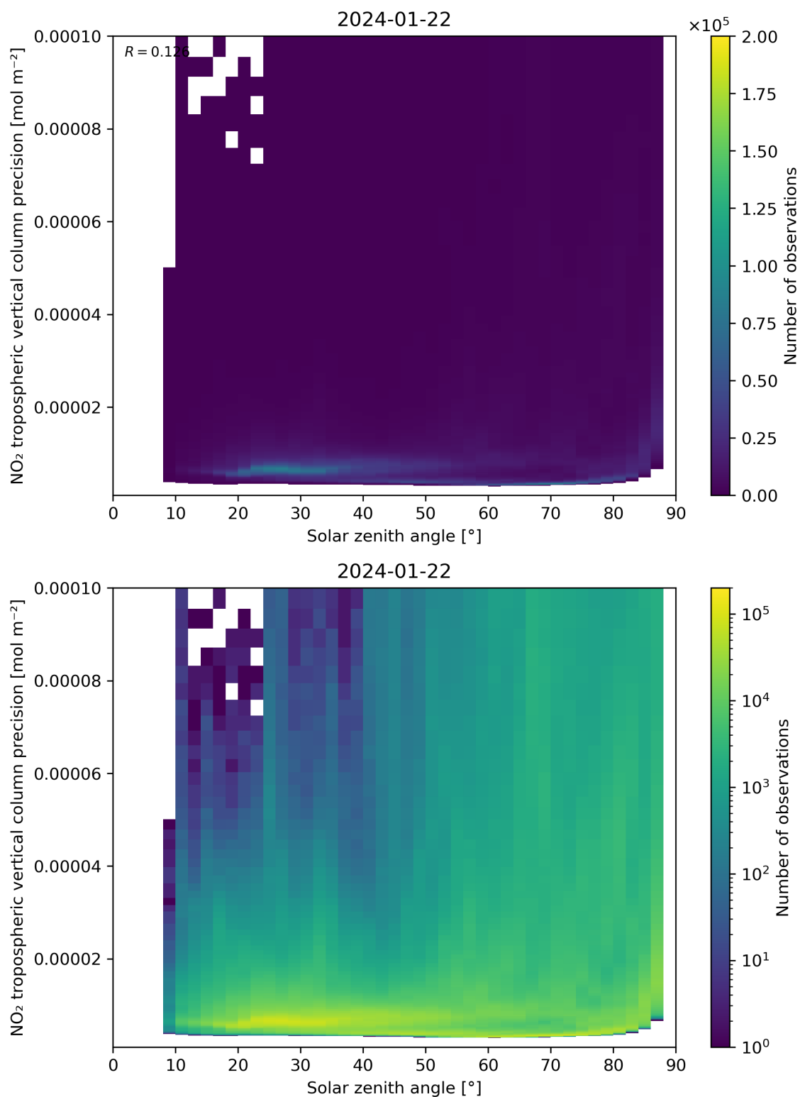
Figure 156: Scatter density plot of “Solar zenith angle” against “NO 2 tropospheric vertical column precision” for 2024-01-21 to 2024-01-23.
