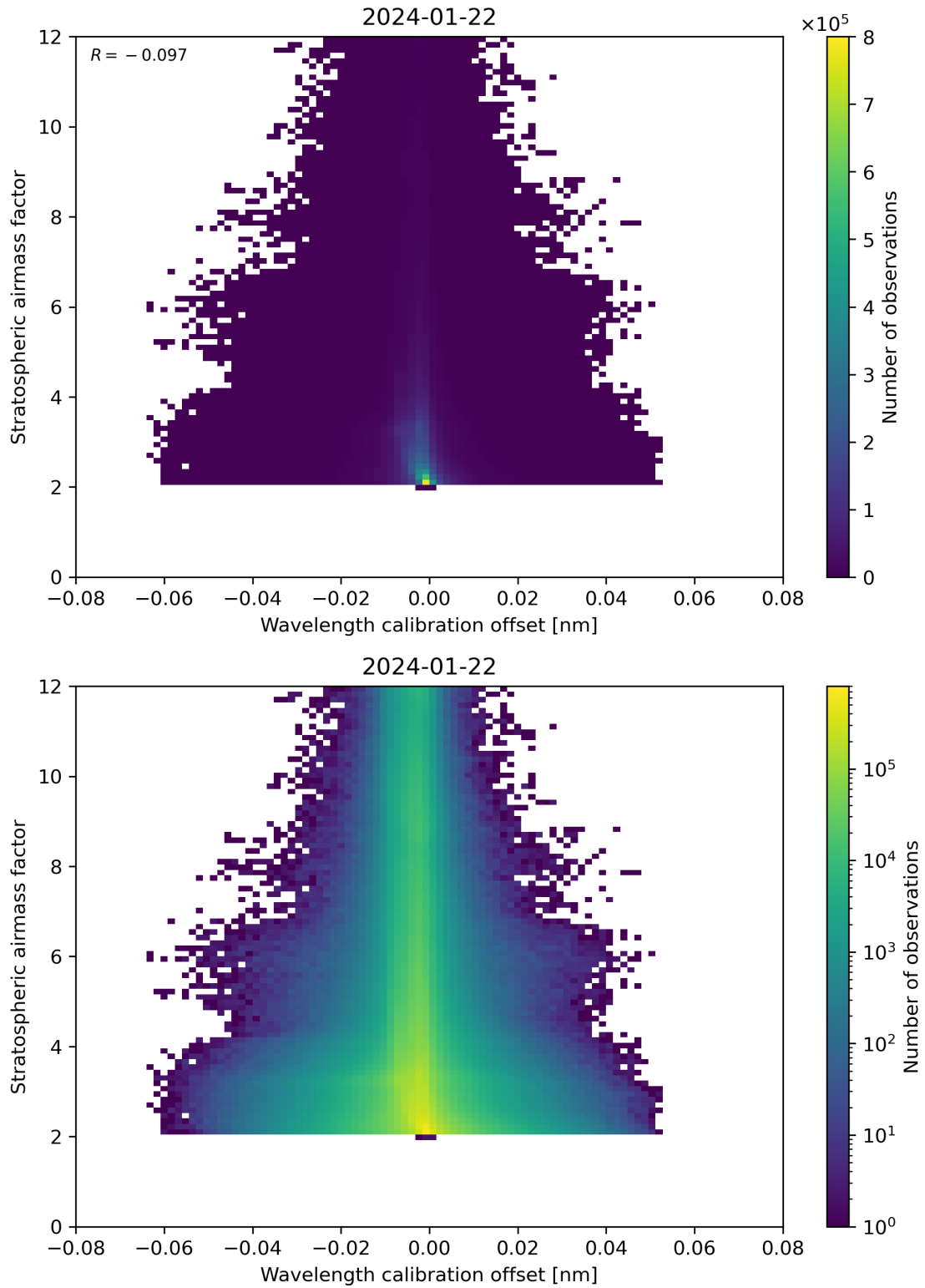
Figure 174: Scatter density plot of “Wavelength calibration offset” against “Stratospheric airmass factor” for 2024-01-21 to 2024-01-23.
