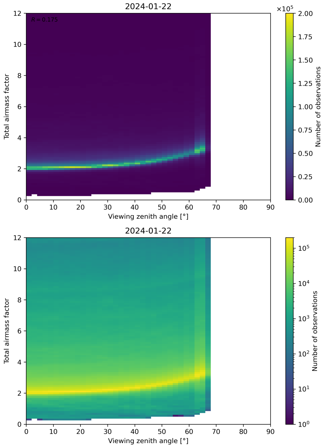
Figure 160: Scatter density plot of “Viewing zenith angle” against “Total airmass factor” for 2024-01-21 to 2024-01-23.
