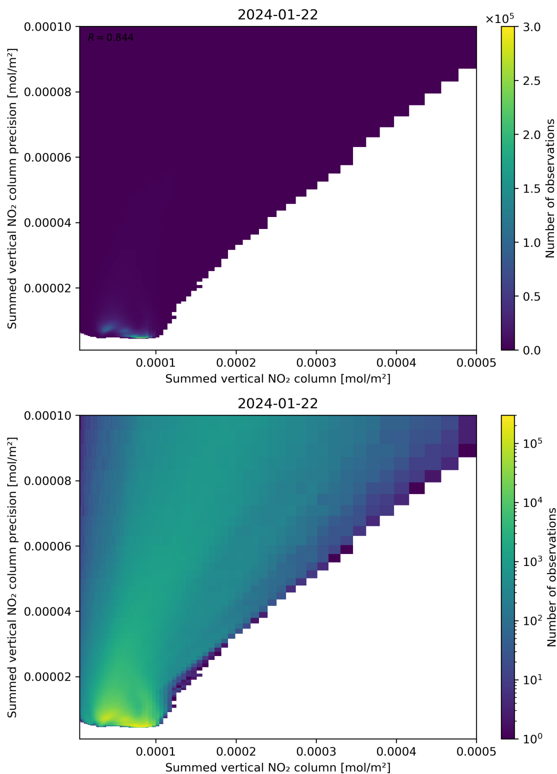
Figure 105: Scatter density plot of “Summed vertical NO 2 column” against “Summed vertical NO 2 column precision” for 2024-01-21 to 2024-01-23.
