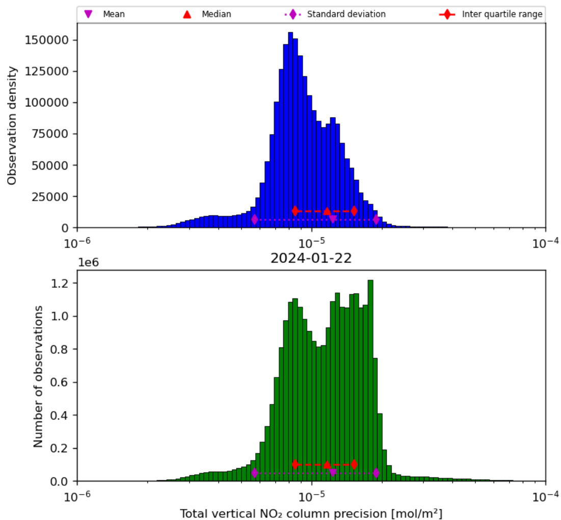
Figure 39: Histogram of “Total vertical NO 2 column precision” for 2024-01-21 to 2024-01-23
