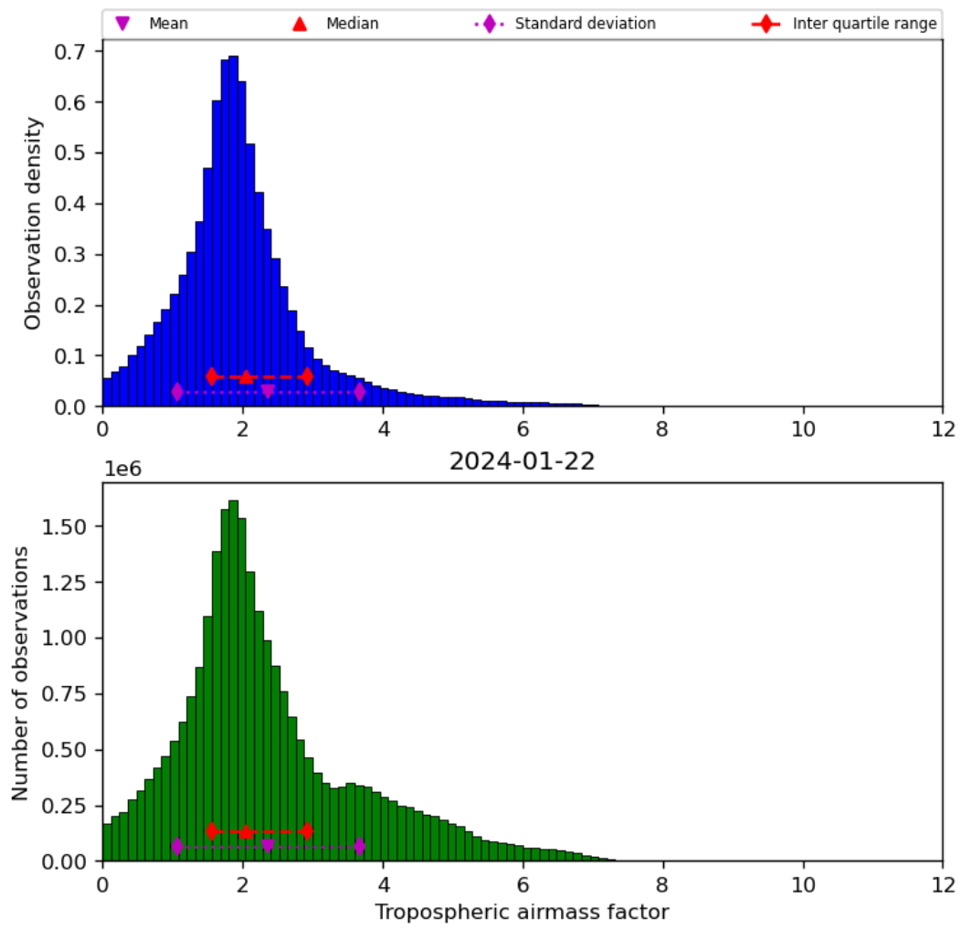
Figure 31: Histogram of “Tropospheric airmass factor” for 2024-01-21 to 2024-01-23
