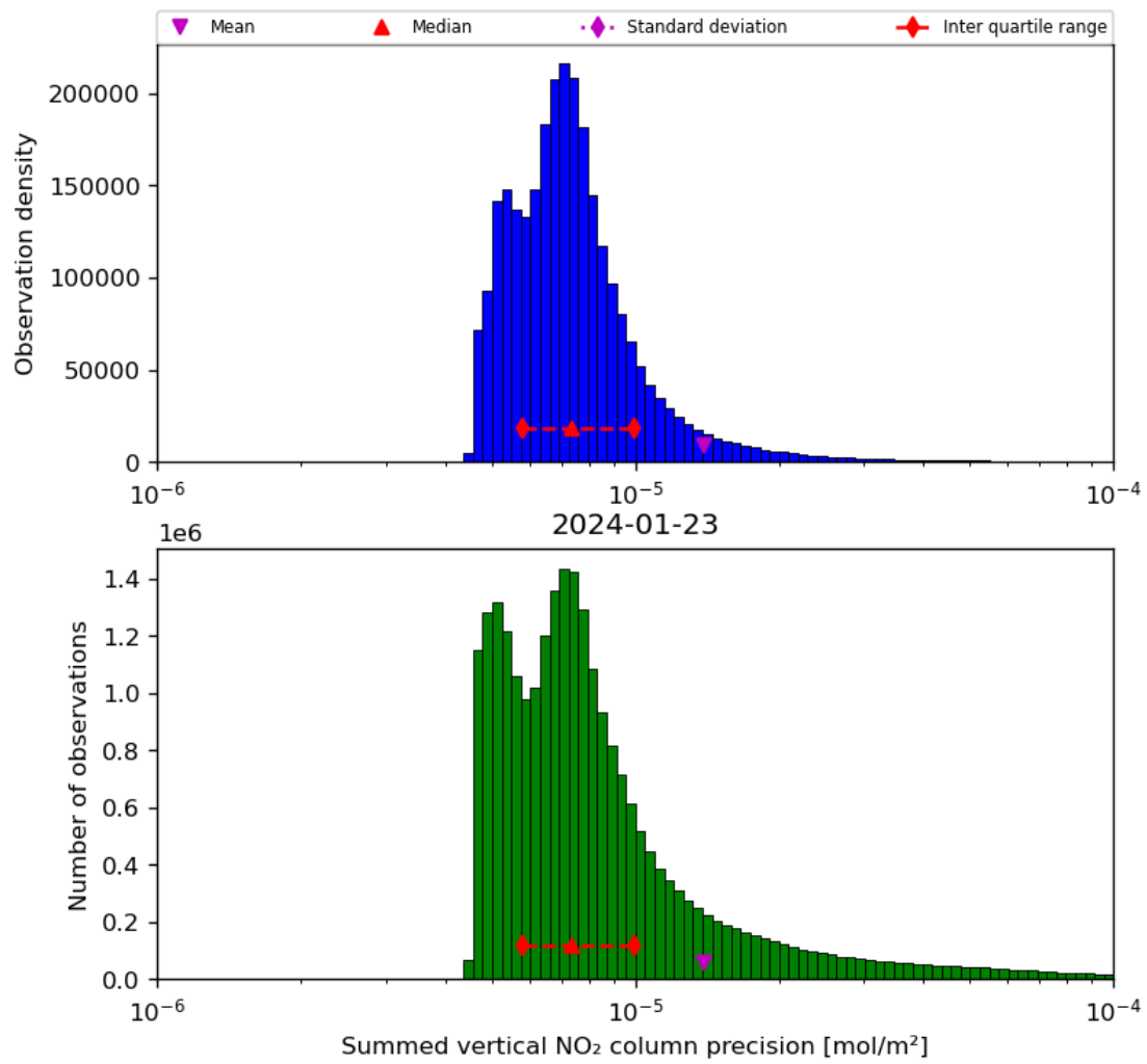
Figure 41: Histogram of "Summed vertical NO 2 column precision" for 2024-01-22 to 2024-01-24
