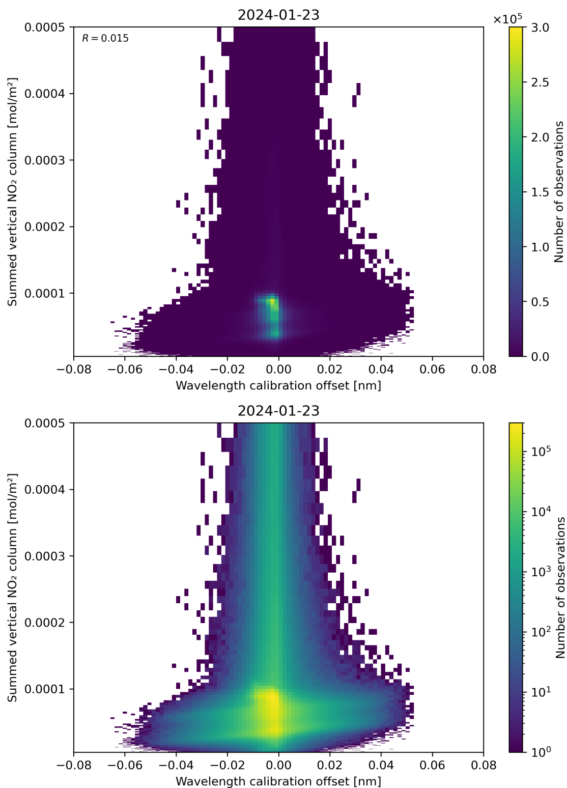
Figure 177: Scatter density plot of “Wavelength calibration offset” against “Summed vertical NO 2 column” for 2024-01-22 to 2024-01-24.
