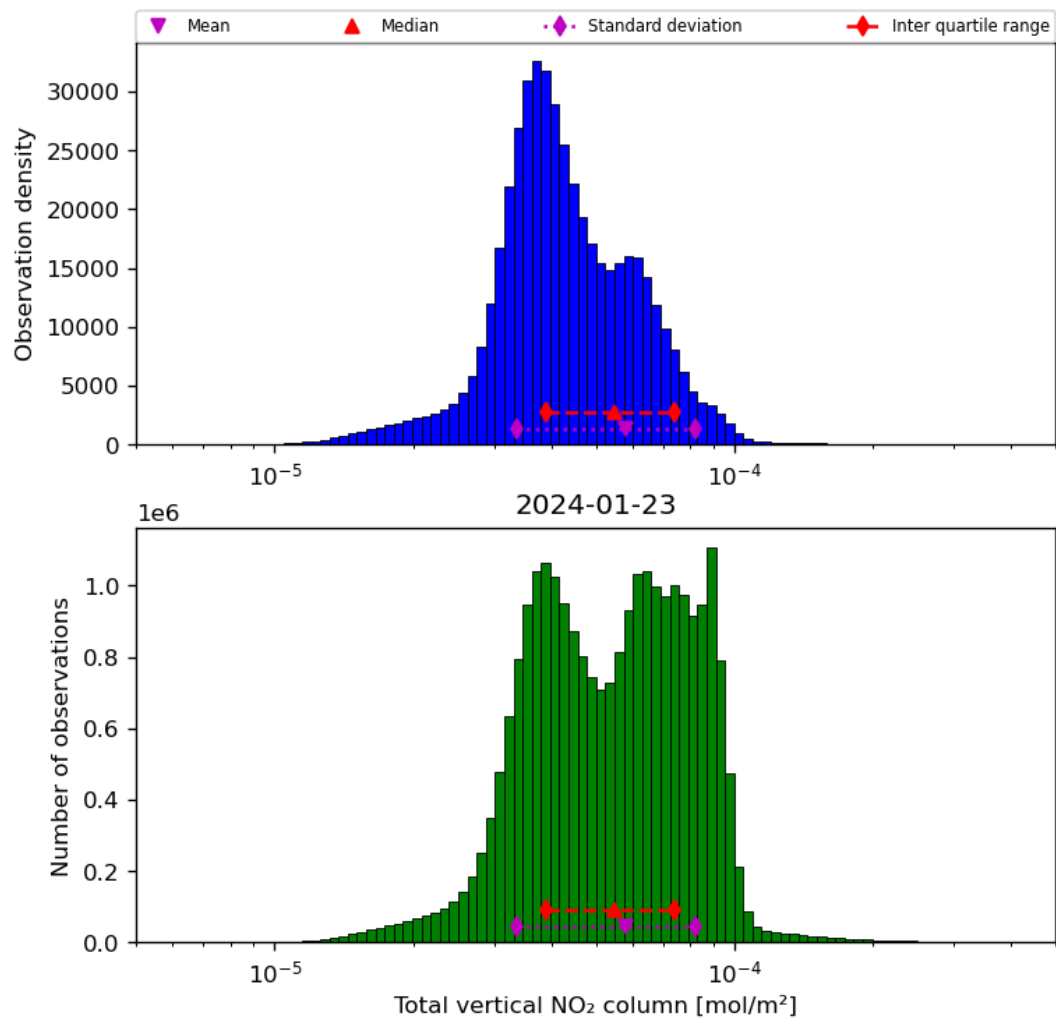
Figure 38: Histogram of “Total vertical NO 2 column” for 2024-01-22 to 2024-01-24
