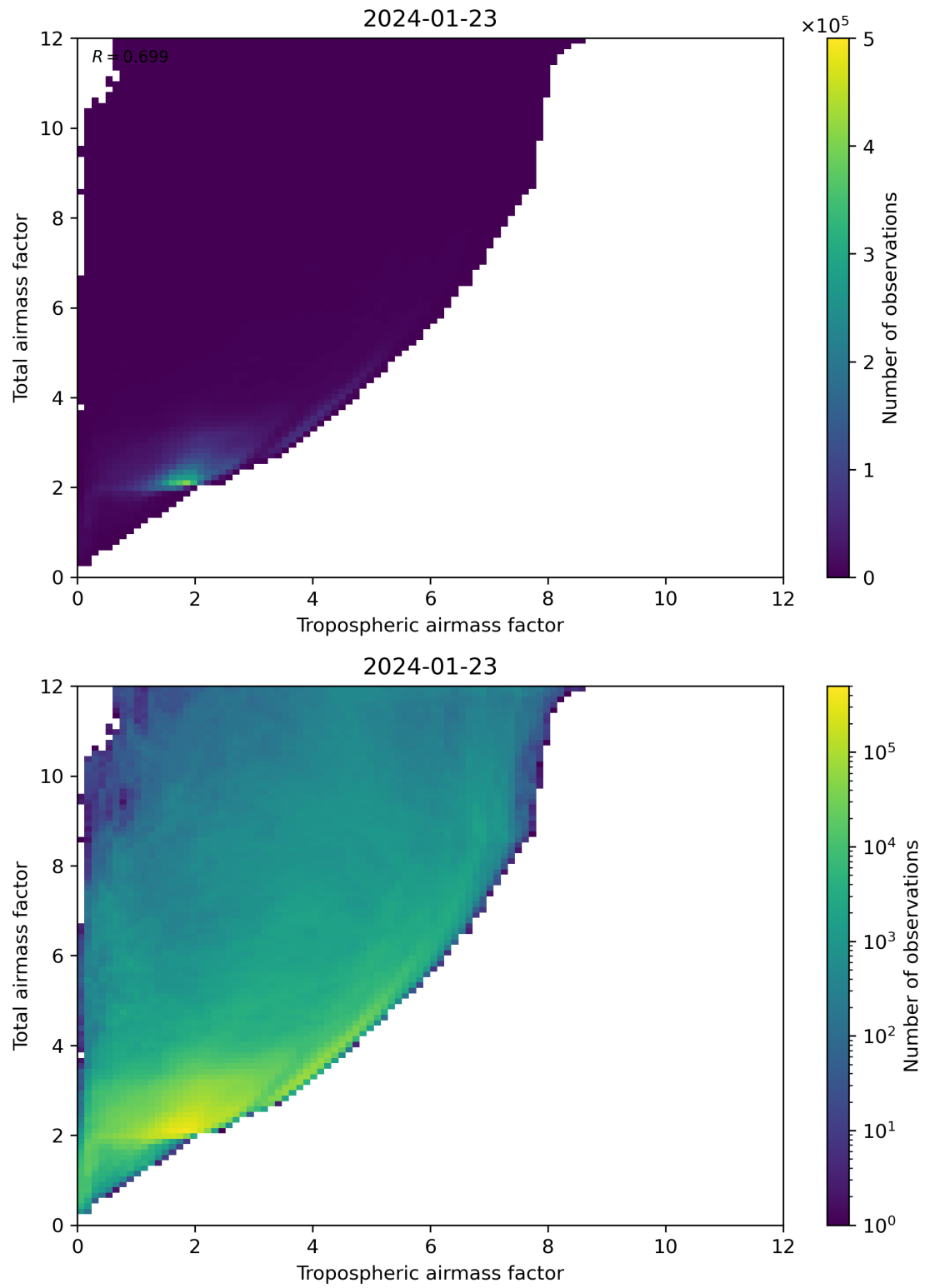
Figure 72: Scatter density plot of “Tropospheric airmass factor” against “Total airmass factor” for 2024-01-22 to 2024-01-24.
