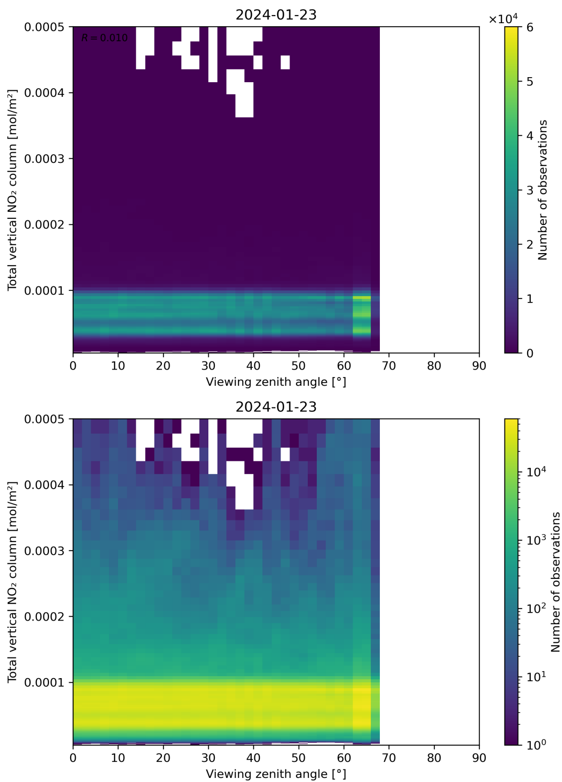
Figure 167: Scatter density plot of “Viewing zenith angle” against “Total vertical NO 2 column” for 2024-01-22 to 2024-01-24.
