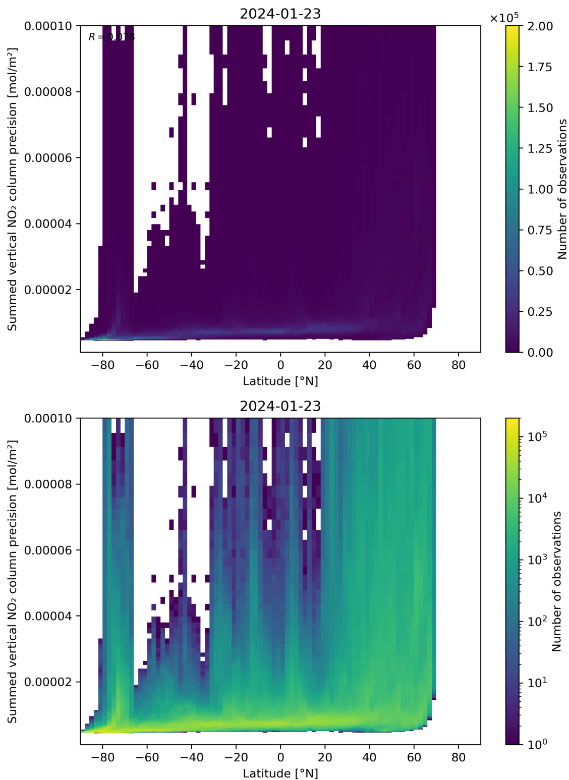
Figure 89: Scatter density plot of “Latitude” against “Summed vertical NO 2 column precision” for 2024-01-22 to 2024-01-24.
