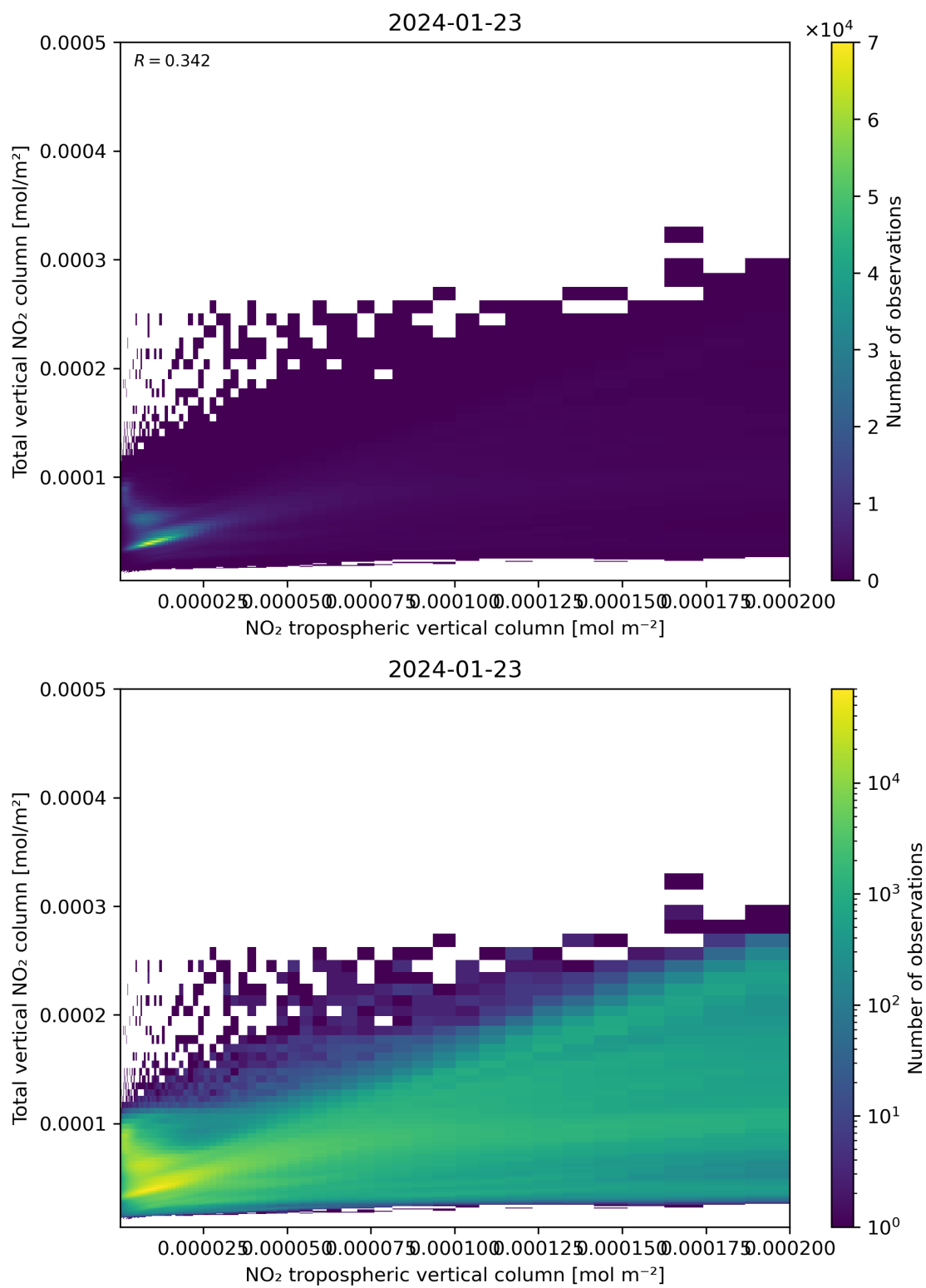
Figure 128: Scatter density plot of “NO 2 tropospheric vertical column” against “Total vertical NO 2 column” for 2024-01-22 to 2024-01-24.
