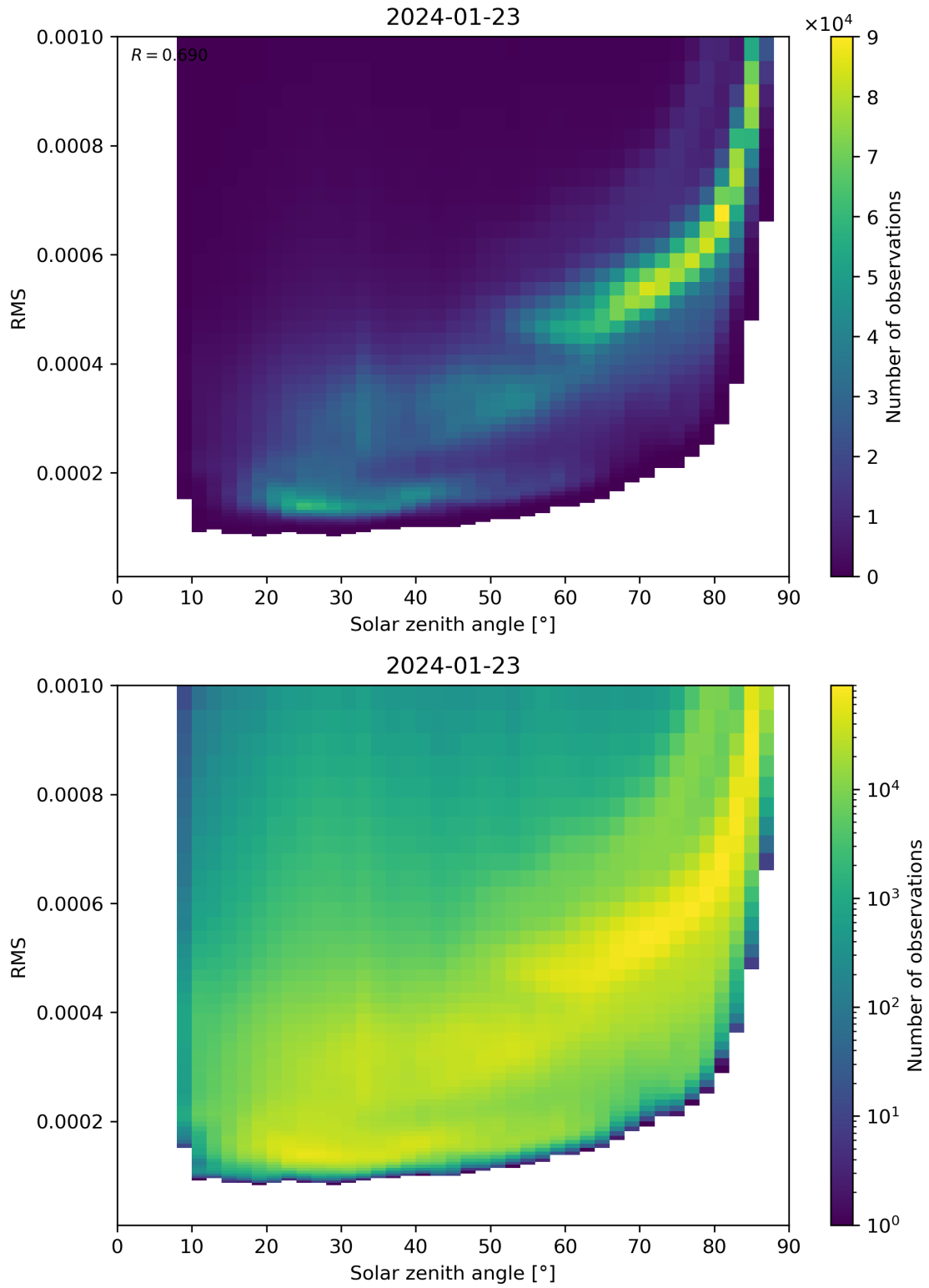
Figure 157: Scatter density plot of “Solar zenith angle” against “RMS” for 2024-01-22 to 2024-01-24.
