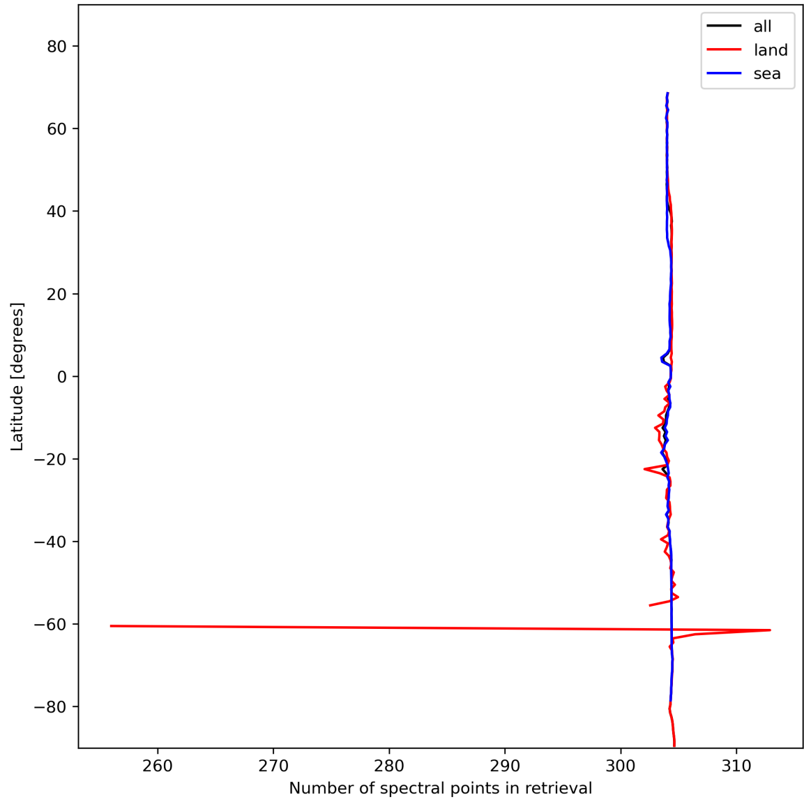
Figure 16: Zonal average of “Number of spectral points in retrieval” for 2024-01-22 to 2024-01-24.
