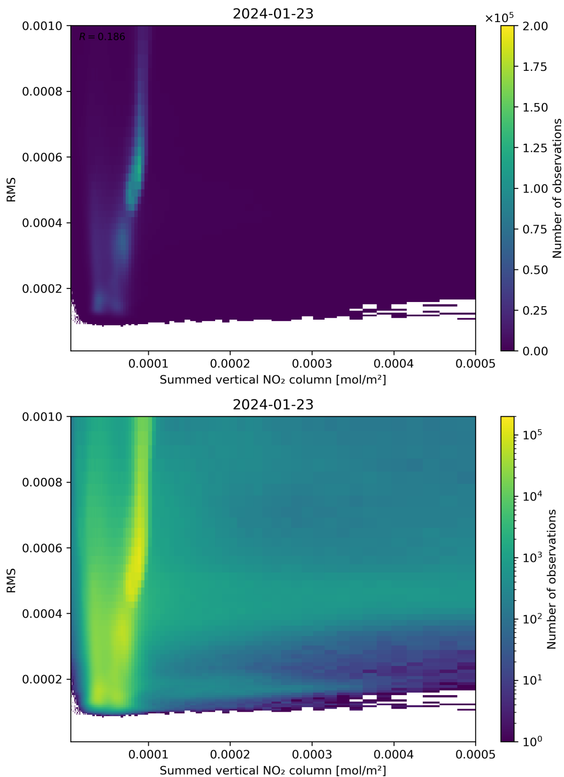
Figure 109: Scatter density plot of “Summed vertical NO 2 column” against “RMS” for 2024-01-22 to 2024-01-24.
