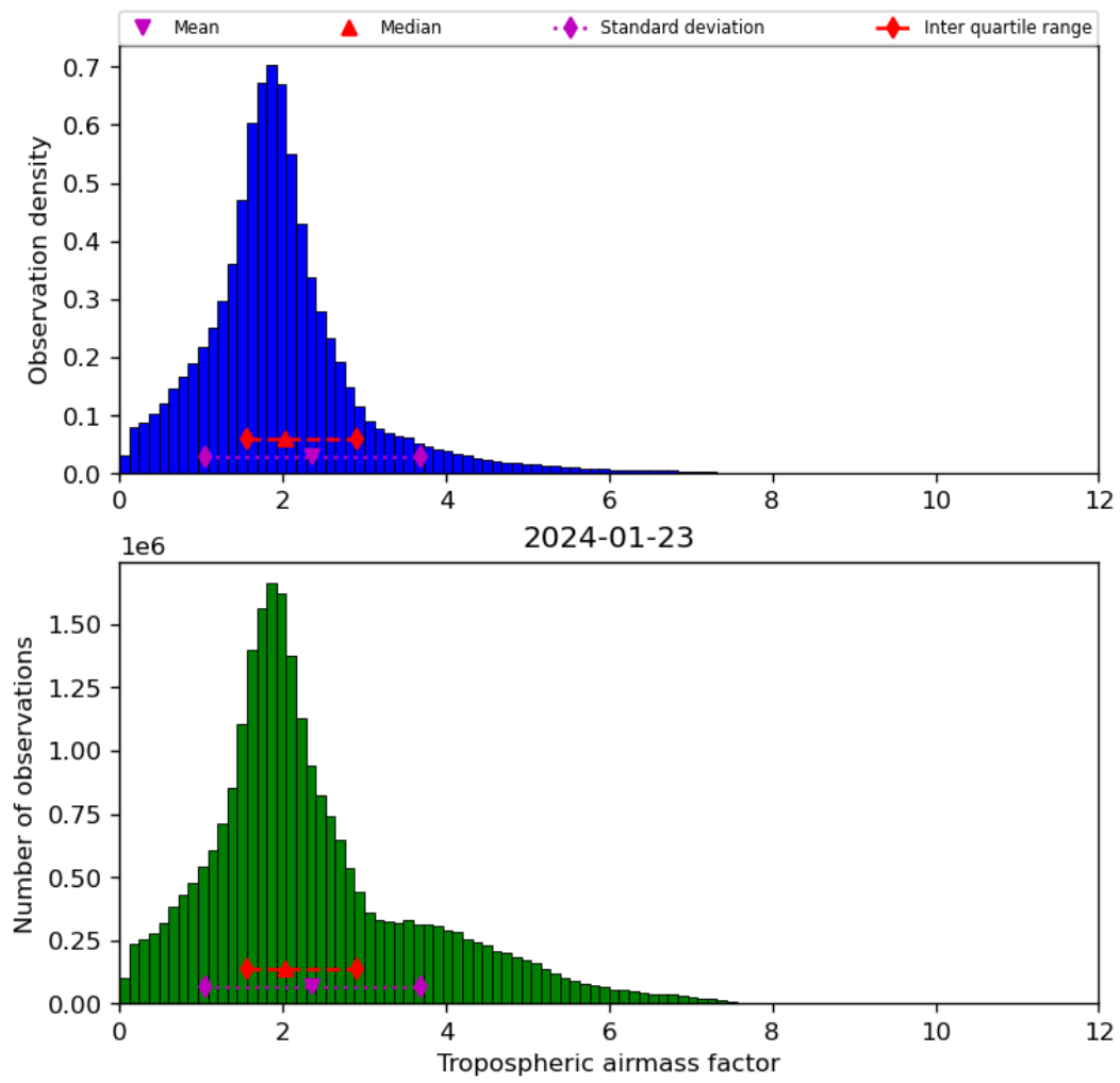
Figure 31: Histogram of “Tropospheric airmass factor” for 2024-01-22 to 2024-01-24
