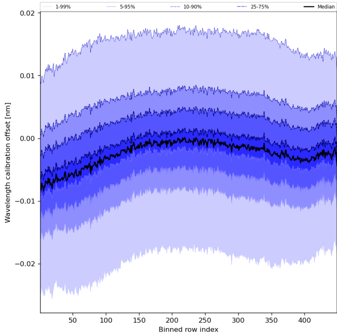
Figure 52: Along track statistics of “Wavelength calibration offset” for 2024-01-22 to 2024-01-24
