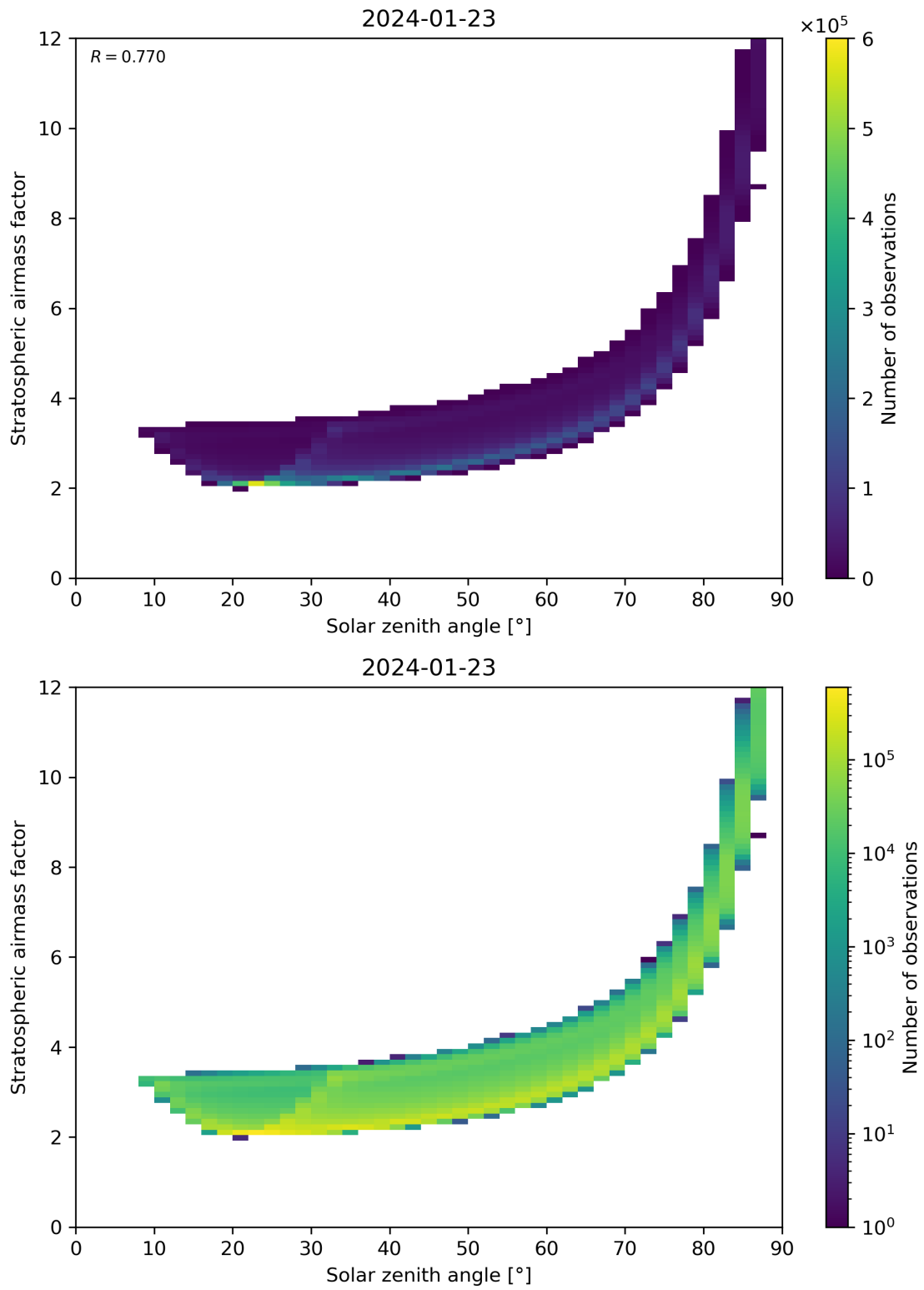
Figure 145: Scatter density plot of “Solar zenith angle” against “Stratospheric airmass factor” for 2024-01-22 to 2024-01-24.
