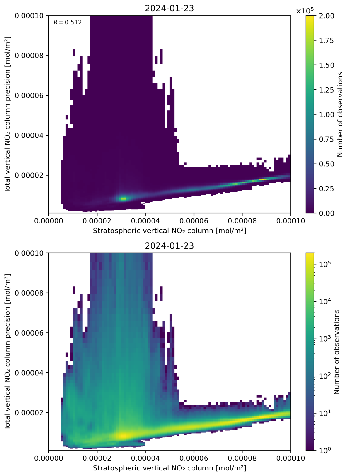
Figure 101: Scatter density plot of “Stratospheric vertical NO 2 column” against “Total vertical NO 2 column precision” for 2024-01-22 to 2024-01-24.
