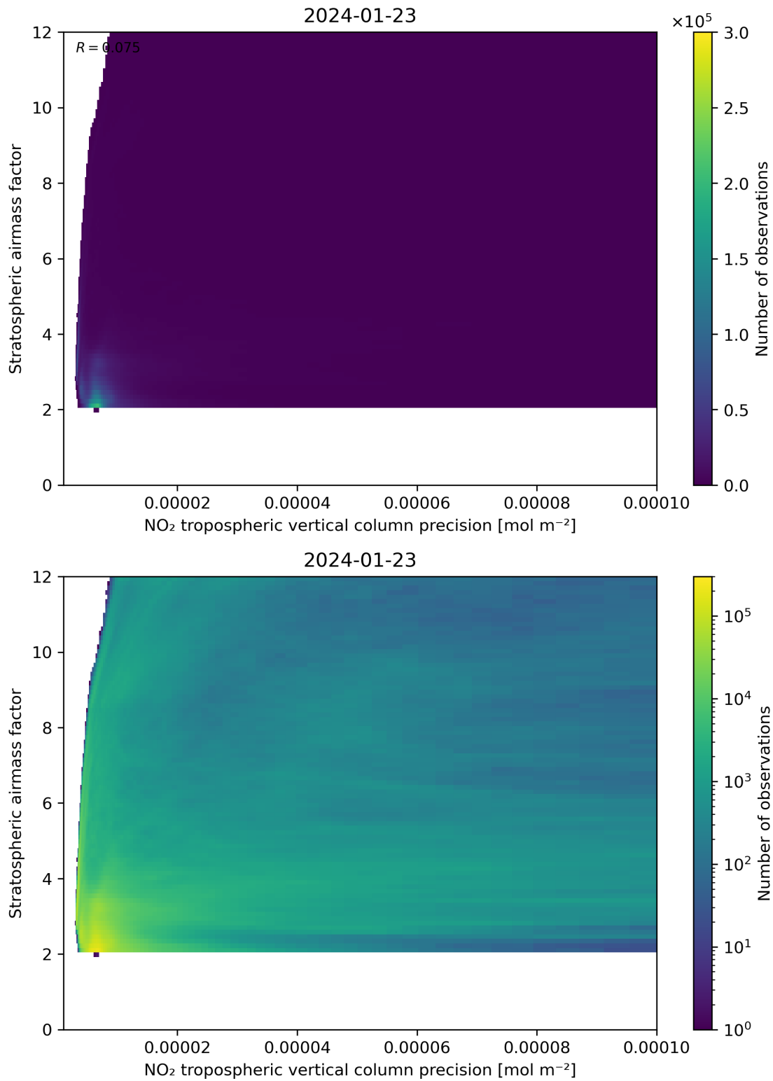
Figure 131: Scatter density plot of “NO 2 tropospheric vertical column precision” against “Stratospheric airmass factor” for 2024-01-22 to 2024-01-24.
