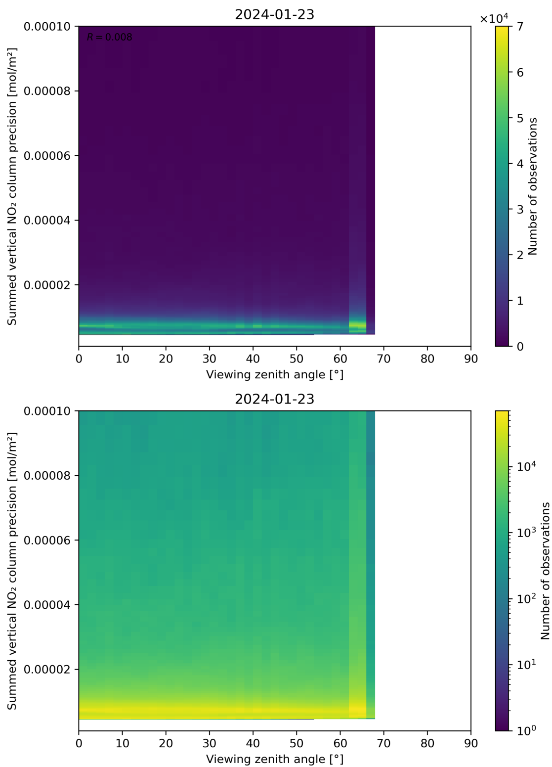
Figure 166: Scatter density plot of “Viewing zenith angle” against “Summed vertical NO 2 column precision” for 2024-01-22 to 2024-01-24.
