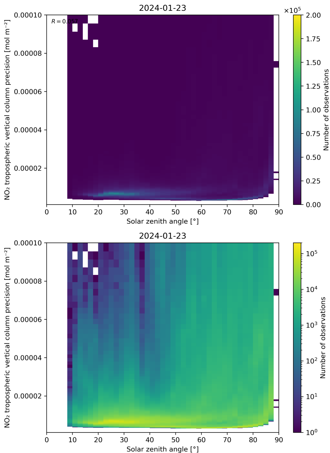
Figure 156: Scatter density plot of “Solar zenith angle” against “NO 2 tropospheric vertical column precision” for 2024-01-22 to 2024-01-24.
