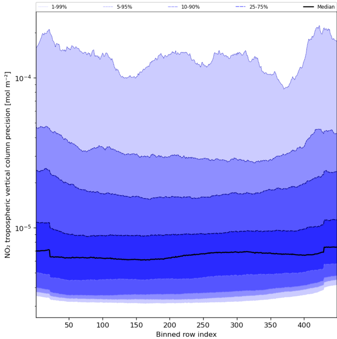
Figure 47: Along track statistics of “NO 2 tropospheric vertical column precision” for 2024-01-22 to 2024-01-24
