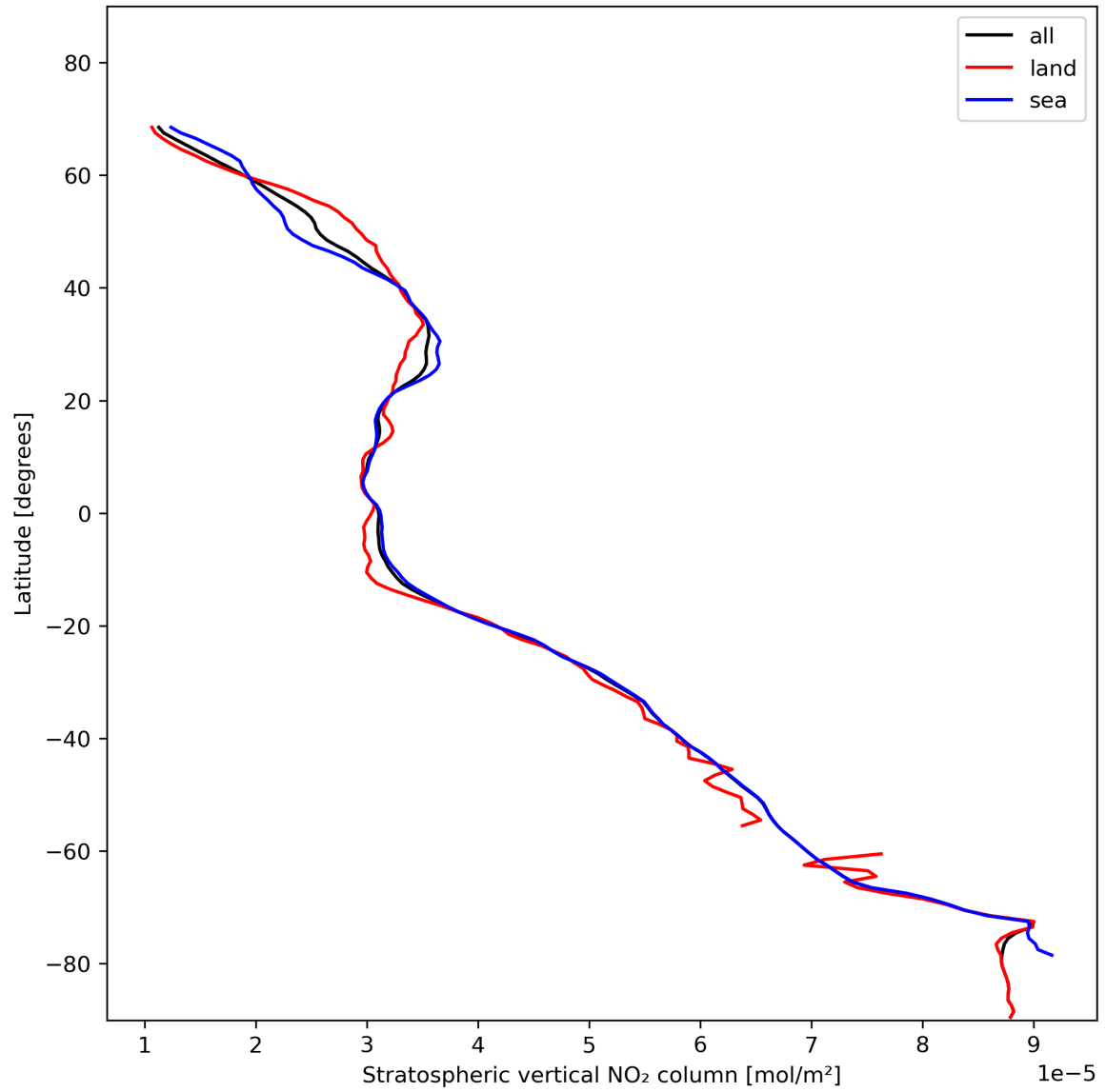
Figure 19: Zonal average of “Stratospheric vertical NO 2 column” for 2024-01-22 to 2024-01-24.
