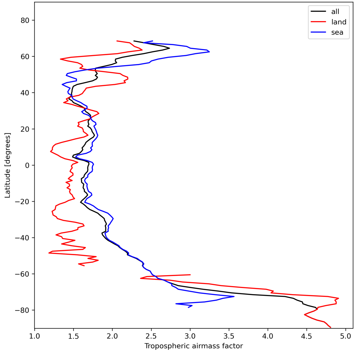
Figure 14: Zonal average of “Tropospheric airmass factor” for 2024-01-22 to 2024-01-24.
