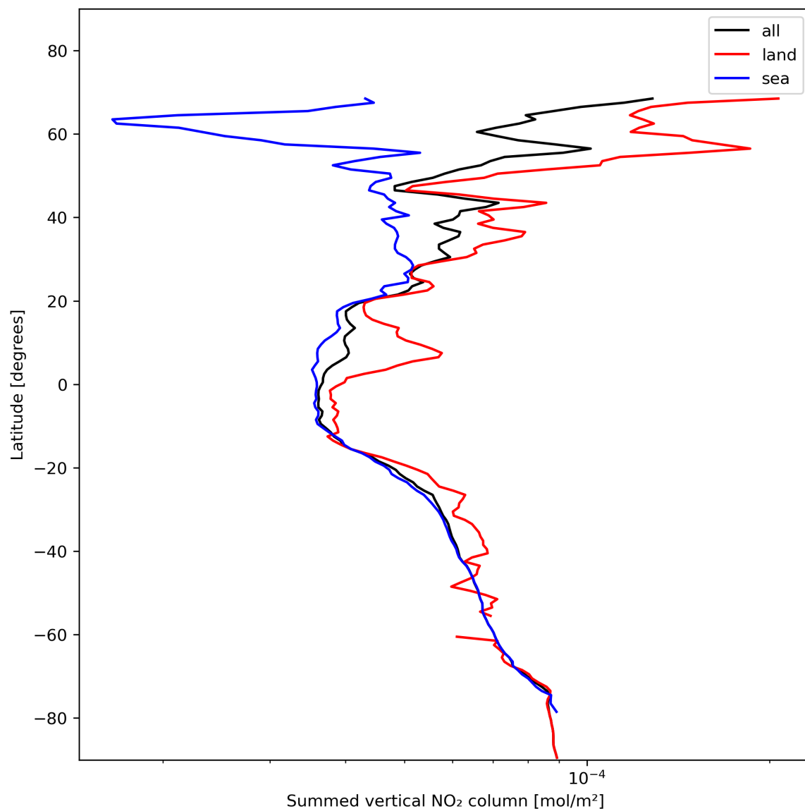
Figure 23: Zonal average of “Summed vertical NO 2 column” for 2024-01-22 to 2024-01-24.
