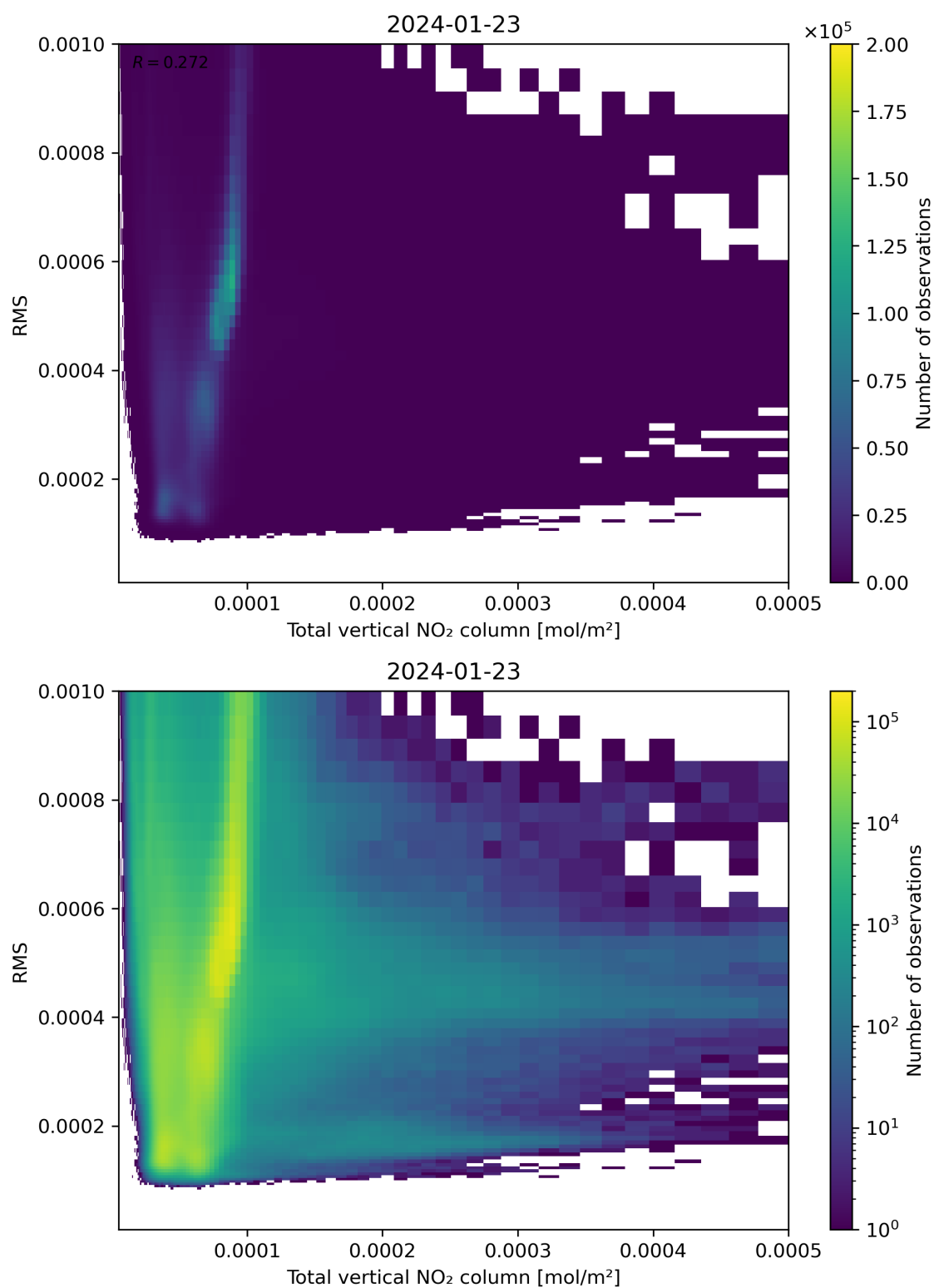
Figure 120: Scatter density plot of “Total vertical NO 2 column” against “RMS” for 2024-01-22 to 2024-01-24.
