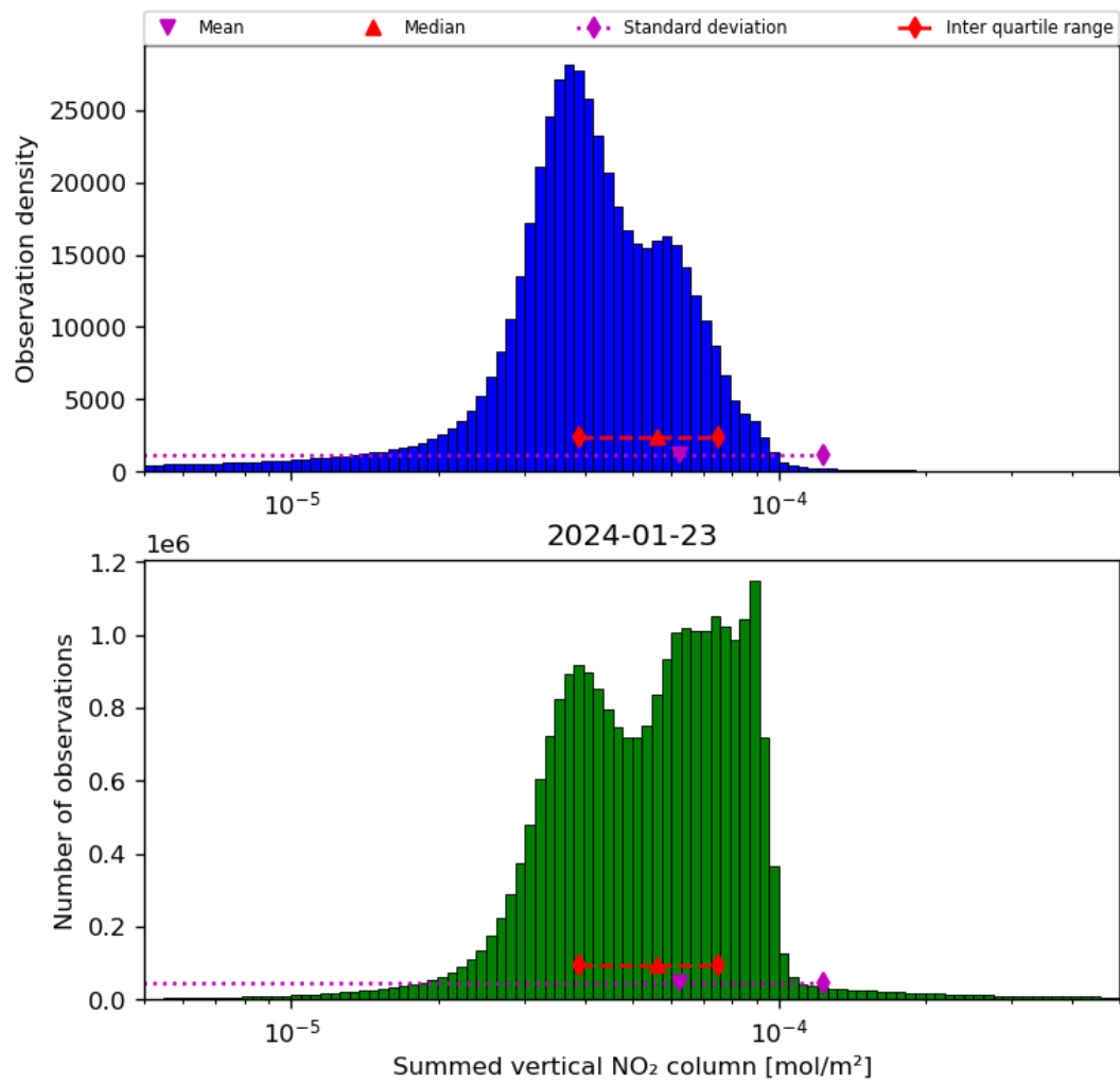
Figure 40: Histogram of “Summed vertical NO 2 column” for 2024-01-22 to 2024-01-24
