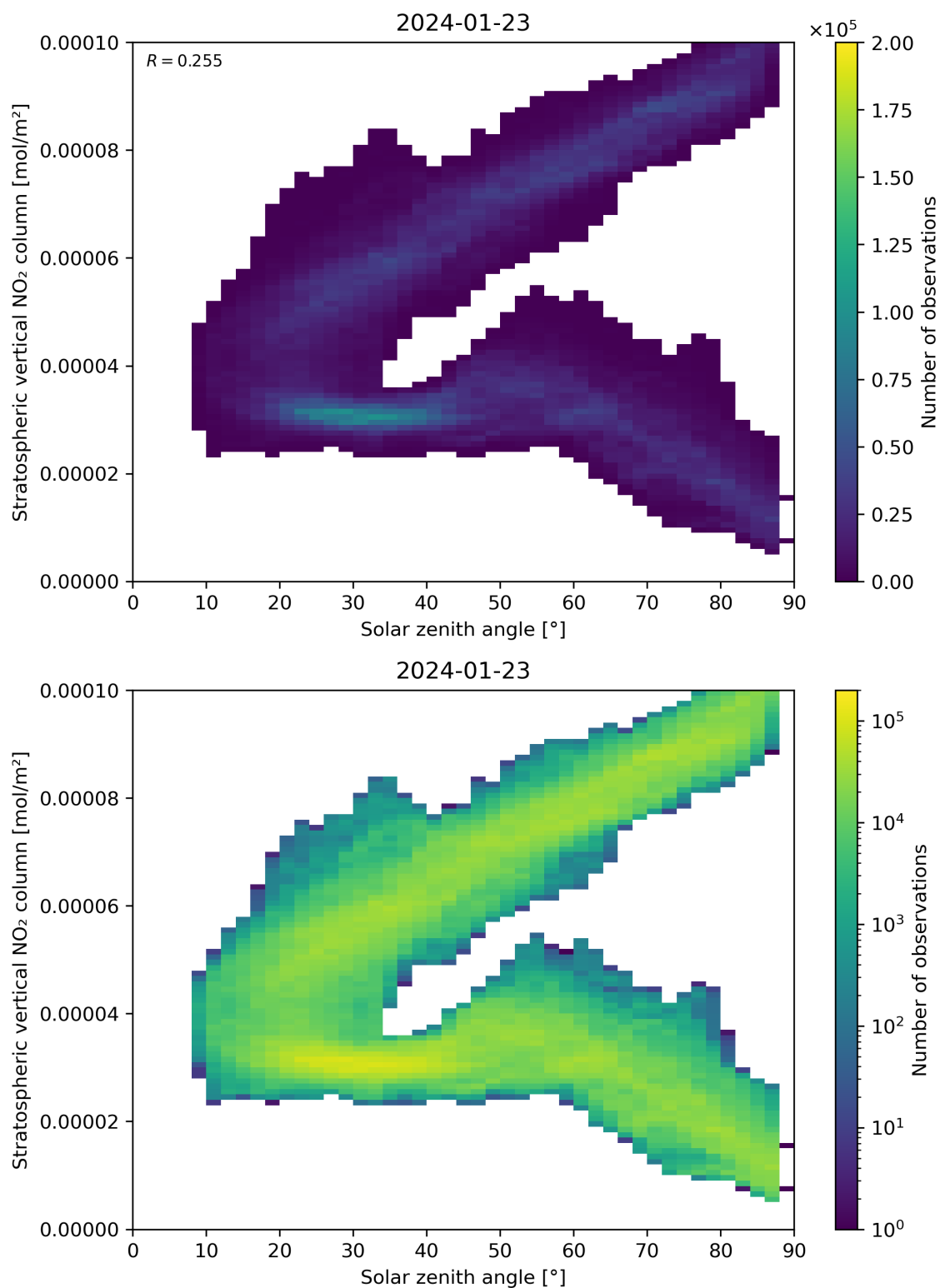
Figure 150: Scatter density plot of “Solar zenith angle” against “Stratospheric vertical NO 2 column” for 2024-01-22 to 2024-01-24.
