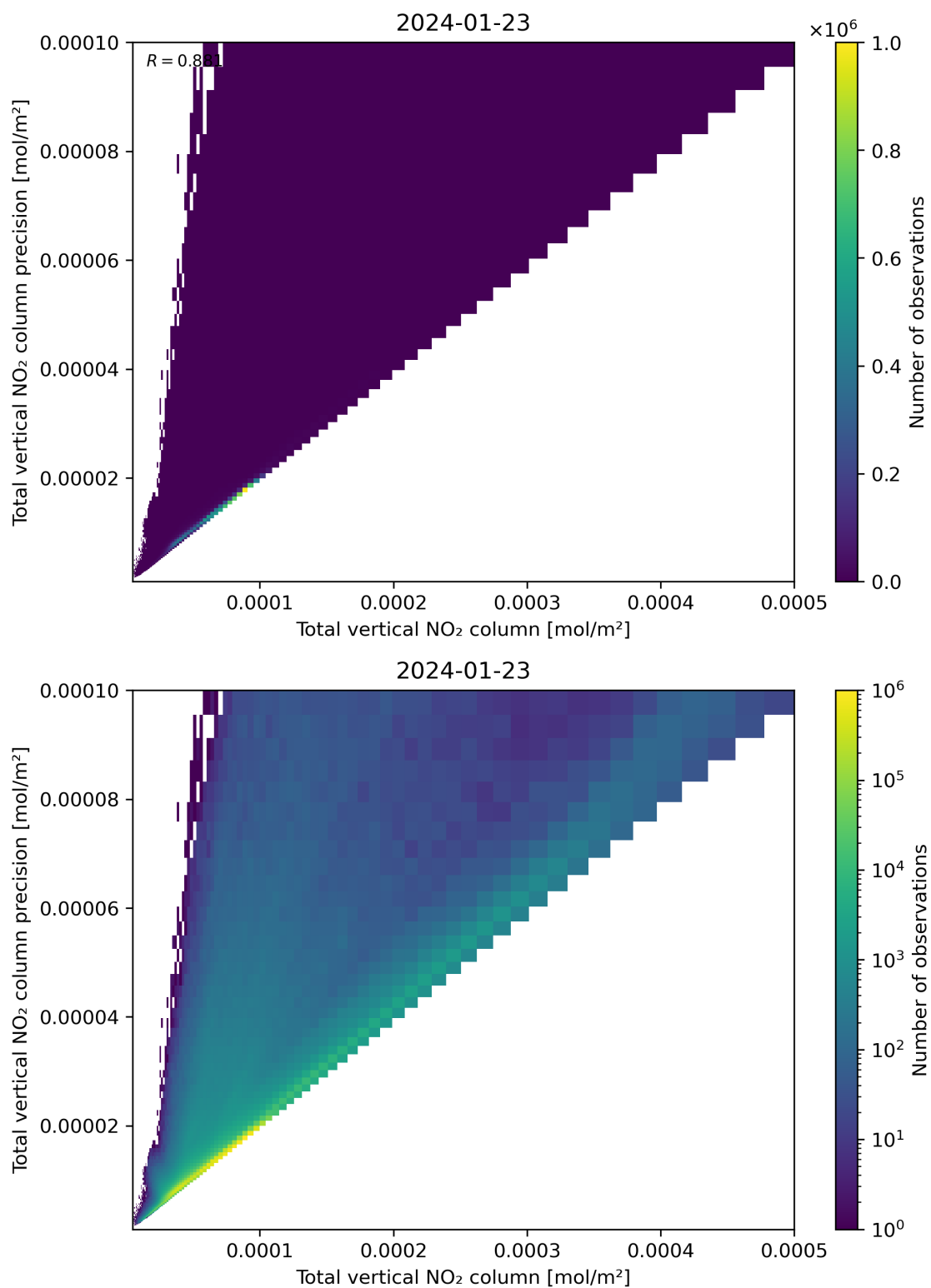
Figure 114: Scatter density plot of “Total vertical NO 2 column” against “Total vertical NO 2 column precision” for 2024-01-22 to 2024-01-24.
