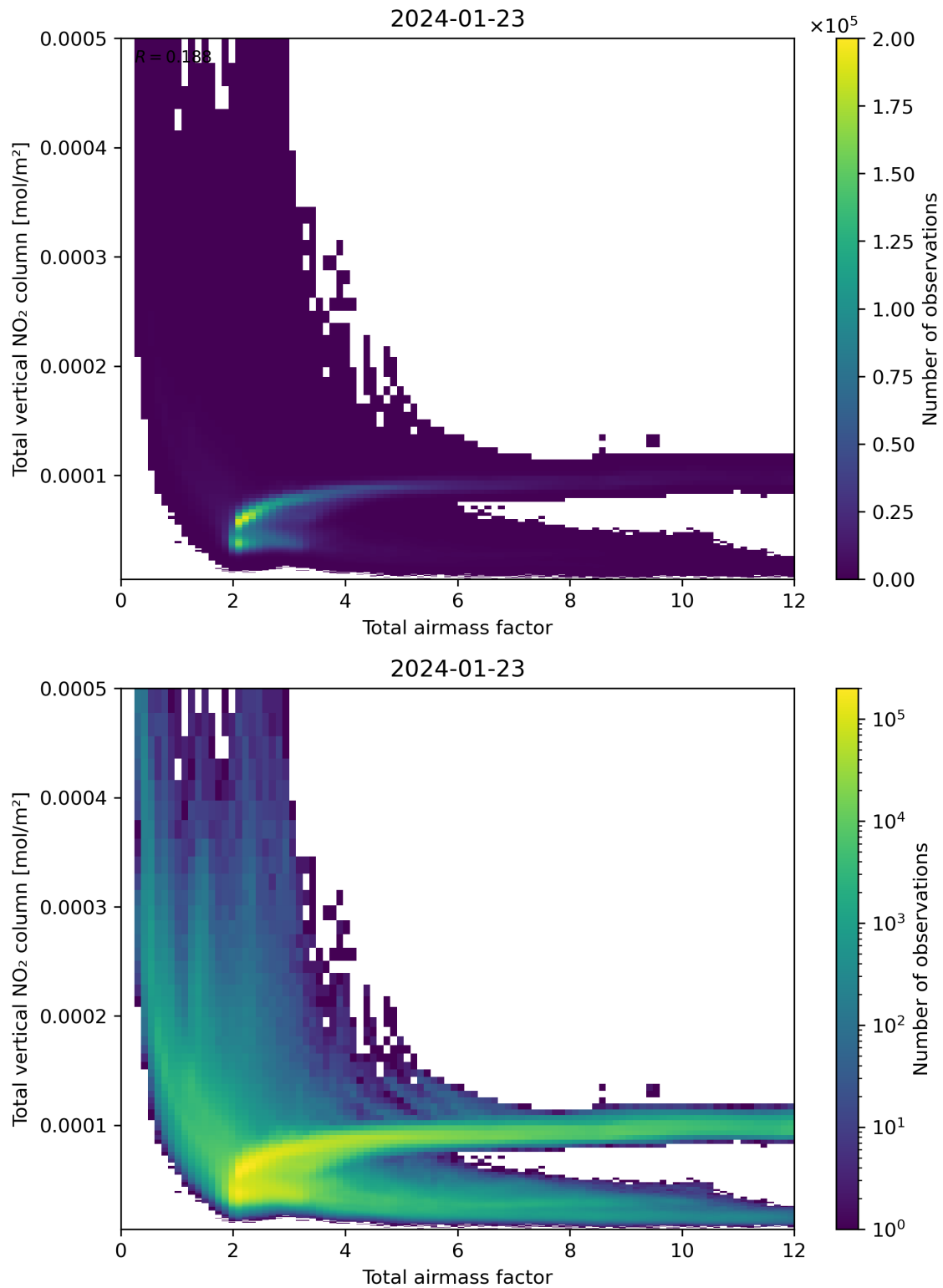
Figure 67: Scatter density plot of “Total airmass factor” against “Total vertical NO 2 column” for 2024-01-22 to 2024-01-24.
