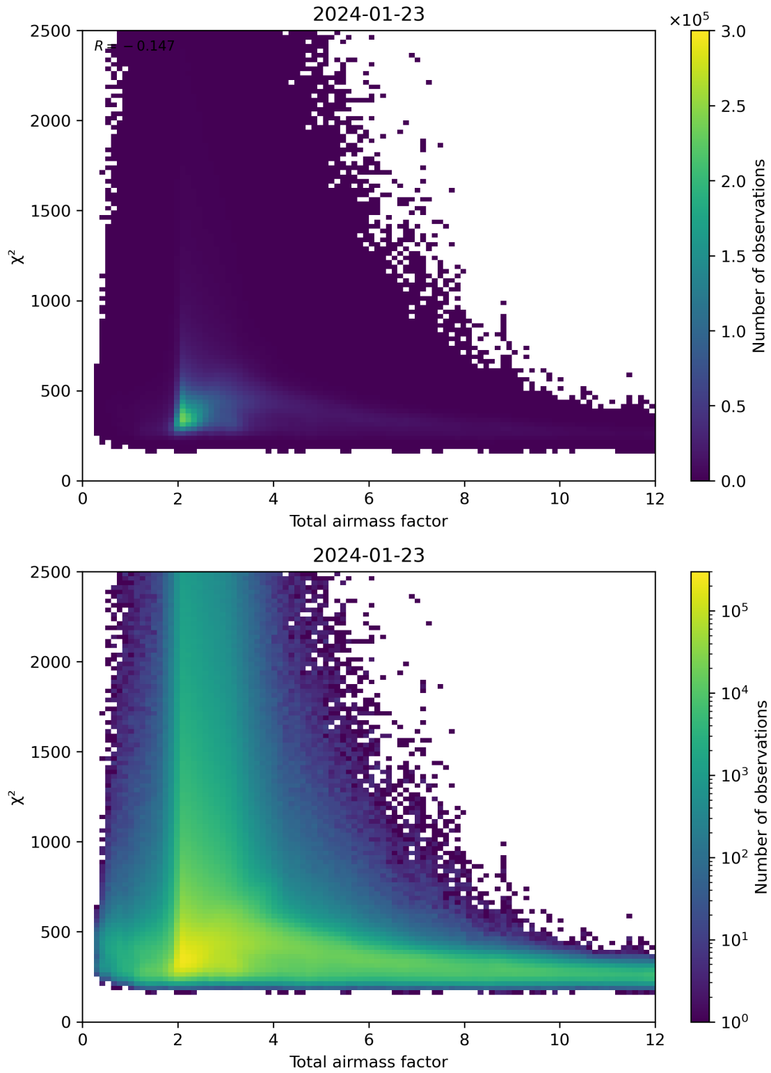
Figure 63: Scatter density plot of “Total airmass factor” against “ \chi^2 ” for 2024-01-22 to 2024-01-24.
