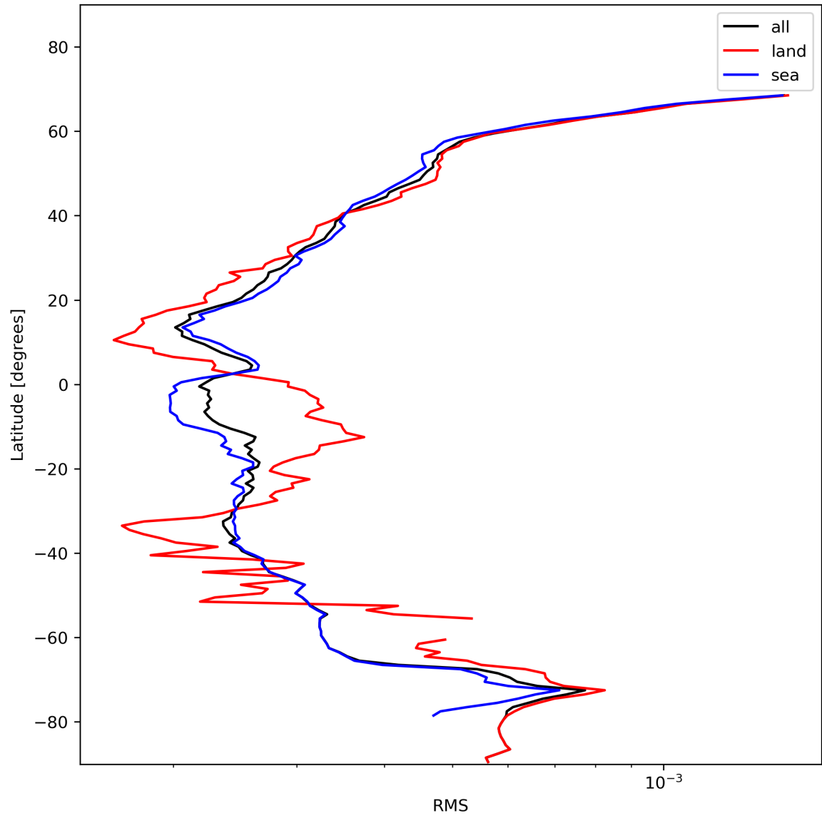
Figure 26: Zonal average of “RMS” for 2024-01-22 to 2024-01-24.
