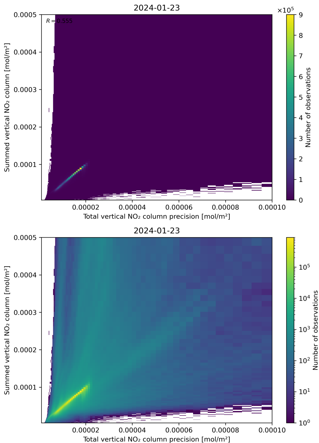
Figure 117: Scatter density plot of “Total vertical NO 2 column precision” against “Summed vertical NO 2 column” for 2024-01-22 to 2024-01-24.
