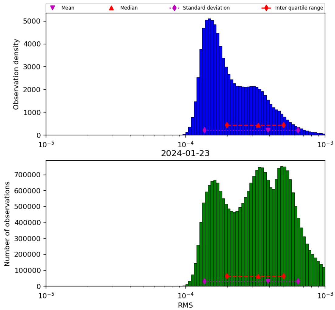
Figure 43: Histogram of “RMS” for 2024-01-22 to 2024-01-24
