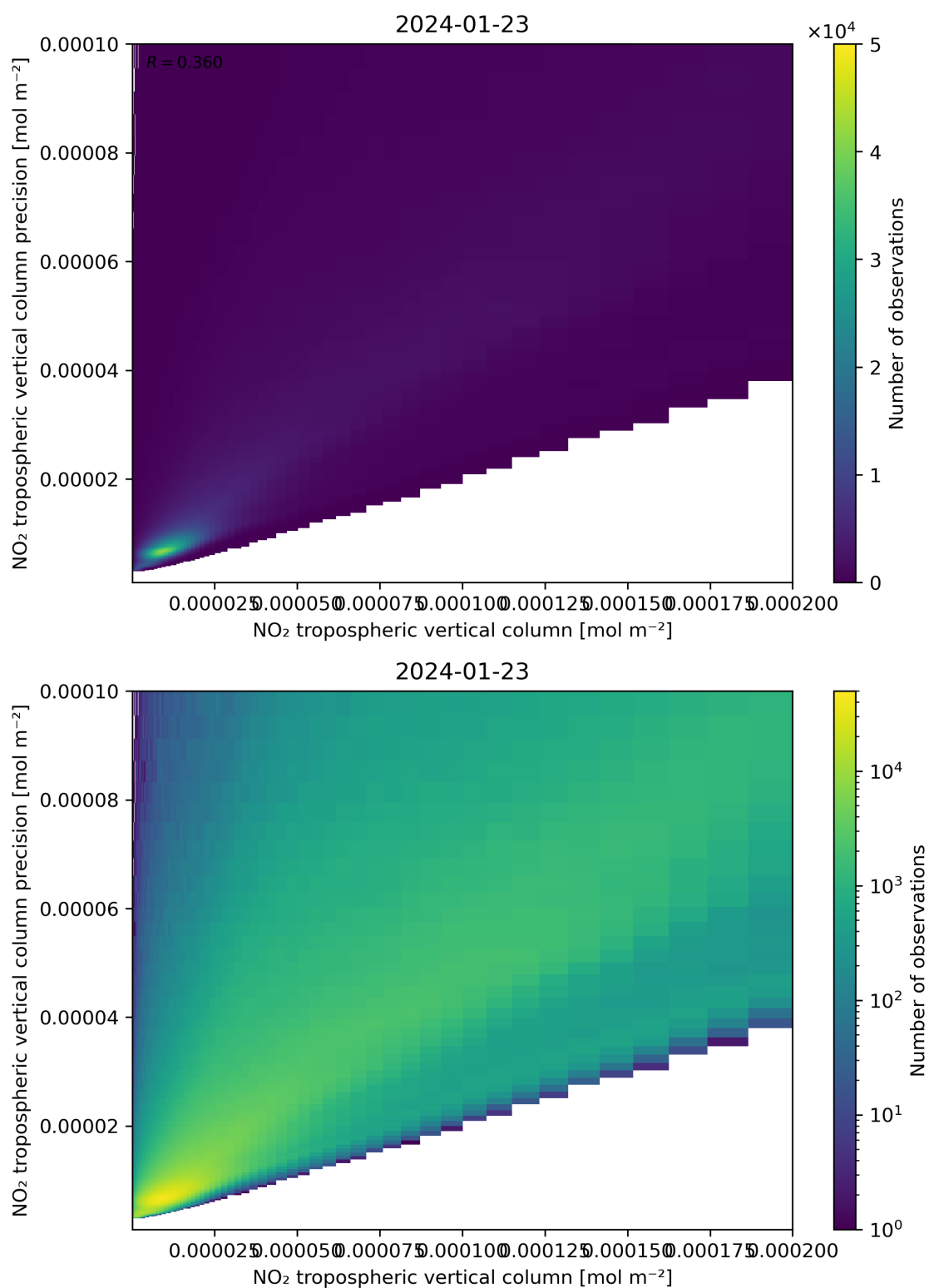
Figure 130: Scatter density plot of “NO 2 tropospheric vertical column” against “NO 2 tropospheric vertical column precision” for 2024-01-22 to 2024-01-24.
