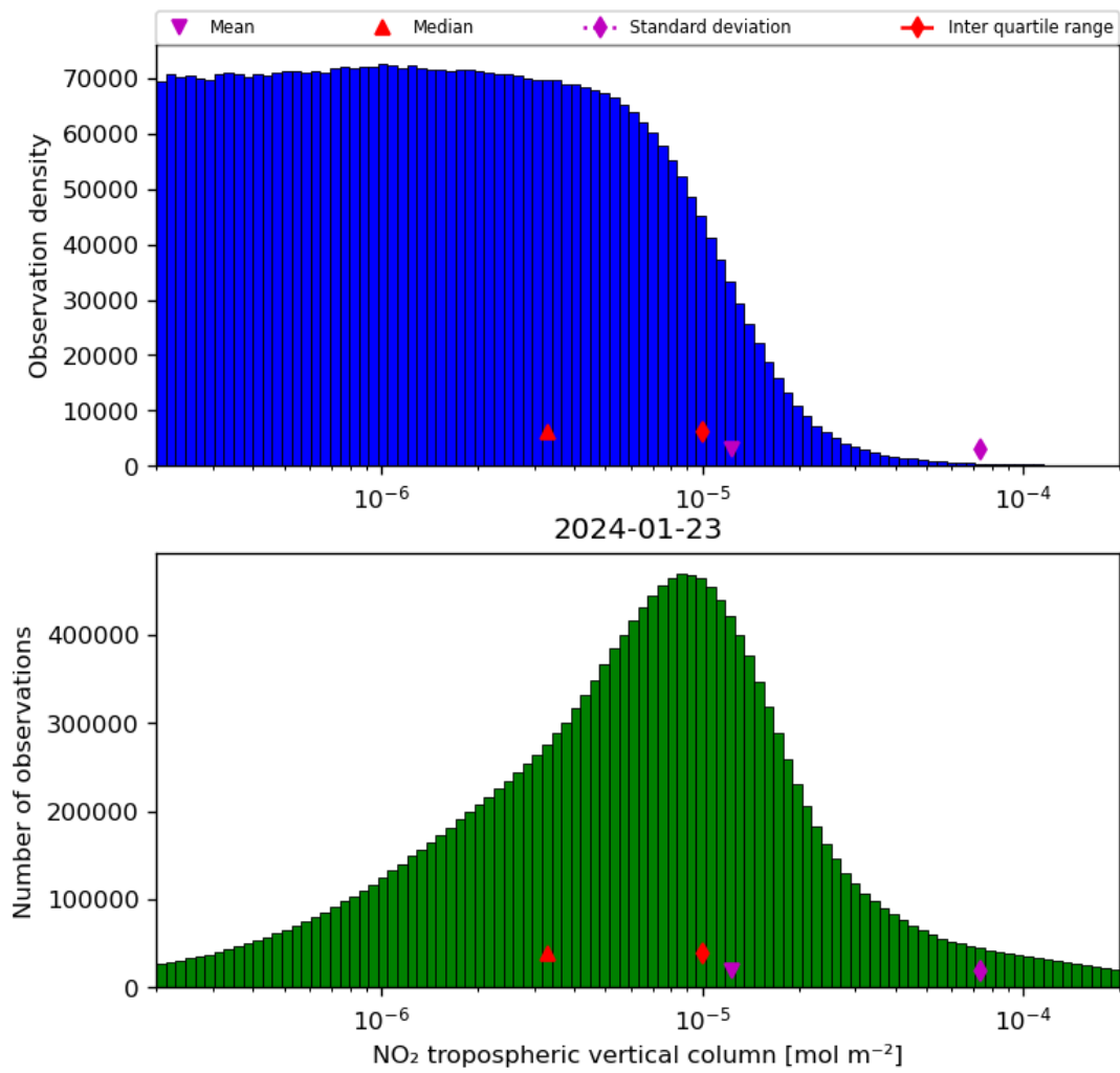
Figure 29: Histogram of “NO 2 tropospheric vertical column” for 2024-01-22 to 2024-01-24
