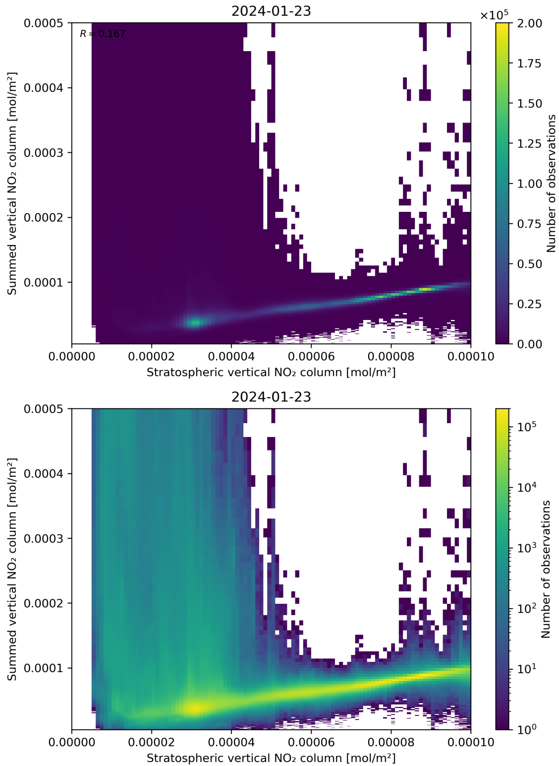
Figure 98: Scatter density plot of “Stratospheric vertical NO 2 column” against “Summed vertical NO 2 column” for 2024-01-22 to 2024-01-24.
