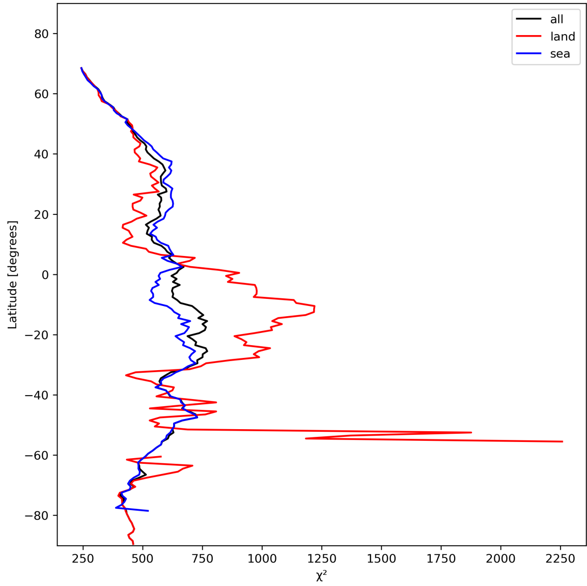
Figure 25: Zonal average of “ \chi^2 ” for 2024-01-22 to 2024-01-24.
