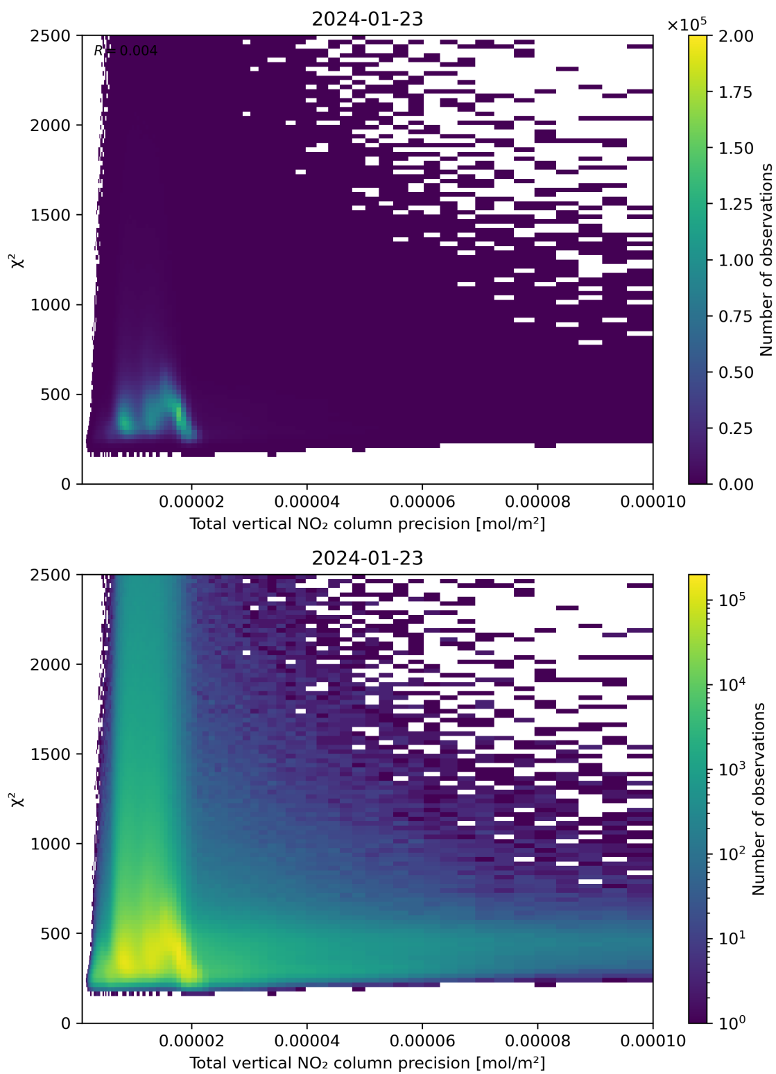
Figure 116: Scatter density plot of “Total vertical NO 2 column precision” against “ \chi^2 ” for 2024-01-22 to 2024-01-24.
