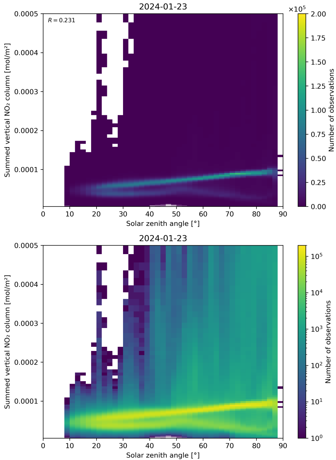
Figure 151: Scatter density plot of “Solar zenith angle” against “Summed vertical NO 2 column” for 2024-01-22 to 2024-01-24.
