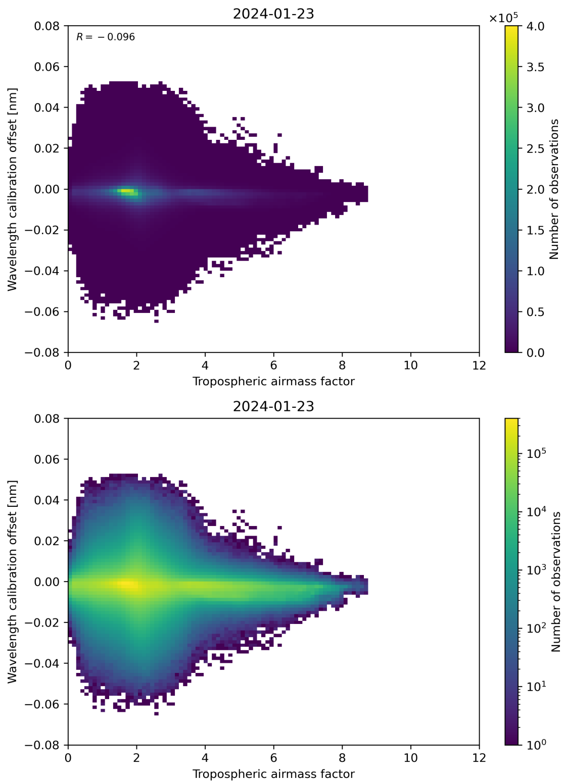
Figure 80: Scatter density plot of “Tropospheric airmass factor” against “Wavelength calibration offset” for 2024-01-22 to 2024-01-24.
