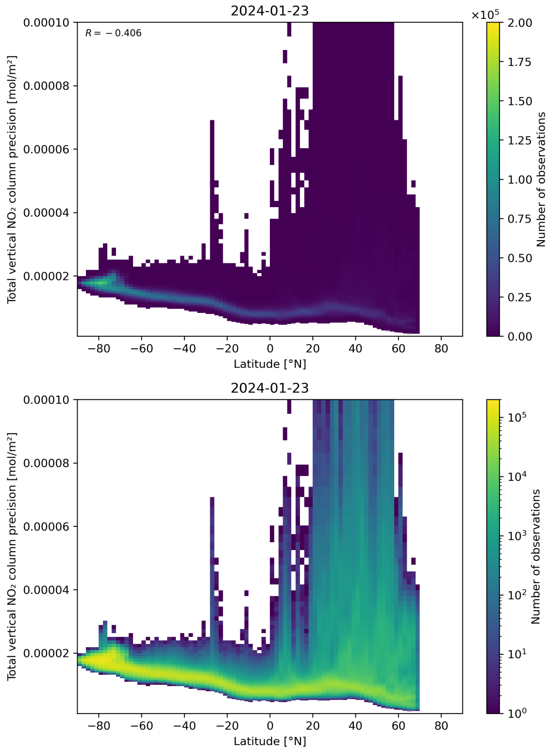
Figure 91: Scatter density plot of “Latitude” against “Total vertical NO 2 column precision” for 2024-01-22 to 2024-01-24.
