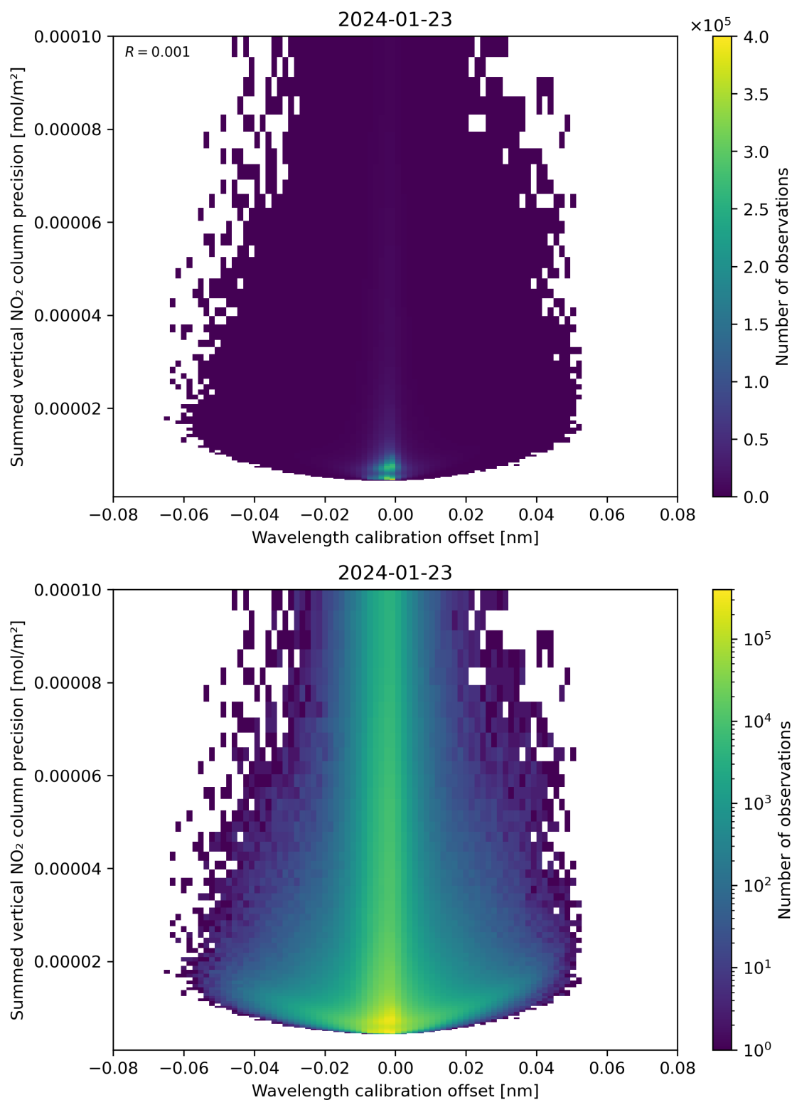
Figure 178: Scatter density plot of “Wavelength calibration offset” against “Summed vertical NO 2 column precision” for 2024-01-22 to 2024-01-24.
