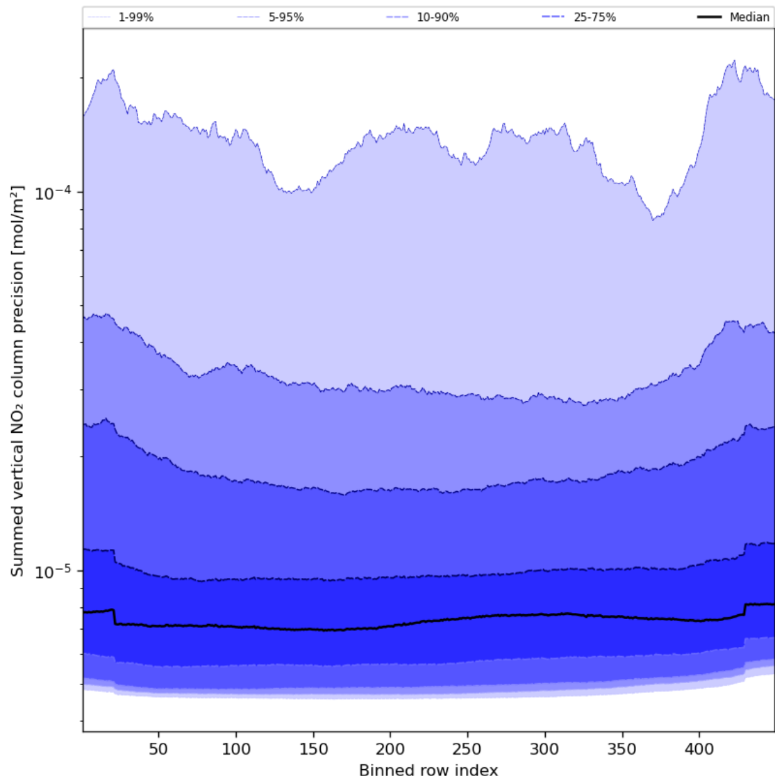
Figure 58: Along track statistics of “Summed vertical NO 2 column precision” for 2024-01-22 to 2024-01-24
