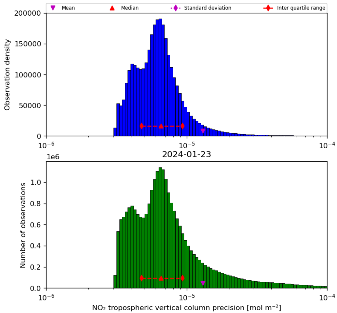
Figure 30: Histogram of “NO 2 tropospheric vertical column precision” for 2024-01-22 to 2024-01-24
