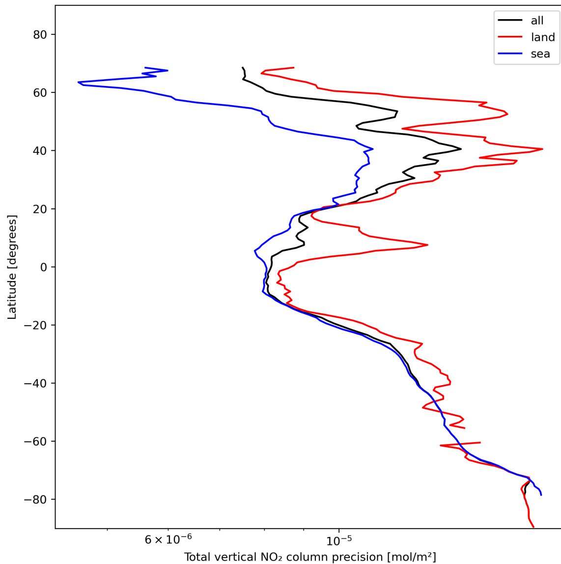
Figure 22: Zonal average of “Total vertical NO 2 column precision” for 2024-01-22 to 2024-01-24.
