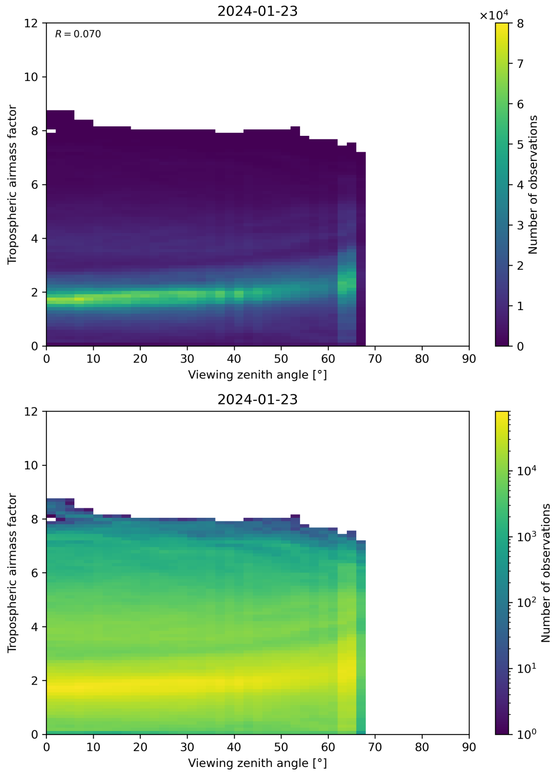
Figure 161: Scatter density plot of “Viewing zenith angle” against “Tropospheric airmass factor” for 2024-01-22 to 2024-01-24.
