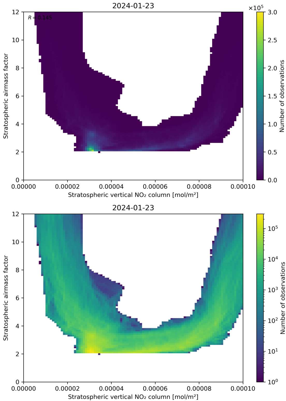
Figure 96: Scatter density plot of “Stratospheric vertical NO 2 column” against “Stratospheric airmass factor” for 2024-01-22 to 2024-01-24.
