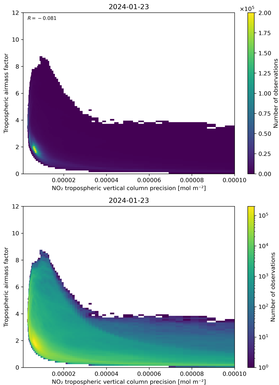
Figure 133: Scatter density plot of “NO 2 tropospheric vertical column precision” against “Tropospheric airmass factor” for 2024-01-22 to 2024-01-24.
