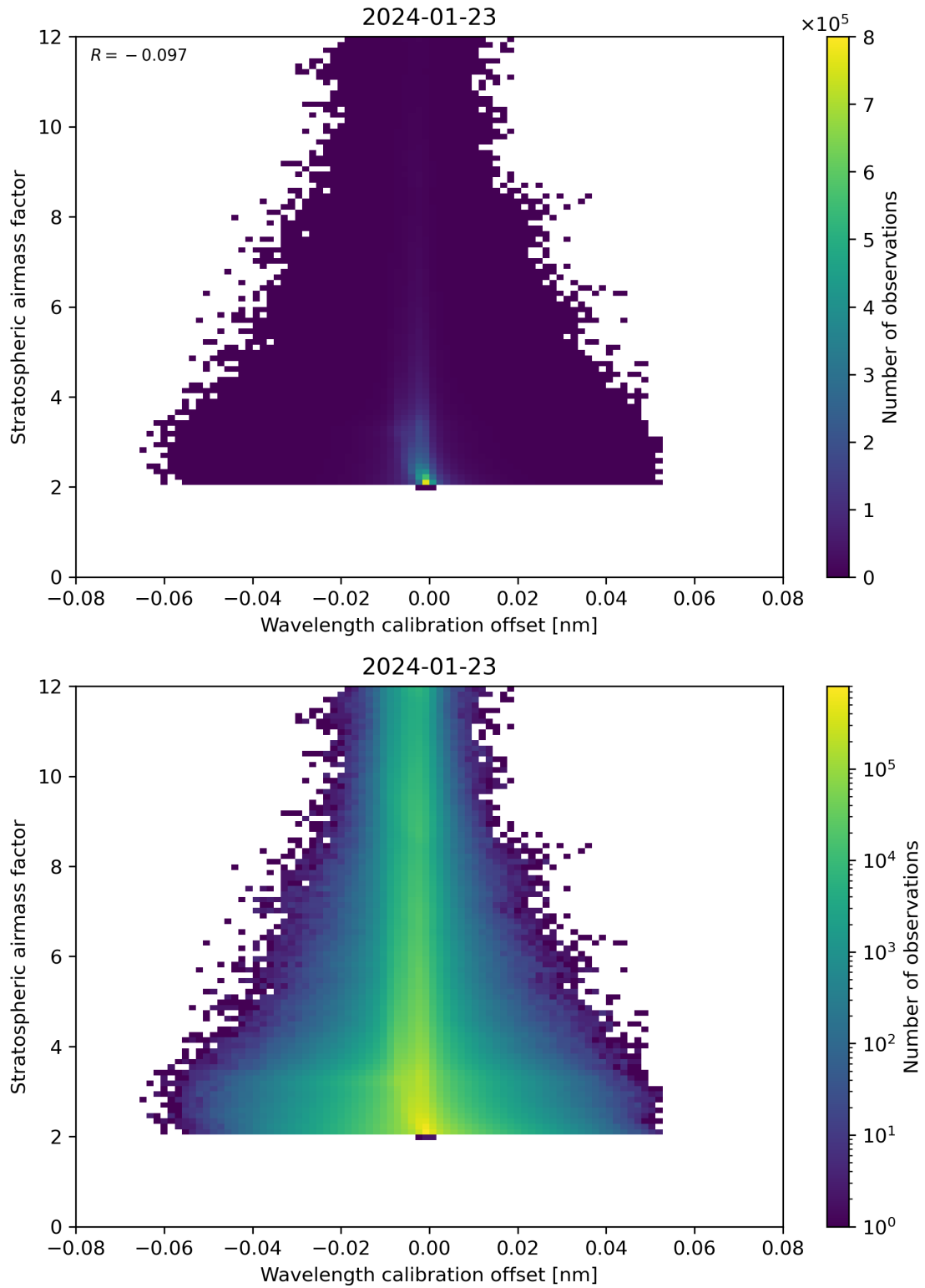
Figure 174: Scatter density plot of “Wavelength calibration offset” against “Stratospheric airmass factor” for 2024-01-22 to 2024-01-24.
