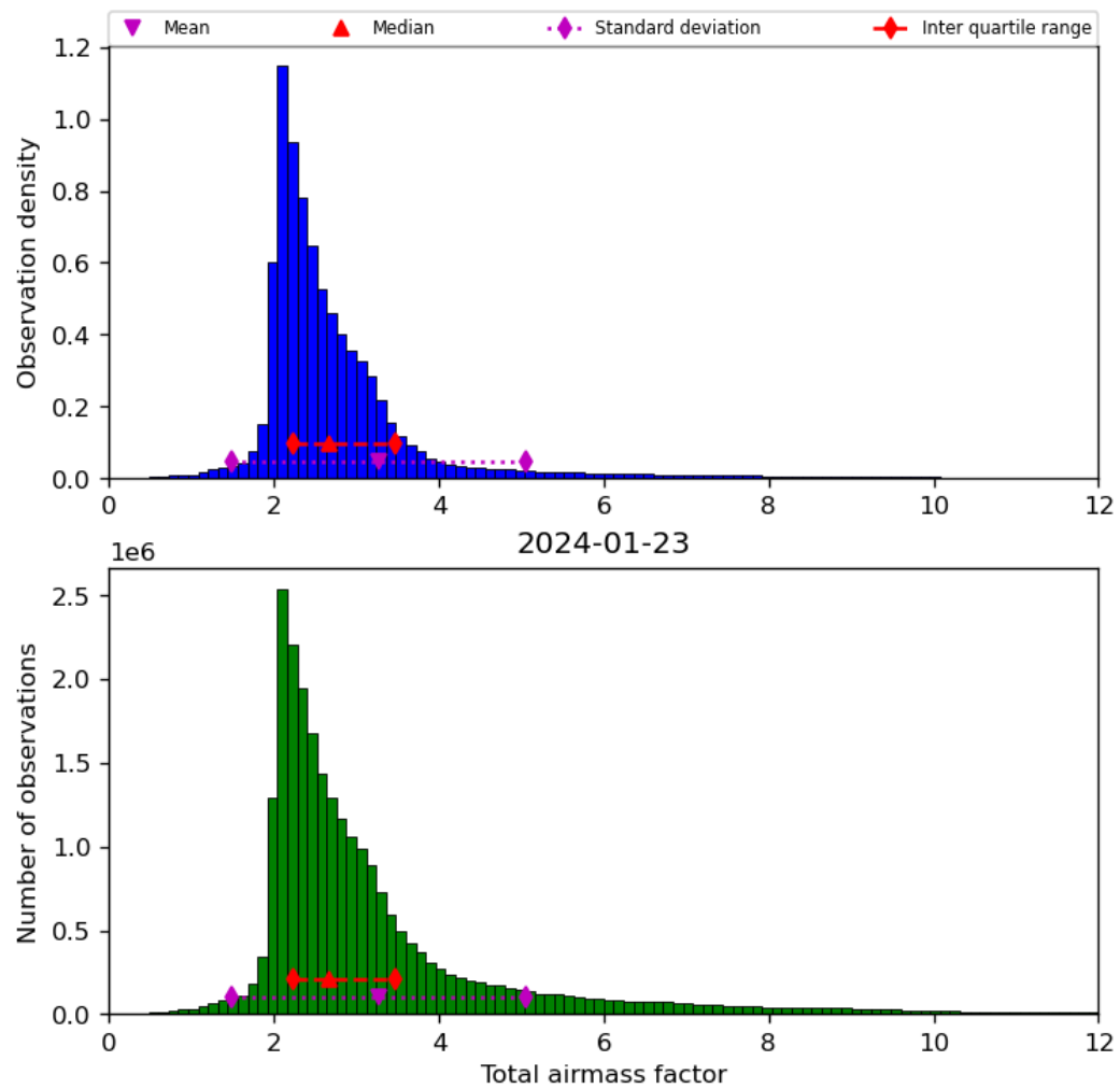
Figure 32: Histogram of “Total airmass factor” for 2024-01-22 to 2024-01-24
