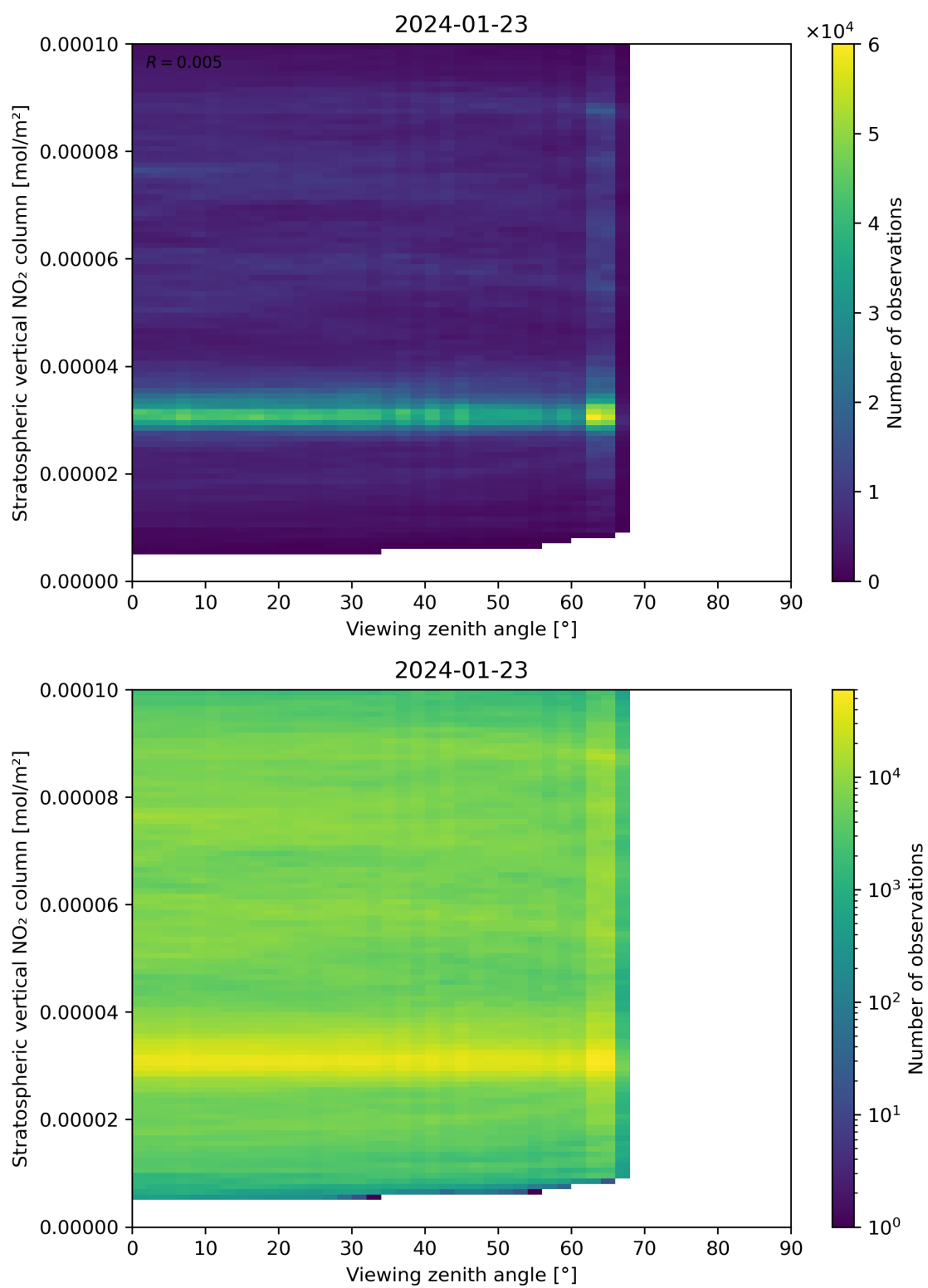
Figure 164: Scatter density plot of “Viewing zenith angle” against “Stratospheric vertical NO 2 column” for 2024-01-22 to 2024-01-24.
