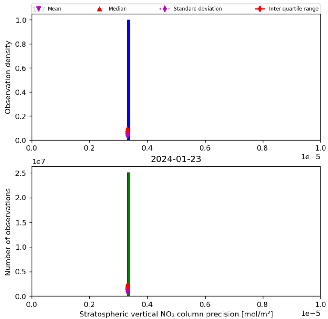
Figure 37: Histogram of “Stratospheric vertical NO 2 column precision” for 2024-01-22 to 2024-01-24
