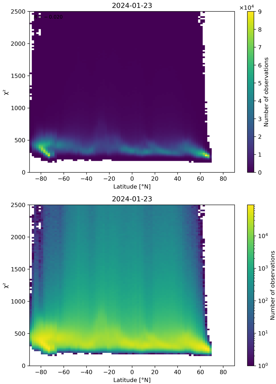
Figure 86: Scatter density plot of “Latitude” against “ \chi^2 ” for 2024-01-22 to 2024-01-24.
