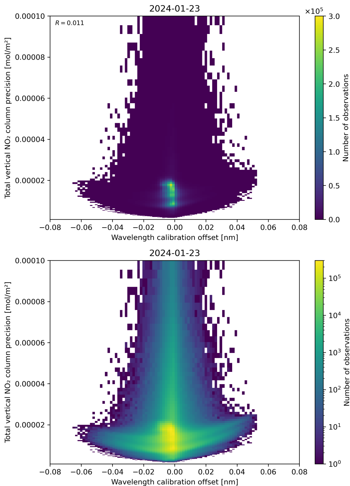
Figure 180: Scatter density plot of “Wavelength calibration offset” against “Total vertical NO 2 column precision” for 2024-01-22 to 2024-01-24.
