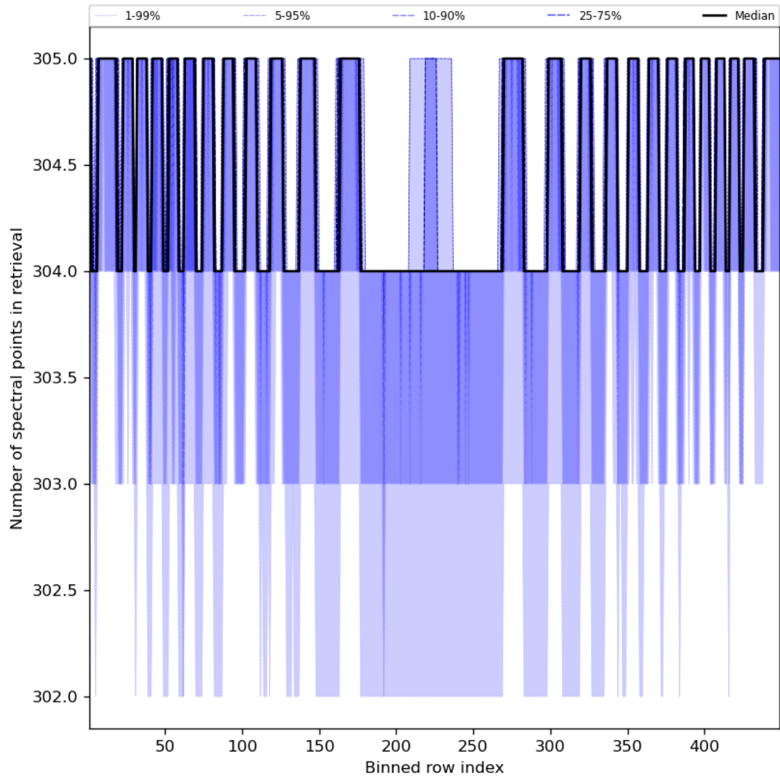
Figure 50: Along track statistics of “Number of spectral points in retrieval” for 2024-01-22 to 2024-01-24
