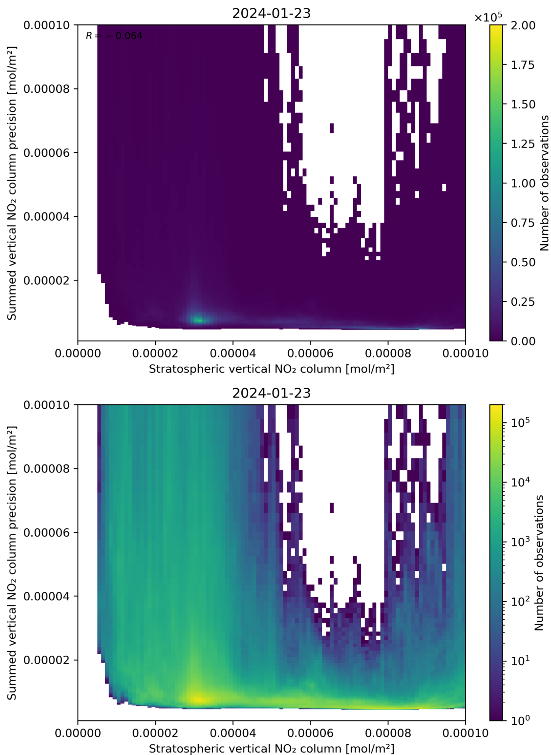
Figure 99: Scatter density plot of “Stratospheric vertical NO 2 column” against “Summed vertical NO 2 column precision” for 2024-01-22 to 2024-01-24.
