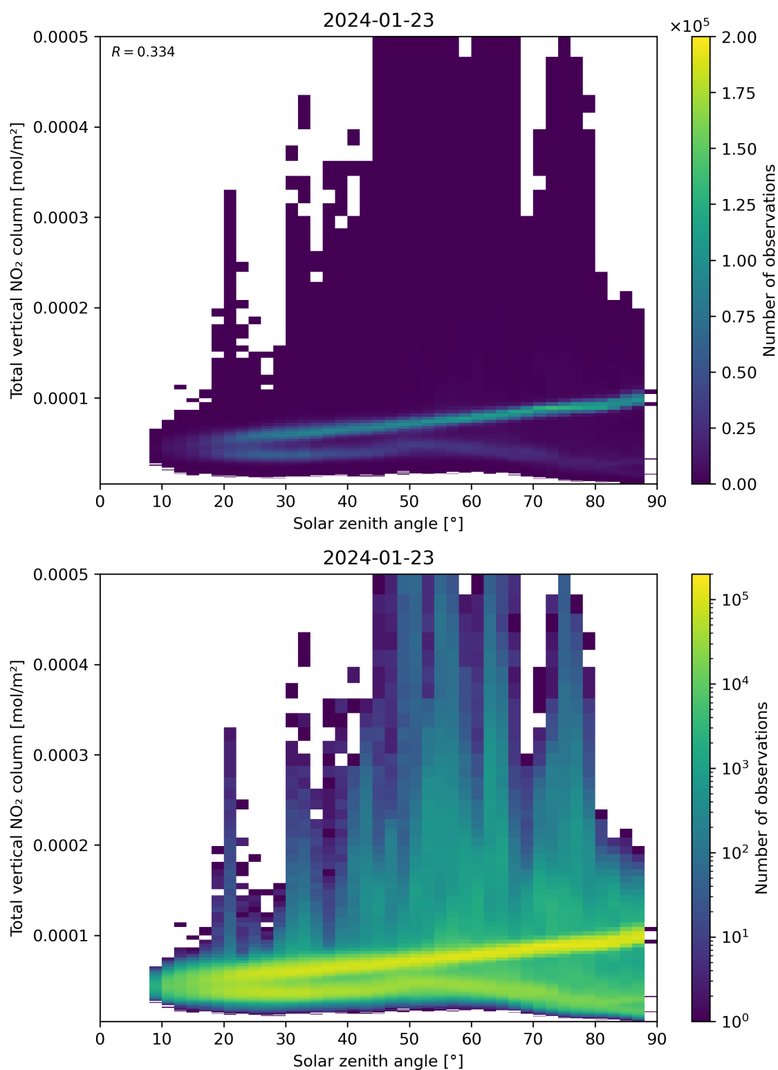
Figure 153: Scatter density plot of “Solar zenith angle” against “Total vertical NO 2 column” for 2024-01-22 to 2024-01-24.
