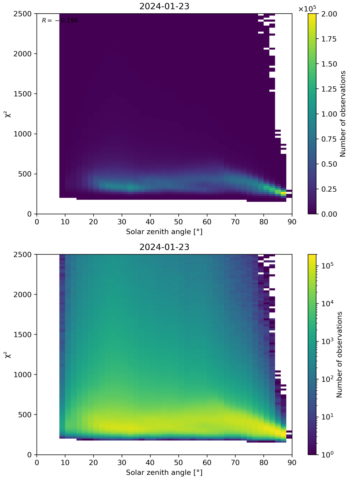
Figure 148: Scatter density plot of “Solar zenith angle” against “ \chi^2 ” for 2024-01-22 to 2024-01-24.
