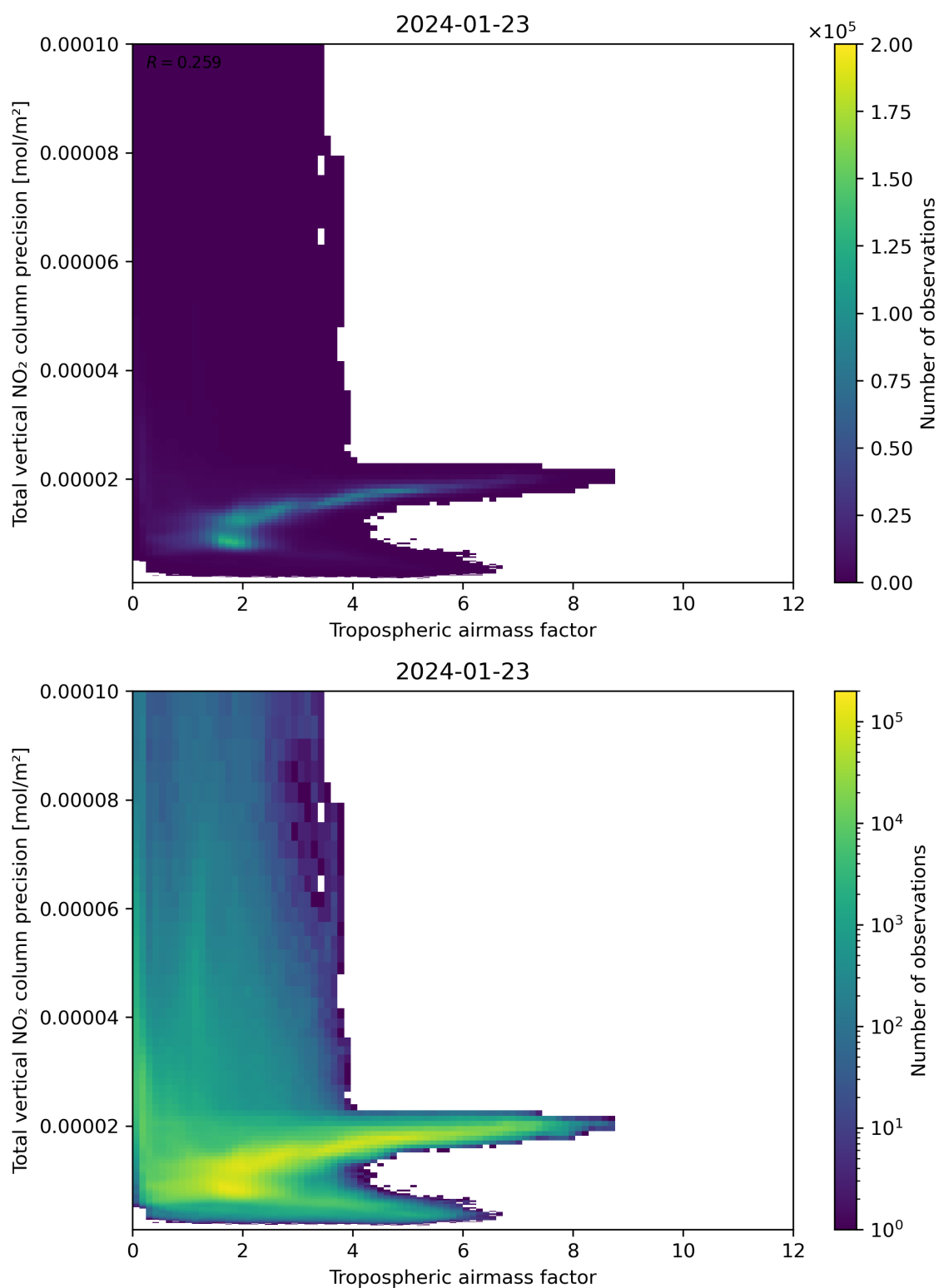
Figure 78: Scatter density plot of “Tropospheric air mass factor” against “Total vertical NO 2 column precision” for 2024-01-22 to 2024-01-24.
