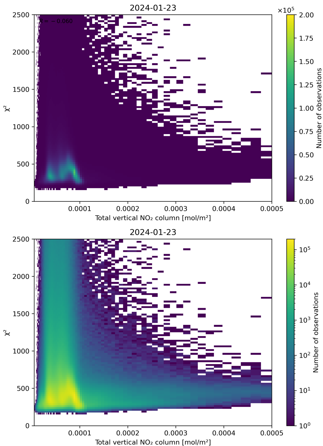
Figure 111: Scatter density plot of “Total vertical NO 2 column” against “ \chi^2 ” for 2024-01-22 to 2024-01-24.
