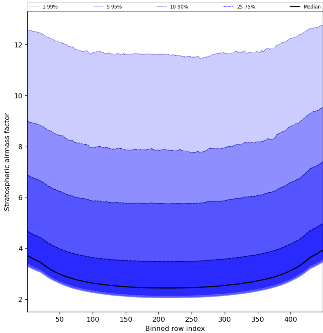
Figure 61: Along track statistics of “Stratospheric airmass factor” for 2024-01-22 to 2024-01-24
