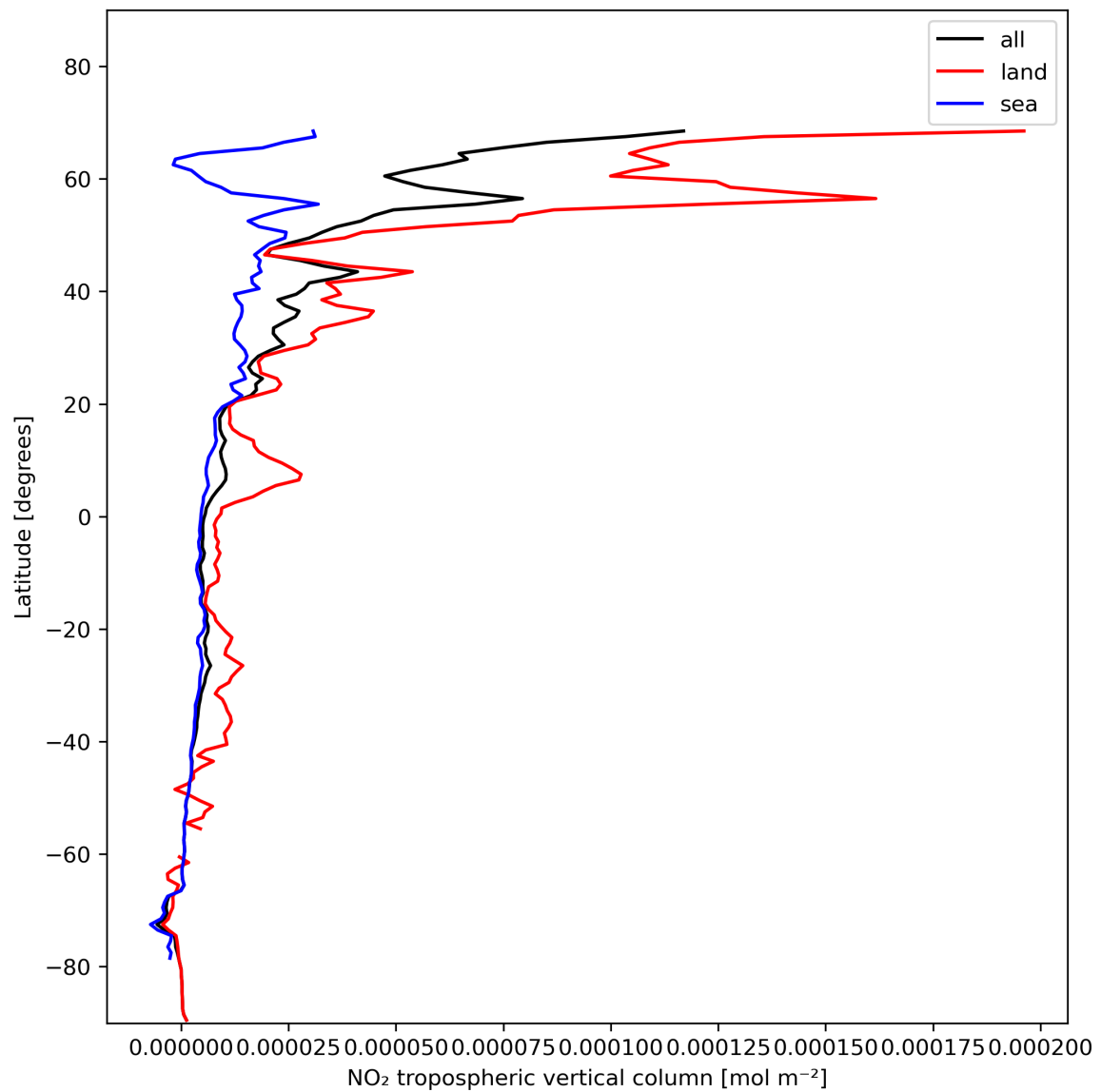
Figure 12: Zonal average of “NO 2 tropospheric vertical column” for 2024-01-22 to 2024-01-24.
