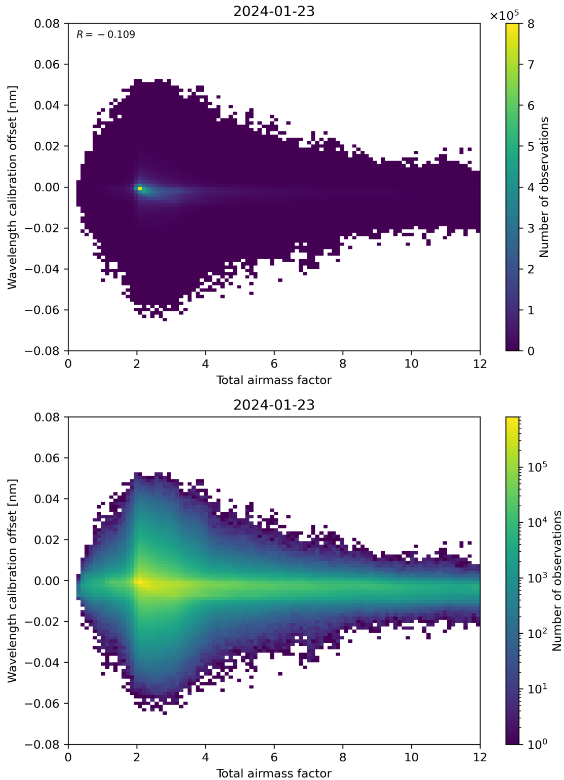
Figure 70: Scatter density plot of “Total airmass factor” against “Wavelength calibration offset” for 2024-01-22 to 2024-01-24.
