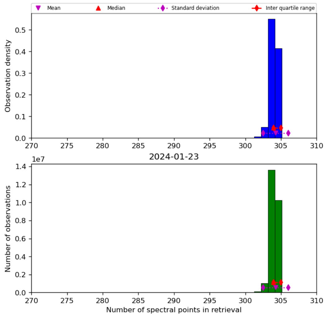
Figure 33: Histogram of “Number of spectral points in retrieval” for 2024-01-22 to 2024-01-24
