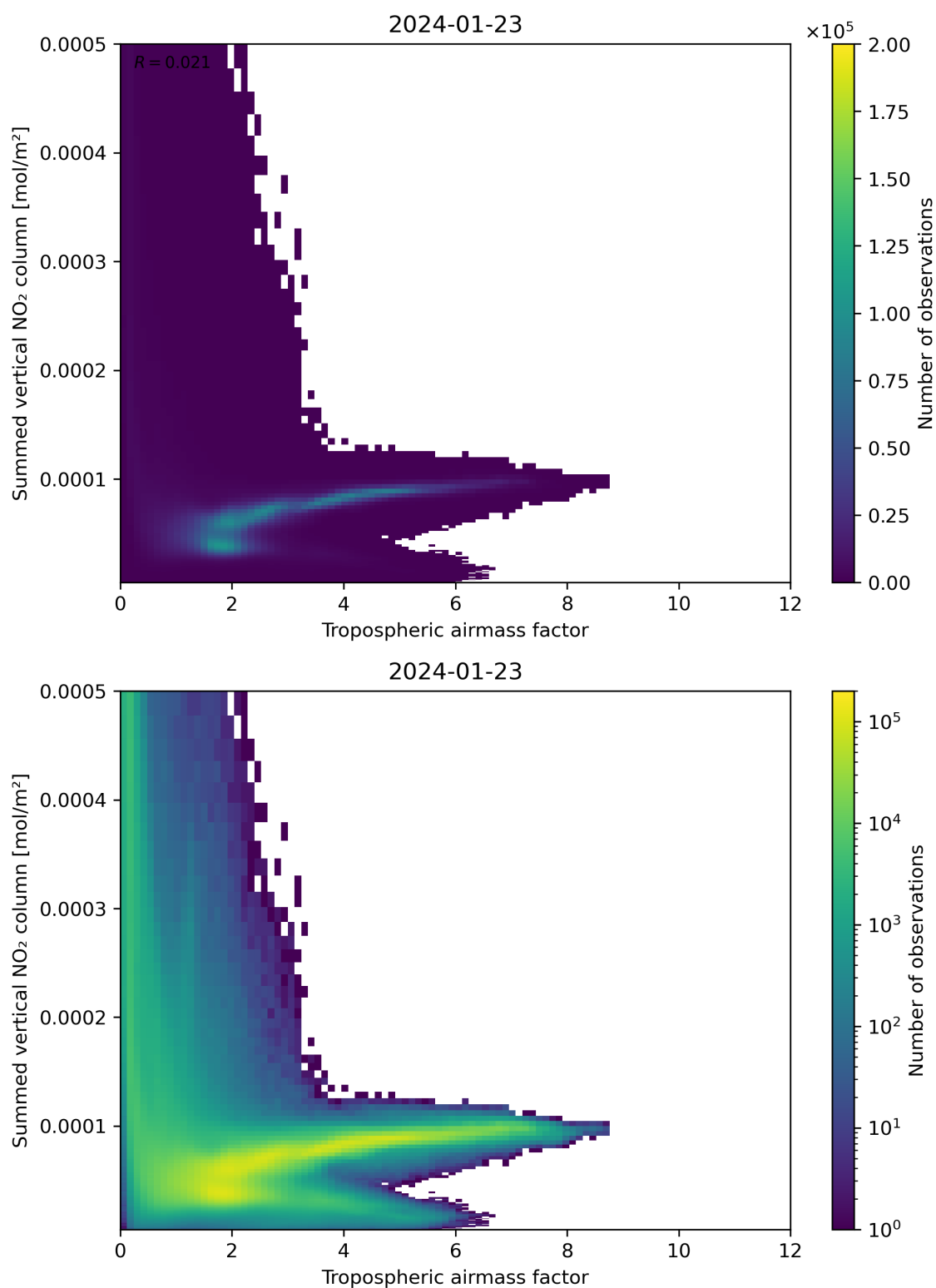
Figure 75: Scatter density plot of “Tropospheric airmass factor” against “Summed vertical NO 2 column” for 2024-01-22 to 2024-01-24.
