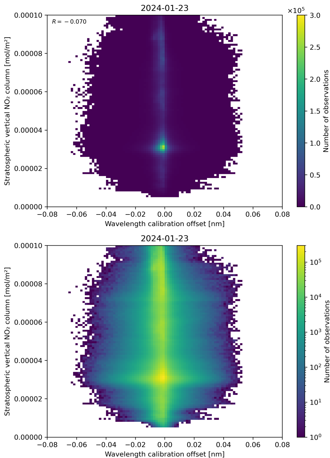
Figure 176: Scatter density plot of “Wavelength calibration offset” against “Stratospheric vertical NO 2 column” for 2024-01-22 to 2024-01-24.
