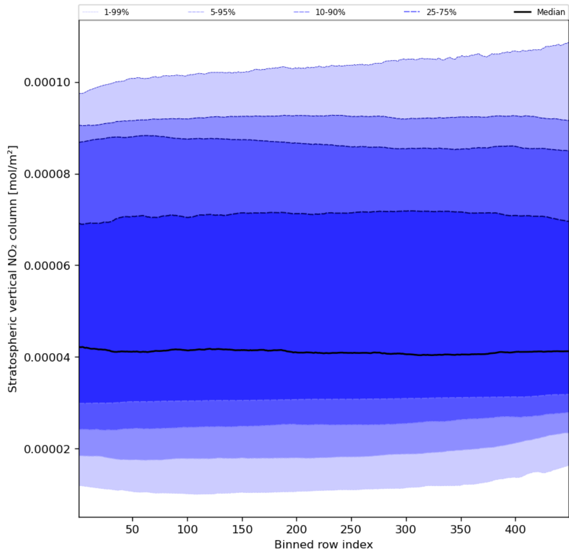
Figure 53: Along track statistics of “Stratospheric vertical NO 2 column” for 2024-01-22 to 2024-01-24
