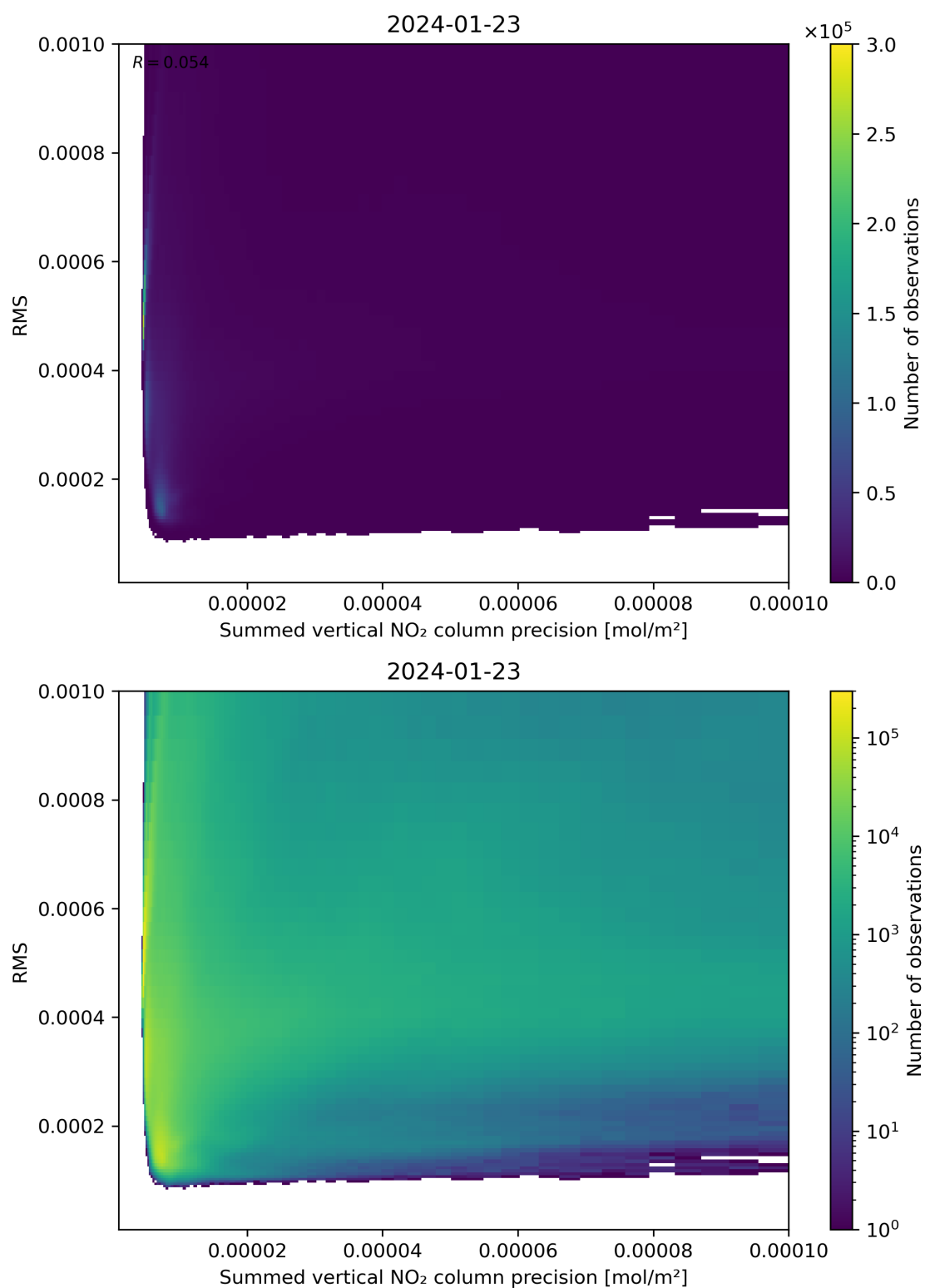
Figure 108: Scatter density plot of “Summed vertical NO 2 column precision” against “RMS” for 2024-01-22 to 2024-01-24.
