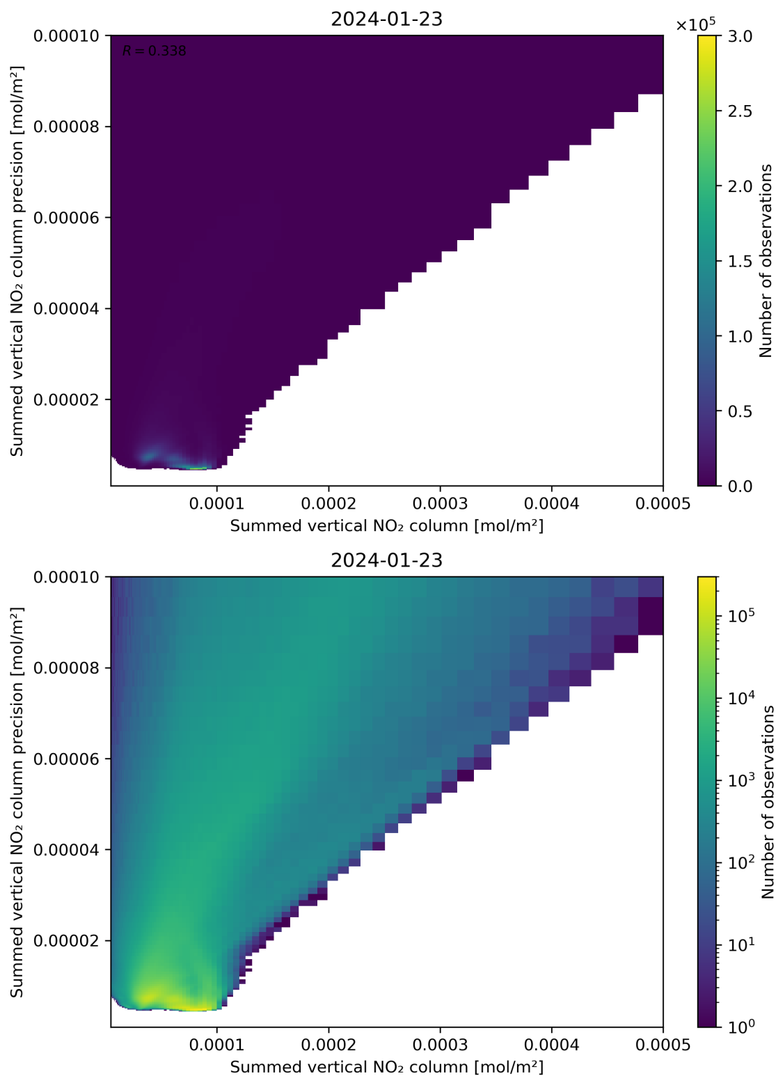
Figure 105: Scatter density plot of “Summed vertical NO 2 column” against “Summed vertical NO 2 column precision” for 2024-01-22 to 2024-01-24.
