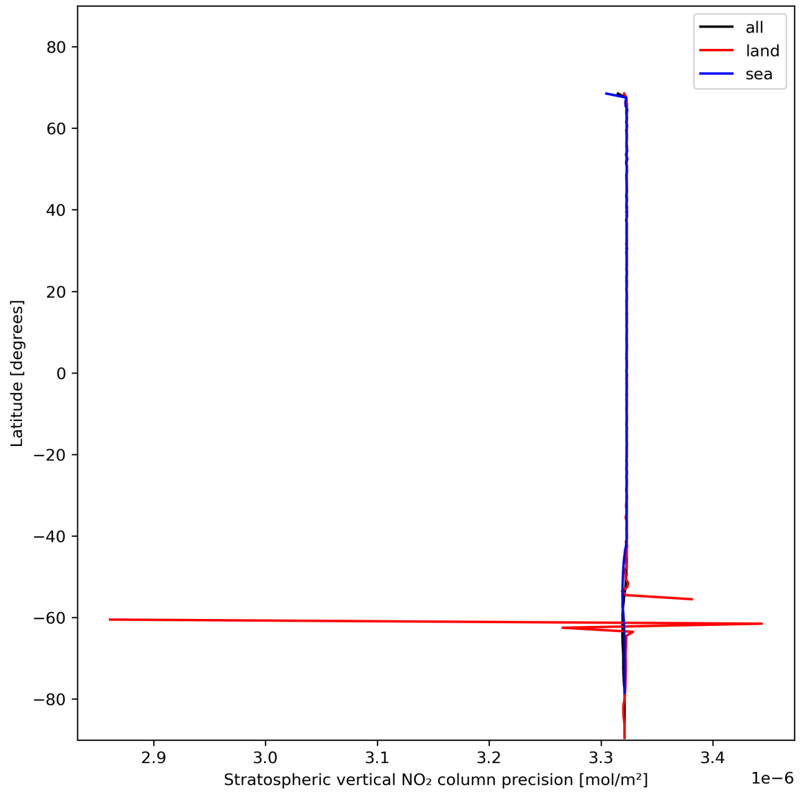
Figure 20: Zonal average of “Stratospheric vertical NO 2 column precision” for 2024-01-22 to 2024-01-24.
