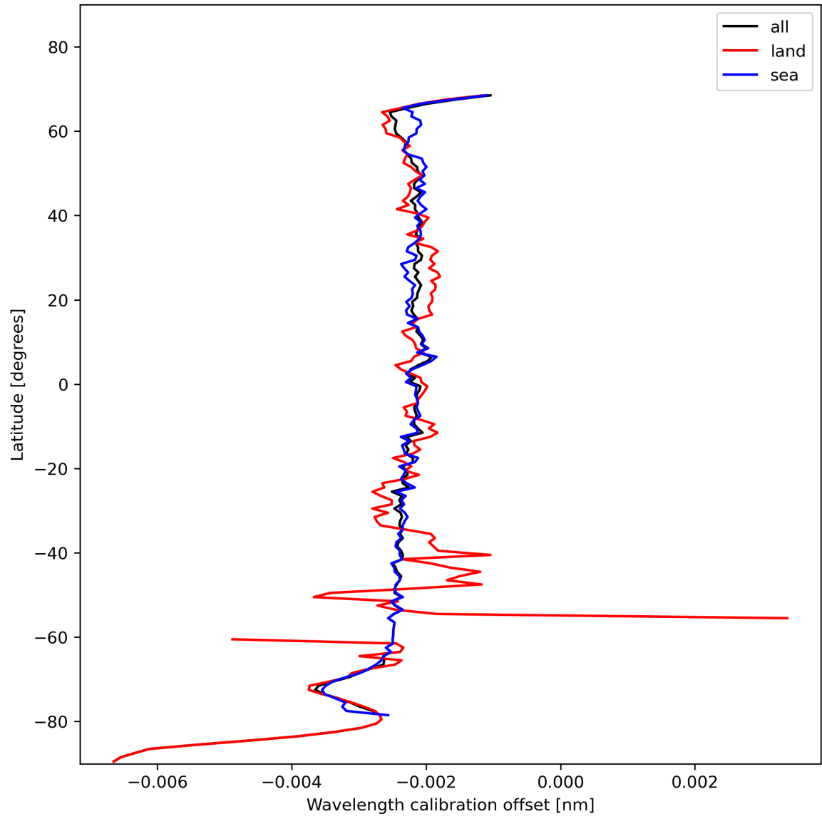
Figure 18: Zonal average of “Wavelength calibration offset” for 2024-01-22 to 2024-01-24.
