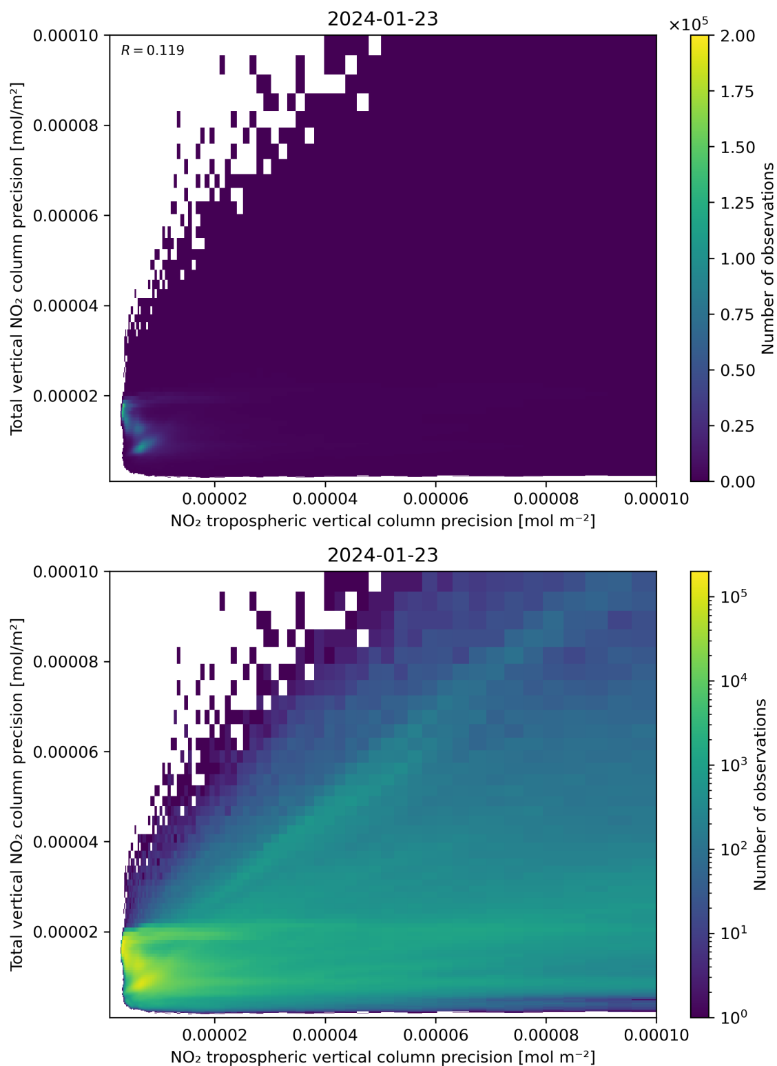
Figure 139: Scatter density plot of “NO 2 tropospheric vertical column precision” against “Total vertical NO 2 column precision” for 2024-01-22 to 2024-01-24.
