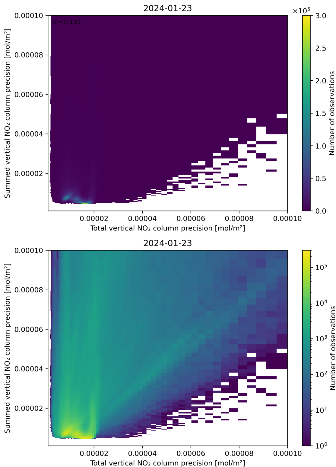
Figure 118: Scatter density plot of “Total vertical NO 2 column precision” against “Summed vertical NO 2 column precision” for 2024-01-22 to 2024-01-24.
