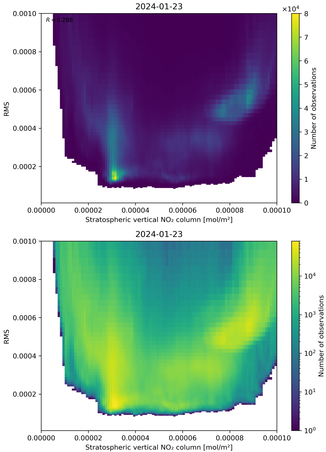
Figure 102: Scatter density plot of “Stratospheric vertical NO 2 column” against “RMS” for 2024-01-22 to 2024-01-24.
