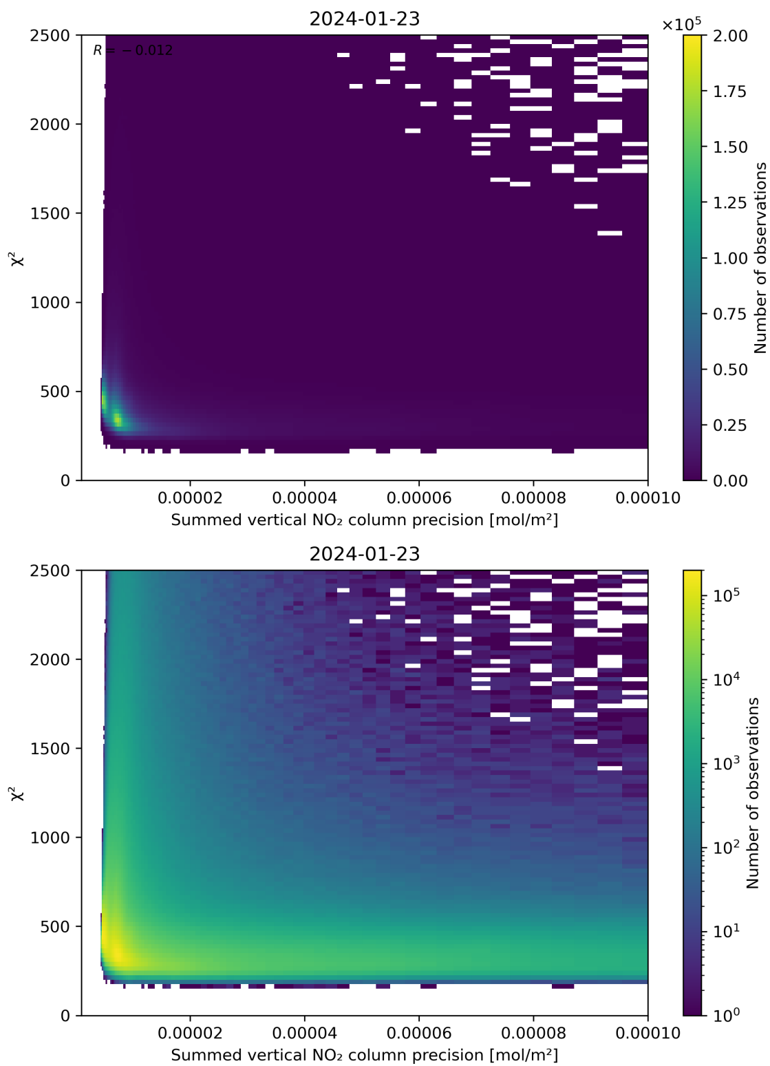
Figure 107: Scatter density plot of “Summed vertical NO 2 column precision” against “ \chi^2 ” for 2024-01-22 to 2024-01-24.
