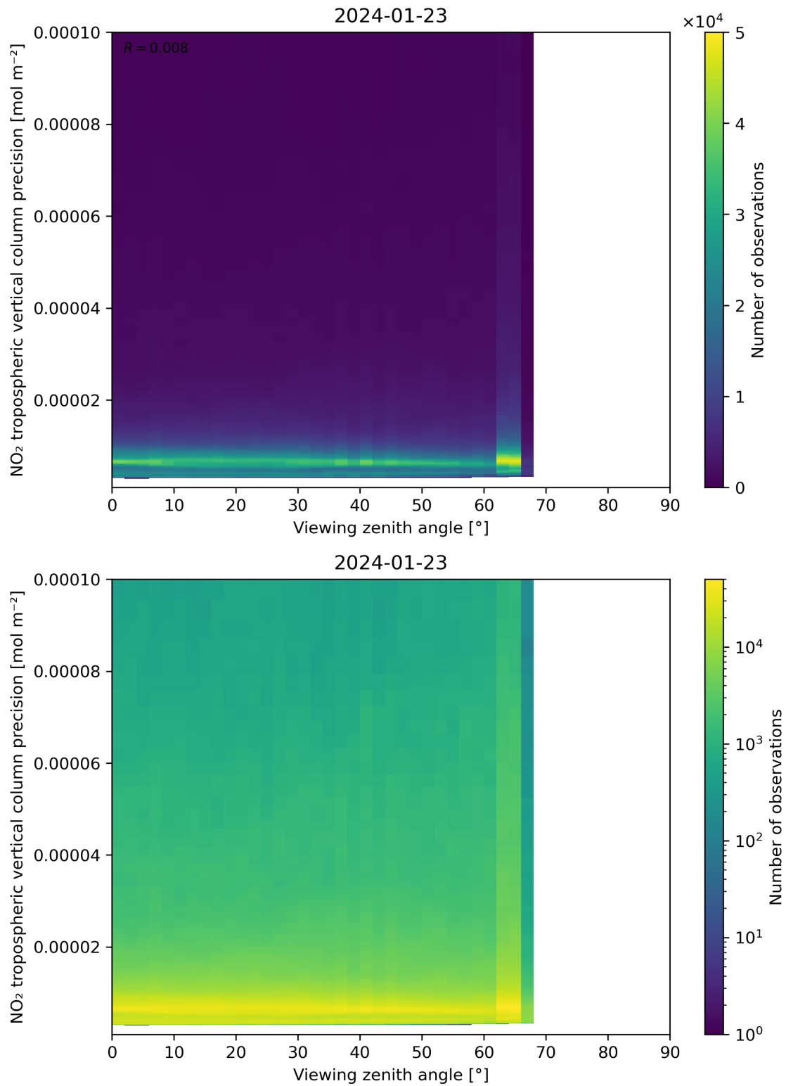
Figure 170: Scatter density plot of “Viewing zenith angle” against “NO 2 tropospheric vertical column precision” for 2024-01-22 to 2024-01-24.
