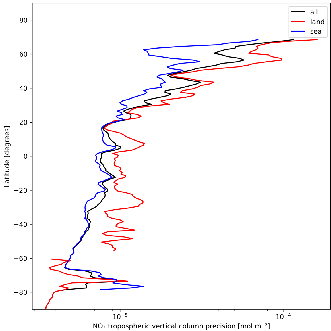
Figure 13: Zonal average of “NO 2 tropospheric vertical column precision” for 2024-01-22 to 2024-01-24.
