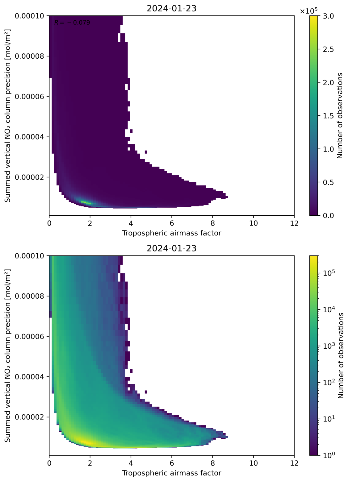
Figure 76: Scatter density plot of “Tropospheric air mass factor” against “Summed vertical NO 2 column precision” for 2024-01-22 to 2024-01-24.
