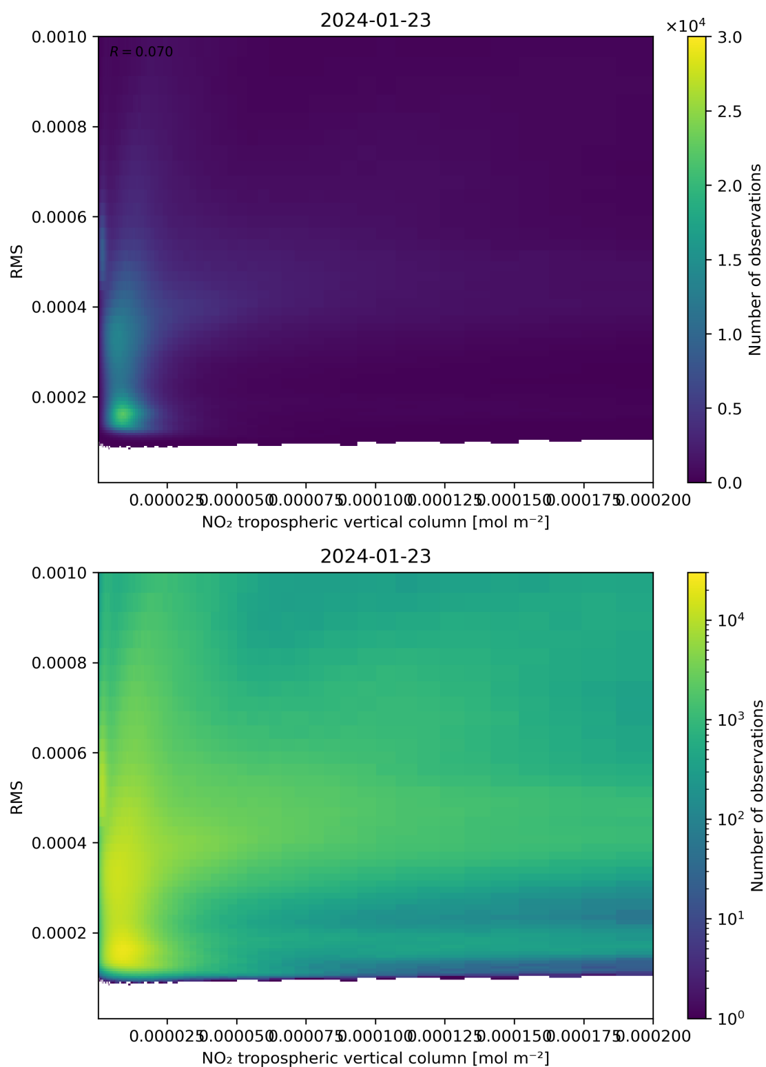
Figure 142: Scatter density plot of “NO 2 tropospheric vertical column” against “RMS” for 2024-01-22 to 2024-01-24.
