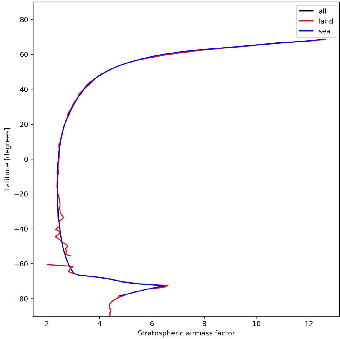
Figure 27: Zonal average of “Stratospheric airmass factor” for 2024-01-22 to 2024-01-24.
