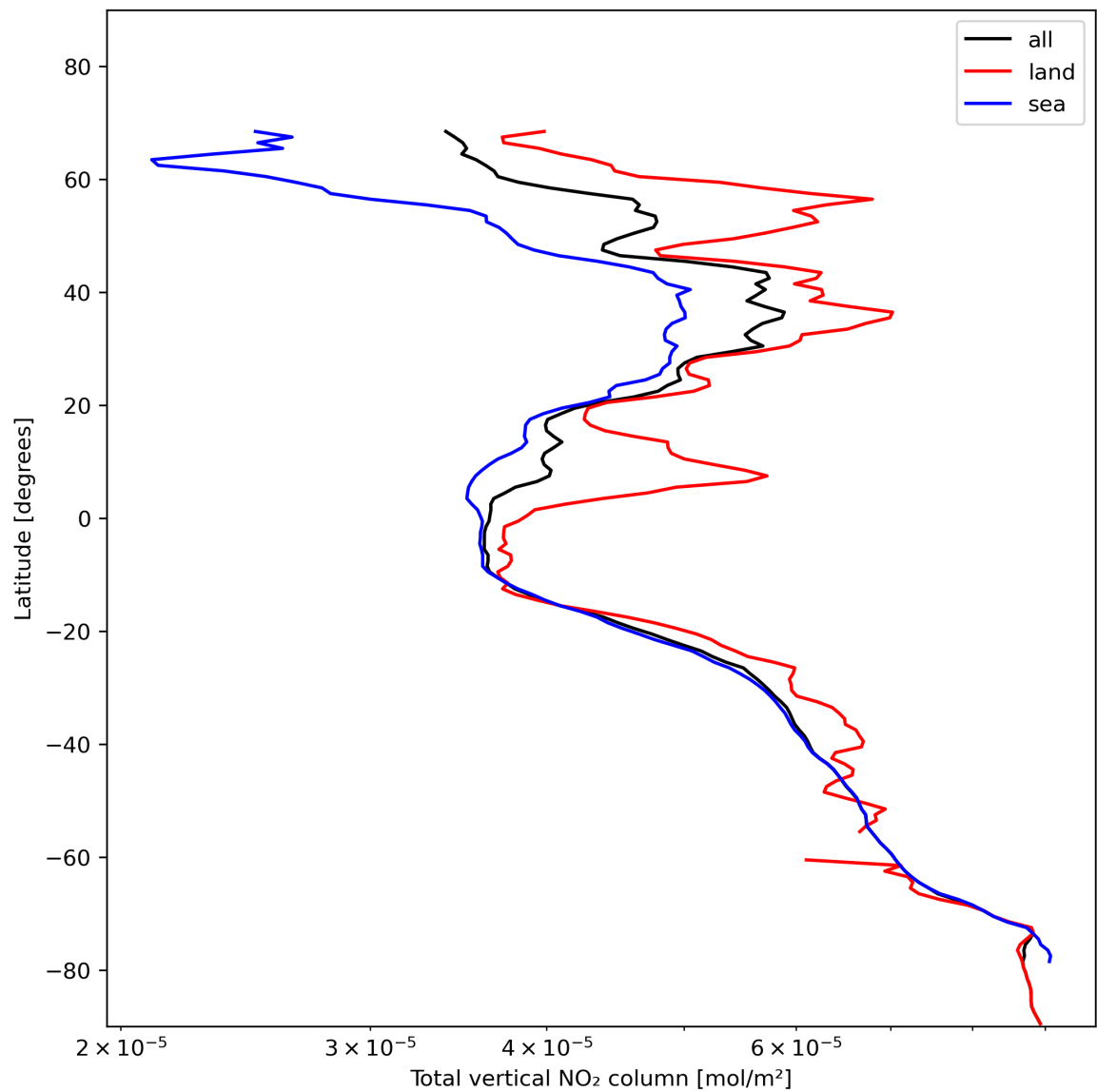
Figure 21: Zonal average of “Total vertical NO 2 column” for 2024-01-22 to 2024-01-24.
