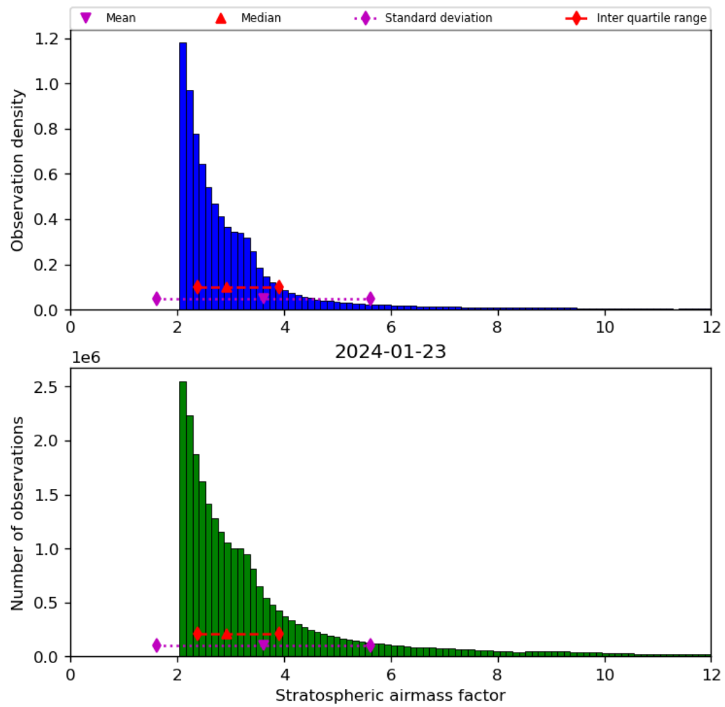
Figure 44: Histogram of “Stratospheric airmass factor” for 2024-01-22 to 2024-01-24
