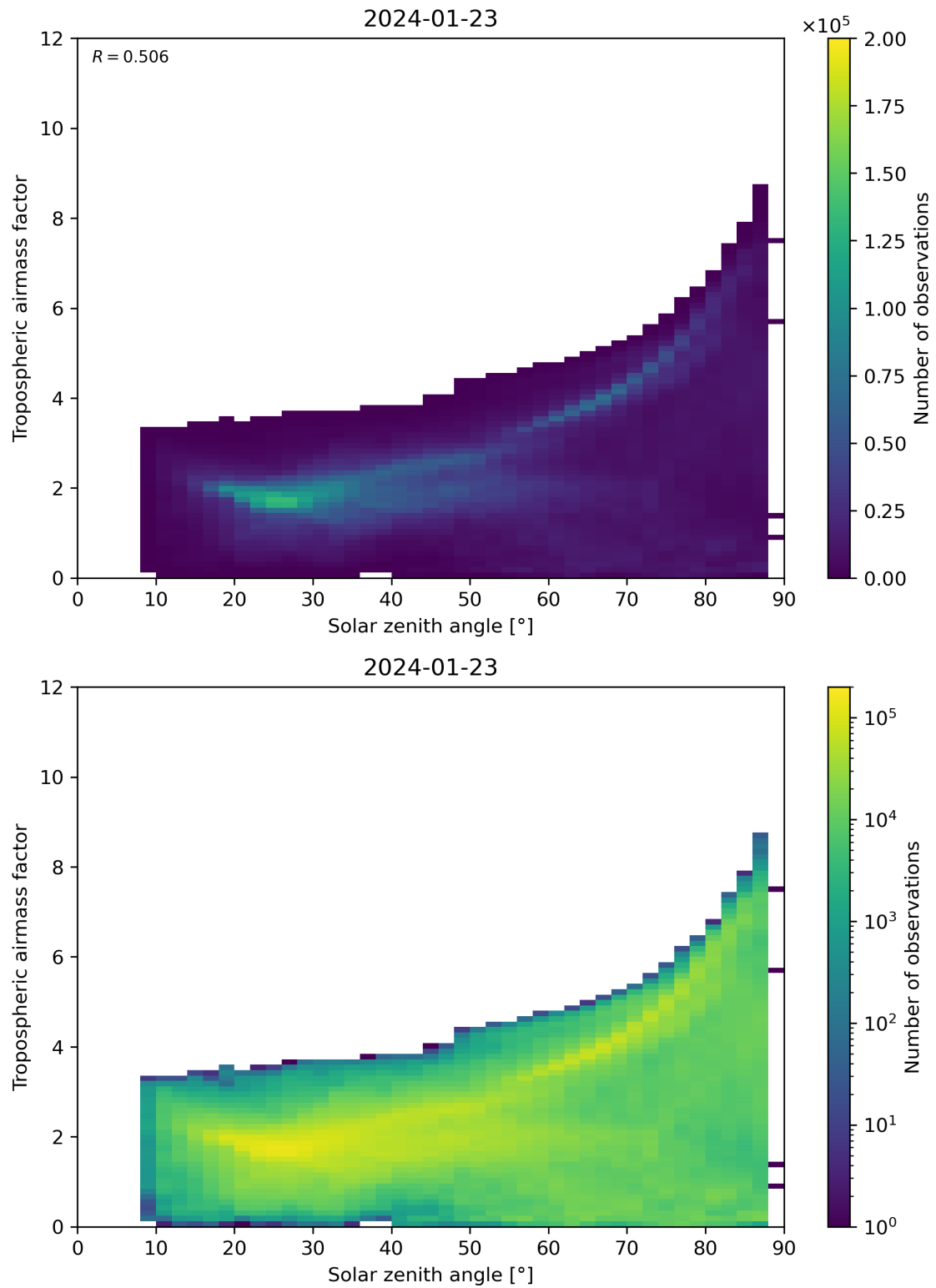
Figure 147: Scatter density plot of “Solar zenith angle” against “Tropospheric airmass factor” for 2024-01-22 to 2024-01-24.
