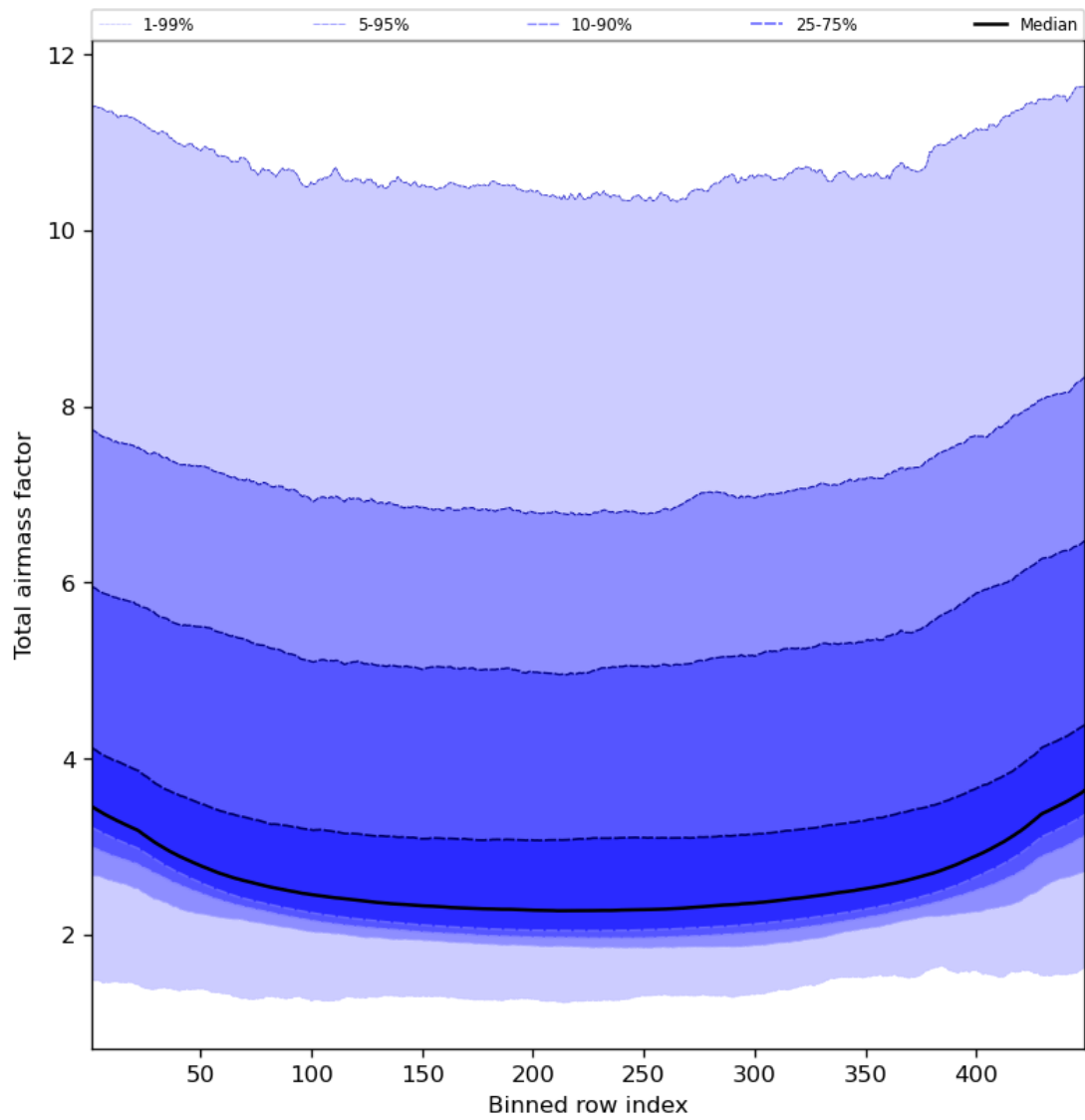
Figure 49: Along track statistics of “Total airmass factor” for 2024-01-22 to 2024-01-24
