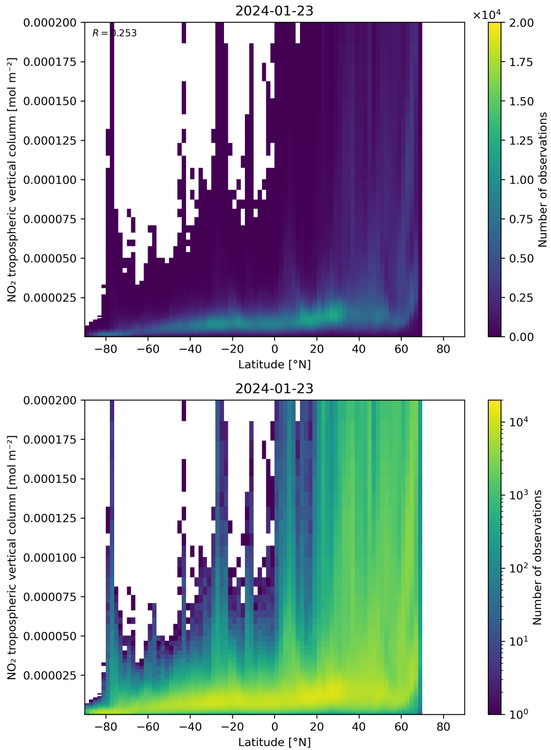
Figure 92: Scatter density plot of “Latitude” against “NO 2 tropospheric vertical column” for 2024-01-22 to 2024-01-24.
