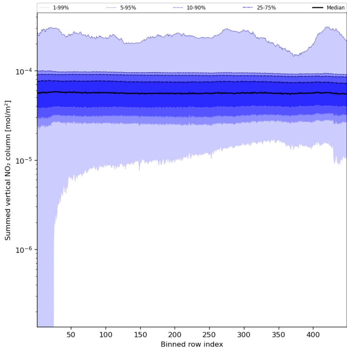
Figure 57: Along track statistics of “Summed vertical NO 2 column” for 2024-01-22 to 2024-01-24
