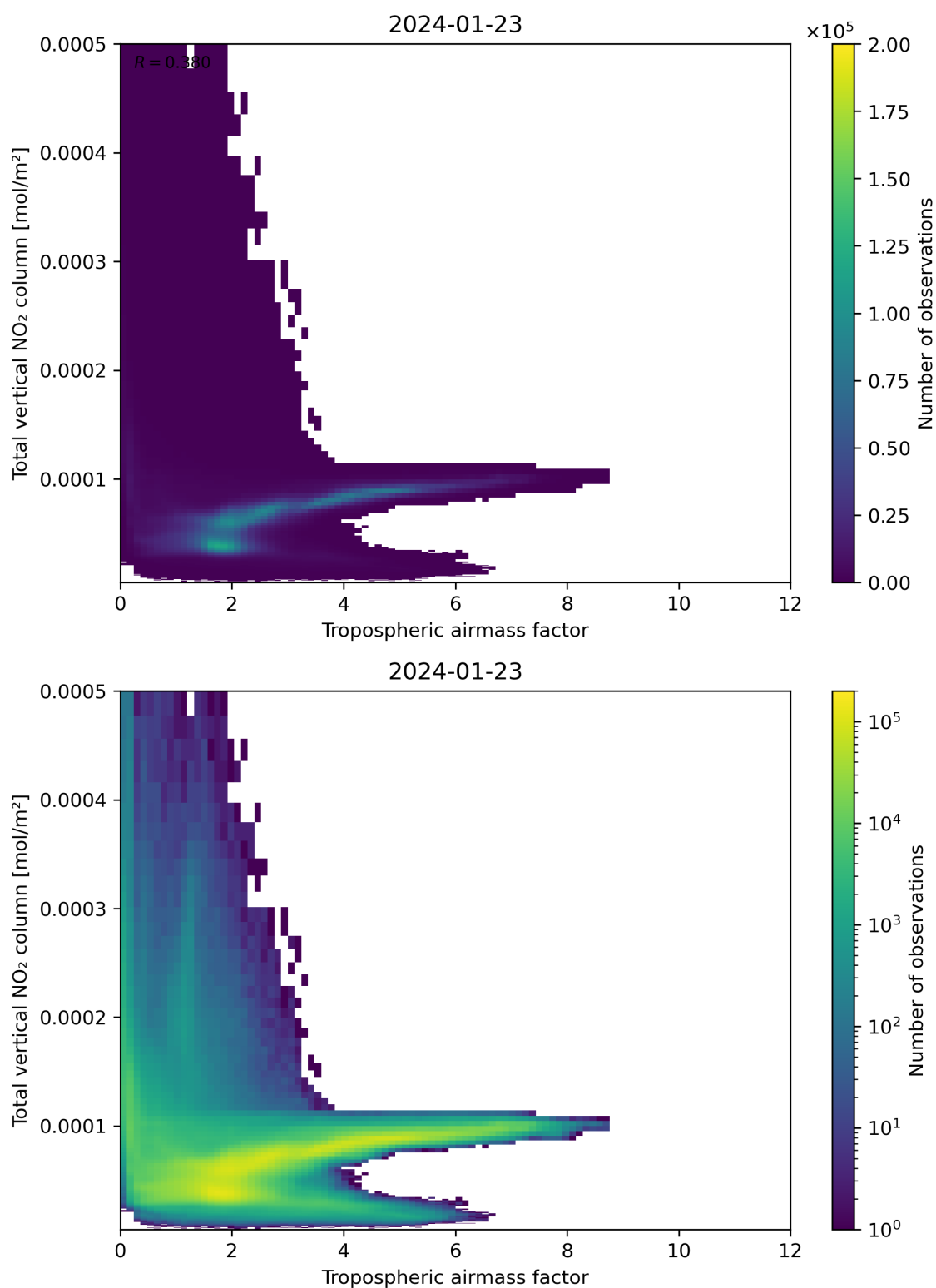
Figure 77: Scatter density plot of “Tropospheric airmass factor” against “Total vertical NO 2 column” for 2024-01-22 to 2024-01-24.
