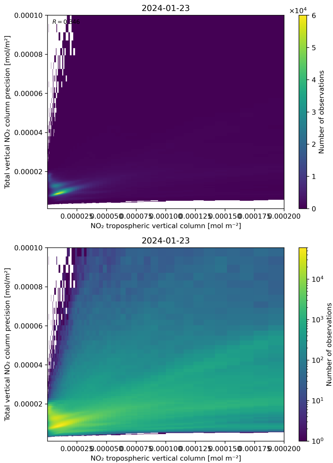
Figure 129: Scatter density plot of “NO 2 tropospheric vertical column” against “Total vertical NO 2 column precision” for 2024-01-22 to 2024-01-24.
