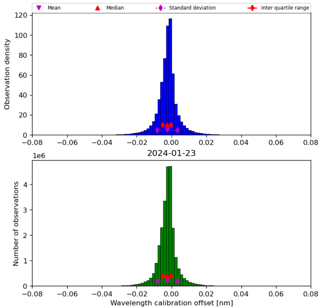
Figure 35: Histogram of “Wavelength calibration offset” for 2024-01-22 to 2024-01-24
