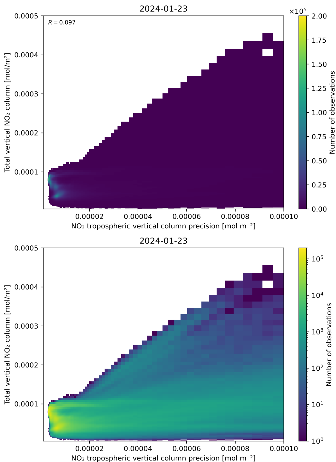
Figure 138: Scatter density plot of “NO 2 tropospheric vertical column precision” against “Total vertical NO 2 column” for 2024-01-22 to 2024-01-24.
