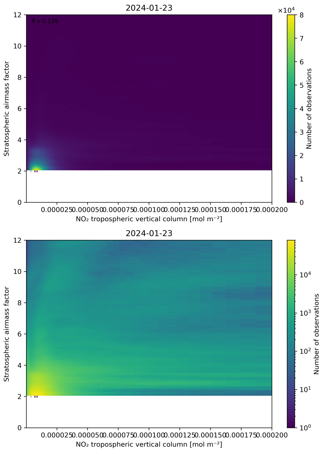
Figure 121: Scatter density plot of “NO 2 tropospheric vertical column” against “Stratospheric airmass factor” for 2024-01-22 to 2024-01-24.
