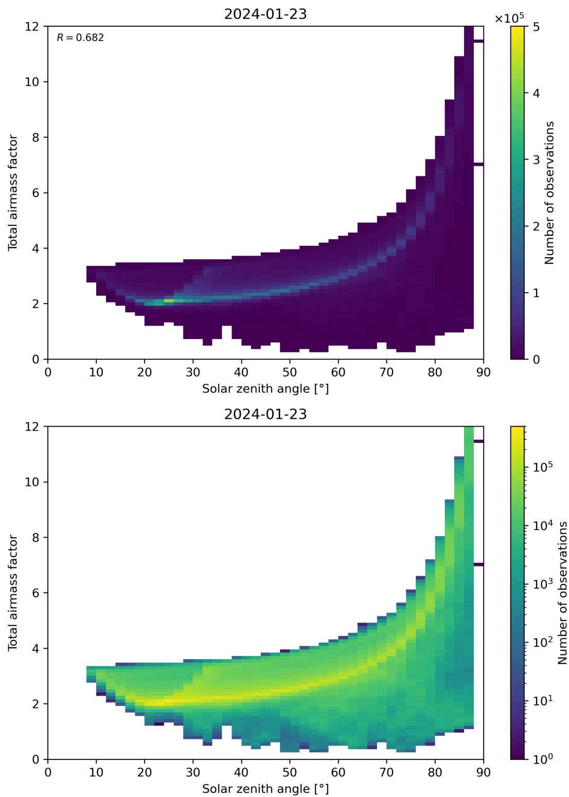
Figure 146: Scatter density plot of “Solar zenith angle” against “Total air mass factor” for 2024-01-22 to 2024-01-24.
