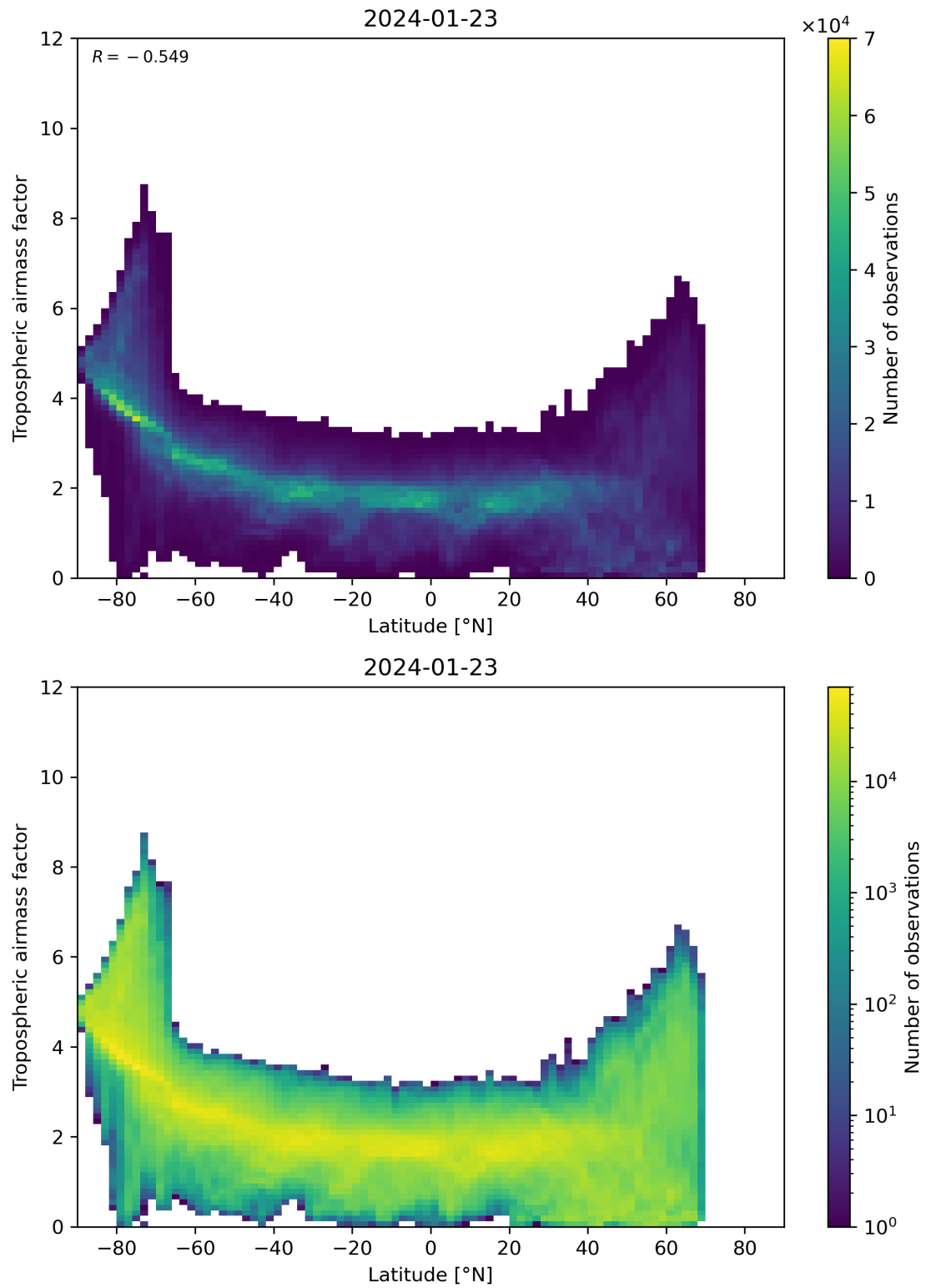
Figure 85: Scatter density plot of “Latitude” against “Tropospheric airmass factor” for 2024-01-22 to 2024-01-24.
