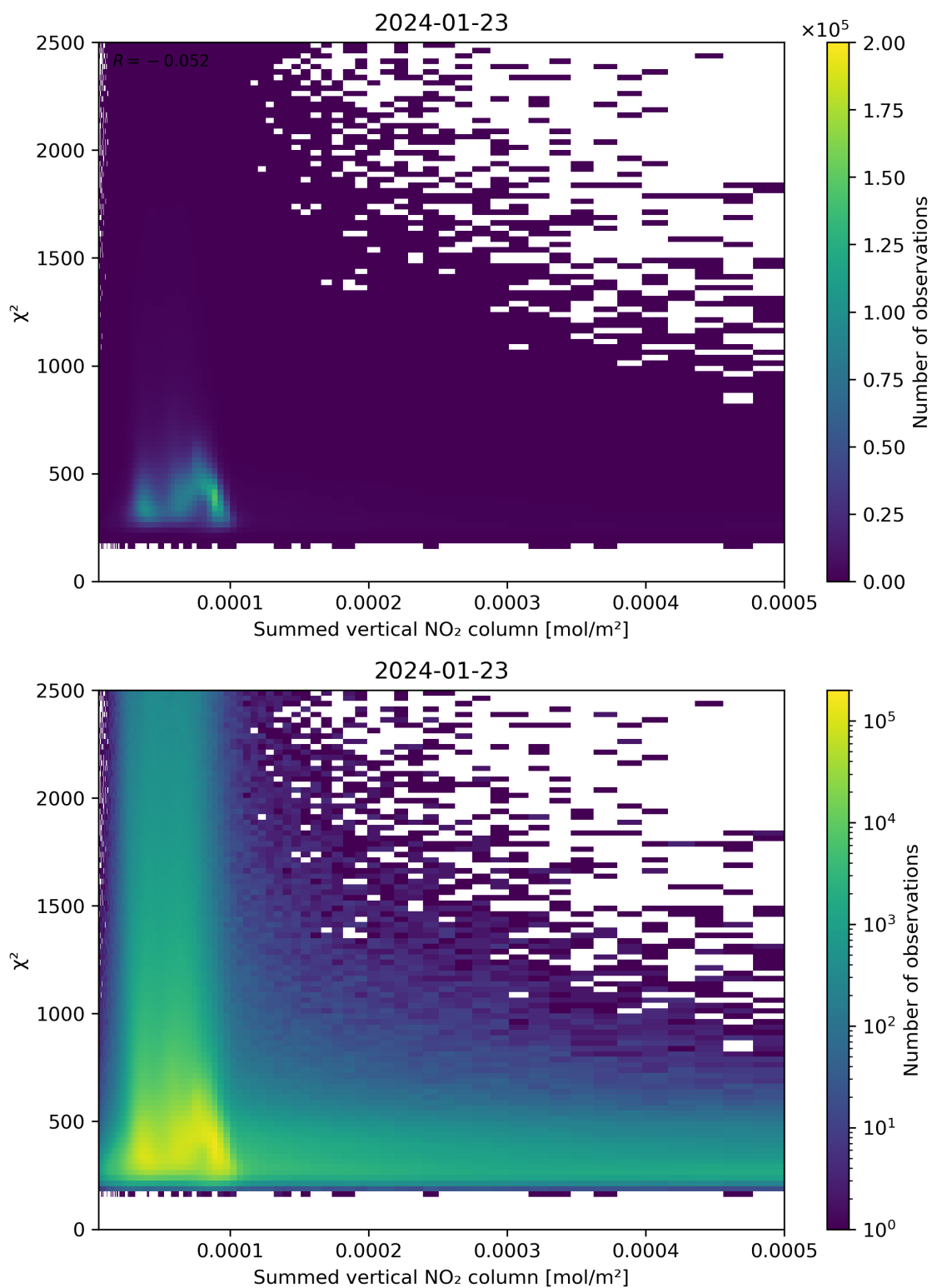
Figure 104: Scatter density plot of “Summed vertical NO 2 column” against “ \chi^2 ” for 2024-01-22 to 2024-01-24.
