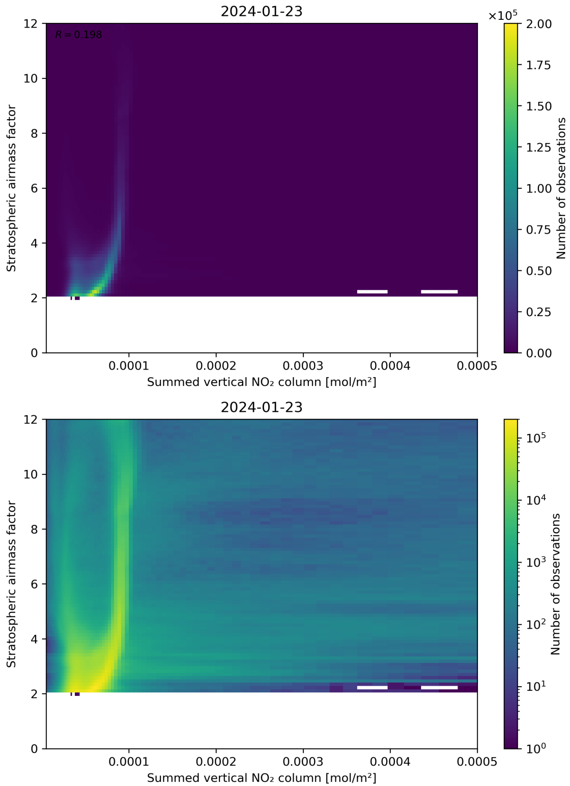
Figure 103: Scatter density plot of “Summed vertical NO 2 column” against “Stratospheric airmass factor” for 2024-01-22 to 2024-01-24.
