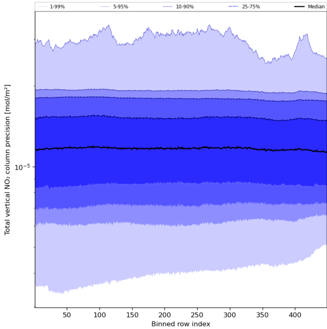
Figure 56: Along track statistics of “Total vertical NO 2 column precision” for 2024-01-22 to 2024-01-24
