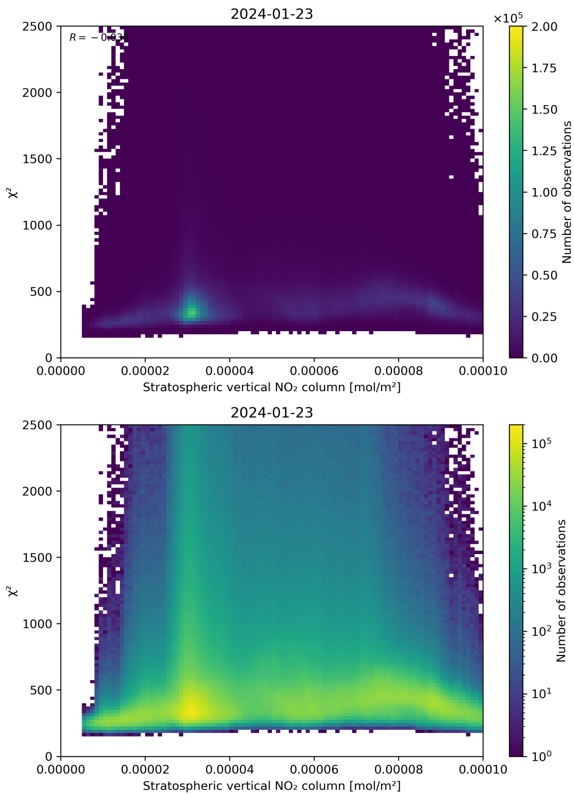
Figure 97: Scatter density plot of “Stratospheric vertical NO 2 column” against “ \chi^2 ” for 2024-01-22 to 2024-01-24.
