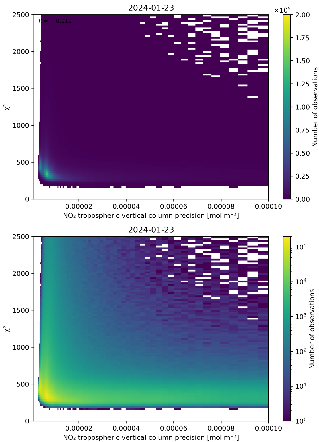
Figure 134: Scatter density plot of “NO 2 tropospheric vertical column precision” against “ \chi^2 ” for 2024-01-22 to 2024-01-24.
