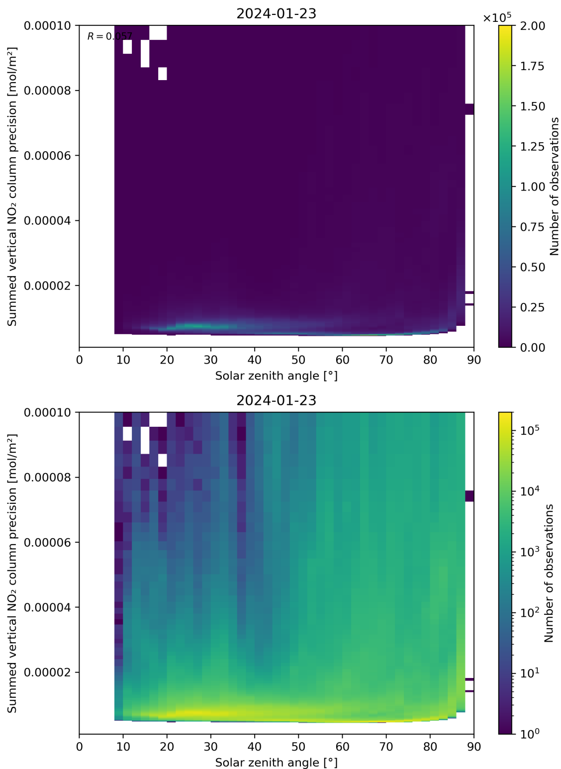
Figure 152: Scatter density plot of “Solar zenith angle” against “Summed vertical NO 2 column precision” for 2024-01-22 to 2024-01-24.
