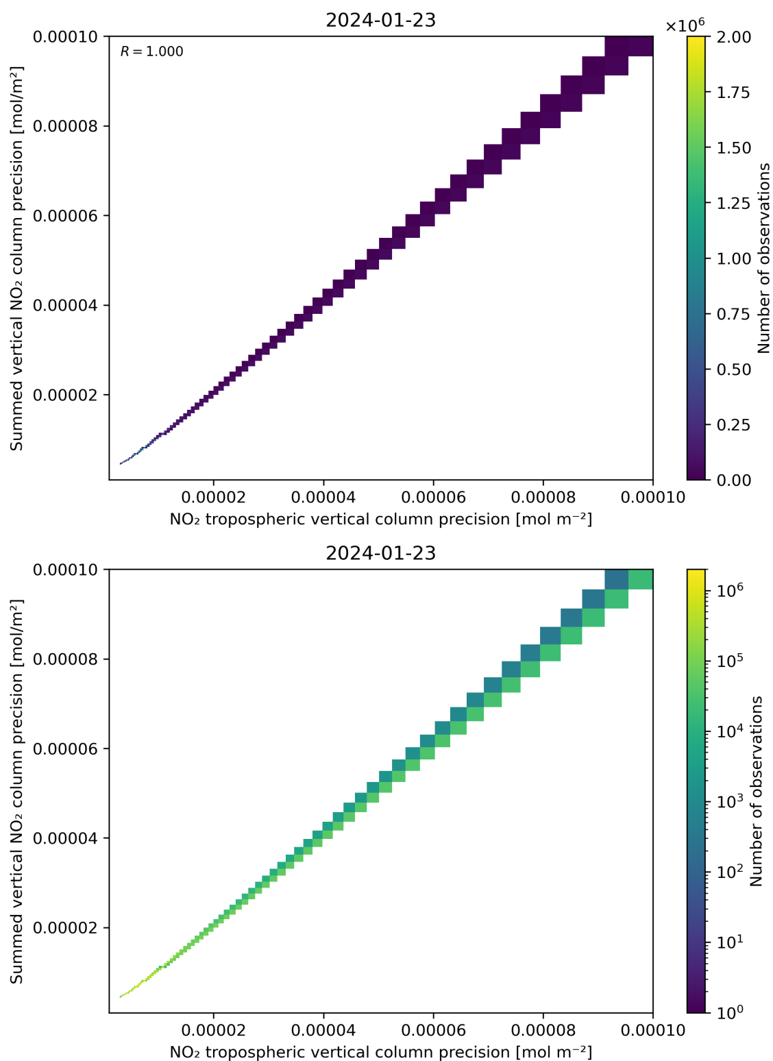
Figure 137: Scatter density plot of “NO 2 tropospheric vertical column precision” against “Summed vertical NO 2 column precision” for 2024-01-22 to 2024-01-24.
