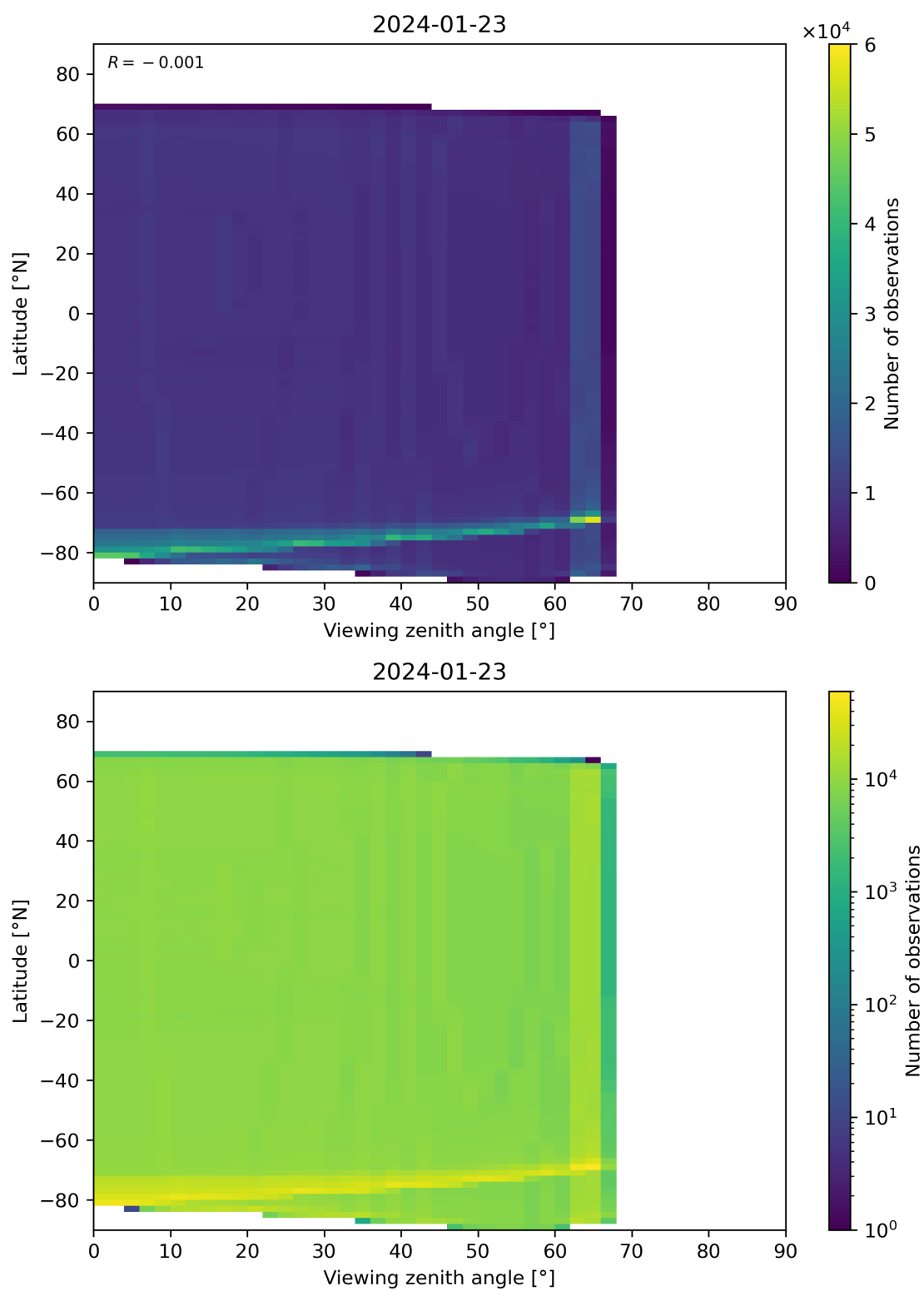
Figure 163: Scatter density plot of “Viewing zenith angle” against “Latitude” for 2024-01-22 to 2024-01-24.
