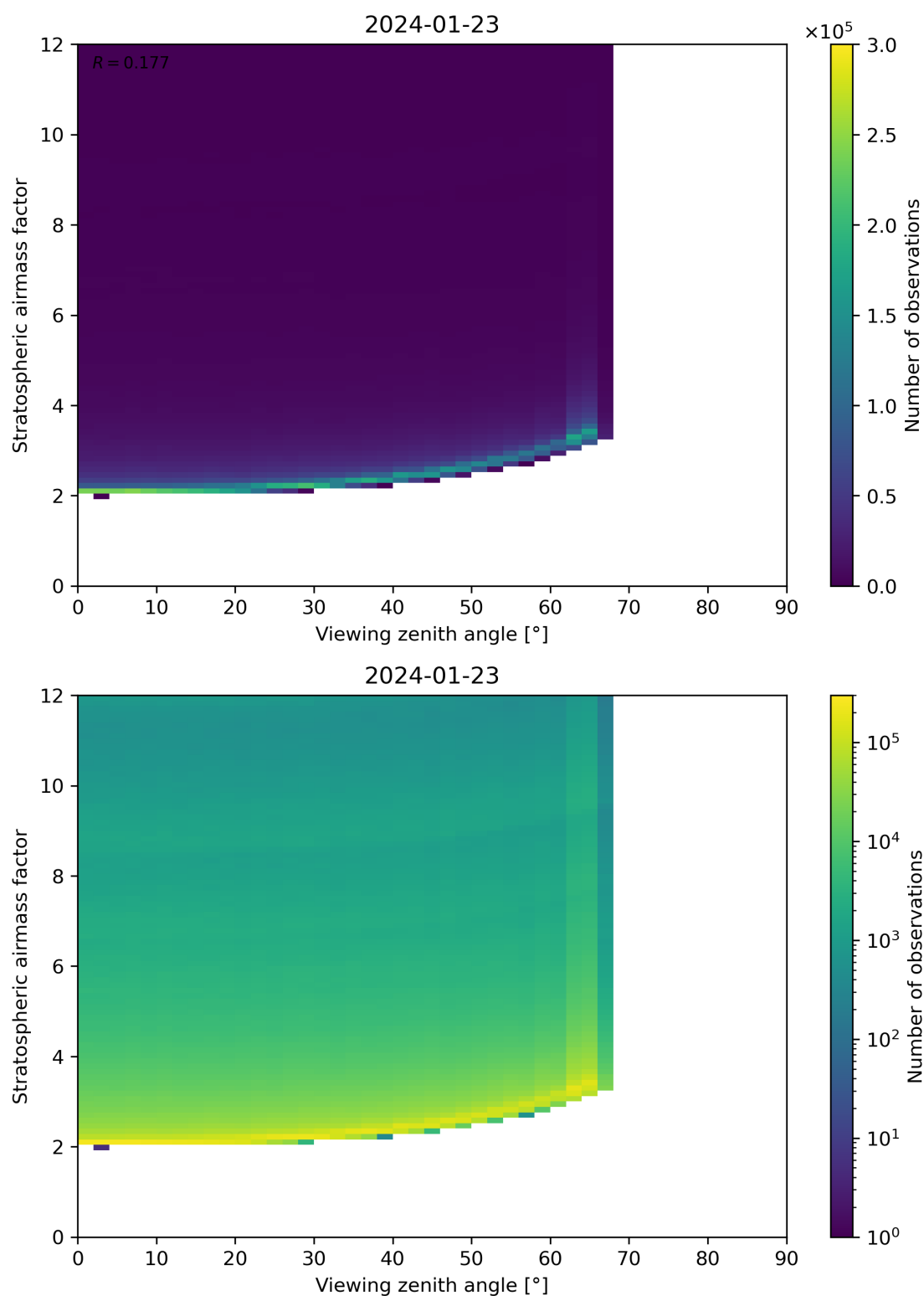
Figure 159: Scatter density plot of “Viewing zenith angle” against “Stratospheric airmass factor” for 2024-01-22 to 2024-01-24.
