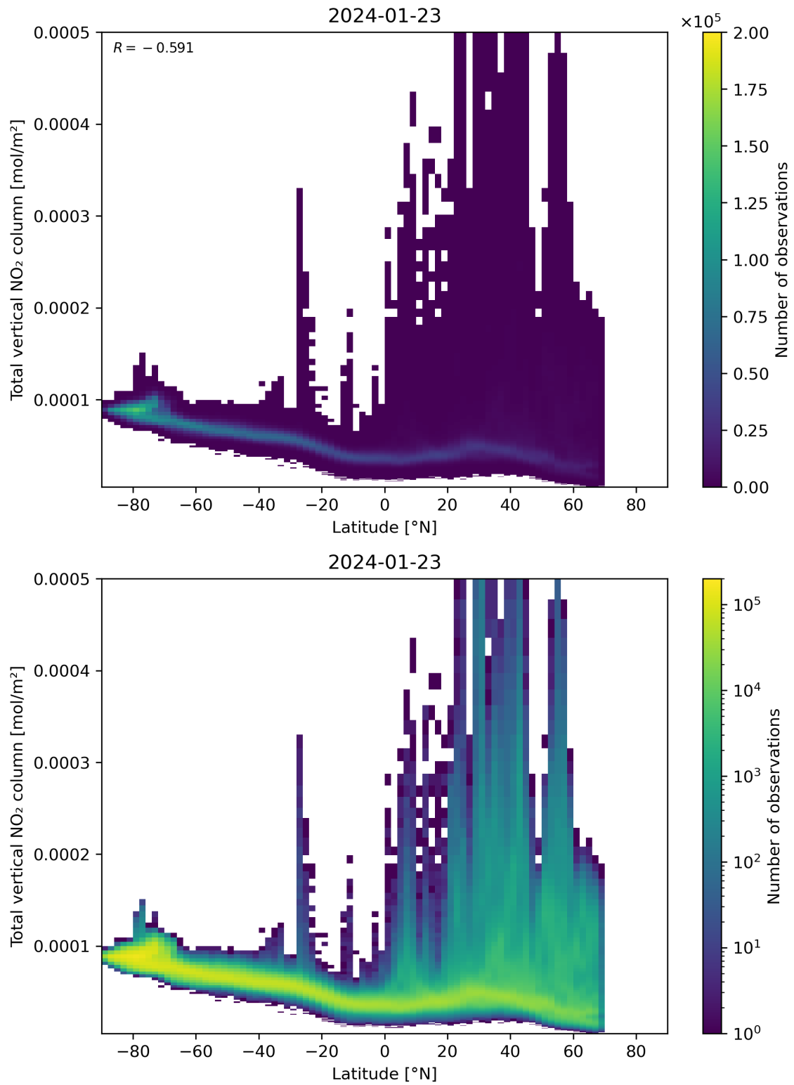
Figure 90: Scatter density plot of “Latitude” against “Total vertical NO 2 column” for 2024-01-22 to 2024-01-24.
