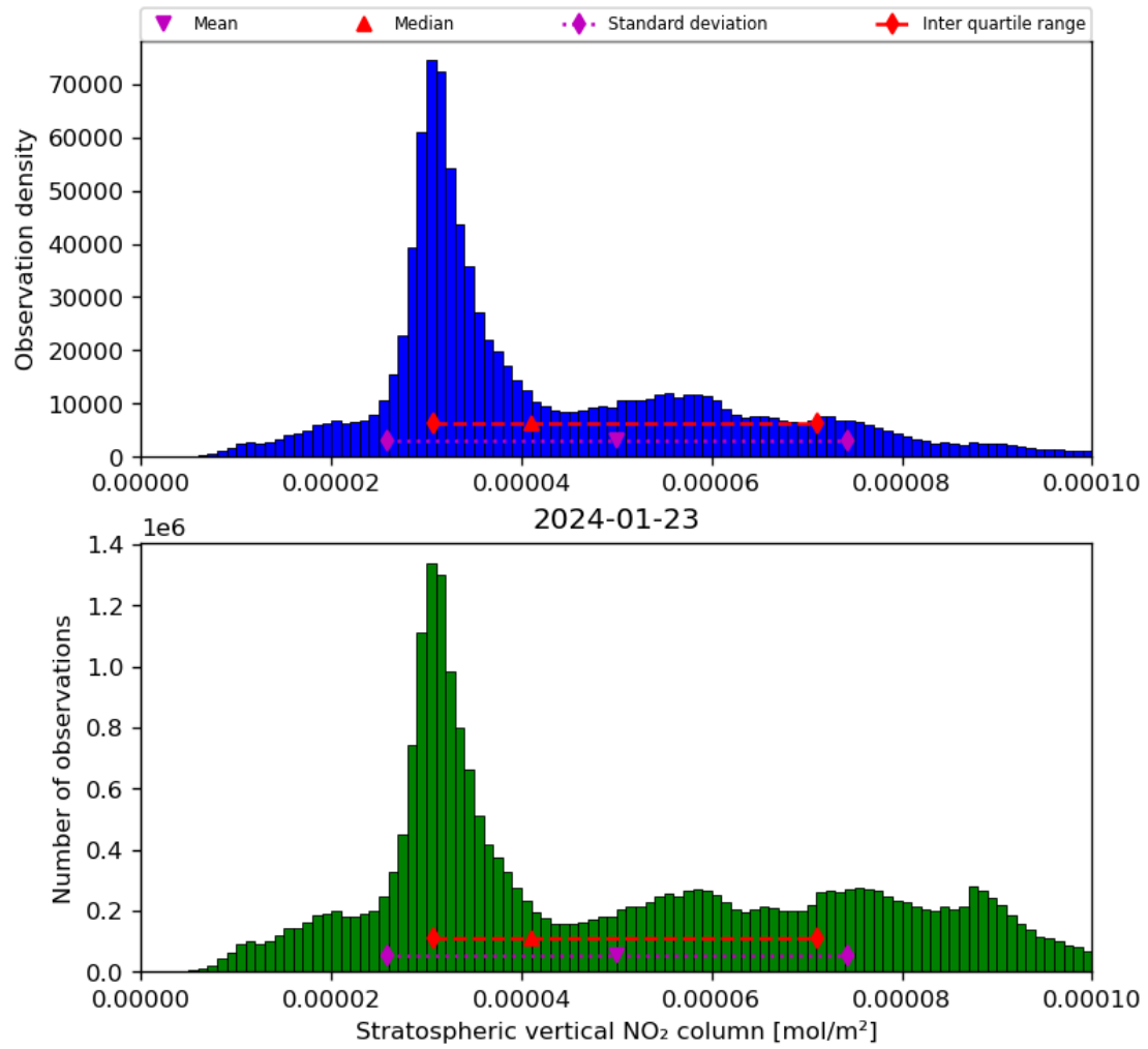
Figure 36: Histogram of “Stratospheric vertical NO 2 column” for 2024-01-22 to 2024-01-24
