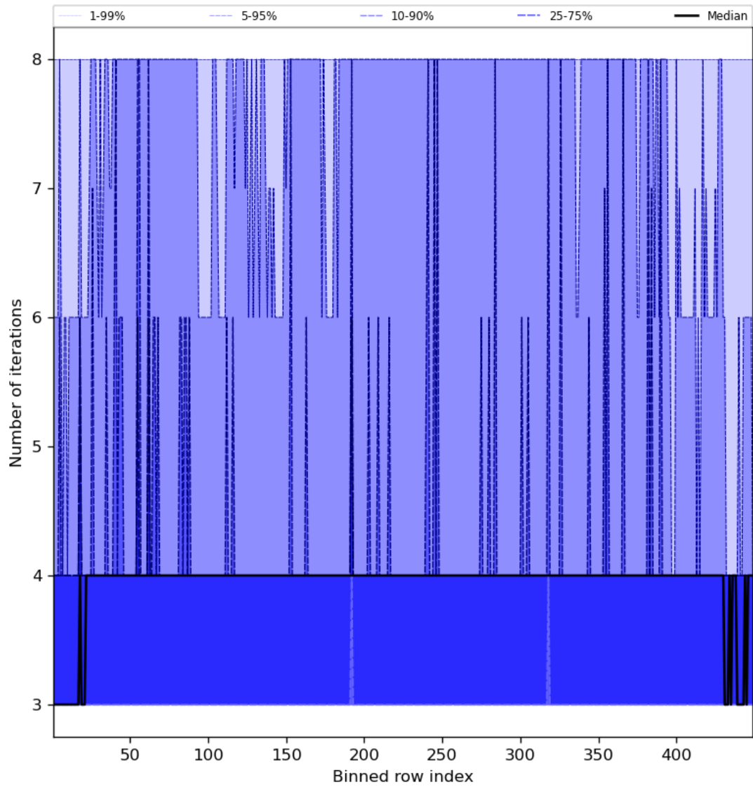
Figure 51: Along track statistics of “Number of iterations” for 2024-01-22 to 2024-01-24
