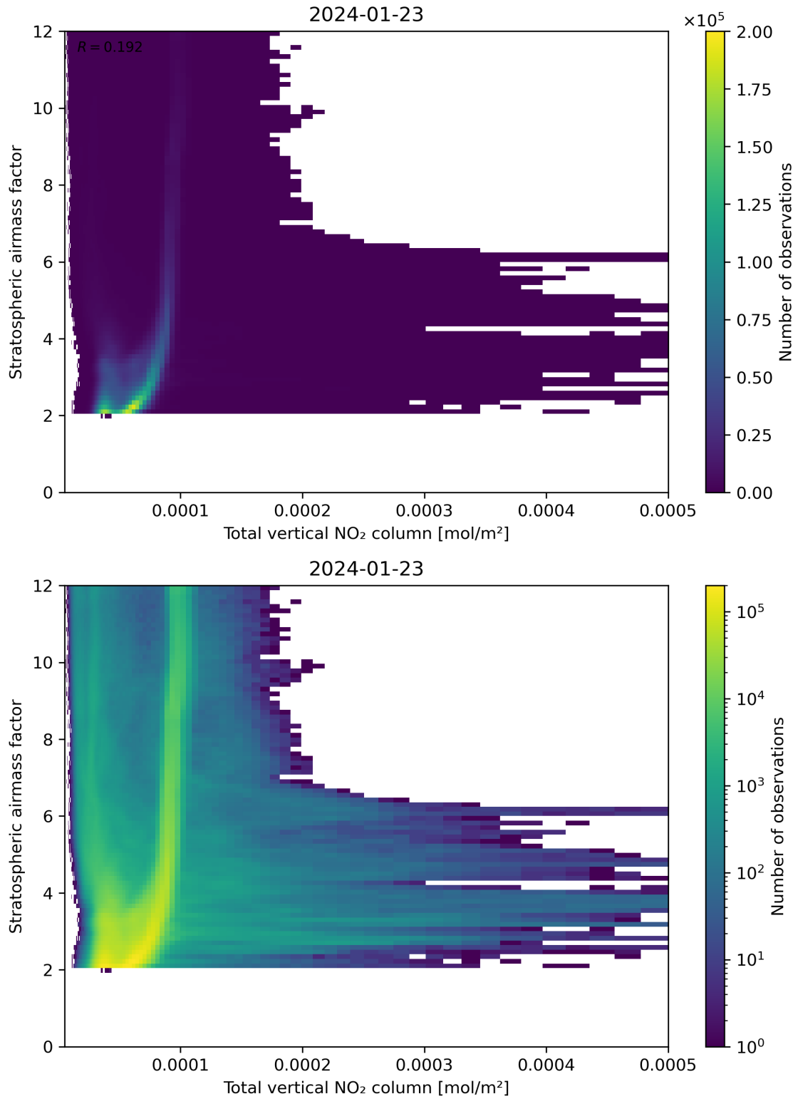
Figure 110: Scatter density plot of “Total vertical NO 2 column” against “Stratospheric airmass factor” for 2024-01-22 to 2024-01-24.
