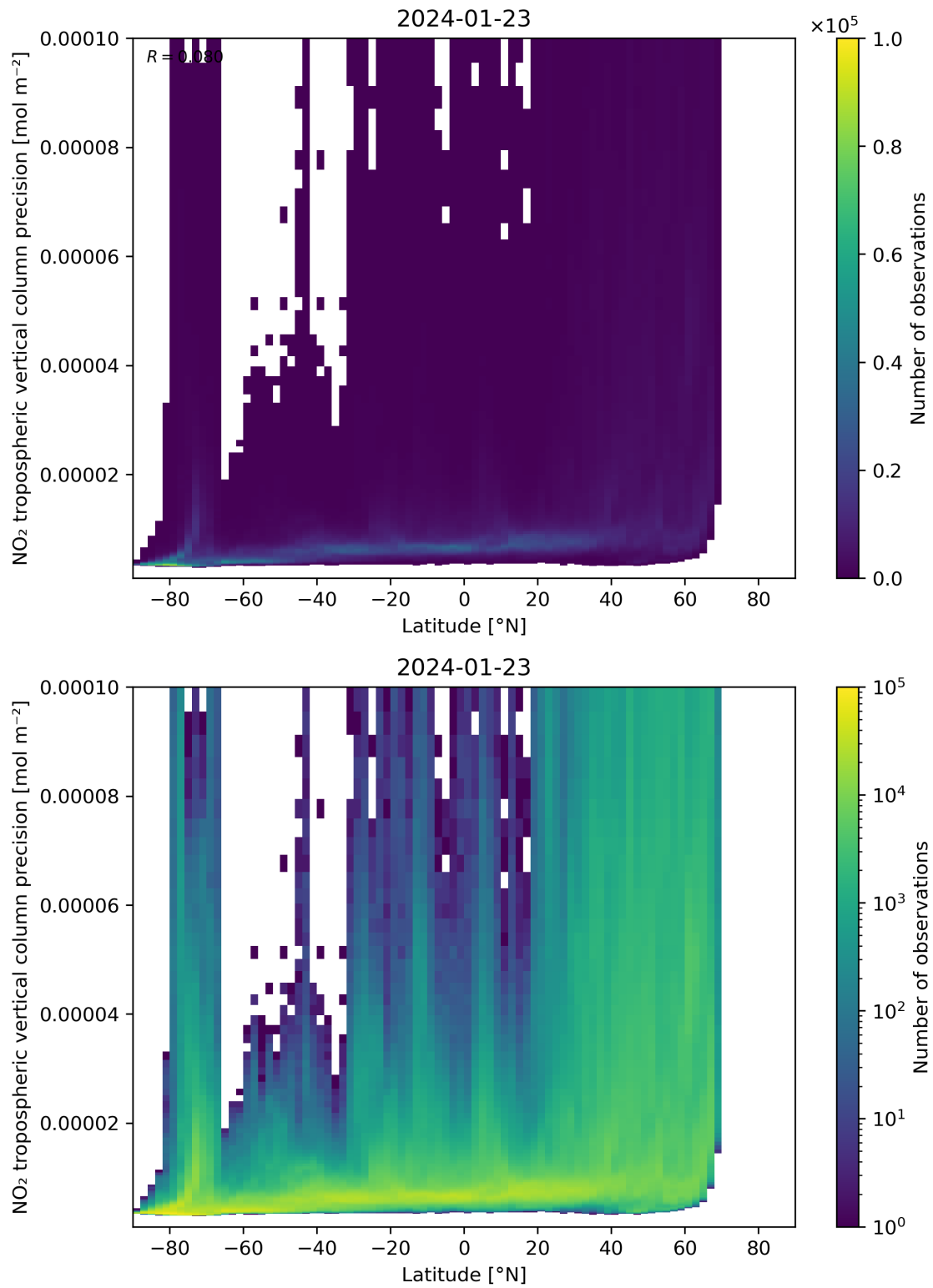
Figure 93: Scatter density plot of “Latitude” against “NO 2 tropospheric vertical column precision” for 2024-01-22 to 2024-01-24.
