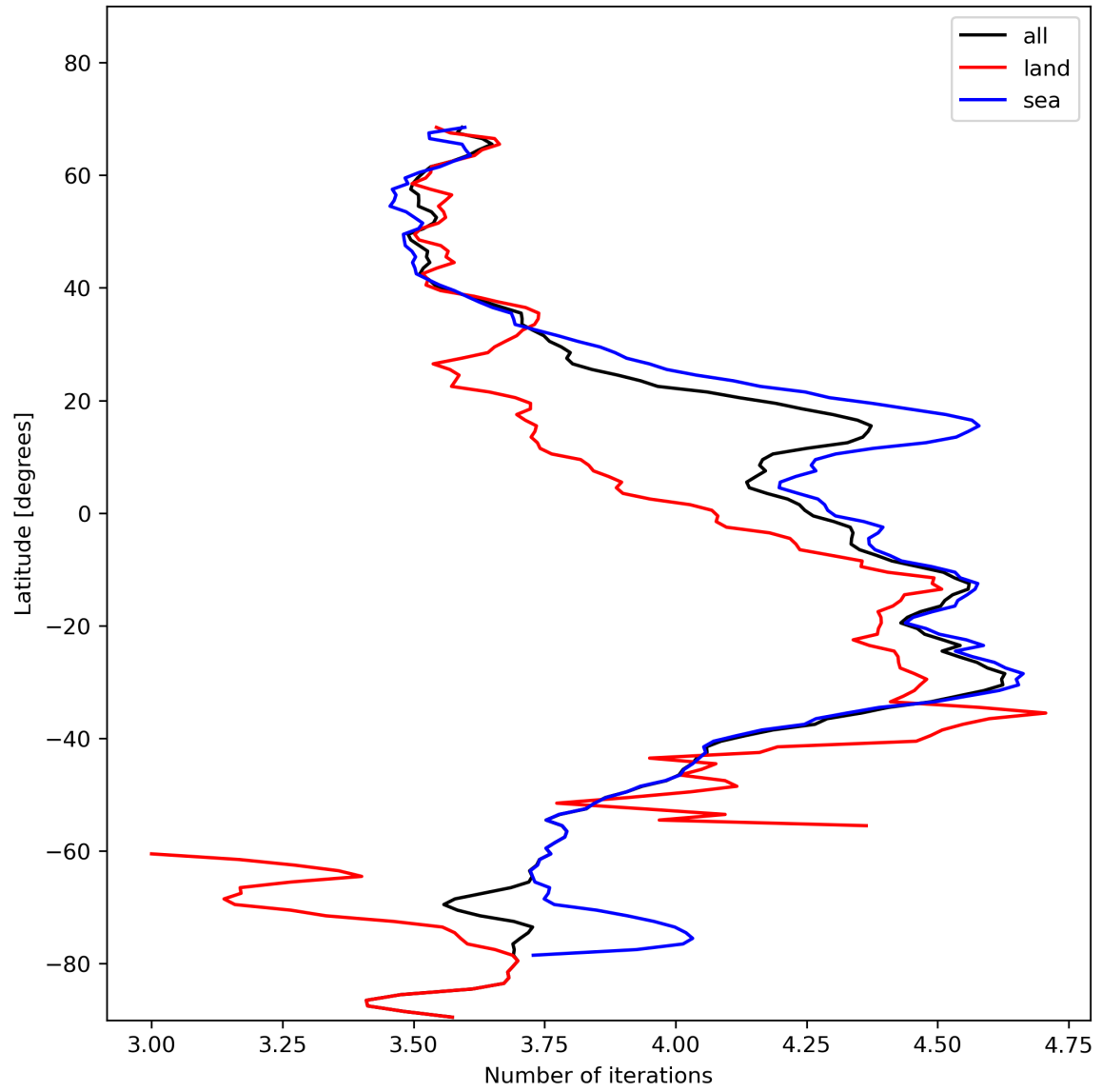
Figure 17: Zonal average of “Number of iterations” for 2024-01-22 to 2024-01-24.
