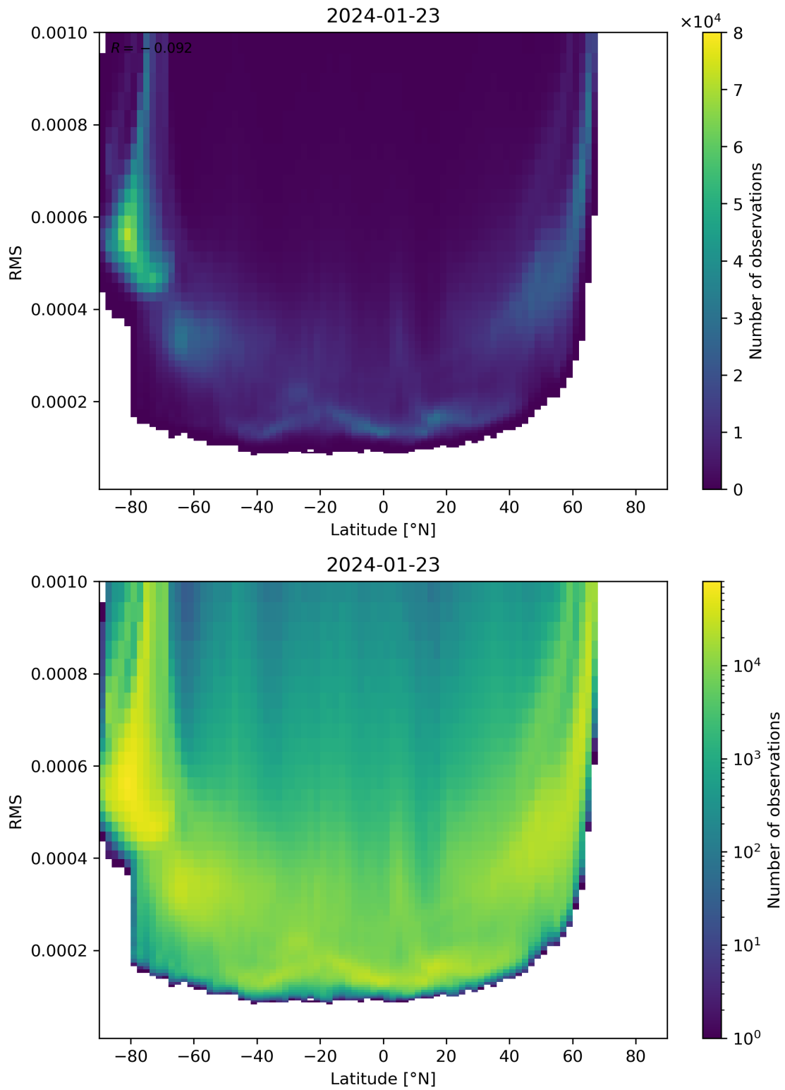
Figure 94: Scatter density plot of “Latitude” against “RMS” for 2024-01-22 to 2024-01-24.
