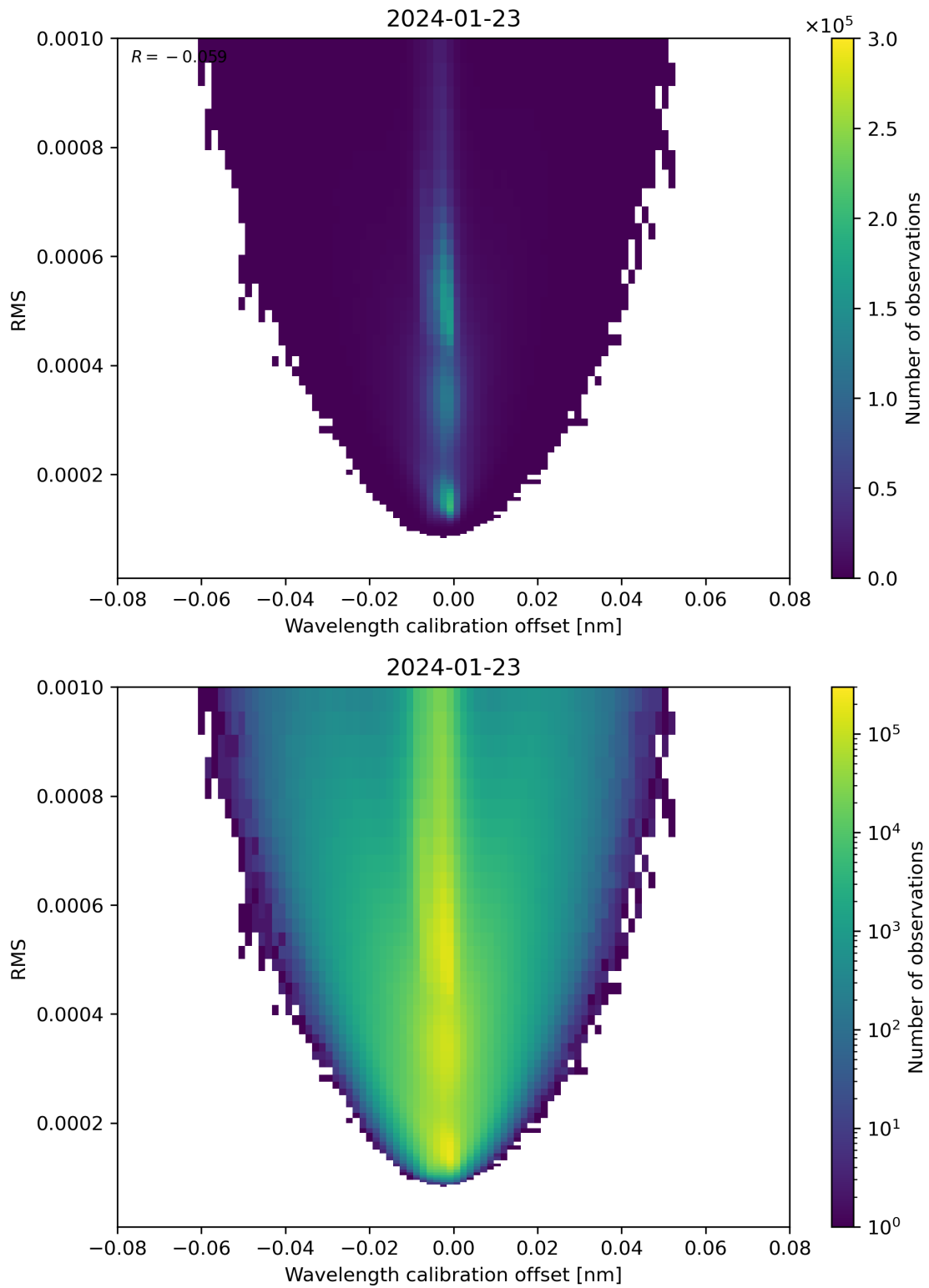
Figure 181: Scatter density plot of “Wavelength calibration offset” against “RMS” for 2024-01-22 to 2024-01-24.
