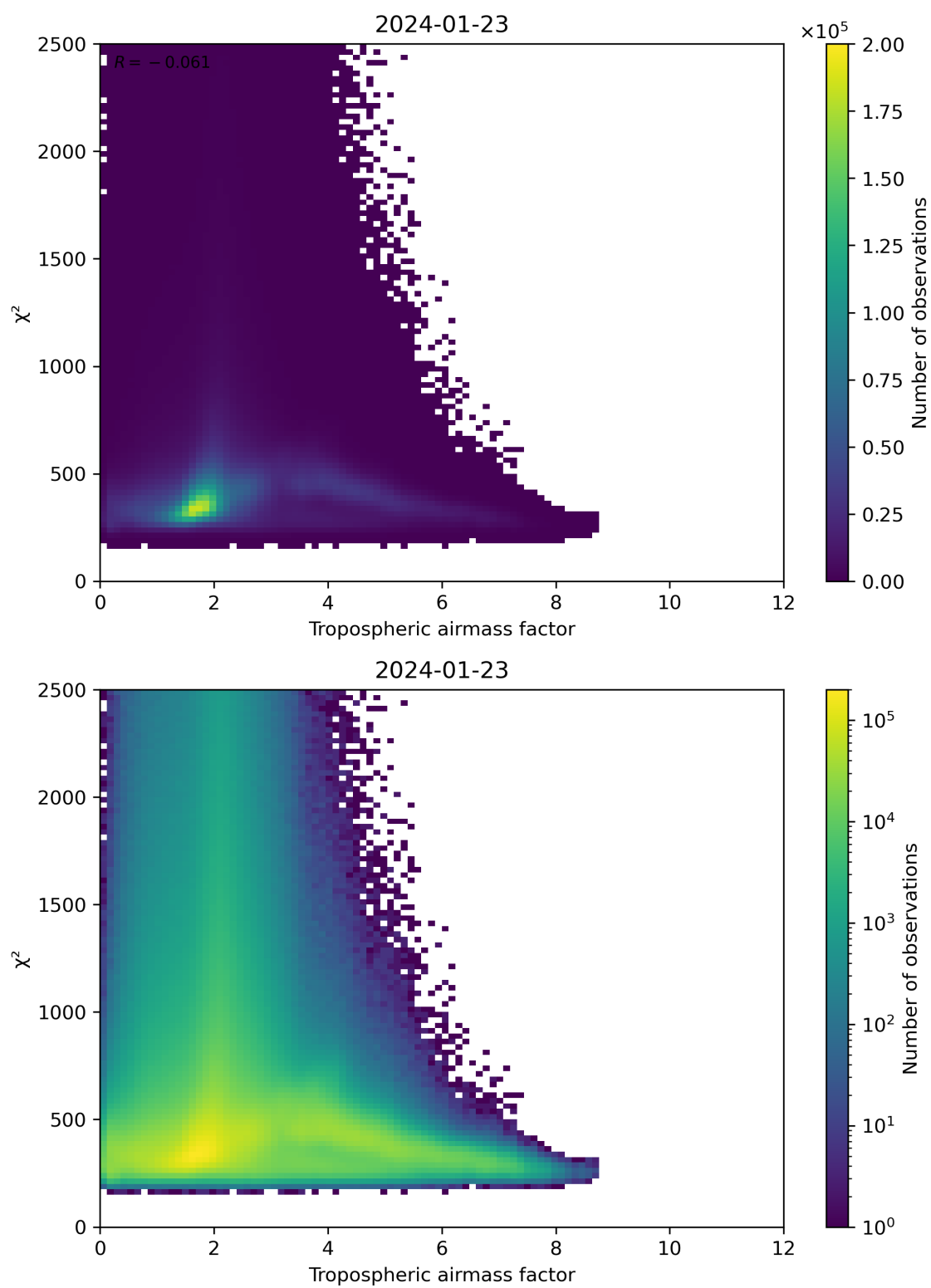
Figure 73: Scatter density plot of “Tropospheric airmass factor” against “ \chi^2 ” for 2024-01-22 to 2024-01-24.
