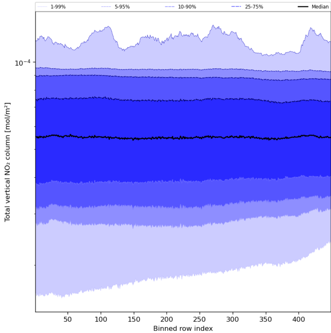
Figure 55: Along track statistics of “Total vertical NO 2 column” for 2024-01-22 to 2024-01-24
