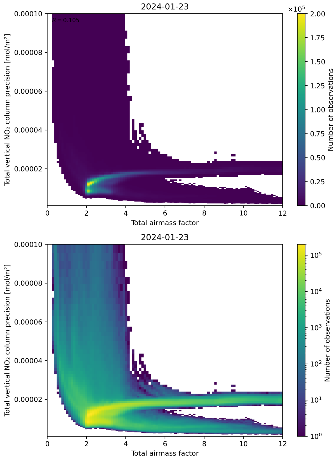
Figure 68: Scatter density plot of “Total airmass factor” against “Total vertical NO 2 column precision” for 2024-01-22 to 2024-01-24.
