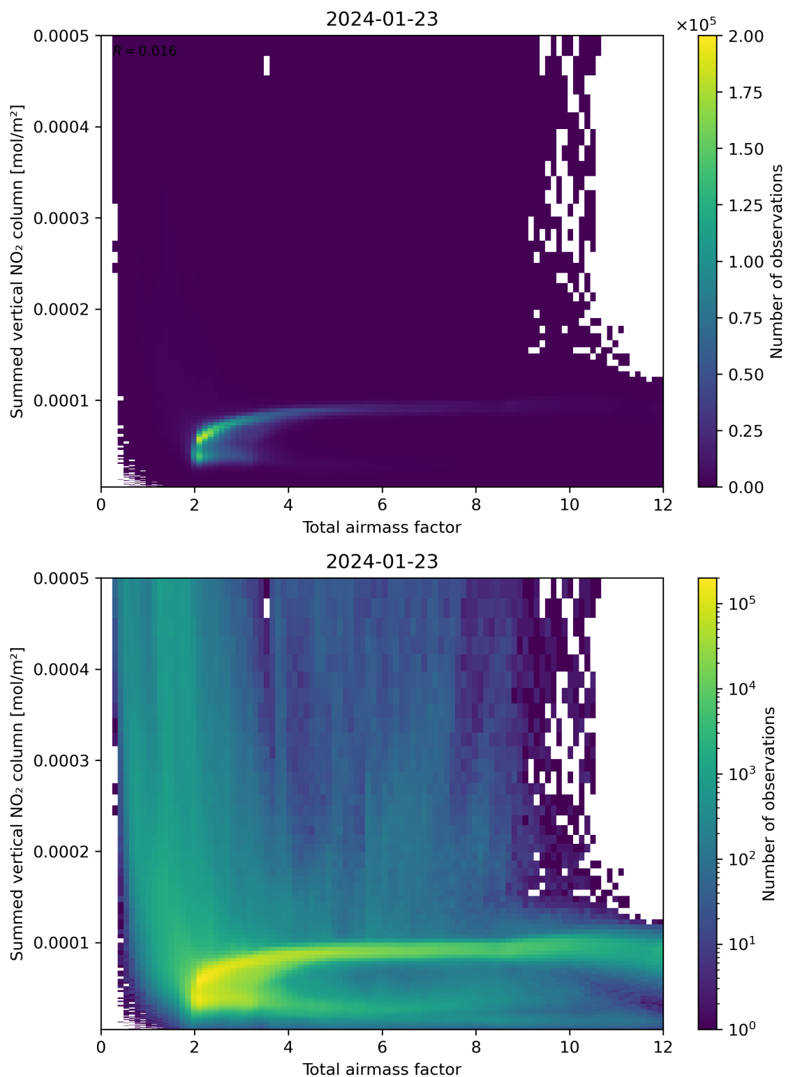
Figure 65: Scatter density plot of “Total airmass factor” against “Summed vertical NO 2 column” for 2024-01-22 to 2024-01-24.
