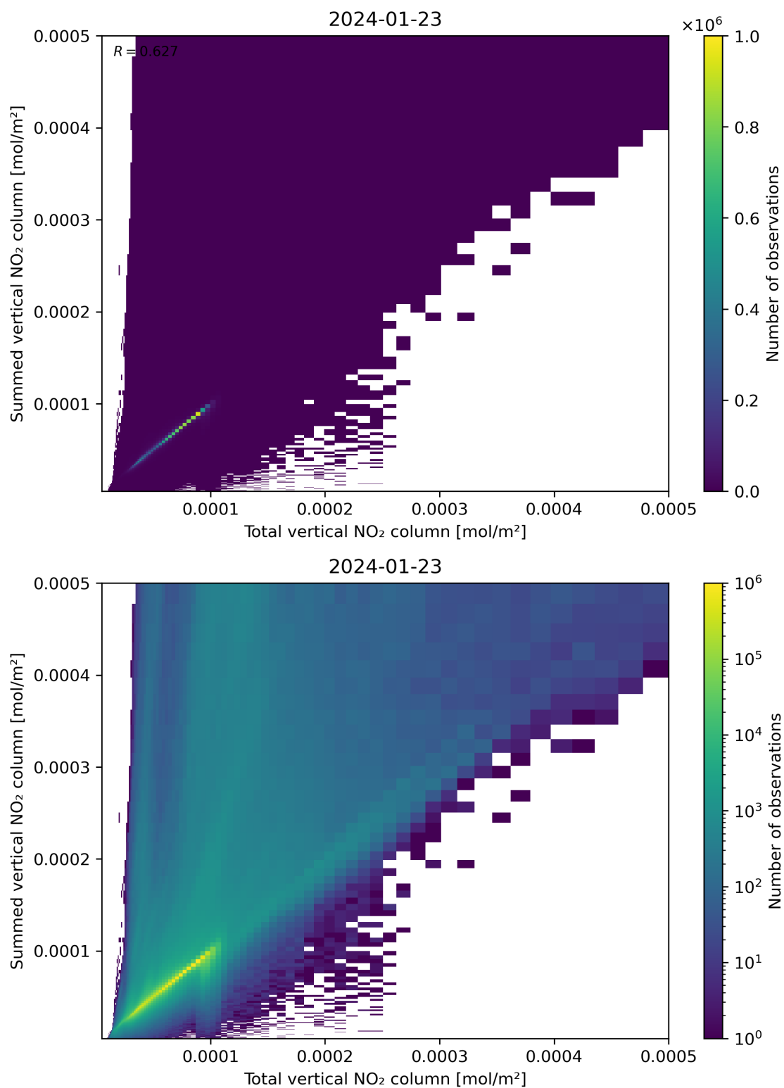
Figure 112: Scatter density plot of “Total vertical NO 2 column” against “Summed vertical NO 2 column” for 2024-01-22 to 2024-01-24.
