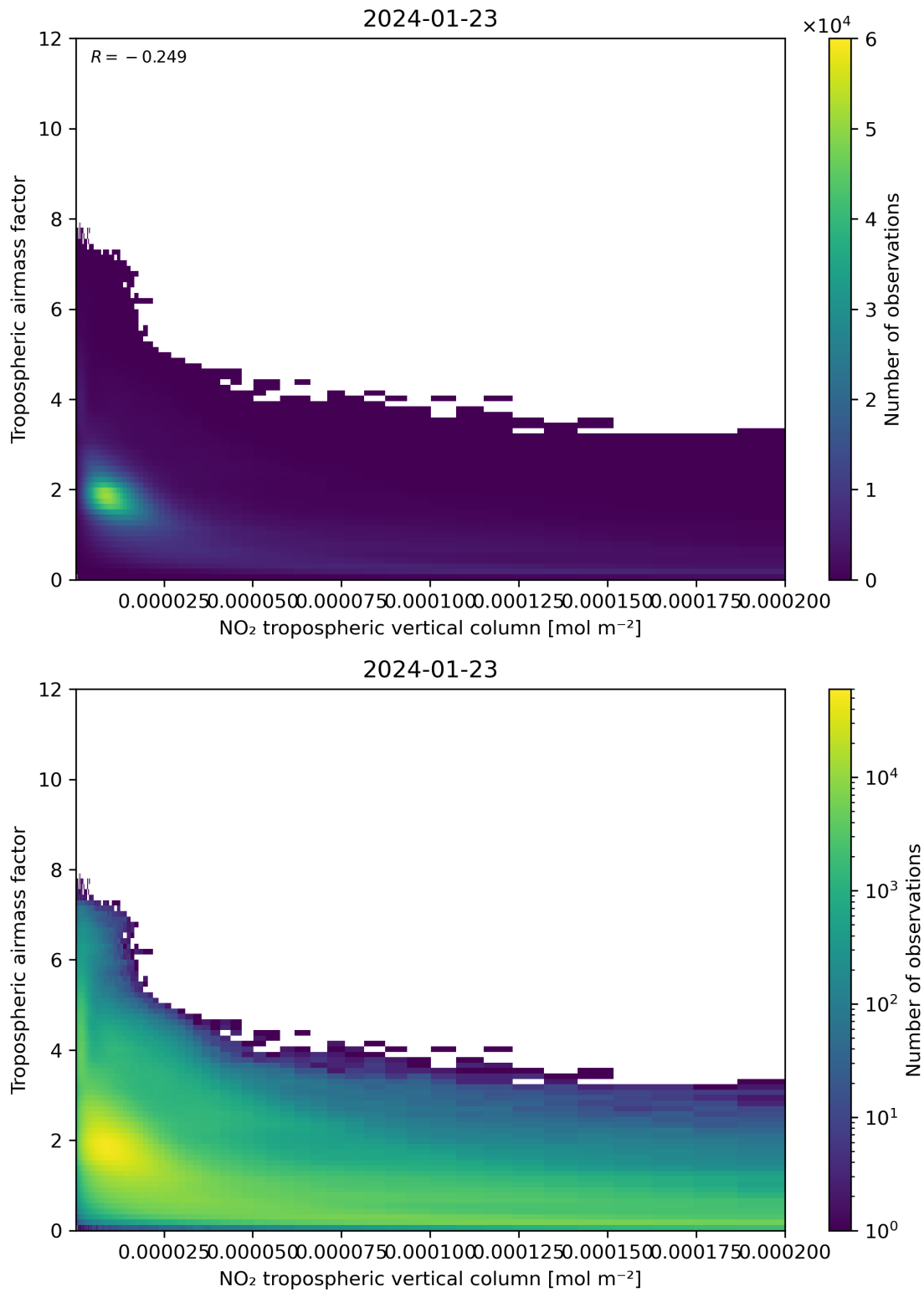
Figure 123: Scatter density plot of “NO 2 tropospheric vertical column” against “Tropospheric airmass factor” for 2024-01-22 to 2024-01-24.
