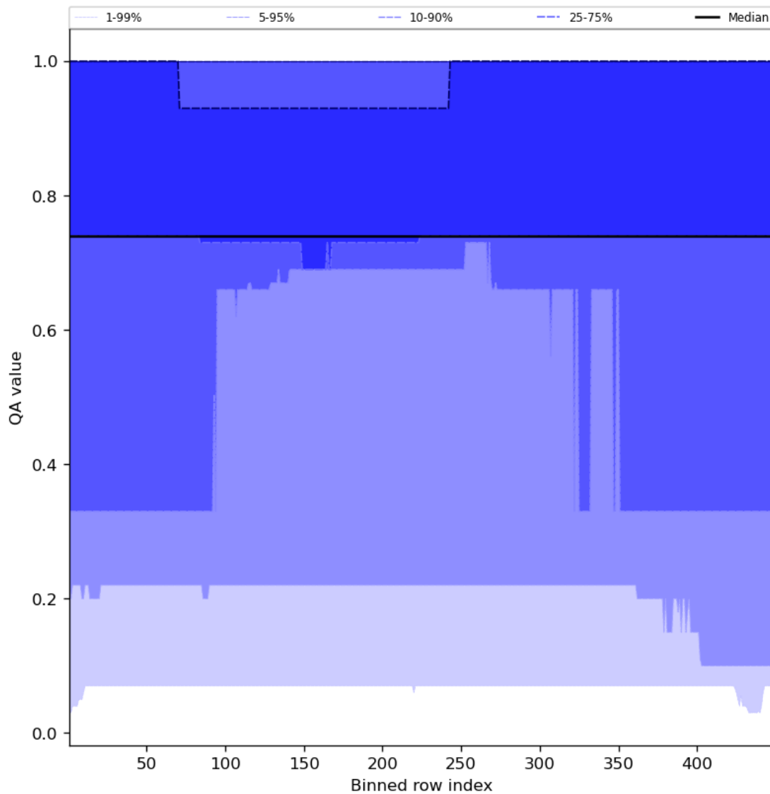
Figure 45: Along track statistics of “QA value” for 2024-01-22 to 2024-01-24
