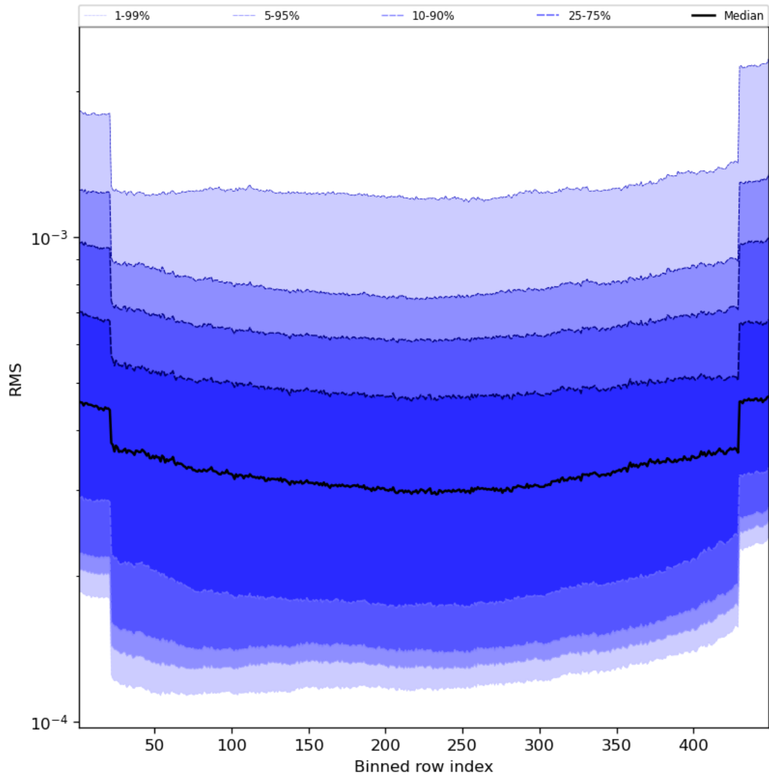
Figure 60: Along track statistics of “RMS” for 2024-01-22 to 2024-01-24
