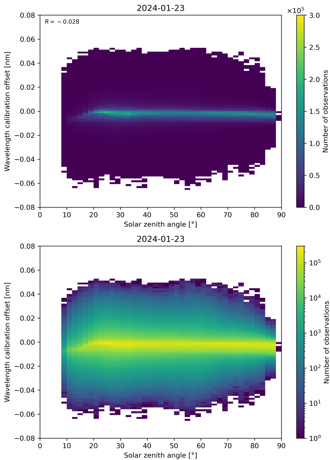
Figure 158: Scatter density plot of “Solar zenith angle” against “Wavelength calibration offset” for 2024-01-22 to 2024-01-24.
