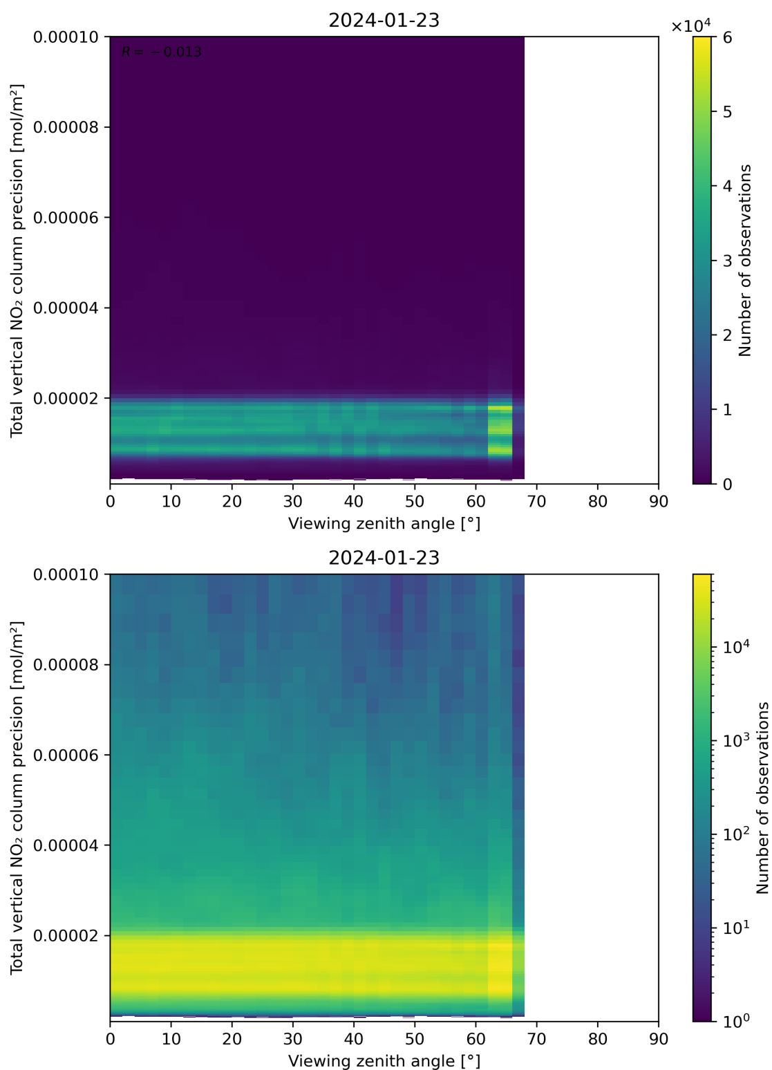
Figure 168: Scatter density plot of “Viewing zenith angle” against “Total vertical NO 2 column precision” for 2024-01-22 to 2024-01-24.
