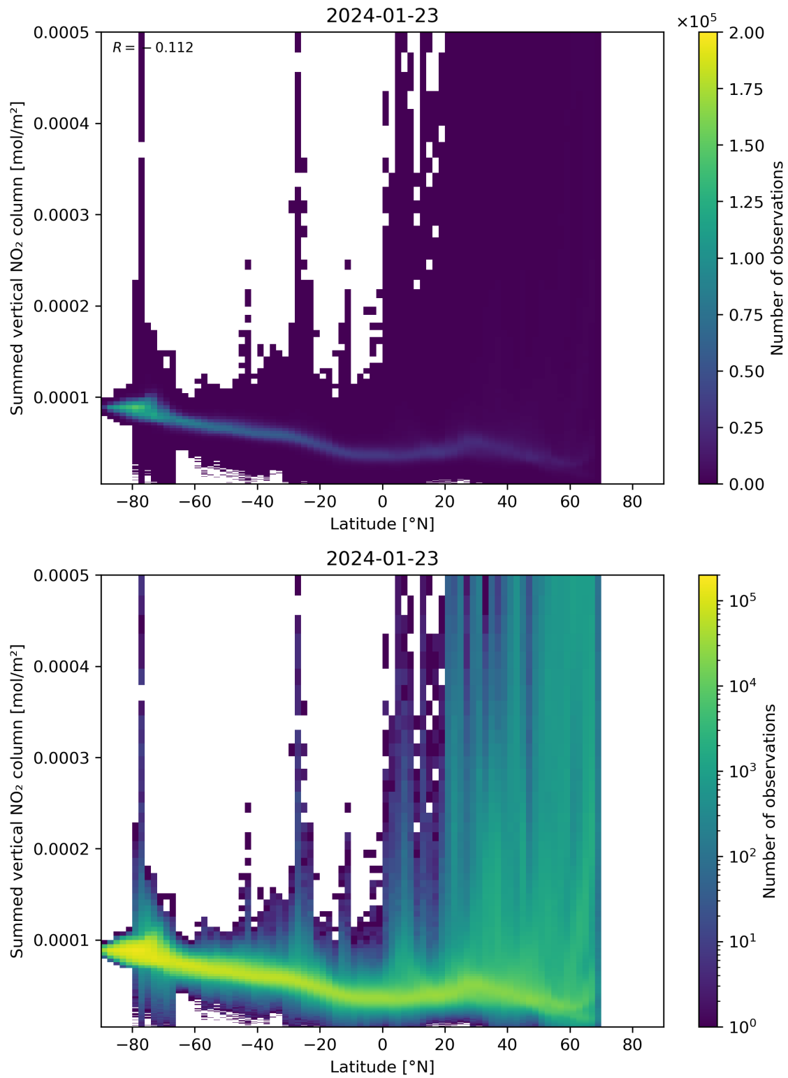
Figure 88: Scatter density plot of “Latitude” against “Summed vertical NO 2 column” for 2024-01-22 to 2024-01-24.
