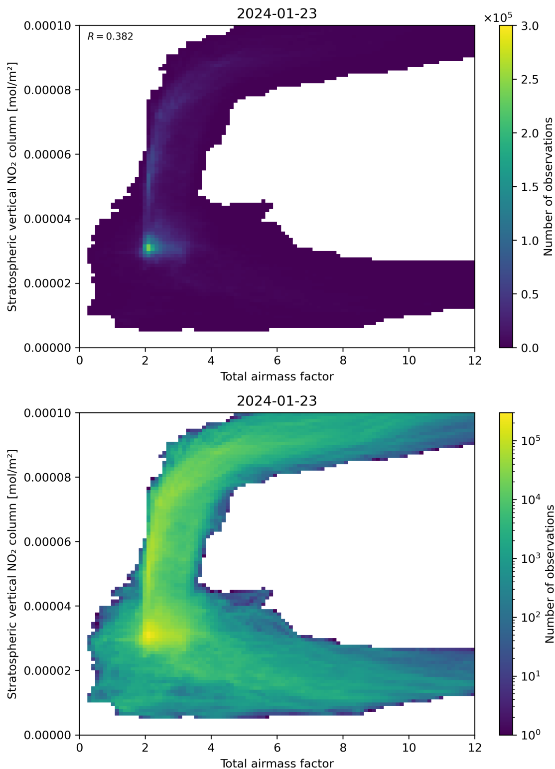
Figure 64: Scatter density plot of “Total airmass factor” against “Stratospheric vertical NO 2 column” for 2024-01-22 to 2024-01-24.
