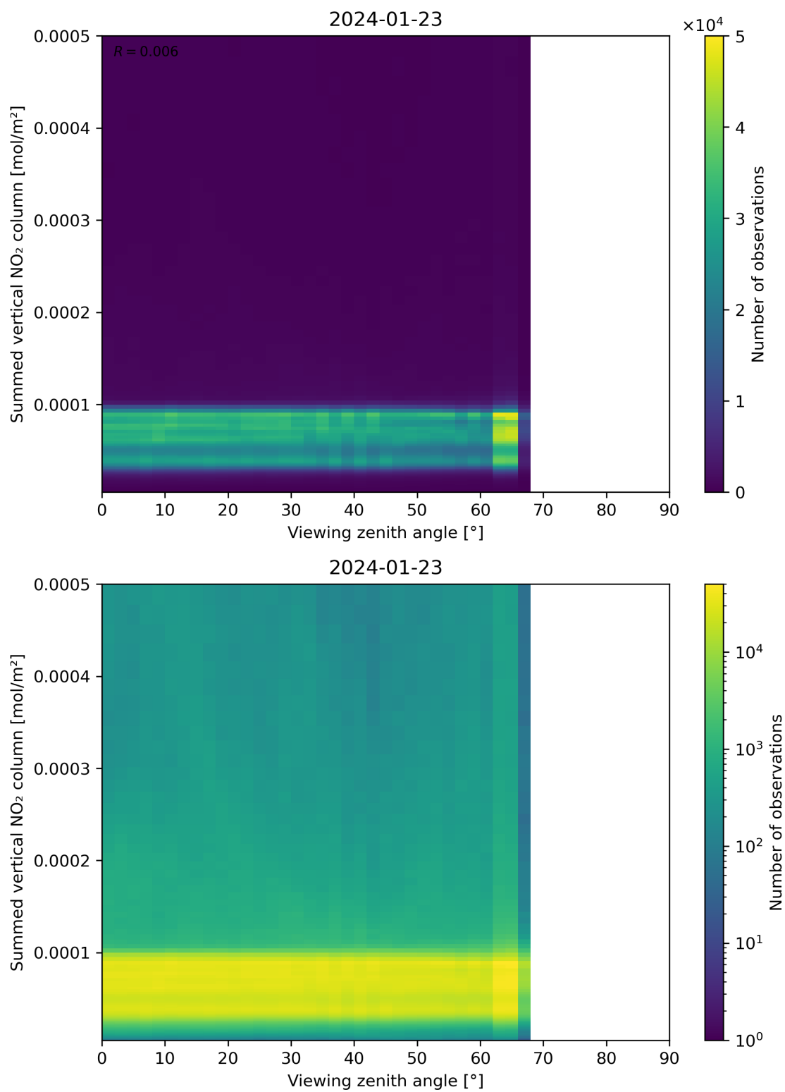
Figure 165: Scatter density plot of “Viewing zenith angle” against “Summed vertical NO 2 column” for 2024-01-22 to 2024-01-24.
