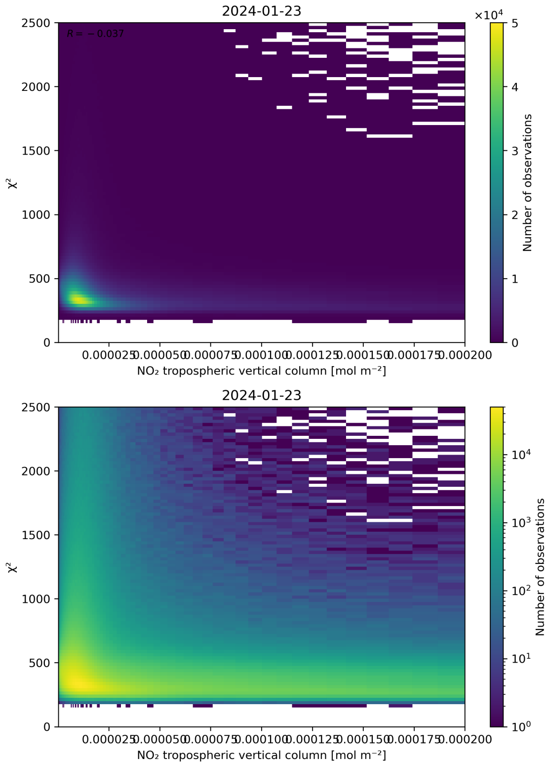
Figure 124: Scatter density plot of “NO 2 tropospheric vertical column” against “ \chi^2 ” for 2024-01-22 to 2024-01-24.
