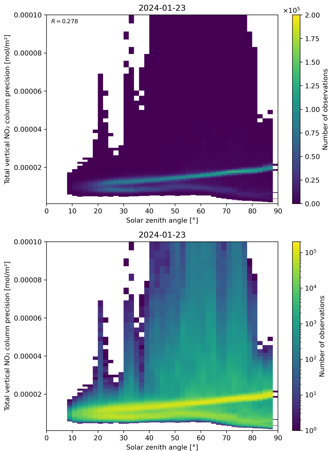
Figure 154: Scatter density plot of “Solar zenith angle” against “Total vertical NO 2 column precision” for 2024-01-22 to 2024-01-24.
