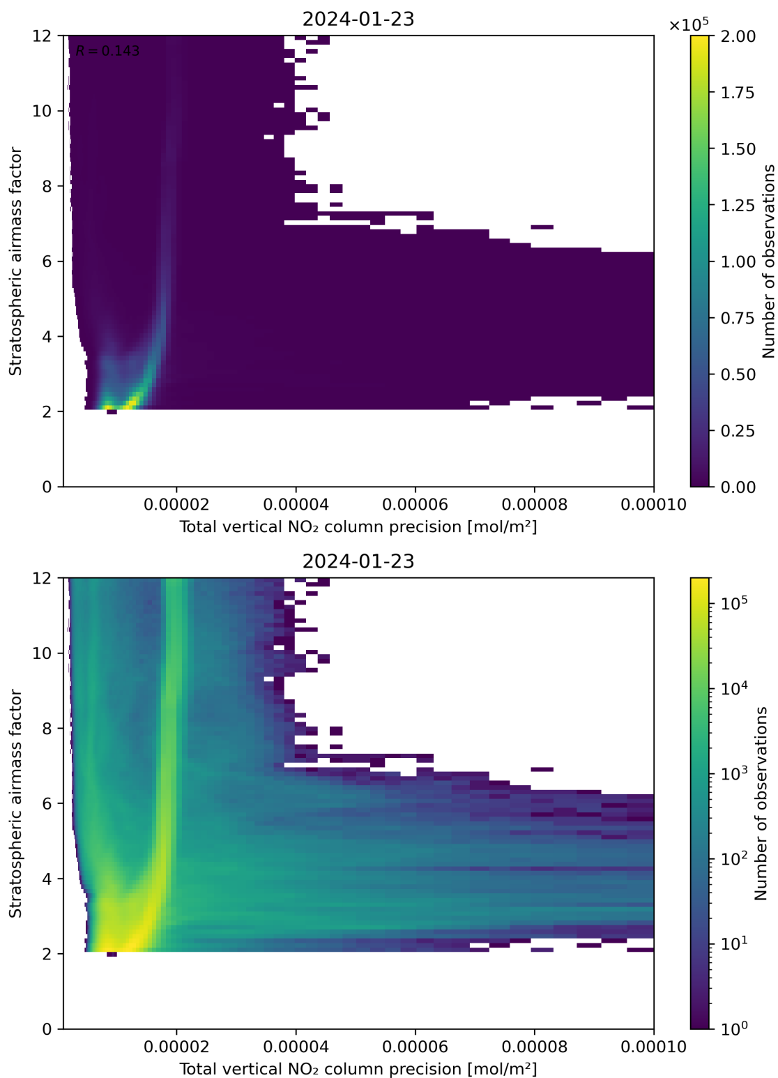
Figure 115: Scatter density plot of “Total vertical NO 2 column precision” against “Stratospheric air mass factor” for 2024-01-22 to 2024-01-24.
