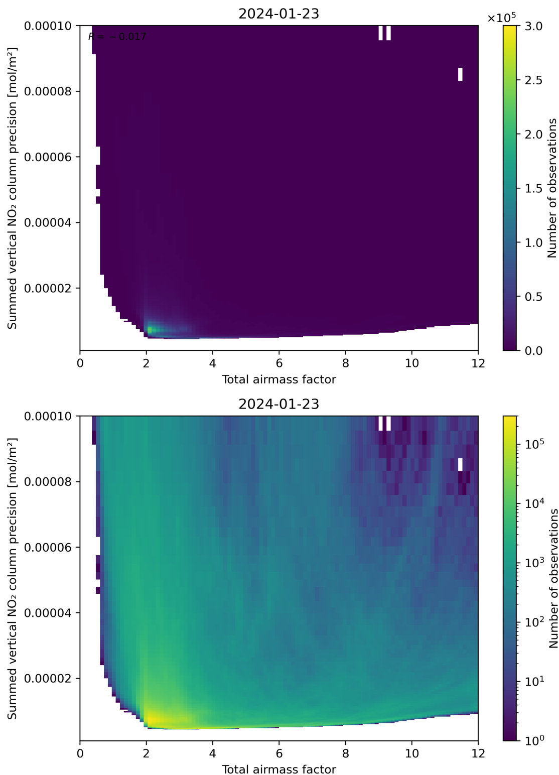
Figure 66: Scatter density plot of “Total airmass factor” against “Summed vertical NO 2 column precision” for 2024-01-22 to 2024-01-24.
