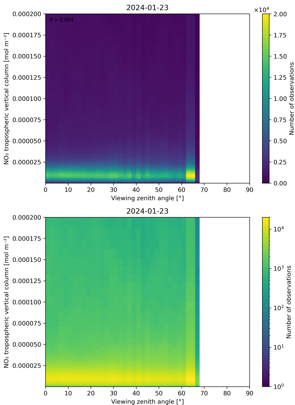
Figure 169: Scatter density plot of “Viewing zenith angle” against “NO 2 tropospheric vertical column” for 2024-01-22 to 2024-01-24.
