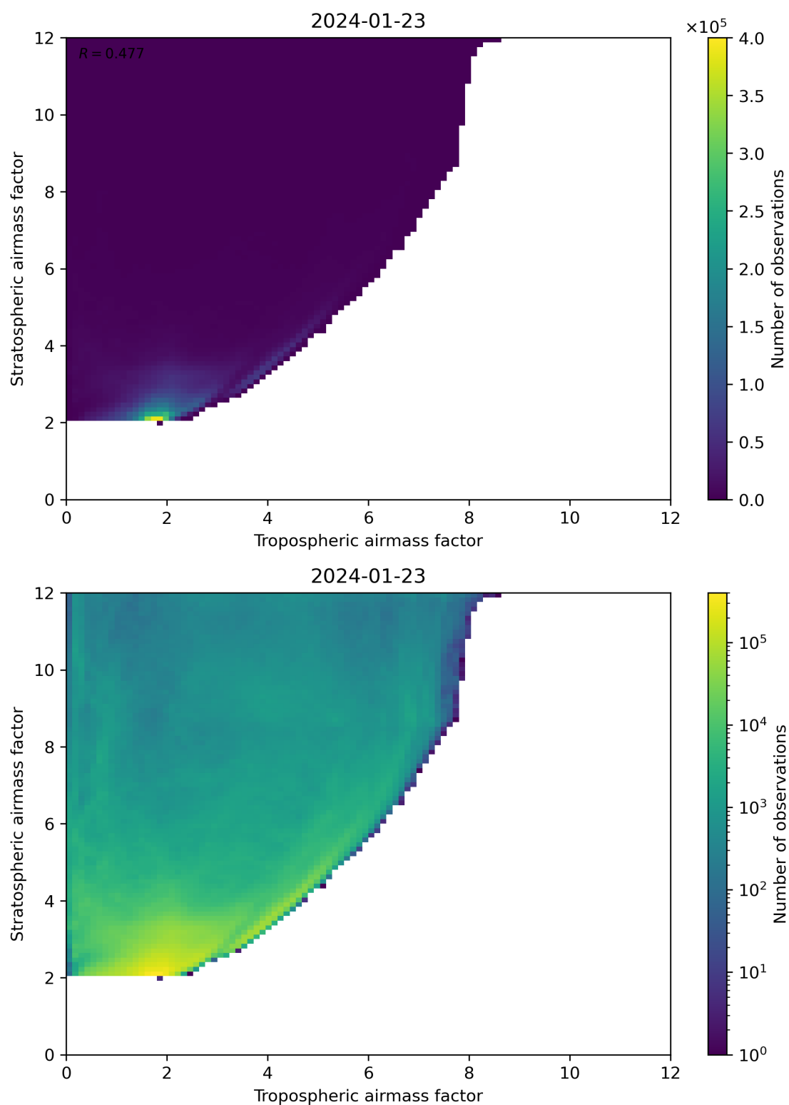
Figure 71: Scatter density plot of “Tropospheric airmass factor” against “Stratospheric airmass factor” for 2024-01-22 to 2024-01-24.
