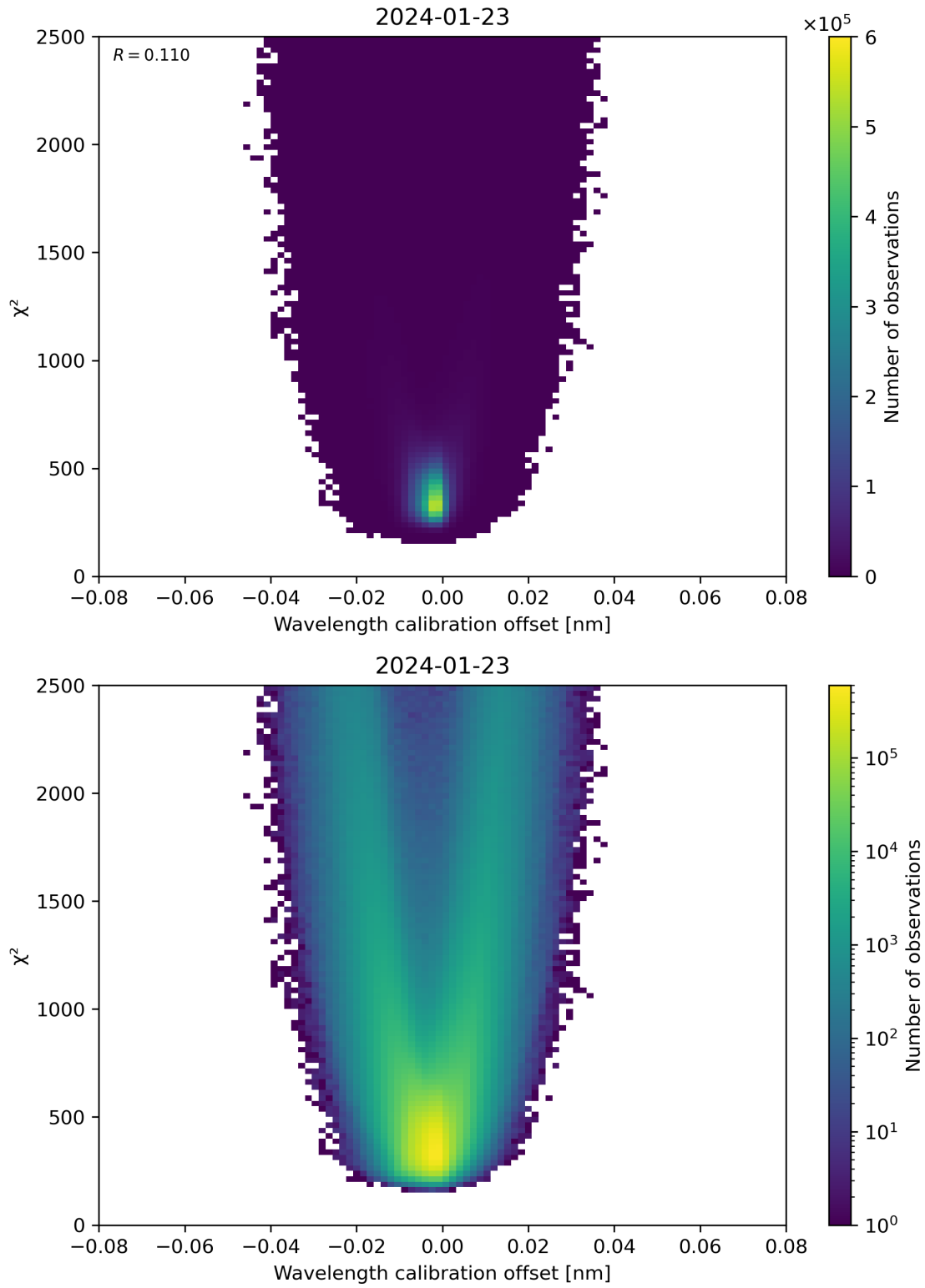
Figure 175: Scatter density plot of “Wavelength calibration offset” against “ \chi^2 ” for 2024-01-22 to 2024-01-24.
