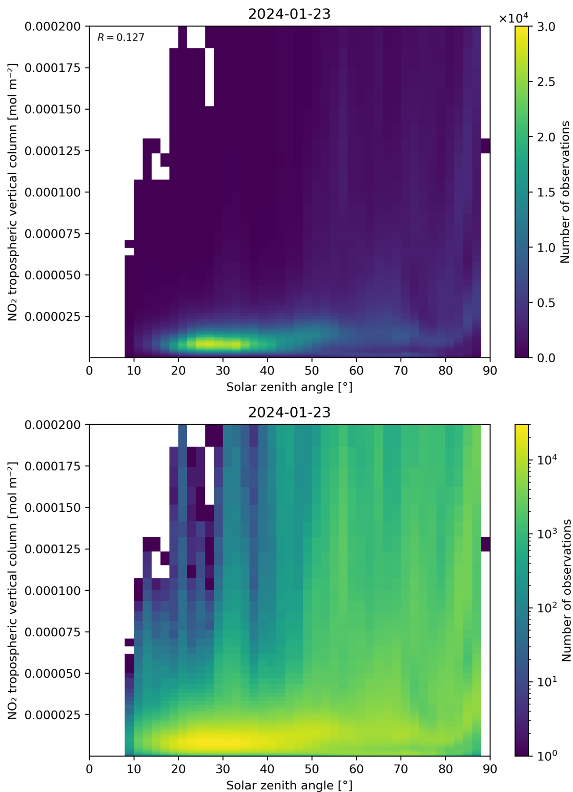
Figure 155: Scatter density plot of “Solar zenith angle” against “NO 2 tropospheric vertical column” for 2024-01-22 to 2024-01-24.
