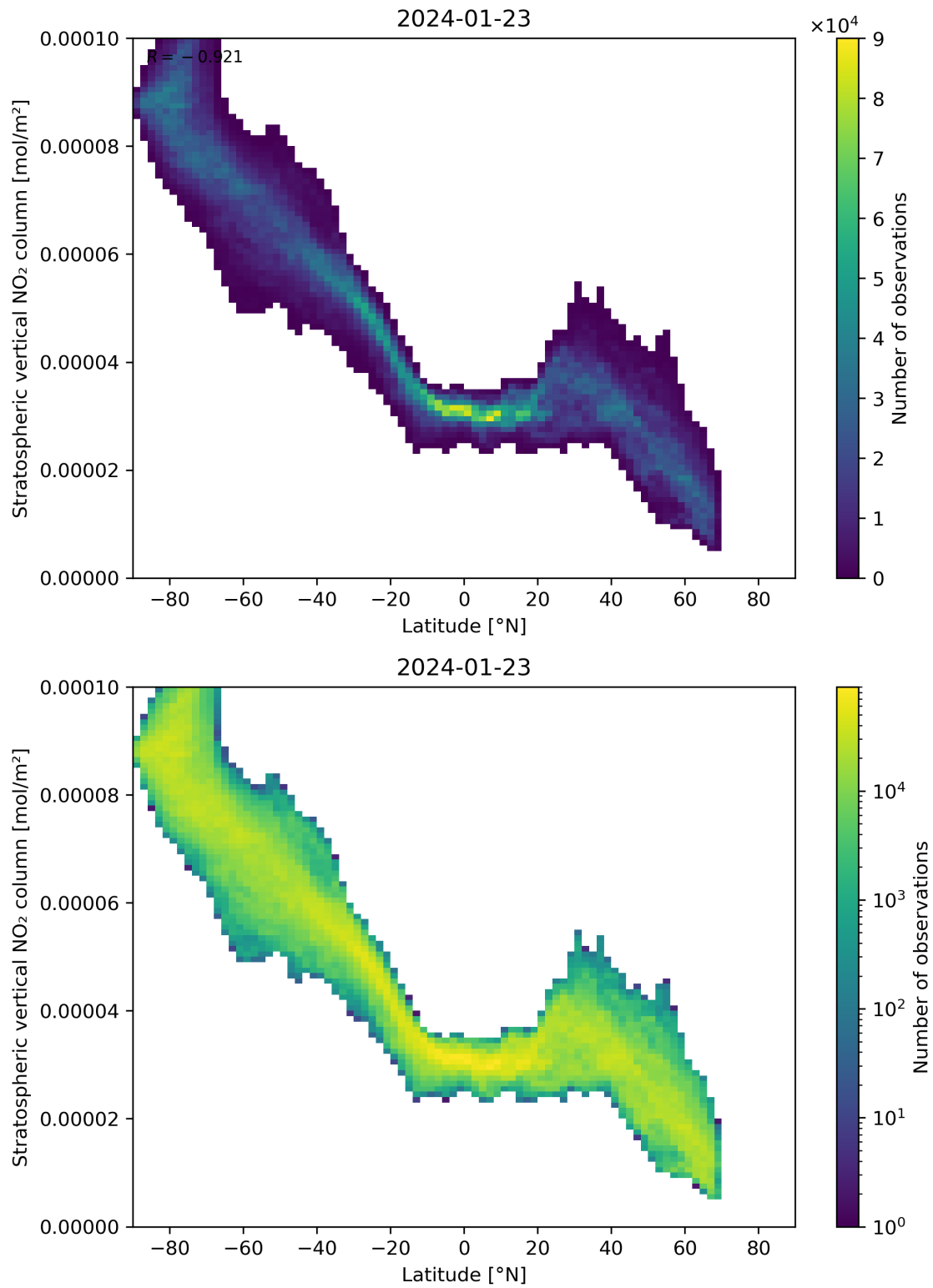
Figure 87: Scatter density plot of “Latitude” against “Stratospheric vertical NO 2 column” for 2024-01-22 to 2024-01-24.
