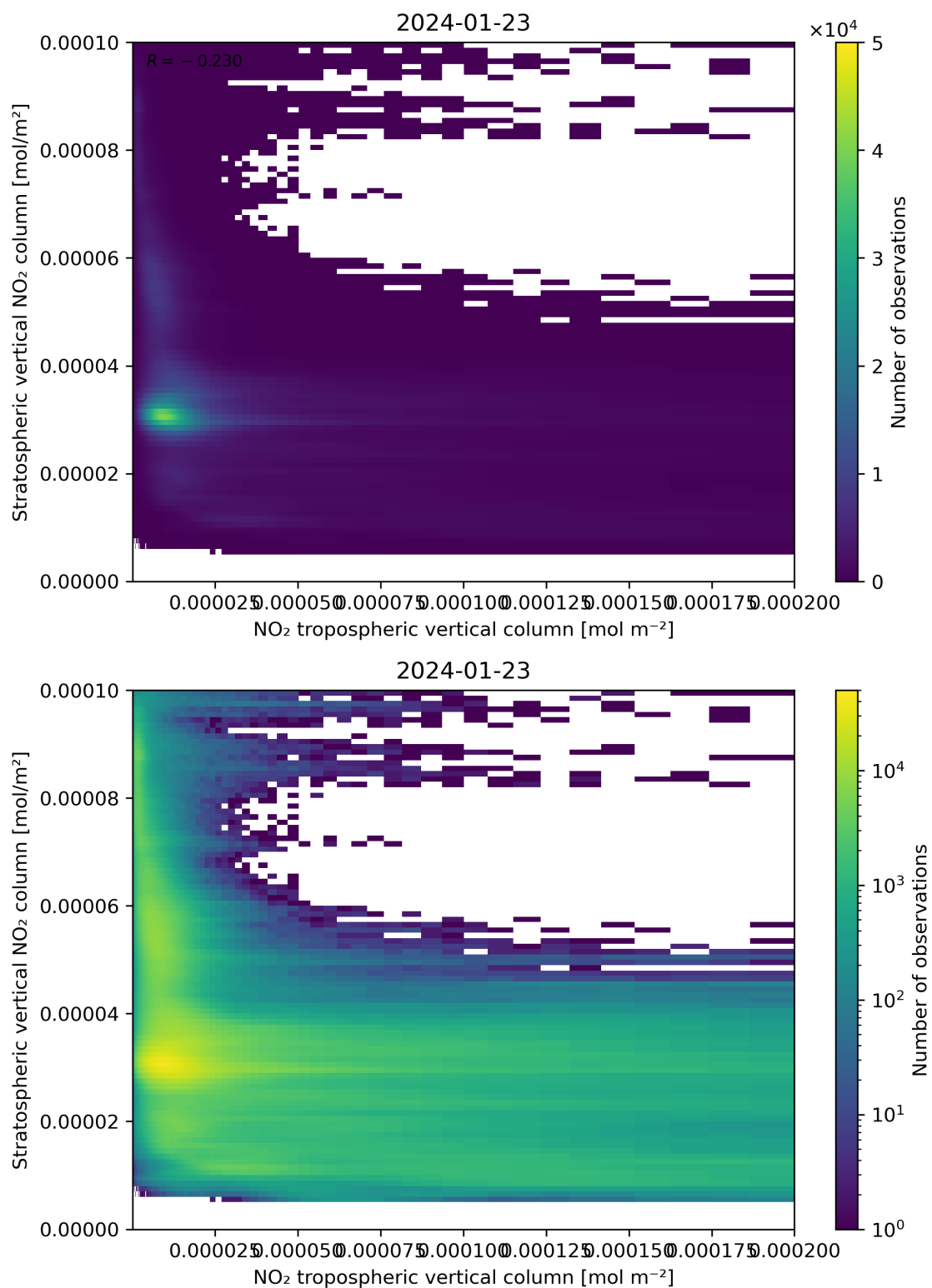
Figure 125: Scatter density plot of “NO 2 tropospheric vertical column” against “Stratospheric vertical NO 2 column” for 2024-01-22 to 2024-01-24.
