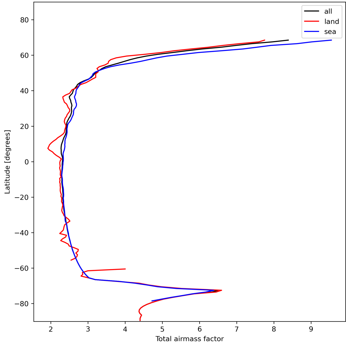
Figure 15: Zonal average of “Total airmass factor” for 2024-01-22 to 2024-01-24.
