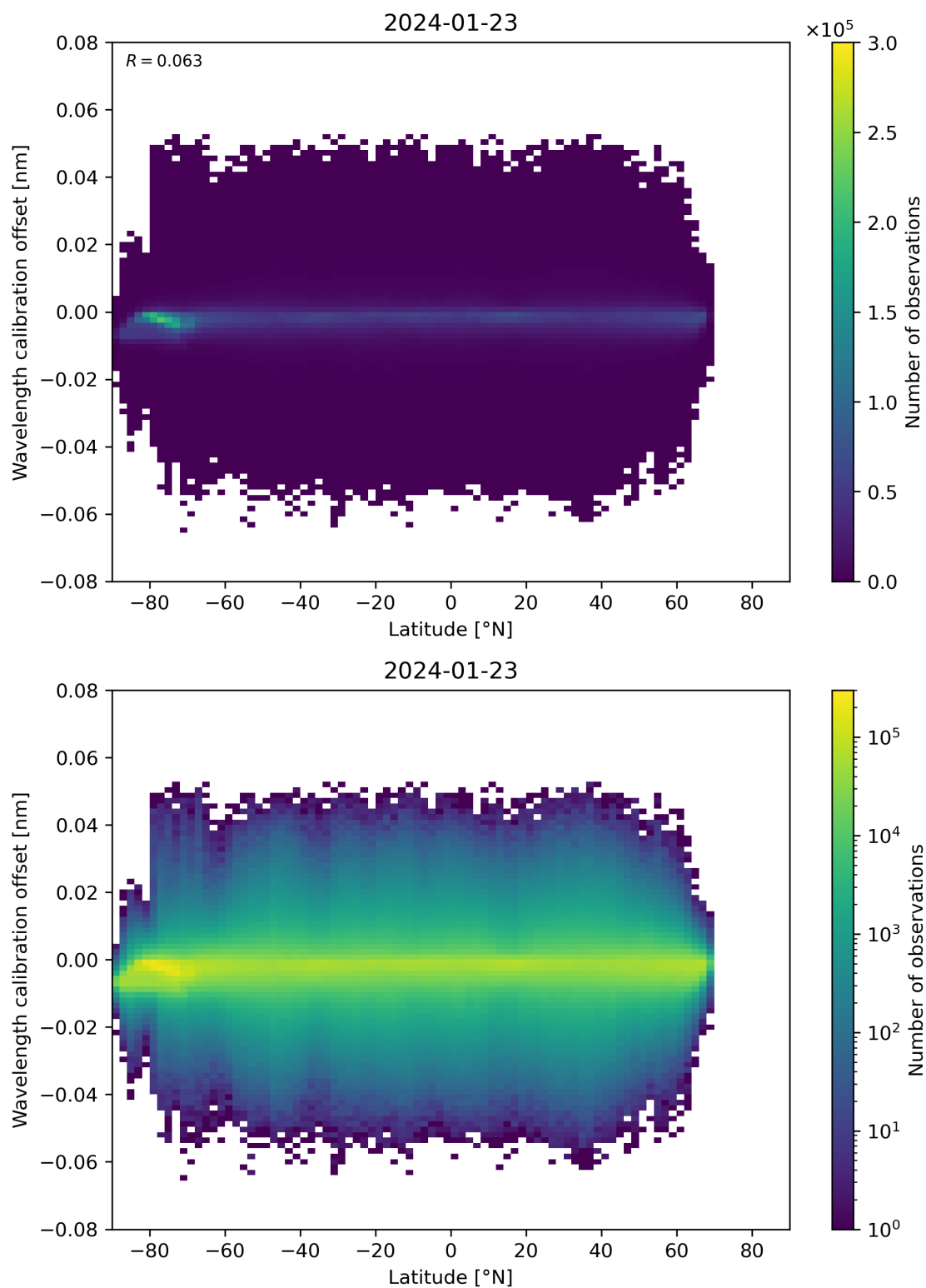
Figure 95: Scatter density plot of “Latitude” against “Wavelength calibration offset” for 2024-01-22 to 2024-01-24.
