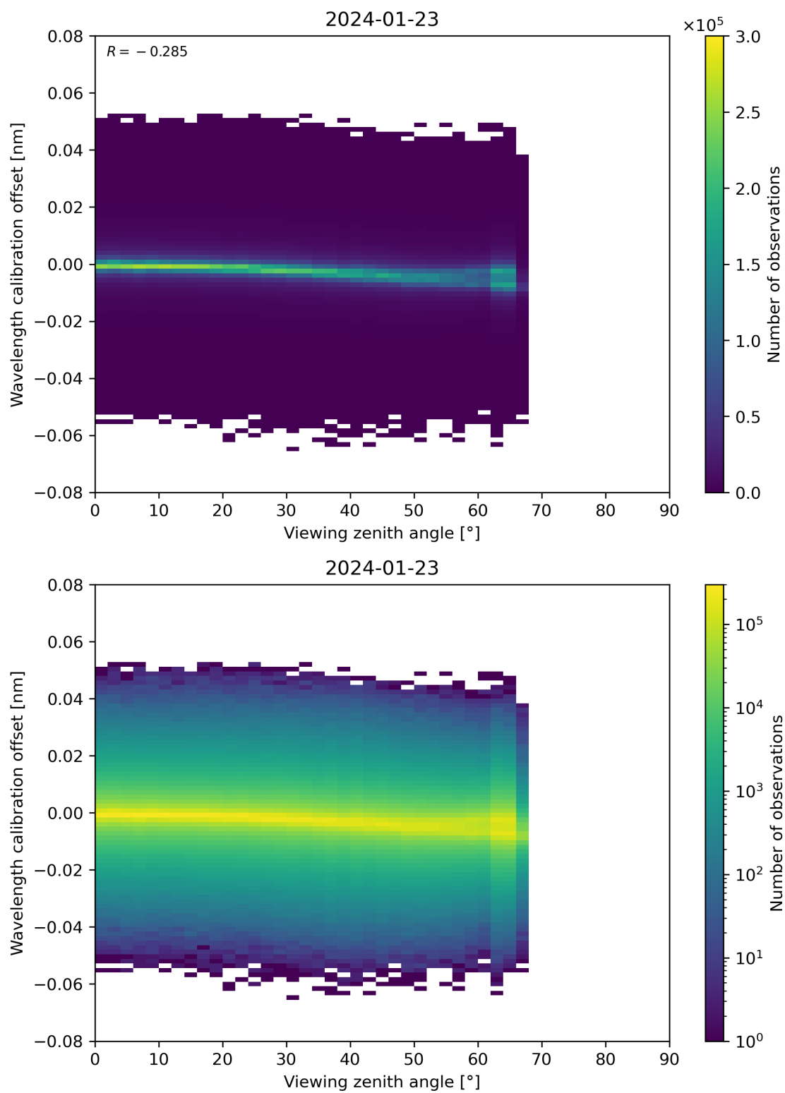
Figure 173: Scatter density plot of “Viewing zenith angle” against “Wavelength calibration offset” for 2024-01-22 to 2024-01-24.
