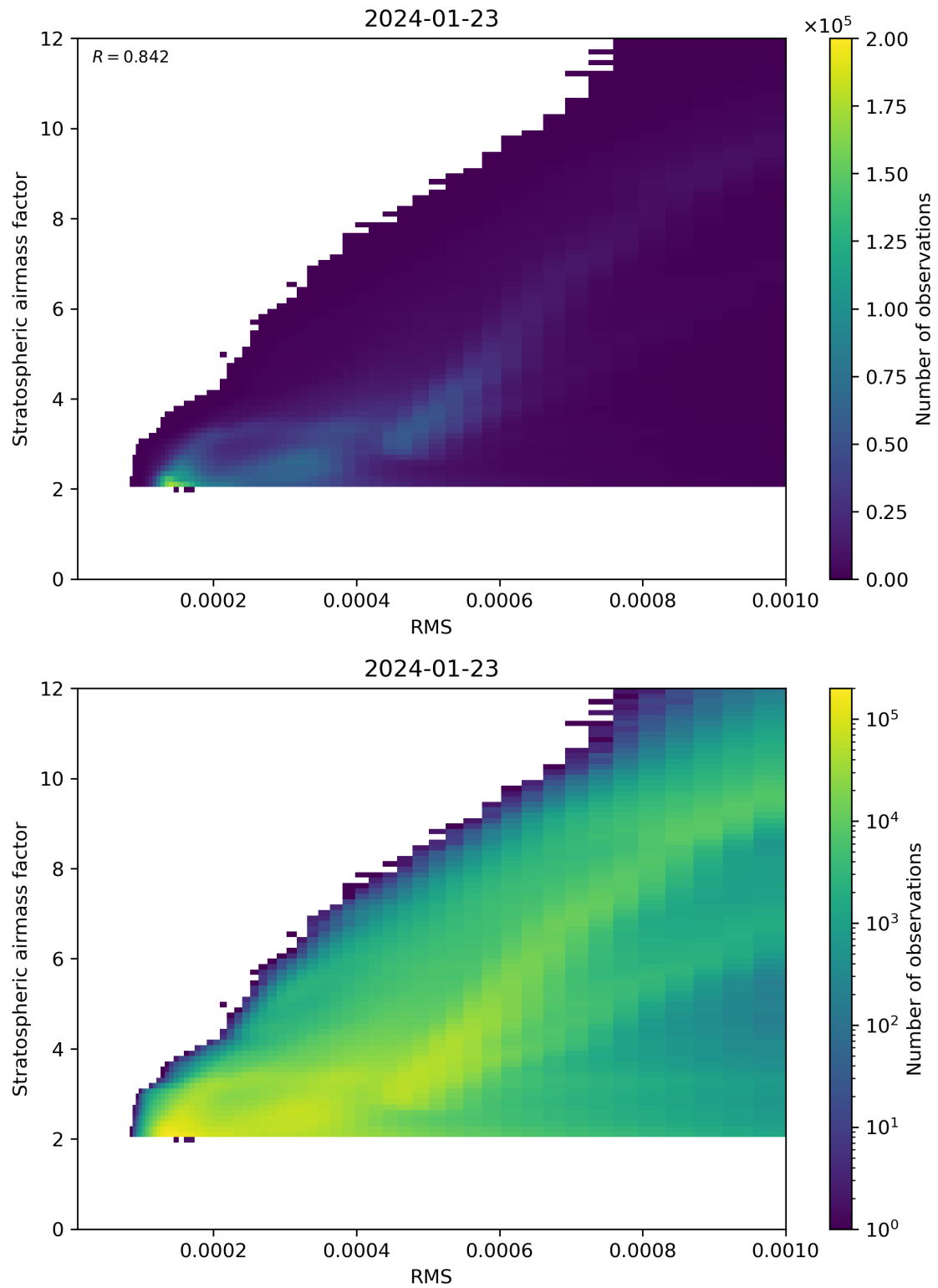
Figure 144: Scatter density plot of “RMS” against “Stratospheric airmass factor” for 2024-01-22 to 2024-01-24.
