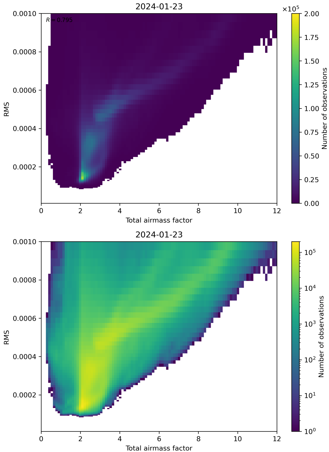
Figure 69: Scatter density plot of “Total airmass factor” against “RMS” for 2024-01-22 to 2024-01-24.
