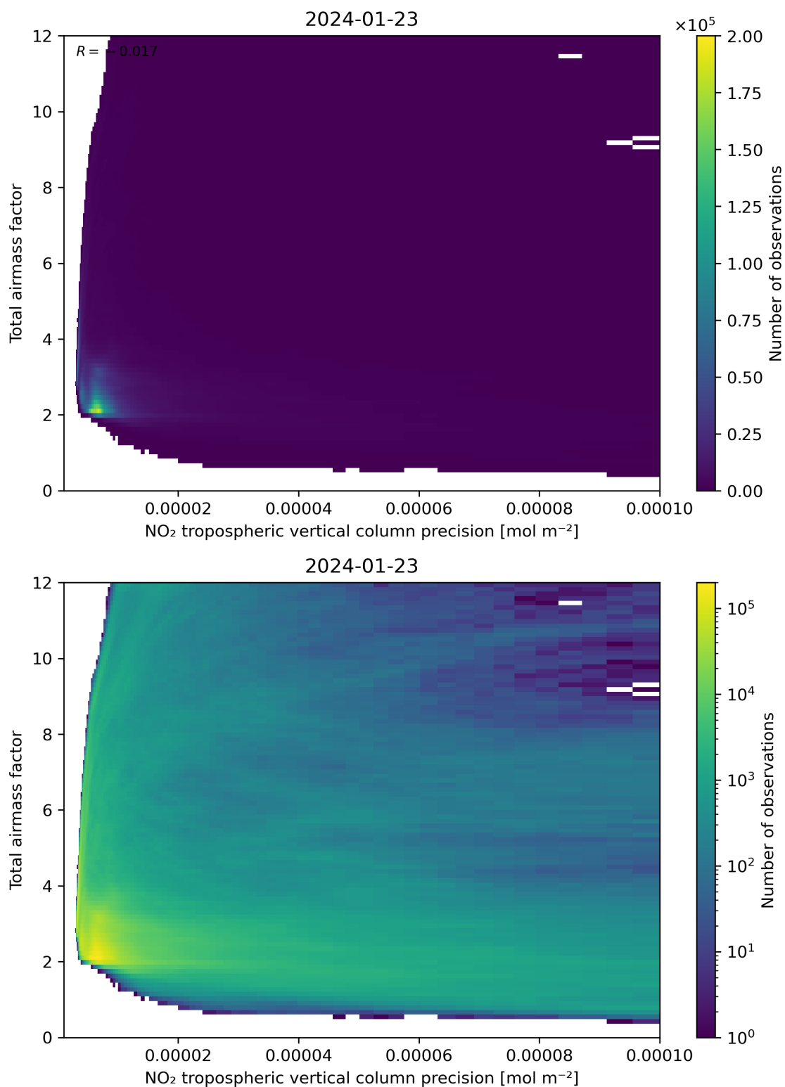
Figure 132: Scatter density plot of “NO 2 tropospheric vertical column precision” against “Total air mass factor” for 2024-01-22 to 2024-01-24.
