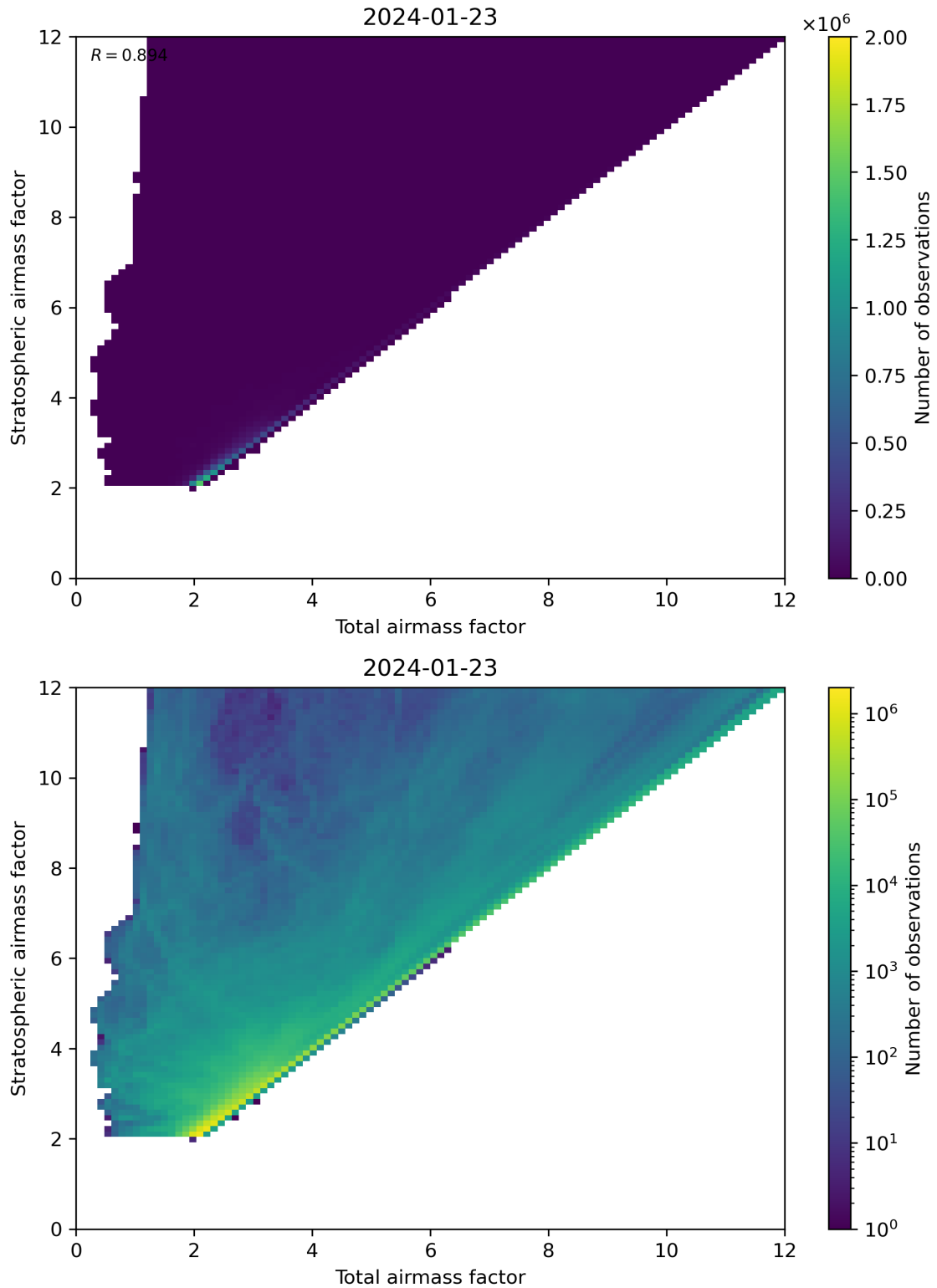
Figure 62: Scatter density plot of “Total airmass factor” against “Stratospheric airmass factor” for 2024-01-22 to 2024-01-24.
