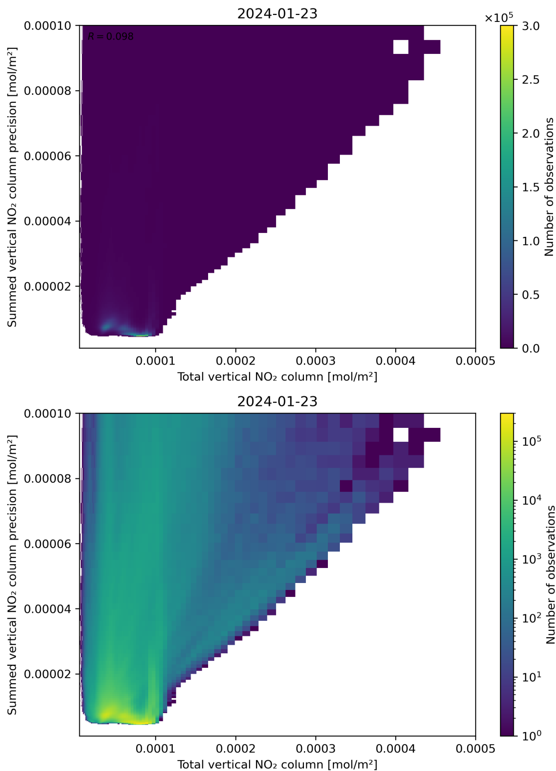
Figure 113: Scatter density plot of “Total vertical NO 2 column” against “Summed vertical NO 2 column precision” for 2024-01-22 to 2024-01-24.
