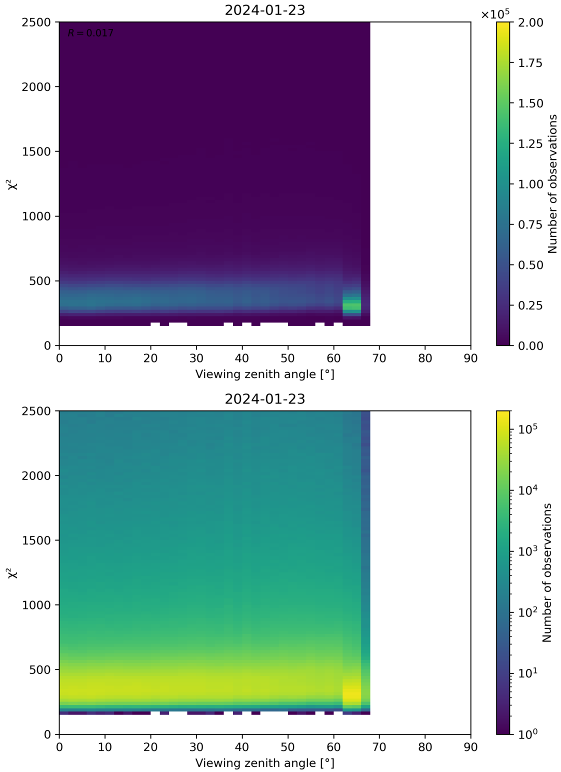
Figure 162: Scatter density plot of “Viewing zenith angle” against “ \chi^2 ” for 2024-01-22 to 2024-01-24.
