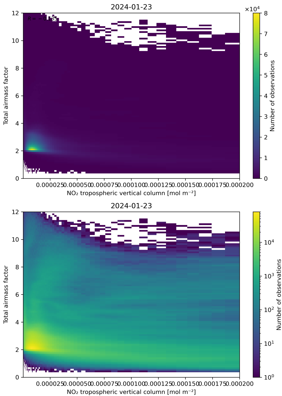
Figure 122: Scatter density plot of “NO 2 tropospheric vertical column” against “Total air mass factor” for 2024-01-22 to 2024-01-24.
