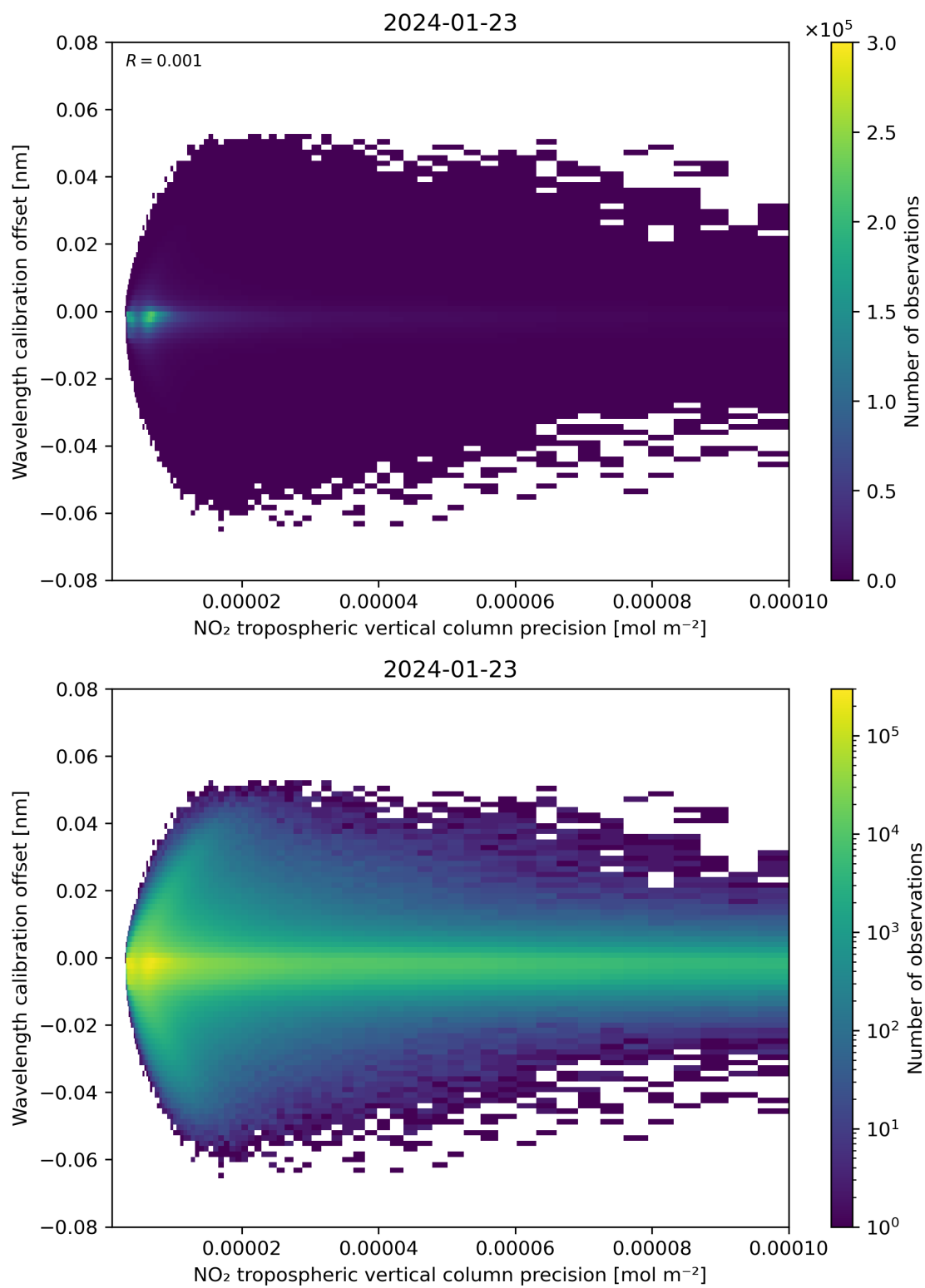
Figure 141: Scatter density plot of “NO 2 tropospheric vertical column precision” against “Wavelength calibration offset” for 2024-01-22 to 2024-01-24.
