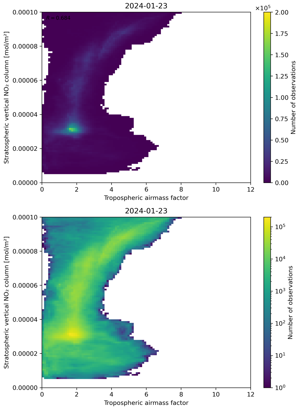
Figure 74: Scatter density plot of “Tropospheric air mass factor” against “Stratospheric vertical NO 2 column” for 2024-01-22 to 2024-01-24.
