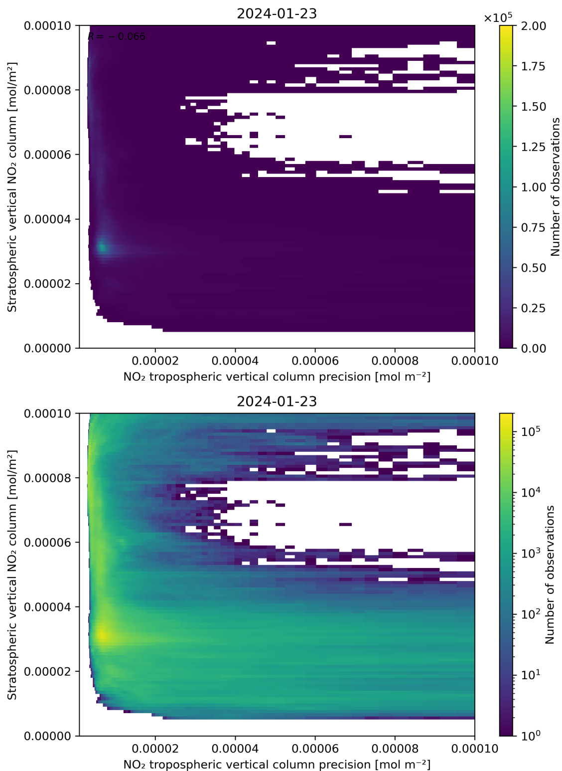
Figure 135: Scatter density plot of “NO 2 tropospheric vertical column precision” against “Stratospheric vertical NO 2 column” for 2024-01-22 to 2024-01-24.
