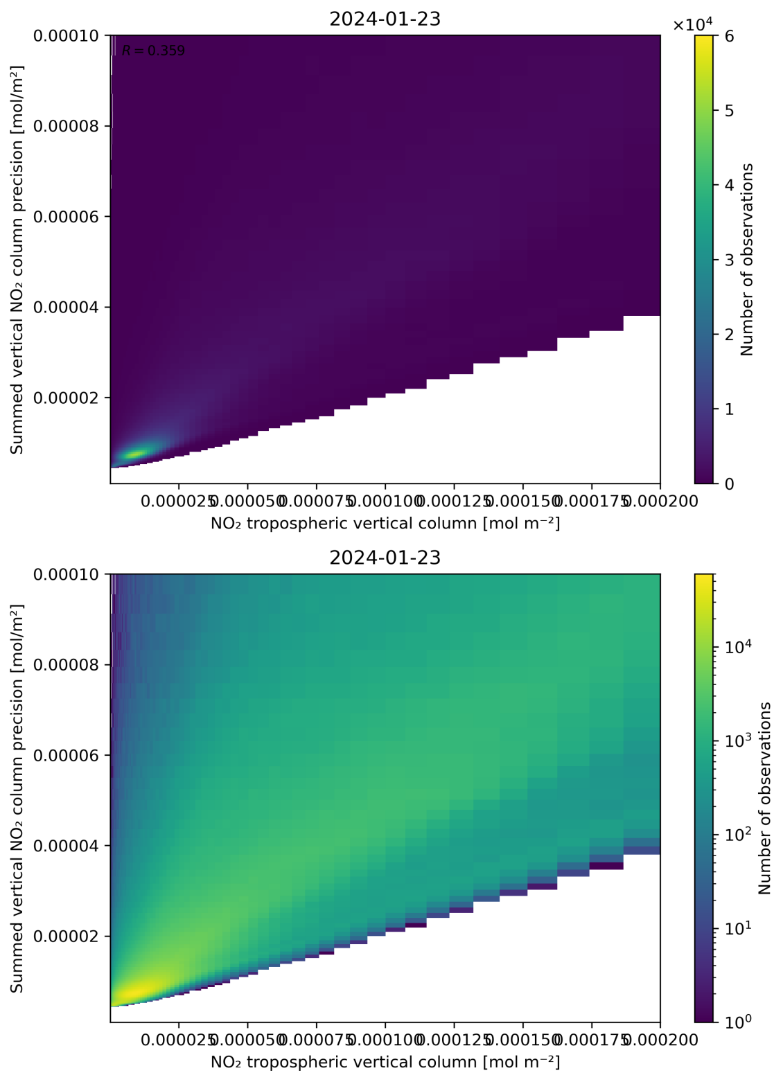
Figure 127: Scatter density plot of “NO 2 tropospheric vertical column” against “Summed vertical NO 2 column precision” for 2024-01-22 to 2024-01-24.
