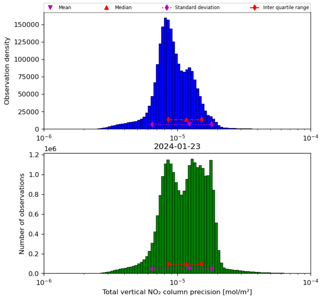
Figure 39: Histogram of “Total vertical NO 2 column precision” for 2024-01-22 to 2024-01-24
