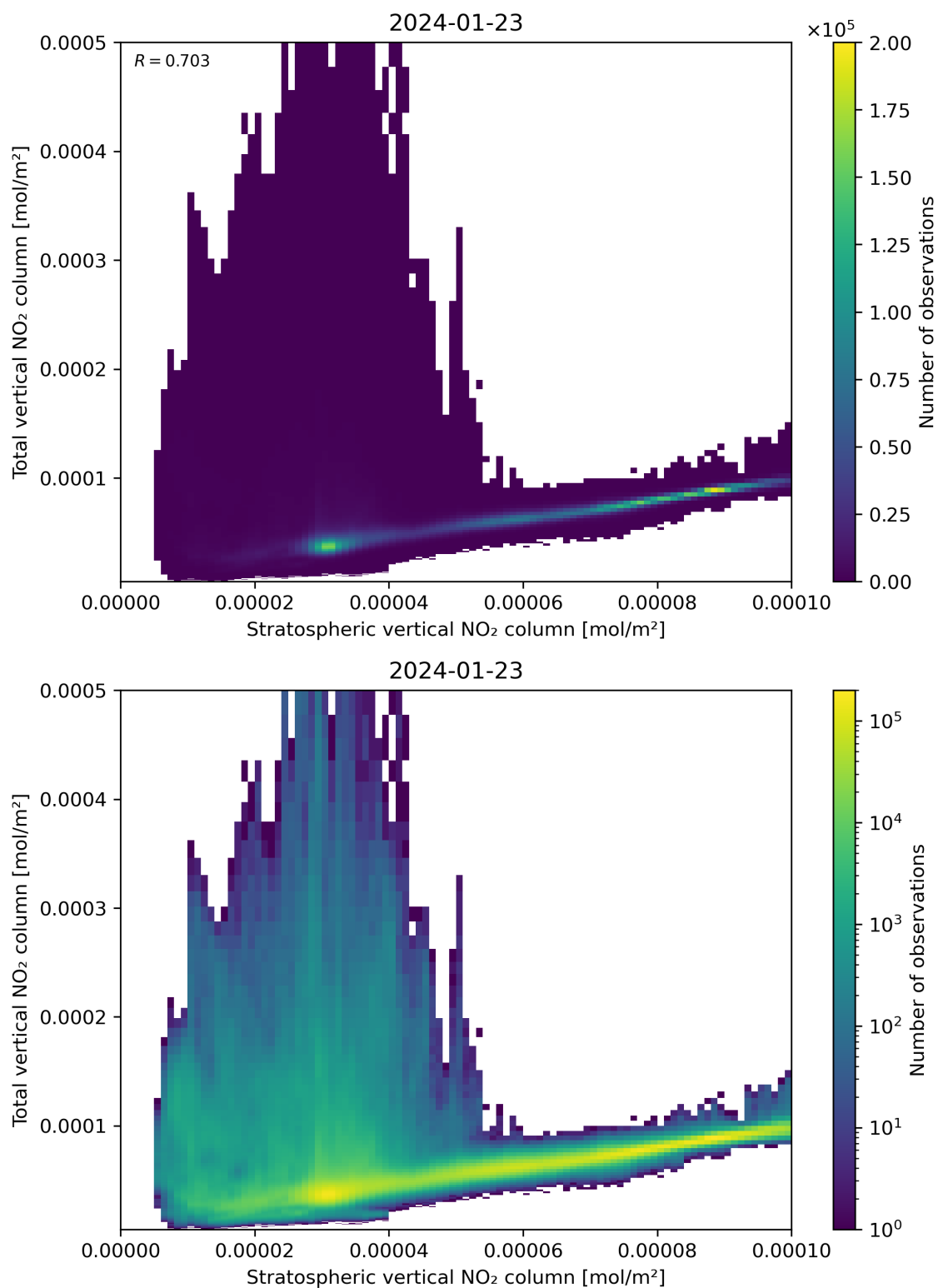
Figure 100: Scatter density plot of “Stratospheric vertical NO 2 column” against “Total vertical NO 2 column” for 2024-01-22 to 2024-01-24.
