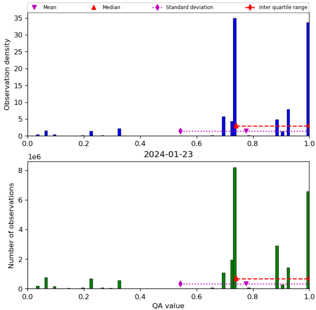
Figure 28: Histogram of “QA value” for 2024-01-22 to 2024-01-24
