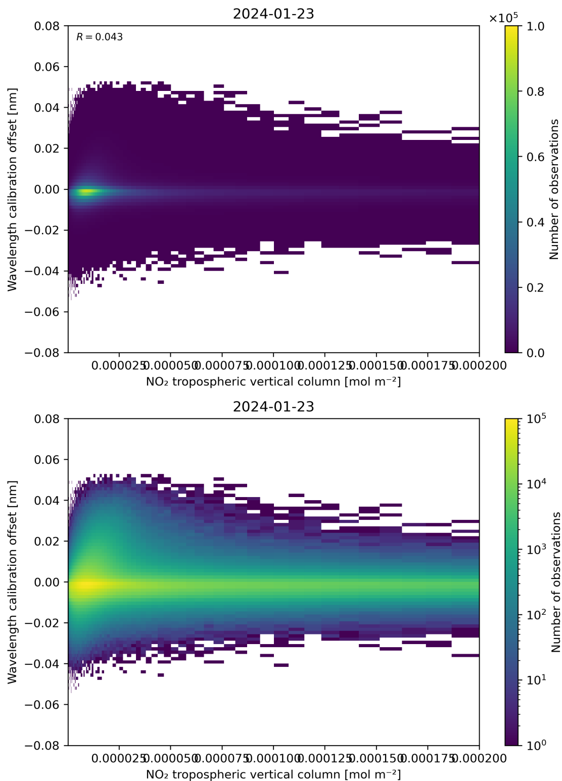
Figure 143: Scatter density plot of “NO 2 tropospheric vertical column” against “Wavelength calibration offset” for 2024-01-22 to 2024-01-24.
