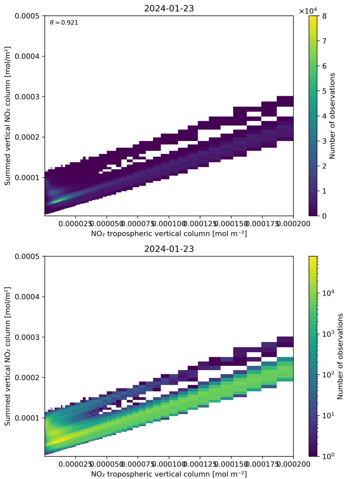
Figure 126: Scatter density plot of “NO 2 tropospheric vertical column” against “Summed vertical NO 2 column” for 2024-01-22 to 2024-01-24.
