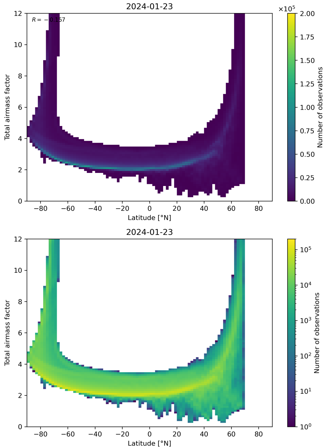
Figure 84: Scatter density plot of “Latitude” against “Total airmass factor” for 2024-01-22 to 2024-01-24.
