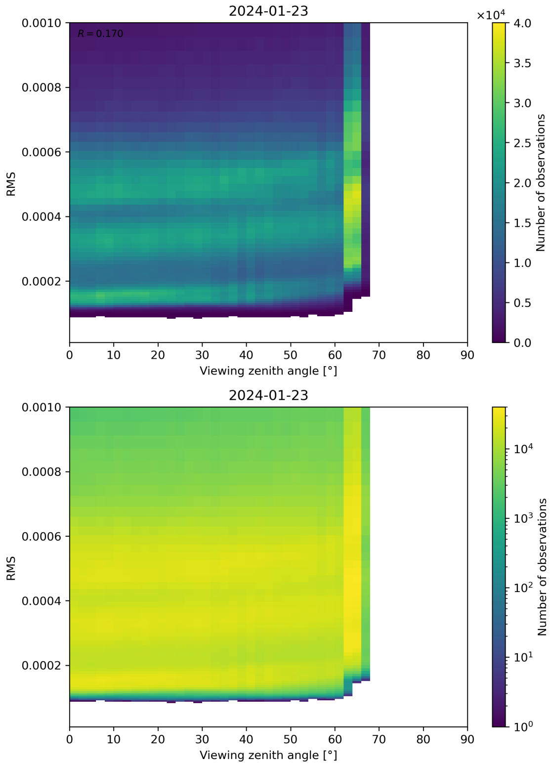
Figure 171: Scatter density plot of “Viewing zenith angle” against “RMS” for 2024-01-22 to 2024-01-24.
