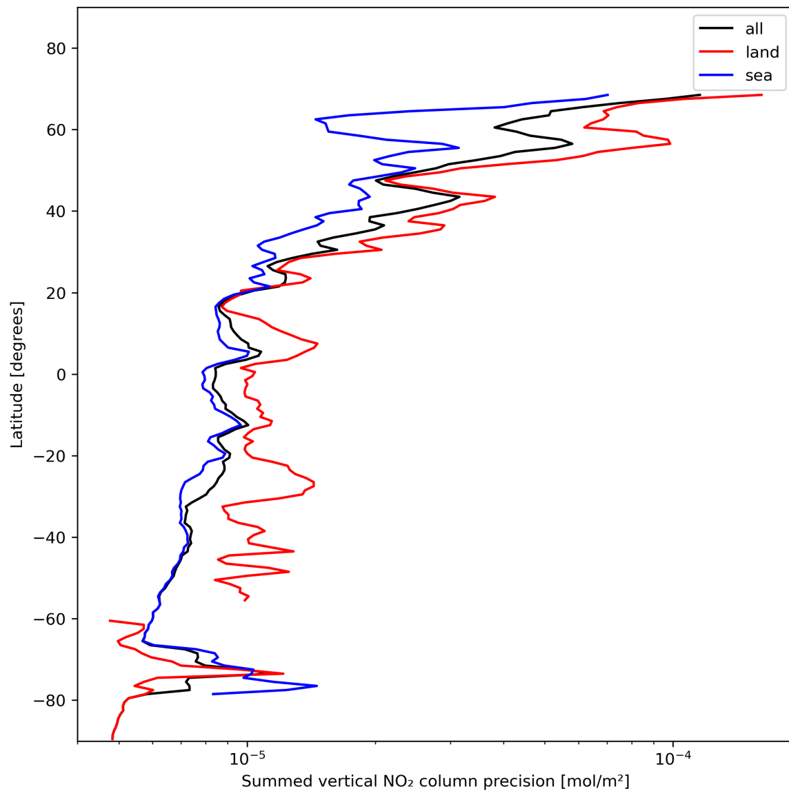
Figure 24: Zonal average of “Summed vertical NO 2 column precision” for 2024-01-22 to 2024-01-24.
