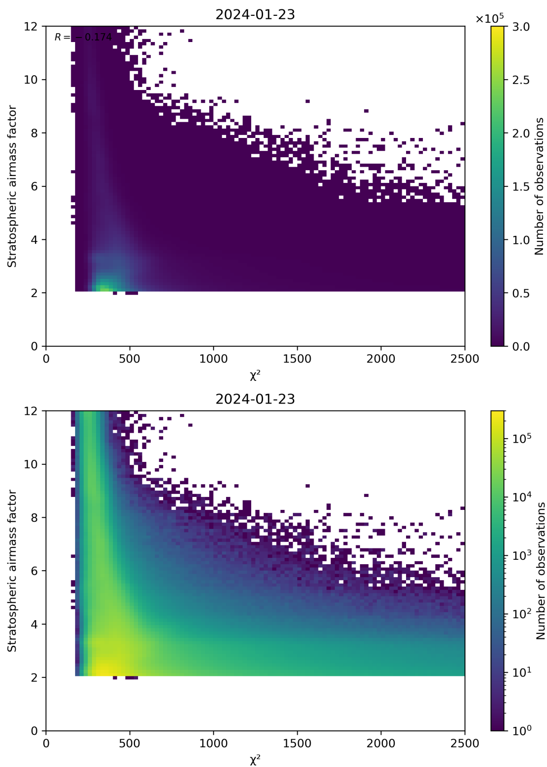
Figure 81: Scatter density plot of “ \chi^2 ” against “Stratospheric airmass factor” for 2024-01-22 to 2024-01-24.
