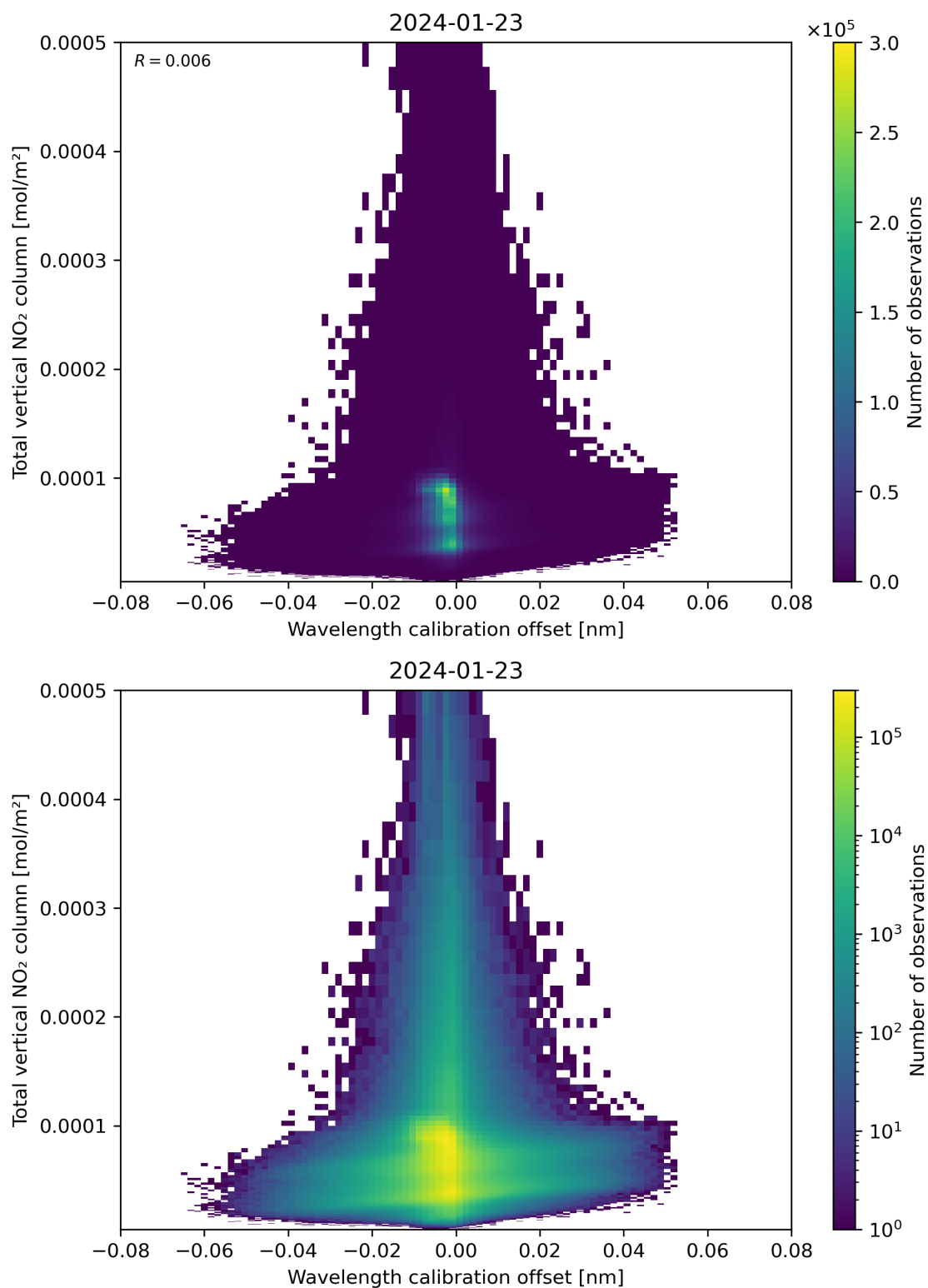
Figure 179: Scatter density plot of “Wavelength calibration offset” against “Total vertical NO 2 column” for 2024-01-22 to 2024-01-24.
