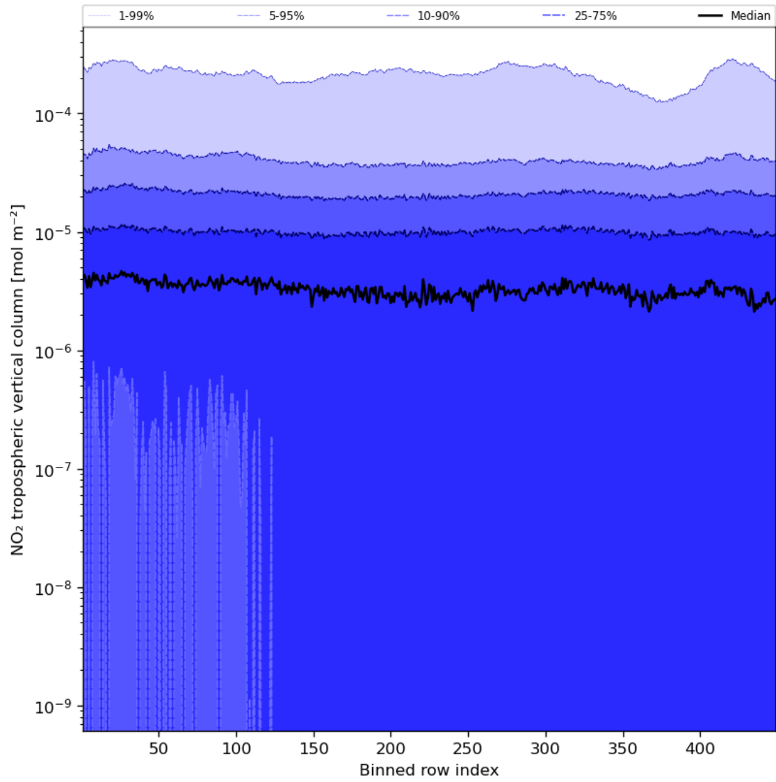
Figure 46: Along track statistics of “NO 2 tropospheric vertical column” for 2024-01-22 to 2024-01-24
