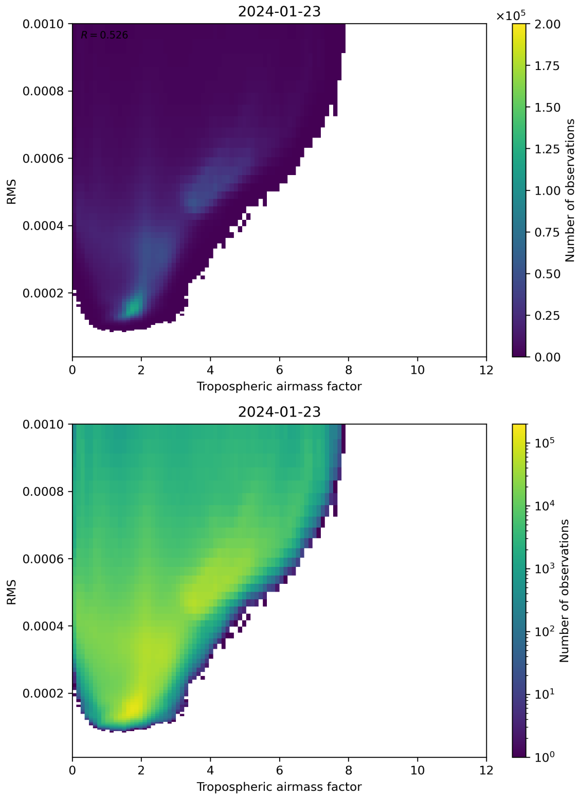
Figure 79: Scatter density plot of “Tropospheric airmass factor” against “RMS” for 2024-01-22 to 2024-01-24.
