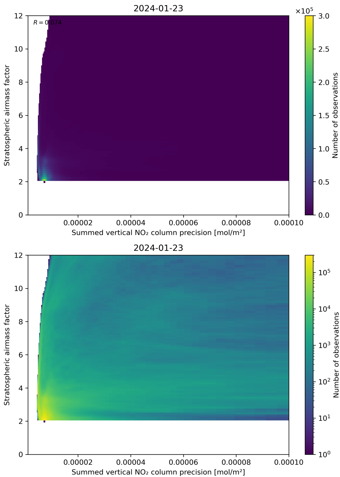
Figure 106: Scatter density plot of “Summed vertical NO 2 column precision” against “Stratospheric airmass factor” for 2024-01-22 to 2024-01-24.
