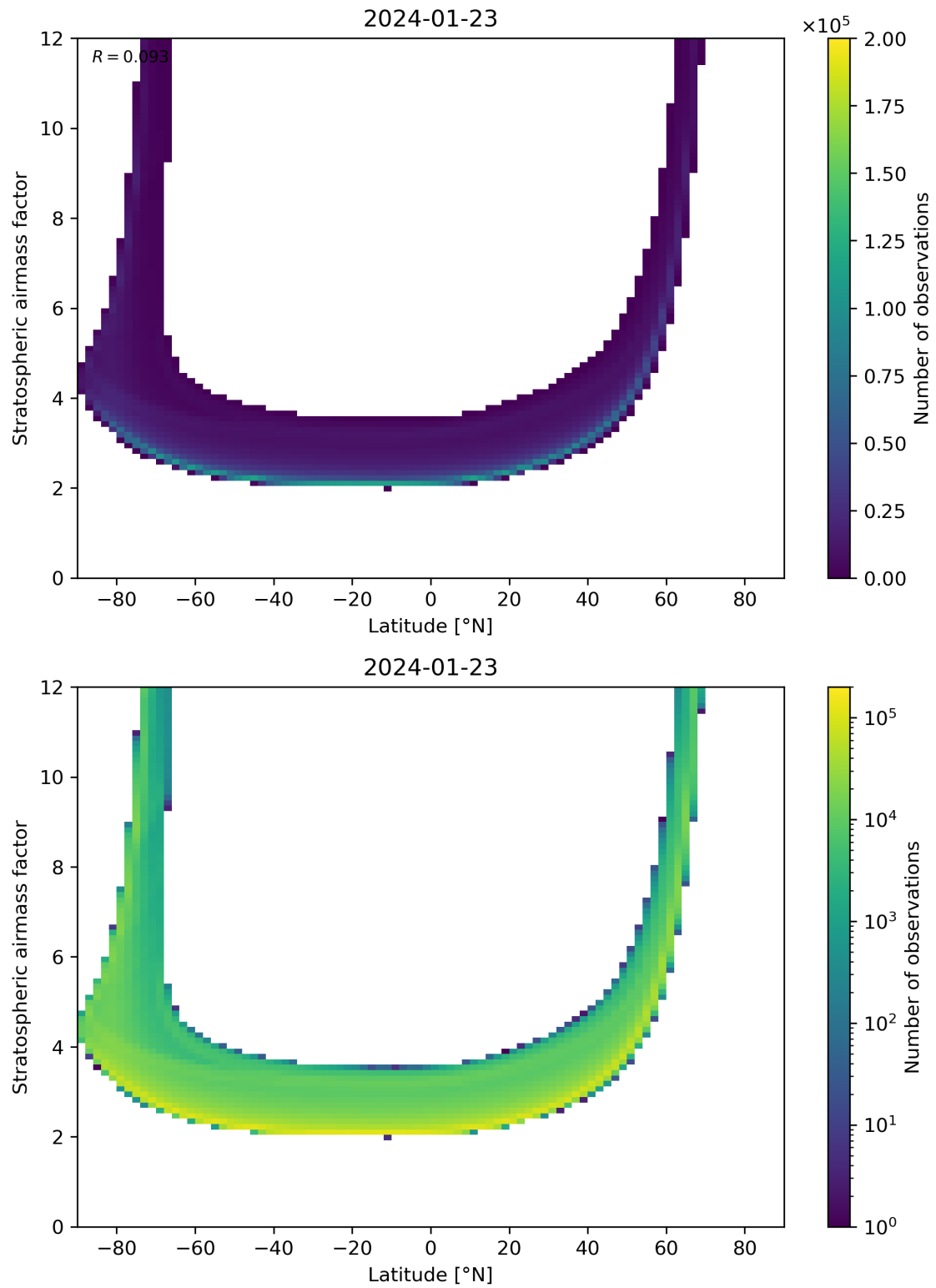
Figure 83: Scatter density plot of “Latitude” against “Stratospheric airmass factor” for 2024-01-22 to 2024-01-24.
