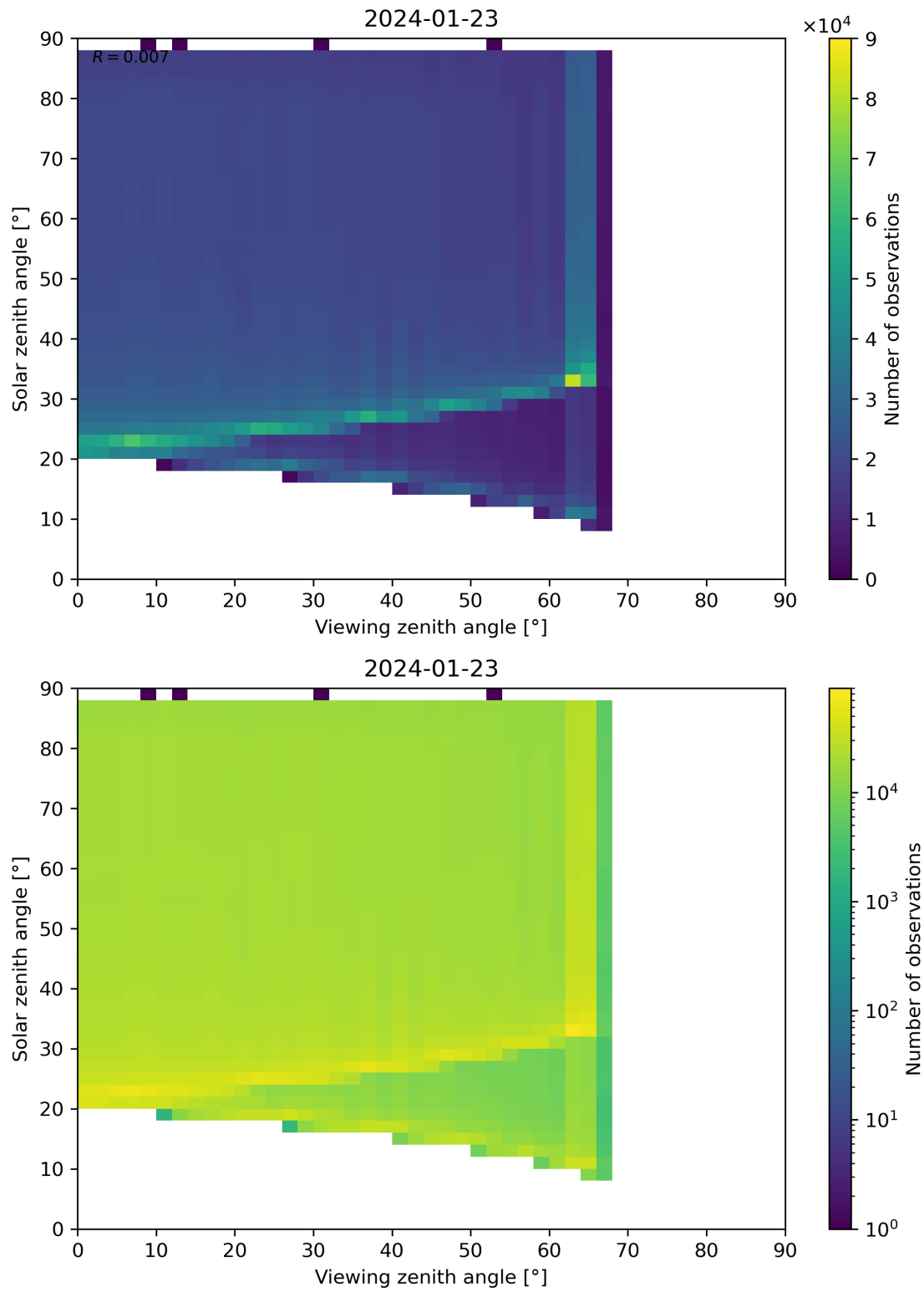
Figure 172: Scatter density plot of “Viewing zenith angle” against “Solar zenith angle” for 2024-01-22 to 2024-01-24.
