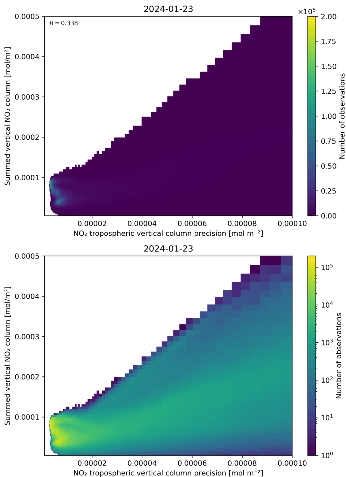
Figure 136: Scatter density plot of “NO 2 tropospheric vertical column precision” against “Summed vertical NO 2 column” for 2024-01-22 to 2024-01-24.
