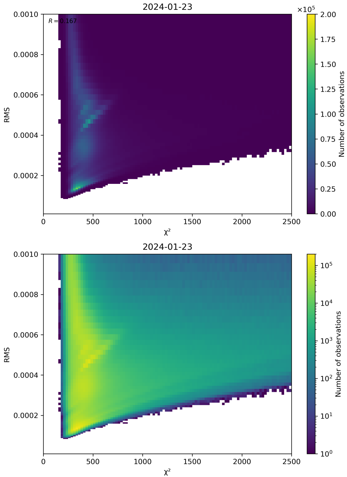
Figure 82: Scatter density plot of “ \chi^2 ” against “RMS” for 2024-01-22 to 2024-01-24.
