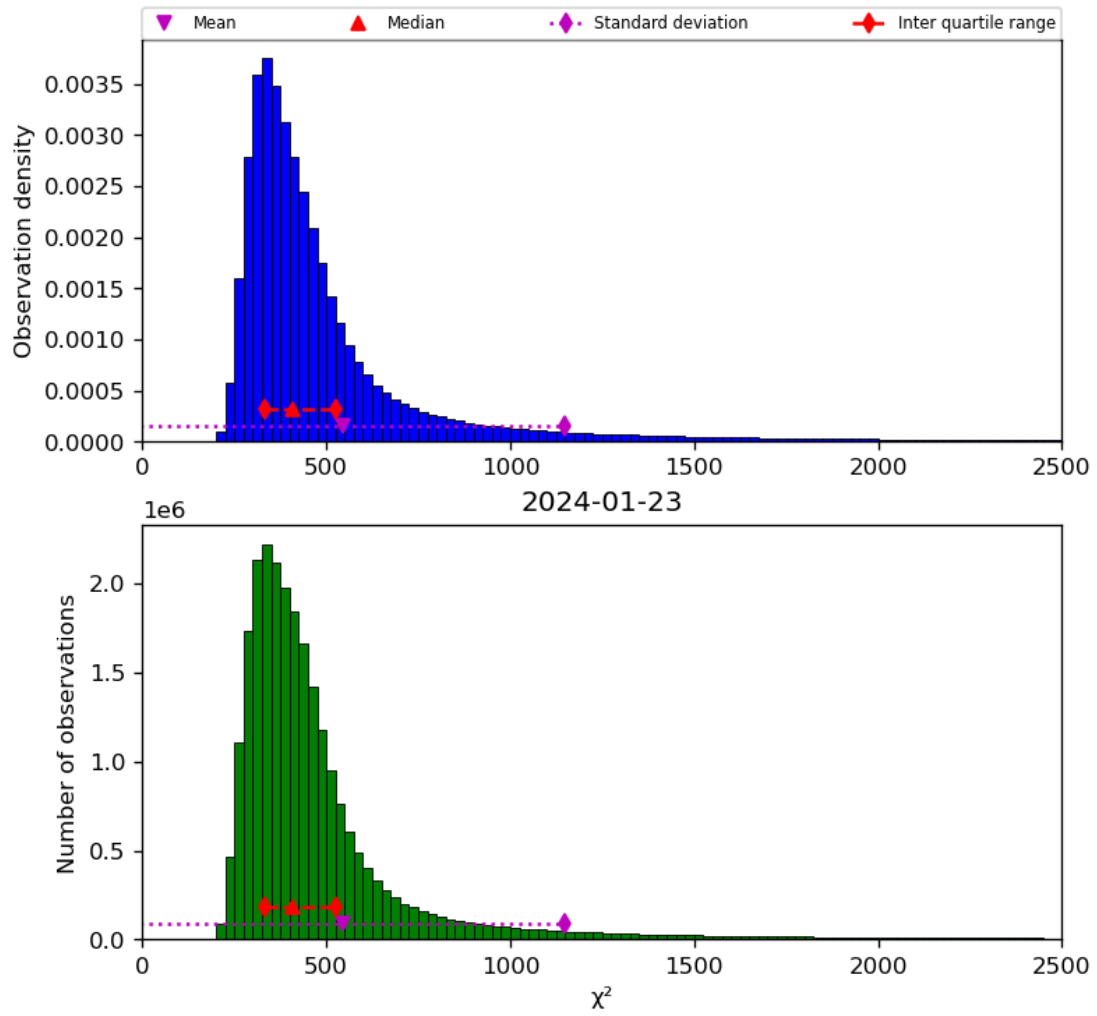
Figure 42: Histogram of “ \chi^2 ” for 2024-01-22 to 2024-01-24
