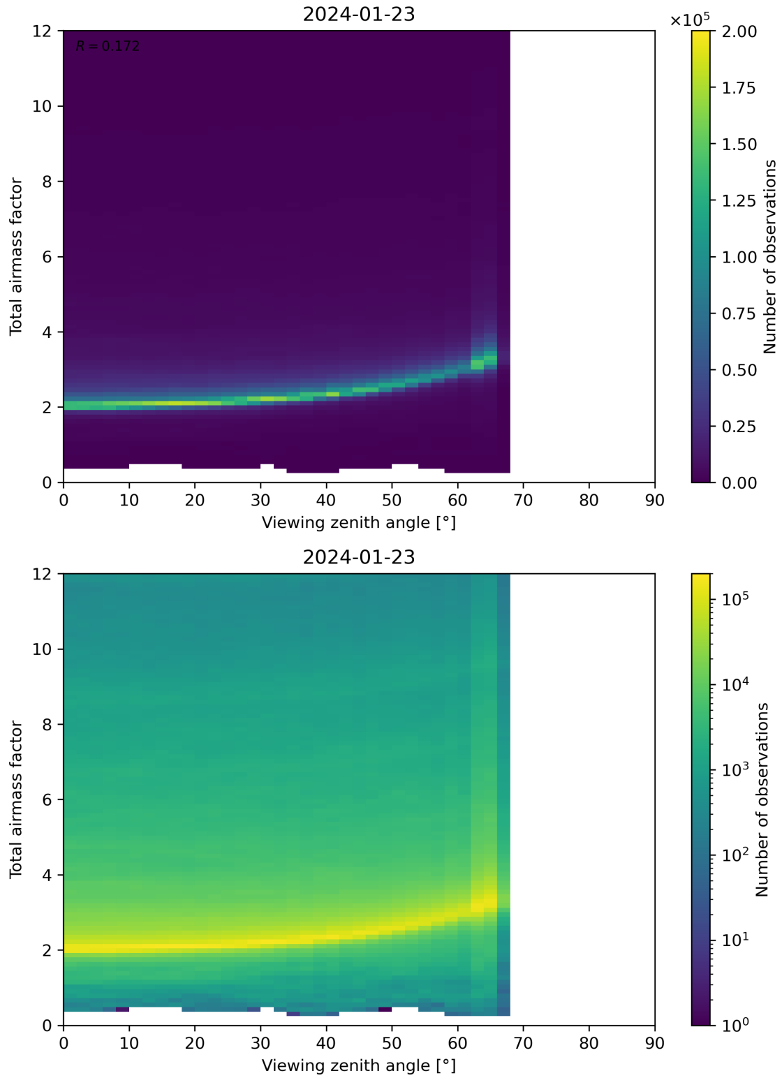
Figure 160: Scatter density plot of “Viewing zenith angle” against “Total airmass factor” for 2024-01-22 to 2024-01-24.
