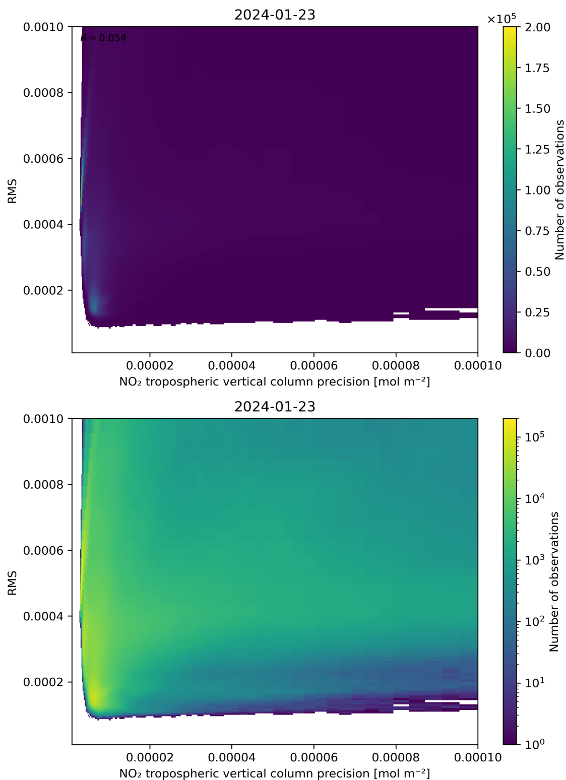
Figure 140: Scatter density plot of “NO 2 tropospheric vertical column precision” against “RMS” for 2024-01-22 to 2024-01-24.
