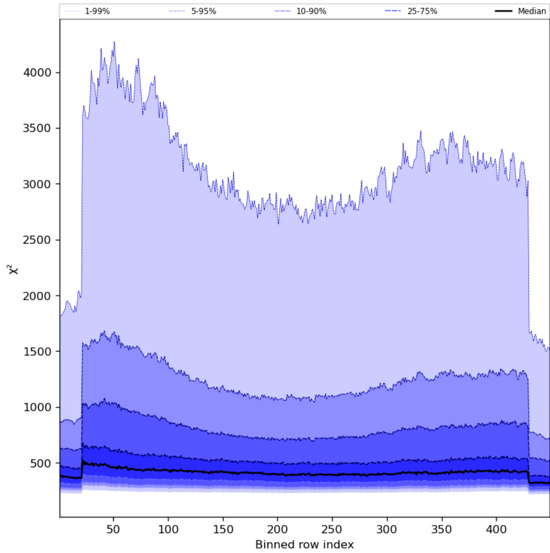
Figure 59: Along track statistics of “ \chi^2 ” for 2024-01-22 to 2024-01-24
