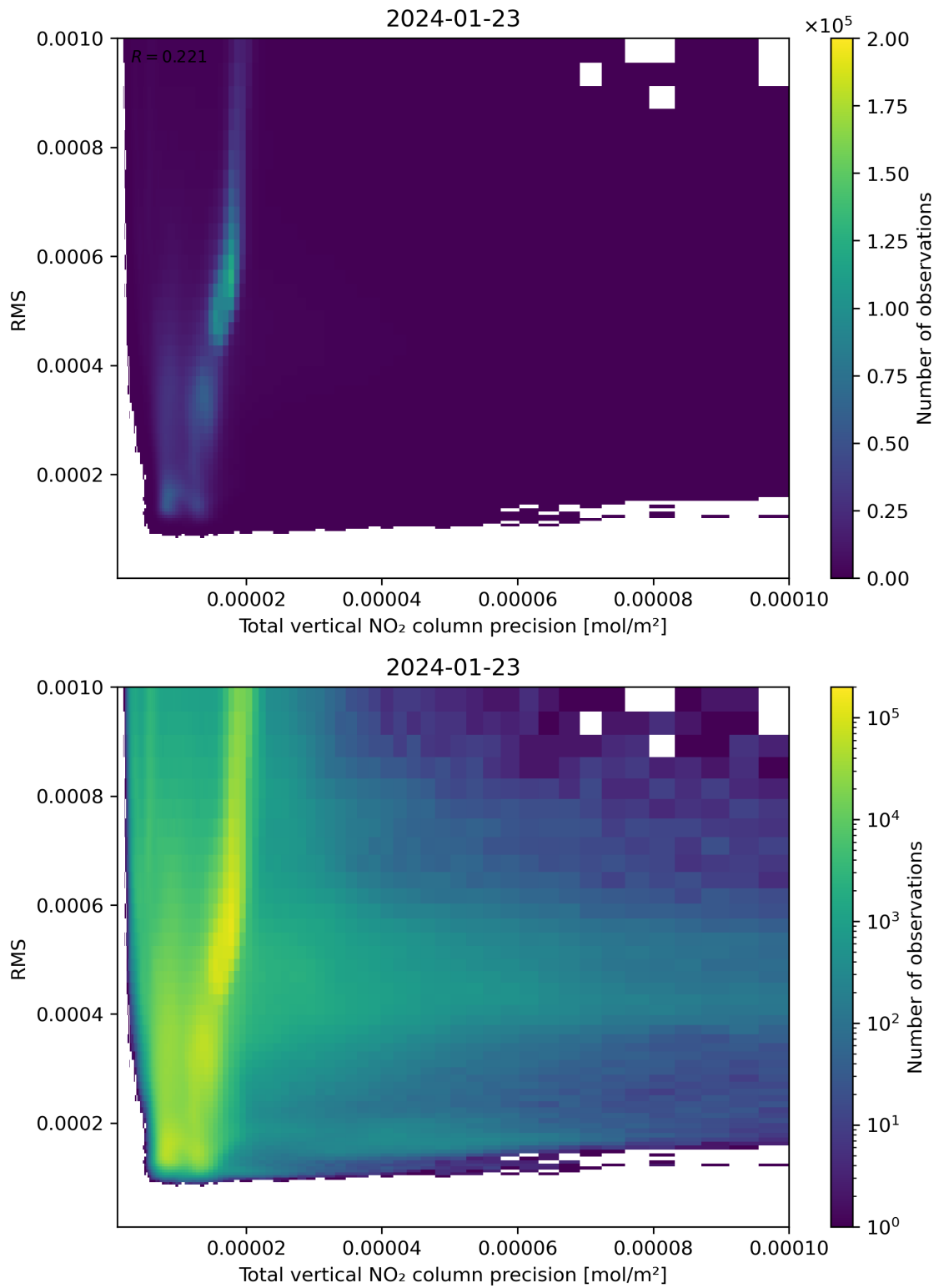
Figure 119: Scatter density plot of “Total vertical NO 2 column precision” against “RMS” for 2024-01-22 to 2024-01-24.
