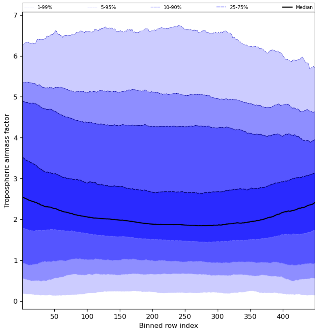
Figure 48: Along track statistics of “Tropospheric air mass factor” for 2024-01-22 to 2024-01-24
