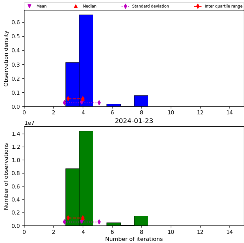
Figure 34: Histogram of “Number of iterations” for 2024-01-22 to 2024-01-24
