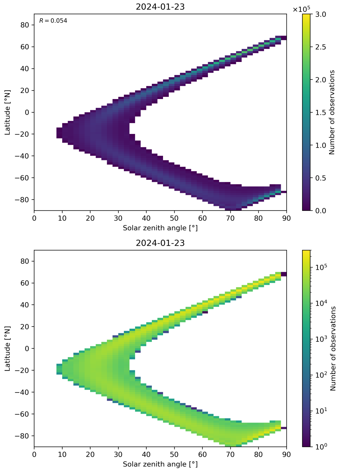
Figure 149: Scatter density plot of “Solar zenith angle” against “Latitude” for 2024-01-22 to 2024-01-24.
