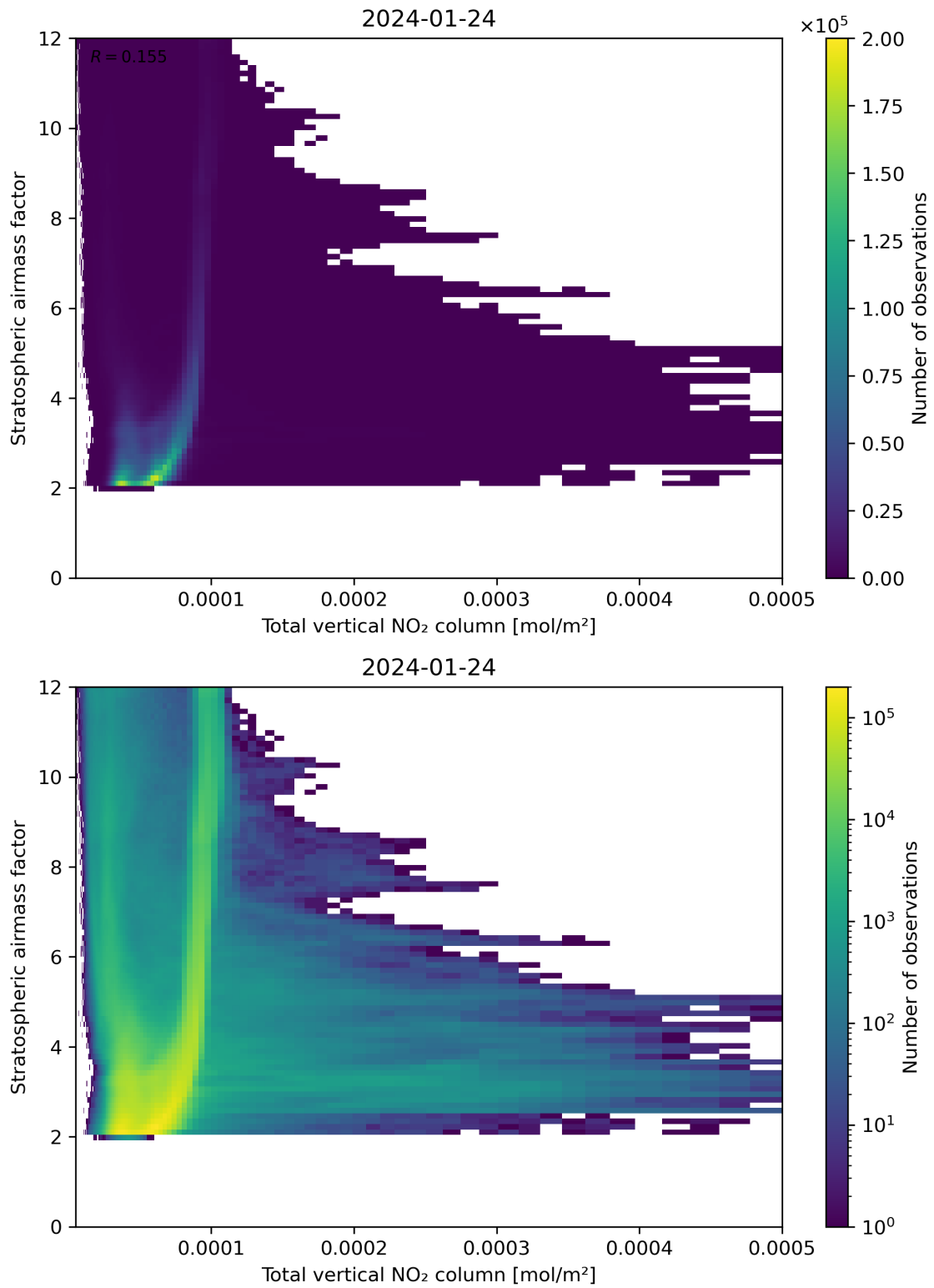
Figure 110: Scatter density plot of “Total vertical NO 2 column” against “Stratospheric air mass factor” for 2024-01-23 to 2024-01-25.
