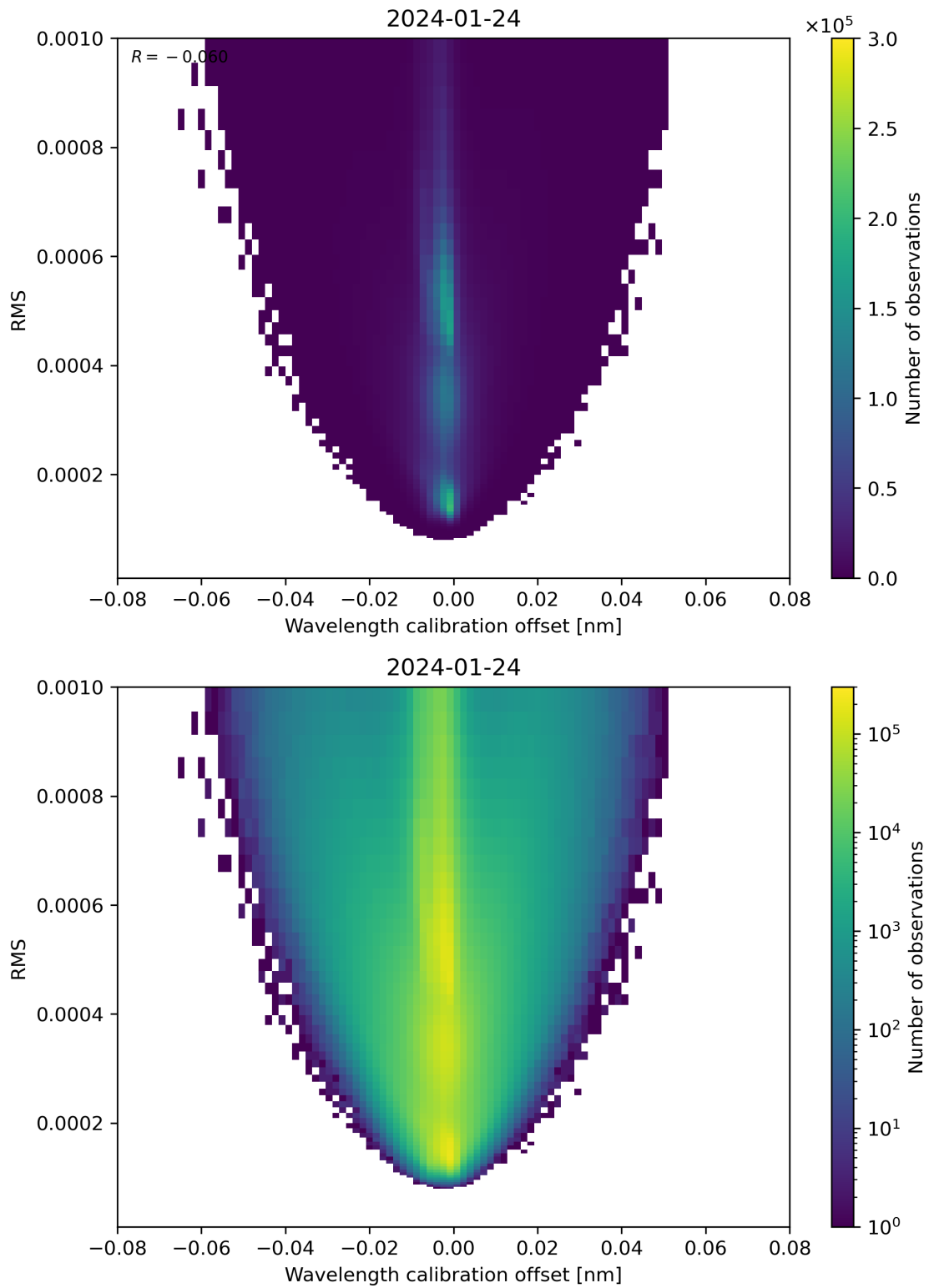
Figure 181: Scatter density plot of “Wavelength calibration offset” against “RMS” for 2024-01-23 to 2024-01-25.
