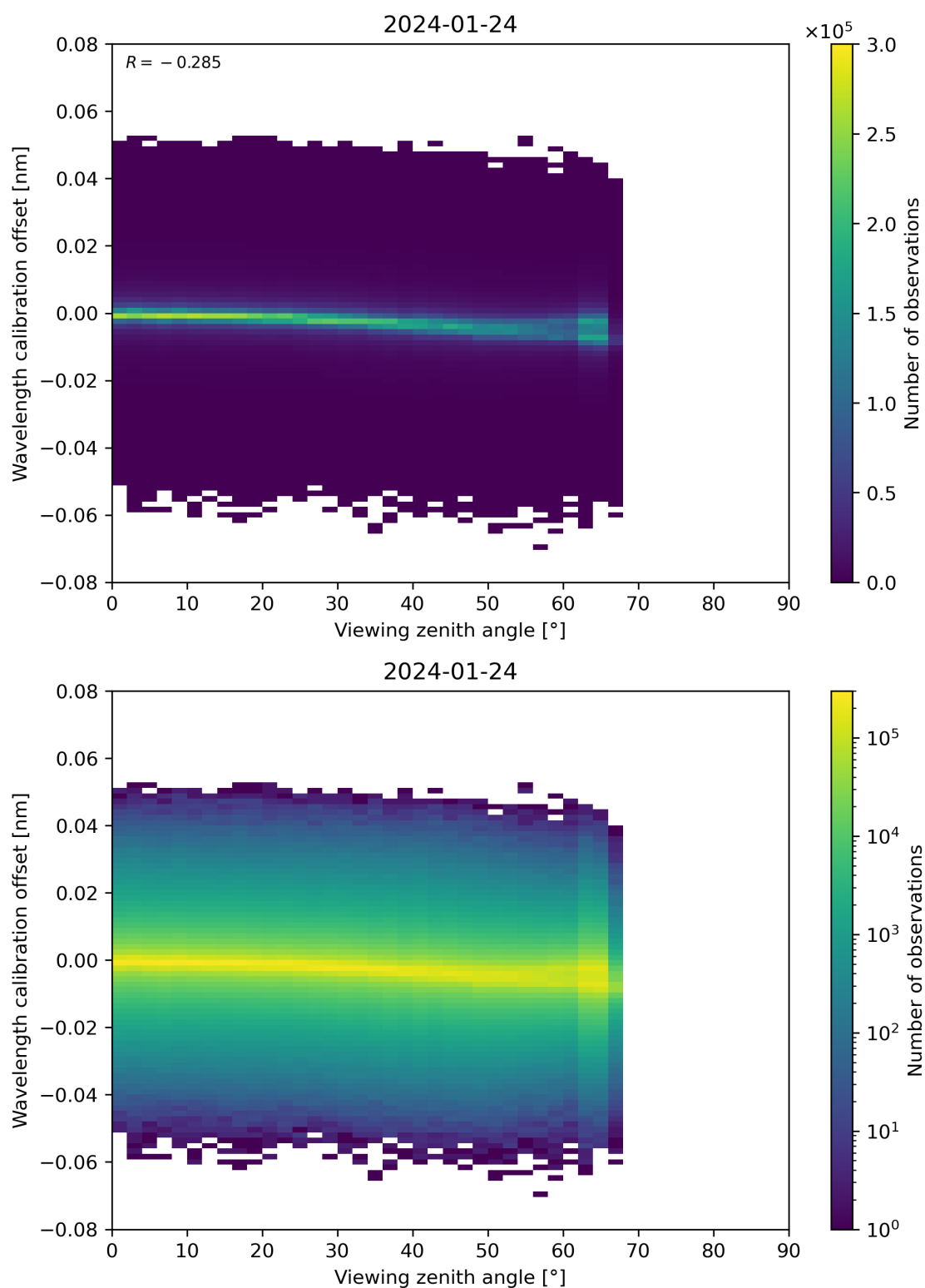
Figure 173: Scatter density plot of “Viewing zenith angle” against “Wavelength calibration offset” for 2024-01-23 to 2024-01-25.
