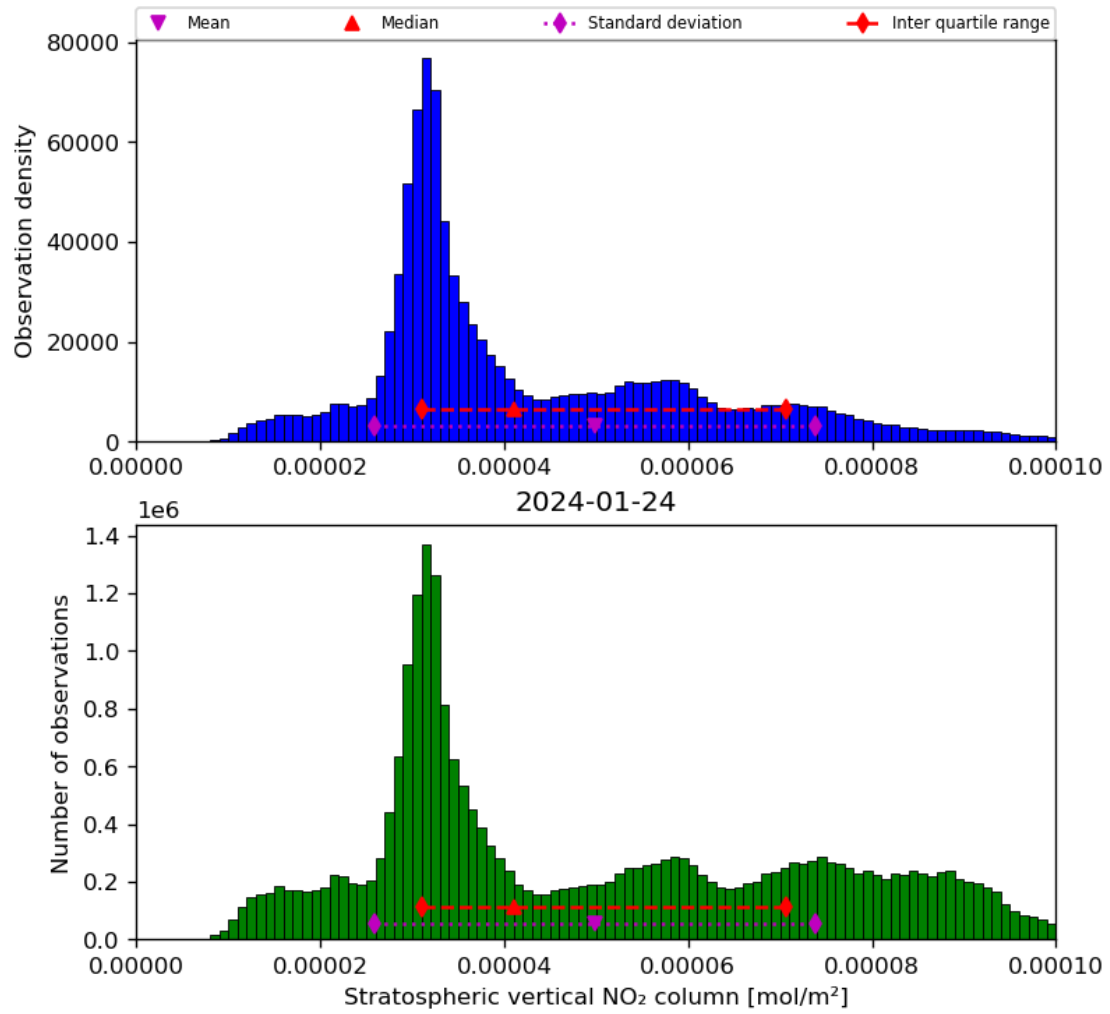
Figure 36: Histogram of “Stratospheric vertical NO 2 column” for 2024-01-23 to 2024-01-25
