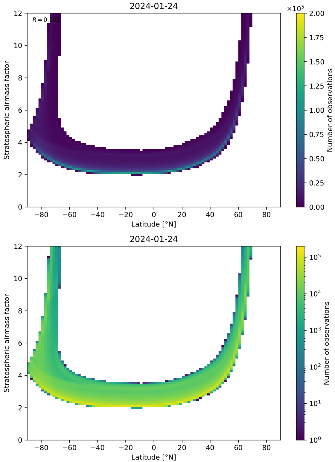
Figure 83: Scatter density plot of “Latitude” against “Stratospheric airmass factor” for 2024-01-23 to 2024-01-25.
