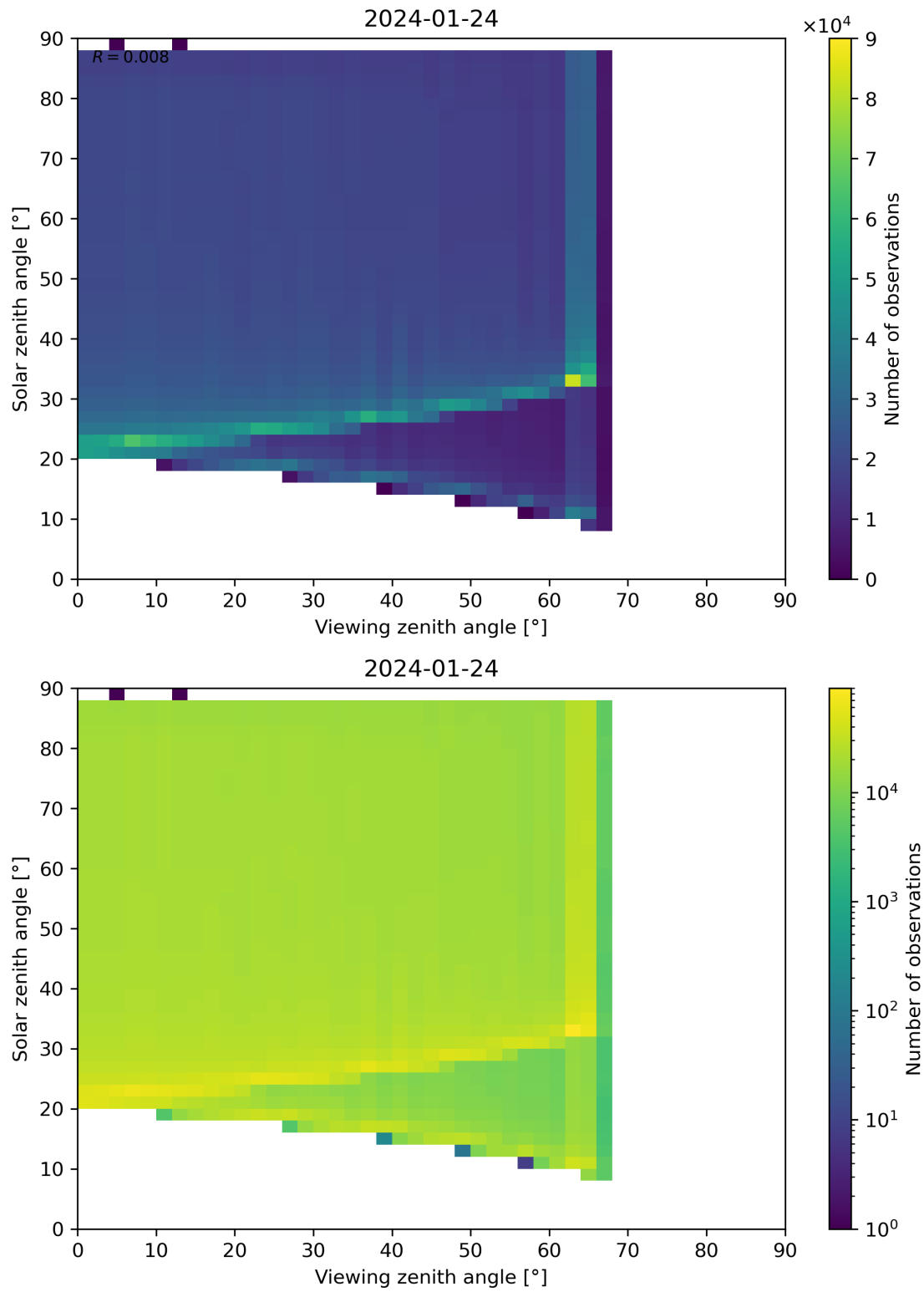
Figure 172: Scatter density plot of “Viewing zenith angle” against “Solar zenith angle” for 2024-01-23 to 2024-01-25.
