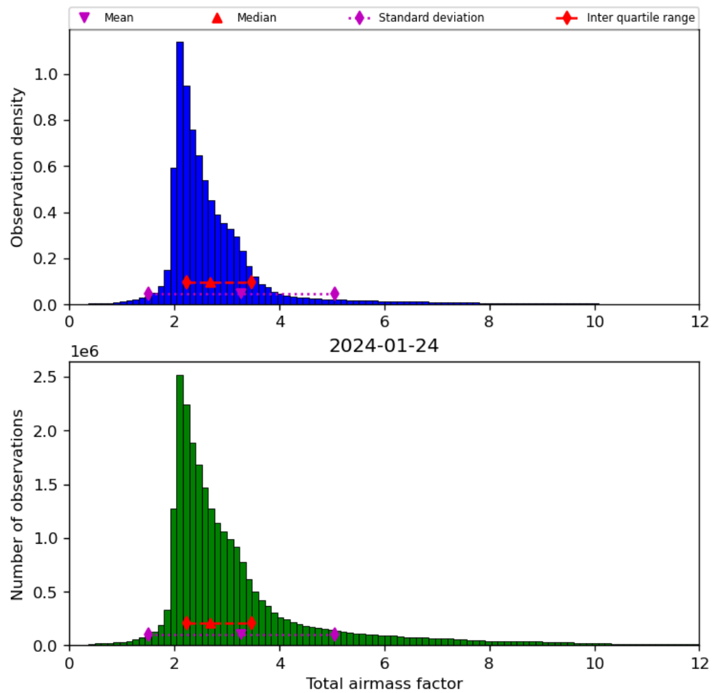
Figure 32: Histogram of “Total airmass factor” for 2024-01-23 to 2024-01-25
