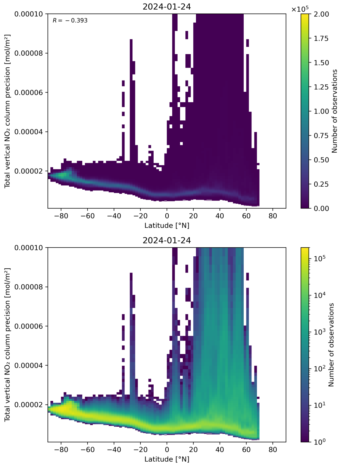
Figure 91: Scatter density plot of “Latitude” against “Total vertical NO 2 column precision” for 2024-01-23 to 2024-01-25.
