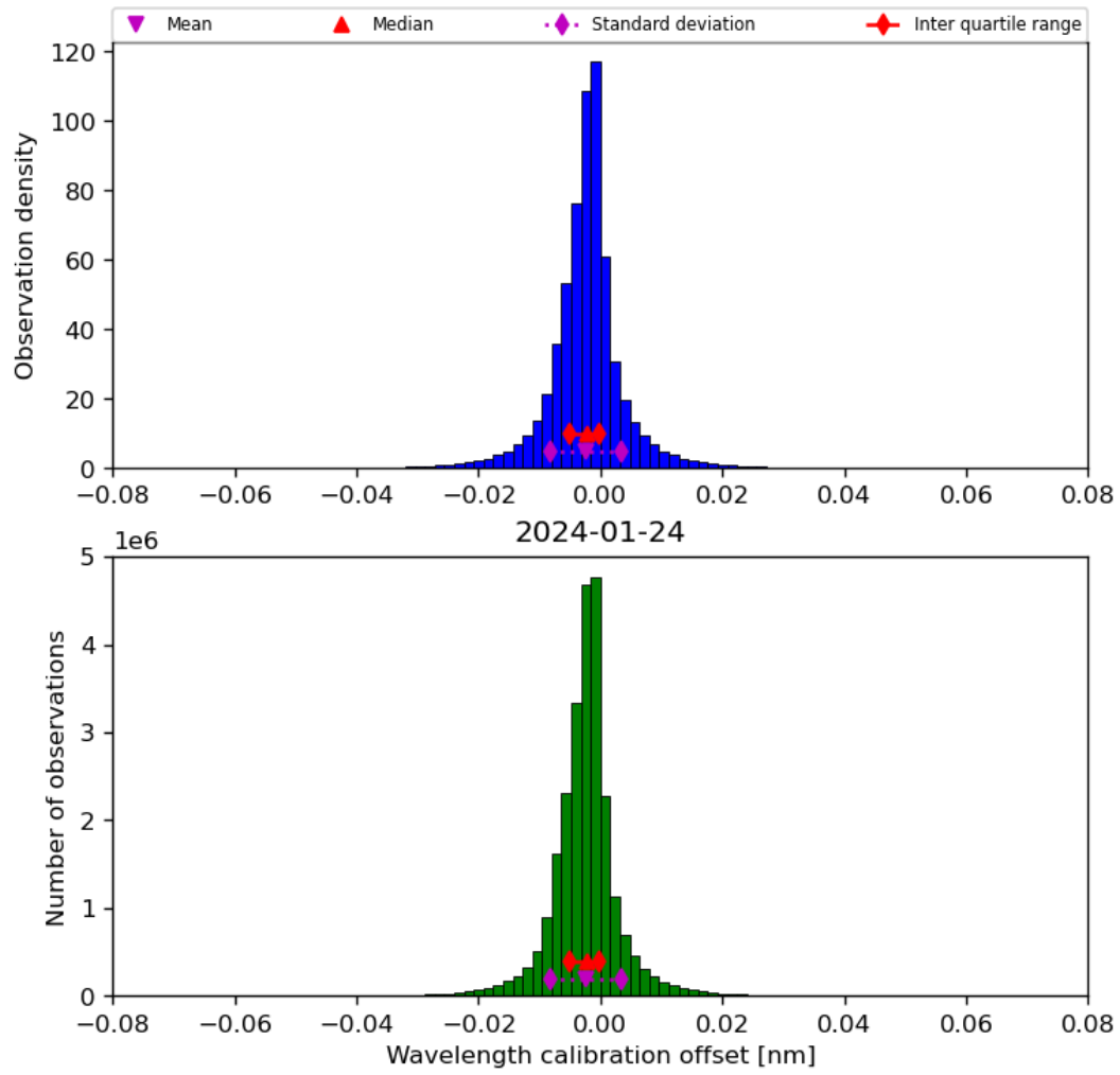
Figure 35: Histogram of “Wavelength calibration offset” for 2024-01-23 to 2024-01-25
