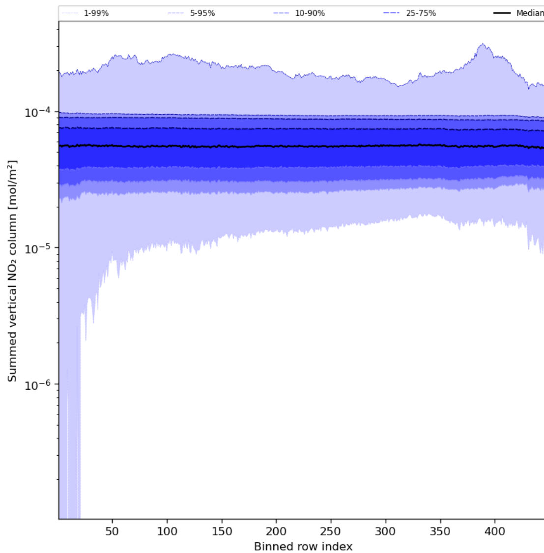
Figure 57: Along track statistics of “Summed vertical NO 2 column” for 2024-01-23 to 2024-01-25
