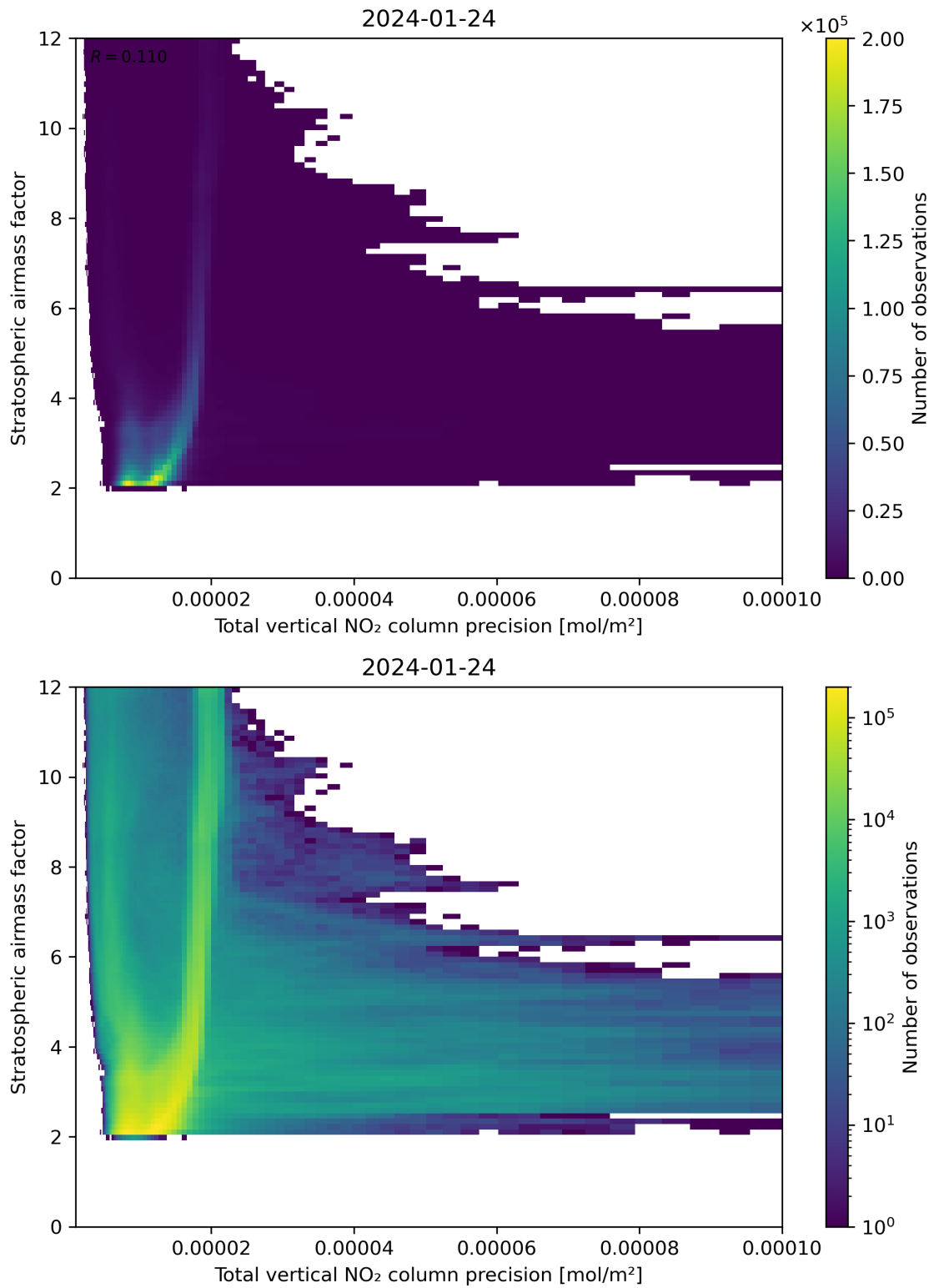
Figure 115: Scatter density plot of “Total vertical NO 2 column precision” against “Stratospheric air mass factor” for 2024-01-23 to 2024-01-25.
