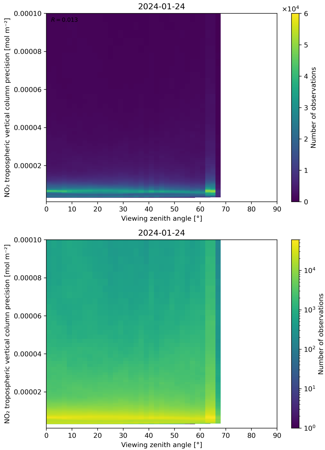
Figure 170: Scatter density plot of “Viewing zenith angle” against “NO 2 tropospheric vertical column precision” for 2024-01-23 to 2024-01-25.
