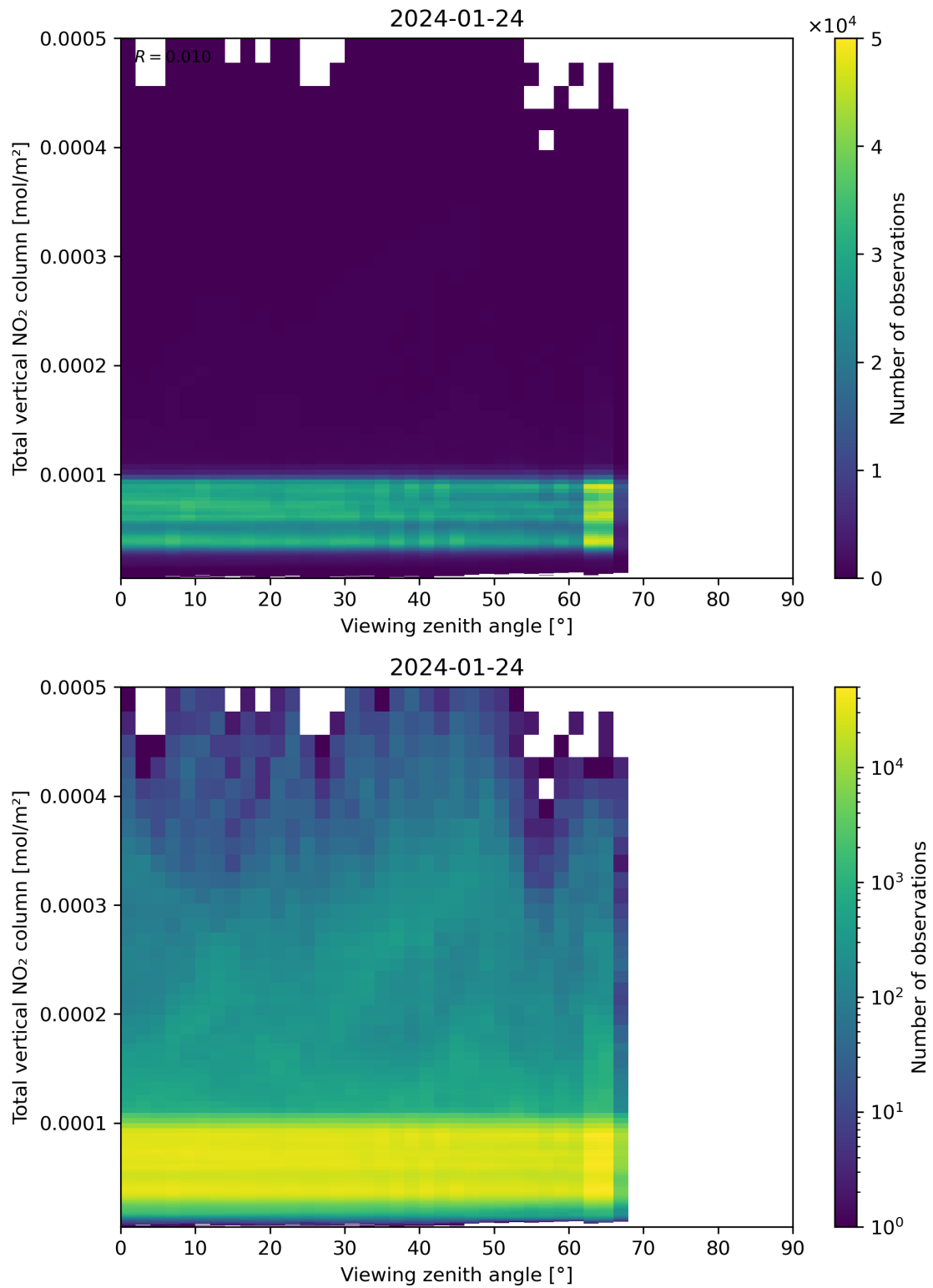
Figure 167: Scatter density plot of “Viewing zenith angle” against “Total vertical NO 2 column” for 2024-01-23 to 2024-01-25.
