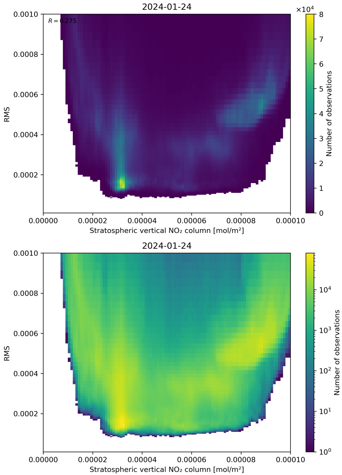
Figure 102: Scatter density plot of “Stratospheric vertical NO 2 column” against “RMS” for 2024-01-23 to 2024-01-25.
