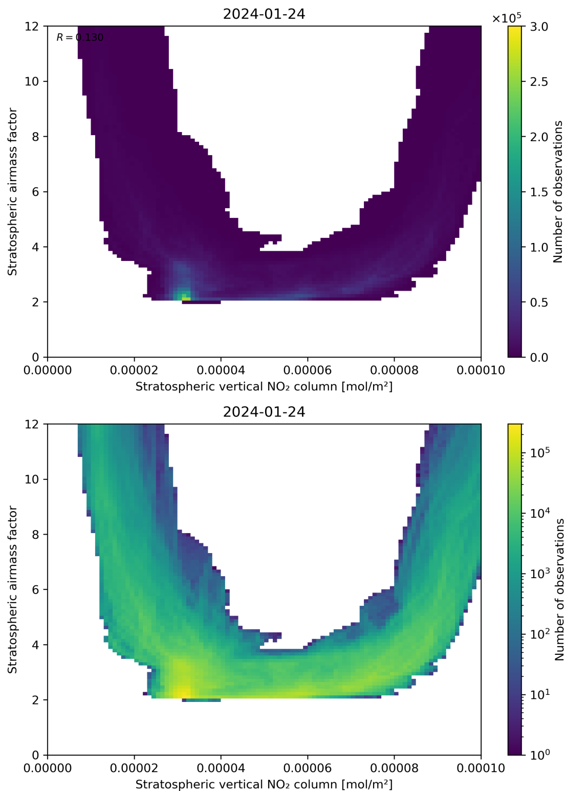
Figure 96: Scatter density plot of “Stratospheric vertical NO 2 column” against “Stratospheric airmass factor” for 2024-01-23 to 2024-01-25.
