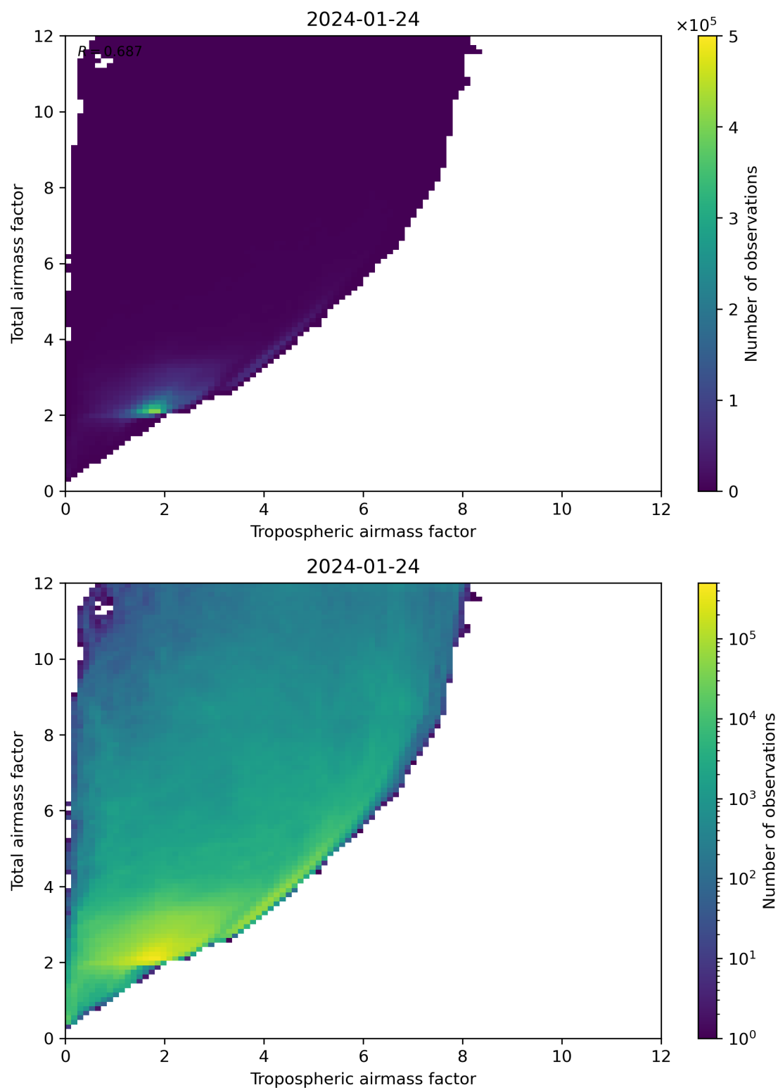
Figure 72: Scatter density plot of “Tropospheric airmass factor” against “Total airmass factor” for 2024-01-23 to 2024-01-25.
