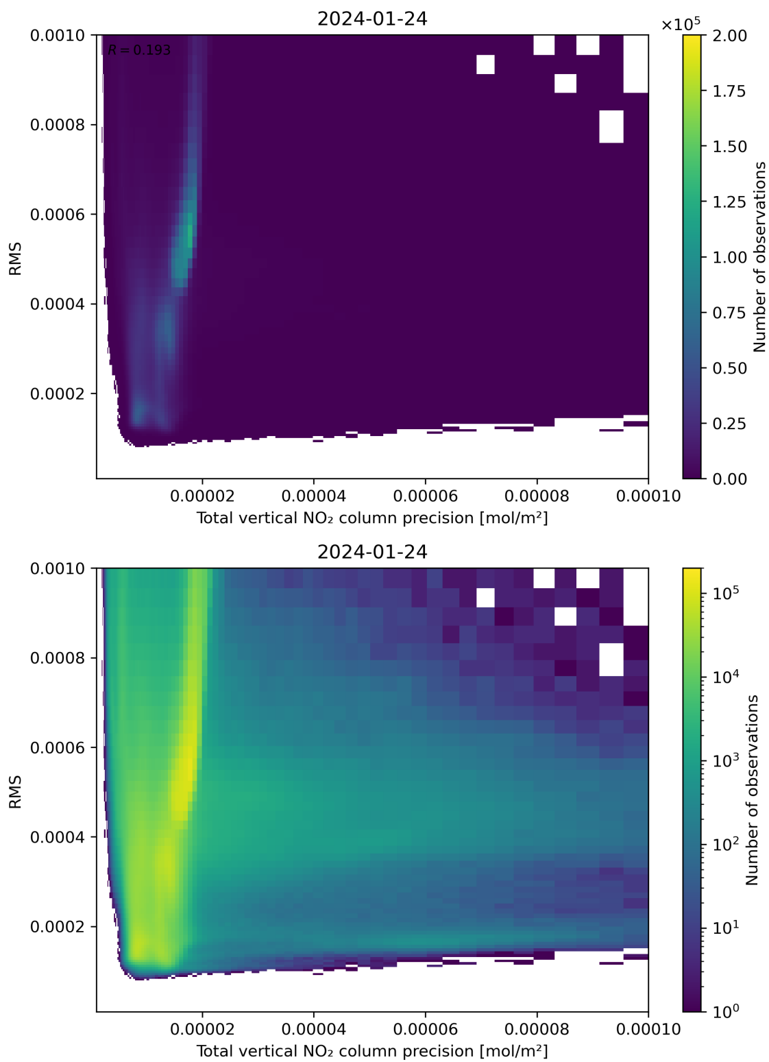
Figure 119: Scatter density plot of “Total vertical NO 2 column precision” against “RMS” for 2024-01-23 to 2024-01-25.
