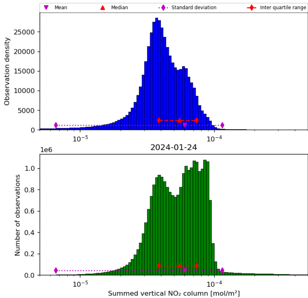
Figure 40: Histogram of “Summed vertical NO 2 column” for 2024-01-23 to 2024-01-25
