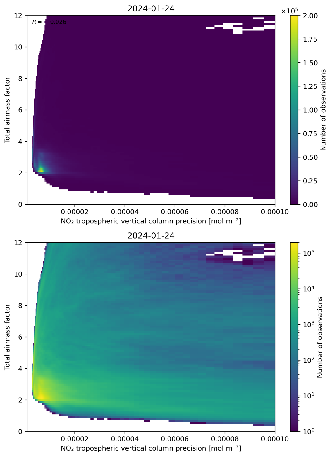
Figure 132: Scatter density plot of “NO 2 tropospheric vertical column precision” against “Total air mass factor” for 2024-01-23 to 2024-01-25.
