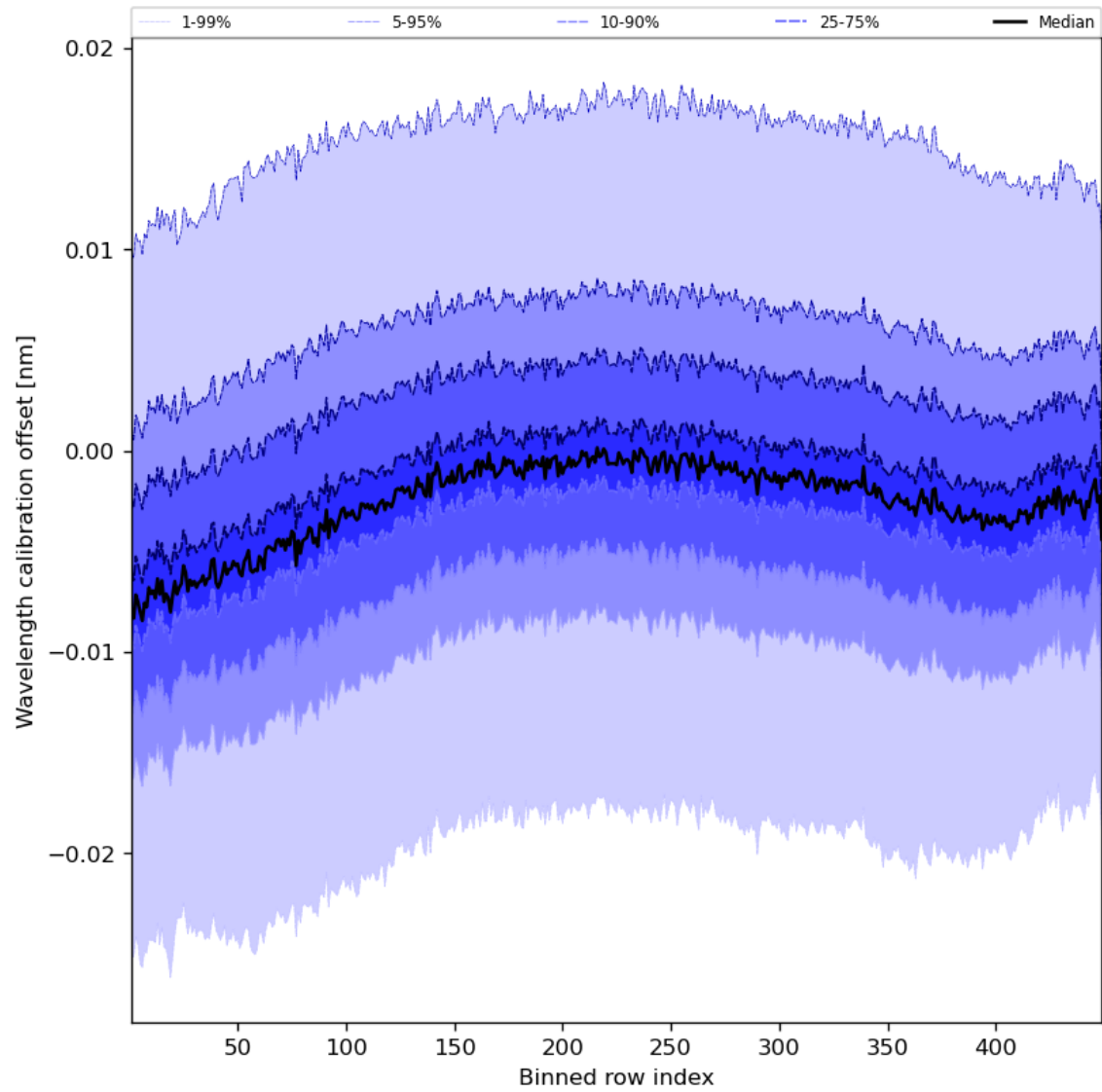
Figure 52: Along track statistics of “Wavelength calibration offset” for 2024-01-23 to 2024-01-25
