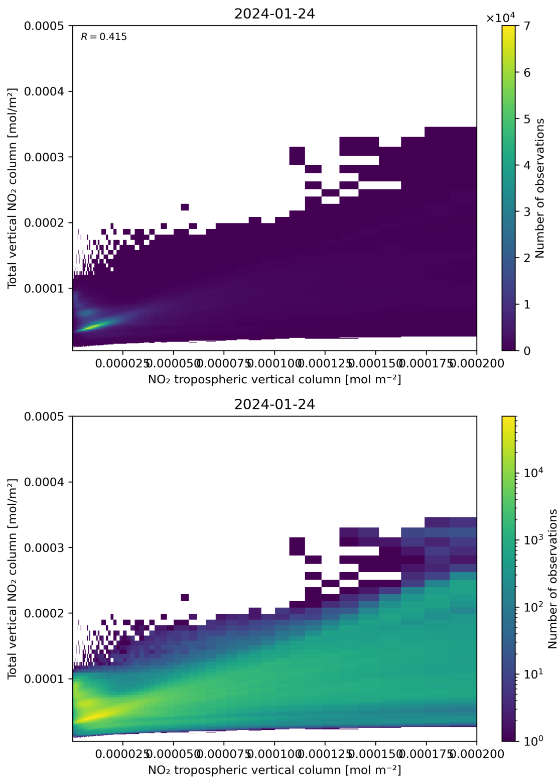
Figure 128: Scatter density plot of “NO 2 tropospheric vertical column” against “Total vertical NO 2 column” for 2024-01-23 to 2024-01-25.
