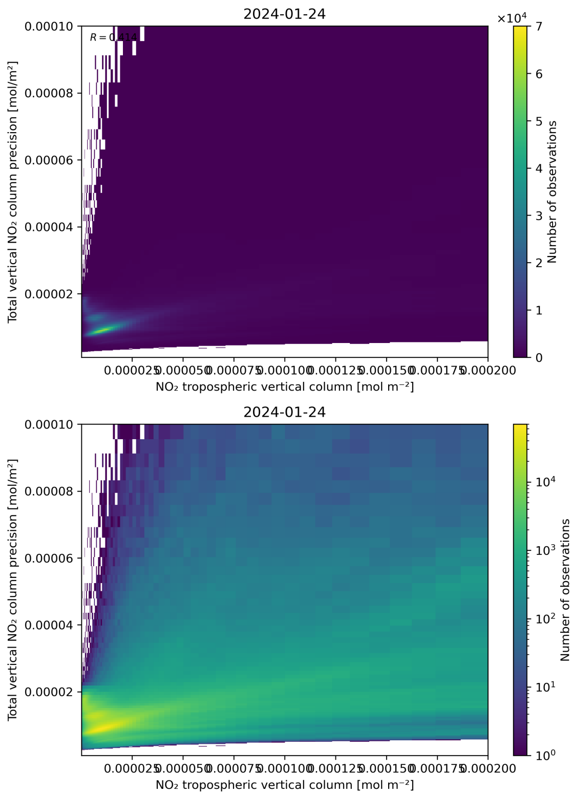
Figure 129: Scatter density plot of “NO 2 tropospheric vertical column” against “Total vertical NO 2 column precision” for 2024-01-23 to 2024-01-25.
