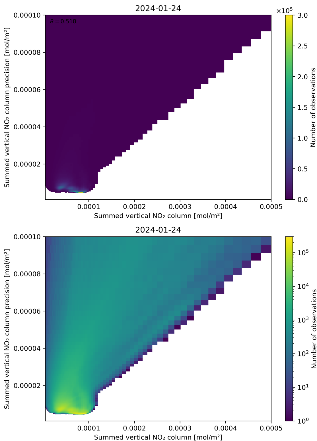
Figure 105: Scatter density plot of “Summed vertical NO 2 column” against “Summed vertical NO 2 column precision” for 2024-01-23 to 2024-01-25.
