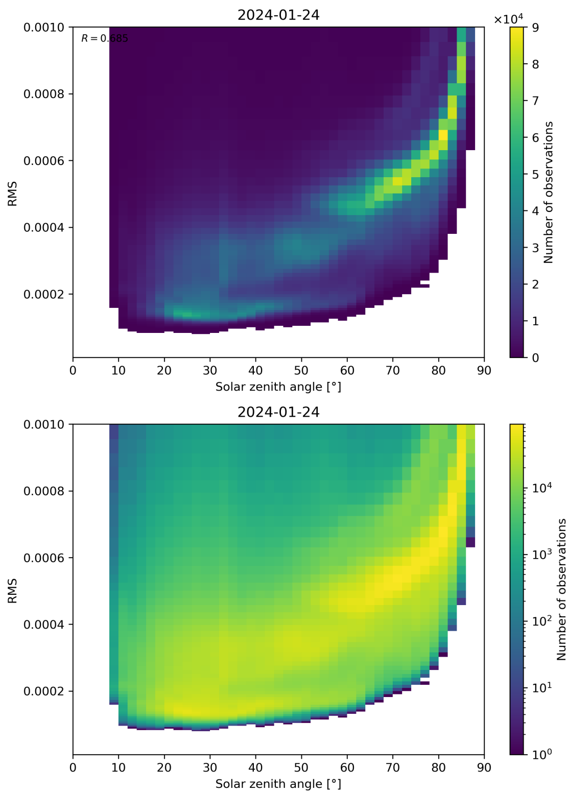
Figure 157: Scatter density plot of “Solar zenith angle” against “RMS” for 2024-01-23 to 2024-01-25.
