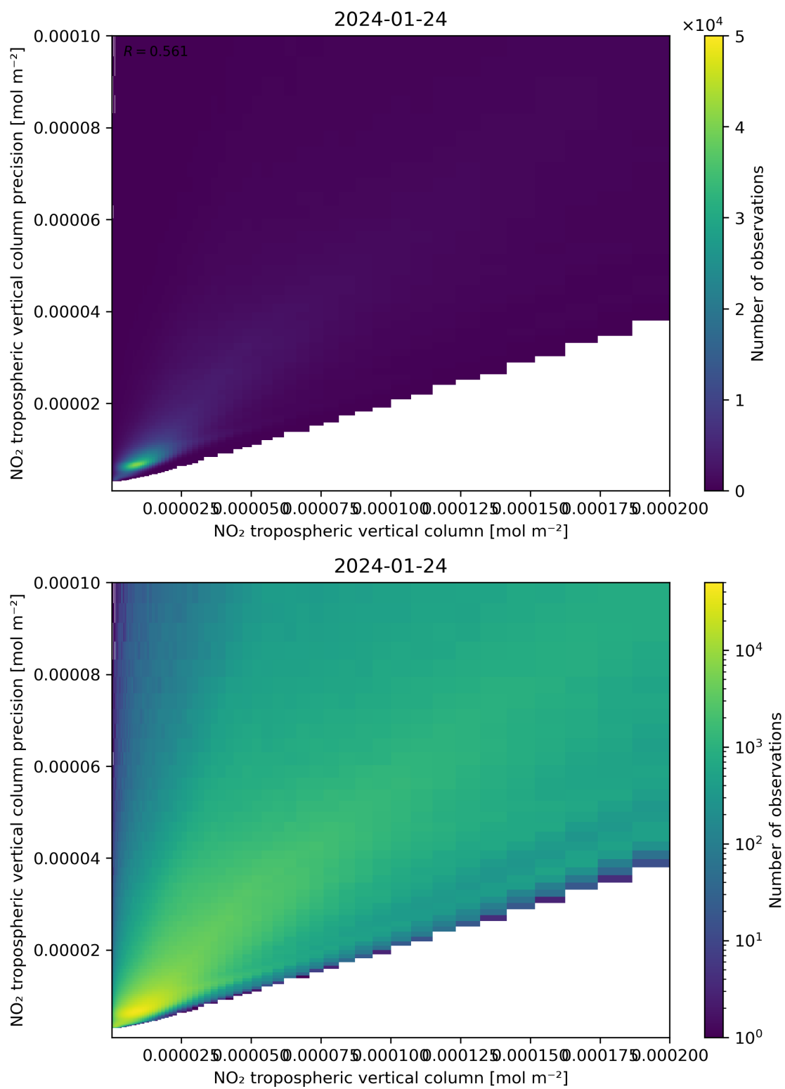
Figure 130: Scatter density plot of “NO 2 tropospheric vertical column” against “NO 2 tropospheric vertical column precision” for 2024-01-23 to 2024-01-25.
