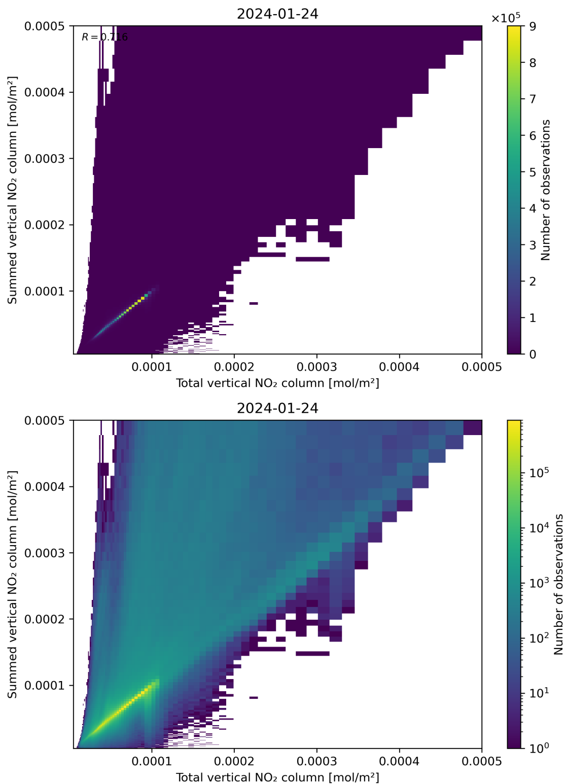
Figure 112: Scatter density plot of “Total vertical NO 2 column” against “Summed vertical NO 2 column” for 2024-01-23 to 2024-01-25.
