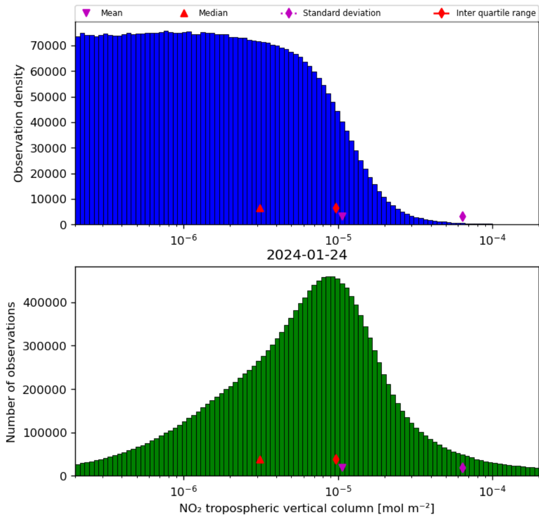
Figure 29: Histogram of “NO 2 tropospheric vertical column” for 2024-01-23 to 2024-01-25
