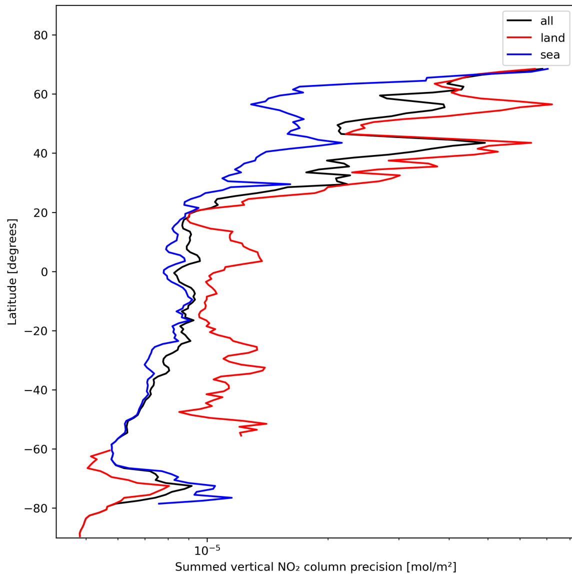
Figure 24: Zonal average of “Summed vertical NO 2 column precision” for 2024-01-23 to 2024-01-25.
