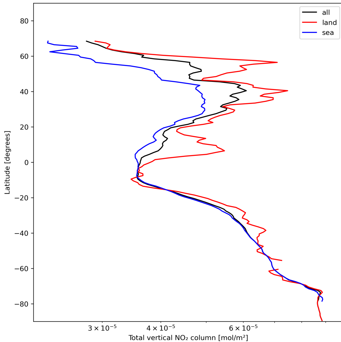
Figure 21: Zonal average of “Total vertical NO 2 column” for 2024-01-23 to 2024-01-25.
