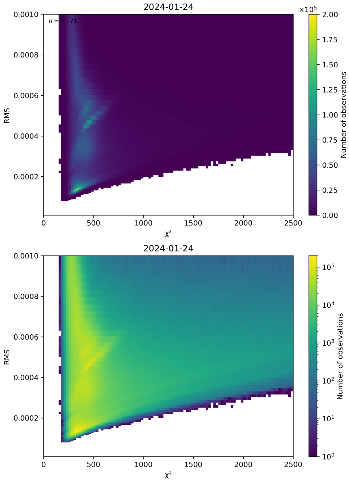
Figure 82: Scatter density plot of “ \chi^2 ” against “RMS” for 2024-01-23 to 2024-01-25.
