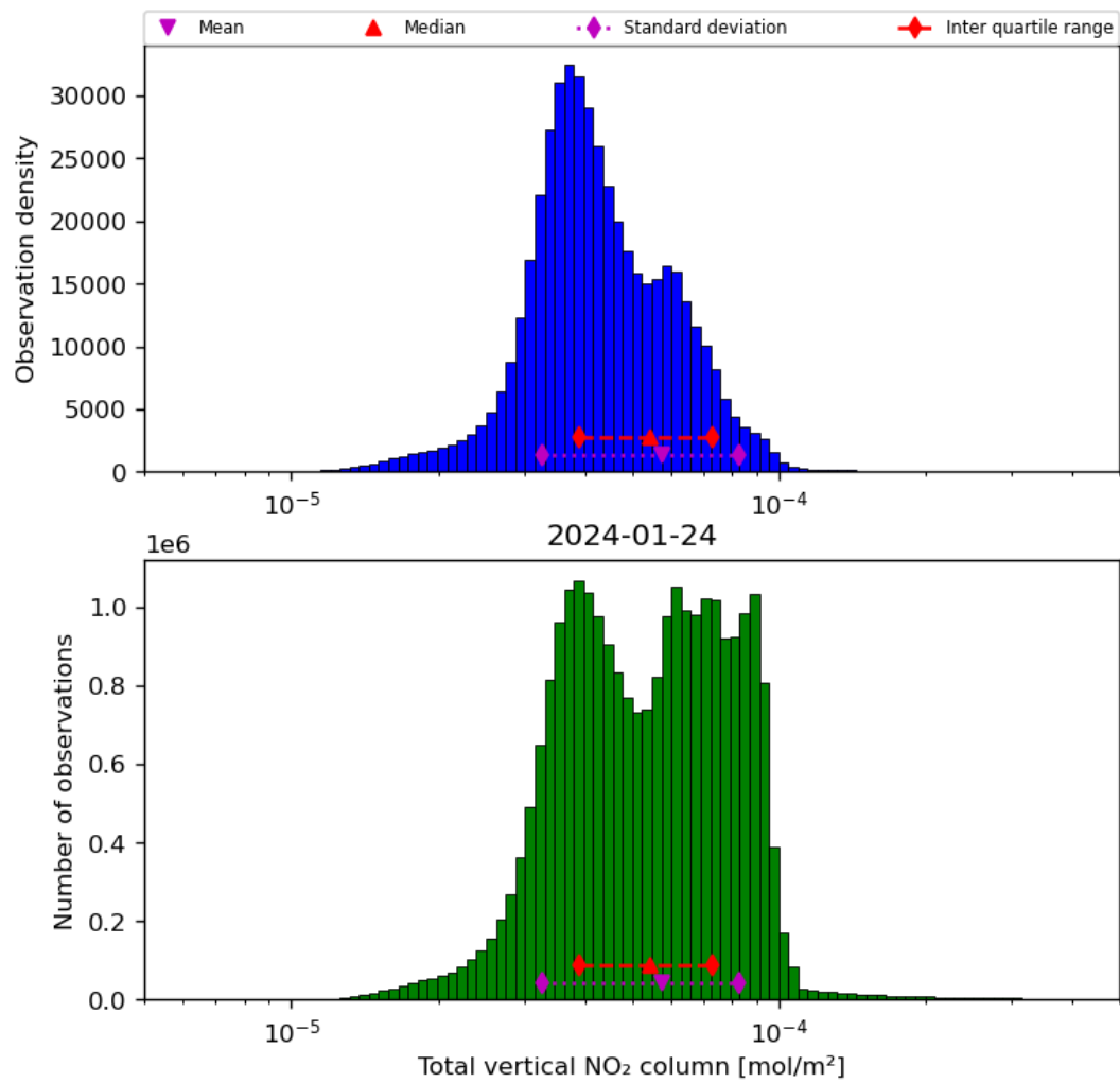
Figure 38: Histogram of “Total vertical NO 2 column” for 2024-01-23 to 2024-01-25
