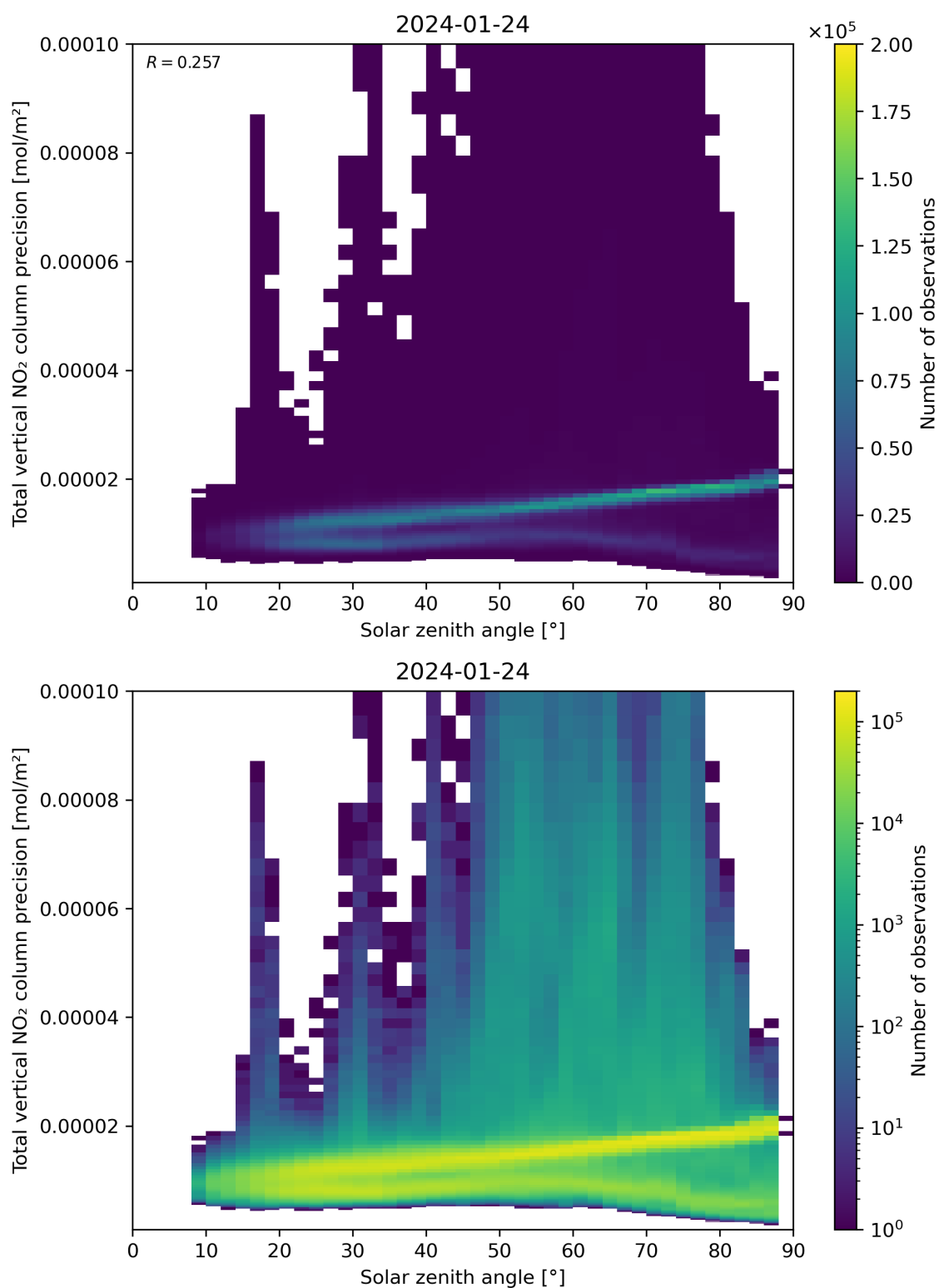
Figure 154: Scatter density plot of “Solar zenith angle” against “Total vertical NO 2 column precision” for 2024-01-23 to 2024-01-25.
