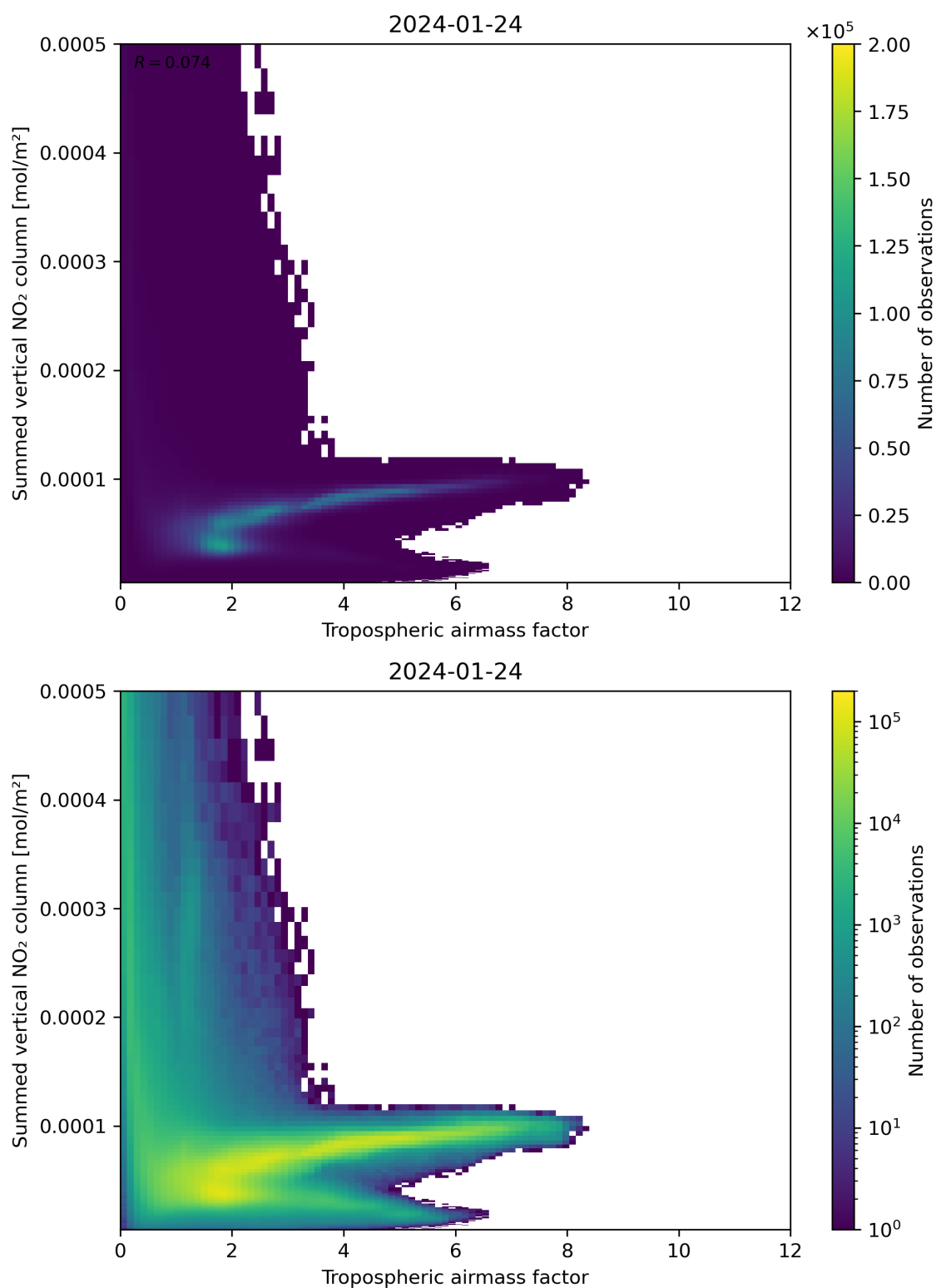
Figure 75: Scatter density plot of “Tropospheric air mass factor” against “Summed vertical NO 2 column” for 2024-01-23 to 2024-01-25.
