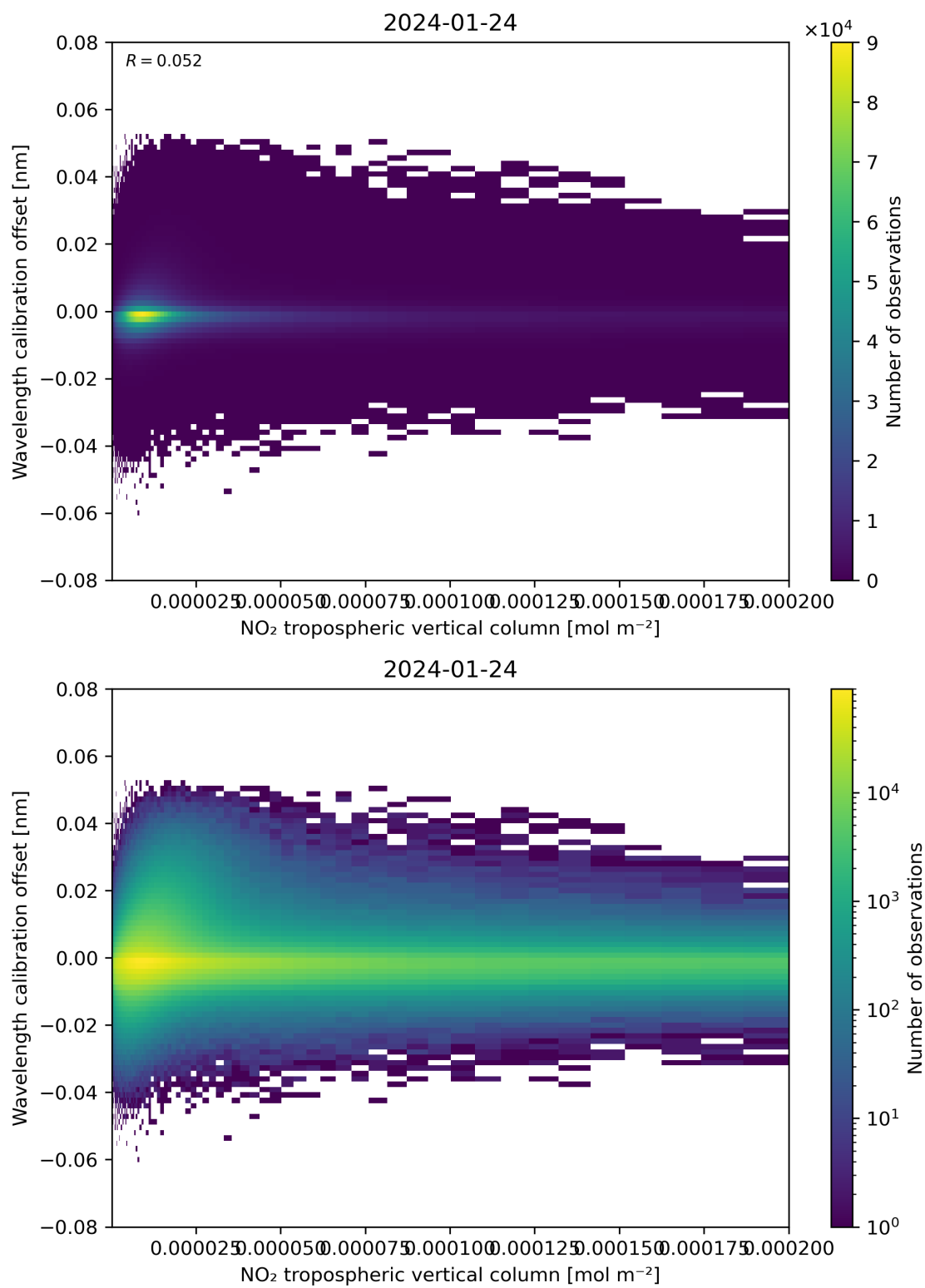
Figure 143: Scatter density plot of “NO 2 tropospheric vertical column” against “Wavelength calibration offset” for 2024-01-23 to 2024-01-25.
