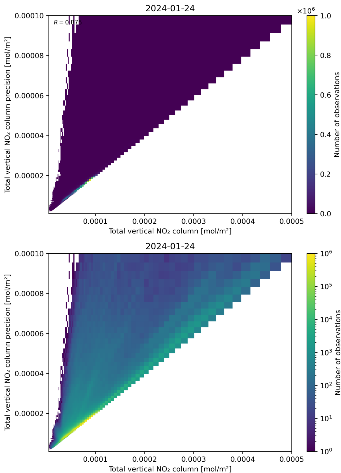
Figure 114: Scatter density plot of “Total vertical NO 2 column” against “Total vertical NO 2 column precision” for 2024-01-23 to 2024-01-25.
