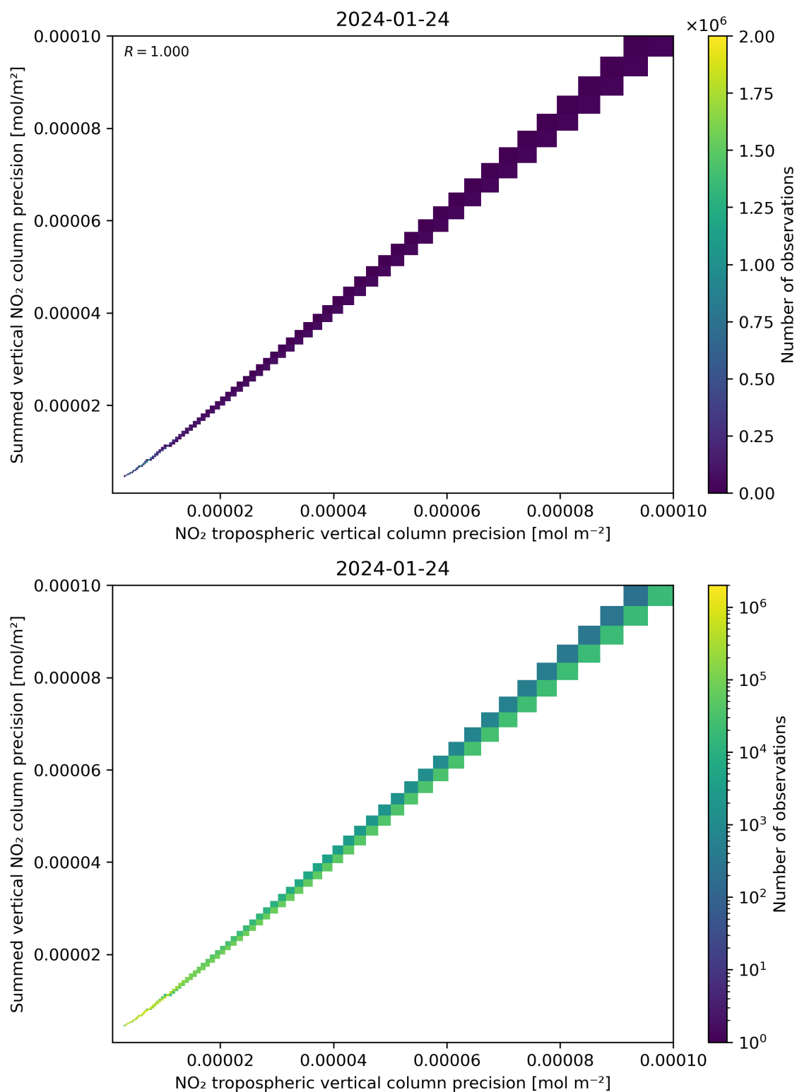
Figure 137: Scatter density plot of “NO 2 tropospheric vertical column precision” against “Summed vertical NO 2 column precision” for 2024-01-23 to 2024-01-25.
