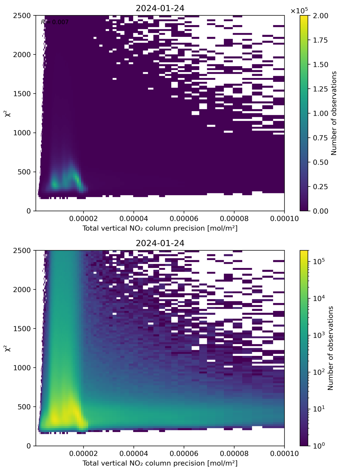
Figure 116: Scatter density plot of “Total vertical NO 2 column precision” against “ \chi^2 ” for 2024-01-23 to 2024-01-25.
