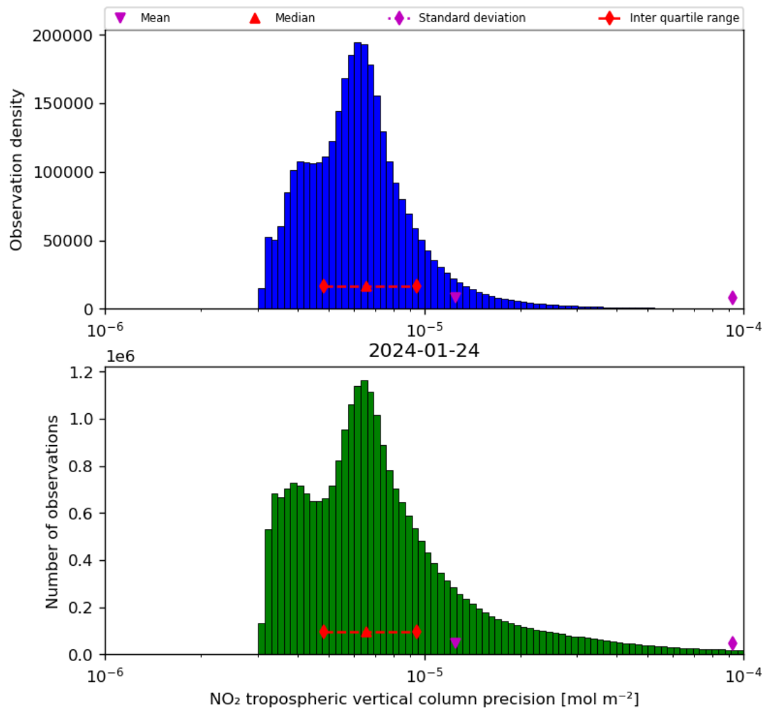
Figure 30: Histogram of “NO 2 tropospheric vertical column precision” for 2024-01-23 to 2024-01-25
