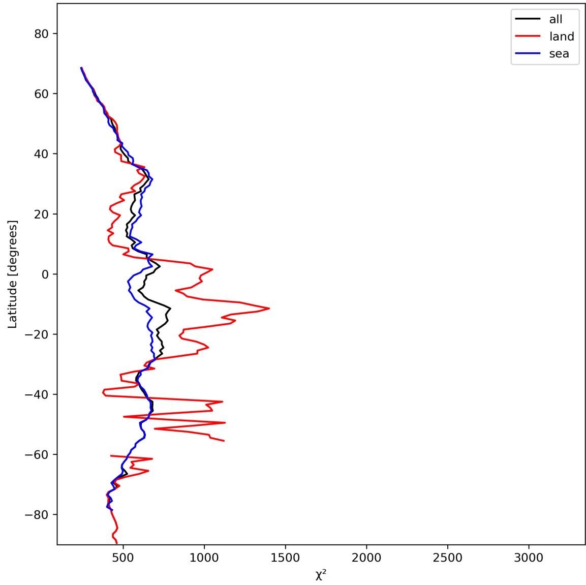
Figure 25: Zonal average of “ \chi^2 ” for 2024-01-23 to 2024-01-25.
