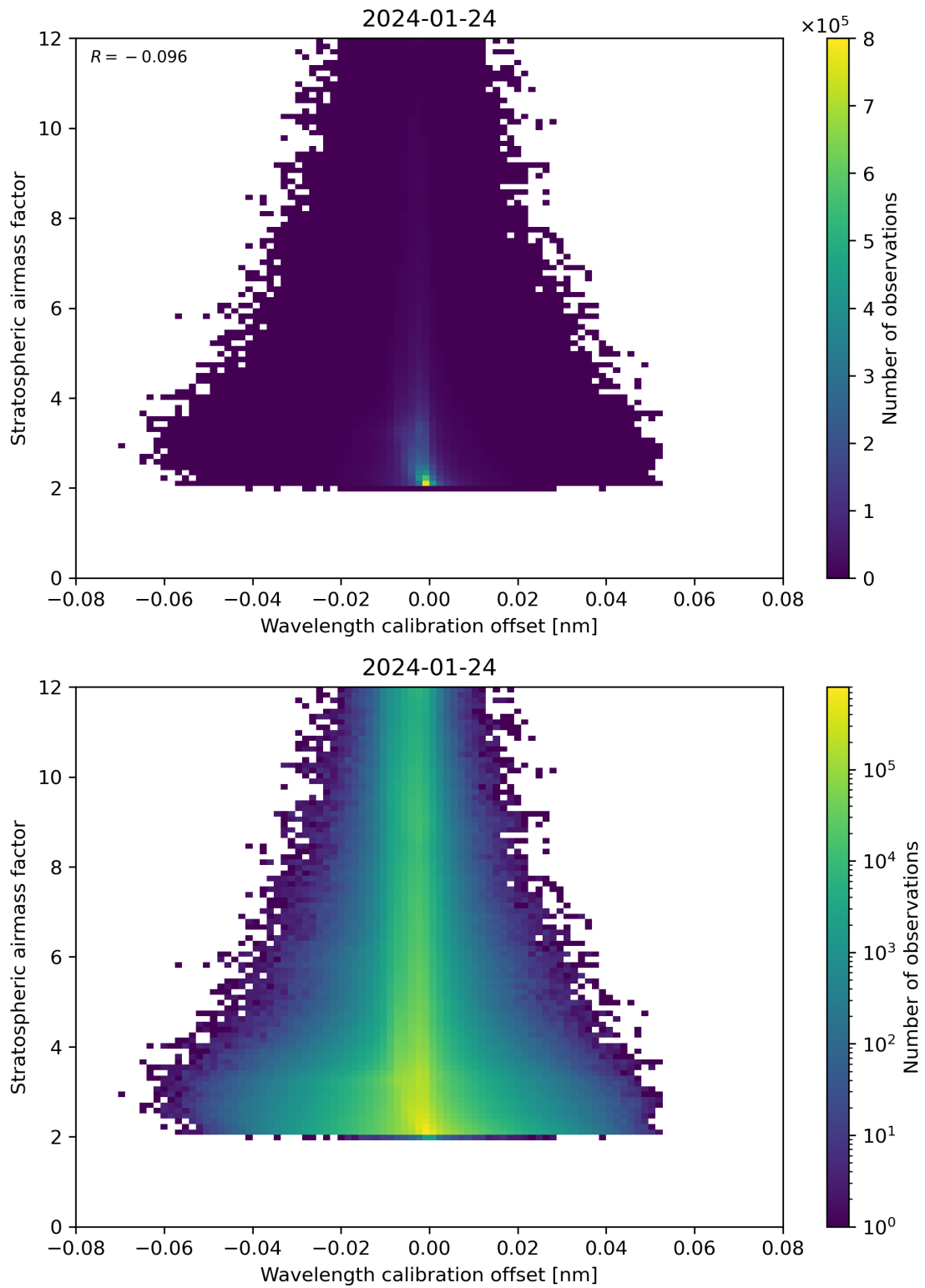
Figure 174: Scatter density plot of “Wavelength calibration offset” against “Stratospheric airmass factor” for 2024-01-23 to 2024-01-25.
