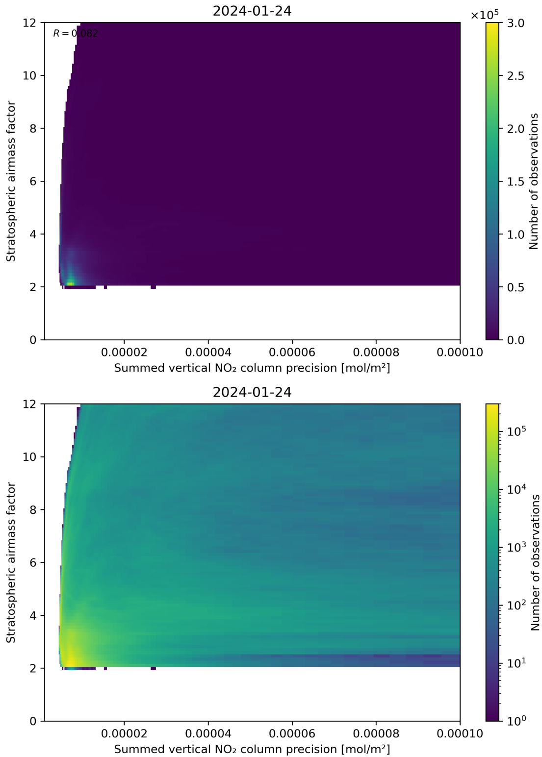
Figure 106: Scatter density plot of “Summed vertical NO 2 column precision” against “Stratospheric airmass factor” for 2024-01-23 to 2024-01-25.
