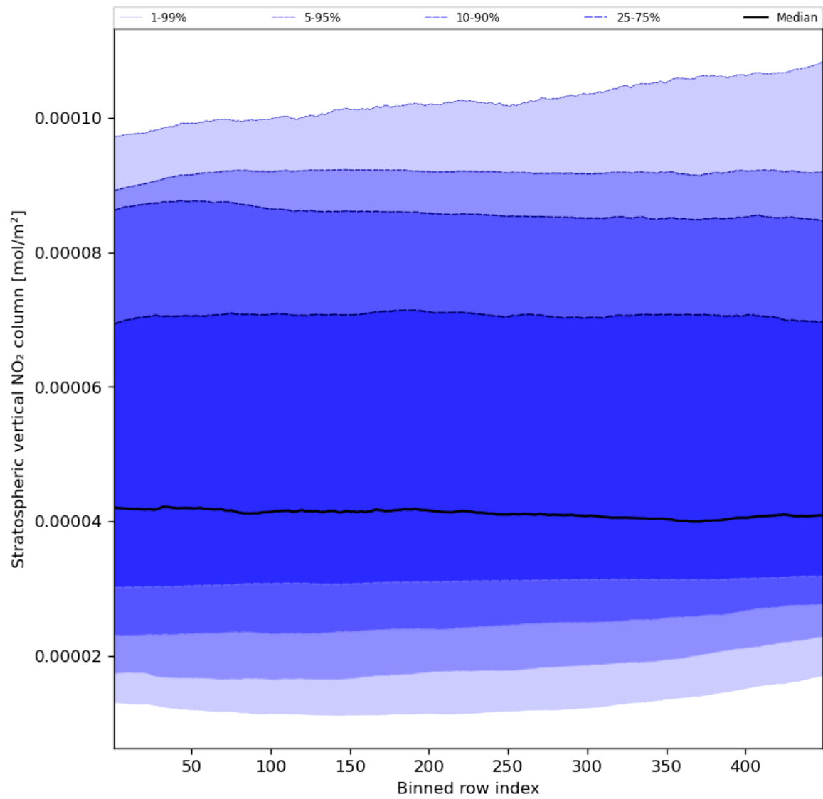
Figure 53: Along track statistics of “Stratospheric vertical NO 2 column” for 2024-01-23 to 2024-01-25
