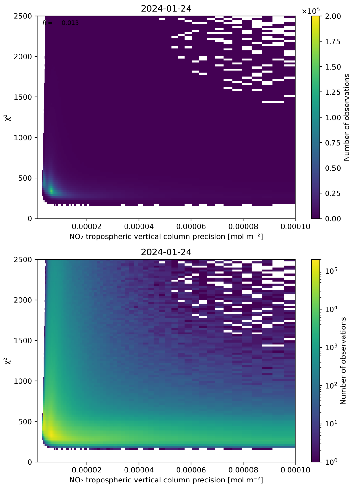
Figure 134: Scatter density plot of “NO 2 tropospheric vertical column precision” against “ \chi^2 ” for 2024-01-23 to 2024-01-25.
