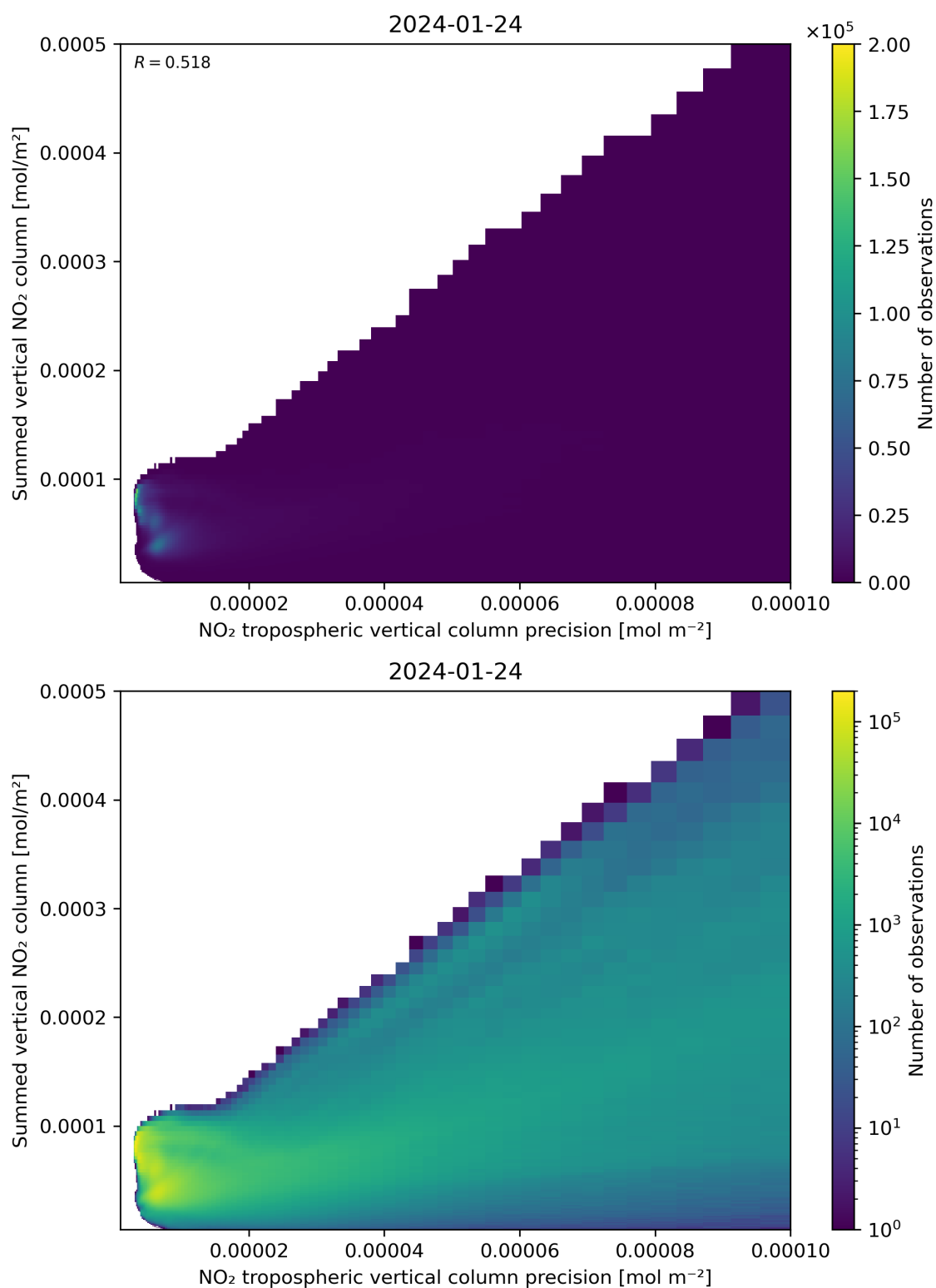
Figure 136: Scatter density plot of “NO 2 tropospheric vertical column precision” against “Summed vertical NO 2 column” for 2024-01-23 to 2024-01-25.
