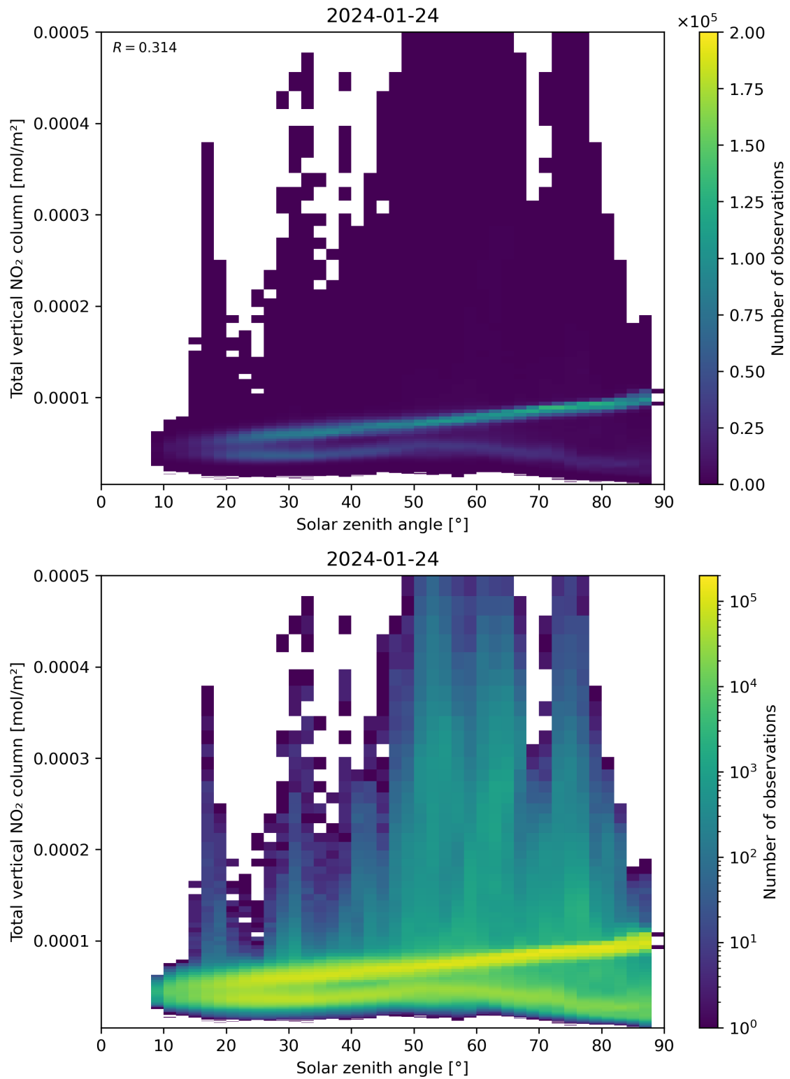
Figure 153: Scatter density plot of “Solar zenith angle” against “Total vertical NO 2 column” for 2024-01-23 to 2024-01-25.
