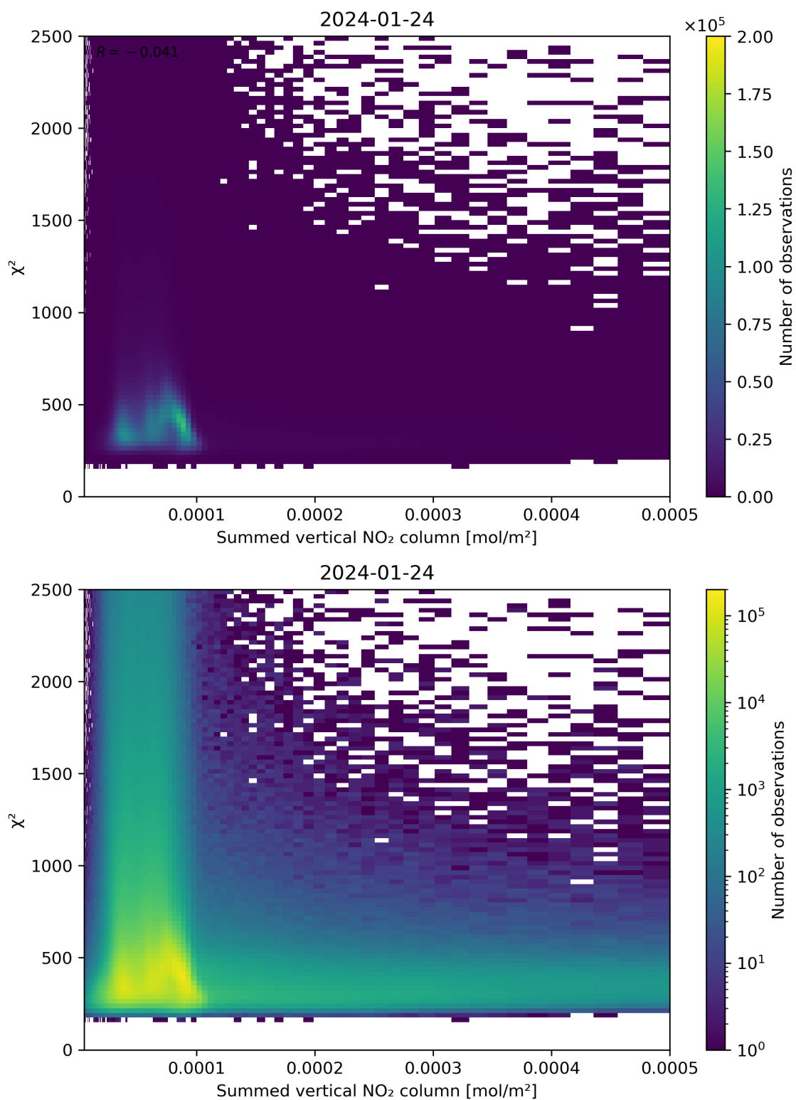
Figure 104: Scatter density plot of “Summed vertical NO 2 column” against “ \chi^2 ” for 2024-01-23 to 2024-01-25.
