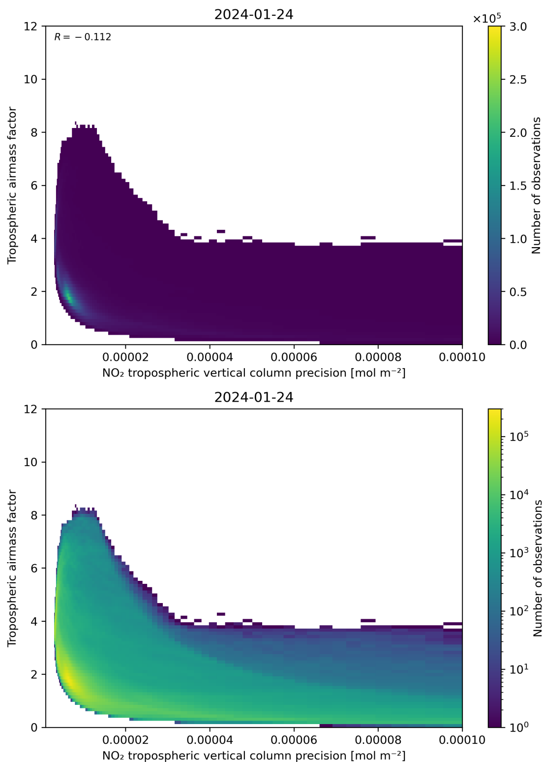
Figure 133: Scatter density plot of “NO 2 tropospheric vertical column precision” against “Tropospheric airmass factor” for 2024-01-23 to 2024-01-25.
