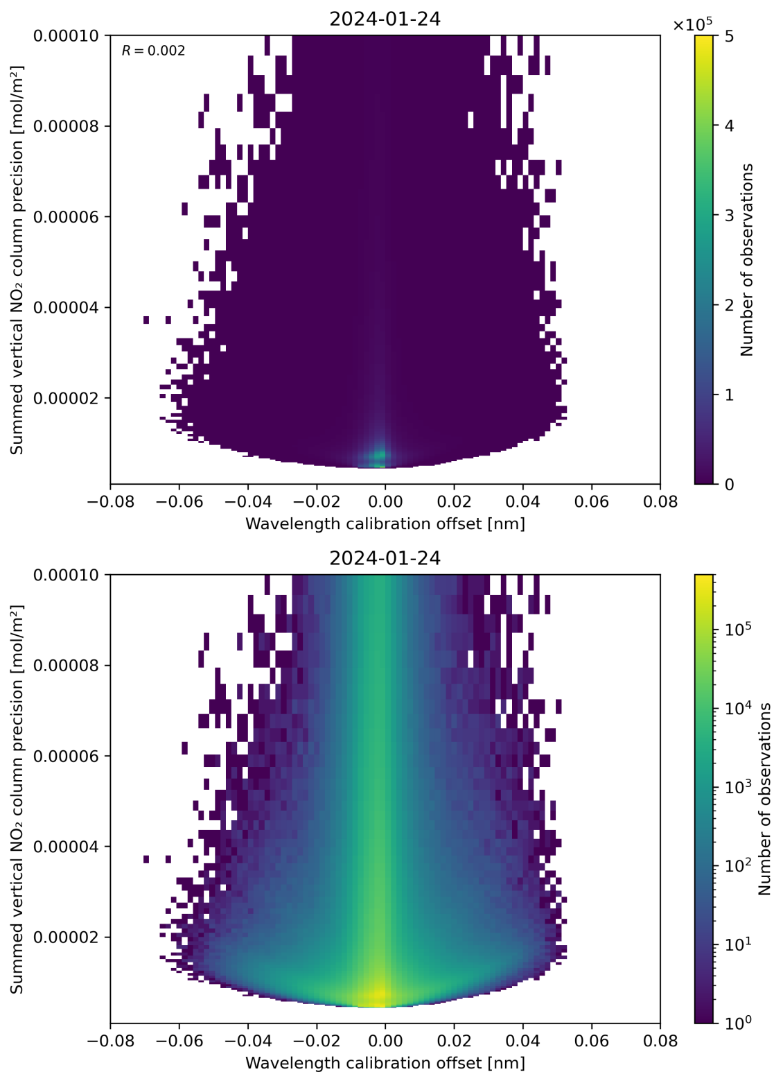
Figure 178: Scatter density plot of “Wavelength calibration offset” against “Summed vertical NO 2 column precision” for 2024-01-23 to 2024-01-25.
