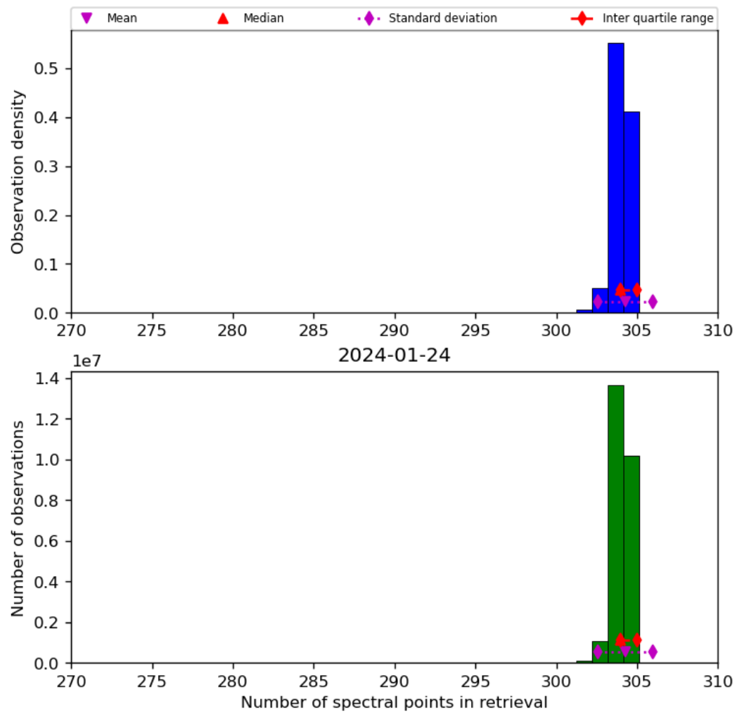
Figure 33: Histogram of “Number of spectral points in retrieval” for 2024-01-23 to 2024-01-25
