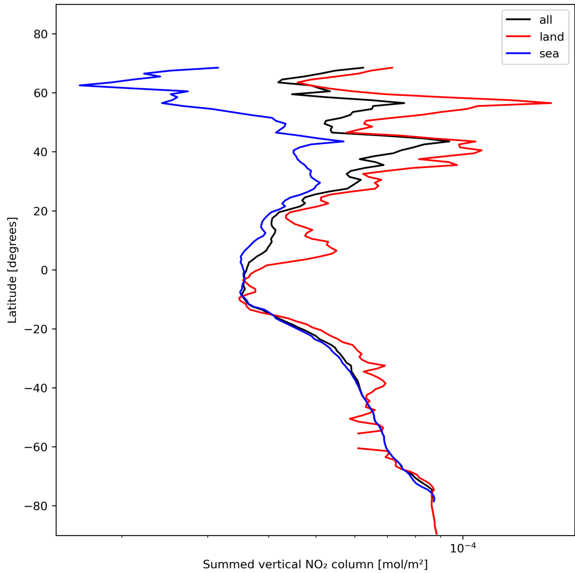
Figure 23: Zonal average of “Summed vertical NO 2 column” for 2024-01-23 to 2024-01-25.
