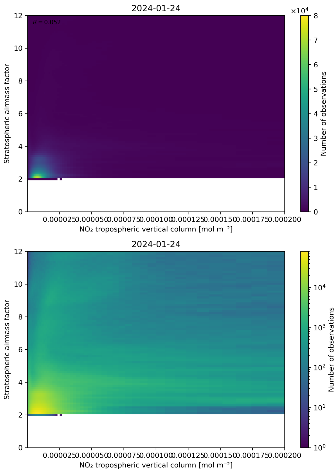
Figure 121: Scatter density plot of “NO 2 tropospheric vertical column” against “Stratospheric airmass factor” for 2024-01-23 to 2024-01-25.
