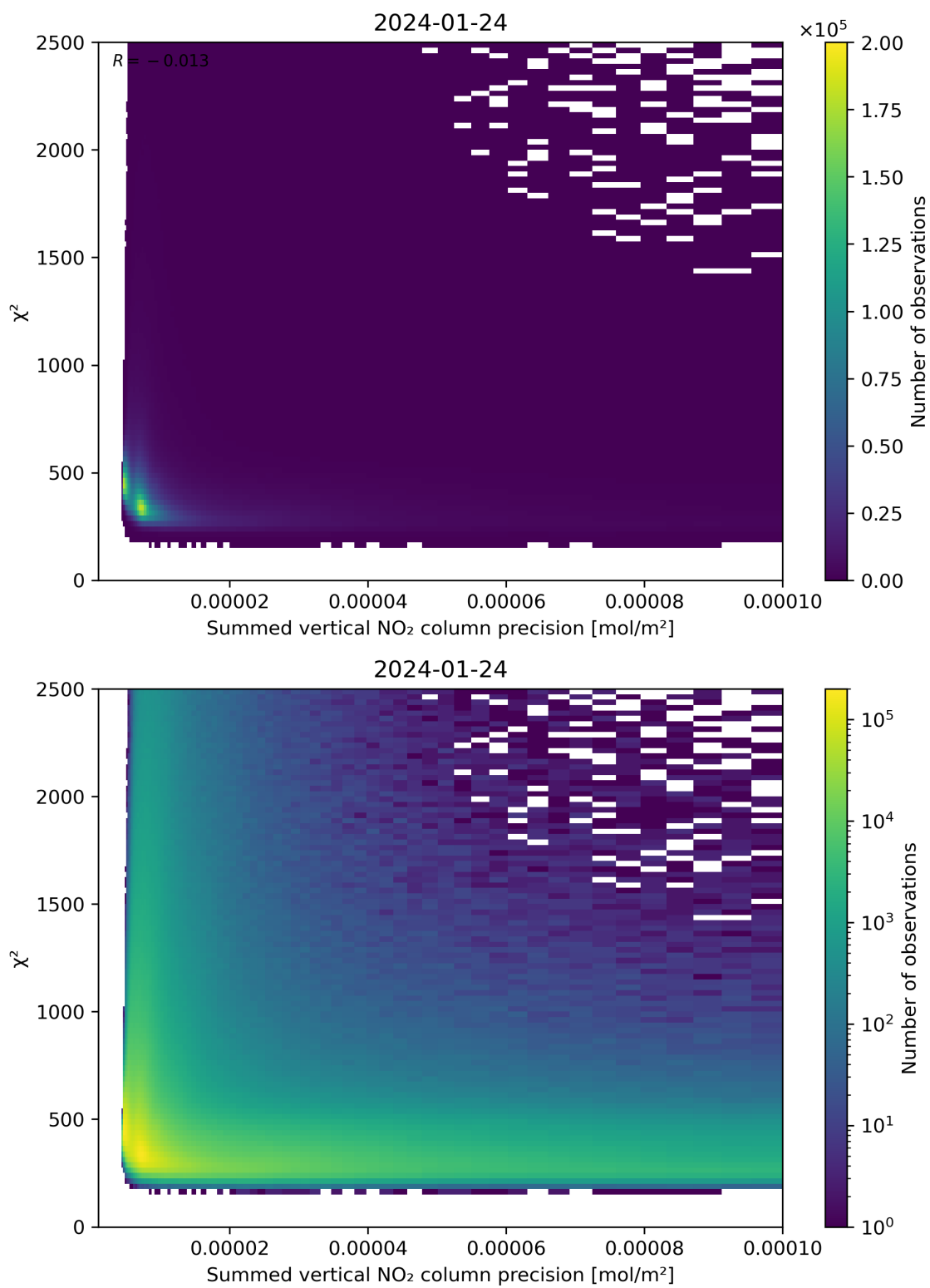
Figure 107: Scatter density plot of “Summed vertical NO 2 column precision” against “ \chi^2 ” for 2024-01-23 to 2024-01-25.
