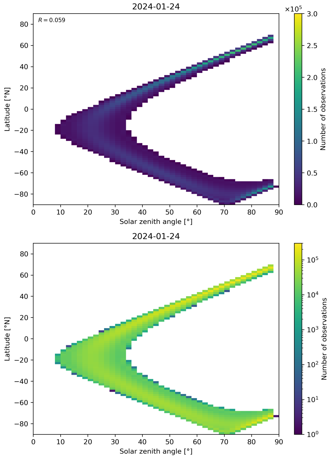
Figure 149: Scatter density plot of “Solar zenith angle” against “Latitude” for 2024-01-23 to 2024-01-25.
