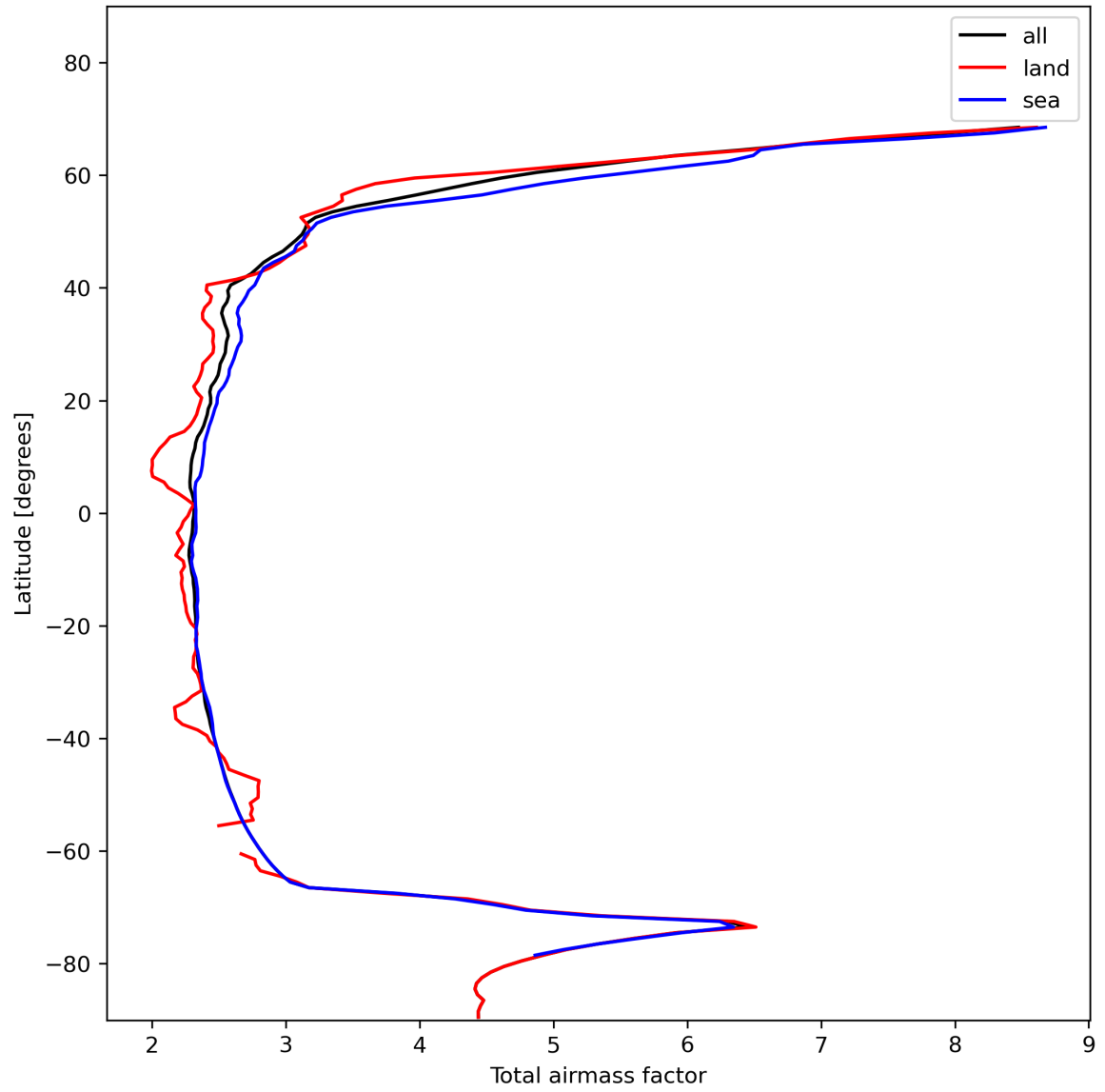
Figure 15: Zonal average of “Total airmass factor” for 2024-01-23 to 2024-01-25.
