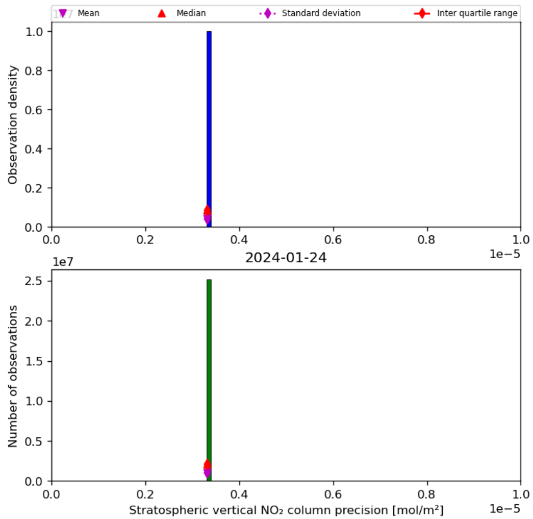
Figure 37: Histogram of “Stratospheric vertical NO 2 column precision” for 2024-01-23 to 2024-01-25
