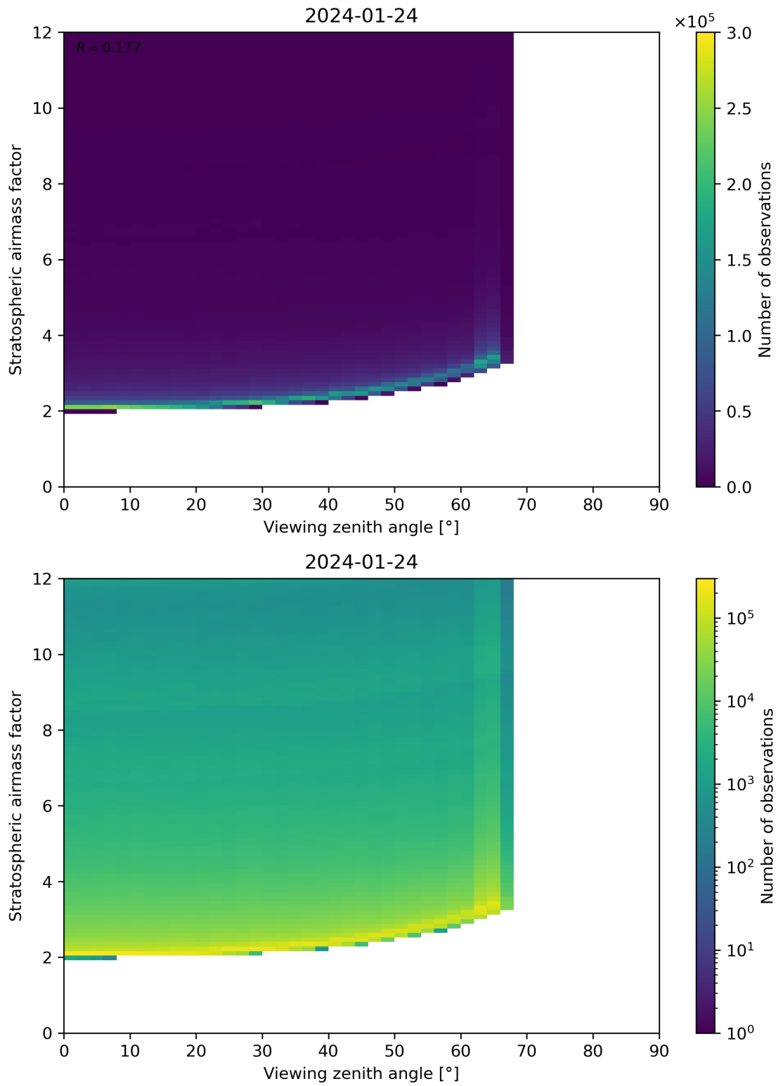
Figure 159: Scatter density plot of “Viewing zenith angle” against “Stratospheric airmass factor” for 2024-01-23 to 2024-01-25.
