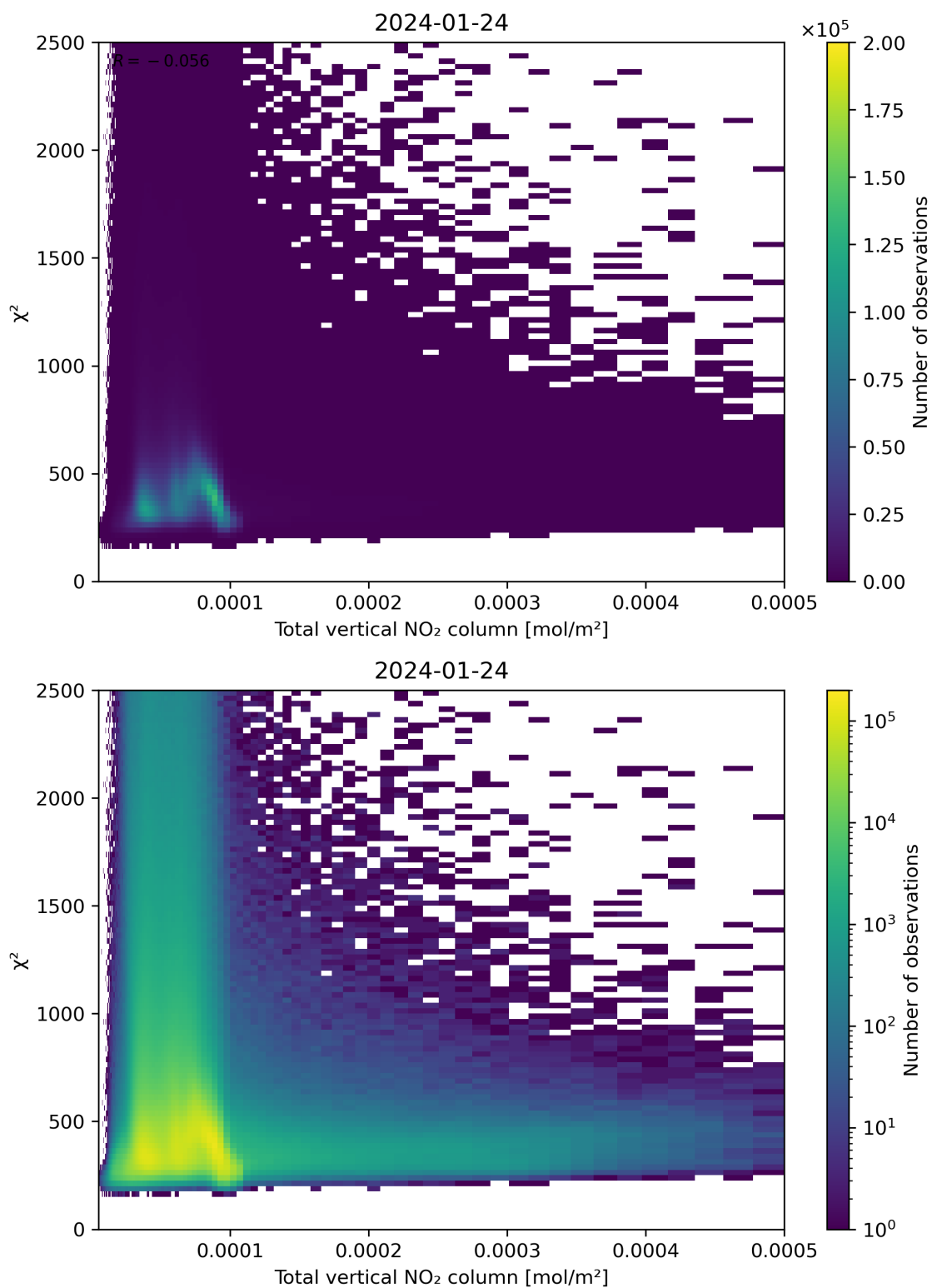
Figure 111: Scatter density plot of “Total vertical NO 2 column” against “ \chi^2 ” for 2024-01-23 to 2024-01-25.
