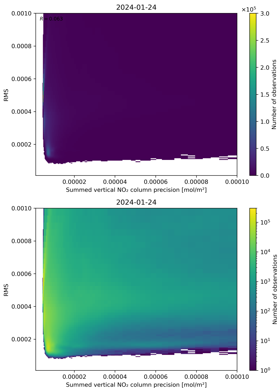
Figure 108: Scatter density plot of “Summed vertical NO 2 column precision” against “RMS” for 2024-01-23 to 2024-01-25.
