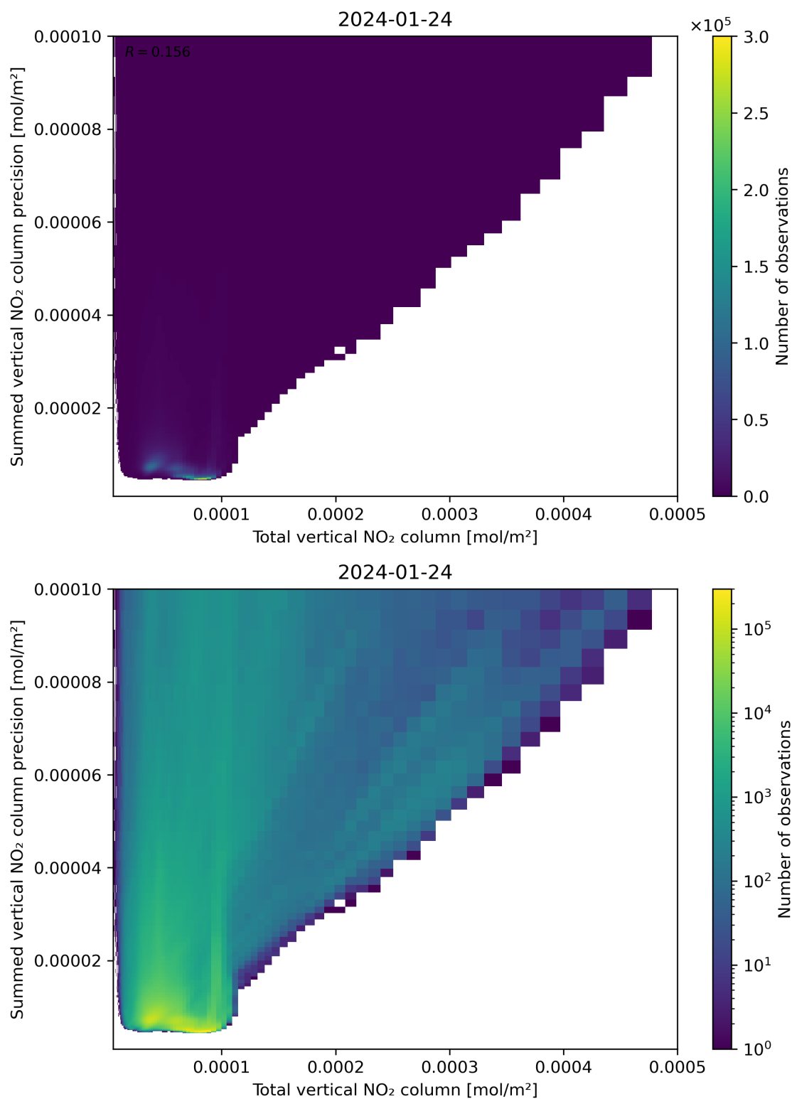
Figure 113: Scatter density plot of “Total vertical NO 2 column” against “Summed vertical NO 2 column precision” for 2024-01-23 to 2024-01-25.
