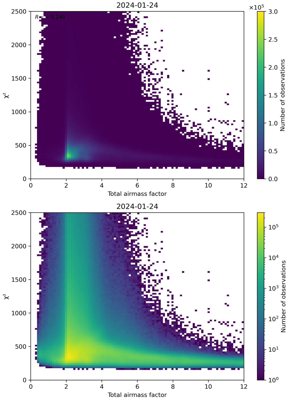
Figure 63: Scatter density plot of “Total airmass factor” against “ \chi^2 ” for 2024-01-23 to 2024-01-25.
