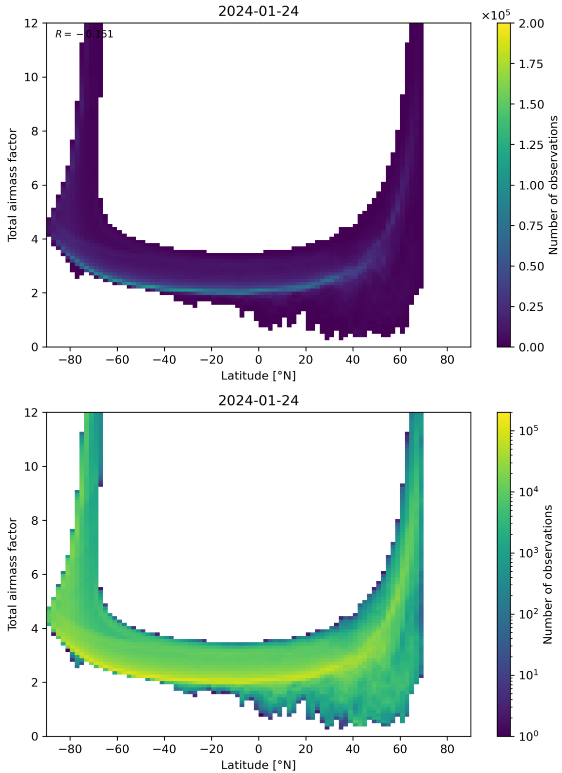
Figure 84: Scatter density plot of “Latitude” against “Total airmass factor” for 2024-01-23 to 2024-01-25.
