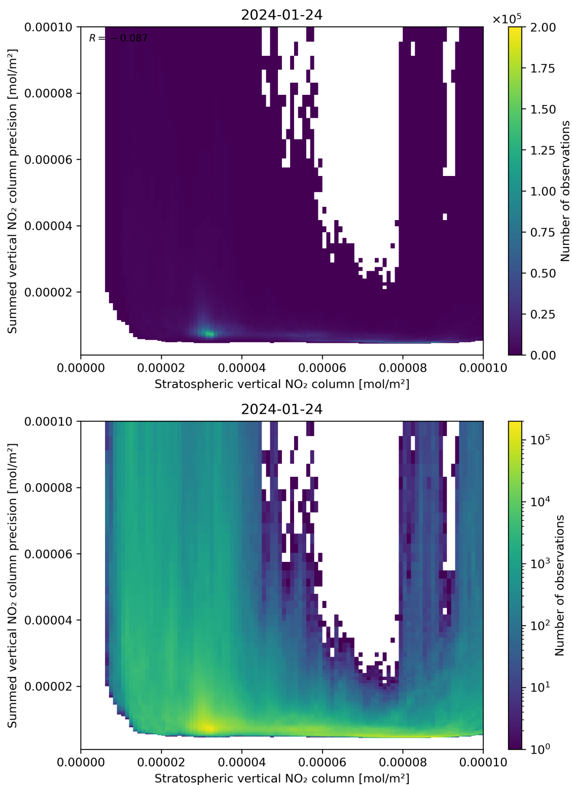
Figure 99: Scatter density plot of “Stratospheric vertical NO 2 column” against “Summed vertical NO 2 column precision” for 2024-01-23 to 2024-01-25.
