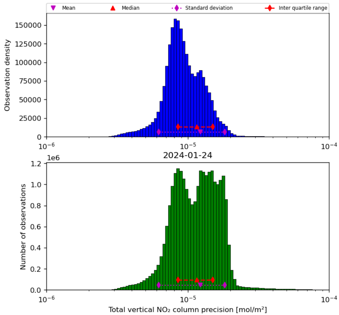
Figure 39: Histogram of “Total vertical NO 2 column precision” for 2024-01-23 to 2024-01-25
