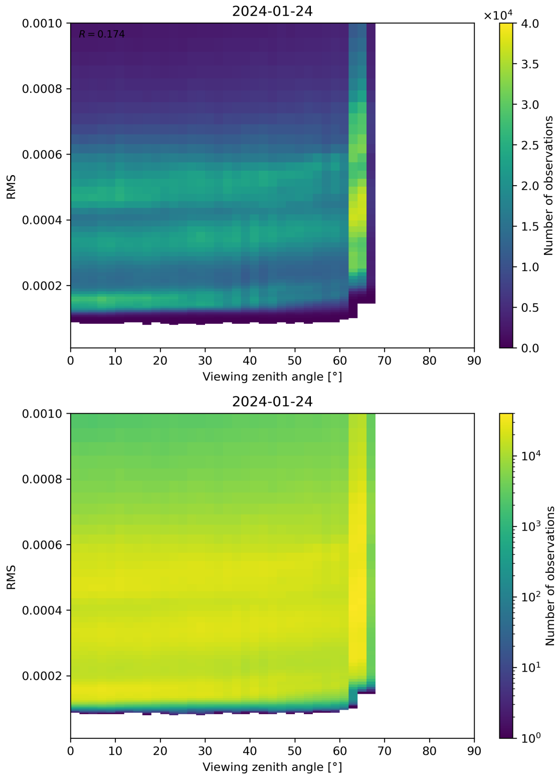
Figure 171: Scatter density plot of “Viewing zenith angle” against “RMS” for 2024-01-23 to 2024-01-25.
