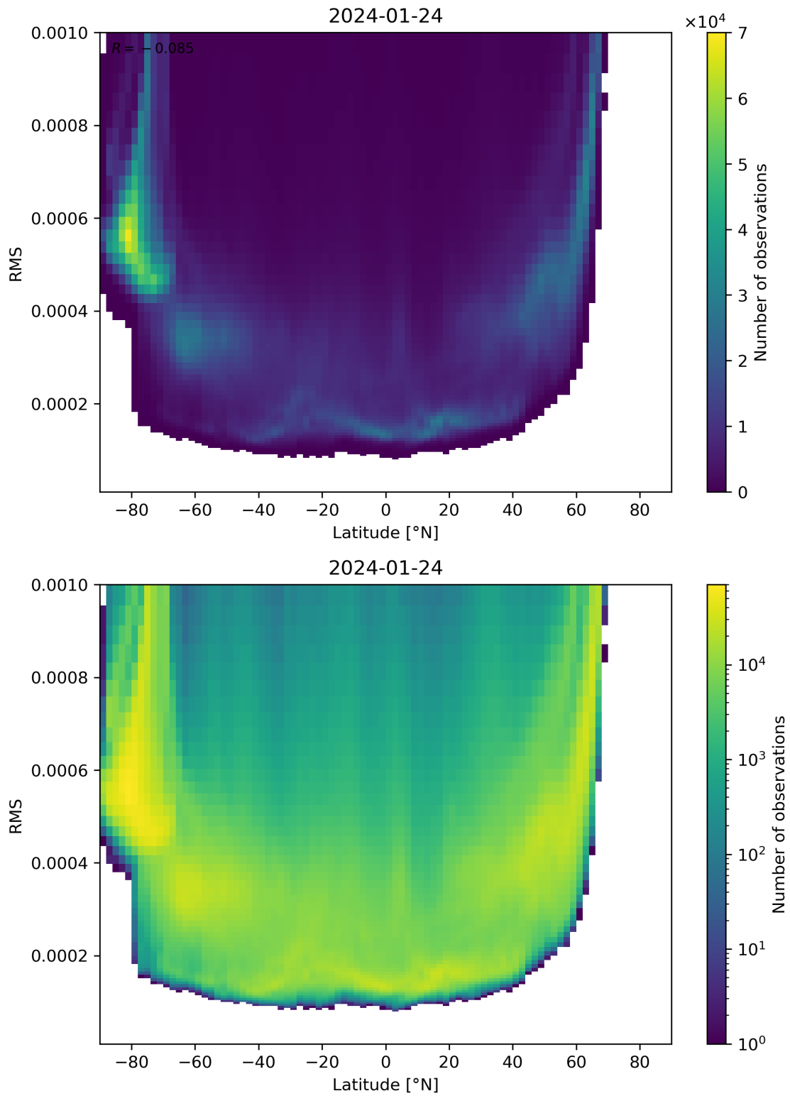
Figure 94: Scatter density plot of “Latitude” against “RMS” for 2024-01-23 to 2024-01-25.
