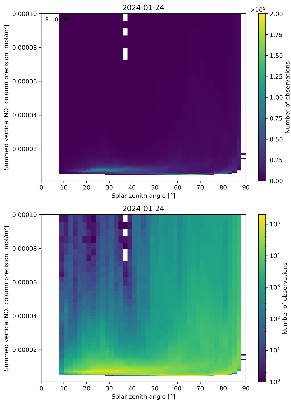
Figure 152: Scatter density plot of “Solar zenith angle” against “Summed vertical NO 2 column precision” for 2024-01-23 to 2024-01-25.
