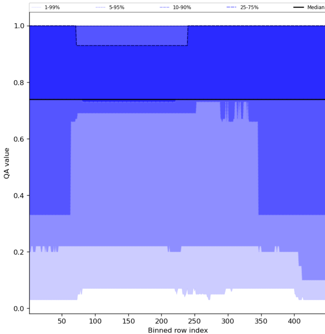
Figure 45: Along track statistics of “QA value” for 2024-01-23 to 2024-01-25
