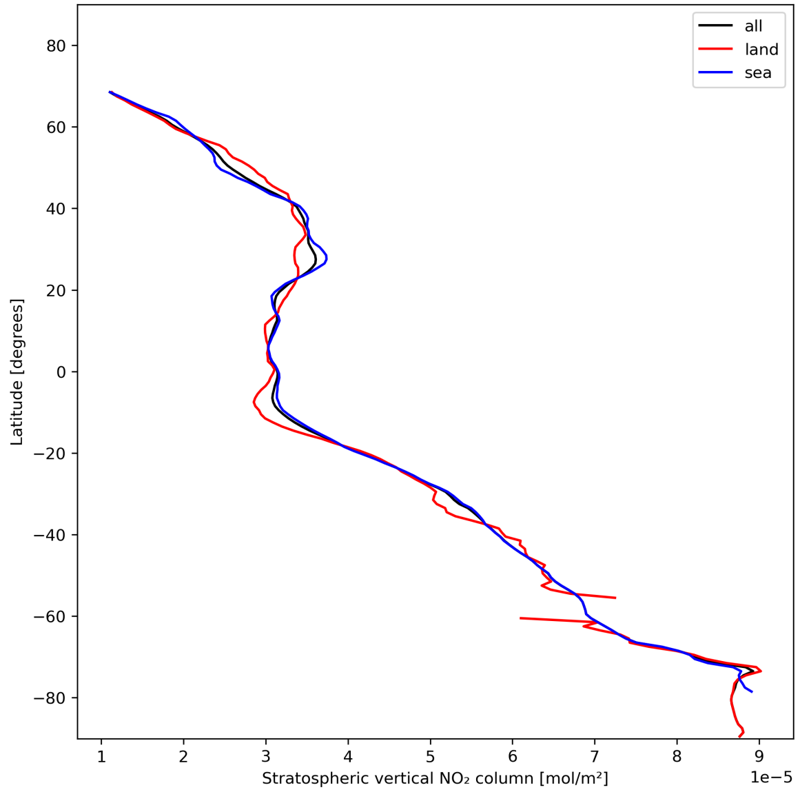
Figure 19: Zonal average of “Stratospheric vertical NO 2 column” for 2024-01-23 to 2024-01-25.
