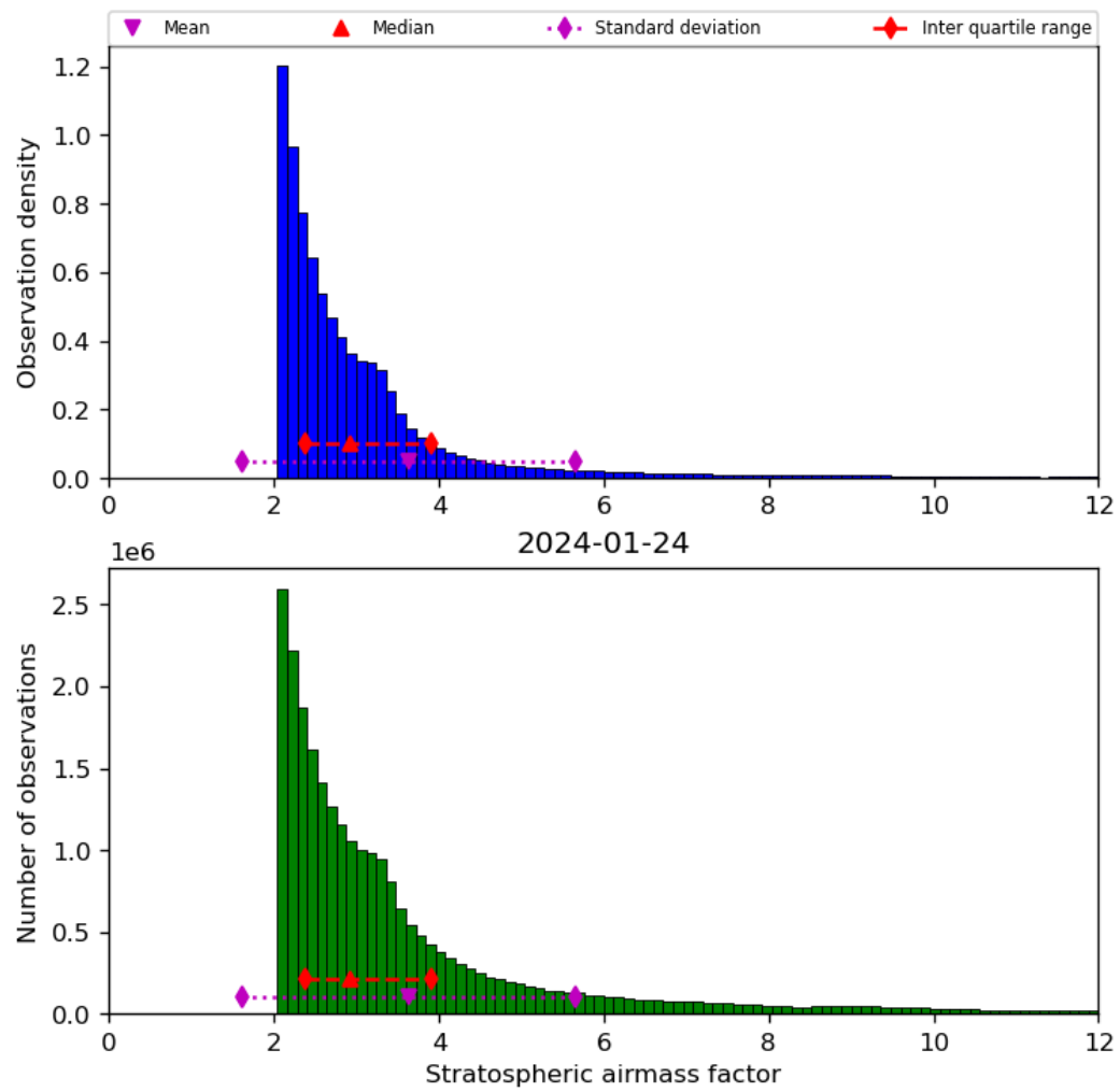
Figure 44: Histogram of “Stratospheric airmass factor” for 2024-01-23 to 2024-01-25
