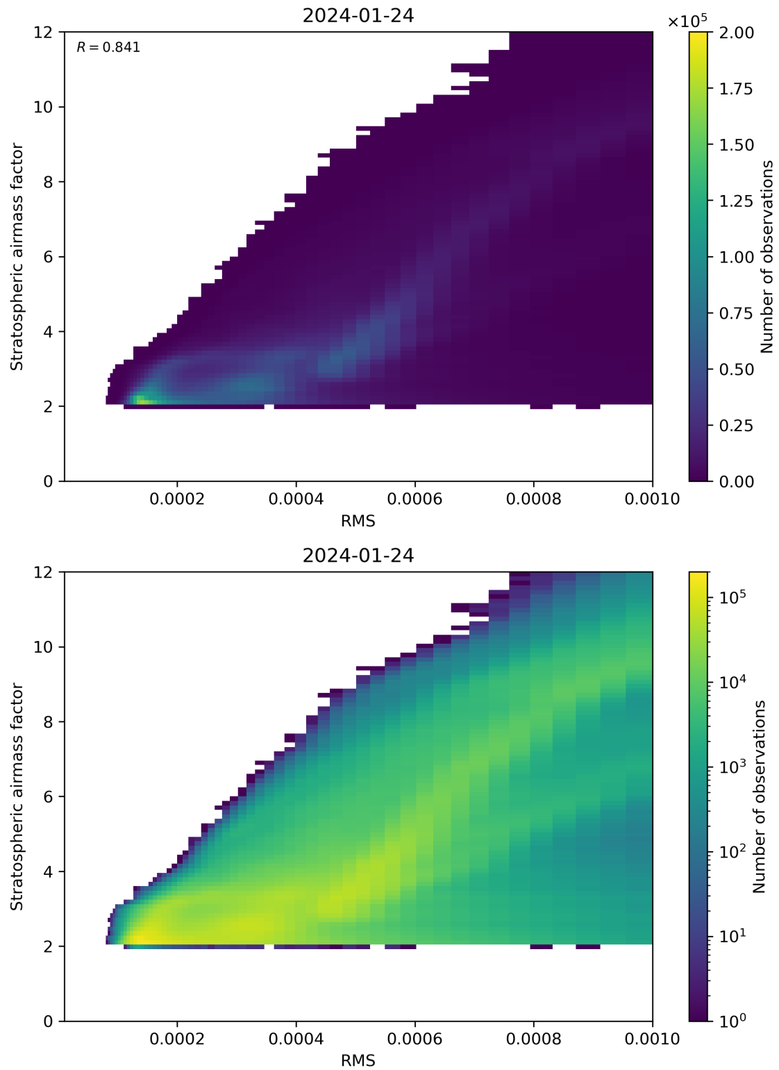
Figure 144: Scatter density plot of “RMS” against “Stratospheric airmass factor” for 2024-01-23 to 2024-01-25.
