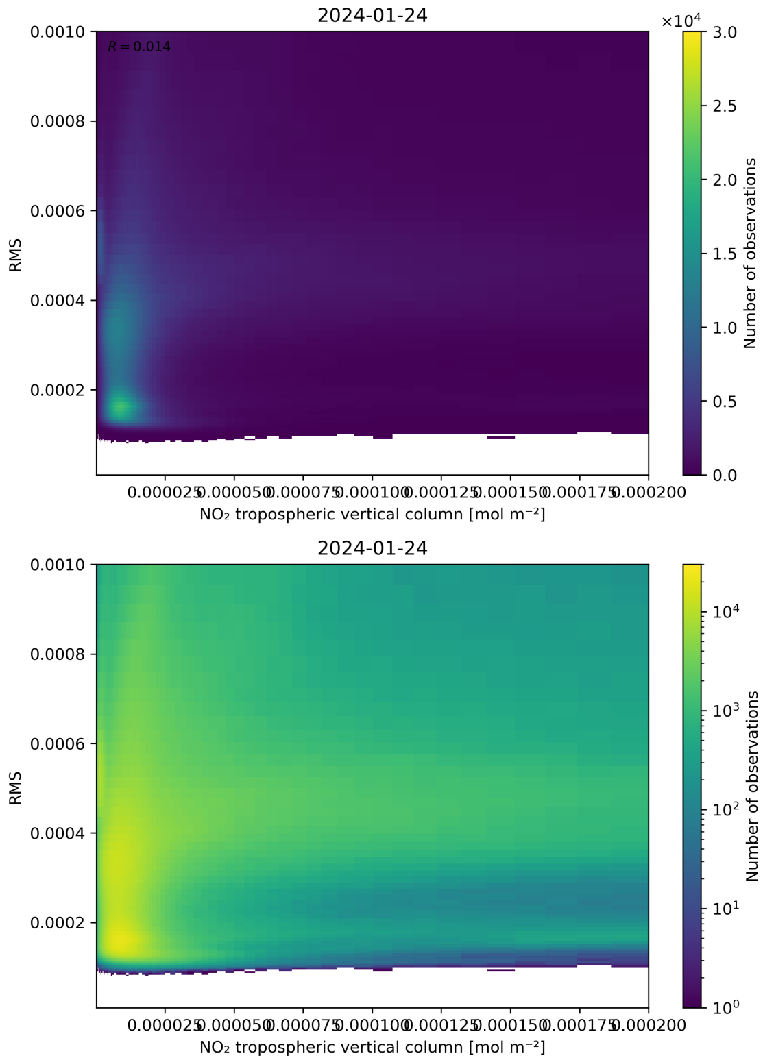
Figure 142: Scatter density plot of “NO 2 tropospheric vertical column” against “RMS” for 2024-01-23 to 2024-01-25.
