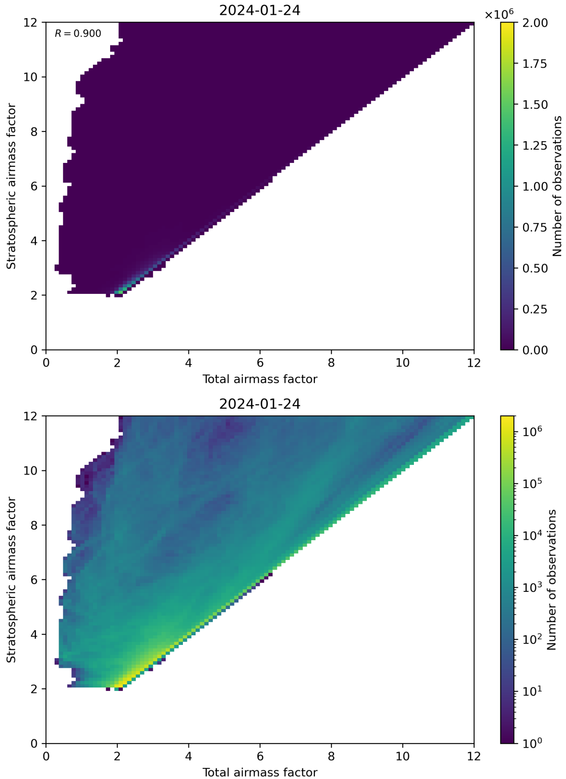
Figure 62: Scatter density plot of “Total airmass factor” against “Stratospheric airmass factor” for 2024-01-23 to 2024-01-25.
