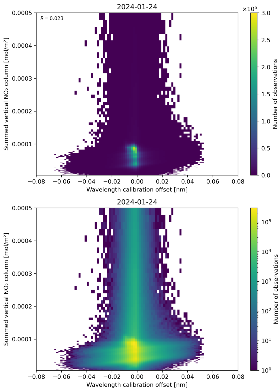
Figure 177: Scatter density plot of “Wavelength calibration offset” against “Summed vertical NO 2 column” for 2024-01-23 to 2024-01-25.
