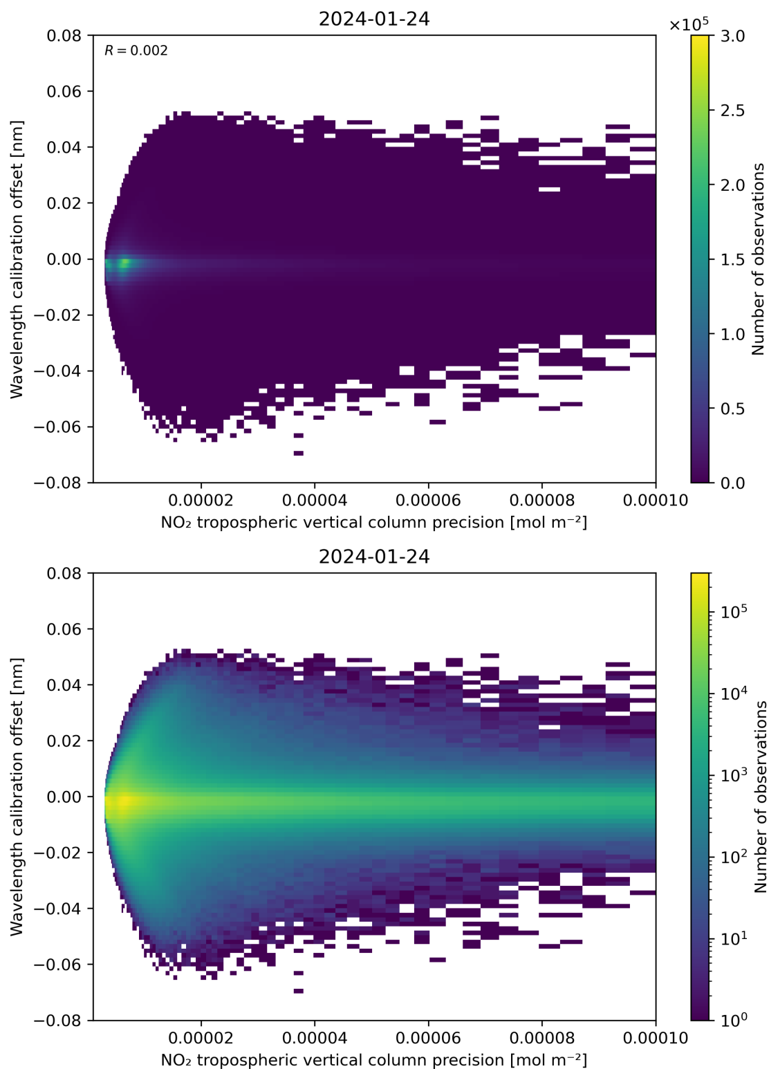
Figure 141: Scatter density plot of “NO 2 tropospheric vertical column precision” against “Wavelength calibration offset” for 2024-01-23 to 2024-01-25.
