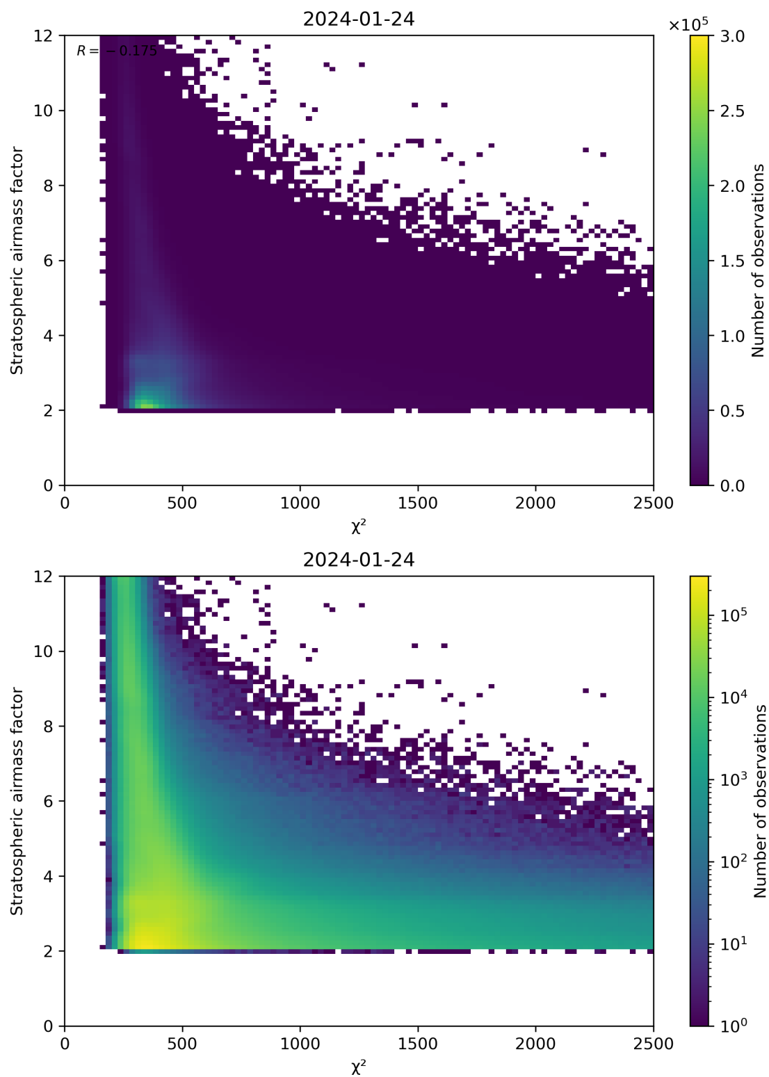
Figure 81: Scatter density plot of “ \chi^2 ” against “Stratospheric airmass factor” for 2024-01-23 to 2024-01-25.
