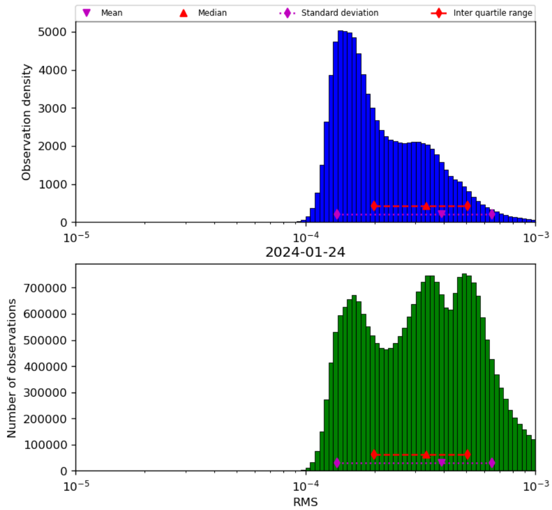
Figure 43: Histogram of “RMS” for 2024-01-23 to 2024-01-25
