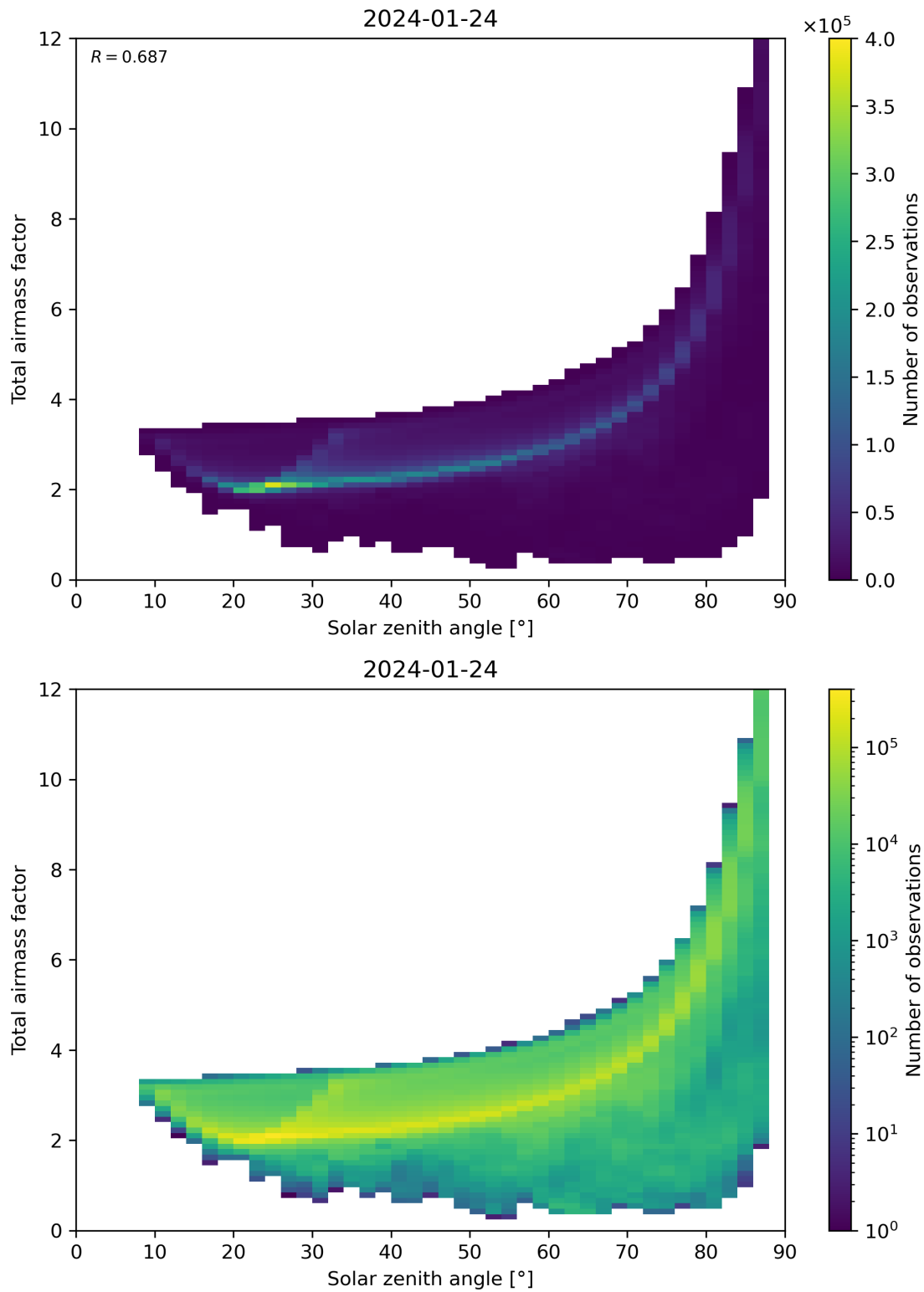
Figure 146: Scatter density plot of “Solar zenith angle” against “Total air mass factor” for 2024-01-23 to 2024-01-25.
