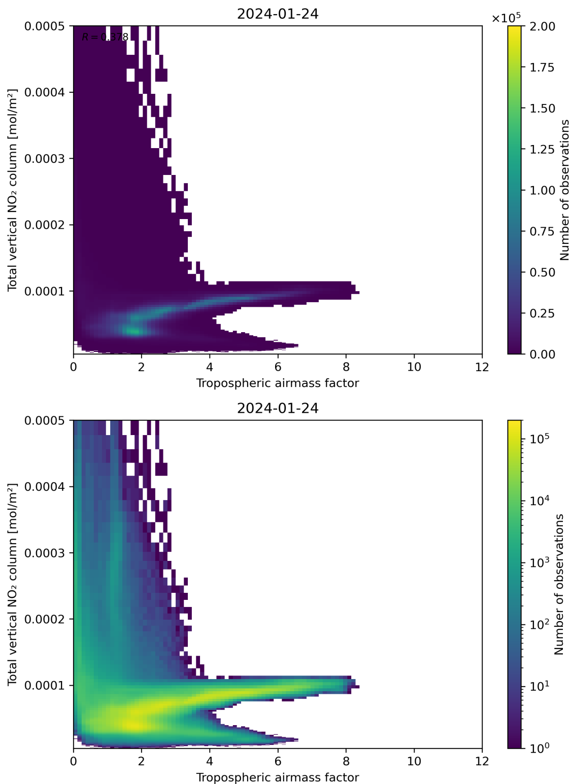
Figure 77: Scatter density plot of “Tropospheric airmass factor” against “Total vertical NO 2 column” for 2024-01-23 to 2024-01-25.
