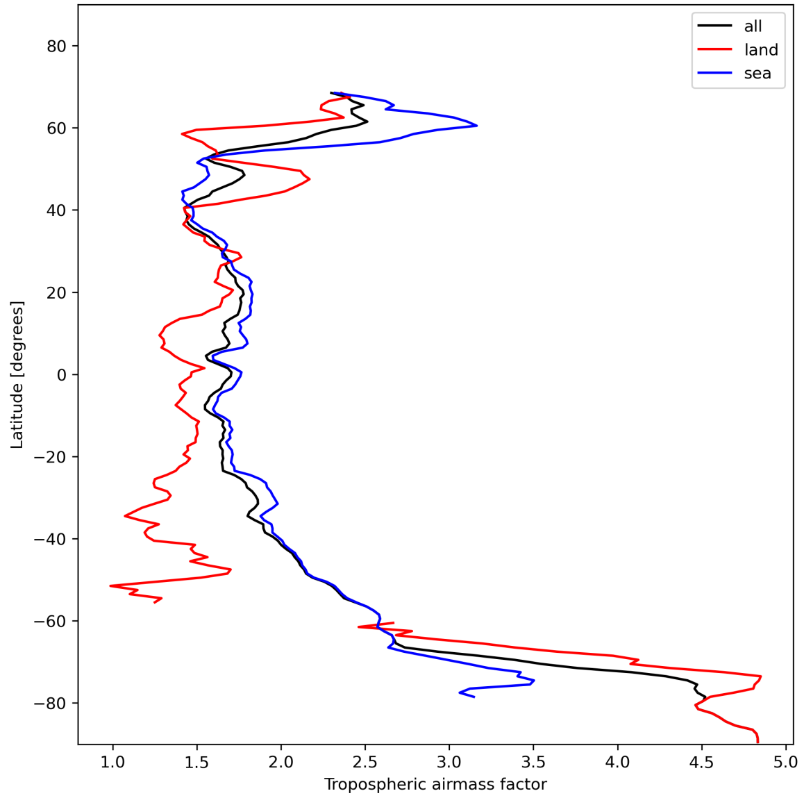
Figure 14: Zonal average of “Tropospheric airmass factor” for 2024-01-23 to 2024-01-25.
