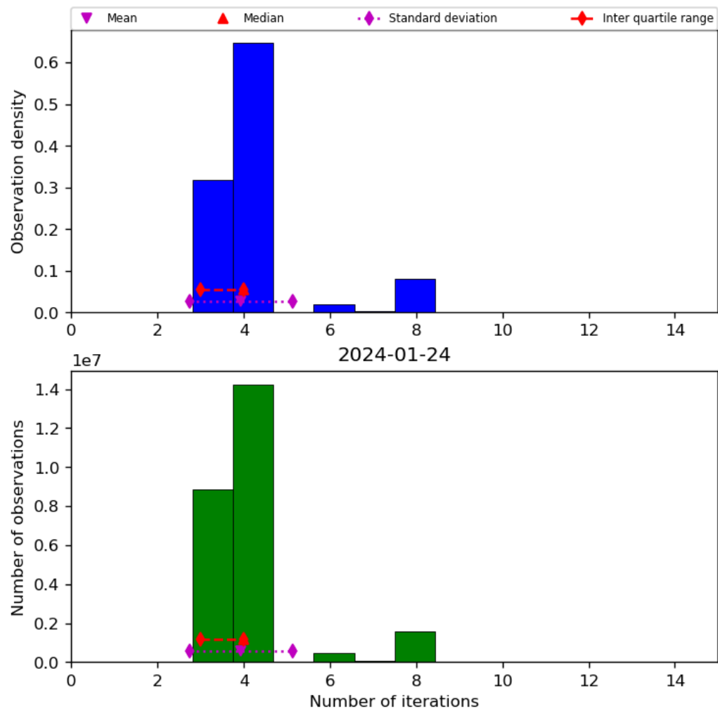
Figure 34: Histogram of “Number of iterations” for 2024-01-23 to 2024-01-25
