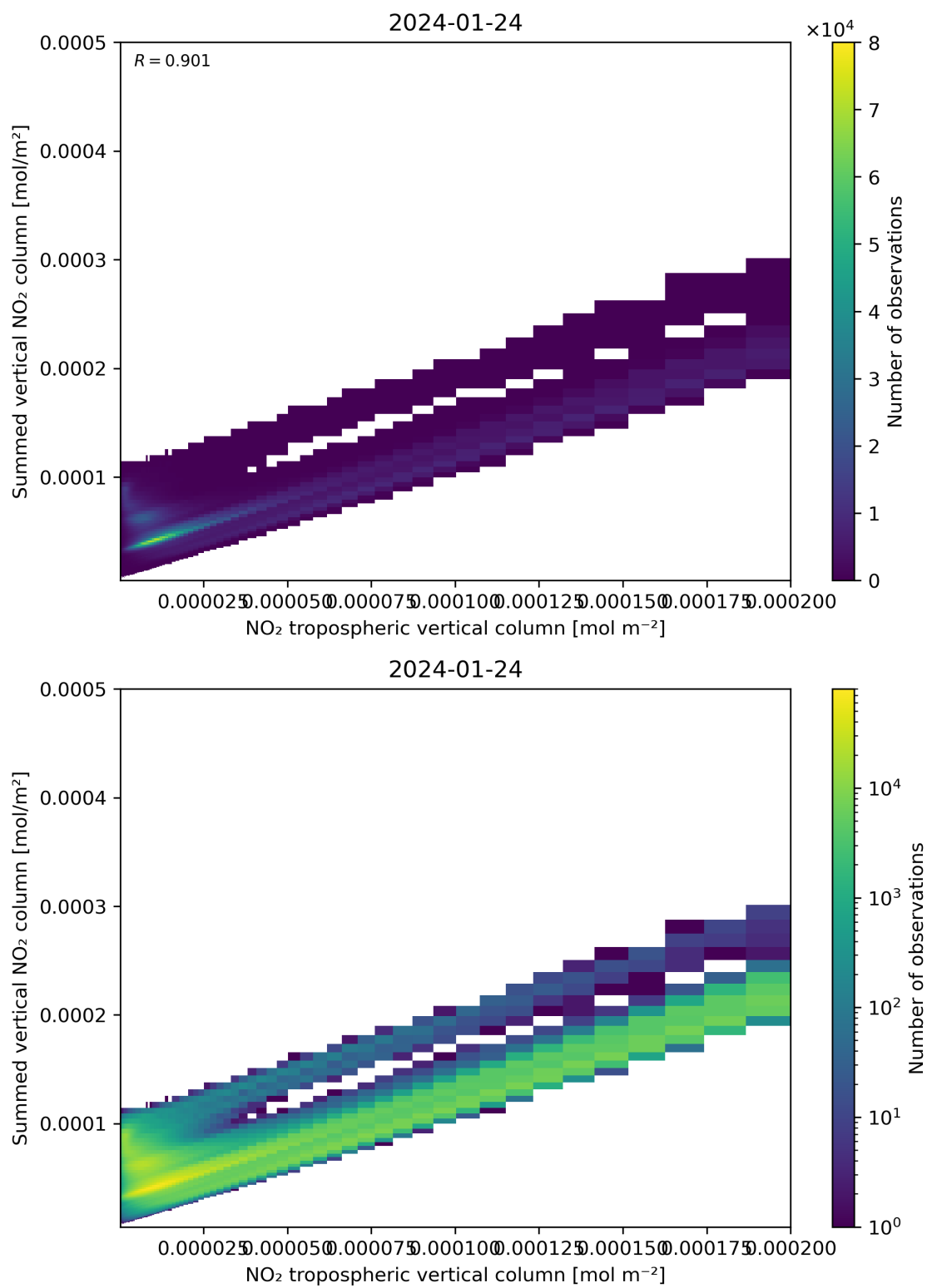
Figure 126: Scatter density plot of “NO 2 tropospheric vertical column” against “Summed vertical NO 2 column” for 2024-01-23 to 2024-01-25.
