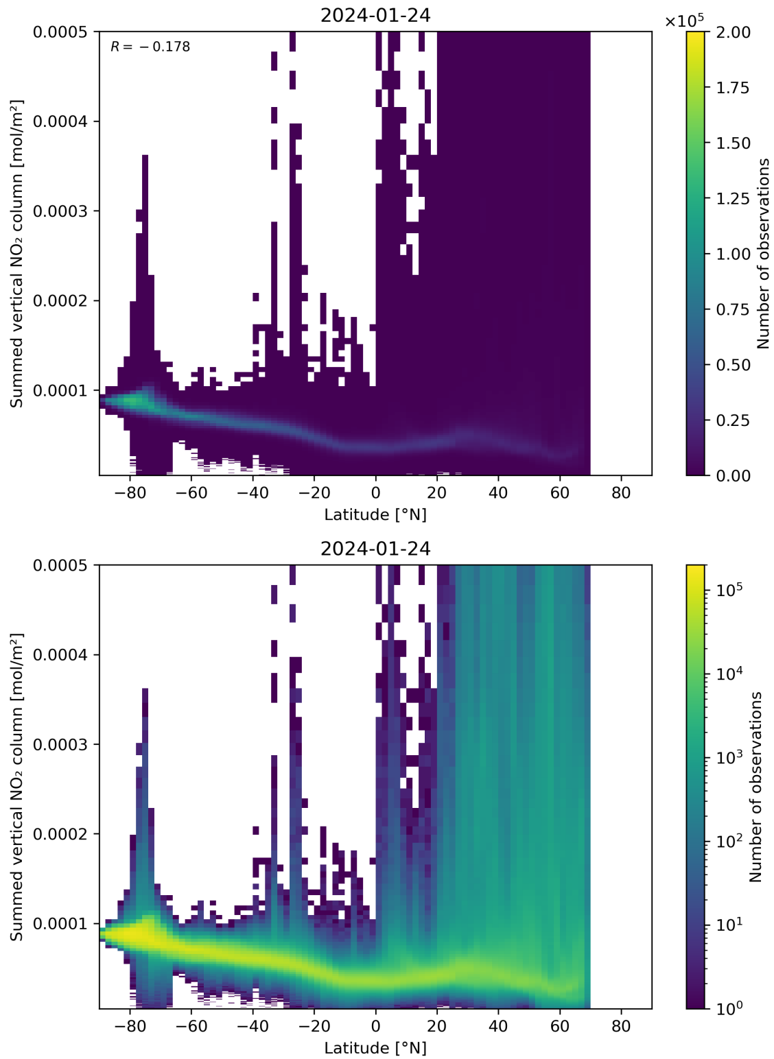
Figure 88: Scatter density plot of “Latitude” against “Summed vertical NO 2 column” for 2024-01-23 to 2024-01-25.
