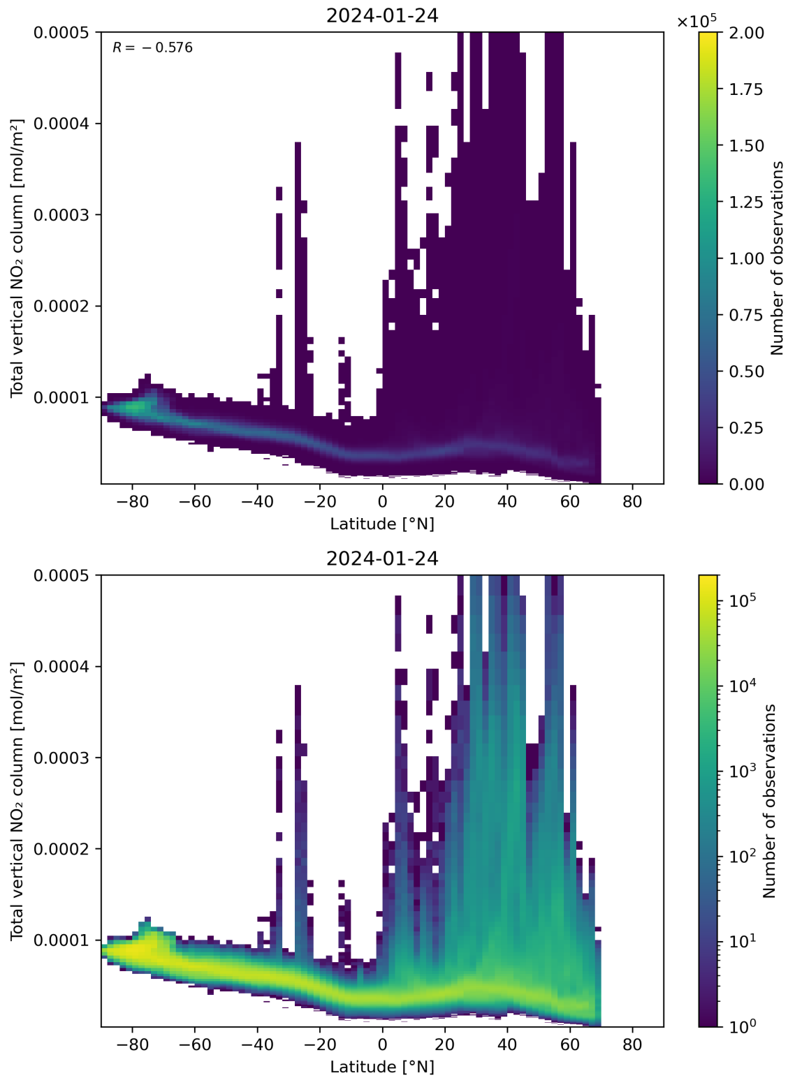
Figure 90: Scatter density plot of “Latitude” against “Total vertical NO 2 column” for 2024-01-23 to 2024-01-25.
