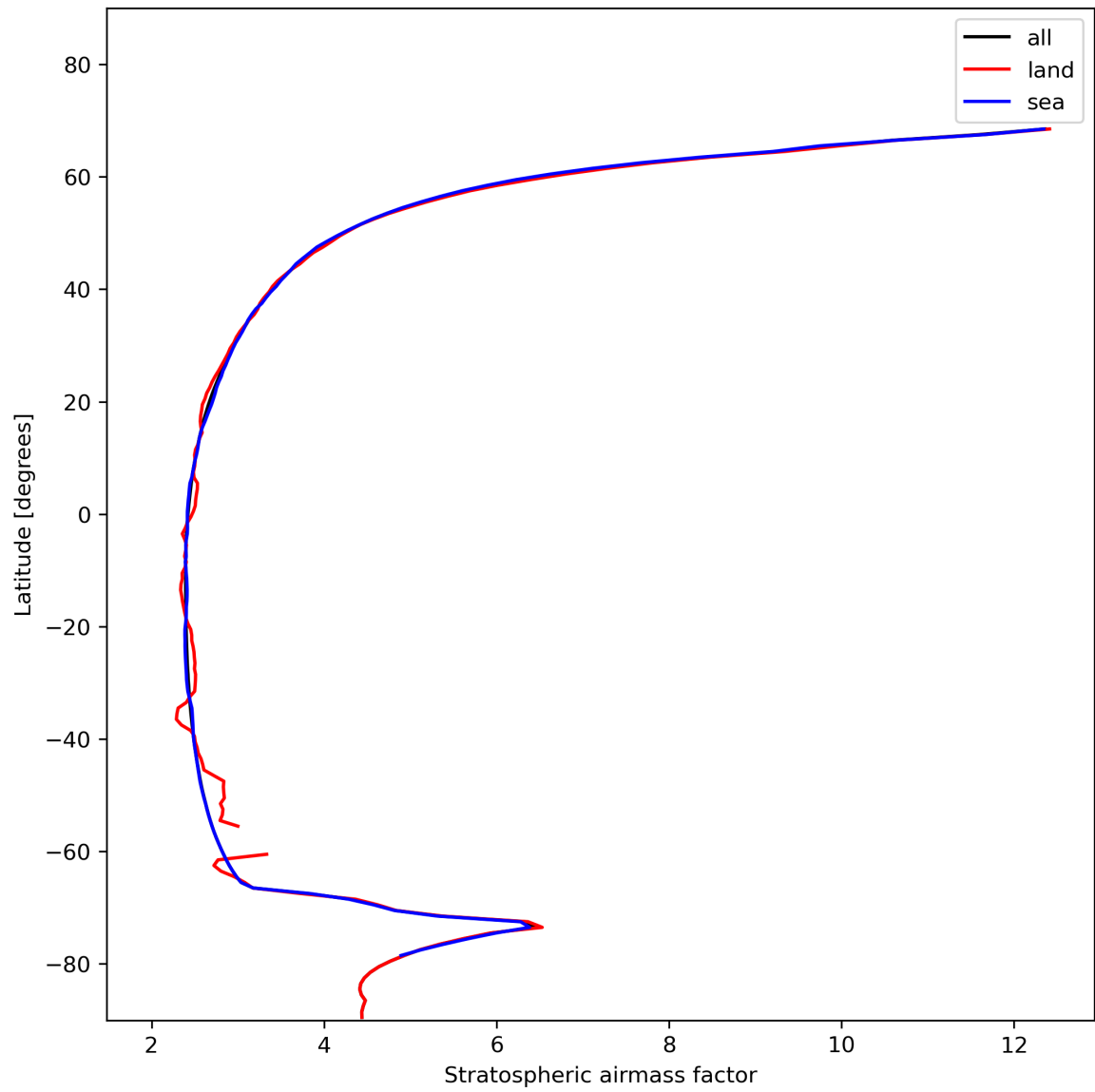
Figure 27: Zonal average of “Stratospheric airmass factor” for 2024-01-23 to 2024-01-25.
