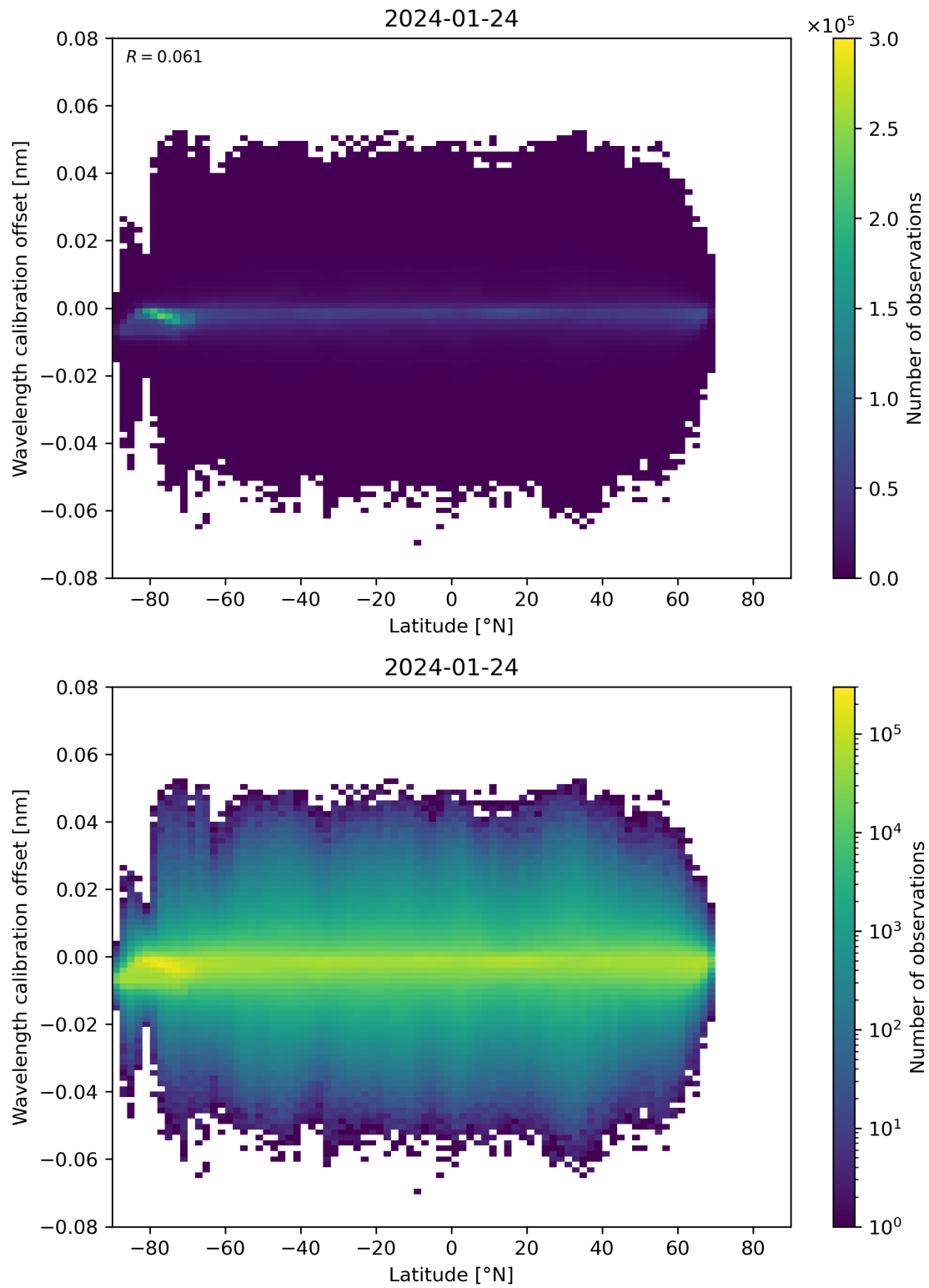
Figure 95: Scatter density plot of “Latitude” against “Wavelength calibration offset” for 2024-01-23 to 2024-01-25.
