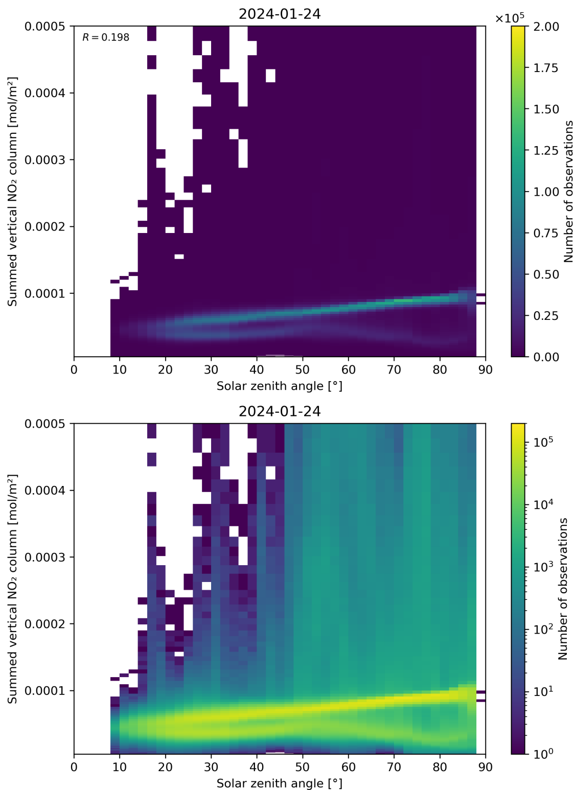
Figure 151: Scatter density plot of “Solar zenith angle” against “Summed vertical NO 2 column” for 2024-01-23 to 2024-01-25.
