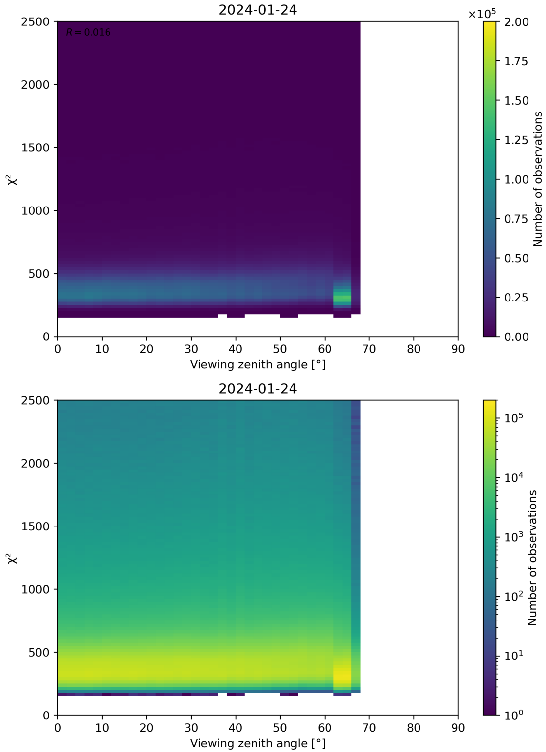
Figure 162: Scatter density plot of “Viewing zenith angle” against “ \chi^2 ” for 2024-01-23 to 2024-01-25.
