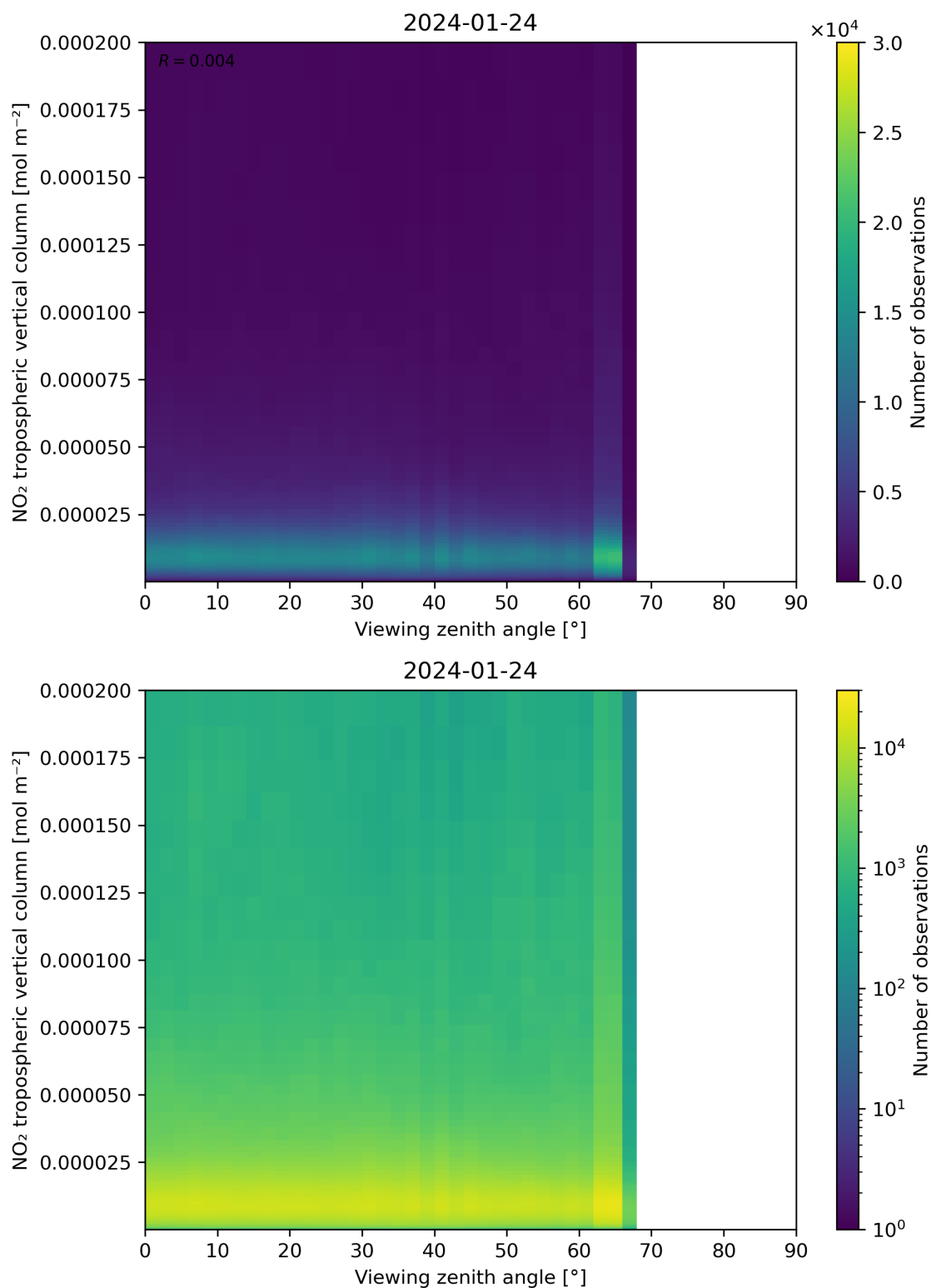
Figure 169: Scatter density plot of “Viewing zenith angle” against “NO 2 tropospheric vertical column” for 2024-01-23 to 2024-01-25.
