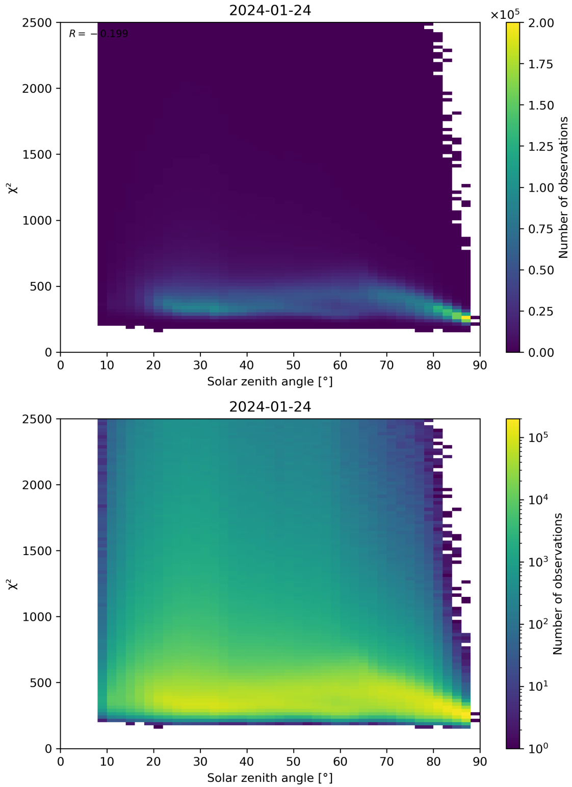
Figure 148: Scatter density plot of “Solar zenith angle” against “ \chi^2 ” for 2024-01-23 to 2024-01-25.
