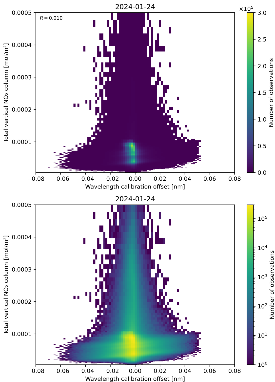
Figure 179: Scatter density plot of “Wavelength calibration offset” against “Total vertical NO 2 column” for 2024-01-23 to 2024-01-25.
