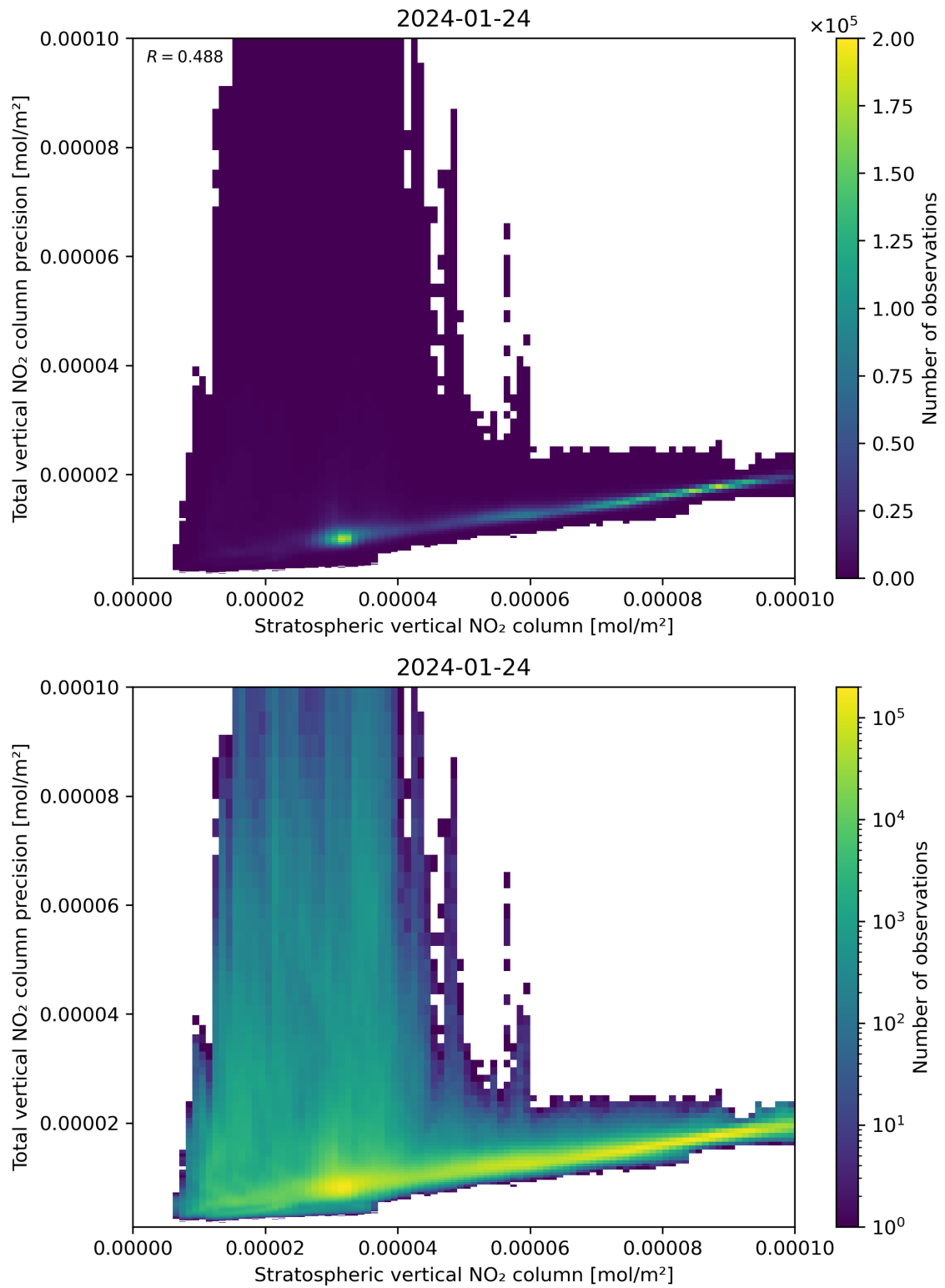
Figure 101: Scatter density plot of “Stratospheric vertical NO 2 column” against “Total vertical NO 2 column precision” for 2024-01-23 to 2024-01-25.
