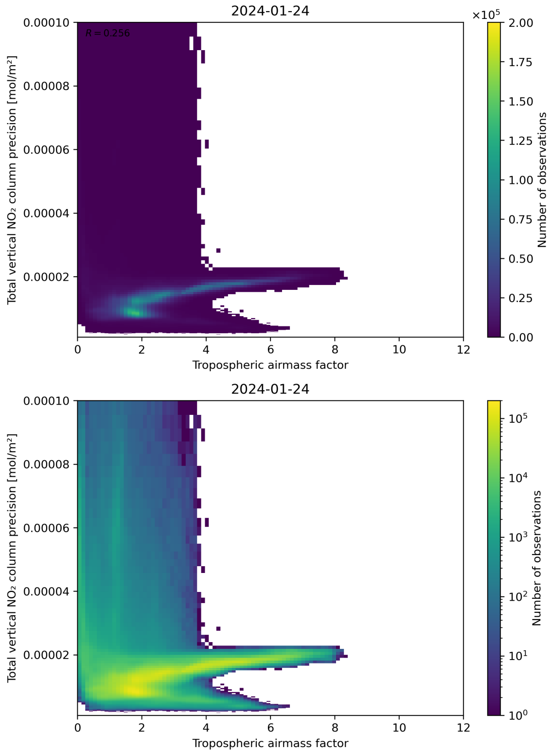
Figure 78: Scatter density plot of “Tropospheric air mass factor” against “Total vertical NO 2 column precision” for 2024-01-23 to 2024-01-25.
