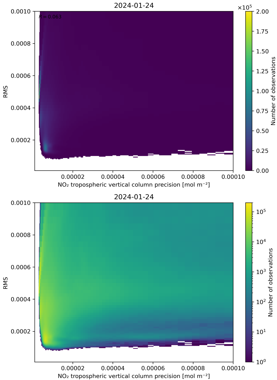
Figure 140: Scatter density plot of “NO 2 tropospheric vertical column precision” against “RMS” for 2024-01-23 to 2024-01-25.
