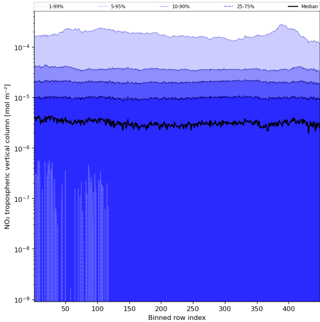
Figure 46: Along track statistics of “NO 2 tropospheric vertical column” for 2024-01-23 to 2024-01-25
