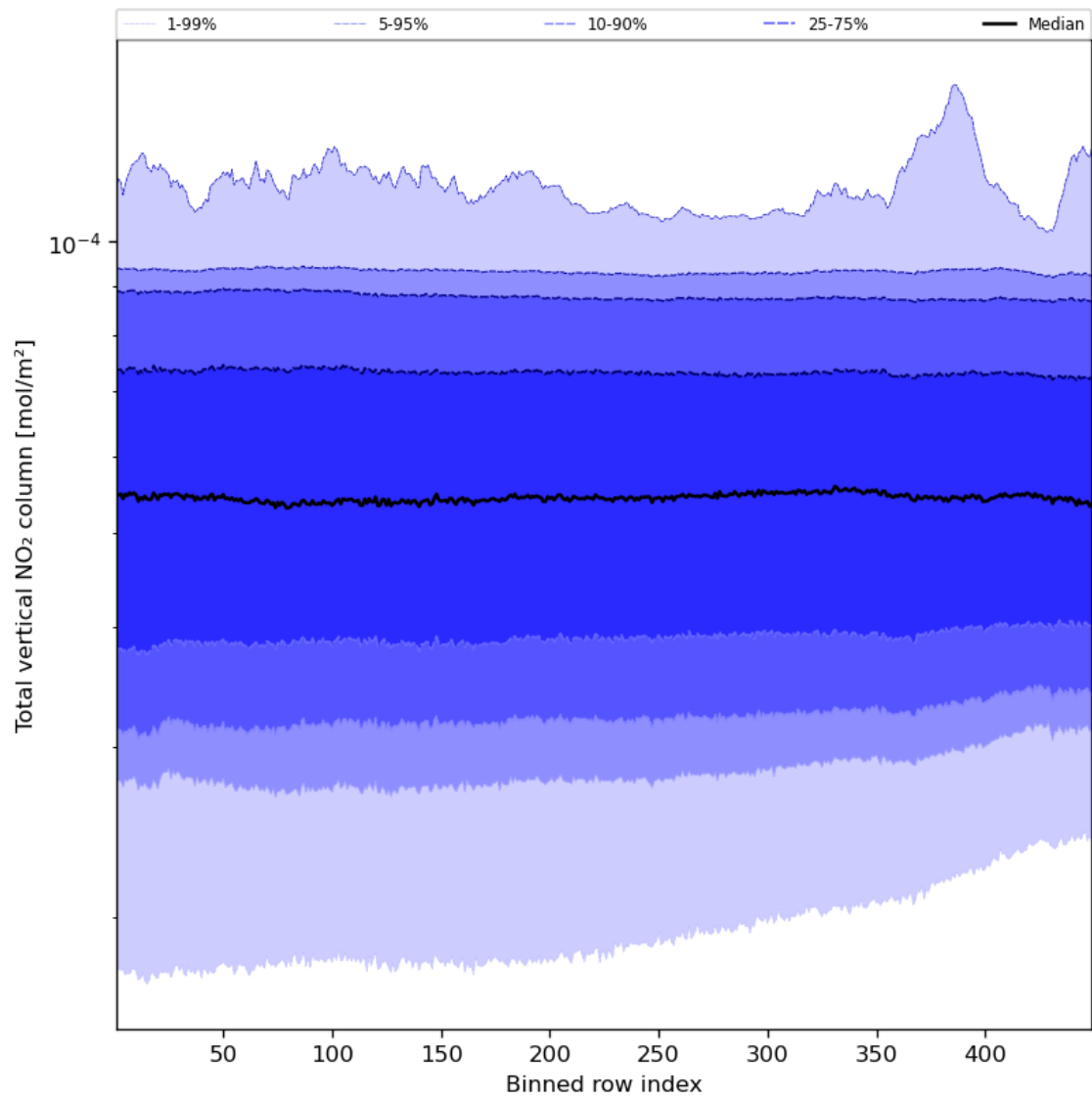
Figure 55: Along track statistics of “Total vertical NO 2 column” for 2024-01-23 to 2024-01-25
