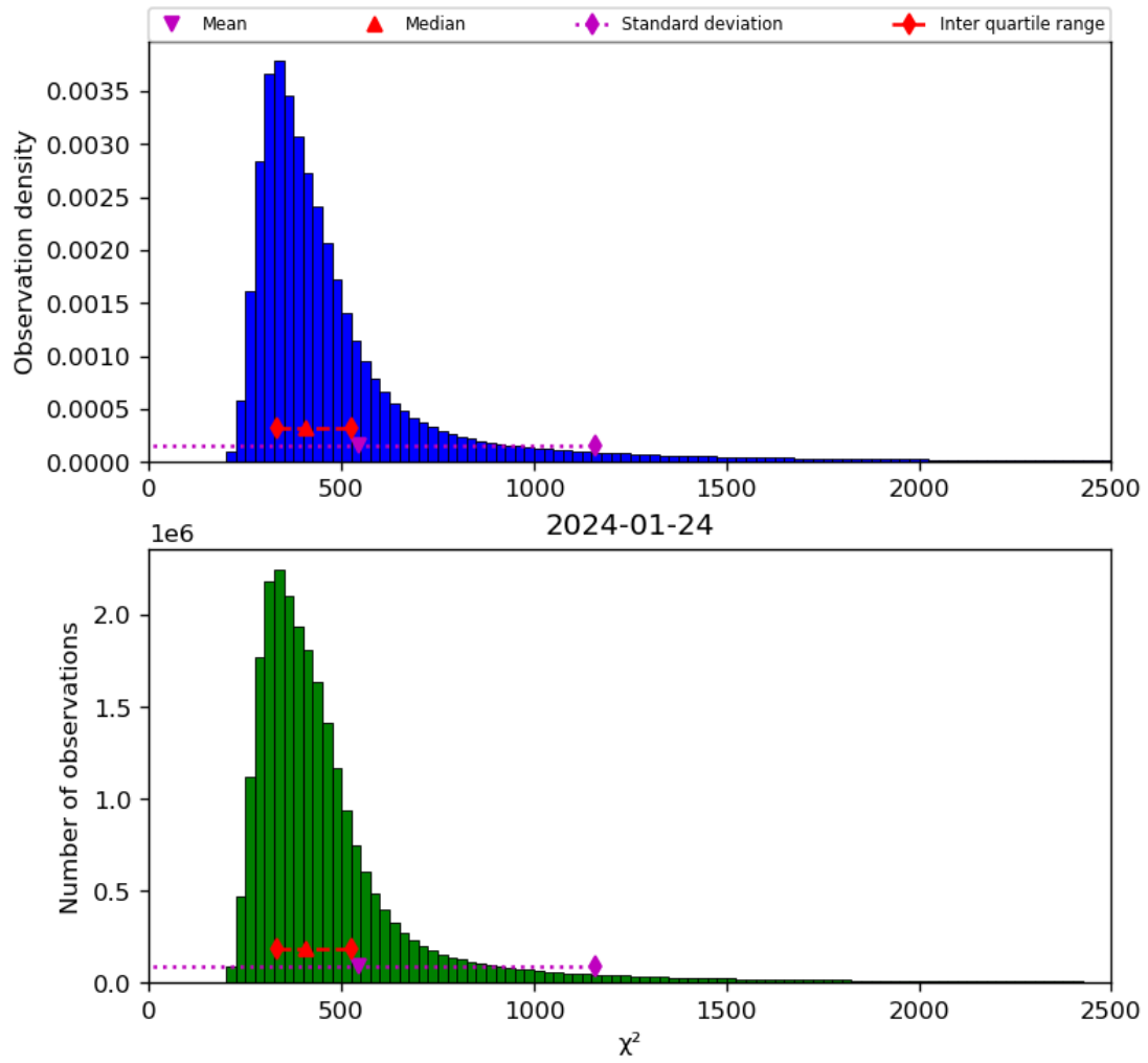
Figure 42: Histogram of “ \chi^2 ” for 2024-01-23 to 2024-01-25
