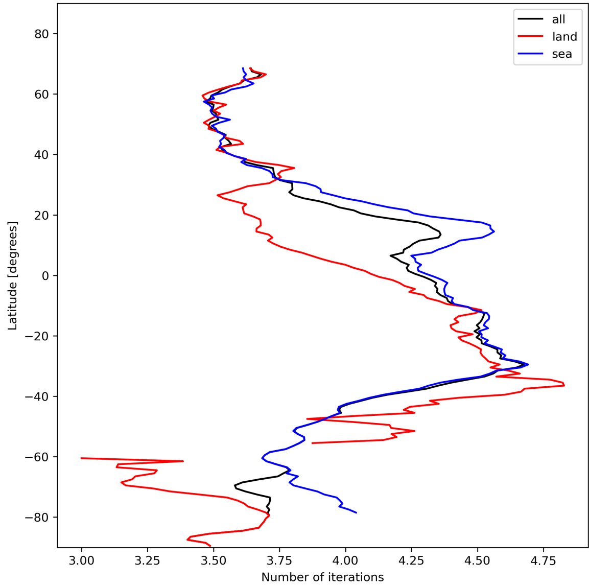
Figure 17: Zonal average of “Number of iterations” for 2024-01-23 to 2024-01-25.
