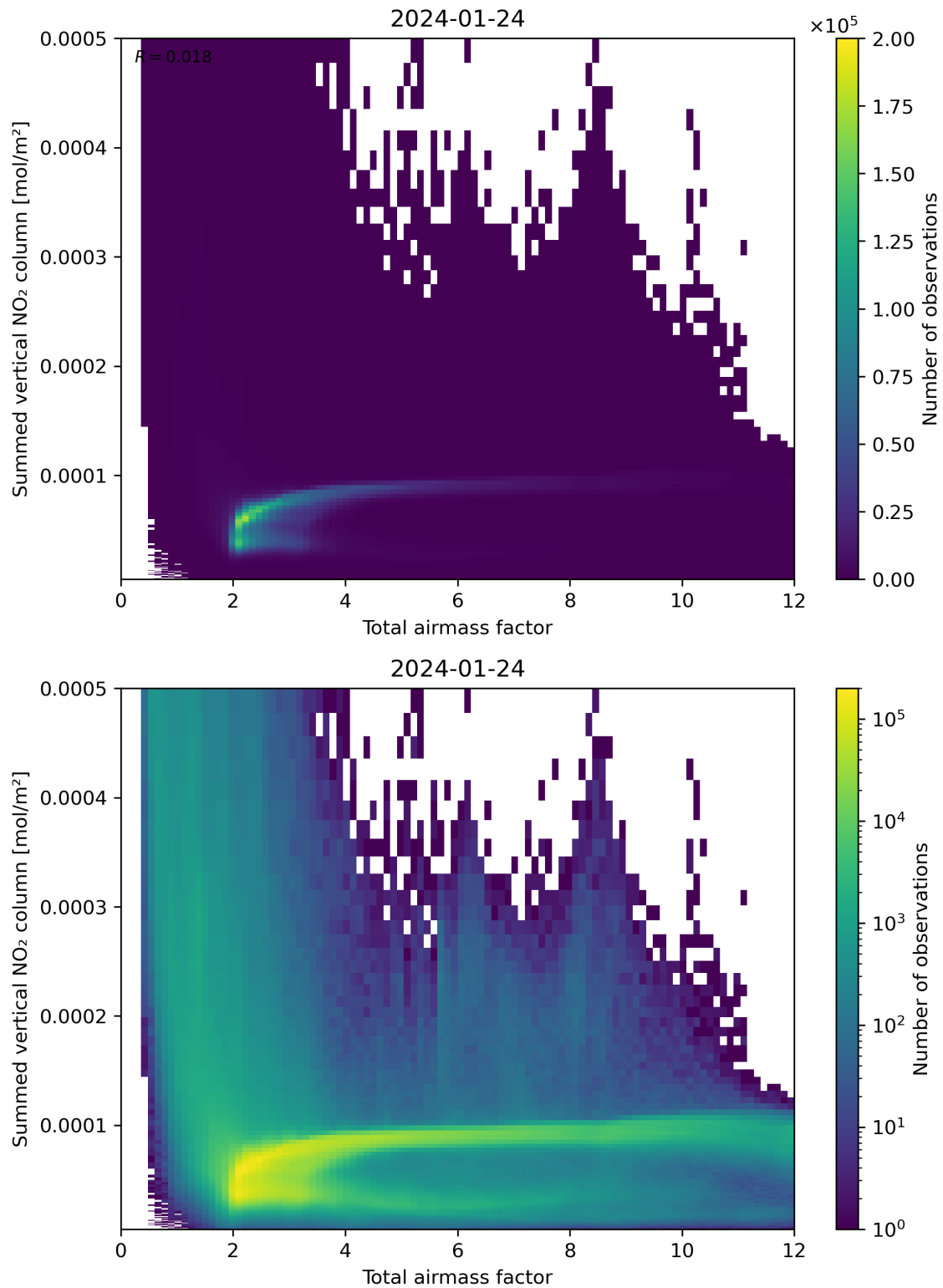
Figure 65: Scatter density plot of “Total airmass factor” against “Summed vertical NO 2 column” for 2024-01-23 to 2024-01-25.
