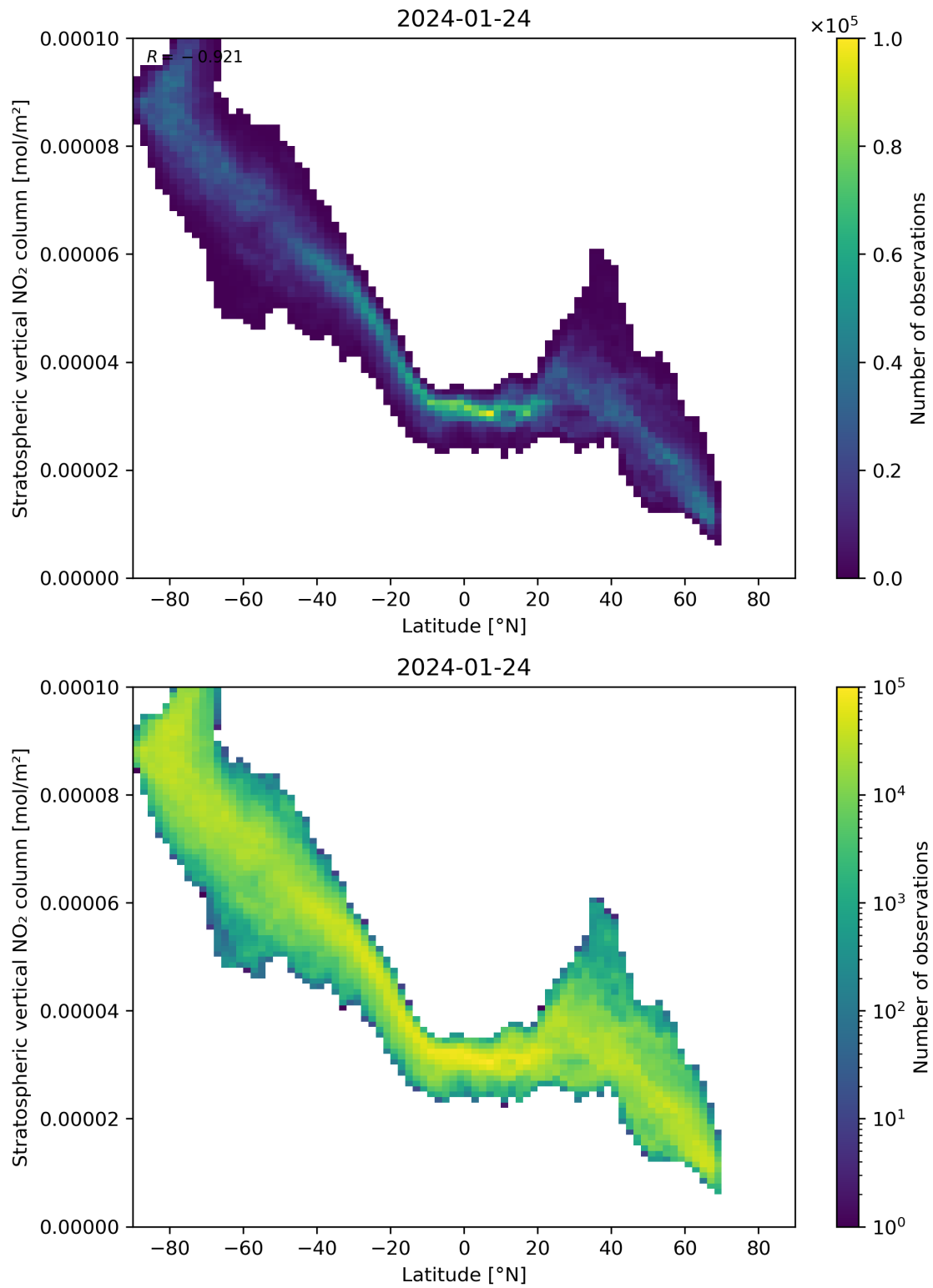
Figure 87: Scatter density plot of “Latitude” against “Stratospheric vertical NO 2 column” for 2024-01-23 to 2024-01-25.
