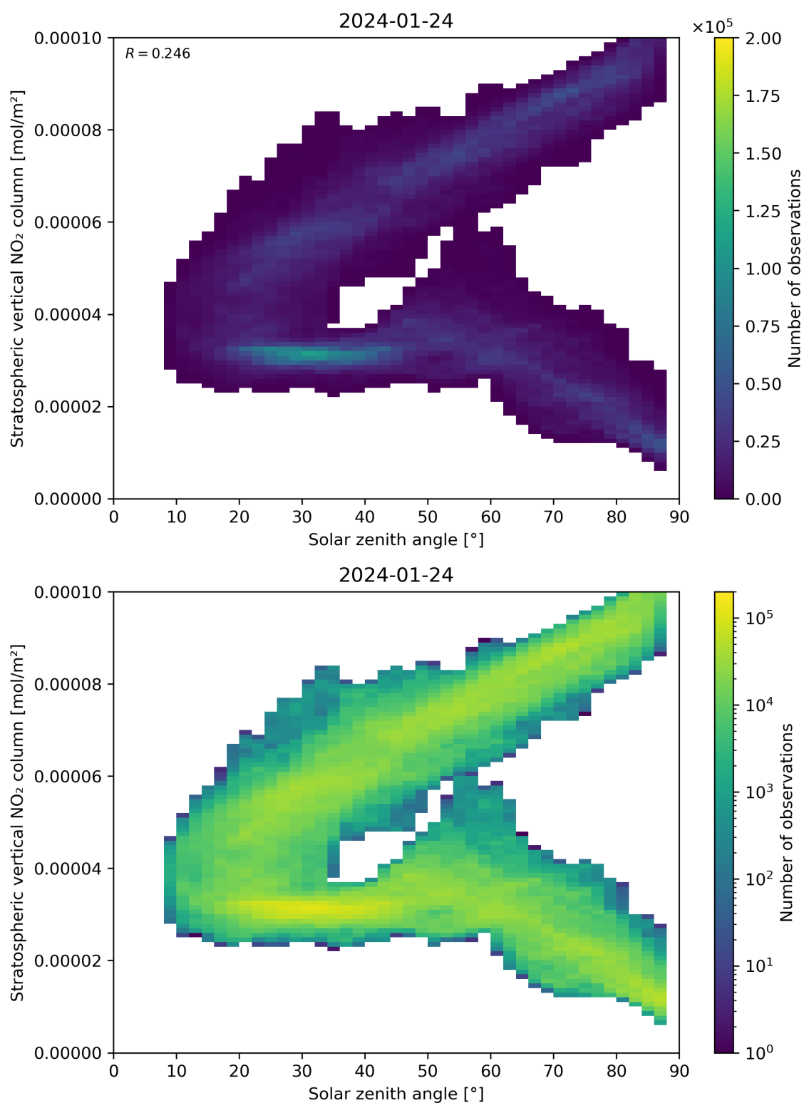
Figure 150: Scatter density plot of “Solar zenith angle” against “Stratospheric vertical NO 2 column” for 2024-01-23 to 2024-01-25.
