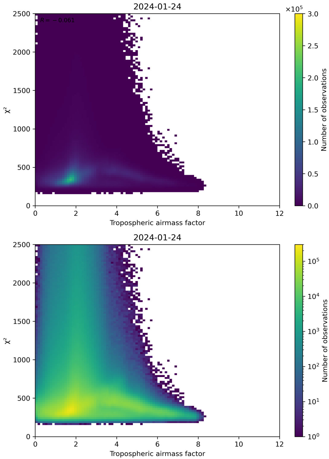
Figure 73: Scatter density plot of “Tropospheric airmass factor” against “ \chi^2 ” for 2024-01-23 to 2024-01-25.
