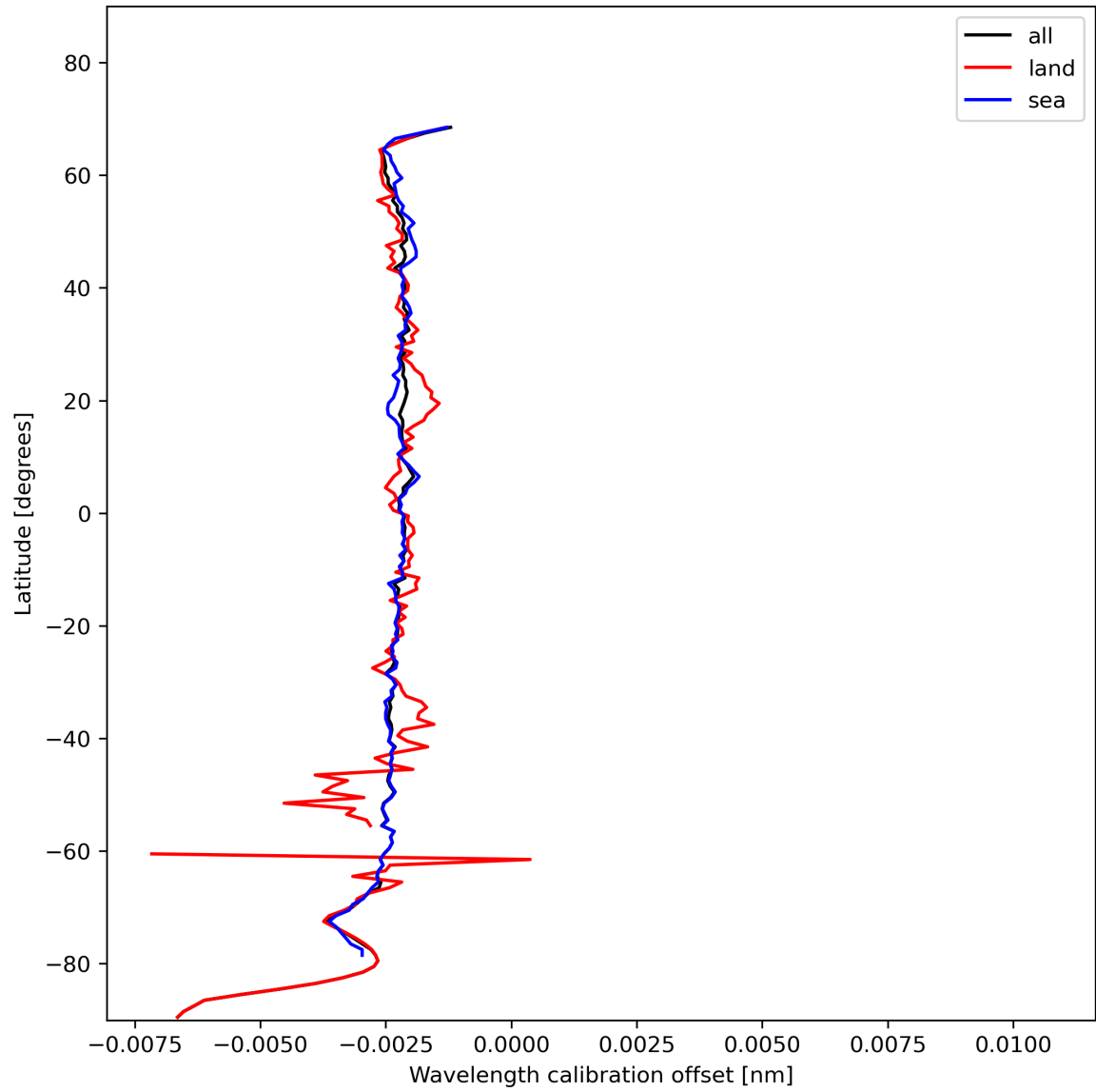
Figure 18: Zonal average of “Wavelength calibration offset” for 2024-01-23 to 2024-01-25.
