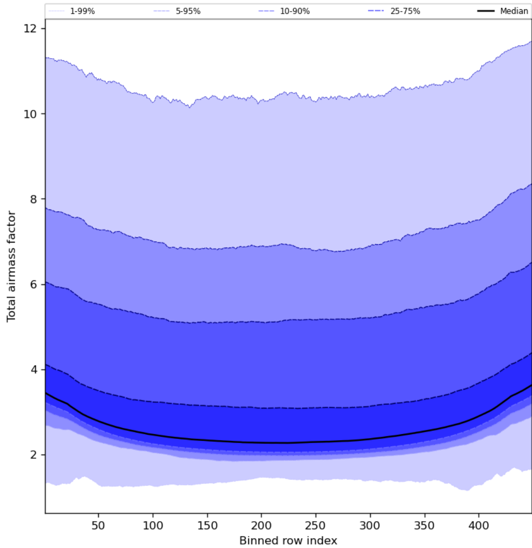
Figure 49: Along track statistics of “Total airmass factor” for 2024-01-23 to 2024-01-25
