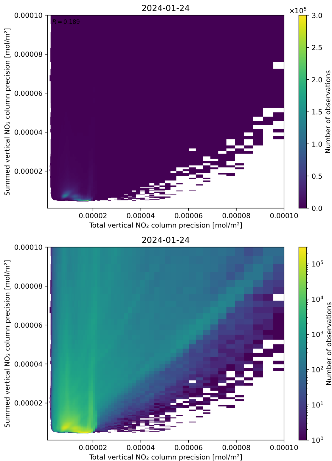
Figure 118: Scatter density plot of “Total vertical NO 2 column precision” against “Summed vertical NO 2 column precision” for 2024-01-23 to 2024-01-25.
