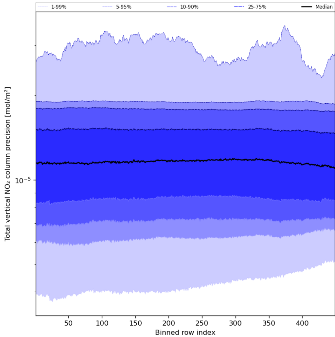
Figure 56: Along track statistics of “Total vertical NO 2 column precision” for 2024-01-23 to 2024-01-25
