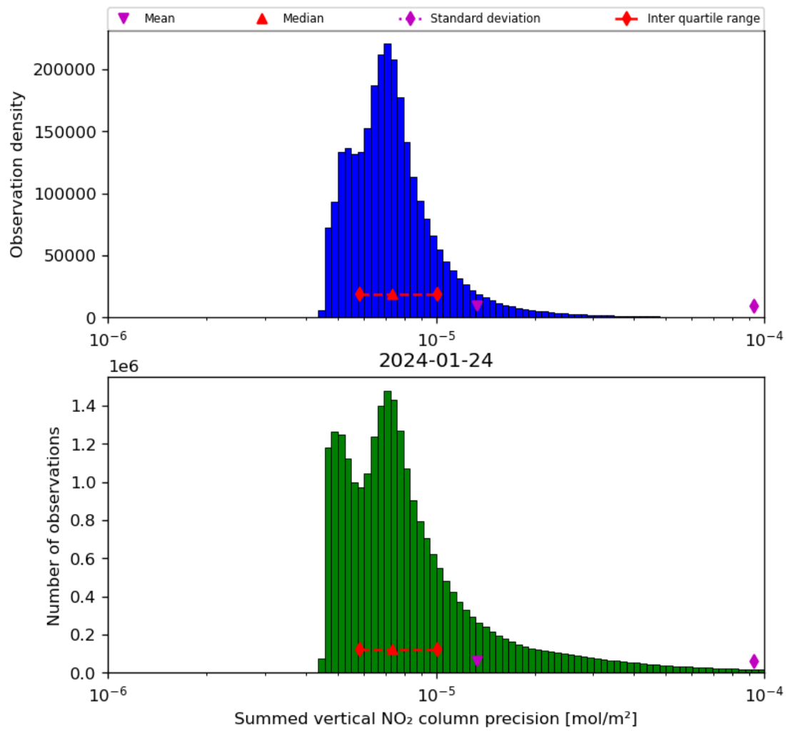
Figure 41: Histogram of “Summed vertical NO 2 column precision” for 2024-01-23 to 2024-01-25
