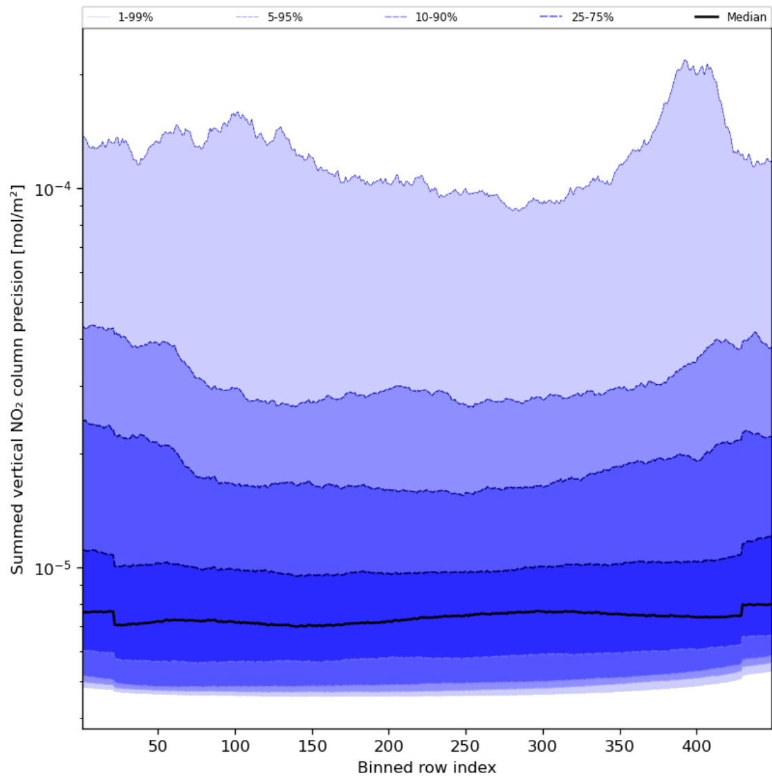
Figure 58: Along track statistics of “Summed vertical NO 2 column precision” for 2024-01-23 to 2024-01-25
