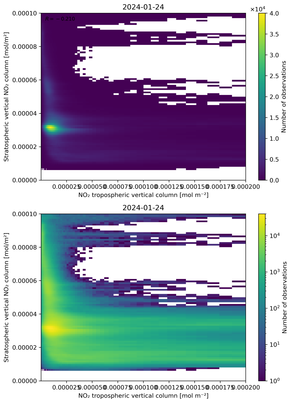
Figure 125: Scatter density plot of “NO 2 tropospheric vertical column” against “Stratospheric vertical NO 2 column” for 2024-01-23 to 2024-01-25.
