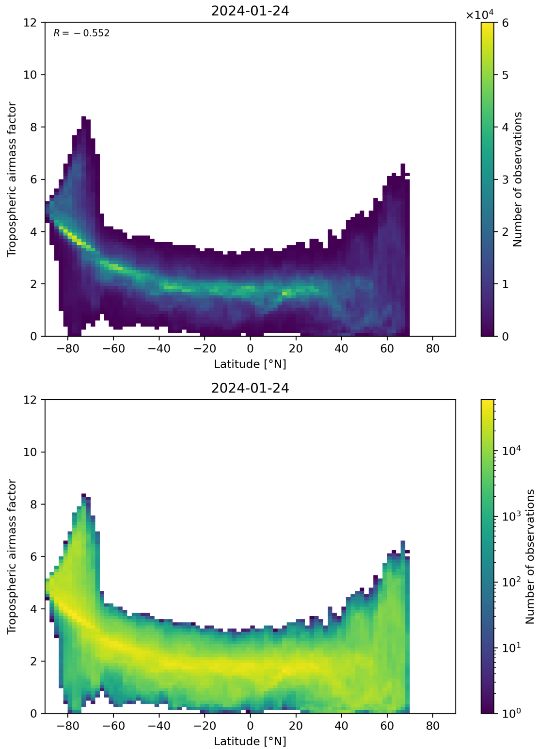
Figure 85: Scatter density plot of “Latitude” against “Tropospheric air mass factor” for 2024-01-23 to 2024-01-25.
