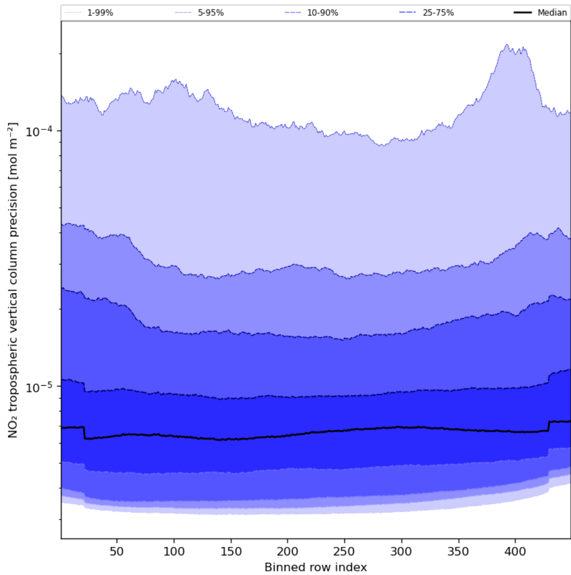
Figure 47: Along track statistics of “NO 2 tropospheric vertical column precision” for 2024-01-23 to 2024-01-25
