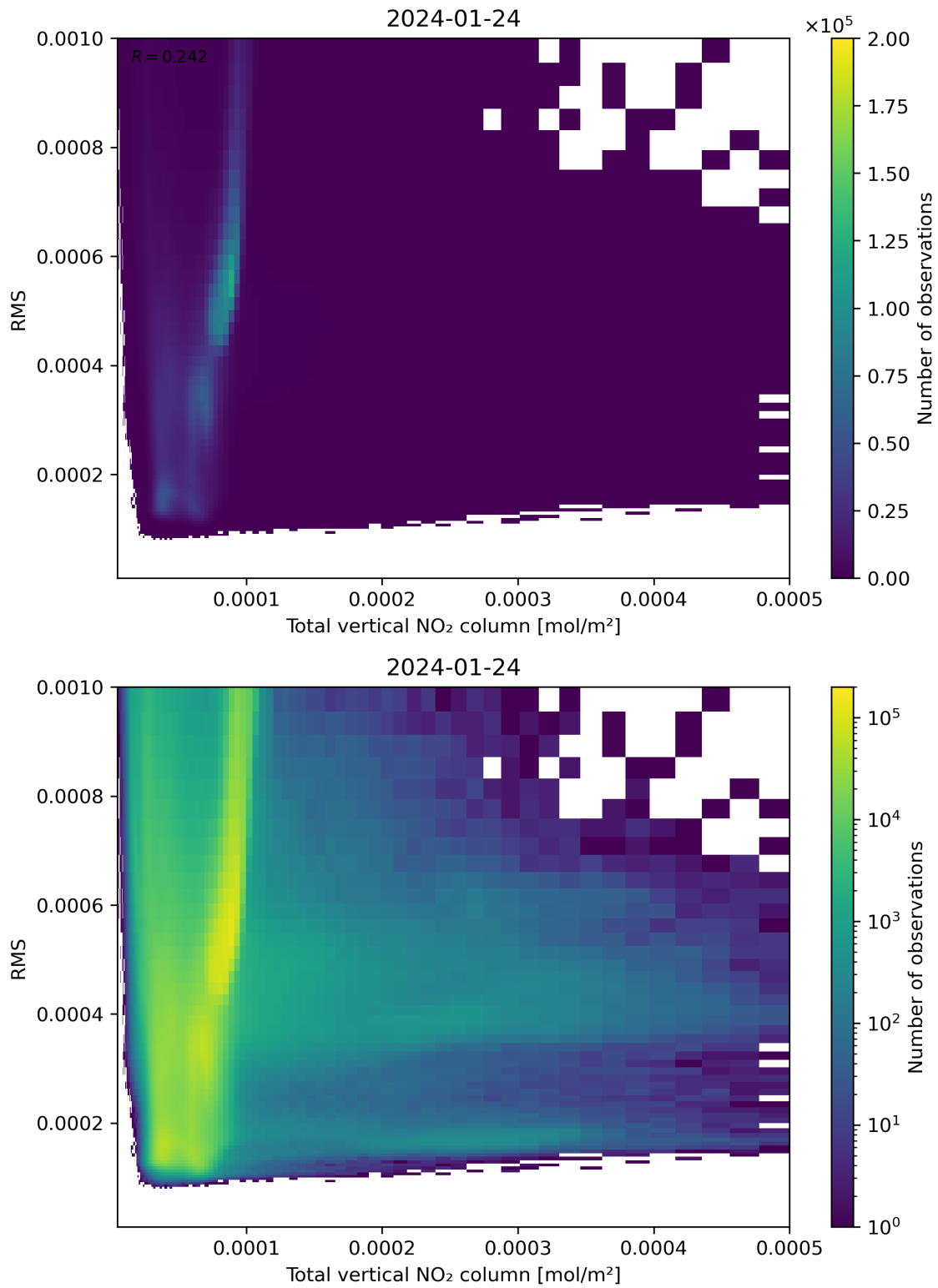
Figure 120: Scatter density plot of “Total vertical NO 2 column” against “RMS” for 2024-01-23 to 2024-01-25.
