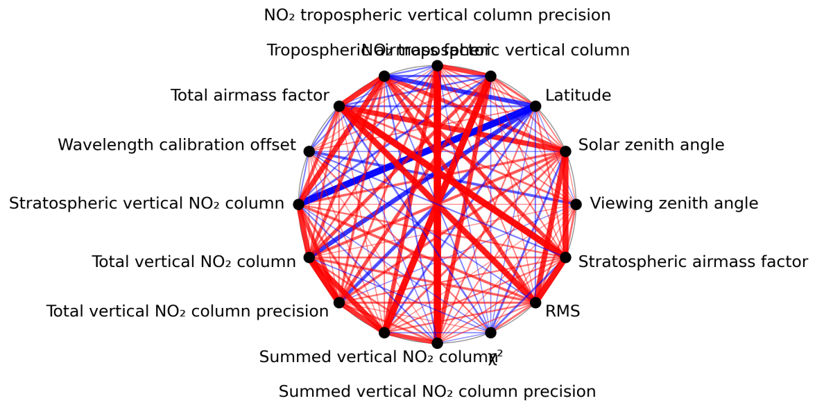
Figure 1: Map of correlation graph for 2024-01-23 to 2024-01-25.
