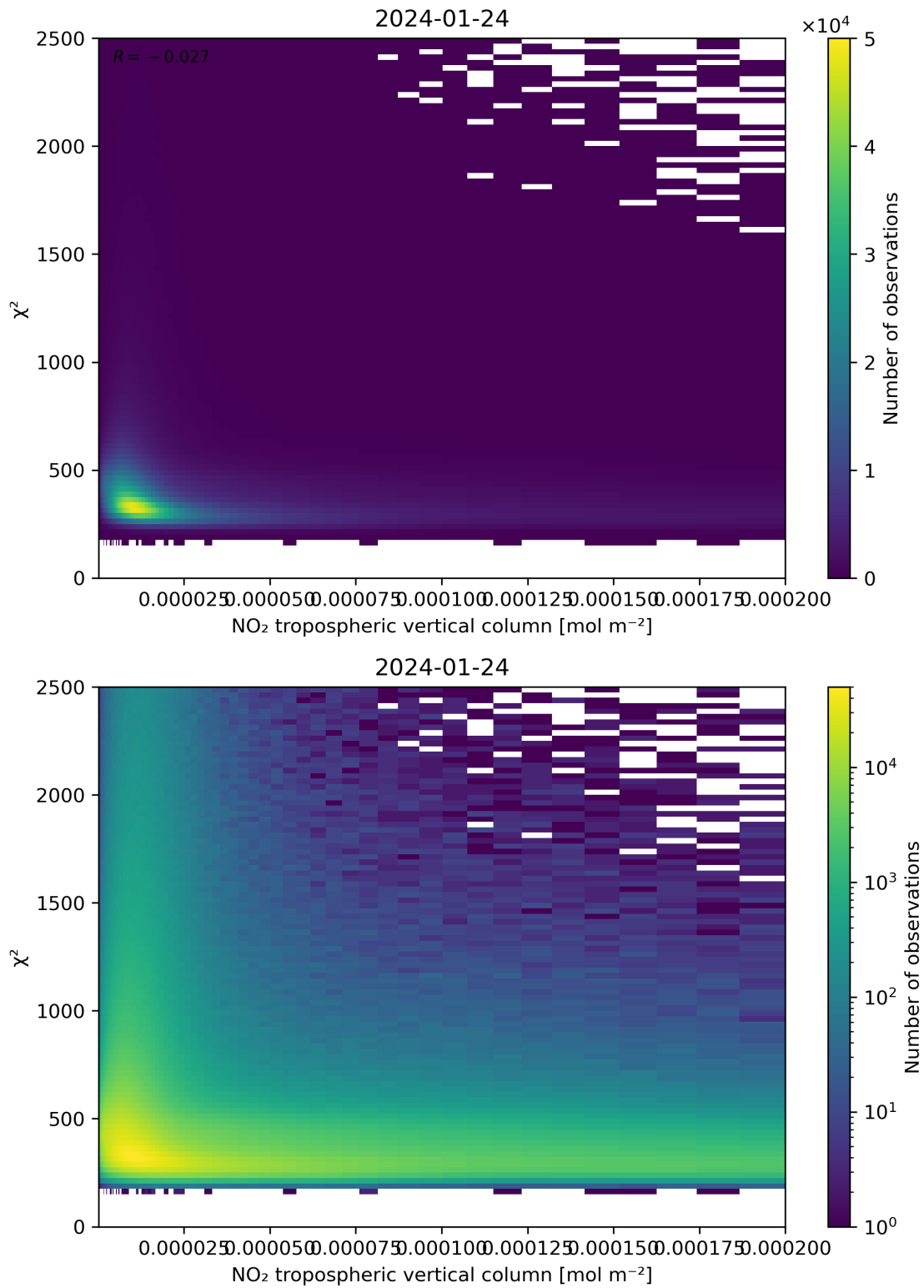
Figure 124: Scatter density plot of “NO 2 tropospheric vertical column” against “ \chi^2 ” for 2024-01-23 to 2024-01-25.
