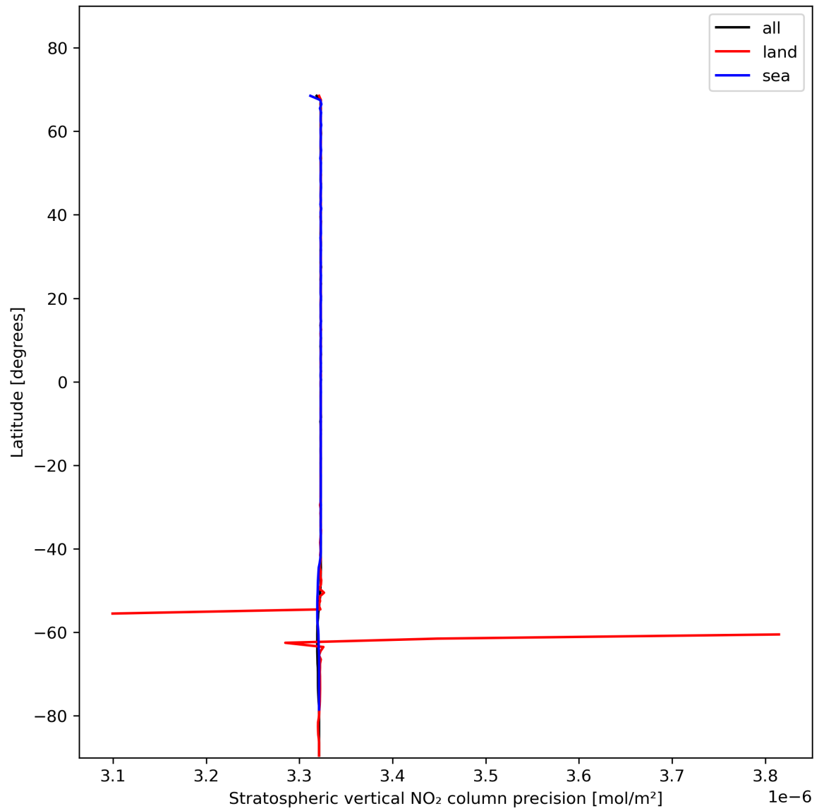
Figure 20: Zonal average of “Stratospheric vertical NO 2 column precision” for 2024-01-23 to 2024-01-25.
