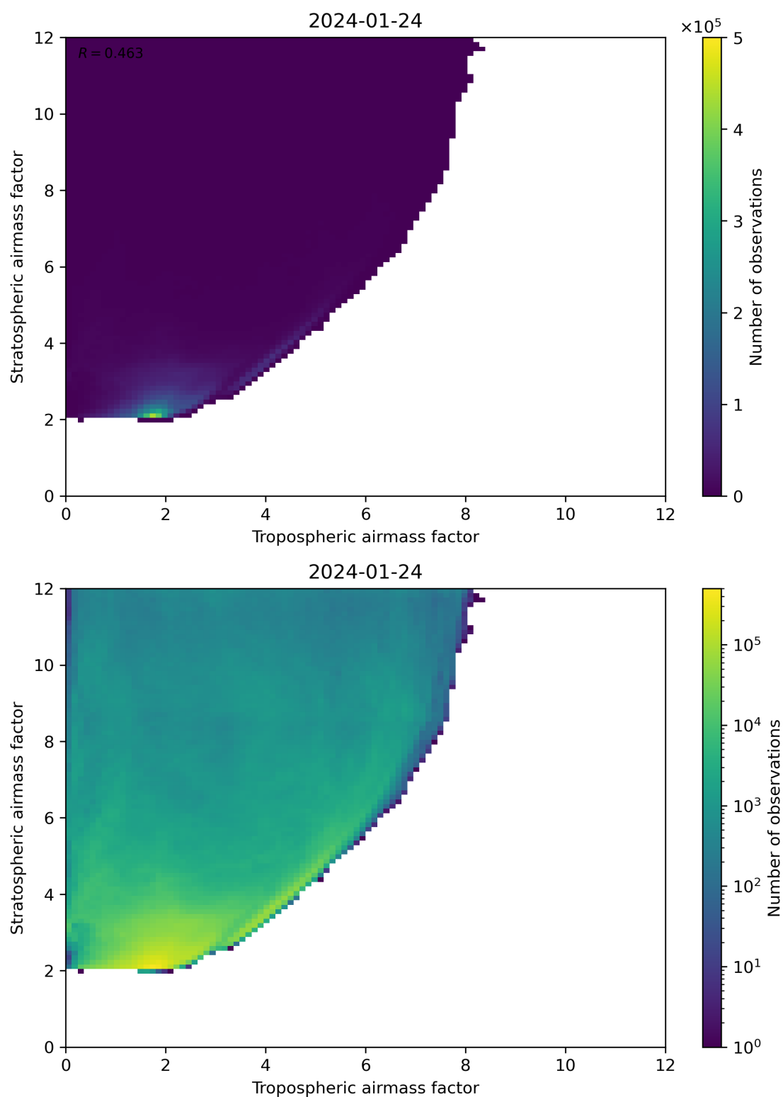
Figure 71: Scatter density plot of “Tropospheric airmass factor” against “Stratospheric airmass factor” for 2024-01-23 to 2024-01-25.
