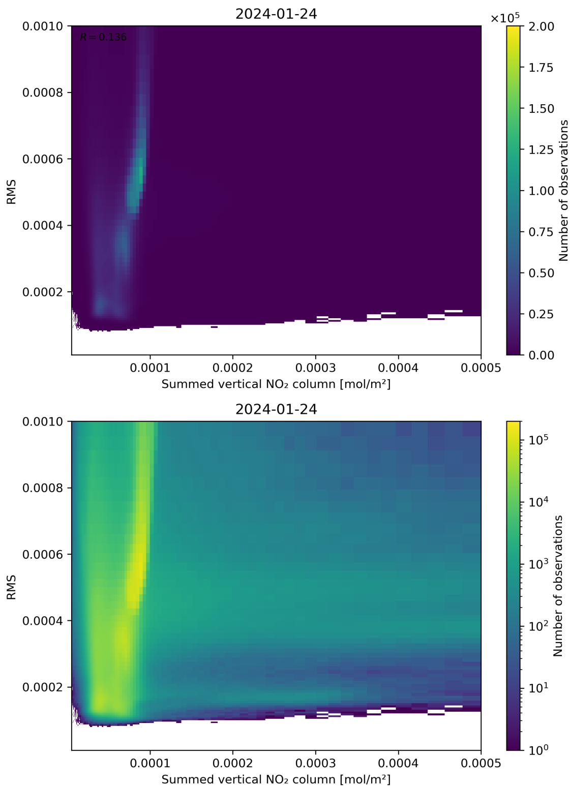
Figure 109: Scatter density plot of “Summed vertical NO 2 column” against “RMS” for 2024-01-23 to 2024-01-25.
