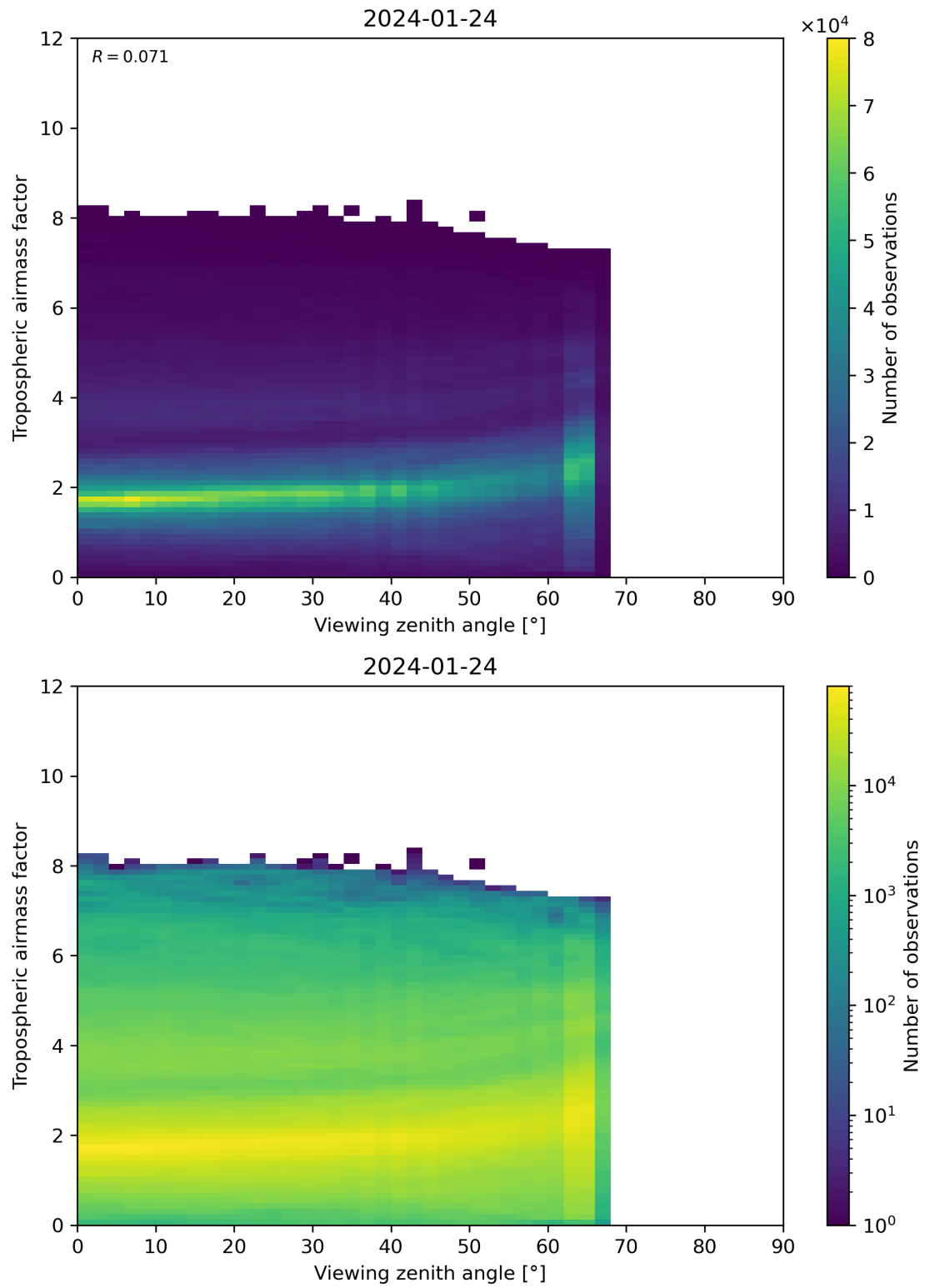
Figure 161: Scatter density plot of “Viewing zenith angle” against “Tropospheric airmass factor” for 2024-01-23 to 2024-01-25.
