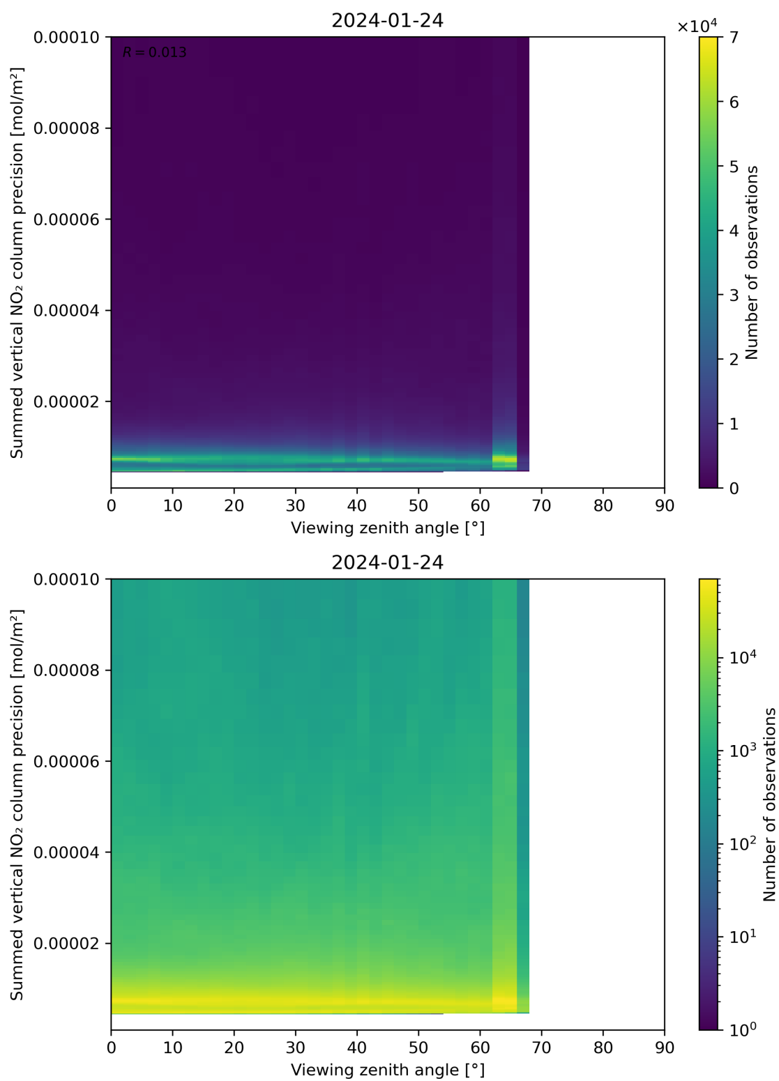
Figure 166: Scatter density plot of “Viewing zenith angle” against “Summed vertical NO 2 column precision” for 2024-01-23 to 2024-01-25.
