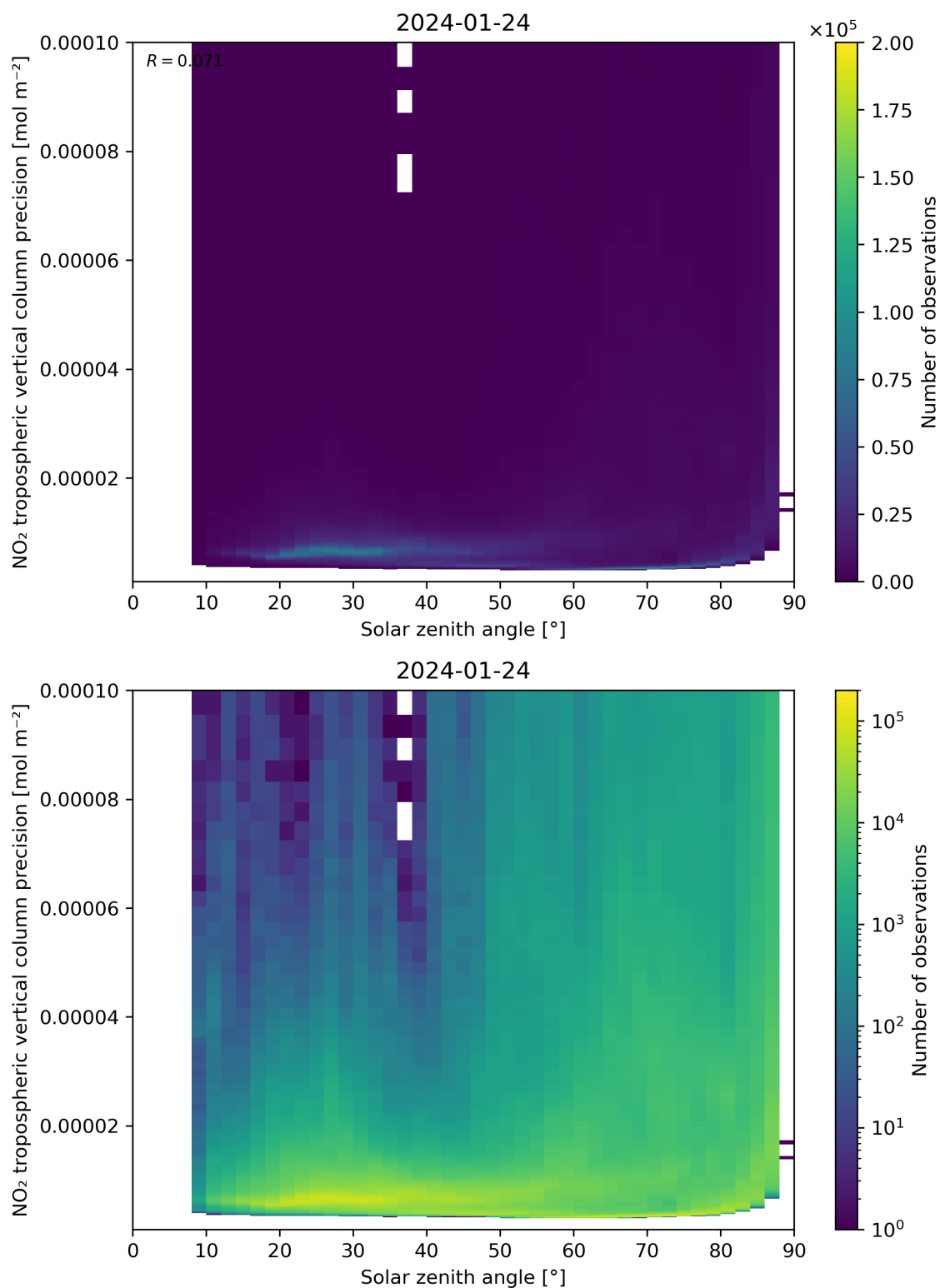
Figure 156: Scatter density plot of “Solar zenith angle” against “NO 2 tropospheric vertical column precision” for 2024-01-23 to 2024-01-25.
