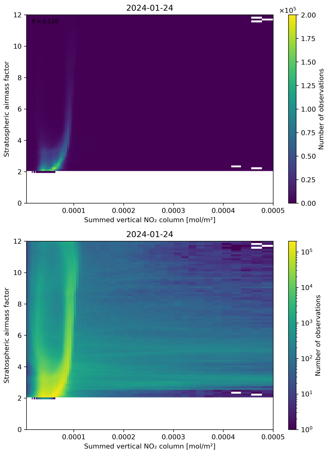
Figure 103: Scatter density plot of “Summed vertical NO 2 column” against “Stratospheric airmass factor” for 2024-01-23 to 2024-01-25.
