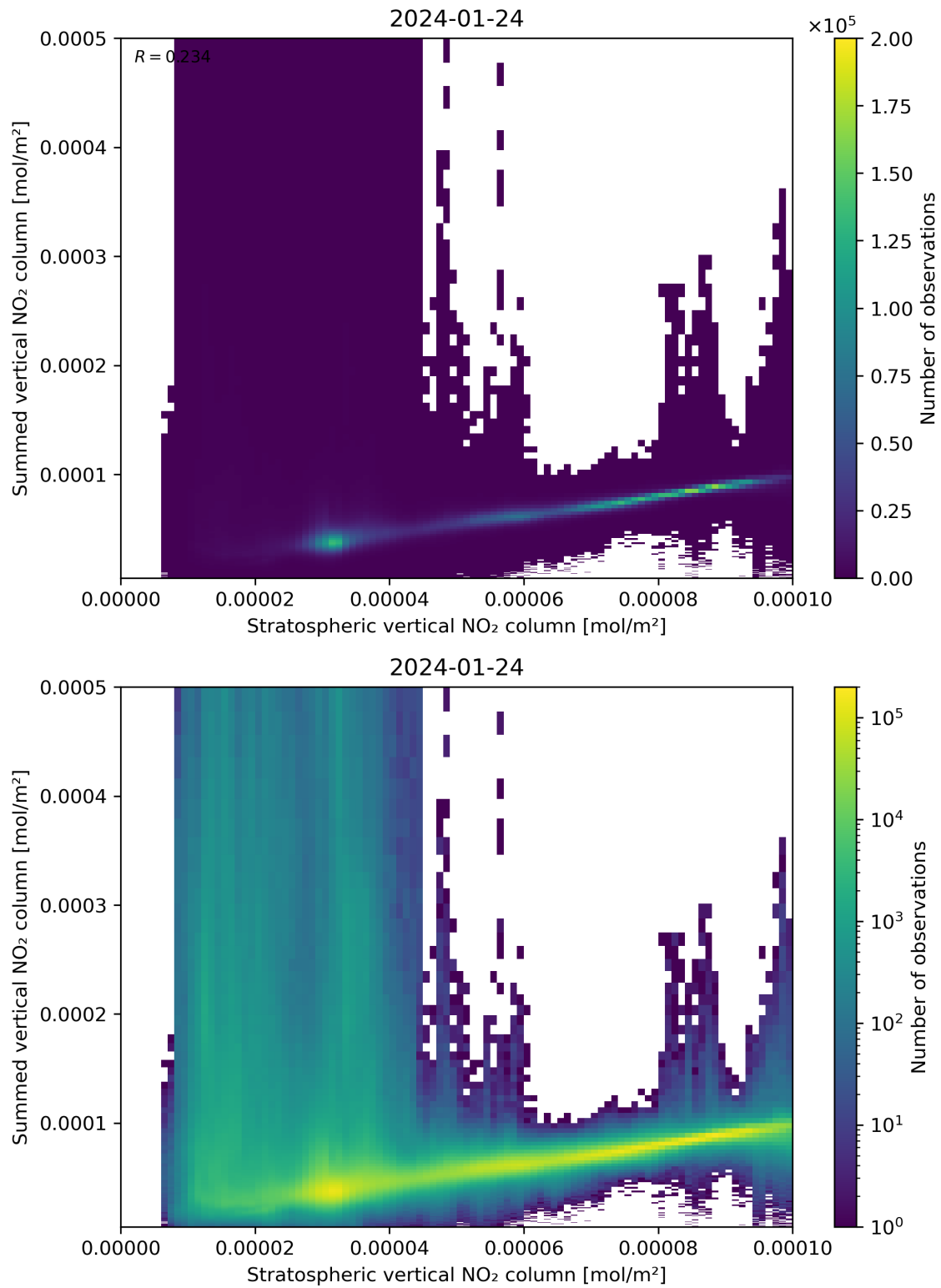
Figure 98: Scatter density plot of “Stratospheric vertical NO 2 column” against “Summed vertical NO 2 column” for 2024-01-23 to 2024-01-25.
