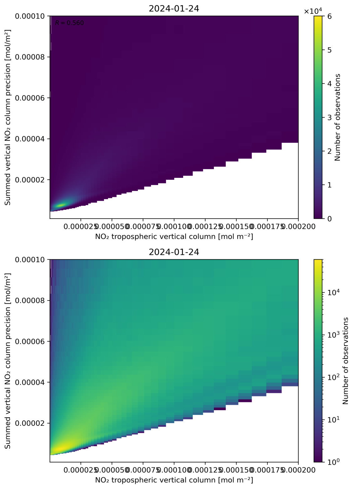
Figure 127: Scatter density plot of “NO 2 tropospheric vertical column” against “Summed vertical NO 2 column precision” for 2024-01-23 to 2024-01-25.
