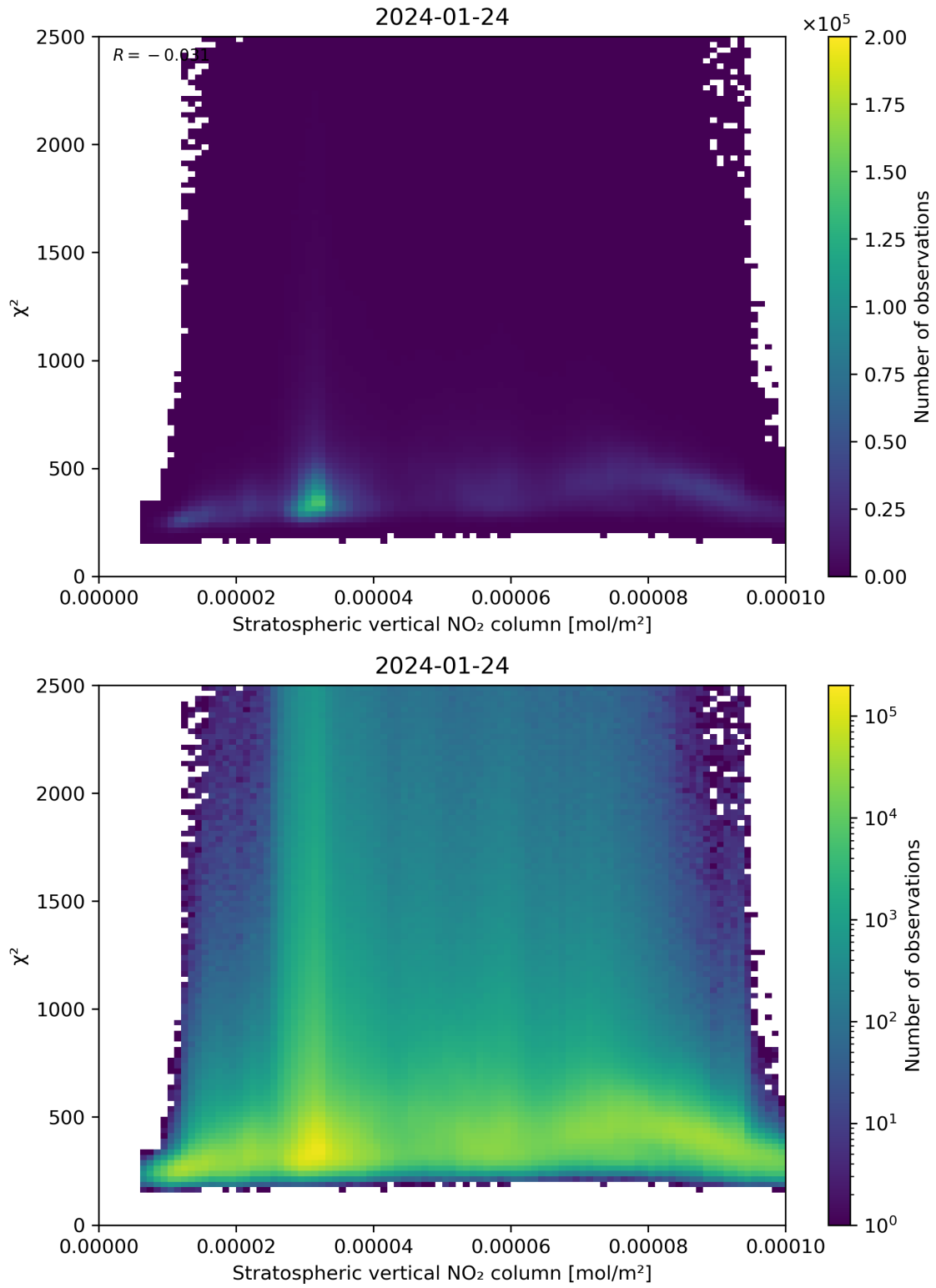
Figure 97: Scatter density plot of “Stratospheric vertical NO 2 column” against “ \chi^2 ” for 2024-01-23 to 2024-01-25.
