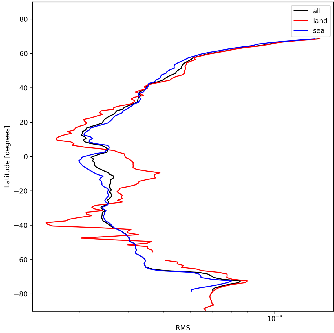
Figure 26: Zonal average of “RMS” for 2024-01-23 to 2024-01-25.
