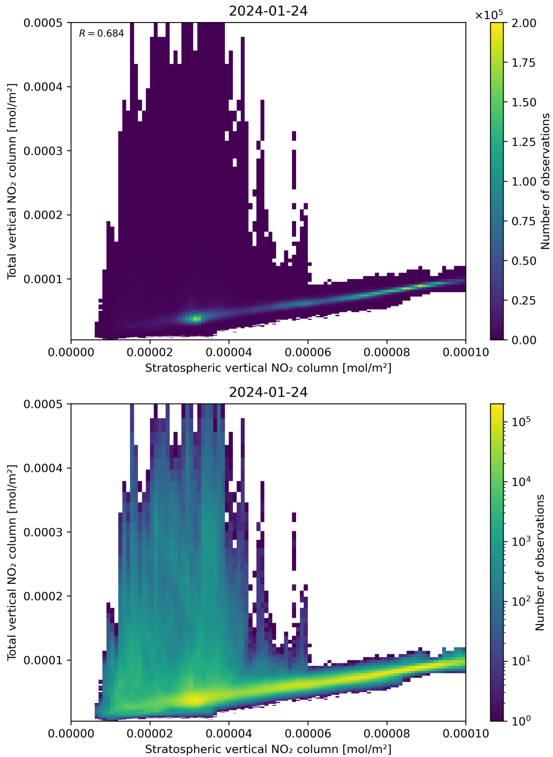
Figure 100: Scatter density plot of “Stratospheric vertical NO 2 column” against “Total vertical NO 2 column” for 2024-01-23 to 2024-01-25.
