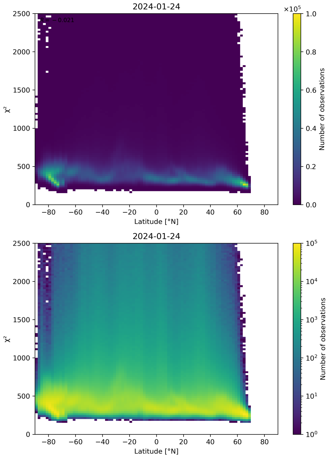
Figure 86: Scatter density plot of “Latitude” against “ \chi^2 ” for 2024-01-23 to 2024-01-25.
