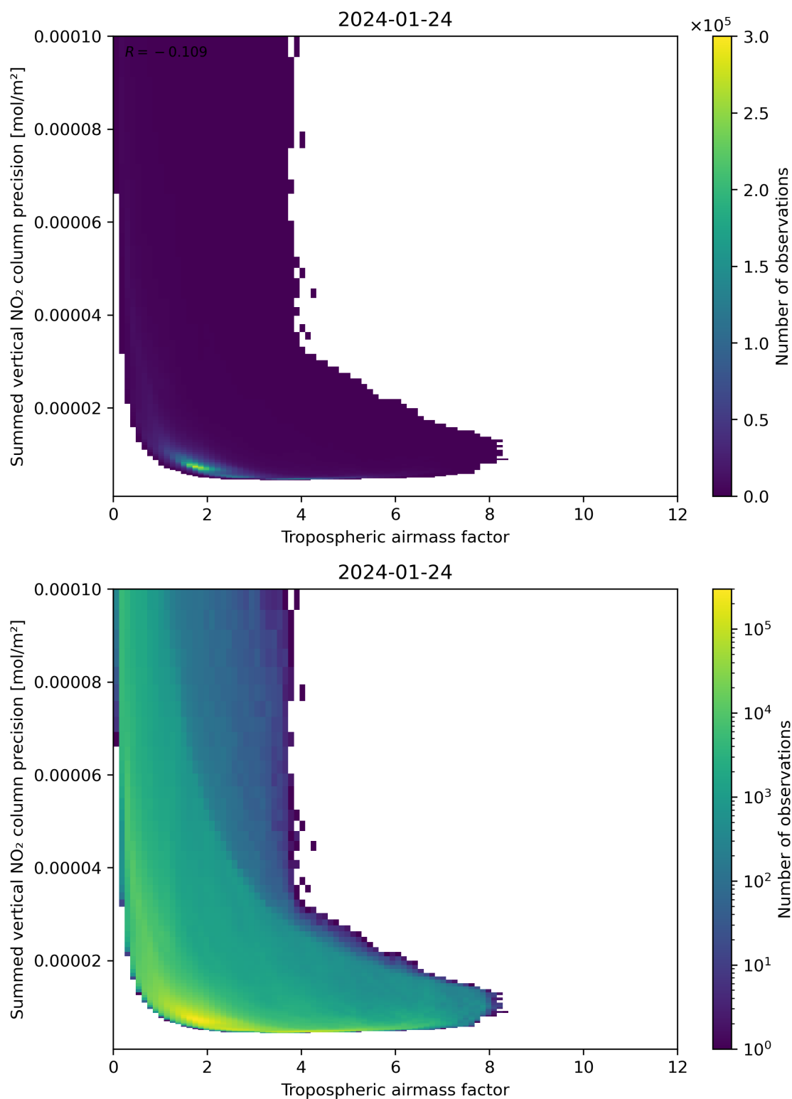
Figure 76: Scatter density plot of “Tropospheric air mass factor” against “Summed vertical NO 2 column precision” for 2024-01-23 to 2024-01-25.
