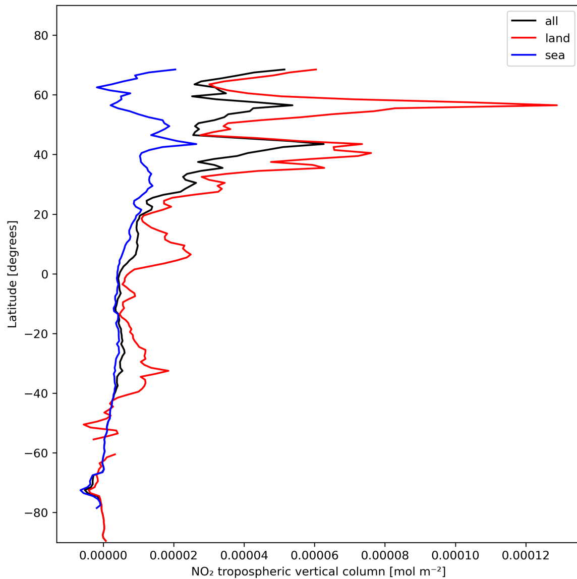
Figure 12: Zonal average of “NO 2 tropospheric vertical column” for 2024-01-23 to 2024-01-25.
