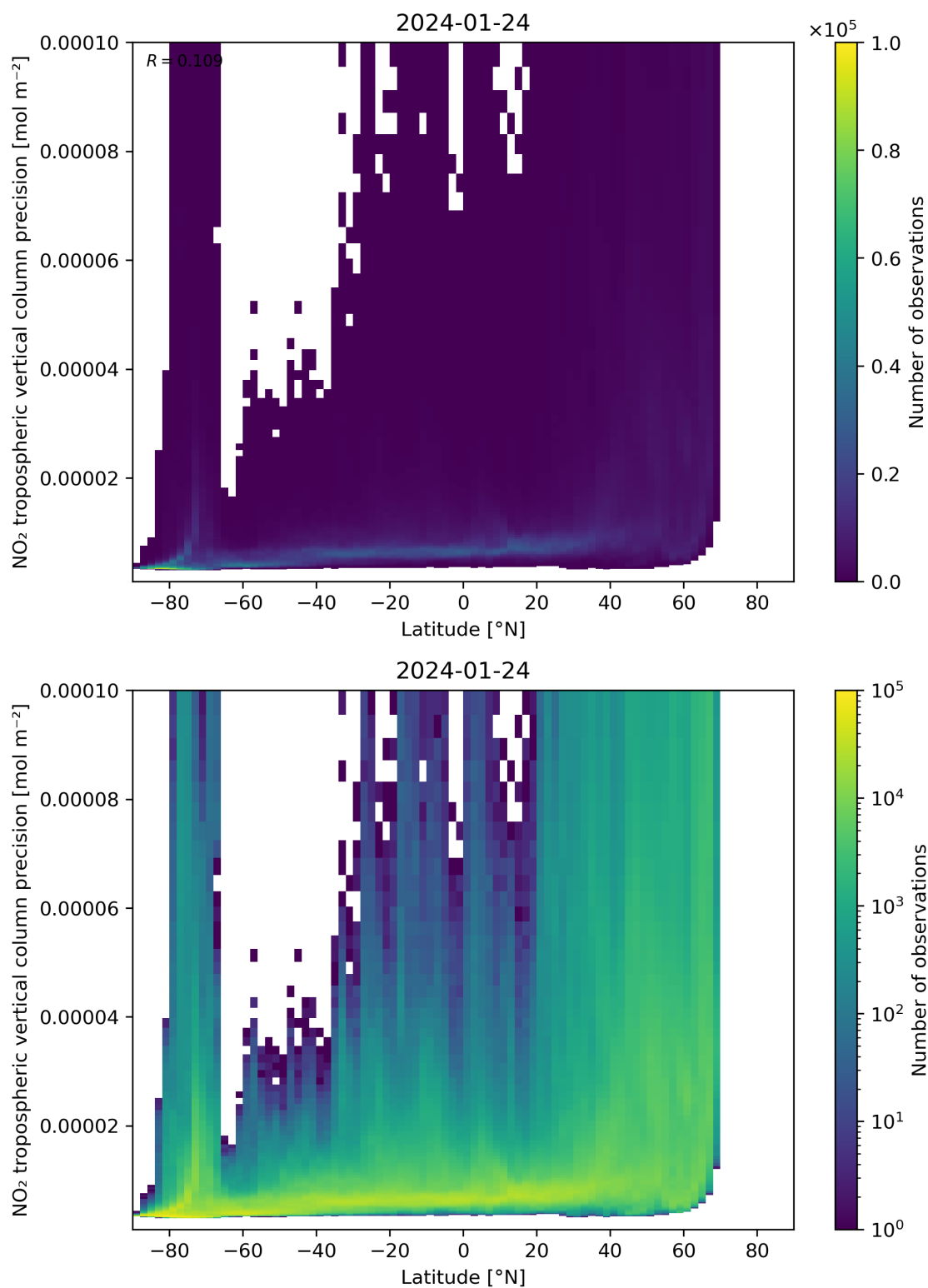
Figure 93: Scatter density plot of “Latitude” against “NO 2 tropospheric vertical column precision” for 2024-01-23 to 2024-01-25.
