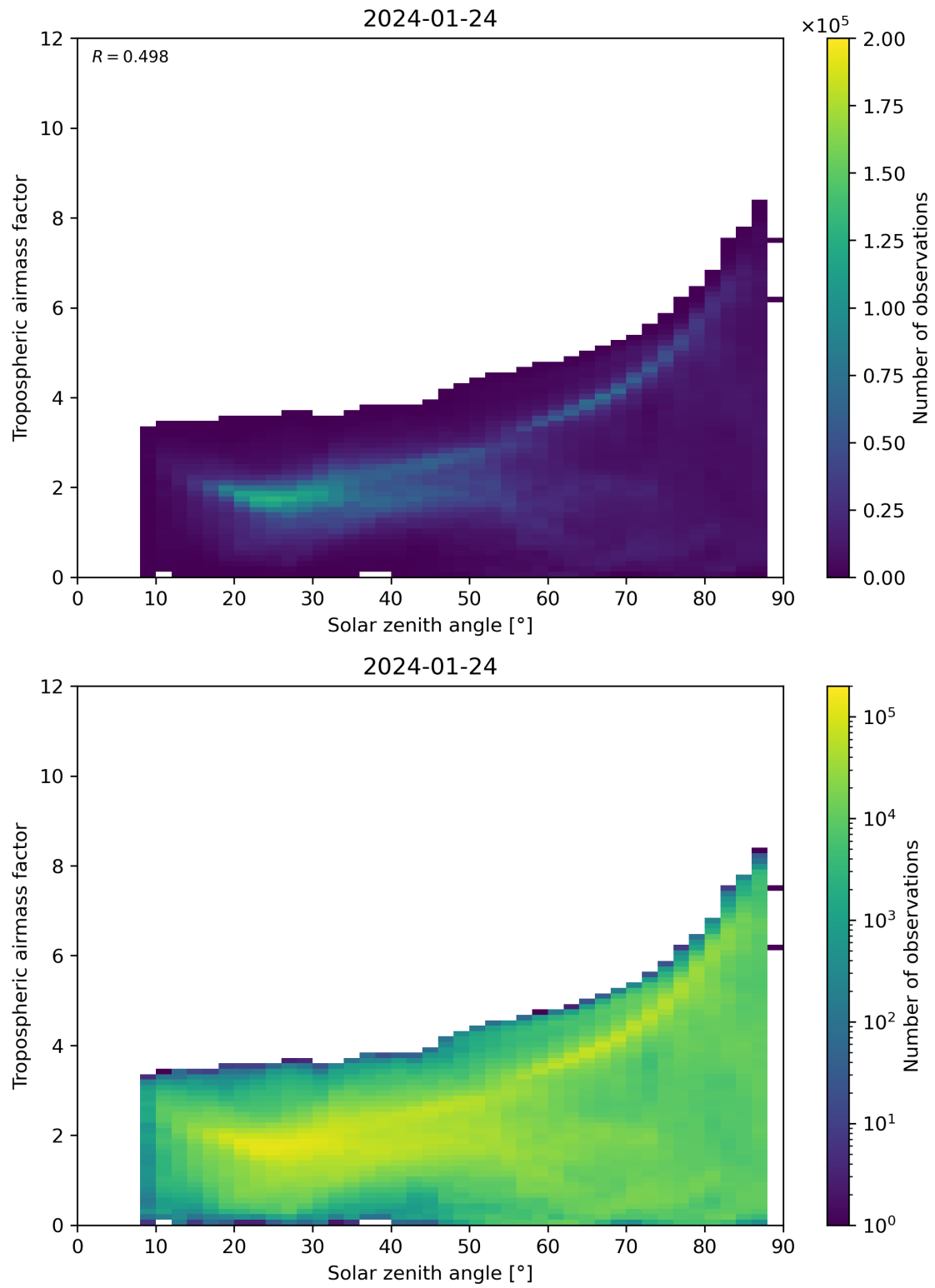
Figure 147: Scatter density plot of “Solar zenith angle” against “Tropospheric airmass factor” for 2024-01-23 to 2024-01-25.
