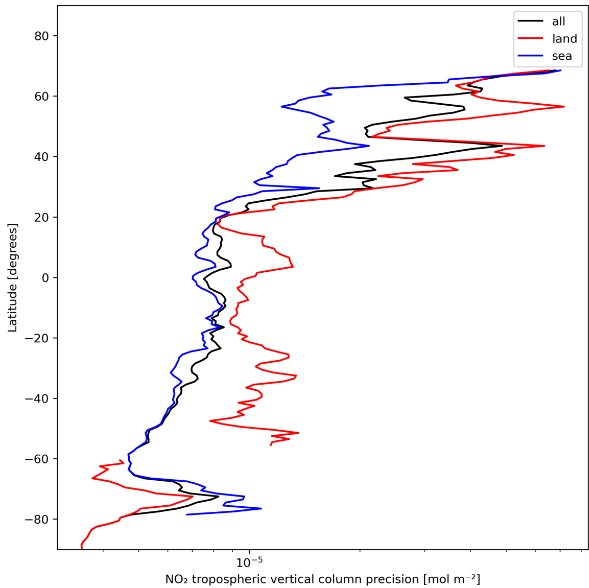
Figure 13: Zonal average of “NO 2 tropospheric vertical column precision” for 2024-01-23 to 2024-01-25.
