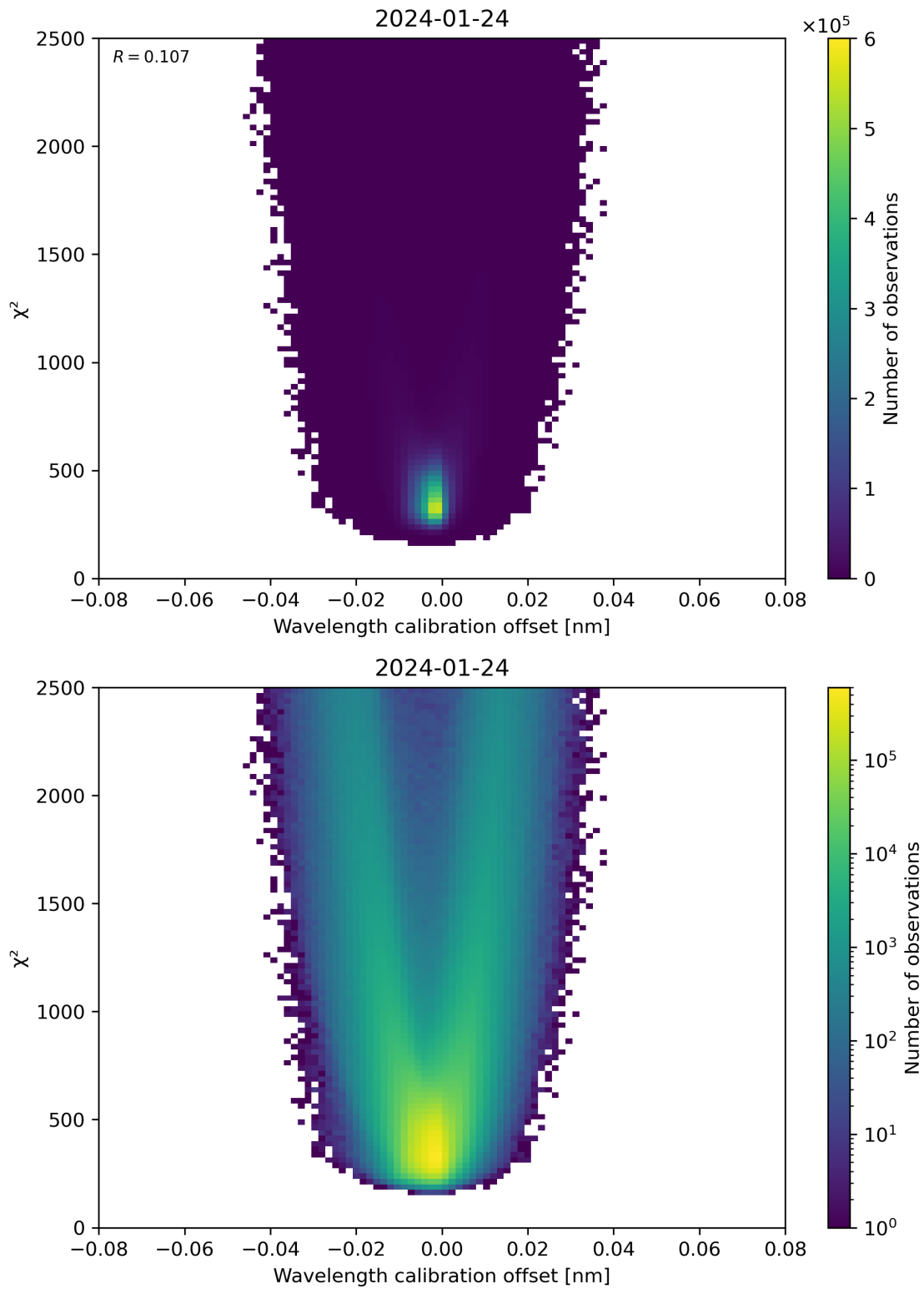
Figure 175: Scatter density plot of “Wavelength calibration offset” against “ \chi^2 ” for 2024-01-23 to 2024-01-25.
