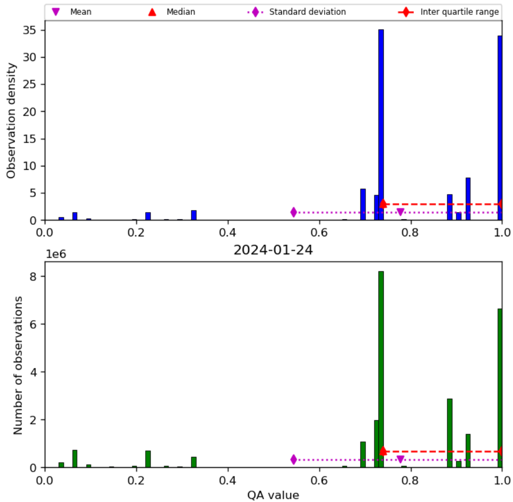
Figure 28: Histogram of “QA value” for 2024-01-23 to 2024-01-25
