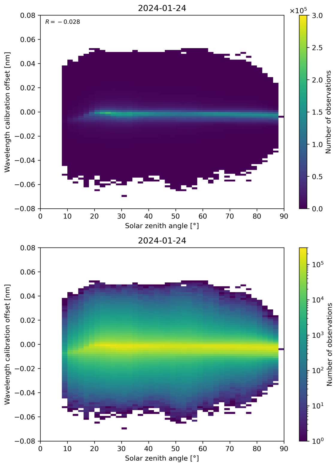
Figure 158: Scatter density plot of “Solar zenith angle” against “Wavelength calibration offset” for 2024-01-23 to 2024-01-25.
