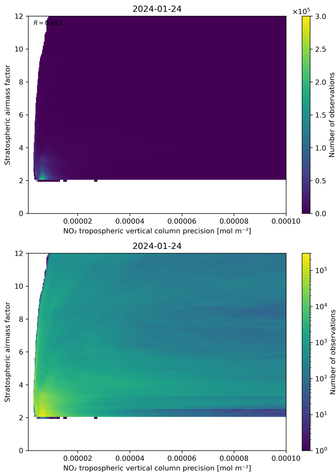
Figure 131: Scatter density plot of “NO 2 tropospheric vertical column precision” against “Stratospheric airmass factor” for 2024-01-23 to 2024-01-25.
