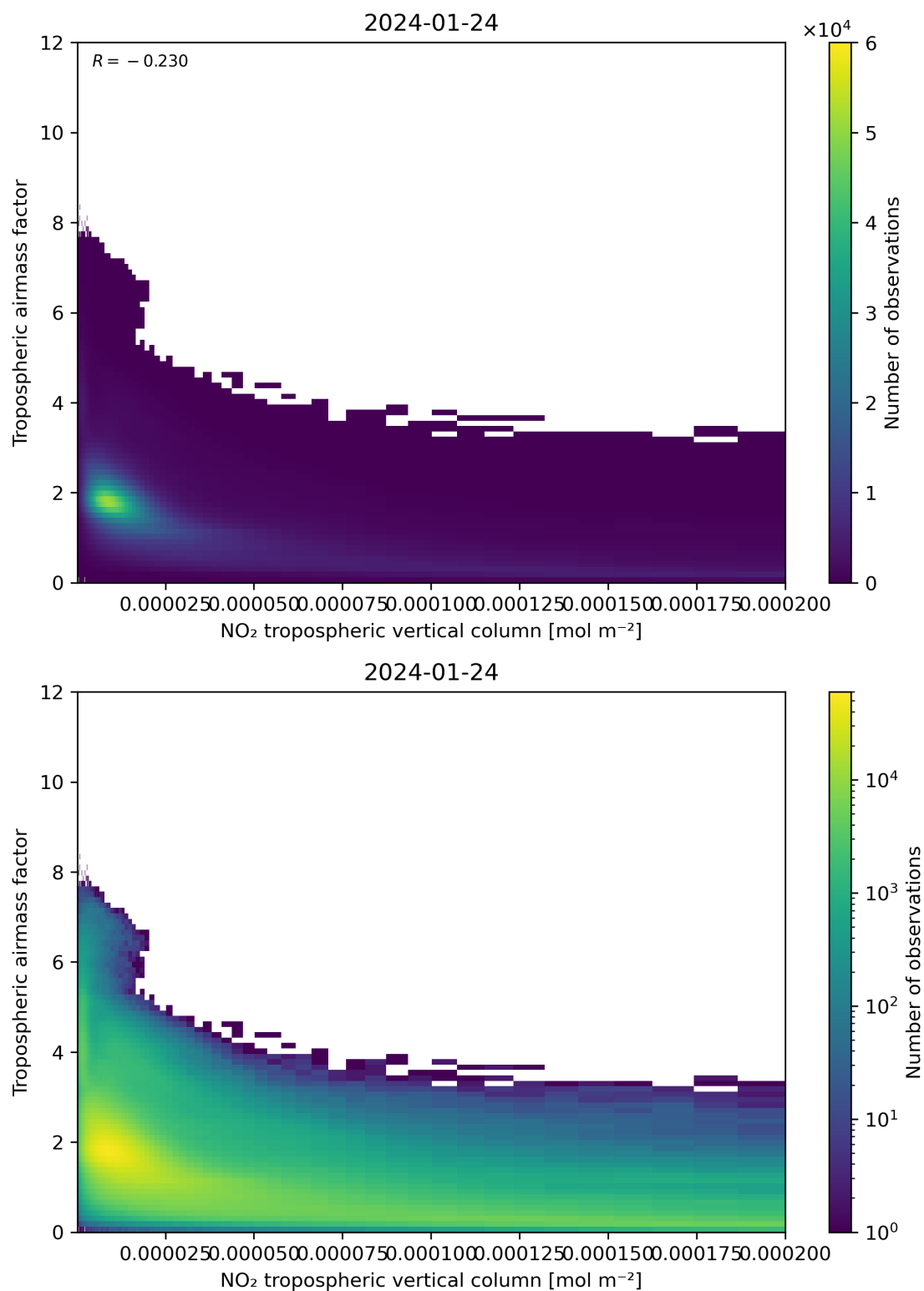
Figure 123: Scatter density plot of “NO 2 tropospheric vertical column” against “Tropospheric airmass factor” for 2024-01-23 to 2024-01-25.
