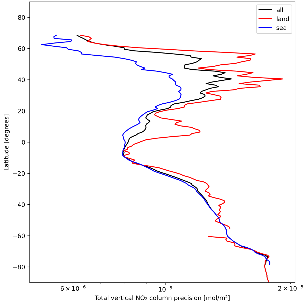
Figure 22: Zonal average of “Total vertical NO 2 column precision” for 2024-01-23 to 2024-01-25.
