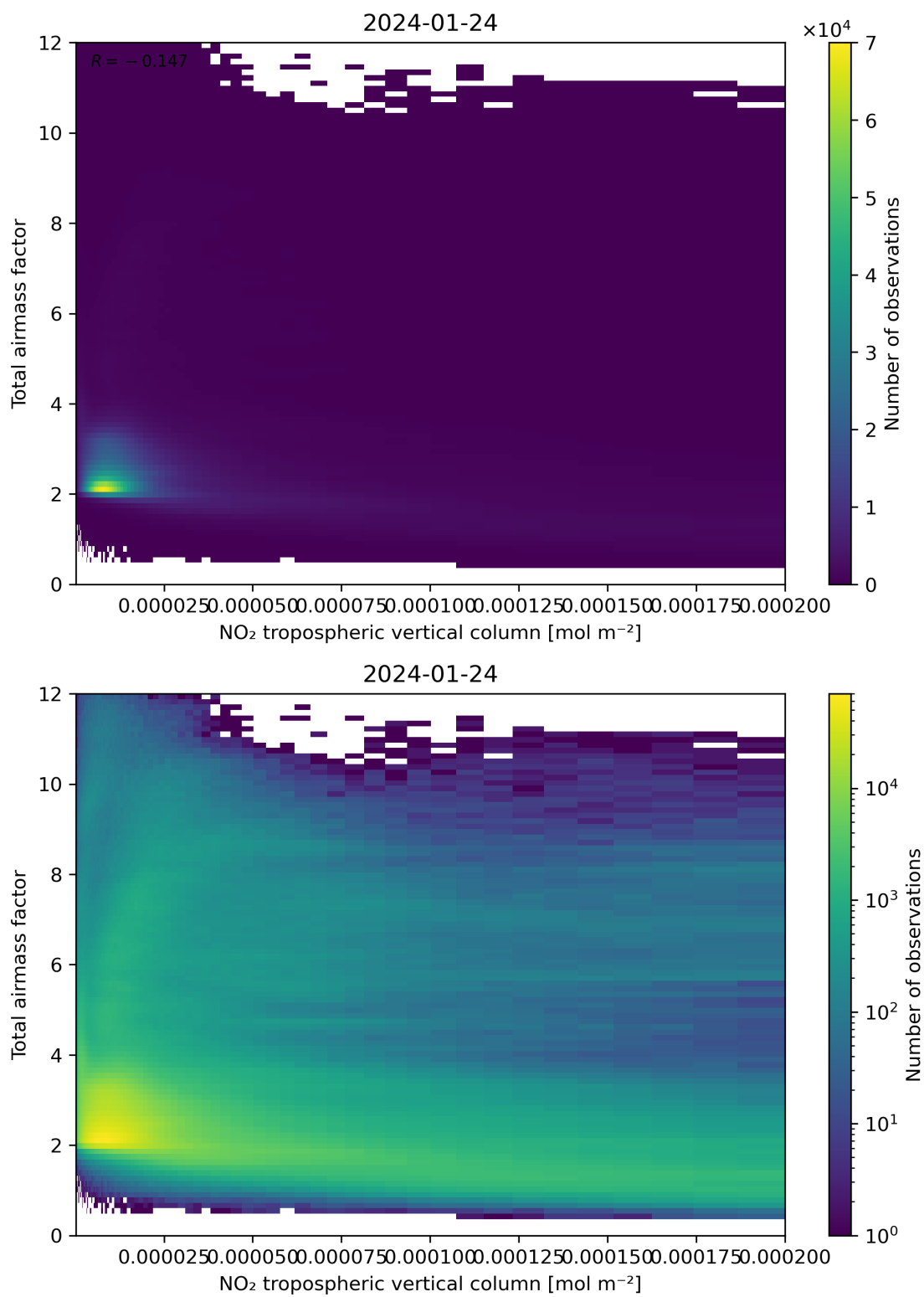
Figure 122: Scatter density plot of “NO 2 tropospheric vertical column” against “Total air mass factor” for 2024-01-23 to 2024-01-25.
