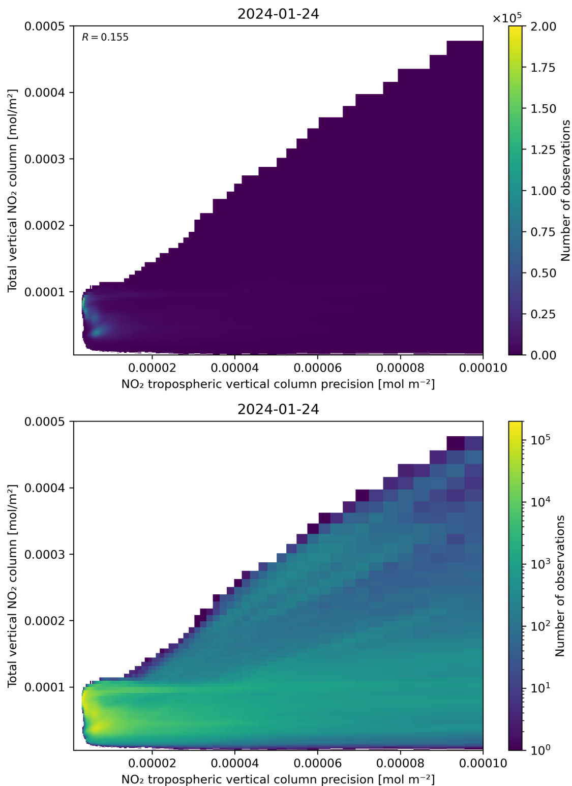
Figure 138: Scatter density plot of “NO 2 tropospheric vertical column precision” against “Total vertical NO 2 column” for 2024-01-23 to 2024-01-25.
