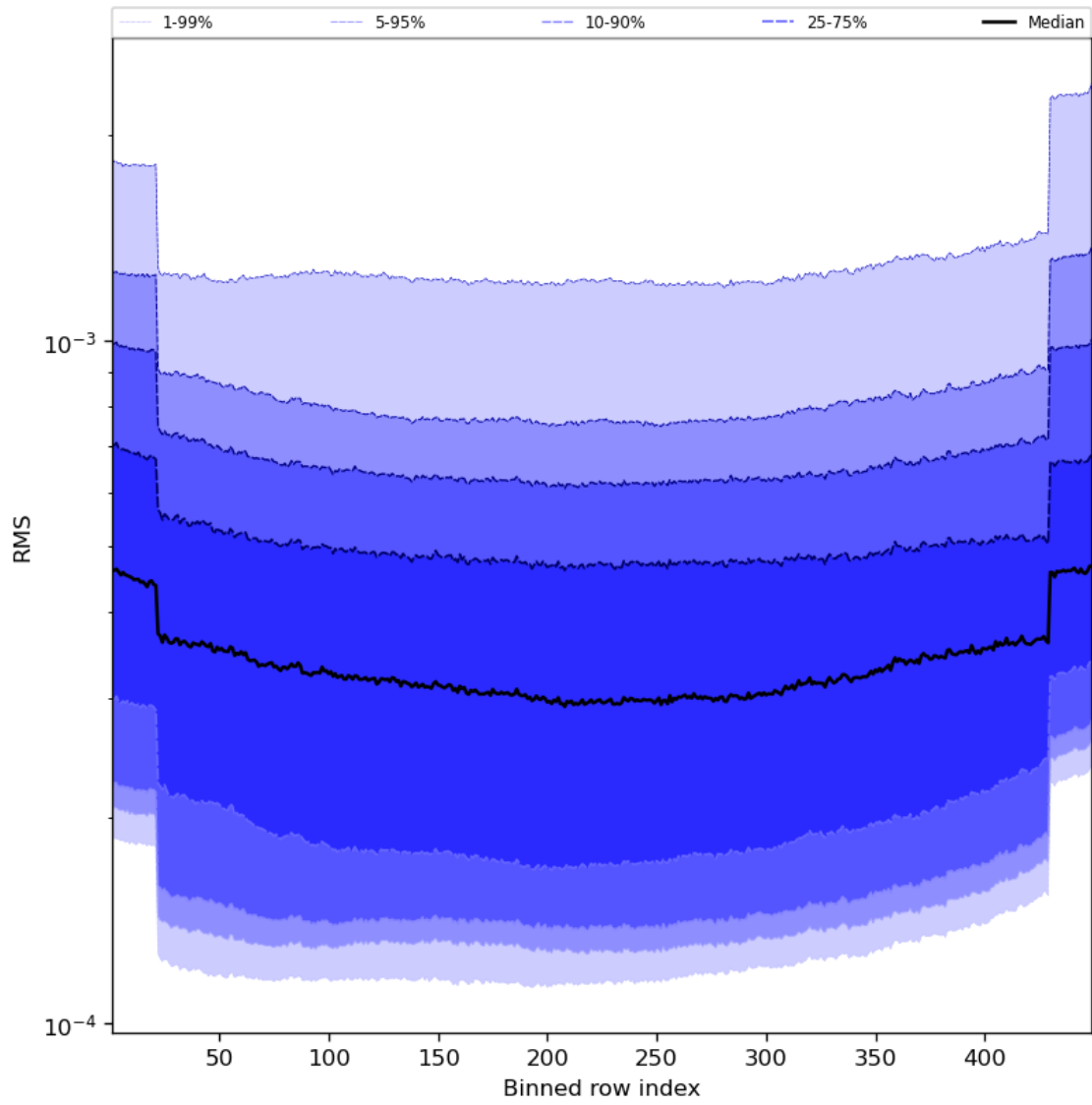
Figure 60: Along track statistics of “RMS” for 2024-01-23 to 2024-01-25
