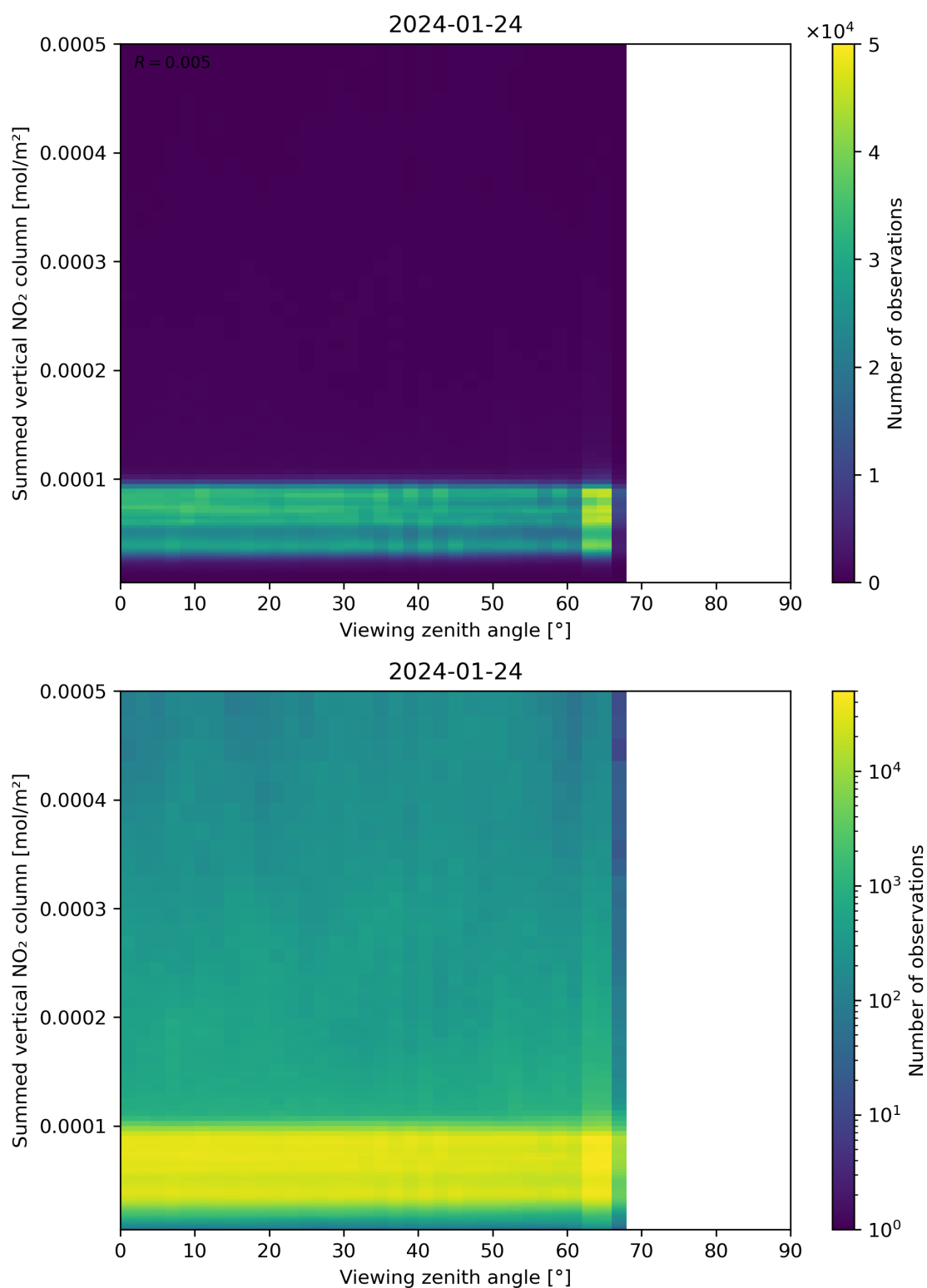
Figure 165: Scatter density plot of “Viewing zenith angle” against “Summed vertical NO 2 column” for 2024-01-23 to 2024-01-25.
