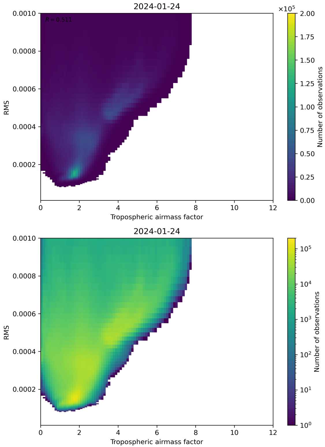
Figure 79: Scatter density plot of “Tropospheric airmass factor” against “RMS” for 2024-01-23 to 2024-01-25.
