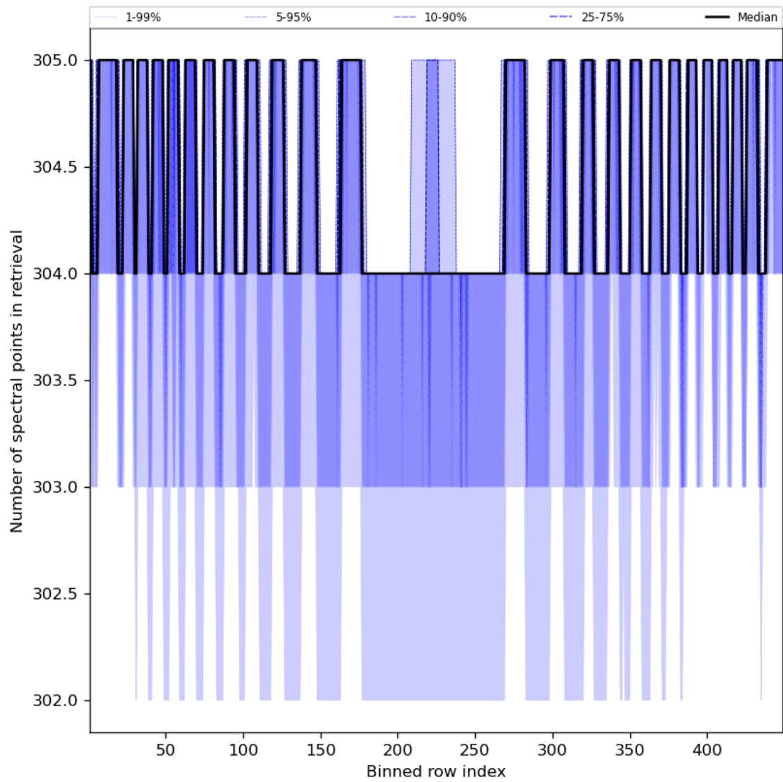
Figure 50: Along track statistics of “Number of spectral points in retrieval” for 2024-01-23 to 2024-01-25
