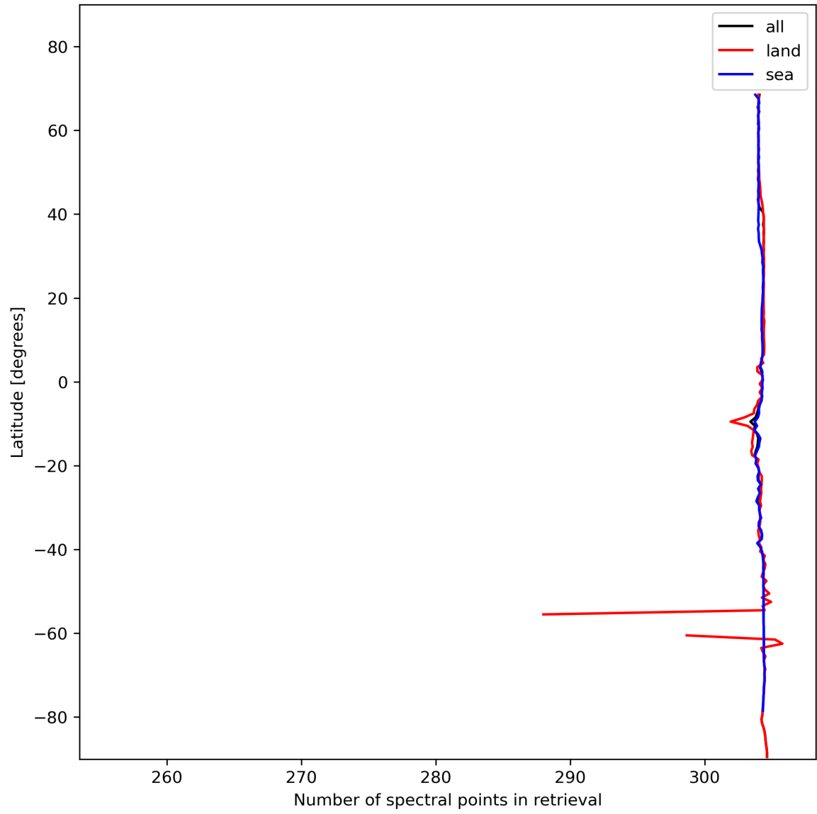
Figure 16: Zonal average of “Number of spectral points in retrieval” for 2024-01-23 to 2024-01-25.
