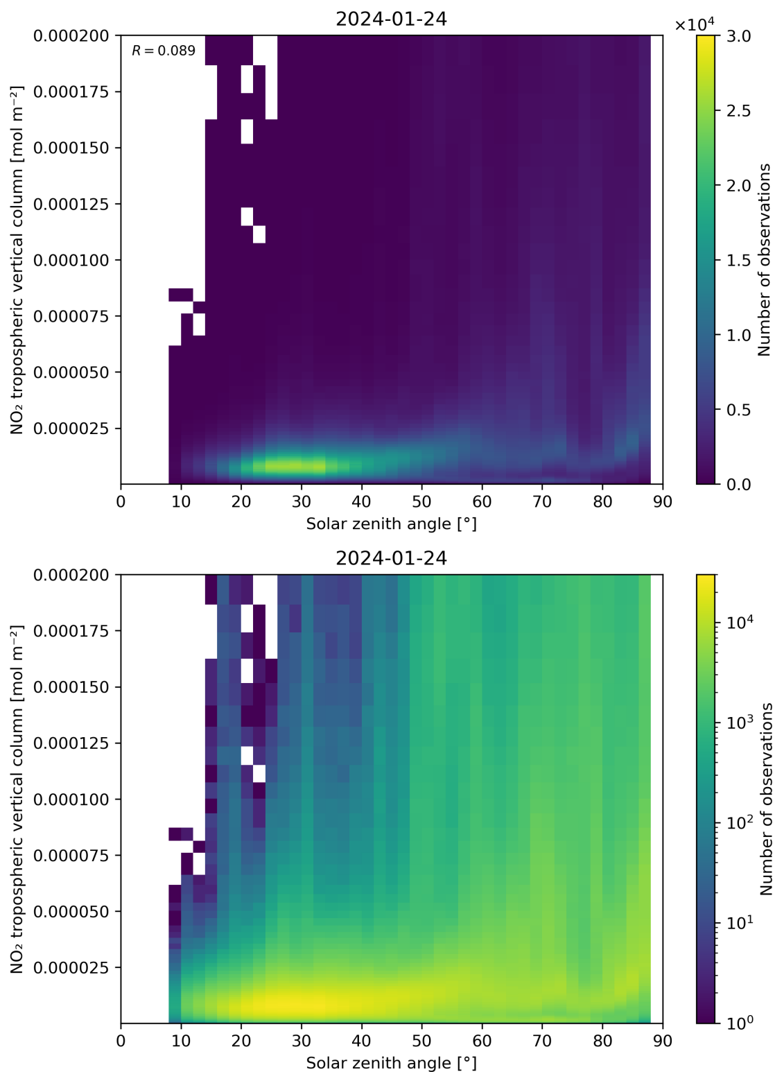
Figure 155: Scatter density plot of “Solar zenith angle” against “NO 2 tropospheric vertical column” for 2024-01-23 to 2024-01-25.
