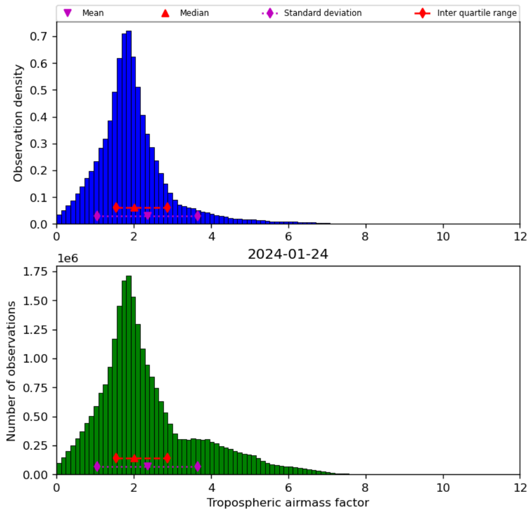
Figure 31: Histogram of “Tropospheric airmass factor” for 2024-01-23 to 2024-01-25
