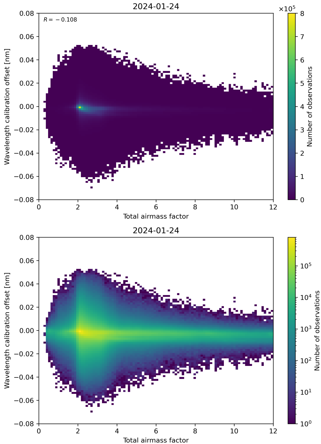
Figure 70: Scatter density plot of “Total airmass factor” against “Wavelength calibration offset” for 2024-01-23 to 2024-01-25.
