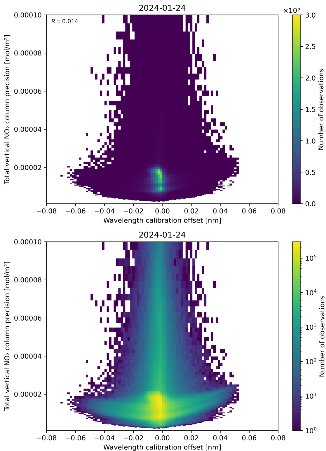
Figure 180: Scatter density plot of “Wavelength calibration offset” against “Total vertical NO 2 column precision” for 2024-01-23 to 2024-01-25.
