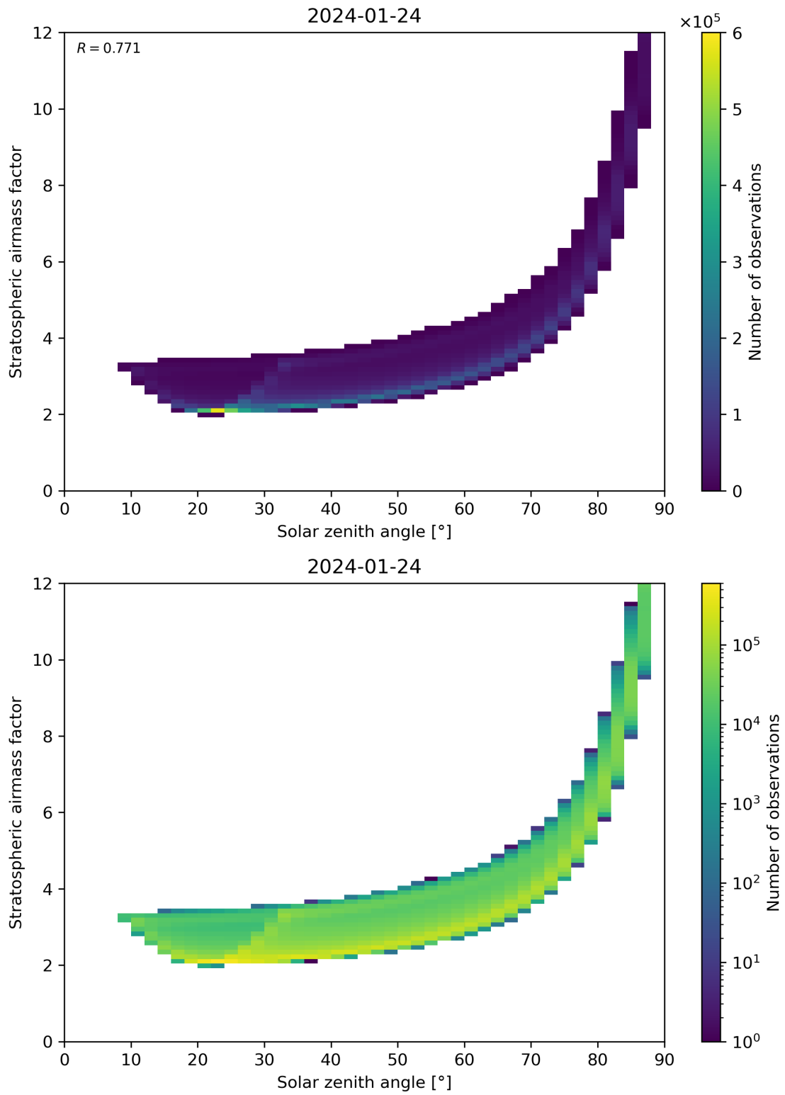
Figure 145: Scatter density plot of “Solar zenith angle” against “Stratospheric airmass factor” for 2024-01-23 to 2024-01-25.
