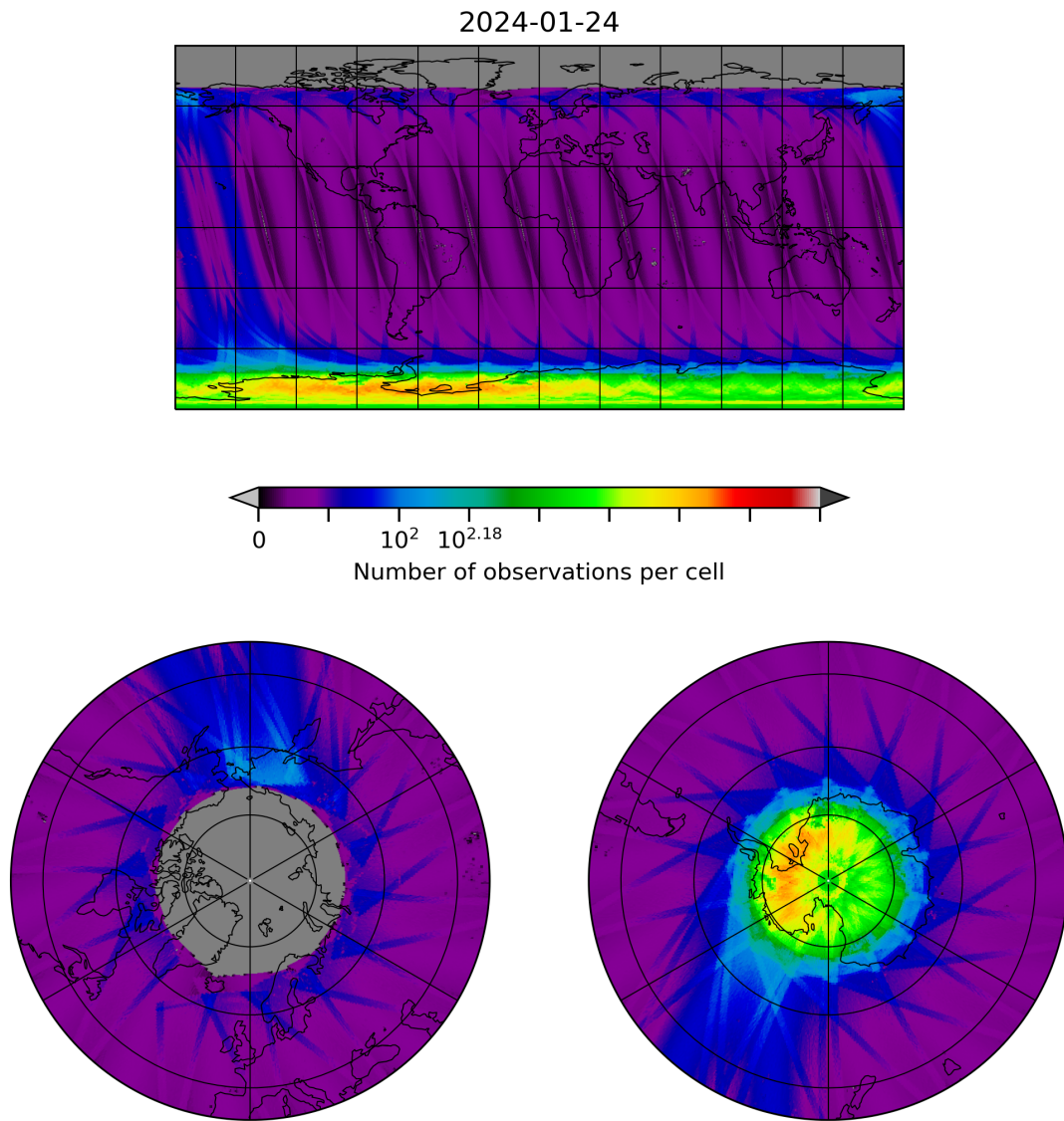
Figure 10: Map of the number of observations for 2024-01-23 to 2024-01-25
