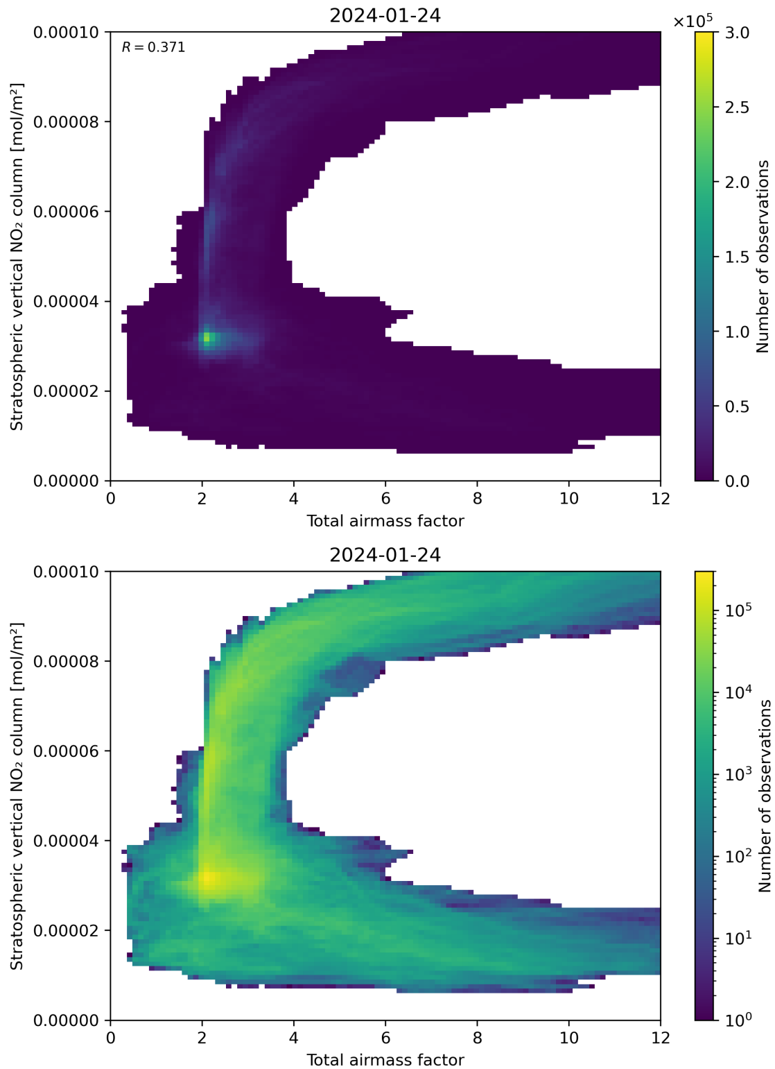
Figure 64: Scatter density plot of “Total airmass factor” against “Stratospheric vertical NO 2 column” for 2024-01-23 to 2024-01-25.
