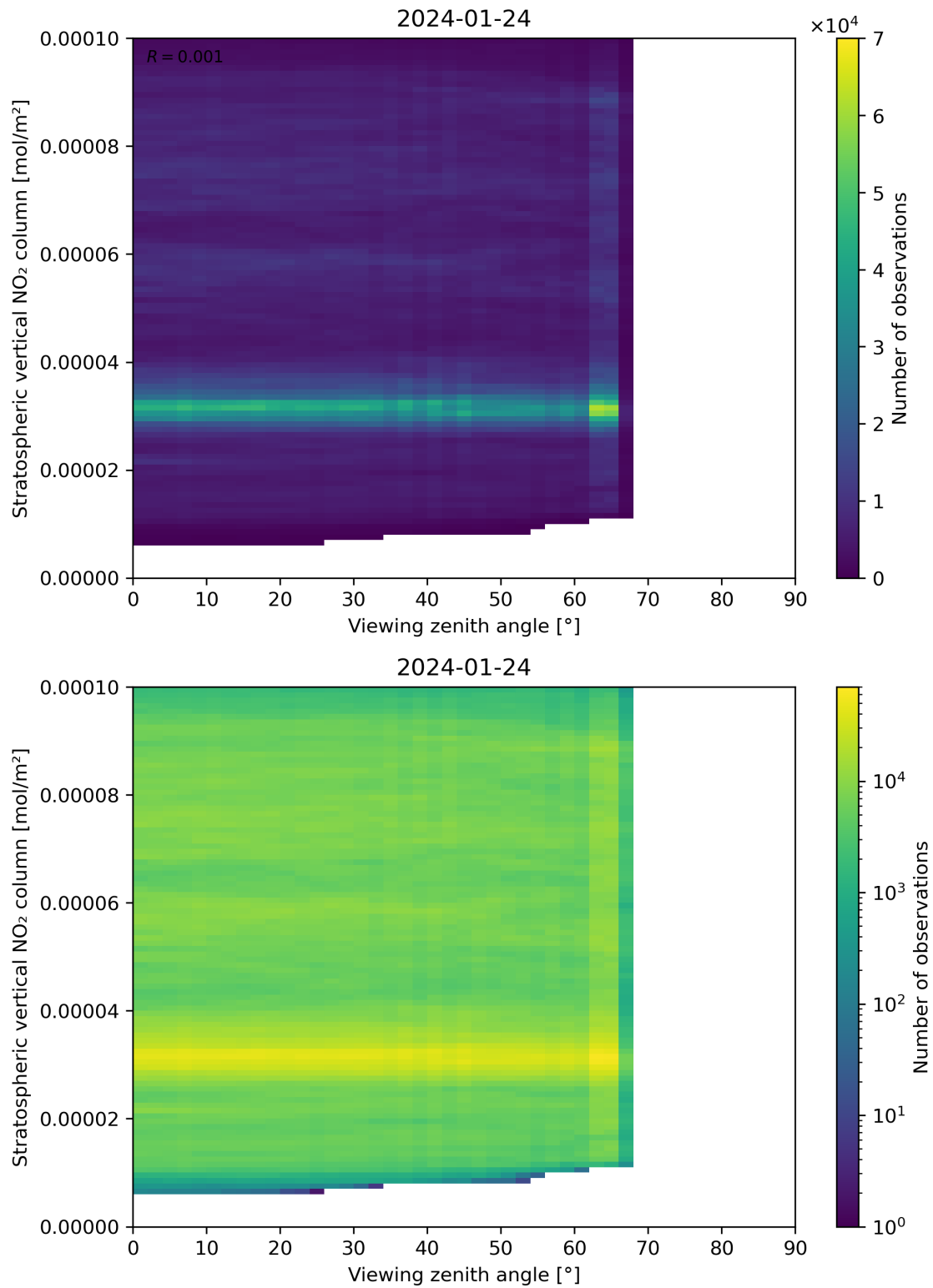
Figure 164: Scatter density plot of “Viewing zenith angle” against “Stratospheric vertical NO 2 column” for 2024-01-23 to 2024-01-25.
