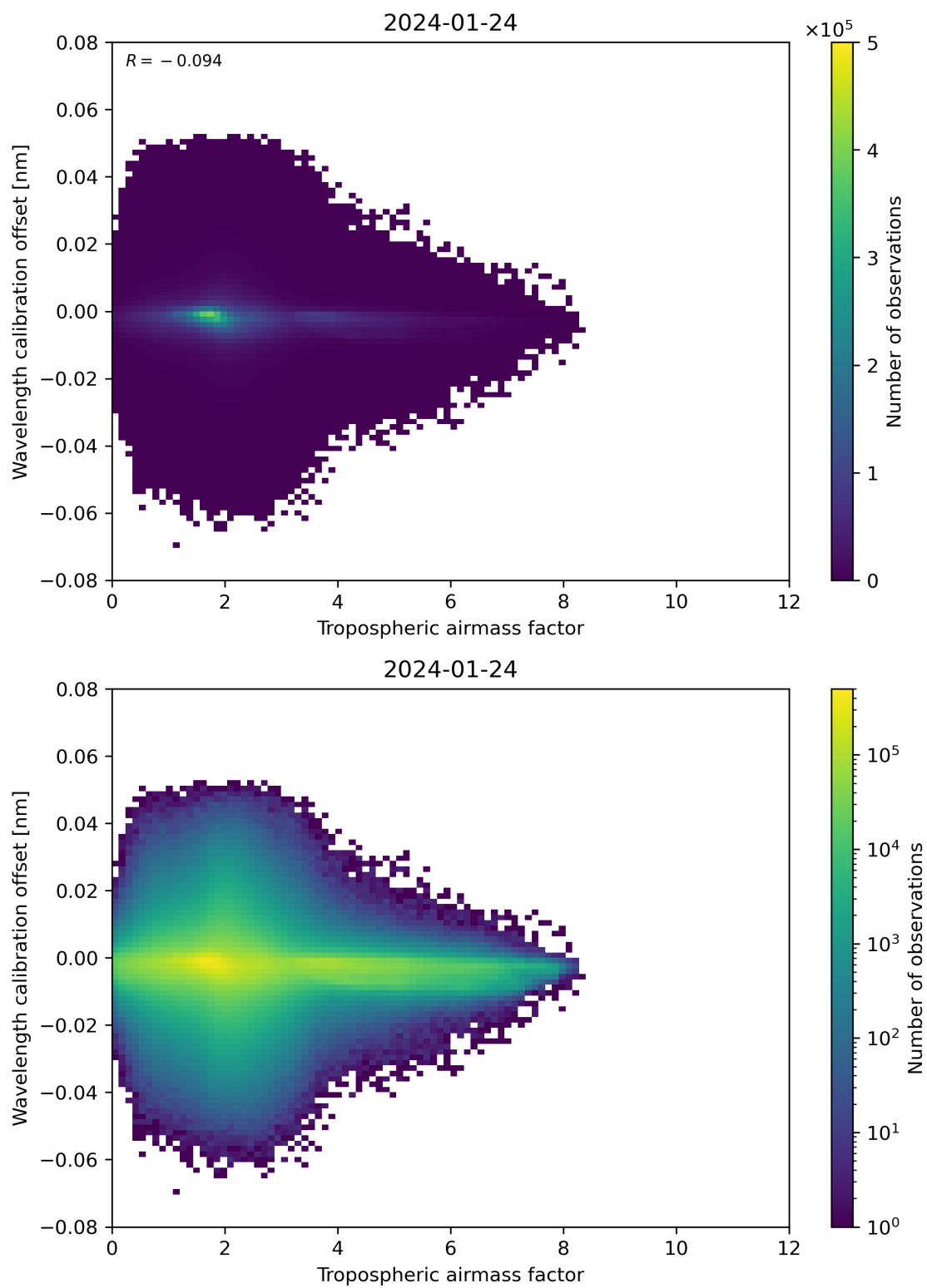
Figure 80: Scatter density plot of “Tropospheric airmass factor” against “Wavelength calibration offset” for 2024-01-23 to 2024-01-25.
