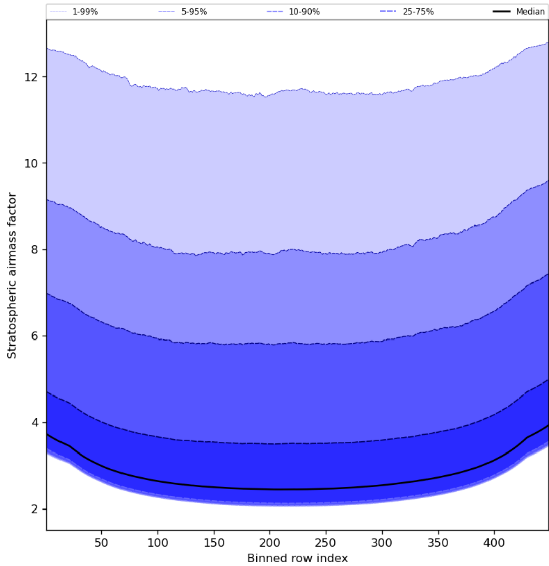
Figure 61: Along track statistics of “Stratospheric airmass factor” for 2024-01-23 to 2024-01-25
