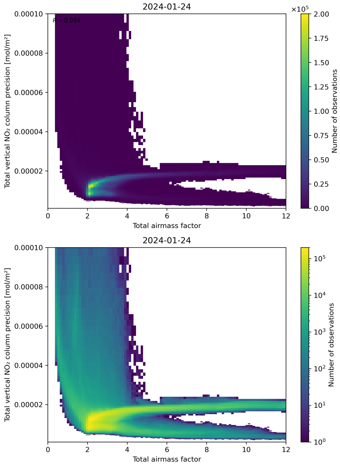
Figure 68: Scatter density plot of “Total airmass factor” against “Total vertical NO 2 column precision” for 2024-01-23 to 2024-01-25.
