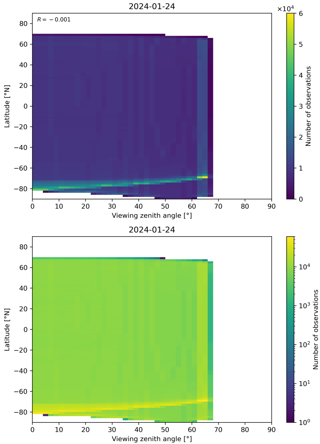
Figure 163: Scatter density plot of “Viewing zenith angle” against “Latitude” for 2024-01-23 to 2024-01-25.
