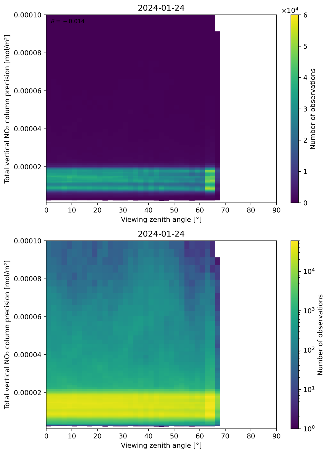
Figure 168: Scatter density plot of “Viewing zenith angle” against “Total vertical NO 2 column precision” for 2024-01-23 to 2024-01-25.
