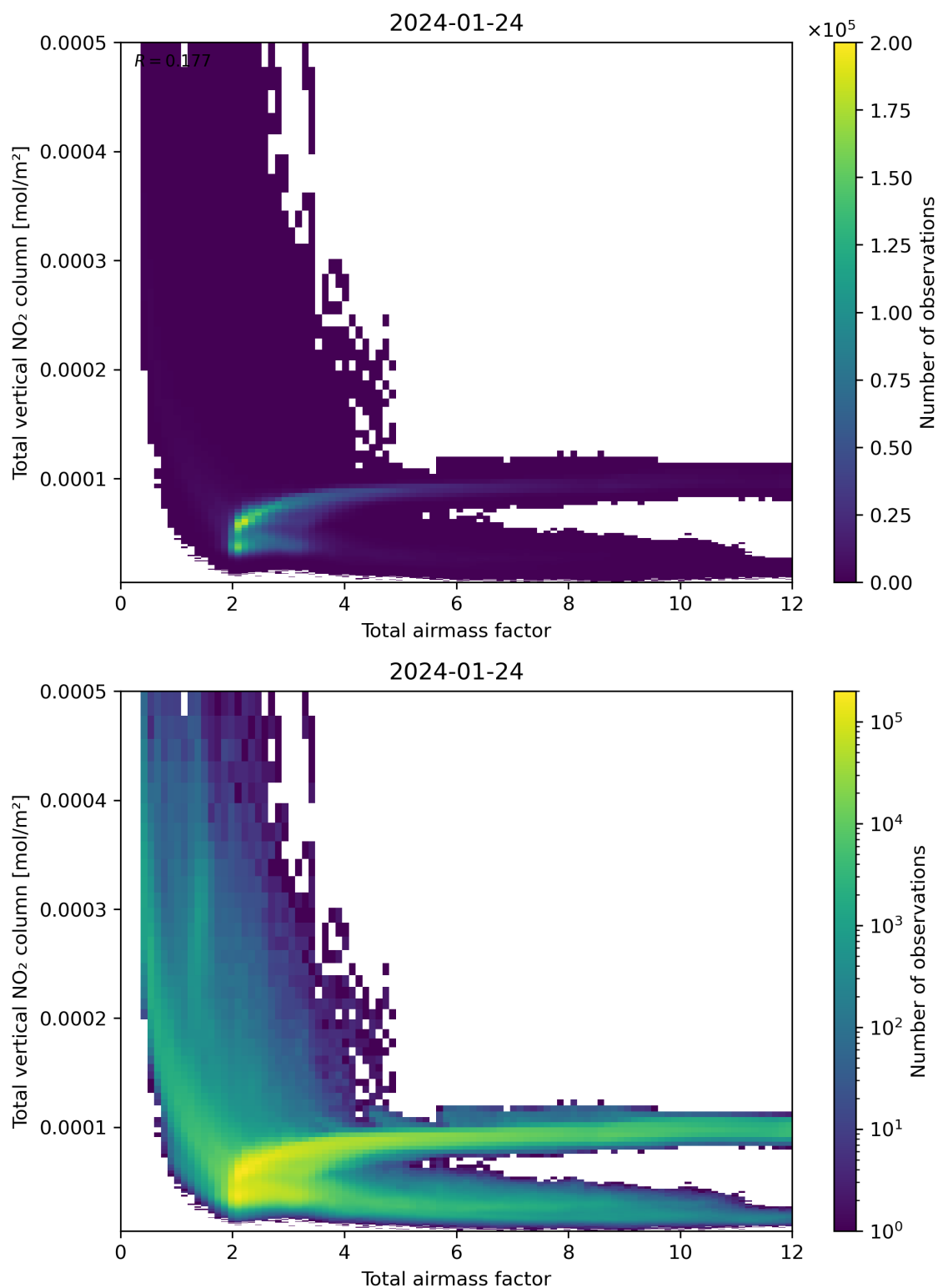
Figure 67: Scatter density plot of “Total airmass factor” against “Total vertical NO 2 column” for 2024-01-23 to 2024-01-25.
