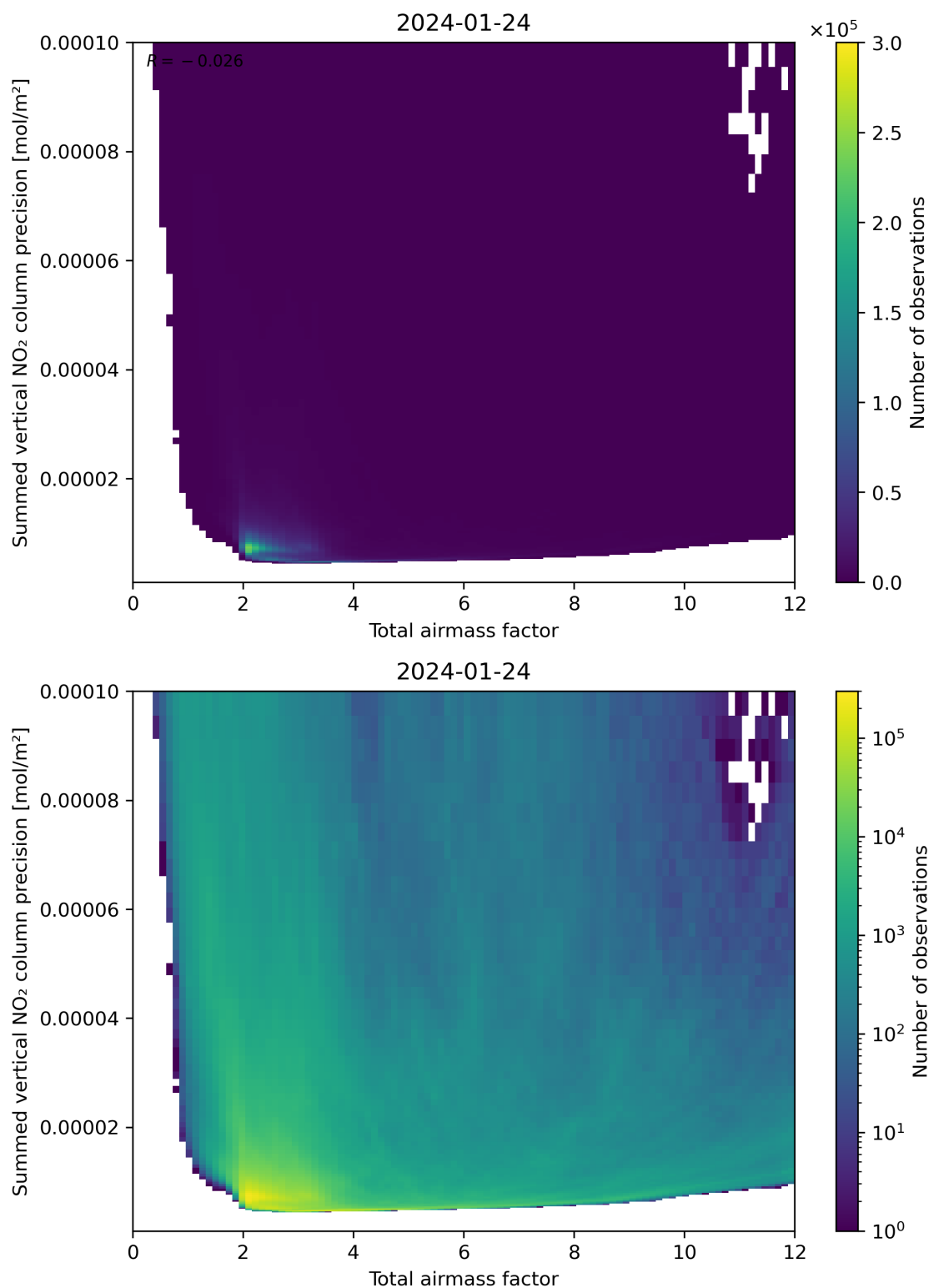
Figure 66: Scatter density plot of “Total airmass factor” against “Summed vertical NO 2 column precision” for 2024-01-23 to 2024-01-25.
