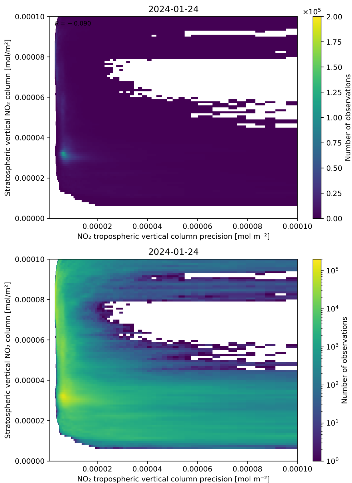
Figure 135: Scatter density plot of “NO 2 tropospheric vertical column precision” against “Stratospheric vertical NO 2 column” for 2024-01-23 to 2024-01-25.
