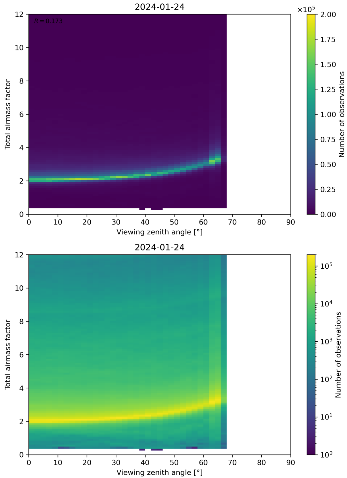
Figure 160: Scatter density plot of “Viewing zenith angle” against “Total airmass factor” for 2024-01-23 to 2024-01-25.
