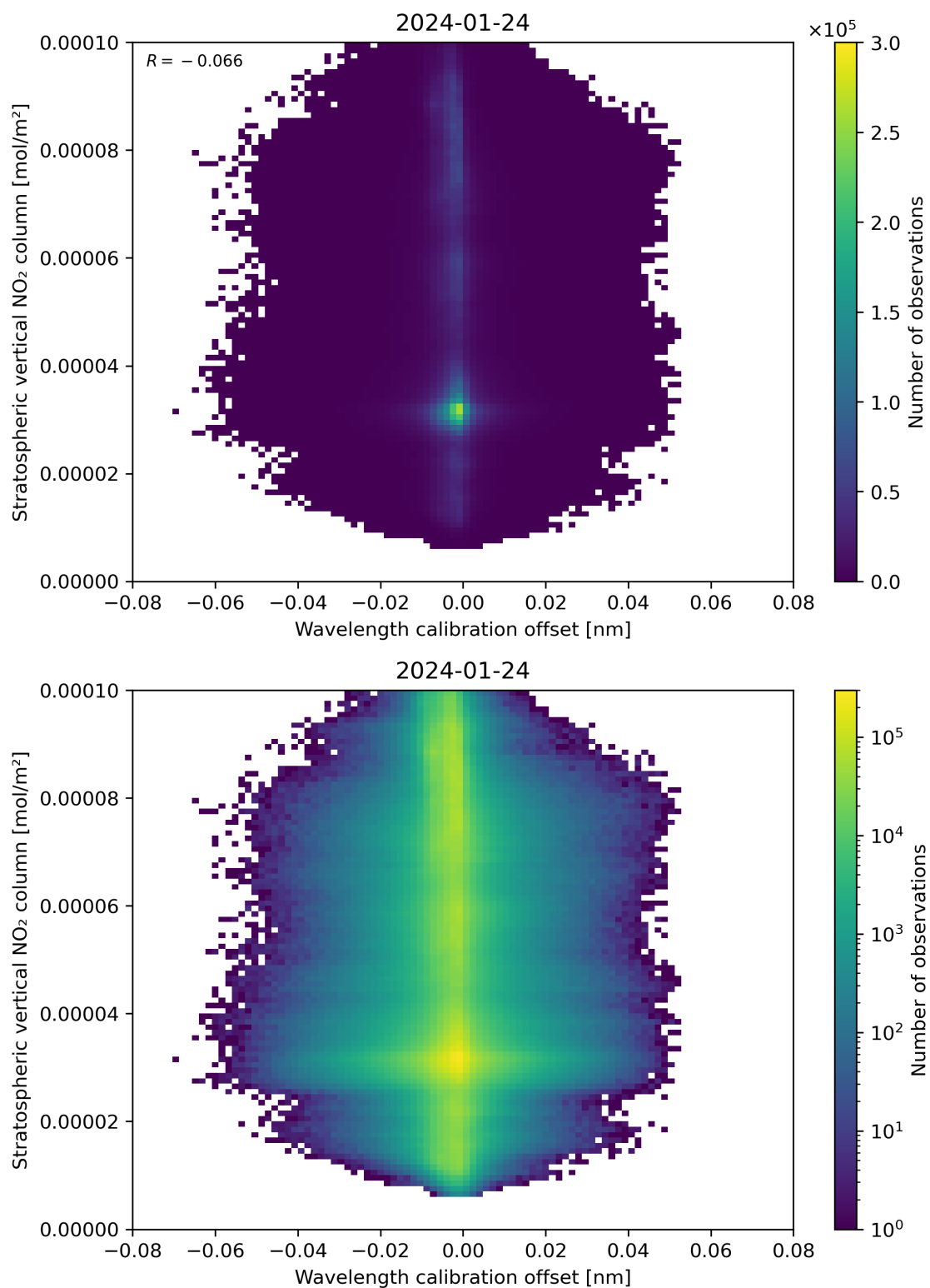
Figure 176: Scatter density plot of “Wavelength calibration offset” against “Stratospheric vertical NO 2 column” for 2024-01-23 to 2024-01-25.
