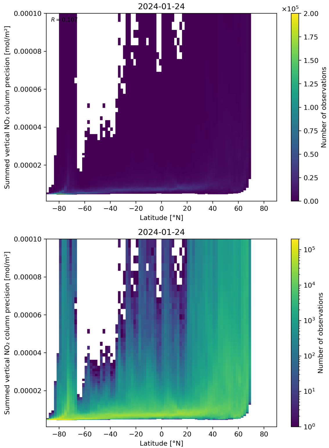
Figure 89: Scatter density plot of “Latitude” against “Summed vertical NO 2 column precision” for 2024-01-23 to 2024-01-25.
