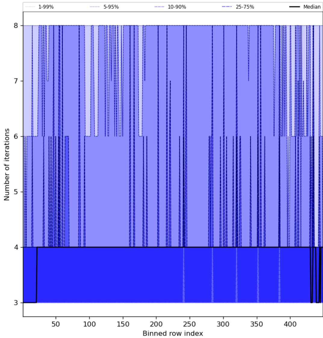
Figure 51: Along track statistics of “Number of iterations” for 2024-01-23 to 2024-01-25
