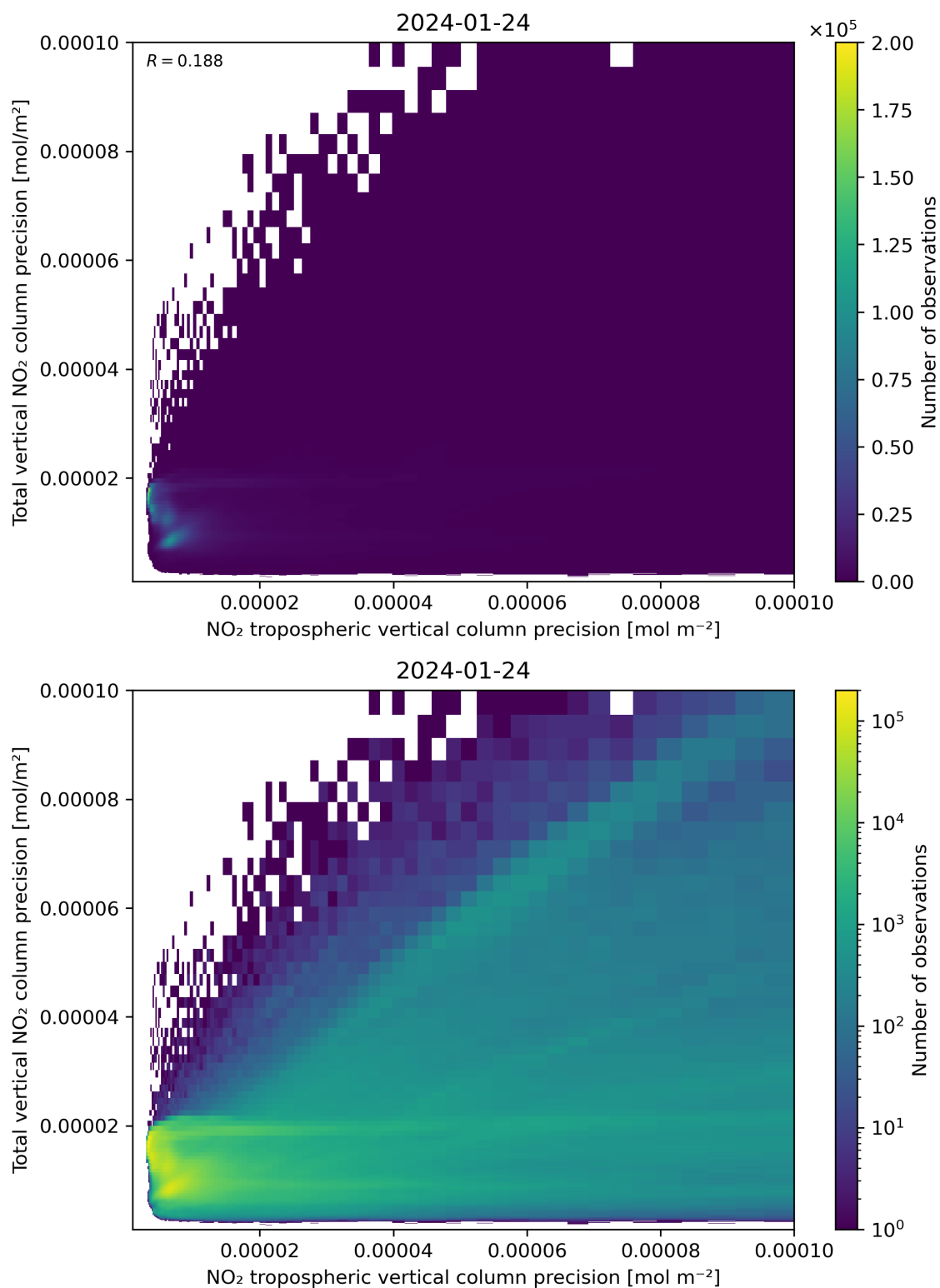
Figure 139: Scatter density plot of “NO 2 tropospheric vertical column precision” against “Total vertical NO 2 column precision” for 2024-01-23 to 2024-01-25.
