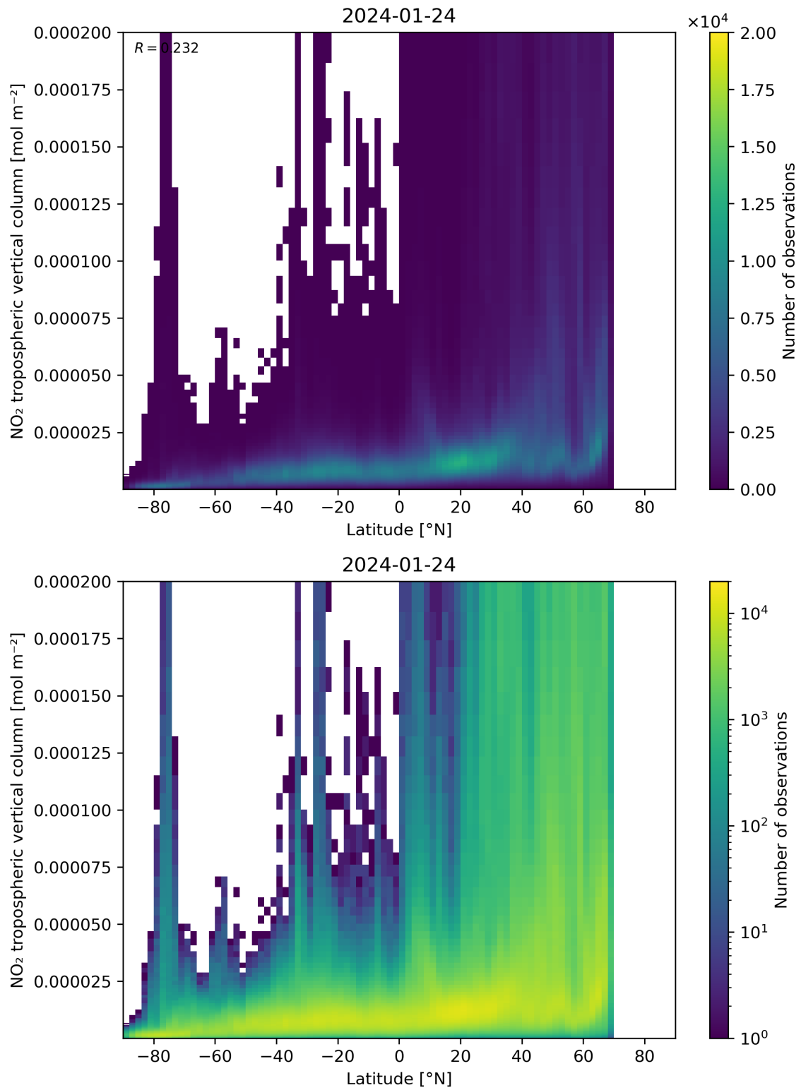
Figure 92: Scatter density plot of “Latitude” against “NO 2 tropospheric vertical column” for 2024-01-23 to 2024-01-25.
