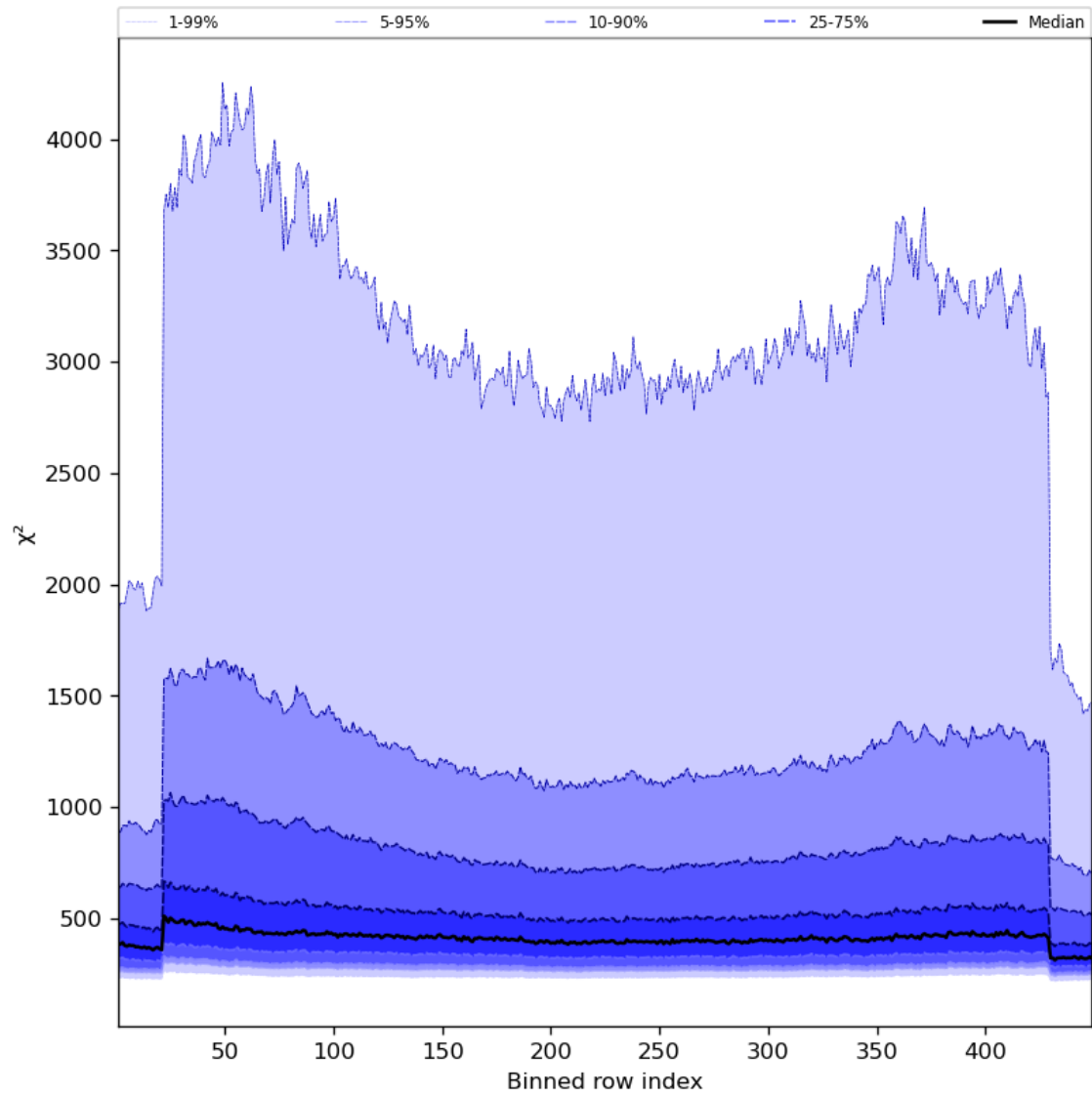
Figure 59: Along track statistics of “ \chi^2 ” for 2024-01-23 to 2024-01-25
