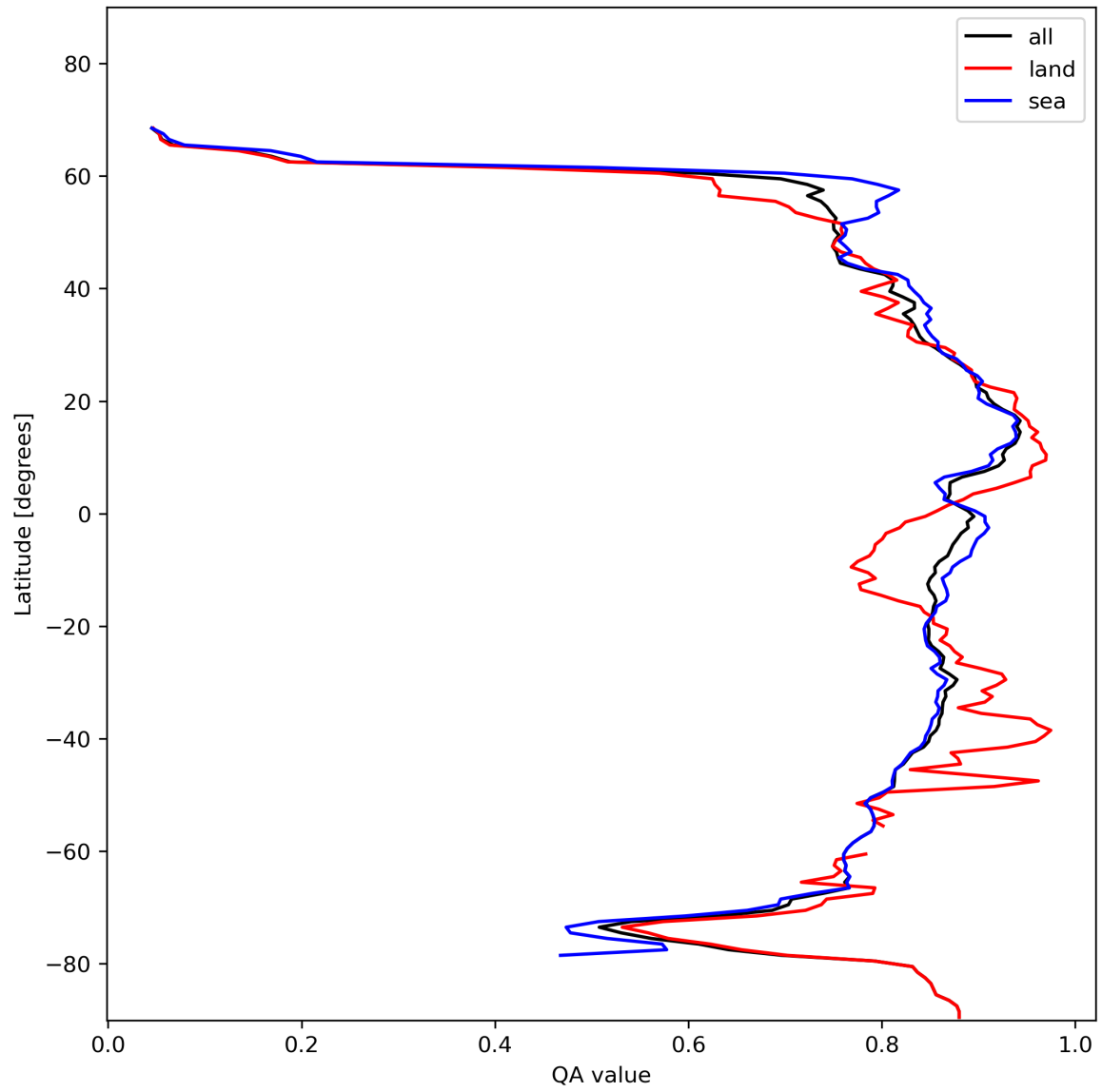
Figure 11: Zonal average of “QA value” for 2024-01-23 to 2024-01-25.
