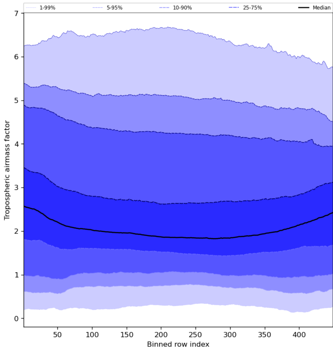
Figure 48: Along track statistics of “Tropospheric air mass factor” for 2024-01-23 to 2024-01-25
