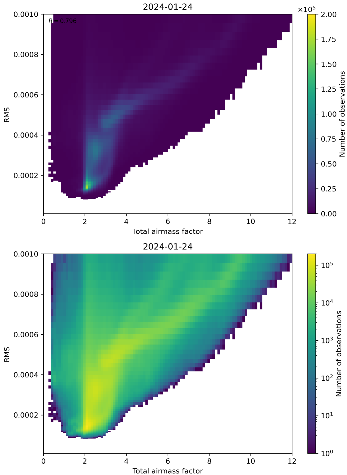
Figure 69: Scatter density plot of “Total airmass factor” against “RMS” for 2024-01-23 to 2024-01-25.
