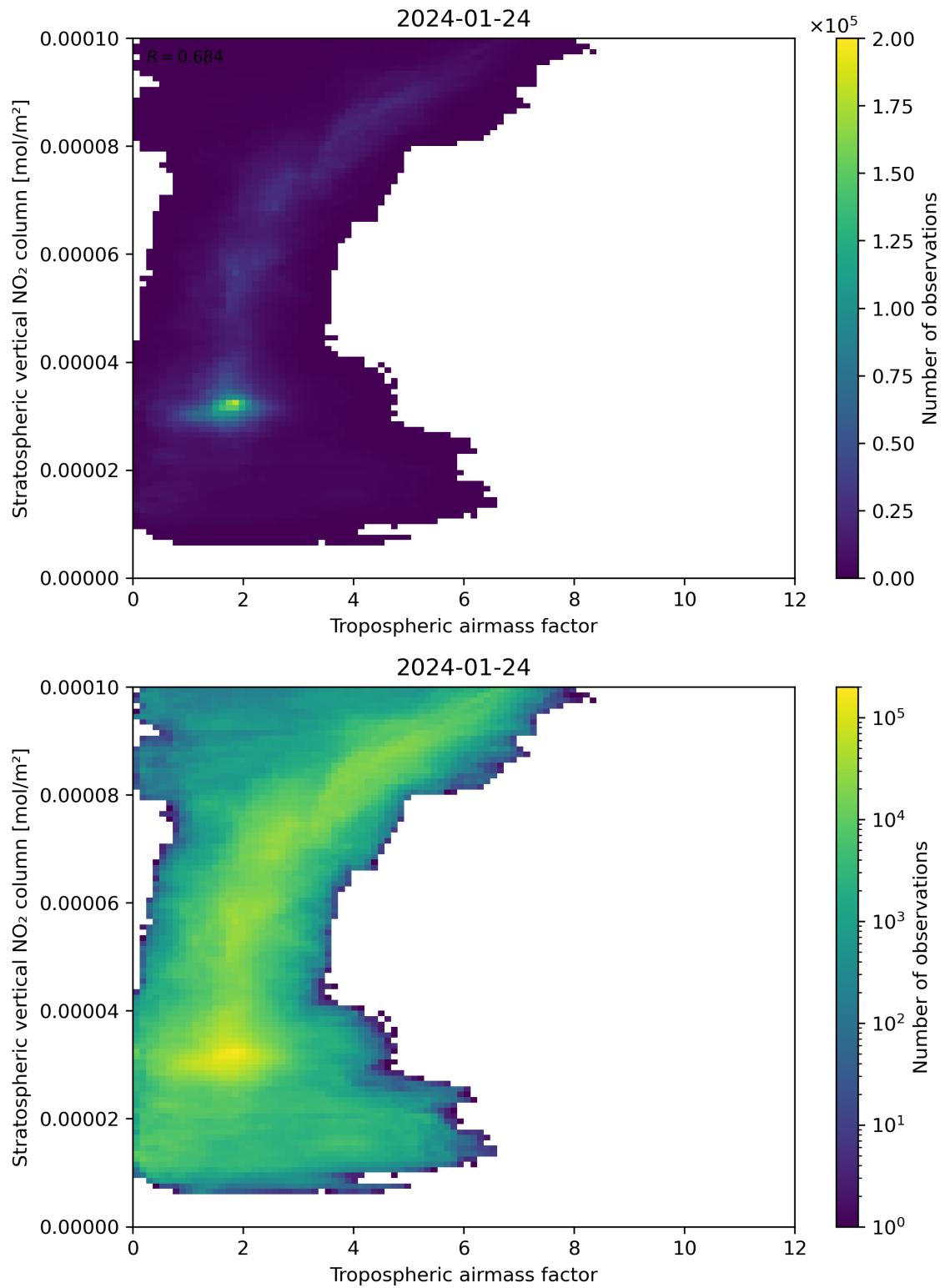
Figure 74: Scatter density plot of “Tropospheric air mass factor” against “Stratospheric vertical NO 2 column” for 2024-01-23 to 2024-01-25.
