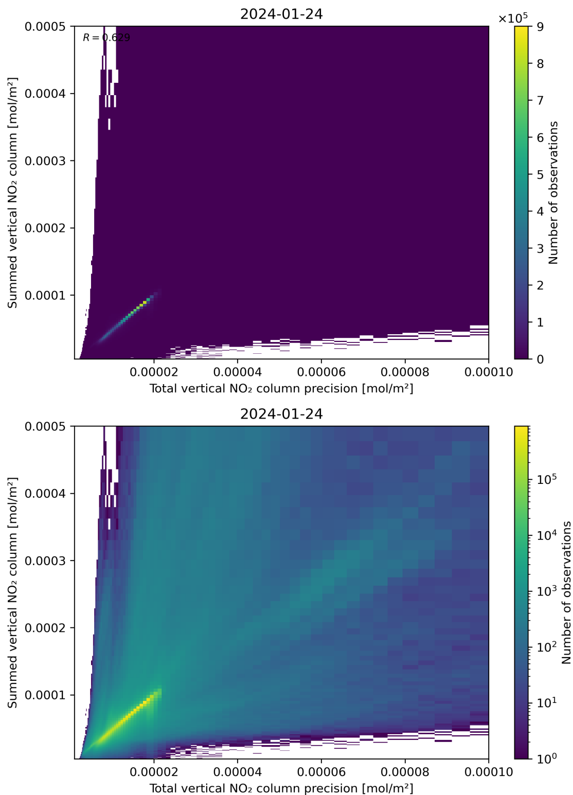
Figure 117: Scatter density plot of “Total vertical NO 2 column precision” against “Summed vertical NO 2 column” for 2024-01-23 to 2024-01-25.
