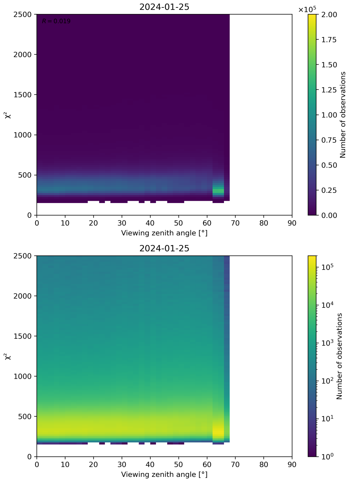
Figure 162: Scatter density plot of “Viewing zenith angle” against “ \chi^2 ” for 2024-01-24 to 2024-01-26.
