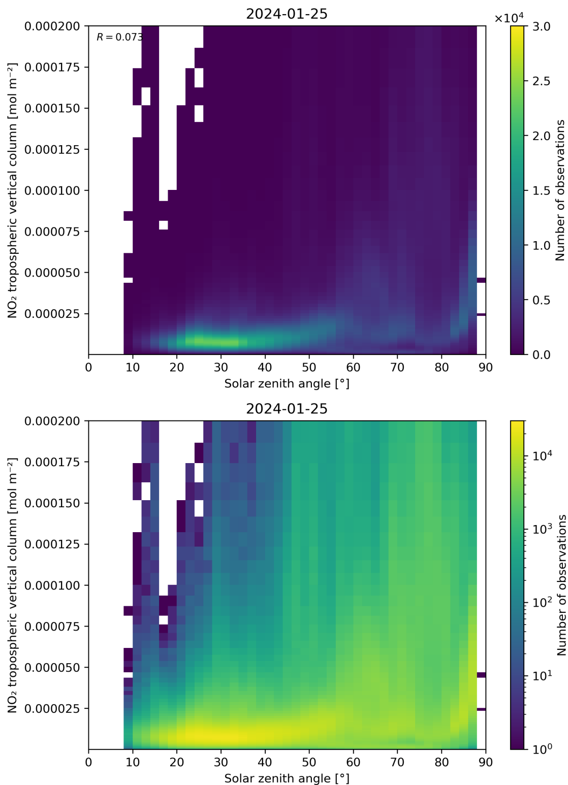
Figure 155: Scatter density plot of “Solar zenith angle” against “NO 2 tropospheric vertical column” for 2024-01-24 to 2024-01-26.
