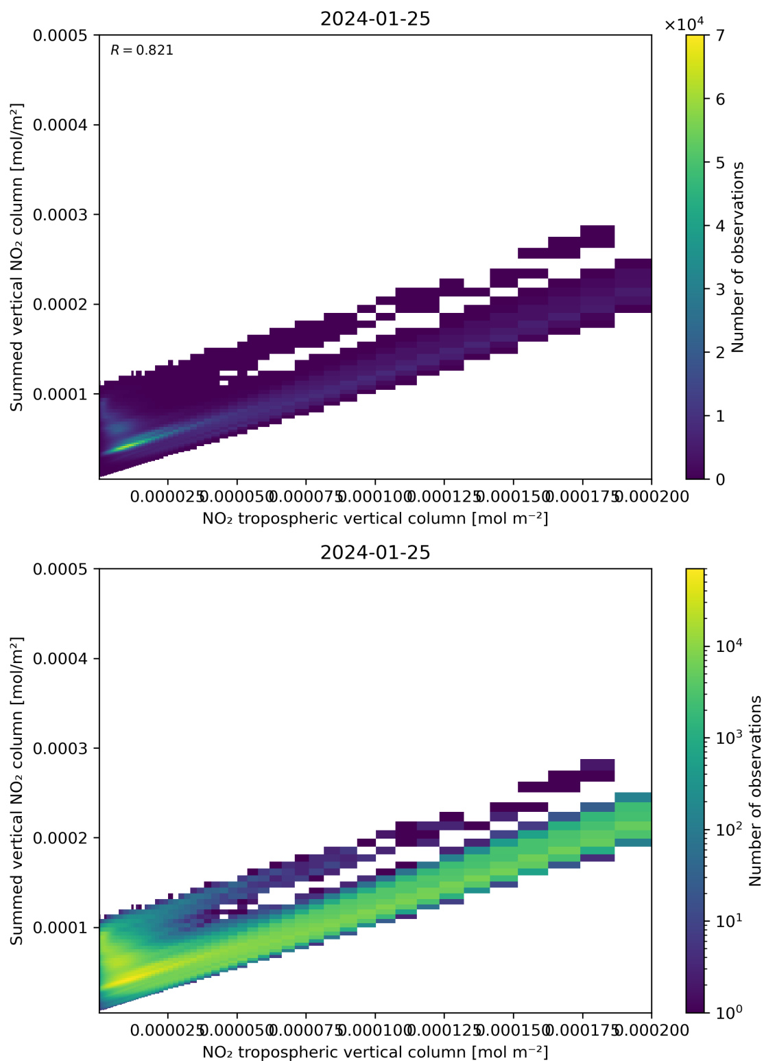
Figure 126: Scatter density plot of “NO 2 tropospheric vertical column” against “Summed vertical NO 2 column” for 2024-01-24 to 2024-01-26.
