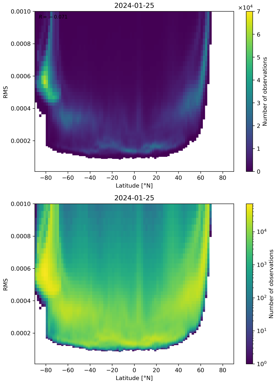
Figure 94: Scatter density plot of “Latitude” against “RMS” for 2024-01-24 to 2024-01-26.
