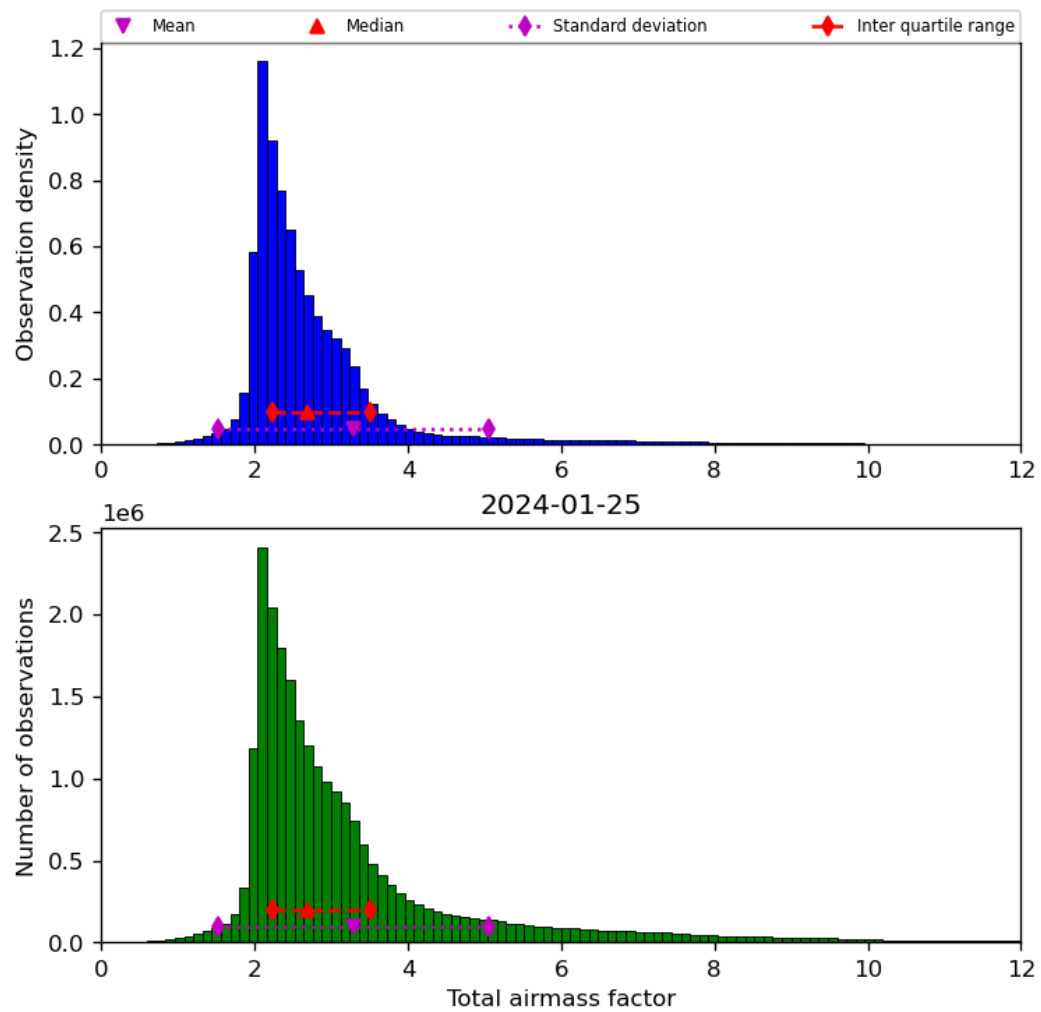
Figure 32: Histogram of “Total airmass factor” for 2024-01-24 to 2024-01-26
