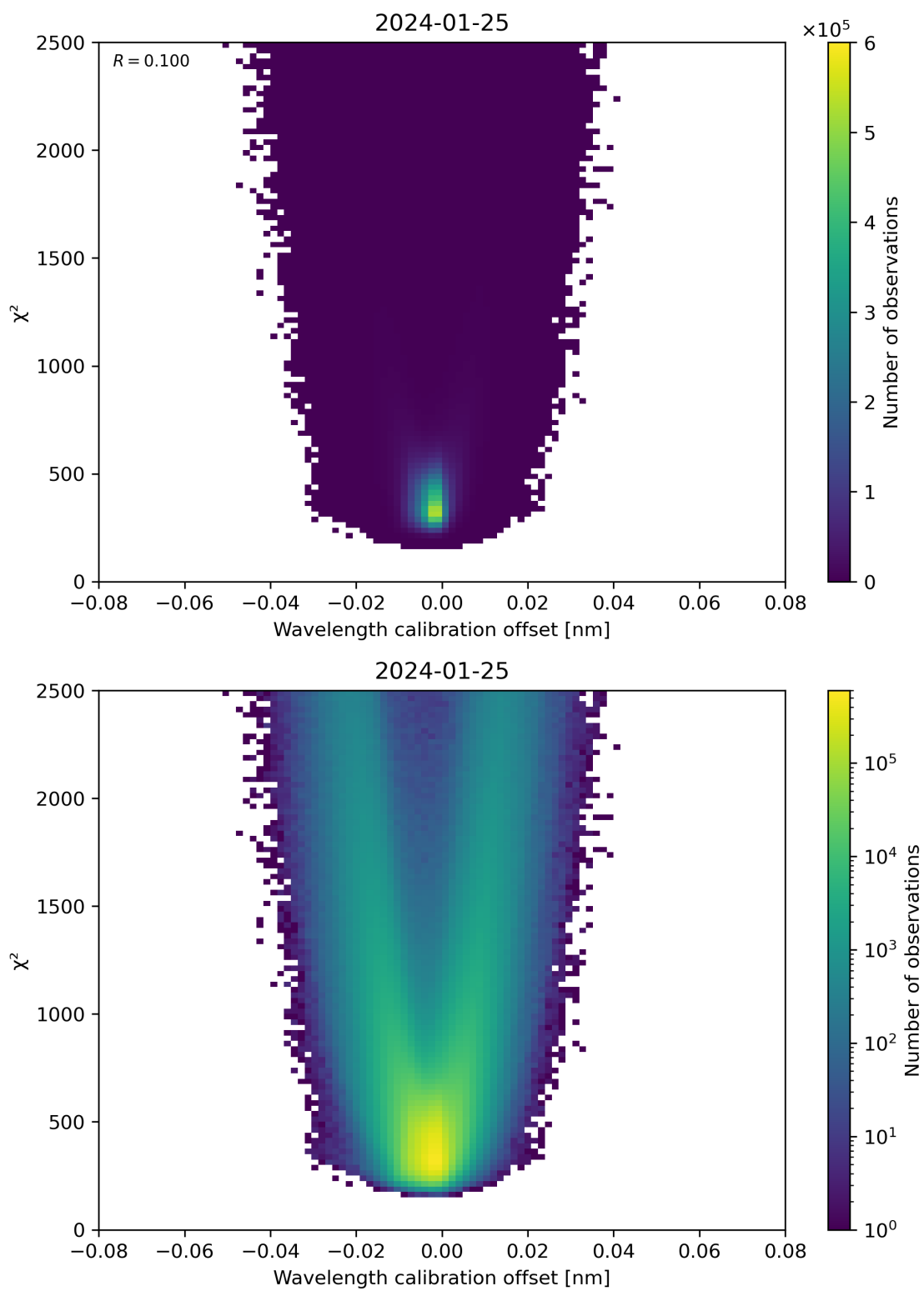
Figure 175: Scatter density plot of “Wavelength calibration offset” against “ \chi^2 ” for 2024-01-24 to 2024-01-26.
