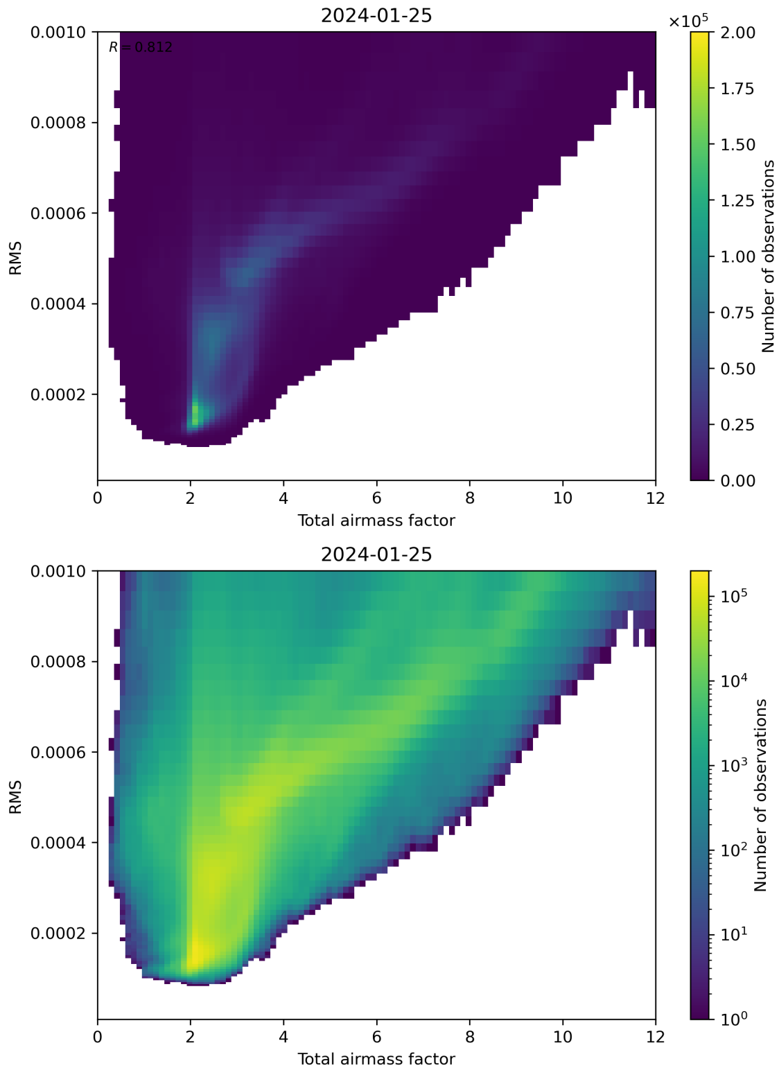
Figure 69: Scatter density plot of “Total airmass factor” against “RMS” for 2024-01-24 to 2024-01-26.
