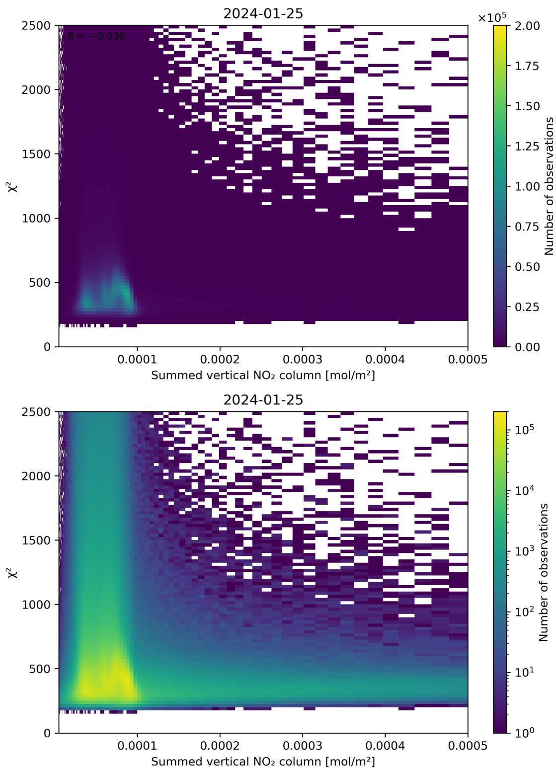
Figure 104: Scatter density plot of “Summed vertical NO 2 column” against “ \chi^2 ” for 2024-01-24 to 2024-01-26.
