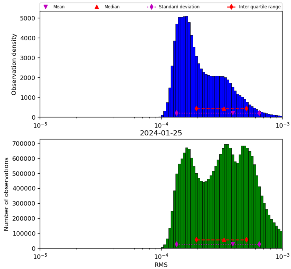
Figure 43: Histogram of “RMS” for 2024-01-24 to 2024-01-26
