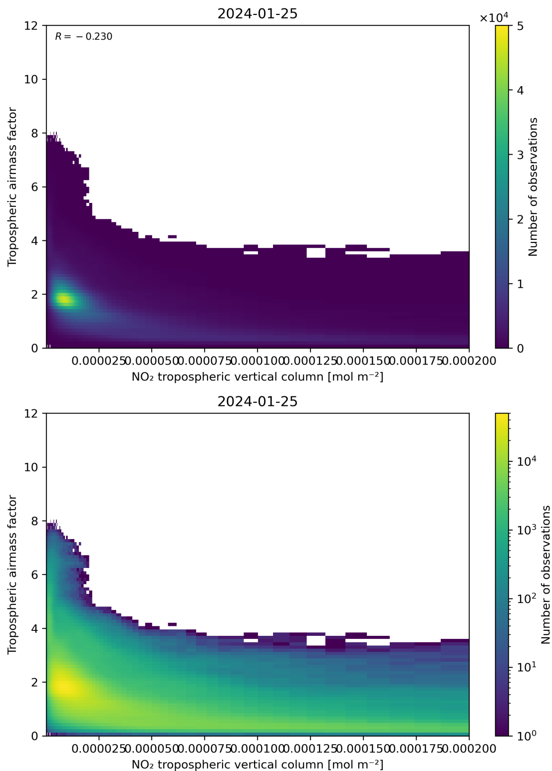
Figure 123: Scatter density plot of “NO 2 tropospheric vertical column” against “Tropospheric air mass factor” for 2024-01-24 to 2024-01-26.
