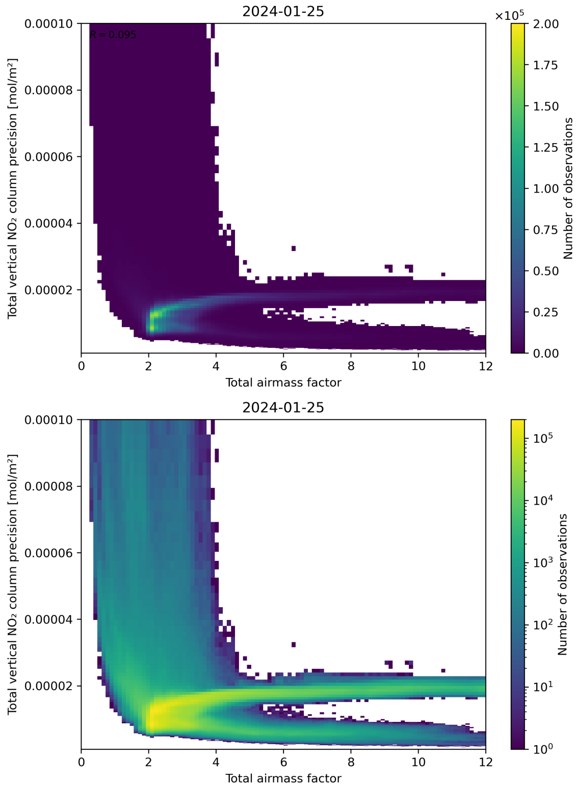
Figure 68: Scatter density plot of “Total airmass factor” against “Total vertical NO 2 column precision” for 2024-01-24 to 2024-01-26.
