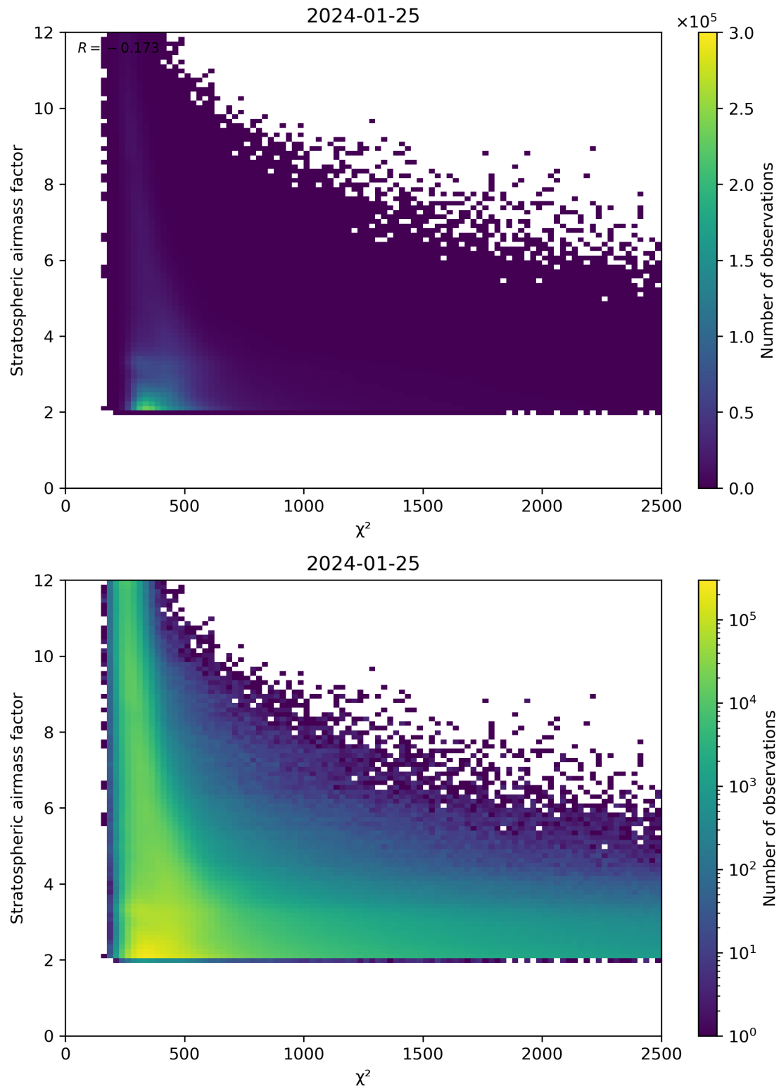
Figure 81: Scatter density plot of “ \chi^2 ” against “Stratospheric airmass factor” for 2024-01-24 to 2024-01-26.
