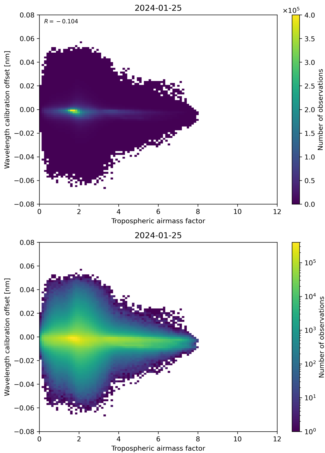
Figure 80: Scatter density plot of “Tropospheric airmass factor” against “Wavelength calibration offset” for 2024-01-24 to 2024-01-26.
