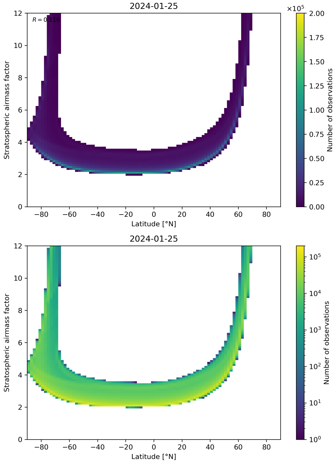
Figure 83: Scatter density plot of “Latitude” against “Stratospheric air mass factor” for 2024-01-24 to 2024-01-26.
