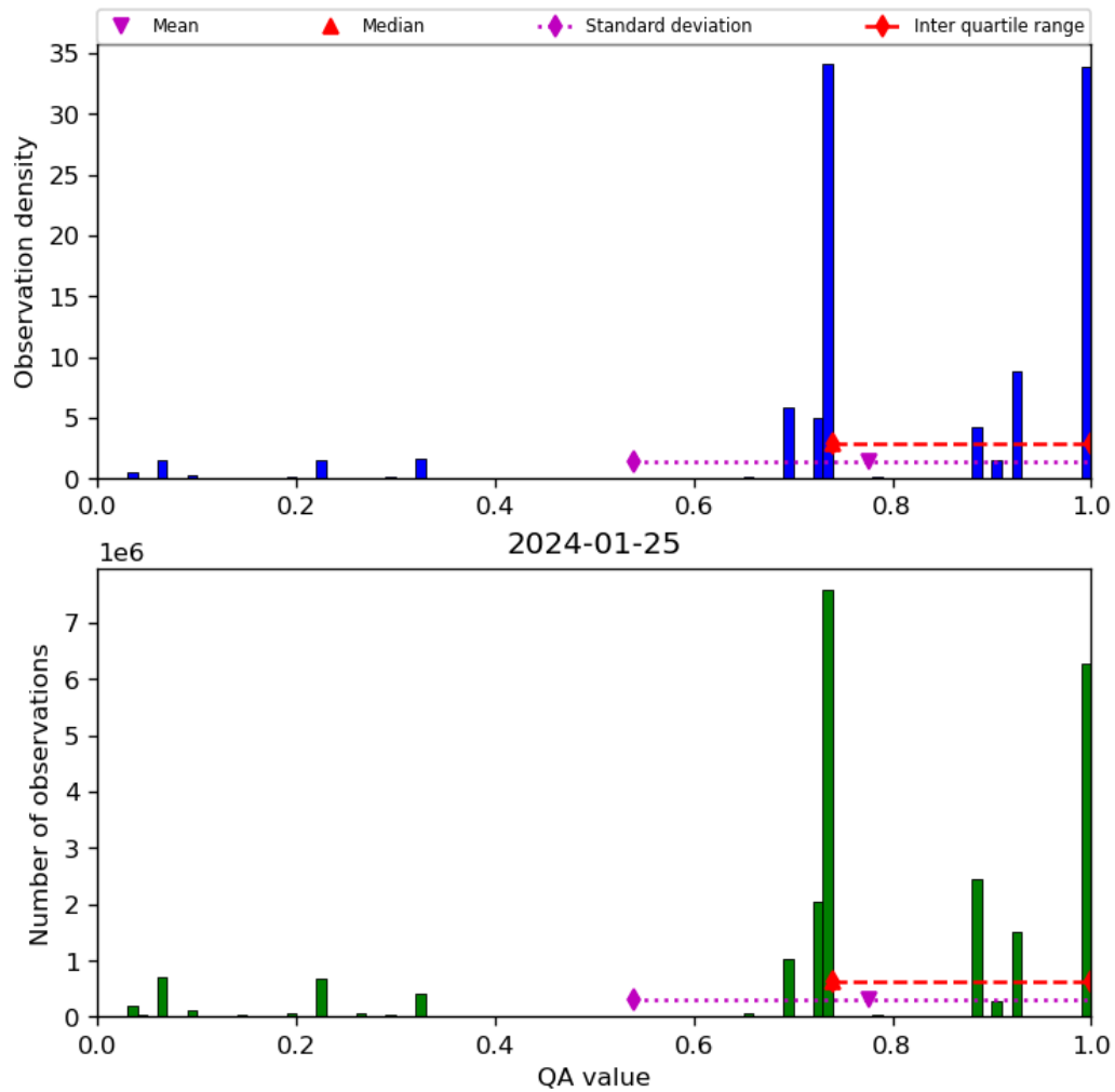
Figure 28: Histogram of “QA value” for 2024-01-24 to 2024-01-26
