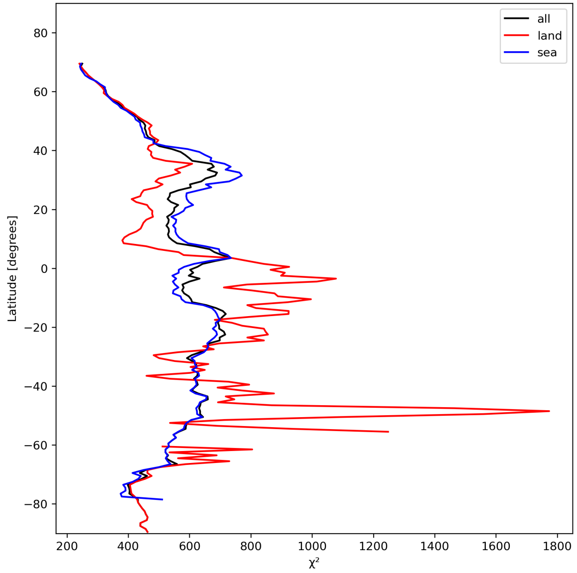
Figure 25: Zonal average of “ \chi^2 ” for 2024-01-24 to 2024-01-26.
