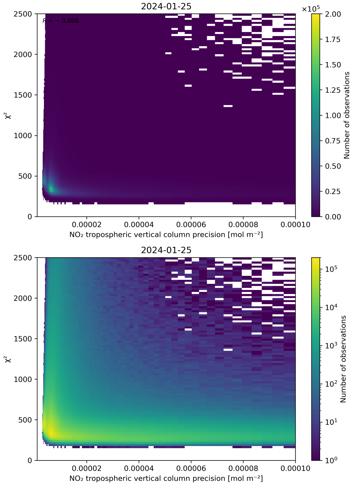
Figure 134: Scatter density plot of “NO 2 tropospheric vertical column precision” against “ \chi^2 ” for 2024-01-24 to 2024-01-26.
