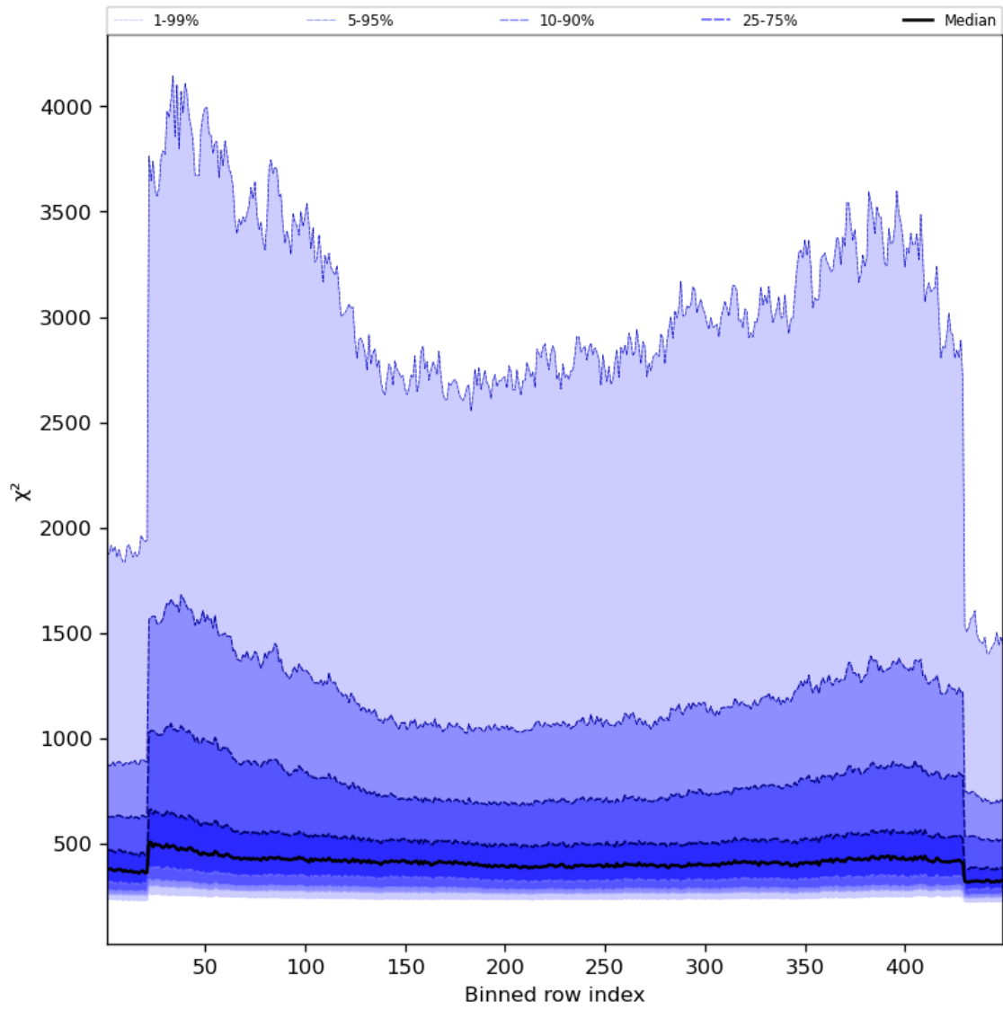
Figure 59: Along track statistics of “ \chi^2 ” for 2024-01-24 to 2024-01-26
