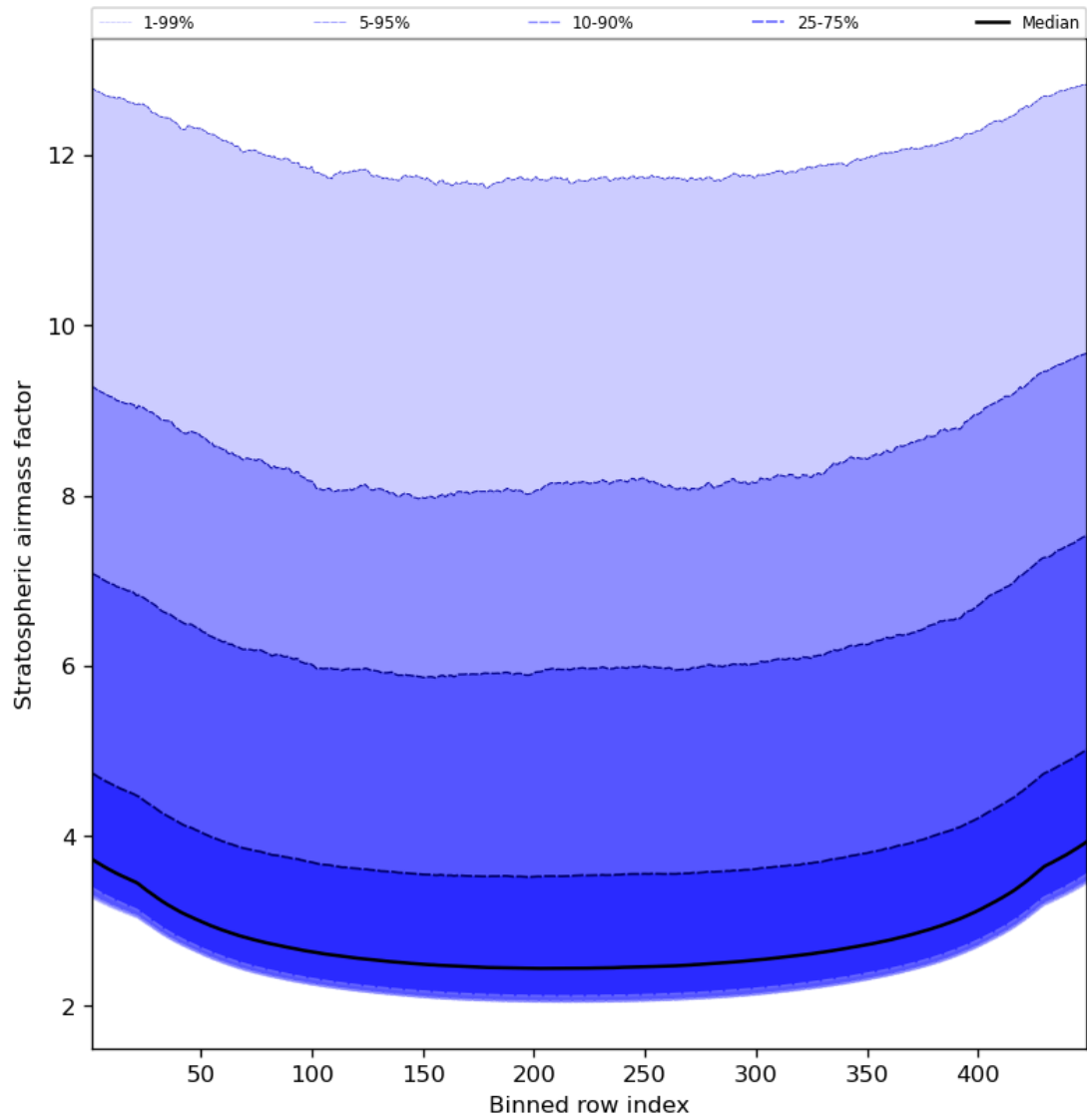
Figure 61: Along track statistics of “Stratospheric airmass factor” for 2024-01-24 to 2024-01-26
