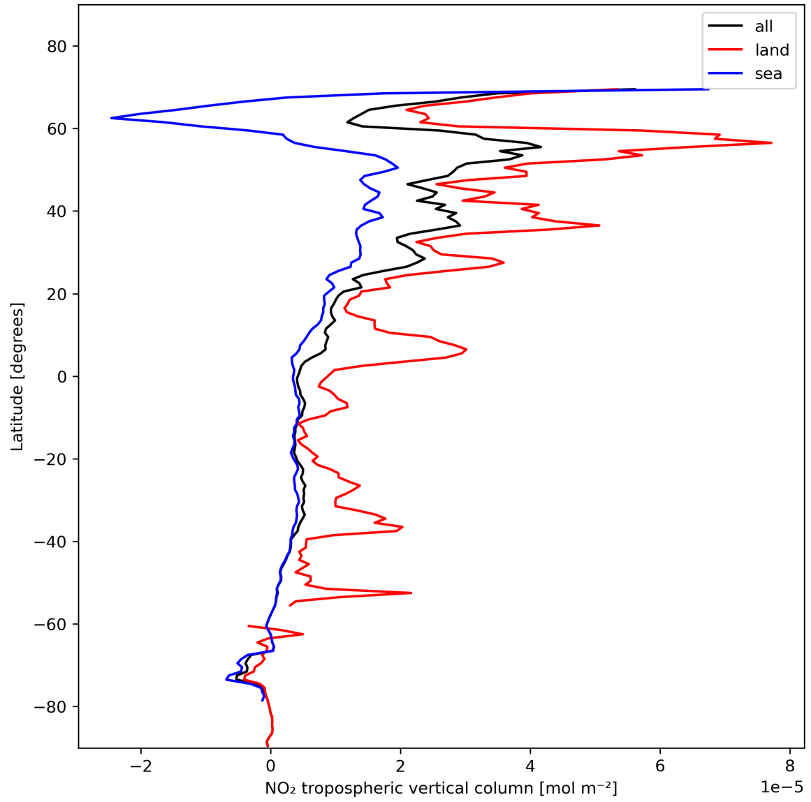
Figure 12: Zonal average of “NO 2 tropospheric vertical column” for 2024-01-24 to 2024-01-26.
