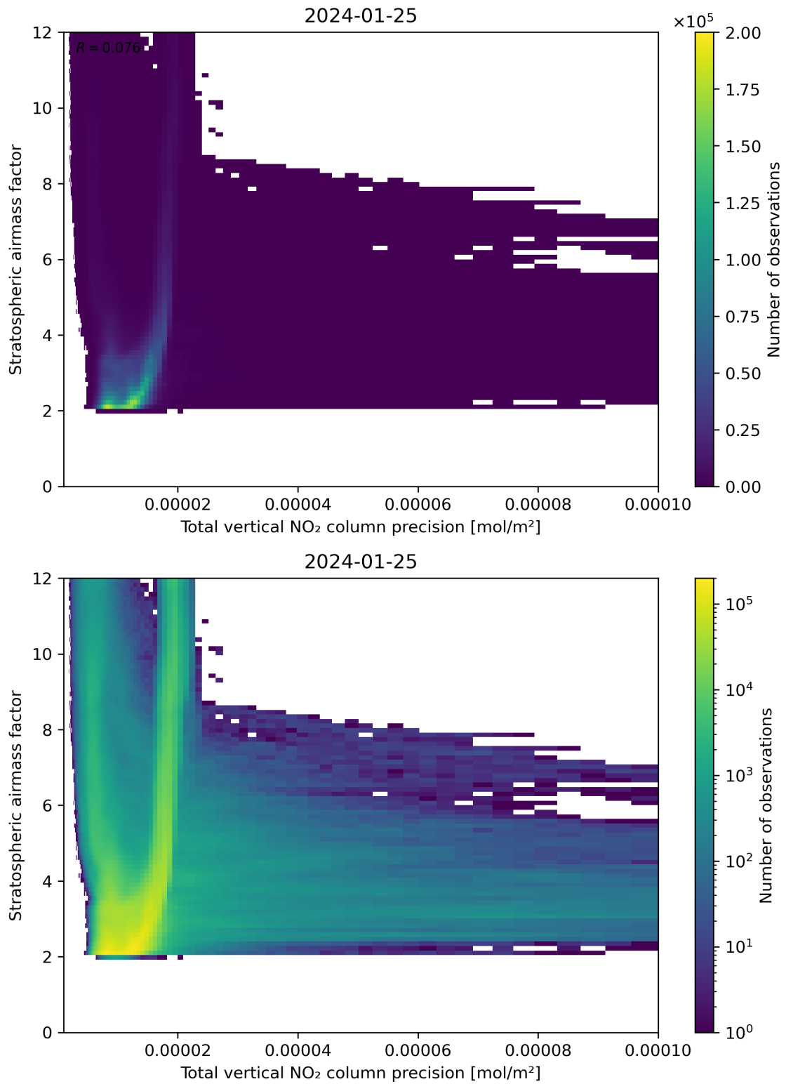
Figure 115: Scatter density plot of “Total vertical NO 2 column precision” against “Stratospheric air mass factor” for 2024-01-24 to 2024-01-26.
