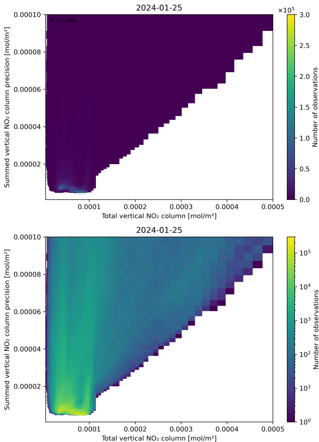
Figure 113: Scatter density plot of “Total vertical NO 2 column” against “Summed vertical NO 2 column precision” for 2024-01-24 to 2024-01-26.
