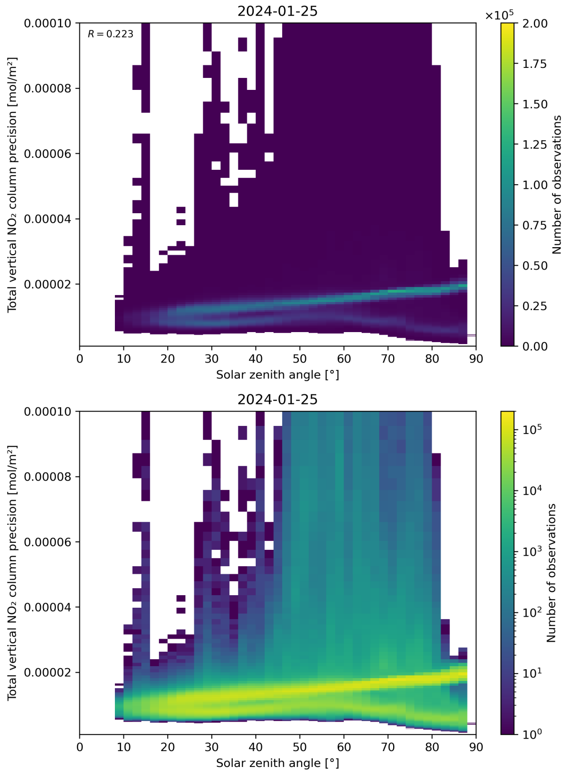
Figure 154: Scatter density plot of “Solar zenith angle” against “Total vertical NO 2 column precision” for 2024-01-24 to 2024-01-26.
