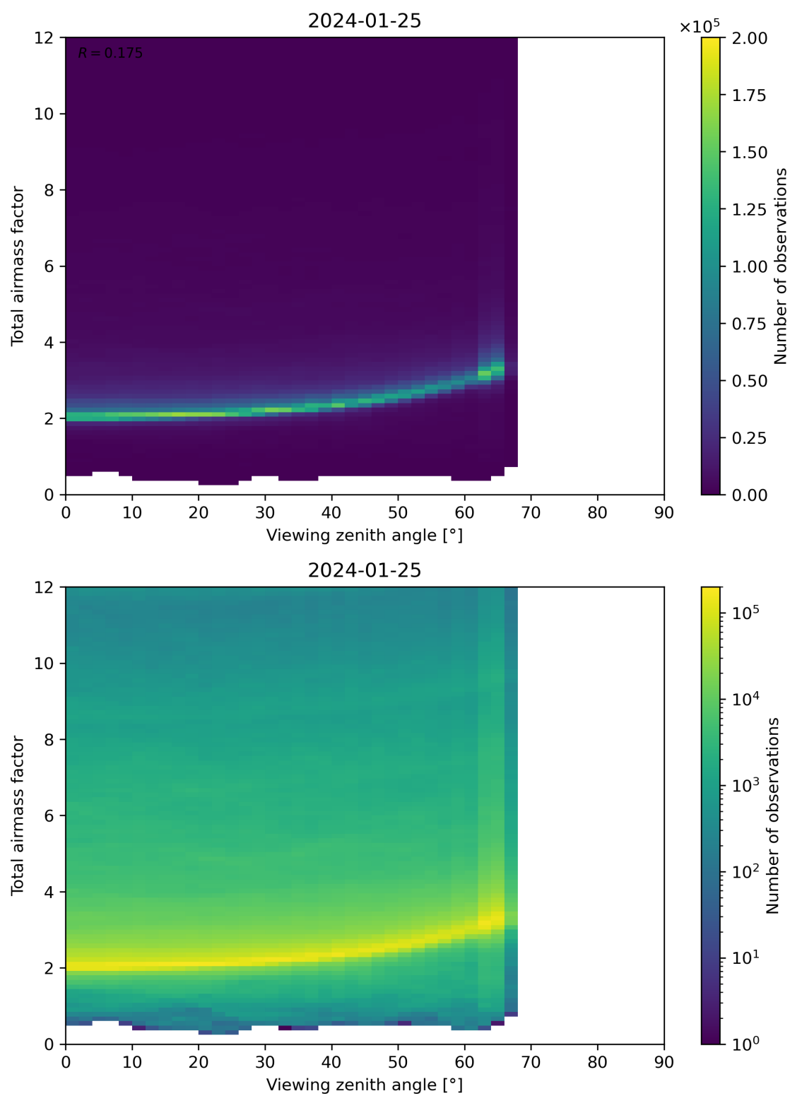
Figure 160: Scatter density plot of “Viewing zenith angle” against “Total airmass factor” for 2024-01-24 to 2024-01-26.
