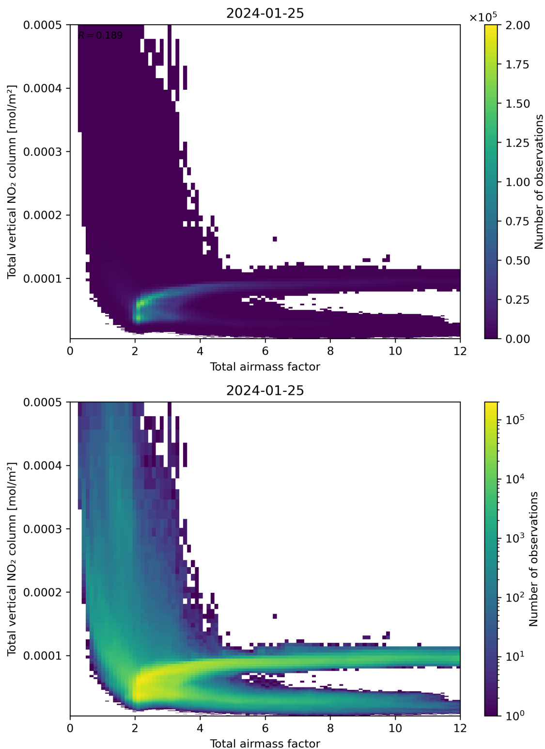
Figure 67: Scatter density plot of “Total airmass factor” against “Total vertical NO 2 column” for 2024-01-24 to 2024-01-26.
