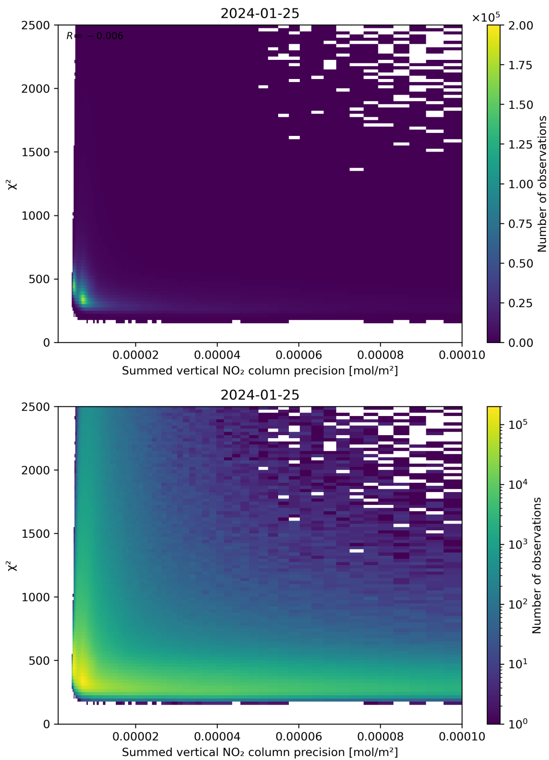
Figure 107: Scatter density plot of “Summed vertical NO 2 column precision” against “ \chi^2 ” for 2024-01-24 to 2024-01-26.
