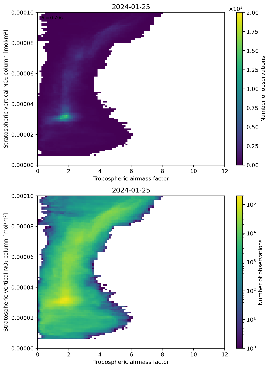
Figure 74: Scatter density plot of “Tropospheric air mass factor” against “Stratospheric vertical NO 2 column” for 2024-01-24 to 2024-01-26.
