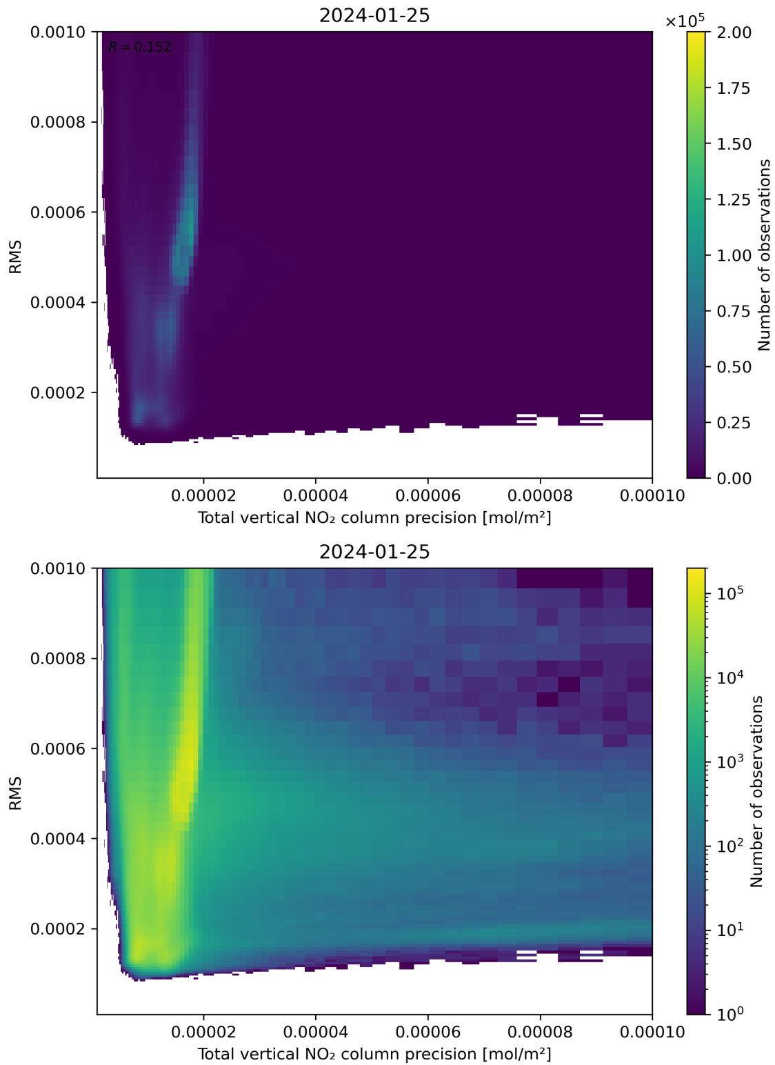
Figure 119: Scatter density plot of “Total vertical NO 2 column precision” against “RMS” for 2024-01-24 to 2024-01-26.
