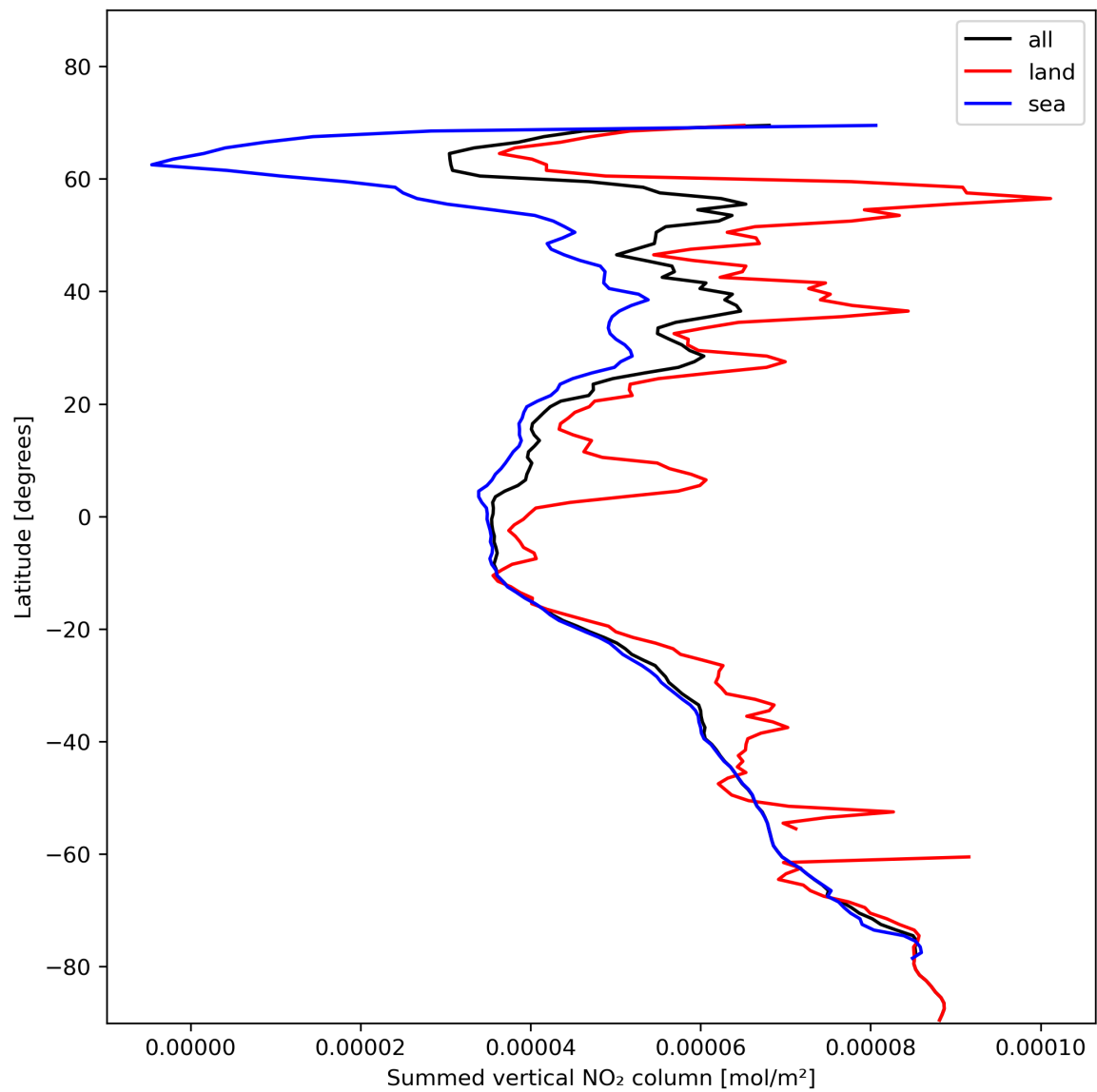
Figure 23: Zonal average of “Summed vertical NO 2 column” for 2024-01-24 to 2024-01-26.
