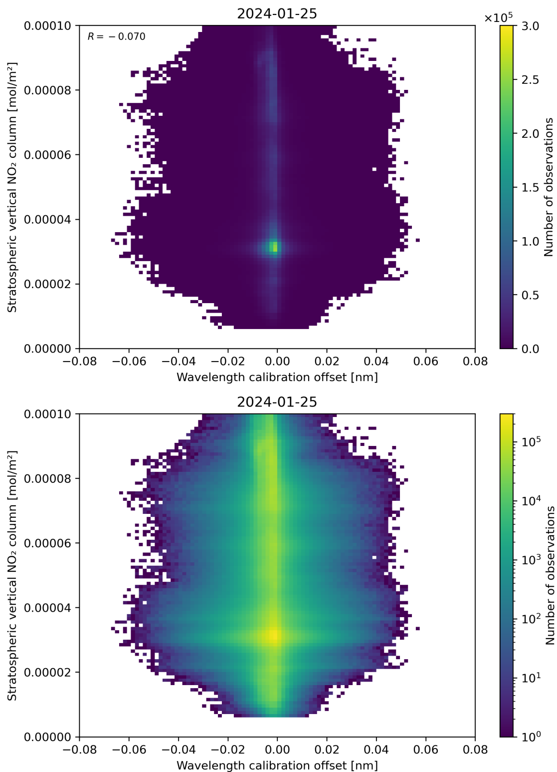
Figure 176: Scatter density plot of “Wavelength calibration offset” against “Stratospheric vertical NO 2 column” for 2024-01-24 to 2024-01-26.
