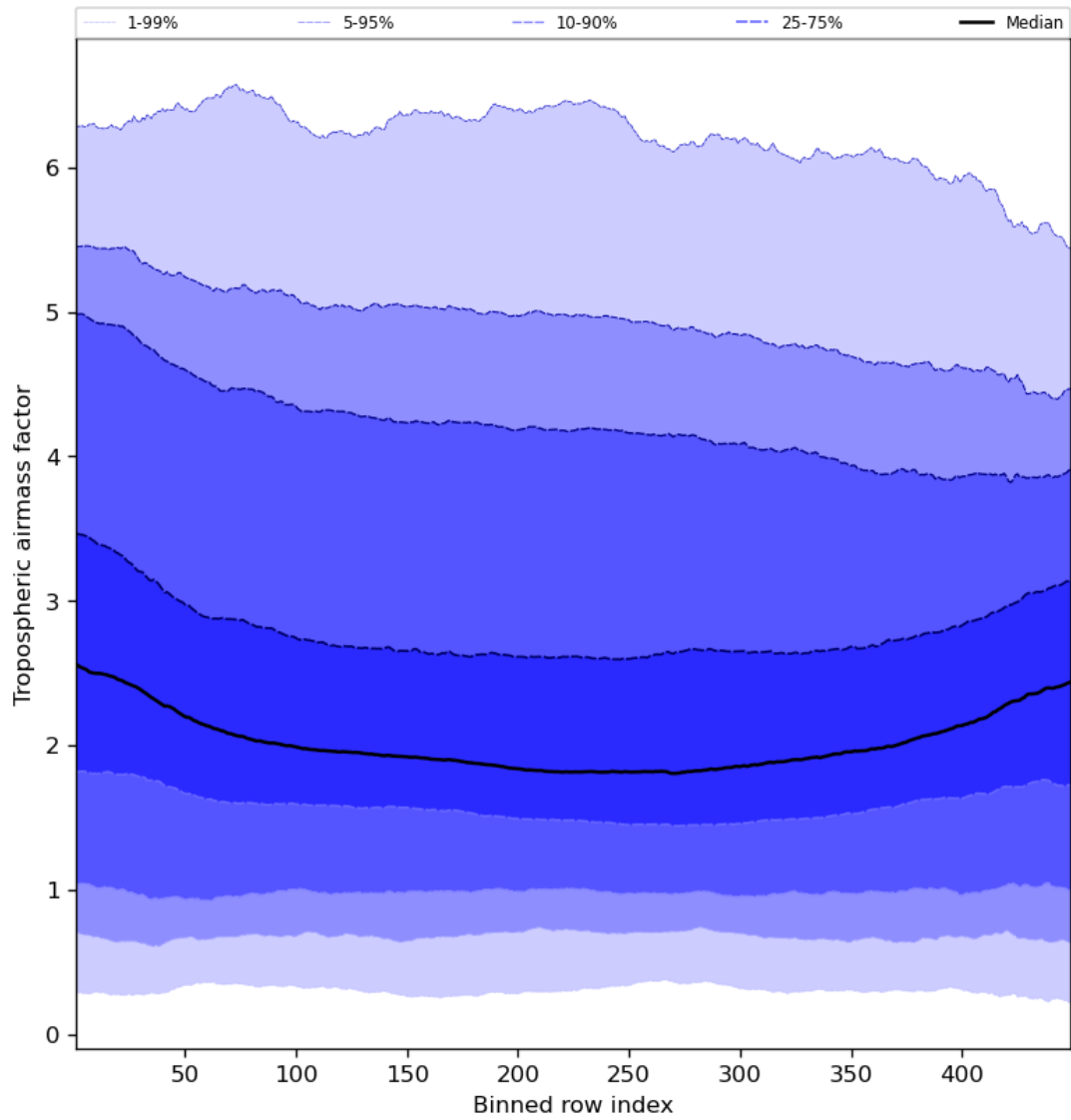
Figure 48: Along track statistics of “Tropospheric airmass factor” for 2024-01-24 to 2024-01-26
