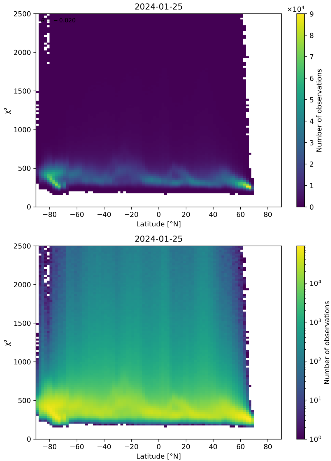
Figure 86: Scatter density plot of “Latitude” against “ \chi^2 ” for 2024-01-24 to 2024-01-26.
