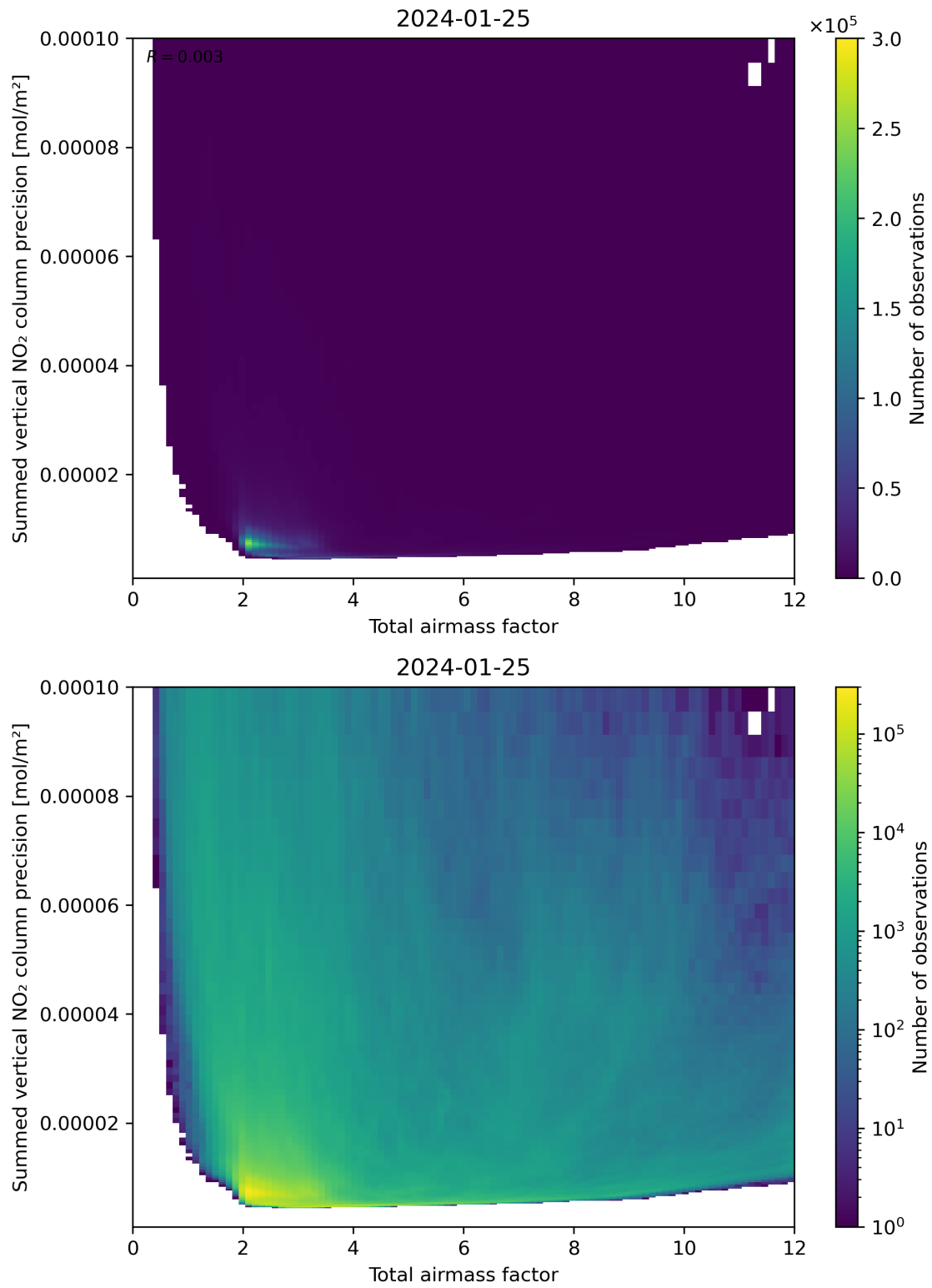
Figure 66: Scatter density plot of “Total airmass factor” against “Summed vertical NO 2 column precision” for 2024-01-24 to 2024-01-26.
