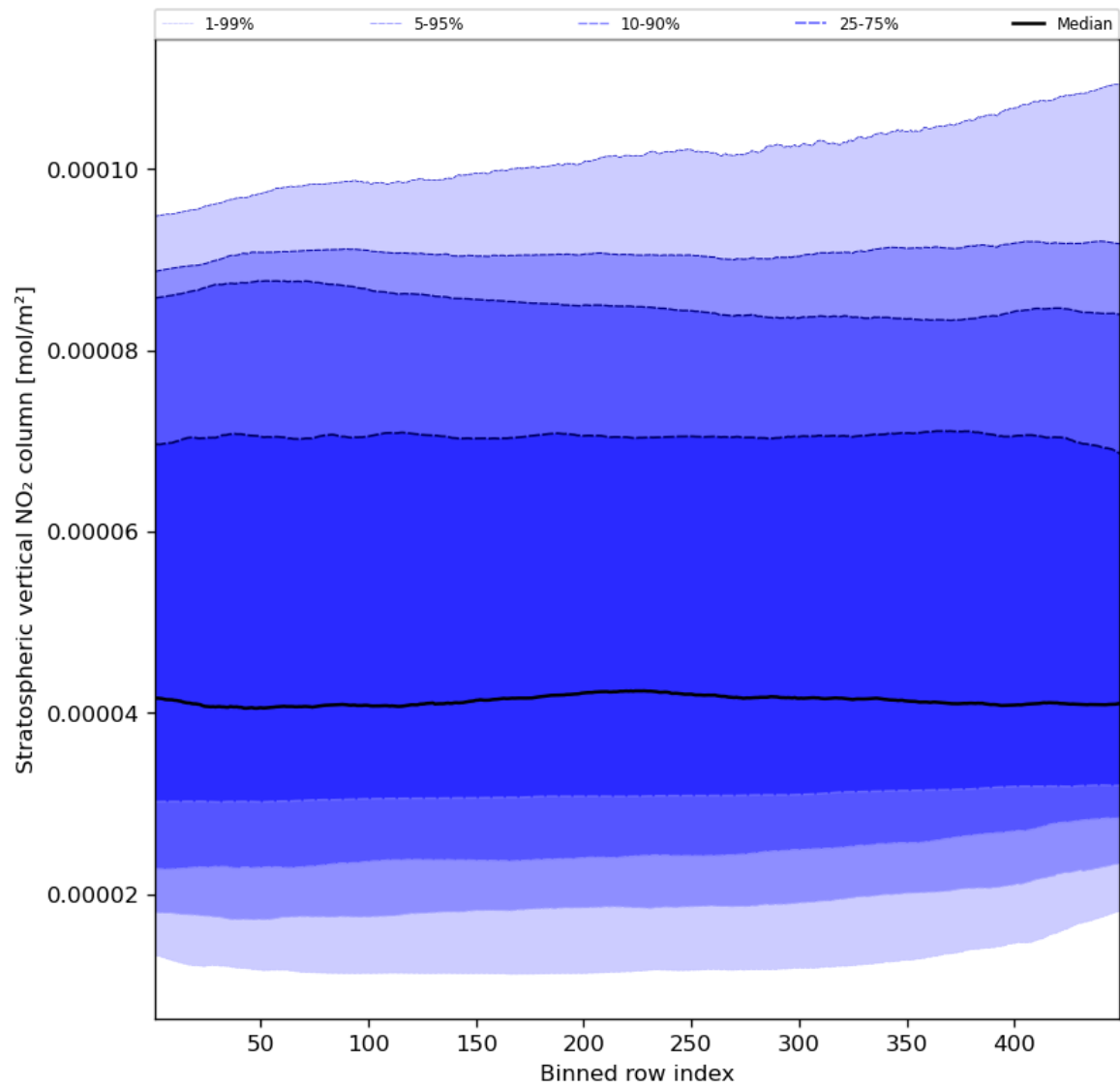
Figure 53: Along track statistics of “Stratospheric vertical NO 2 column” for 2024-01-24 to 2024-01-26
