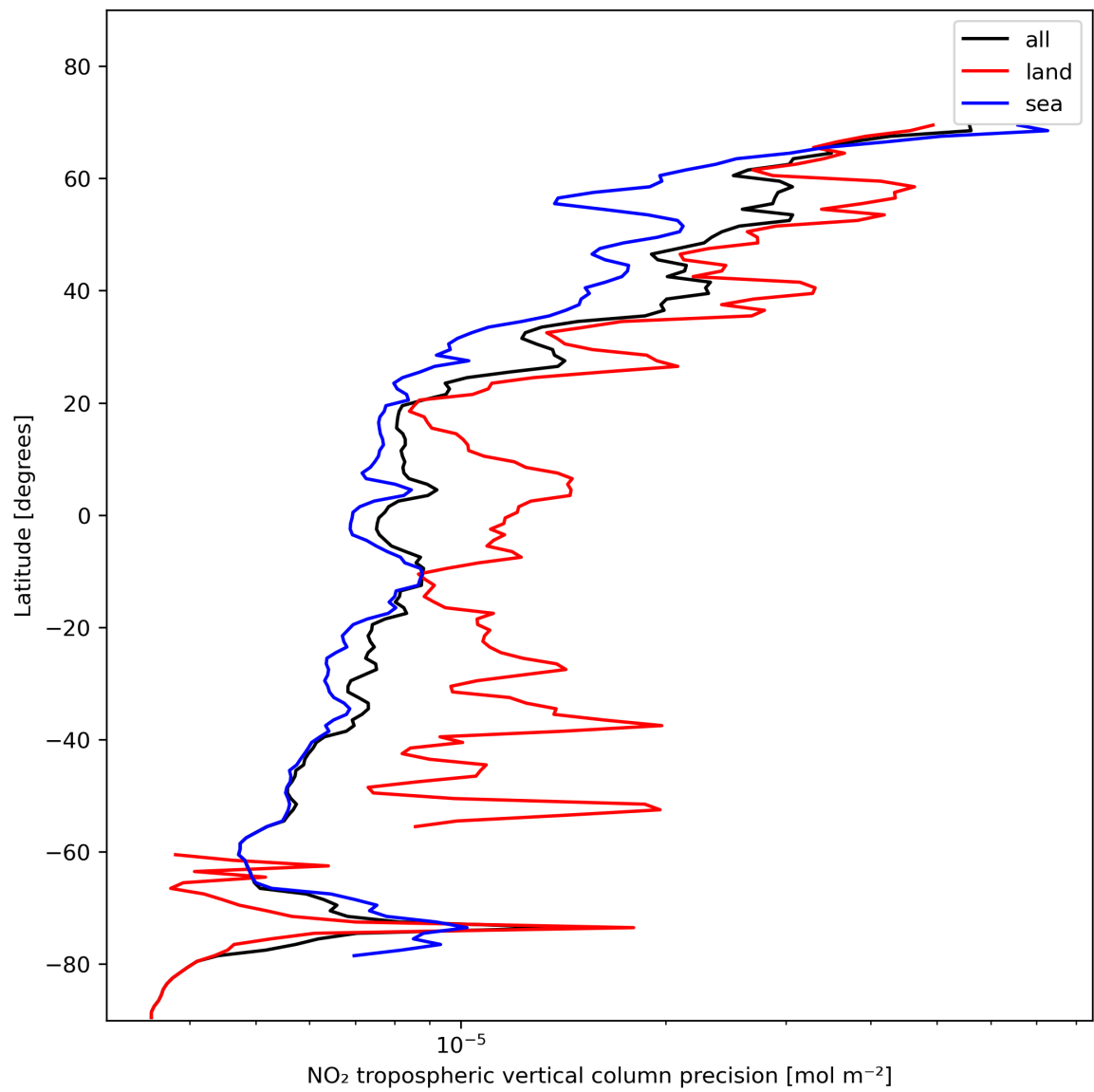
Figure 13: Zonal average of “NO 2 tropospheric vertical column precision” for 2024-01-24 to 2024-01-26.
