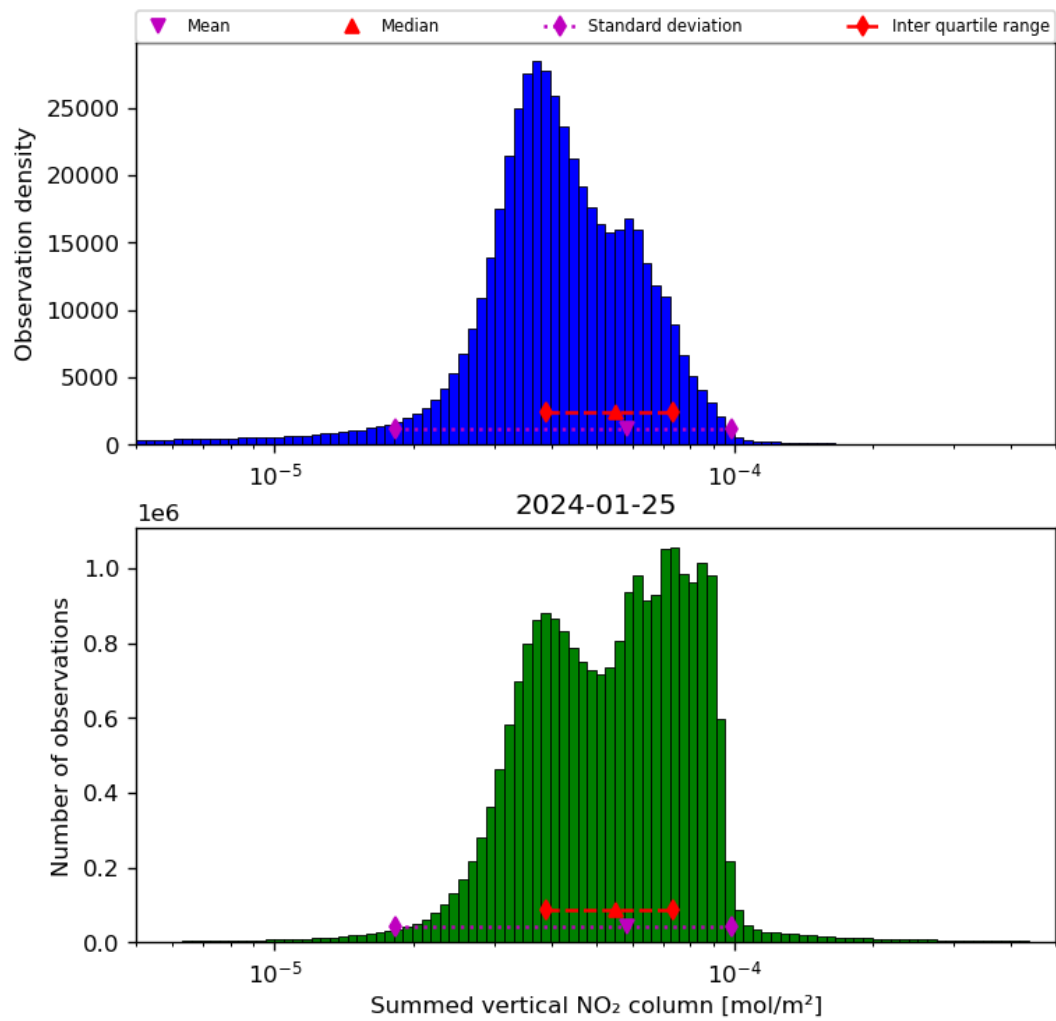
Figure 40: Histogram of “Summed vertical NO 2 column” for 2024-01-24 to 2024-01-26
