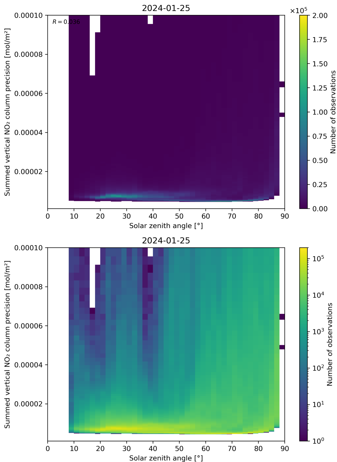
Figure 152: Scatter density plot of “Solar zenith angle” against “Summed vertical NO 2 column precision” for 2024-01-24 to 2024-01-26.
