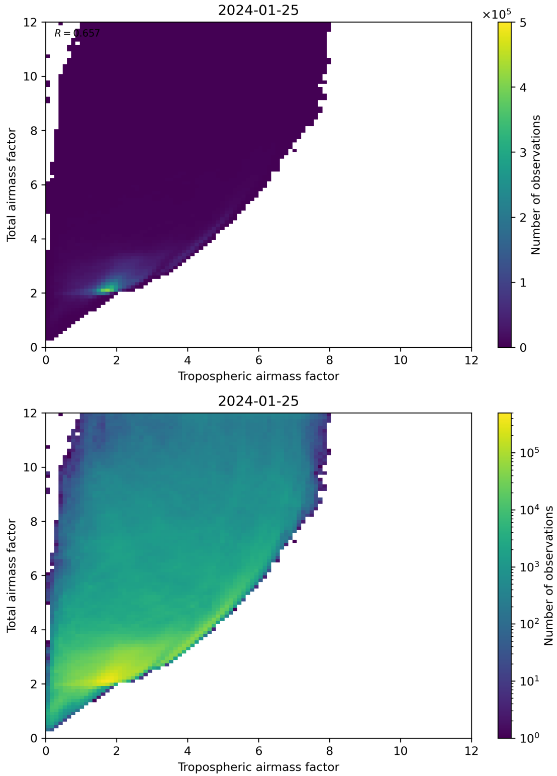
Figure 72: Scatter density plot of “Tropospheric airmass factor” against “Total airmass factor” for 2024-01-24 to 2024-01-26.
