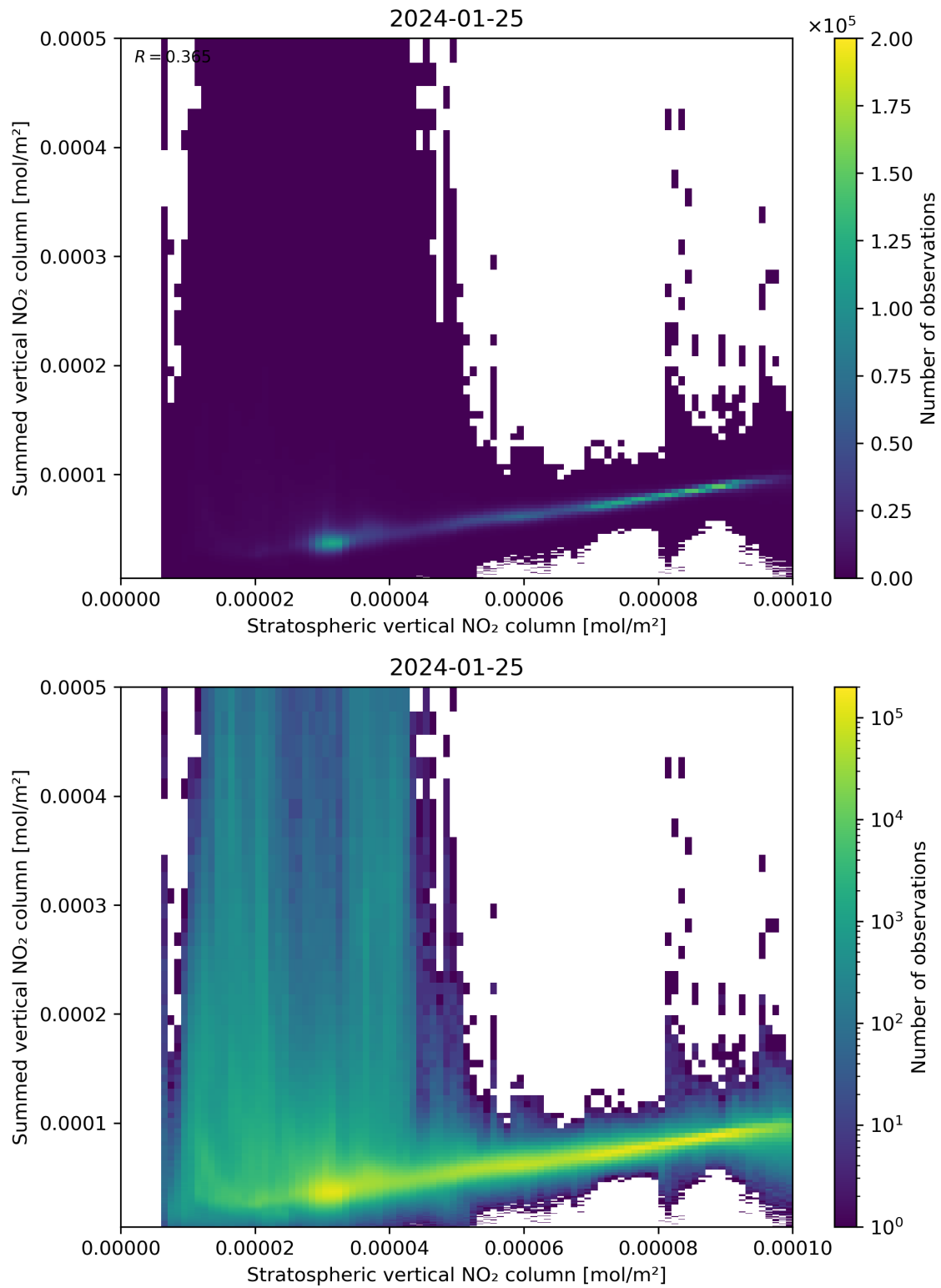
Figure 98: Scatter density plot of “Stratospheric vertical NO 2 column” against “Summed vertical NO 2 column” for 2024-01-24 to 2024-01-26.
