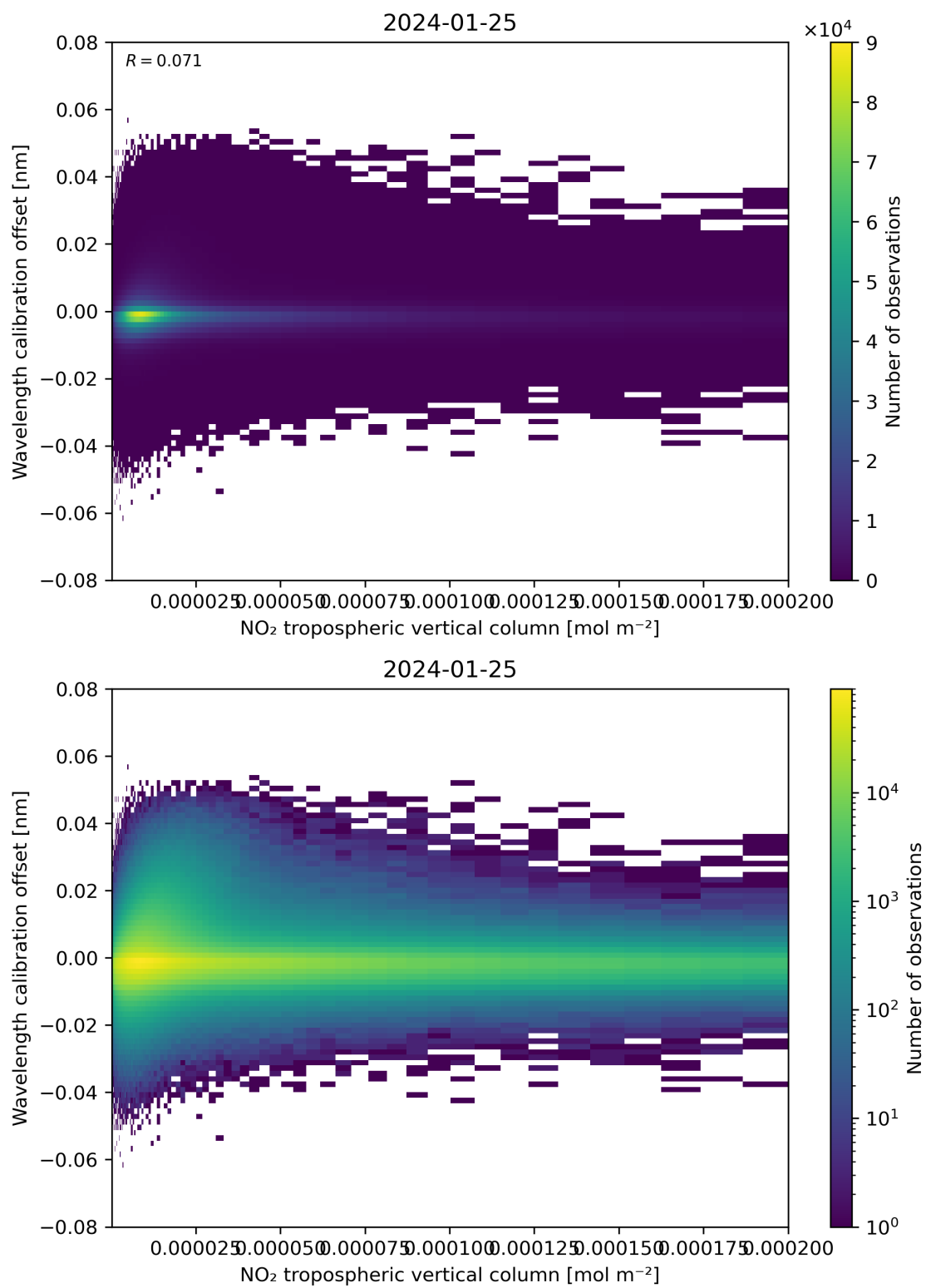
Figure 143: Scatter density plot of “NO 2 tropospheric vertical column” against “Wavelength calibration offset” for 2024-01-24 to 2024-01-26.
