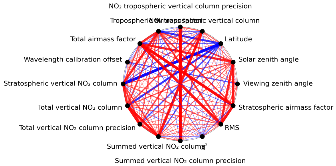
Figure 1: Map of correlation graph for 2024-01-24 to 2024-01-26.
