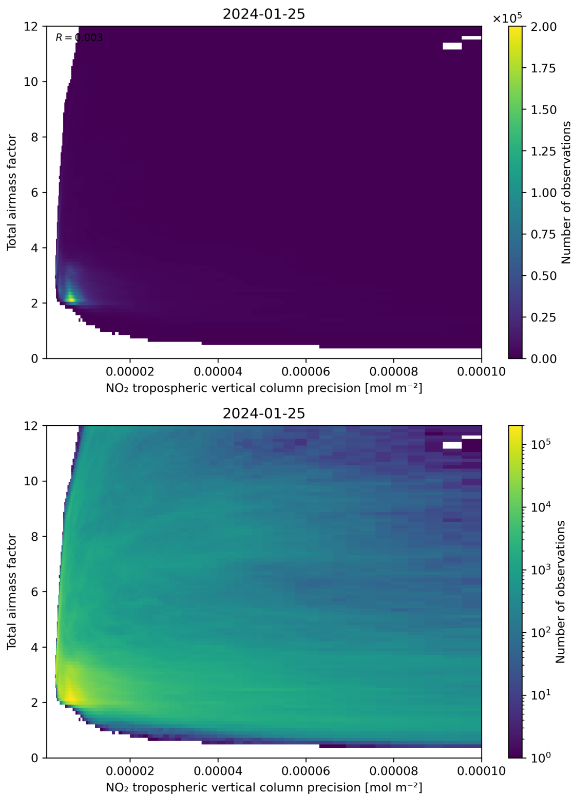
Figure 132: Scatter density plot of “NO 2 tropospheric vertical column precision” against “Total air mass factor” for 2024-01-24 to 2024-01-26.
