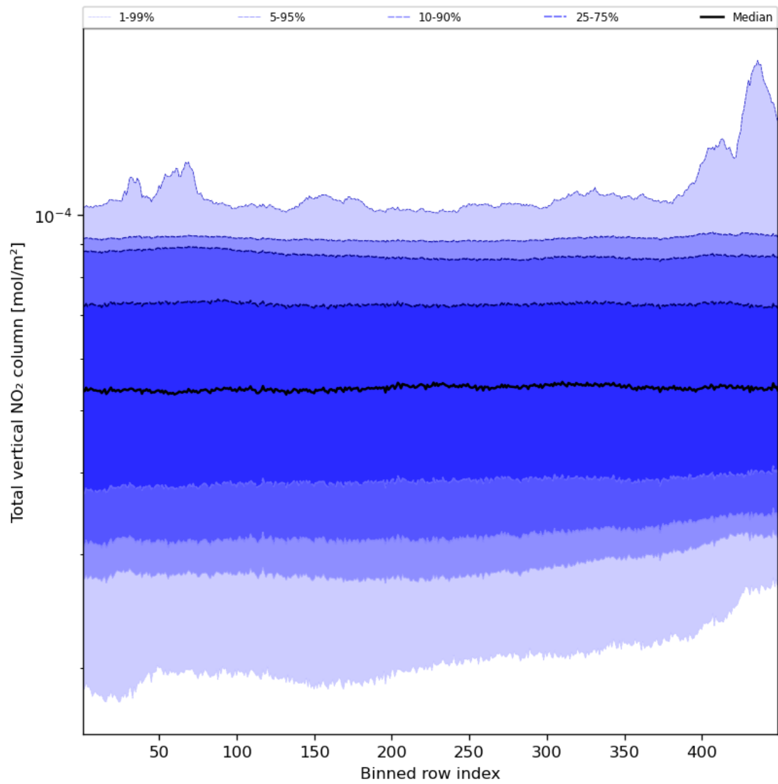
Figure 55: Along track statistics of “Total vertical NO 2 column” for 2024-01-24 to 2024-01-26
