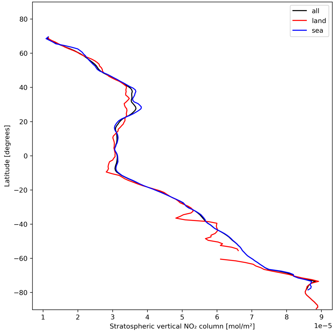
Figure 19: Zonal average of “Stratospheric vertical NO 2 column” for 2024-01-24 to 2024-01-26.
