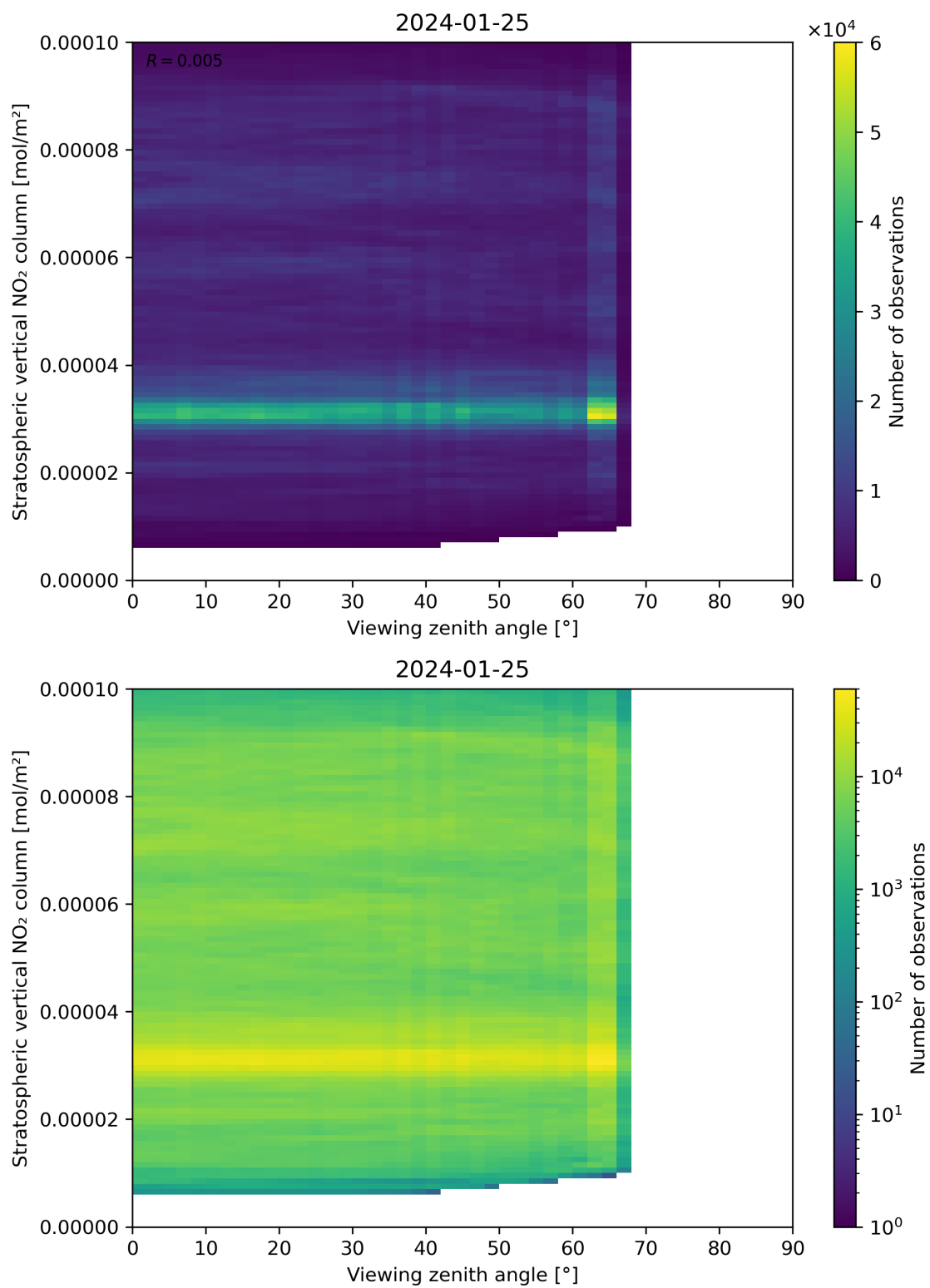
Figure 164: Scatter density plot of “Viewing zenith angle” against “Stratospheric vertical NO 2 column” for 2024-01-24 to 2024-01-26.
