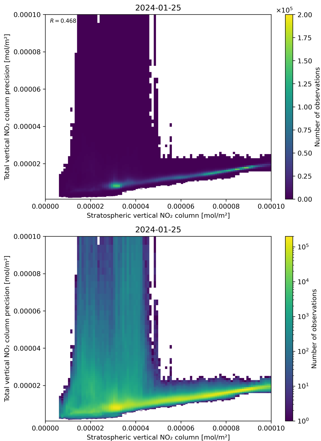
Figure 101: Scatter density plot of “Stratospheric vertical NO 2 column” against “Total vertical NO 2 column precision” for 2024-01-24 to 2024-01-26.
