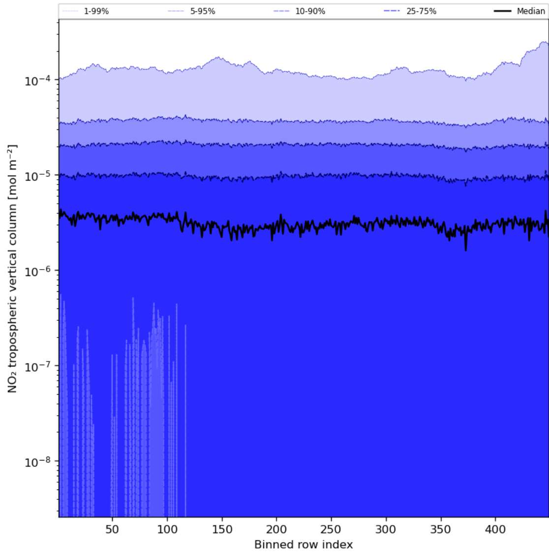
Figure 46: Along track statistics of “NO 2 tropospheric vertical column” for 2024-01-24 to 2024-01-26
