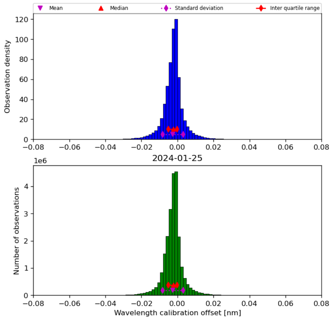
Figure 35: Histogram of “Wavelength calibration offset” for 2024-01-24 to 2024-01-26
