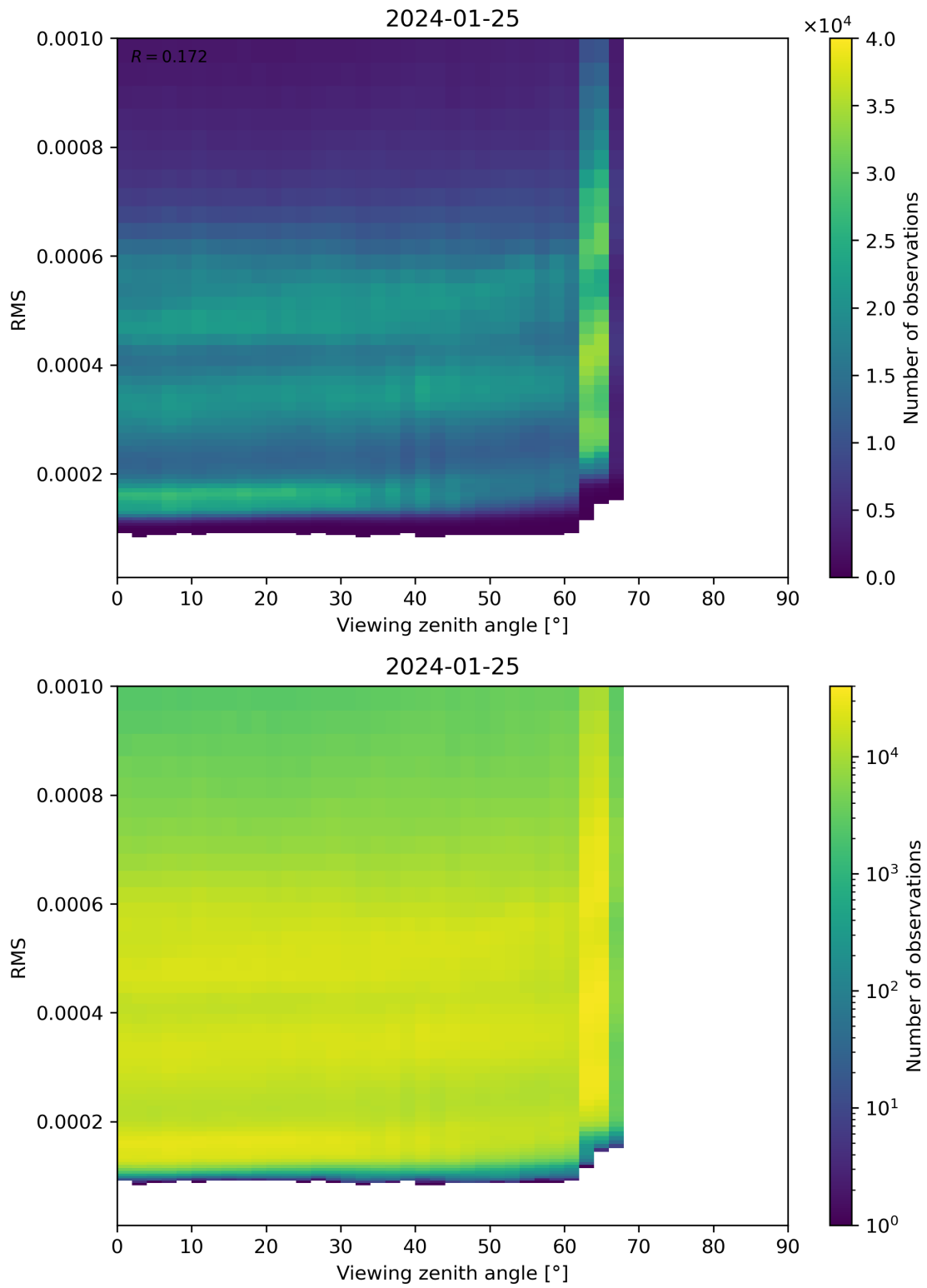
Figure 171: Scatter density plot of “Viewing zenith angle” against “RMS” for 2024-01-24 to 2024-01-26.
