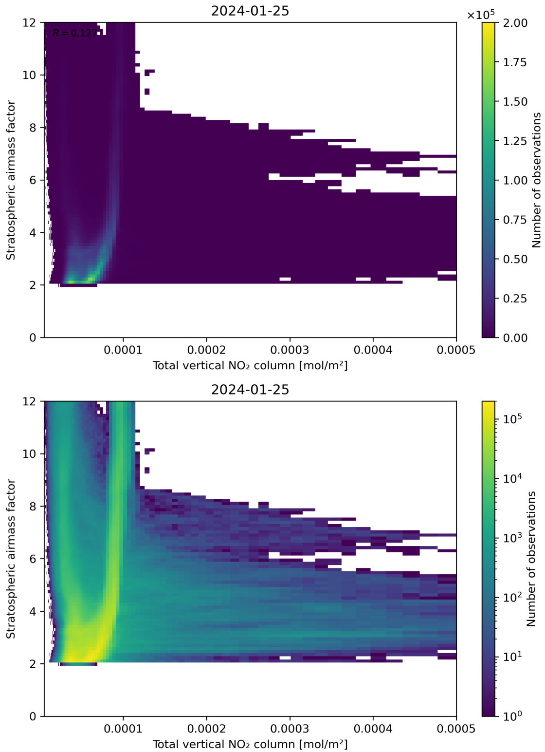
Figure 110: Scatter density plot of “Total vertical NO 2 column” against “Stratospheric air mass factor” for 2024-01-24 to 2024-01-26.
