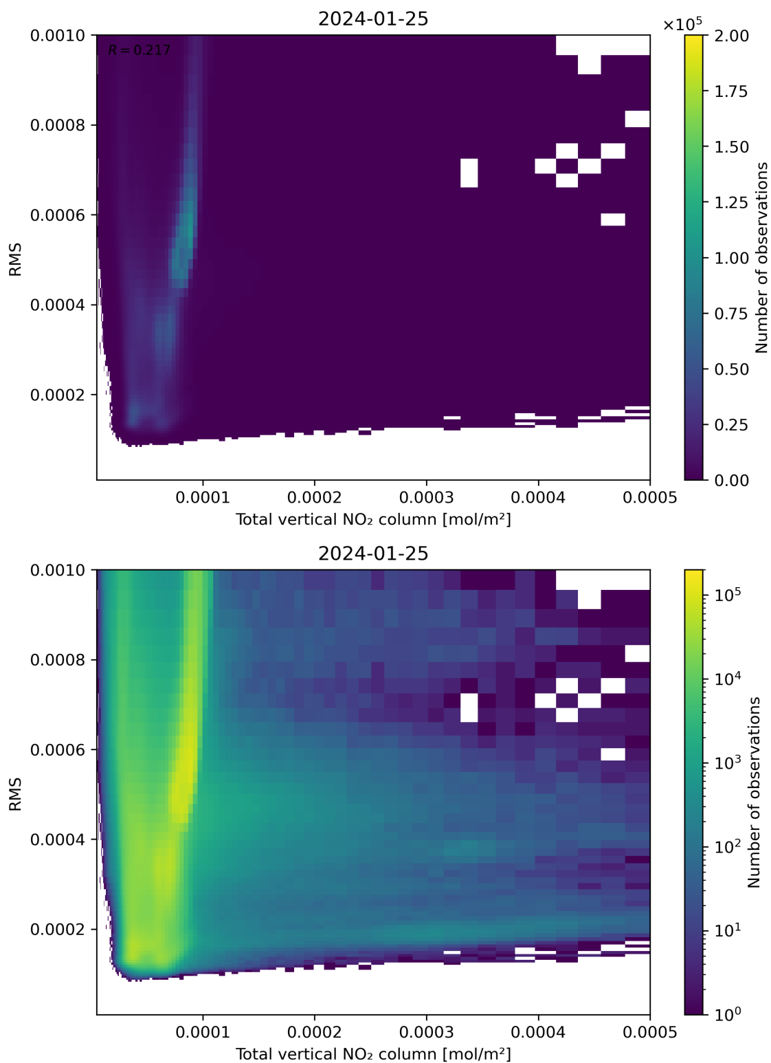
Figure 120: Scatter density plot of “Total vertical NO 2 column” against “RMS” for 2024-01-24 to 2024-01-26.
