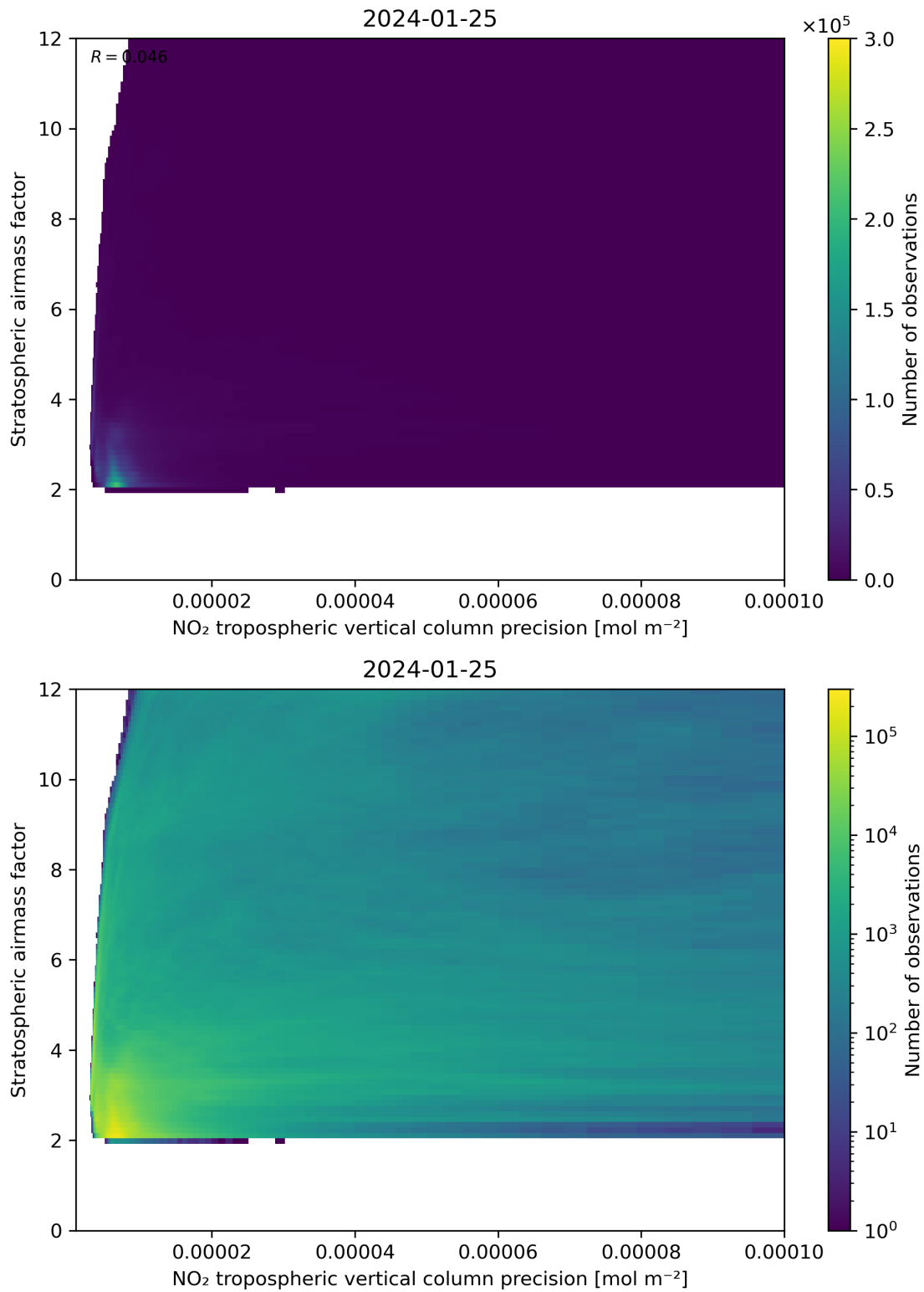
Figure 131: Scatter density plot of “NO 2 tropospheric vertical column precision” against “Stratospheric airmass factor” for 2024-01-24 to 2024-01-26.
