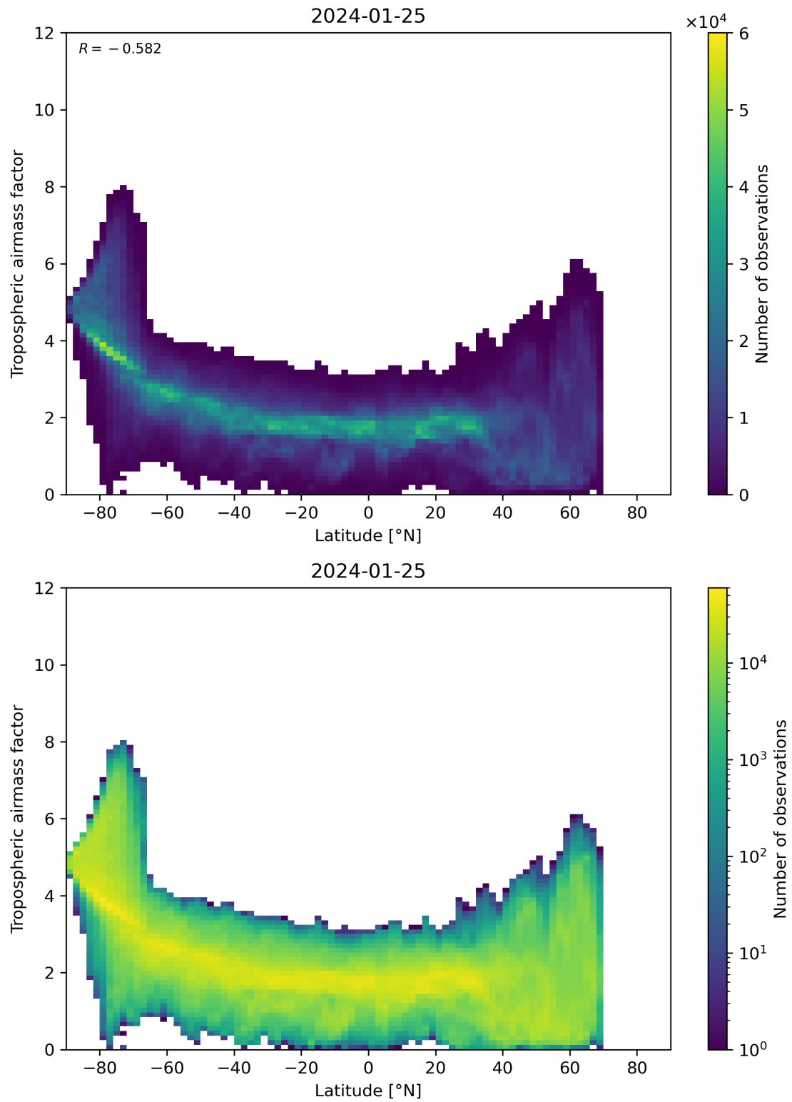
Figure 85: Scatter density plot of “Latitude” against “Tropospheric airmass factor” for 2024-01-24 to 2024-01-26.
