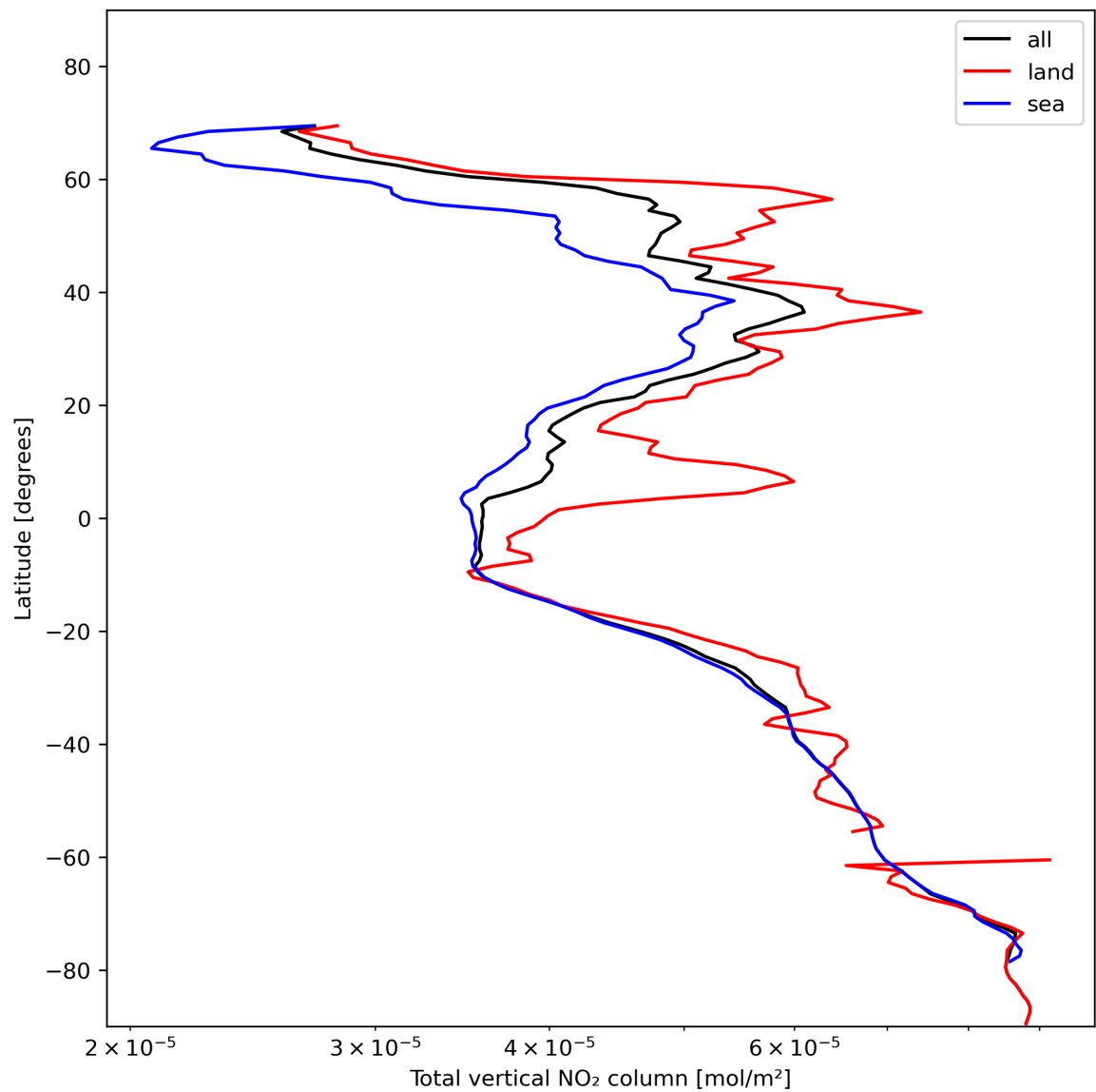
Figure 21: Zonal average of “Total vertical NO 2 column” for 2024-01-24 to 2024-01-26.
