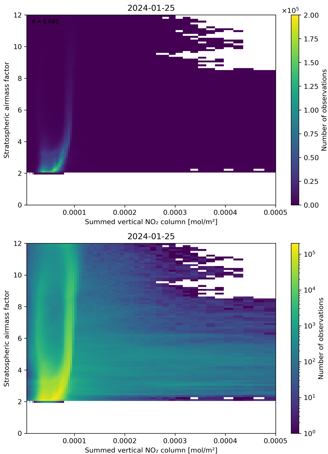
Figure 103: Scatter density plot of “Summed vertical NO 2 column” against “Stratospheric air mass factor” for 2024-01-24 to 2024-01-26.
