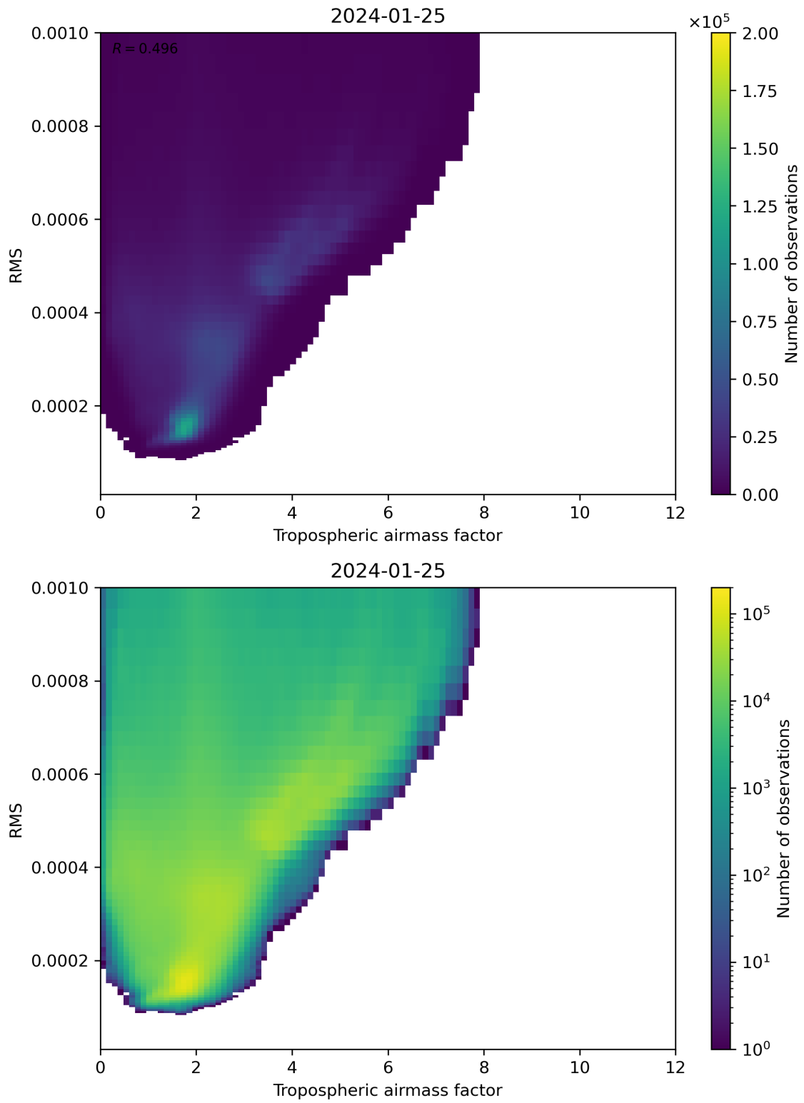
Figure 79: Scatter density plot of “Tropospheric airmass factor” against “RMS” for 2024-01-24 to 2024-01-26.
