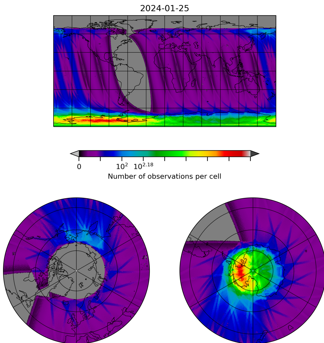
Figure 10: Map of the number of observations for 2024-01-24 to 2024-01-26
