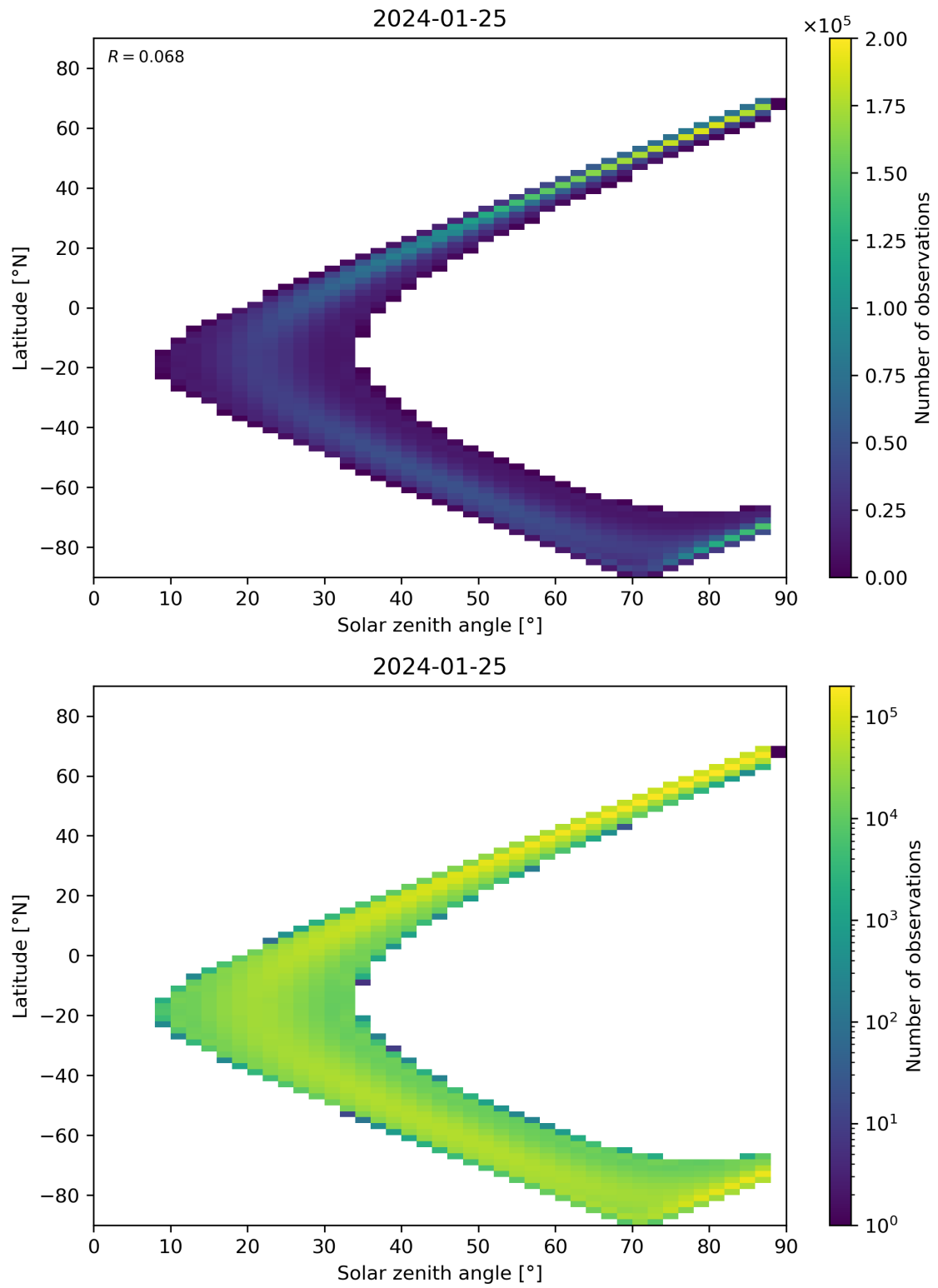
Figure 149: Scatter density plot of “Solar zenith angle” against “Latitude” for 2024-01-24 to 2024-01-26.
