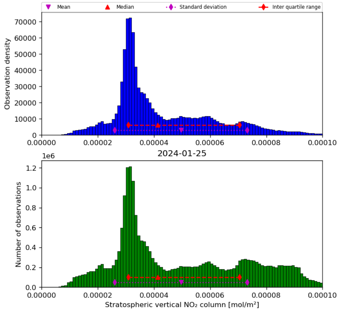
Figure 36: Histogram of “Stratospheric vertical NO 2 column” for 2024-01-24 to 2024-01-26
