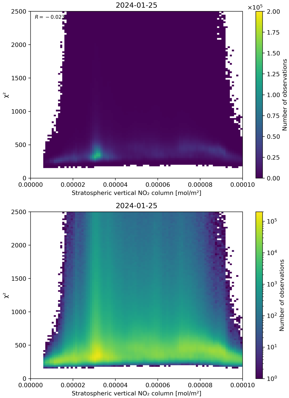
Figure 97: Scatter density plot of “Stratospheric vertical NO 2 column” against “ \chi^2 ” for 2024-01-24 to 2024-01-26.
