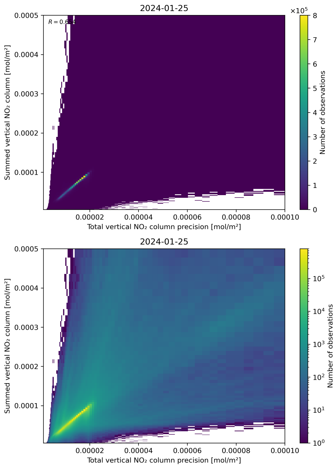
Figure 117: Scatter density plot of “Total vertical NO 2 column precision” against “Summed vertical NO 2 column” for 2024-01-24 to 2024-01-26.
