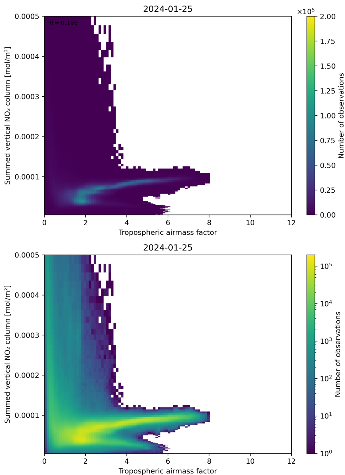
Figure 75: Scatter density plot of “Tropospheric air mass factor” against “Summed vertical NO 2 column” for 2024-01-24 to 2024-01-26.
