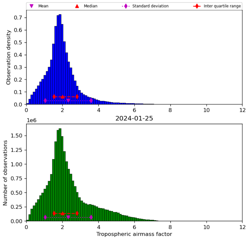
Figure 31: Histogram of “Tropospheric airmass factor” for 2024-01-24 to 2024-01-26
