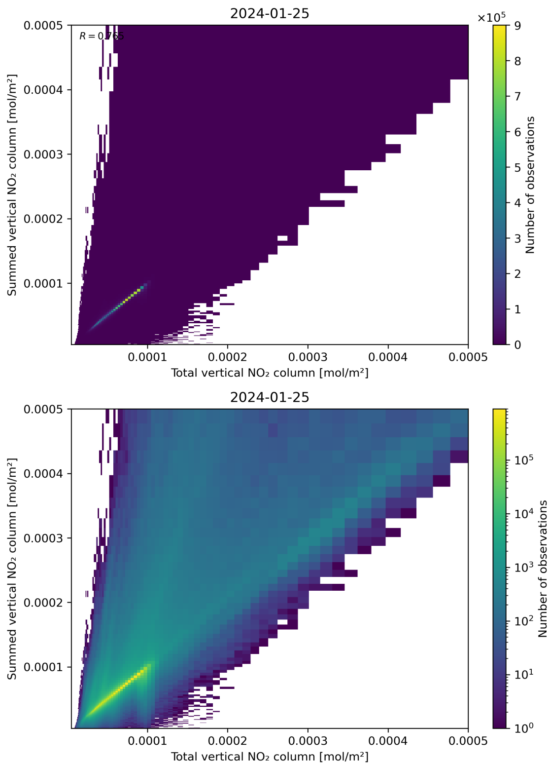
Figure 112: Scatter density plot of “Total vertical NO 2 column” against “Summed vertical NO 2 column” for 2024-01-24 to 2024-01-26.
