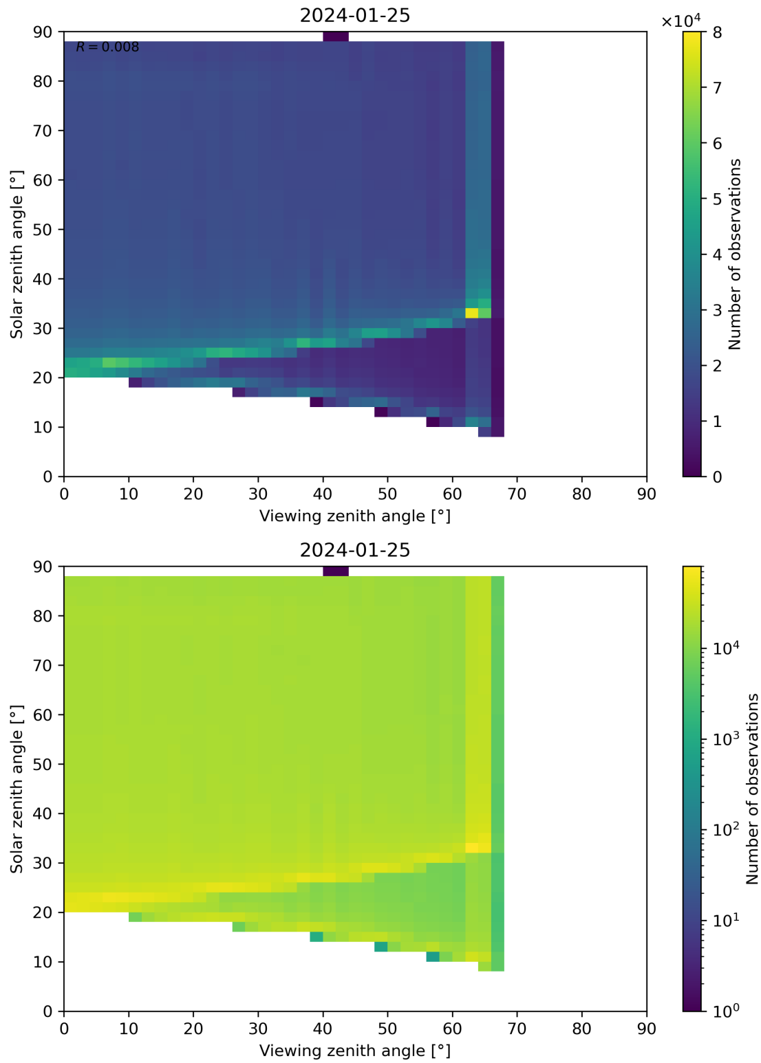
Figure 172: Scatter density plot of “Viewing zenith angle” against “Solar zenith angle” for 2024-01-24 to 2024-01-26.
