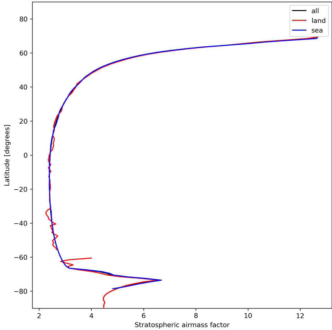
Figure 27: Zonal average of “Stratospheric airmass factor” for 2024-01-24 to 2024-01-26.
