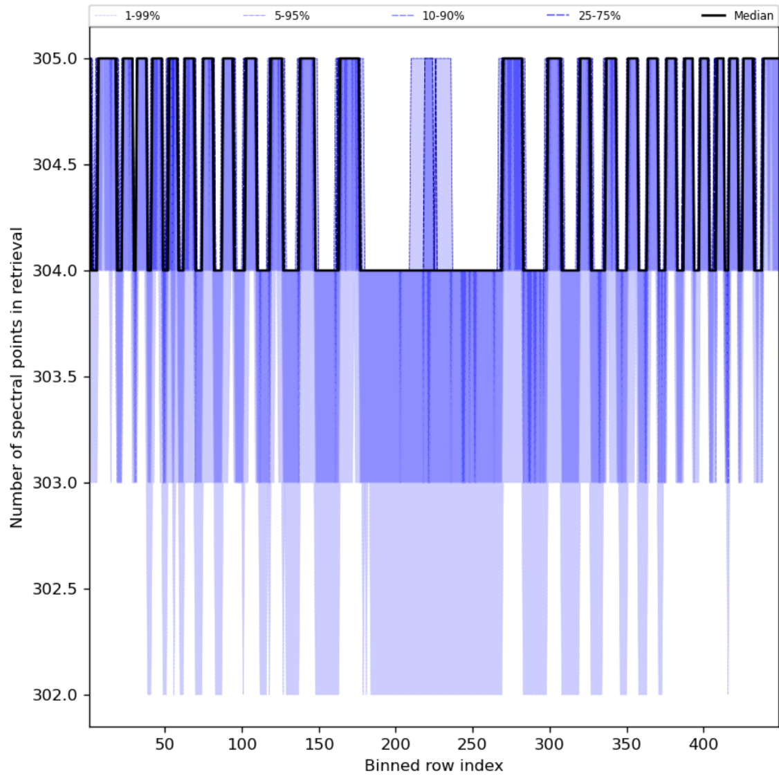
Figure 50: Along track statistics of “Number of spectral points in retrieval” for 2024-01-24 to 2024-01-26
