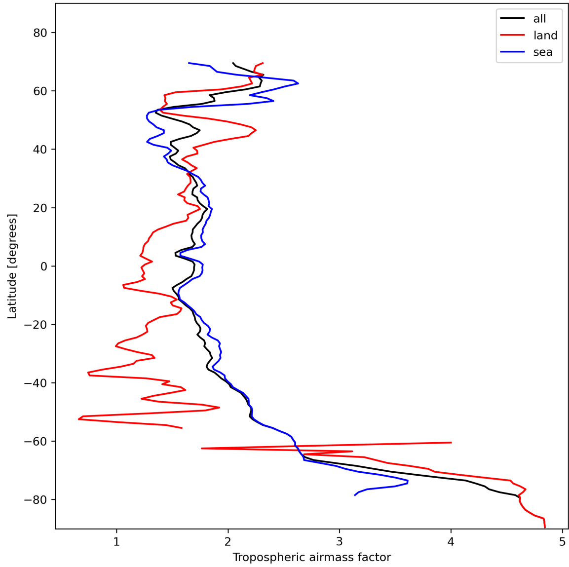
Figure 14: Zonal average of “Tropospheric airmass factor” for 2024-01-24 to 2024-01-26.
