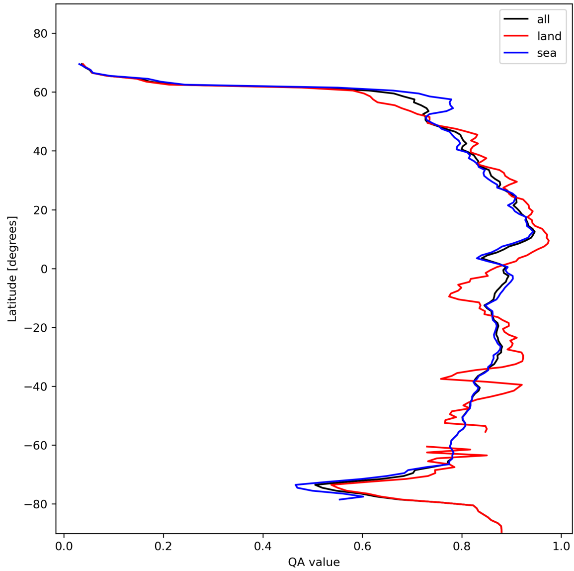
Figure 11: Zonal average of “QA value” for 2024-01-24 to 2024-01-26.
