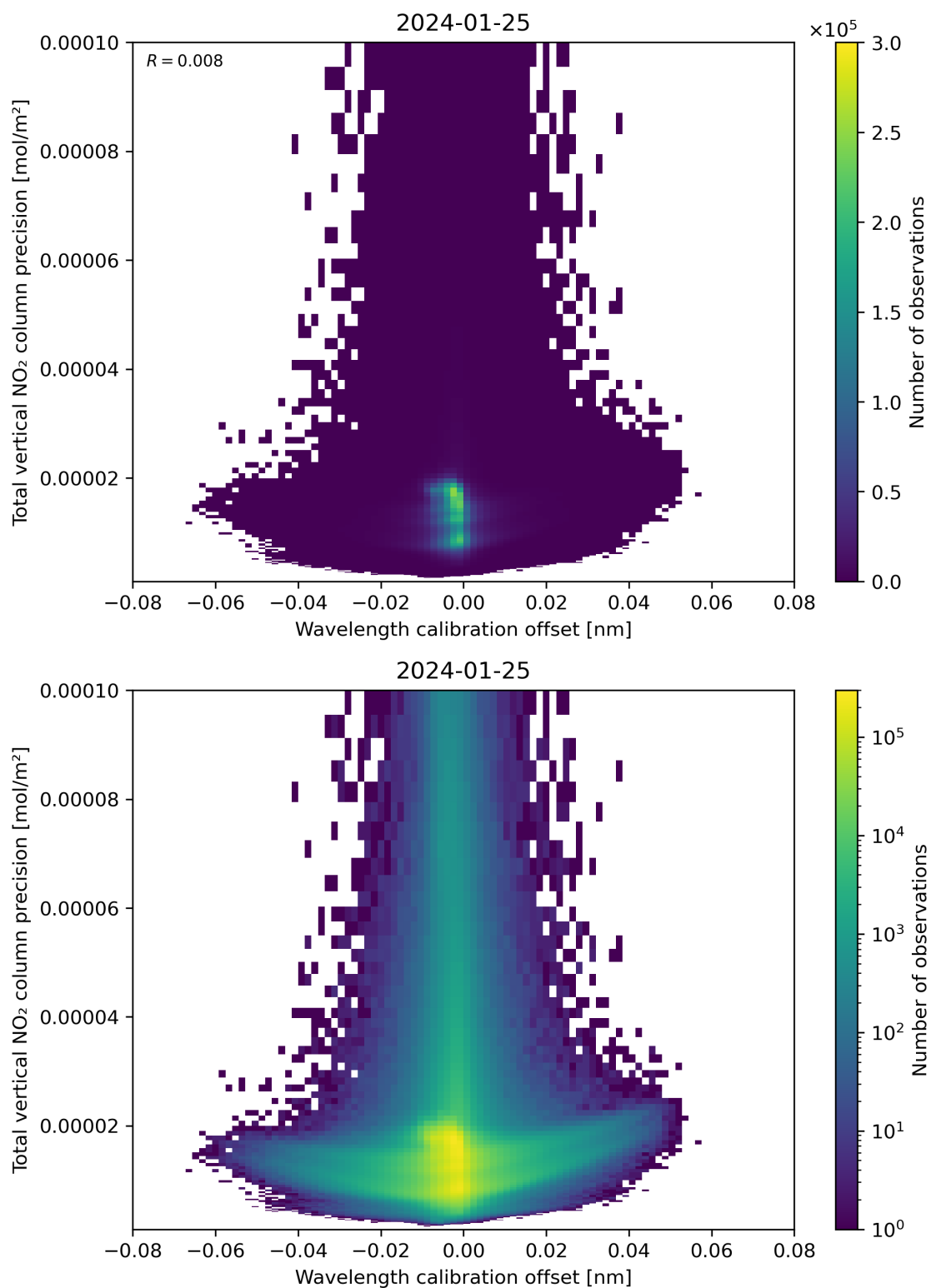
Figure 180: Scatter density plot of “Wavelength calibration offset” against “Total vertical NO 2 column precision” for 2024-01-24 to 2024-01-26.
