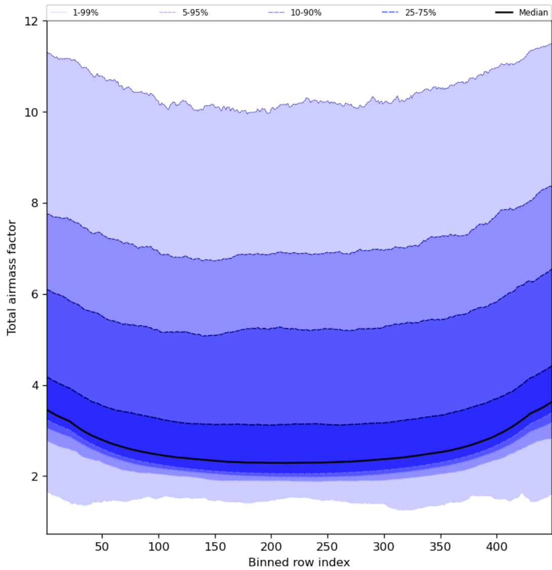
Figure 49: Along track statistics of “Total airmass factor” for 2024-01-24 to 2024-01-26
