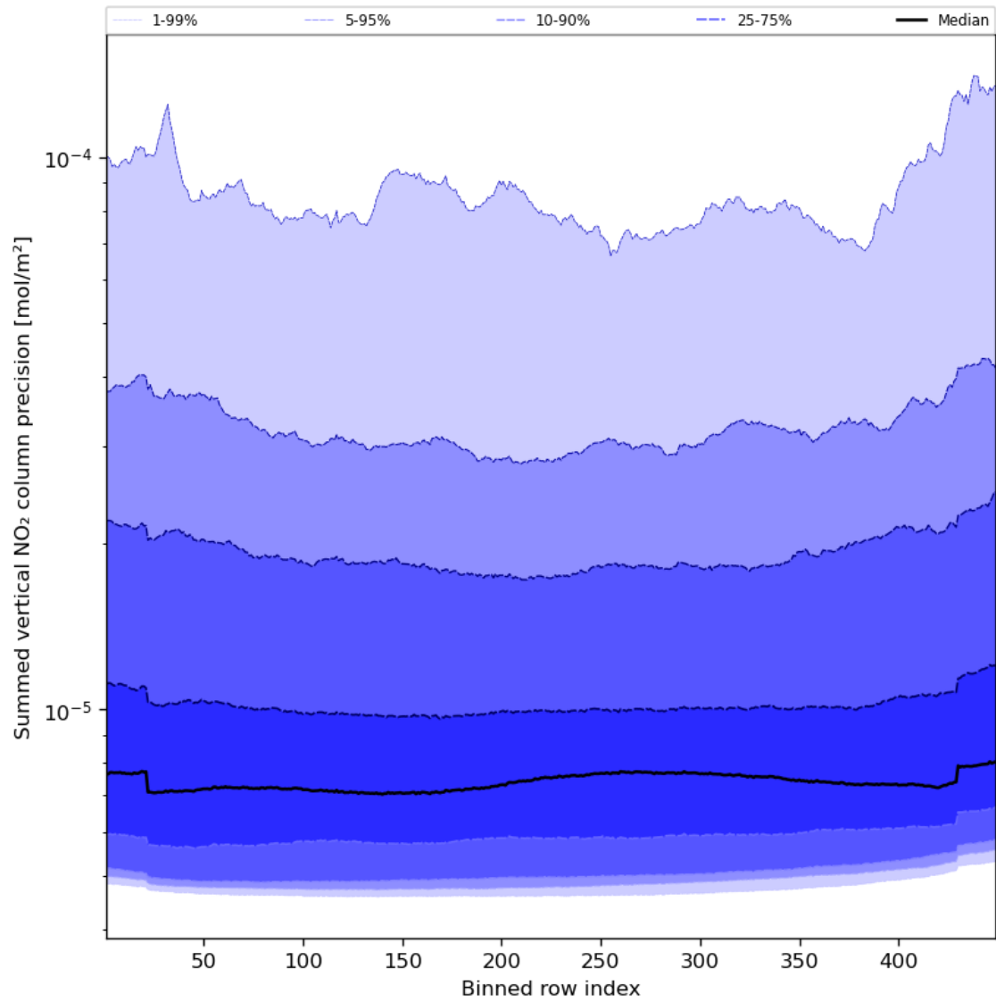
Figure 58: Along track statistics of “Summed vertical NO 2 column precision” for 2024-01-24 to 2024-01-26
