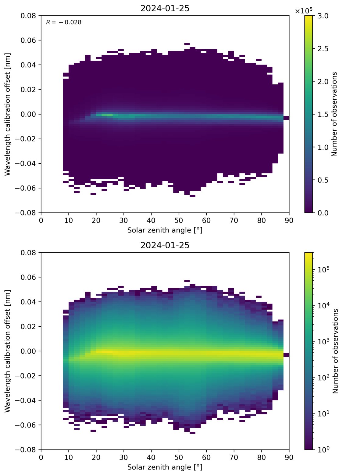
Figure 158: Scatter density plot of “Solar zenith angle” against “Wavelength calibration offset” for 2024-01-24 to 2024-01-26.
