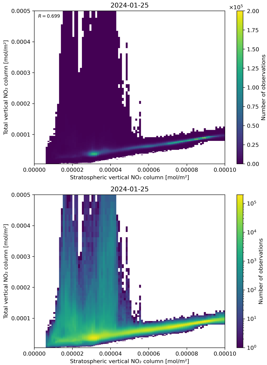
Figure 100: Scatter density plot of “Stratospheric vertical NO 2 column” against “Total vertical NO 2 column” for 2024-01-24 to 2024-01-26.
