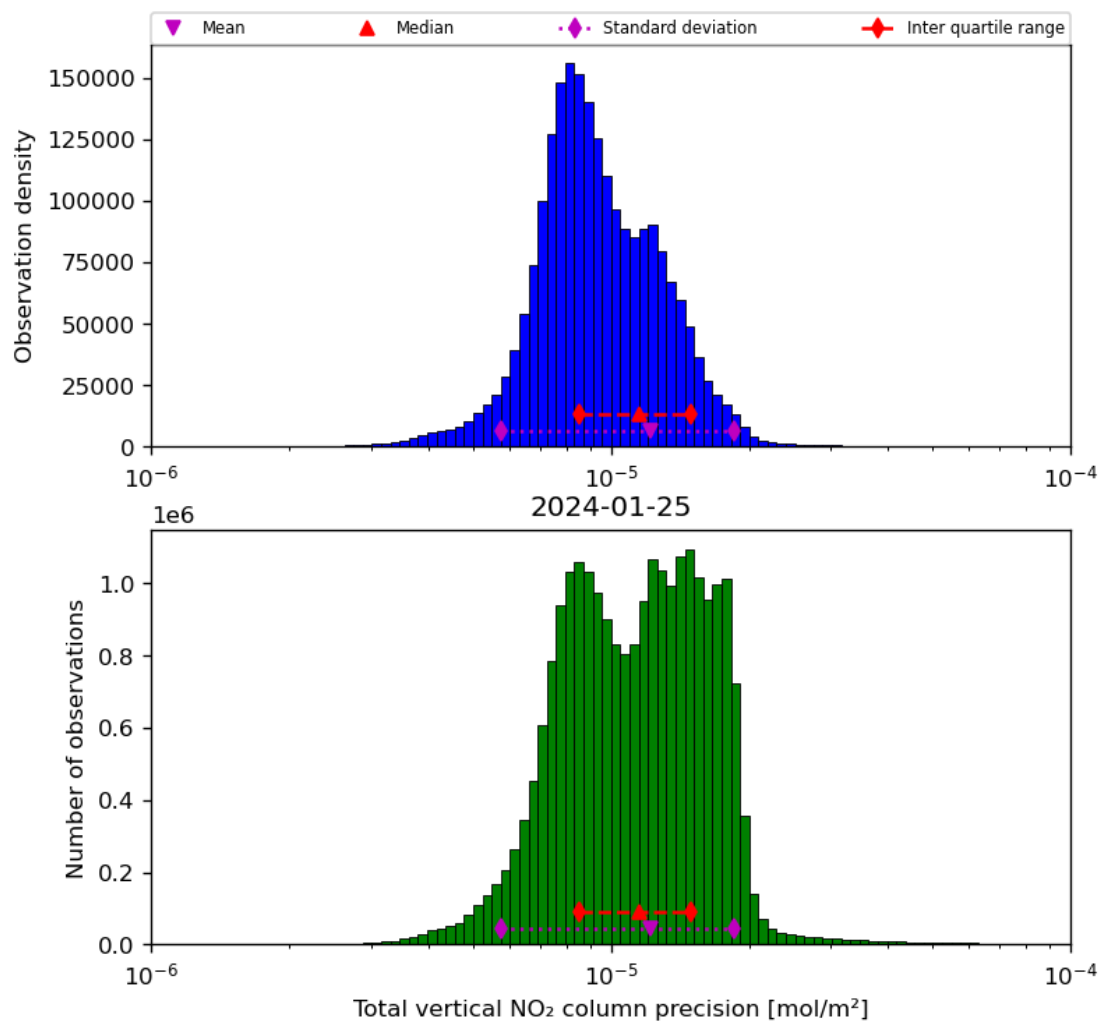
Figure 39: Histogram of “Total vertical NO 2 column precision” for 2024-01-24 to 2024-01-26
