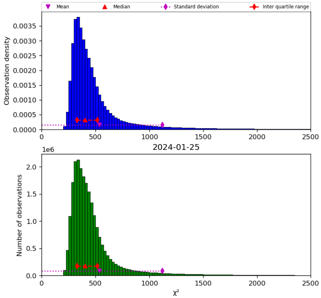
Figure 42: Histogram of " \chi^2 " for 2024-01-24 to 2024-01-26
