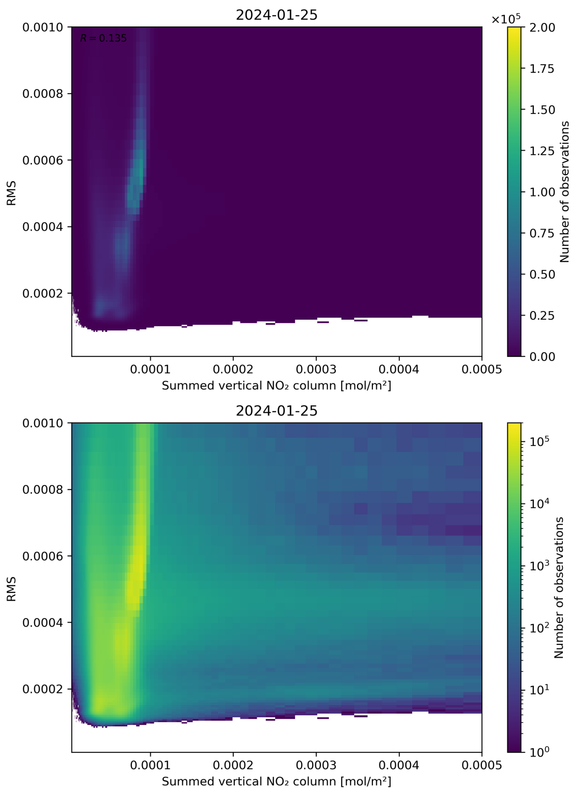
Figure 109: Scatter density plot of “Summed vertical NO 2 column” against “RMS” for 2024-01-24 to 2024-01-26.
