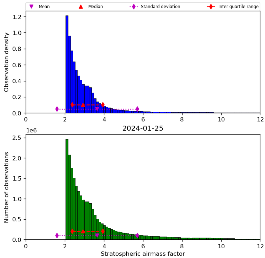
Figure 44: Histogram of “Stratospheric airmass factor” for 2024-01-24 to 2024-01-26
