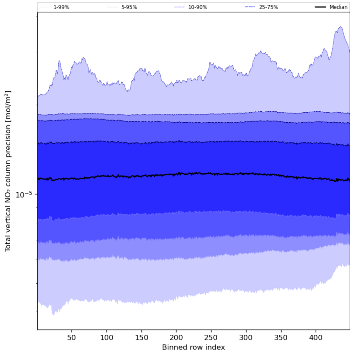
Figure 56: Along track statistics of “Total vertical NO 2 column precision” for 2024-01-24 to 2024-01-26
