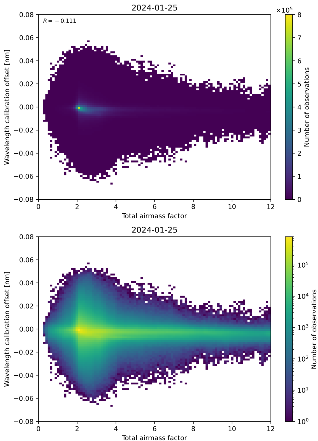
Figure 70: Scatter density plot of “Total airmass factor” against “Wavelength calibration offset” for 2024-01-24 to 2024-01-26.
