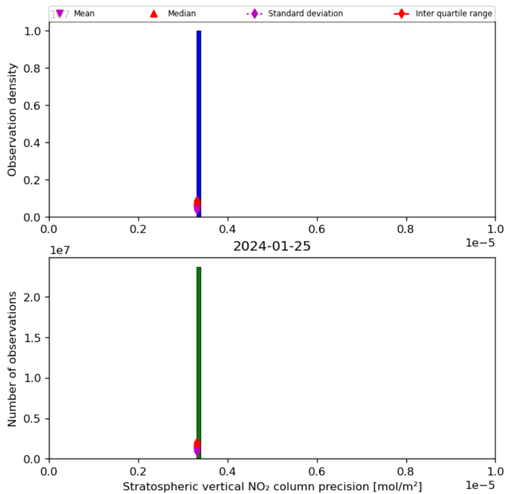
Figure 37: Histogram of “Stratospheric vertical NO 2 column precision” for 2024-01-24 to 2024-01-26
