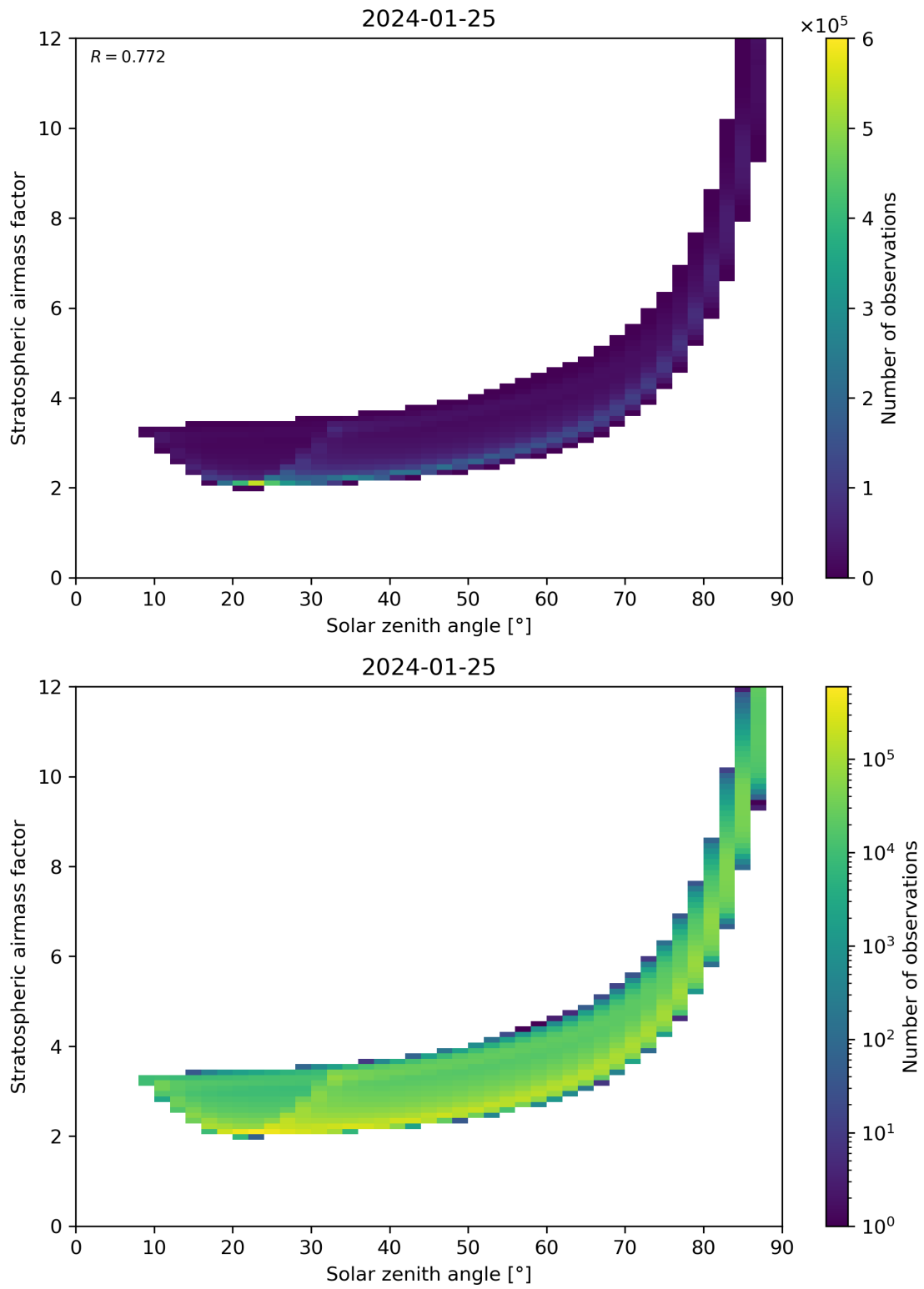
Figure 145: Scatter density plot of “Solar zenith angle” against “Stratospheric airmass factor” for 2024-01-24 to 2024-01-26.
