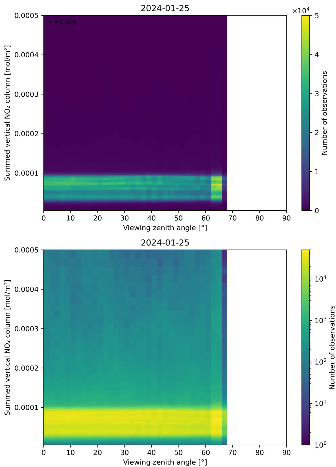
Figure 165: Scatter density plot of “Viewing zenith angle” against “Summed vertical NO 2 column” for 2024-01-24 to 2024-01-26.
