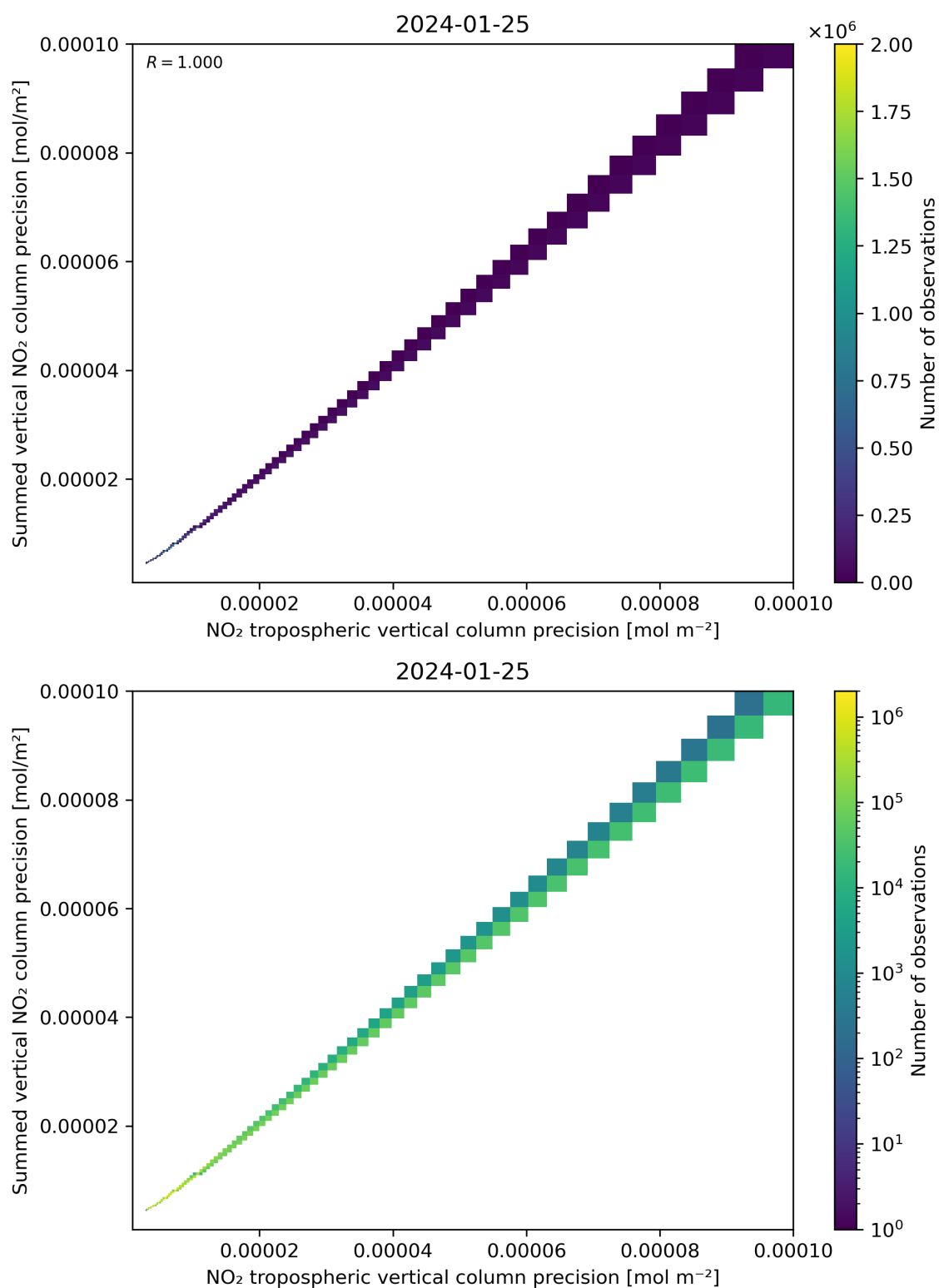
Figure 137: Scatter density plot of “NO 2 tropospheric vertical column precision” against “Summed vertical NO 2 column precision” for 2024-01-24 to 2024-01-26.
