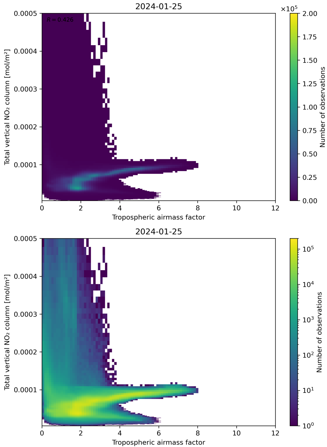
Figure 77: Scatter density plot of “Tropospheric airmass factor” against “Total vertical NO 2 column” for 2024-01-24 to 2024-01-26.
