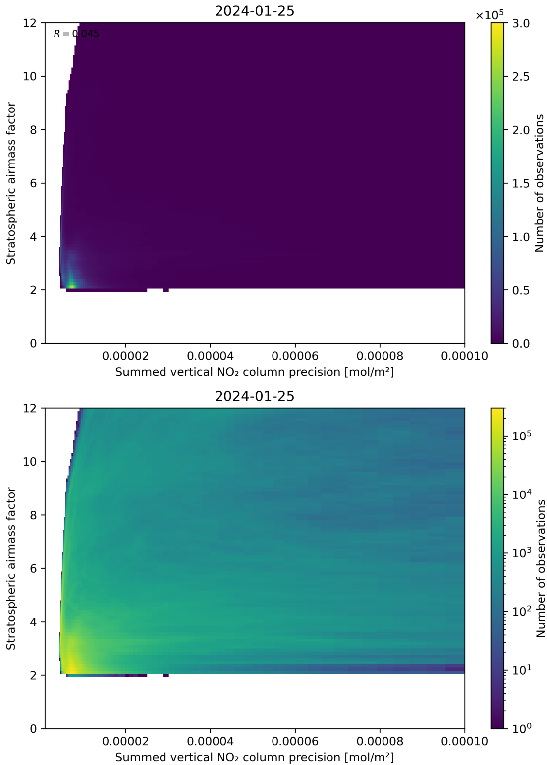
Figure 106: Scatter density plot of “Summed vertical NO 2 column precision” against “Stratospheric airmass factor” for 2024-01-24 to 2024-01-26.
