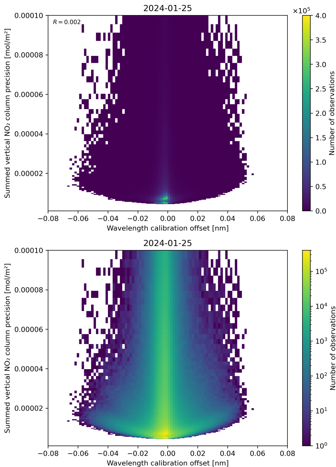
Figure 178: Scatter density plot of “Wavelength calibration offset” against “Summed vertical NO 2 column precision” for 2024-01-24 to 2024-01-26.
