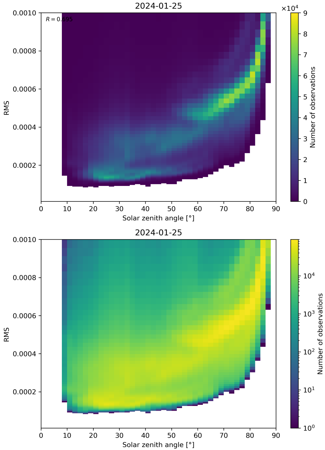
Figure 157: Scatter density plot of “Solar zenith angle” against “RMS” for 2024-01-24 to 2024-01-26.
