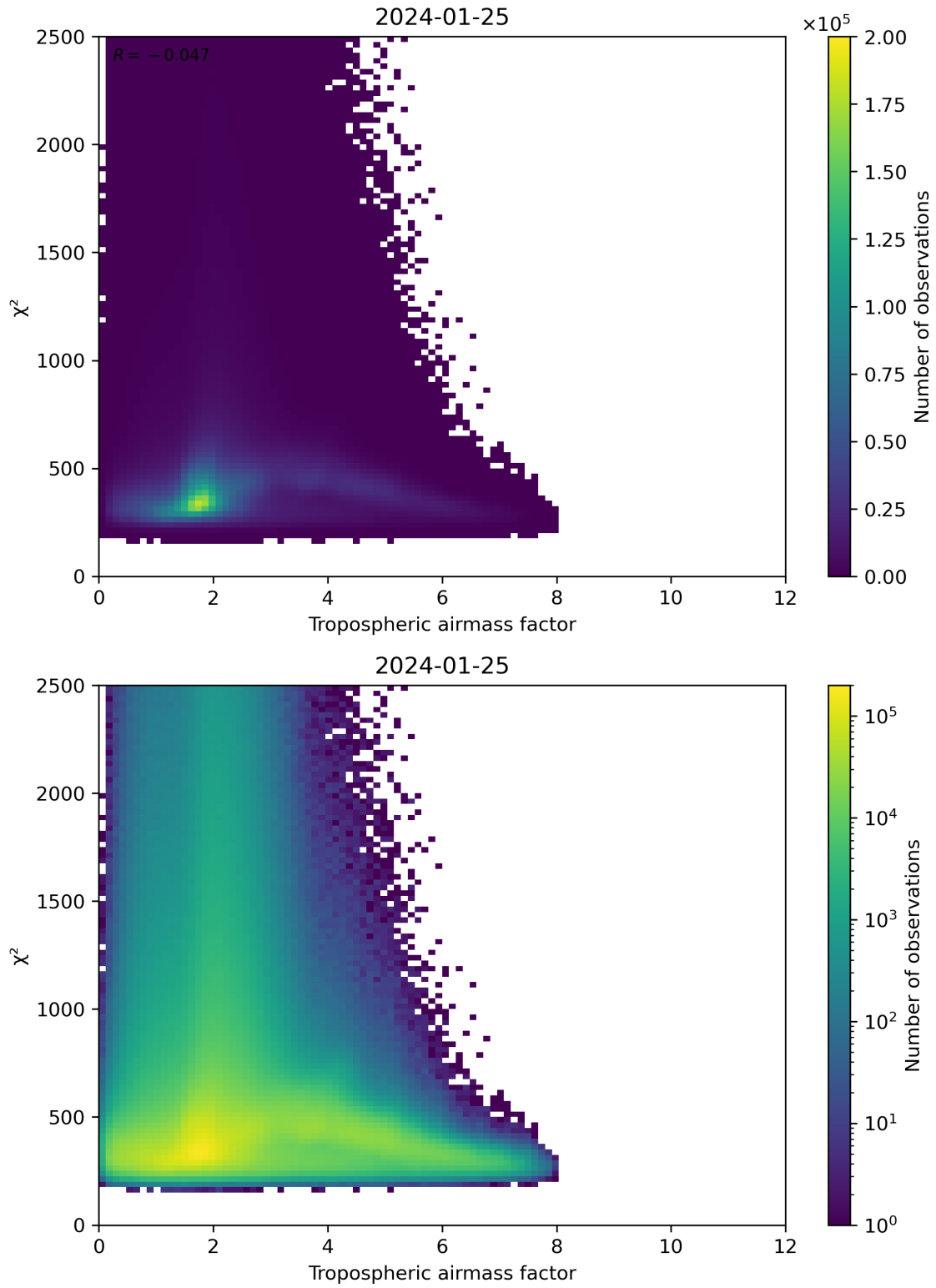
Figure 73: Scatter density plot of “Tropospheric airmass factor” against “ \chi^2 ” for 2024-01-24 to 2024-01-26.
