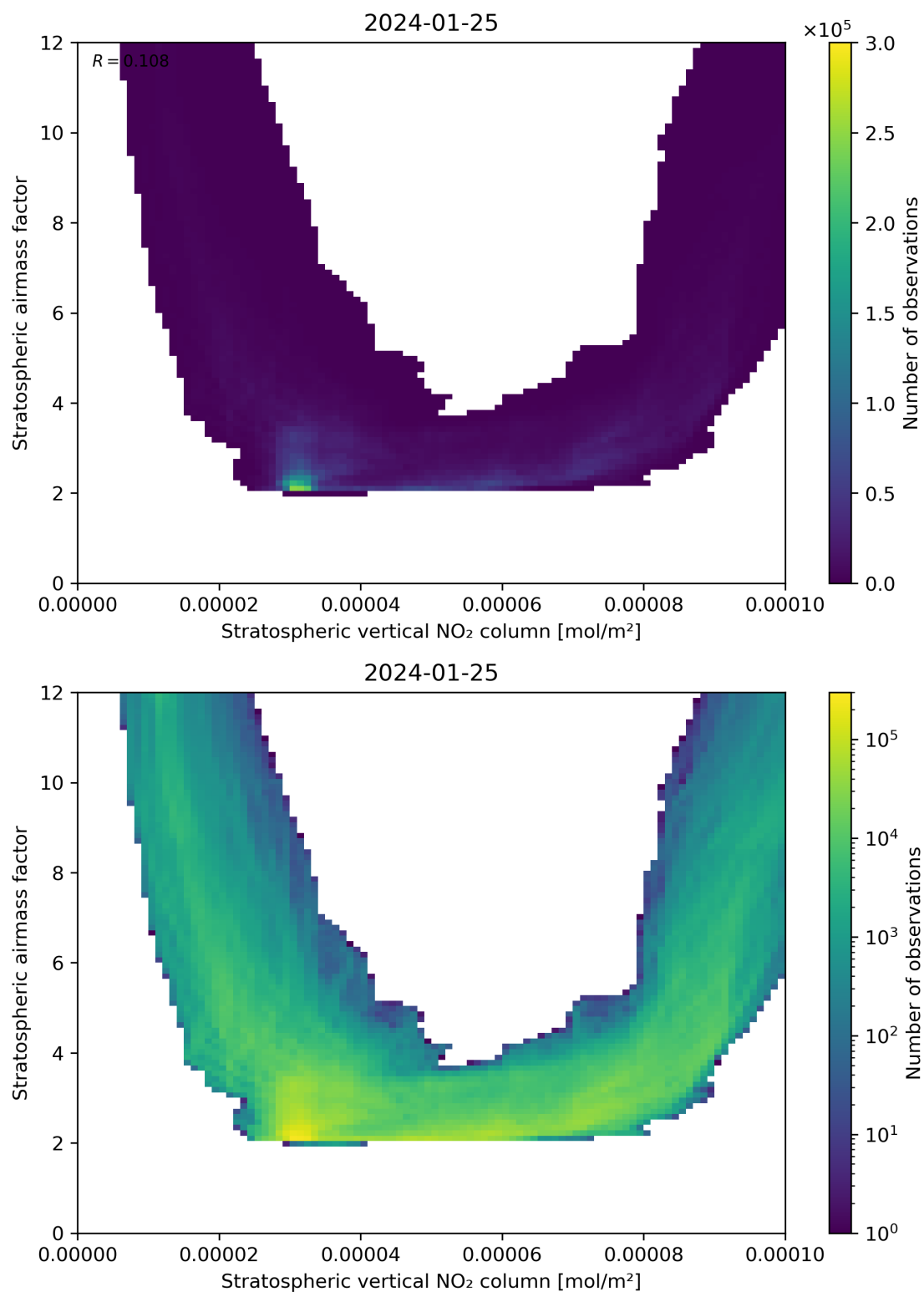
Figure 96: Scatter density plot of “Stratospheric vertical NO 2 column” against “Stratospheric airmass factor” for 2024-01-24 to 2024-01-26.
