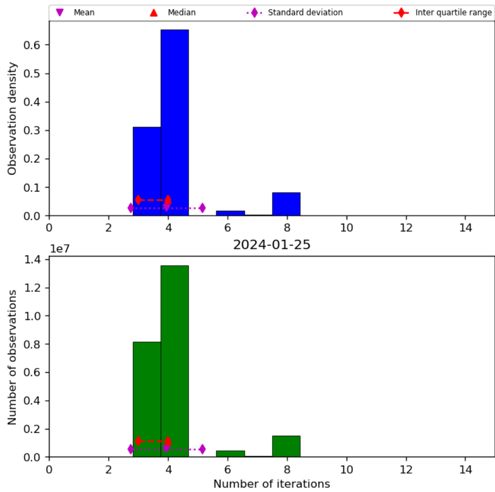
Figure 34: Histogram of “Number of iterations” for 2024-01-24 to 2024-01-26
