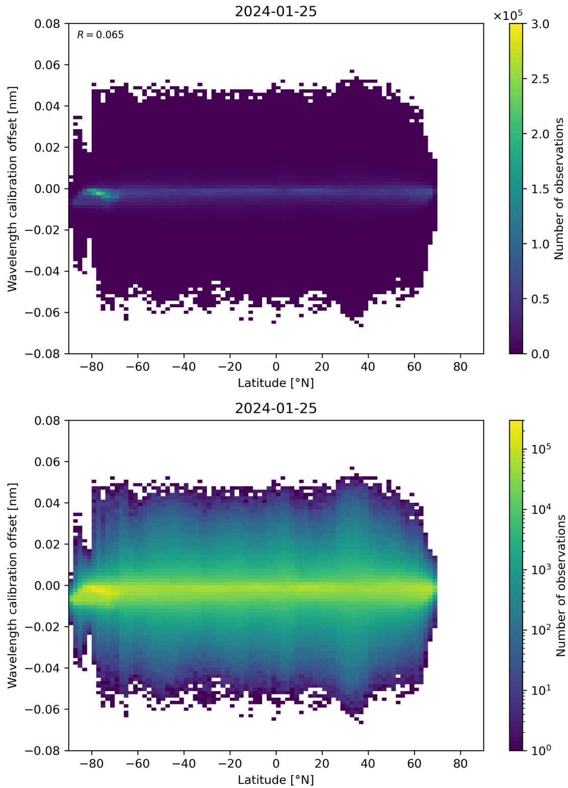
Figure 95: Scatter density plot of “Latitude” against “Wavelength calibration offset” for 2024-01-24 to 2024-01-26.
