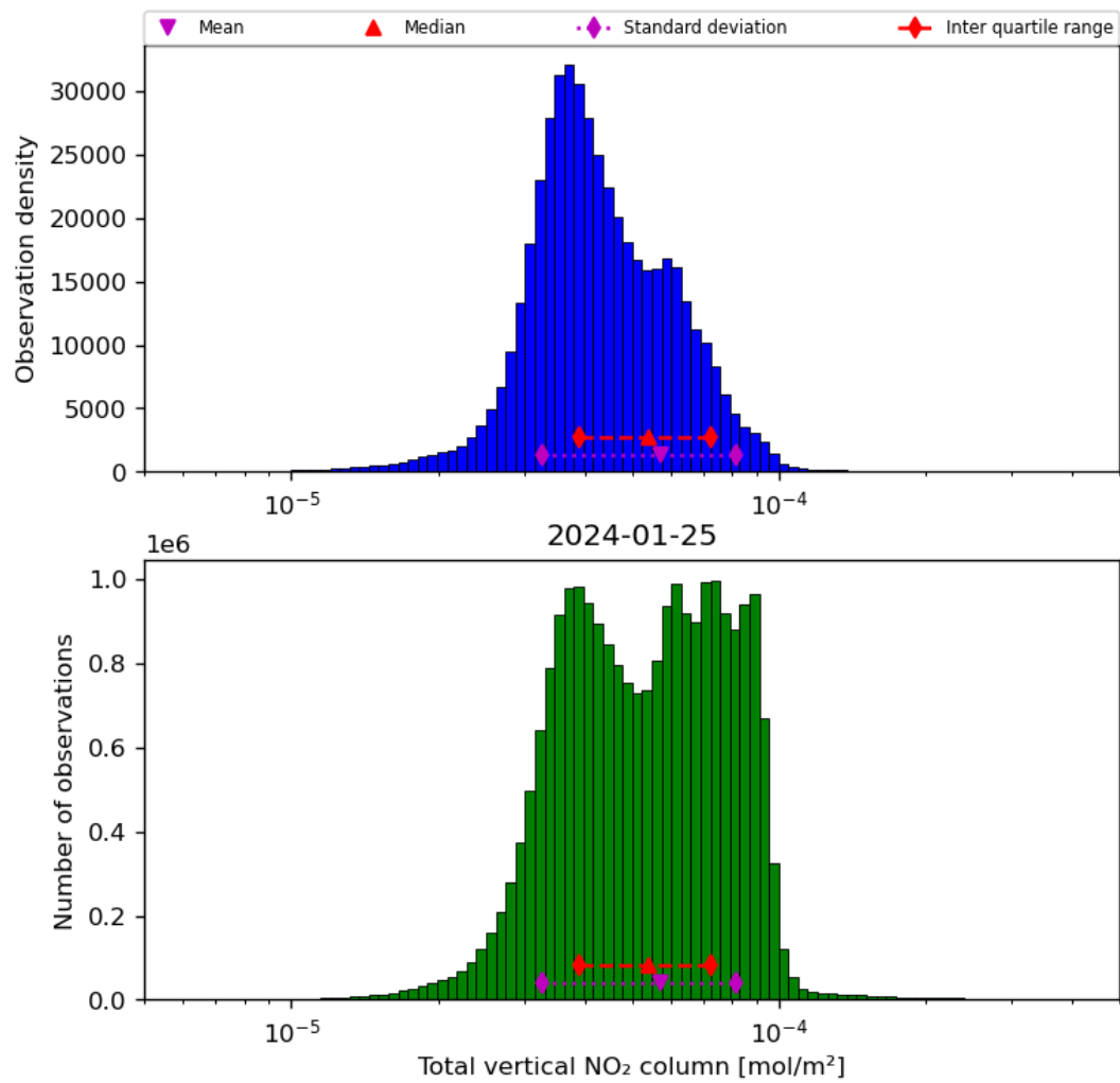
Figure 38: Histogram of "Total vertical NO 2 column" for 2024-01-24 to 2024-01-26
