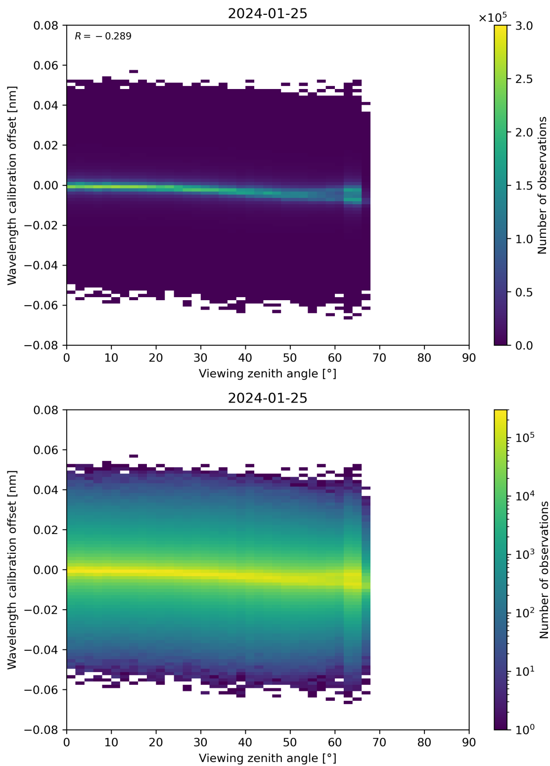
Figure 173: Scatter density plot of “Viewing zenith angle” against “Wavelength calibration offset” for 2024-01-24 to 2024-01-26.
