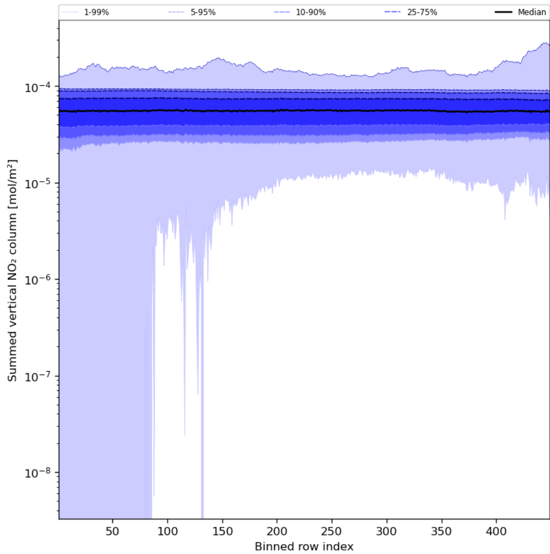
Figure 57: Along track statistics of “Summed vertical NO 2 column” for 2024-01-24 to 2024-01-26
