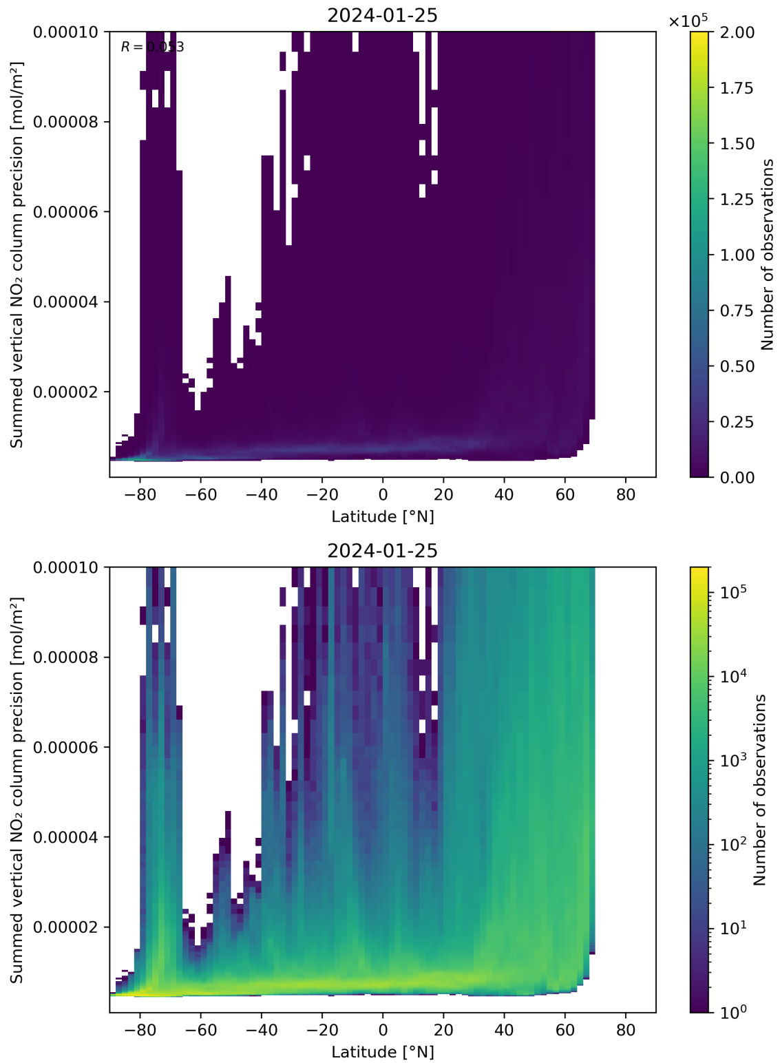
Figure 89: Scatter density plot of “Latitude” against “Summed vertical NO 2 column precision” for 2024-01-24 to 2024-01-26.
