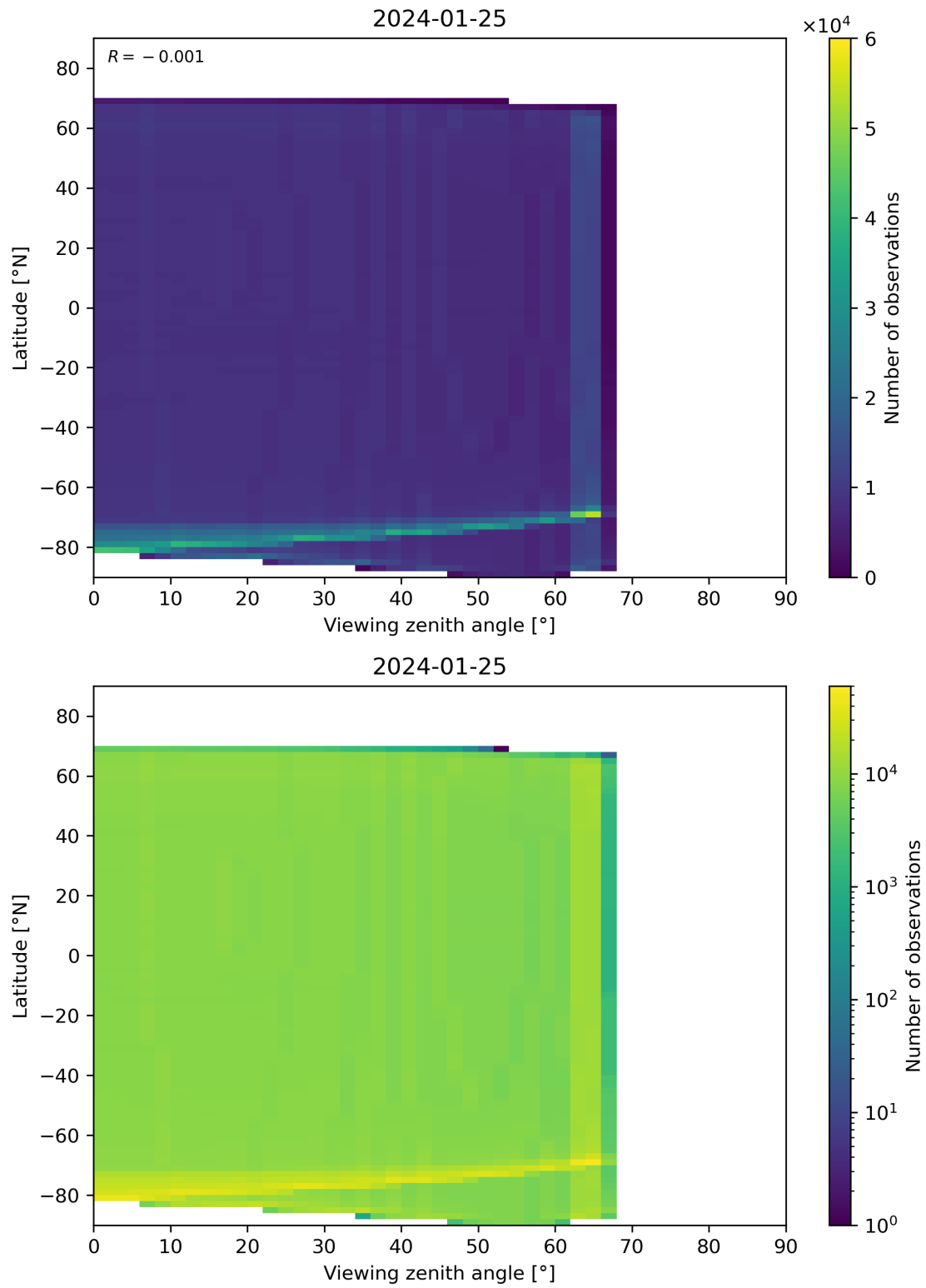
Figure 163: Scatter density plot of “Viewing zenith angle” against “Latitude” for 2024-01-24 to 2024-01-26.
