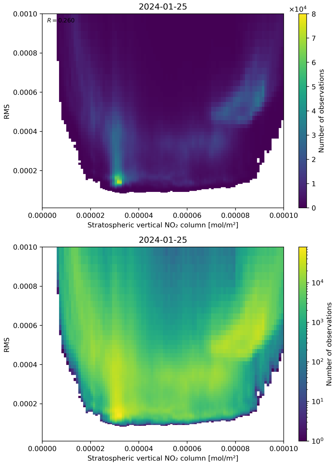
Figure 102: Scatter density plot of “Stratospheric vertical NO 2 column” against “RMS” for 2024-01-24 to 2024-01-26.
