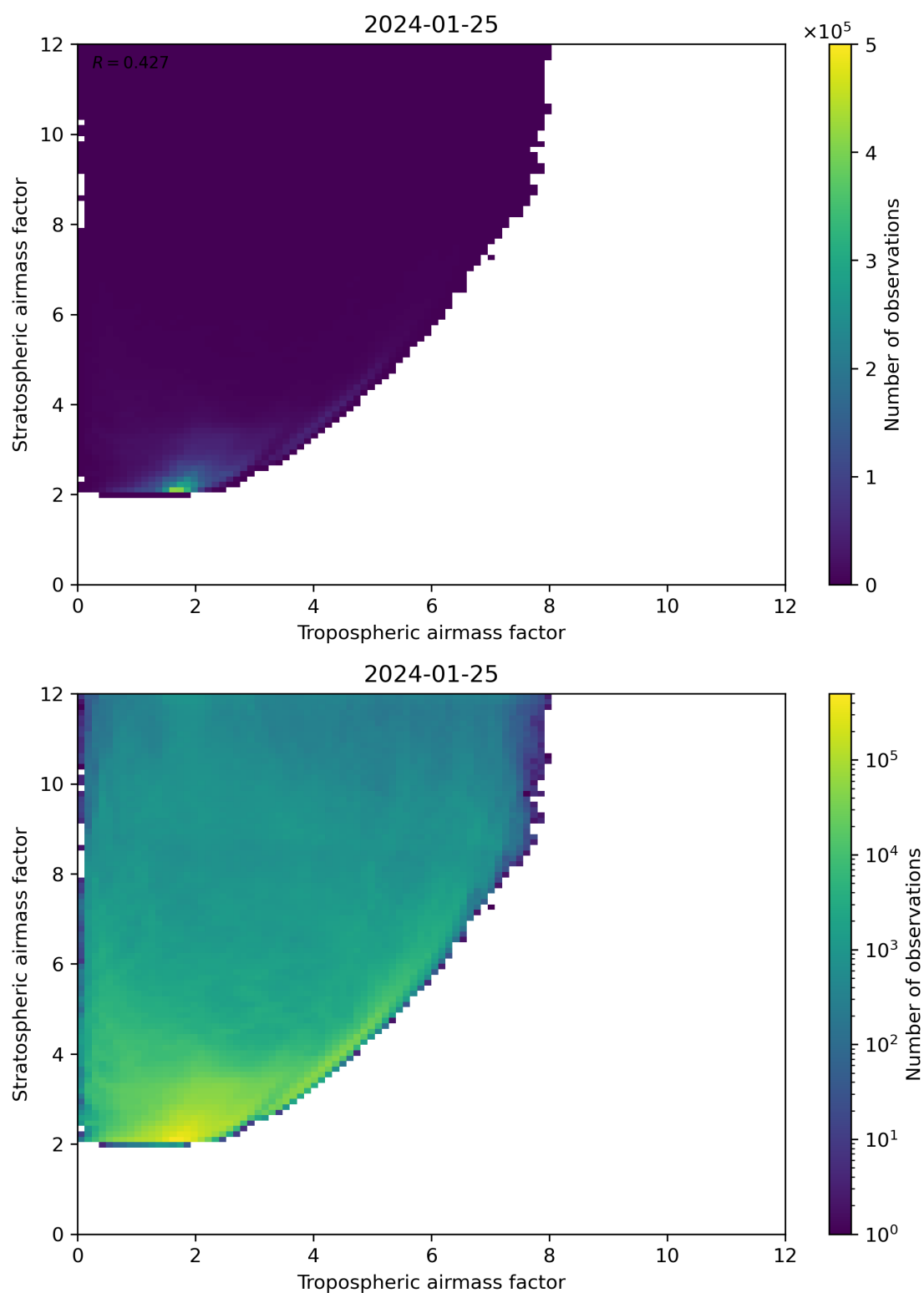
Figure 71: Scatter density plot of “Tropospheric airmass factor” against “Stratospheric airmass factor” for 2024-01-24 to 2024-01-26.
