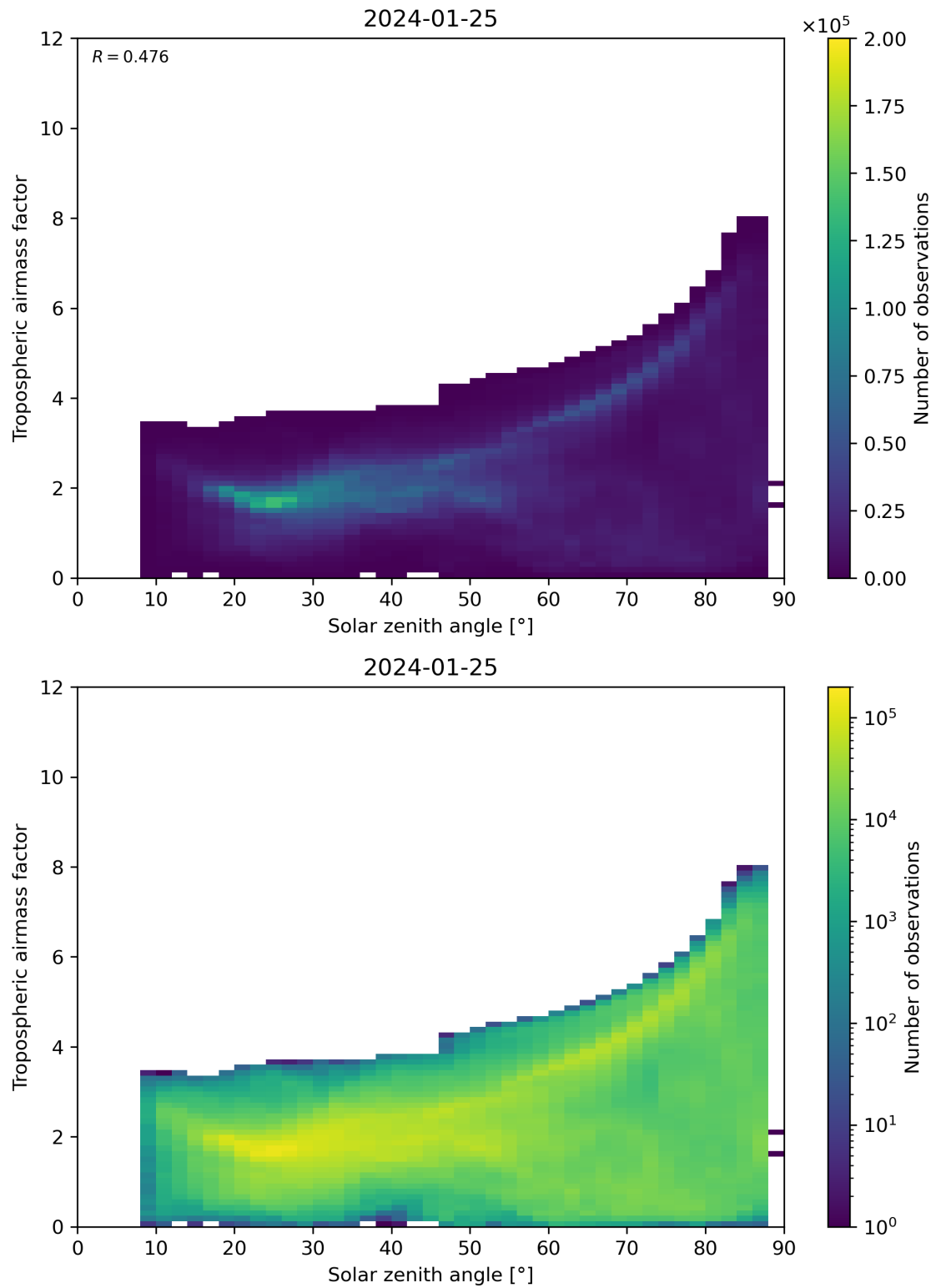
Figure 147: Scatter density plot of “Solar zenith angle” against “Tropospheric airmass factor” for 2024-01-24 to 2024-01-26.
