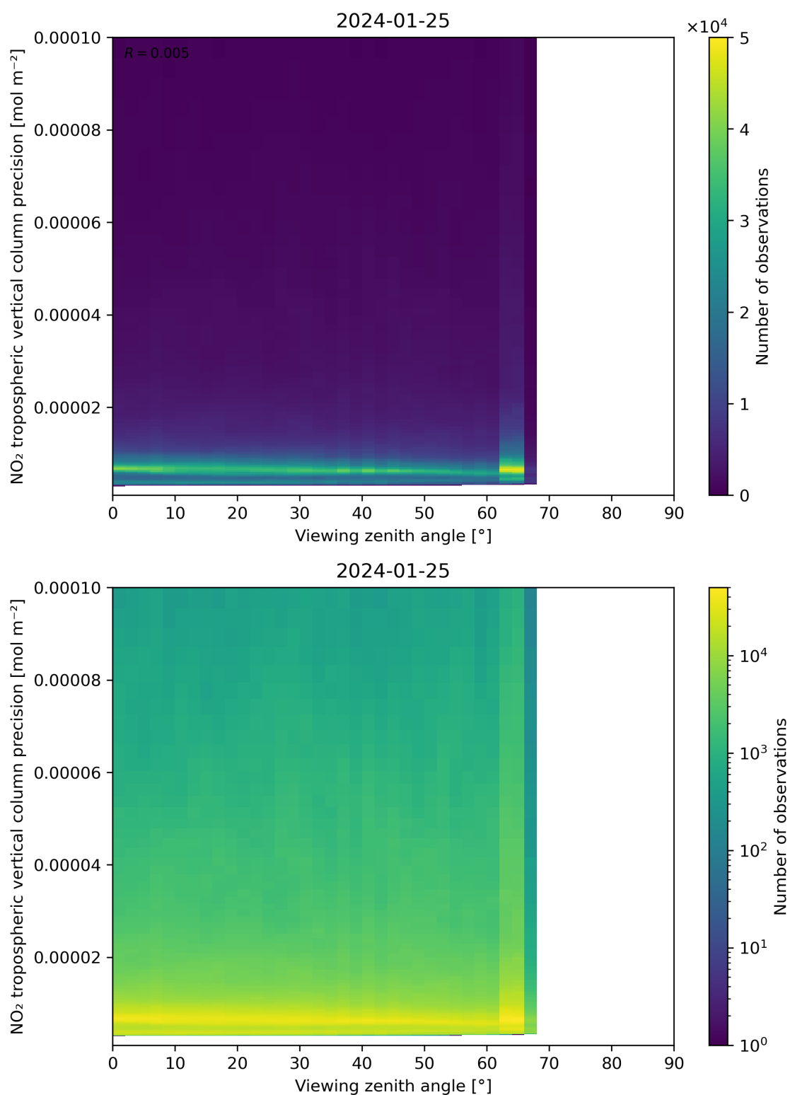
Figure 170: Scatter density plot of “Viewing zenith angle” against “NO 2 tropospheric vertical column precision” for 2024-01-24 to 2024-01-26.
