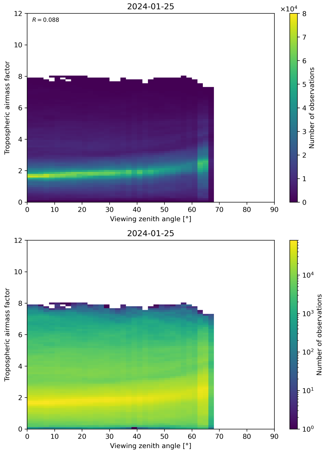
Figure 161: Scatter density plot of “Viewing zenith angle” against “Tropospheric airmass factor” for 2024-01-24 to 2024-01-26.
