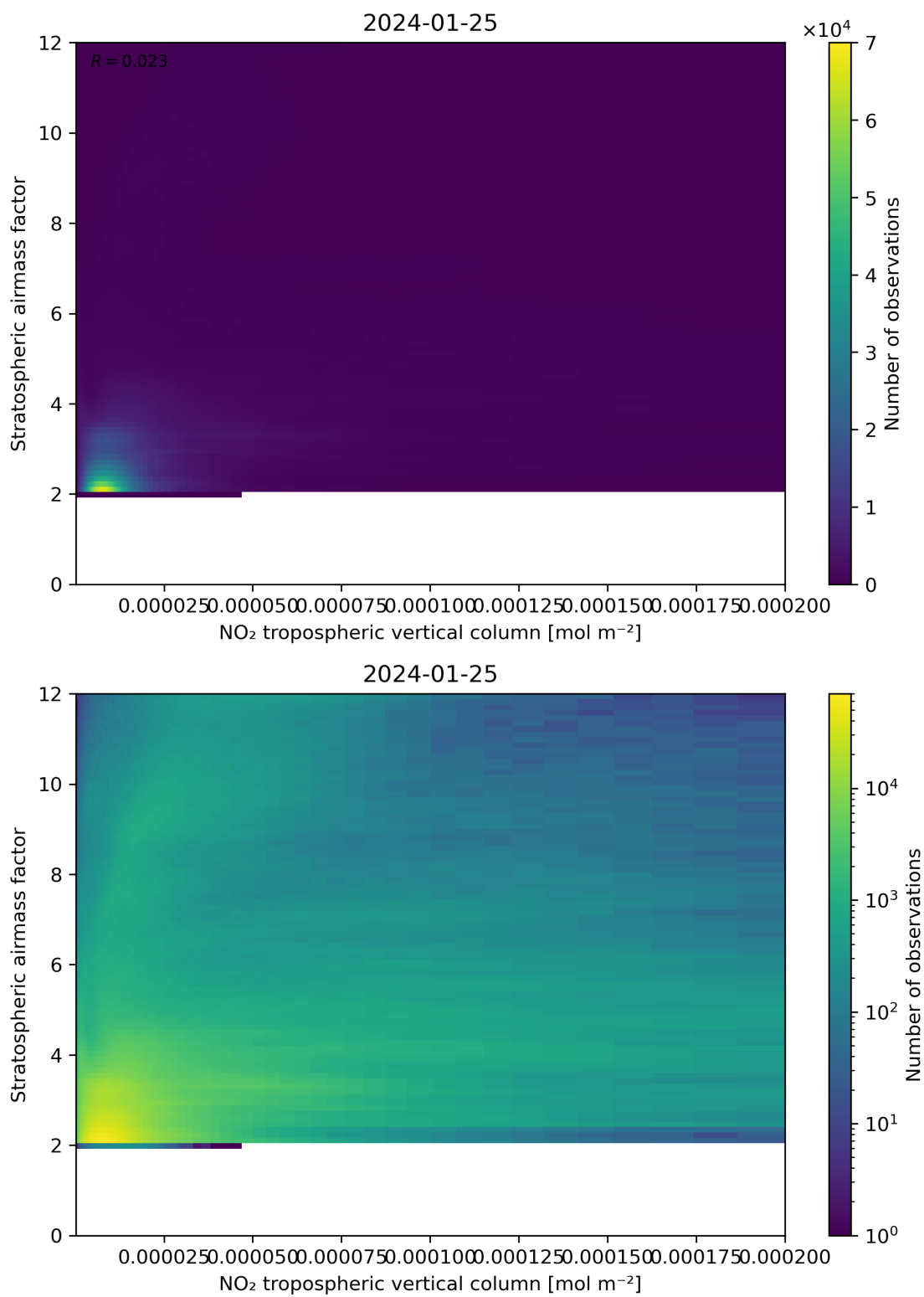
Figure 121: Scatter density plot of “NO 2 tropospheric vertical column” against “Stratospheric airmass factor” for 2024-01-24 to 2024-01-26.
