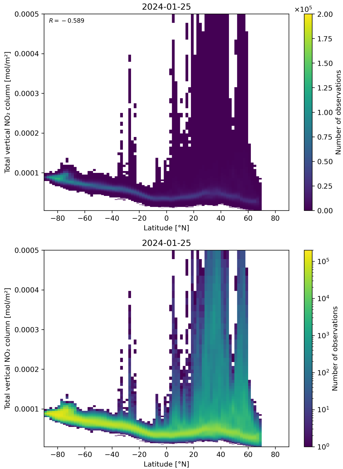
Figure 90: Scatter density plot of “Latitude” against “Total vertical NO 2 column” for 2024-01-24 to 2024-01-26.
