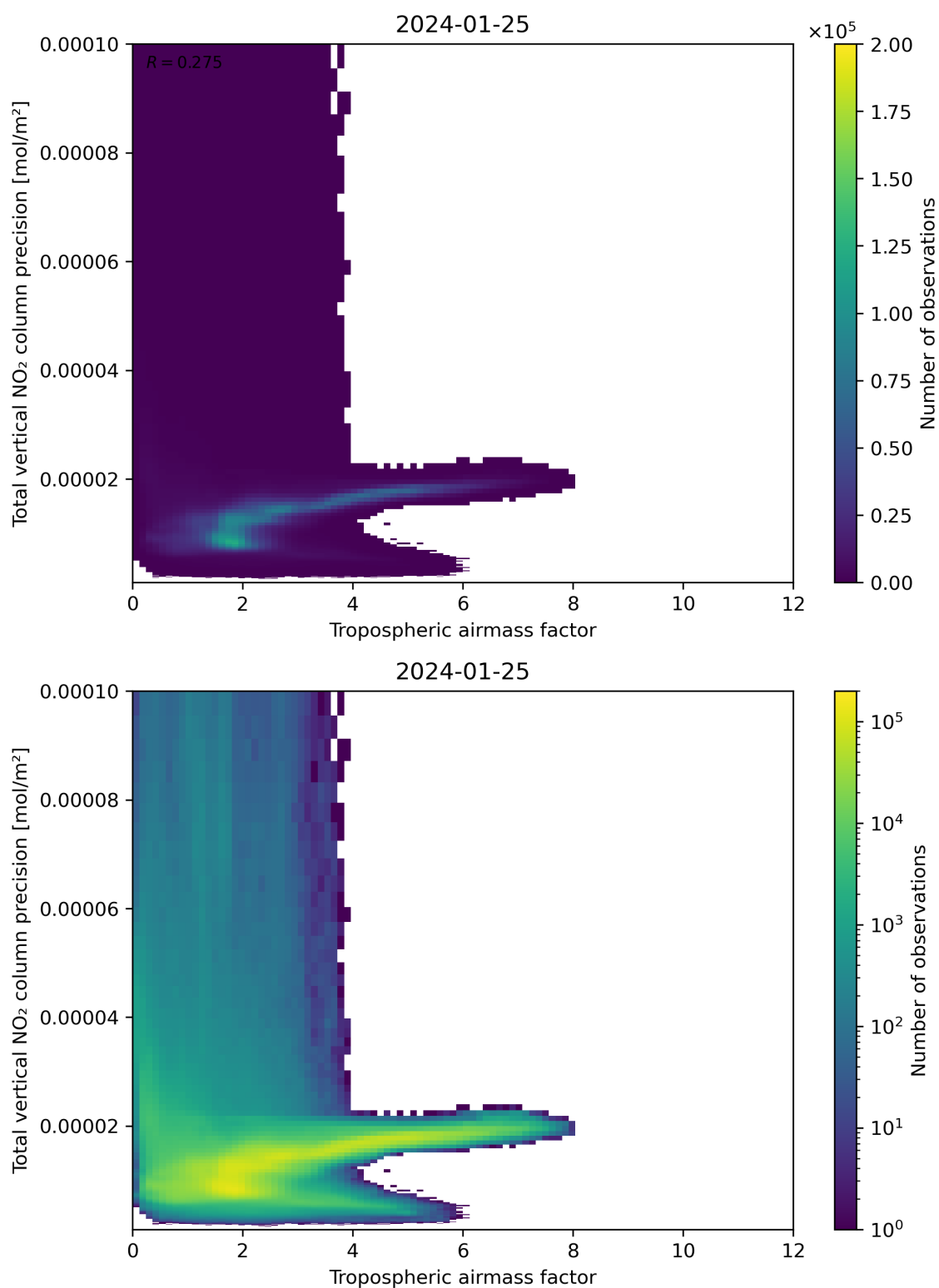
Figure 78: Scatter density plot of “Tropospheric air mass factor” against “Total vertical NO 2 column precision” for 2024-01-24 to 2024-01-26.
