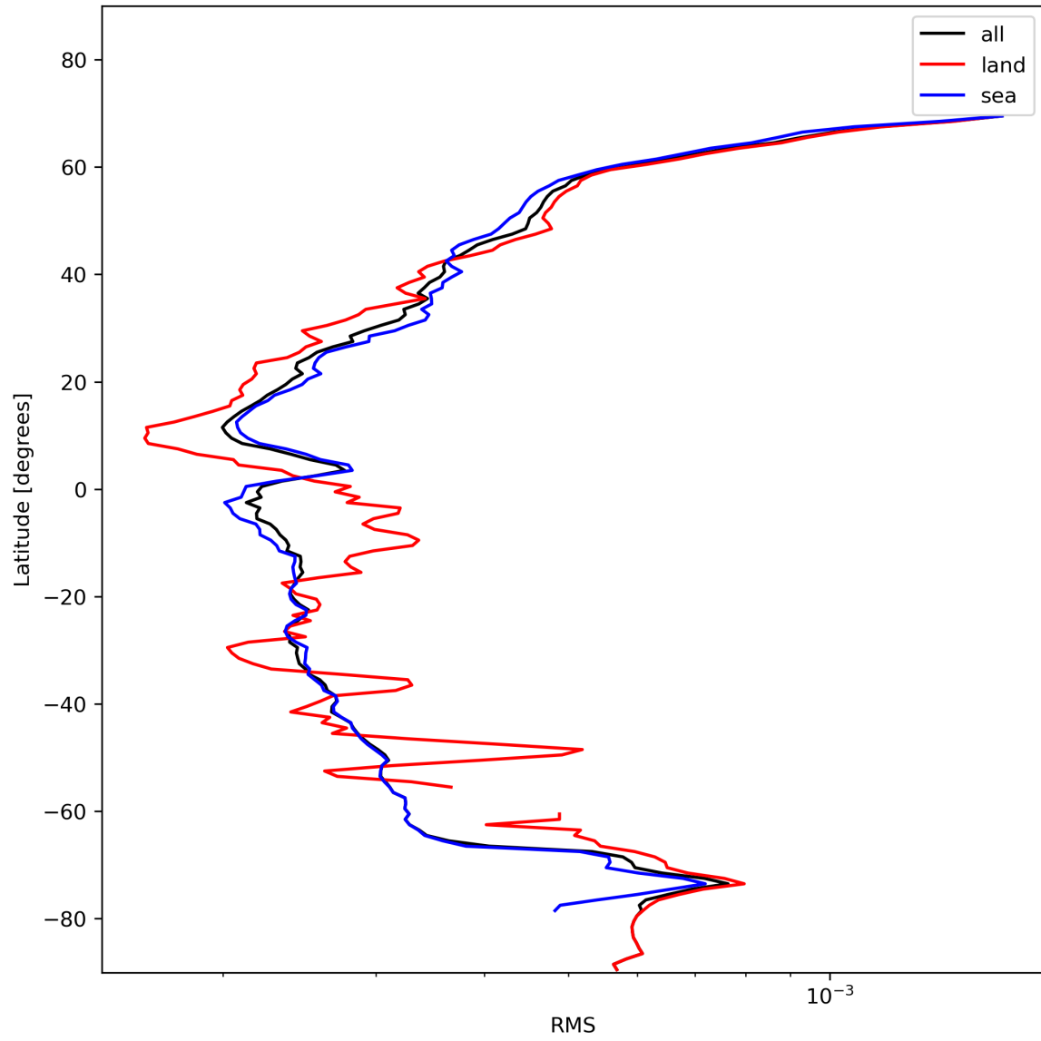
Figure 26: Zonal average of “RMS” for 2024-01-24 to 2024-01-26.
