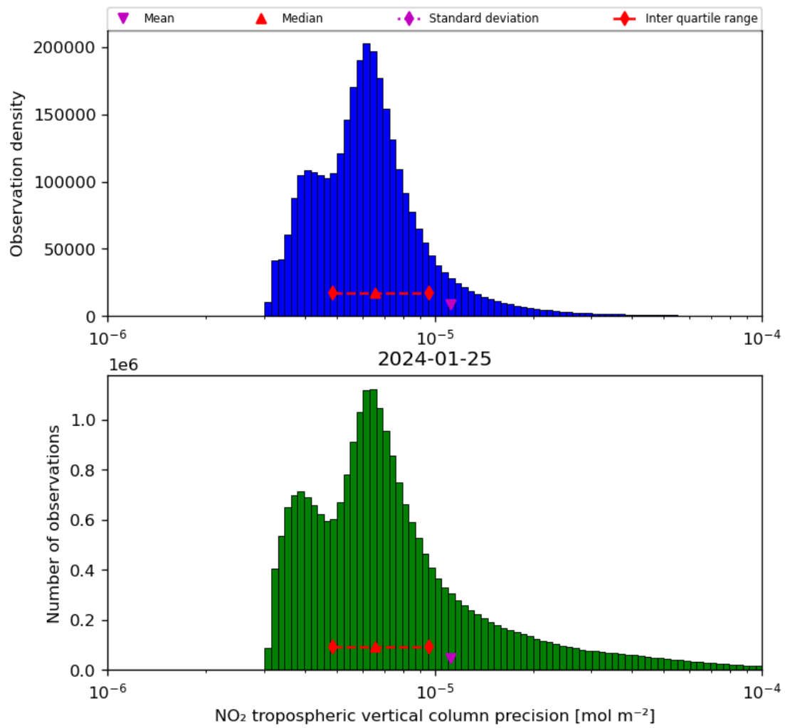
Figure 30: Histogram of “NO 2 tropospheric vertical column precision” for 2024-01-24 to 2024-01-26
