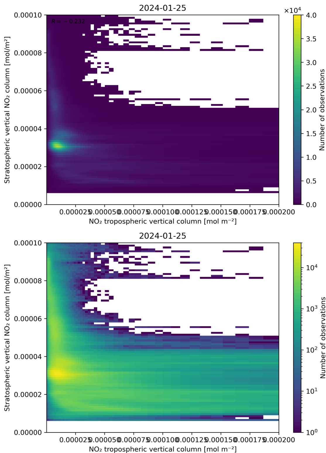
Figure 125: Scatter density plot of “NO 2 tropospheric vertical column” against “Stratospheric vertical NO 2 column” for 2024-01-24 to 2024-01-26.
