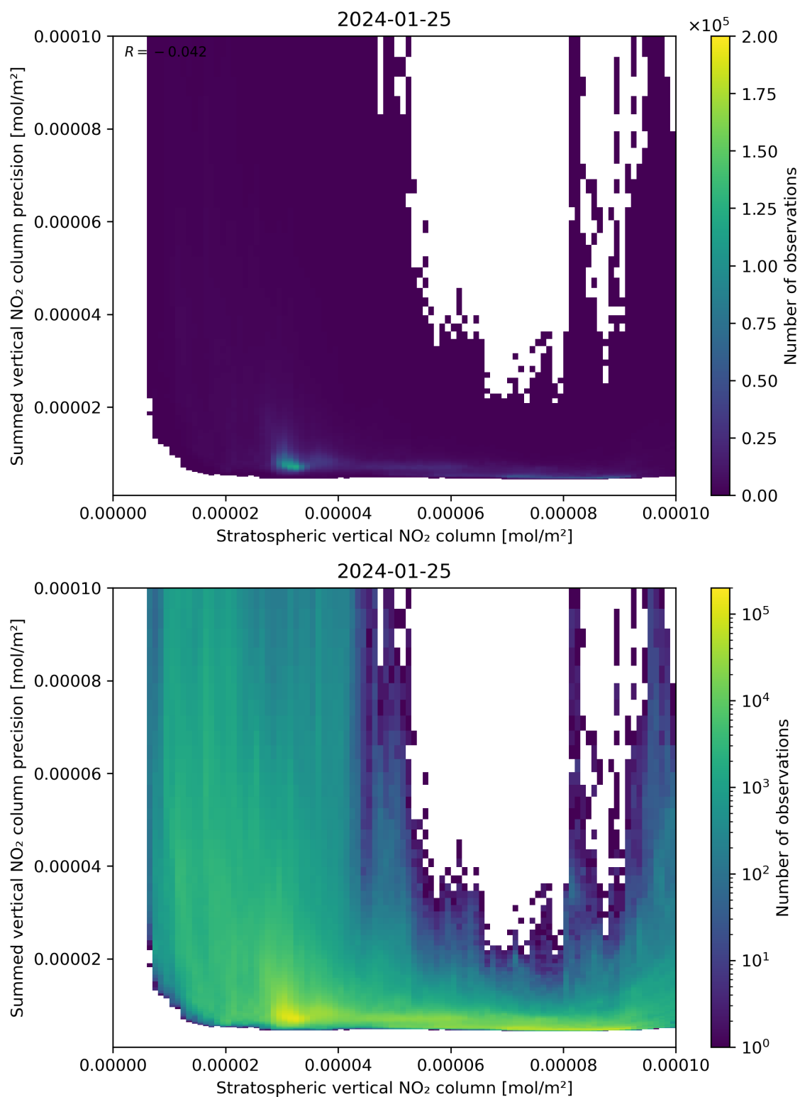
Figure 99: Scatter density plot of “Stratospheric vertical NO 2 column” against “Summed vertical NO 2 column precision” for 2024-01-24 to 2024-01-26.
