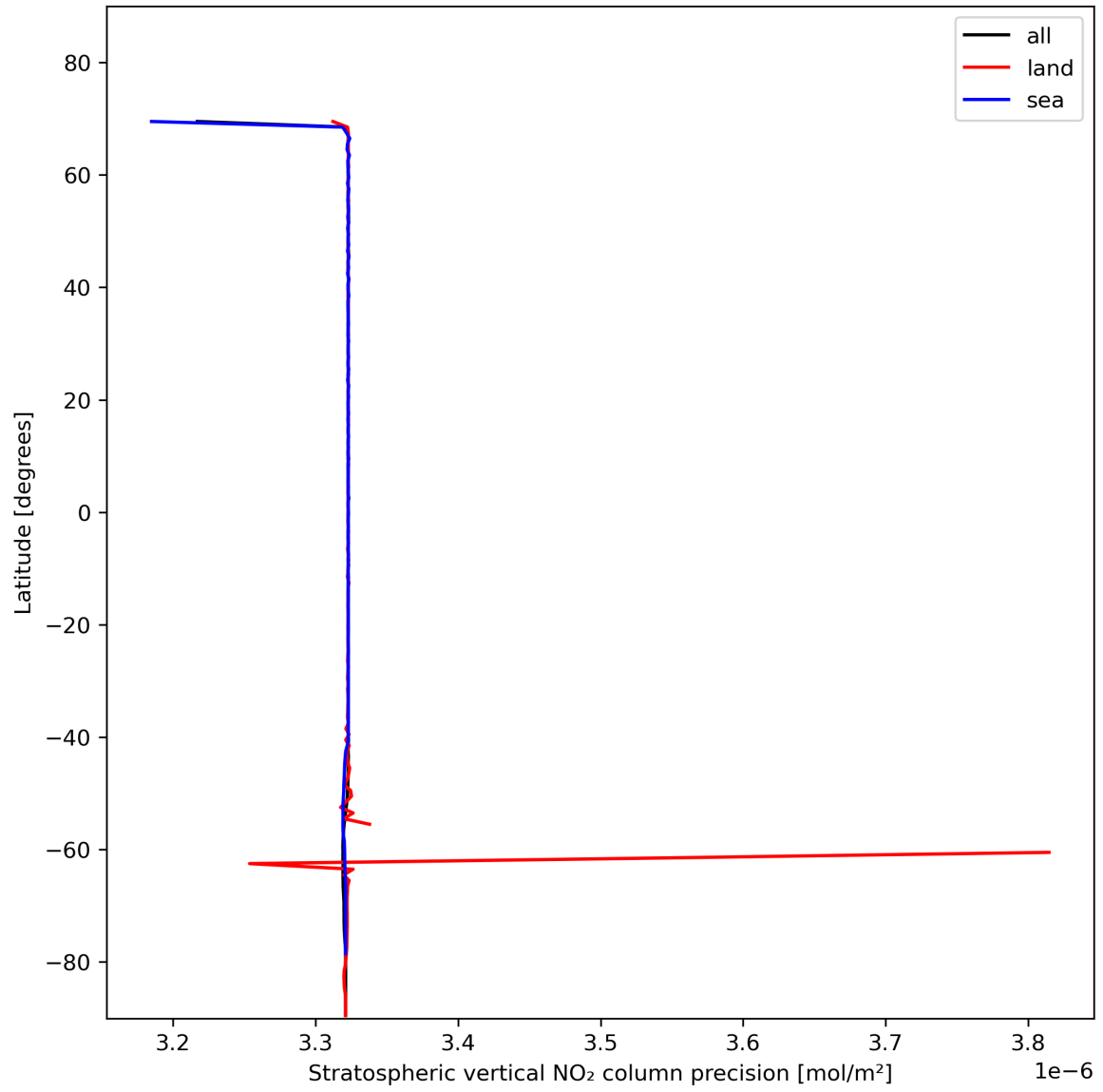
Figure 20: Zonal average of “Stratospheric vertical NO 2 column precision” for 2024-01-24 to 2024-01-26.
