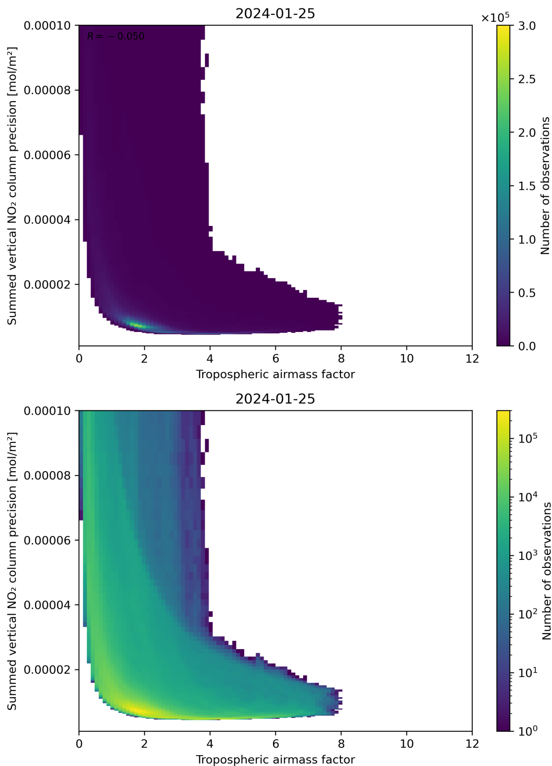
Figure 76: Scatter density plot of “Tropospheric air mass factor” against “Summed vertical NO 2 column precision” for 2024-01-24 to 2024-01-26.
