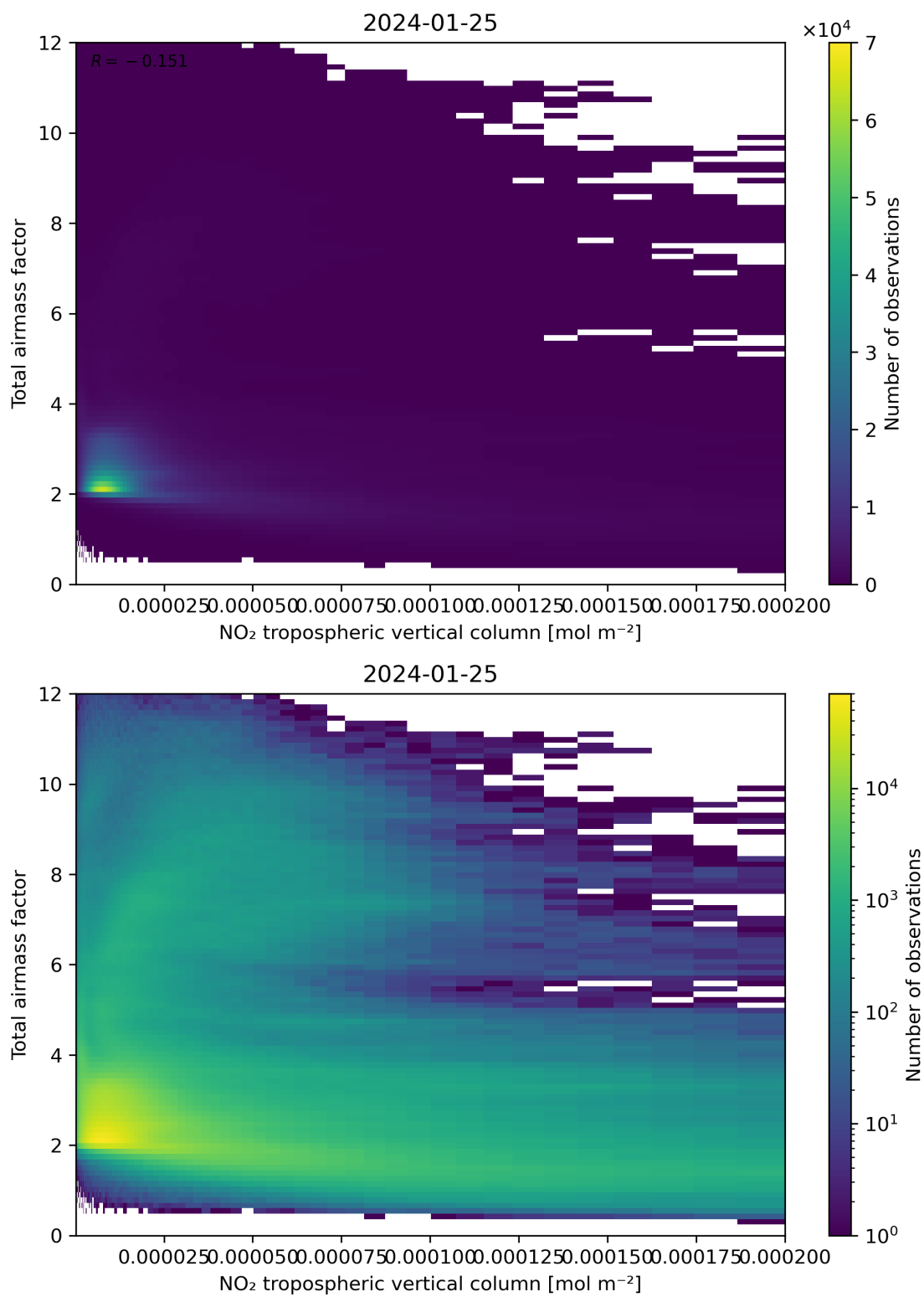
Figure 122: Scatter density plot of “NO 2 tropospheric vertical column” against “Total air mass factor” for 2024-01-24 to 2024-01-26.
