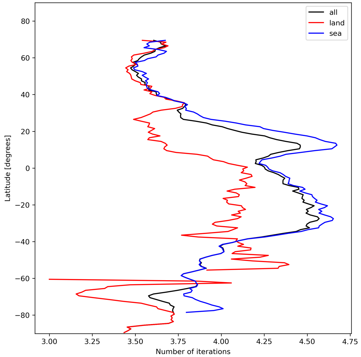
Figure 17: Zonal average of “Number of iterations” for 2024-01-24 to 2024-01-26.
