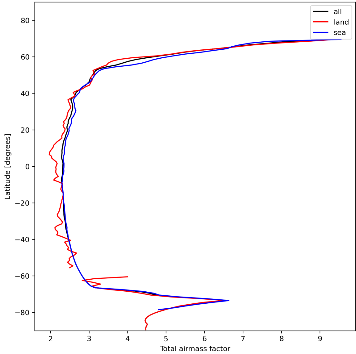
Figure 15: Zonal average of “Total airmass factor” for 2024-01-24 to 2024-01-26.
