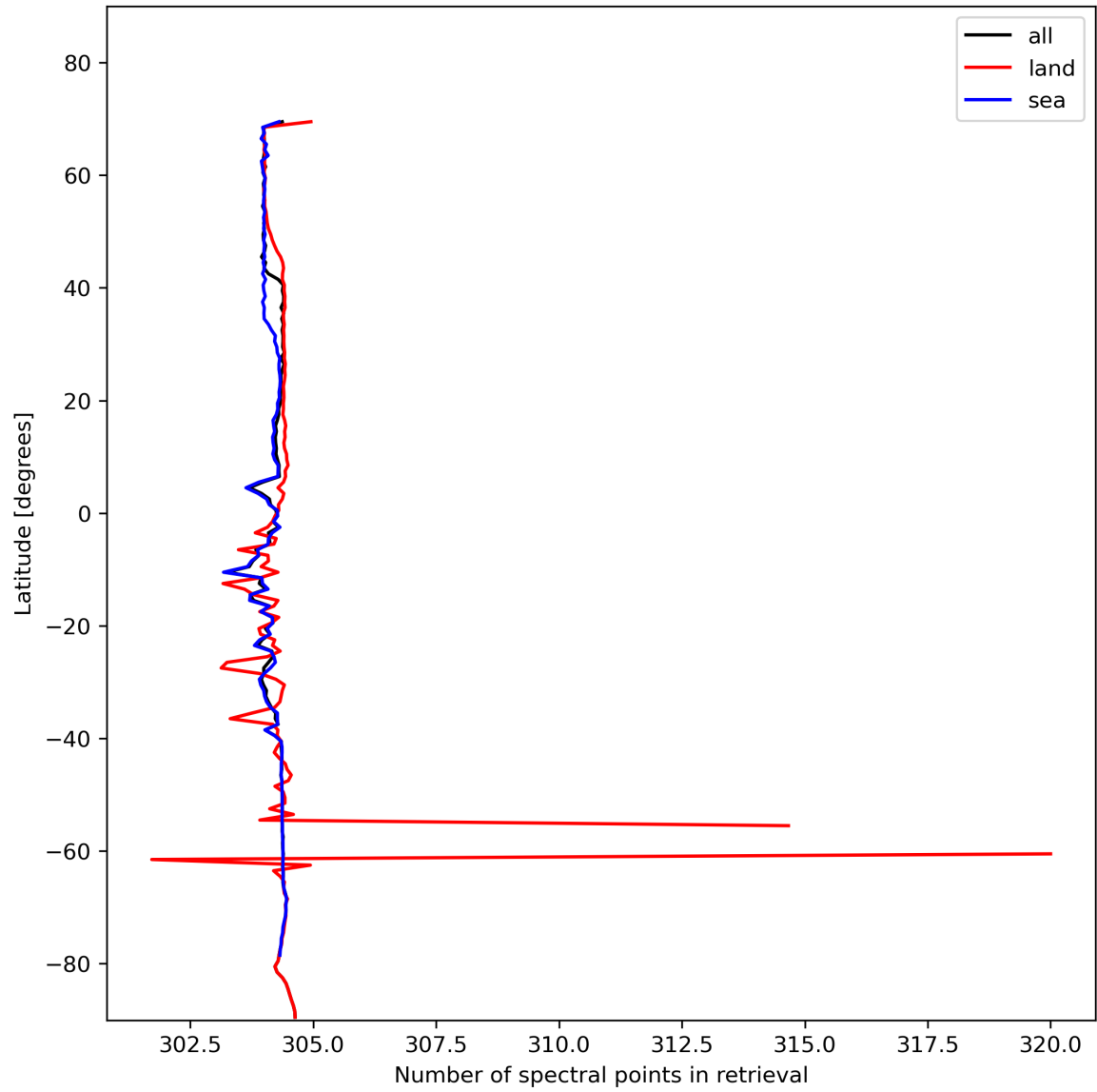
Figure 16: Zonal average of “Number of spectral points in retrieval” for 2024-01-24 to 2024-01-26.
