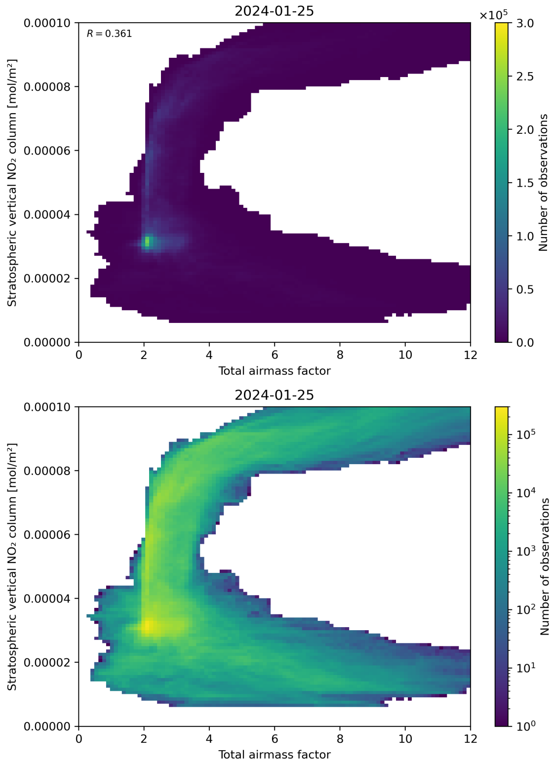
Figure 64: Scatter density plot of “Total airmass factor” against “Stratospheric vertical \text{NO}_2 column” for 2024-01-24 to 2024-01-26.
