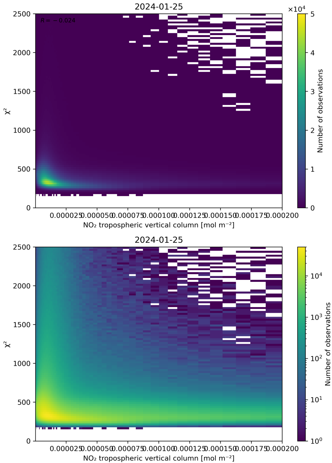
Figure 124: Scatter density plot of “NO 2 tropospheric vertical column” against “ \chi^2 ” for 2024-01-24 to 2024-01-26.
