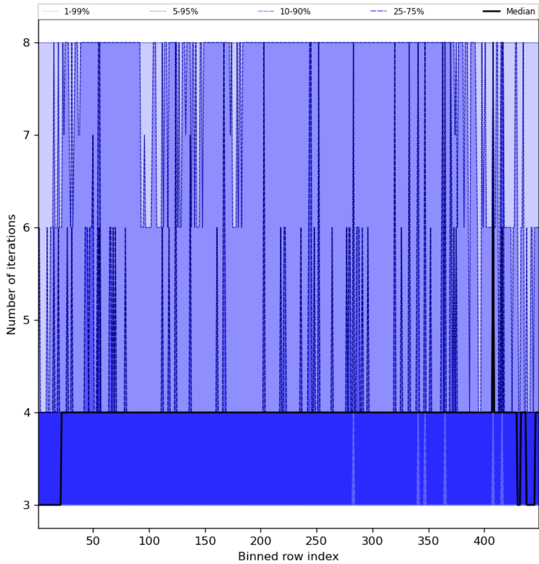
Figure 51: Along track statistics of “Number of iterations” for 2024-01-24 to 2024-01-26
