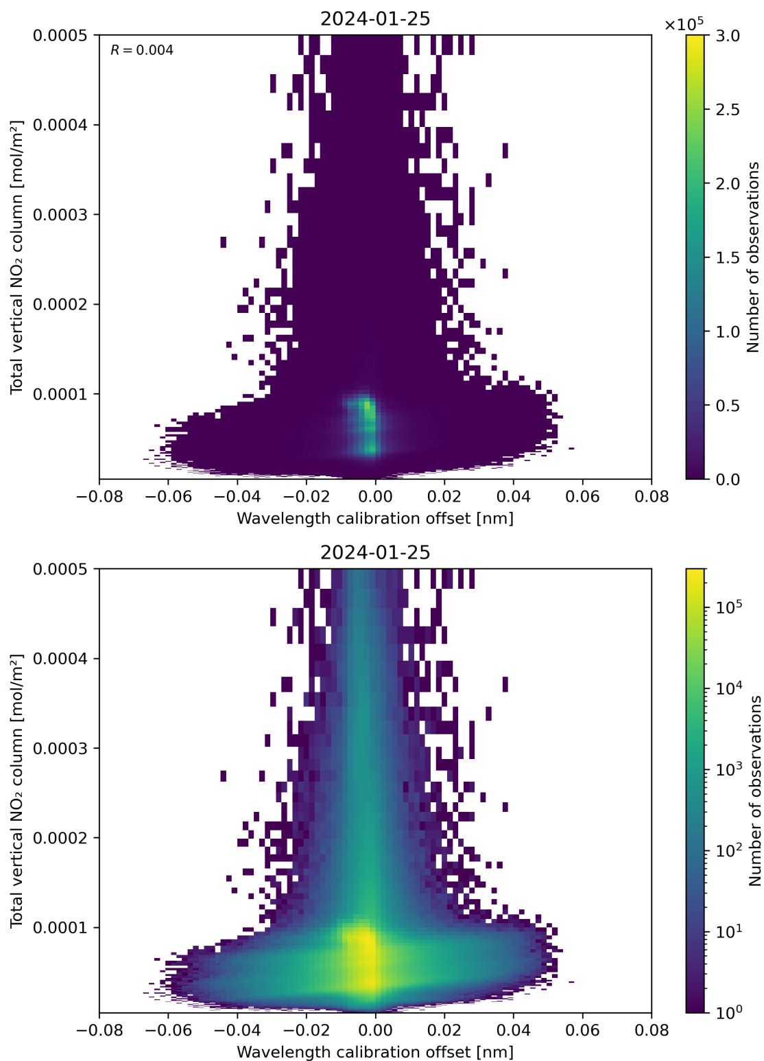
Figure 179: Scatter density plot of “Wavelength calibration offset” against “Total vertical NO 2 column” for 2024-01-24 to 2024-01-26.
