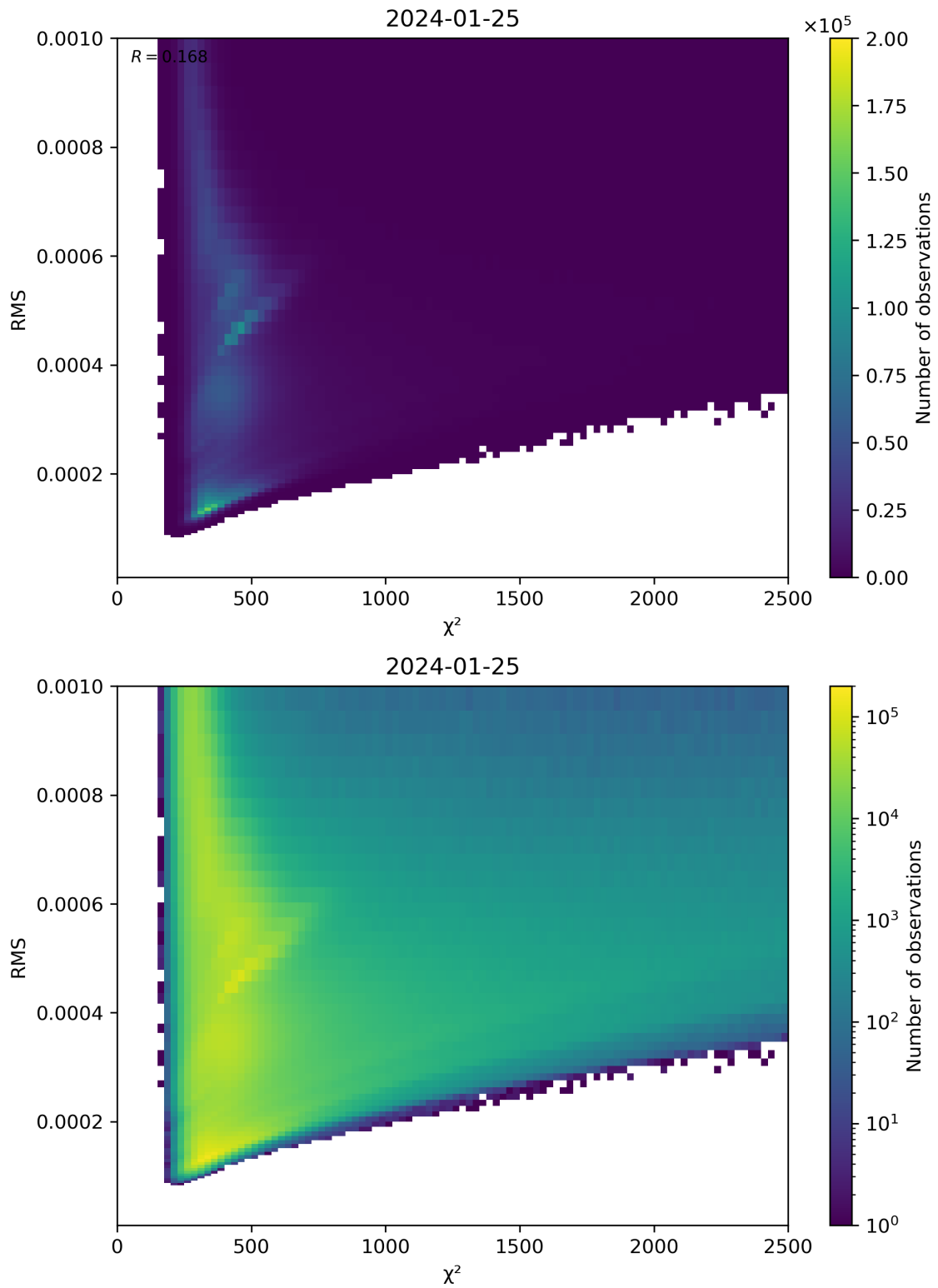
Figure 82: Scatter density plot of “ \chi^2 ” against “RMS” for 2024-01-24 to 2024-01-26.
