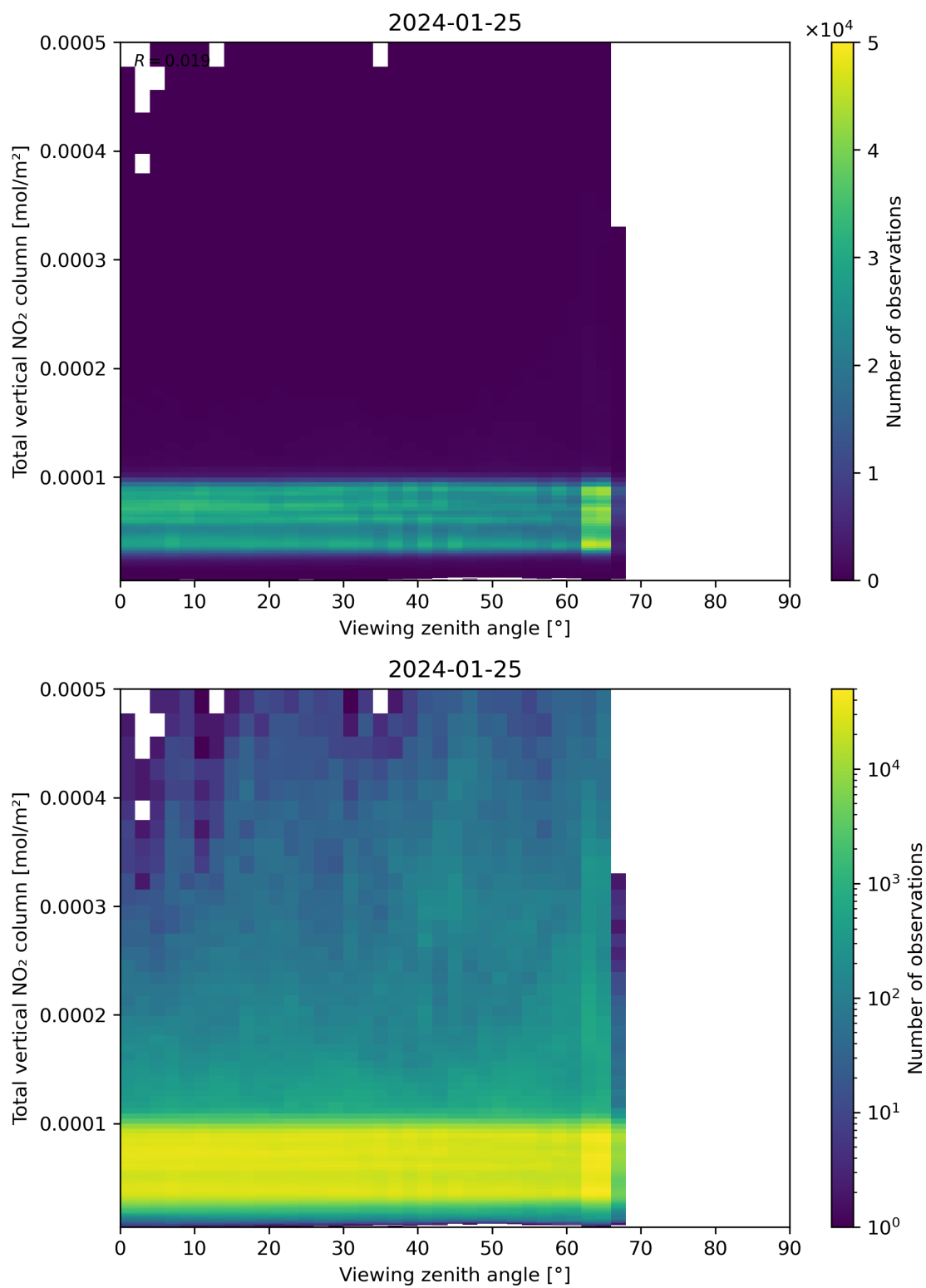
Figure 167: Scatter density plot of “Viewing zenith angle” against “Total vertical NO 2 column” for 2024-01-24 to 2024-01-26.
