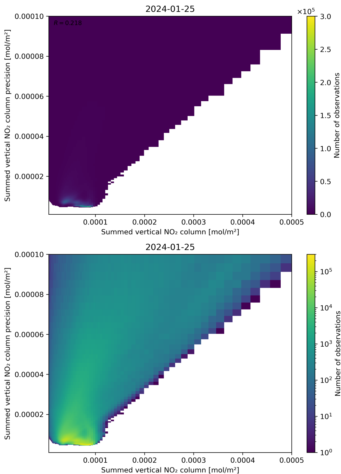
Figure 105: Scatter density plot of “Summed vertical NO 2 column” against “Summed vertical NO 2 column precision” for 2024-01-24 to 2024-01-26.
