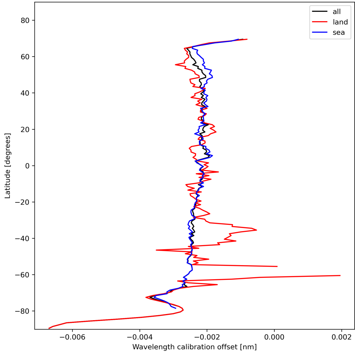
Figure 18: Zonal average of “Wavelength calibration offset” for 2024-01-24 to 2024-01-26.
