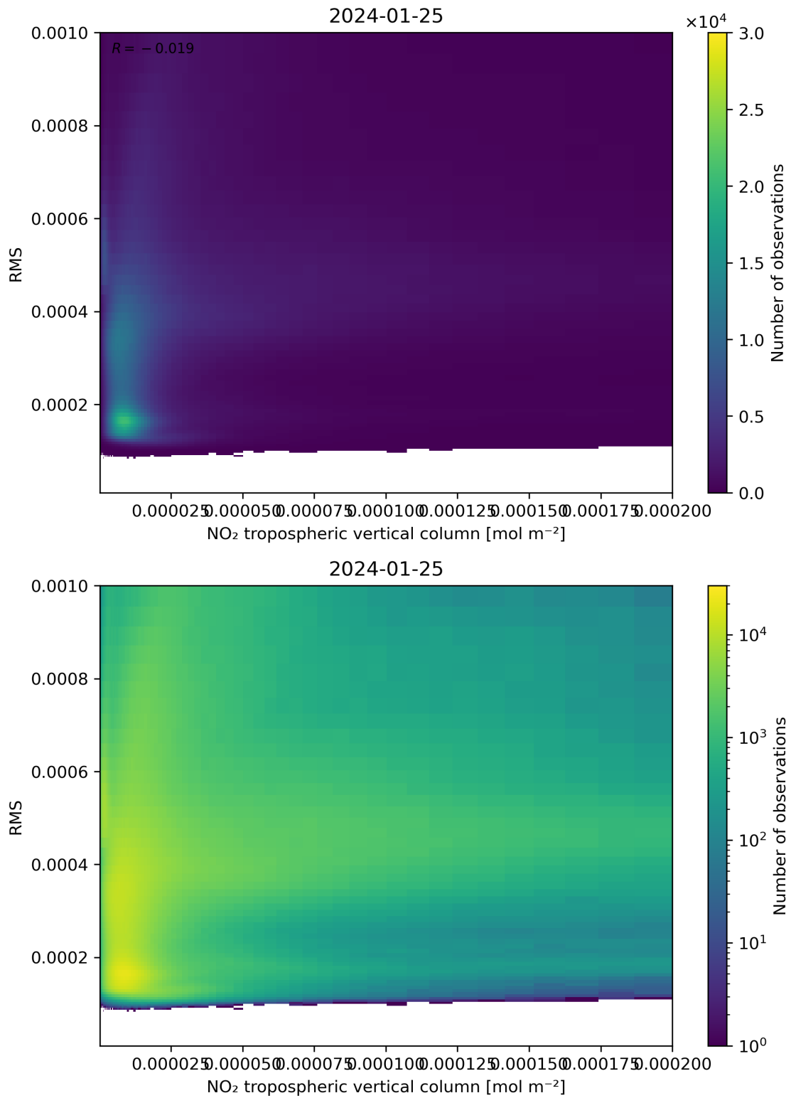
Figure 142: Scatter density plot of “NO 2 tropospheric vertical column” against “RMS” for 2024-01-24 to 2024-01-26.
