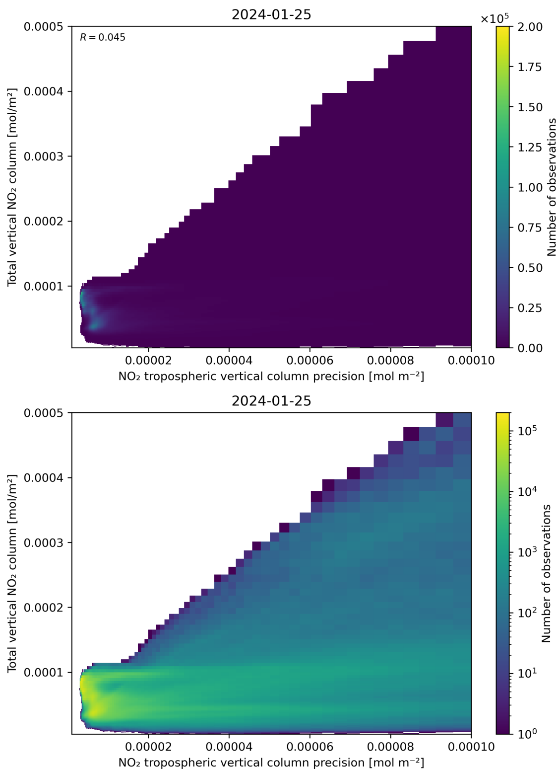
Figure 138: Scatter density plot of “NO 2 tropospheric vertical column precision” against “Total vertical NO 2 column” for 2024-01-24 to 2024-01-26.
