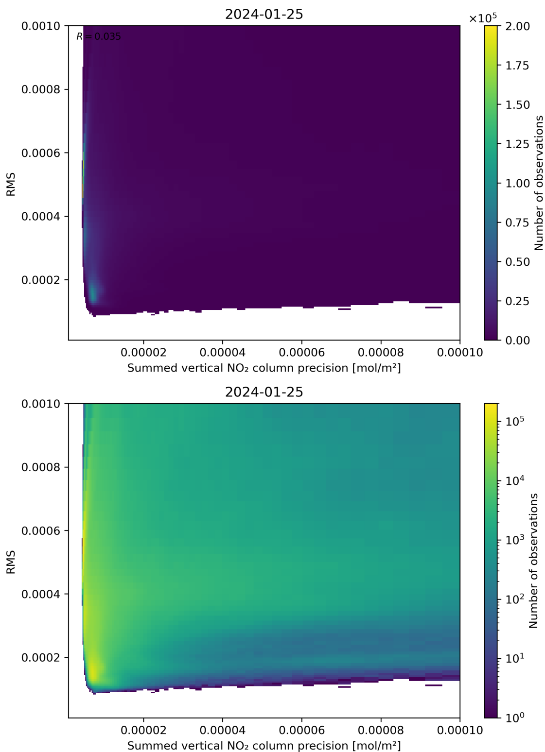
Figure 108: Scatter density plot of “Summed vertical NO 2 column precision” against “RMS” for 2024-01-24 to 2024-01-26.
