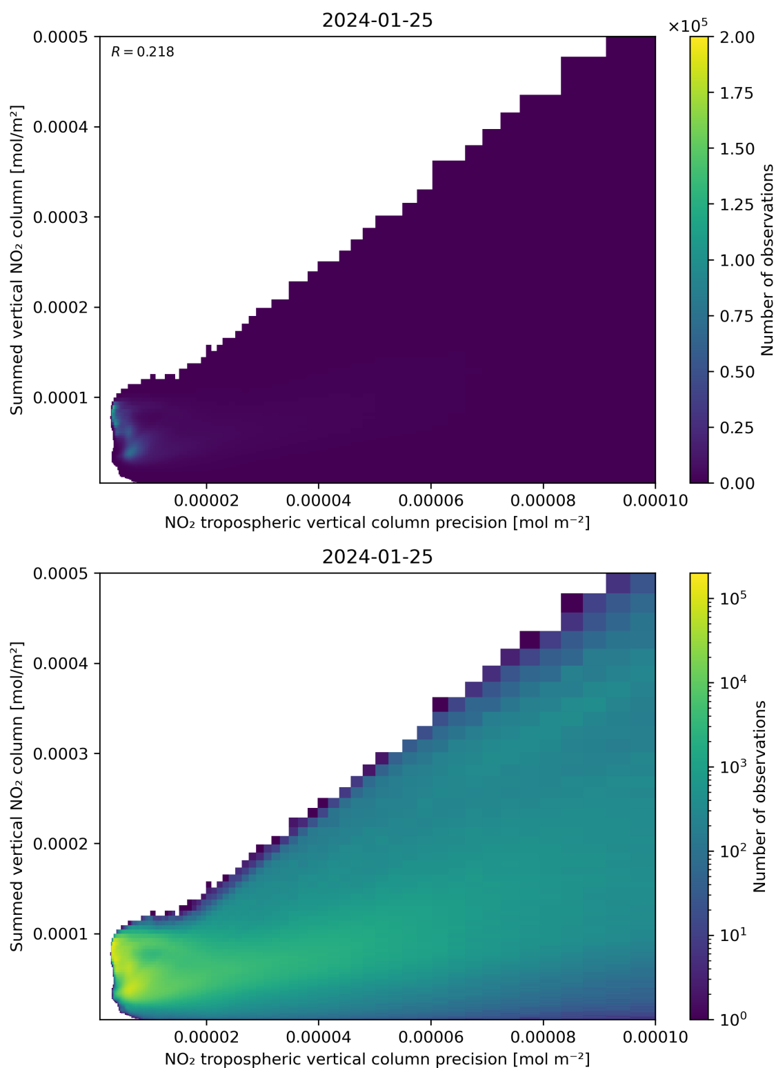
Figure 136: Scatter density plot of “NO 2 tropospheric vertical column precision” against “Summed vertical NO 2 column” for 2024-01-24 to 2024-01-26.
