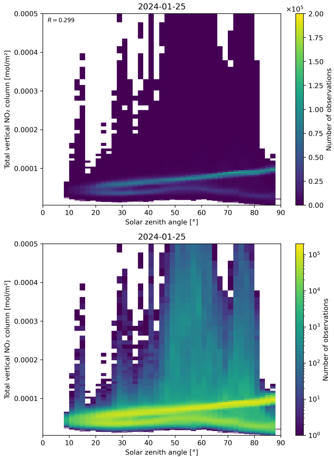
Figure 153: Scatter density plot of “Solar zenith angle” against “Total vertical NO 2 column” for 2024-01-24 to 2024-01-26.
