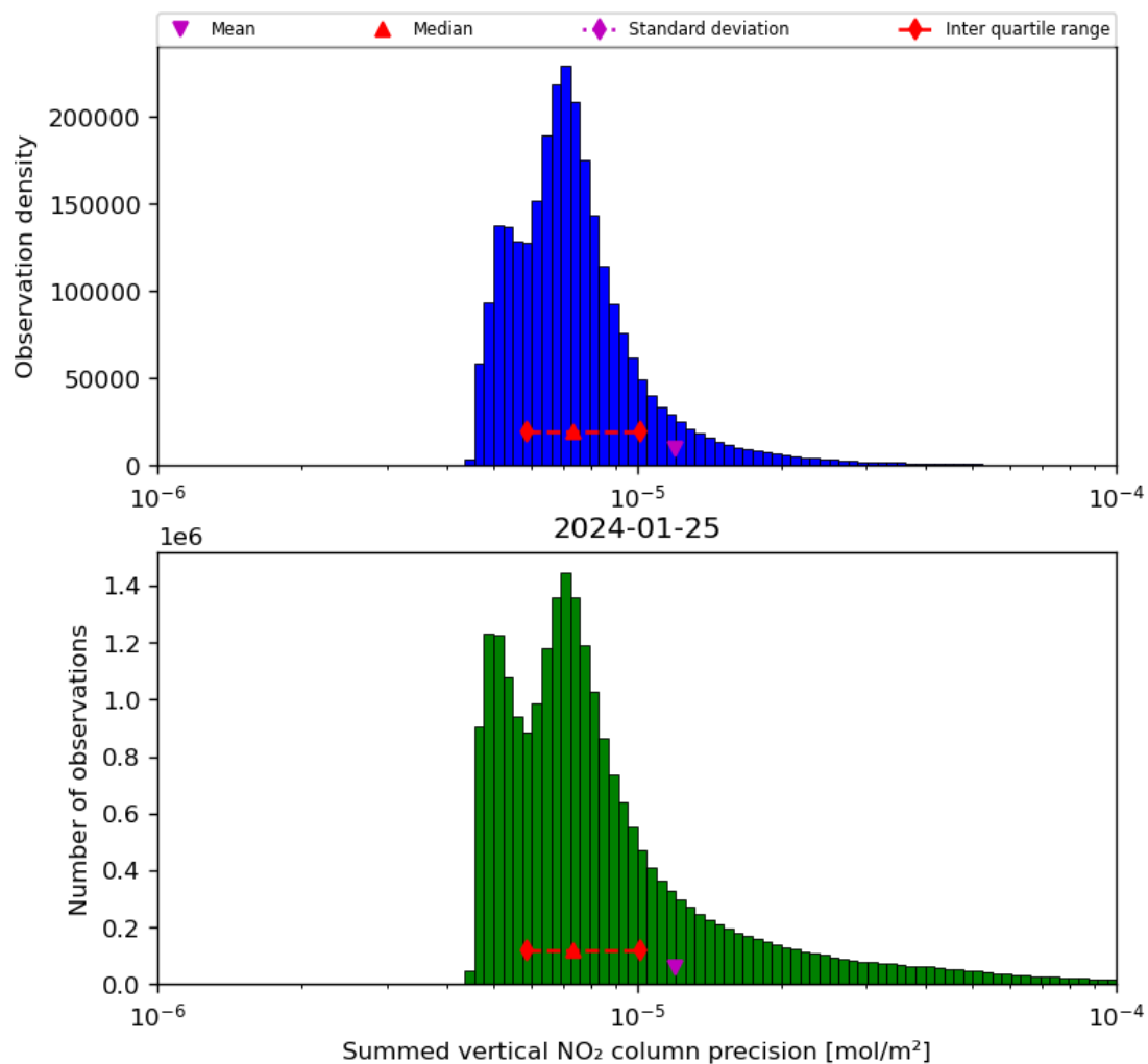
Figure 41: Histogram of “Summed vertical NO 2 column precision” for 2024-01-24 to 2024-01-26
