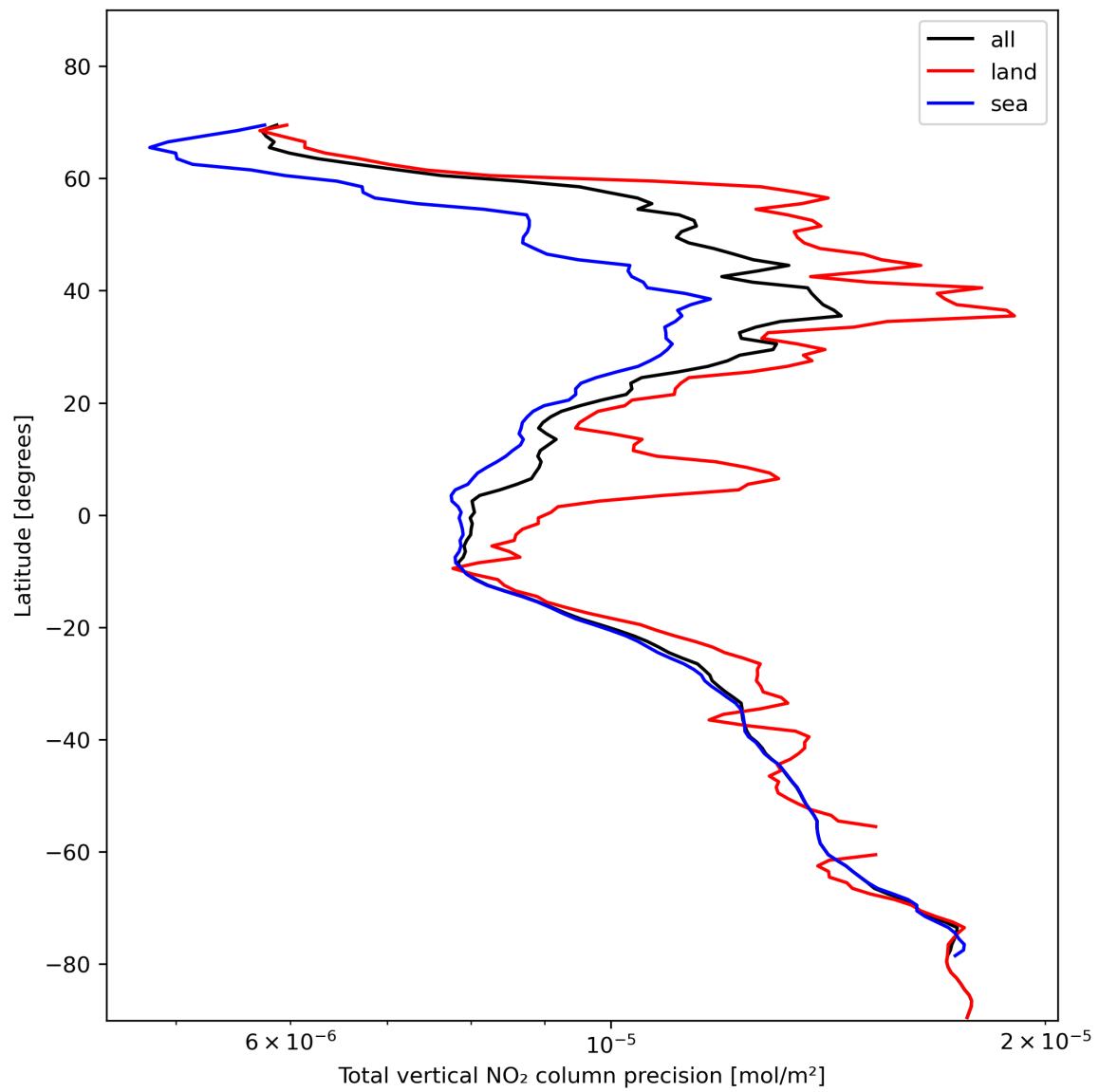
Figure 22: Zonal average of “Total vertical NO 2 column precision” for 2024-01-24 to 2024-01-26.
