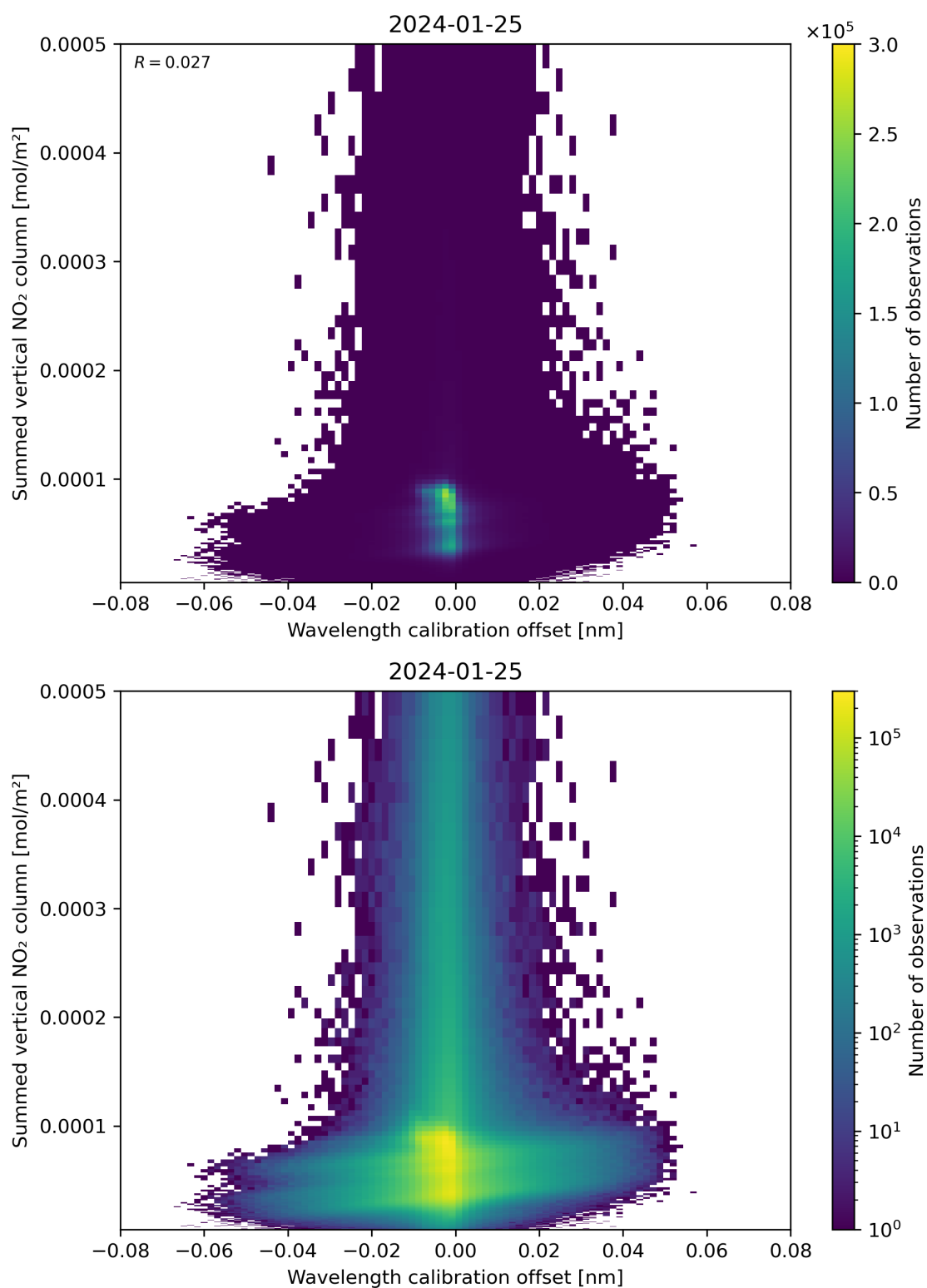
Figure 177: Scatter density plot of “Wavelength calibration offset” against “Summed vertical NO 2 column” for 2024-01-24 to 2024-01-26.
