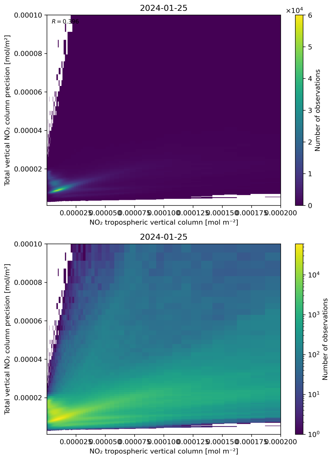
Figure 129: Scatter density plot of “NO 2 tropospheric vertical column” against “Total vertical NO 2 column precision” for 2024-01-24 to 2024-01-26.
