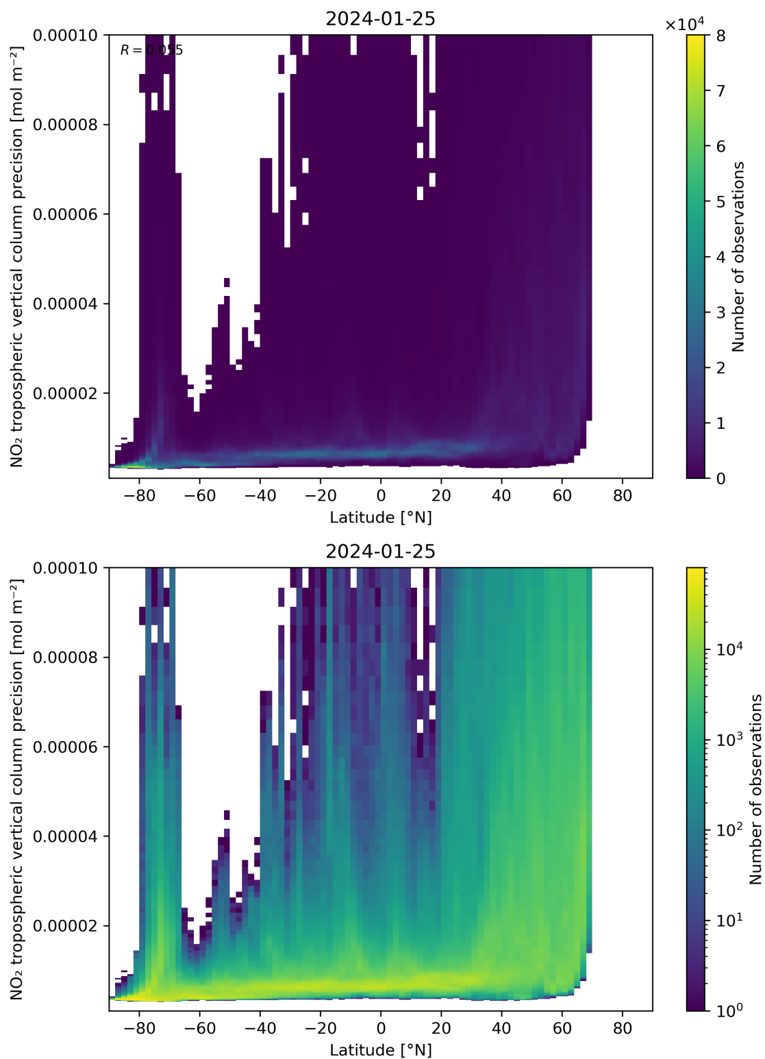
Figure 93: Scatter density plot of “Latitude” against “NO 2 tropospheric vertical column precision” for 2024-01-24 to 2024-01-26.
