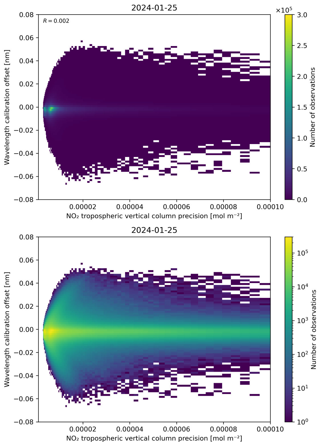
Figure 141: Scatter density plot of “NO 2 tropospheric vertical column precision” against “Wavelength calibration offset” for 2024-01-24 to 2024-01-26.
