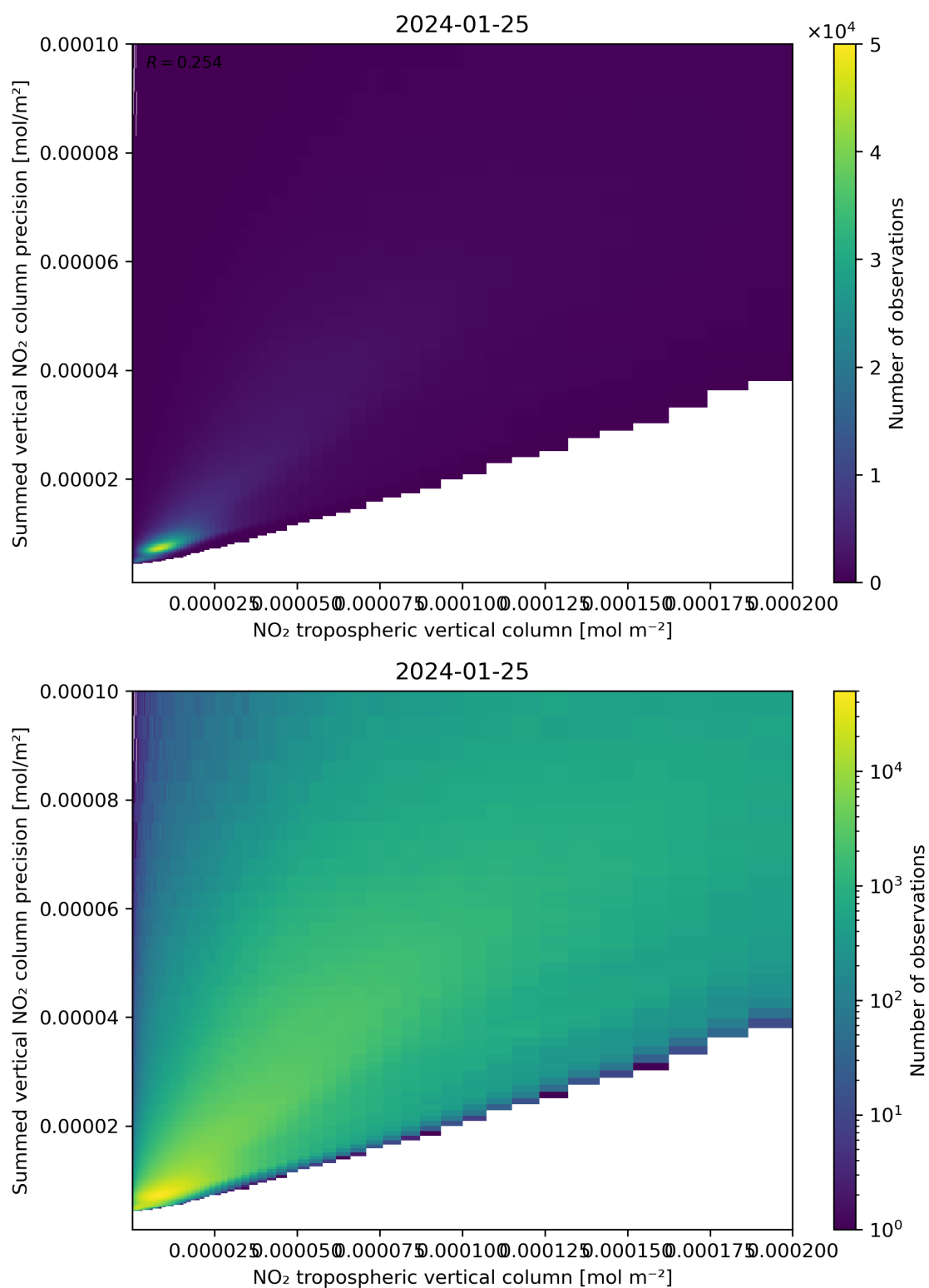
Figure 127: Scatter density plot of “NO 2 tropospheric vertical column” against “Summed vertical NO 2 column precision” for 2024-01-24 to 2024-01-26.
