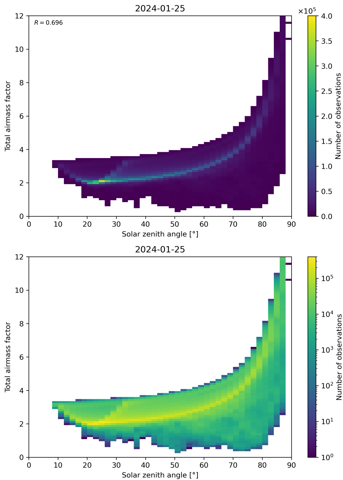
Figure 146: Scatter density plot of “Solar zenith angle” against “Total air mass factor” for 2024-01-24 to 2024-01-26.
