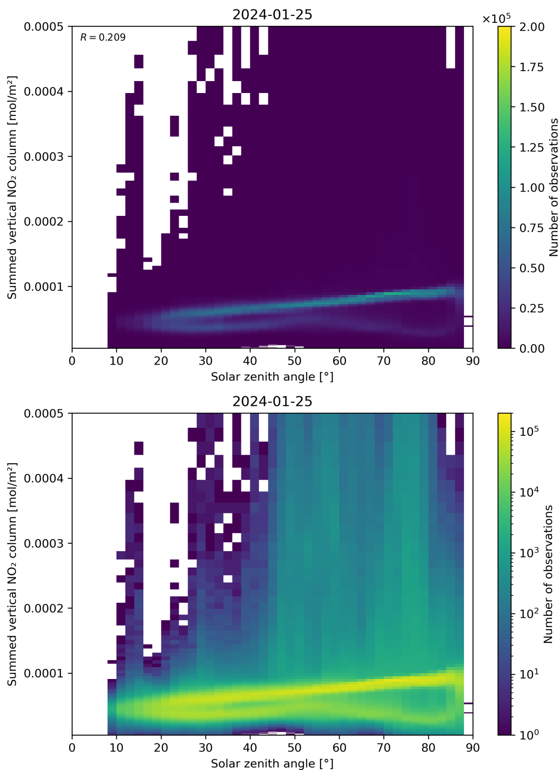
Figure 151: Scatter density plot of “Solar zenith angle” against “Summed vertical NO 2 column” for 2024-01-24 to 2024-01-26.
