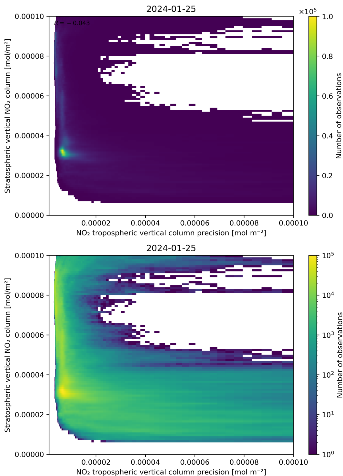
Figure 135: Scatter density plot of “NO 2 tropospheric vertical column precision” against “Stratospheric vertical NO 2 column” for 2024-01-24 to 2024-01-26.
