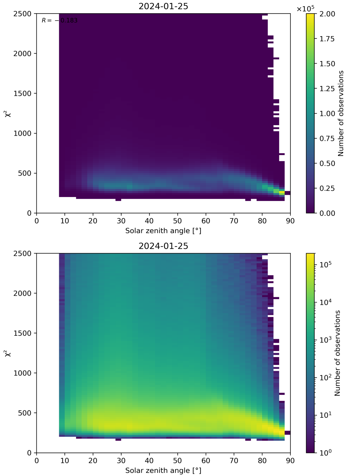
Figure 148: Scatter density plot of “Solar zenith angle” against “ \chi^2 ” for 2024-01-24 to 2024-01-26.
