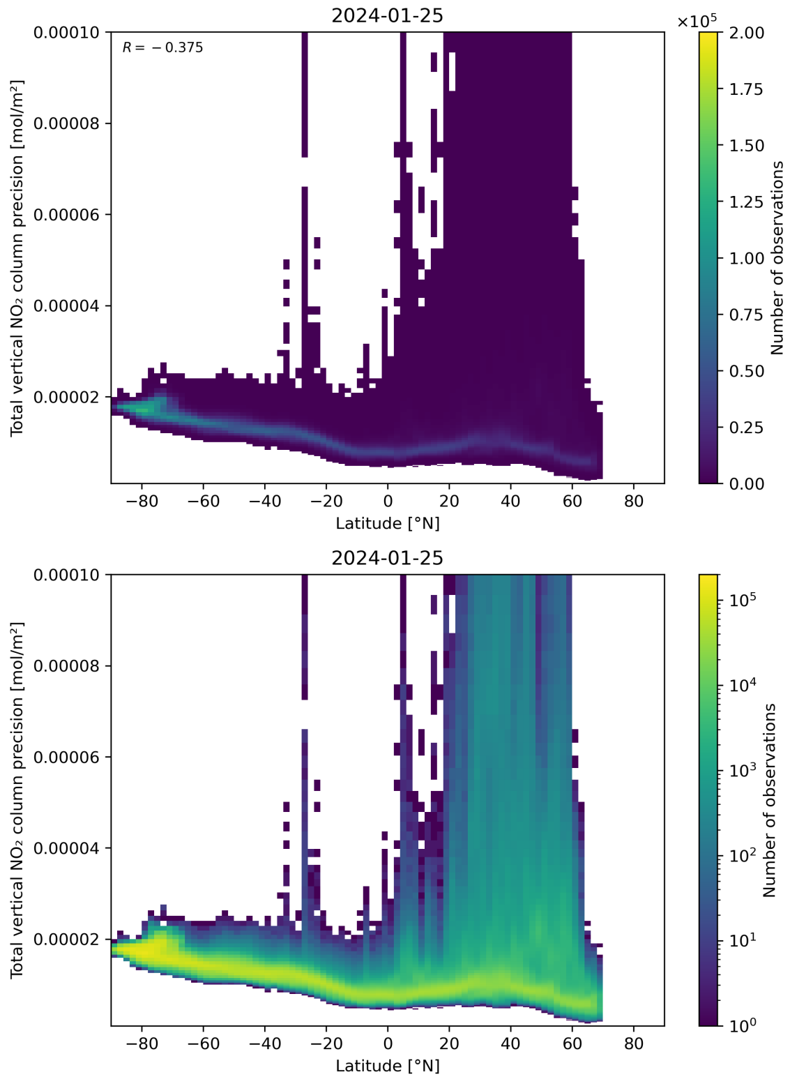
Figure 91: Scatter density plot of “Latitude” against “Total vertical NO 2 column precision” for 2024-01-24 to 2024-01-26.
