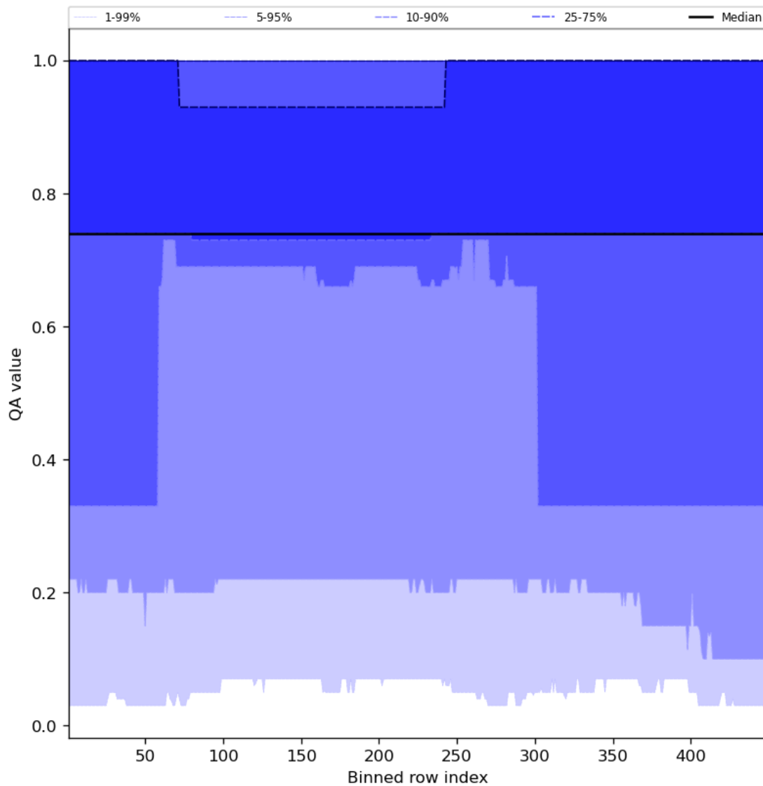
Figure 45: Along track statistics of "QA value" for 2024-01-24 to 2024-01-26
