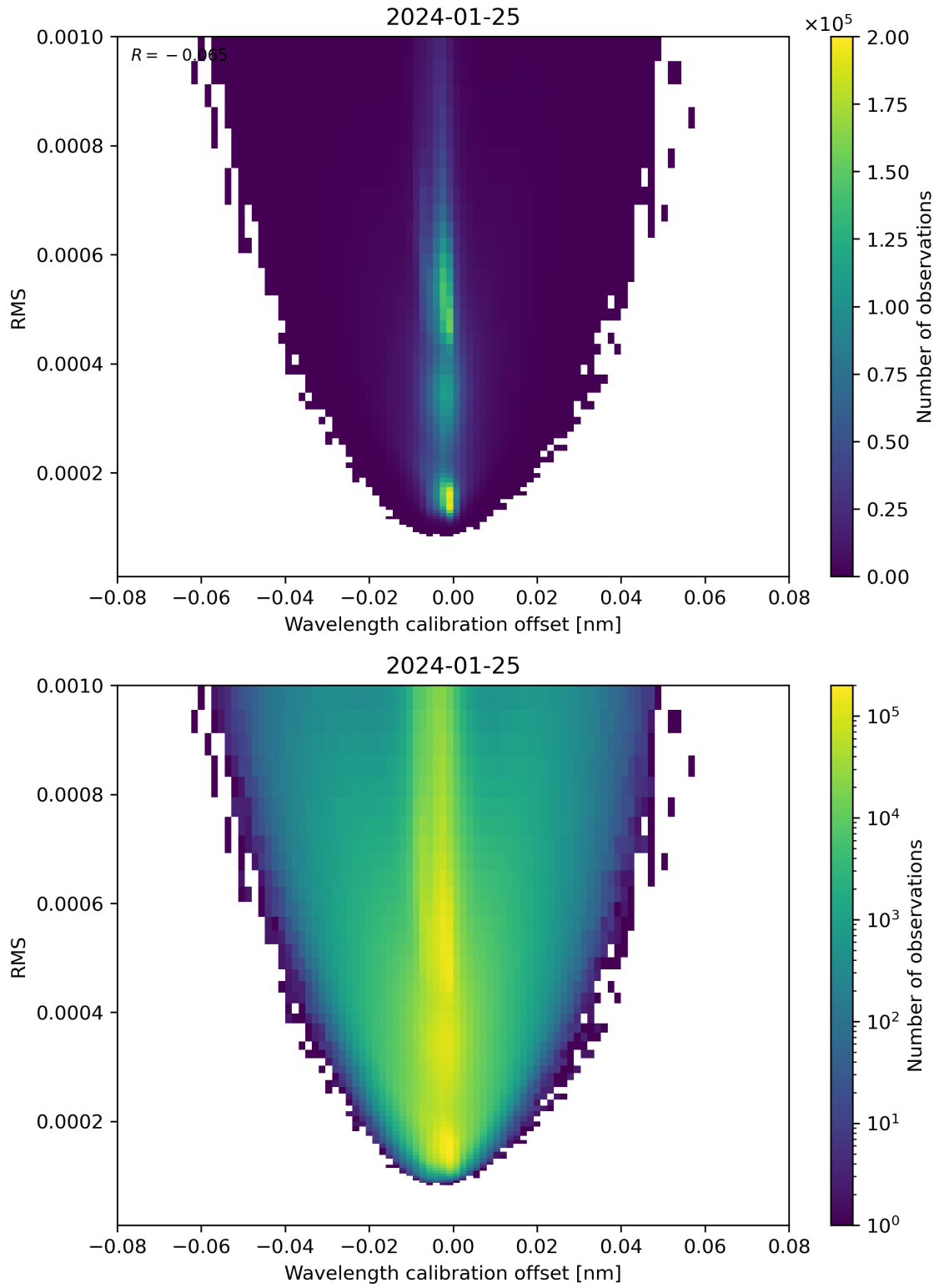
Figure 181: Scatter density plot of “Wavelength calibration offset” against “RMS” for 2024-01-24 to 2024-01-26.
