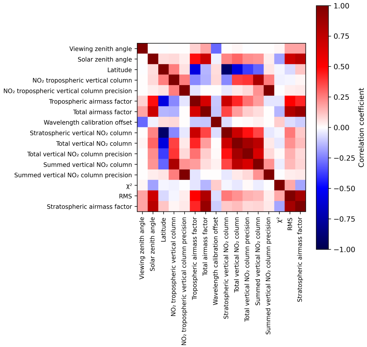
Figure 2: Map of correlation matrix for 2024-01-24 to 2024-01-26.
