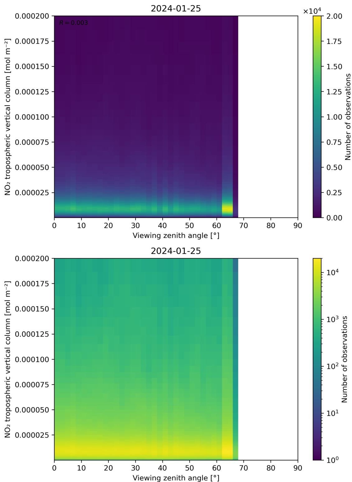
Figure 169: Scatter density plot of “Viewing zenith angle” against “NO 2 tropospheric vertical column” for 2024-01-24 to 2024-01-26.
