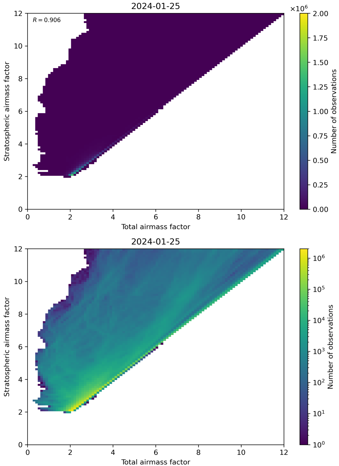
Figure 62: Scatter density plot of “Total air mass factor” against “Stratospheric air mass factor” for 2024-01-24 to 2024-01-26.
