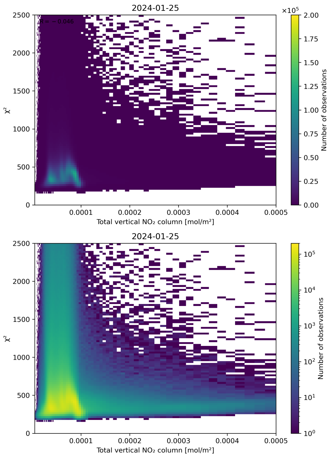
Figure 111: Scatter density plot of “Total vertical NO 2 column” against “ \chi^2 ” for 2024-01-24 to 2024-01-26.
