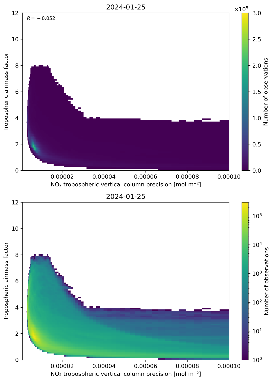
Figure 133: Scatter density plot of “NO 2 tropospheric vertical column precision” against “Tropospheric airmass factor” for 2024-01-24 to 2024-01-26.
