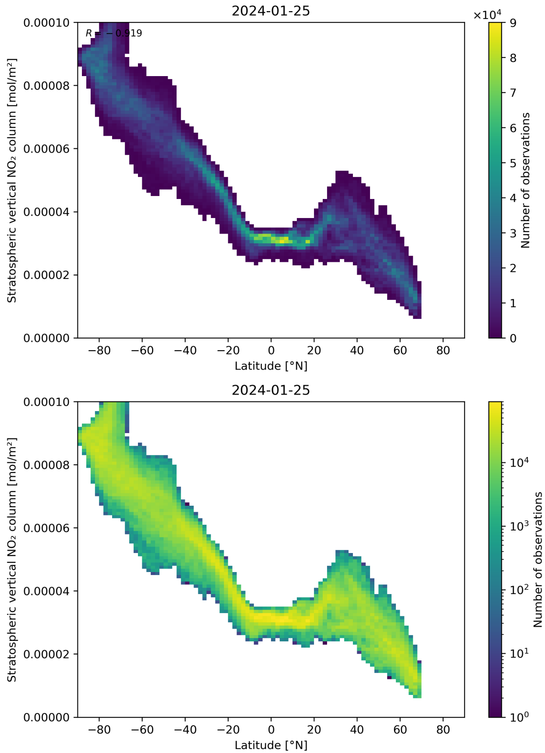
Figure 87: Scatter density plot of “Latitude” against “Stratospheric vertical NO 2 column” for 2024-01-24 to 2024-01-26.
