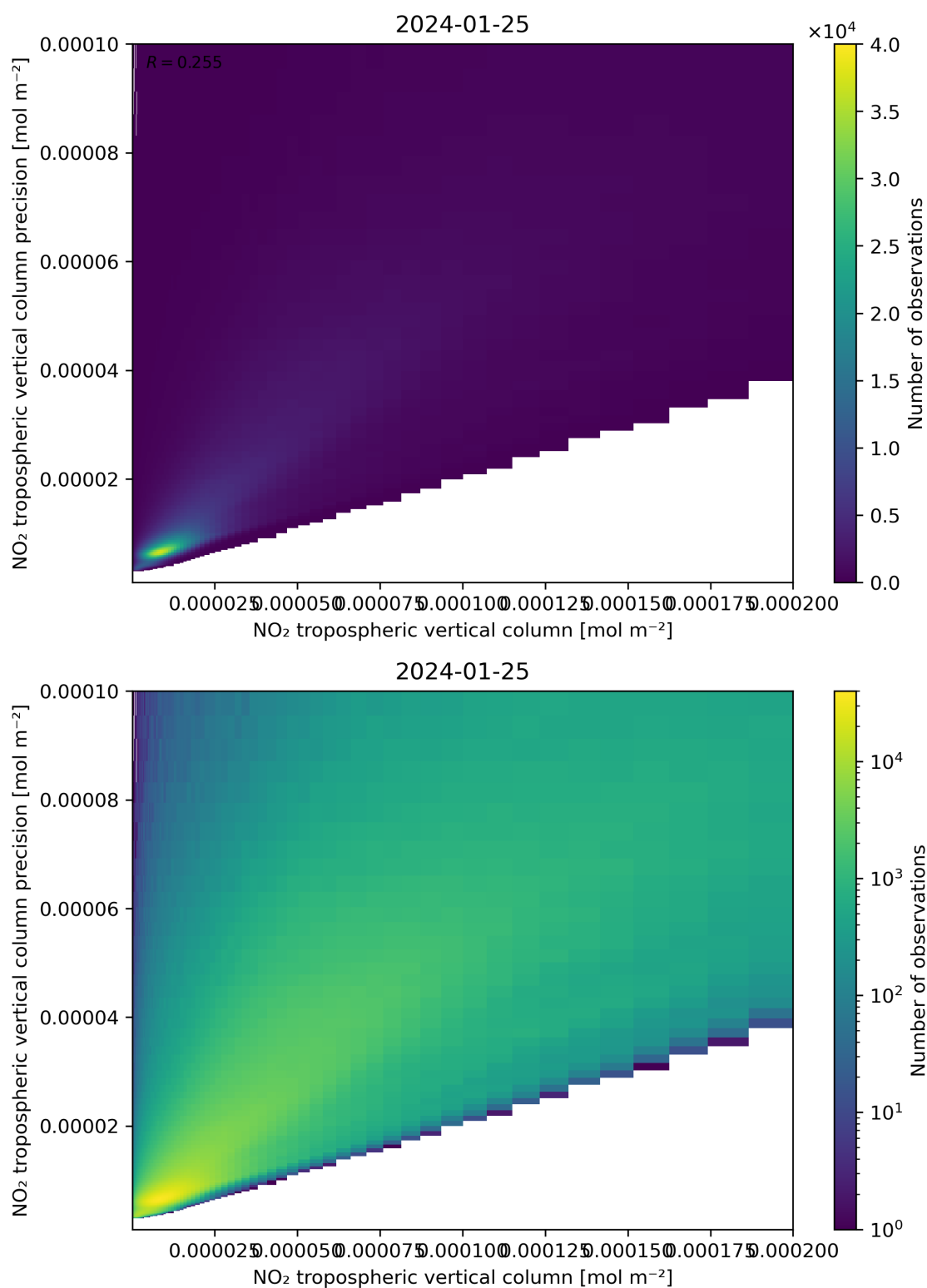
Figure 130: Scatter density plot of “NO 2 tropospheric vertical column” against “NO 2 tropospheric vertical column precision” for 2024-01-24 to 2024-01-26.
