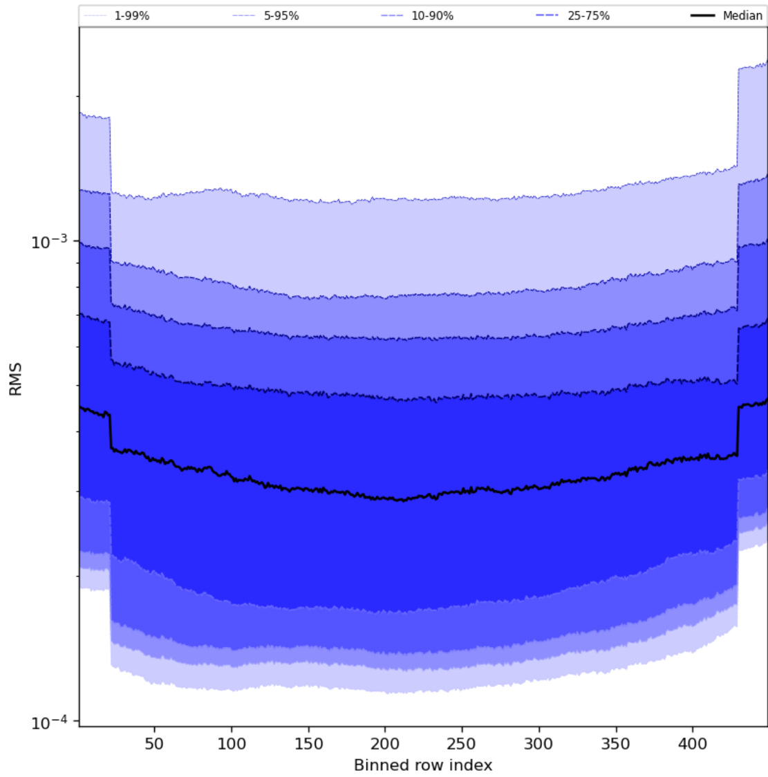
Figure 60: Along track statistics of “RMS” for 2024-01-24 to 2024-01-26
