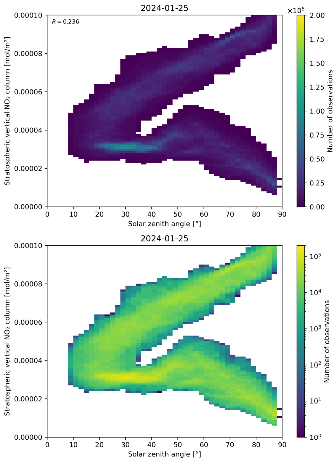
Figure 150: Scatter density plot of “Solar zenith angle” against “Stratospheric vertical \text{NO}_2 column” for 2024-01-24 to 2024-01-26.
