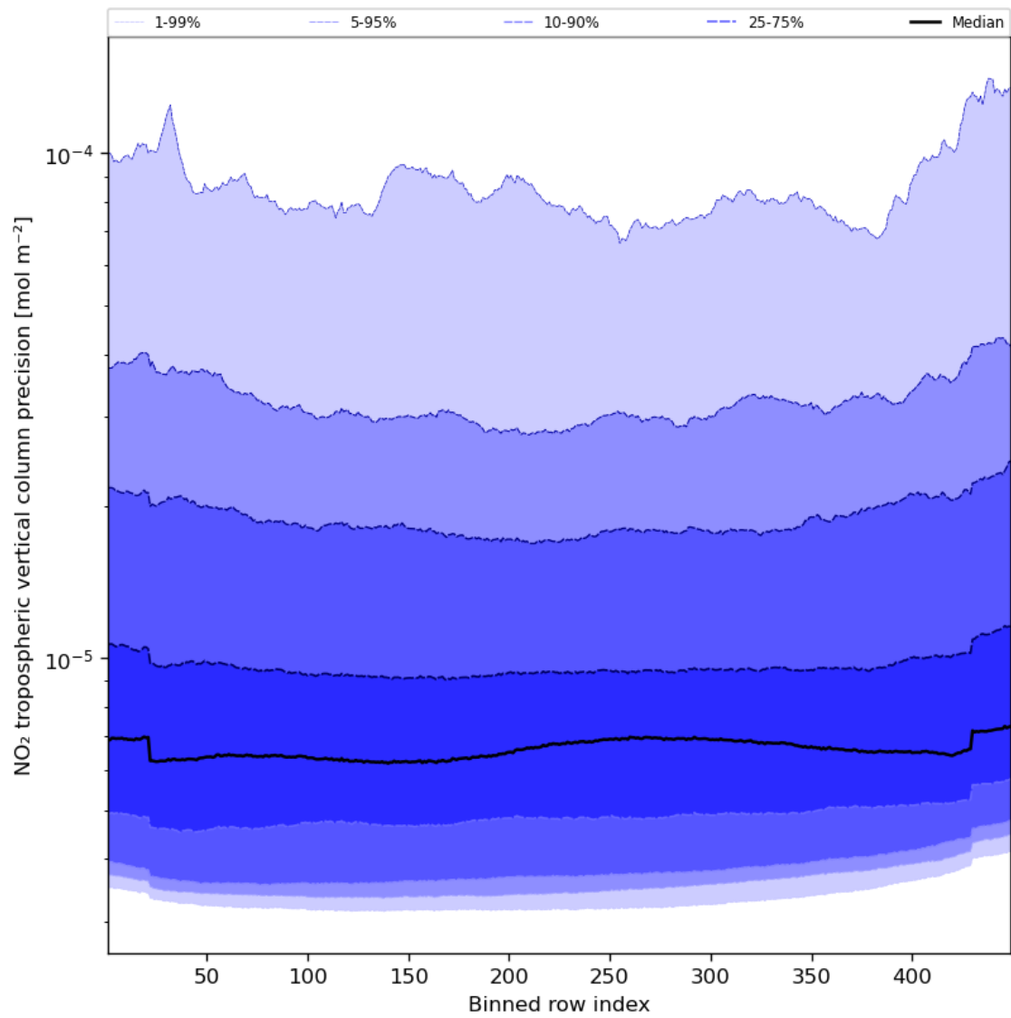
Figure 47: Along track statistics of “NO 2 tropospheric vertical column precision” for 2024-01-24 to 2024-01-26
