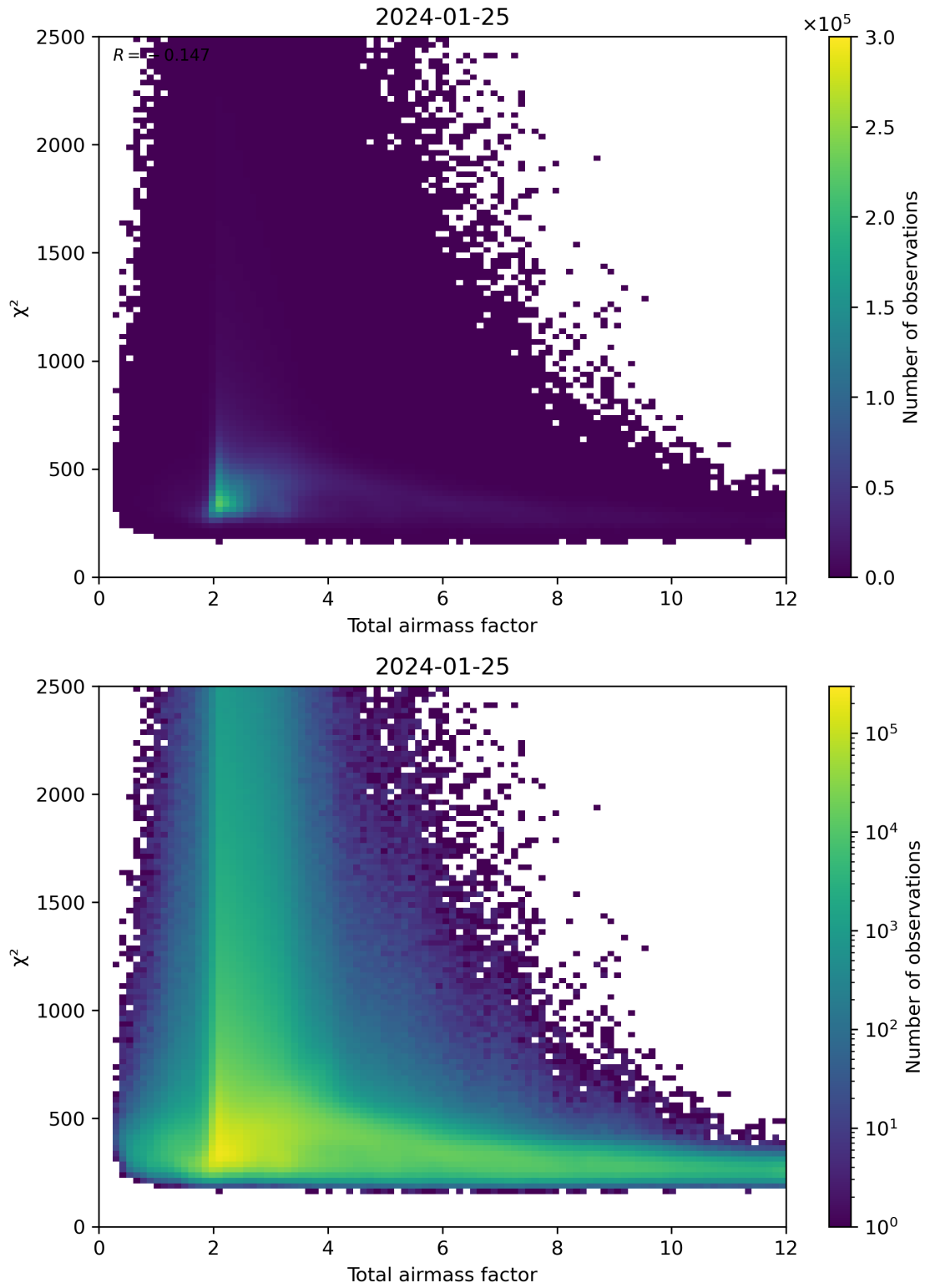
Figure 63: Scatter density plot of “Total airmass factor” against “ \chi^2 ” for 2024-01-24 to 2024-01-26.
