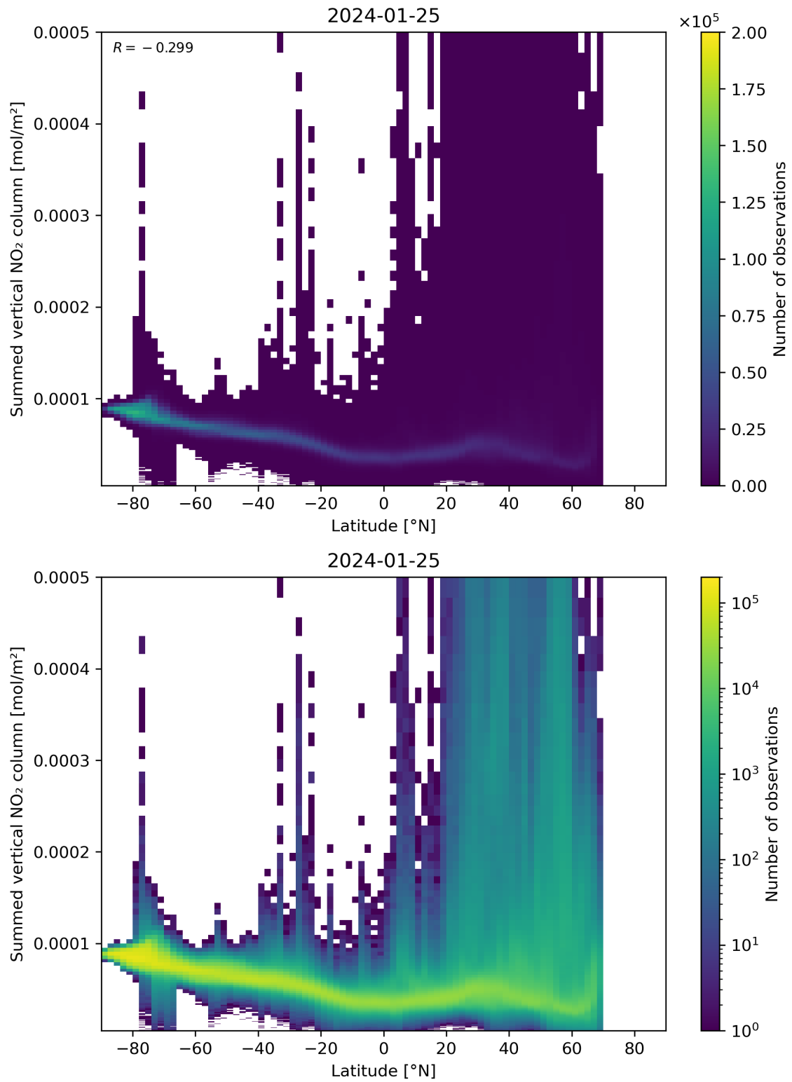
Figure 88: Scatter density plot of “Latitude” against “Summed vertical NO 2 column” for 2024-01-24 to 2024-01-26.
