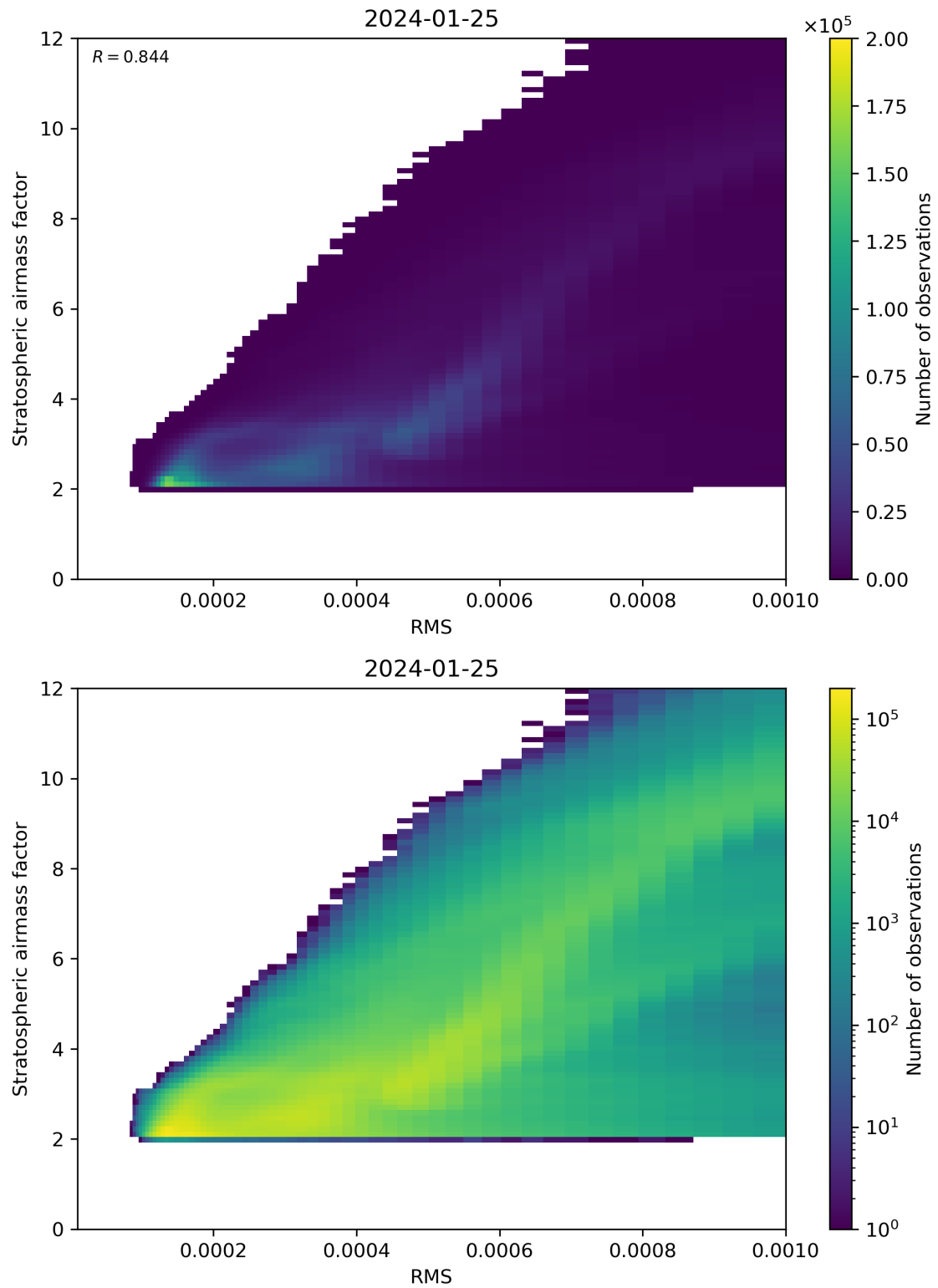
Figure 144: Scatter density plot of “RMS” against “Stratospheric airmass factor” for 2024-01-24 to 2024-01-26.
