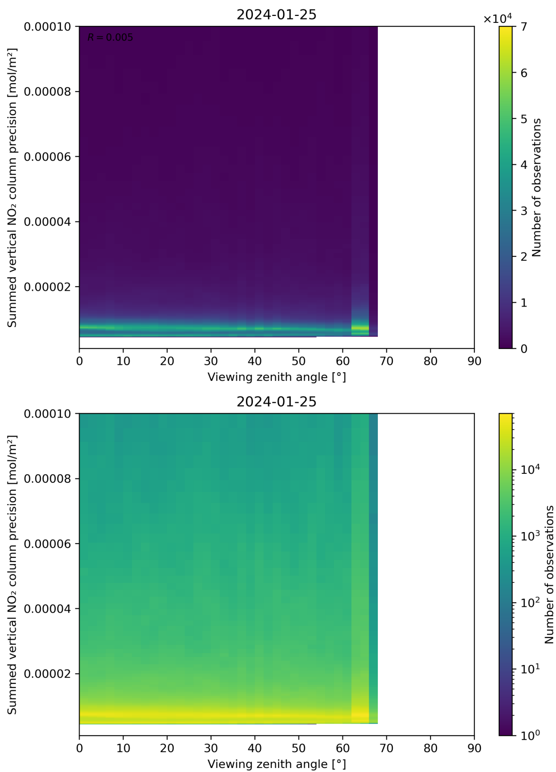
Figure 166: Scatter density plot of “Viewing zenith angle” against “Summed vertical NO 2 column precision” for 2024-01-24 to 2024-01-26.
