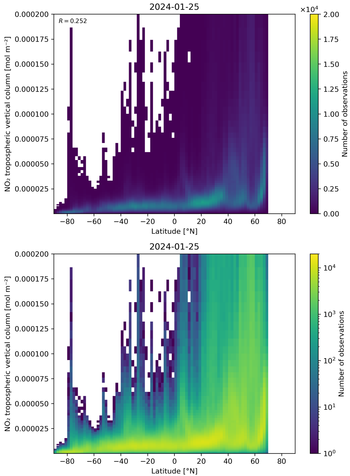
Figure 92: Scatter density plot of “Latitude” against “NO 2 tropospheric vertical column” for 2024-01-24 to 2024-01-26.
