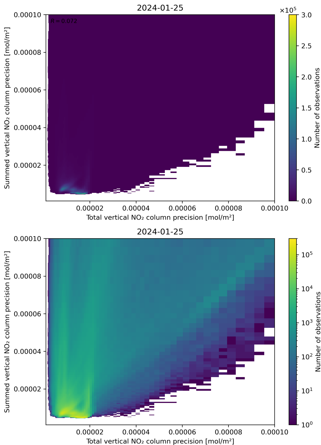
Figure 118: Scatter density plot of “Total vertical NO 2 column precision” against “Summed vertical NO 2 column precision” for 2024-01-24 to 2024-01-26.
