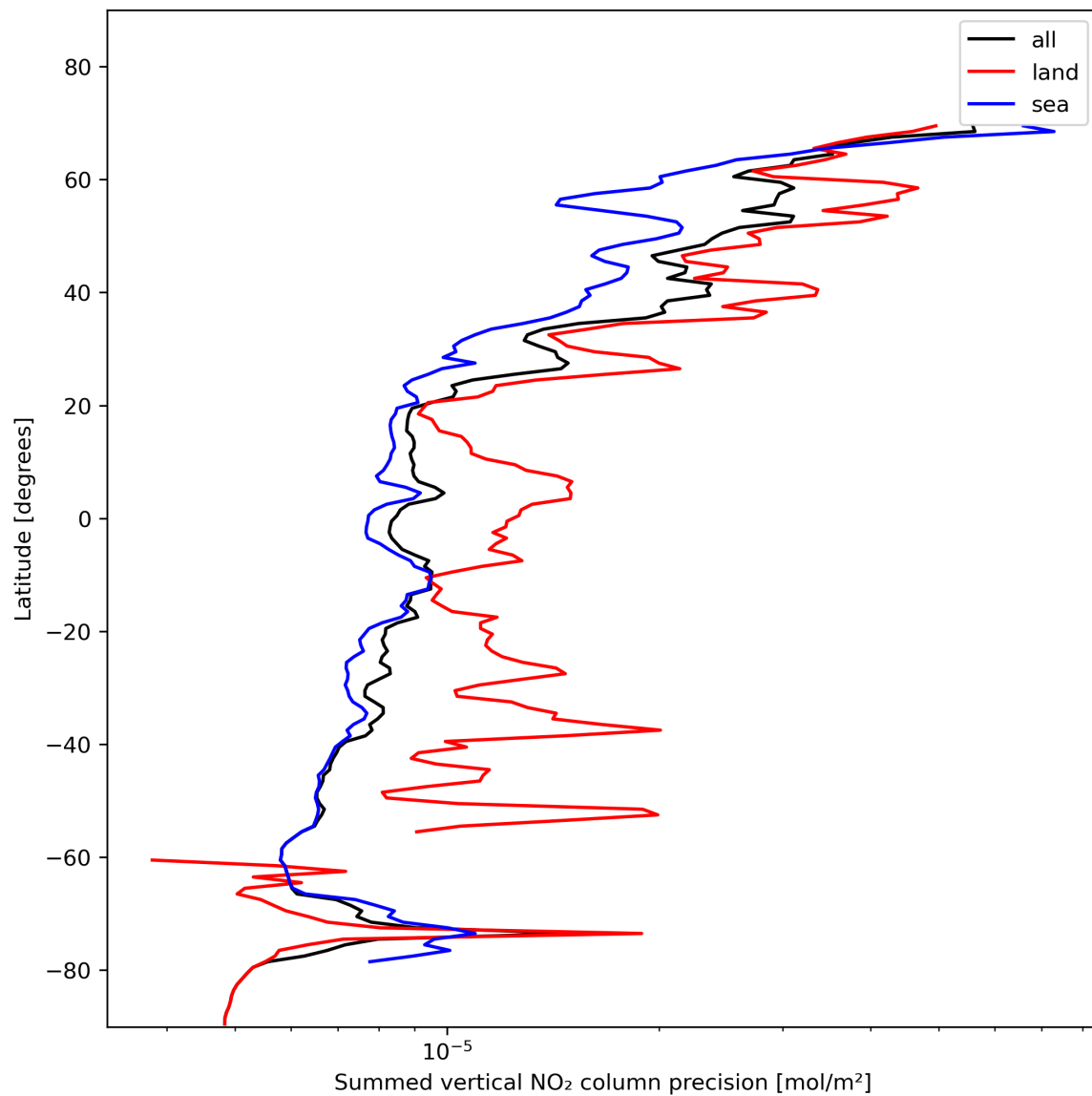
Figure 24: Zonal average of “Summed vertical NO 2 column precision” for 2024-01-24 to 2024-01-26.
