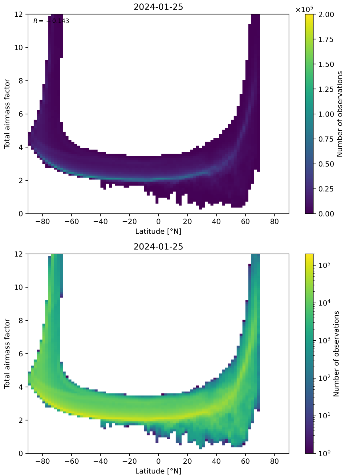
Figure 84: Scatter density plot of “Latitude” against “Total airmass factor” for 2024-01-24 to 2024-01-26.
