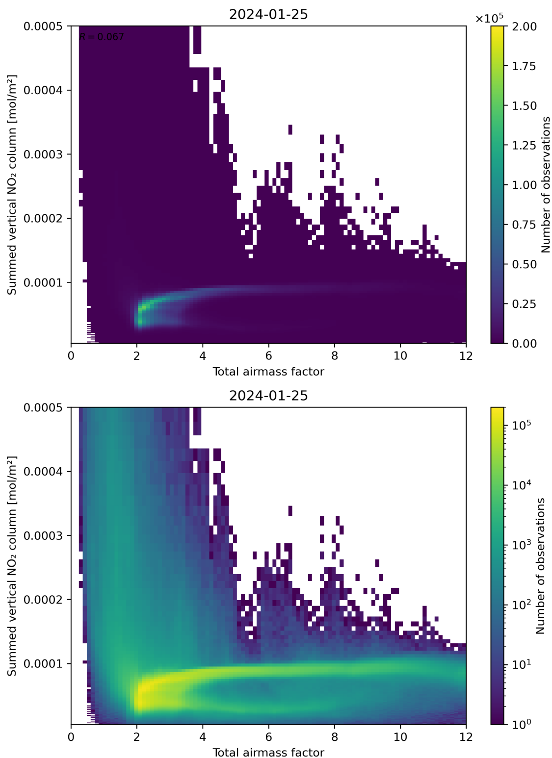
Figure 65: Scatter density plot of “Total airmass factor” against “Summed vertical NO 2 column” for 2024-01-24 to 2024-01-26.
