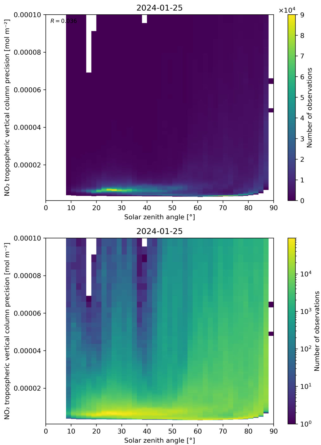
Figure 156: Scatter density plot of “Solar zenith angle” against “NO 2 tropospheric vertical column precision” for 2024-01-24 to 2024-01-26.
