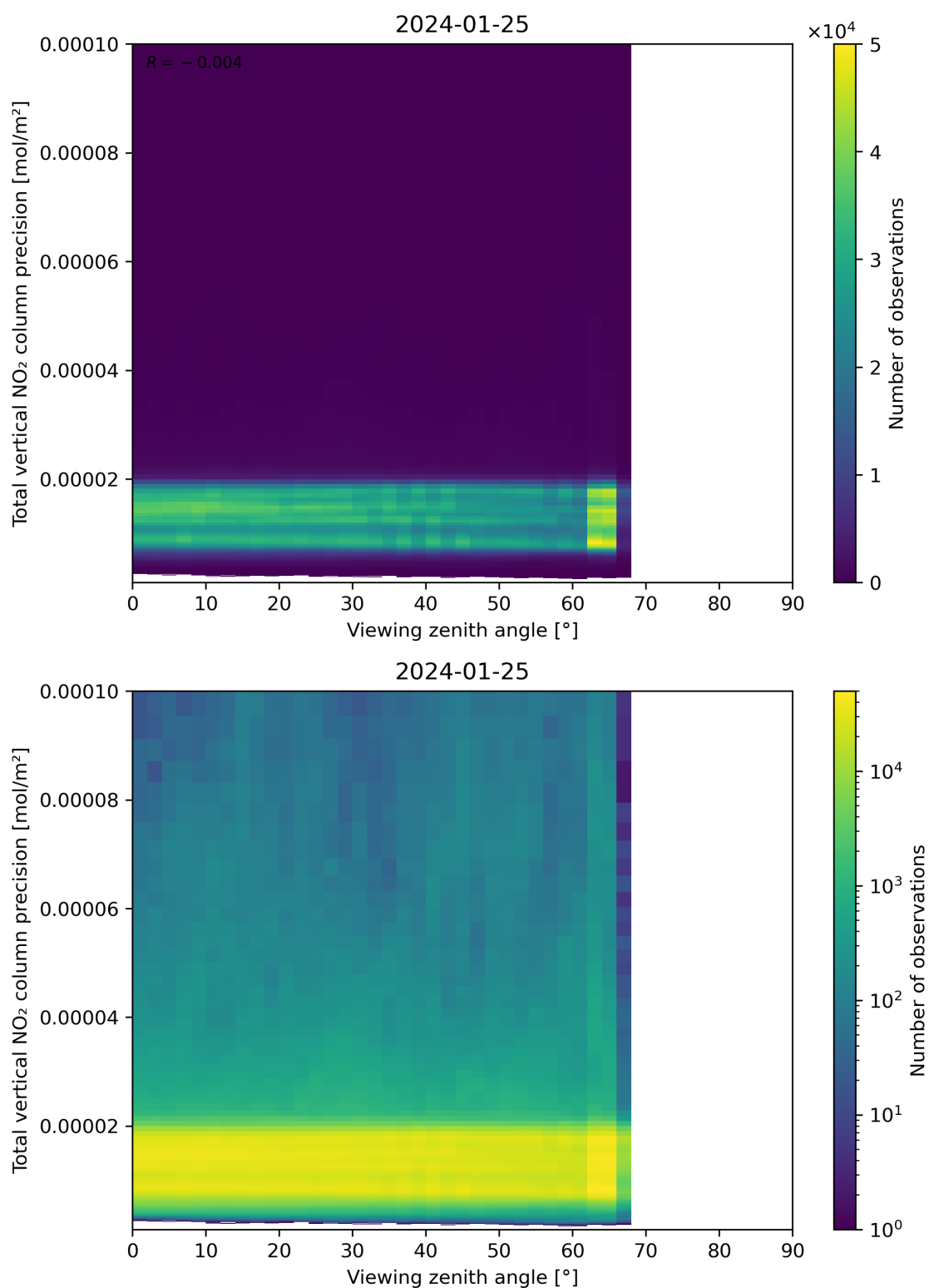
Figure 168: Scatter density plot of “Viewing zenith angle” against “Total vertical NO 2 column precision” for 2024-01-24 to 2024-01-26.
