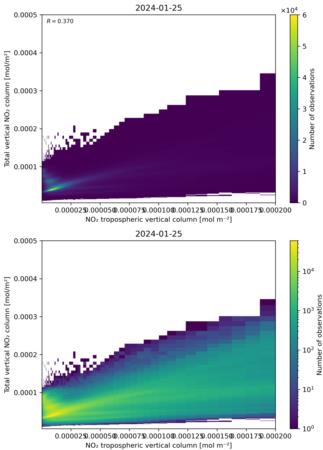
Figure 128: Scatter density plot of “NO 2 tropospheric vertical column” against “Total vertical NO 2 column” for 2024-01-24 to 2024-01-26.
