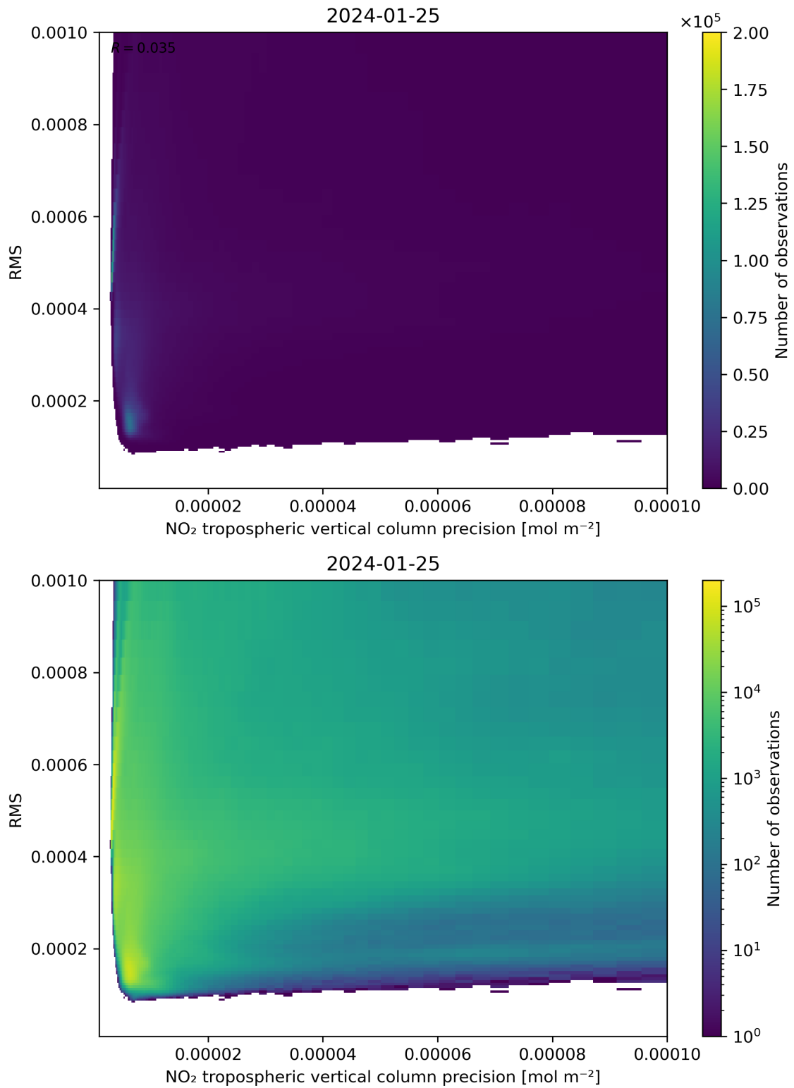
Figure 140: Scatter density plot of “NO 2 tropospheric vertical column precision” against “RMS” for 2024-01-24 to 2024-01-26.
