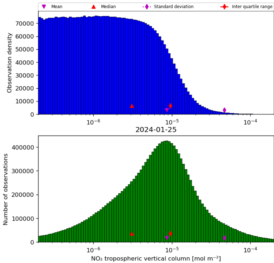
Figure 29: Histogram of “NO 2 tropospheric vertical column” for 2024-01-24 to 2024-01-26
