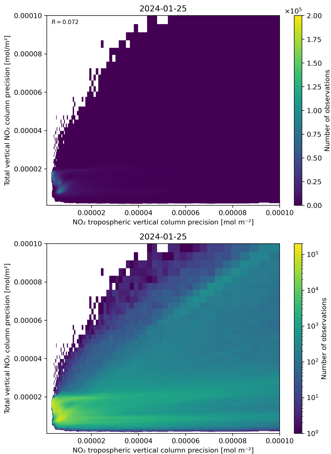
Figure 139: Scatter density plot of “NO 2 tropospheric vertical column precision” against “Total vertical NO 2 column precision” for 2024-01-24 to 2024-01-26.
