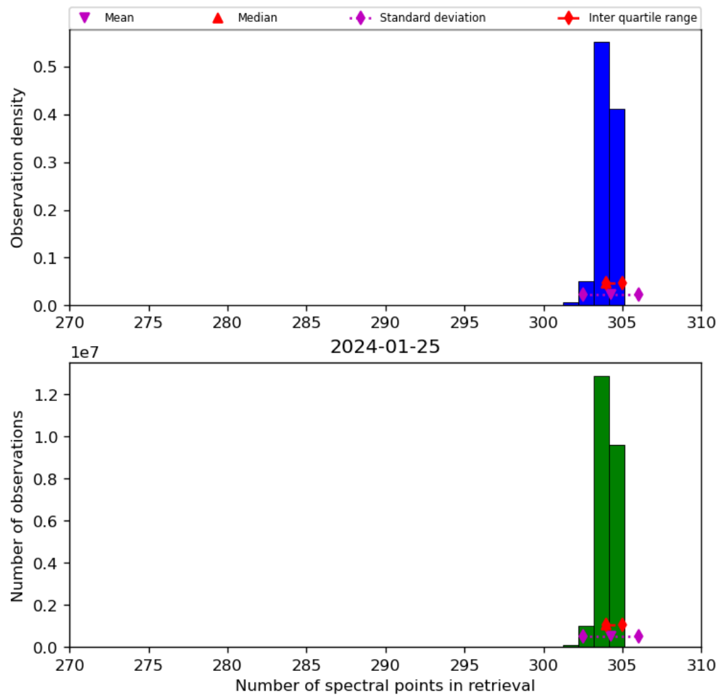
Figure 33: Histogram of “Number of spectral points in retrieval” for 2024-01-24 to 2024-01-26
