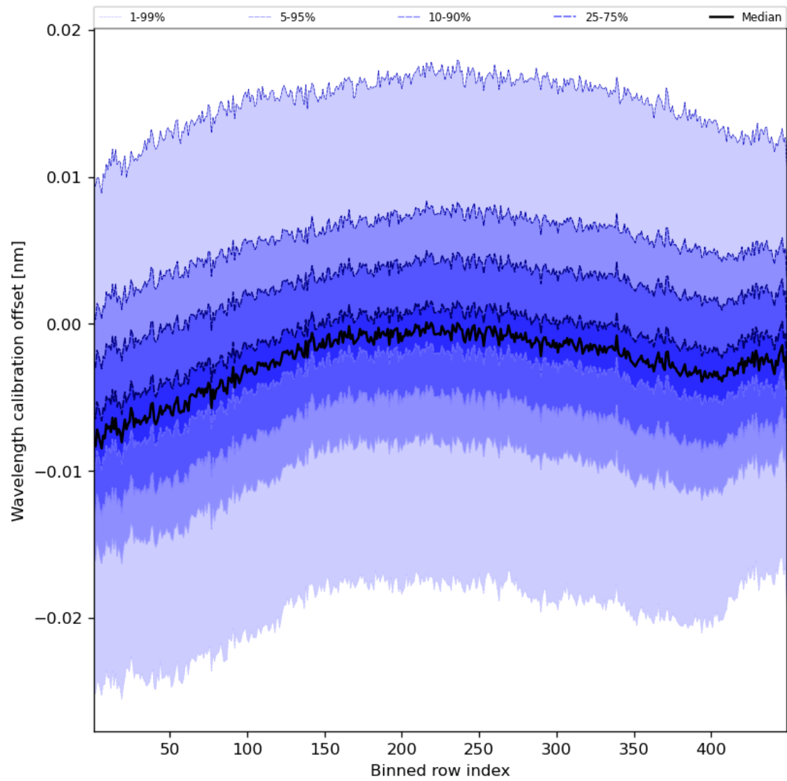
Figure 52: Along track statistics of “Wavelength calibration offset” for 2024-01-24 to 2024-01-26
