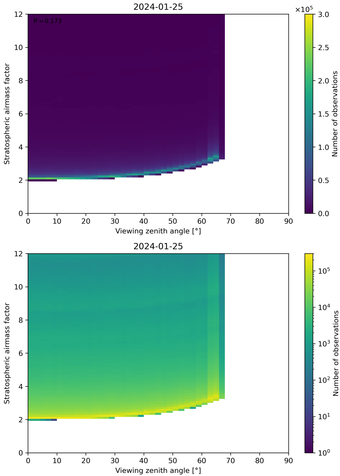
Figure 159: Scatter density plot of “Viewing zenith angle” against “Stratospheric airmass factor” for 2024-01-24 to 2024-01-26.
