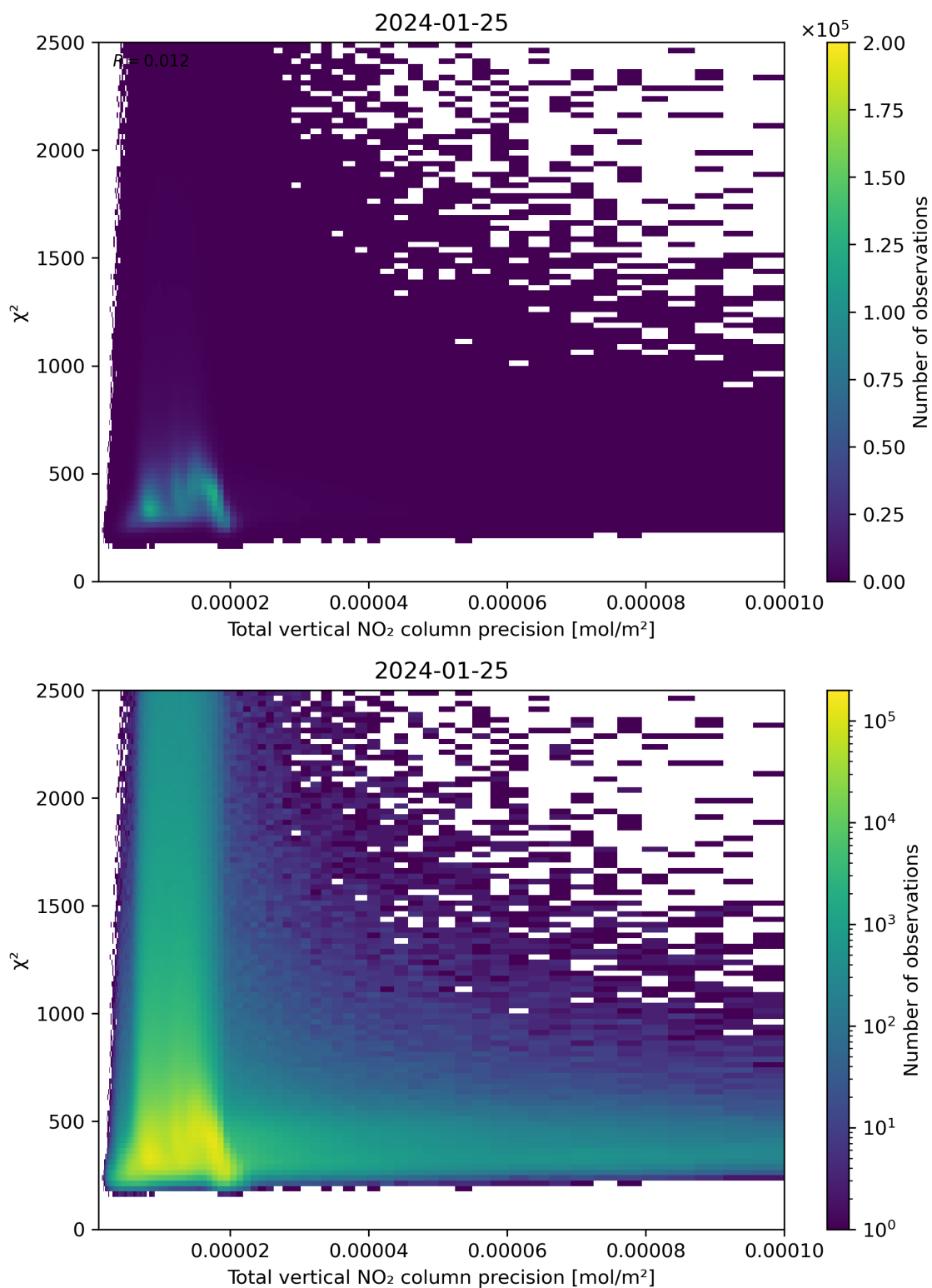
Figure 116: Scatter density plot of “Total vertical NO 2 column precision” against “ \chi^2 ” for 2024-01-24 to 2024-01-26.
