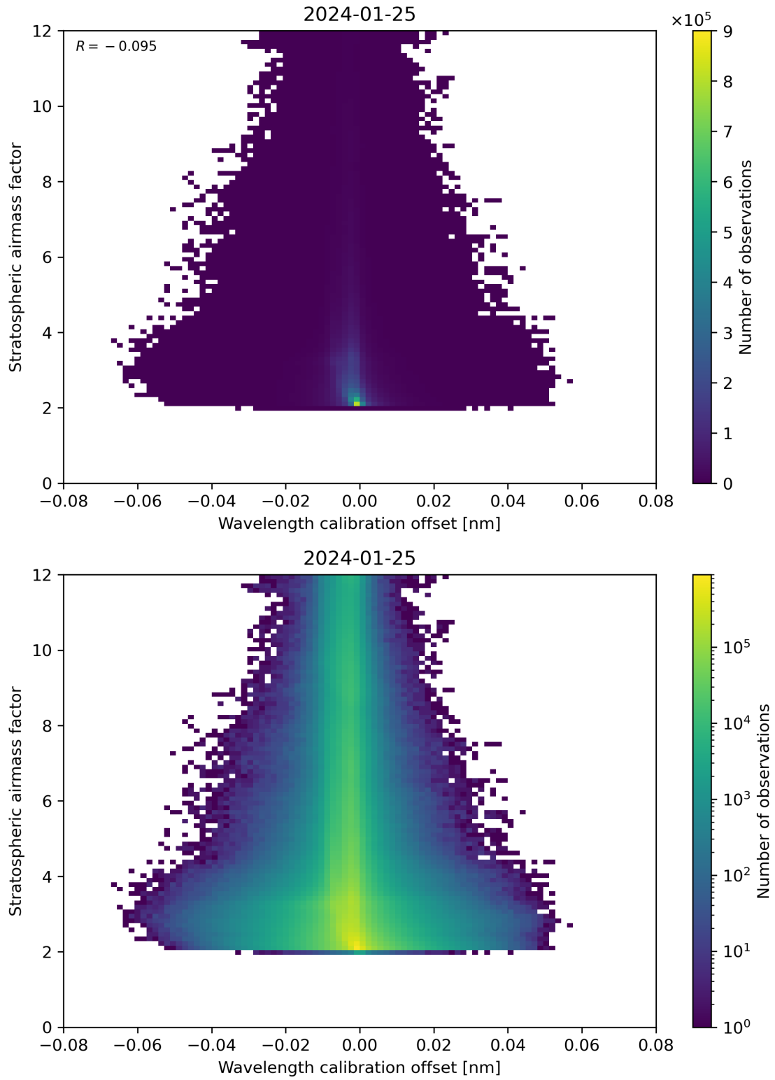
Figure 174: Scatter density plot of “Wavelength calibration offset” against “Stratospheric airmass factor” for 2024-01-24 to 2024-01-26.
