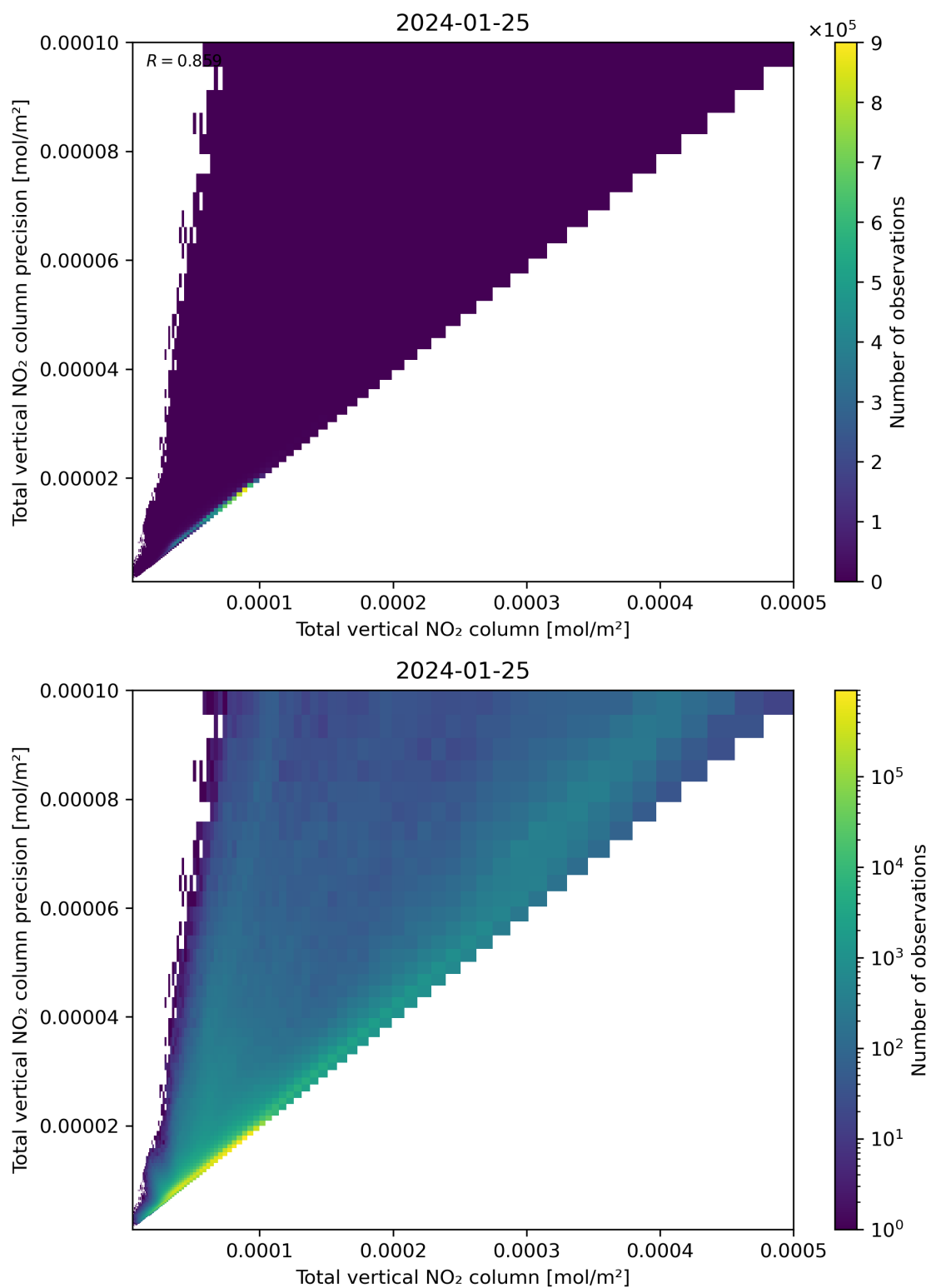
Figure 114: Scatter density plot of “Total vertical NO 2 column” against “Total vertical NO 2 column precision” for 2024-01-24 to 2024-01-26.
