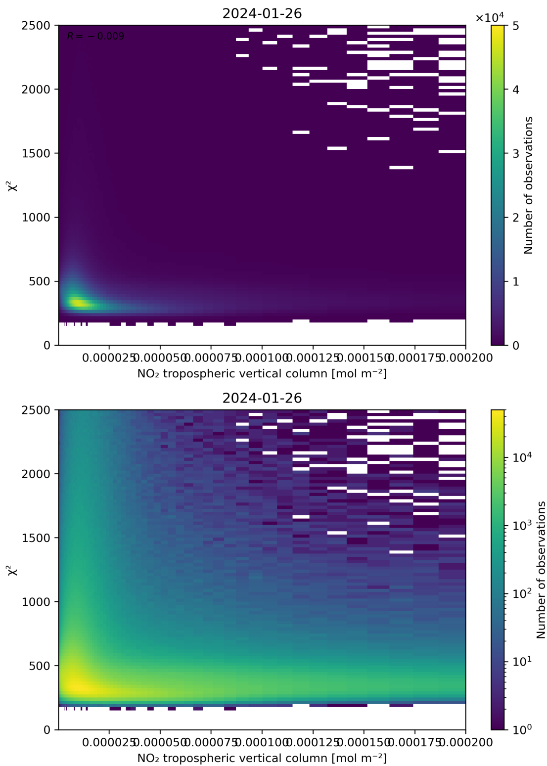
Figure 124: Scatter density plot of “NO 2 tropospheric vertical column” against “ \chi^2 ” for 2024-01-26 to 2024-01-27.
