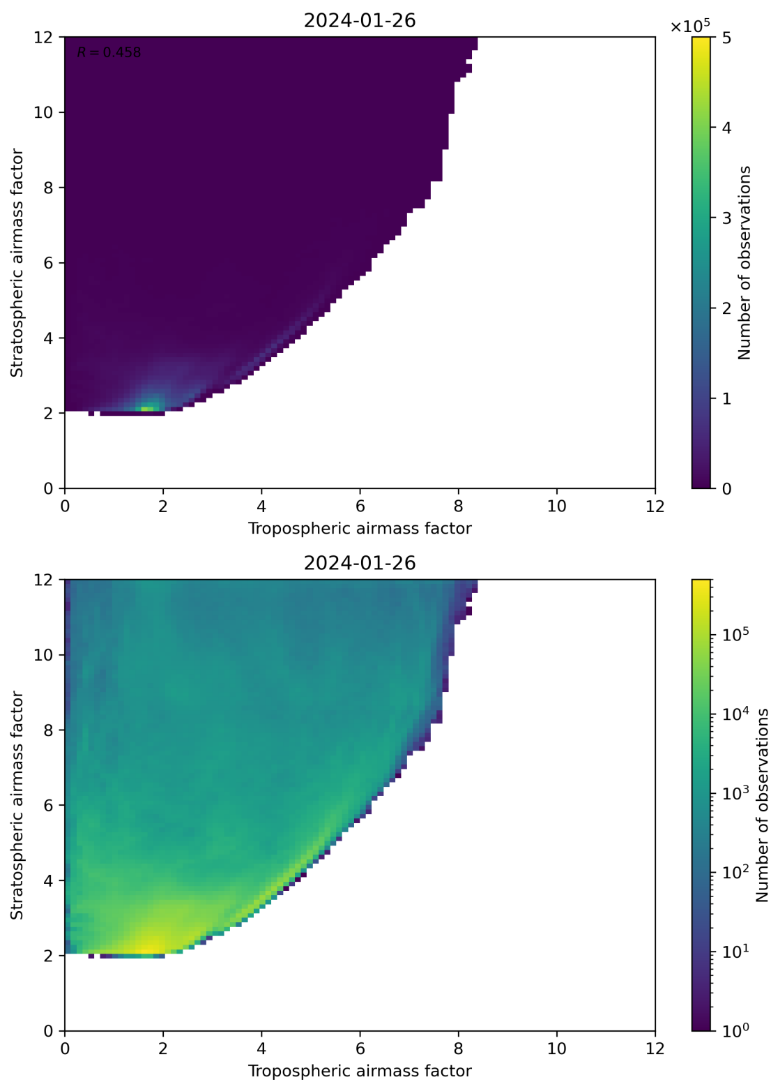
Figure 71: Scatter density plot of “Tropospheric airmass factor” against “Stratospheric airmass factor” for 2024-01-26 to 2024-01-27.
