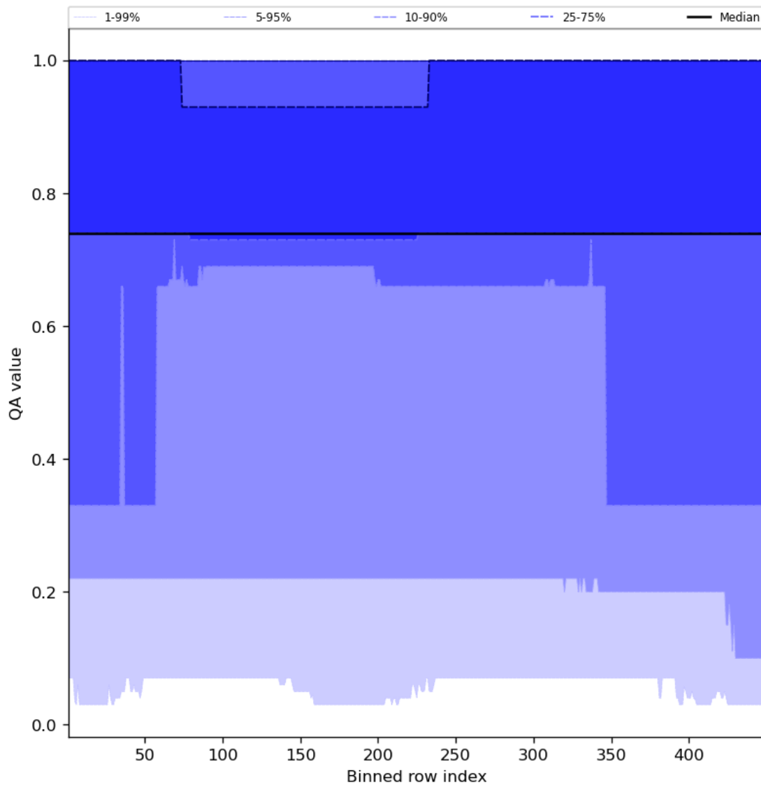
Figure 45: Along track statistics of “QA value” for 2024-01-26 to 2024-01-27
