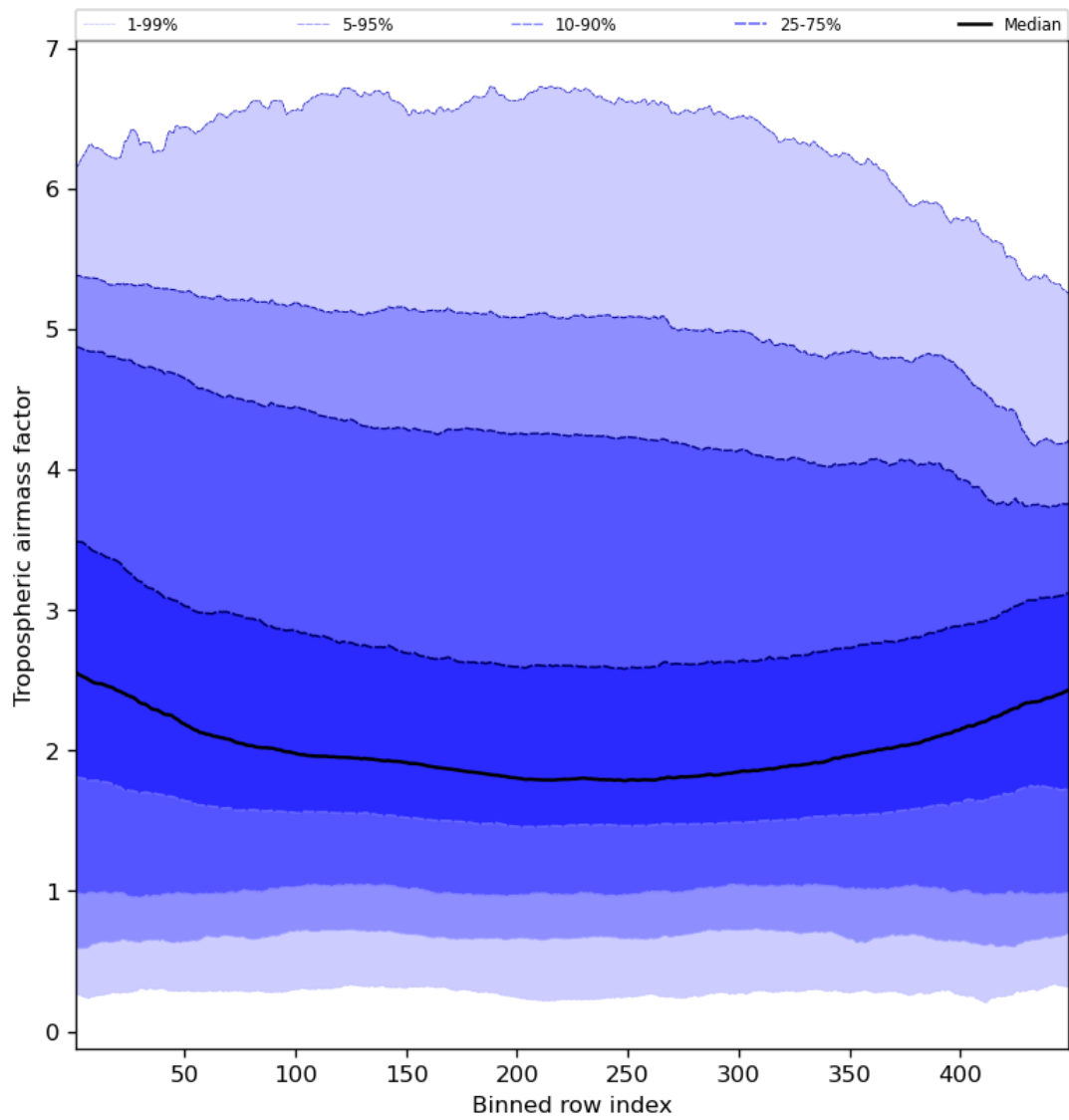
Figure 48: Along track statistics of “Tropospheric air mass factor” for 2024-01-26 to 2024-01-27
