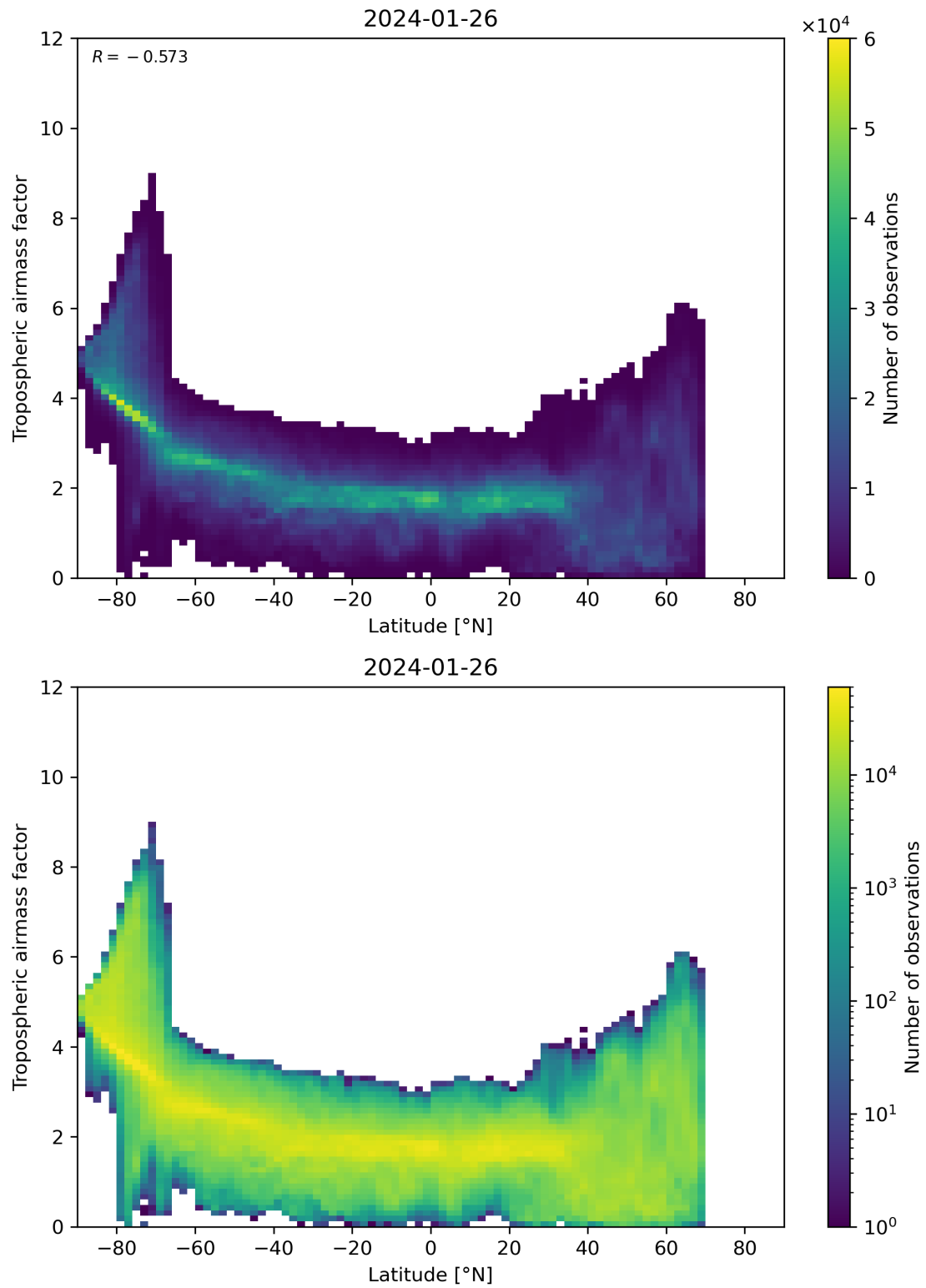
Figure 85: Scatter density plot of “Latitude” against “Tropospheric airmass factor” for 2024-01-26 to 2024-01-27.
