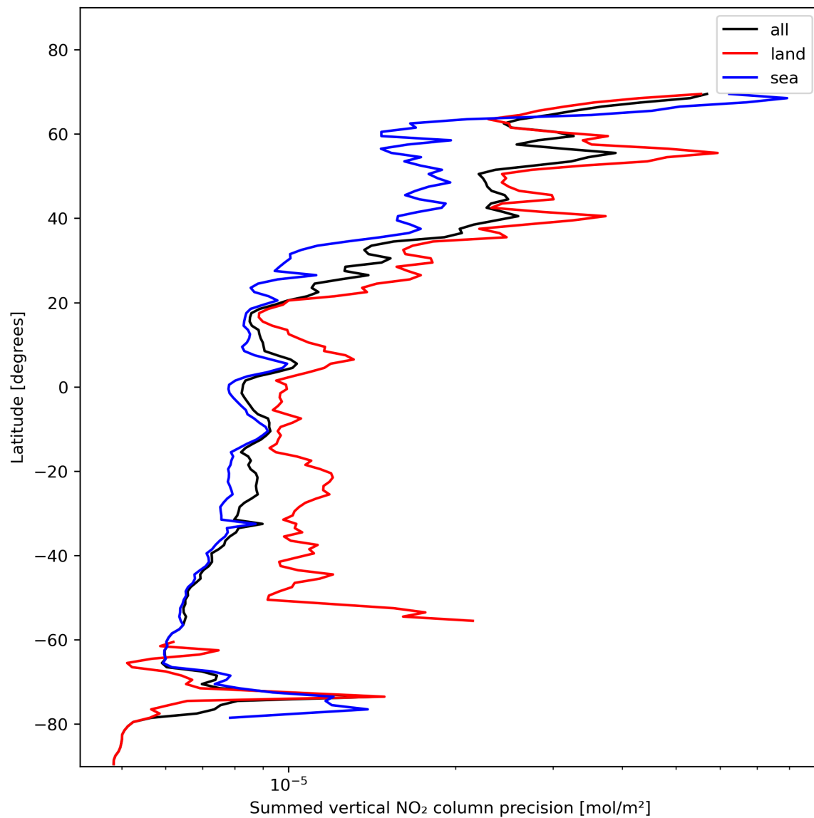
Figure 24: Zonal average of “Summed vertical NO 2 column precision” for 2024-01-26 to 2024-01-27.
