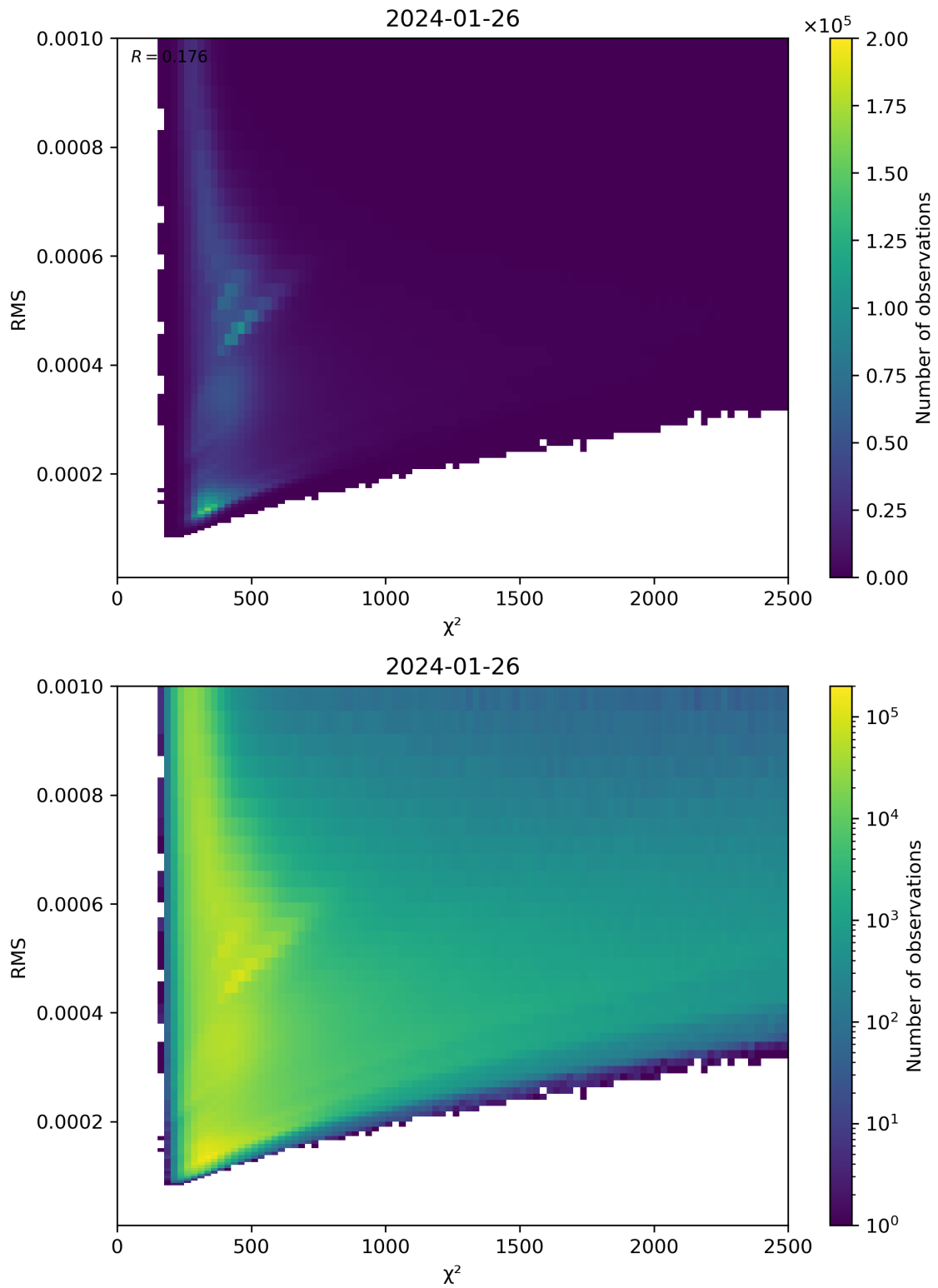
Figure 82: Scatter density plot of “ \chi^2 ” against “RMS” for 2024-01-26 to 2024-01-27.
