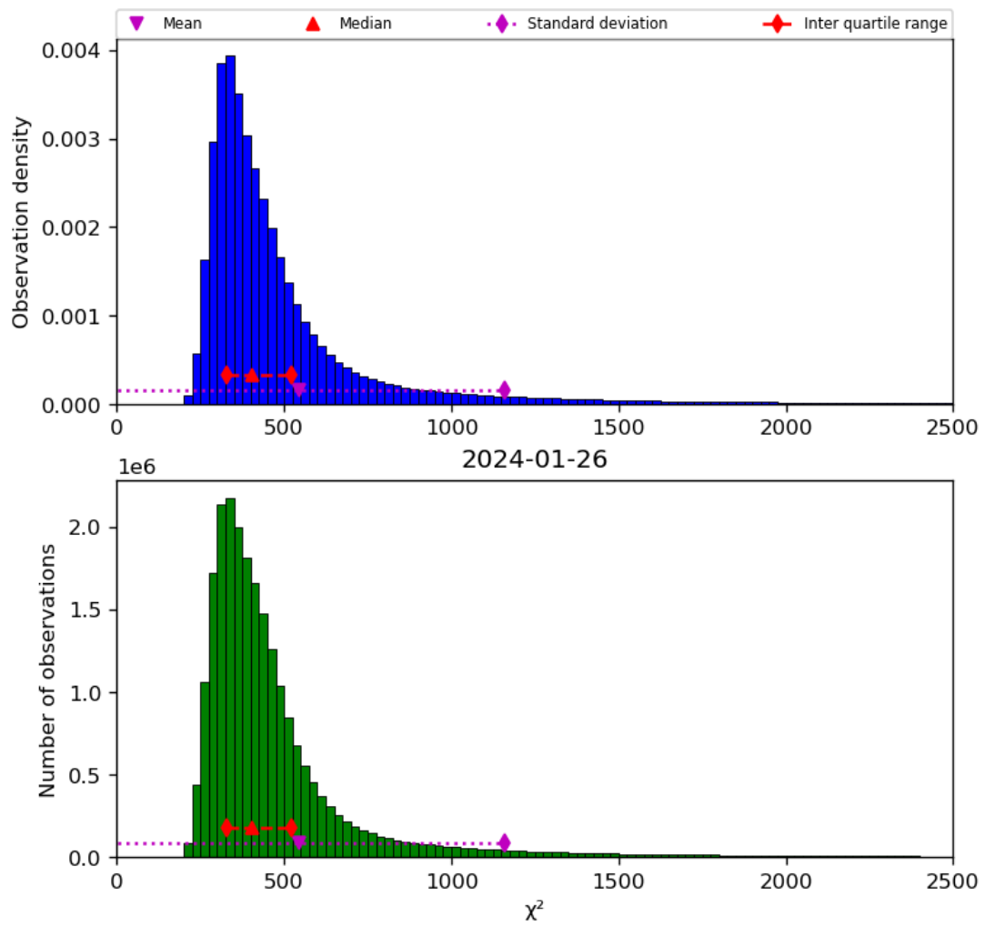
Figure 42: Histogram of “ \chi^2 ” for 2024-01-26 to 2024-01-27
