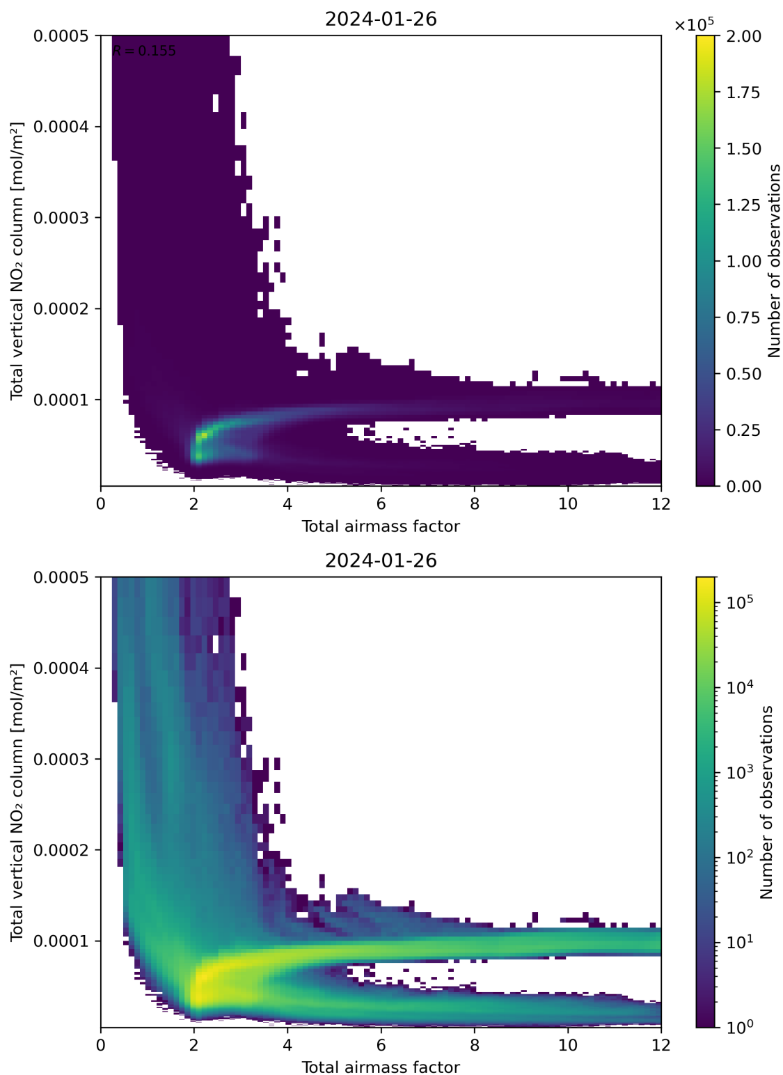
Figure 67: Scatter density plot of “Total airmass factor” against “Total vertical NO 2 column” for 2024-01-26 to 2024-01-27.
