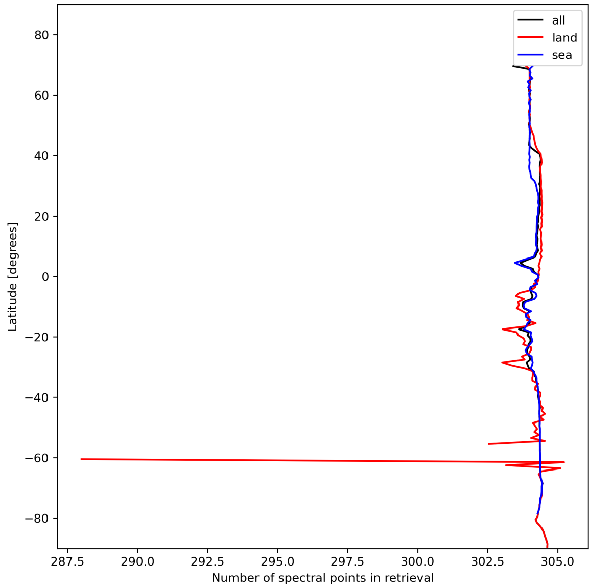
Figure 16: Zonal average of “Number of spectral points in retrieval” for 2024-01-26 to 2024-01-27.
