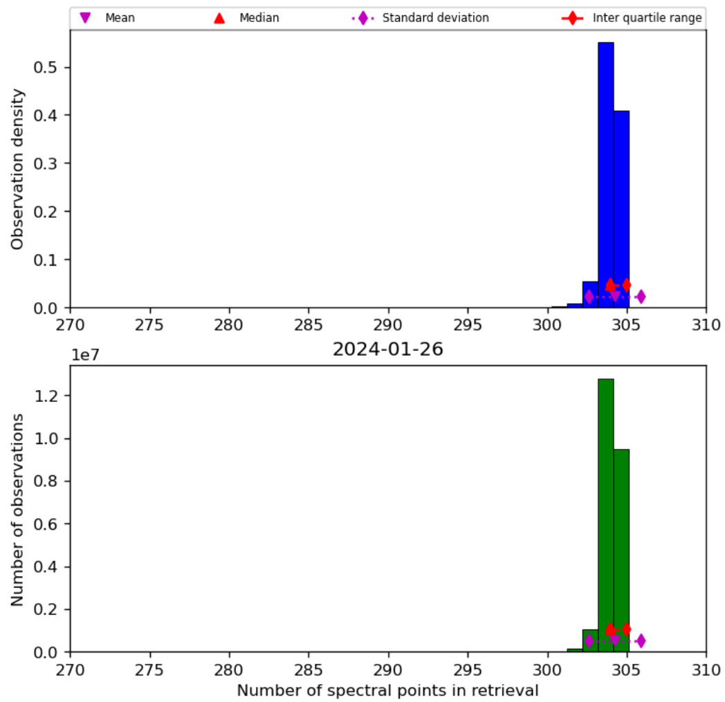
Figure 33: Histogram of “Number of spectral points in retrieval” for 2024-01-26 to 2024-01-27
