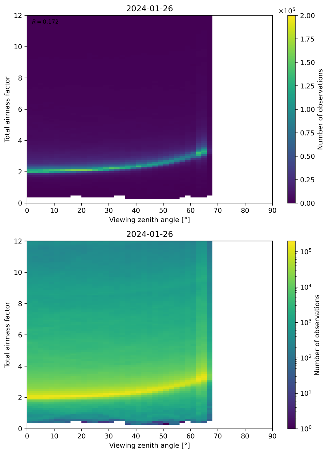
Figure 160: Scatter density plot of “Viewing zenith angle” against “Total airmass factor” for 2024-01-26 to 2024-01-27.
