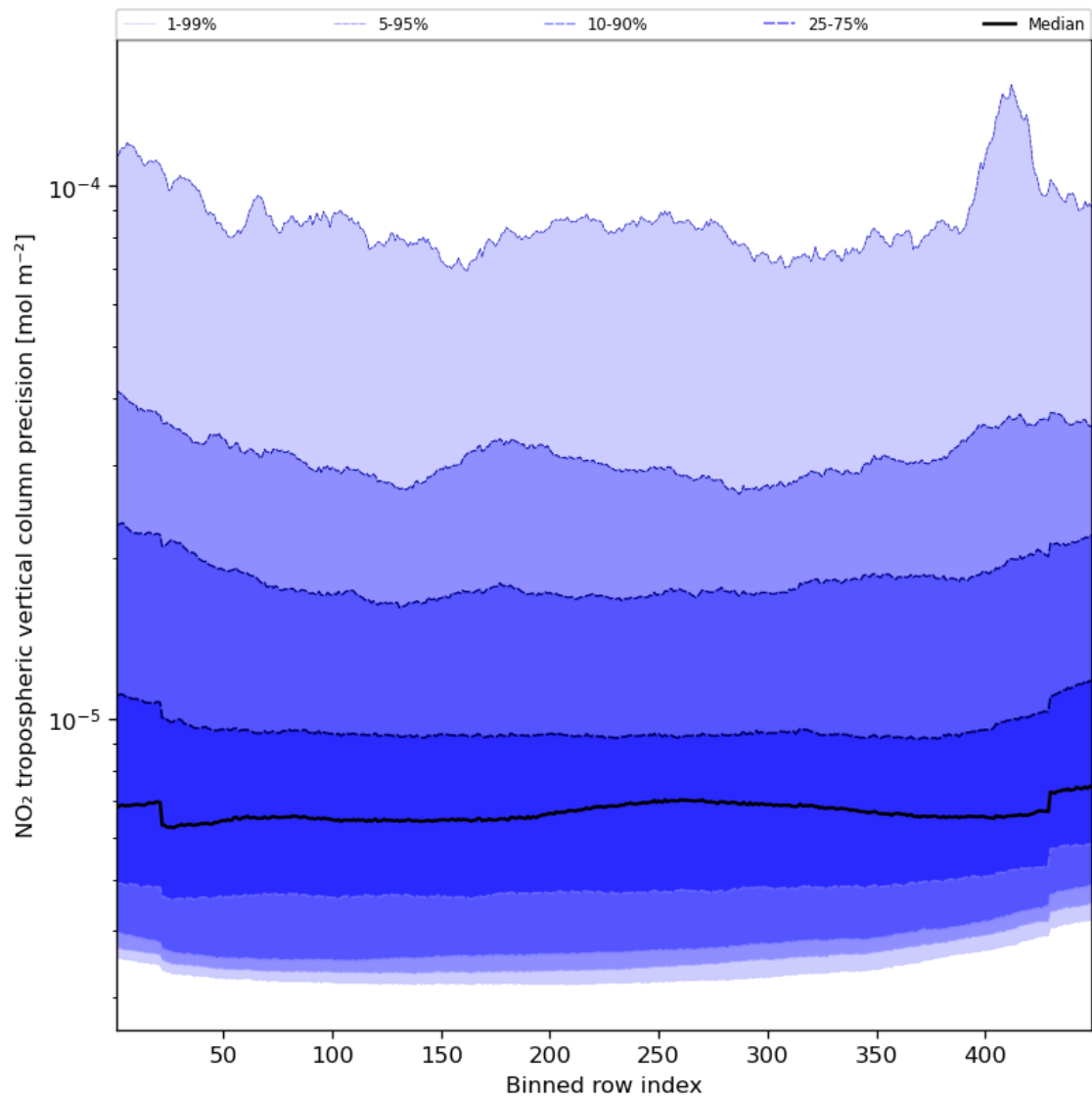
Figure 47: Along track statistics of “NO 2 tropospheric vertical column precision” for 2024-01-26 to 2024-01-27
