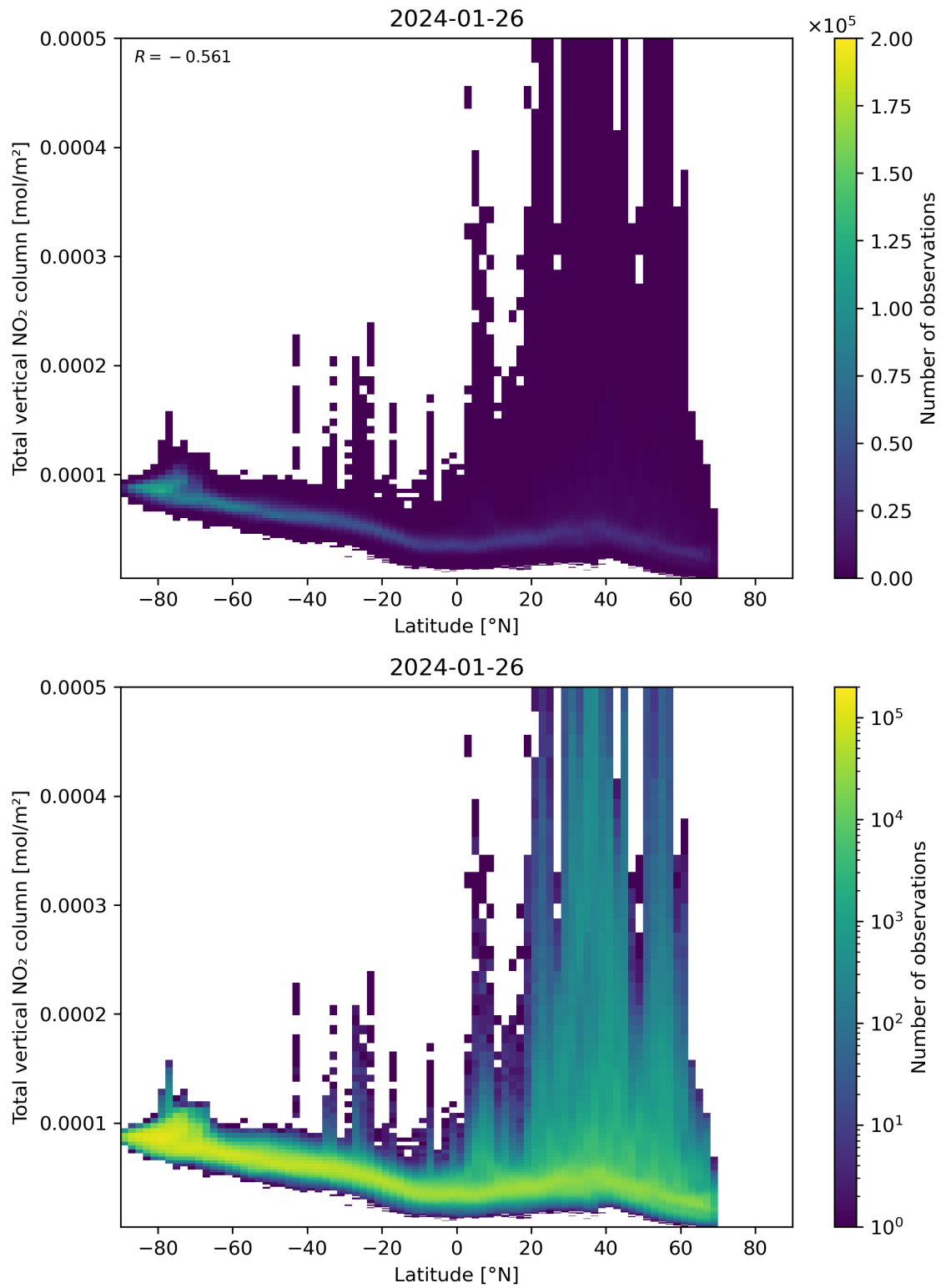
Figure 90: Scatter density plot of “Latitude” against “Total vertical NO 2 column” for 2024-01-26 to 2024-01-27.
