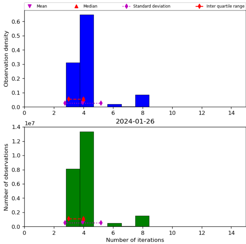
Figure 34: Histogram of “Number of iterations” for 2024-01-26 to 2024-01-27
