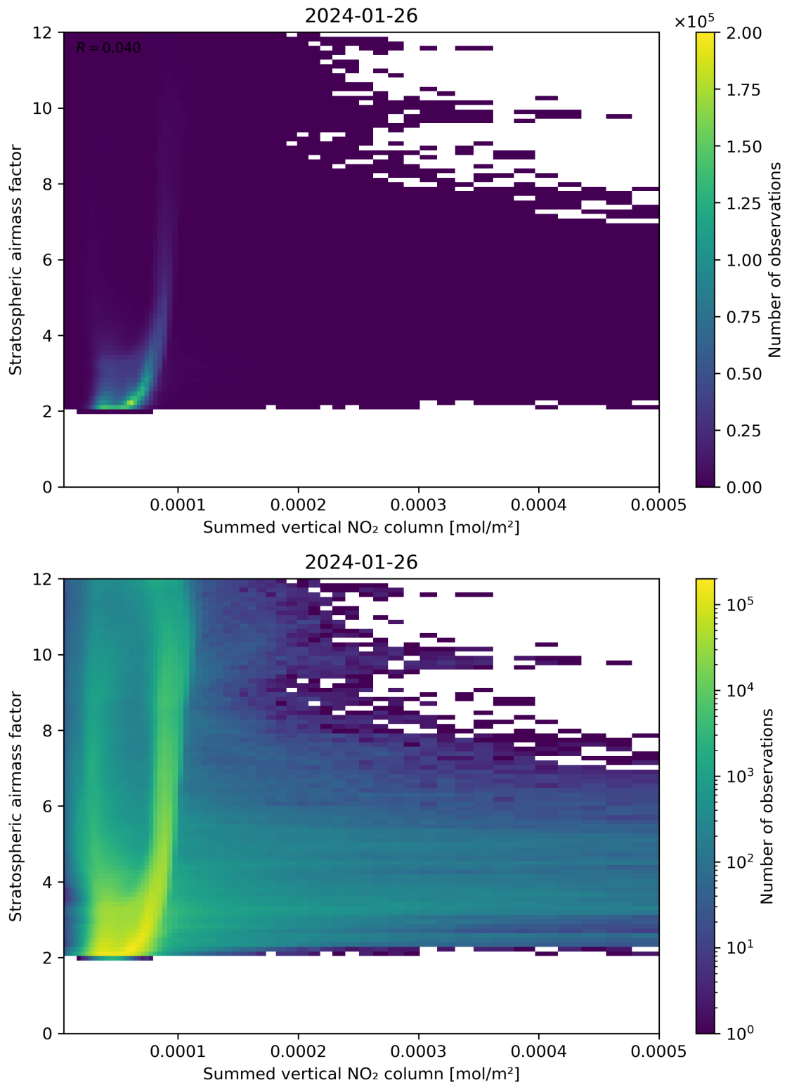
Figure 103: Scatter density plot of “Summed vertical NO 2 column” against “Stratospheric air mass factor” for 2024-01-26 to 2024-01-27.
