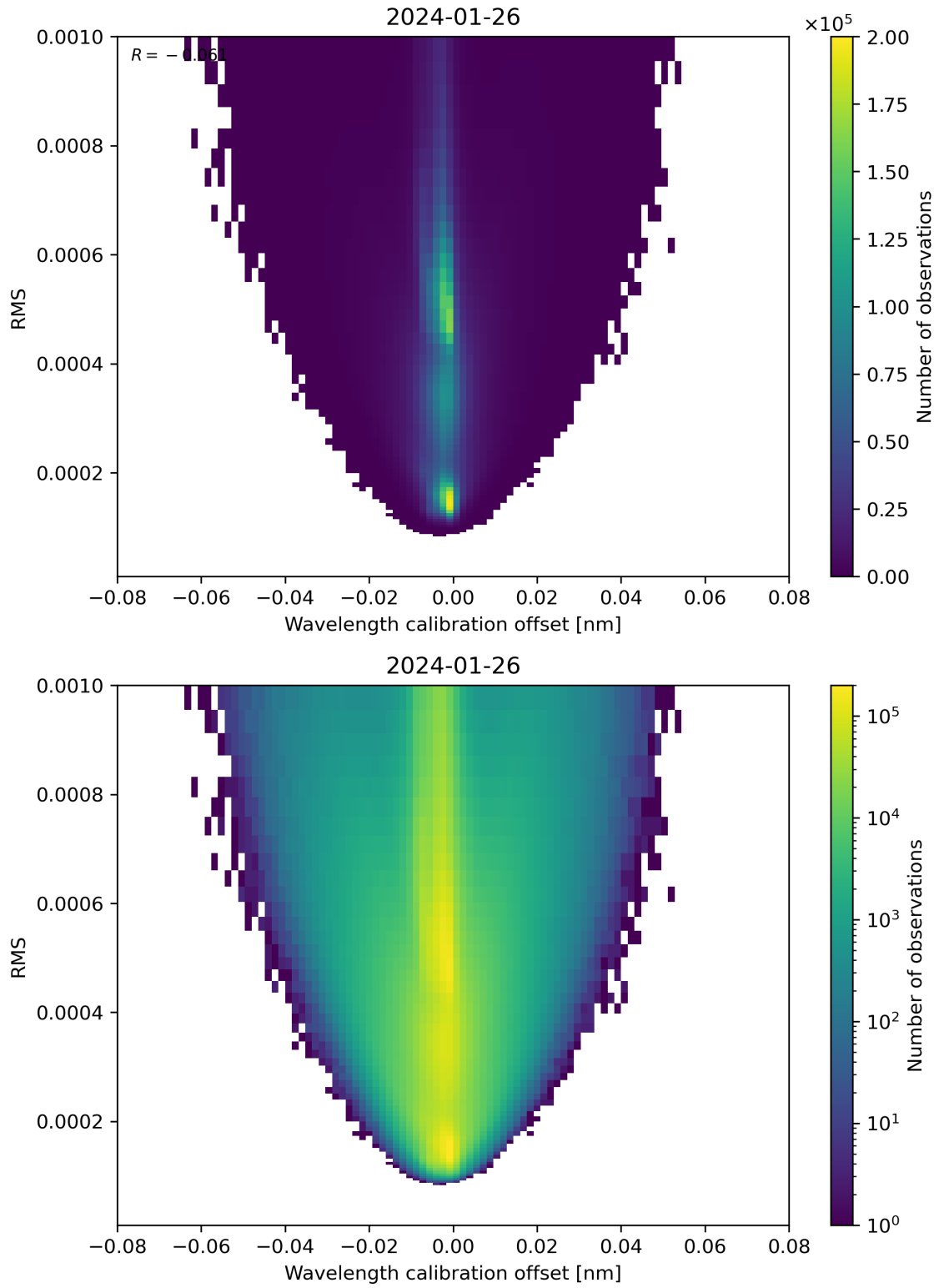
Figure 181: Scatter density plot of “Wavelength calibration offset” against “RMS” for 2024-01-26 to 2024-01-27.
