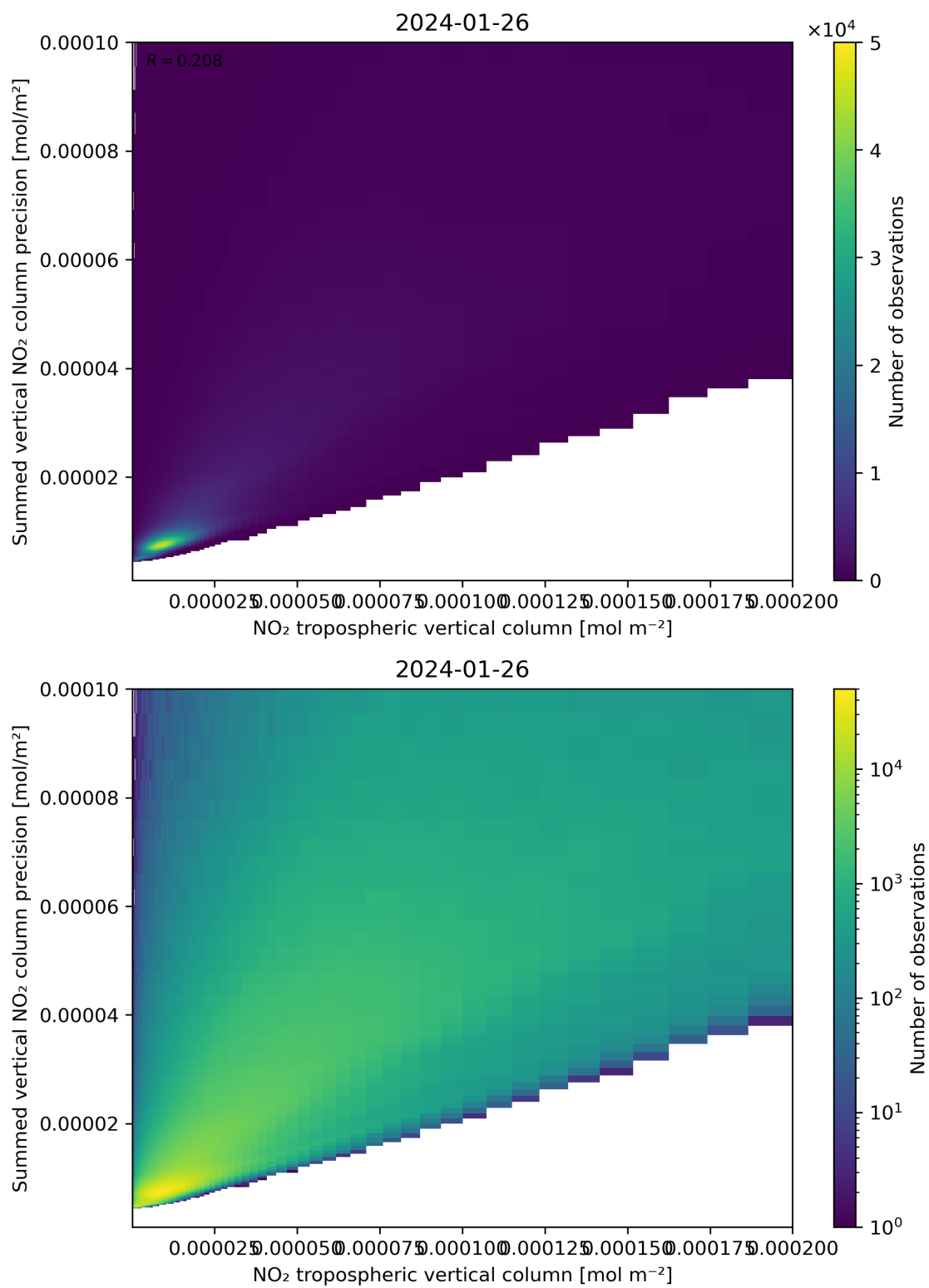
Figure 127: Scatter density plot of “NO 2 tropospheric vertical column” against “Summed vertical NO 2 column precision” for 2024-01-26 to 2024-01-27.
