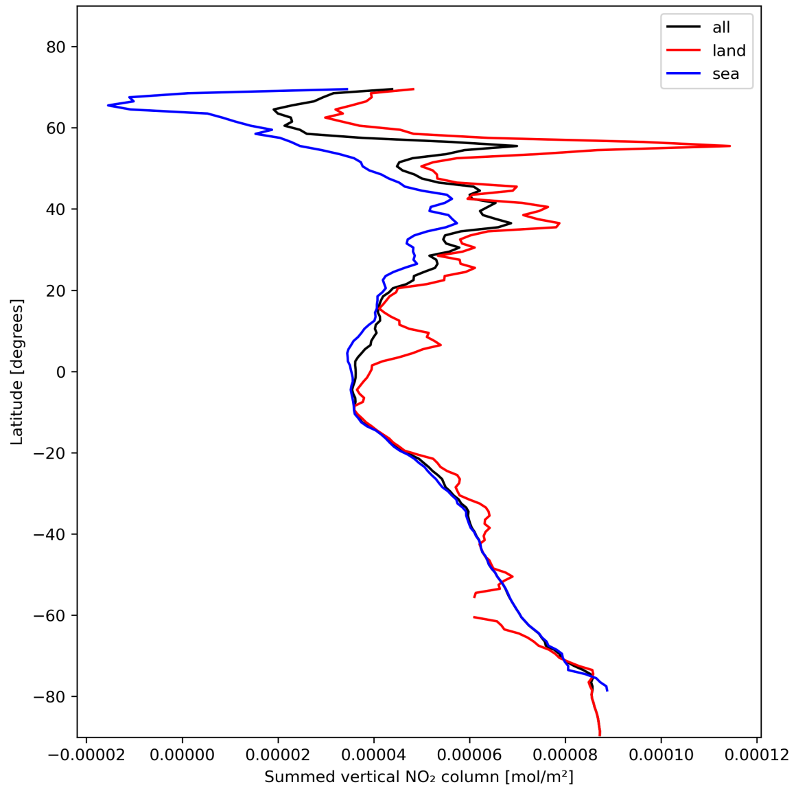
Figure 23: Zonal average of “Summed vertical NO 2 column” for 2024-01-26 to 2024-01-27.
