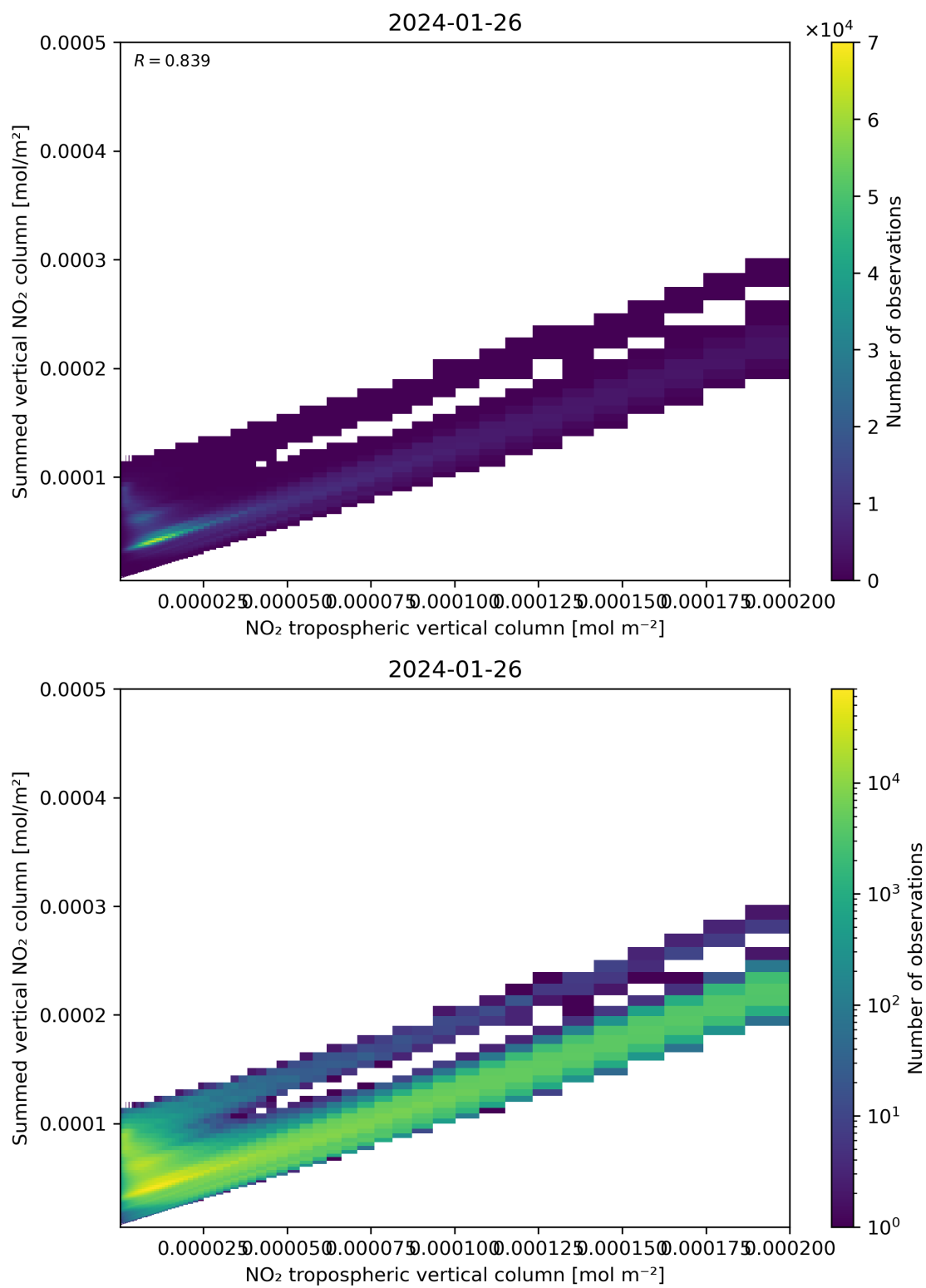
Figure 126: Scatter density plot of “NO 2 tropospheric vertical column” against “Summed vertical NO 2 column” for 2024-01-26 to 2024-01-27.
