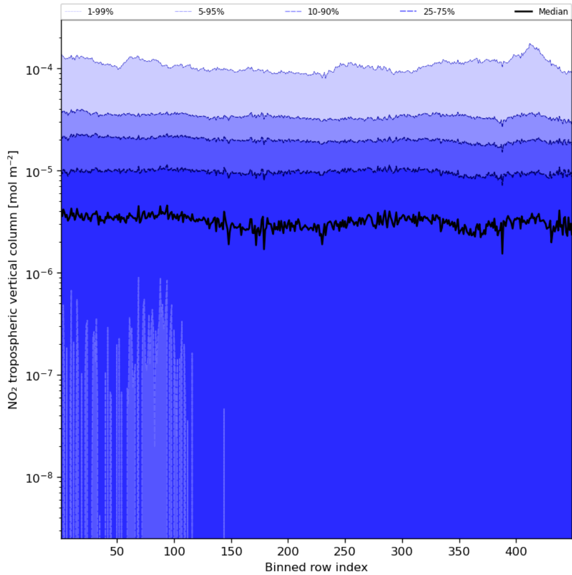
Figure 46: Along track statistics of “NO 2 tropospheric vertical column” for 2024-01-26 to 2024-01-27
