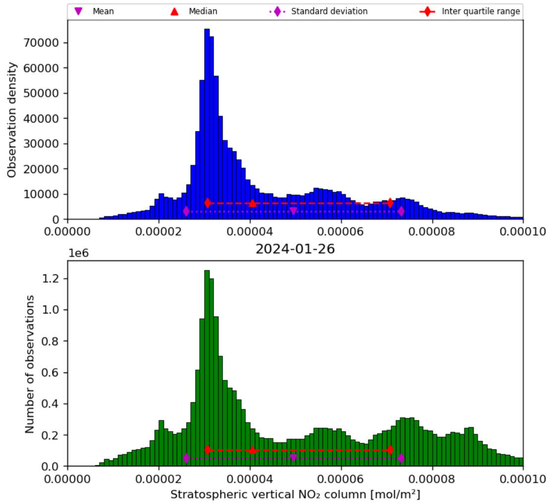
Figure 36: Histogram of “Stratospheric vertical NO 2 column” for 2024-01-26 to 2024-01-27
