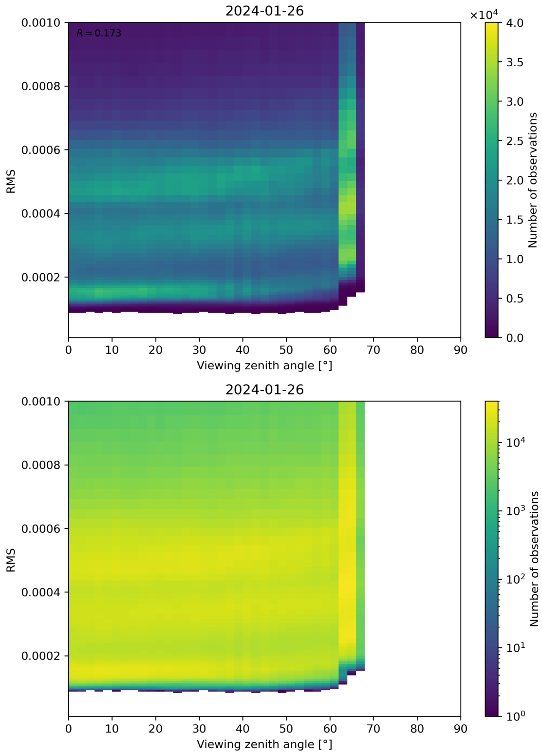
Figure 171: Scatter density plot of “Viewing zenith angle” against “RMS” for 2024-01-26 to 2024-01-27.
