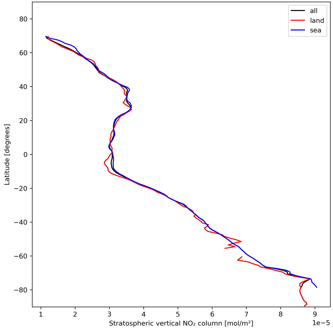
Figure 19: Zonal average of “Stratospheric vertical NO 2 column” for 2024-01-26 to 2024-01-27.
