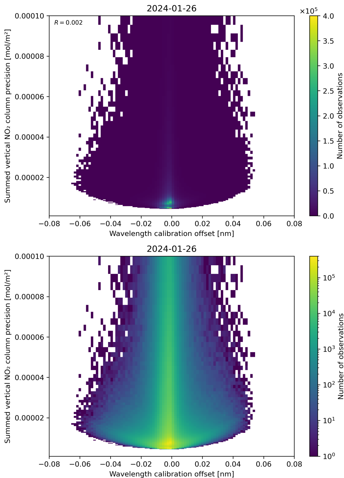
Figure 178: Scatter density plot of “Wavelength calibration offset” against “Summed vertical NO 2 column precision” for 2024-01-26 to 2024-01-27.
