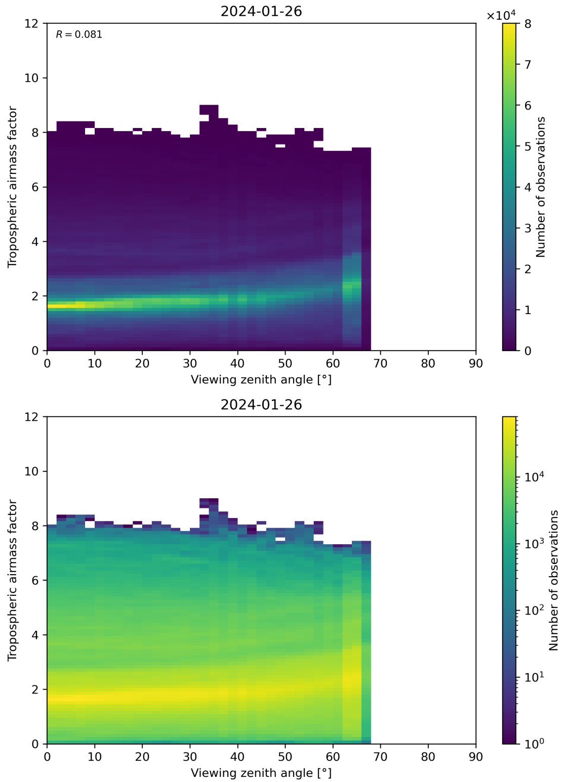
Figure 161: Scatter density plot of “Viewing zenith angle” against “Tropospheric airmass factor” for 2024-01-26 to 2024-01-27.
