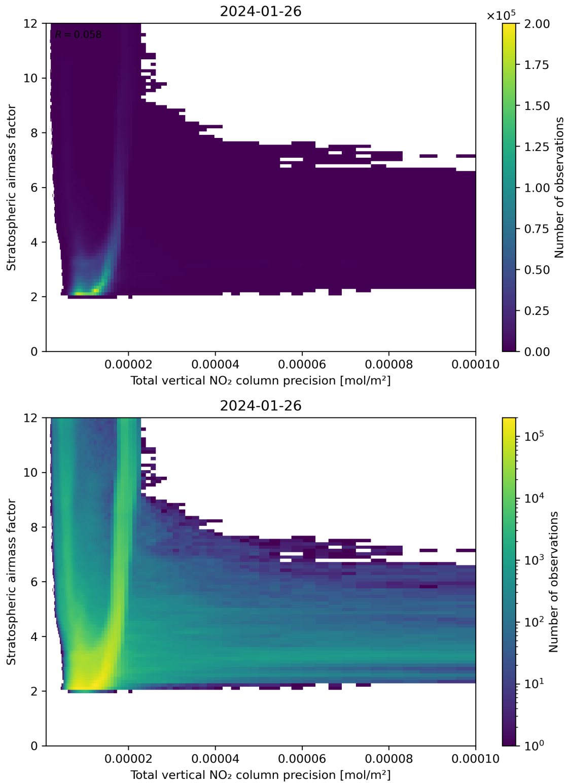
Figure 115: Scatter density plot of “Total vertical NO 2 column precision” against “Stratospheric air mass factor” for 2024-01-26 to 2024-01-27.
