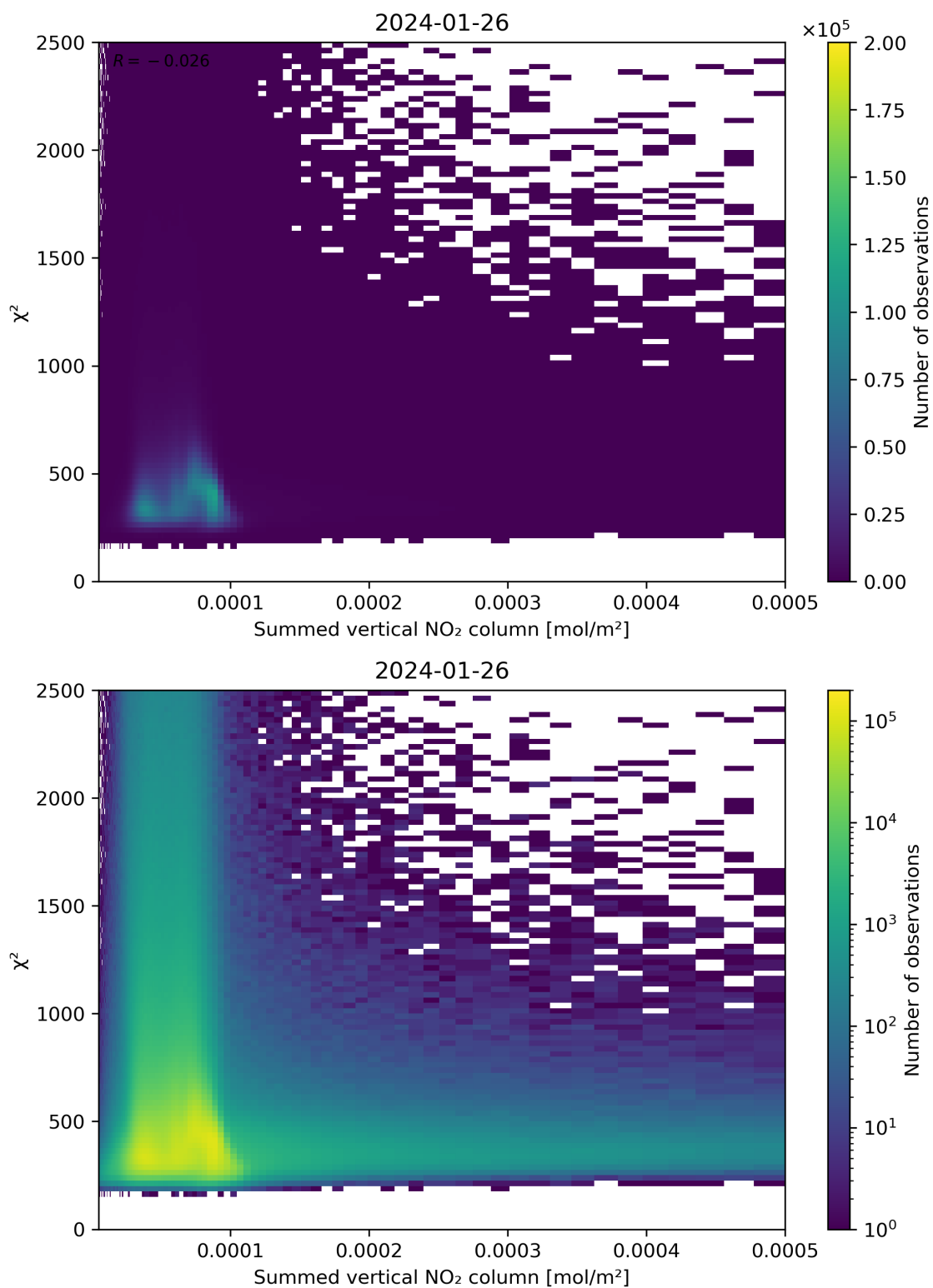
Figure 104: Scatter density plot of “Summed vertical NO 2 column” against “ \chi^2 ” for 2024-01-26 to 2024-01-27.
