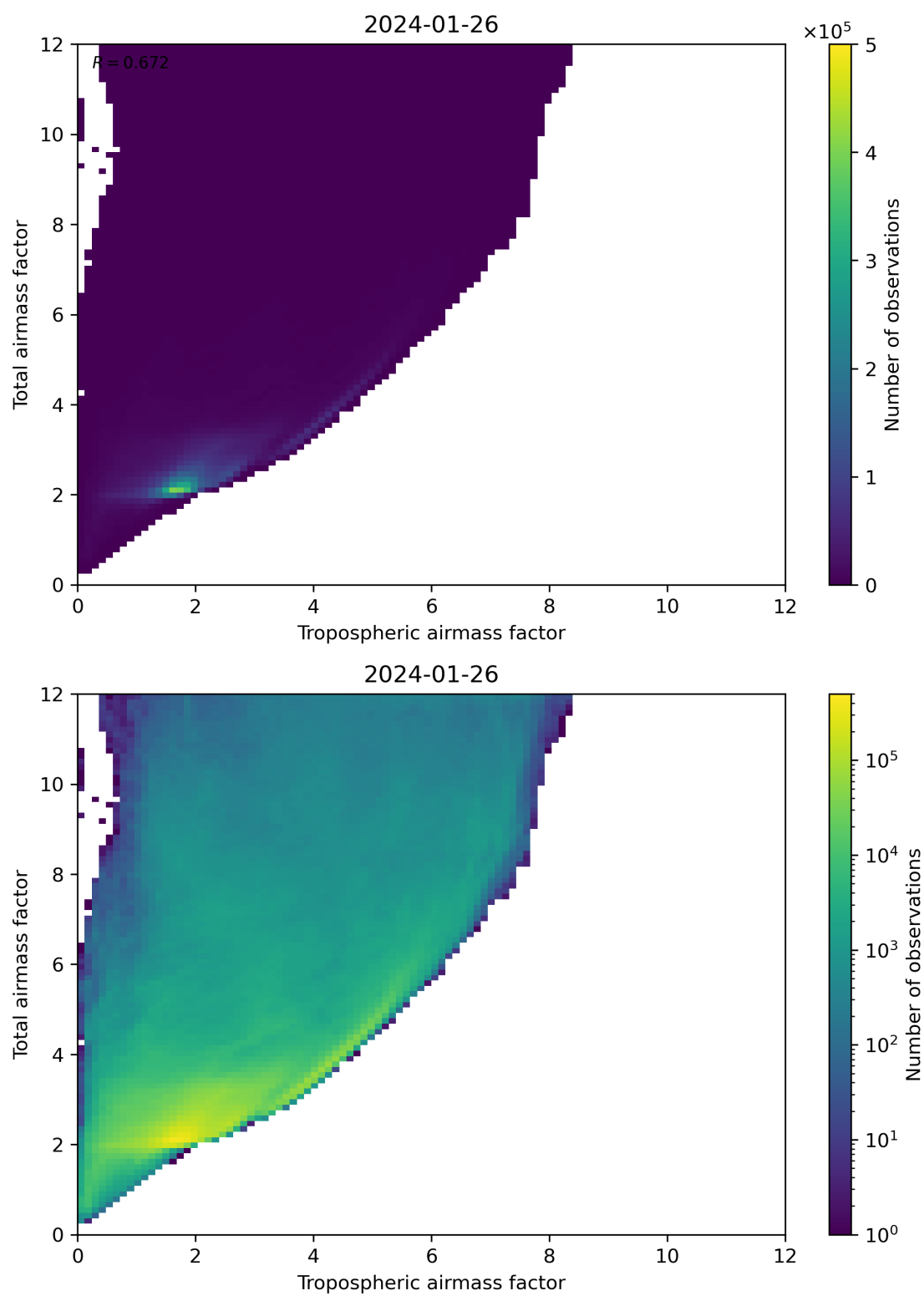
Figure 72: Scatter density plot of “Tropospheric airmass factor” against “Total airmass factor” for 2024-01-26 to 2024-01-27.
