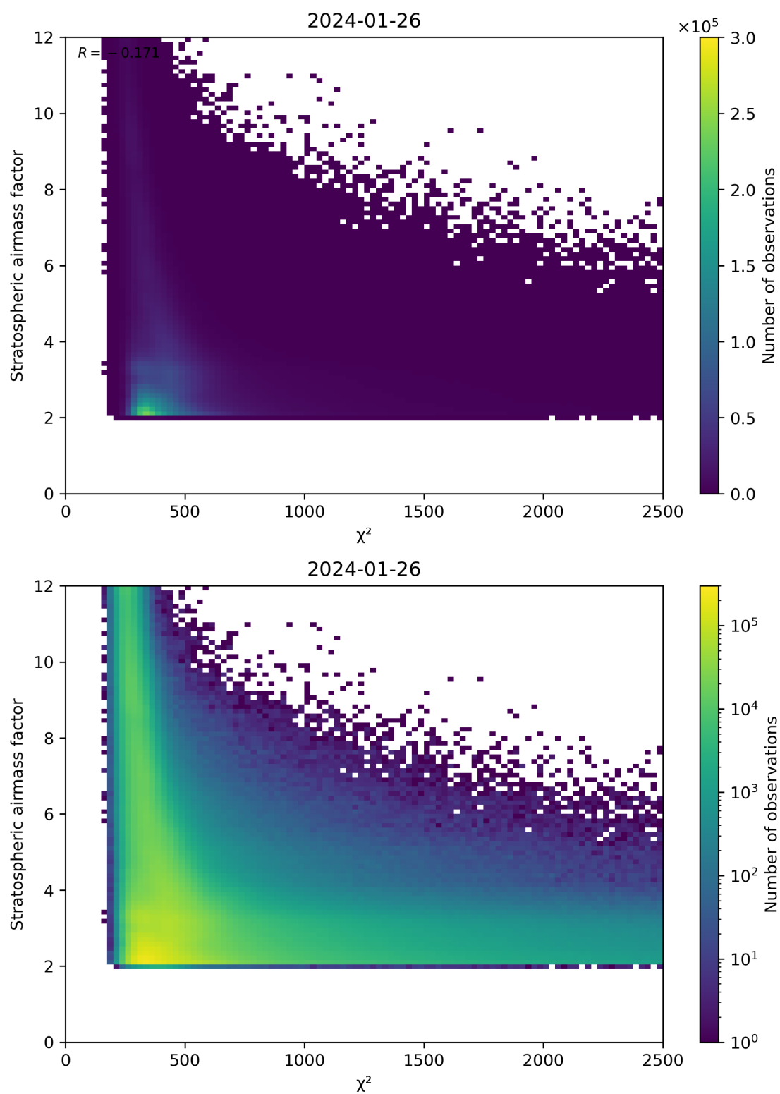
Figure 81: Scatter density plot of “ \chi^2 ” against “Stratospheric airmass factor” for 2024-01-26 to 2024-01-27.
