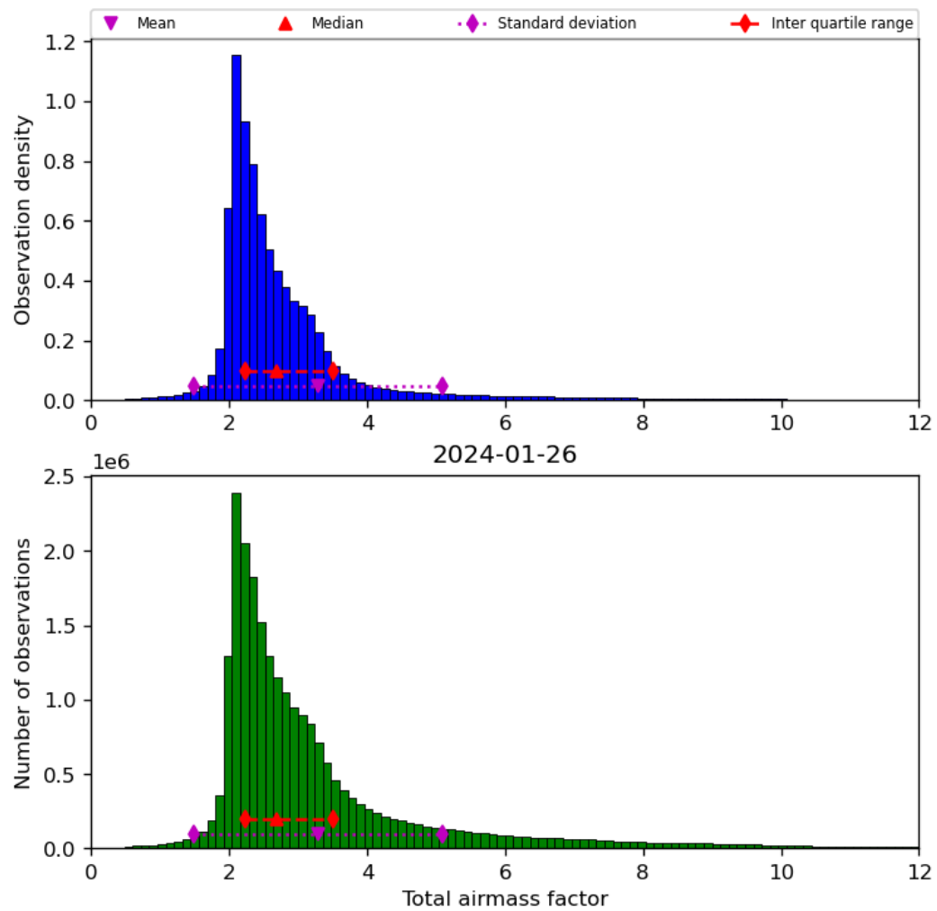
Figure 32: Histogram of “Total airmass factor” for 2024-01-26 to 2024-01-27
