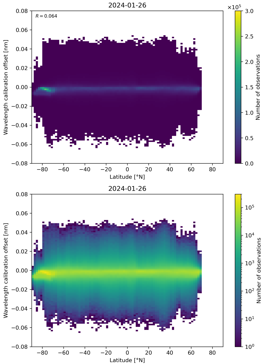
Figure 95: Scatter density plot of “Latitude” against “Wavelength calibration offset” for 2024-01-26 to 2024-01-27.
