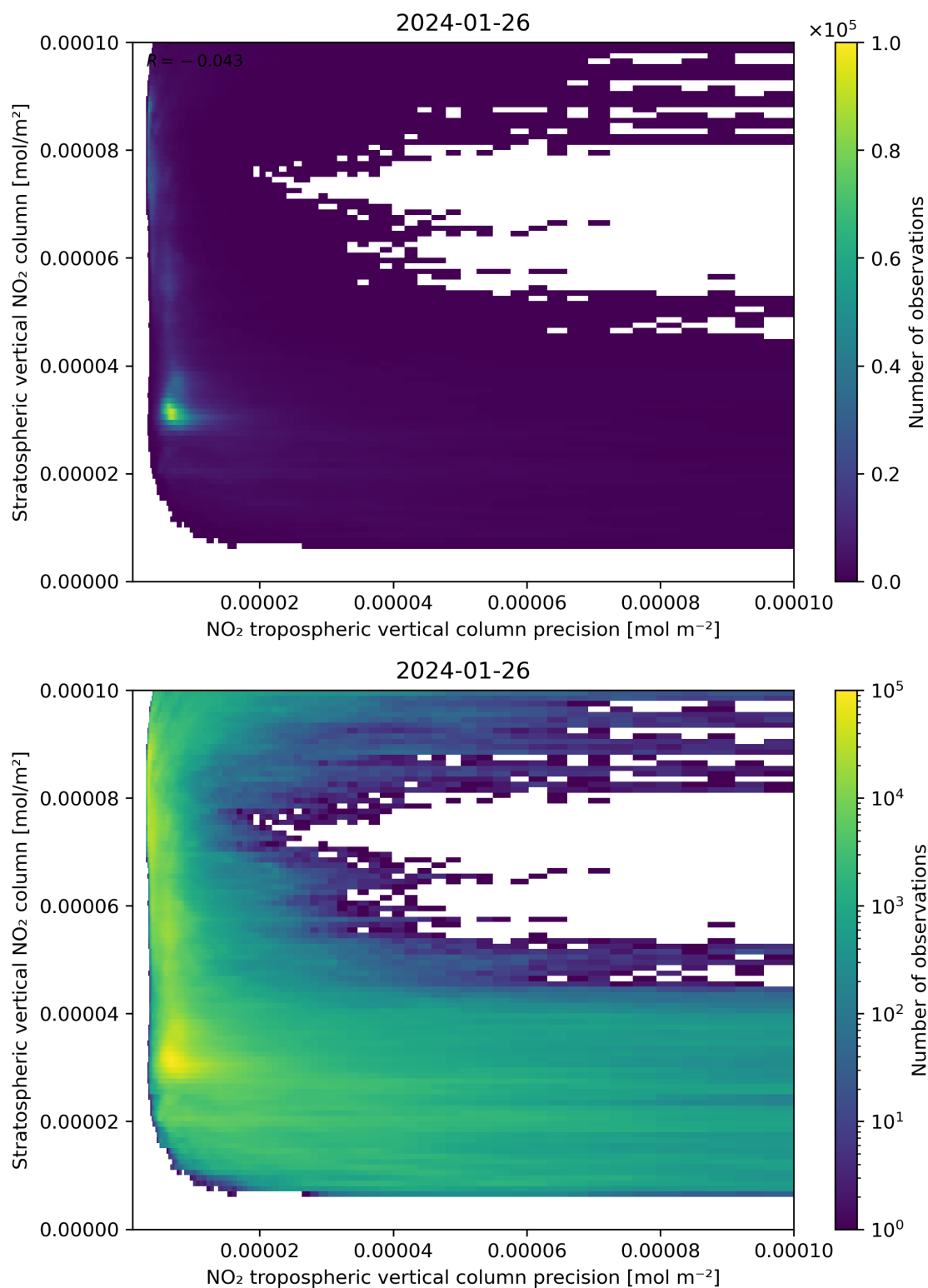
Figure 135: Scatter density plot of “NO 2 tropospheric vertical column precision” against “Stratospheric vertical NO 2 column” for 2024-01-26 to 2024-01-27.
