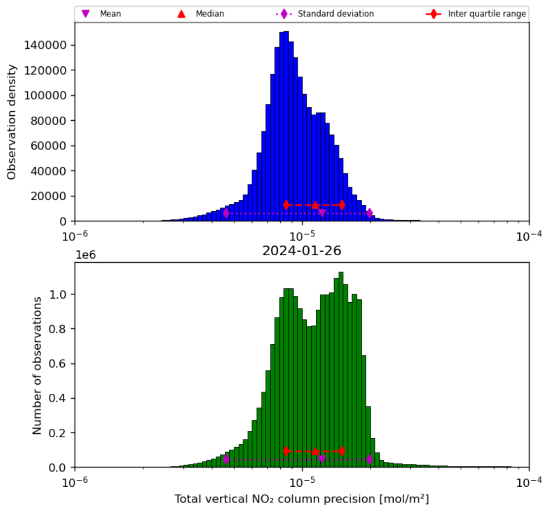
Figure 39: Histogram of “Total vertical NO 2 column precision” for 2024-01-26 to 2024-01-27
