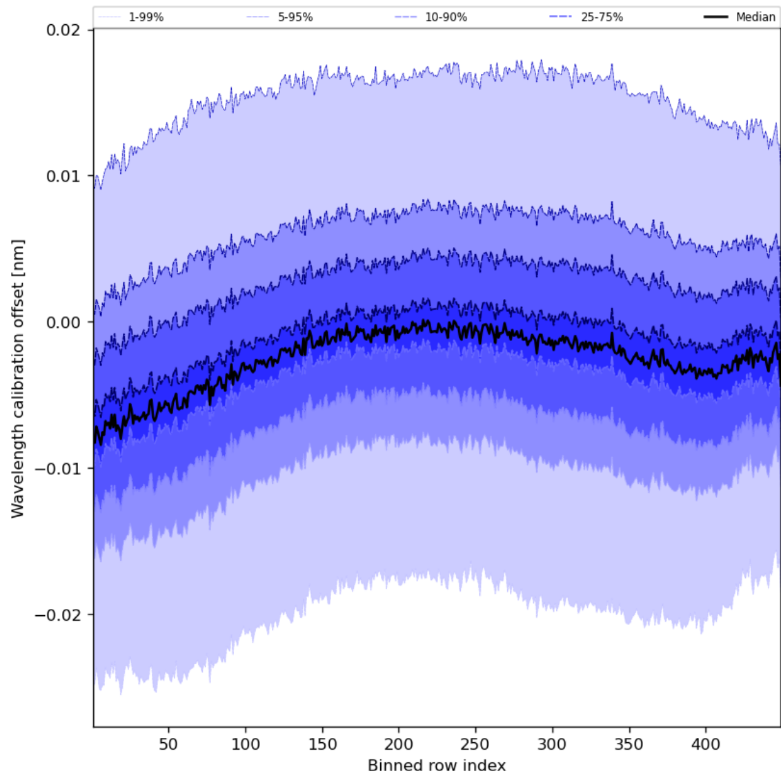
Figure 52: Along track statistics of “Wavelength calibration offset” for 2024-01-26 to 2024-01-27
