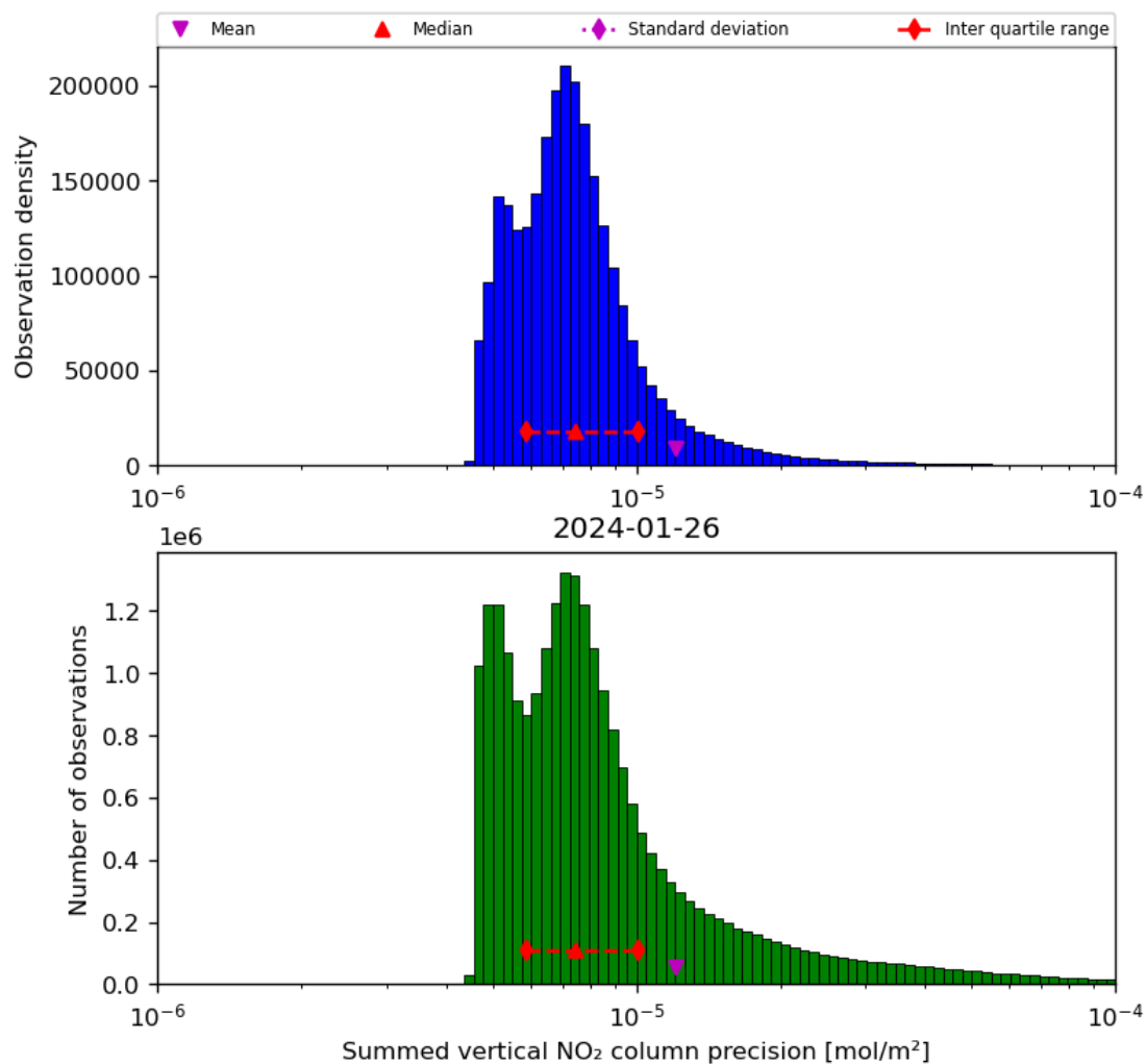
Figure 41: Histogram of “Summed vertical NO 2 column precision” for 2024-01-26 to 2024-01-27
