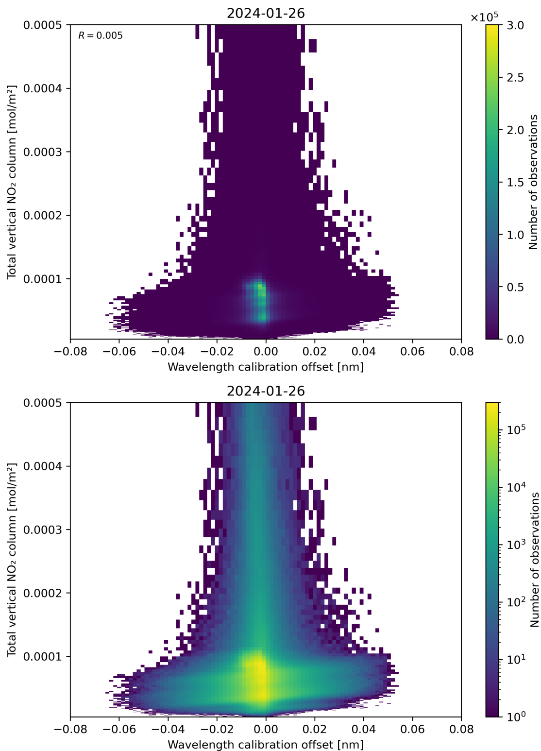
Figure 179: Scatter density plot of “Wavelength calibration offset” against “Total vertical NO 2 column” for 2024-01-26 to 2024-01-27.
