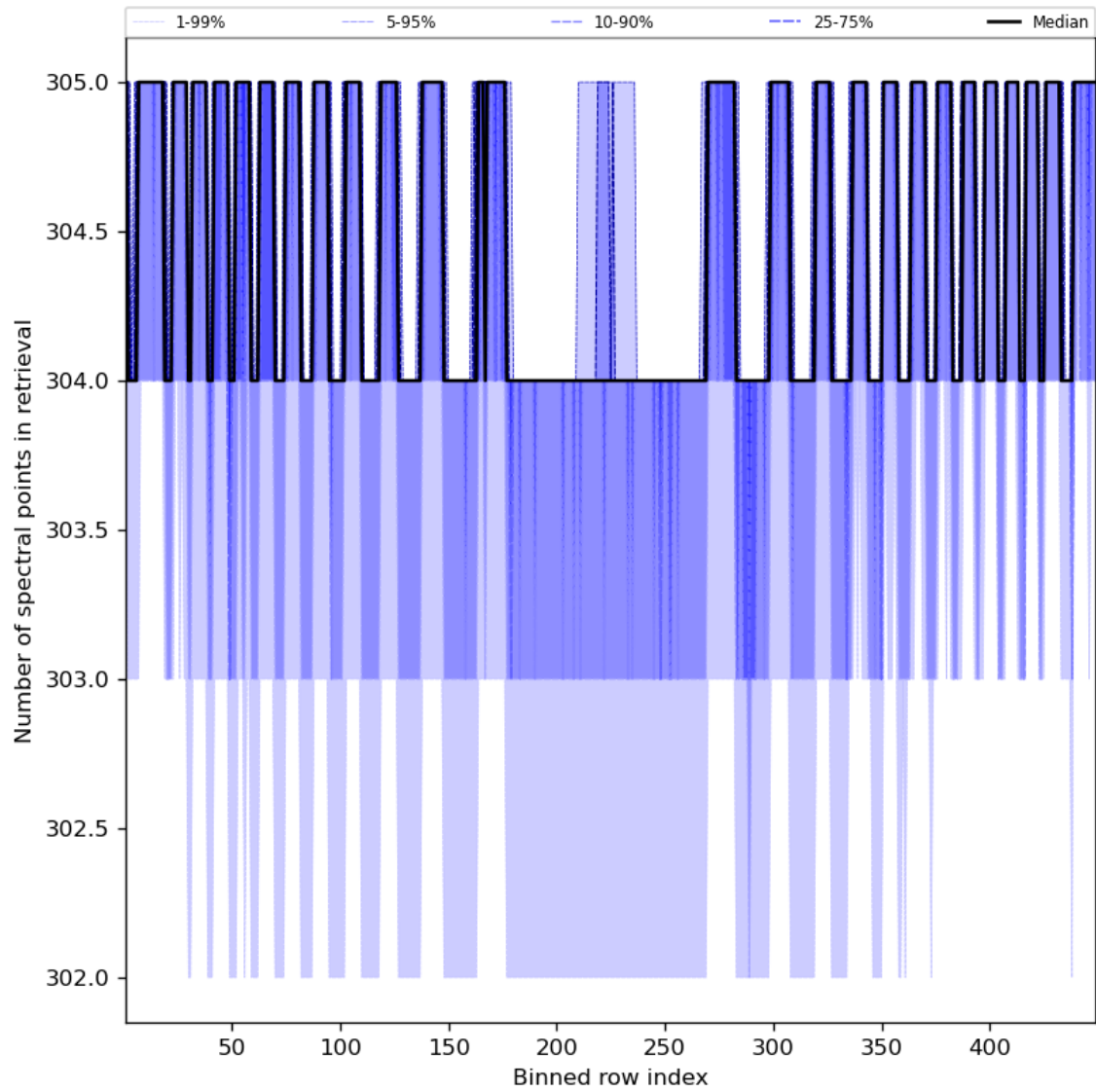
Figure 50: Along track statistics of “Number of spectral points in retrieval” for 2024-01-26 to 2024-01-27
