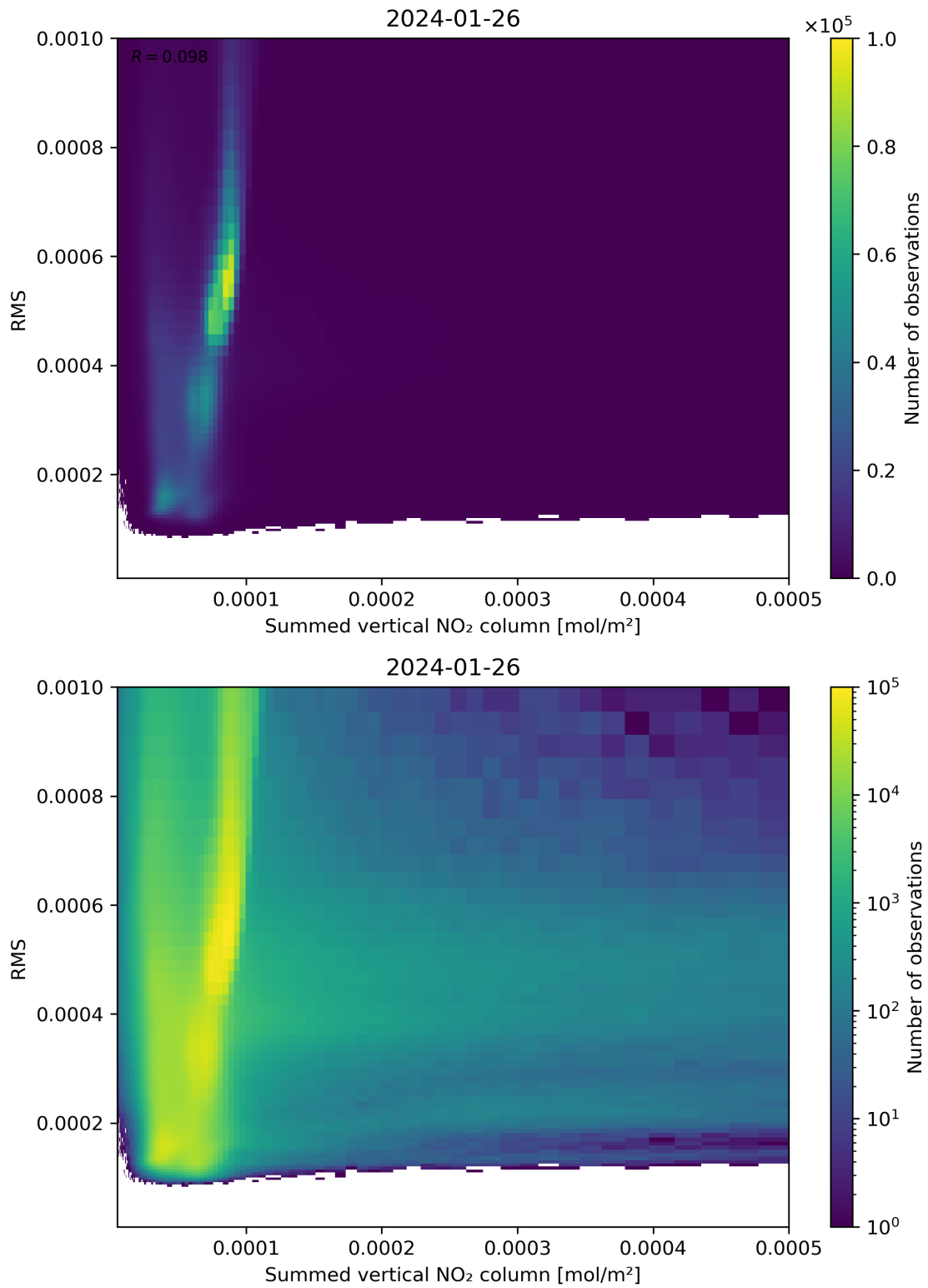
Figure 109: Scatter density plot of “Summed vertical NO 2 column” against “RMS” for 2024-01-26 to 2024-01-27.
