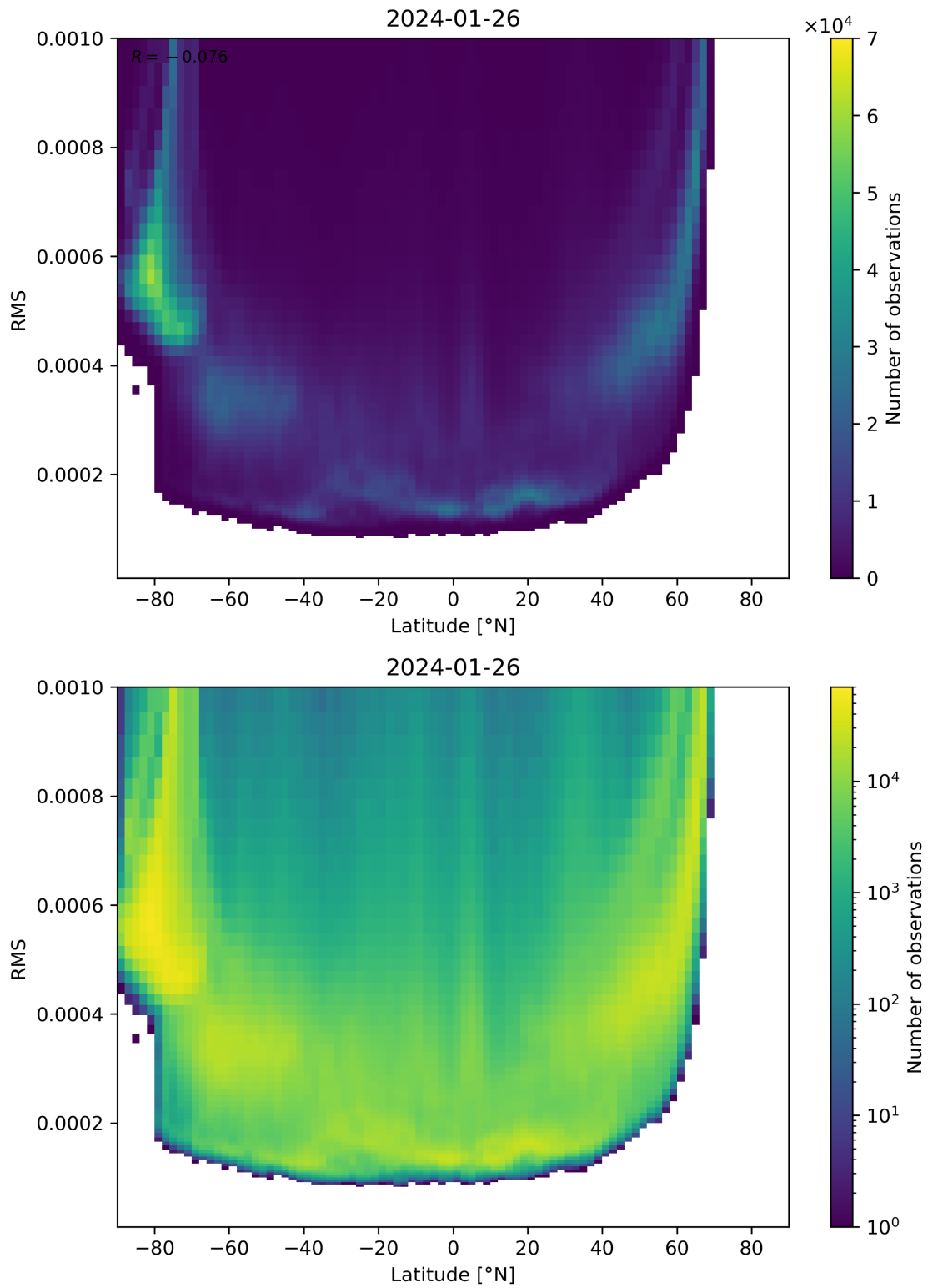
Figure 94: Scatter density plot of “Latitude” against “RMS” for 2024-01-26 to 2024-01-27.
