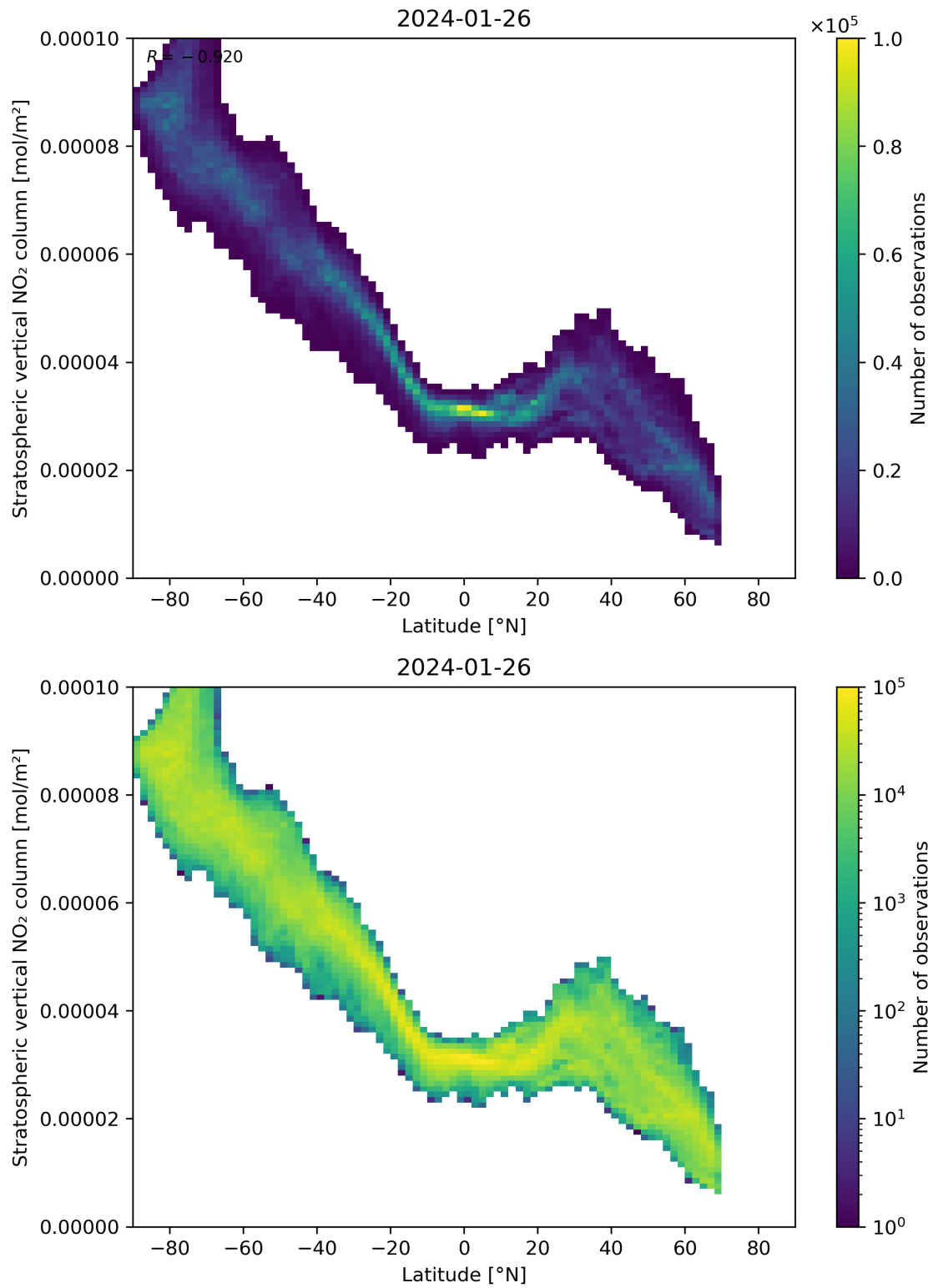
Figure 87: Scatter density plot of “Latitude” against “Stratospheric vertical NO 2 column” for 2024-01-26 to 2024-01-27.
