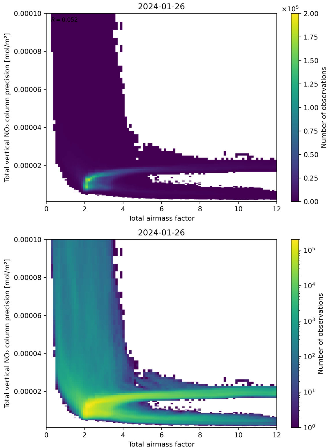
Figure 68: Scatter density plot of “Total airmass factor” against “Total vertical NO 2 column precision” for 2024-01-26 to 2024-01-27.
