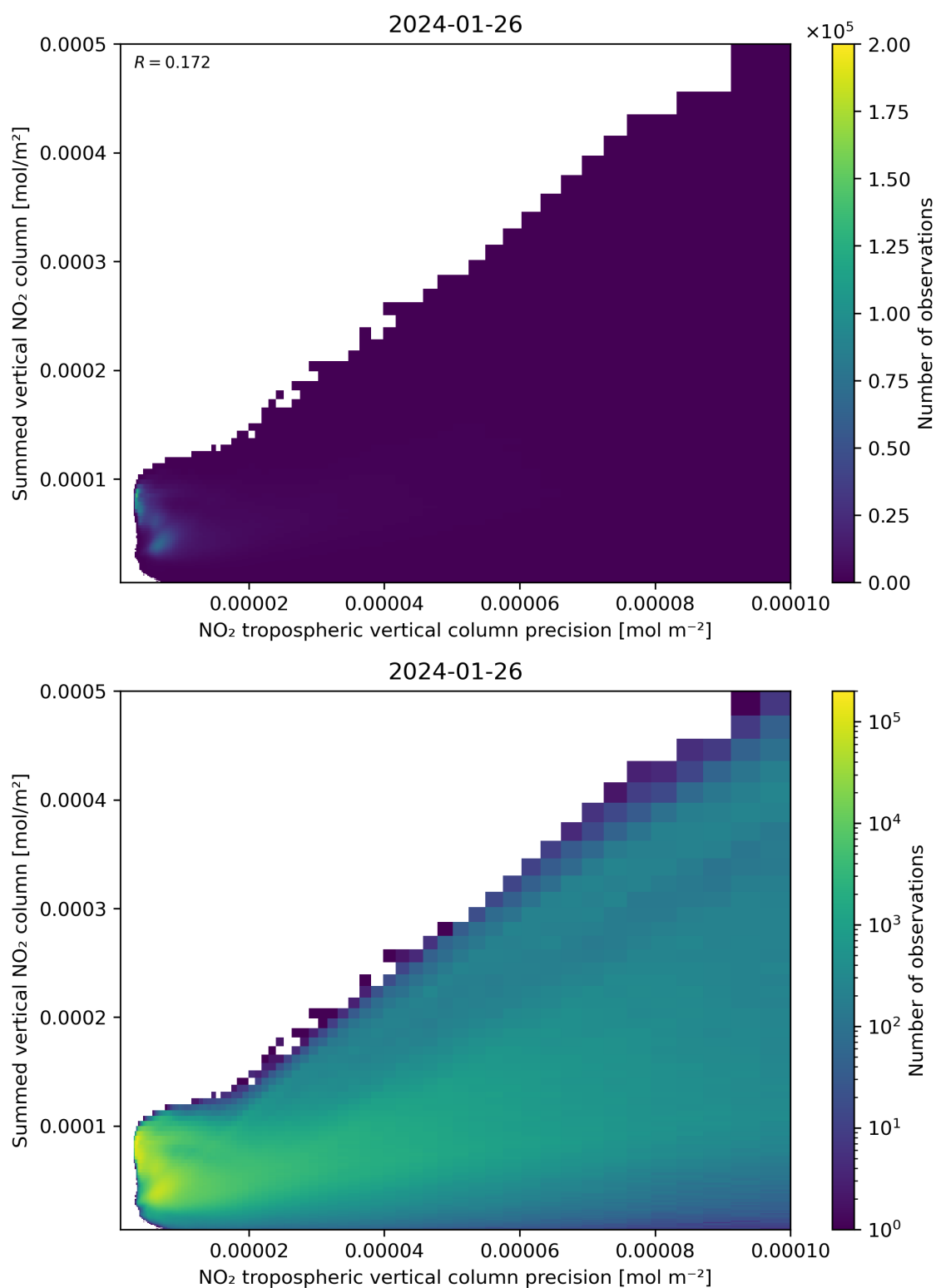
Figure 136: Scatter density plot of “NO 2 tropospheric vertical column precision” against “Summed vertical NO 2 column” for 2024-01-26 to 2024-01-27.
