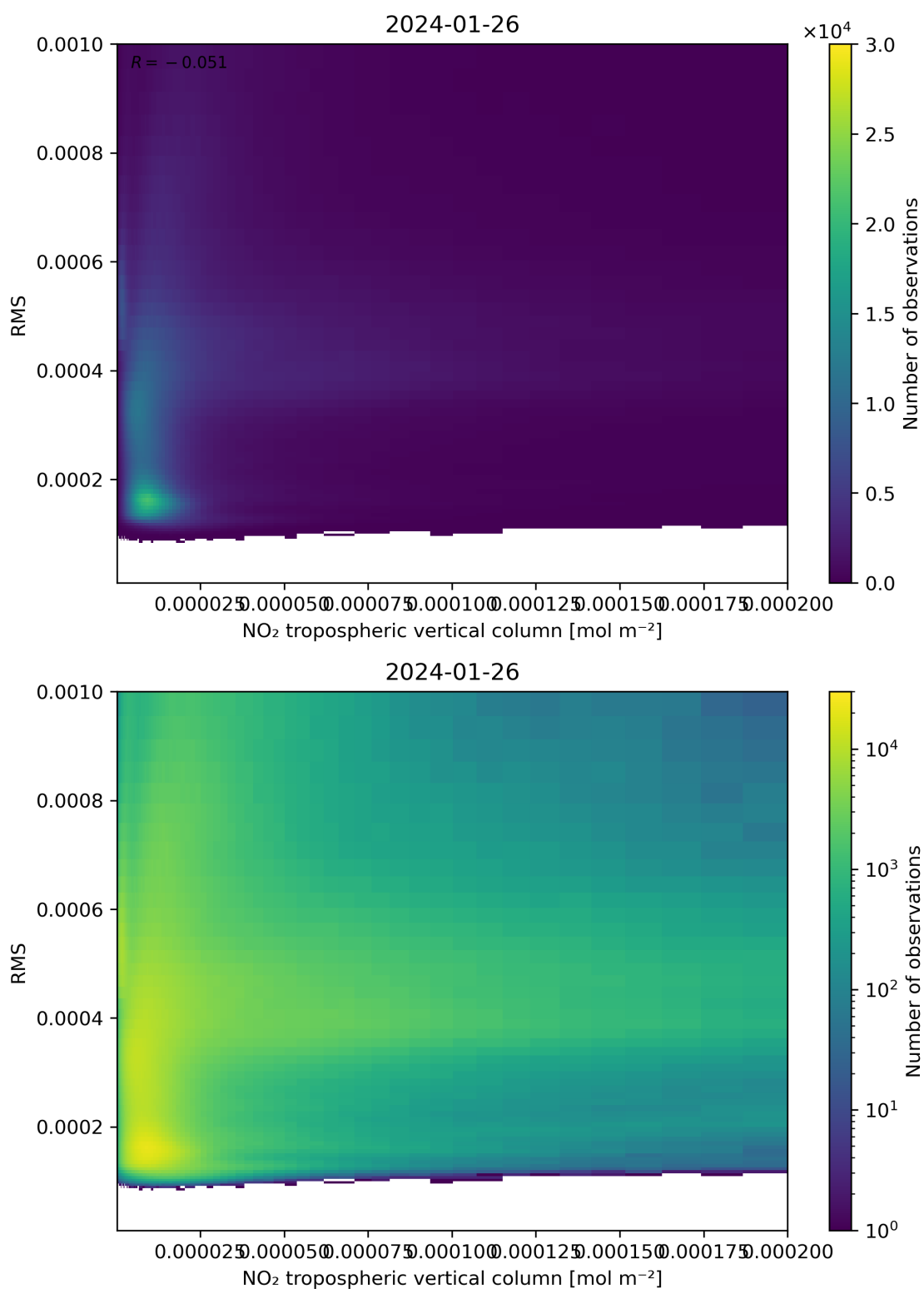
Figure 142: Scatter density plot of “NO 2 tropospheric vertical column” against “RMS” for 2024-01-26 to 2024-01-27.
