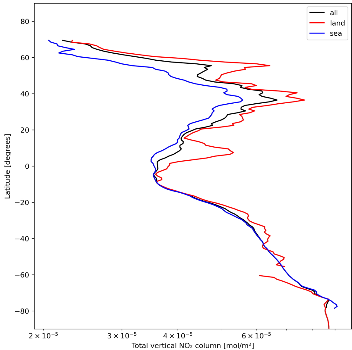
Figure 21: Zonal average of “Total vertical NO 2 column” for 2024-01-26 to 2024-01-27.
