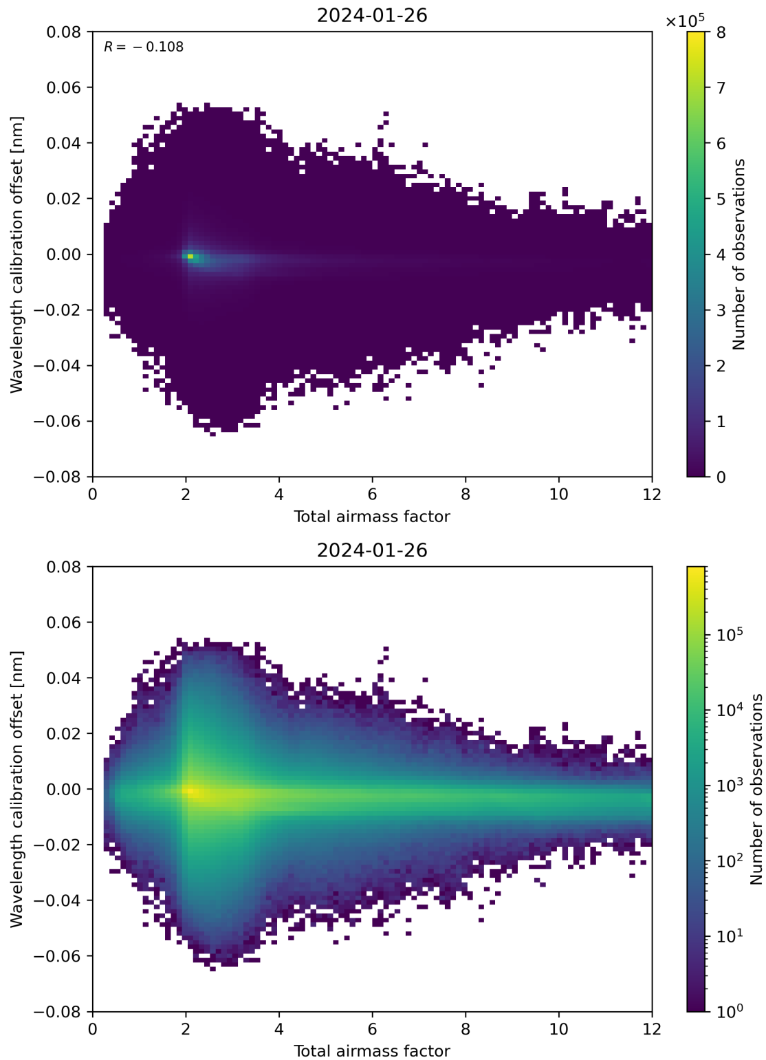
Figure 70: Scatter density plot of “Total airmass factor” against “Wavelength calibration offset” for 2024-01-26 to 2024-01-27.
