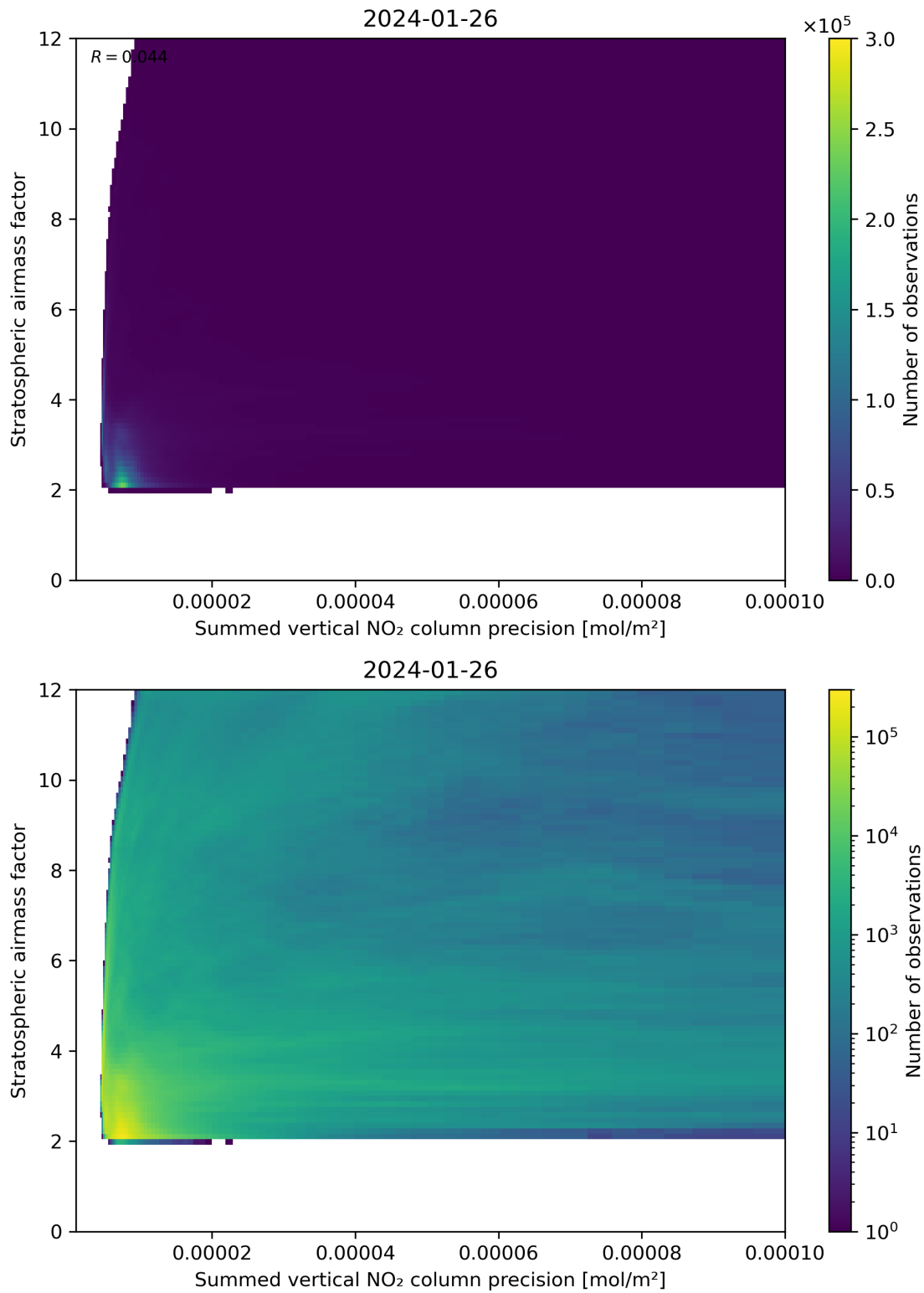
Figure 106: Scatter density plot of “Summed vertical NO 2 column precision” against “Stratospheric airmass factor” for 2024-01-26 to 2024-01-27.
