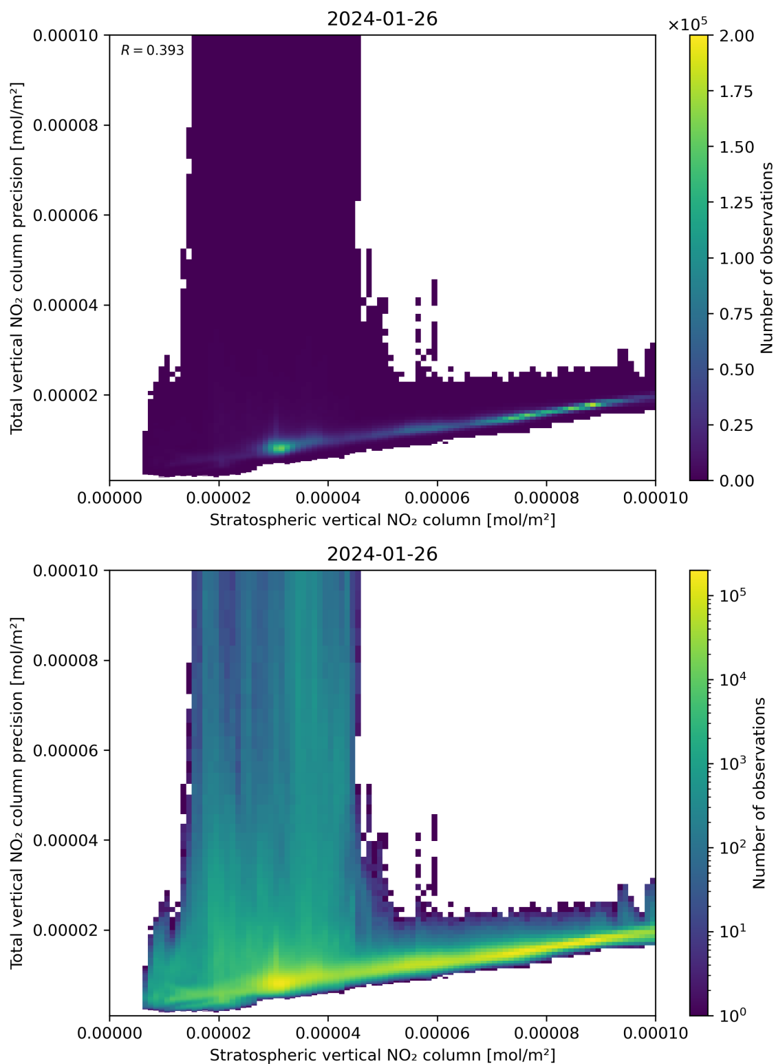
Figure 101: Scatter density plot of “Stratospheric vertical NO 2 column” against “Total vertical NO 2 column precision” for 2024-01-26 to 2024-01-27.
