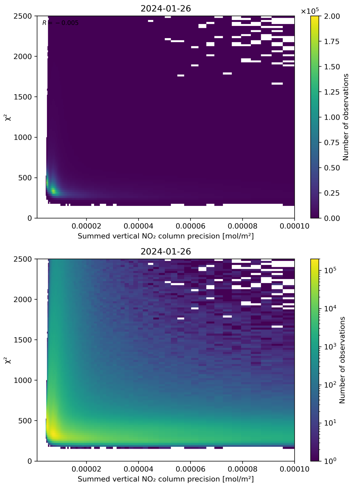
Figure 107: Scatter density plot of “Summed vertical NO 2 column precision” against “ \chi^2 ” for 2024-01-26 to 2024-01-27.
