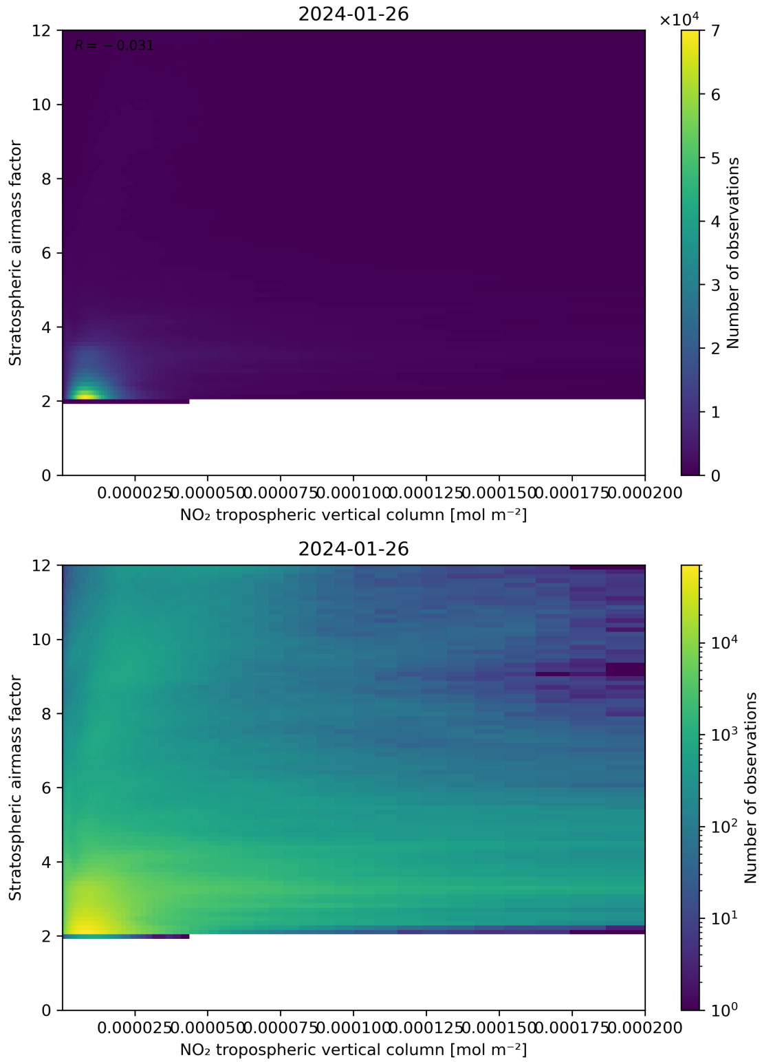
Figure 121: Scatter density plot of “NO 2 tropospheric vertical column” against “Stratospheric airmass factor” for 2024-01-26 to 2024-01-27.
