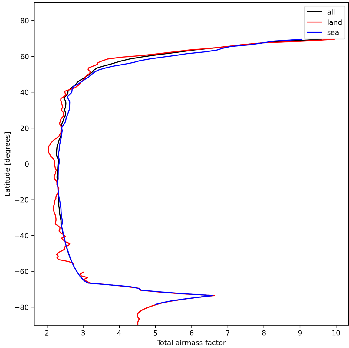
Figure 15: Zonal average of “Total airmass factor” for 2024-01-26 to 2024-01-27.
