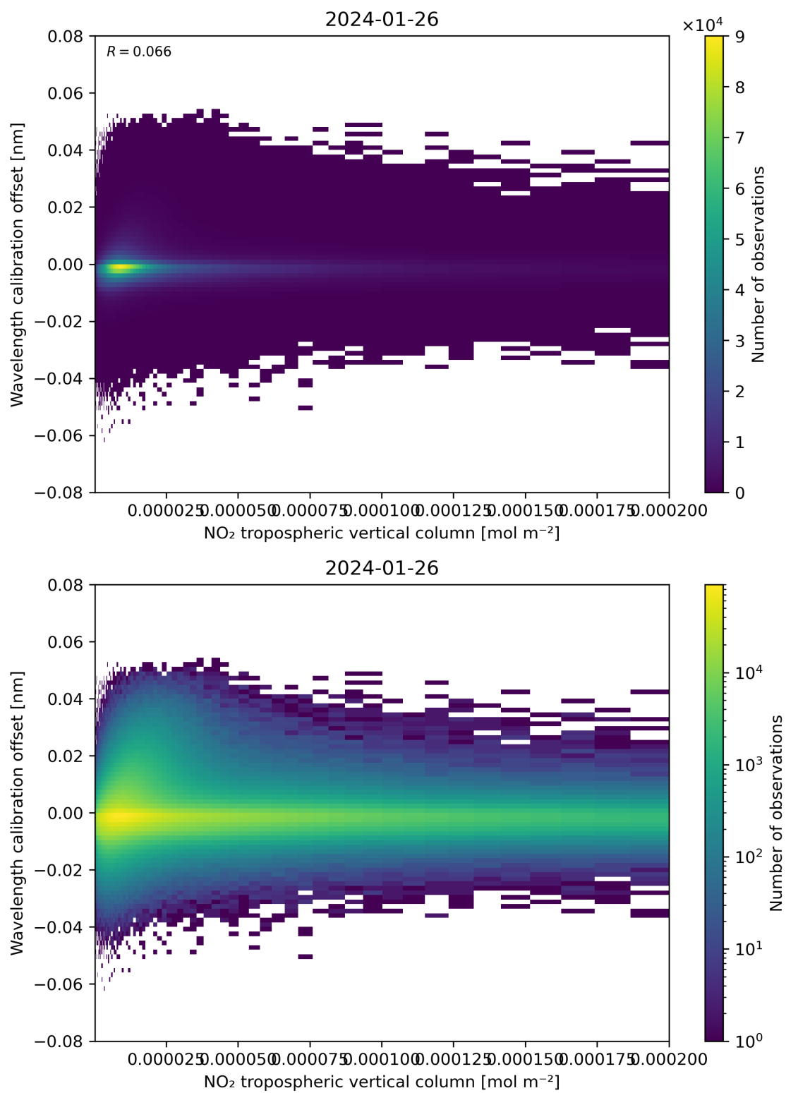
Figure 143: Scatter density plot of “NO 2 tropospheric vertical column” against “Wavelength calibration offset” for 2024-01-26 to 2024-01-27.
