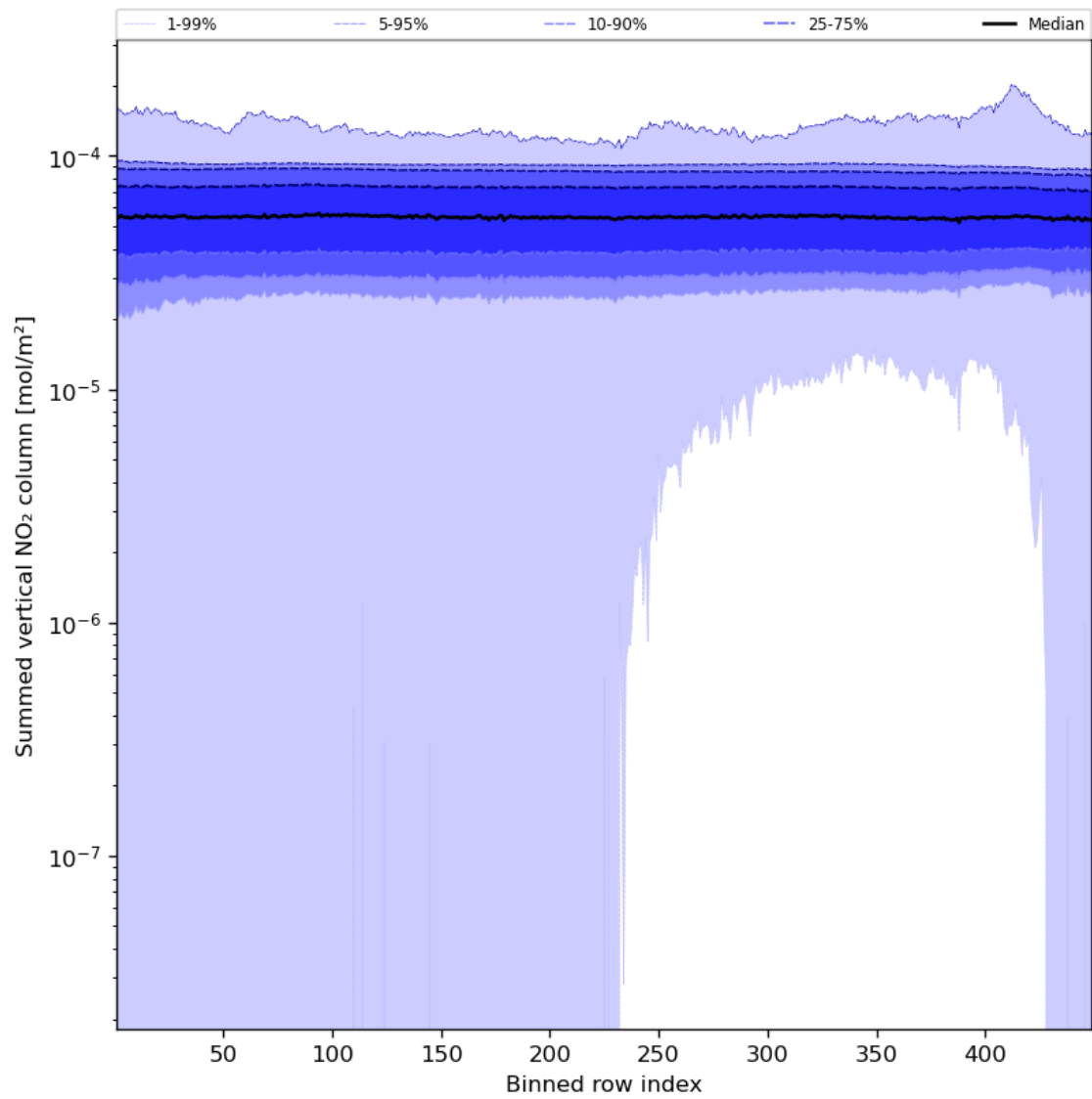
Figure 57: Along track statistics of “Summed vertical NO 2 column” for 2024-01-26 to 2024-01-27
