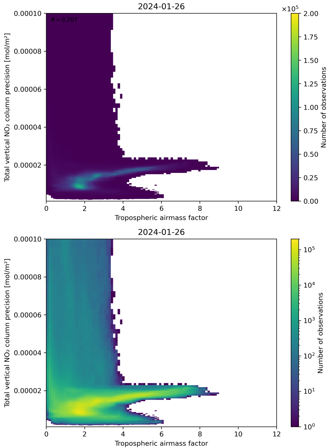
Figure 78: Scatter density plot of “Tropospheric air mass factor” against “Total vertical NO 2 column precision” for 2024-01-26 to 2024-01-27.
