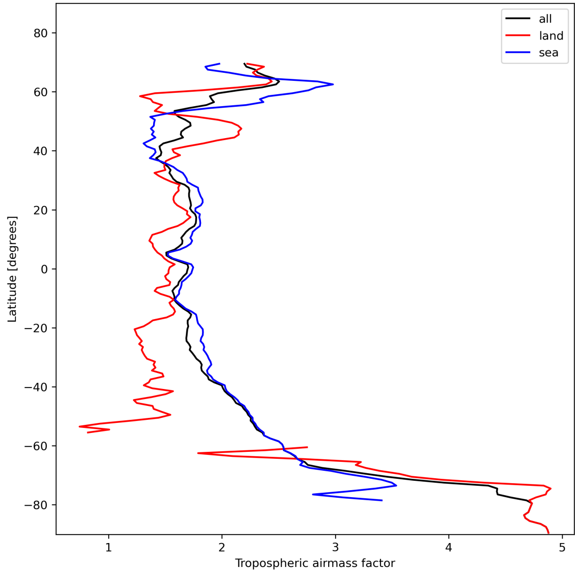
Figure 14: Zonal average of “Tropospheric airmass factor” for 2024-01-26 to 2024-01-27.
