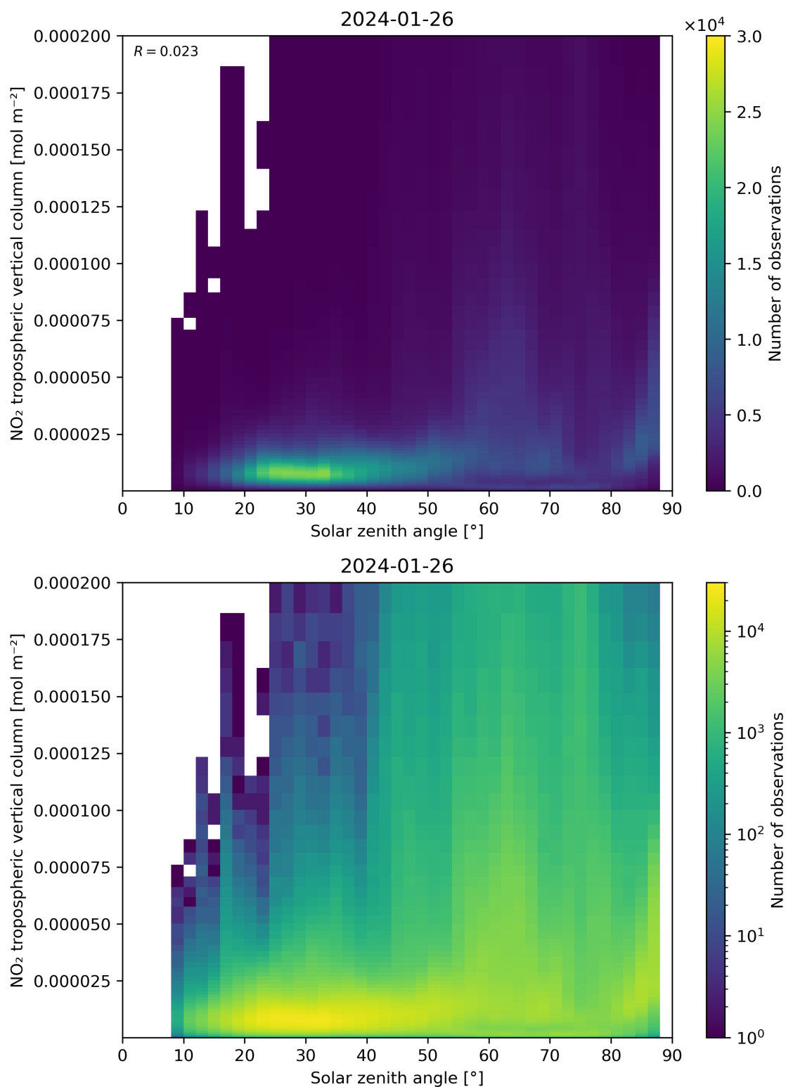
Figure 155: Scatter density plot of “Solar zenith angle” against “NO 2 tropospheric vertical column” for 2024-01-26 to 2024-01-27.
