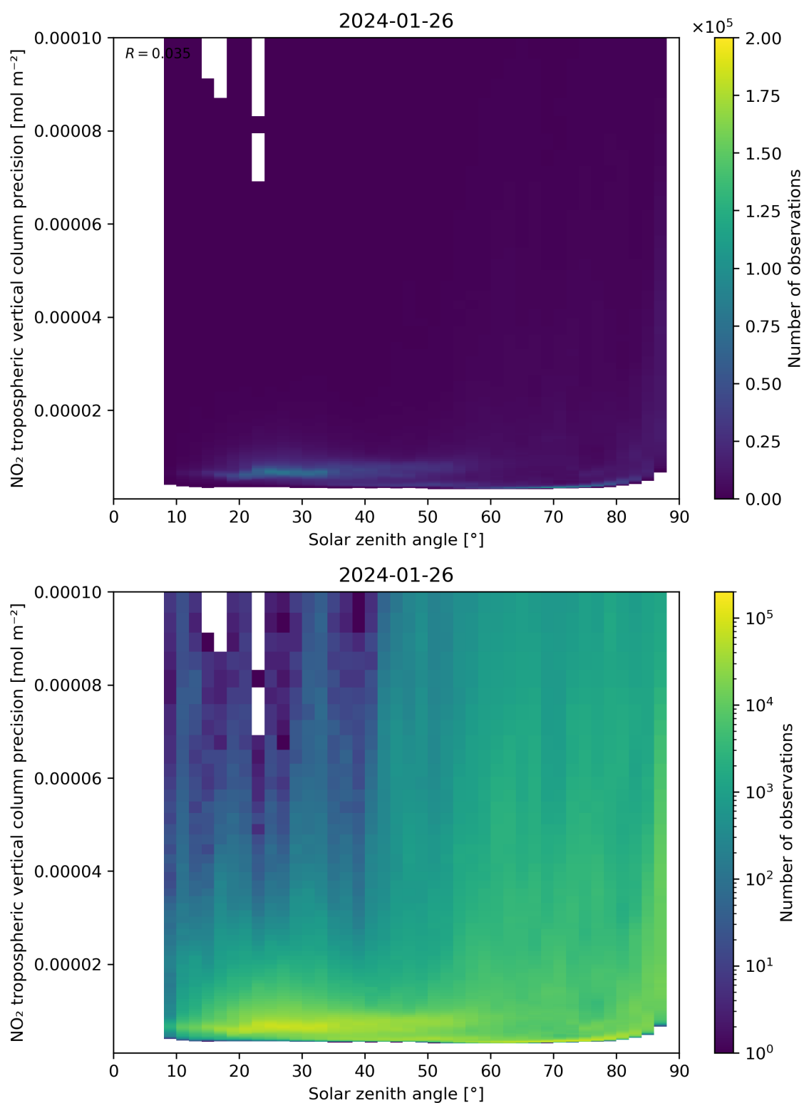
Figure 156: Scatter density plot of “Solar zenith angle” against “NO 2 tropospheric vertical column precision” for 2024-01-26 to 2024-01-27.
