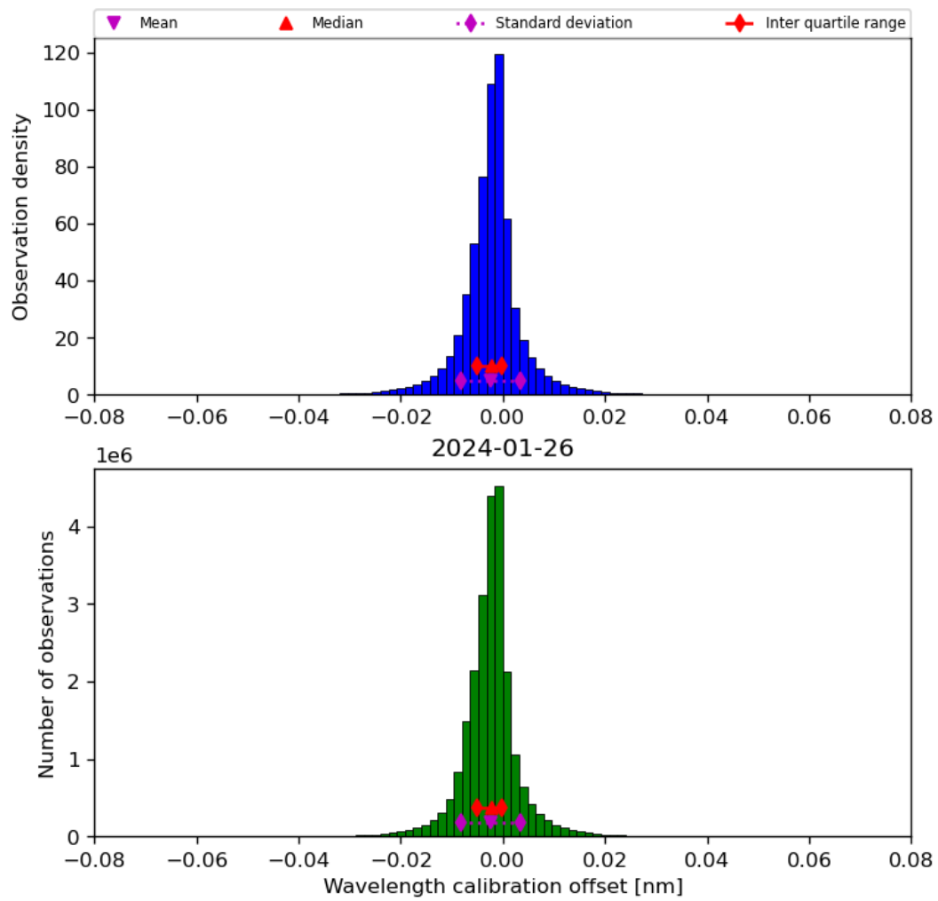
Figure 35: Histogram of “Wavelength calibration offset” for 2024-01-26 to 2024-01-27
