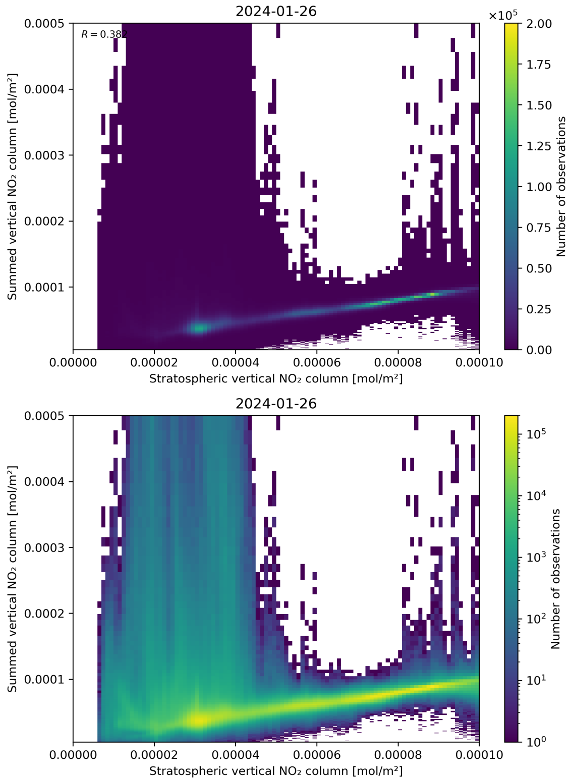
Figure 98: Scatter density plot of “Stratospheric vertical NO 2 column” against “Summed vertical NO 2 column” for 2024-01-26 to 2024-01-27.
