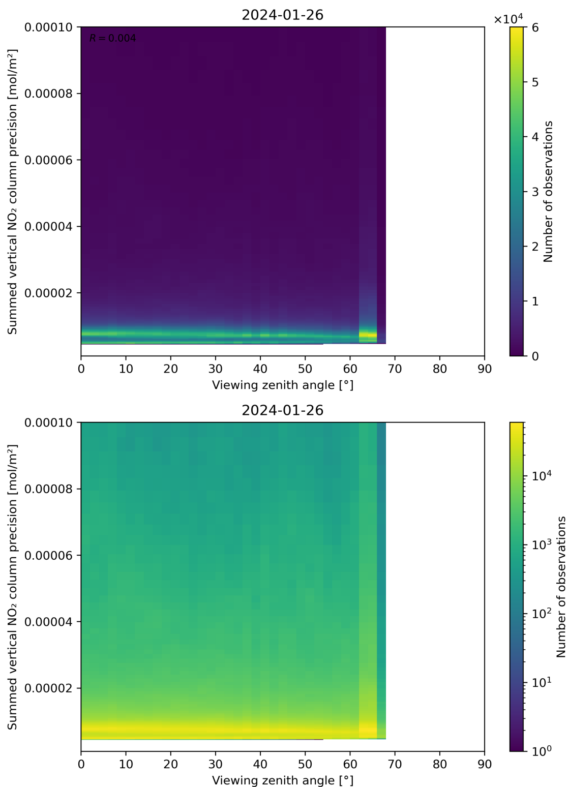
Figure 166: Scatter density plot of “Viewing zenith angle” against “Summed vertical NO 2 column precision” for 2024-01-26 to 2024-01-27.
