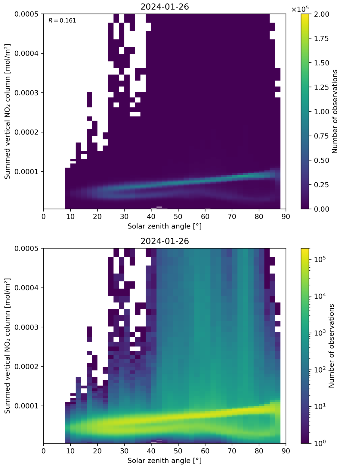
Figure 151: Scatter density plot of “Solar zenith angle” against “Summed vertical NO 2 column” for 2024-01-26 to 2024-01-27.
