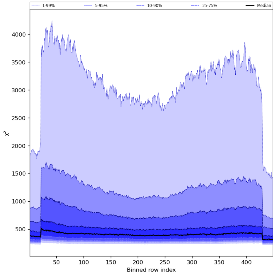
Figure 59: Along track statistics of “ \chi^2 ” for 2024-01-26 to 2024-01-27
