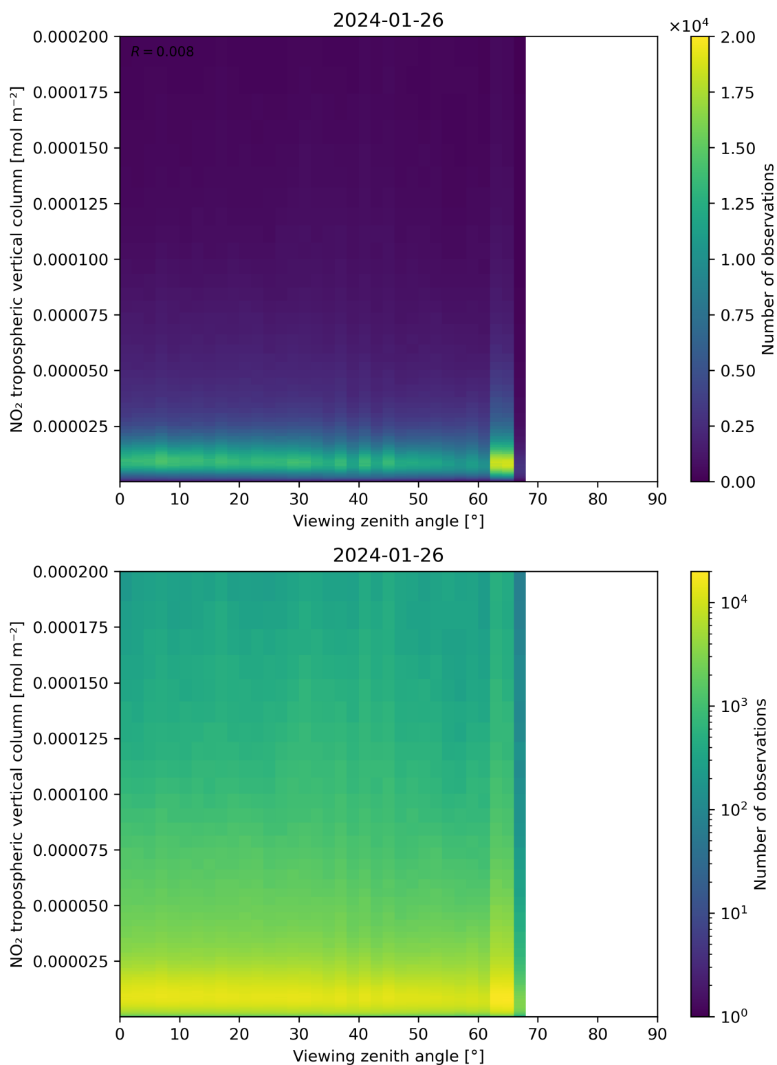
Figure 169: Scatter density plot of “Viewing zenith angle” against “NO 2 tropospheric vertical column” for 2024-01-26 to 2024-01-27.
