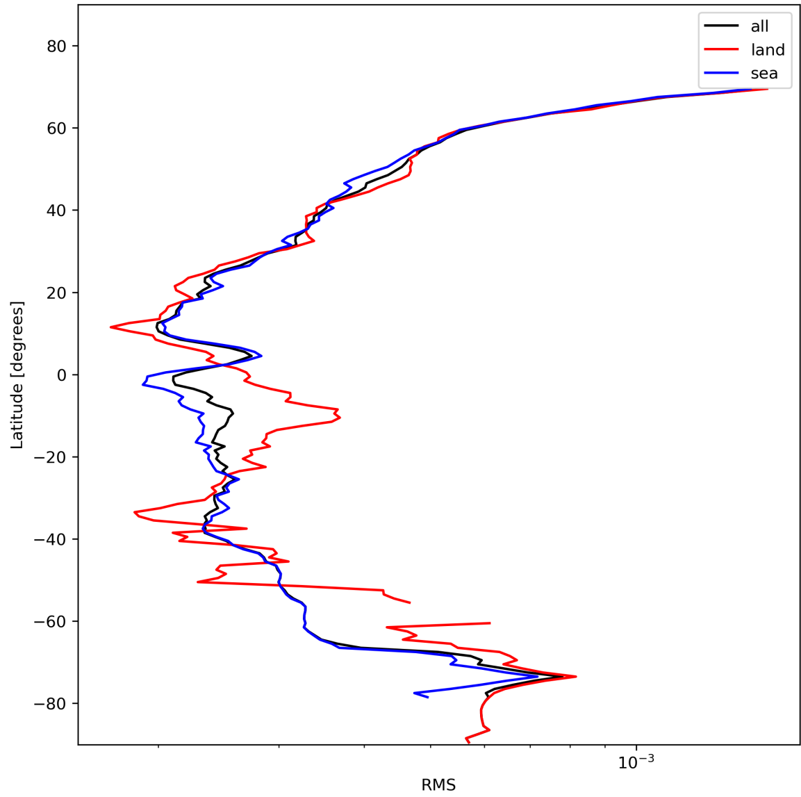
Figure 26: Zonal average of “RMS” for 2024-01-26 to 2024-01-27.
