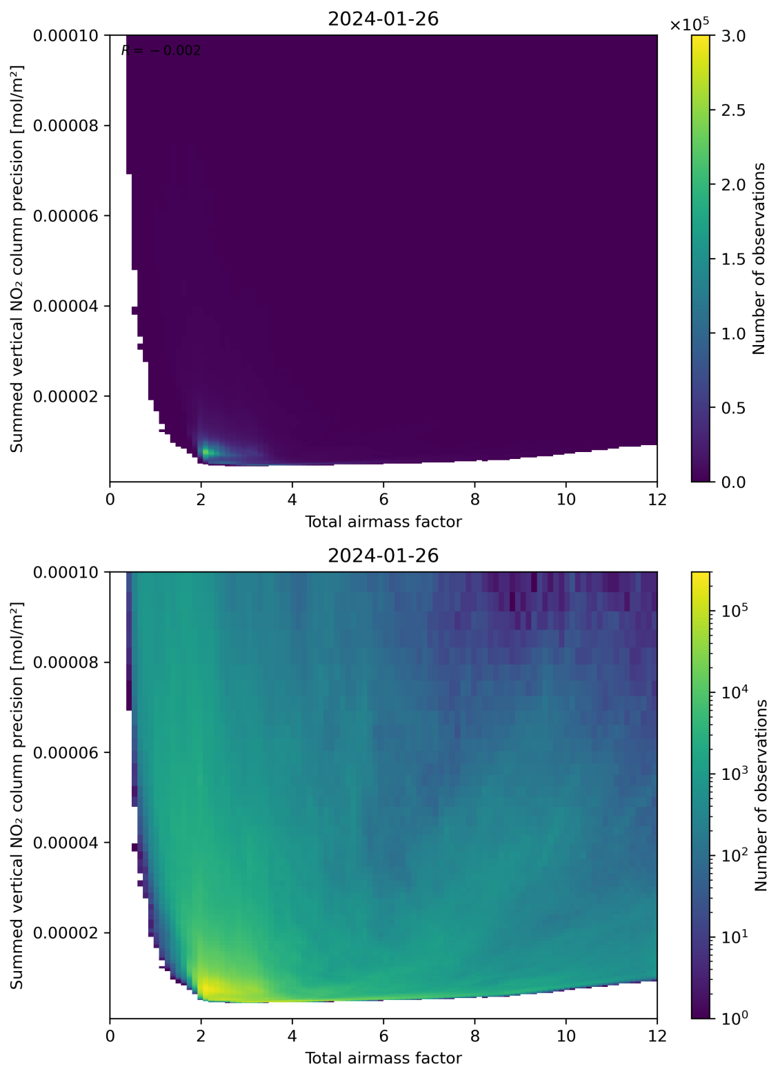
Figure 66: Scatter density plot of “Total airmass factor” against “Summed vertical NO 2 column precision” for 2024-01-26 to 2024-01-27.
