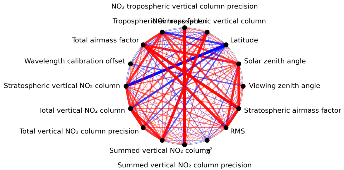
Figure 1: Map of correlation graph for 2024-01-26 to 2024-01-27.
