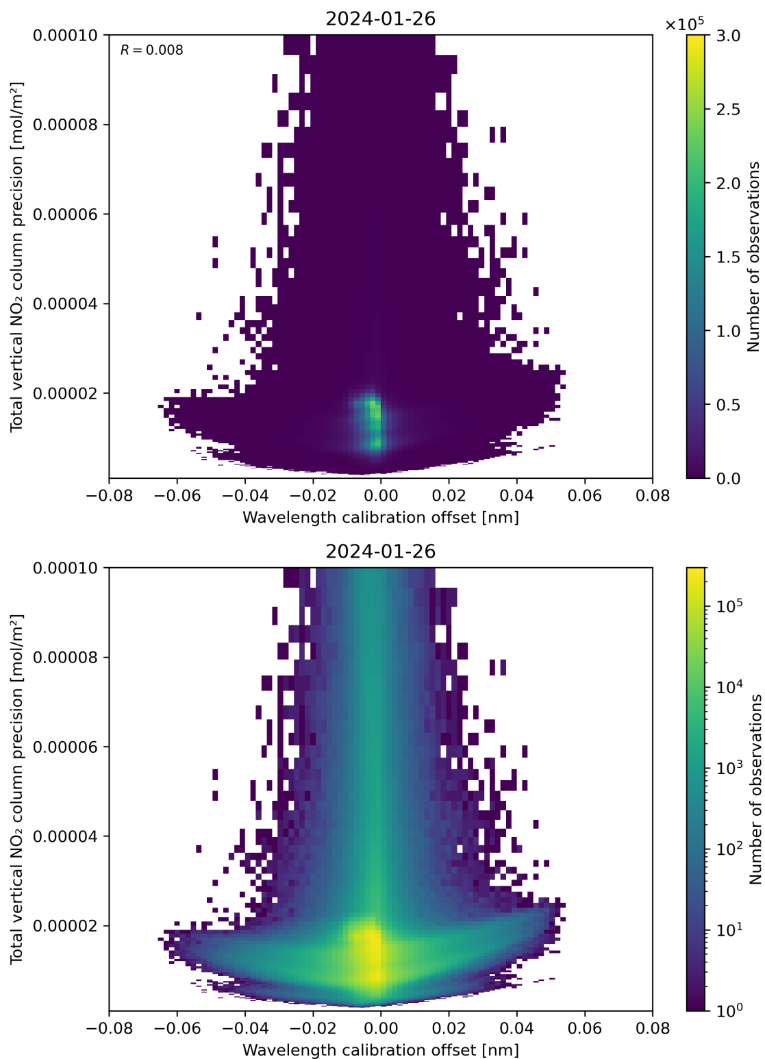
Figure 180: Scatter density plot of “Wavelength calibration offset” against “Total vertical NO 2 column precision” for 2024-01-26 to 2024-01-27.
