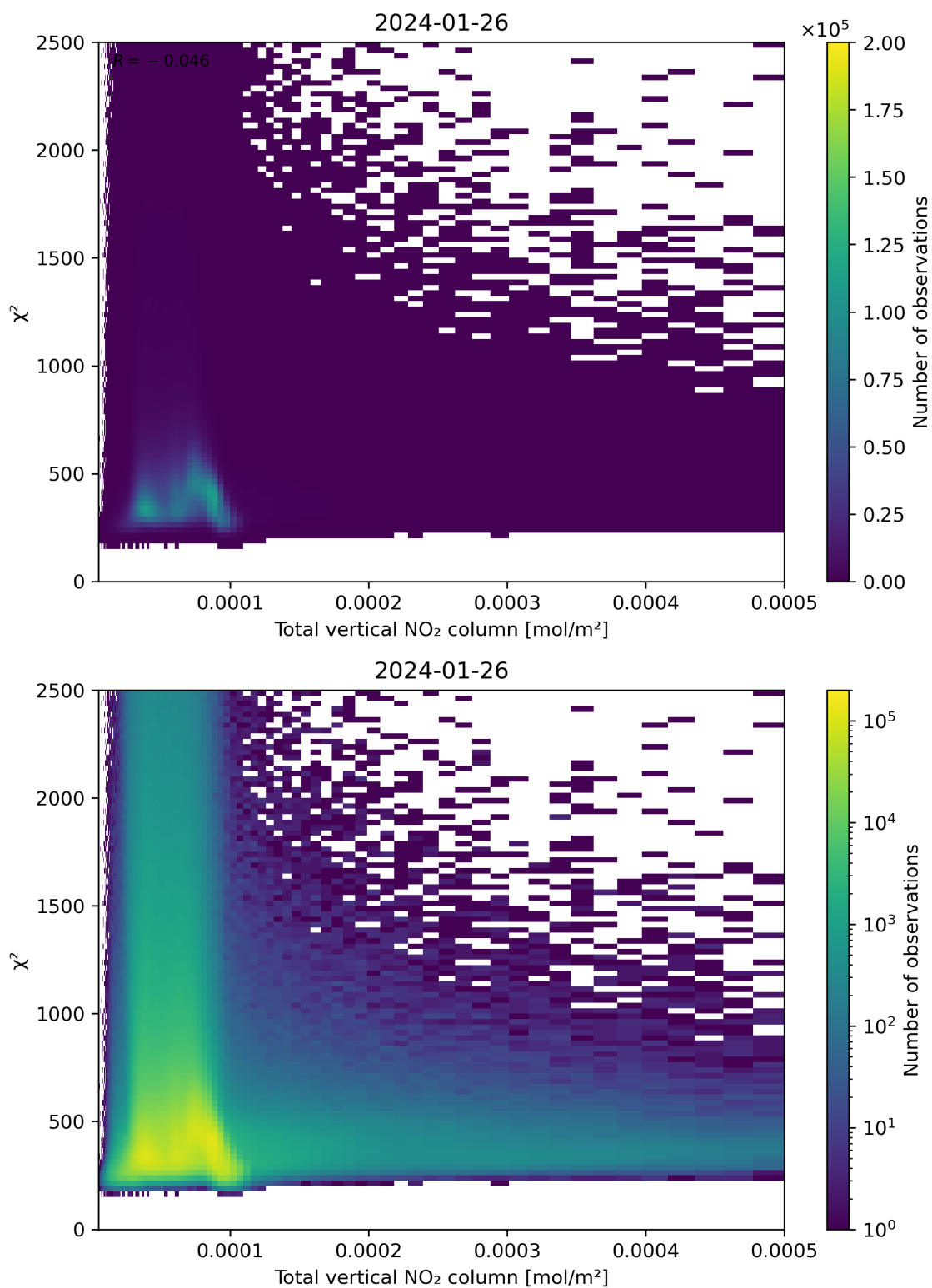
Figure 111: Scatter density plot of “Total vertical NO 2 column” against “ \chi^2 ” for 2024-01-26 to 2024-01-27.
