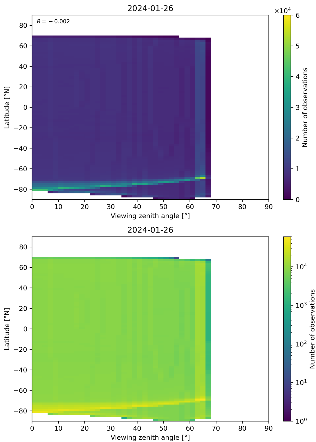
Figure 163: Scatter density plot of “Viewing zenith angle” against “Latitude” for 2024-01-26 to 2024-01-27.
