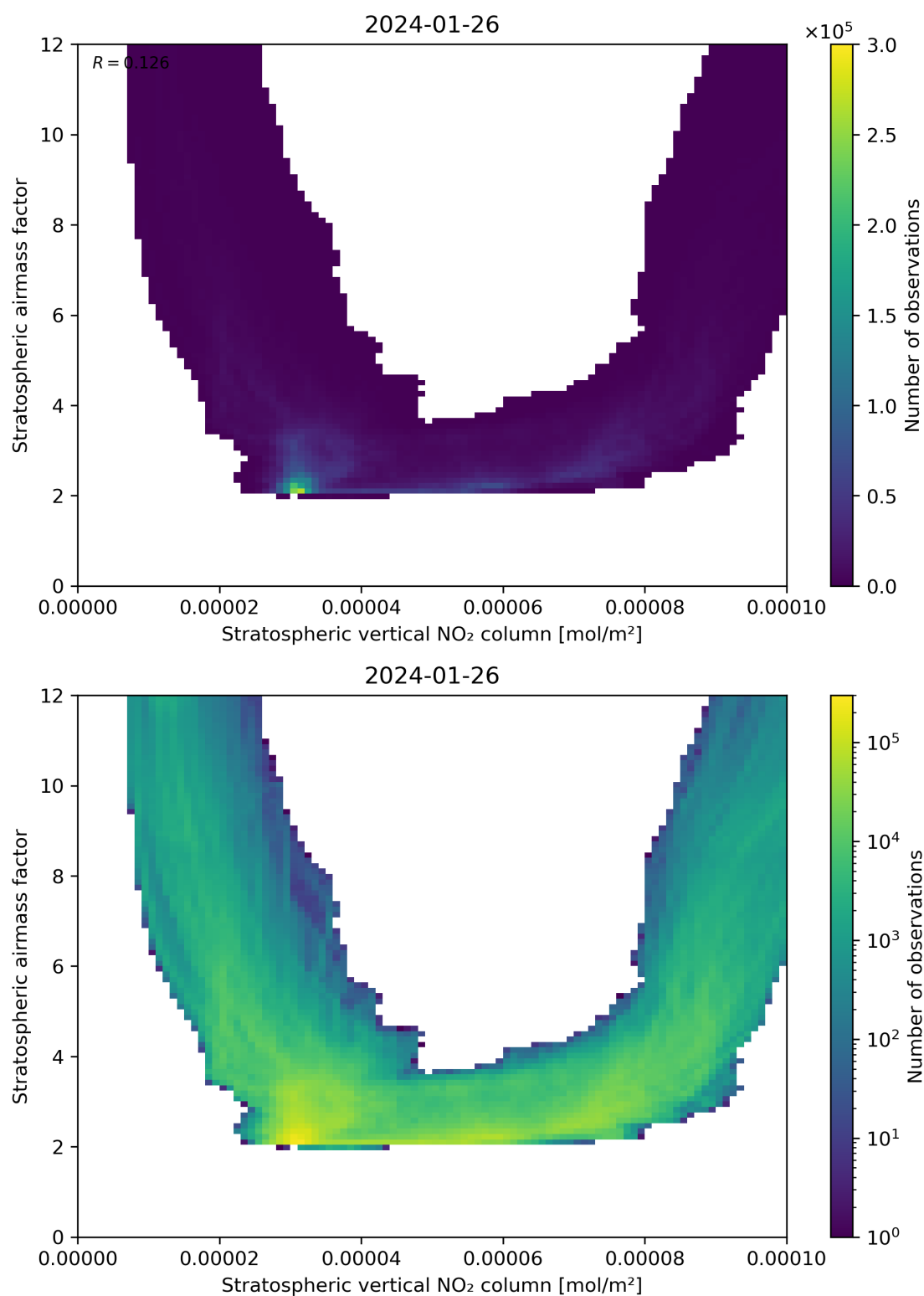
Figure 96: Scatter density plot of “Stratospheric vertical NO 2 column” against “Stratospheric airmass factor” for 2024-01-26 to 2024-01-27.
