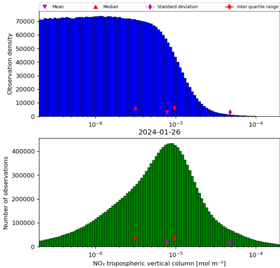
Figure 29: Histogram of “NO 2 tropospheric vertical column” for 2024-01-26 to 2024-01-27
