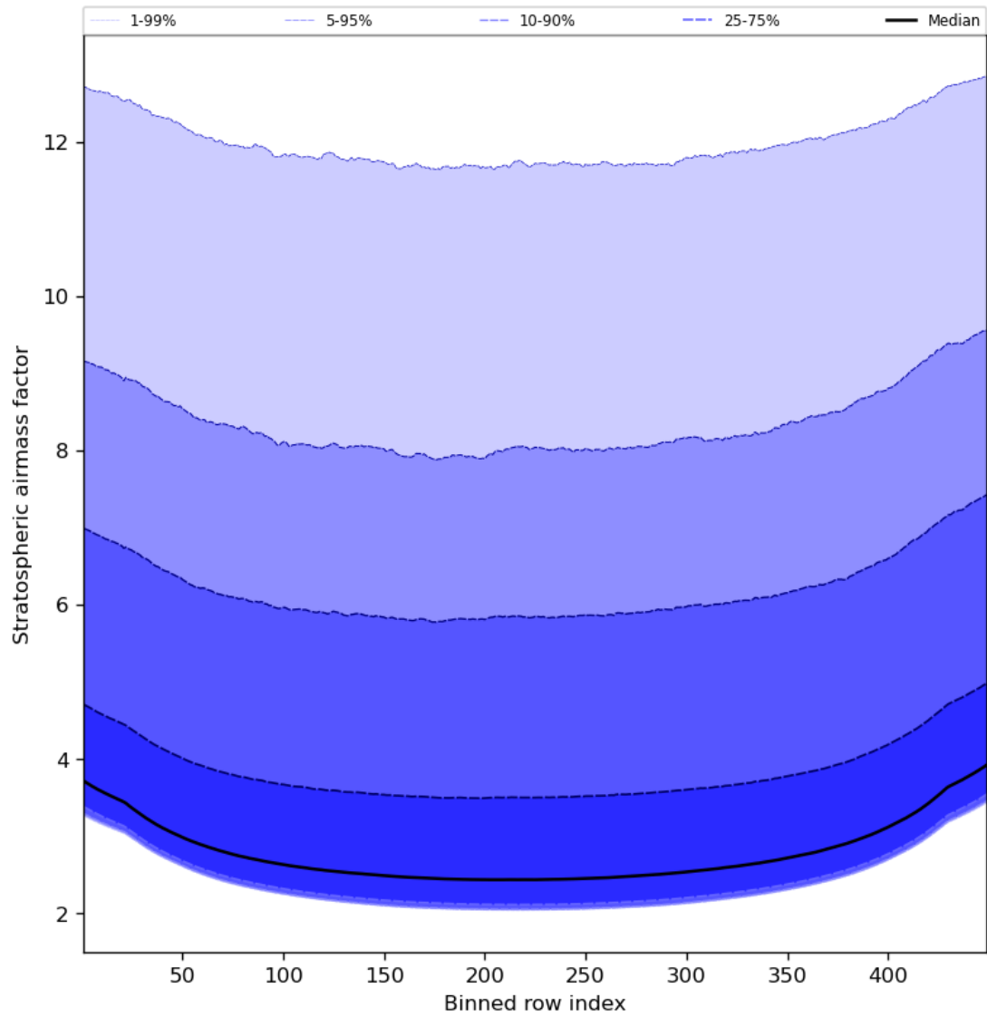
Figure 61: Along track statistics of “Stratospheric airmass factor” for 2024-01-26 to 2024-01-27
