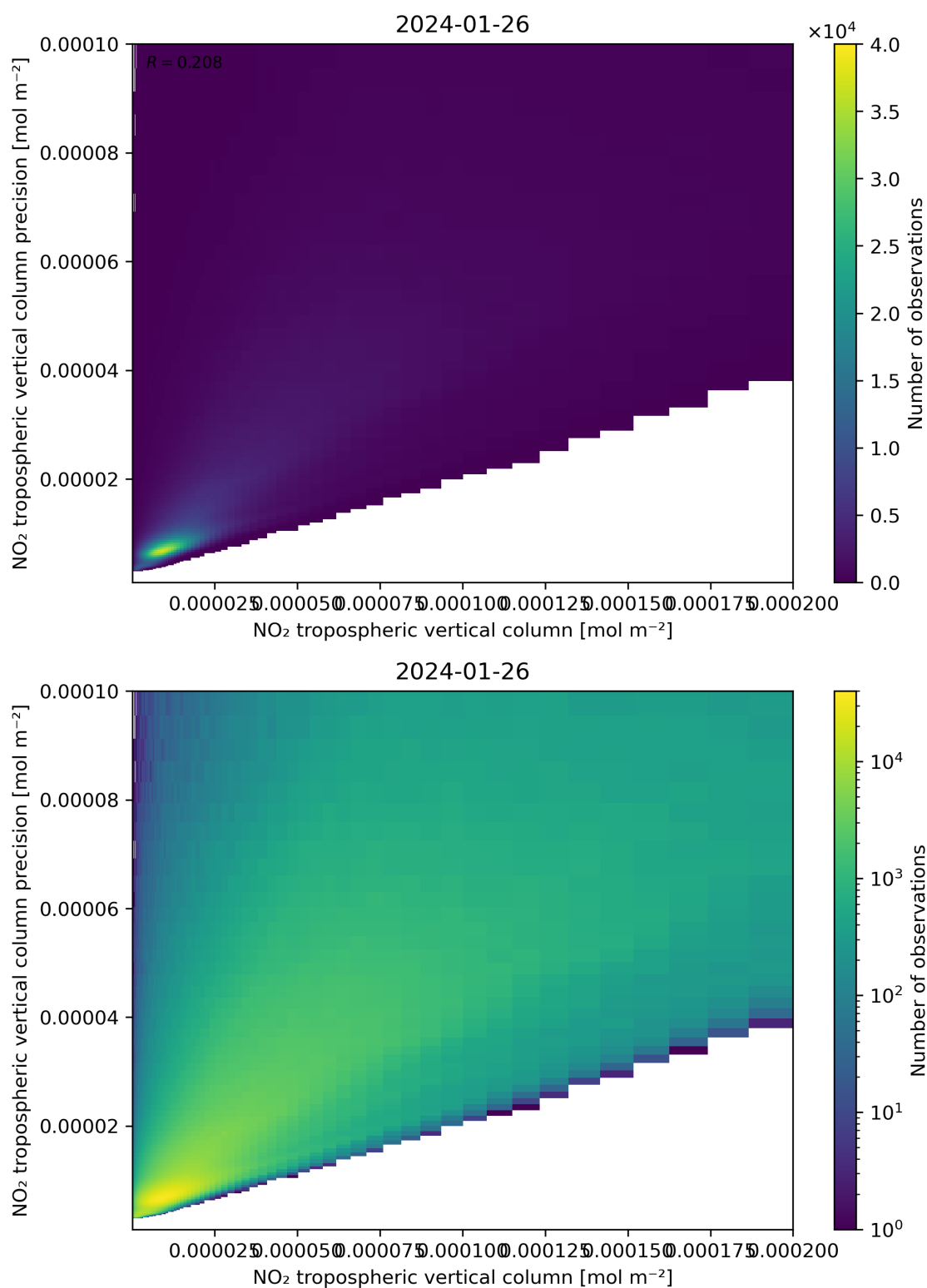
Figure 130: Scatter density plot of “NO 2 tropospheric vertical column” against “NO 2 tropospheric vertical column precision” for 2024-01-26 to 2024-01-27.
