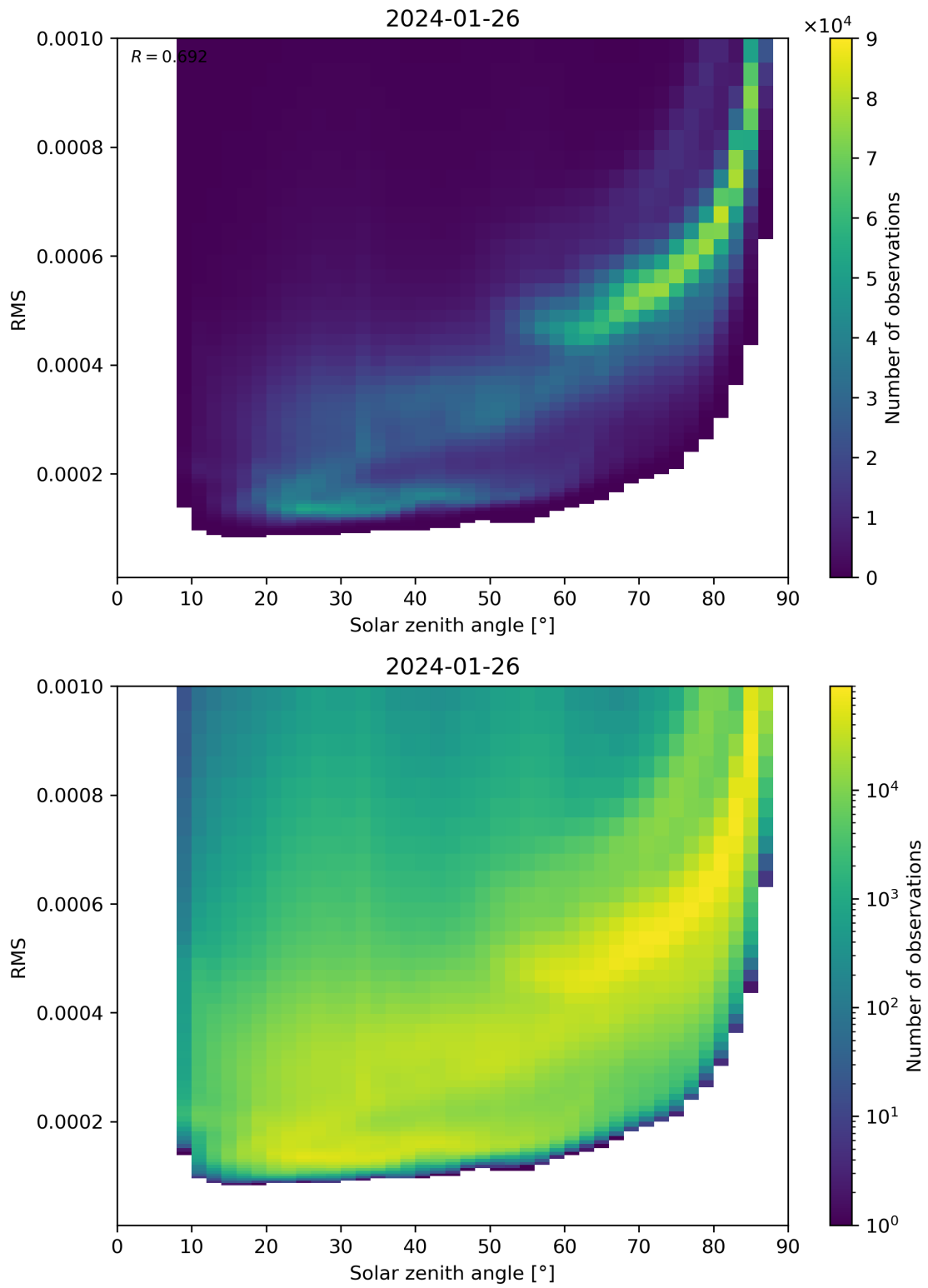
Figure 157: Scatter density plot of “Solar zenith angle” against “RMS” for 2024-01-26 to 2024-01-27.
