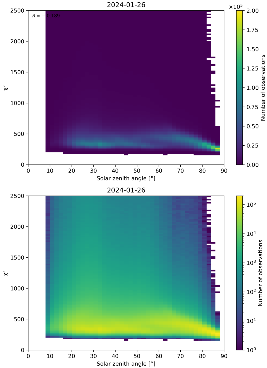
Figure 148: Scatter density plot of “Solar zenith angle” against “ \chi^2 ” for 2024-01-26 to 2024-01-27.
