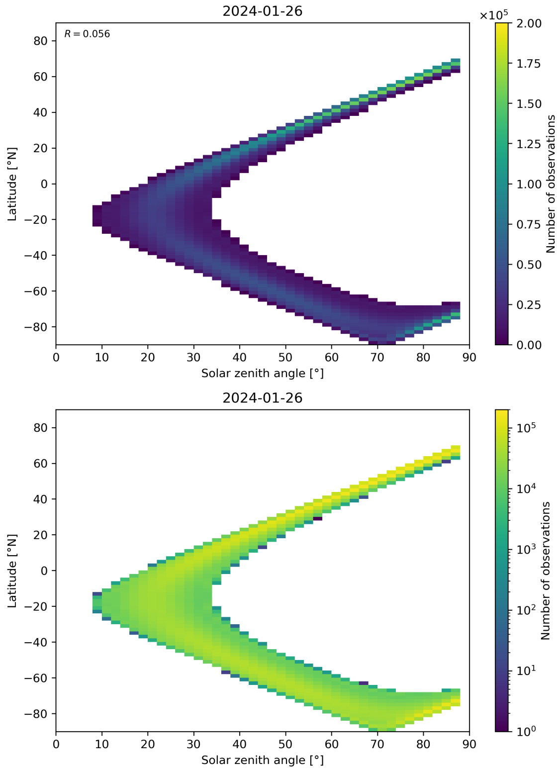
Figure 149: Scatter density plot of “Solar zenith angle” against “Latitude” for 2024-01-26 to 2024-01-27.
