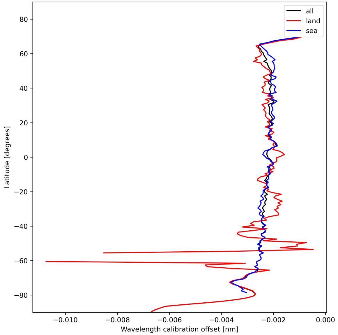
Figure 18: Zonal average of “Wavelength calibration offset” for 2024-01-26 to 2024-01-27.
