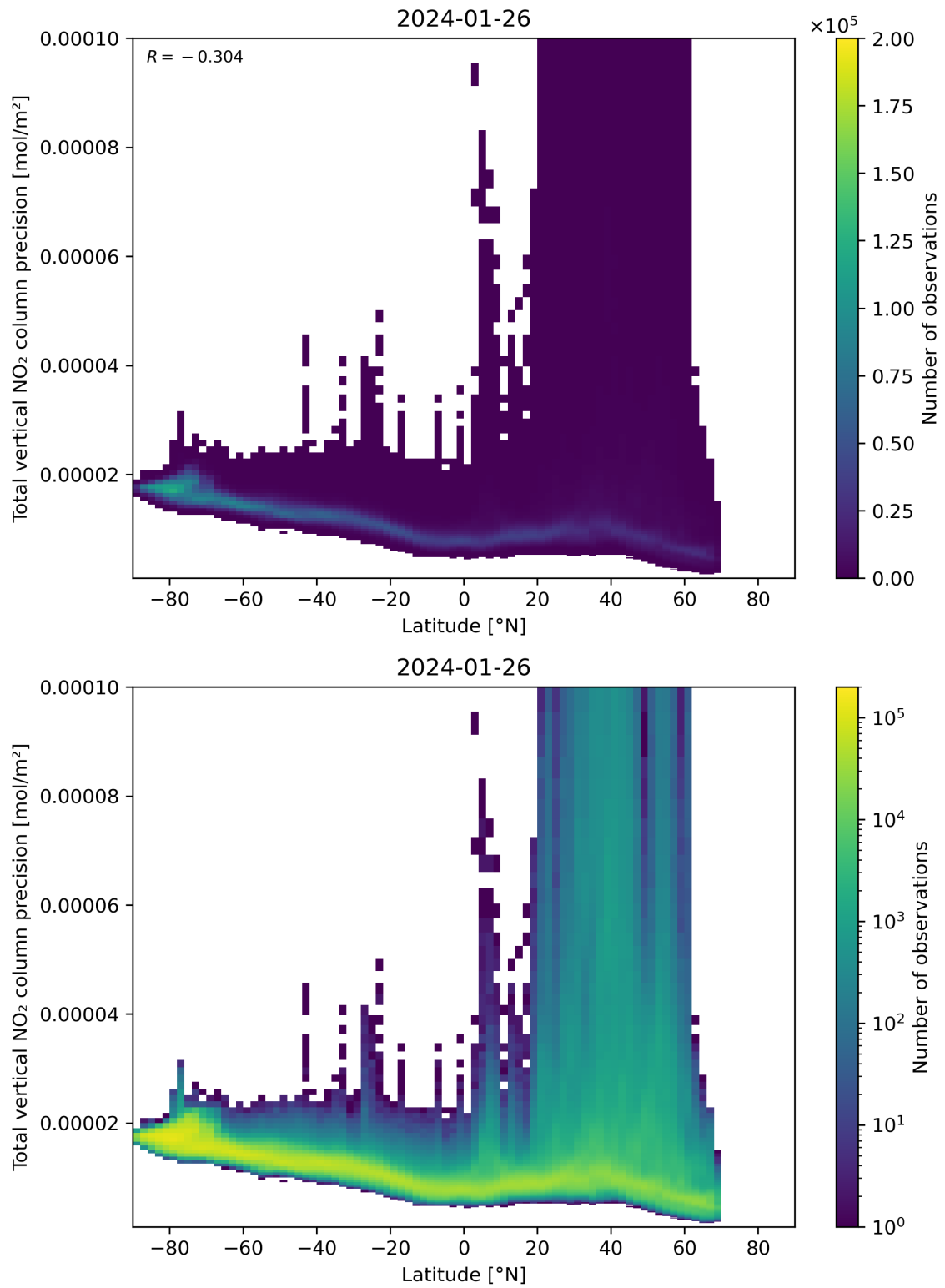
Figure 91: Scatter density plot of “Latitude” against “Total vertical NO 2 column precision” for 2024-01-26 to 2024-01-27.
