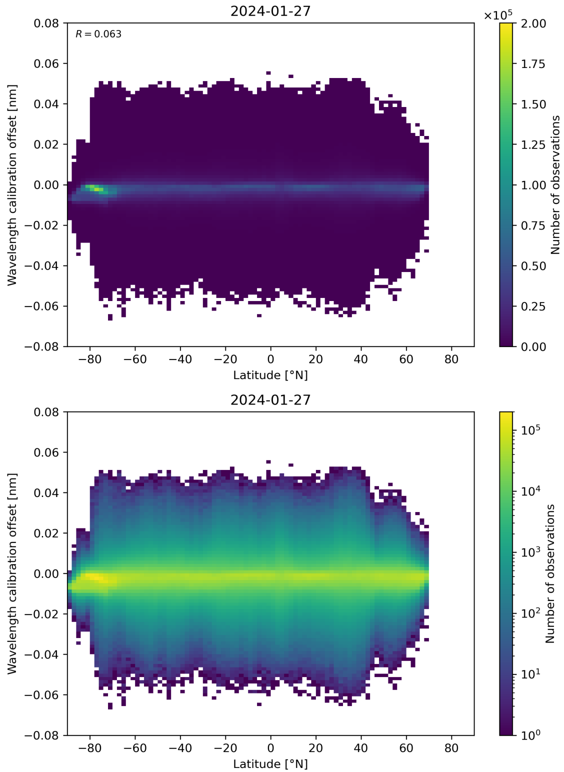
Figure 95: Scatter density plot of “Latitude” against “Wavelength calibration offset” for 2024-01-26 to 2024-01-28.
