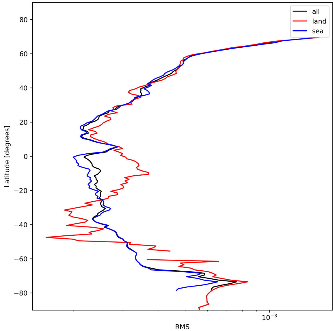
Figure 26: Zonal average of “RMS” for 2024-01-26 to 2024-01-28.
