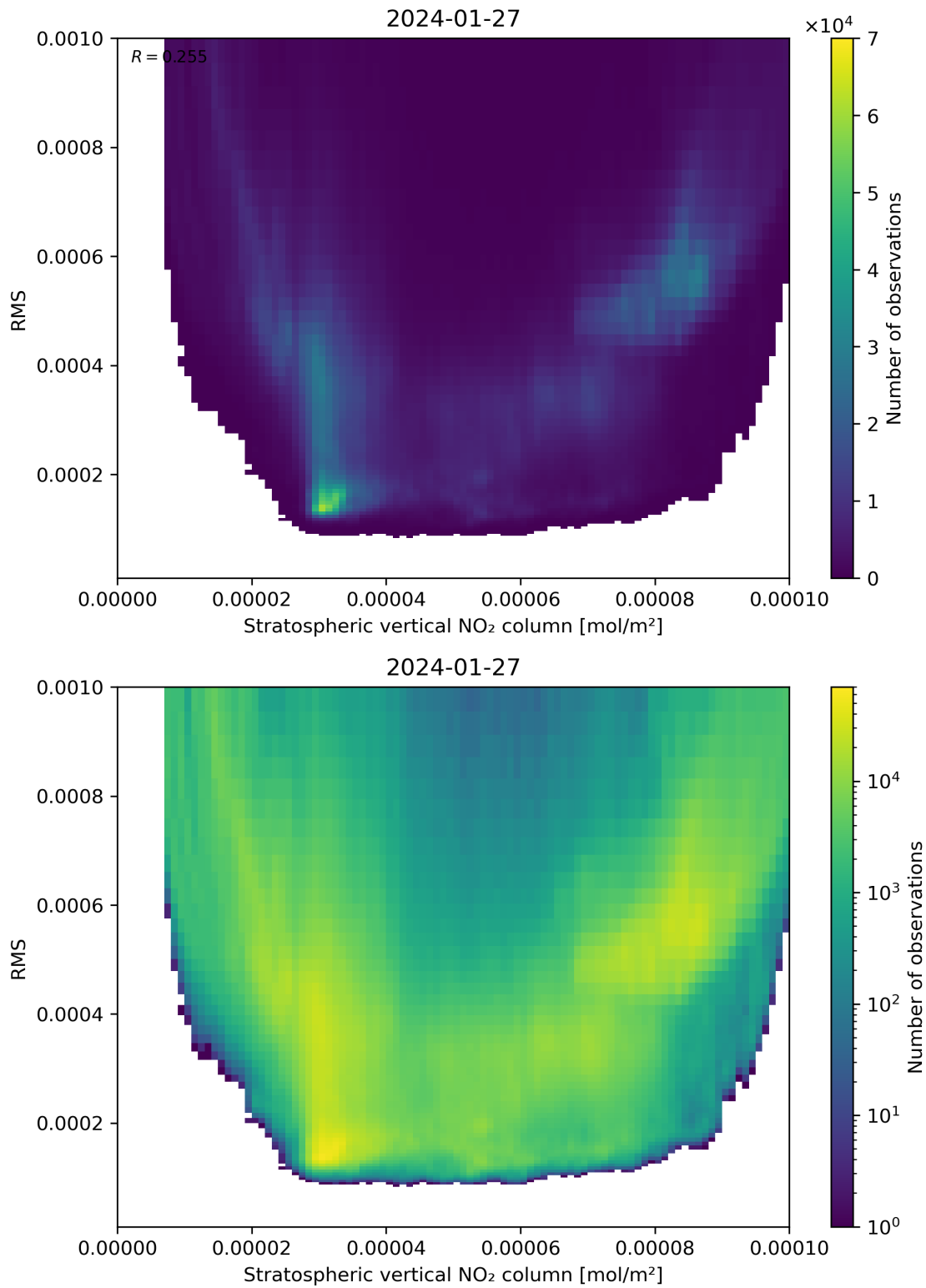
Figure 102: Scatter density plot of “Stratospheric vertical NO 2 column” against “RMS” for 2024-01-26 to 2024-01-28.
