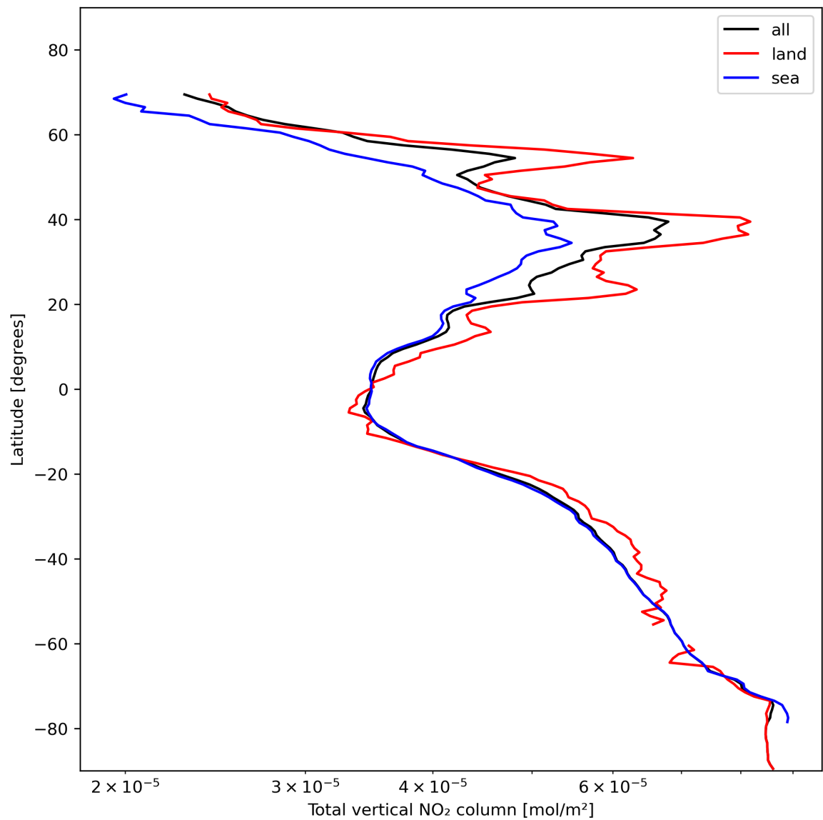
Figure 21: Zonal average of “Total vertical NO 2 column” for 2024-01-26 to 2024-01-28.
