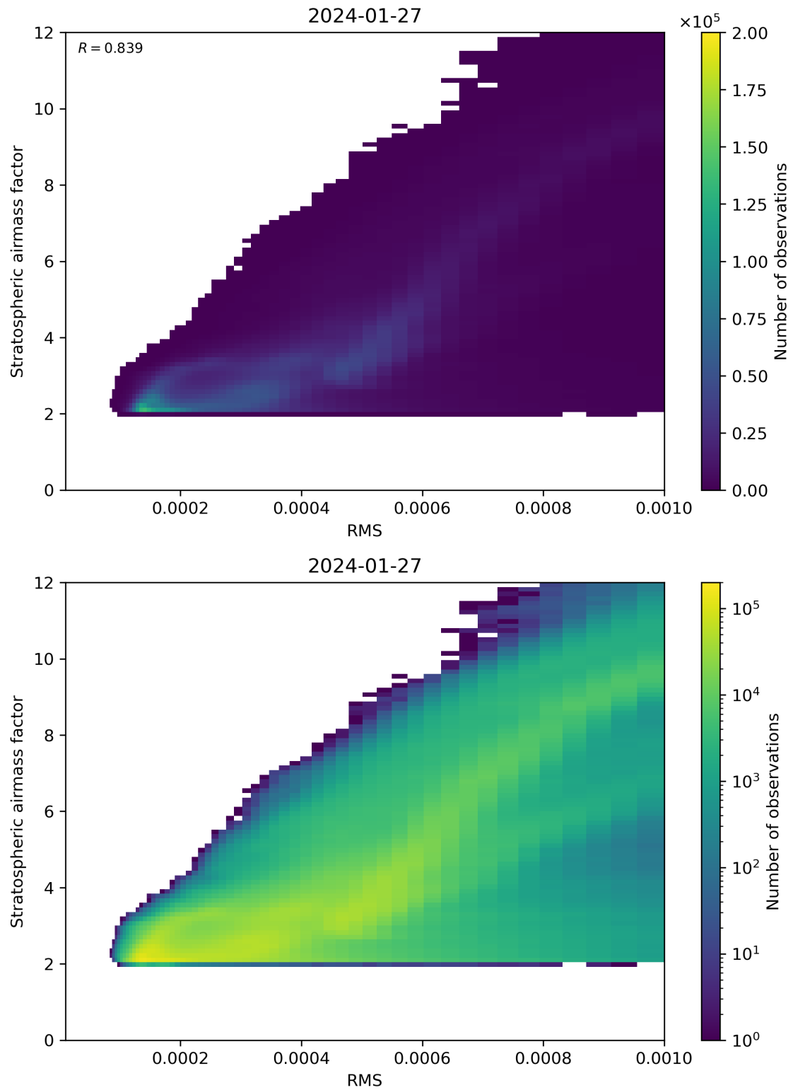
Figure 144: Scatter density plot of “RMS” against “Stratospheric airmass factor” for 2024-01-26 to 2024-01-28.
