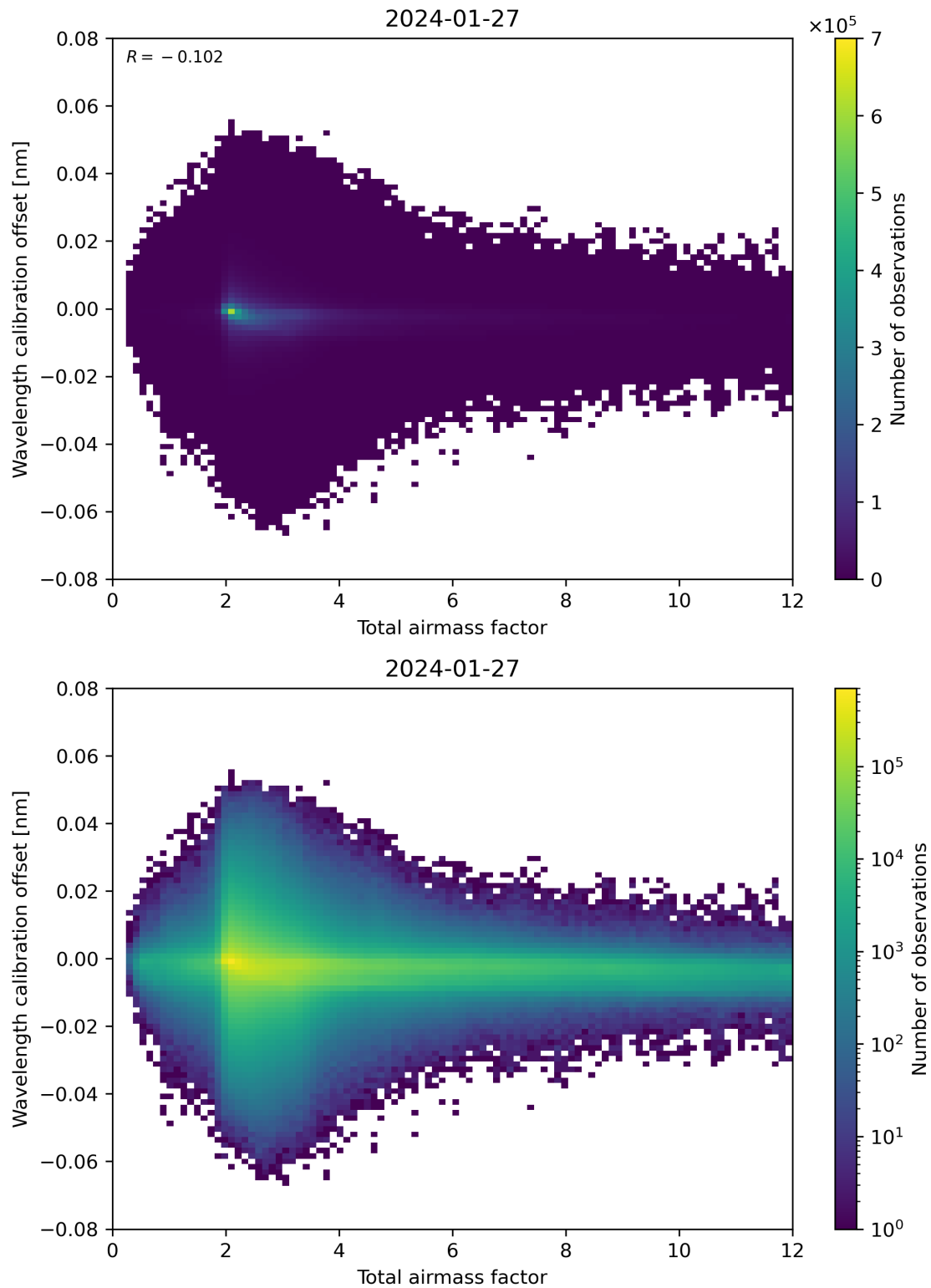
Figure 70: Scatter density plot of “Total airmass factor” against “Wavelength calibration offset” for 2024-01-26 to 2024-01-28.
