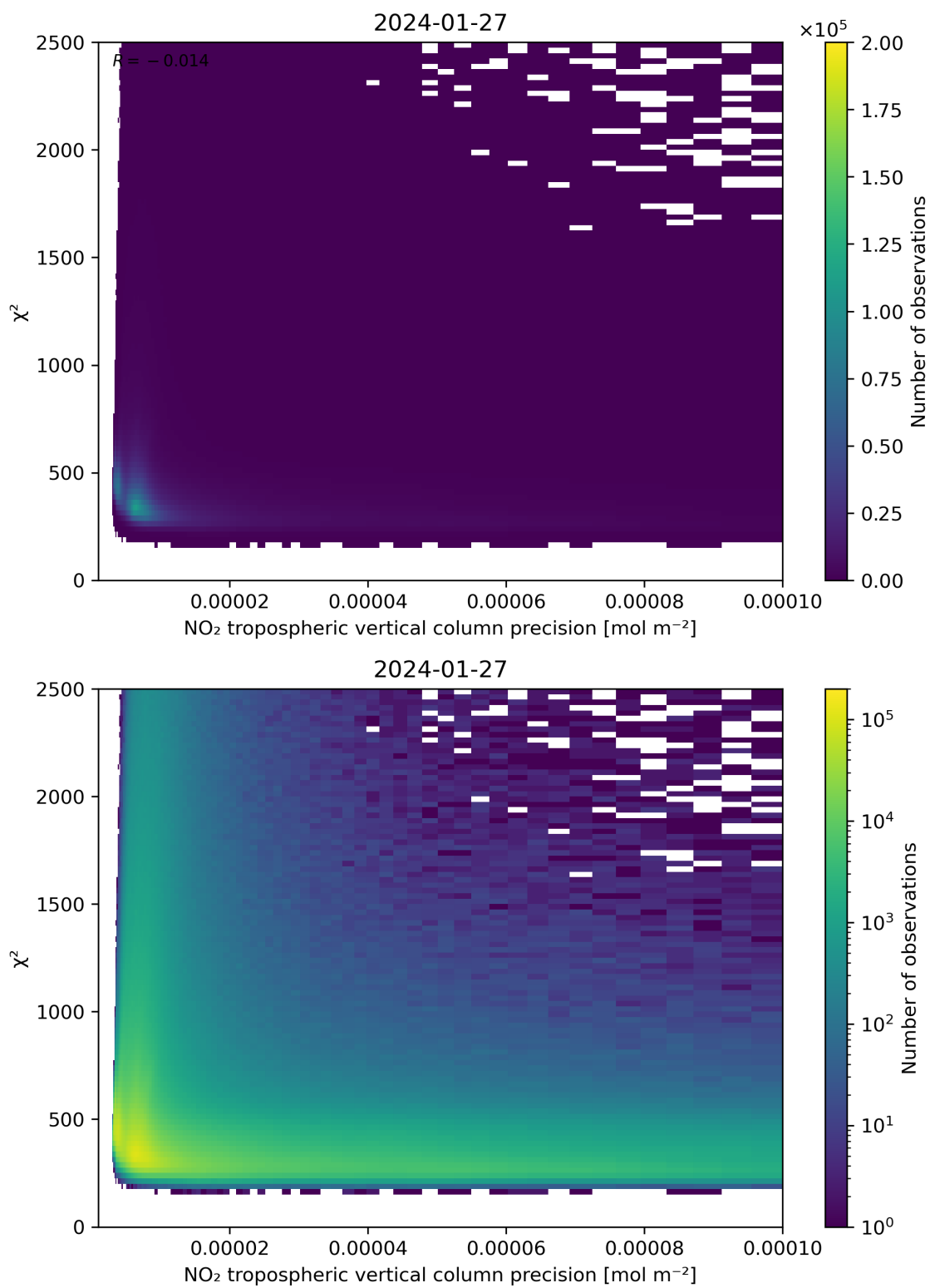
Figure 134: Scatter density plot of “NO 2 tropospheric vertical column precision” against “ \chi^2 ” for 2024-01-26 to 2024-01-28.
