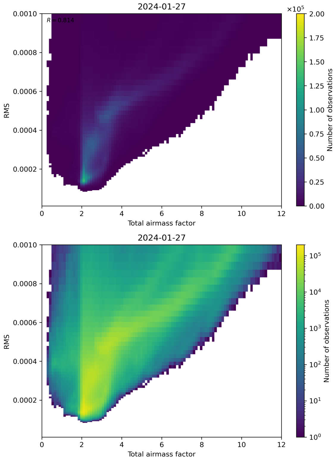
Figure 69: Scatter density plot of “Total airmass factor” against “RMS” for 2024-01-26 to 2024-01-28.
