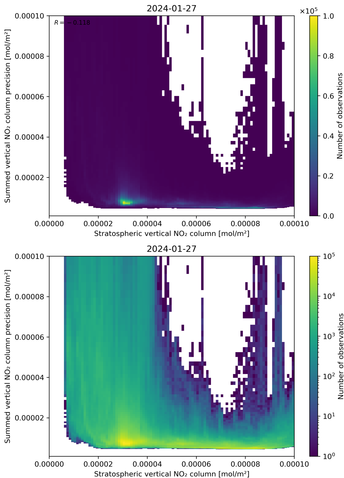
Figure 99: Scatter density plot of “Stratospheric vertical NO 2 column” against “Summed vertical NO 2 column precision” for 2024-01-26 to 2024-01-28.
