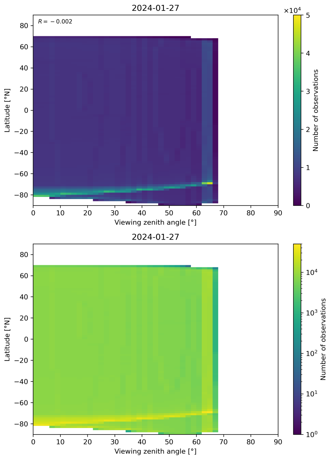
Figure 163: Scatter density plot of “Viewing zenith angle” against “Latitude” for 2024-01-26 to 2024-01-28.
