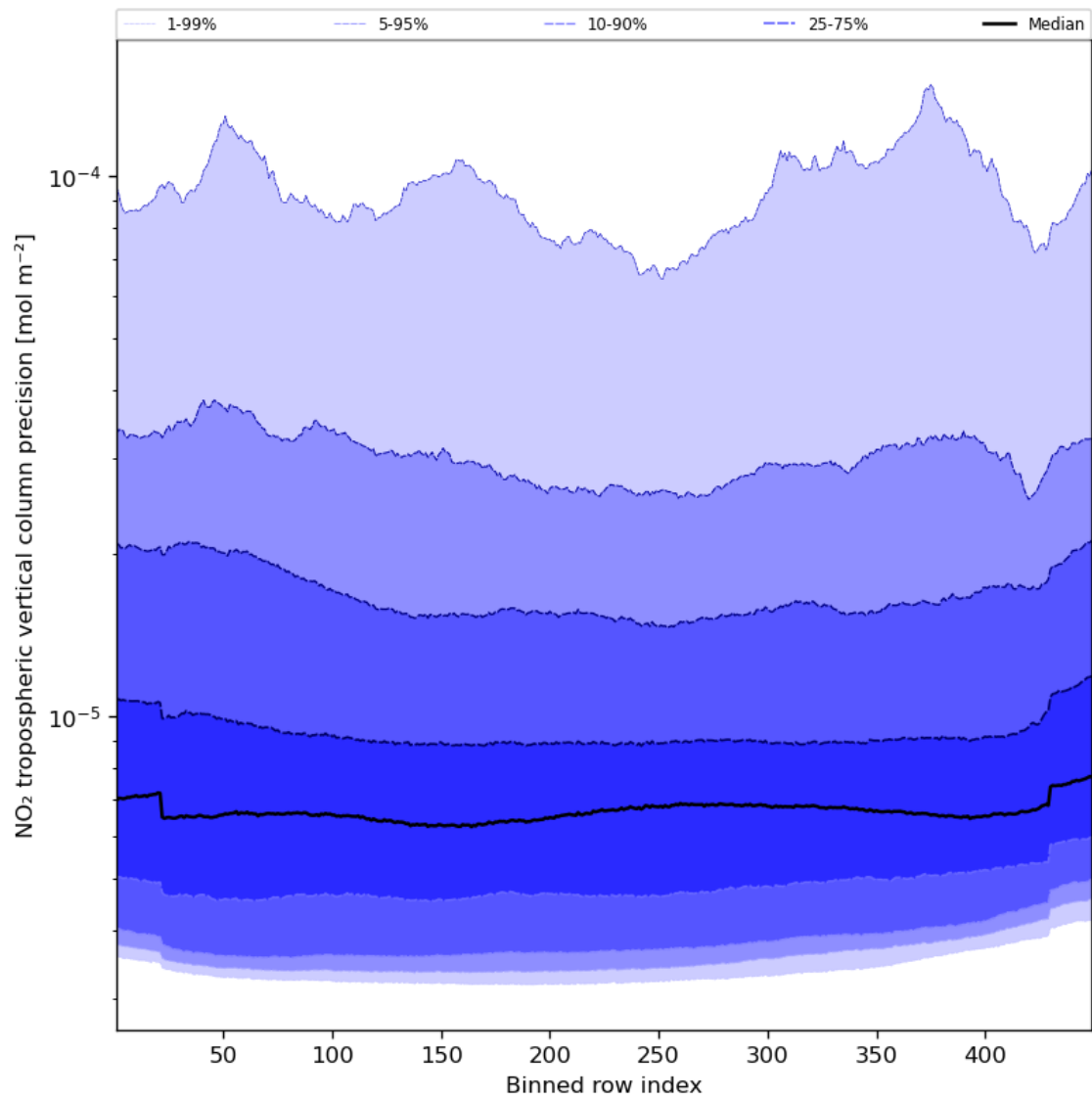
Figure 47: Along track statistics of “NO 2 tropospheric vertical column precision” for 2024-01-26 to 2024-01-28
