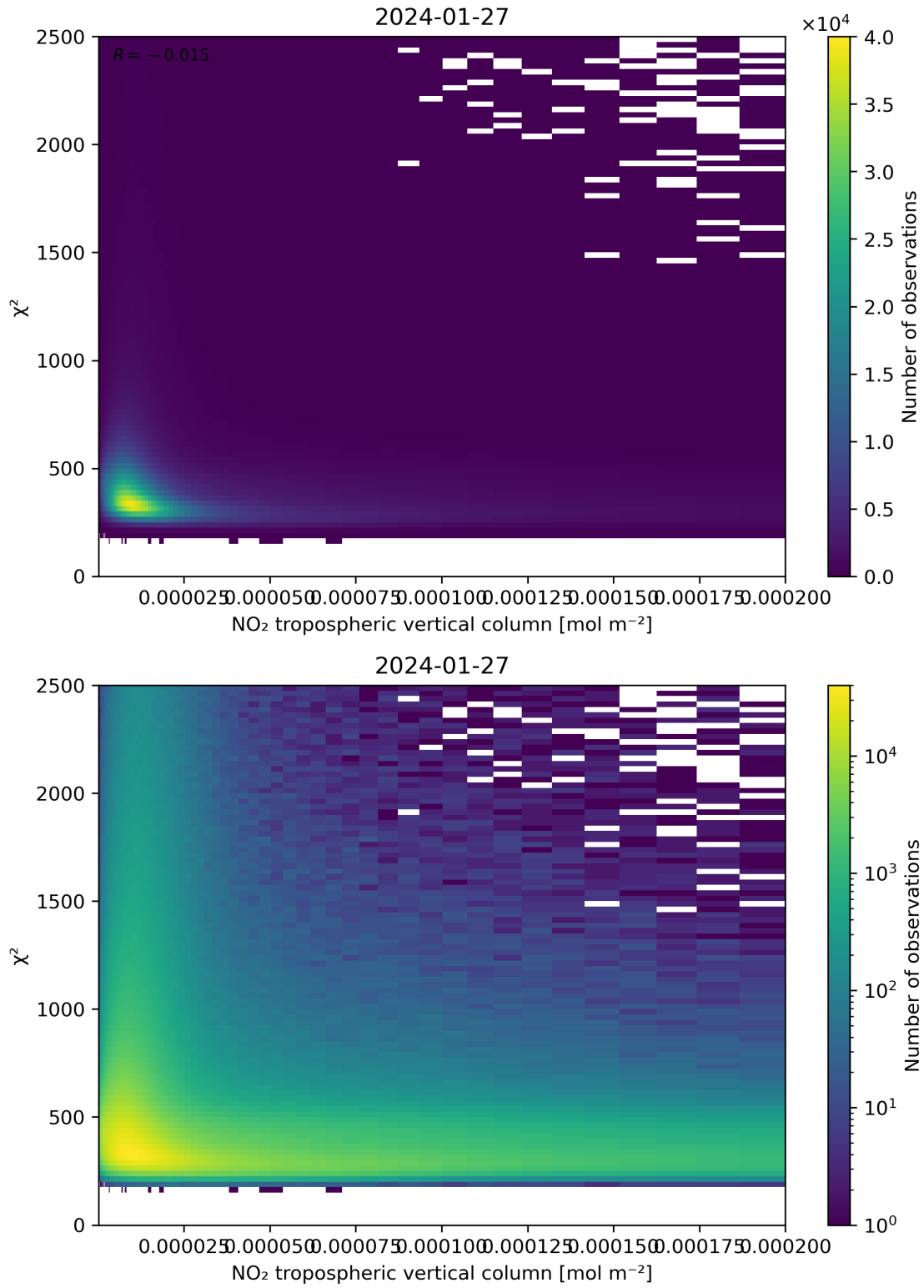
Figure 124: Scatter density plot of “NO 2 tropospheric vertical column” against “ \chi^2 ” for 2024-01-26 to 2024-01-28.
