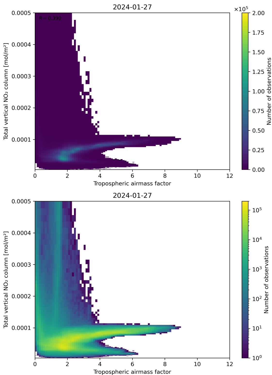
Figure 77: Scatter density plot of “Tropospheric airmass factor” against “Total vertical NO 2 column” for 2024-01-26 to 2024-01-28.
