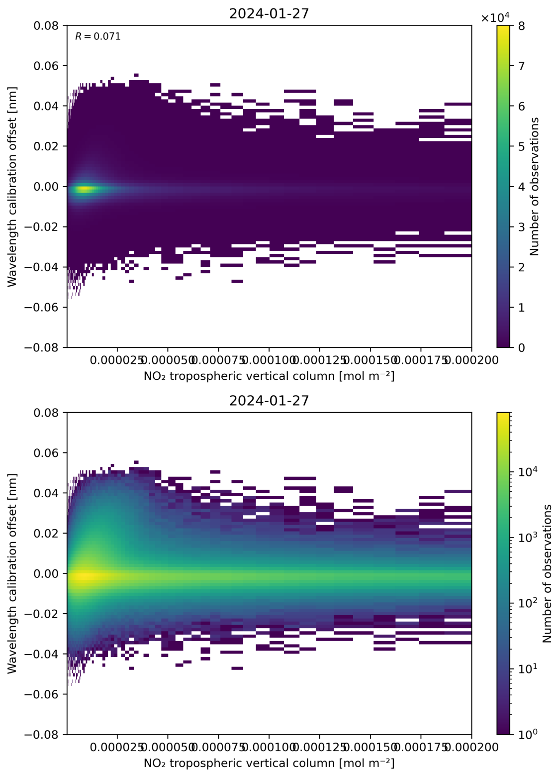
Figure 143: Scatter density plot of “NO 2 tropospheric vertical column” against “Wavelength calibration offset” for 2024-01-26 to 2024-01-28.
