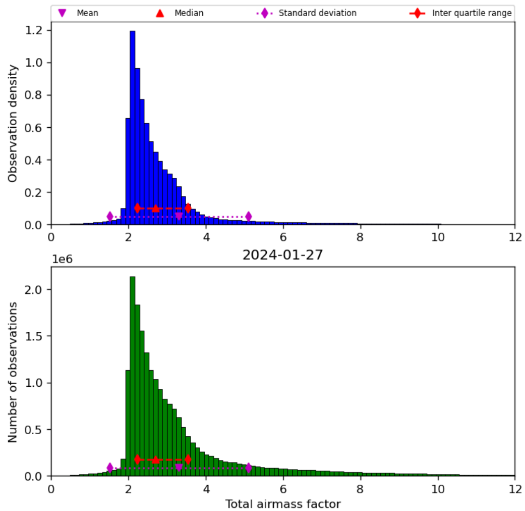
Figure 32: Histogram of “Total airmass factor” for 2024-01-26 to 2024-01-28
