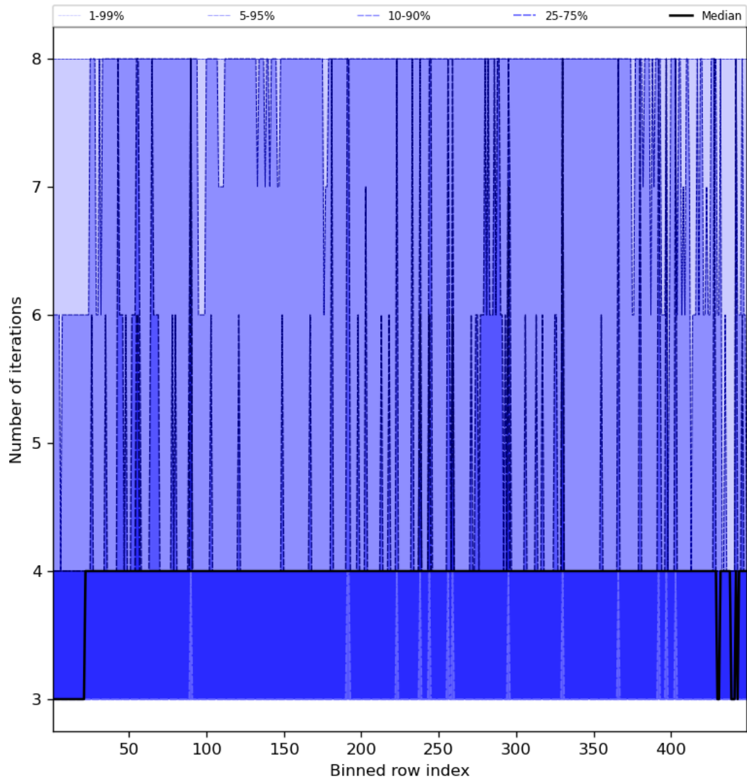
Figure 51: Along track statistics of “Number of iterations” for 2024-01-26 to 2024-01-28
