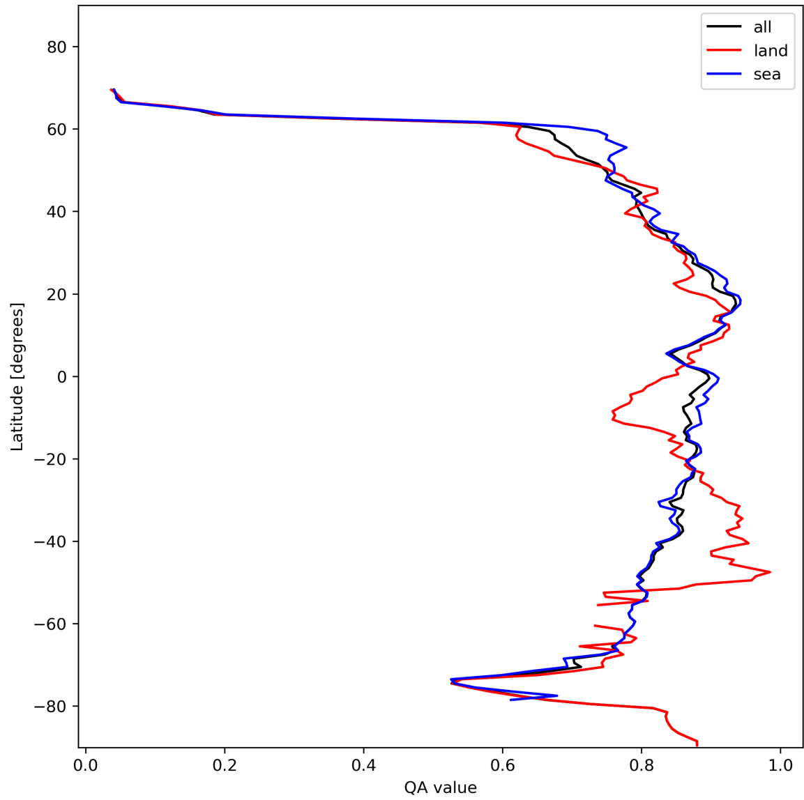
Figure 11: Zonal average of “QA value” for 2024-01-26 to 2024-01-28.
