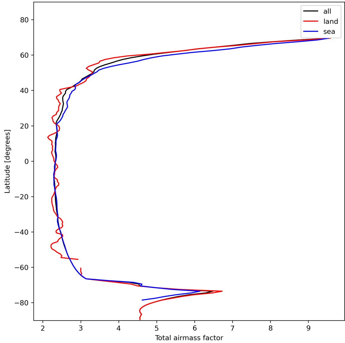
Figure 15: Zonal average of “Total airmass factor” for 2024-01-26 to 2024-01-28.
