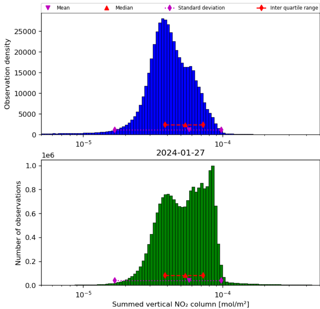
Figure 40: Histogram of “Summed vertical NO 2 column” for 2024-01-26 to 2024-01-28
