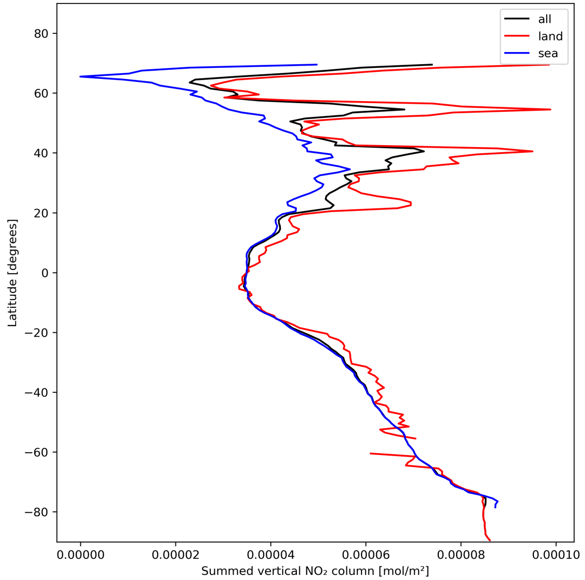
Figure 23: Zonal average of “Summed vertical NO 2 column” for 2024-01-26 to 2024-01-28.
