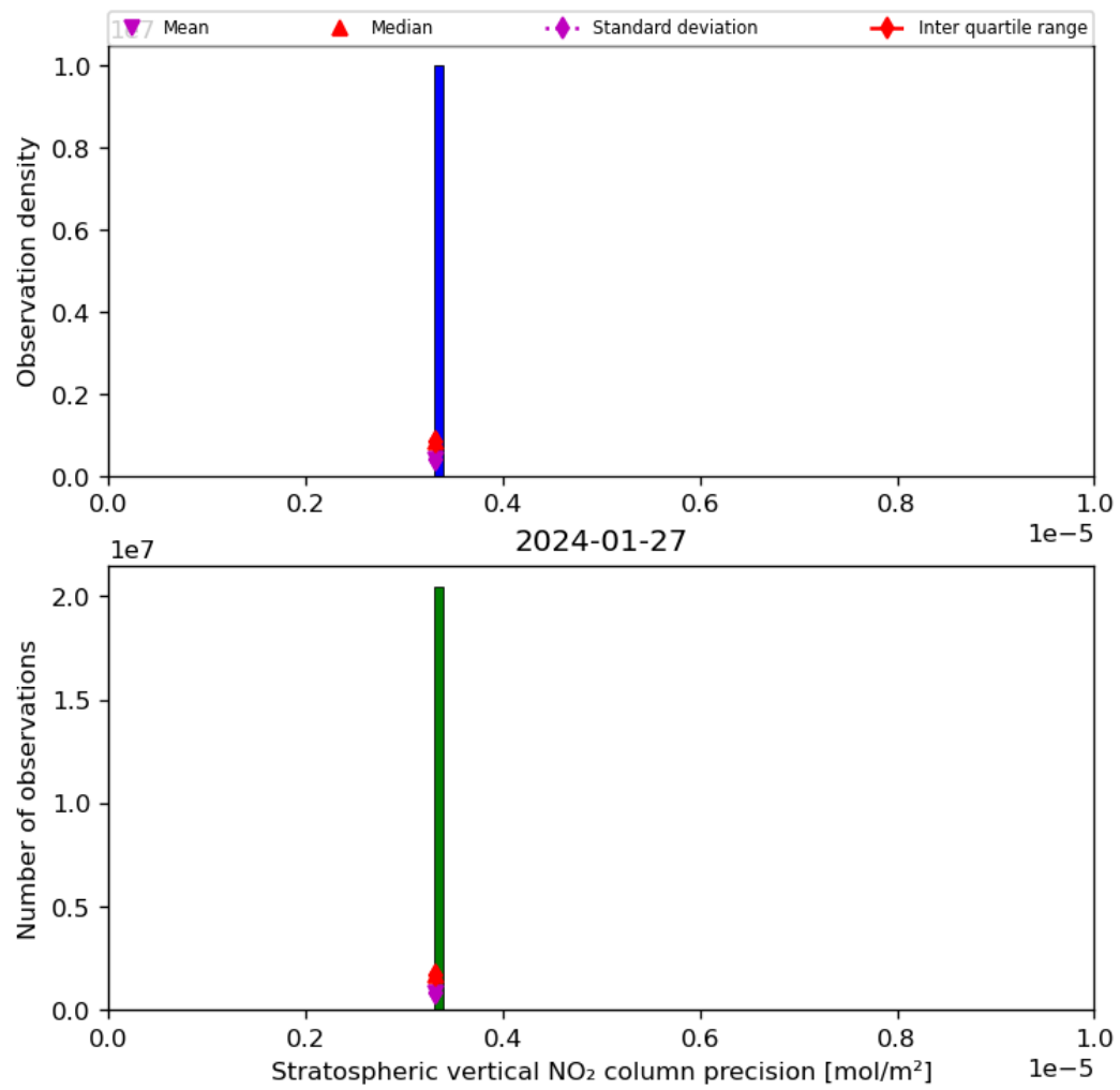
Figure 37: Histogram of “Stratospheric vertical NO 2 column precision” for 2024-01-26 to 2024-01-28
