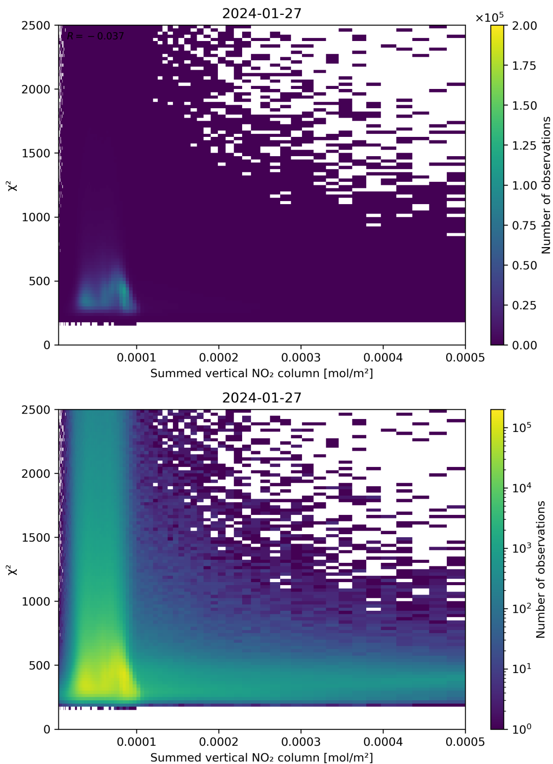
Figure 104: Scatter density plot of “Summed vertical NO 2 column” against “ \chi^2 ” for 2024-01-26 to 2024-01-28.
