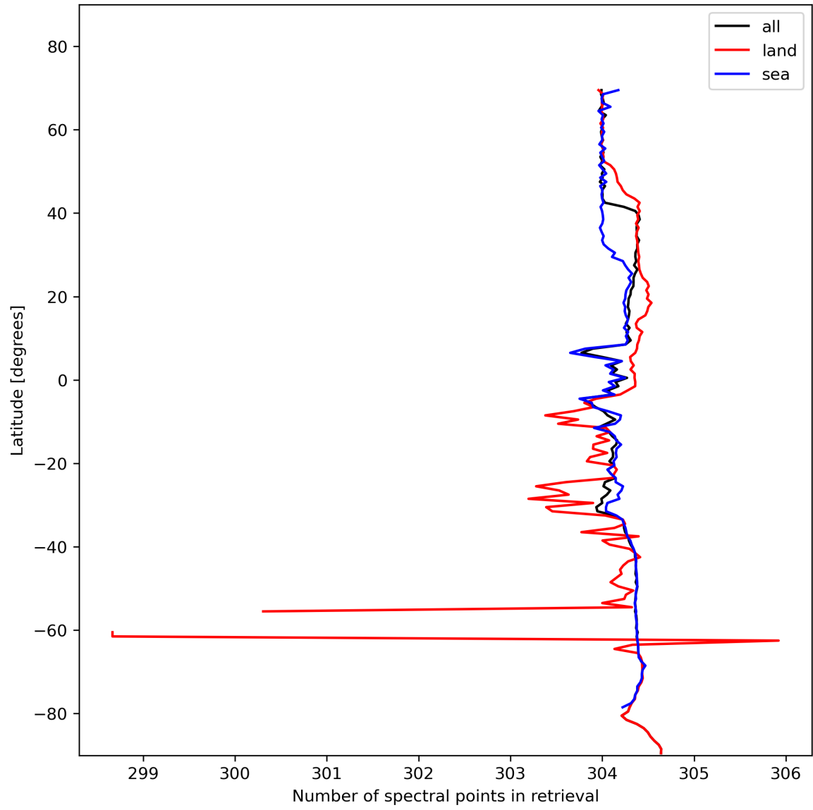
Figure 16: Zonal average of “Number of spectral points in retrieval” for 2024-01-26 to 2024-01-28.
