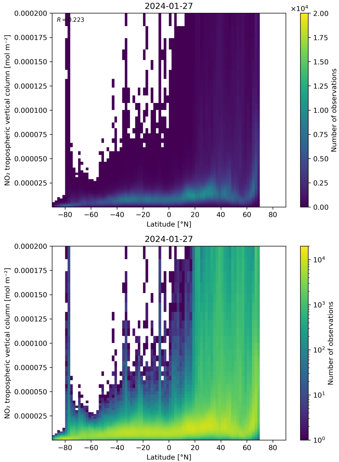
Figure 92: Scatter density plot of “Latitude” against “NO 2 tropospheric vertical column” for 2024-01-26 to 2024-01-28.
