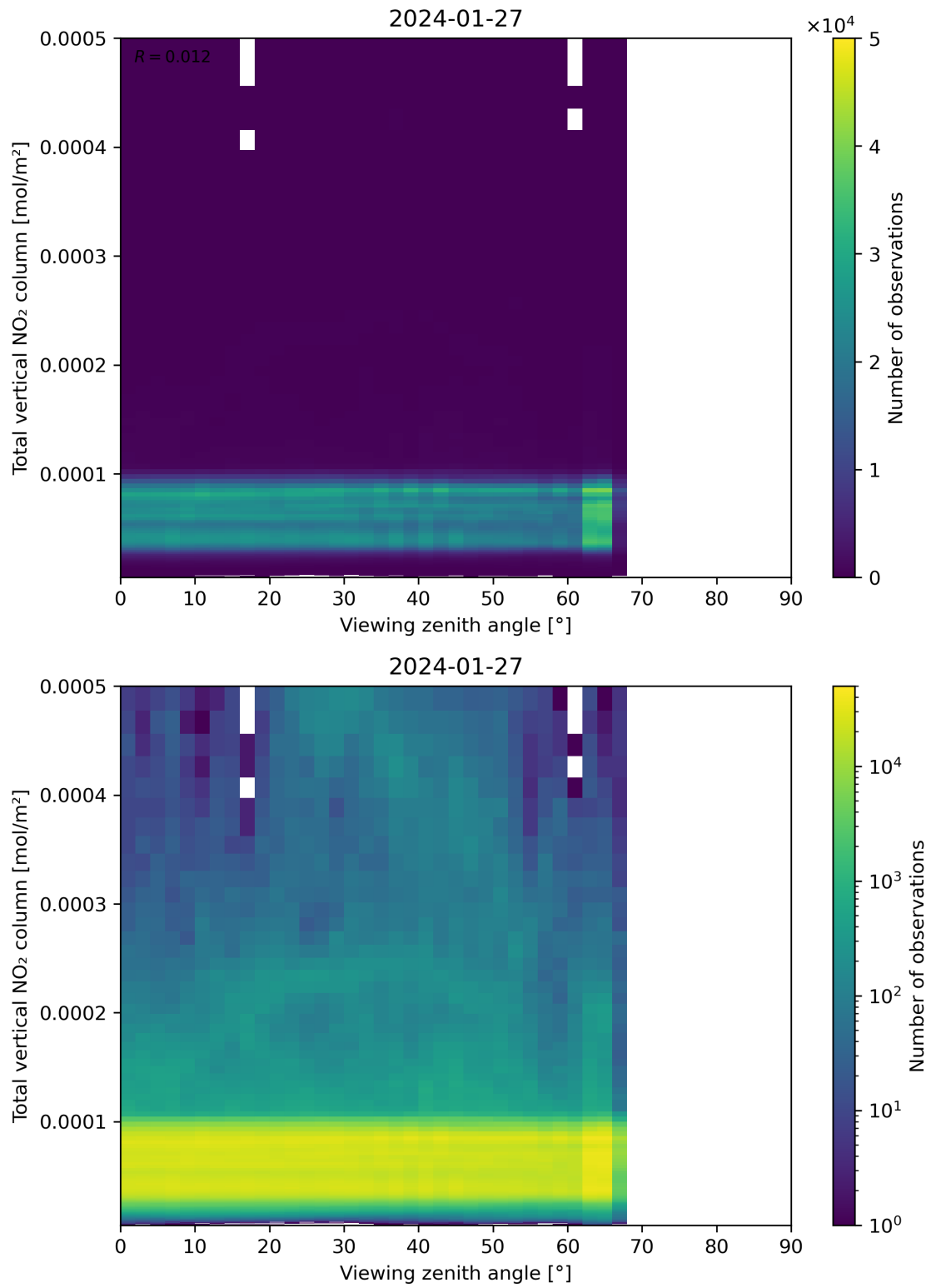
Figure 167: Scatter density plot of “Viewing zenith angle” against “Total vertical NO 2 column” for 2024-01-26 to 2024-01-28.
