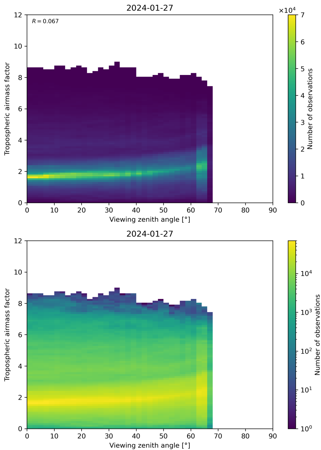
Figure 161: Scatter density plot of “Viewing zenith angle” against “Tropospheric airmass factor” for 2024-01-26 to 2024-01-28.
