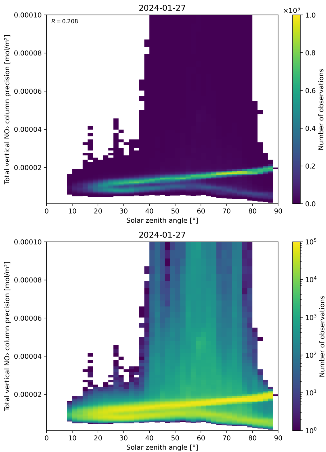
Figure 154: Scatter density plot of “Solar zenith angle” against “Total vertical NO 2 column precision” for 2024-01-26 to 2024-01-28.
