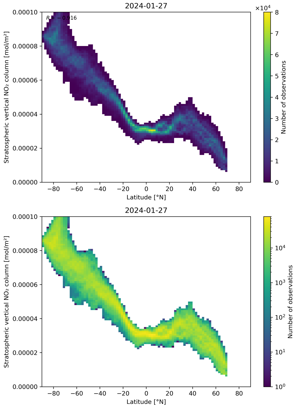
Figure 87: Scatter density plot of “Latitude” against “Stratospheric vertical NO 2 column” for 2024-01-26 to 2024-01-28.
