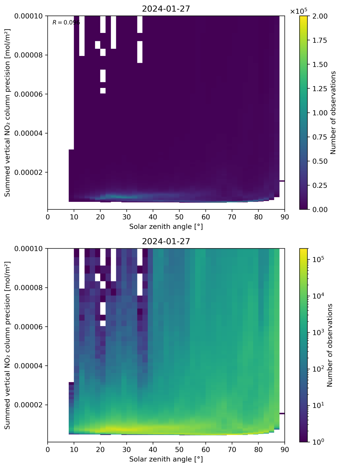
Figure 152: Scatter density plot of “Solar zenith angle” against “Summed vertical NO 2 column precision” for 2024-01-26 to 2024-01-28.
