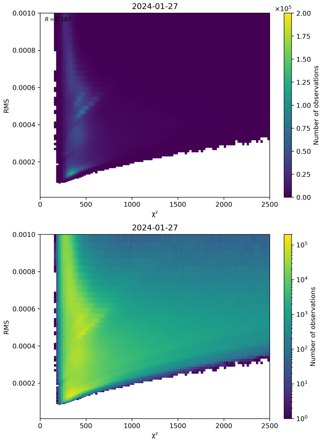
Figure 82: Scatter density plot of “ \chi^2 ” against “RMS” for 2024-01-26 to 2024-01-28.
