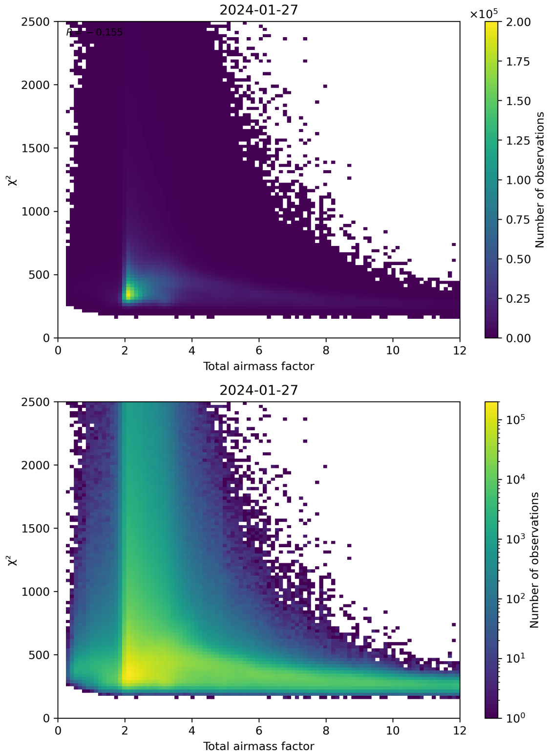
Figure 63: Scatter density plot of “Total airmass factor” against “ \chi^2 ” for 2024-01-26 to 2024-01-28.
