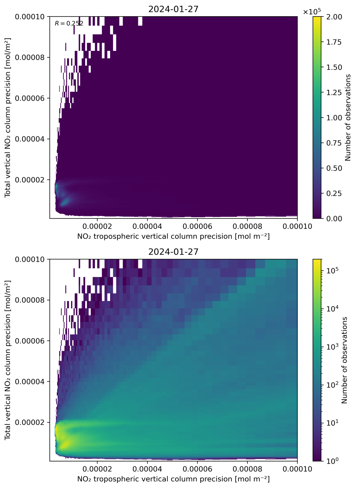
Figure 139: Scatter density plot of “NO 2 tropospheric vertical column precision” against “Total vertical NO 2 column precision” for 2024-01-26 to 2024-01-28.
