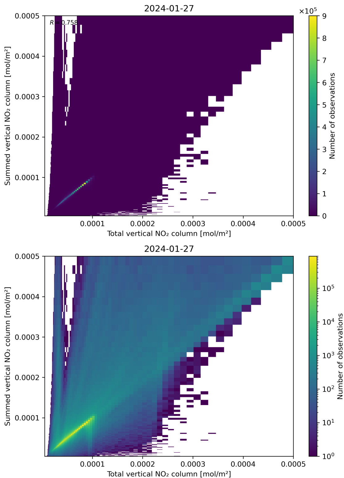
Figure 112: Scatter density plot of “Total vertical NO 2 column” against “Summed vertical NO 2 column” for 2024-01-26 to 2024-01-28.
