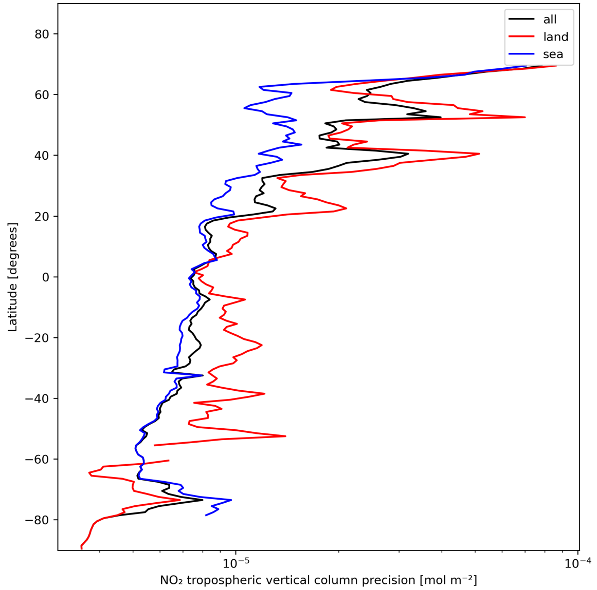
Figure 13: Zonal average of “NO 2 tropospheric vertical column precision” for 2024-01-26 to 2024-01-28.
