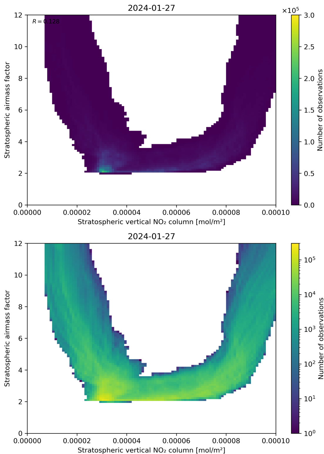
Figure 96: Scatter density plot of “Stratospheric vertical NO 2 column” against “Stratospheric airmass factor” for 2024-01-26 to 2024-01-28.
