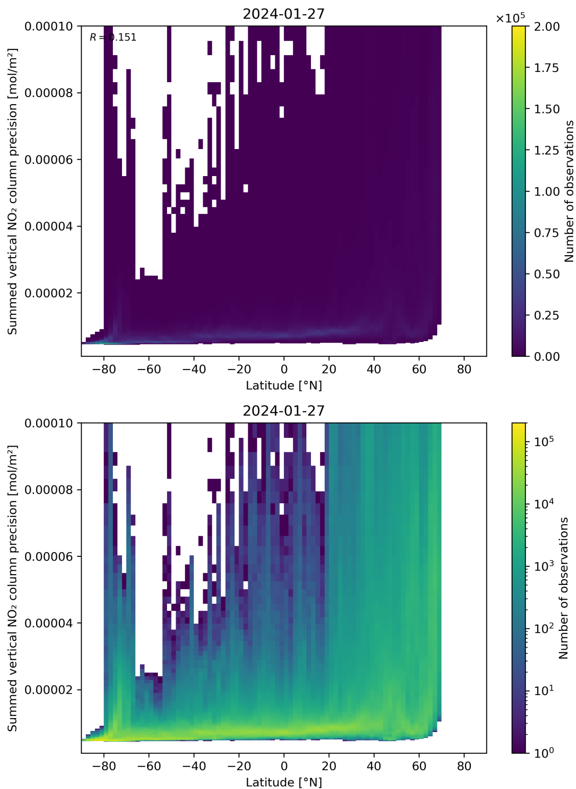
Figure 89: Scatter density plot of “Latitude” against “Summed vertical NO 2 column precision” for 2024-01-26 to 2024-01-28.
