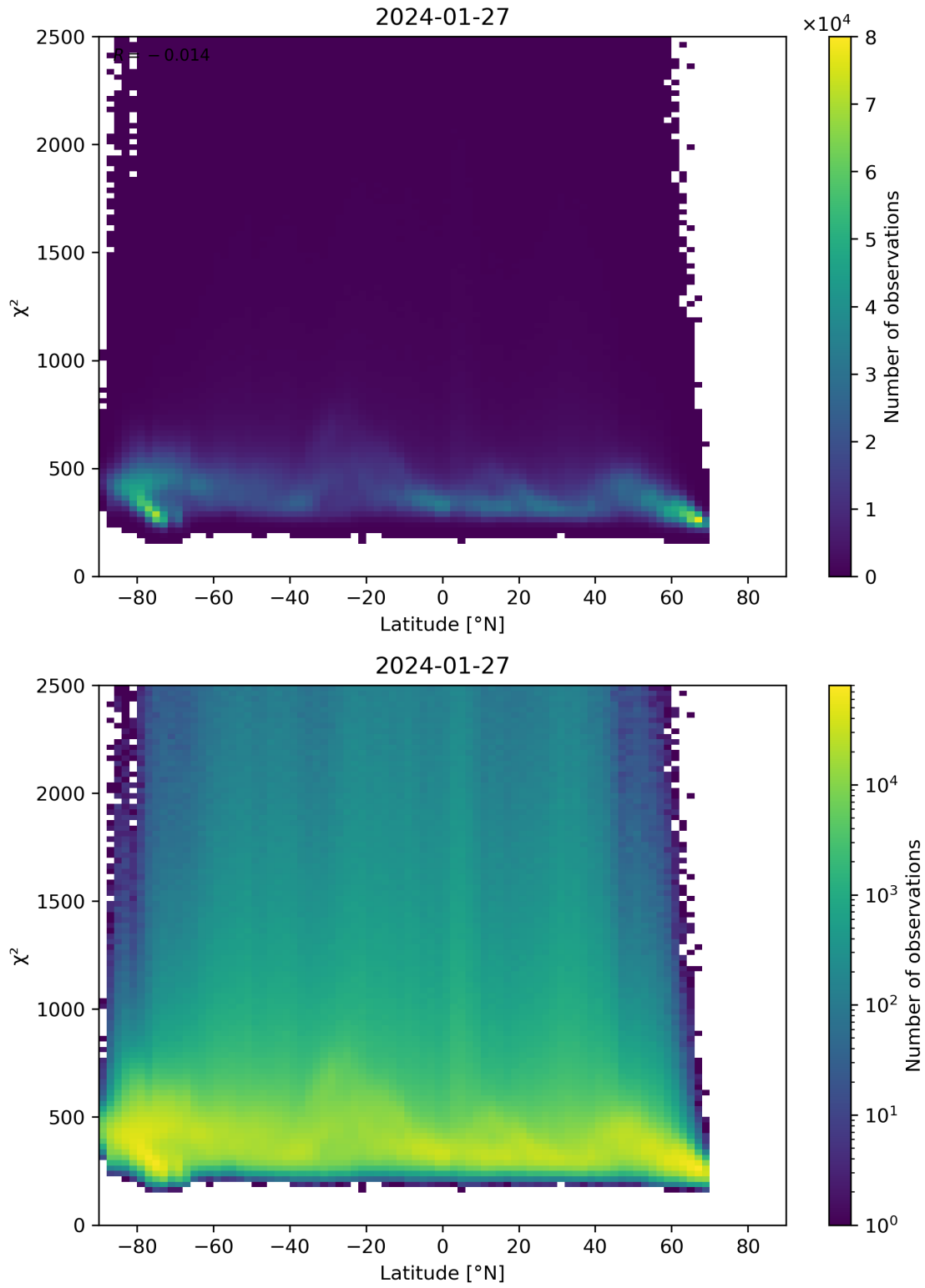
Figure 86: Scatter density plot of “Latitude” against “ \chi^2 ” for 2024-01-26 to 2024-01-28.
