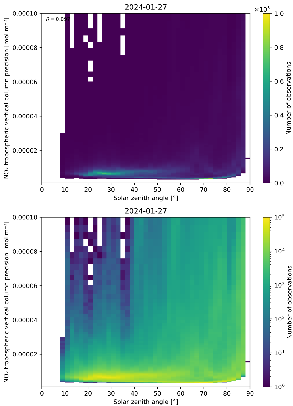
Figure 156: Scatter density plot of “Solar zenith angle” against “NO 2 tropospheric vertical column precision” for 2024-01-26 to 2024-01-28.
