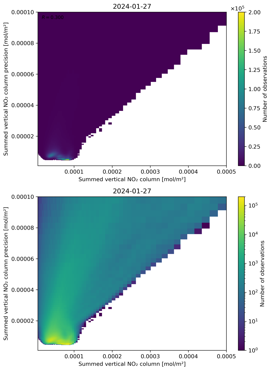
Figure 105: Scatter density plot of “Summed vertical NO 2 column” against “Summed vertical NO 2 column precision” for 2024-01-26 to 2024-01-28.
