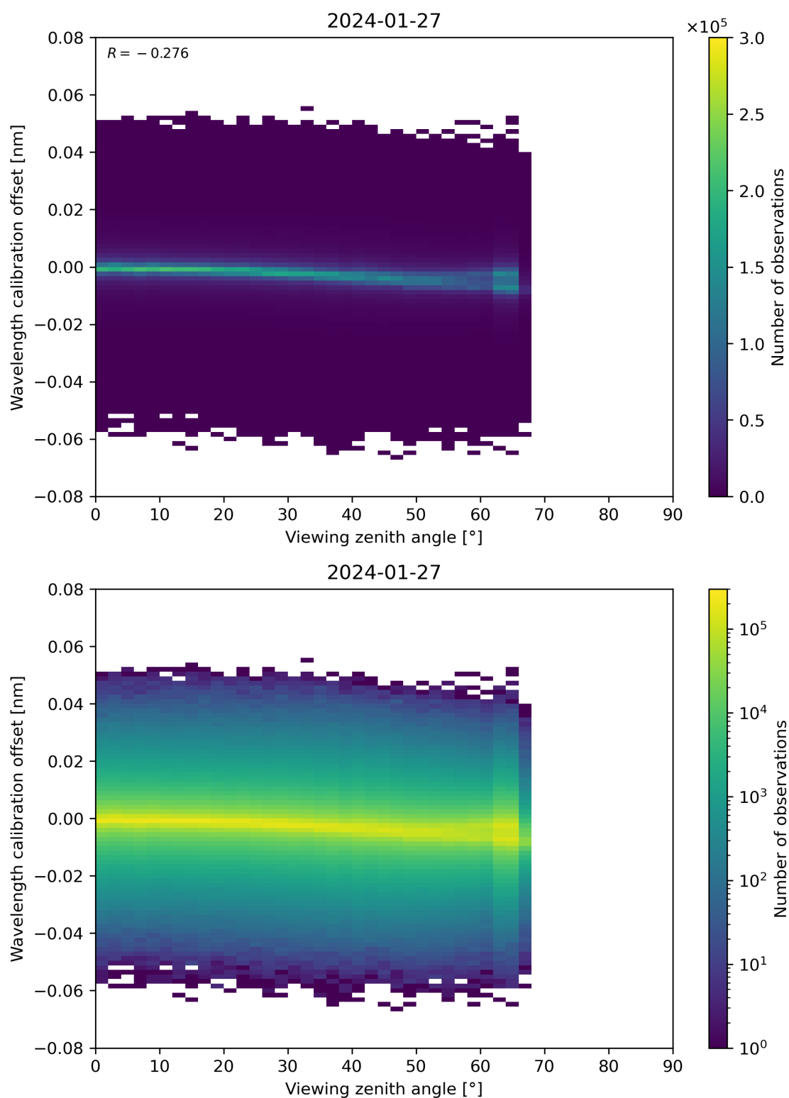
Figure 173: Scatter density plot of “Viewing zenith angle” against “Wavelength calibration offset” for 2024-01-26 to 2024-01-28.
