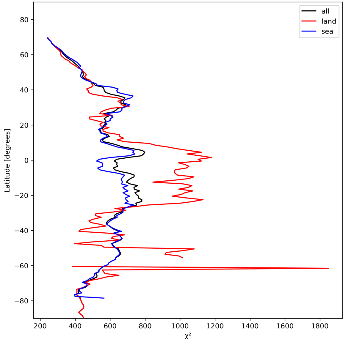
Figure 25: Zonal average of “ \chi^2 ” for 2024-01-26 to 2024-01-28.
