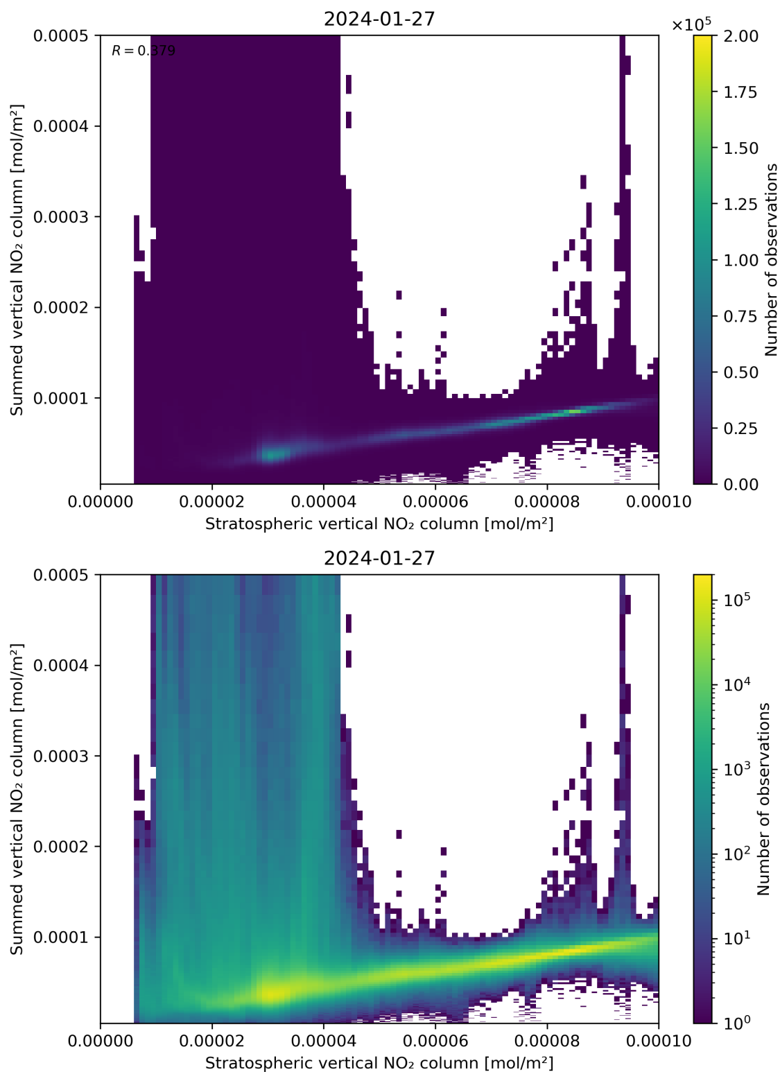
Figure 98: Scatter density plot of “Stratospheric vertical NO 2 column” against “Summed vertical NO 2 column” for 2024-01-26 to 2024-01-28.
