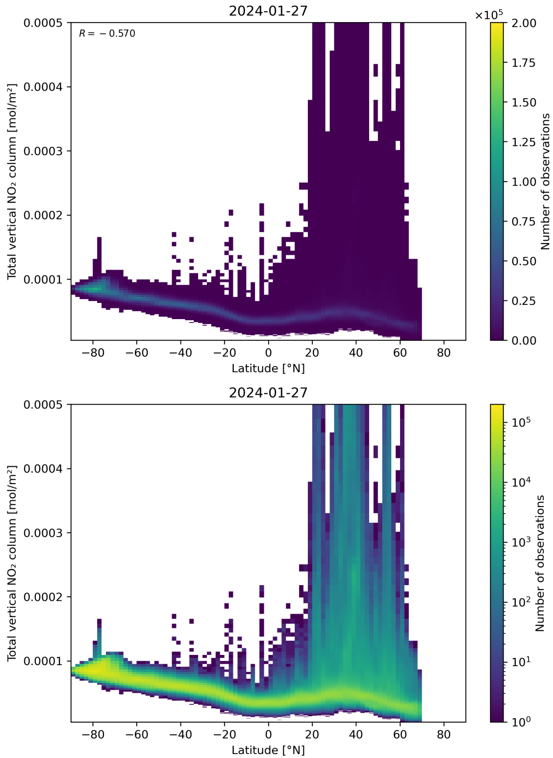
Figure 90: Scatter density plot of “Latitude” against “Total vertical NO 2 column” for 2024-01-26 to 2024-01-28.
