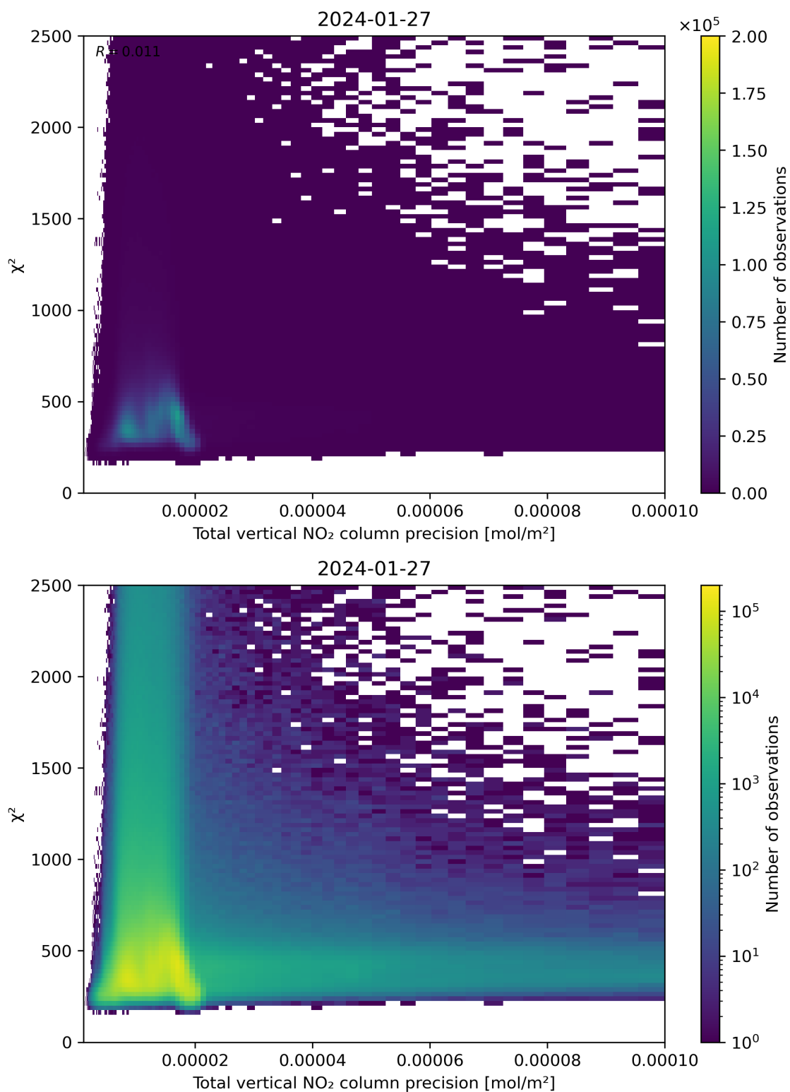
Figure 116: Scatter density plot of “Total vertical NO 2 column precision” against “ \chi^2 ” for 2024-01-26 to 2024-01-28.
