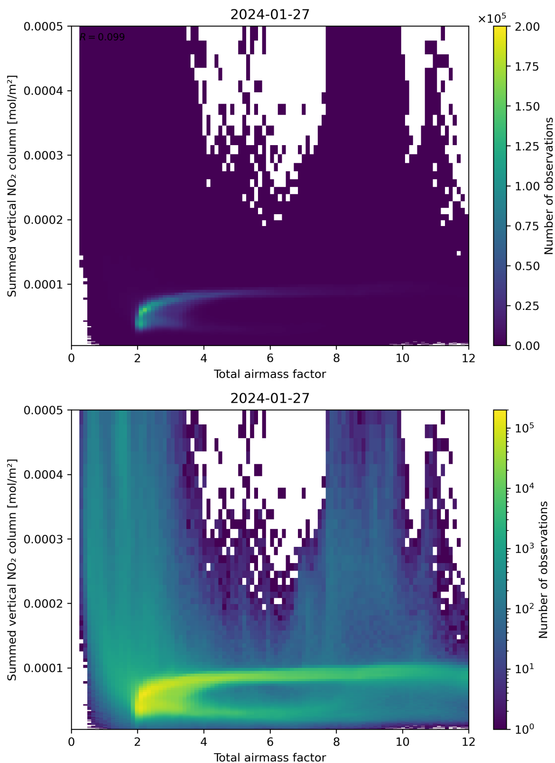
Figure 65: Scatter density plot of “Total airmass factor” against “Summed vertical NO 2 column” for 2024-01-26 to 2024-01-28.
