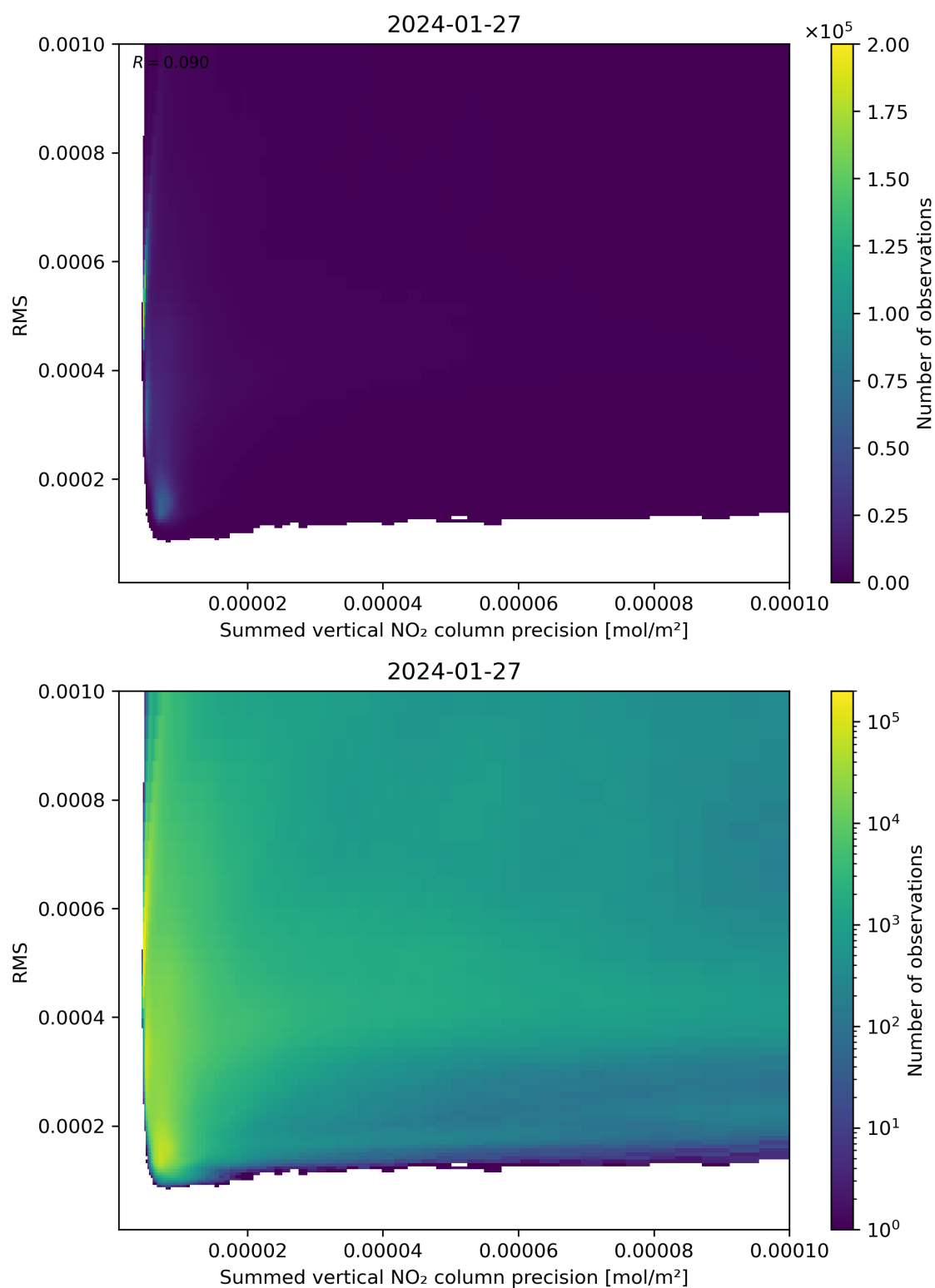
Figure 108: Scatter density plot of “Summed vertical NO 2 column precision” against “RMS” for 2024-01-26 to 2024-01-28.
