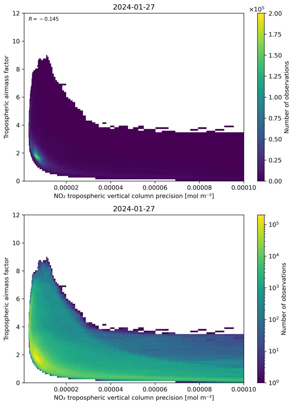
Figure 133: Scatter density plot of “NO 2 tropospheric vertical column precision” against “Tropospheric airmass factor” for 2024-01-26 to 2024-01-28.
