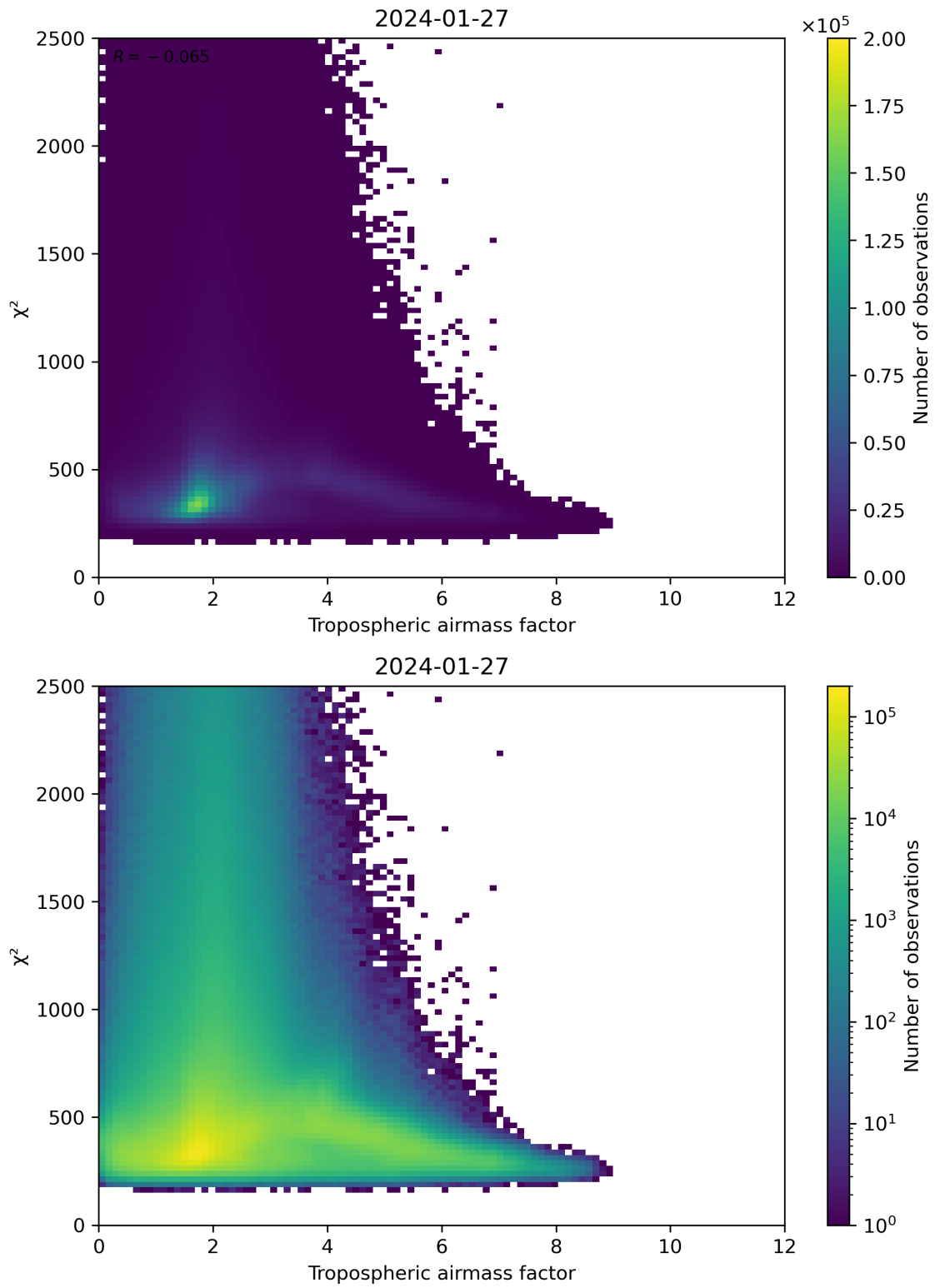
Figure 73: Scatter density plot of “Tropospheric airmass factor” against “ \chi^2 ” for 2024-01-26 to 2024-01-28.
