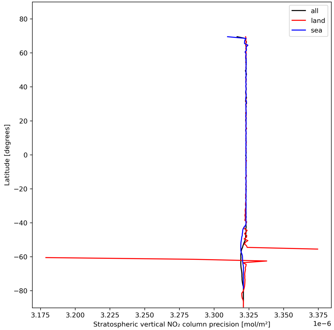
Figure 20: Zonal average of “Stratospheric vertical NO 2 column precision” for 2024-01-26 to 2024-01-28.
