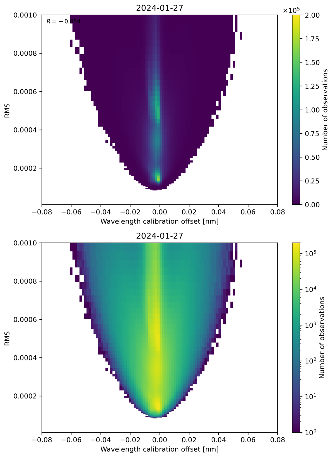
Figure 181: Scatter density plot of “Wavelength calibration offset” against “RMS” for 2024-01-26 to 2024-01-28.
