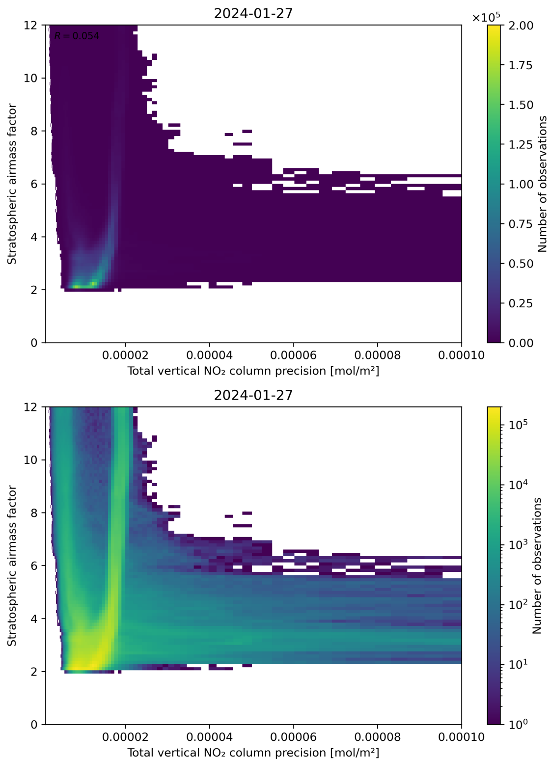
Figure 115: Scatter density plot of “Total vertical NO 2 column precision” against “Stratospheric airmass factor” for 2024-01-26 to 2024-01-28.
