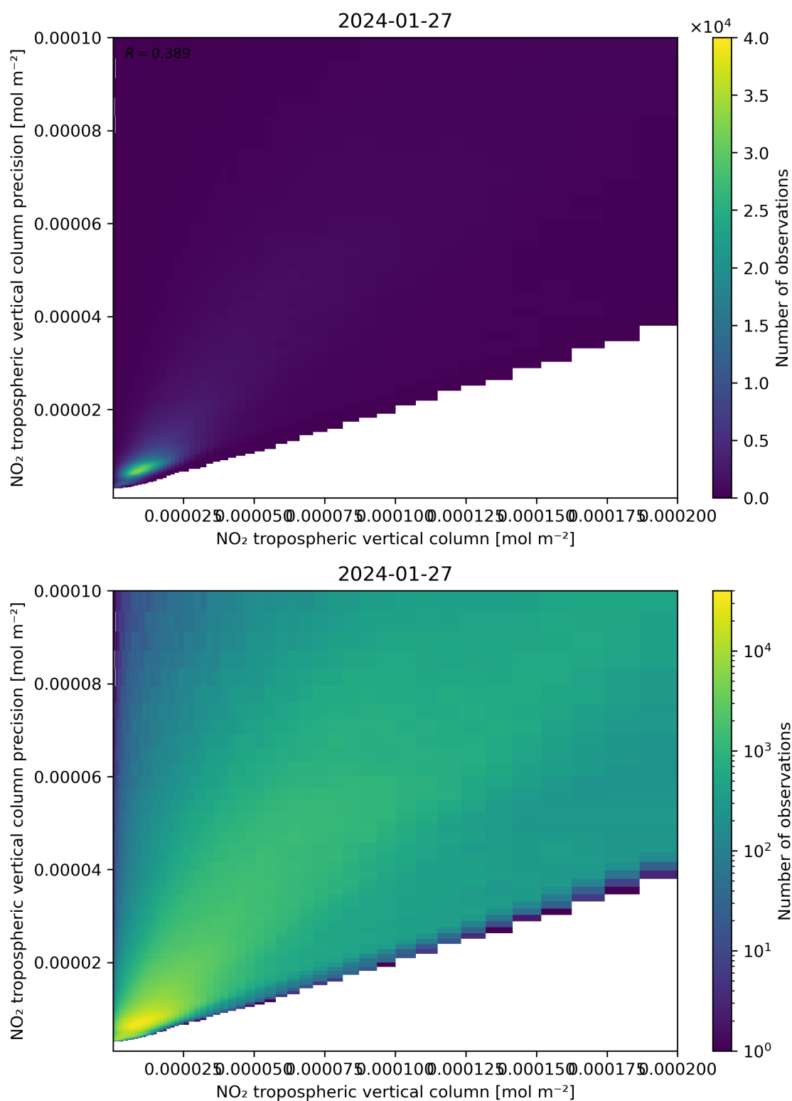
Figure 130: Scatter density plot of “NO 2 tropospheric vertical column” against “NO 2 tropospheric vertical column precision” for 2024-01-26 to 2024-01-28.
