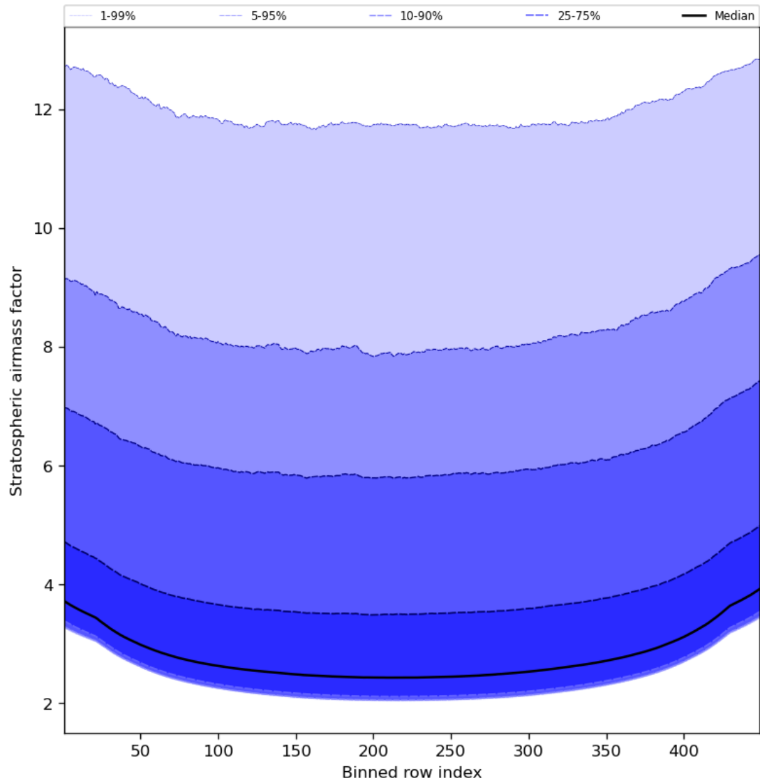
Figure 61: Along track statistics of “Stratospheric airmass factor” for 2024-01-26 to 2024-01-28
