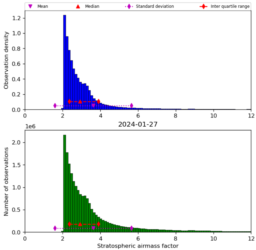
Figure 44: Histogram of “Stratospheric airmass factor” for 2024-01-26 to 2024-01-28
