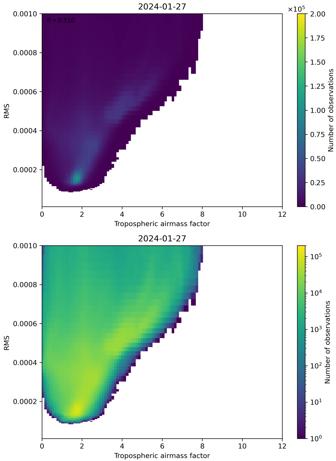
Figure 79: Scatter density plot of “Tropospheric airmass factor” against “RMS” for 2024-01-26 to 2024-01-28.
