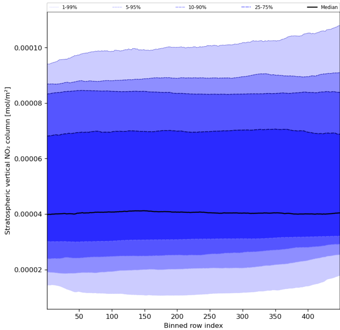
Figure 53: Along track statistics of “Stratospheric vertical NO 2 column” for 2024-01-26 to 2024-01-28
