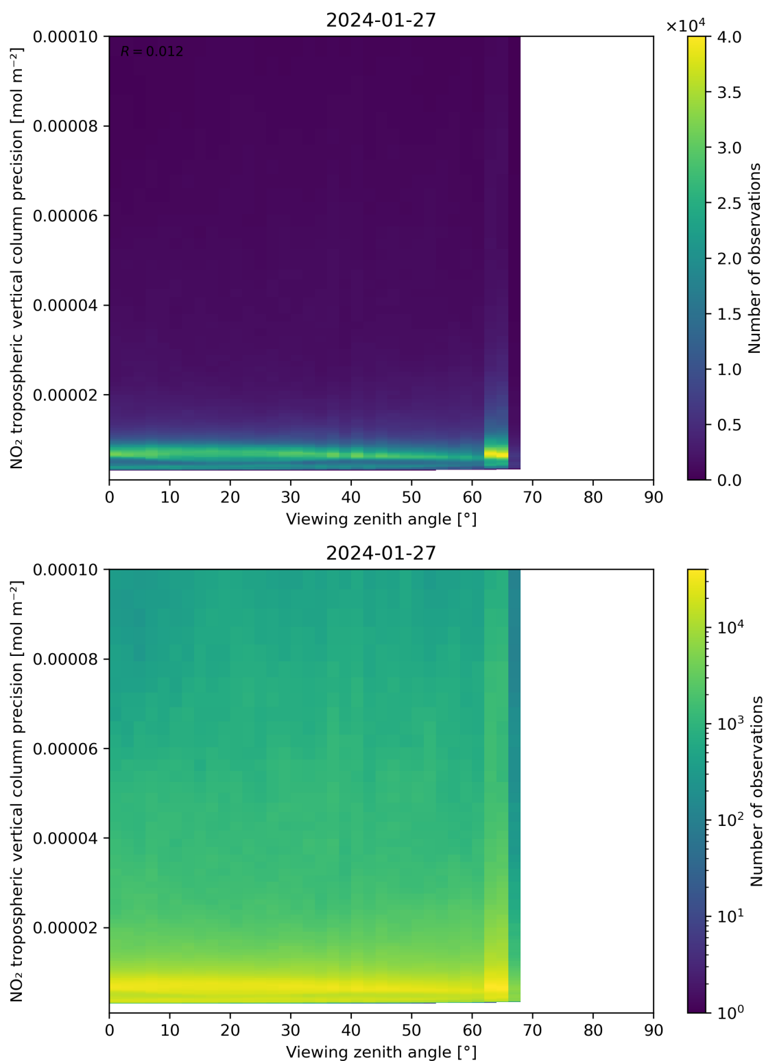
Figure 170: Scatter density plot of “Viewing zenith angle” against “NO 2 tropospheric vertical column precision” for 2024-01-26 to 2024-01-28.
