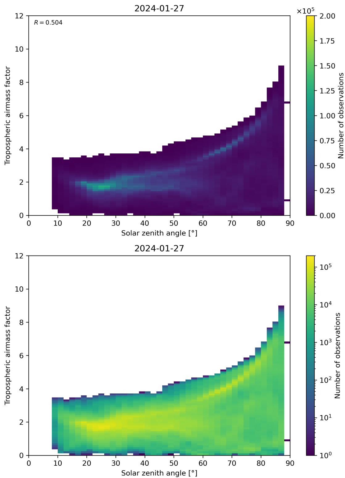
Figure 147: Scatter density plot of “Solar zenith angle” against “Tropospheric airmass factor” for 2024-01-26 to 2024-01-28.
