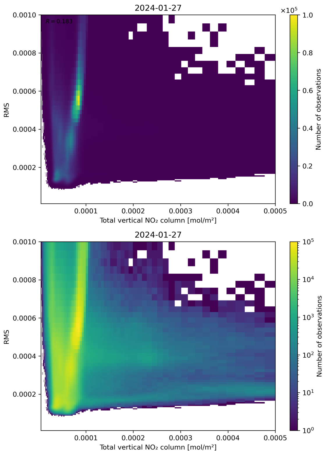
Figure 120: Scatter density plot of “Total vertical NO 2 column” against “RMS” for 2024-01-26 to 2024-01-28.
