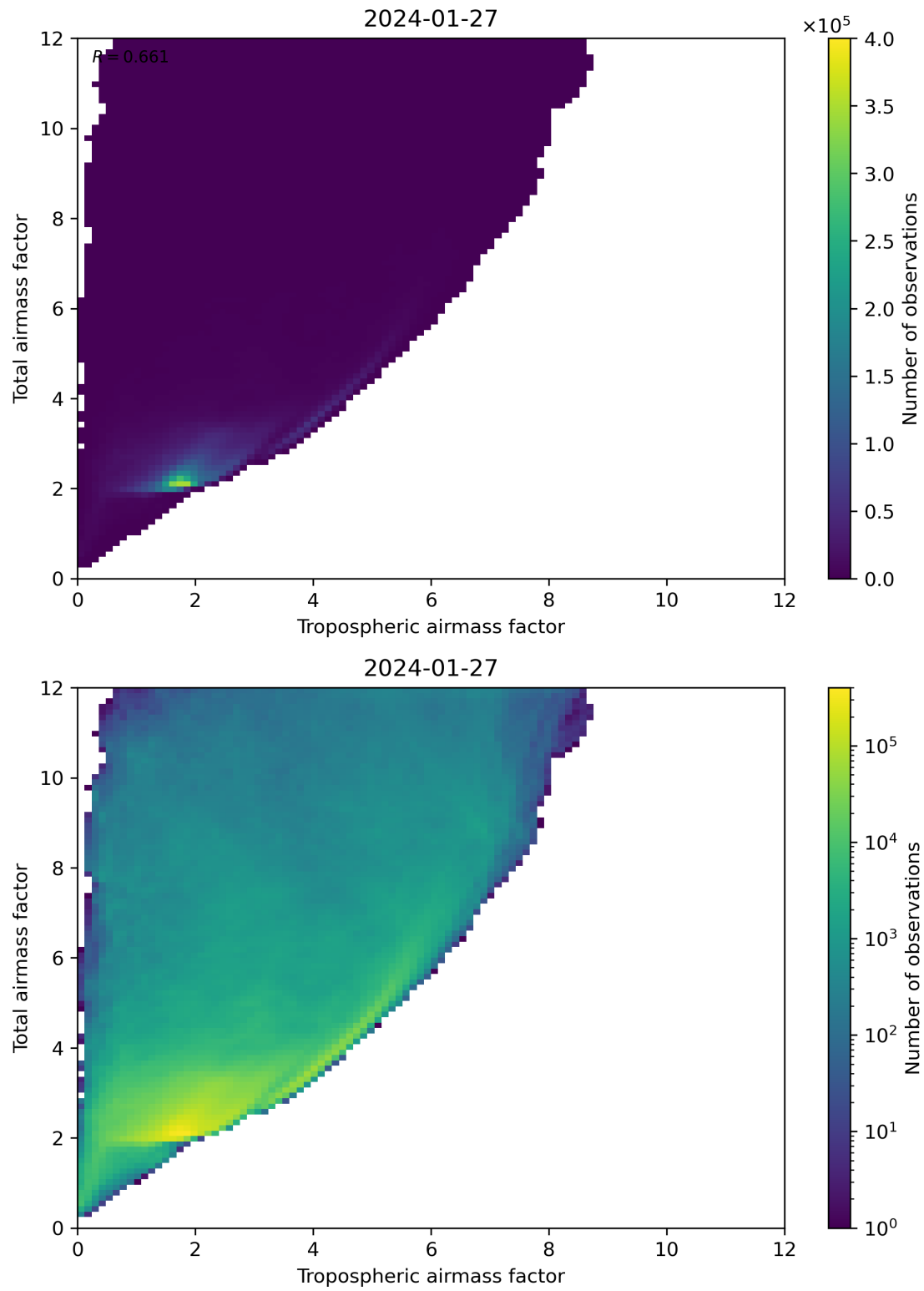
Figure 72: Scatter density plot of “Tropospheric airmass factor” against “Total airmass factor” for 2024-01-26 to 2024-01-28.
