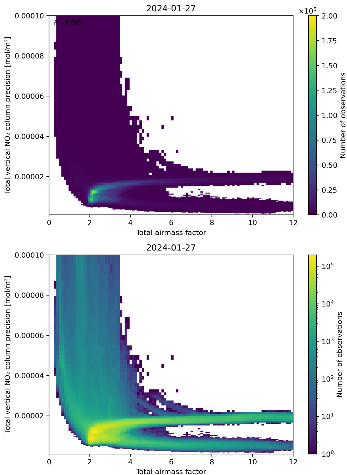
Figure 68: Scatter density plot of “Total airmass factor” against “Total vertical NO 2 column precision” for 2024-01-26 to 2024-01-28.
