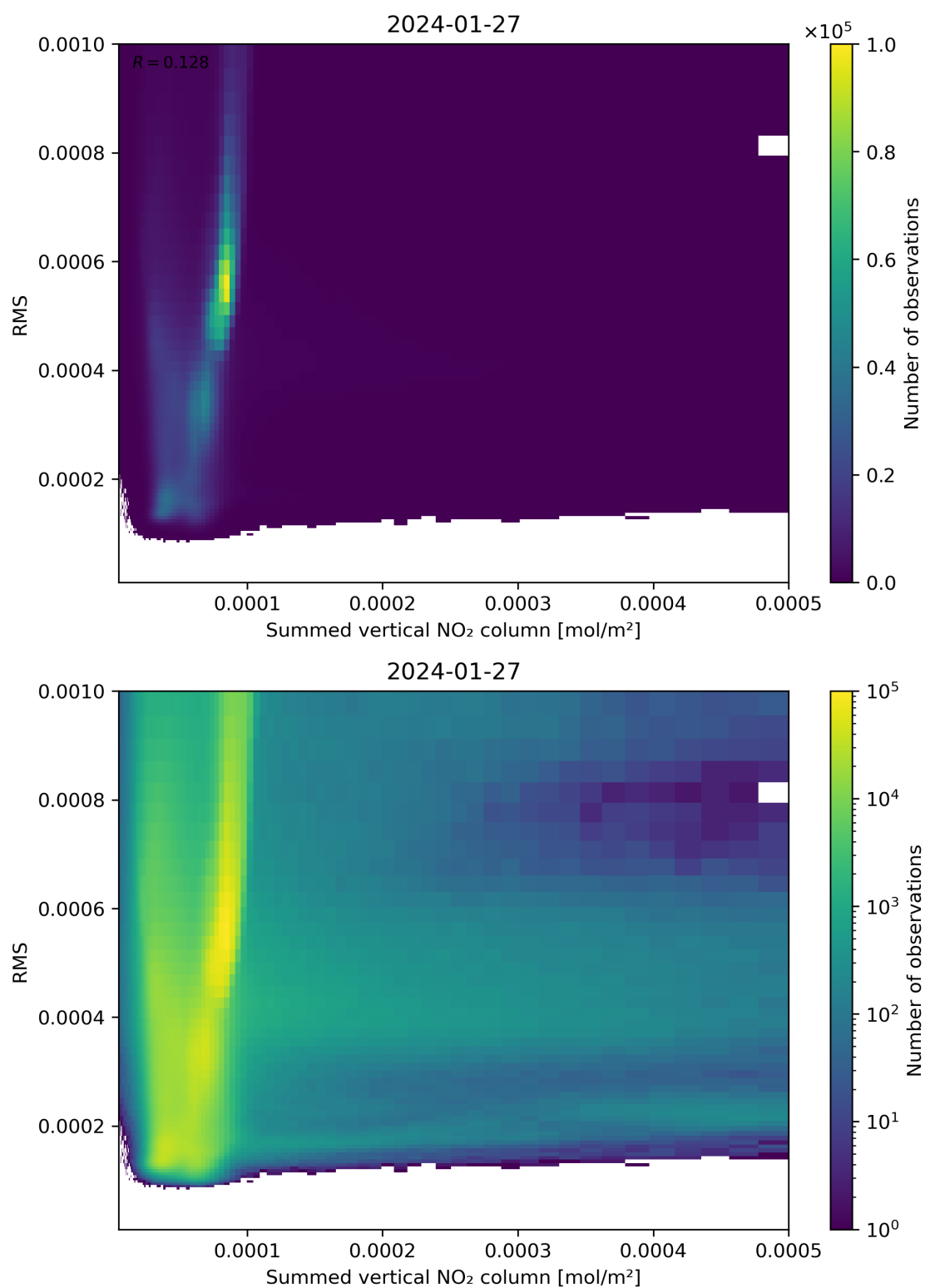
Figure 109: Scatter density plot of “Summed vertical NO 2 column” against “RMS” for 2024-01-26 to 2024-01-28.
