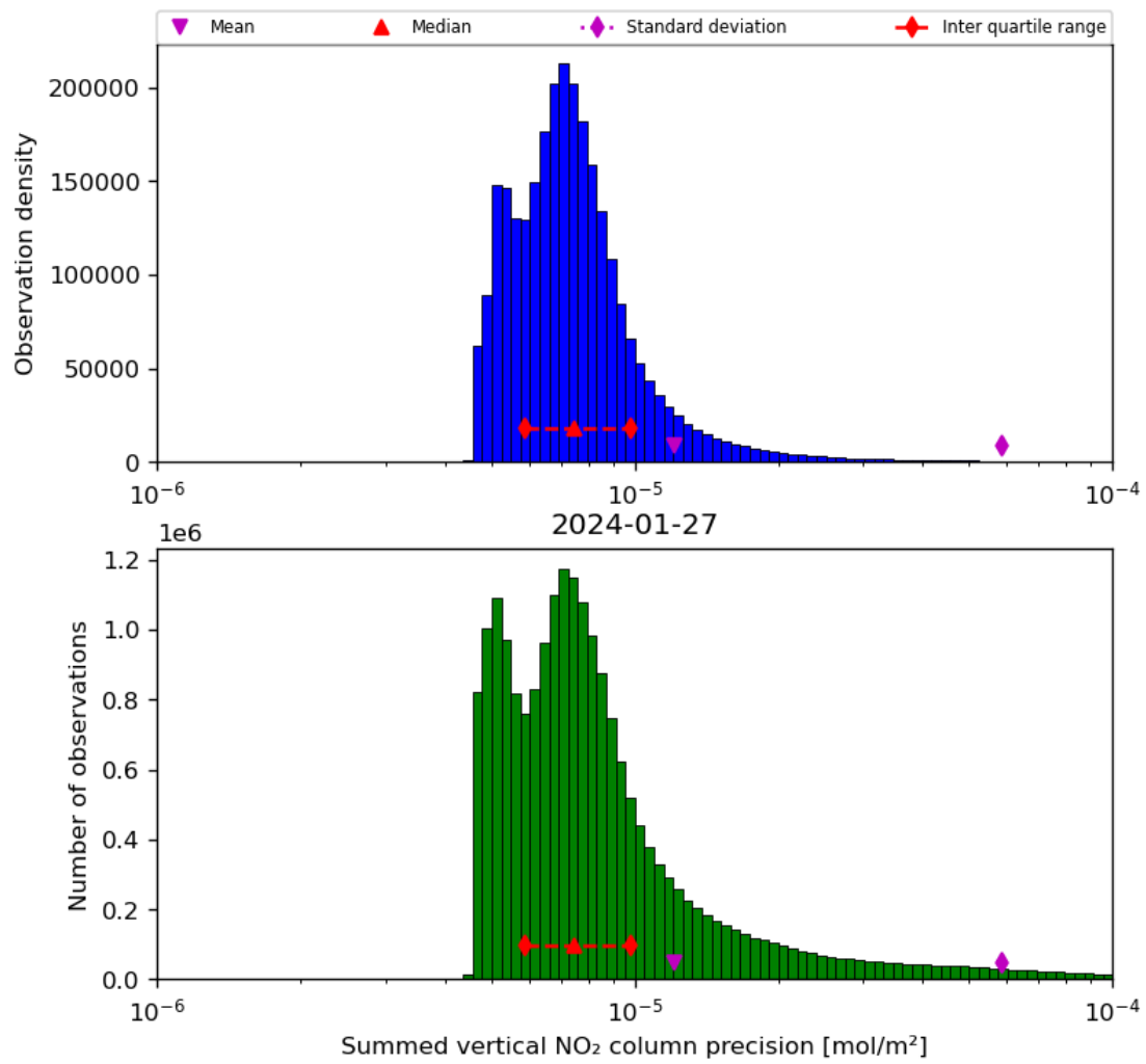
Figure 41: Histogram of “Summed vertical NO 2 column precision” for 2024-01-26 to 2024-01-28
