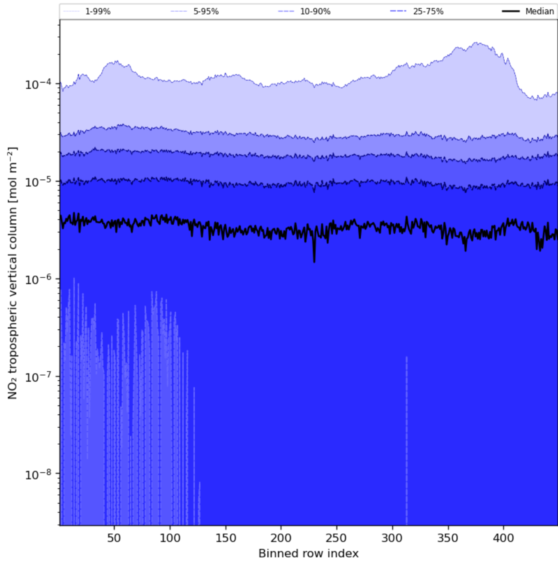
Figure 46: Along track statistics of “NO 2 tropospheric vertical column” for 2024-01-26 to 2024-01-28
