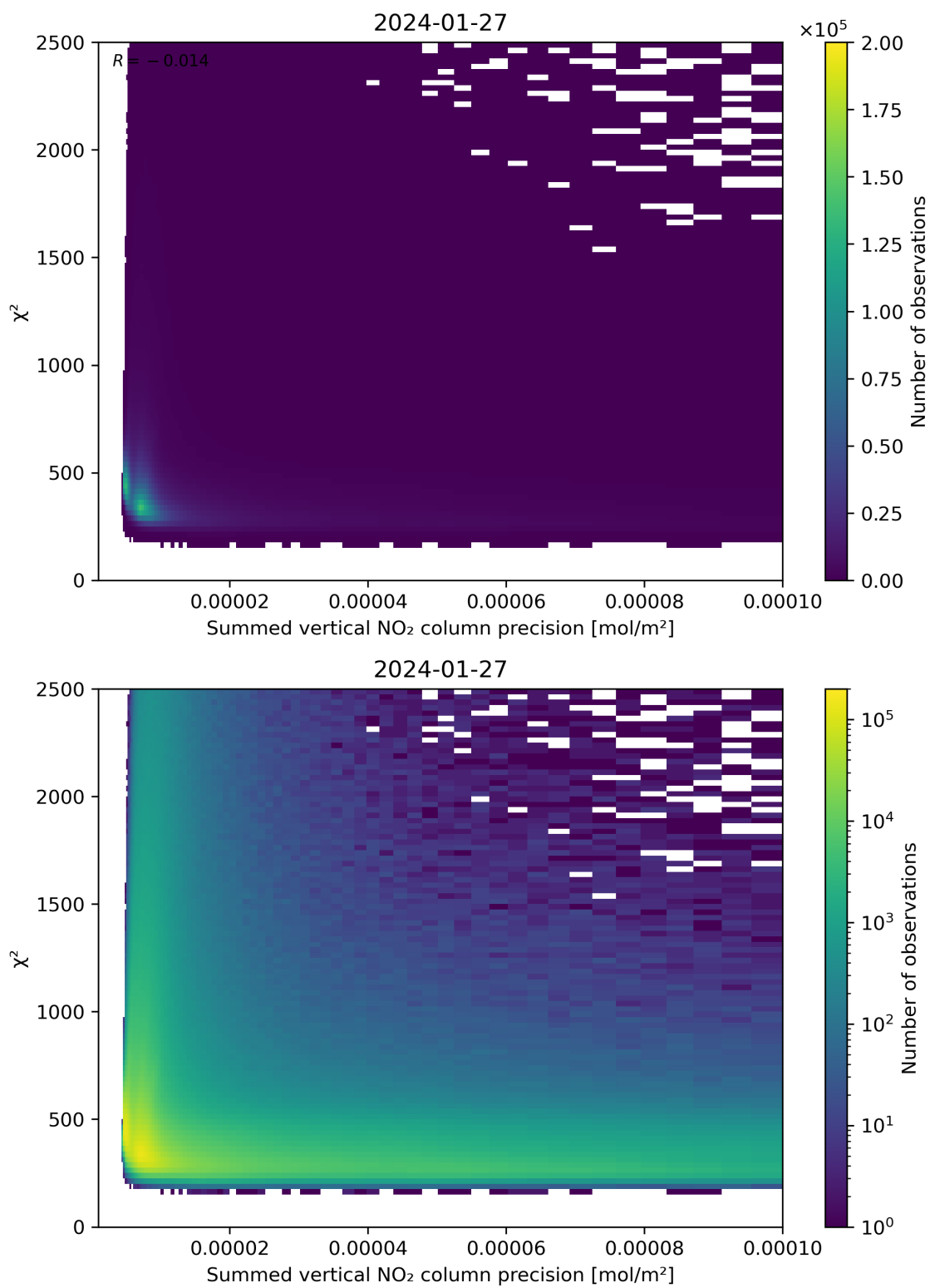
Figure 107: Scatter density plot of “Summed vertical NO 2 column precision” against “ \chi^2 ” for 2024-01-26 to 2024-01-28.
