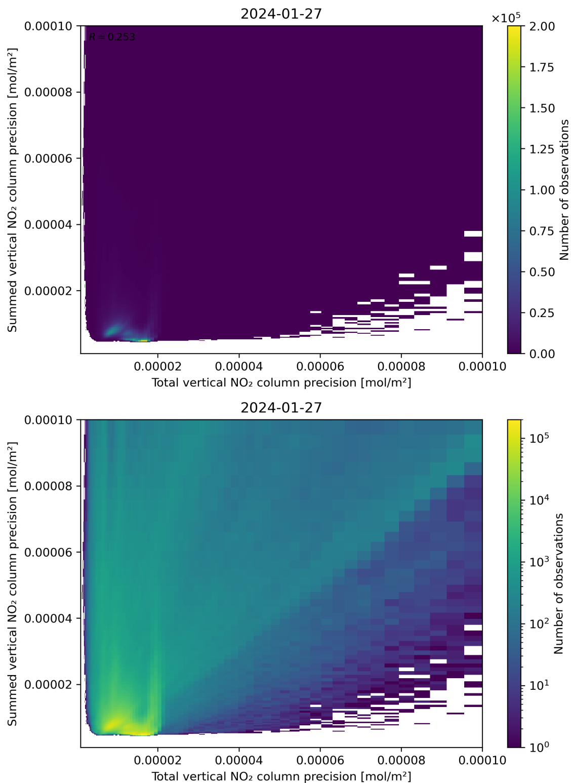
Figure 118: Scatter density plot of “Total vertical NO 2 column precision” against “Summed vertical NO 2 column precision” for 2024-01-26 to 2024-01-28.
