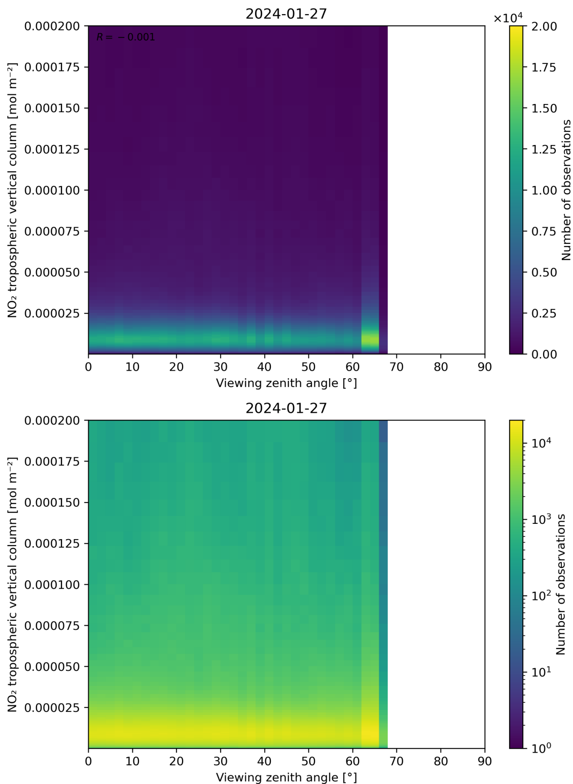
Figure 169: Scatter density plot of “Viewing zenith angle” against “NO 2 tropospheric vertical column” for 2024-01-26 to 2024-01-28.
