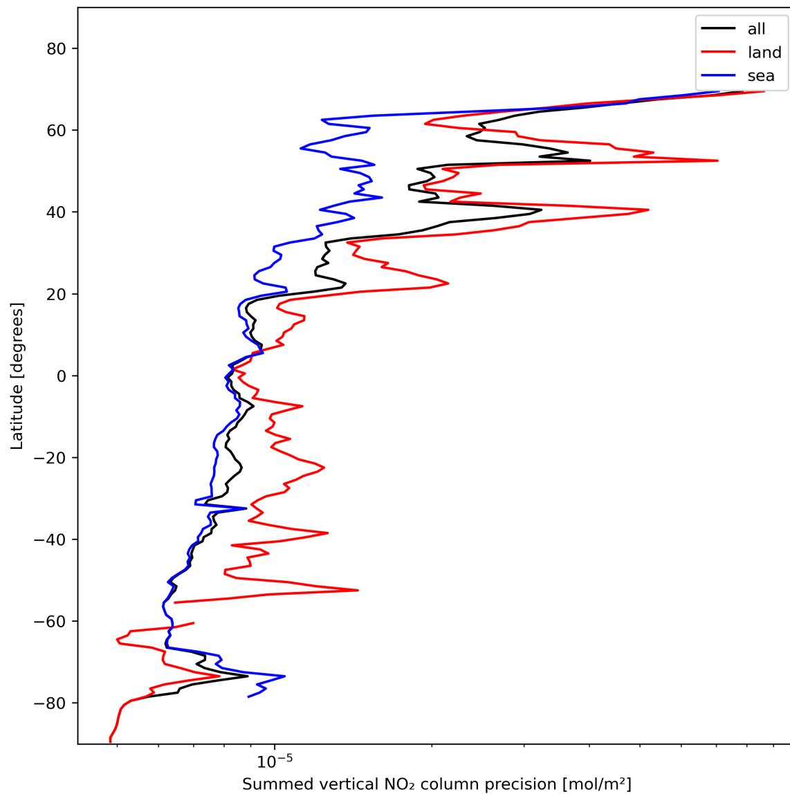
Figure 24: Zonal average of “Summed vertical NO 2 column precision” for 2024-01-26 to 2024-01-28.
