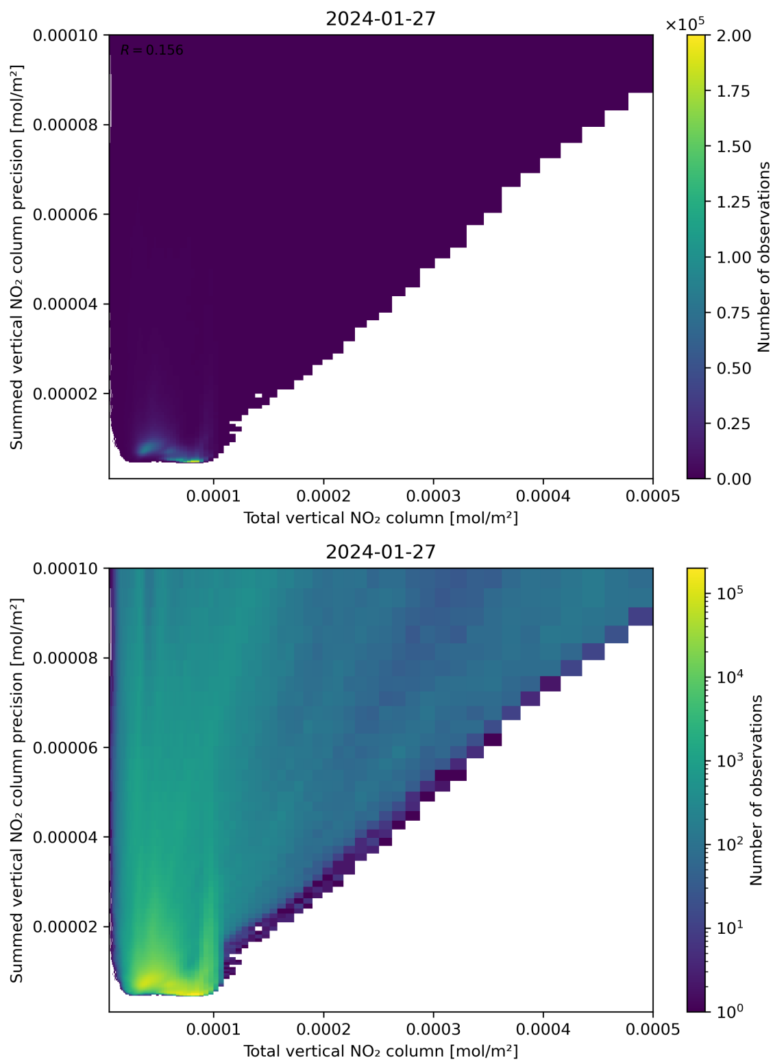
Figure 113: Scatter density plot of “Total vertical NO 2 column” against “Summed vertical NO 2 column precision” for 2024-01-26 to 2024-01-28.
