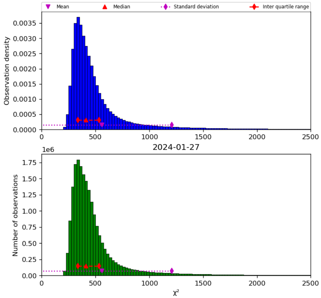
Figure 42: Histogram of " \chi^2 " for 2024-01-26 to 2024-01-28
