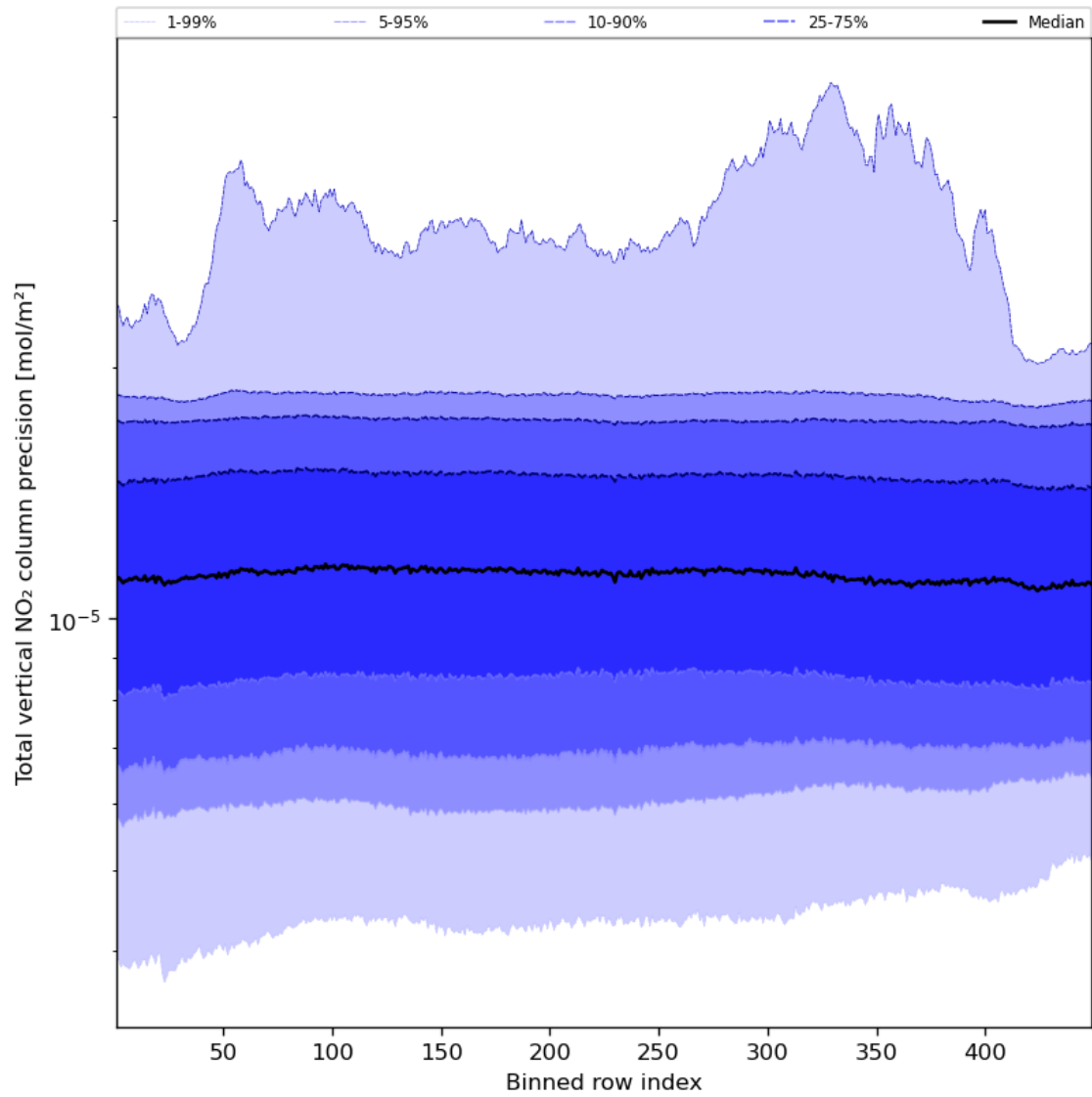
Figure 56: Along track statistics of “Total vertical NO 2 column precision” for 2024-01-26 to 2024-01-28
