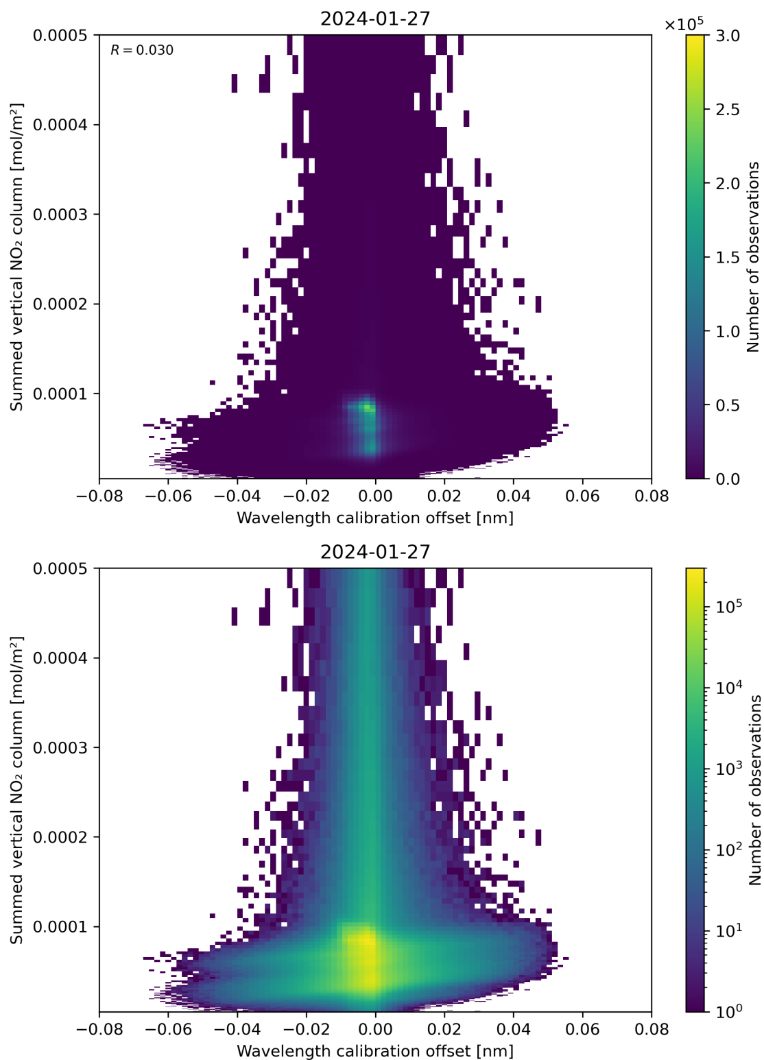
Figure 177: Scatter density plot of “Wavelength calibration offset” against “Summed vertical NO 2 column” for 2024-01-26 to 2024-01-28.
