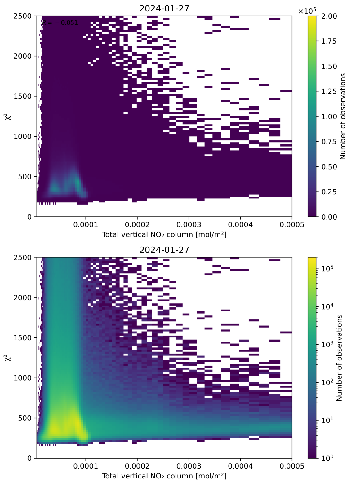
Figure 111: Scatter density plot of “Total vertical NO 2 column” against “ \chi^2 ” for 2024-01-26 to 2024-01-28.
