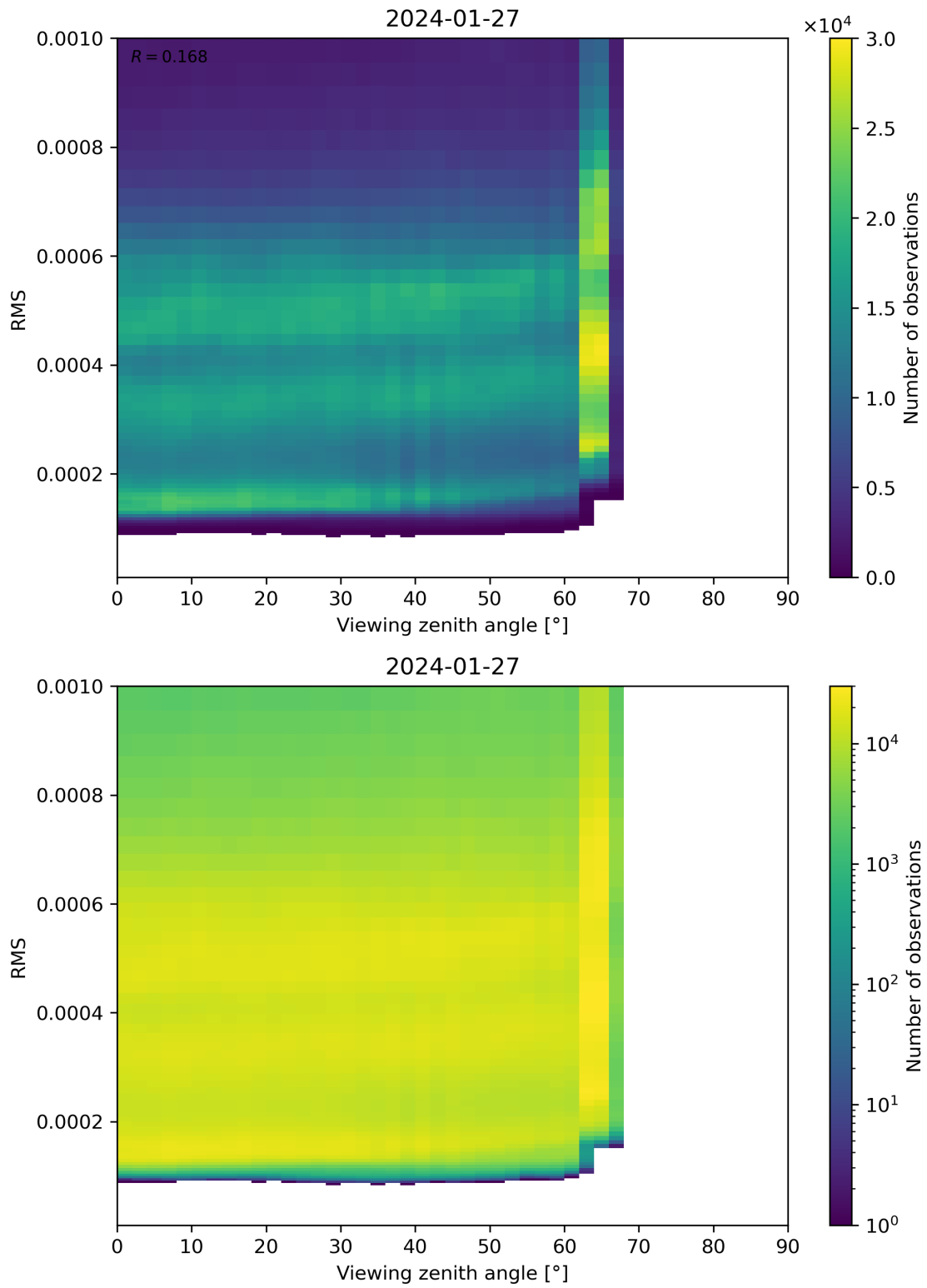
Figure 171: Scatter density plot of “Viewing zenith angle” against “RMS” for 2024-01-26 to 2024-01-28.
