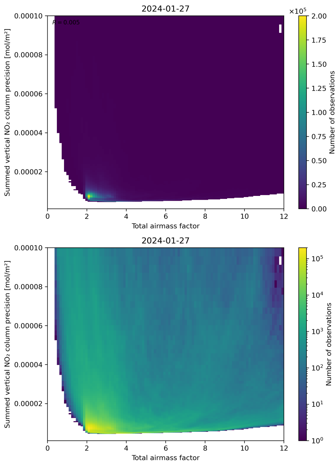
Figure 66: Scatter density plot of “Total airmass factor” against “Summed vertical NO 2 column precision” for 2024-01-26 to 2024-01-28.
