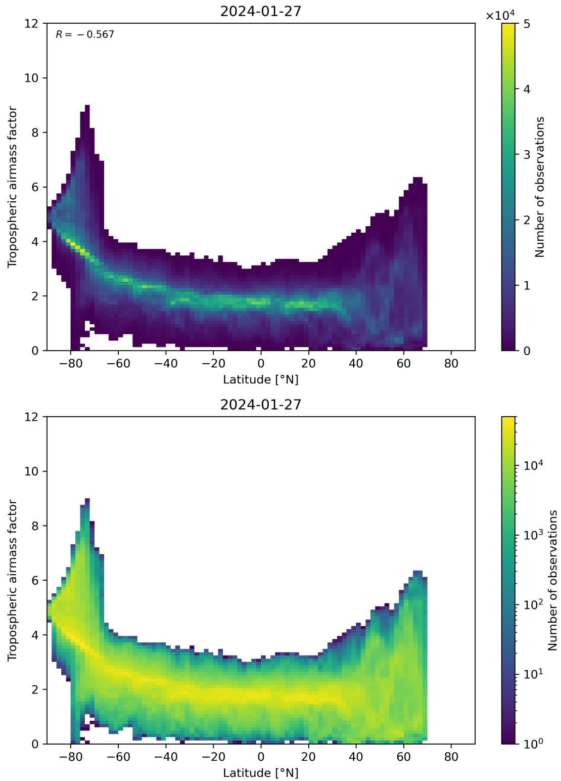
Figure 85: Scatter density plot of “Latitude” against “Tropospheric air mass factor” for 2024-01-26 to 2024-01-28.
