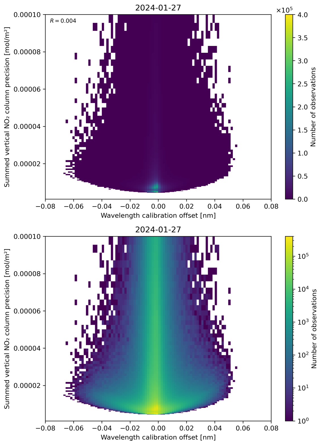
Figure 178: Scatter density plot of “Wavelength calibration offset” against “Summed vertical NO 2 column precision” for 2024-01-26 to 2024-01-28.
