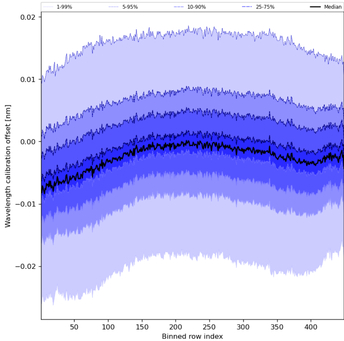
Figure 52: Along track statistics of “Wavelength calibration offset” for 2024-01-26 to 2024-01-28
