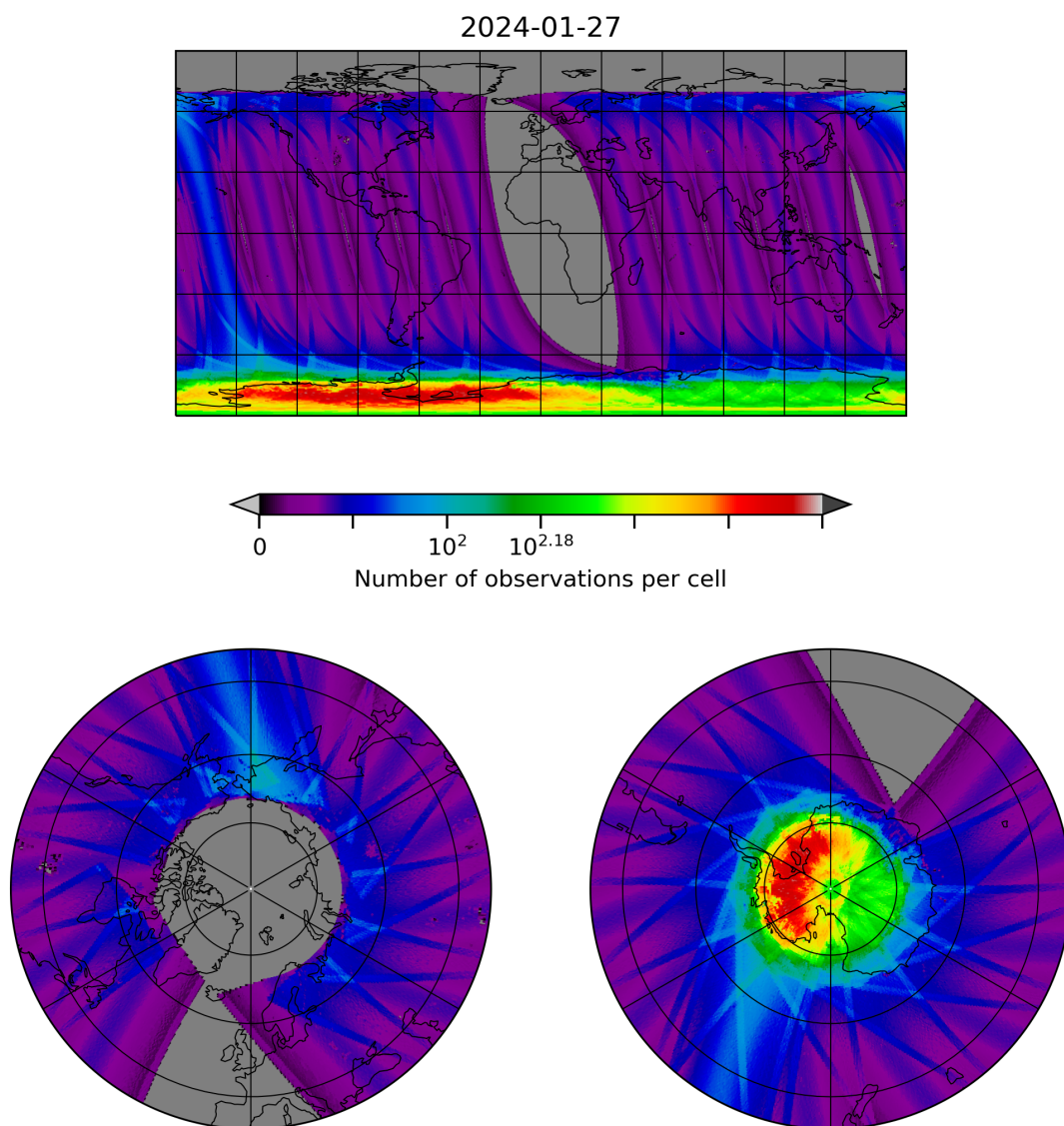
Figure 10: Map of the number of observations for 2024-01-26 to 2024-01-28
