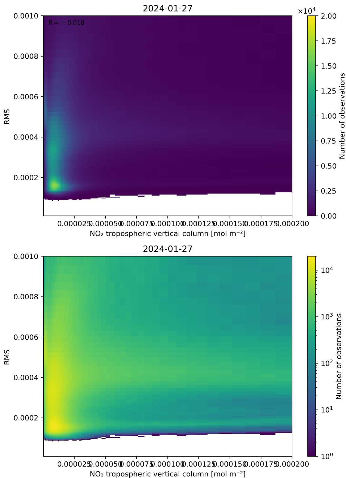
Figure 142: Scatter density plot of “NO 2 tropospheric vertical column” against “RMS” for 2024-01-26 to 2024-01-28.
