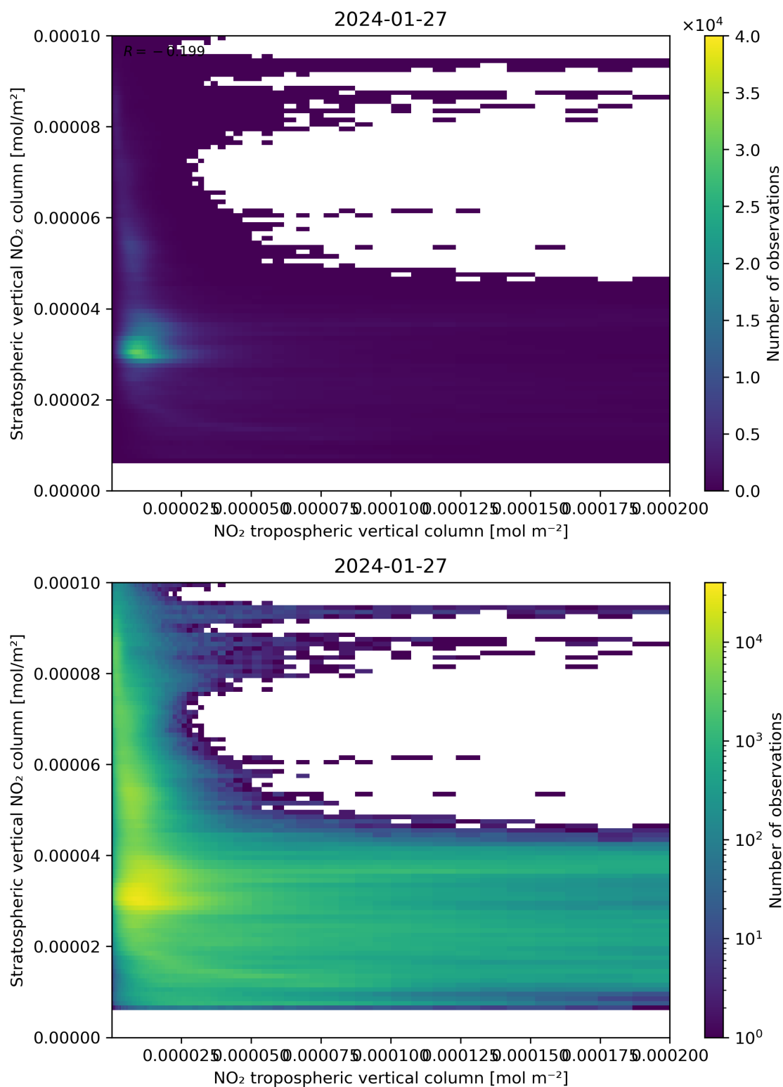
Figure 125: Scatter density plot of “NO 2 tropospheric vertical column” against “Stratospheric vertical NO 2 column” for 2024-01-26 to 2024-01-28.
