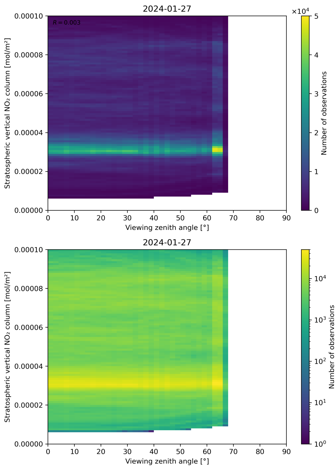
Figure 164: Scatter density plot of “Viewing zenith angle” against “Stratospheric vertical NO 2 column” for 2024-01-26 to 2024-01-28.
