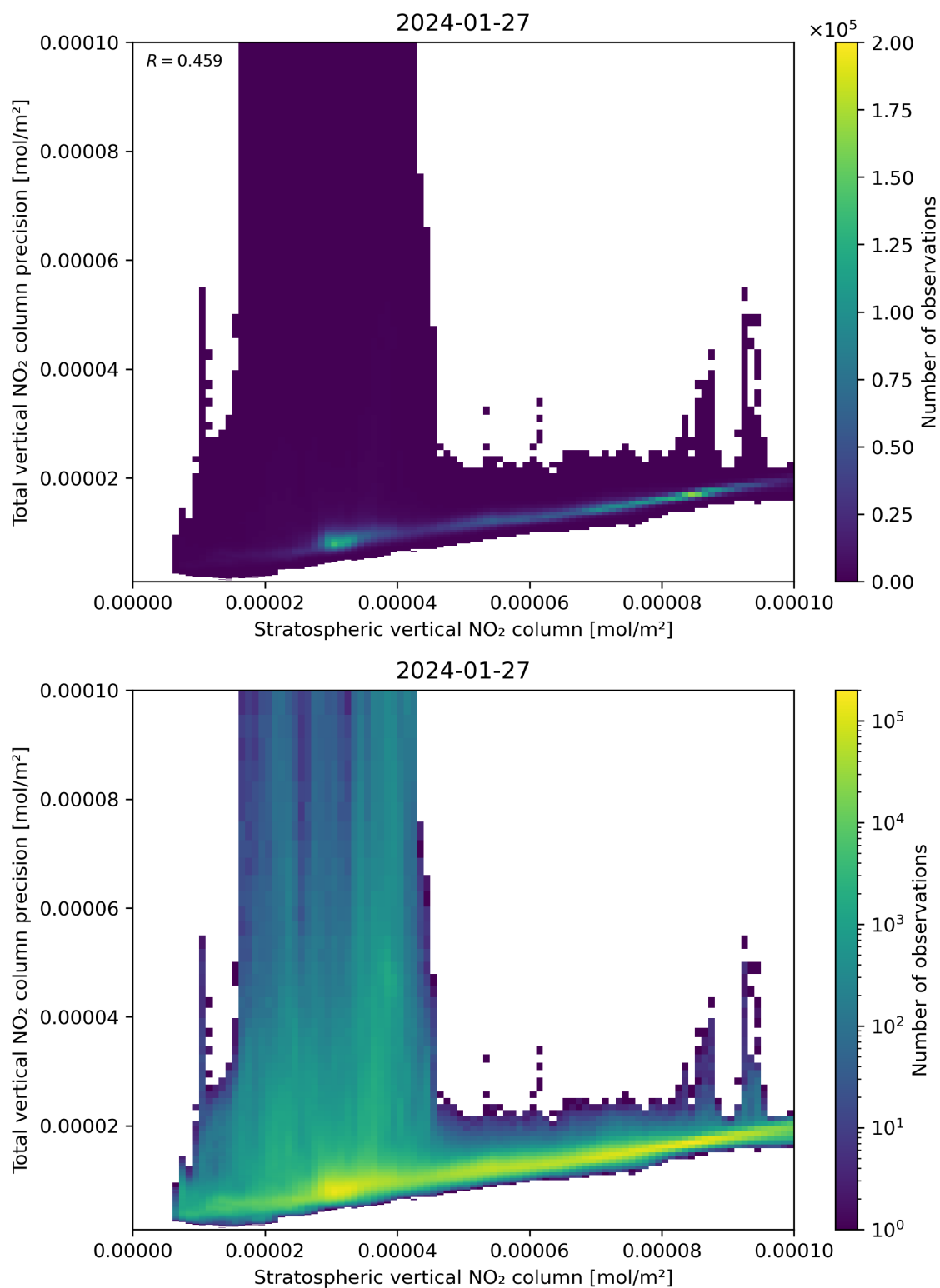
Figure 101: Scatter density plot of “Stratospheric vertical NO 2 column” against “Total vertical NO 2 column precision” for 2024-01-26 to 2024-01-28.
