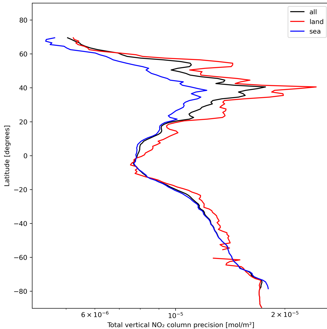
Figure 22: Zonal average of “Total vertical NO 2 column precision” for 2024-01-26 to 2024-01-28.
