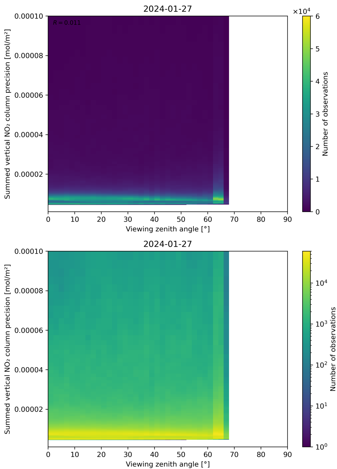
Figure 166: Scatter density plot of “Viewing zenith angle” against “Summed vertical NO 2 column precision” for 2024-01-26 to 2024-01-28.
