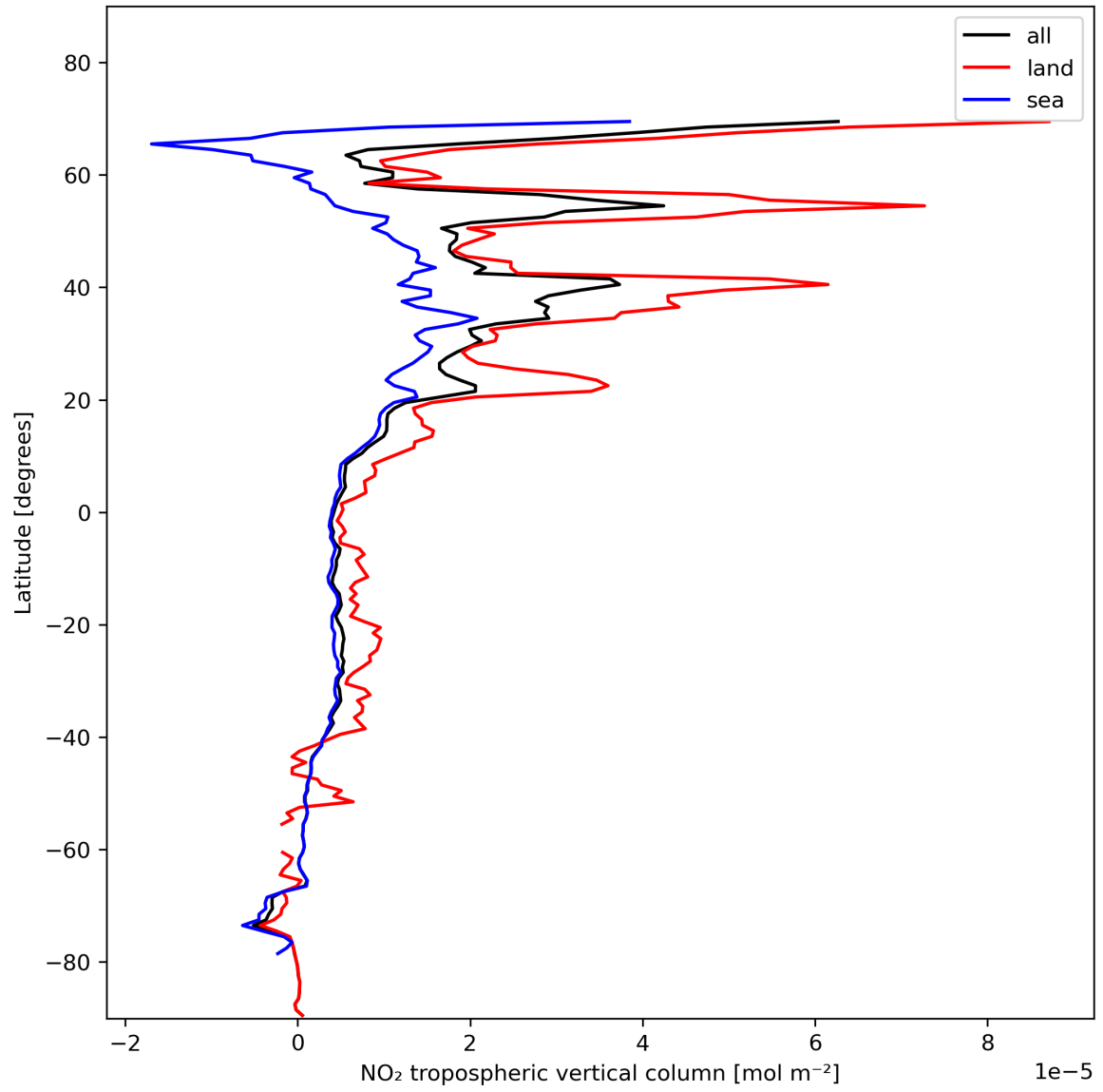
Figure 12: Zonal average of “NO 2 tropospheric vertical column” for 2024-01-26 to 2024-01-28.
