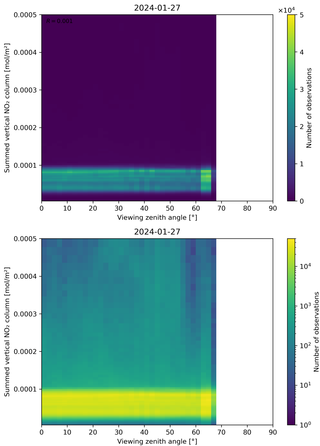
Figure 165: Scatter density plot of “Viewing zenith angle” against “Summed vertical NO 2 column” for 2024-01-26 to 2024-01-28.
