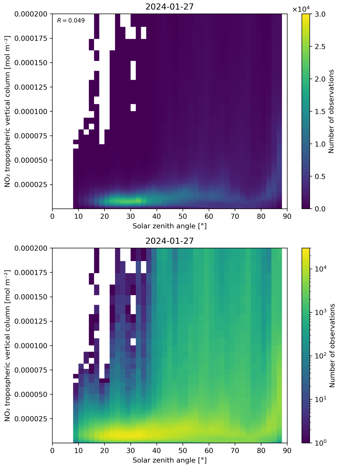
Figure 155: Scatter density plot of “Solar zenith angle” against “NO 2 tropospheric vertical column” for 2024-01-26 to 2024-01-28.
