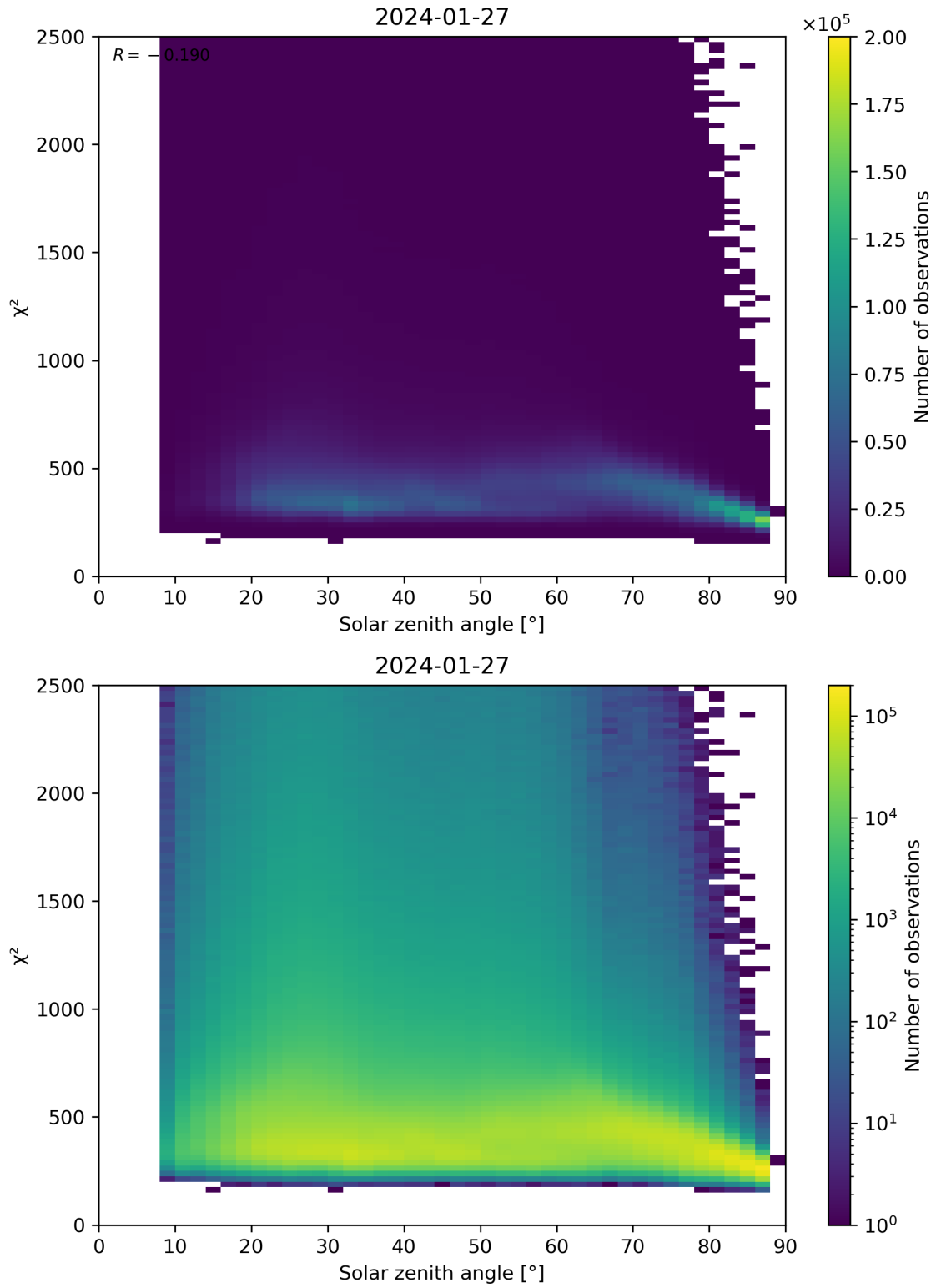
Figure 148: Scatter density plot of “Solar zenith angle” against “ \chi^2 ” for 2024-01-26 to 2024-01-28.
