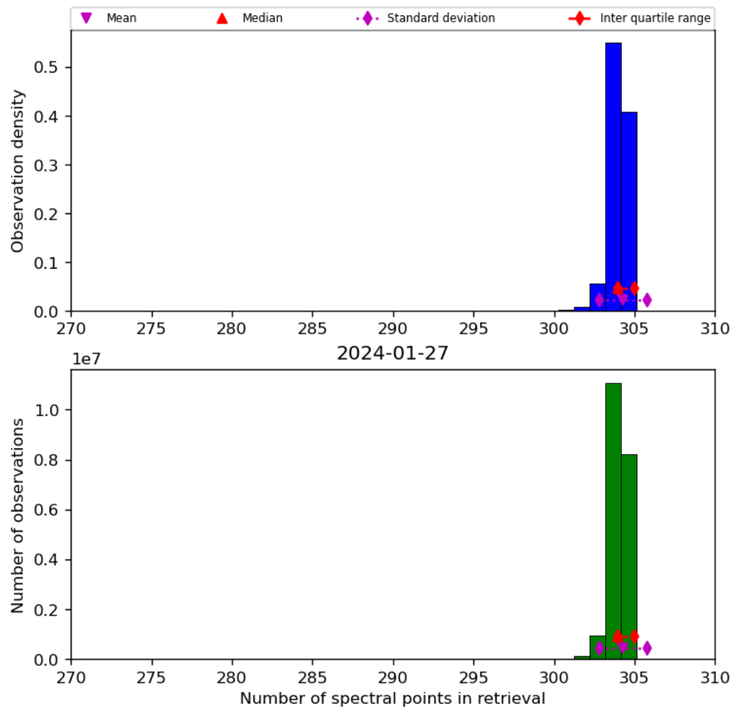
Figure 33: Histogram of “Number of spectral points in retrieval” for 2024-01-26 to 2024-01-28
