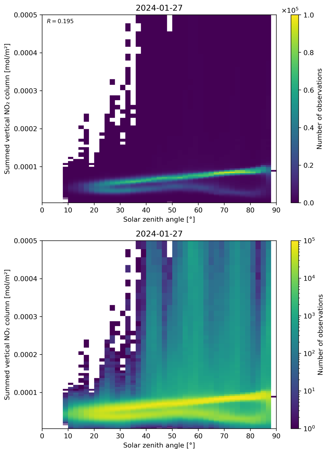
Figure 151: Scatter density plot of “Solar zenith angle” against “Summed vertical NO 2 column” for 2024-01-26 to 2024-01-28.
