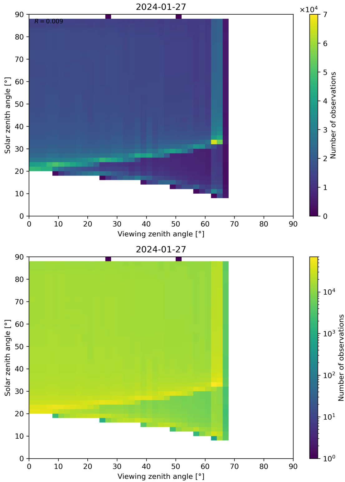
Figure 172: Scatter density plot of “Viewing zenith angle” against “Solar zenith angle” for 2024-01-26 to 2024-01-28.
