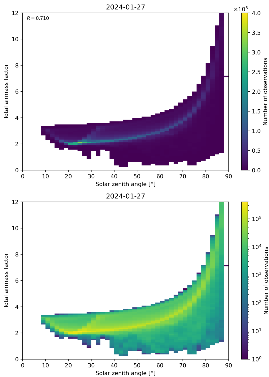
Figure 146: Scatter density plot of “Solar zenith angle” against “Total air mass factor” for 2024-01-26 to 2024-01-28.
