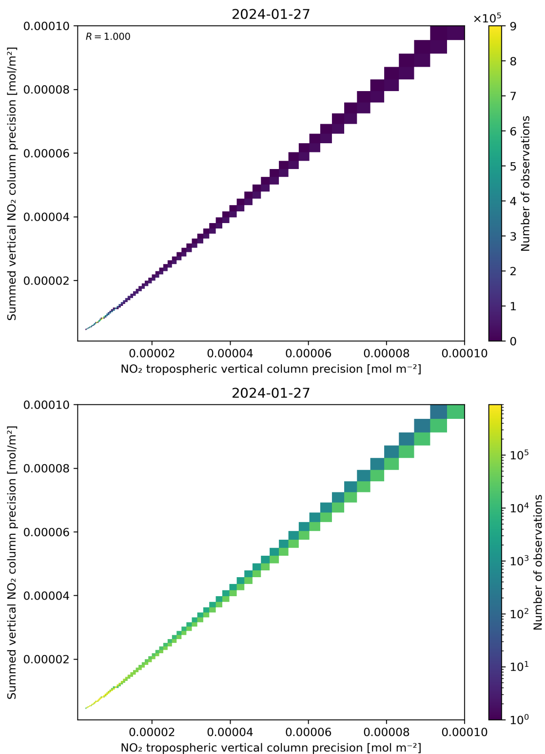
Figure 137: Scatter density plot of “NO 2 tropospheric vertical column precision” against “Summed vertical NO 2 column precision” for 2024-01-26 to 2024-01-28.
