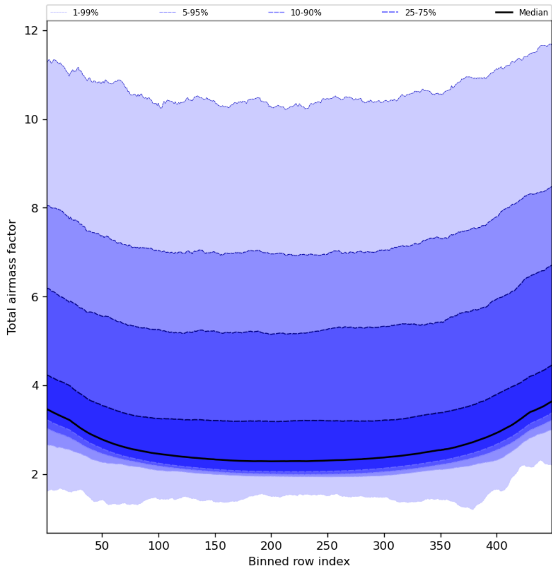
Figure 49: Along track statistics of “Total airmass factor” for 2024-01-26 to 2024-01-28
