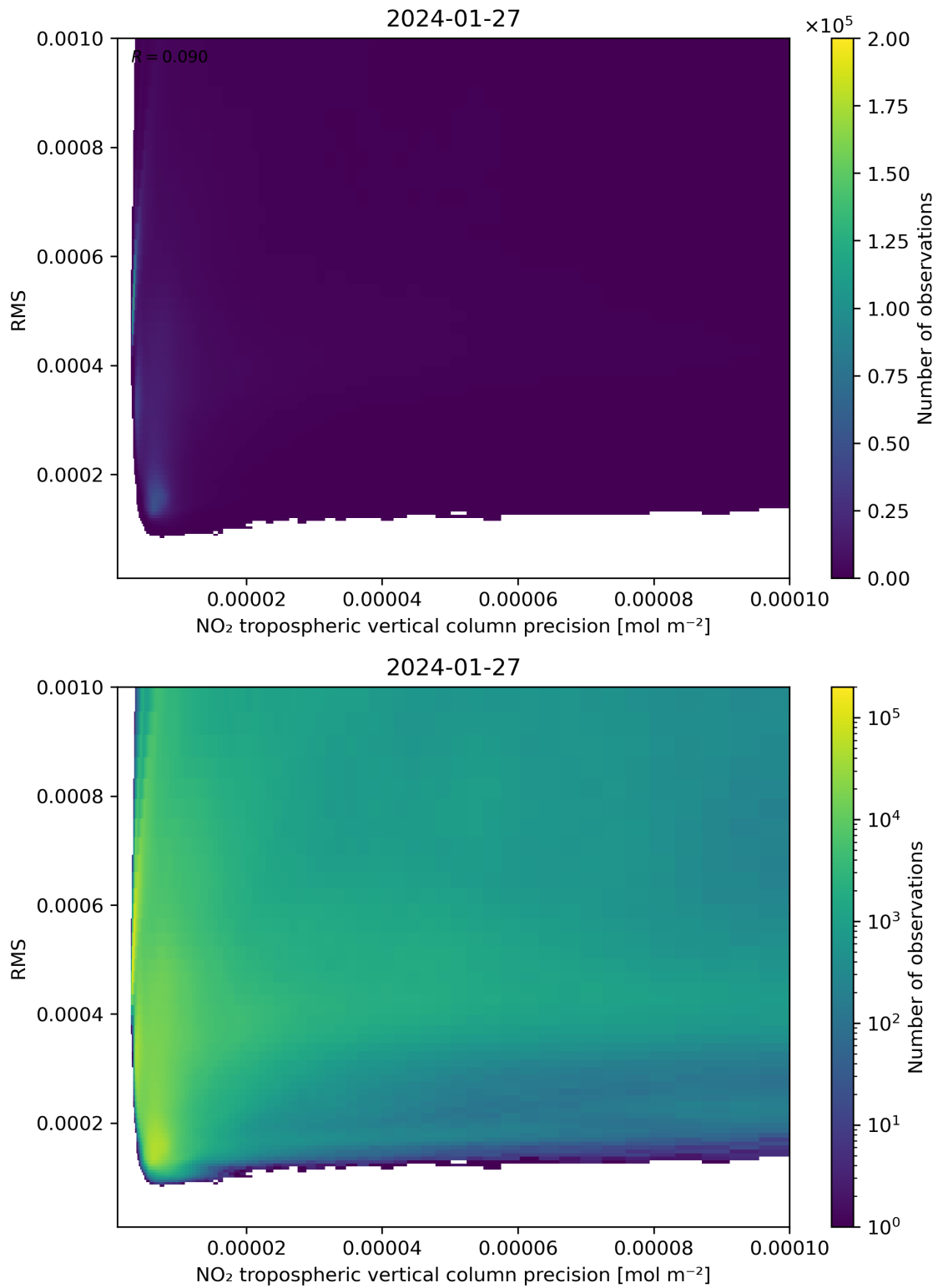
Figure 140: Scatter density plot of “NO 2 tropospheric vertical column precision” against “RMS” for 2024-01-26 to 2024-01-28.
