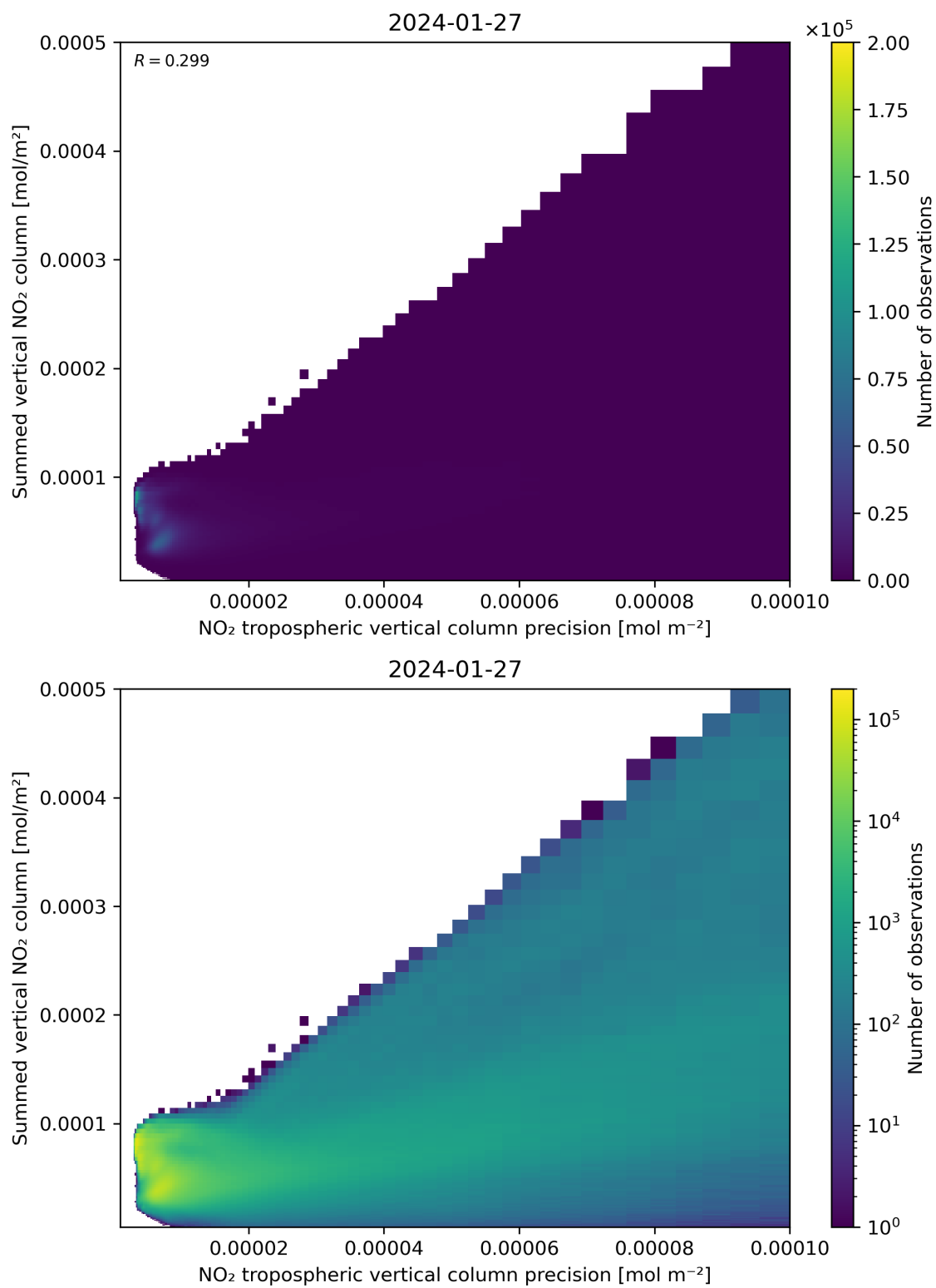
Figure 136: Scatter density plot of “NO 2 tropospheric vertical column precision” against “Summed vertical NO 2 column” for 2024-01-26 to 2024-01-28.
