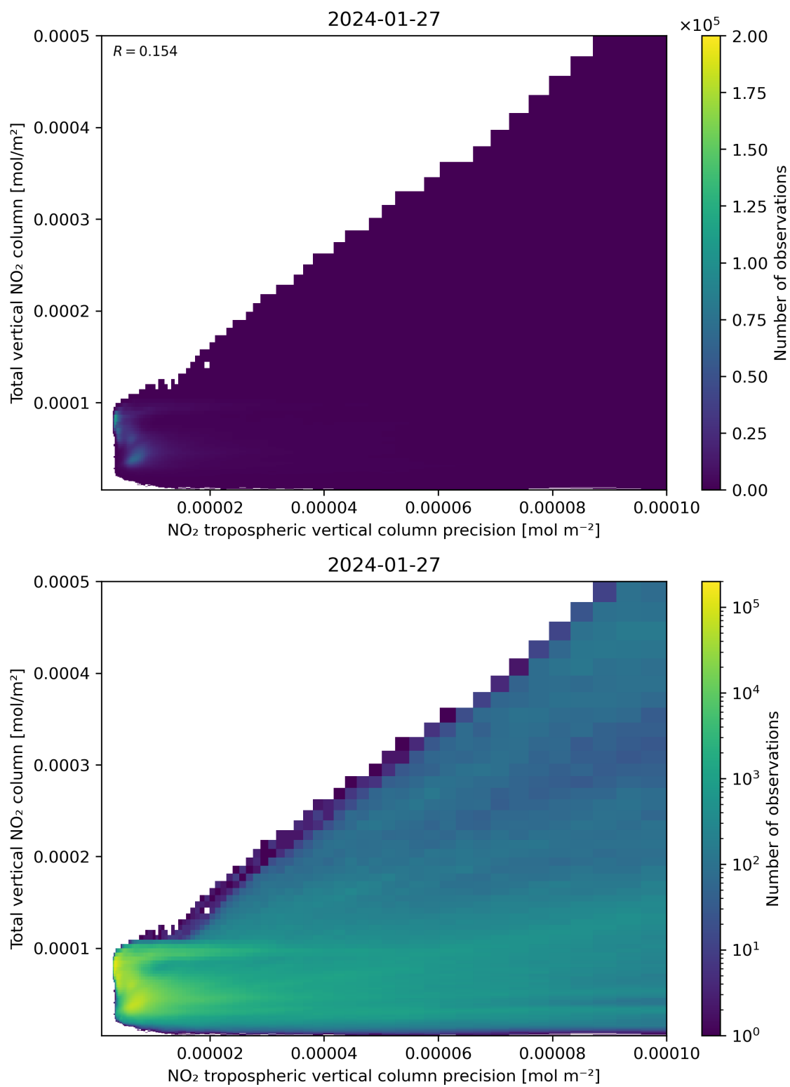
Figure 138: Scatter density plot of “NO 2 tropospheric vertical column precision” against “Total vertical NO 2 column” for 2024-01-26 to 2024-01-28.
