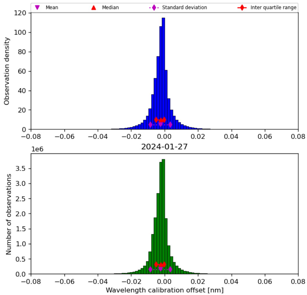
Figure 35: Histogram of “Wavelength calibration offset” for 2024-01-26 to 2024-01-28
