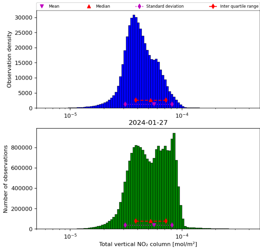
Figure 38: Histogram of “Total vertical NO 2 column” for 2024-01-26 to 2024-01-28
