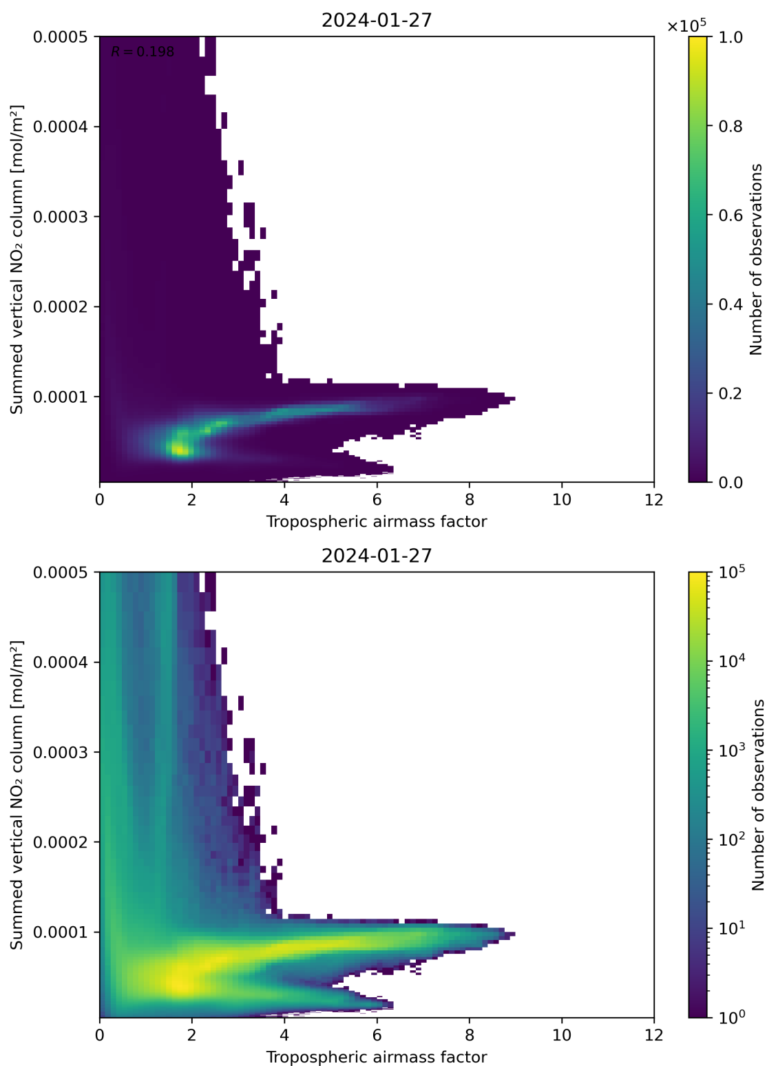
Figure 75: Scatter density plot of “Tropospheric airmass factor” against “Summed vertical NO 2 column” for 2024-01-26 to 2024-01-28.
