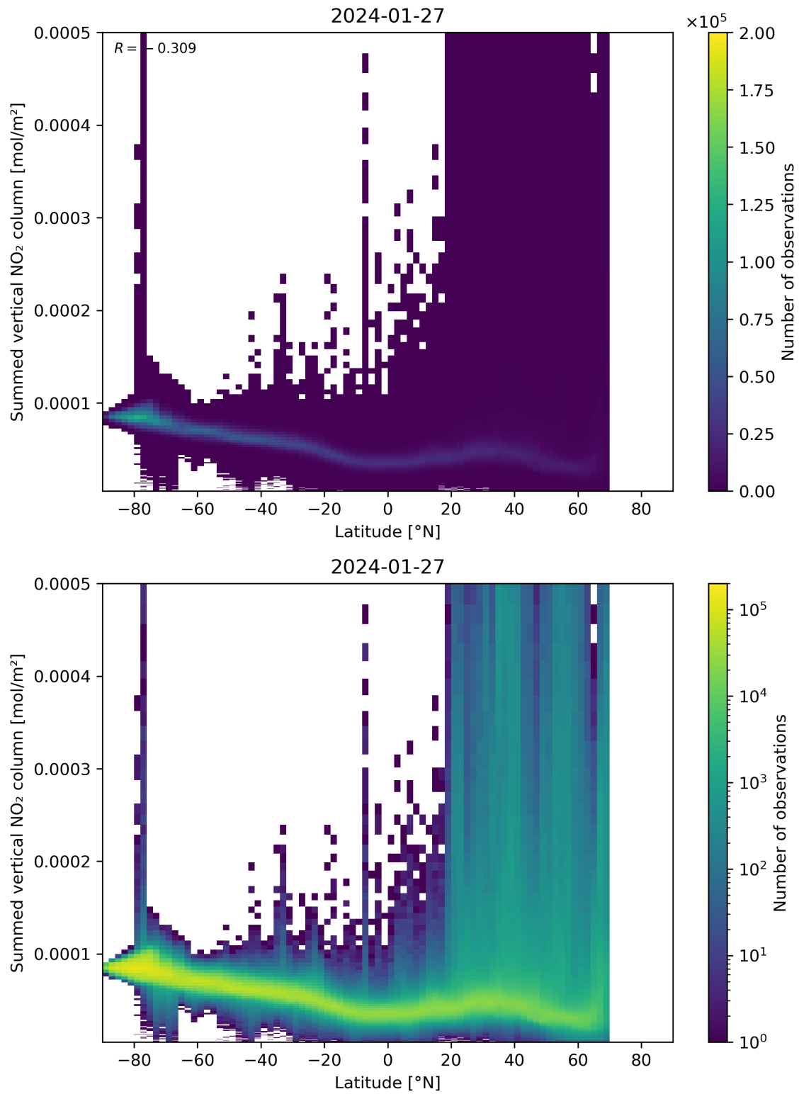
Figure 88: Scatter density plot of “Latitude” against “Summed vertical NO 2 column” for 2024-01-26 to 2024-01-28.
