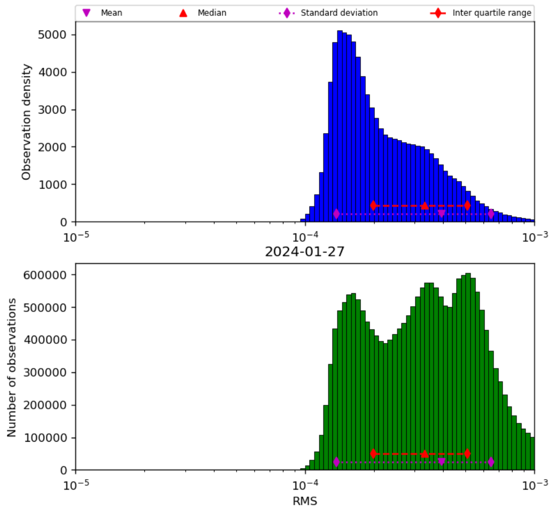
Figure 43: Histogram of “RMS” for 2024-01-26 to 2024-01-28
