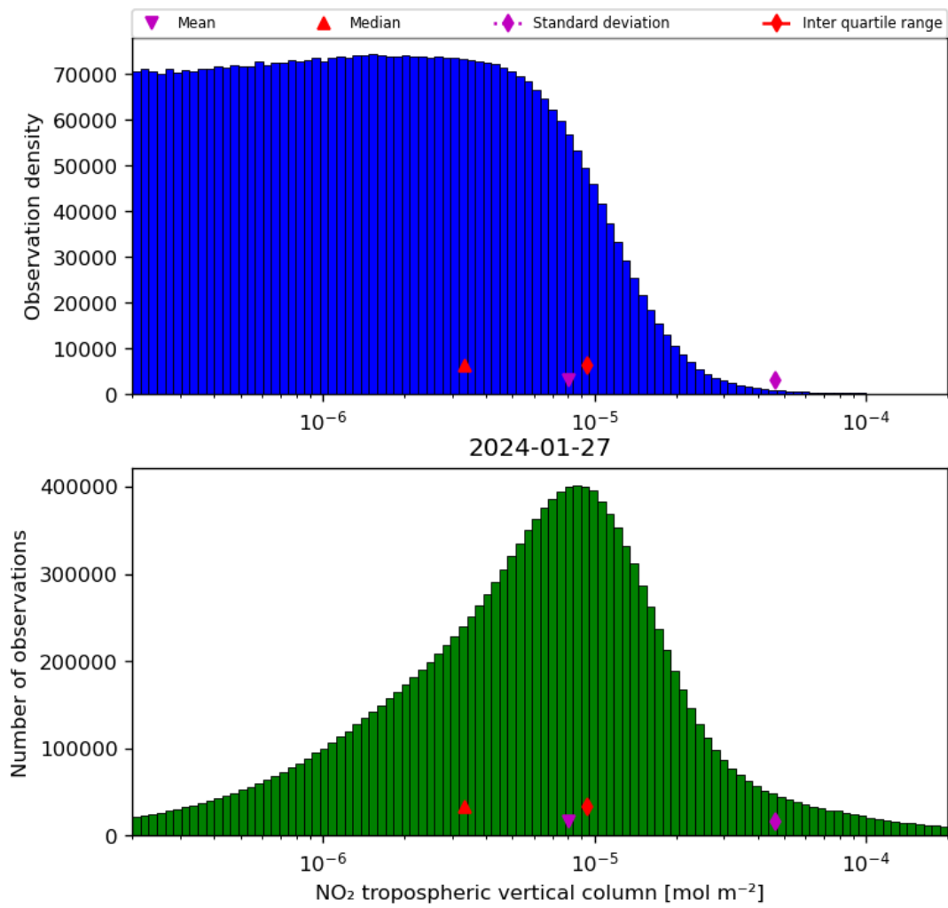
Figure 29: Histogram of “NO 2 tropospheric vertical column” for 2024-01-26 to 2024-01-28
