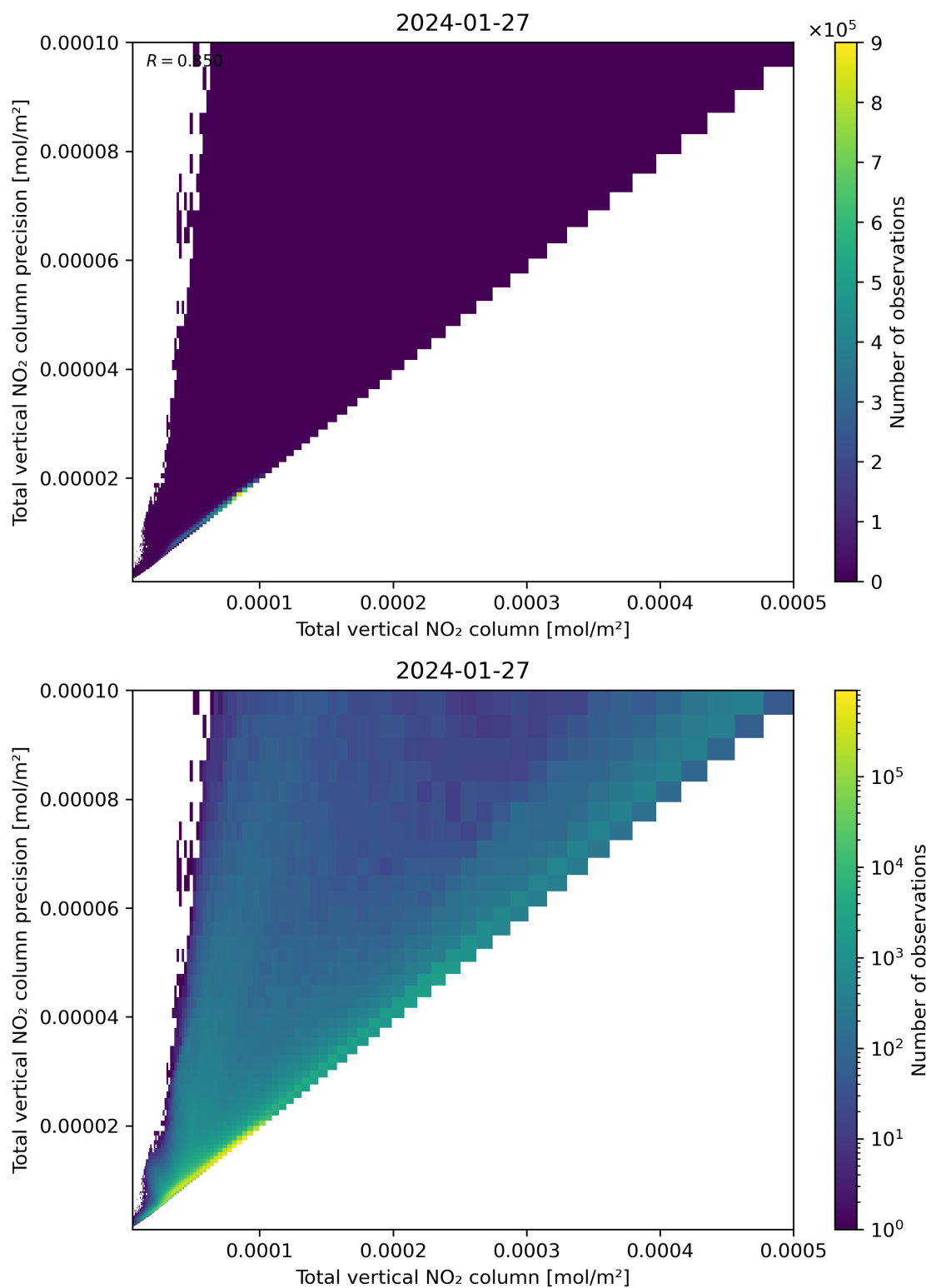
Figure 114: Scatter density plot of “Total vertical NO 2 column” against “Total vertical NO 2 column precision” for 2024-01-26 to 2024-01-28.
