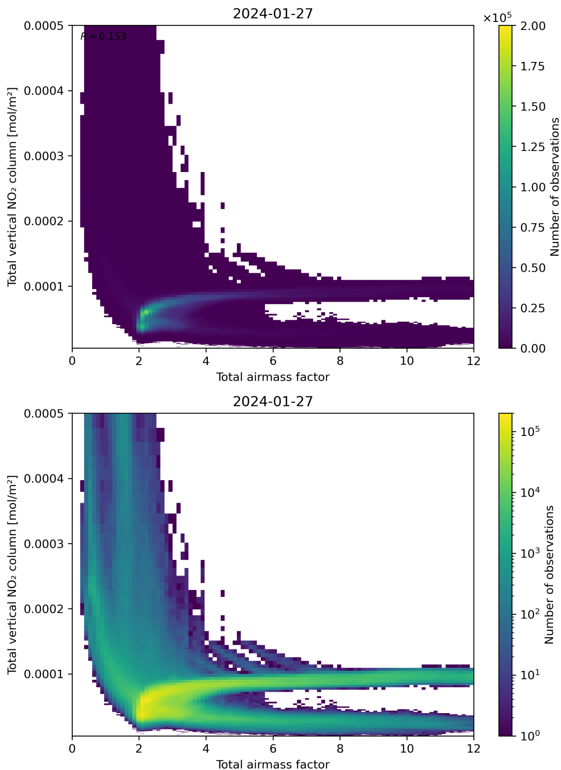
Figure 67: Scatter density plot of “Total airmass factor” against “Total vertical NO 2 column” for 2024-01-26 to 2024-01-28.
