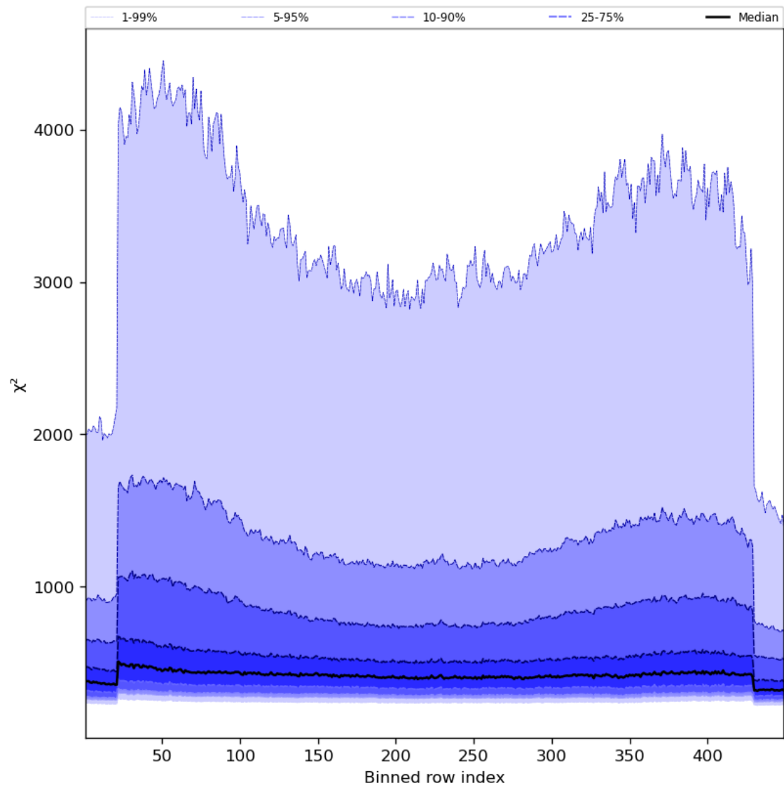
Figure 59: Along track statistics of “ \chi^2 ” for 2024-01-26 to 2024-01-28
