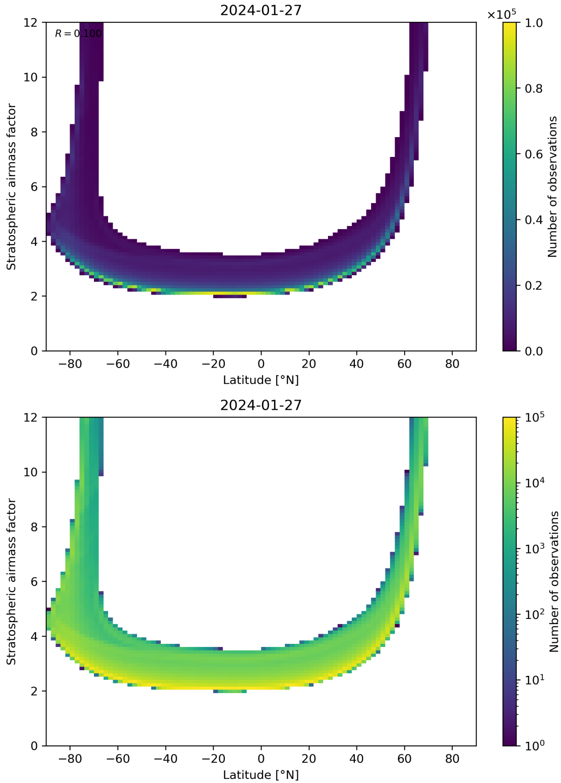
Figure 83: Scatter density plot of “Latitude” against “Stratospheric air mass factor” for 2024-01-26 to 2024-01-28.
