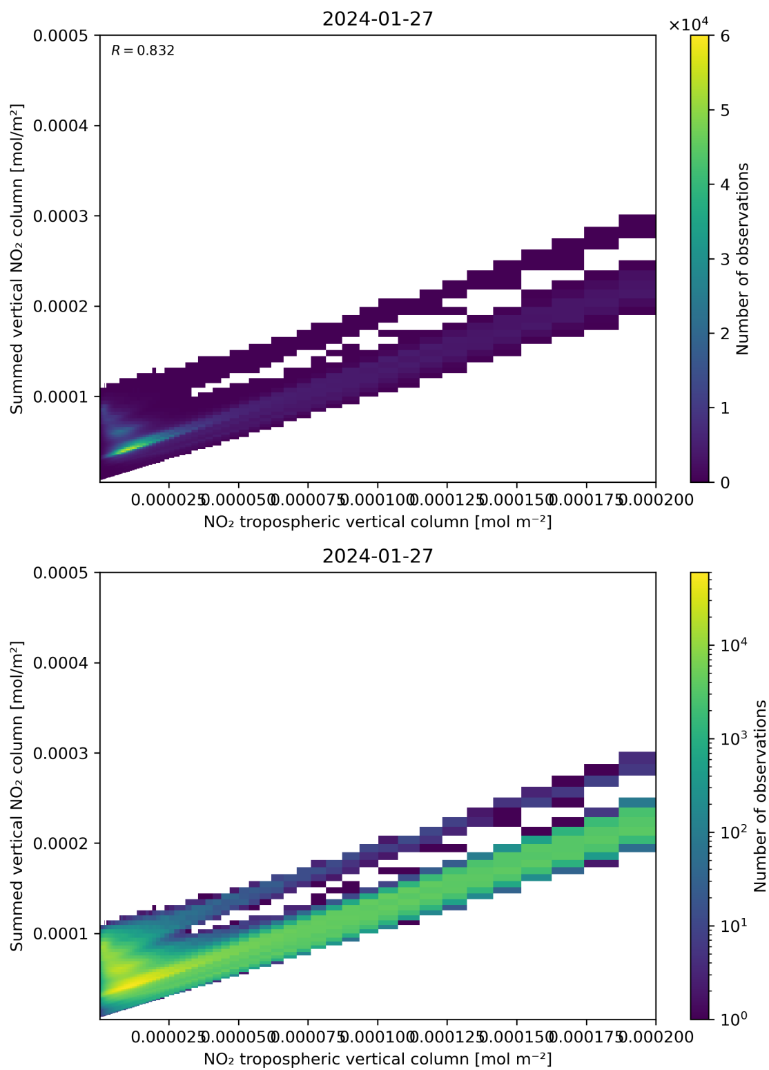
Figure 126: Scatter density plot of “NO 2 tropospheric vertical column” against “Summed vertical NO 2 column” for 2024-01-26 to 2024-01-28.
