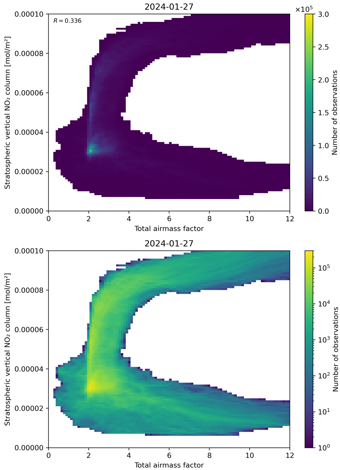
Figure 64: Scatter density plot of “Total airmass factor” against “Stratospheric vertical NO 2 column” for 2024-01-26 to 2024-01-28.
