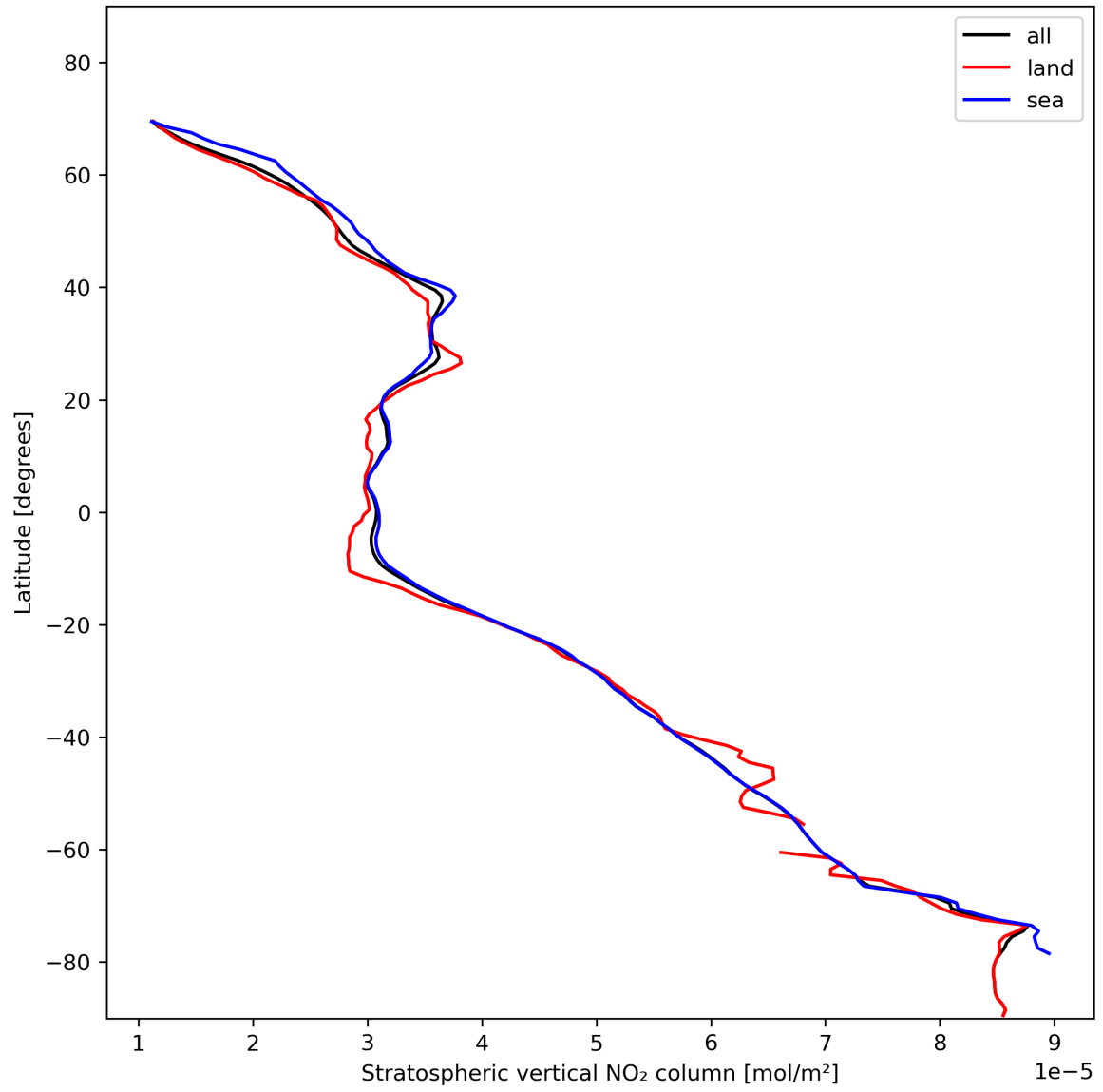
Figure 19: Zonal average of “Stratospheric vertical NO 2 column” for 2024-01-26 to 2024-01-28.
