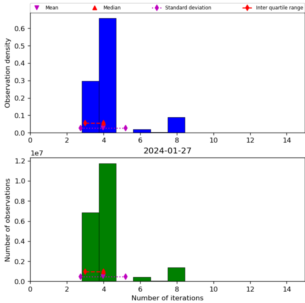
Figure 34: Histogram of “Number of iterations” for 2024-01-26 to 2024-01-28
