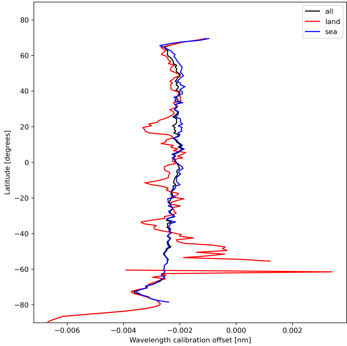
Figure 18: Zonal average of “Wavelength calibration offset” for 2024-01-26 to 2024-01-28.
