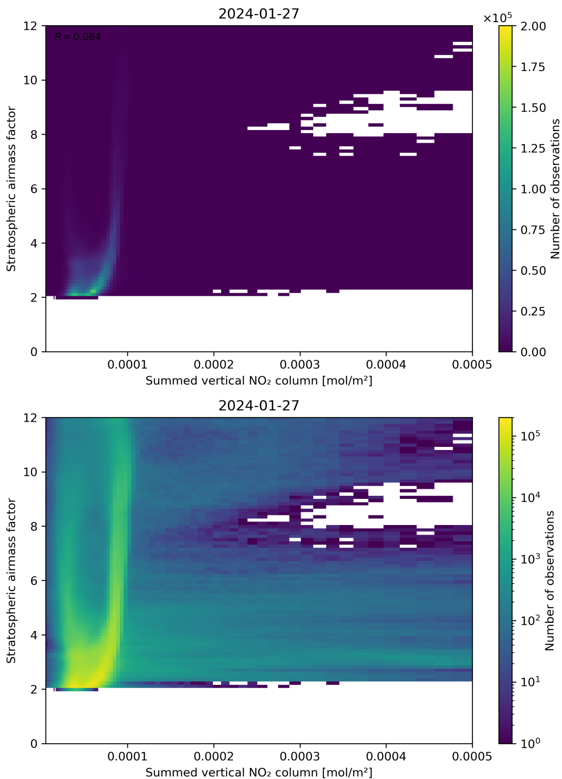
Figure 103: Scatter density plot of “Summed vertical NO 2 column” against “Stratospheric airmass factor” for 2024-01-26 to 2024-01-28.
