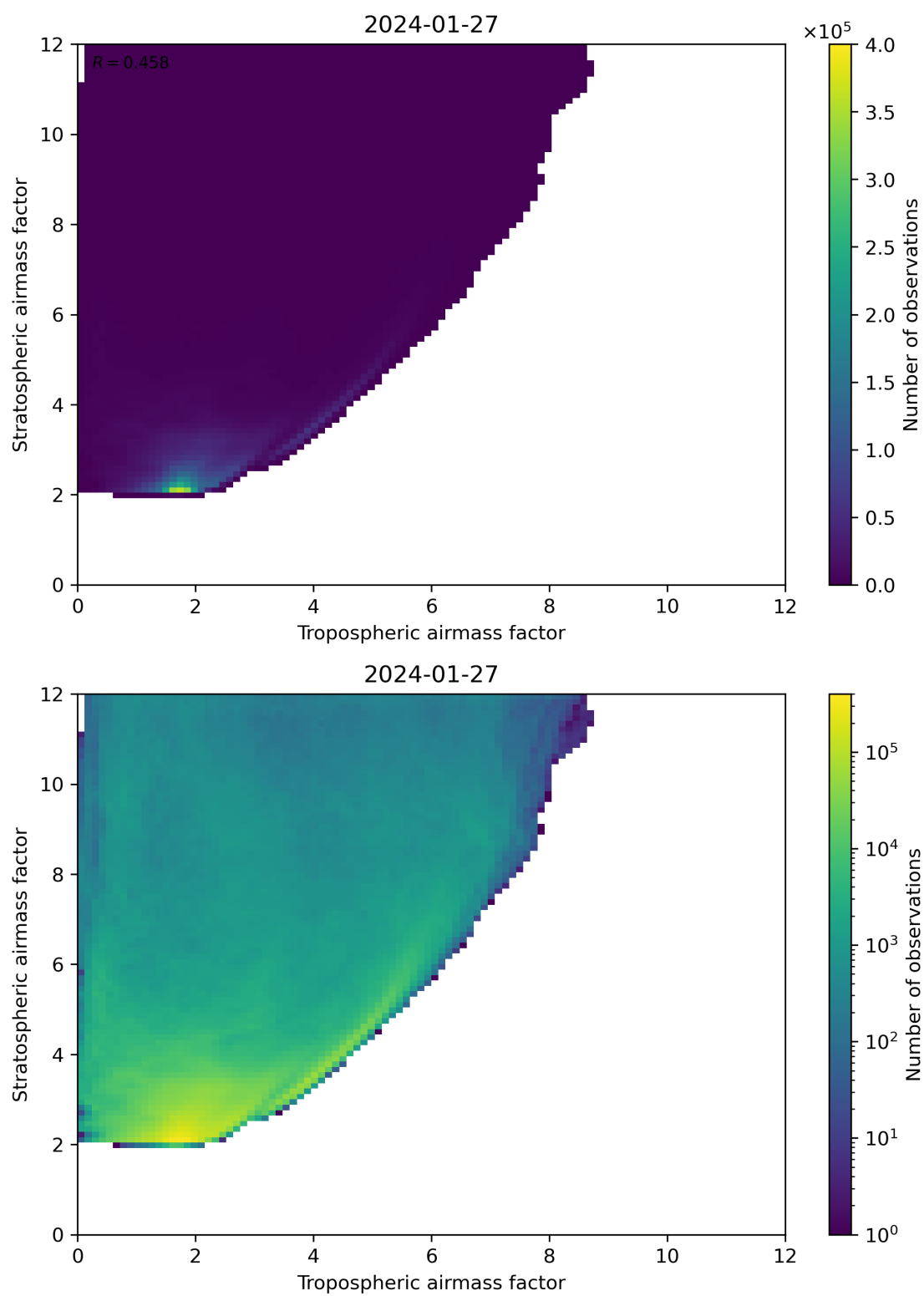
Figure 71: Scatter density plot of “Tropospheric airmass factor” against “Stratospheric airmass factor” for 2024-01-26 to 2024-01-28.
