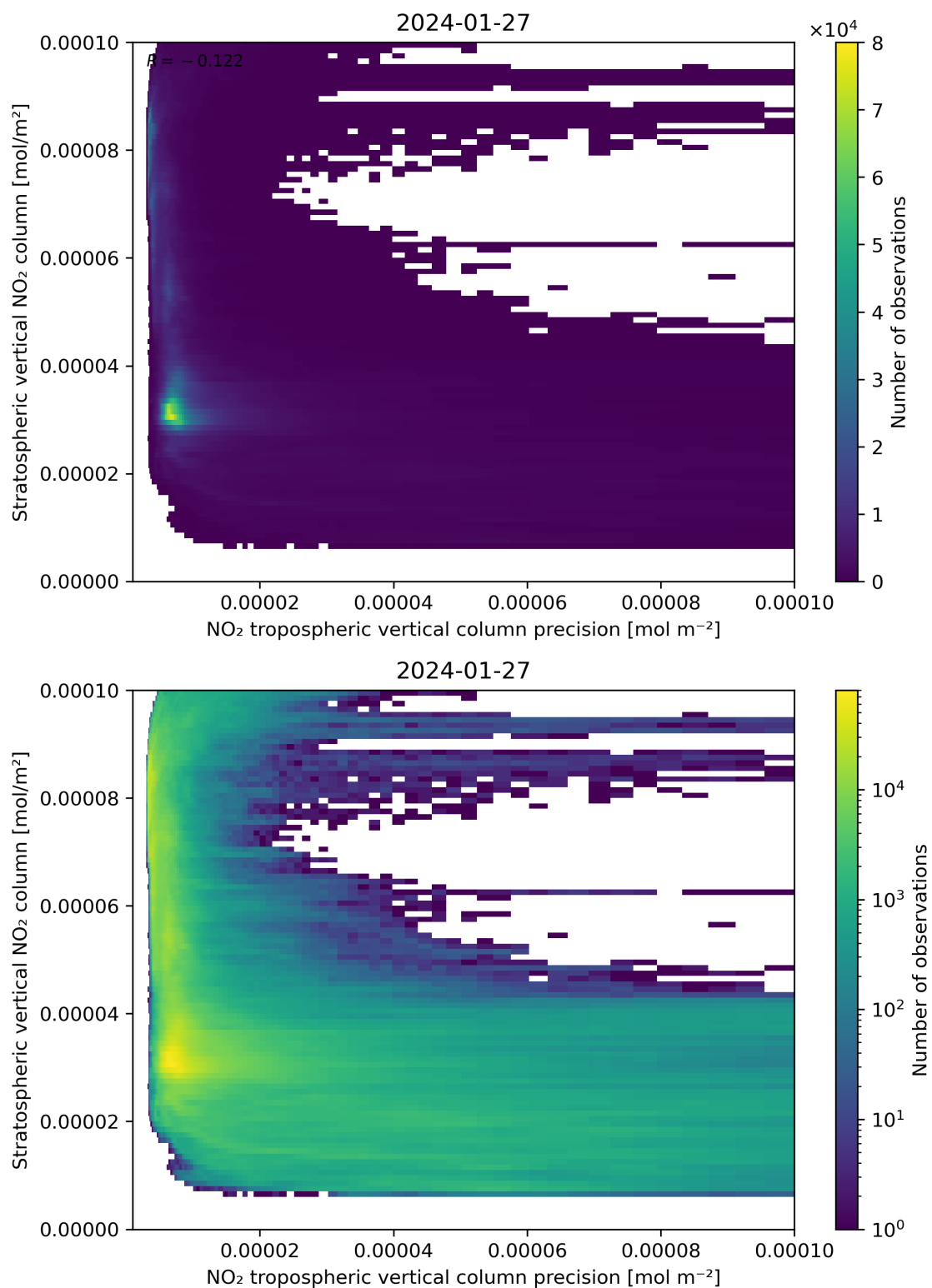
Figure 135: Scatter density plot of “NO 2 tropospheric vertical column precision” against “Stratospheric vertical NO 2 column” for 2024-01-26 to 2024-01-28.
