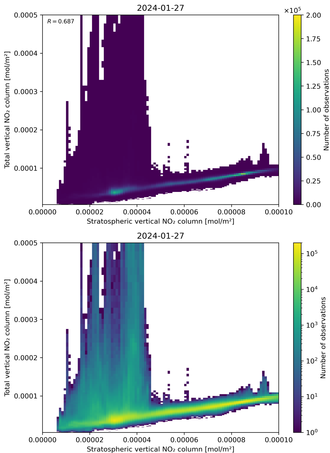
Figure 100: Scatter density plot of “Stratospheric vertical NO 2 column” against “Total vertical NO 2 column” for 2024-01-26 to 2024-01-28.
