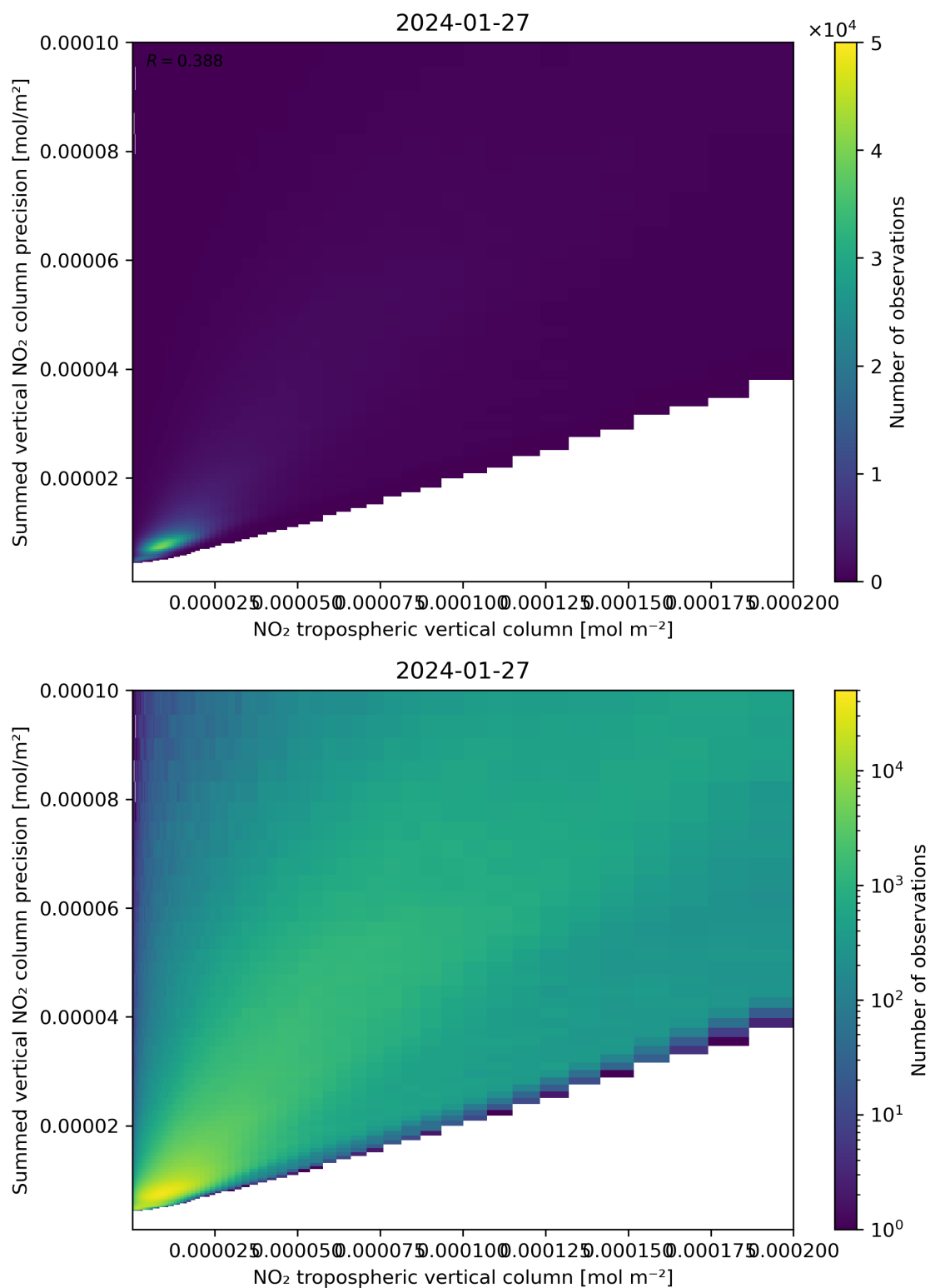
Figure 127: Scatter density plot of “NO 2 tropospheric vertical column” against “Summed vertical NO 2 column precision” for 2024-01-26 to 2024-01-28.
