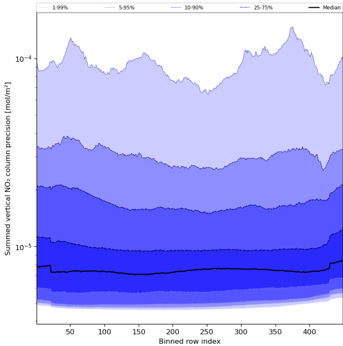
Figure 58: Along track statistics of “Summed vertical NO 2 column precision” for 2024-01-26 to 2024-01-28
