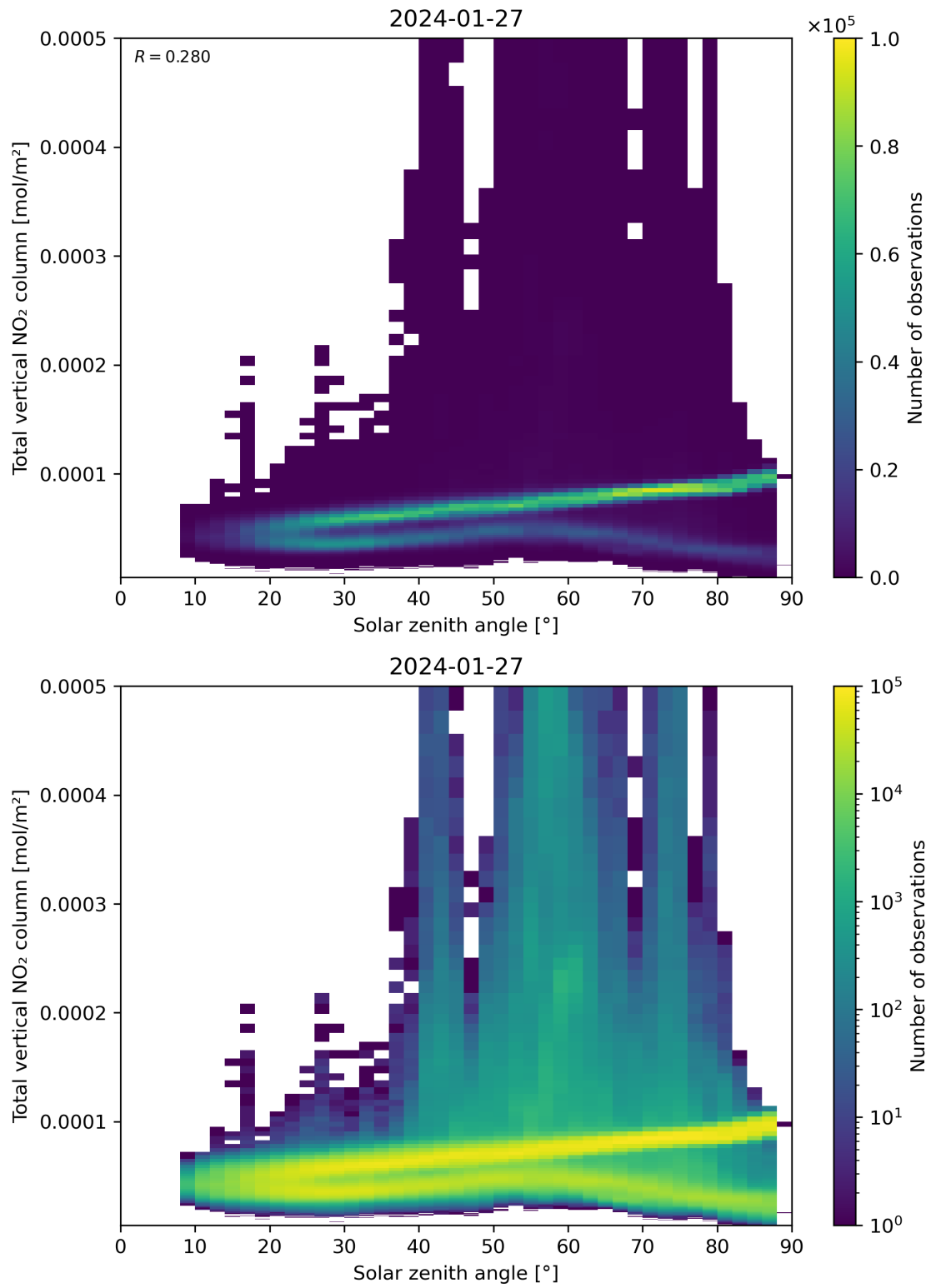
Figure 153: Scatter density plot of “Solar zenith angle” against “Total vertical NO 2 column” for 2024-01-26 to 2024-01-28.
