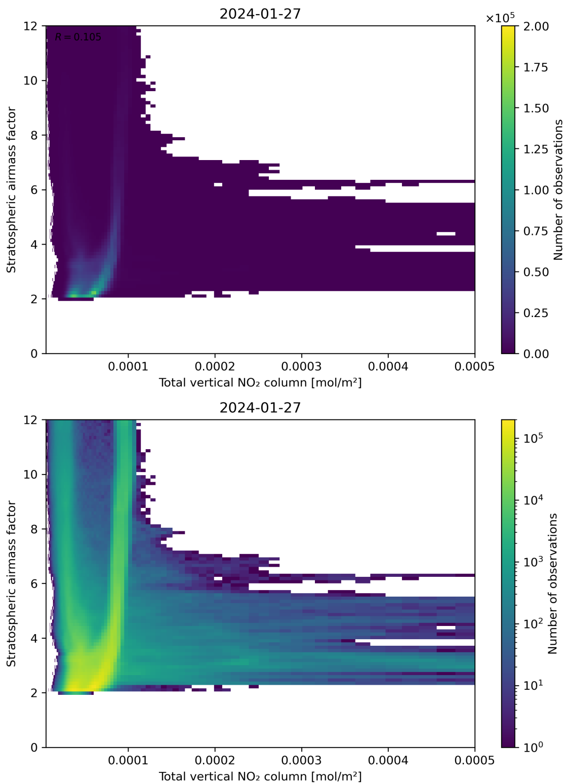
Figure 110: Scatter density plot of “Total vertical NO 2 column” against “Stratospheric airmass factor” for 2024-01-26 to 2024-01-28.
