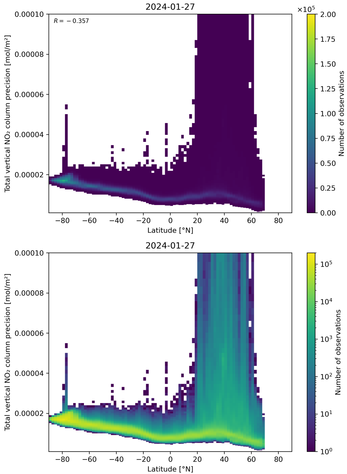
Figure 91: Scatter density plot of “Latitude” against “Total vertical NO 2 column precision” for 2024-01-26 to 2024-01-28.
