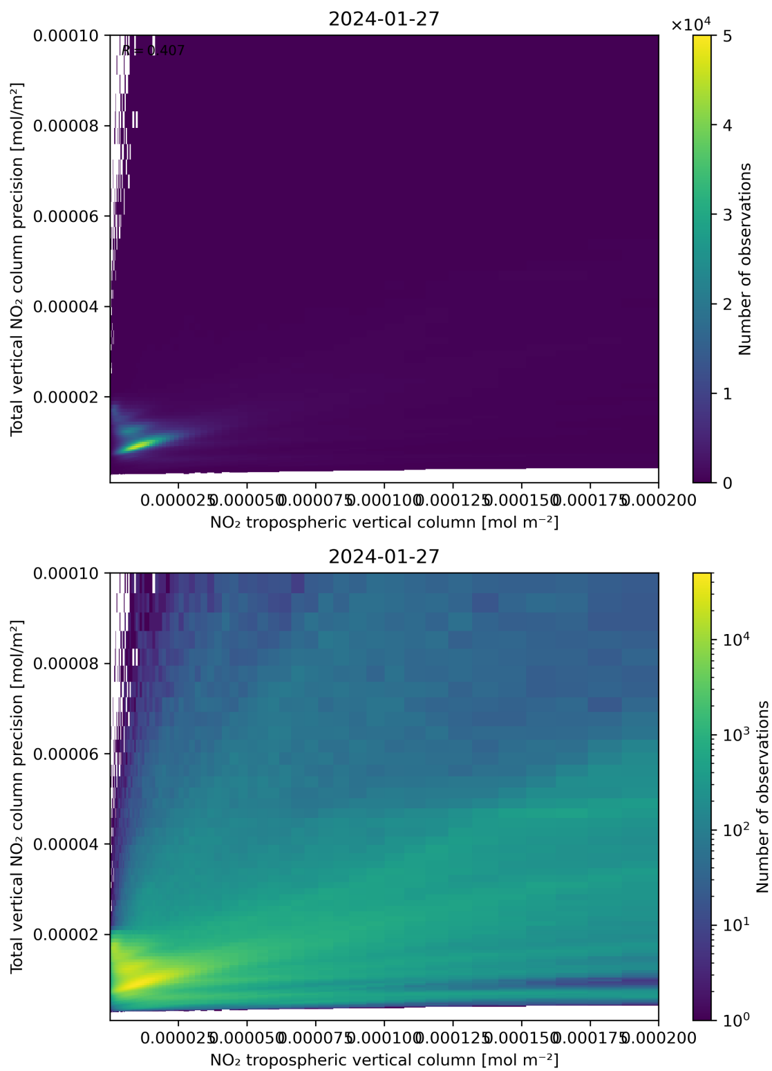
Figure 129: Scatter density plot of “NO 2 tropospheric vertical column” against “Total vertical NO 2 column precision” for 2024-01-26 to 2024-01-28.
