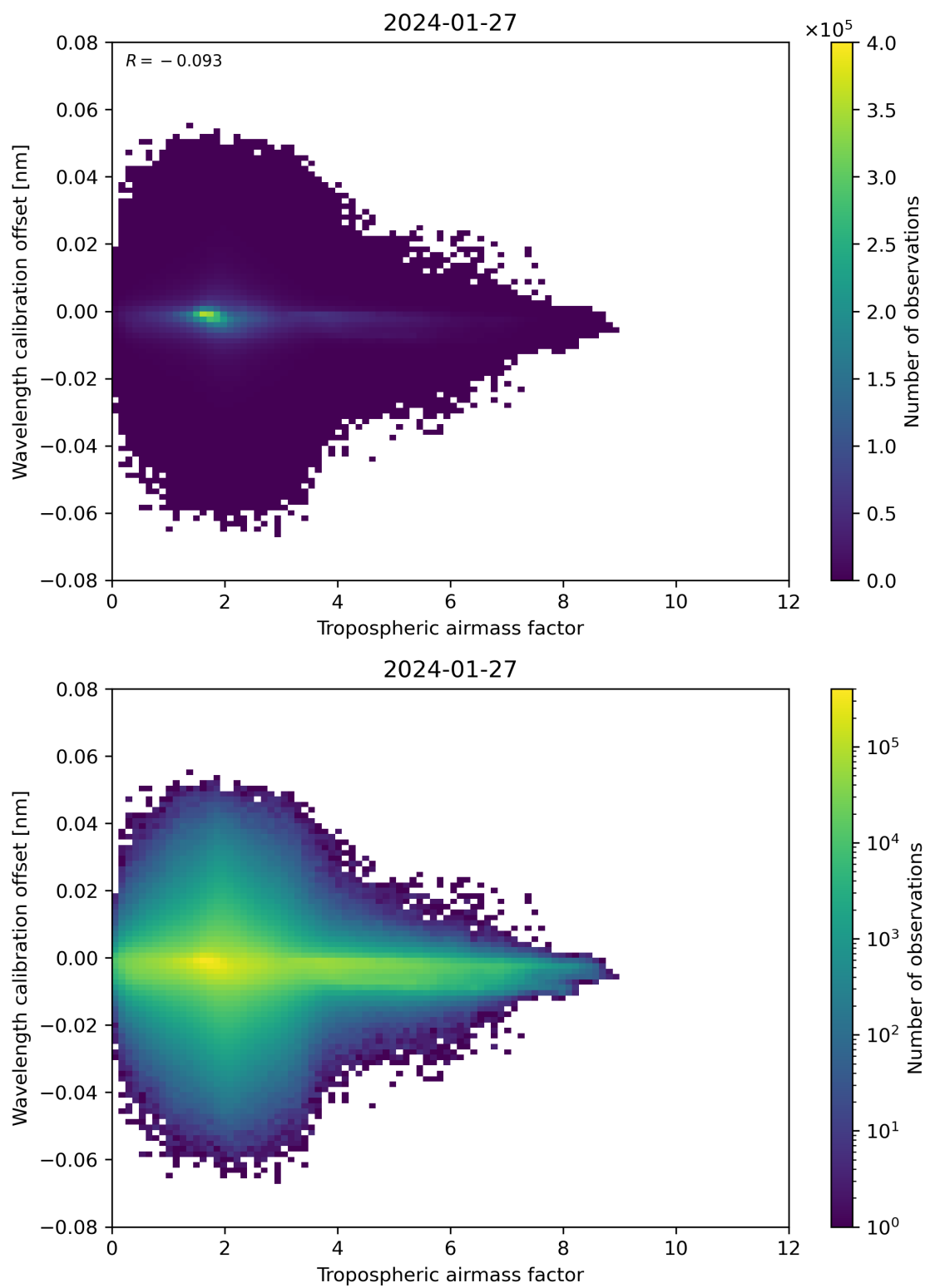
Figure 80: Scatter density plot of “Tropospheric airmass factor” against “Wavelength calibration offset” for 2024-01-26 to 2024-01-28.
