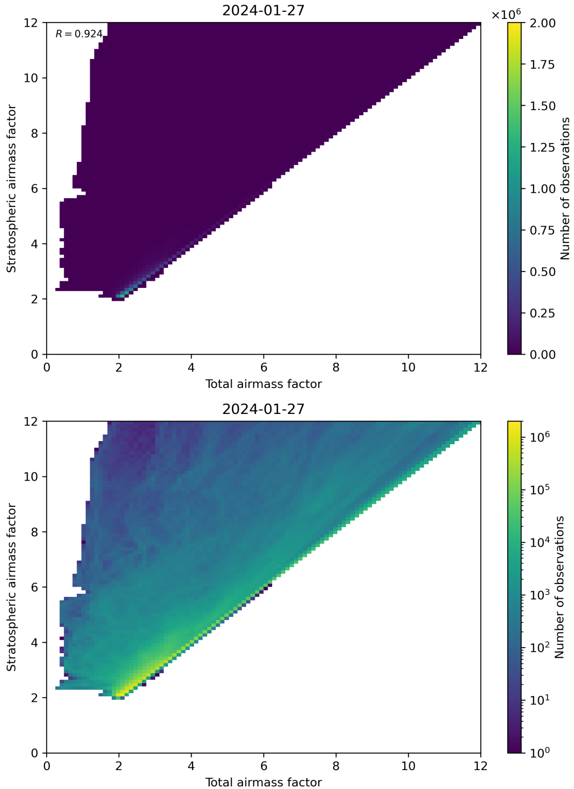
Figure 62: Scatter density plot of “Total airmass factor” against “Stratospheric airmass factor” for 2024-01-26 to 2024-01-28.
