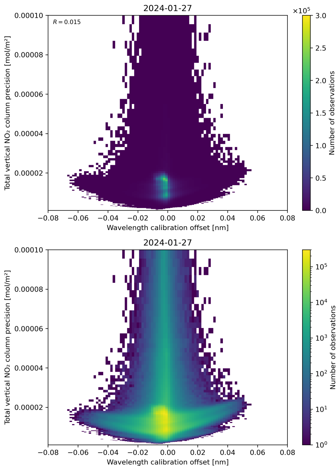
Figure 180: Scatter density plot of “Wavelength calibration offset” against “Total vertical NO 2 column precision” for 2024-01-26 to 2024-01-28.
