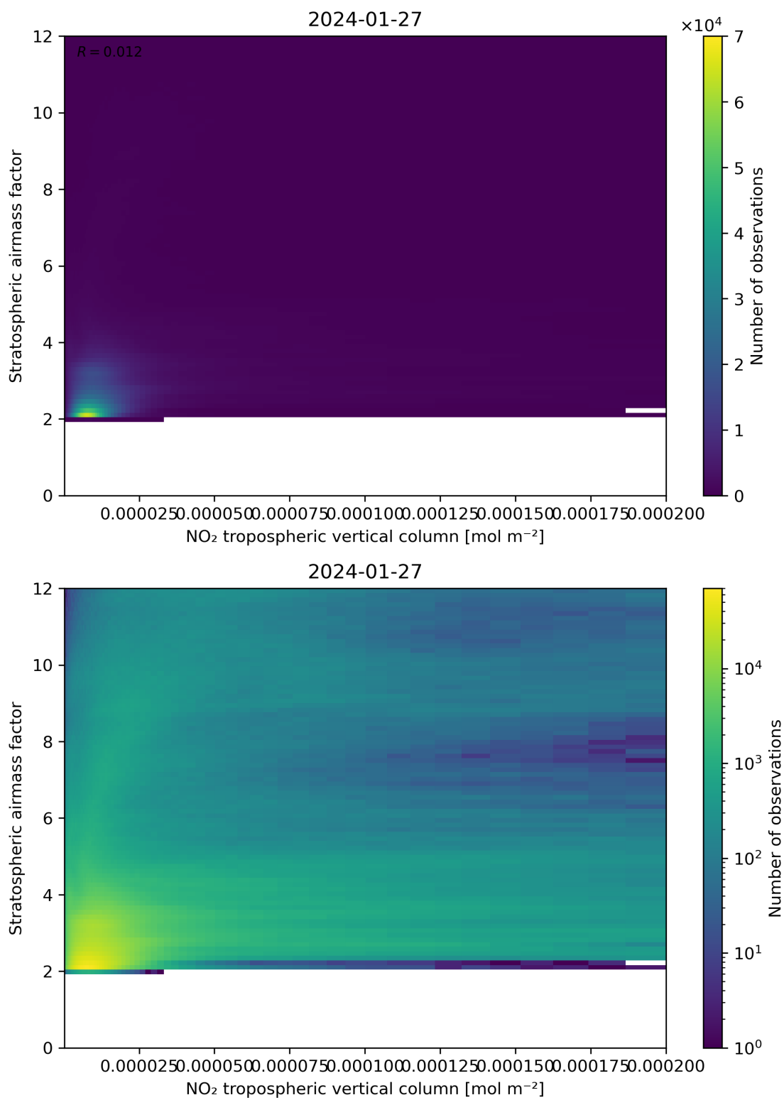
Figure 121: Scatter density plot of “NO 2 tropospheric vertical column” against “Stratospheric airmass factor” for 2024-01-26 to 2024-01-28.
