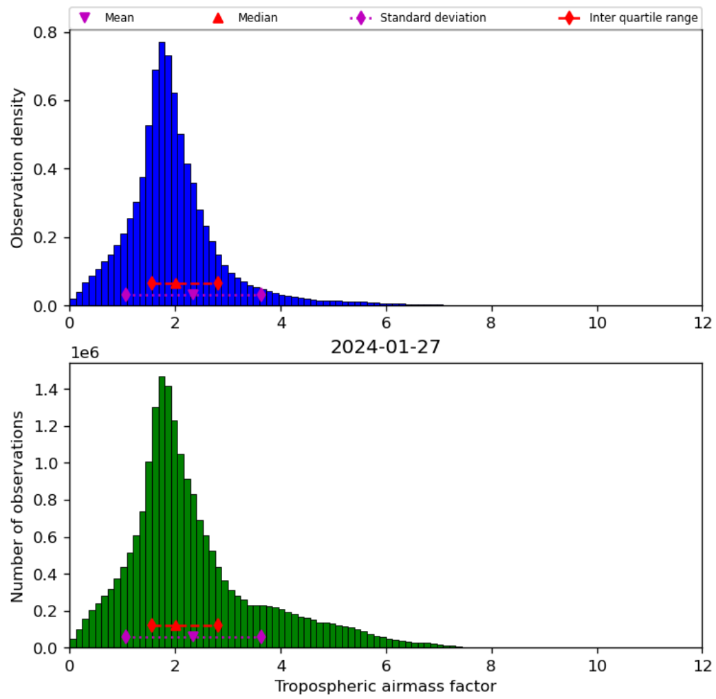
Figure 31: Histogram of “Tropospheric airmass factor” for 2024-01-26 to 2024-01-28
