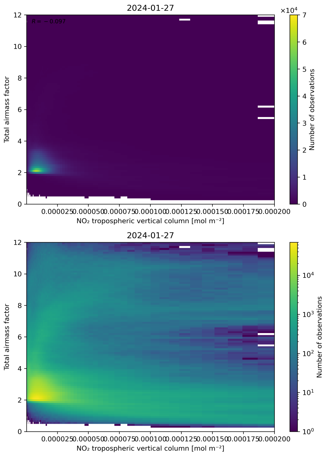
Figure 122: Scatter density plot of “NO 2 tropospheric vertical column” against “Total air mass factor” for 2024-01-26 to 2024-01-28.
