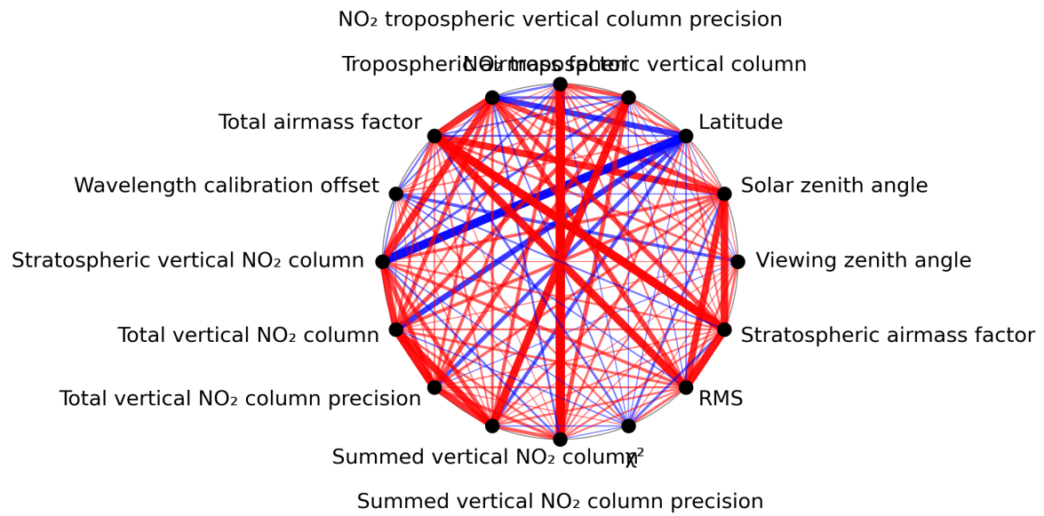
Figure 1: Map of correlation graph for 2024-01-26 to 2024-01-28.
