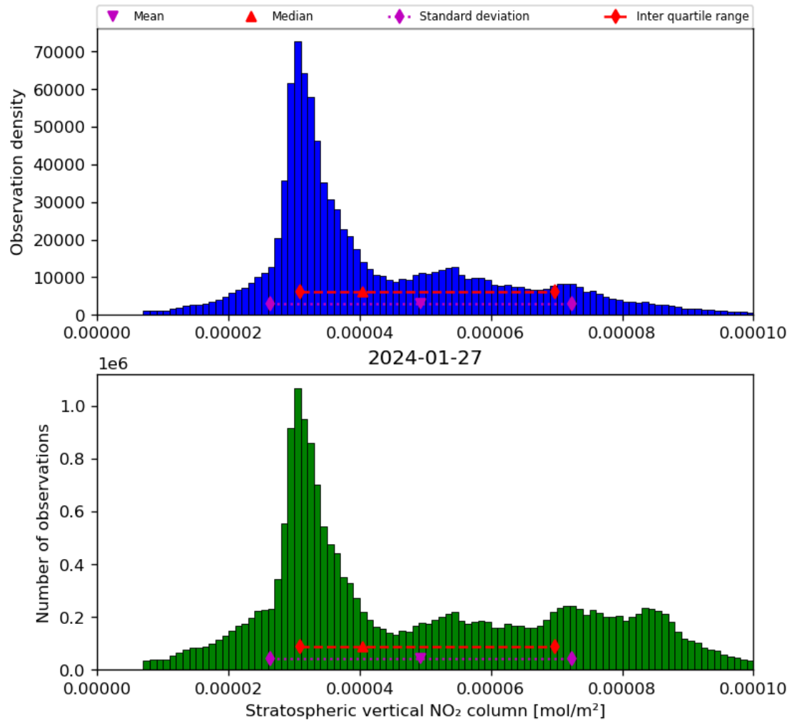
Figure 36: Histogram of “Stratospheric vertical NO 2 column” for 2024-01-26 to 2024-01-28
