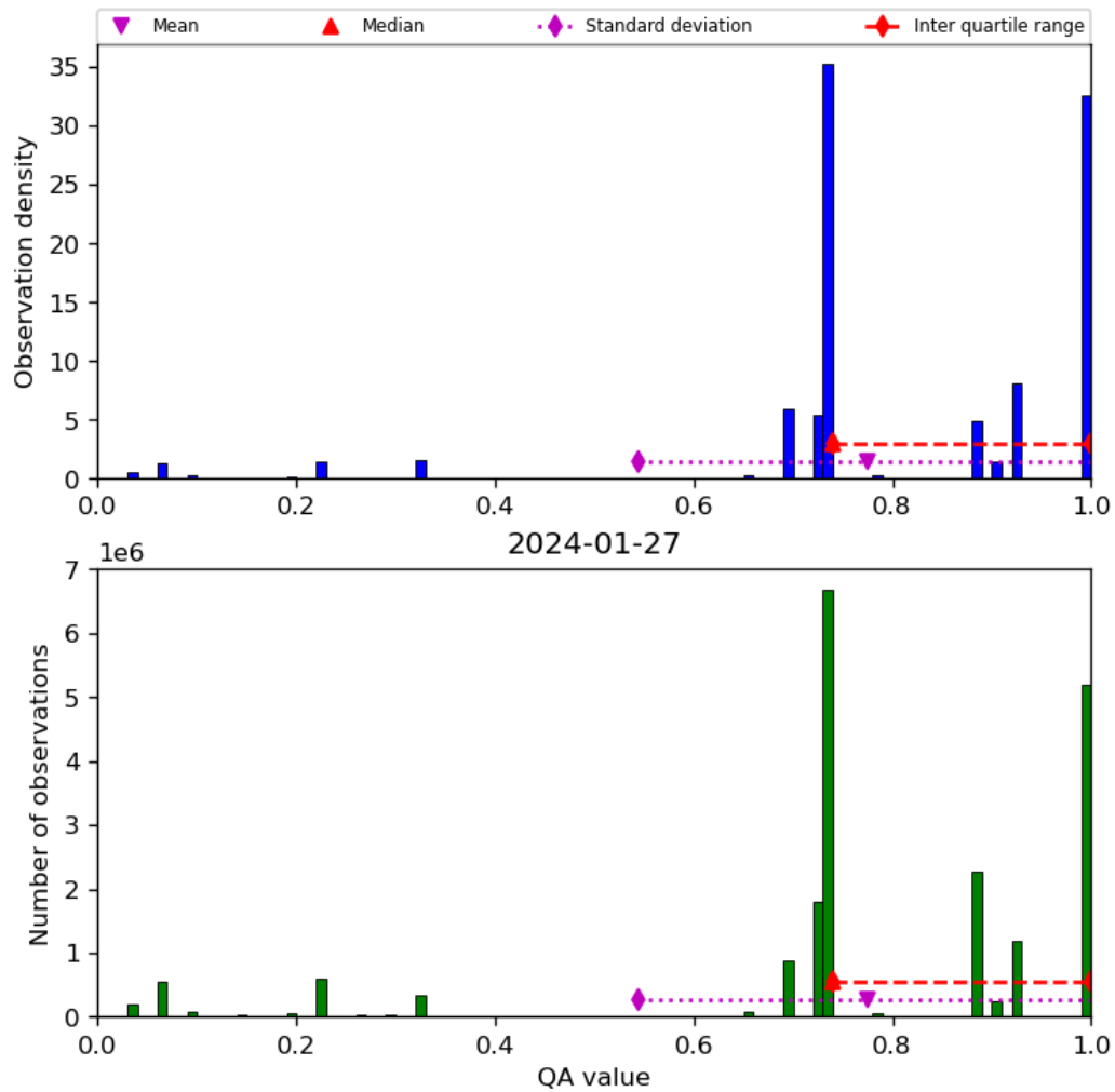
Figure 28: Histogram of “QA value” for 2024-01-26 to 2024-01-28
