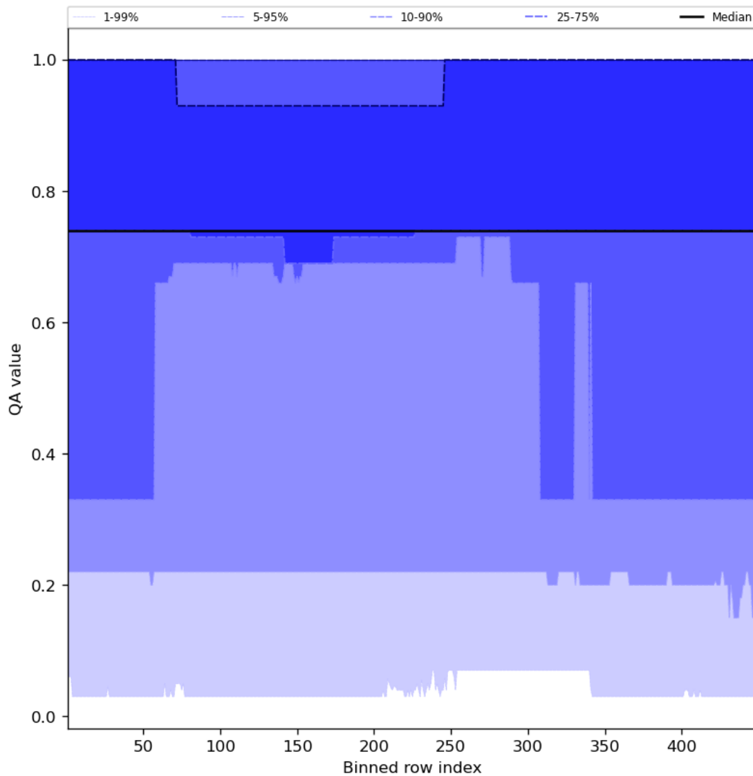
Figure 45: Along track statistics of “QA value” for 2024-01-26 to 2024-01-28
