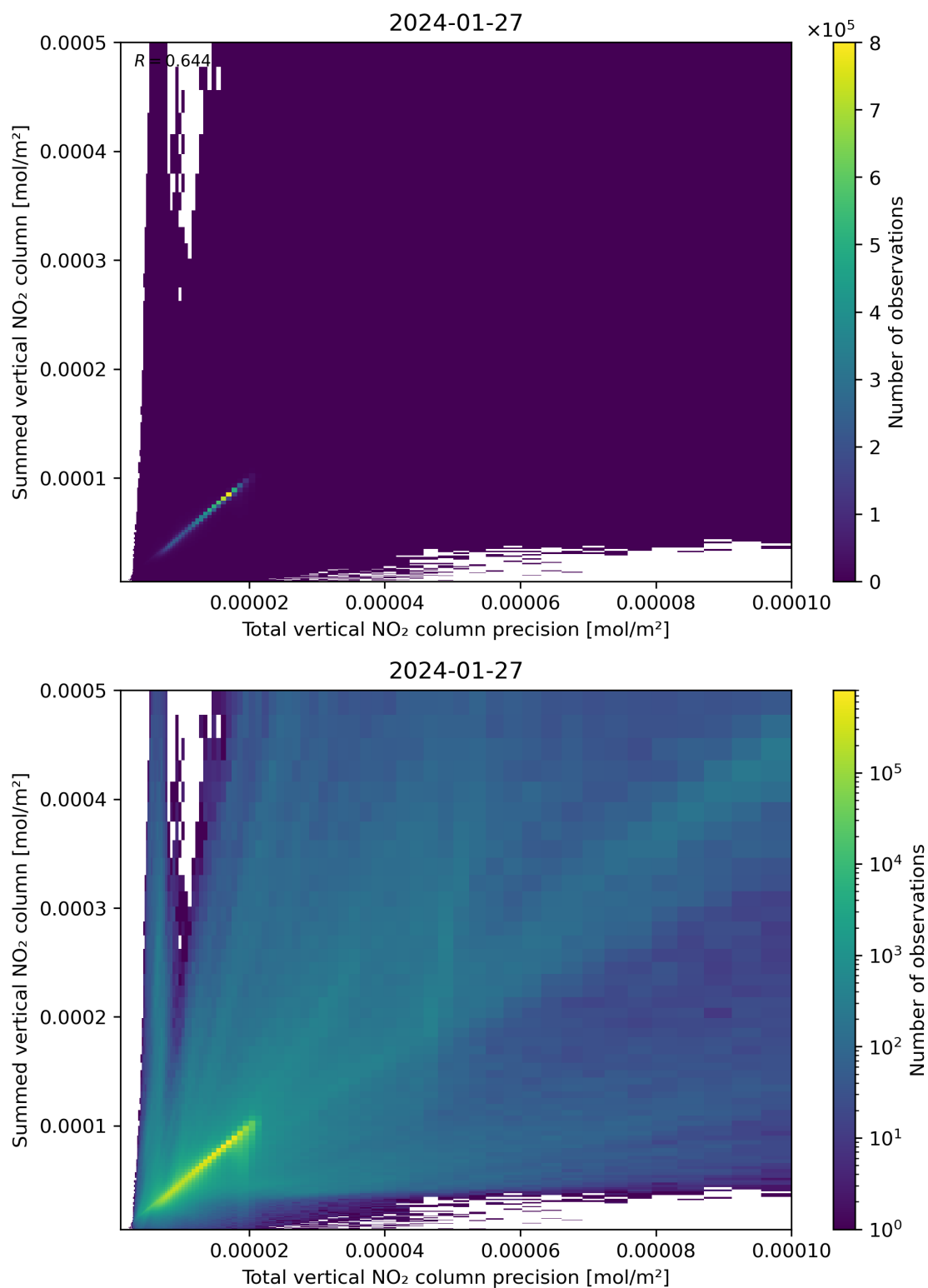
Figure 117: Scatter density plot of “Total vertical NO 2 column precision” against “Summed vertical NO 2 column” for 2024-01-26 to 2024-01-28.
