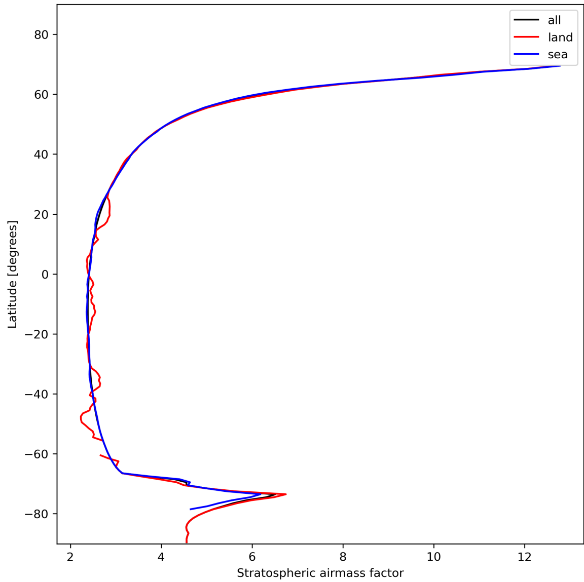
Figure 27: Zonal average of “Stratospheric air mass factor” for 2024-01-26 to 2024-01-28.
