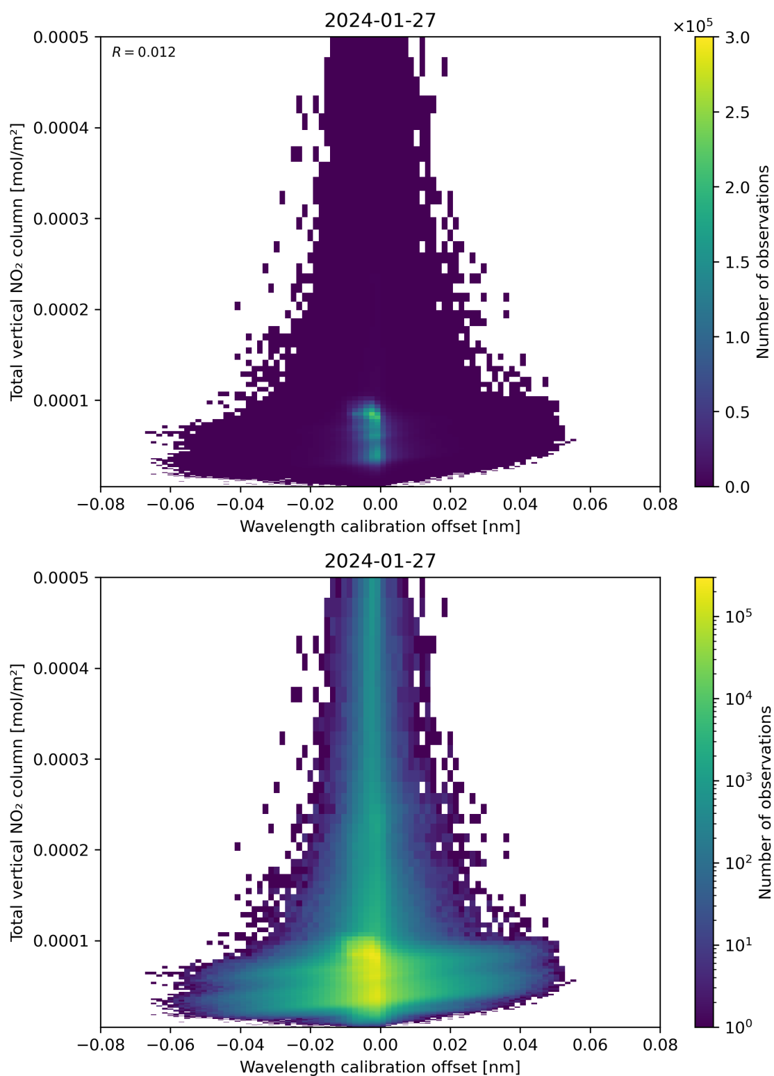
Figure 179: Scatter density plot of “Wavelength calibration offset” against “Total vertical NO 2 column” for 2024-01-26 to 2024-01-28.
