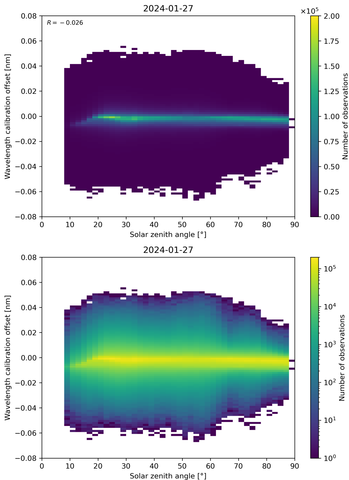
Figure 158: Scatter density plot of “Solar zenith angle” against “Wavelength calibration offset” for 2024-01-26 to 2024-01-28.
