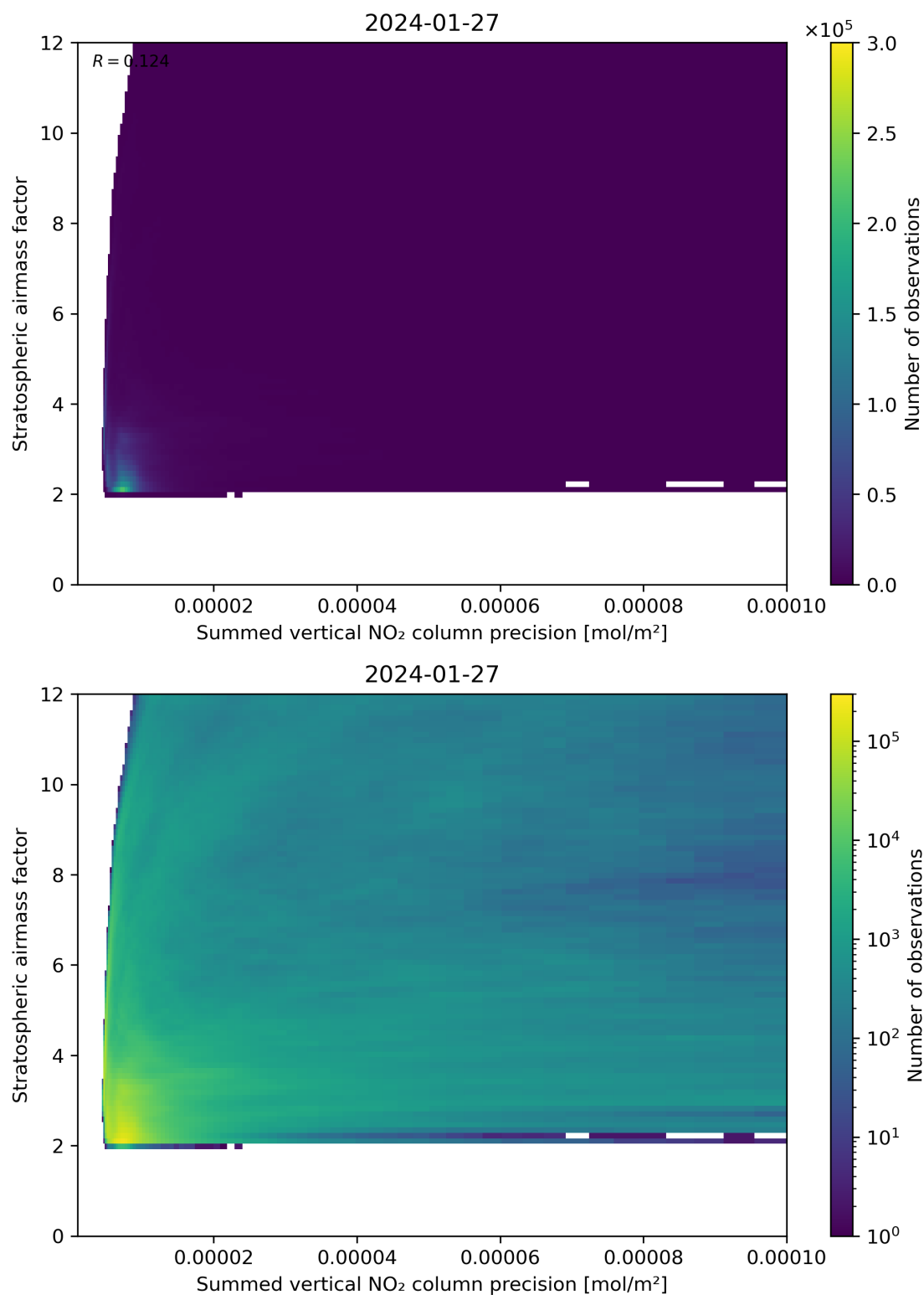
Figure 106: Scatter density plot of “Summed vertical NO 2 column precision” against “Stratospheric airmass factor” for 2024-01-26 to 2024-01-28.
