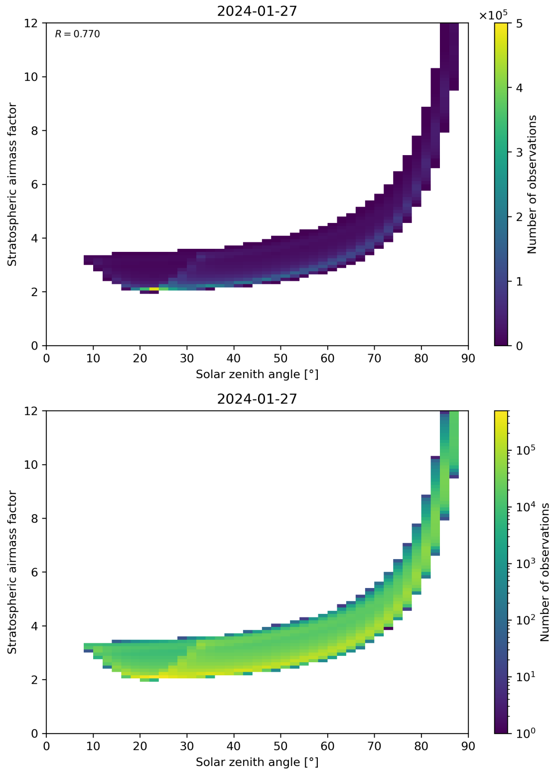
Figure 145: Scatter density plot of “Solar zenith angle” against “Stratospheric airmass factor” for 2024-01-26 to 2024-01-28.
