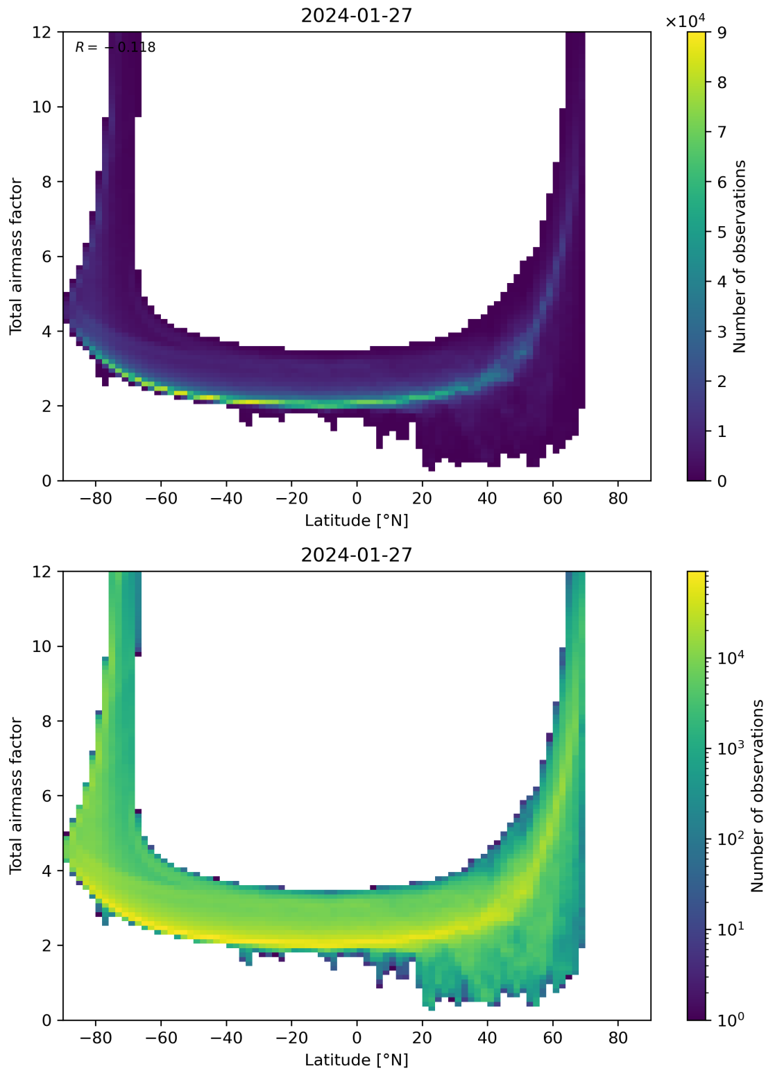
Figure 84: Scatter density plot of “Latitude” against “Total airmass factor” for 2024-01-26 to 2024-01-28.
