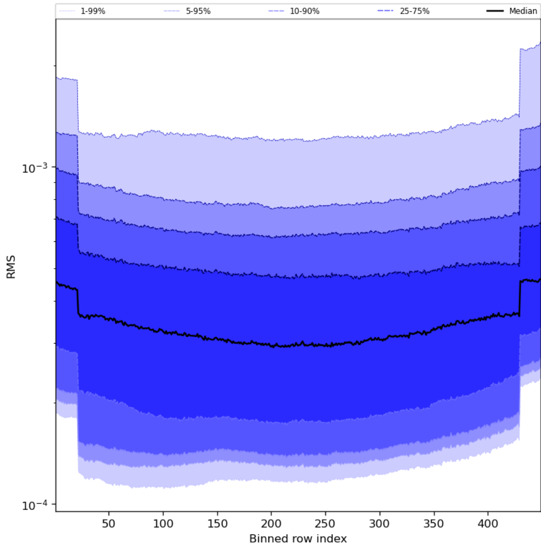
Figure 60: Along track statistics of “RMS” for 2024-01-26 to 2024-01-28
