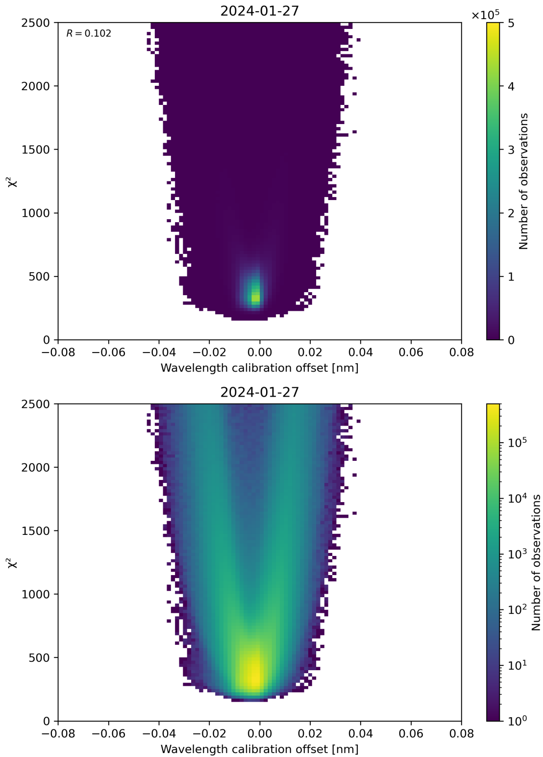
Figure 175: Scatter density plot of “Wavelength calibration offset” against “ \chi^2 ” for 2024-01-26 to 2024-01-28.
