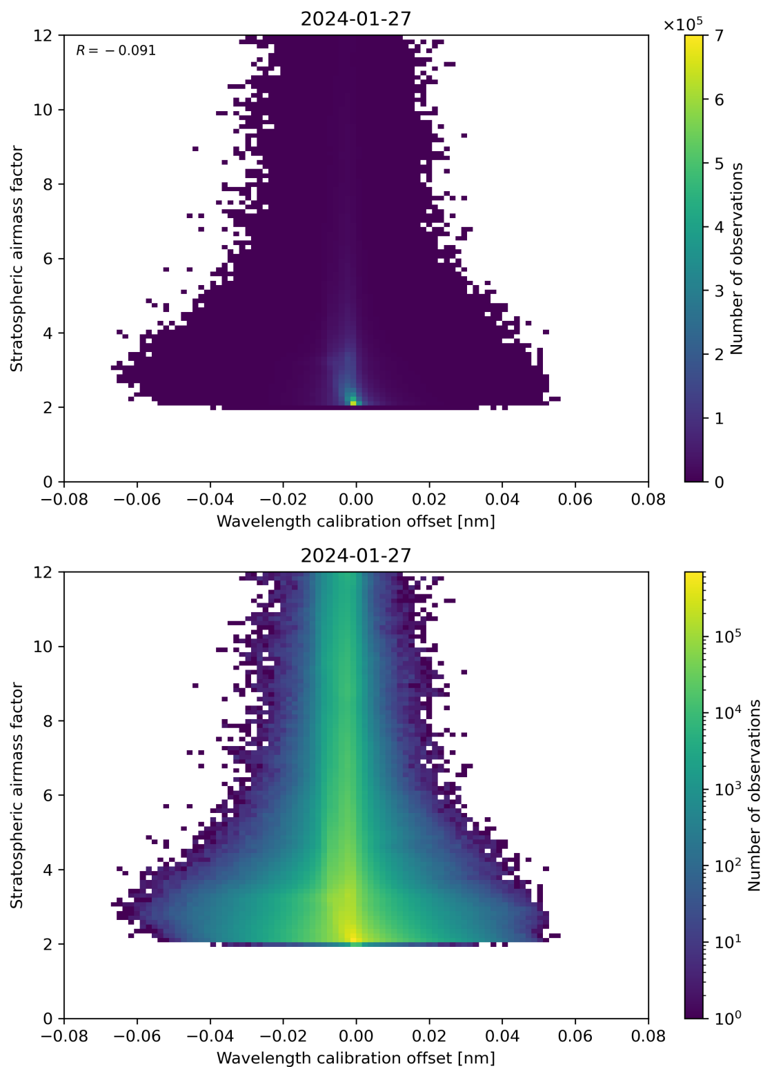
Figure 174: Scatter density plot of “Wavelength calibration offset” against “Stratospheric air mass factor” for 2024-01-26 to 2024-01-28.
