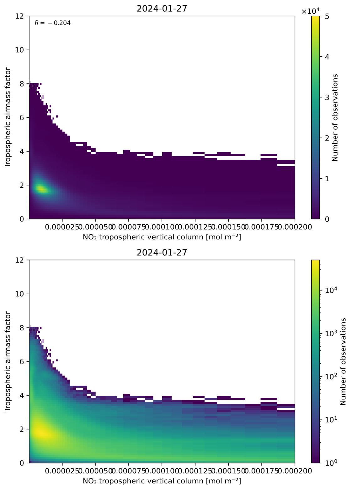
Figure 123: Scatter density plot of “NO 2 tropospheric vertical column” against “Tropospheric air mass factor” for 2024-01-26 to 2024-01-28.
