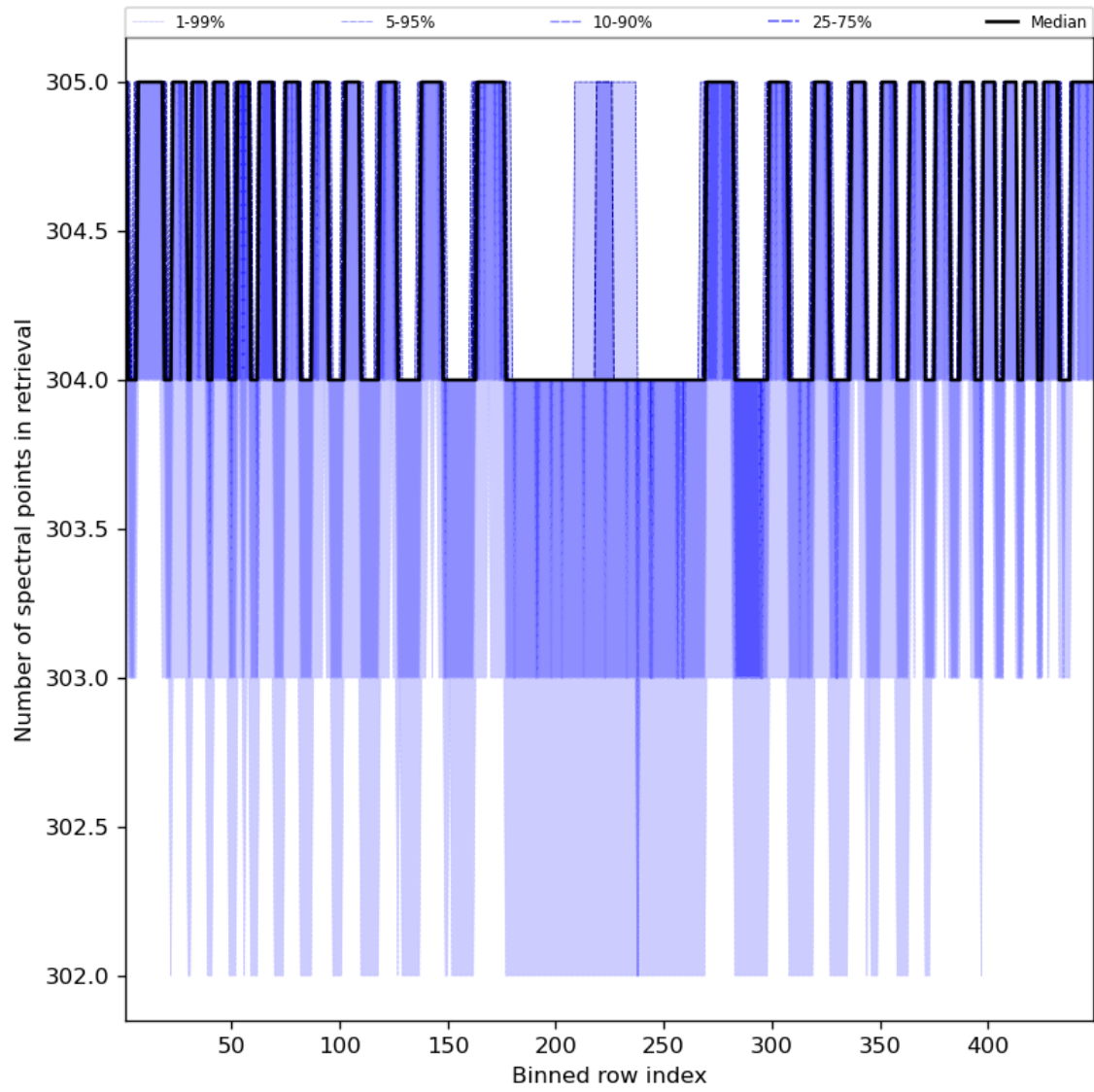
Figure 50: Along track statistics of “Number of spectral points in retrieval” for 2024-01-26 to 2024-01-28
