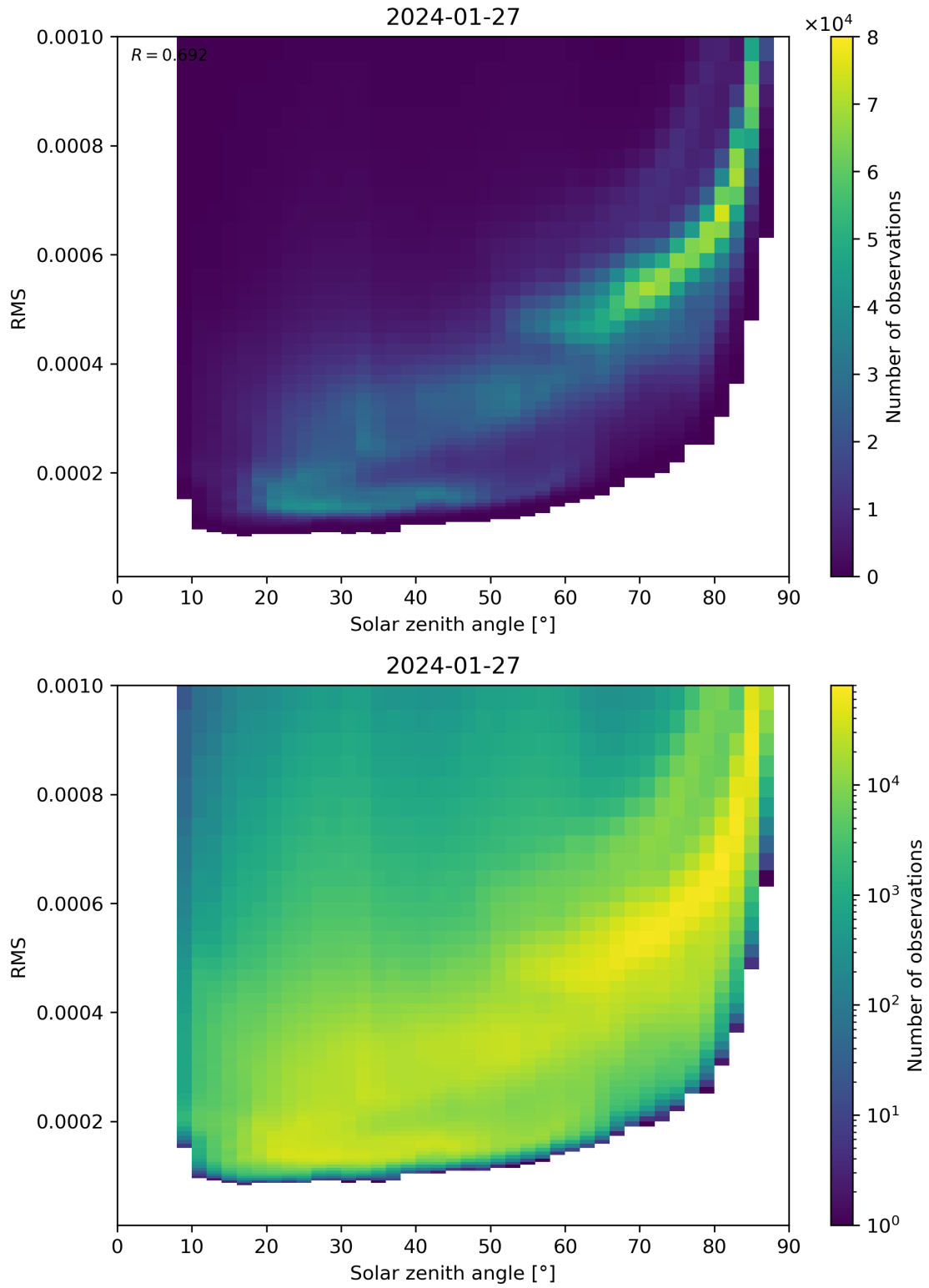
Figure 157: Scatter density plot of “Solar zenith angle” against “RMS” for 2024-01-26 to 2024-01-28.
