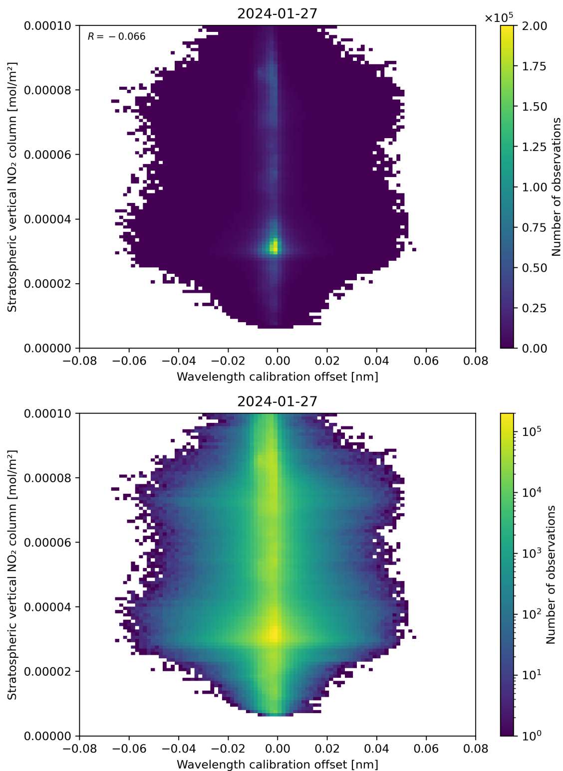
Figure 176: Scatter density plot of “Wavelength calibration offset” against “Stratospheric vertical NO 2 column” for 2024-01-26 to 2024-01-28.
