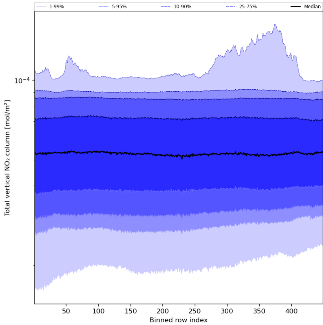
Figure 55: Along track statistics of “Total vertical NO 2 column” for 2024-01-26 to 2024-01-28
