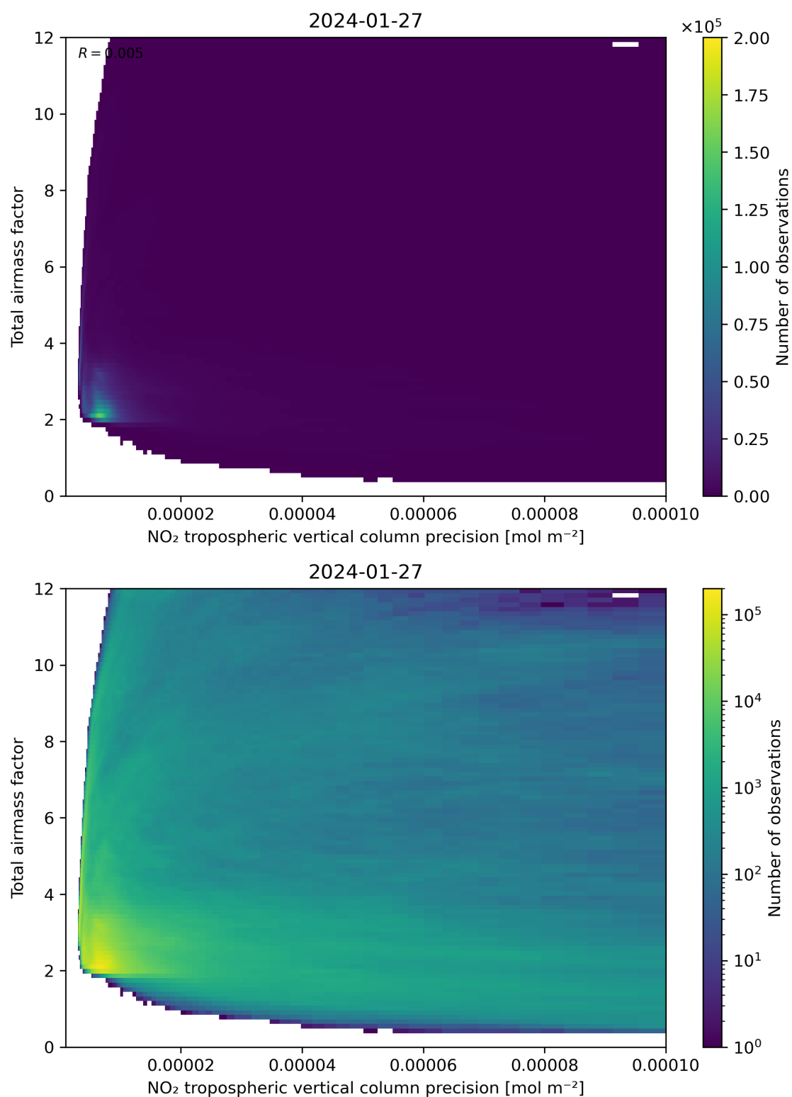
Figure 132: Scatter density plot of “NO 2 tropospheric vertical column precision” against “Total air mass factor” for 2024-01-26 to 2024-01-28.
