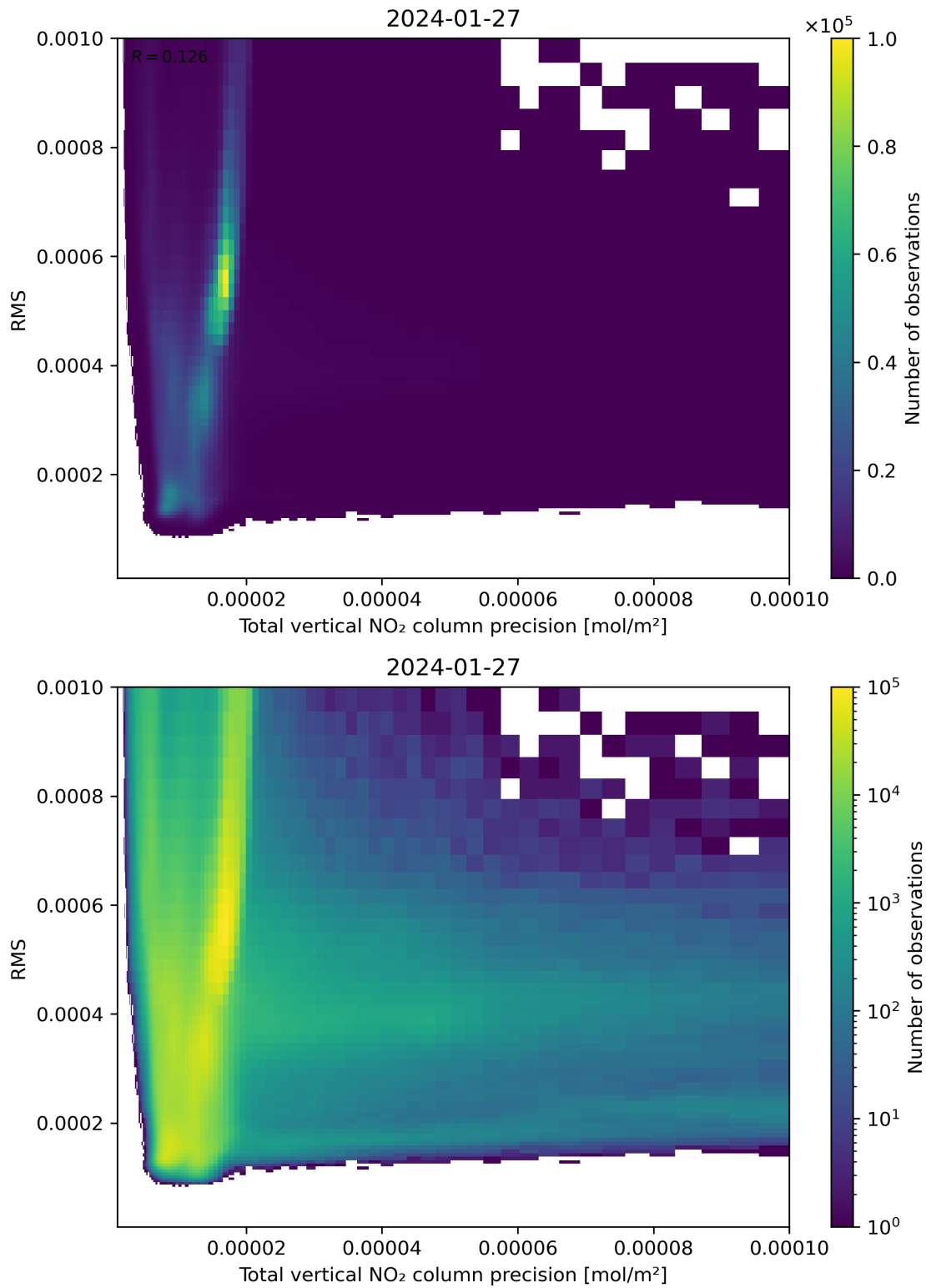
Figure 119: Scatter density plot of “Total vertical NO 2 column precision” against “RMS” for 2024-01-26 to 2024-01-28.
