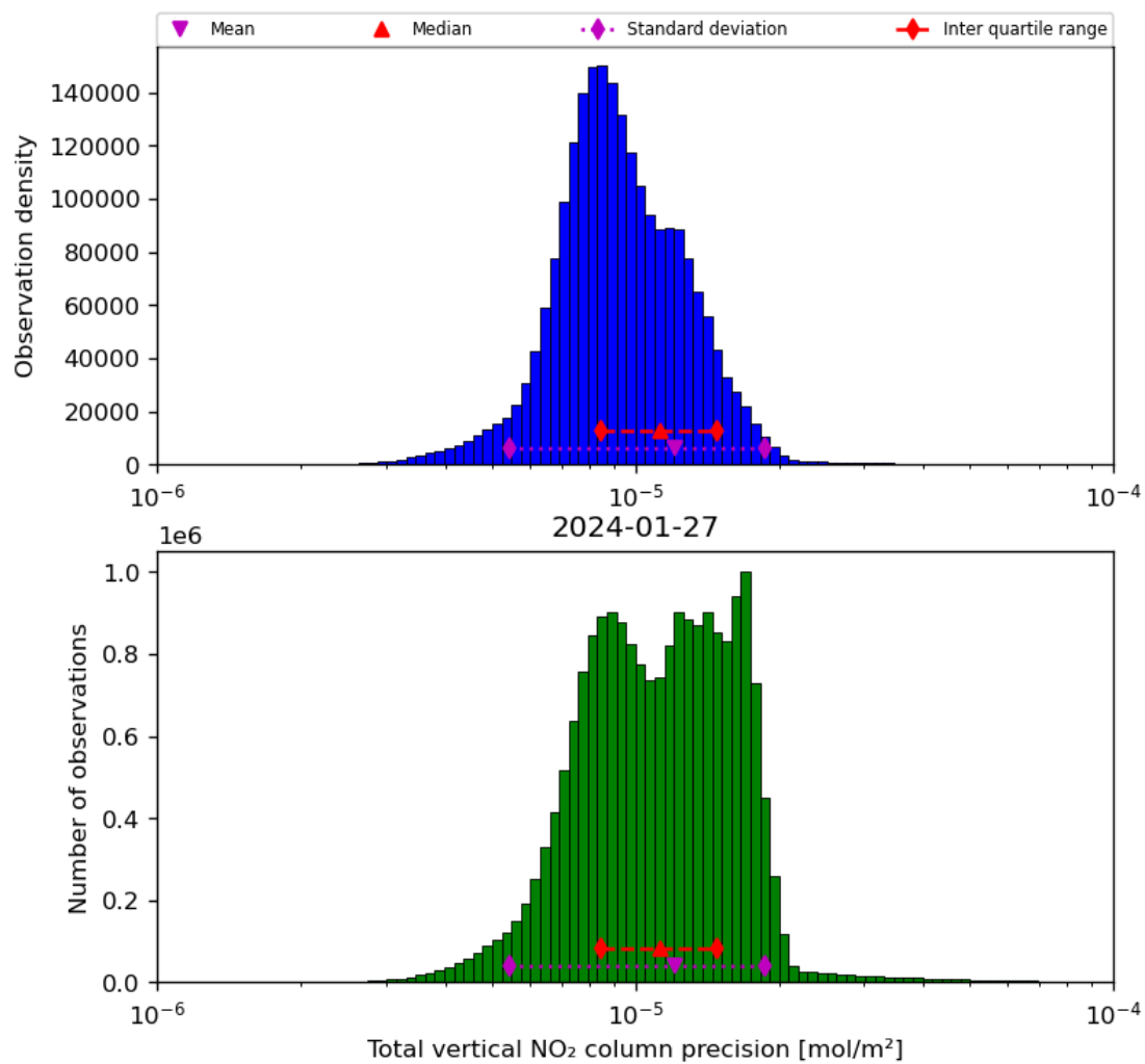
Figure 39: Histogram of “Total vertical NO 2 column precision” for 2024-01-26 to 2024-01-28
