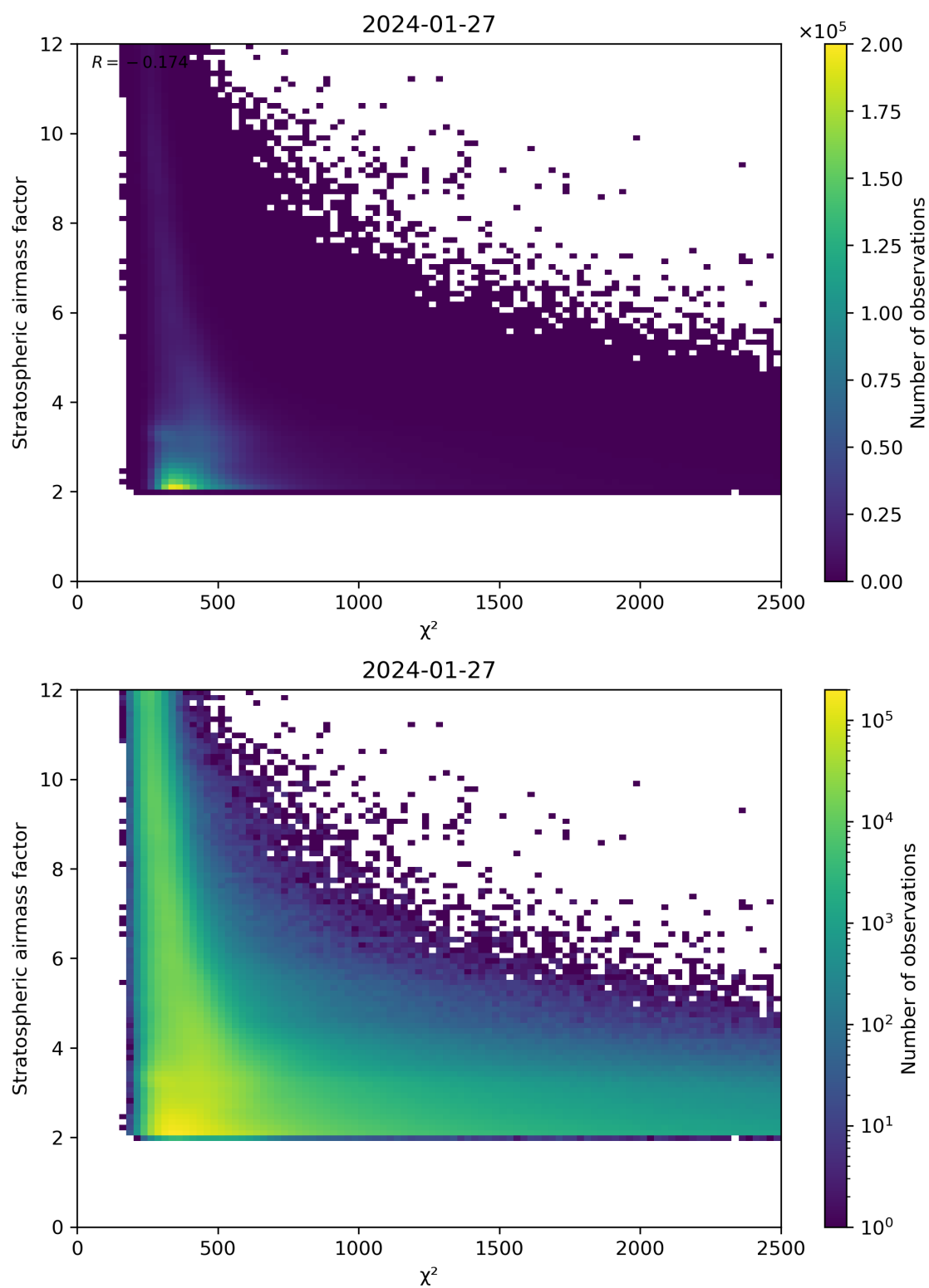
Figure 81: Scatter density plot of “ \chi^2 ” against “Stratospheric airmass factor” for 2024-01-26 to 2024-01-28.
