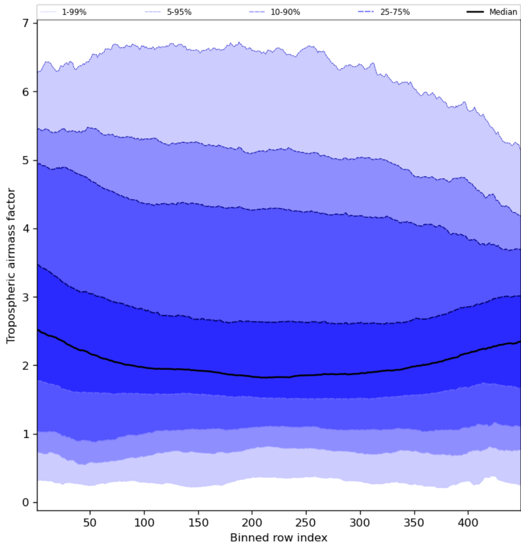
Figure 48: Along track statistics of “Tropospheric air mass factor” for 2024-01-26 to 2024-01-28
