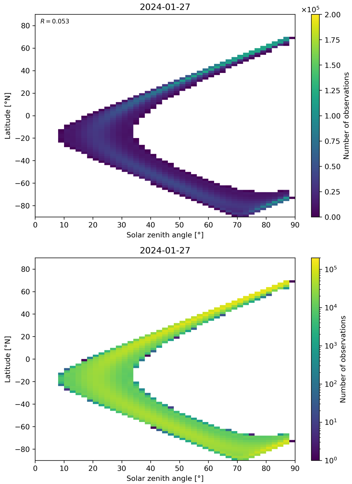
Figure 149: Scatter density plot of “Solar zenith angle” against “Latitude” for 2024-01-26 to 2024-01-28.
