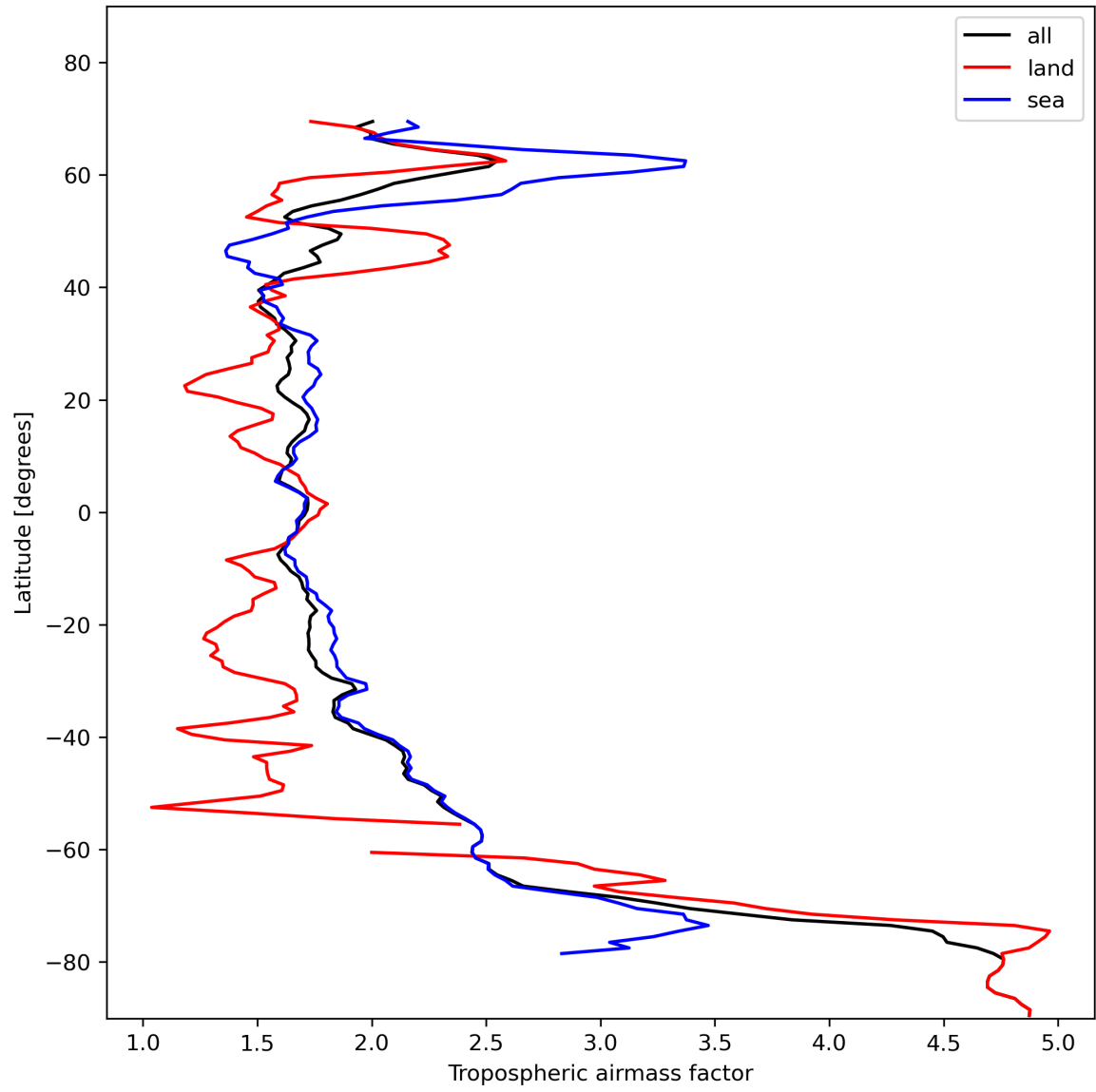
Figure 14: Zonal average of “Tropospheric airmass factor” for 2024-01-26 to 2024-01-28.
