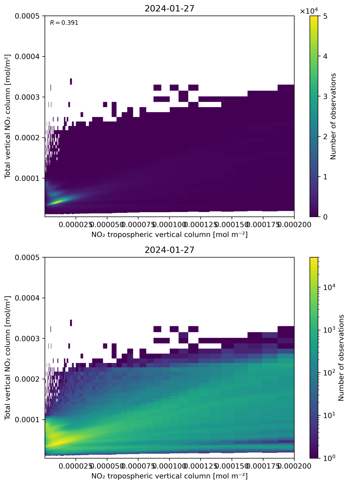
Figure 128: Scatter density plot of “NO 2 tropospheric vertical column” against “Total vertical NO 2 column” for 2024-01-26 to 2024-01-28.
