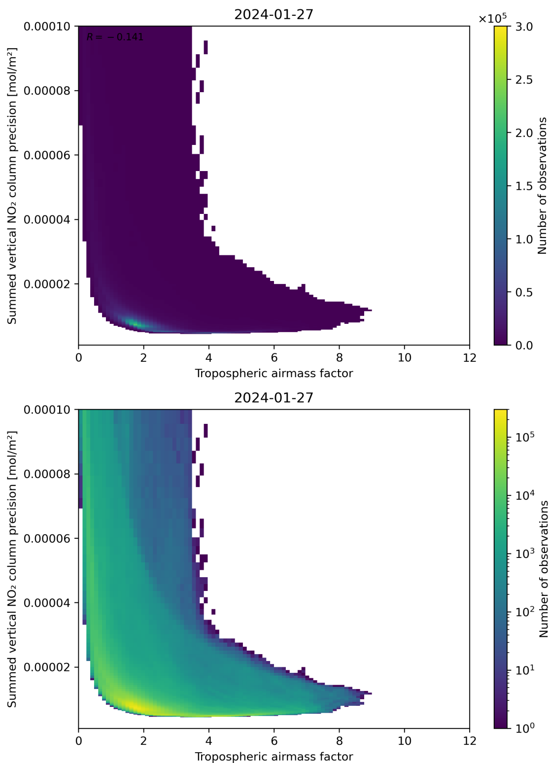
Figure 76: Scatter density plot of “Tropospheric air mass factor” against “Summed vertical NO 2 column precision” for 2024-01-26 to 2024-01-28.
