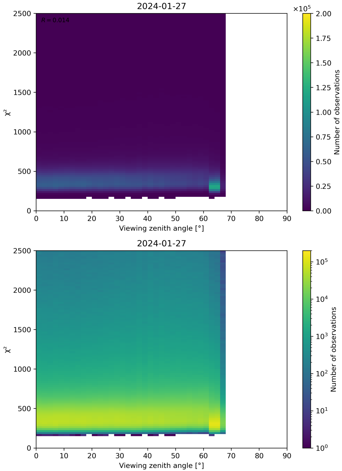
Figure 162: Scatter density plot of “Viewing zenith angle” against “ \chi^2 ” for 2024-01-26 to 2024-01-28.
