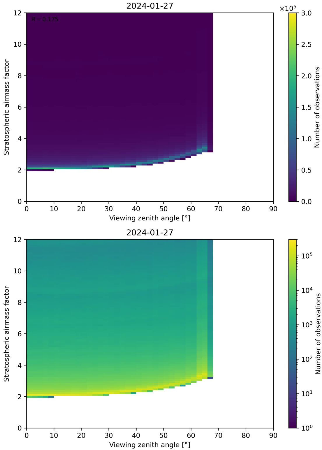
Figure 159: Scatter density plot of “Viewing zenith angle” against “Stratospheric airmass factor” for 2024-01-26 to 2024-01-28.
