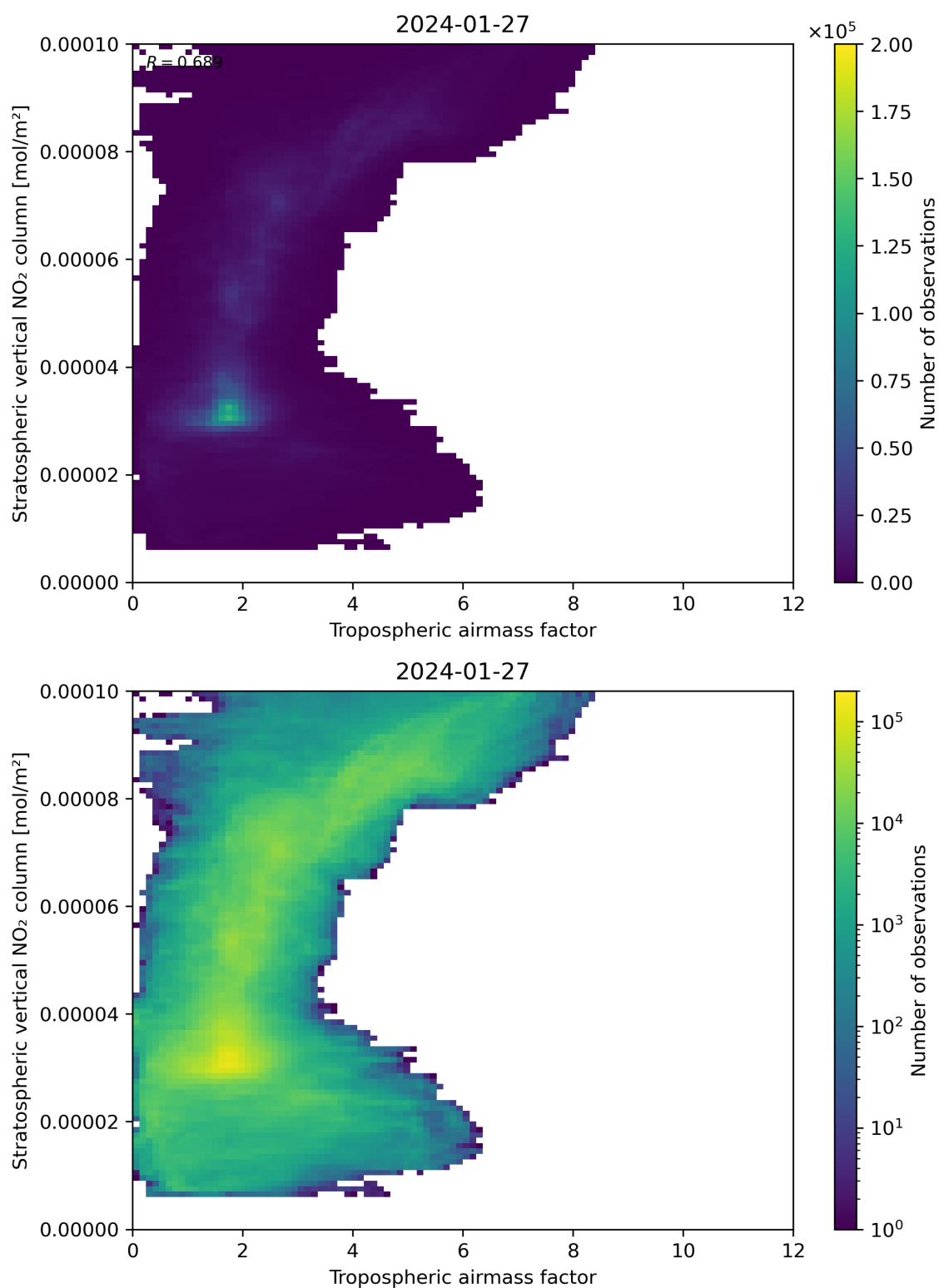
Figure 74: Scatter density plot of “Tropospheric airmass factor” against “Stratospheric vertical NO 2 column” for 2024-01-26 to 2024-01-28.
