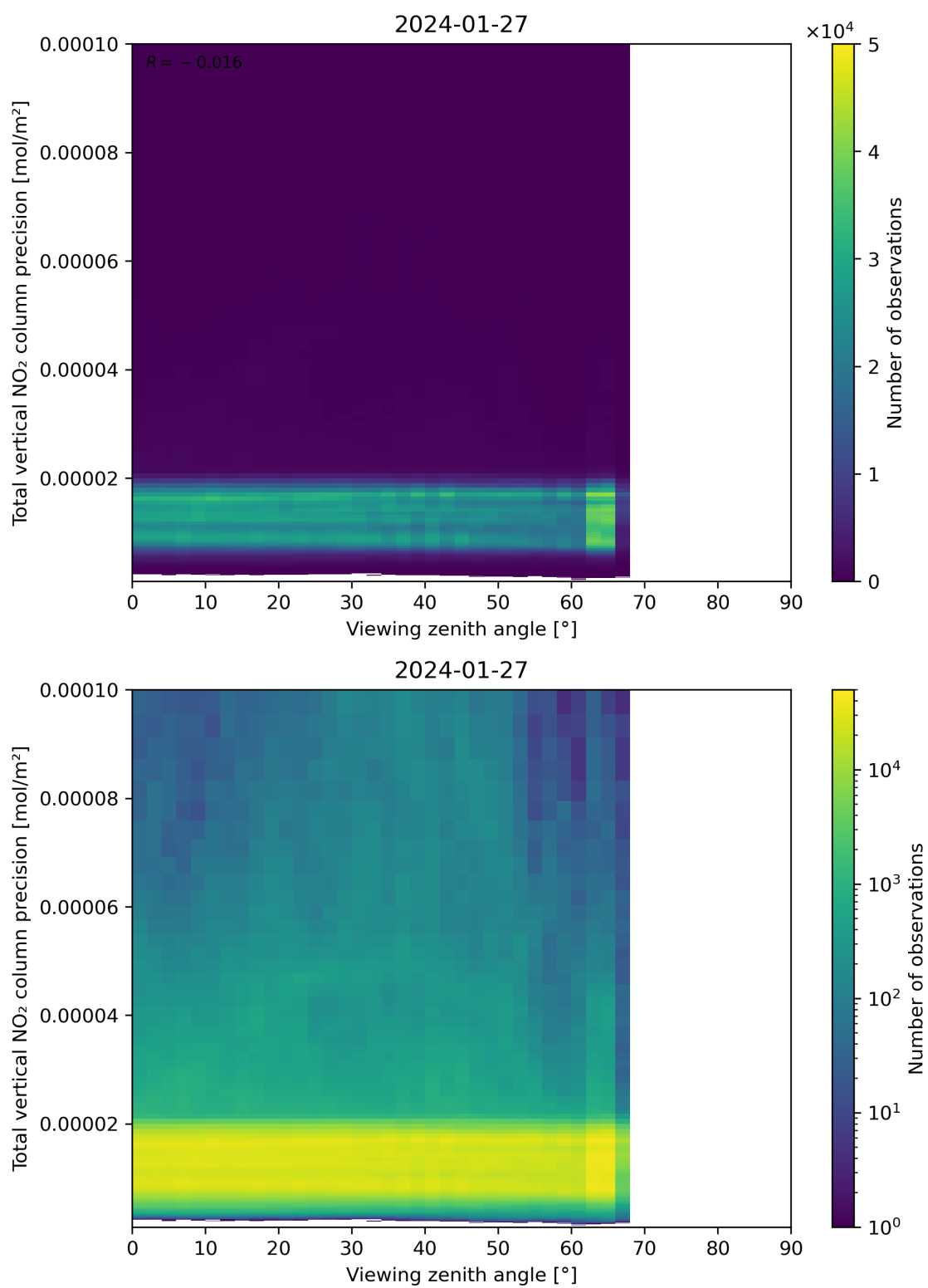
Figure 168: Scatter density plot of “Viewing zenith angle” against “Total vertical NO 2 column precision” for 2024-01-26 to 2024-01-28.
