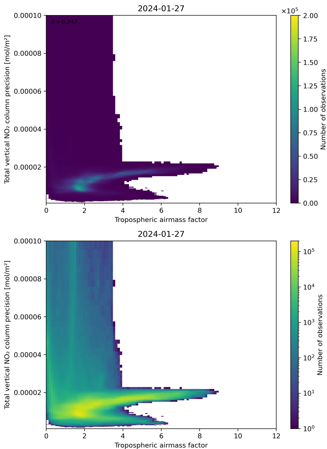
Figure 78: Scatter density plot of “Tropospheric air mass factor” against “Total vertical NO 2 column precision” for 2024-01-26 to 2024-01-28.
