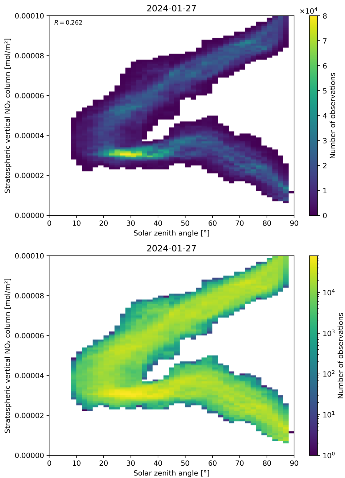
Figure 150: Scatter density plot of “Solar zenith angle” against “Stratospheric vertical NO 2 column” for 2024-01-26 to 2024-01-28.
