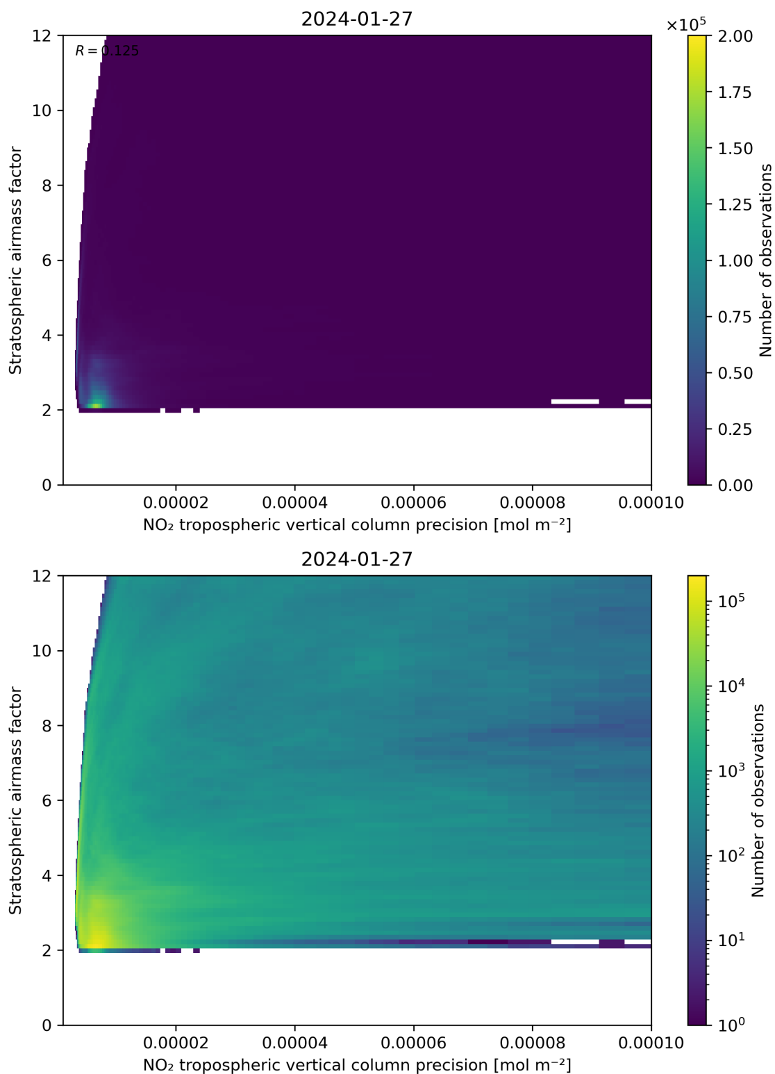
Figure 131: Scatter density plot of “NO 2 tropospheric vertical column precision” against “Stratospheric airmass factor” for 2024-01-26 to 2024-01-28.
