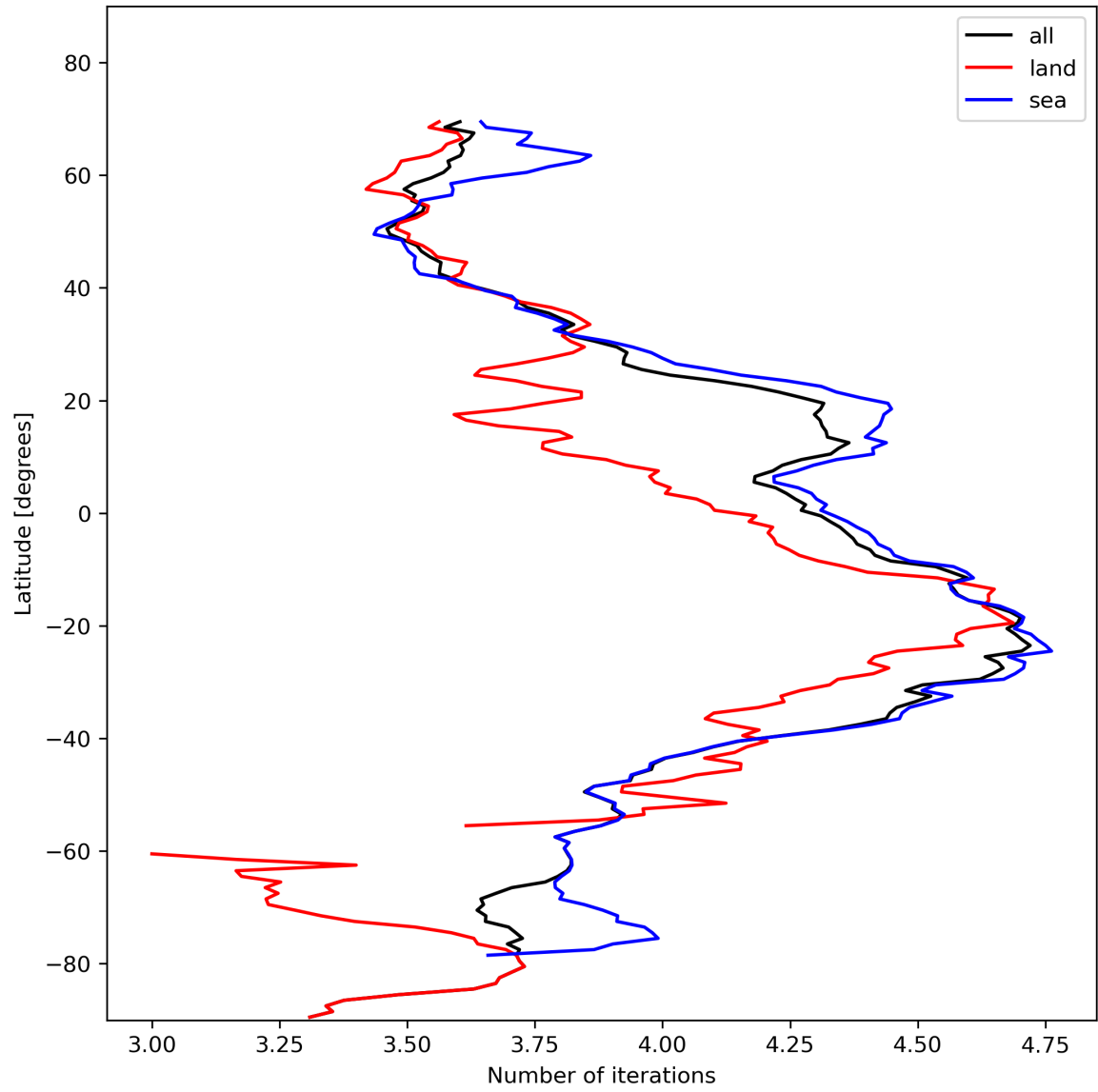
Figure 17: Zonal average of “Number of iterations” for 2024-01-26 to 2024-01-28.
