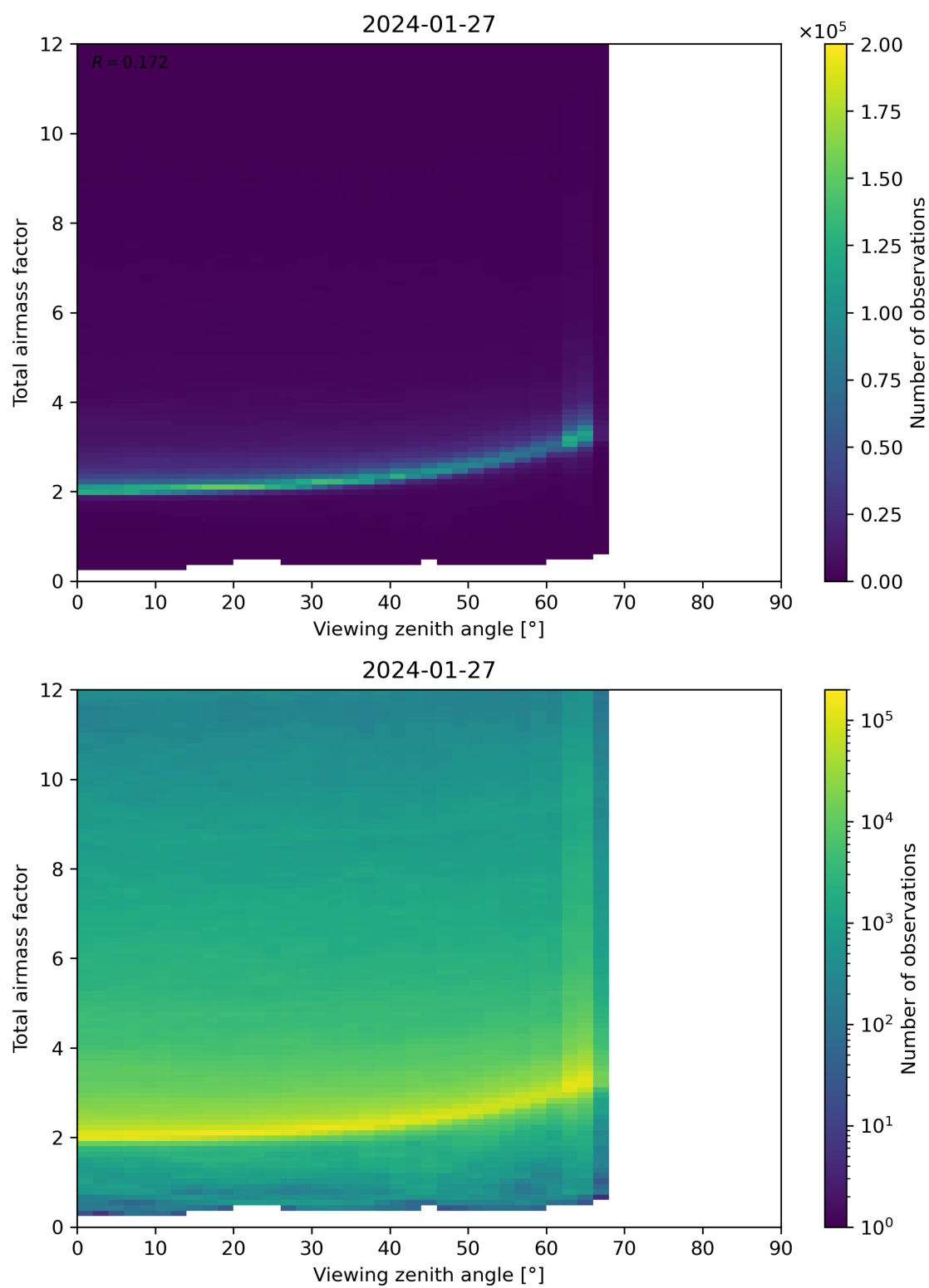
Figure 160: Scatter density plot of “Viewing zenith angle” against “Total airmass factor” for 2024-01-26 to 2024-01-28.
