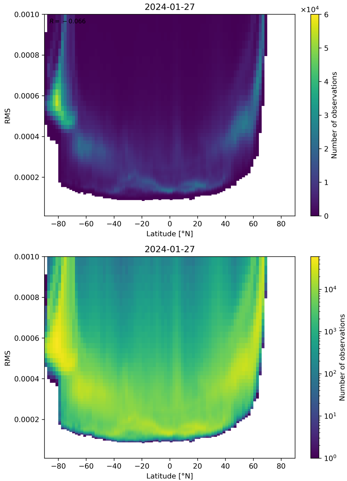
Figure 94: Scatter density plot of “Latitude” against “RMS” for 2024-01-26 to 2024-01-28.
