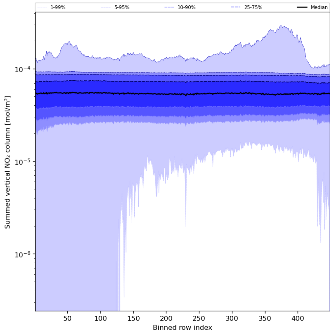
Figure 57: Along track statistics of “Summed vertical NO 2 column” for 2024-01-26 to 2024-01-28
