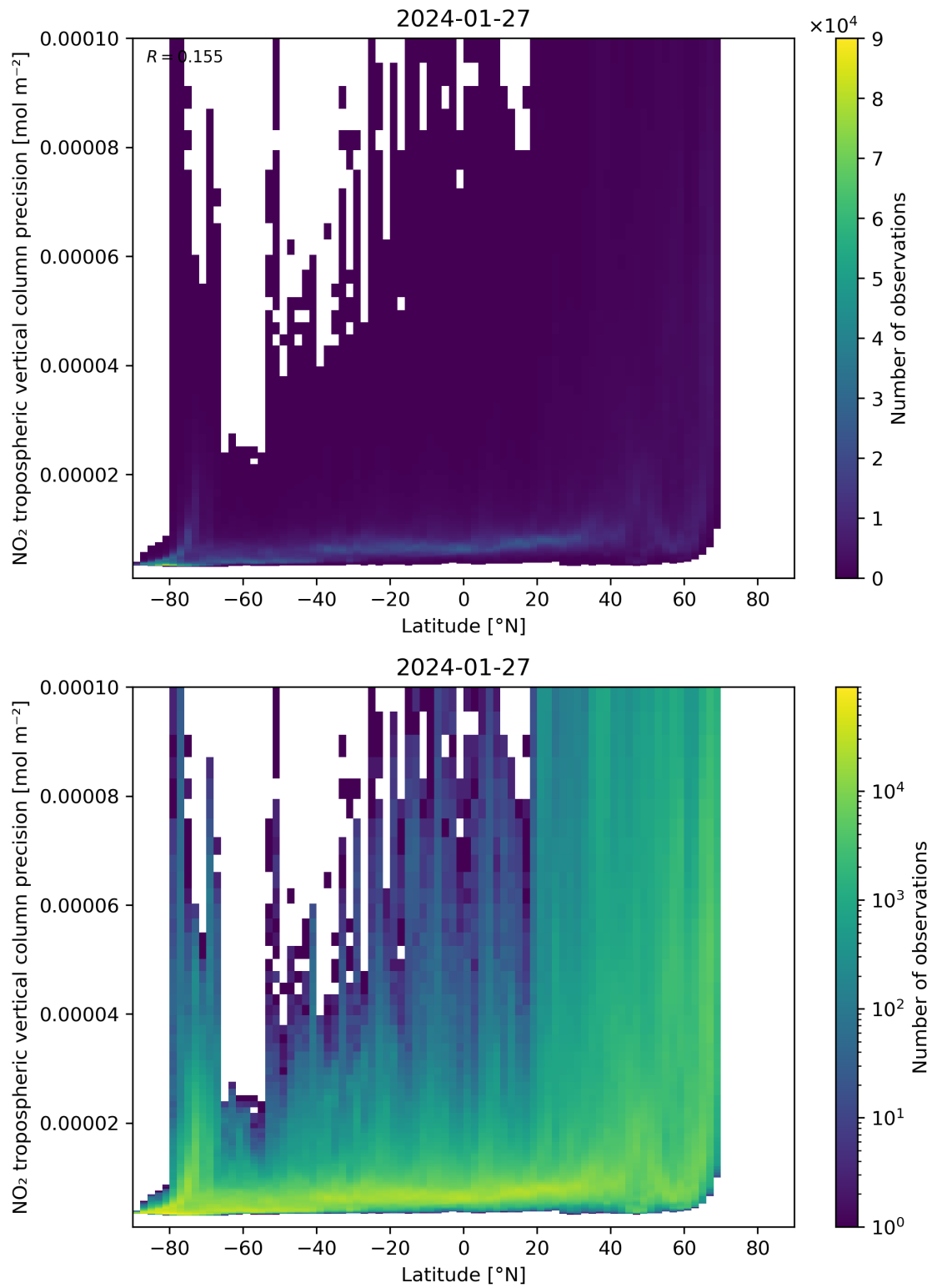
Figure 93: Scatter density plot of “Latitude” against “NO 2 tropospheric vertical column precision” for 2024-01-26 to 2024-01-28.
