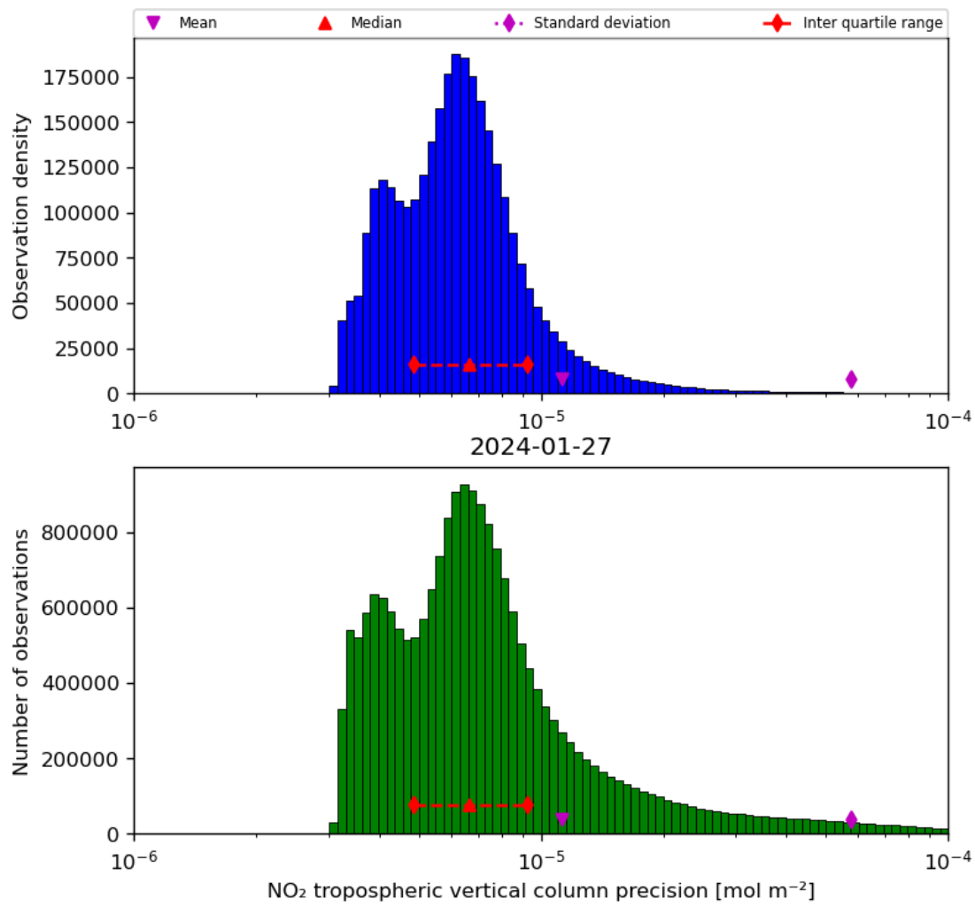
Figure 30: Histogram of “NO 2 tropospheric vertical column precision” for 2024-01-26 to 2024-01-28
