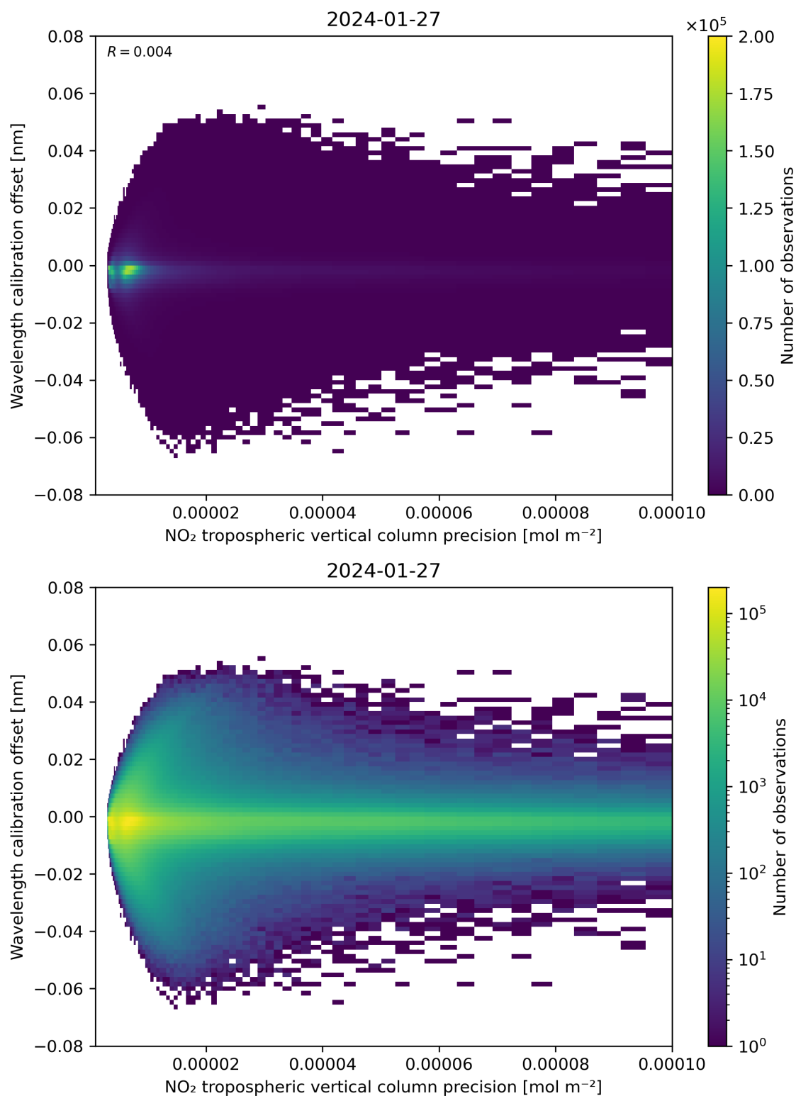
Figure 141: Scatter density plot of “NO 2 tropospheric vertical column precision” against “Wavelength calibration offset” for 2024-01-26 to 2024-01-28.
