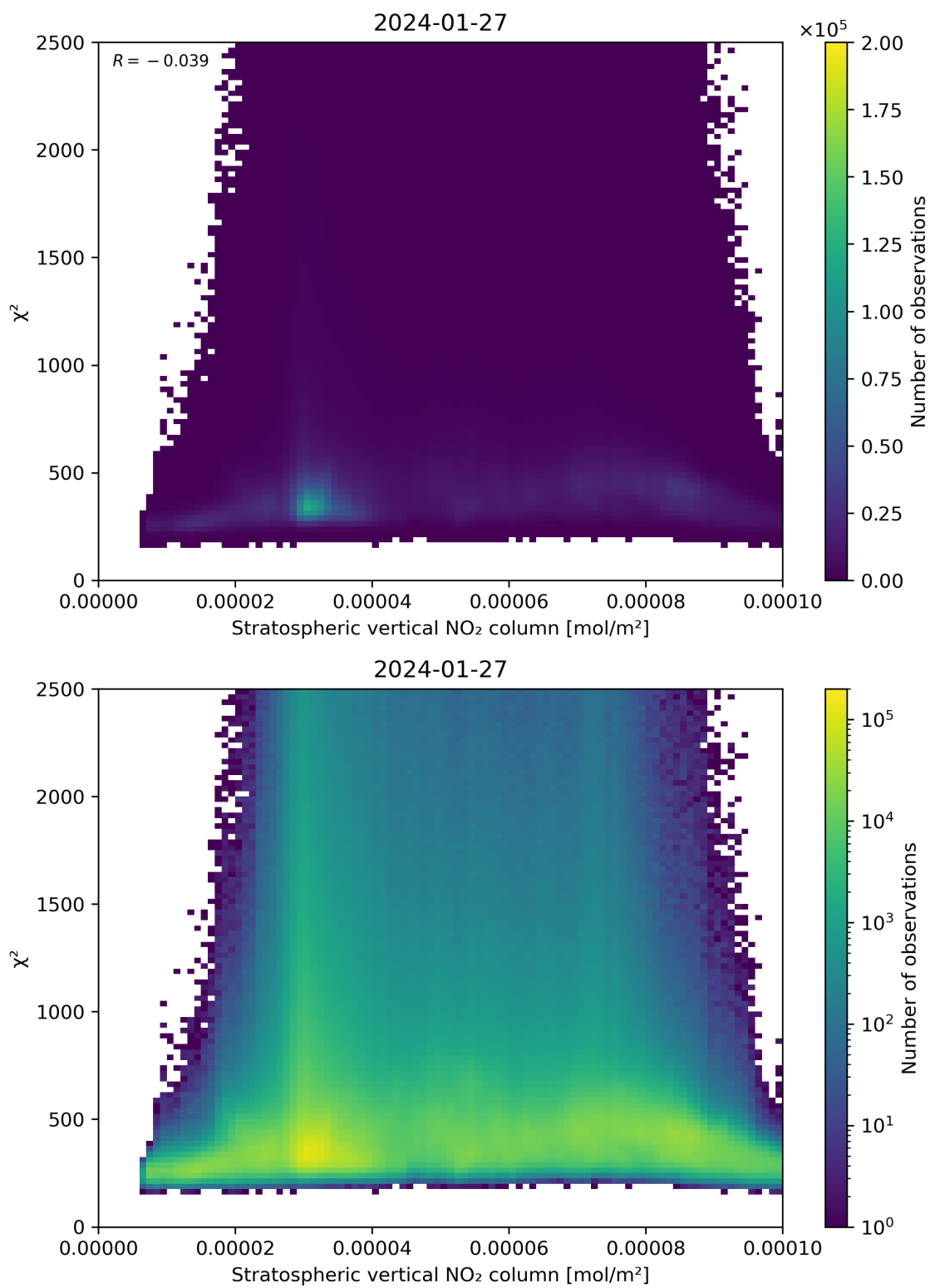
Figure 97: Scatter density plot of “Stratospheric vertical NO 2 column” against “ \chi^2 ” for 2024-01-26 to 2024-01-28.
