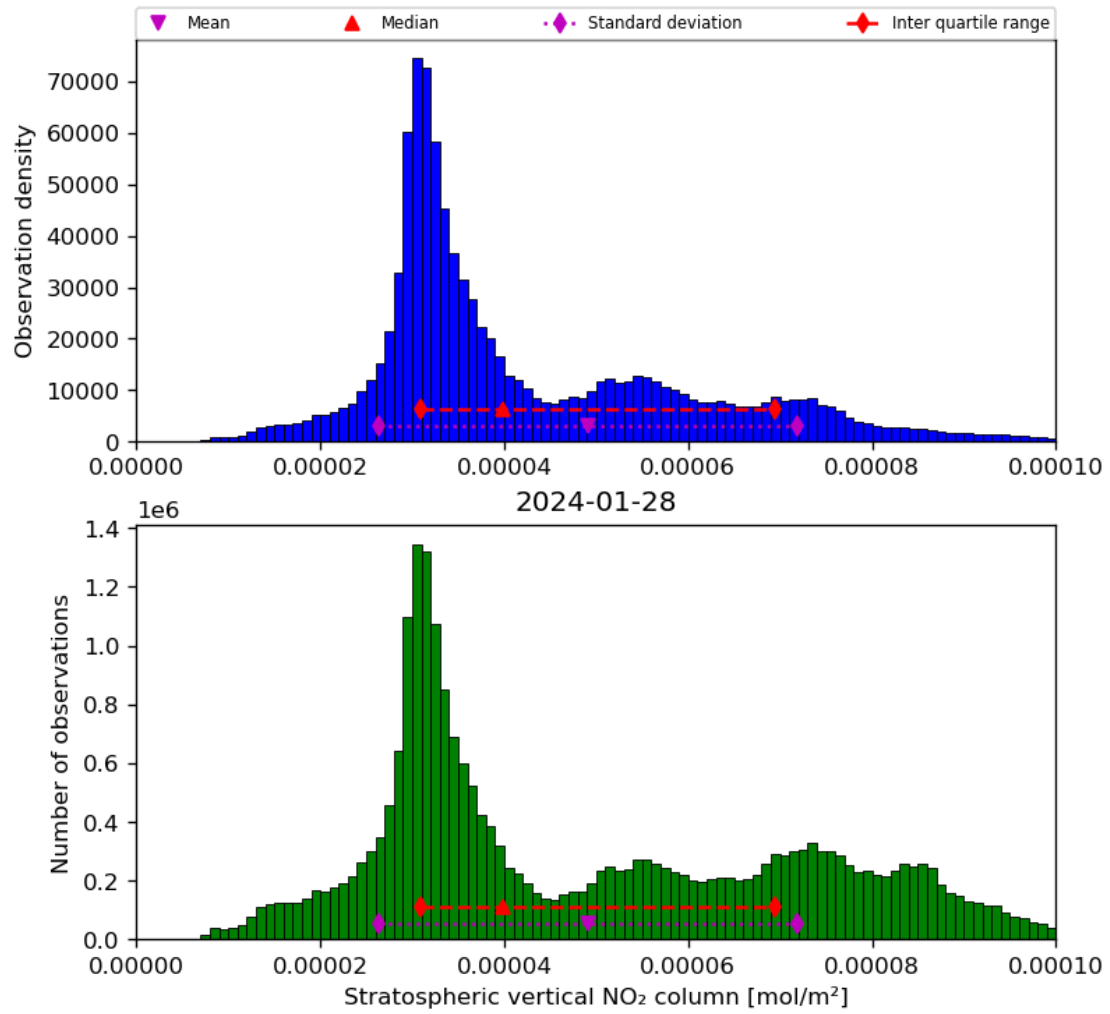
Figure 36: Histogram of “Stratospheric vertical NO 2 column” for 2024-01-27 to 2024-01-29
