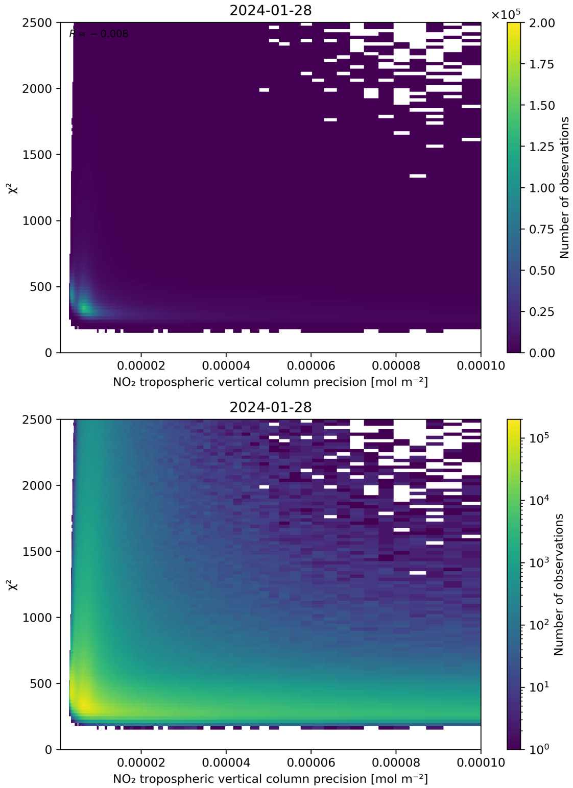
Figure 134: Scatter density plot of “NO 2 tropospheric vertical column precision” against “ \chi^2 ” for 2024-01-27 to 2024-01-29.
