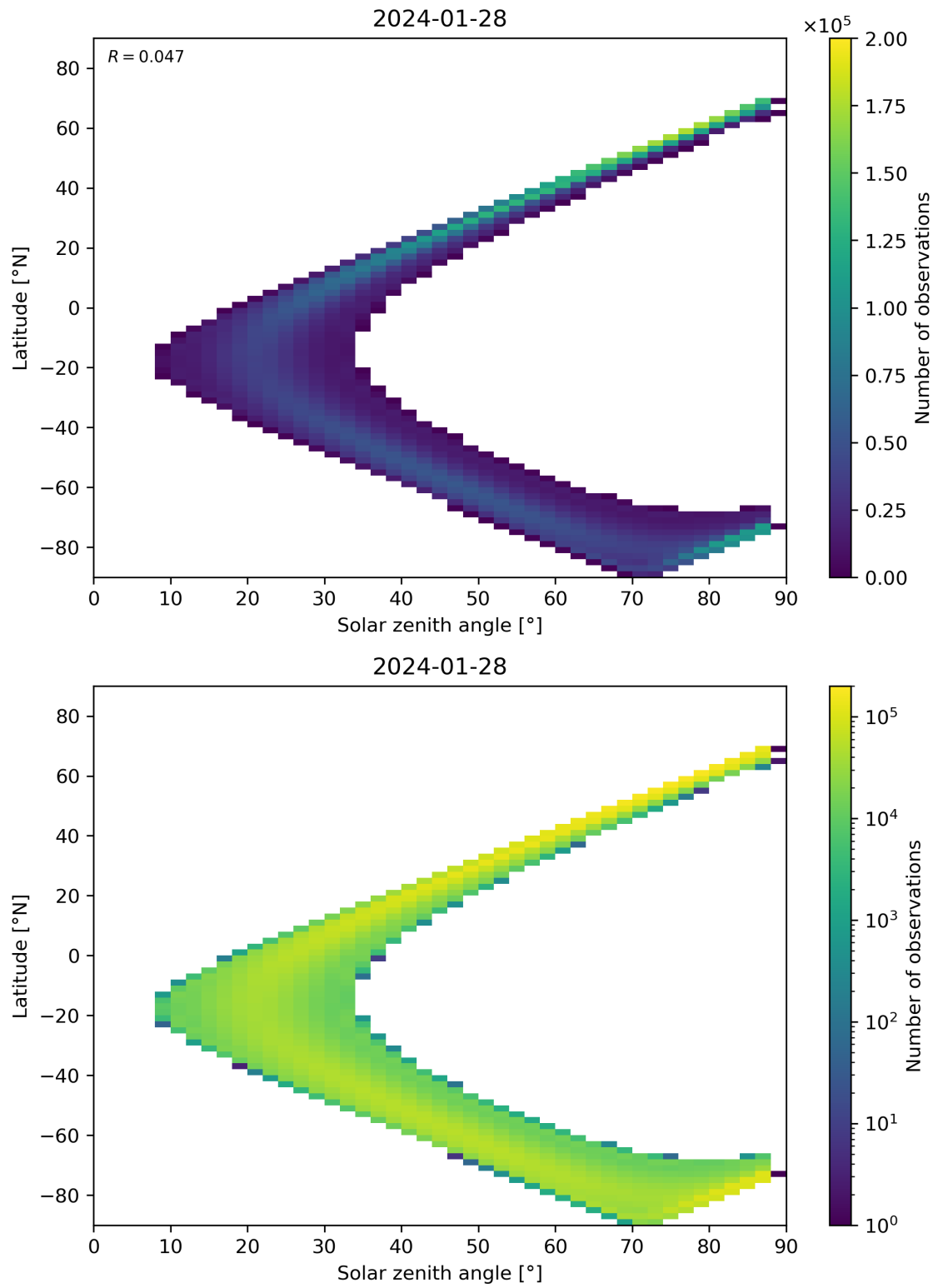
Figure 149: Scatter density plot of “Solar zenith angle” against “Latitude” for 2024-01-27 to 2024-01-29.
