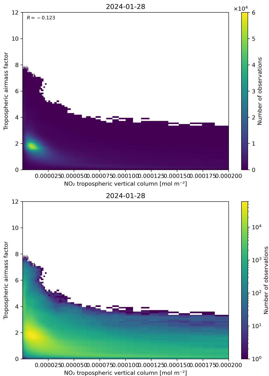
Figure 123: Scatter density plot of “NO 2 tropospheric vertical column” against “Tropospheric air mass factor” for 2024-01-27 to 2024-01-29.
