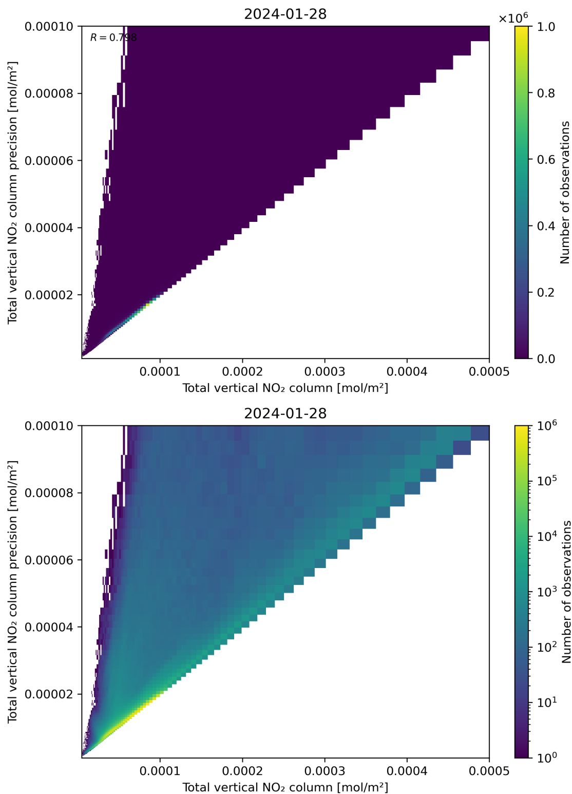
Figure 114: Scatter density plot of “Total vertical NO 2 column” against “Total vertical NO 2 column precision” for 2024-01-27 to 2024-01-29.
