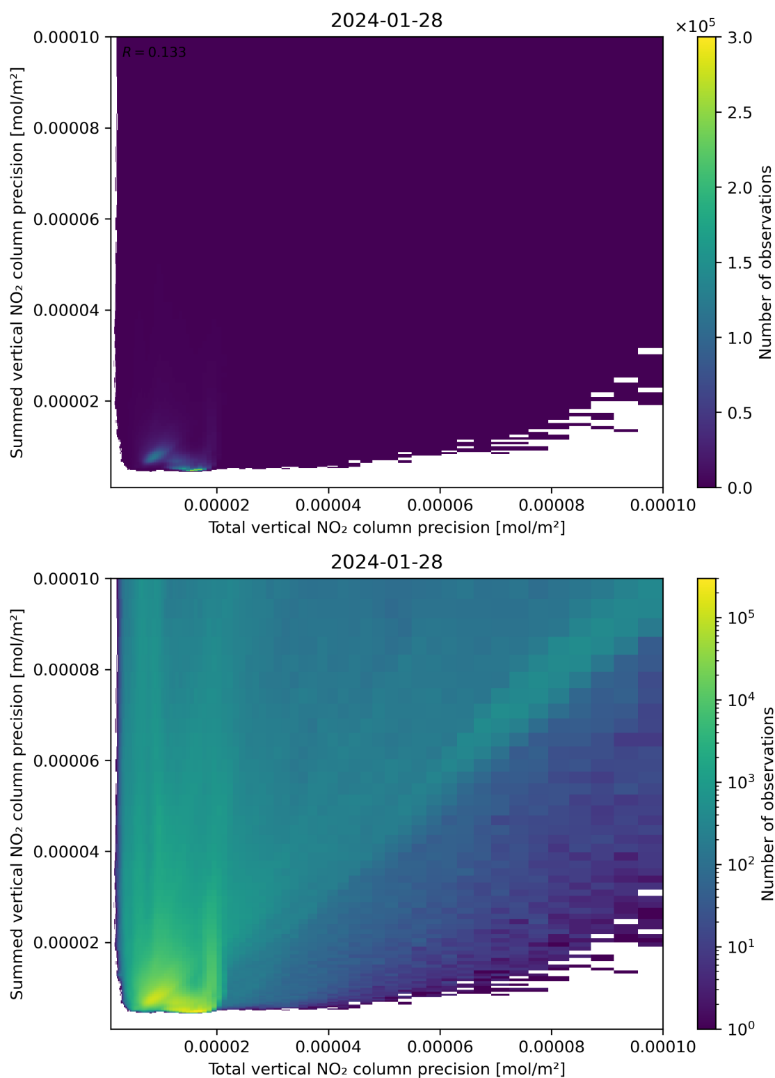
Figure 118: Scatter density plot of “Total vertical NO 2 column precision” against “Summed vertical NO 2 column precision” for 2024-01-27 to 2024-01-29.
