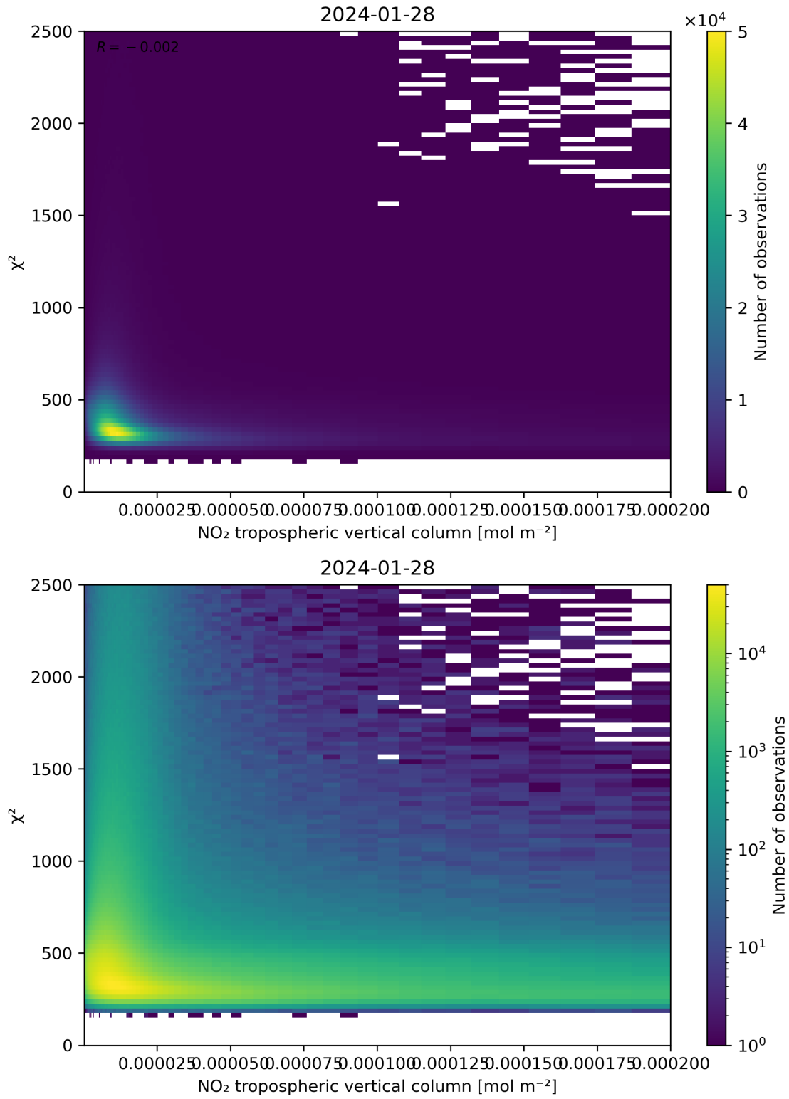
Figure 124: Scatter density plot of “NO 2 tropospheric vertical column” against “ \chi^2 ” for 2024-01-27 to 2024-01-29.
