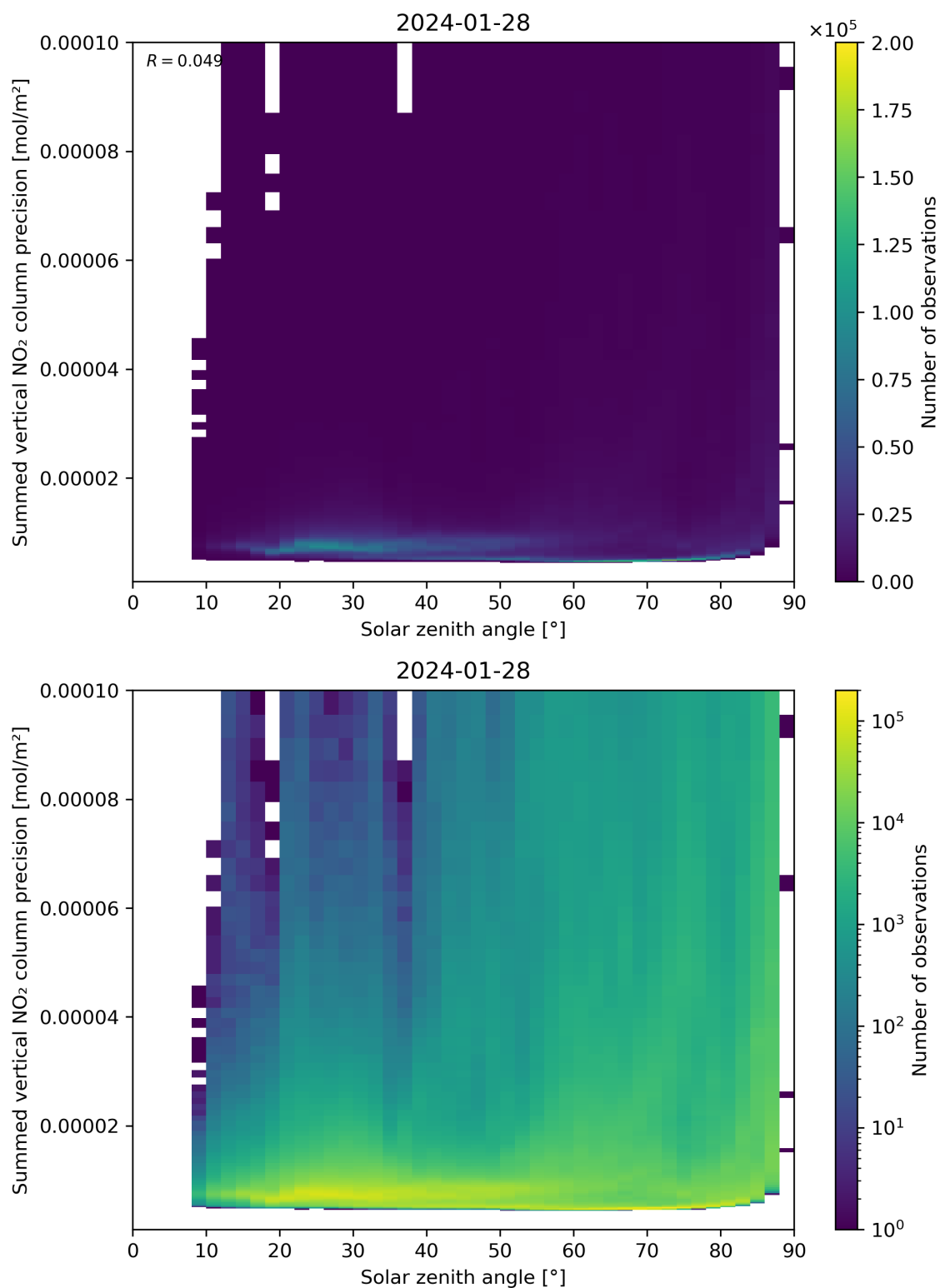
Figure 152: Scatter density plot of “Solar zenith angle” against “Summed vertical NO 2 column precision” for 2024-01-27 to 2024-01-29.
