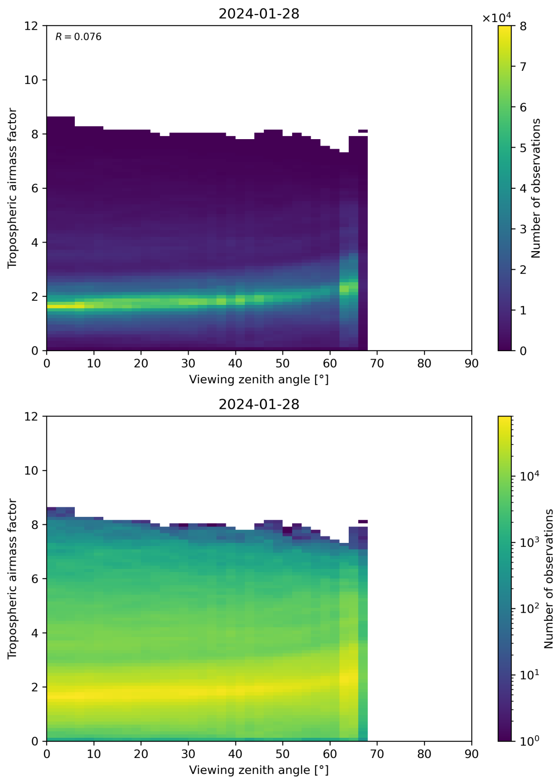
Figure 161: Scatter density plot of “Viewing zenith angle” against “Tropospheric airmass factor” for 2024-01-27 to 2024-01-29.
