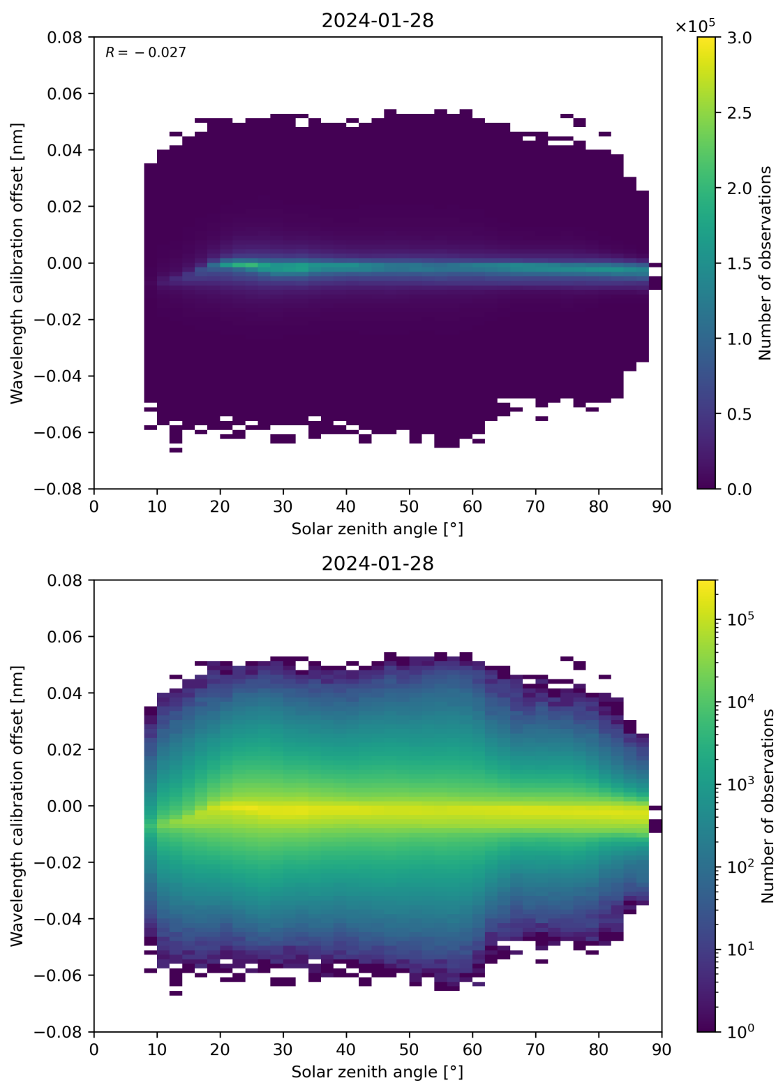
Figure 158: Scatter density plot of “Solar zenith angle” against “Wavelength calibration offset” for 2024-01-27 to 2024-01-29.
