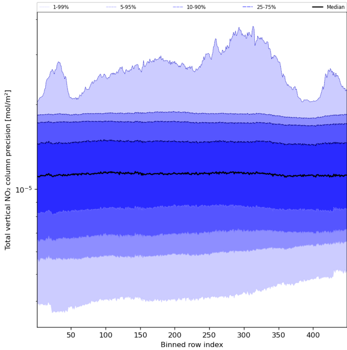
Figure 56: Along track statistics of “Total vertical NO 2 column precision” for 2024-01-27 to 2024-01-29
