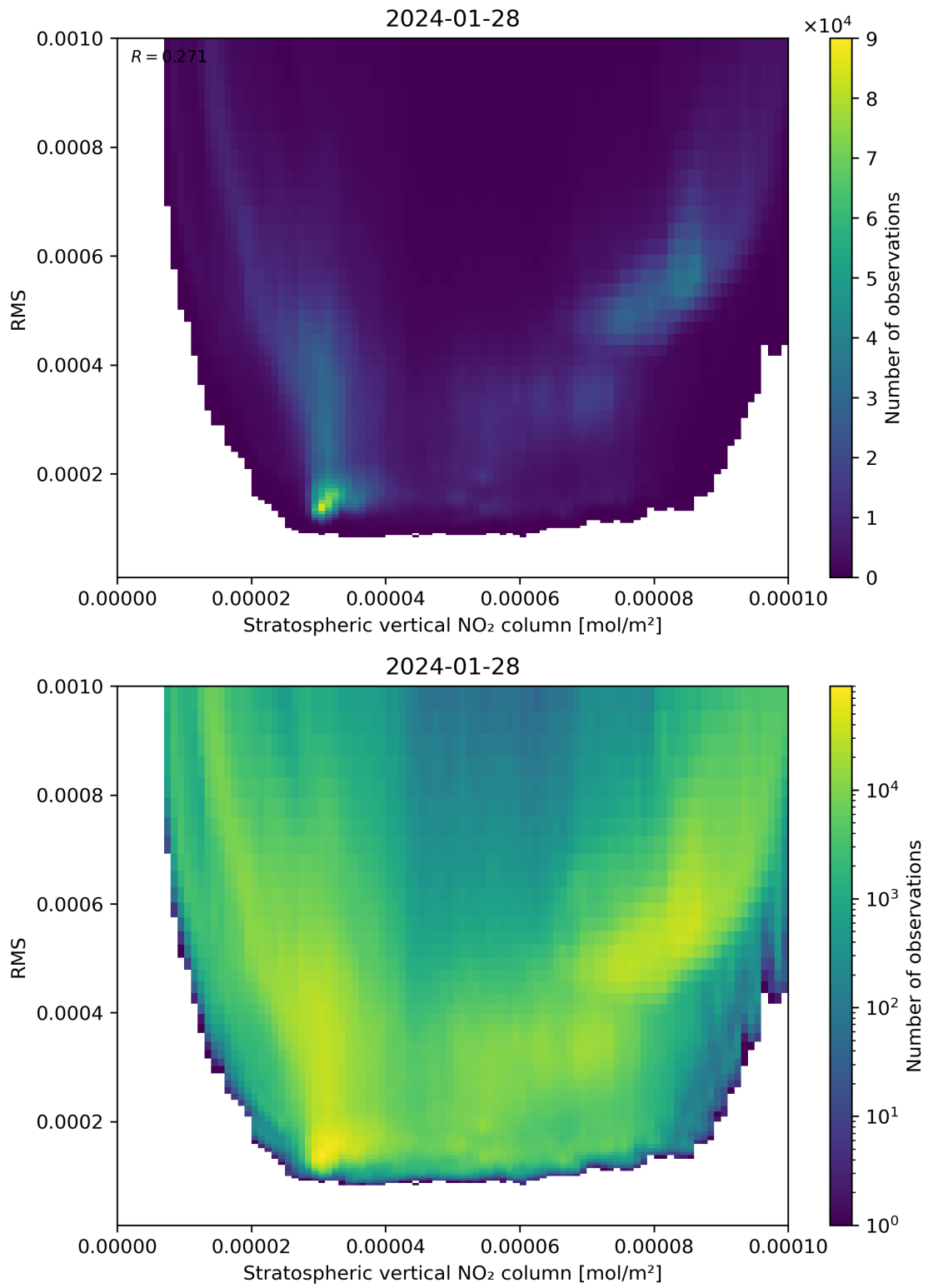
Figure 102: Scatter density plot of “Stratospheric vertical NO 2 column” against “RMS” for 2024-01-27 to 2024-01-29.
