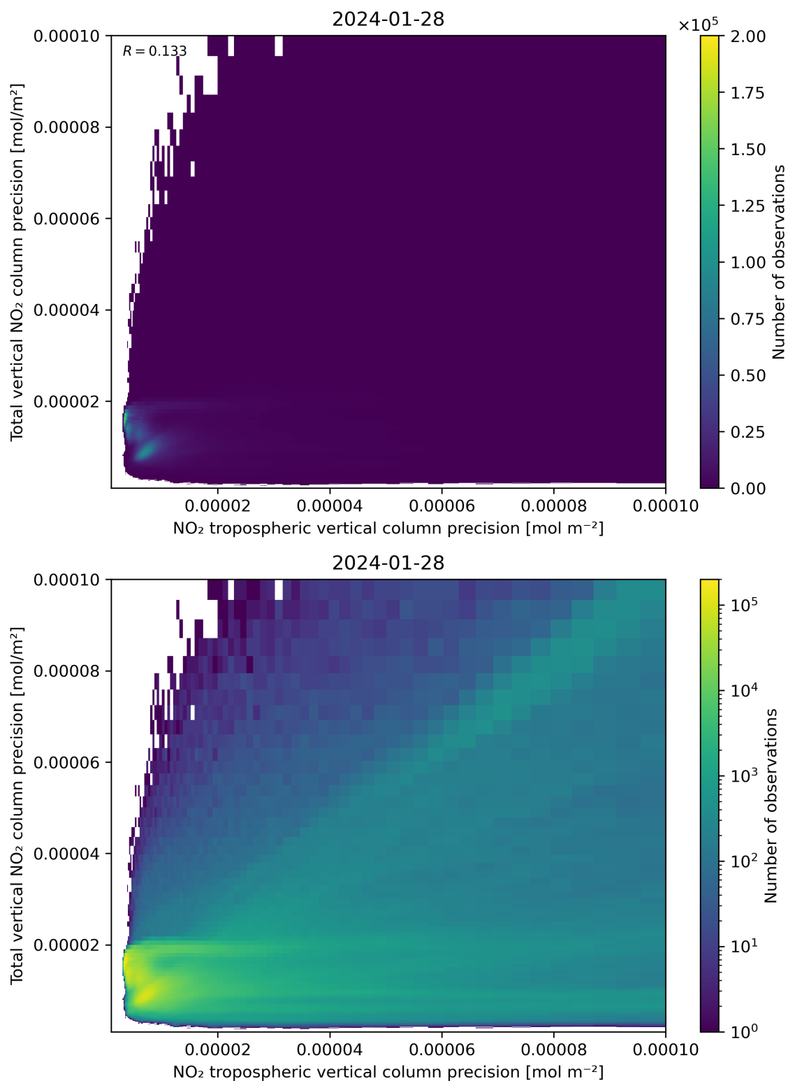
Figure 139: Scatter density plot of “NO 2 tropospheric vertical column precision” against “Total vertical NO 2 column precision” for 2024-01-27 to 2024-01-29.
