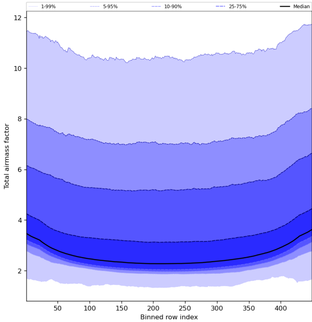
Figure 49: Along track statistics of “Total airmass factor” for 2024-01-27 to 2024-01-29
