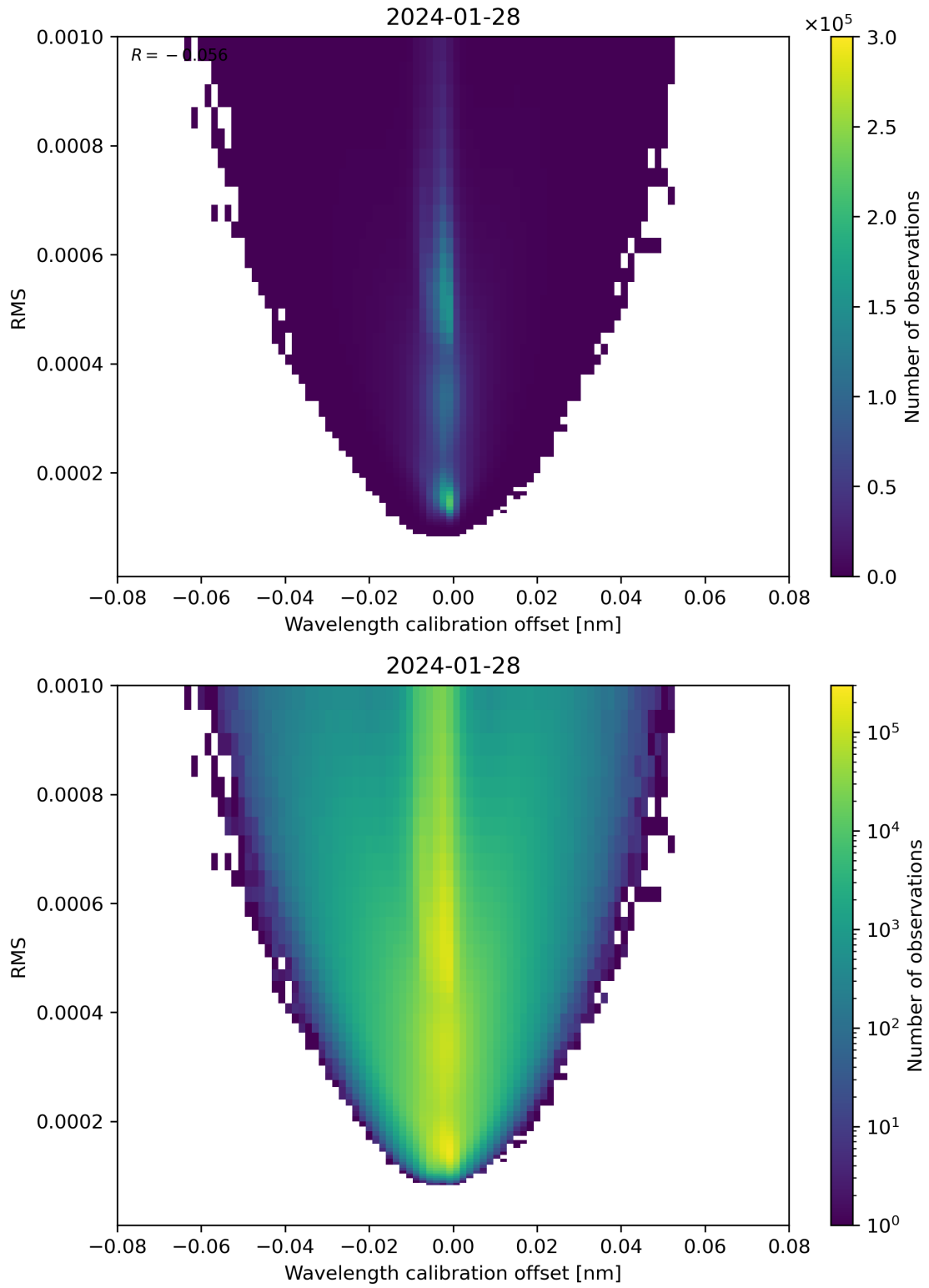
Figure 181: Scatter density plot of “Wavelength calibration offset” against “RMS” for 2024-01-27 to 2024-01-29.
