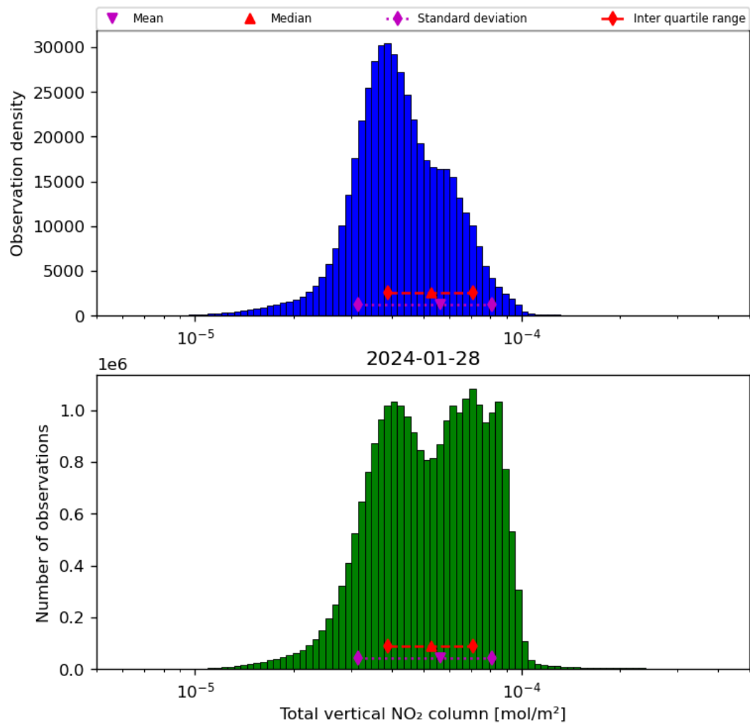
Figure 38: Histogram of “Total vertical NO 2 column” for 2024-01-27 to 2024-01-29
