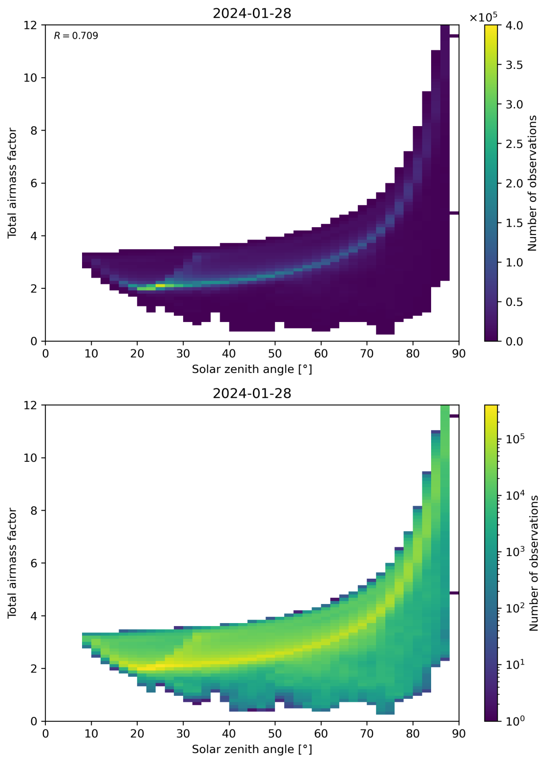
Figure 146: Scatter density plot of “Solar zenith angle” against “Total air mass factor” for 2024-01-27 to 2024-01-29.
