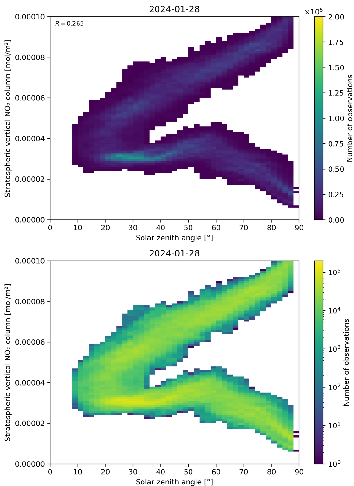
Figure 150: Scatter density plot of “Solar zenith angle” against “Stratospheric vertical NO 2 column” for 2024-01-27 to 2024-01-29.
