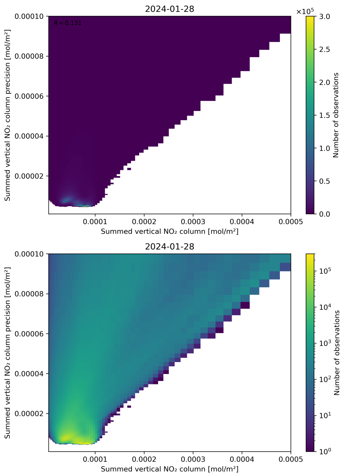
Figure 105: Scatter density plot of “Summed vertical NO 2 column” against “Summed vertical NO 2 column precision” for 2024-01-27 to 2024-01-29.
