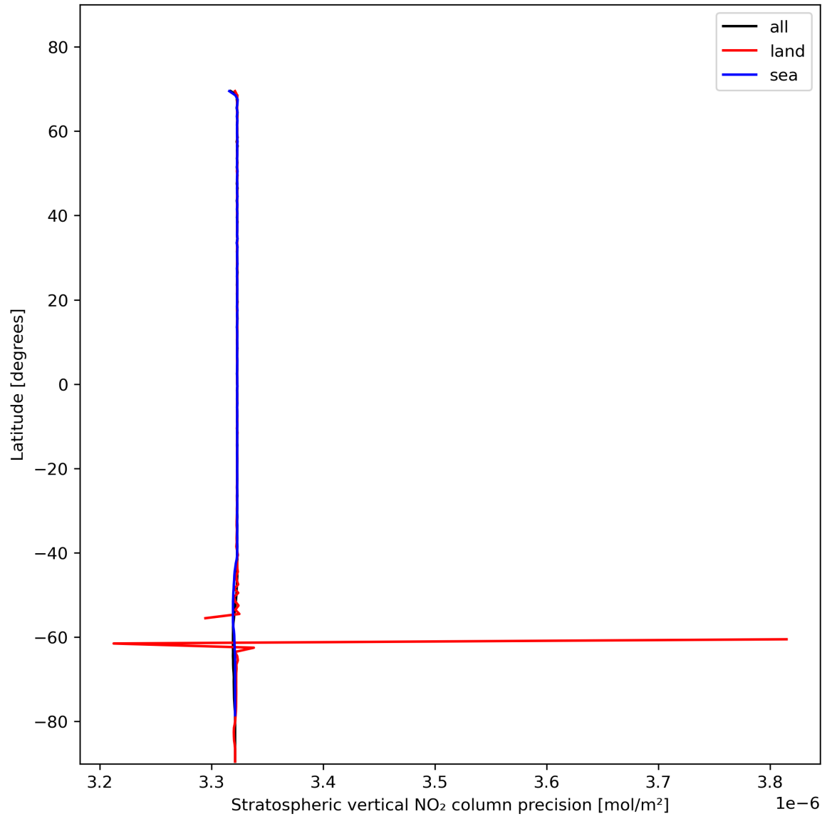
Figure 20: Zonal average of “Stratospheric vertical NO 2 column precision” for 2024-01-27 to 2024-01-29.
