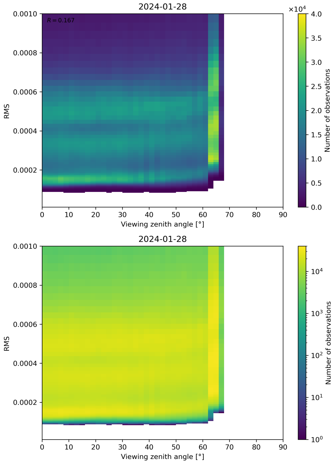
Figure 171: Scatter density plot of “Viewing zenith angle” against “RMS” for 2024-01-27 to 2024-01-29.
