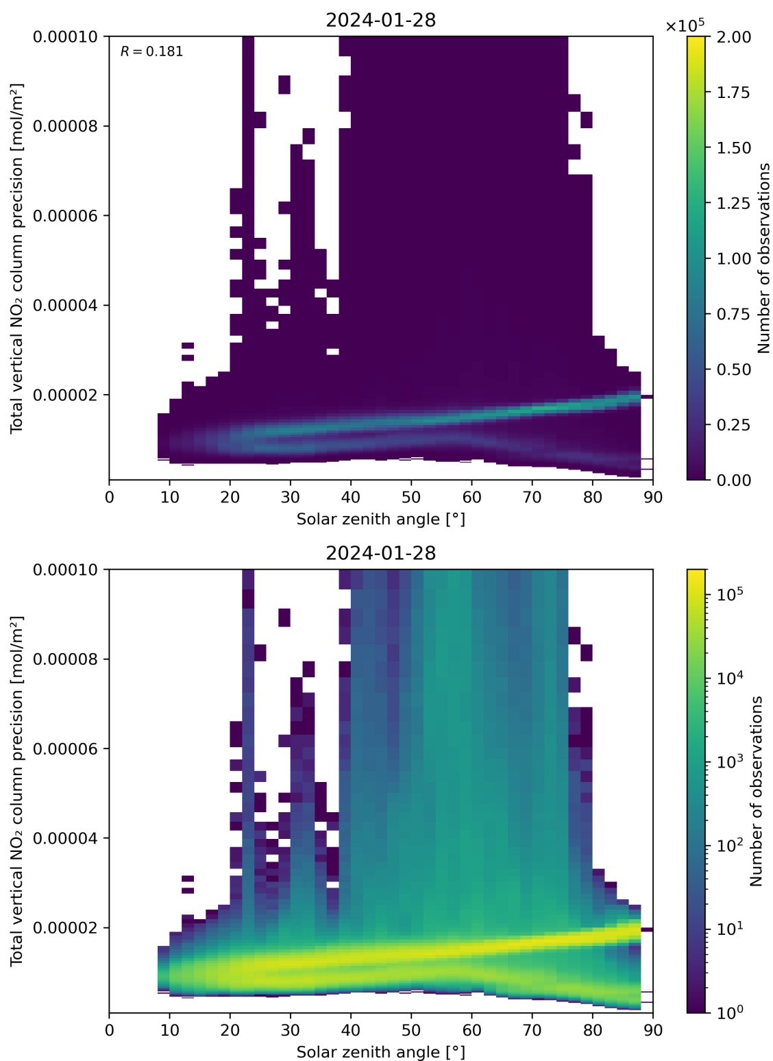
Figure 154: Scatter density plot of “Solar zenith angle” against “Total vertical NO 2 column precision” for 2024-01-27 to 2024-01-29.
