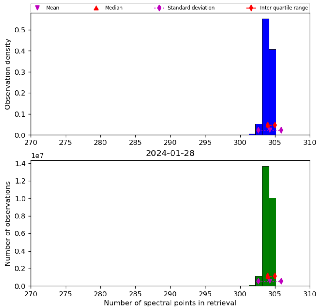
Figure 33: Histogram of “Number of spectral points in retrieval” for 2024-01-27 to 2024-01-29
