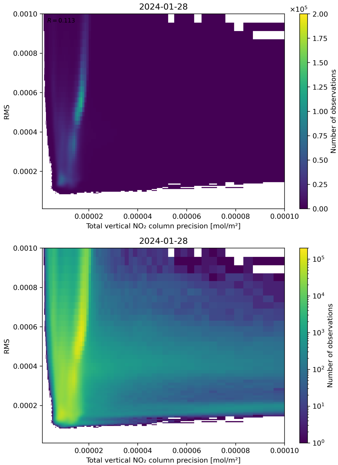
Figure 119: Scatter density plot of “Total vertical NO 2 column precision” against “RMS” for 2024-01-27 to 2024-01-29.
