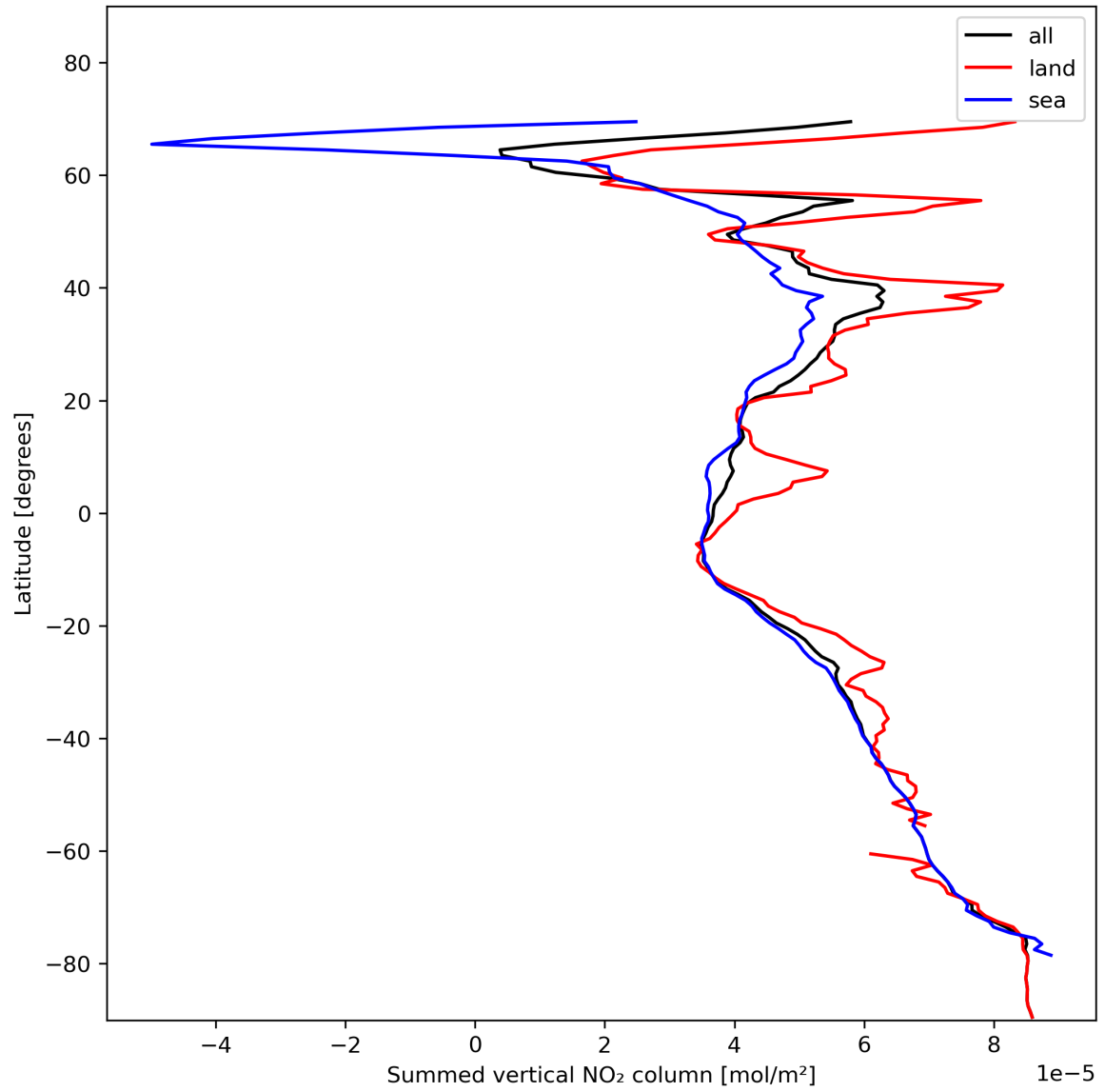
Figure 23: Zonal average of “Summed vertical NO 2 column” for 2024-01-27 to 2024-01-29.
