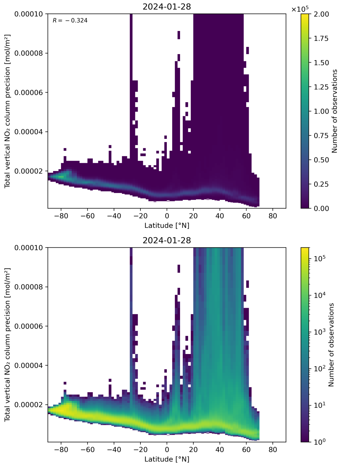
Figure 91: Scatter density plot of “Latitude” against “Total vertical NO 2 column precision” for 2024-01-27 to 2024-01-29.
