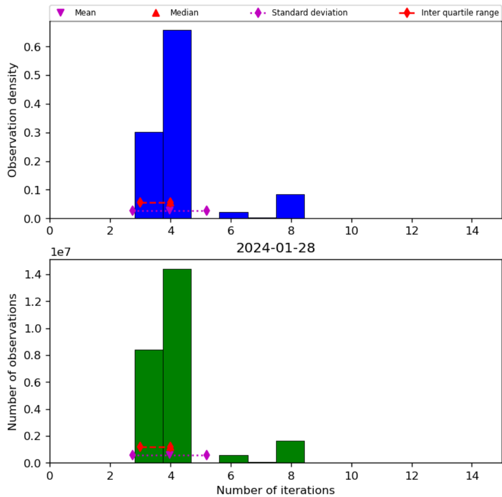
Figure 34: Histogram of “Number of iterations” for 2024-01-27 to 2024-01-29
