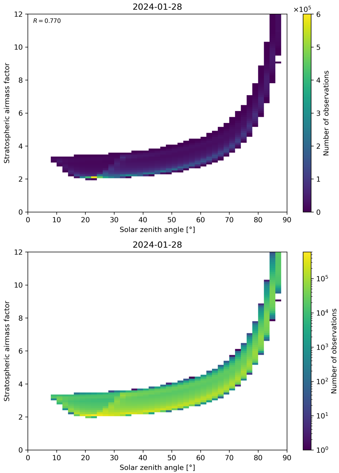
Figure 145: Scatter density plot of “Solar zenith angle” against “Stratospheric airmass factor” for 2024-01-27 to 2024-01-29.
