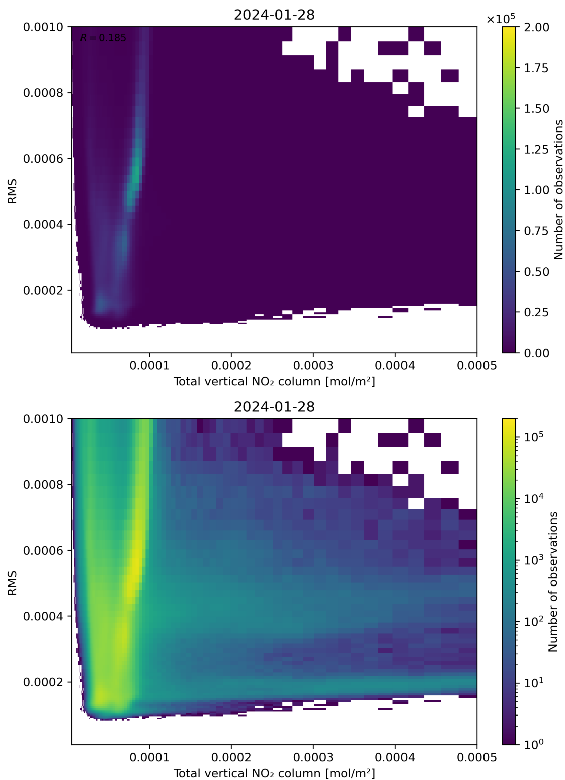
Figure 120: Scatter density plot of “Total vertical NO 2 column” against “RMS” for 2024-01-27 to 2024-01-29.
