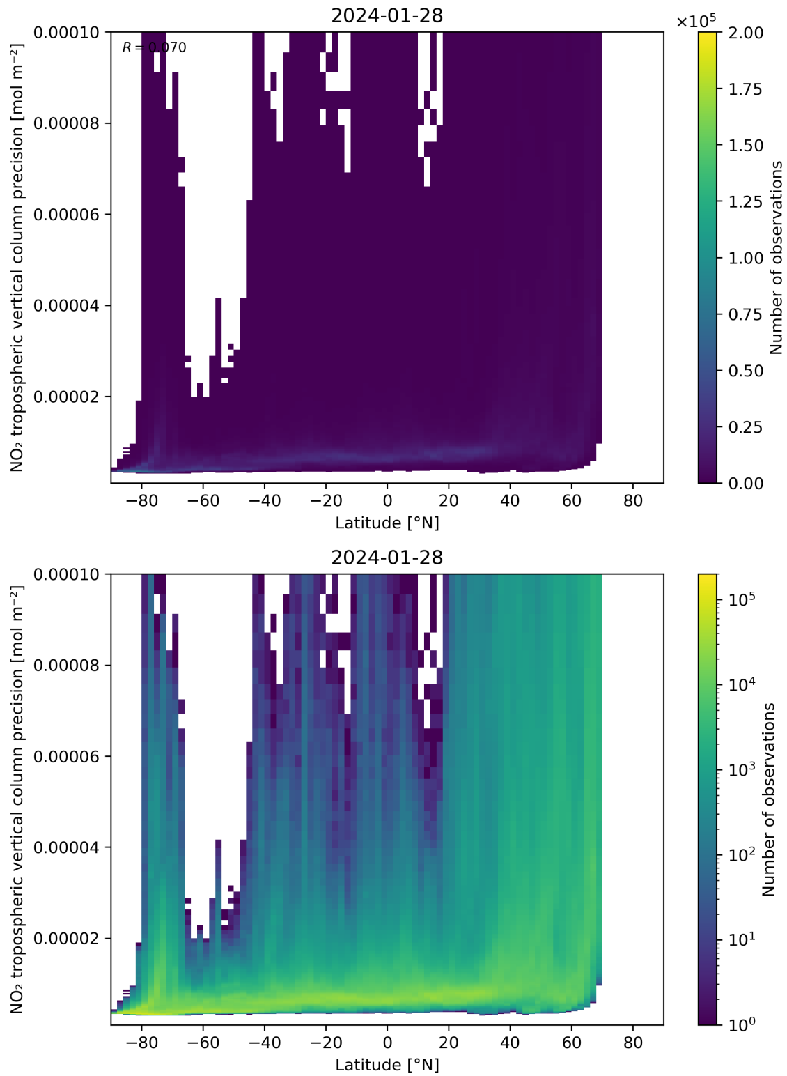
Figure 93: Scatter density plot of “Latitude” against “NO 2 tropospheric vertical column precision” for 2024-01-27 to 2024-01-29.
