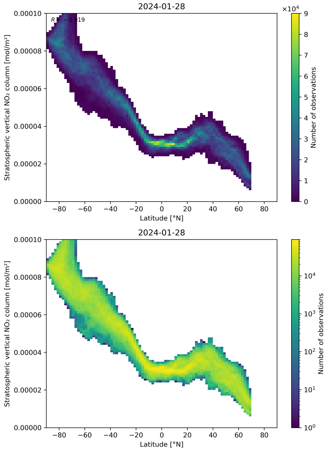
Figure 87: Scatter density plot of “Latitude” against “Stratospheric vertical NO 2 column” for 2024-01-27 to 2024-01-29.
