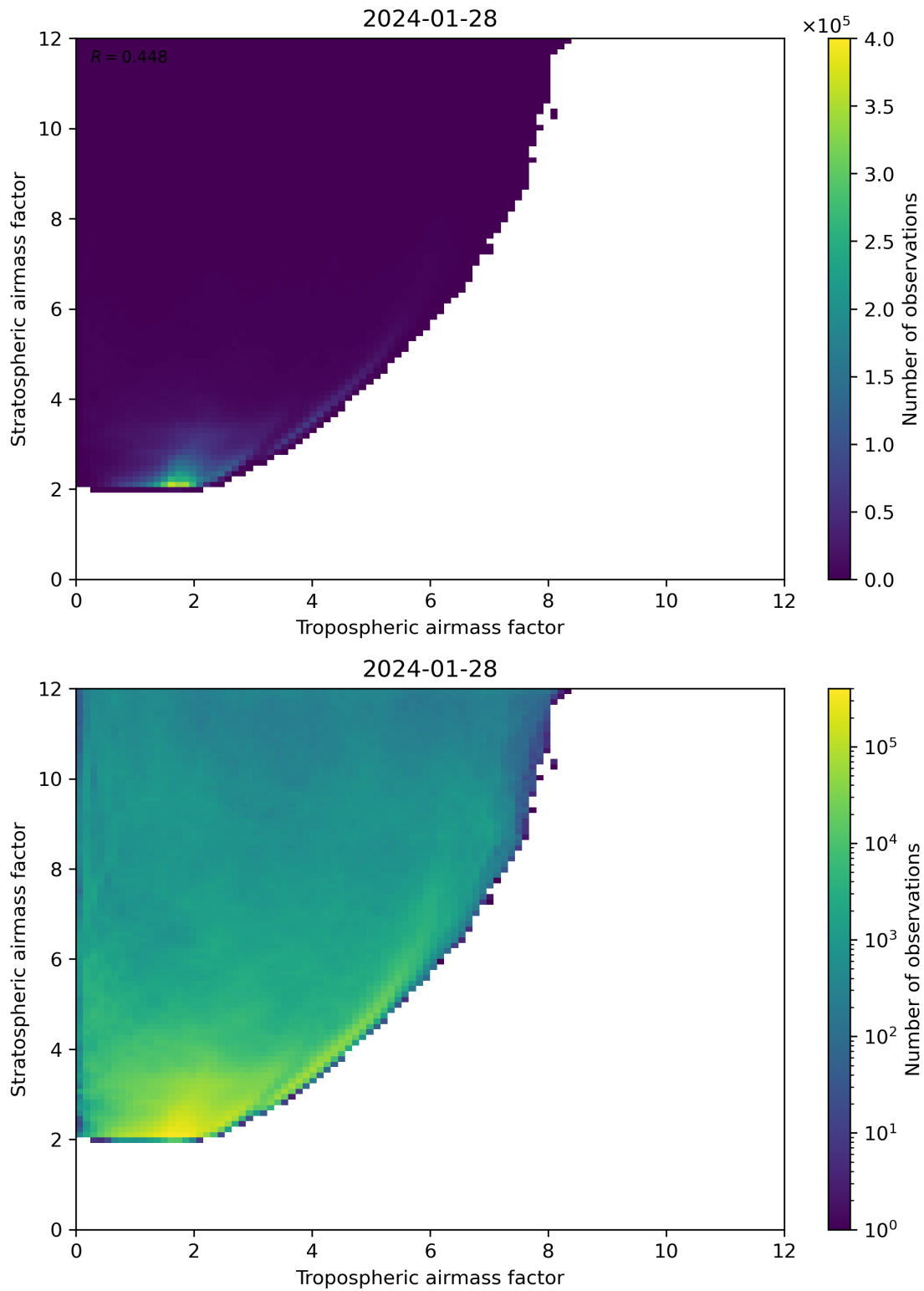
Figure 71: Scatter density plot of “Tropospheric airmass factor” against “Stratospheric airmass factor” for 2024-01-27 to 2024-01-29.
