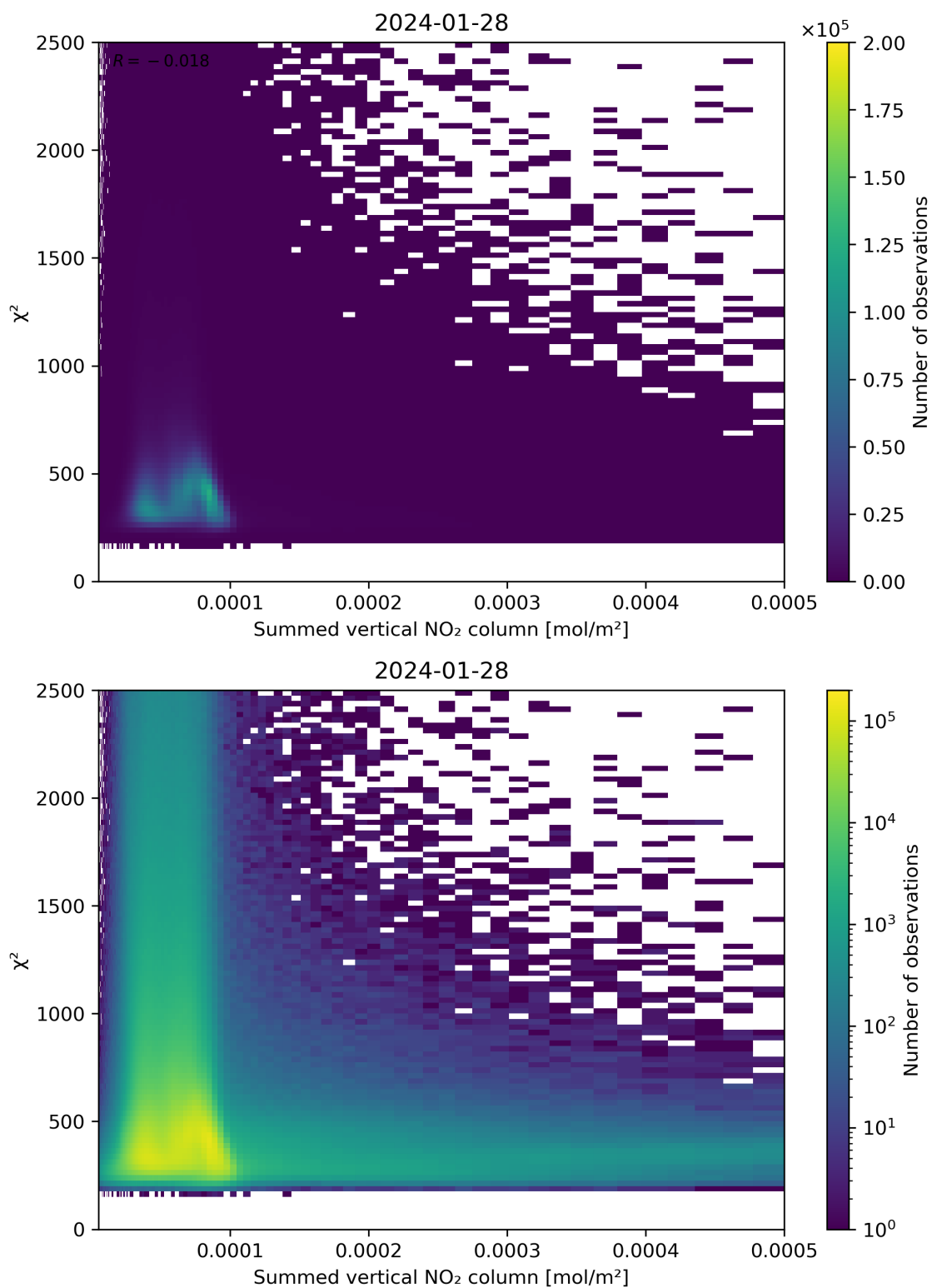
Figure 104: Scatter density plot of “Summed vertical NO 2 column” against “ \chi^2 ” for 2024-01-27 to 2024-01-29.
