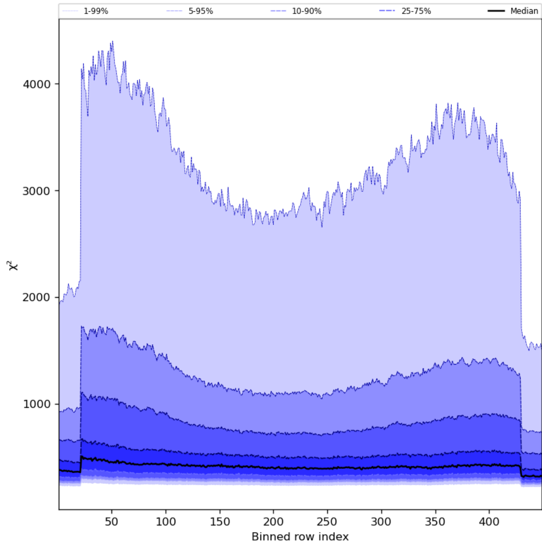
Figure 59: Along track statistics of “ \chi^2 ” for 2024-01-27 to 2024-01-29
