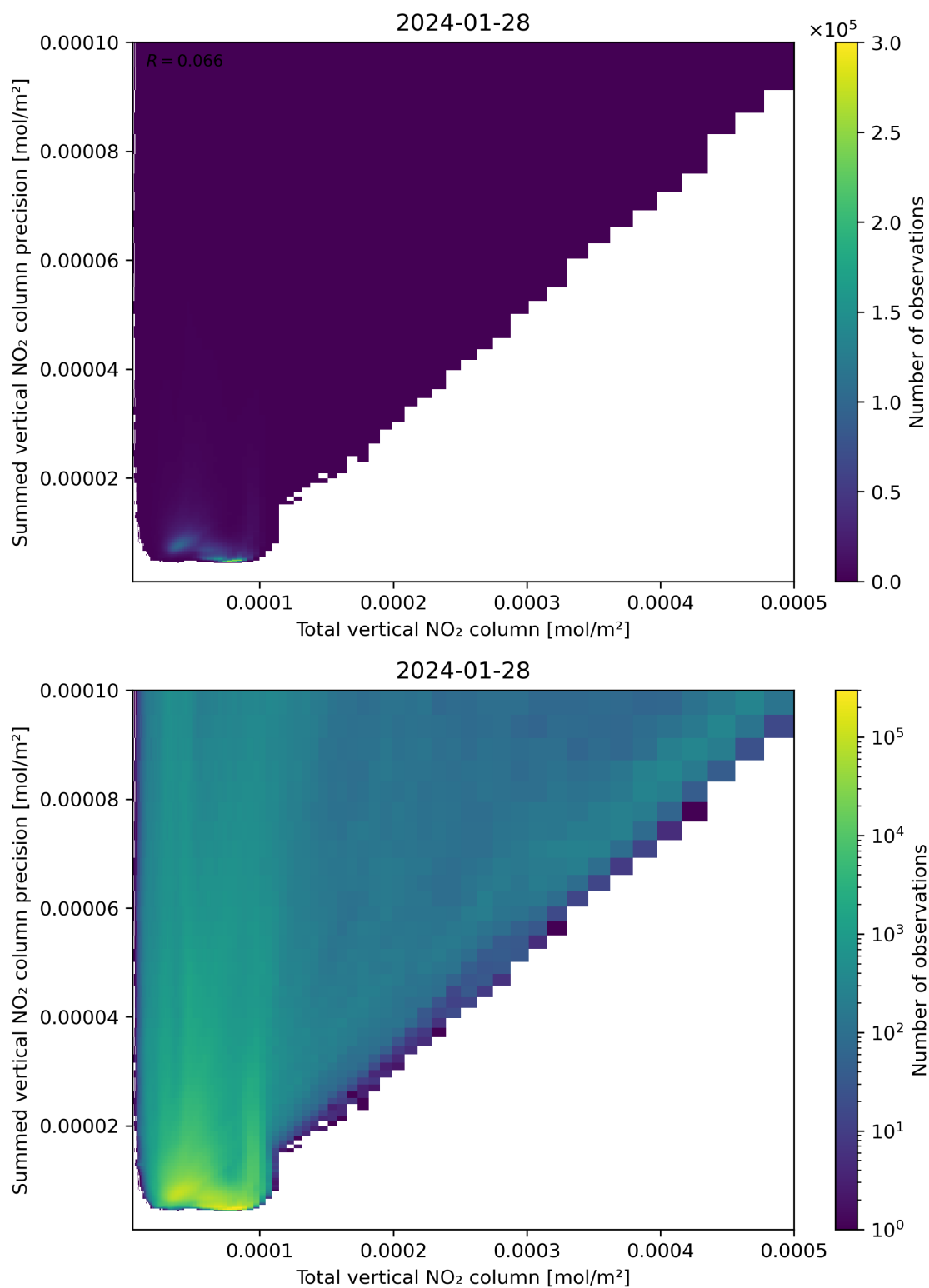
Figure 113: Scatter density plot of “Total vertical NO 2 column” against “Summed vertical NO 2 column precision” for 2024-01-27 to 2024-01-29.
