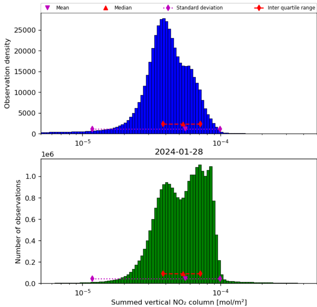
Figure 40: Histogram of “Summed vertical NO 2 column” for 2024-01-27 to 2024-01-29
