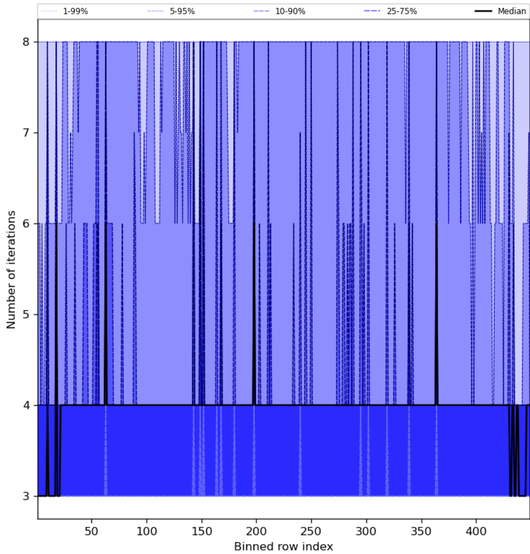
Figure 51: Along track statistics of “Number of iterations” for 2024-01-27 to 2024-01-29
