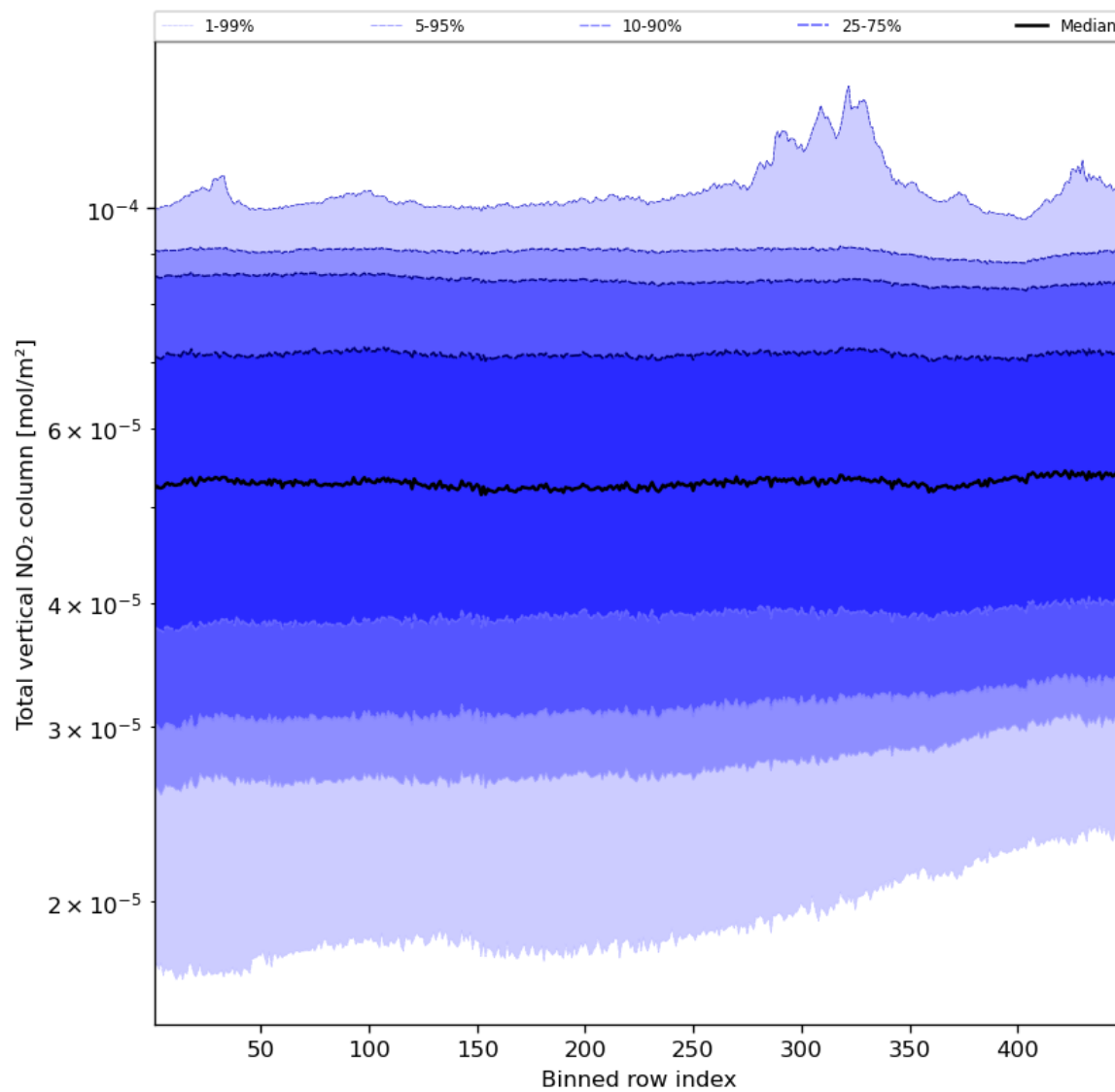
Figure 55: Along track statistics of “Total vertical NO 2 column” for 2024-01-27 to 2024-01-29
