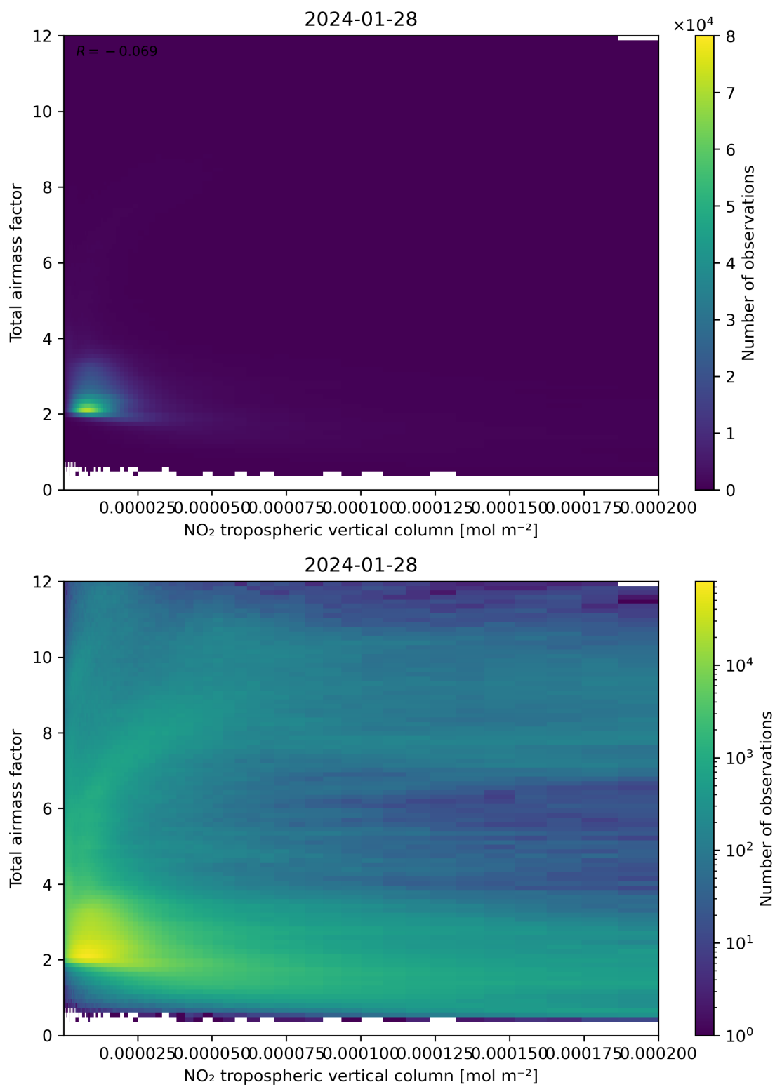
Figure 122: Scatter density plot of “NO 2 tropospheric vertical column” against “Total air mass factor” for 2024-01-27 to 2024-01-29.
