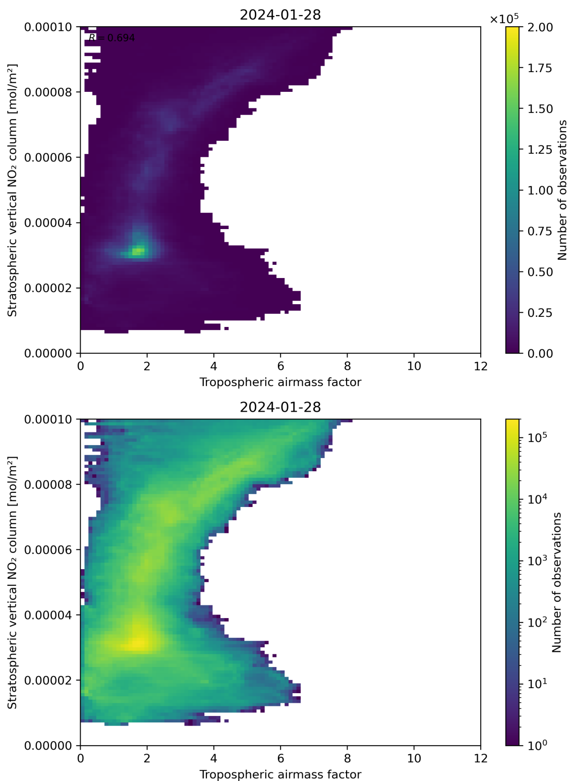
Figure 74: Scatter density plot of “Tropospheric air mass factor” against “Stratospheric vertical NO 2 column” for 2024-01-27 to 2024-01-29.
