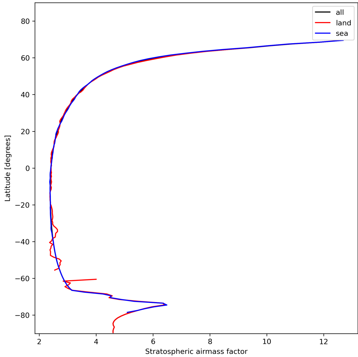
Figure 27: Zonal average of “Stratospheric airmass factor” for 2024-01-27 to 2024-01-29.
