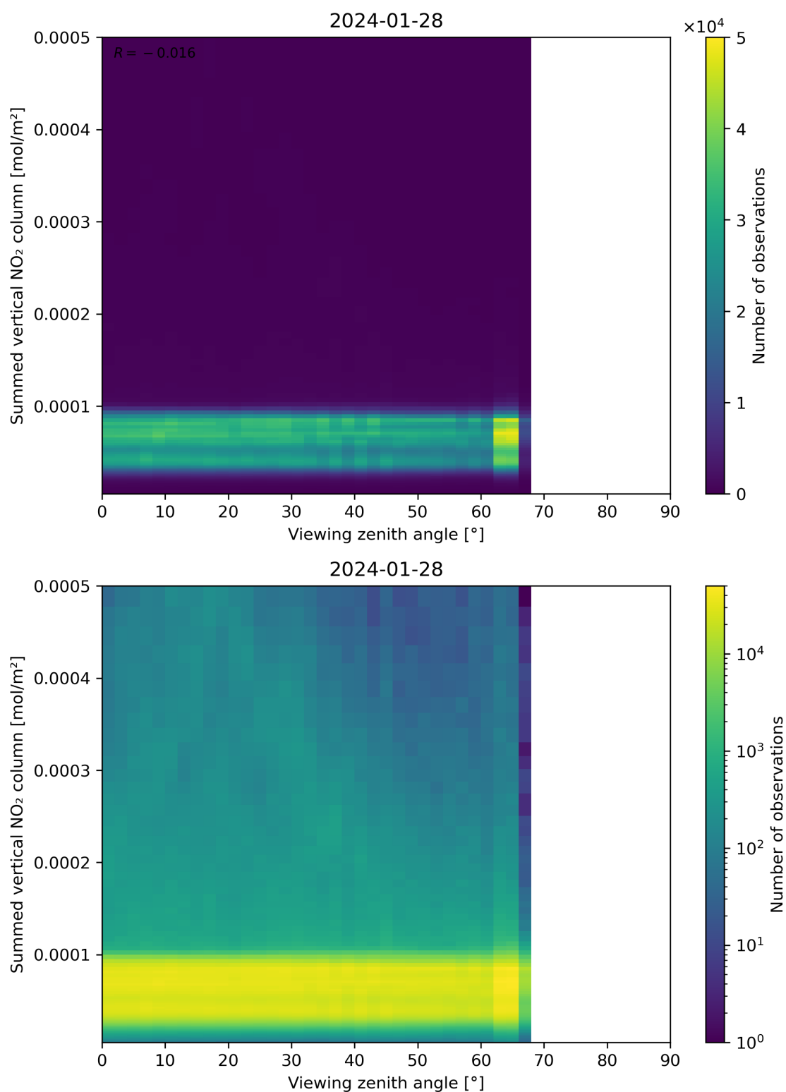
Figure 165: Scatter density plot of “Viewing zenith angle” against “Summed vertical NO 2 column” for 2024-01-27 to 2024-01-29.
