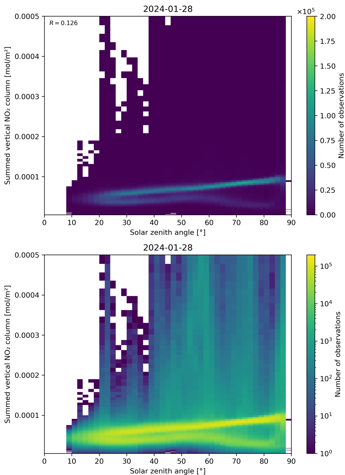
Figure 151: Scatter density plot of “Solar zenith angle” against “Summed vertical NO 2 column” for 2024-01-27 to 2024-01-29.
