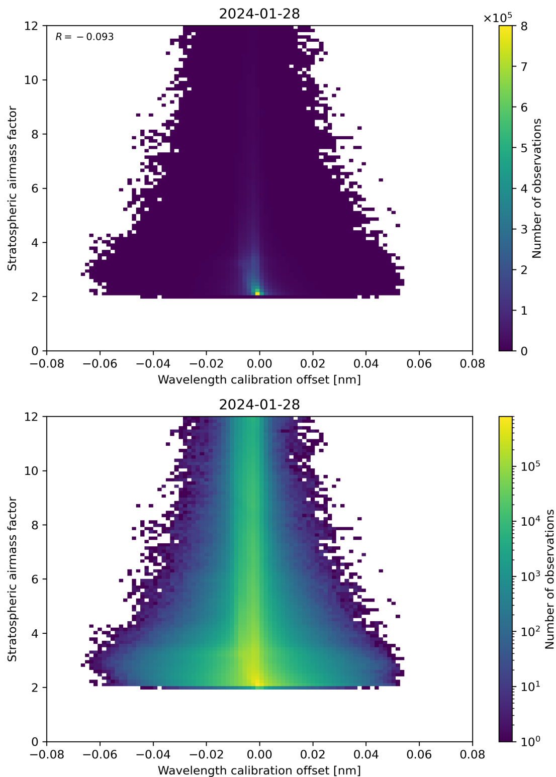
Figure 174: Scatter density plot of “Wavelength calibration offset” against “Stratospheric air mass factor” for 2024-01-27 to 2024-01-29.
