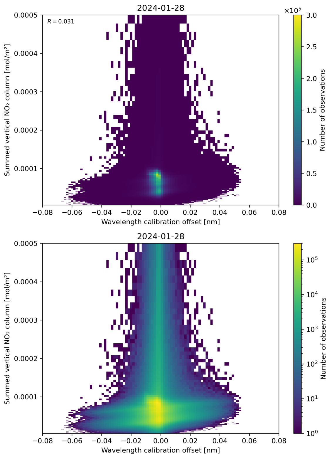
Figure 177: Scatter density plot of “Wavelength calibration offset” against “Summed vertical NO 2 column” for 2024-01-27 to 2024-01-29.
