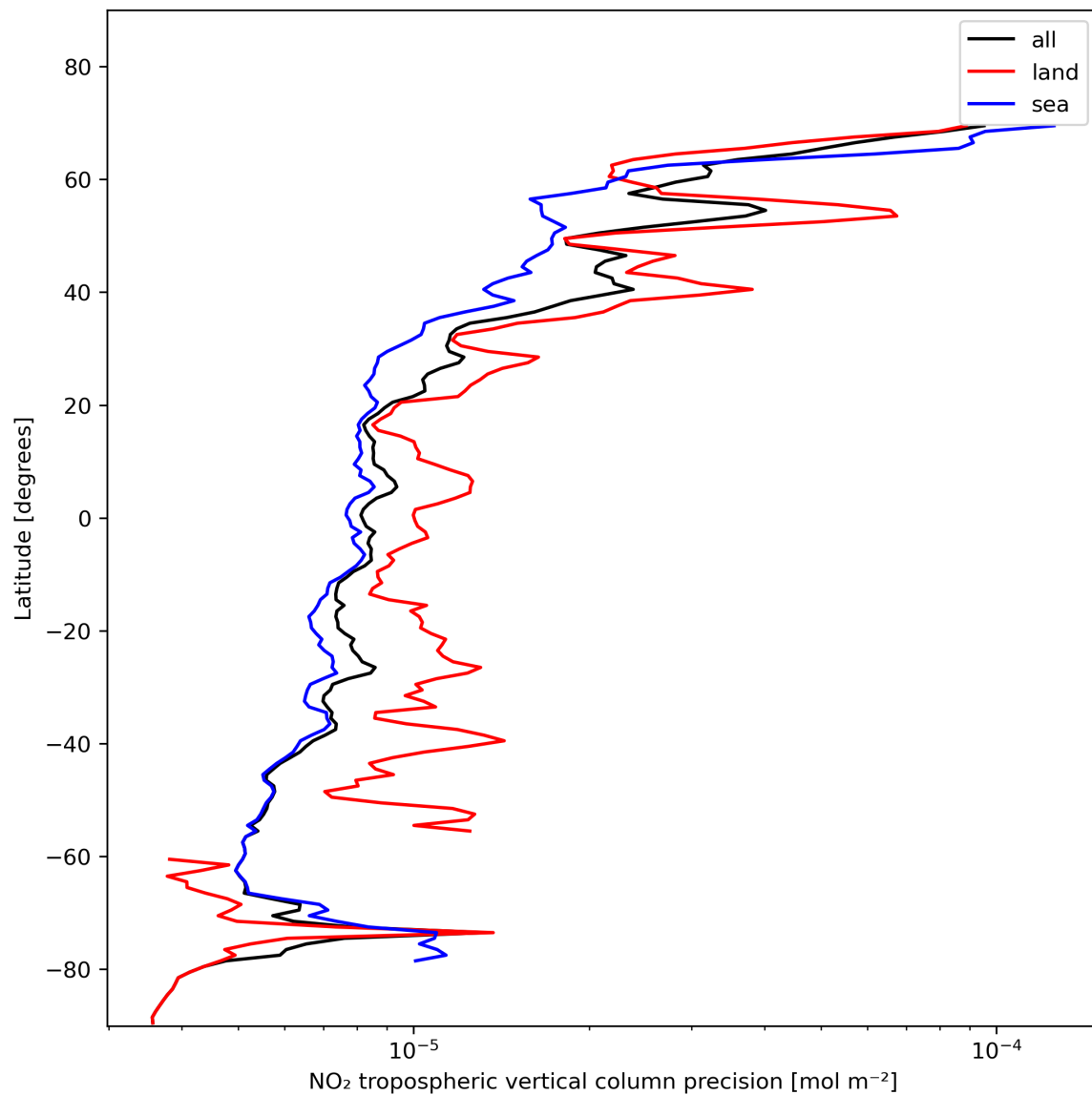
Figure 13: Zonal average of “NO 2 tropospheric vertical column precision” for 2024-01-27 to 2024-01-29.
