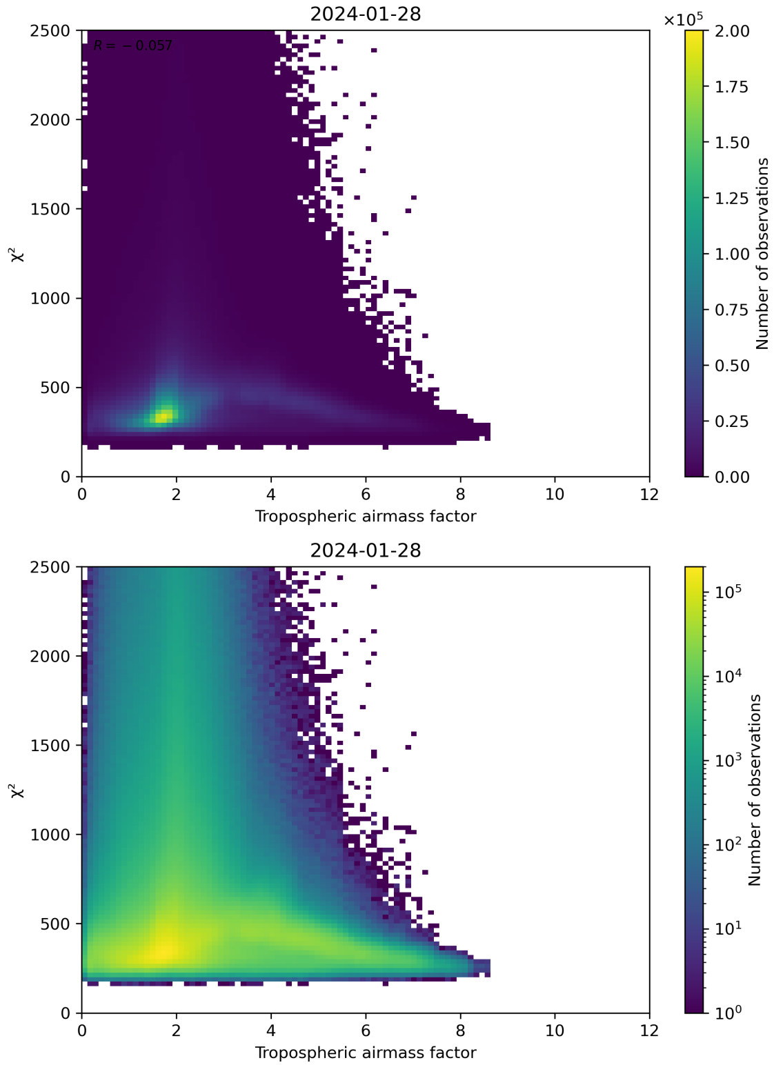
Figure 73: Scatter density plot of “Tropospheric airmass factor” against “ \chi^2 ” for 2024-01-27 to 2024-01-29.
