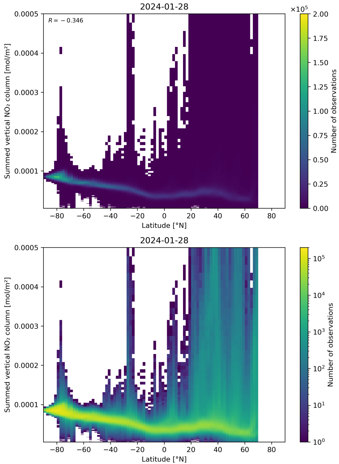
Figure 88: Scatter density plot of “Latitude” against “Summed vertical NO 2 column” for 2024-01-27 to 2024-01-29.
