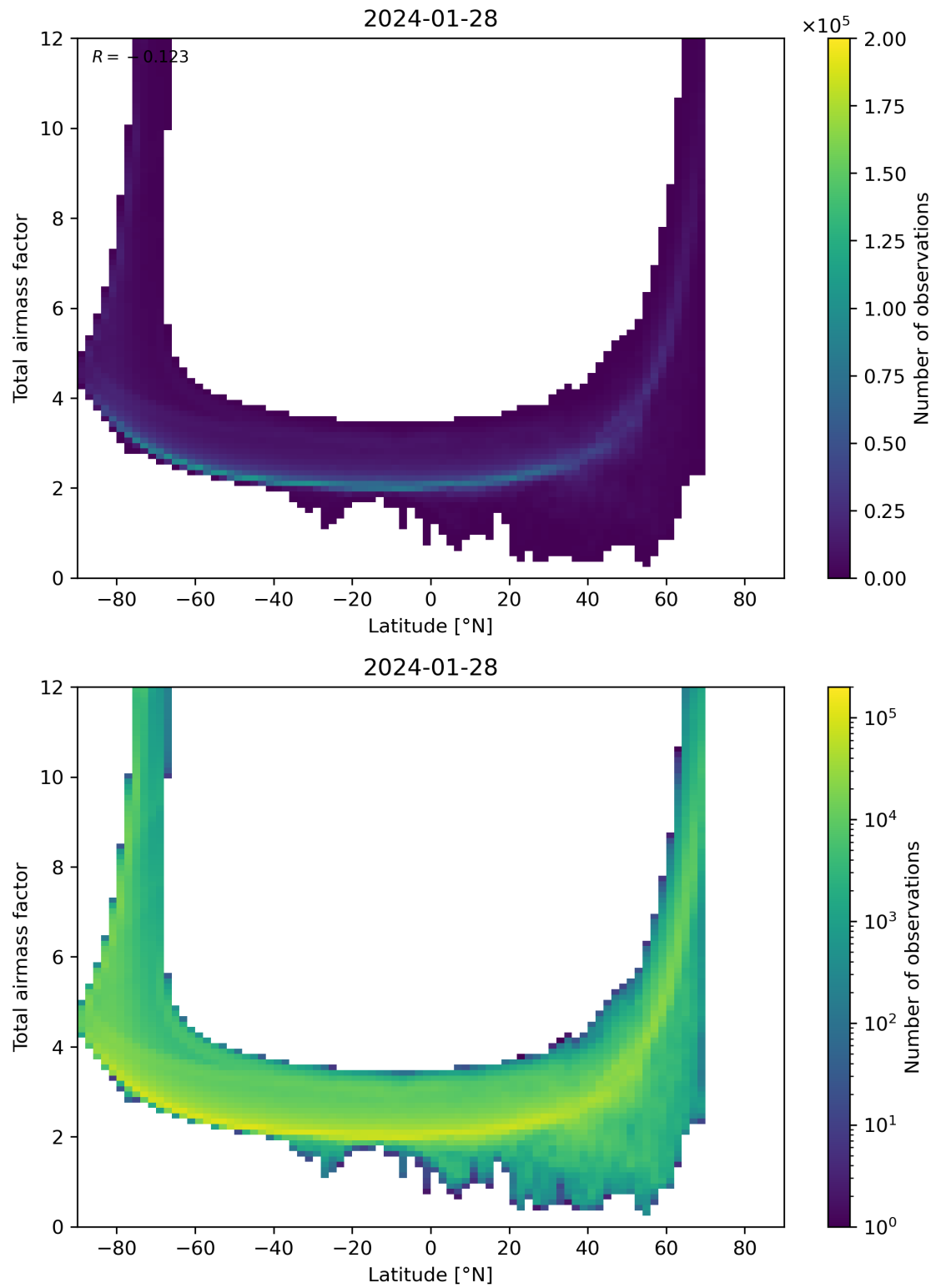
Figure 84: Scatter density plot of “Latitude” against “Total airmass factor” for 2024-01-27 to 2024-01-29.
