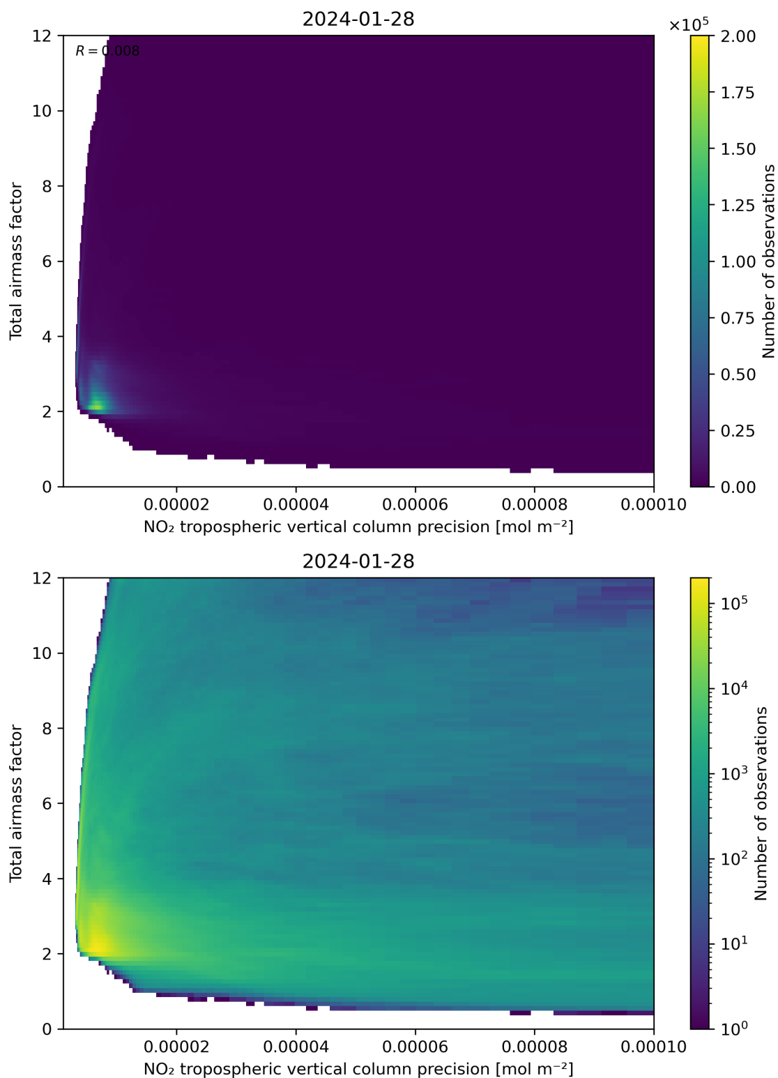
Figure 132: Scatter density plot of “NO 2 tropospheric vertical column precision” against “Total air mass factor” for 2024-01-27 to 2024-01-29.
