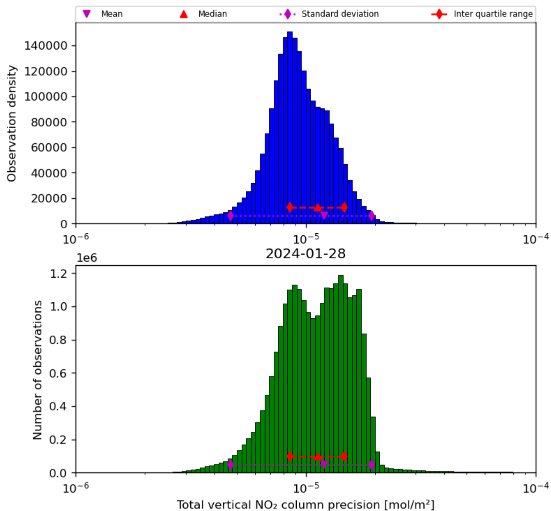
Figure 39: Histogram of "Total vertical NO 2 column precision" for 2024-01-27 to 2024-01-29
