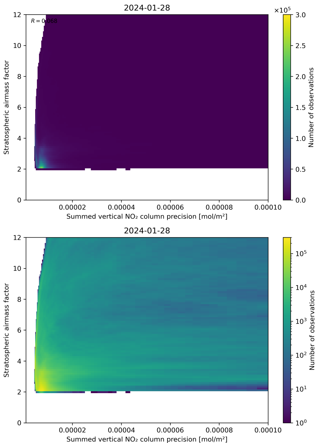
Figure 106: Scatter density plot of “Summed vertical NO 2 column precision” against “Stratospheric airmass factor” for 2024-01-27 to 2024-01-29.
