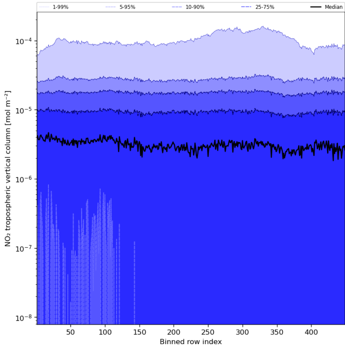
Figure 46: Along track statistics of “NO 2 tropospheric vertical column” for 2024-01-27 to 2024-01-29
