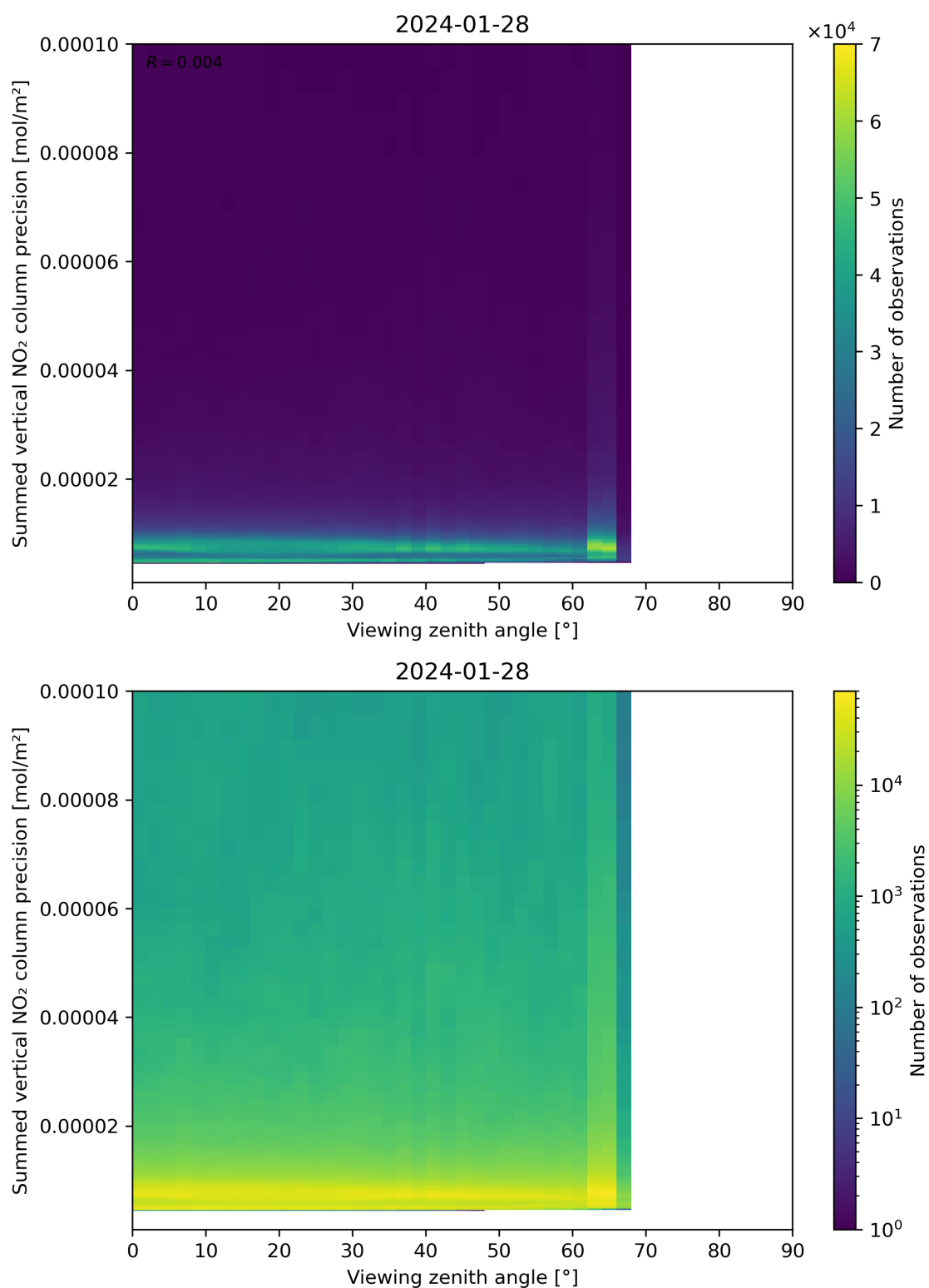
Figure 166: Scatter density plot of “Viewing zenith angle” against “Summed vertical NO 2 column precision” for 2024-01-27 to 2024-01-29.
