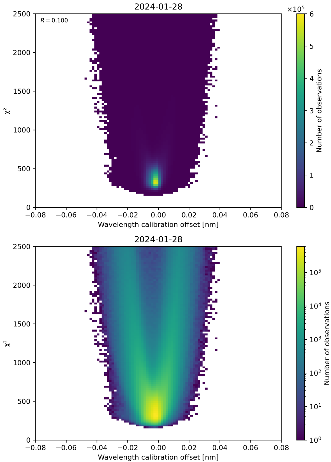
Figure 175: Scatter density plot of “Wavelength calibration offset” against “ \chi^2 ” for 2024-01-27 to 2024-01-29.
