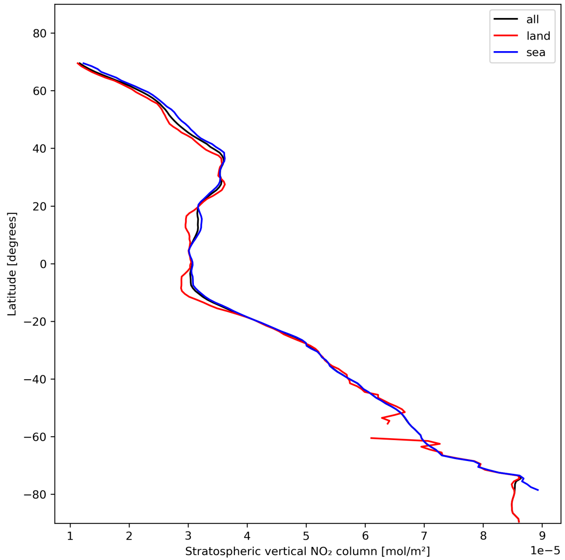
Figure 19: Zonal average of “Stratospheric vertical NO 2 column” for 2024-01-27 to 2024-01-29.
