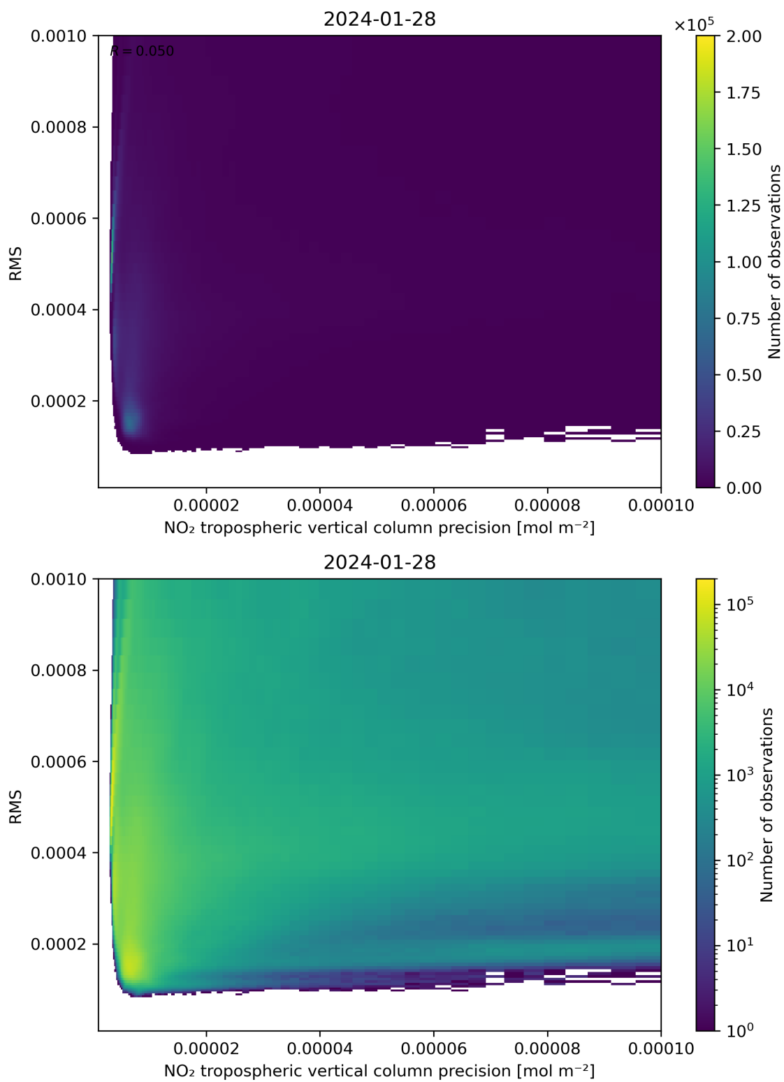
Figure 140: Scatter density plot of “NO 2 tropospheric vertical column precision” against “RMS” for 2024-01-27 to 2024-01-29.
