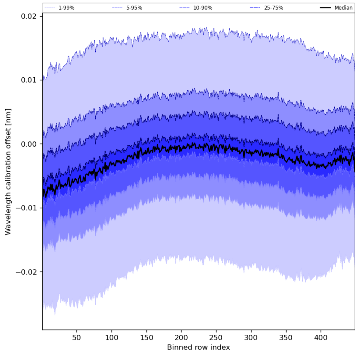
Figure 52: Along track statistics of “Wavelength calibration offset” for 2024-01-27 to 2024-01-29
