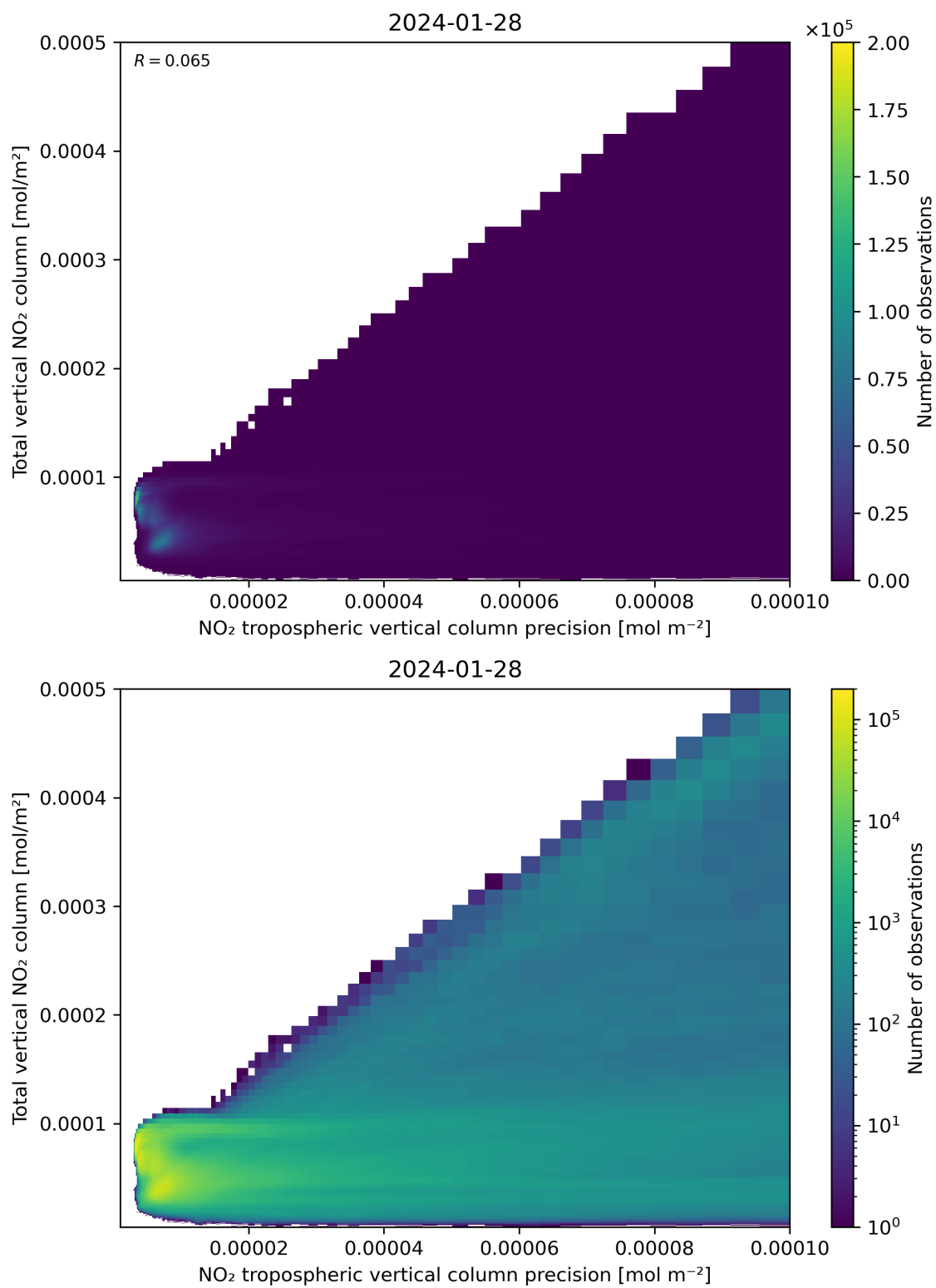
Figure 138: Scatter density plot of “NO 2 tropospheric vertical column precision” against “Total vertical NO 2 column” for 2024-01-27 to 2024-01-29.
