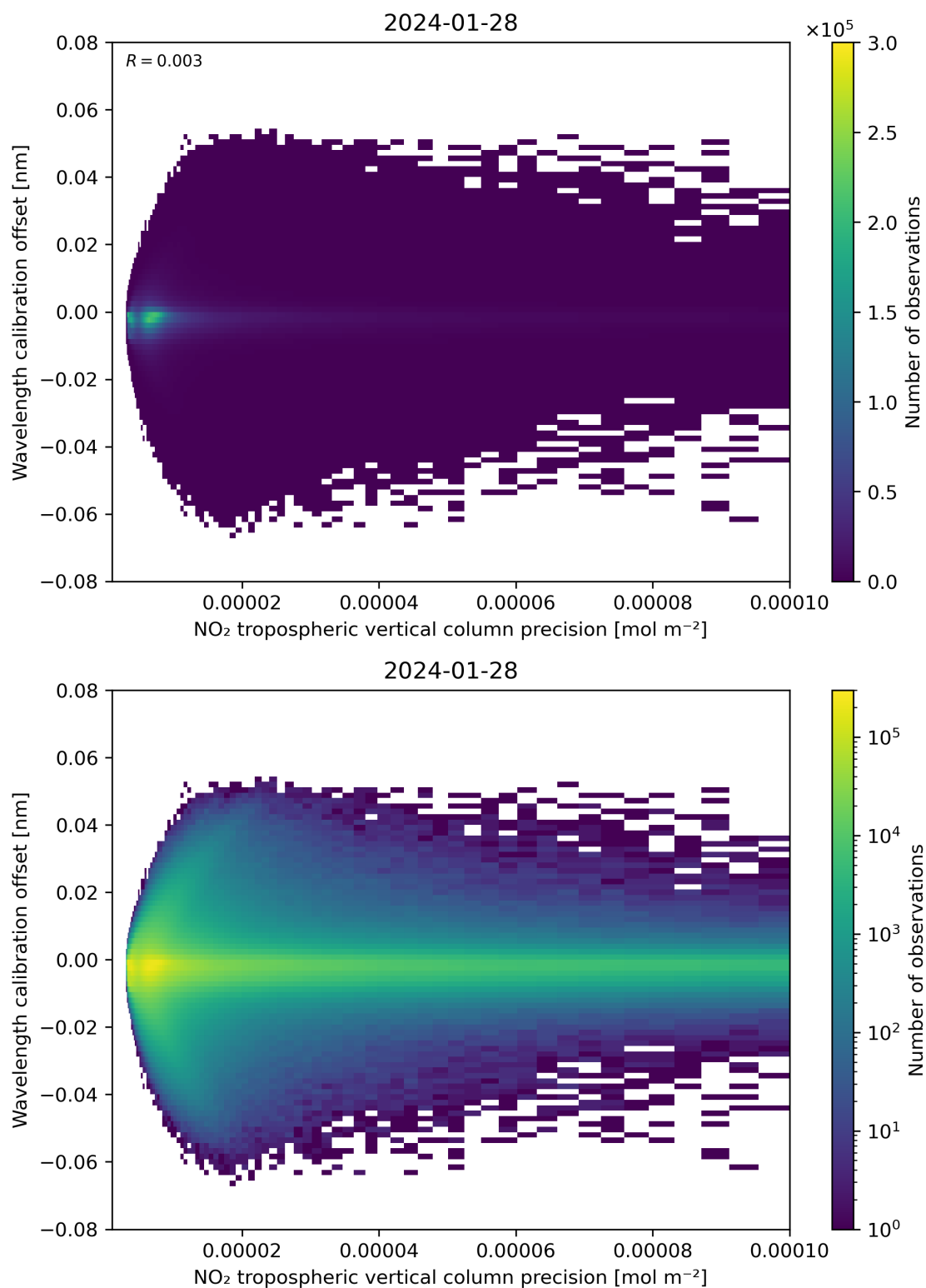
Figure 141: Scatter density plot of “NO 2 tropospheric vertical column precision” against “Wavelength calibration offset” for 2024-01-27 to 2024-01-29.
