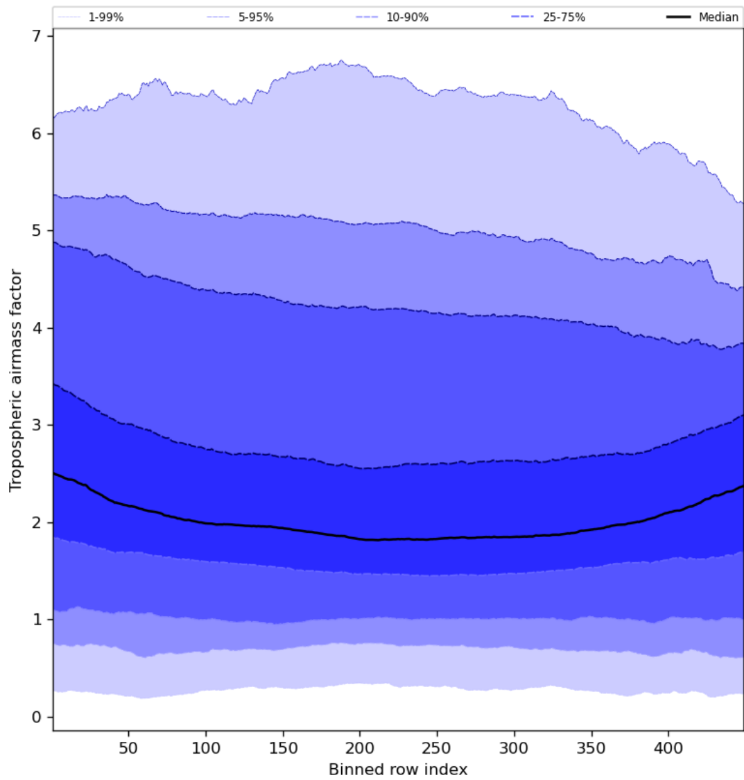
Figure 48: Along track statistics of “Tropospheric air mass factor” for 2024-01-27 to 2024-01-29
