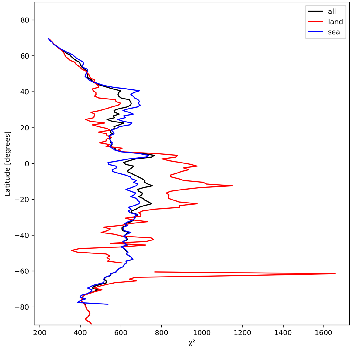
Figure 25: Zonal average of “ \chi^2 ” for 2024-01-27 to 2024-01-29.
