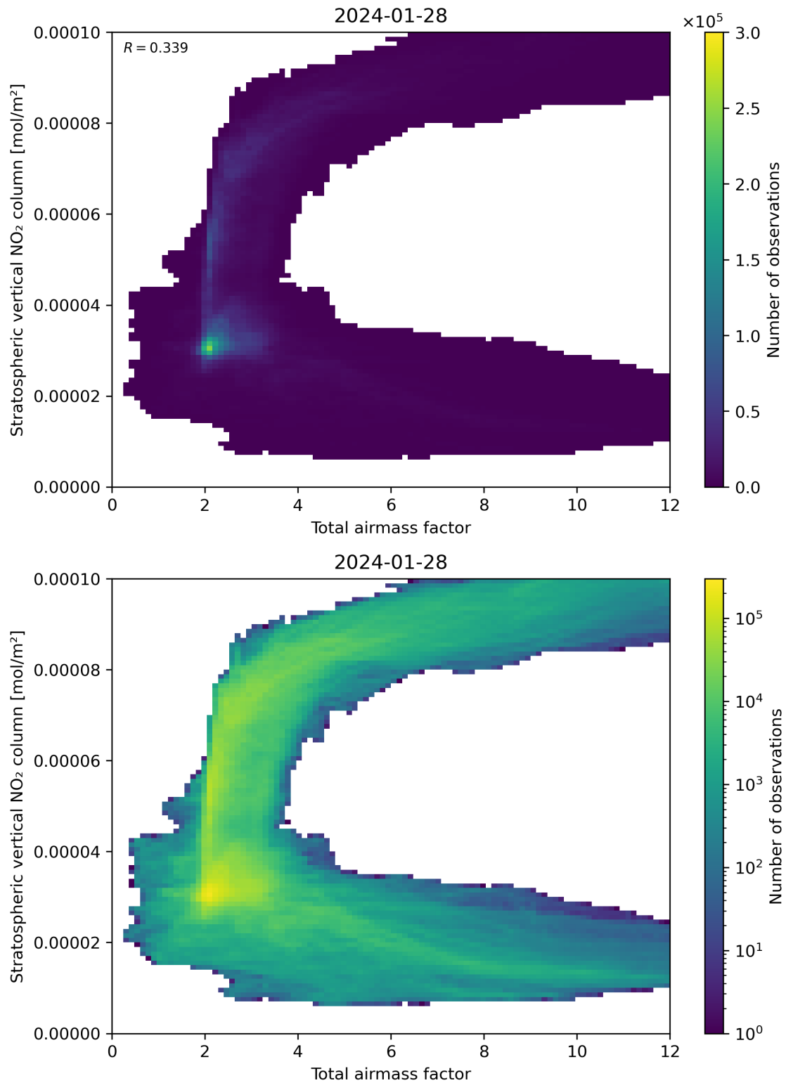
Figure 64: Scatter density plot of “Total airmass factor” against “Stratospheric vertical NO 2 column” for 2024-01-27 to 2024-01-29.
