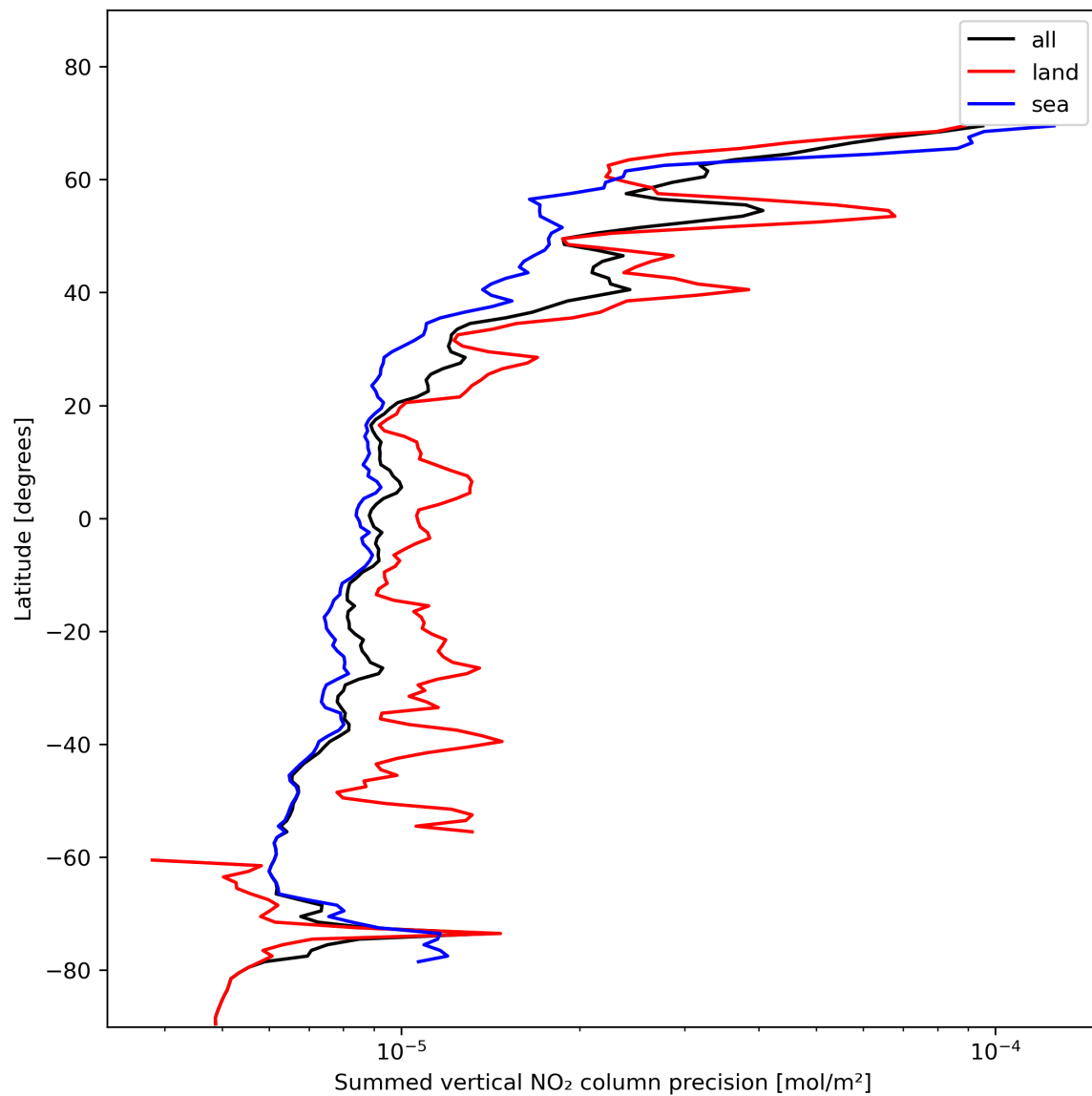
Figure 24: Zonal average of “Summed vertical NO 2 column precision” for 2024-01-27 to 2024-01-29.
