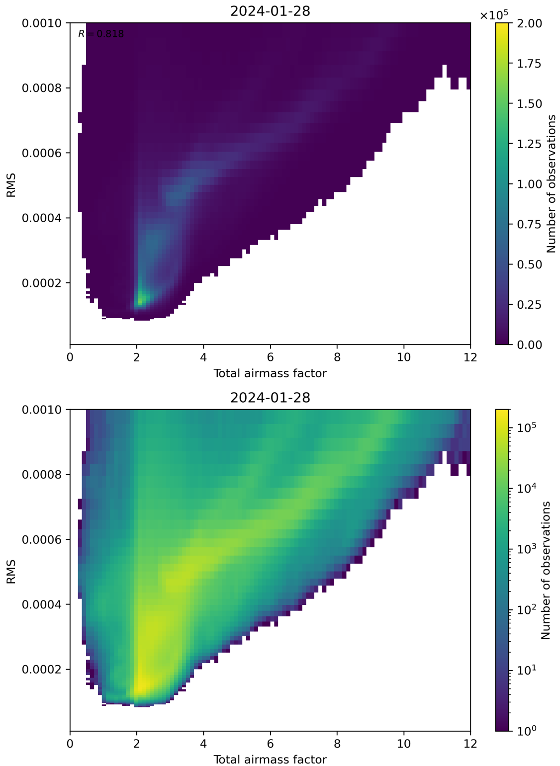
Figure 69: Scatter density plot of “Total airmass factor” against “RMS” for 2024-01-27 to 2024-01-29.
