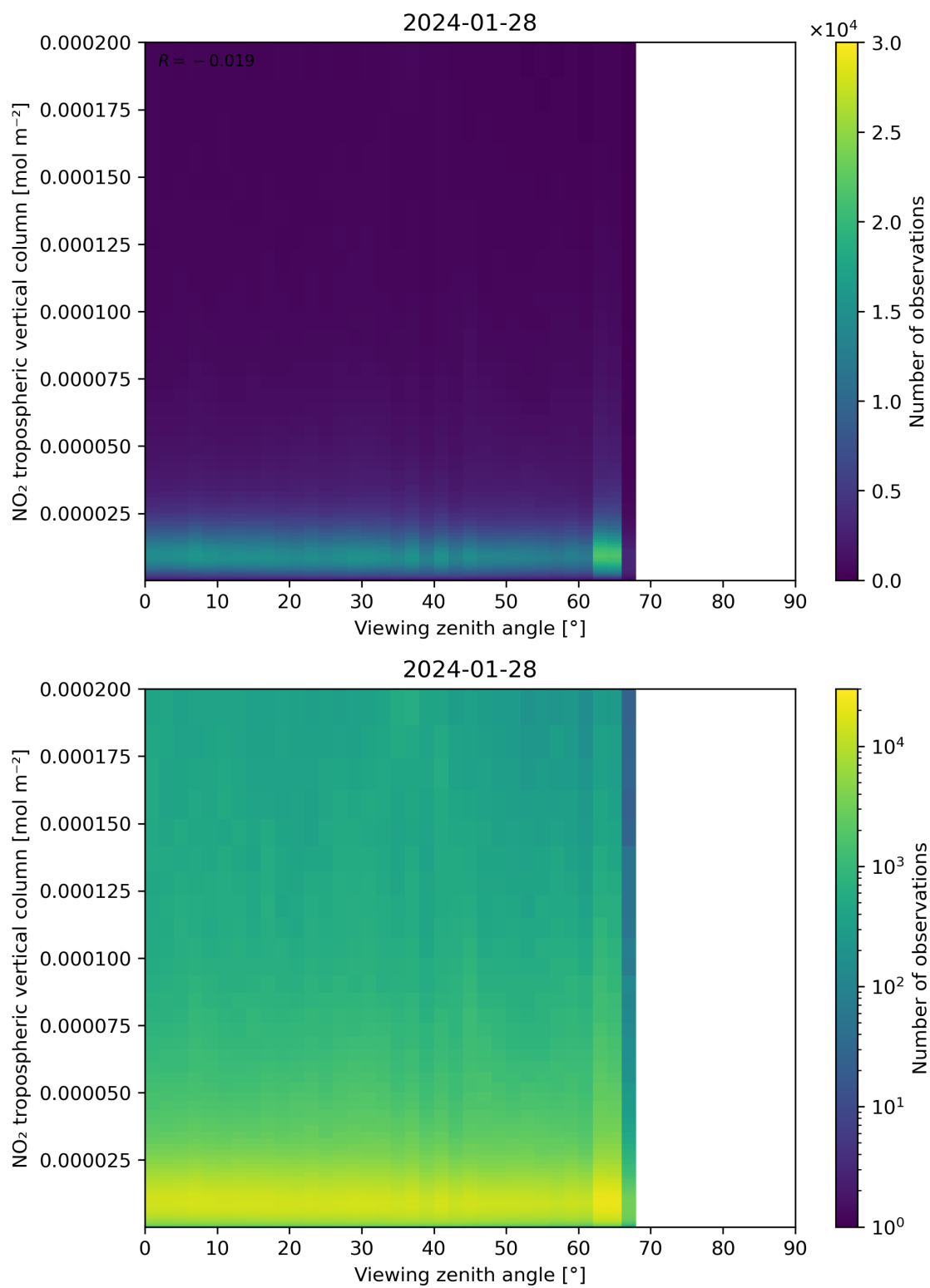
Figure 169: Scatter density plot of “Viewing zenith angle” against “NO 2 tropospheric vertical column” for 2024-01-27 to 2024-01-29.
