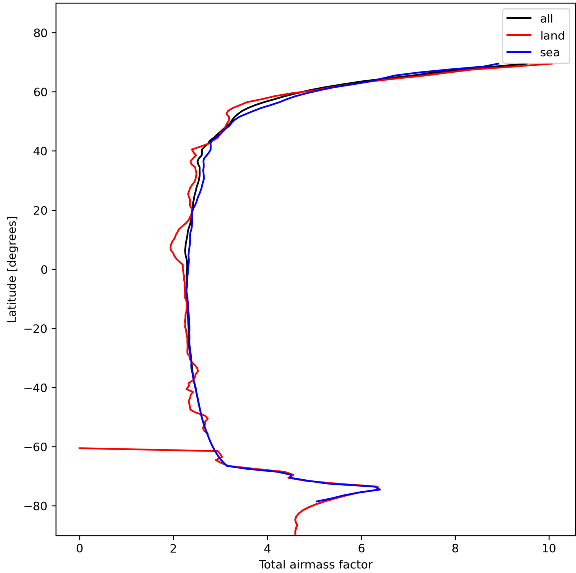
Figure 15: Zonal average of “Total airmass factor” for 2024-01-27 to 2024-01-29.
