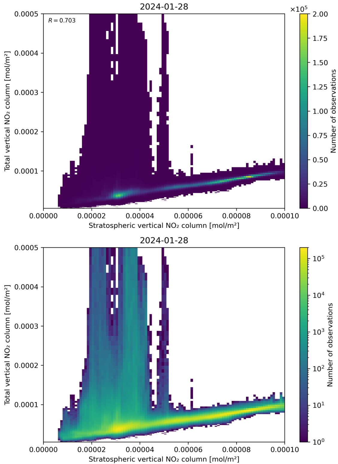
Figure 100: Scatter density plot of “Stratospheric vertical NO 2 column” against “Total vertical NO 2 column” for 2024-01-27 to 2024-01-29.
