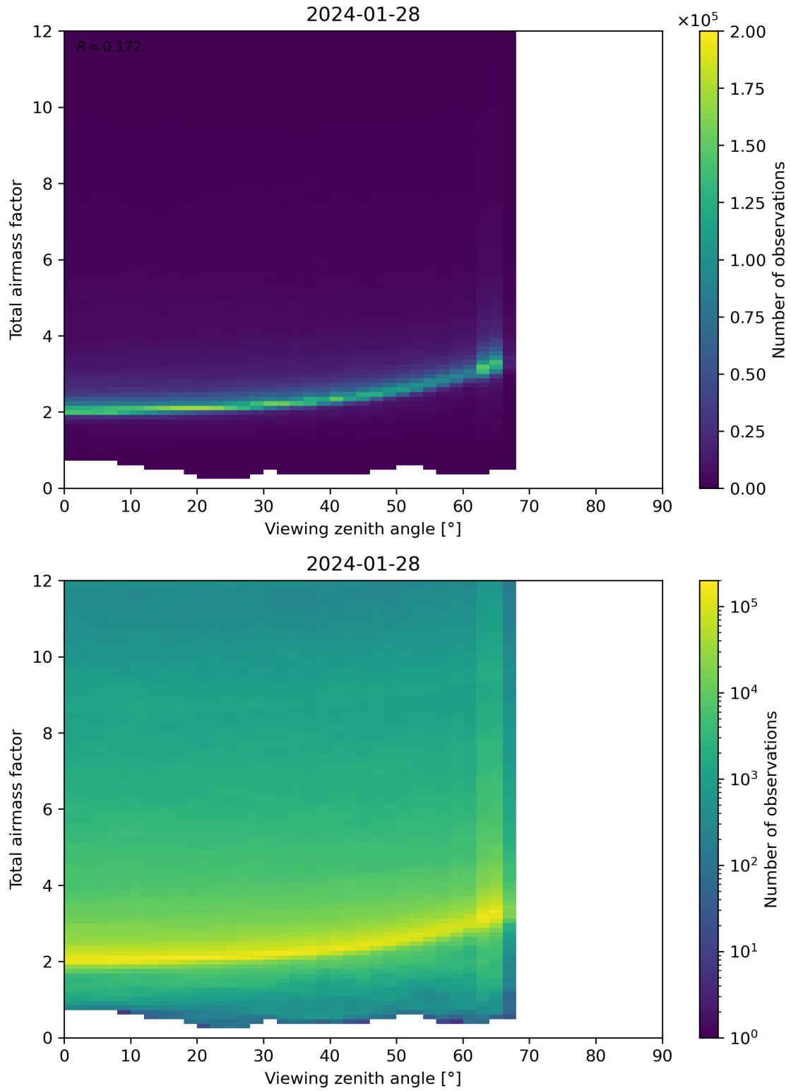
Figure 160: Scatter density plot of “Viewing zenith angle” against “Total airmass factor” for 2024-01-27 to 2024-01-29.
