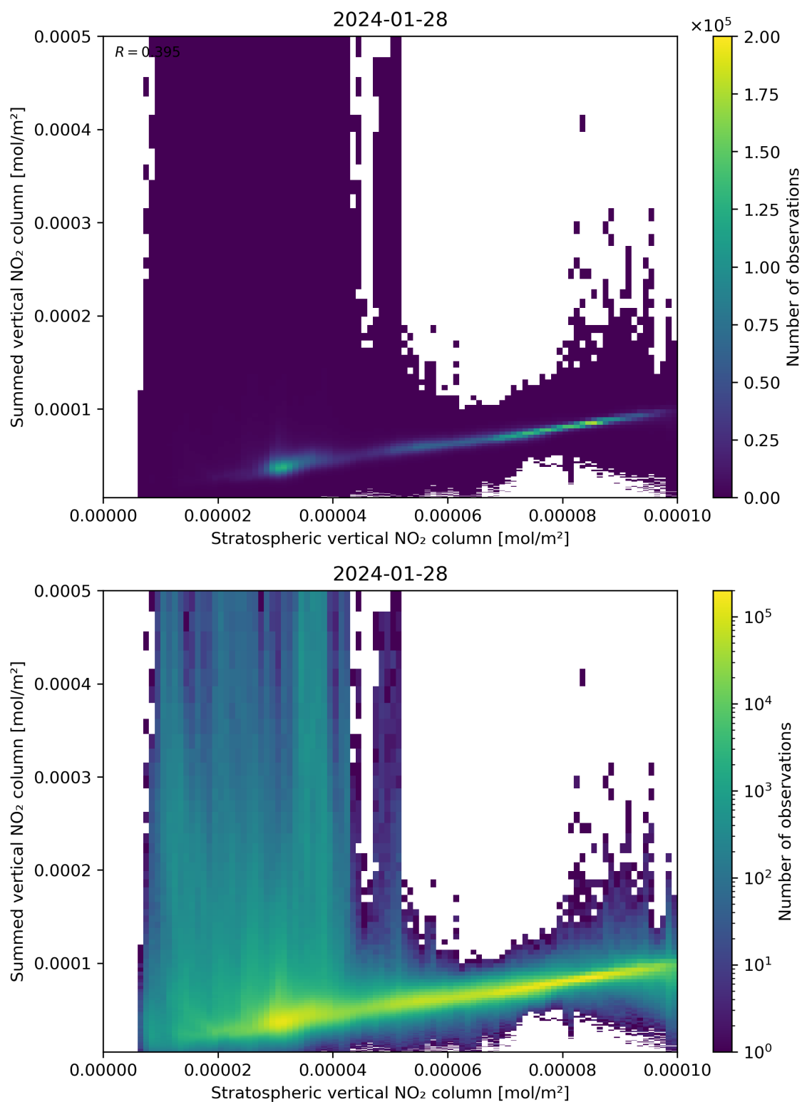
Figure 98: Scatter density plot of “Stratospheric vertical NO 2 column” against “Summed vertical NO 2 column” for 2024-01-27 to 2024-01-29.
