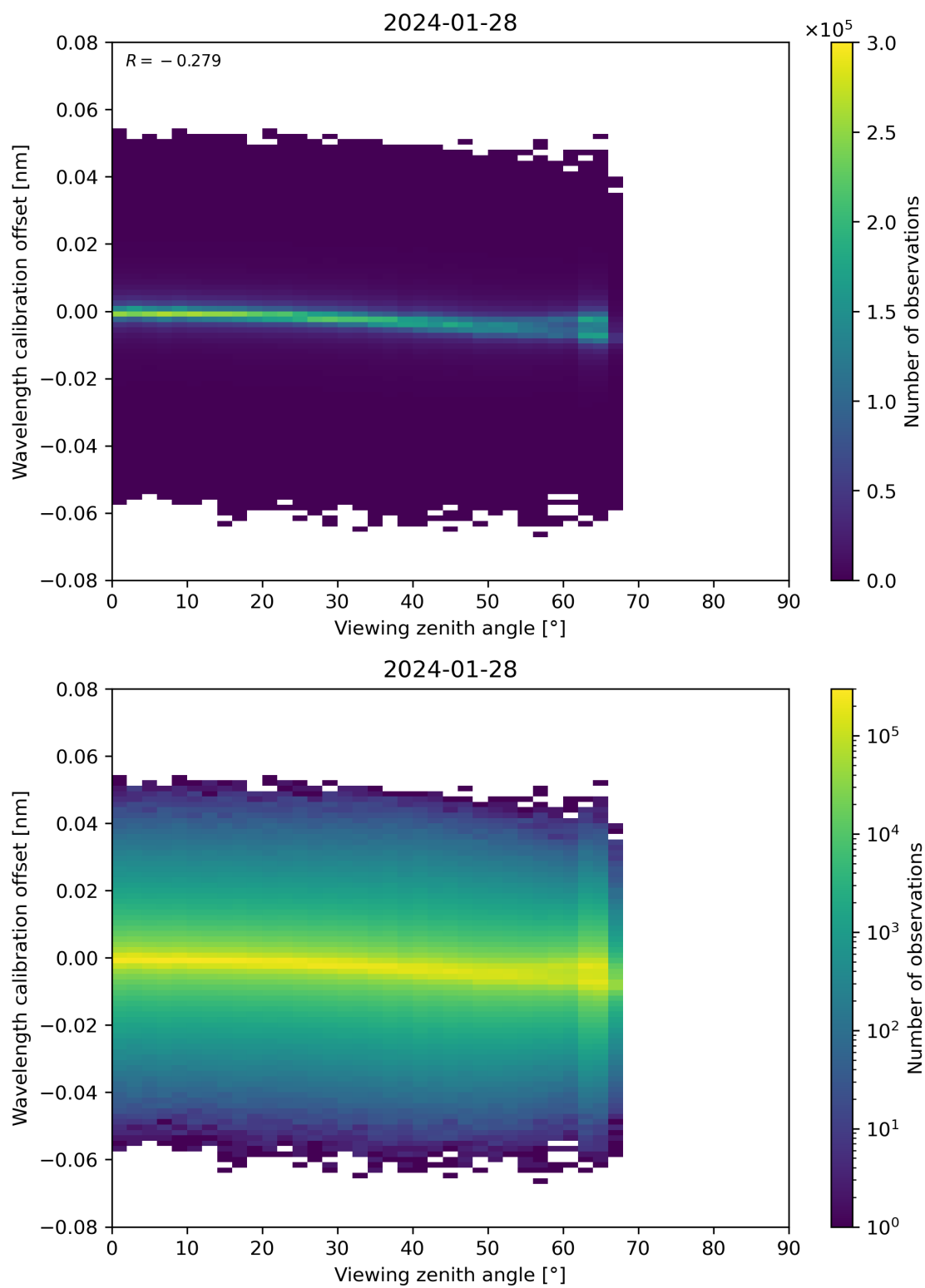
Figure 173: Scatter density plot of “Viewing zenith angle” against “Wavelength calibration offset” for 2024-01-27 to 2024-01-29.
