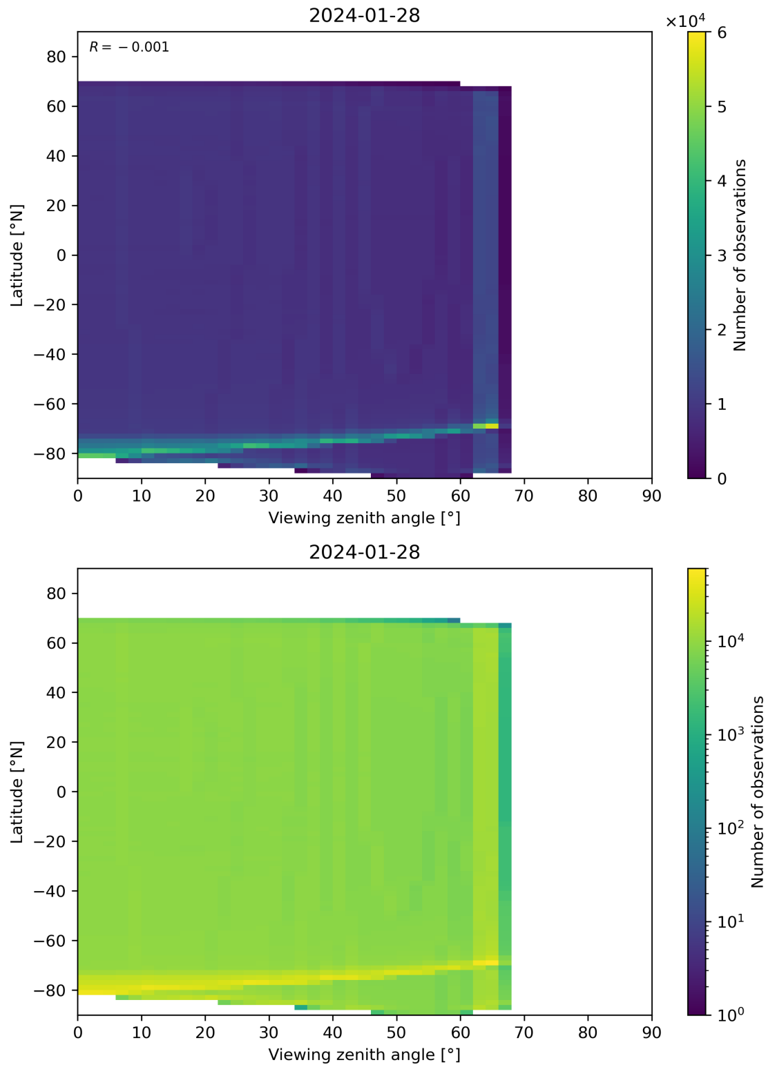
Figure 163: Scatter density plot of “Viewing zenith angle” against “Latitude” for 2024-01-27 to 2024-01-29.
