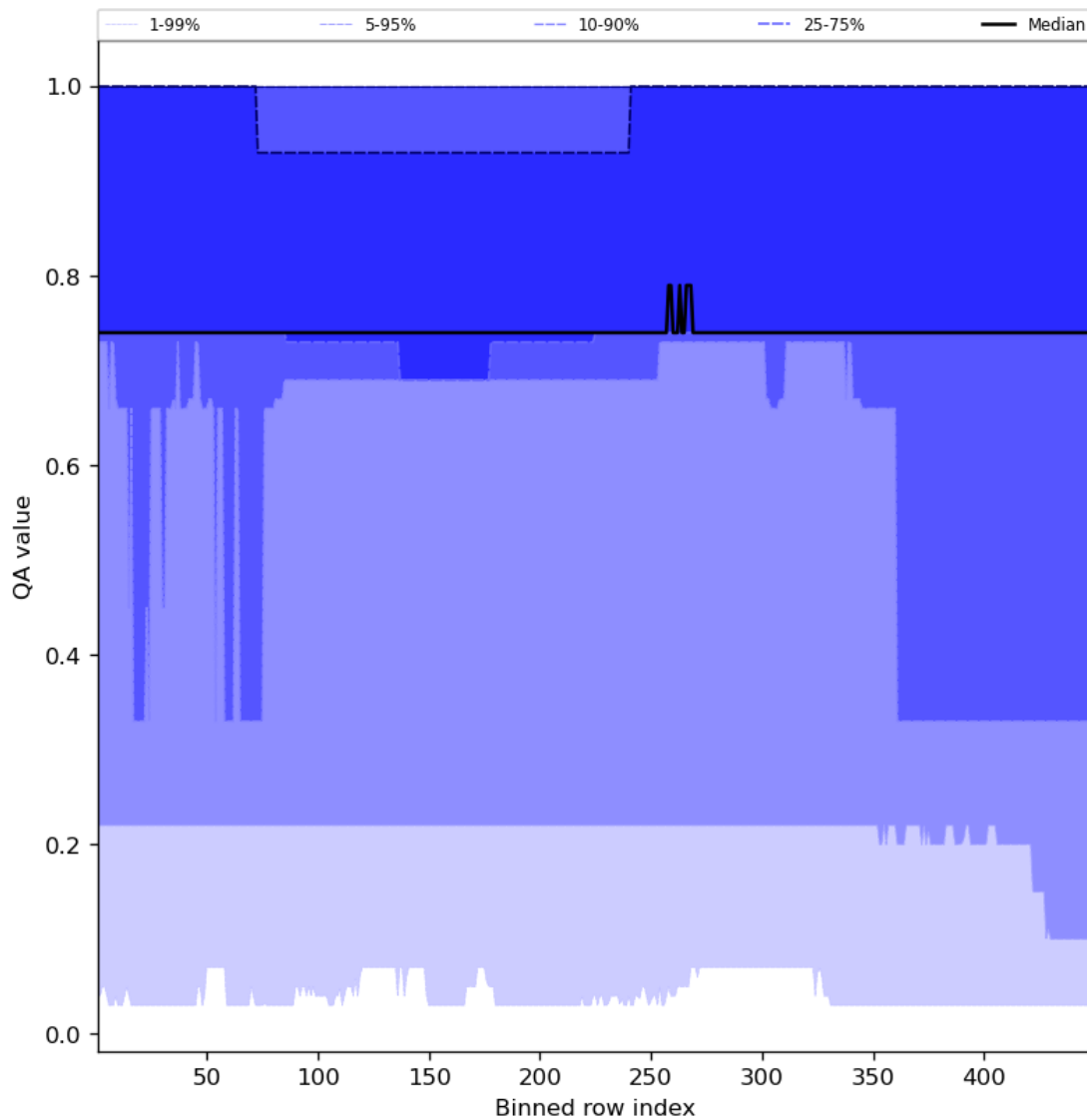
Figure 45: Along track statistics of “QA value” for 2024-01-27 to 2024-01-29
