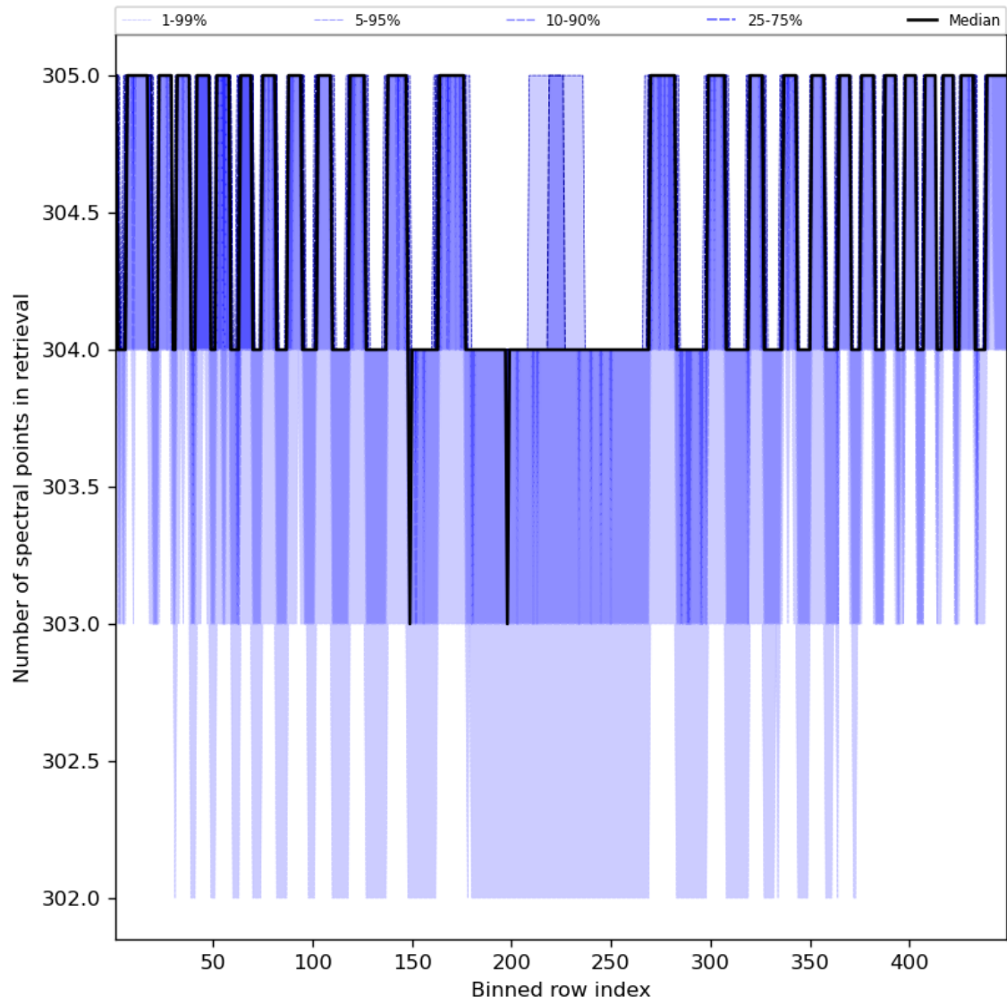
Figure 50: Along track statistics of “Number of spectral points in retrieval” for 2024-01-27 to 2024-01-29
