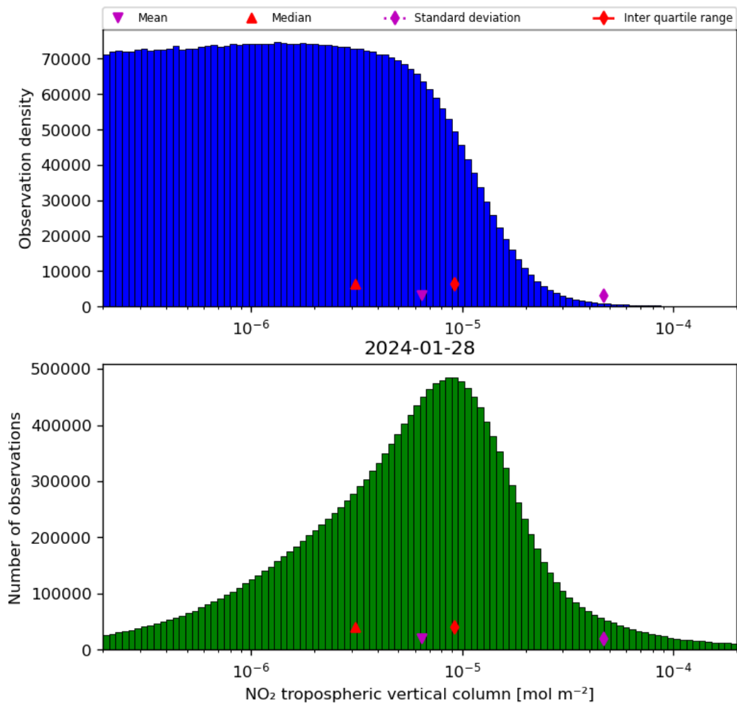
Figure 29: Histogram of “NO 2 tropospheric vertical column” for 2024-01-27 to 2024-01-29
