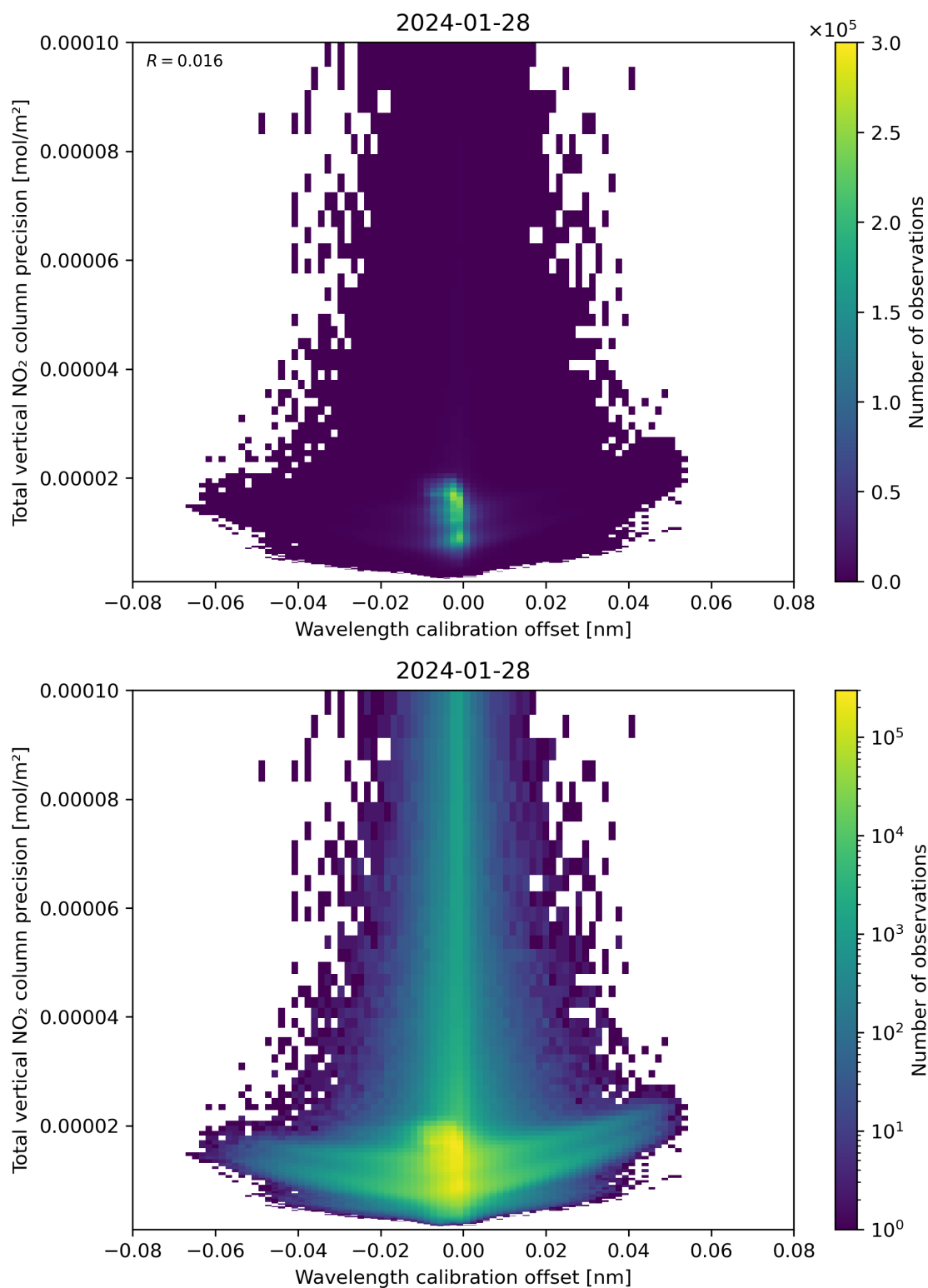
Figure 180: Scatter density plot of “Wavelength calibration offset” against “Total vertical NO 2 column precision” for 2024-01-27 to 2024-01-29.
