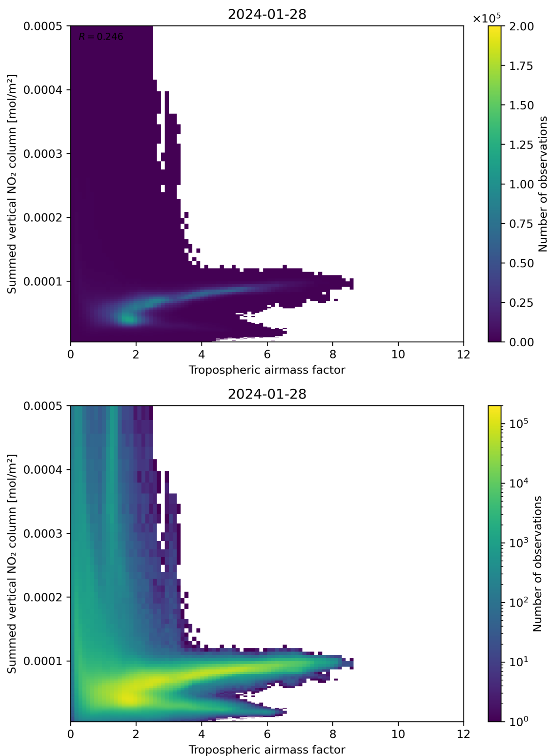
Figure 75: Scatter density plot of “Tropospheric airmass factor” against “Summed vertical NO 2 column” for 2024-01-27 to 2024-01-29.
