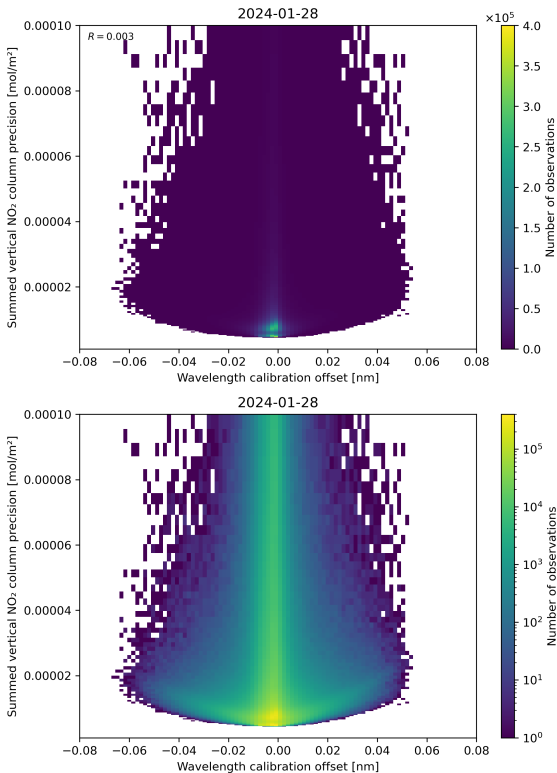
Figure 178: Scatter density plot of “Wavelength calibration offset” against “Summed vertical NO 2 column precision” for 2024-01-27 to 2024-01-29.
