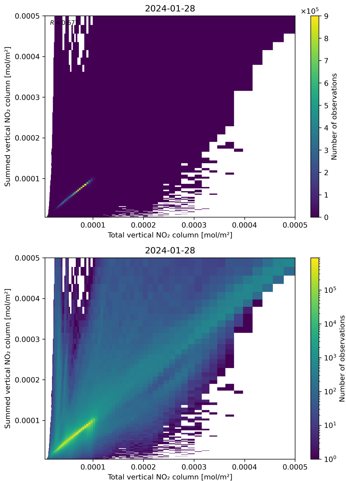
Figure 112: Scatter density plot of “Total vertical NO 2 column” against “Summed vertical NO 2 column” for 2024-01-27 to 2024-01-29.
