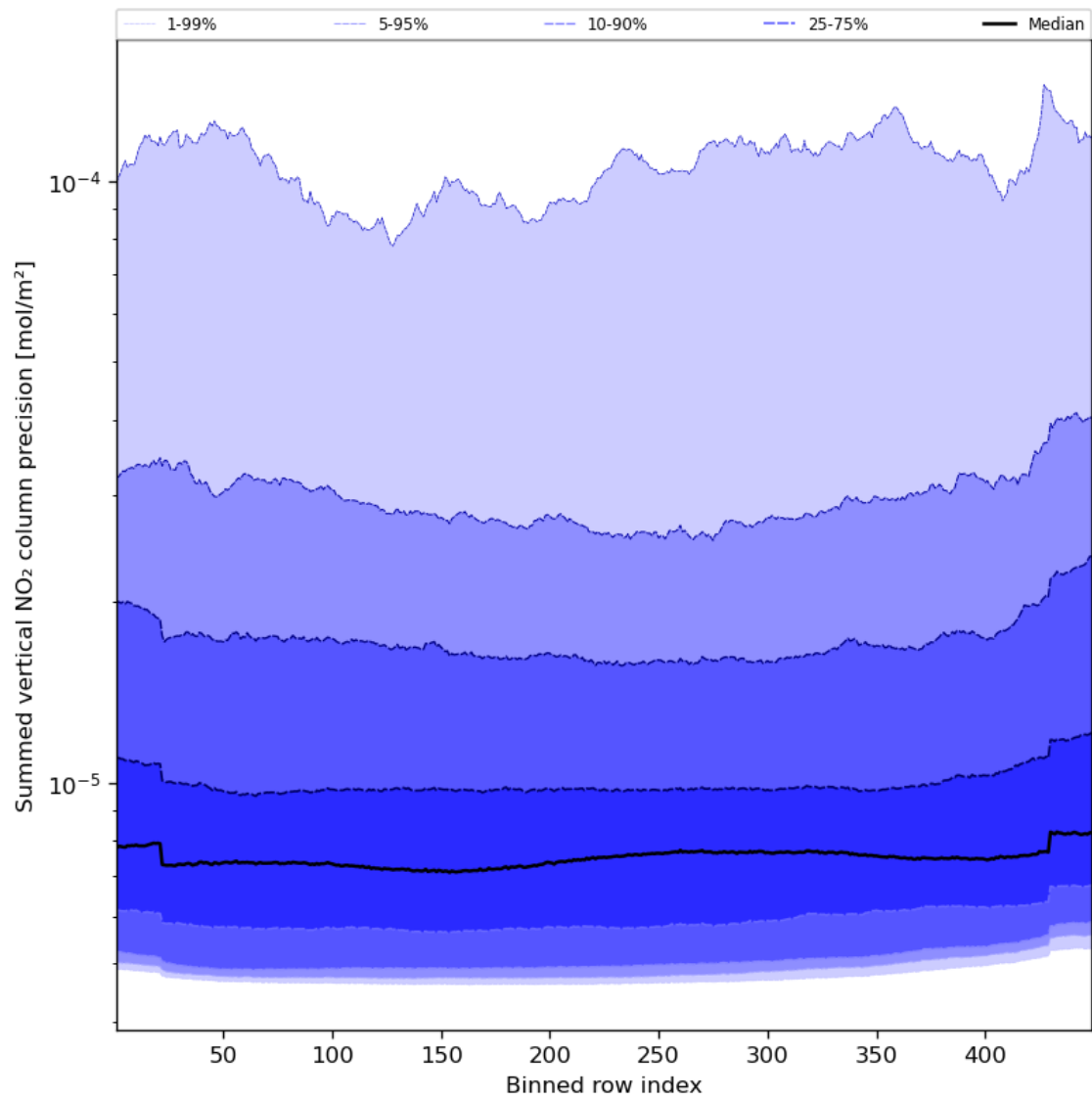
Figure 58: Along track statistics of “Summed vertical NO 2 column precision” for 2024-01-27 to 2024-01-29
