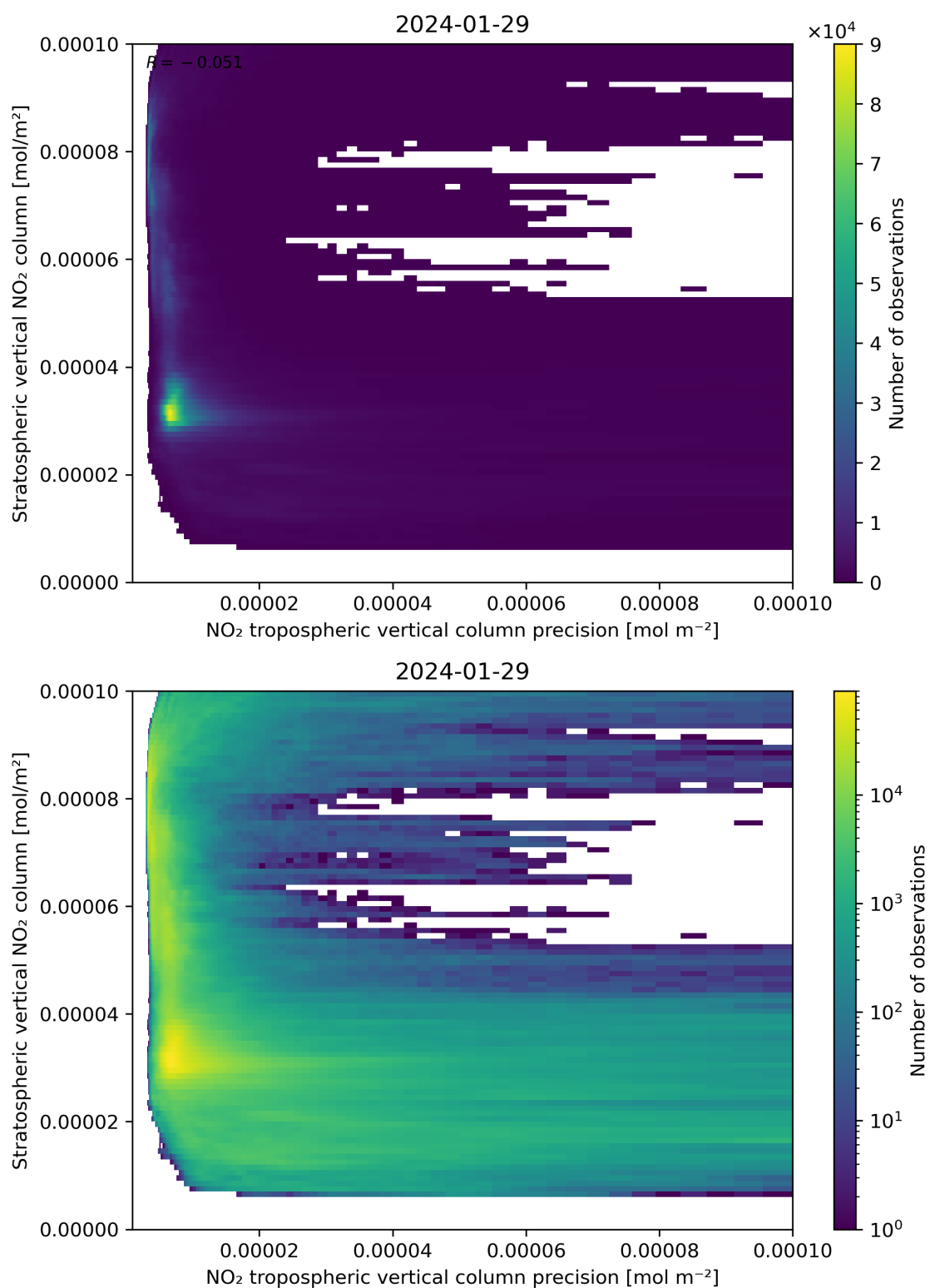
Figure 135: Scatter density plot of “NO 2 tropospheric vertical column precision” against “Stratospheric vertical NO 2 column” for 2024-01-28 to 2024-01-30.
