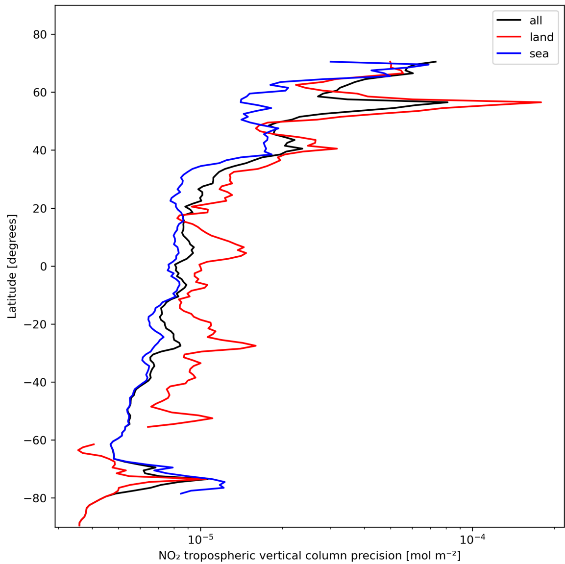
Figure 13: Zonal average of “NO 2 tropospheric vertical column precision” for 2024-01-28 to 2024-01-30.
