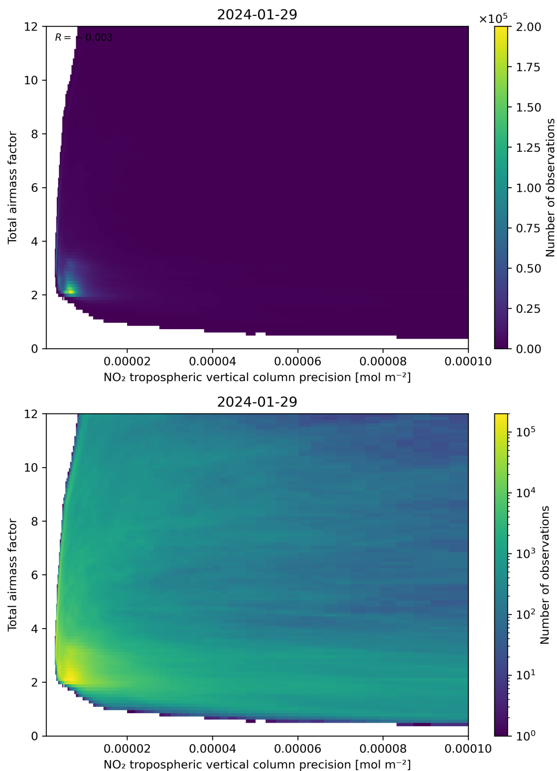
Figure 132: Scatter density plot of “NO 2 tropospheric vertical column precision” against “Total air mass factor” for 2024-01-28 to 2024-01-30.
