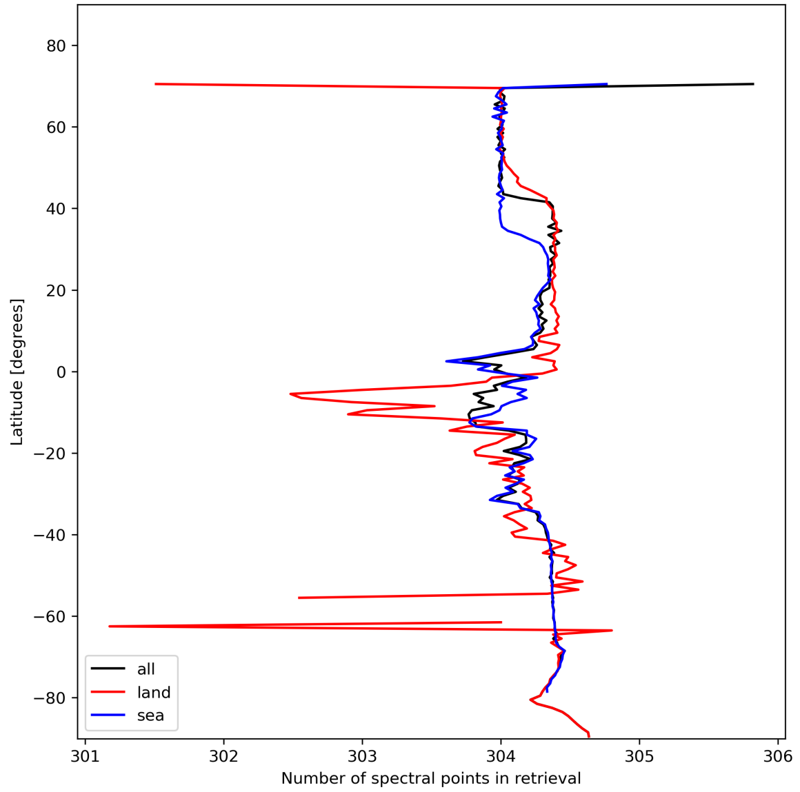
Figure 16: Zonal average of “Number of spectral points in retrieval” for 2024-01-28 to 2024-01-30.
