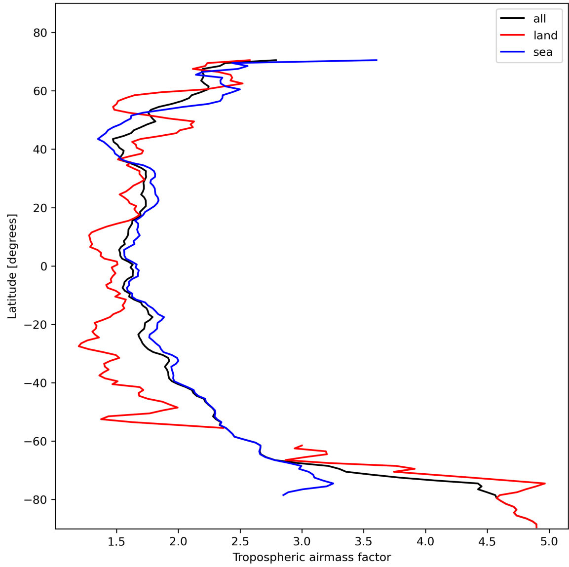
Figure 14: Zonal average of “Tropospheric airmass factor” for 2024-01-28 to 2024-01-30.
