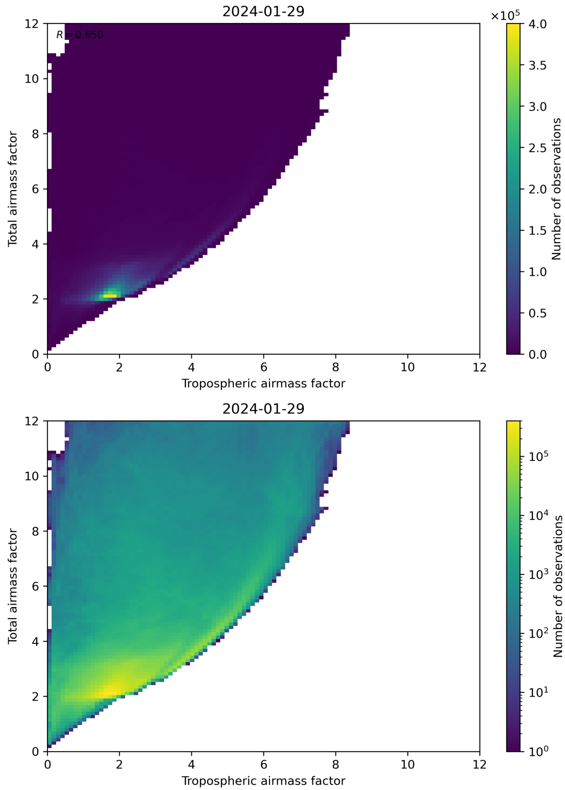
Figure 72: Scatter density plot of “Tropospheric airmass factor” against “Total airmass factor” for 2024-01-28 to 2024-01-30.
