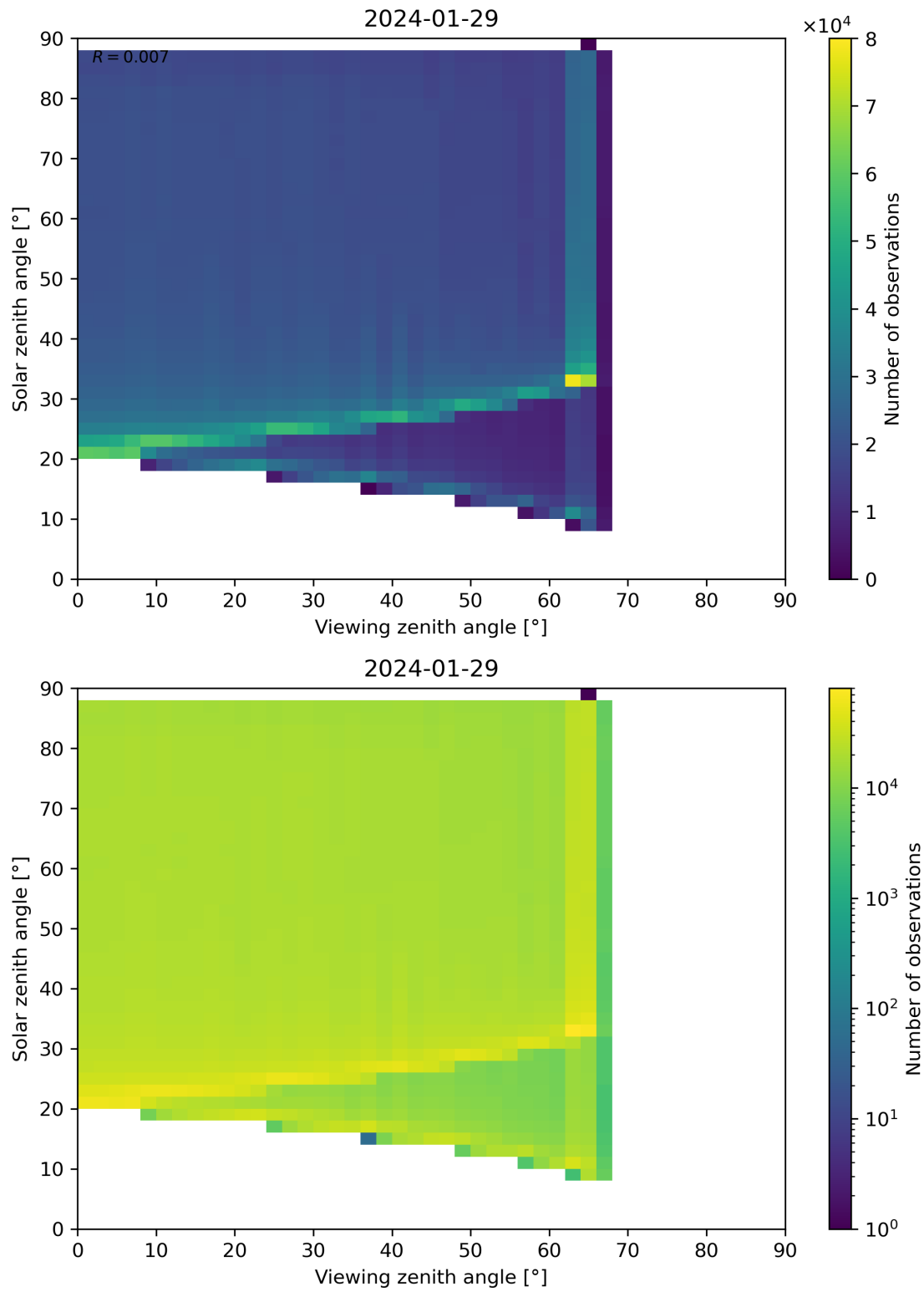
Figure 172: Scatter density plot of “Viewing zenith angle” against “Solar zenith angle” for 2024-01-28 to 2024-01-30.
