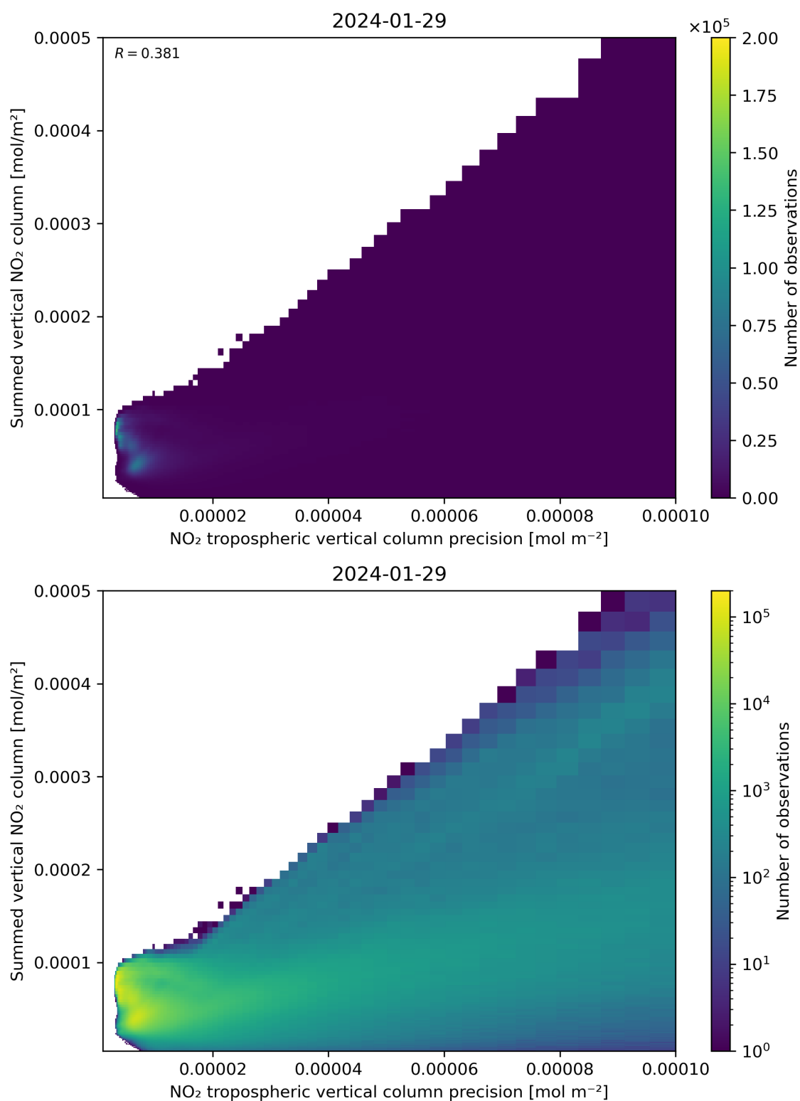
Figure 136: Scatter density plot of “NO 2 tropospheric vertical column precision” against “Summed vertical NO 2 column” for 2024-01-28 to 2024-01-30.
