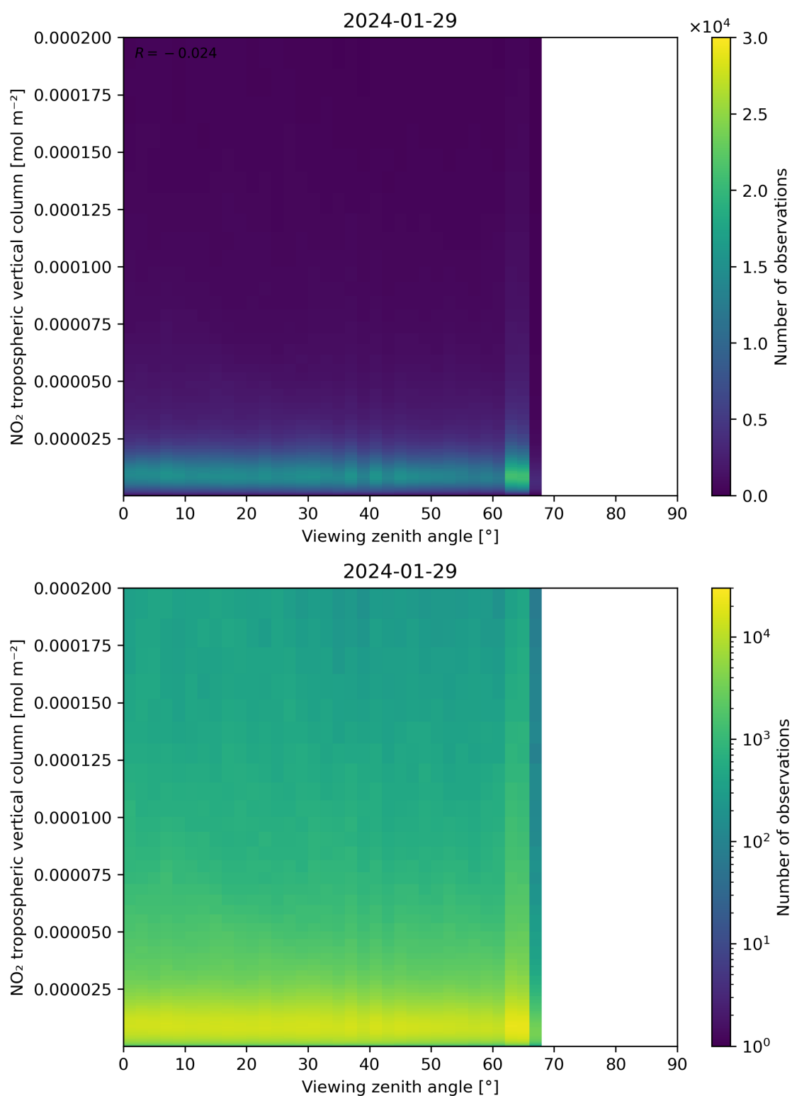
Figure 169: Scatter density plot of “Viewing zenith angle” against “NO 2 tropospheric vertical column” for 2024-01-28 to 2024-01-30.
