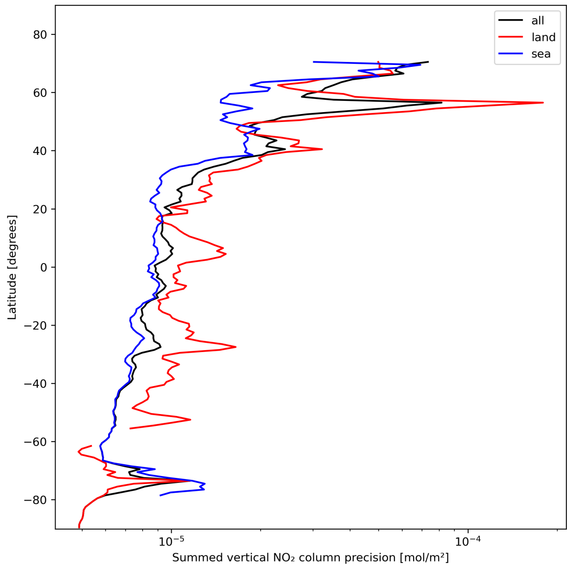
Figure 24: Zonal average of “Summed vertical NO 2 column precision” for 2024-01-28 to 2024-01-30.
