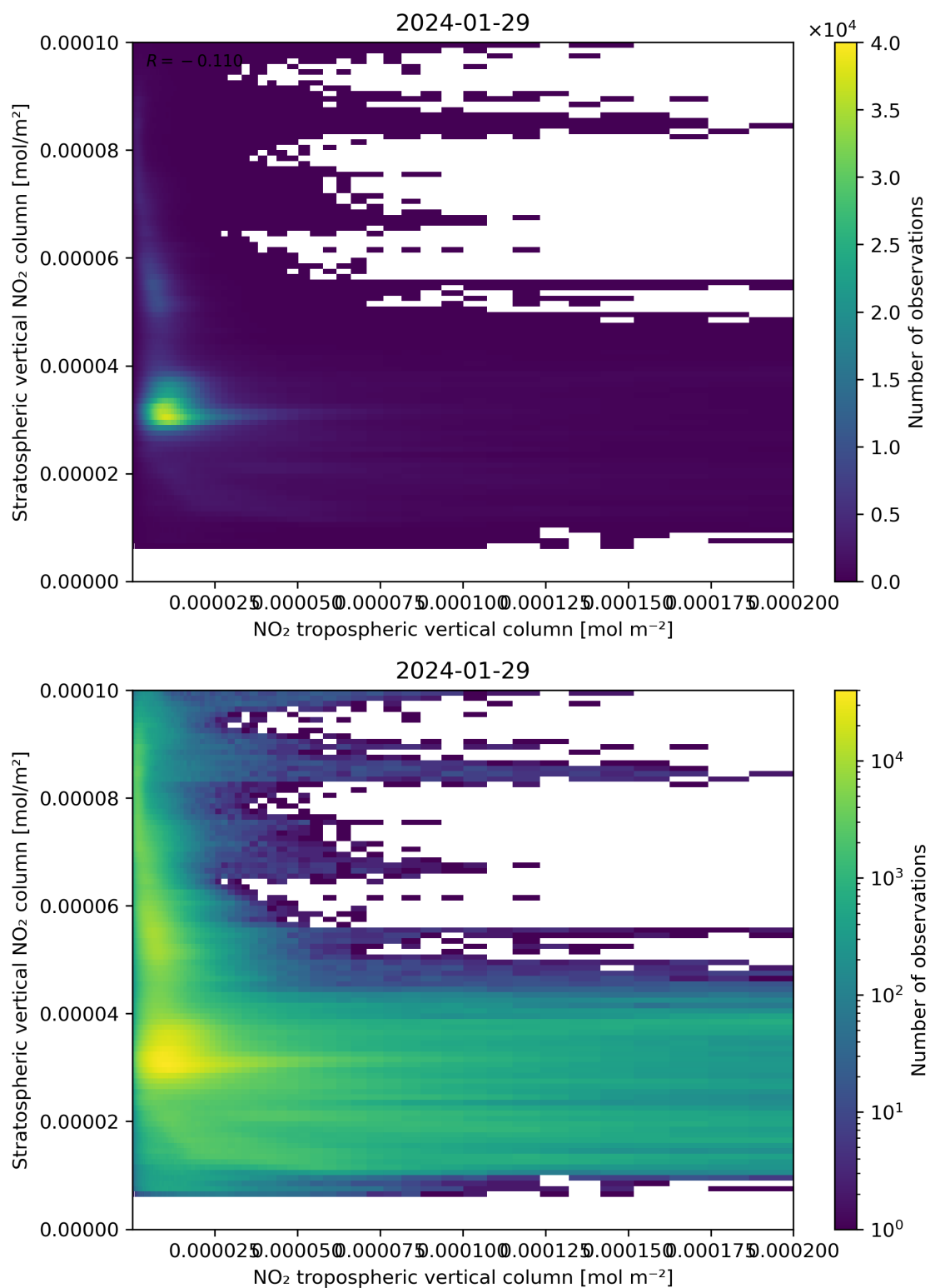
Figure 125: Scatter density plot of “NO 2 tropospheric vertical column” against “Stratospheric vertical NO 2 column” for 2024-01-28 to 2024-01-30.
