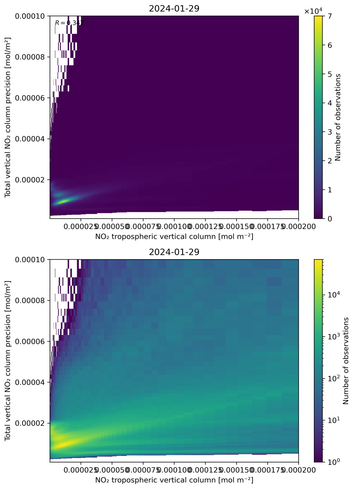
Figure 129: Scatter density plot of “NO 2 tropospheric vertical column” against “Total vertical NO 2 column precision” for 2024-01-28 to 2024-01-30.
