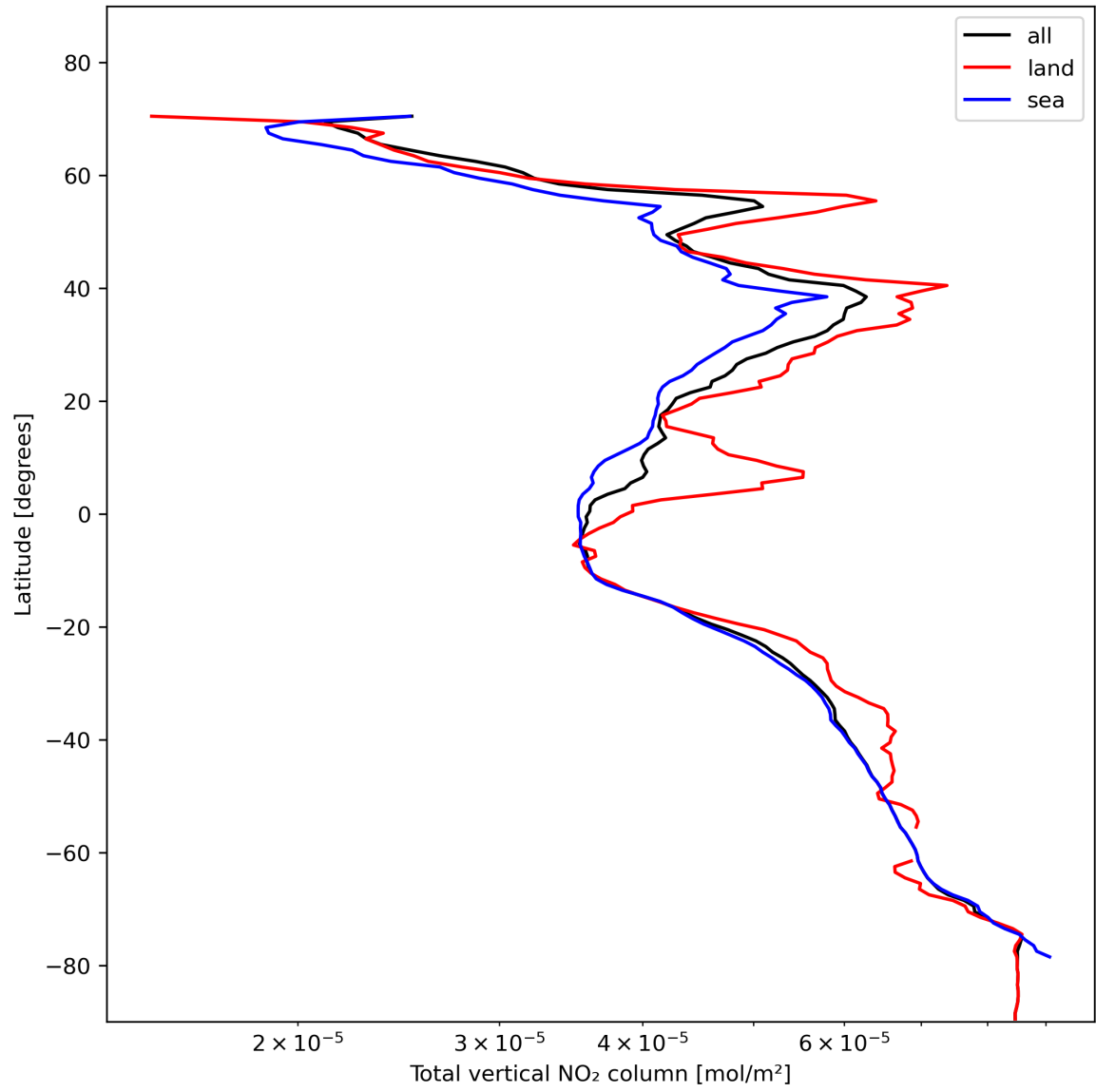
Figure 21: Zonal average of “Total vertical NO 2 column” for 2024-01-28 to 2024-01-30.
