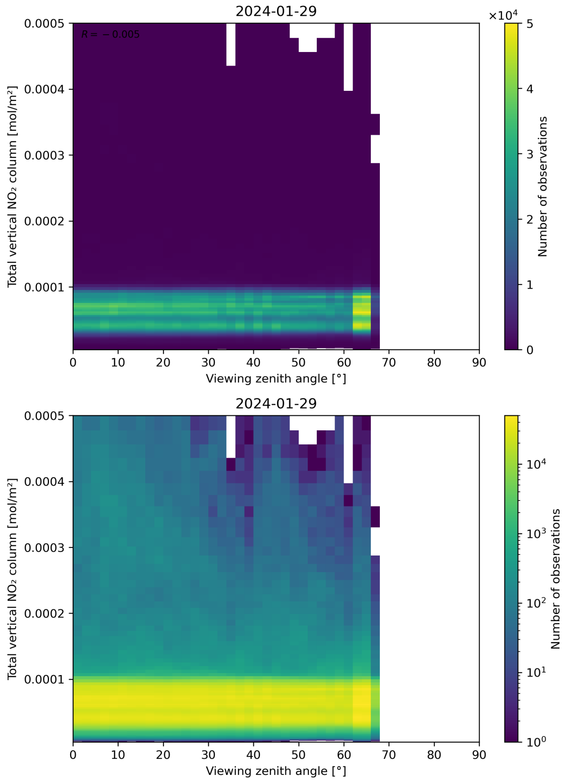
Figure 167: Scatter density plot of “Viewing zenith angle” against “Total vertical NO 2 column” for 2024-01-28 to 2024-01-30.
