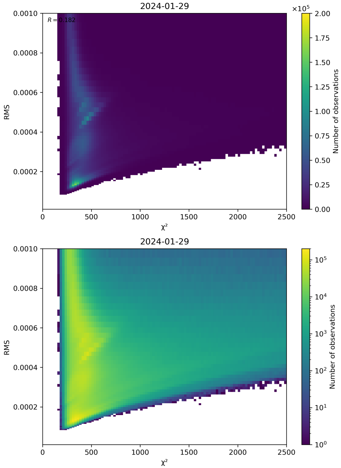
Figure 82: Scatter density plot of “ \chi^2 ” against “RMS” for 2024-01-28 to 2024-01-30.
