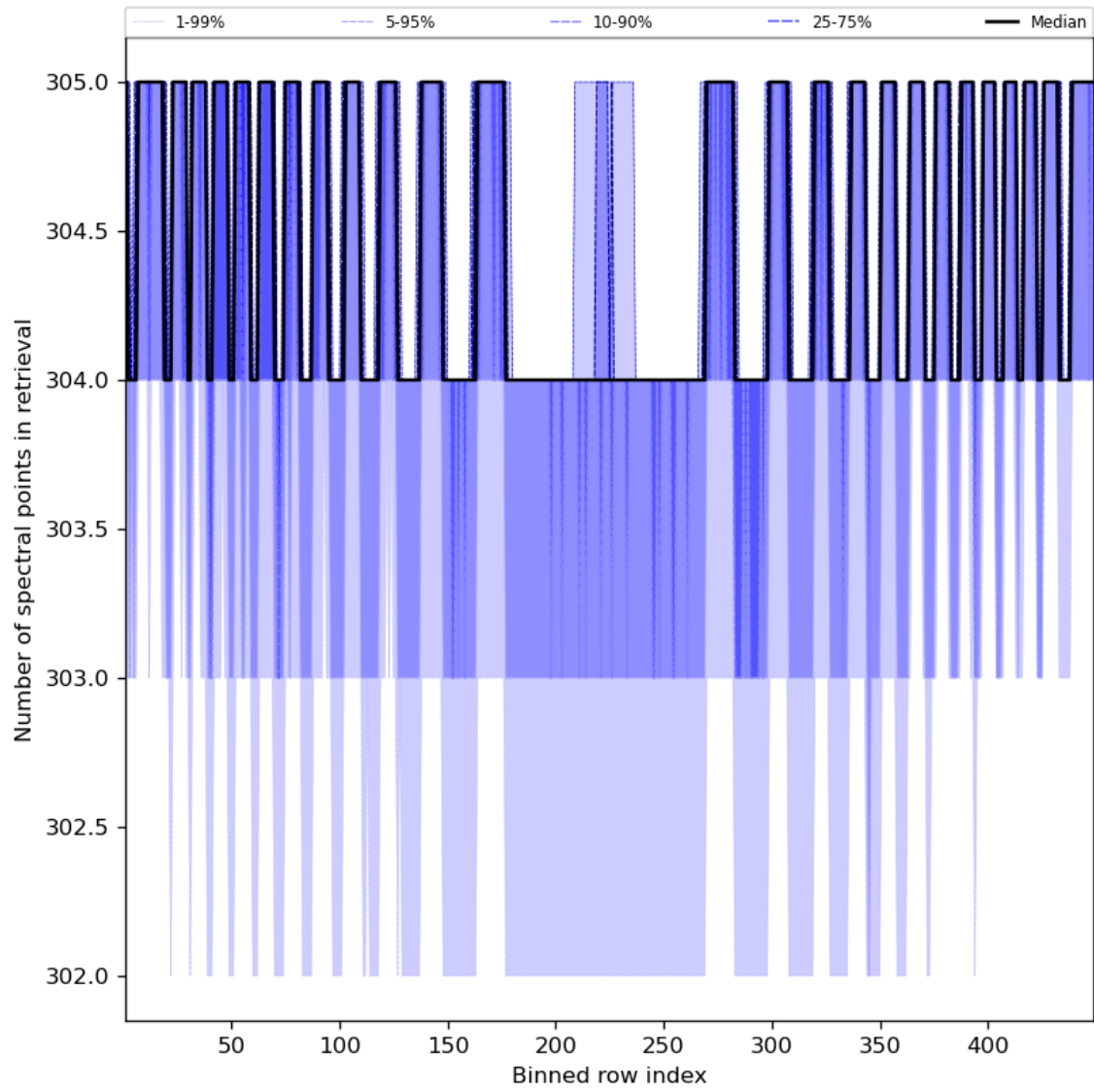
Figure 50: Along track statistics of “Number of spectral points in retrieval” for 2024-01-28 to 2024-01-30
