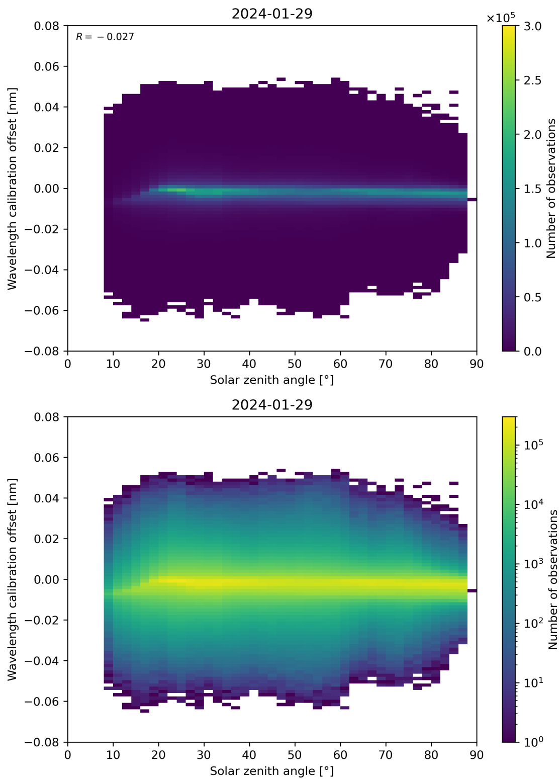
Figure 158: Scatter density plot of “Solar zenith angle” against “Wavelength calibration offset” for 2024-01-28 to 2024-01-30.
