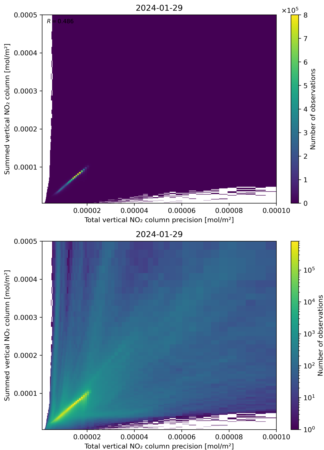
Figure 117: Scatter density plot of “Total vertical NO 2 column precision” against “Summed vertical NO 2 column” for 2024-01-28 to 2024-01-30.
