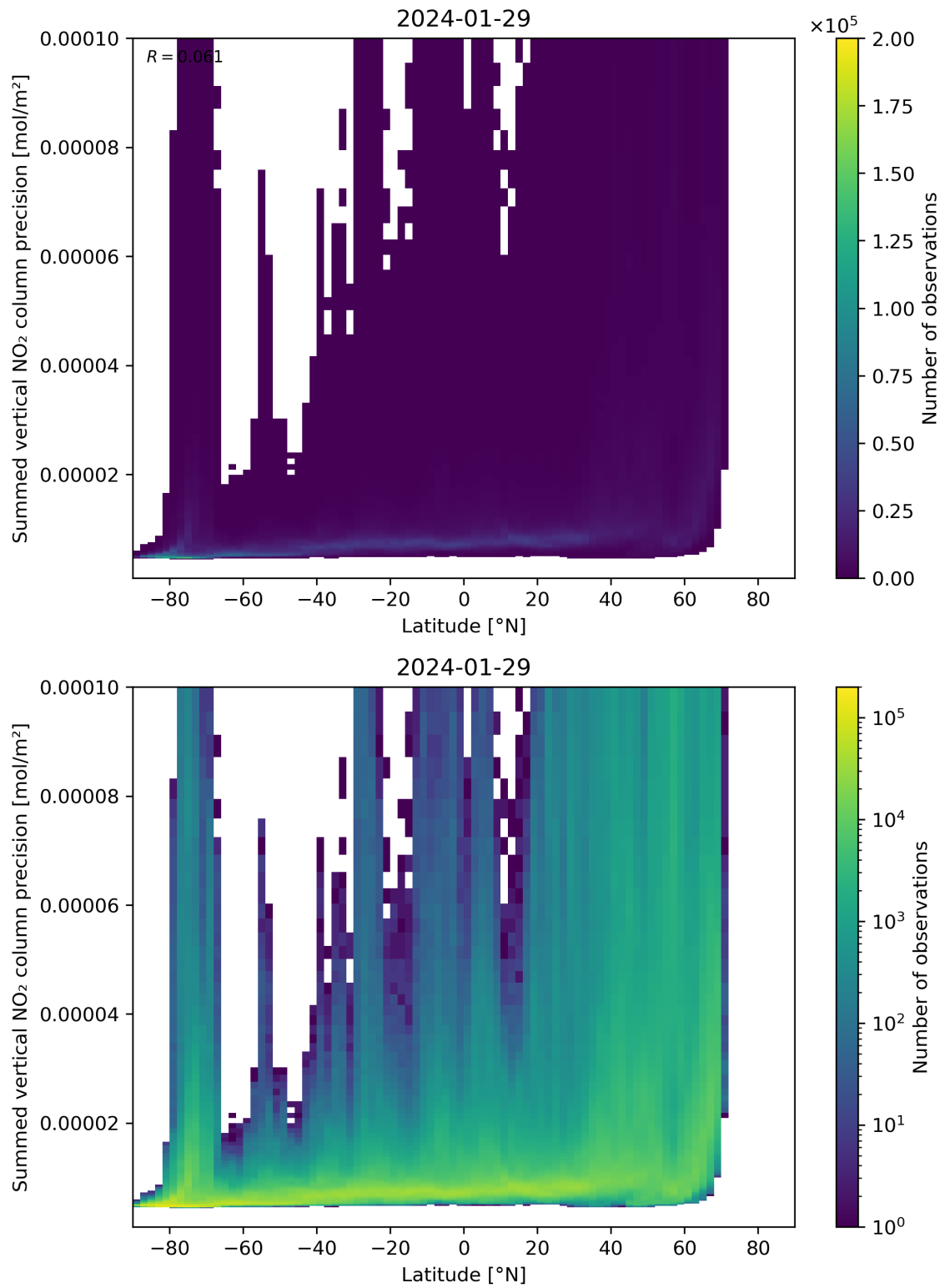
Figure 89: Scatter density plot of “Latitude” against “Summed vertical NO 2 column precision” for 2024-01-28 to 2024-01-30.
