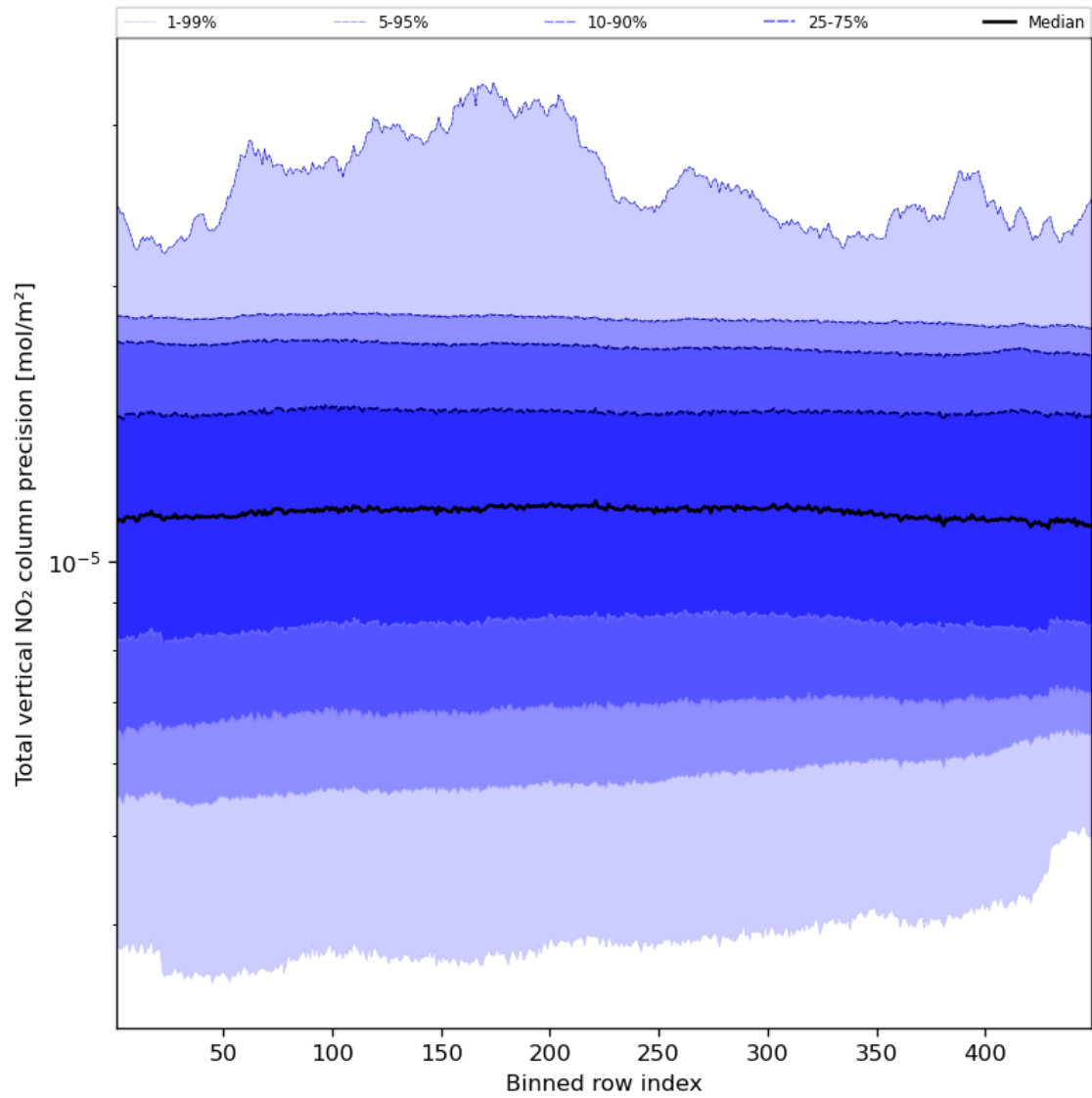
Figure 56: Along track statistics of “Total vertical NO 2 column precision” for 2024-01-28 to 2024-01-30
