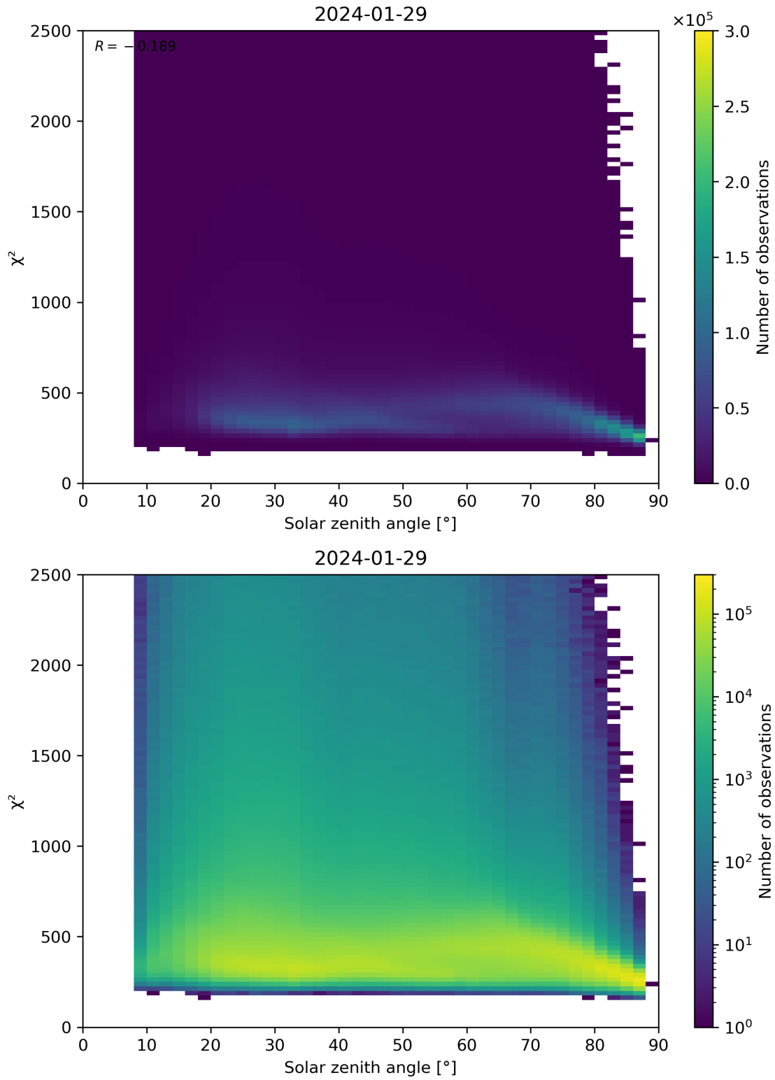
Figure 148: Scatter density plot of “Solar zenith angle” against “ \chi^2 ” for 2024-01-28 to 2024-01-30.
