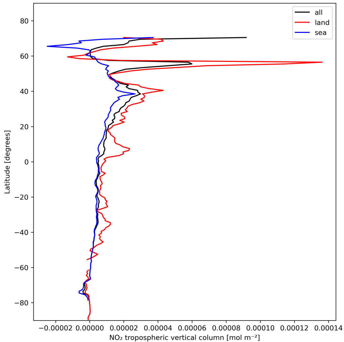
Figure 12: Zonal average of “NO 2 tropospheric vertical column” for 2024-01-28 to 2024-01-30.
