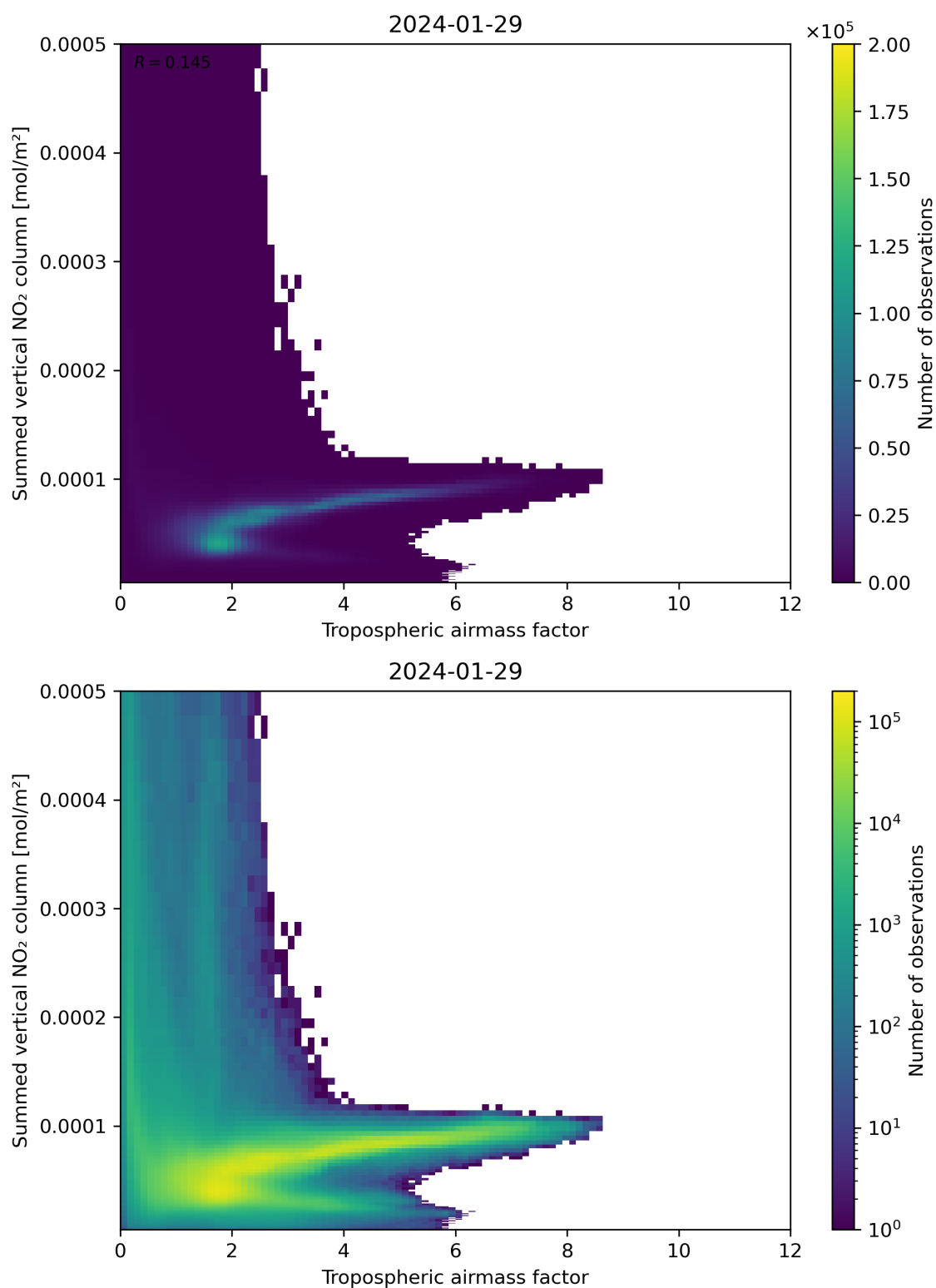
Figure 75: Scatter density plot of “Tropospheric airmass factor” against “Summed vertical NO 2 column” for 2024-01-28 to 2024-01-30.
