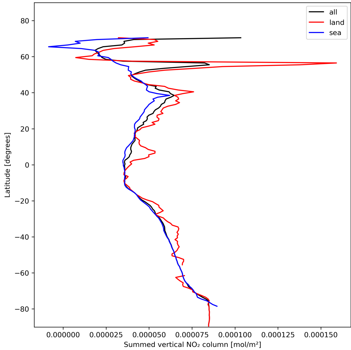
Figure 23: Zonal average of “Summed vertical NO 2 column” for 2024-01-28 to 2024-01-30.
