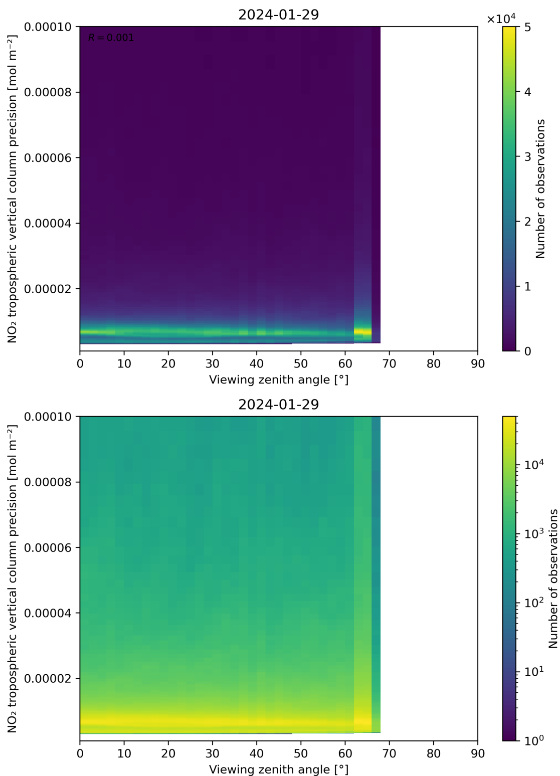
Figure 170: Scatter density plot of “Viewing zenith angle” against “NO 2 tropospheric vertical column precision” for 2024-01-28 to 2024-01-30.
