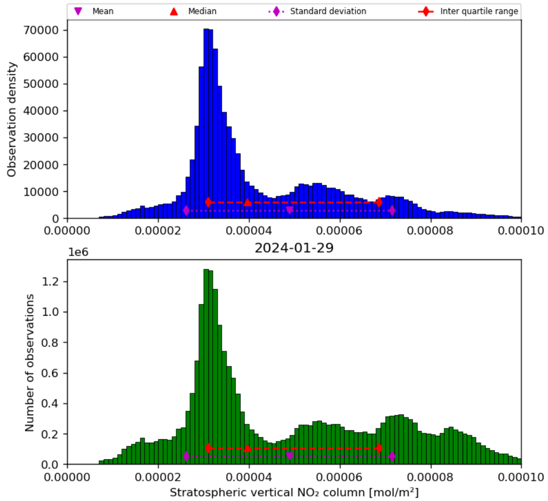
Figure 36: Histogram of “Stratospheric vertical NO 2 column” for 2024-01-28 to 2024-01-30
