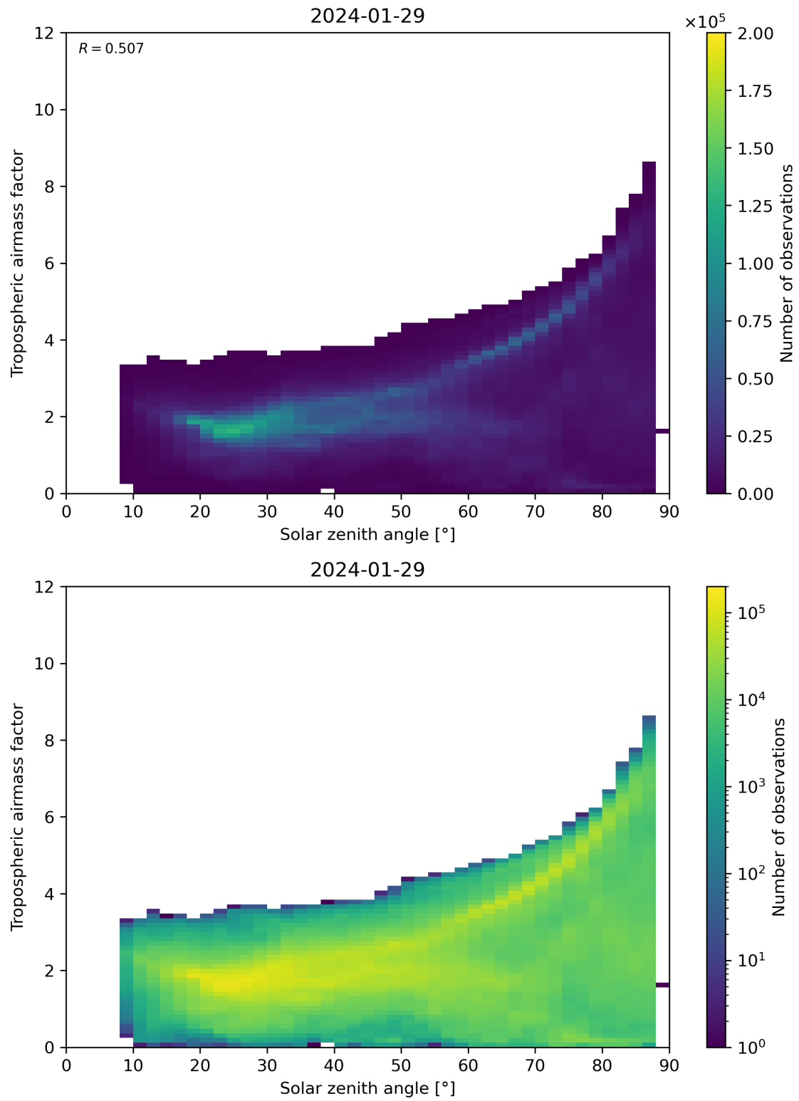
Figure 147: Scatter density plot of “Solar zenith angle” against “Tropospheric airmass factor” for 2024-01-28 to 2024-01-30.
