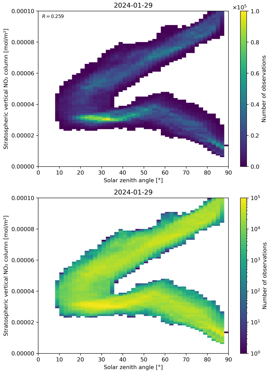
Figure 150: Scatter density plot of “Solar zenith angle” against “Stratospheric vertical NO 2 column” for 2024-01-28 to 2024-01-30.
