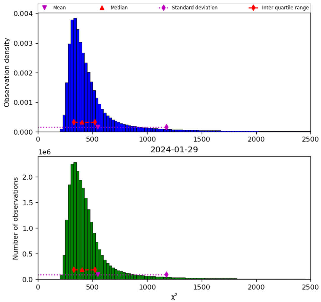
Figure 42: Histogram of " \chi^2 " for 2024-01-28 to 2024-01-30
