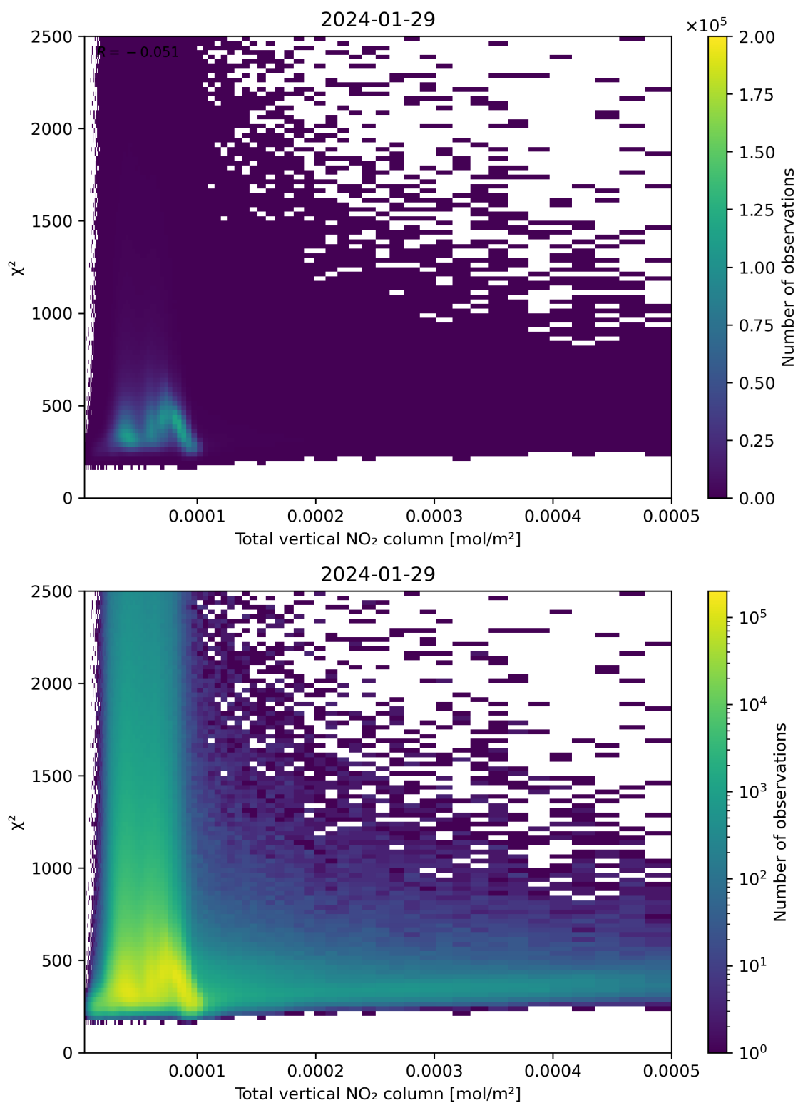
Figure 111: Scatter density plot of “Total vertical NO 2 column” against “ \chi^2 ” for 2024-01-28 to 2024-01-30.
