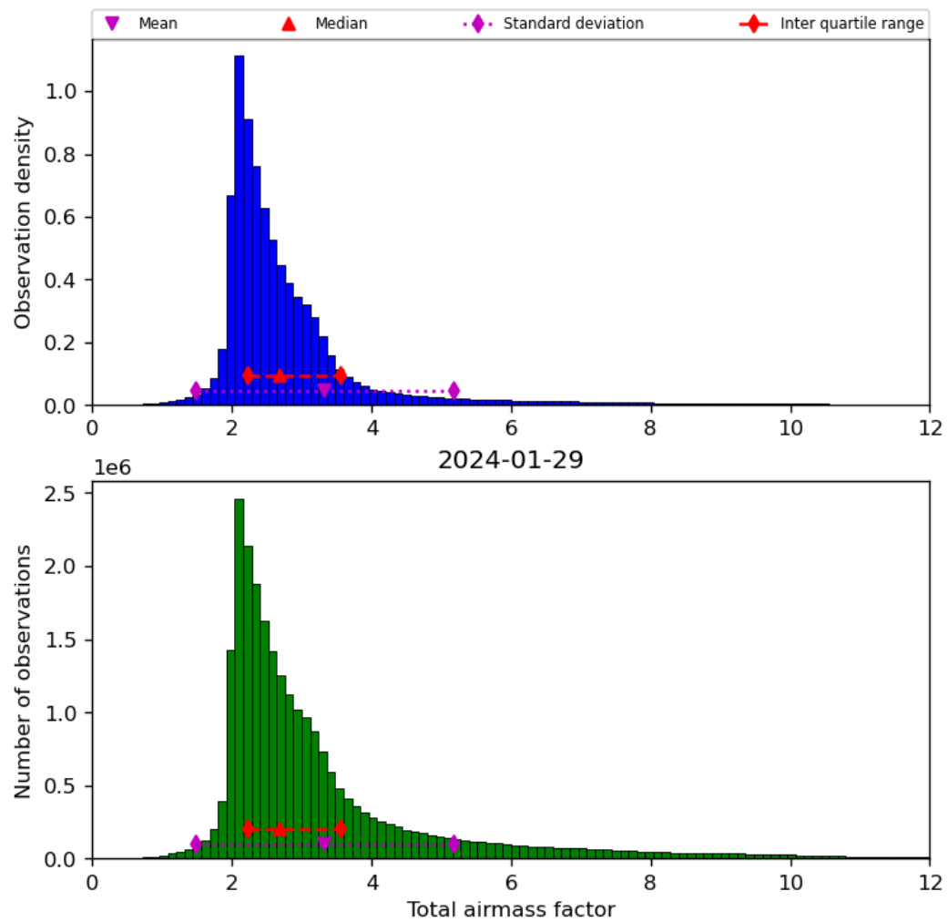
Figure 32: Histogram of “Total airmass factor” for 2024-01-28 to 2024-01-30
