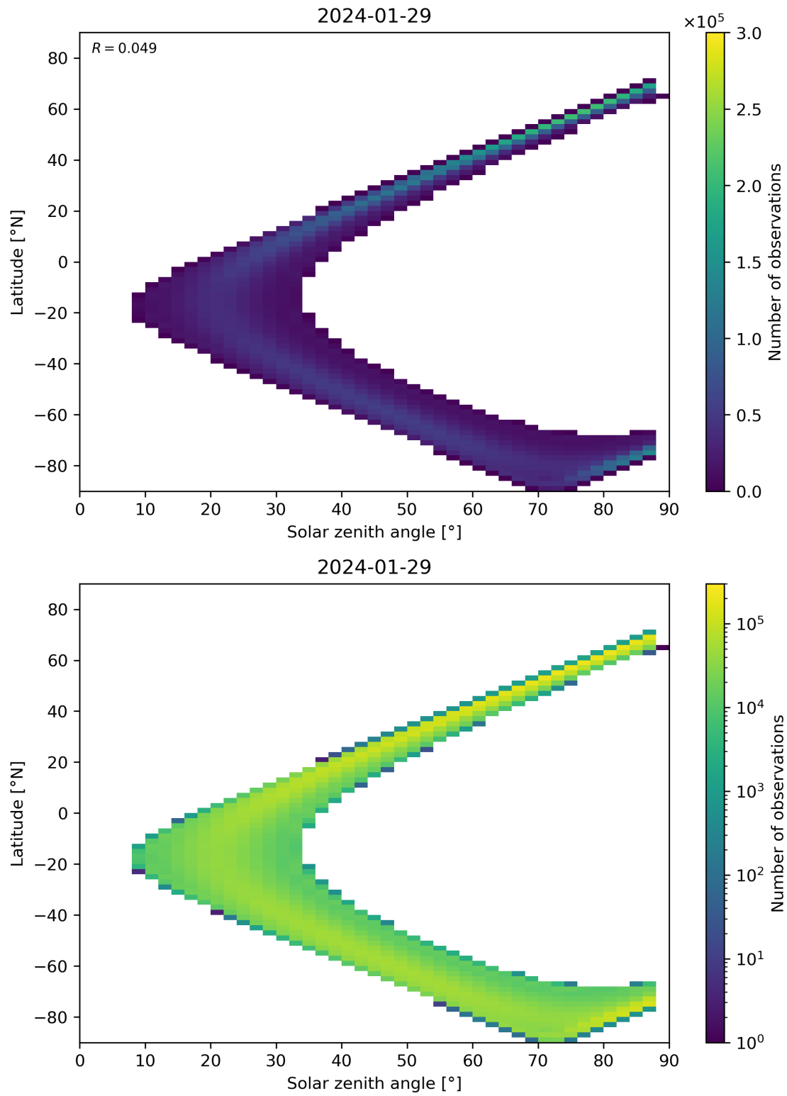
Figure 149: Scatter density plot of “Solar zenith angle” against “Latitude” for 2024-01-28 to 2024-01-30.
