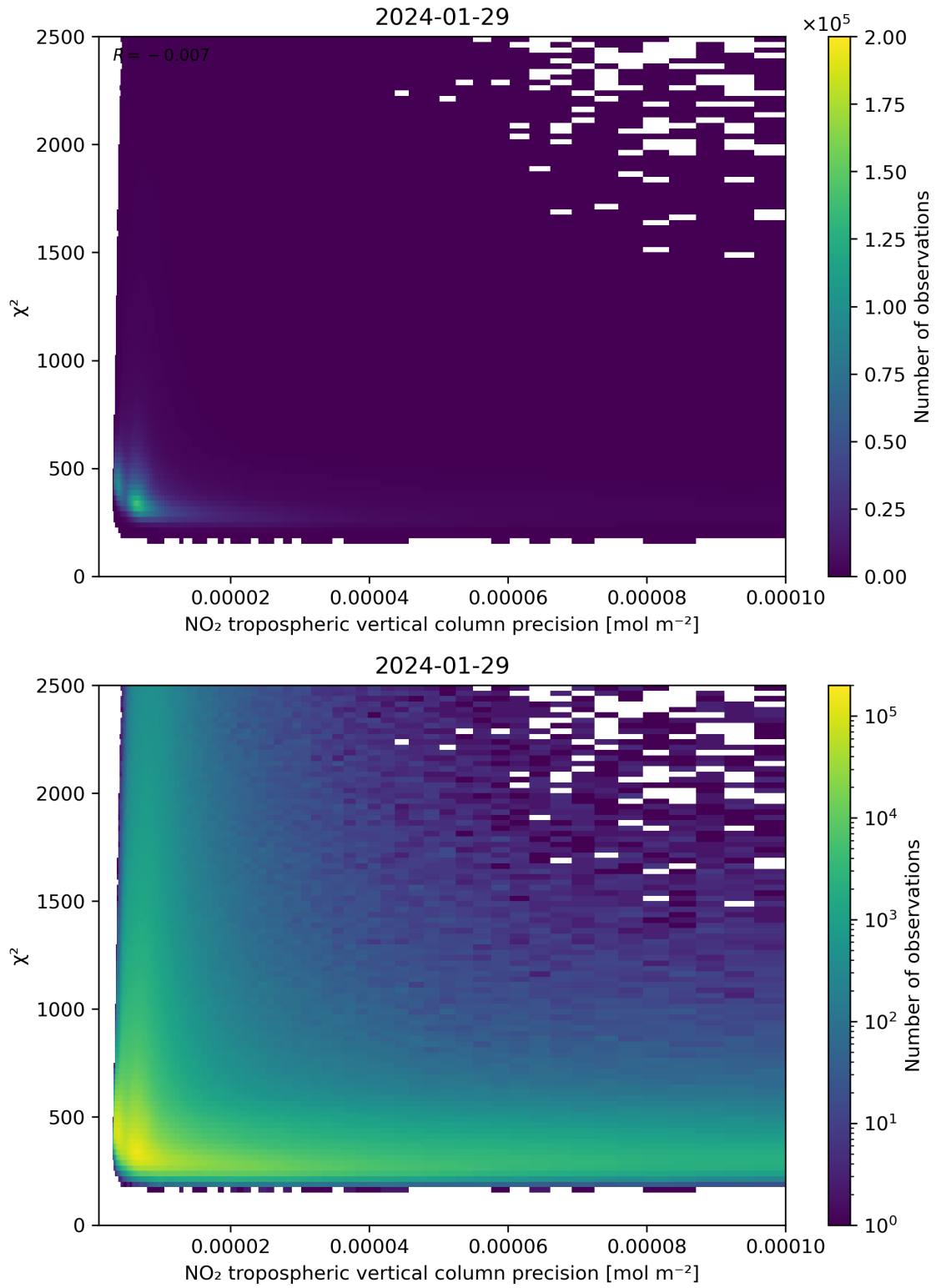
Figure 134: Scatter density plot of “NO 2 tropospheric vertical column precision” against “ \chi^2 ” for 2024-01-28 to 2024-01-30.
