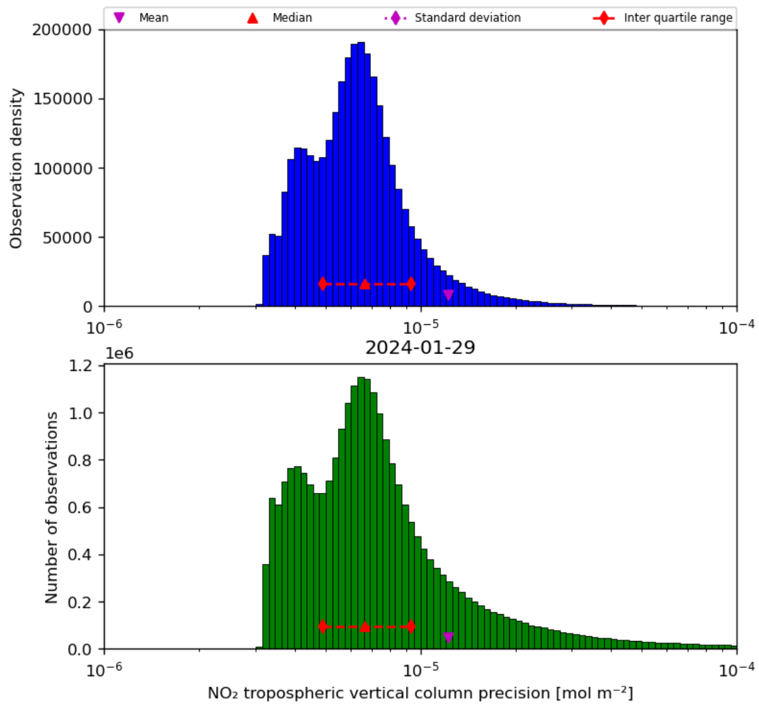
Figure 30: Histogram of “NO 2 tropospheric vertical column precision” for 2024-01-28 to 2024-01-30
