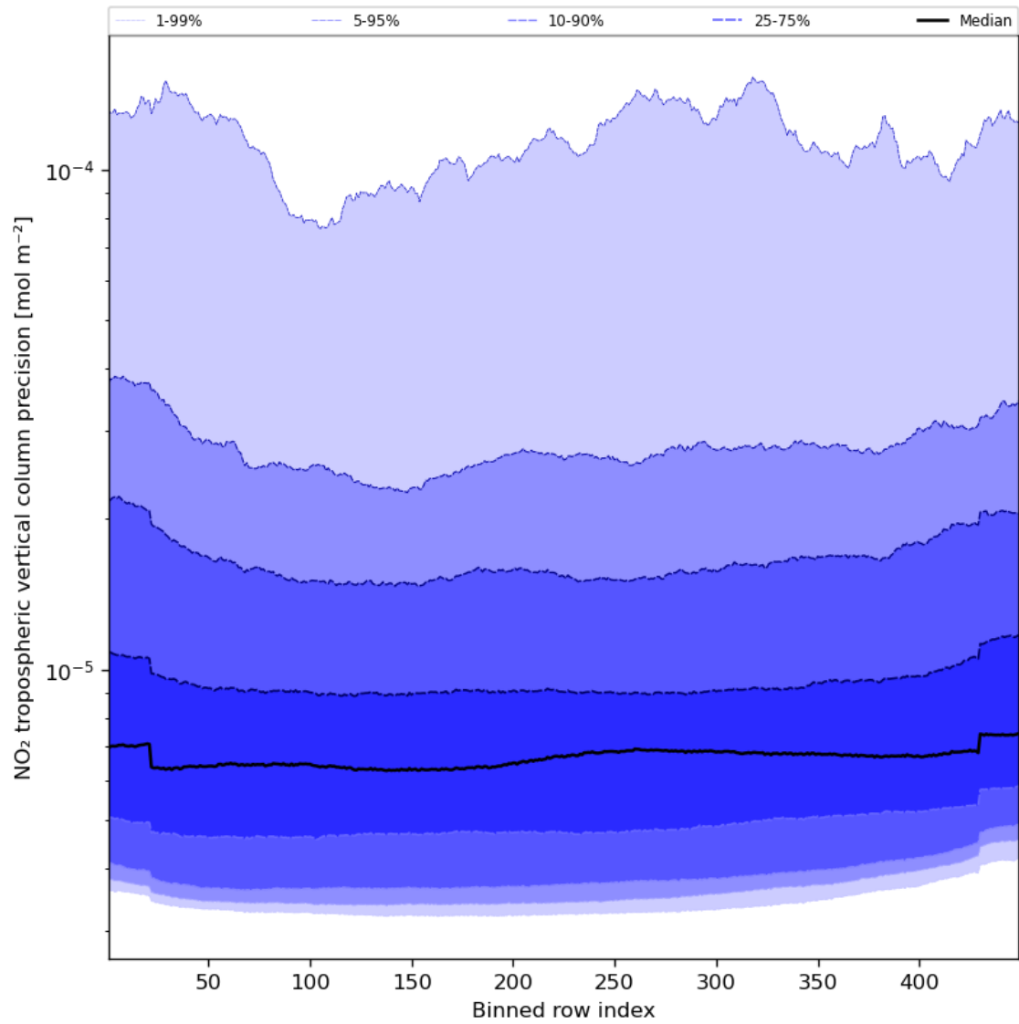
Figure 47: Along track statistics of “NO 2 tropospheric vertical column precision” for 2024-01-28 to 2024-01-30
