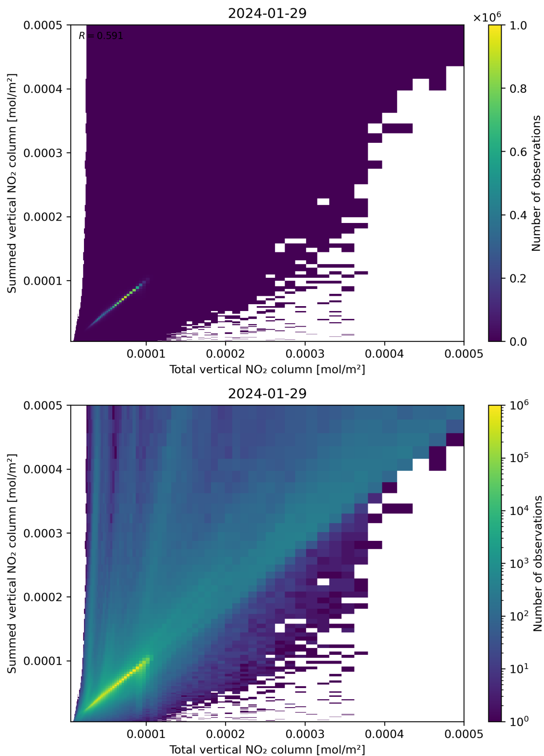
Figure 112: Scatter density plot of “Total vertical NO 2 column” against “Summed vertical NO 2 column” for 2024-01-28 to 2024-01-30.
