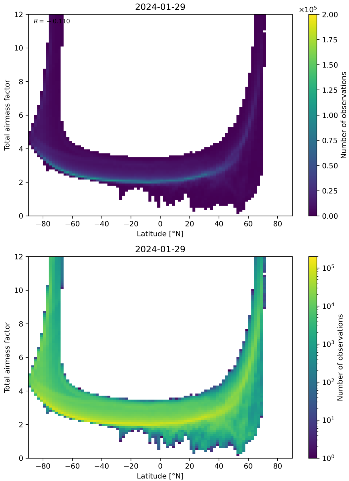
Figure 84: Scatter density plot of “Latitude” against “Total airmass factor” for 2024-01-28 to 2024-01-30.
