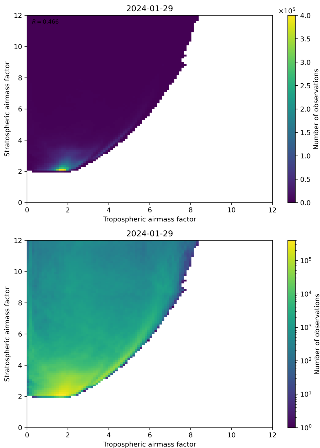
Figure 71: Scatter density plot of “Tropospheric airmass factor” against “Stratospheric airmass factor” for 2024-01-28 to 2024-01-30.
