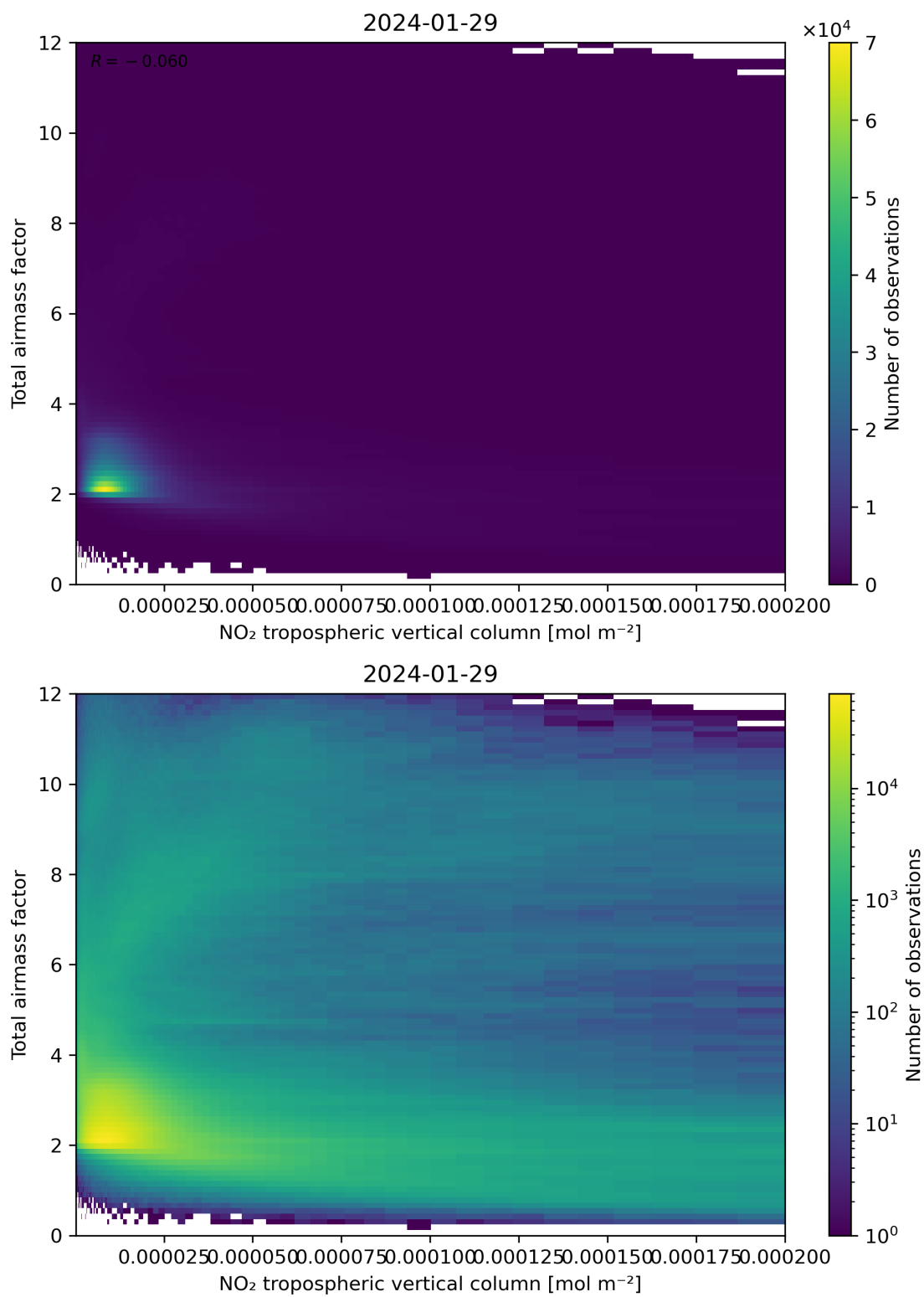
Figure 122: Scatter density plot of “NO 2 tropospheric vertical column” against “Total air mass factor” for 2024-01-28 to 2024-01-30.
