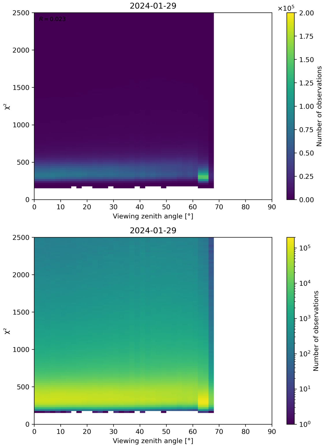
Figure 162: Scatter density plot of “Viewing zenith angle” against “ \chi^2 ” for 2024-01-28 to 2024-01-30.
