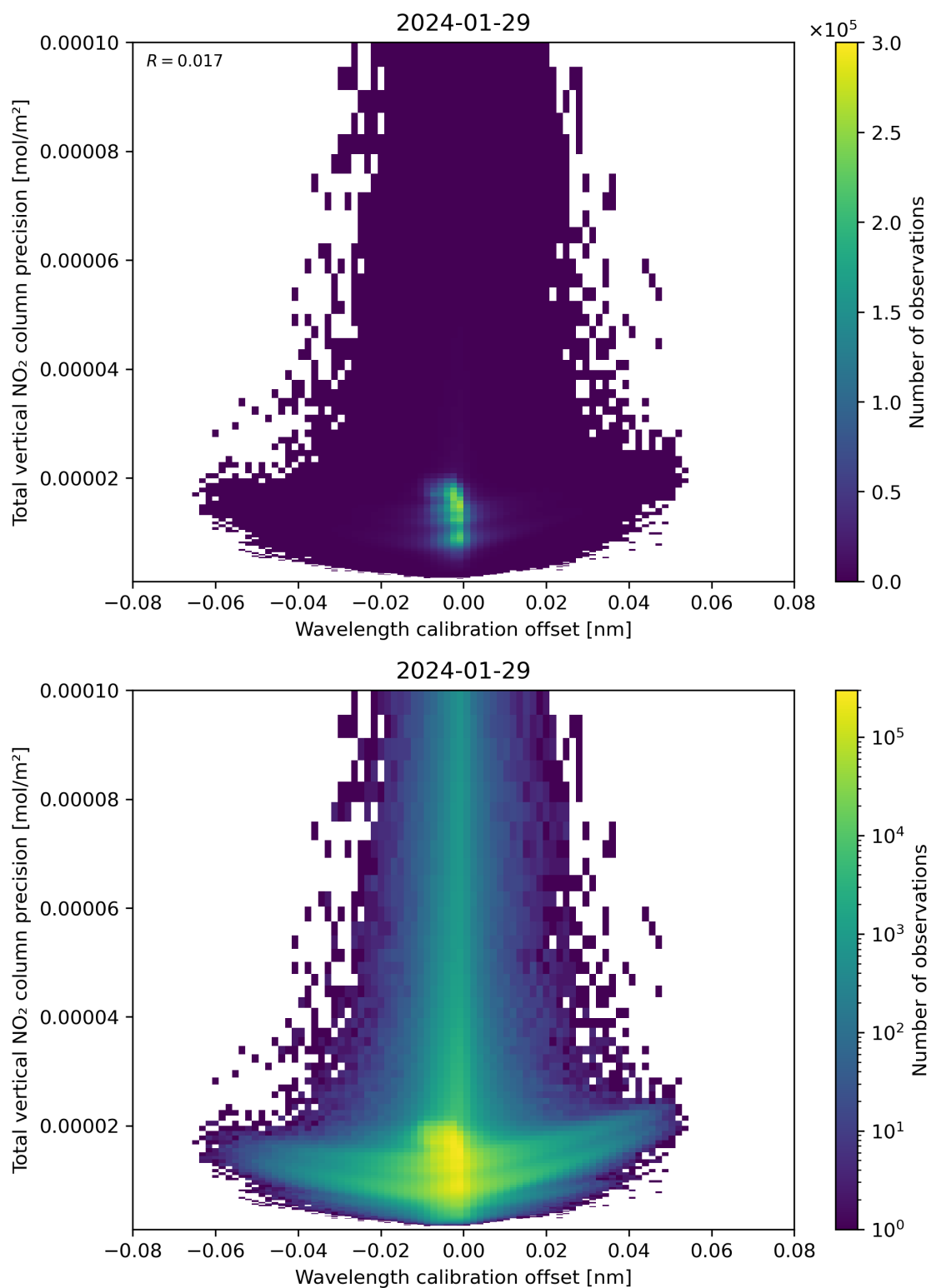
Figure 180: Scatter density plot of “Wavelength calibration offset” against “Total vertical NO 2 column precision” for 2024-01-28 to 2024-01-30.
