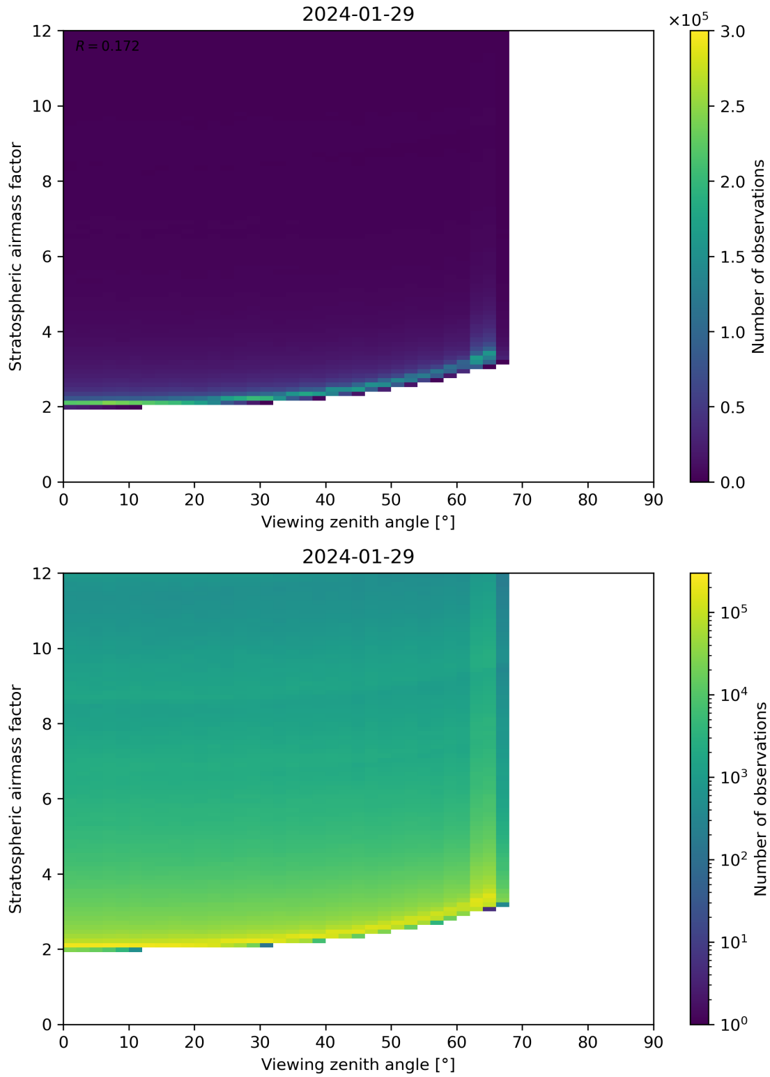
Figure 159: Scatter density plot of “Viewing zenith angle” against “Stratospheric airmass factor” for 2024-01-28 to 2024-01-30.
