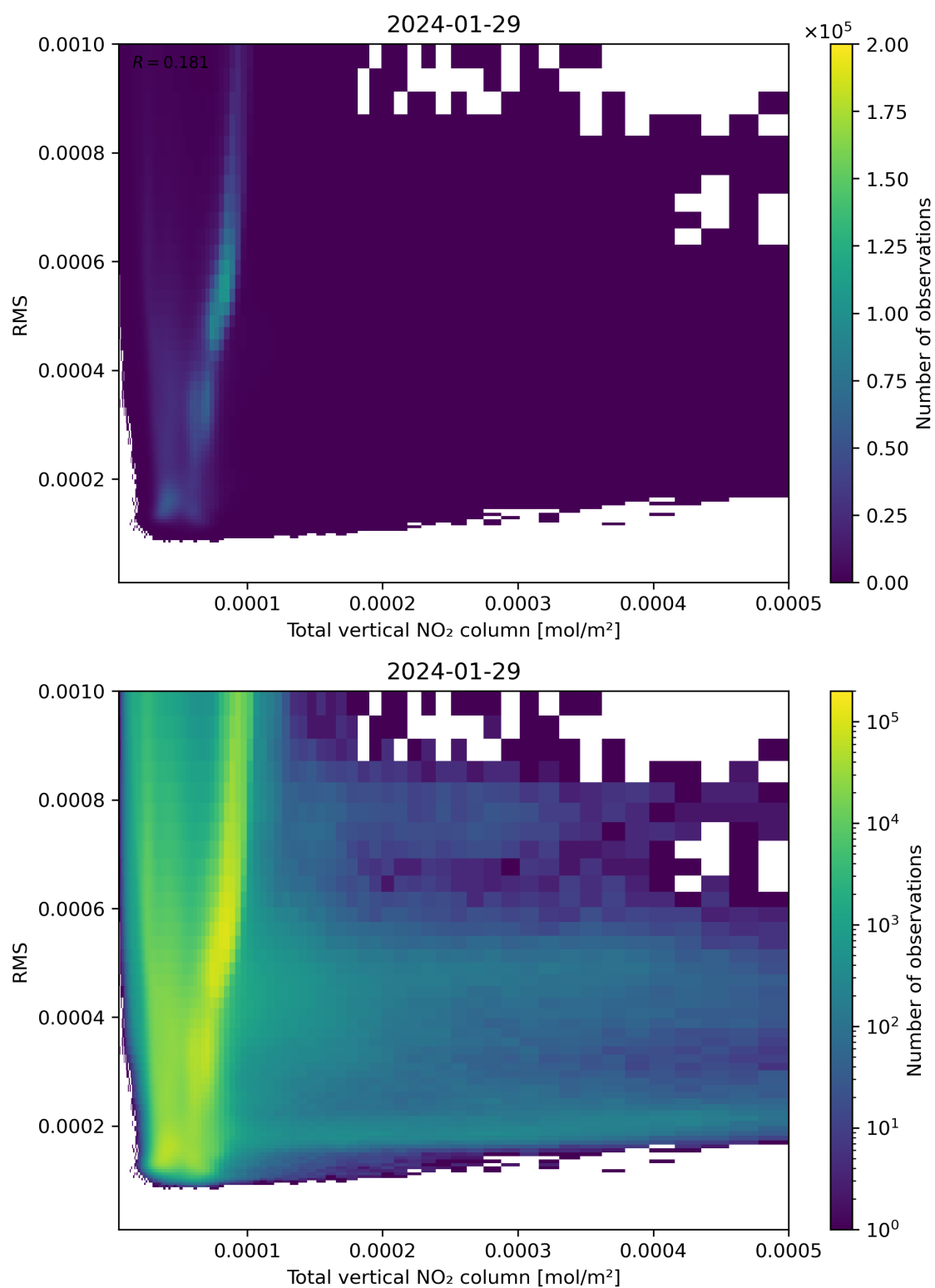
Figure 120: Scatter density plot of “Total vertical NO 2 column” against “RMS” for 2024-01-28 to 2024-01-30.
