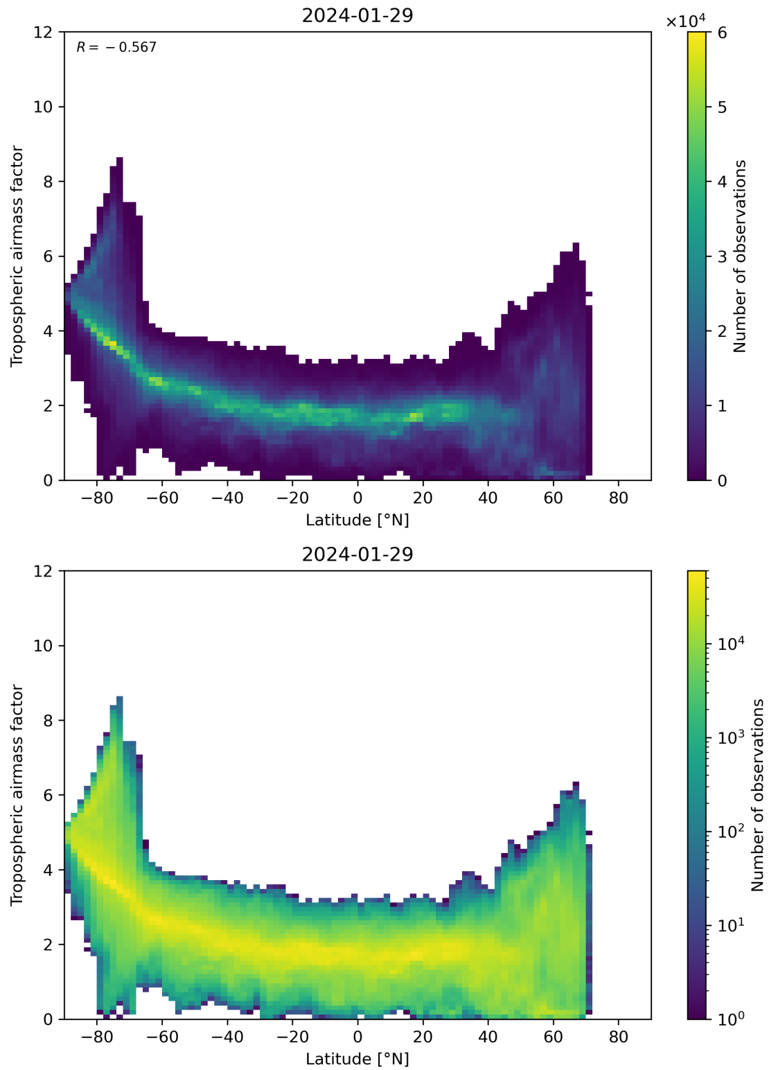
Figure 85: Scatter density plot of “Latitude” against “Tropospheric airmass factor” for 2024-01-28 to 2024-01-30.
