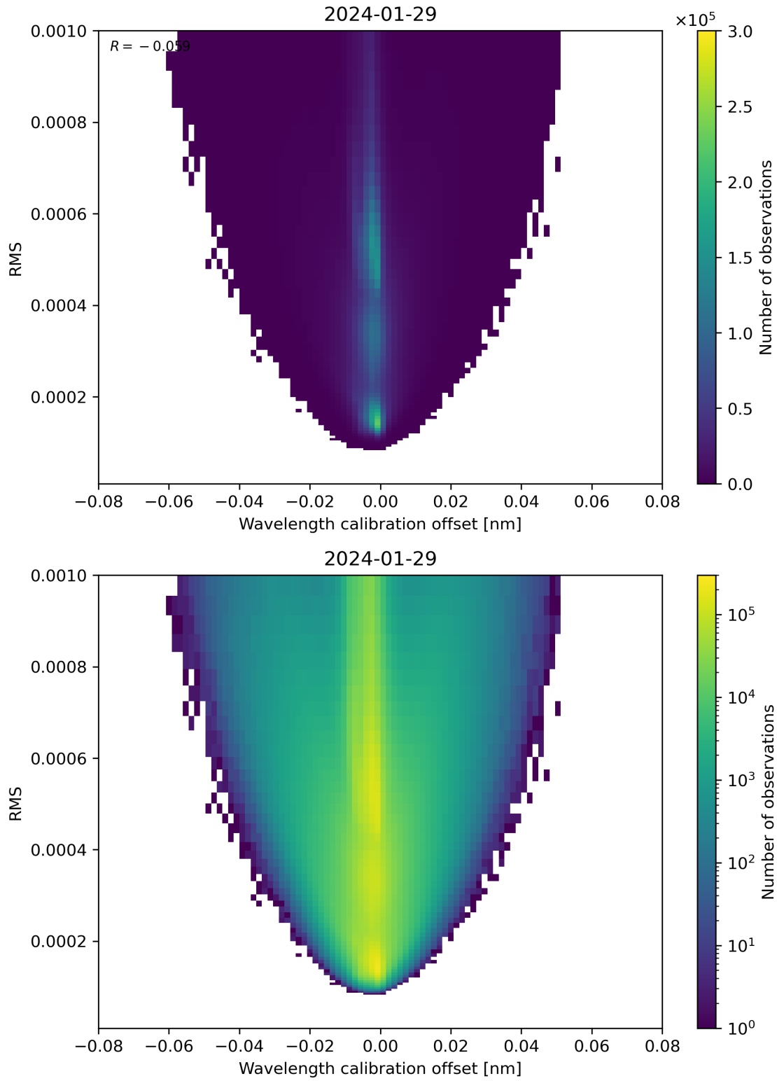
Figure 181: Scatter density plot of “Wavelength calibration offset” against “RMS” for 2024-01-28 to 2024-01-30.
