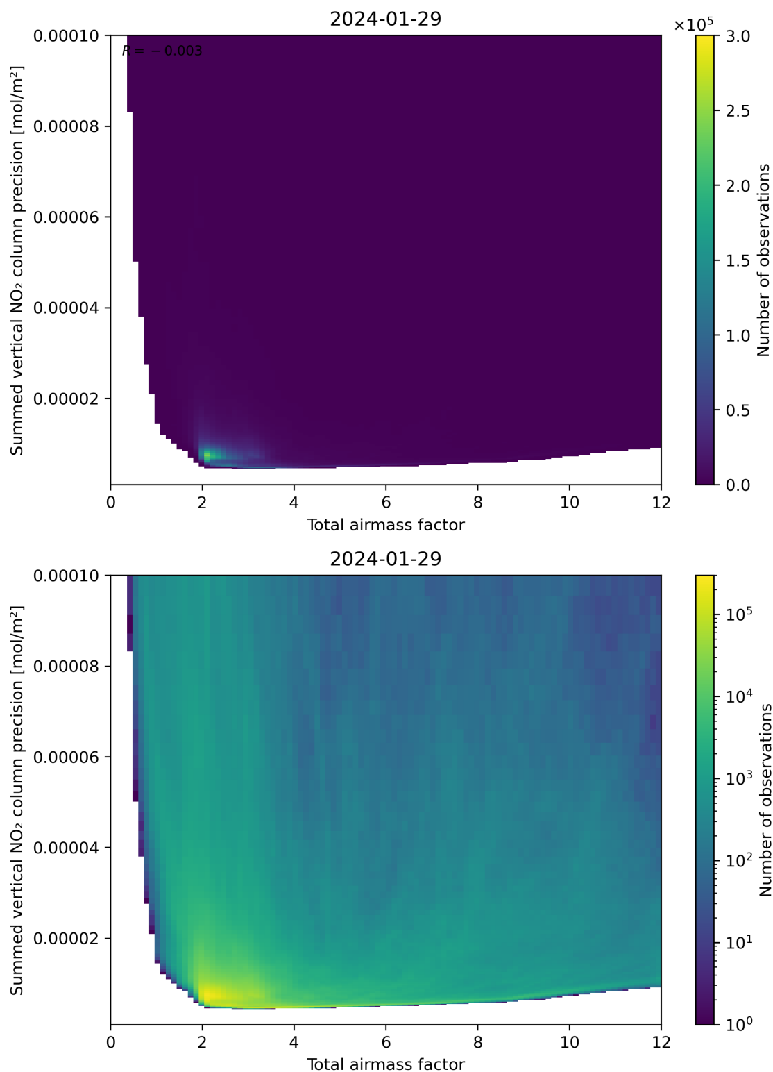
Figure 66: Scatter density plot of “Total airmass factor” against “Summed vertical NO 2 column precision” for 2024-01-28 to 2024-01-30.
