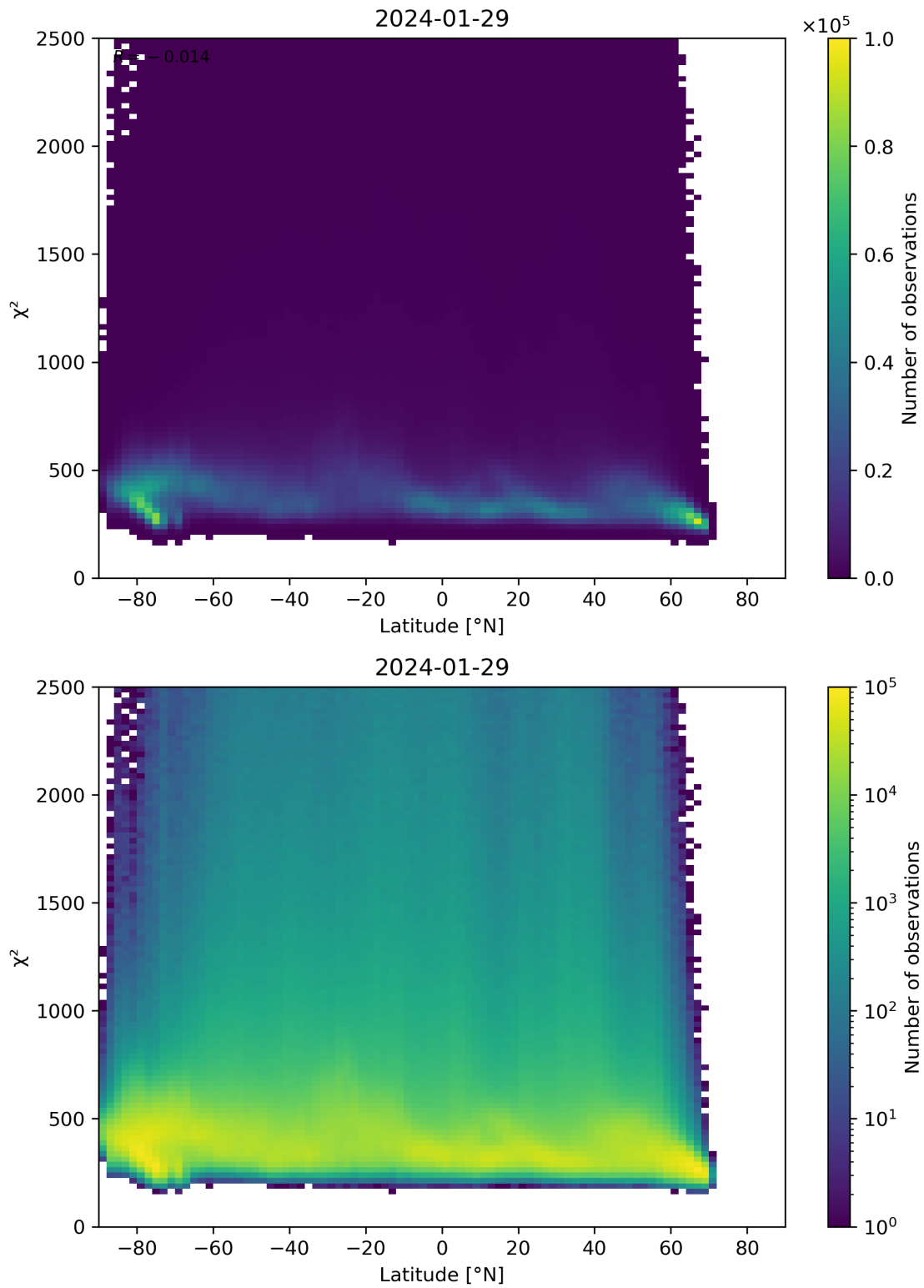
Figure 86: Scatter density plot of “Latitude” against “ \chi^2 ” for 2024-01-28 to 2024-01-30.
