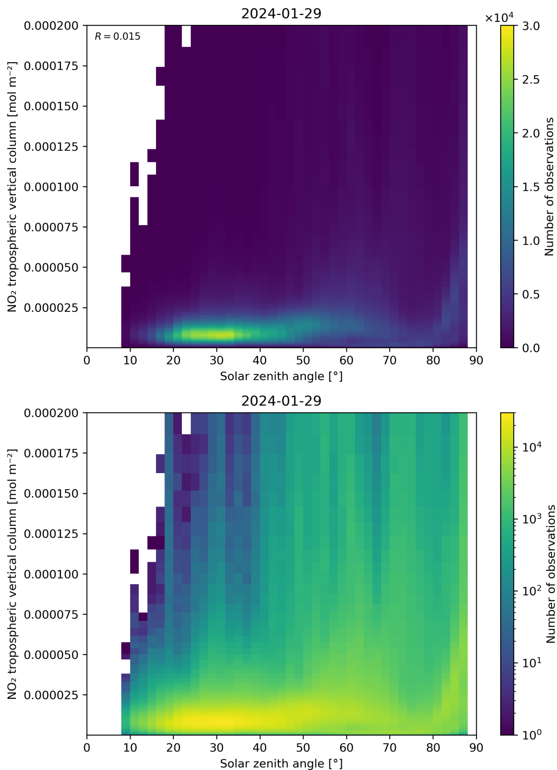
Figure 155: Scatter density plot of “Solar zenith angle” against “NO 2 tropospheric vertical column” for 2024-01-28 to 2024-01-30.
