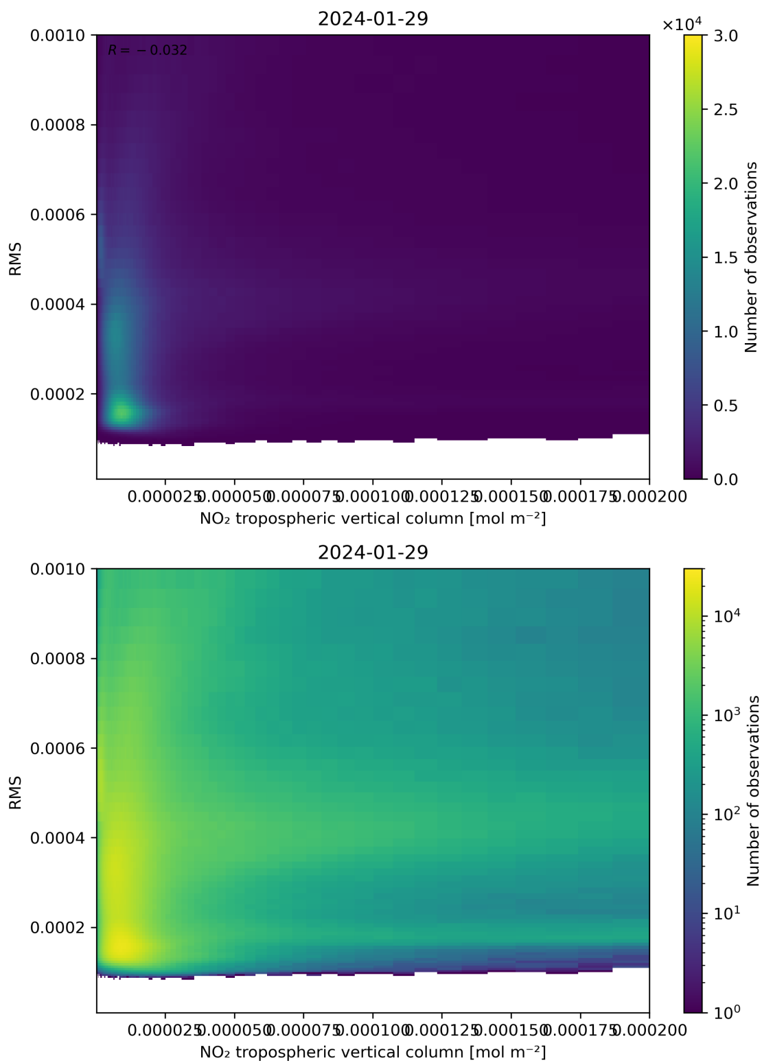
Figure 142: Scatter density plot of “NO 2 tropospheric vertical column” against “RMS” for 2024-01-28 to 2024-01-30.
