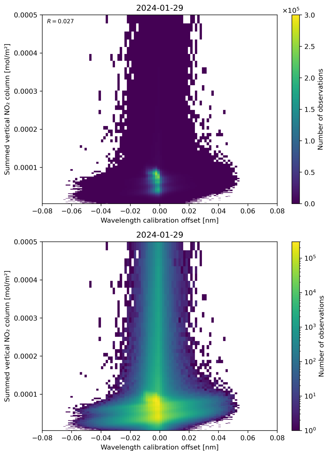
Figure 177: Scatter density plot of “Wavelength calibration offset” against “Summed vertical NO 2 column” for 2024-01-28 to 2024-01-30.
