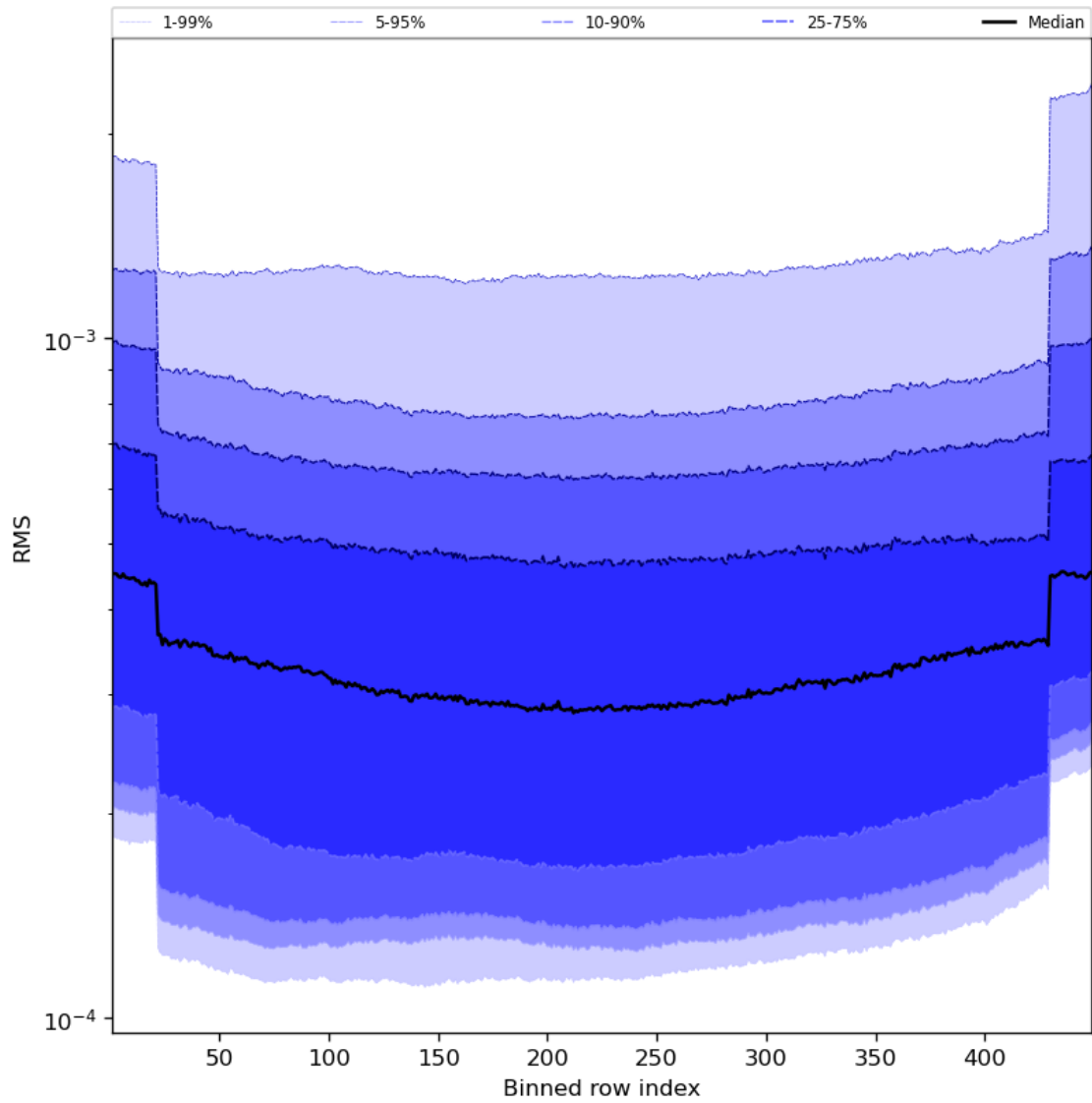
Figure 60: Along track statistics of “RMS” for 2024-01-28 to 2024-01-30
