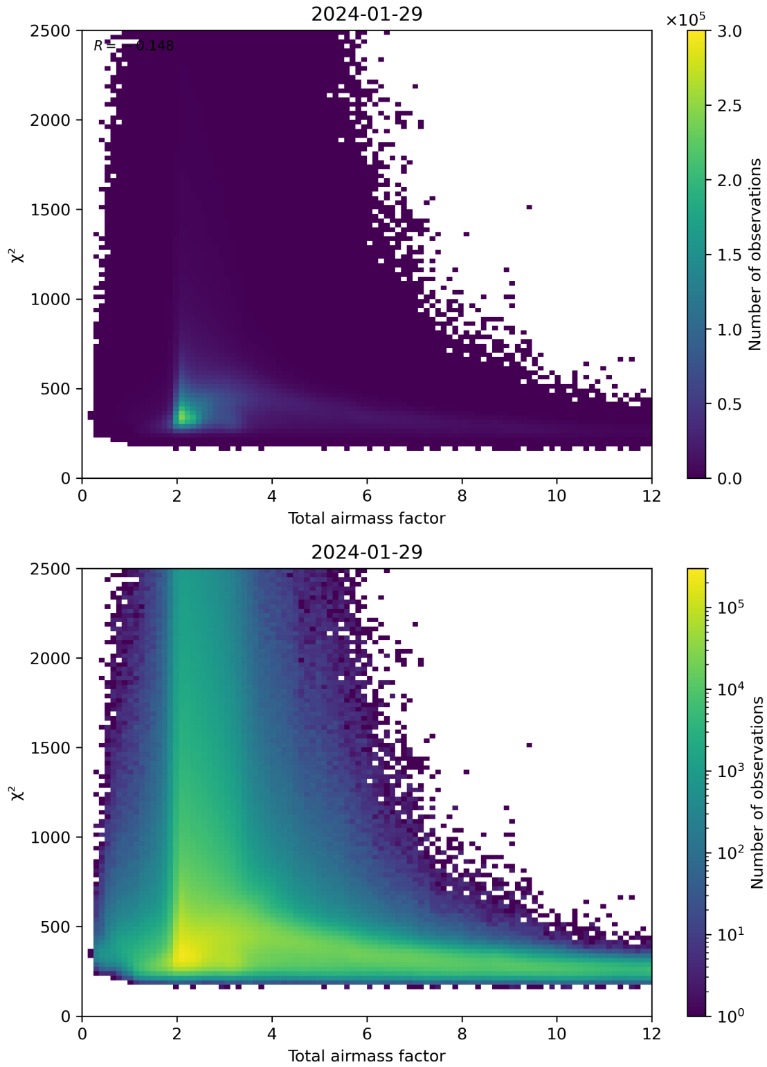
Figure 63: Scatter density plot of “Total airmass factor” against “ \chi^2 ” for 2024-01-28 to 2024-01-30.
