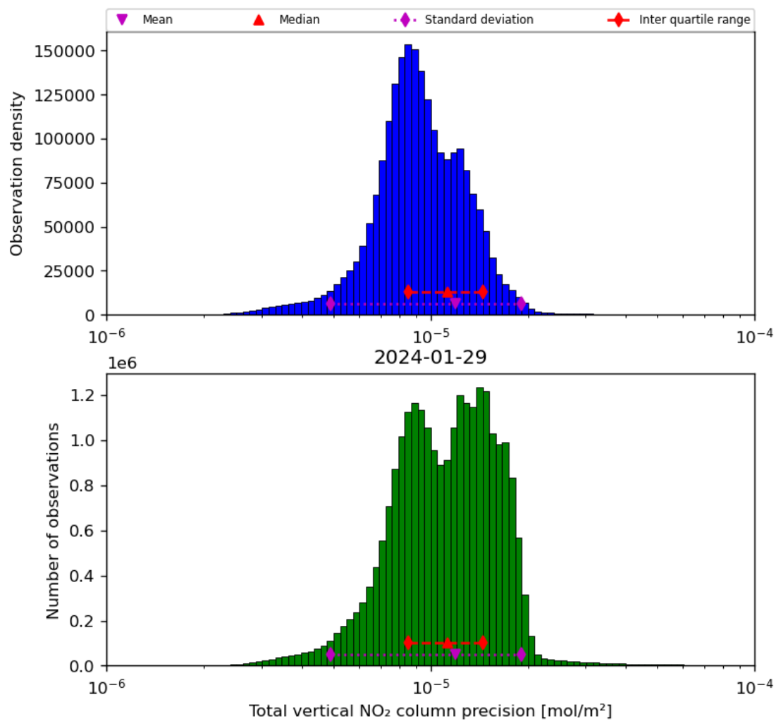
Figure 39: Histogram of “Total vertical NO 2 column precision” for 2024-01-28 to 2024-01-30
