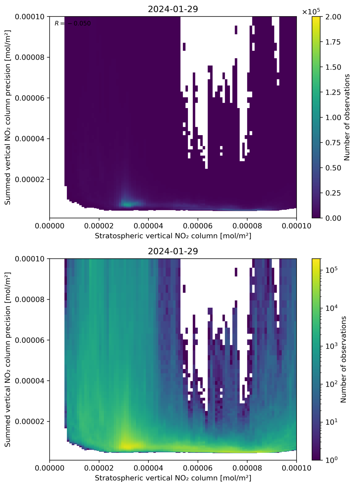
Figure 99: Scatter density plot of “Stratospheric vertical NO 2 column” against “Summed vertical NO 2 column precision” for 2024-01-28 to 2024-01-30.
