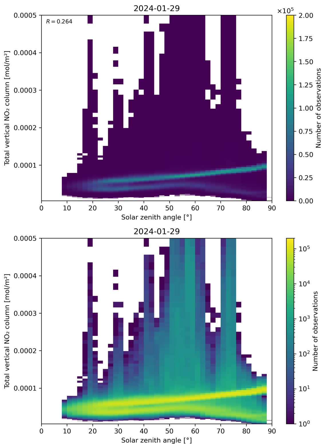
Figure 153: Scatter density plot of “Solar zenith angle” against “Total vertical NO 2 column” for 2024-01-28 to 2024-01-30.
