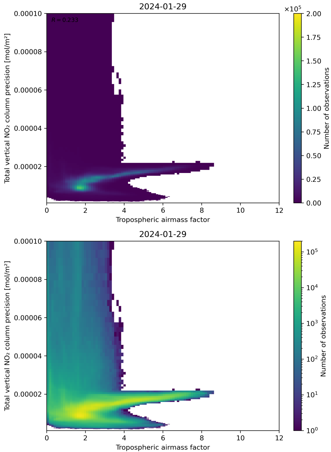
Figure 78: Scatter density plot of “Tropospheric air mass factor” against “Total vertical NO 2 column precision” for 2024-01-28 to 2024-01-30.
