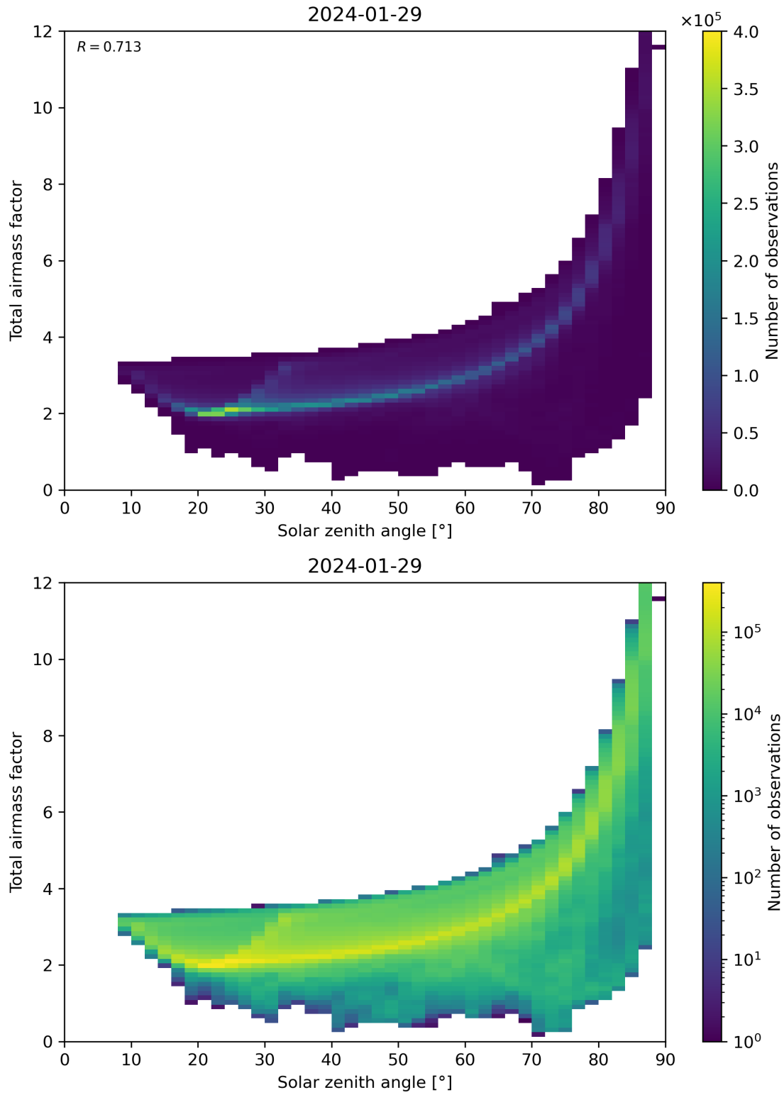
Figure 146: Scatter density plot of “Solar zenith angle” against “Total air mass factor” for 2024-01-28 to 2024-01-30.
