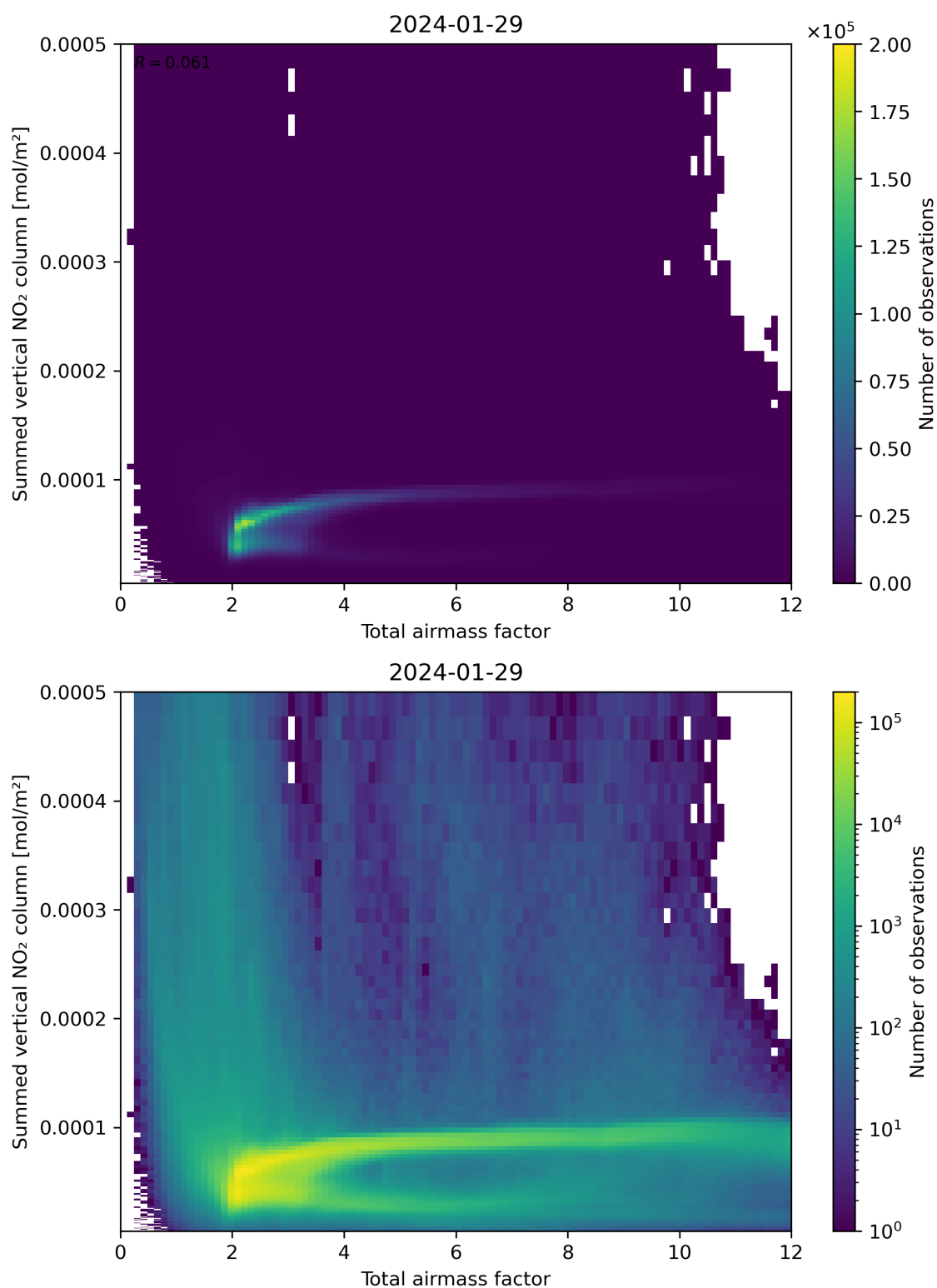
Figure 65: Scatter density plot of “Total airmass factor” against “Summed vertical NO 2 column” for 2024-01-28 to 2024-01-30.
