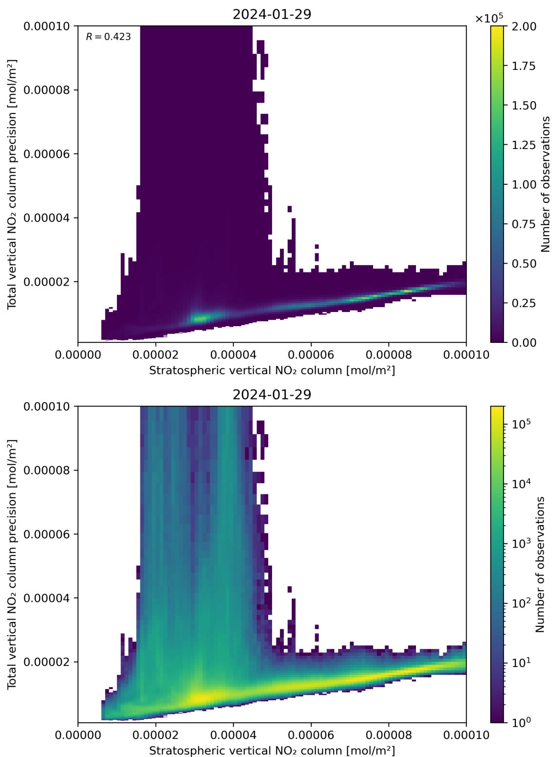
Figure 101: Scatter density plot of “Stratospheric vertical NO 2 column” against “Total vertical NO 2 column precision” for 2024-01-28 to 2024-01-30.
