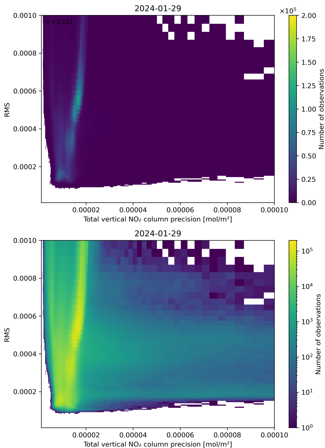
Figure 119: Scatter density plot of “Total vertical NO 2 column precision” against “RMS” for 2024-01-28 to 2024-01-30.
