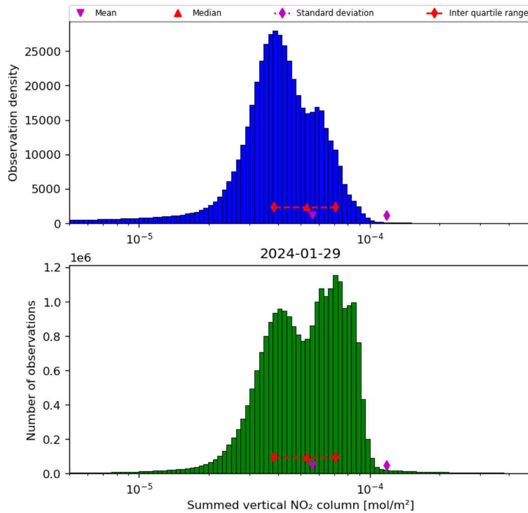
Figure 40: Histogram of “Summed vertical NO 2 column” for 2024-01-28 to 2024-01-30
