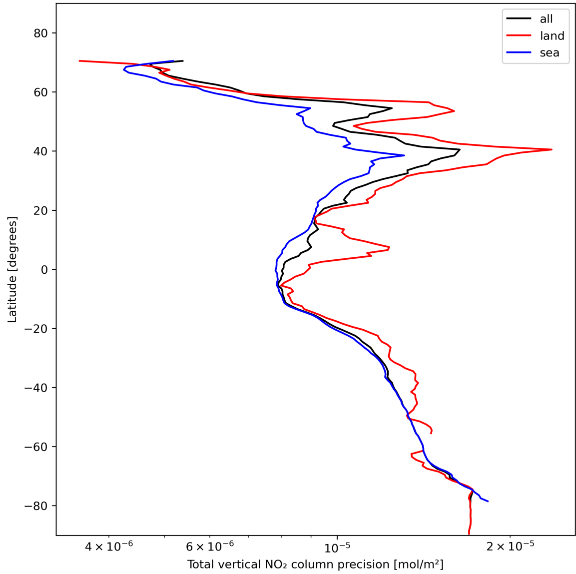
Figure 22: Zonal average of “Total vertical NO 2 column precision” for 2024-01-28 to 2024-01-30.
