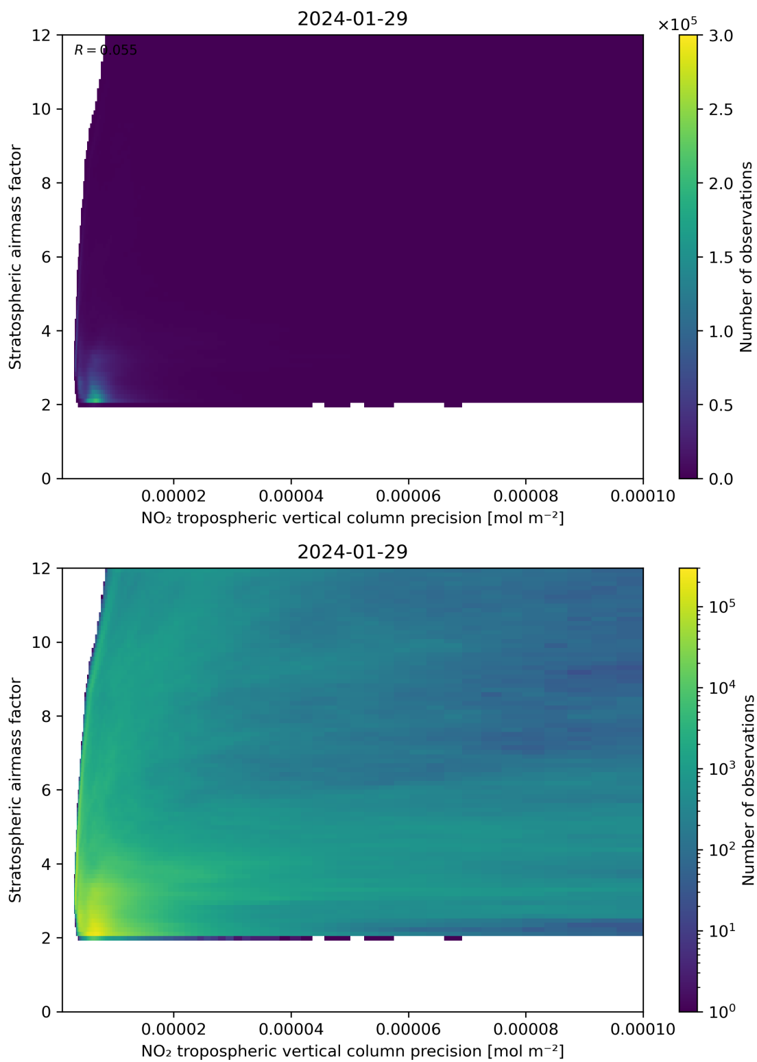
Figure 131: Scatter density plot of “NO 2 tropospheric vertical column precision” against “Stratospheric airmass factor” for 2024-01-28 to 2024-01-30.
