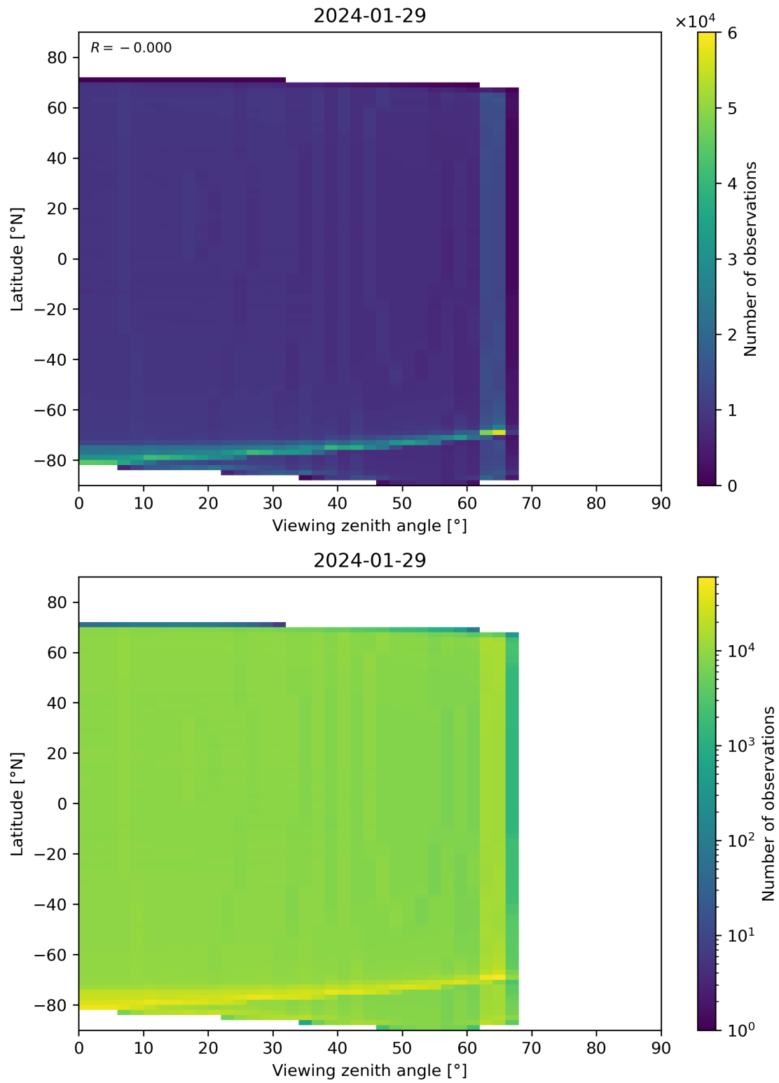
Figure 163: Scatter density plot of “Viewing zenith angle” against “Latitude” for 2024-01-28 to 2024-01-30.
