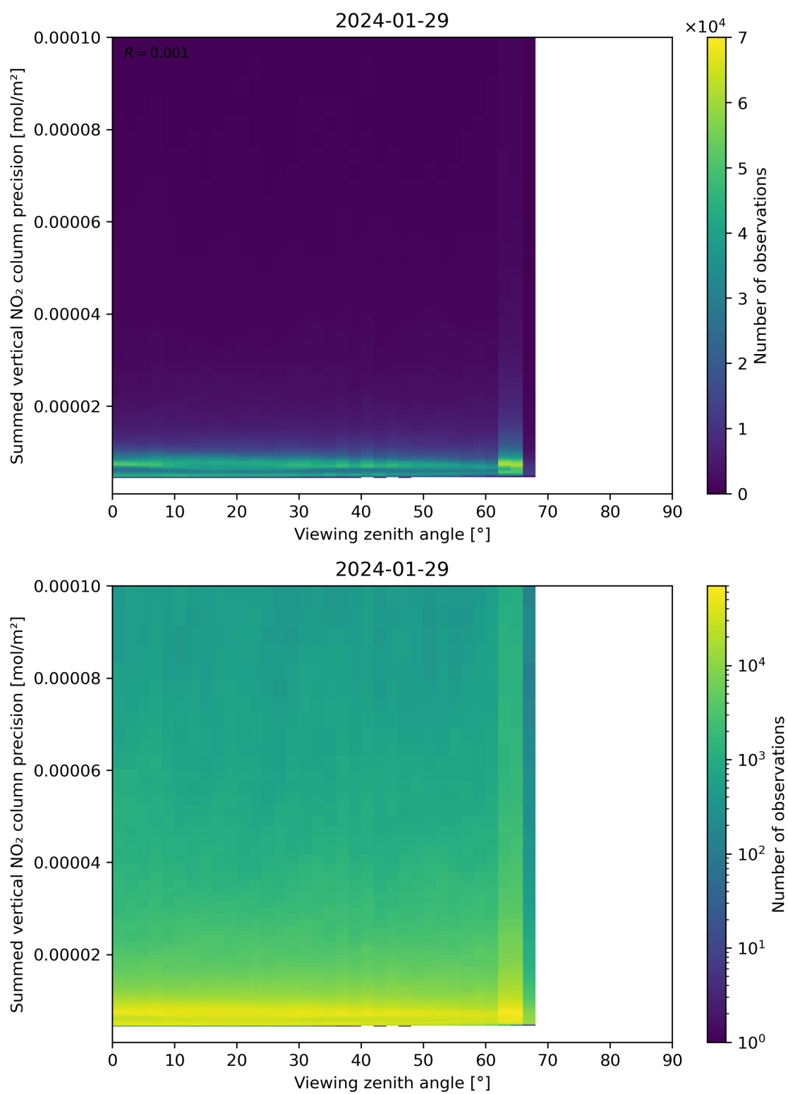
Figure 166: Scatter density plot of “Viewing zenith angle” against “Summed vertical NO 2 column precision” for 2024-01-28 to 2024-01-30.
