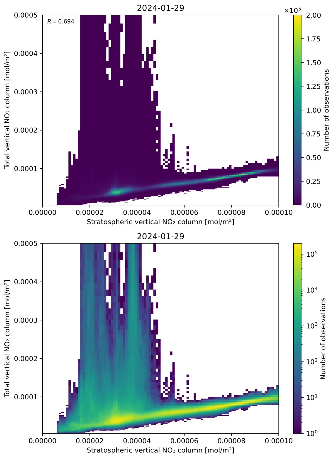
Figure 100: Scatter density plot of “Stratospheric vertical NO 2 column” against “Total vertical NO 2 column” for 2024-01-28 to 2024-01-30.
