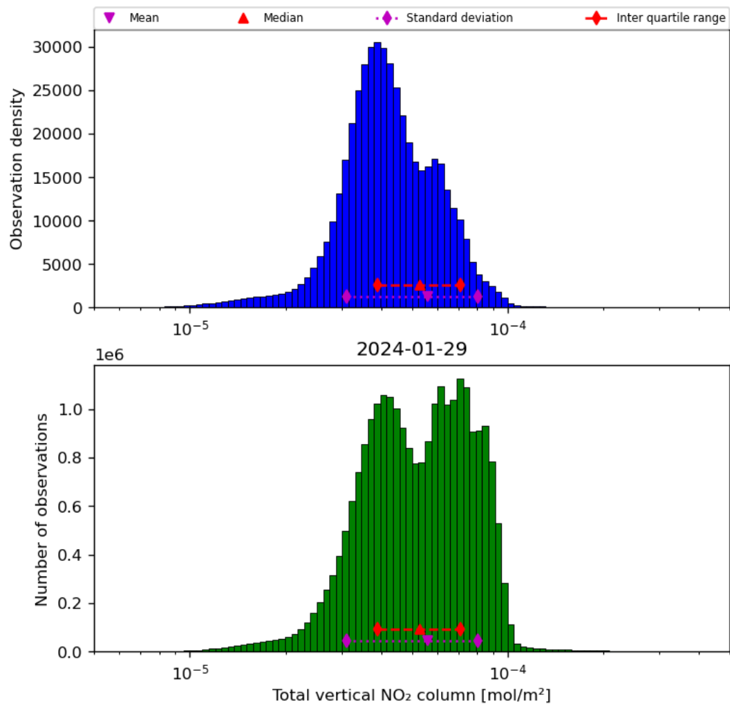
Figure 38: Histogram of “Total vertical NO 2 column” for 2024-01-28 to 2024-01-30
