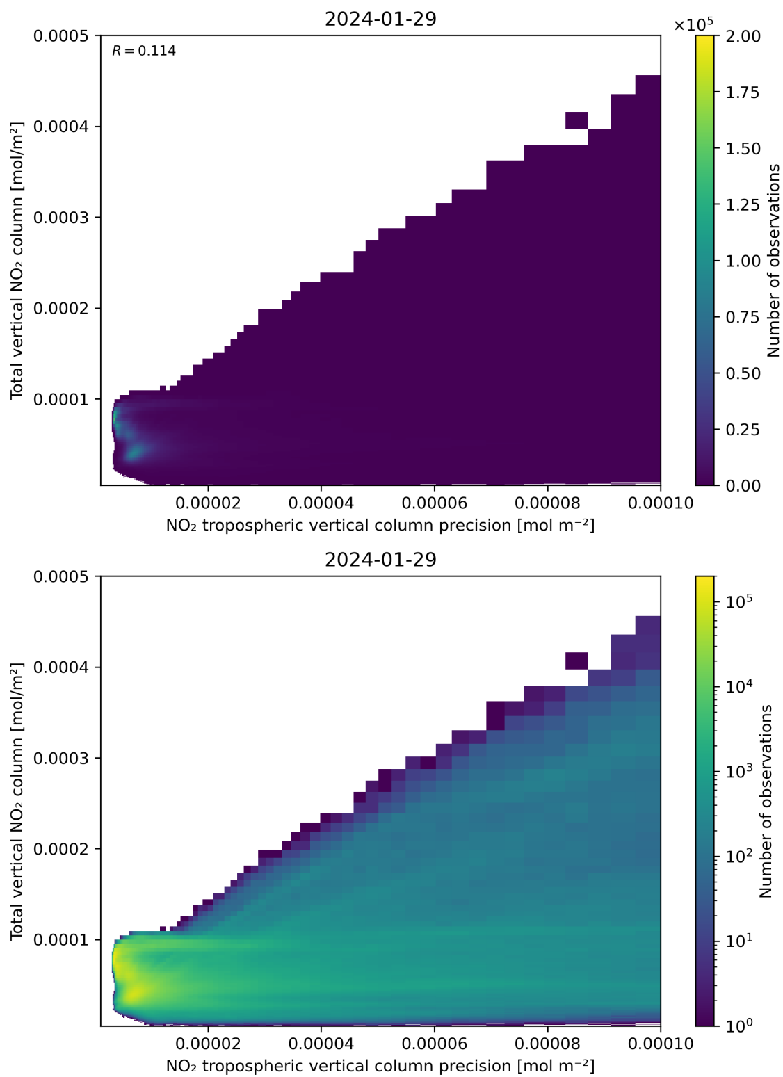
Figure 138: Scatter density plot of “NO 2 tropospheric vertical column precision” against “Total vertical NO 2 column” for 2024-01-28 to 2024-01-30.
