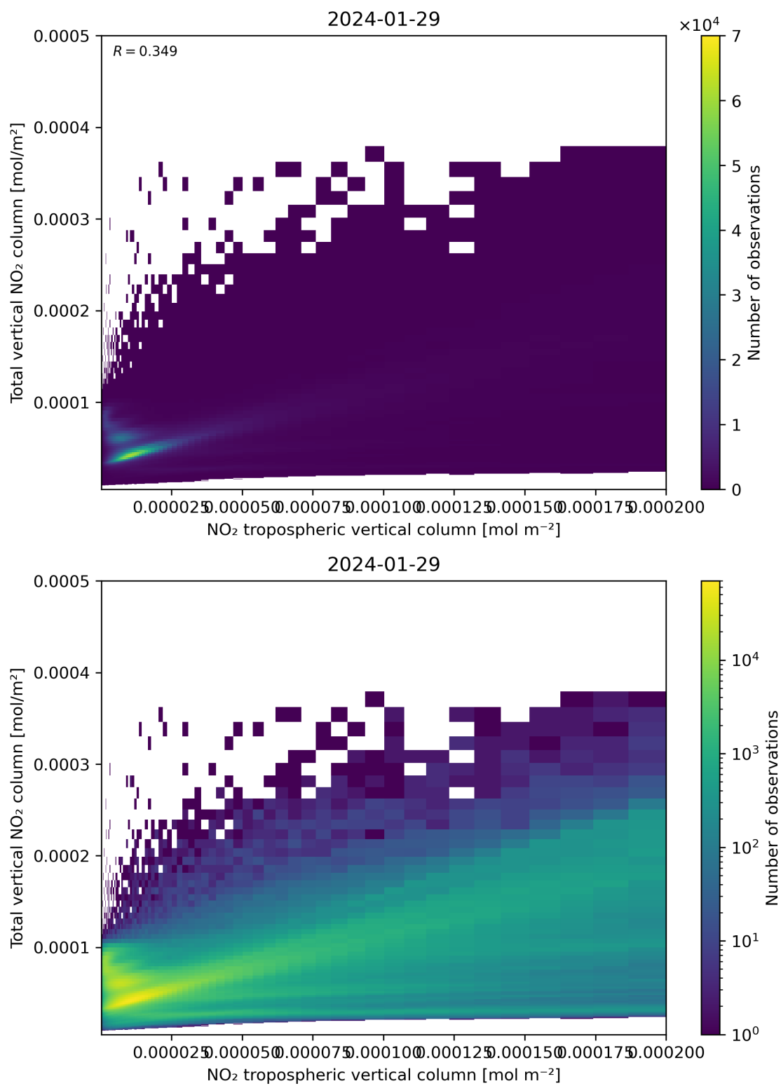
Figure 128: Scatter density plot of “NO 2 tropospheric vertical column” against “Total vertical NO 2 column” for 2024-01-28 to 2024-01-30.
