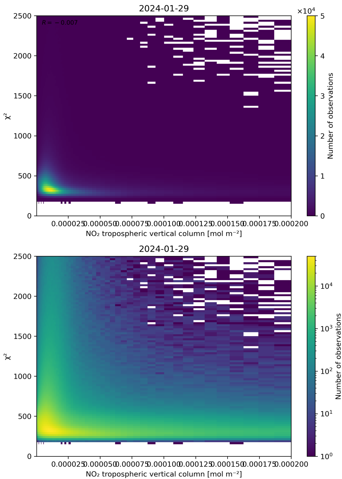
Figure 124: Scatter density plot of “NO 2 tropospheric vertical column” against “ \chi^2 ” for 2024-01-28 to 2024-01-30.
