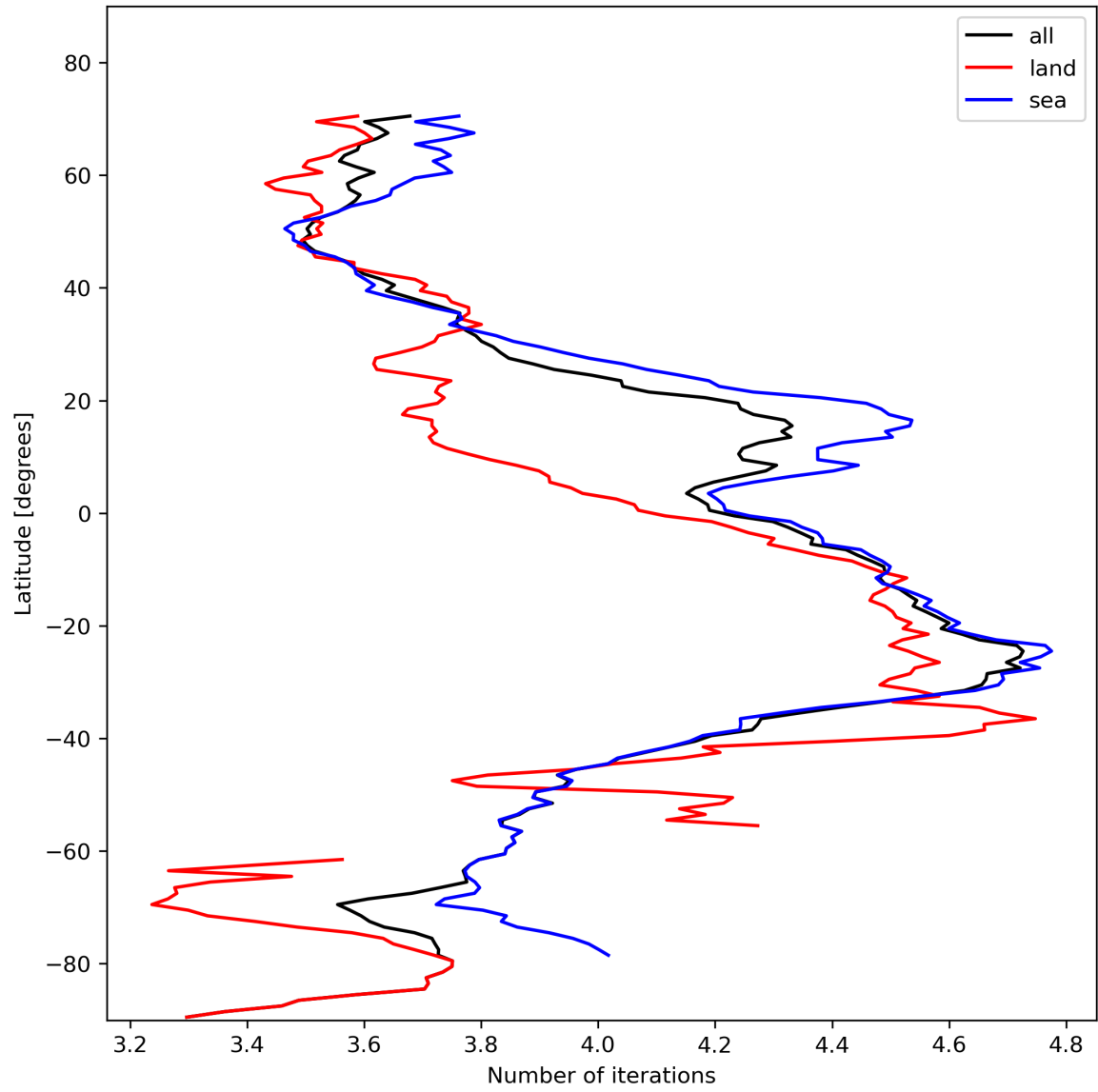
Figure 17: Zonal average of “Number of iterations” for 2024-01-28 to 2024-01-30.
