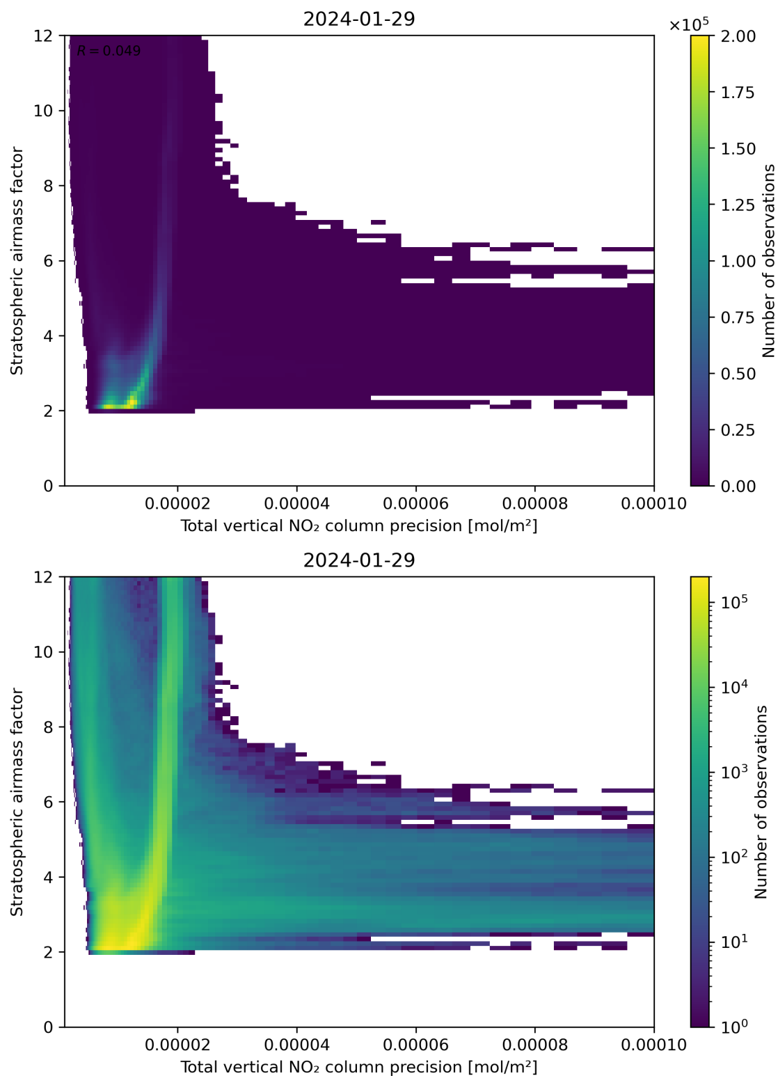
Figure 115: Scatter density plot of “Total vertical NO 2 column precision” against “Stratospheric airmass factor” for 2024-01-28 to 2024-01-30.
