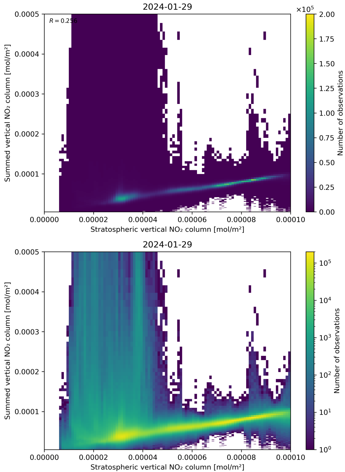
Figure 98: Scatter density plot of “Stratospheric vertical NO 2 column” against “Summed vertical NO 2 column” for 2024-01-28 to 2024-01-30.
