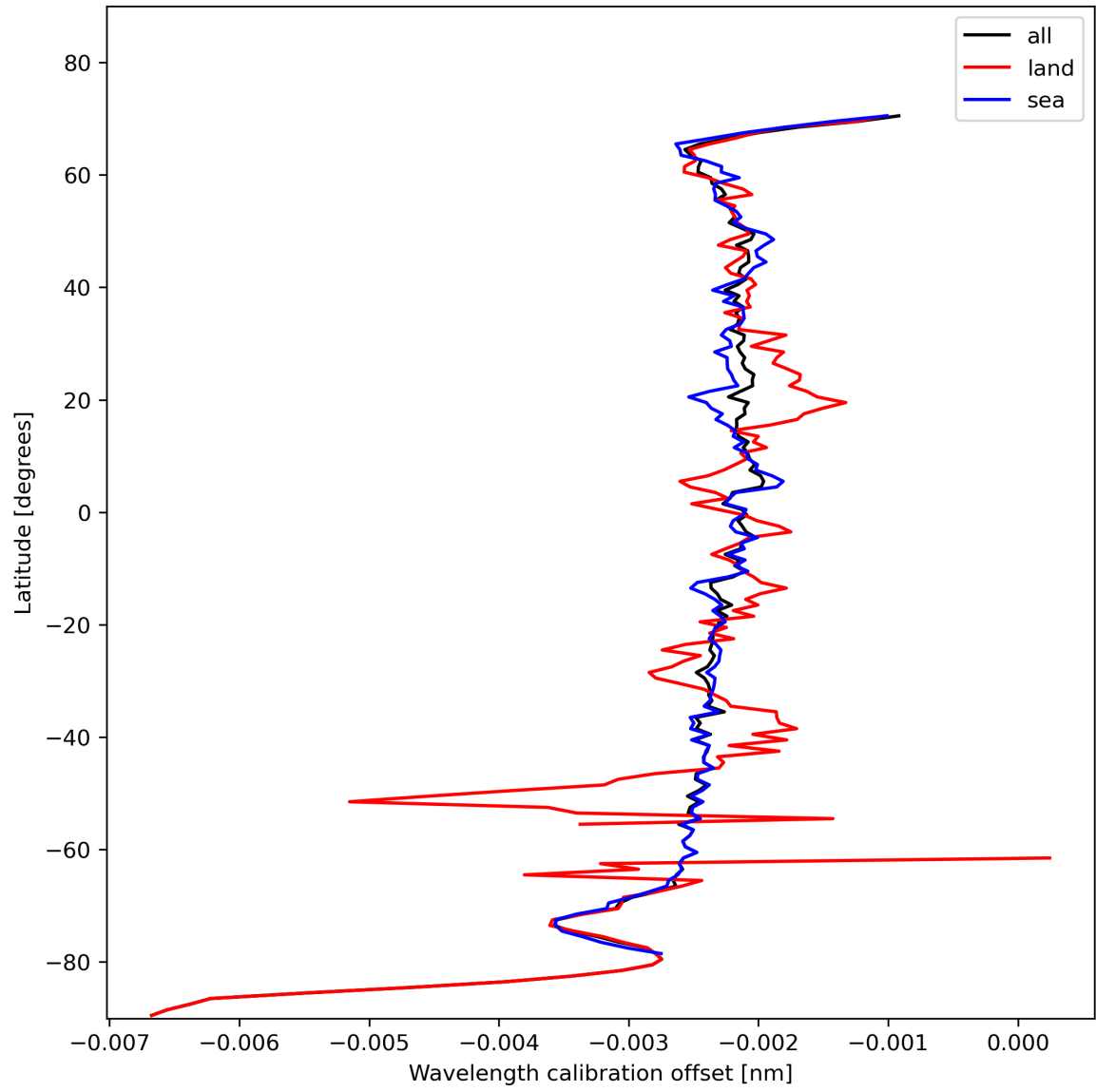
Figure 18: Zonal average of “Wavelength calibration offset” for 2024-01-28 to 2024-01-30.
