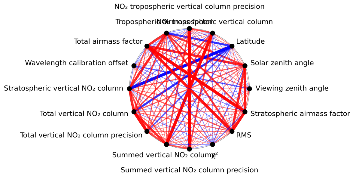
Figure 1: Map of correlation graph for 2024-01-28 to 2024-01-30.
