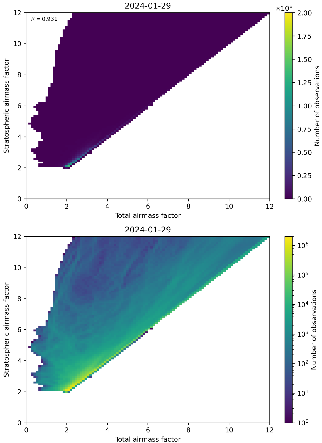
Figure 62: Scatter density plot of “Total airmass factor” against “Stratospheric airmass factor” for 2024-01-28 to 2024-01-30.
