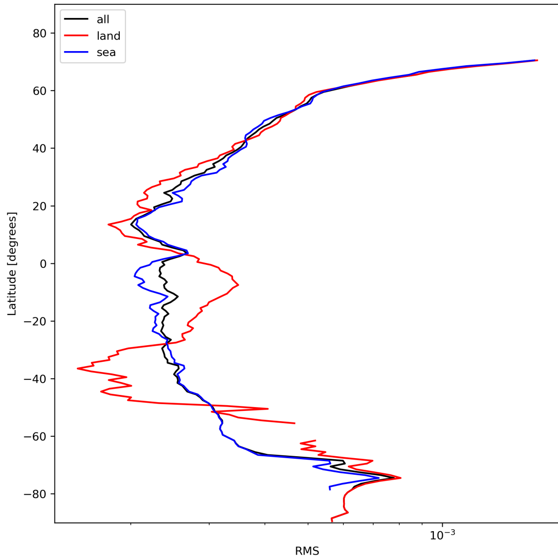
Figure 26: Zonal average of “RMS” for 2024-01-28 to 2024-01-30.
