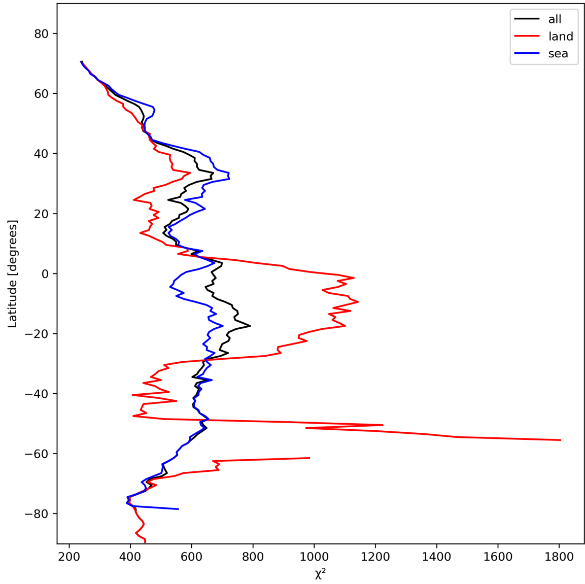
Figure 25: Zonal average of “ \chi^2 ” for 2024-01-28 to 2024-01-30.
