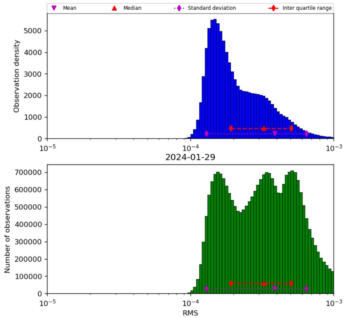
Figure 43: Histogram of “RMS” for 2024-01-28 to 2024-01-30
