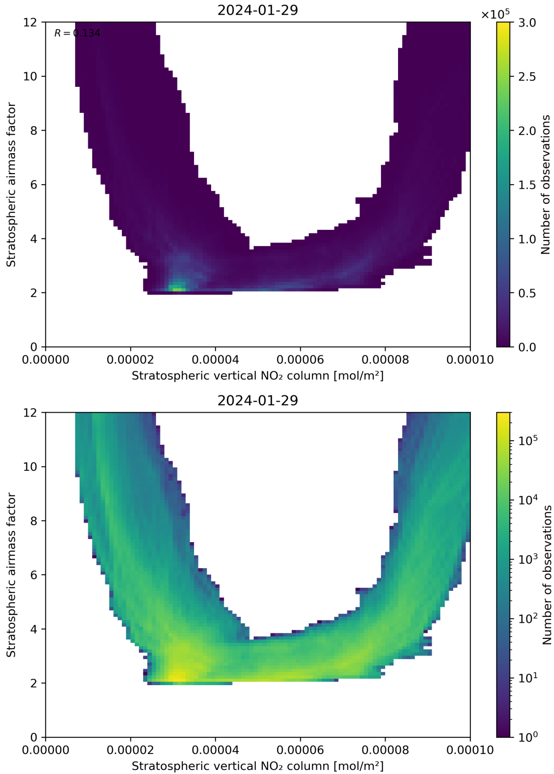
Figure 96: Scatter density plot of “Stratospheric vertical NO 2 column” against “Stratospheric airmass factor” for 2024-01-28 to 2024-01-30.
