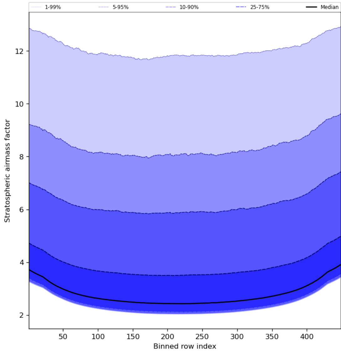
Figure 61: Along track statistics of “Stratospheric airmass factor” for 2024-01-28 to 2024-01-30
