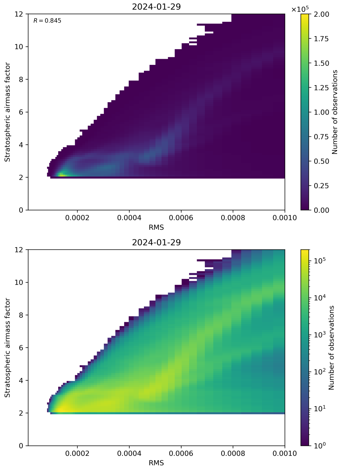
Figure 144: Scatter density plot of “RMS” against “Stratospheric airmass factor” for 2024-01-28 to 2024-01-30.
