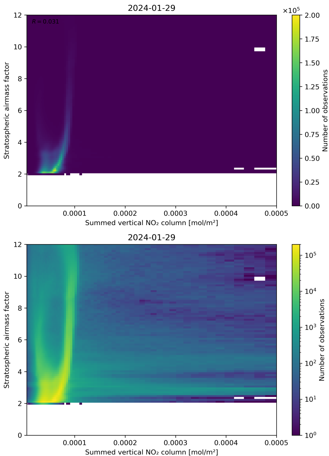
Figure 103: Scatter density plot of “Summed vertical NO 2 column” against “Stratospheric airmass factor” for 2024-01-28 to 2024-01-30.
