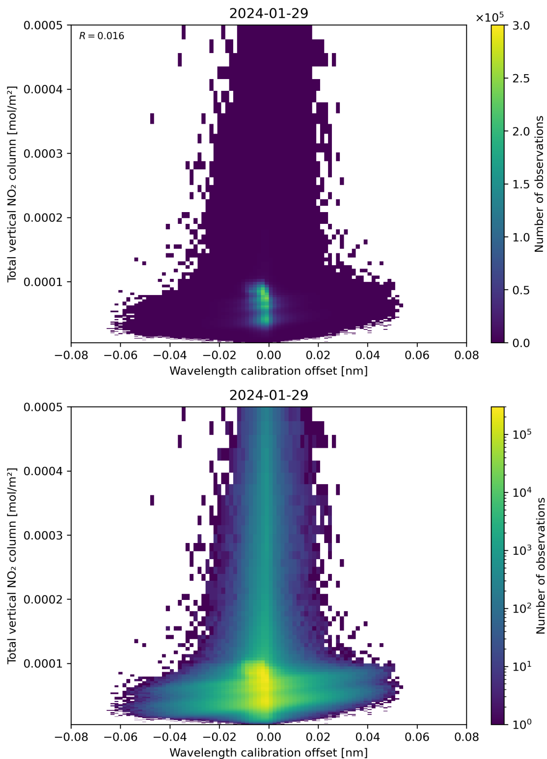
Figure 179: Scatter density plot of “Wavelength calibration offset” against “Total vertical NO 2 column” for 2024-01-28 to 2024-01-30.
