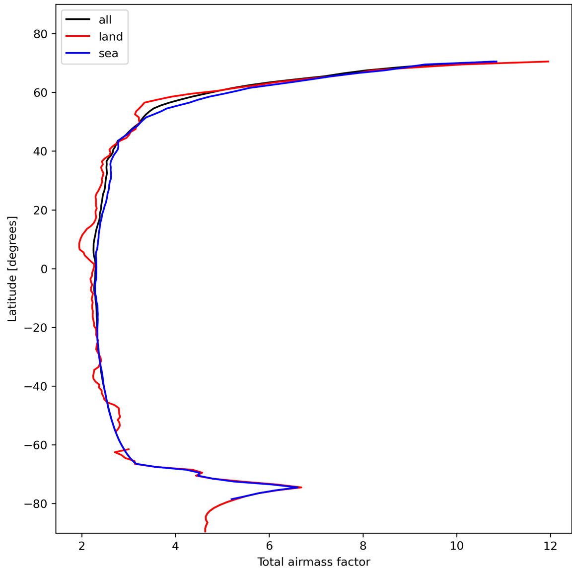
Figure 15: Zonal average of “Total airmass factor” for 2024-01-28 to 2024-01-30.
