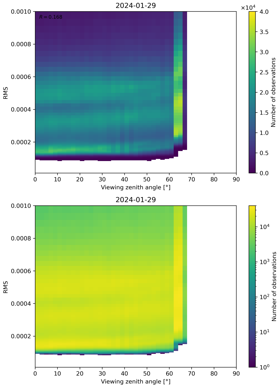
Figure 171: Scatter density plot of “Viewing zenith angle” against “RMS” for 2024-01-28 to 2024-01-30.
