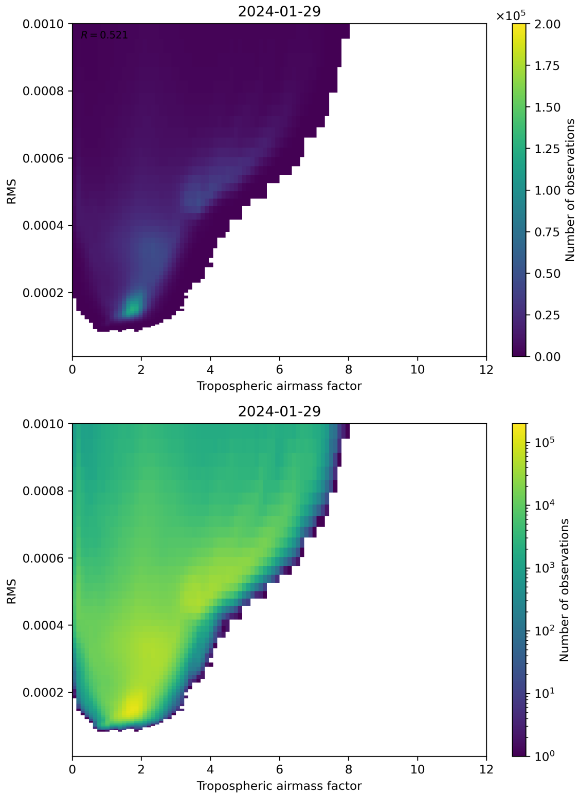
Figure 79: Scatter density plot of “Tropospheric airmass factor” against “RMS” for 2024-01-28 to 2024-01-30.
