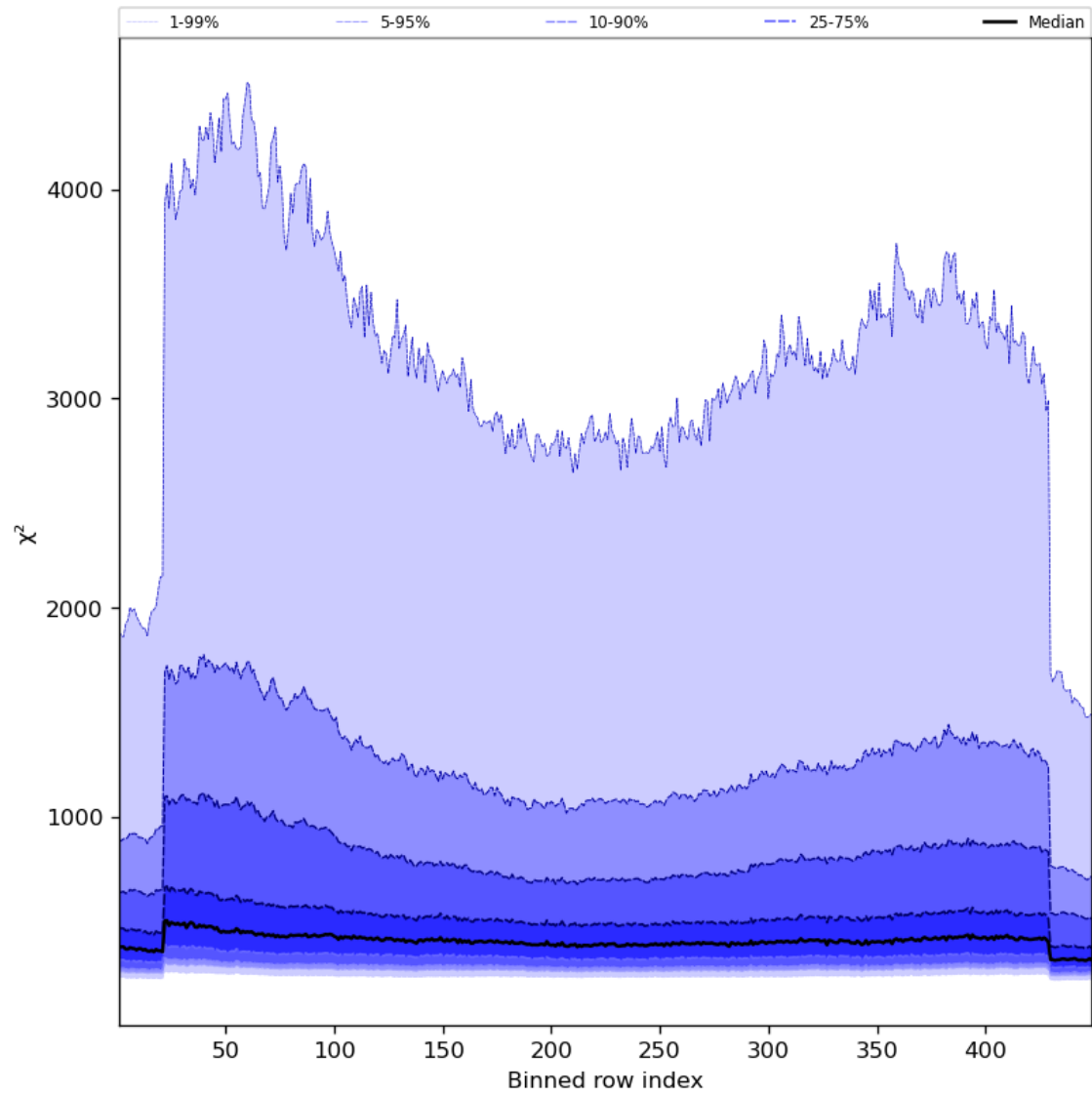
Figure 59: Along track statistics of “ \chi^2 ” for 2024-01-28 to 2024-01-30
