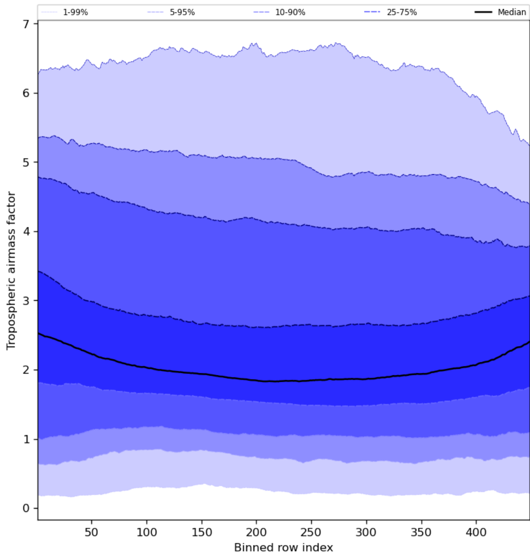
Figure 48: Along track statistics of “Tropospheric air mass factor” for 2024-01-28 to 2024-01-30
