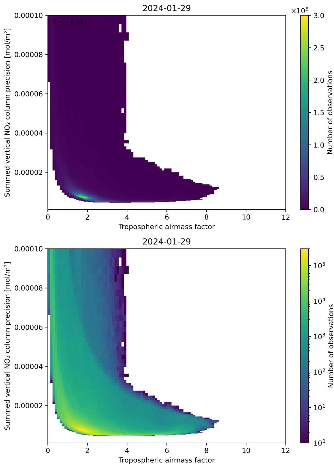
Figure 76: Scatter density plot of “Tropospheric air mass factor” against “Summed vertical NO 2 column precision” for 2024-01-28 to 2024-01-30.
