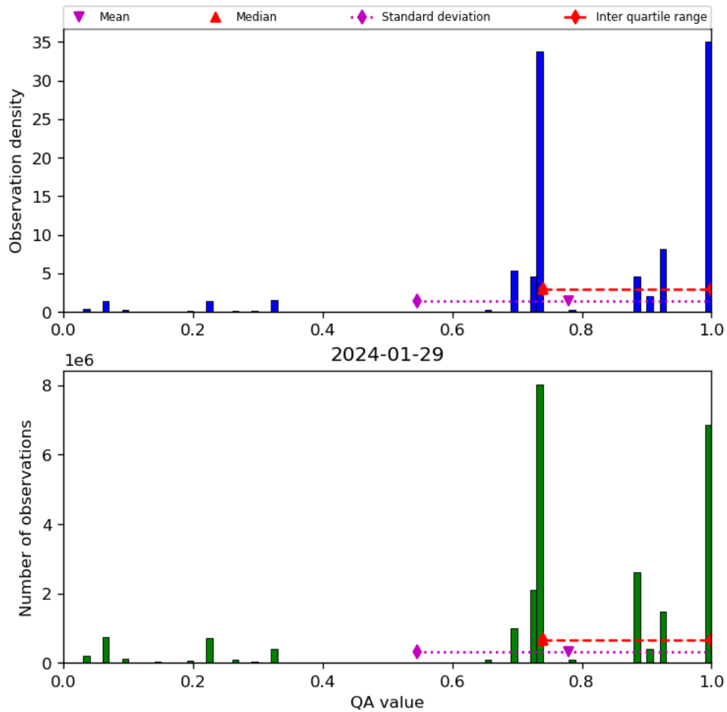
Figure 28: Histogram of “QA value” for 2024-01-28 to 2024-01-30
