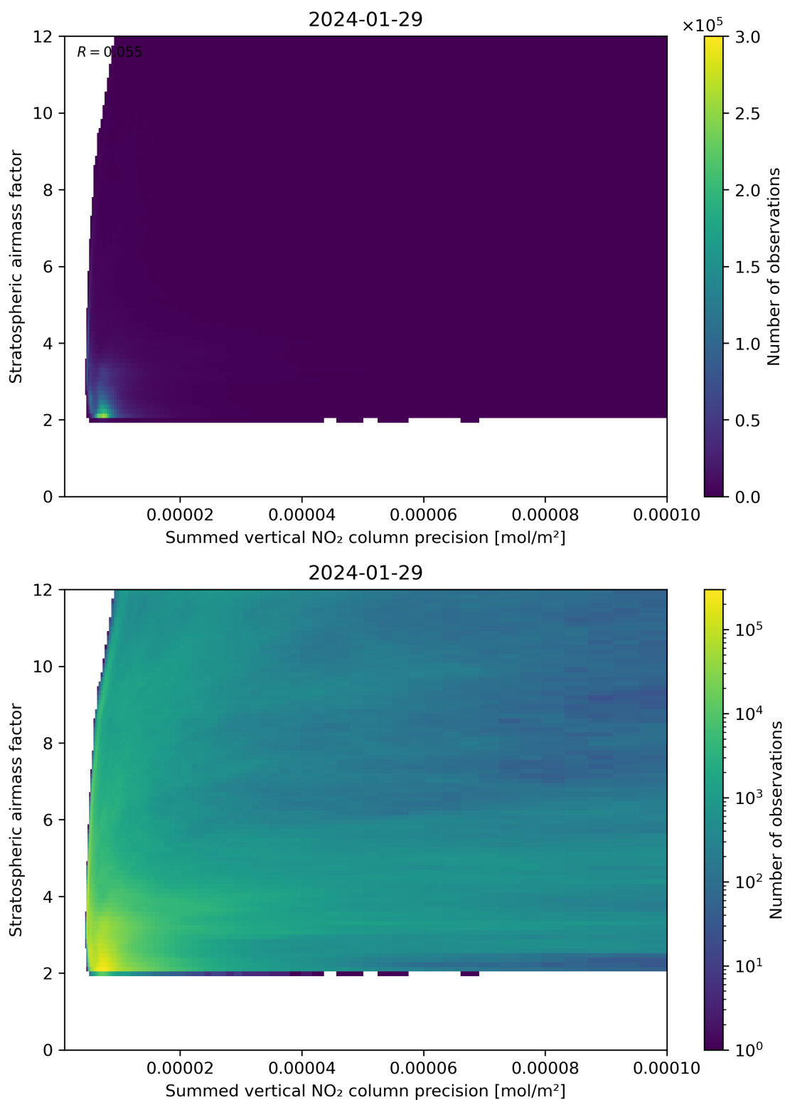
Figure 106: Scatter density plot of “Summed vertical NO 2 column precision” against “Stratospheric airmass factor” for 2024-01-28 to 2024-01-30.
