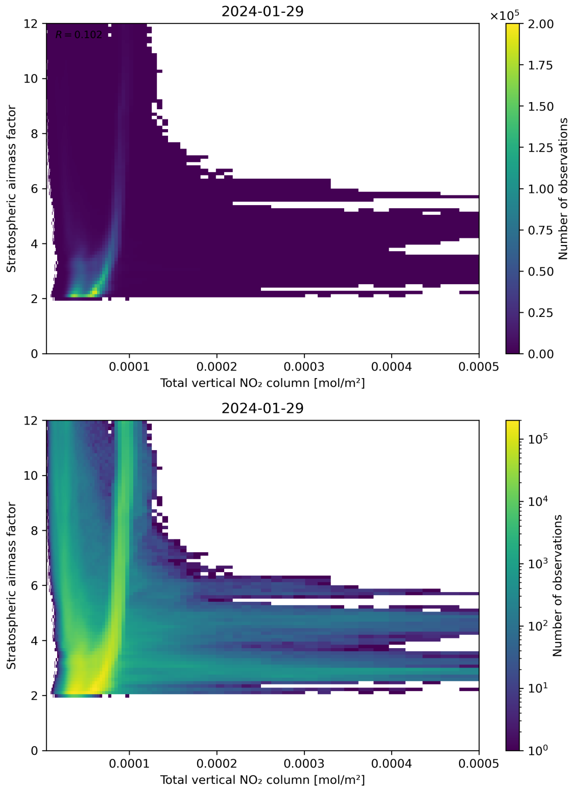
Figure 110: Scatter density plot of “Total vertical NO 2 column” against “Stratospheric airmass factor” for 2024-01-28 to 2024-01-30.
