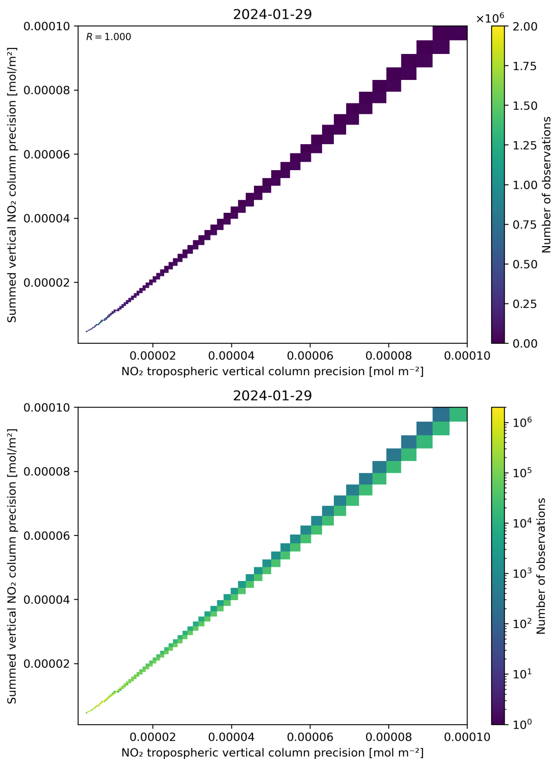
Figure 137: Scatter density plot of “NO 2 tropospheric vertical column precision” against “Summed vertical NO 2 column precision” for 2024-01-28 to 2024-01-30.
