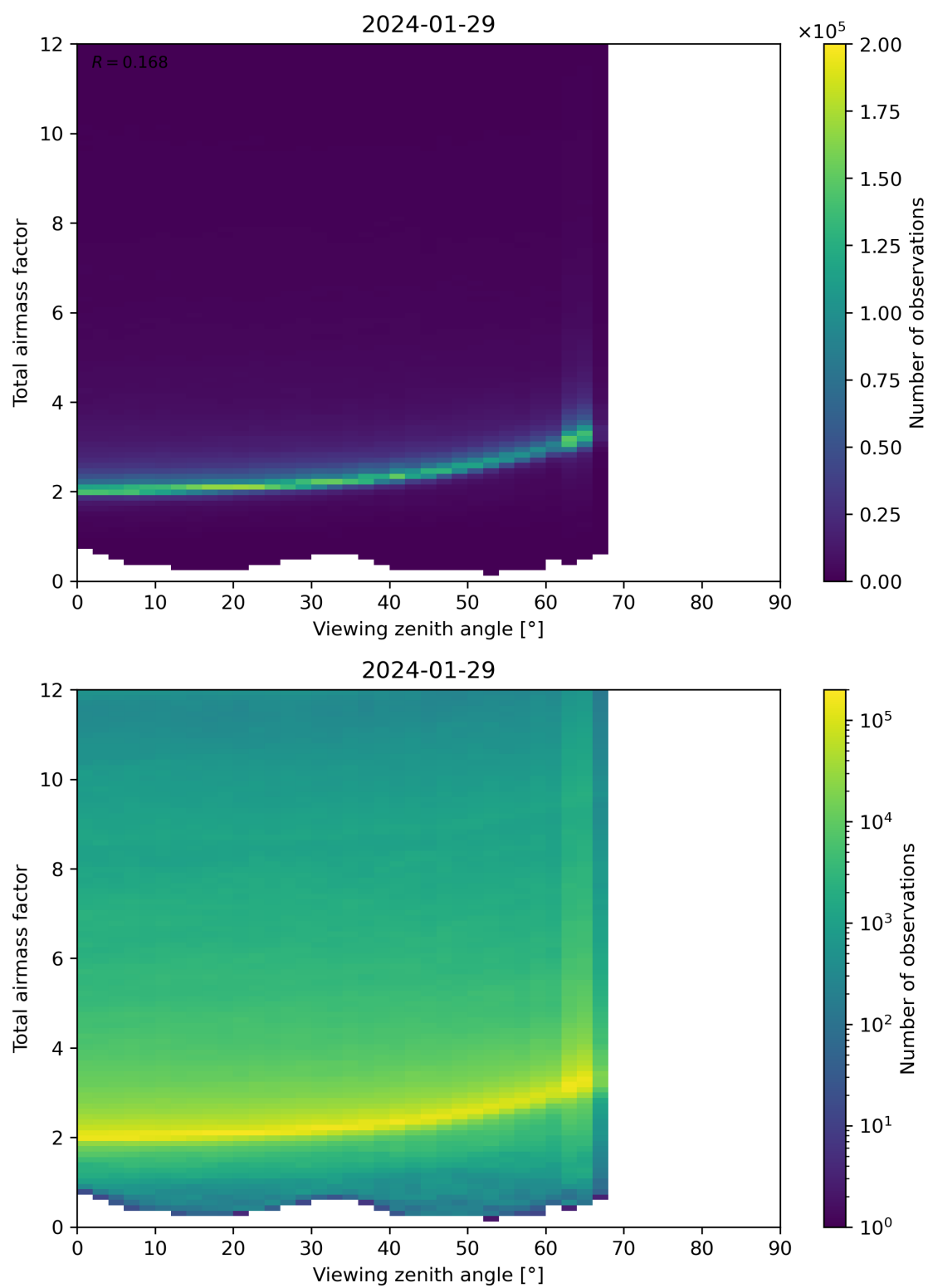
Figure 160: Scatter density plot of “Viewing zenith angle” against “Total airmass factor” for 2024-01-28 to 2024-01-30.
