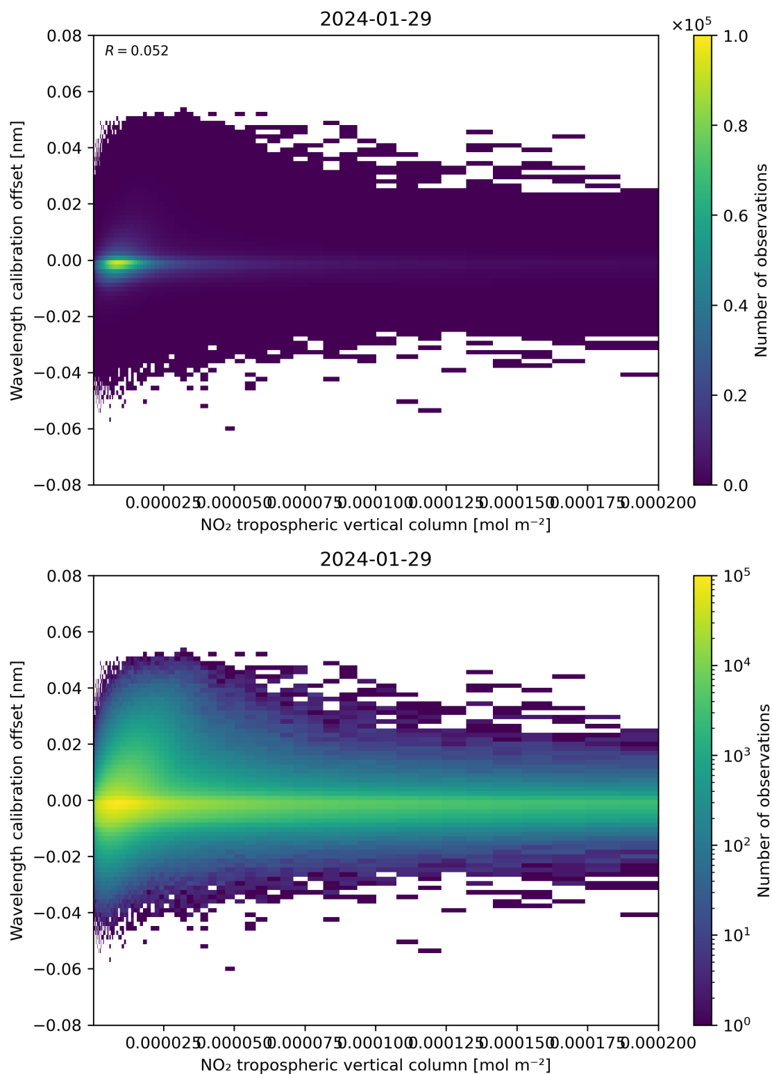
Figure 143: Scatter density plot of “NO 2 tropospheric vertical column” against “Wavelength calibration offset” for 2024-01-28 to 2024-01-30.
