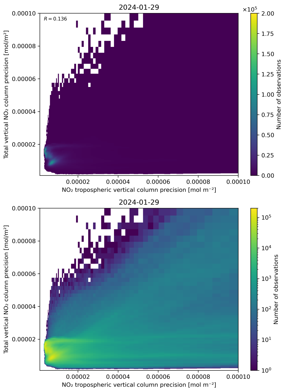
Figure 139: Scatter density plot of “NO 2 tropospheric vertical column precision” against “Total vertical NO 2 column precision” for 2024-01-28 to 2024-01-30.
