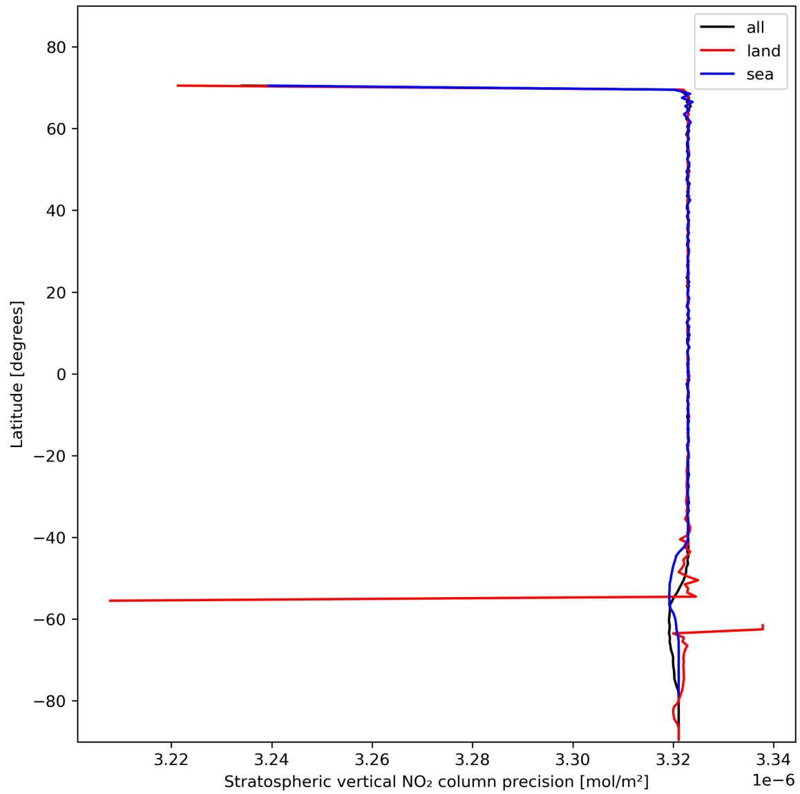
Figure 20: Zonal average of “Stratospheric vertical NO 2 column precision” for 2024-01-28 to 2024-01-30.
