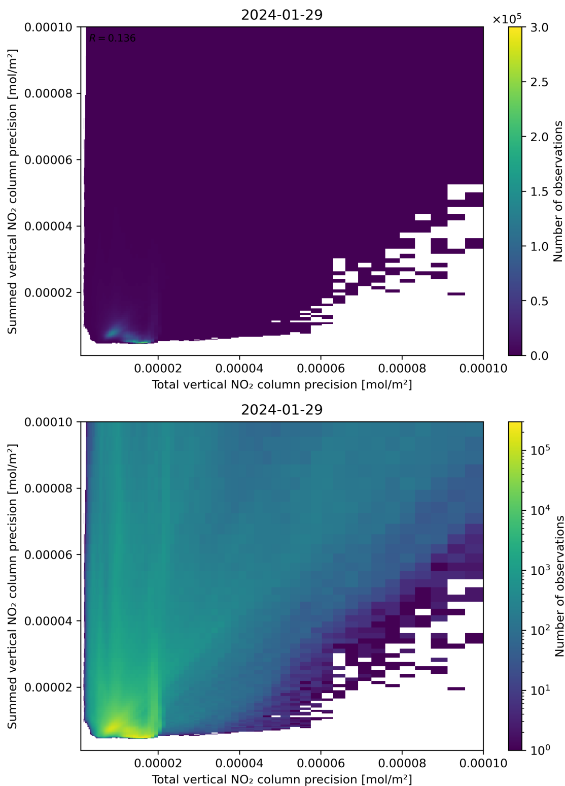
Figure 118: Scatter density plot of “Total vertical NO 2 column precision” against “Summed vertical NO 2 column precision” for 2024-01-28 to 2024-01-30.
