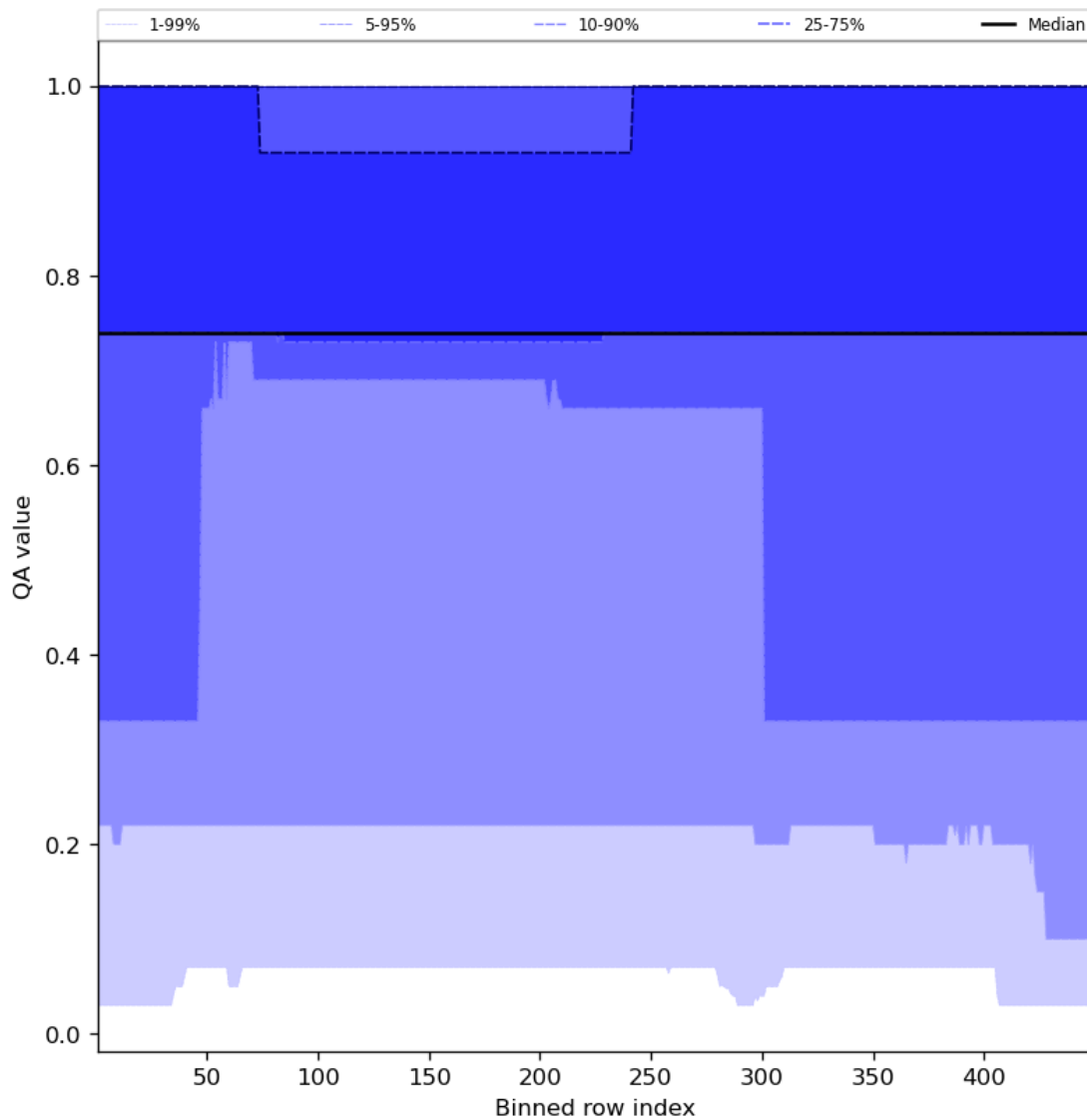
Figure 45: Along track statistics of “QA value” for 2024-01-28 to 2024-01-30
