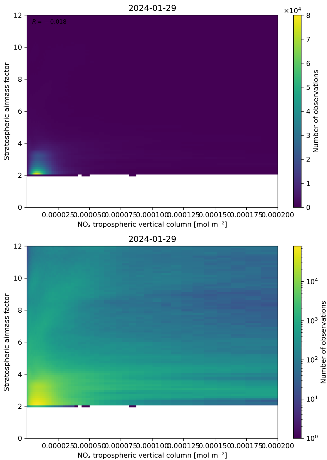
Figure 121: Scatter density plot of “NO 2 tropospheric vertical column” against “Stratospheric airmass factor” for 2024-01-28 to 2024-01-30.
