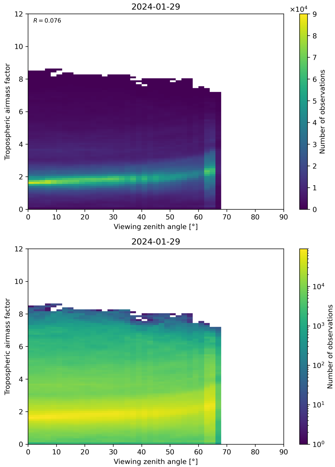
Figure 161: Scatter density plot of “Viewing zenith angle” against “Tropospheric airmass factor” for 2024-01-28 to 2024-01-30.
