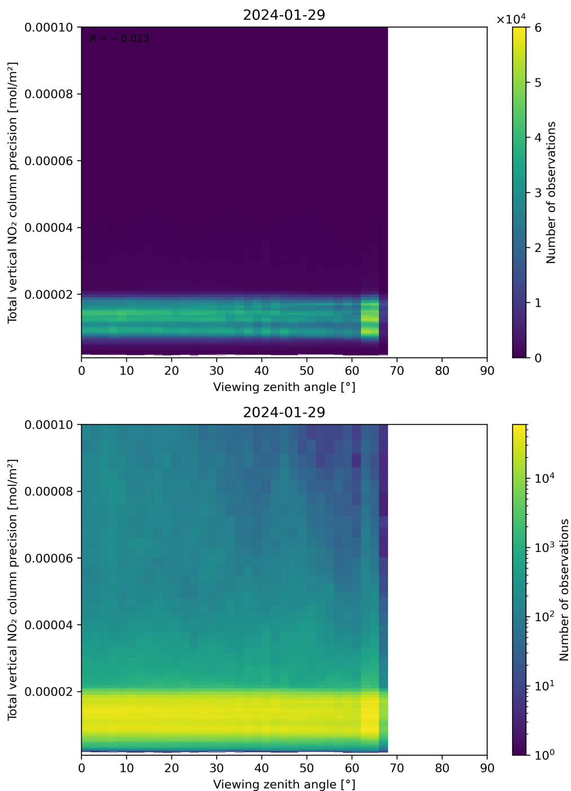
Figure 168: Scatter density plot of “Viewing zenith angle” against “Total vertical NO 2 column precision” for 2024-01-28 to 2024-01-30.
