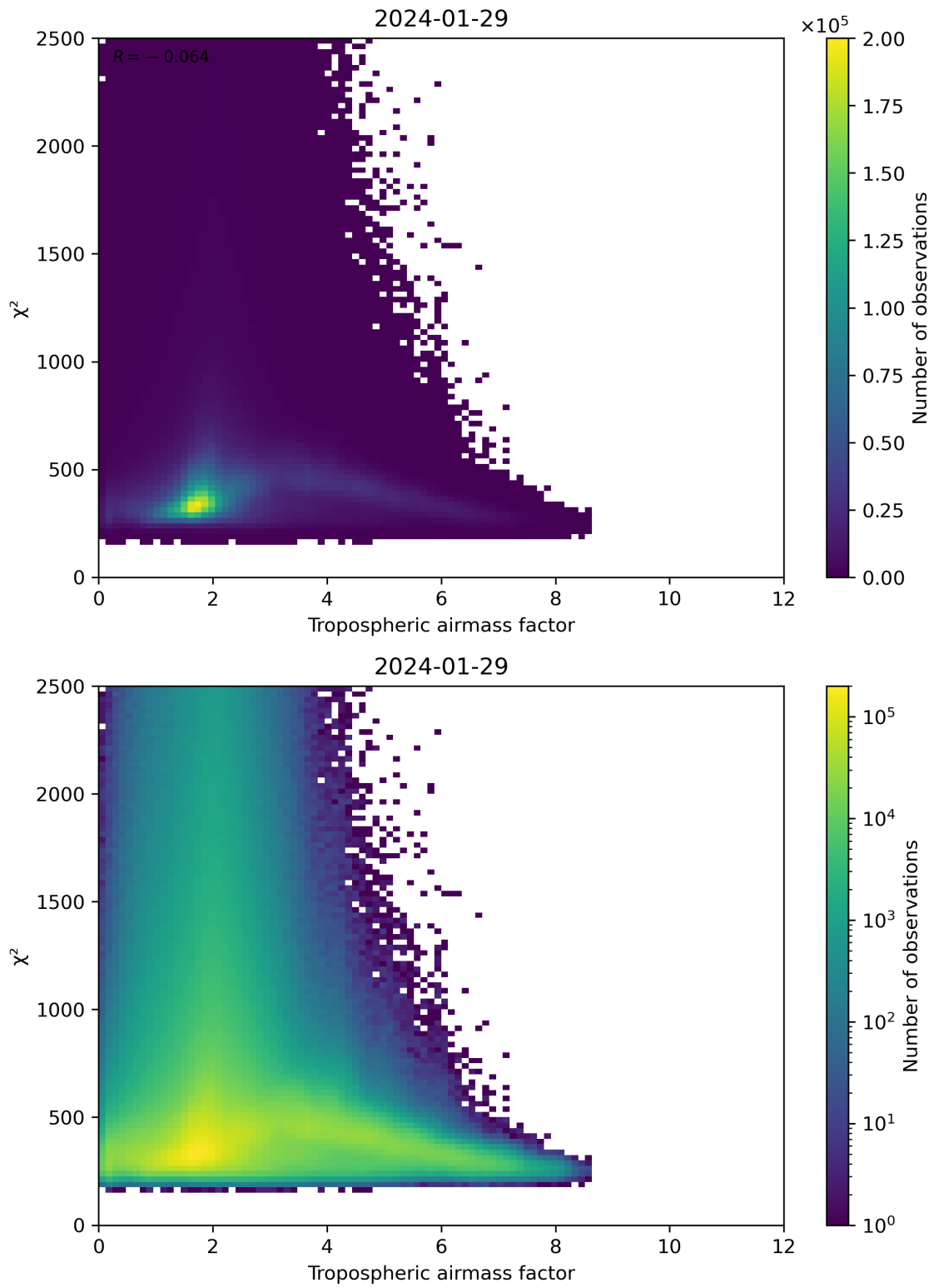
Figure 73: Scatter density plot of “Tropospheric airmass factor” against “ \chi^2 ” for 2024-01-28 to 2024-01-30.
