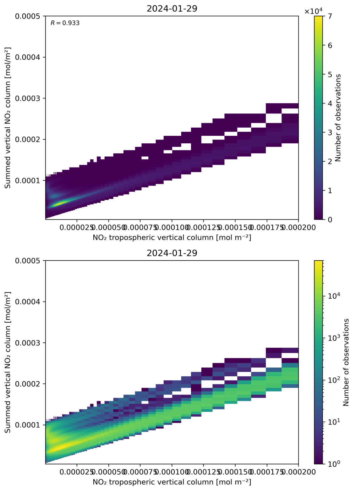
Figure 126: Scatter density plot of “NO 2 tropospheric vertical column” against “Summed vertical NO 2 column” for 2024-01-28 to 2024-01-30.
