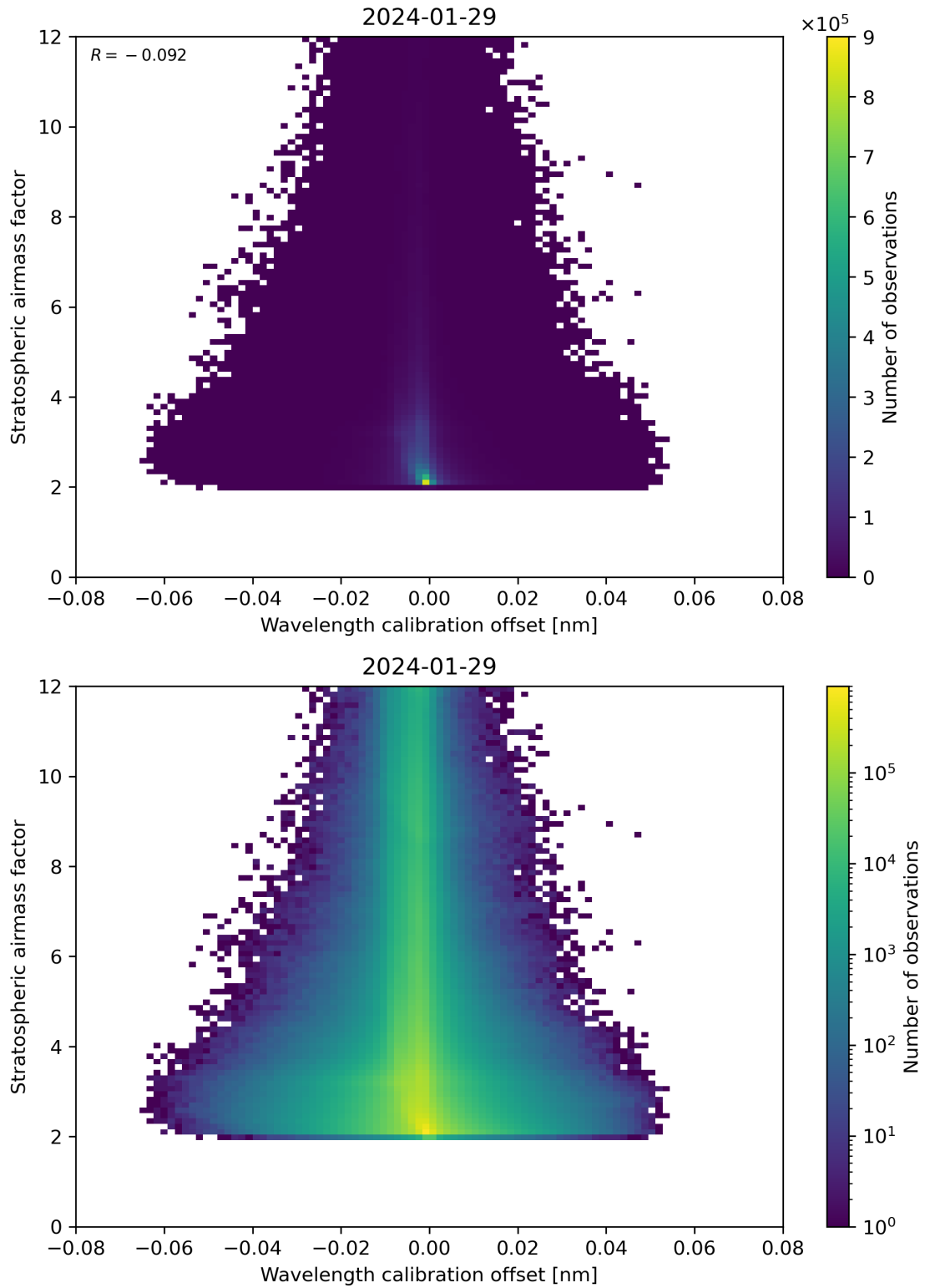
Figure 174: Scatter density plot of “Wavelength calibration offset” against “Stratospheric airmass factor” for 2024-01-28 to 2024-01-30.
