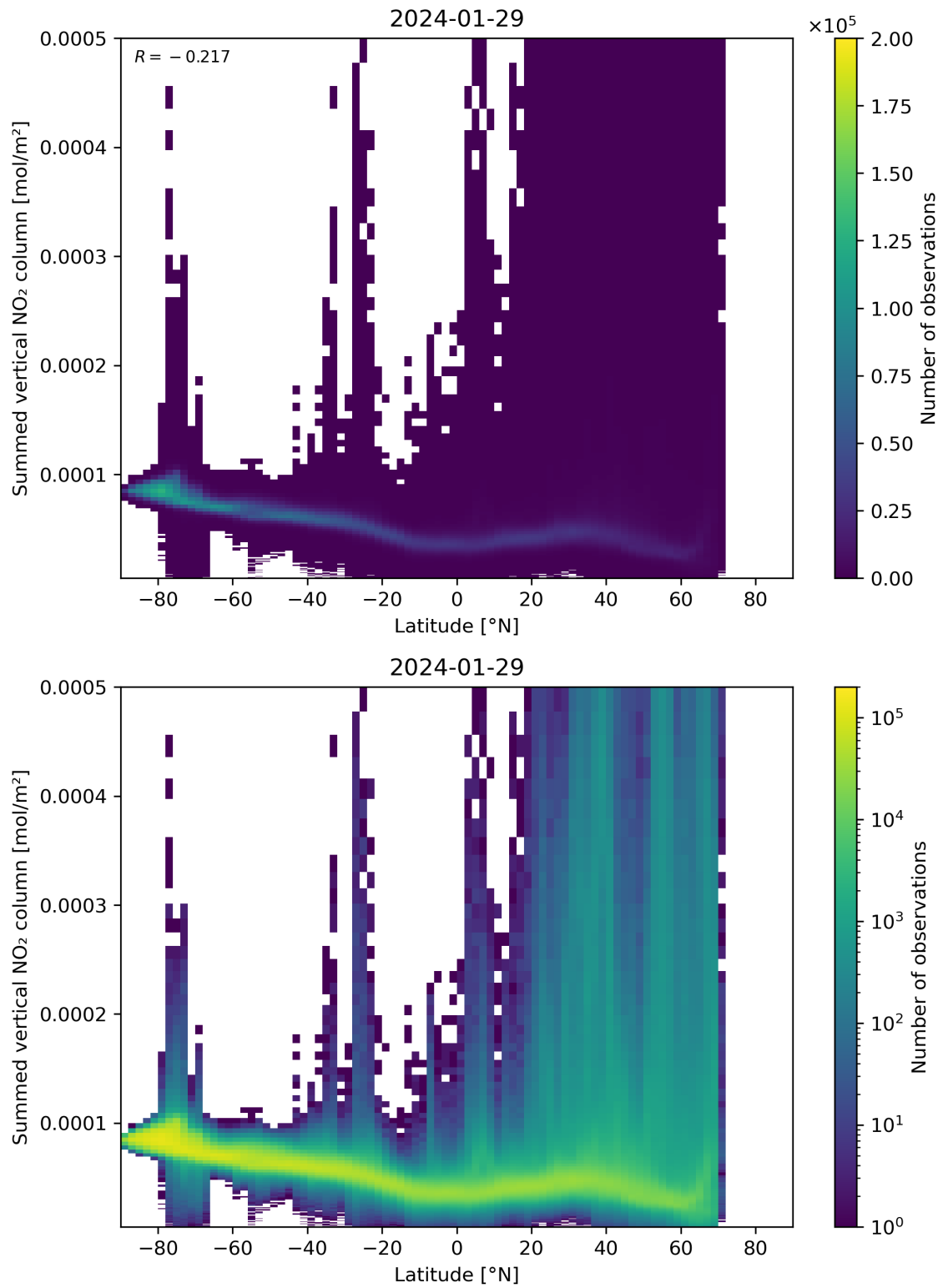
Figure 88: Scatter density plot of “Latitude” against “Summed vertical NO 2 column” for 2024-01-28 to 2024-01-30.
