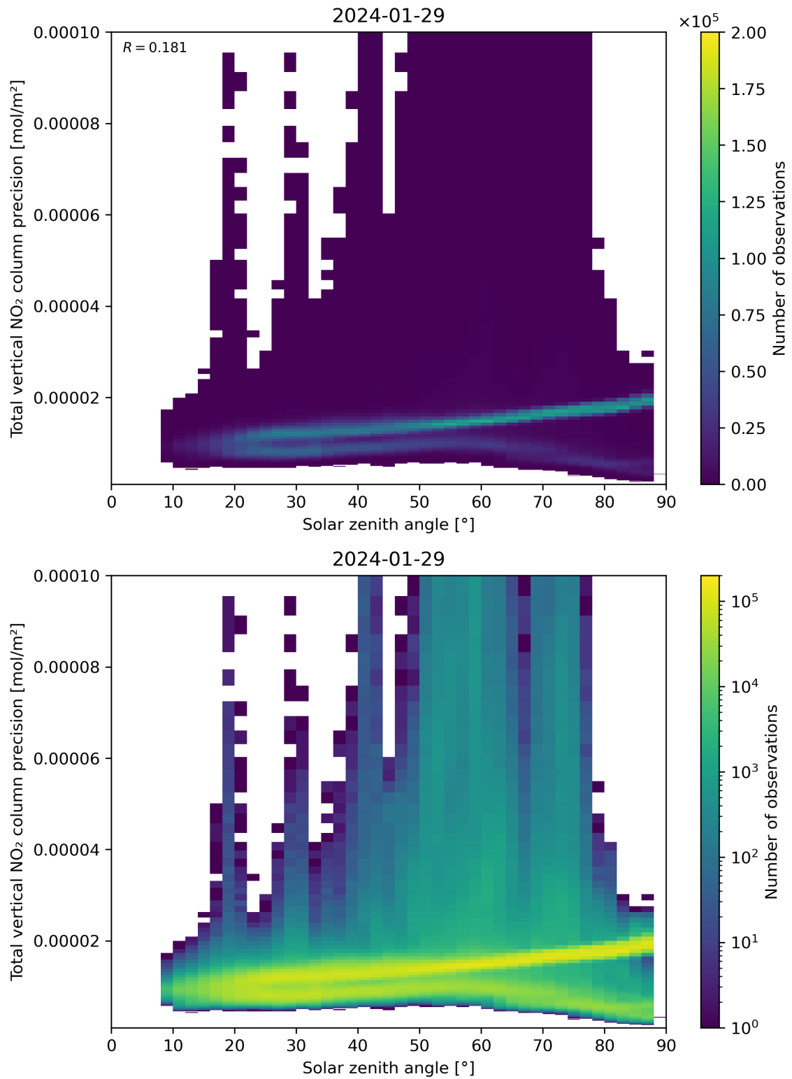
Figure 154: Scatter density plot of “Solar zenith angle” against “Total vertical NO 2 column precision” for 2024-01-28 to 2024-01-30.
