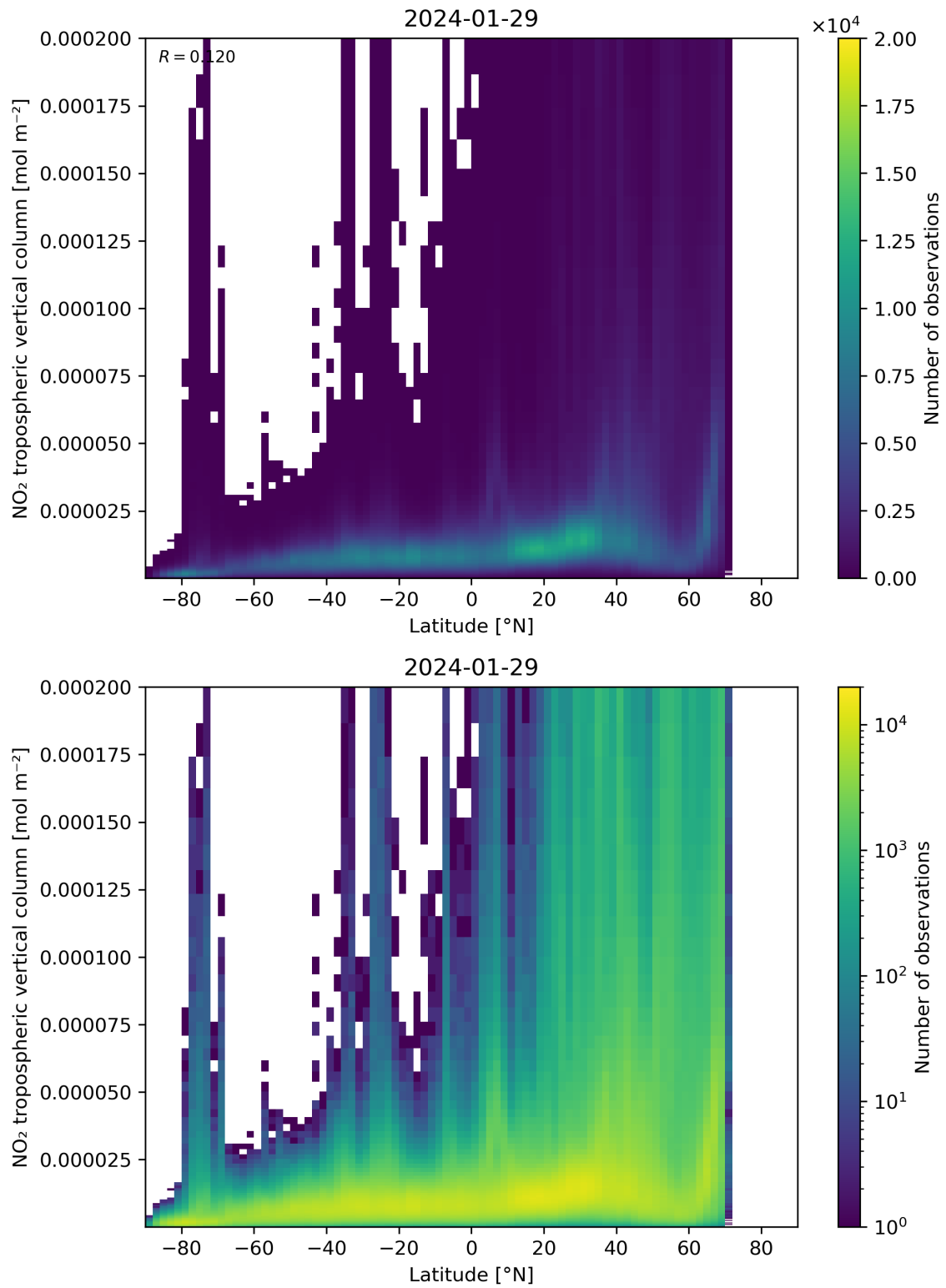
Figure 92: Scatter density plot of “Latitude” against “NO 2 tropospheric vertical column” for 2024-01-28 to 2024-01-30.
