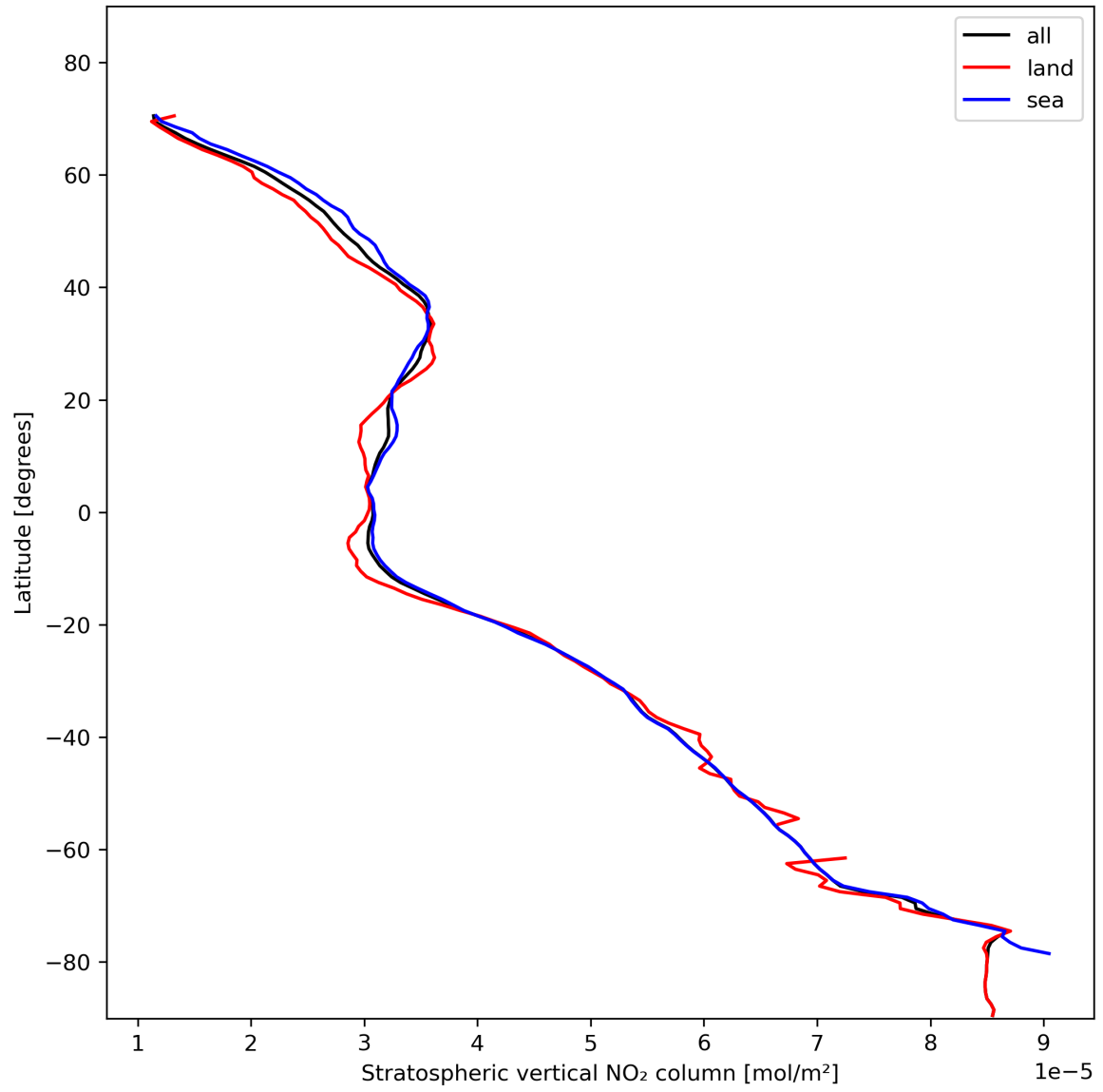
Figure 19: Zonal average of “Stratospheric vertical NO 2 column” for 2024-01-28 to 2024-01-30.
