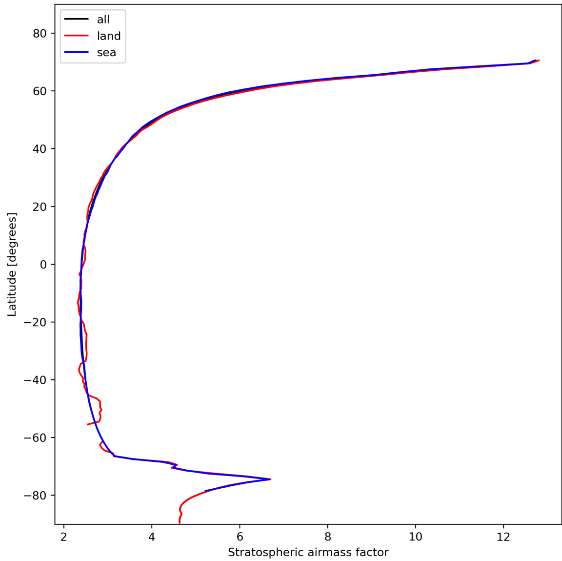
Figure 27: Zonal average of “Stratospheric airmass factor” for 2024-01-28 to 2024-01-30.
