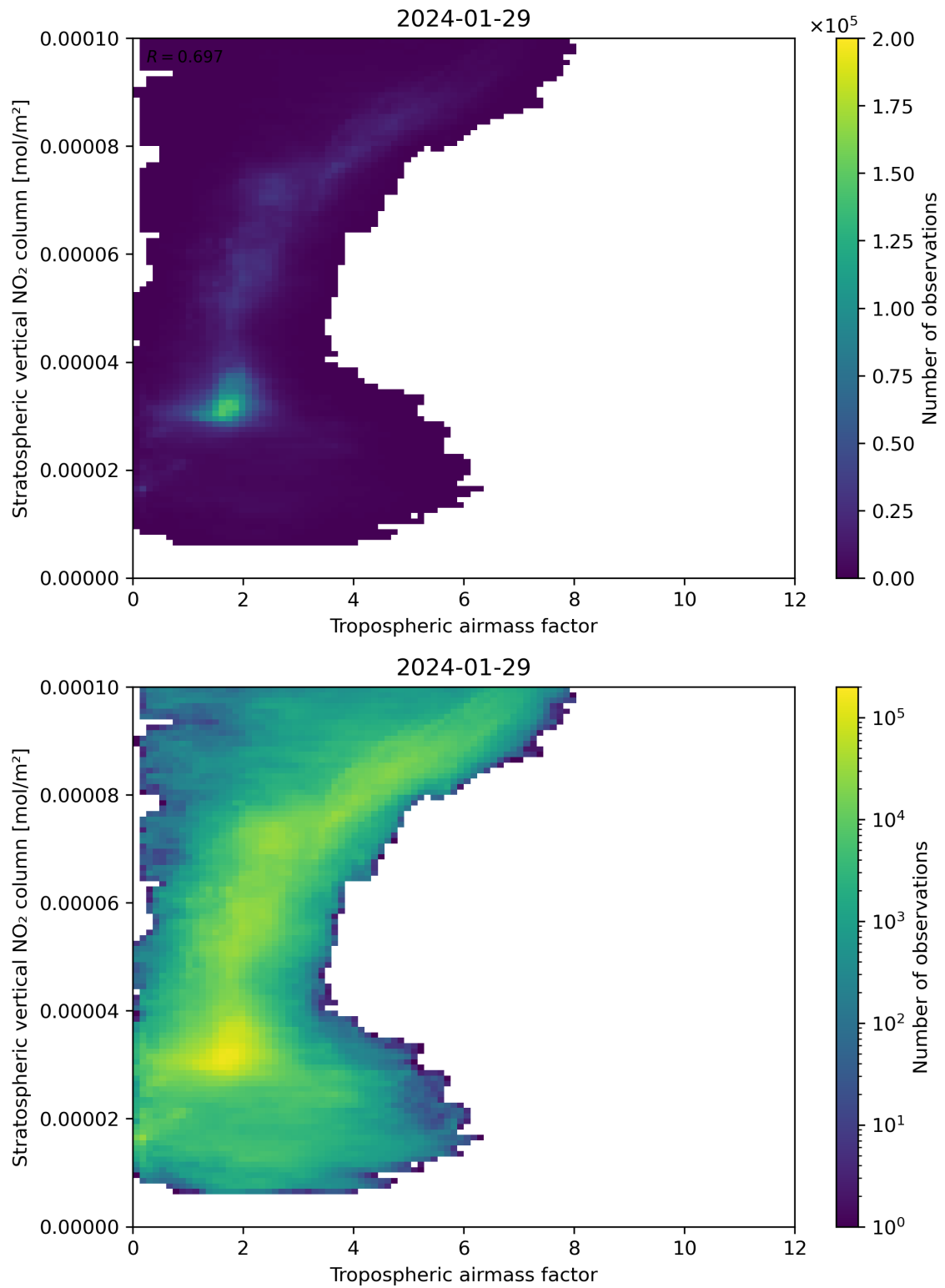
Figure 74: Scatter density plot of “Tropospheric air mass factor” against “Stratospheric vertical NO 2 column” for 2024-01-28 to 2024-01-30.
