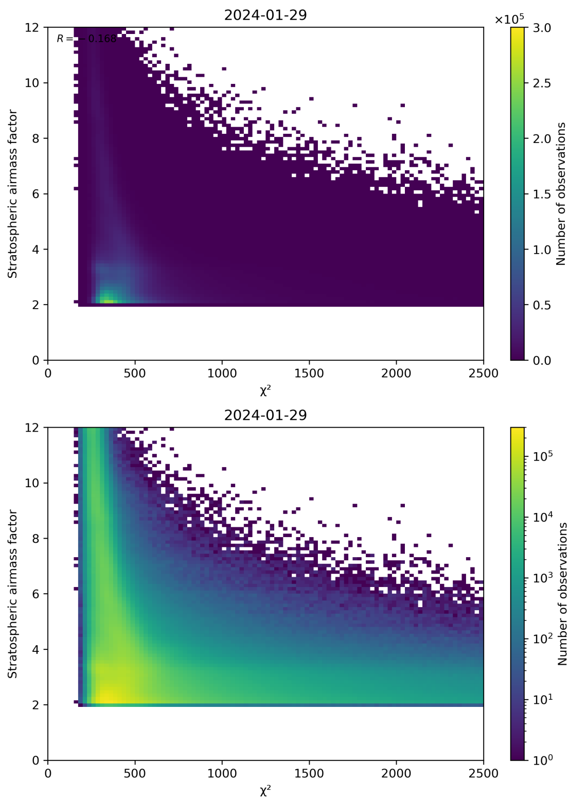
Figure 81: Scatter density plot of “ \chi^2 ” against “Stratospheric airmass factor” for 2024-01-28 to 2024-01-30.
