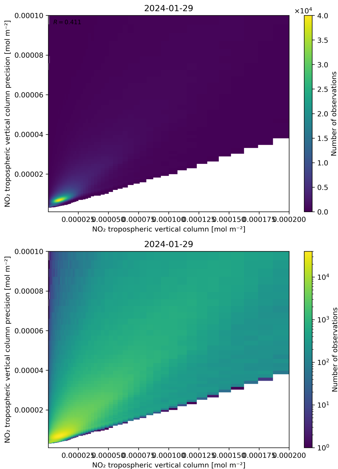
Figure 130: Scatter density plot of “NO 2 tropospheric vertical column” against “NO 2 tropospheric vertical column precision” for 2024-01-28 to 2024-01-30.
