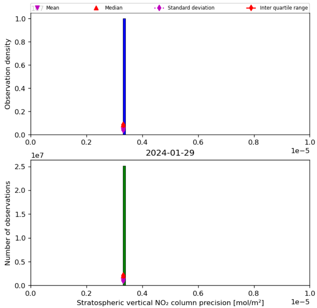
Figure 37: Histogram of “Stratospheric vertical NO 2 column precision” for 2024-01-28 to 2024-01-30
