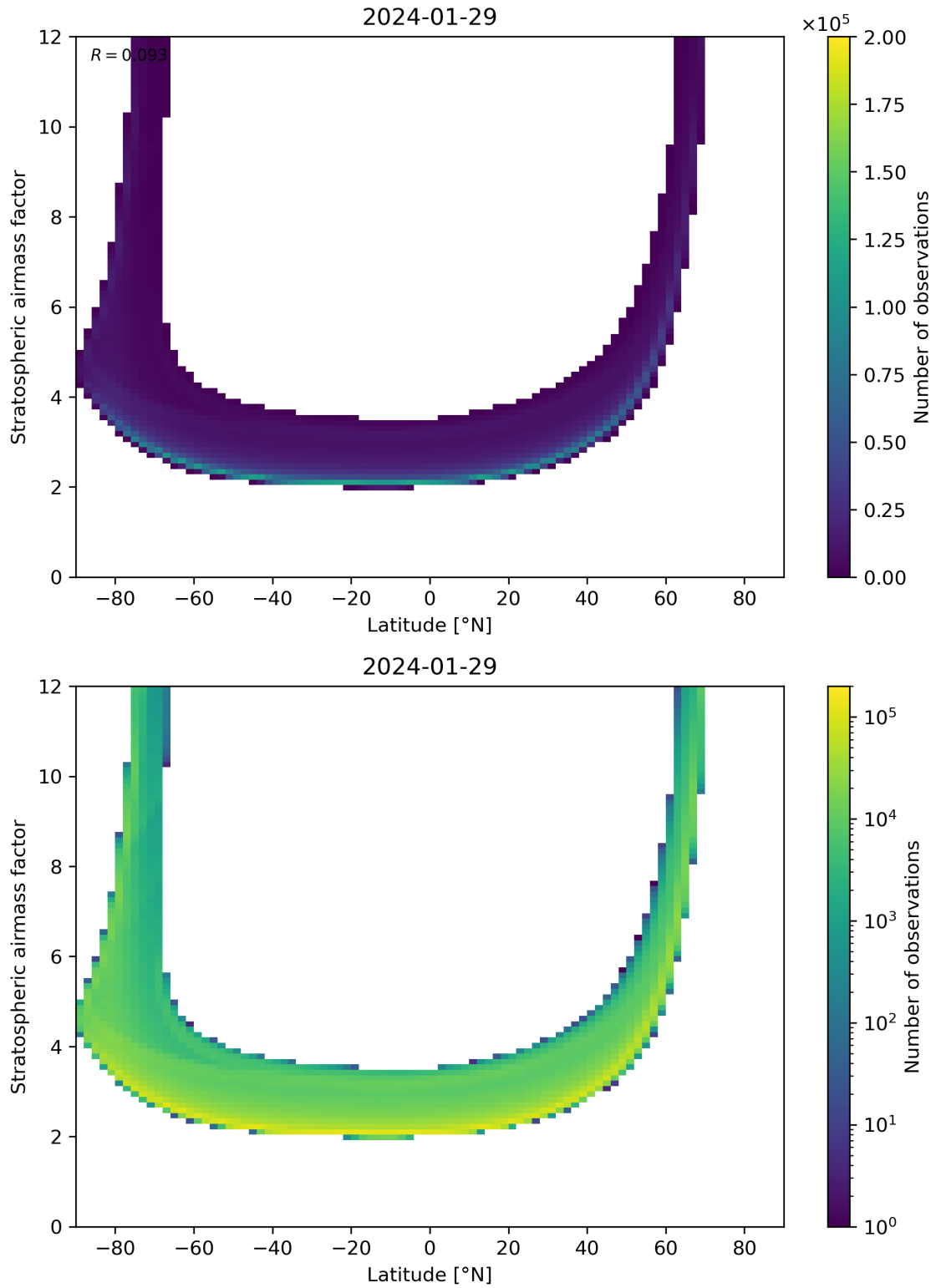
Figure 83: Scatter density plot of “Latitude” against “Stratospheric air mass factor” for 2024-01-28 to 2024-01-30.
