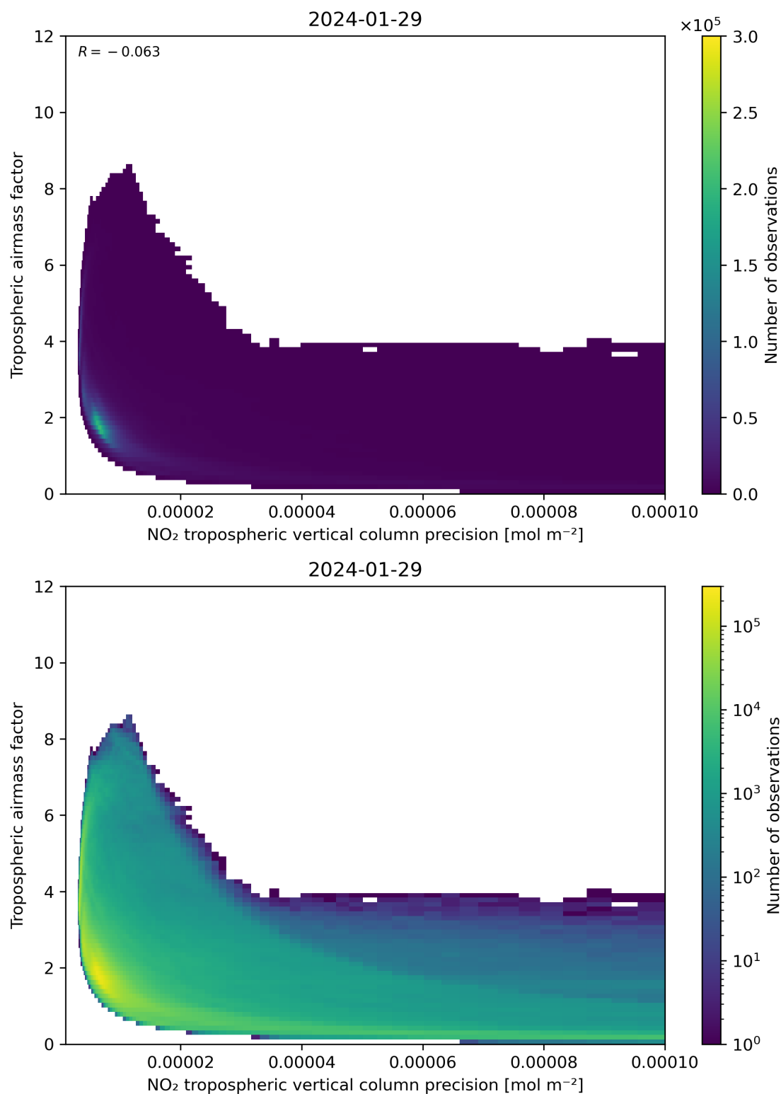
Figure 133: Scatter density plot of “NO 2 tropospheric vertical column precision” against “Tropospheric airmass factor” for 2024-01-28 to 2024-01-30.
