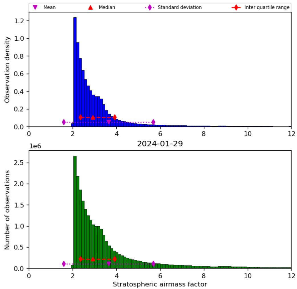
Figure 44: Histogram of “Stratospheric airmass factor” for 2024-01-28 to 2024-01-30
