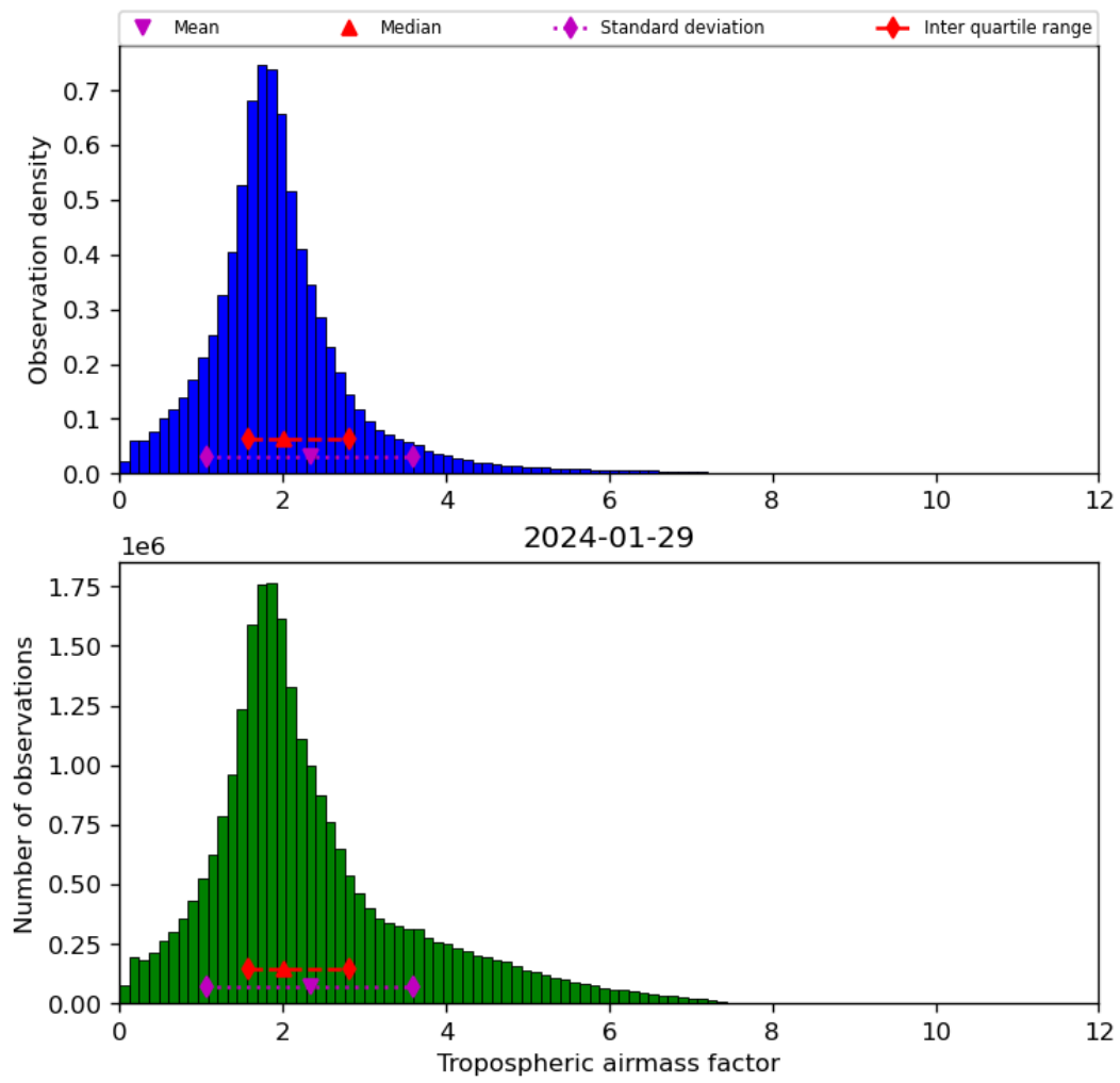
Figure 31: Histogram of “Tropospheric airmass factor” for 2024-01-28 to 2024-01-30
