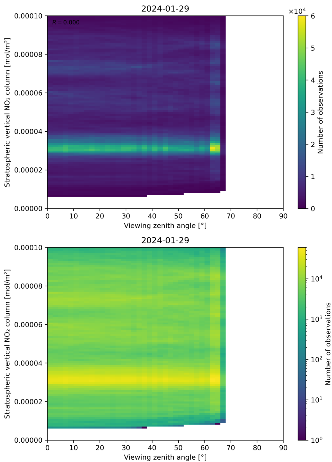
Figure 164: Scatter density plot of “Viewing zenith angle” against “Stratospheric vertical NO 2 column” for 2024-01-28 to 2024-01-30.
