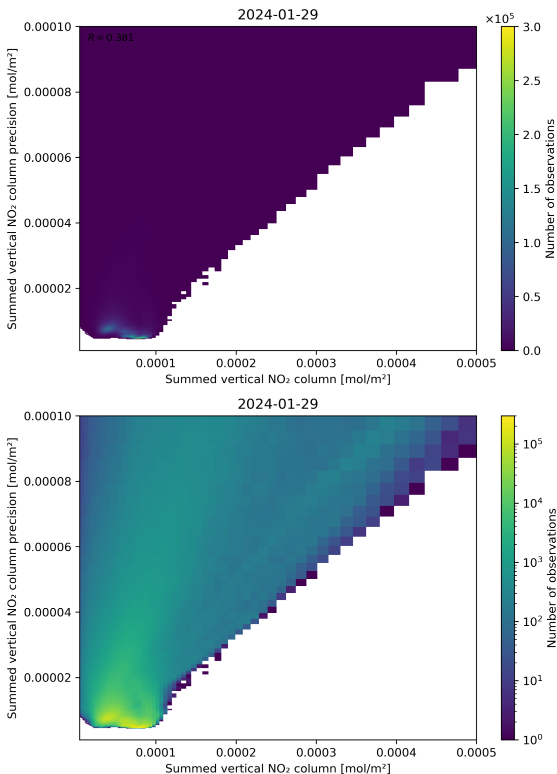
Figure 105: Scatter density plot of “Summed vertical NO 2 column” against “Summed vertical NO 2 column precision” for 2024-01-28 to 2024-01-30.
