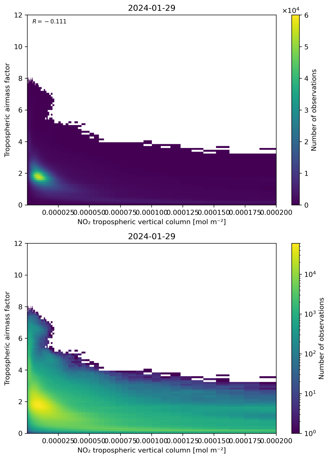
Figure 123: Scatter density plot of “NO 2 tropospheric vertical column” against “Tropospheric air mass factor” for 2024-01-28 to 2024-01-30.
