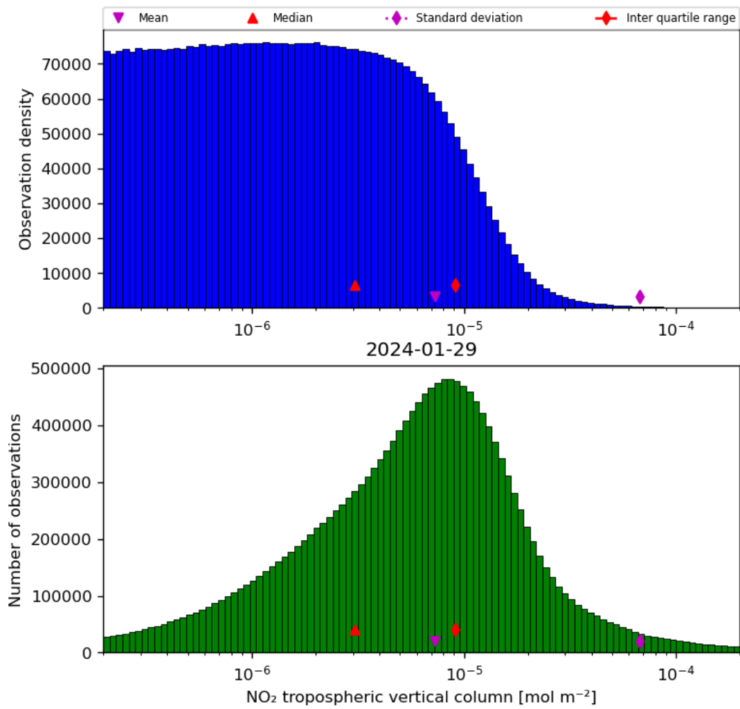
Figure 29: Histogram of “ \text{NO}_2 tropospheric vertical column” for 2024-01-28 to 2024-01-30
