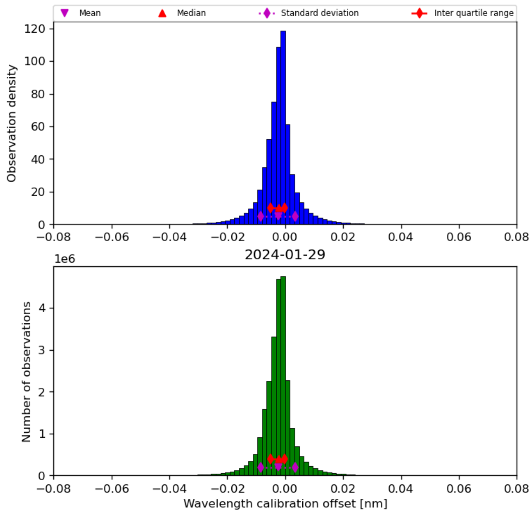
Figure 35: Histogram of “Wavelength calibration offset” for 2024-01-28 to 2024-01-30
