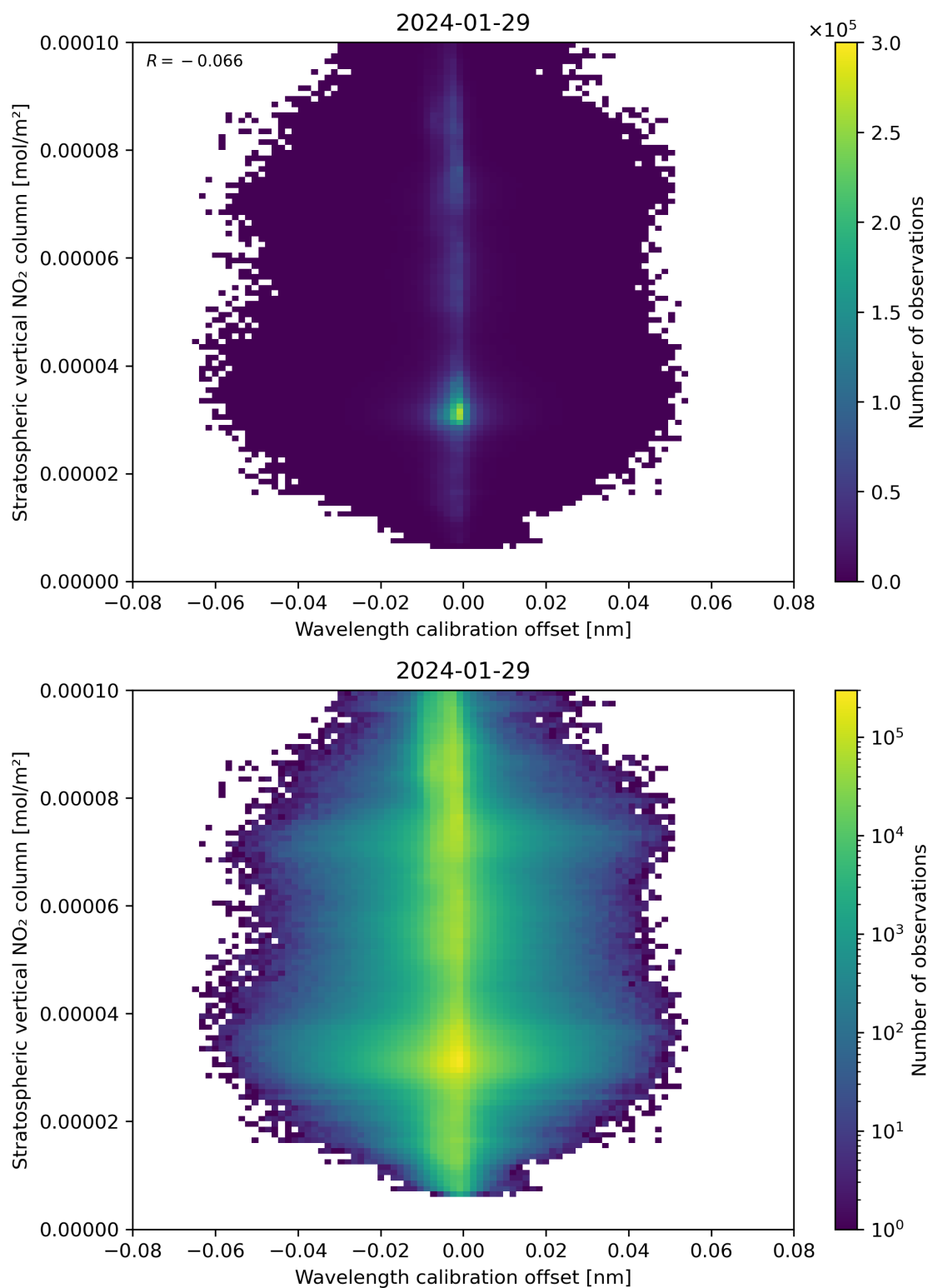
Figure 176: Scatter density plot of “Wavelength calibration offset” against “Stratospheric vertical NO 2 column” for 2024-01-28 to 2024-01-30.
