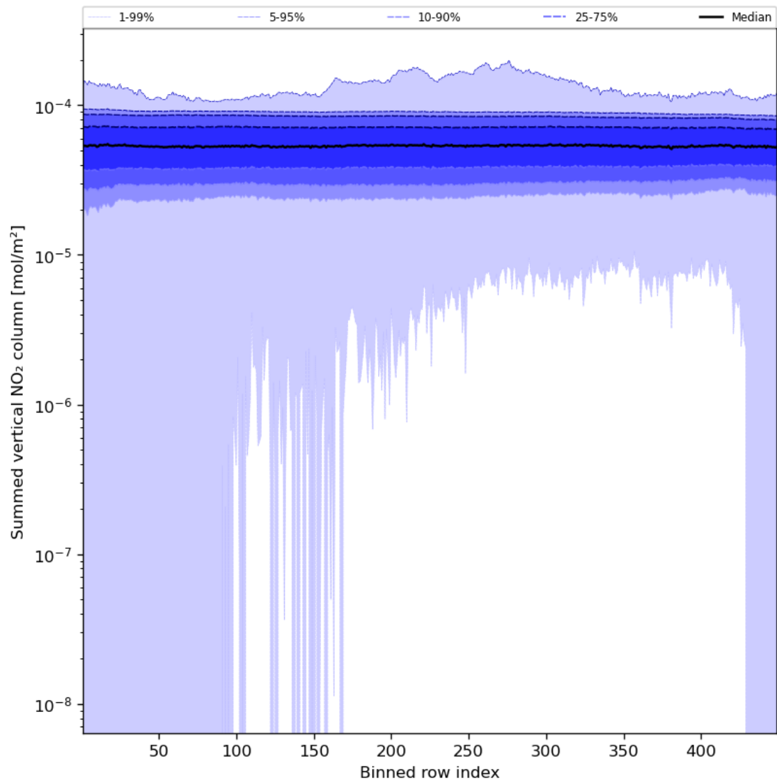
Figure 57: Along track statistics of “Summed vertical NO 2 column” for 2024-01-28 to 2024-01-30
