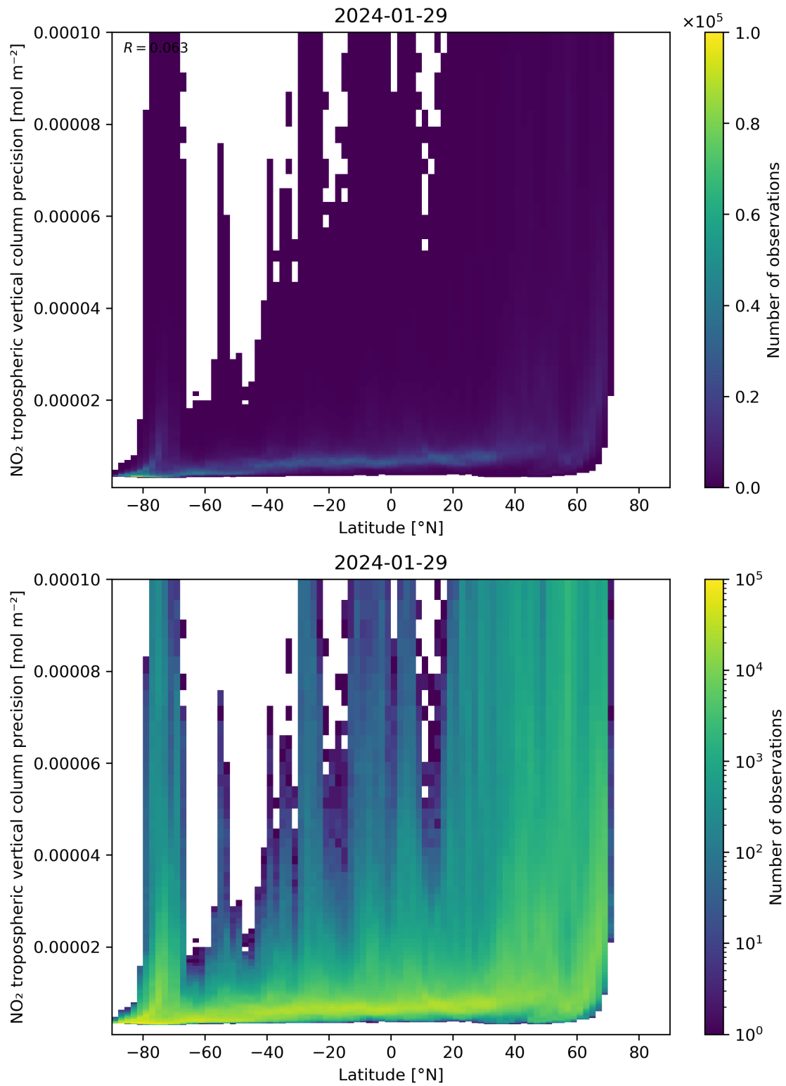
Figure 93: Scatter density plot of “Latitude” against “NO 2 tropospheric vertical column precision” for 2024-01-28 to 2024-01-30.
