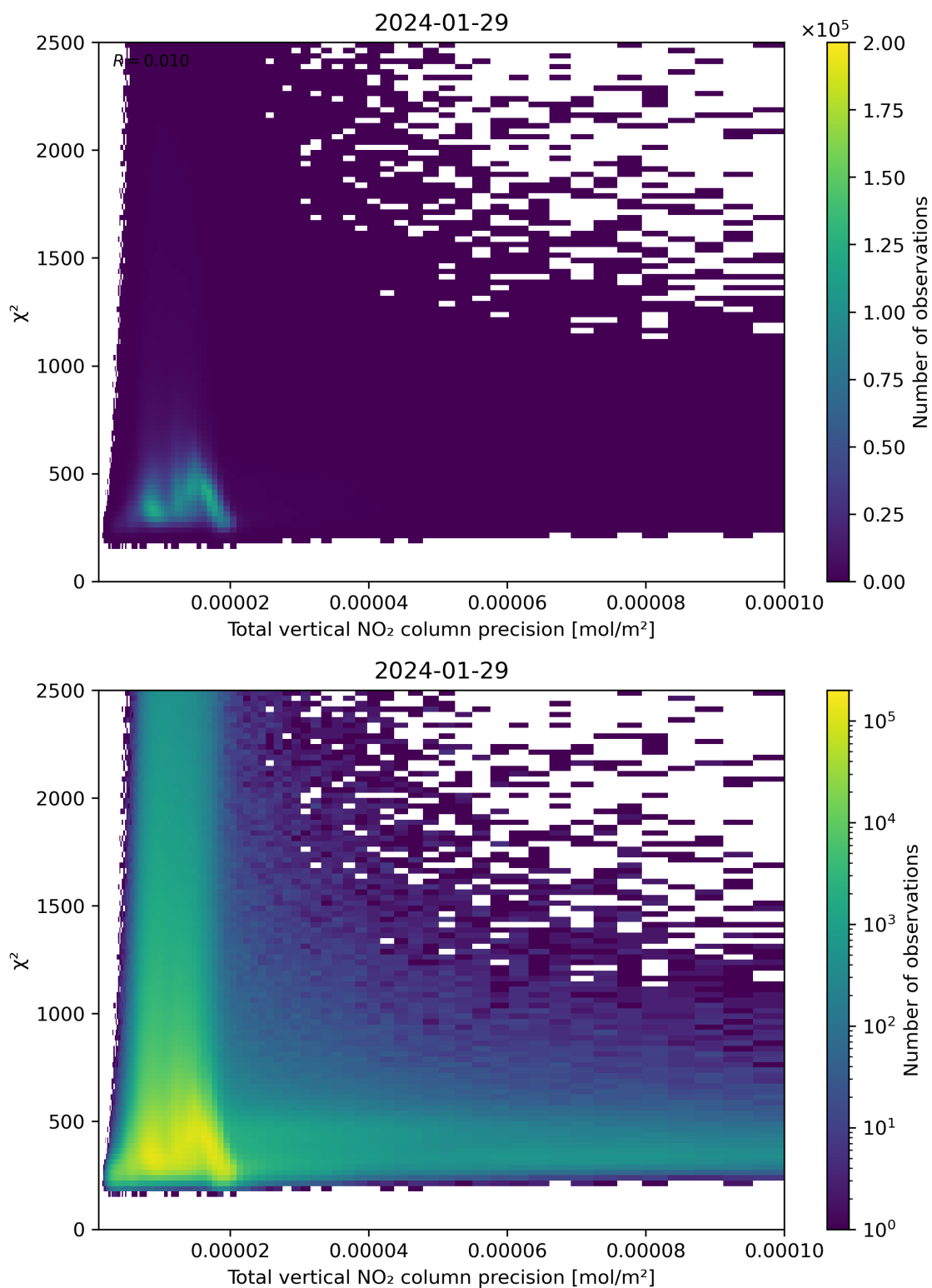
Figure 116: Scatter density plot of “Total vertical NO 2 column precision” against “ \chi^2 ” for 2024-01-28 to 2024-01-30.
