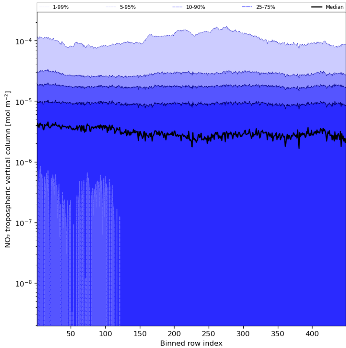
Figure 46: Along track statistics of “NO 2 tropospheric vertical column” for 2024-01-28 to 2024-01-30
