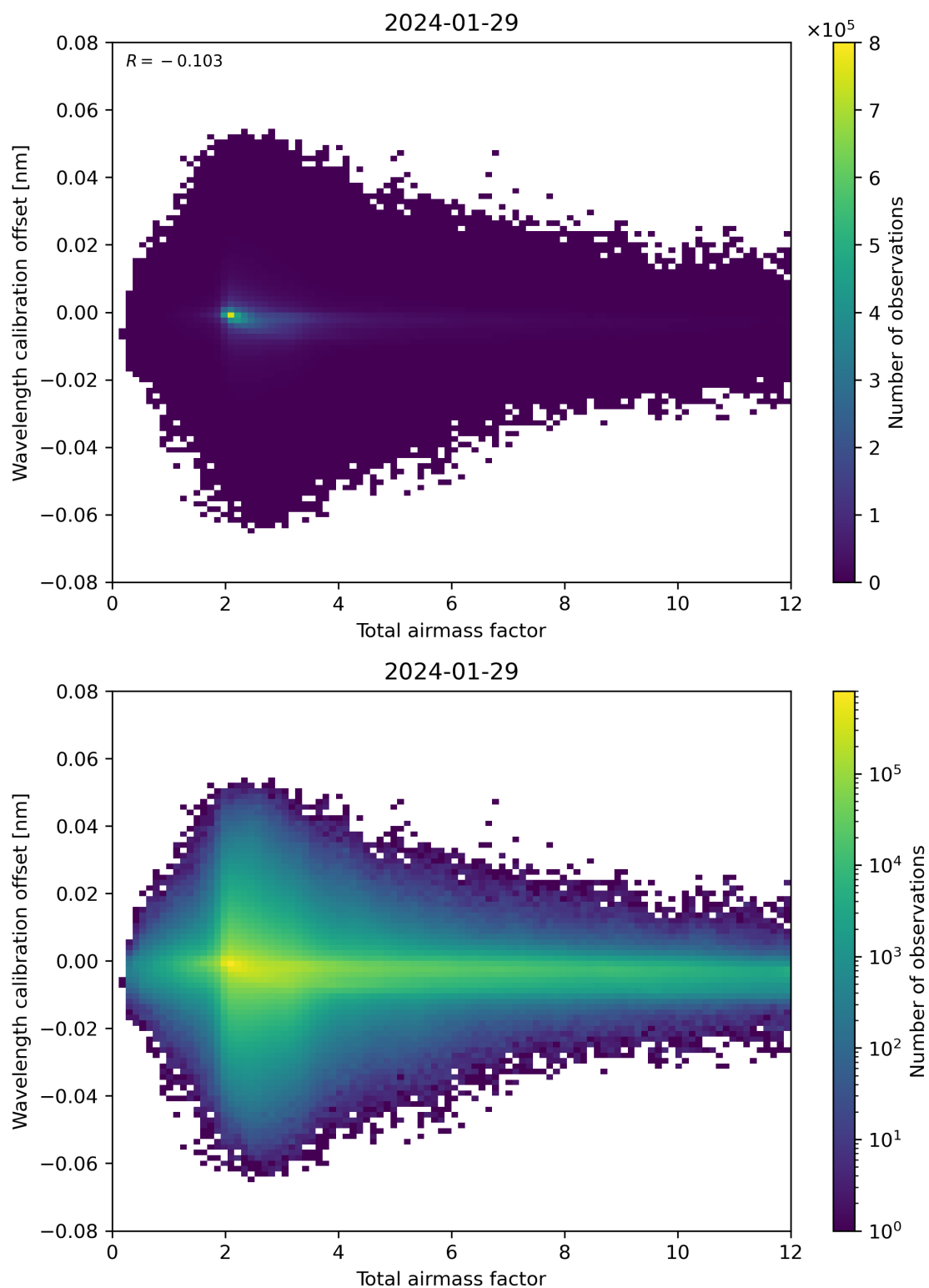
Figure 70: Scatter density plot of “Total airmass factor” against “Wavelength calibration offset” for 2024-01-28 to 2024-01-30.
