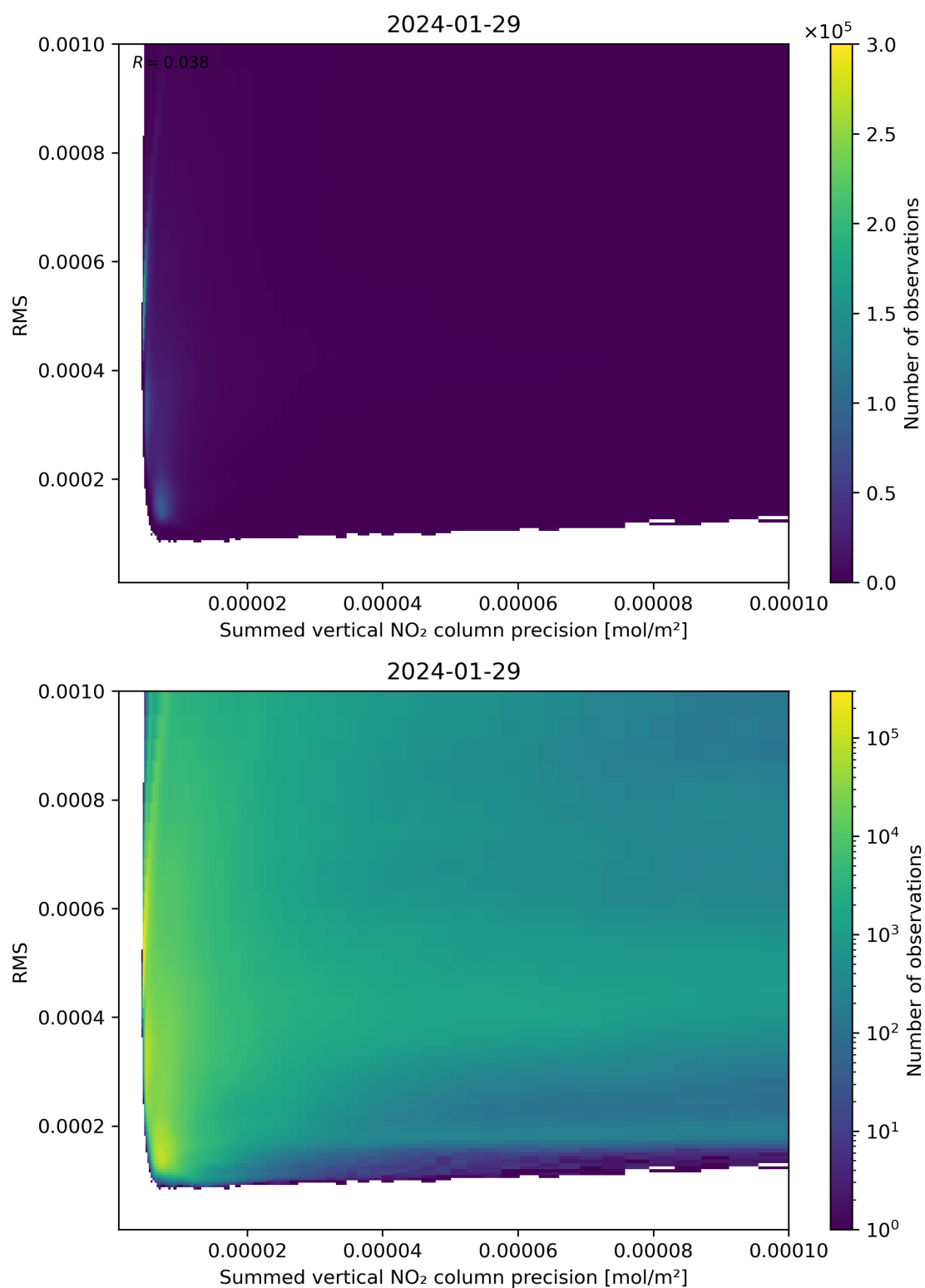
Figure 108: Scatter density plot of “Summed vertical NO 2 column precision” against “RMS” for 2024-01-28 to 2024-01-30.
