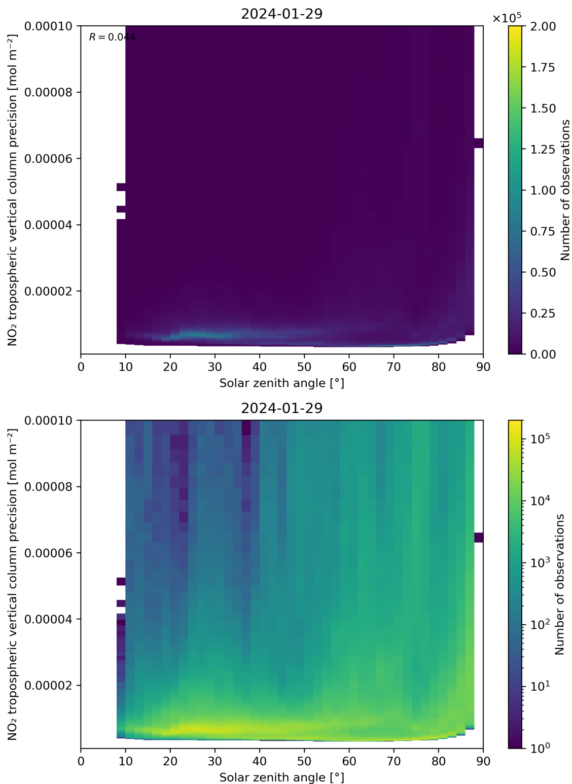
Figure 156: Scatter density plot of “Solar zenith angle” against “NO 2 tropospheric vertical column precision” for 2024-01-28 to 2024-01-30.
