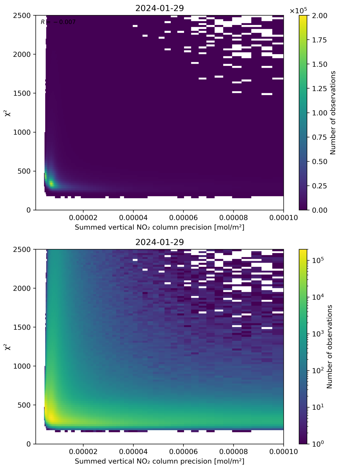
Figure 107: Scatter density plot of “Summed vertical NO 2 column precision” against “ \chi^2 ” for 2024-01-28 to 2024-01-30.
