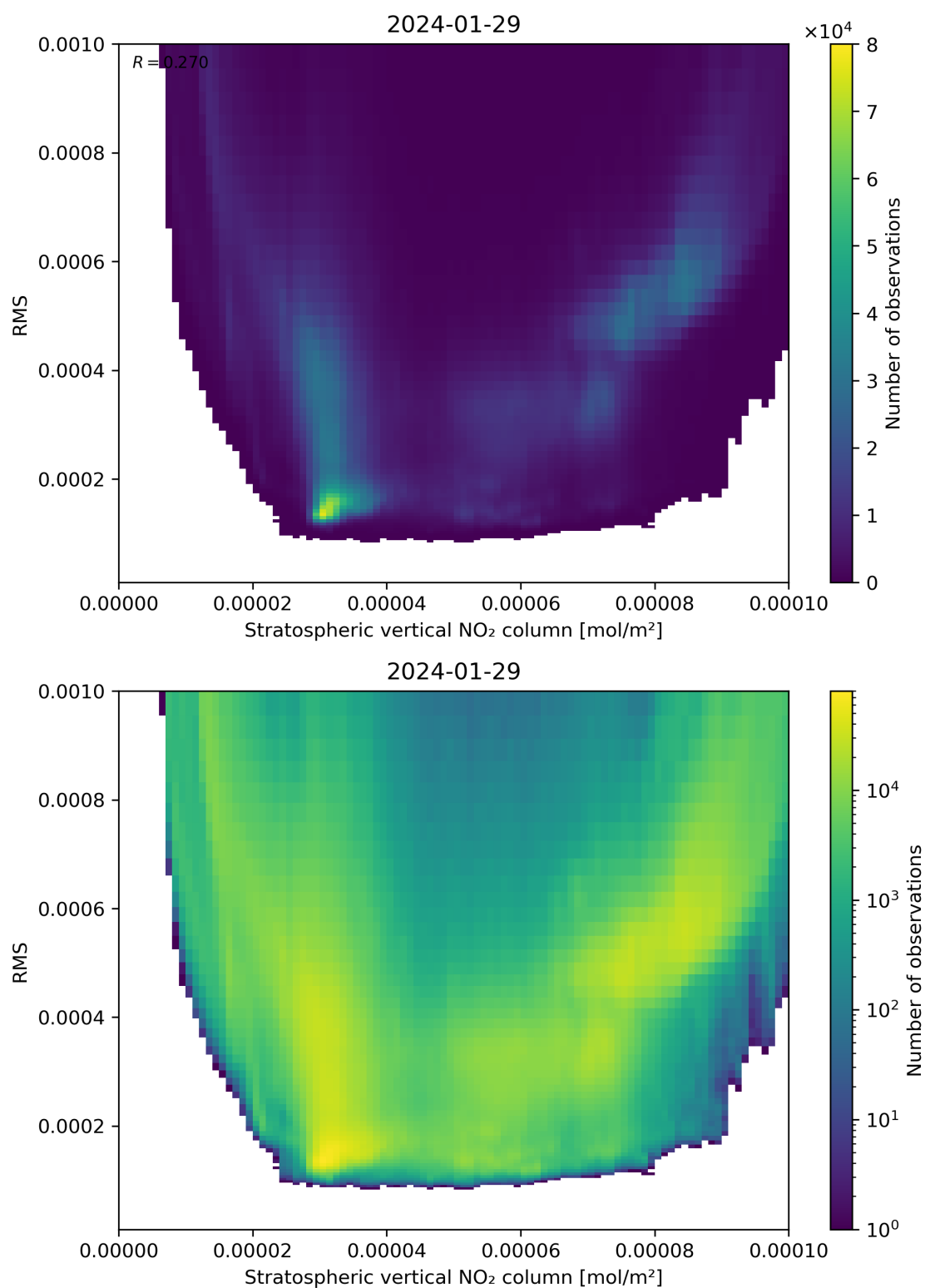
Figure 102: Scatter density plot of “Stratospheric vertical NO 2 column” against “RMS” for 2024-01-28 to 2024-01-30.
