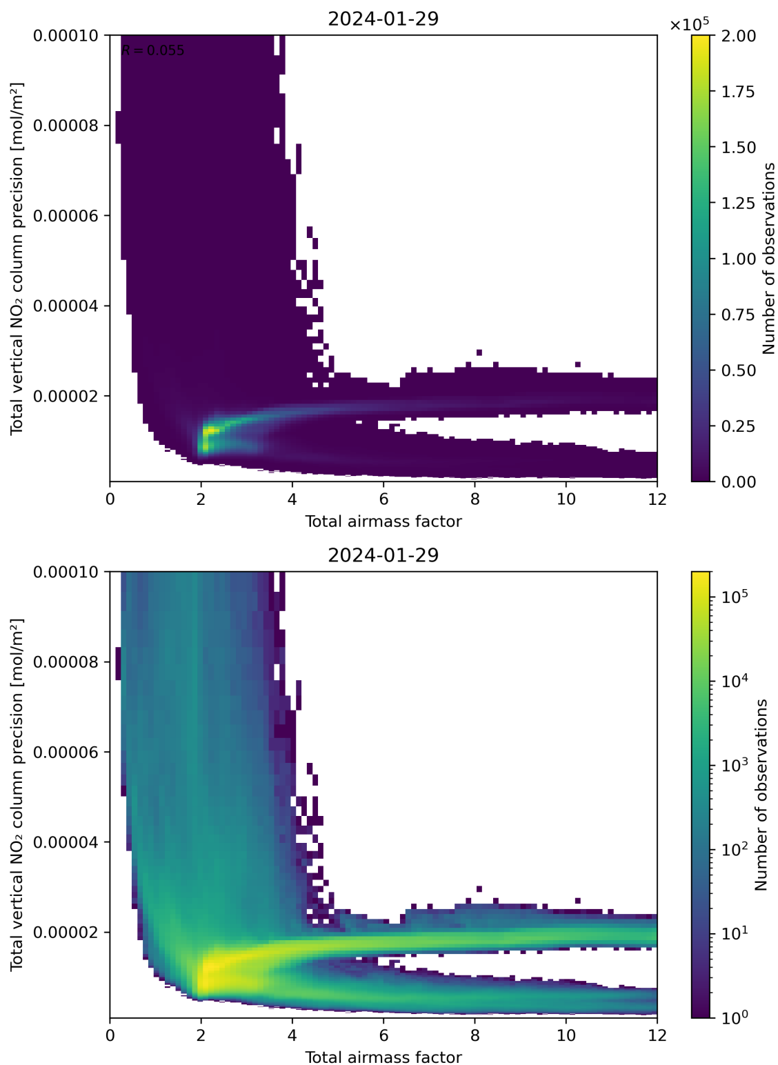
Figure 68: Scatter density plot of “Total airmass factor” against “Total vertical NO 2 column precision” for 2024-01-28 to 2024-01-30.
