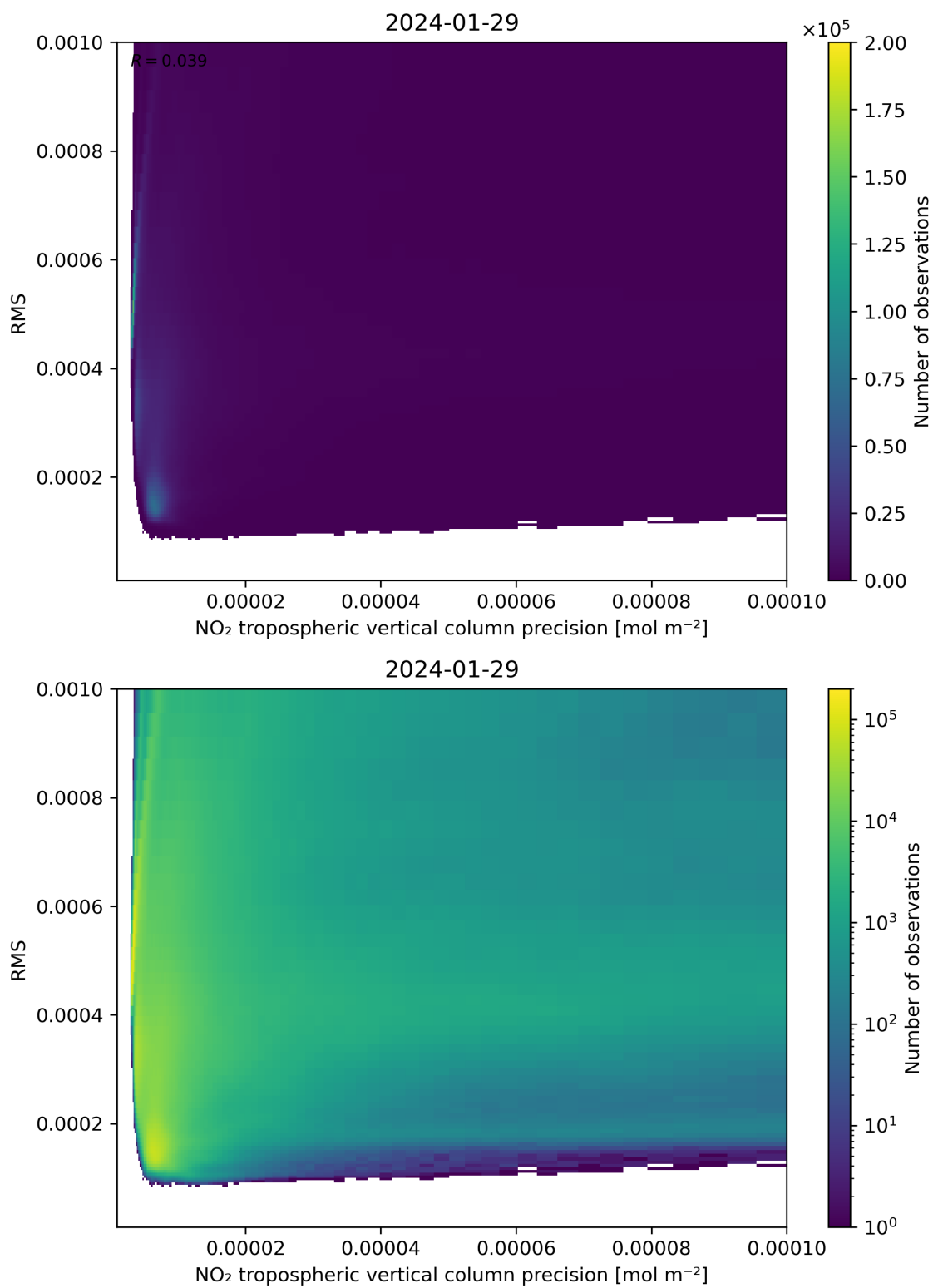
Figure 140: Scatter density plot of “NO 2 tropospheric vertical column precision” against “RMS” for 2024-01-28 to 2024-01-30.
