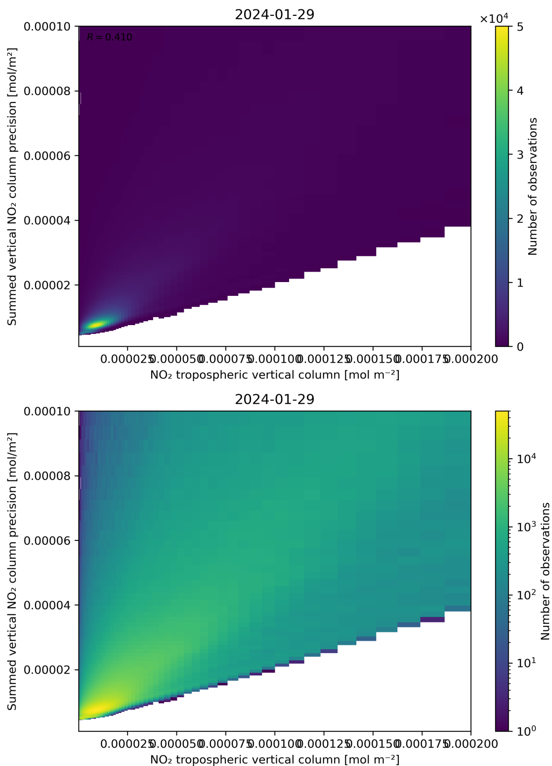
Figure 127: Scatter density plot of “NO 2 tropospheric vertical column” against “Summed vertical NO 2 column precision” for 2024-01-28 to 2024-01-30.
