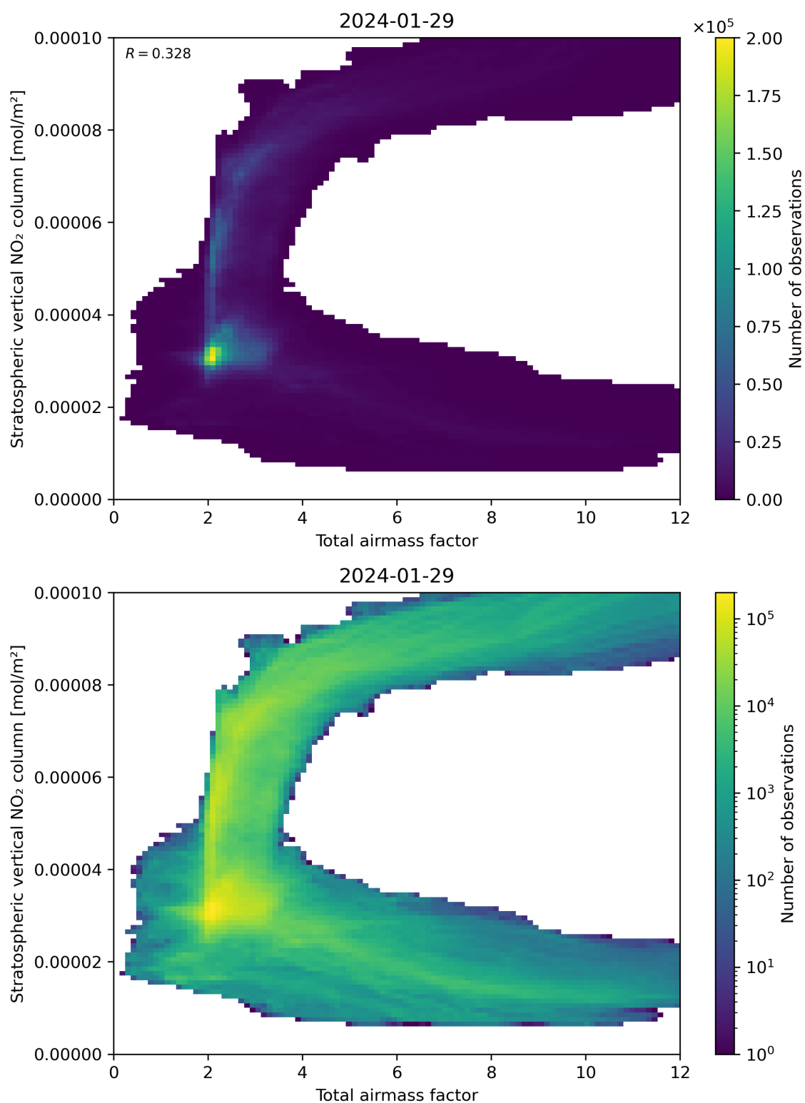
Figure 64: Scatter density plot of “Total airmass factor” against “Stratospheric vertical \text{NO}_2 column” for 2024-01-28 to 2024-01-30.
