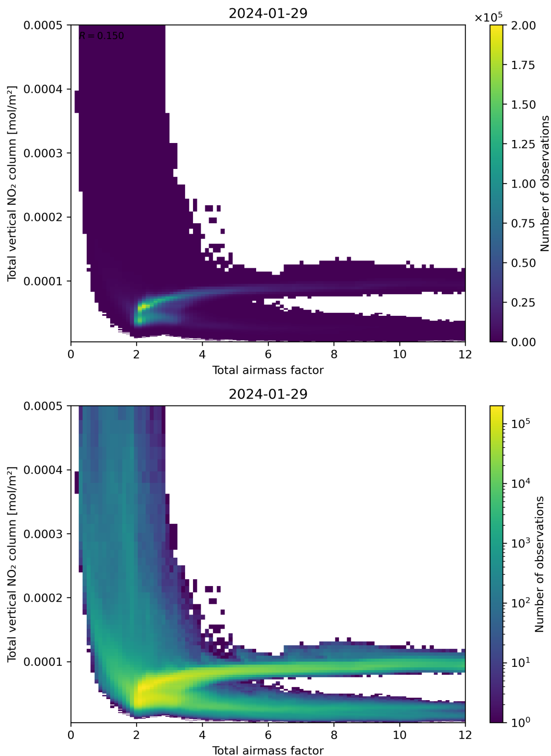
Figure 67: Scatter density plot of “Total airmass factor” against “Total vertical NO 2 column” for 2024-01-28 to 2024-01-30.
