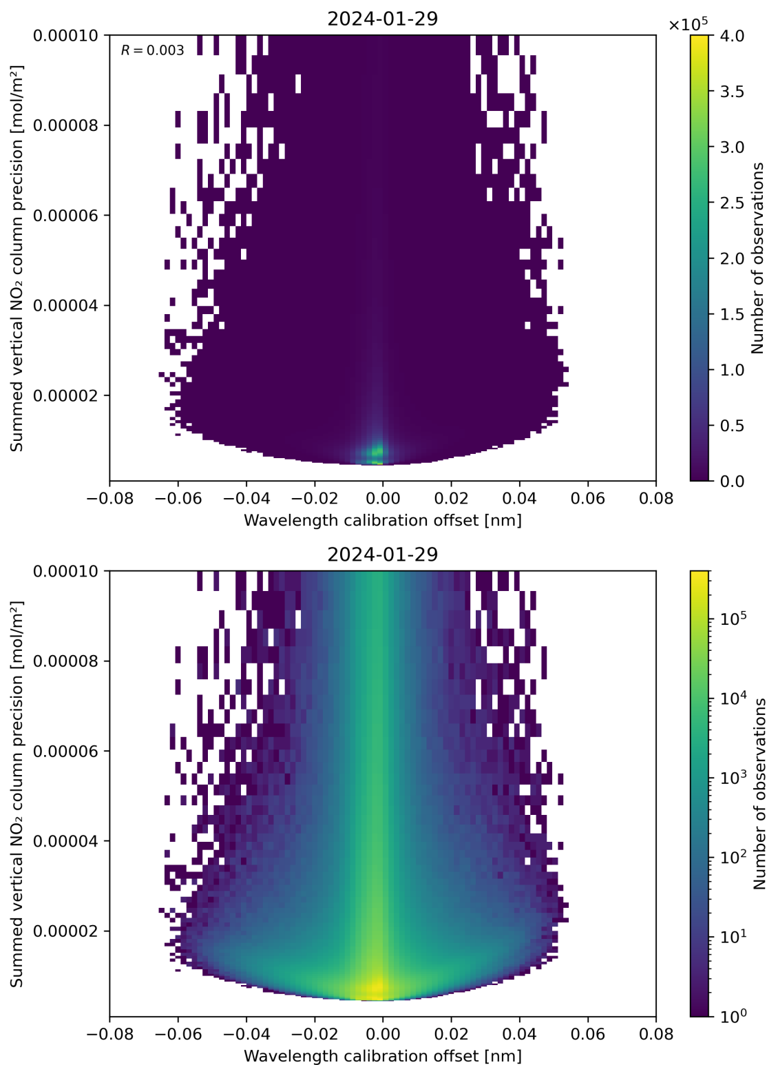
Figure 178: Scatter density plot of “Wavelength calibration offset” against “Summed vertical NO 2 column precision” for 2024-01-28 to 2024-01-30.
