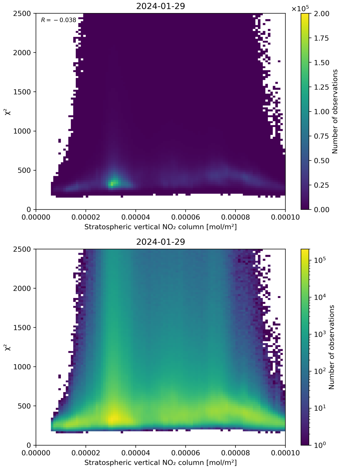
Figure 97: Scatter density plot of “Stratospheric vertical NO 2 column” against “ \chi^2 ” for 2024-01-28 to 2024-01-30.
