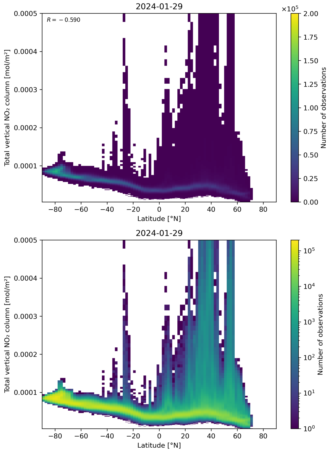
Figure 90: Scatter density plot of “Latitude” against “Total vertical NO 2 column” for 2024-01-28 to 2024-01-30.
