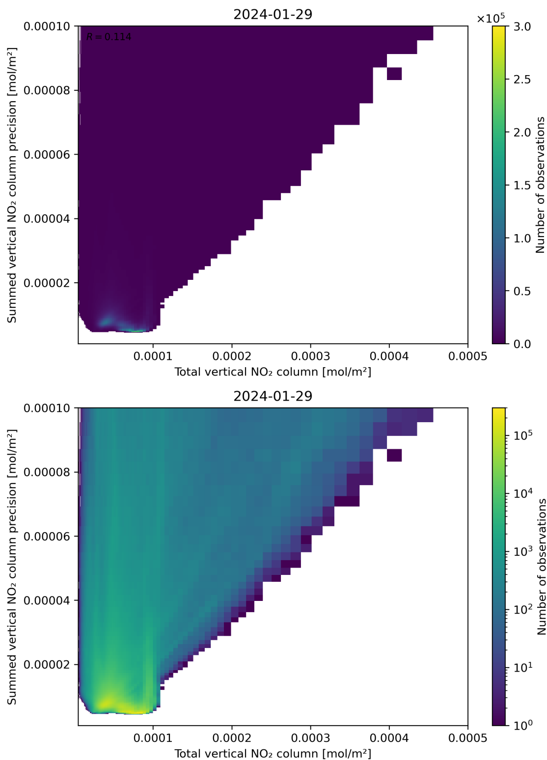
Figure 113: Scatter density plot of “Total vertical NO 2 column” against “Summed vertical NO 2 column precision” for 2024-01-28 to 2024-01-30.
