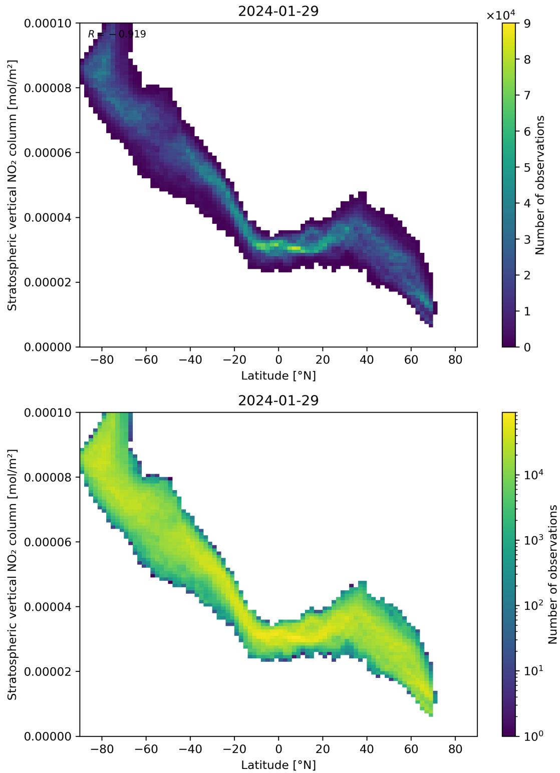
Figure 87: Scatter density plot of “Latitude” against “Stratospheric vertical NO 2 column” for 2024-01-28 to 2024-01-30.
