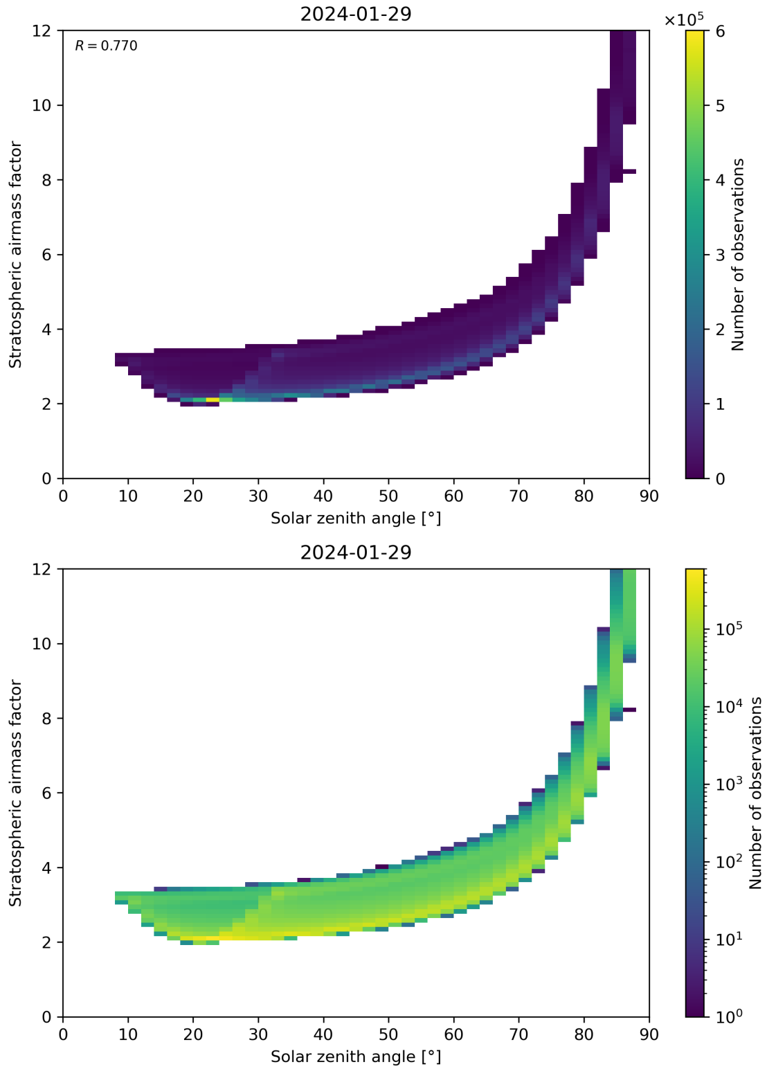
Figure 145: Scatter density plot of “Solar zenith angle” against “Stratospheric airmass factor” for 2024-01-28 to 2024-01-30.
