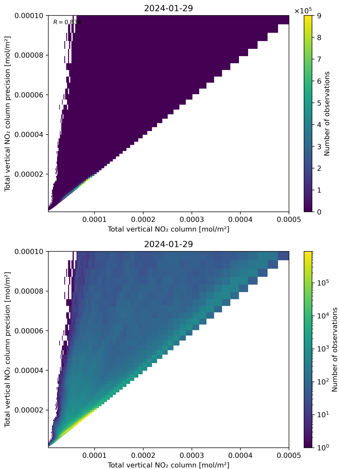
Figure 114: Scatter density plot of “Total vertical NO 2 column” against “Total vertical NO 2 column precision” for 2024-01-28 to 2024-01-30.
