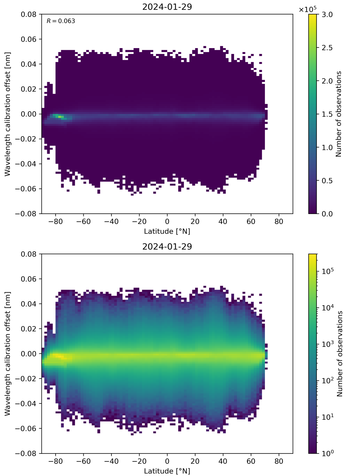
Figure 95: Scatter density plot of “Latitude” against “Wavelength calibration offset” for 2024-01-28 to 2024-01-30.
