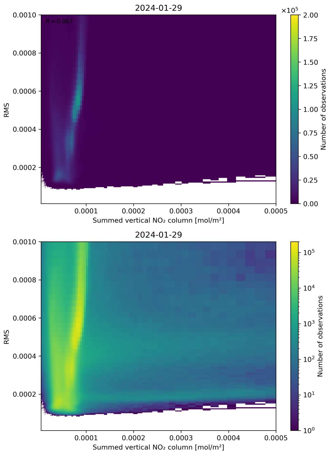
Figure 109: Scatter density plot of “Summed vertical NO 2 column” against “RMS” for 2024-01-28 to 2024-01-30.
