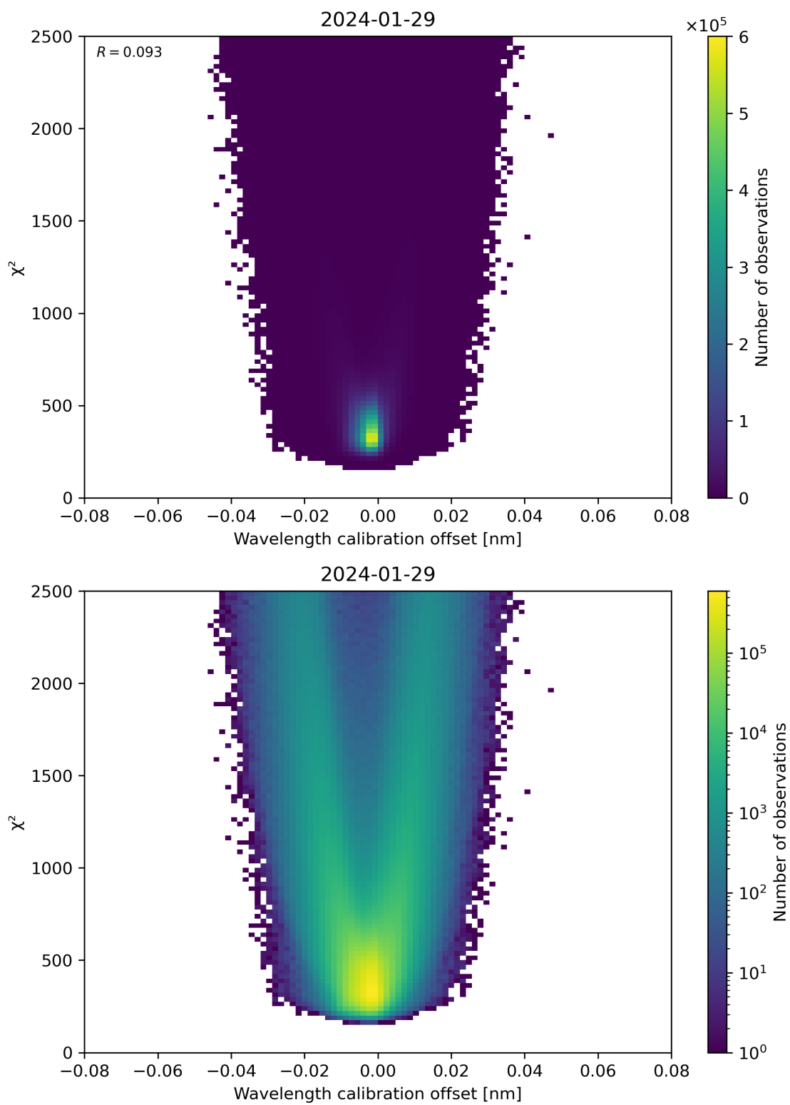
Figure 175: Scatter density plot of “Wavelength calibration offset” against “ \chi^2 ” for 2024-01-28 to 2024-01-30.
