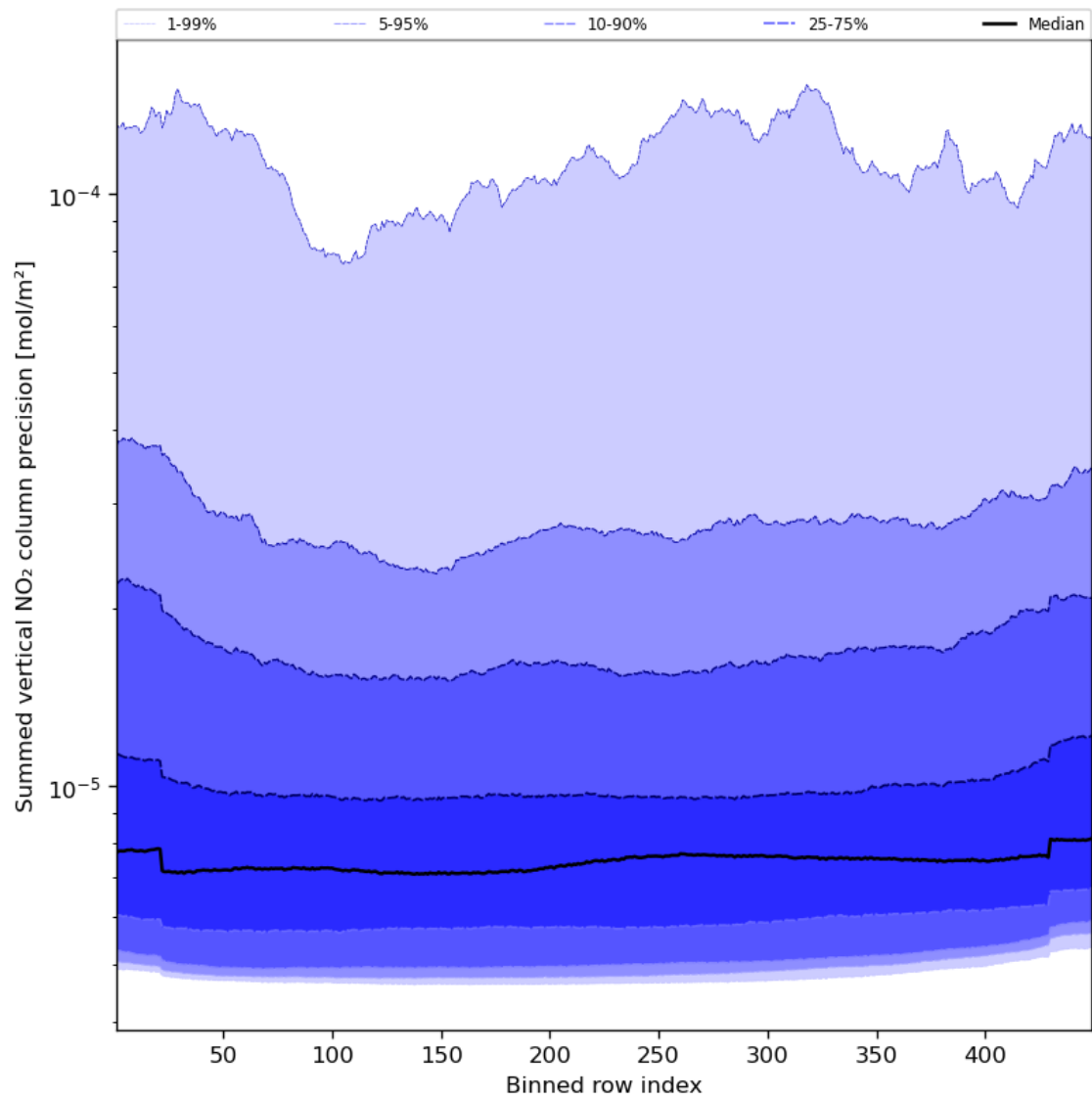
Figure 58: Along track statistics of “Summed vertical NO 2 column precision” for 2024-01-28 to 2024-01-30
