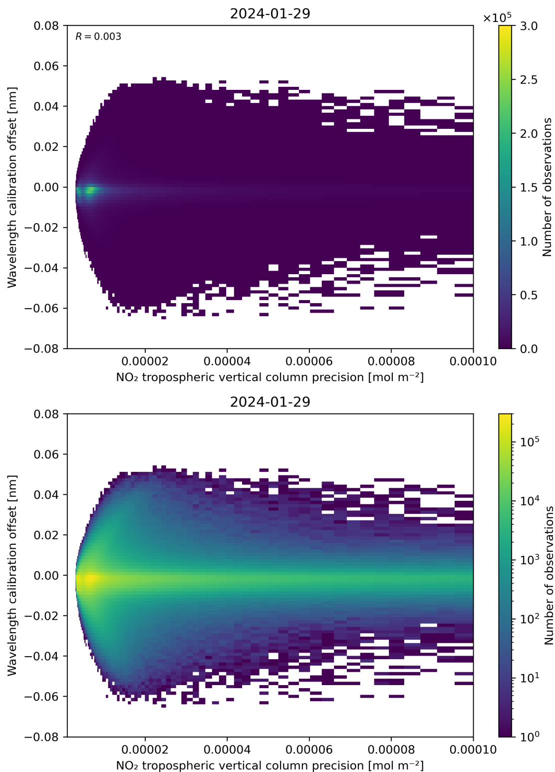
Figure 141: Scatter density plot of “NO 2 tropospheric vertical column precision” against “Wavelength calibration offset” for 2024-01-28 to 2024-01-30.
