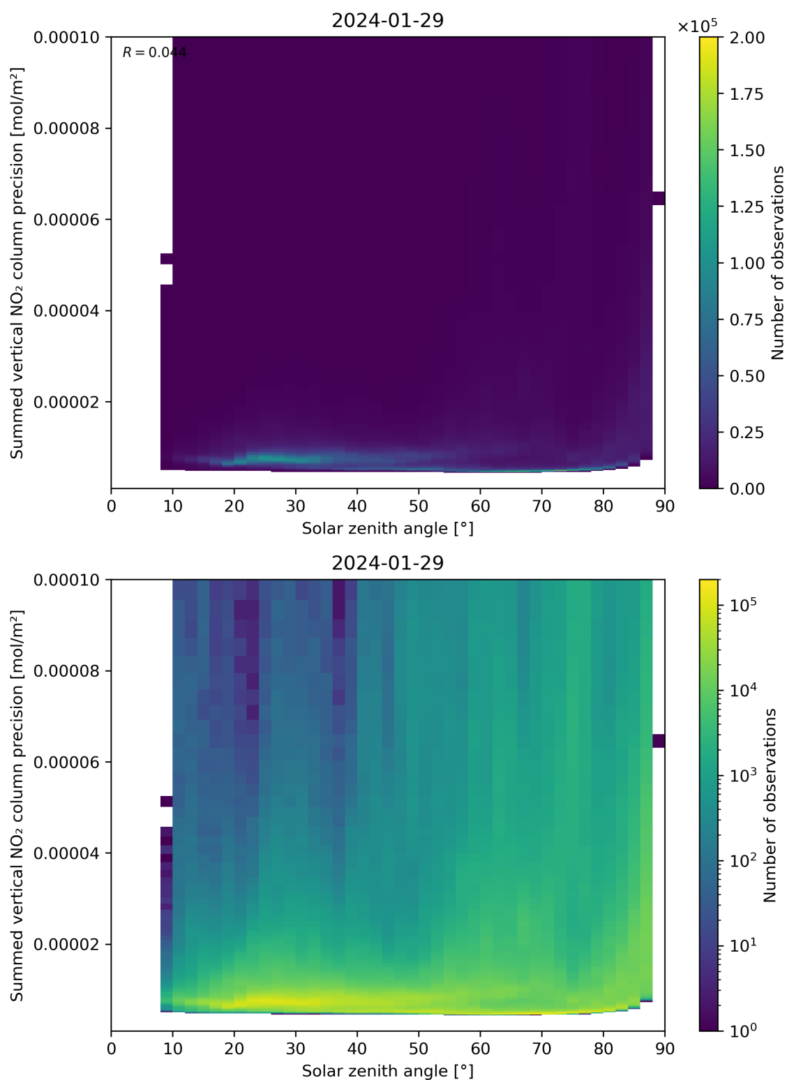
Figure 152: Scatter density plot of “Solar zenith angle” against “Summed vertical NO 2 column precision” for 2024-01-28 to 2024-01-30.
