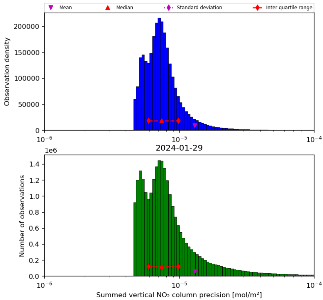
Figure 41: Histogram of "Summed vertical NO 2 column precision" for 2024-01-28 to 2024-01-30
