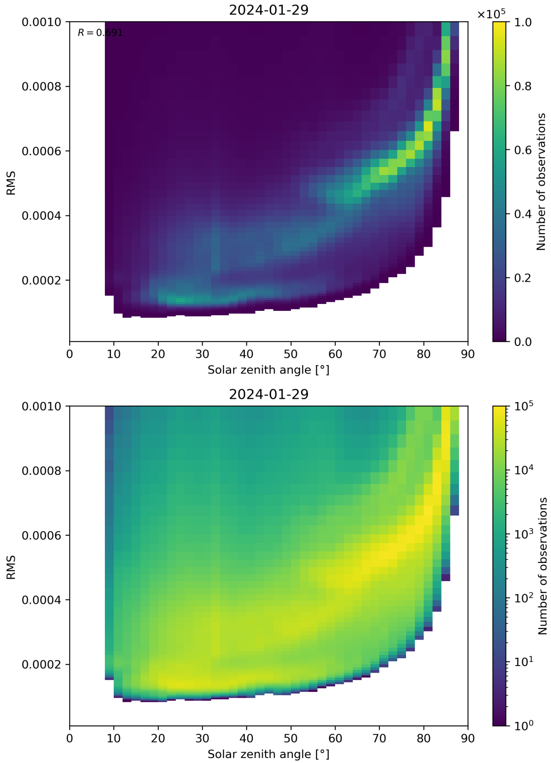
Figure 157: Scatter density plot of “Solar zenith angle” against “RMS” for 2024-01-28 to 2024-01-30.
