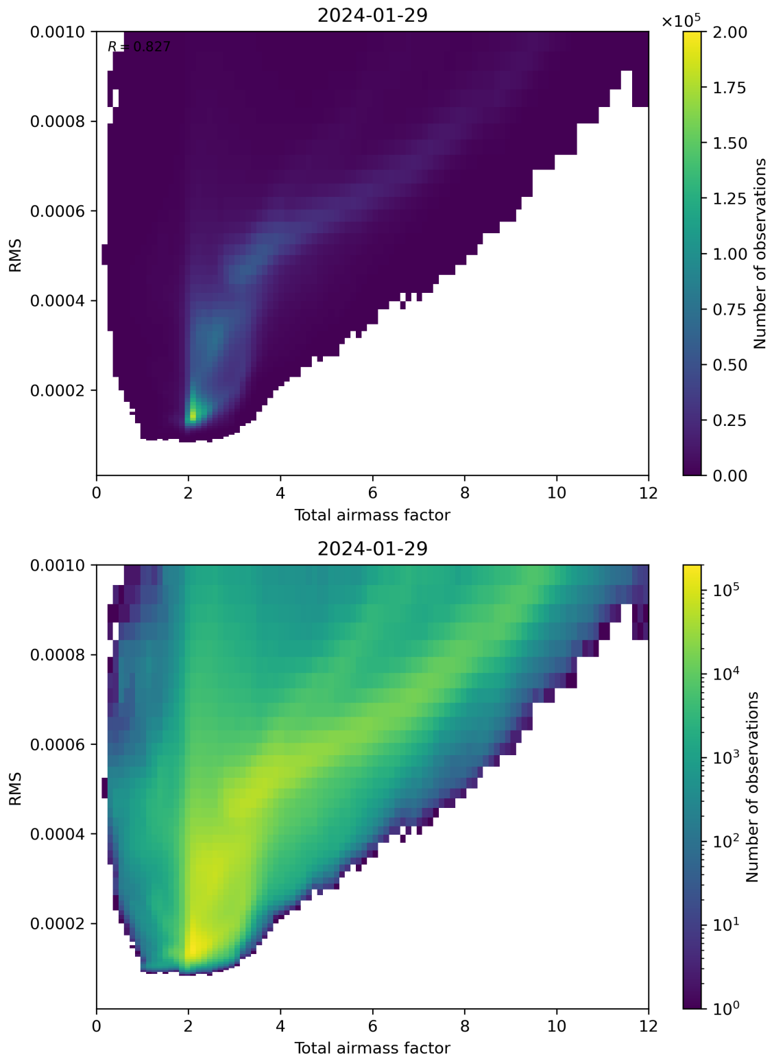
Figure 69: Scatter density plot of “Total airmass factor” against “RMS” for 2024-01-28 to 2024-01-30.
