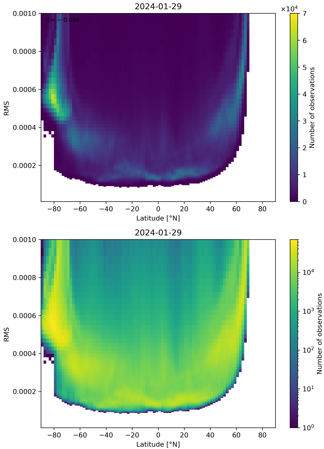
Figure 94: Scatter density plot of “Latitude” against “RMS” for 2024-01-28 to 2024-01-30.
