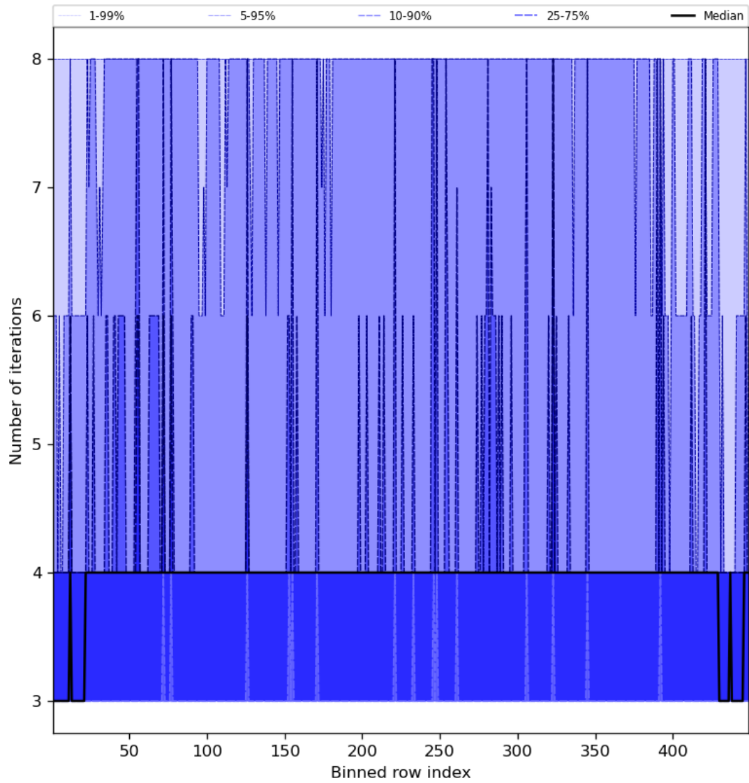
Figure 51: Along track statistics of “Number of iterations” for 2024-01-28 to 2024-01-30
