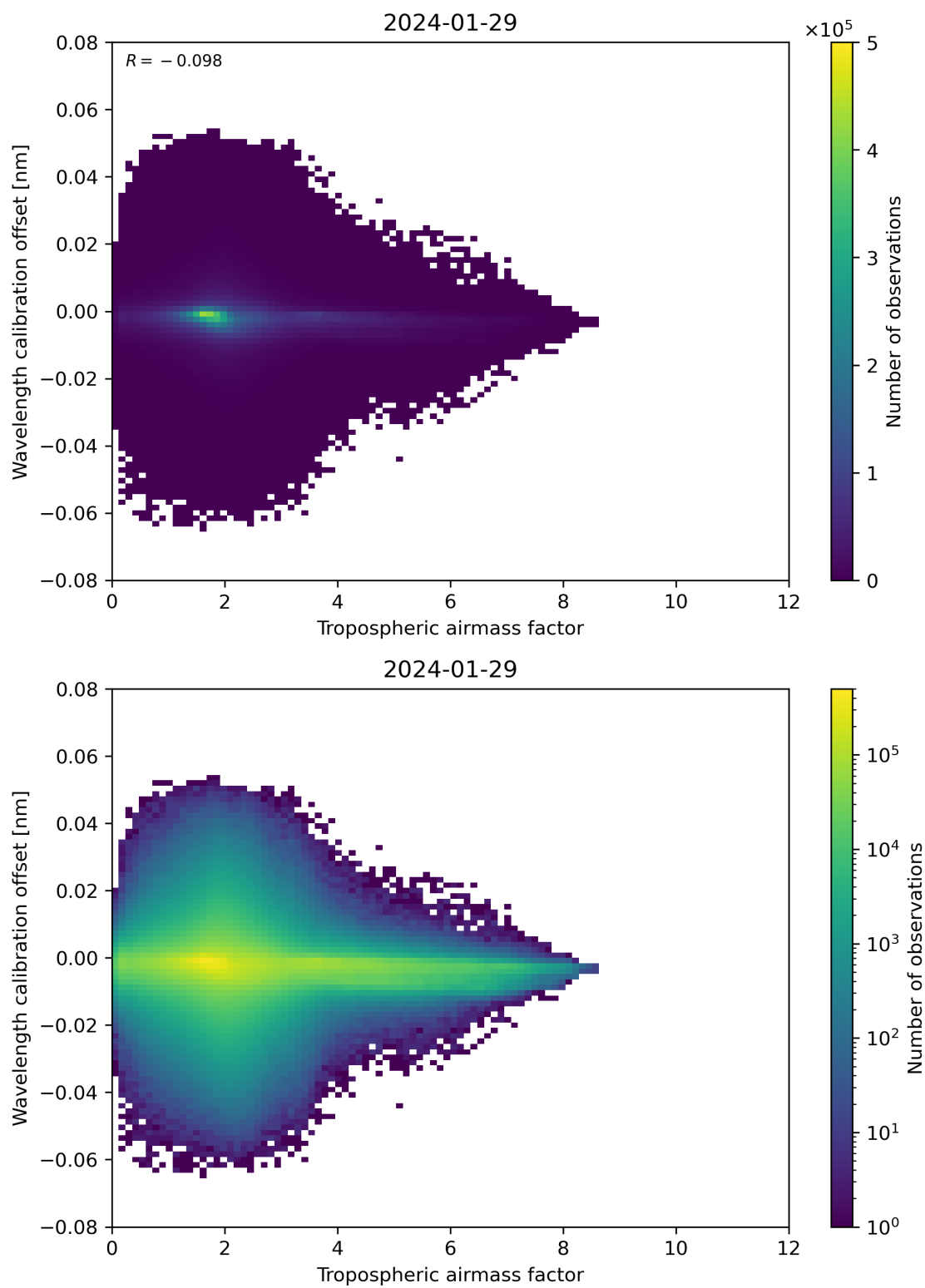
Figure 80: Scatter density plot of “Tropospheric airmass factor” against “Wavelength calibration offset” for 2024-01-28 to 2024-01-30.
