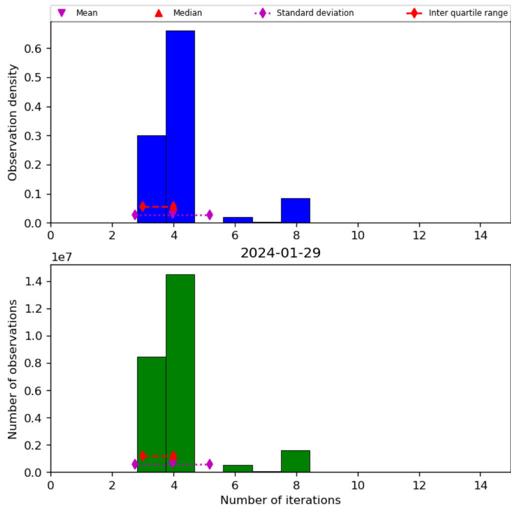
Figure 34: Histogram of “Number of iterations” for 2024-01-28 to 2024-01-30
