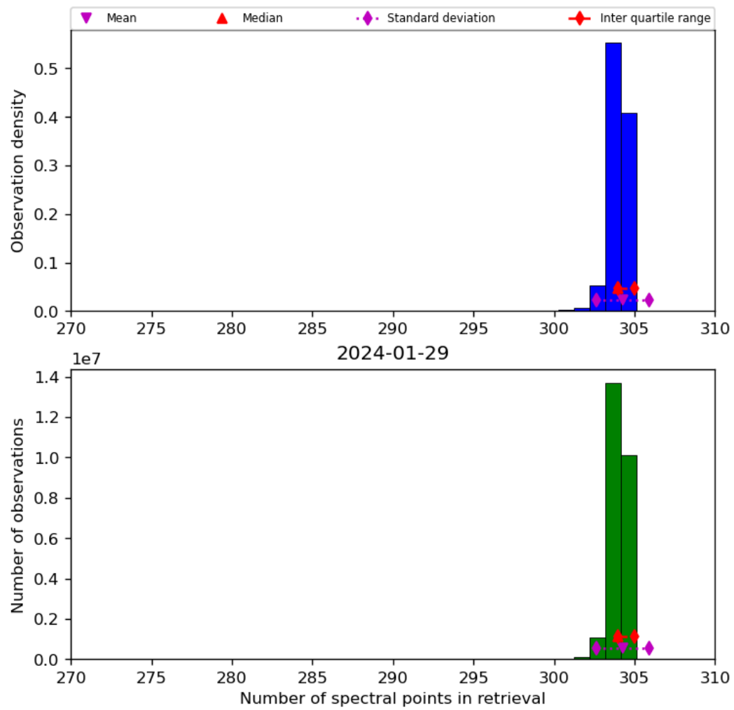
Figure 33: Histogram of “Number of spectral points in retrieval” for 2024-01-28 to 2024-01-30
