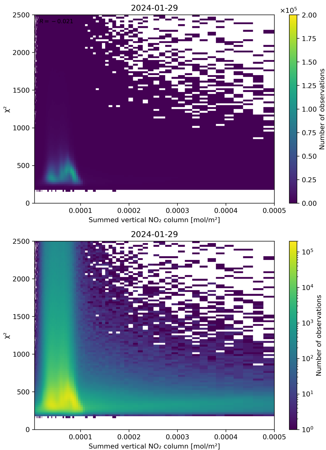
Figure 104: Scatter density plot of “Summed vertical NO 2 column” against “ \chi^2 ” for 2024-01-28 to 2024-01-30.
