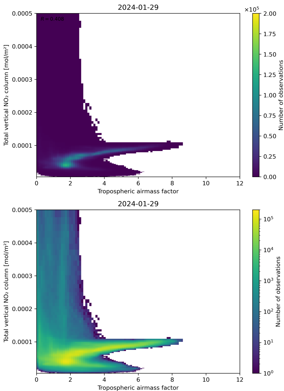
Figure 77: Scatter density plot of “Tropospheric airmass factor” against “Total vertical NO 2 column” for 2024-01-28 to 2024-01-30.
