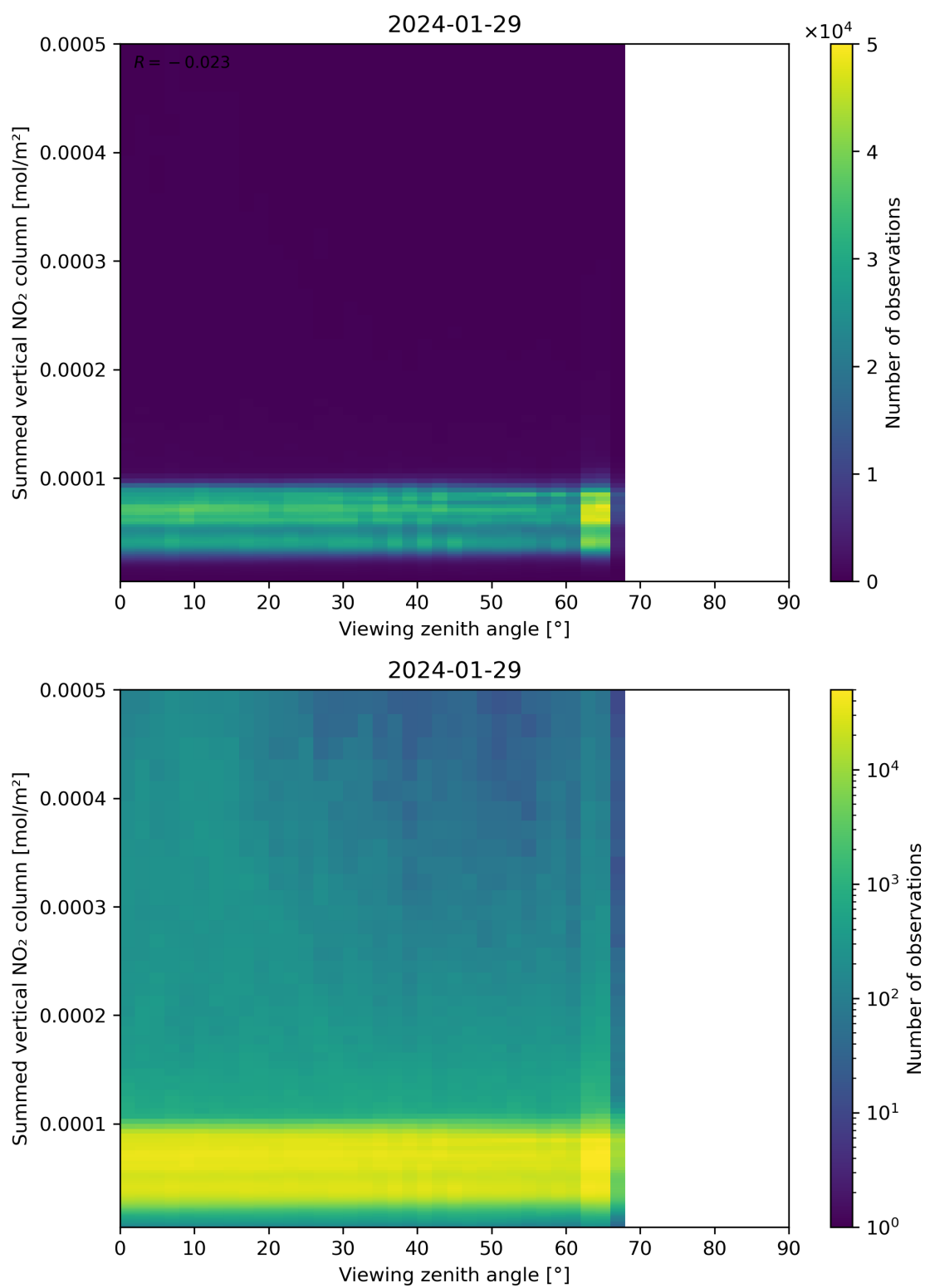
Figure 165: Scatter density plot of “Viewing zenith angle” against “Summed vertical NO 2 column” for 2024-01-28 to 2024-01-30.
