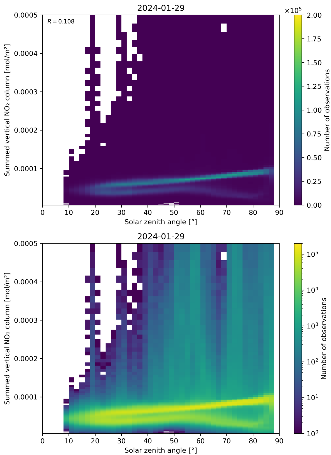
Figure 151: Scatter density plot of “Solar zenith angle” against “Summed vertical NO 2 column” for 2024-01-28 to 2024-01-30.
