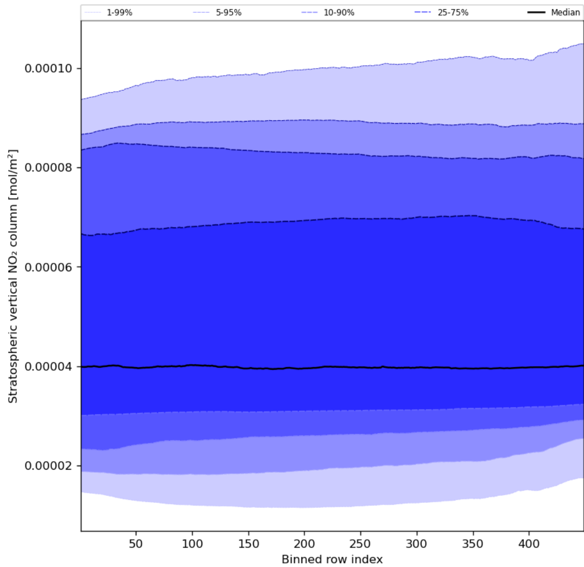
Figure 53: Along track statistics of “Stratospheric vertical NO 2 column” for 2024-01-28 to 2024-01-30
