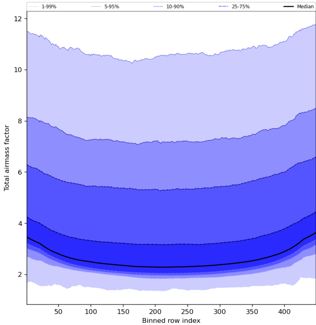
Figure 49: Along track statistics of “Total airmass factor” for 2024-01-28 to 2024-01-30
