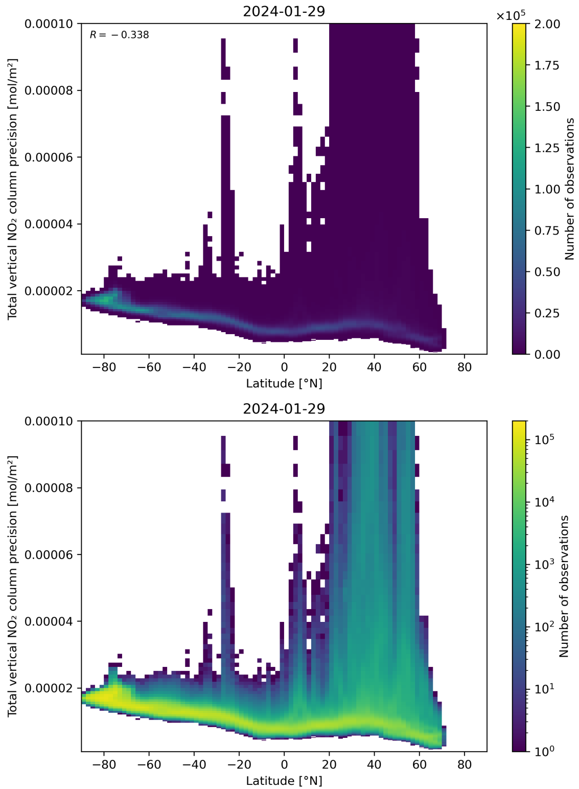
Figure 91: Scatter density plot of “Latitude” against “Total vertical NO 2 column precision” for 2024-01-28 to 2024-01-30.
