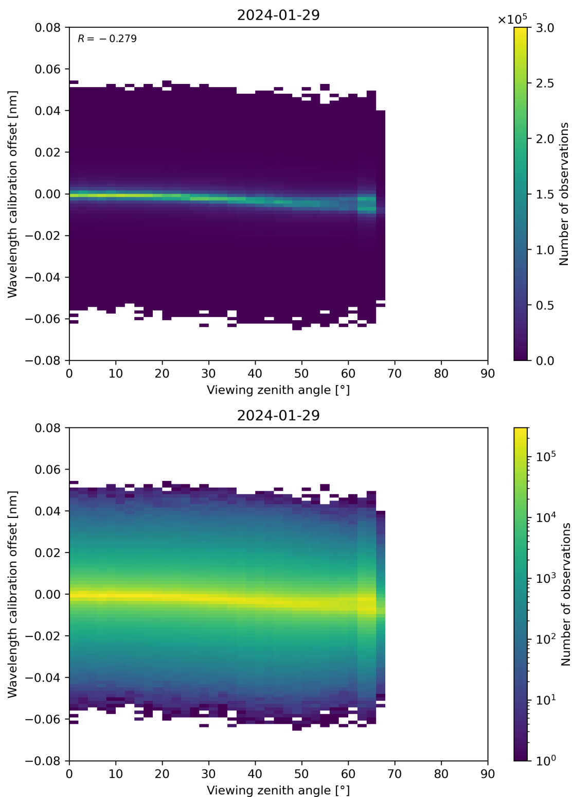
Figure 173: Scatter density plot of “Viewing zenith angle” against “Wavelength calibration offset” for 2024-01-28 to 2024-01-30.
