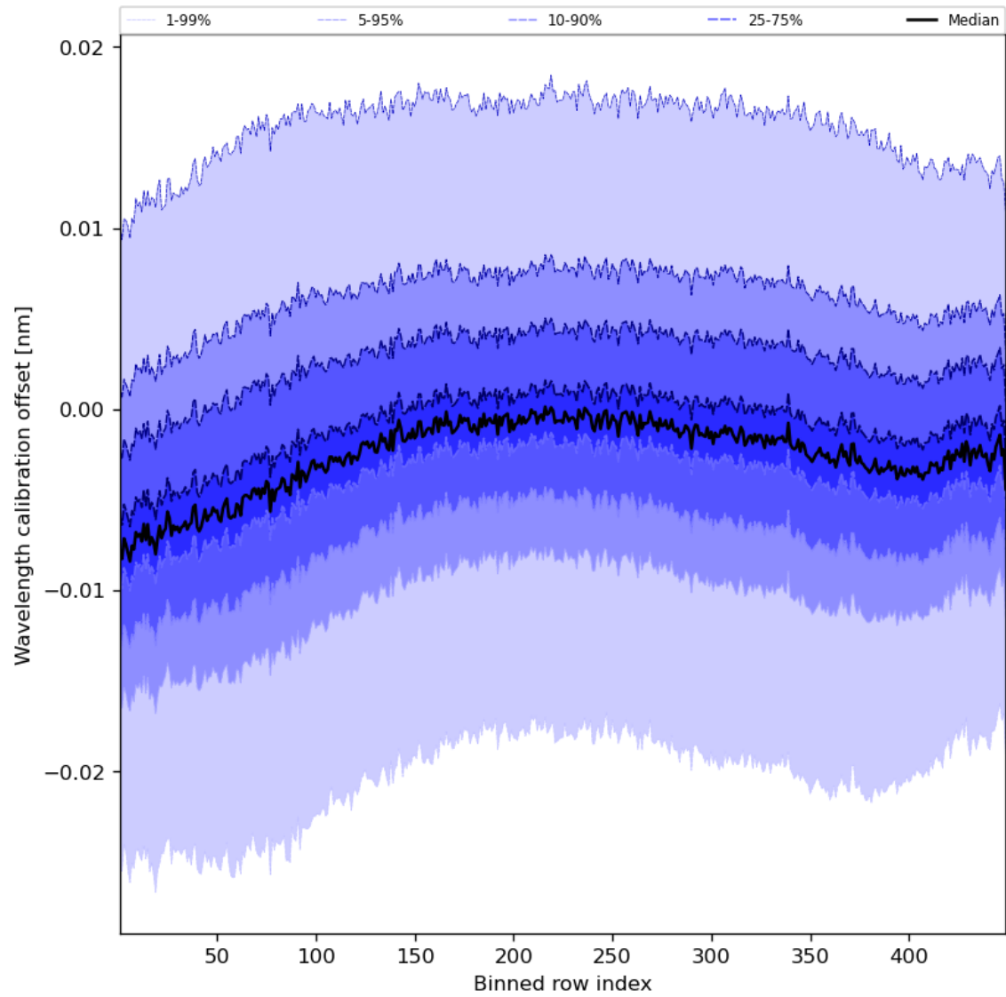
Figure 52: Along track statistics of “Wavelength calibration offset” for 2024-01-28 to 2024-01-30
