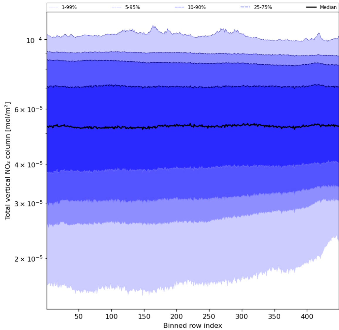
Figure 55: Along track statistics of “Total vertical NO 2 column” for 2024-01-28 to 2024-01-30
