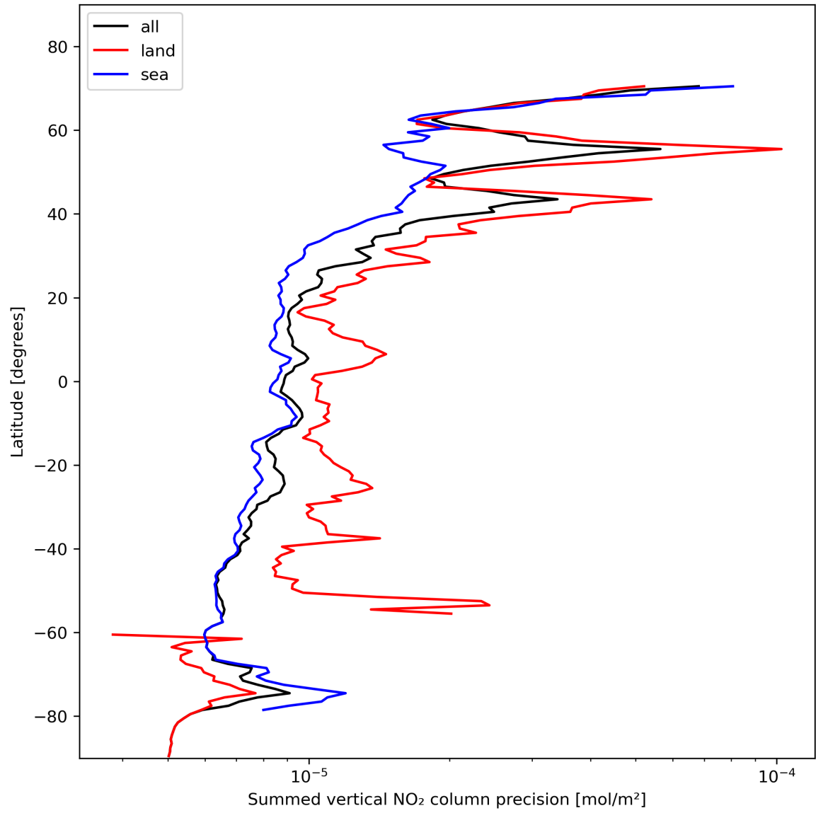
Figure 24: Zonal average of “Summed vertical NO 2 column precision” for 2024-01-29 to 2024-01-31.
