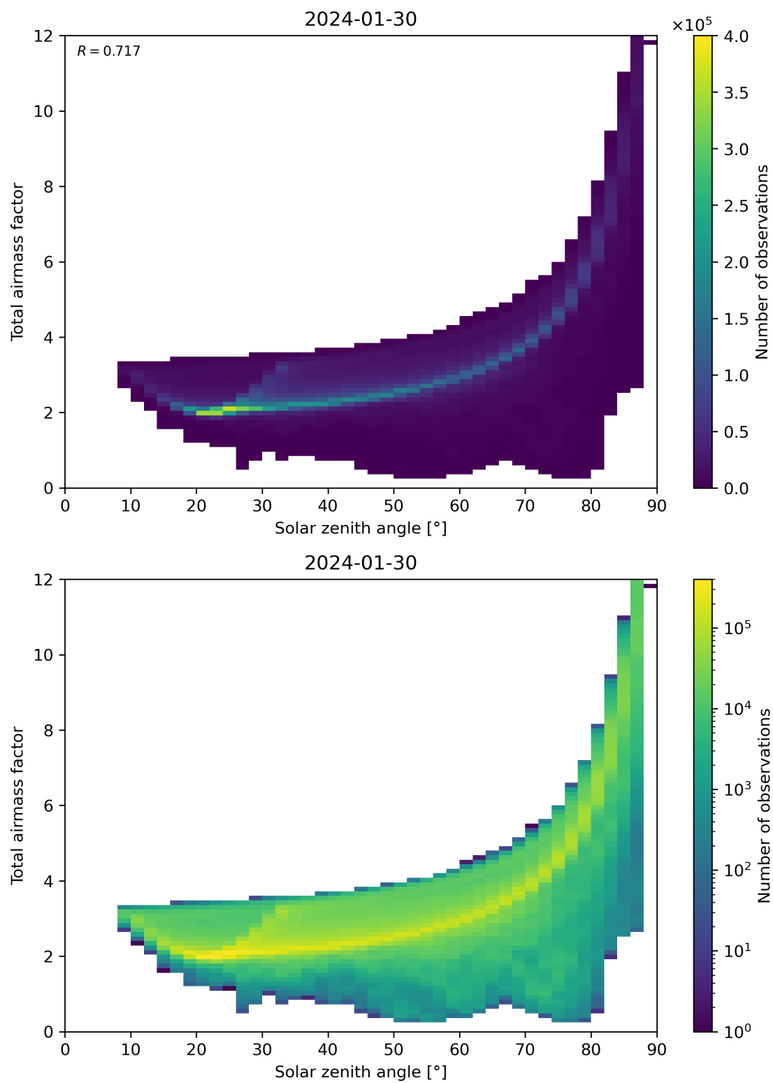
Figure 146: Scatter density plot of “Solar zenith angle” against “Total air mass factor” for 2024-01-29 to 2024-01-31.
