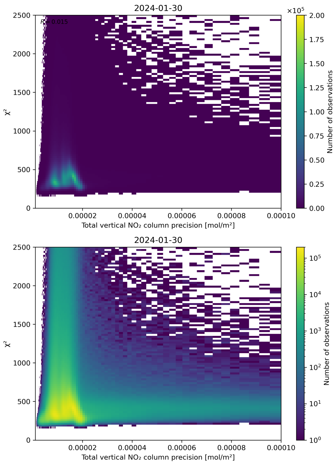
Figure 116: Scatter density plot of “Total vertical NO 2 column precision” against “ \chi^2 ” for 2024-01-29 to 2024-01-31.
