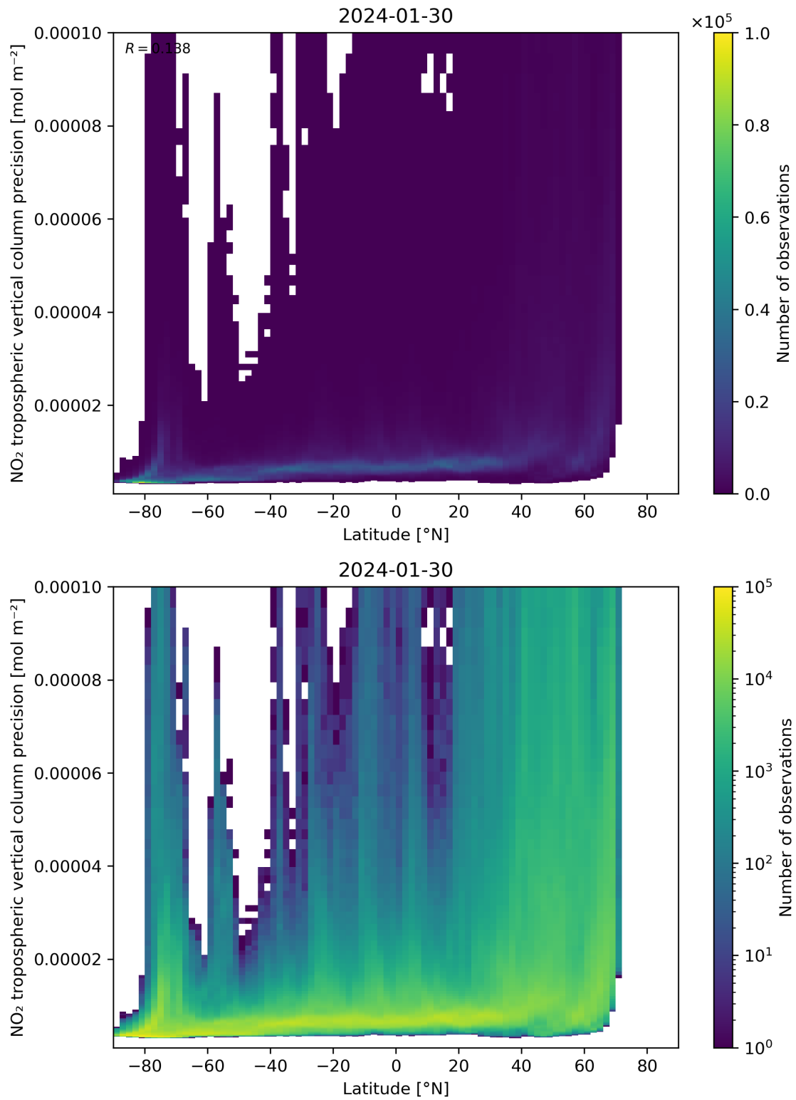
Figure 93: Scatter density plot of “Latitude” against “NO 2 tropospheric vertical column precision” for 2024-01-29 to 2024-01-31.
