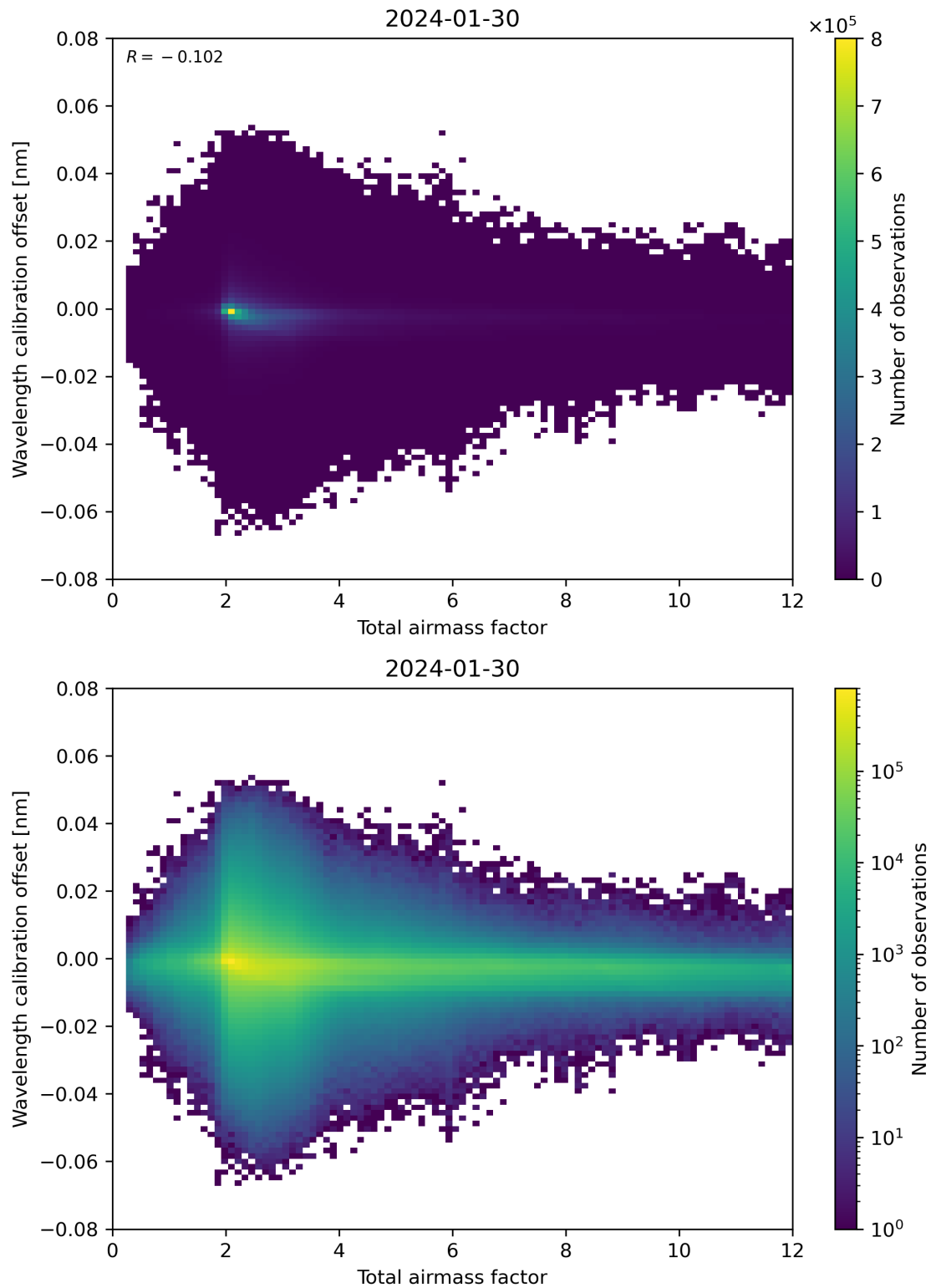
Figure 70: Scatter density plot of “Total airmass factor” against “Wavelength calibration offset” for 2024-01-29 to 2024-01-31.
