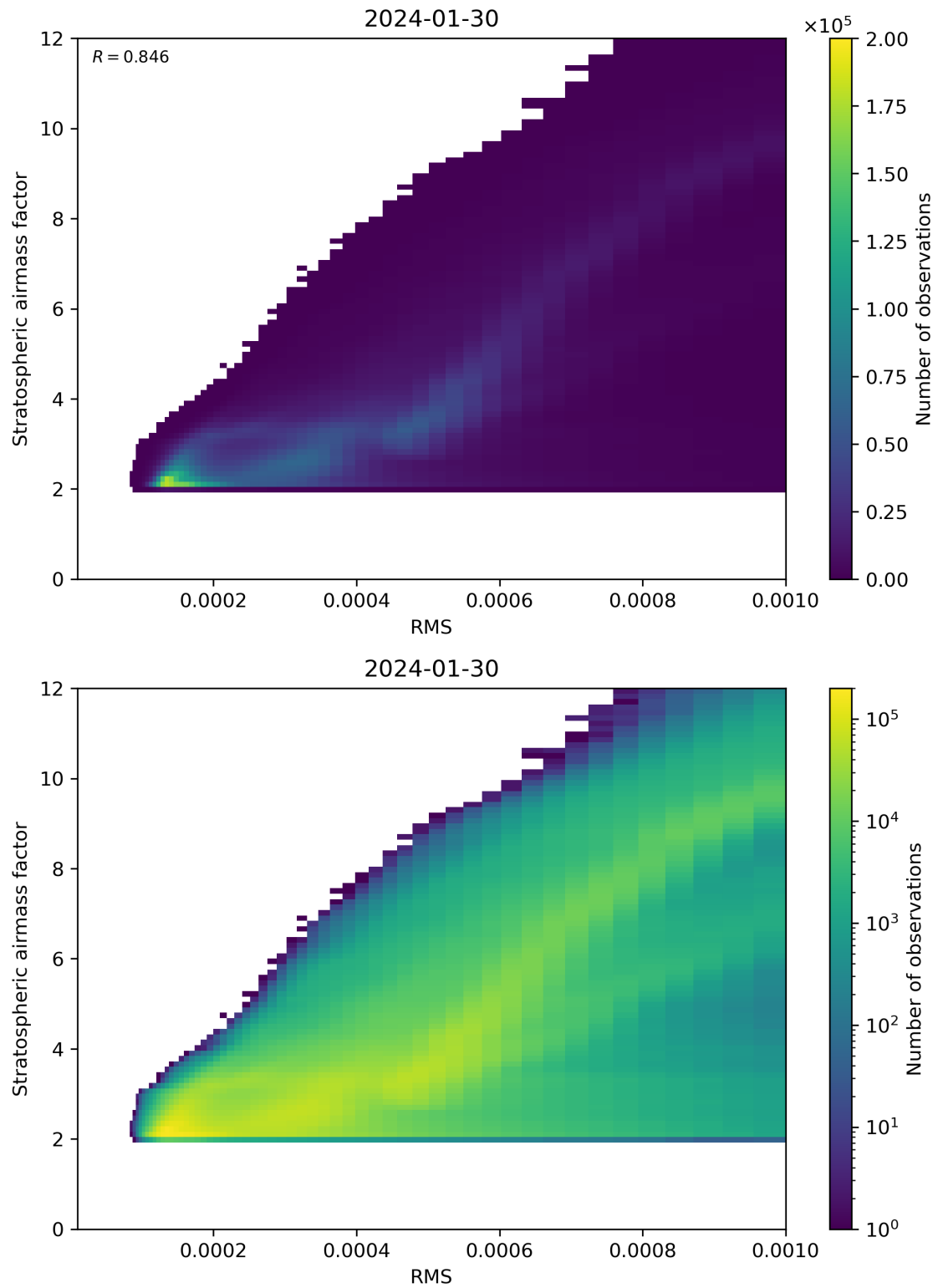
Figure 144: Scatter density plot of “RMS” against “Stratospheric airmass factor” for 2024-01-29 to 2024-01-31.
