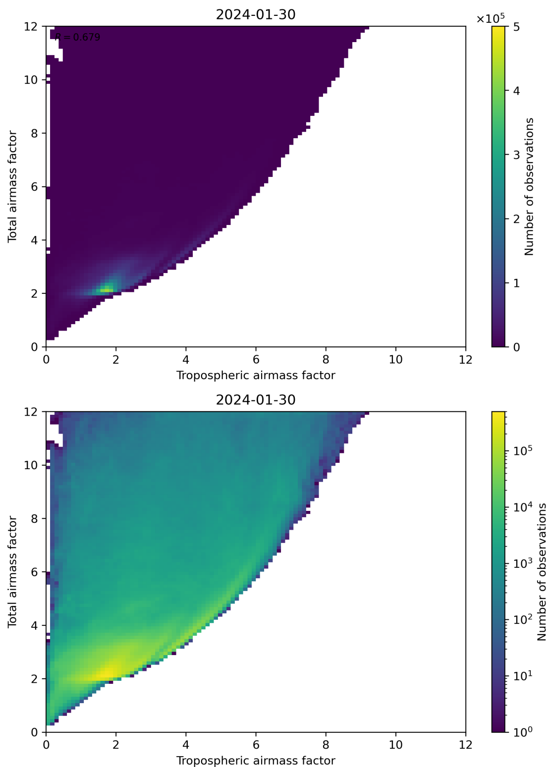
Figure 72: Scatter density plot of “Tropospheric airmass factor” against “Total airmass factor” for 2024-01-29 to 2024-01-31.
