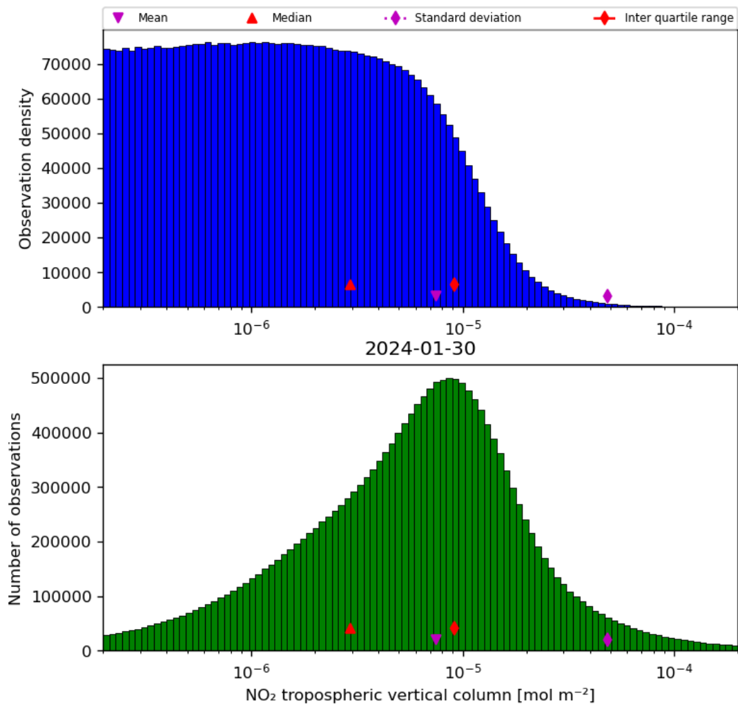
Figure 29: Histogram of “NO 2 tropospheric vertical column” for 2024-01-29 to 2024-01-31
