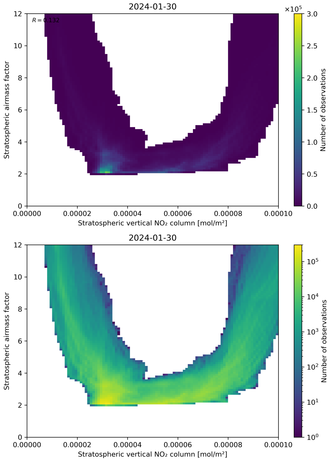
Figure 96: Scatter density plot of “Stratospheric vertical NO 2 column” against “Stratospheric airmass factor” for 2024-01-29 to 2024-01-31.
