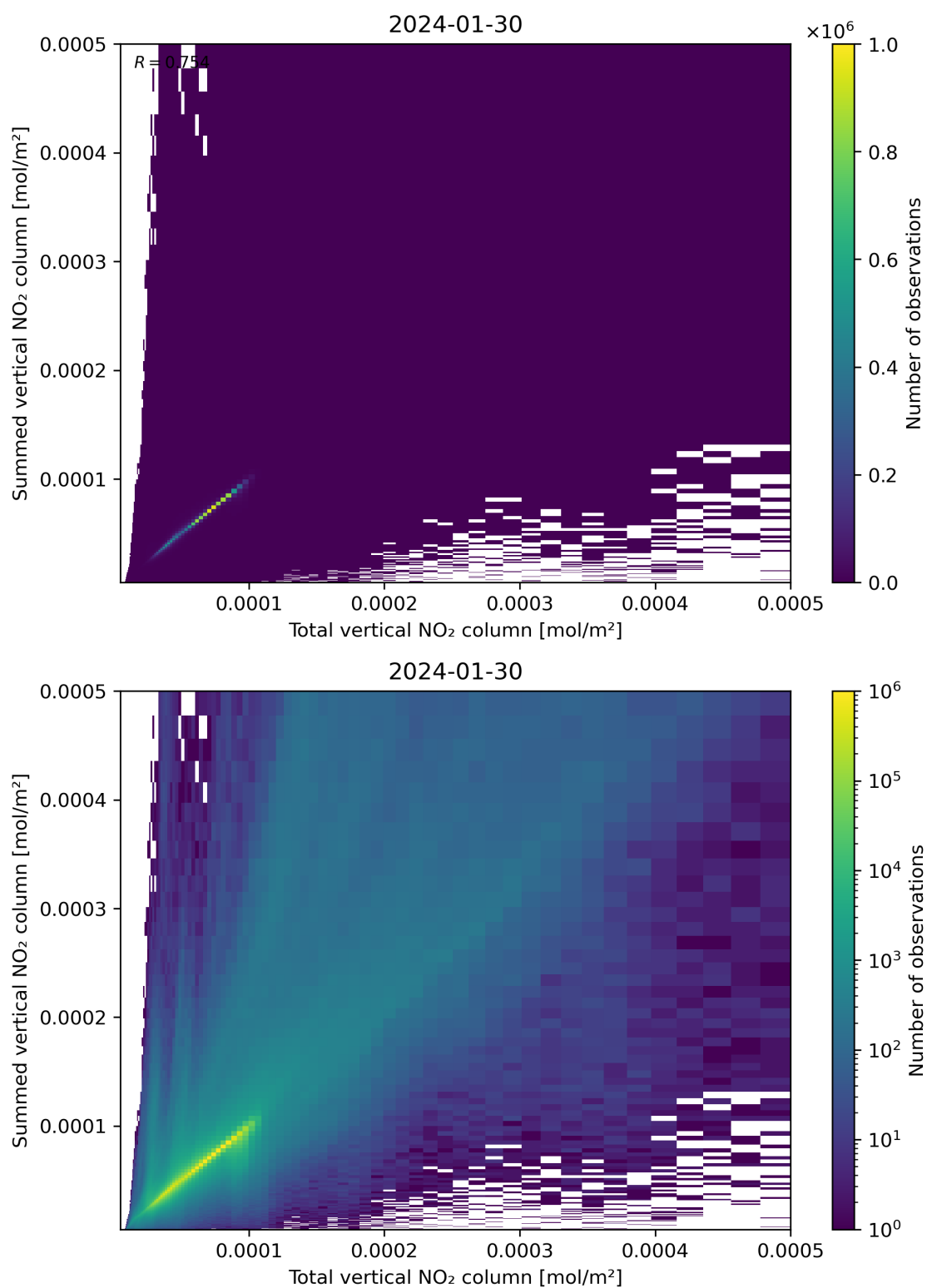
Figure 112: Scatter density plot of “Total vertical NO 2 column” against “Summed vertical NO 2 column” for 2024-01-29 to 2024-01-31.
