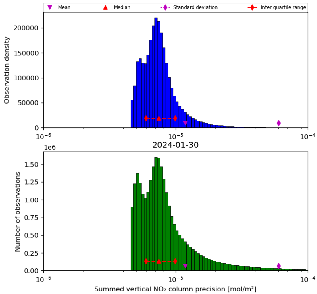
Figure 41: Histogram of “Summed vertical NO 2 column precision” for 2024-01-29 to 2024-01-31
