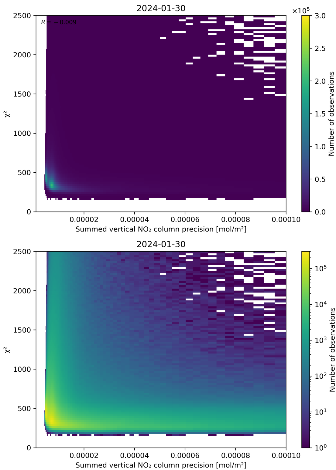
Figure 107: Scatter density plot of “Summed vertical NO 2 column precision” against “ \chi^2 ” for 2024-01-29 to 2024-01-31.
