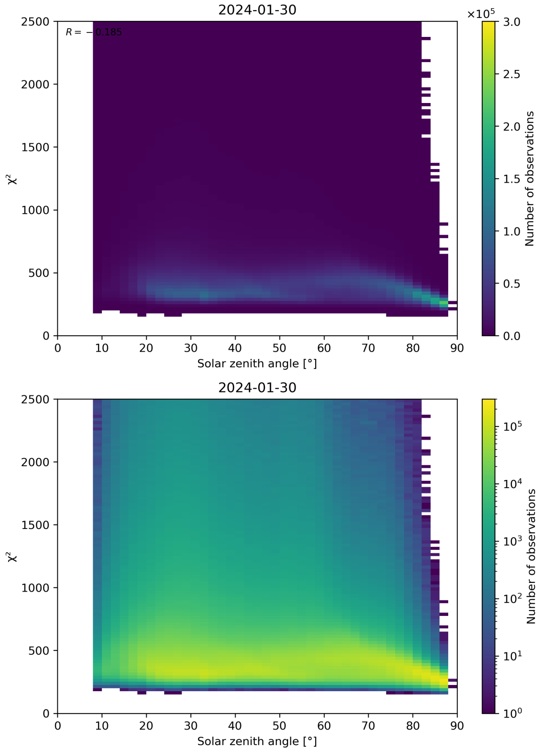
Figure 148: Scatter density plot of “Solar zenith angle” against “ \chi^2 ” for 2024-01-29 to 2024-01-31.
