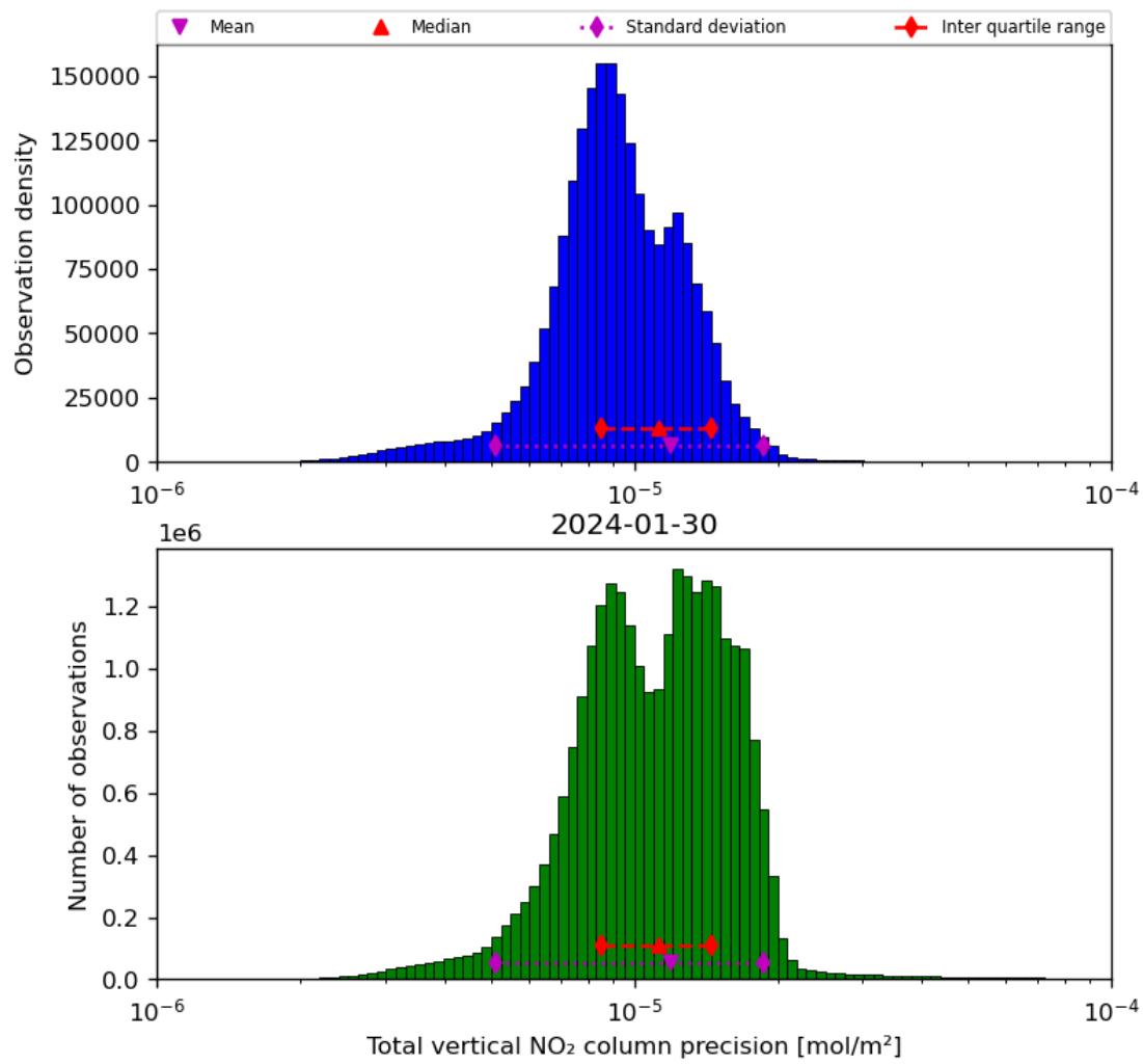
Figure 39: Histogram of “Total vertical NO 2 column precision” for 2024-01-29 to 2024-01-31
