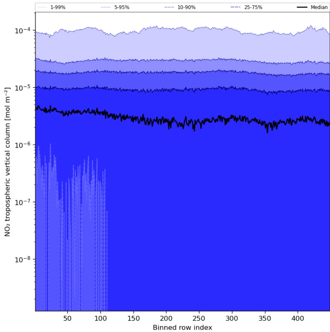
Figure 46: Along track statistics of “NO 2 tropospheric vertical column” for 2024-01-29 to 2024-01-31
