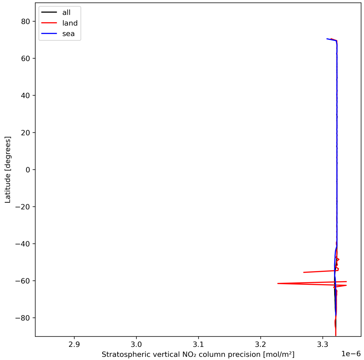
Figure 20: Zonal average of “Stratospheric vertical NO 2 column precision” for 2024-01-29 to 2024-01-31.
