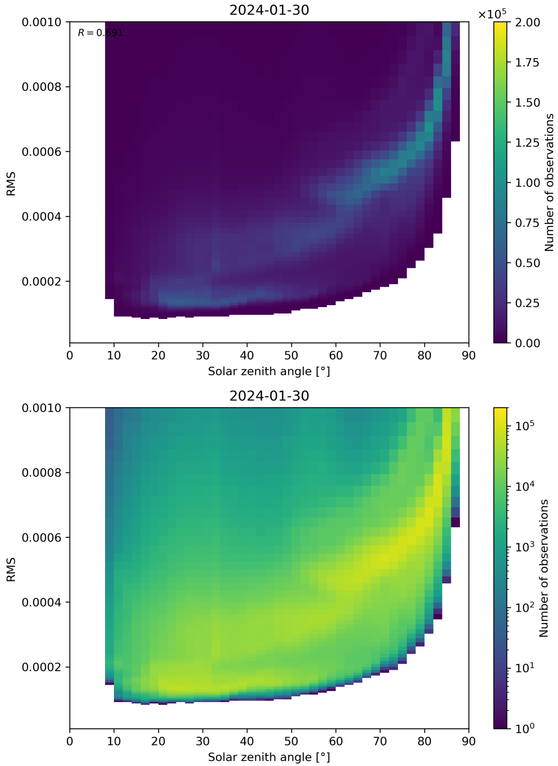
Figure 157: Scatter density plot of “Solar zenith angle” against “RMS” for 2024-01-29 to 2024-01-31.
