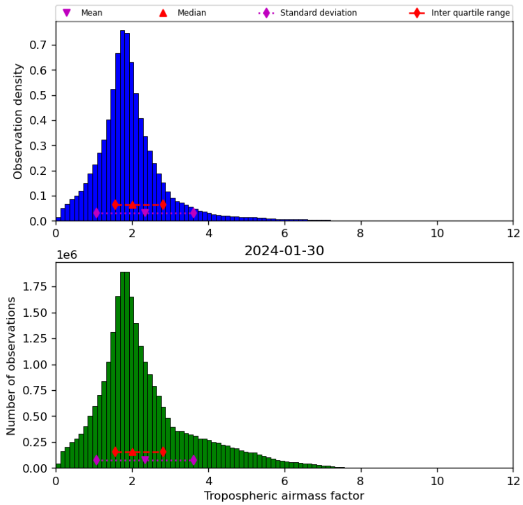
Figure 31: Histogram of “Tropospheric airmass factor” for 2024-01-29 to 2024-01-31
