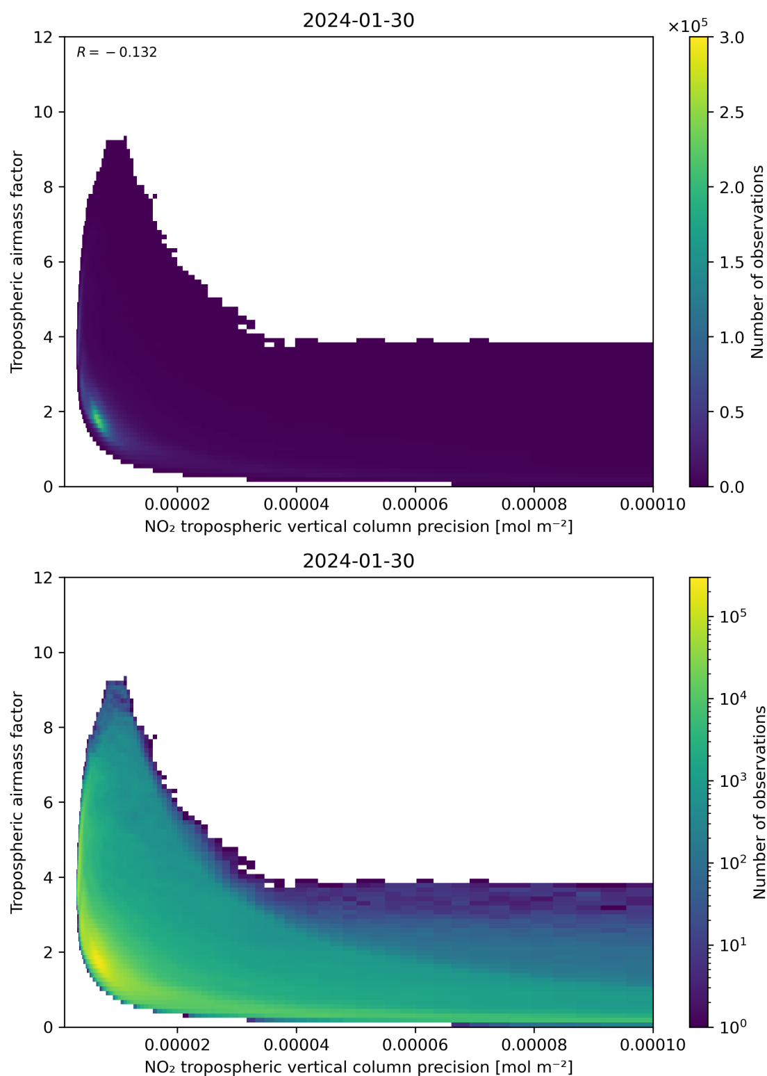
Figure 133: Scatter density plot of “NO 2 tropospheric vertical column precision” against “Tropospheric airmass factor” for 2024-01-29 to 2024-01-31.
