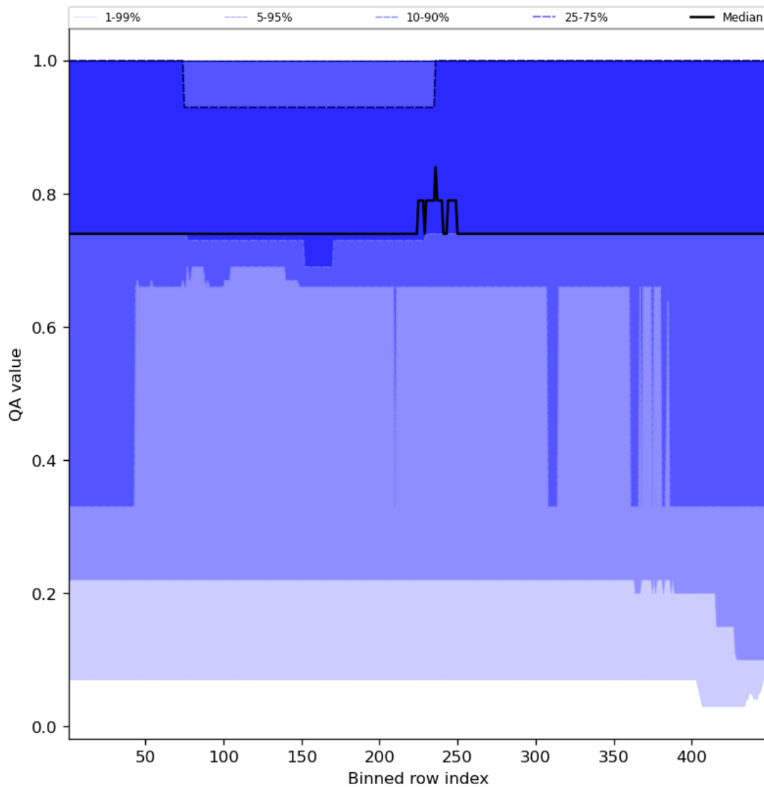
Figure 45: Along track statistics of “QA value” for 2024-01-29 to 2024-01-31
