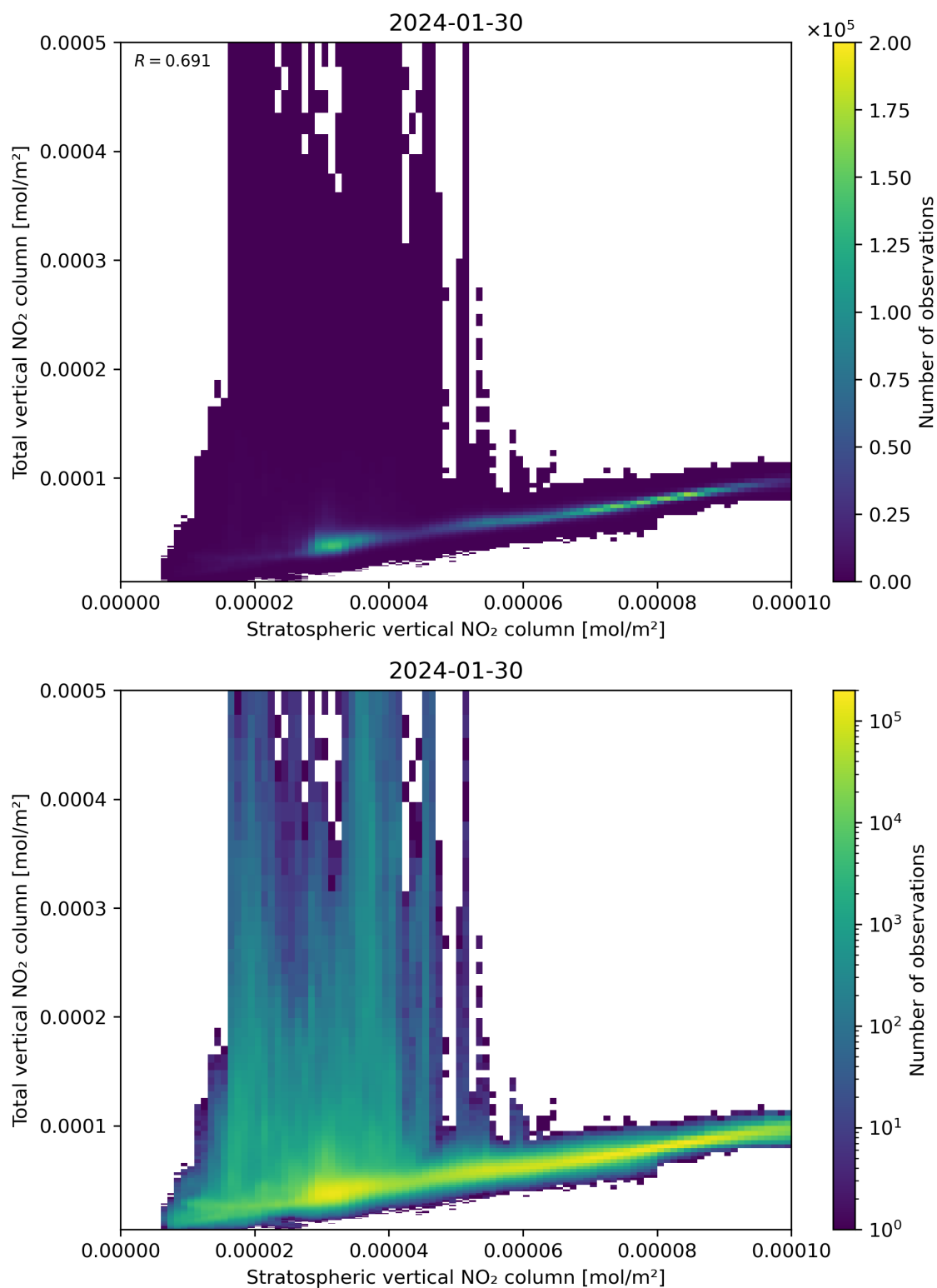
Figure 100: Scatter density plot of “Stratospheric vertical NO 2 column” against “Total vertical NO 2 column” for 2024-01-29 to 2024-01-31.
