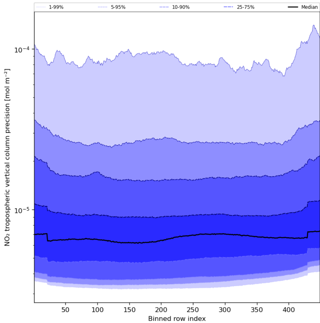
Figure 47: Along track statistics of “NO 2 tropospheric vertical column precision” for 2024-01-29 to 2024-01-31
