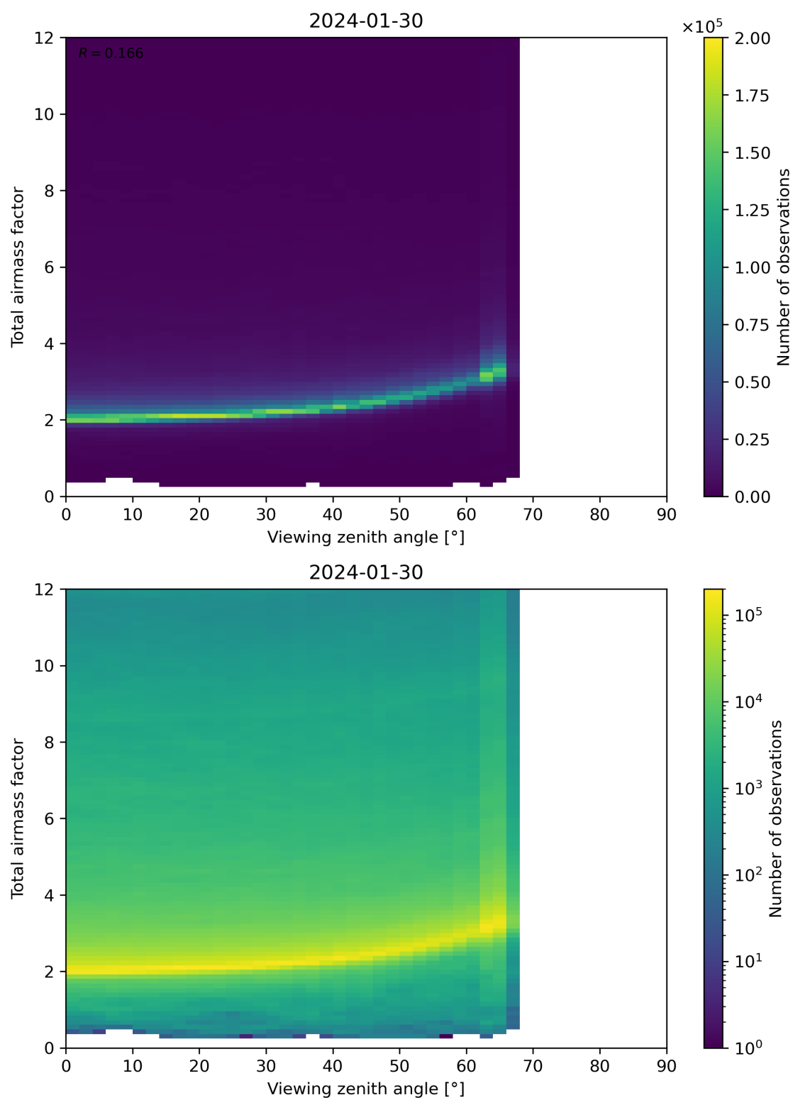
Figure 160: Scatter density plot of “Viewing zenith angle” against “Total airmass factor” for 2024-01-29 to 2024-01-31.
