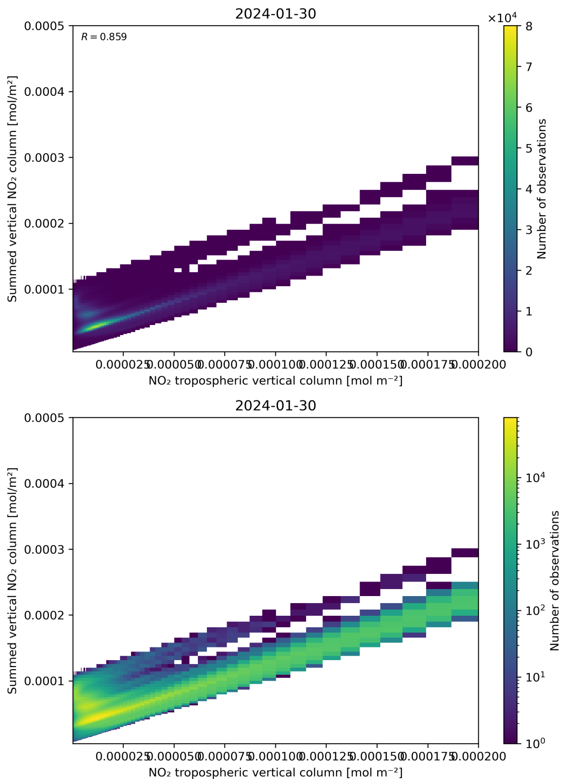
Figure 126: Scatter density plot of “NO 2 tropospheric vertical column” against “Summed vertical NO 2 column” for 2024-01-29 to 2024-01-31.
