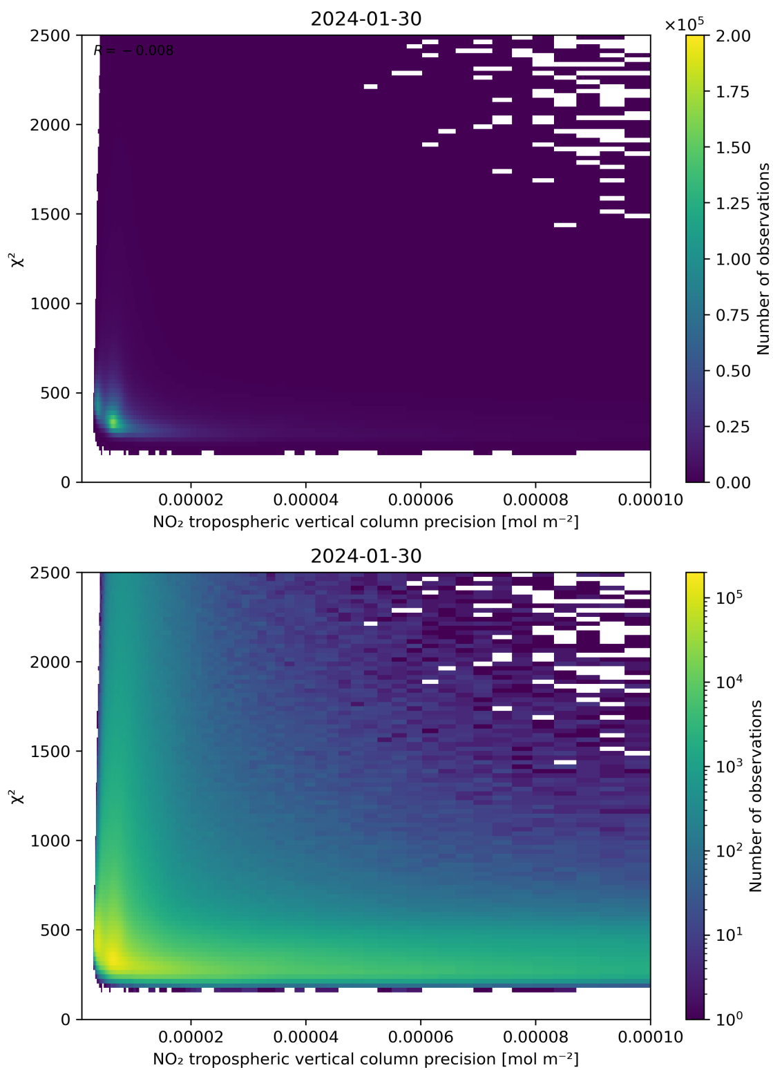
Figure 134: Scatter density plot of “NO 2 tropospheric vertical column precision” against “ \chi^2 ” for 2024-01-29 to 2024-01-31.
