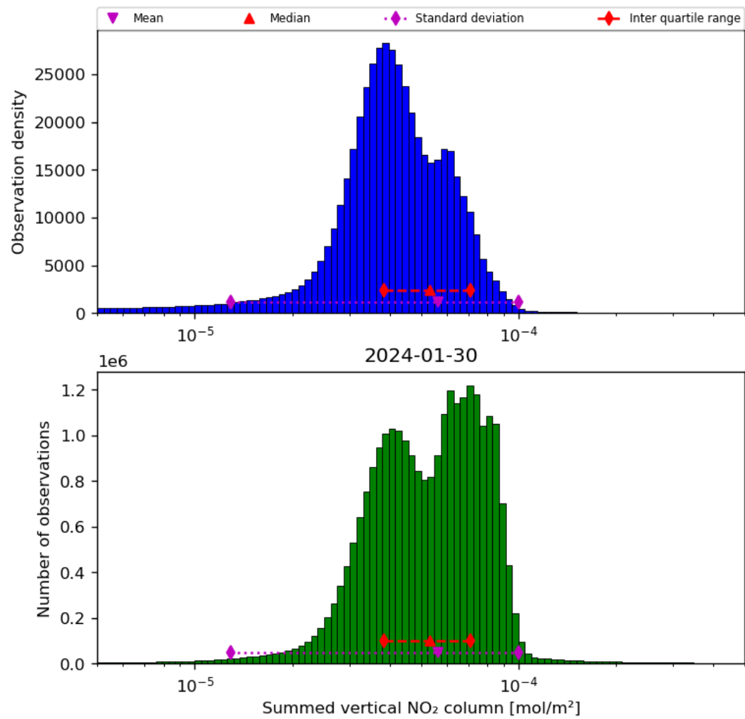
Figure 40: Histogram of “Summed vertical NO 2 column” for 2024-01-29 to 2024-01-31
