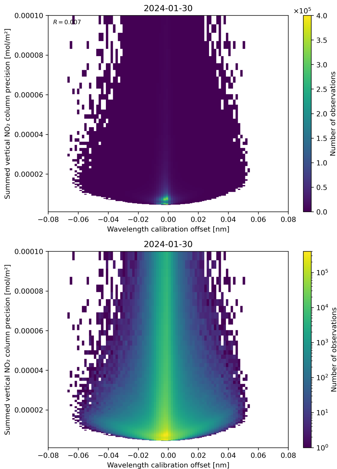
Figure 178: Scatter density plot of “Wavelength calibration offset” against “Summed vertical NO 2 column precision” for 2024-01-29 to 2024-01-31.
