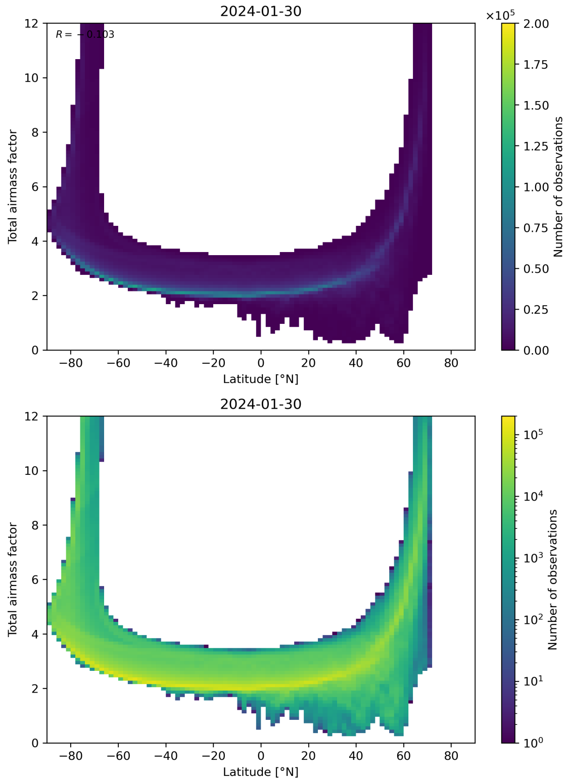
Figure 84: Scatter density plot of “Latitude” against “Total airmass factor” for 2024-01-29 to 2024-01-31.
