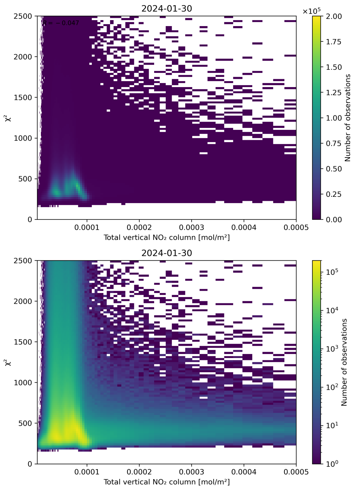
Figure 111: Scatter density plot of “Total vertical NO 2 column” against “ \chi^2 ” for 2024-01-29 to 2024-01-31.
