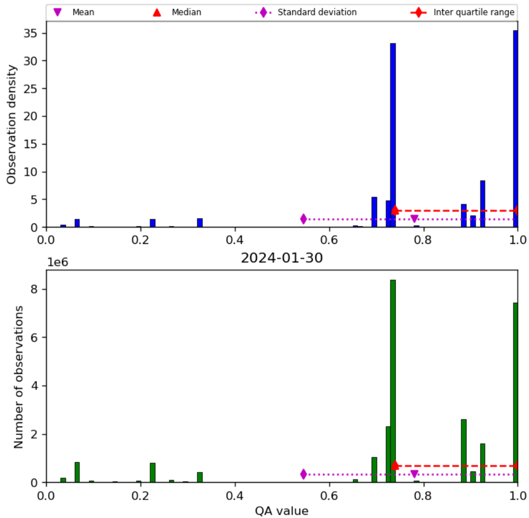
Figure 28: Histogram of “QA value” for 2024-01-29 to 2024-01-31
