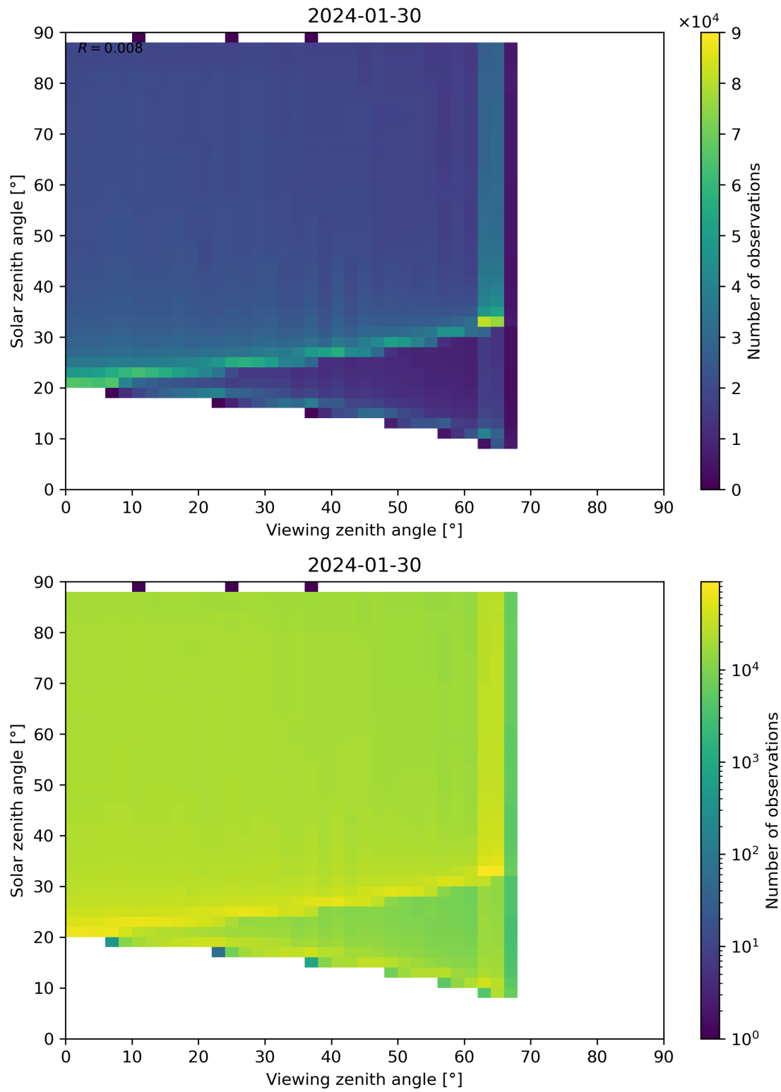
Figure 172: Scatter density plot of “Viewing zenith angle” against “Solar zenith angle” for 2024-01-29 to 2024-01-31.
