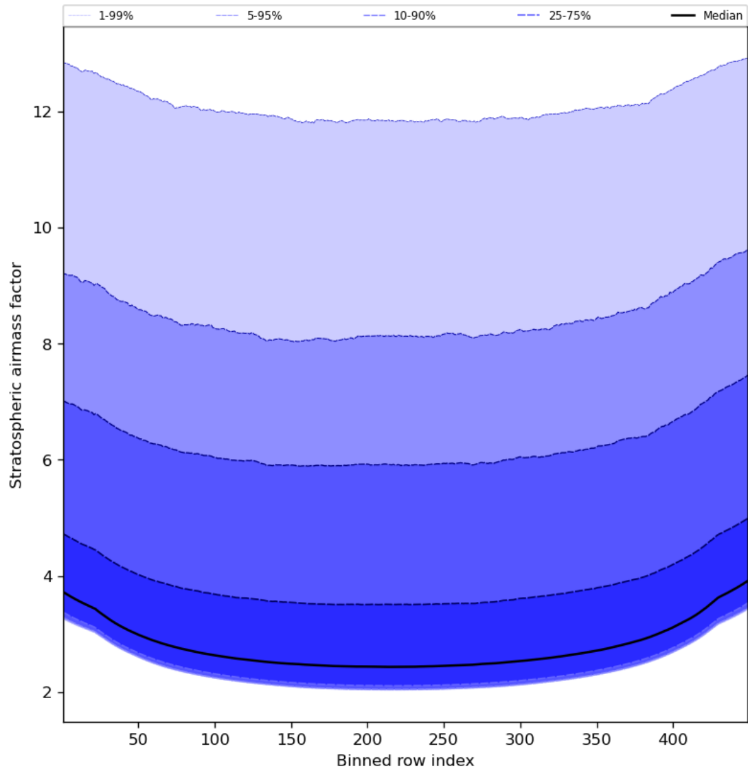
Figure 61: Along track statistics of “Stratospheric airmass factor” for 2024-01-29 to 2024-01-31
