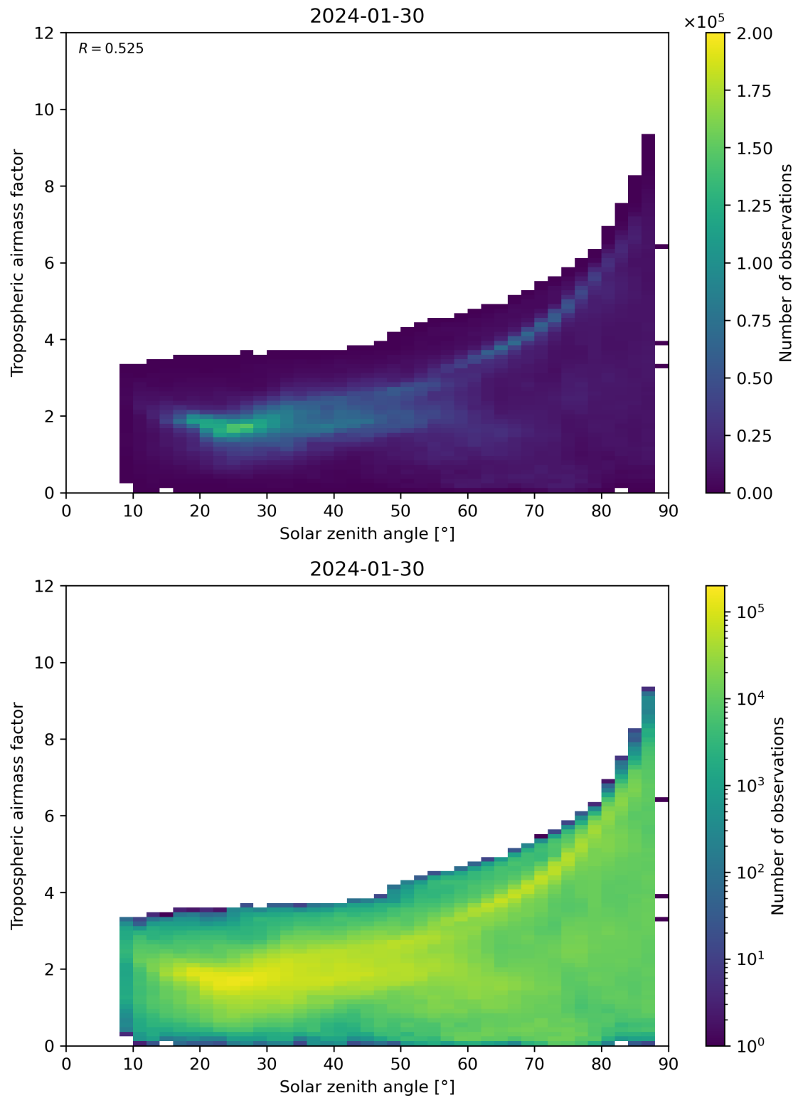
Figure 147: Scatter density plot of “Solar zenith angle” against “Tropospheric airmass factor” for 2024-01-29 to 2024-01-31.
