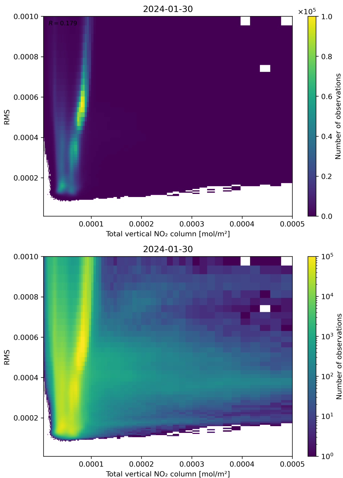
Figure 120: Scatter density plot of “Total vertical NO 2 column” against “RMS” for 2024-01-29 to 2024-01-31.
