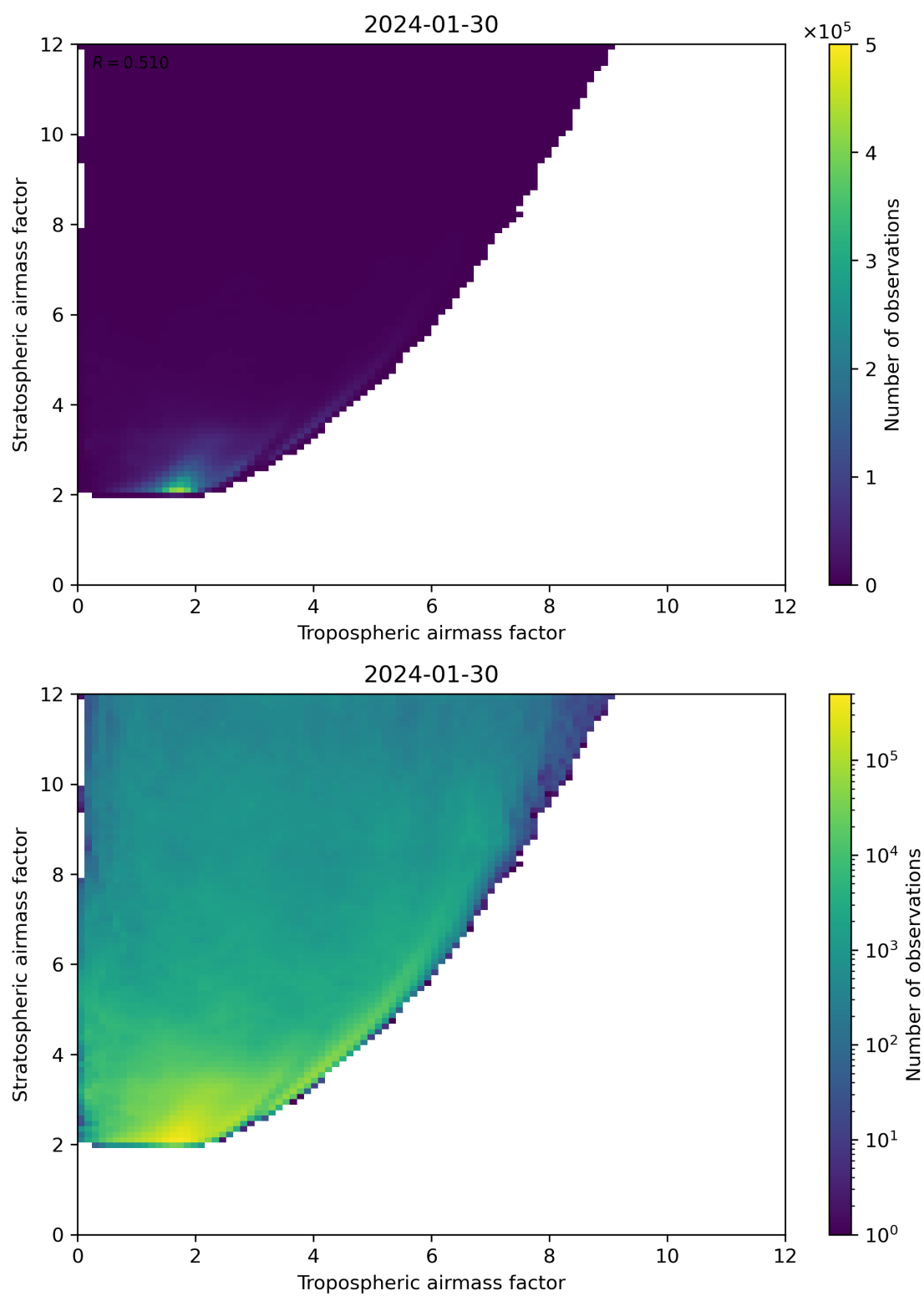
Figure 71: Scatter density plot of “Tropospheric airmass factor” against “Stratospheric airmass factor” for 2024-01-29 to 2024-01-31.
