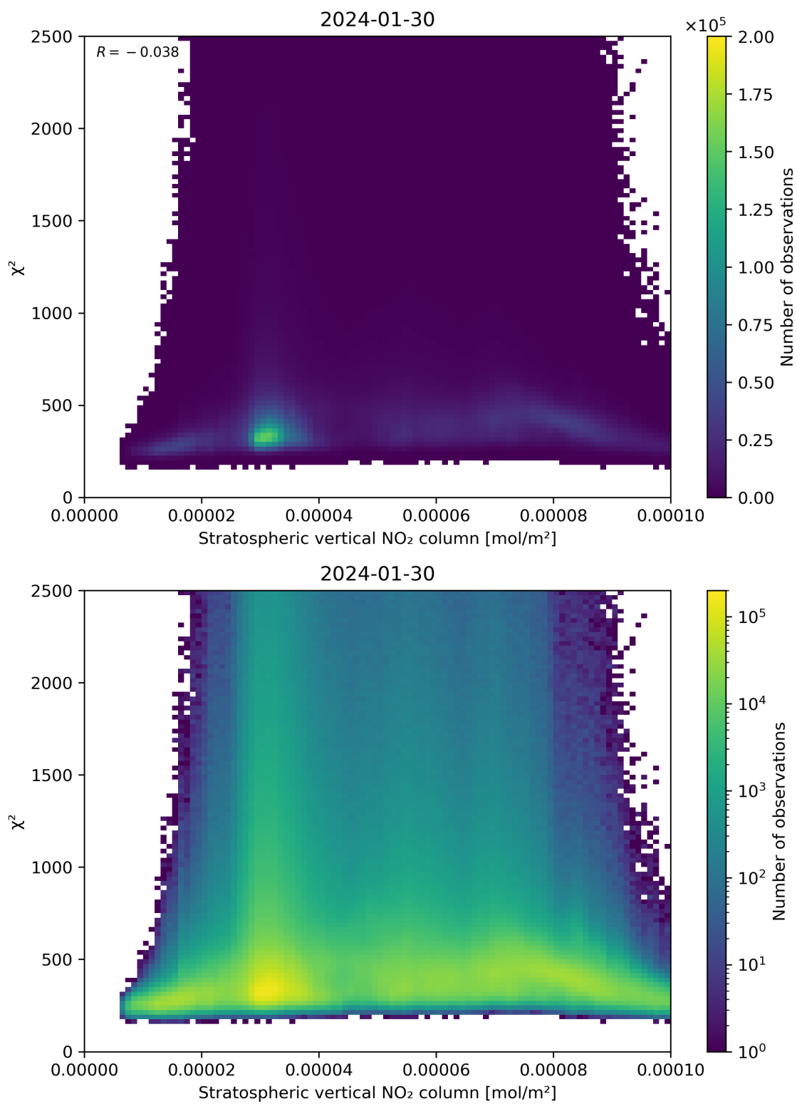
Figure 97: Scatter density plot of “Stratospheric vertical NO 2 column” against “ \chi^2 ” for 2024-01-29 to 2024-01-31.
