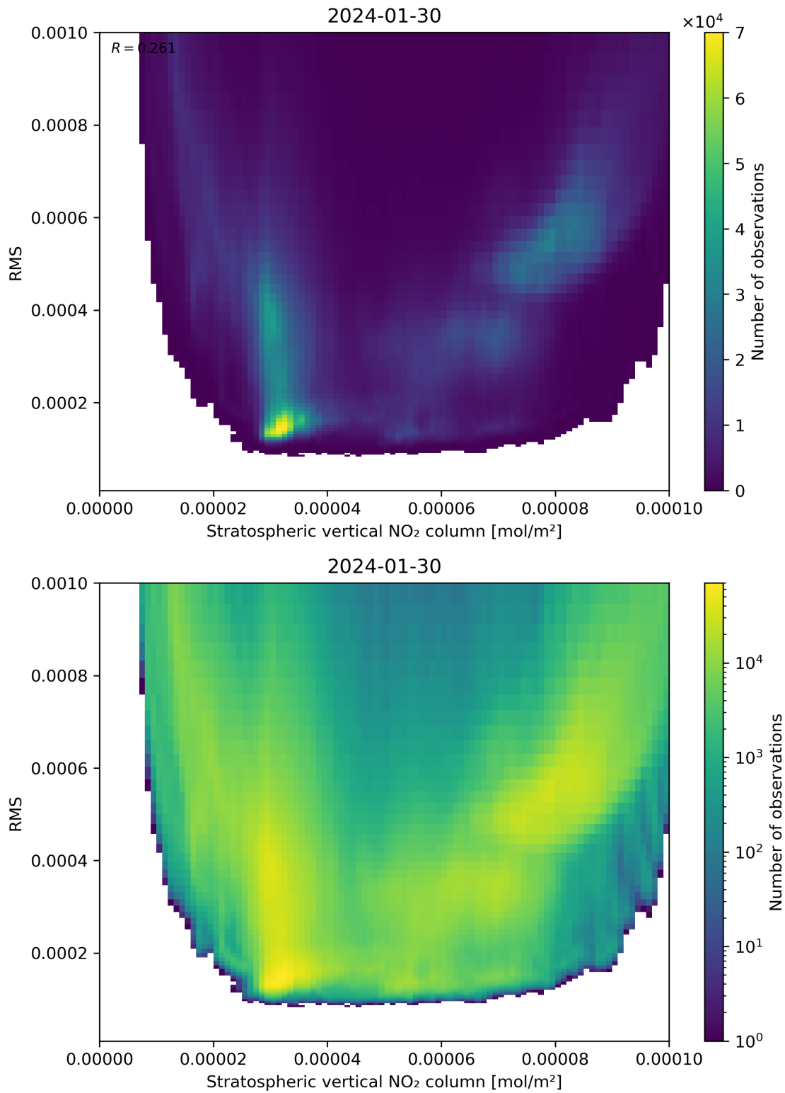
Figure 102: Scatter density plot of “Stratospheric vertical NO 2 column” against “RMS” for 2024-01-29 to 2024-01-31.
