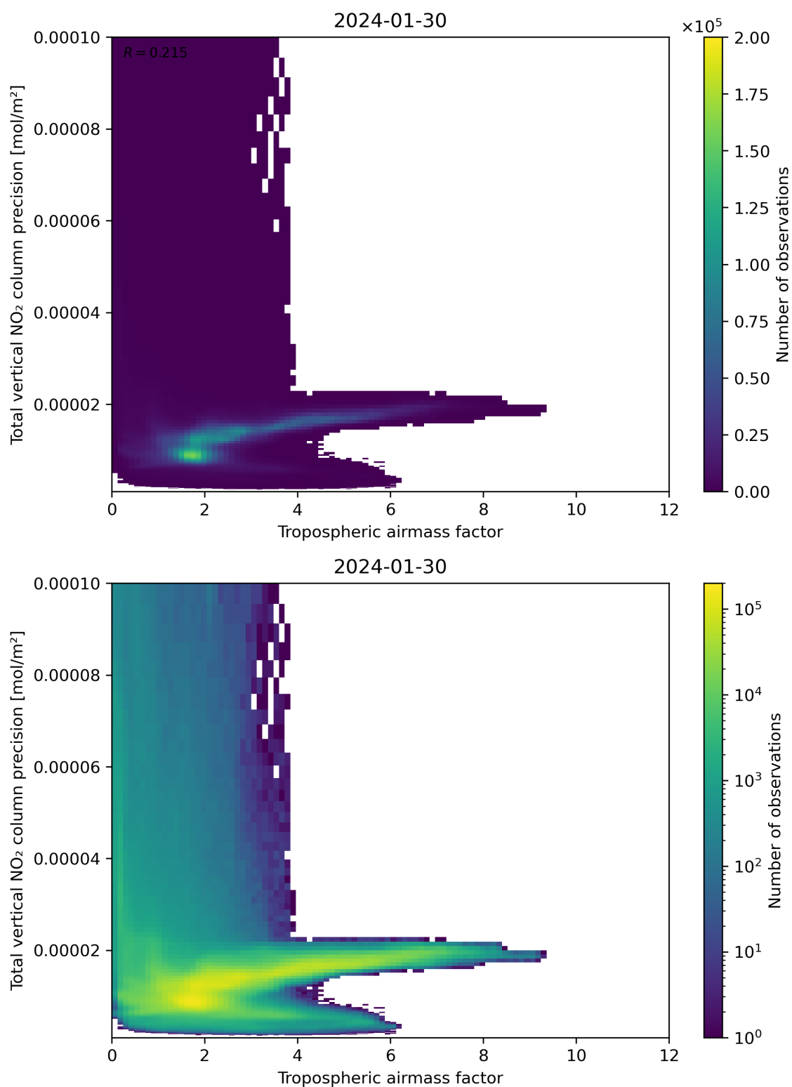
Figure 78: Scatter density plot of “Tropospheric air mass factor” against “Total vertical NO 2 column precision” for 2024-01-29 to 2024-01-31.
