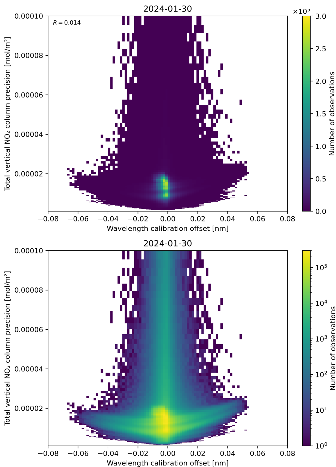
Figure 180: Scatter density plot of “Wavelength calibration offset” against “Total vertical NO 2 column precision” for 2024-01-29 to 2024-01-31.
