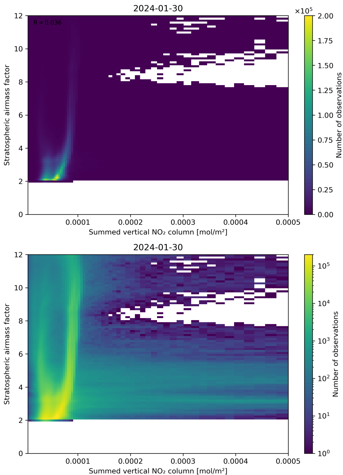
Figure 103: Scatter density plot of “Summed vertical NO 2 column” against “Stratospheric air mass factor” for 2024-01-29 to 2024-01-31.
