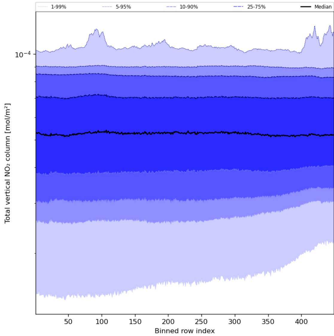
Figure 55: Along track statistics of “Total vertical NO 2 column” for 2024-01-29 to 2024-01-31
