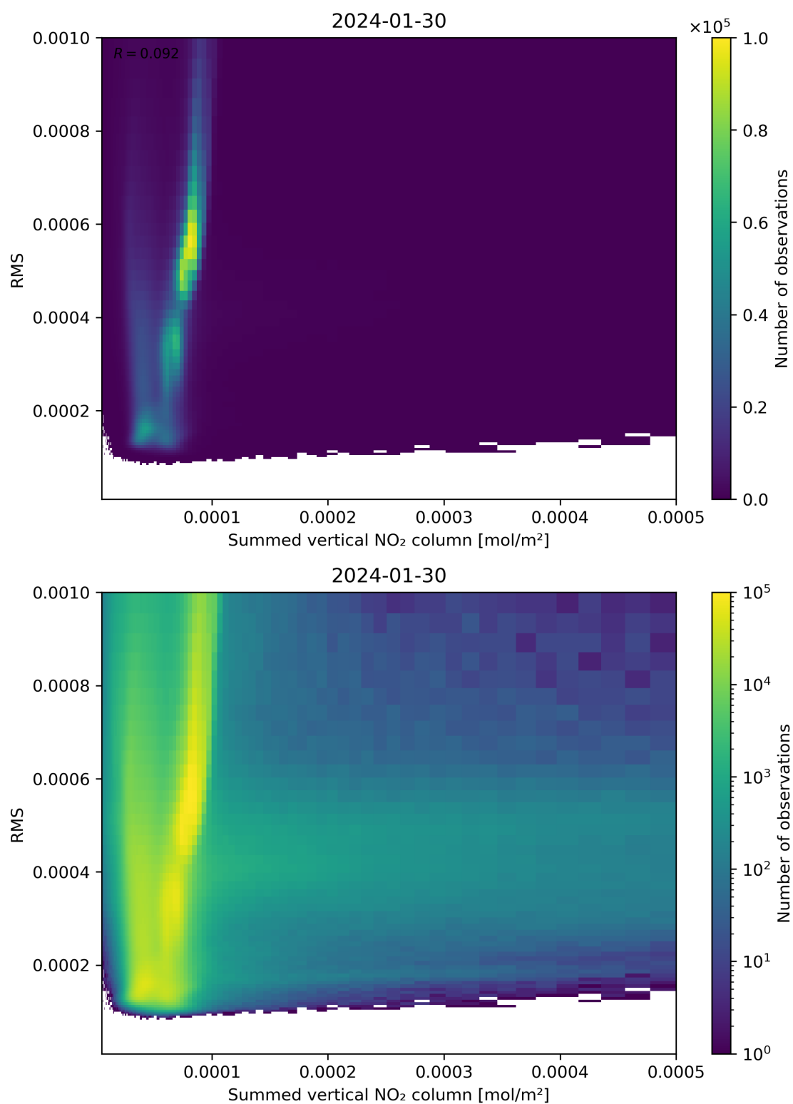
Figure 109: Scatter density plot of “Summed vertical NO 2 column” against “RMS” for 2024-01-29 to 2024-01-31.
