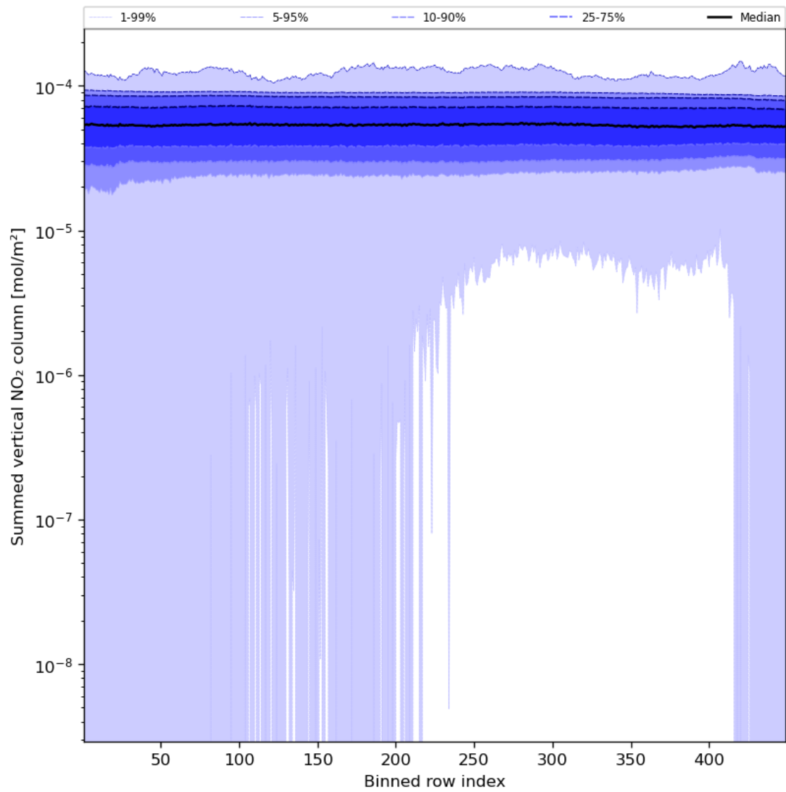
Figure 57: Along track statistics of “Summed vertical NO 2 column” for 2024-01-29 to 2024-01-31
