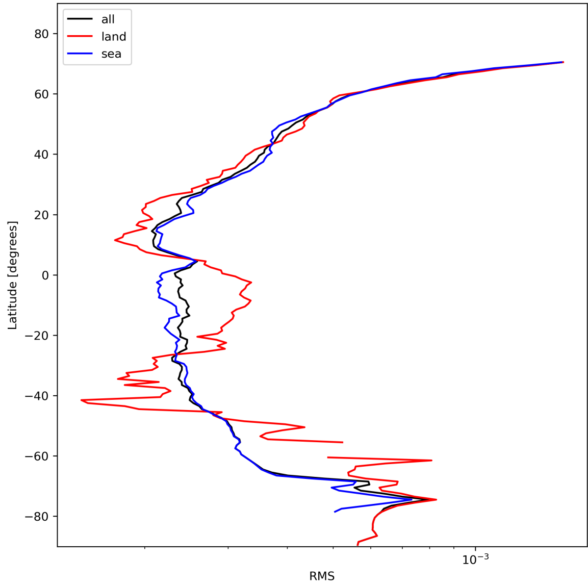
Figure 26: Zonal average of “RMS” for 2024-01-29 to 2024-01-31.
