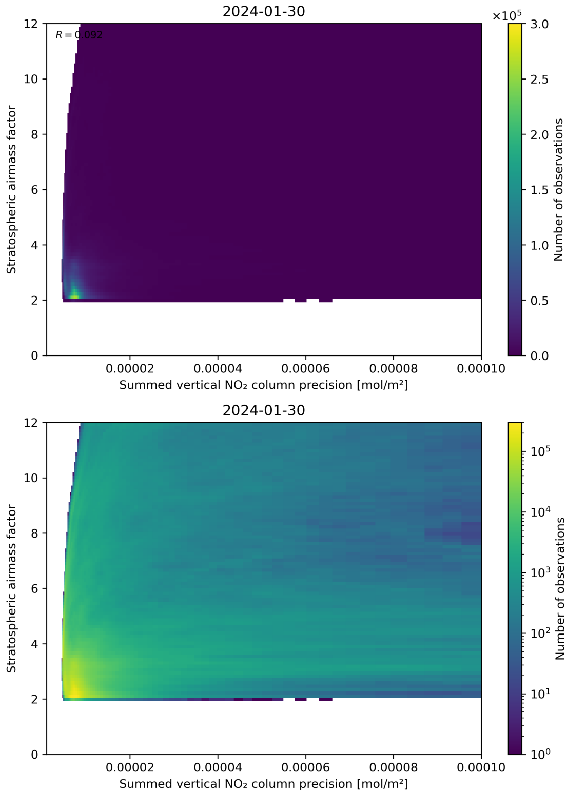
Figure 106: Scatter density plot of “Summed vertical NO 2 column precision” against “Stratospheric airmass factor” for 2024-01-29 to 2024-01-31.
