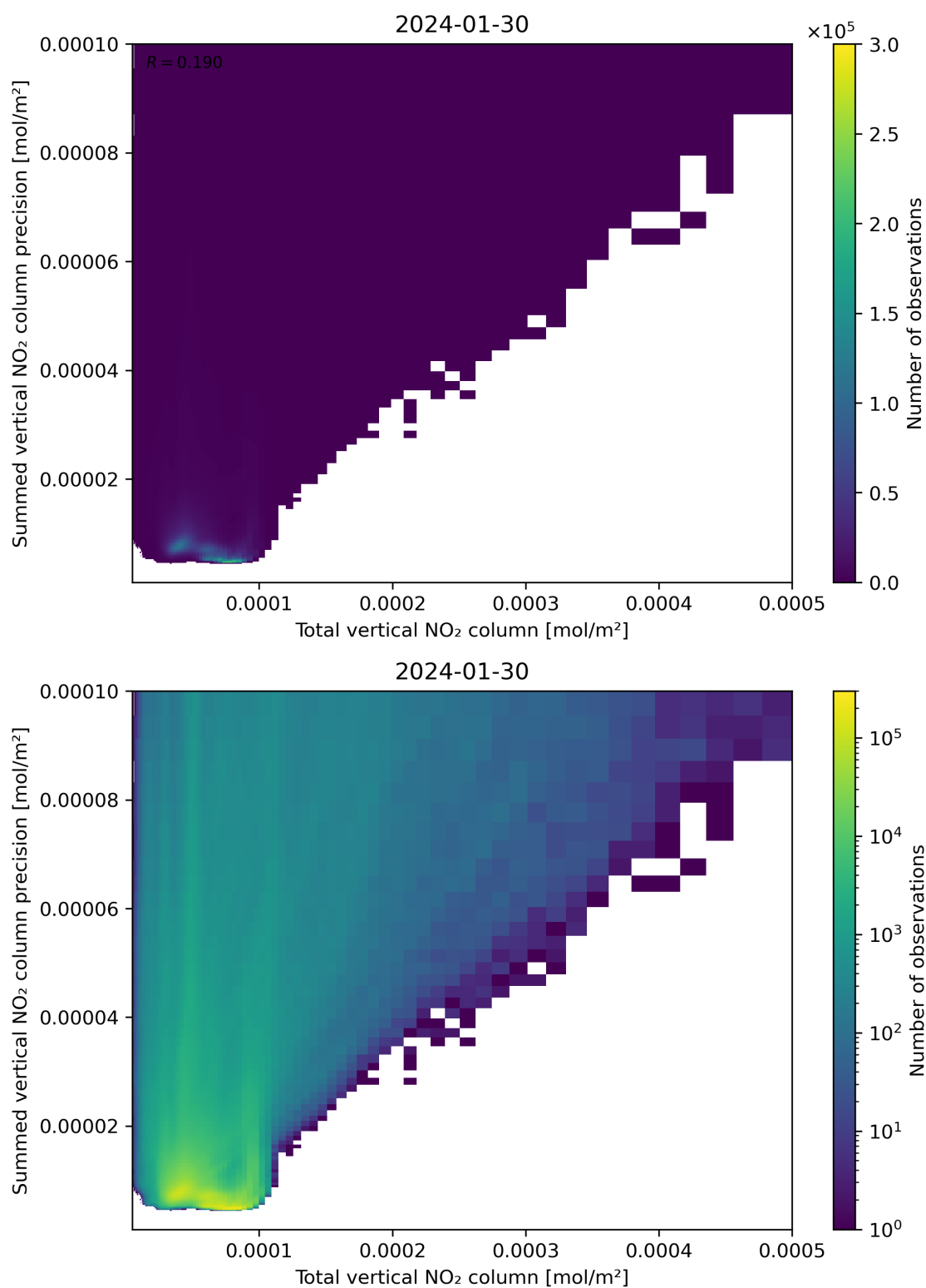
Figure 113: Scatter density plot of “Total vertical NO 2 column” against “Summed vertical NO 2 column precision” for 2024-01-29 to 2024-01-31.
