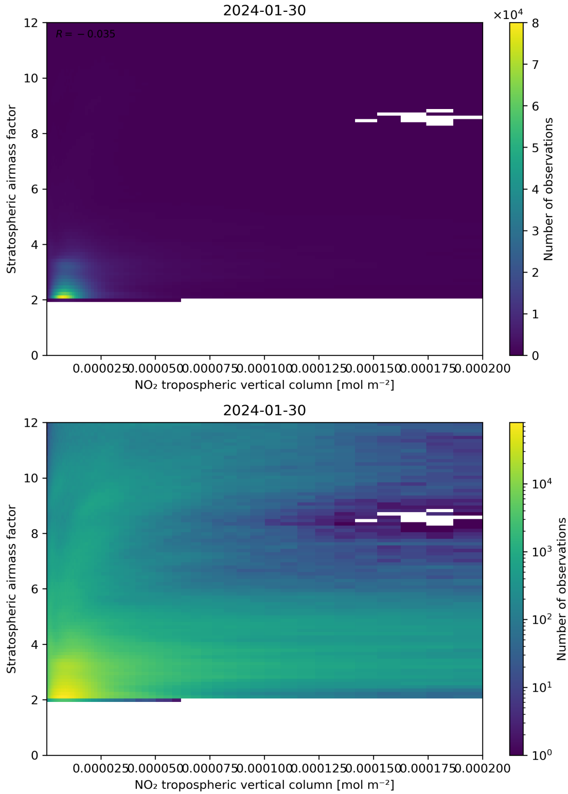
Figure 121: Scatter density plot of “NO 2 tropospheric vertical column” against “Stratospheric air mass factor” for 2024-01-29 to 2024-01-31.
