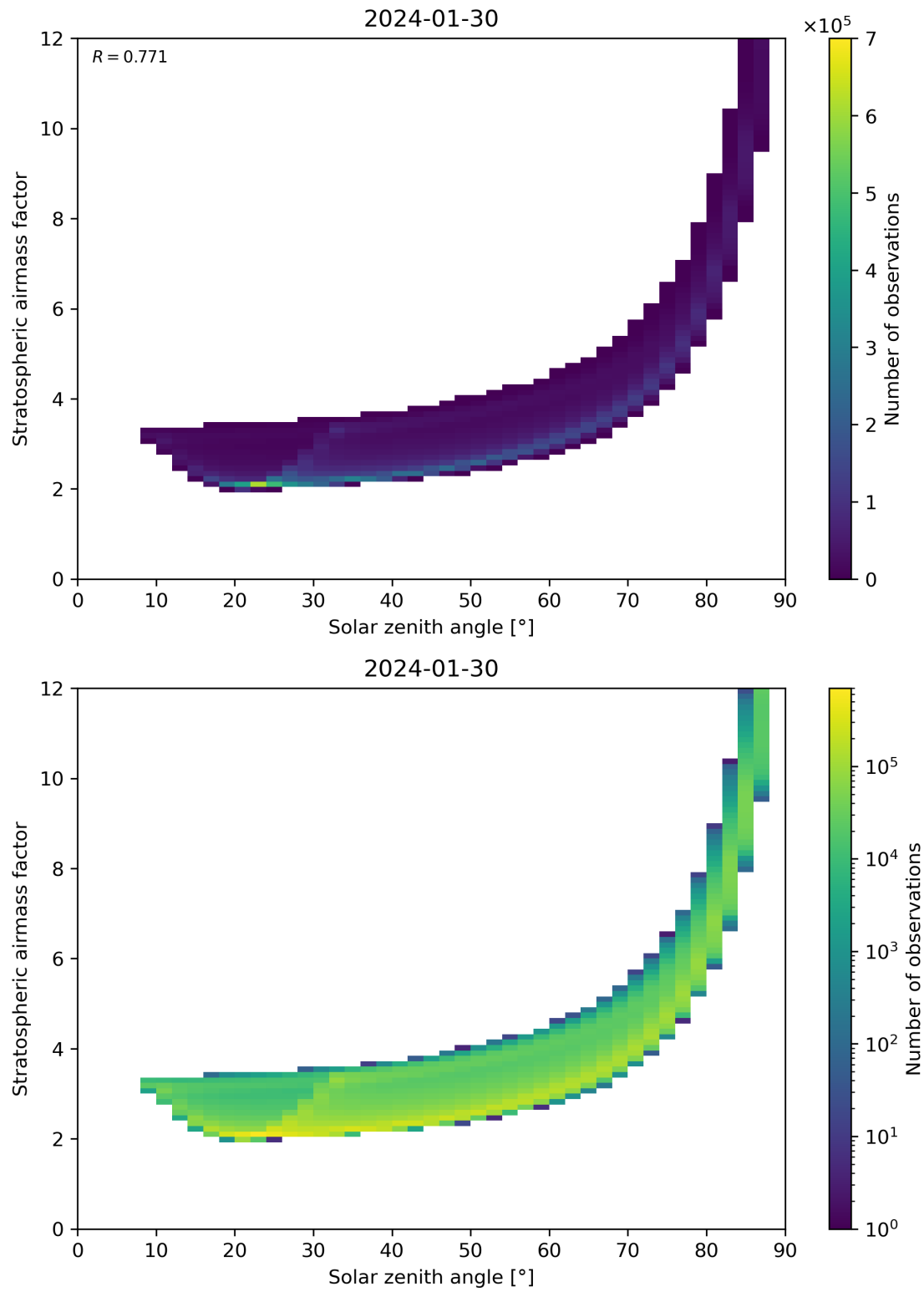
Figure 145: Scatter density plot of “Solar zenith angle” against “Stratospheric airmass factor” for 2024-01-29 to 2024-01-31.
