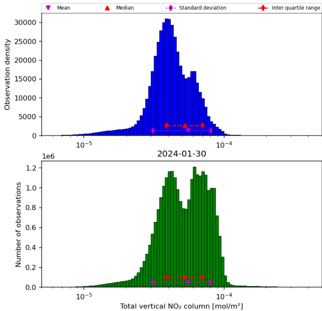
Figure 38: Histogram of "Total vertical NO 2 column" for 2024-01-29 to 2024-01-31
