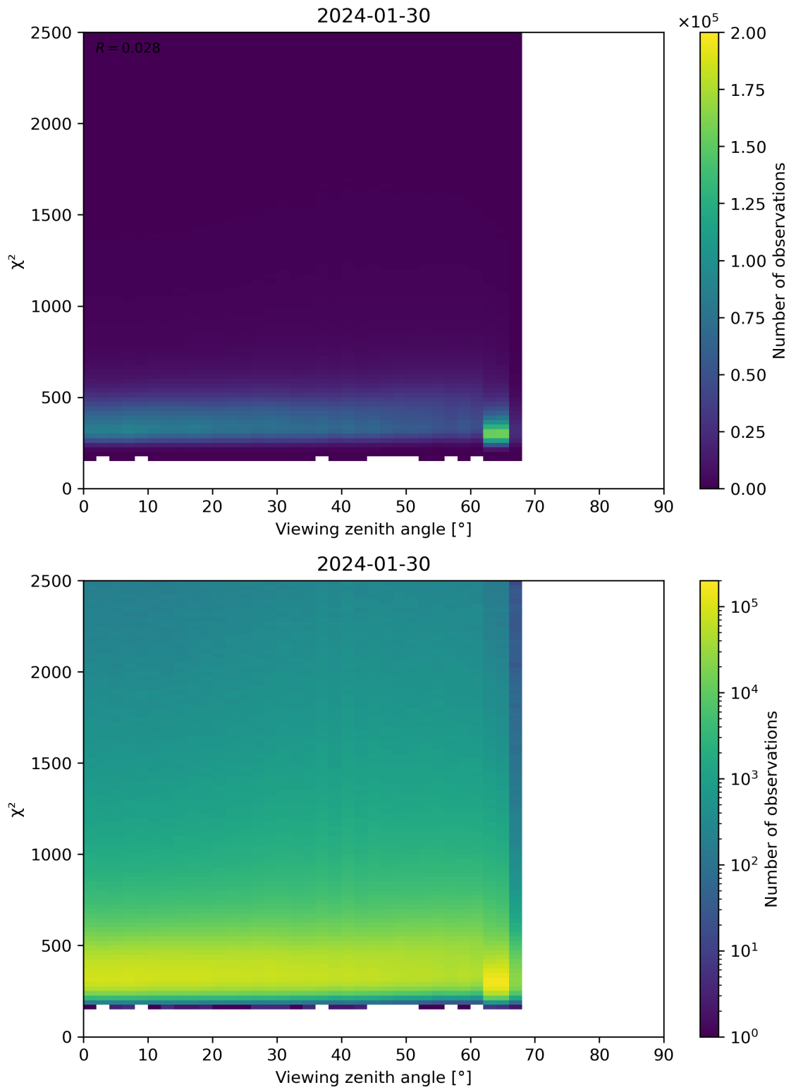
Figure 162: Scatter density plot of “Viewing zenith angle” against “ \chi^2 ” for 2024-01-29 to 2024-01-31.
