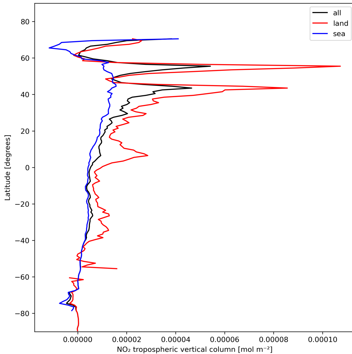
Figure 12: Zonal average of “NO 2 tropospheric vertical column” for 2024-01-29 to 2024-01-31.
