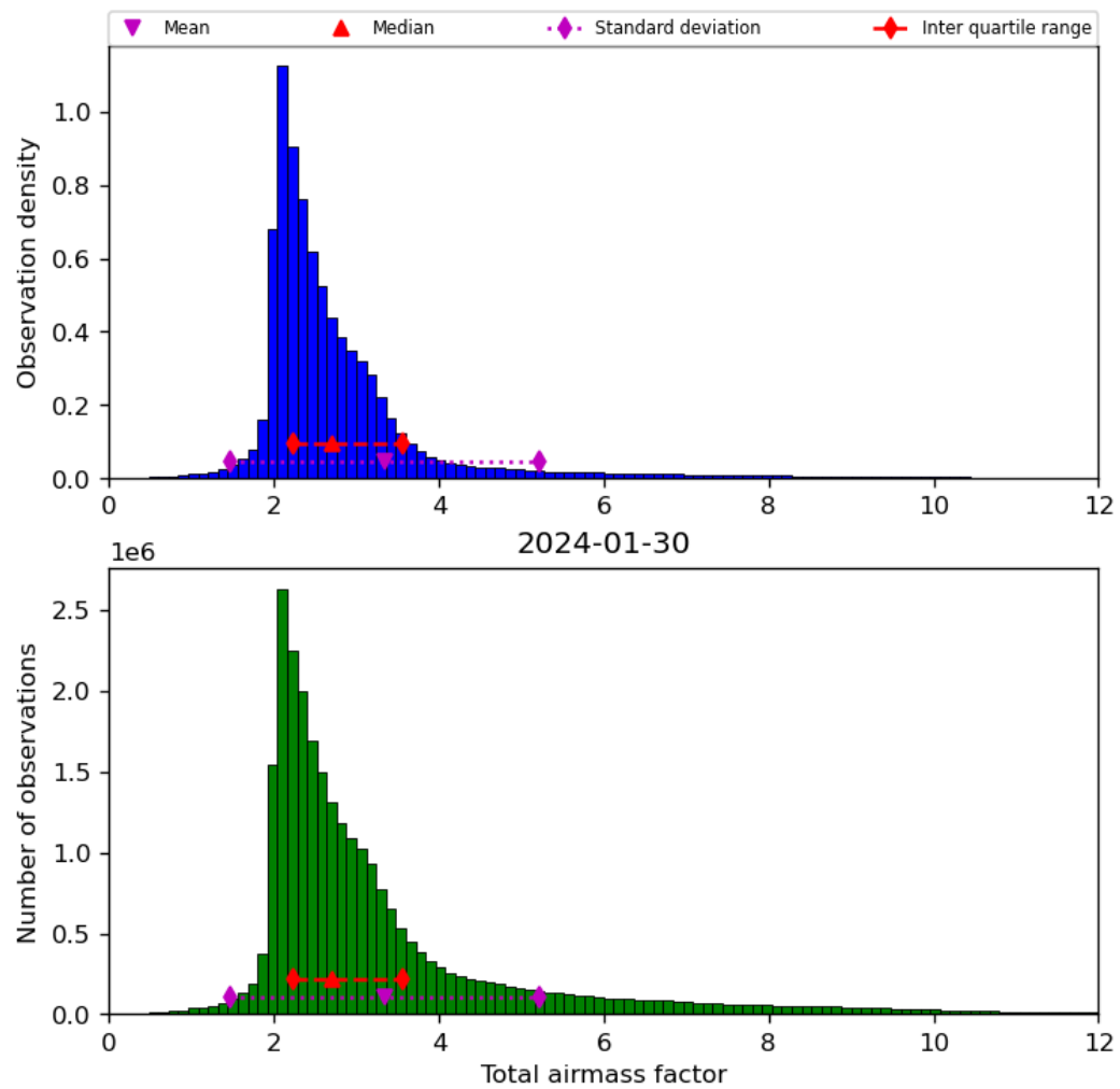
Figure 32: Histogram of “Total airmass factor” for 2024-01-29 to 2024-01-31
