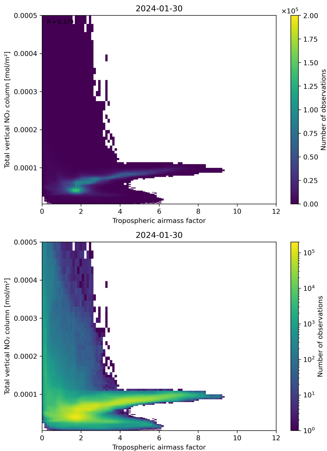
Figure 77: Scatter density plot of “Tropospheric airmass factor” against “Total vertical NO 2 column” for 2024-01-29 to 2024-01-31.
