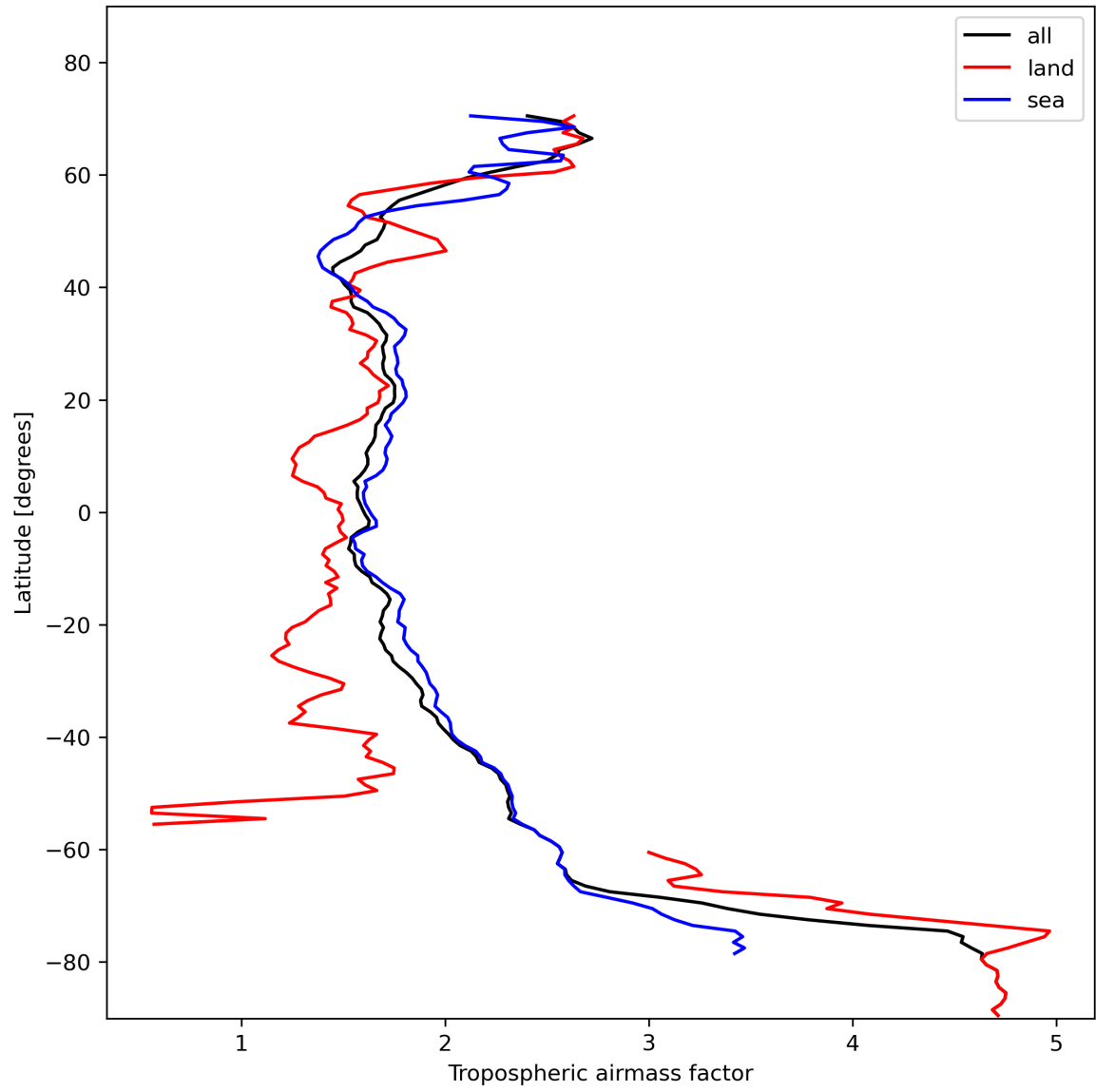
Figure 14: Zonal average of “Tropospheric airmass factor” for 2024-01-29 to 2024-01-31.
