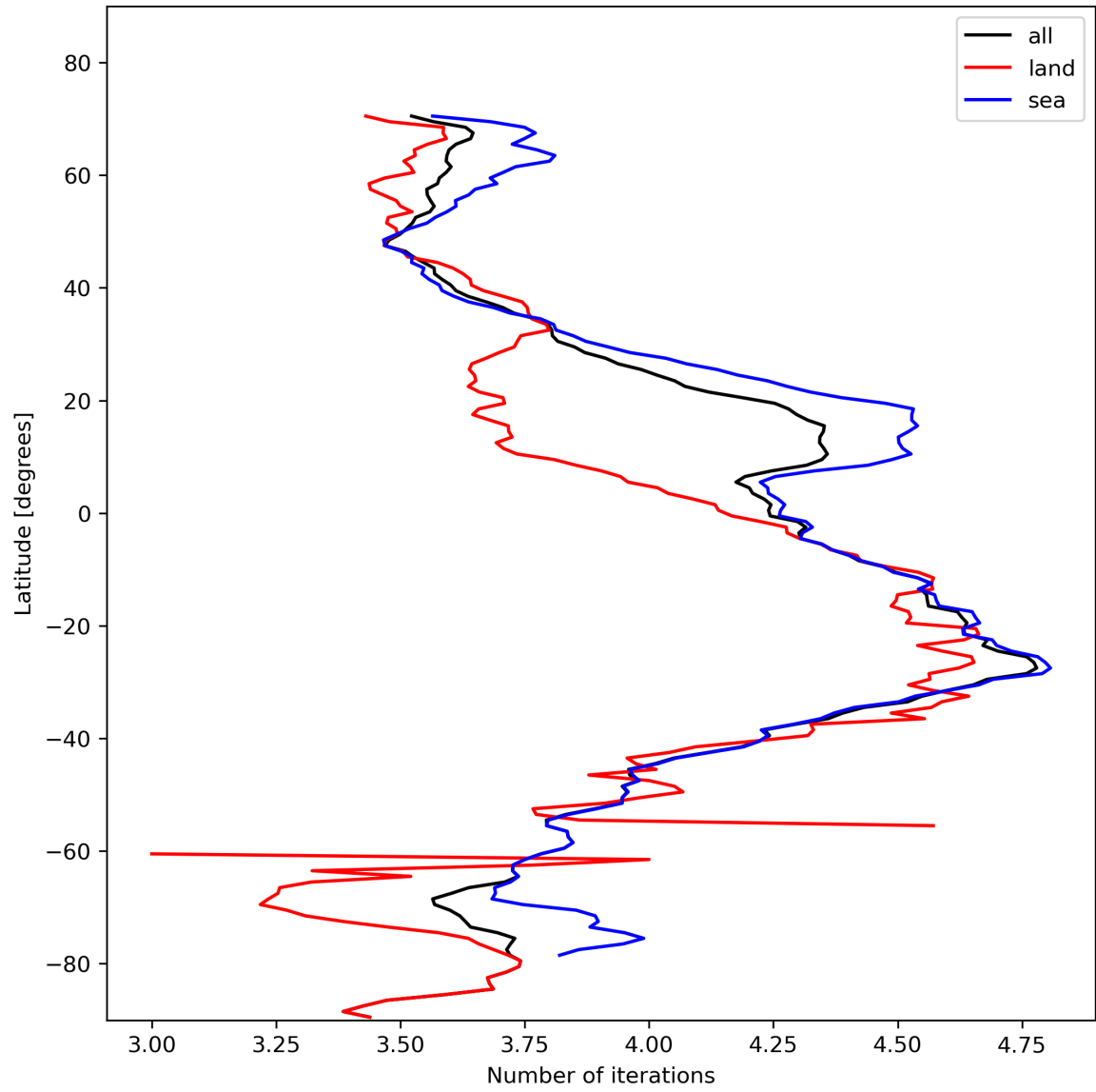
Figure 17: Zonal average of “Number of iterations” for 2024-01-29 to 2024-01-31.
