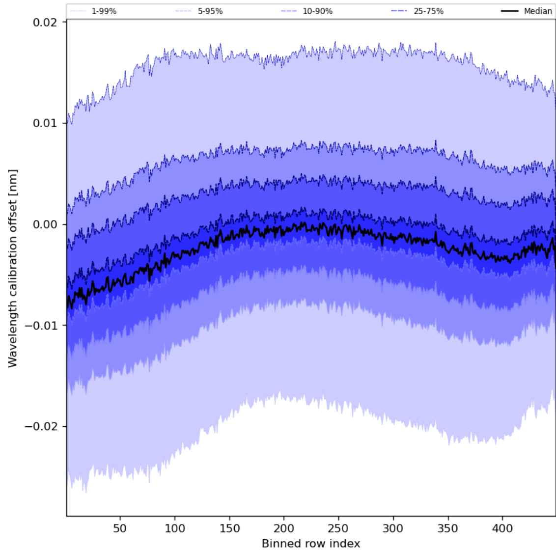
Figure 52: Along track statistics of “Wavelength calibration offset” for 2024-01-29 to 2024-01-31
