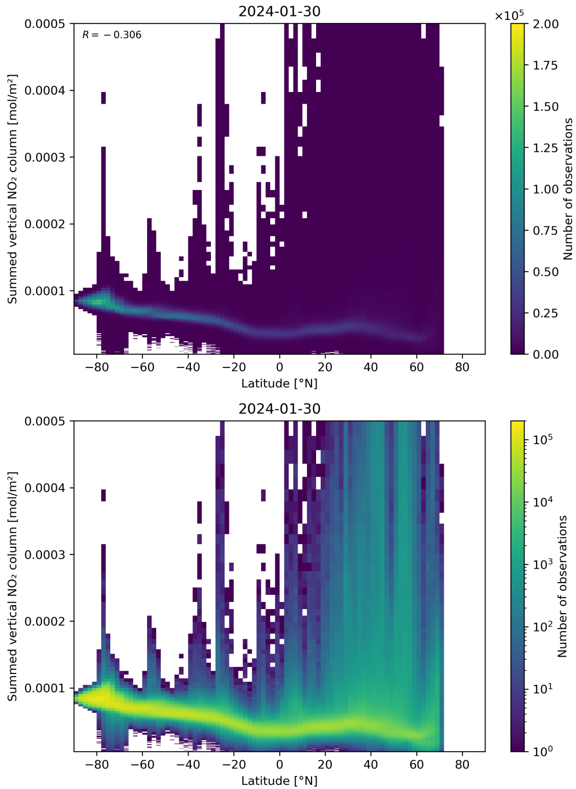
Figure 88: Scatter density plot of “Latitude” against “Summed vertical NO 2 column” for 2024-01-29 to 2024-01-31.
