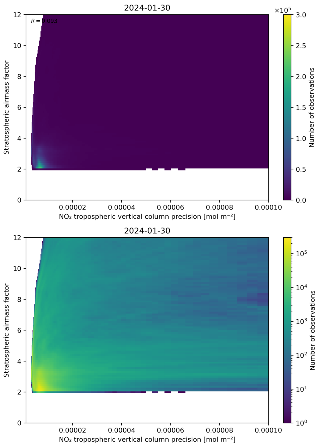
Figure 131: Scatter density plot of “NO 2 tropospheric vertical column precision” against “Stratospheric airmass factor” for 2024-01-29 to 2024-01-31.
