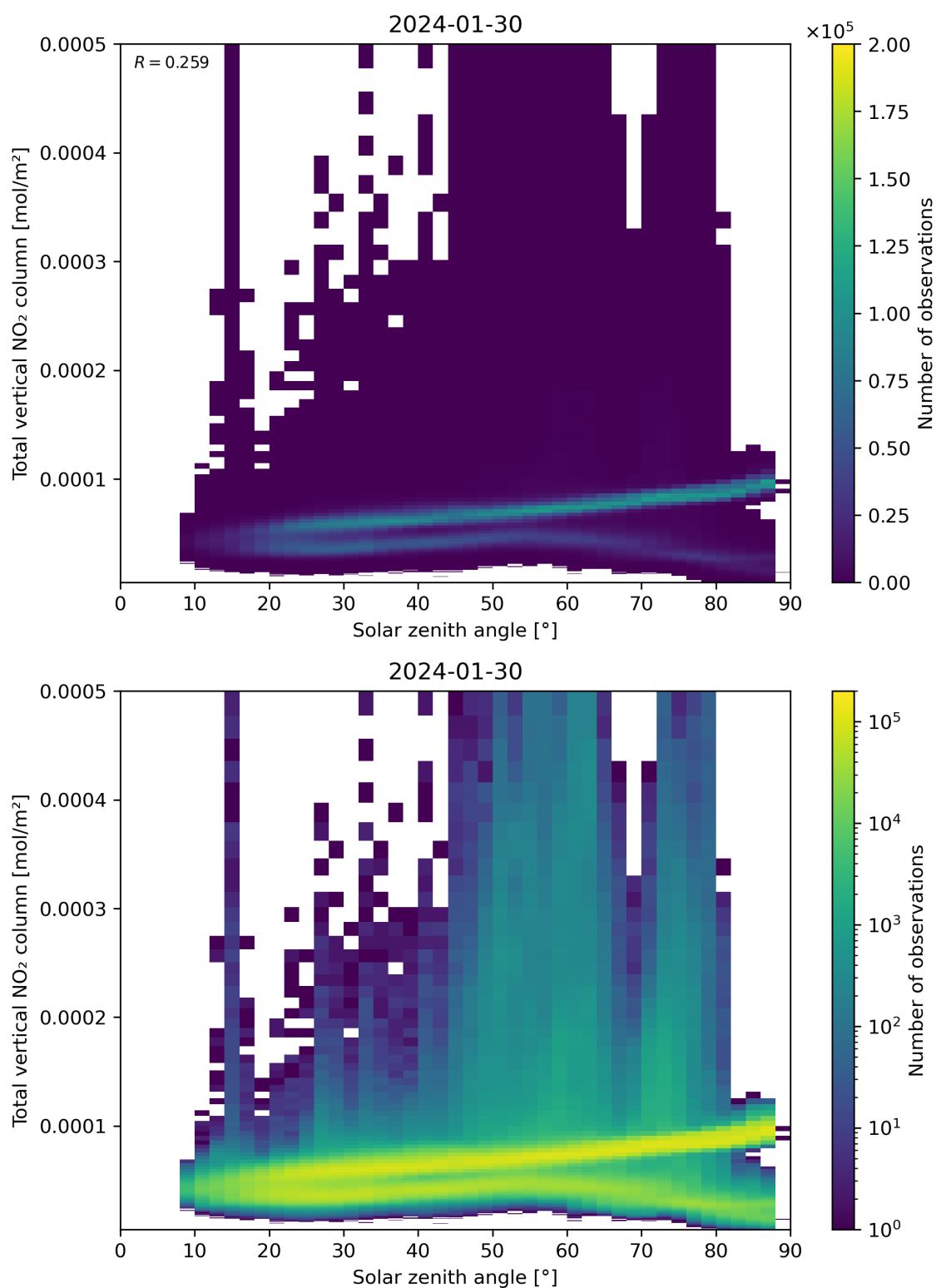
Figure 153: Scatter density plot of “Solar zenith angle” against “Total vertical NO 2 column” for 2024-01-29 to 2024-01-31.
