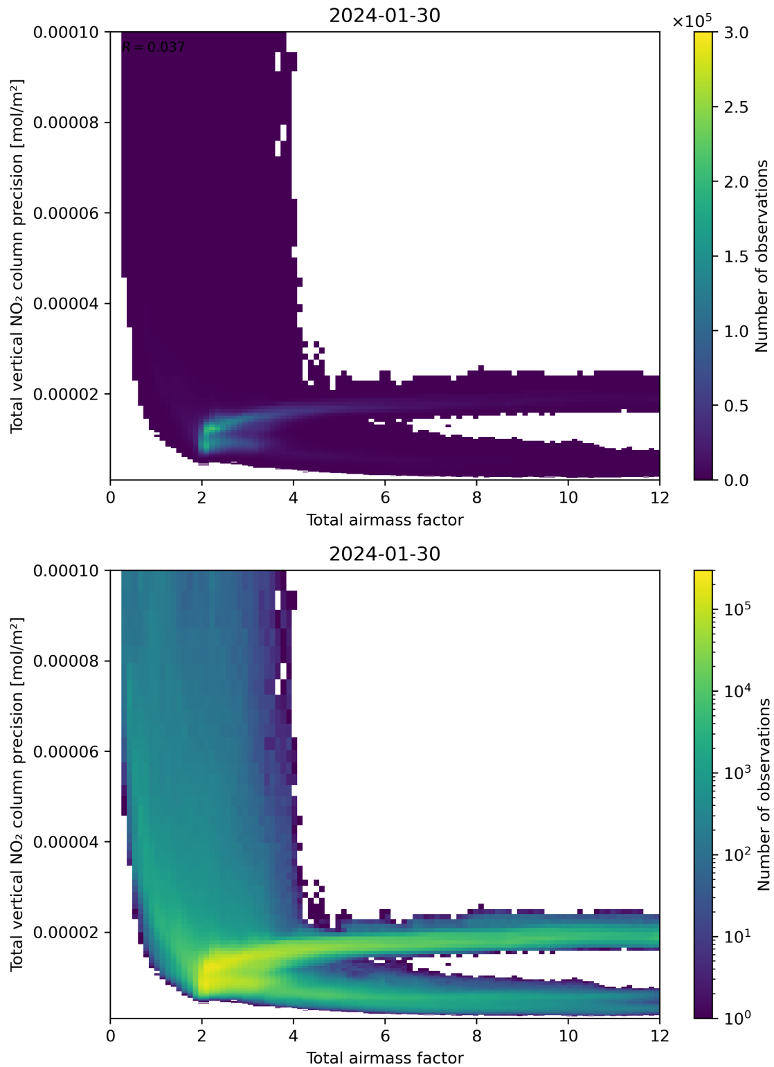
Figure 68: Scatter density plot of “Total airmass factor” against “Total vertical NO 2 column precision” for 2024-01-29 to 2024-01-31.
