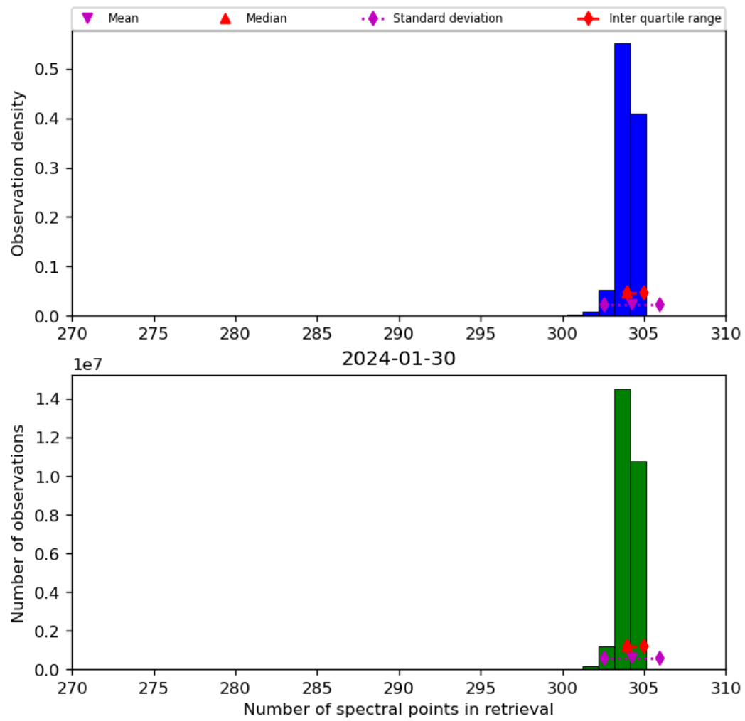
Figure 33: Histogram of “Number of spectral points in retrieval” for 2024-01-29 to 2024-01-31
