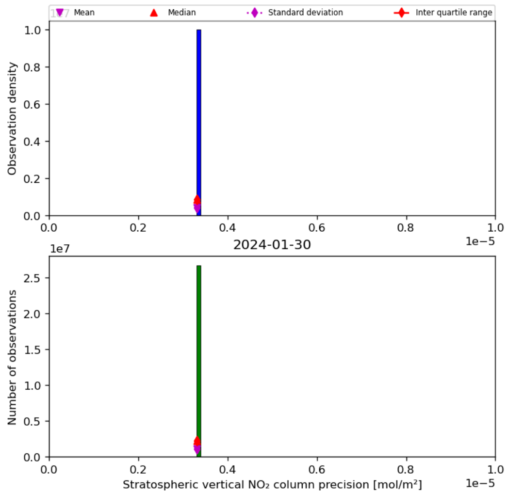
Figure 37: Histogram of “Stratospheric vertical NO 2 column precision” for 2024-01-29 to 2024-01-31
