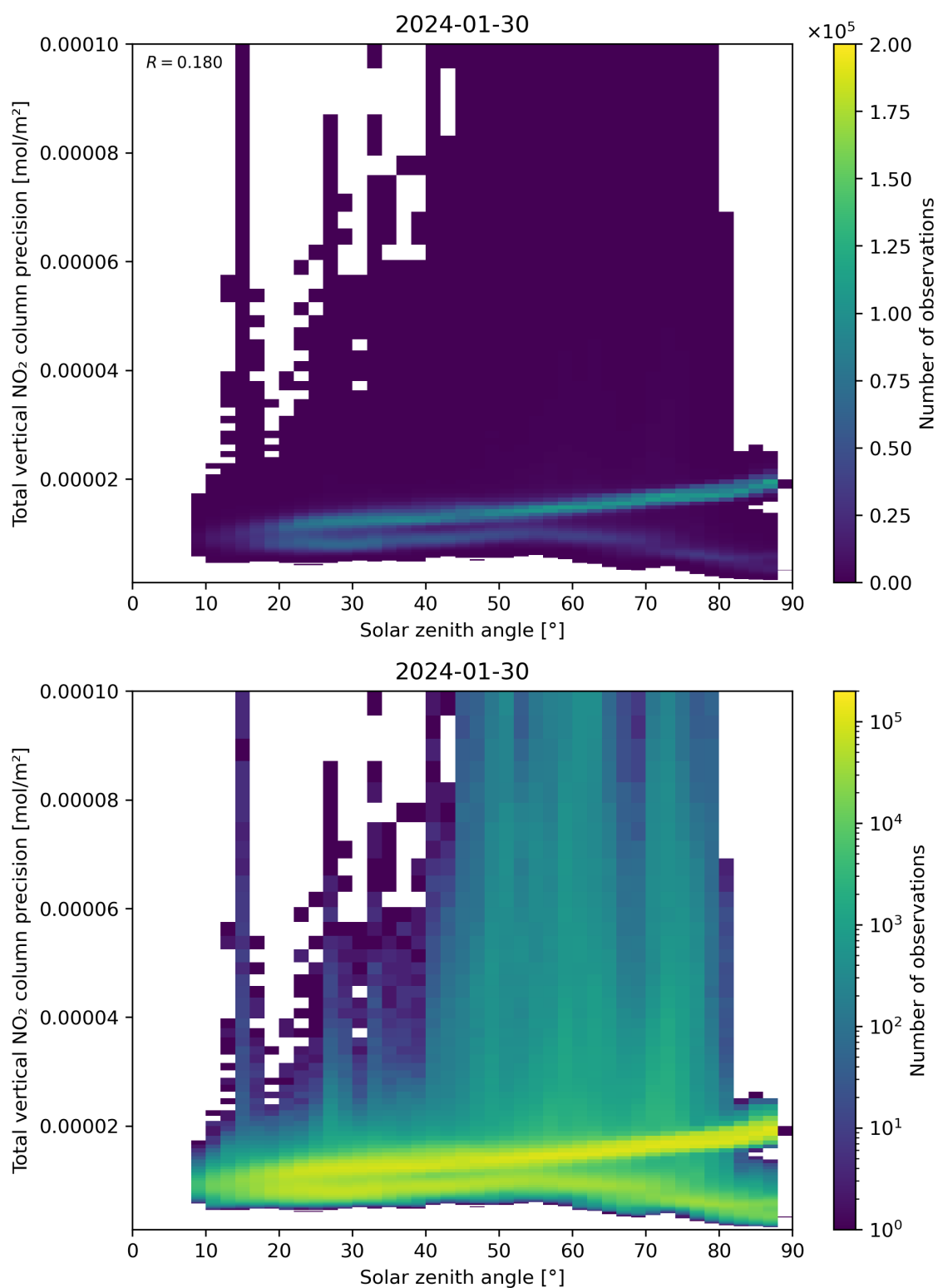
Figure 154: Scatter density plot of “Solar zenith angle” against “Total vertical NO 2 column precision” for 2024-01-29 to 2024-01-31.
