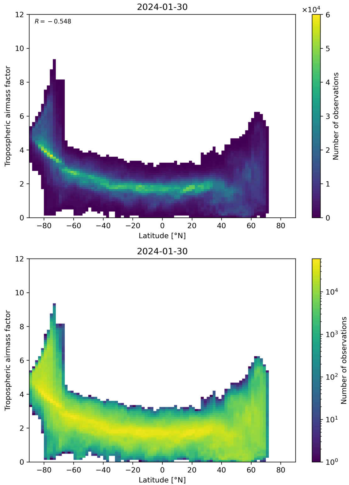
Figure 85: Scatter density plot of “Latitude” against “Tropospheric airmass factor” for 2024-01-29 to 2024-01-31.
