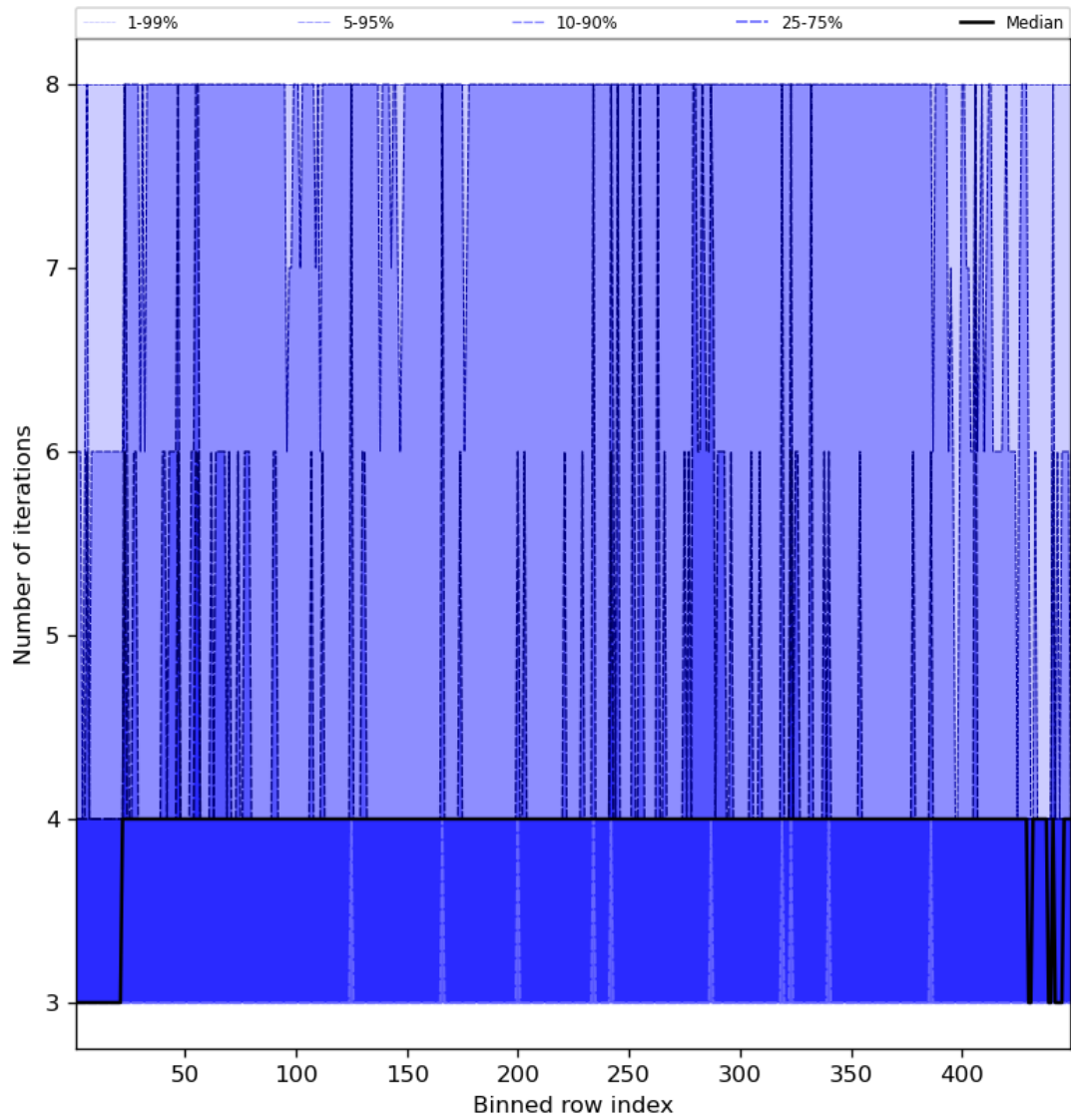
Figure 51: Along track statistics of “Number of iterations” for 2024-01-29 to 2024-01-31
