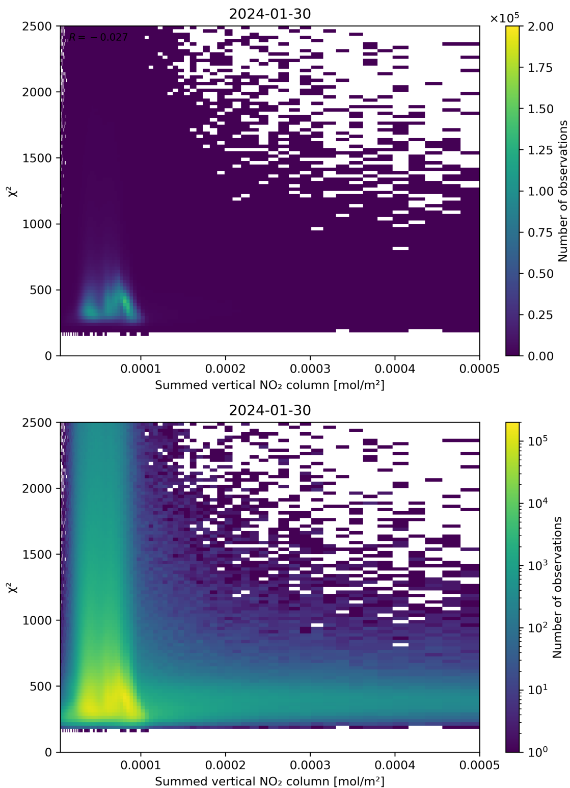
Figure 104: Scatter density plot of “Summed vertical NO 2 column” against “ \chi^2 ” for 2024-01-29 to 2024-01-31.
