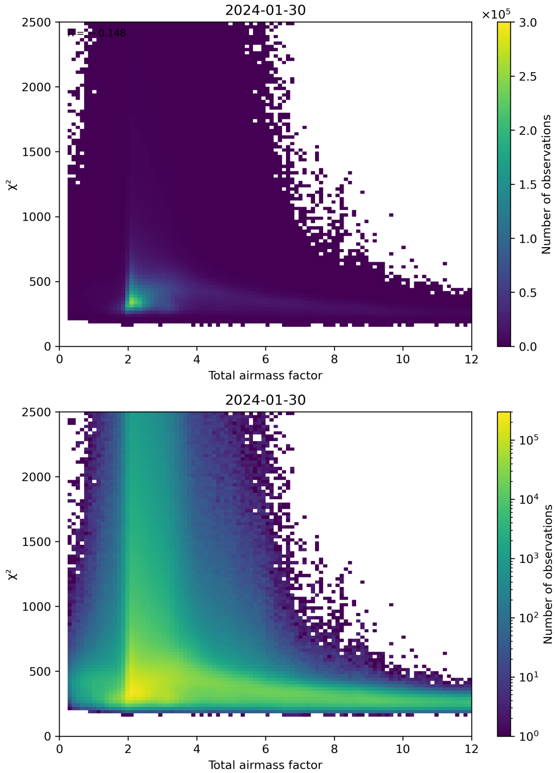
Figure 63: Scatter density plot of “Total airmass factor” against “ \chi^2 ” for 2024-01-29 to 2024-01-31.
