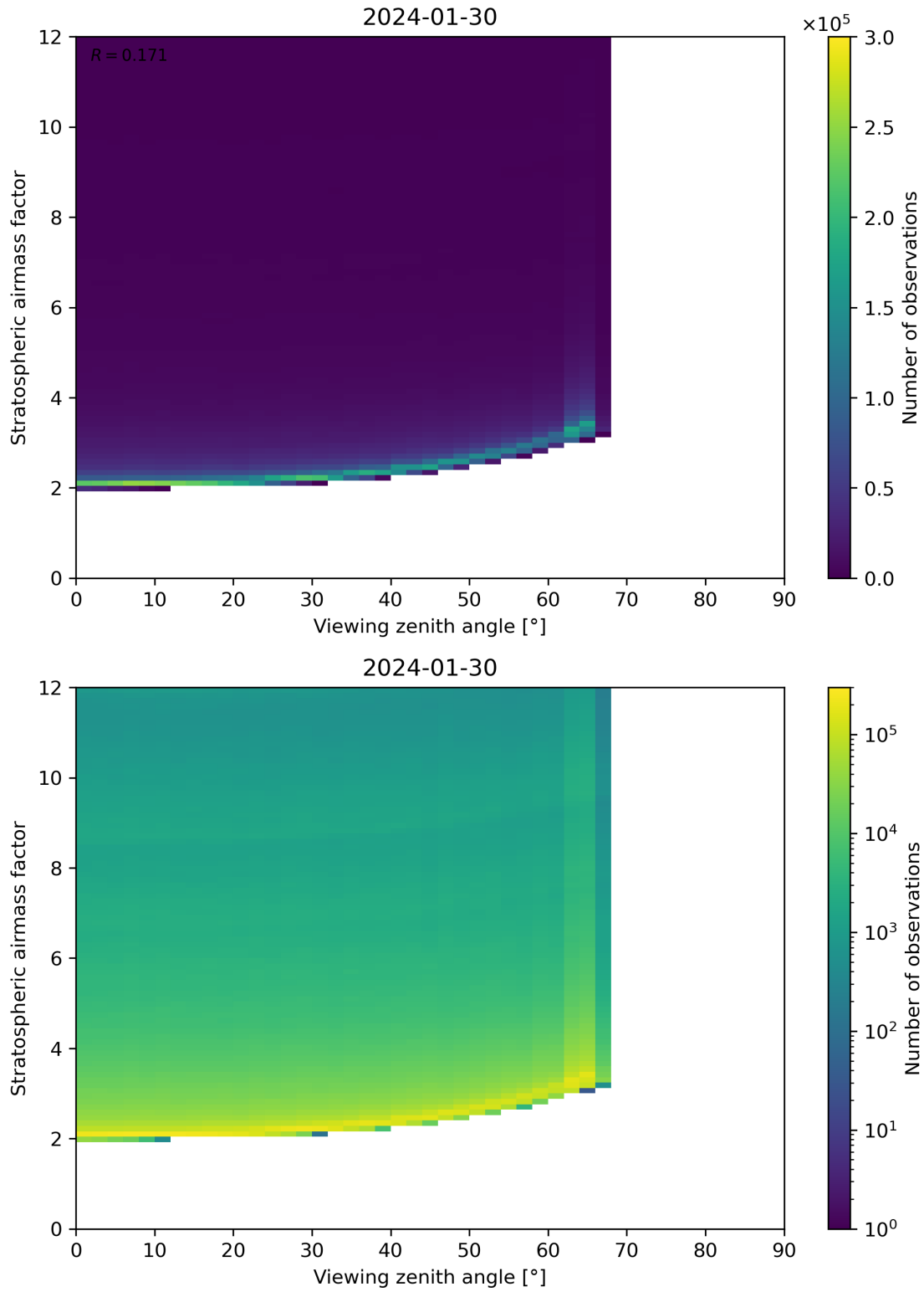
Figure 159: Scatter density plot of “Viewing zenith angle” against “Stratospheric airmass factor” for 2024-01-29 to 2024-01-31.
