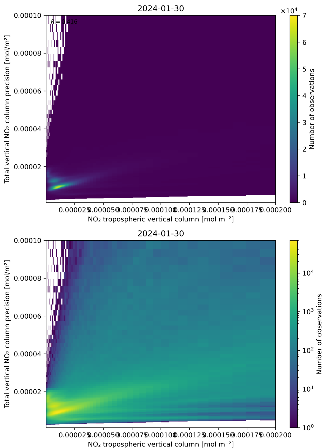
Figure 129: Scatter density plot of “NO 2 tropospheric vertical column” against “Total vertical NO 2 column precision” for 2024-01-29 to 2024-01-31.
