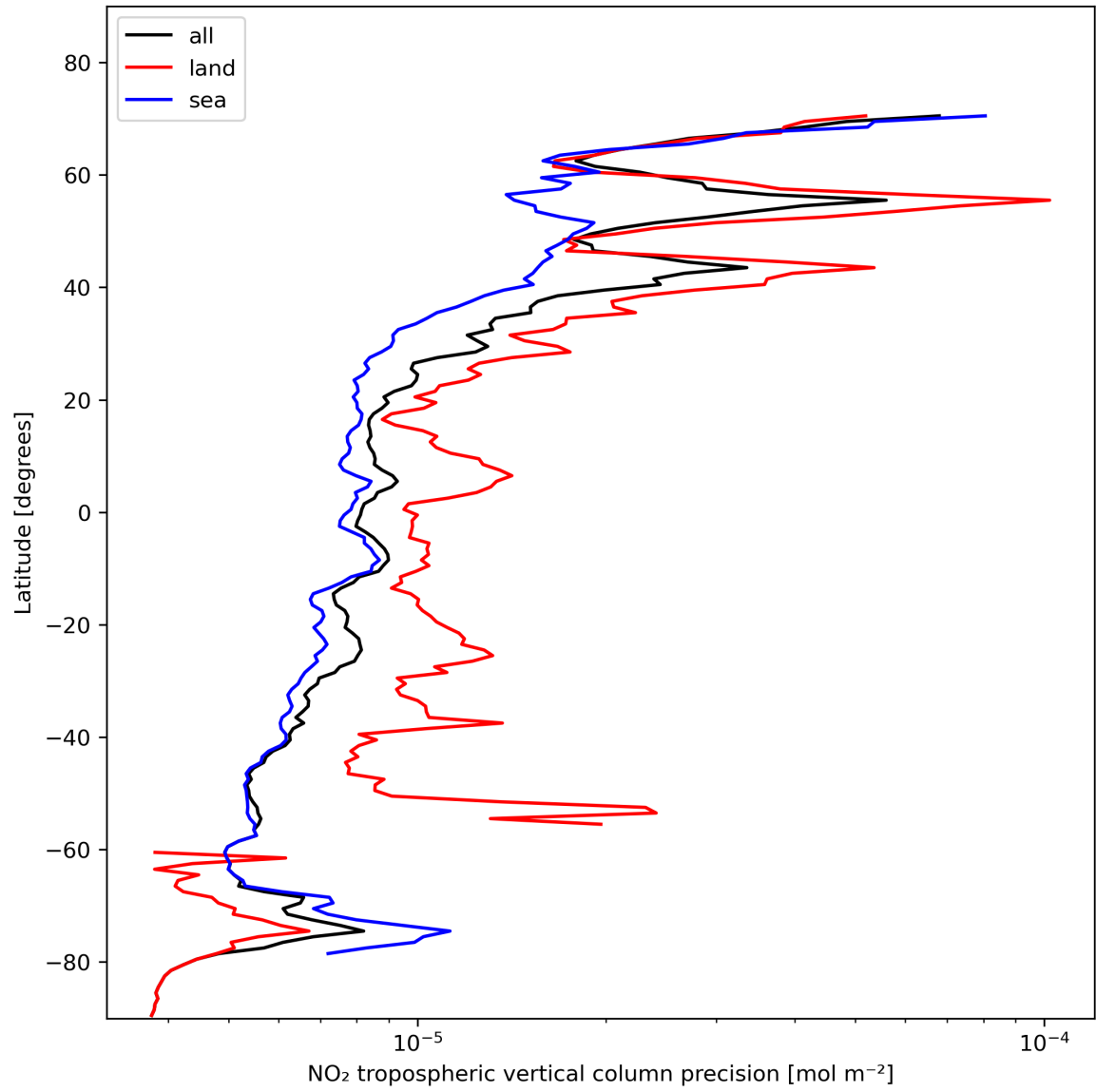
Figure 13: Zonal average of “NO 2 tropospheric vertical column precision” for 2024-01-29 to 2024-01-31.
