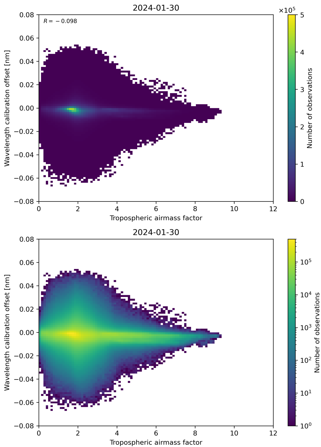
Figure 80: Scatter density plot of “Tropospheric airmass factor” against “Wavelength calibration offset” for 2024-01-29 to 2024-01-31.
