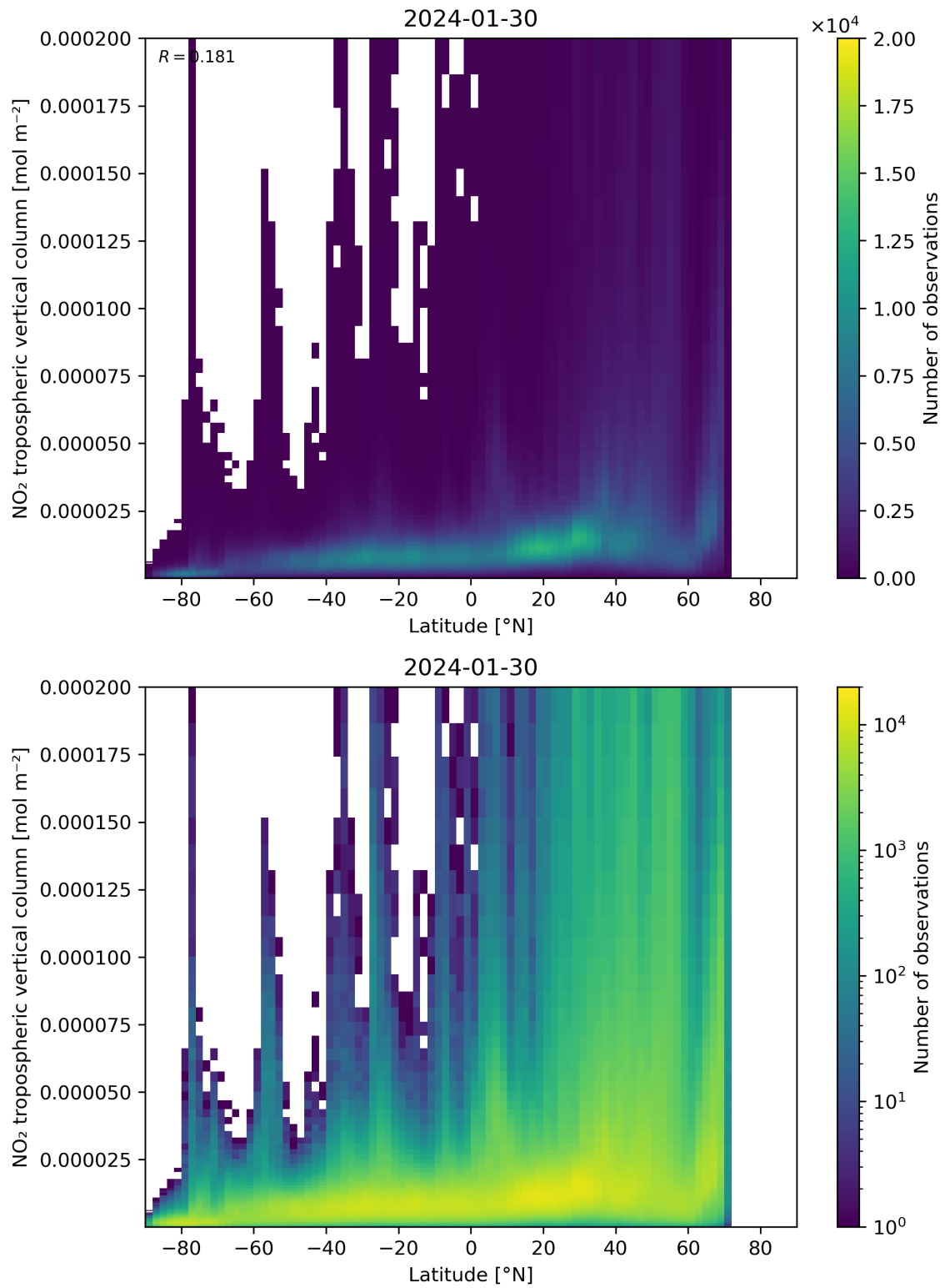
Figure 92: Scatter density plot of “Latitude” against “NO 2 tropospheric vertical column” for 2024-01-29 to 2024-01-31.
