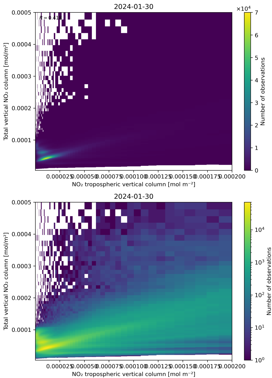
Figure 128: Scatter density plot of “NO 2 tropospheric vertical column” against “Total vertical NO 2 column” for 2024-01-29 to 2024-01-31.
