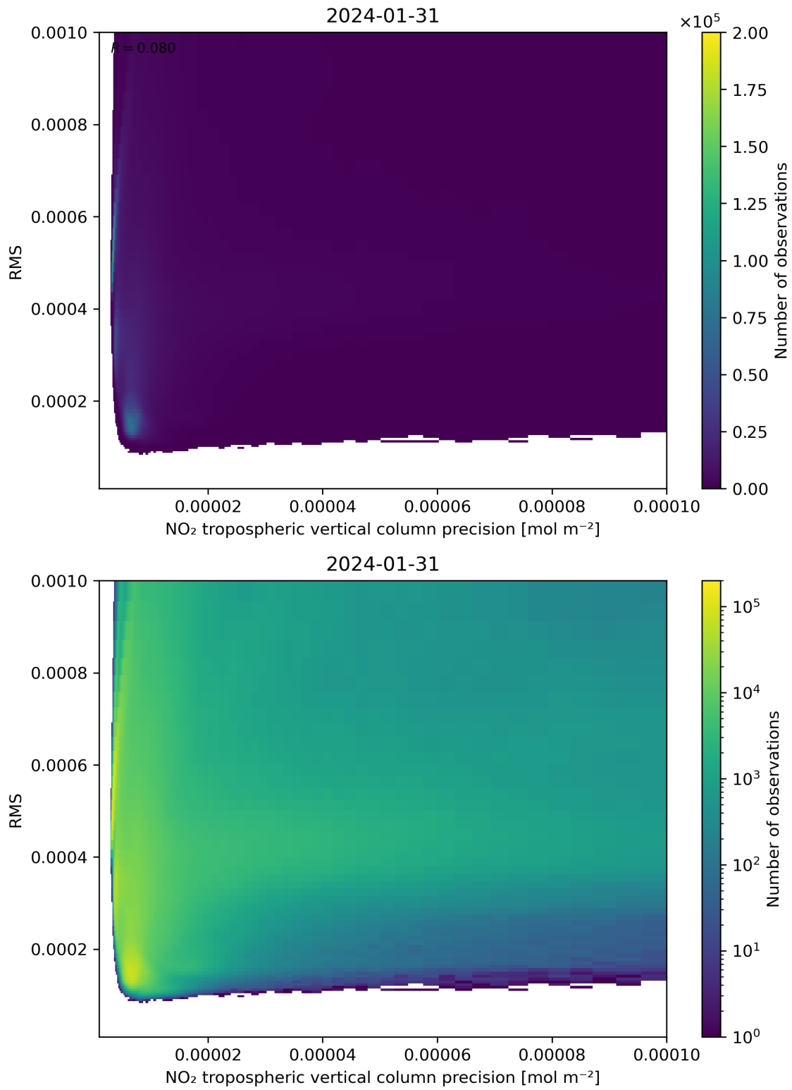
Figure 140: Scatter density plot of “NO 2 tropospheric vertical column precision” against “RMS” for 2024-01-31 to 2024-02-01.
