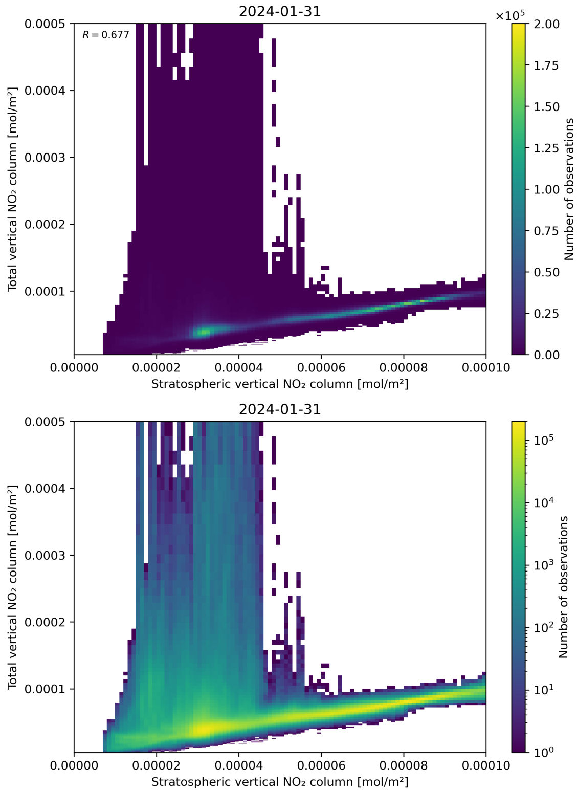
Figure 100: Scatter density plot of “Stratospheric vertical NO 2 column” against “Total vertical NO 2 column” for 2024-01-31 to 2024-02-01.
