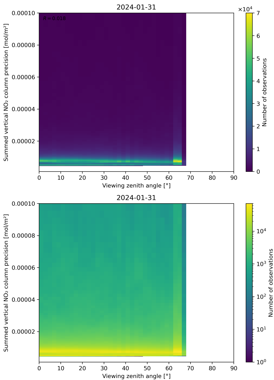
Figure 166: Scatter density plot of “Viewing zenith angle” against “Summed vertical NO 2 column precision” for 2024-01-31 to 2024-02-01.
