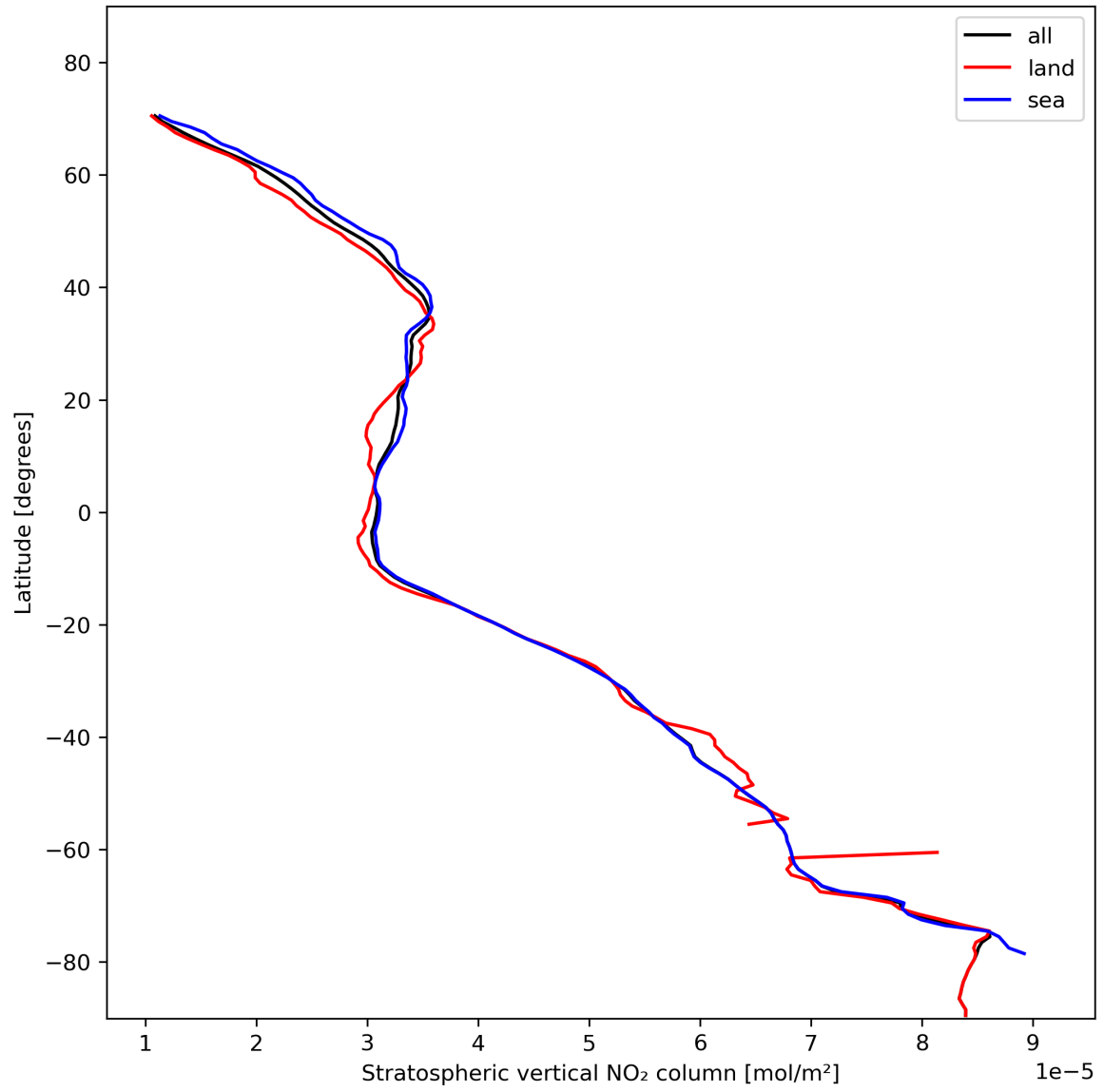
Figure 19: Zonal average of “Stratospheric vertical NO 2 column” for 2024-01-31 to 2024-02-01.
