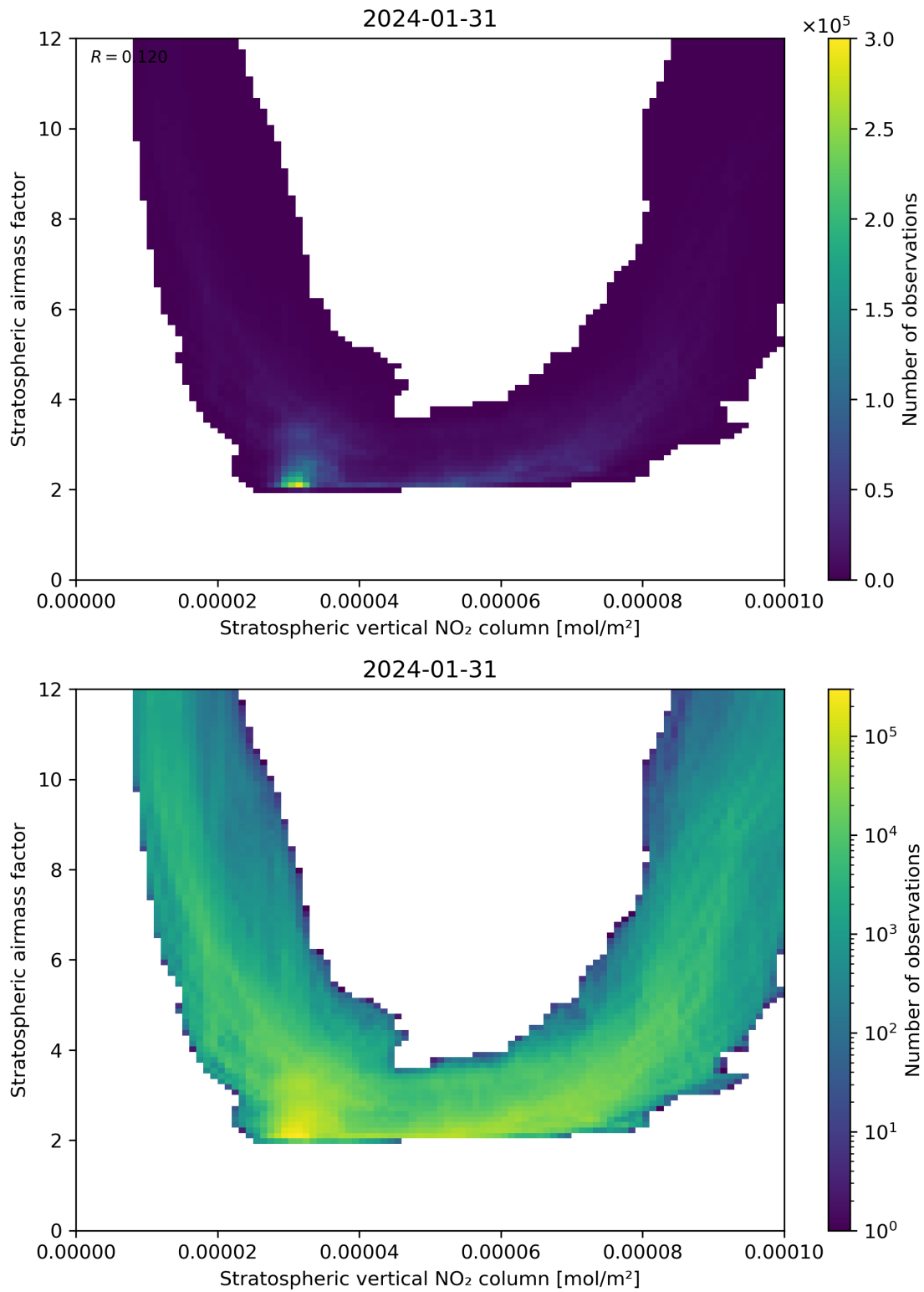
Figure 96: Scatter density plot of “Stratospheric vertical NO 2 column” against “Stratospheric airmass factor” for 2024-01-31 to 2024-02-01.
