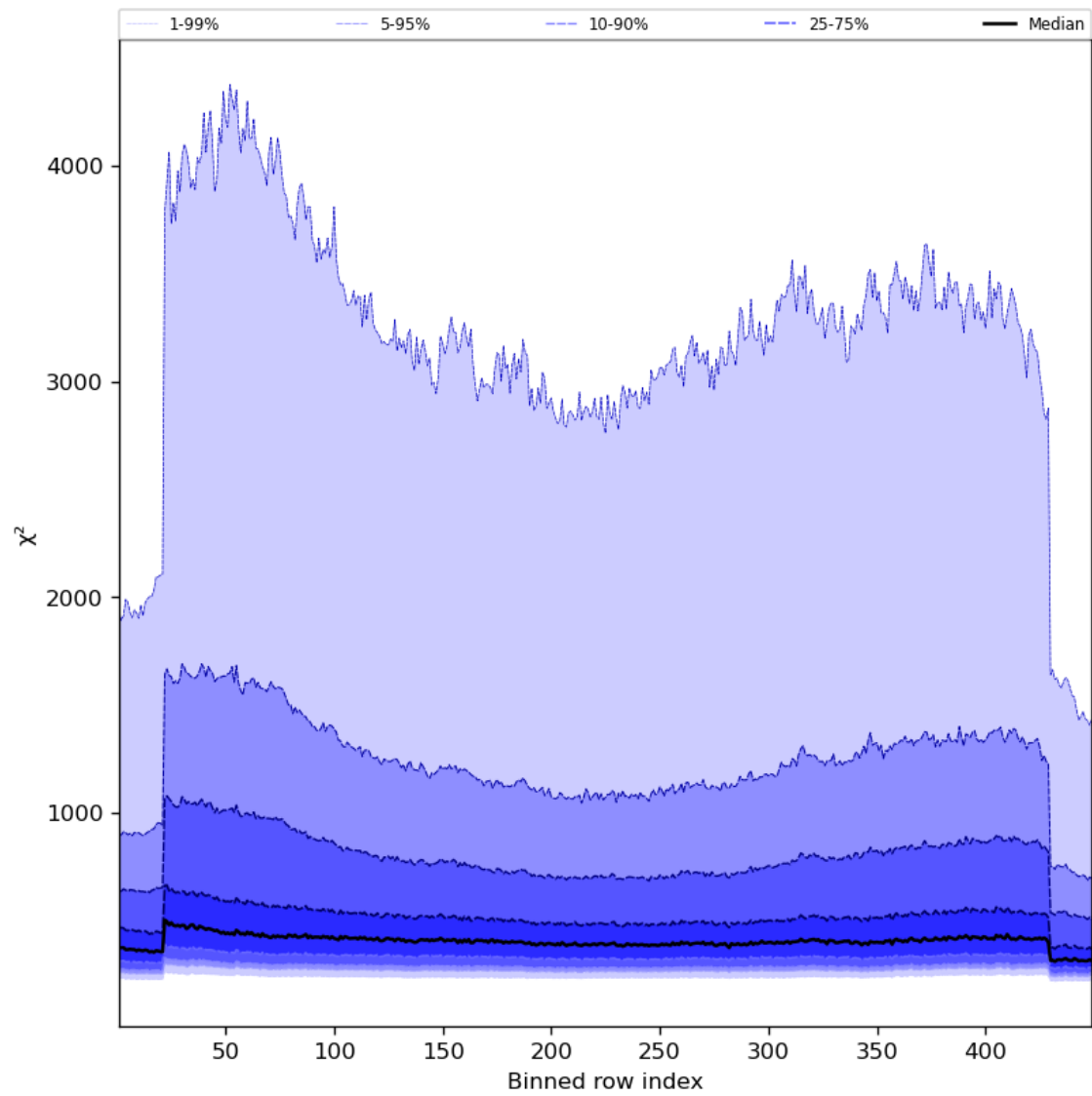
Figure 59: Along track statistics of “ \chi^2 ” for 2024-01-31 to 2024-02-01
