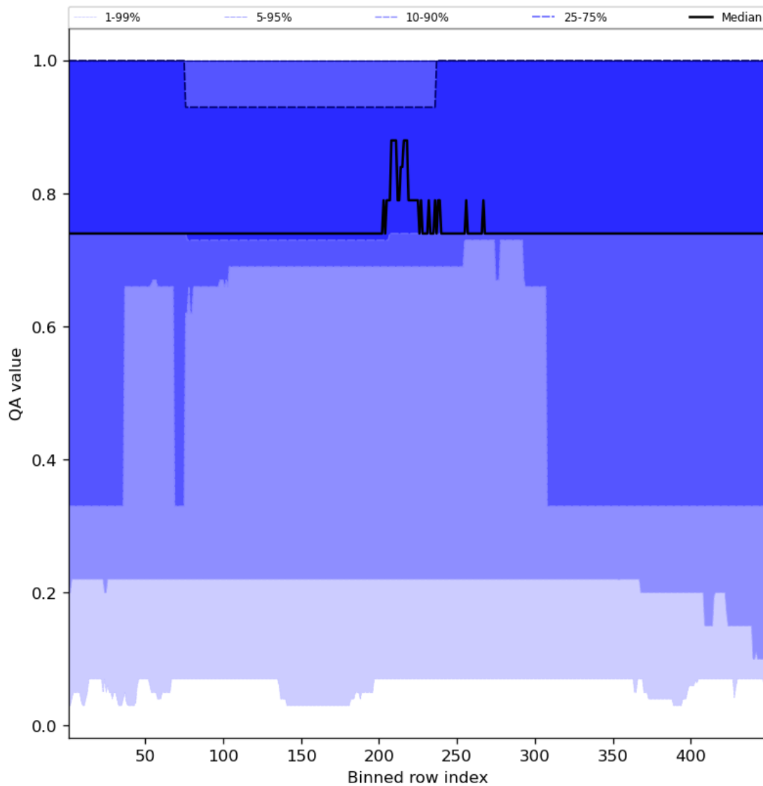
Figure 45: Along track statistics of “QA value” for 2024-01-31 to 2024-02-01
