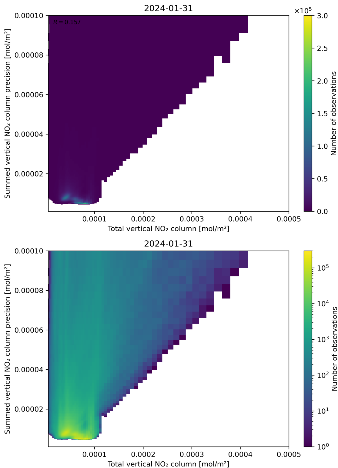
Figure 113: Scatter density plot of “Total vertical NO 2 column” against “Summed vertical NO 2 column precision” for 2024-01-31 to 2024-02-01.
