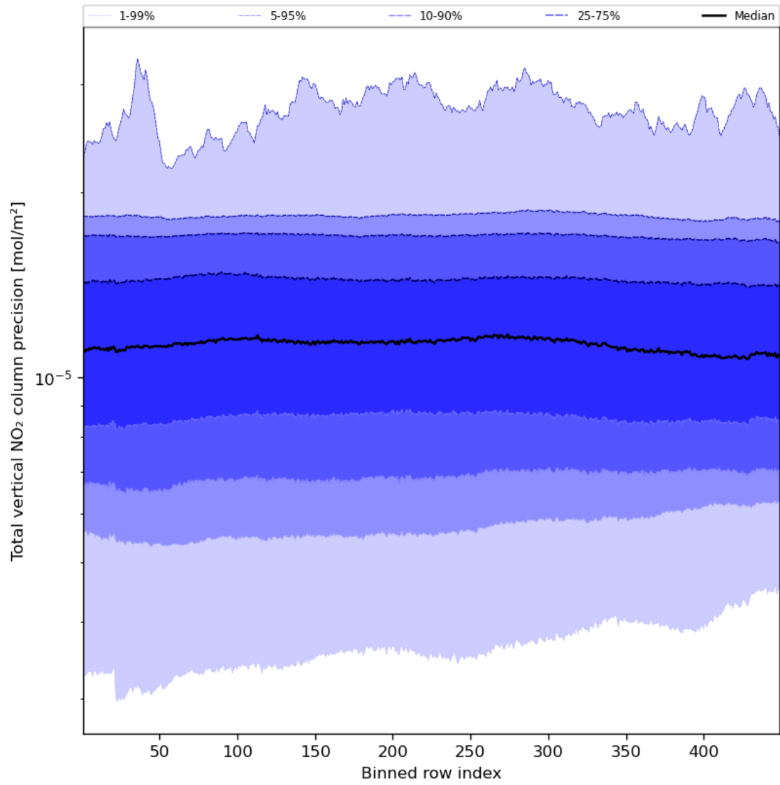
Figure 56: Along track statistics of "Total vertical NO 2 column precision" for 2024-01-31 to 2024-02-01
