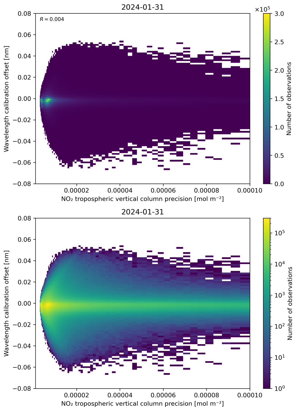
Figure 141: Scatter density plot of “NO 2 tropospheric vertical column precision” against “Wavelength calibration offset” for 2024-01-31 to 2024-02-01.
