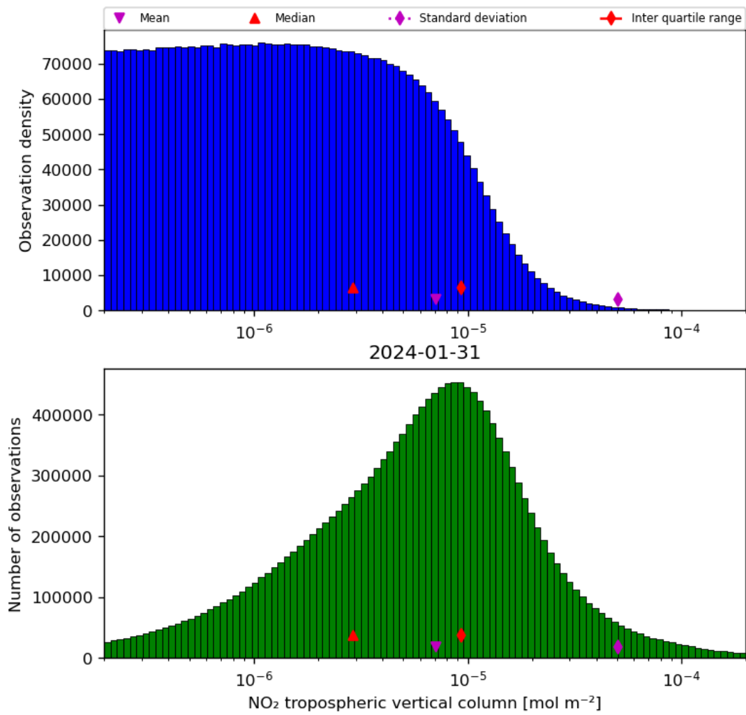
Figure 29: Histogram of “NO 2 tropospheric vertical column” for 2024-01-31 to 2024-02-01
