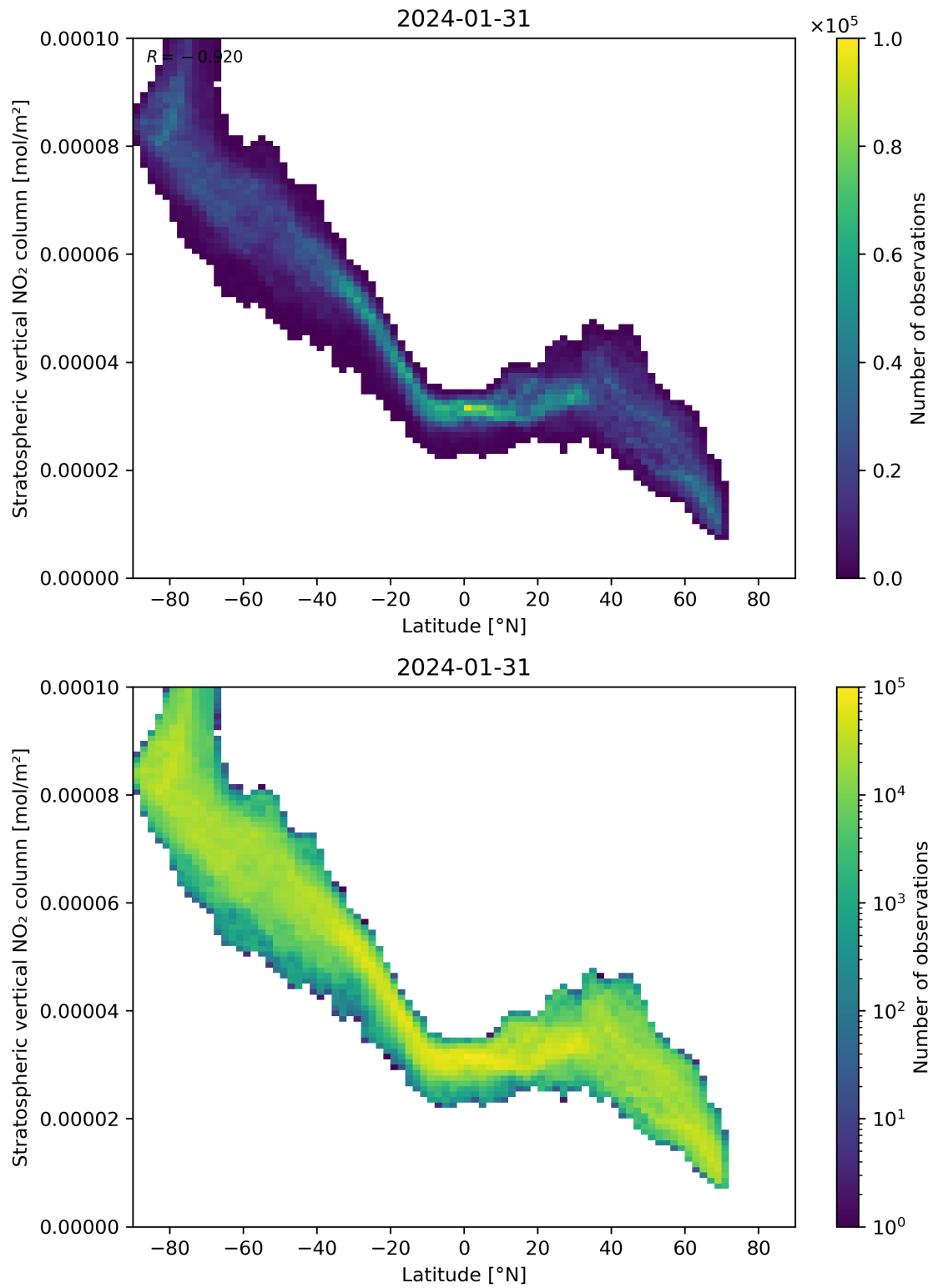
Figure 87: Scatter density plot of “Latitude” against “Stratospheric vertical NO 2 column” for 2024-01-31 to 2024-02-01.
