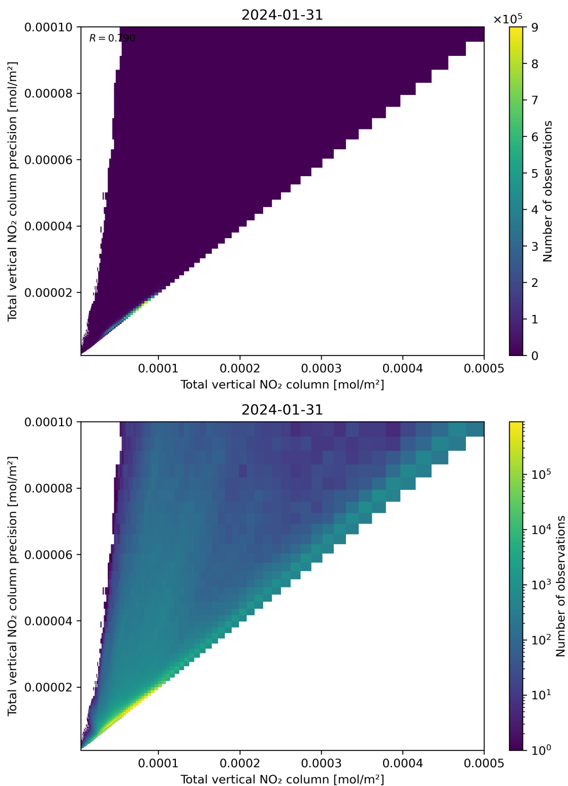
Figure 114: Scatter density plot of “Total vertical NO 2 column” against “Total vertical NO 2 column precision” for 2024-01-31 to 2024-02-01.
