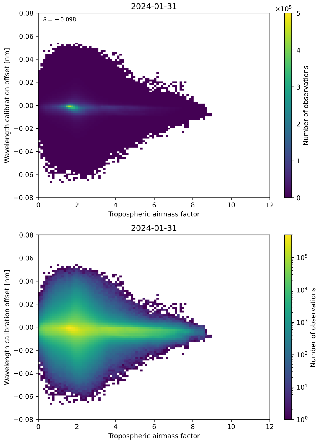
Figure 80: Scatter density plot of “Tropospheric airmass factor” against “Wavelength calibration offset” for 2024-01-31 to 2024-02-01.
