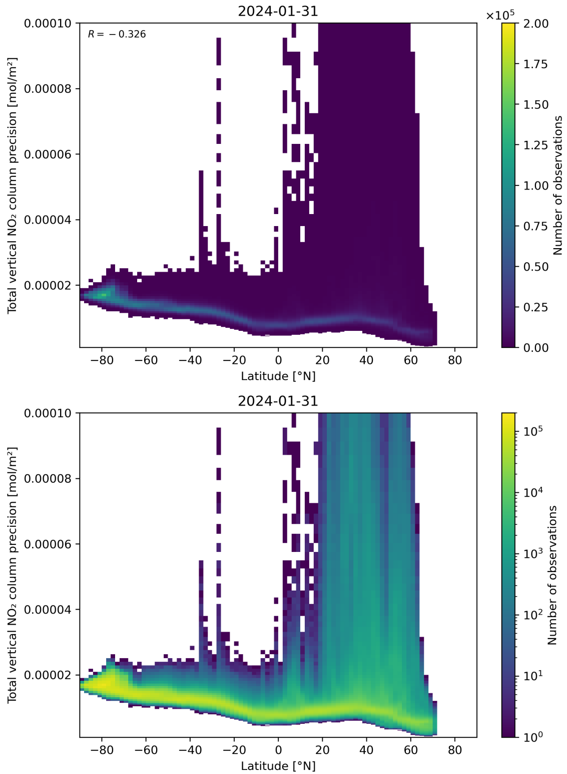
Figure 91: Scatter density plot of “Latitude” against “Total vertical NO 2 column precision” for 2024-01-31 to 2024-02-01.
