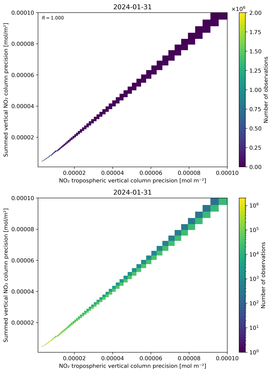
Figure 137: Scatter density plot of “NO 2 tropospheric vertical column precision” against “Summed vertical NO 2 column precision” for 2024-01-31 to 2024-02-01.
