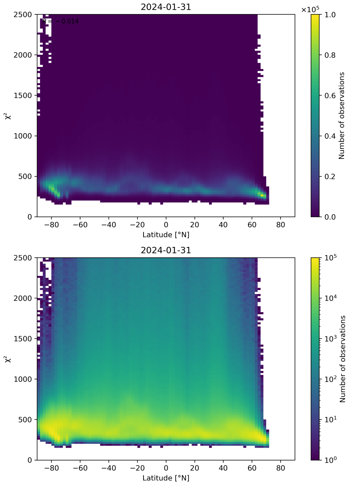
Figure 86: Scatter density plot of “Latitude” against “ \chi^2 ” for 2024-01-31 to 2024-02-01.
