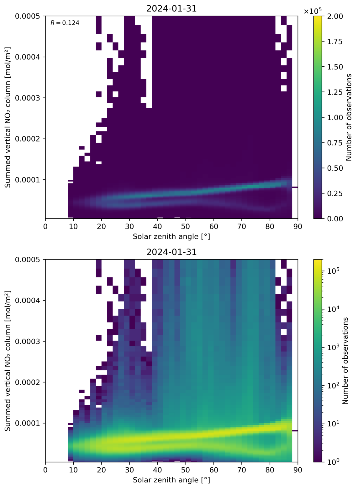
Figure 151: Scatter density plot of “Solar zenith angle” against “Summed vertical NO 2 column” for 2024-01-31 to 2024-02-01.
