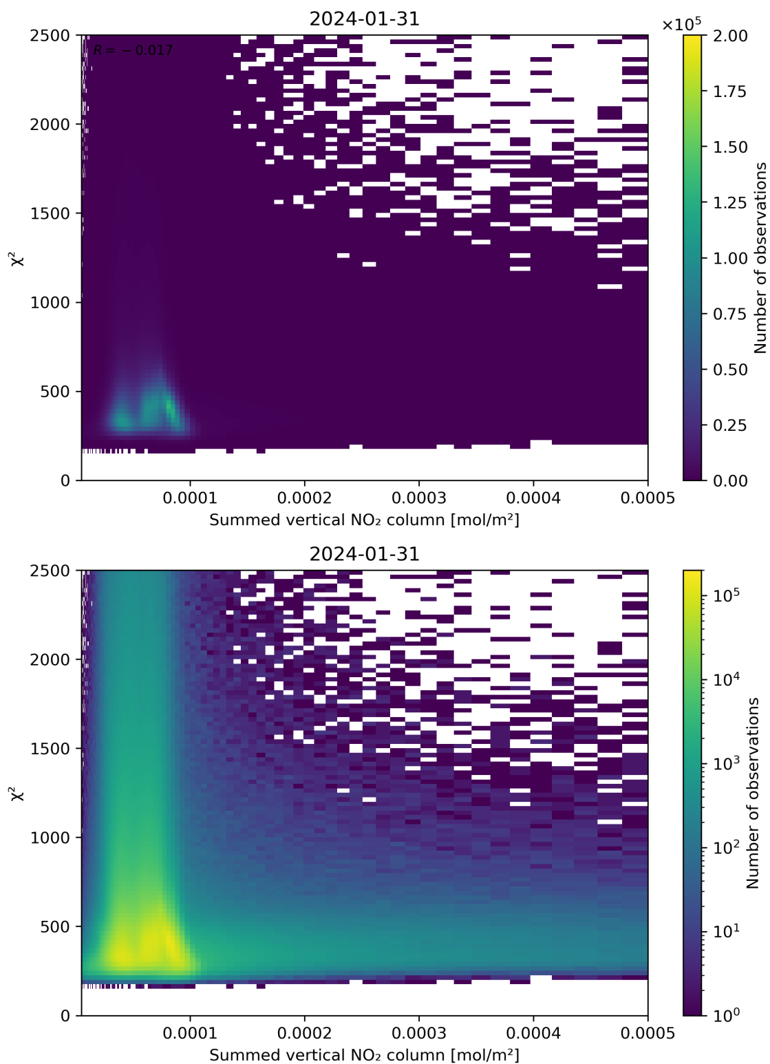
Figure 104: Scatter density plot of “Summed vertical NO 2 column” against “ \chi^2 ” for 2024-01-31 to 2024-02-01.
