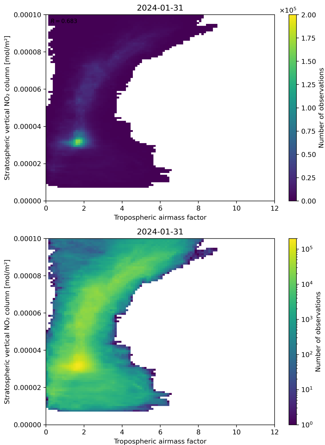
Figure 74: Scatter density plot of “Tropospheric air mass factor” against “Stratospheric vertical NO 2 column” for 2024-01-31 to 2024-02-01.
