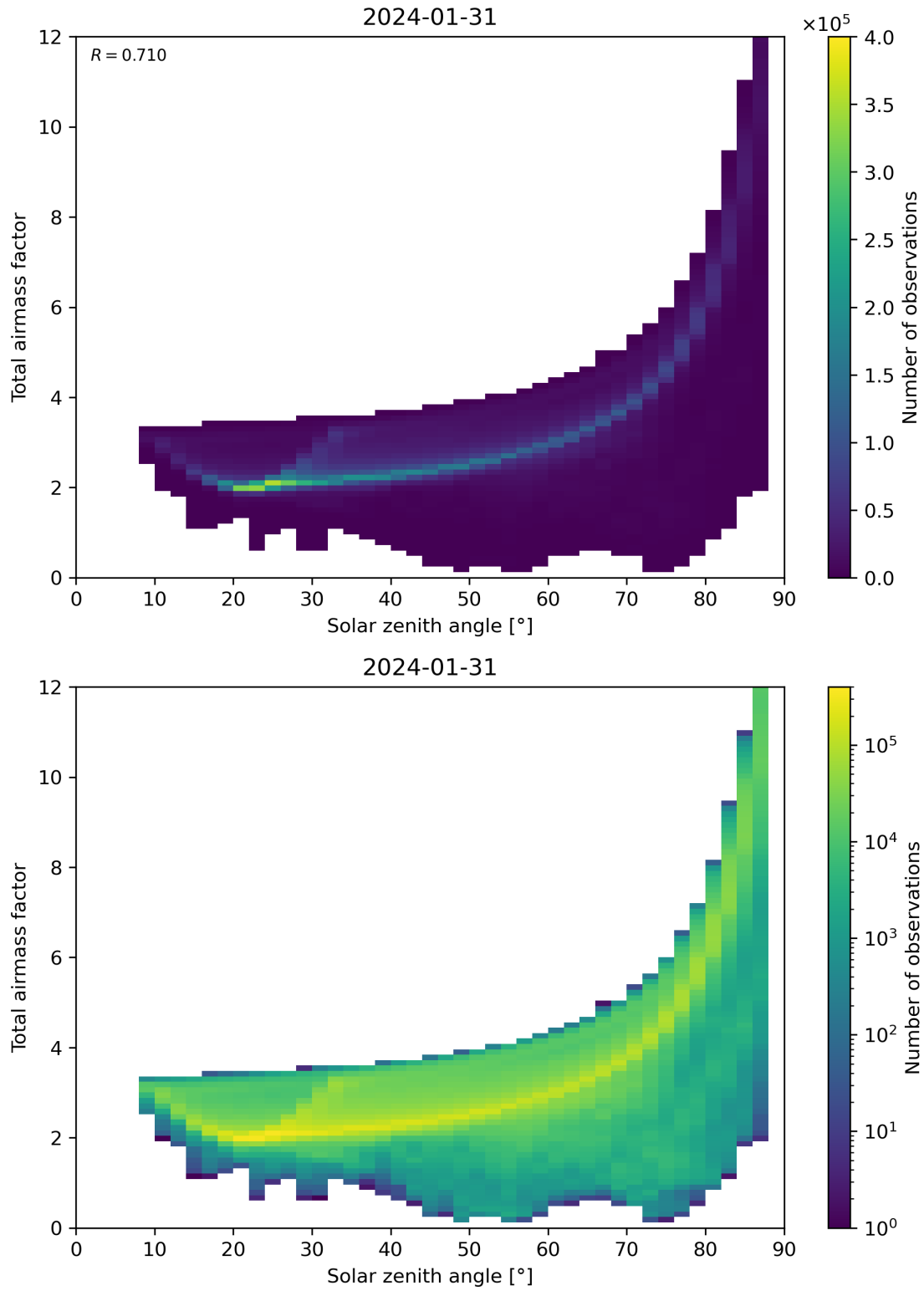
Figure 146: Scatter density plot of “Solar zenith angle” against “Total air mass factor” for 2024-01-31 to 2024-02-01.
