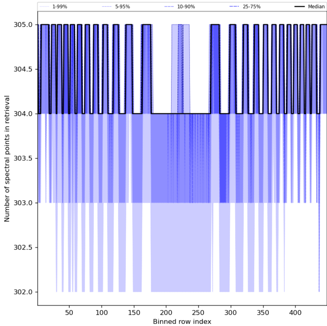
Figure 50: Along track statistics of “Number of spectral points in retrieval” for 2024-01-31 to 2024-02-01
