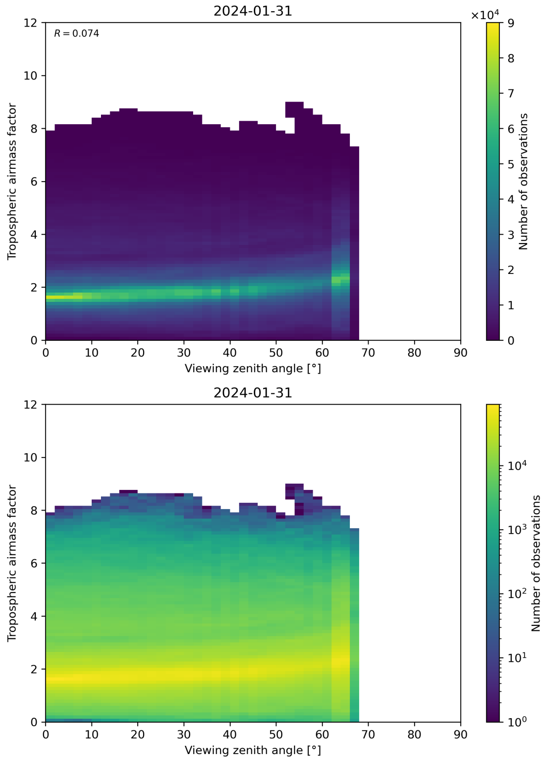
Figure 161: Scatter density plot of “Viewing zenith angle” against “Tropospheric airmass factor” for 2024-01-31 to 2024-02-01.
