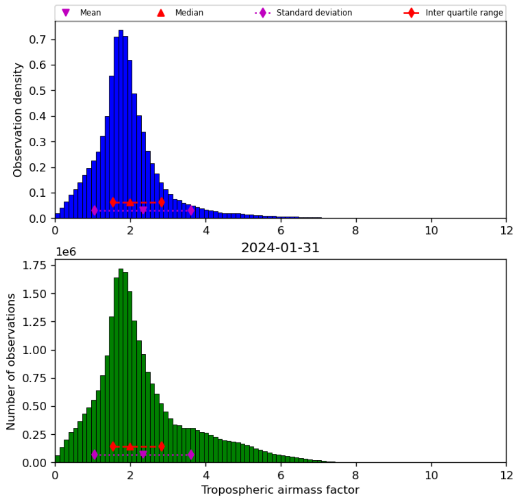
Figure 31: Histogram of “Tropospheric airmass factor” for 2024-01-31 to 2024-02-01
