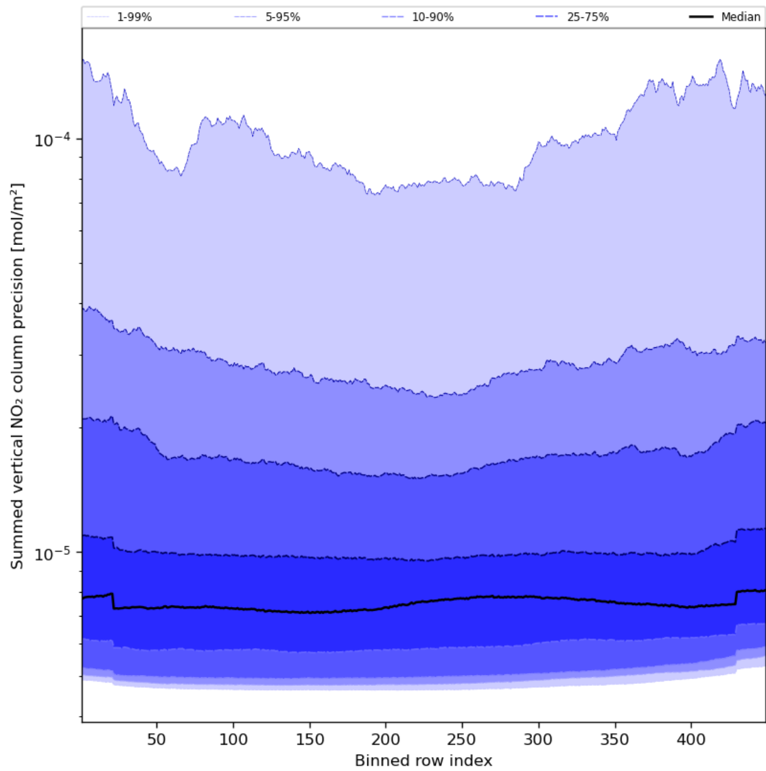
Figure 58: Along track statistics of “Summed vertical NO 2 column precision” for 2024-01-31 to 2024-02-01
