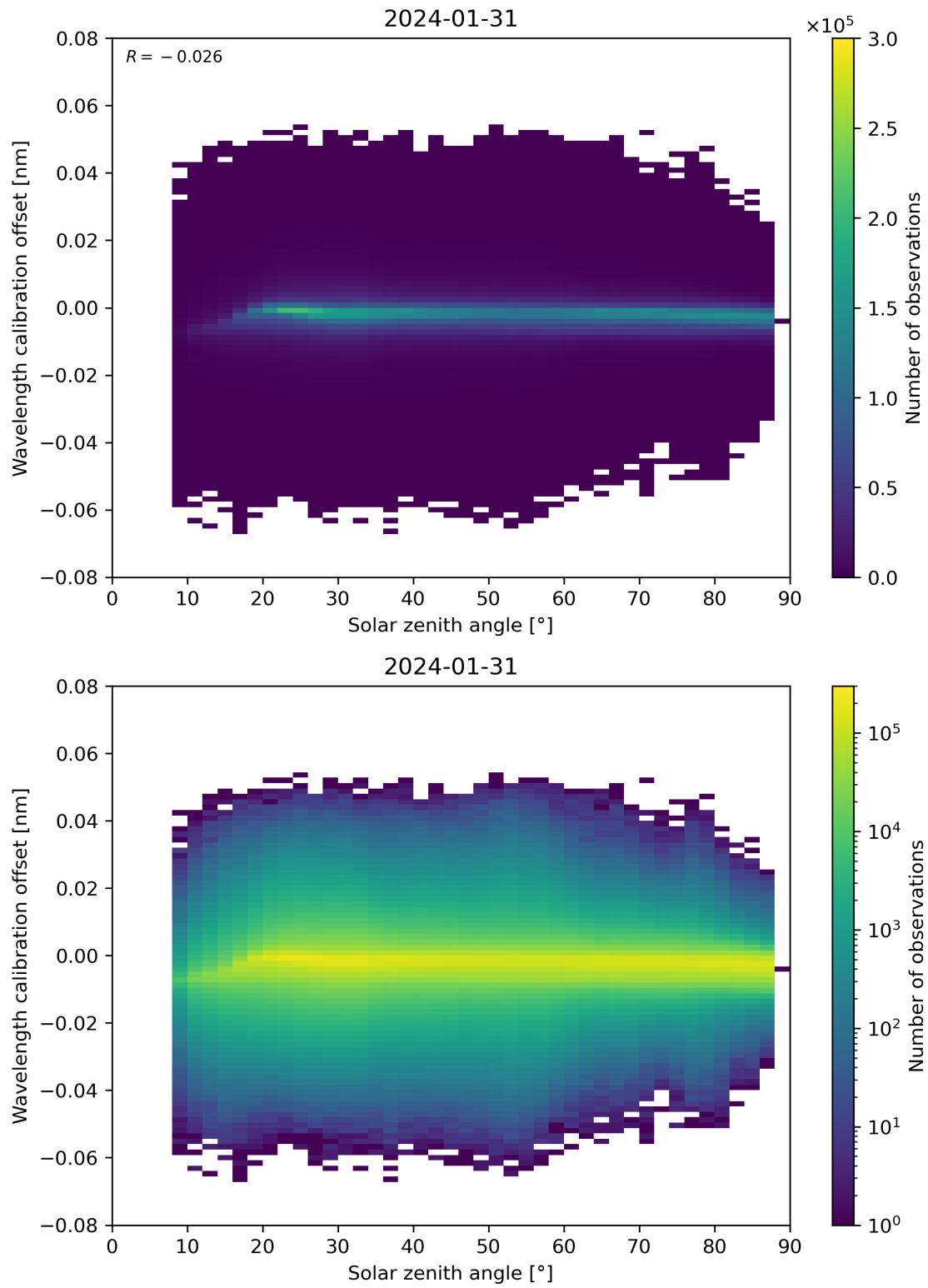
Figure 158: Scatter density plot of “Solar zenith angle” against “Wavelength calibration offset” for 2024-01-31 to 2024-02-01.
