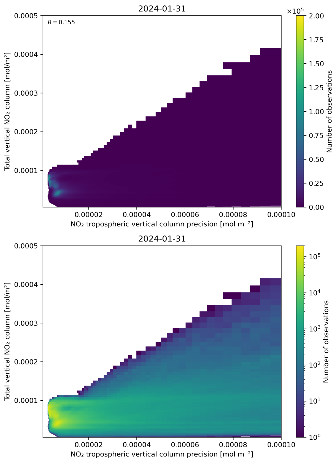
Figure 138: Scatter density plot of “NO 2 tropospheric vertical column precision” against “Total vertical NO 2 column” for 2024-01-31 to 2024-02-01.
