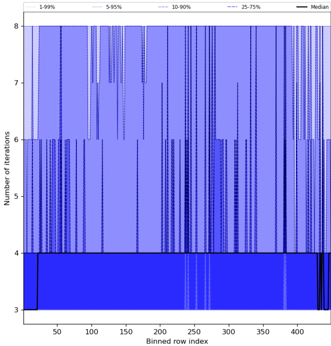
Figure 51: Along track statistics of “Number of iterations” for 2024-01-31 to 2024-02-01
