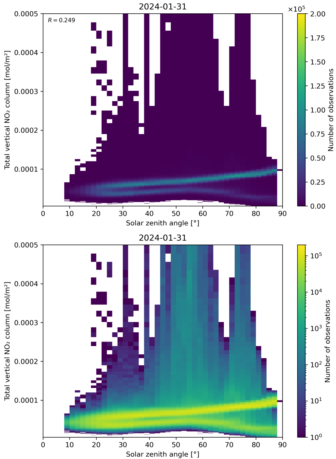
Figure 153: Scatter density plot of “Solar zenith angle” against “Total vertical NO 2 column” for 2024-01-31 to 2024-02-01.
