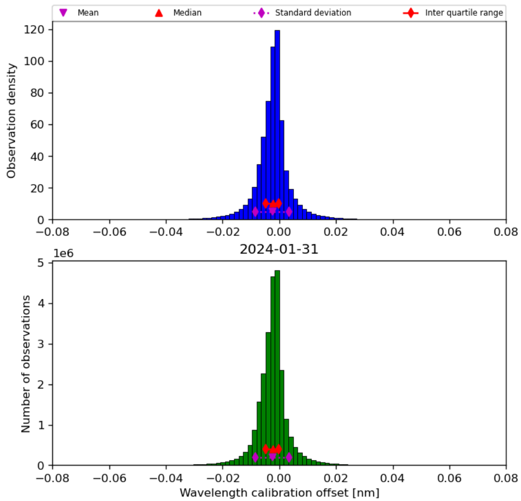
Figure 35: Histogram of “Wavelength calibration offset” for 2024-01-31 to 2024-02-01
