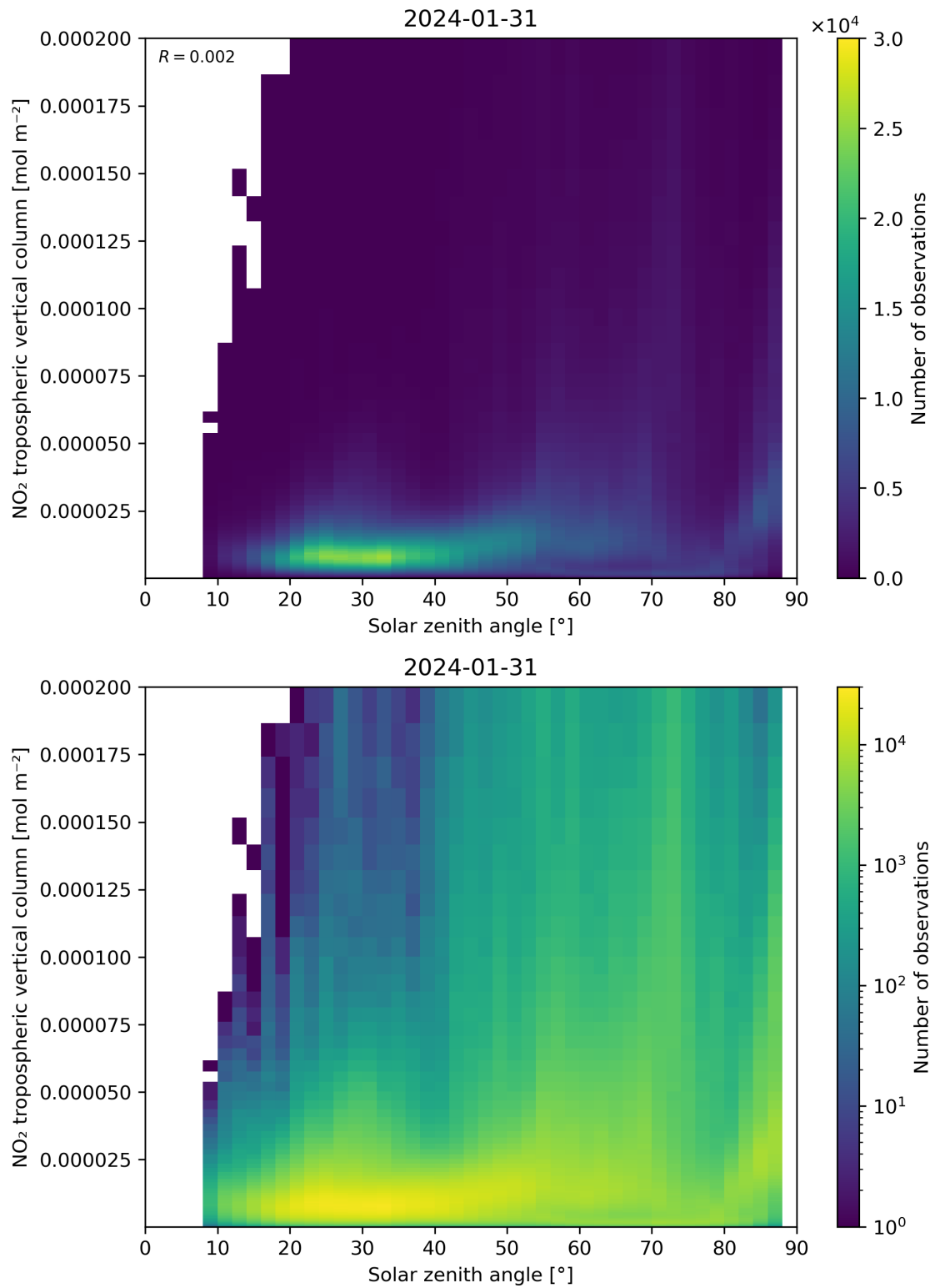
Figure 155: Scatter density plot of “Solar zenith angle” against “NO 2 tropospheric vertical column” for 2024-01-31 to 2024-02-01.
