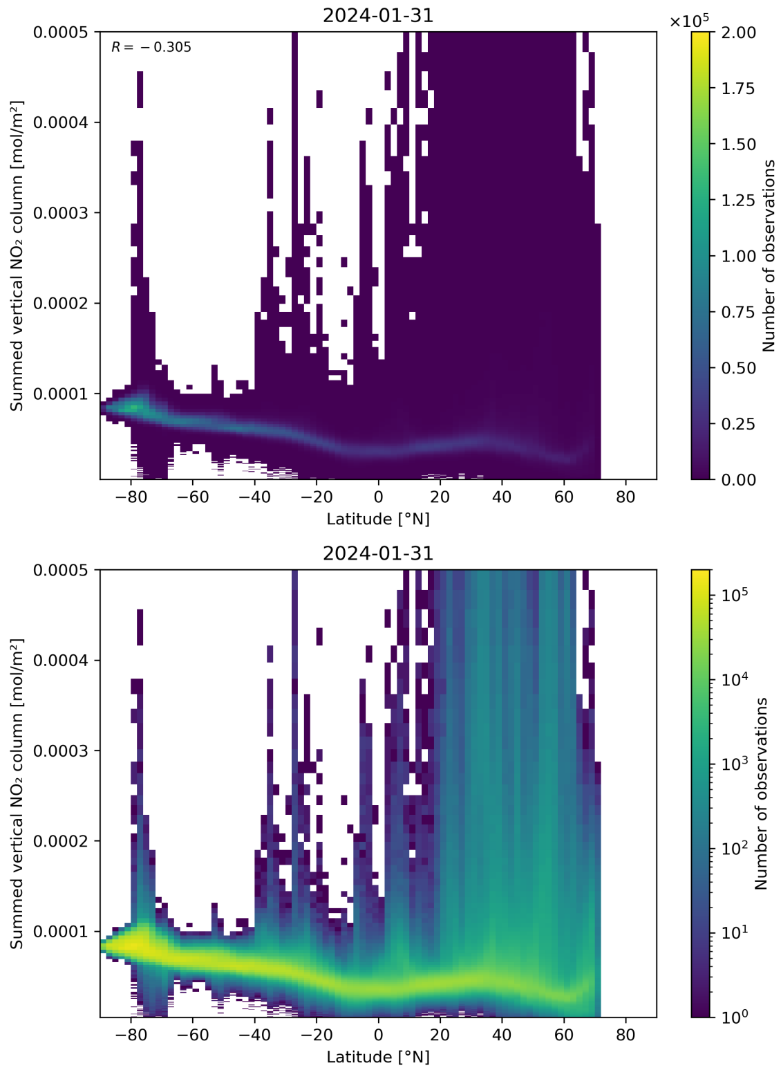
Figure 88: Scatter density plot of “Latitude” against “Summed vertical NO 2 column” for 2024-01-31 to 2024-02-01.
