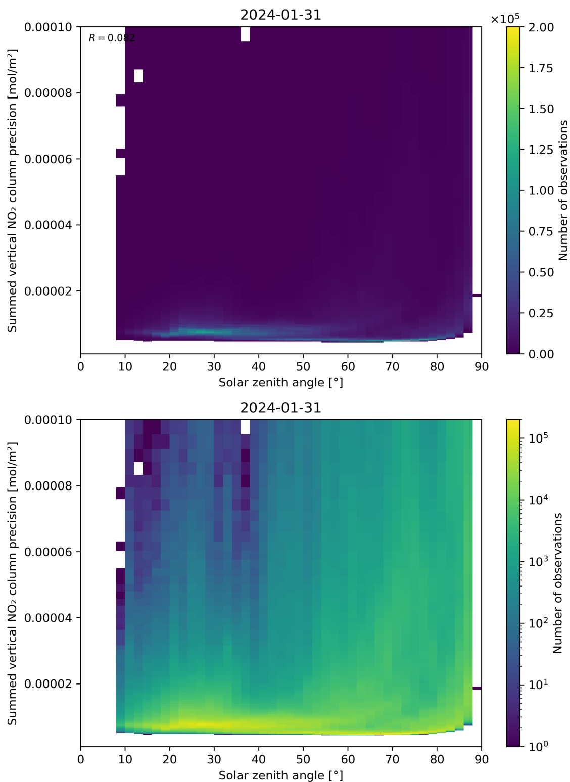
Figure 152: Scatter density plot of “Solar zenith angle” against “Summed vertical NO 2 column precision” for 2024-01-31 to 2024-02-01.
