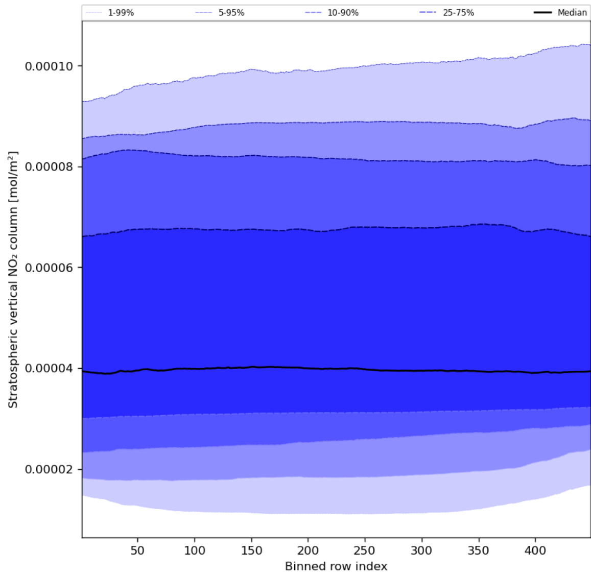
Figure 53: Along track statistics of “Stratospheric vertical NO 2 column” for 2024-01-31 to 2024-02-01
