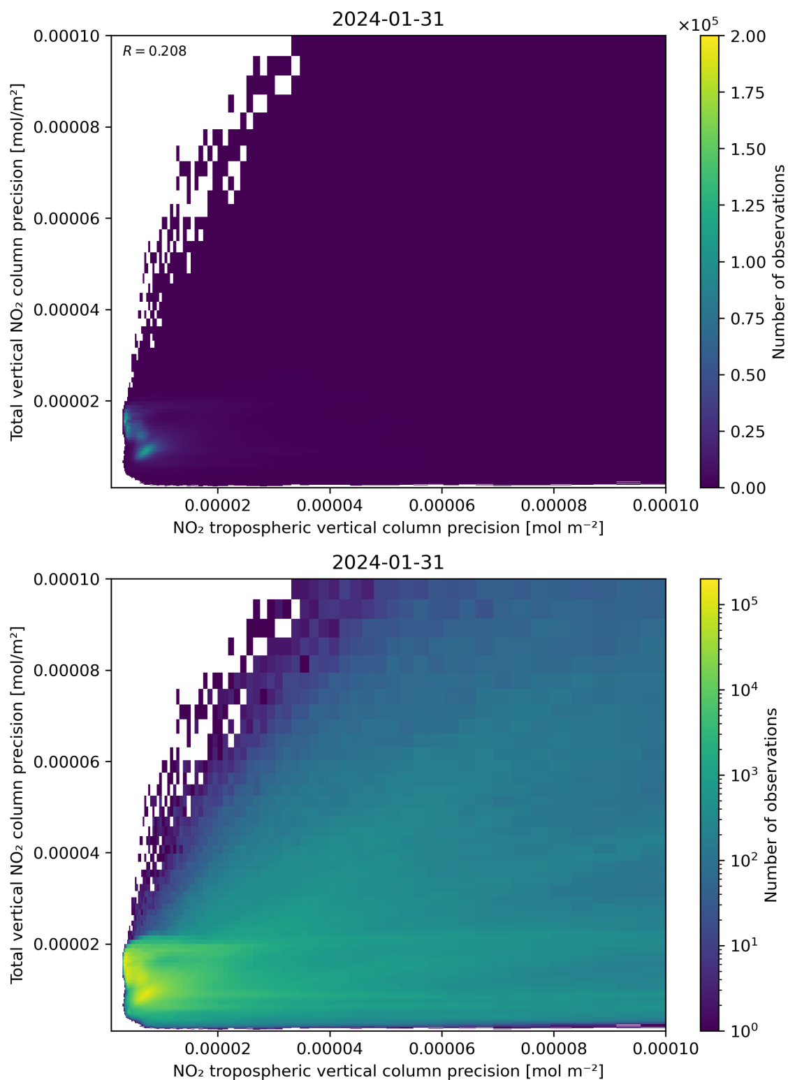
Figure 139: Scatter density plot of “NO 2 tropospheric vertical column precision” against “Total vertical NO 2 column precision” for 2024-01-31 to 2024-02-01.
