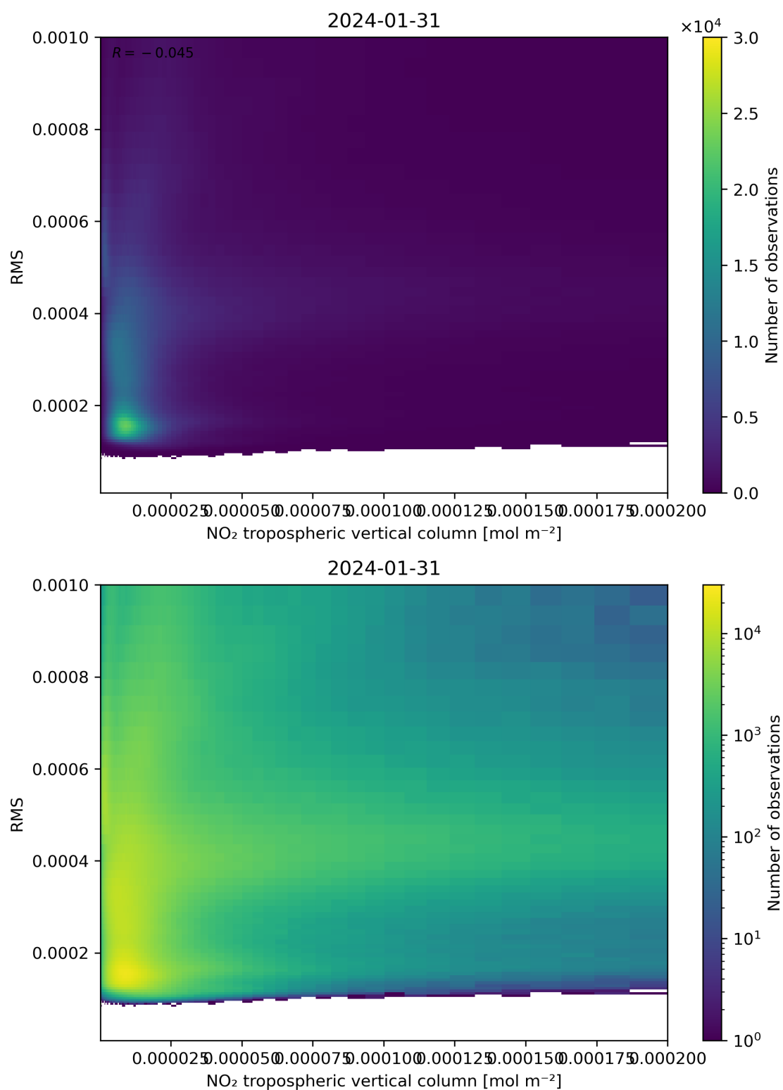
Figure 142: Scatter density plot of “NO 2 tropospheric vertical column” against “RMS” for 2024-01-31 to 2024-02-01.
