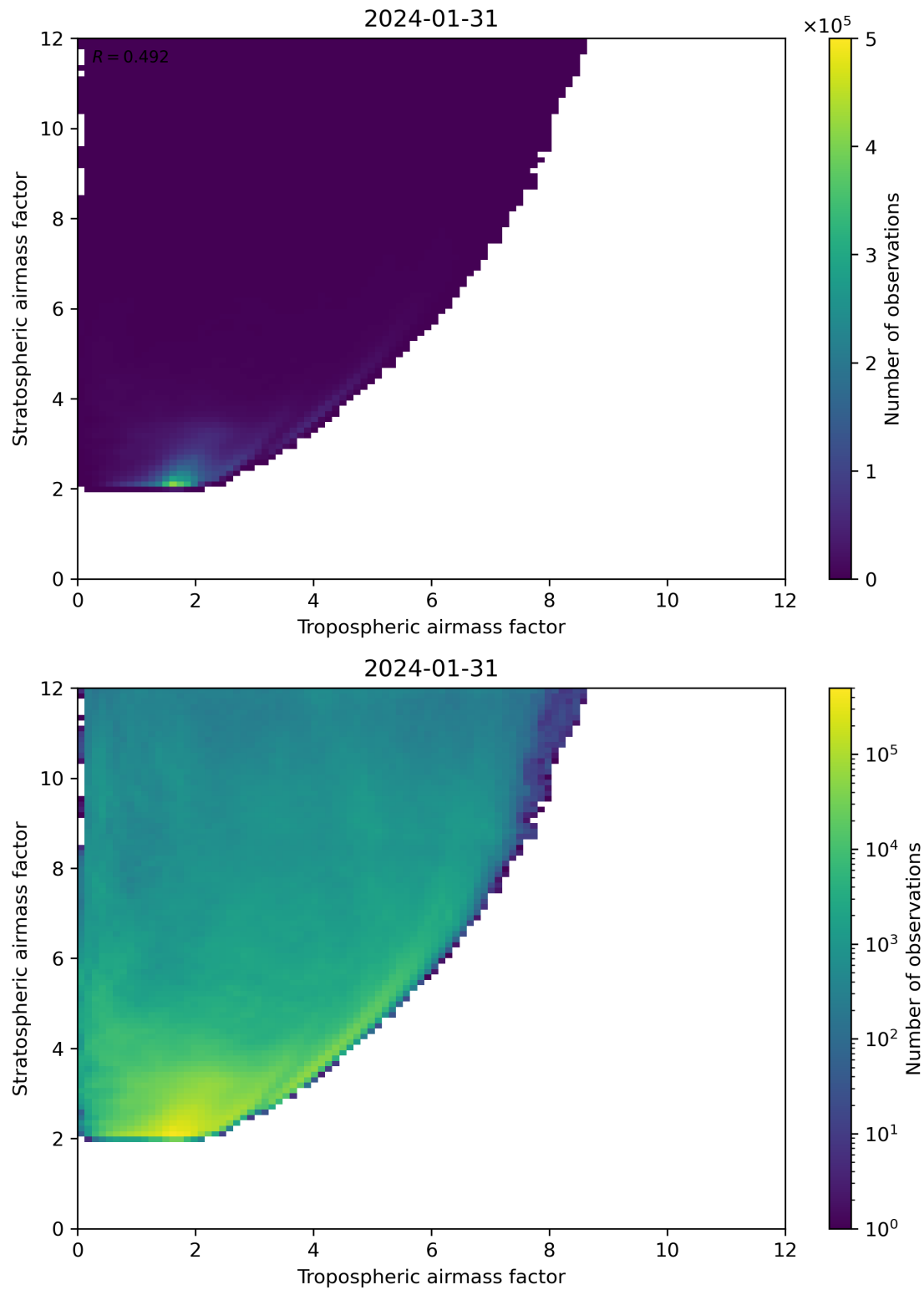
Figure 71: Scatter density plot of “Tropospheric airmass factor” against “Stratospheric airmass factor” for 2024-01-31 to 2024-02-01.
