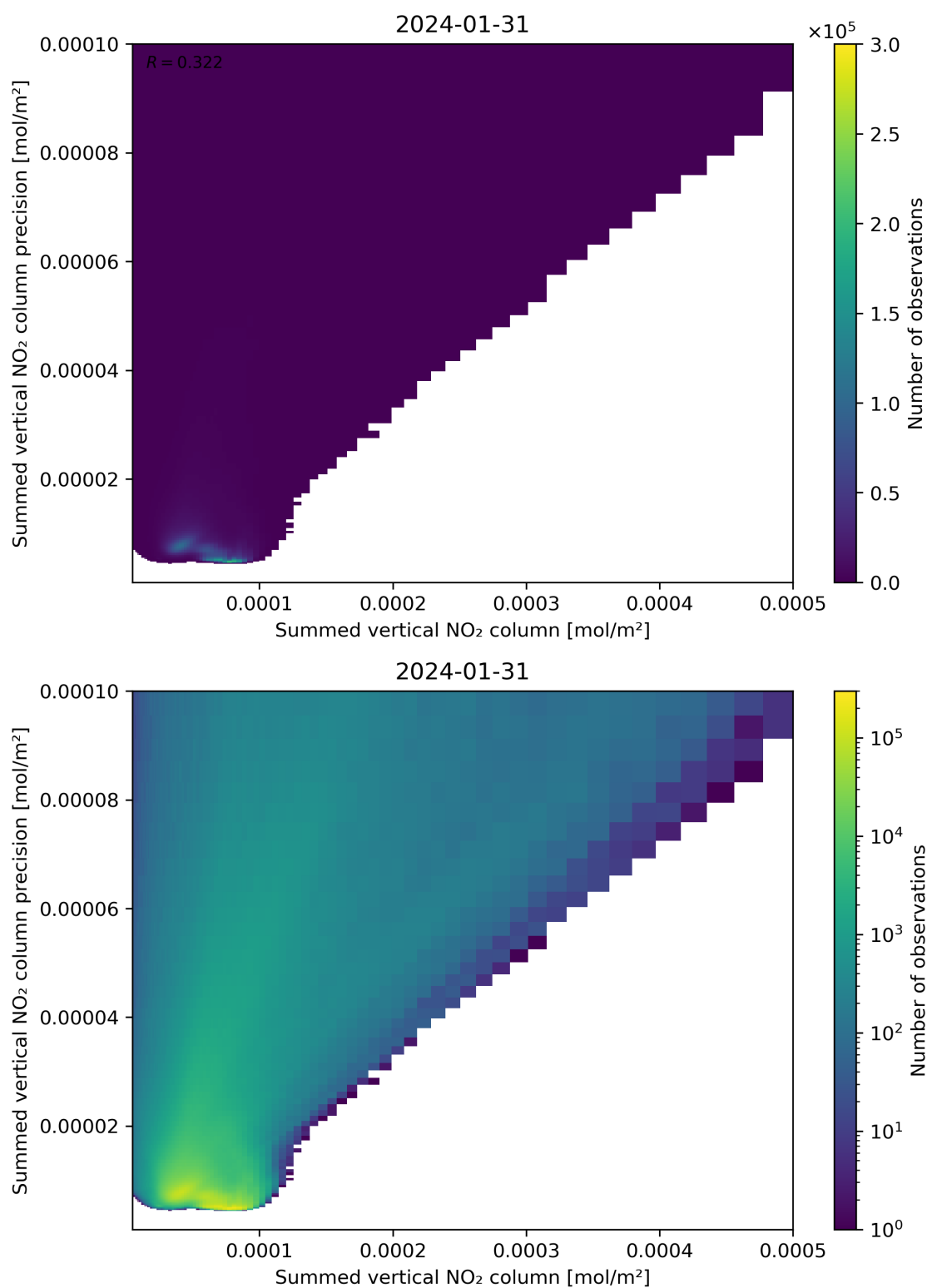
Figure 105: Scatter density plot of “Summed vertical NO 2 column” against “Summed vertical NO 2 column precision” for 2024-01-31 to 2024-02-01.
