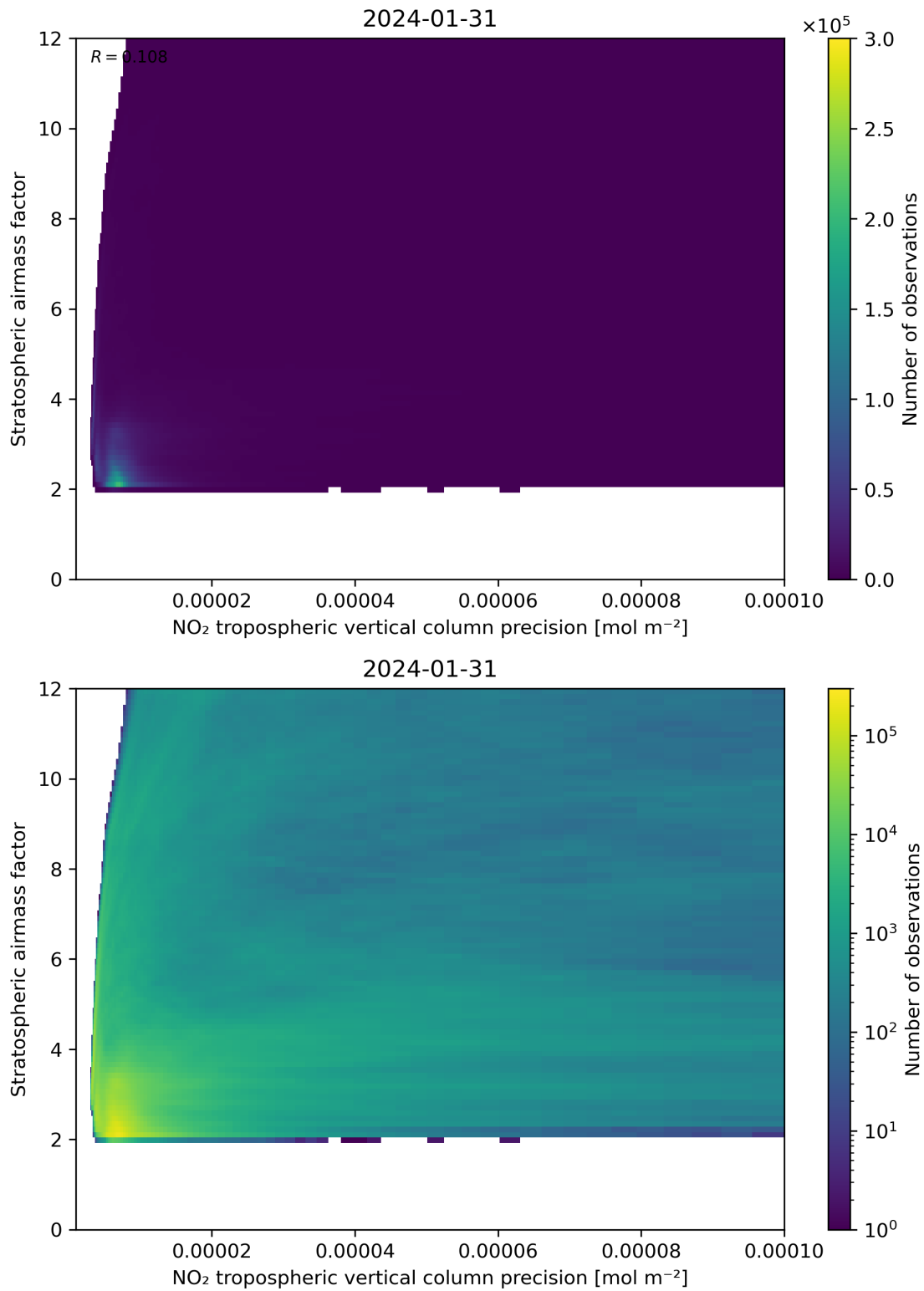
Figure 131: Scatter density plot of “NO 2 tropospheric vertical column precision” against “Stratospheric airmass factor” for 2024-01-31 to 2024-02-01.
