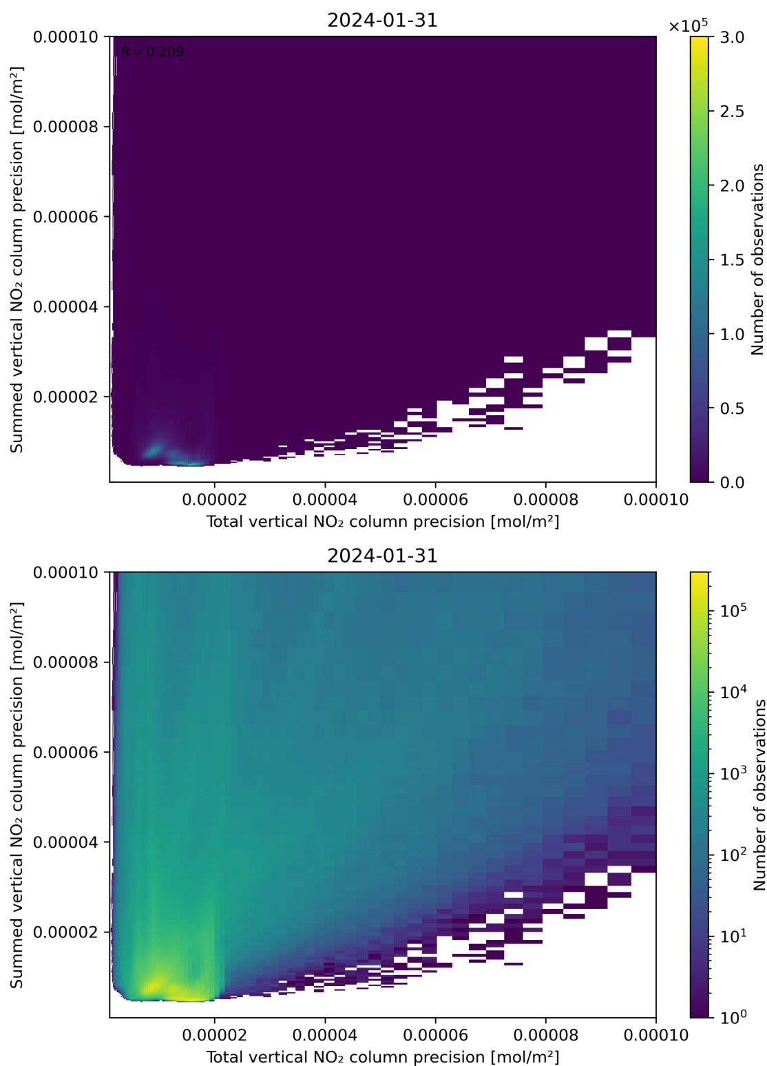
Figure 118: Scatter density plot of “Total vertical NO 2 column precision” against “Summed vertical NO 2 column precision” for 2024-01-31 to 2024-02-01.
