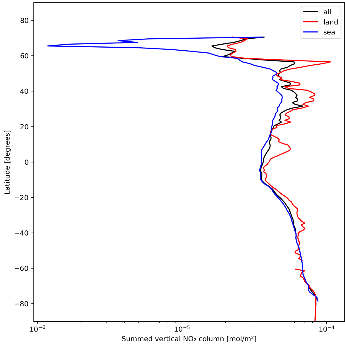
Figure 23: Zonal average of “Summed vertical NO 2 column” for 2024-01-31 to 2024-02-01.
