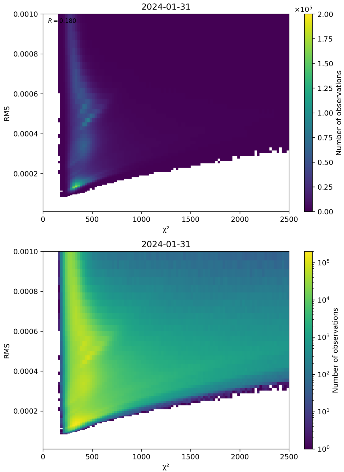
Figure 82: Scatter density plot of “ \chi^2 ” against “RMS” for 2024-01-31 to 2024-02-01.
