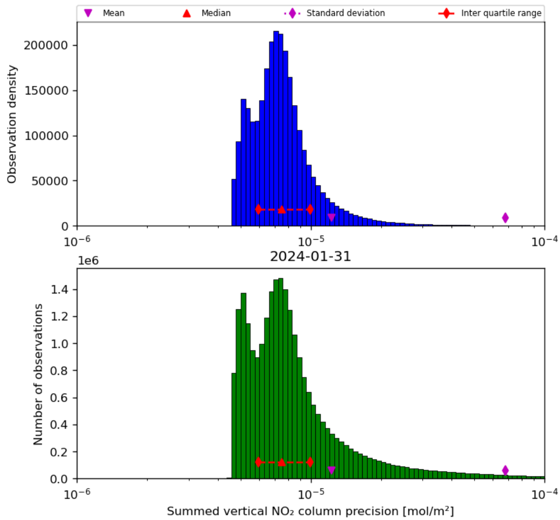
Figure 41: Histogram of "Summed vertical NO 2 column precision" for 2024-01-31 to 2024-02-01
