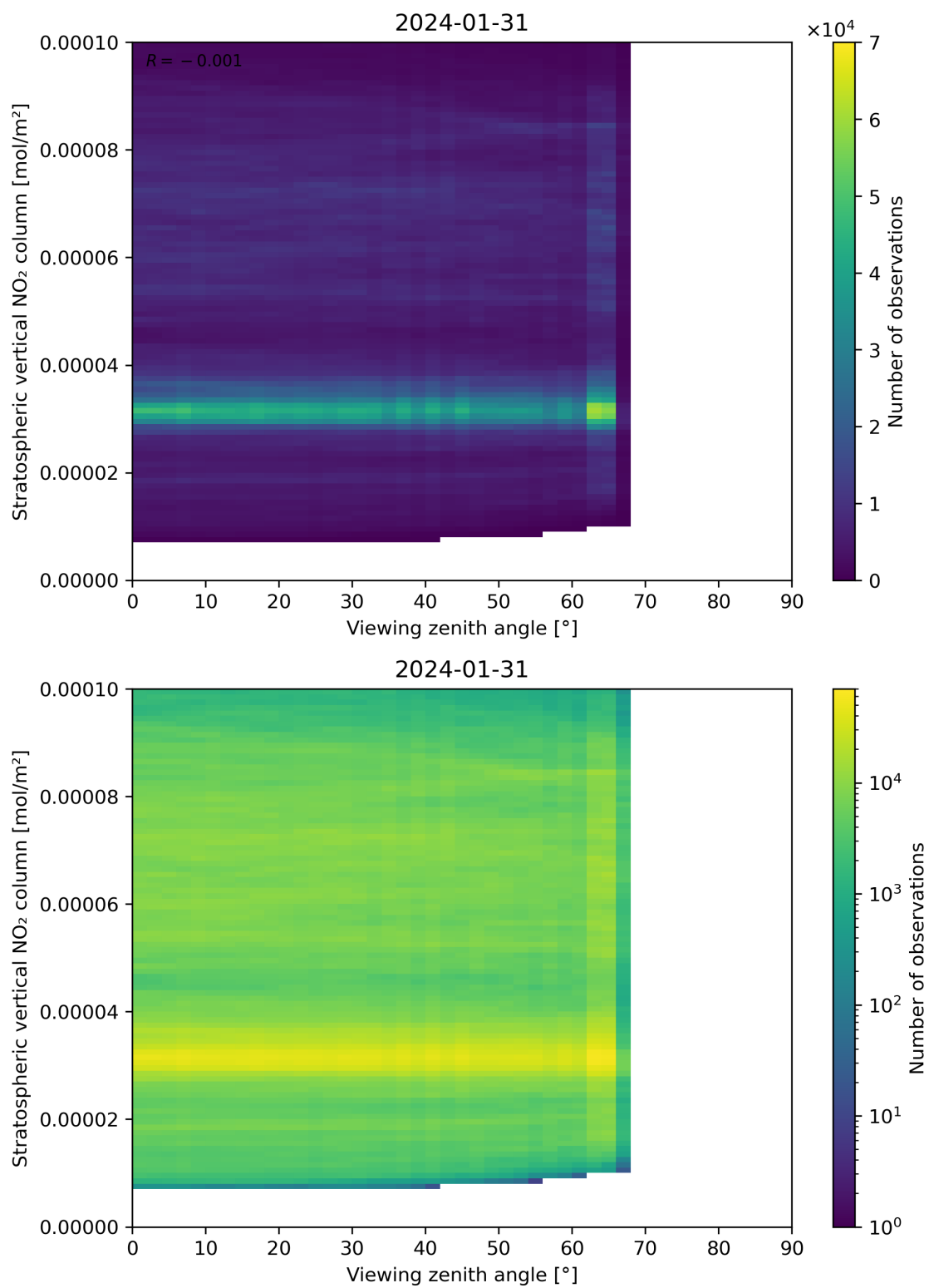
Figure 164: Scatter density plot of “Viewing zenith angle” against “Stratospheric vertical NO 2 column” for 2024-01-31 to 2024-02-01.
