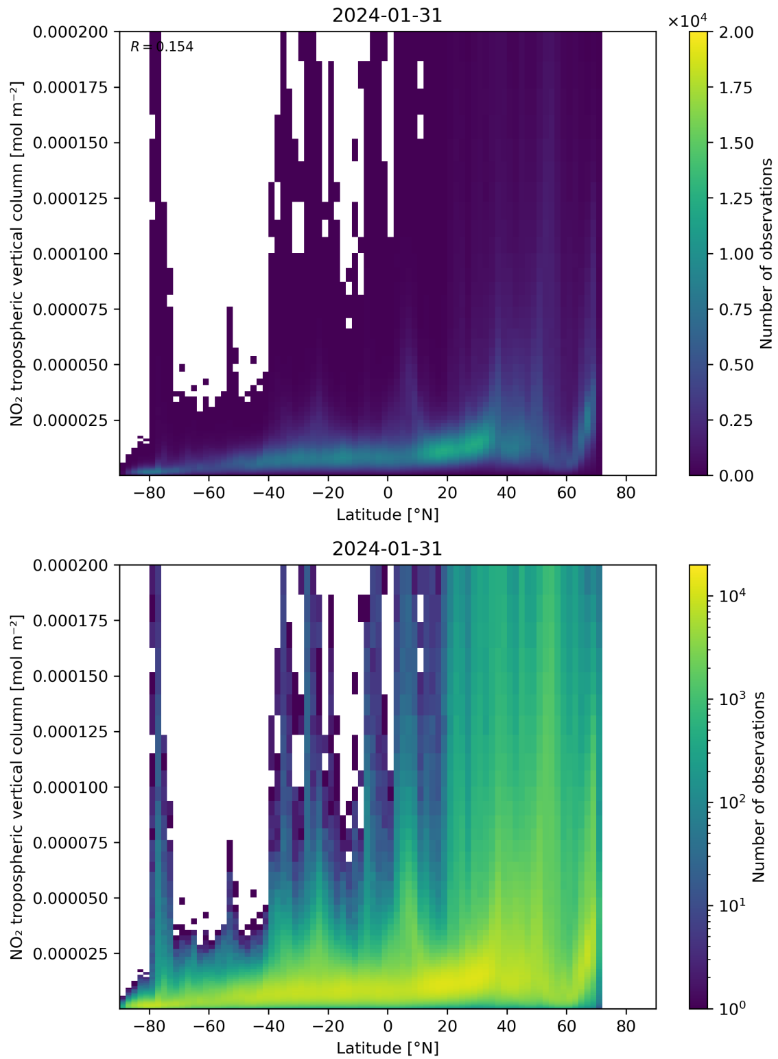
Figure 92: Scatter density plot of “Latitude” against “NO 2 tropospheric vertical column” for 2024-01-31 to 2024-02-01.
