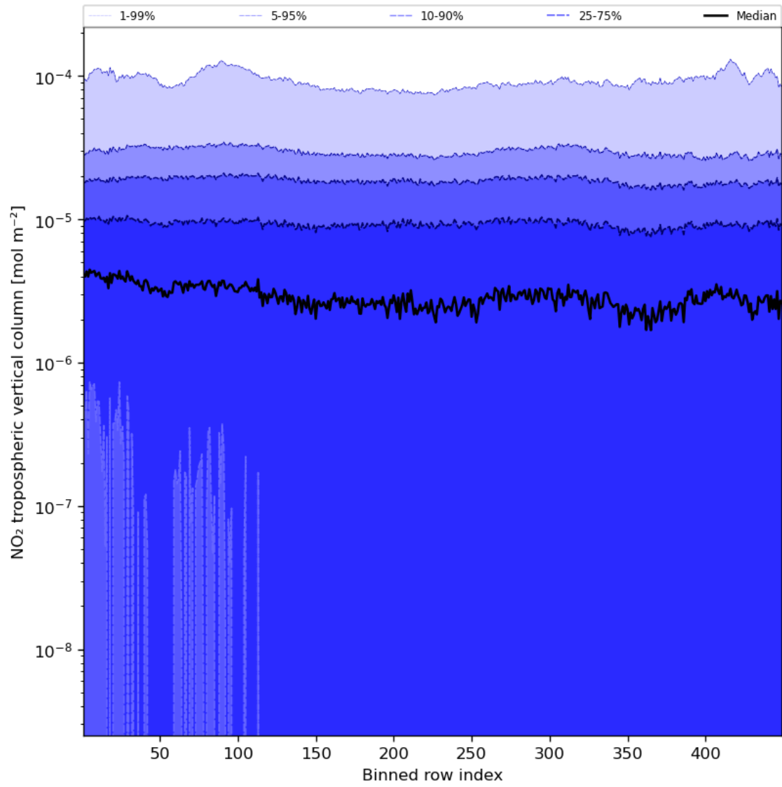
Figure 46: Along track statistics of “NO 2 tropospheric vertical column” for 2024-01-31 to 2024-02-01
