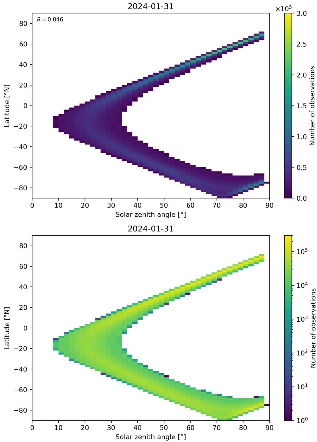
Figure 149: Scatter density plot of “Solar zenith angle” against “Latitude” for 2024-01-31 to 2024-02-01.
