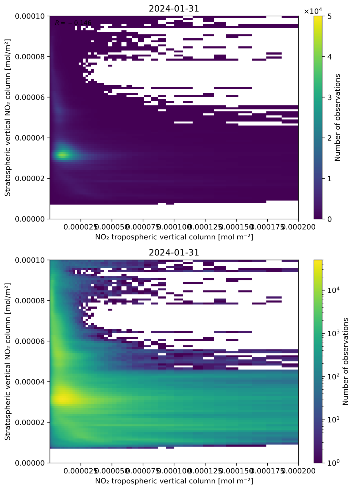
Figure 125: Scatter density plot of “NO 2 tropospheric vertical column” against “Stratospheric vertical NO 2 column” for 2024-01-31 to 2024-02-01.
