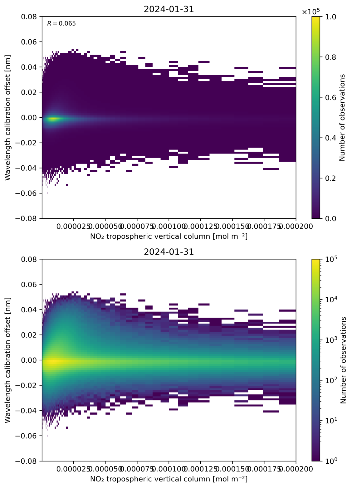
Figure 143: Scatter density plot of “NO 2 tropospheric vertical column” against “Wavelength calibration offset” for 2024-01-31 to 2024-02-01.
