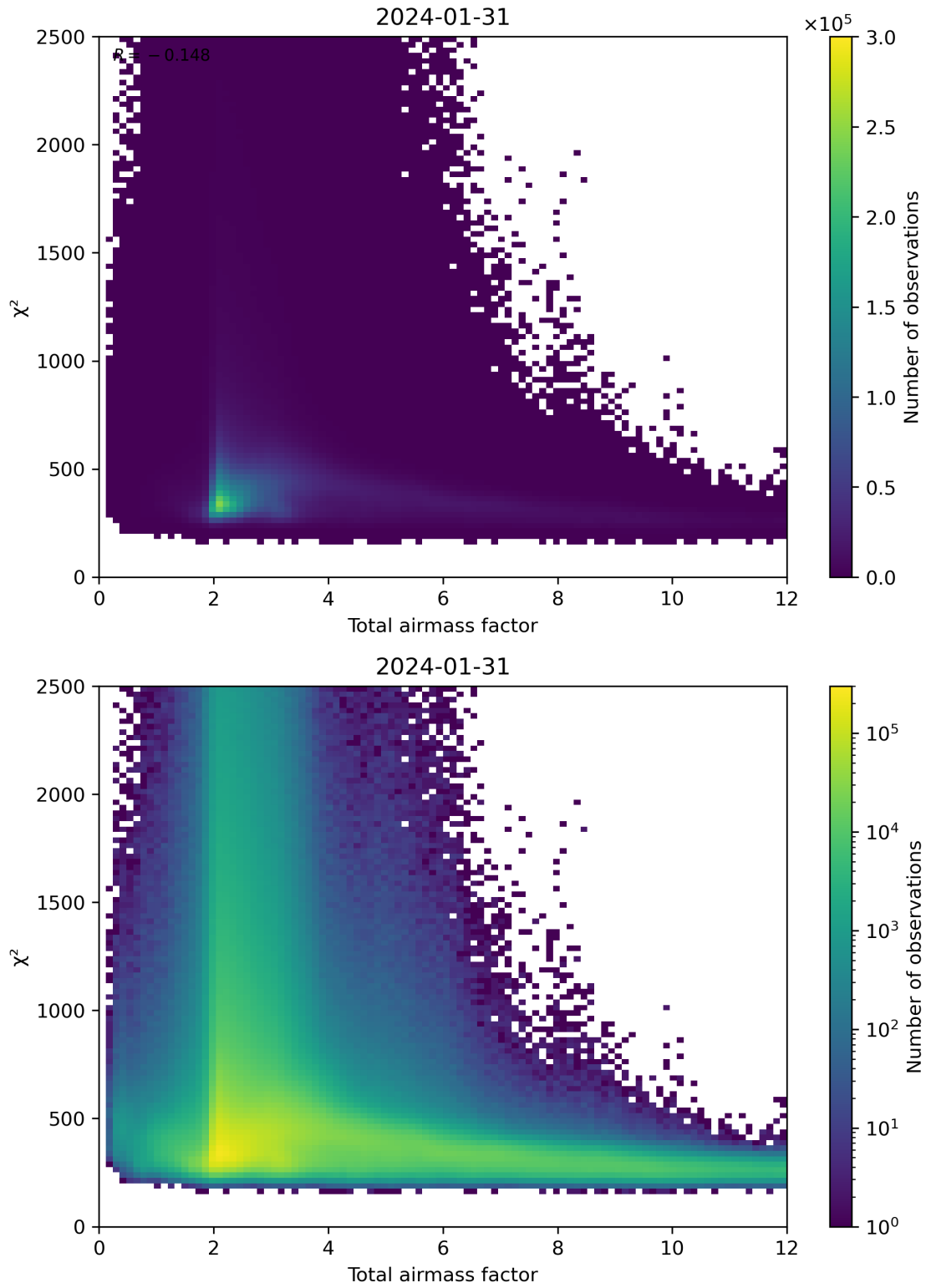
Figure 63: Scatter density plot of “Total airmass factor” against “ \chi^2 ” for 2024-01-31 to 2024-02-01.
