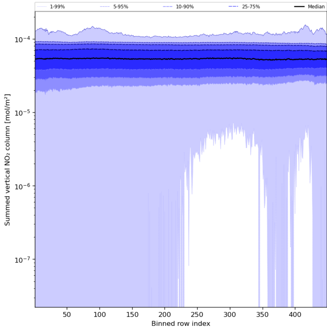
Figure 57: Along track statistics of “Summed vertical NO 2 column” for 2024-01-31 to 2024-02-01
