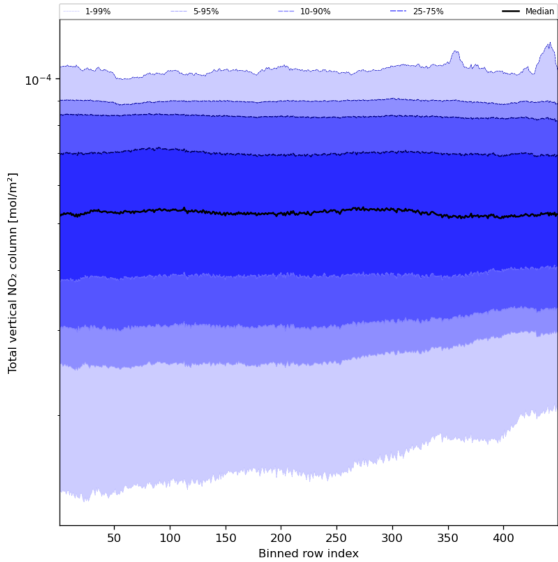
Figure 55: Along track statistics of “Total vertical NO 2 column” for 2024-01-31 to 2024-02-01
