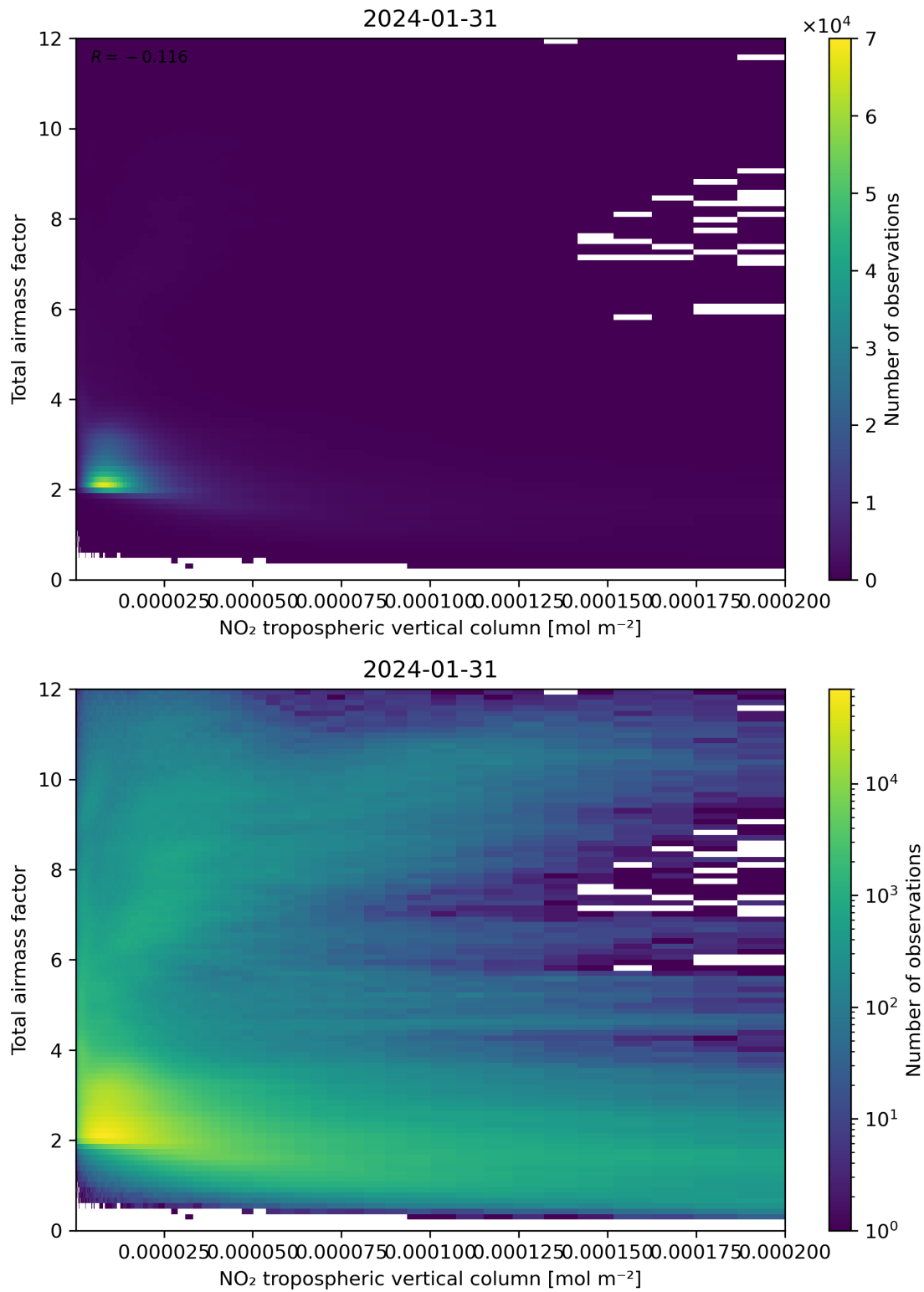
Figure 122: Scatter density plot of “NO 2 tropospheric vertical column” against “Total air mass factor” for 2024-01-31 to 2024-02-01.
