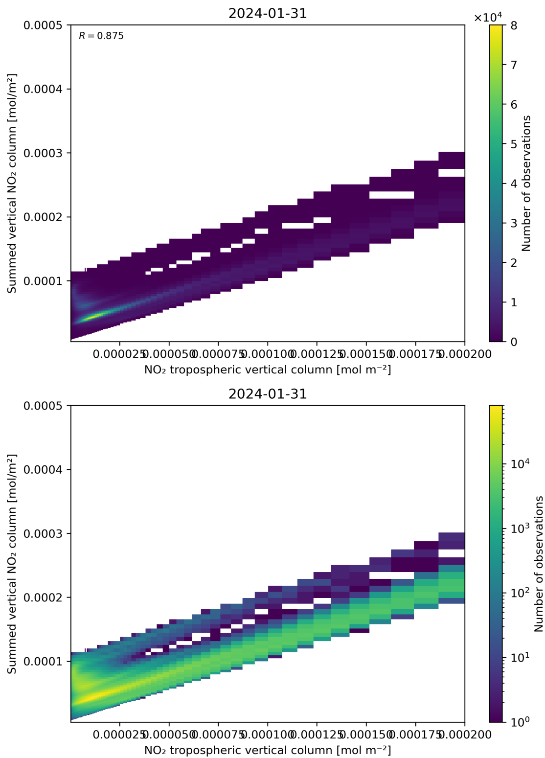
Figure 126: Scatter density plot of “NO 2 tropospheric vertical column” against “Summed vertical NO 2 column” for 2024-01-31 to 2024-02-01.
