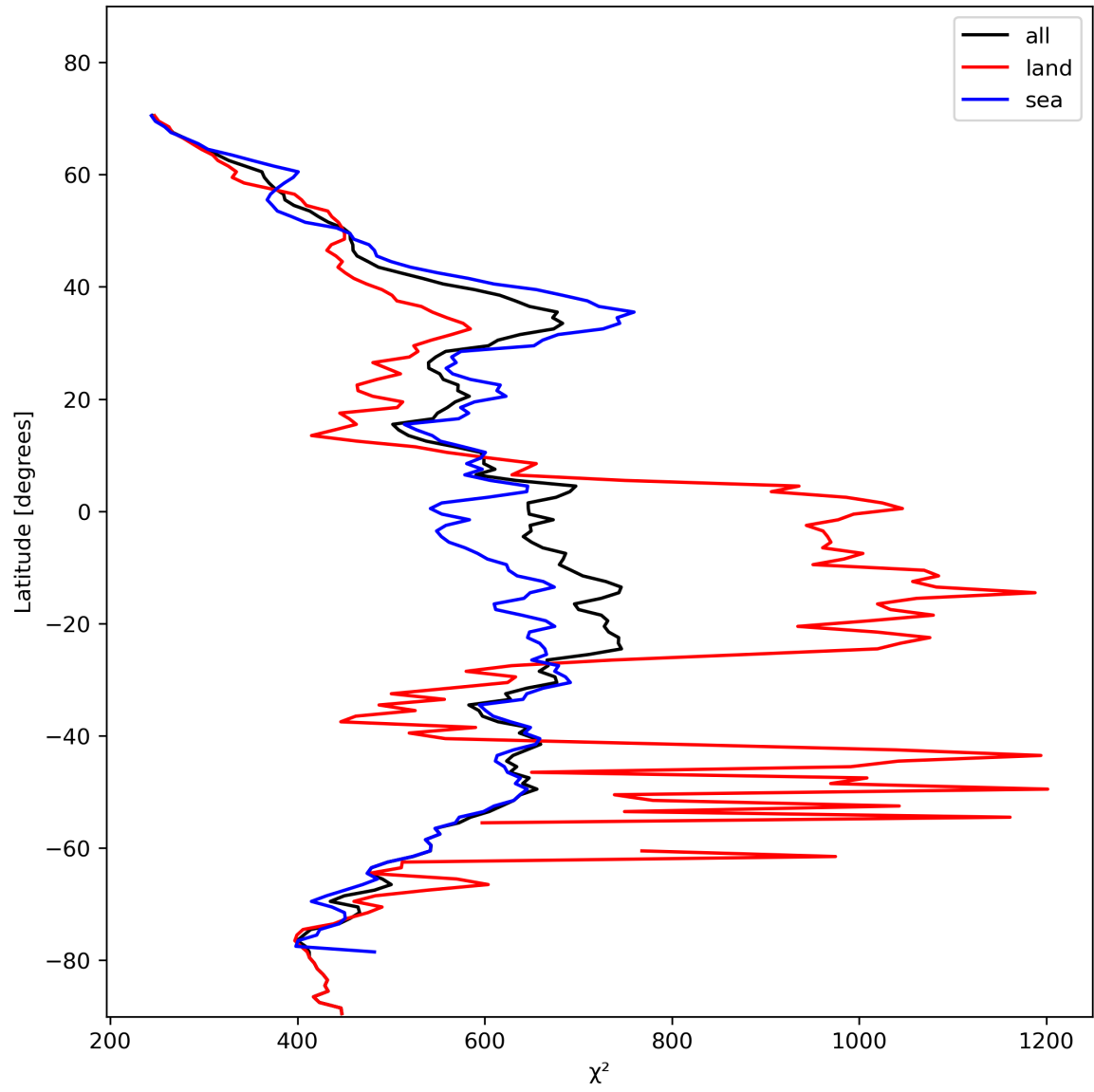
Figure 25: Zonal average of “ \chi^2 ” for 2024-01-31 to 2024-02-01.
