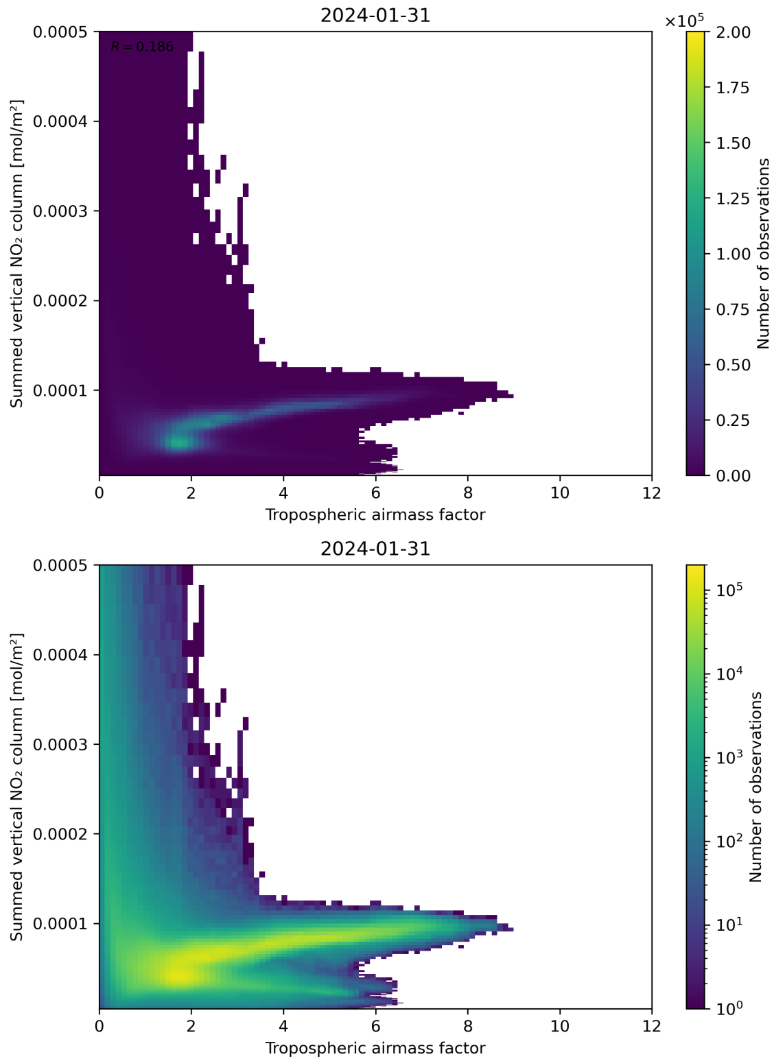
Figure 75: Scatter density plot of “Tropospheric airmass factor” against “Summed vertical NO 2 column” for 2024-01-31 to 2024-02-01.
