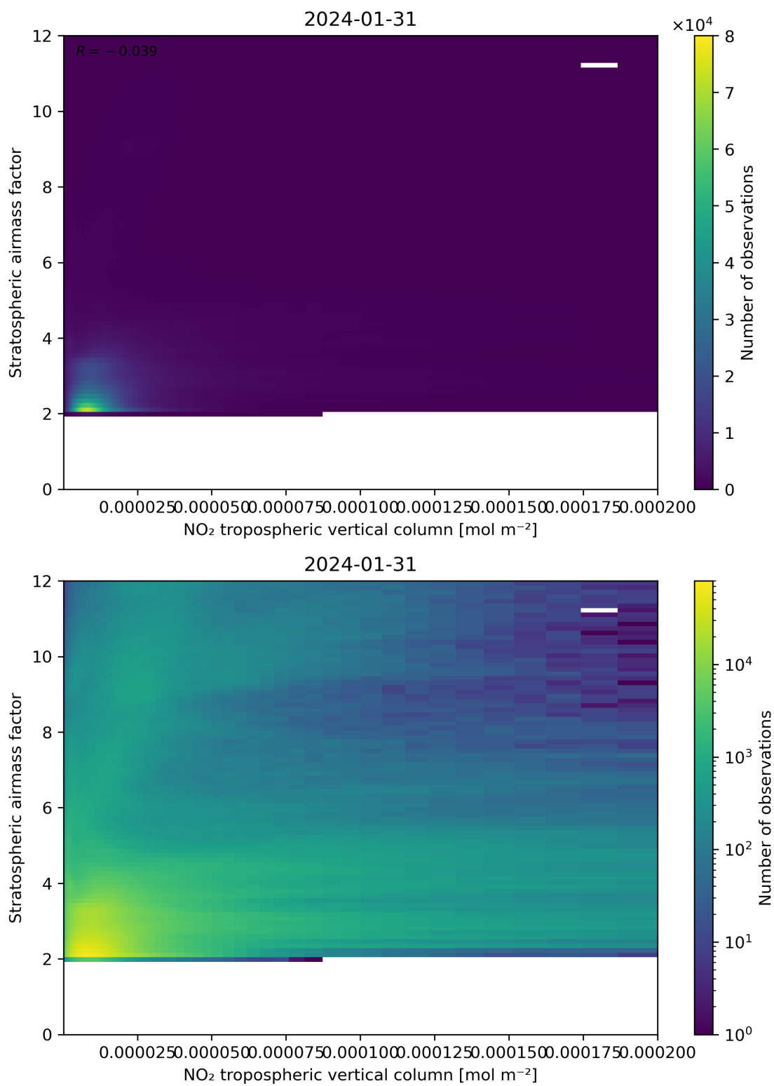
Figure 121: Scatter density plot of “NO 2 tropospheric vertical column” against “Stratospheric airmass factor” for 2024-01-31 to 2024-02-01.
