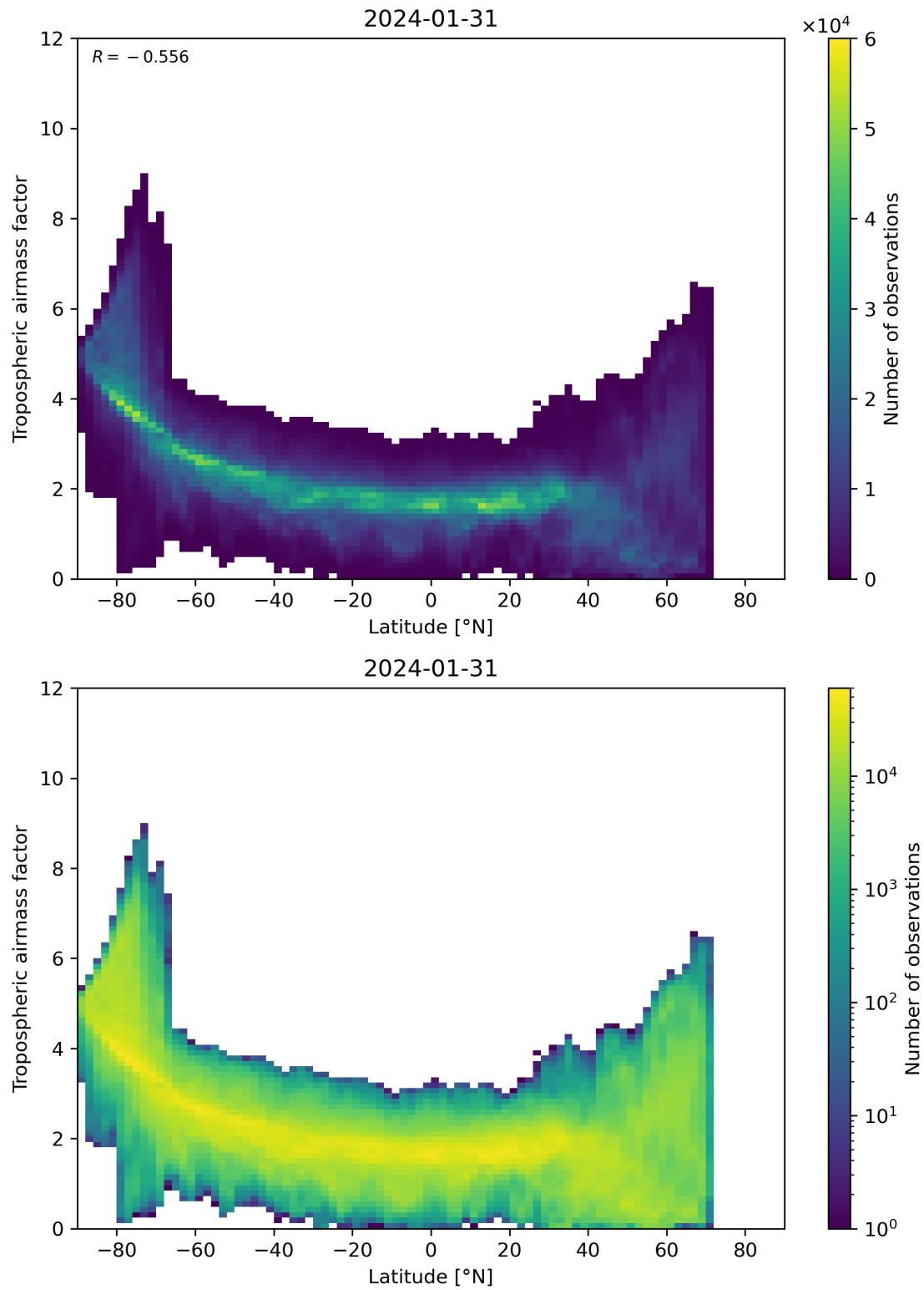
Figure 85: Scatter density plot of “Latitude” against “Tropospheric airmass factor” for 2024-01-31 to 2024-02-01.
