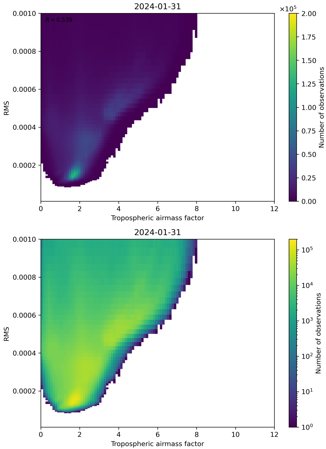
Figure 79: Scatter density plot of “Tropospheric airmass factor” against “RMS” for 2024-01-31 to 2024-02-01.
