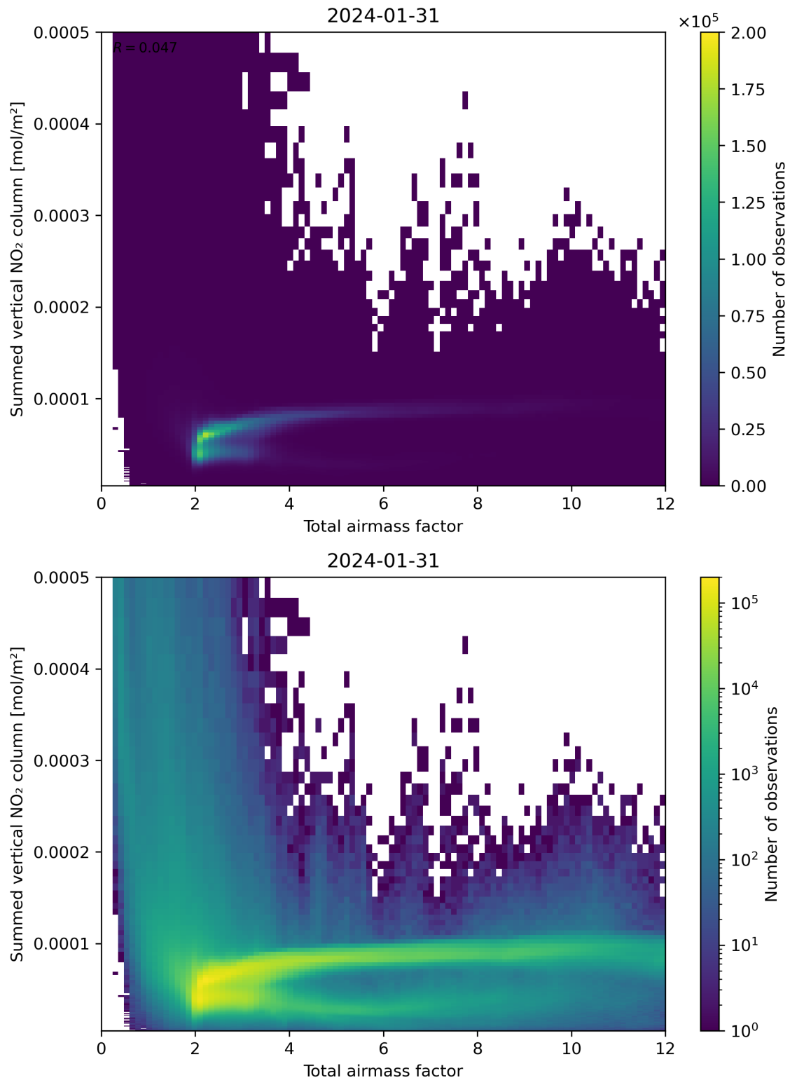
Figure 65: Scatter density plot of “Total airmass factor” against “Summed vertical NO 2 column” for 2024-01-31 to 2024-02-01.
