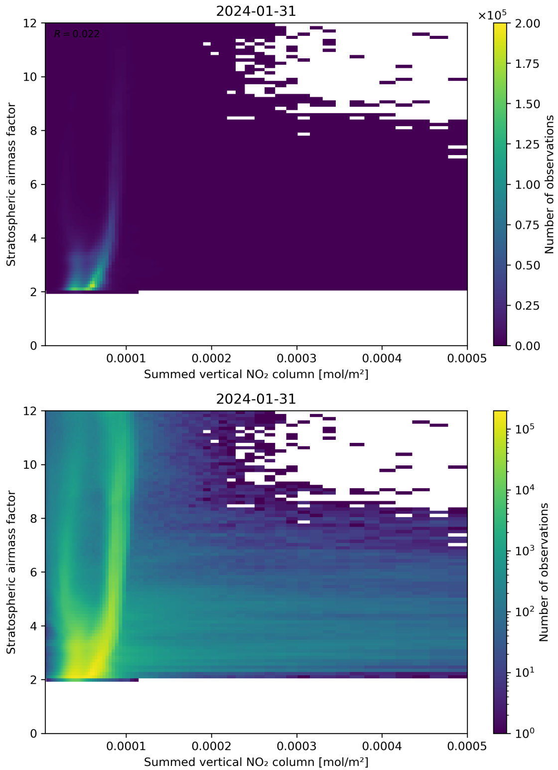
Figure 103: Scatter density plot of “Summed vertical NO 2 column” against “Stratospheric air mass factor” for 2024-01-31 to 2024-02-01.
