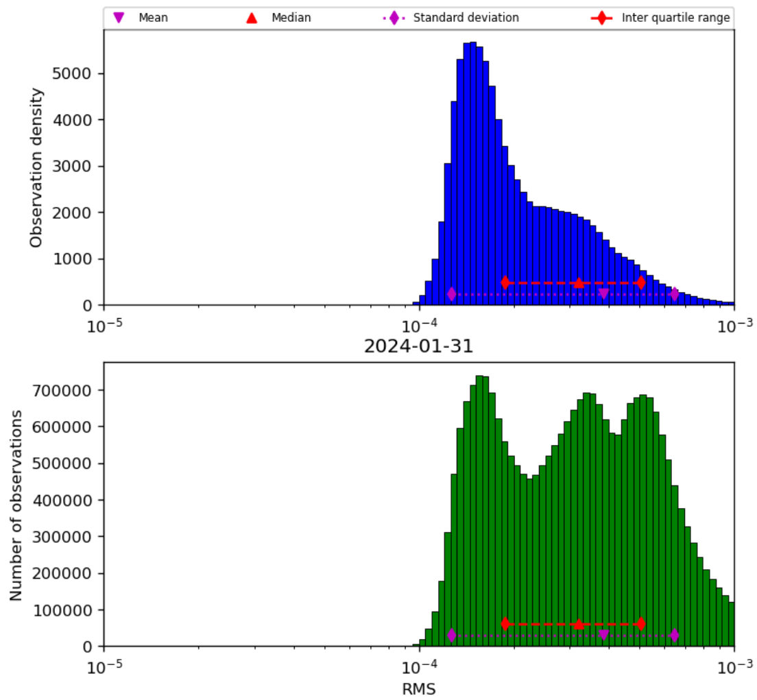
Figure 43: Histogram of “RMS” for 2024-01-31 to 2024-02-01
