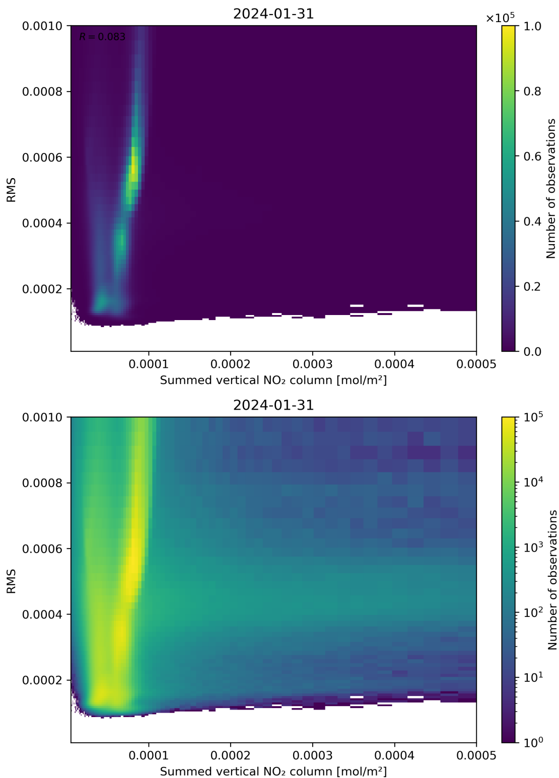
Figure 109: Scatter density plot of “Summed vertical NO 2 column” against “RMS” for 2024-01-31 to 2024-02-01.
