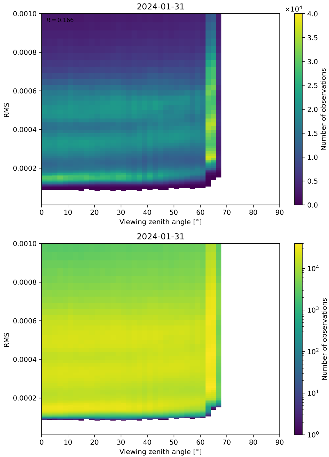
Figure 171: Scatter density plot of “Viewing zenith angle” against “RMS” for 2024-01-31 to 2024-02-01.
