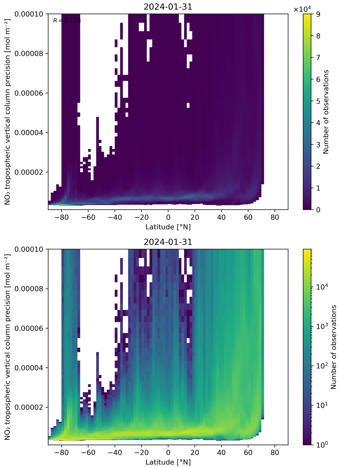
Figure 93: Scatter density plot of “Latitude” against “NO 2 tropospheric vertical column precision” for 2024-01-31 to 2024-02-01.
