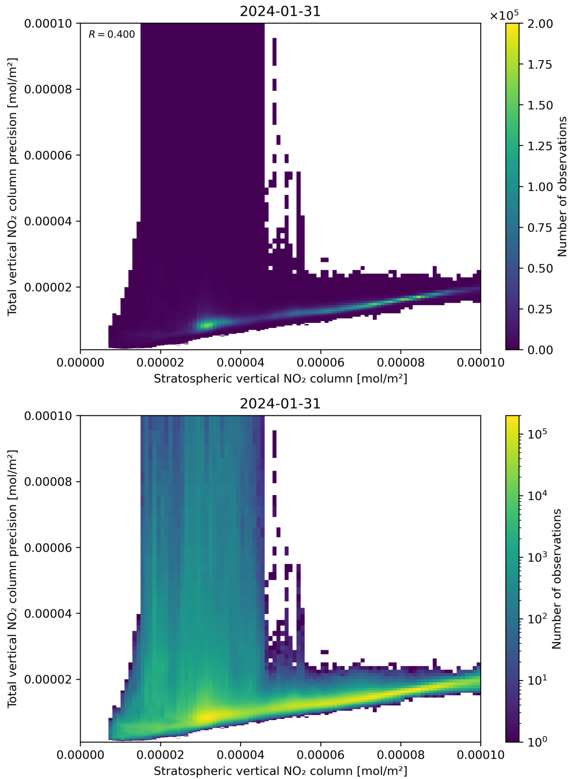
Figure 101: Scatter density plot of “Stratospheric vertical NO 2 column” against “Total vertical NO 2 column precision” for 2024-01-31 to 2024-02-01.
