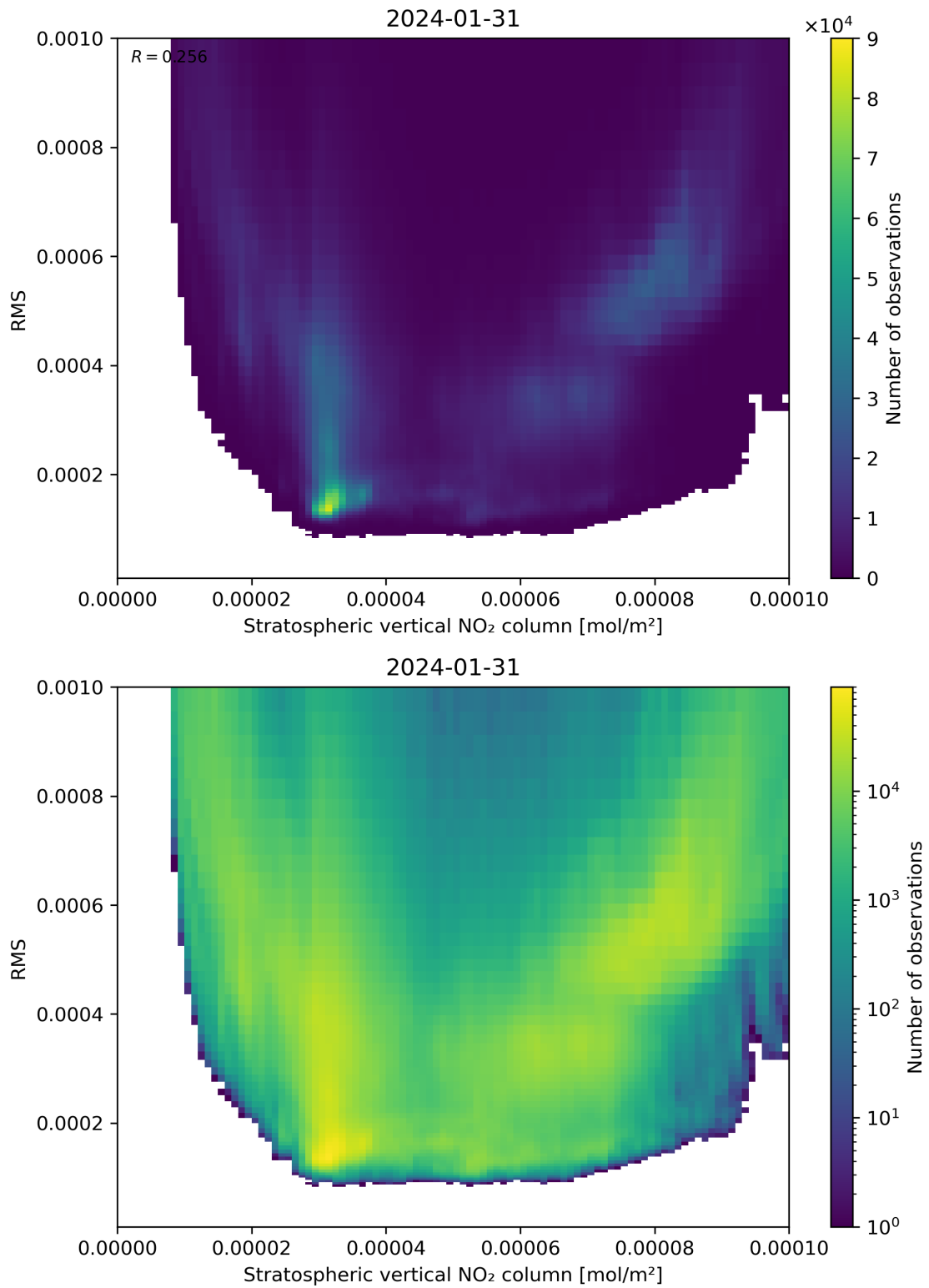
Figure 102: Scatter density plot of “Stratospheric vertical NO 2 column” against “RMS” for 2024-01-31 to 2024-02-01.
