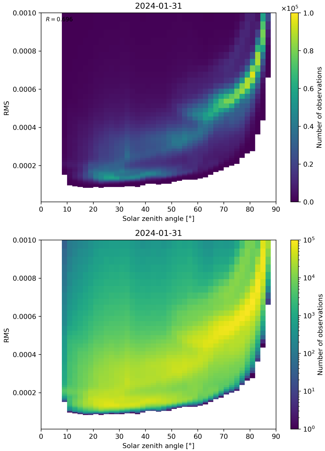
Figure 157: Scatter density plot of “Solar zenith angle” against “RMS” for 2024-01-31 to 2024-02-01.
