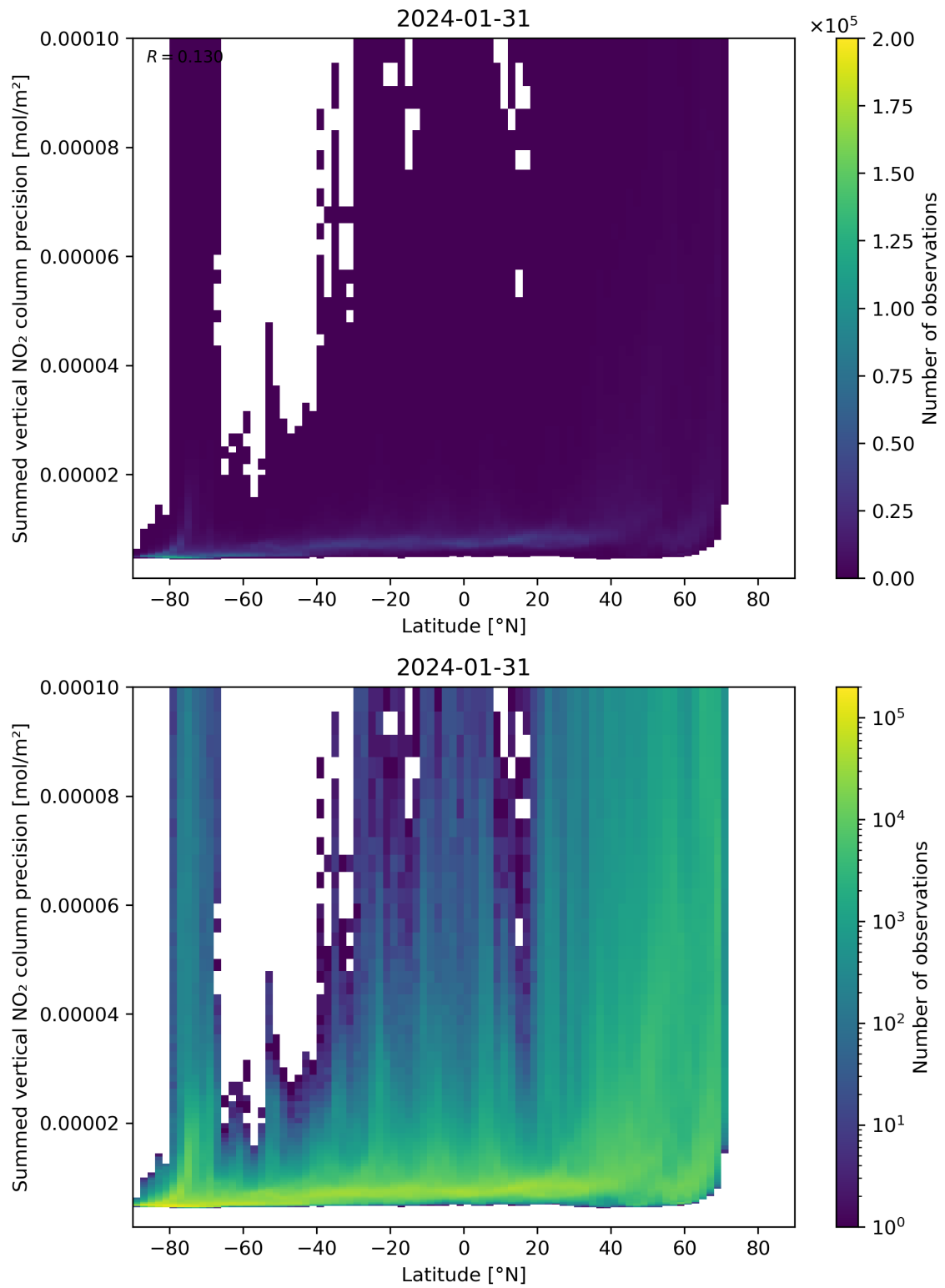
Figure 89: Scatter density plot of “Latitude” against “Summed vertical NO 2 column precision” for 2024-01-31 to 2024-02-01.
