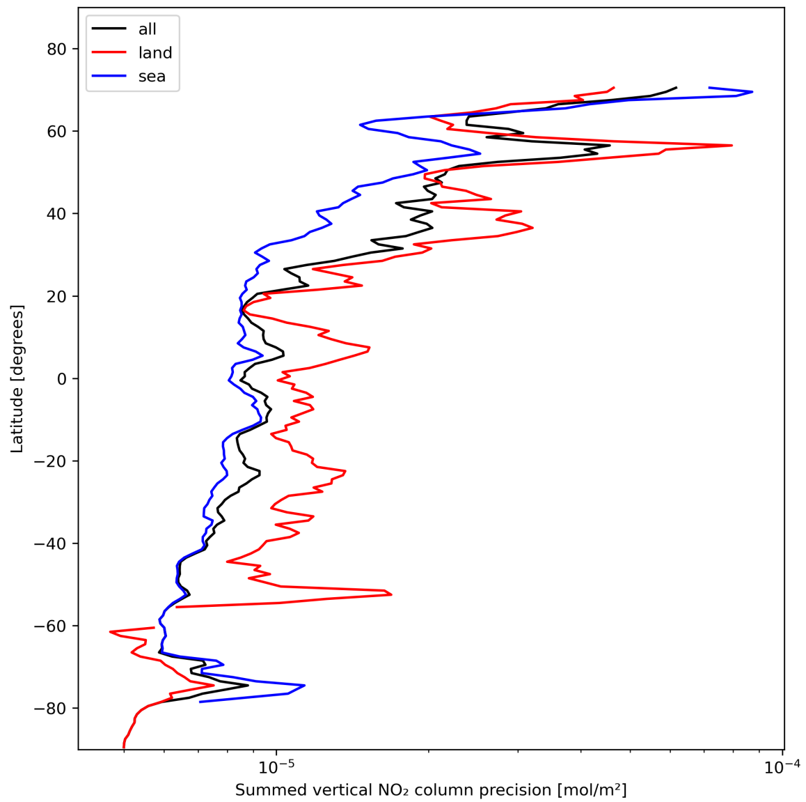
Figure 24: Zonal average of “Summed vertical NO 2 column precision” for 2024-01-31 to 2024-02-01.
