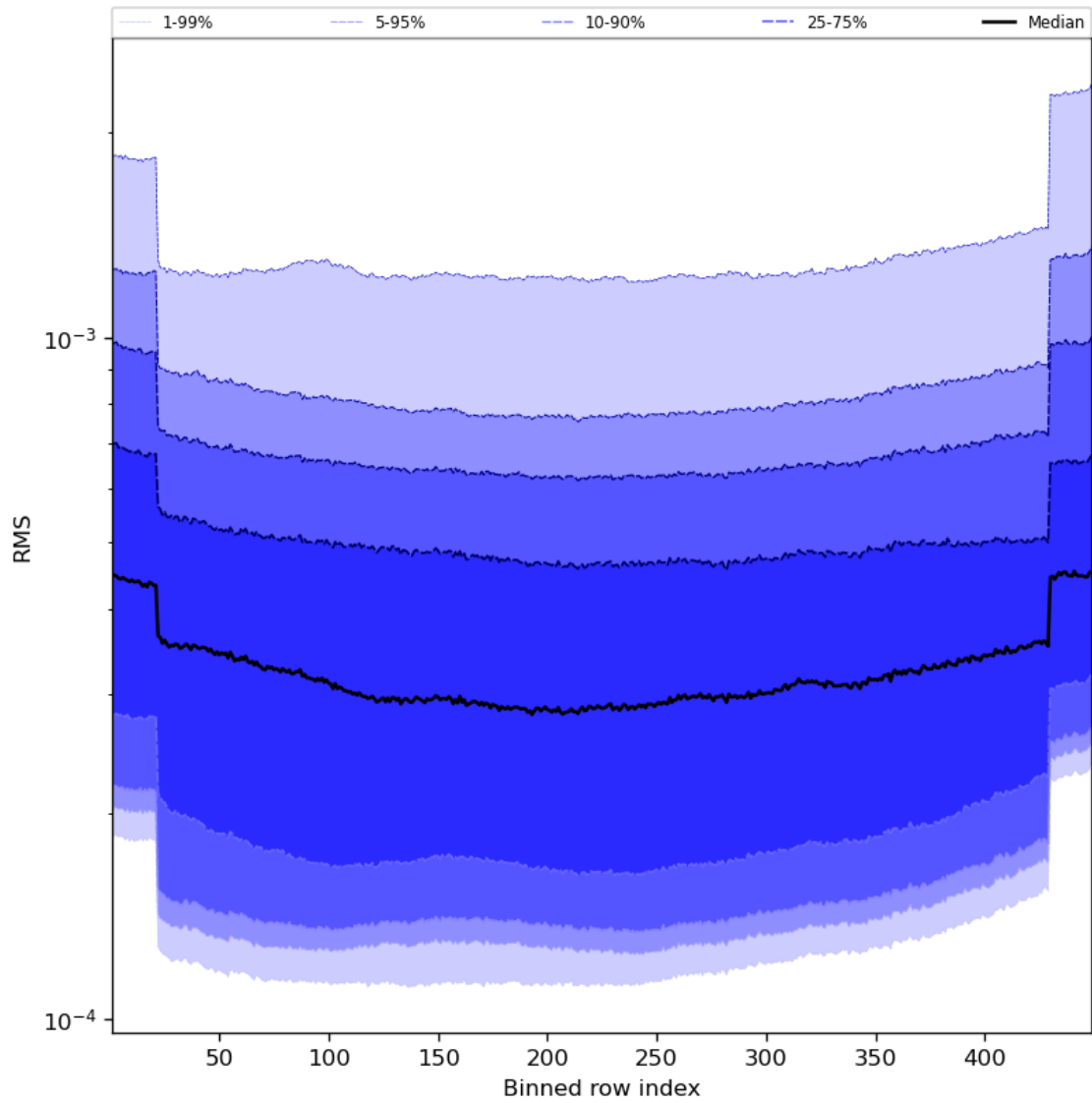
Figure 60: Along track statistics of “RMS” for 2024-01-31 to 2024-02-01
