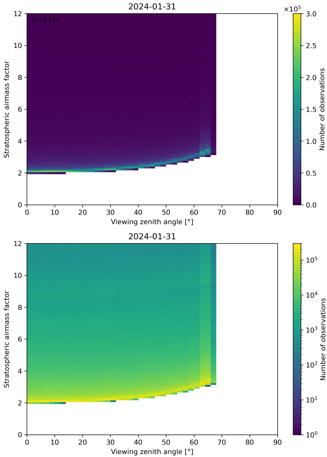
Figure 159: Scatter density plot of “Viewing zenith angle” against “Stratospheric airmass factor” for 2024-01-31 to 2024-02-01.
