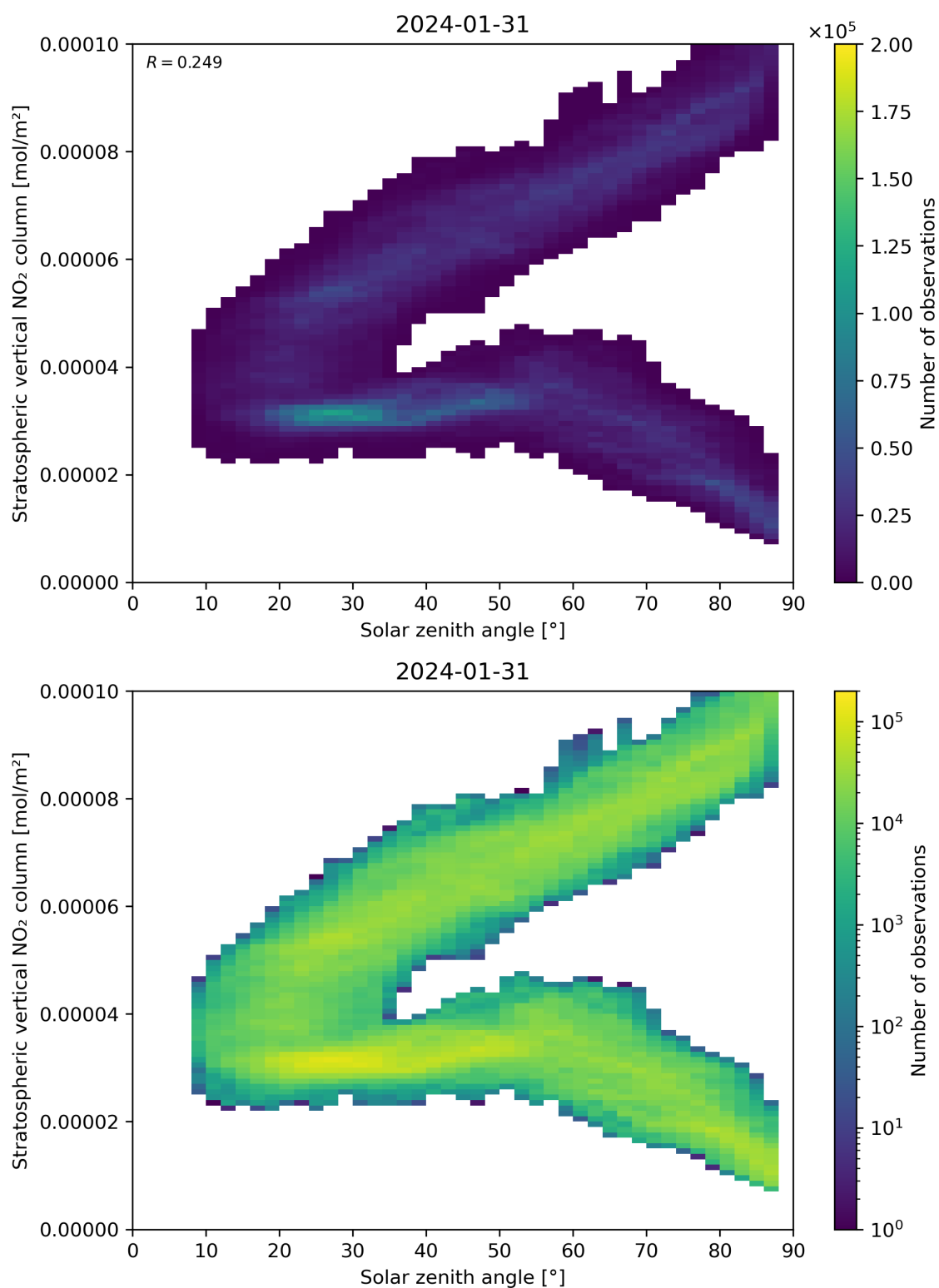
Figure 150: Scatter density plot of “Solar zenith angle” against “Stratospheric vertical NO 2 column” for 2024-01-31 to 2024-02-01.
