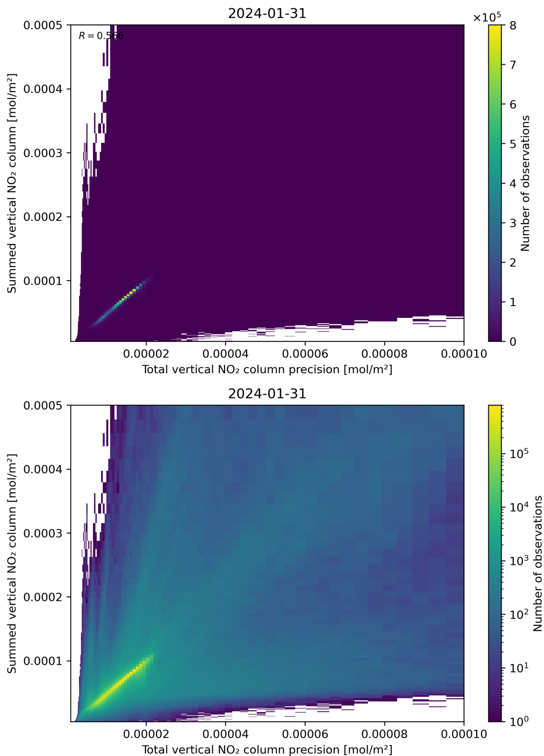
Figure 117: Scatter density plot of “Total vertical NO 2 column precision” against “Summed vertical NO 2 column” for 2024-01-31 to 2024-02-01.
