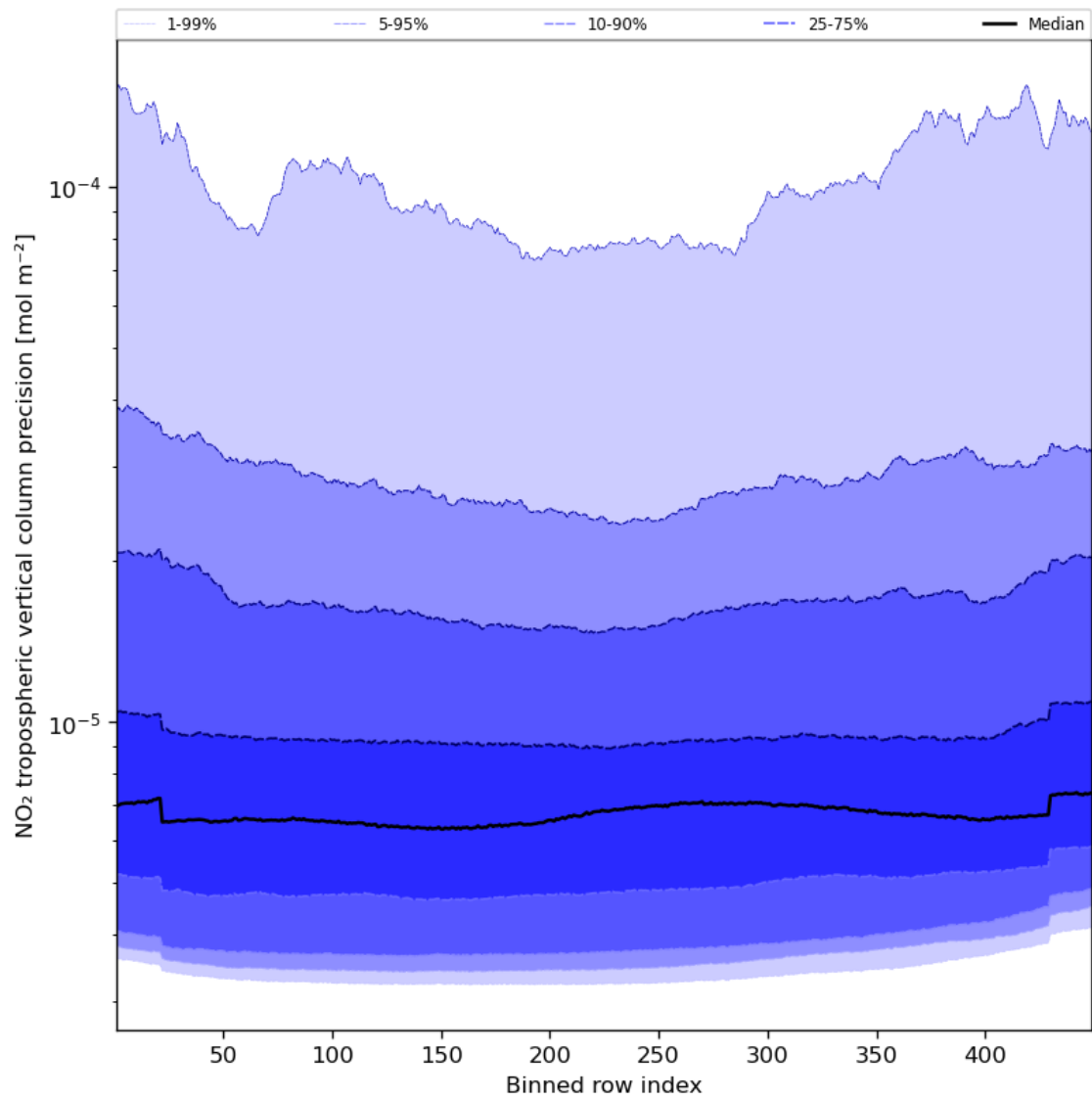
Figure 47: Along track statistics of “NO 2 tropospheric vertical column precision” for 2024-01-31 to 2024-02-01
