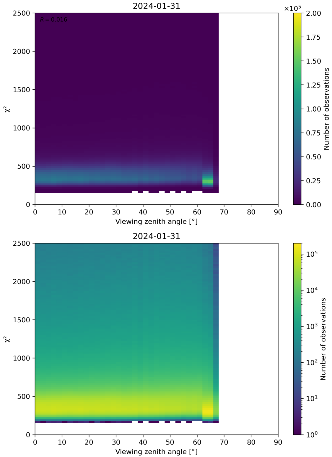
Figure 162: Scatter density plot of “Viewing zenith angle” against “ \chi^2 ” for 2024-01-31 to 2024-02-01.
