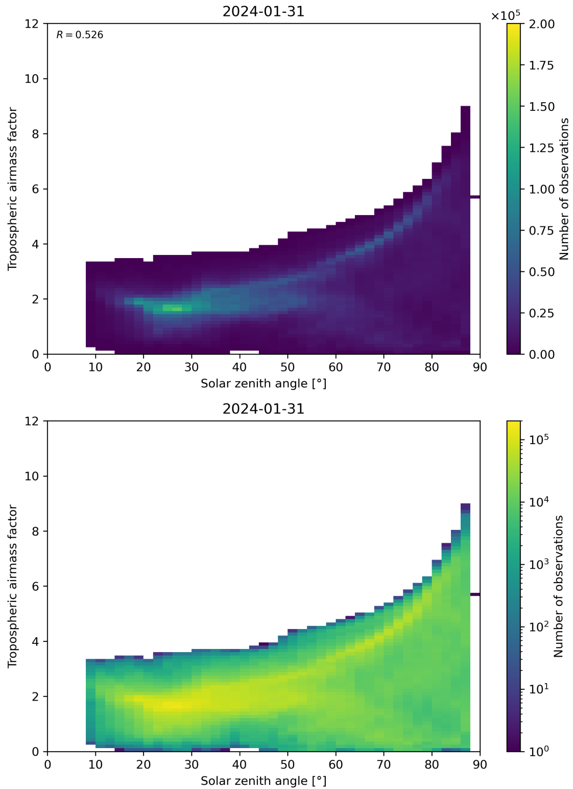
Figure 147: Scatter density plot of “Solar zenith angle” against “Tropospheric airmass factor” for 2024-01-31 to 2024-02-01.
