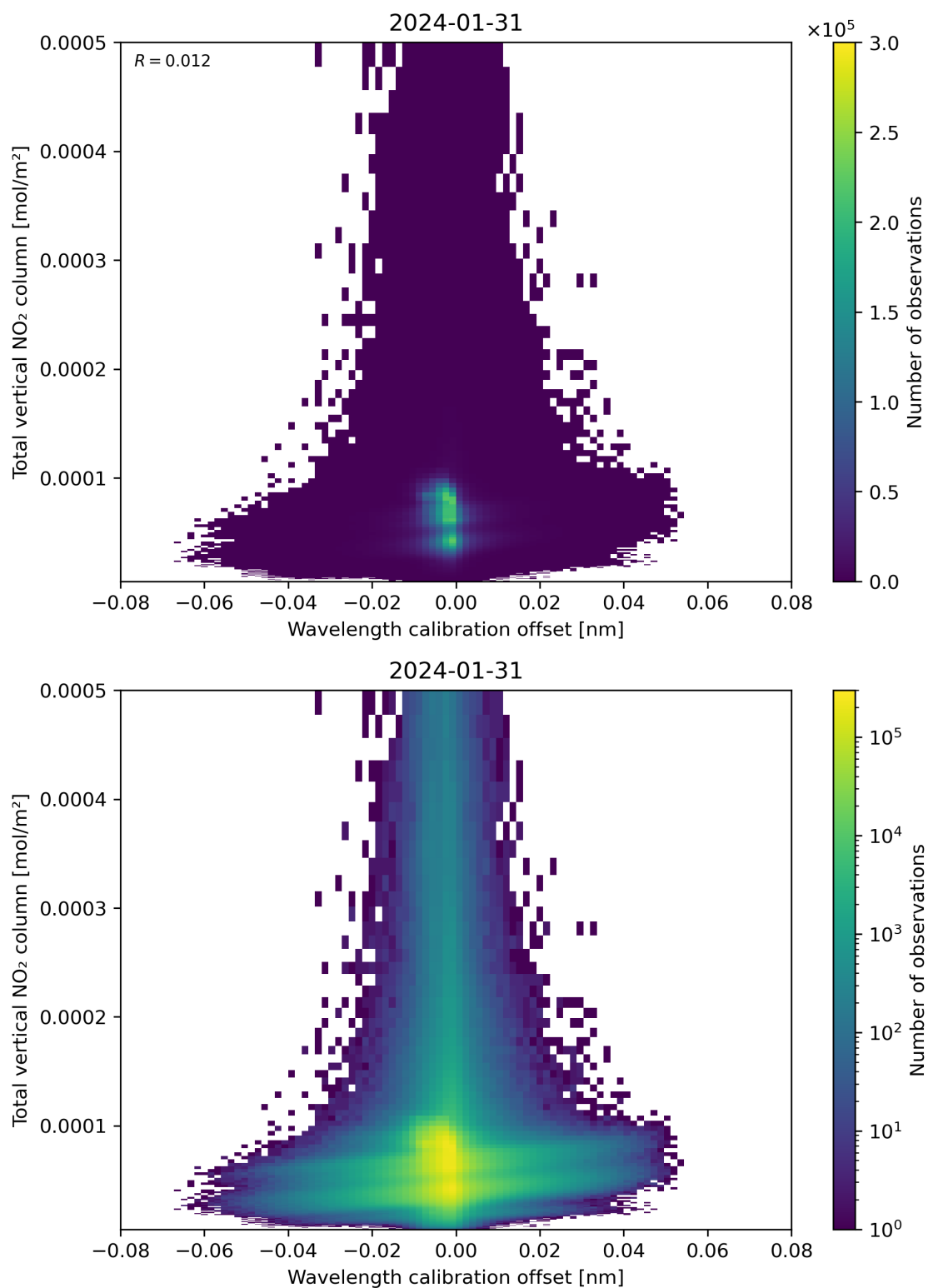
Figure 179: Scatter density plot of “Wavelength calibration offset” against “Total vertical NO 2 column” for 2024-01-31 to 2024-02-01.
