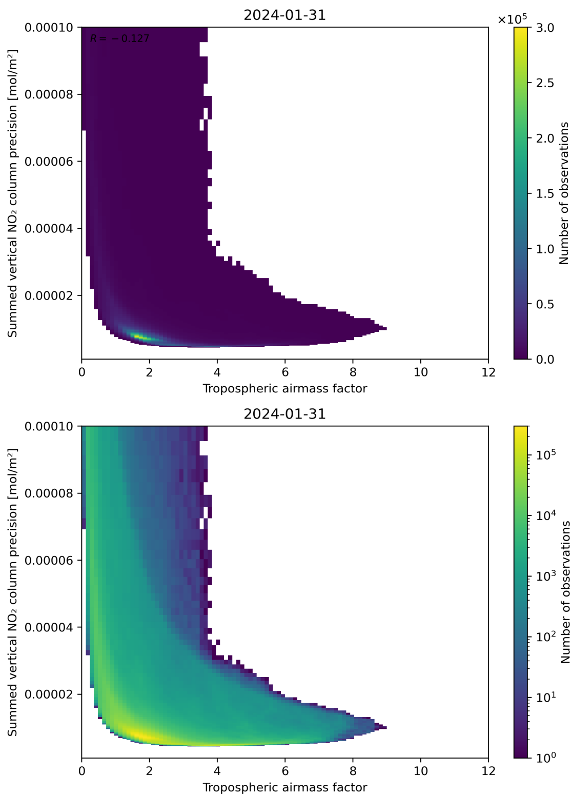
Figure 76: Scatter density plot of “Tropospheric air mass factor” against “Summed vertical NO 2 column precision” for 2024-01-31 to 2024-02-01.
