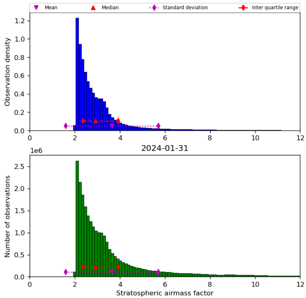
Figure 44: Histogram of “Stratospheric airmass factor” for 2024-01-31 to 2024-02-01
