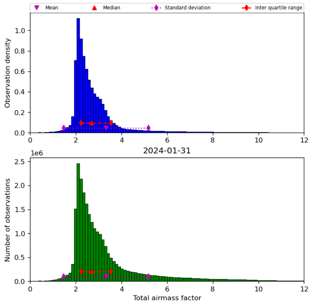
Figure 32: Histogram of “Total airmass factor” for 2024-01-31 to 2024-02-01
