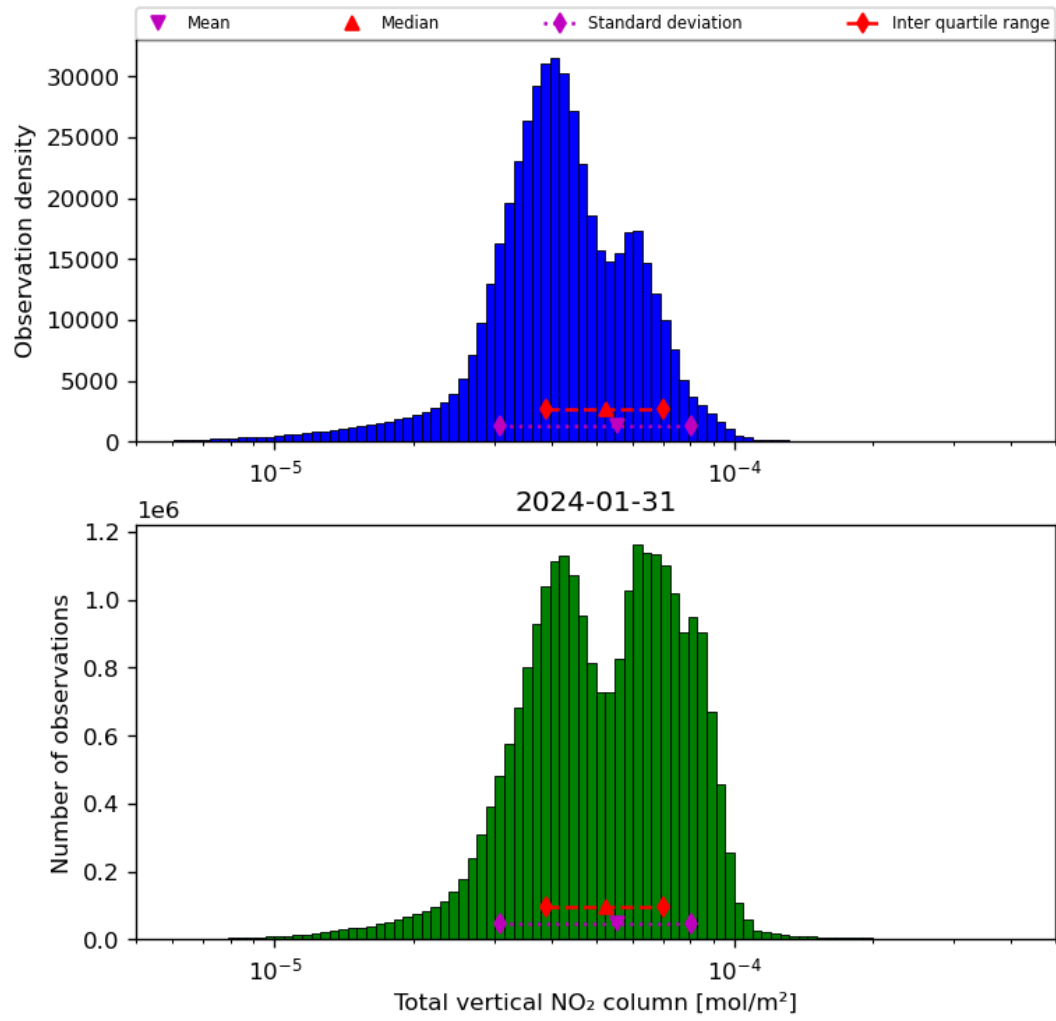
Figure 38: Histogram of “Total vertical NO 2 column” for 2024-01-31 to 2024-02-01
