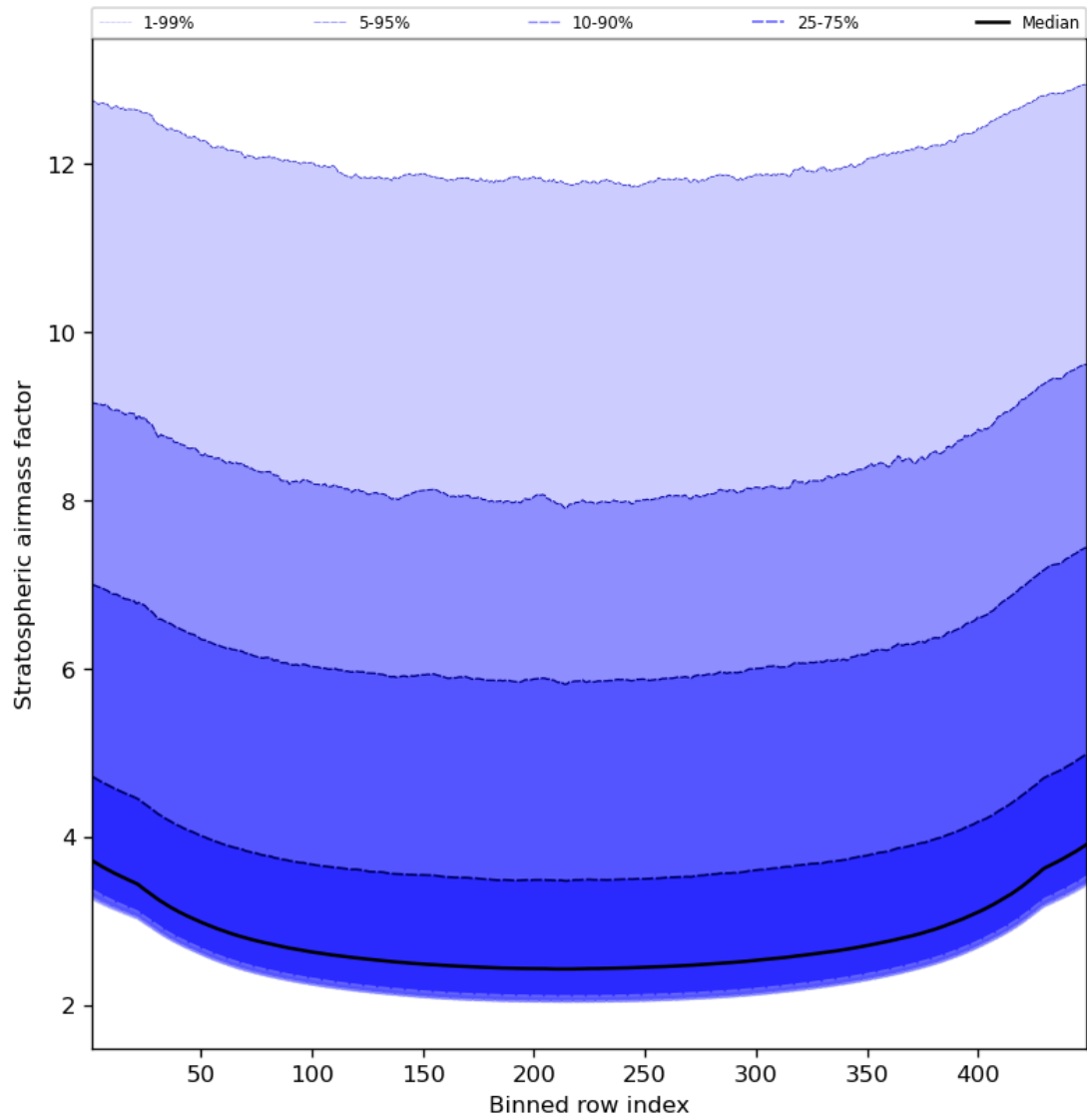
Figure 61: Along track statistics of “Stratospheric airmass factor” for 2024-01-31 to 2024-02-01
