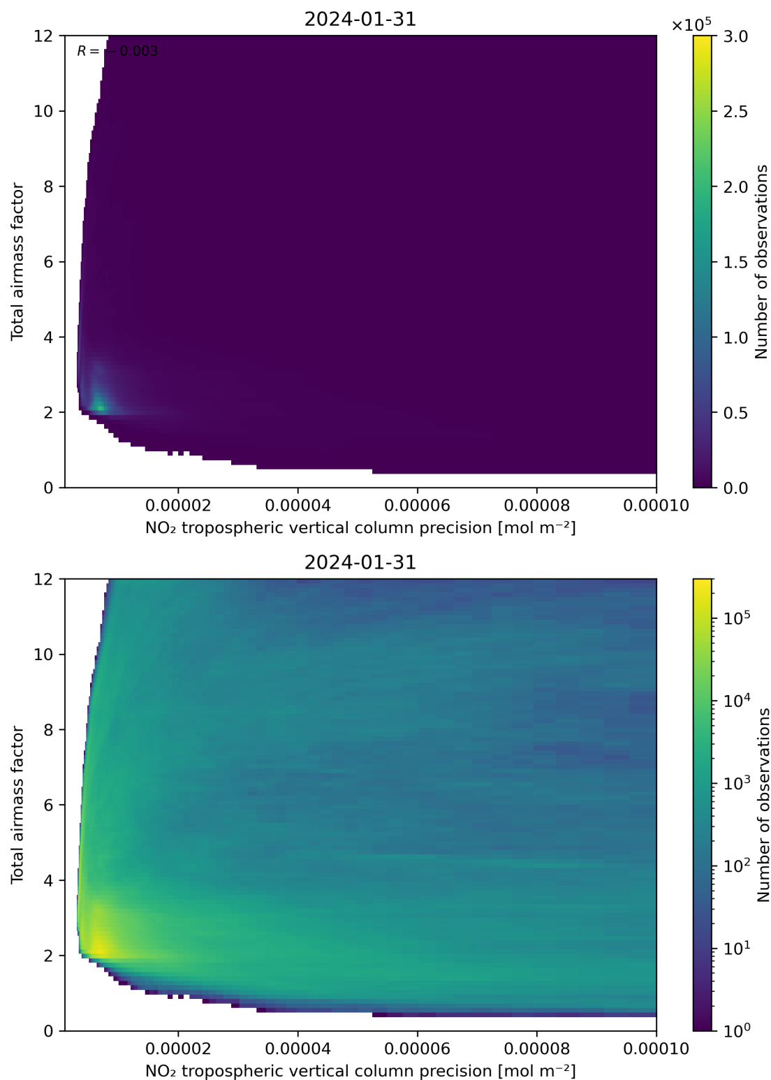
Figure 132: Scatter density plot of “NO 2 tropospheric vertical column precision” against “Total air mass factor” for 2024-01-31 to 2024-02-01.
