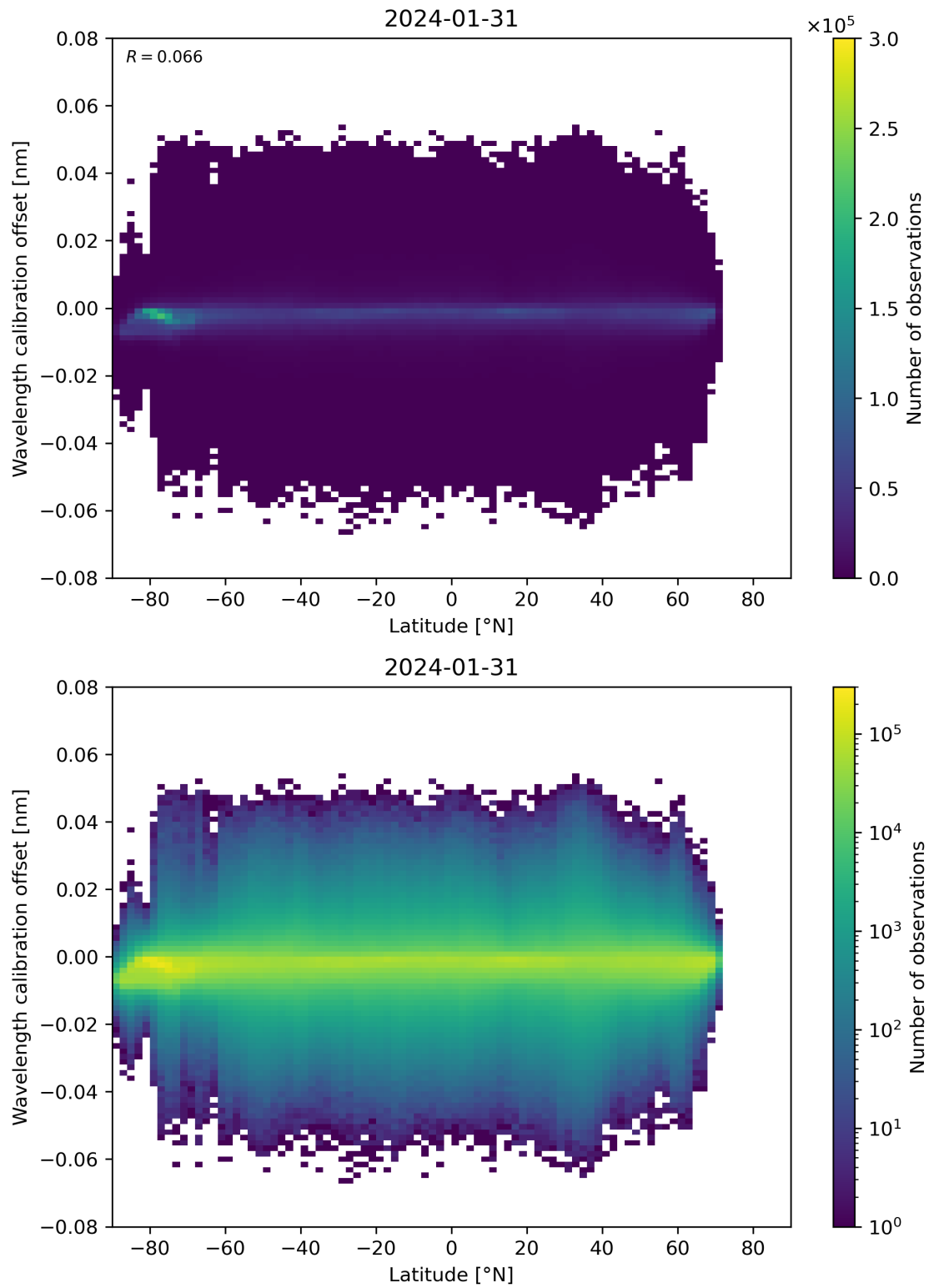
Figure 95: Scatter density plot of “Latitude” against “Wavelength calibration offset” for 2024-01-31 to 2024-02-01.
