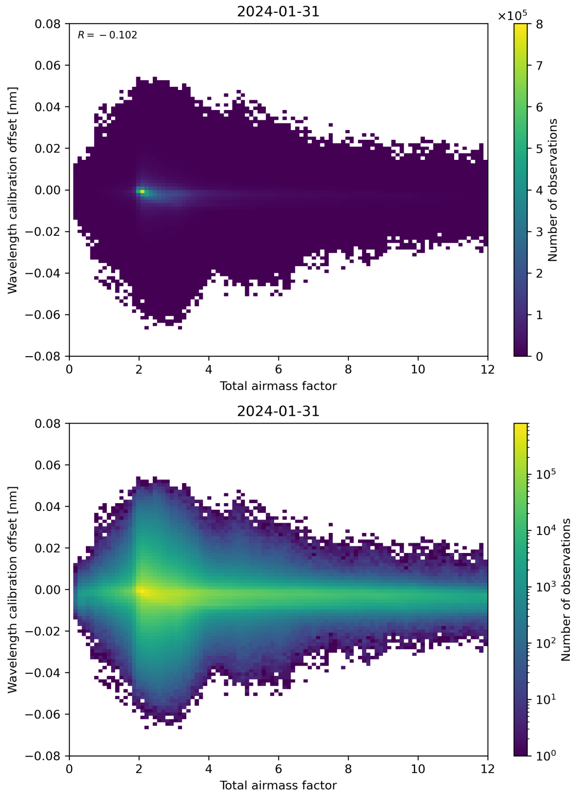
Figure 70: Scatter density plot of “Total airmass factor” against “Wavelength calibration offset” for 2024-01-31 to 2024-02-01.
