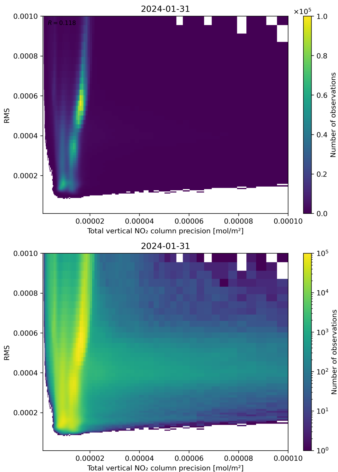
Figure 119: Scatter density plot of “Total vertical NO 2 column precision” against “RMS” for 2024-01-31 to 2024-02-01.
