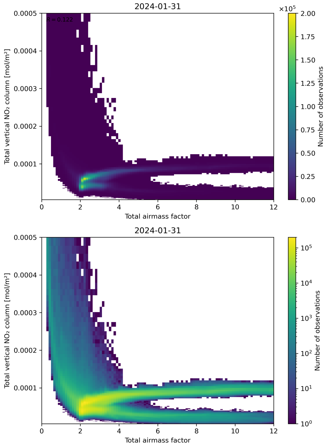
Figure 67: Scatter density plot of “Total airmass factor” against “Total vertical NO 2 column” for 2024-01-31 to 2024-02-01.
