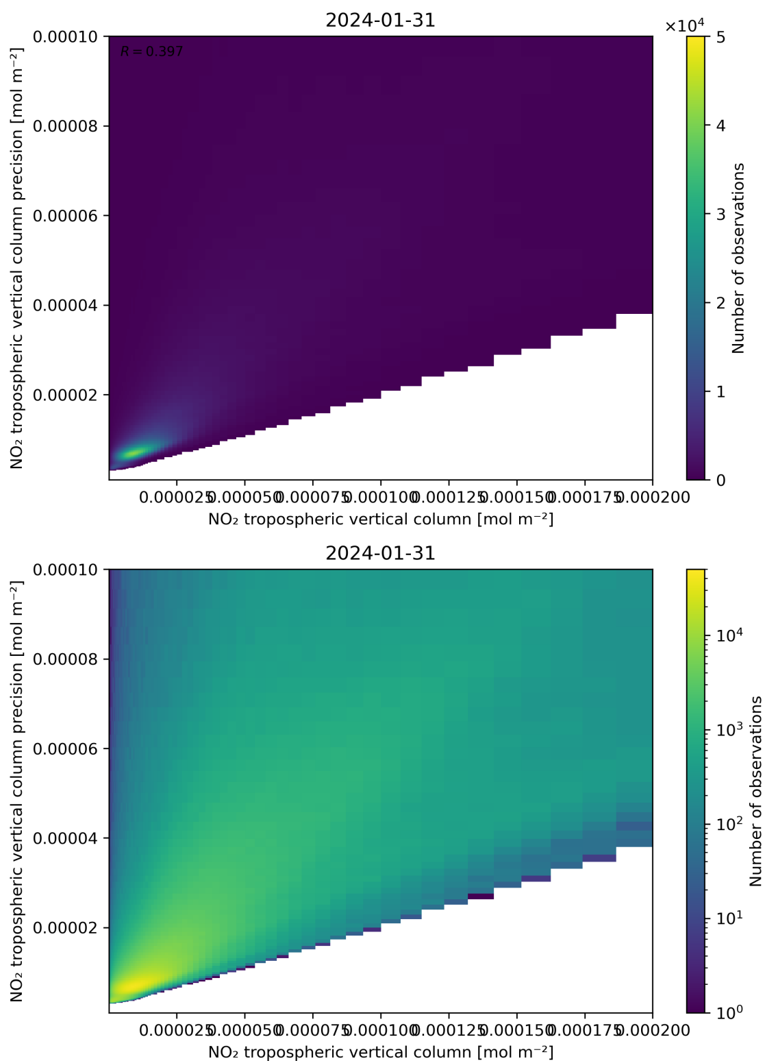
Figure 130: Scatter density plot of “NO 2 tropospheric vertical column” against “NO 2 tropospheric vertical column precision” for 2024-01-31 to 2024-02-01.
