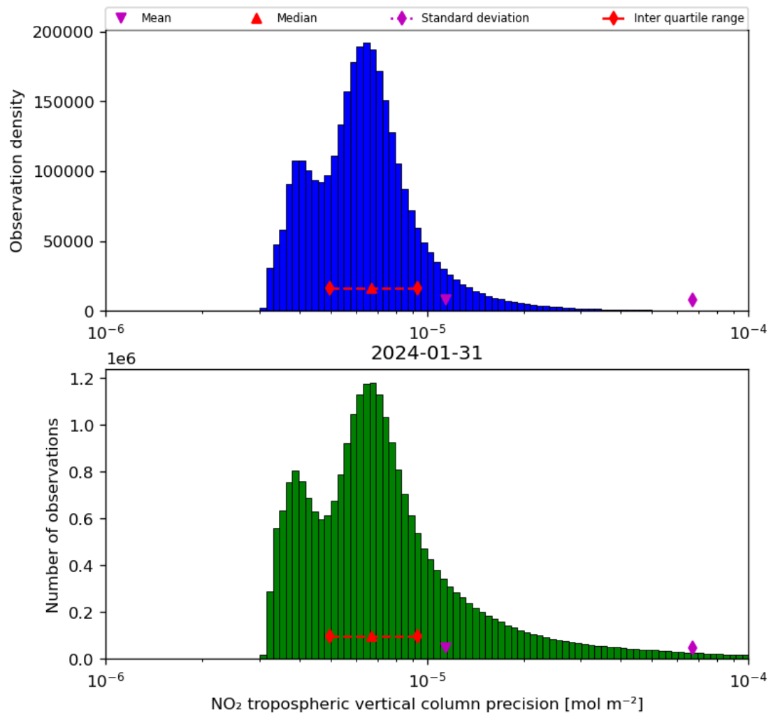
Figure 30: Histogram of “NO 2 tropospheric vertical column precision” for 2024-01-31 to 2024-02-01
