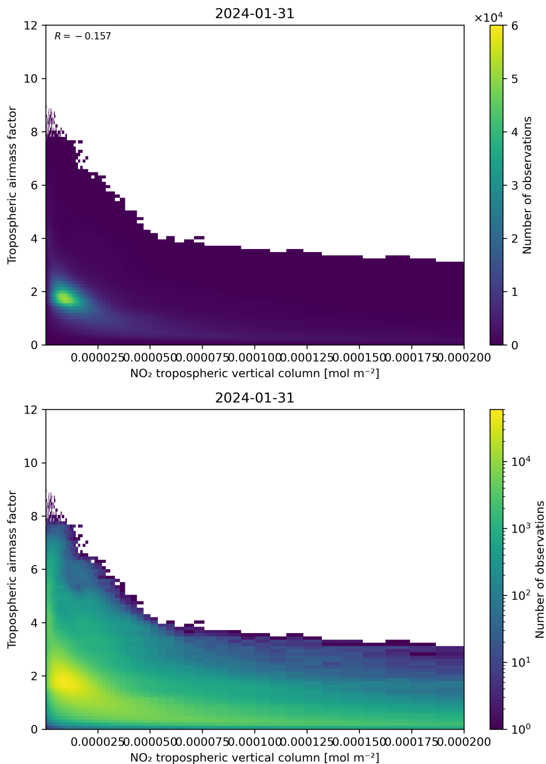
Figure 123: Scatter density plot of “NO 2 tropospheric vertical column” against “Tropospheric air mass factor” for 2024-01-31 to 2024-02-01.
