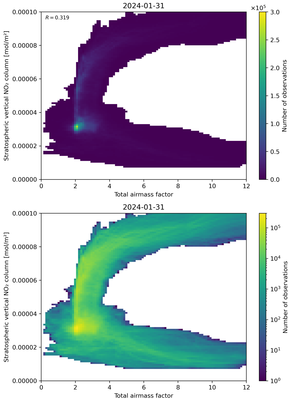
Figure 64: Scatter density plot of “Total airmass factor” against “Stratospheric vertical \text{NO}_2 column” for 2024-01-31 to 2024-02-01.
