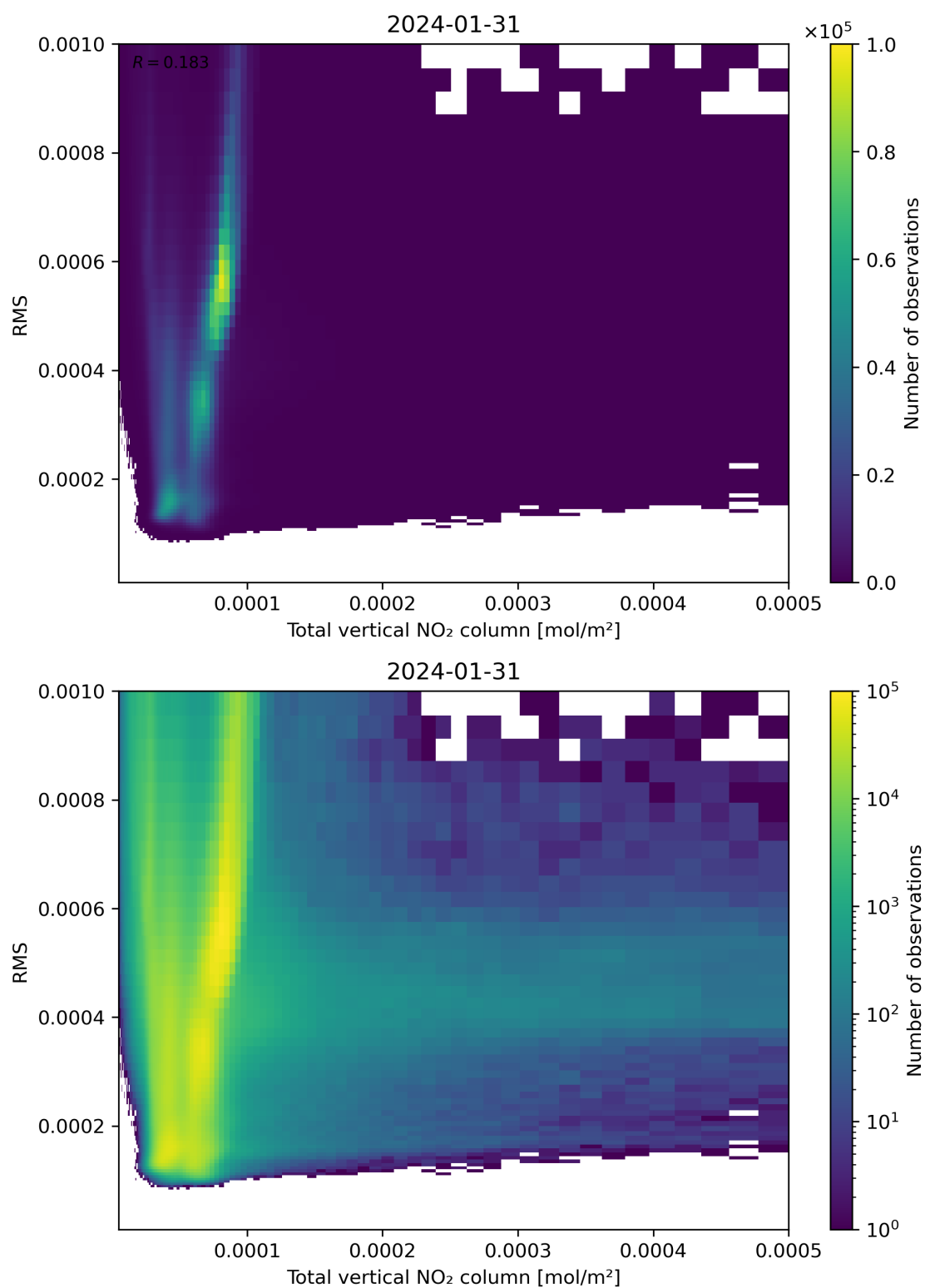
Figure 120: Scatter density plot of “Total vertical NO 2 column” against “RMS” for 2024-01-31 to 2024-02-01.
