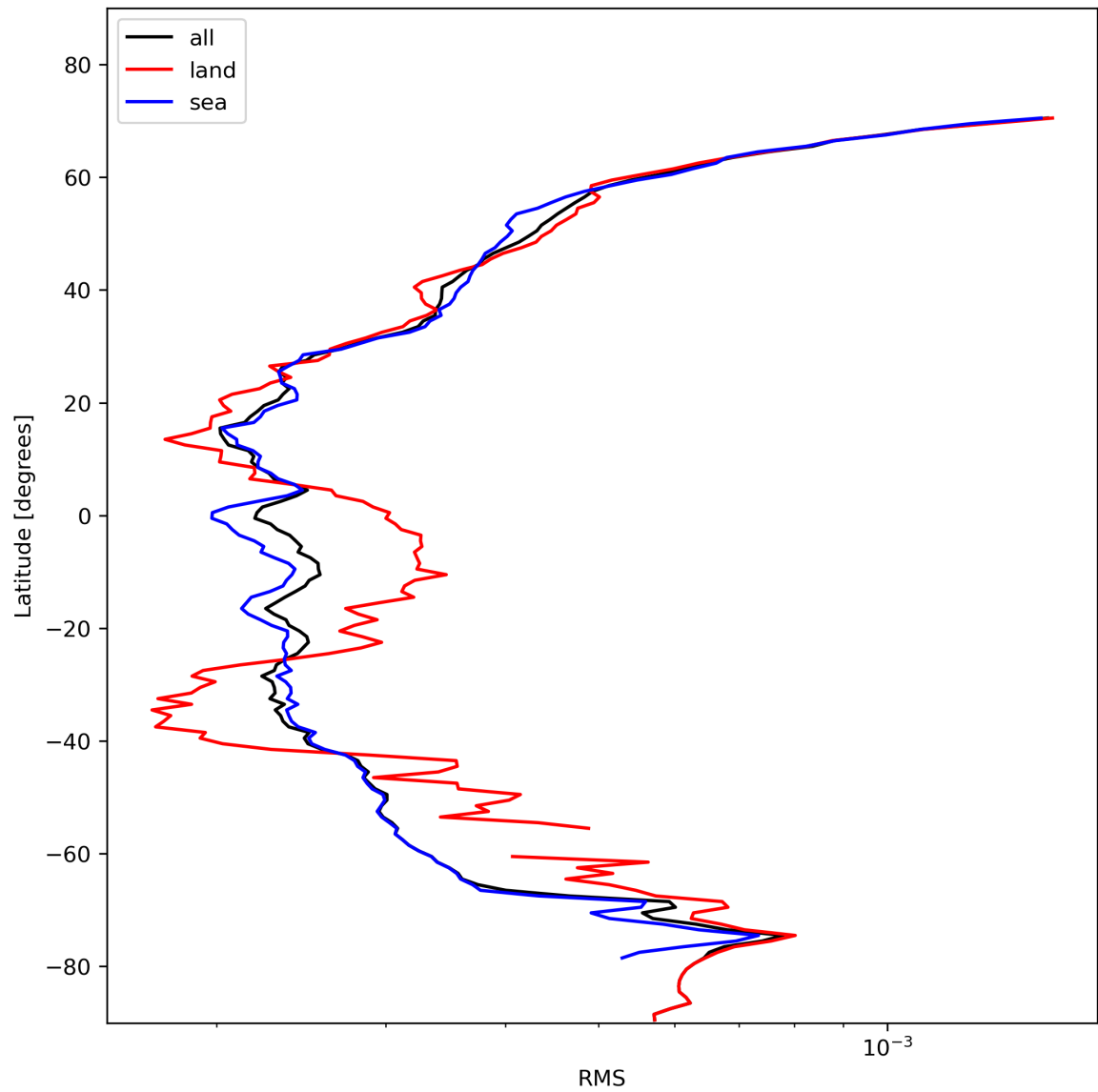
Figure 26: Zonal average of “RMS” for 2024-01-31 to 2024-02-01.
