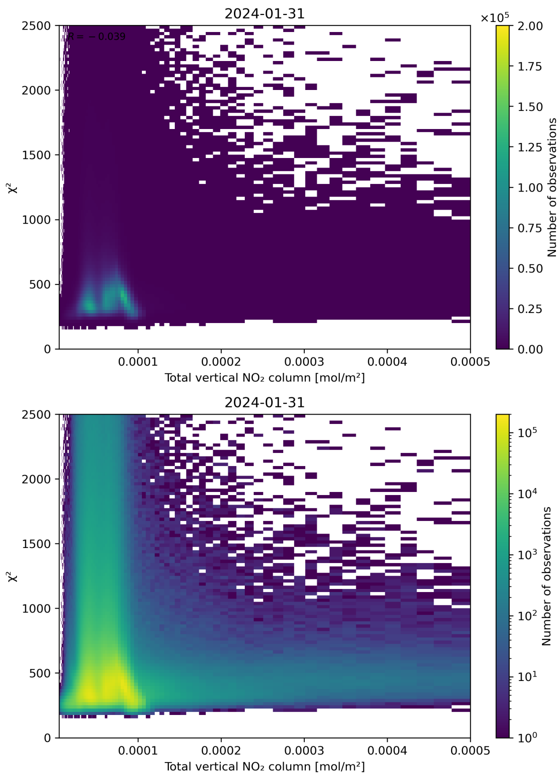
Figure 111: Scatter density plot of “Total vertical NO 2 column” against “ \chi^2 ” for 2024-01-31 to 2024-02-01.
