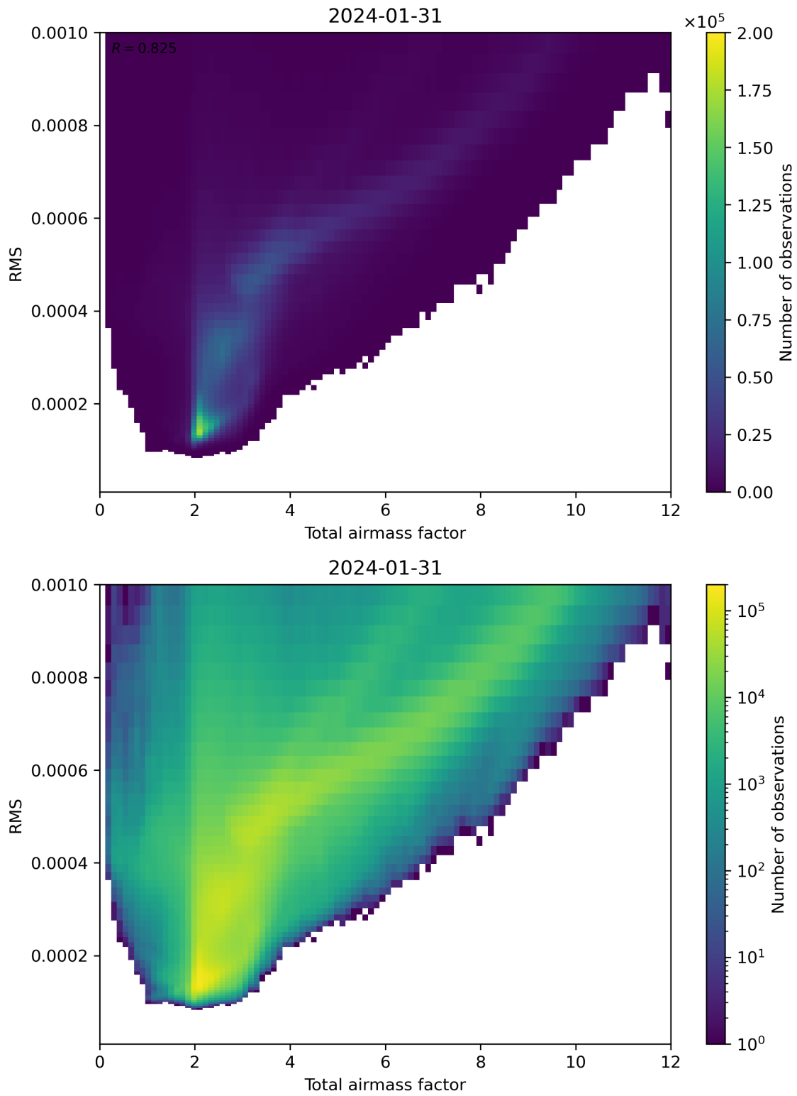
Figure 69: Scatter density plot of “Total airmass factor” against “RMS” for 2024-01-31 to 2024-02-01.
