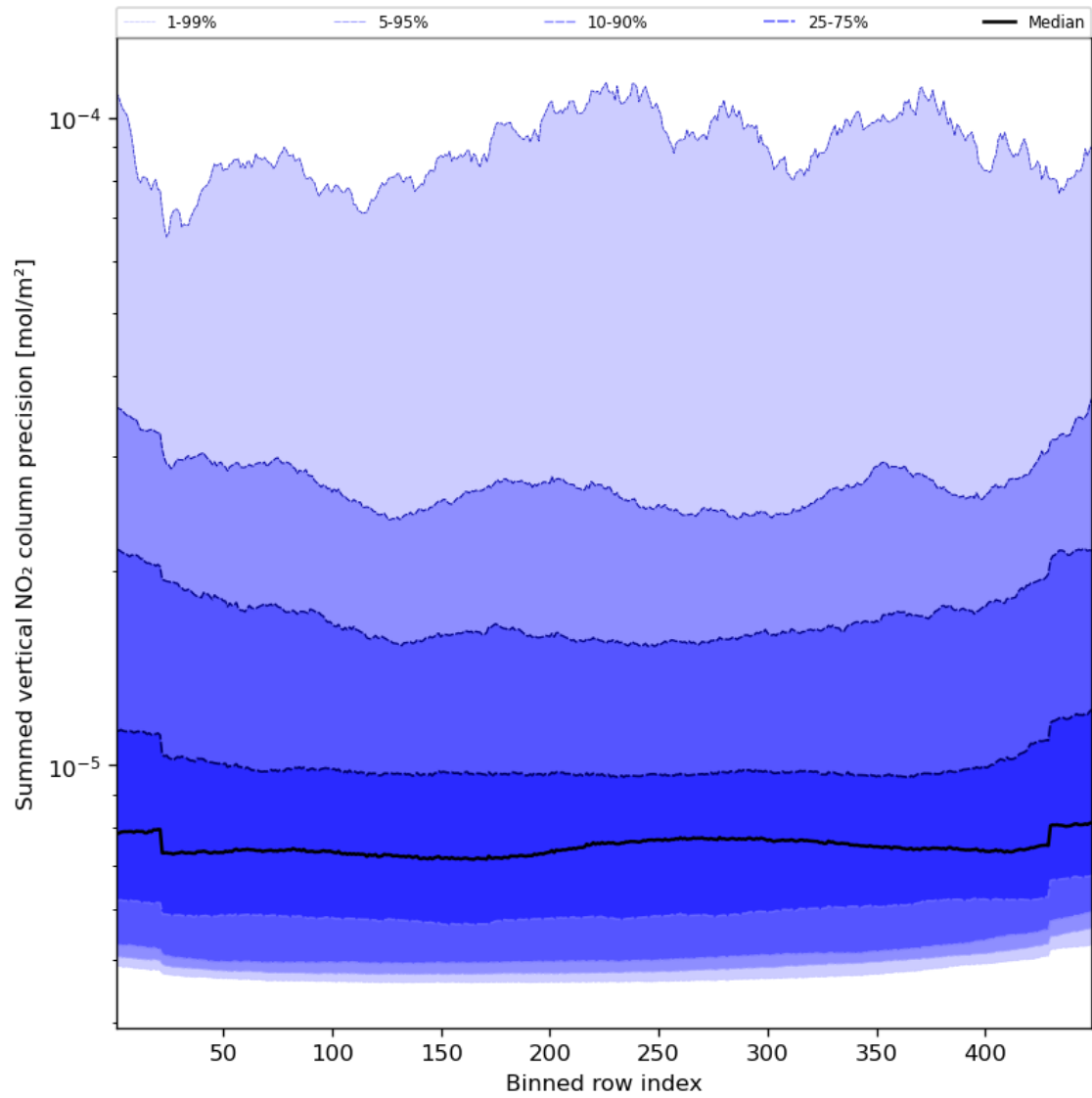
Figure 58: Along track statistics of “Summed vertical NO 2 column precision” for 2024-01-31 to 2024-02-02
