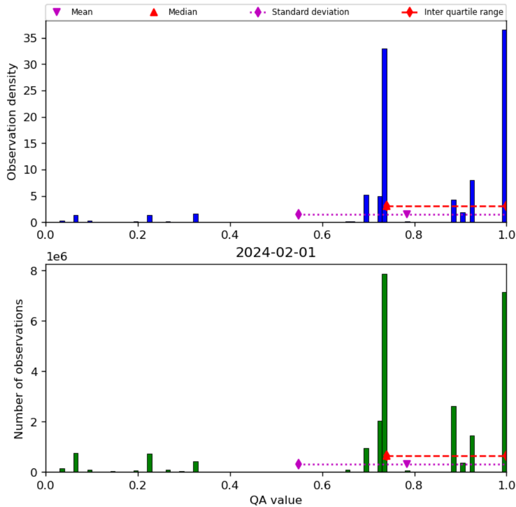
Figure 28: Histogram of “QA value” for 2024-01-31 to 2024-02-02
