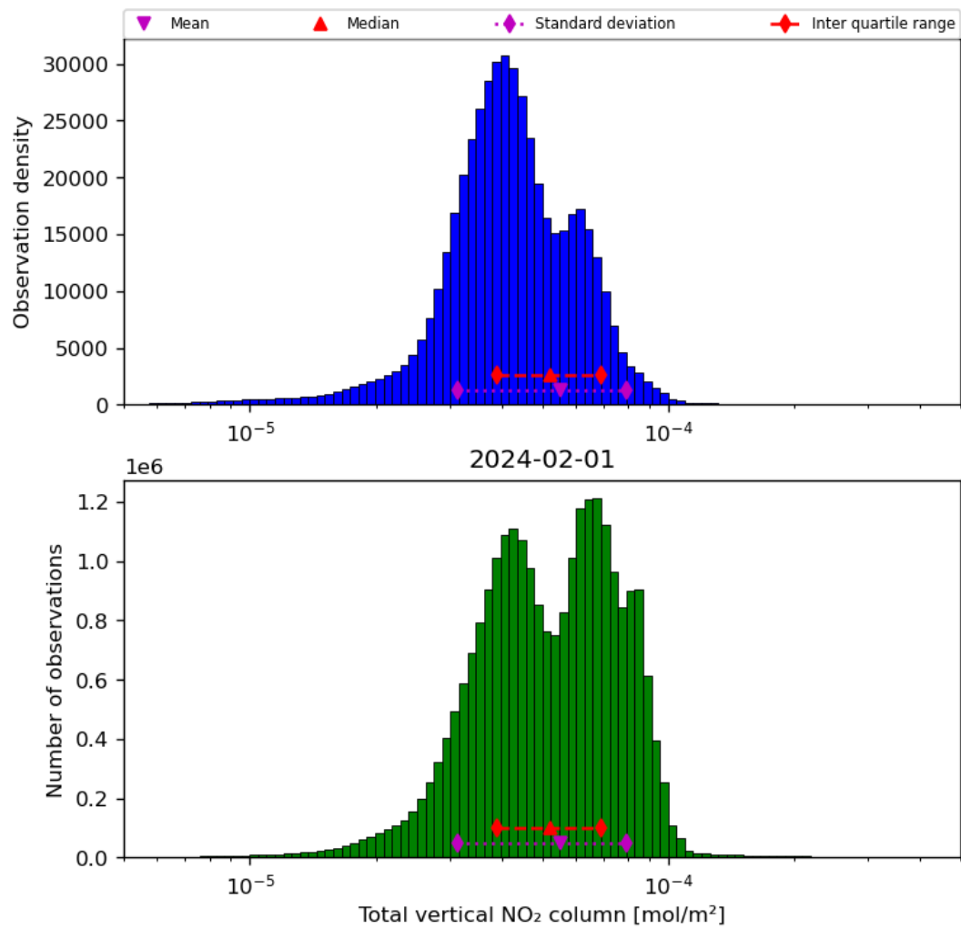
Figure 38: Histogram of “Total vertical NO 2 column” for 2024-01-31 to 2024-02-02
