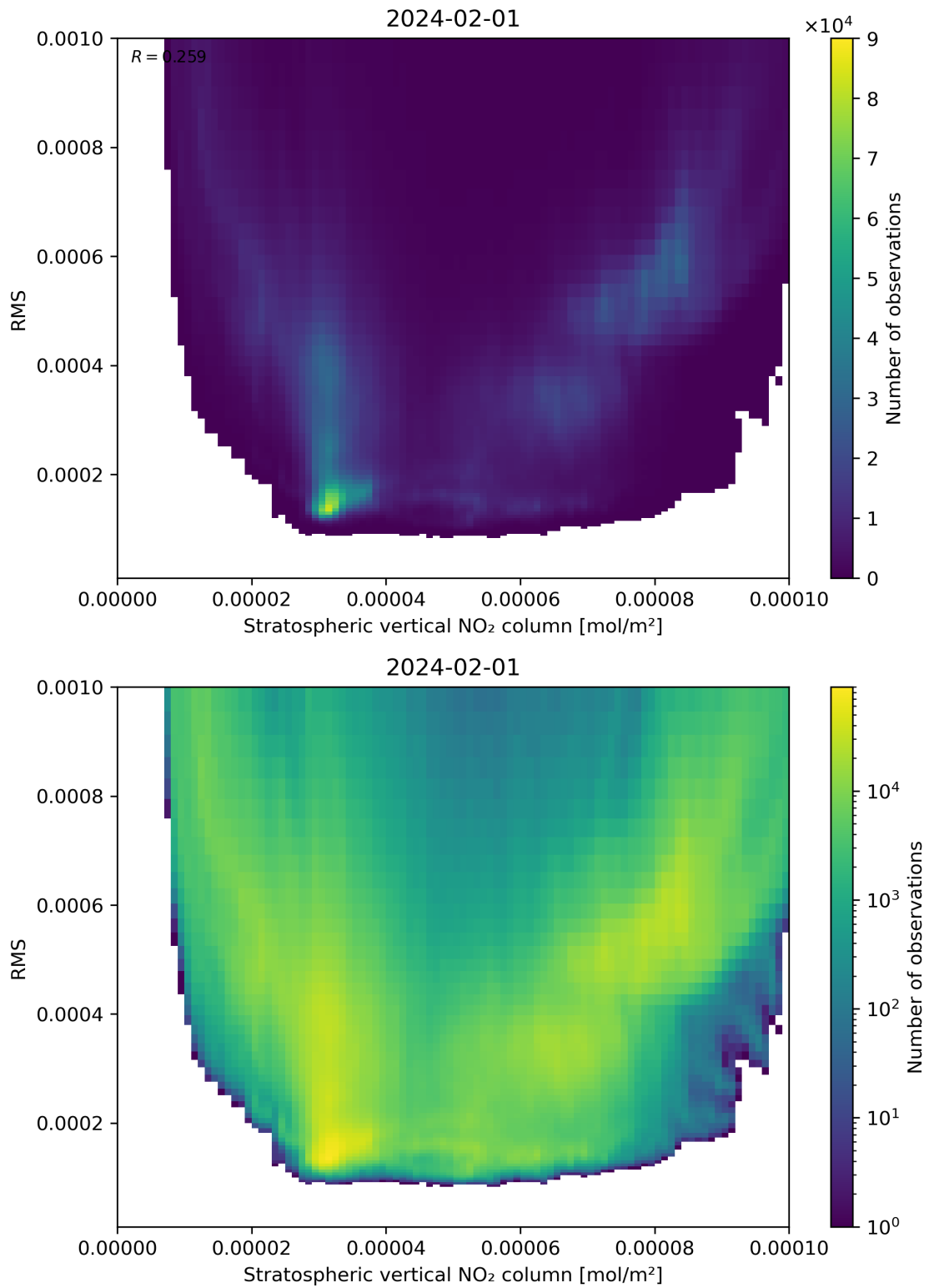
Figure 102: Scatter density plot of “Stratospheric vertical NO 2 column” against “RMS” for 2024-01-31 to 2024-02-02.
