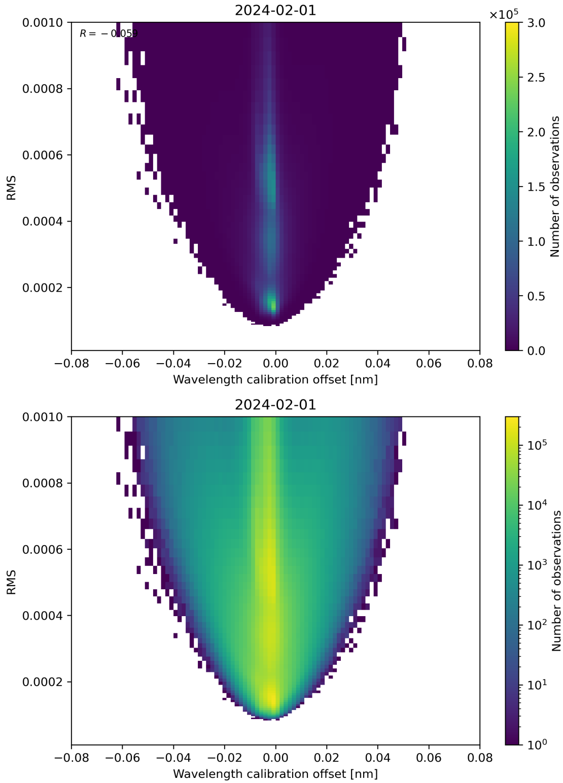
Figure 181: Scatter density plot of “Wavelength calibration offset” against “RMS” for 2024-01-31 to 2024-02-02.
