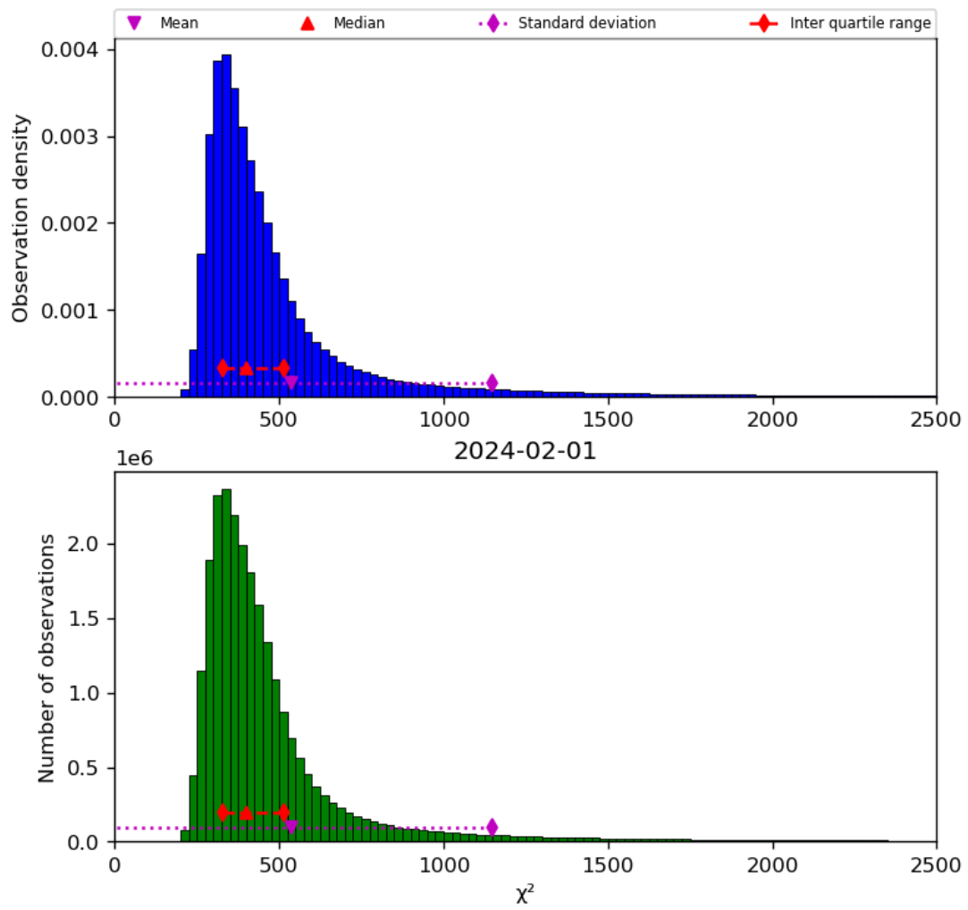
Figure 42: Histogram of " \chi^2 " for 2024-01-31 to 2024-02-02
