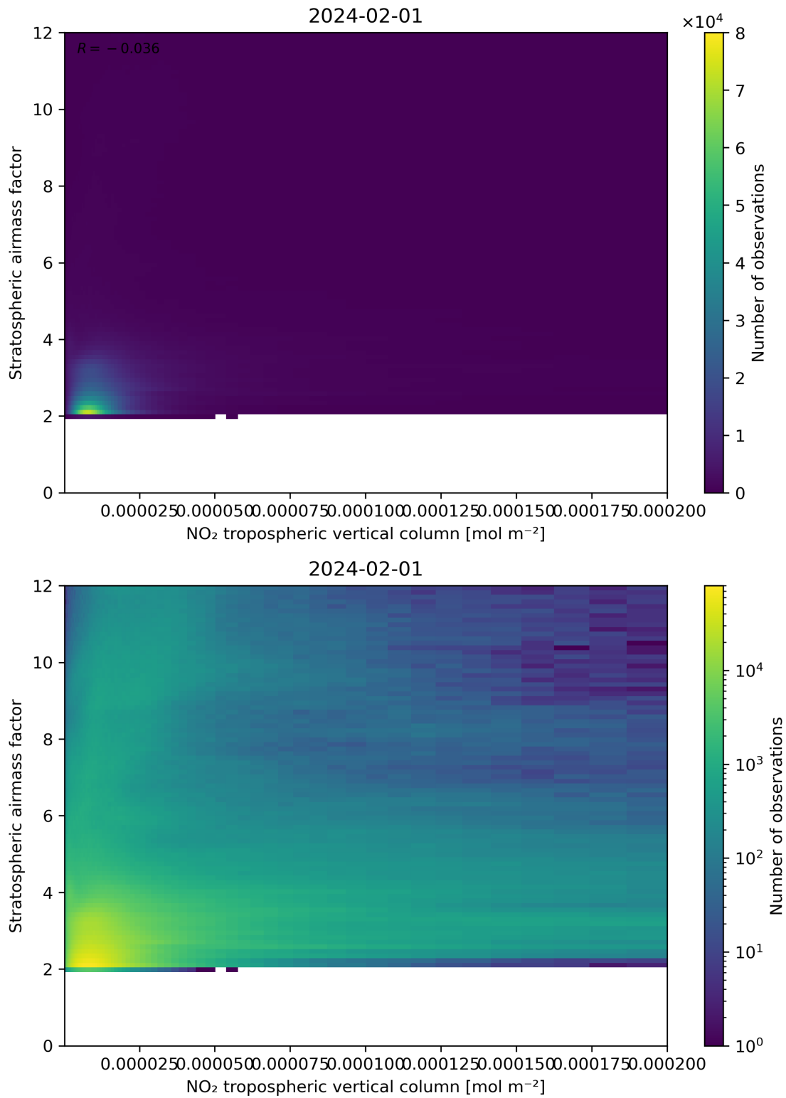
Figure 121: Scatter density plot of “NO 2 tropospheric vertical column” against “Stratospheric airmass factor” for 2024-01-31 to 2024-02-02.
