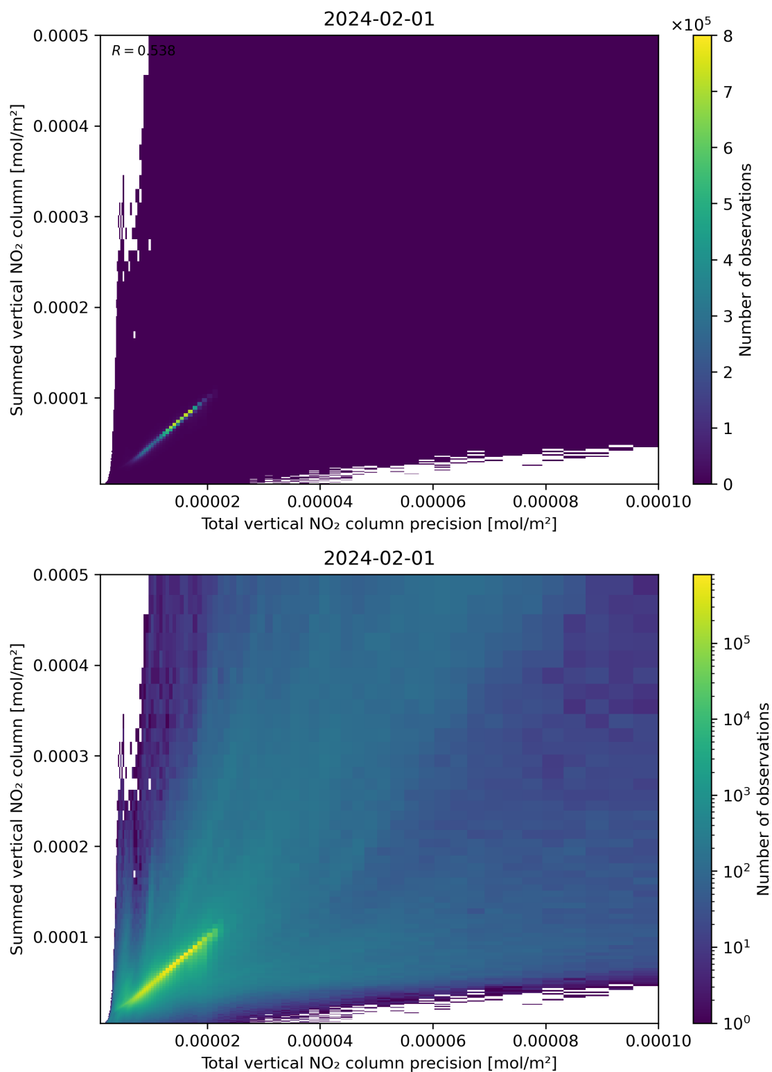
Figure 117: Scatter density plot of “Total vertical NO 2 column precision” against “Summed vertical NO 2 column” for 2024-01-31 to 2024-02-02.
