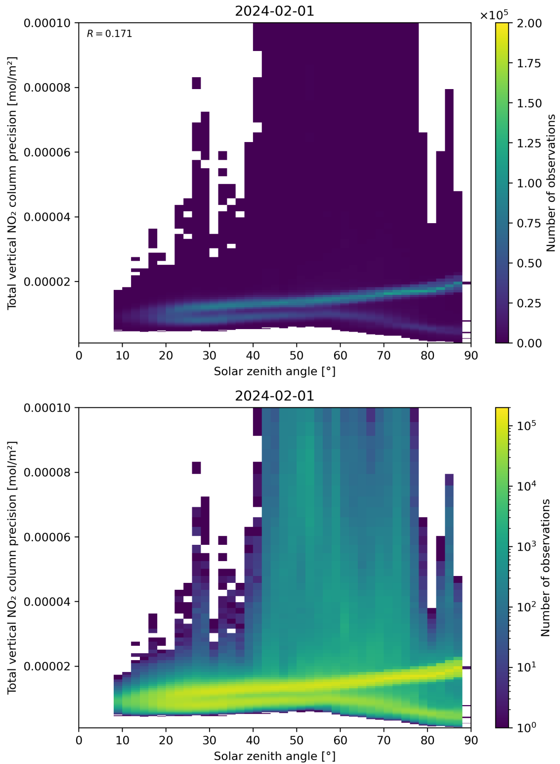
Figure 154: Scatter density plot of “Solar zenith angle” against “Total vertical NO 2 column precision” for 2024-01-31 to 2024-02-02.
