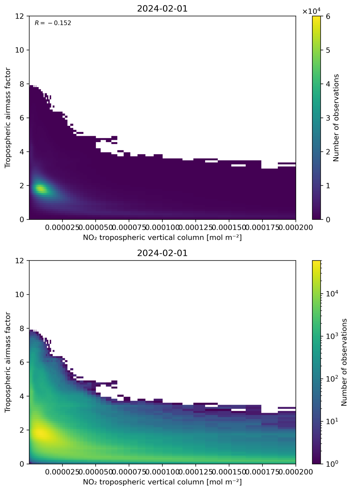
Figure 123: Scatter density plot of “NO 2 tropospheric vertical column” against “Tropospheric air mass factor” for 2024-01-31 to 2024-02-02.
