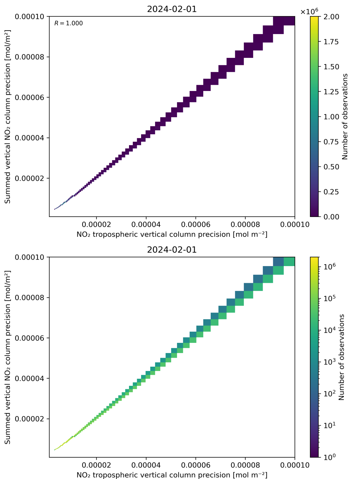
Figure 137: Scatter density plot of “NO 2 tropospheric vertical column precision” against “Summed vertical NO 2 column precision” for 2024-01-31 to 2024-02-02.
