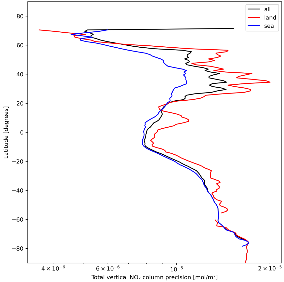
Figure 22: Zonal average of “Total vertical NO 2 column precision” for 2024-01-31 to 2024-02-02.
