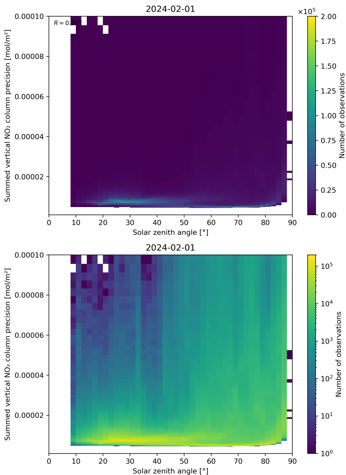
Figure 152: Scatter density plot of “Solar zenith angle” against “Summed vertical NO 2 column precision” for 2024-01-31 to 2024-02-02.
