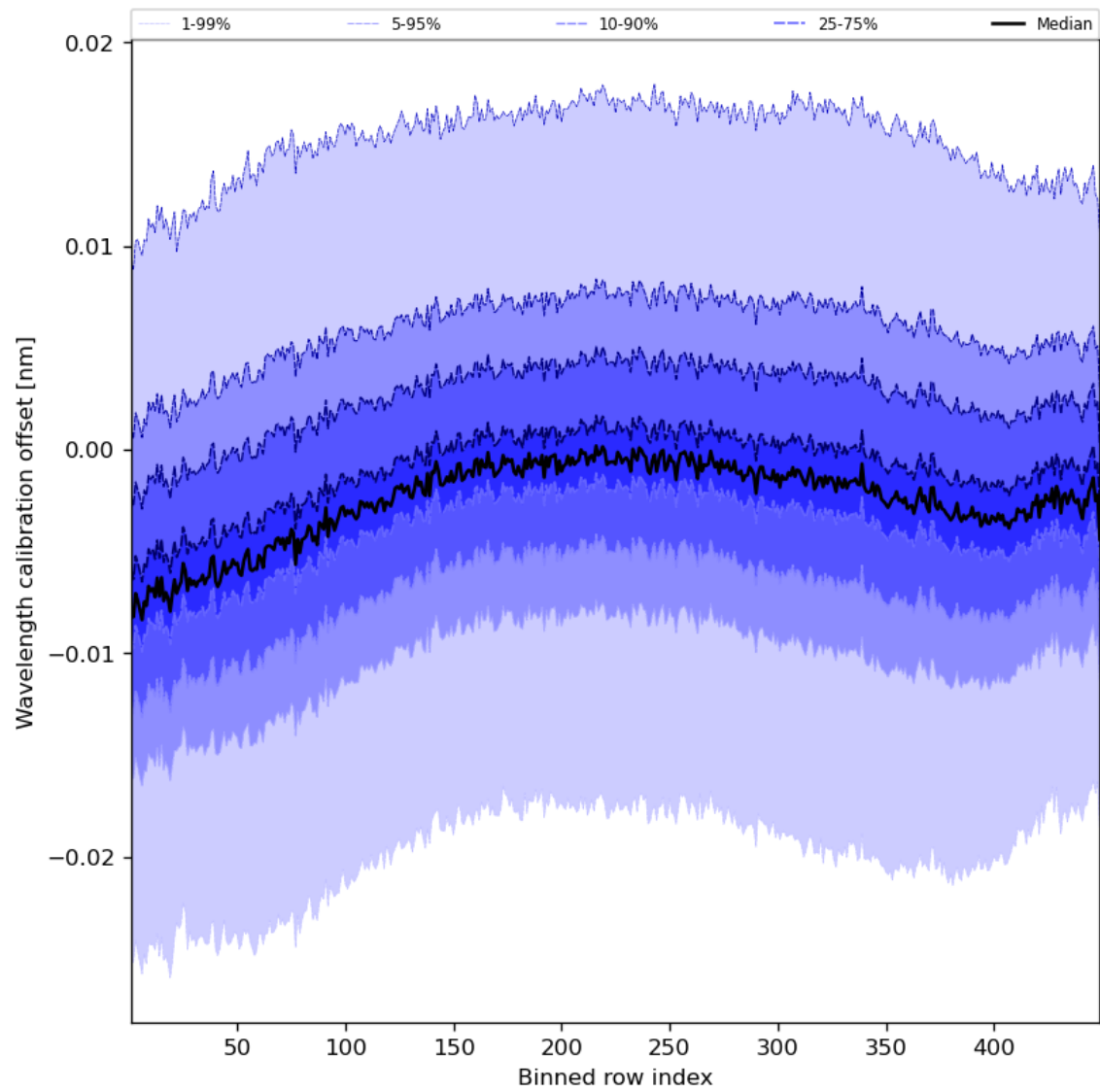
Figure 52: Along track statistics of “Wavelength calibration offset” for 2024-01-31 to 2024-02-02
