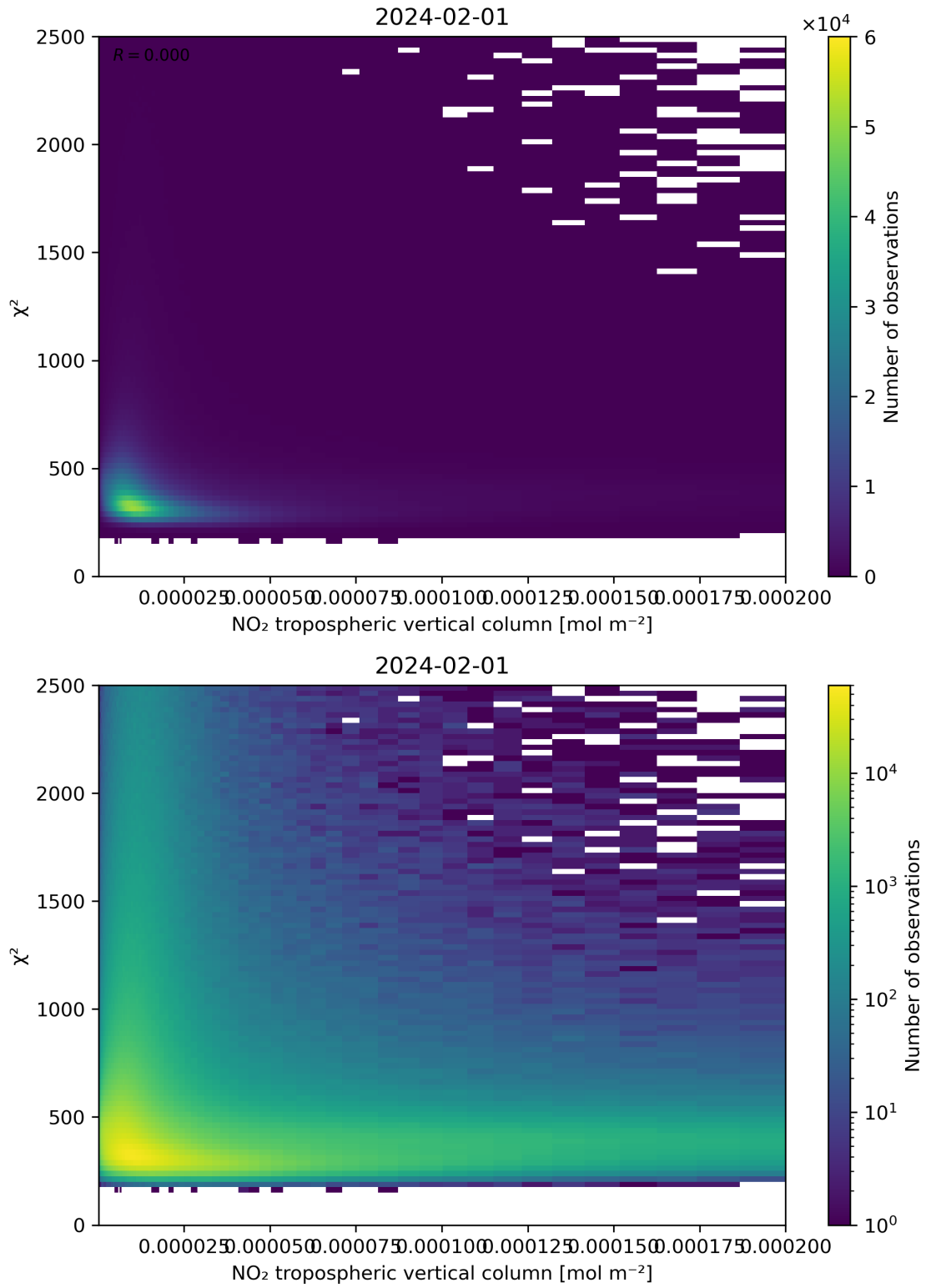
Figure 124: Scatter density plot of “NO 2 tropospheric vertical column” against “ \chi^2 ” for 2024-01-31 to 2024-02-02.
