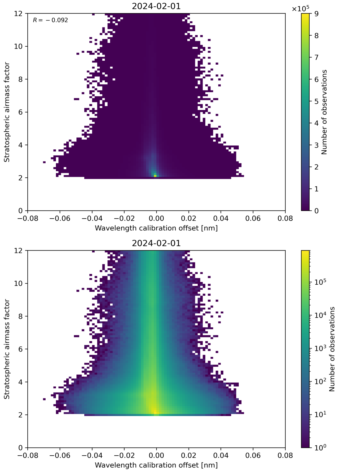
Figure 174: Scatter density plot of “Wavelength calibration offset” against “Stratospheric air mass factor” for 2024-01-31 to 2024-02-02.
