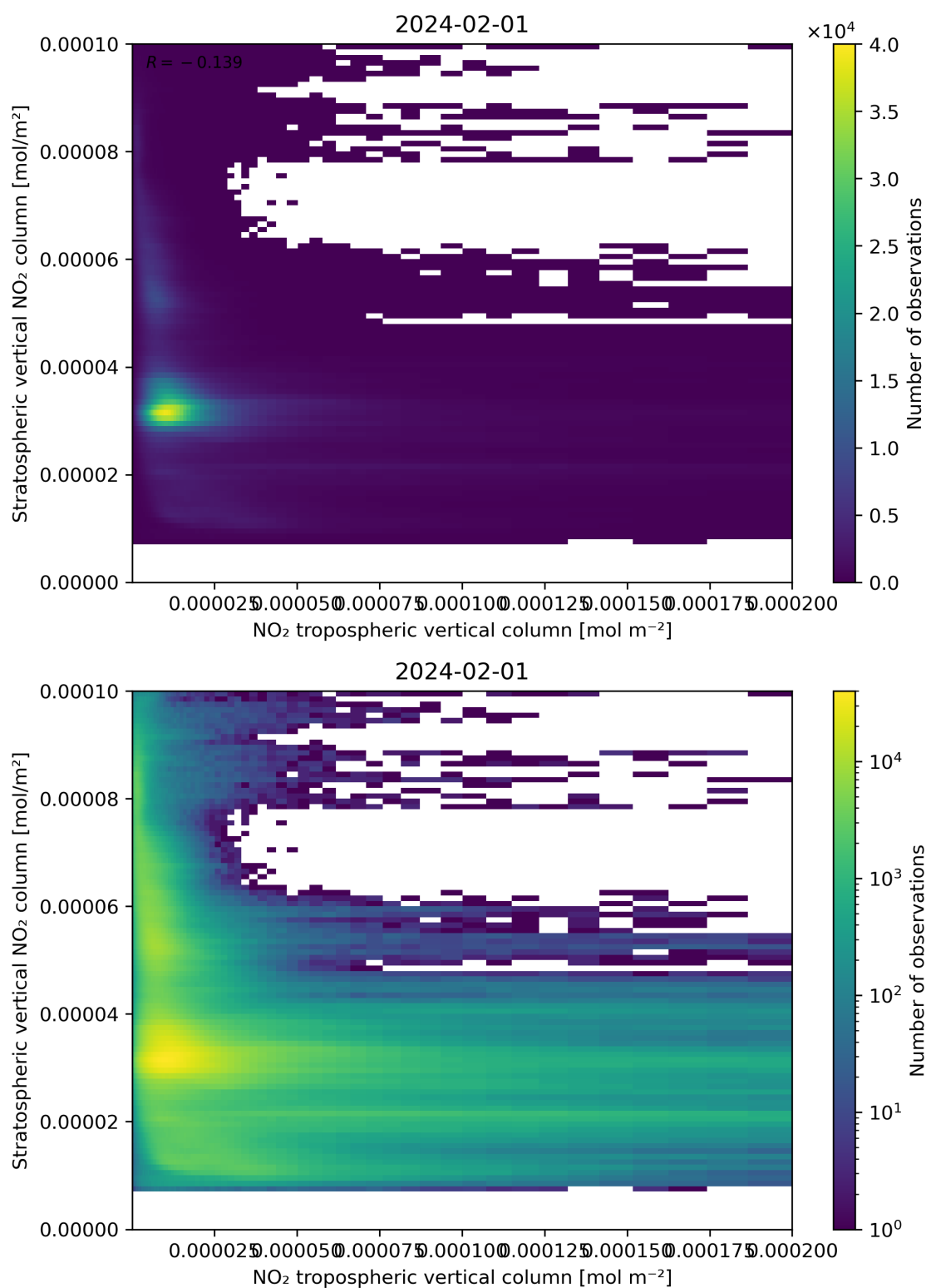
Figure 125: Scatter density plot of “NO 2 tropospheric vertical column” against “Stratospheric vertical NO 2 column” for 2024-01-31 to 2024-02-02.
