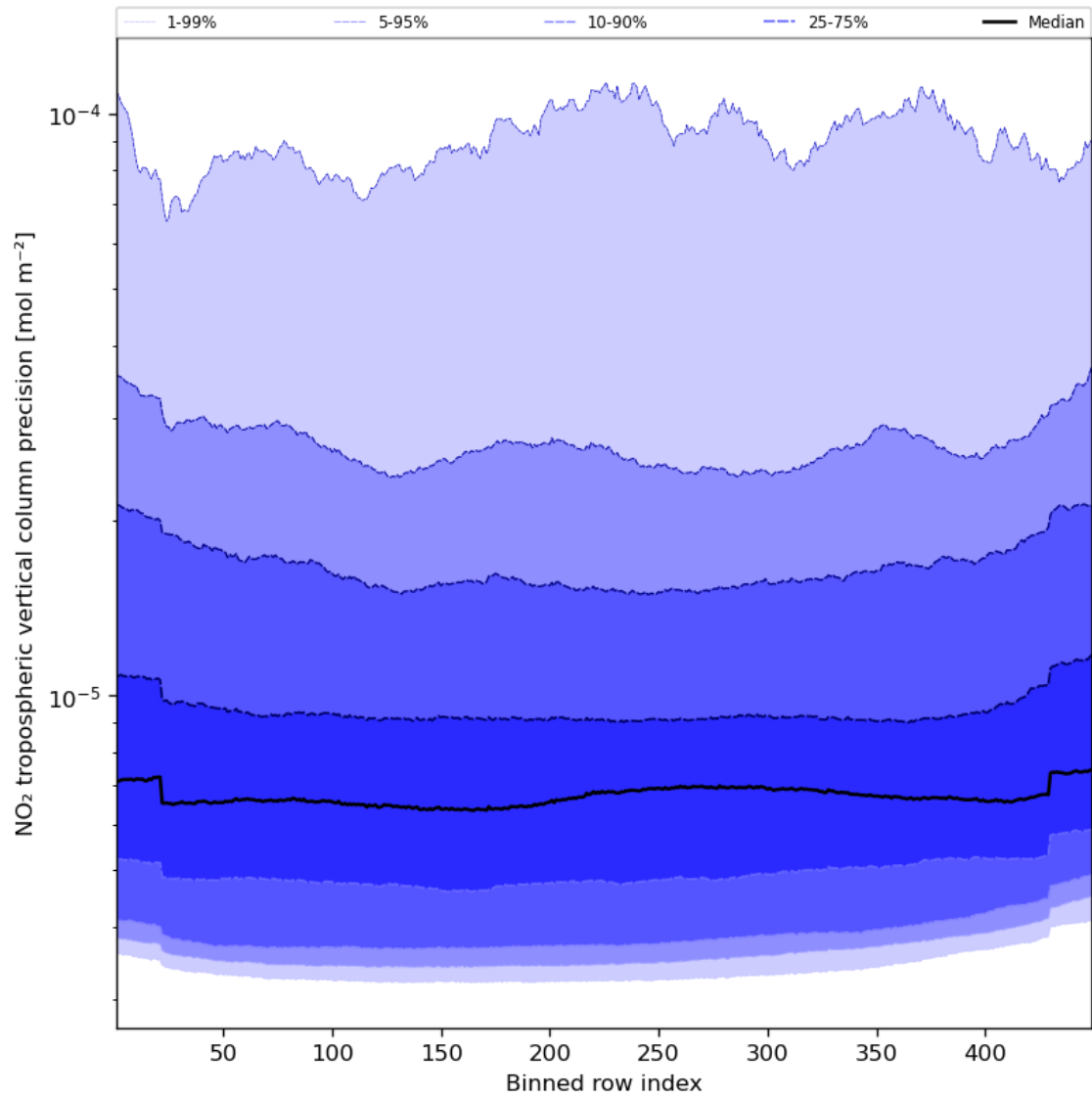
Figure 47: Along track statistics of “NO 2 tropospheric vertical column precision” for 2024-01-31 to 2024-02-02
