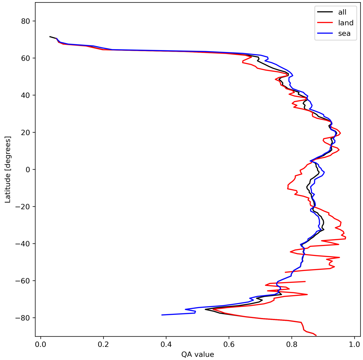
Figure 11: Zonal average of “QA value” for 2024-01-31 to 2024-02-02.
