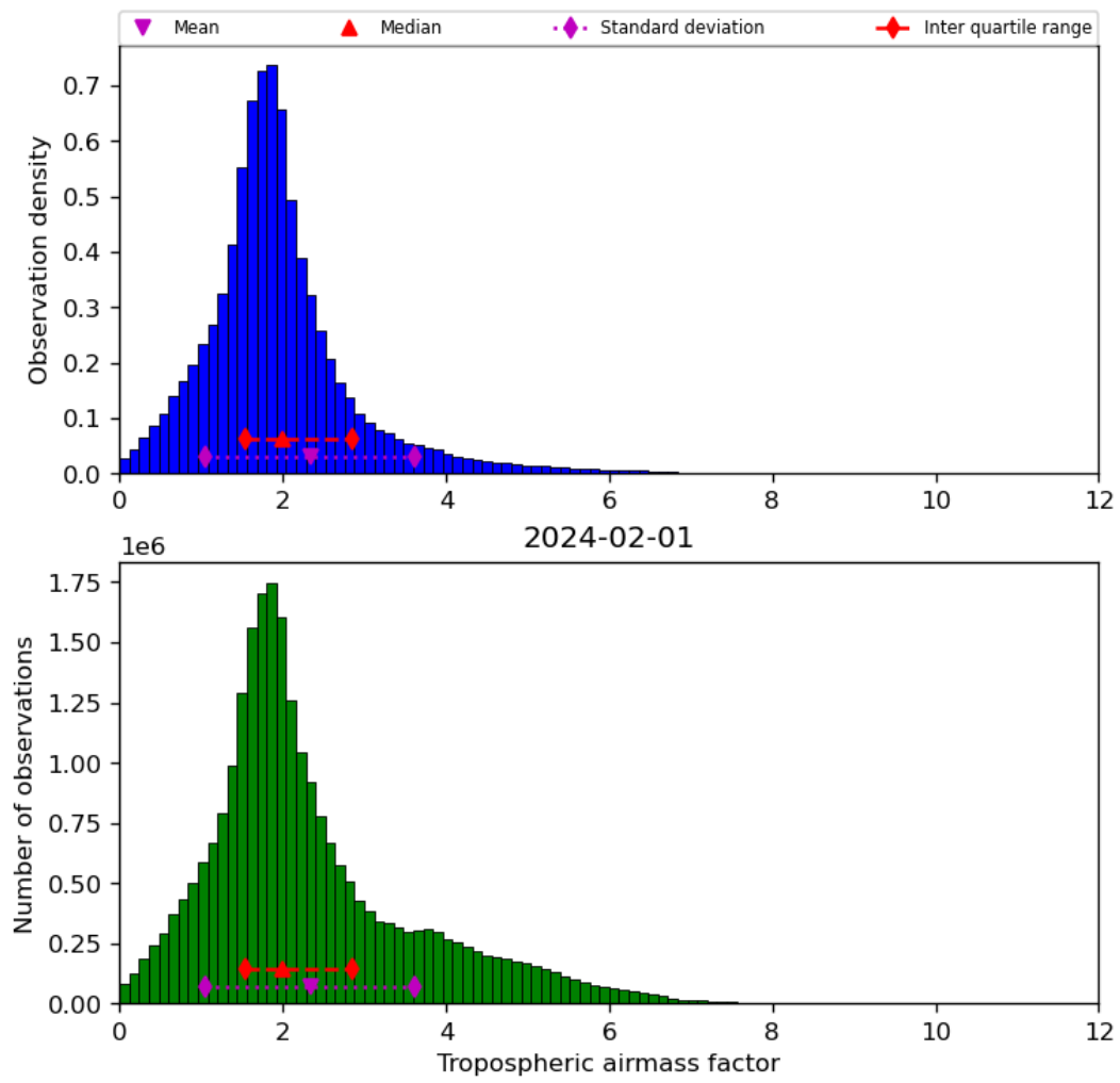
Figure 31: Histogram of “Tropospheric airmass factor” for 2024-01-31 to 2024-02-02
