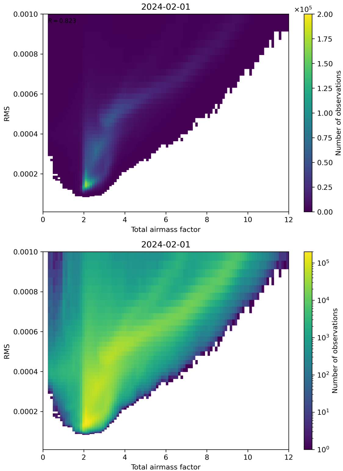
Figure 69: Scatter density plot of “Total airmass factor” against “RMS” for 2024-01-31 to 2024-02-02.
