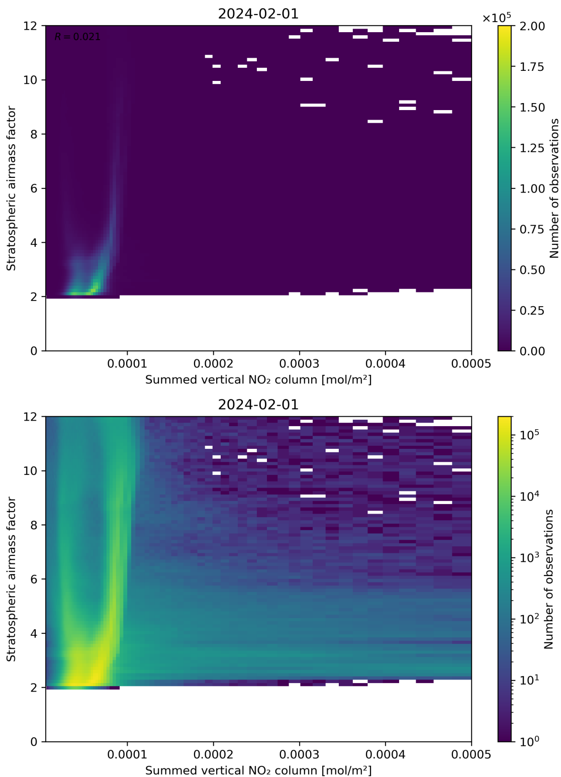
Figure 103: Scatter density plot of “Summed vertical NO 2 column” against “Stratospheric air mass factor” for 2024-01-31 to 2024-02-02.
