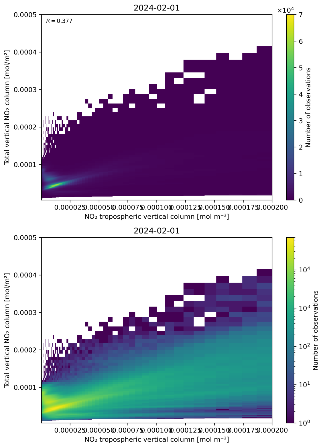
Figure 128: Scatter density plot of “NO 2 tropospheric vertical column” against “Total vertical NO 2 column” for 2024-01-31 to 2024-02-02.
