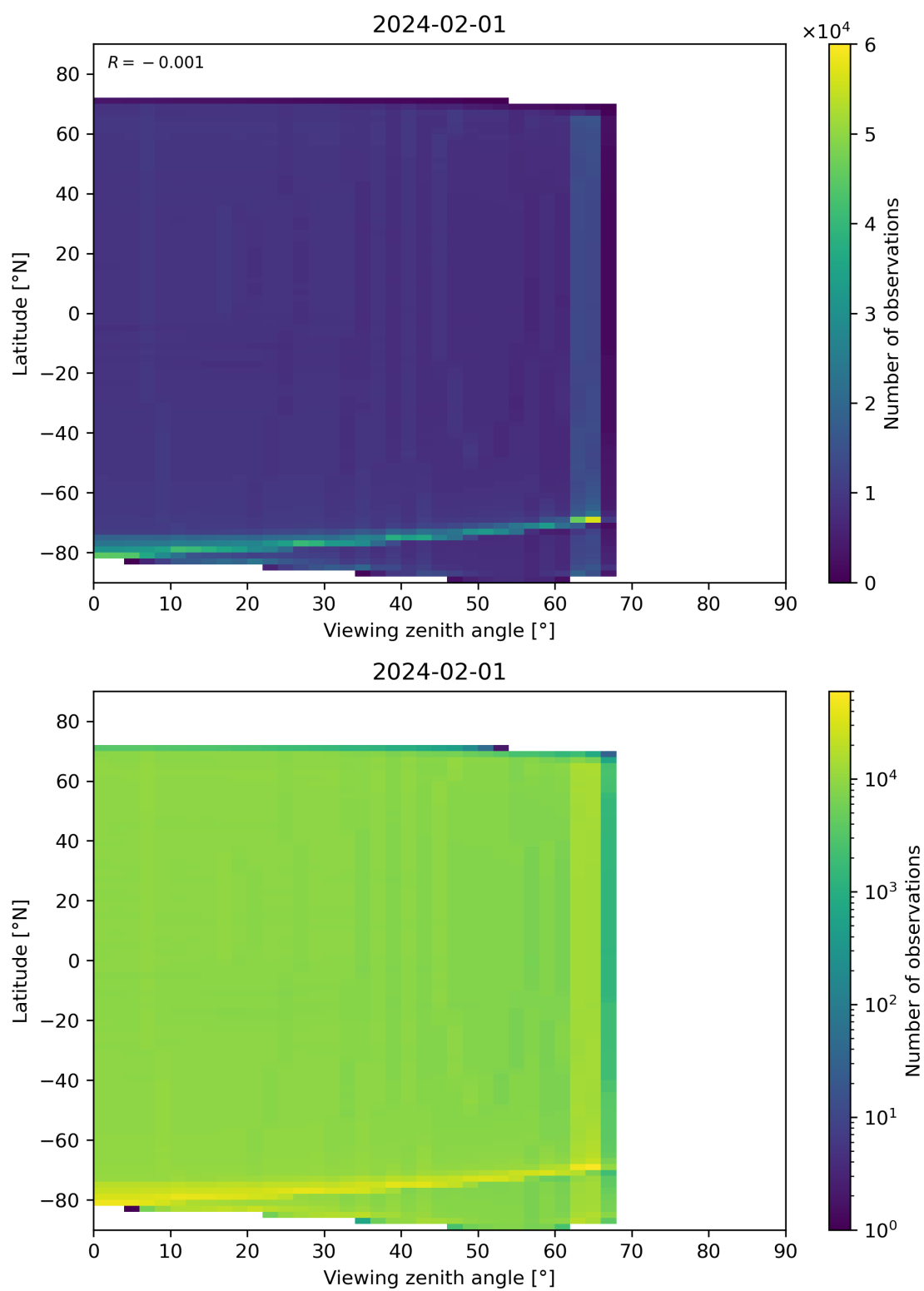
Figure 163: Scatter density plot of “Viewing zenith angle” against “Latitude” for 2024-01-31 to 2024-02-02.
