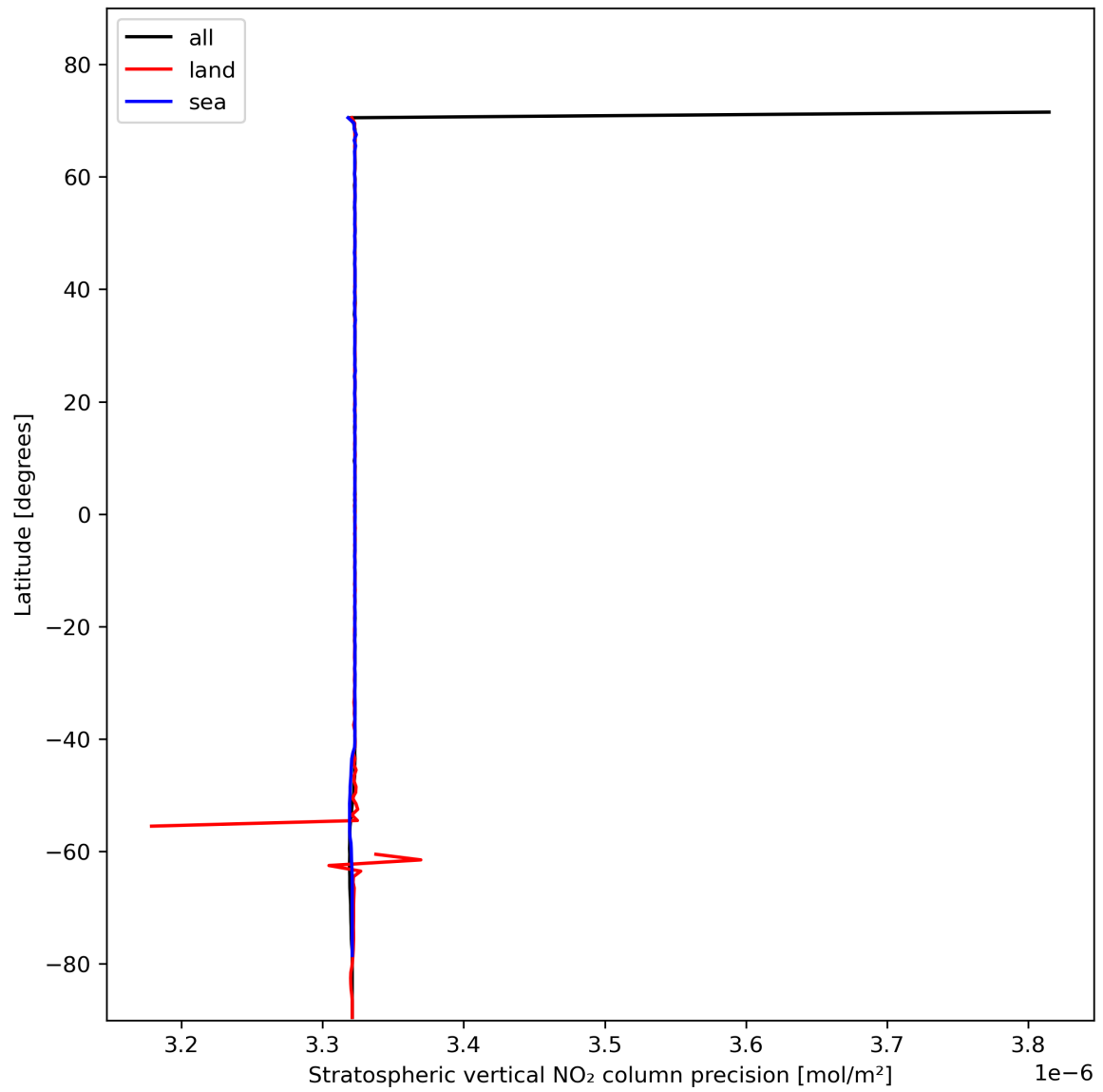
Figure 20: Zonal average of “Stratospheric vertical NO 2 column precision” for 2024-01-31 to 2024-02-02.
