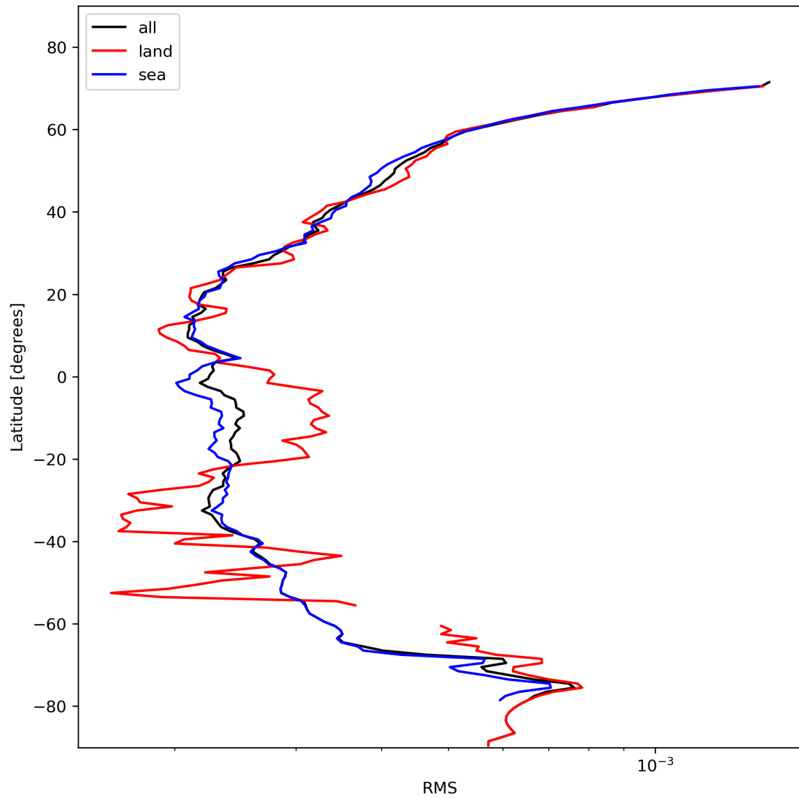
Figure 26: Zonal average of “RMS” for 2024-01-31 to 2024-02-02.
