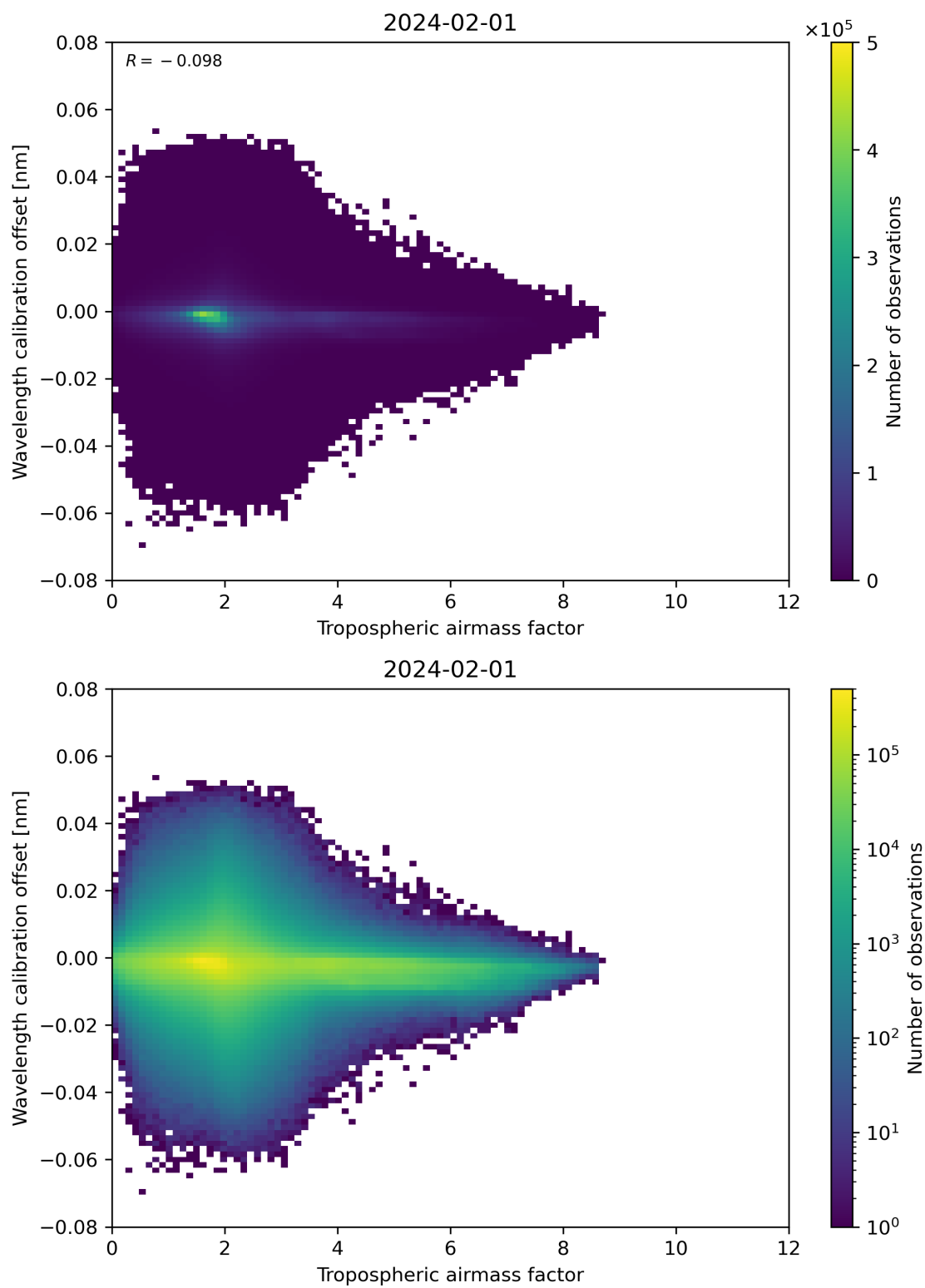
Figure 80: Scatter density plot of “Tropospheric air mass factor” against “Wavelength calibration offset” for 2024-01-31 to 2024-02-02.
