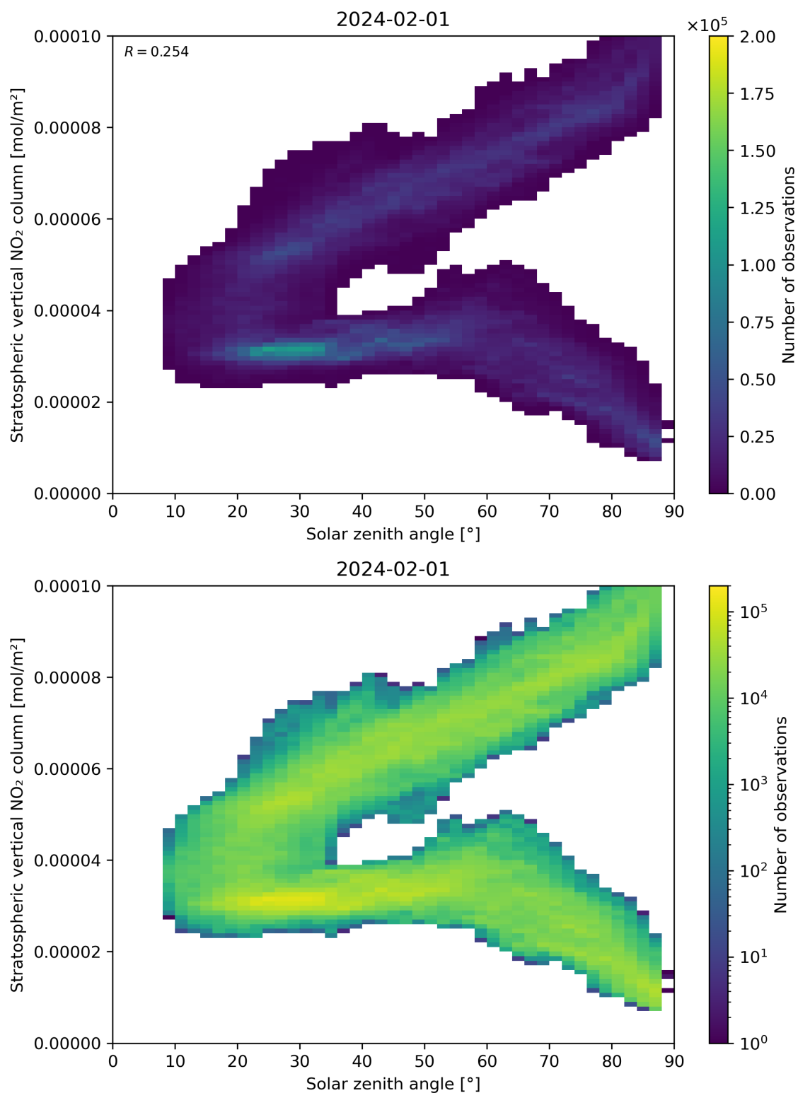
Figure 150: Scatter density plot of “Solar zenith angle” against “Stratospheric vertical NO 2 column” for 2024-01-31 to 2024-02-02.
