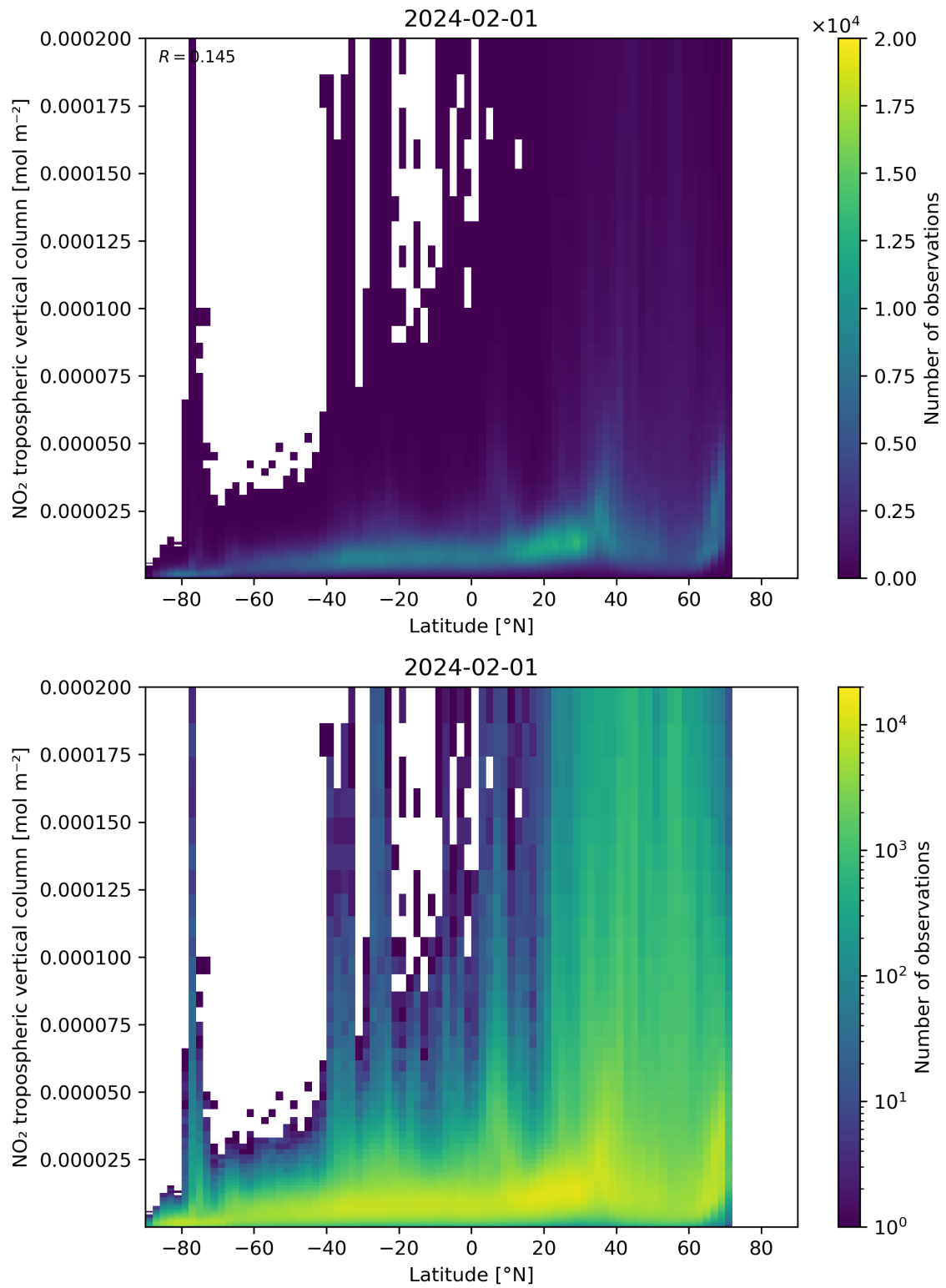
Figure 92: Scatter density plot of “Latitude” against “NO 2 tropospheric vertical column” for 2024-01-31 to 2024-02-02.
