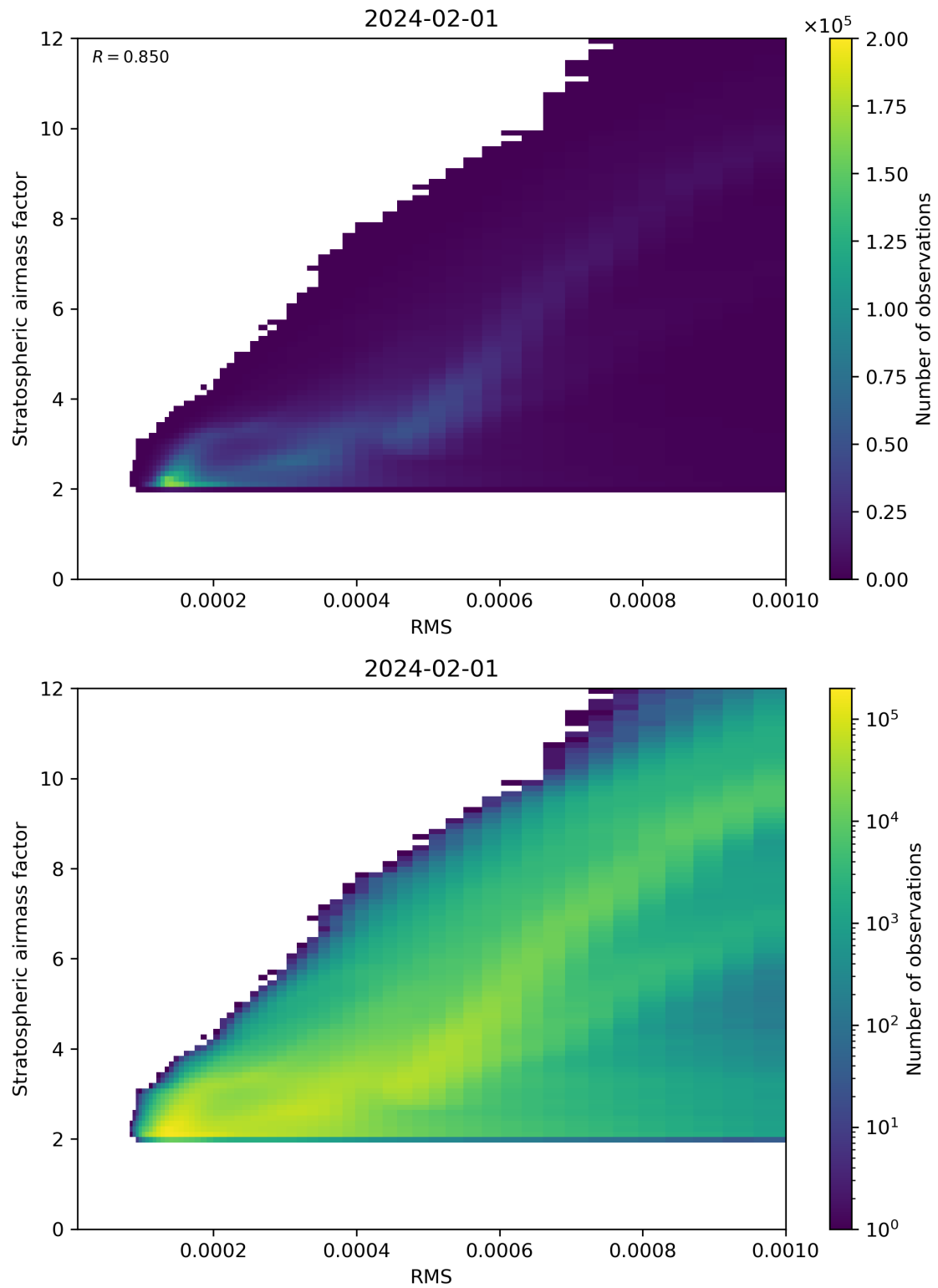
Figure 144: Scatter density plot of “RMS” against “Stratospheric airmass factor” for 2024-01-31 to 2024-02-02.
