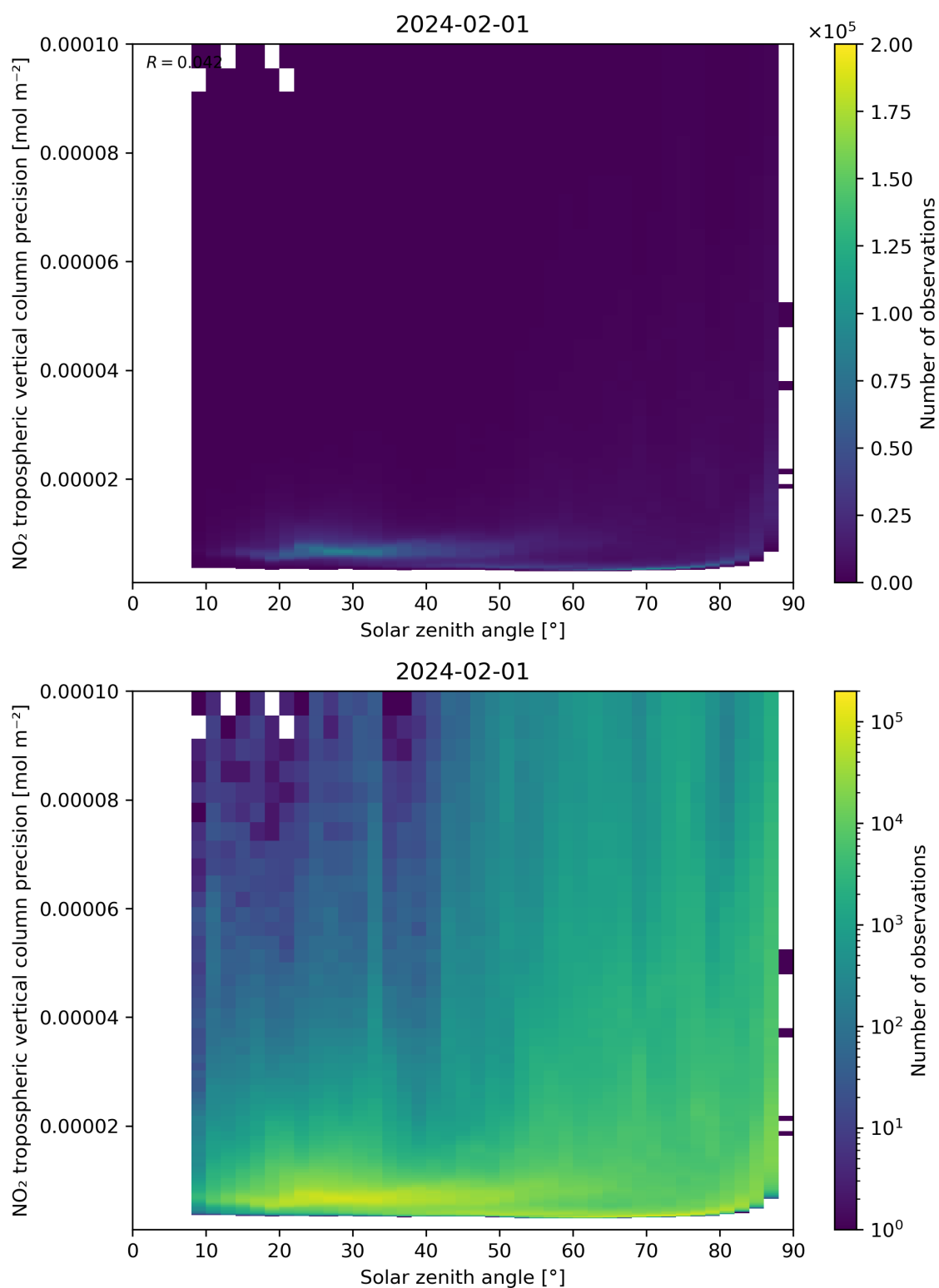
Figure 156: Scatter density plot of “Solar zenith angle” against “NO 2 tropospheric vertical column precision” for 2024-01-31 to 2024-02-02.
