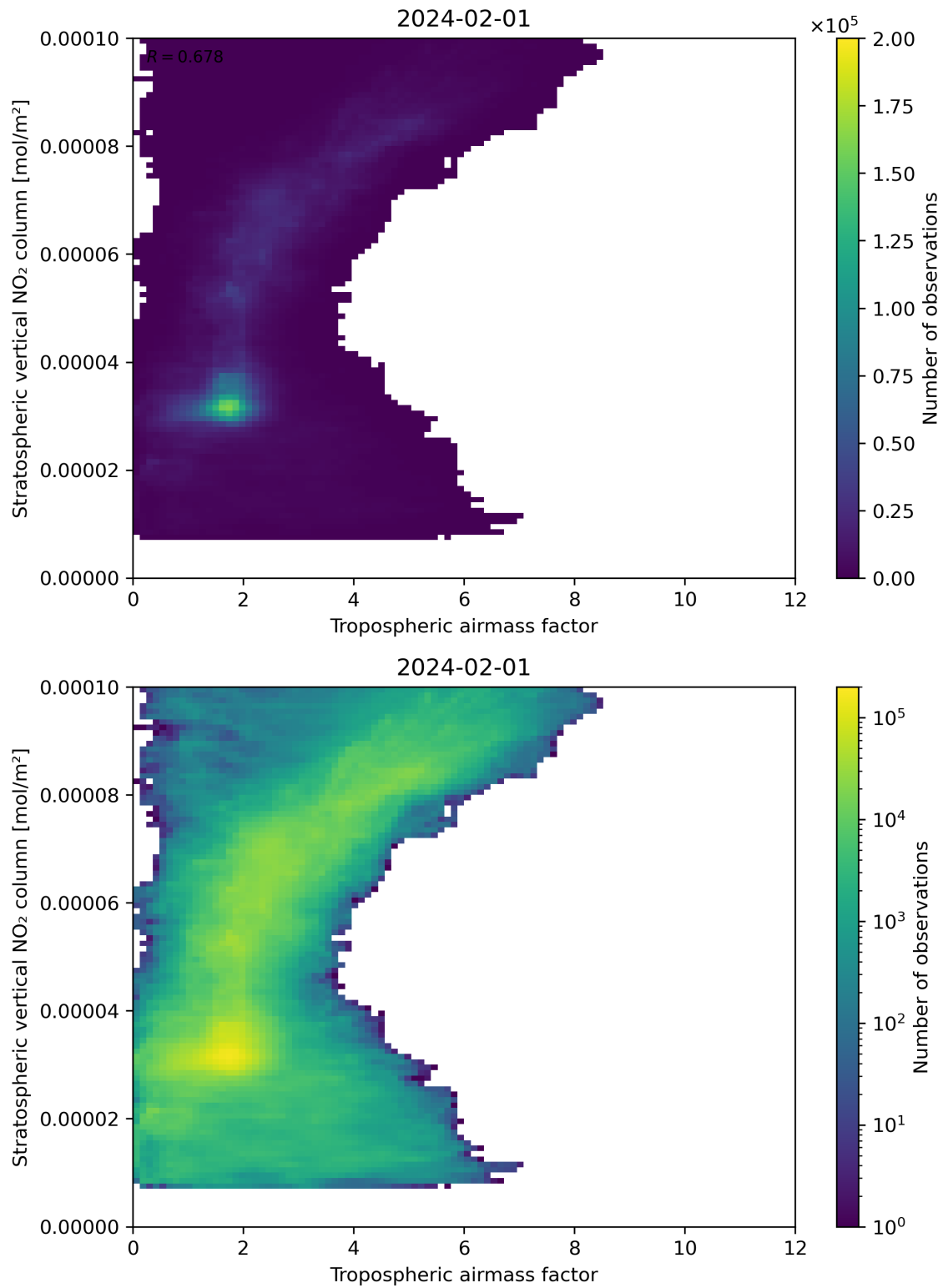
Figure 74: Scatter density plot of “Tropospheric air mass factor” against “Stratospheric vertical NO 2 column” for 2024-01-31 to 2024-02-02.
