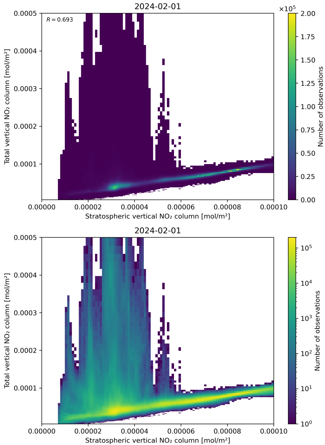
Figure 100: Scatter density plot of “Stratospheric vertical NO 2 column” against “Total vertical NO 2 column” for 2024-01-31 to 2024-02-02.
