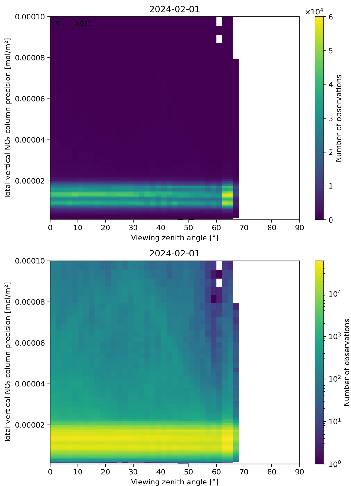
Figure 168: Scatter density plot of “Viewing zenith angle” against “Total vertical NO 2 column precision” for 2024-01-31 to 2024-02-02.
