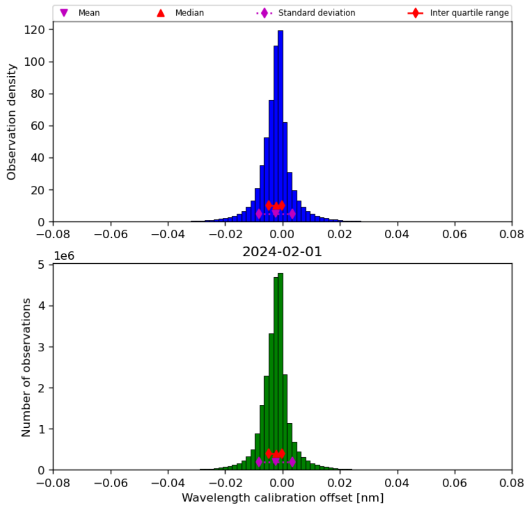
Figure 35: Histogram of “Wavelength calibration offset” for 2024-01-31 to 2024-02-02
