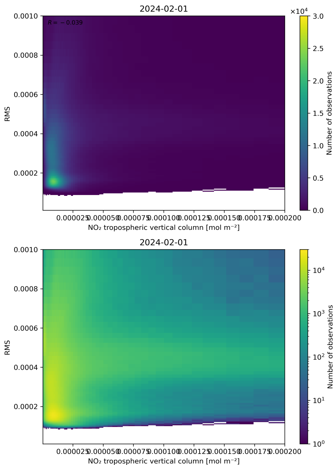
Figure 142: Scatter density plot of “NO 2 tropospheric vertical column” against “RMS” for 2024-01-31 to 2024-02-02.
