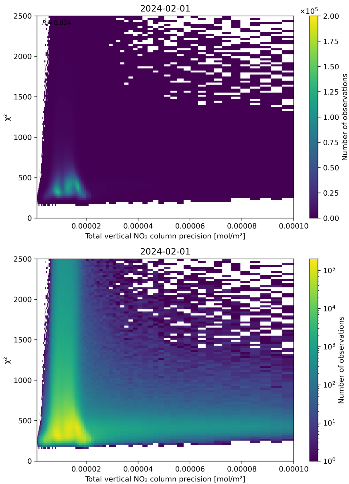
Figure 116: Scatter density plot of "Total vertical NO 2 column precision" against " \chi^2 " for 2024-01-31 to 2024-02-02.
