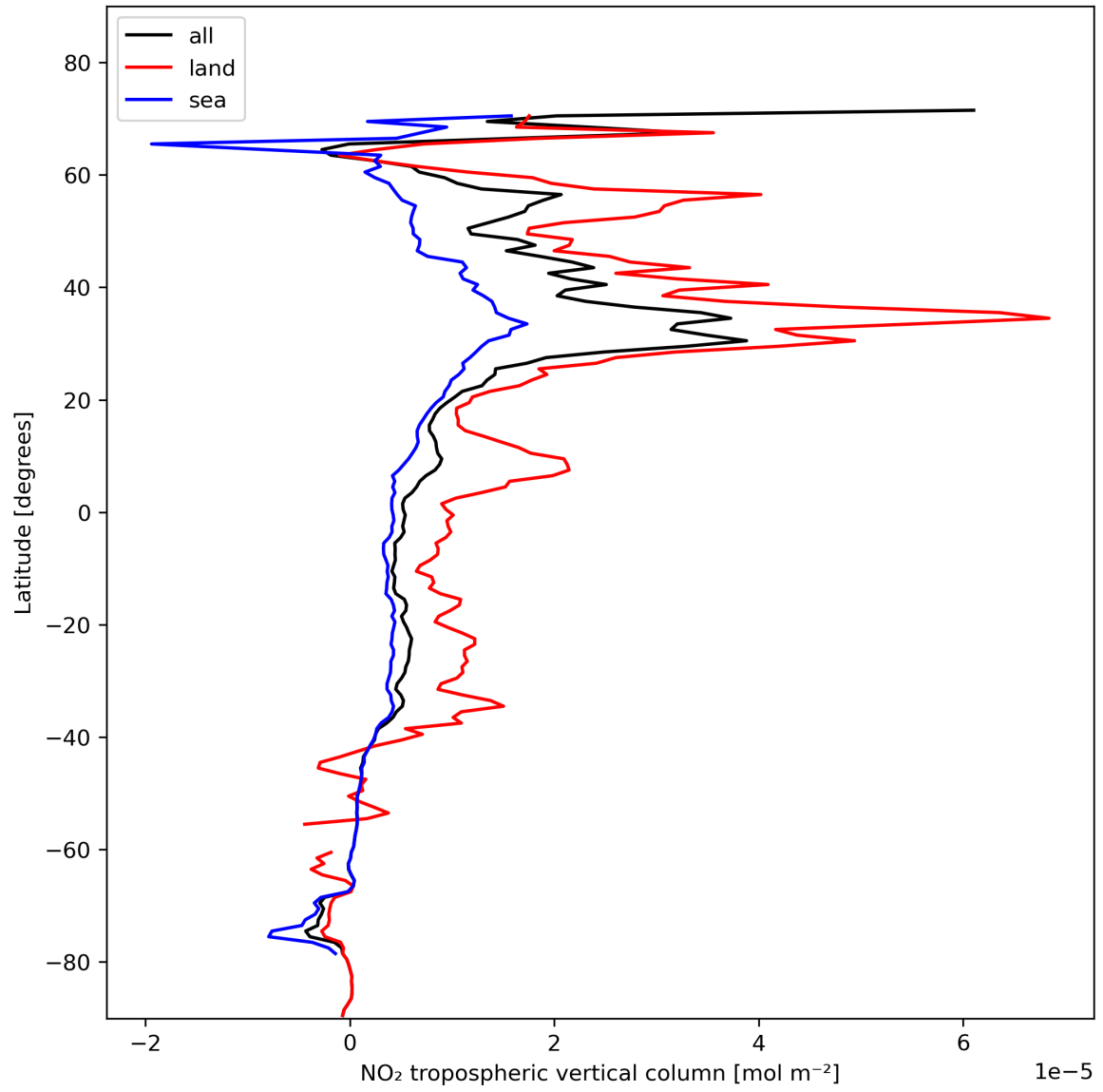
Figure 12: Zonal average of “NO 2 tropospheric vertical column” for 2024-01-31 to 2024-02-02.
