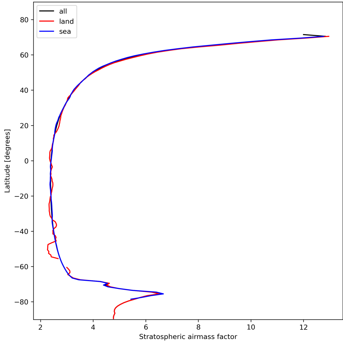
Figure 27: Zonal average of “Stratospheric air mass factor” for 2024-01-31 to 2024-02-02.
