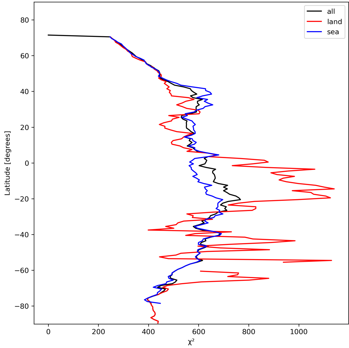
Figure 25: Zonal average of “ \chi^2 ” for 2024-01-31 to 2024-02-02.
