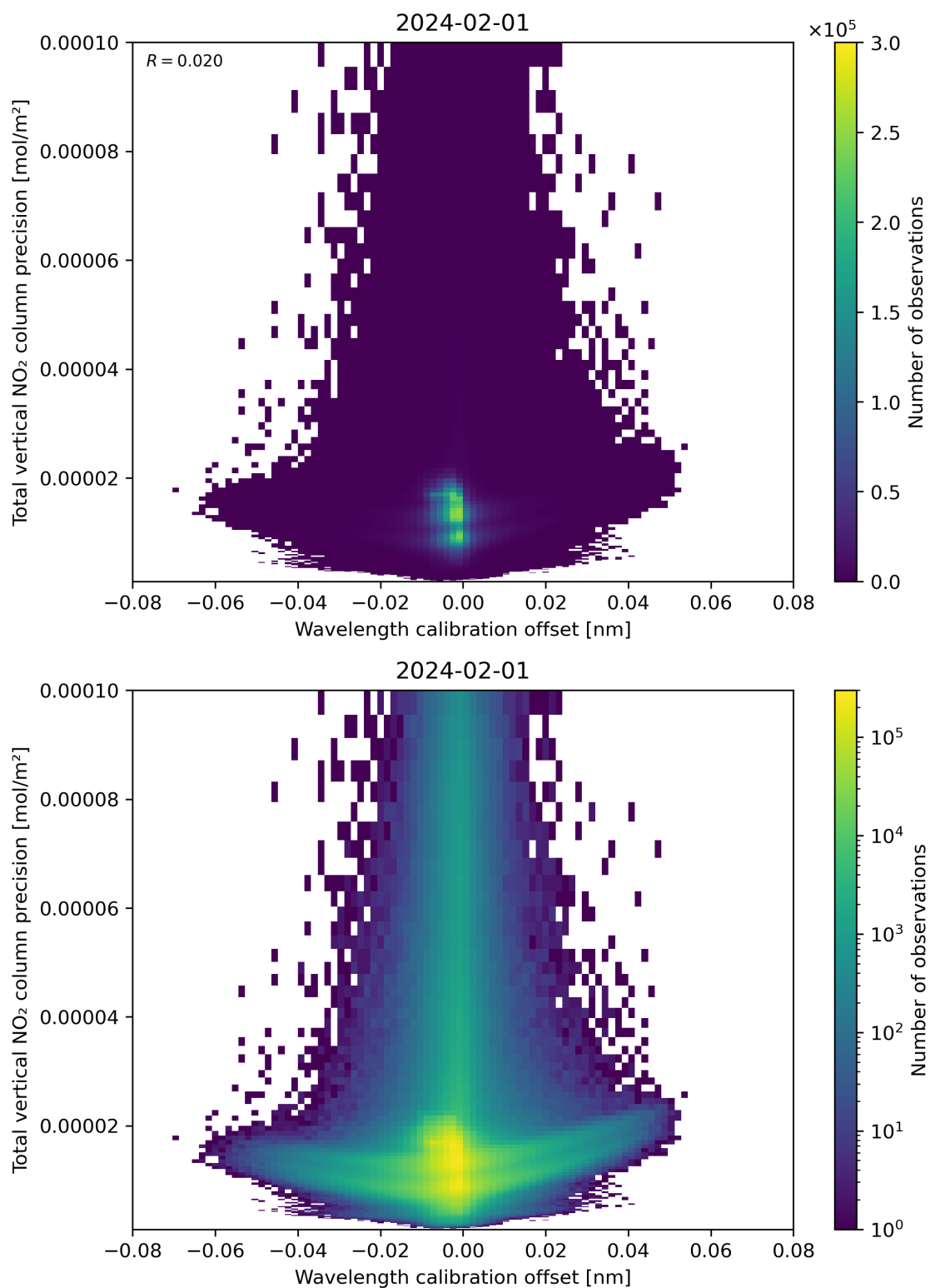
Figure 180: Scatter density plot of “Wavelength calibration offset” against “Total vertical NO 2 column precision” for 2024-01-31 to 2024-02-02.
