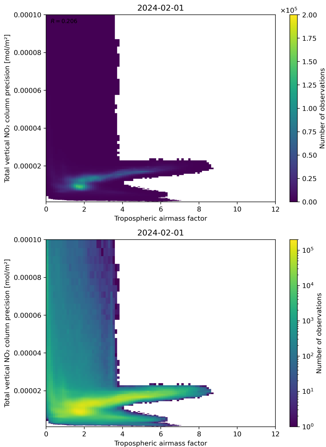
Figure 78: Scatter density plot of “Tropospheric air mass factor” against “Total vertical NO 2 column precision” for 2024-01-31 to 2024-02-02.
