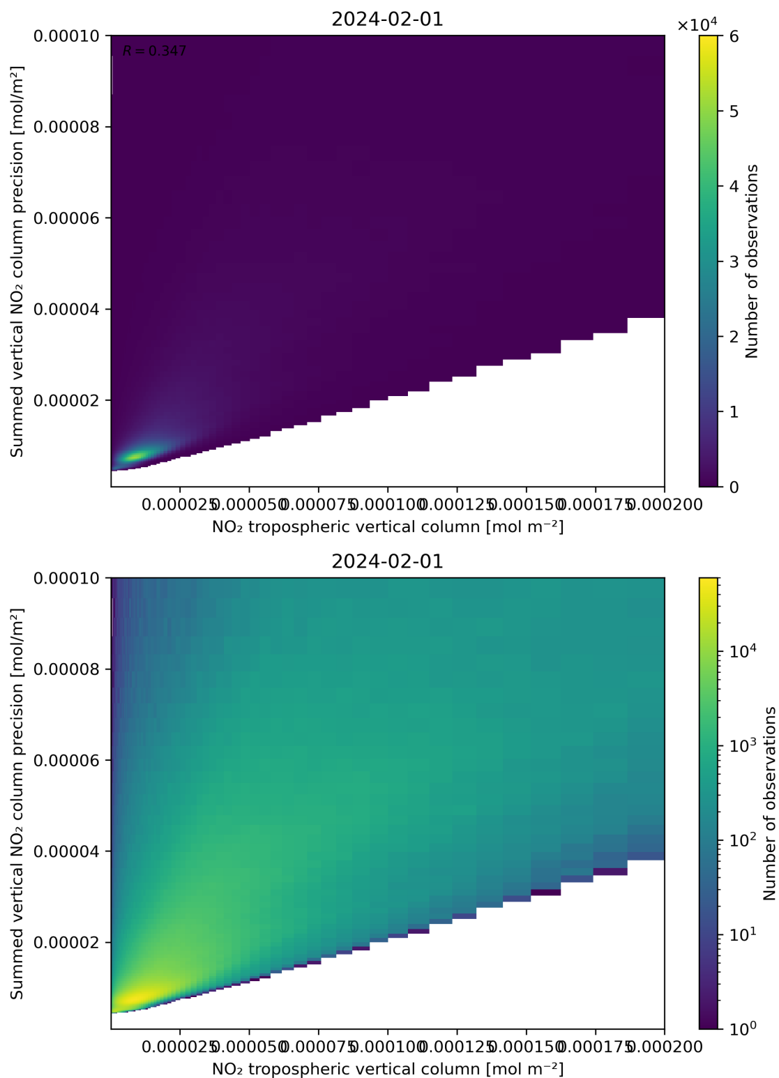
Figure 127: Scatter density plot of “NO 2 tropospheric vertical column” against “Summed vertical NO 2 column precision” for 2024-01-31 to 2024-02-02.
