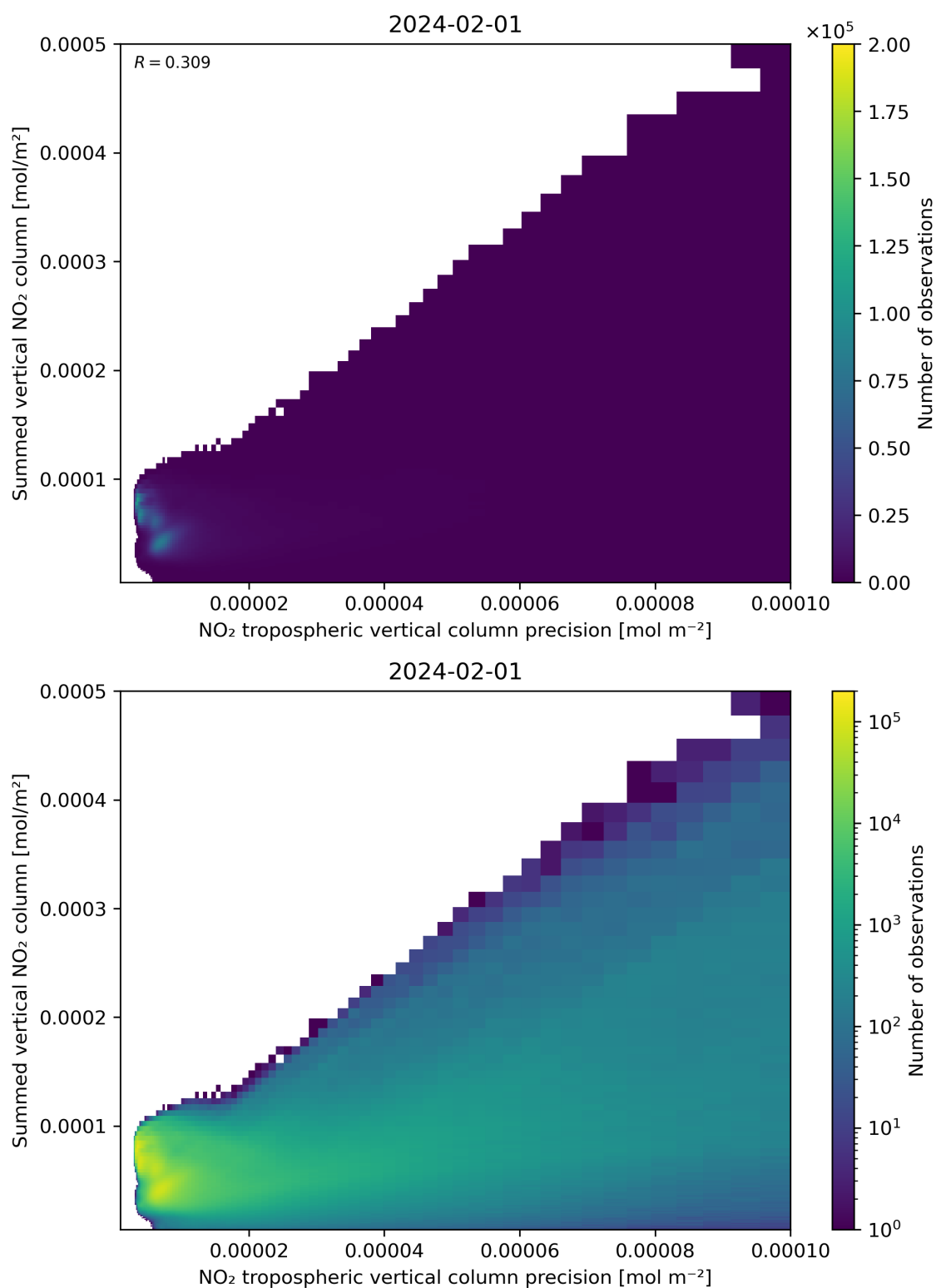
Figure 136: Scatter density plot of “NO 2 tropospheric vertical column precision” against “Summed vertical NO 2 column” for 2024-01-31 to 2024-02-02.
