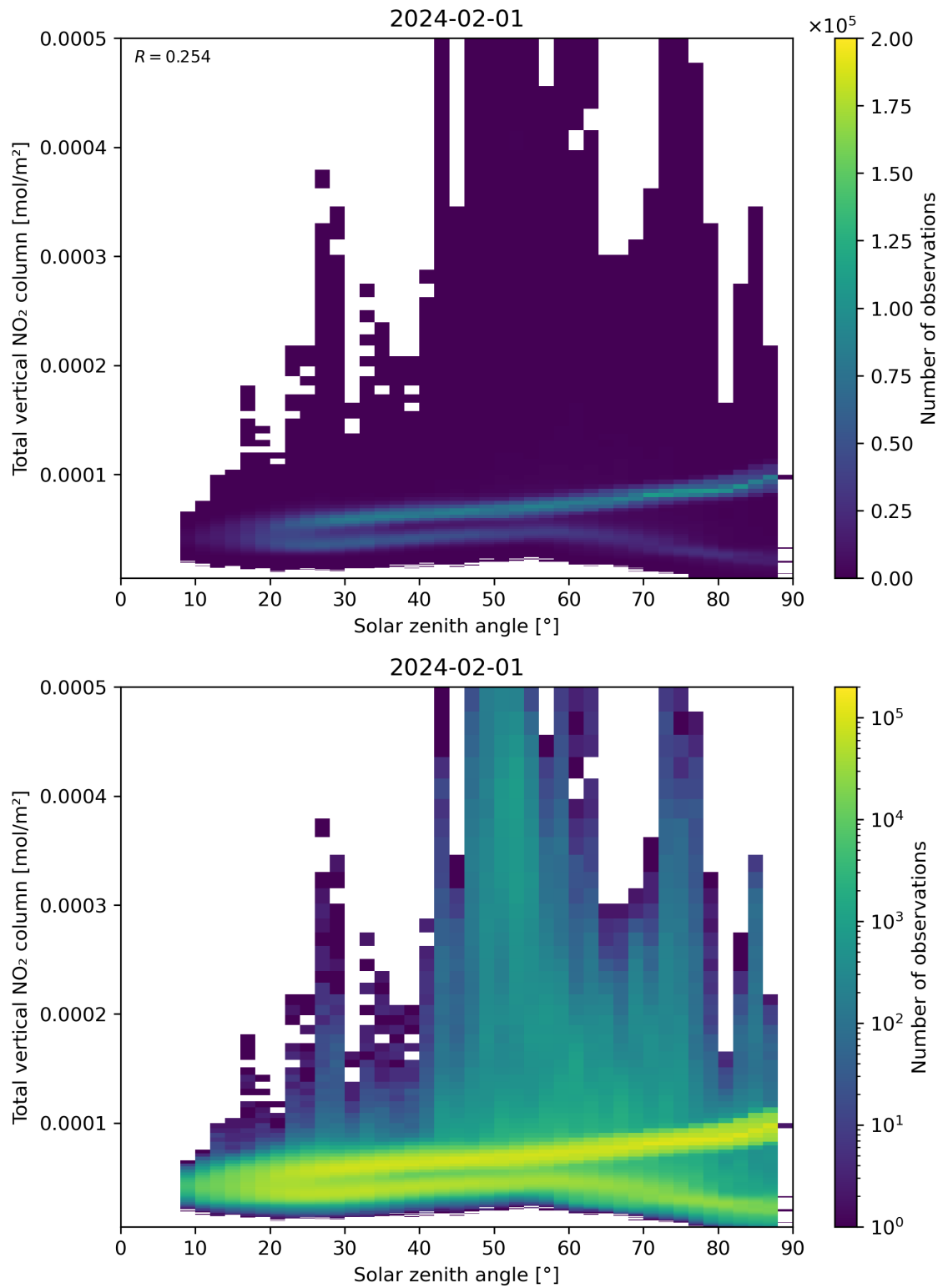
Figure 153: Scatter density plot of “Solar zenith angle” against “Total vertical NO 2 column” for 2024-01-31 to 2024-02-02.
