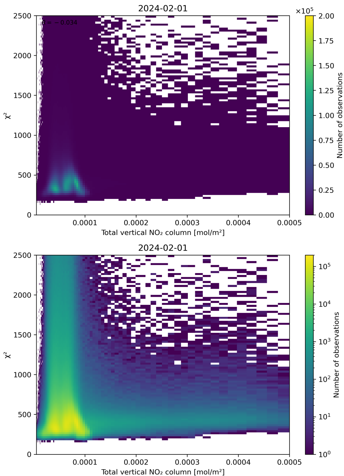
Figure 111: Scatter density plot of “Total vertical NO 2 column” against “ \chi^2 ” for 2024-01-31 to 2024-02-02.
