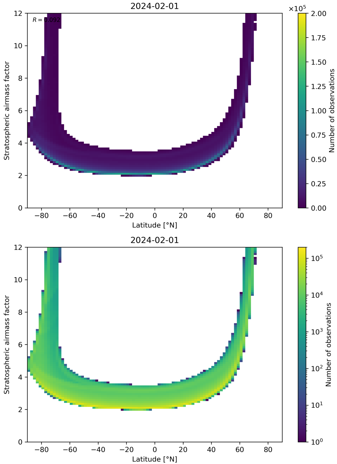
Figure 83: Scatter density plot of “Latitude” against “Stratospheric air mass factor” for 2024-01-31 to 2024-02-02.
