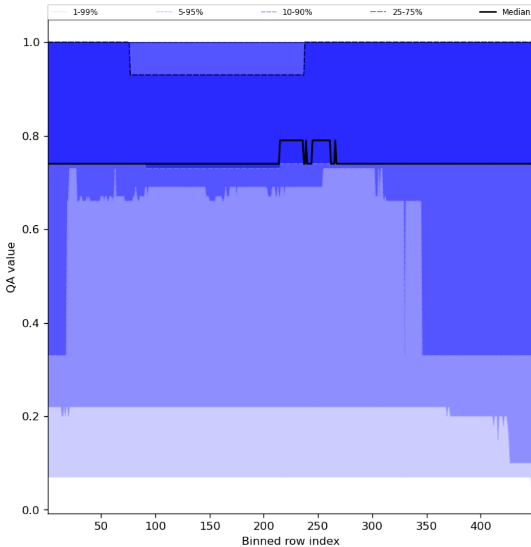
Figure 45: Along track statistics of “QA value” for 2024-01-31 to 2024-02-02
