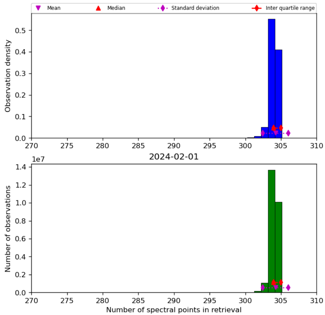
Figure 33: Histogram of “Number of spectral points in retrieval” for 2024-01-31 to 2024-02-02
