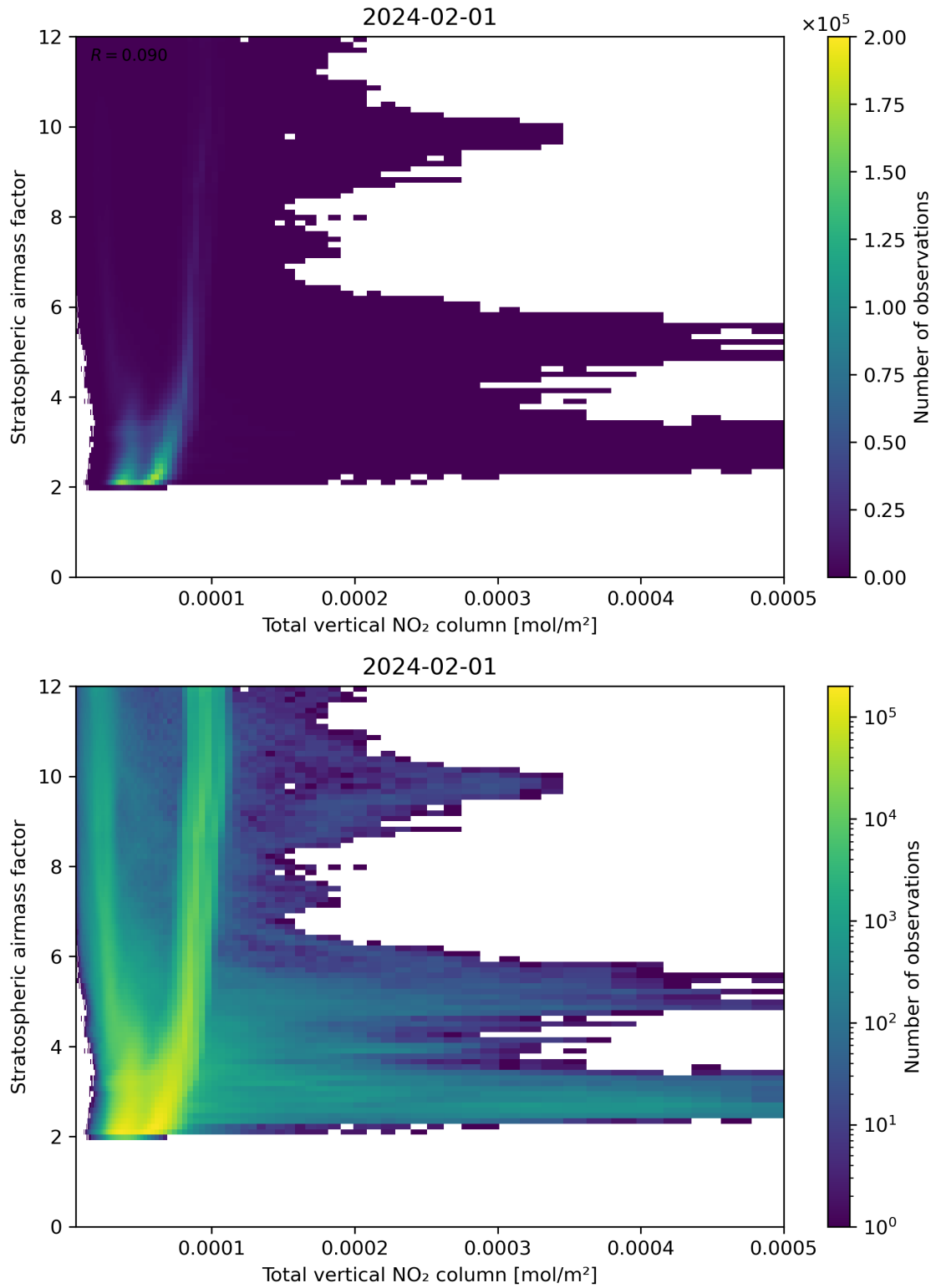
Figure 110: Scatter density plot of “Total vertical NO 2 column” against “Stratospheric airmass factor” for 2024-01-31 to 2024-02-02.
