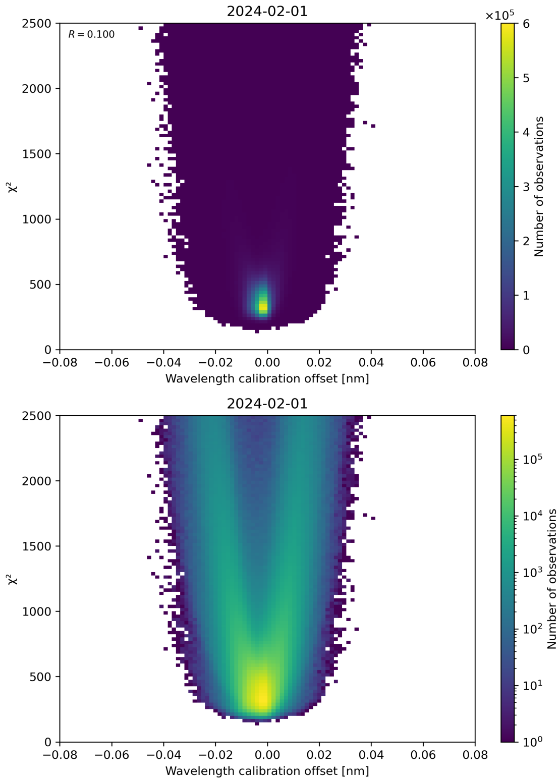
Figure 175: Scatter density plot of “Wavelength calibration offset” against “ \chi^2 ” for 2024-01-31 to 2024-02-02.
