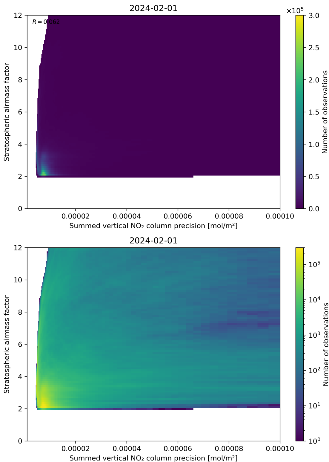
Figure 106: Scatter density plot of “Summed vertical NO 2 column precision” against “Stratospheric airmass factor” for 2024-01-31 to 2024-02-02.
