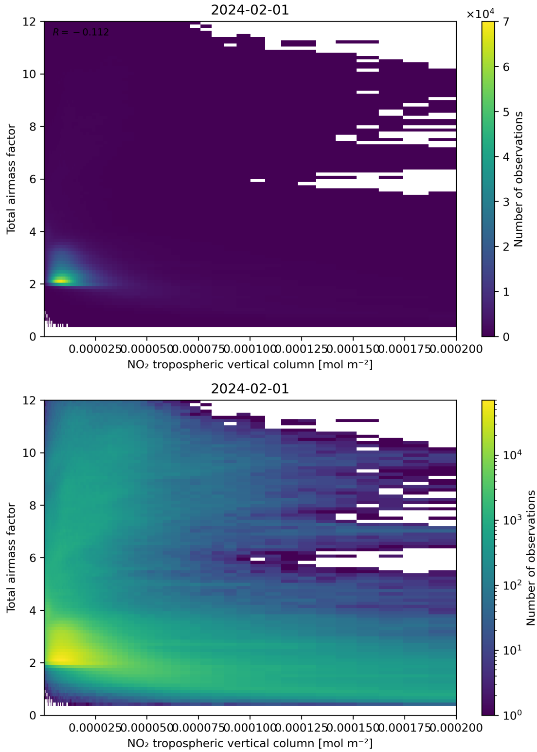
Figure 122: Scatter density plot of “NO 2 tropospheric vertical column” against “Total air mass factor” for 2024-01-31 to 2024-02-02.
