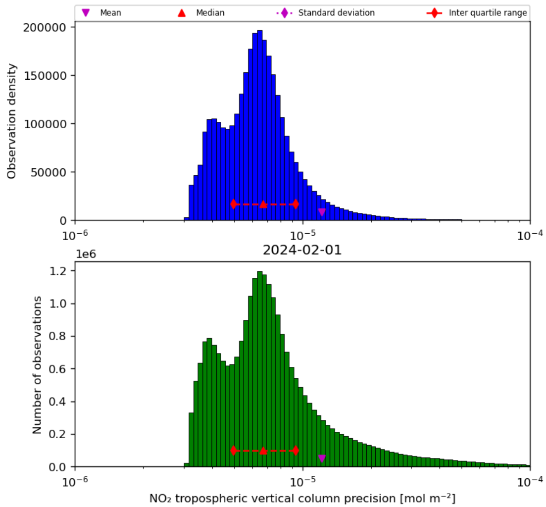
Figure 30: Histogram of “NO 2 tropospheric vertical column precision” for 2024-01-31 to 2024-02-02
