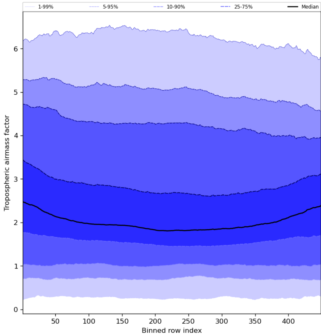
Figure 48: Along track statistics of “Tropospheric airmass factor” for 2024-01-31 to 2024-02-02
