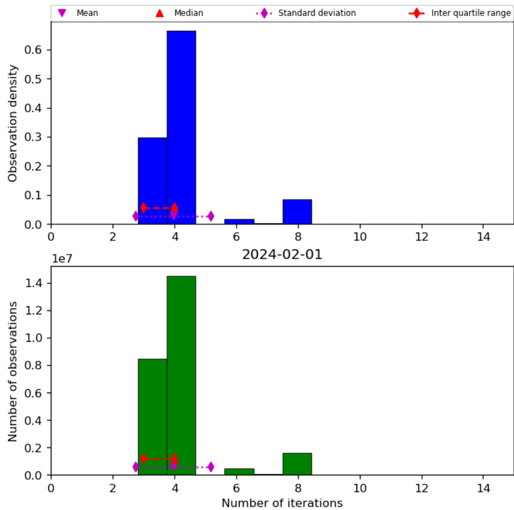
Figure 34: Histogram of “Number of iterations” for 2024-01-31 to 2024-02-02
