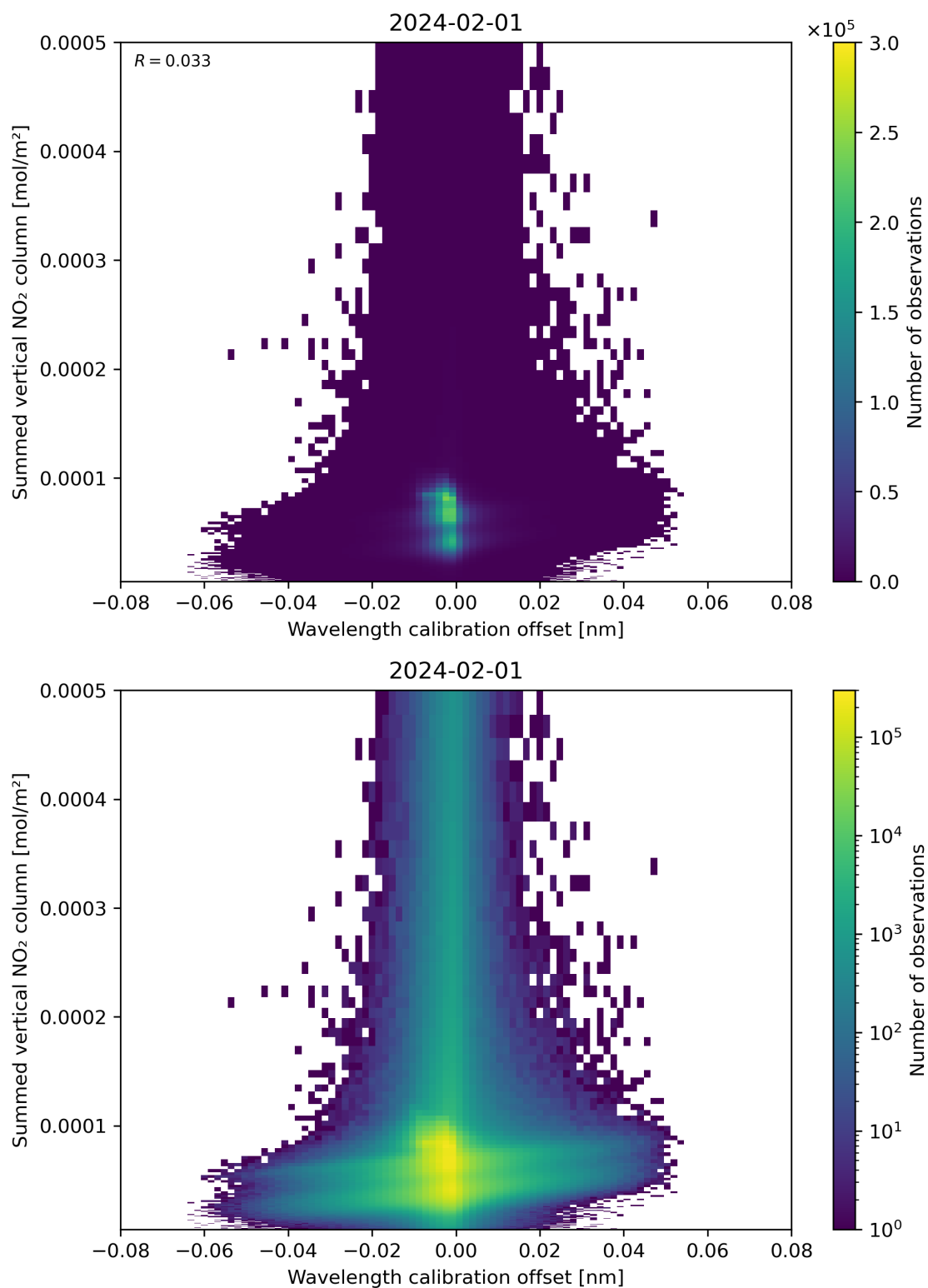
Figure 177: Scatter density plot of “Wavelength calibration offset” against “Summed vertical NO 2 column” for 2024-01-31 to 2024-02-02.
