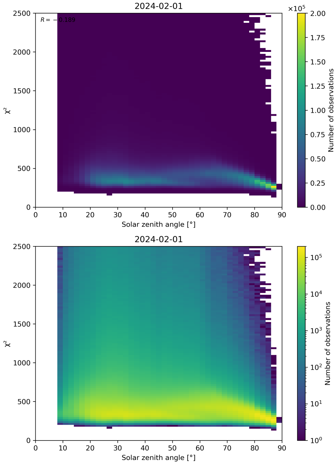
Figure 148: Scatter density plot of “Solar zenith angle” against “ \chi^2 ” for 2024-01-31 to 2024-02-02.
