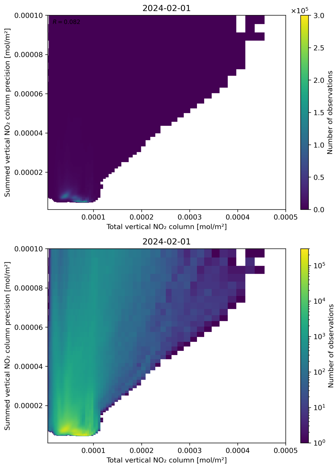
Figure 113: Scatter density plot of “Total vertical NO 2 column” against “Summed vertical NO 2 column precision” for 2024-01-31 to 2024-02-02.
