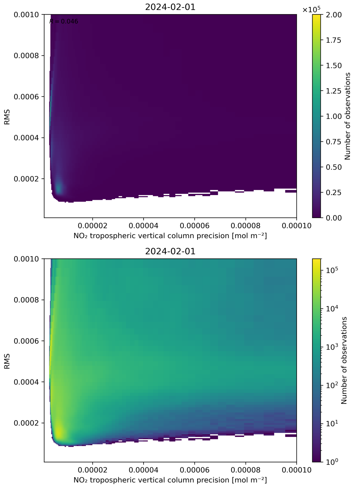
Figure 140: Scatter density plot of “NO 2 tropospheric vertical column precision” against “RMS” for 2024-01-31 to 2024-02-02.
