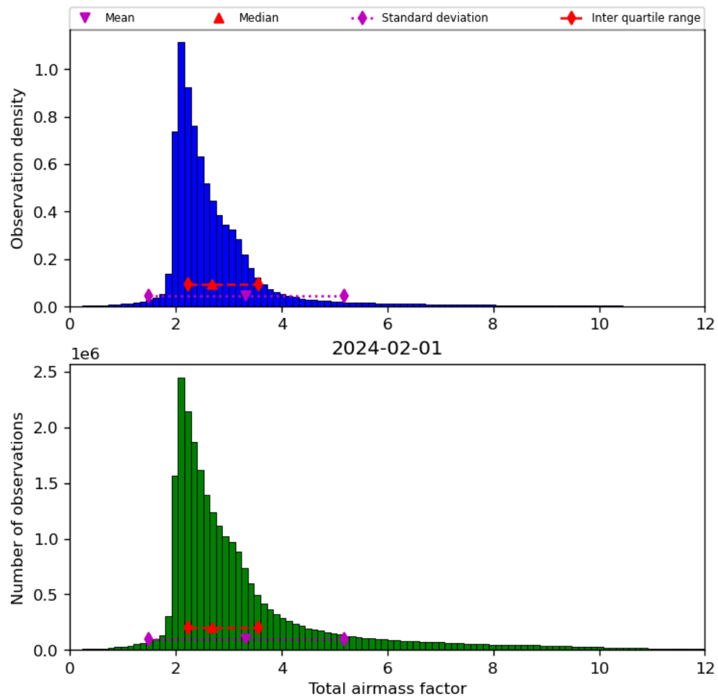
Figure 32: Histogram of “Total airmass factor” for 2024-01-31 to 2024-02-02
