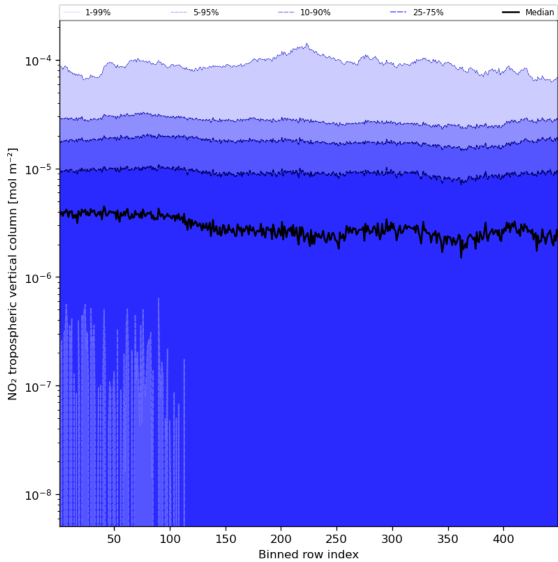
Figure 46: Along track statistics of “NO 2 tropospheric vertical column” for 2024-01-31 to 2024-02-02
