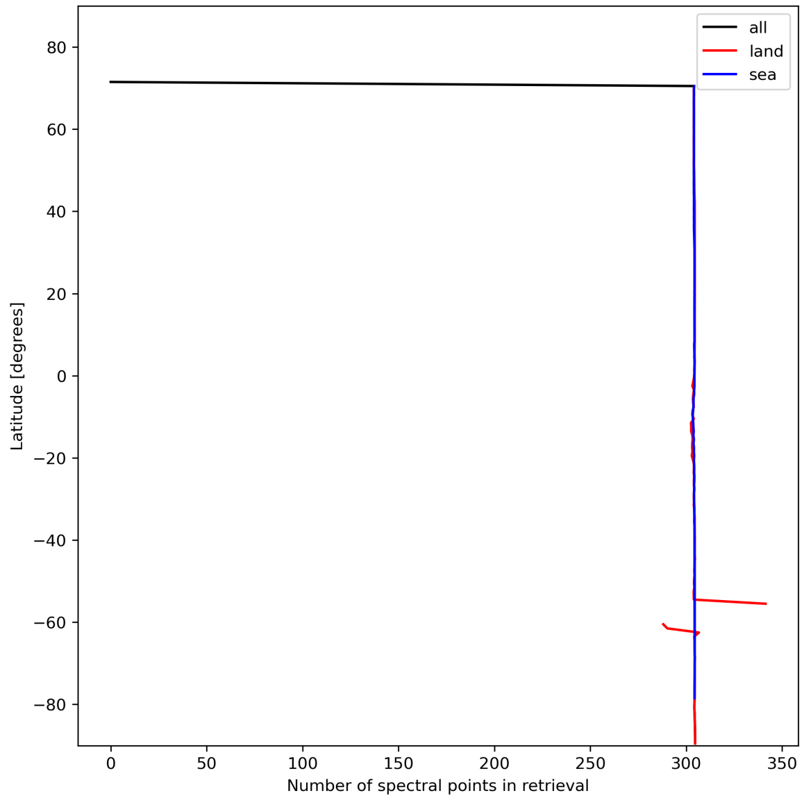
Figure 16: Zonal average of “Number of spectral points in retrieval” for 2024-01-31 to 2024-02-02.
