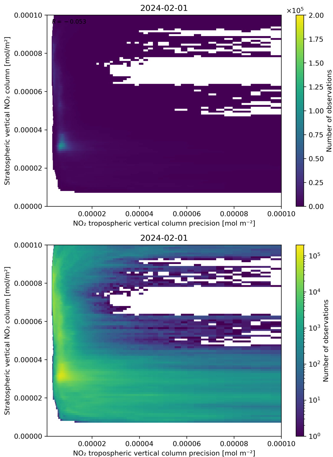
Figure 135: Scatter density plot of “NO 2 tropospheric vertical column precision” against “Stratospheric vertical NO 2 column” for 2024-01-31 to 2024-02-02.
