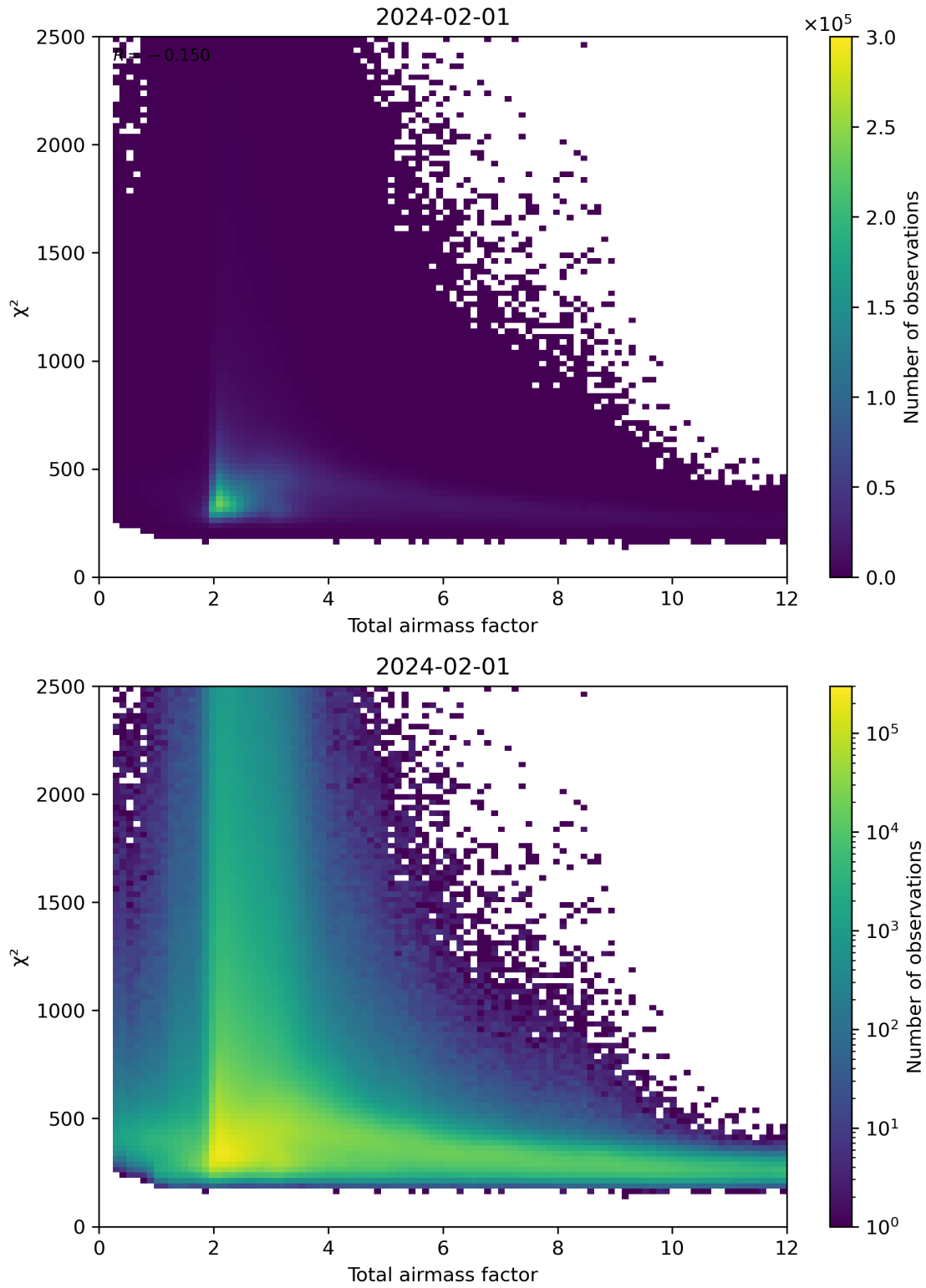
Figure 63: Scatter density plot of “Total airmass factor” against “ \chi^2 ” for 2024-01-31 to 2024-02-02.
