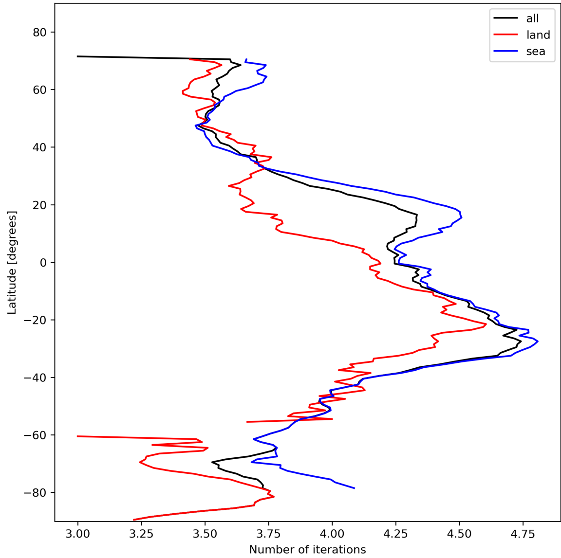
Figure 17: Zonal average of “Number of iterations” for 2024-01-31 to 2024-02-02.
