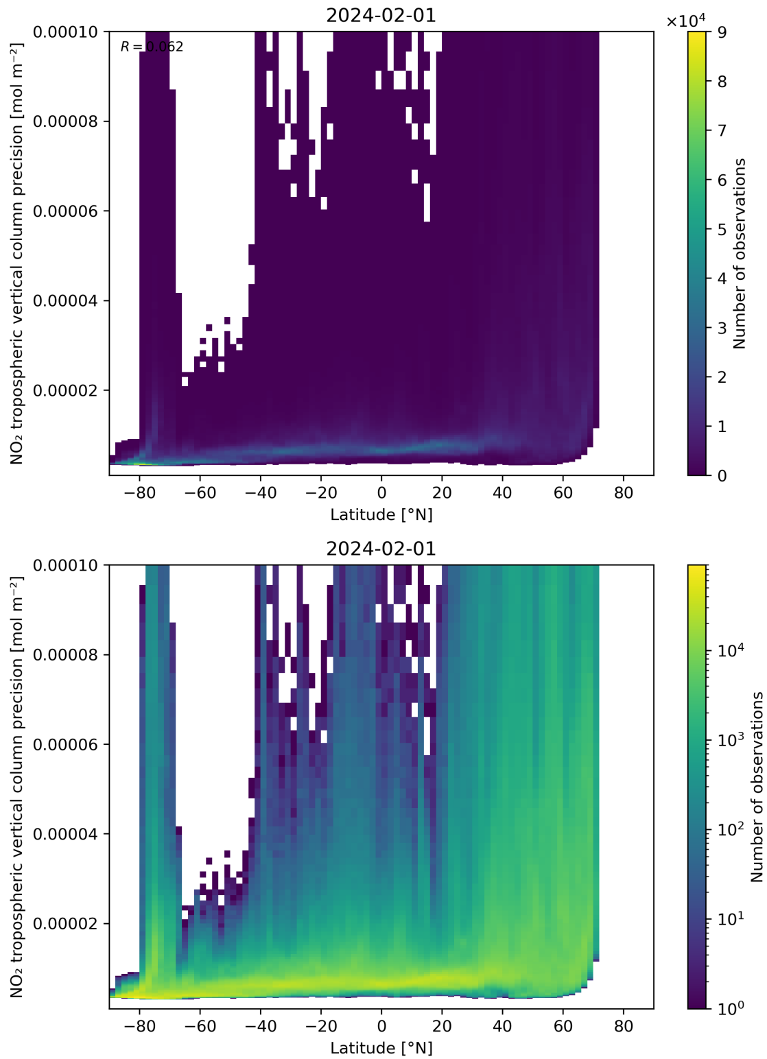
Figure 93: Scatter density plot of “Latitude” against “NO 2 tropospheric vertical column precision” for 2024-01-31 to 2024-02-02.
