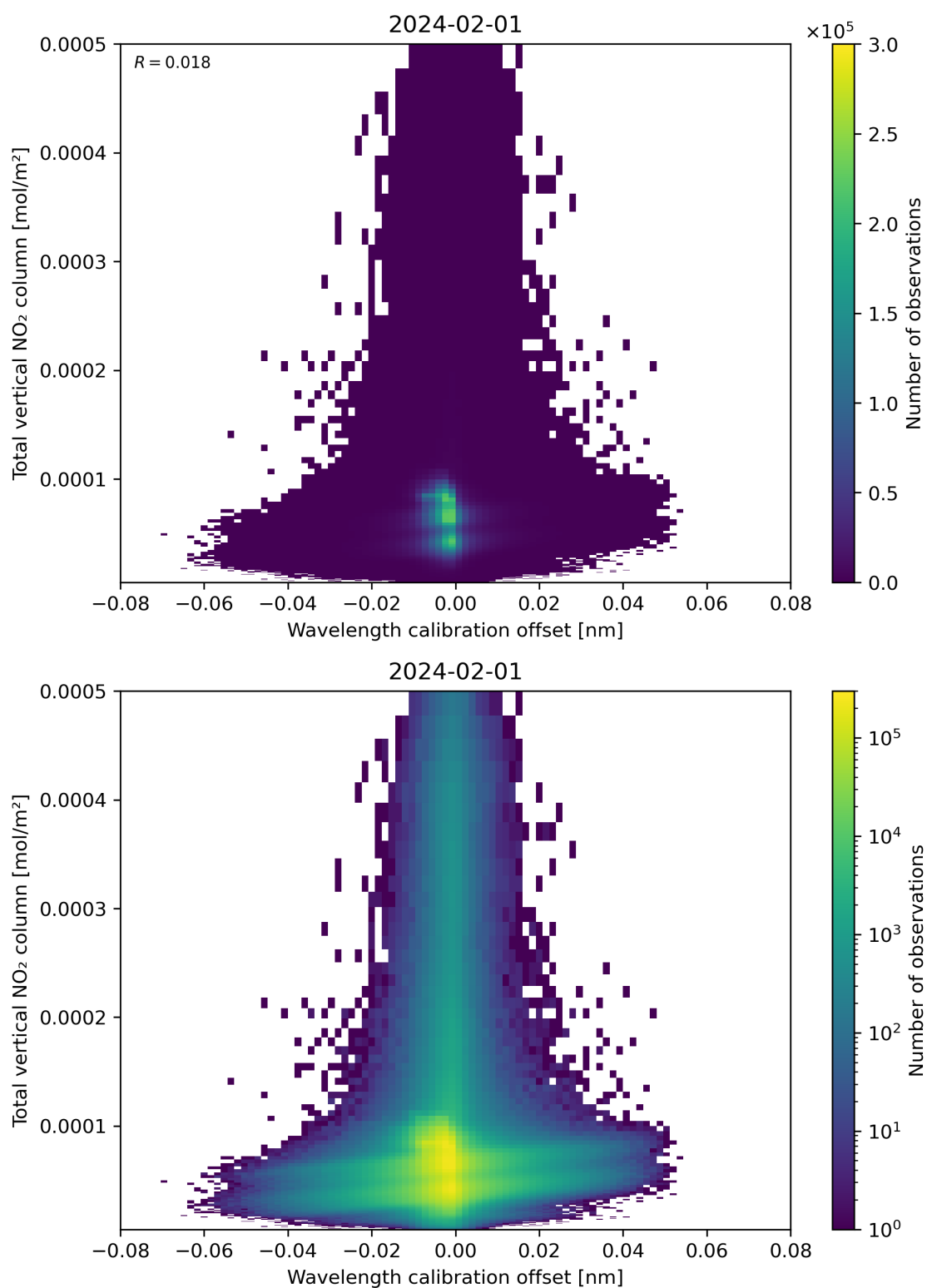
Figure 179: Scatter density plot of “Wavelength calibration offset” against “Total vertical NO 2 column” for 2024-01-31 to 2024-02-02.
