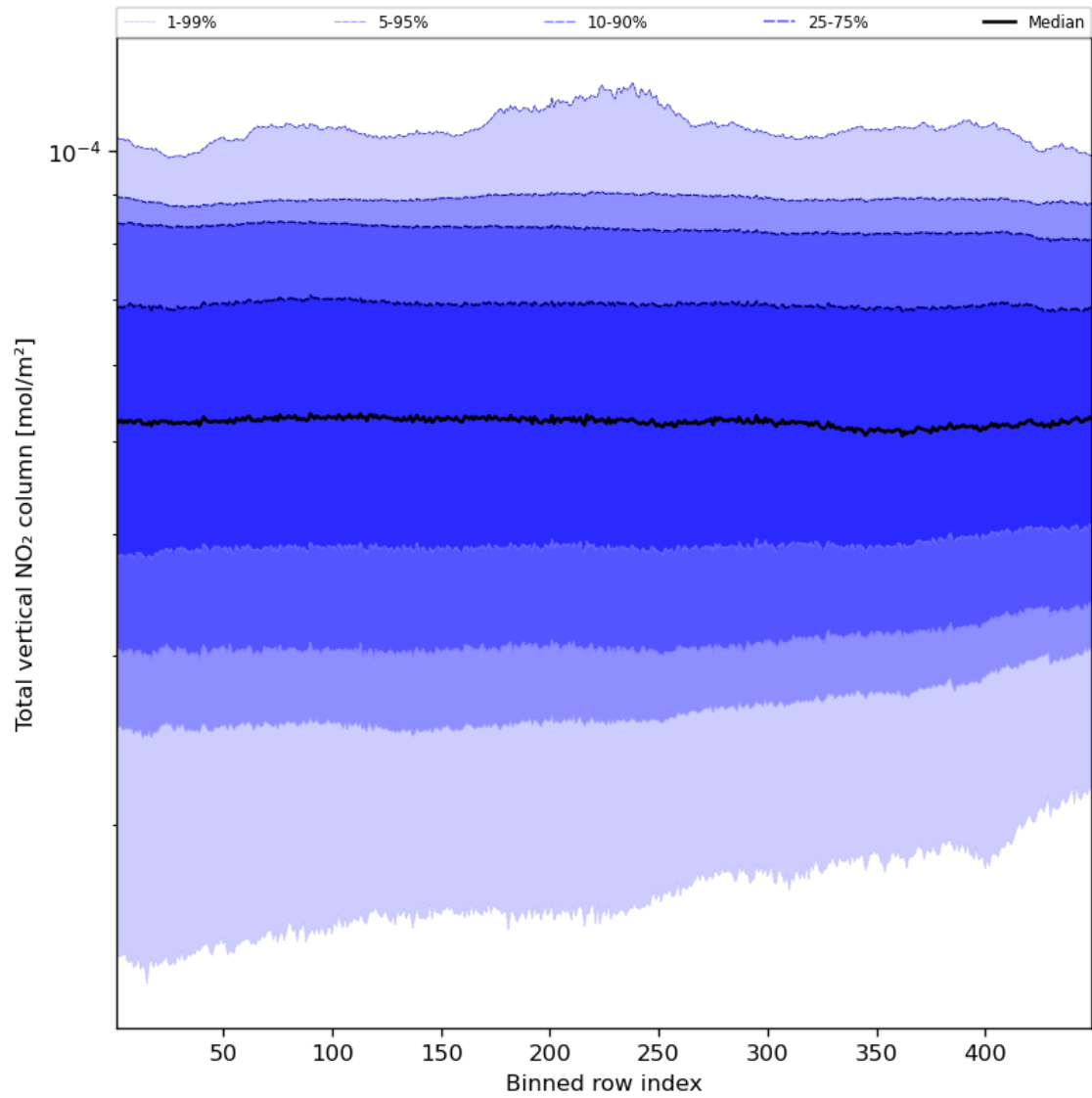
Figure 55: Along track statistics of “Total vertical NO 2 column” for 2024-01-31 to 2024-02-02
