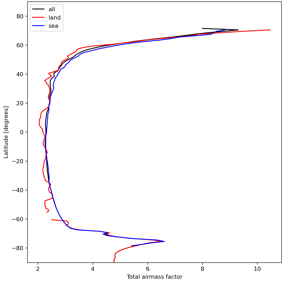
Figure 15: Zonal average of “Total airmass factor” for 2024-01-31 to 2024-02-02.
