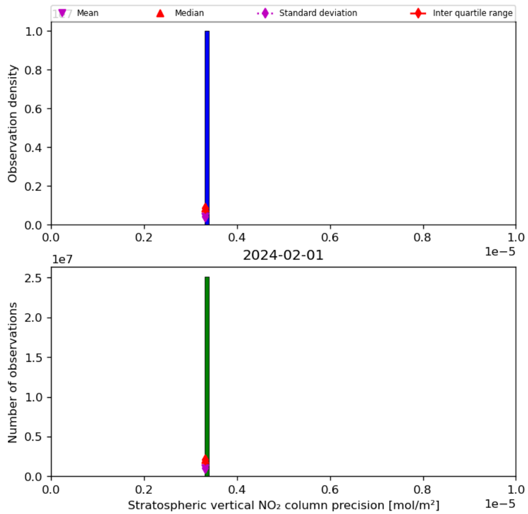
Figure 37: Histogram of “Stratospheric vertical NO 2 column precision” for 2024-01-31 to 2024-02-02
