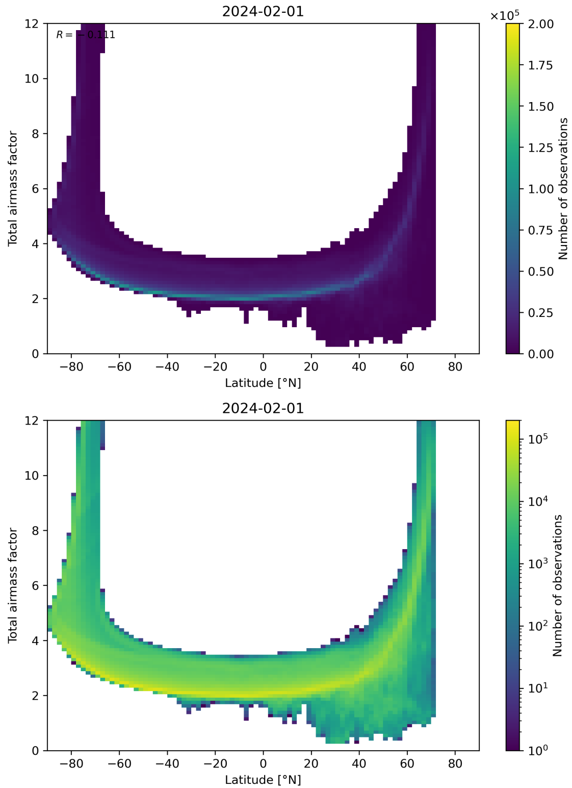
Figure 84: Scatter density plot of “Latitude” against “Total airmass factor” for 2024-01-31 to 2024-02-02.
