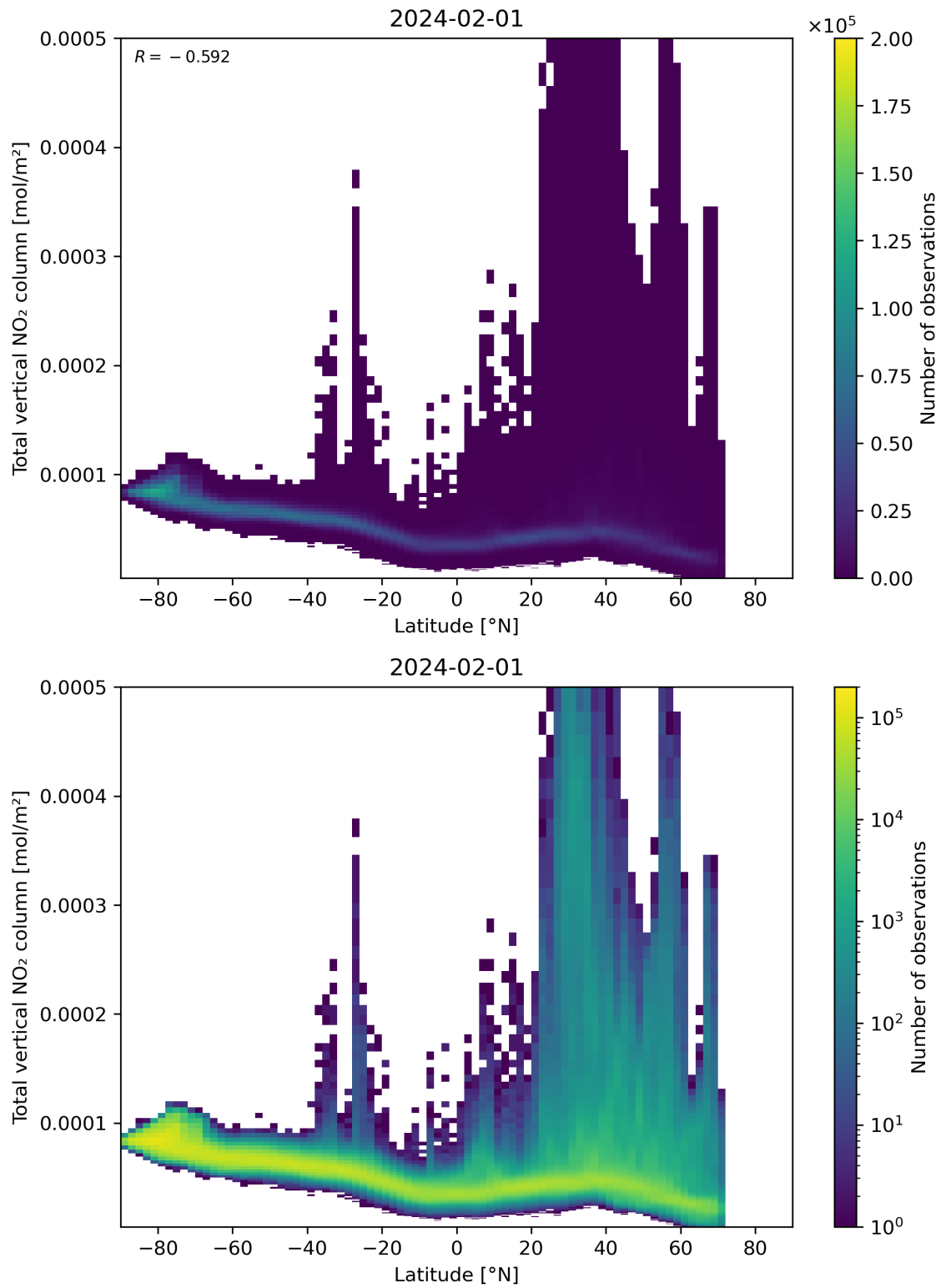
Figure 90: Scatter density plot of “Latitude” against “Total vertical NO 2 column” for 2024-01-31 to 2024-02-02.
