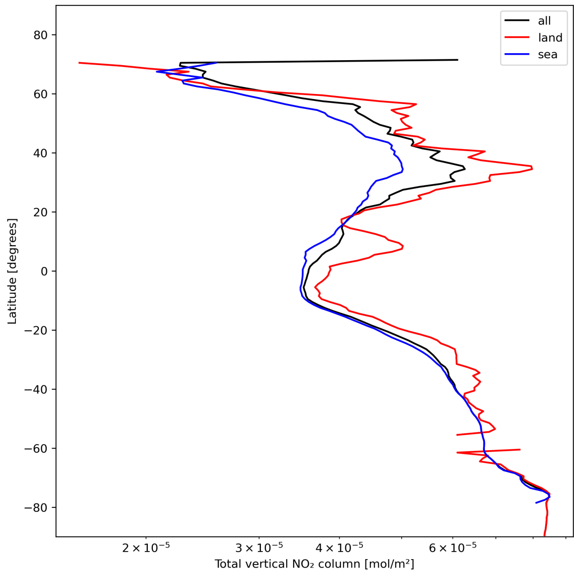
Figure 21: Zonal average of “Total vertical NO 2 column” for 2024-01-31 to 2024-02-02.
