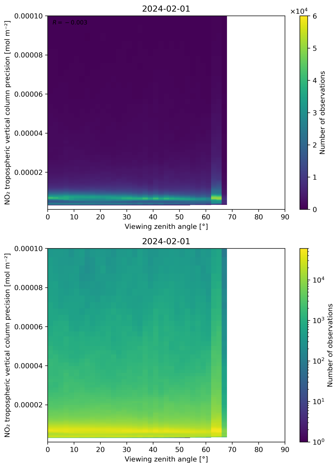
Figure 170: Scatter density plot of “Viewing zenith angle” against “NO 2 tropospheric vertical column precision” for 2024-01-31 to 2024-02-02.
