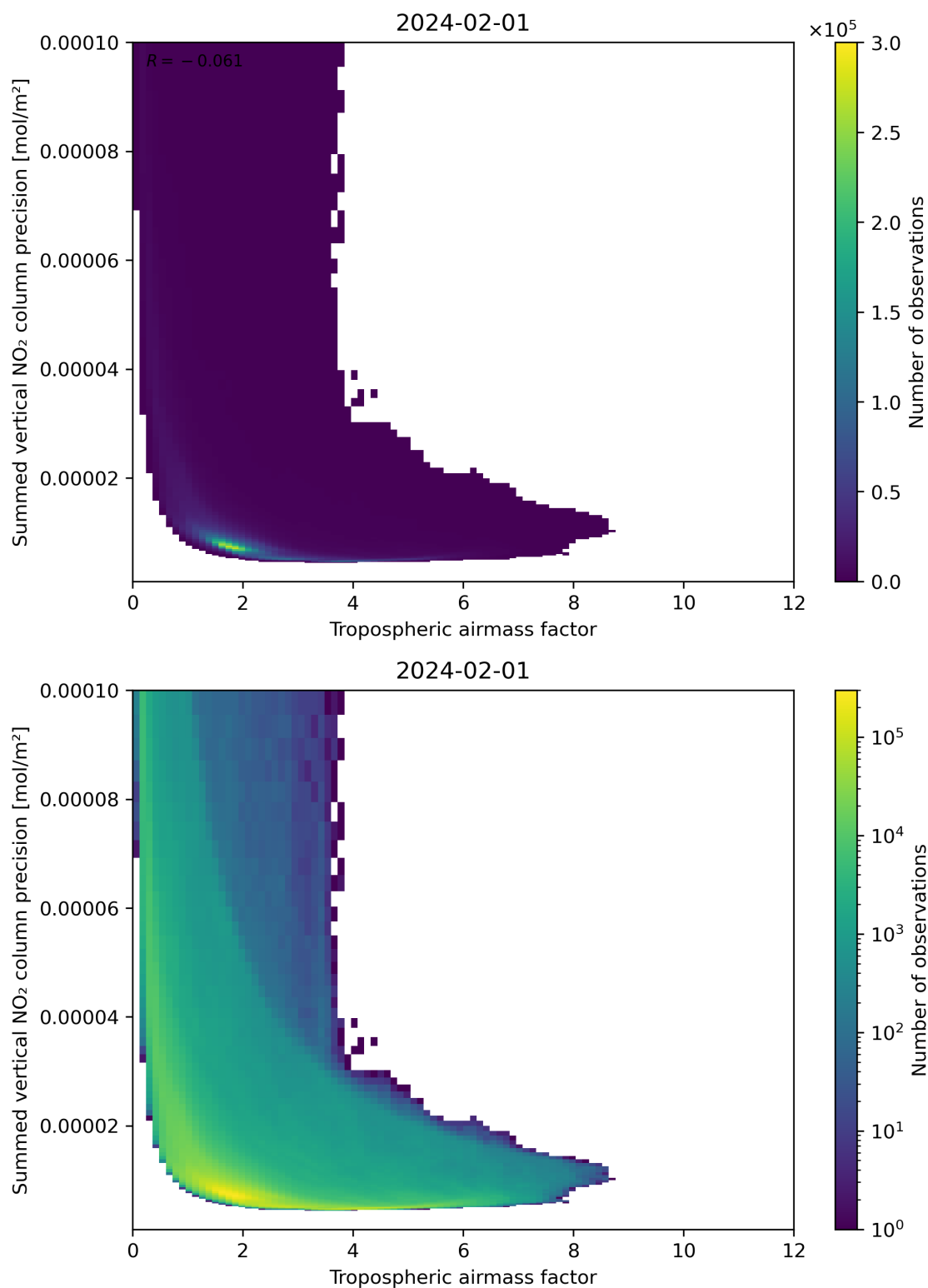
Figure 76: Scatter density plot of “Tropospheric air mass factor” against “Summed vertical NO 2 column precision” for 2024-01-31 to 2024-02-02.
