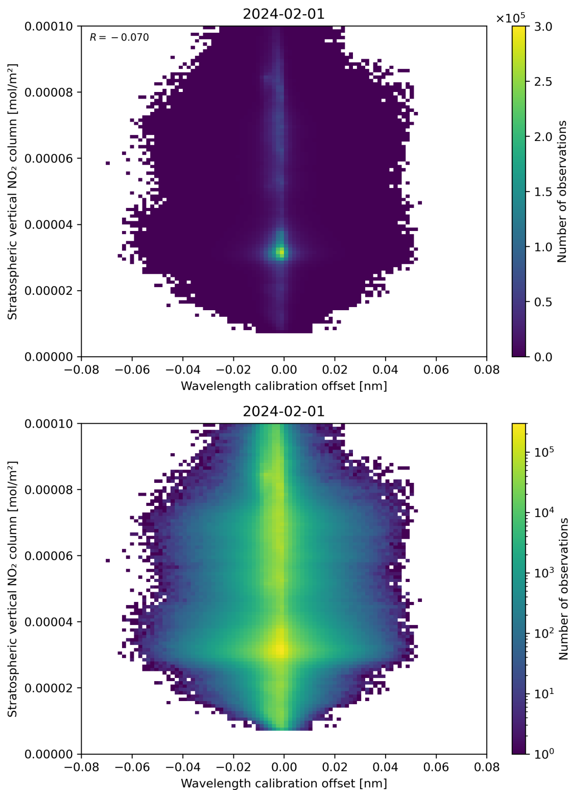
Figure 176: Scatter density plot of “Wavelength calibration offset” against “Stratospheric vertical NO 2 column” for 2024-01-31 to 2024-02-02.
