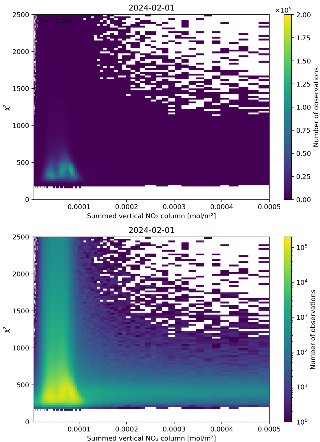
Figure 104: Scatter density plot of “Summed vertical NO 2 column” against “ \chi^2 ” for 2024-01-31 to 2024-02-02.
