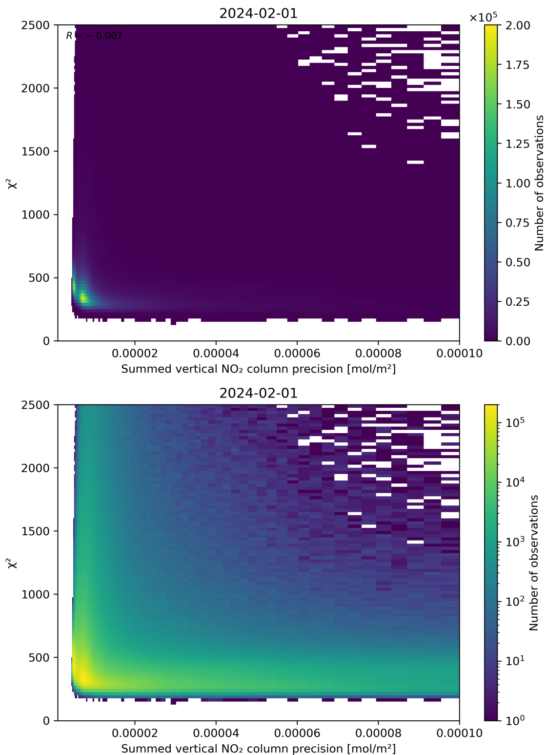
Figure 107: Scatter density plot of “Summed vertical NO 2 column precision” against “ \chi^2 ” for 2024-01-31 to 2024-02-02.
