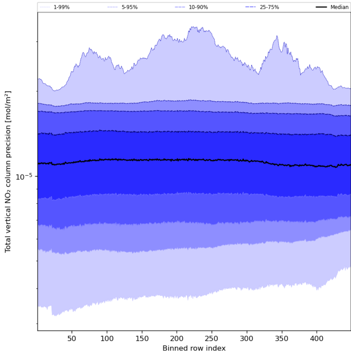
Figure 56: Along track statistics of “Total vertical NO 2 column precision” for 2024-01-31 to 2024-02-02
