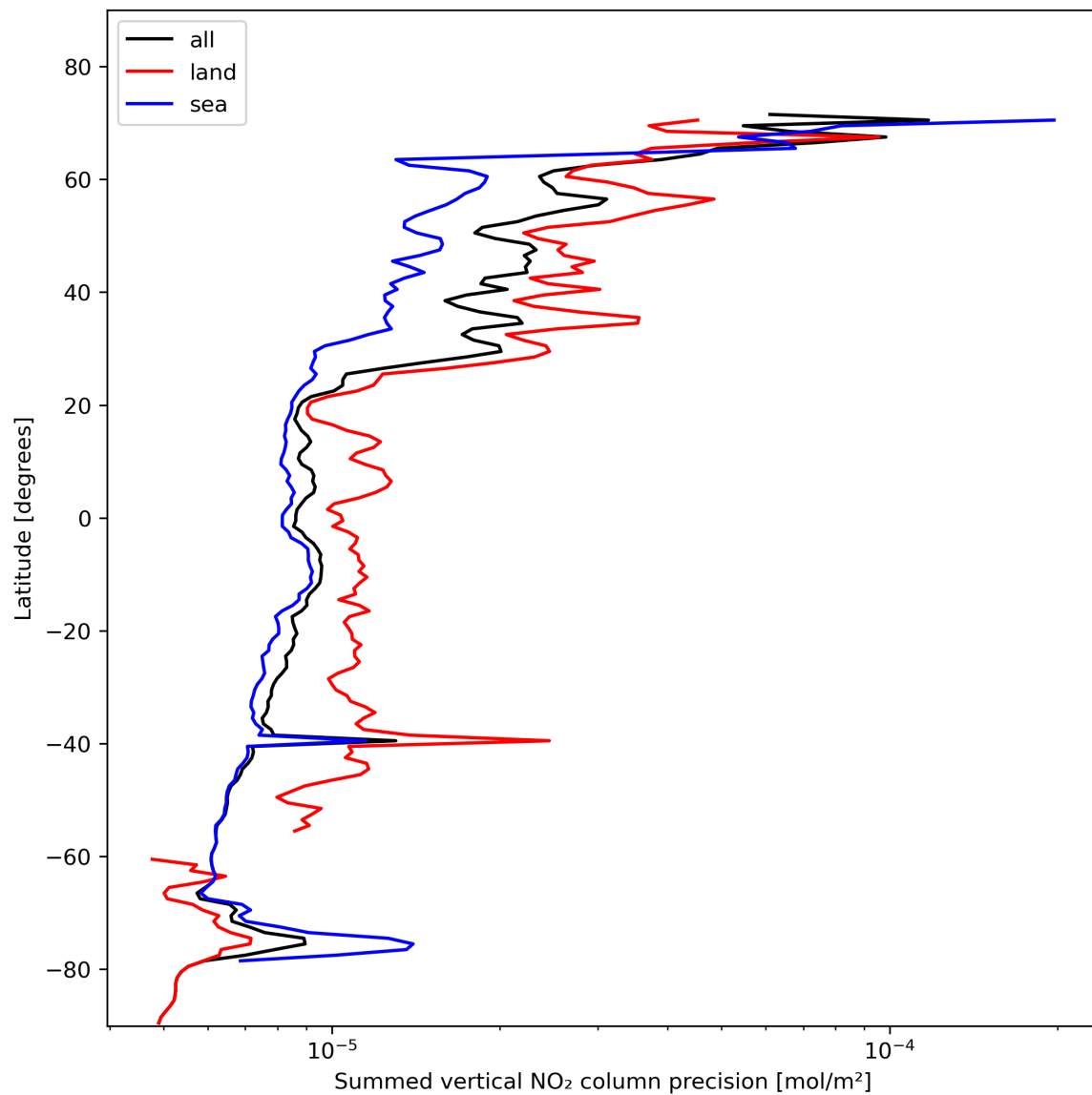
Figure 24: Zonal average of “Summed vertical NO 2 column precision” for 2024-01-31 to 2024-02-02.
