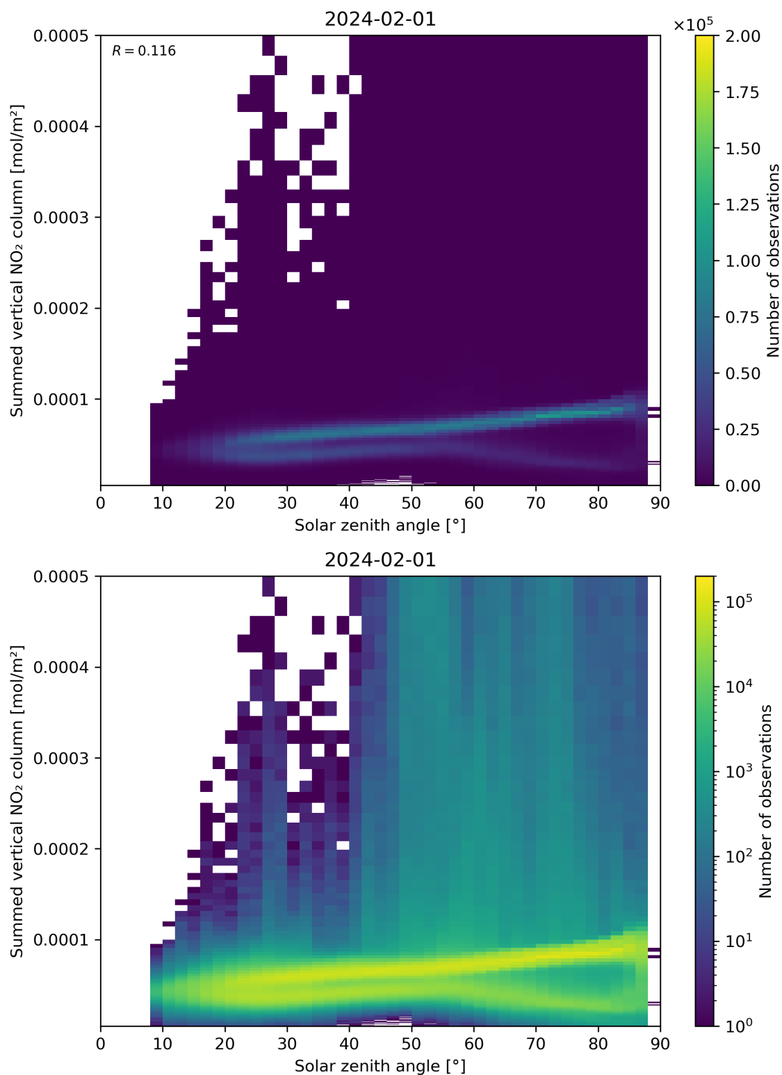
Figure 151: Scatter density plot of “Solar zenith angle” against “Summed vertical NO 2 column” for 2024-01-31 to 2024-02-02.
