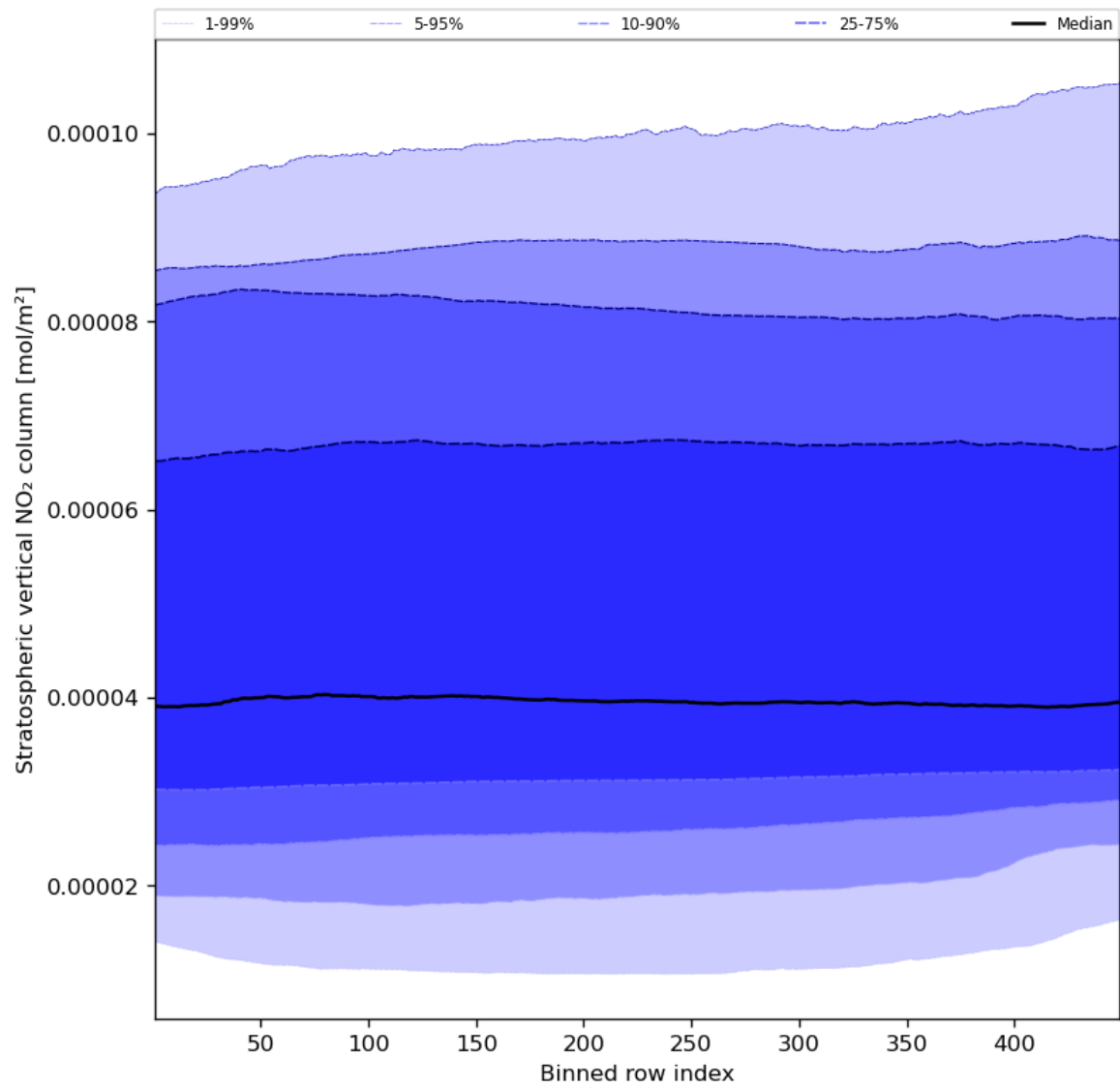
Figure 53: Along track statistics of “Stratospheric vertical NO 2 column” for 2024-01-31 to 2024-02-02
