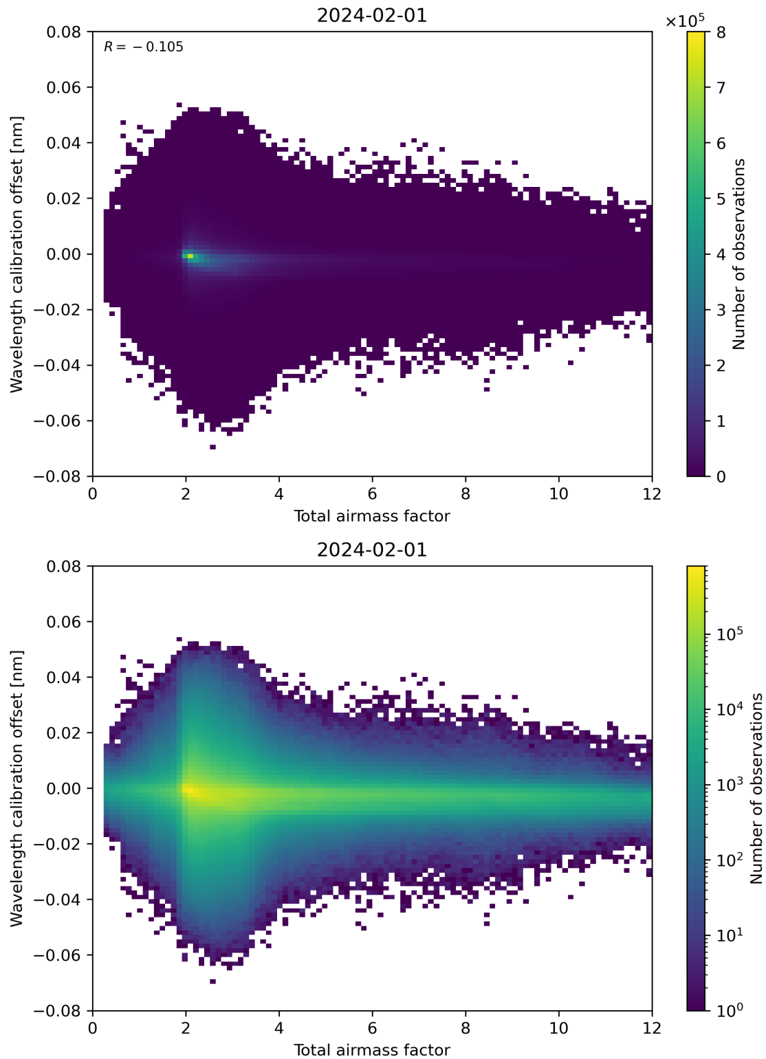
Figure 70: Scatter density plot of “Total airmass factor” against “Wavelength calibration offset” for 2024-01-31 to 2024-02-02.
