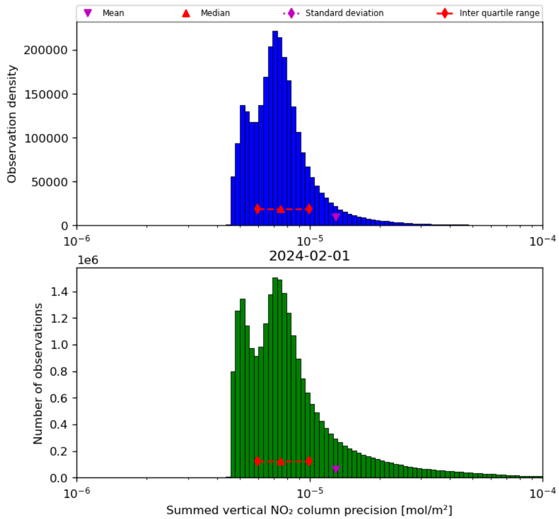
Figure 41: Histogram of "Summed vertical NO 2 column precision" for 2024-01-31 to 2024-02-02
