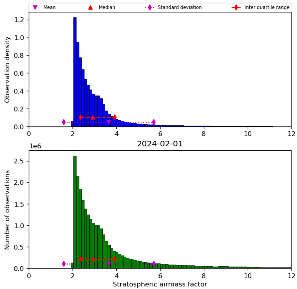
Figure 44: Histogram of “Stratospheric airmass factor” for 2024-01-31 to 2024-02-02
