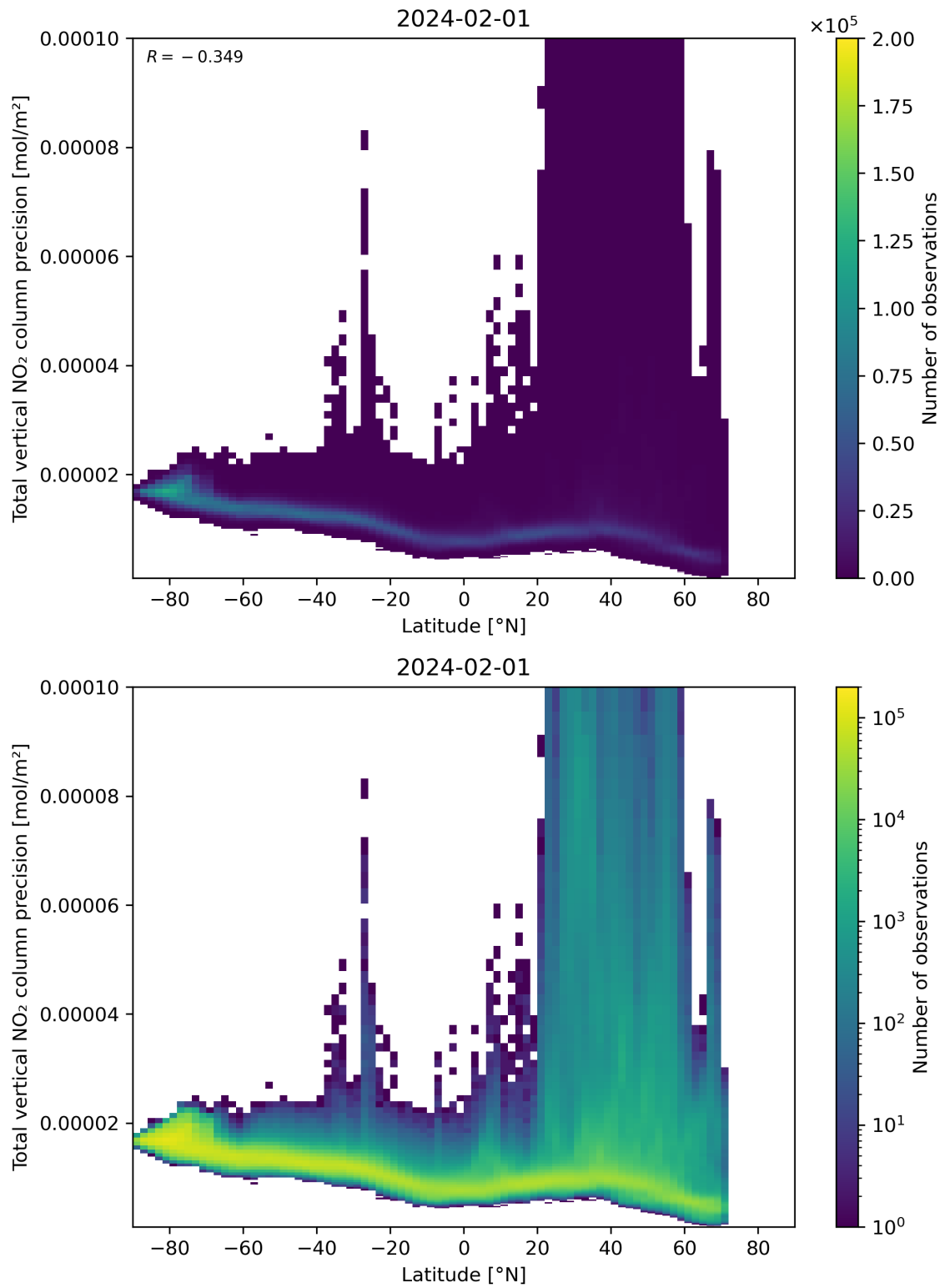
Figure 91: Scatter density plot of “Latitude” against “Total vertical NO 2 column precision” for 2024-01-31 to 2024-02-02.
