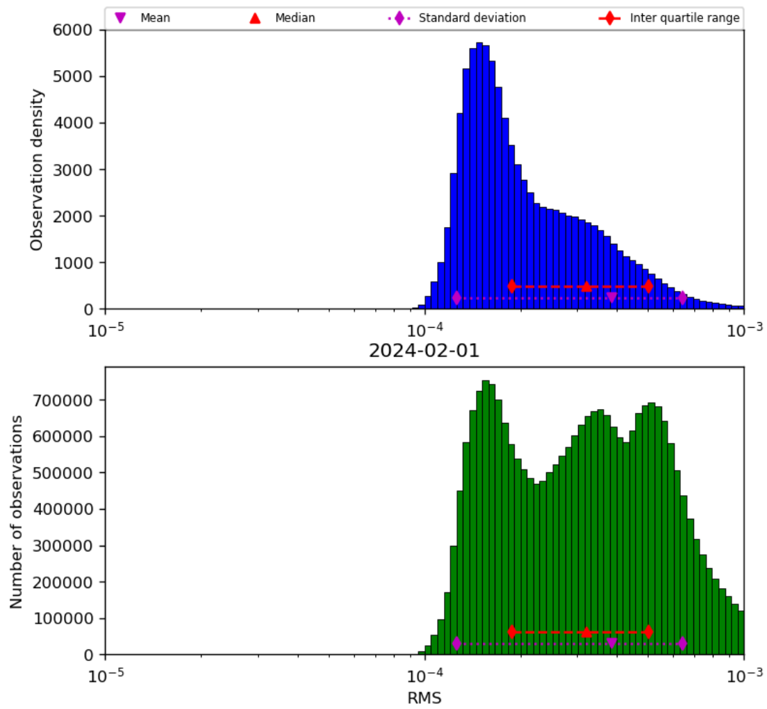
Figure 43: Histogram of “RMS” for 2024-01-31 to 2024-02-02
