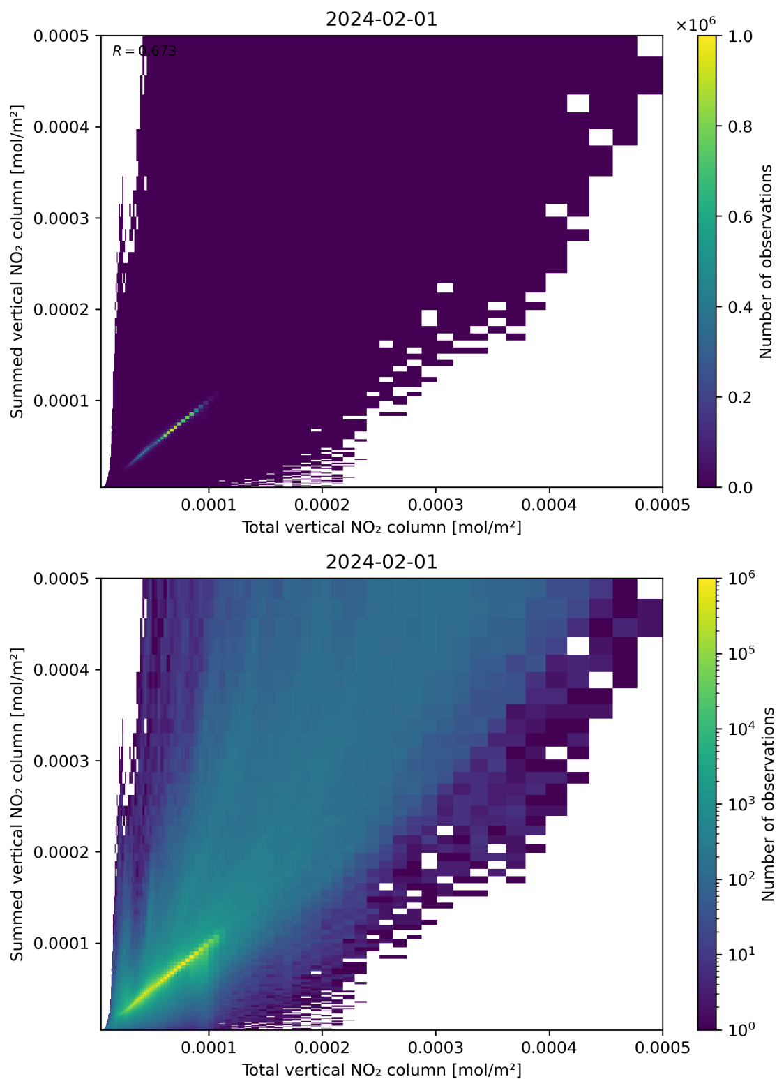
Figure 112: Scatter density plot of “Total vertical NO 2 column” against “Summed vertical NO 2 column” for 2024-01-31 to 2024-02-02.
