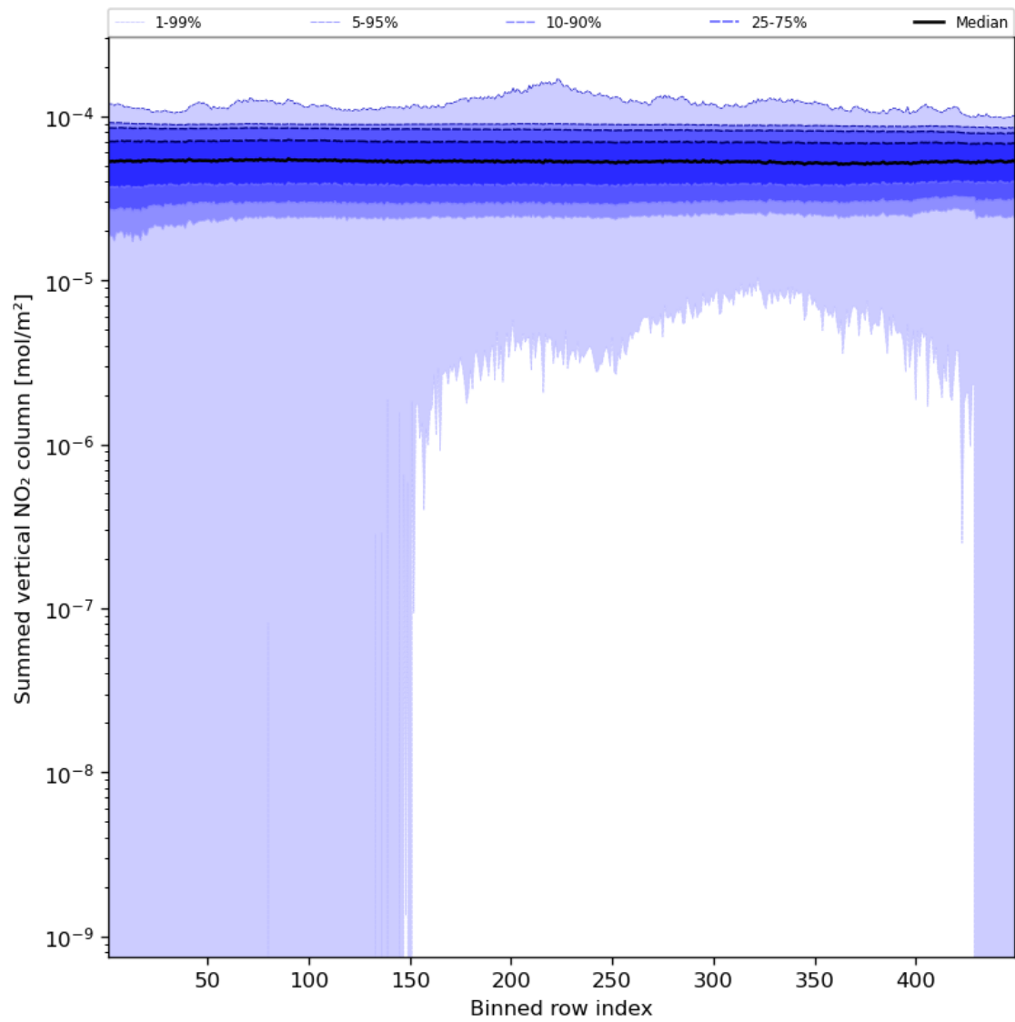
Figure 57: Along track statistics of “Summed vertical NO 2 column” for 2024-01-31 to 2024-02-02
