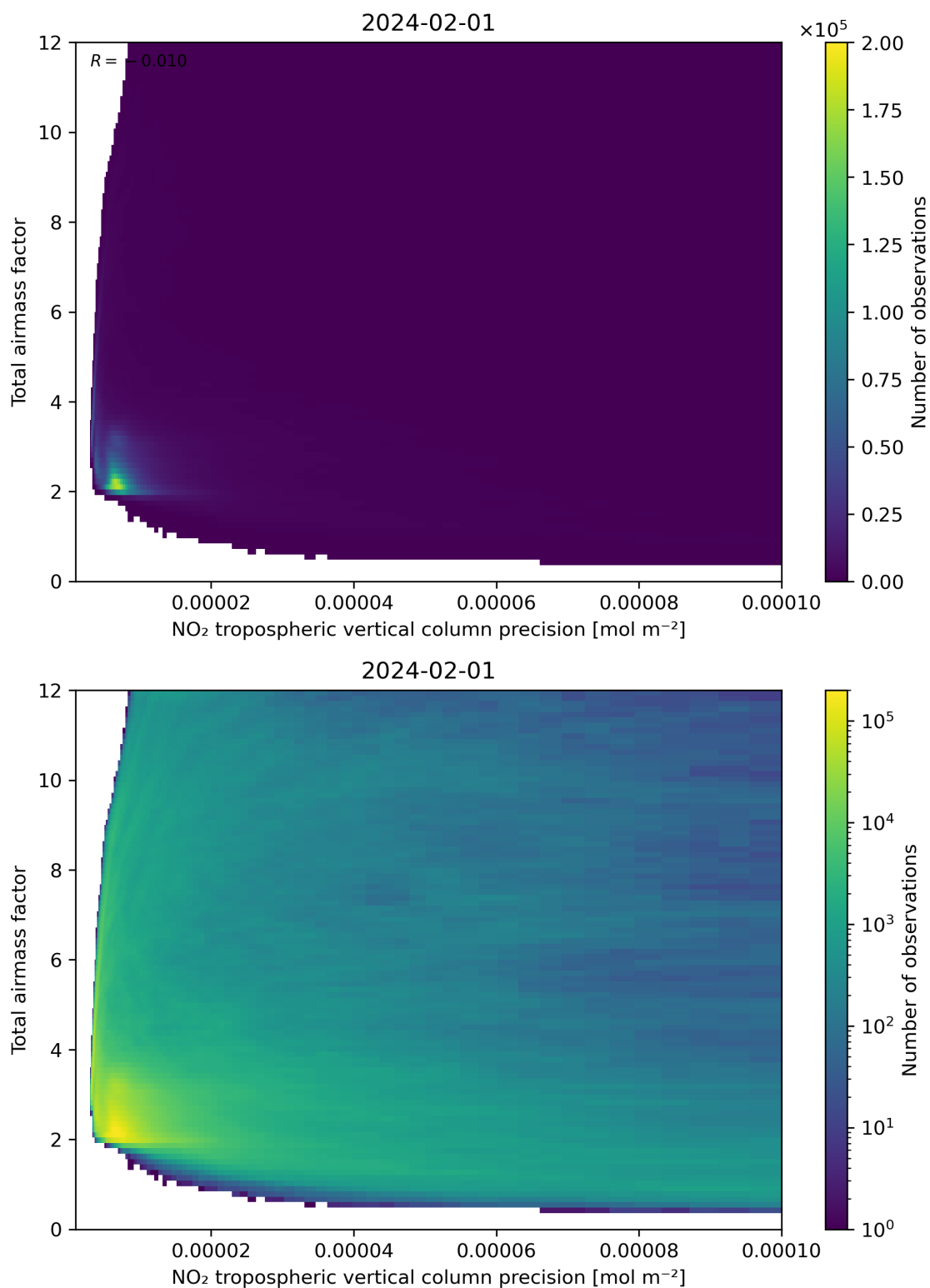
Figure 132: Scatter density plot of “NO 2 tropospheric vertical column precision” against “Total air mass factor” for 2024-01-31 to 2024-02-02.
