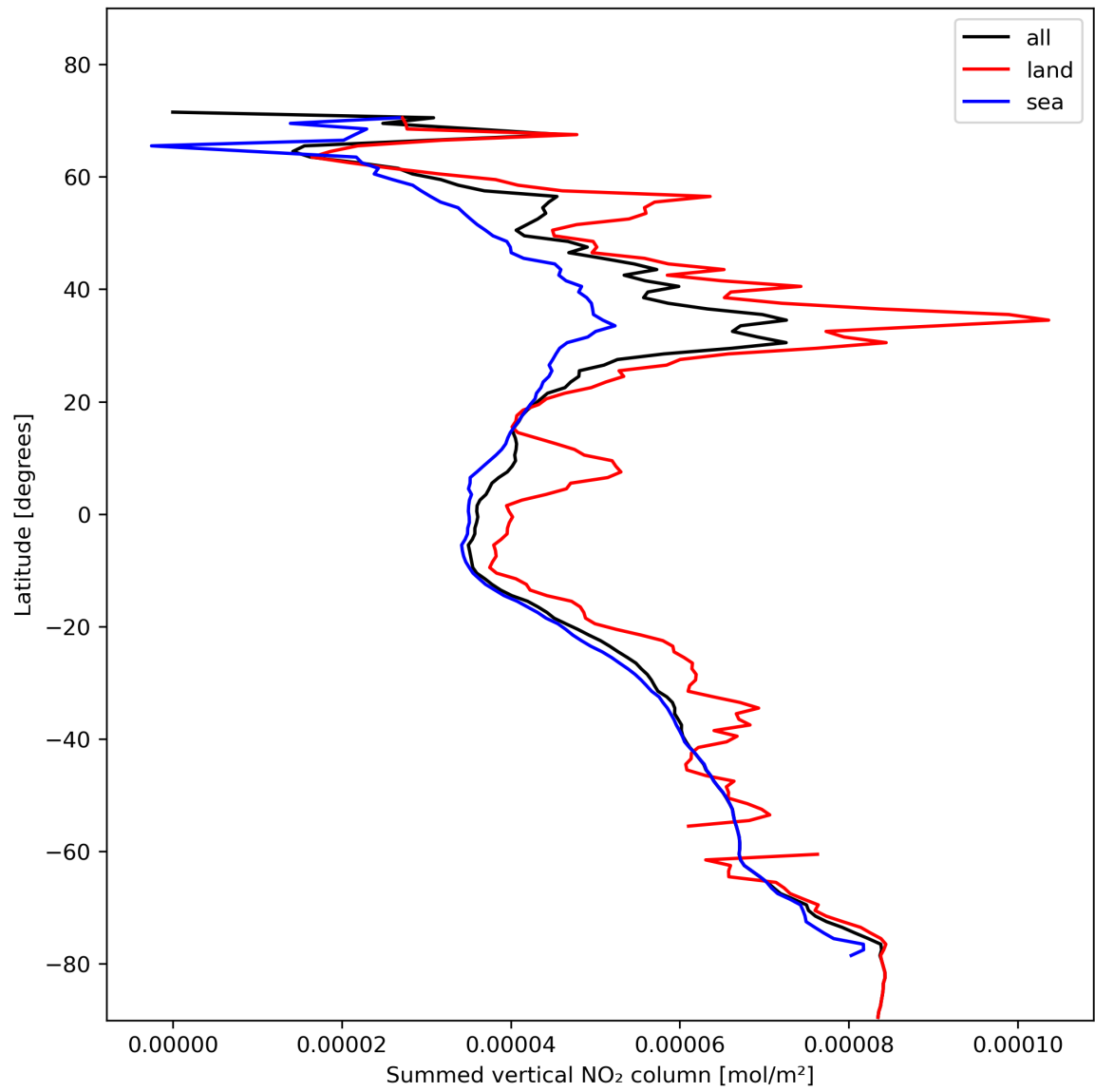
Figure 23: Zonal average of “Summed vertical NO 2 column” for 2024-01-31 to 2024-02-02.
