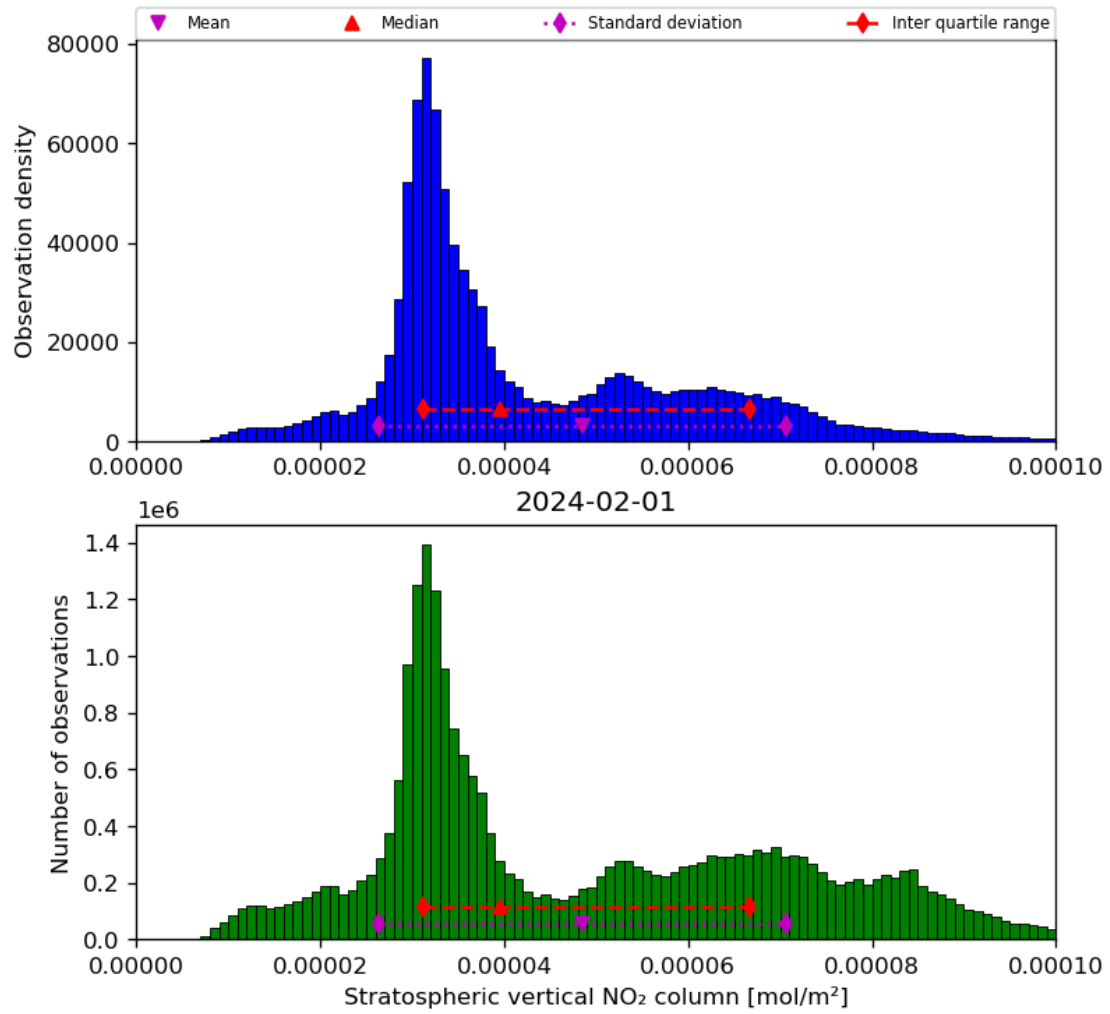
Figure 36: Histogram of “Stratospheric vertical NO 2 column” for 2024-01-31 to 2024-02-02
