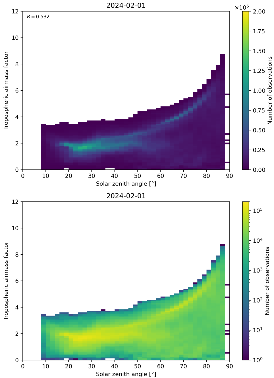
Figure 147: Scatter density plot of “Solar zenith angle” against “Tropospheric airmass factor” for 2024-01-31 to 2024-02-02.
