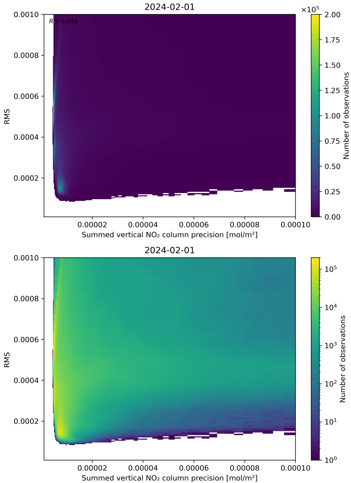
Figure 108: Scatter density plot of “Summed vertical NO 2 column precision” against “RMS” for 2024-01-31 to 2024-02-02.
