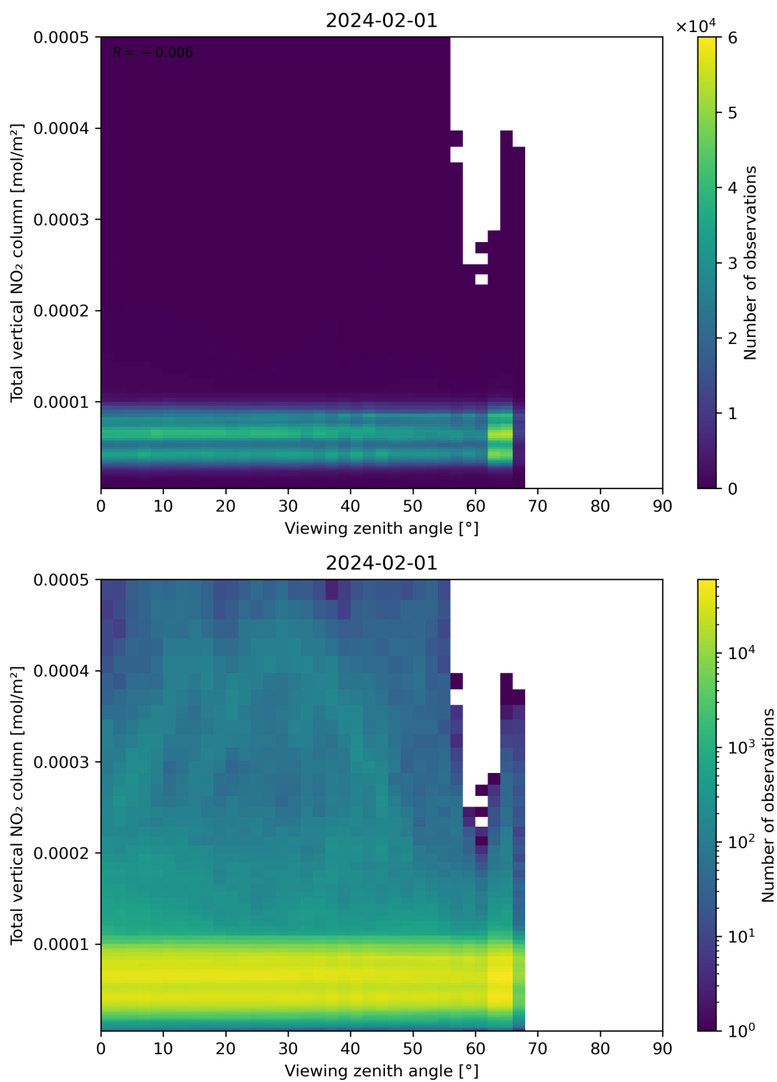
Figure 167: Scatter density plot of “Viewing zenith angle” against “Total vertical NO 2 column” for 2024-01-31 to 2024-02-02.
