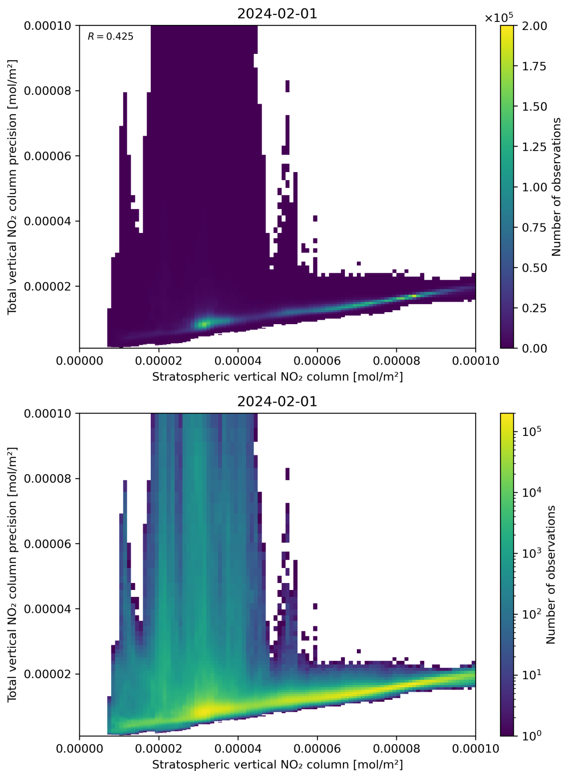
Figure 101: Scatter density plot of “Stratospheric vertical NO 2 column” against “Total vertical NO 2 column precision” for 2024-01-31 to 2024-02-02.
