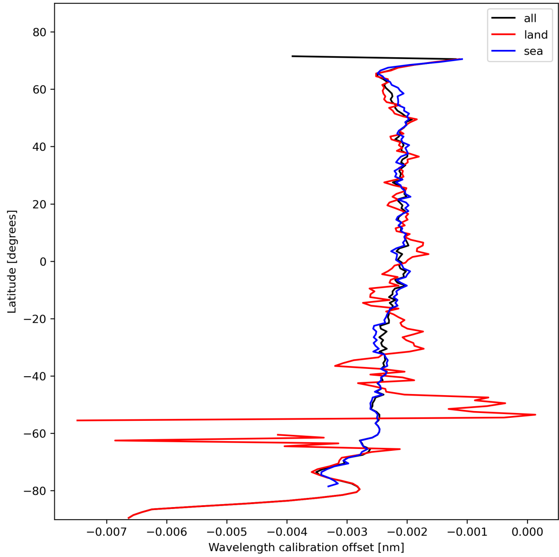
Figure 18: Zonal average of “Wavelength calibration offset” for 2024-01-31 to 2024-02-02.
