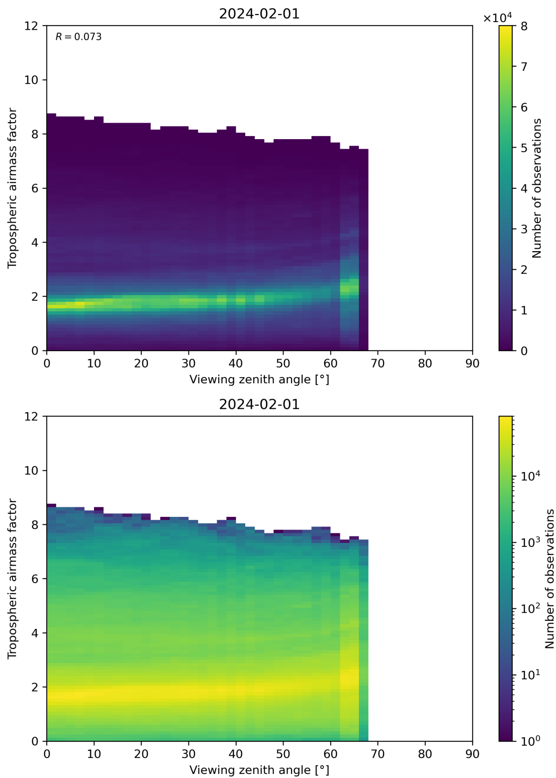
Figure 161: Scatter density plot of “Viewing zenith angle” against “Tropospheric airmass factor” for 2024-01-31 to 2024-02-02.
