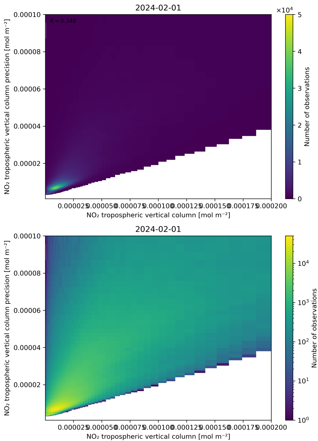
Figure 130: Scatter density plot of “NO 2 tropospheric vertical column” against “NO 2 tropospheric vertical column precision” for 2024-01-31 to 2024-02-02.
