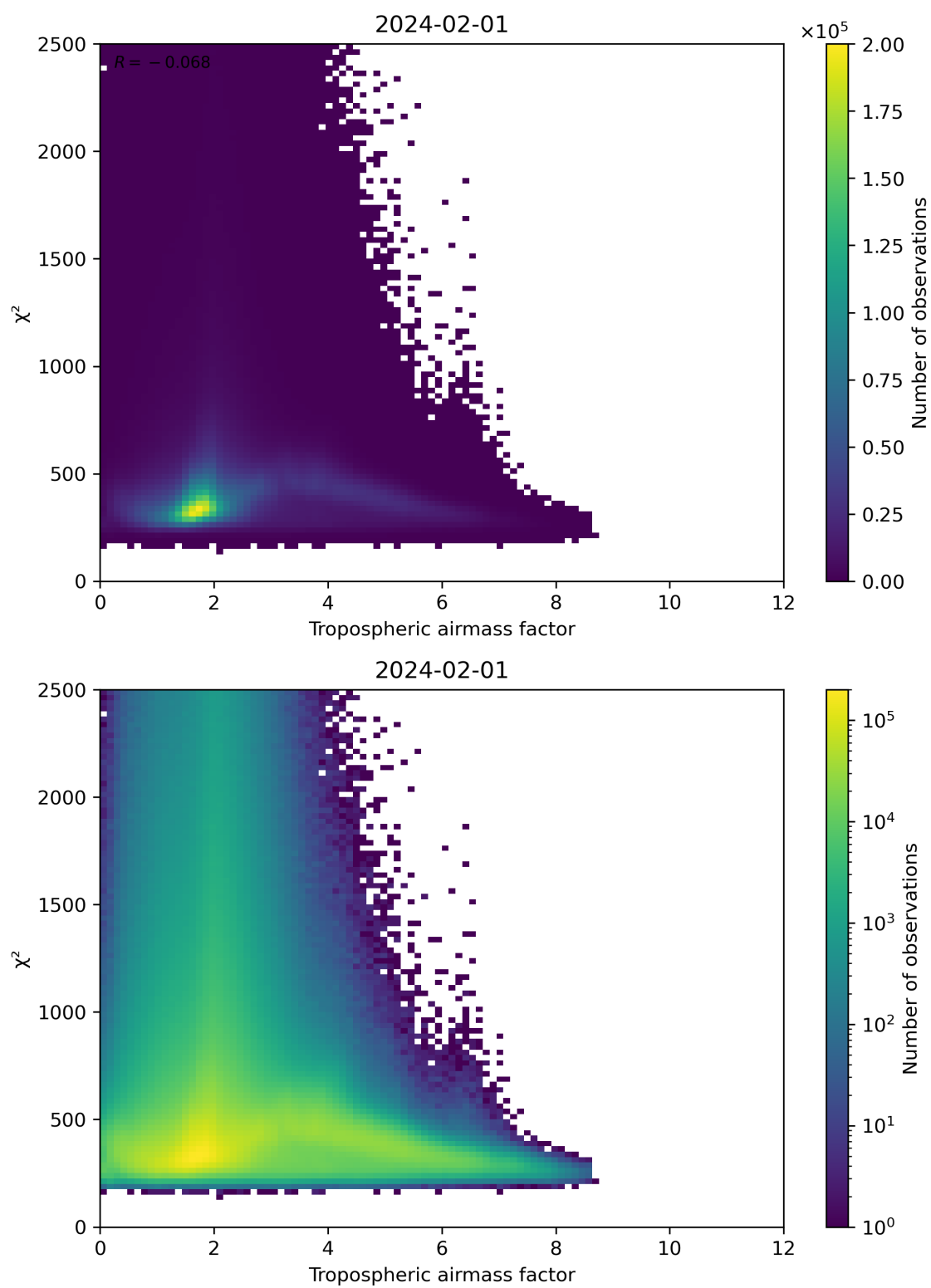
Figure 73: Scatter density plot of “Tropospheric airmass factor” against “ \chi^2 ” for 2024-01-31 to 2024-02-02.
