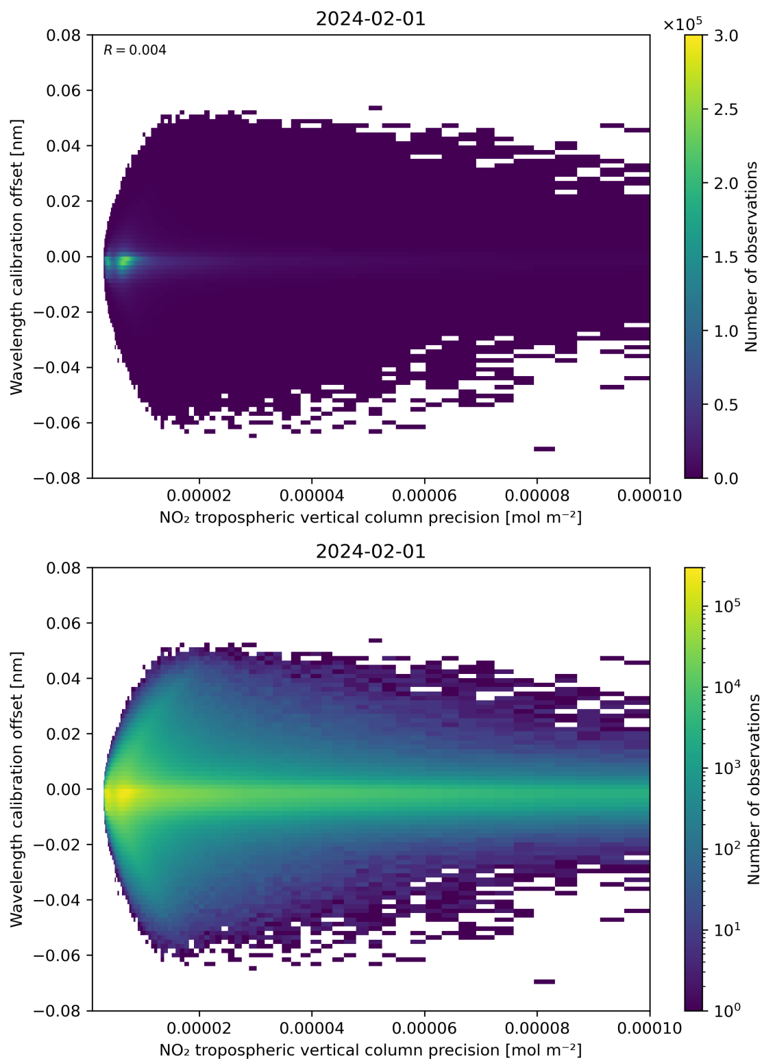
Figure 141: Scatter density plot of “NO 2 tropospheric vertical column precision” against “Wavelength calibration offset” for 2024-01-31 to 2024-02-02.
