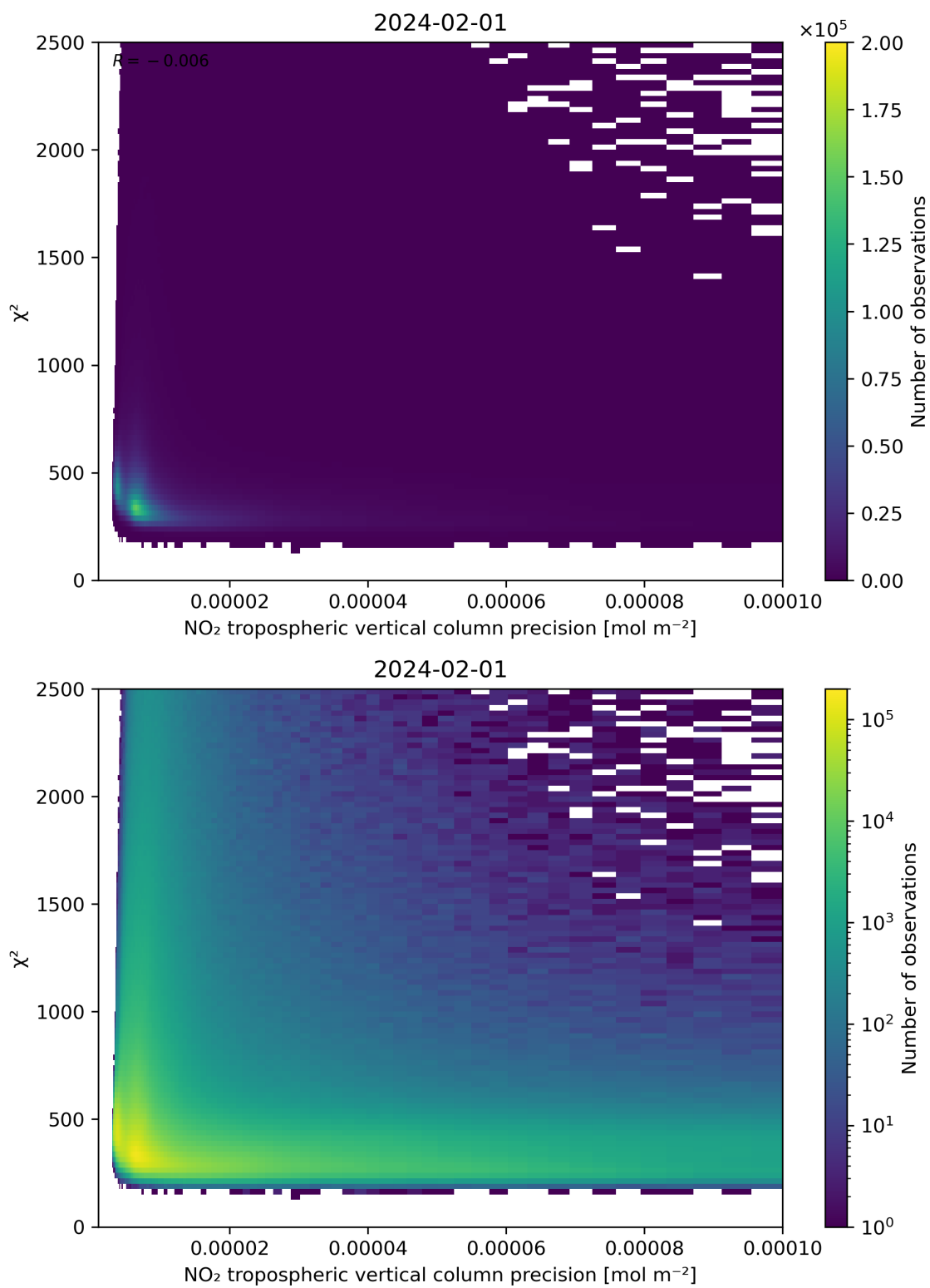
Figure 134: Scatter density plot of “NO 2 tropospheric vertical column precision” against “ \chi^2 ” for 2024-01-31 to 2024-02-02.
