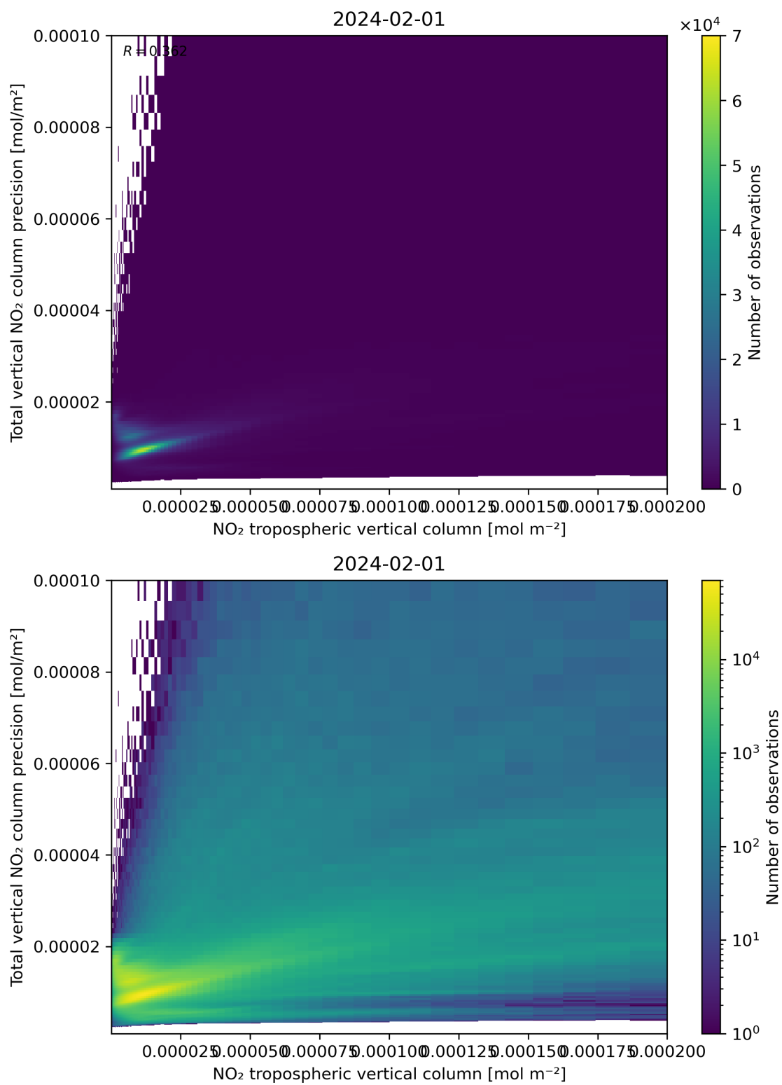
Figure 129: Scatter density plot of “NO 2 tropospheric vertical column” against “Total vertical NO 2 column precision” for 2024-01-31 to 2024-02-02.
