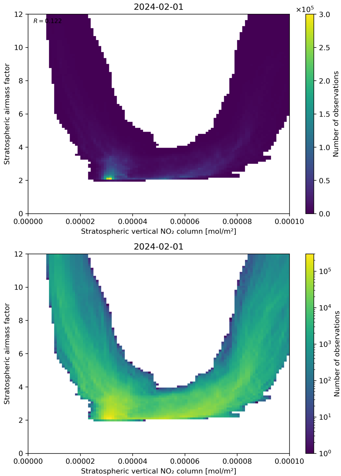
Figure 96: Scatter density plot of “Stratospheric vertical NO 2 column” against “Stratospheric airmass factor” for 2024-01-31 to 2024-02-02.
