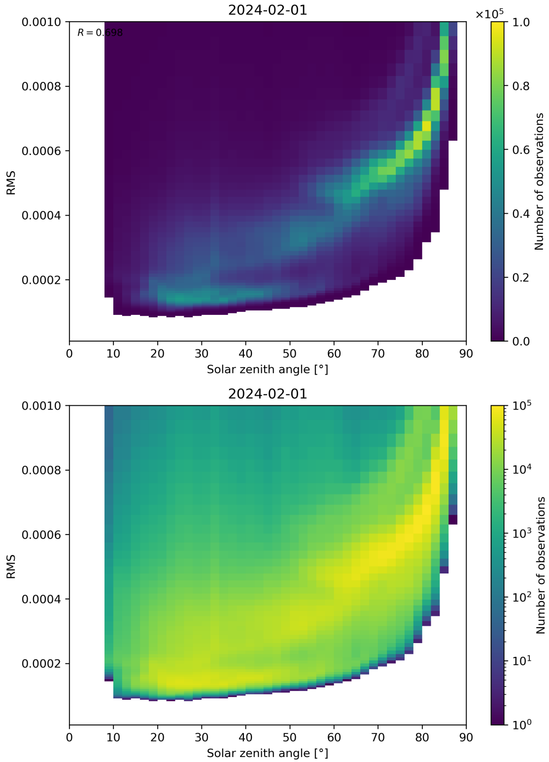
Figure 157: Scatter density plot of “Solar zenith angle” against “RMS” for 2024-01-31 to 2024-02-02.
