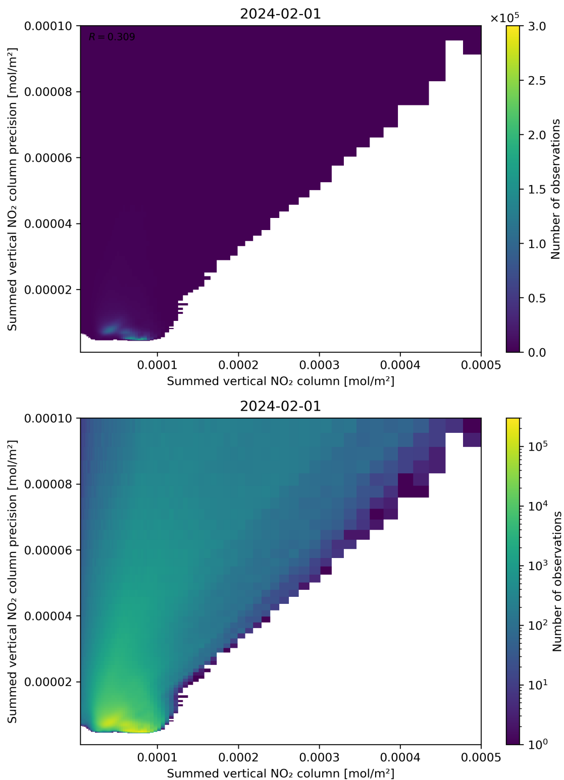
Figure 105: Scatter density plot of “Summed vertical NO 2 column” against “Summed vertical NO 2 column precision” for 2024-01-31 to 2024-02-02.
