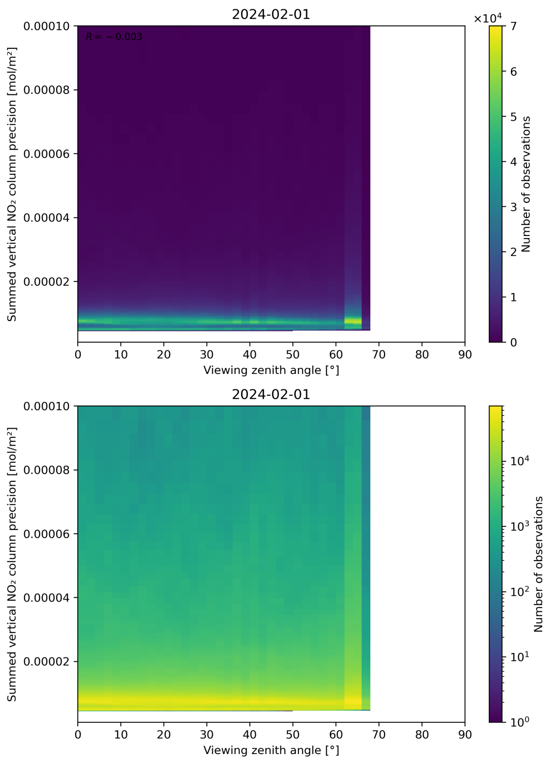
Figure 166: Scatter density plot of “Viewing zenith angle” against “Summed vertical NO 2 column precision” for 2024-01-31 to 2024-02-02.
