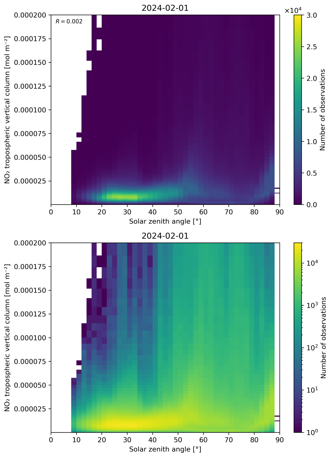
Figure 155: Scatter density plot of “Solar zenith angle” against “NO 2 tropospheric vertical column” for 2024-01-31 to 2024-02-02.
