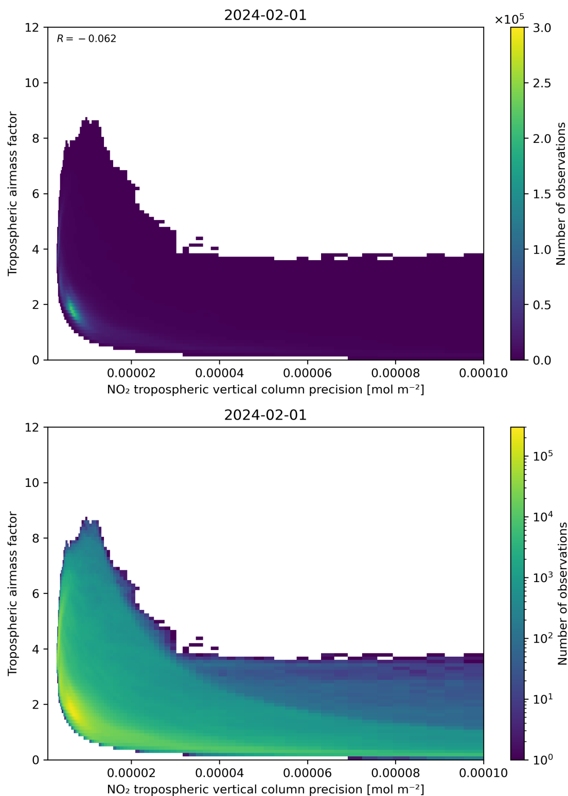
Figure 133: Scatter density plot of “NO 2 tropospheric vertical column precision” against “Tropospheric airmass factor” for 2024-01-31 to 2024-02-02.
