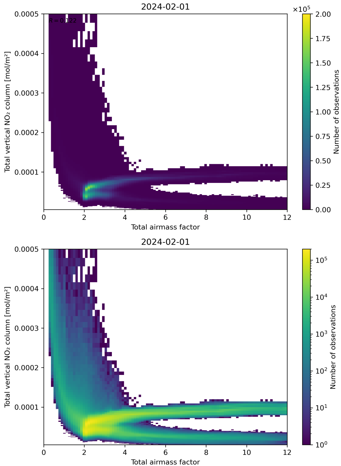
Figure 67: Scatter density plot of “Total airmass factor” against “Total vertical NO 2 column” for 2024-01-31 to 2024-02-02.
