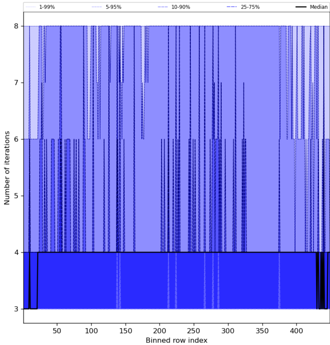
Figure 51: Along track statistics of “Number of iterations” for 2024-01-31 to 2024-02-02
