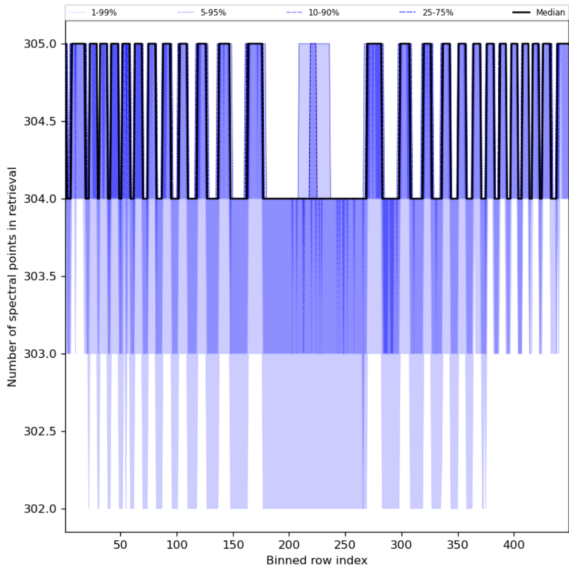
Figure 50: Along track statistics of “Number of spectral points in retrieval” for 2024-01-31 to 2024-02-02
