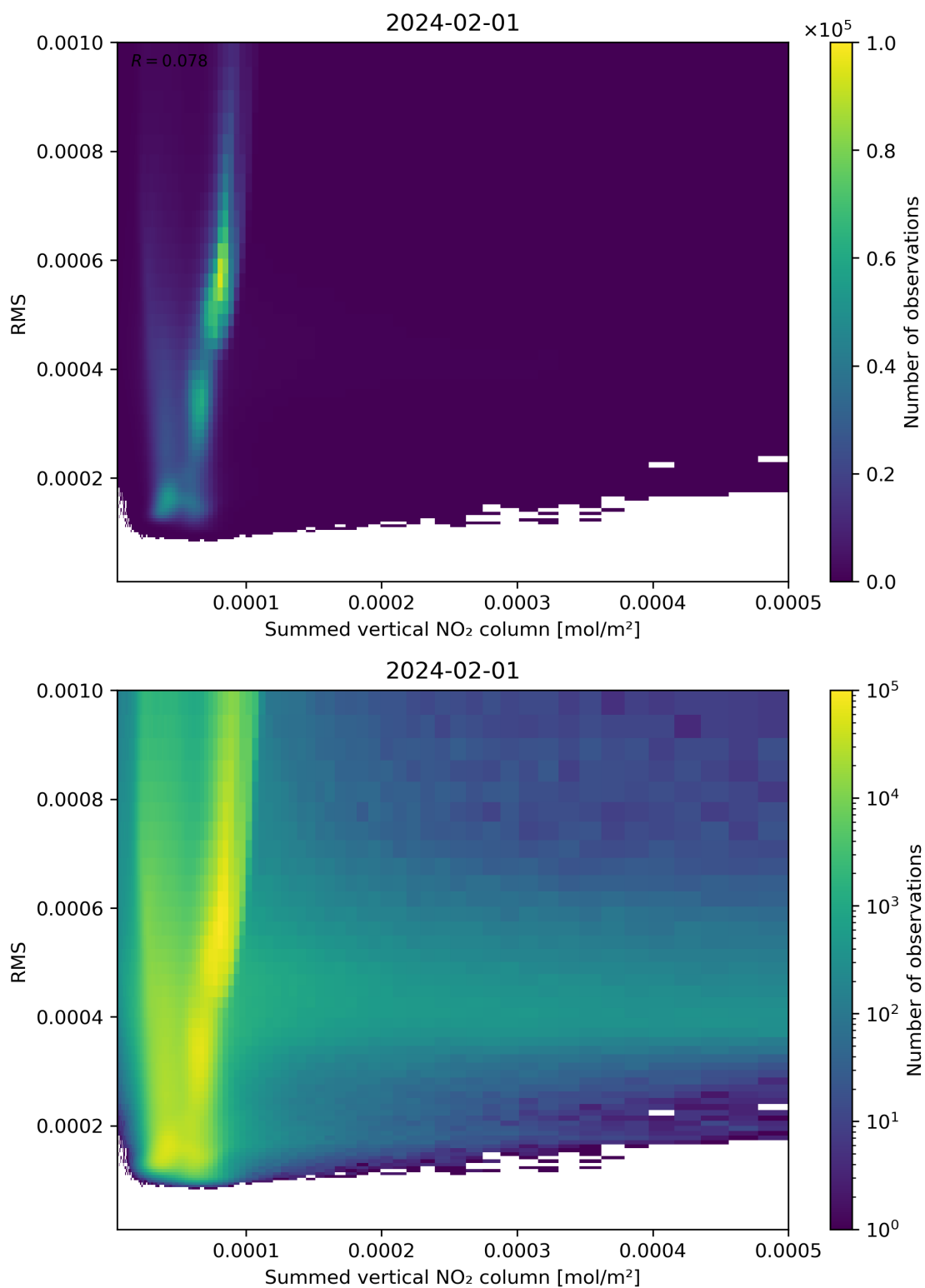
Figure 109: Scatter density plot of “Summed vertical NO 2 column” against “RMS” for 2024-01-31 to 2024-02-02.
