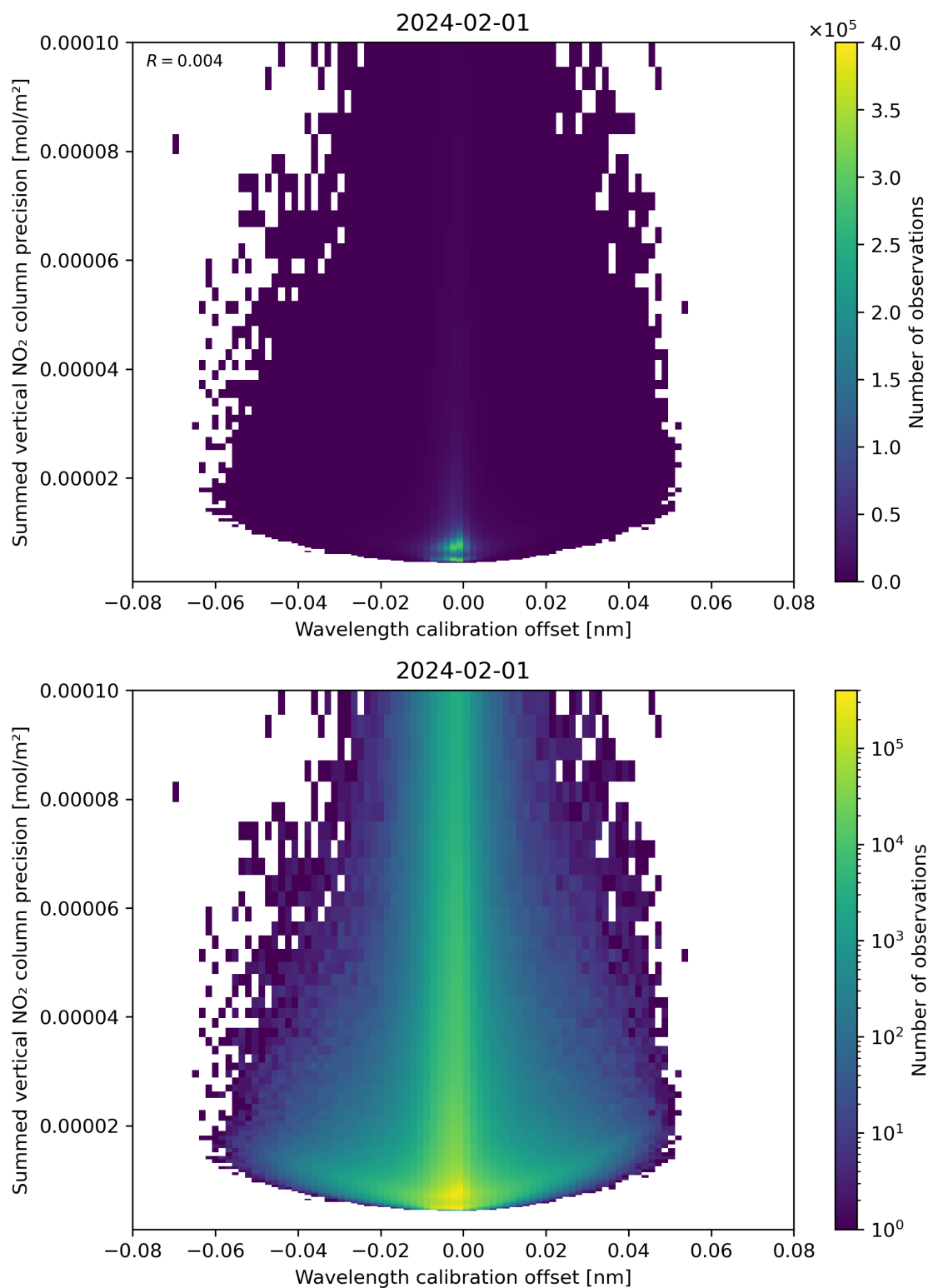
Figure 178: Scatter density plot of “Wavelength calibration offset” against “Summed vertical NO 2 column precision” for 2024-01-31 to 2024-02-02.
