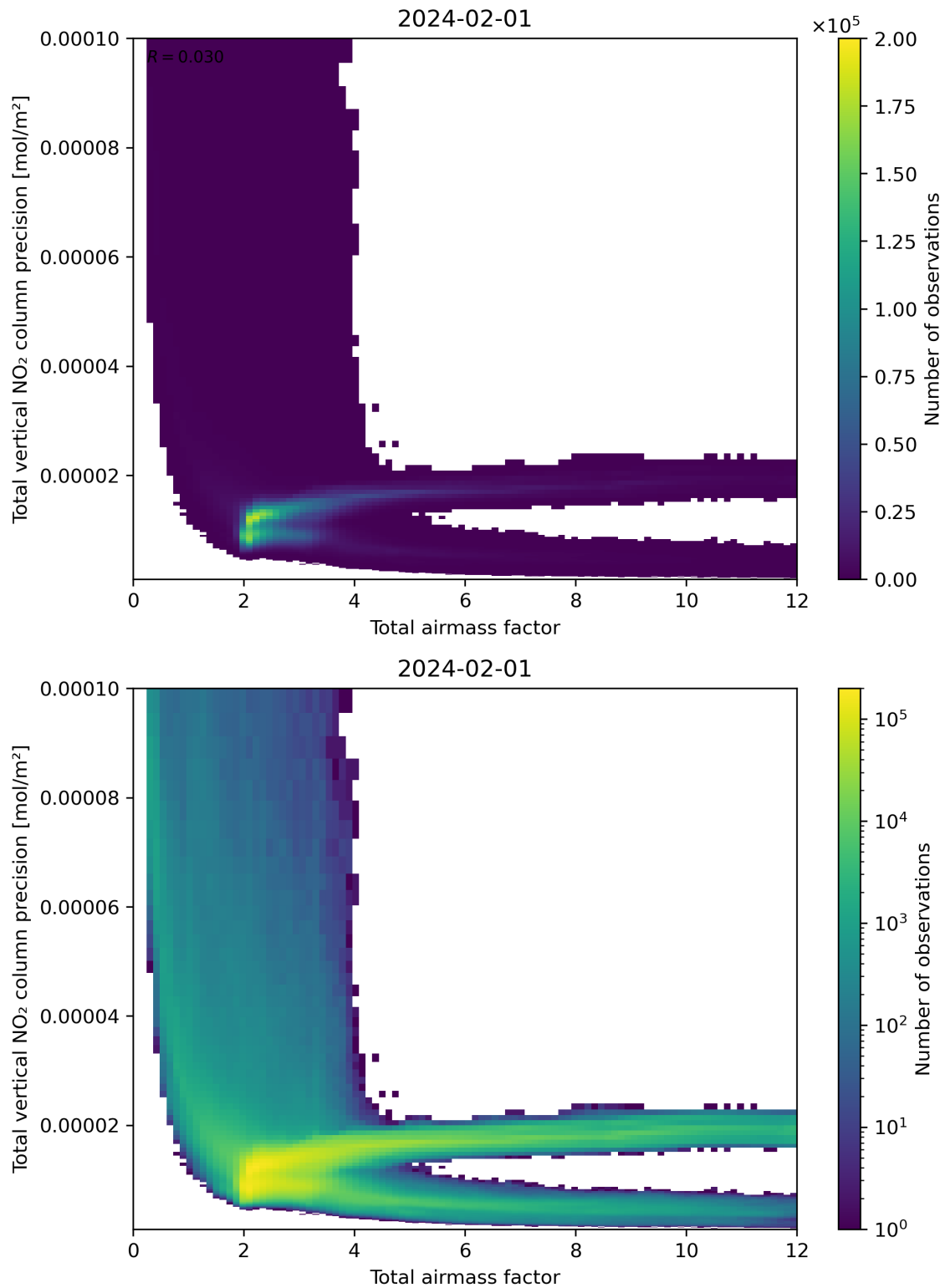
Figure 68: Scatter density plot of “Total airmass factor” against “Total vertical NO 2 column precision” for 2024-01-31 to 2024-02-02.
