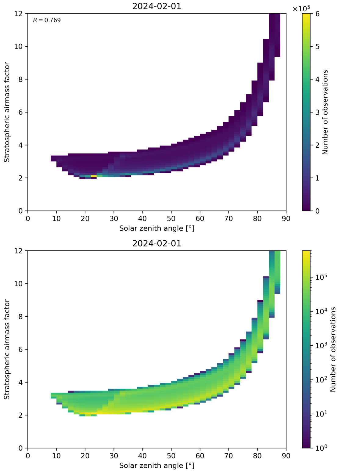
Figure 145: Scatter density plot of “Solar zenith angle” against “Stratospheric airmass factor” for 2024-01-31 to 2024-02-02.
