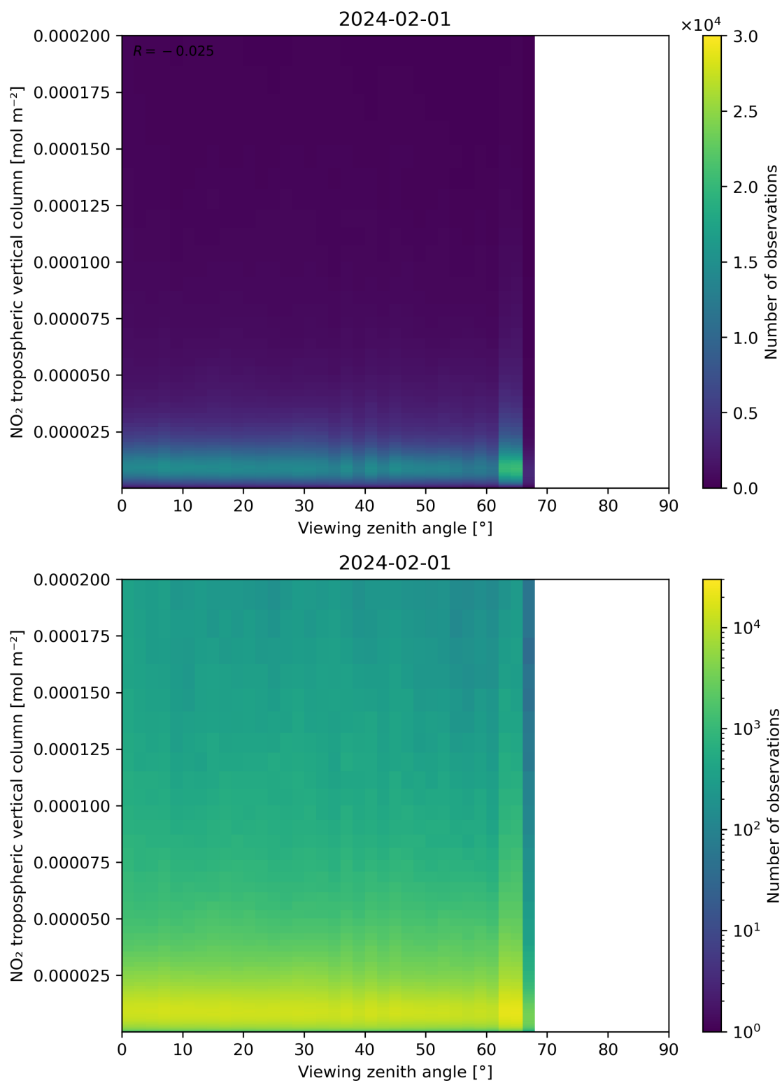
Figure 169: Scatter density plot of “Viewing zenith angle” against “NO 2 tropospheric vertical column” for 2024-01-31 to 2024-02-02.
