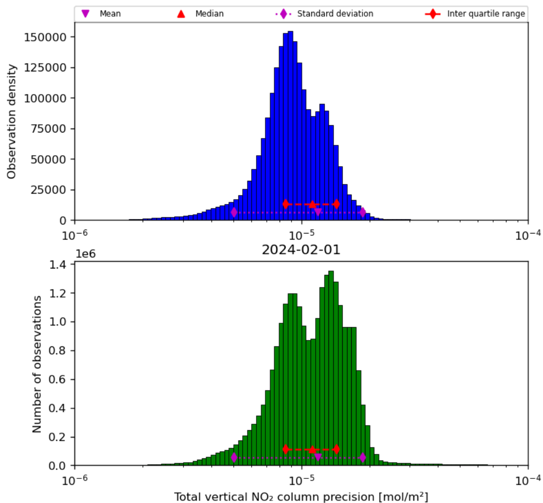
Figure 39: Histogram of “Total vertical NO 2 column precision” for 2024-01-31 to 2024-02-02
