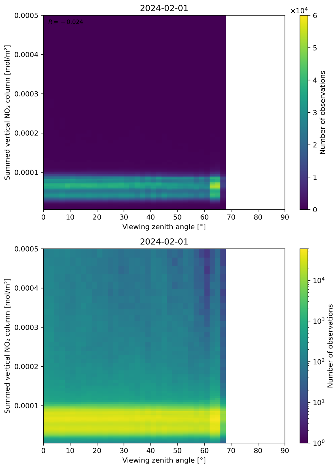
Figure 165: Scatter density plot of “Viewing zenith angle” against “Summed vertical NO 2 column” for 2024-01-31 to 2024-02-02.
