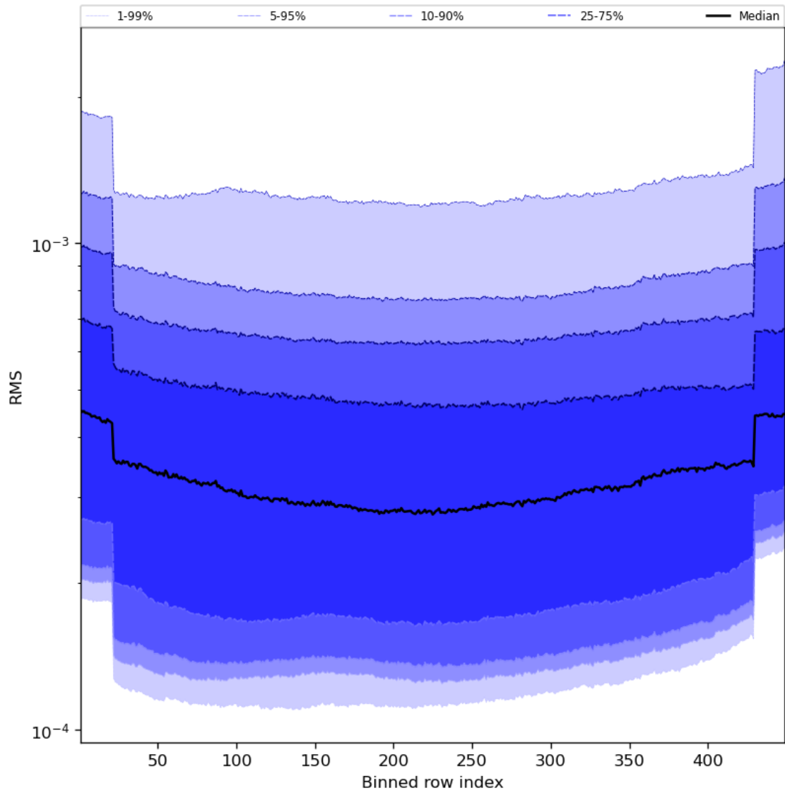
Figure 60: Along track statistics of “RMS” for 2024-01-31 to 2024-02-02
