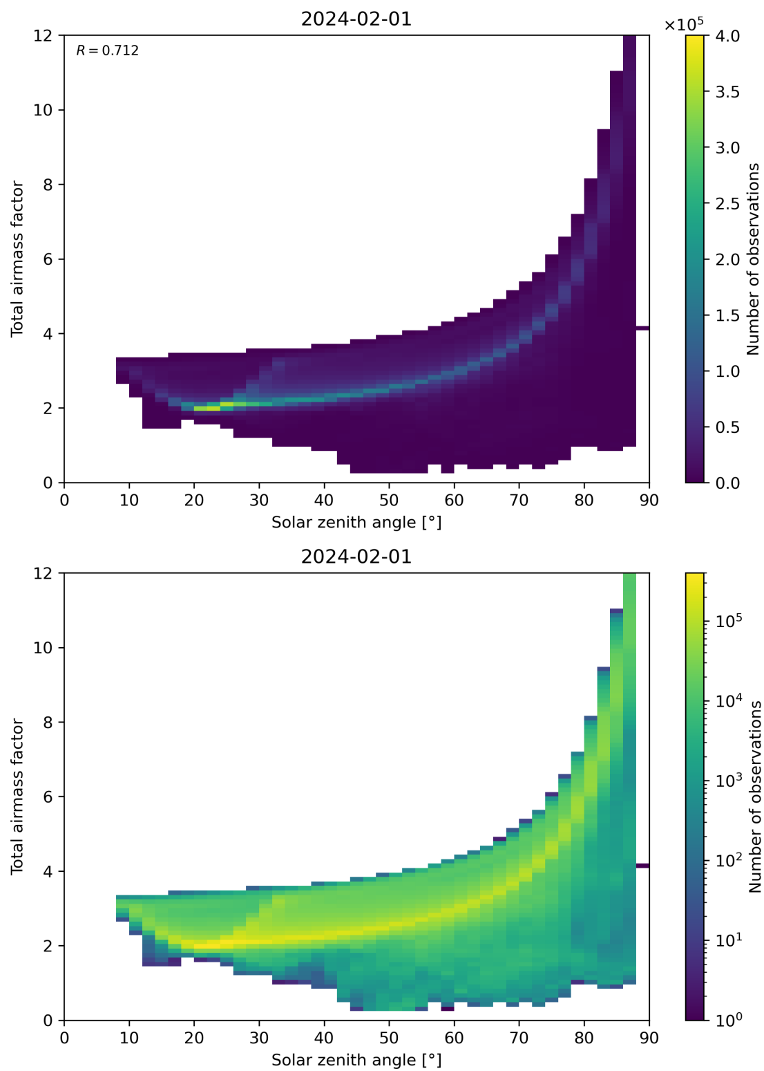
Figure 146: Scatter density plot of “Solar zenith angle” against “Total air mass factor” for 2024-01-31 to 2024-02-02.
