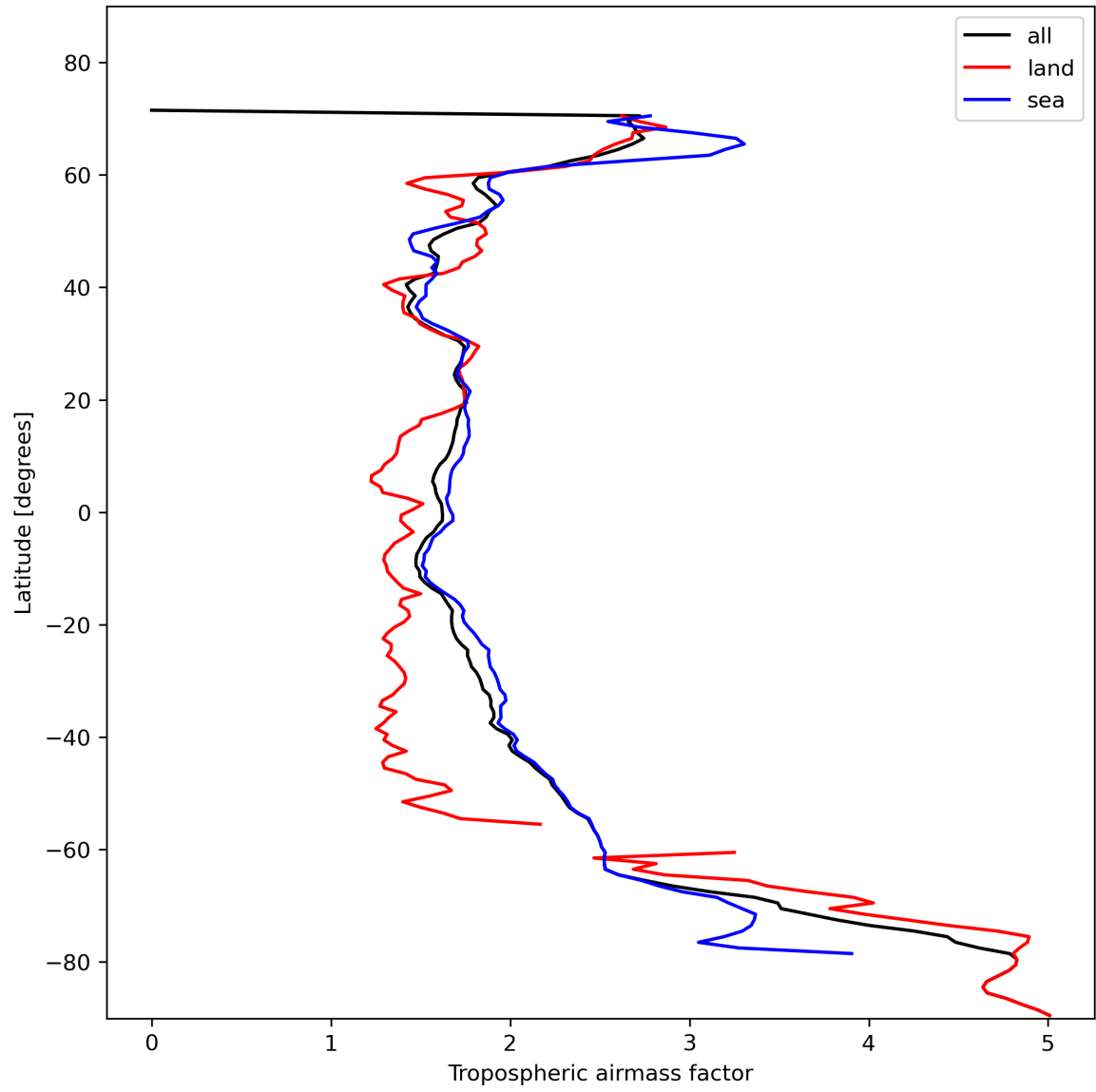
Figure 14: Zonal average of “Tropospheric airmass factor” for 2024-01-31 to 2024-02-02.
