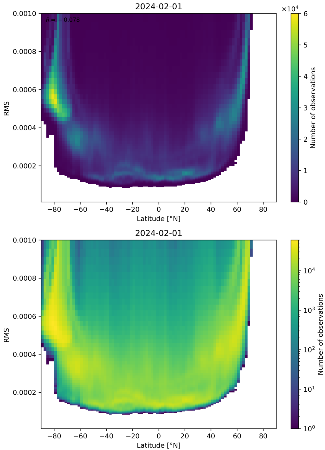
Figure 94: Scatter density plot of “Latitude” against “RMS” for 2024-01-31 to 2024-02-02.
