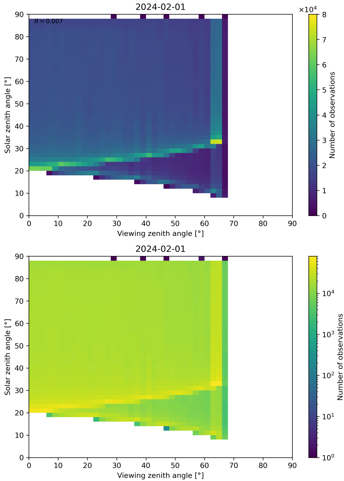
Figure 172: Scatter density plot of “Viewing zenith angle” against “Solar zenith angle” for 2024-01-31 to 2024-02-02.
