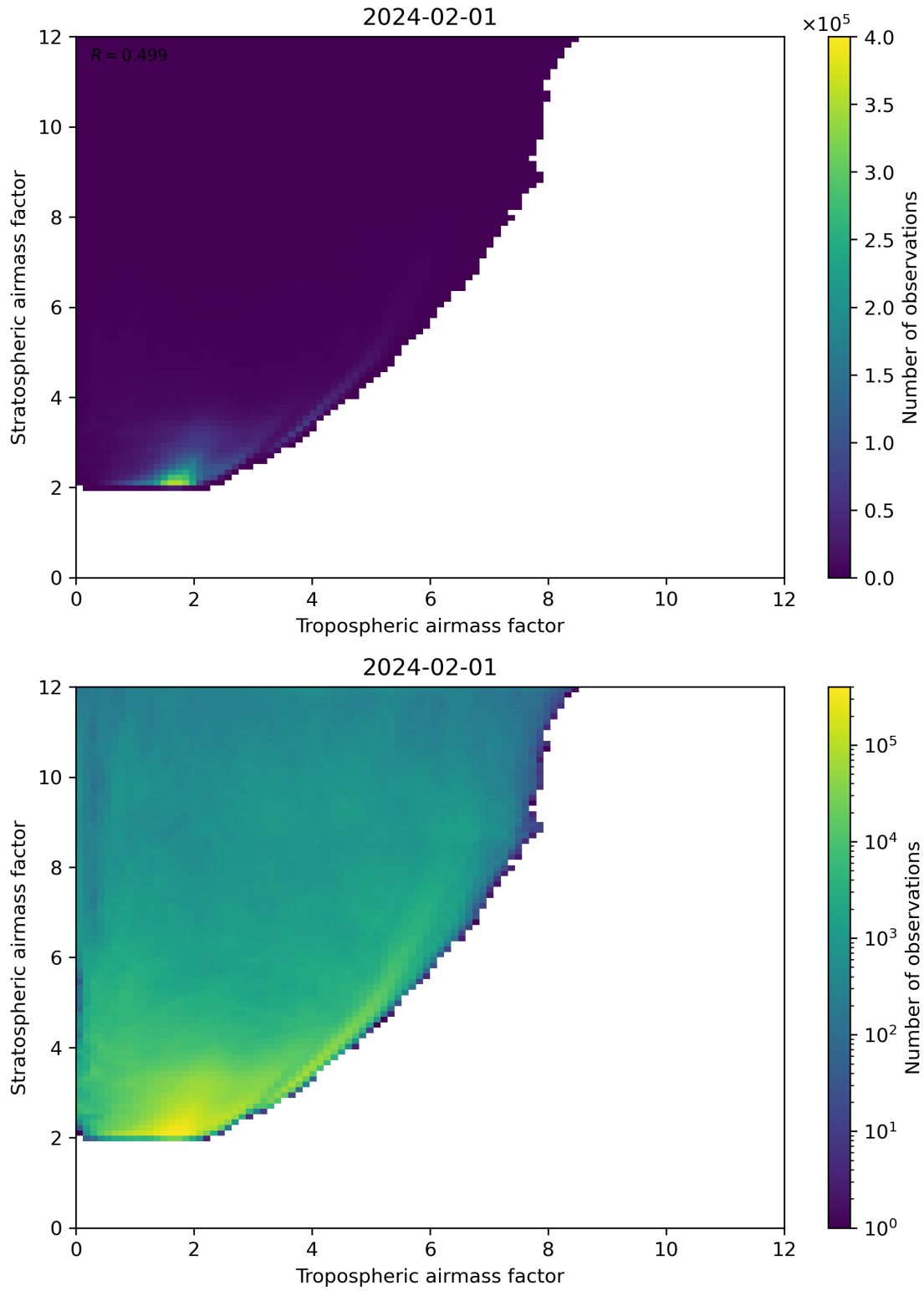
Figure 71: Scatter density plot of “Tropospheric airmass factor” against “Stratospheric airmass factor” for 2024-01-31 to 2024-02-02.
