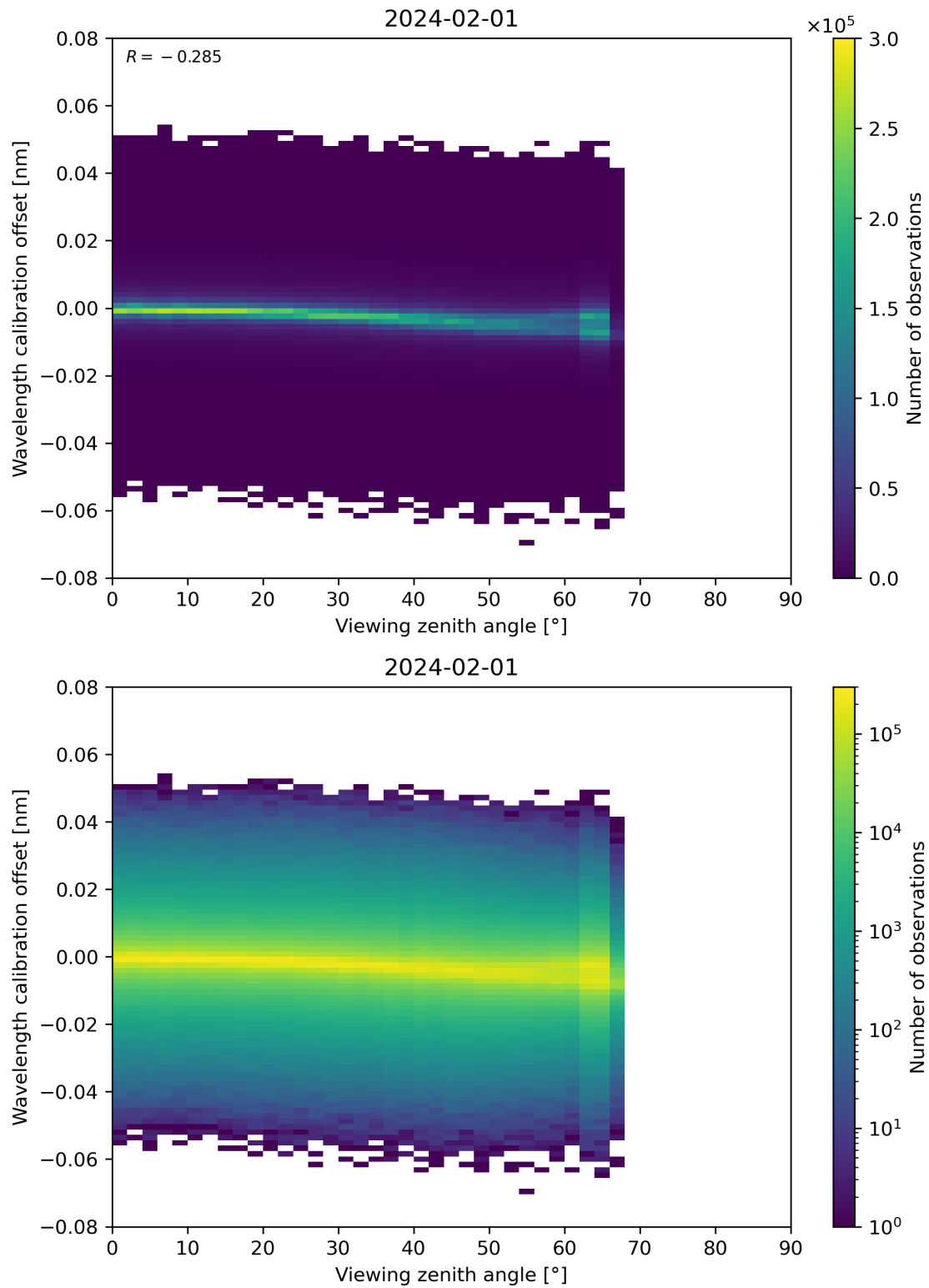
Figure 173: Scatter density plot of “Viewing zenith angle” against “Wavelength calibration offset” for 2024-01-31 to 2024-02-02.
