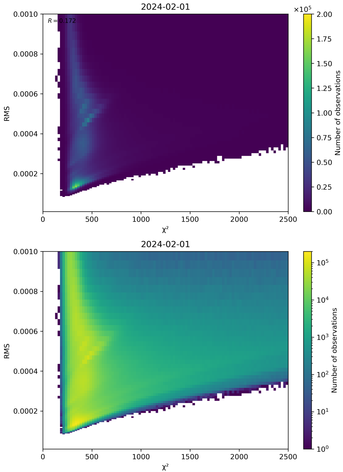
Figure 82: Scatter density plot of “ \chi^2 ” against “RMS” for 2024-01-31 to 2024-02-02.
