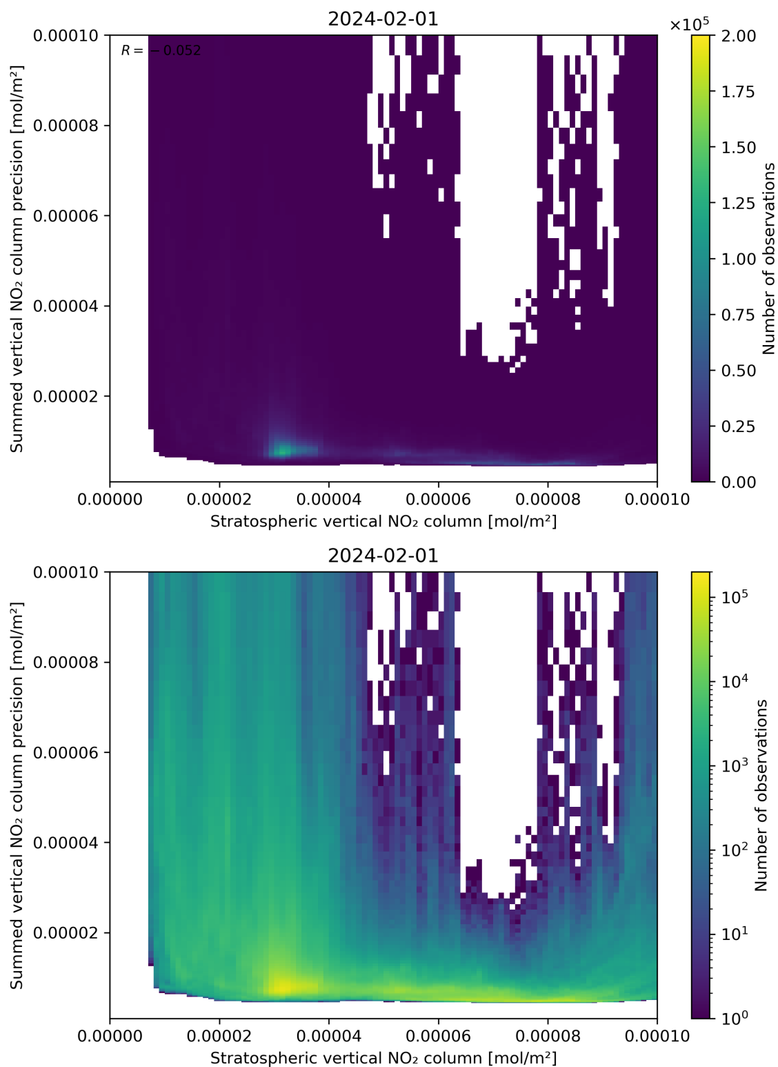
Figure 99: Scatter density plot of “Stratospheric vertical NO 2 column” against “Summed vertical NO 2 column precision” for 2024-01-31 to 2024-02-02.
