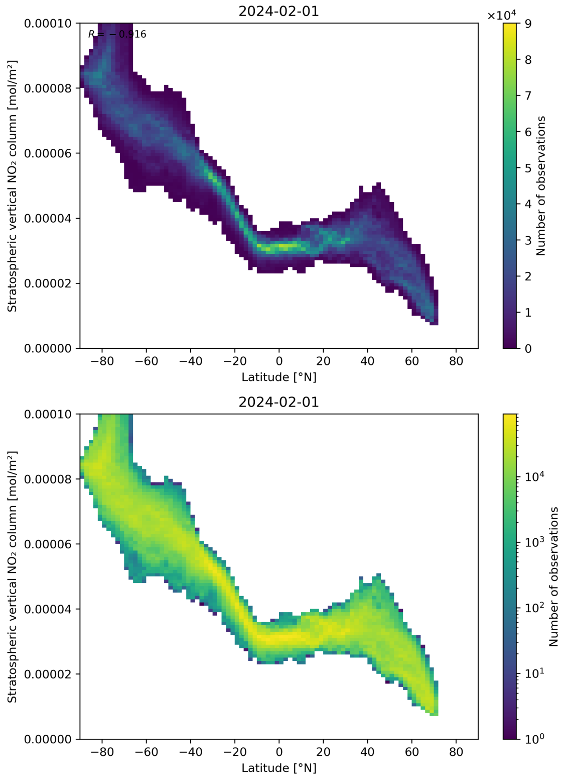
Figure 87: Scatter density plot of “Latitude” against “Stratospheric vertical NO 2 column” for 2024-01-31 to 2024-02-02.
