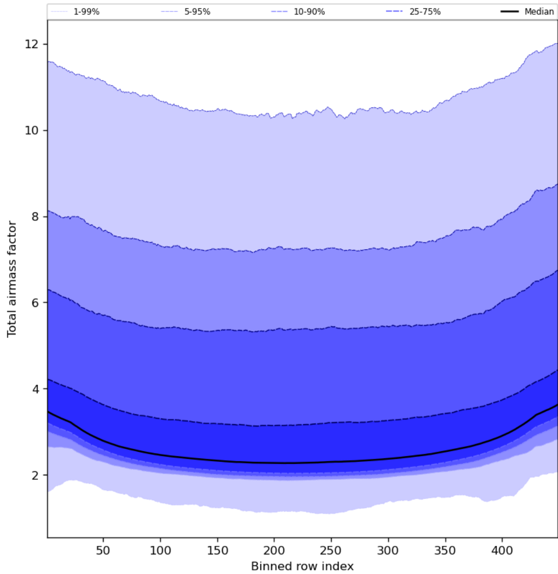
Figure 49: Along track statistics of “Total airmass factor” for 2024-01-31 to 2024-02-02
