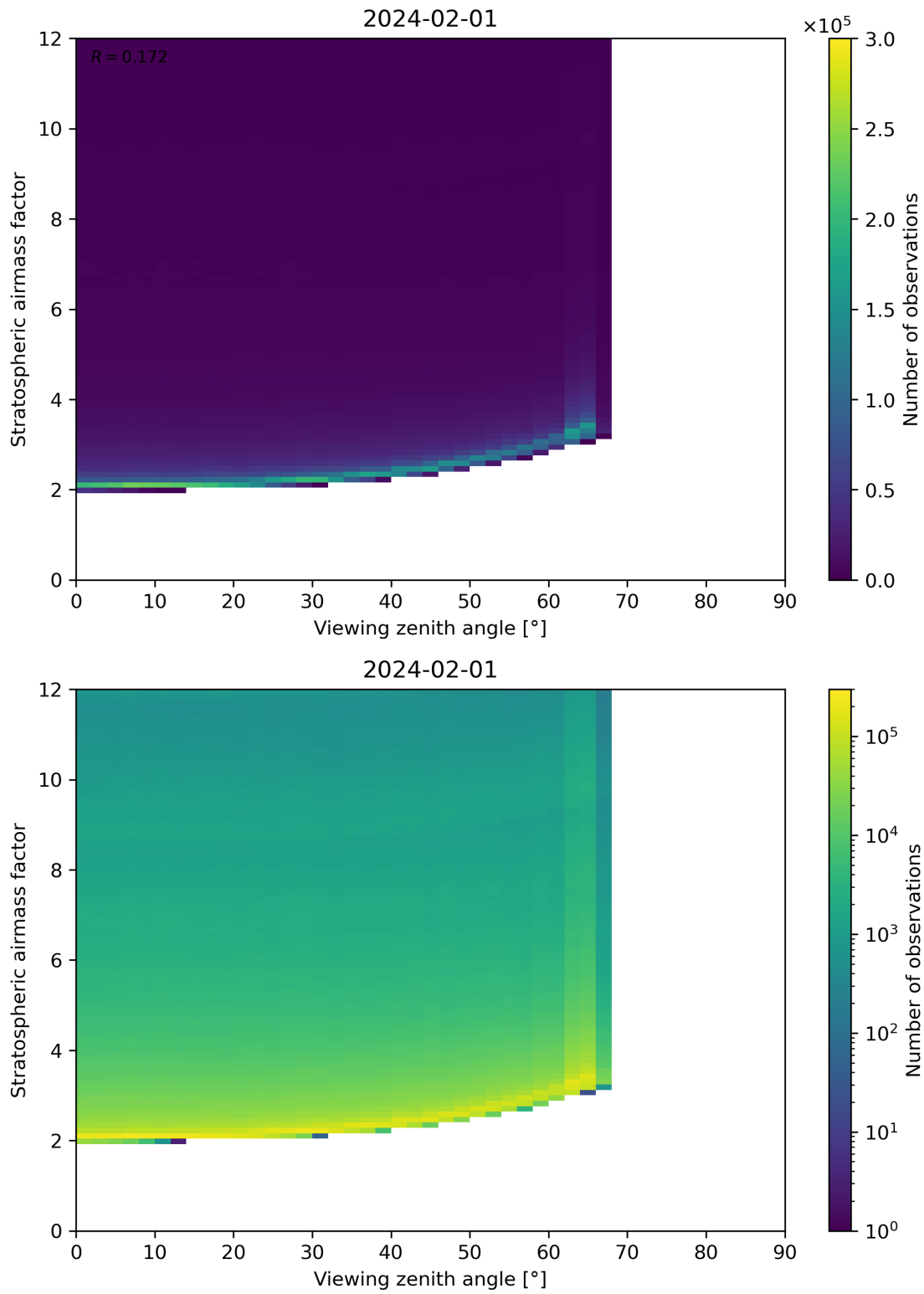
Figure 159: Scatter density plot of “Viewing zenith angle” against “Stratospheric airmass factor” for 2024-01-31 to 2024-02-02.
