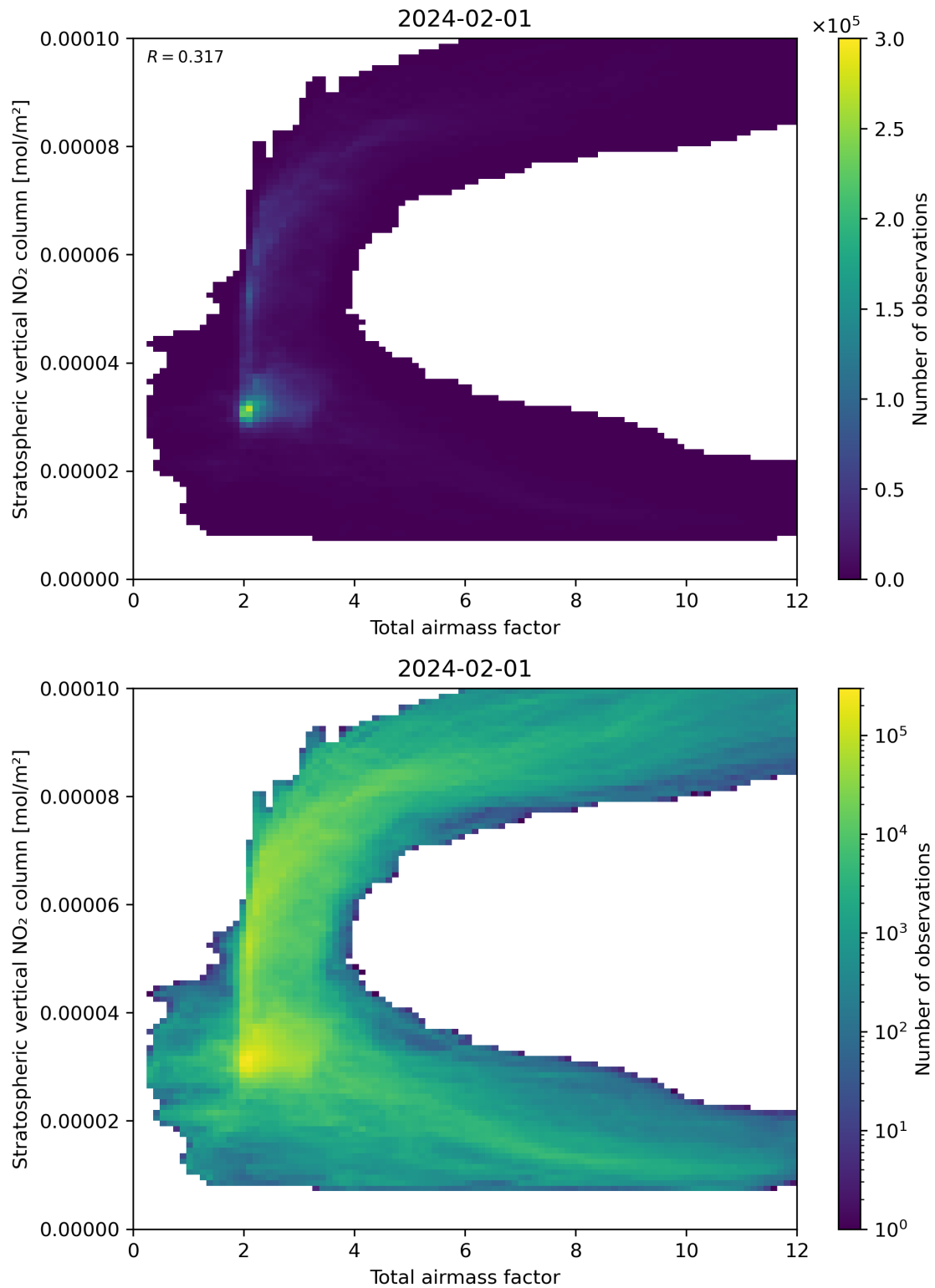
Figure 64: Scatter density plot of “Total airmass factor” against “Stratospheric vertical NO 2 column” for 2024-01-31 to 2024-02-02.
