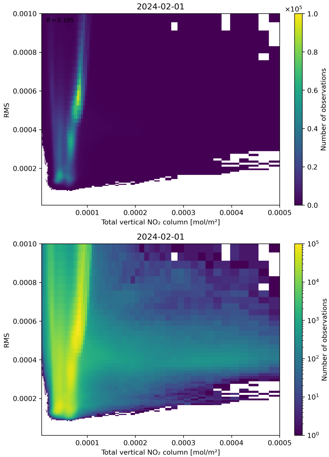
Figure 120: Scatter density plot of “Total vertical NO 2 column” against “RMS” for 2024-01-31 to 2024-02-02.
