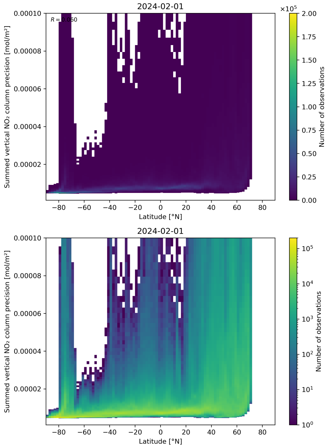
Figure 89: Scatter density plot of “Latitude” against “Summed vertical NO 2 column precision” for 2024-01-31 to 2024-02-02.
