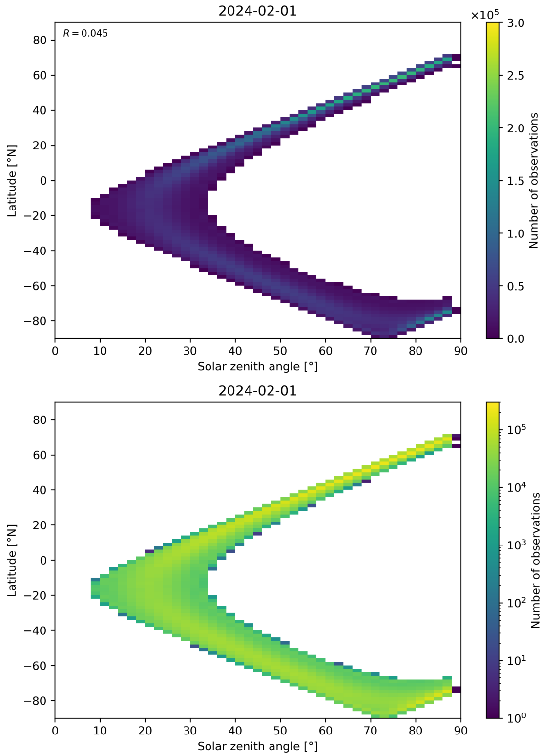
Figure 149: Scatter density plot of “Solar zenith angle” against “Latitude” for 2024-01-31 to 2024-02-02.
