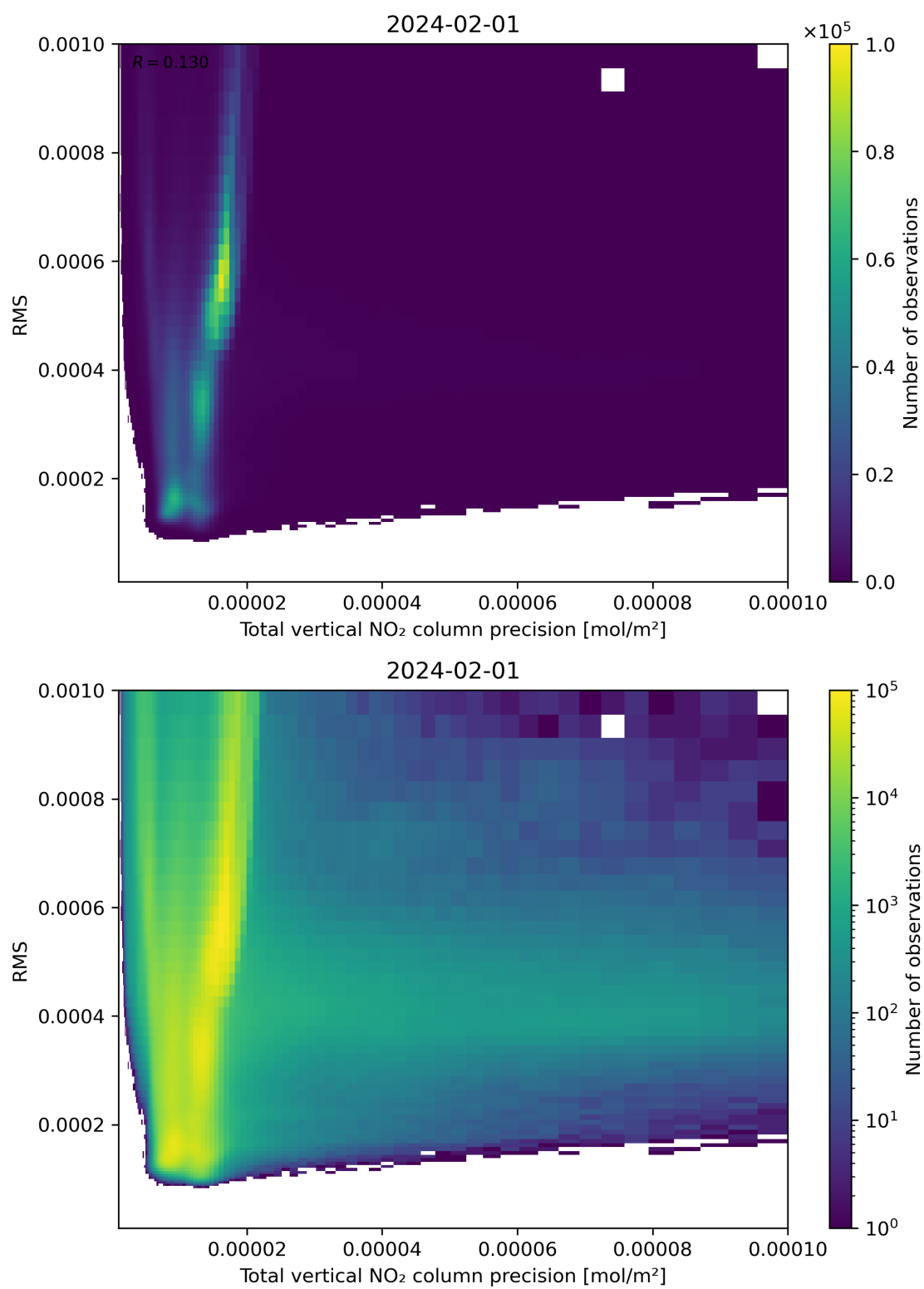
Figure 119: Scatter density plot of “Total vertical NO 2 column precision” against “RMS” for 2024-01-31 to 2024-02-02.
