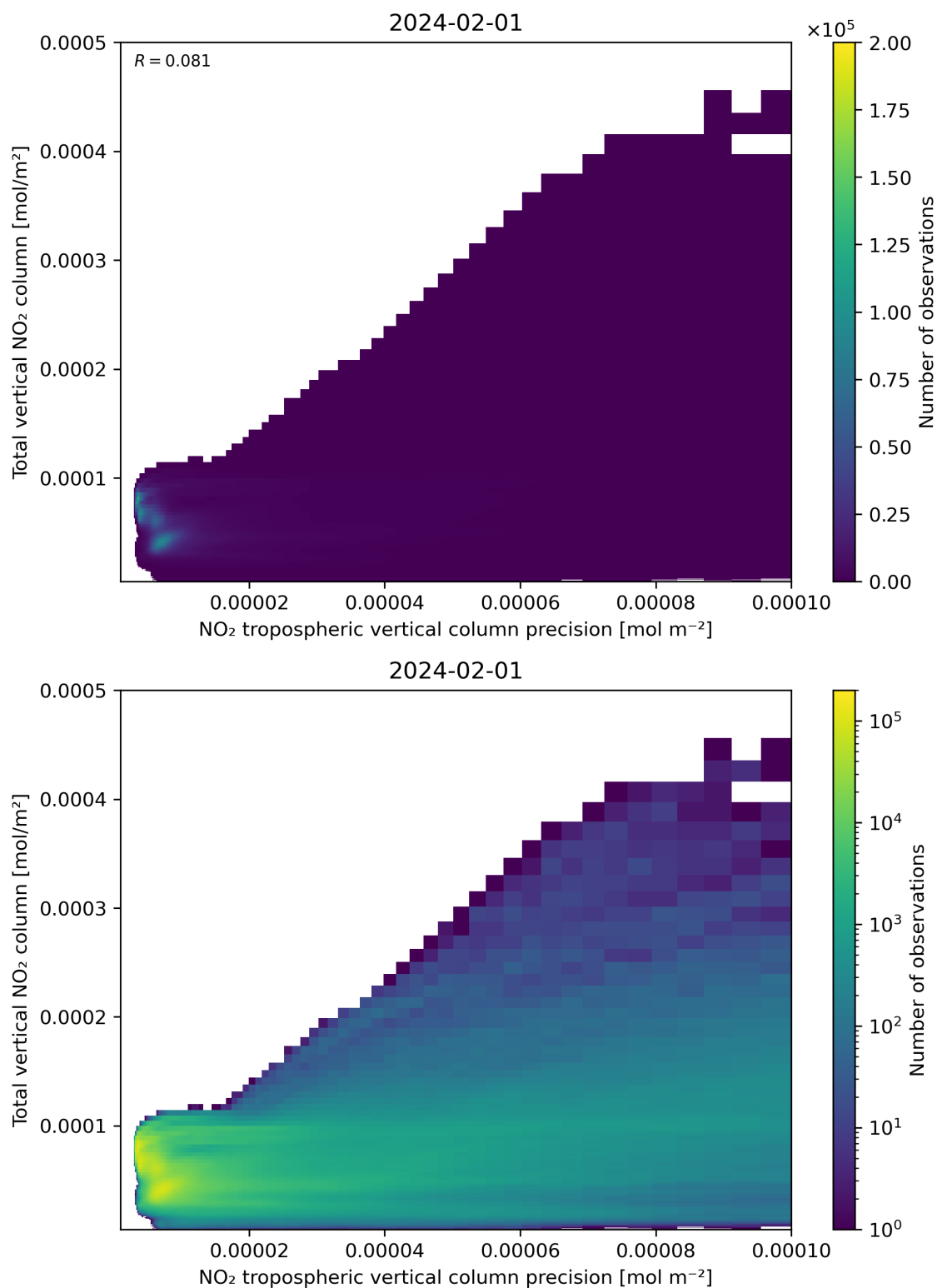
Figure 138: Scatter density plot of “NO 2 tropospheric vertical column precision” against “Total vertical NO 2 column” for 2024-01-31 to 2024-02-02.
