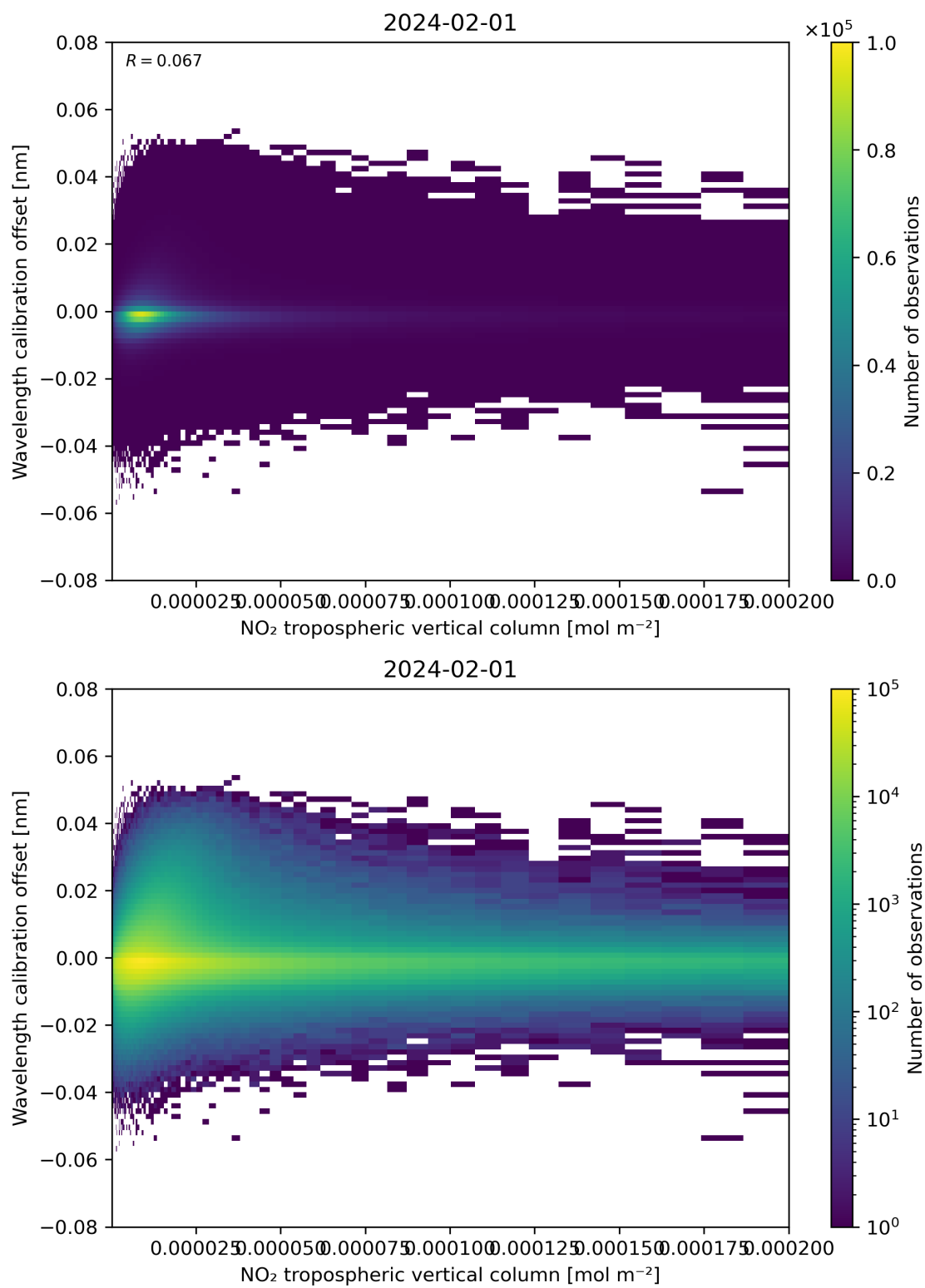
Figure 143: Scatter density plot of “NO 2 tropospheric vertical column” against “Wavelength calibration offset” for 2024-01-31 to 2024-02-02.
