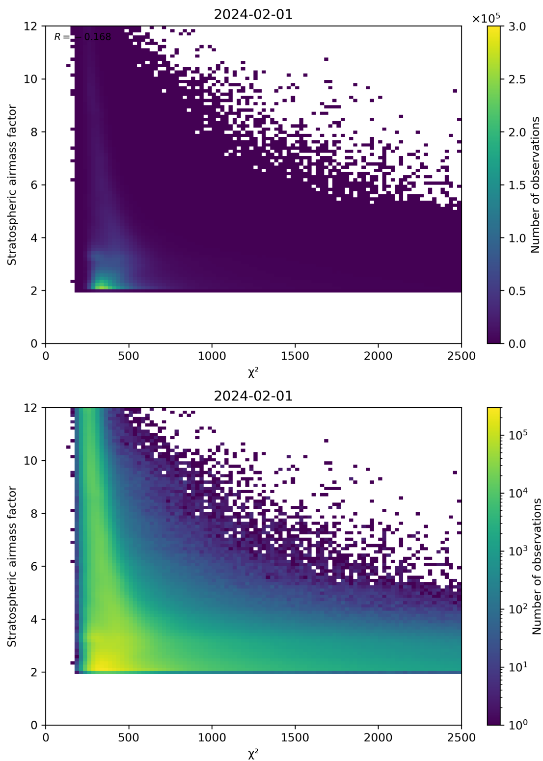
Figure 81: Scatter density plot of “ \chi^2 ” against “Stratospheric airmass factor” for 2024-01-31 to 2024-02-02.
