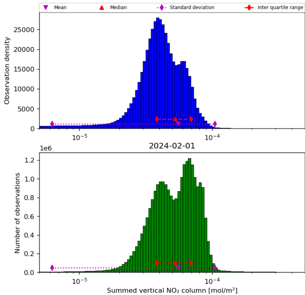
Figure 40: Histogram of “Summed vertical NO 2 column” for 2024-01-31 to 2024-02-02
