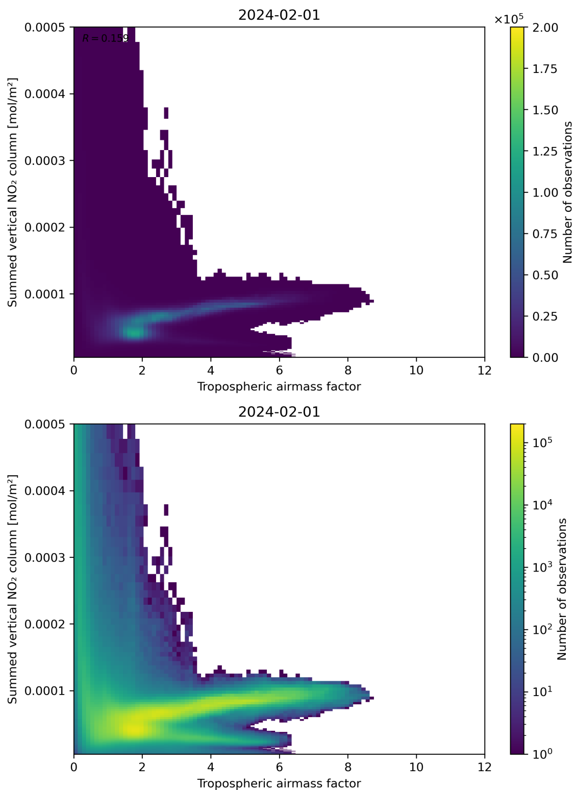
Figure 75: Scatter density plot of “Tropospheric airmass factor” against “Summed vertical NO 2 column” for 2024-01-31 to 2024-02-02.
