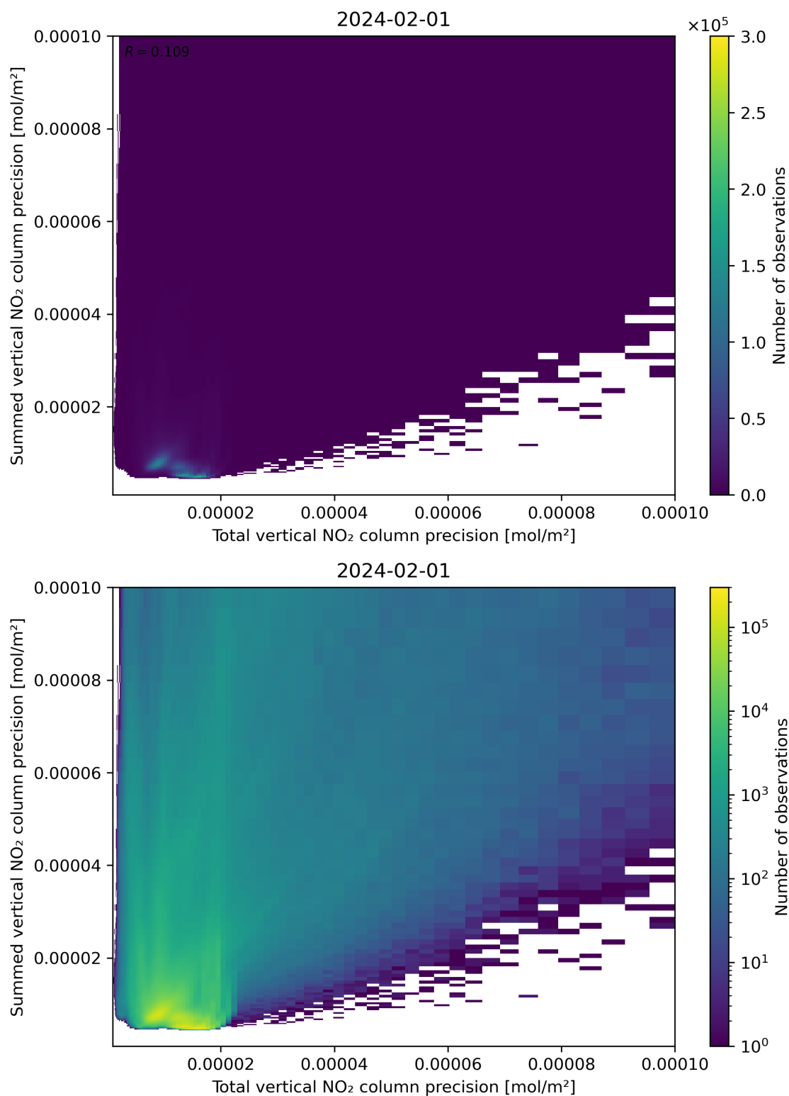
Figure 118: Scatter density plot of “Total vertical NO 2 column precision” against “Summed vertical NO 2 column precision” for 2024-01-31 to 2024-02-02.
