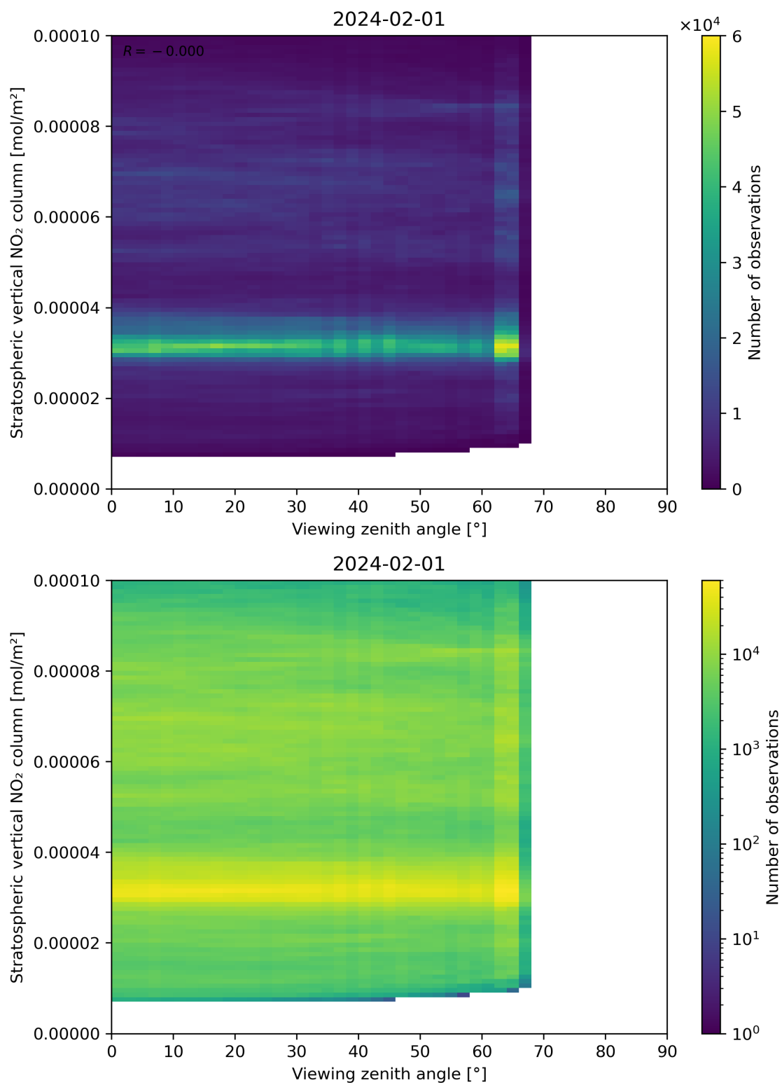
Figure 164: Scatter density plot of “Viewing zenith angle” against “Stratospheric vertical NO 2 column” for 2024-01-31 to 2024-02-02.
