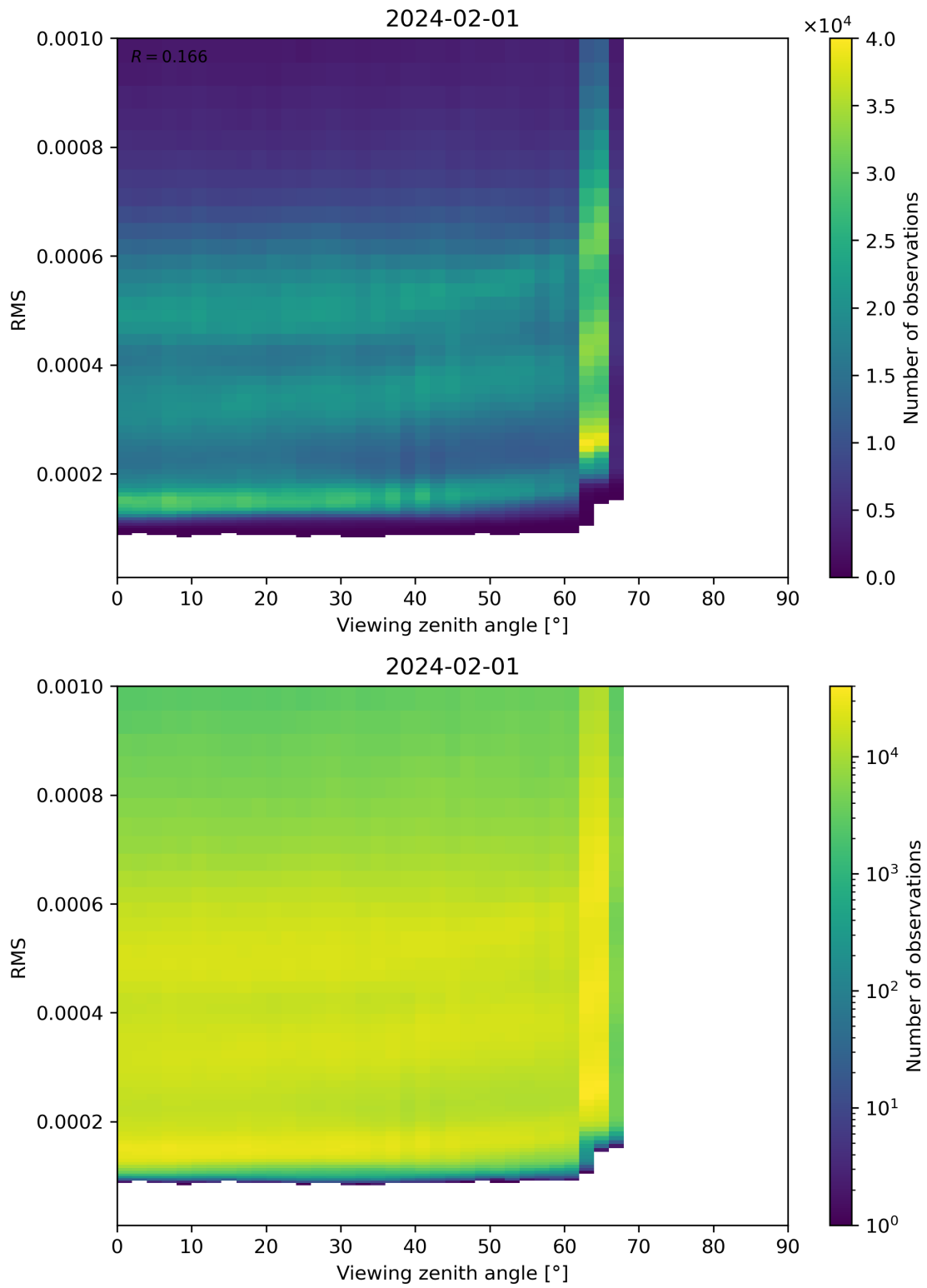
Figure 171: Scatter density plot of “Viewing zenith angle” against “RMS” for 2024-01-31 to 2024-02-02.
