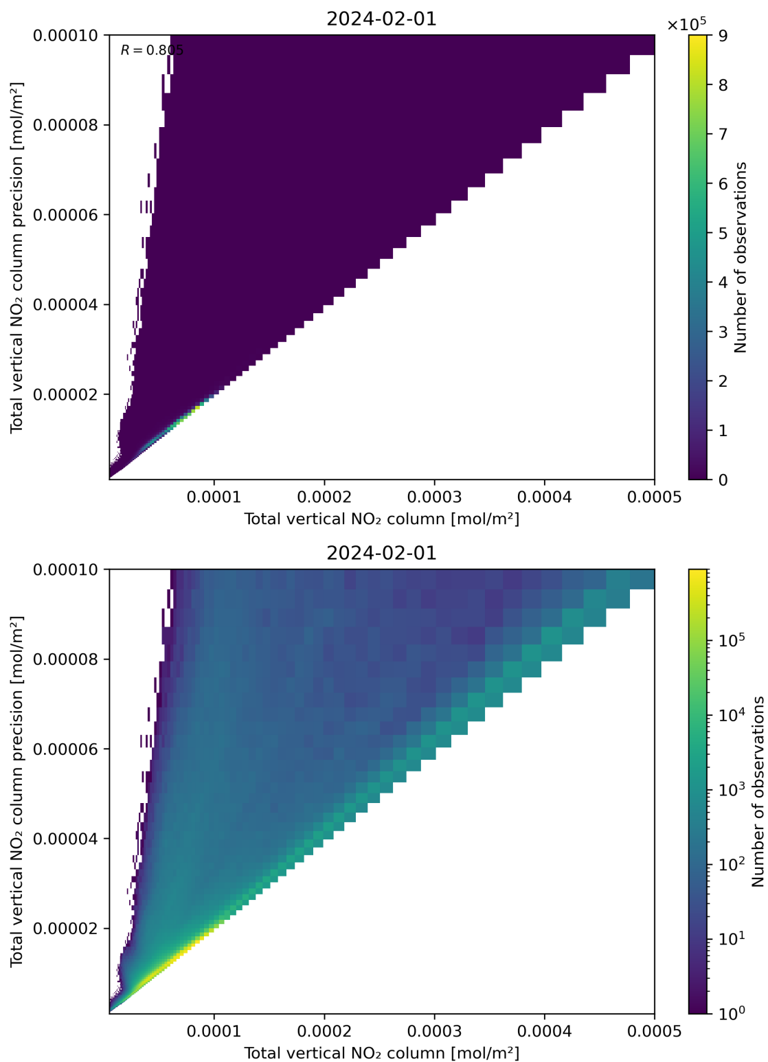
Figure 114: Scatter density plot of “Total vertical NO 2 column” against “Total vertical NO 2 column precision” for 2024-01-31 to 2024-02-02.
