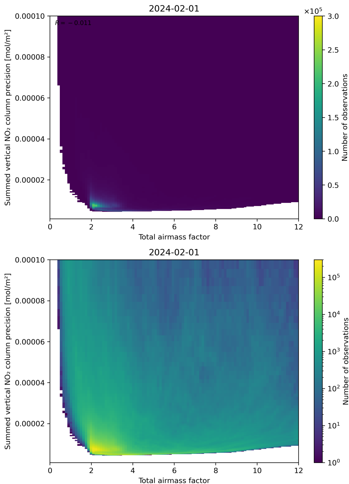
Figure 66: Scatter density plot of “Total airmass factor” against “Summed vertical NO 2 column precision” for 2024-01-31 to 2024-02-02.
