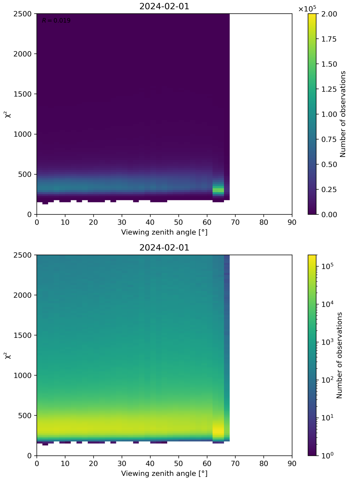
Figure 162: Scatter density plot of “Viewing zenith angle” against “ \chi^2 ” for 2024-01-31 to 2024-02-02.
