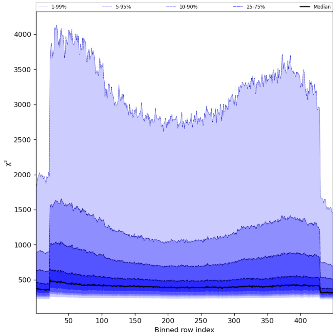
Figure 59: Along track statistics of “ \chi^2 ” for 2024-01-31 to 2024-02-02
