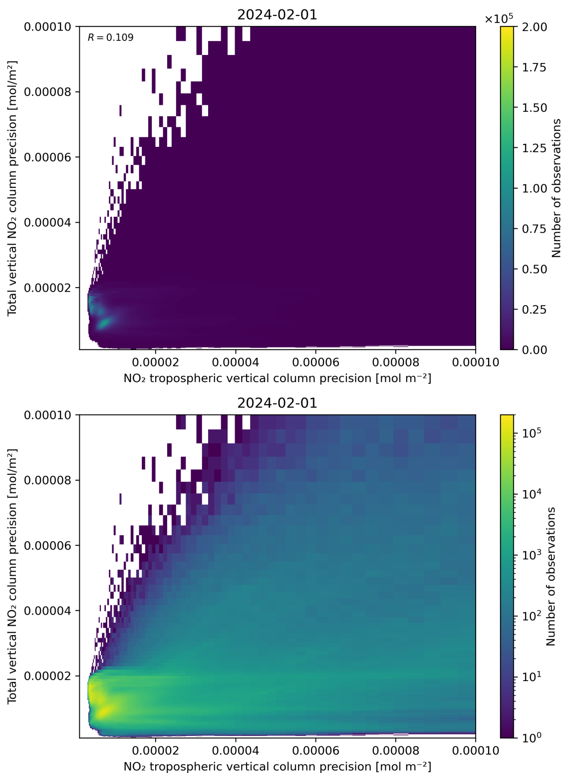
Figure 139: Scatter density plot of “NO 2 tropospheric vertical column precision” against “Total vertical NO 2 column precision” for 2024-01-31 to 2024-02-02.
