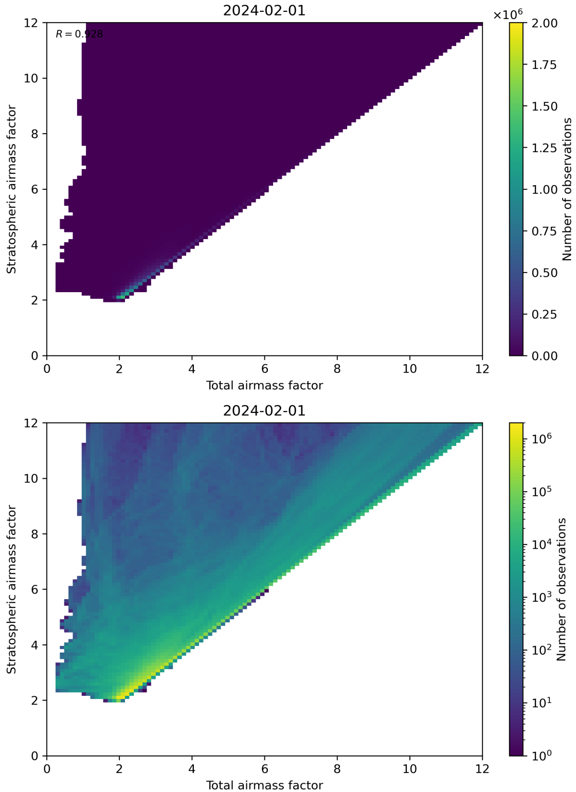
Figure 62: Scatter density plot of “Total airmass factor” against “Stratospheric airmass factor” for 2024-01-31 to 2024-02-02.
