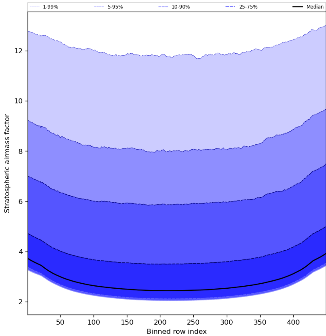
Figure 61: Along track statistics of “Stratospheric airmass factor” for 2024-01-31 to 2024-02-02
