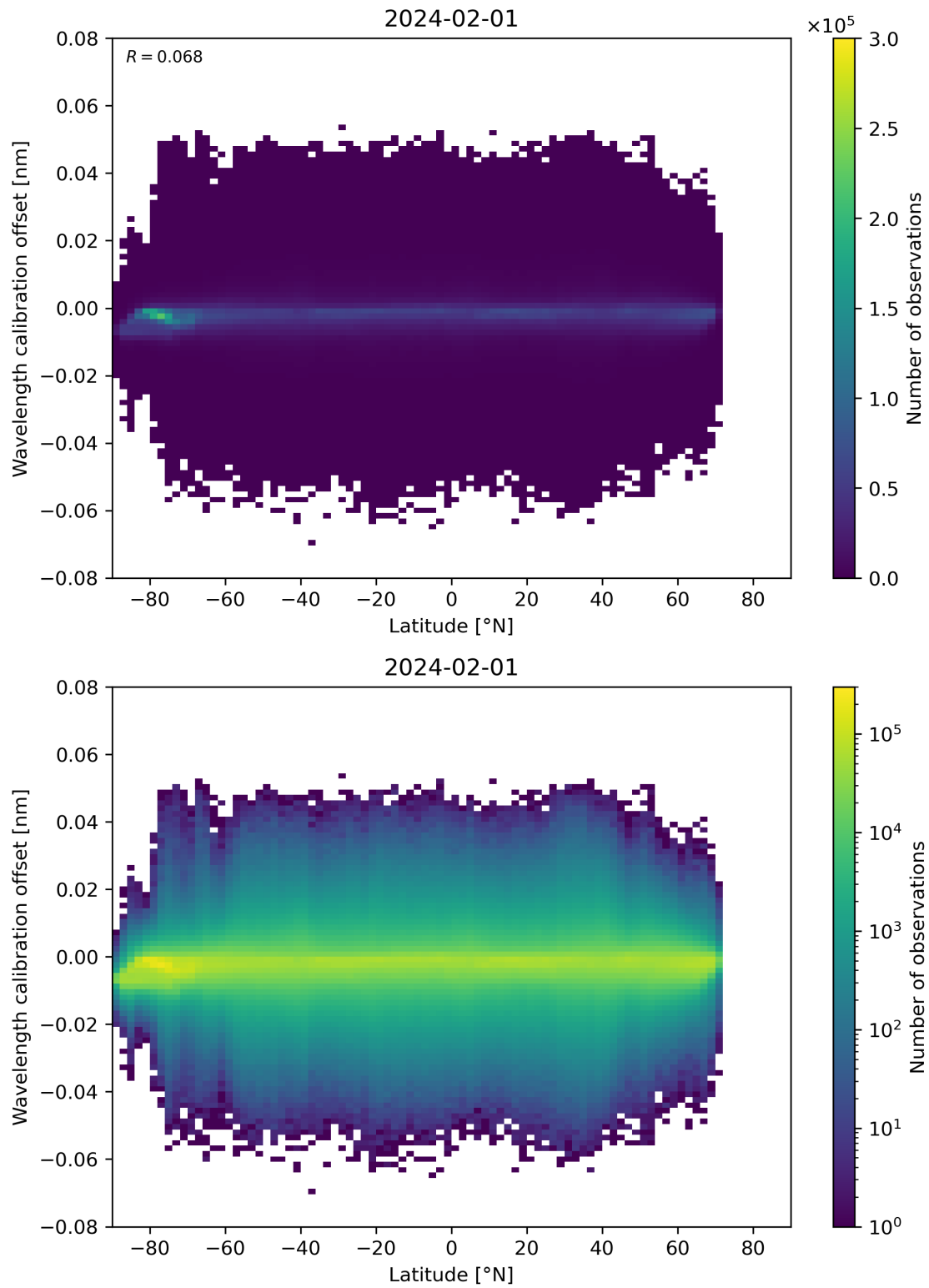
Figure 95: Scatter density plot of “Latitude” against “Wavelength calibration offset” for 2024-01-31 to 2024-02-02.
