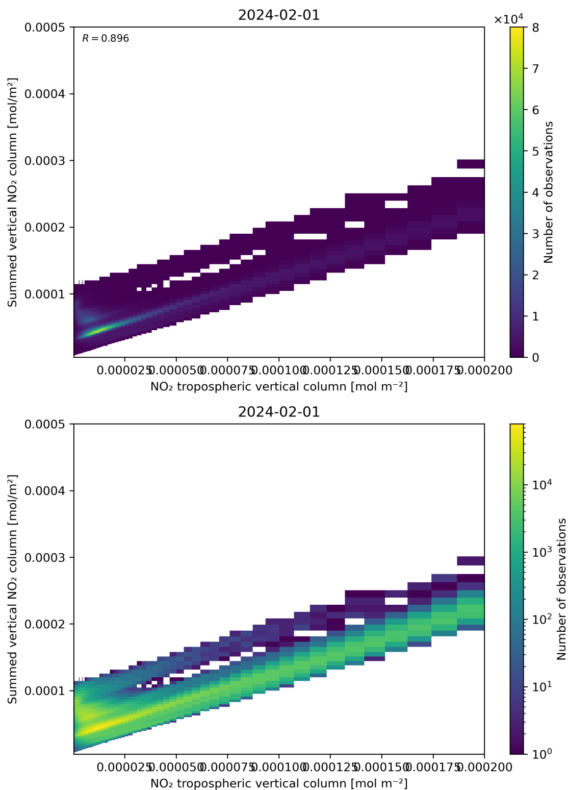
Figure 126: Scatter density plot of “NO 2 tropospheric vertical column” against “Summed vertical NO 2 column” for 2024-01-31 to 2024-02-02.
