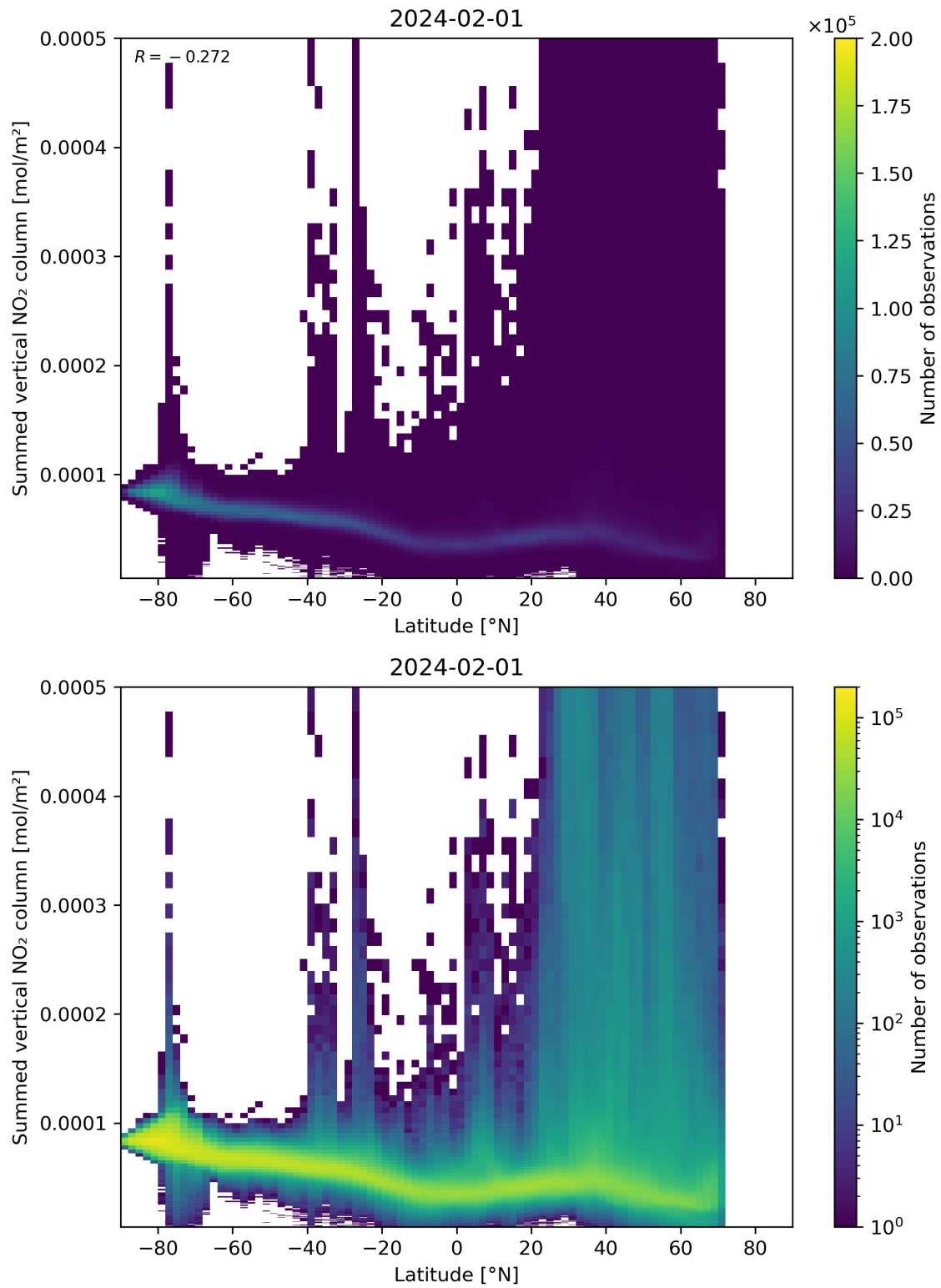
Figure 88: Scatter density plot of “Latitude” against “Summed vertical NO 2 column” for 2024-01-31 to 2024-02-02.
