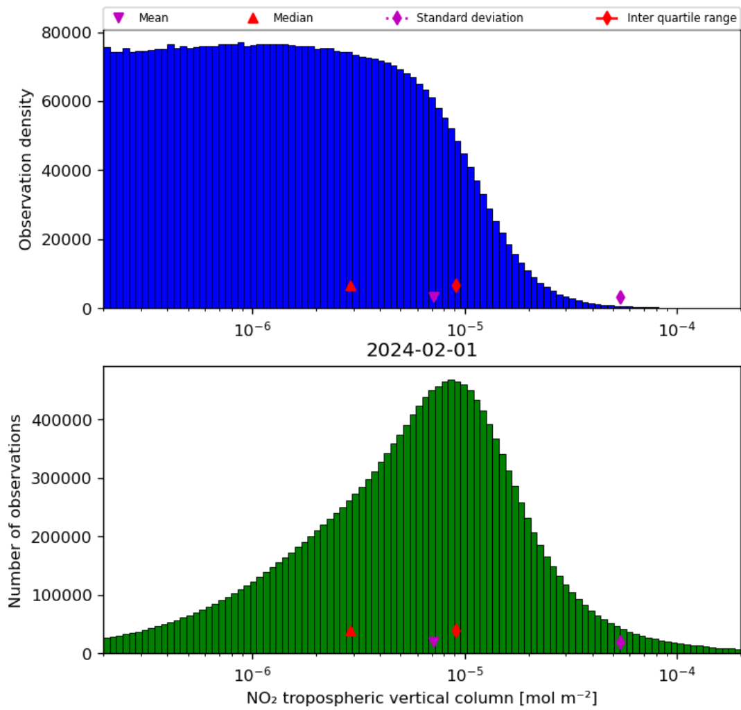
Figure 29: Histogram of “ \text{NO}_2 tropospheric vertical column” for 2024-01-31 to 2024-02-02
