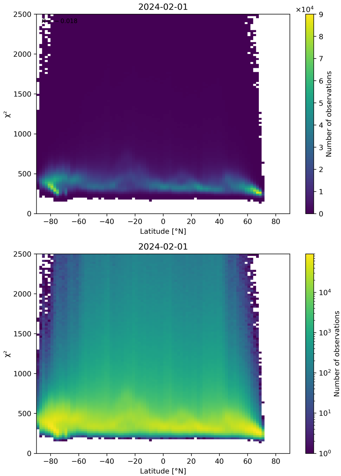
Figure 86: Scatter density plot of “Latitude” against “ \chi^2 ” for 2024-01-31 to 2024-02-02.
