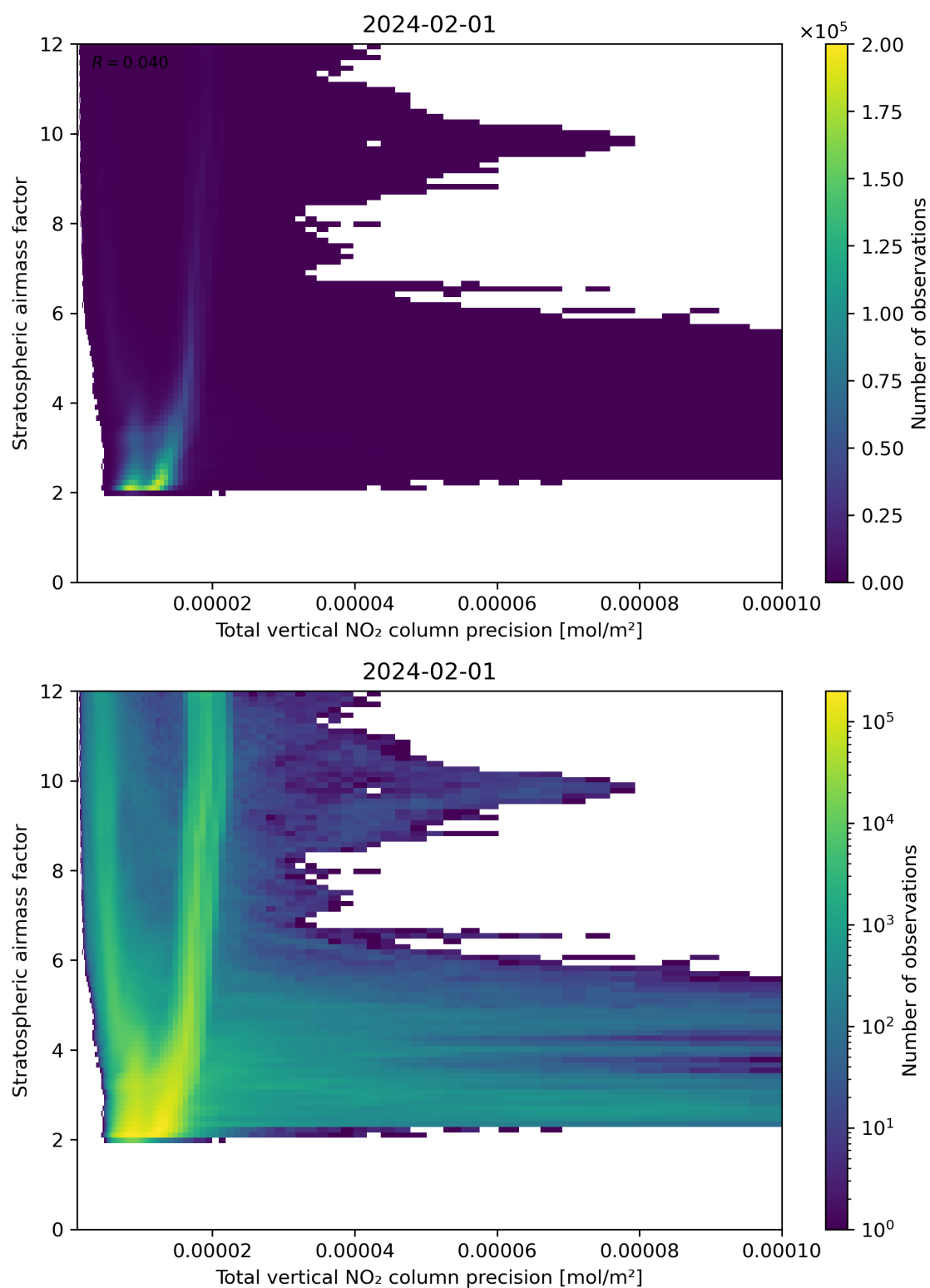
Figure 115: Scatter density plot of “Total vertical NO 2 column precision” against “Stratospheric air mass factor” for 2024-01-31 to 2024-02-02.
