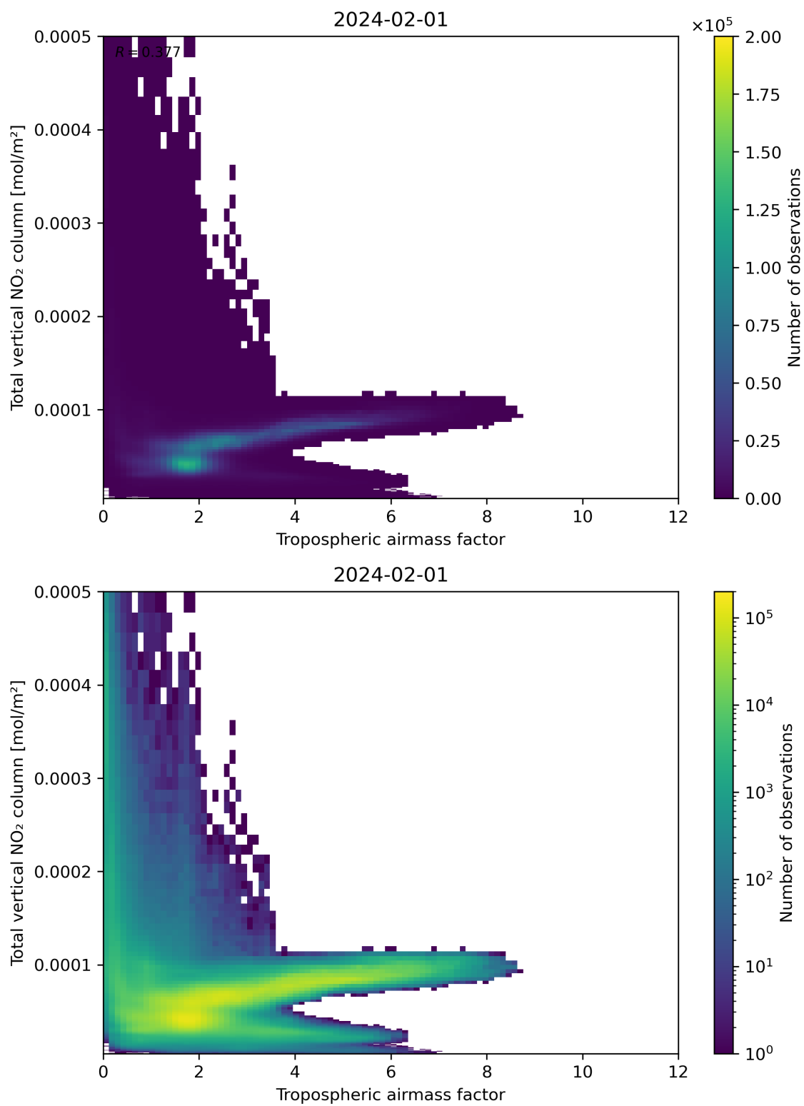
Figure 77: Scatter density plot of “Tropospheric airmass factor” against “Total vertical NO 2 column” for 2024-01-31 to 2024-02-02.
