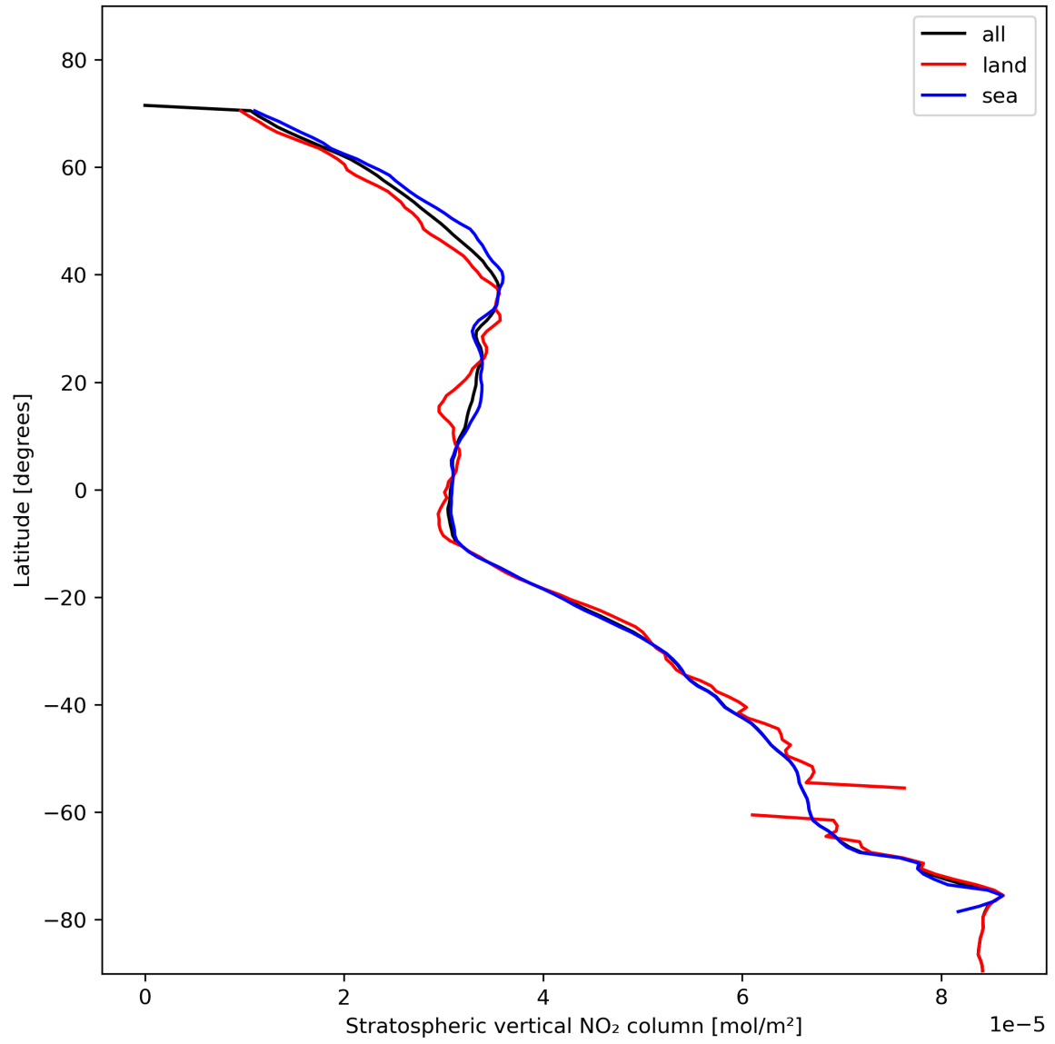
Figure 19: Zonal average of “Stratospheric vertical NO 2 column” for 2024-01-31 to 2024-02-02.
