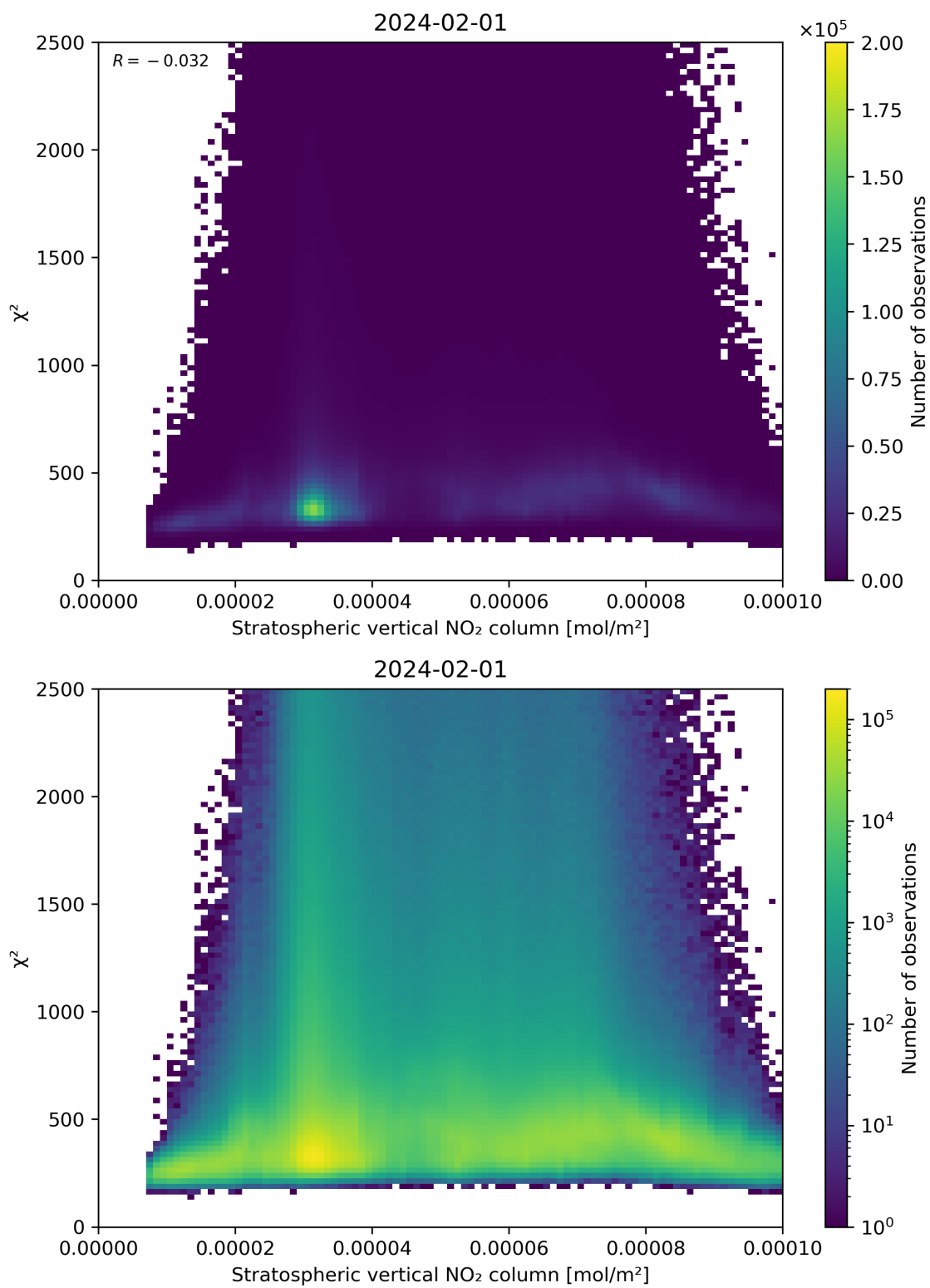
Figure 97: Scatter density plot of “Stratospheric vertical NO 2 column” against “ \chi^2 ” for 2024-01-31 to 2024-02-02.
