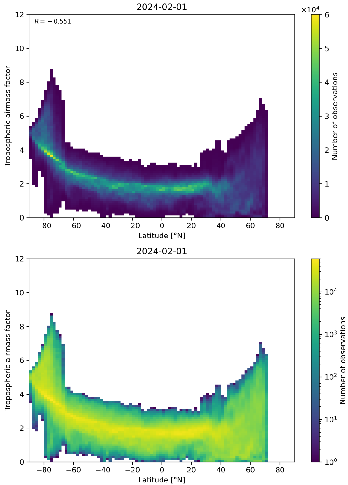
Figure 85: Scatter density plot of “Latitude” against “Tropospheric airmass factor” for 2024-01-31 to 2024-02-02.
