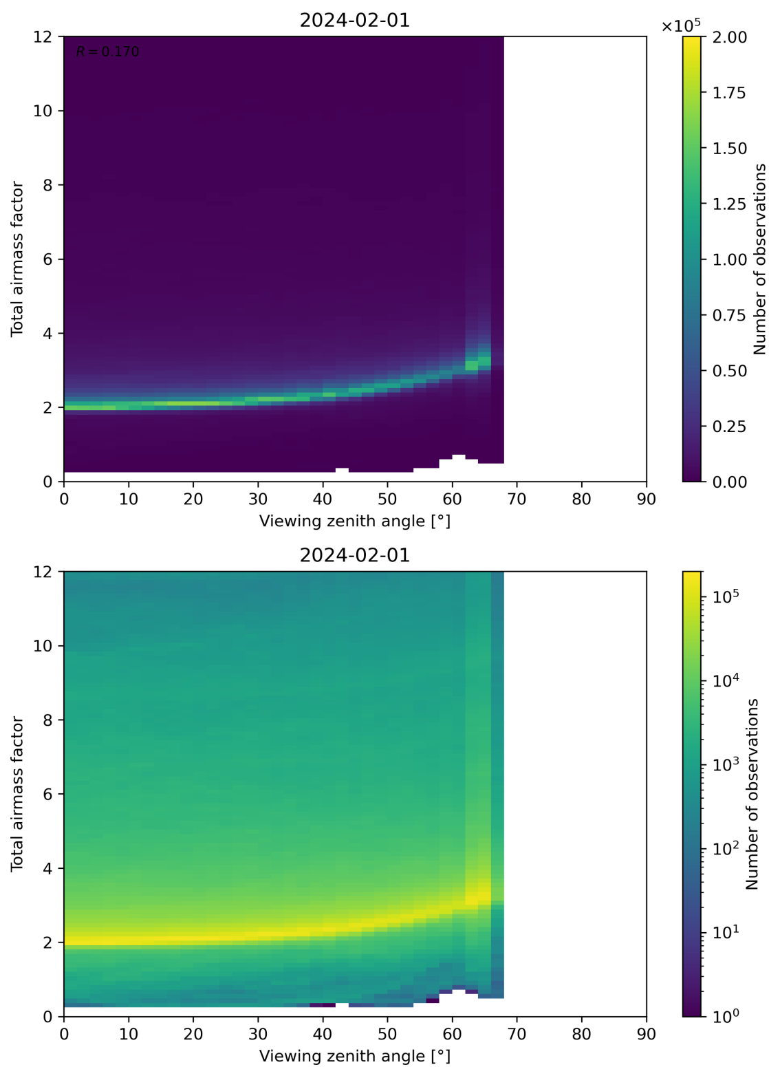
Figure 160: Scatter density plot of “Viewing zenith angle” against “Total airmass factor” for 2024-01-31 to 2024-02-02.
