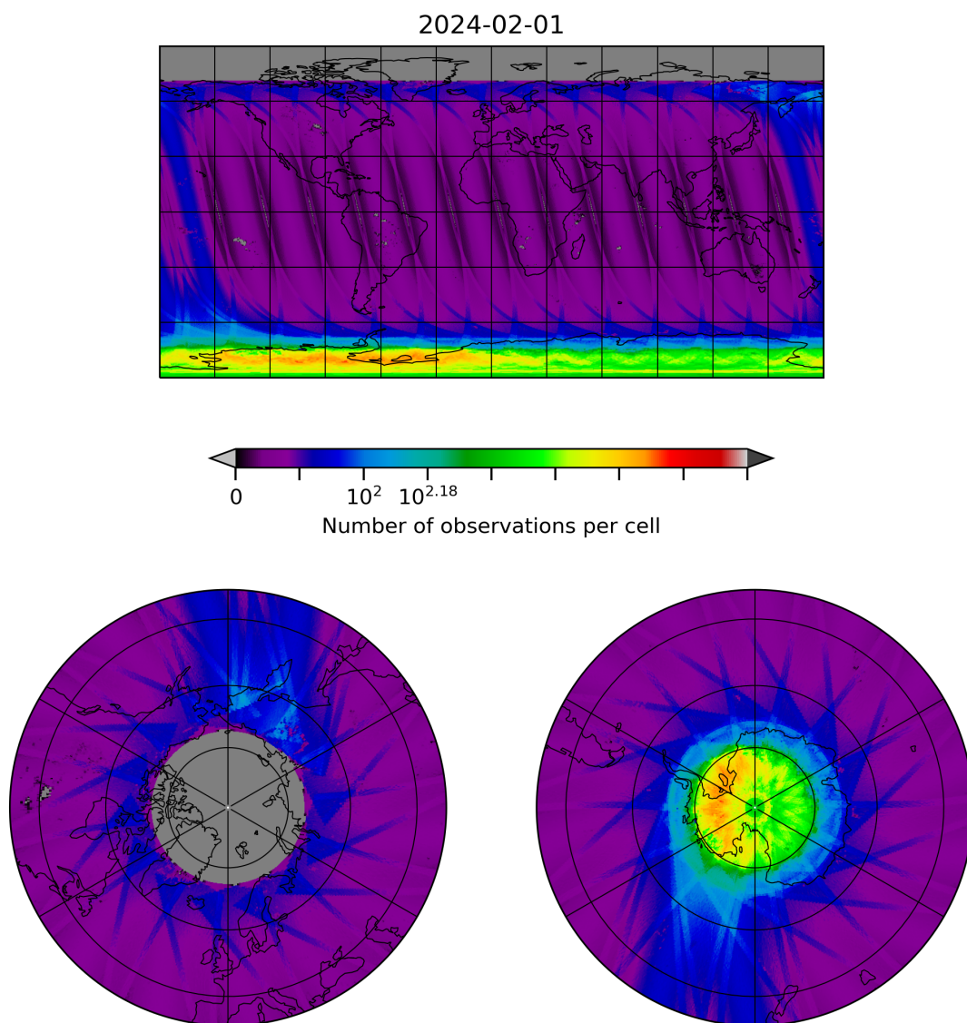
Figure 10: Map of the number of observations for 2024-01-31 to 2024-02-02
