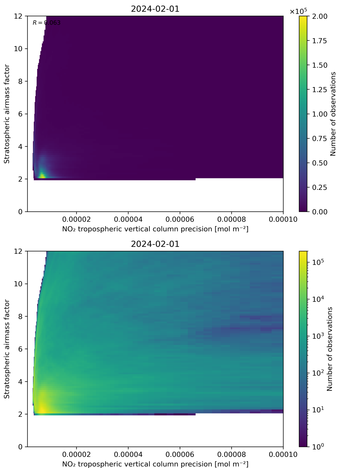
Figure 131: Scatter density plot of “NO 2 tropospheric vertical column precision” against “Stratospheric airmass factor” for 2024-01-31 to 2024-02-02.
