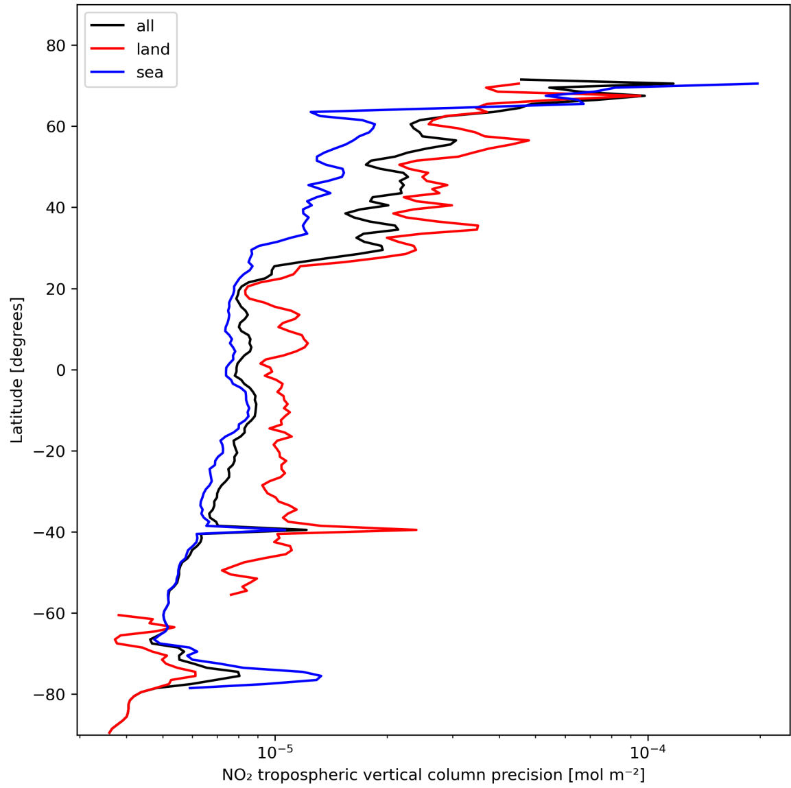
Figure 13: Zonal average of “NO 2 tropospheric vertical column precision” for 2024-01-31 to 2024-02-02.
