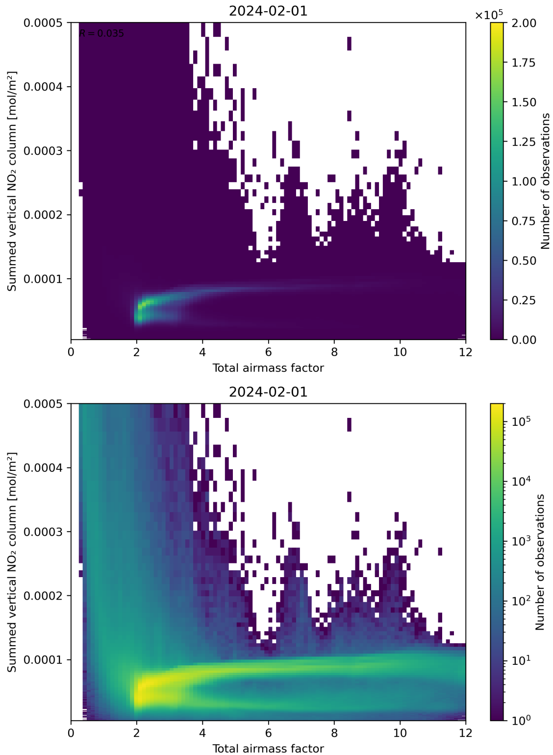
Figure 65: Scatter density plot of “Total airmass factor” against “Summed vertical NO 2 column” for 2024-01-31 to 2024-02-02.
