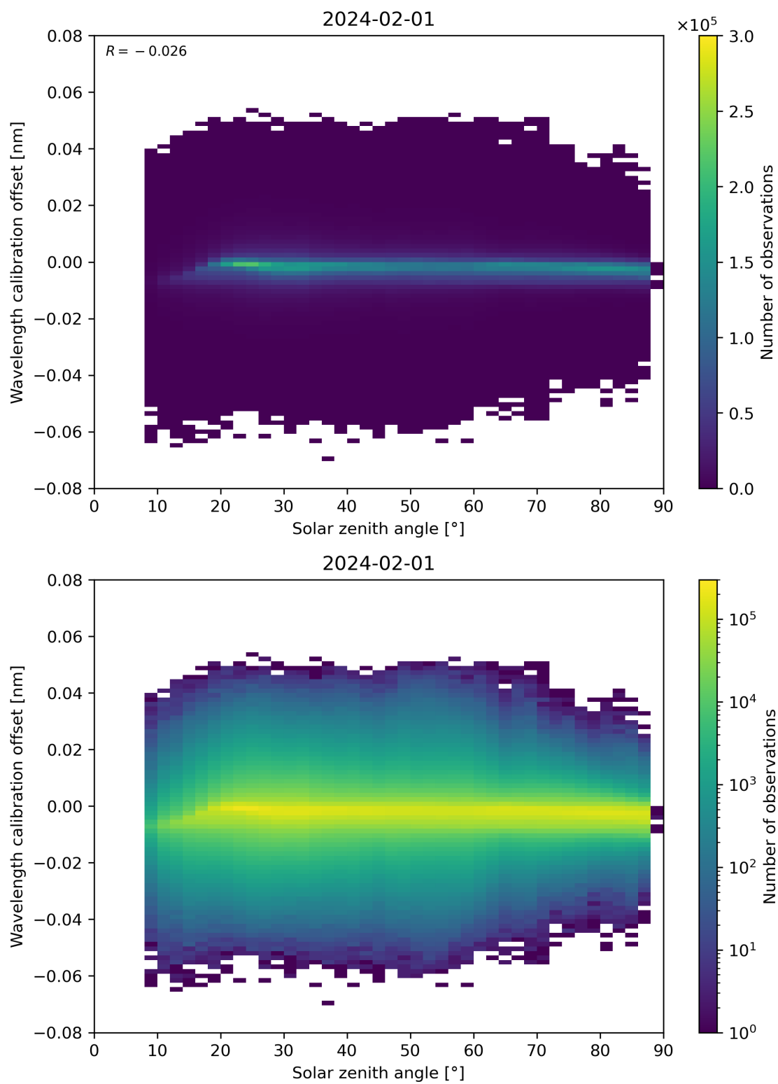
Figure 158: Scatter density plot of “Solar zenith angle” against “Wavelength calibration offset” for 2024-01-31 to 2024-02-02.
