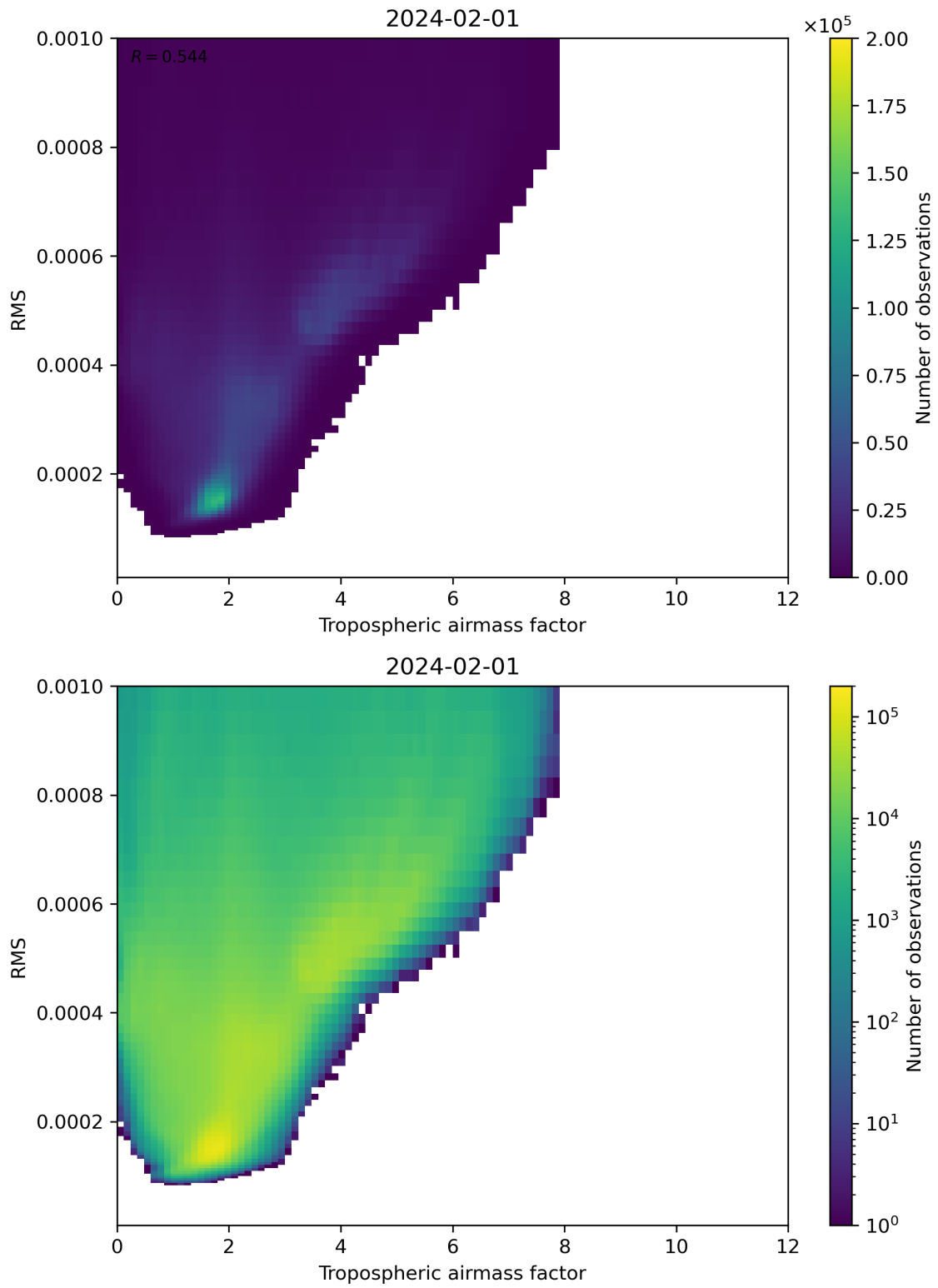
Figure 79: Scatter density plot of “Tropospheric airmass factor” against “RMS” for 2024-01-31 to 2024-02-02.
