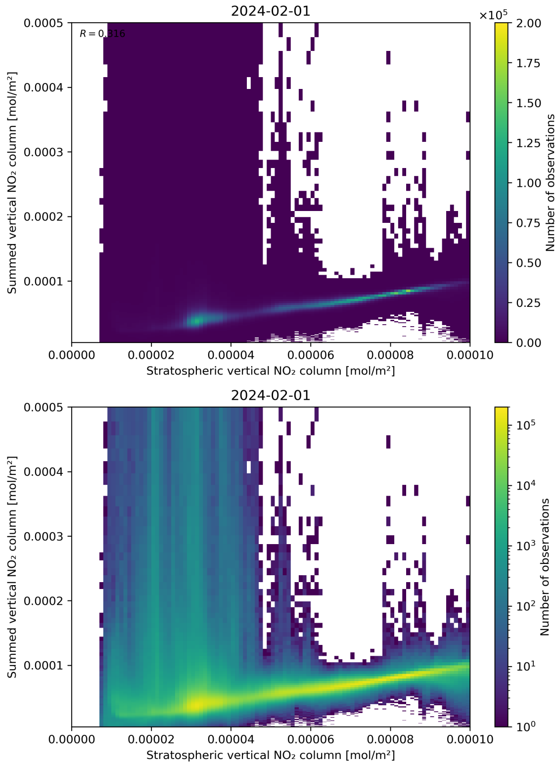
Figure 98: Scatter density plot of “Stratospheric vertical NO 2 column” against “Summed vertical NO 2 column” for 2024-01-31 to 2024-02-02.
