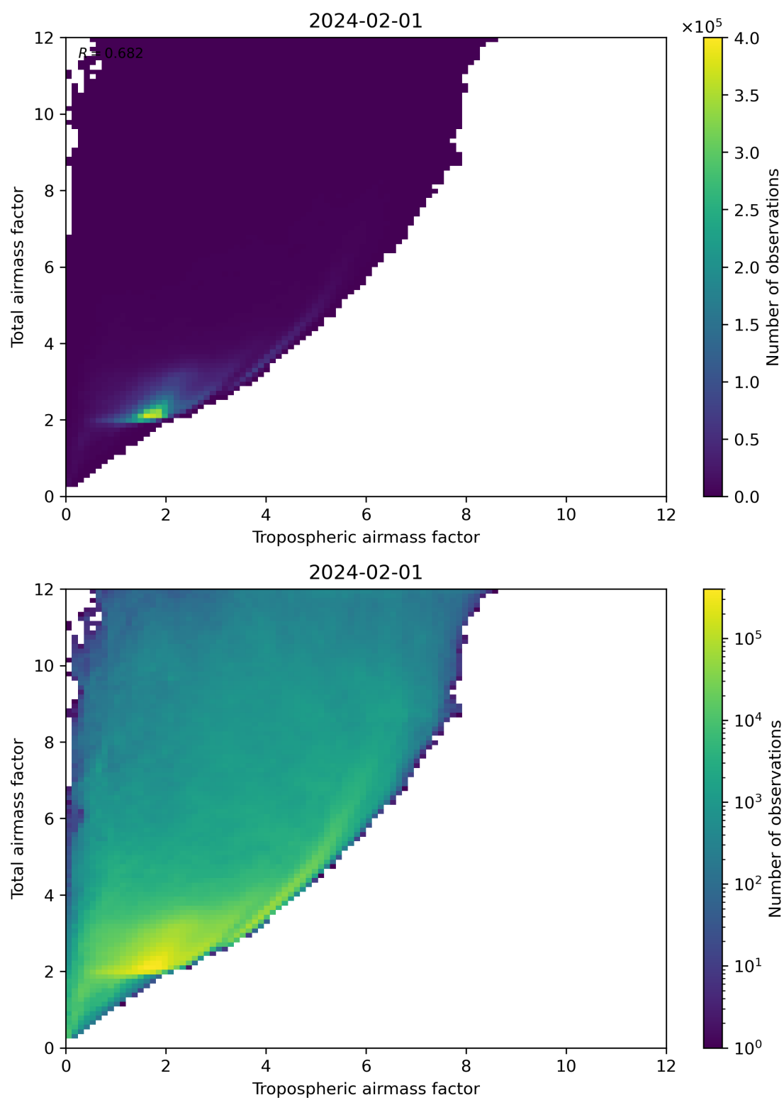
Figure 72: Scatter density plot of “Tropospheric airmass factor” against “Total airmass factor” for 2024-01-31 to 2024-02-02.
