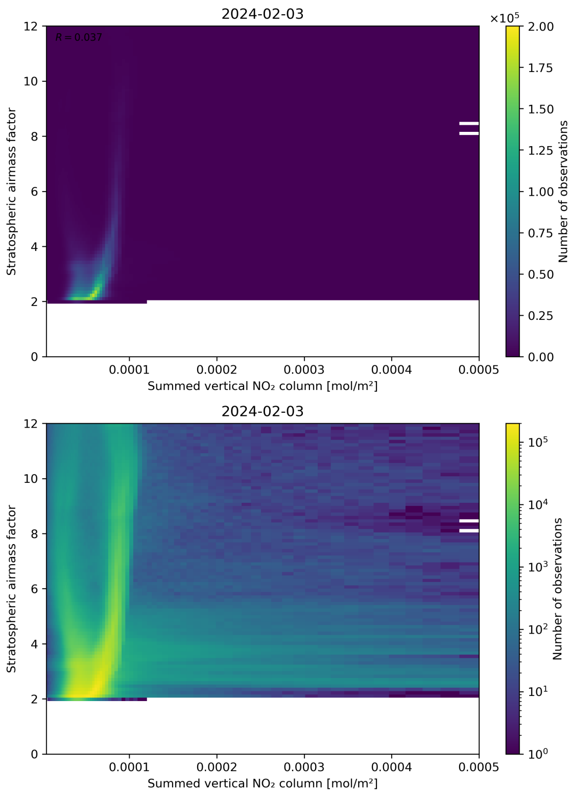
Figure 103: Scatter density plot of “Summed vertical NO 2 column” against “Stratospheric air mass factor” for 2024-02-02 to 2024-02-04.
