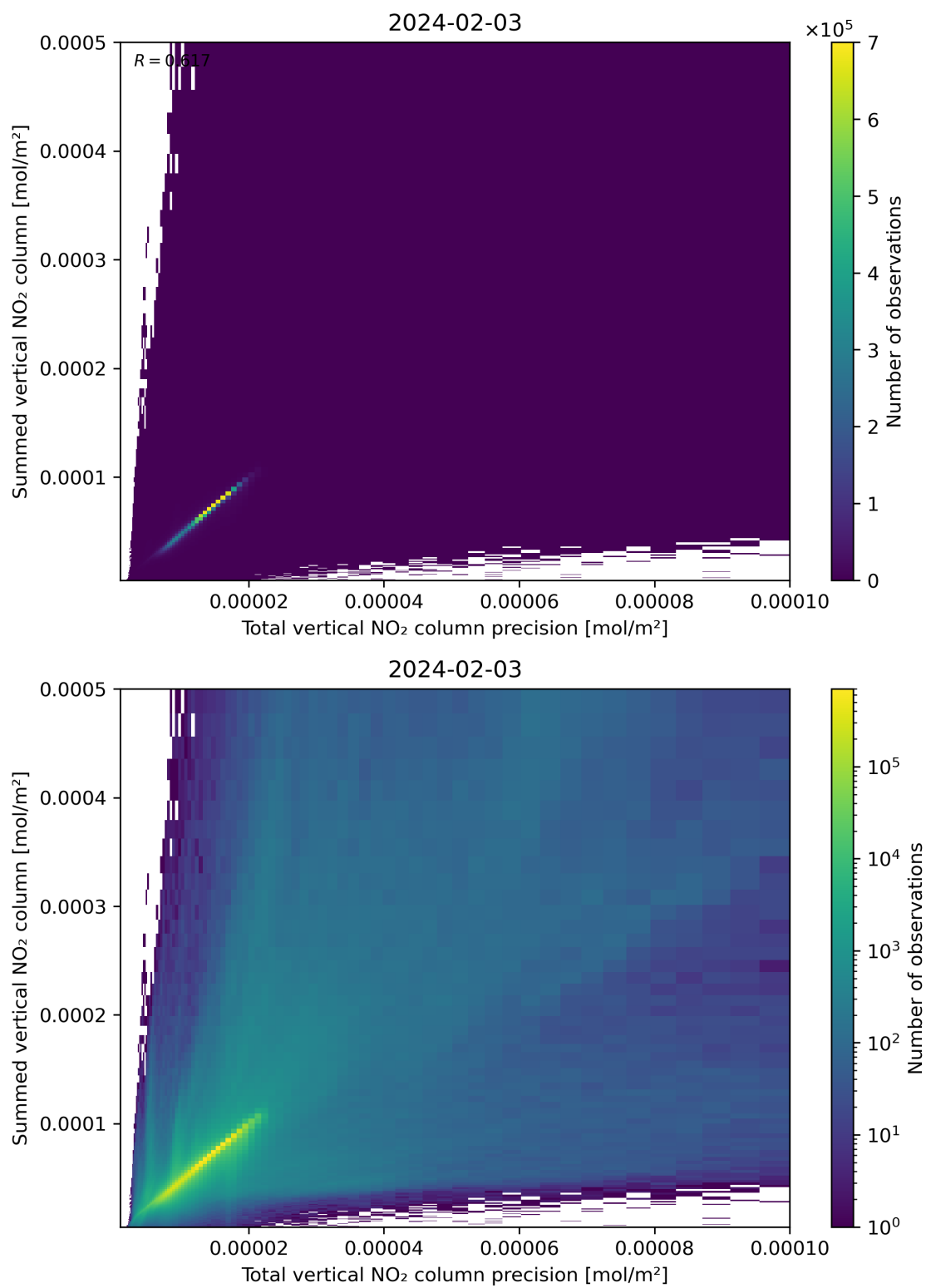
Figure 117: Scatter density plot of “Total vertical NO 2 column precision” against “Summed vertical NO 2 column” for 2024-02-02 to 2024-02-04.
