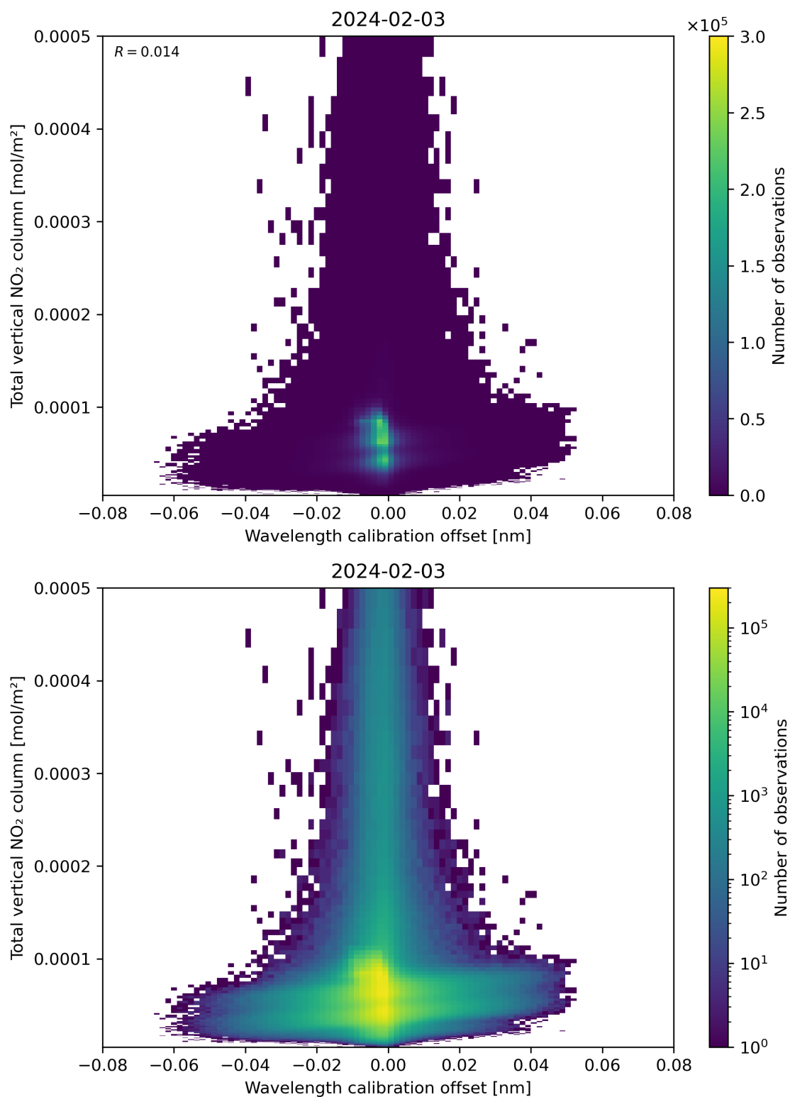
Figure 179: Scatter density plot of “Wavelength calibration offset” against “Total vertical NO 2 column” for 2024-02-02 to 2024-02-04.
