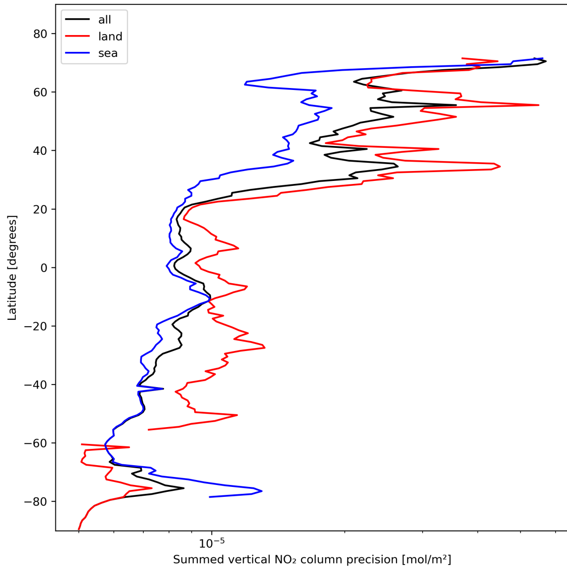
Figure 24: Zonal average of “Summed vertical NO 2 column precision” for 2024-02-02 to 2024-02-04.
