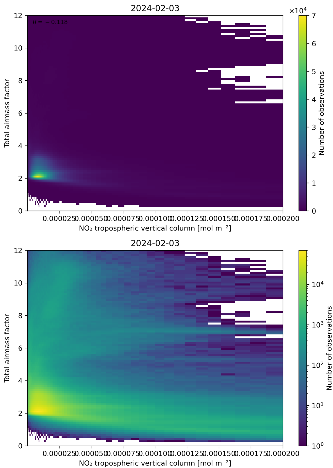
Figure 122: Scatter density plot of “NO 2 tropospheric vertical column” against “Total air mass factor” for 2024-02-02 to 2024-02-04.
