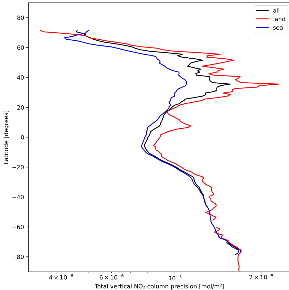
Figure 22: Zonal average of “Total vertical NO 2 column precision” for 2024-02-02 to 2024-02-04.
