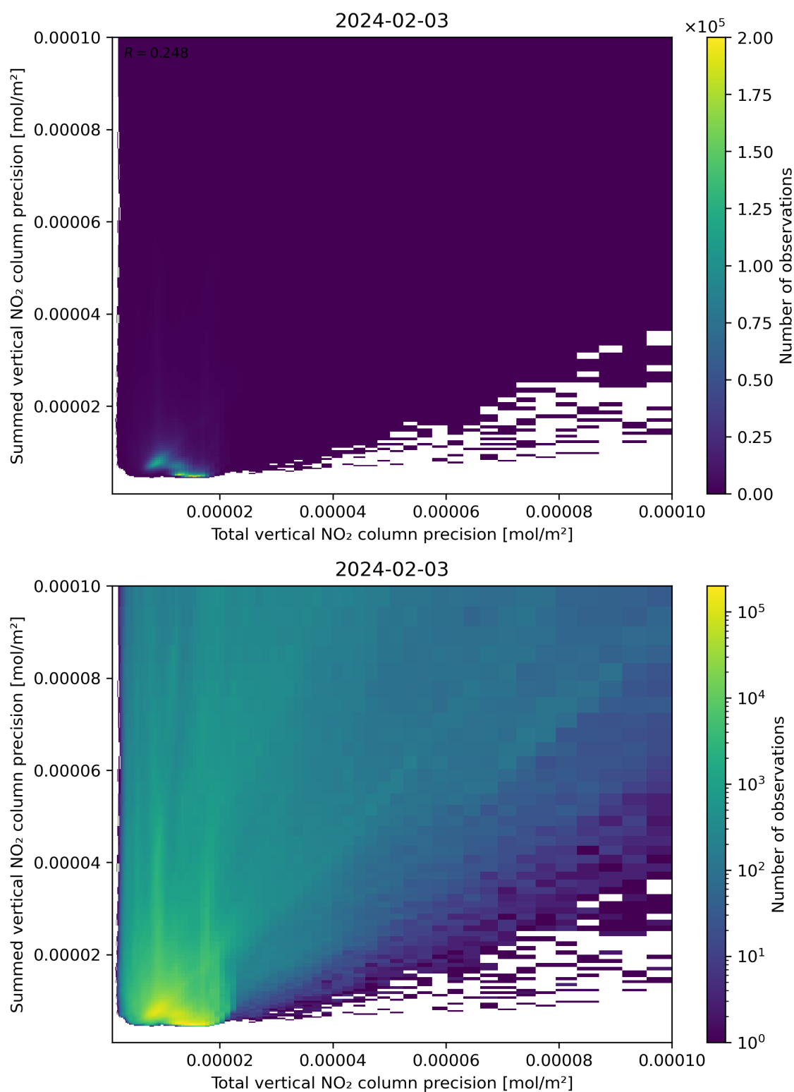
Figure 118: Scatter density plot of “Total vertical NO 2 column precision” against “Summed vertical NO 2 column precision” for 2024-02-02 to 2024-02-04.
