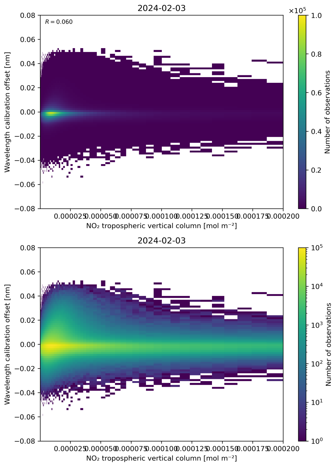
Figure 143: Scatter density plot of “NO 2 tropospheric vertical column” against “Wavelength calibration offset” for 2024-02-02 to 2024-02-04.
