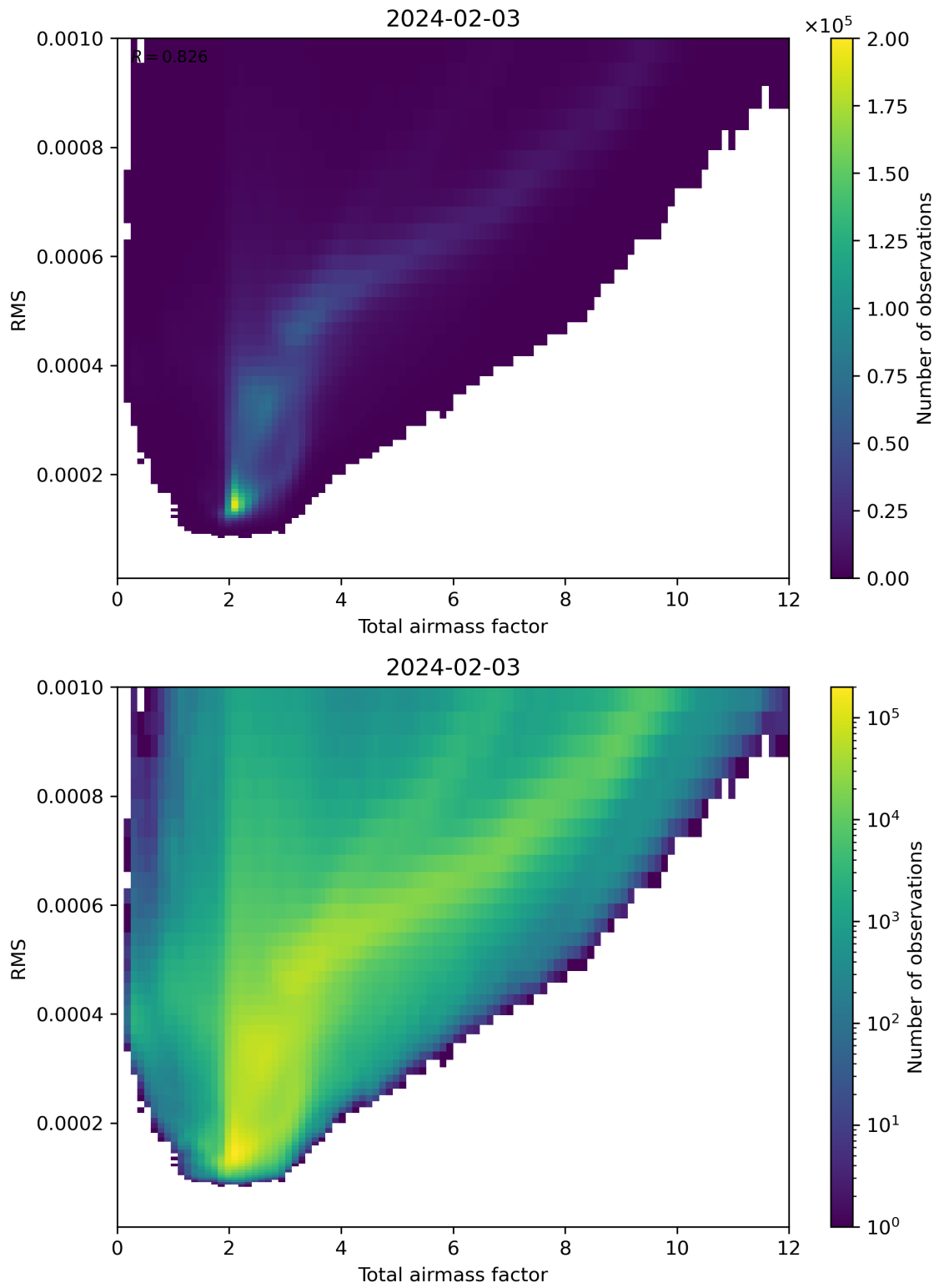
Figure 69: Scatter density plot of “Total airmass factor” against “RMS” for 2024-02-02 to 2024-02-04.
