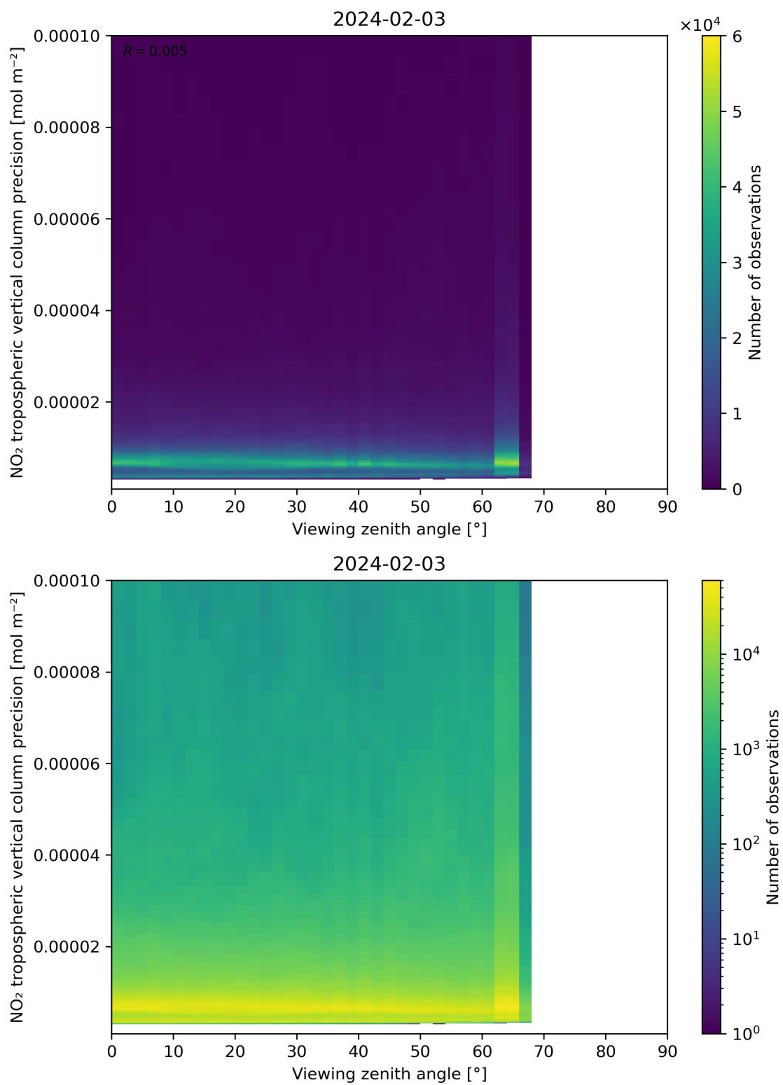
Figure 170: Scatter density plot of “Viewing zenith angle” against “NO 2 tropospheric vertical column precision” for 2024-02-02 to 2024-02-04.
