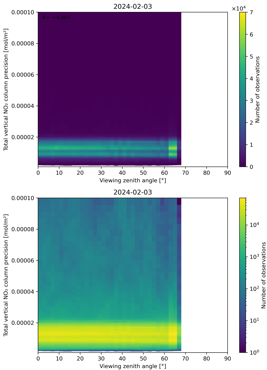
Figure 168: Scatter density plot of “Viewing zenith angle” against “Total vertical NO 2 column precision” for 2024-02-02 to 2024-02-04.
