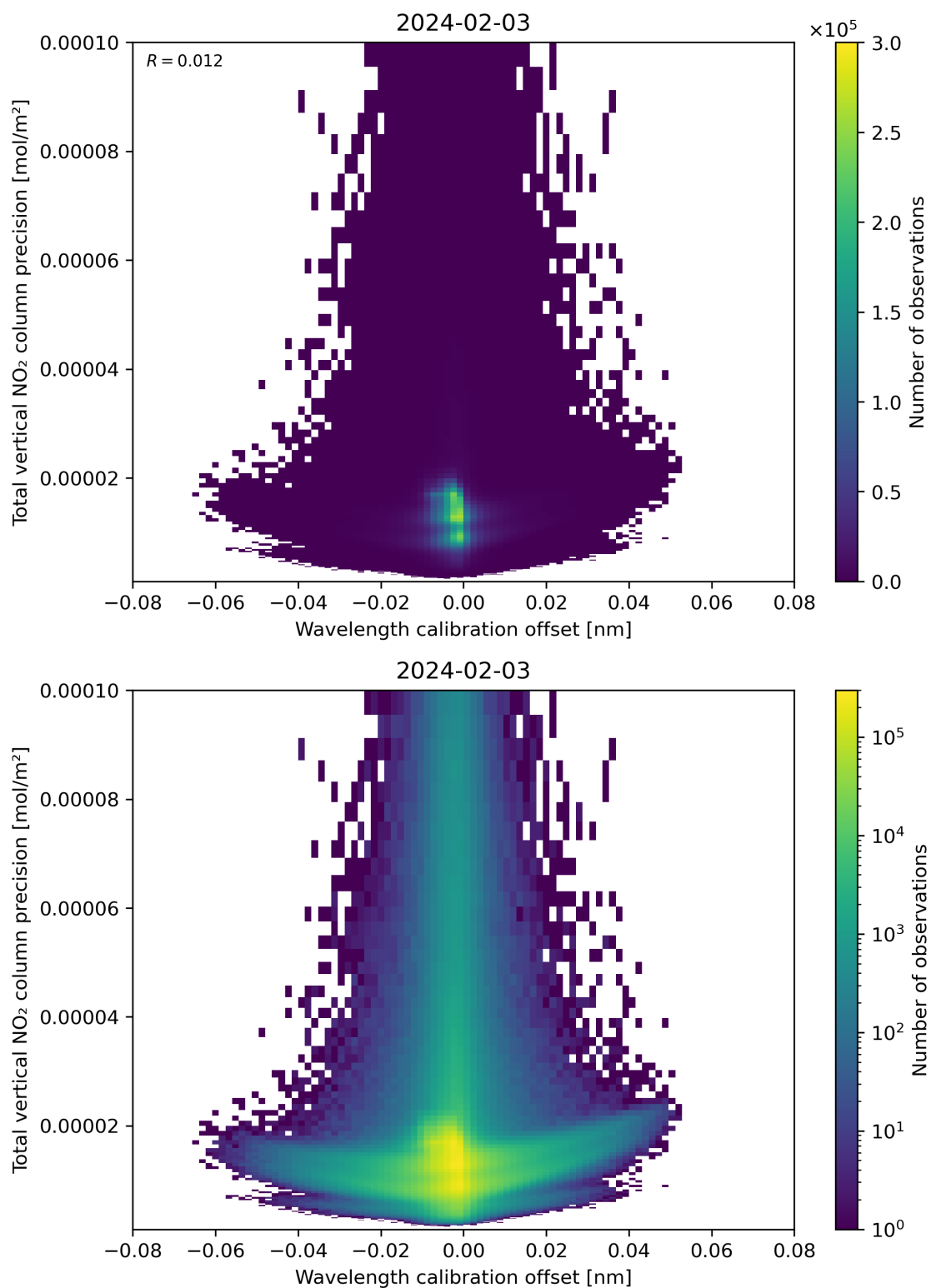
Figure 180: Scatter density plot of “Wavelength calibration offset” against “Total vertical NO 2 column precision” for 2024-02-02 to 2024-02-04.
