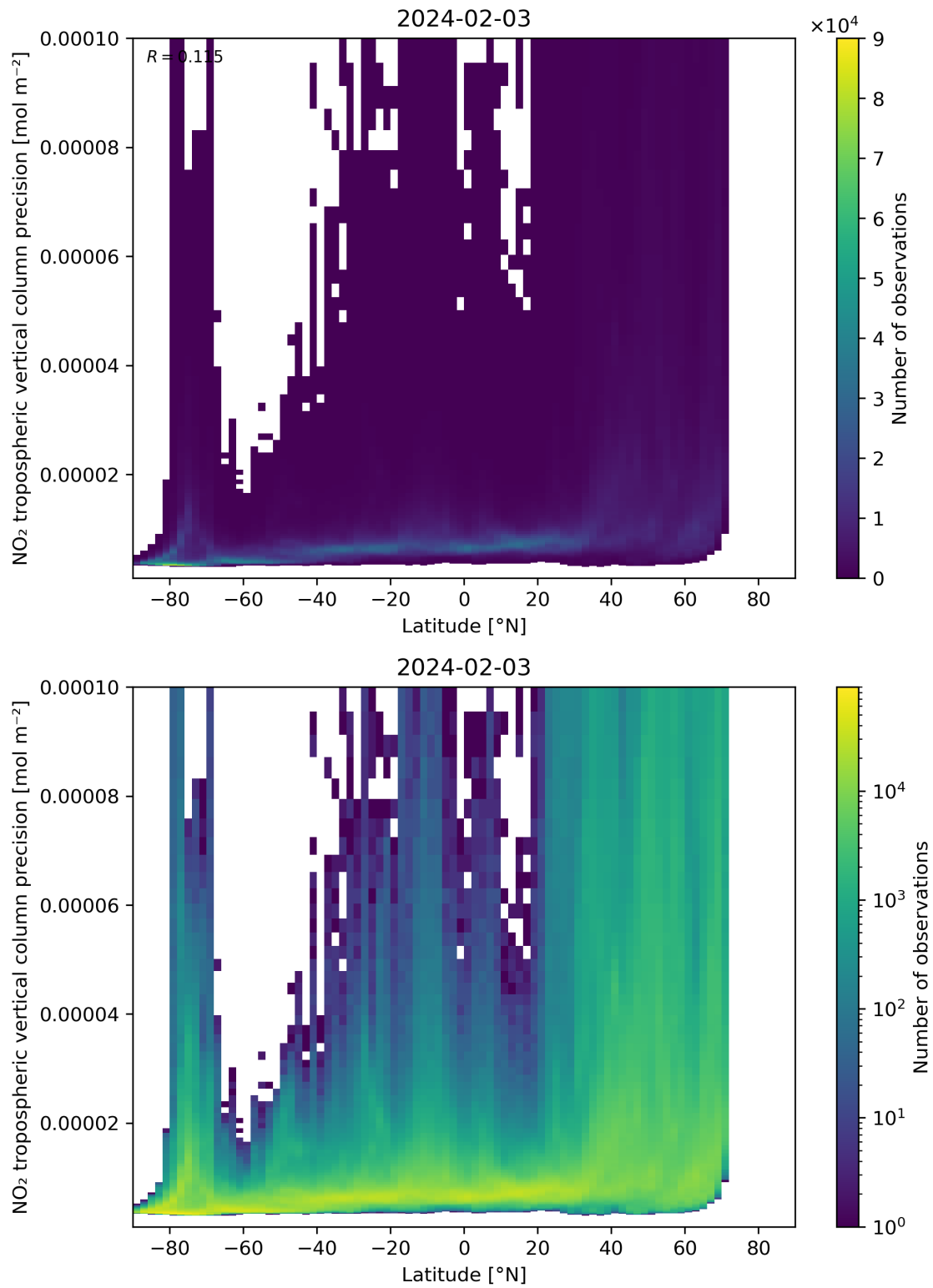
Figure 93: Scatter density plot of “Latitude” against “NO 2 tropospheric vertical column precision” for 2024-02-02 to 2024-02-04.
