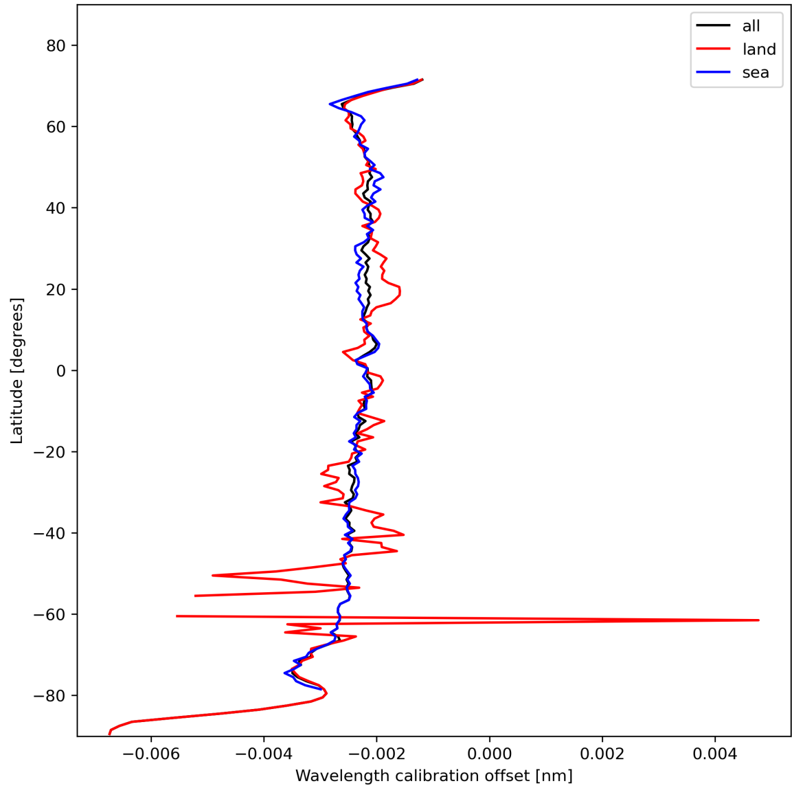
Figure 18: Zonal average of “Wavelength calibration offset” for 2024-02-02 to 2024-02-04.
