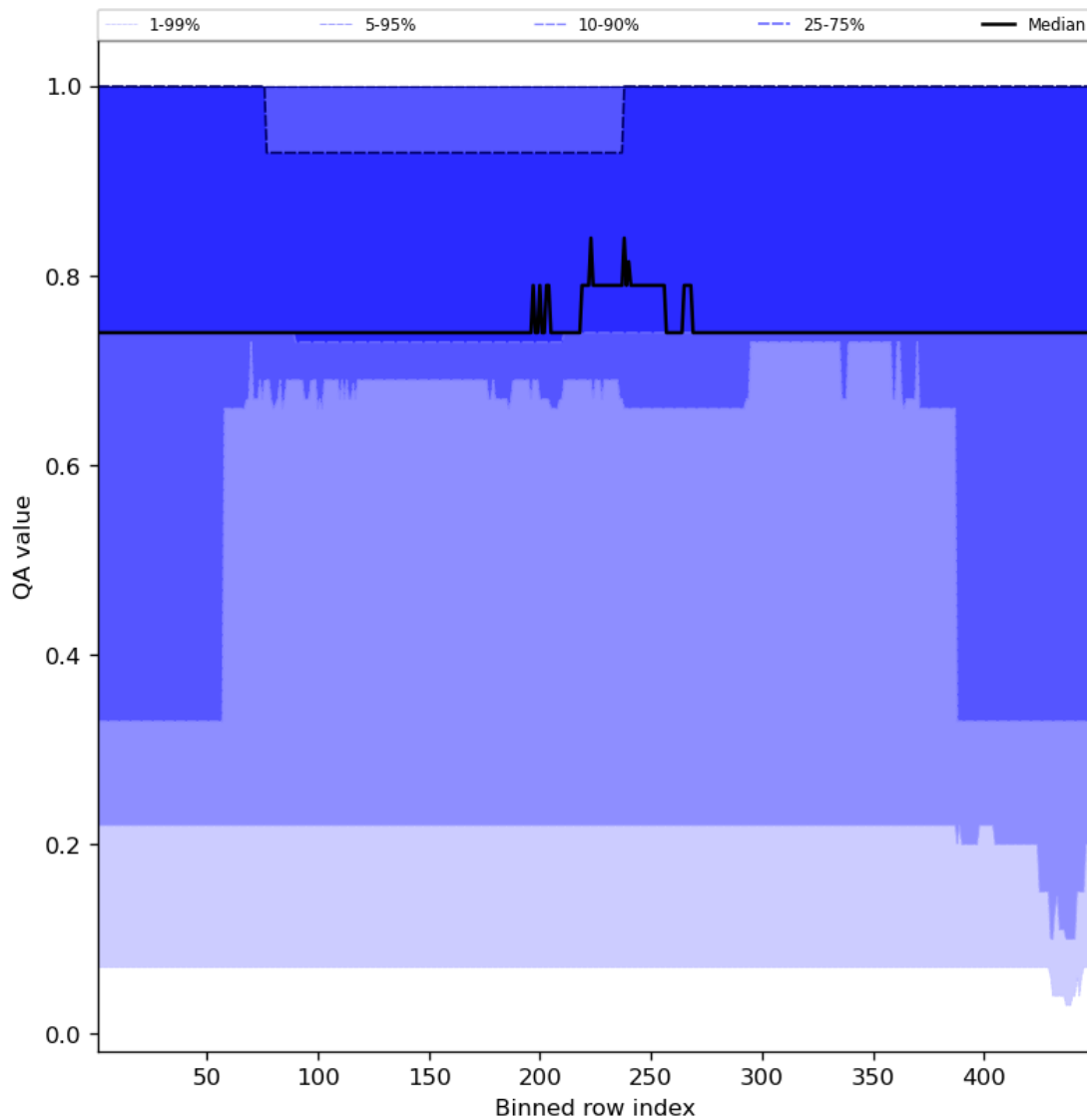
Figure 45: Along track statistics of “QA value” for 2024-02-02 to 2024-02-04
