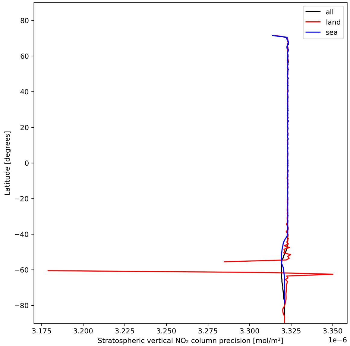
Figure 20: Zonal average of “Stratospheric vertical NO 2 column precision” for 2024-02-02 to 2024-02-04.
