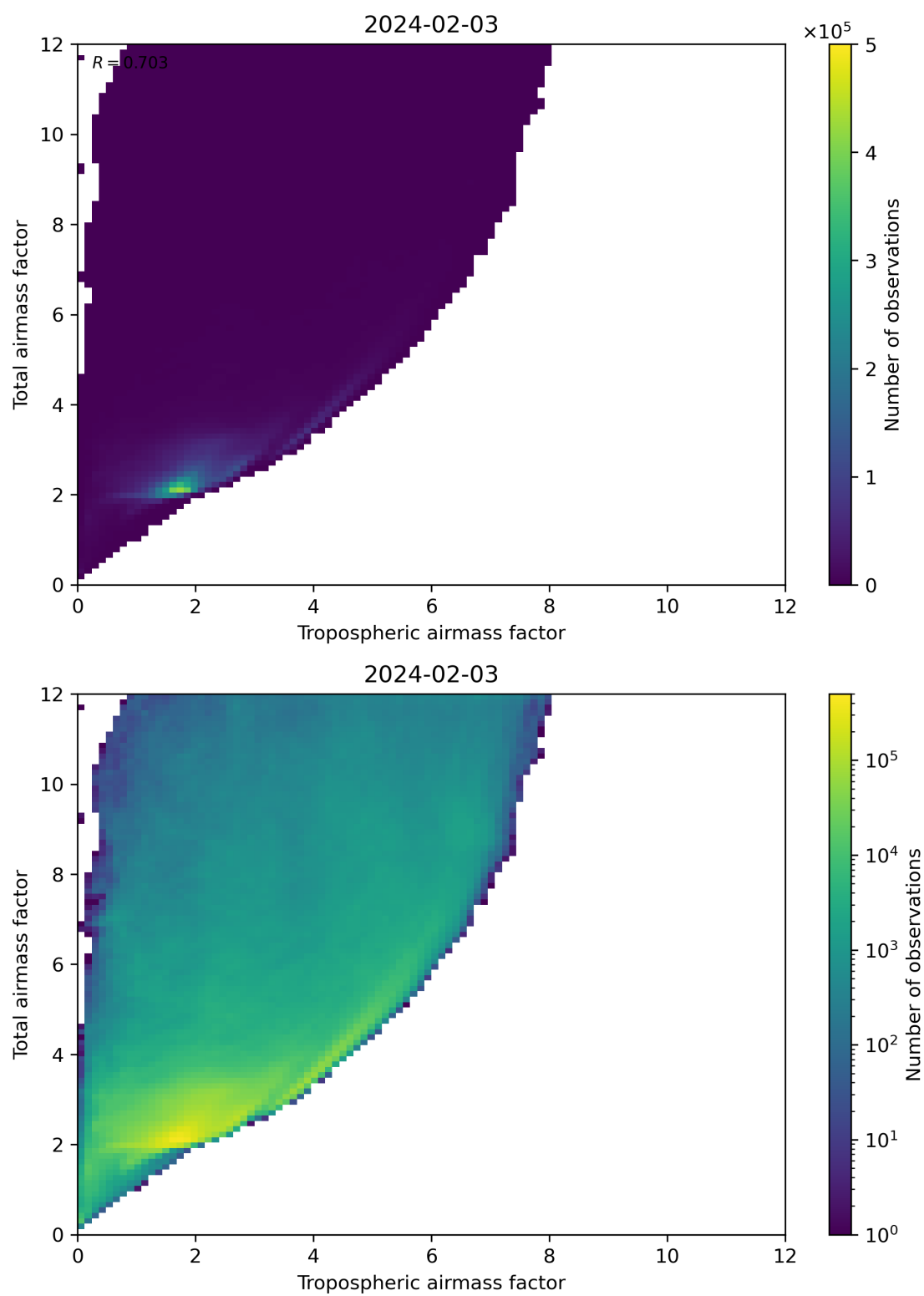
Figure 72: Scatter density plot of “Tropospheric airmass factor” against “Total airmass factor” for 2024-02-02 to 2024-02-04.
