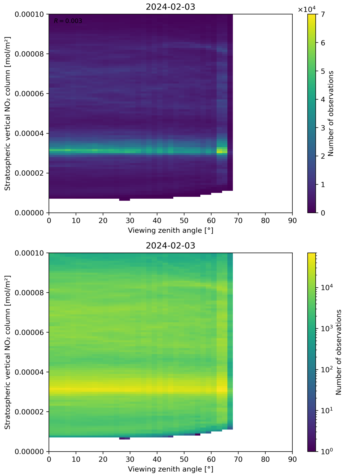
Figure 164: Scatter density plot of “Viewing zenith angle” against “Stratospheric vertical NO 2 column” for 2024-02-02 to 2024-02-04.
