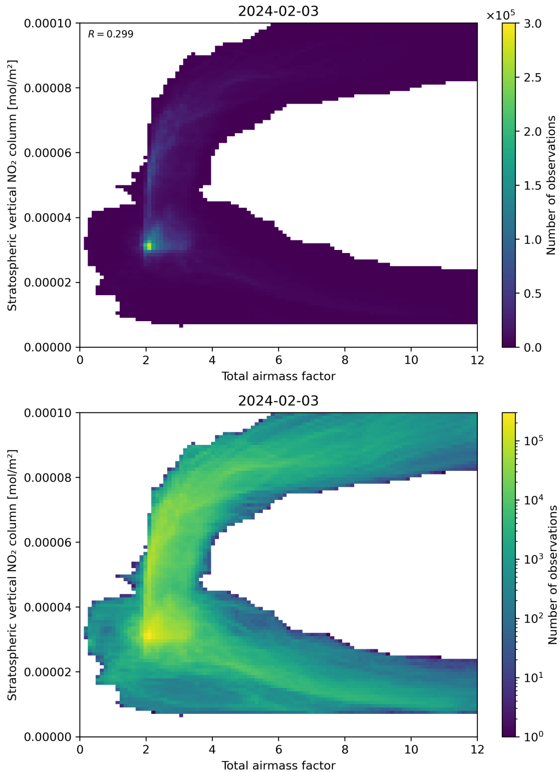
Figure 64: Scatter density plot of “Total airmass factor” against “Stratospheric vertical \text{NO}_2 column” for 2024-02-02 to 2024-02-04.
