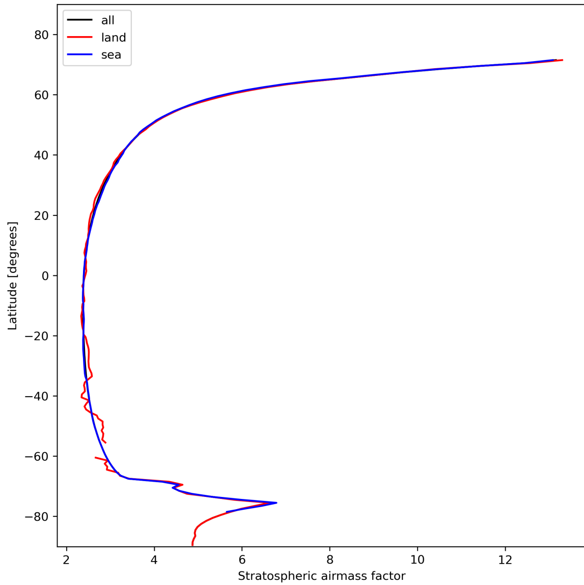
Figure 27: Zonal average of “Stratospheric air mass factor” for 2024-02-02 to 2024-02-04.
