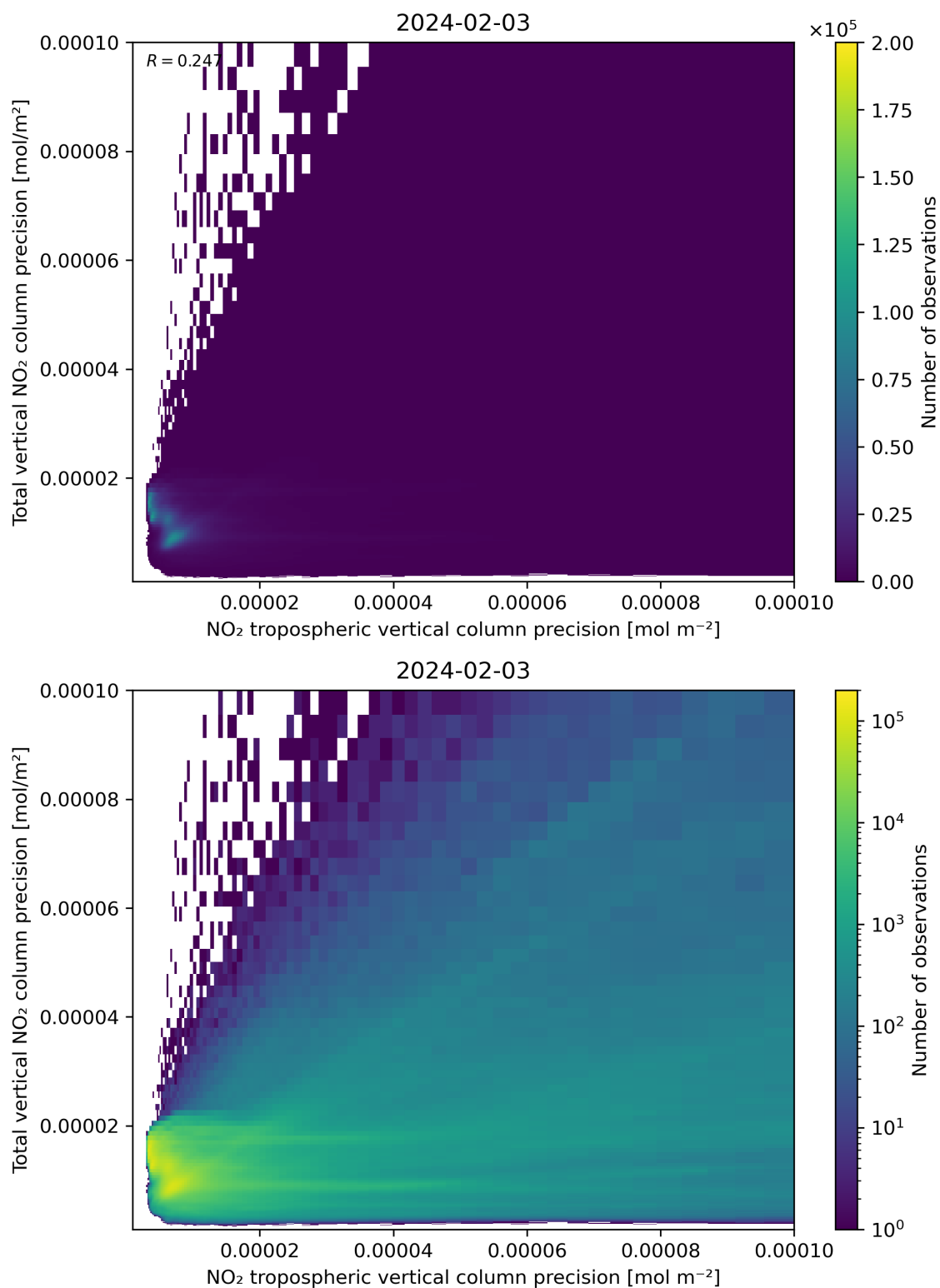
Figure 139: Scatter density plot of “NO 2 tropospheric vertical column precision” against “Total vertical NO 2 column precision” for 2024-02-02 to 2024-02-04.
