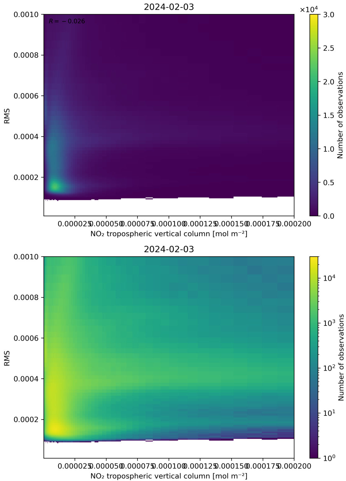
Figure 142: Scatter density plot of “NO 2 tropospheric vertical column” against “RMS” for 2024-02-02 to 2024-02-04.
