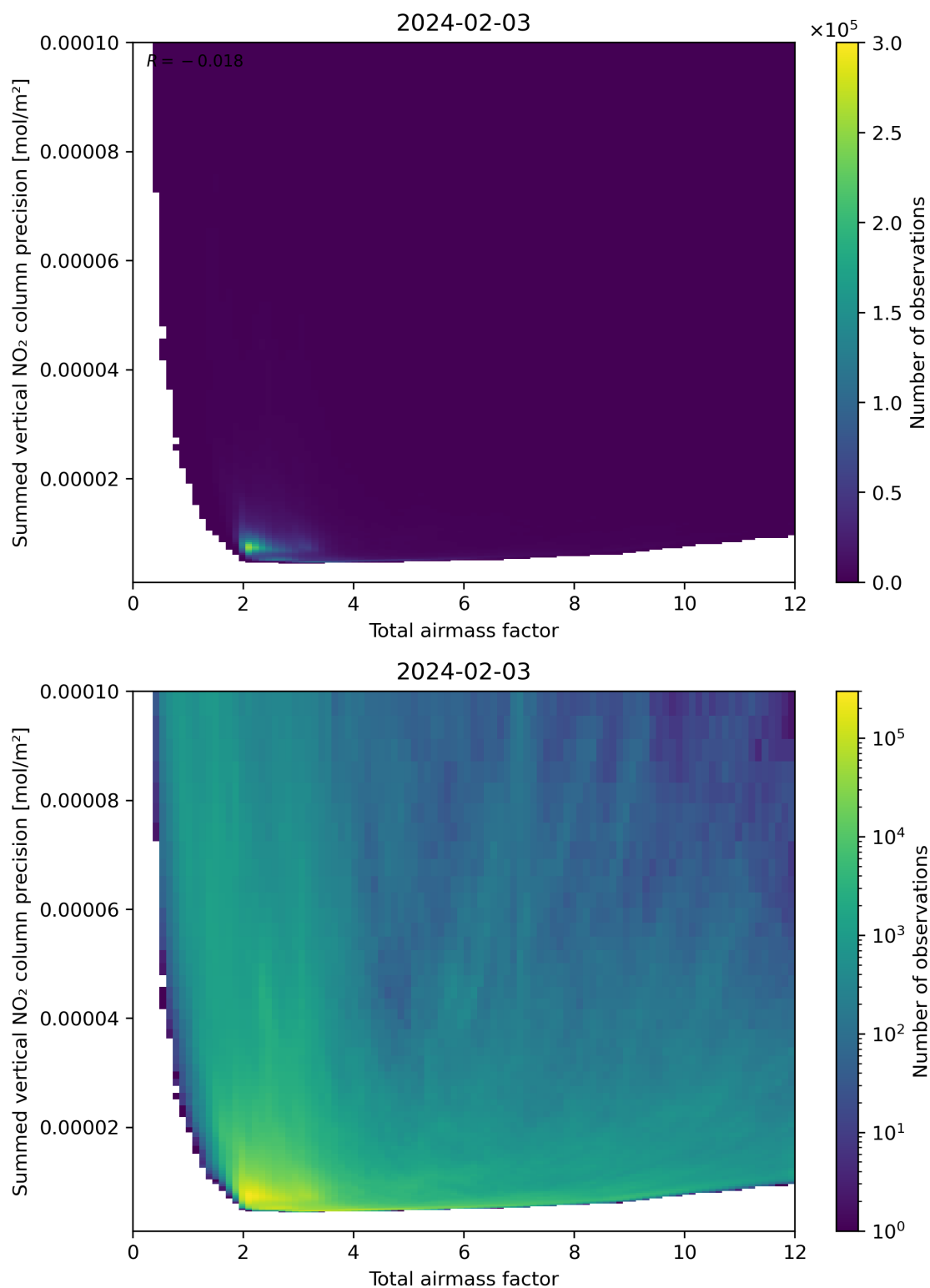
Figure 66: Scatter density plot of “Total airmass factor” against “Summed vertical NO 2 column precision” for 2024-02-02 to 2024-02-04.
