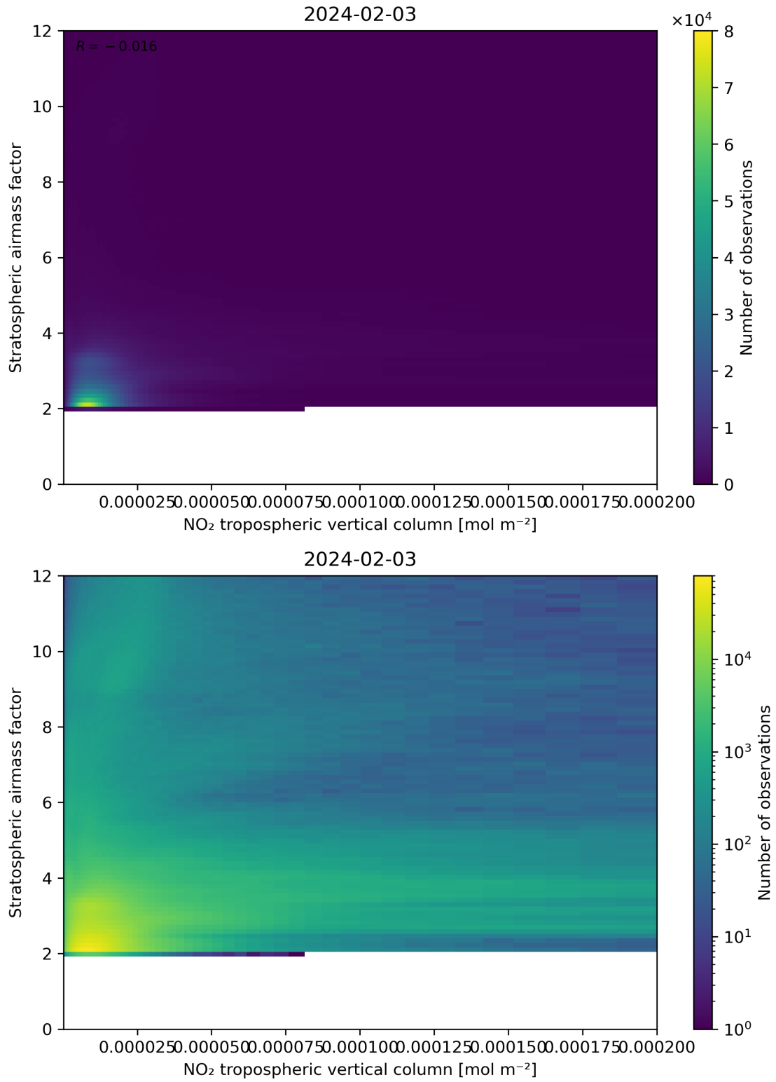
Figure 121: Scatter density plot of “NO 2 tropospheric vertical column” against “Stratospheric airmass factor” for 2024-02-02 to 2024-02-04.
