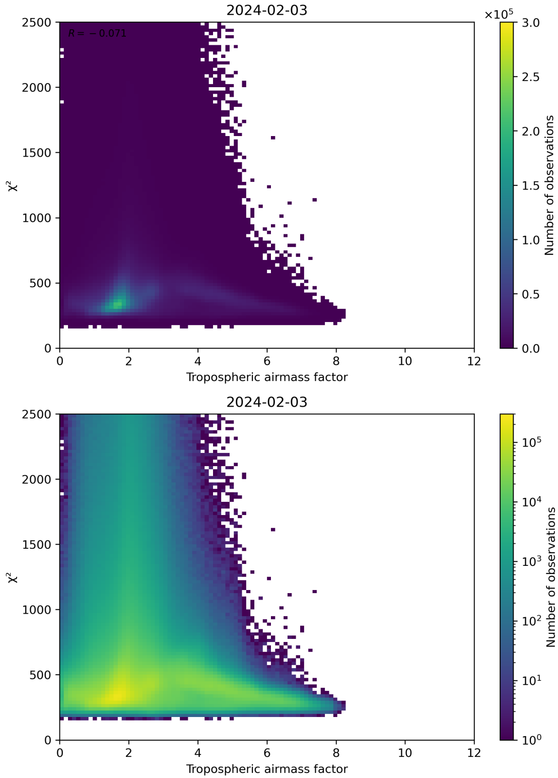
Figure 73: Scatter density plot of “Tropospheric airmass factor” against “ \chi^2 ” for 2024-02-02 to 2024-02-04.
