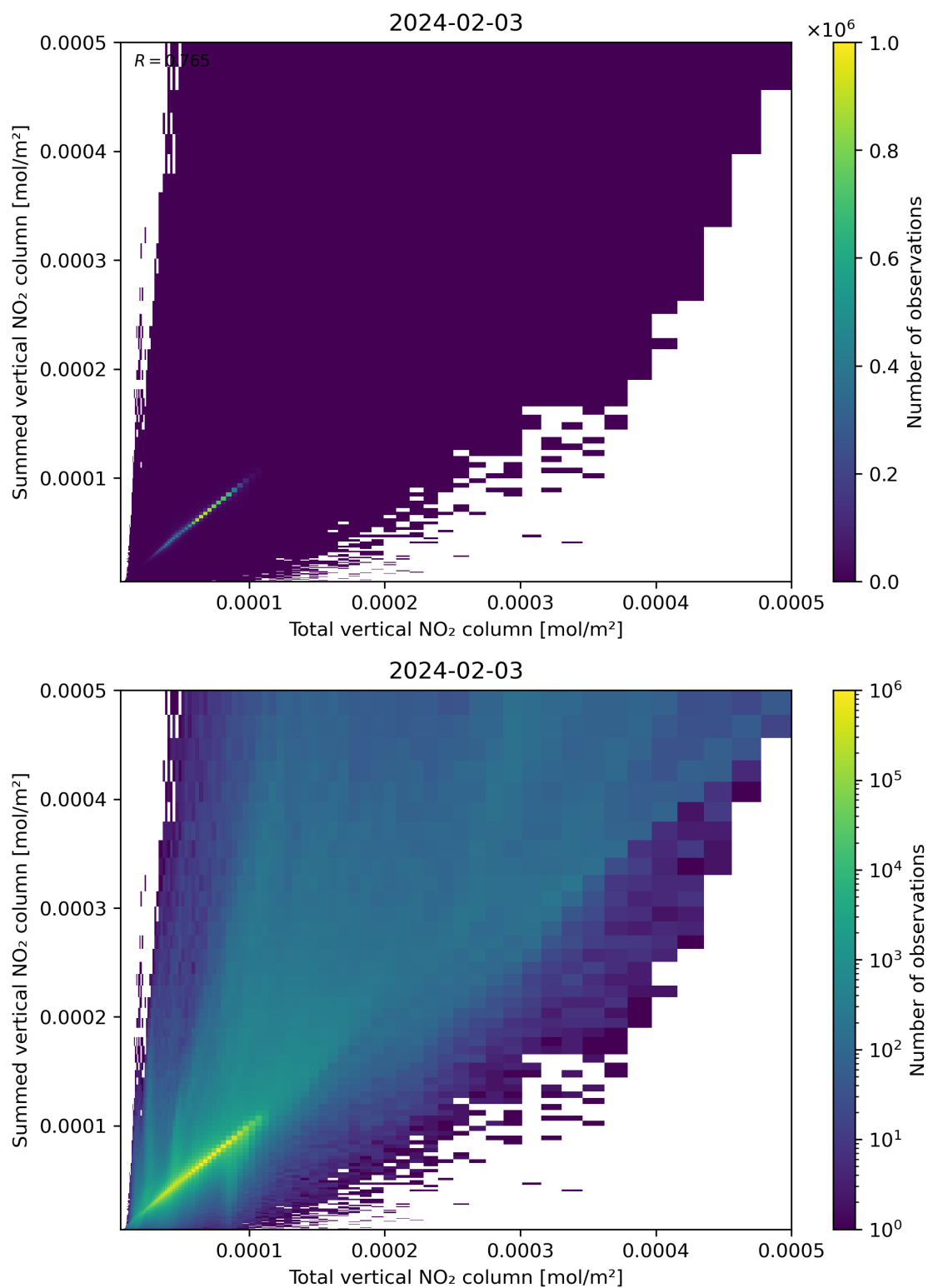
Figure 112: Scatter density plot of “Total vertical NO 2 column” against “Summed vertical NO 2 column” for 2024-02-02 to 2024-02-04.
