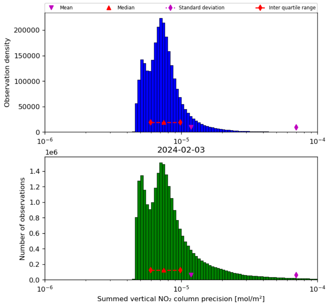
Figure 41: Histogram of "Summed vertical NO 2 column precision" for 2024-02-02 to 2024-02-04
