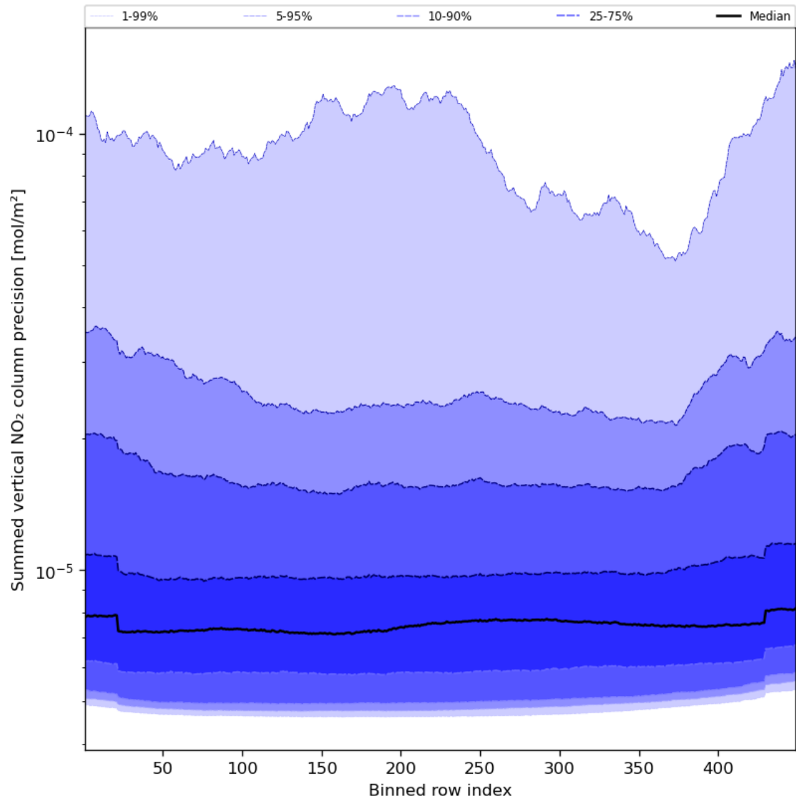
Figure 58: Along track statistics of “Summed vertical NO 2 column precision” for 2024-02-02 to 2024-02-04
