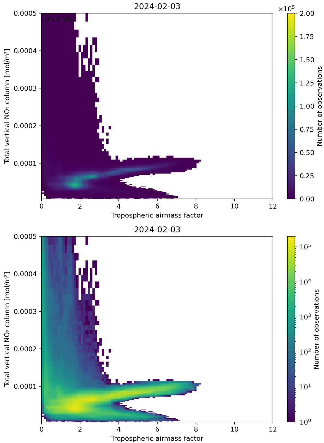
Figure 77: Scatter density plot of “Tropospheric airmass factor” against “Total vertical NO 2 column” for 2024-02-02 to 2024-02-04.
