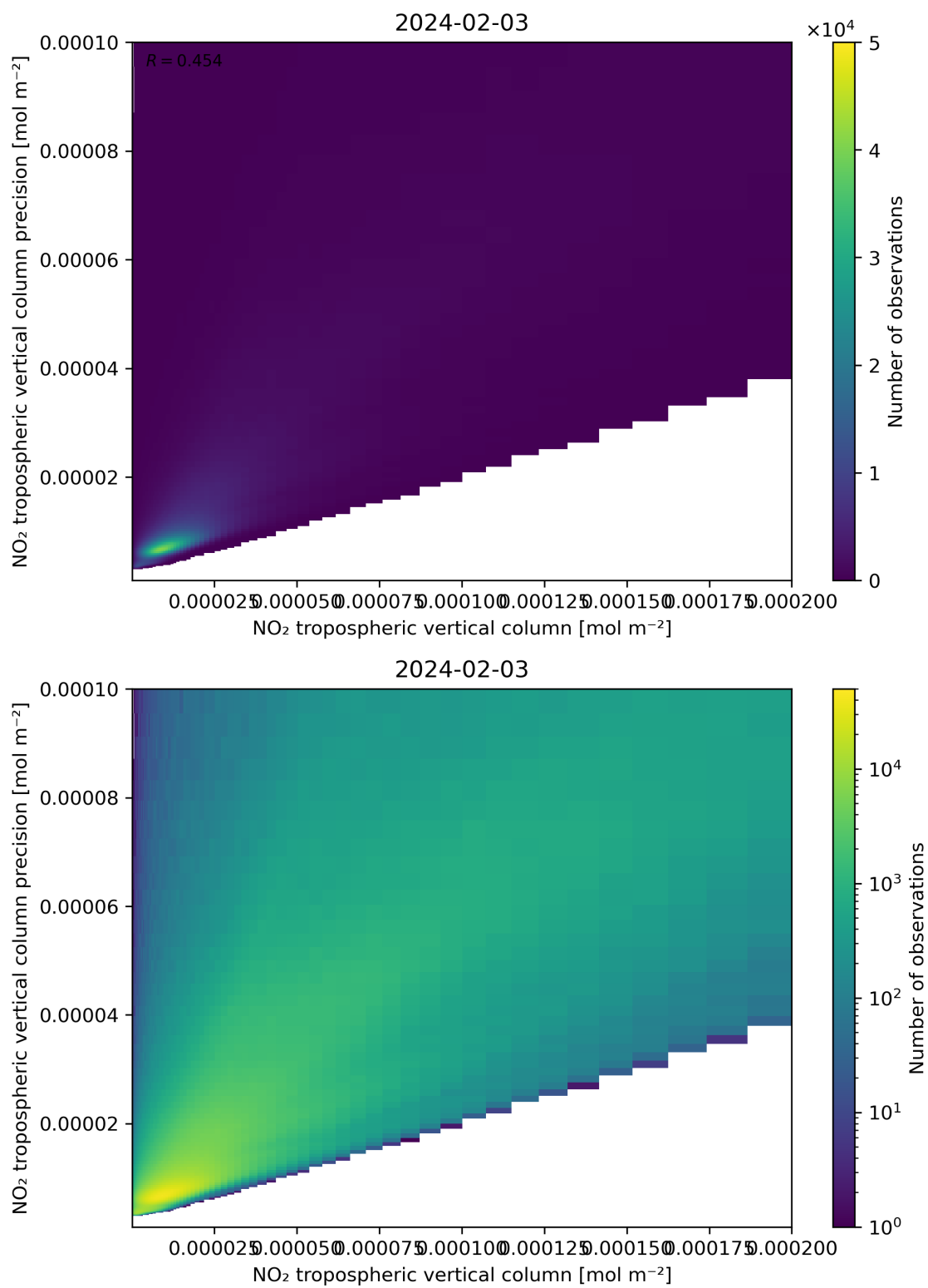
Figure 130: Scatter density plot of “NO 2 tropospheric vertical column” against “NO 2 tropospheric vertical column precision” for 2024-02-02 to 2024-02-04.
