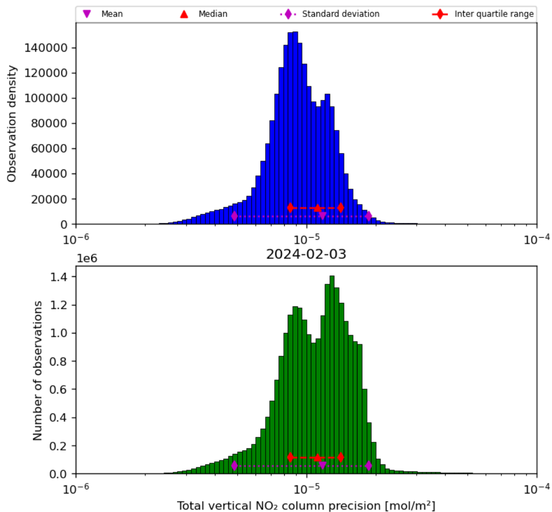
Figure 39: Histogram of “Total vertical NO 2 column precision” for 2024-02-02 to 2024-02-04
