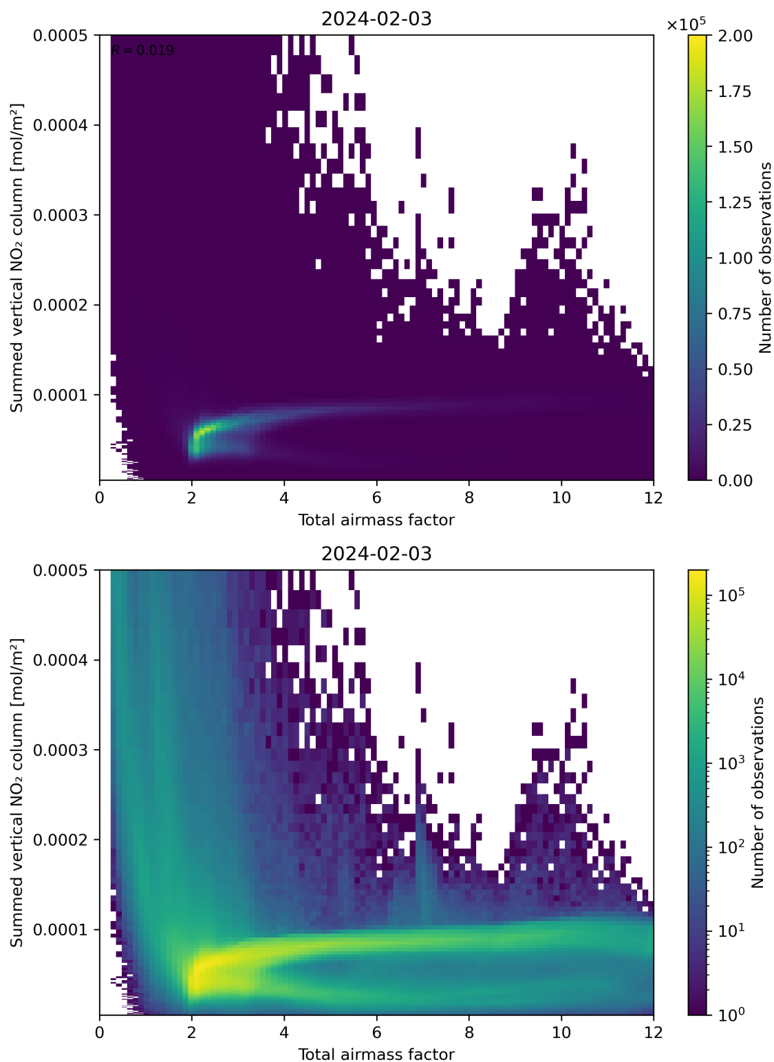
Figure 65: Scatter density plot of “Total airmass factor” against “Summed vertical NO 2 column” for 2024-02-02 to 2024-02-04.
