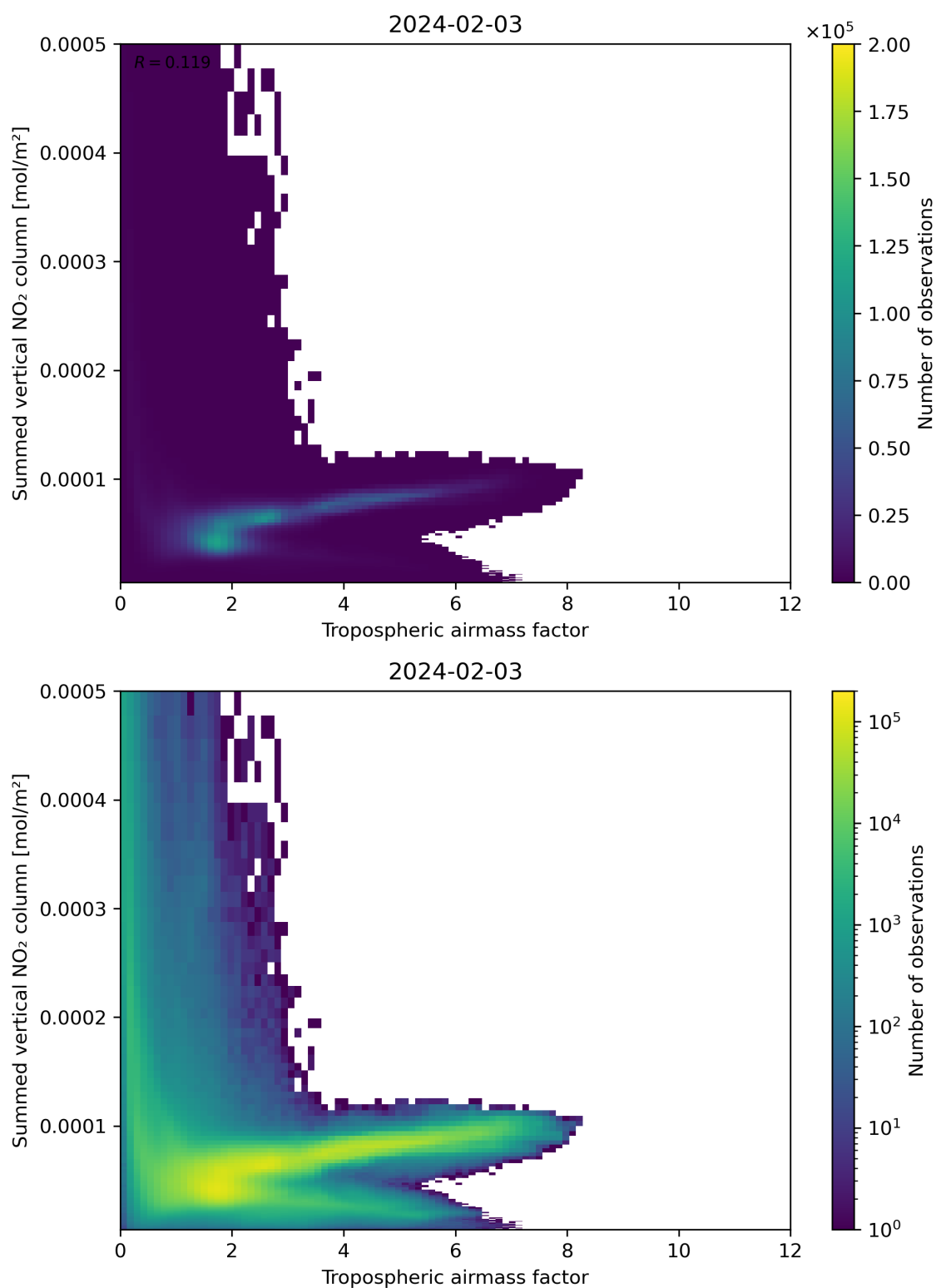
Figure 75: Scatter density plot of “Tropospheric airmass factor” against “Summed vertical NO 2 column” for 2024-02-02 to 2024-02-04.
