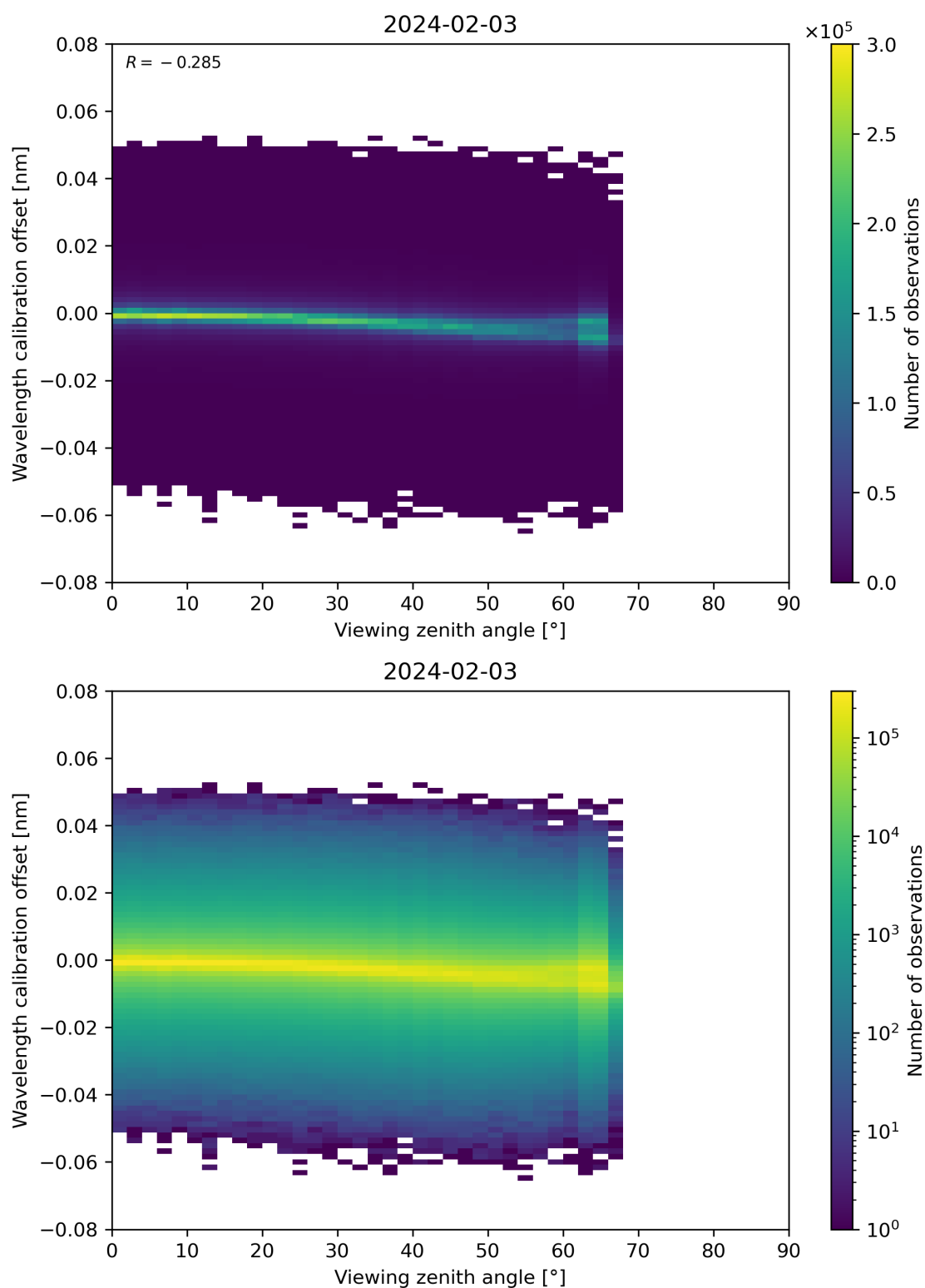
Figure 173: Scatter density plot of “Viewing zenith angle” against “Wavelength calibration offset” for 2024-02-02 to 2024-02-04.
