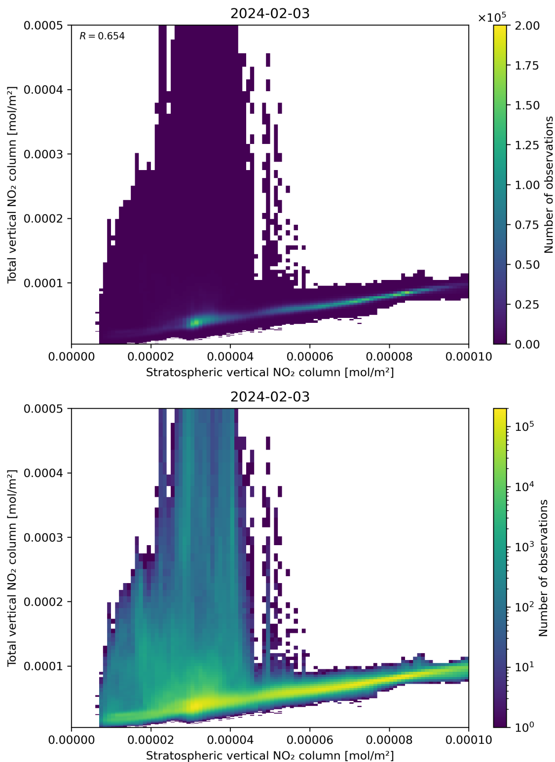
Figure 100: Scatter density plot of “Stratospheric vertical NO 2 column” against “Total vertical NO 2 column” for 2024-02-02 to 2024-02-04.
