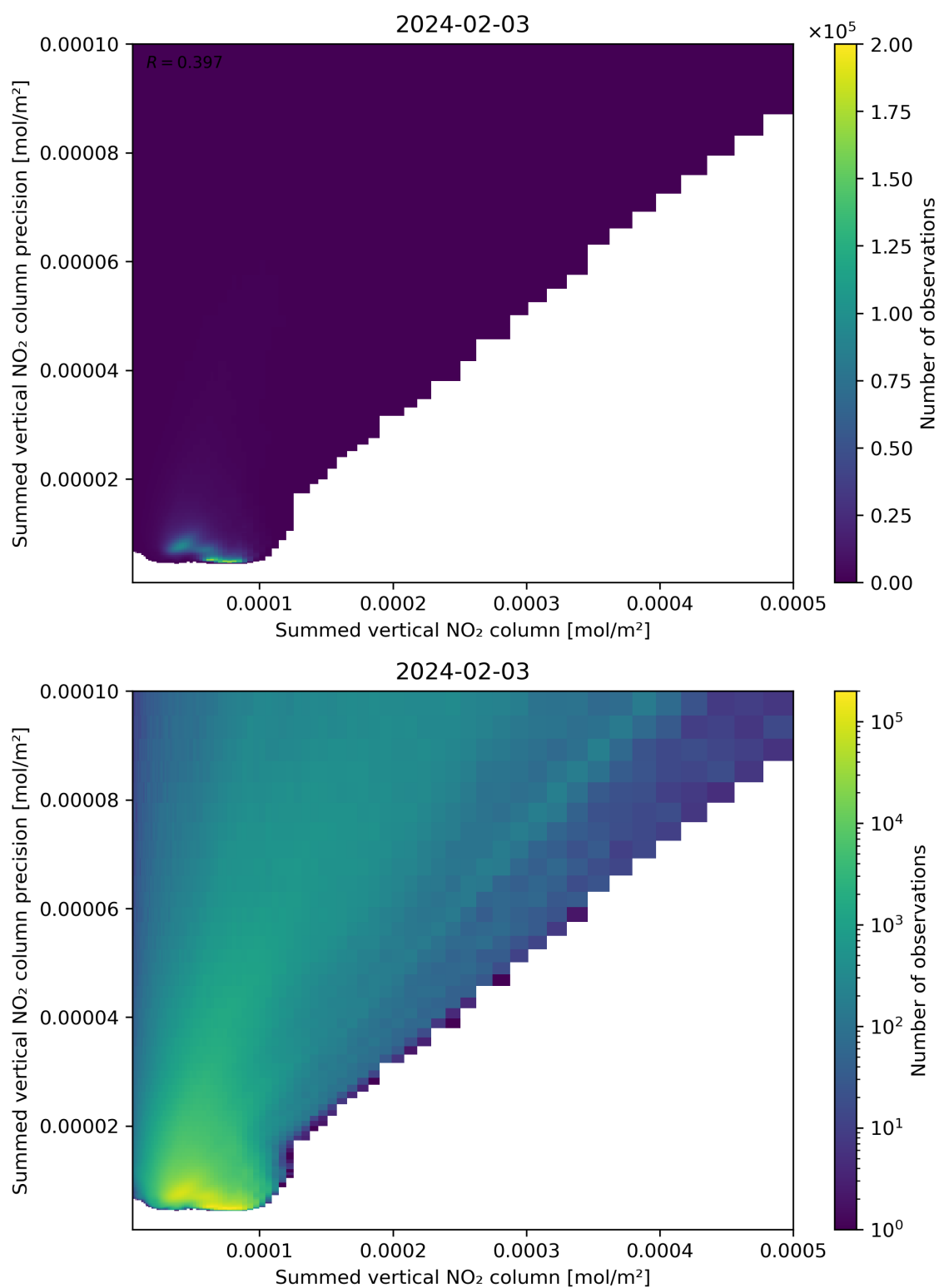
Figure 105: Scatter density plot of “Summed vertical NO 2 column” against “Summed vertical NO 2 column precision” for 2024-02-02 to 2024-02-04.
