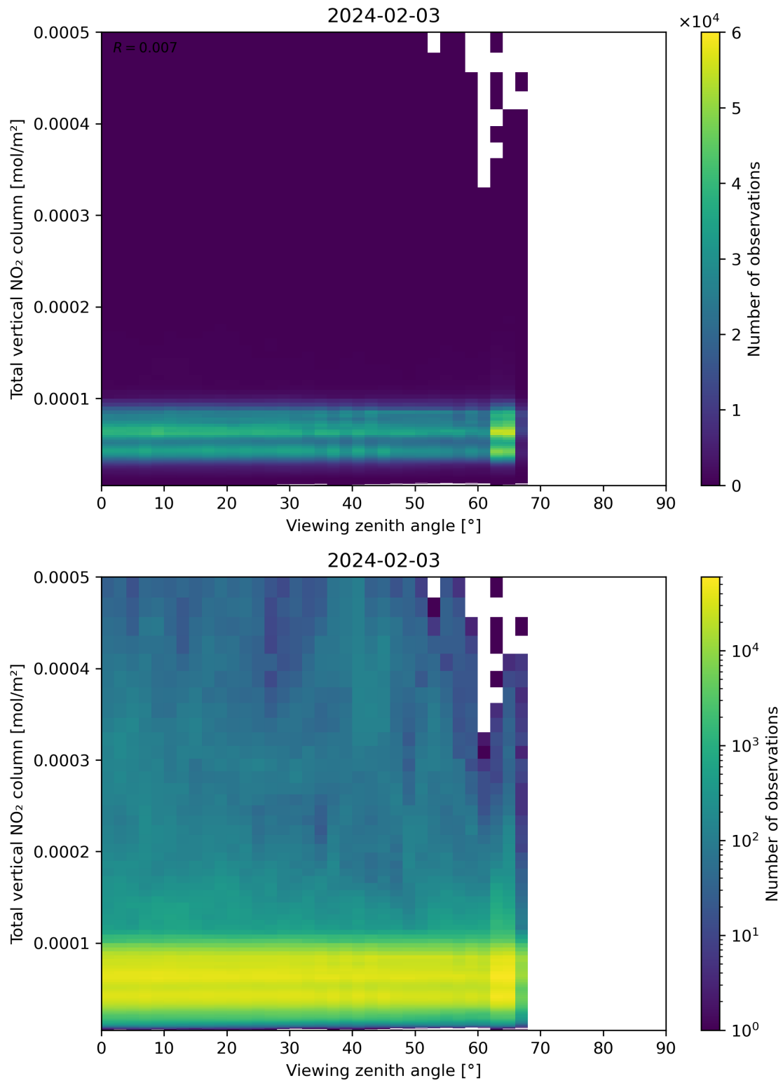
Figure 167: Scatter density plot of “Viewing zenith angle” against “Total vertical NO 2 column” for 2024-02-02 to 2024-02-04.
