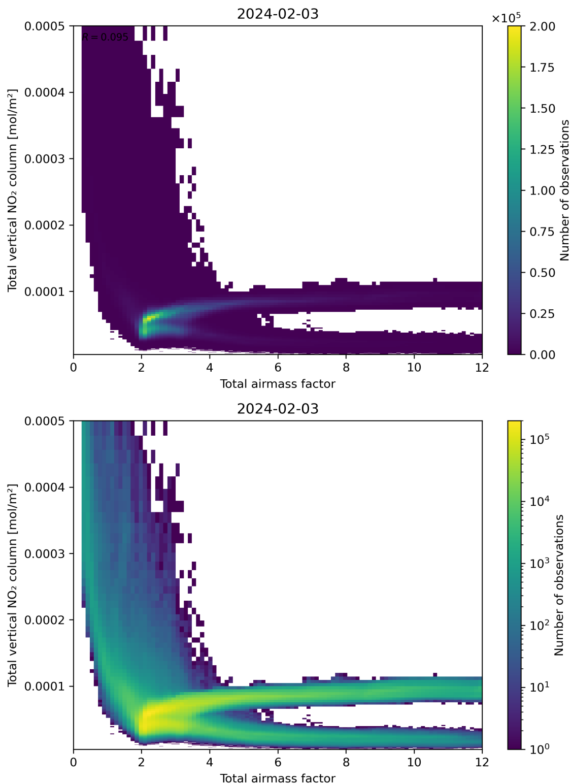
Figure 67: Scatter density plot of “Total airmass factor” against “Total vertical NO 2 column” for 2024-02-02 to 2024-02-04.
