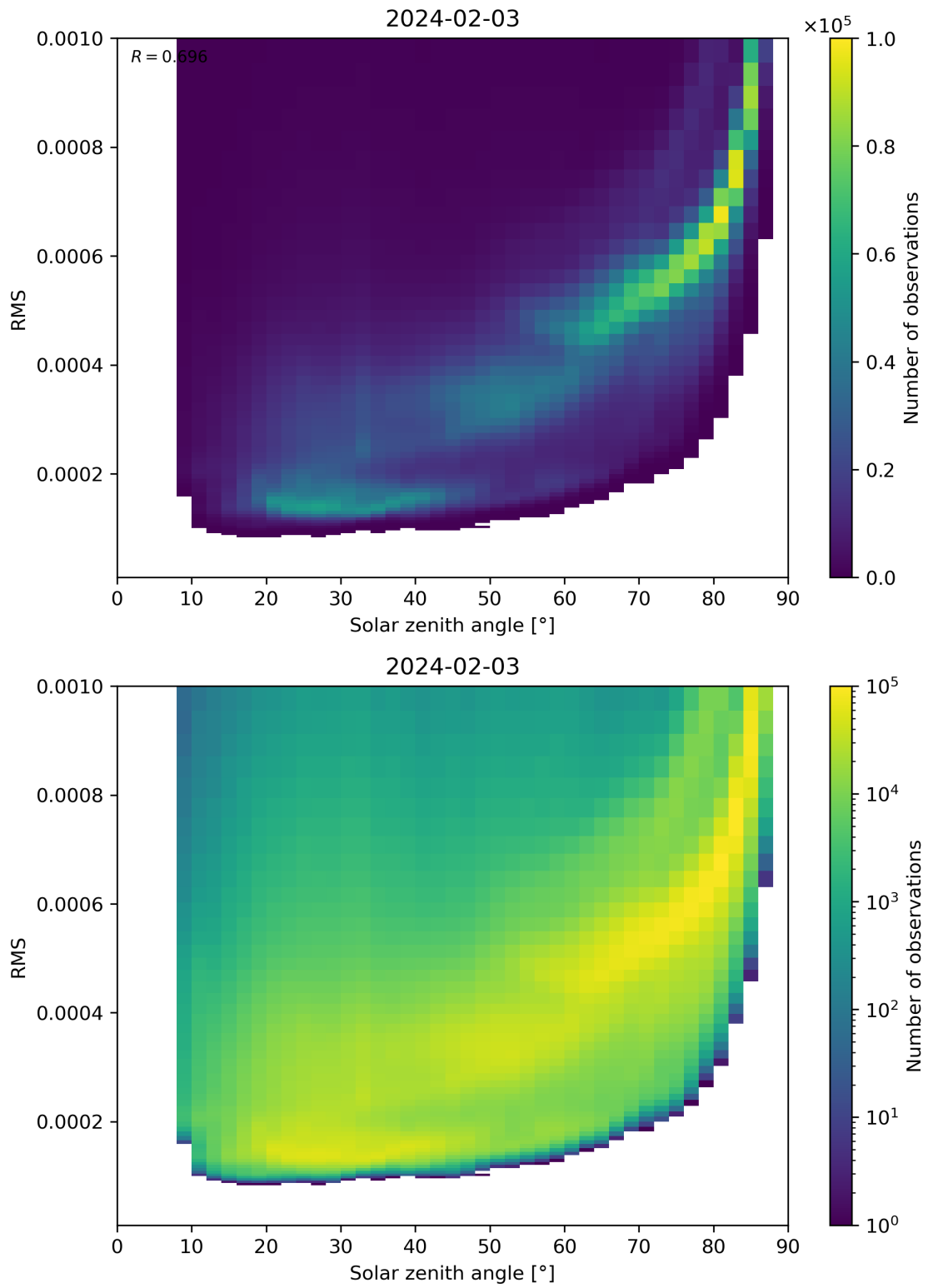
Figure 157: Scatter density plot of “Solar zenith angle” against “RMS” for 2024-02-02 to 2024-02-04.
