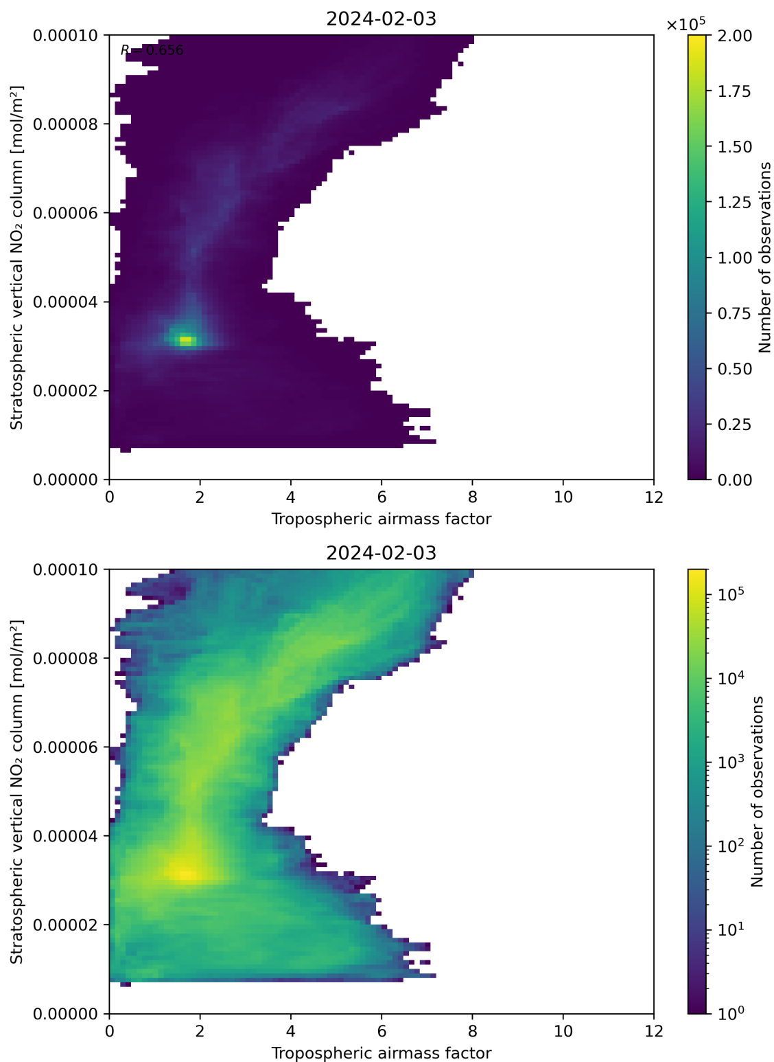
Figure 74: Scatter density plot of “Tropospheric air mass factor” against “Stratospheric vertical NO 2 column” for 2024-02-02 to 2024-02-04.
