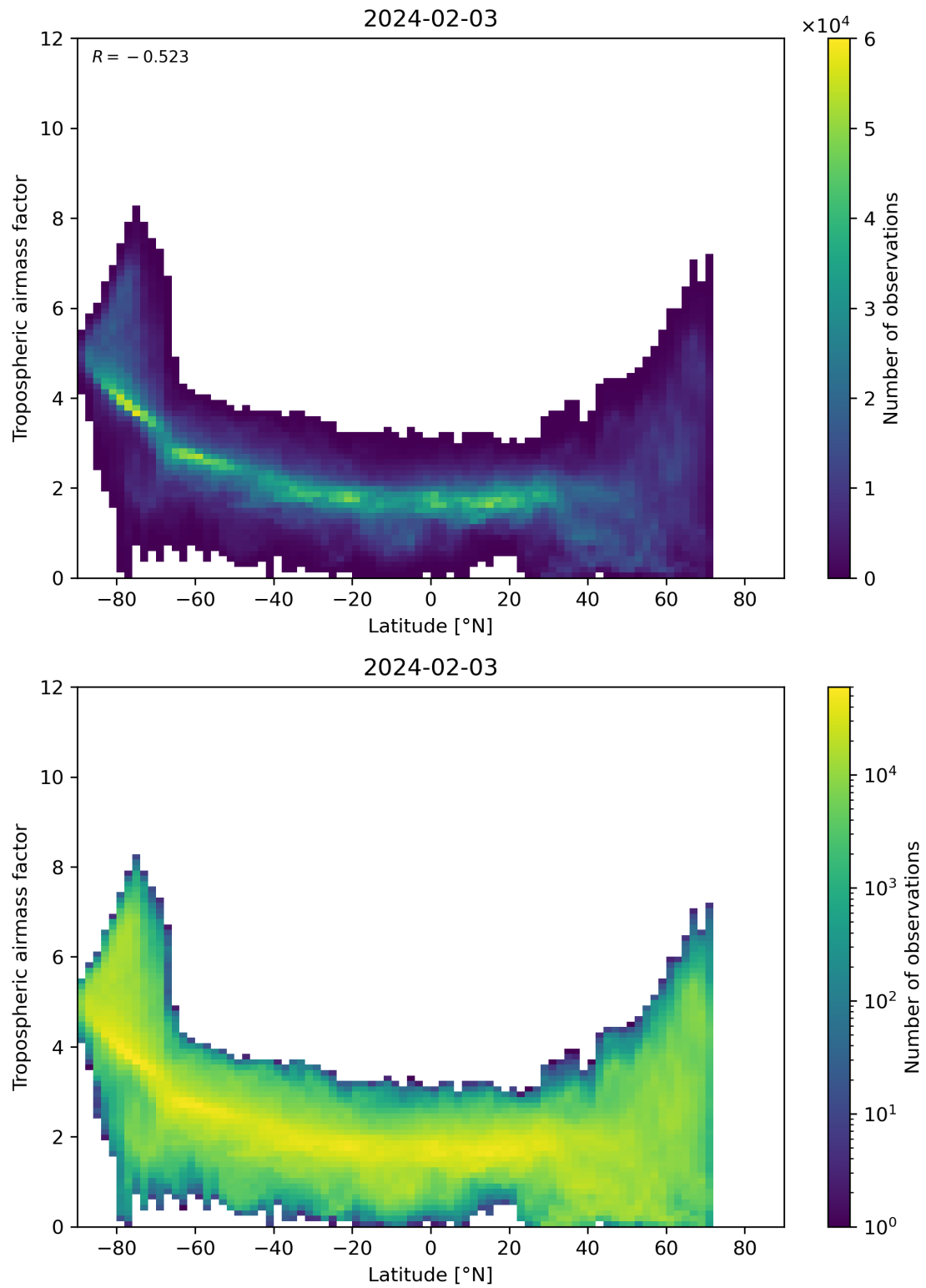
Figure 85: Scatter density plot of “Latitude” against “Tropospheric airmass factor” for 2024-02-02 to 2024-02-04.
