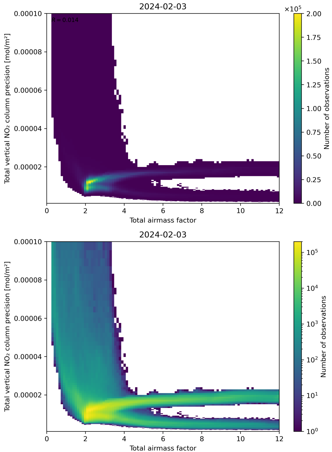
Figure 68: Scatter density plot of “Total airmass factor” against “Total vertical NO 2 column precision” for 2024-02-02 to 2024-02-04.
