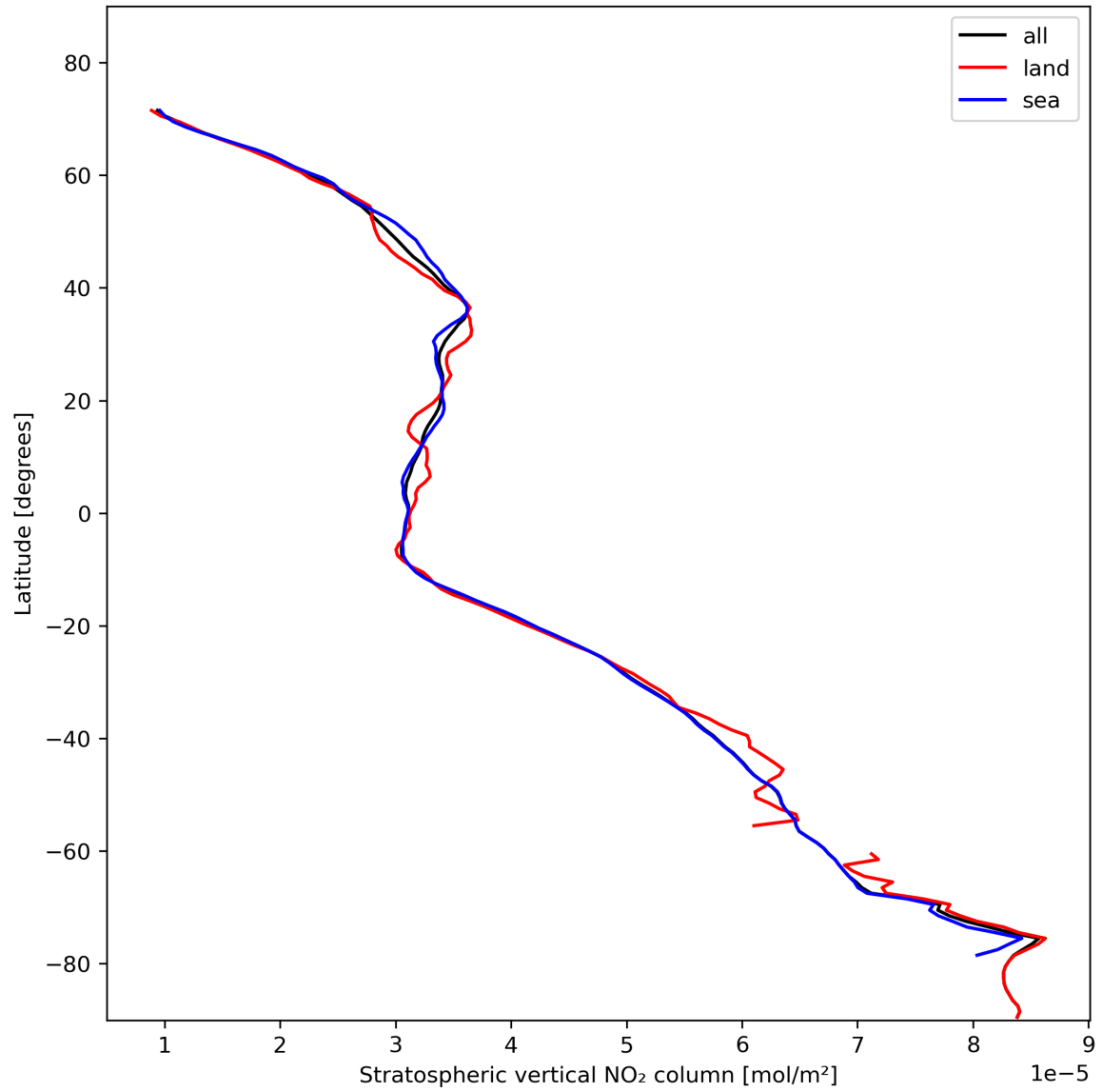
Figure 19: Zonal average of “Stratospheric vertical NO 2 column” for 2024-02-02 to 2024-02-04.
