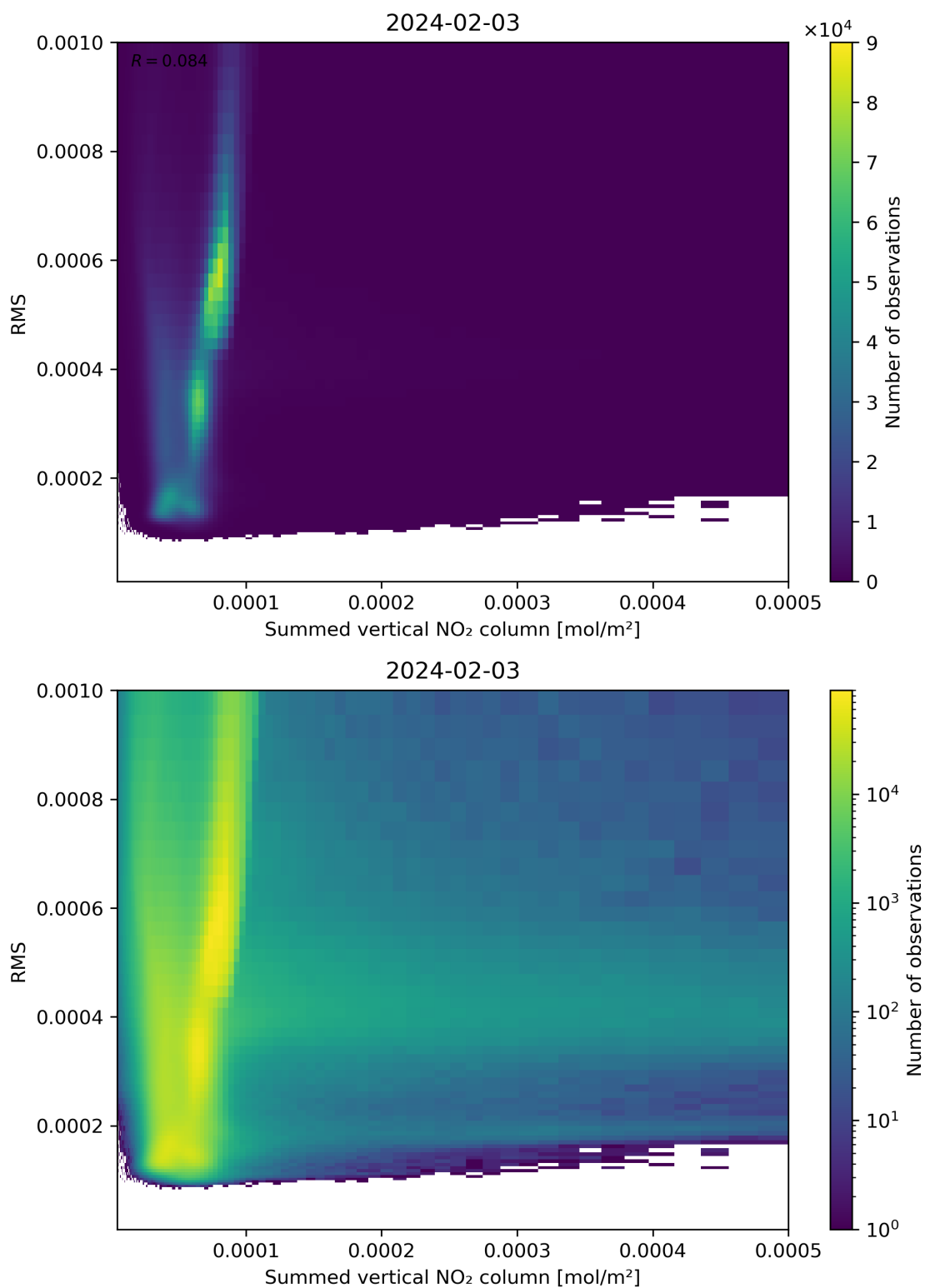
Figure 109: Scatter density plot of “Summed vertical NO 2 column” against “RMS” for 2024-02-02 to 2024-02-04.
