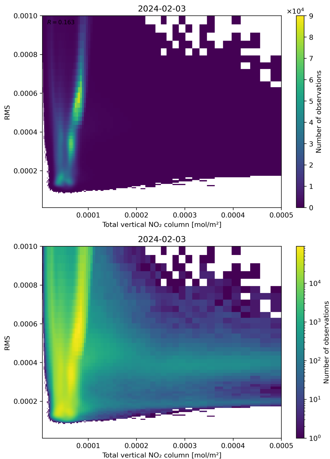
Figure 120: Scatter density plot of “Total vertical NO 2 column” against “RMS” for 2024-02-02 to 2024-02-04.
