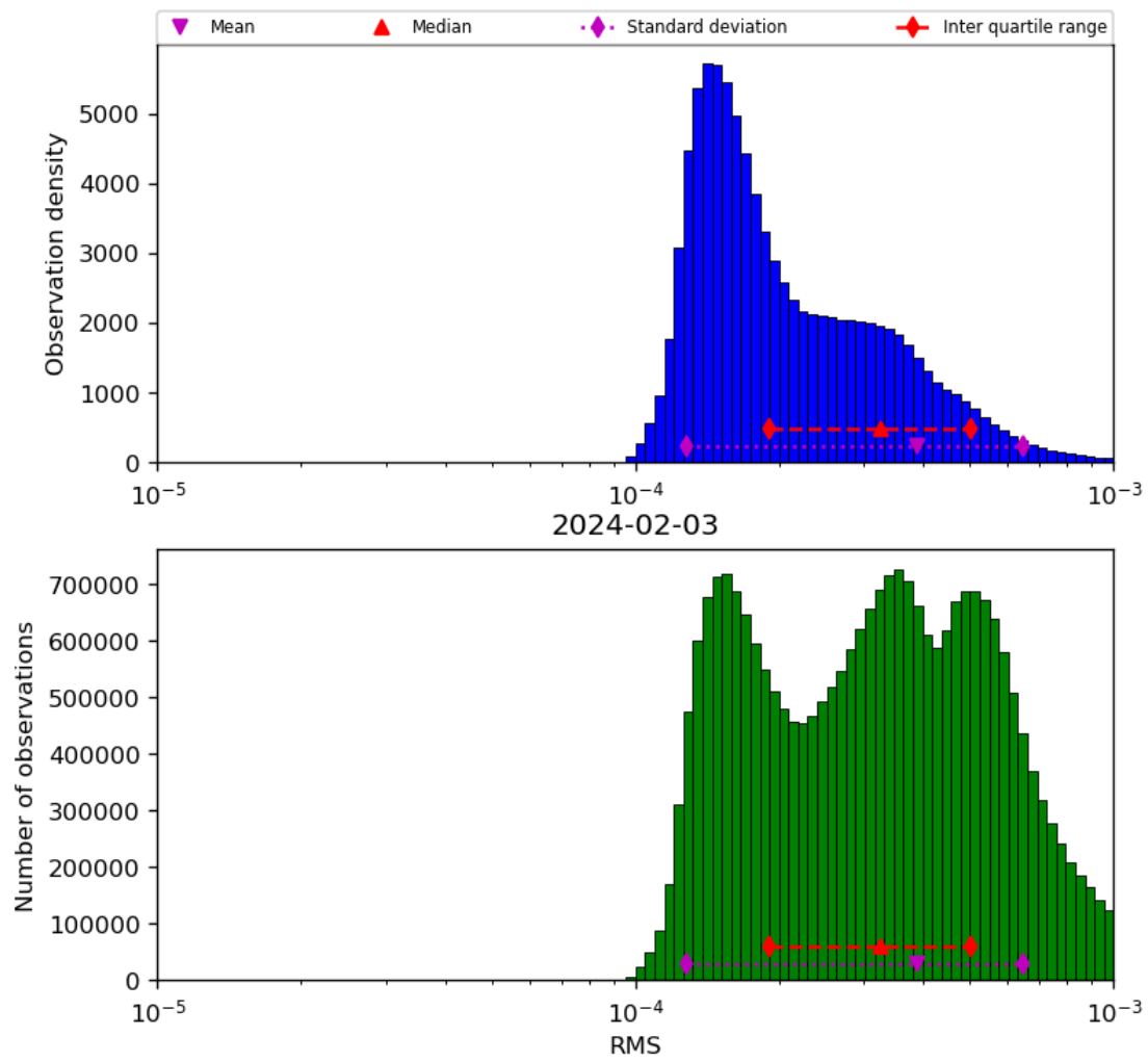
Figure 43: Histogram of “RMS” for 2024-02-02 to 2024-02-04
