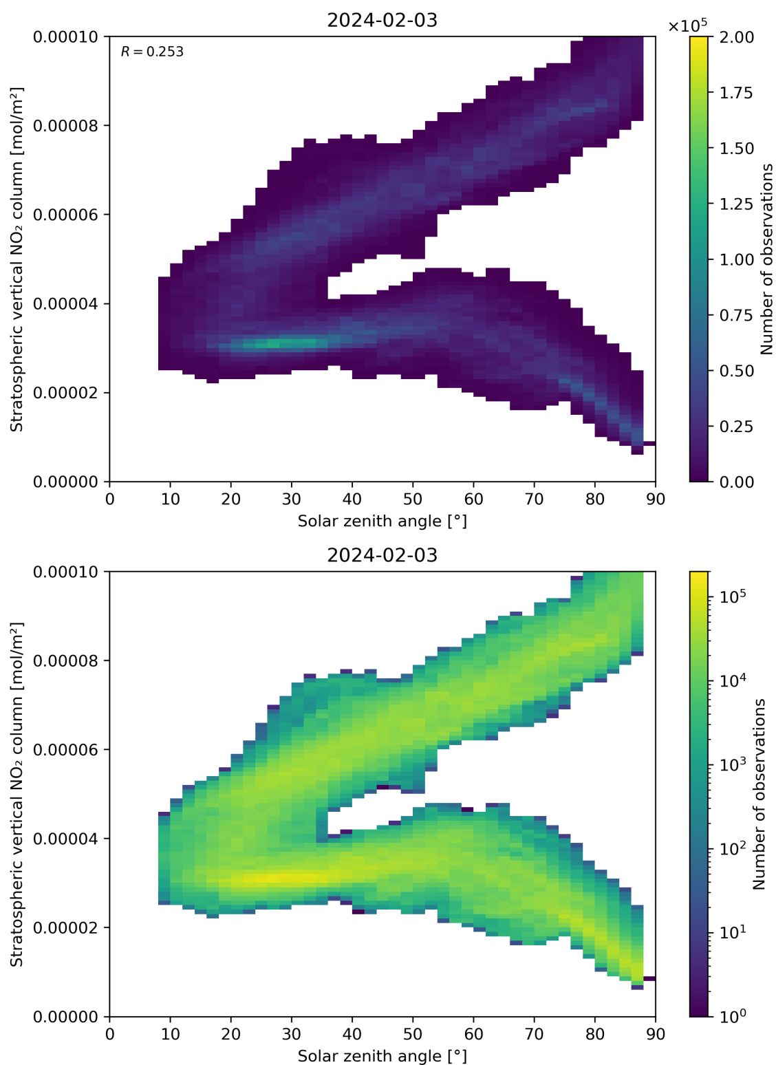
Figure 150: Scatter density plot of “Solar zenith angle” against “Stratospheric vertical NO 2 column” for 2024-02-02 to 2024-02-04.
