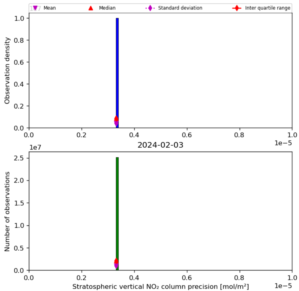
Figure 37: Histogram of “Stratospheric vertical NO 2 column precision” for 2024-02-02 to 2024-02-04
