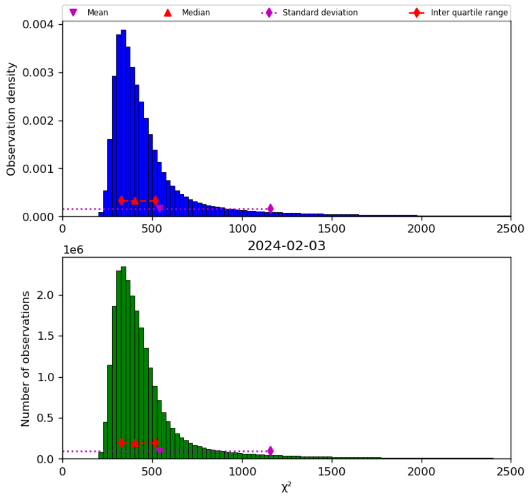
Figure 42: Histogram of “ \chi^2 ” for 2024-02-02 to 2024-02-04
