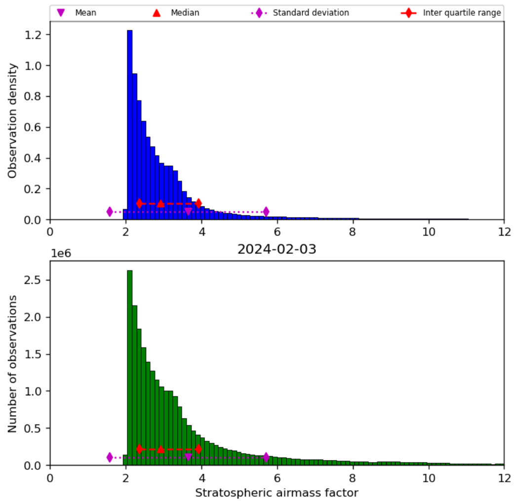
Figure 44: Histogram of “Stratospheric airmass factor” for 2024-02-02 to 2024-02-04
