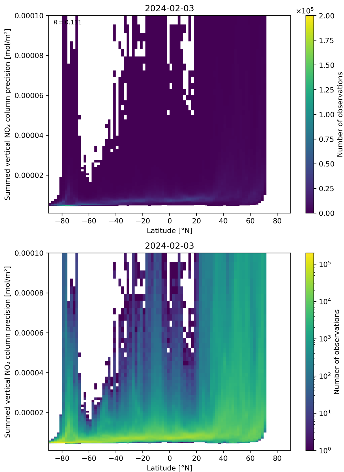
Figure 89: Scatter density plot of “Latitude” against “Summed vertical NO 2 column precision” for 2024-02-02 to 2024-02-04.
