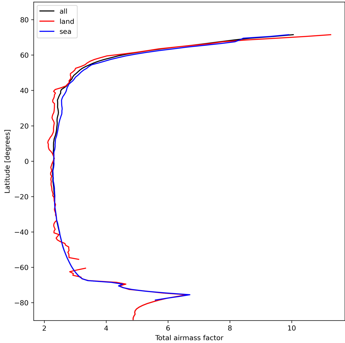
Figure 15: Zonal average of “Total airmass factor” for 2024-02-02 to 2024-02-04.
