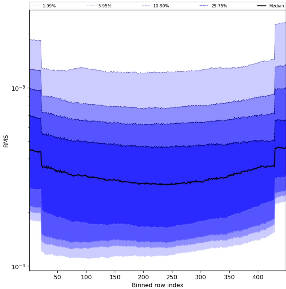
Figure 60: Along track statistics of “RMS” for 2024-02-02 to 2024-02-04
