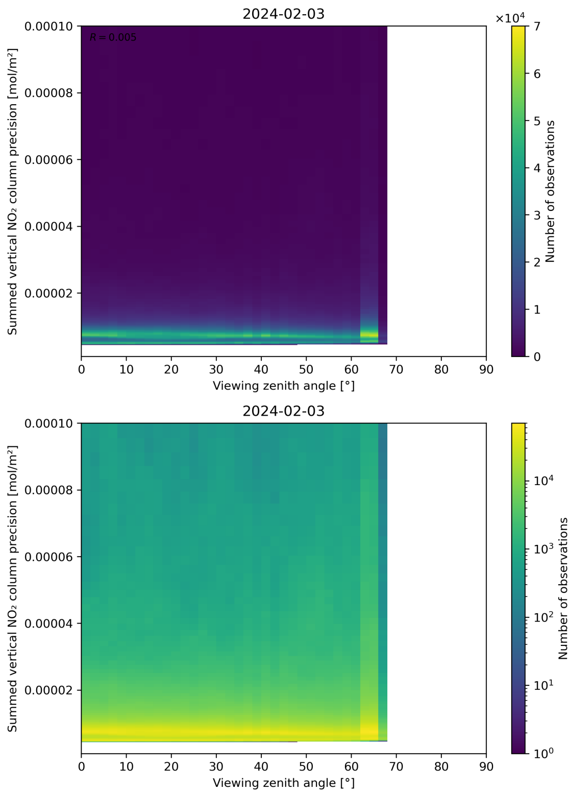
Figure 166: Scatter density plot of “Viewing zenith angle” against “Summed vertical NO 2 column precision” for 2024-02-02 to 2024-02-04.
