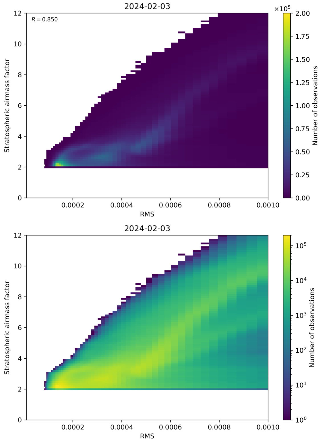
Figure 144: Scatter density plot of “RMS” against “Stratospheric airmass factor” for 2024-02-02 to 2024-02-04.
