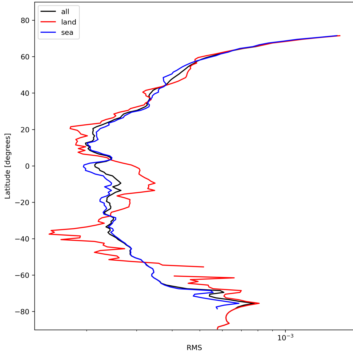
Figure 26: Zonal average of “RMS” for 2024-02-02 to 2024-02-04.
