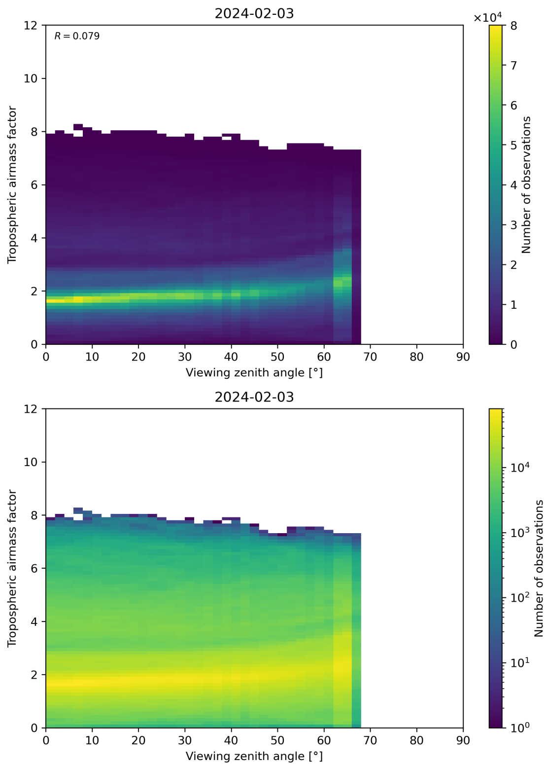
Figure 161: Scatter density plot of “Viewing zenith angle” against “Tropospheric airmass factor” for 2024-02-02 to 2024-02-04.
