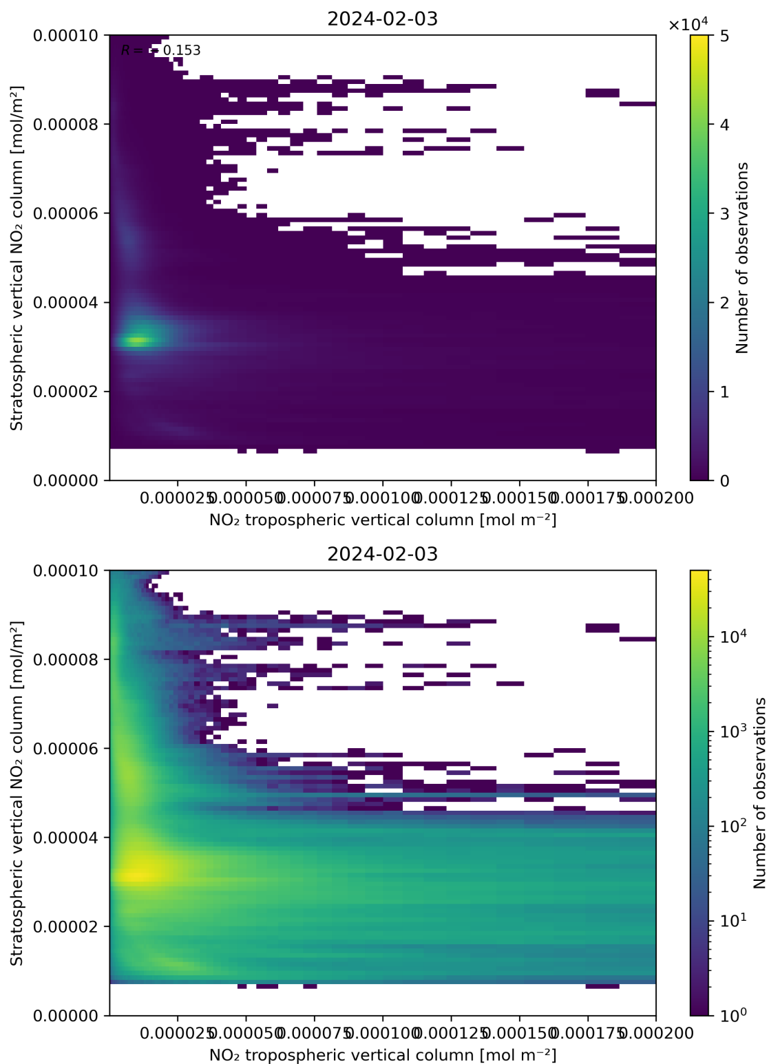
Figure 125: Scatter density plot of “NO 2 tropospheric vertical column” against “Stratospheric vertical NO 2 column” for 2024-02-02 to 2024-02-04.
