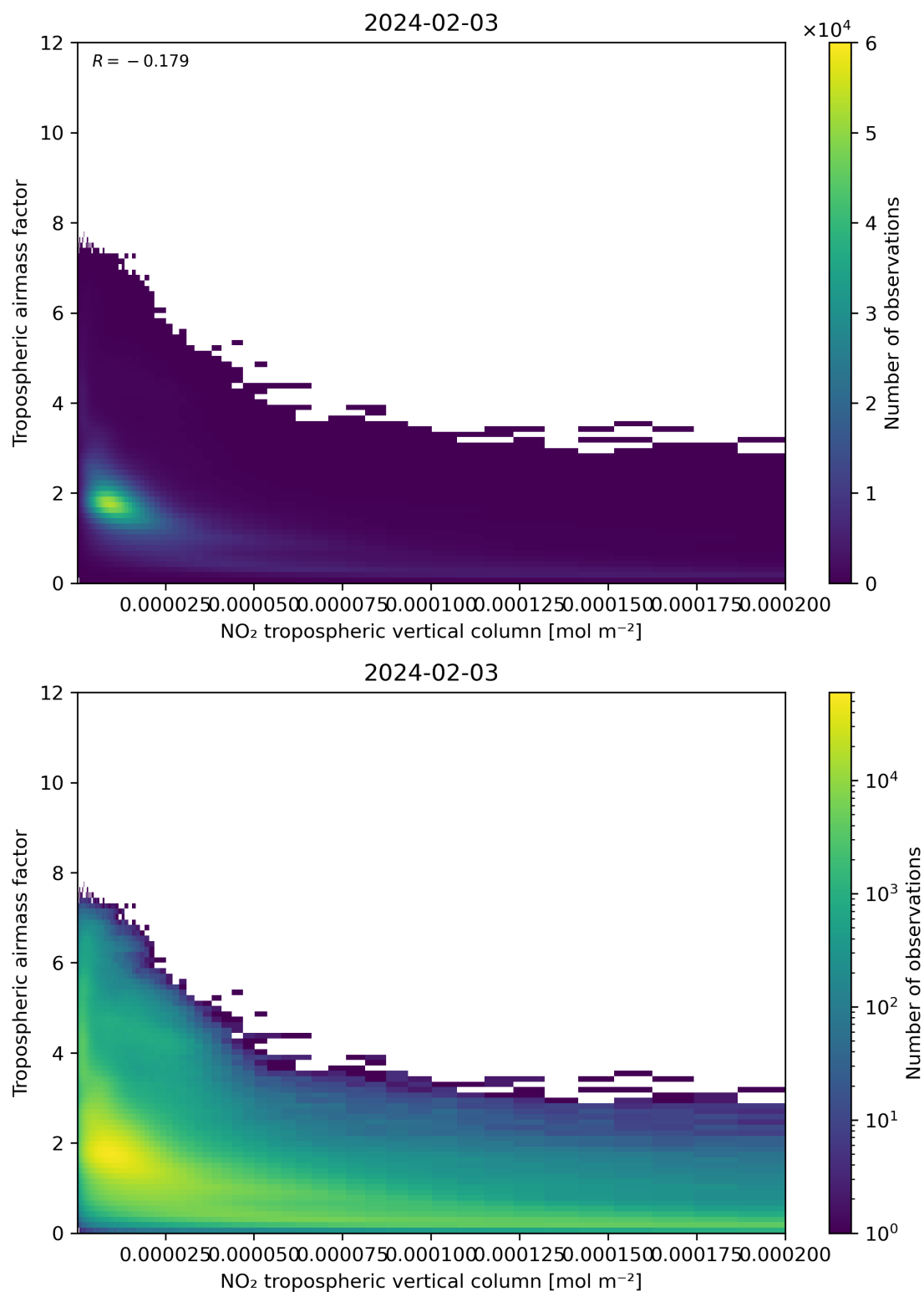
Figure 123: Scatter density plot of “NO 2 tropospheric vertical column” against “Tropospheric air mass factor” for 2024-02-02 to 2024-02-04.
