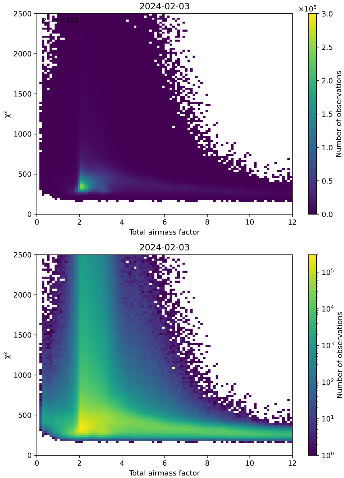
Figure 63: Scatter density plot of “Total airmass factor” against “ \chi^2 ” for 2024-02-02 to 2024-02-04.
