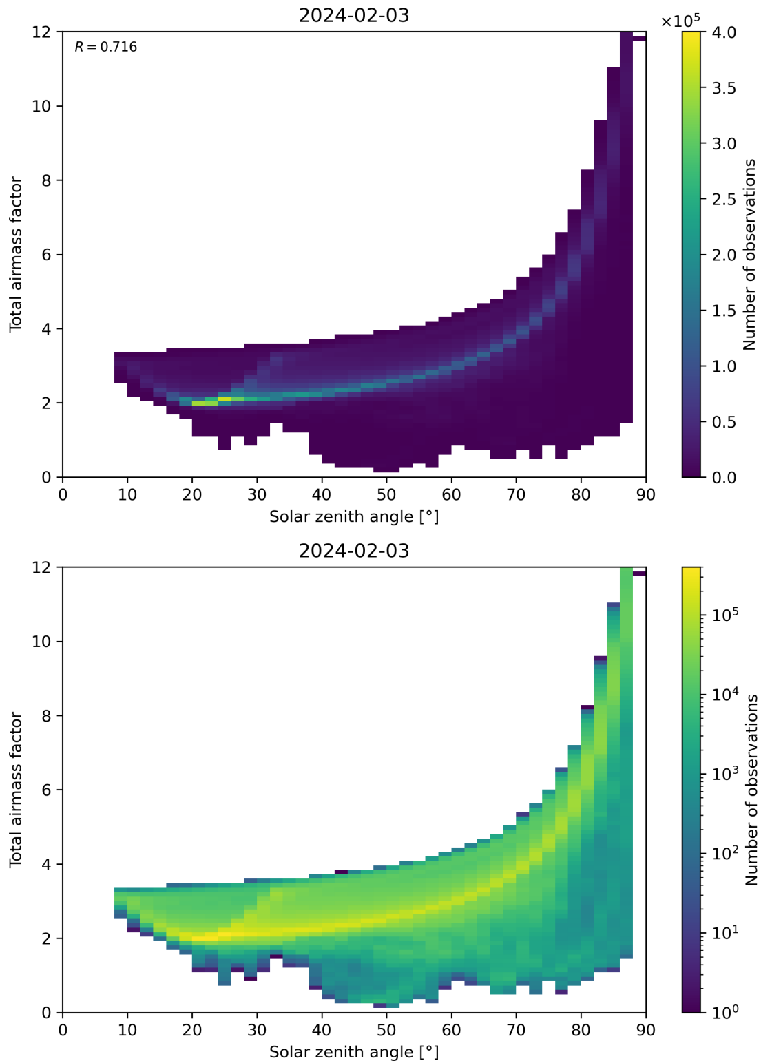
Figure 146: Scatter density plot of “Solar zenith angle” against “Total air mass factor” for 2024-02-02 to 2024-02-04.
