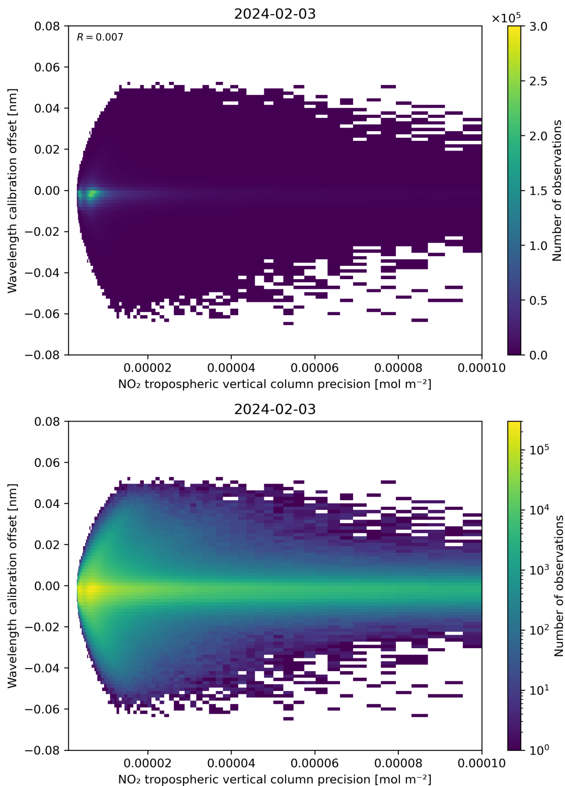
Figure 141: Scatter density plot of “NO 2 tropospheric vertical column precision” against “Wavelength calibration offset” for 2024-02-02 to 2024-02-04.
