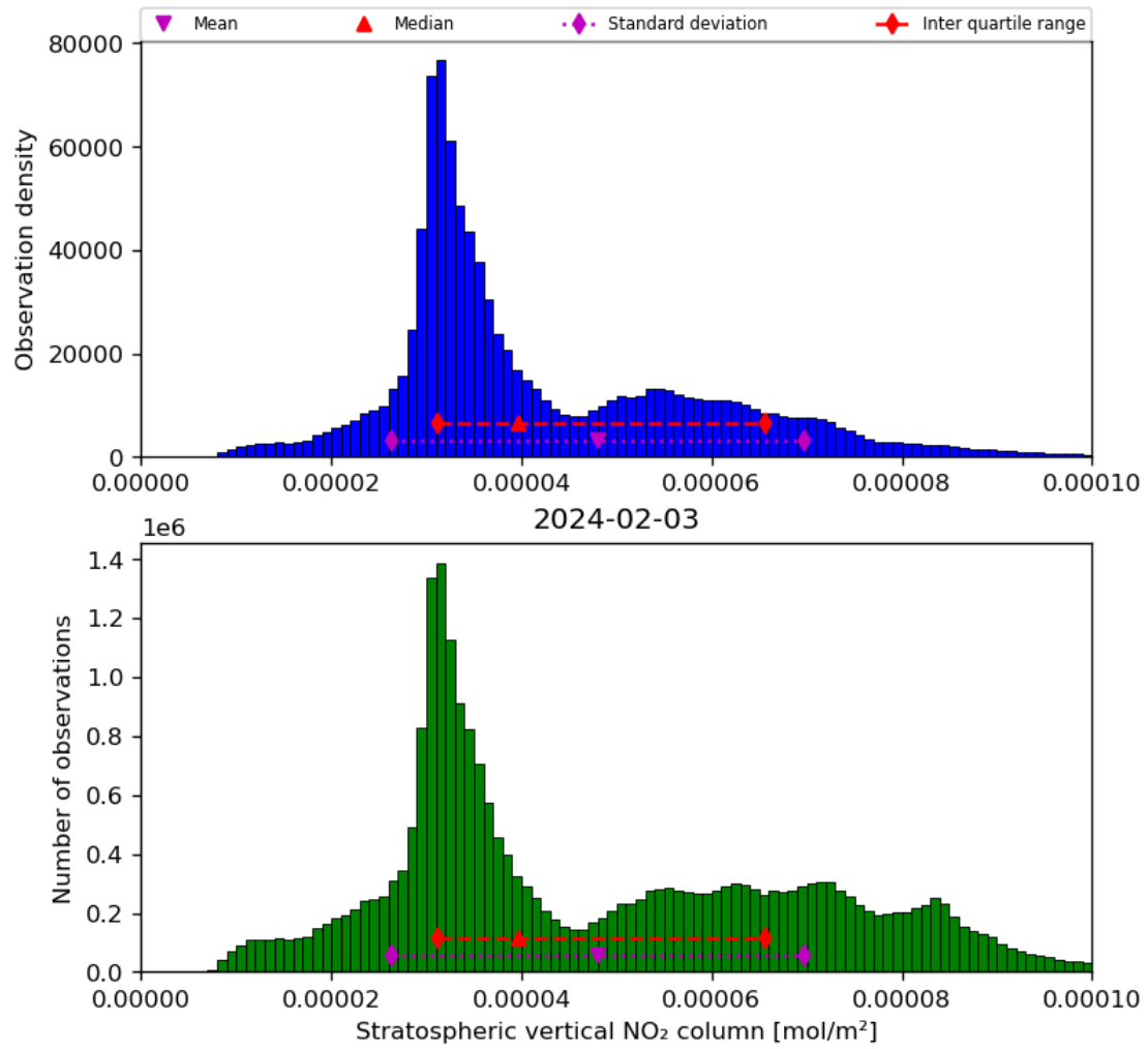
Figure 36: Histogram of “Stratospheric vertical NO 2 column” for 2024-02-02 to 2024-02-04
