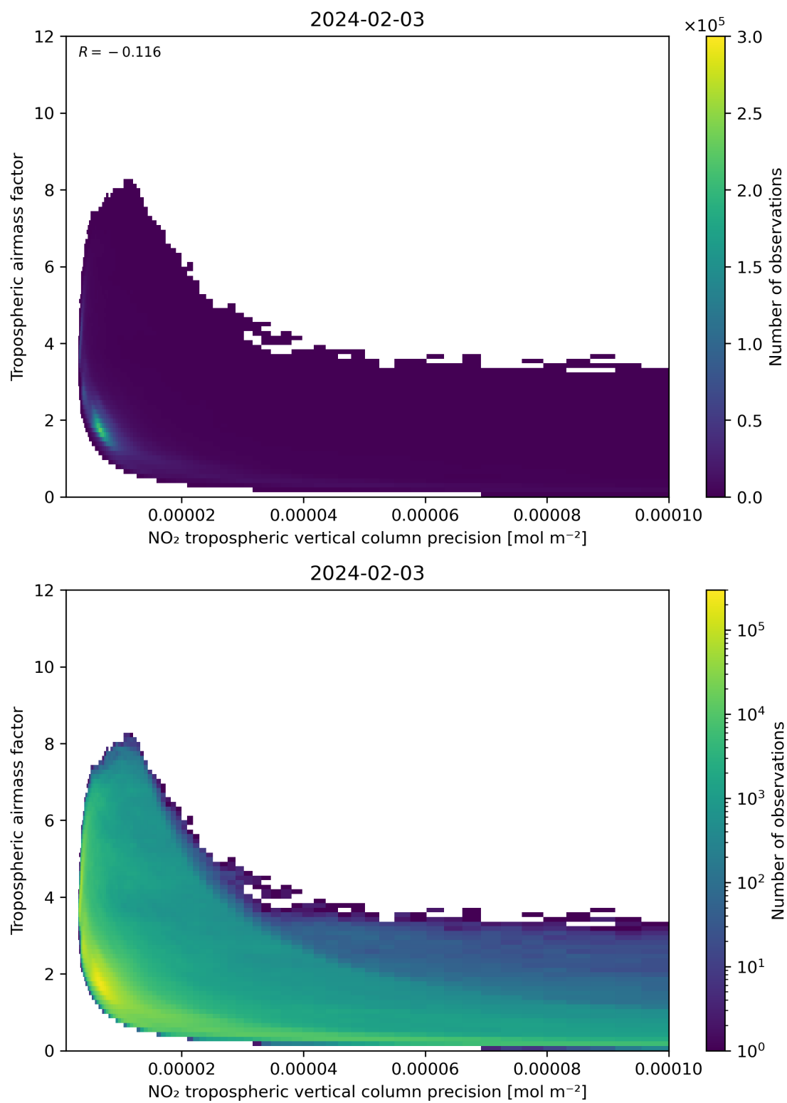
Figure 133: Scatter density plot of “NO 2 tropospheric vertical column precision” against “Tropospheric airmass factor” for 2024-02-02 to 2024-02-04.
