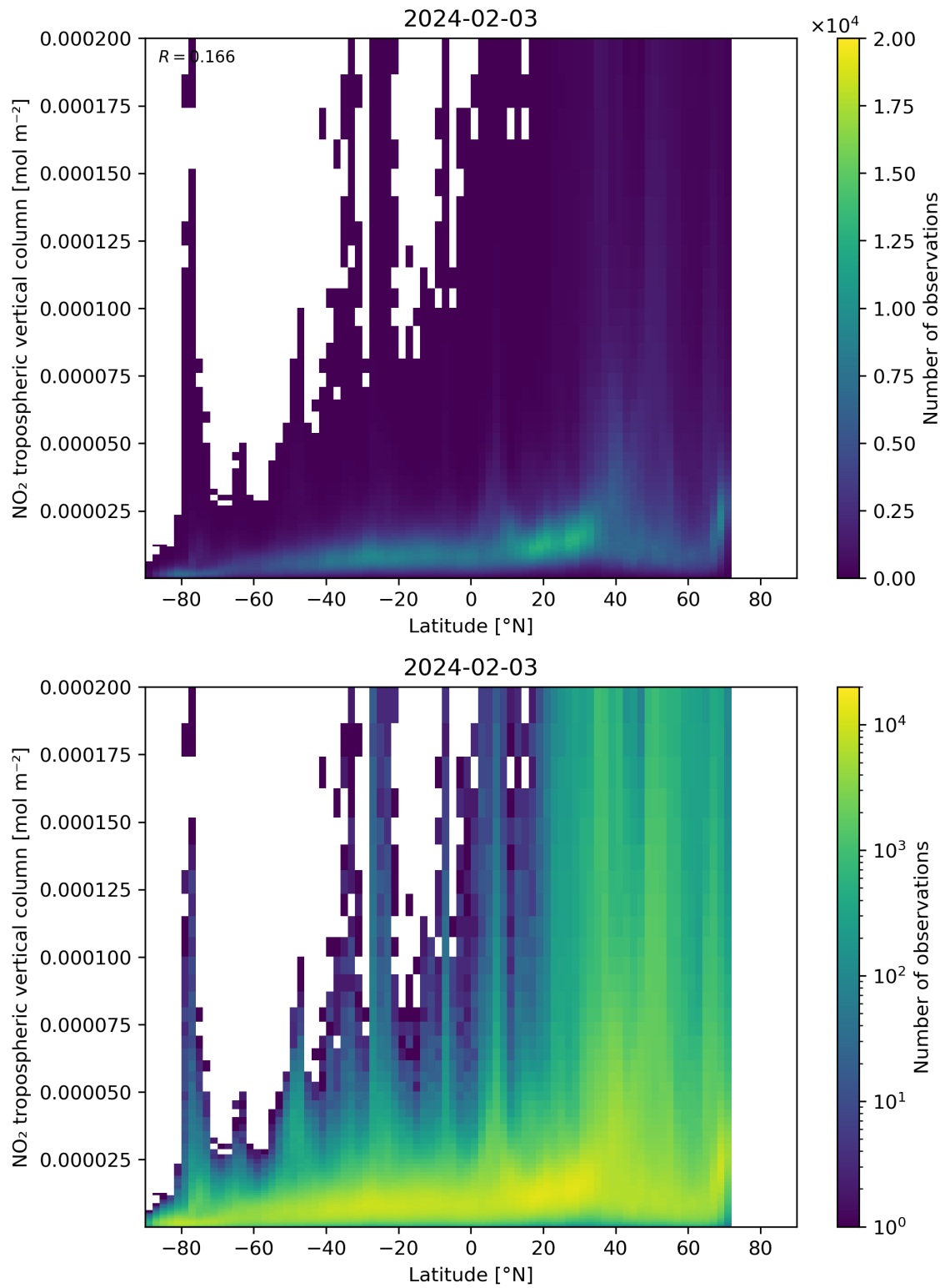
Figure 92: Scatter density plot of “Latitude” against “NO 2 tropospheric vertical column” for 2024-02-02 to 2024-02-04.
