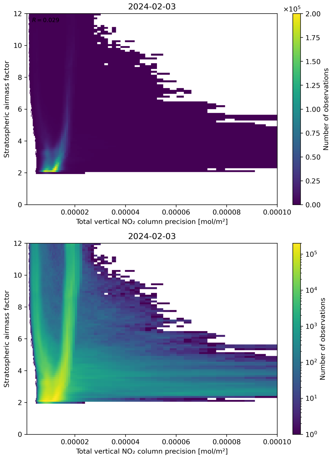
Figure 115: Scatter density plot of “Total vertical NO 2 column precision” against “Stratospheric air mass factor” for 2024-02-02 to 2024-02-04.
