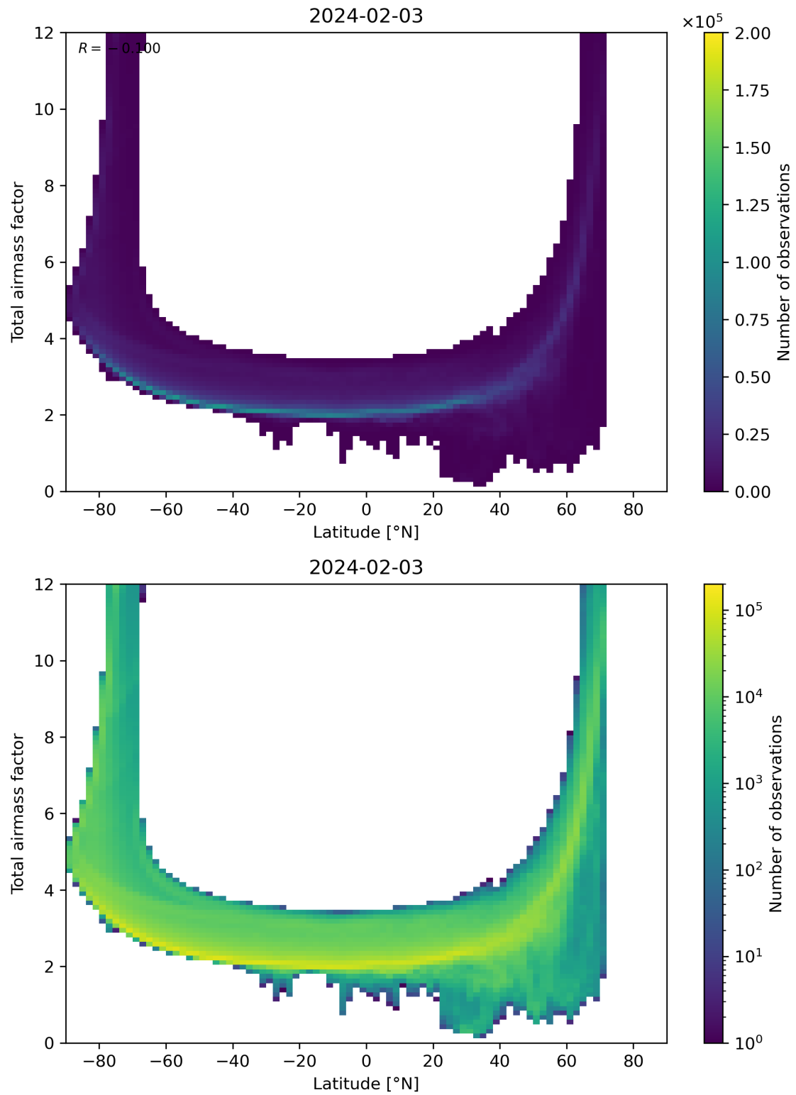
Figure 84: Scatter density plot of “Latitude” against “Total airmass factor” for 2024-02-02 to 2024-02-04.
