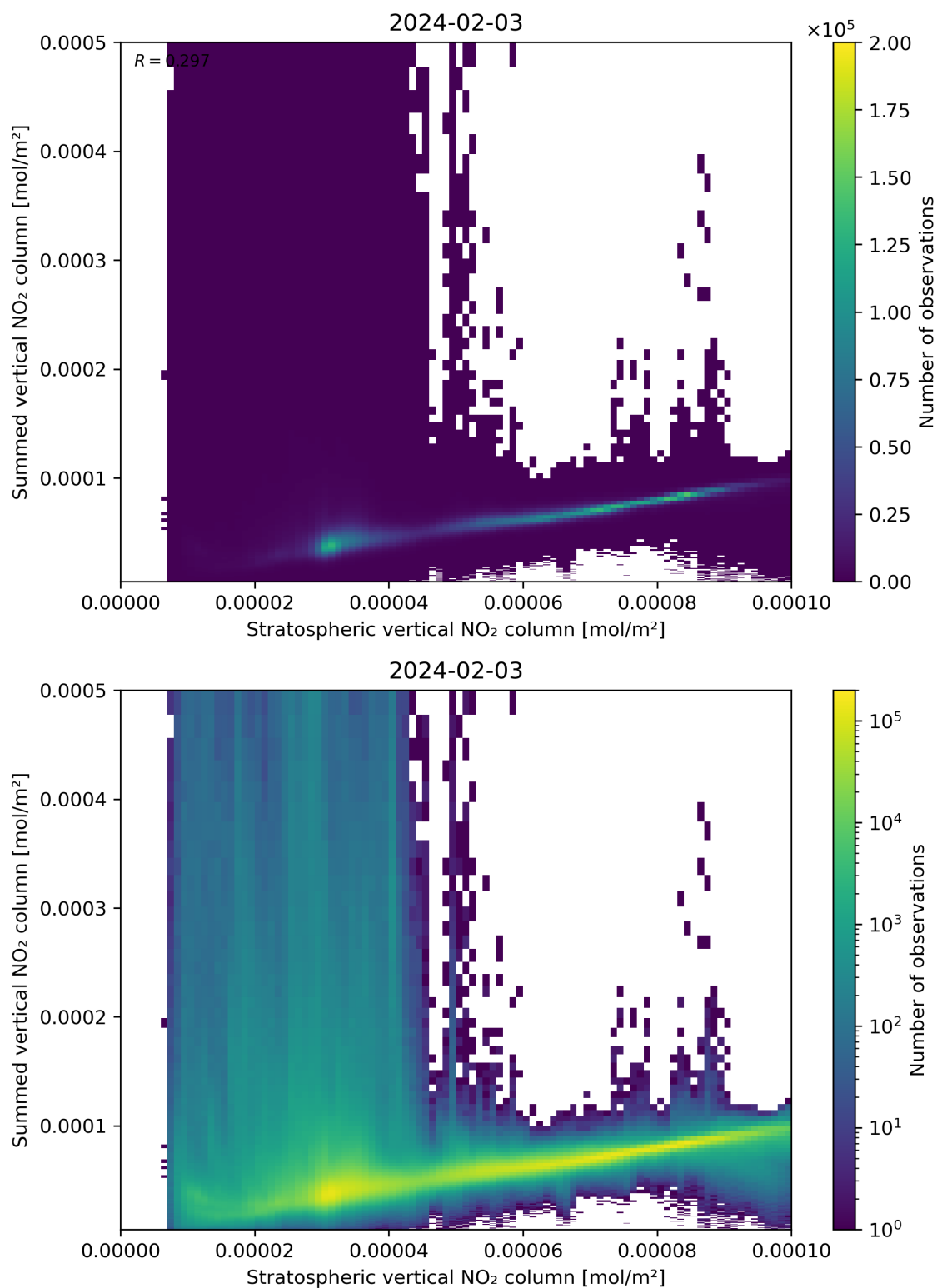
Figure 98: Scatter density plot of “Stratospheric vertical NO 2 column” against “Summed vertical NO 2 column” for 2024-02-02 to 2024-02-04.
