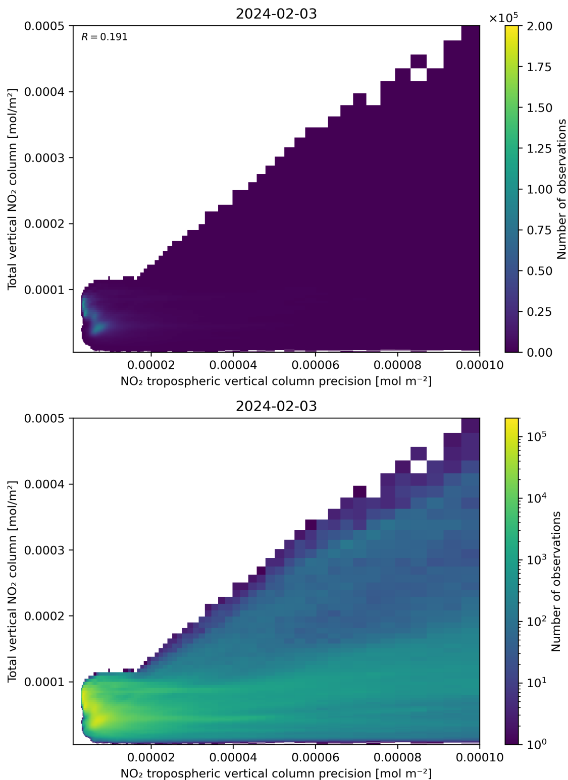
Figure 138: Scatter density plot of “NO 2 tropospheric vertical column precision” against “Total vertical NO 2 column” for 2024-02-02 to 2024-02-04.
