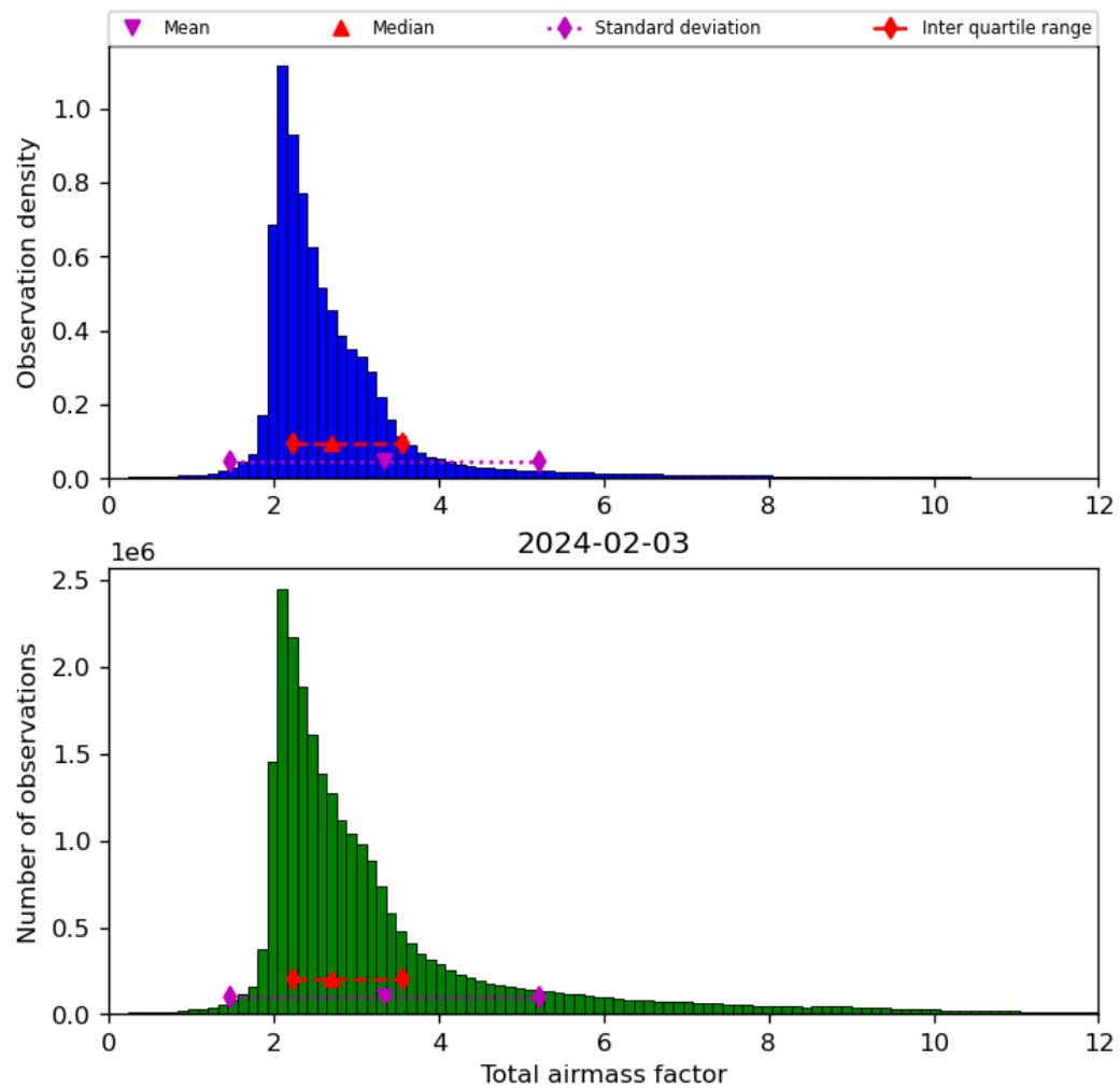
Figure 32: Histogram of “Total airmass factor” for 2024-02-02 to 2024-02-04
