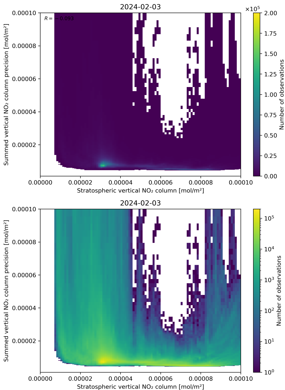
Figure 99: Scatter density plot of “Stratospheric vertical NO 2 column” against “Summed vertical NO 2 column precision” for 2024-02-02 to 2024-02-04.
