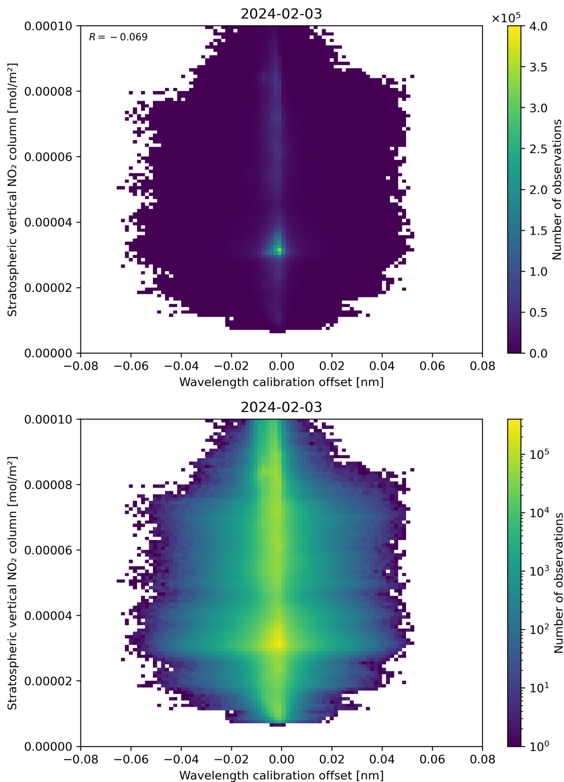
Figure 176: Scatter density plot of “Wavelength calibration offset” against “Stratospheric vertical NO 2 column” for 2024-02-02 to 2024-02-04.
