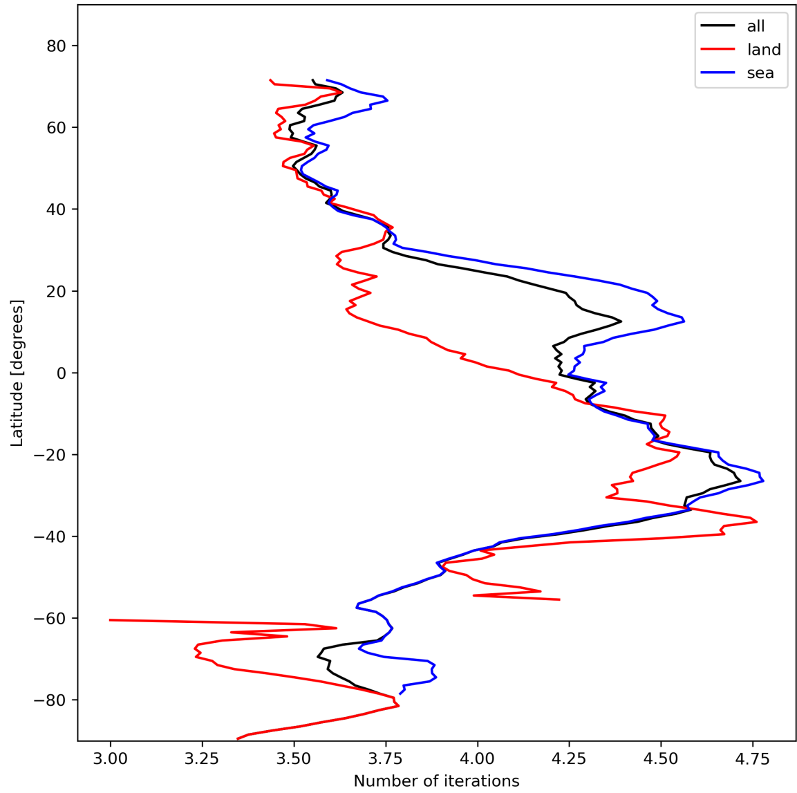
Figure 17: Zonal average of “Number of iterations” for 2024-02-02 to 2024-02-04.
