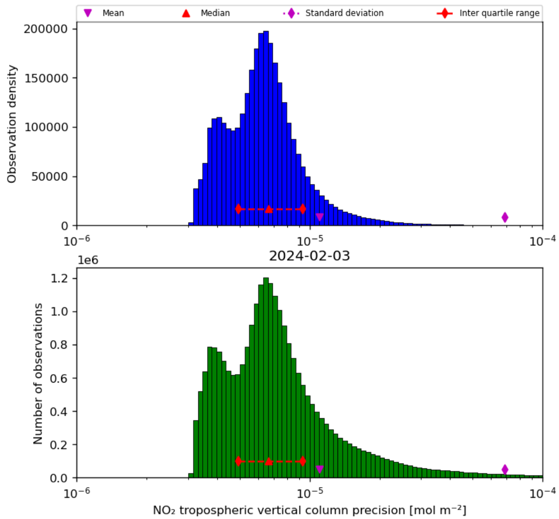
Figure 30: Histogram of “NO 2 tropospheric vertical column precision” for 2024-02-02 to 2024-02-04
