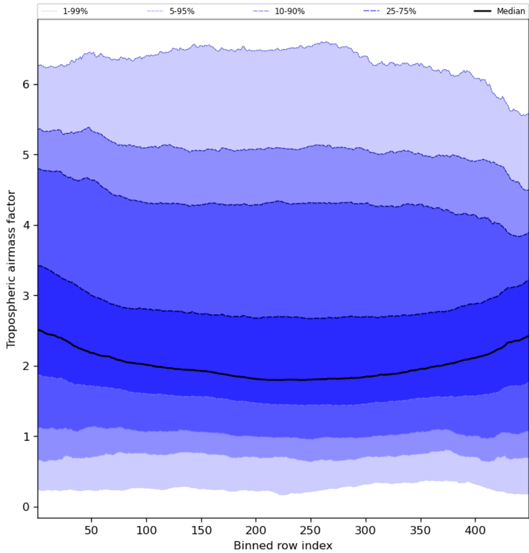
Figure 48: Along track statistics of “Tropospheric airmass factor” for 2024-02-02 to 2024-02-04
