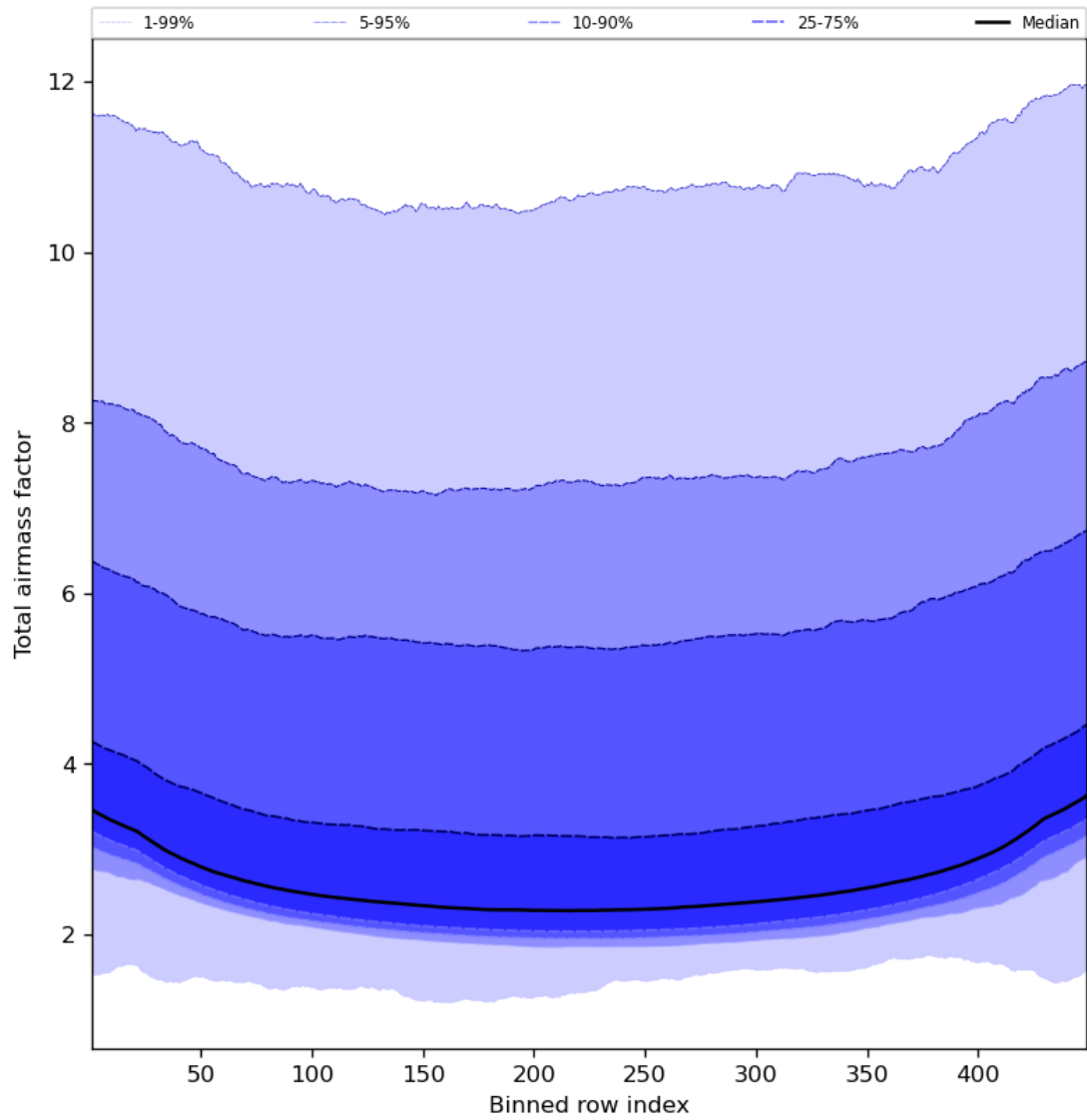
Figure 49: Along track statistics of “Total airmass factor” for 2024-02-02 to 2024-02-04
