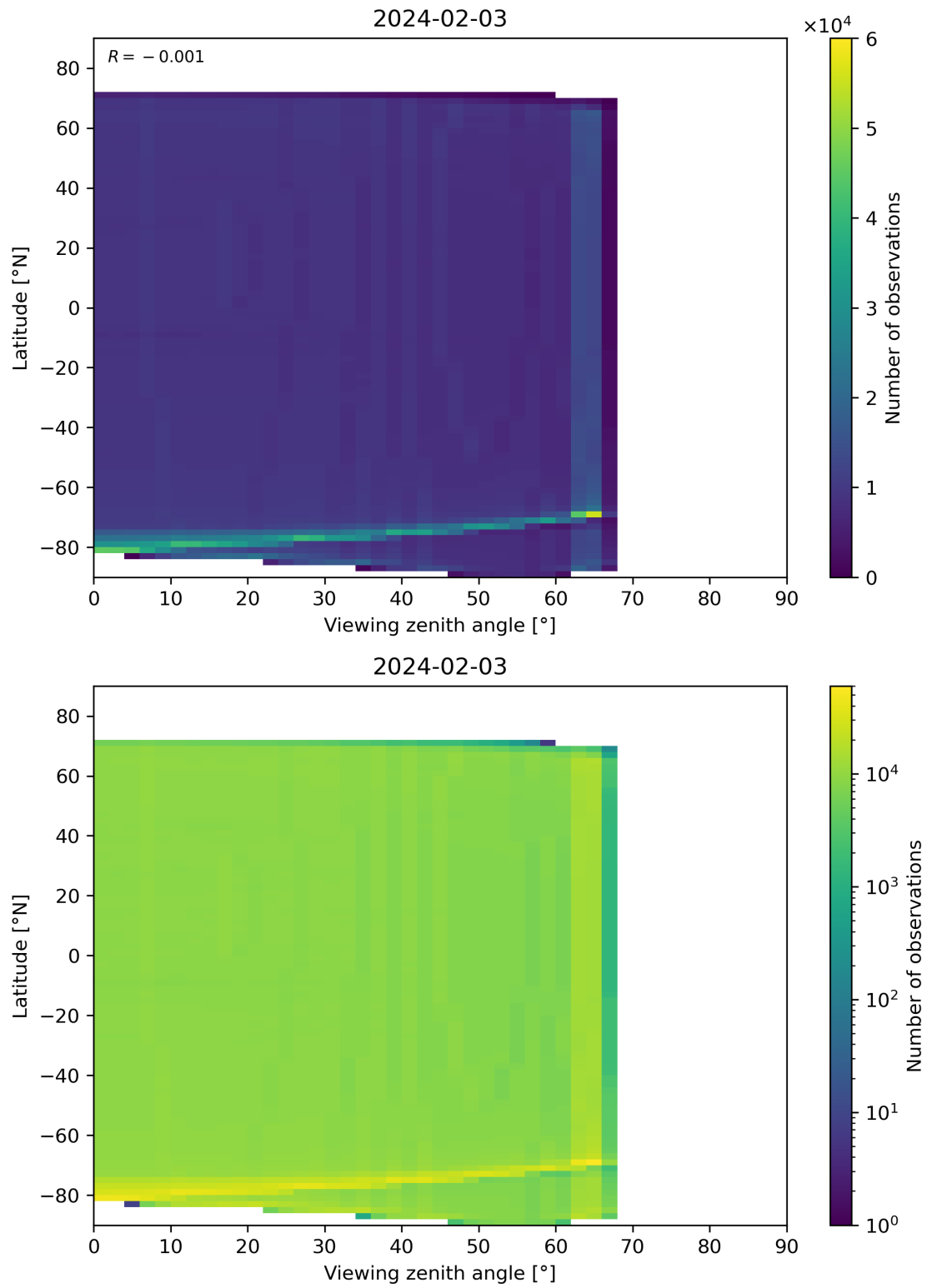
Figure 163: Scatter density plot of “Viewing zenith angle” against “Latitude” for 2024-02-02 to 2024-02-04.
