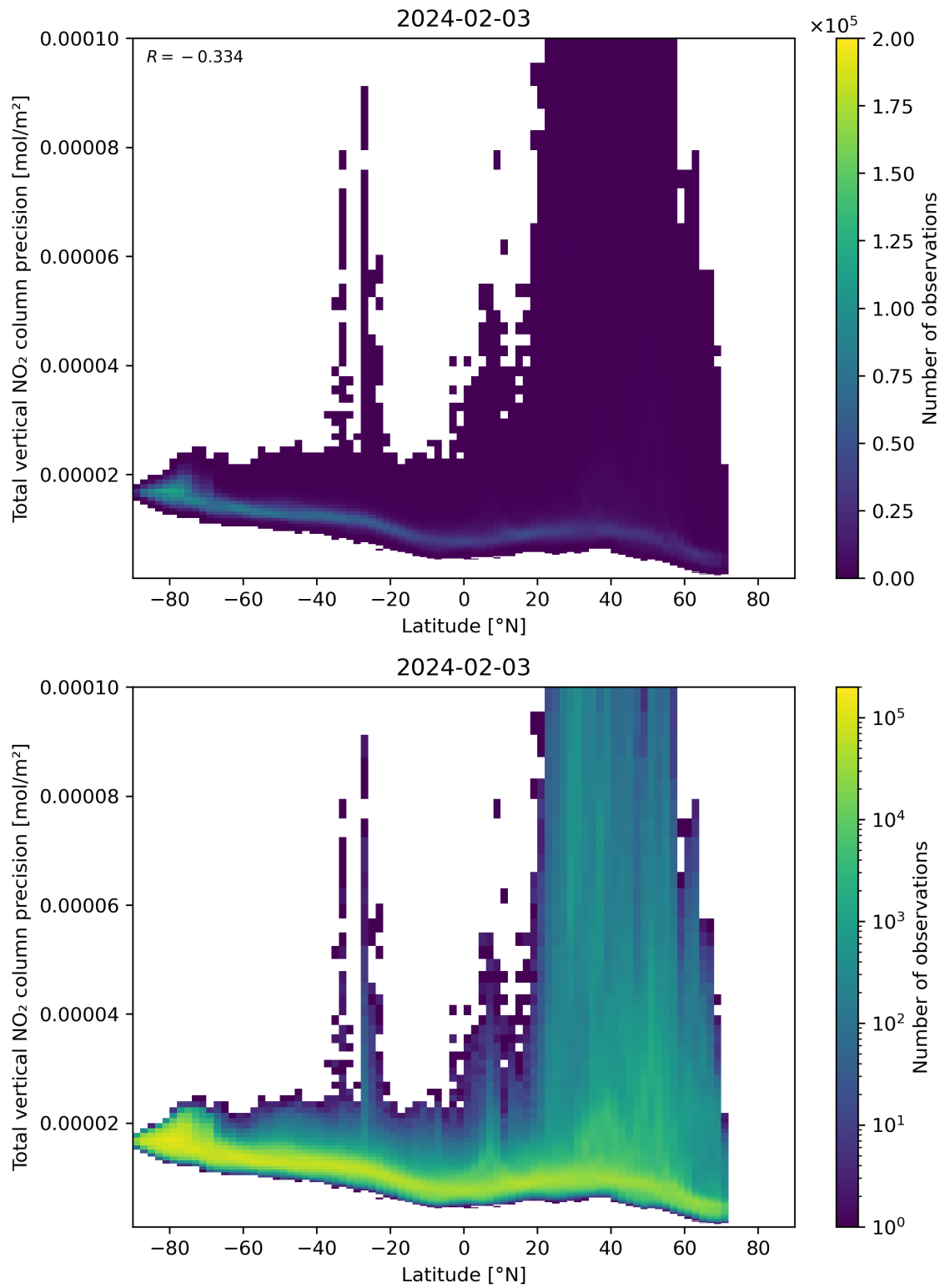
Figure 91: Scatter density plot of “Latitude” against “Total vertical NO 2 column precision” for 2024-02-02 to 2024-02-04.
