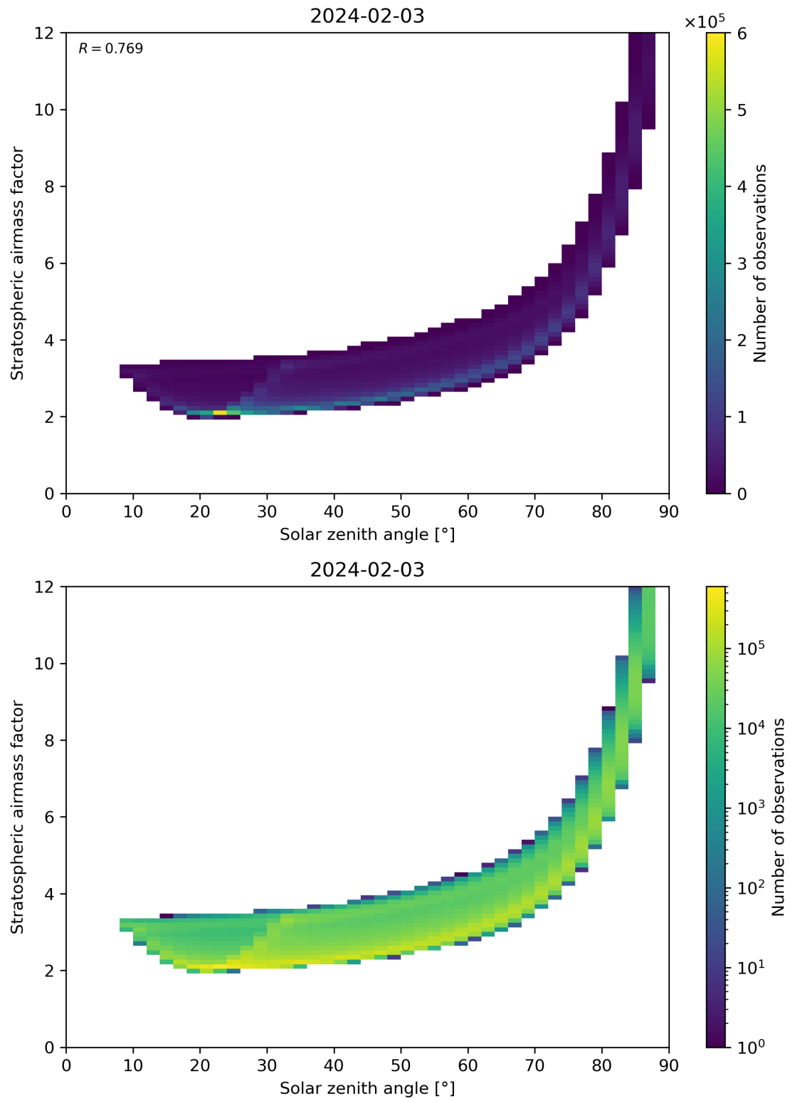
Figure 145: Scatter density plot of “Solar zenith angle” against “Stratospheric airmass factor” for 2024-02-02 to 2024-02-04.
