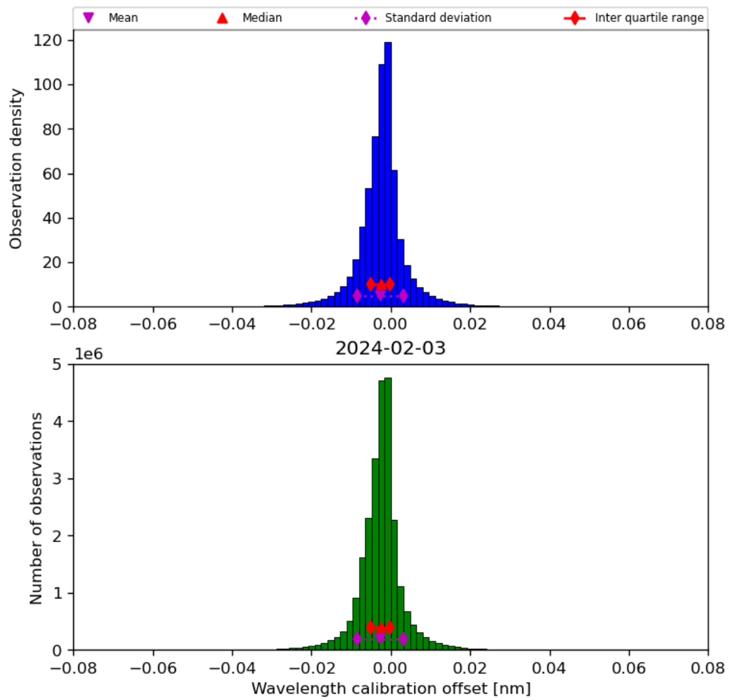
Figure 35: Histogram of “Wavelength calibration offset” for 2024-02-02 to 2024-02-04
