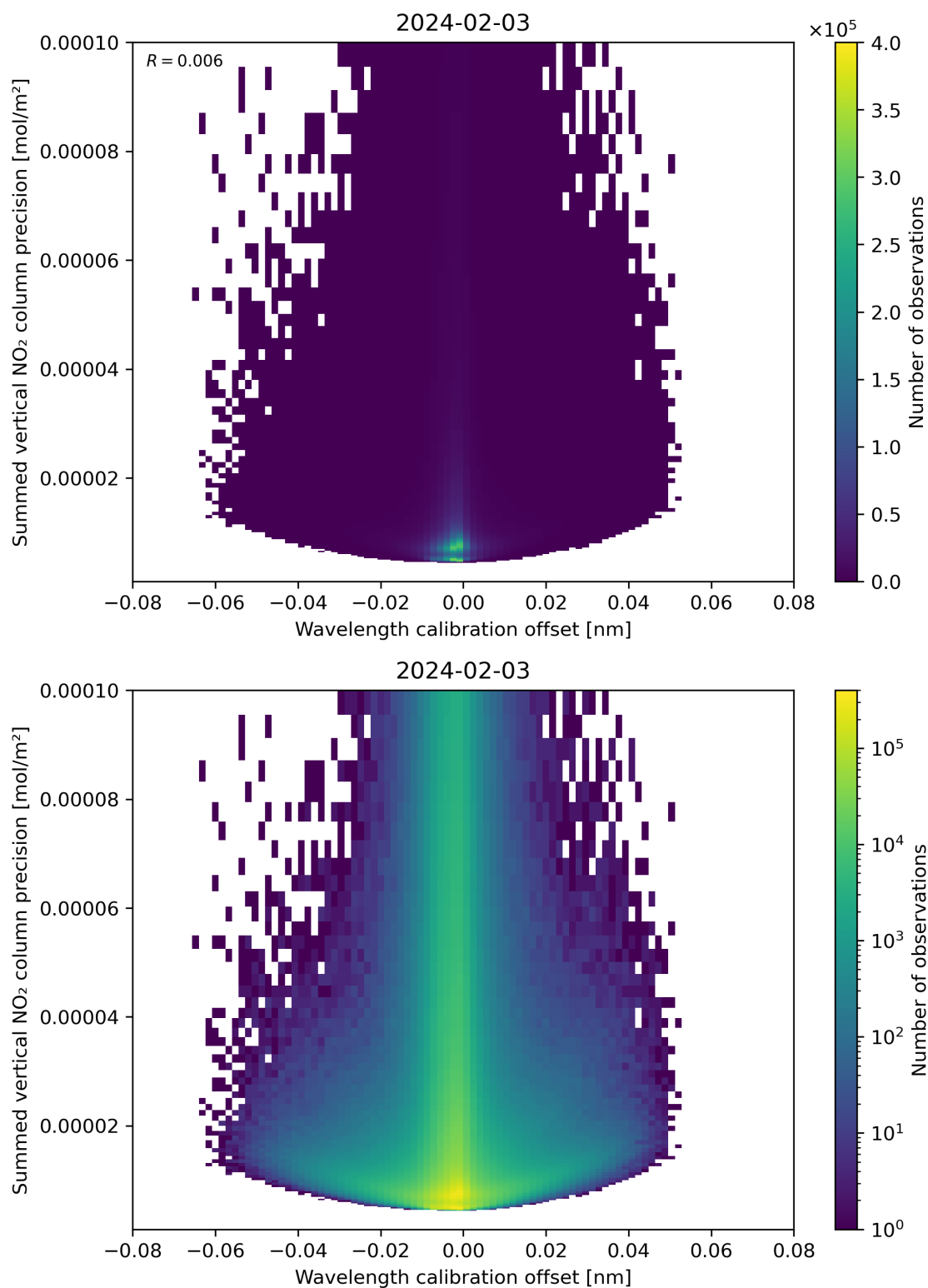
Figure 178: Scatter density plot of “Wavelength calibration offset” against “Summed vertical NO 2 column precision” for 2024-02-02 to 2024-02-04.
