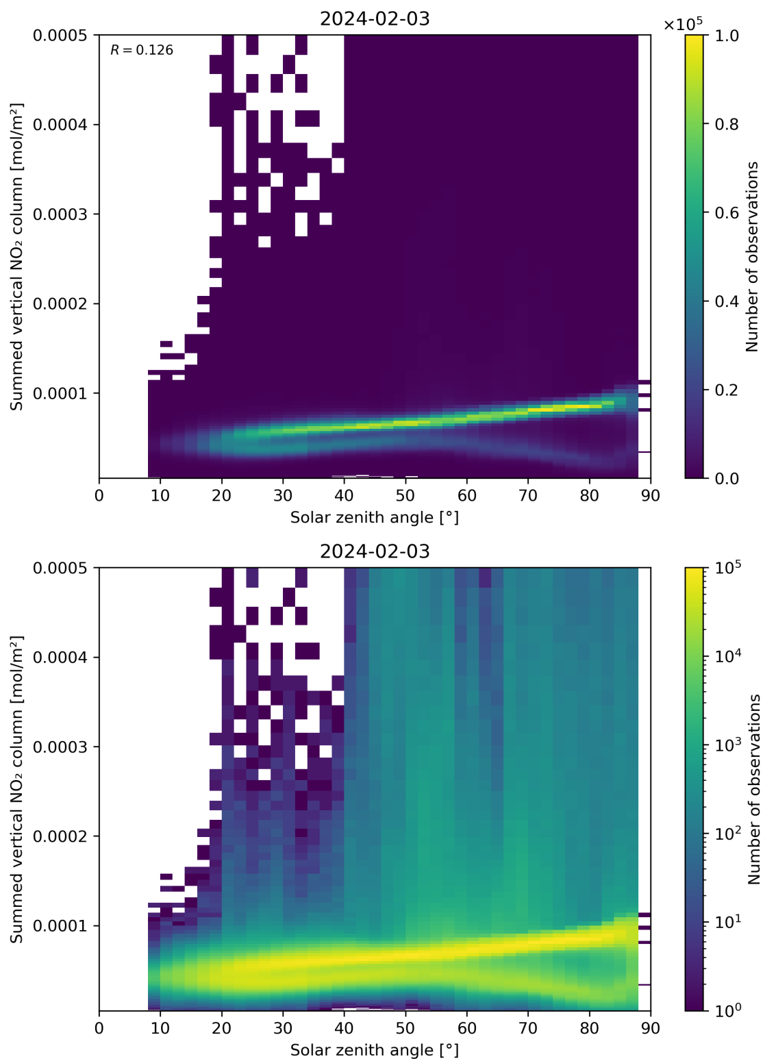
Figure 151: Scatter density plot of “Solar zenith angle” against “Summed vertical NO 2 column” for 2024-02-02 to 2024-02-04.
