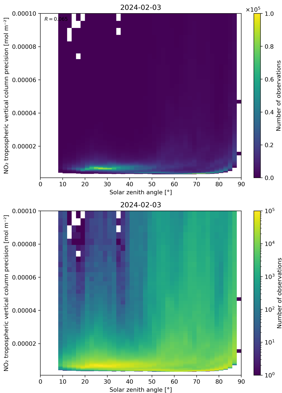
Figure 156: Scatter density plot of “Solar zenith angle” against “NO 2 tropospheric vertical column precision” for 2024-02-02 to 2024-02-04.
