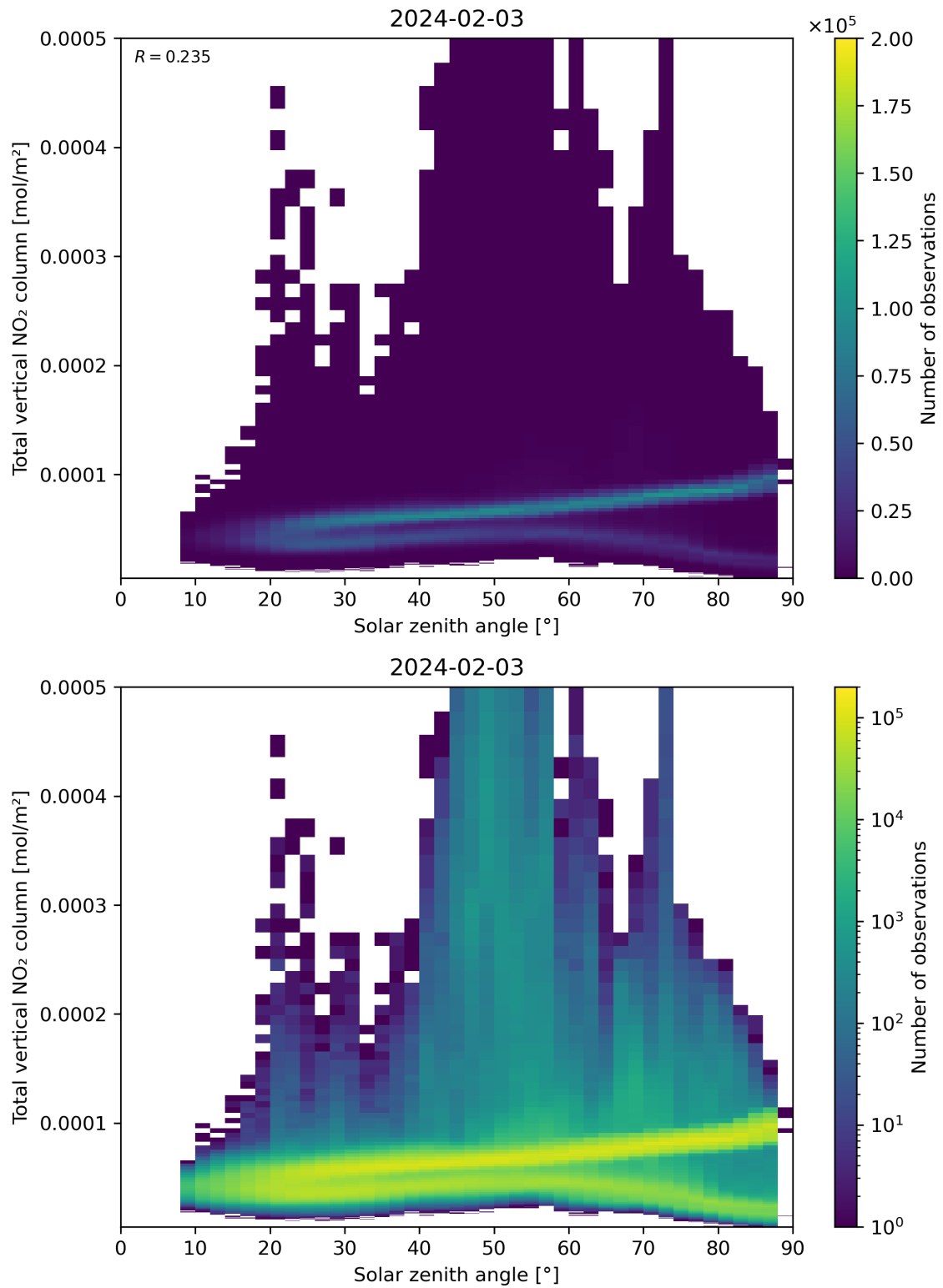
Figure 153: Scatter density plot of “Solar zenith angle” against “Total vertical NO 2 column” for 2024-02-02 to 2024-02-04.
