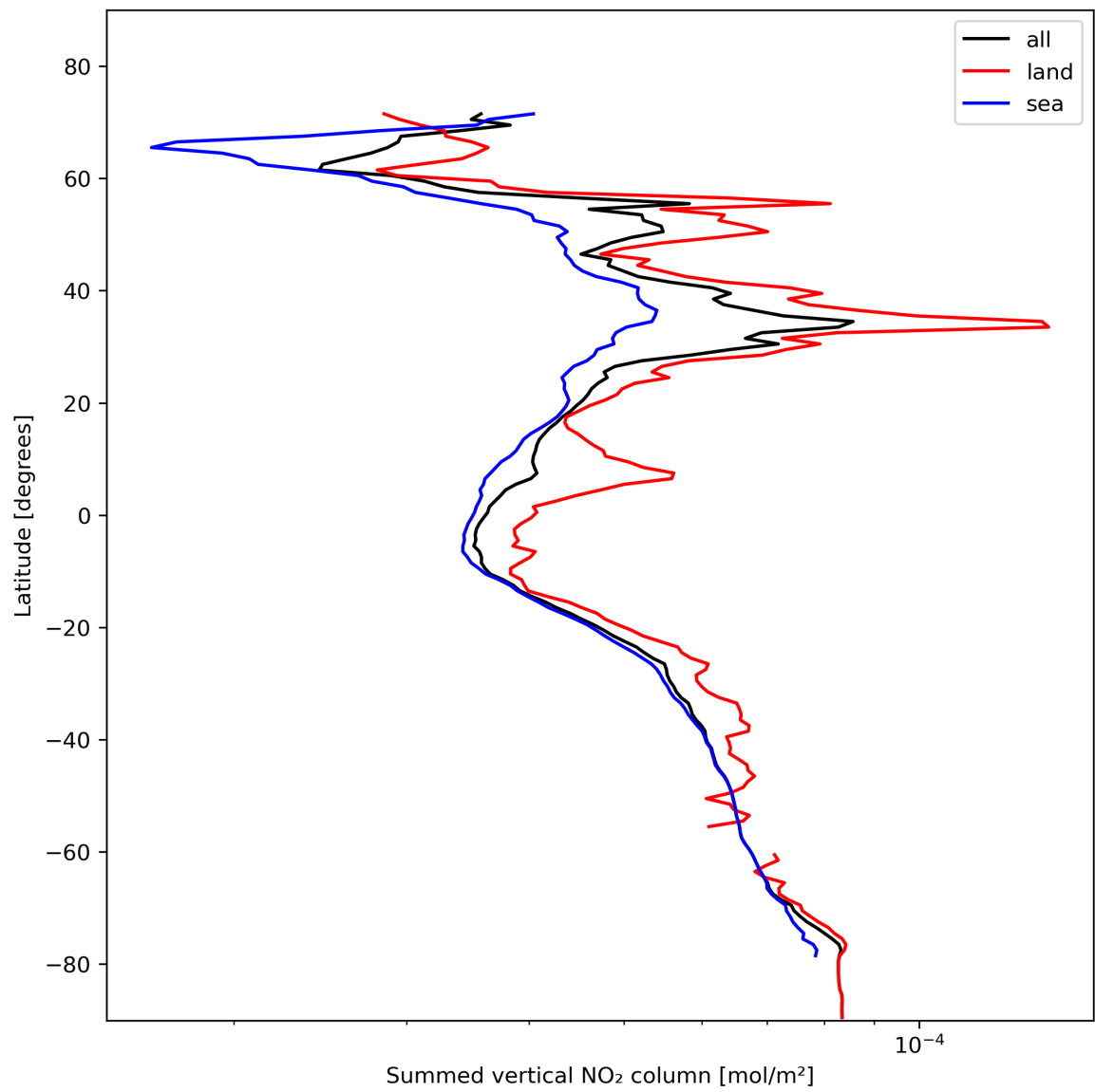
Figure 23: Zonal average of “Summed vertical NO 2 column” for 2024-02-02 to 2024-02-04.
