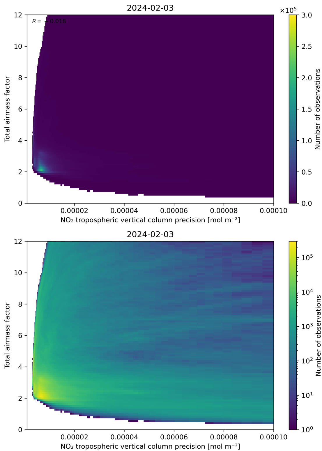
Figure 132: Scatter density plot of “NO 2 tropospheric vertical column precision” against “Total airmass factor” for 2024-02-02 to 2024-02-04.
