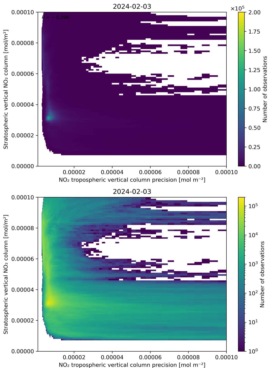
Figure 135: Scatter density plot of “NO 2 tropospheric vertical column precision” against “Stratospheric vertical NO 2 column” for 2024-02-02 to 2024-02-04.
