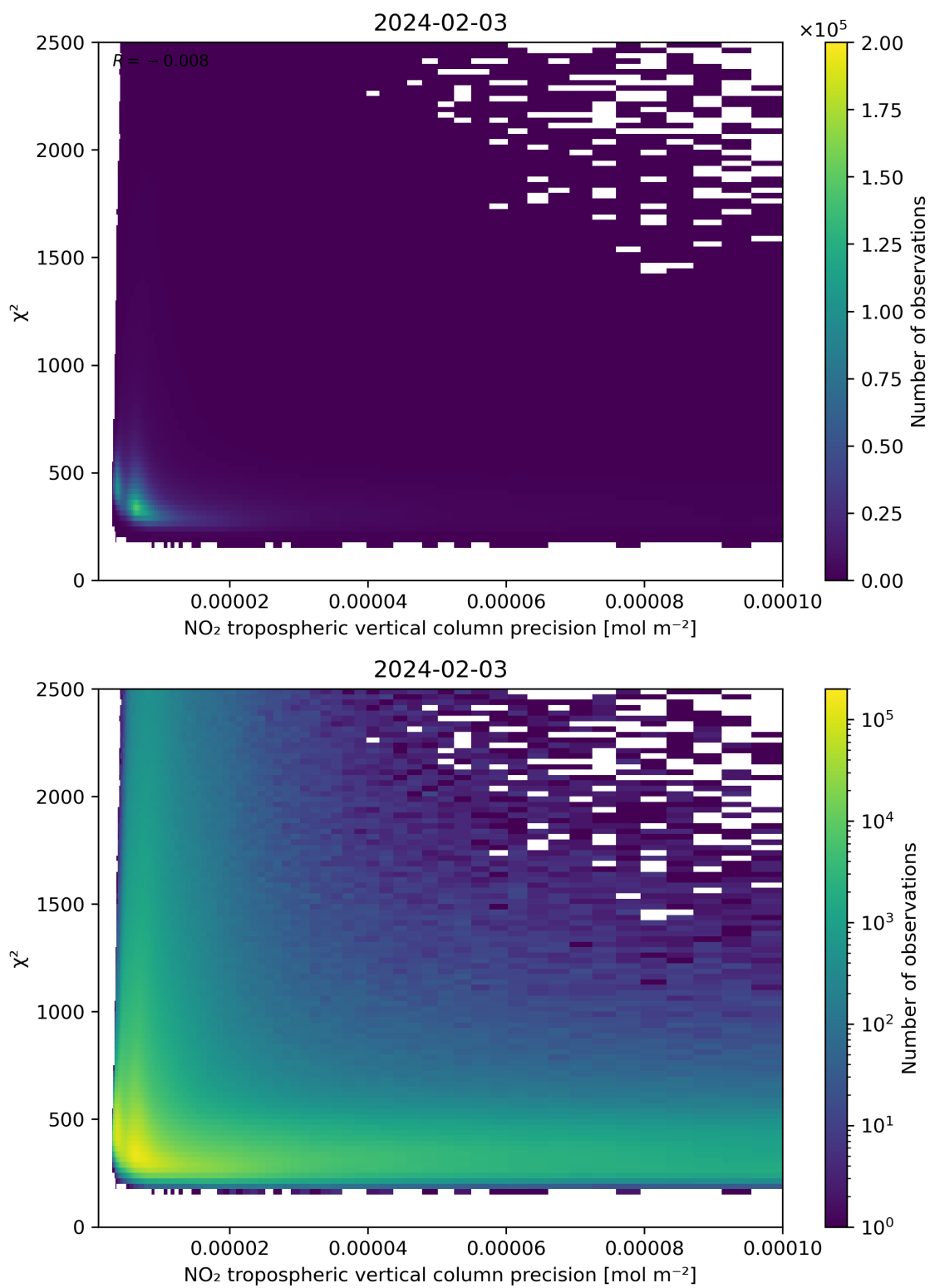
Figure 134: Scatter density plot of “NO 2 tropospheric vertical column precision” against “ \chi^2 ” for 2024-02-02 to 2024-02-04.
