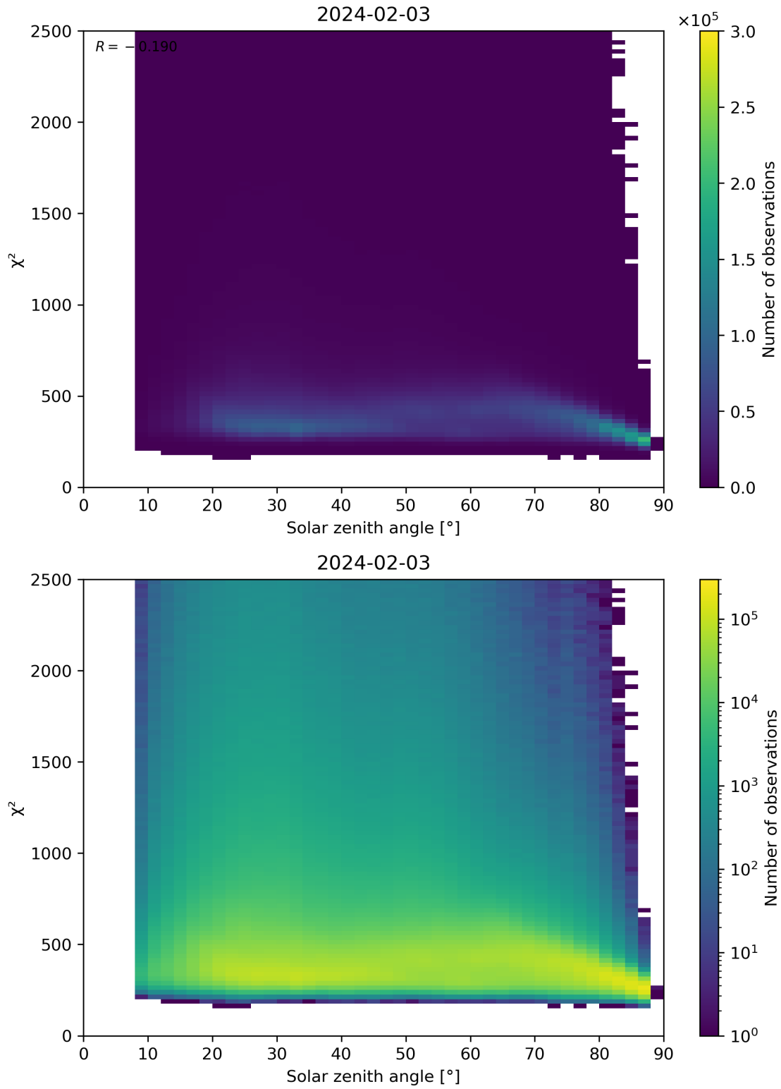
Figure 148: Scatter density plot of “Solar zenith angle” against “ \chi^2 ” for 2024-02-02 to 2024-02-04.
