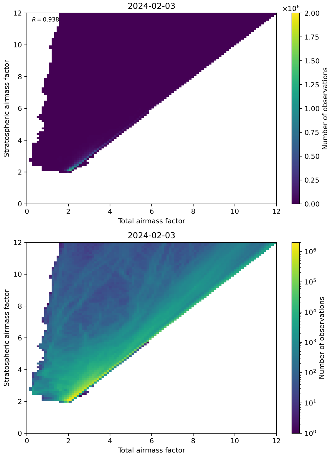
Figure 62: Scatter density plot of “Total airmass factor” against “Stratospheric airmass factor” for 2024-02-02 to 2024-02-04.
