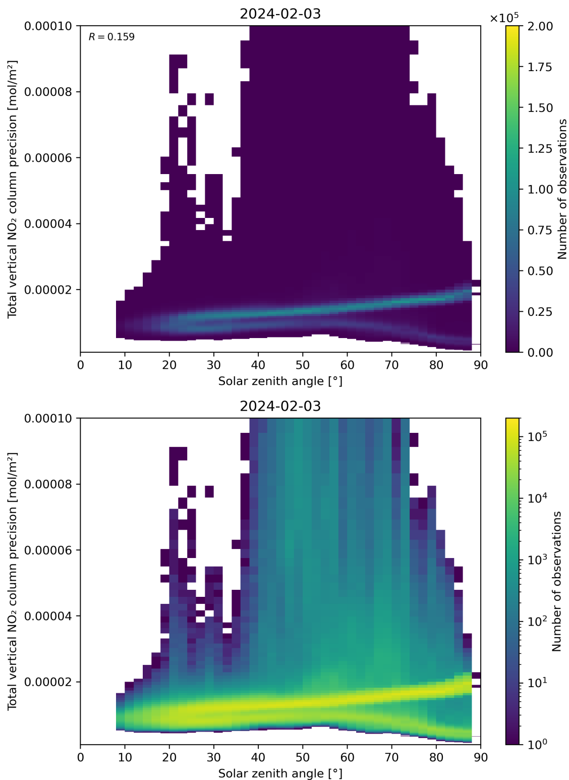
Figure 154: Scatter density plot of “Solar zenith angle” against “Total vertical NO 2 column precision” for 2024-02-02 to 2024-02-04.
