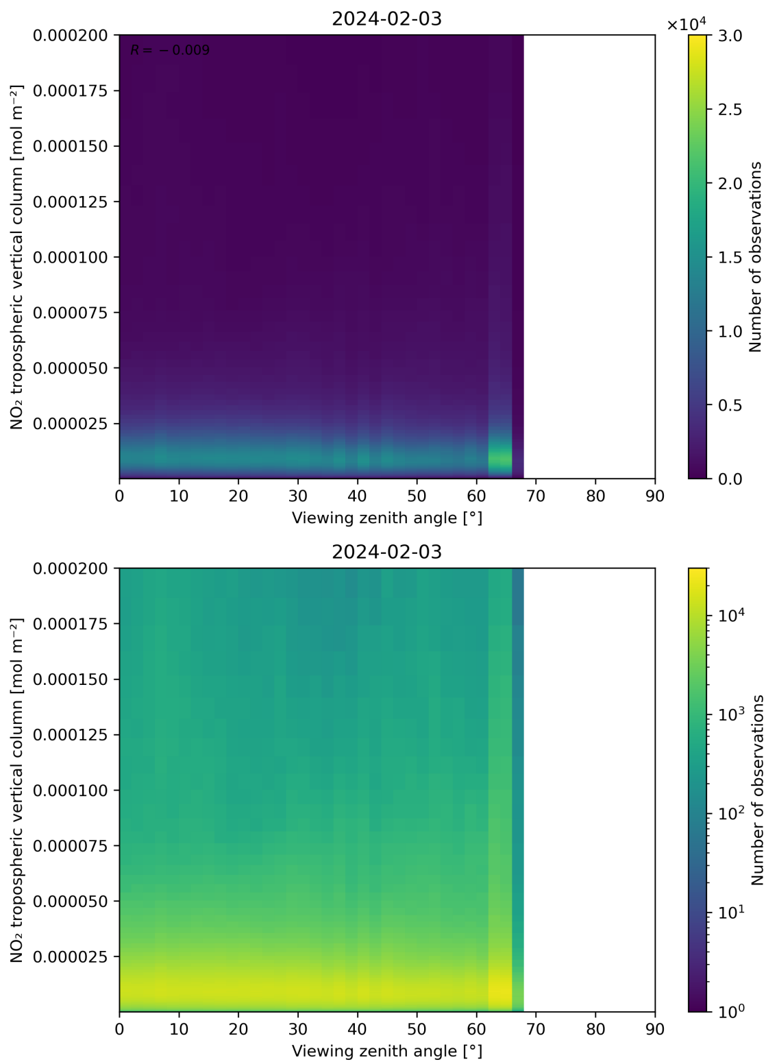
Figure 169: Scatter density plot of “Viewing zenith angle” against “NO 2 tropospheric vertical column” for 2024-02-02 to 2024-02-04.
