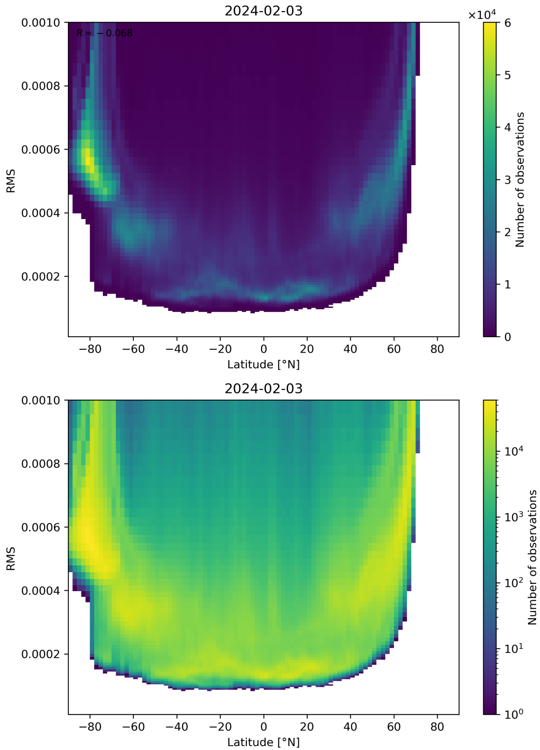
Figure 94: Scatter density plot of “Latitude” against “RMS” for 2024-02-02 to 2024-02-04.
