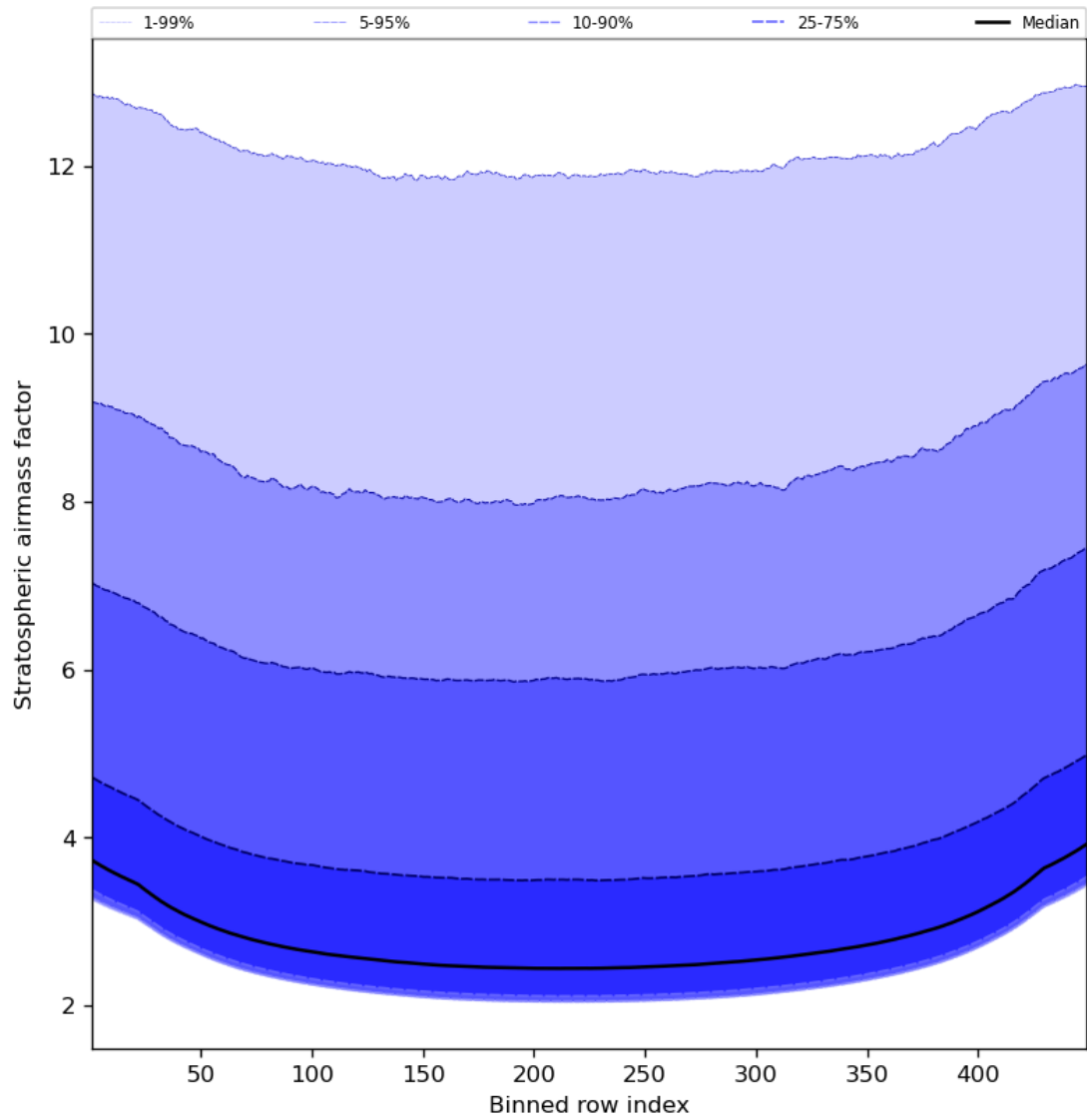
Figure 61: Along track statistics of “Stratospheric airmass factor” for 2024-02-02 to 2024-02-04
