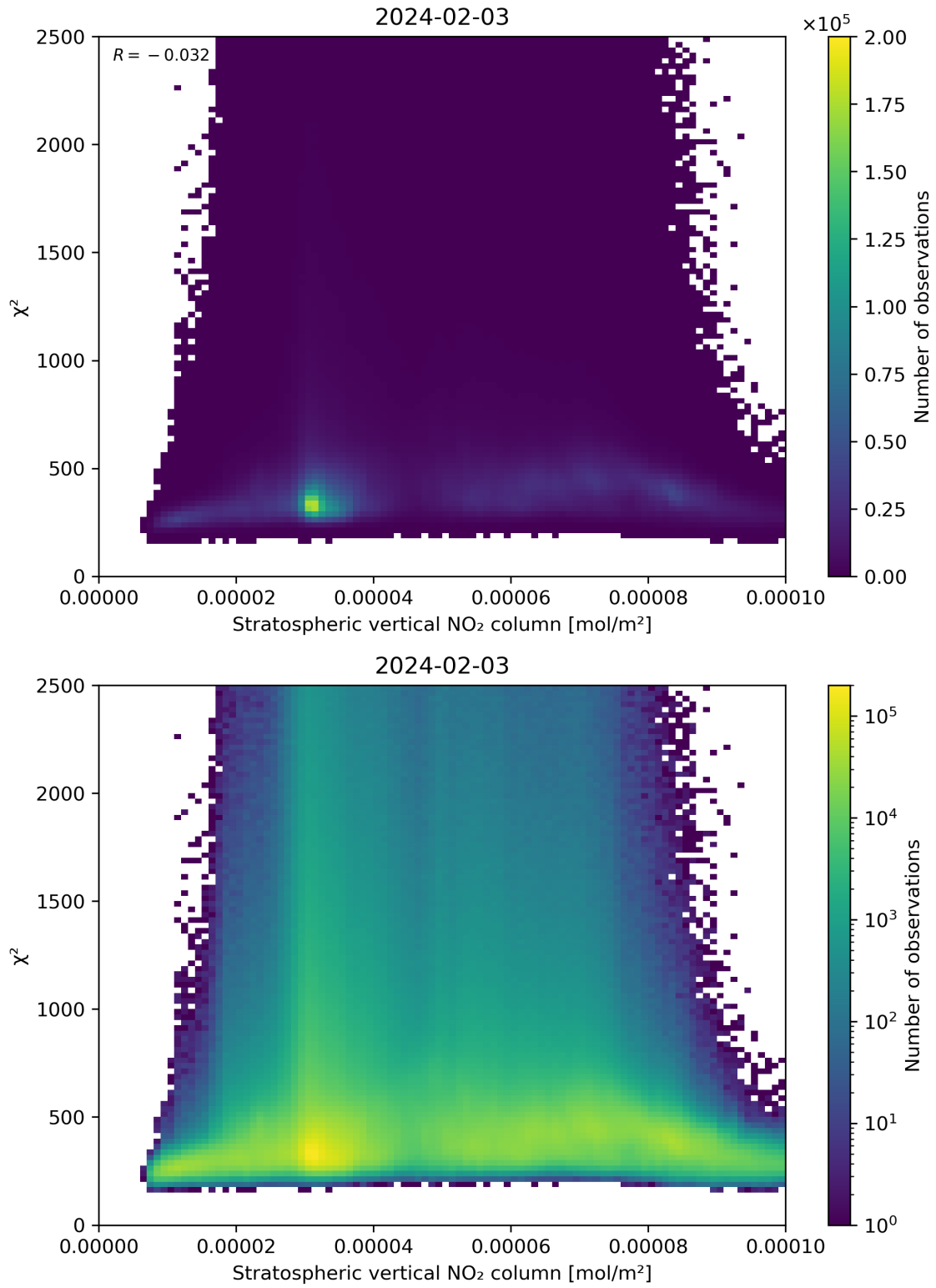
Figure 97: Scatter density plot of “Stratospheric vertical NO 2 column” against “ \chi^2 ” for 2024-02-02 to 2024-02-04.
