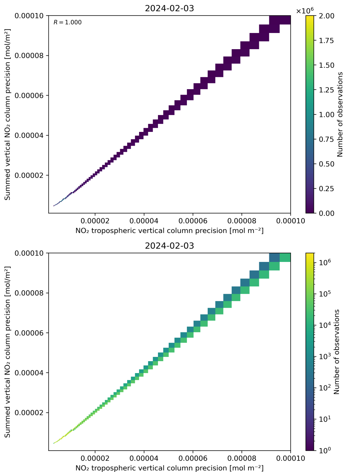
Figure 137: Scatter density plot of “NO 2 tropospheric vertical column precision” against “Summed vertical NO 2 column precision” for 2024-02-02 to 2024-02-04.
