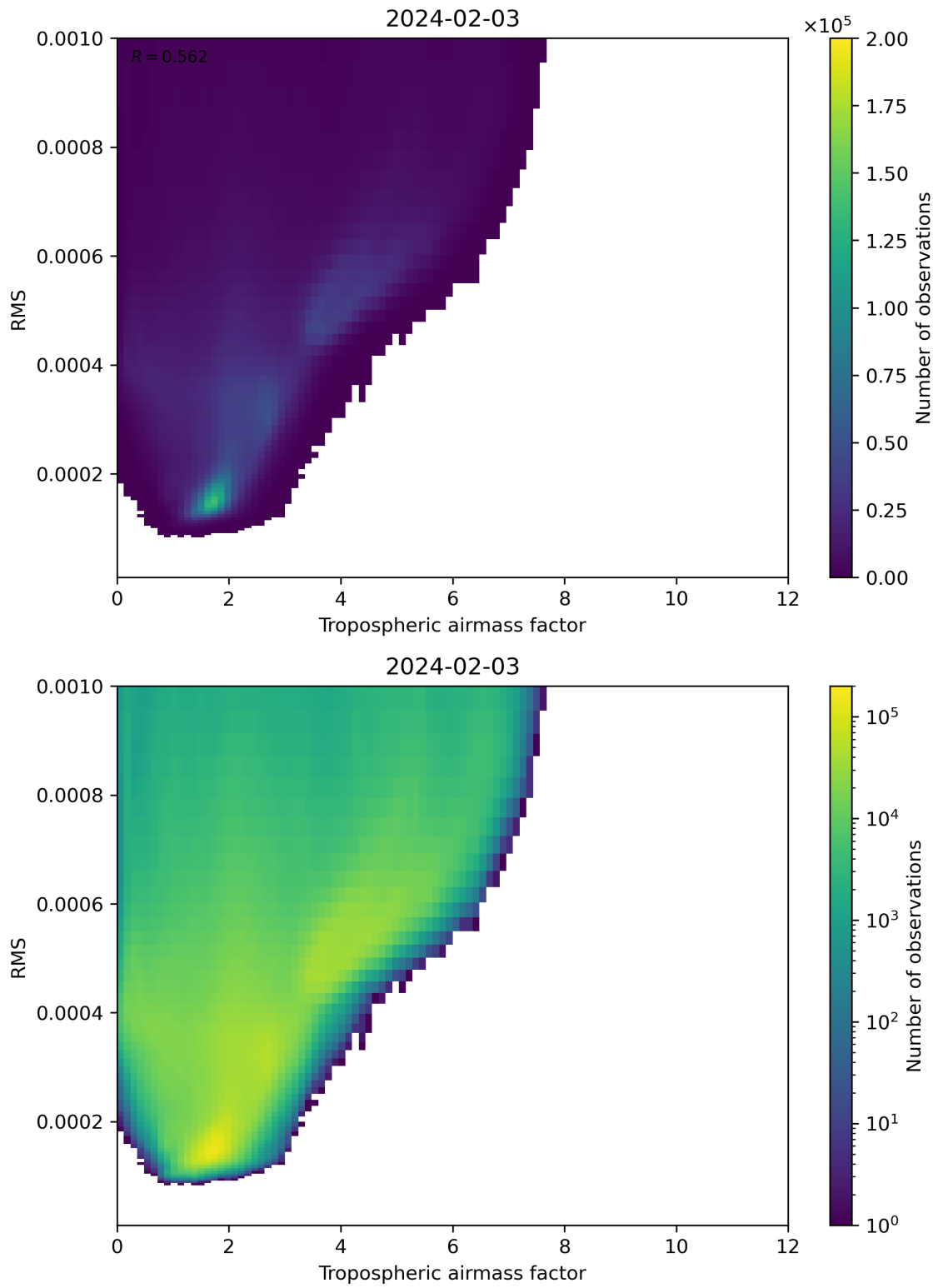
Figure 79: Scatter density plot of “Tropospheric airmass factor” against “RMS” for 2024-02-02 to 2024-02-04.
