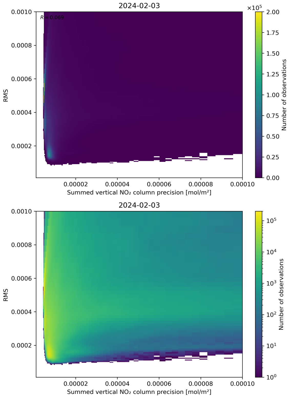
Figure 108: Scatter density plot of “Summed vertical NO 2 column precision” against “RMS” for 2024-02-02 to 2024-02-04.
