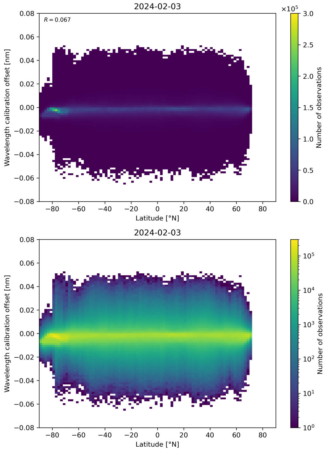
Figure 95: Scatter density plot of “Latitude” against “Wavelength calibration offset” for 2024-02-02 to 2024-02-04.
