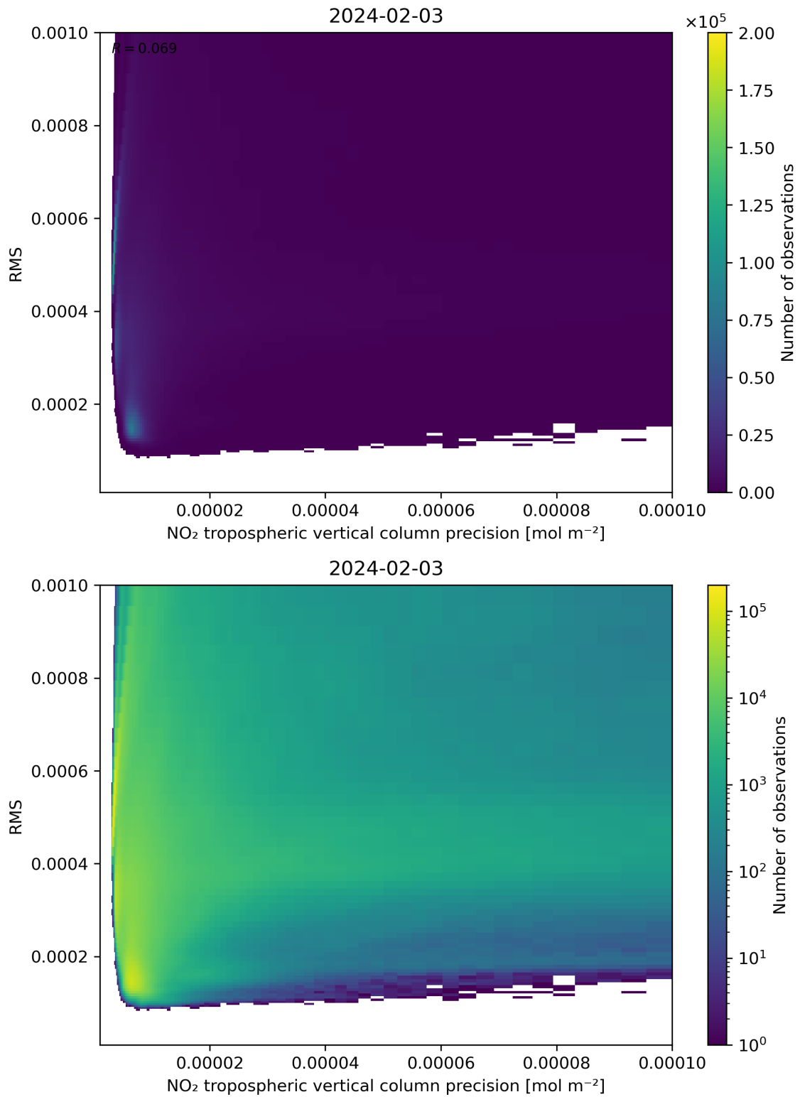
Figure 140: Scatter density plot of “NO 2 tropospheric vertical column precision” against “RMS” for 2024-02-02 to 2024-02-04.
