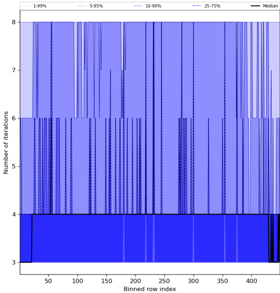
Figure 51: Along track statistics of “Number of iterations” for 2024-02-02 to 2024-02-04
