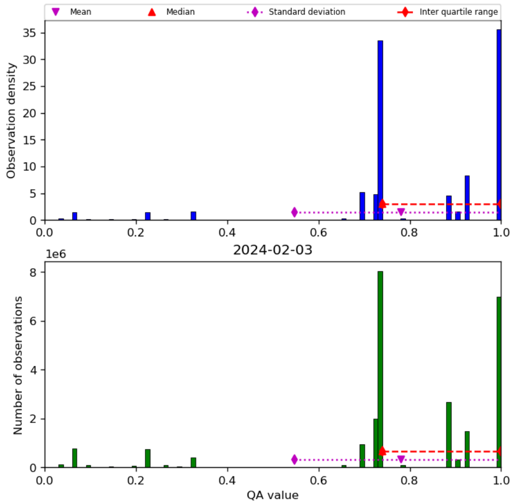
Figure 28: Histogram of “QA value” for 2024-02-02 to 2024-02-04
