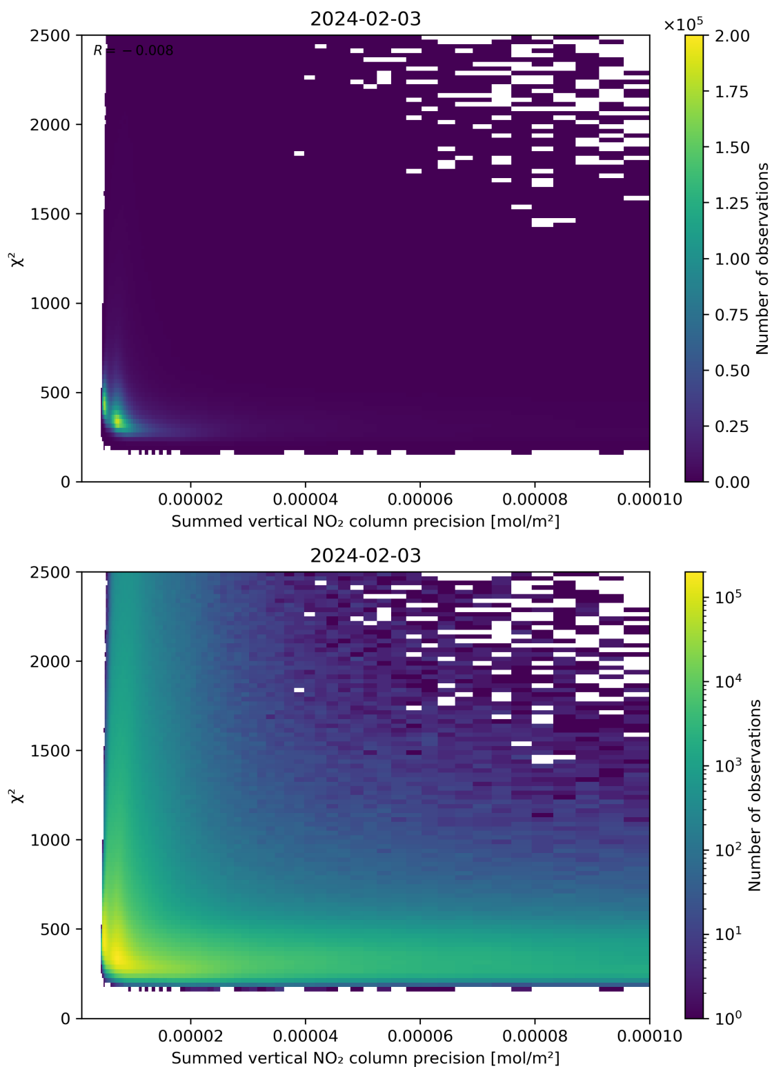
Figure 107: Scatter density plot of “Summed vertical NO 2 column precision” against “ \chi^2 ” for 2024-02-02 to 2024-02-04.
