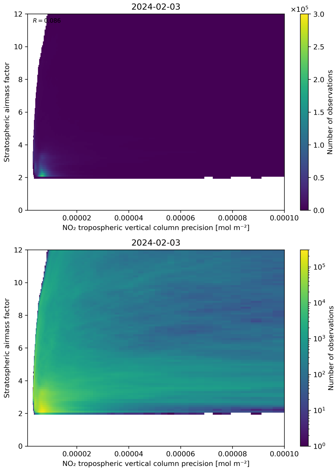
Figure 131: Scatter density plot of “NO 2 tropospheric vertical column precision” against “Stratospheric airmass factor” for 2024-02-02 to 2024-02-04.
