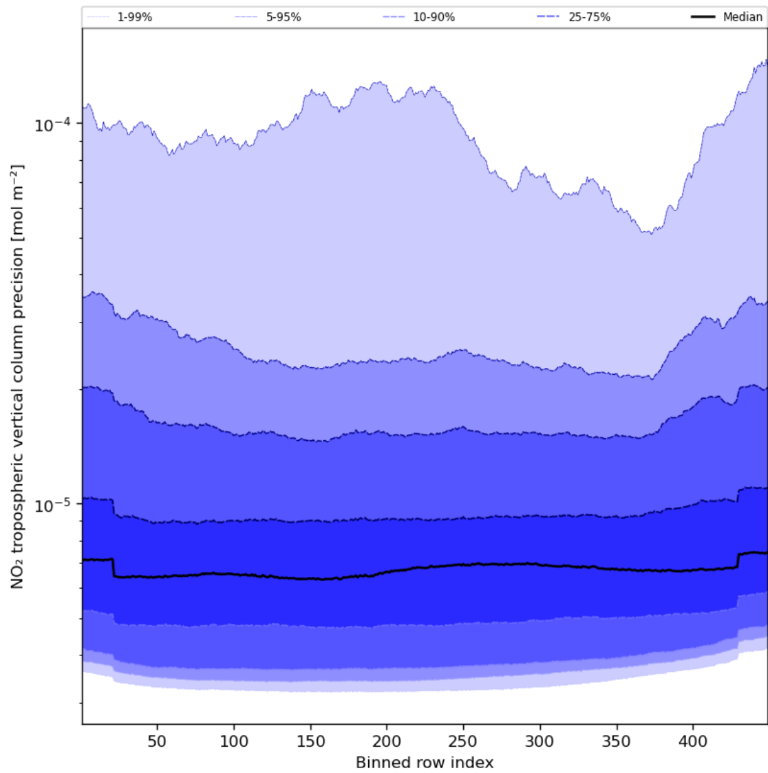
Figure 47: Along track statistics of “NO 2 tropospheric vertical column precision” for 2024-02-02 to 2024-02-04
