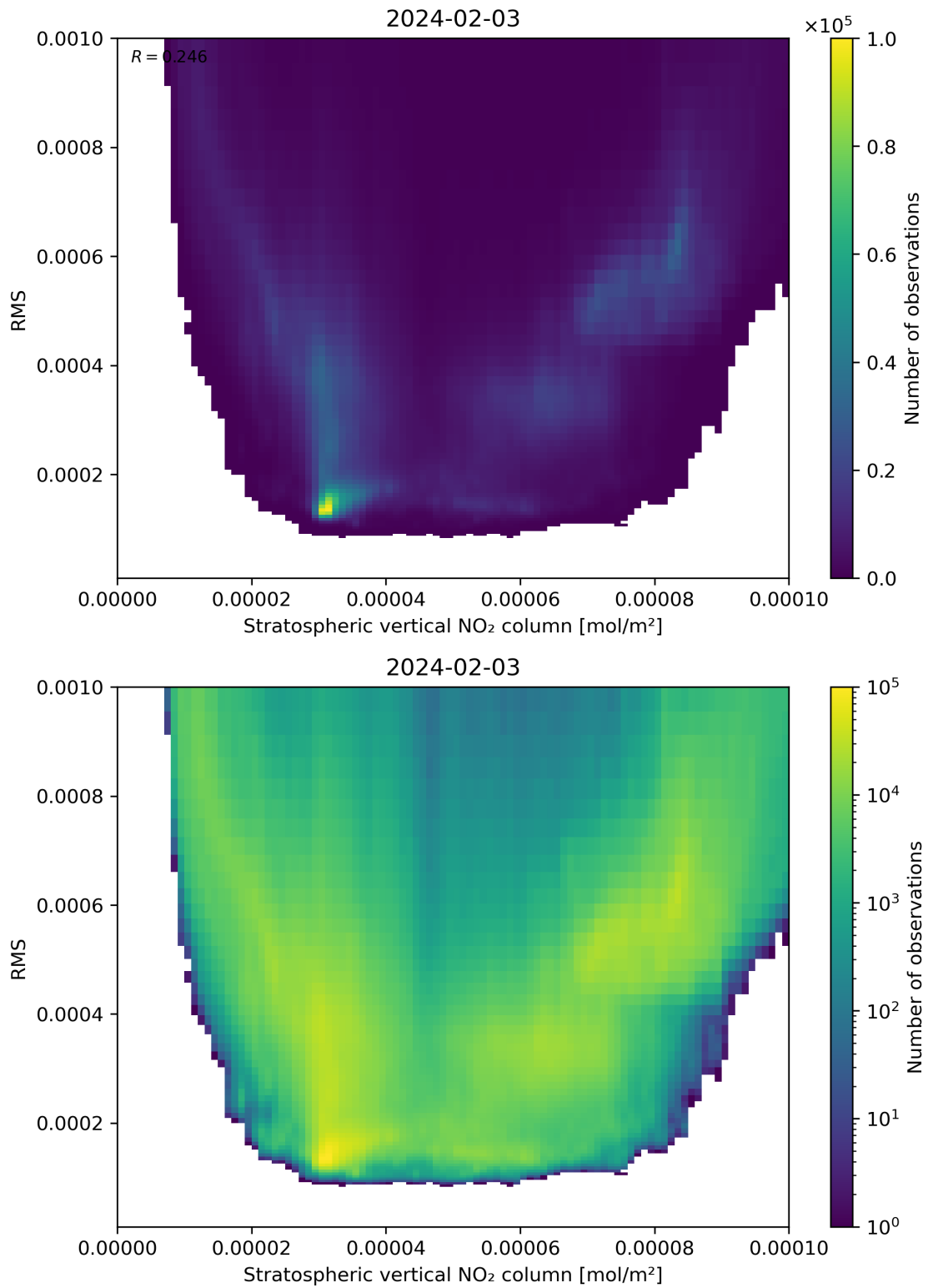
Figure 102: Scatter density plot of “Stratospheric vertical NO 2 column” against “RMS” for 2024-02-02 to 2024-02-04.
