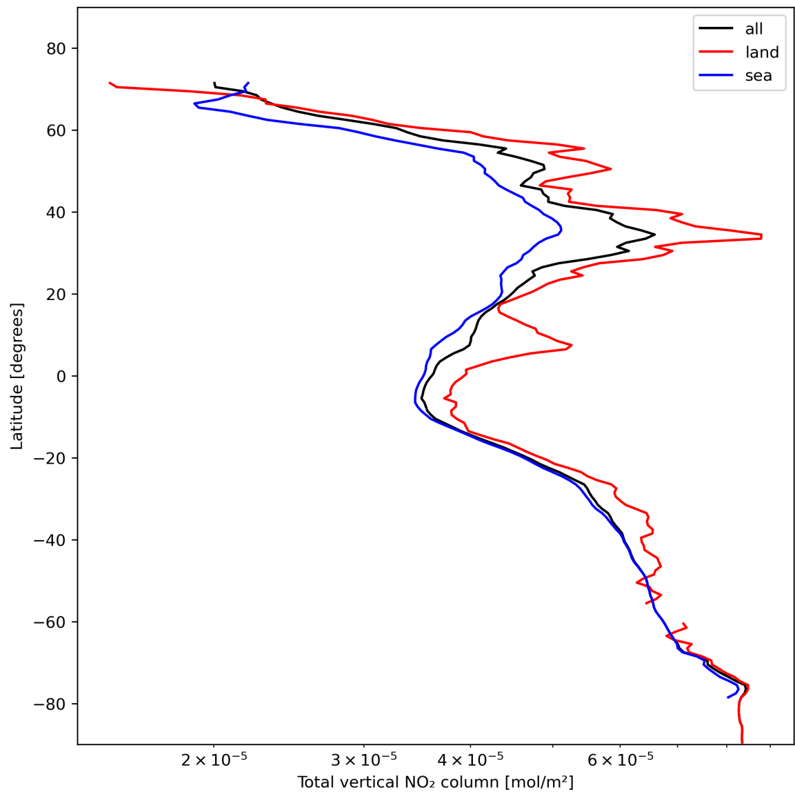
Figure 21: Zonal average of “Total vertical NO 2 column” for 2024-02-02 to 2024-02-04.
