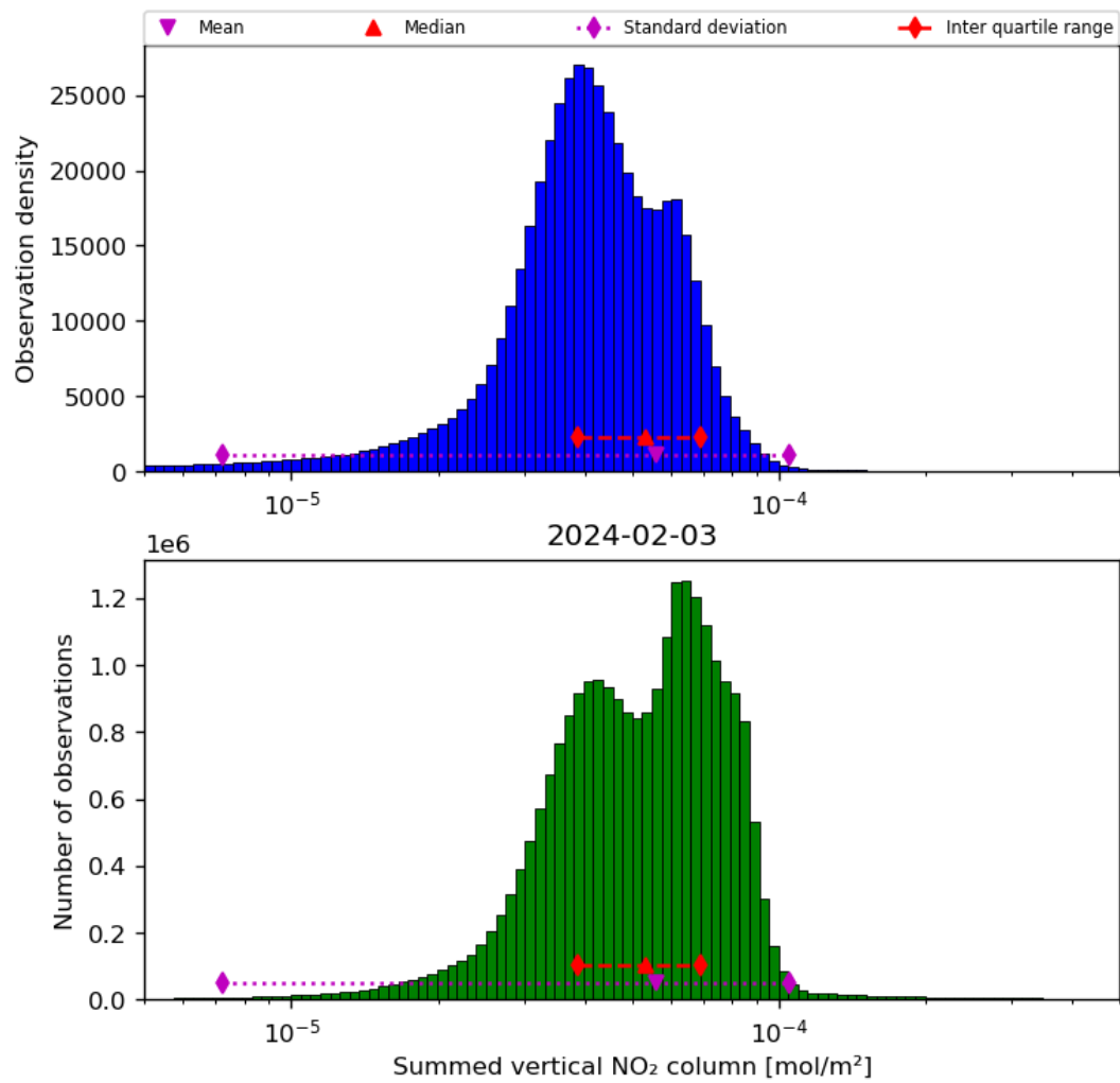
Figure 40: Histogram of “Summed vertical NO 2 column” for 2024-02-02 to 2024-02-04
