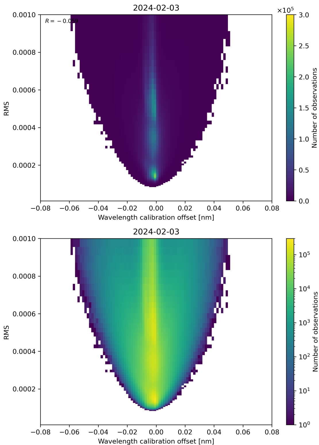
Figure 181: Scatter density plot of “Wavelength calibration offset” against “RMS” for 2024-02-02 to 2024-02-04.
