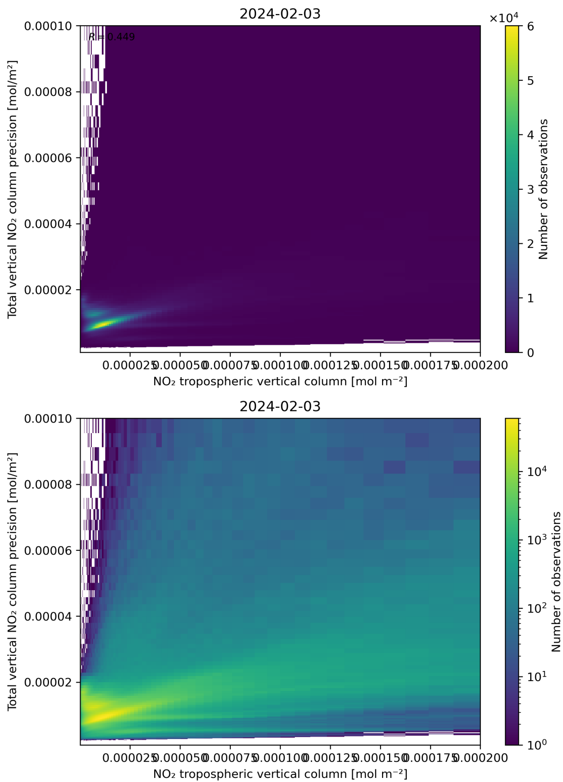
Figure 129: Scatter density plot of “NO 2 tropospheric vertical column” against “Total vertical NO 2 column precision” for 2024-02-02 to 2024-02-04.
