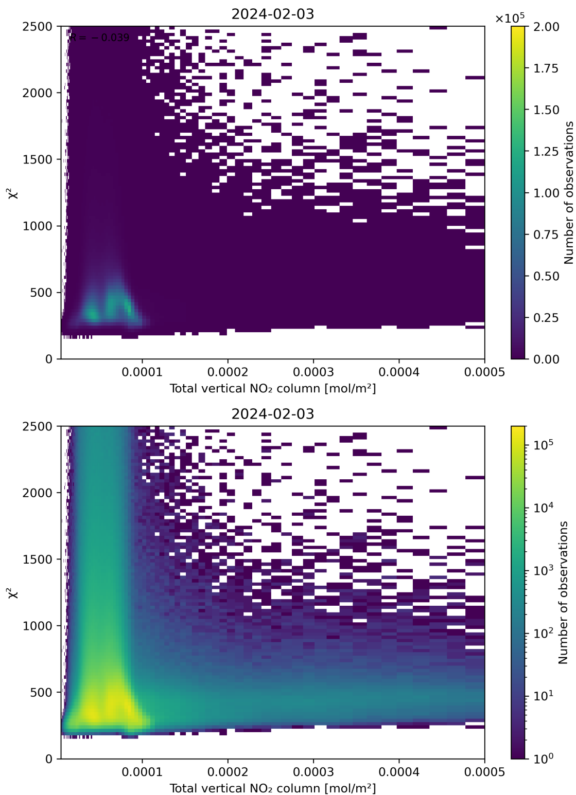
Figure 111: Scatter density plot of “Total vertical NO 2 column” against “ \chi^2 ” for 2024-02-02 to 2024-02-04.
