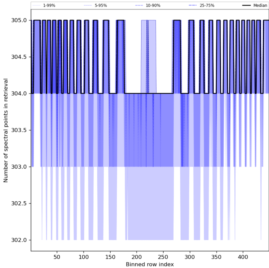
Figure 50: Along track statistics of “Number of spectral points in retrieval” for 2024-02-02 to 2024-02-04
