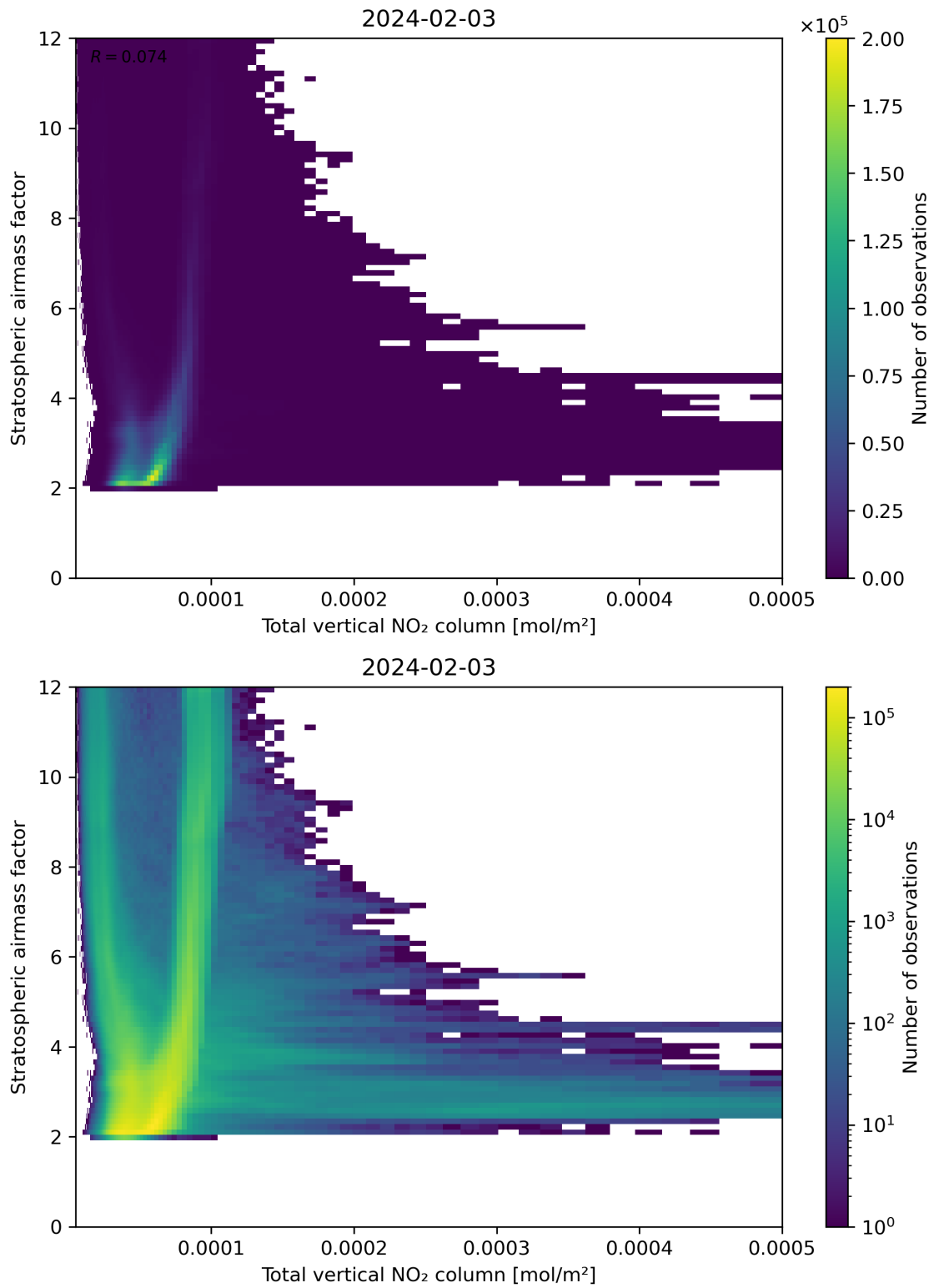
Figure 110: Scatter density plot of “Total vertical NO 2 column” against “Stratospheric airmass factor” for 2024-02-02 to 2024-02-04.
