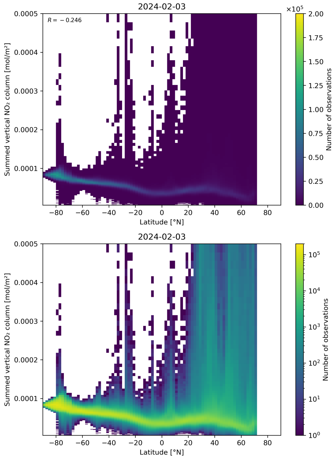
Figure 88: Scatter density plot of “Latitude” against “Summed vertical NO 2 column” for 2024-02-02 to 2024-02-04.
