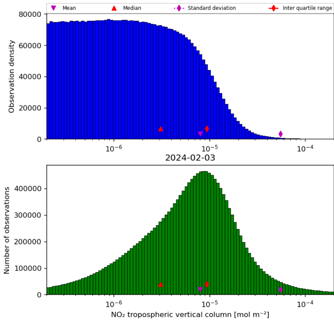
Figure 29: Histogram of “NO 2 tropospheric vertical column” for 2024-02-02 to 2024-02-04
