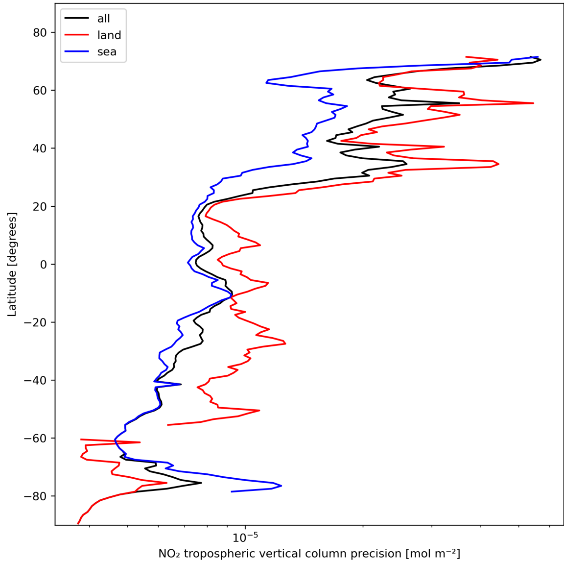
Figure 13: Zonal average of “NO 2 tropospheric vertical column precision” for 2024-02-02 to 2024-02-04.
