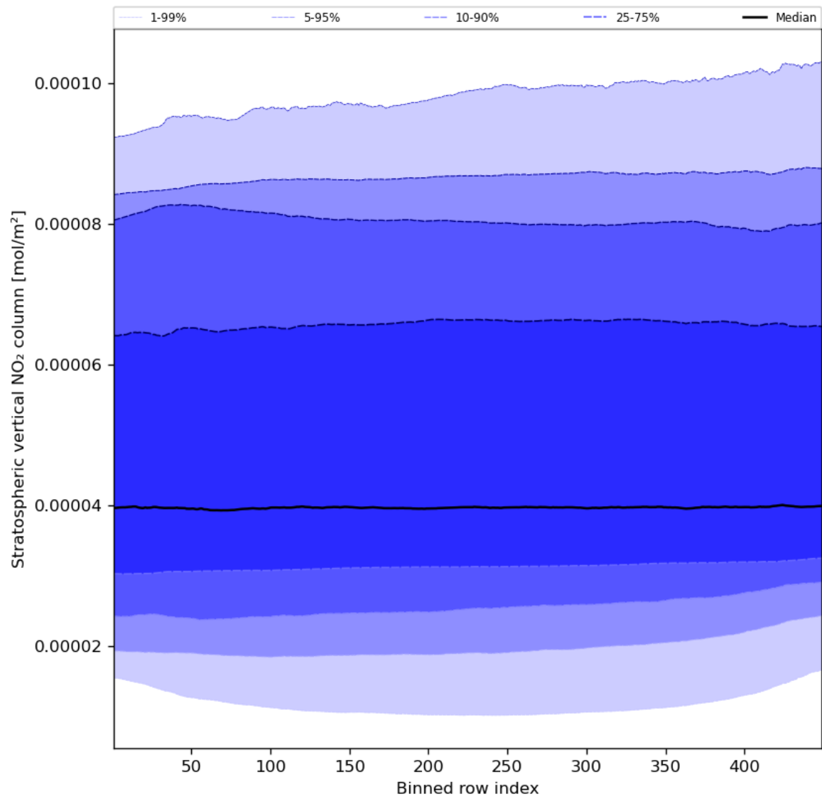
Figure 53: Along track statistics of “Stratospheric vertical NO 2 column” for 2024-02-02 to 2024-02-04
