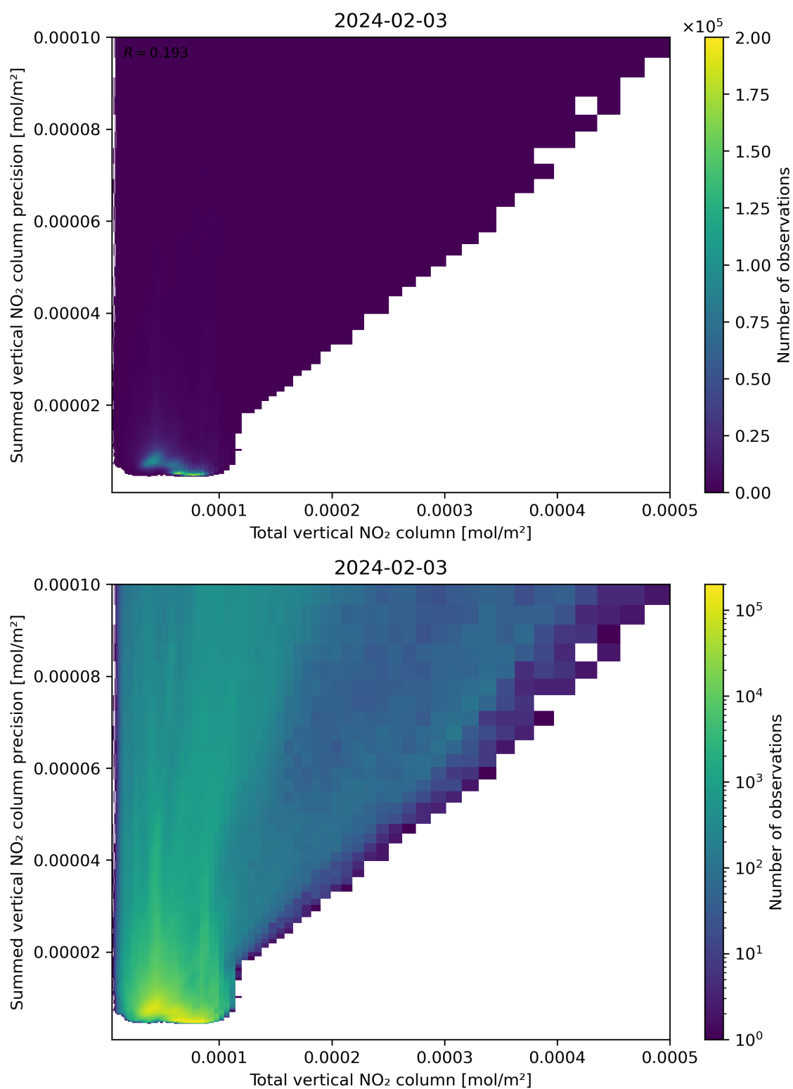
Figure 113: Scatter density plot of “Total vertical NO 2 column” against “Summed vertical NO 2 column precision” for 2024-02-02 to 2024-02-04.
