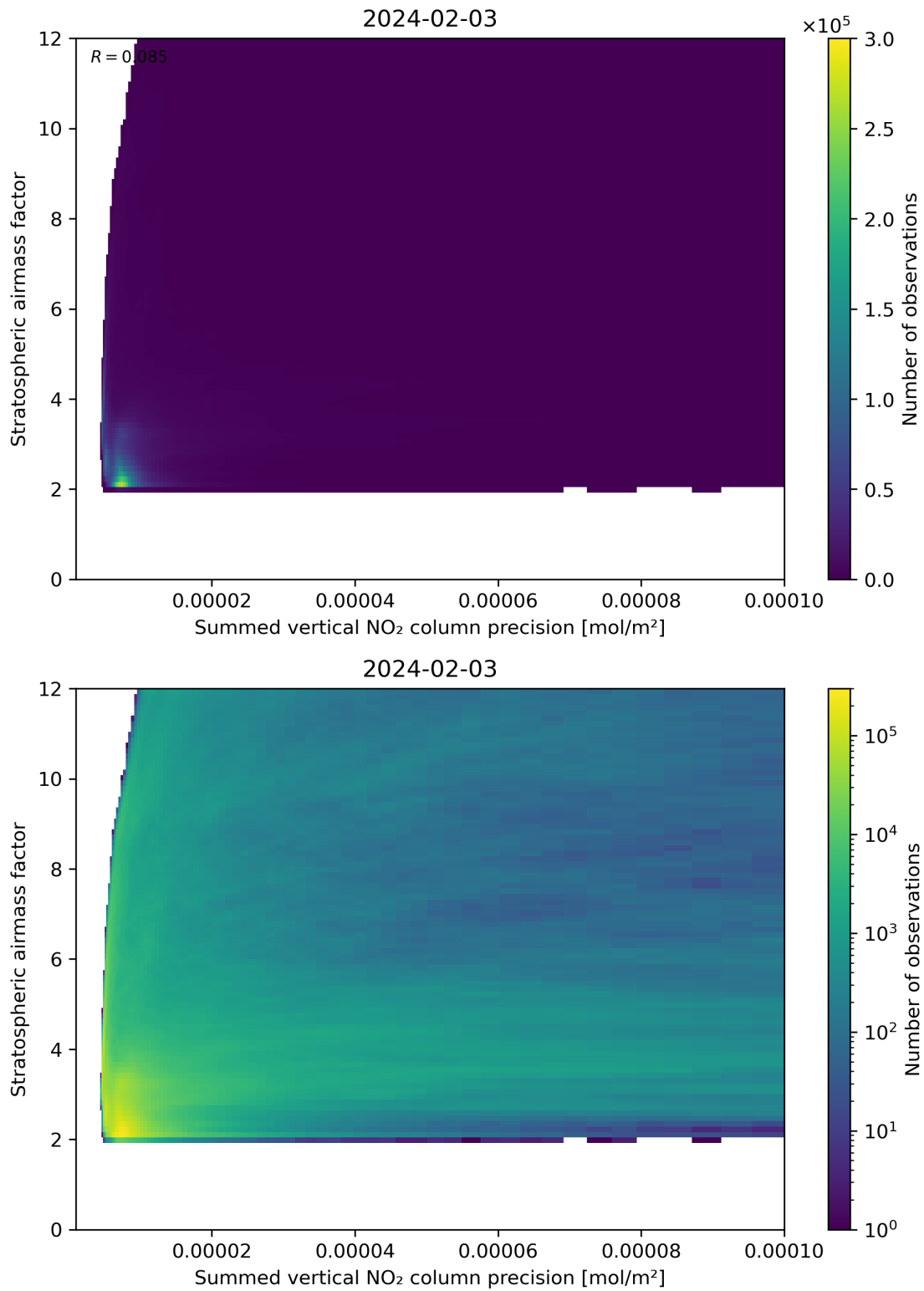
Figure 106: Scatter density plot of “Summed vertical NO 2 column precision” against “Stratospheric airmass factor” for 2024-02-02 to 2024-02-04.
