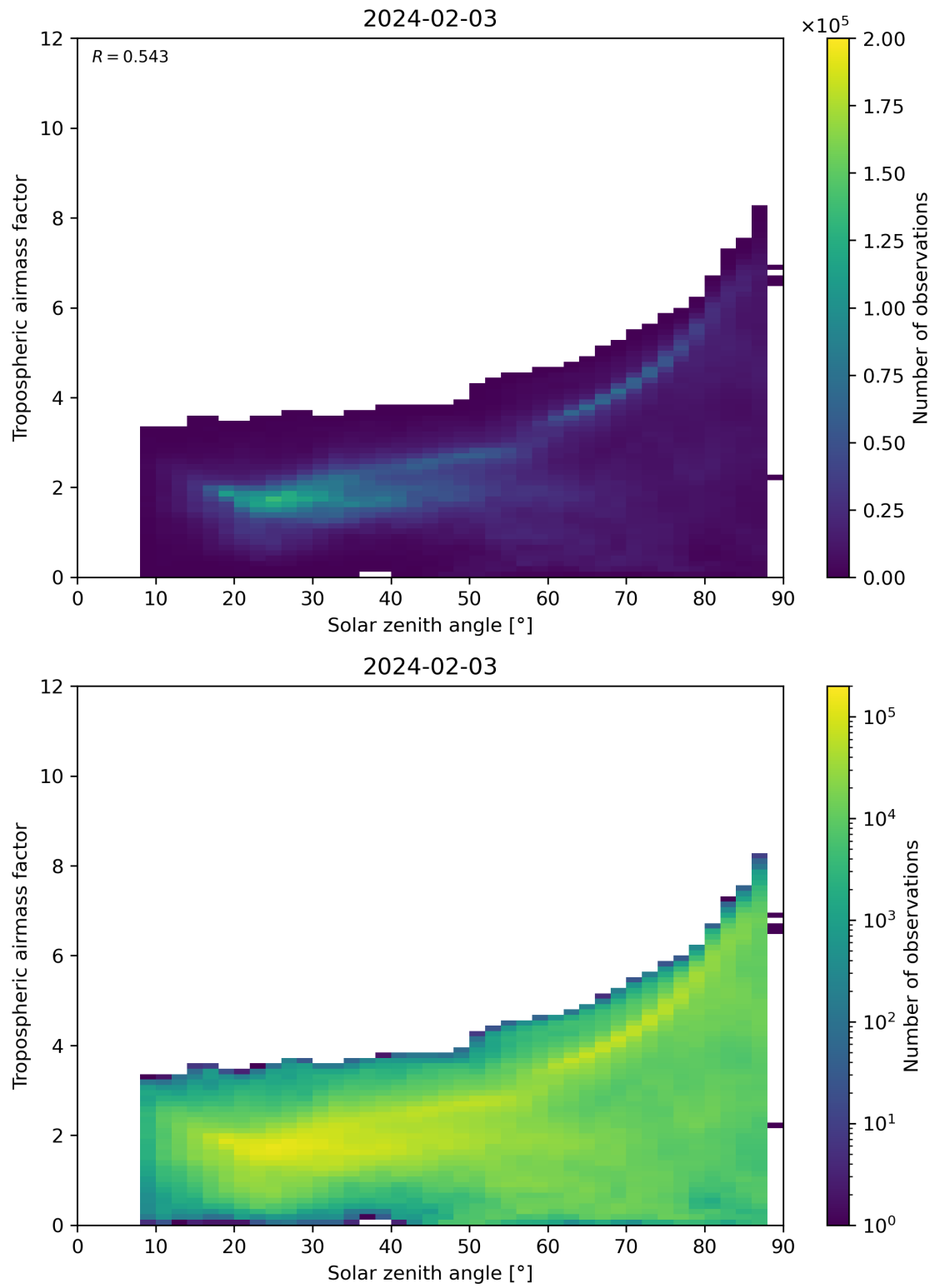
Figure 147: Scatter density plot of “Solar zenith angle” against “Tropospheric airmass factor” for 2024-02-02 to 2024-02-04.
