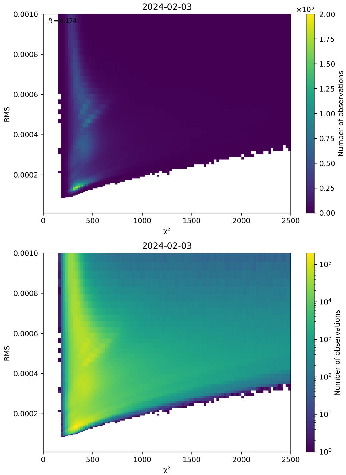
Figure 82: Scatter density plot of “ \chi^2 ” against “RMS” for 2024-02-02 to 2024-02-04.
