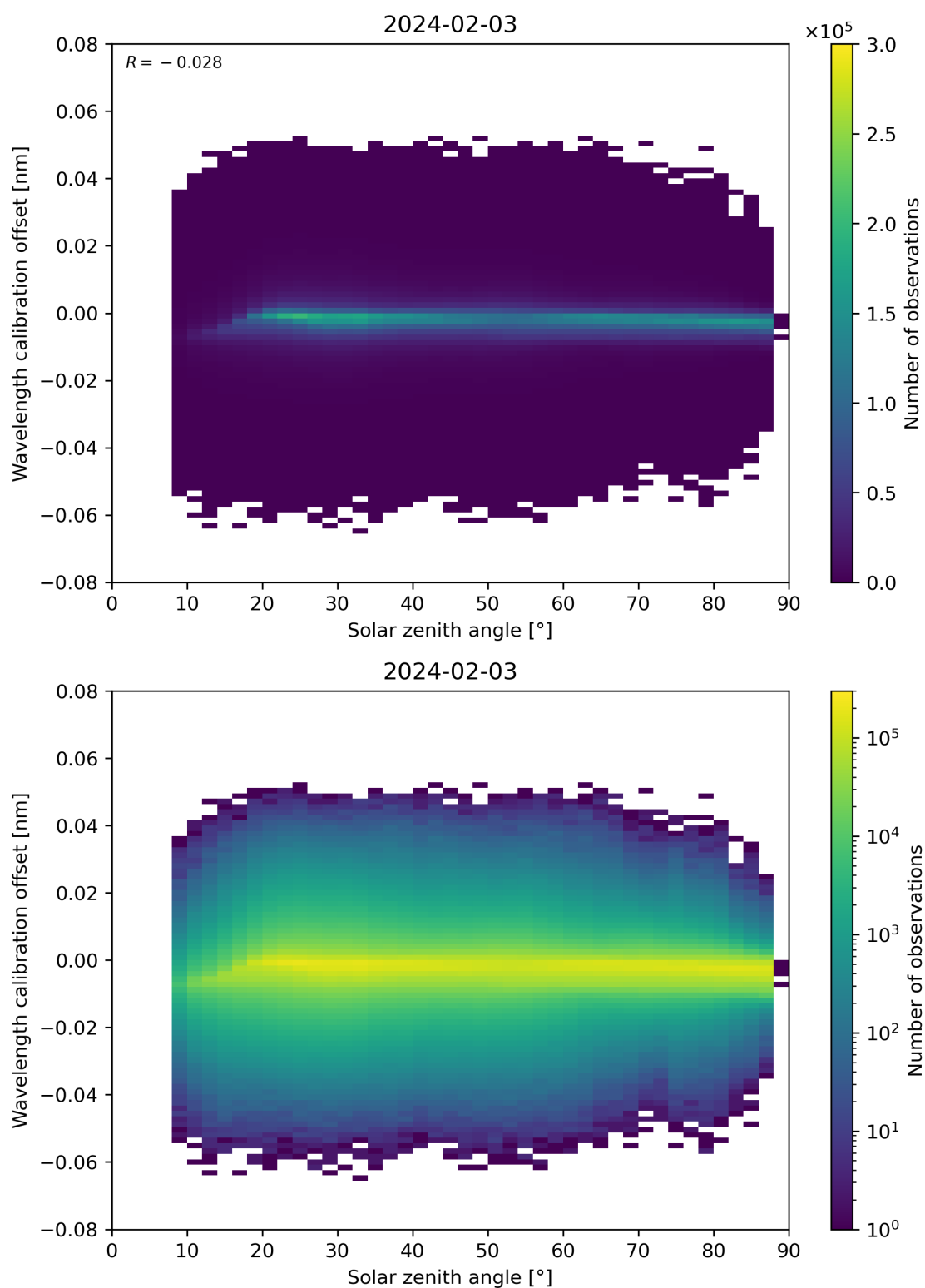
Figure 158: Scatter density plot of “Solar zenith angle” against “Wavelength calibration offset” for 2024-02-02 to 2024-02-04.
