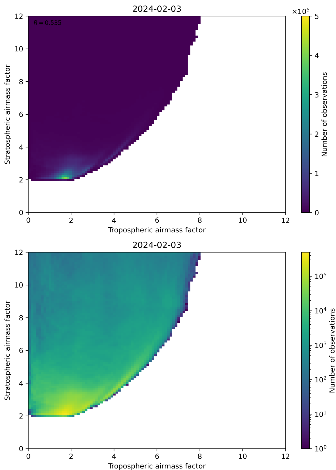
Figure 71: Scatter density plot of “Tropospheric airmass factor” against “Stratospheric airmass factor” for 2024-02-02 to 2024-02-04.
