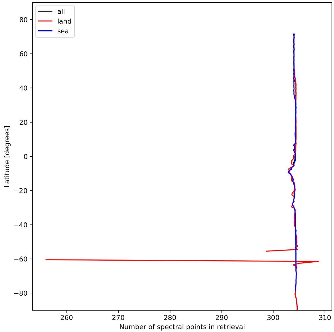
Figure 16: Zonal average of “Number of spectral points in retrieval” for 2024-02-02 to 2024-02-04.
