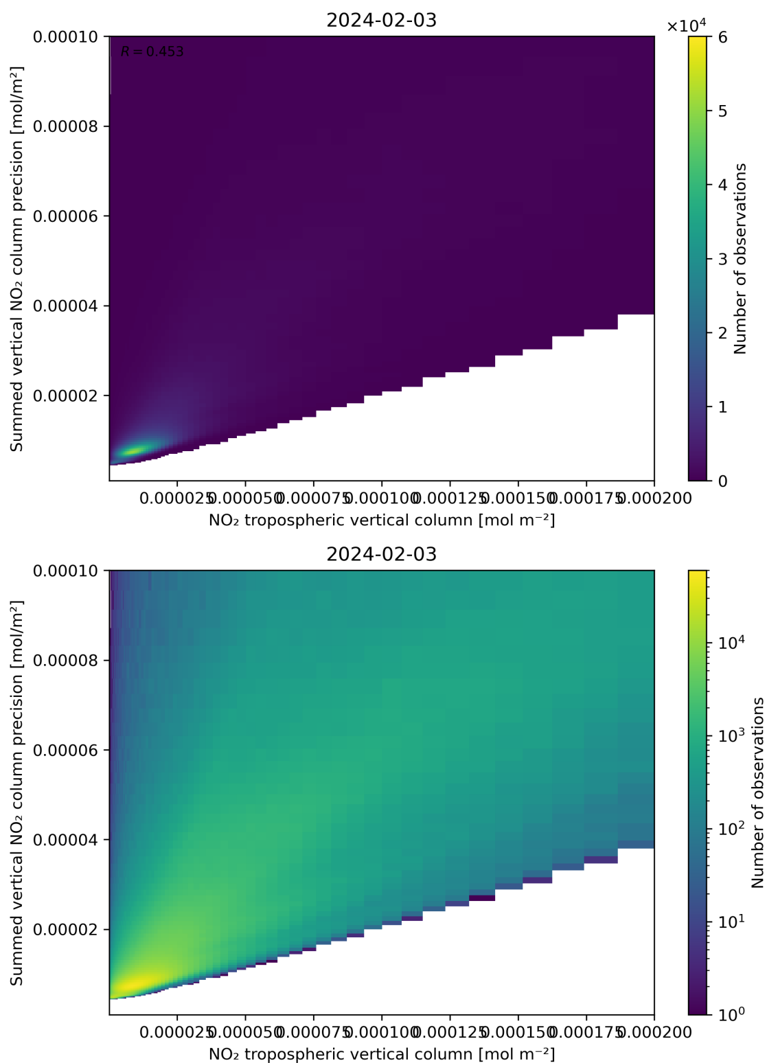
Figure 127: Scatter density plot of “NO 2 tropospheric vertical column” against “Summed vertical NO 2 column precision” for 2024-02-02 to 2024-02-04.
