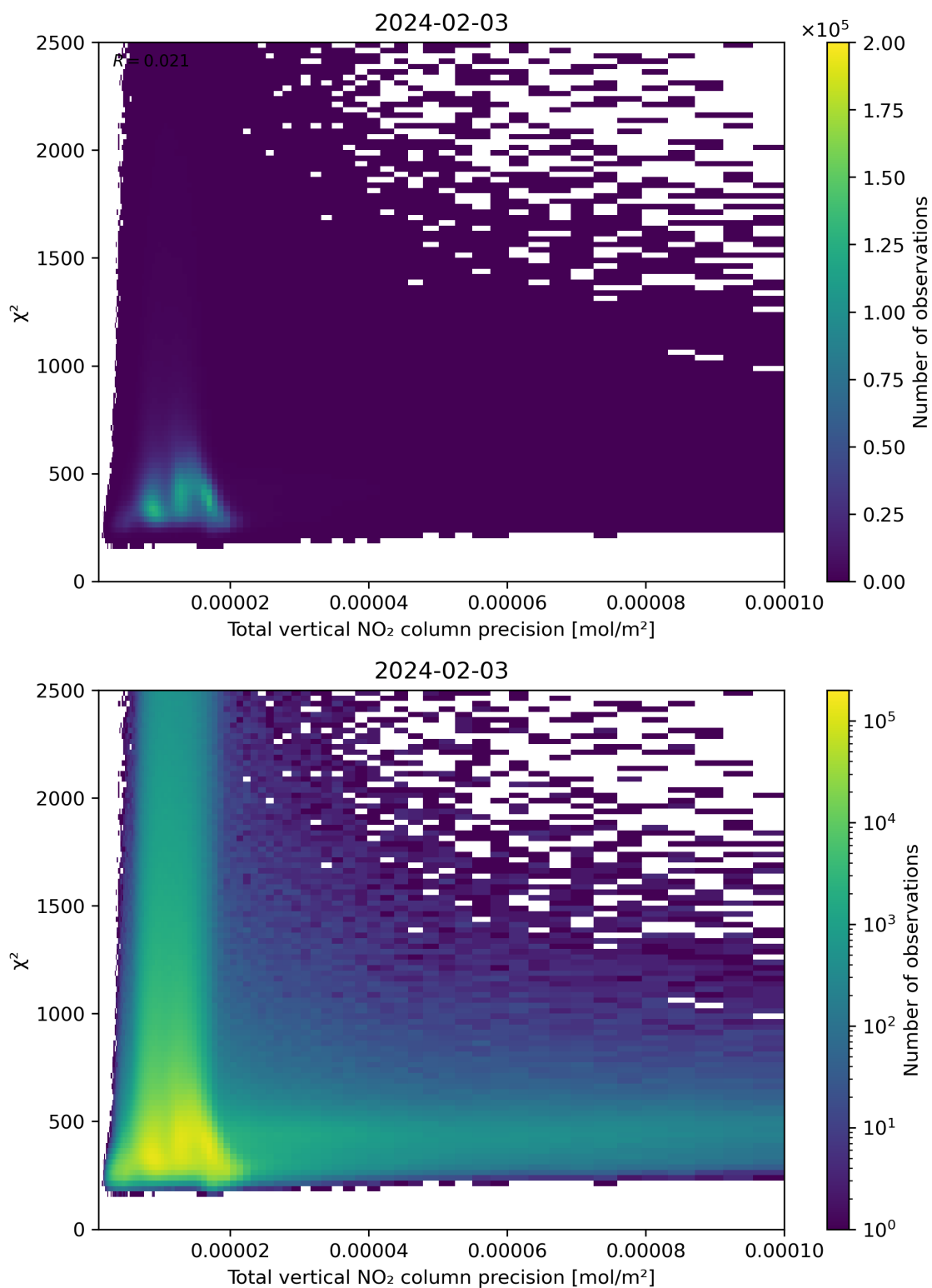
Figure 116: Scatter density plot of "Total vertical NO 2 column precision" against " \chi^2 " for 2024-02-02 to 2024-02-04.
