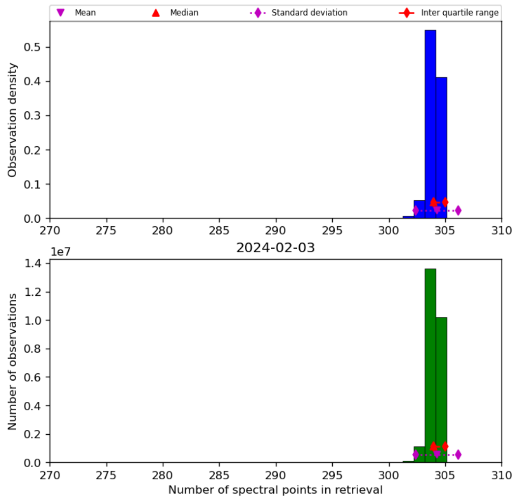
Figure 33: Histogram of “Number of spectral points in retrieval” for 2024-02-02 to 2024-02-04
