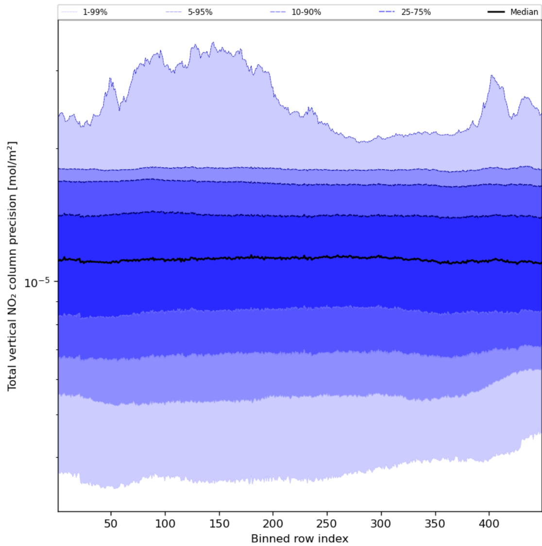
Figure 56: Along track statistics of “Total vertical NO 2 column precision” for 2024-02-02 to 2024-02-04
