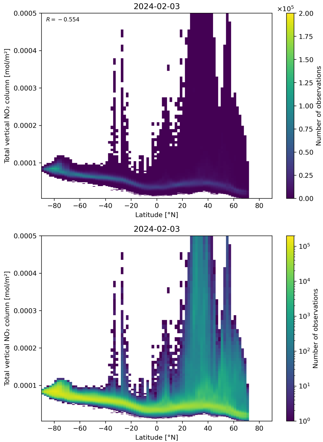
Figure 90: Scatter density plot of “Latitude” against “Total vertical NO 2 column” for 2024-02-02 to 2024-02-04.
