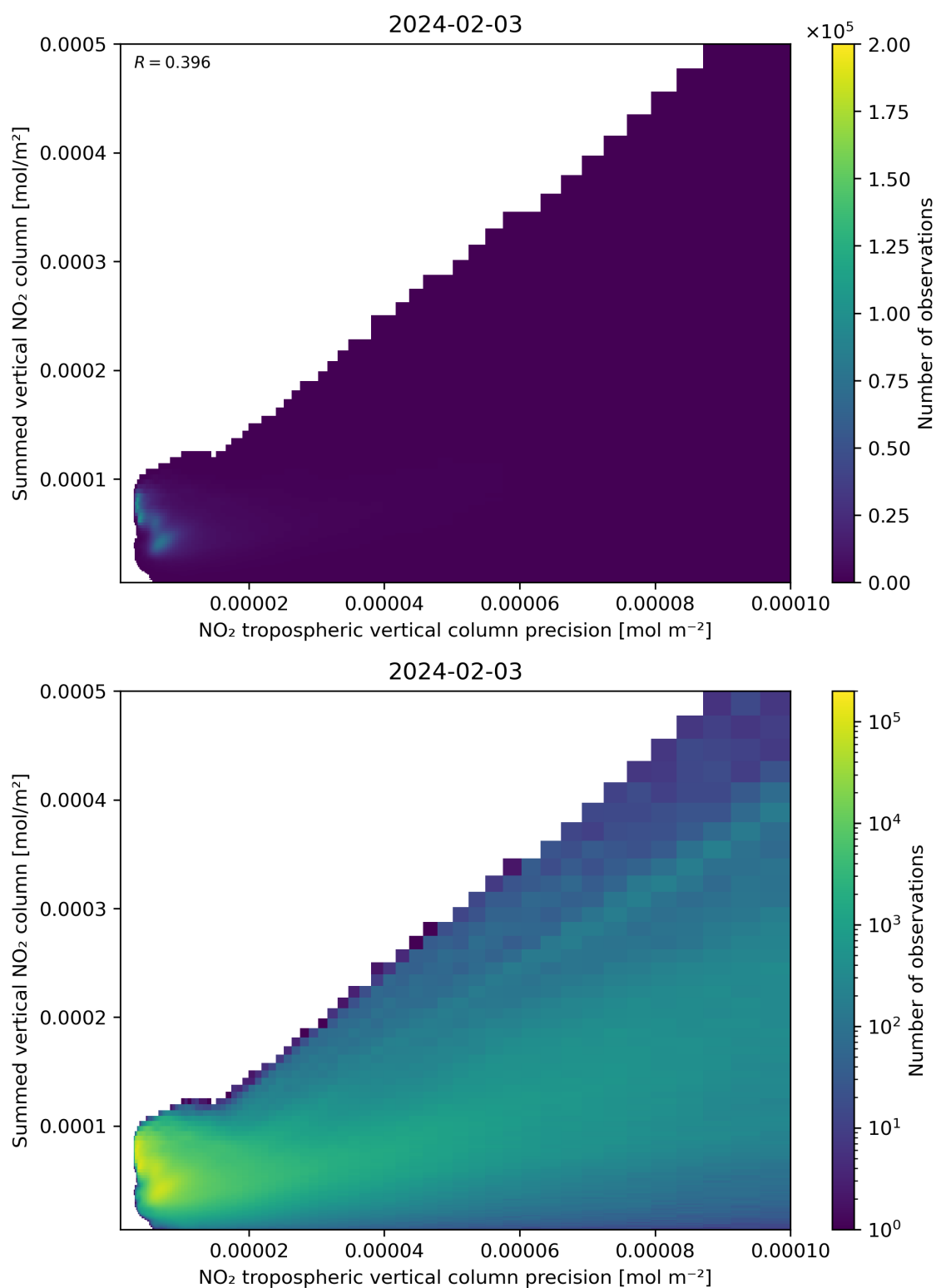
Figure 136: Scatter density plot of “NO 2 tropospheric vertical column precision” against “Summed vertical NO 2 column” for 2024-02-02 to 2024-02-04.
