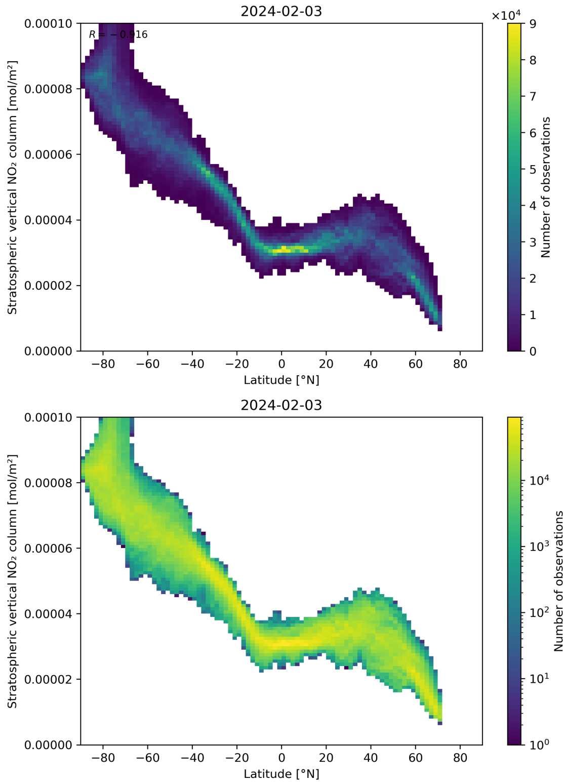
Figure 87: Scatter density plot of “Latitude” against “Stratospheric vertical NO 2 column” for 2024-02-02 to 2024-02-04.
