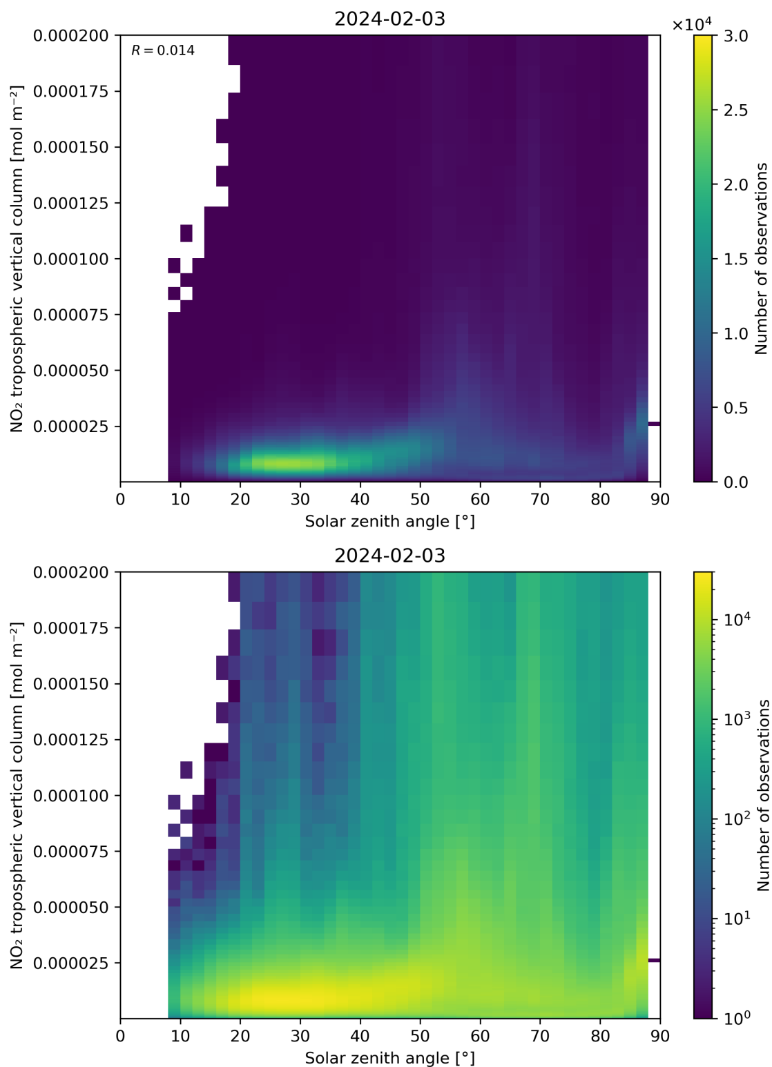
Figure 155: Scatter density plot of “Solar zenith angle” against “NO 2 tropospheric vertical column” for 2024-02-02 to 2024-02-04.
