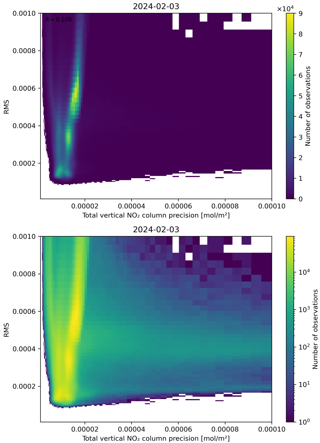
Figure 119: Scatter density plot of “Total vertical NO 2 column precision” against “RMS” for 2024-02-02 to 2024-02-04.
