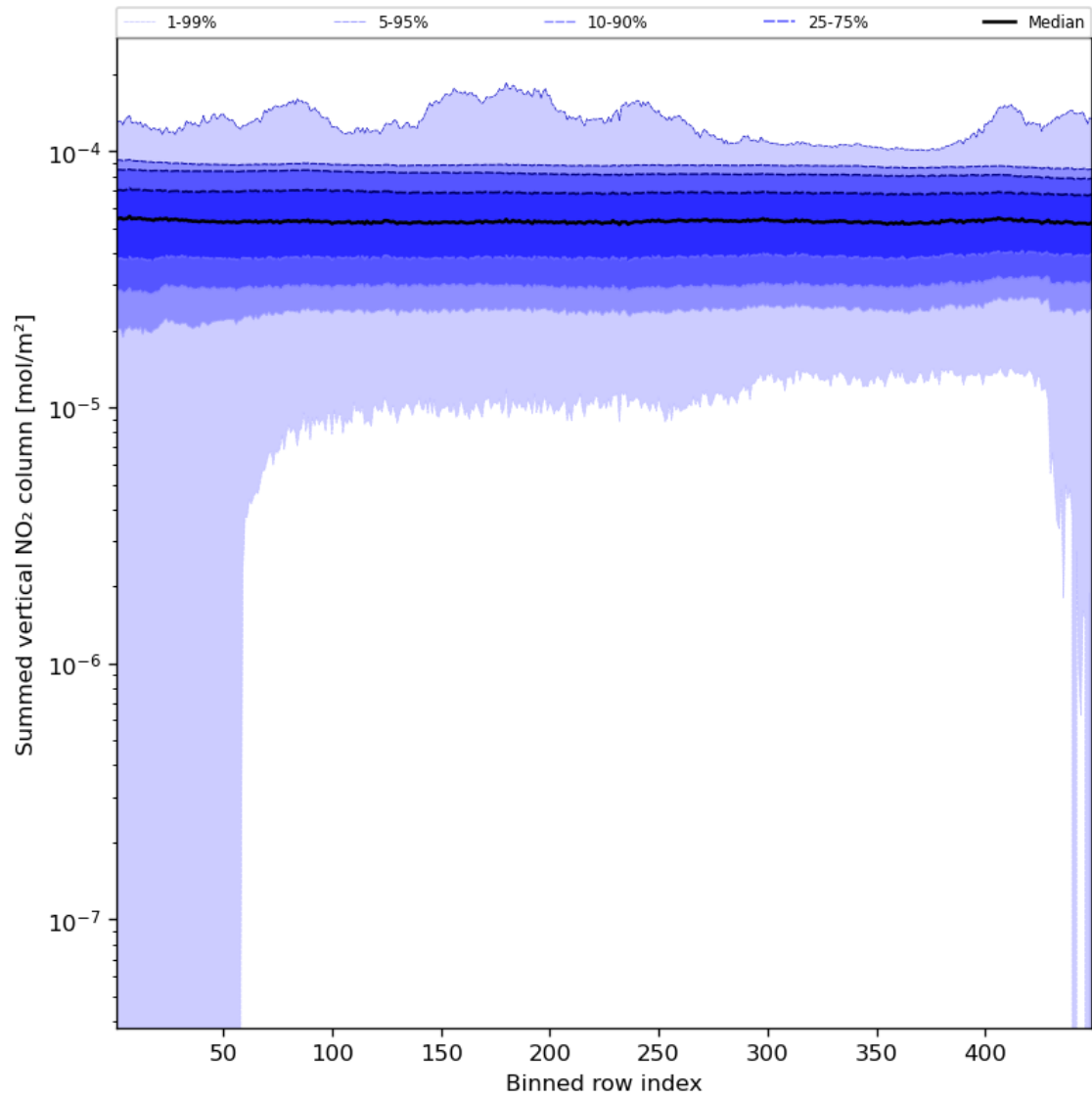
Figure 57: Along track statistics of “Summed vertical NO 2 column” for 2024-02-02 to 2024-02-04
