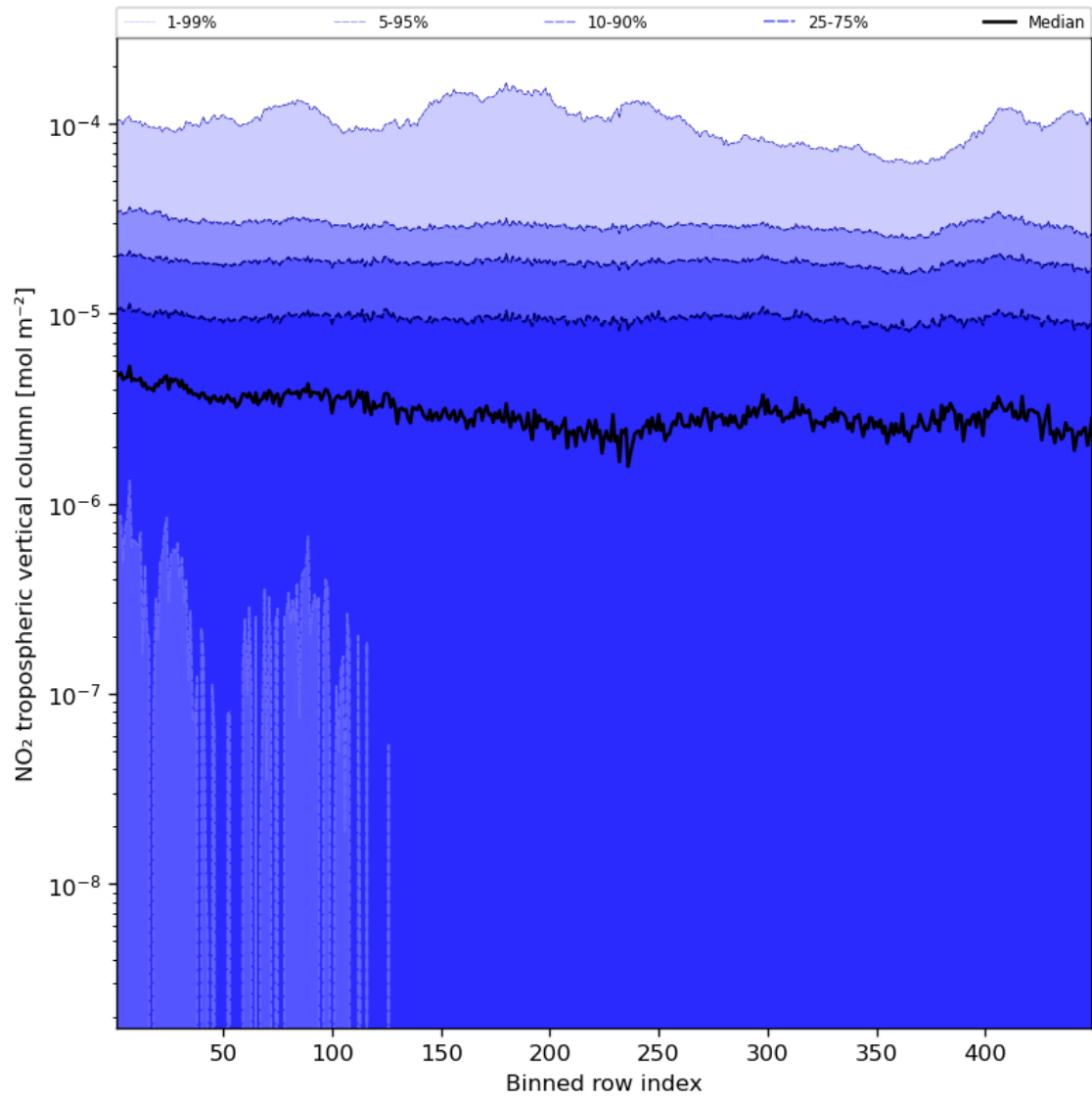
Figure 46: Along track statistics of “NO 2 tropospheric vertical column” for 2024-02-02 to 2024-02-04
