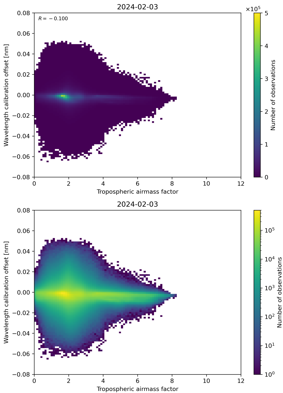
Figure 80: Scatter density plot of “Tropospheric airmass factor” against “Wavelength calibration offset” for 2024-02-02 to 2024-02-04.
