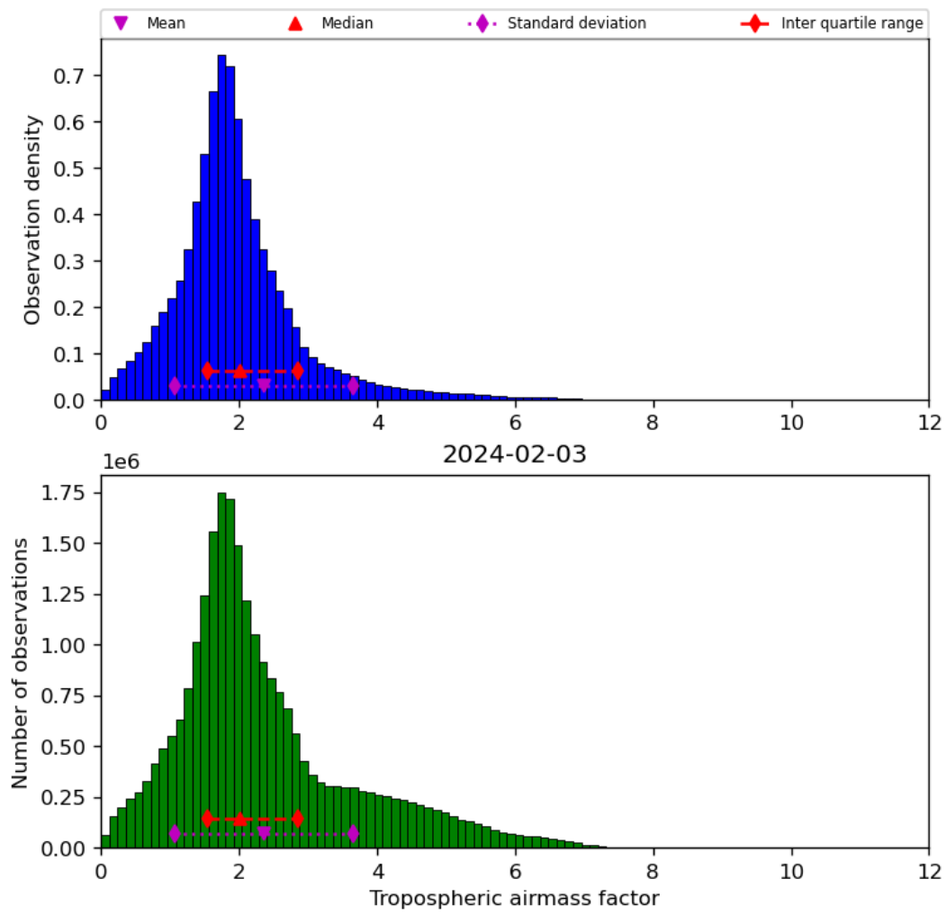
Figure 31: Histogram of “Tropospheric airmass factor” for 2024-02-02 to 2024-02-04
