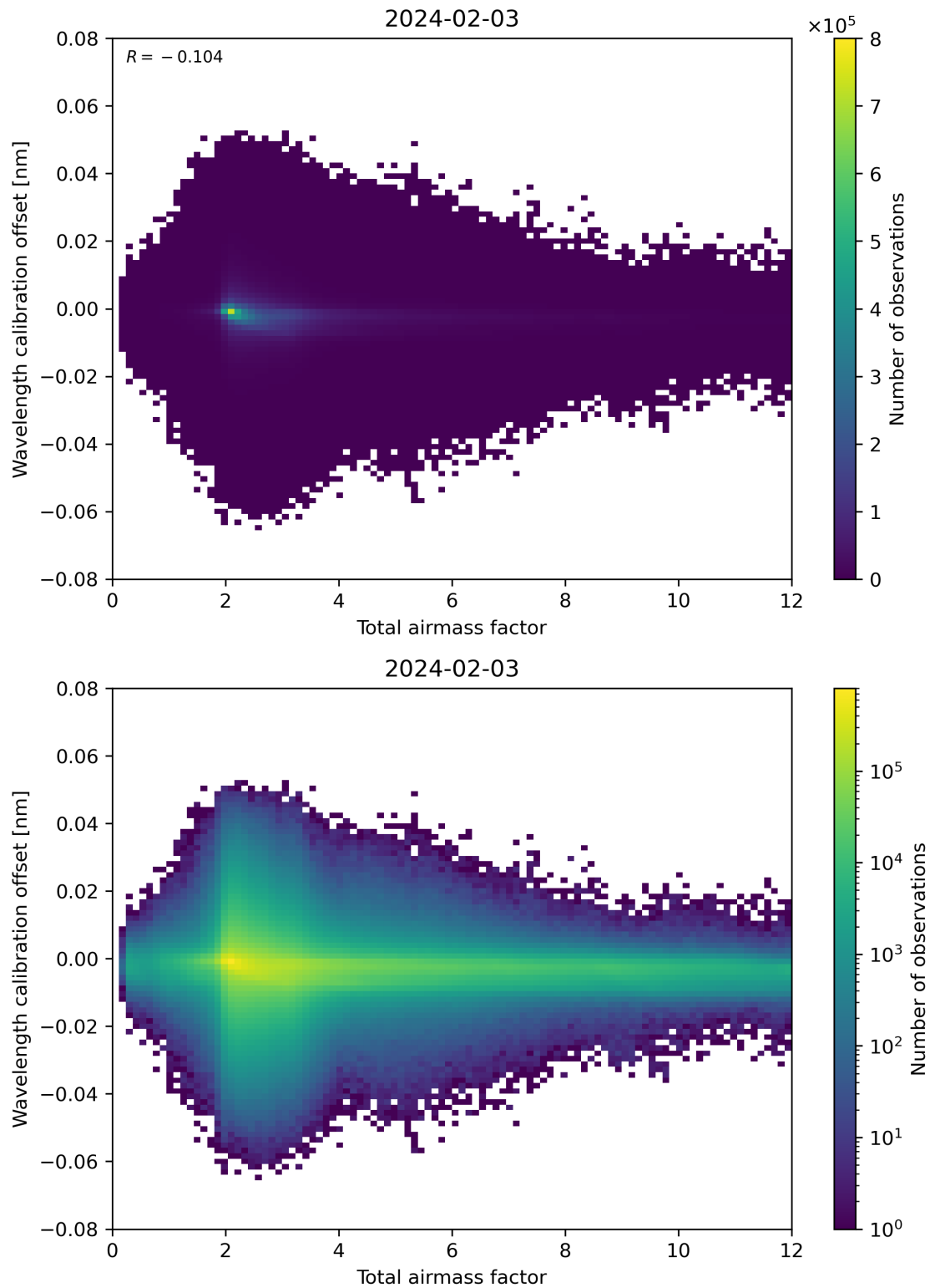
Figure 70: Scatter density plot of “Total airmass factor” against “Wavelength calibration offset” for 2024-02-02 to 2024-02-04.
