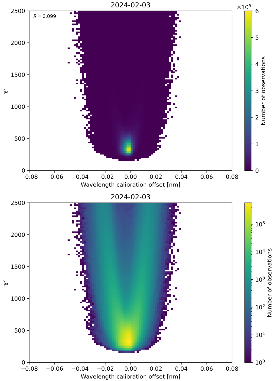
Figure 175: Scatter density plot of “Wavelength calibration offset” against “ \chi^2 ” for 2024-02-02 to 2024-02-04.
