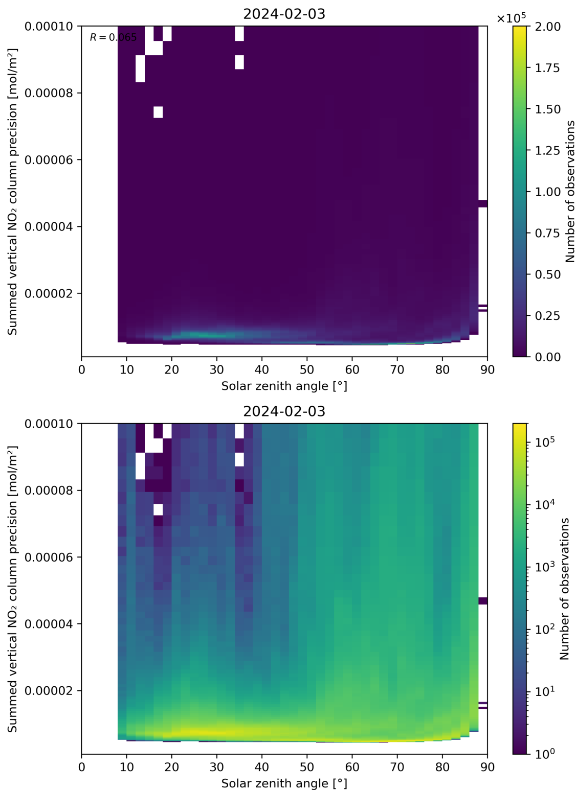
Figure 152: Scatter density plot of “Solar zenith angle” against “Summed vertical NO 2 column precision” for 2024-02-02 to 2024-02-04.
