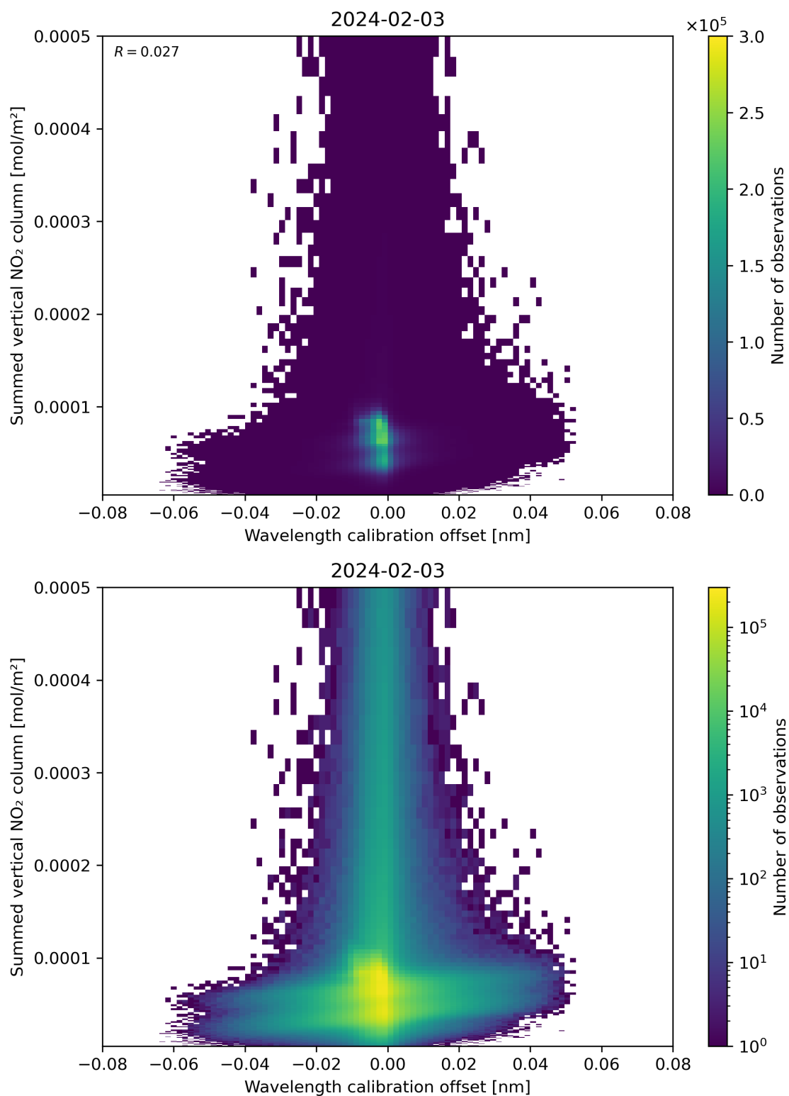
Figure 177: Scatter density plot of “Wavelength calibration offset” against “Summed vertical NO 2 column” for 2024-02-02 to 2024-02-04.
