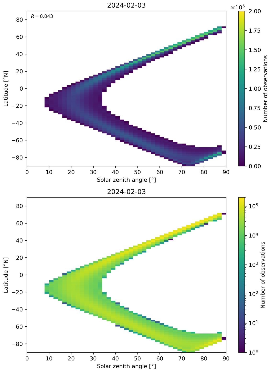
Figure 149: Scatter density plot of “Solar zenith angle” against “Latitude” for 2024-02-02 to 2024-02-04.
