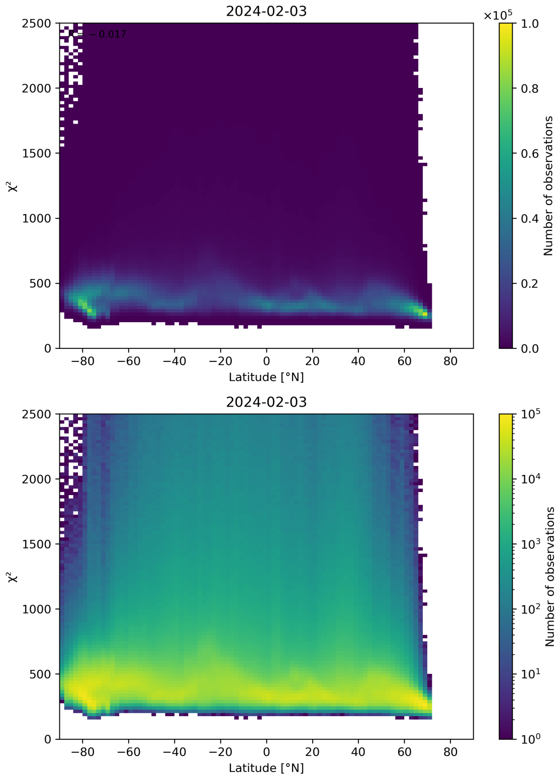
Figure 86: Scatter density plot of “Latitude” against “ \chi^2 ” for 2024-02-02 to 2024-02-04.
