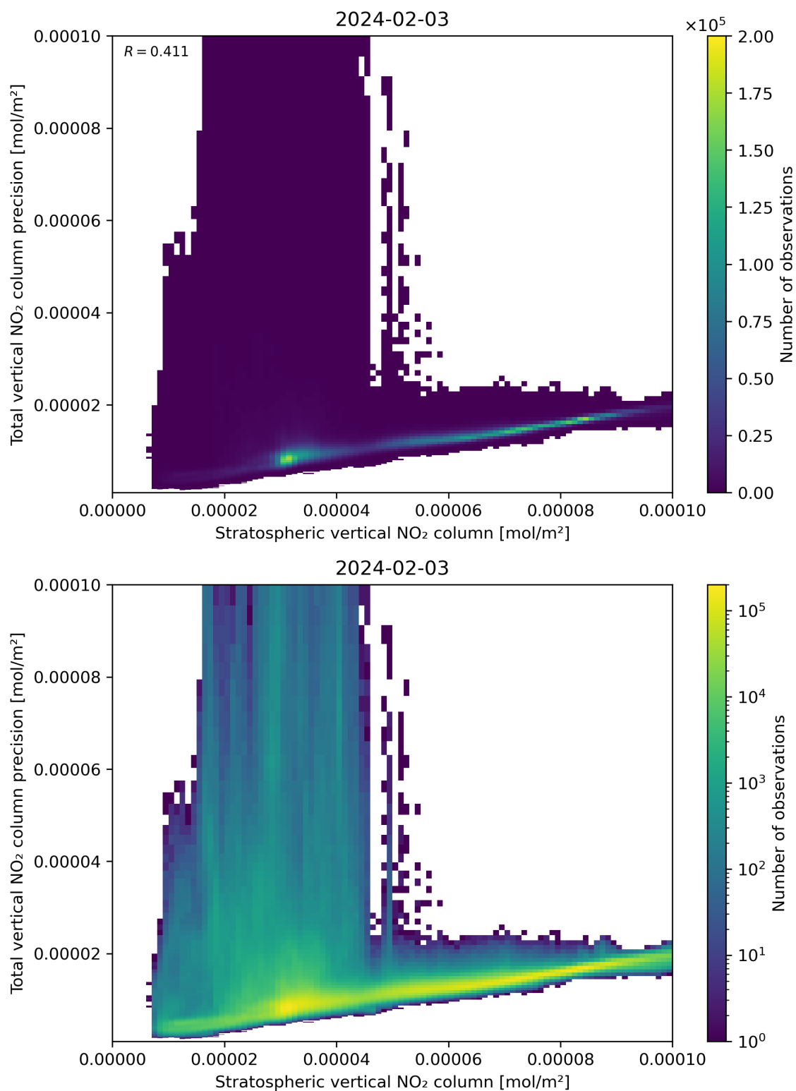
Figure 101: Scatter density plot of “Stratospheric vertical NO 2 column” against “Total vertical NO 2 column precision” for 2024-02-02 to 2024-02-04.
