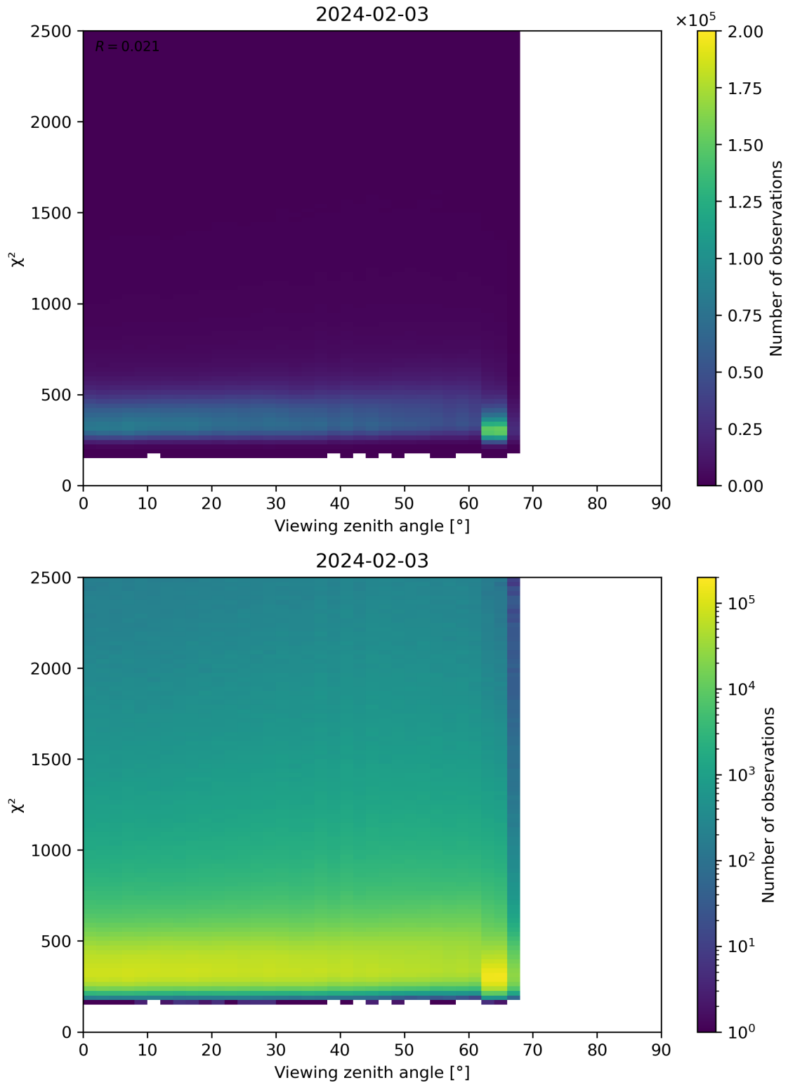
Figure 162: Scatter density plot of “Viewing zenith angle” against “ \chi^2 ” for 2024-02-02 to 2024-02-04.
