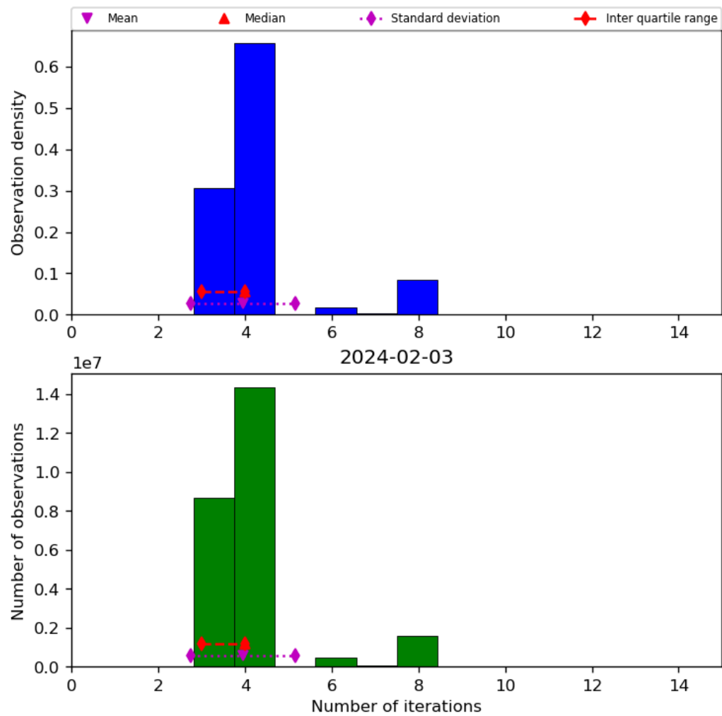
Figure 34: Histogram of “Number of iterations” for 2024-02-02 to 2024-02-04
