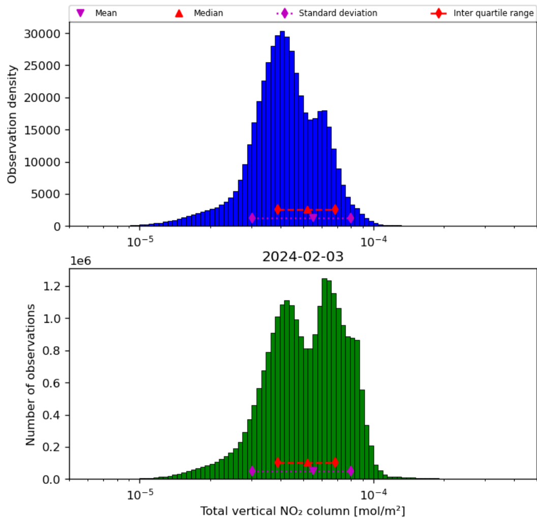
Figure 38: Histogram of “Total vertical NO 2 column” for 2024-02-02 to 2024-02-04
