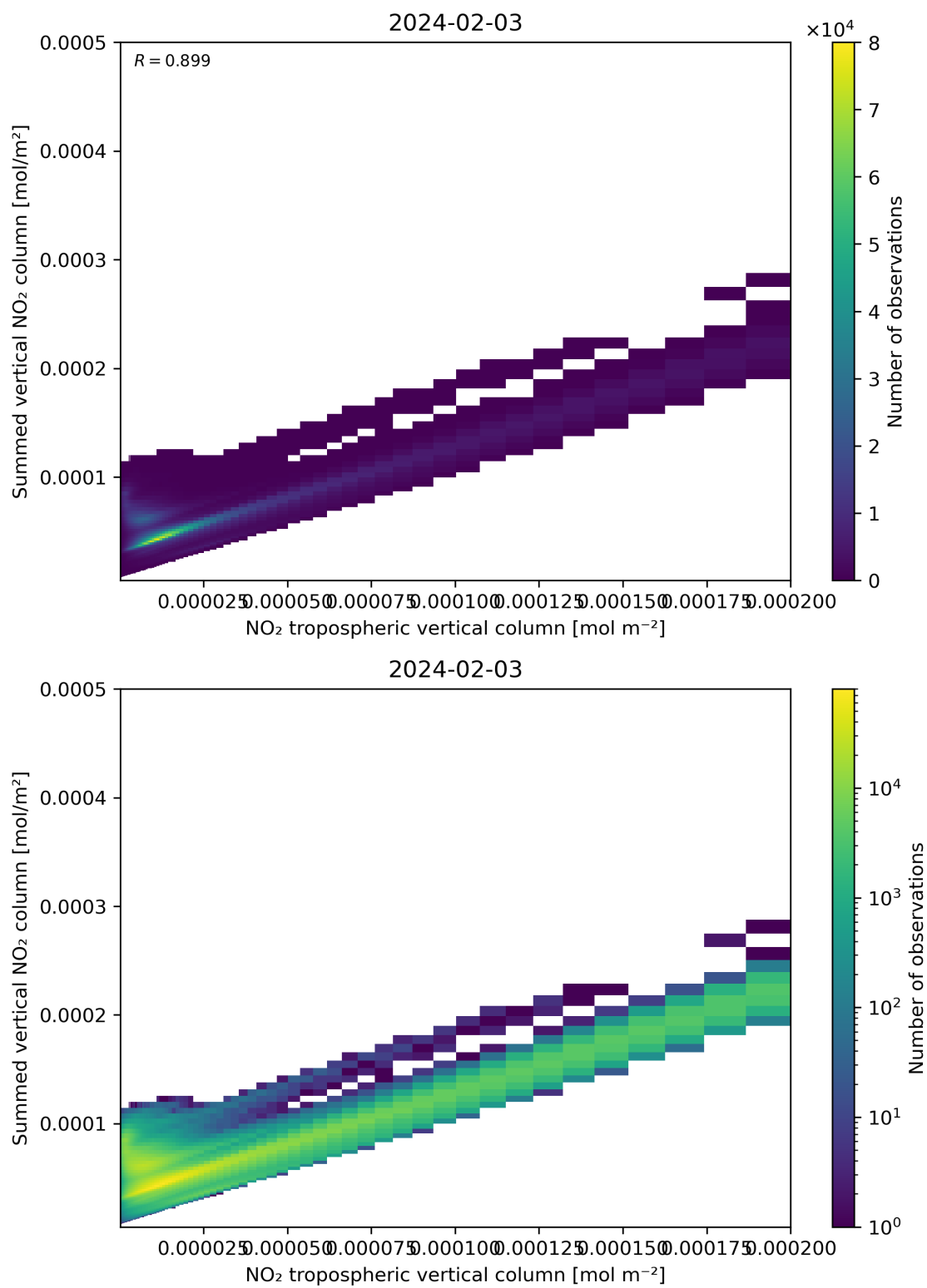
Figure 126: Scatter density plot of “NO 2 tropospheric vertical column” against “Summed vertical NO 2 column” for 2024-02-02 to 2024-02-04.
