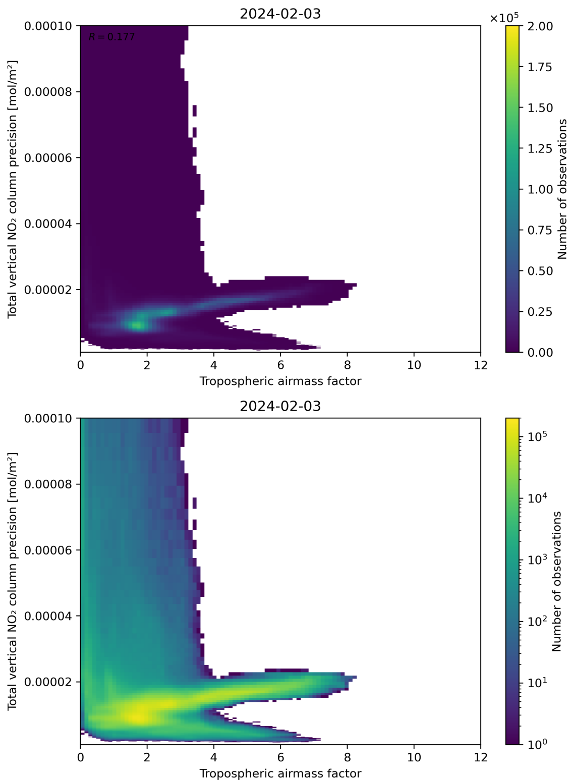
Figure 78: Scatter density plot of “Tropospheric air mass factor” against “Total vertical NO 2 column precision” for 2024-02-02 to 2024-02-04.
