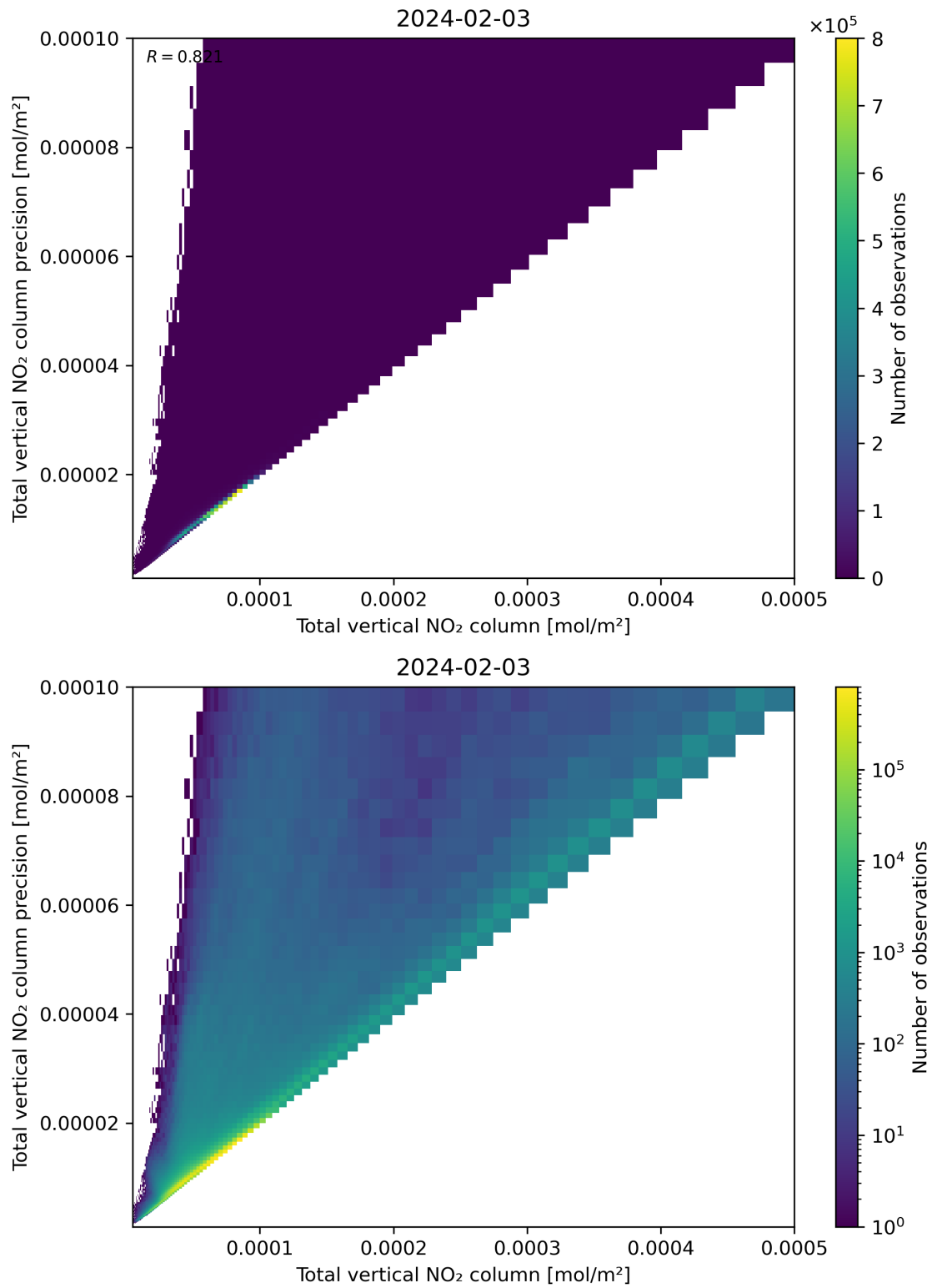
Figure 114: Scatter density plot of “Total vertical NO 2 column” against “Total vertical NO 2 column precision” for 2024-02-02 to 2024-02-04.
