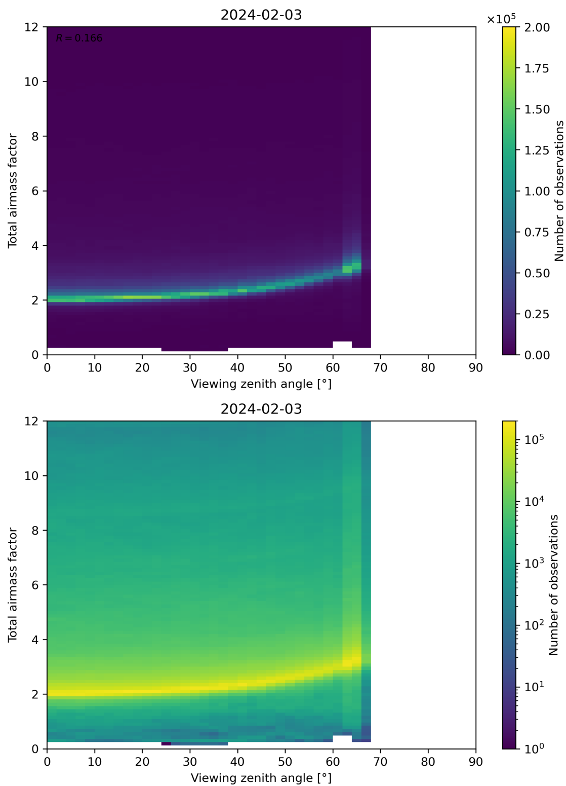
Figure 160: Scatter density plot of “Viewing zenith angle” against “Total airmass factor” for 2024-02-02 to 2024-02-04.
