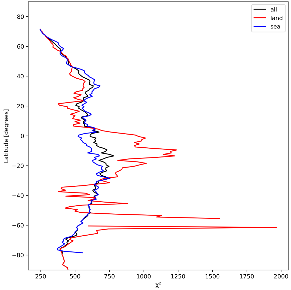
Figure 25: Zonal average of “ \chi^2 ” for 2024-02-02 to 2024-02-04.
