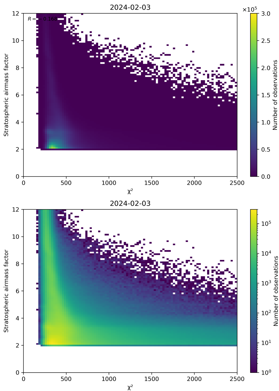
Figure 81: Scatter density plot of “ \chi^2 ” against “Stratospheric airmass factor” for 2024-02-02 to 2024-02-04.
