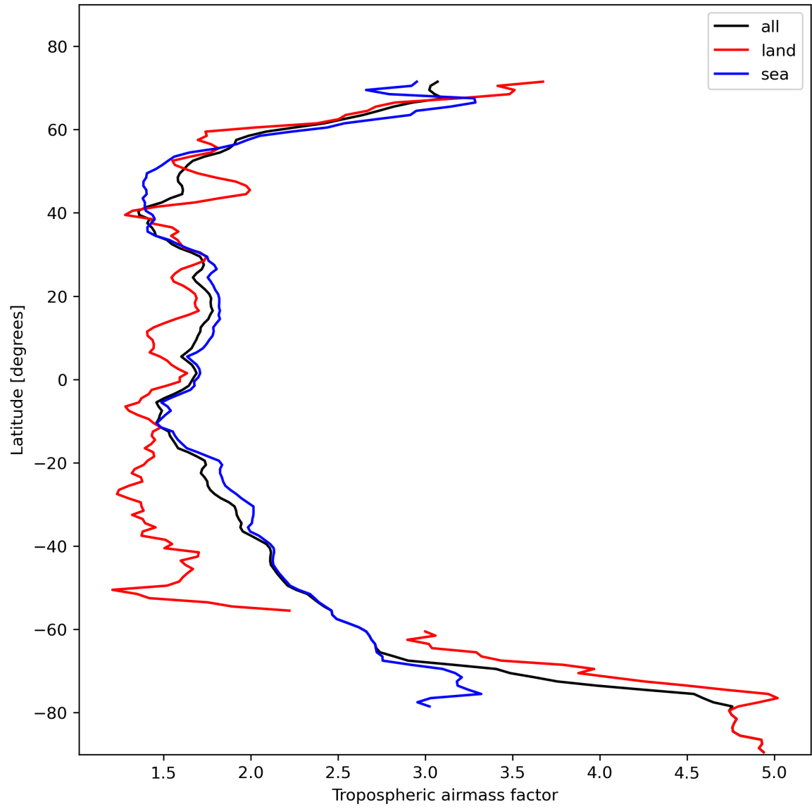
Figure 14: Zonal average of “Tropospheric airmass factor” for 2024-02-02 to 2024-02-04.
