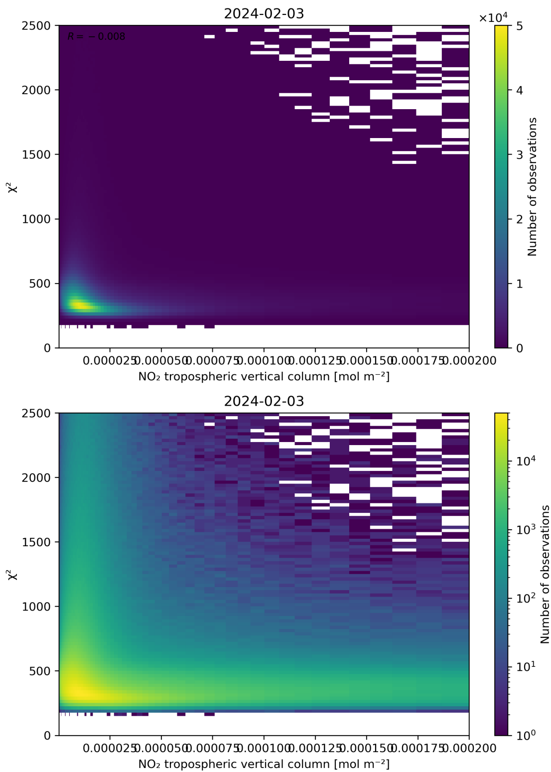
Figure 124: Scatter density plot of “NO 2 tropospheric vertical column” against “ \chi^2 ” for 2024-02-02 to 2024-02-04.
