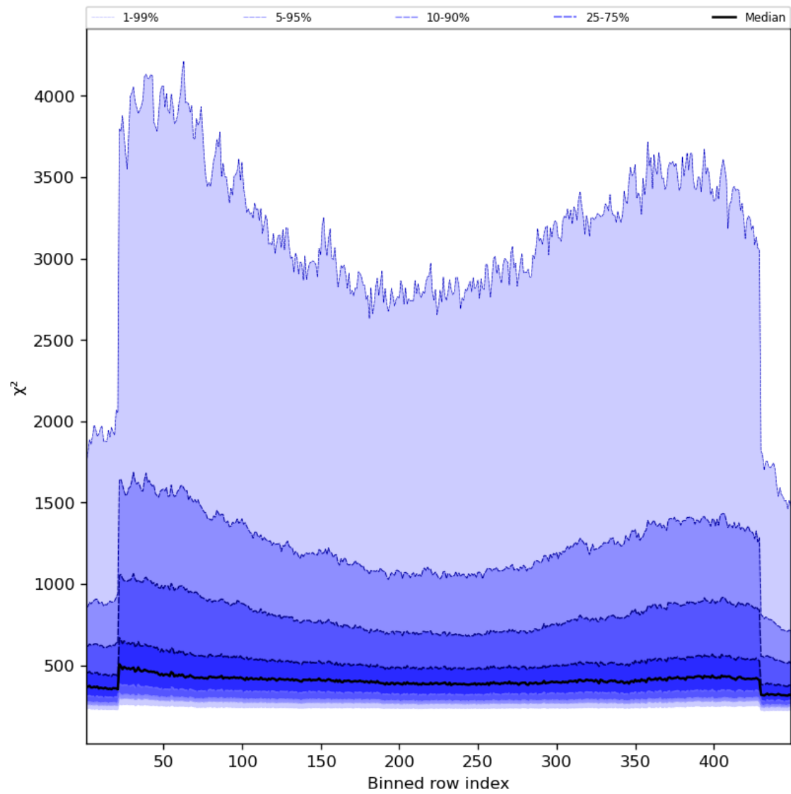
Figure 59: Along track statistics of “ \chi^2 ” for 2024-02-02 to 2024-02-04
