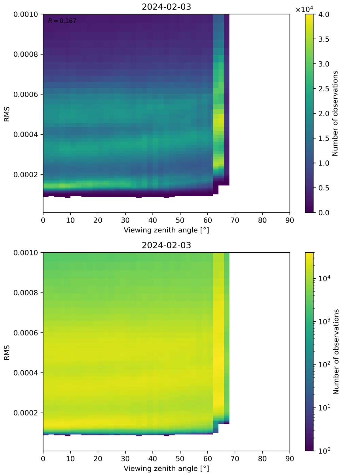
Figure 171: Scatter density plot of “Viewing zenith angle” against “RMS” for 2024-02-02 to 2024-02-04.
