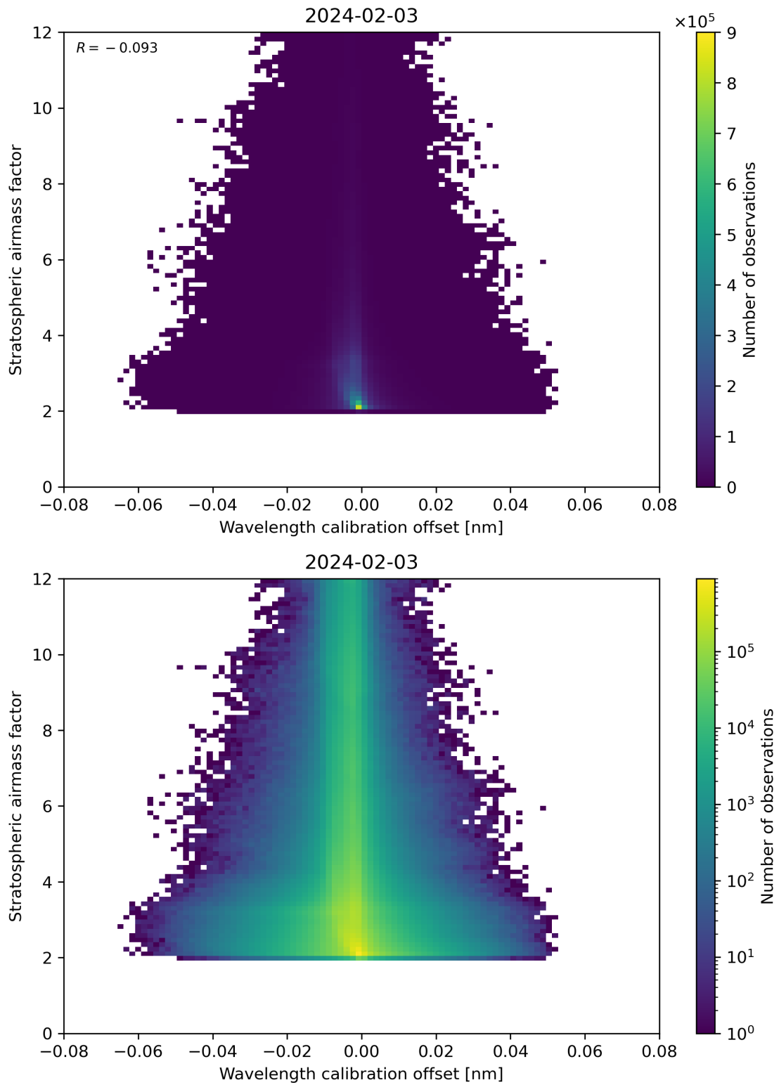
Figure 174: Scatter density plot of “Wavelength calibration offset” against “Stratospheric air mass factor” for 2024-02-02 to 2024-02-04.
