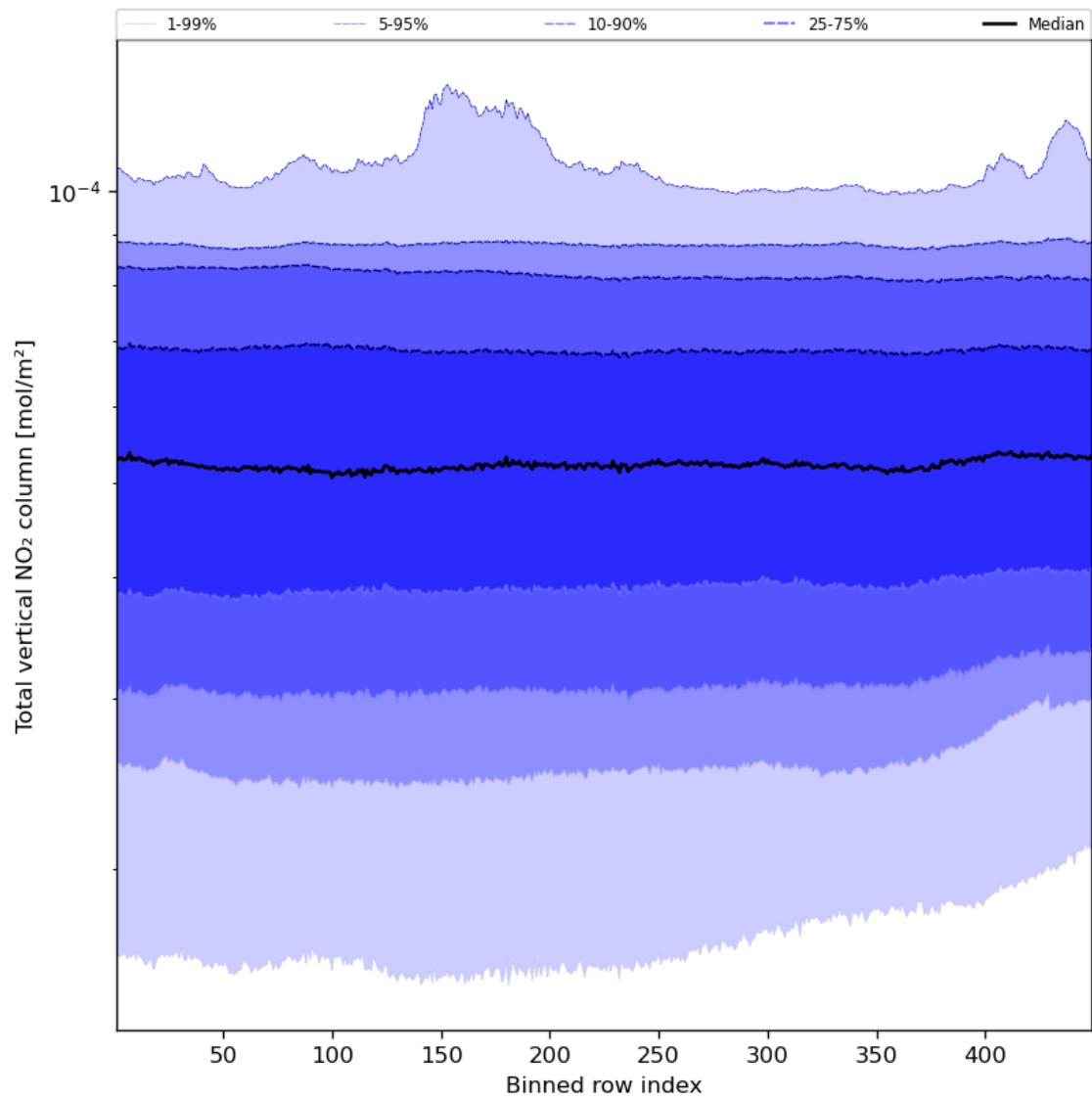
Figure 55: Along track statistics of “Total vertical NO 2 column” for 2024-02-02 to 2024-02-04
