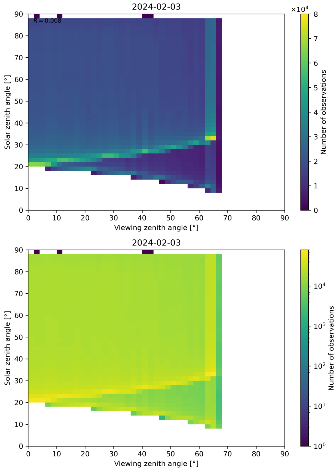
Figure 172: Scatter density plot of “Viewing zenith angle” against “Solar zenith angle” for 2024-02-02 to 2024-02-04.
