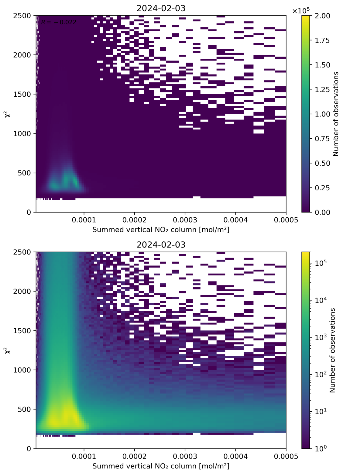
Figure 104: Scatter density plot of “Summed vertical NO 2 column” against “ \chi^2 ” for 2024-02-02 to 2024-02-04.
