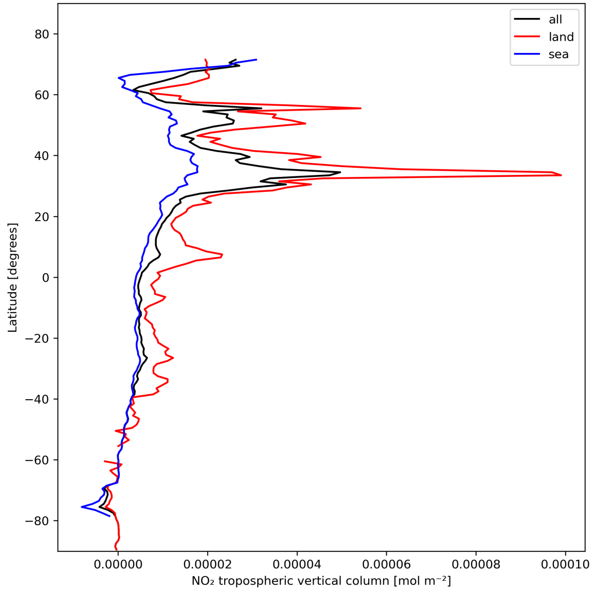
Figure 12: Zonal average of “NO 2 tropospheric vertical column” for 2024-02-02 to 2024-02-04.
