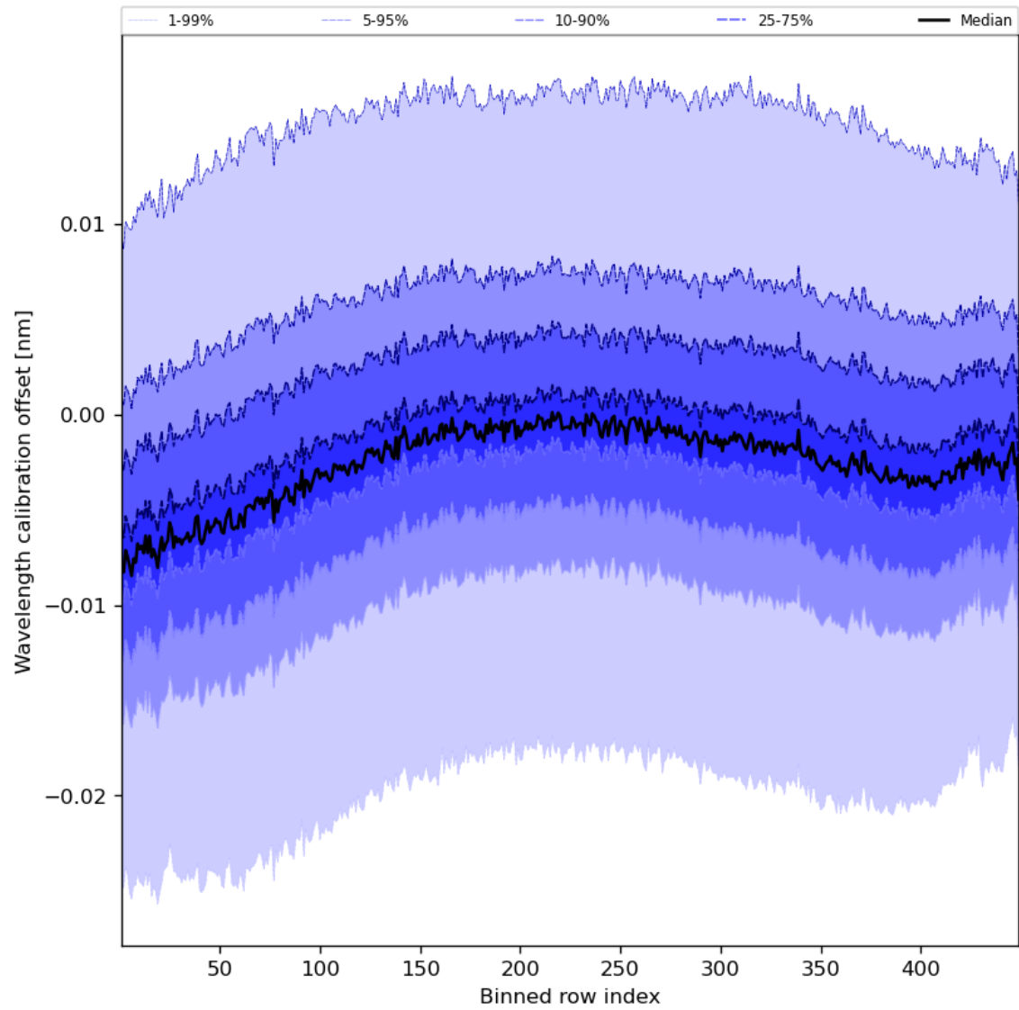
Figure 52: Along track statistics of “Wavelength calibration offset” for 2024-02-02 to 2024-02-04
