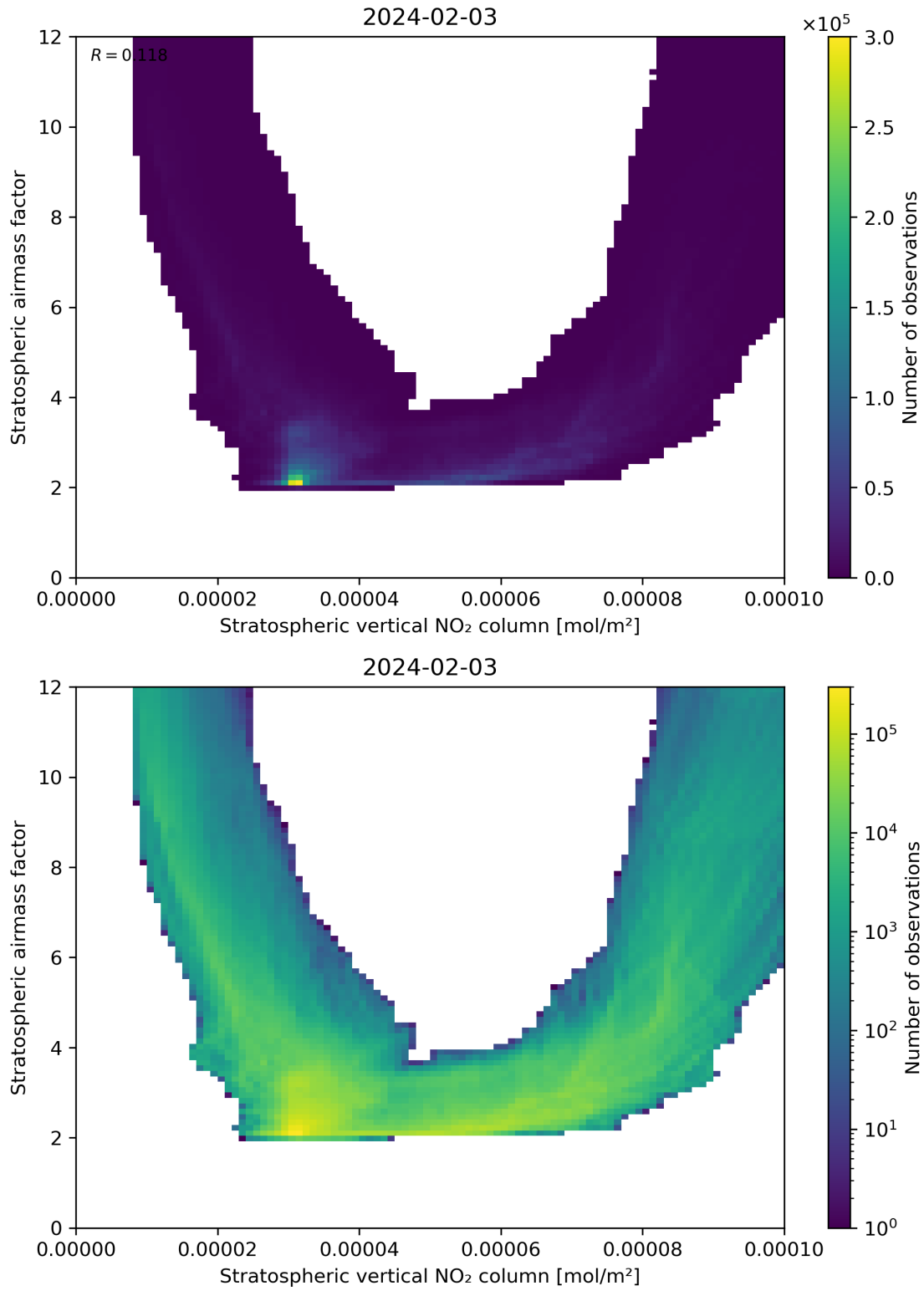
Figure 96: Scatter density plot of “Stratospheric vertical NO 2 column” against “Stratospheric airmass factor” for 2024-02-02 to 2024-02-04.
