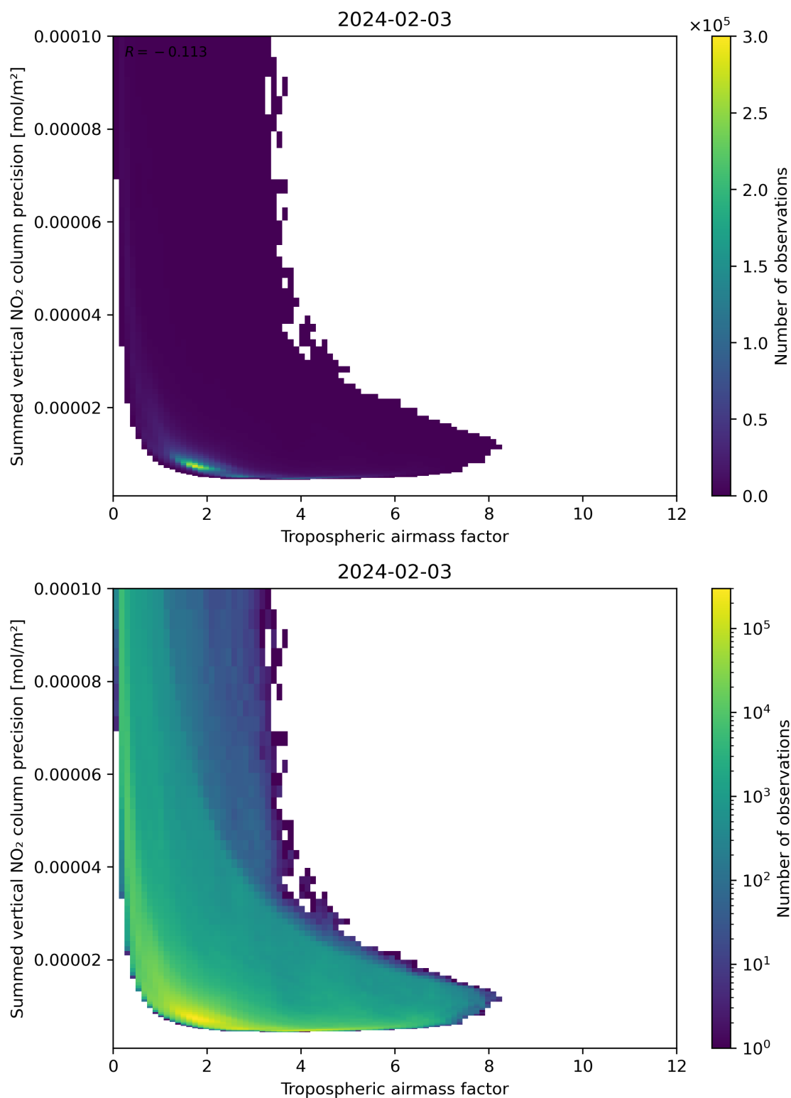
Figure 76: Scatter density plot of “Tropospheric air mass factor” against “Summed vertical NO 2 column precision” for 2024-02-02 to 2024-02-04.
