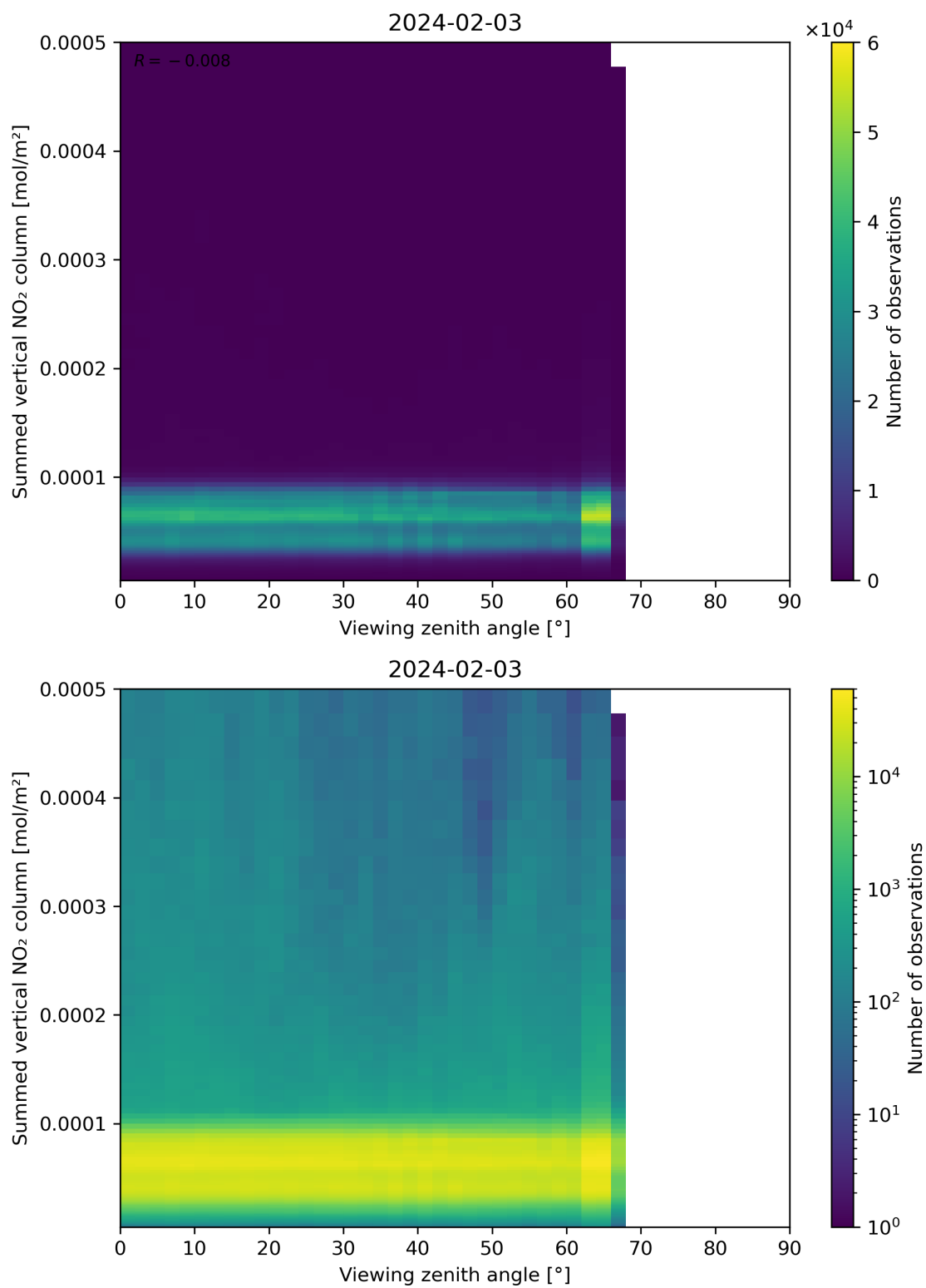
Figure 165: Scatter density plot of “Viewing zenith angle” against “Summed vertical NO 2 column” for 2024-02-02 to 2024-02-04.
