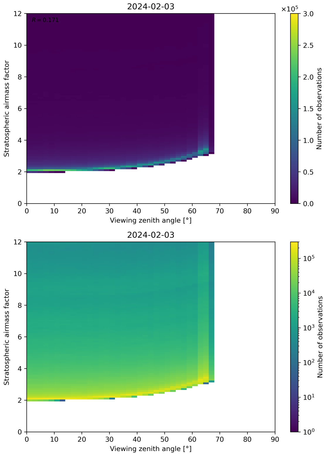
Figure 159: Scatter density plot of “Viewing zenith angle” against “Stratospheric airmass factor” for 2024-02-02 to 2024-02-04.
