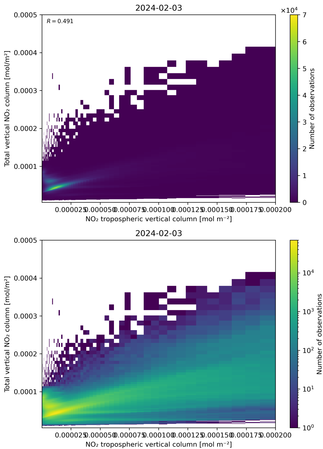
Figure 128: Scatter density plot of “NO 2 tropospheric vertical column” against “Total vertical NO 2 column” for 2024-02-02 to 2024-02-04.
