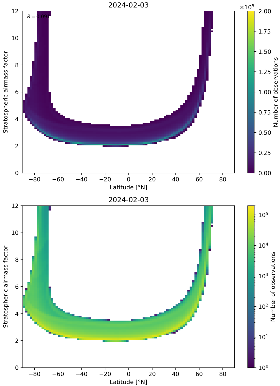
Figure 83: Scatter density plot of “Latitude” against “Stratospheric airmass factor” for 2024-02-02 to 2024-02-04.
