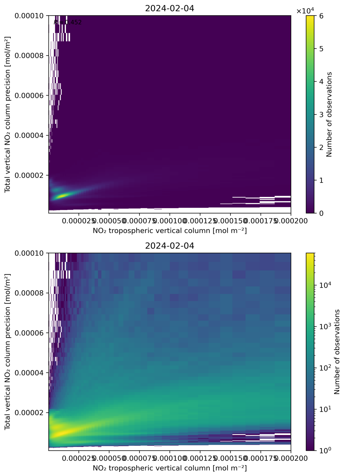
Figure 129: Scatter density plot of “NO 2 tropospheric vertical column” against “Total vertical NO 2 column precision” for 2024-02-03 to 2024-02-05.
