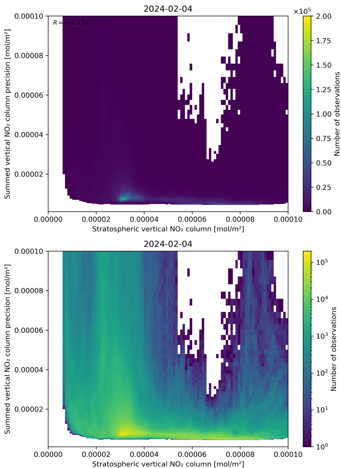
Figure 99: Scatter density plot of “Stratospheric vertical NO 2 column” against “Summed vertical NO 2 column precision” for 2024-02-03 to 2024-02-05.
