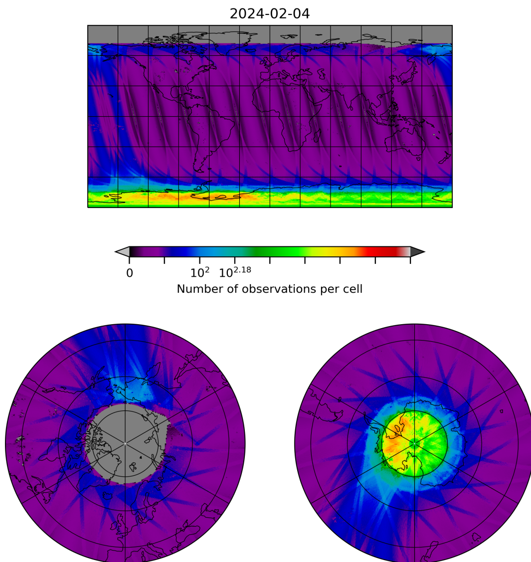
Figure 10: Map of the number of observations for 2024-02-03 to 2024-02-05
