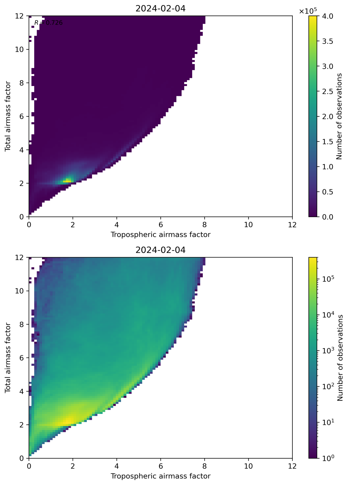
Figure 72: Scatter density plot of “Tropospheric airmass factor” against “Total airmass factor” for 2024-02-03 to 2024-02-05.
