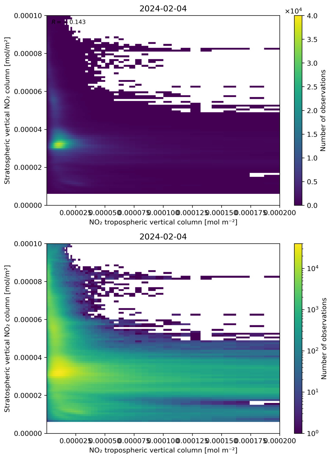
Figure 125: Scatter density plot of “NO 2 tropospheric vertical column” against “Stratospheric vertical NO 2 column” for 2024-02-03 to 2024-02-05.
