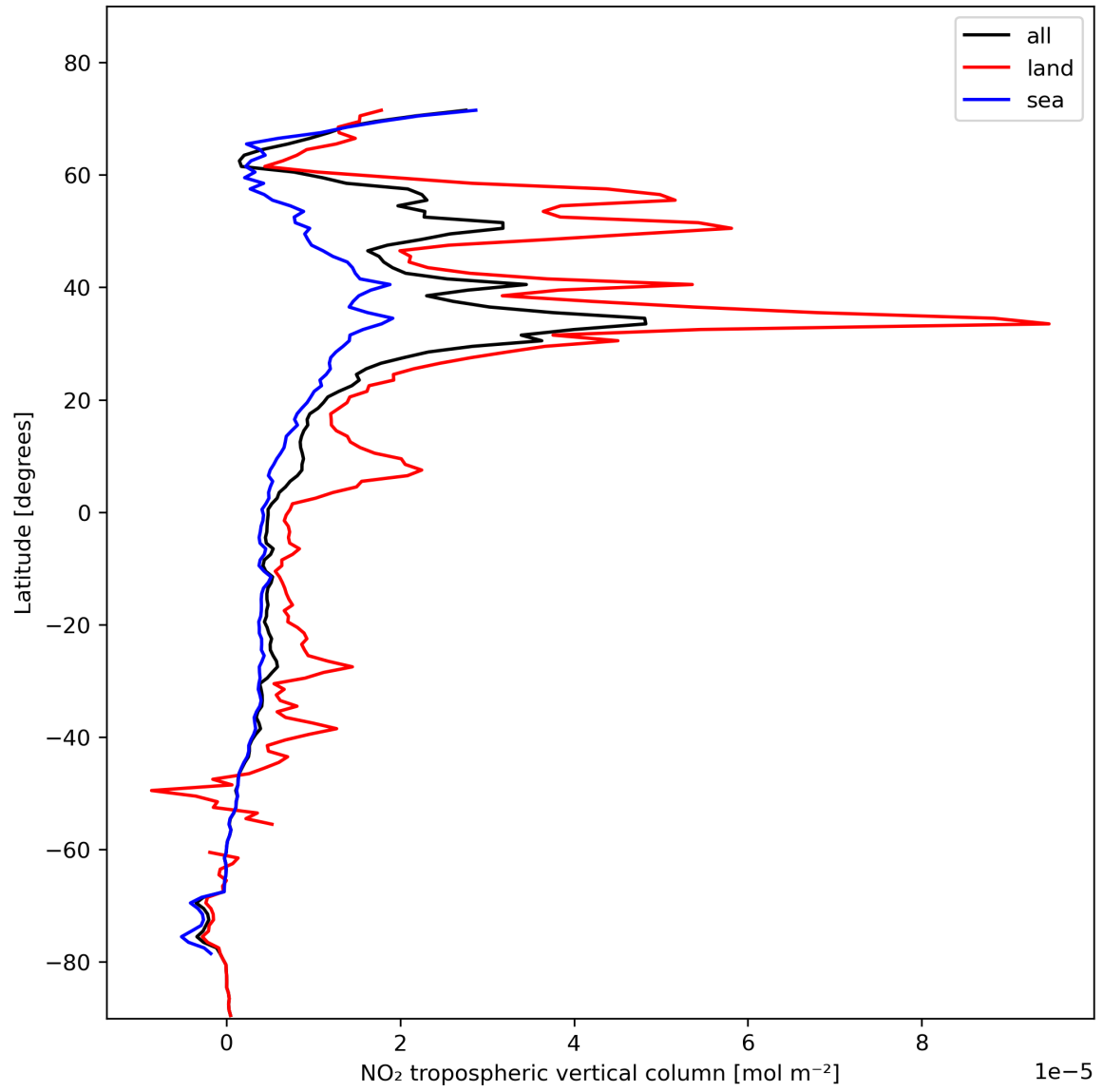
Figure 12: Zonal average of “NO 2 tropospheric vertical column” for 2024-02-03 to 2024-02-05.
