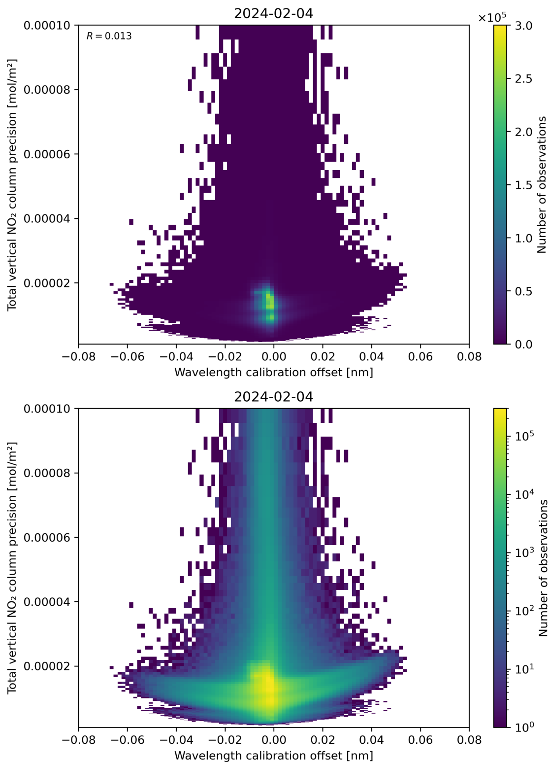
Figure 180: Scatter density plot of “Wavelength calibration offset” against “Total vertical NO 2 column precision” for 2024-02-03 to 2024-02-05.
