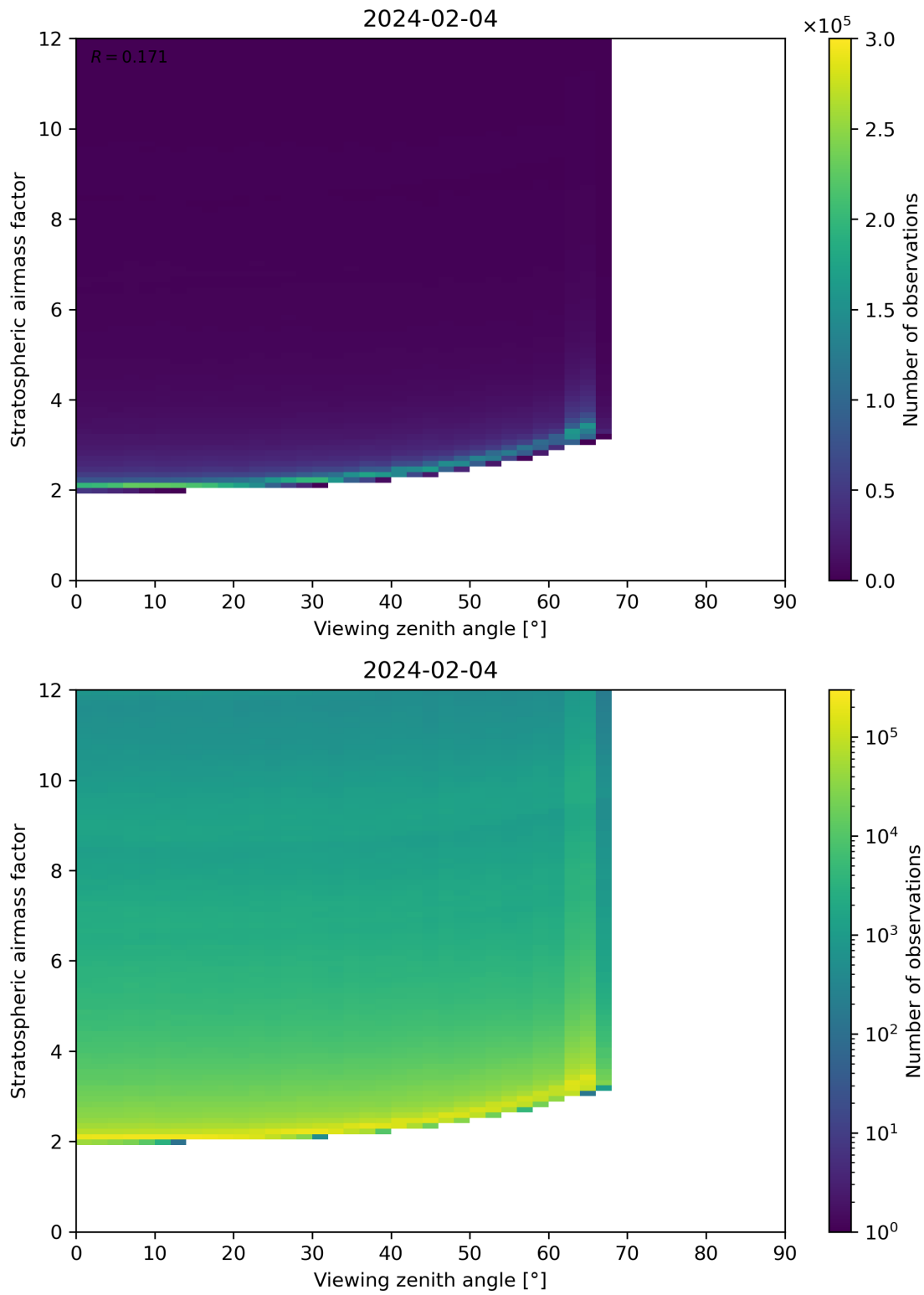
Figure 159: Scatter density plot of “Viewing zenith angle” against “Stratospheric airmass factor” for 2024-02-03 to 2024-02-05.
