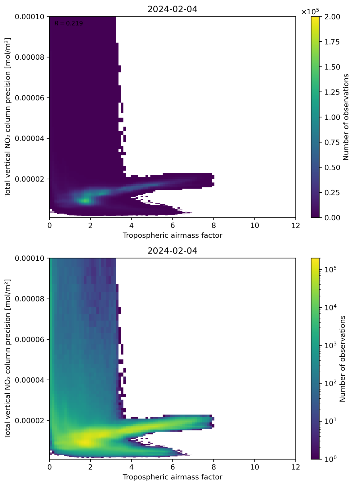
Figure 78: Scatter density plot of “Tropospheric air mass factor” against “Total vertical NO 2 column precision” for 2024-02-03 to 2024-02-05.
