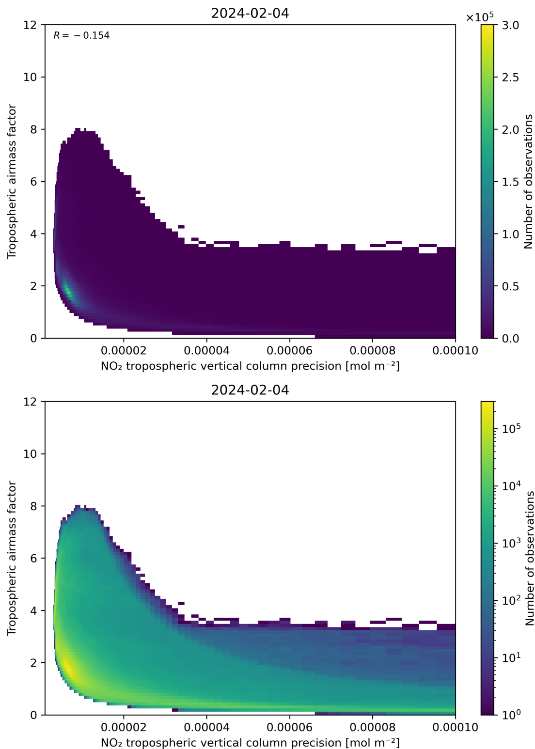
Figure 133: Scatter density plot of “NO 2 tropospheric vertical column precision” against “Tropospheric airmass factor” for 2024-02-03 to 2024-02-05.
