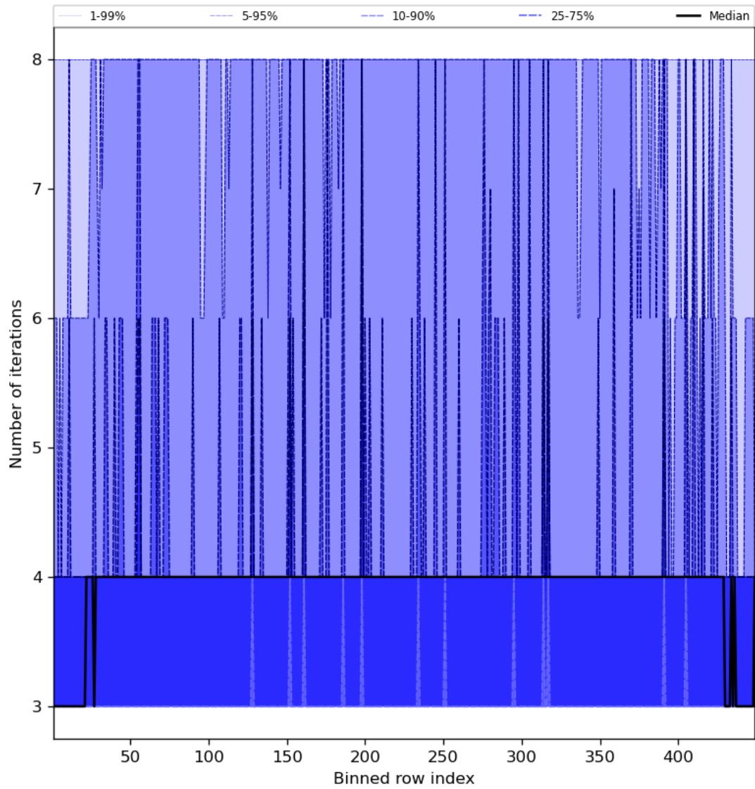
Figure 51: Along track statistics of “Number of iterations” for 2024-02-03 to 2024-02-05
