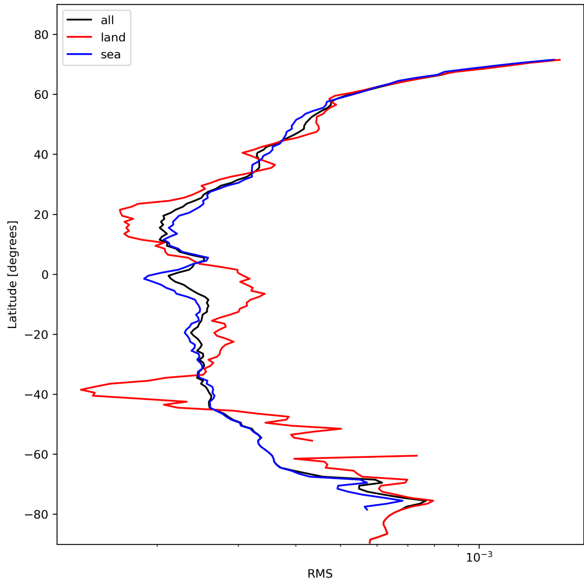
Figure 26: Zonal average of “RMS” for 2024-02-03 to 2024-02-05.
