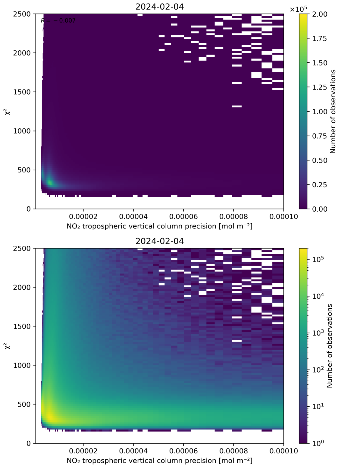
Figure 134: Scatter density plot of “NO 2 tropospheric vertical column precision” against “ \chi^2 ” for 2024-02-03 to 2024-02-05.
