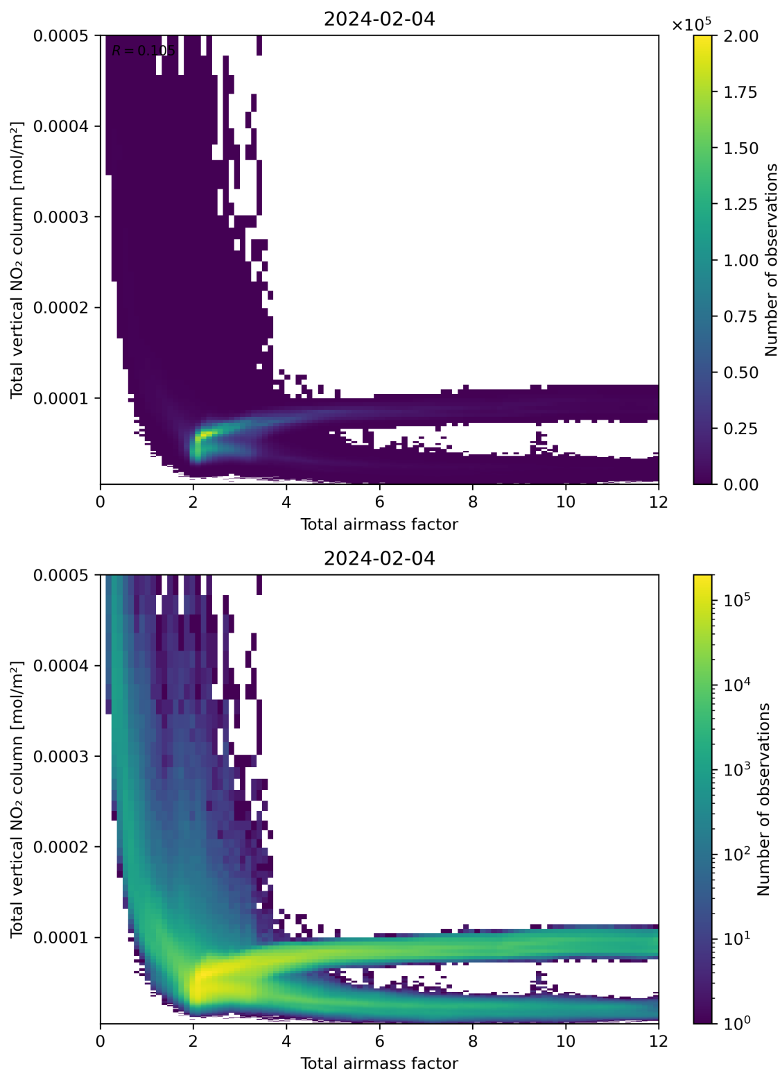
Figure 67: Scatter density plot of “Total airmass factor” against “Total vertical NO 2 column” for 2024-02-03 to 2024-02-05.
