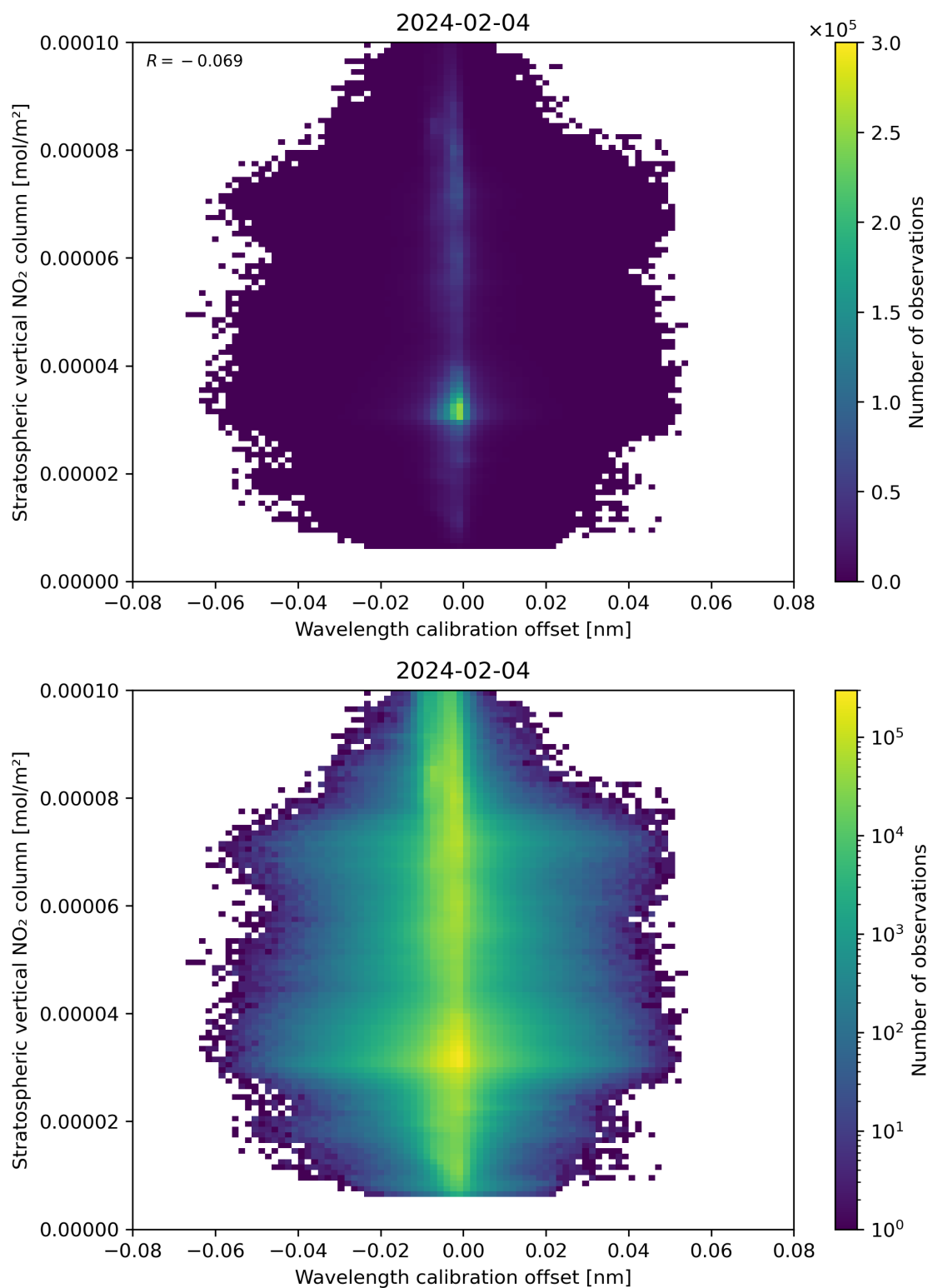
Figure 176: Scatter density plot of “Wavelength calibration offset” against “Stratospheric vertical NO 2 column” for 2024-02-03 to 2024-02-05.
