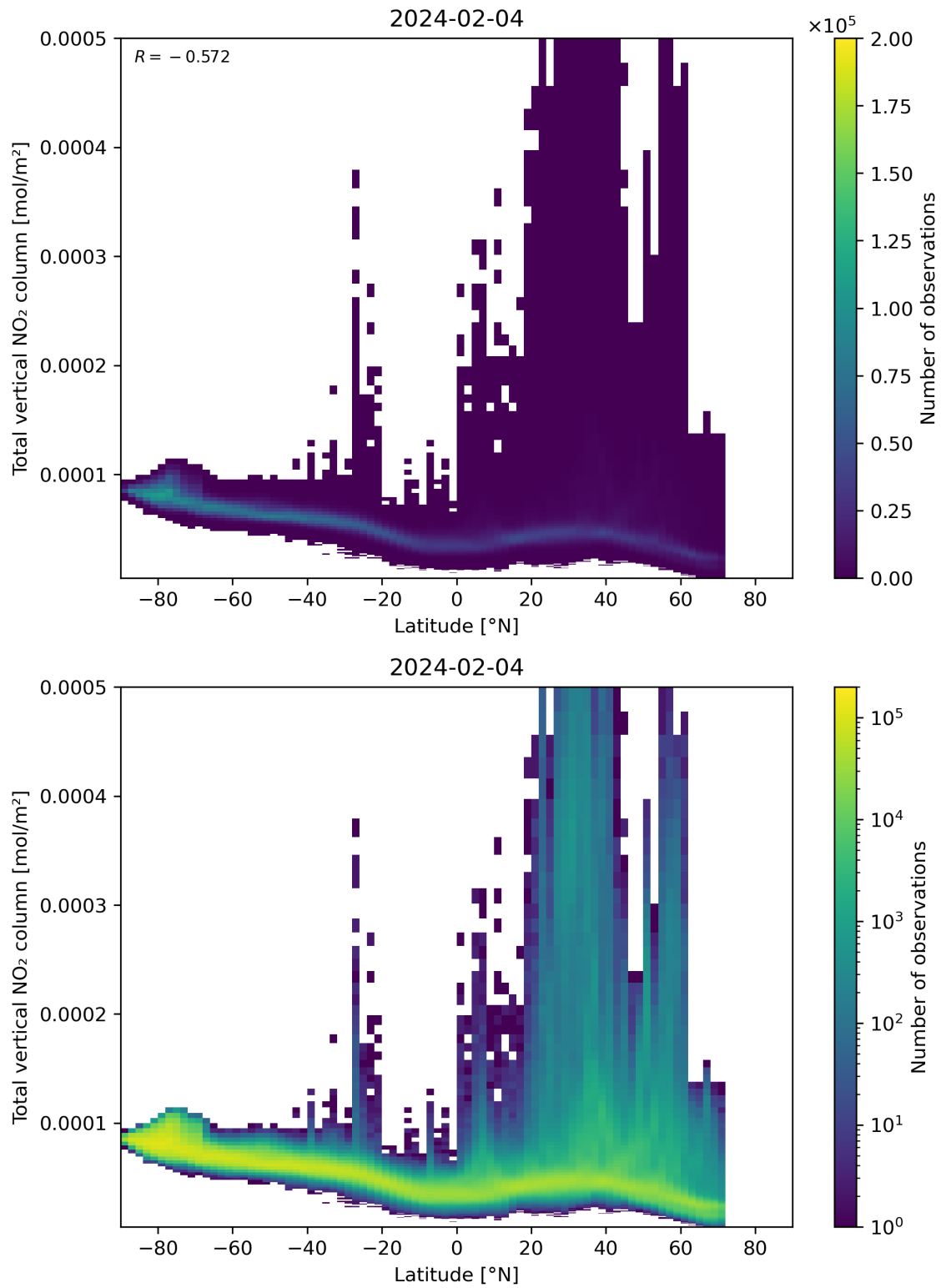
Figure 90: Scatter density plot of “Latitude” against “Total vertical NO 2 column” for 2024-02-03 to 2024-02-05.
