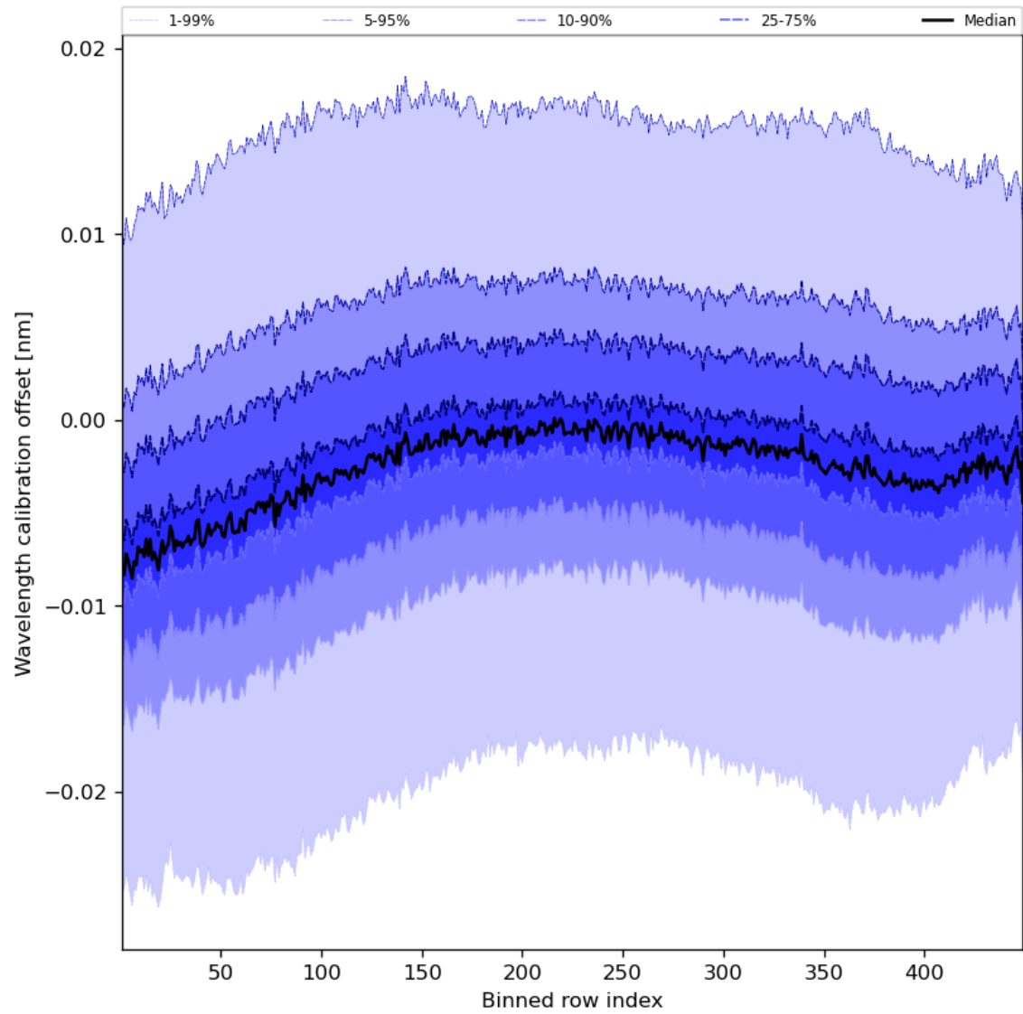
Figure 52: Along track statistics of “Wavelength calibration offset” for 2024-02-03 to 2024-02-05
