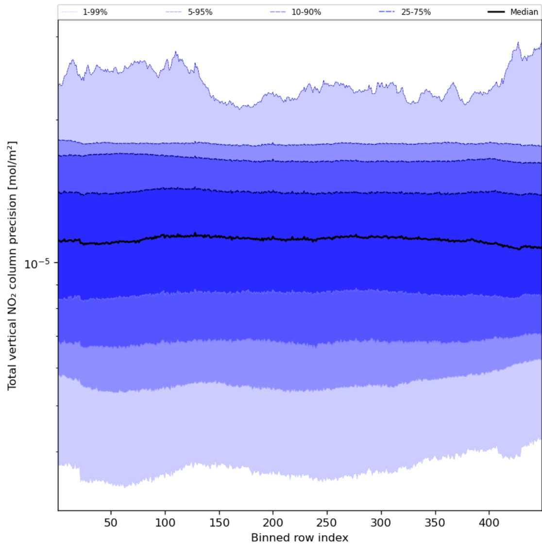
Figure 56: Along track statistics of “Total vertical NO 2 column precision” for 2024-02-03 to 2024-02-05
