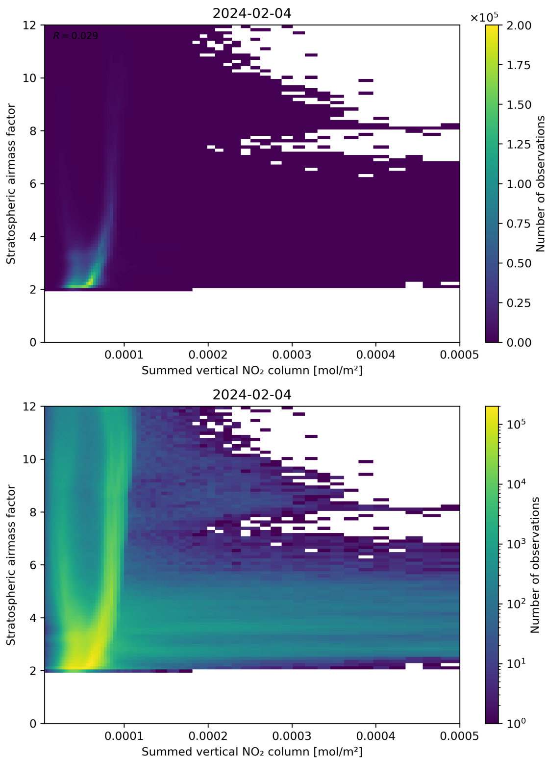
Figure 103: Scatter density plot of “Summed vertical NO 2 column” against “Stratospheric air mass factor” for 2024-02-03 to 2024-02-05.
