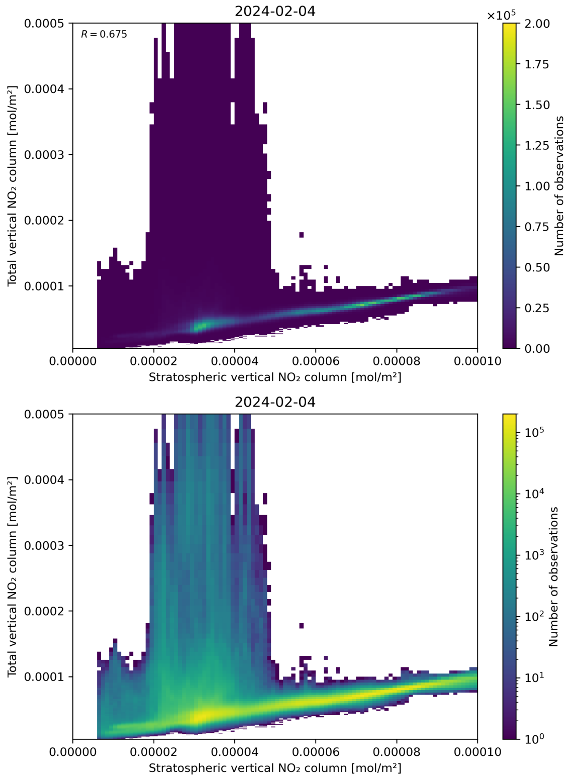
Figure 100: Scatter density plot of “Stratospheric vertical NO 2 column” against “Total vertical NO 2 column” for 2024-02-03 to 2024-02-05.
