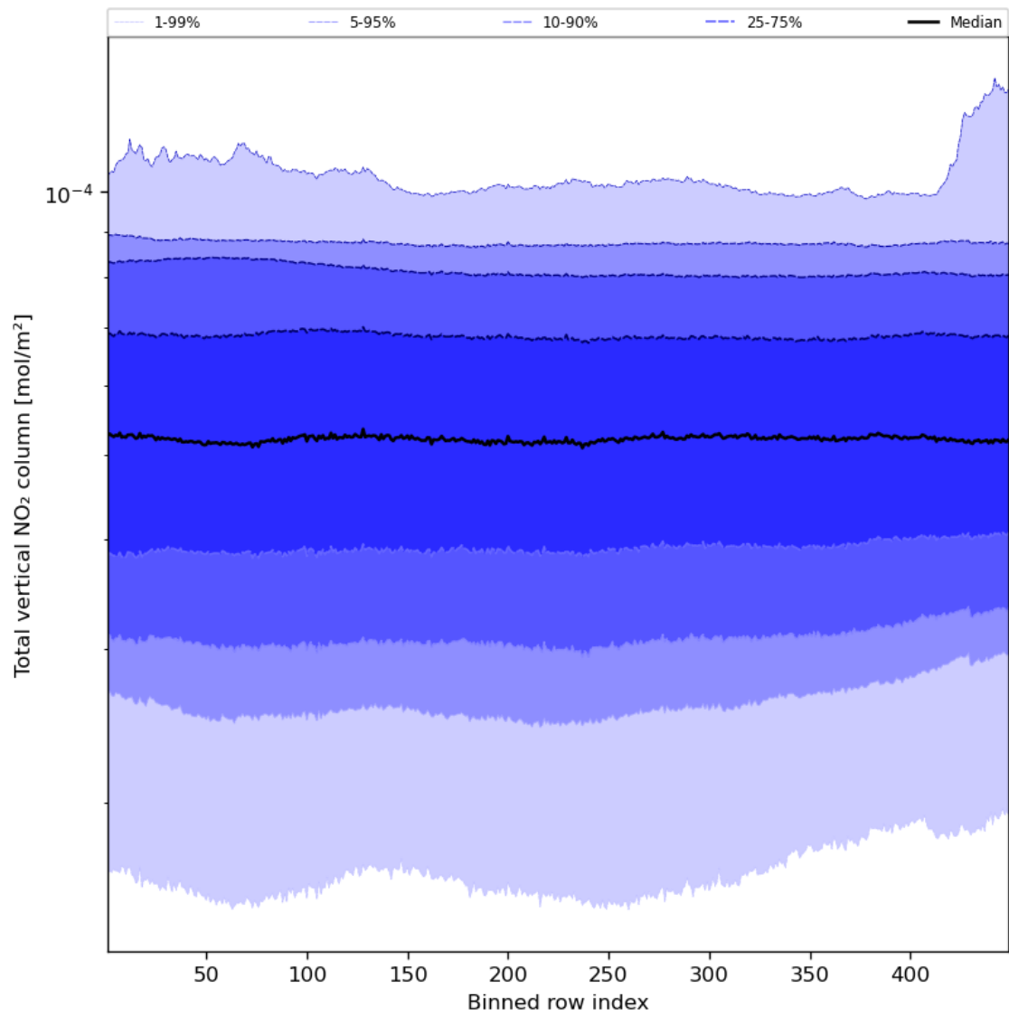
Figure 55: Along track statistics of “Total vertical NO 2 column” for 2024-02-03 to 2024-02-05
