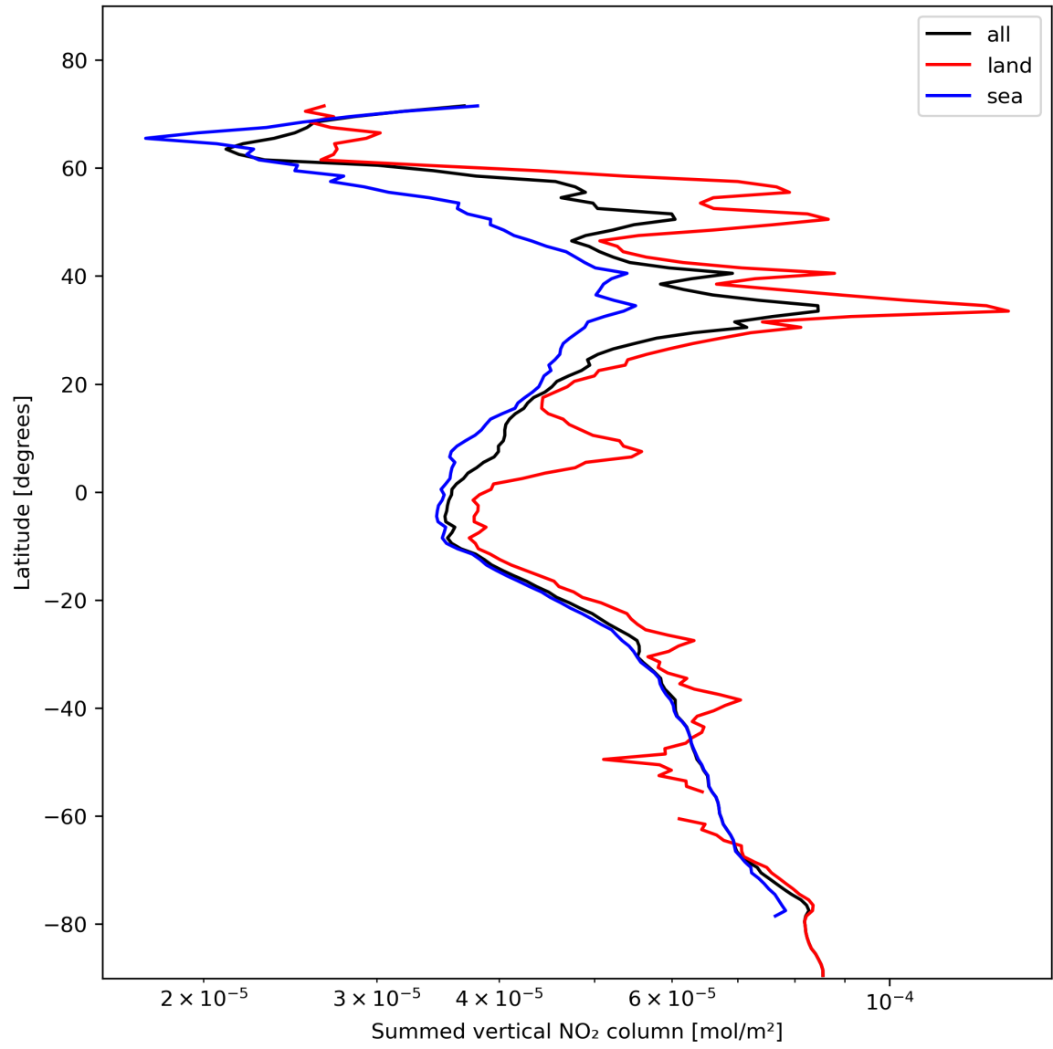
Figure 23: Zonal average of “Summed vertical NO 2 column” for 2024-02-03 to 2024-02-05.
