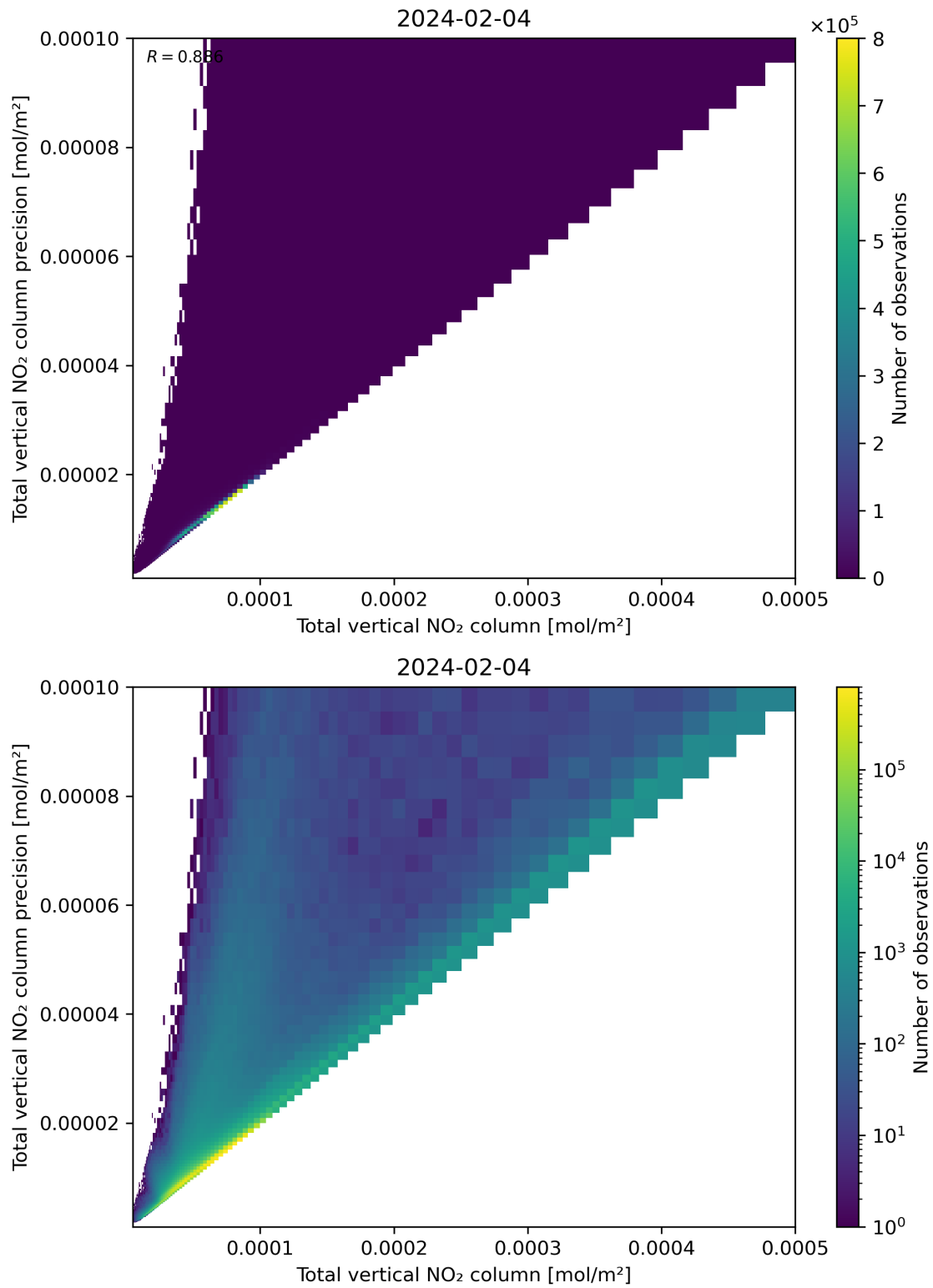
Figure 114: Scatter density plot of “Total vertical NO 2 column” against “Total vertical NO 2 column precision” for 2024-02-03 to 2024-02-05.
