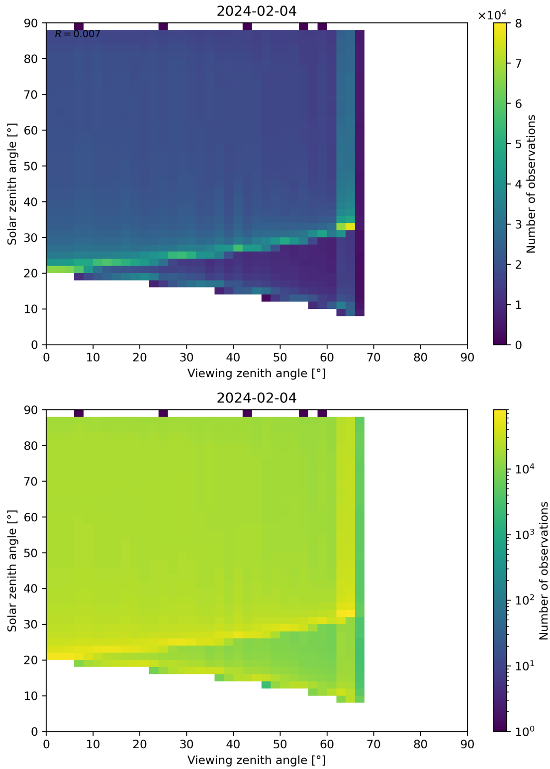
Figure 172: Scatter density plot of “Viewing zenith angle” against “Solar zenith angle” for 2024-02-03 to 2024-02-05.
