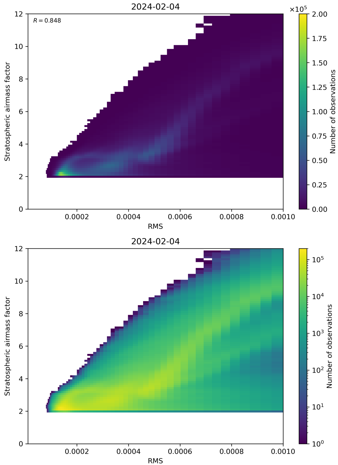
Figure 144: Scatter density plot of “RMS” against “Stratospheric airmass factor” for 2024-02-03 to 2024-02-05.
