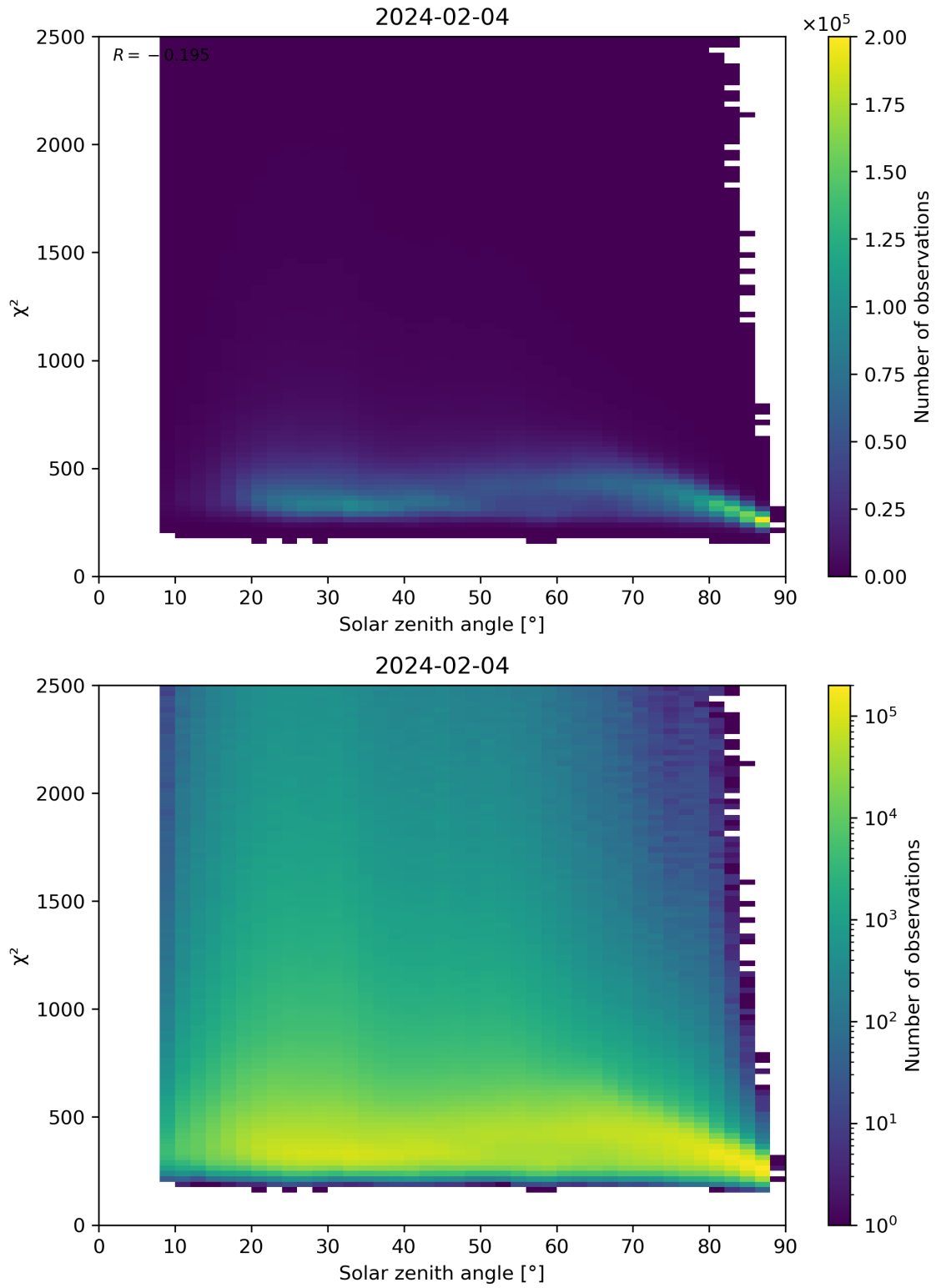
Figure 148: Scatter density plot of “Solar zenith angle” against “ \chi^2 ” for 2024-02-03 to 2024-02-05.
