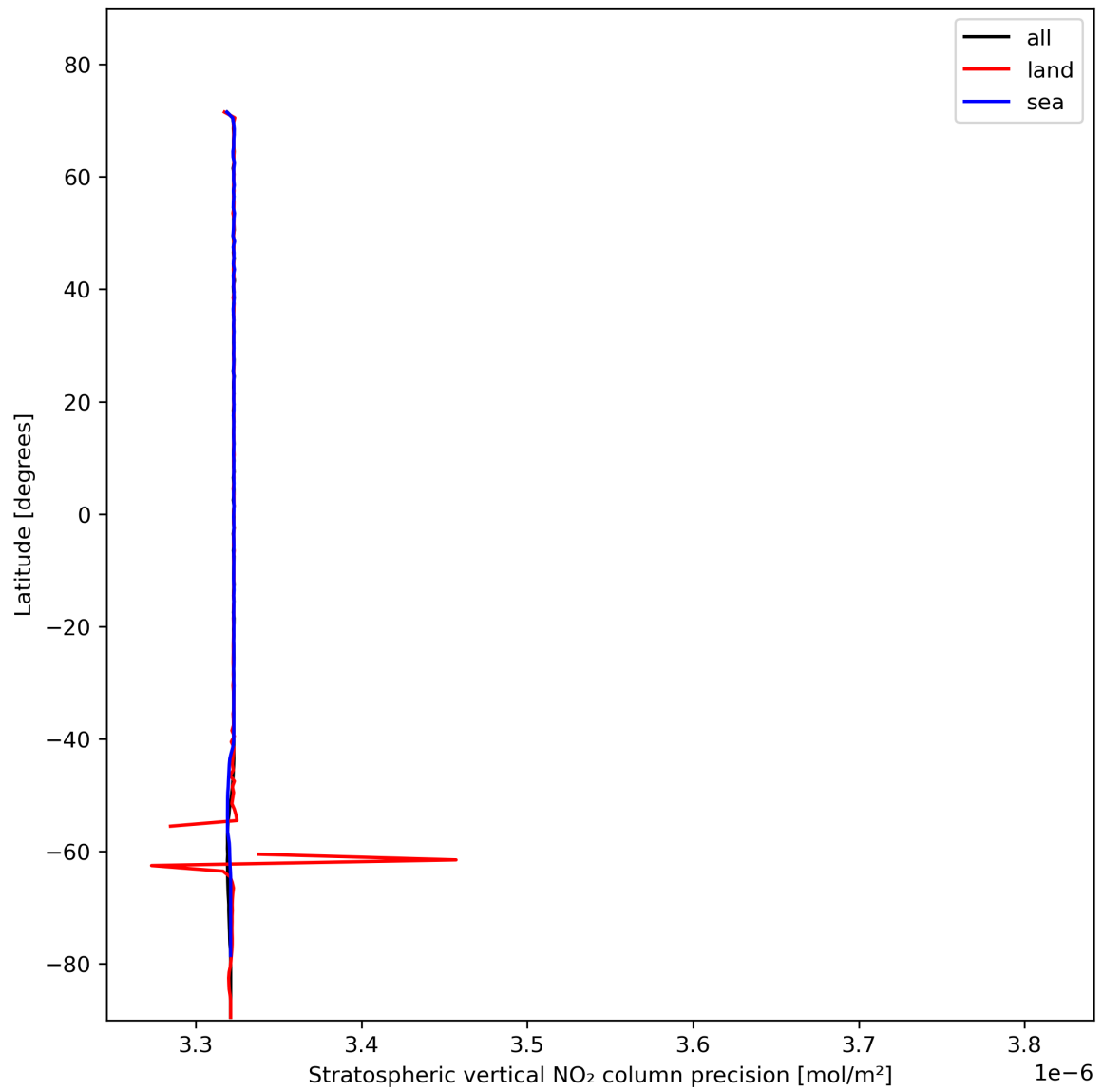
Figure 20: Zonal average of “Stratospheric vertical NO 2 column precision” for 2024-02-03 to 2024-02-05.
