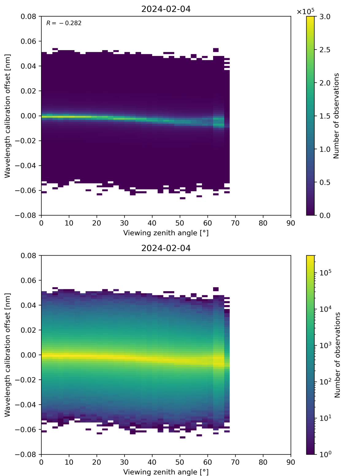
Figure 173: Scatter density plot of “Viewing zenith angle” against “Wavelength calibration offset” for 2024-02-03 to 2024-02-05.
