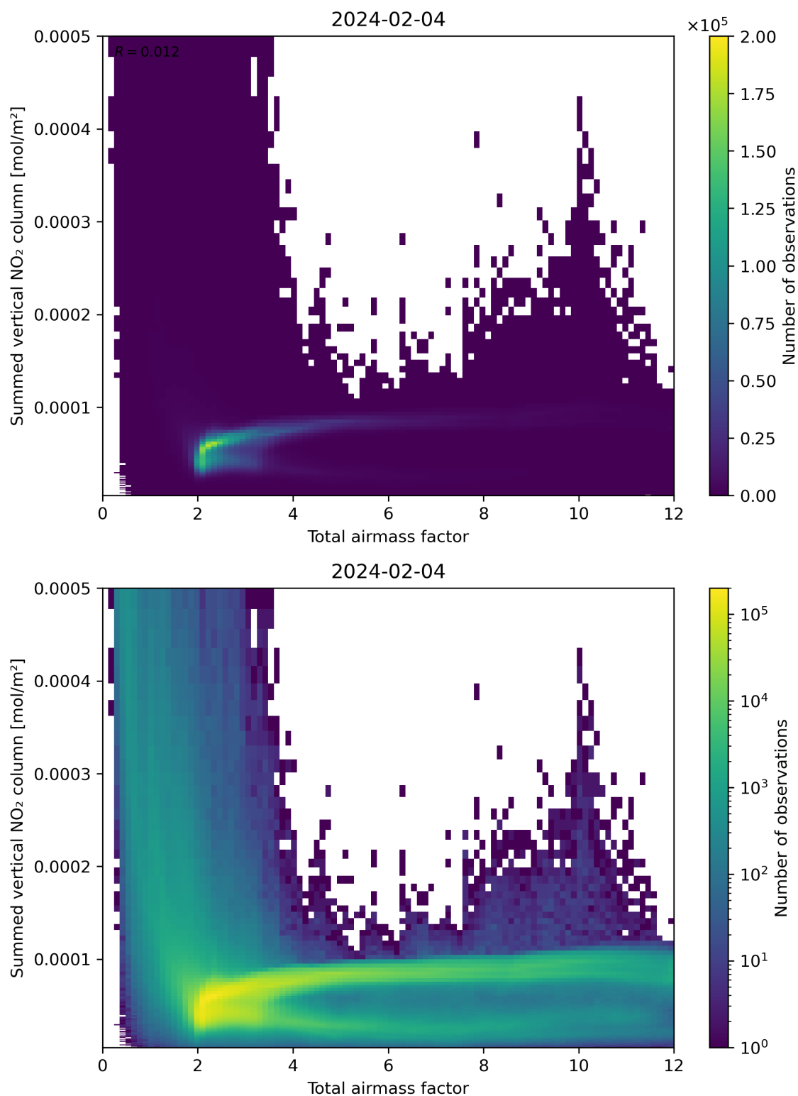
Figure 65: Scatter density plot of “Total airmass factor” against “Summed vertical NO 2 column” for 2024-02-03 to 2024-02-05.
