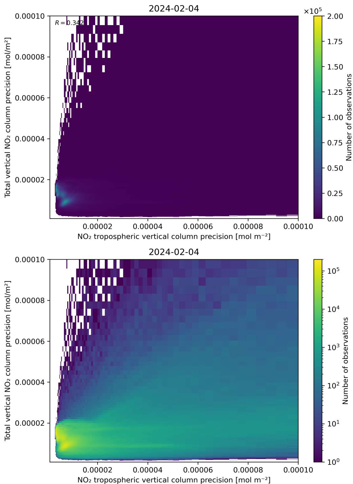
Figure 139: Scatter density plot of “NO 2 tropospheric vertical column precision” against “Total vertical NO 2 column precision” for 2024-02-03 to 2024-02-05.
