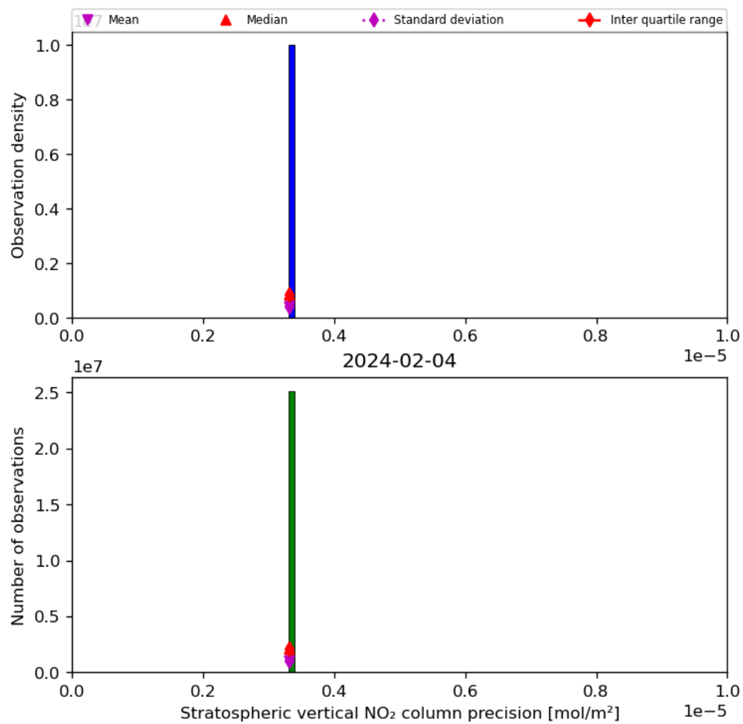
Figure 37: Histogram of “Stratospheric vertical NO 2 column precision” for 2024-02-03 to 2024-02-05
