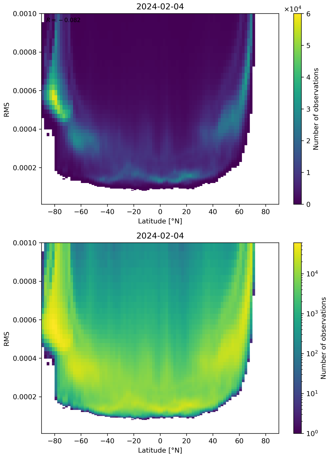
Figure 94: Scatter density plot of “Latitude” against “RMS” for 2024-02-03 to 2024-02-05.
