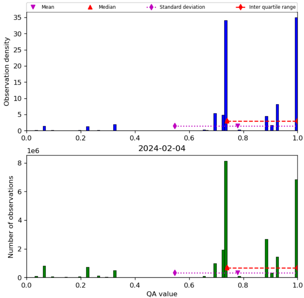
Figure 28: Histogram of “QA value” for 2024-02-03 to 2024-02-05
