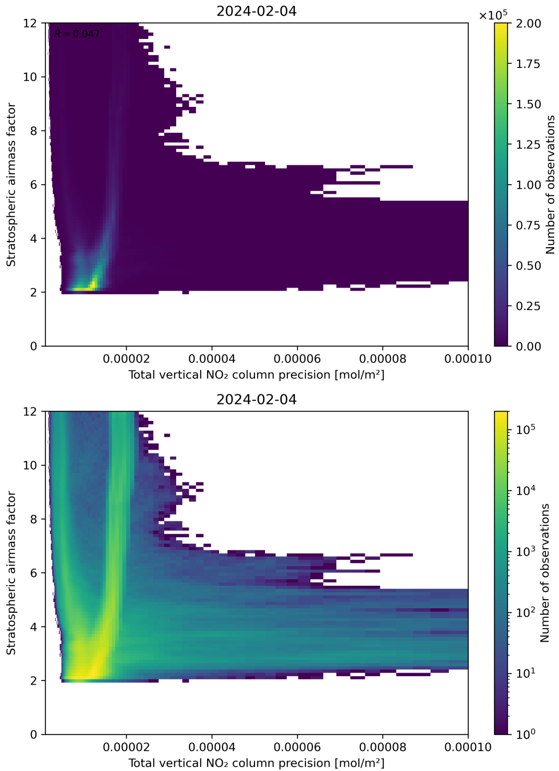
Figure 115: Scatter density plot of “Total vertical NO 2 column precision” against “Stratospheric air mass factor” for 2024-02-03 to 2024-02-05.
