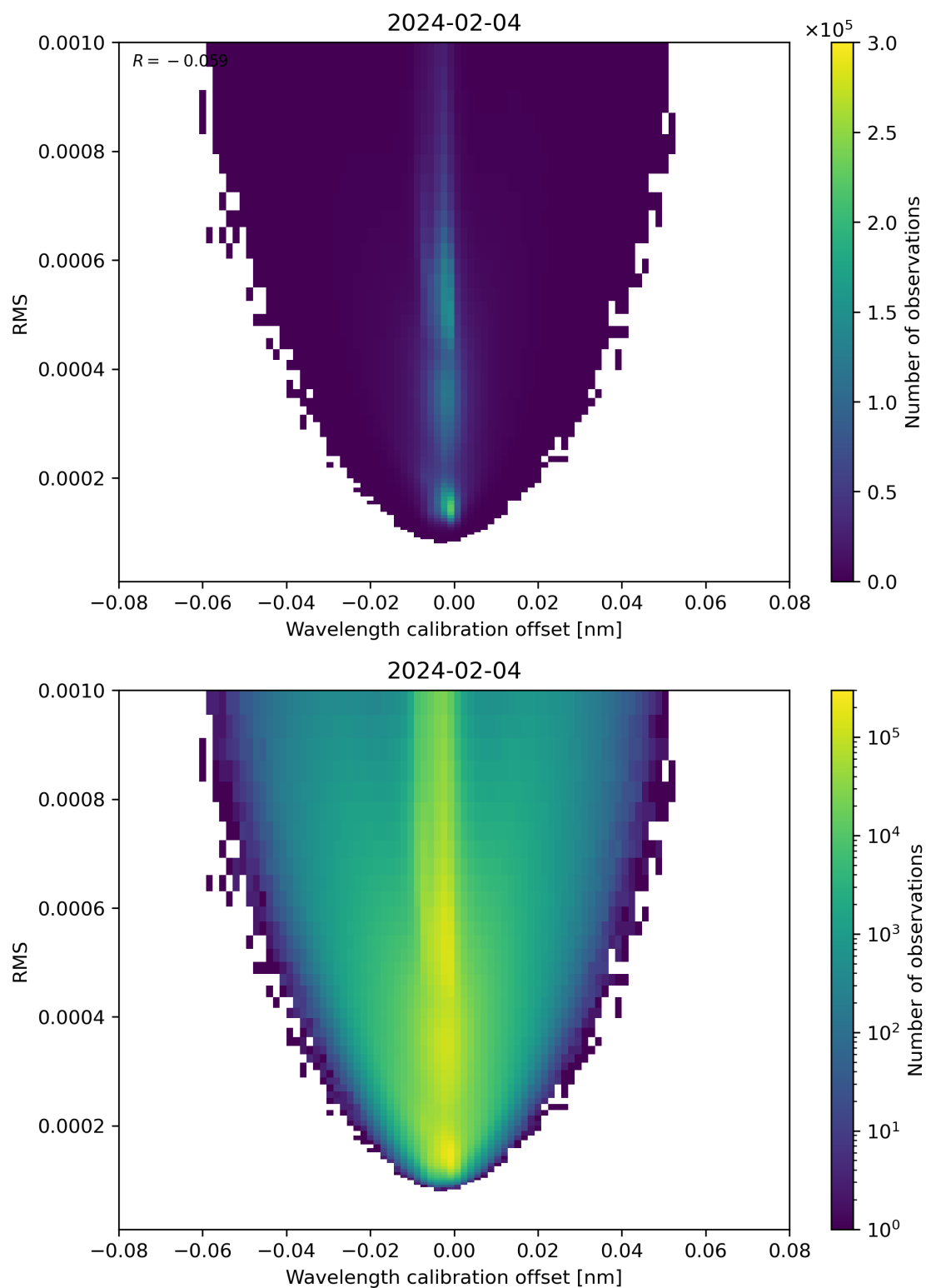
Figure 181: Scatter density plot of “Wavelength calibration offset” against “RMS” for 2024-02-03 to 2024-02-05.
