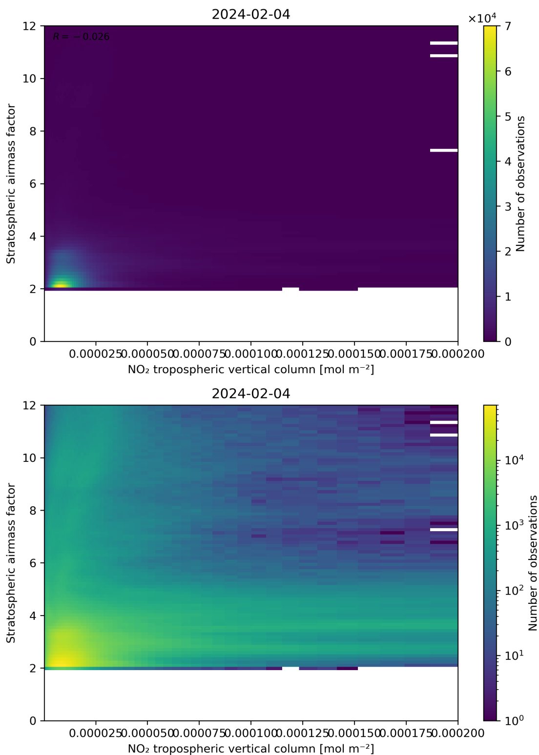
Figure 121: Scatter density plot of “NO 2 tropospheric vertical column” against “Stratospheric airmass factor” for 2024-02-03 to 2024-02-05.
