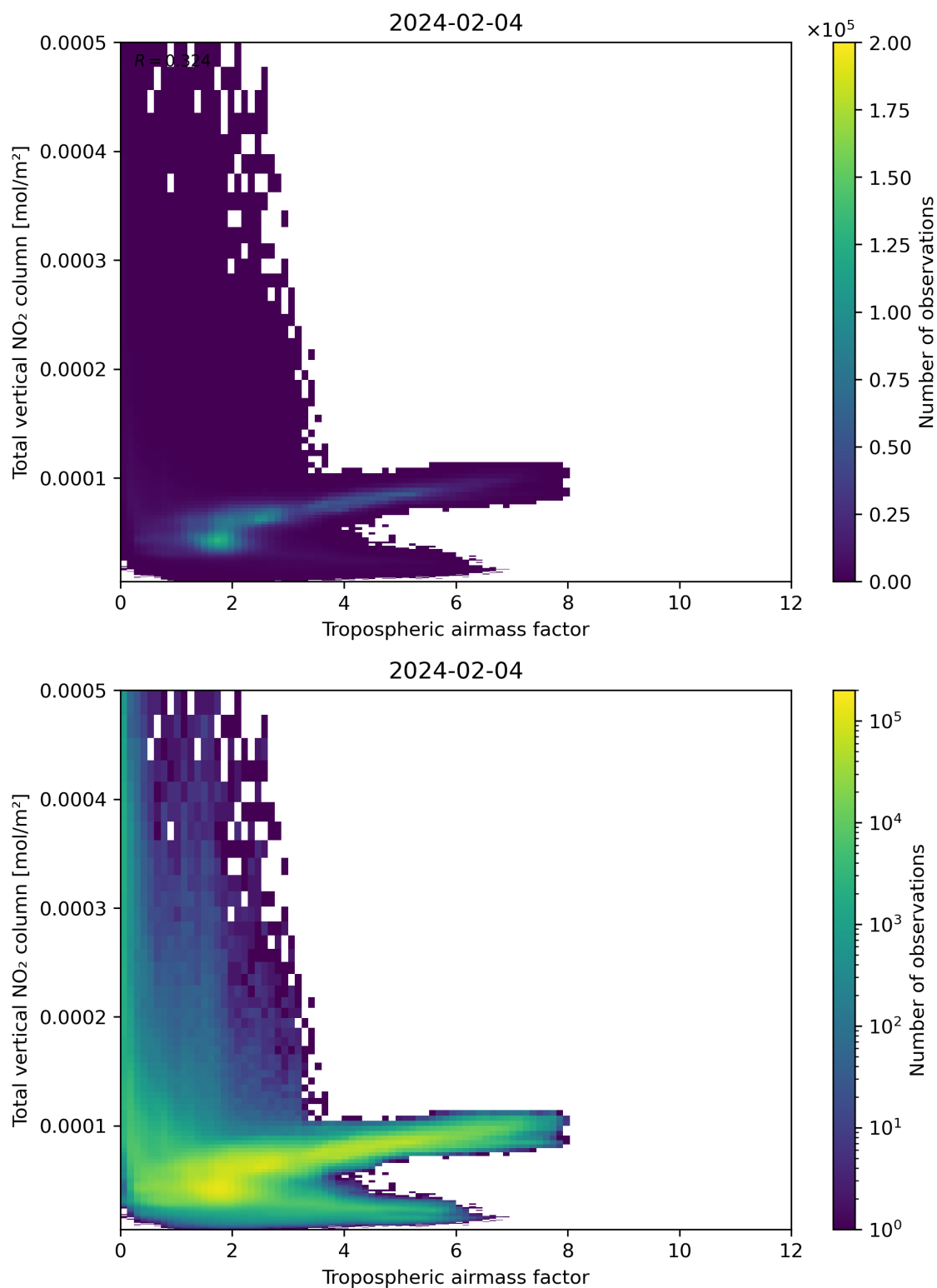
Figure 77: Scatter density plot of “Tropospheric airmass factor” against “Total vertical NO 2 column” for 2024-02-03 to 2024-02-05.
