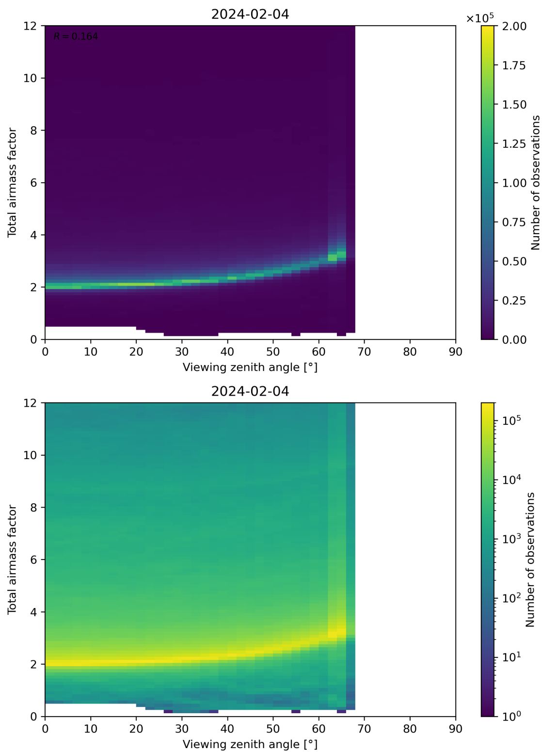
Figure 160: Scatter density plot of “Viewing zenith angle” against “Total airmass factor” for 2024-02-03 to 2024-02-05.
