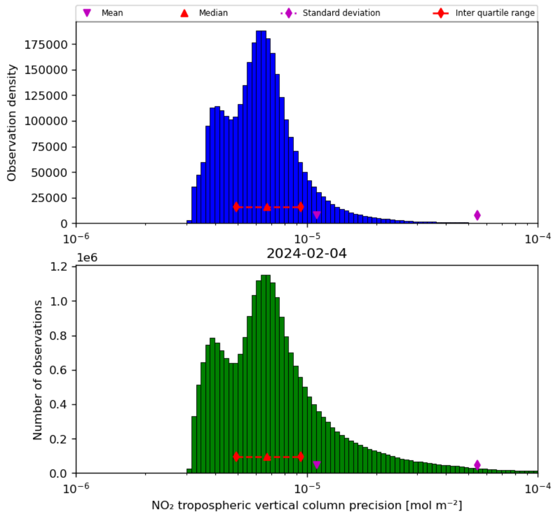
Figure 30: Histogram of “NO 2 tropospheric vertical column precision” for 2024-02-03 to 2024-02-05
