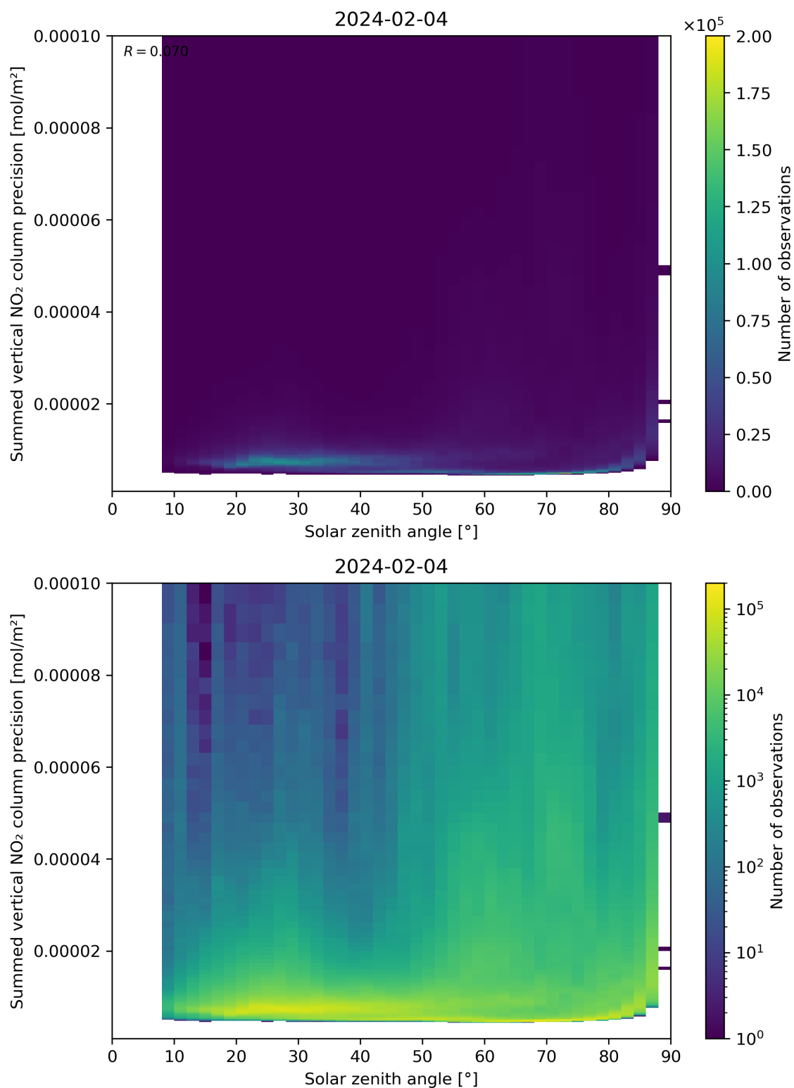
Figure 152: Scatter density plot of “Solar zenith angle” against “Summed vertical NO 2 column precision” for 2024-02-03 to 2024-02-05.
