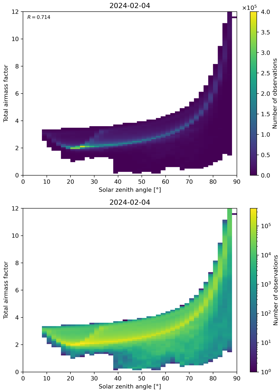
Figure 146: Scatter density plot of “Solar zenith angle” against “Total air mass factor” for 2024-02-03 to 2024-02-05.
