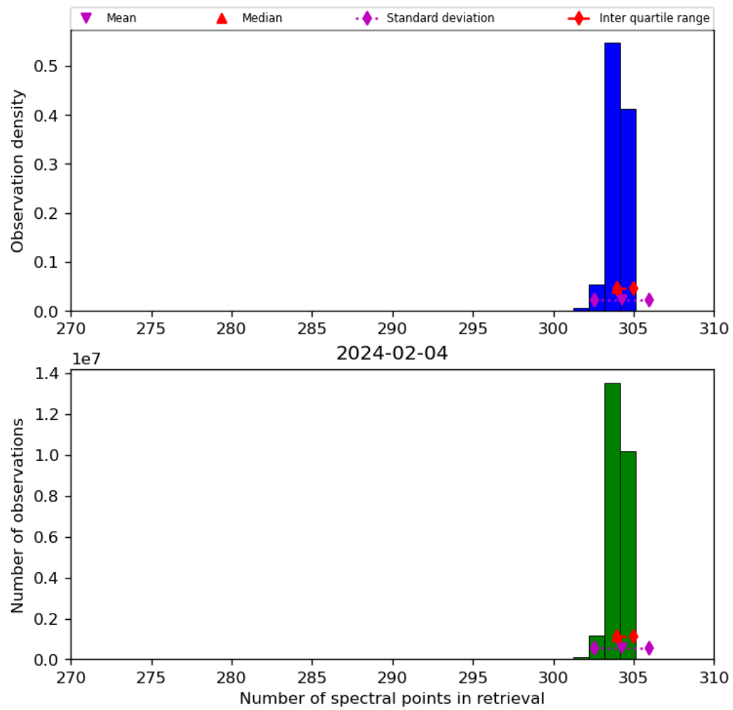
Figure 33: Histogram of “Number of spectral points in retrieval” for 2024-02-03 to 2024-02-05
