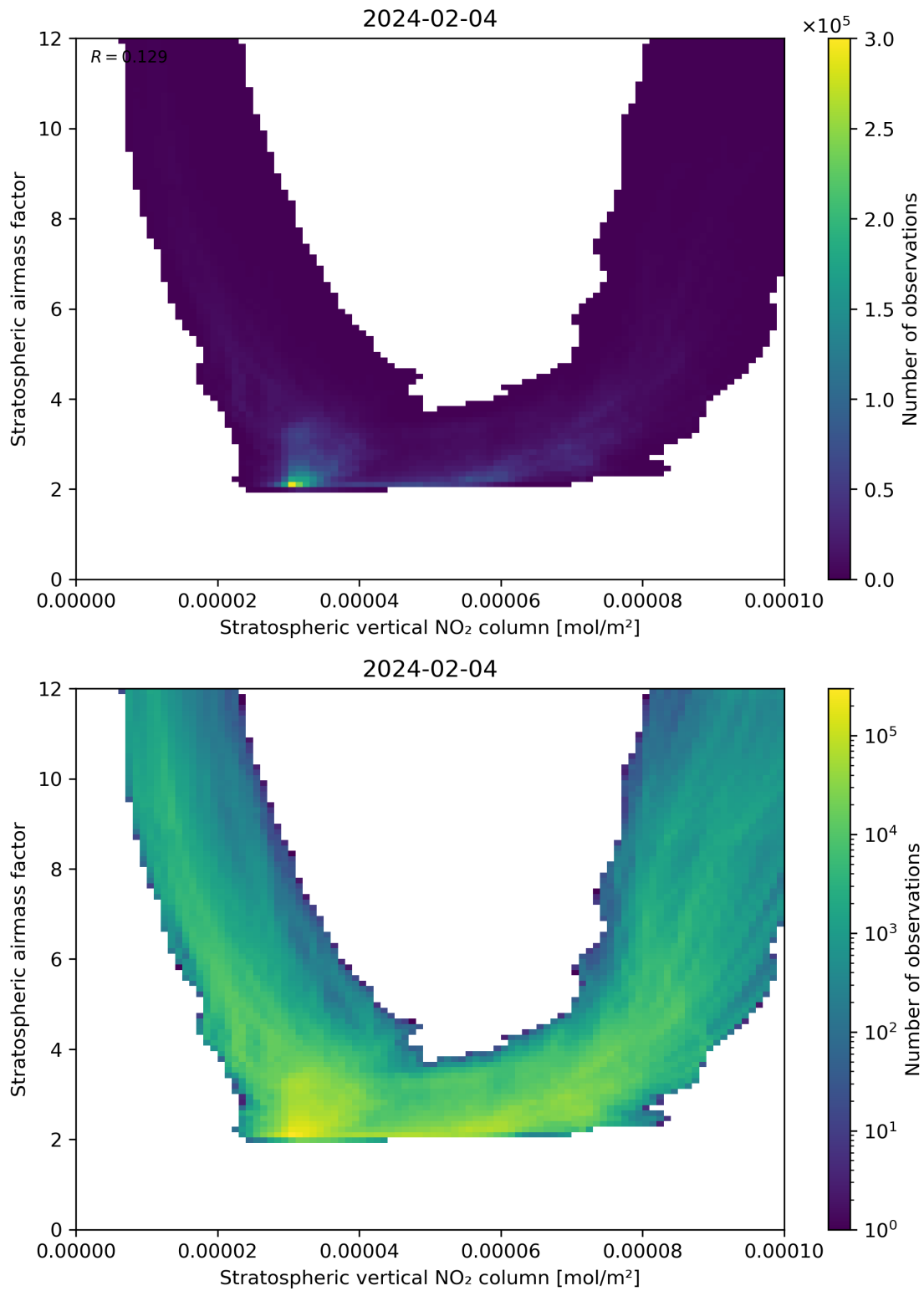
Figure 96: Scatter density plot of “Stratospheric vertical NO 2 column” against “Stratospheric airmass factor” for 2024-02-03 to 2024-02-05.
