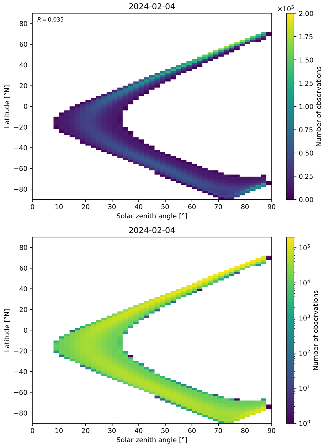
Figure 149: Scatter density plot of “Solar zenith angle” against “Latitude” for 2024-02-03 to 2024-02-05.
