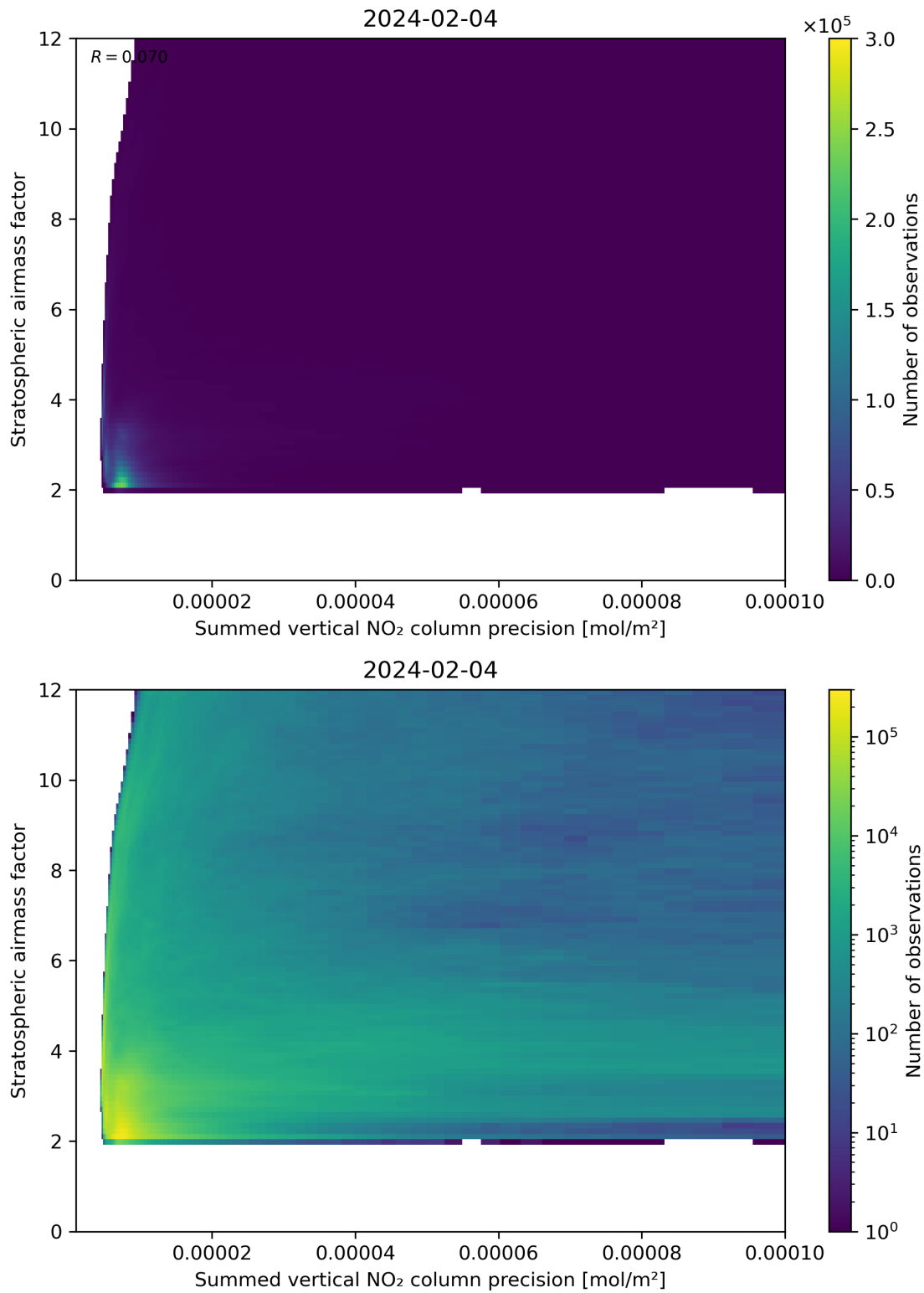
Figure 106: Scatter density plot of “Summed vertical NO 2 column precision” against “Stratospheric airmass factor” for 2024-02-03 to 2024-02-05.
