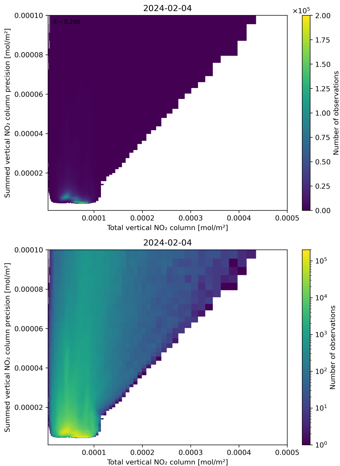
Figure 113: Scatter density plot of “Total vertical NO 2 column” against “Summed vertical NO 2 column precision” for 2024-02-03 to 2024-02-05.
