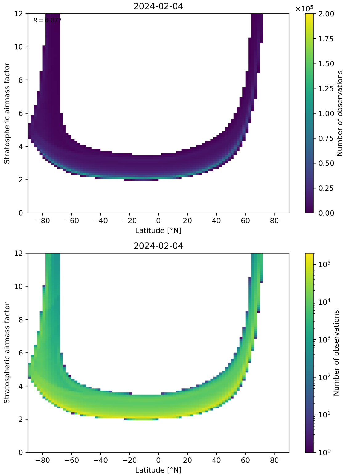
Figure 83: Scatter density plot of “Latitude” against “Stratospheric airmass factor” for 2024-02-03 to 2024-02-05.
