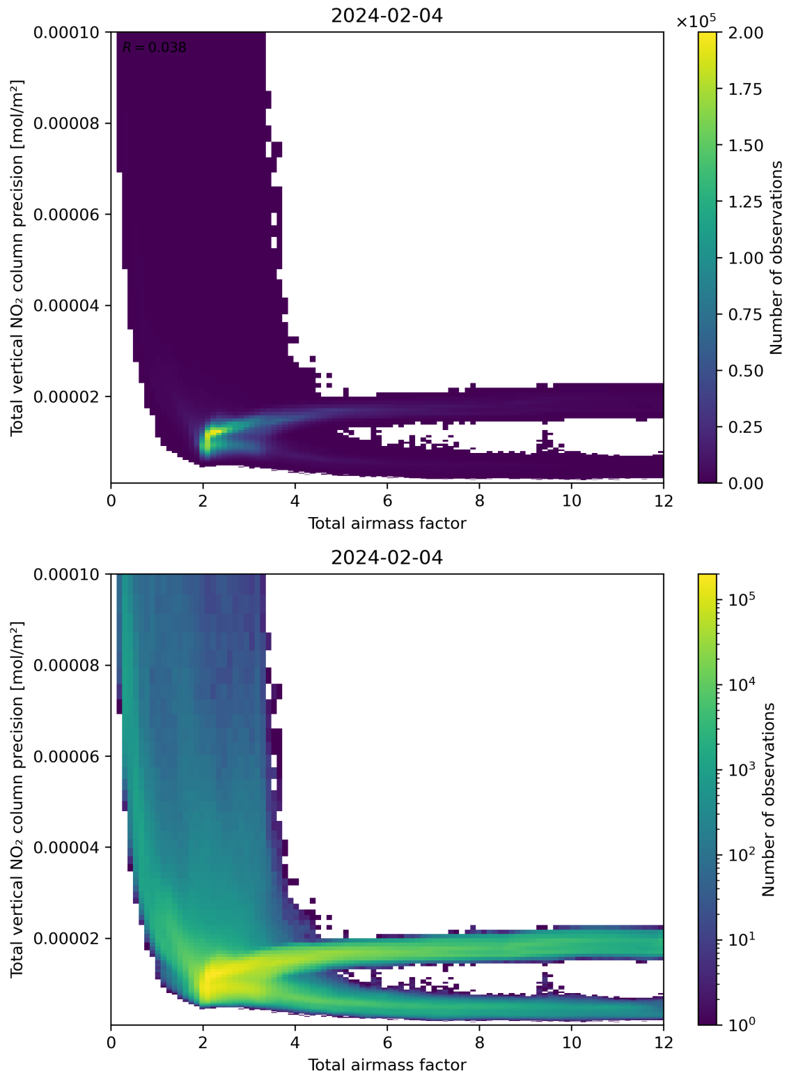
Figure 68: Scatter density plot of “Total airmass factor” against “Total vertical NO 2 column precision” for 2024-02-03 to 2024-02-05.
