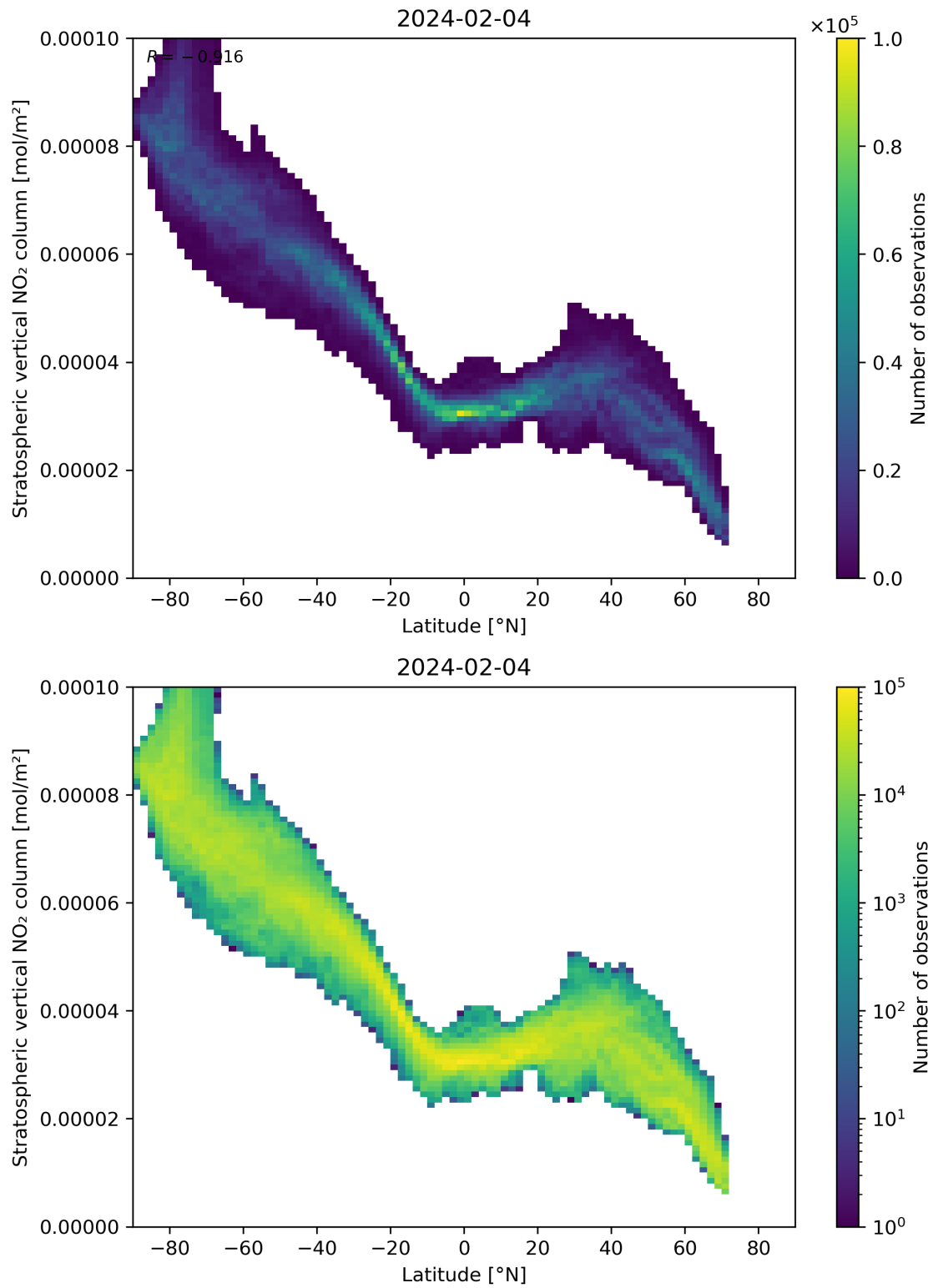
Figure 87: Scatter density plot of “Latitude” against “Stratospheric vertical NO 2 column” for 2024-02-03 to 2024-02-05.
