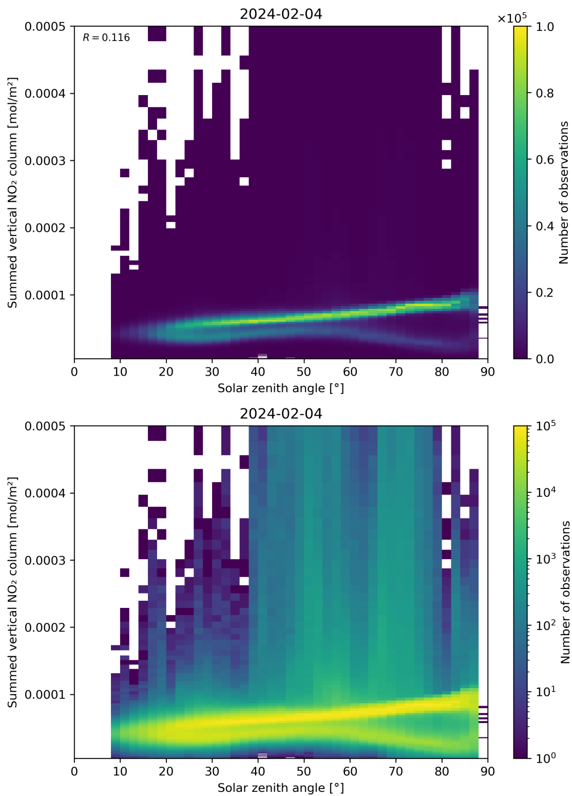
Figure 151: Scatter density plot of “Solar zenith angle” against “Summed vertical NO 2 column” for 2024-02-03 to 2024-02-05.
