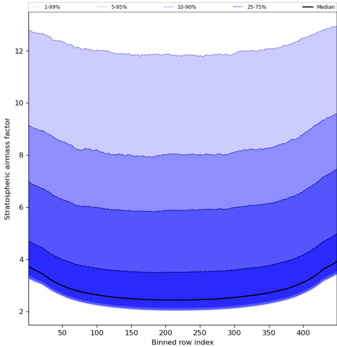
Figure 61: Along track statistics of “Stratospheric airmass factor” for 2024-02-03 to 2024-02-05
