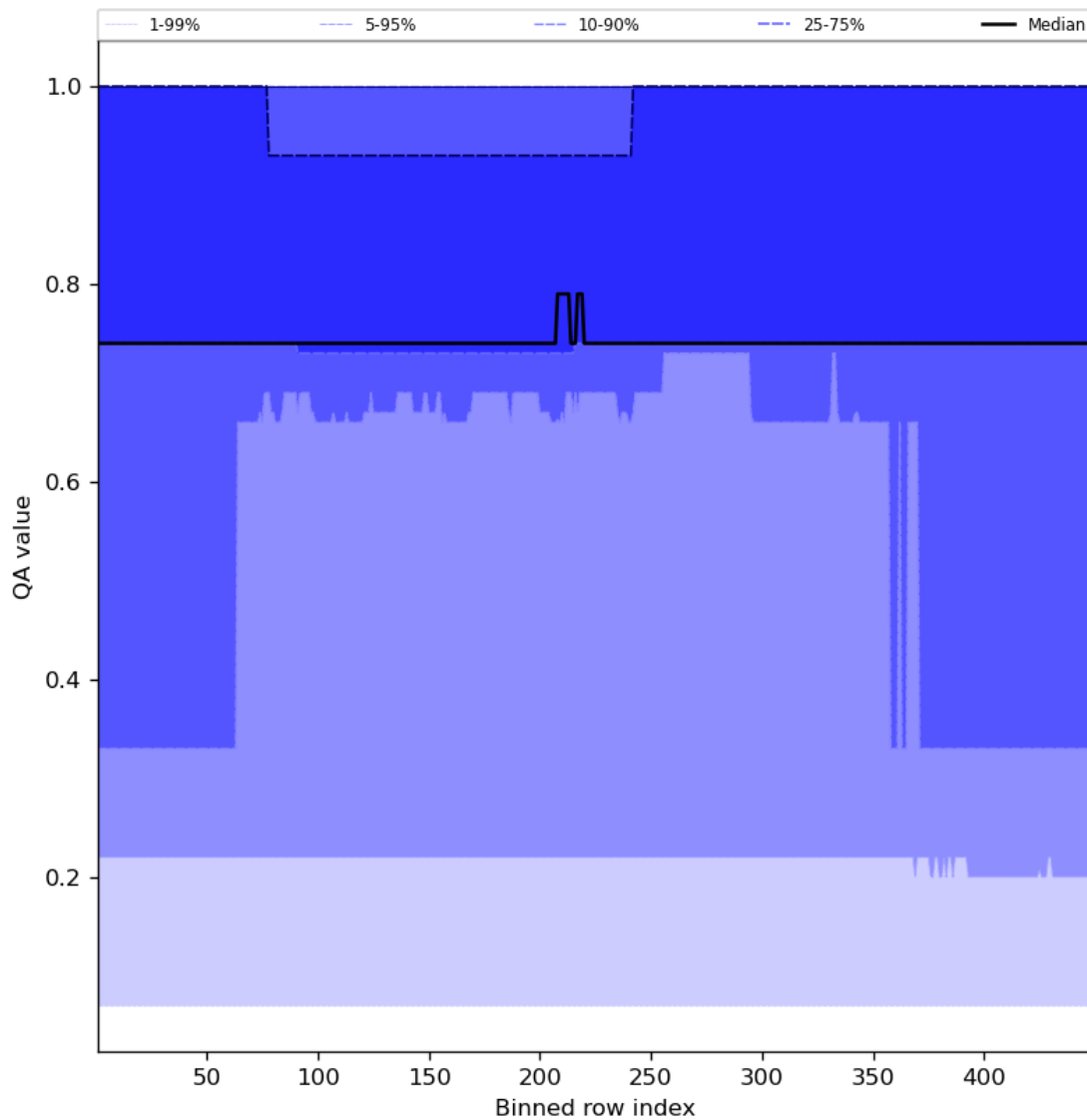
Figure 45: Along track statistics of “QA value” for 2024-02-03 to 2024-02-05
