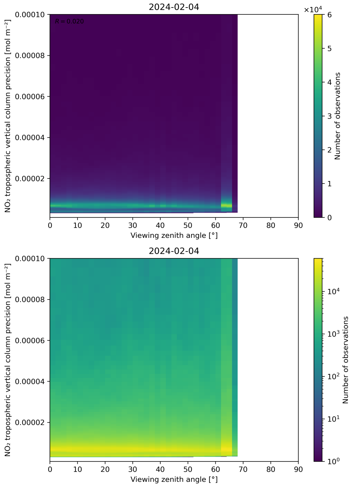
Figure 170: Scatter density plot of “Viewing zenith angle” against “NO 2 tropospheric vertical column precision” for 2024-02-03 to 2024-02-05.
