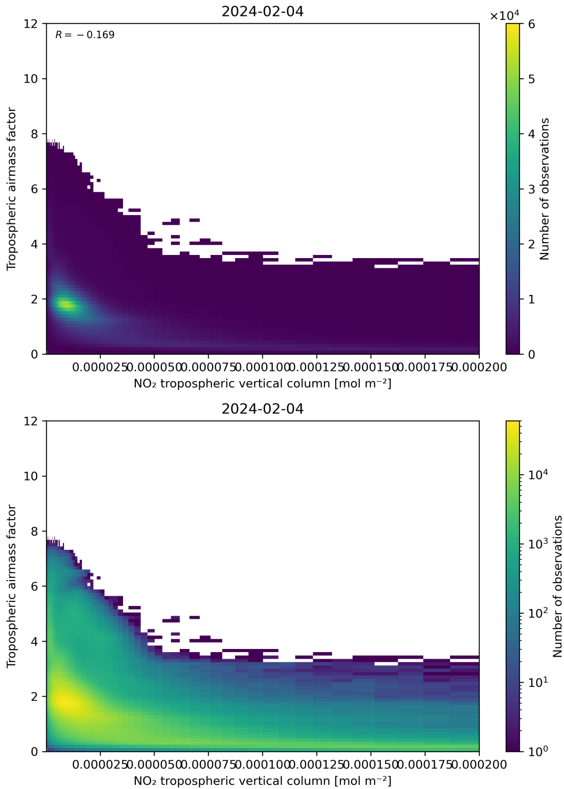
Figure 123: Scatter density plot of “NO 2 tropospheric vertical column” against “Tropospheric air mass factor” for 2024-02-03 to 2024-02-05.
