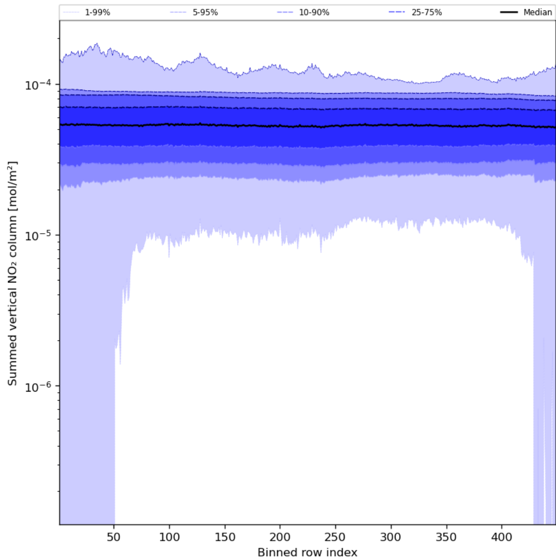
Figure 57: Along track statistics of “Summed vertical NO 2 column” for 2024-02-03 to 2024-02-05
