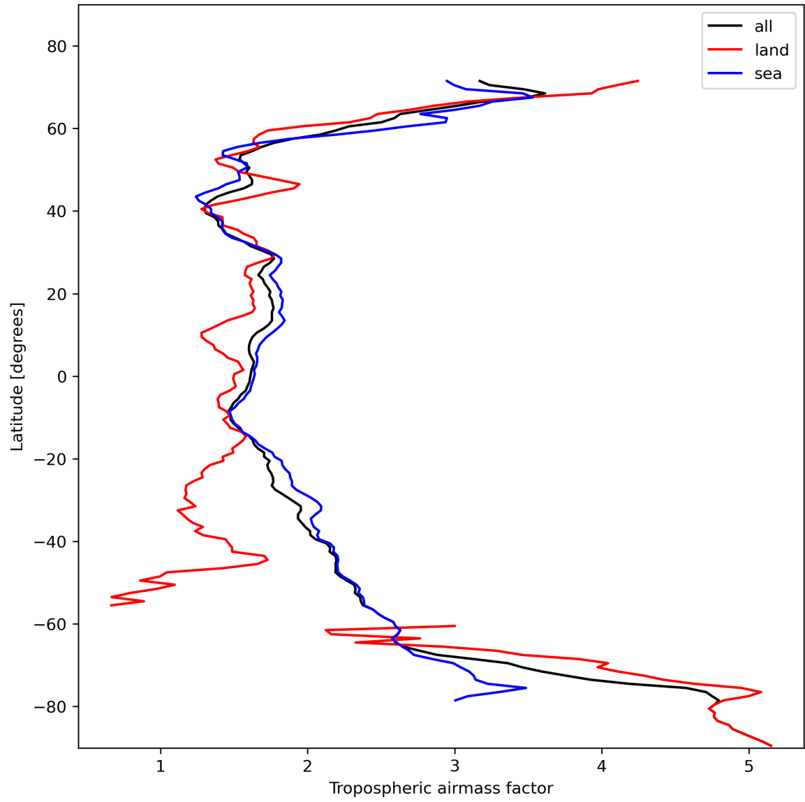
Figure 14: Zonal average of “Tropospheric airmass factor” for 2024-02-03 to 2024-02-05.
