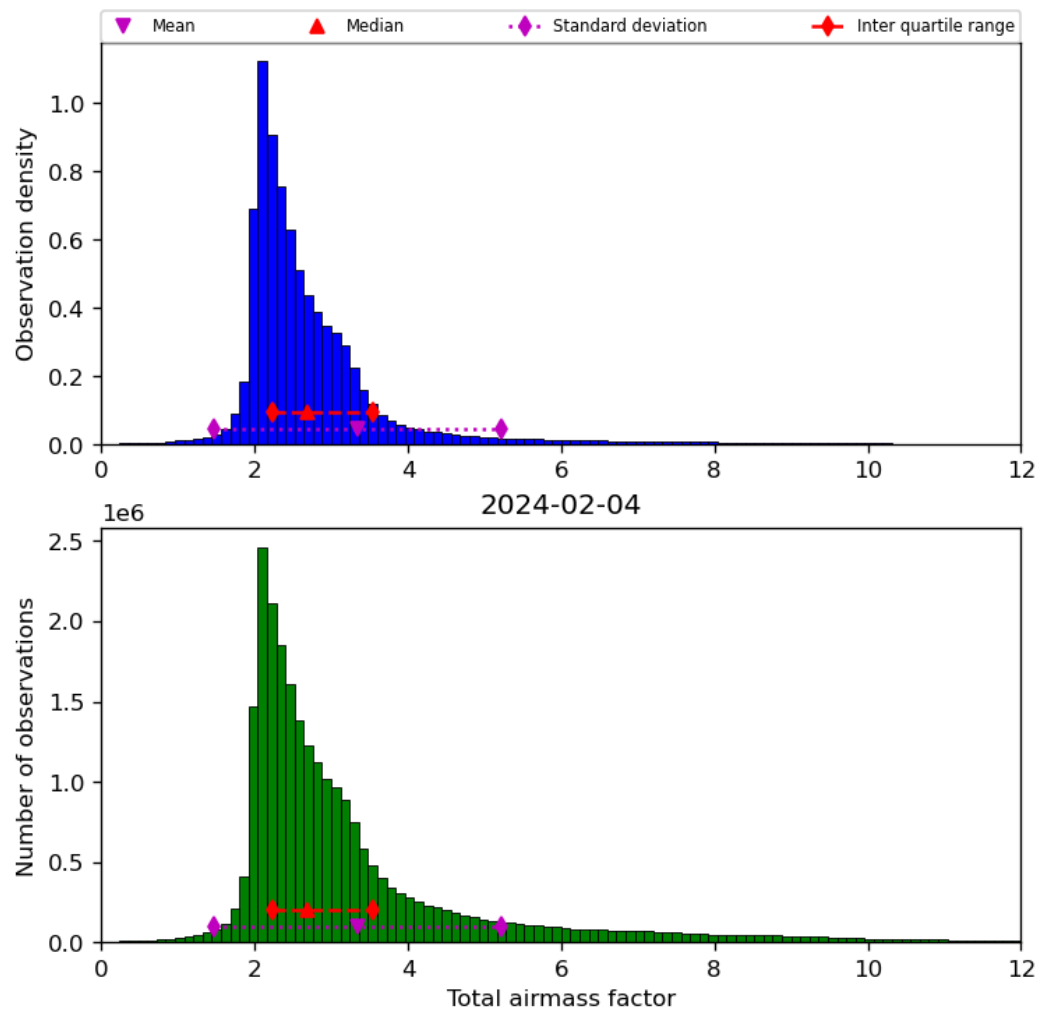
Figure 32: Histogram of “Total airmass factor” for 2024-02-03 to 2024-02-05
