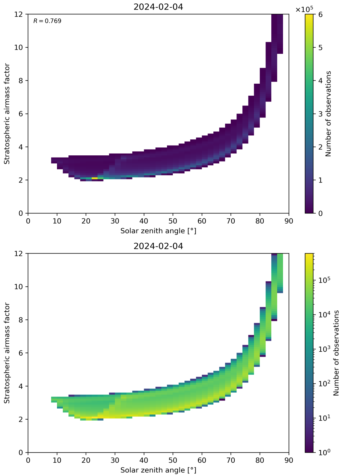
Figure 145: Scatter density plot of “Solar zenith angle” against “Stratospheric airmass factor” for 2024-02-03 to 2024-02-05.
