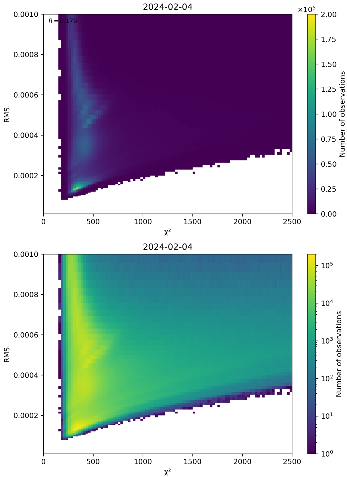
Figure 82: Scatter density plot of “ \chi^2 ” against “RMS” for 2024-02-03 to 2024-02-05.
