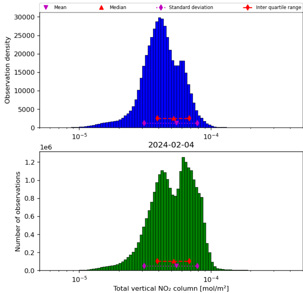
Figure 38: Histogram of “Total vertical NO 2 column” for 2024-02-03 to 2024-02-05
