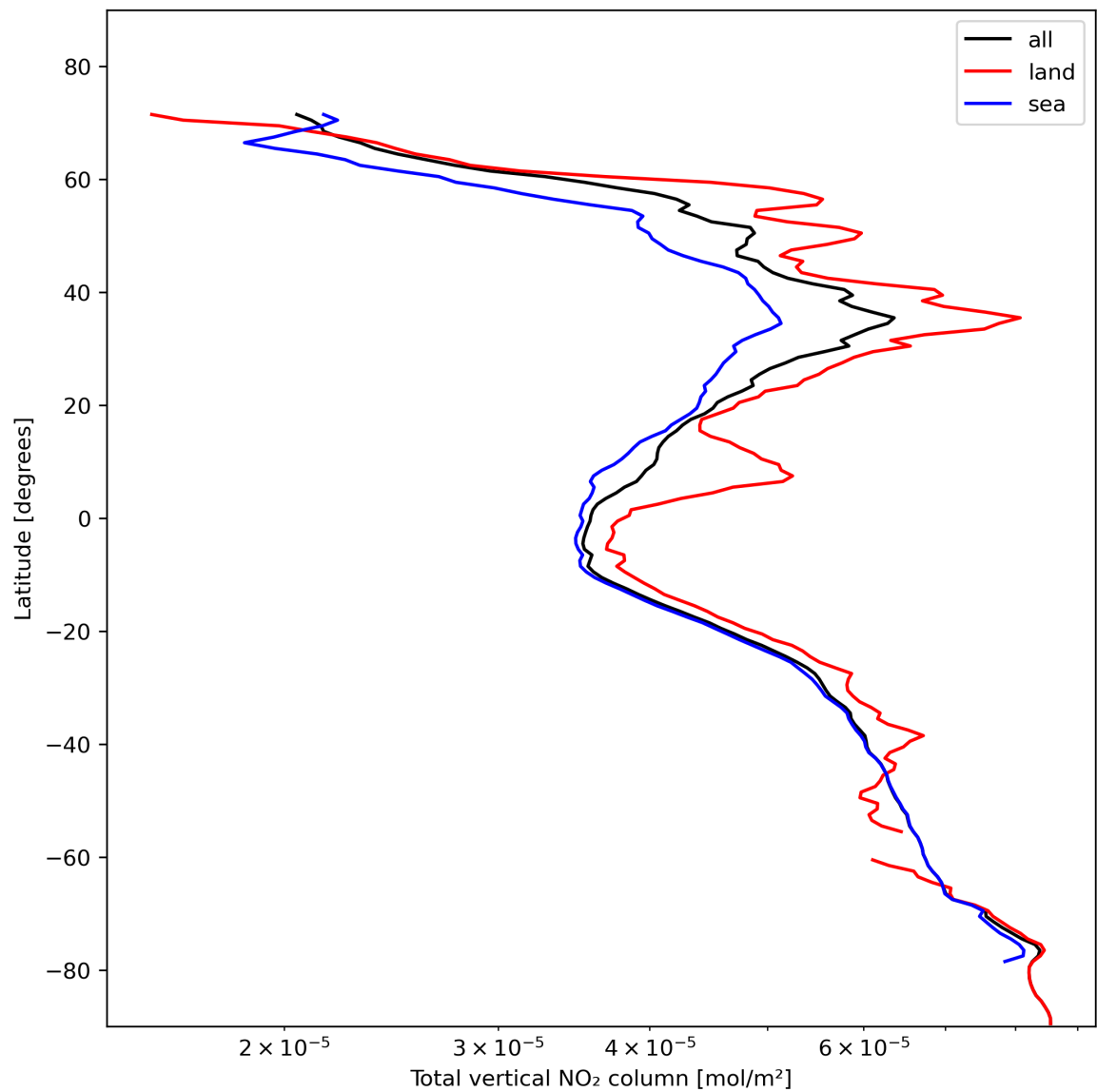
Figure 21: Zonal average of “Total vertical NO 2 column” for 2024-02-03 to 2024-02-05.
