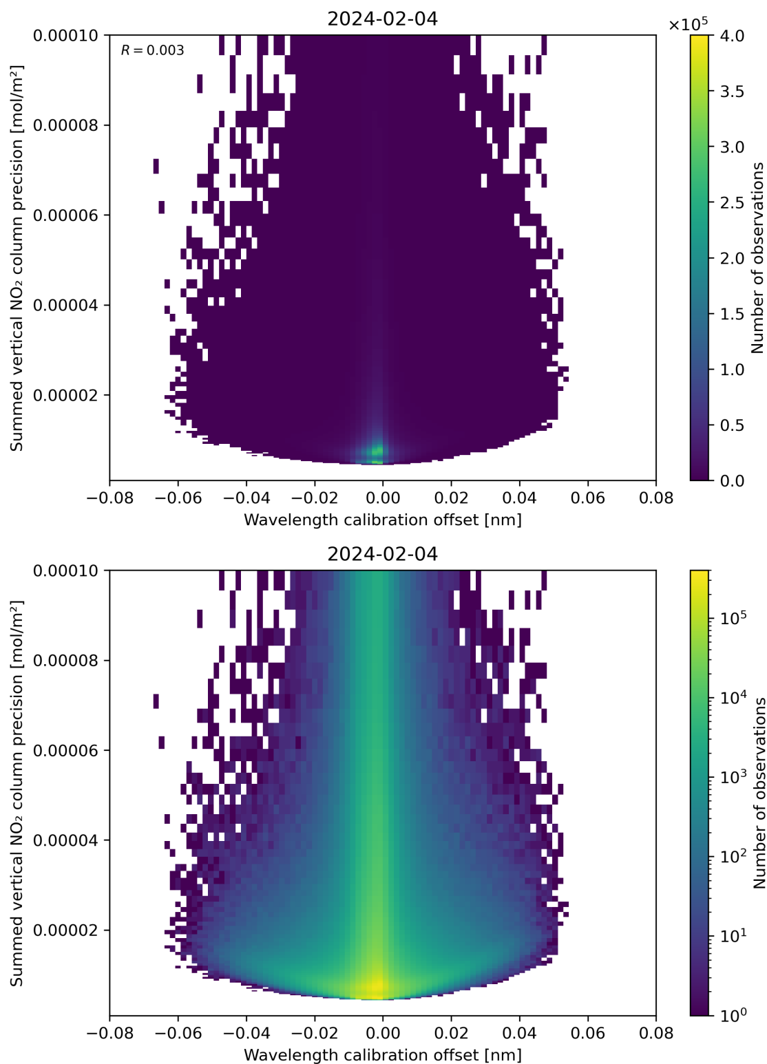
Figure 178: Scatter density plot of “Wavelength calibration offset” against “Summed vertical NO 2 column precision” for 2024-02-03 to 2024-02-05.
