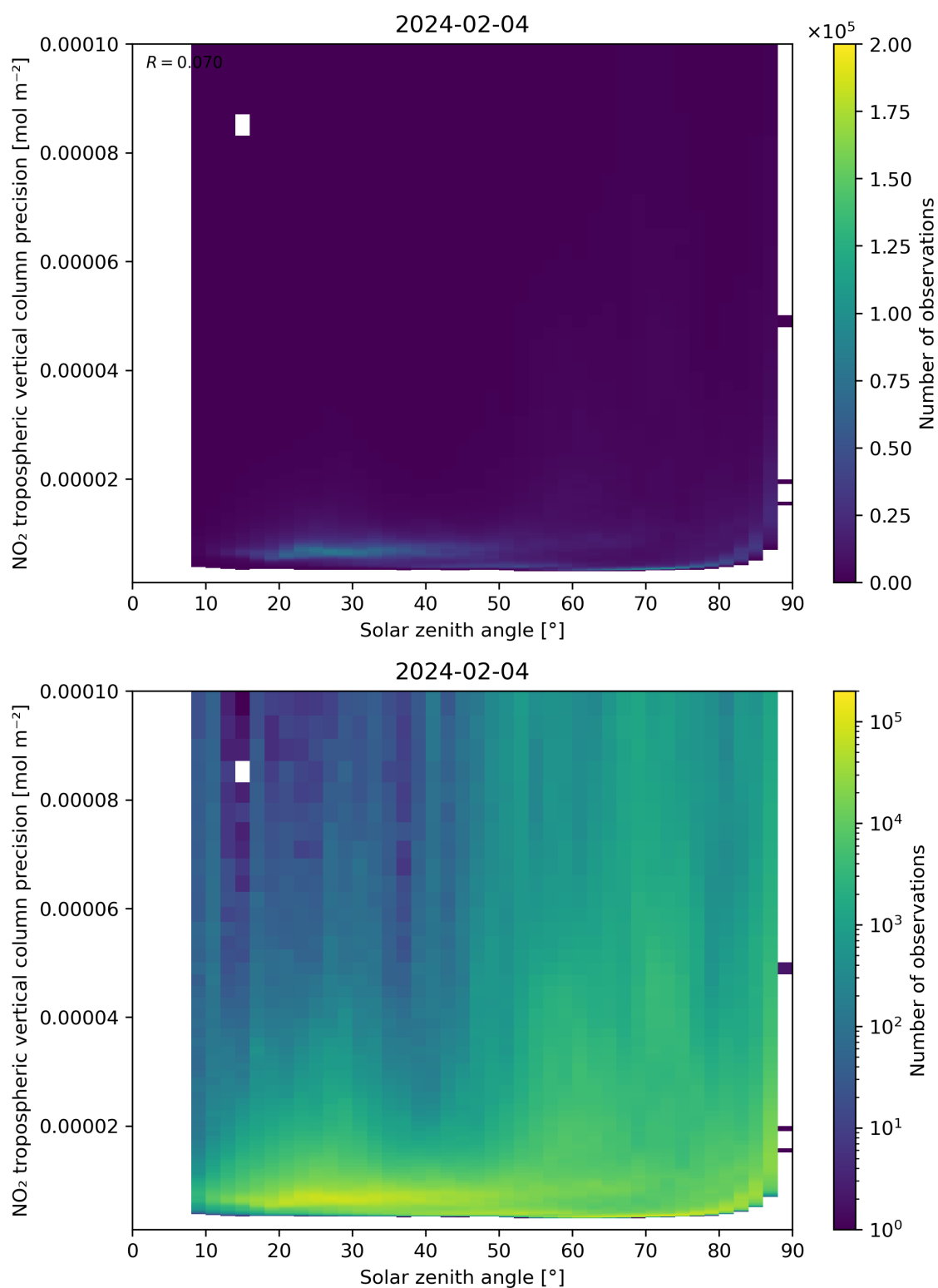
Figure 156: Scatter density plot of “Solar zenith angle” against “NO 2 tropospheric vertical column precision” for 2024-02-03 to 2024-02-05.
