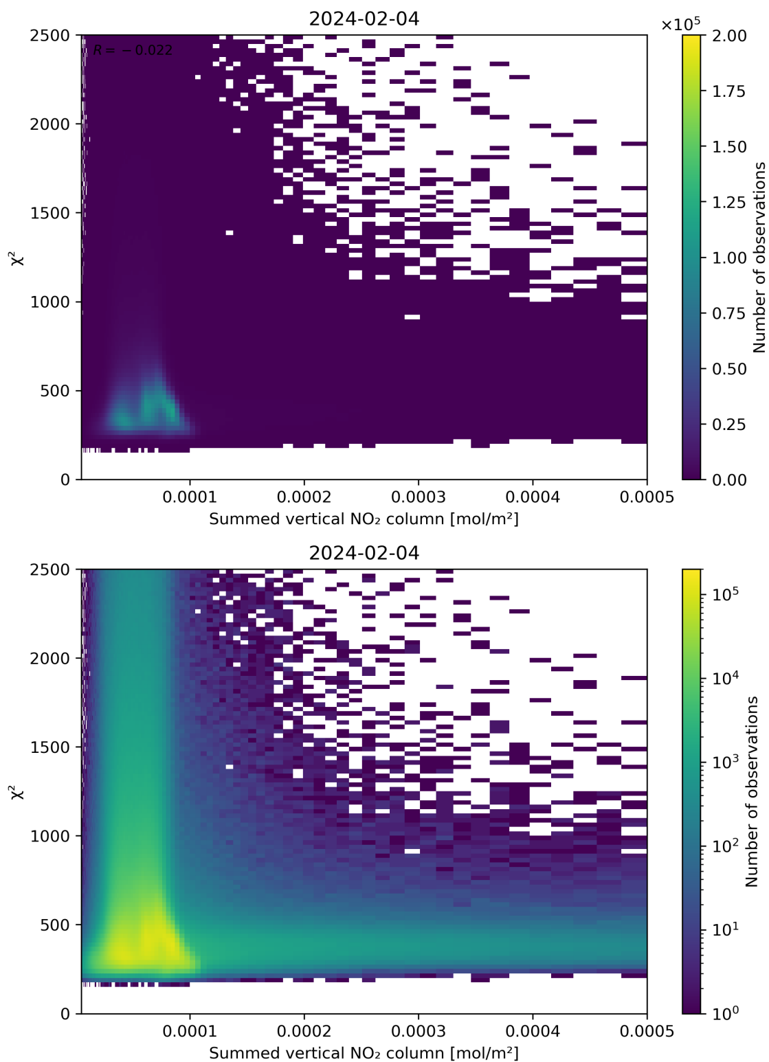
Figure 104: Scatter density plot of “Summed vertical NO 2 column” against “ \chi^2 ” for 2024-02-03 to 2024-02-05.
