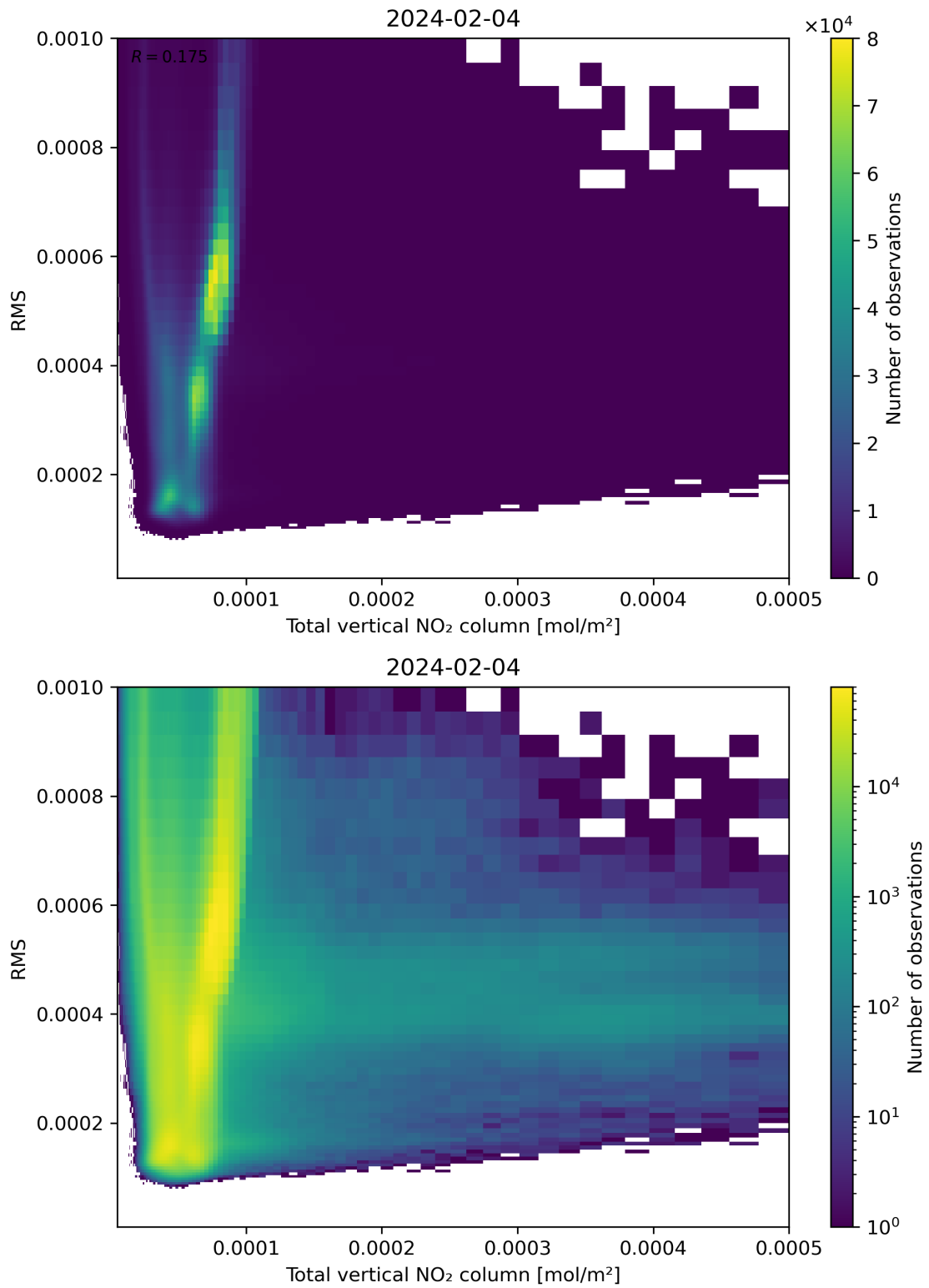
Figure 120: Scatter density plot of “Total vertical NO 2 column” against “RMS” for 2024-02-03 to 2024-02-05.
