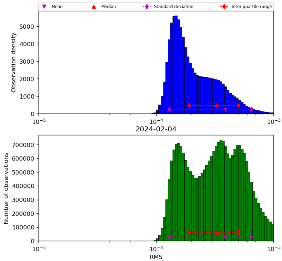
Figure 43: Histogram of “RMS” for 2024-02-03 to 2024-02-05
