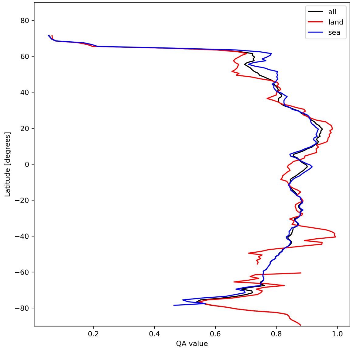
Figure 11: Zonal average of “QA value” for 2024-02-03 to 2024-02-05.
