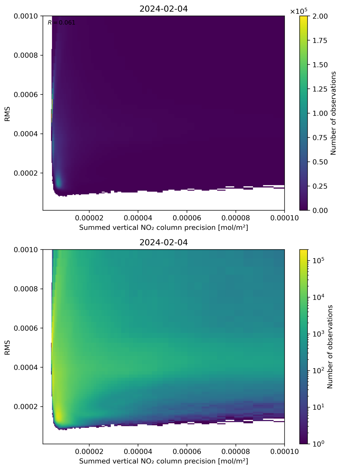
Figure 108: Scatter density plot of “Summed vertical NO 2 column precision” against “RMS” for 2024-02-03 to 2024-02-05.
