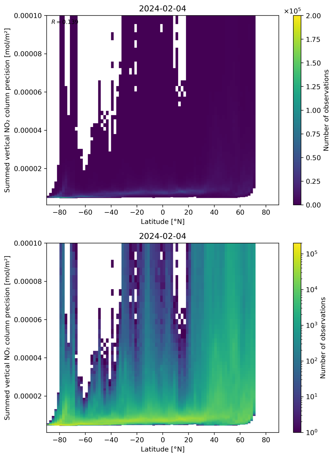
Figure 89: Scatter density plot of “Latitude” against “Summed vertical NO 2 column precision” for 2024-02-03 to 2024-02-05.
