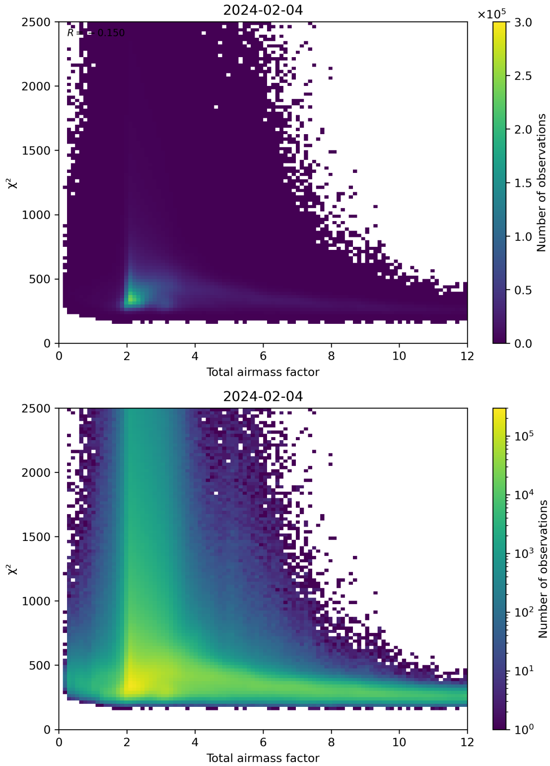
Figure 63: Scatter density plot of “Total airmass factor” against “ \chi^2 ” for 2024-02-03 to 2024-02-05.
