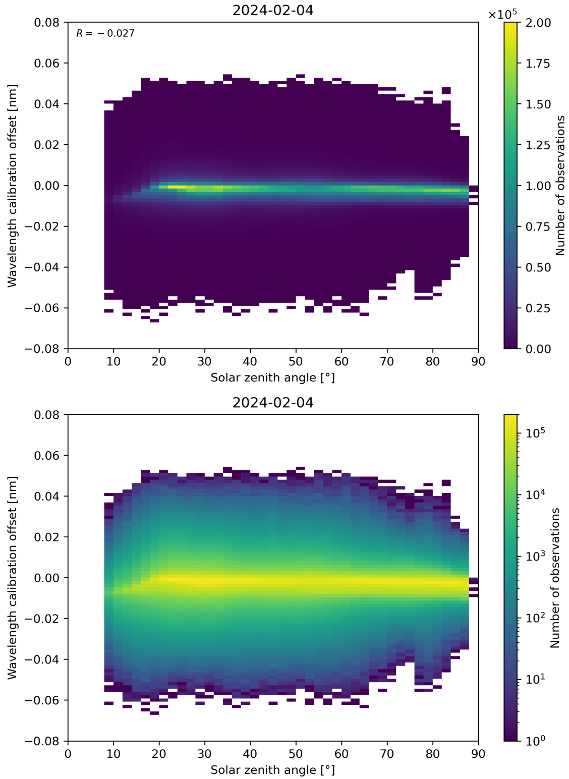
Figure 158: Scatter density plot of “Solar zenith angle” against “Wavelength calibration offset” for 2024-02-03 to 2024-02-05.
