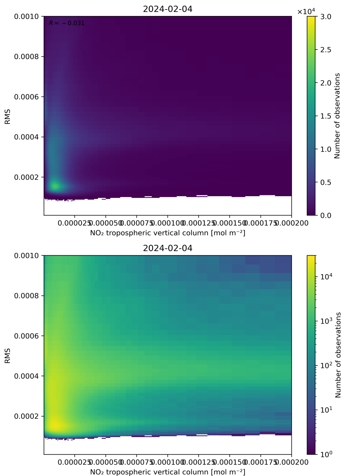
Figure 142: Scatter density plot of “NO 2 tropospheric vertical column” against “RMS” for 2024-02-03 to 2024-02-05.
