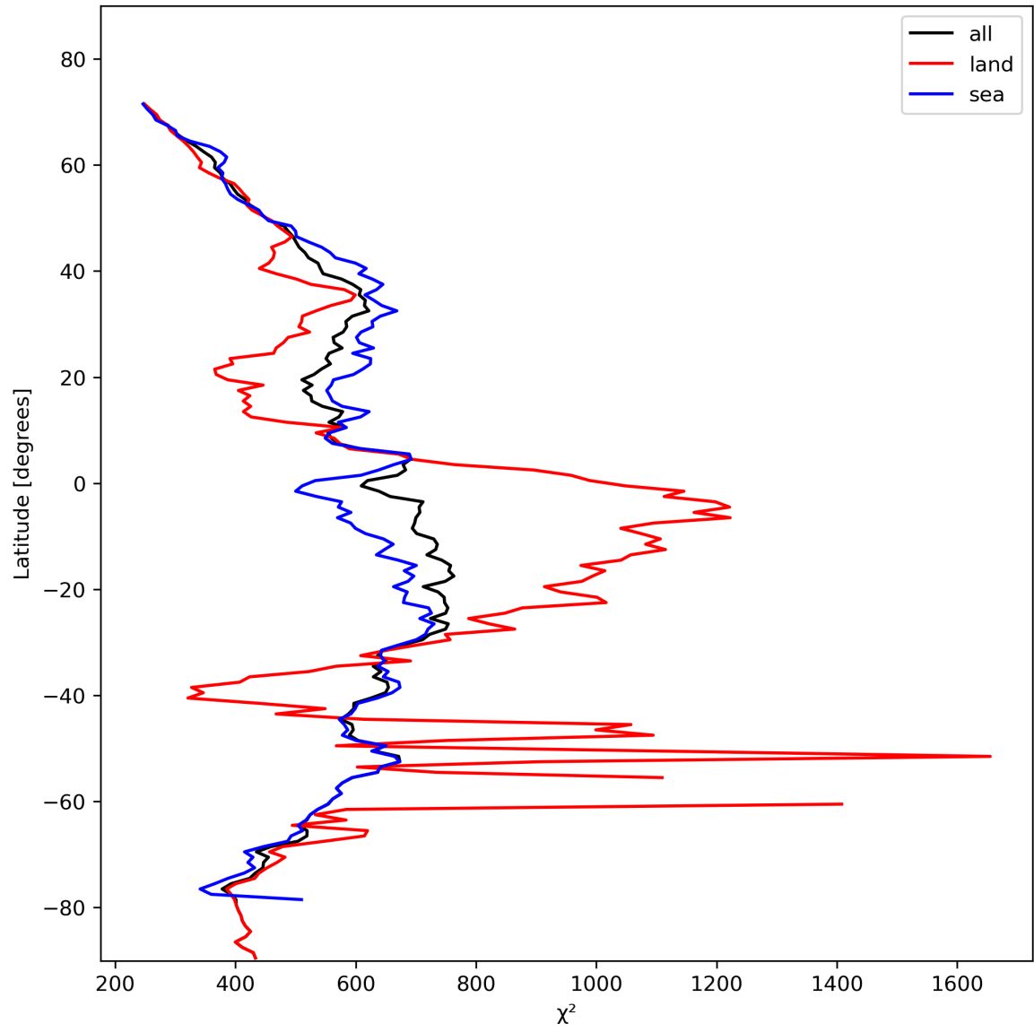
Figure 25: Zonal average of “ \chi^2 ” for 2024-02-03 to 2024-02-05.
