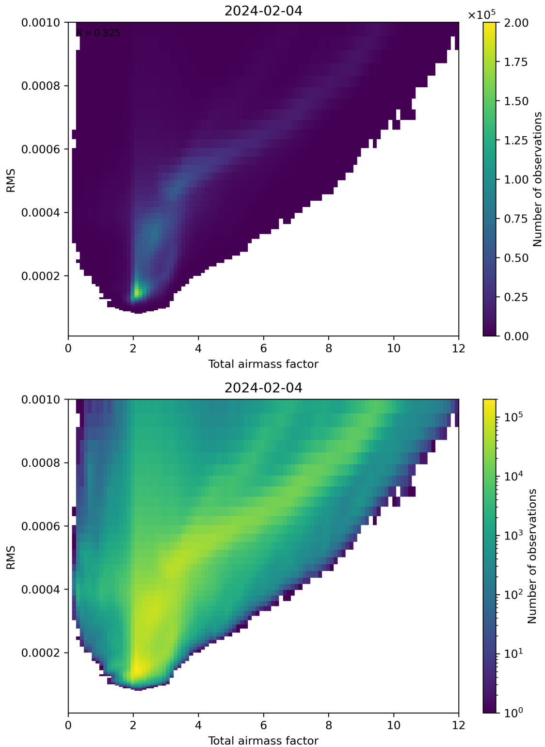
Figure 69: Scatter density plot of “Total airmass factor” against “RMS” for 2024-02-03 to 2024-02-05.
