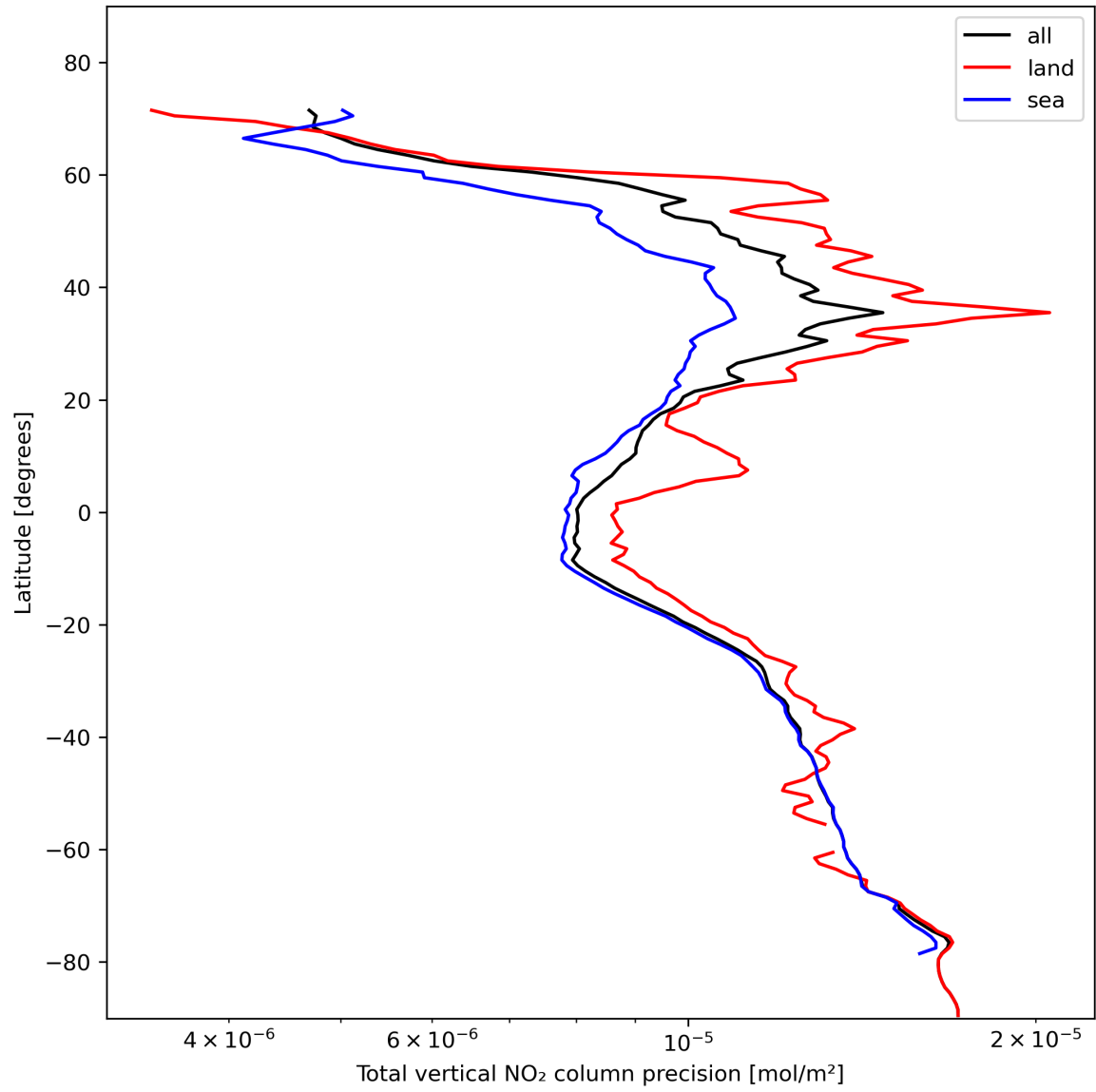
Figure 22: Zonal average of “Total vertical NO 2 column precision” for 2024-02-03 to 2024-02-05.
