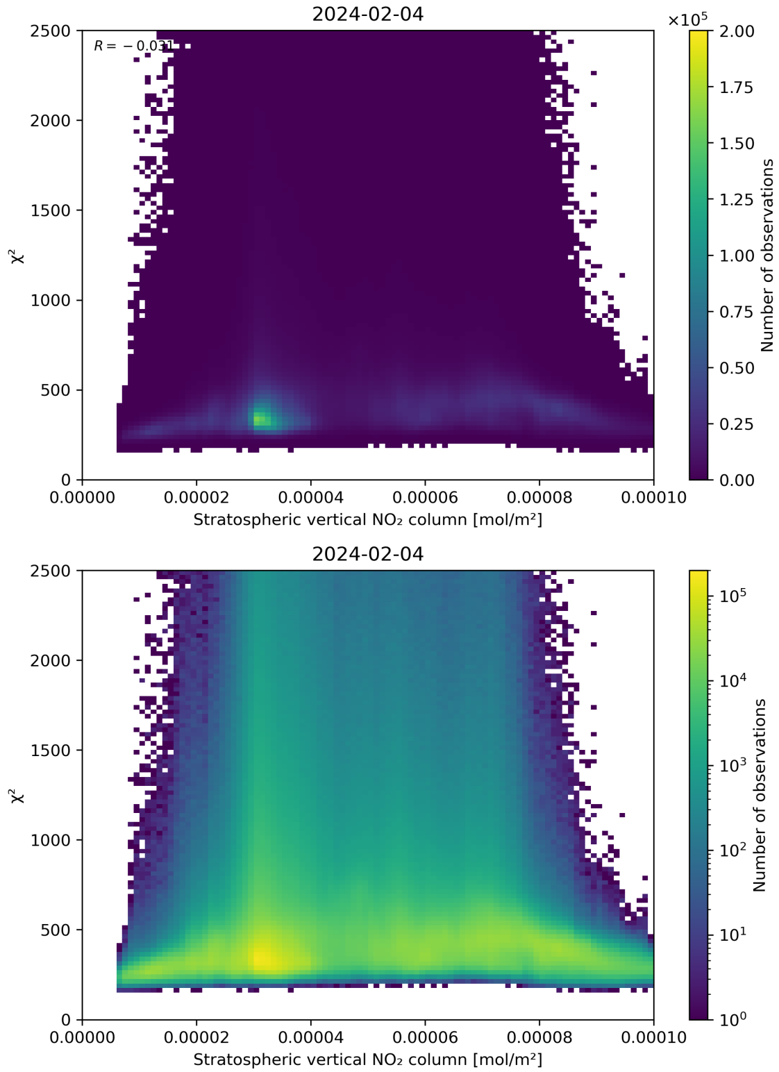
Figure 97: Scatter density plot of “Stratospheric vertical NO 2 column” against “ \chi^2 ” for 2024-02-03 to 2024-02-05.
