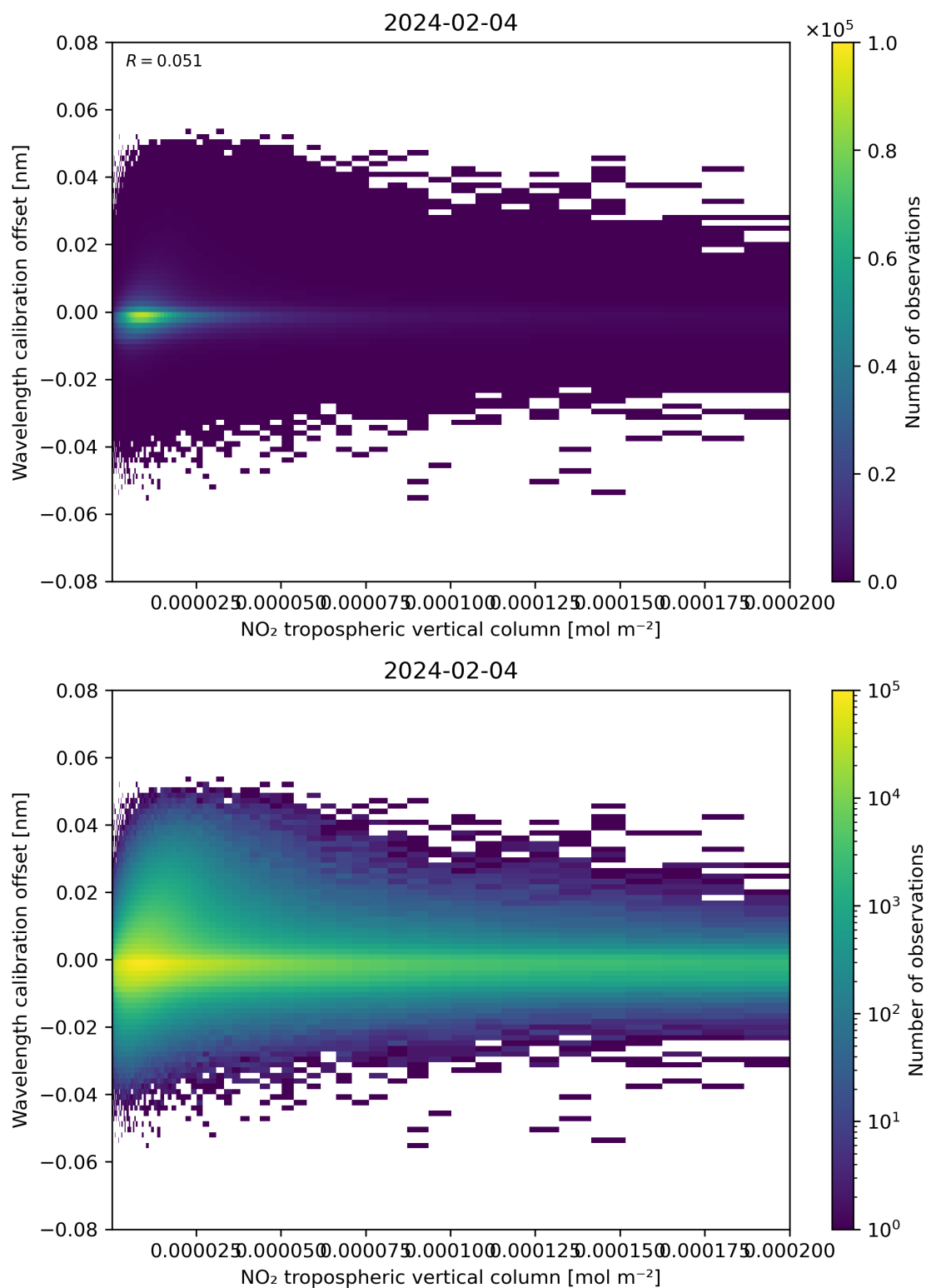
Figure 143: Scatter density plot of “NO 2 tropospheric vertical column” against “Wavelength calibration offset” for 2024-02-03 to 2024-02-05.
