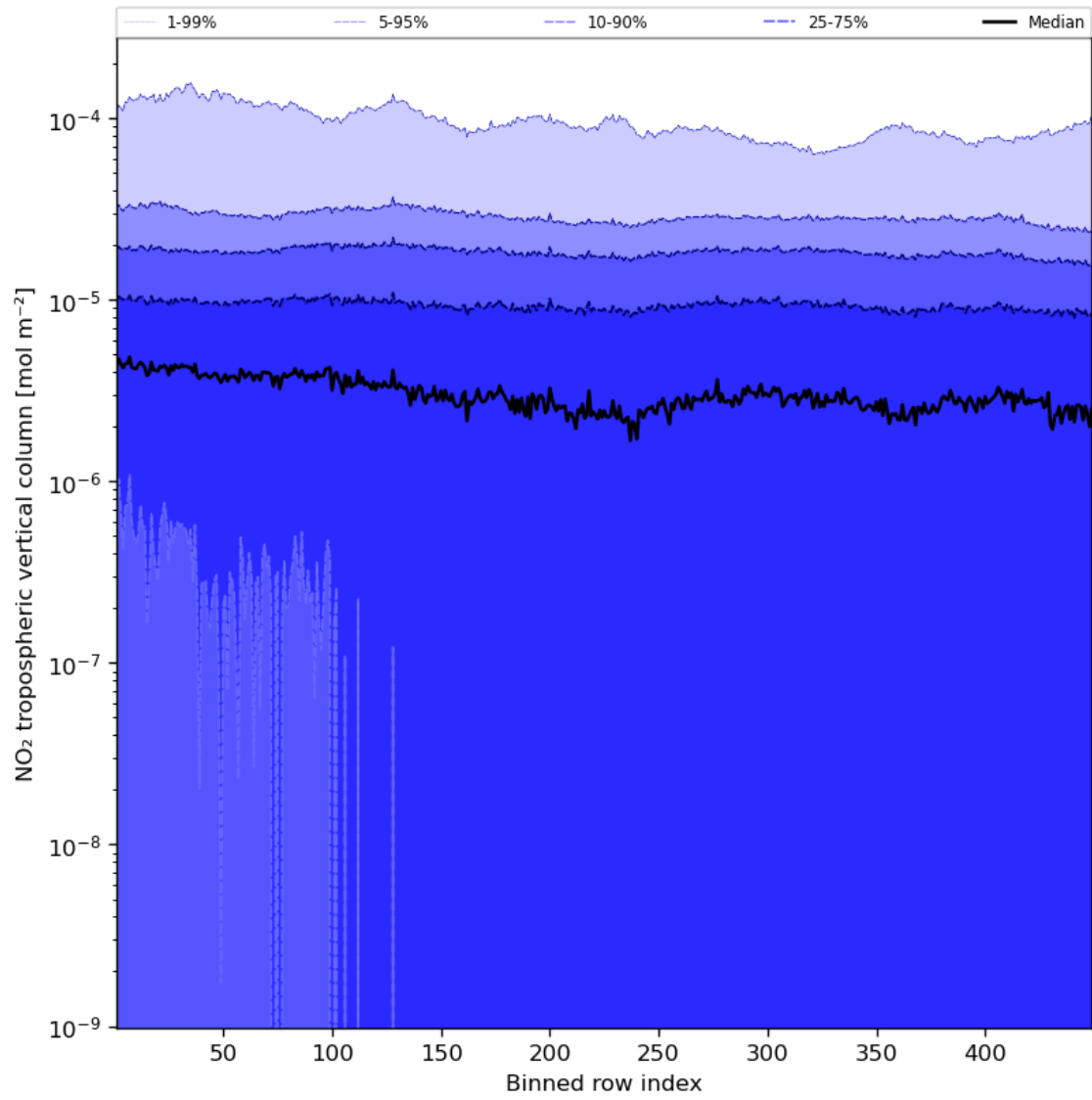
Figure 46: Along track statistics of “NO 2 tropospheric vertical column” for 2024-02-03 to 2024-02-05
