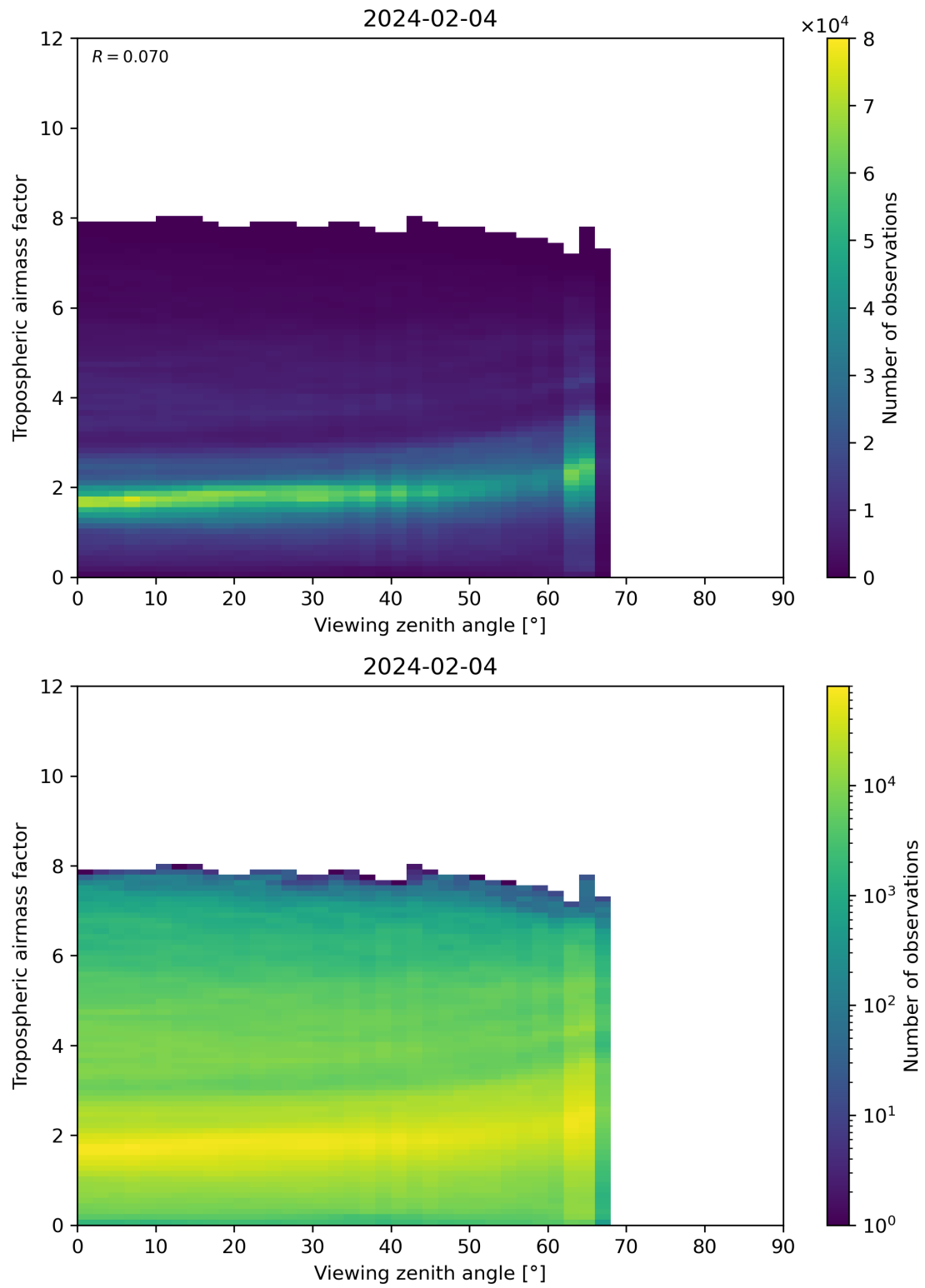
Figure 161: Scatter density plot of “Viewing zenith angle” against “Tropospheric airmass factor” for 2024-02-03 to 2024-02-05.
