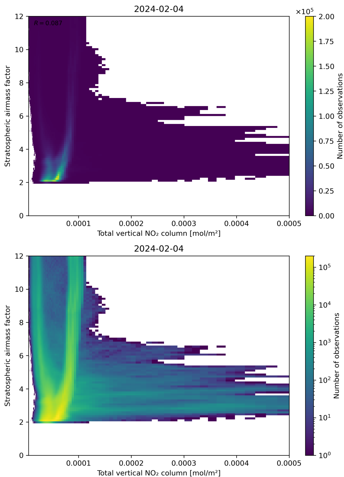
Figure 110: Scatter density plot of “Total vertical NO 2 column” against “Stratospheric air mass factor” for 2024-02-03 to 2024-02-05.
