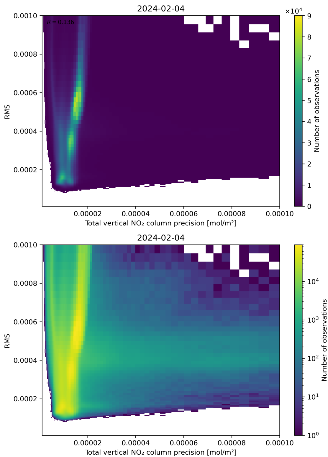
Figure 119: Scatter density plot of “Total vertical NO 2 column precision” against “RMS” for 2024-02-03 to 2024-02-05.
