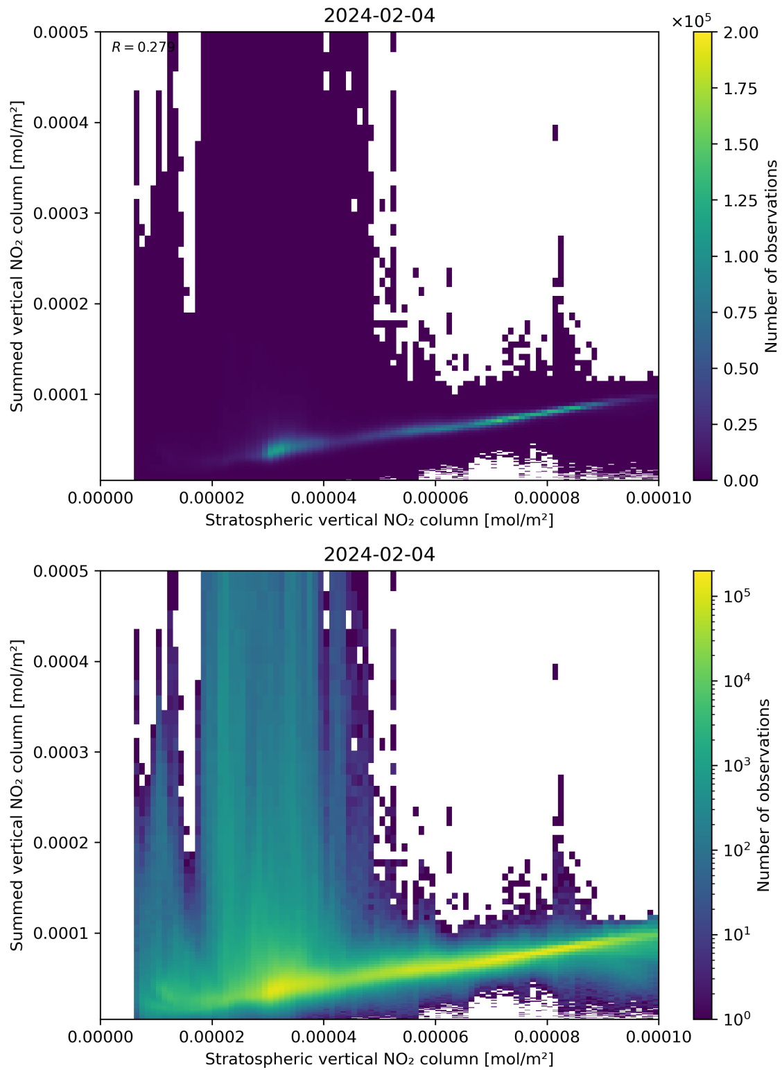
Figure 98: Scatter density plot of “Stratospheric vertical NO 2 column” against “Summed vertical NO 2 column” for 2024-02-03 to 2024-02-05.
