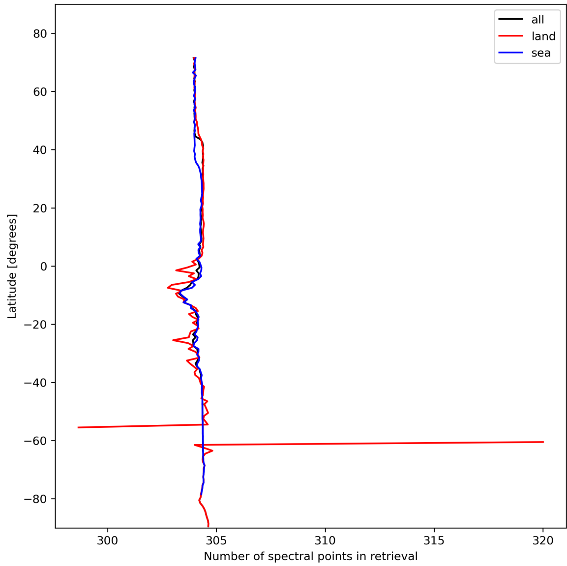
Figure 16: Zonal average of “Number of spectral points in retrieval” for 2024-02-03 to 2024-02-05.
