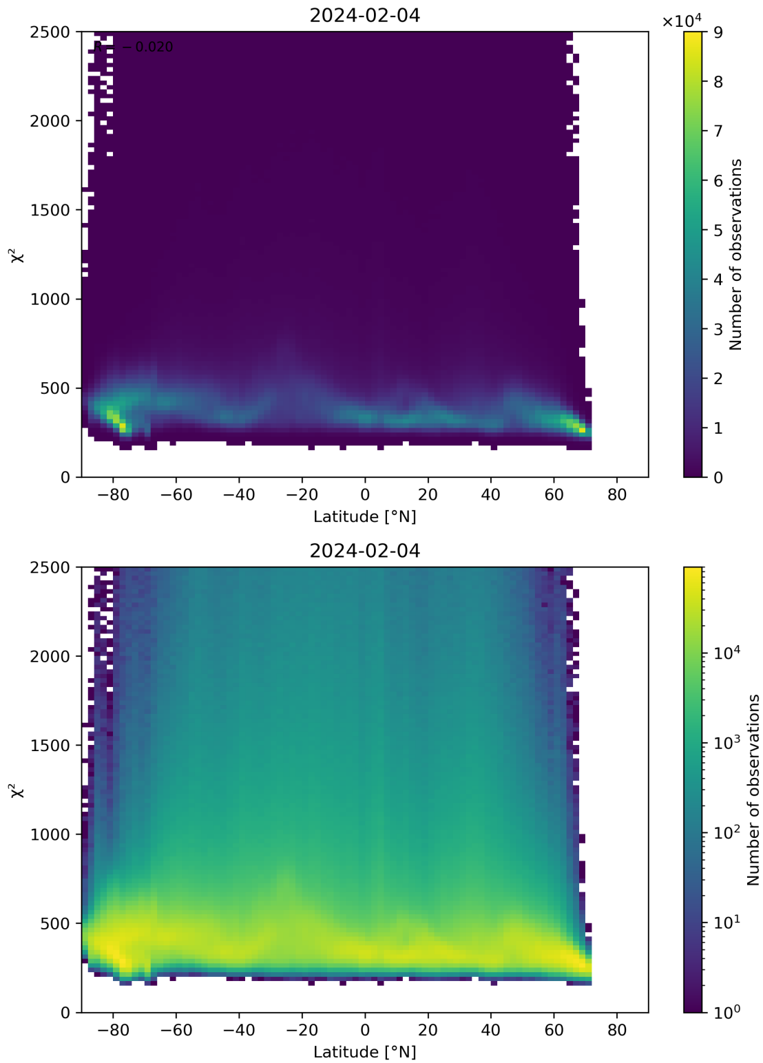
Figure 86: Scatter density plot of “Latitude” against “ \chi^2 ” for 2024-02-03 to 2024-02-05.
