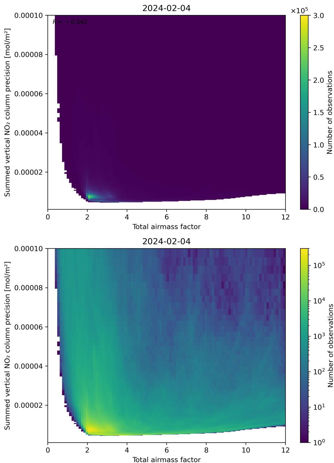
Figure 66: Scatter density plot of “Total airmass factor” against “Summed vertical NO 2 column precision” for 2024-02-03 to 2024-02-05.
