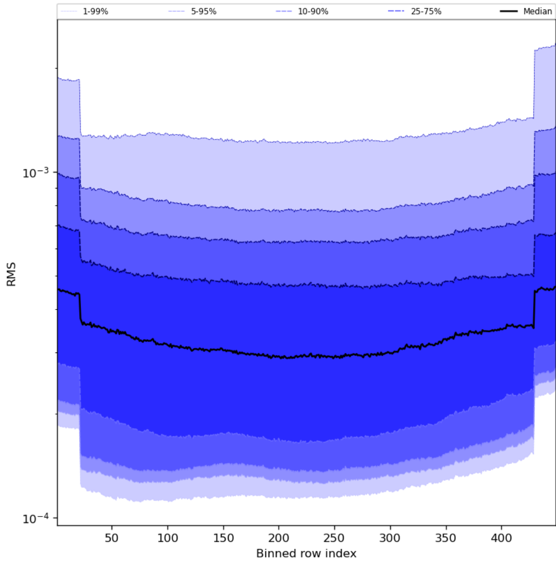
Figure 60: Along track statistics of “RMS” for 2024-02-03 to 2024-02-05
