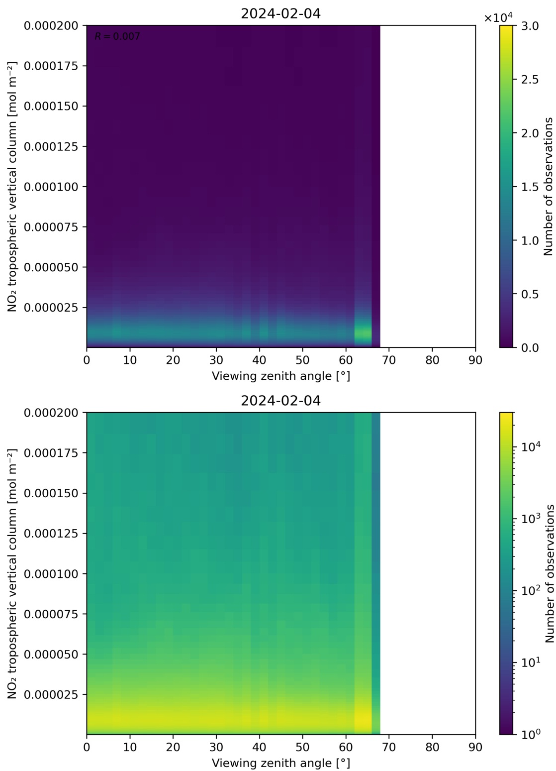
Figure 169: Scatter density plot of “Viewing zenith angle” against “NO 2 tropospheric vertical column” for 2024-02-03 to 2024-02-05.
