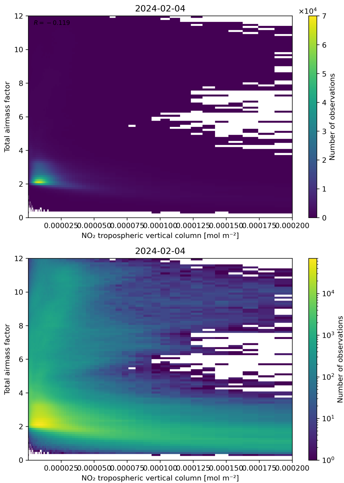
Figure 122: Scatter density plot of “NO 2 tropospheric vertical column” against “Total air mass factor” for 2024-02-03 to 2024-02-05.
