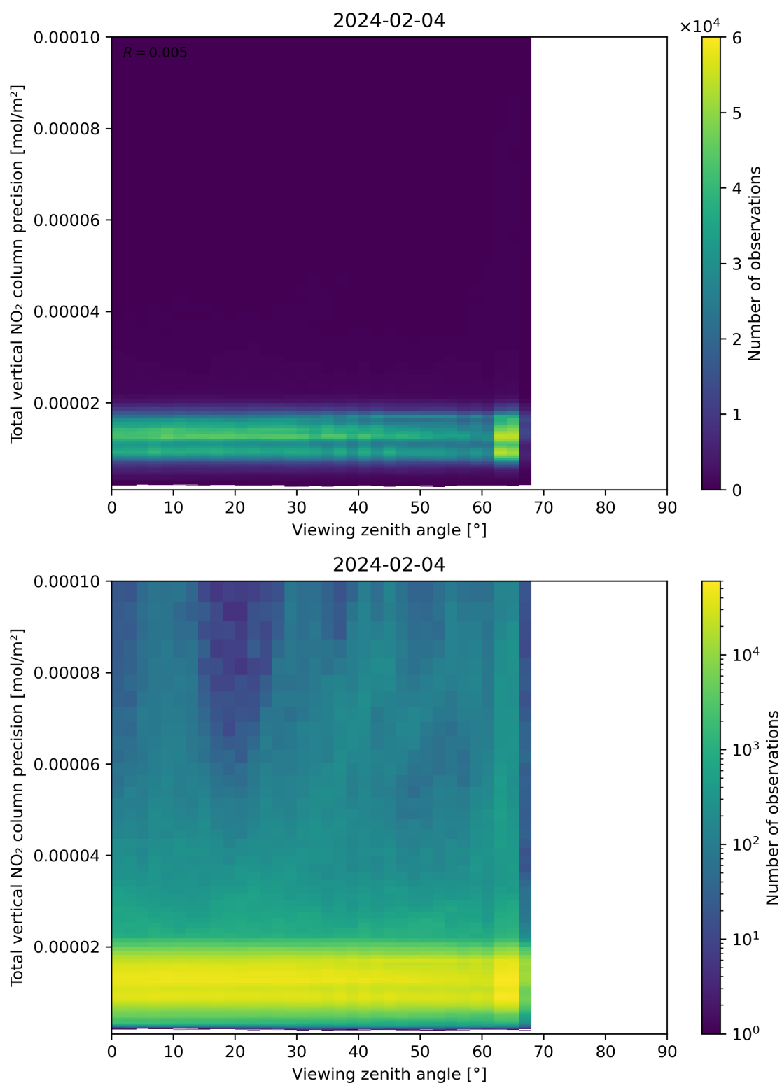
Figure 168: Scatter density plot of “Viewing zenith angle” against “Total vertical NO 2 column precision” for 2024-02-03 to 2024-02-05.
