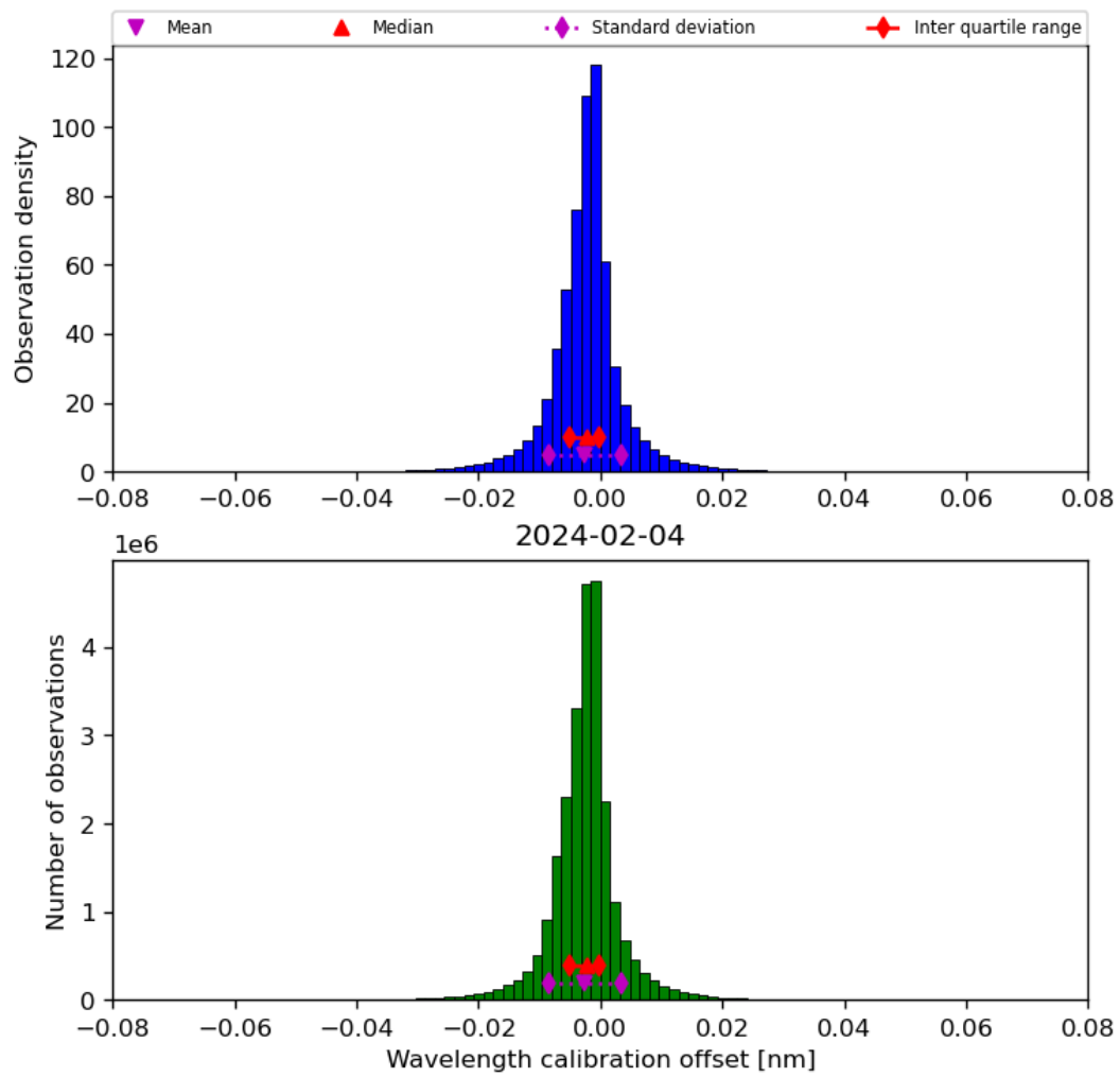
Figure 35: Histogram of “Wavelength calibration offset” for 2024-02-03 to 2024-02-05
