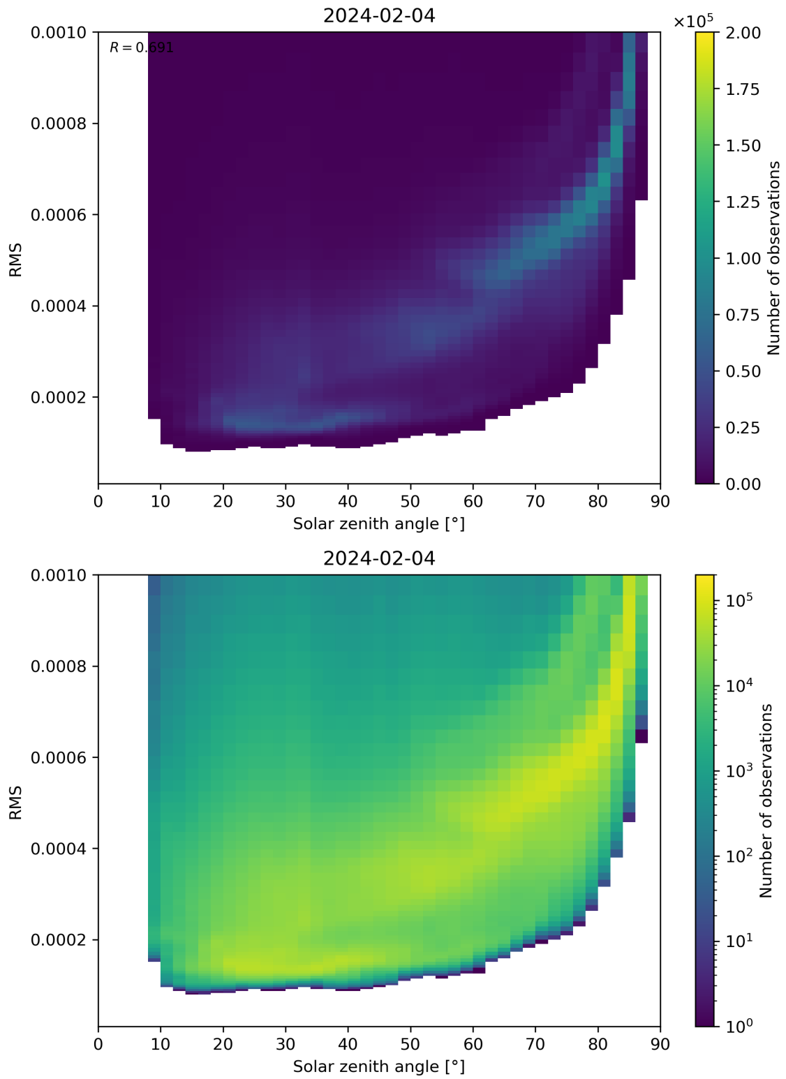
Figure 157: Scatter density plot of “Solar zenith angle” against “RMS” for 2024-02-03 to 2024-02-05.
