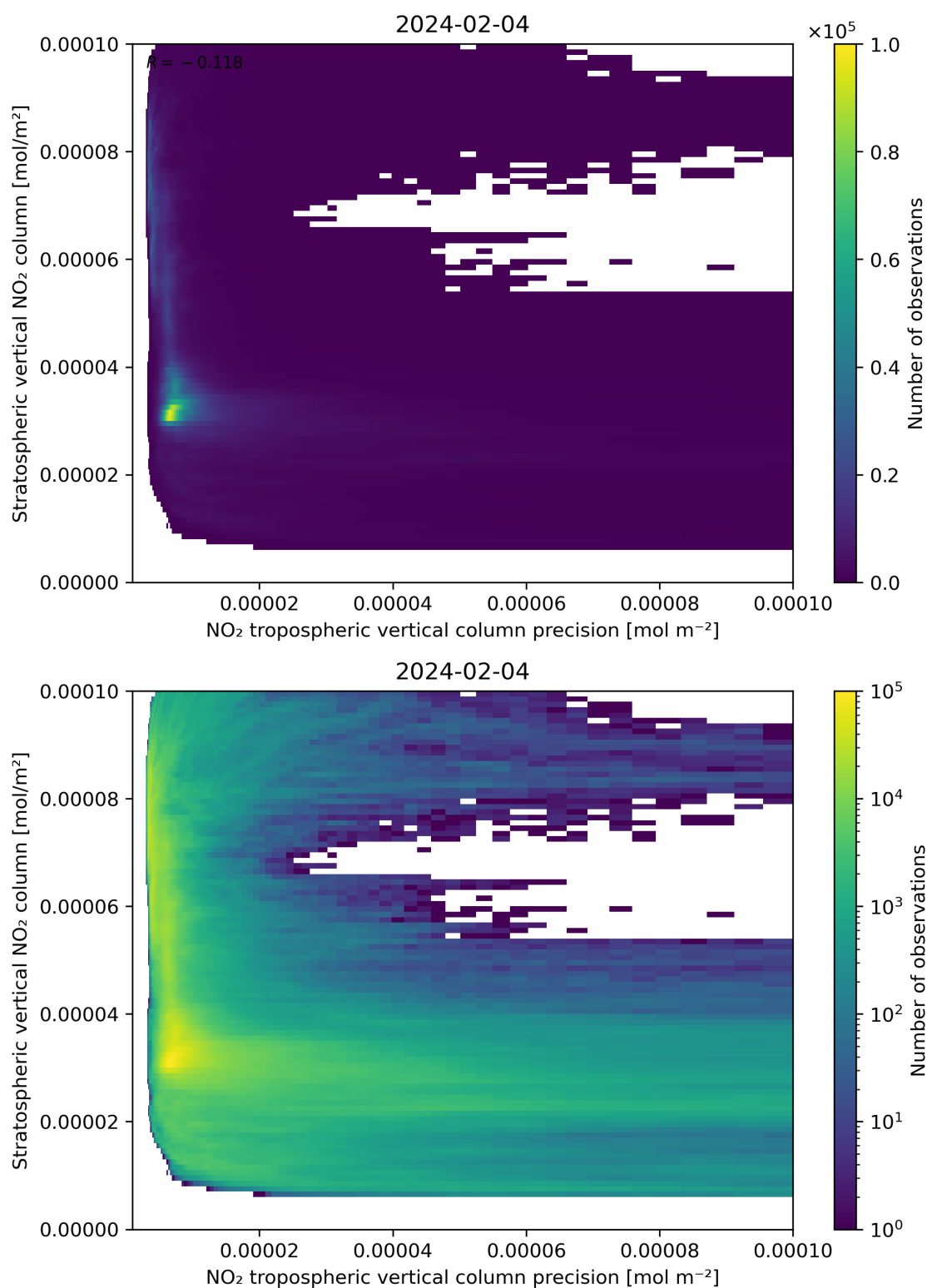
Figure 135: Scatter density plot of “NO 2 tropospheric vertical column precision” against “Stratospheric vertical NO 2 column” for 2024-02-03 to 2024-02-05.
