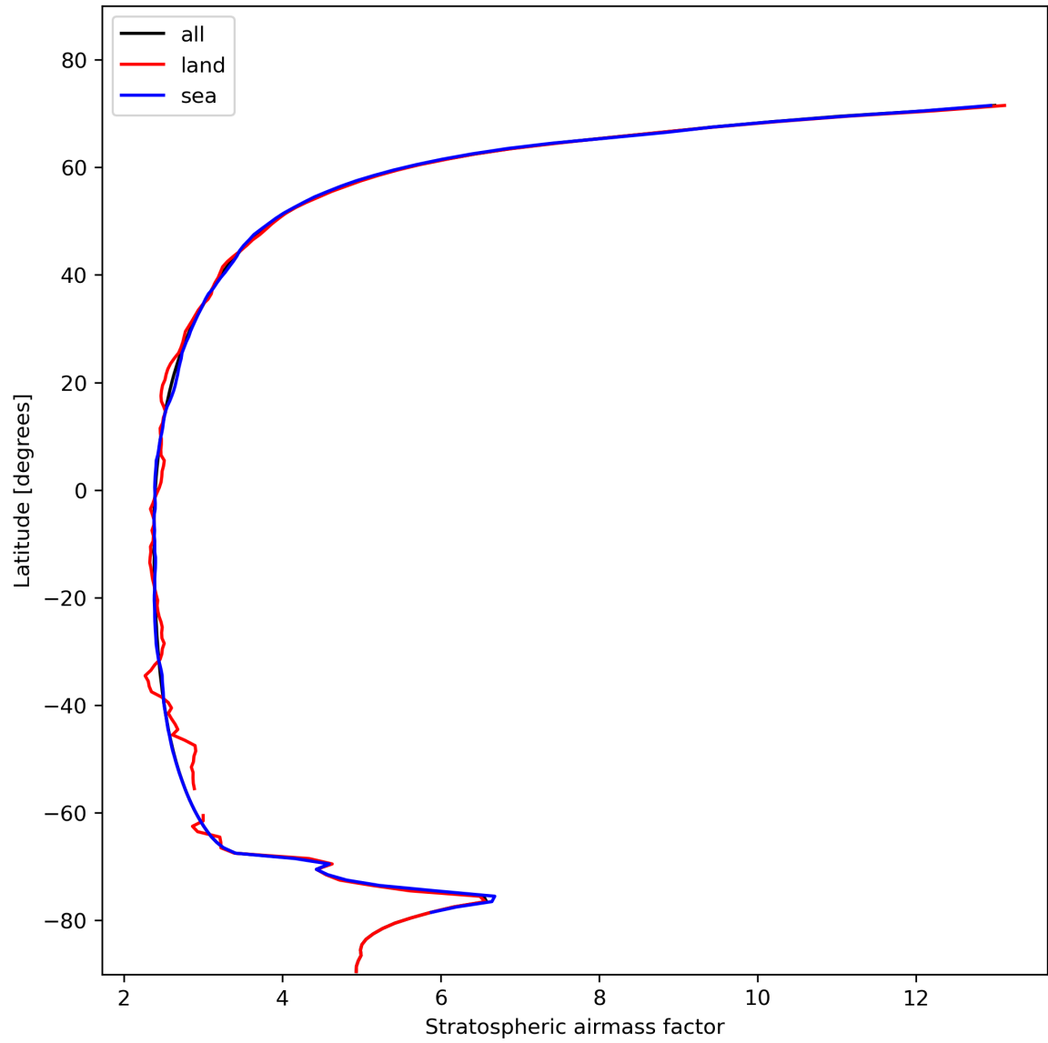
Figure 27: Zonal average of “Stratospheric air mass factor” for 2024-02-03 to 2024-02-05.
