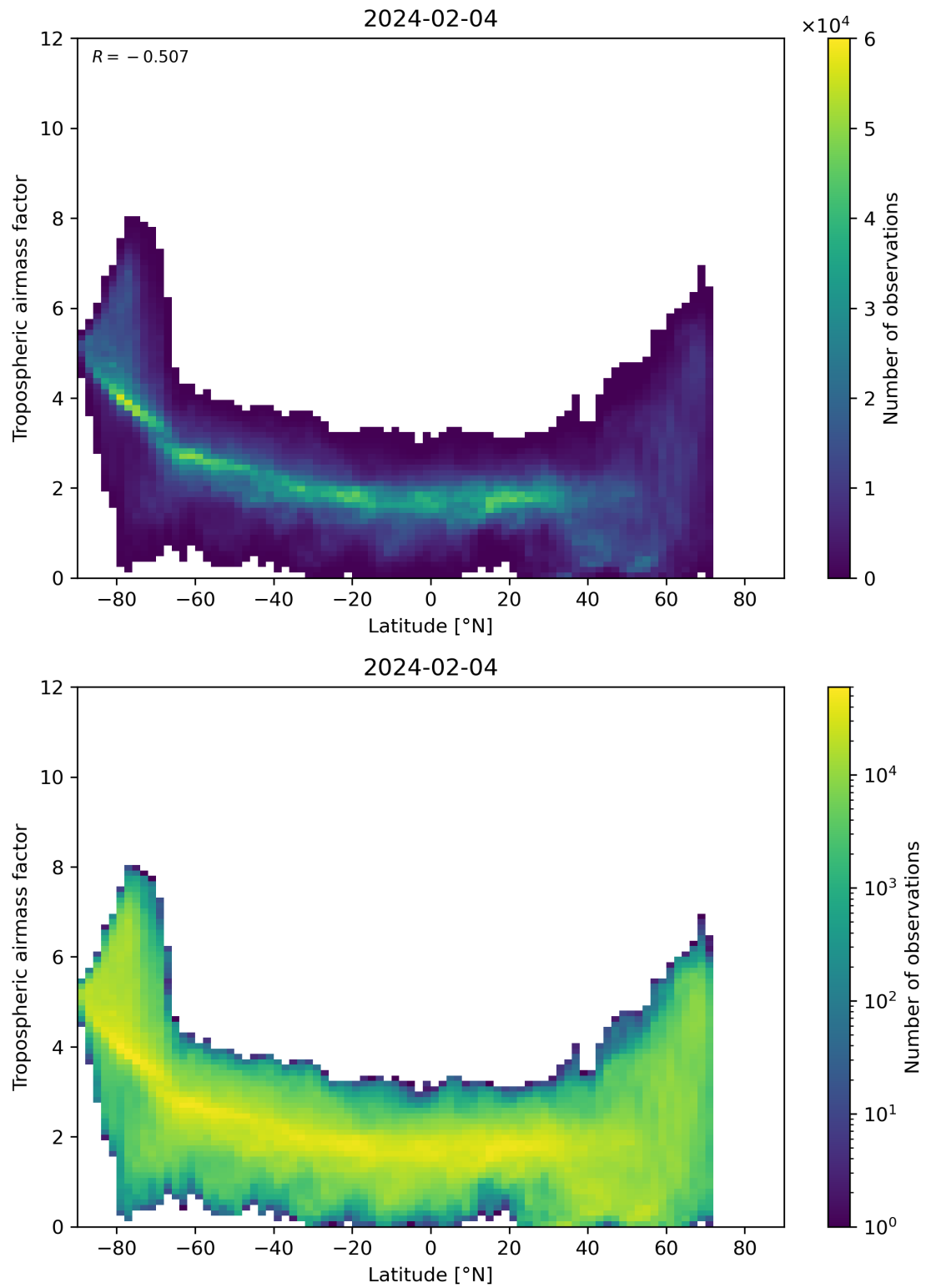
Figure 85: Scatter density plot of “Latitude” against “Tropospheric airmass factor” for 2024-02-03 to 2024-02-05.
