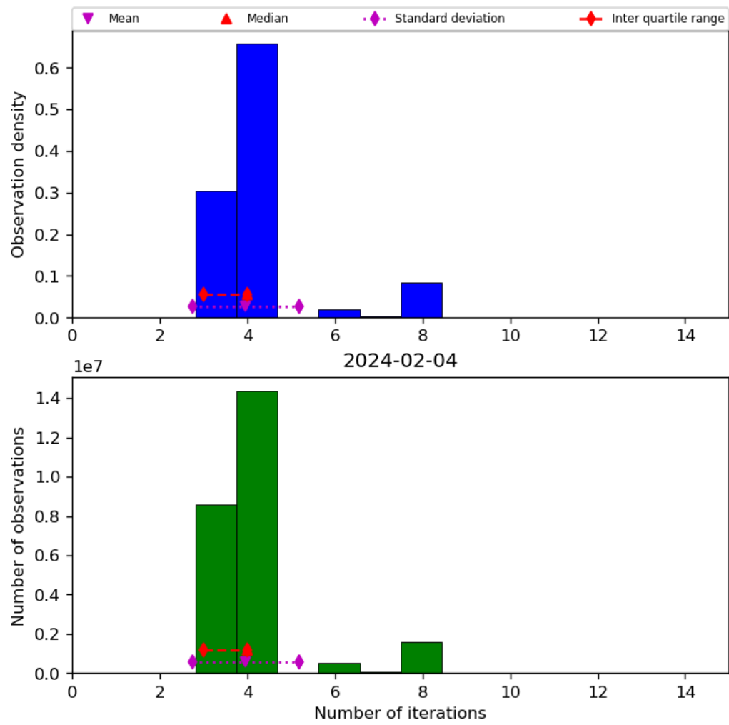
Figure 34: Histogram of “Number of iterations” for 2024-02-03 to 2024-02-05
