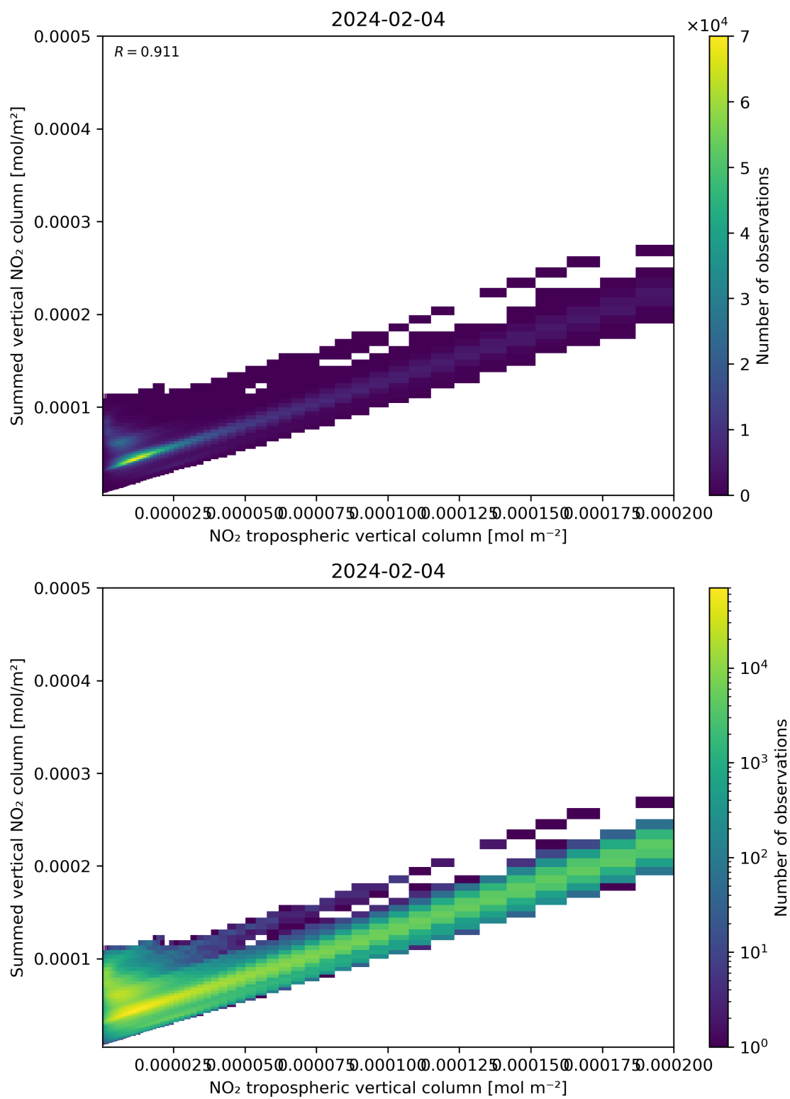
Figure 126: Scatter density plot of “NO 2 tropospheric vertical column” against “Summed vertical NO 2 column” for 2024-02-03 to 2024-02-05.
