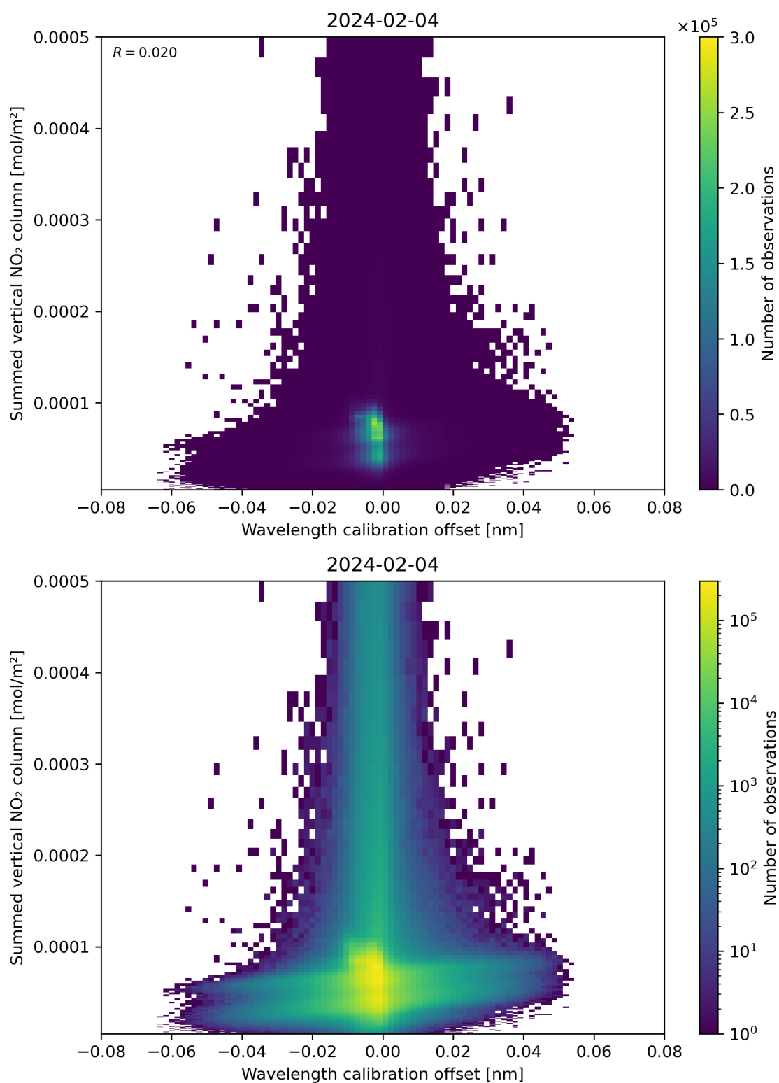
Figure 177: Scatter density plot of “Wavelength calibration offset” against “Summed vertical NO 2 column” for 2024-02-03 to 2024-02-05.
