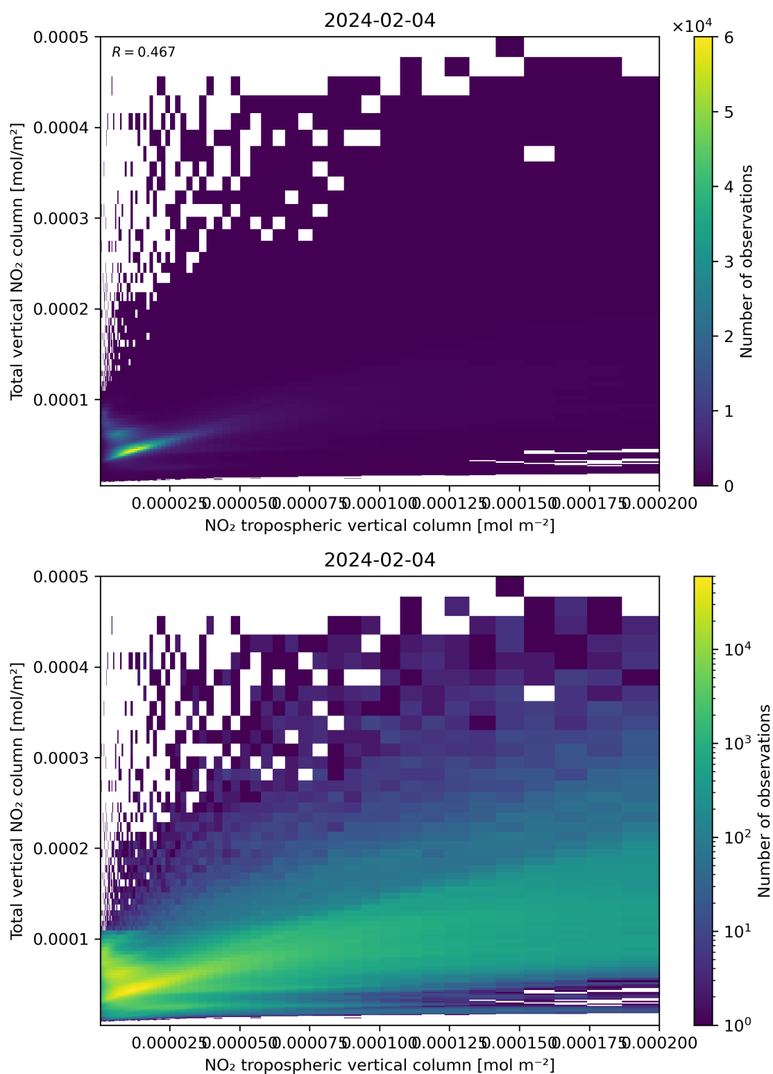
Figure 128: Scatter density plot of “NO 2 tropospheric vertical column” against “Total vertical NO 2 column” for 2024-02-03 to 2024-02-05.
