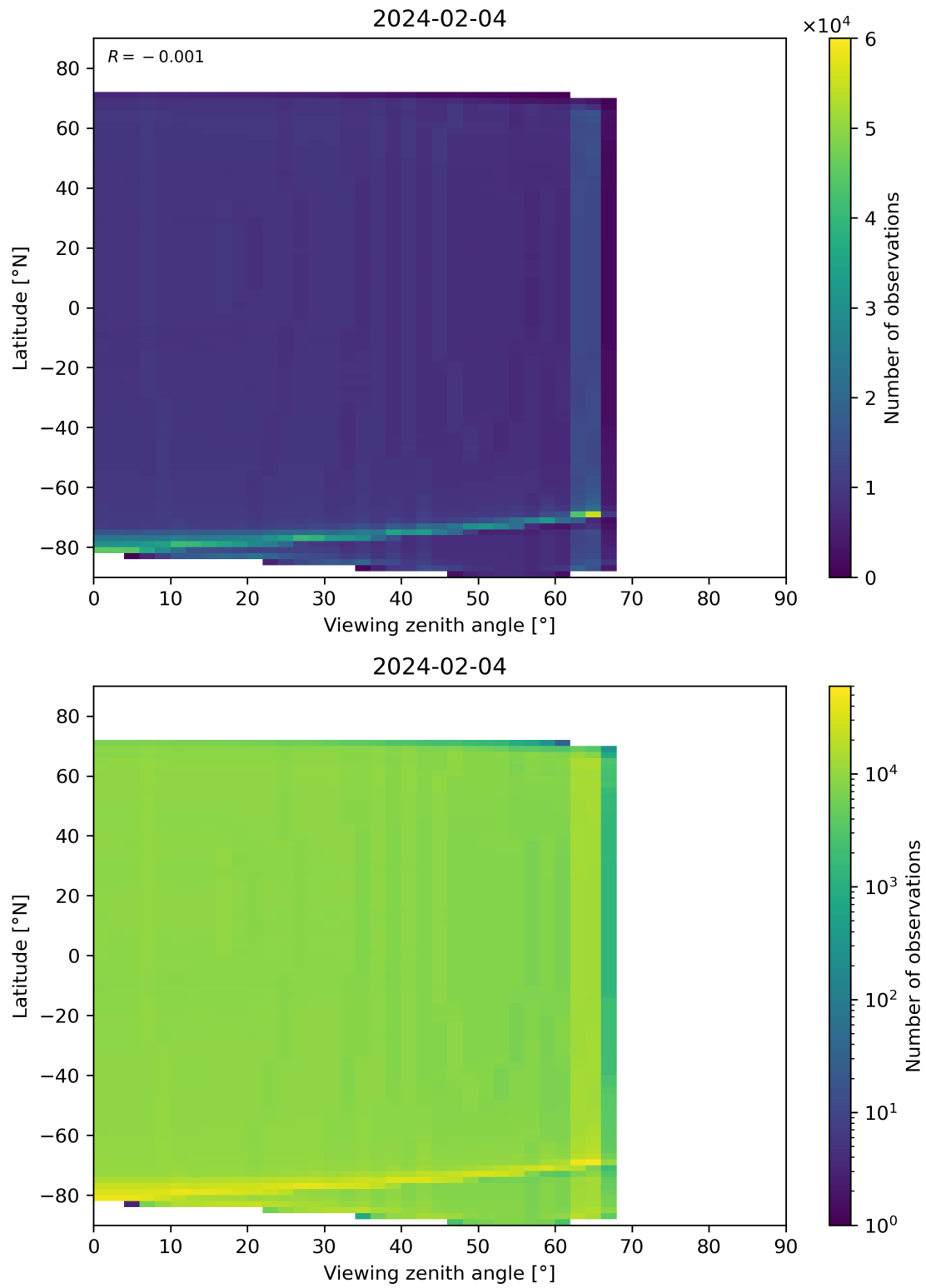
Figure 163: Scatter density plot of “Viewing zenith angle” against “Latitude” for 2024-02-03 to 2024-02-05.
