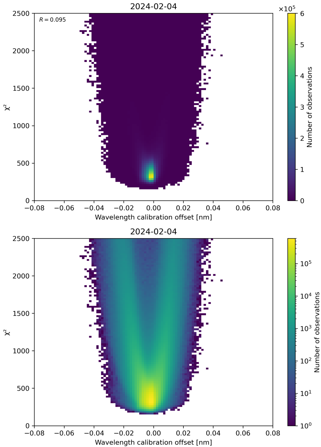
Figure 175: Scatter density plot of “Wavelength calibration offset” against “ \chi^2 ” for 2024-02-03 to 2024-02-05.
