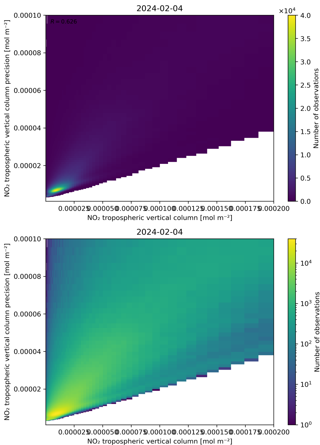
Figure 130: Scatter density plot of “NO 2 tropospheric vertical column” against “NO 2 tropospheric vertical column precision” for 2024-02-03 to 2024-02-05.
