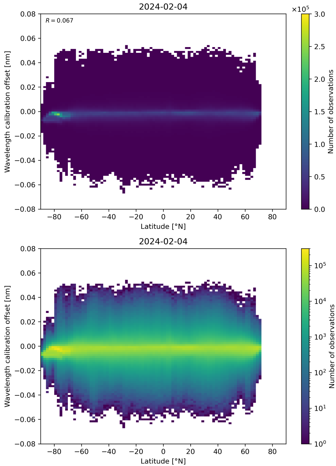
Figure 95: Scatter density plot of “Latitude” against “Wavelength calibration offset” for 2024-02-03 to 2024-02-05.
