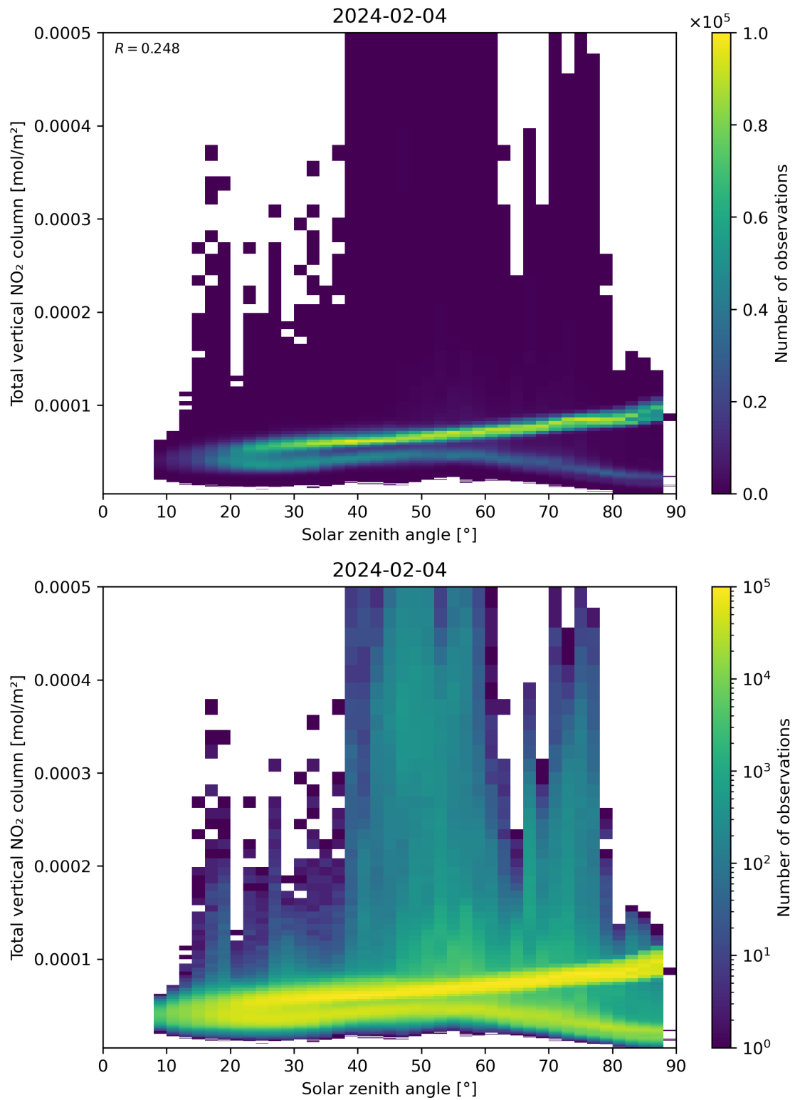
Figure 153: Scatter density plot of “Solar zenith angle” against “Total vertical NO 2 column” for 2024-02-03 to 2024-02-05.
