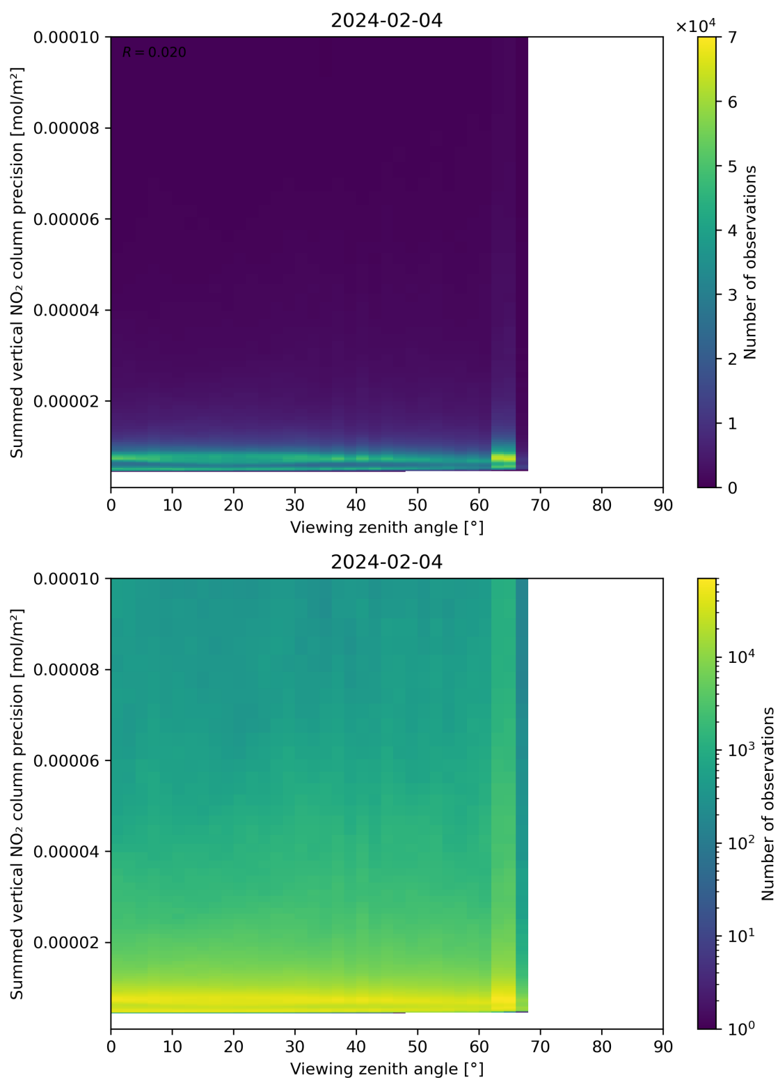
Figure 166: Scatter density plot of “Viewing zenith angle” against “Summed vertical NO 2 column precision” for 2024-02-03 to 2024-02-05.
