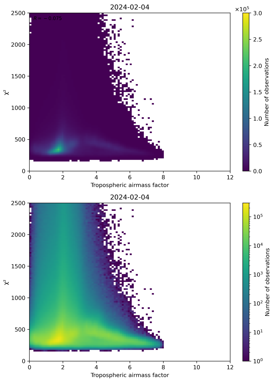
Figure 73: Scatter density plot of “Tropospheric airmass factor” against “ \chi^2 ” for 2024-02-03 to 2024-02-05.
