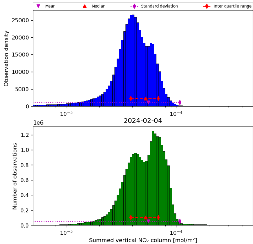
Figure 40: Histogram of "Summed vertical NO 2 column" for 2024-02-03 to 2024-02-05
