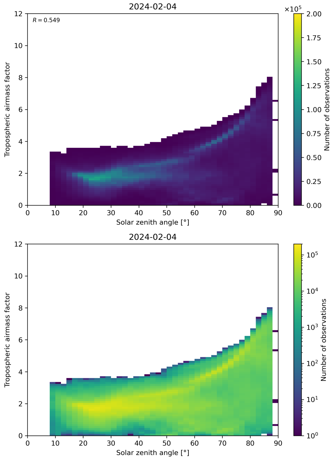
Figure 147: Scatter density plot of “Solar zenith angle” against “Tropospheric airmass factor” for 2024-02-03 to 2024-02-05.
