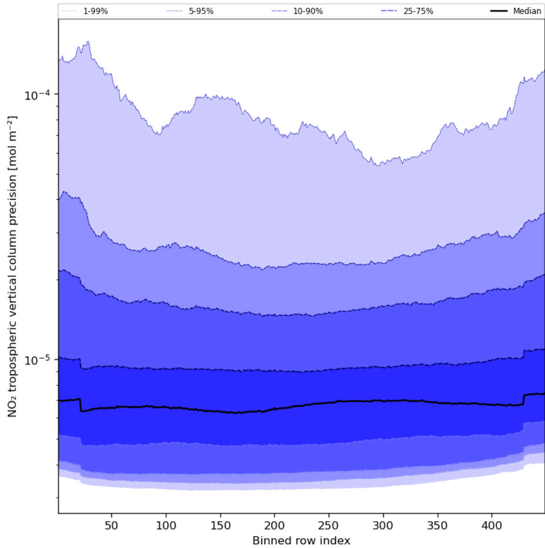
Figure 47: Along track statistics of “NO 2 tropospheric vertical column precision” for 2024-02-03 to 2024-02-05
