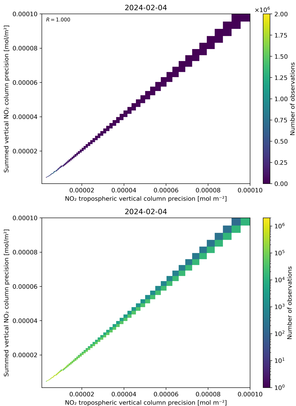
Figure 137: Scatter density plot of “NO 2 tropospheric vertical column precision” against “Summed vertical NO 2 column precision” for 2024-02-03 to 2024-02-05.
