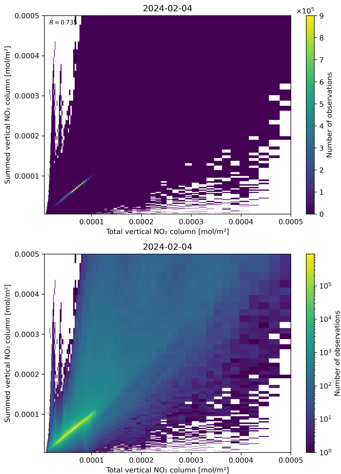
Figure 112: Scatter density plot of “Total vertical NO 2 column” against “Summed vertical NO 2 column” for 2024-02-03 to 2024-02-05.
