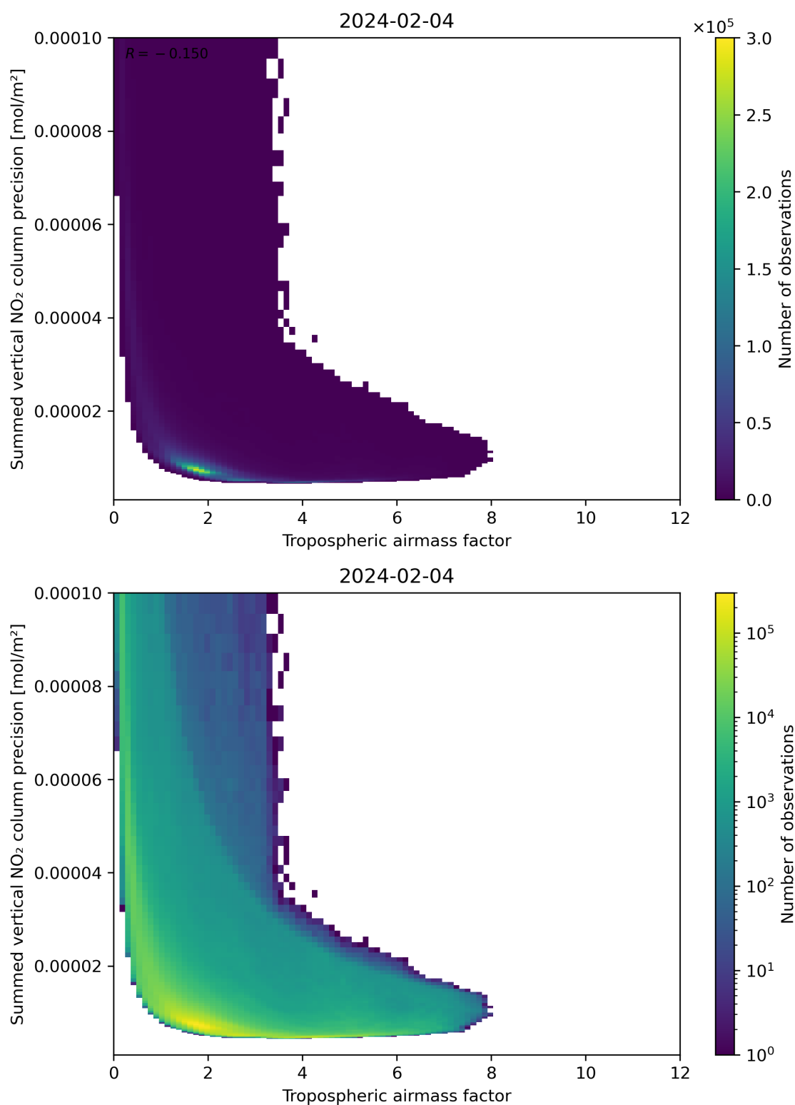
Figure 76: Scatter density plot of “Tropospheric air mass factor” against “Summed vertical NO 2 column precision” for 2024-02-03 to 2024-02-05.
