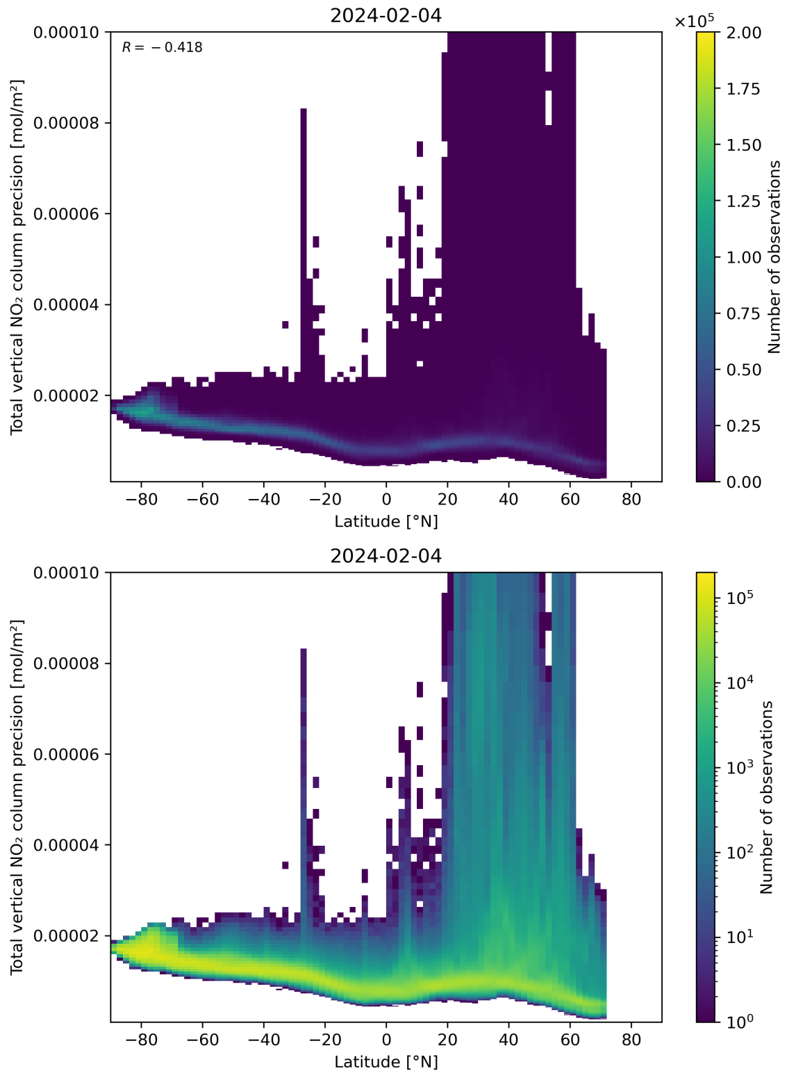
Figure 91: Scatter density plot of “Latitude” against “Total vertical NO 2 column precision” for 2024-02-03 to 2024-02-05.
