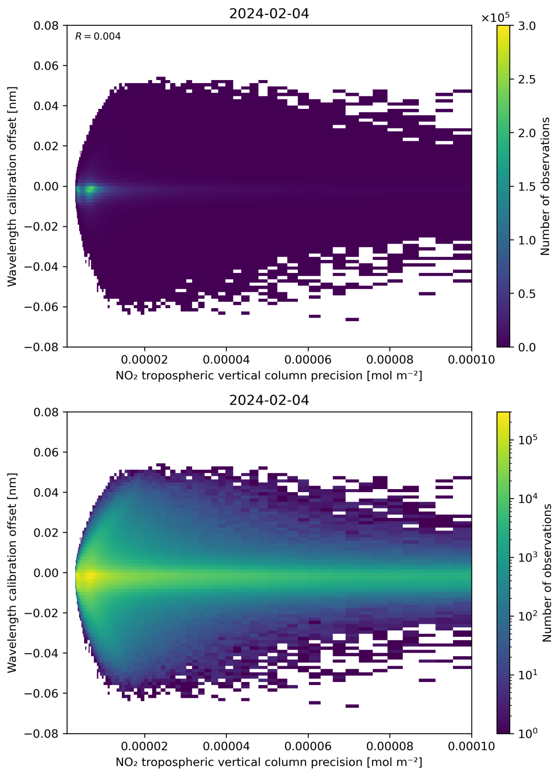
Figure 141: Scatter density plot of “NO 2 tropospheric vertical column precision” against “Wavelength calibration offset” for 2024-02-03 to 2024-02-05.
