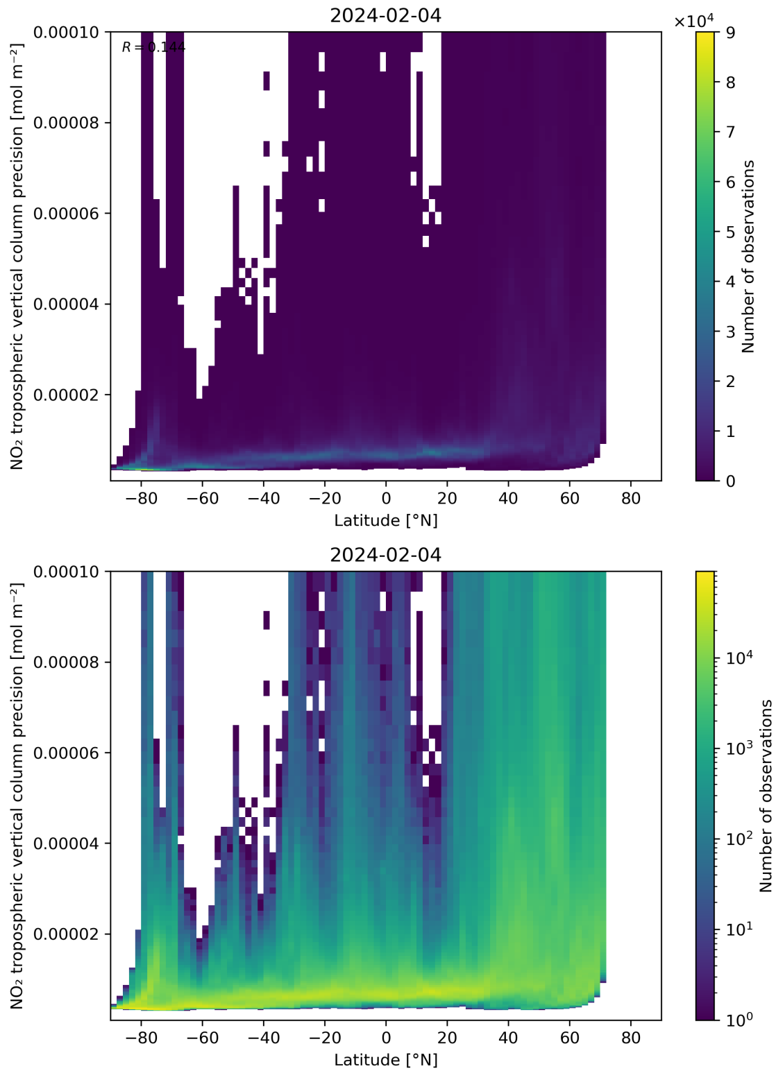
Figure 93: Scatter density plot of “Latitude” against “NO 2 tropospheric vertical column precision” for 2024-02-03 to 2024-02-05.
