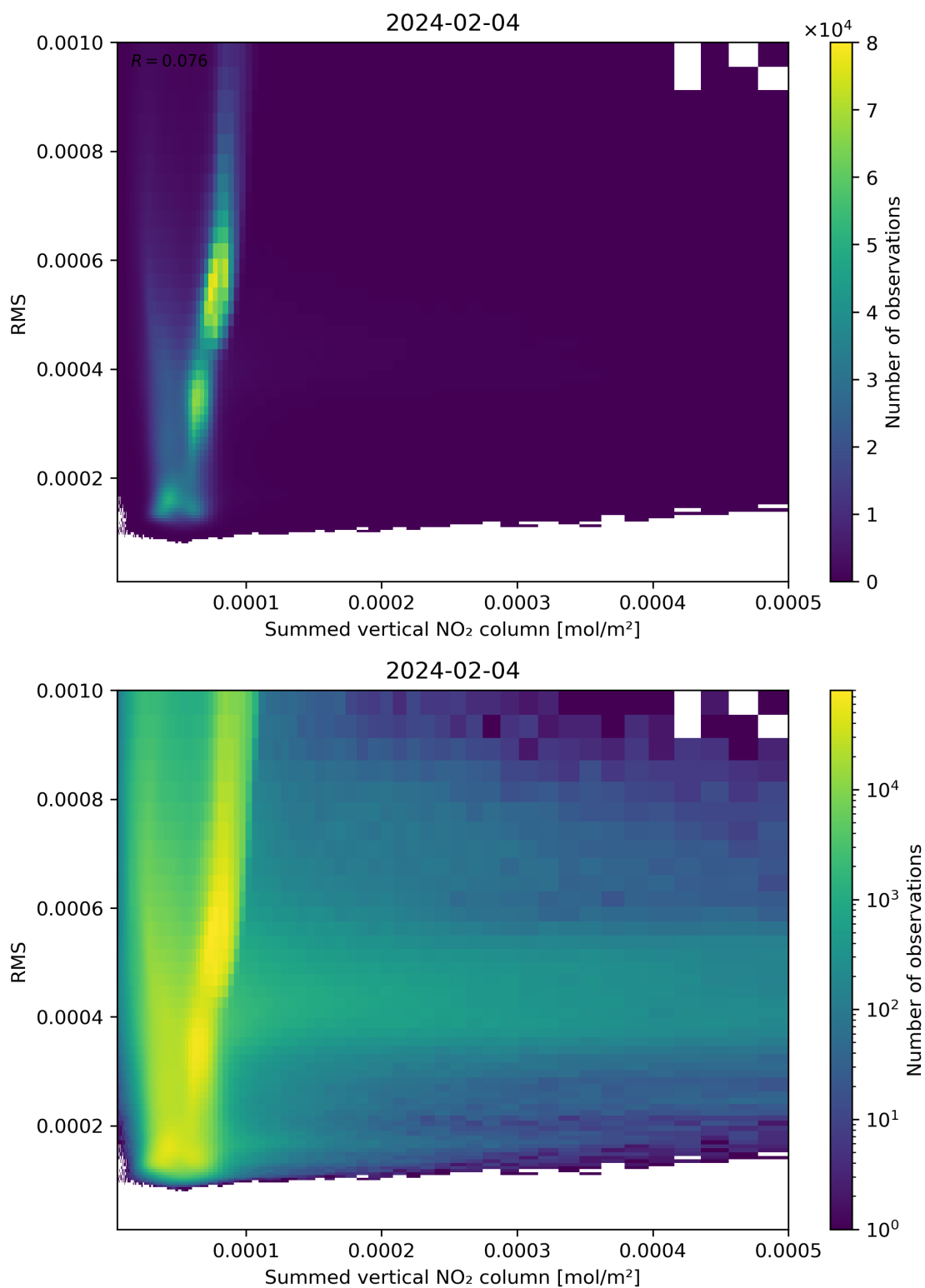
Figure 109: Scatter density plot of “Summed vertical NO 2 column” against “RMS” for 2024-02-03 to 2024-02-05.
