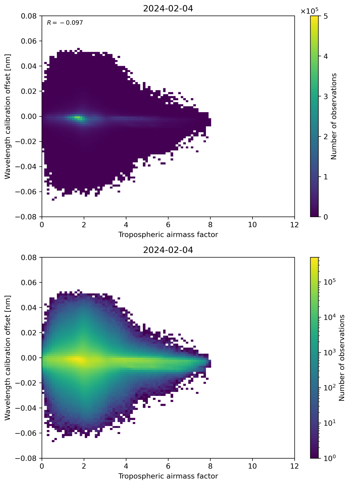
Figure 80: Scatter density plot of “Tropospheric air mass factor” against “Wavelength calibration offset” for 2024-02-03 to 2024-02-05.
