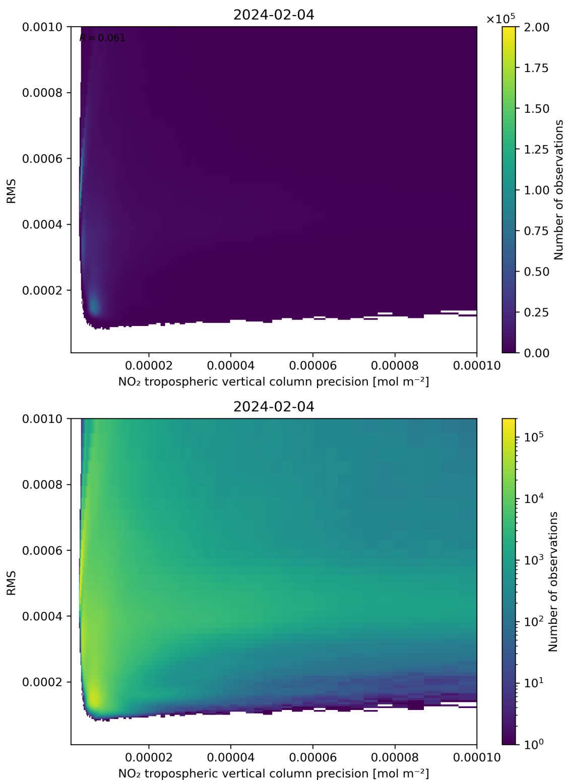
Figure 140: Scatter density plot of “NO 2 tropospheric vertical column precision” against “RMS” for 2024-02-03 to 2024-02-05.
