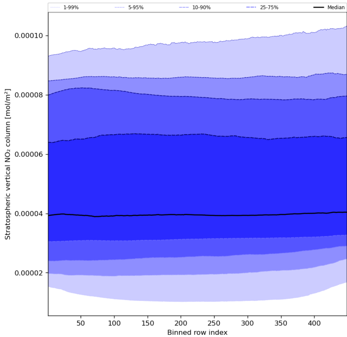
Figure 53: Along track statistics of “Stratospheric vertical NO 2 column” for 2024-02-03 to 2024-02-05
