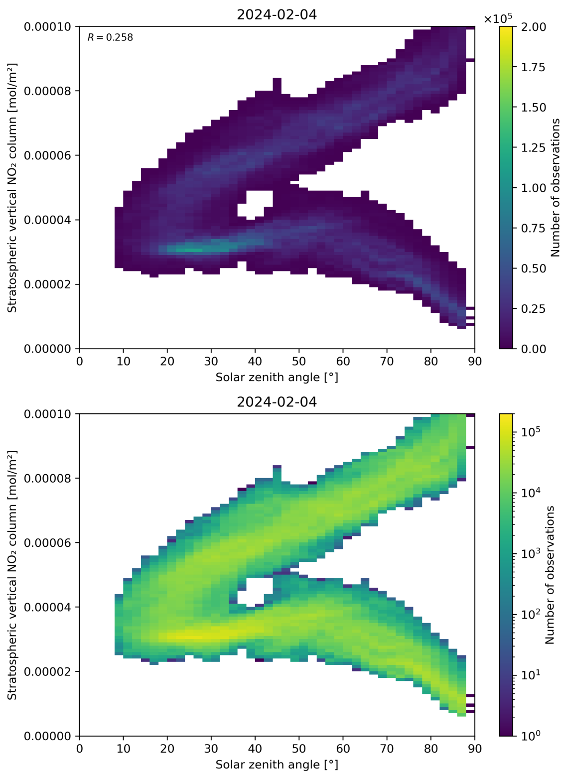
Figure 150: Scatter density plot of “Solar zenith angle” against “Stratospheric vertical NO 2 column” for 2024-02-03 to 2024-02-05.
