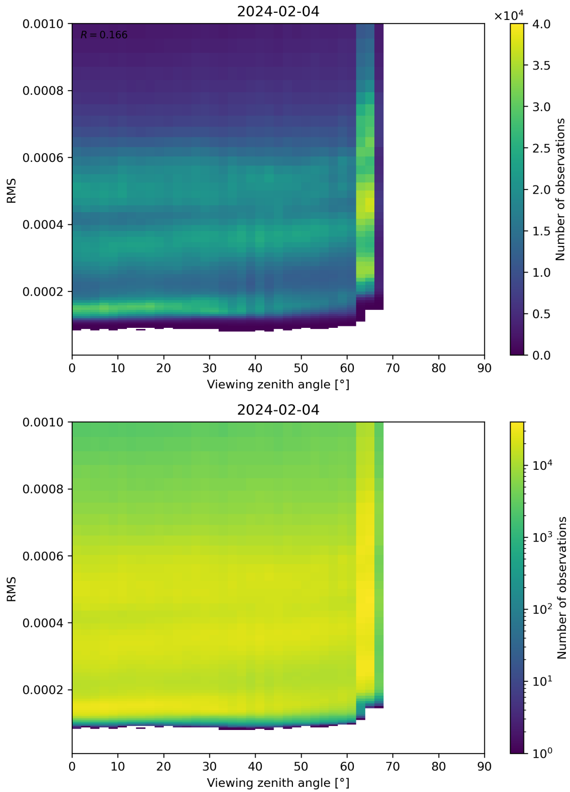
Figure 171: Scatter density plot of “Viewing zenith angle” against “RMS” for 2024-02-03 to 2024-02-05.
