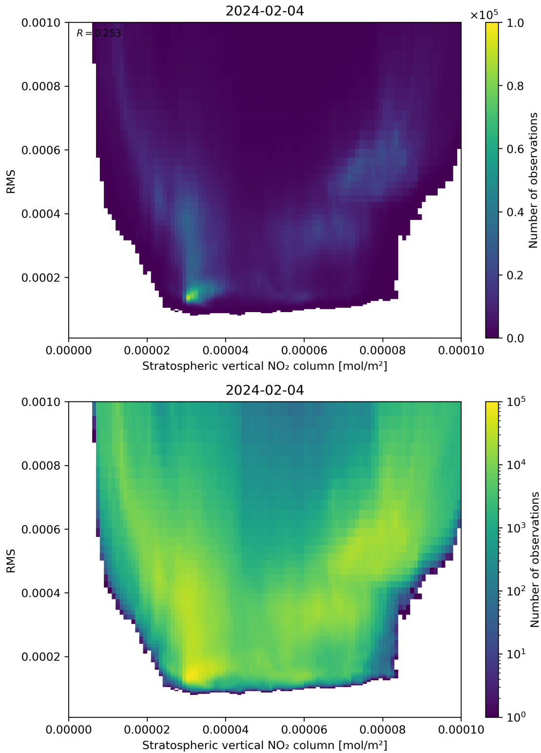
Figure 102: Scatter density plot of “Stratospheric vertical NO 2 column” against “RMS” for 2024-02-03 to 2024-02-05.
