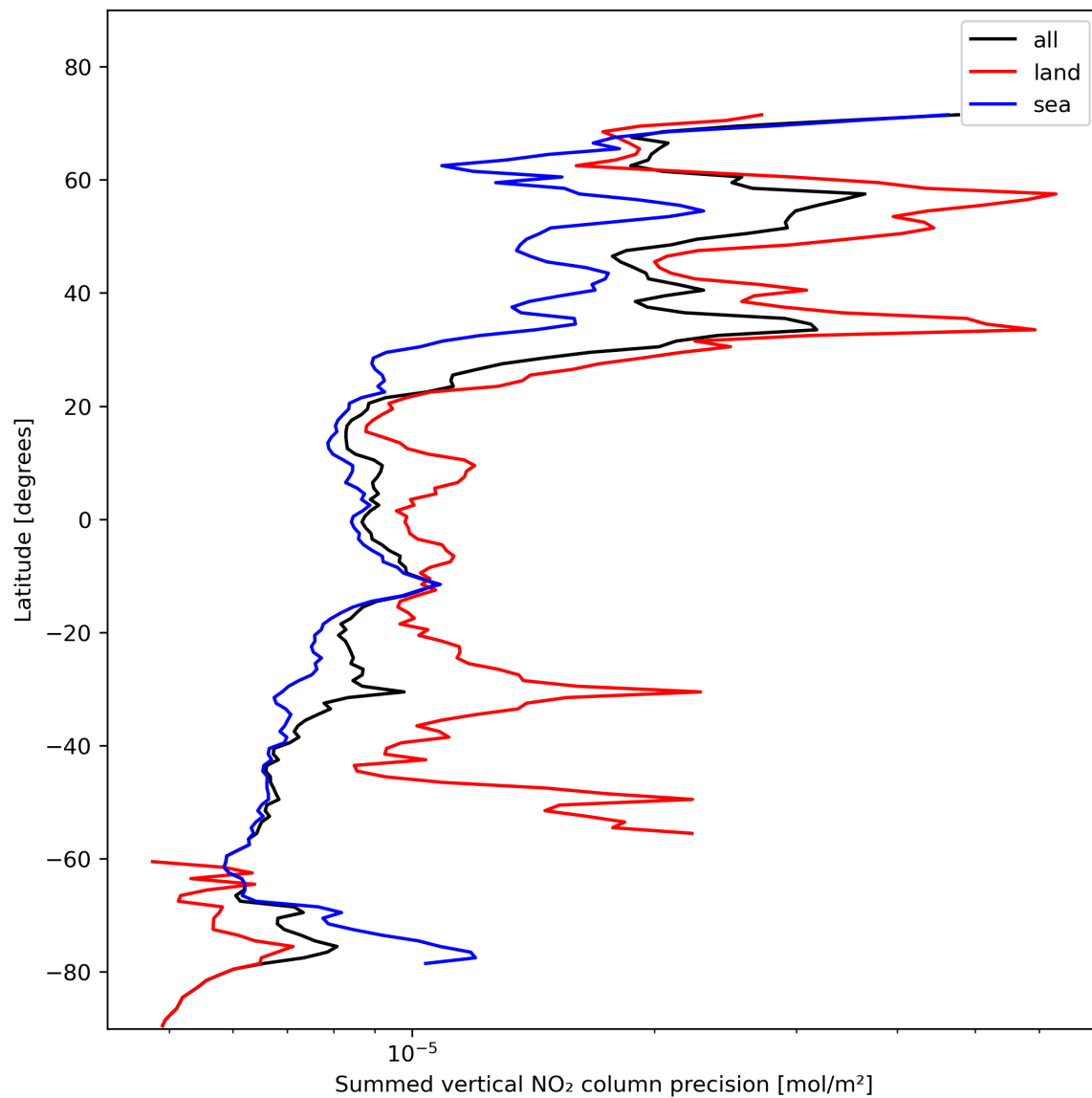
Figure 24: Zonal average of “Summed vertical NO 2 column precision” for 2024-02-03 to 2024-02-05.
