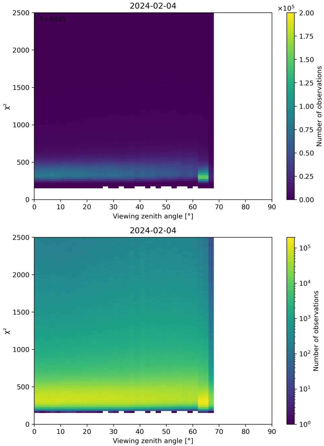
Figure 162: Scatter density plot of “Viewing zenith angle” against “ \chi^2 ” for 2024-02-03 to 2024-02-05.
