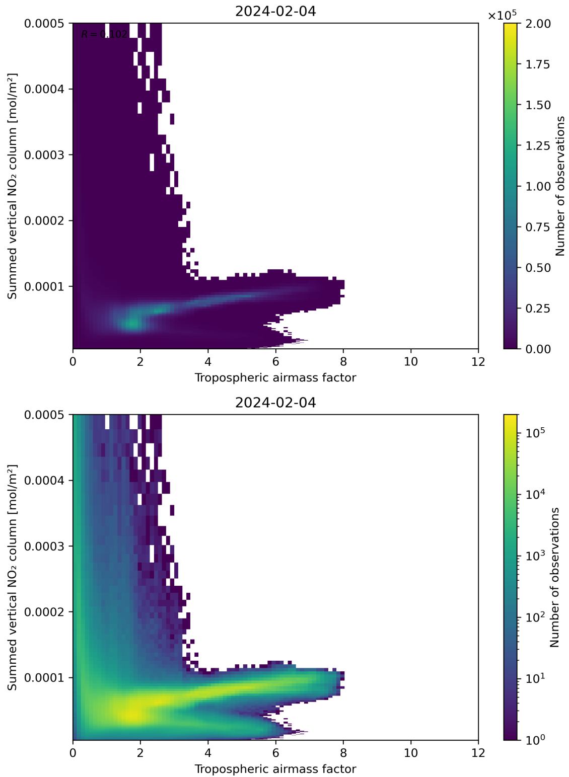
Figure 75: Scatter density plot of “Tropospheric airmass factor” against “Summed vertical NO 2 column” for 2024-02-03 to 2024-02-05.
