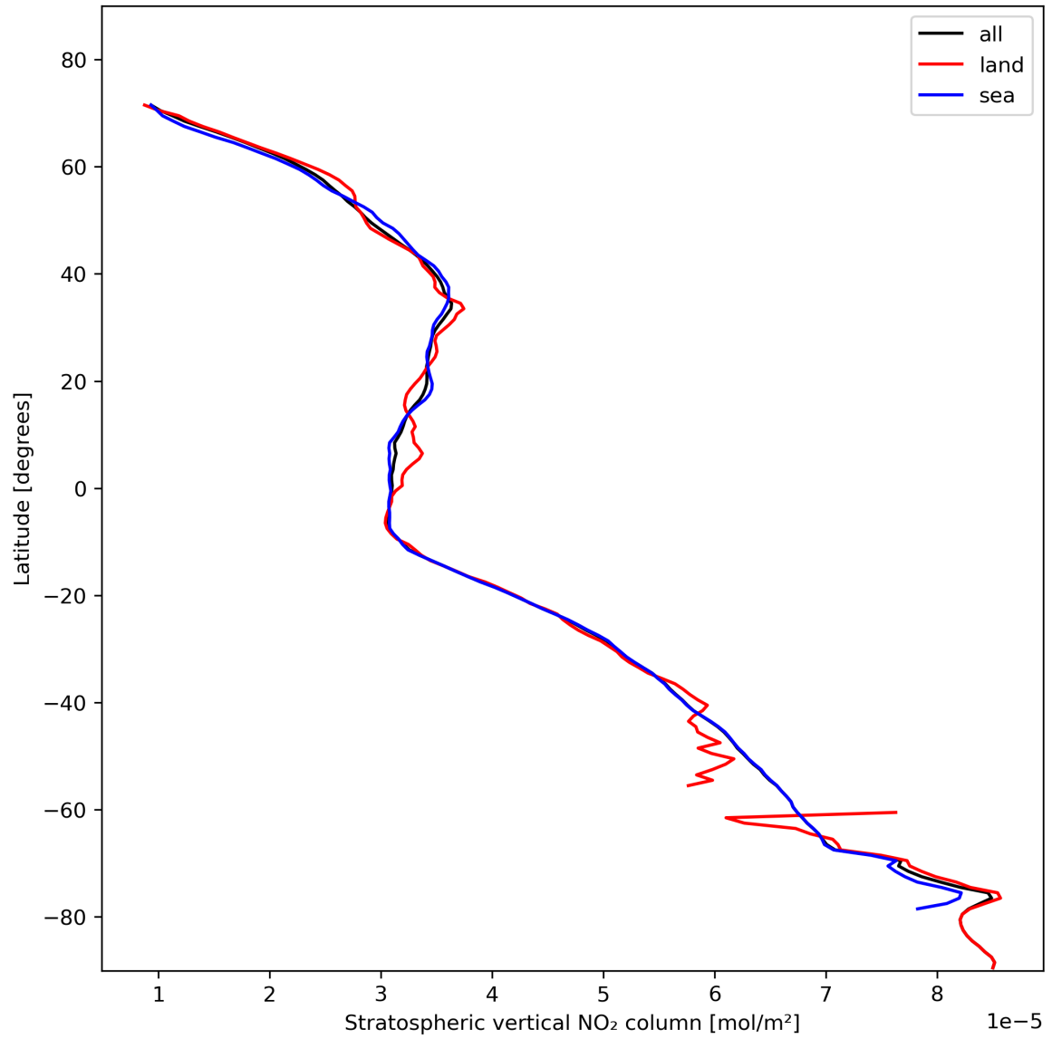
Figure 19: Zonal average of “Stratospheric vertical NO 2 column” for 2024-02-03 to 2024-02-05.
