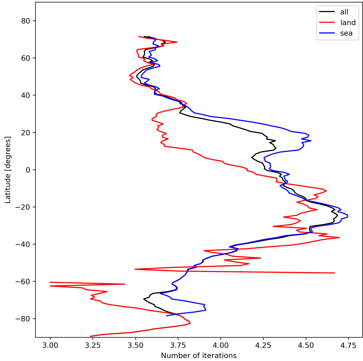
Figure 17: Zonal average of “Number of iterations” for 2024-02-03 to 2024-02-05.
