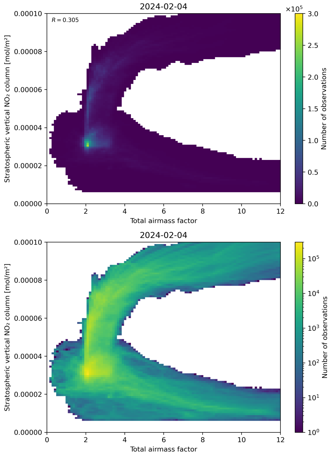
Figure 64: Scatter density plot of “Total airmass factor” against “Stratospheric vertical \text{NO}_2 column” for 2024-02-03 to 2024-02-05.
