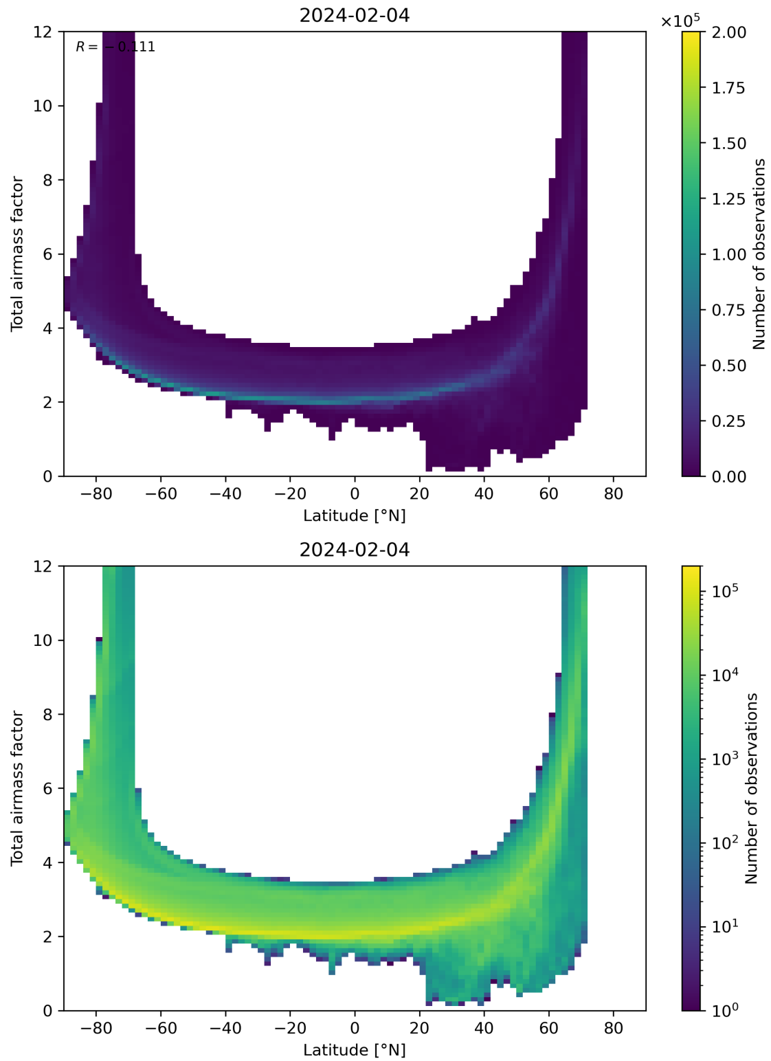
Figure 84: Scatter density plot of “Latitude” against “Total airmass factor” for 2024-02-03 to 2024-02-05.
