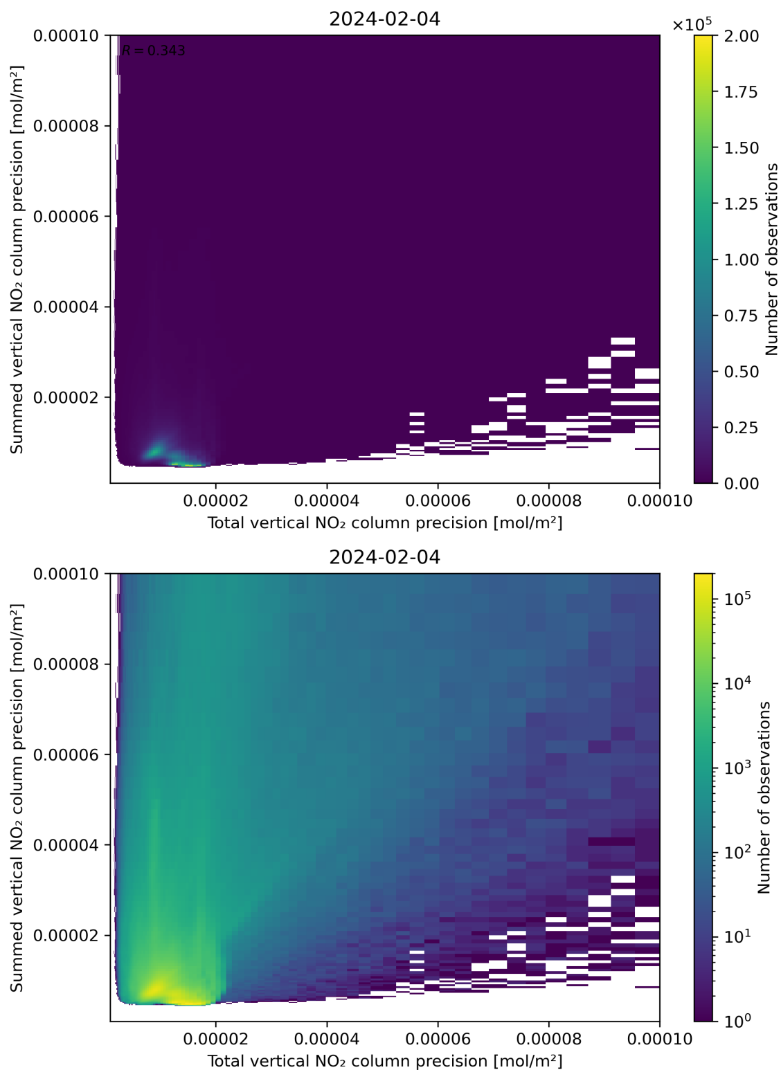
Figure 118: Scatter density plot of “Total vertical NO 2 column precision” against “Summed vertical NO 2 column precision” for 2024-02-03 to 2024-02-05.
