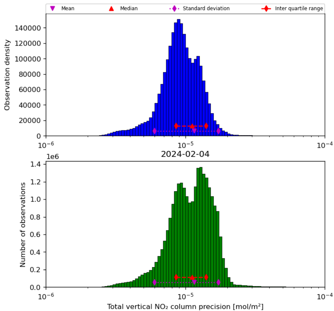
Figure 39: Histogram of “Total vertical NO 2 column precision” for 2024-02-03 to 2024-02-05
