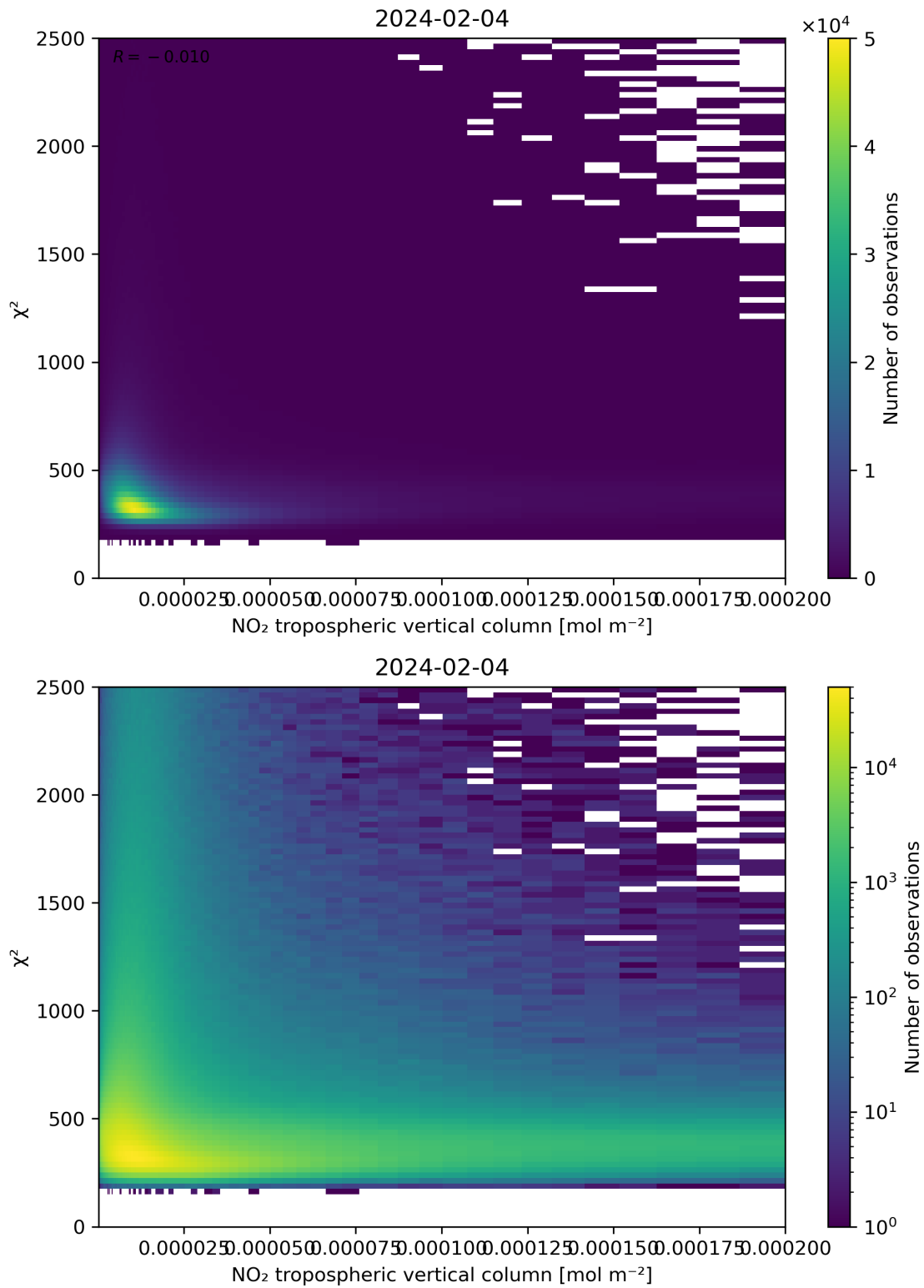
Figure 124: Scatter density plot of “NO 2 tropospheric vertical column” against “ \chi^2 ” for 2024-02-03 to 2024-02-05.
