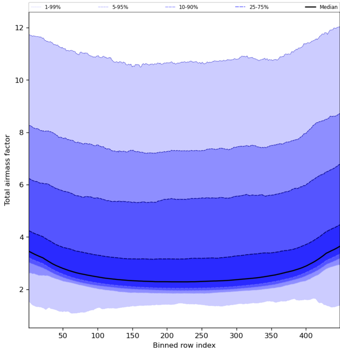
Figure 49: Along track statistics of “Total airmass factor” for 2024-02-03 to 2024-02-05
