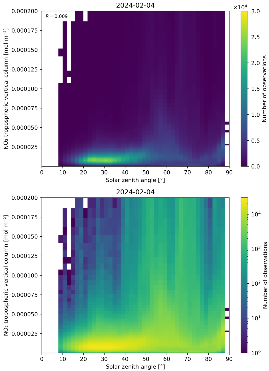
Figure 155: Scatter density plot of “Solar zenith angle” against “NO 2 tropospheric vertical column” for 2024-02-03 to 2024-02-05.
