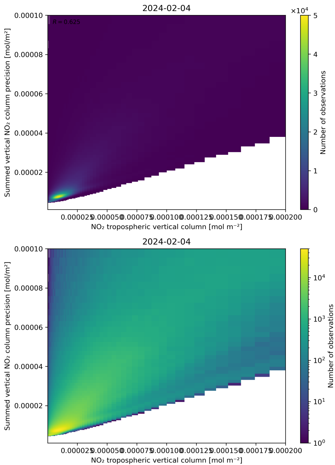
Figure 127: Scatter density plot of “NO 2 tropospheric vertical column” against “Summed vertical NO 2 column precision” for 2024-02-03 to 2024-02-05.
