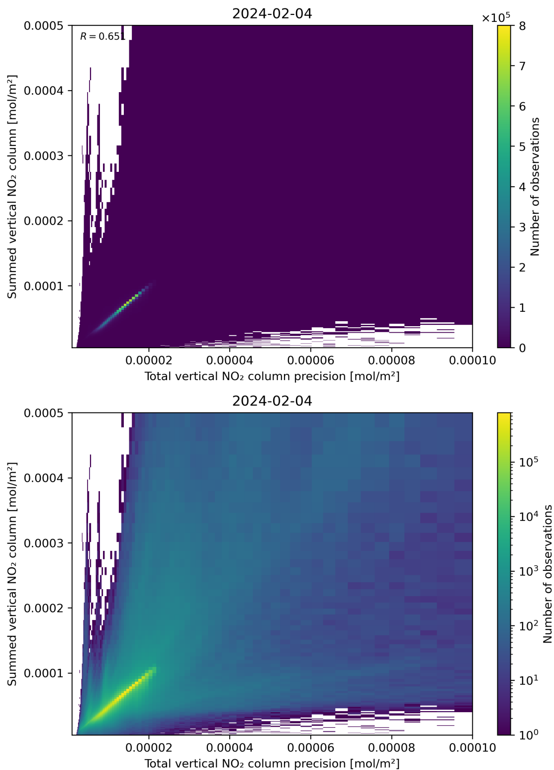
Figure 117: Scatter density plot of “Total vertical NO 2 column precision” against “Summed vertical NO 2 column” for 2024-02-03 to 2024-02-05.
