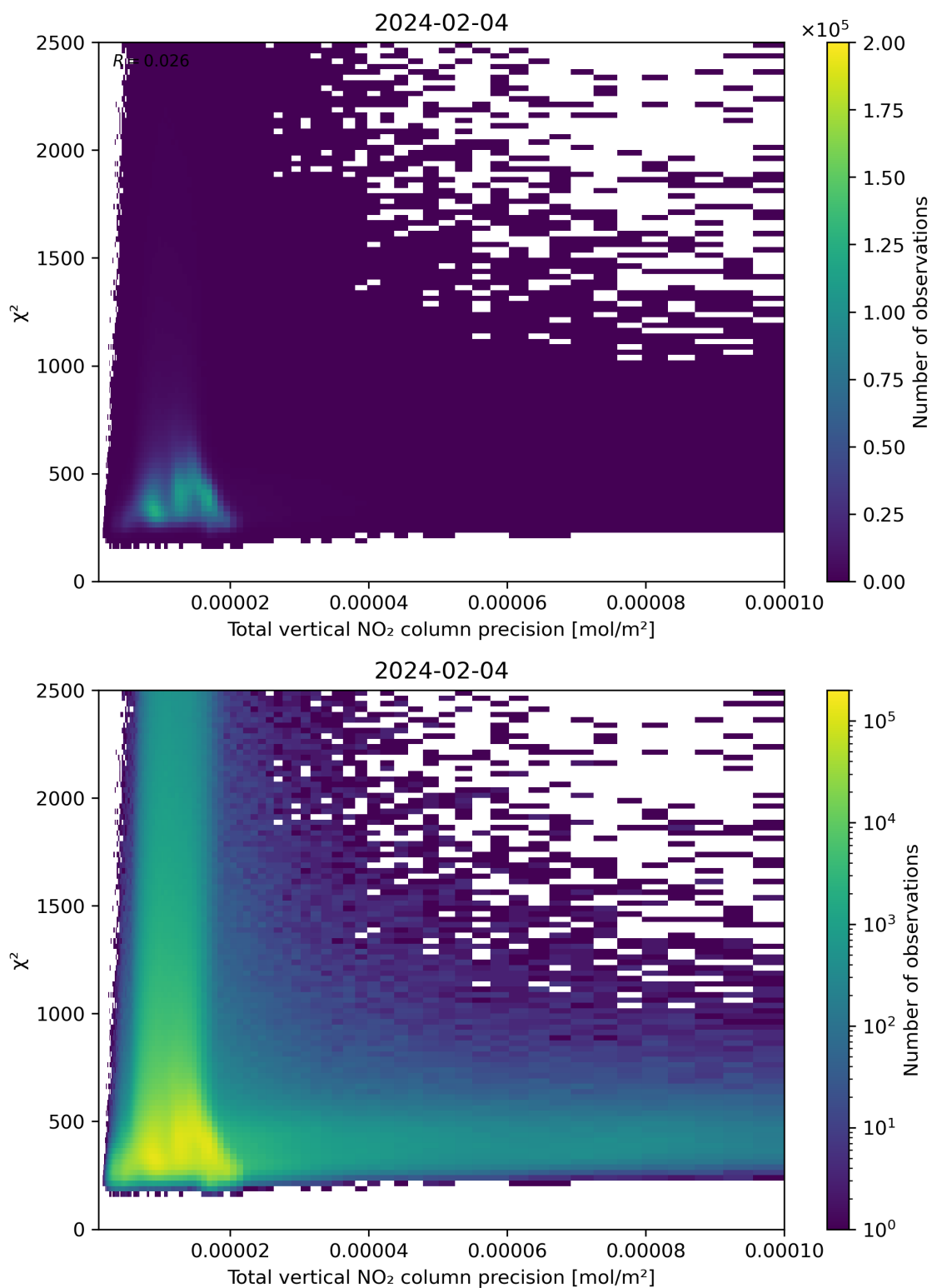
Figure 116: Scatter density plot of "Total vertical NO 2 column precision" against " \chi^2 " for 2024-02-03 to 2024-02-05.
