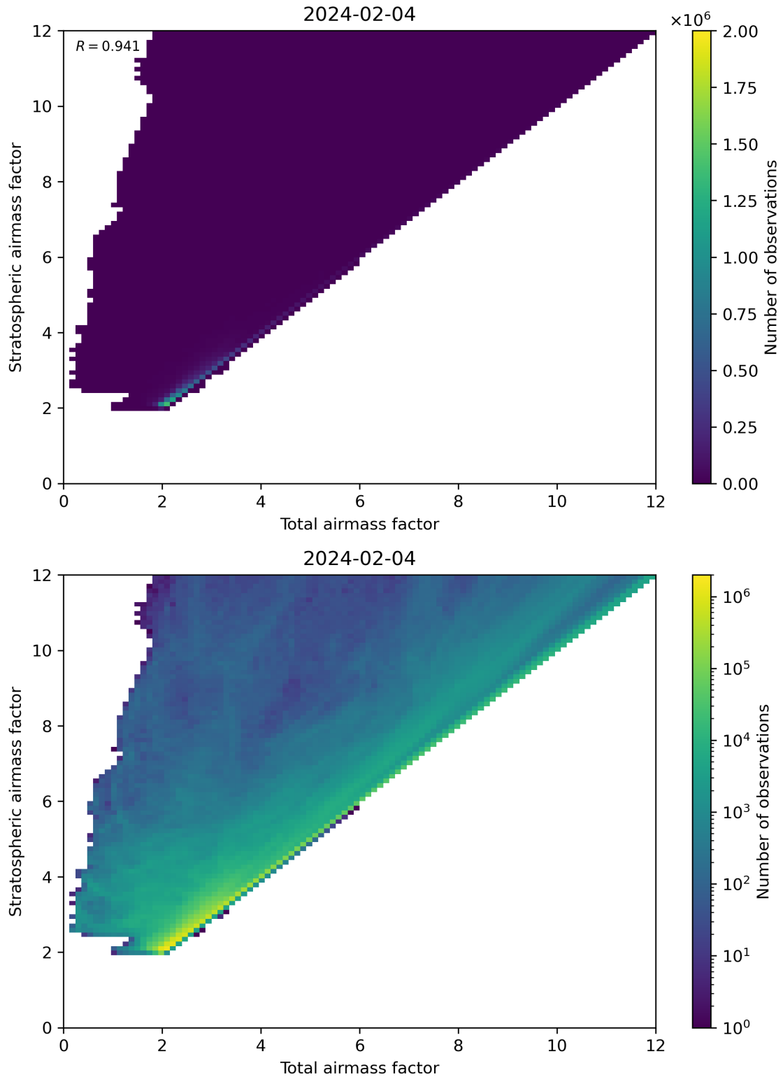
Figure 62: Scatter density plot of “Total airmass factor” against “Stratospheric airmass factor” for 2024-02-03 to 2024-02-05.
