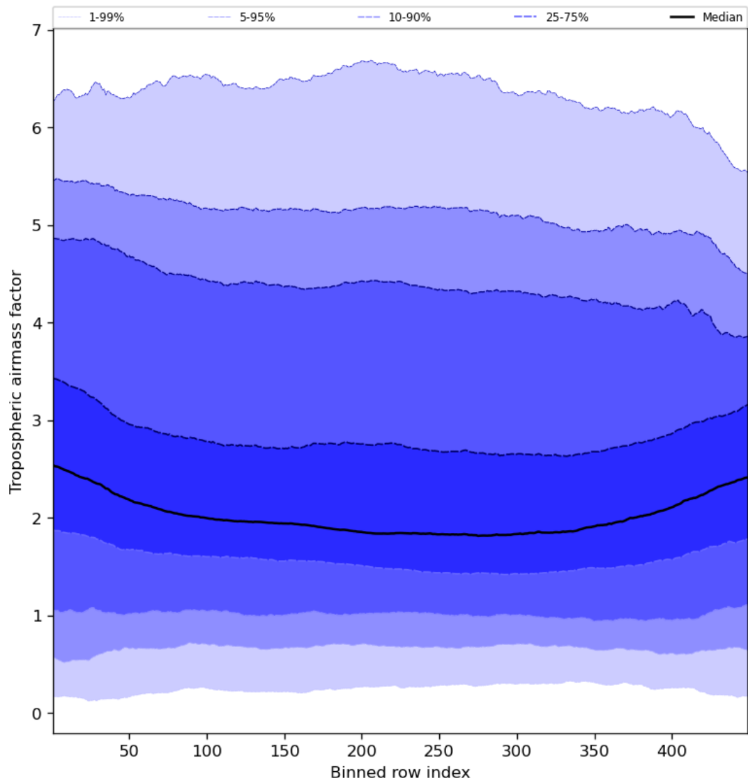
Figure 48: Along track statistics of “Tropospheric airmass factor” for 2024-02-03 to 2024-02-05
