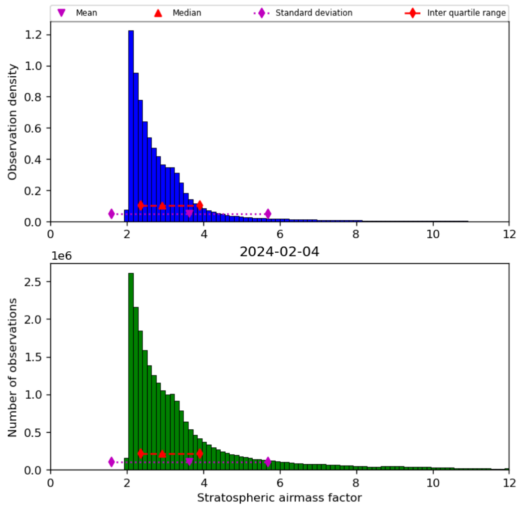
Figure 44: Histogram of “Stratospheric airmass factor” for 2024-02-03 to 2024-02-05
