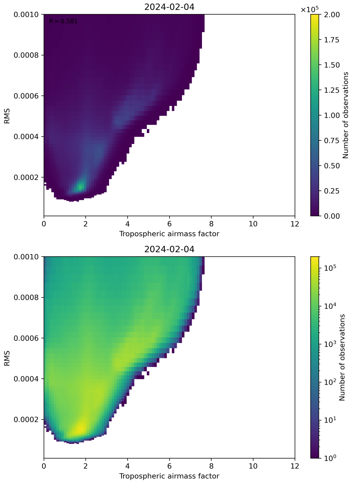
Figure 79: Scatter density plot of “Tropospheric airmass factor” against “RMS” for 2024-02-03 to 2024-02-05.
