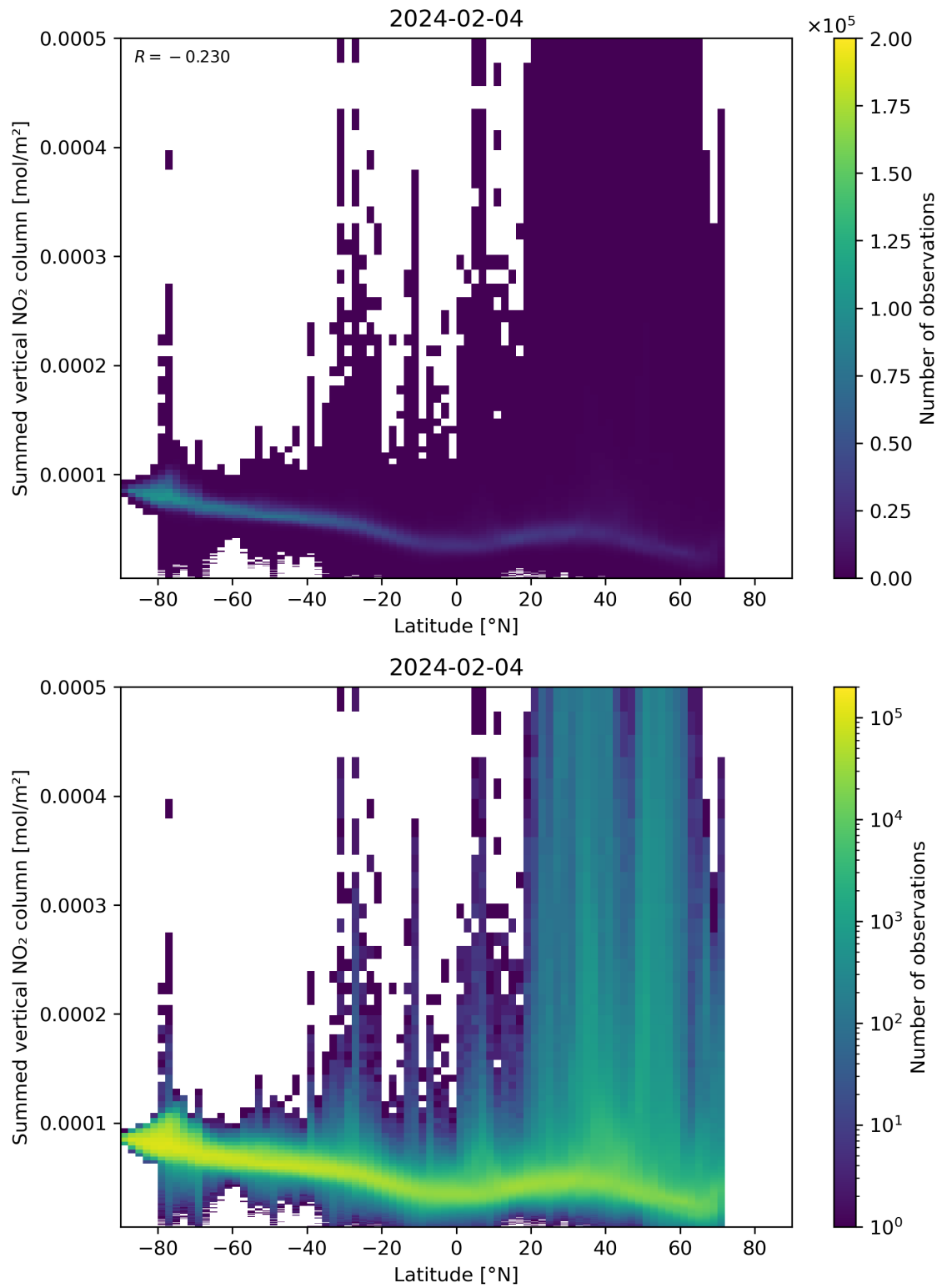
Figure 88: Scatter density plot of “Latitude” against “Summed vertical NO 2 column” for 2024-02-03 to 2024-02-05.
