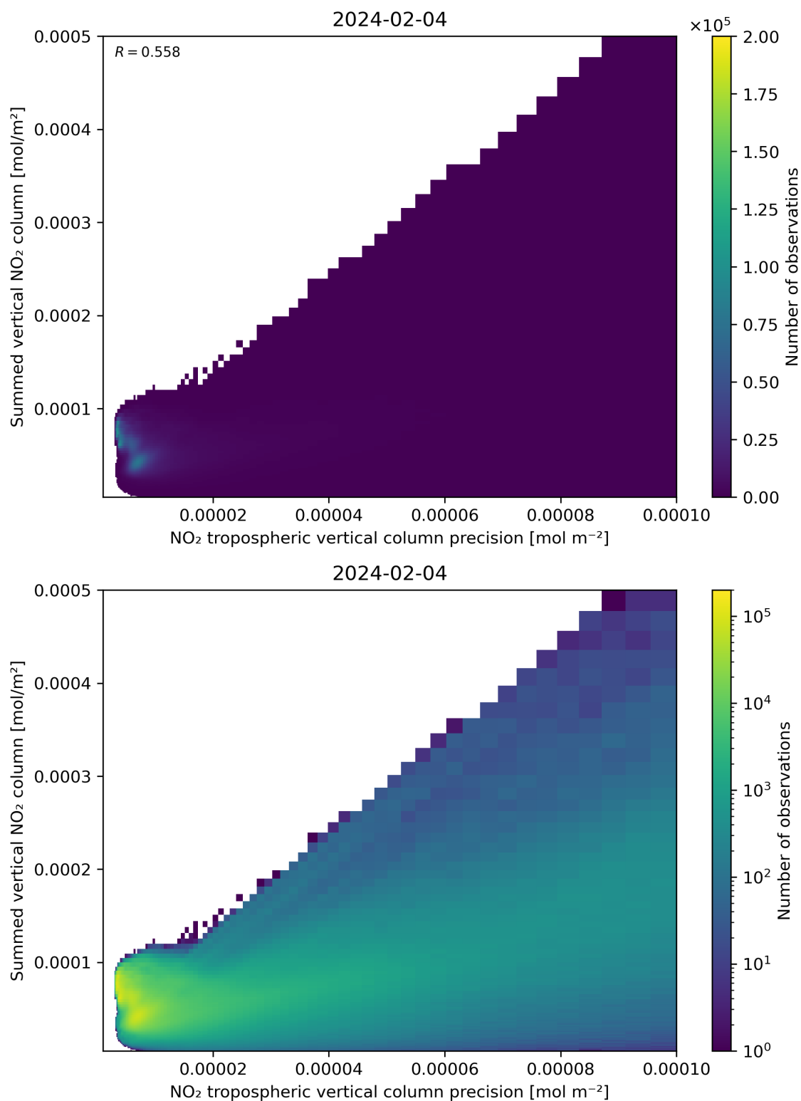
Figure 136: Scatter density plot of “NO 2 tropospheric vertical column precision” against “Summed vertical NO 2 column” for 2024-02-03 to 2024-02-05.
