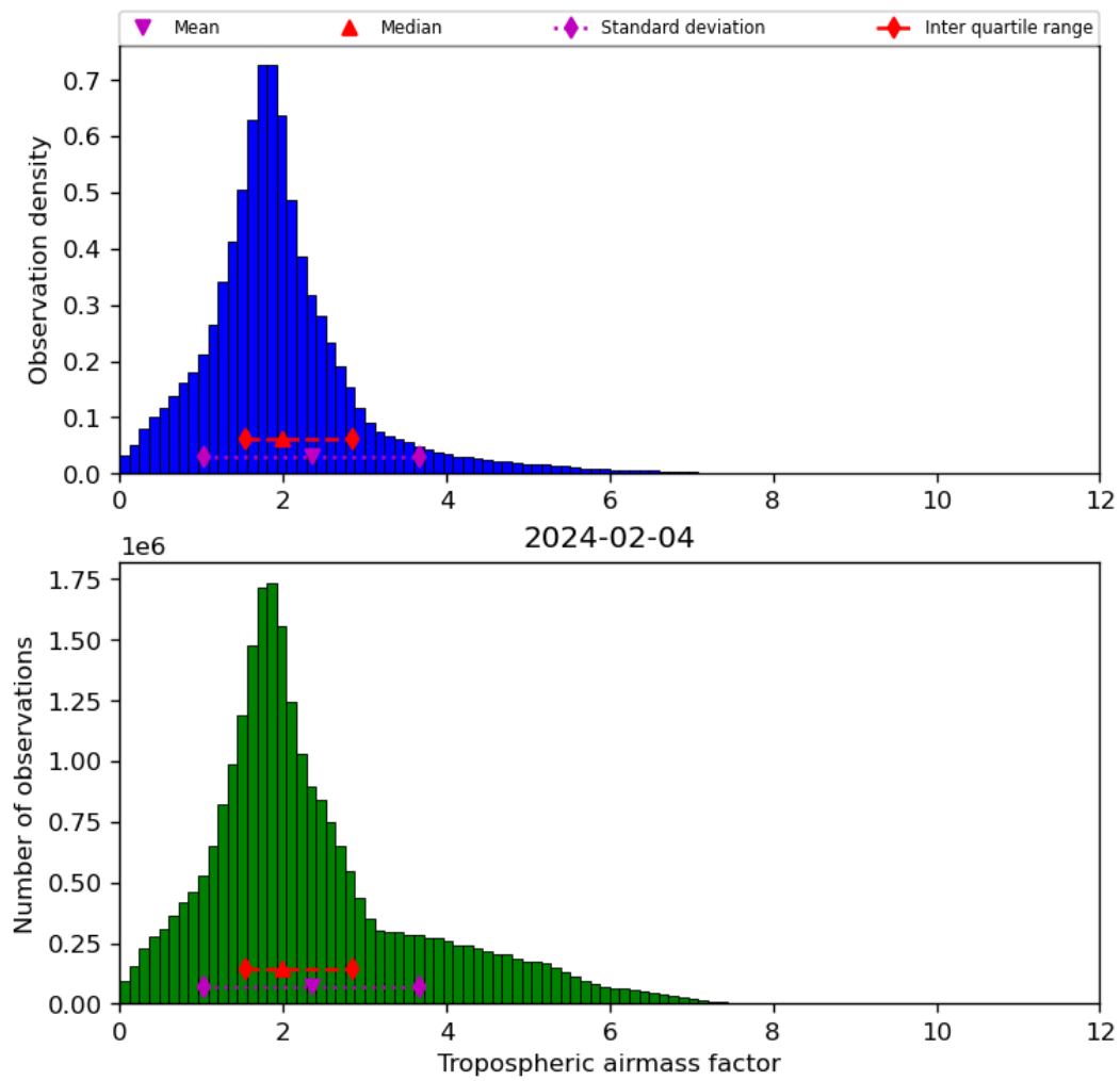
Figure 31: Histogram of “Tropospheric airmass factor” for 2024-02-03 to 2024-02-05
