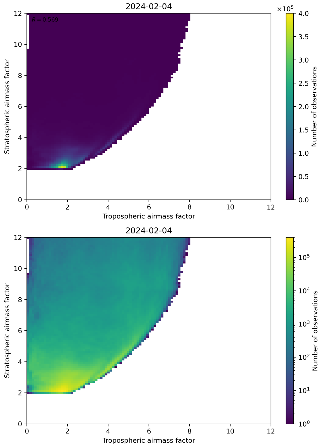
Figure 71: Scatter density plot of “Tropospheric airmass factor” against “Stratospheric airmass factor” for 2024-02-03 to 2024-02-05.
