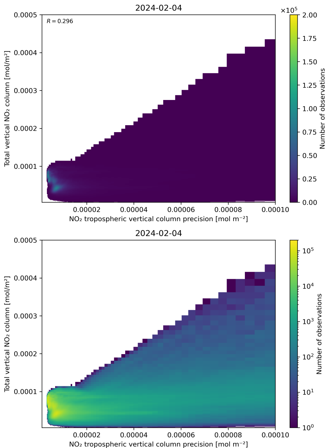
Figure 138: Scatter density plot of “NO 2 tropospheric vertical column precision” against “Total vertical NO 2 column” for 2024-02-03 to 2024-02-05.
