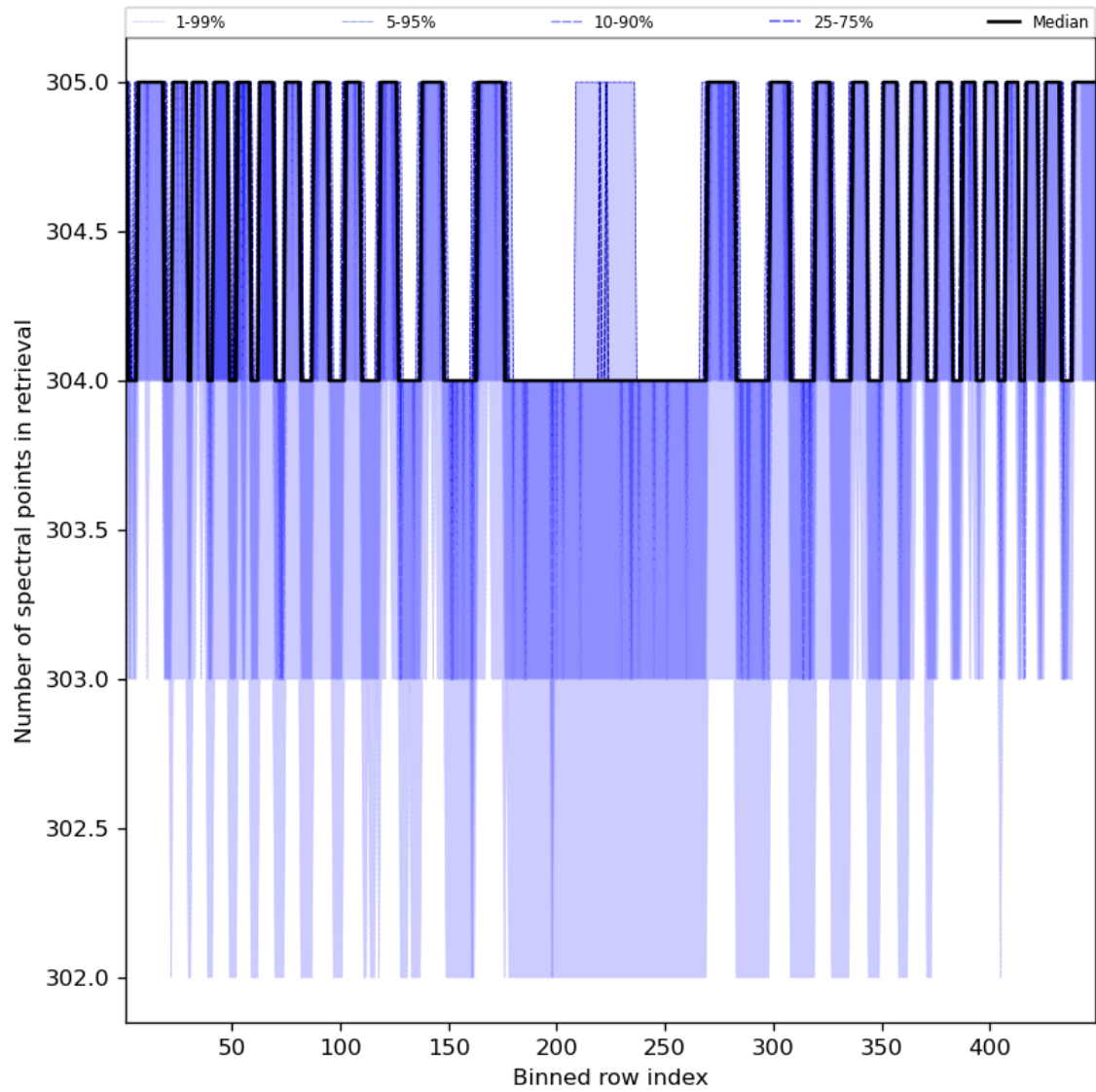
Figure 50: Along track statistics of “Number of spectral points in retrieval” for 2024-02-03 to 2024-02-05
