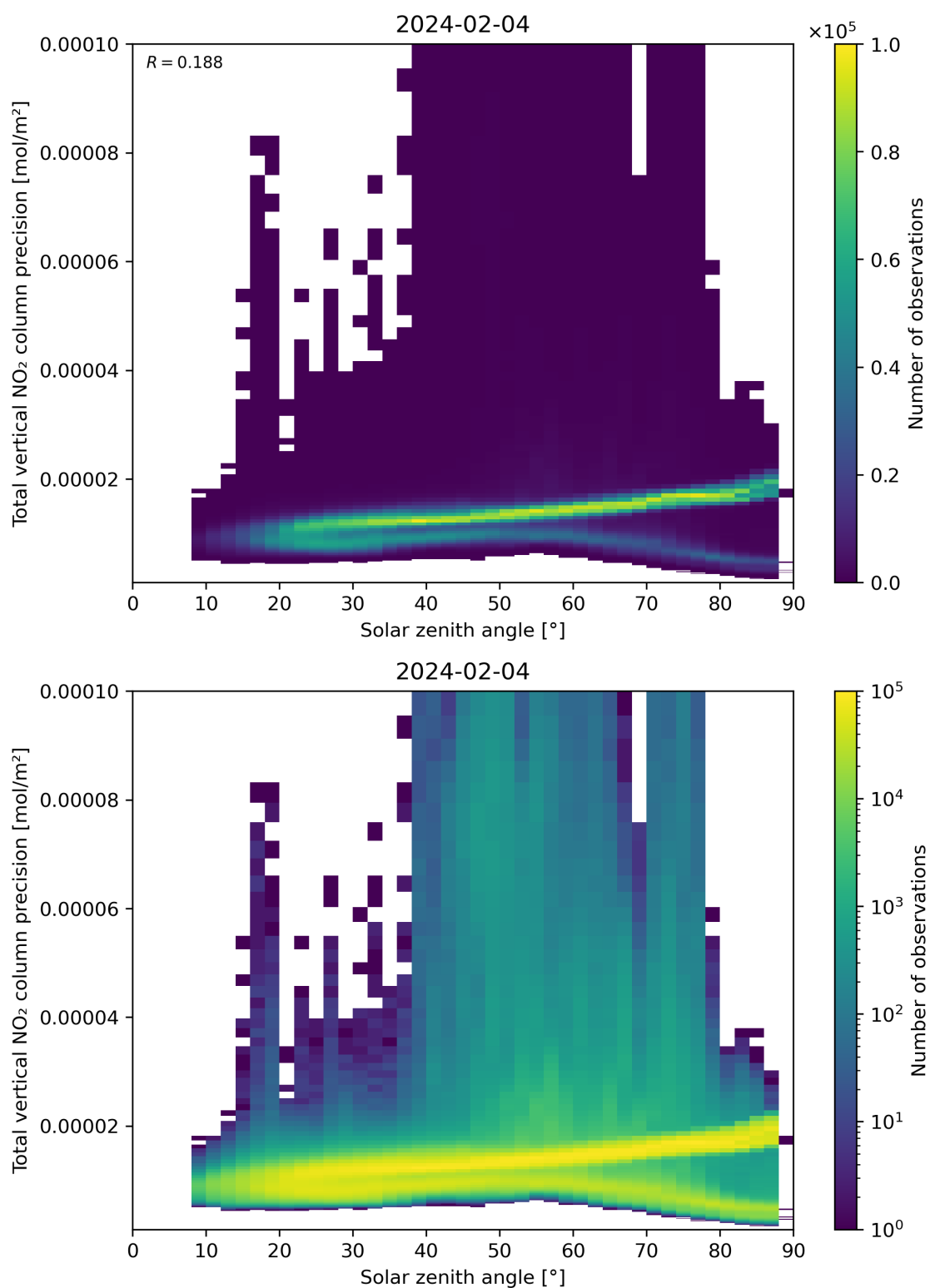
Figure 154: Scatter density plot of “Solar zenith angle” against “Total vertical NO 2 column precision” for 2024-02-03 to 2024-02-05.
