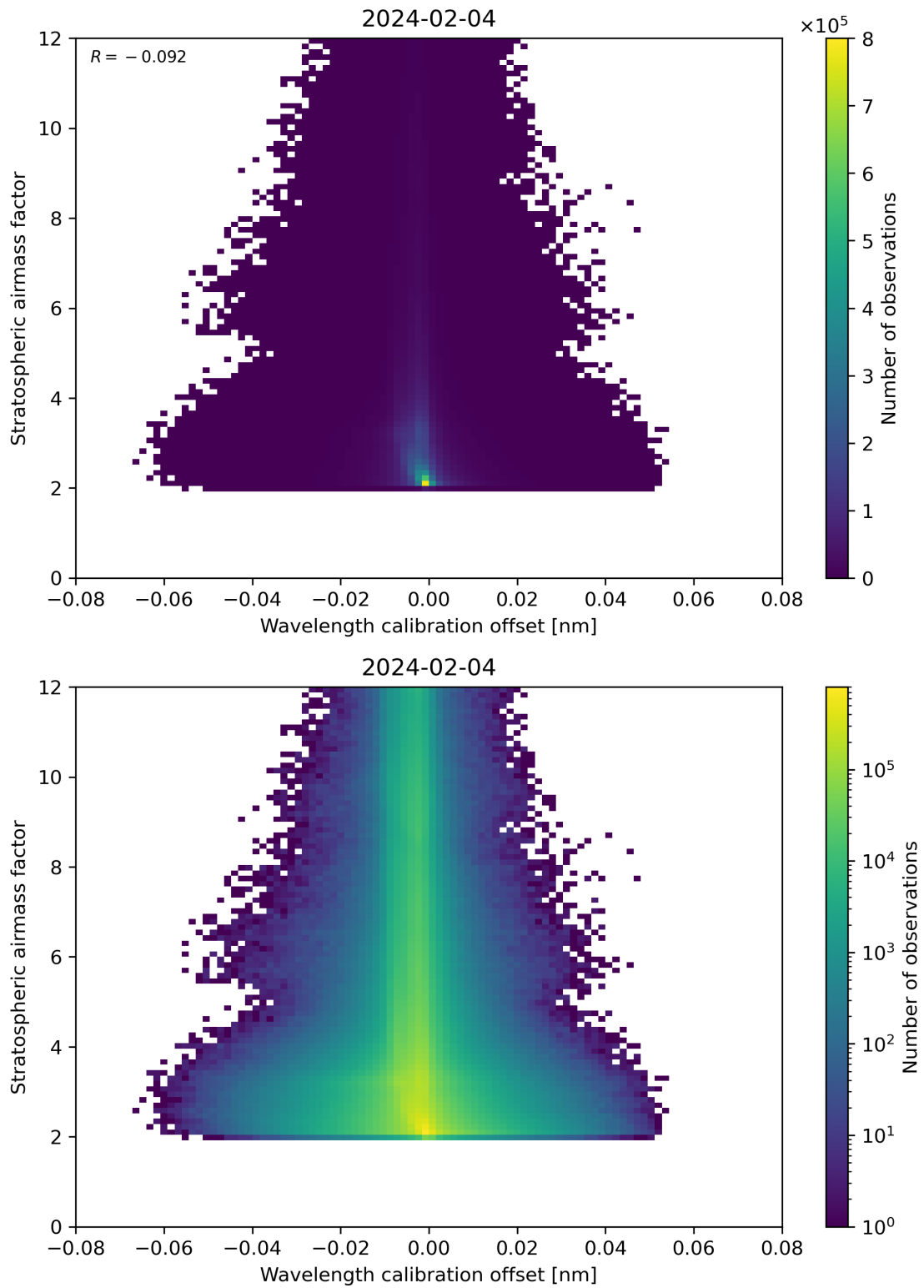
Figure 174: Scatter density plot of “Wavelength calibration offset” against “Stratospheric airmass factor” for 2024-02-03 to 2024-02-05.
