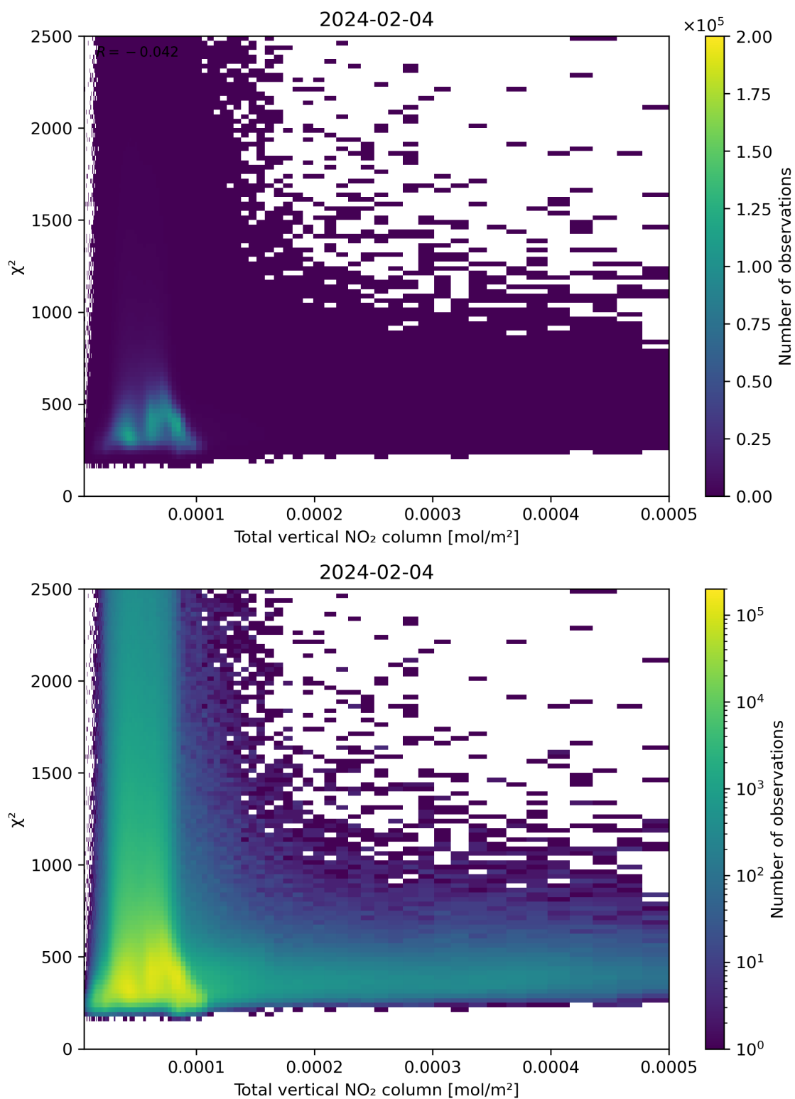
Figure 111: Scatter density plot of “Total vertical NO 2 column” against “ \chi^2 ” for 2024-02-03 to 2024-02-05.
