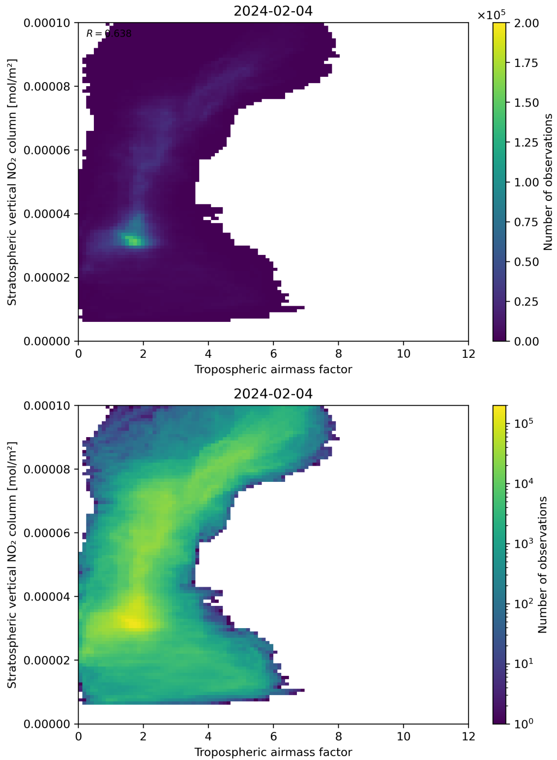
Figure 74: Scatter density plot of “Tropospheric air mass factor” against “Stratospheric vertical NO 2 column” for 2024-02-03 to 2024-02-05.
