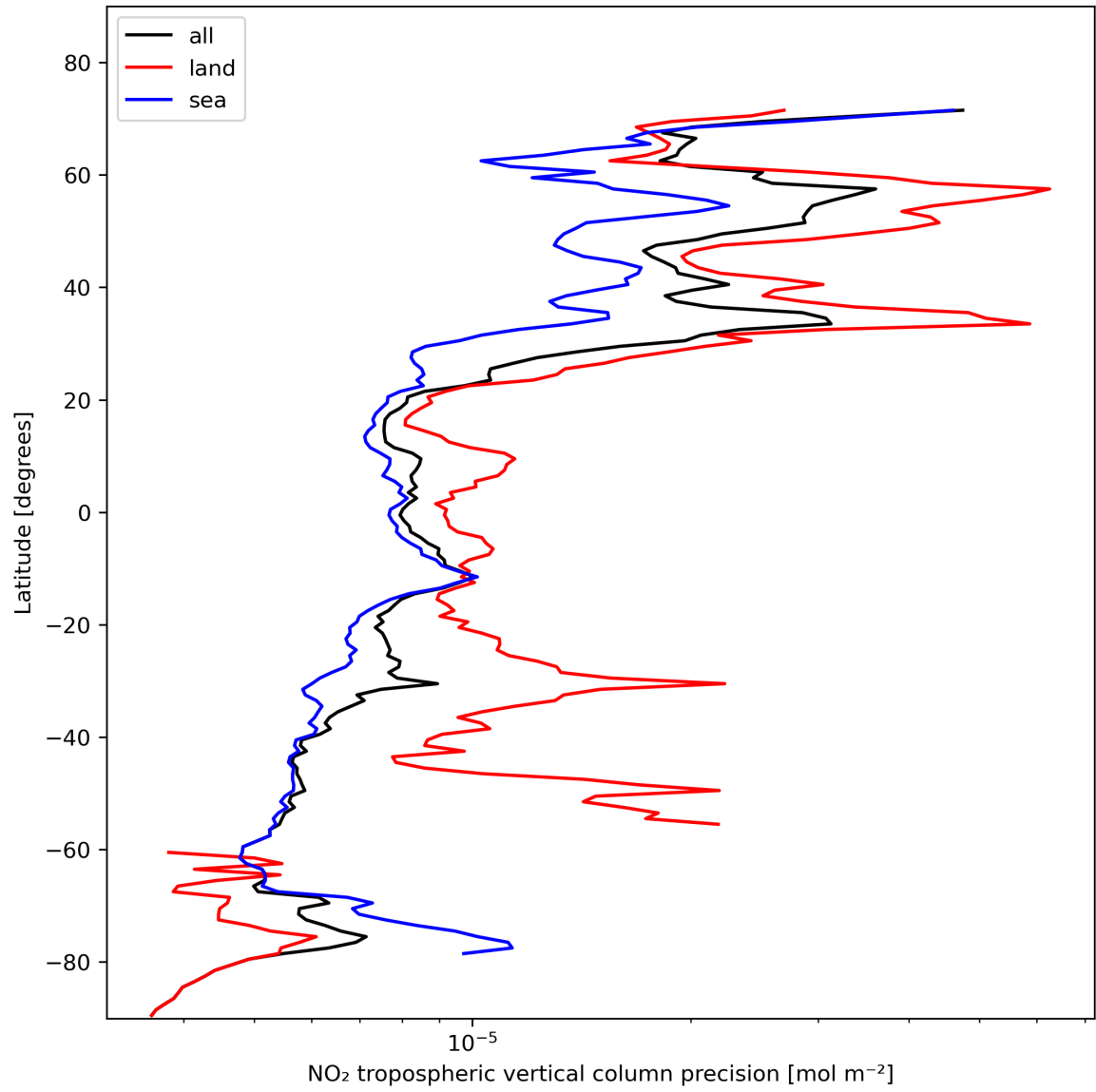
Figure 13: Zonal average of “NO 2 tropospheric vertical column precision” for 2024-02-03 to 2024-02-05.
