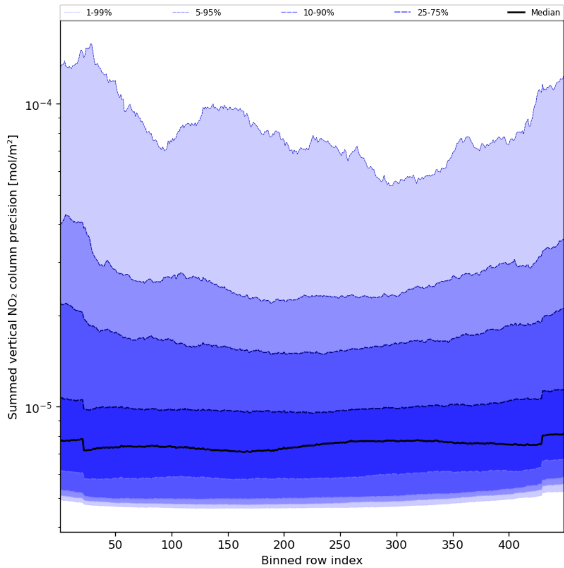
Figure 58: Along track statistics of “Summed vertical NO 2 column precision” for 2024-02-03 to 2024-02-05
