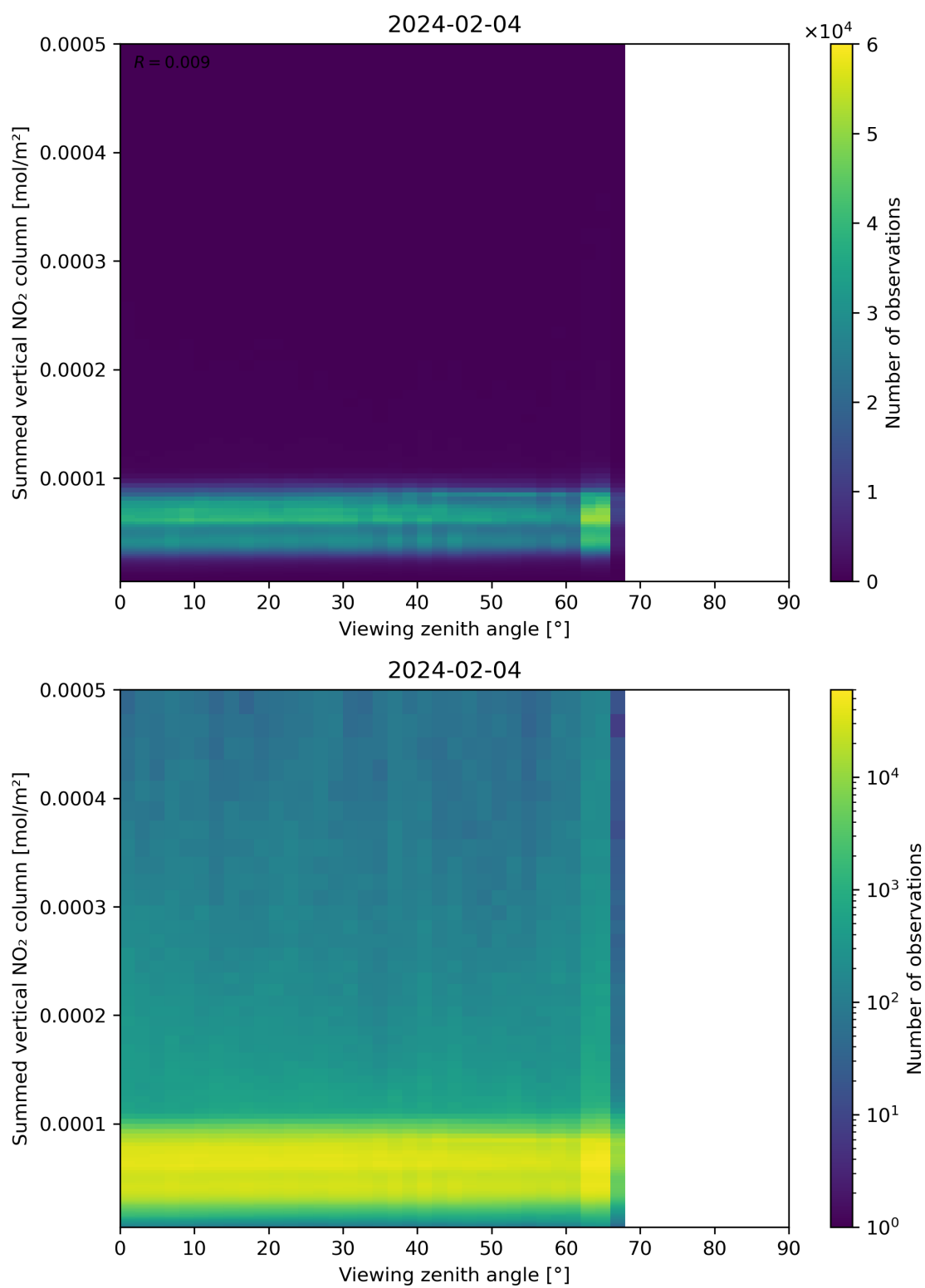
Figure 165: Scatter density plot of “Viewing zenith angle” against “Summed vertical NO 2 column” for 2024-02-03 to 2024-02-05.
