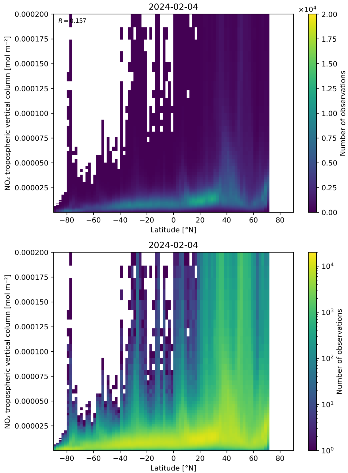
Figure 92: Scatter density plot of “Latitude” against “NO 2 tropospheric vertical column” for 2024-02-03 to 2024-02-05.
