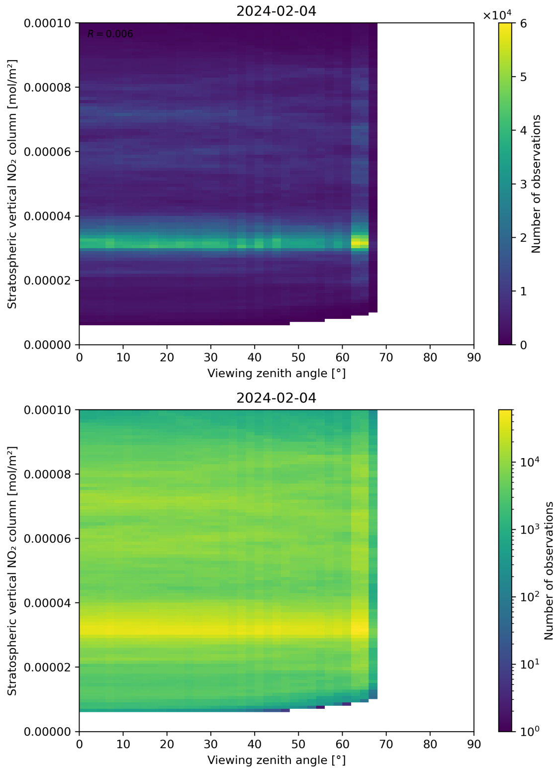
Figure 164: Scatter density plot of “Viewing zenith angle” against “Stratospheric vertical NO 2 column” for 2024-02-03 to 2024-02-05.
