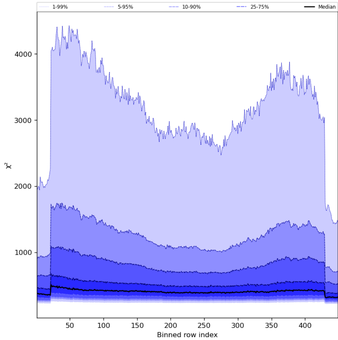
Figure 59: Along track statistics of “ \chi^2 ” for 2024-02-03 to 2024-02-05
