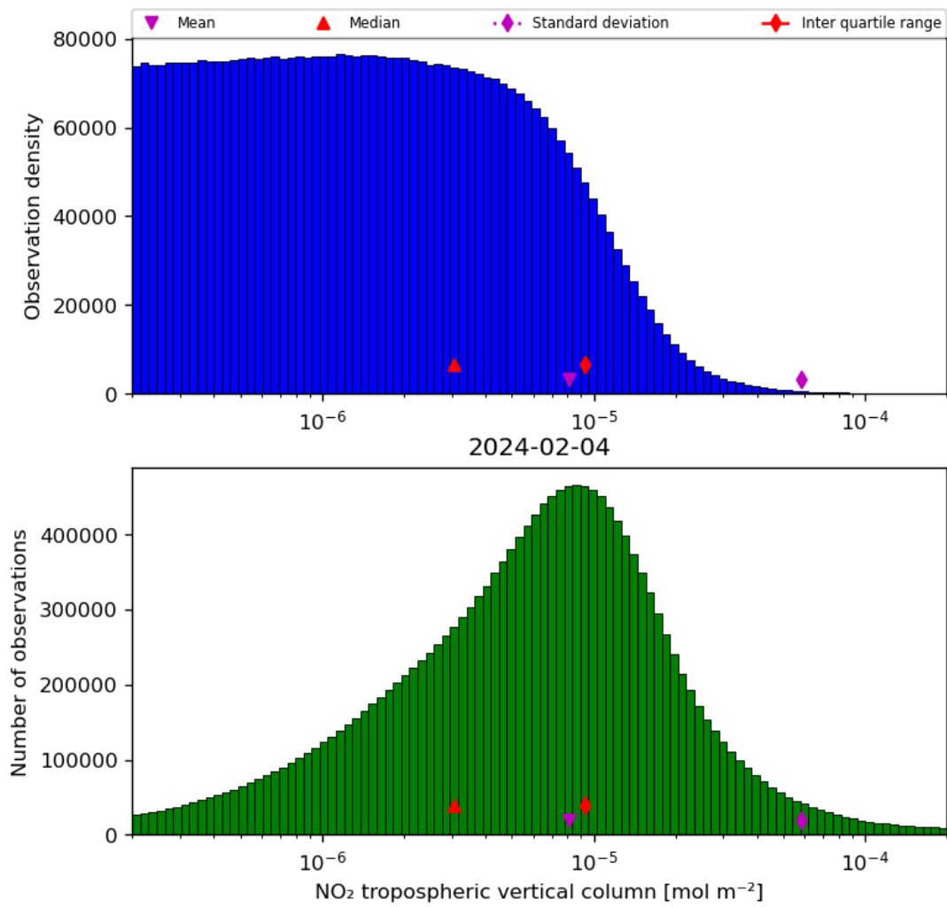
Figure 29: Histogram of “NO 2 tropospheric vertical column” for 2024-02-03 to 2024-02-05
