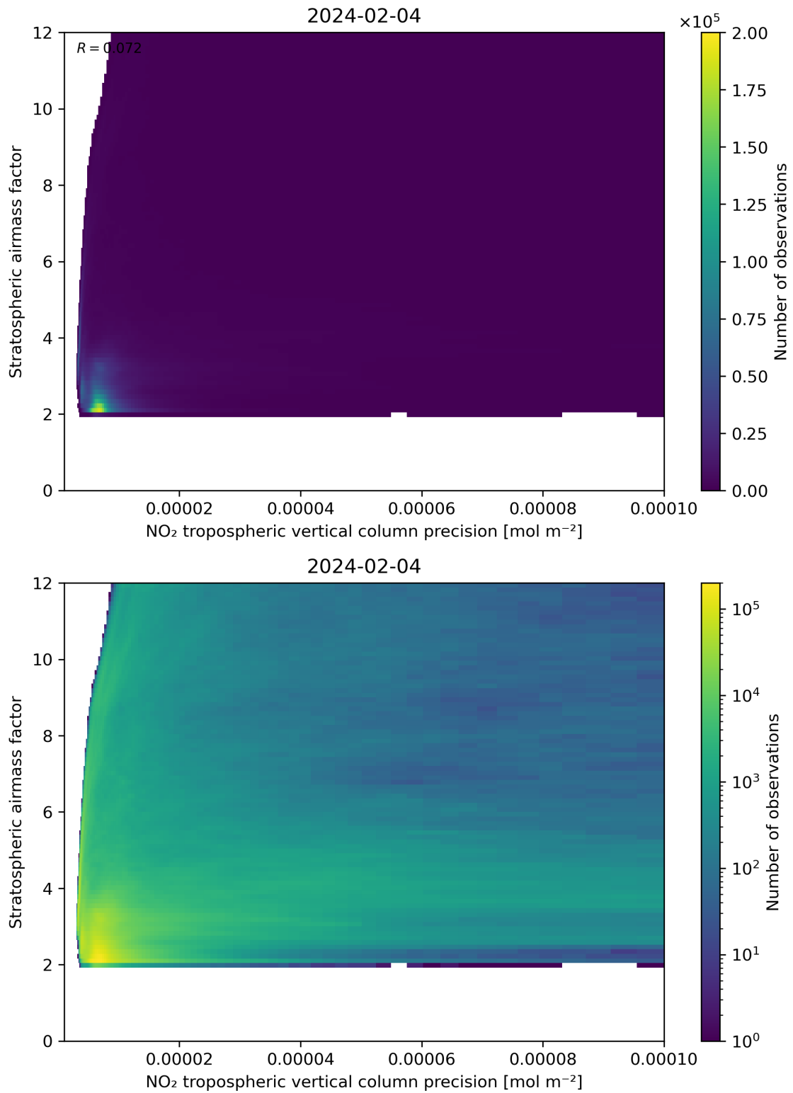
Figure 131: Scatter density plot of “NO 2 tropospheric vertical column precision” against “Stratospheric airmass factor” for 2024-02-03 to 2024-02-05.
