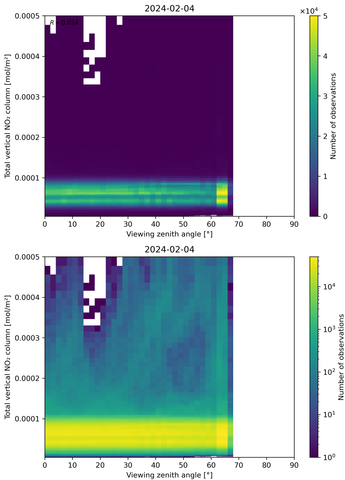
Figure 167: Scatter density plot of “Viewing zenith angle” against “Total vertical NO 2 column” for 2024-02-03 to 2024-02-05.
