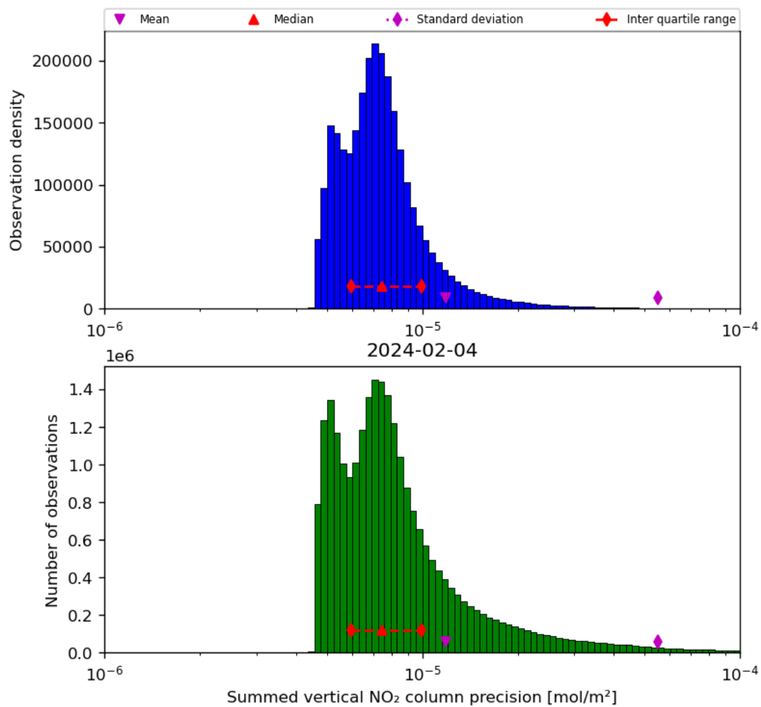
Figure 41: Histogram of “Summed vertical NO 2 column precision” for 2024-02-03 to 2024-02-05
