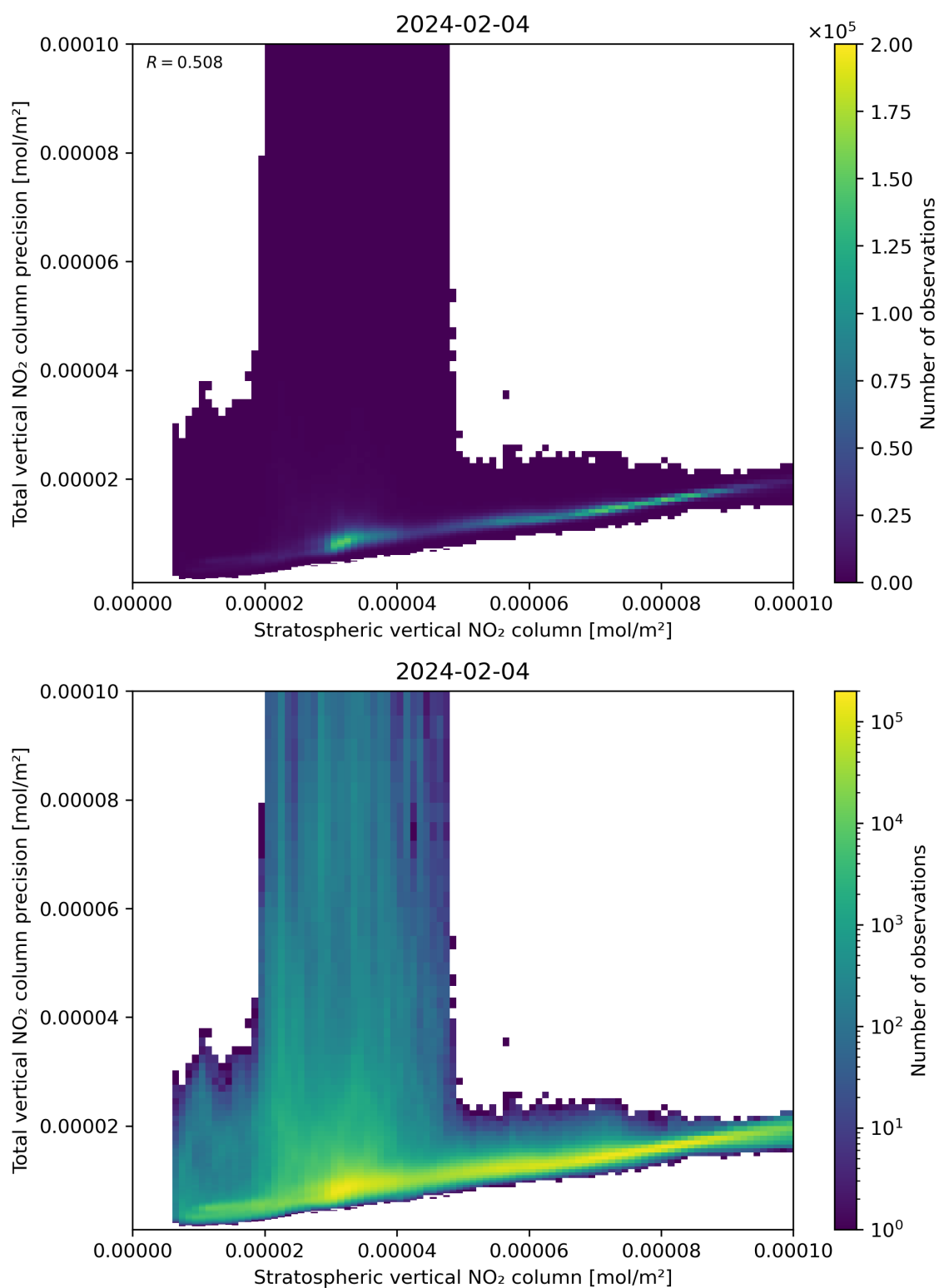
Figure 101: Scatter density plot of “Stratospheric vertical NO 2 column” against “Total vertical NO 2 column precision” for 2024-02-03 to 2024-02-05.
