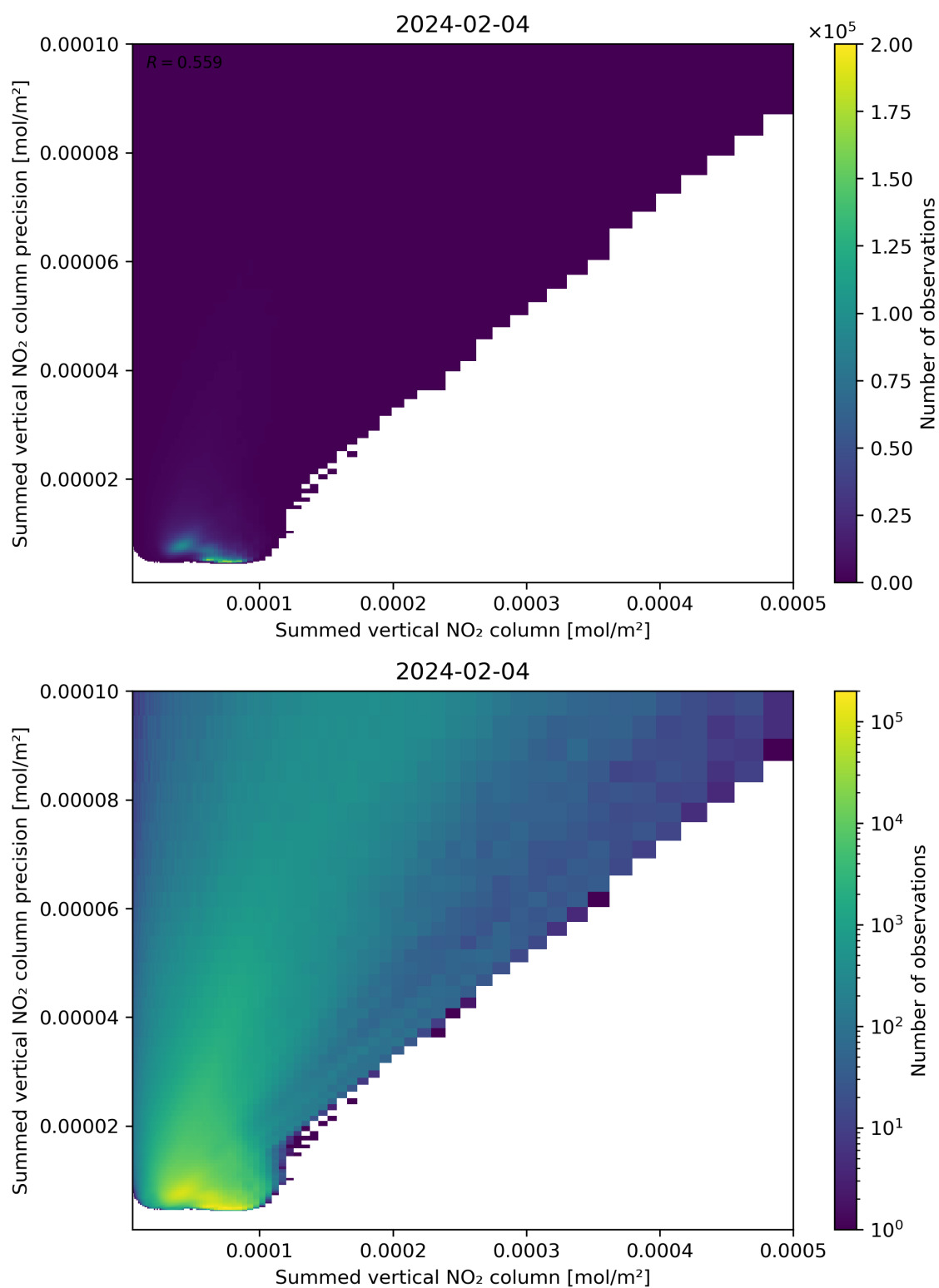
Figure 105: Scatter density plot of “Summed vertical NO 2 column” against “Summed vertical NO 2 column precision” for 2024-02-03 to 2024-02-05.
