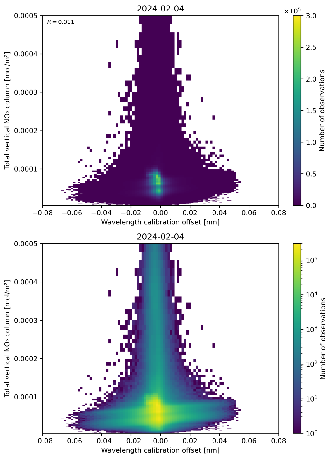
Figure 179: Scatter density plot of “Wavelength calibration offset” against “Total vertical NO 2 column” for 2024-02-03 to 2024-02-05.
