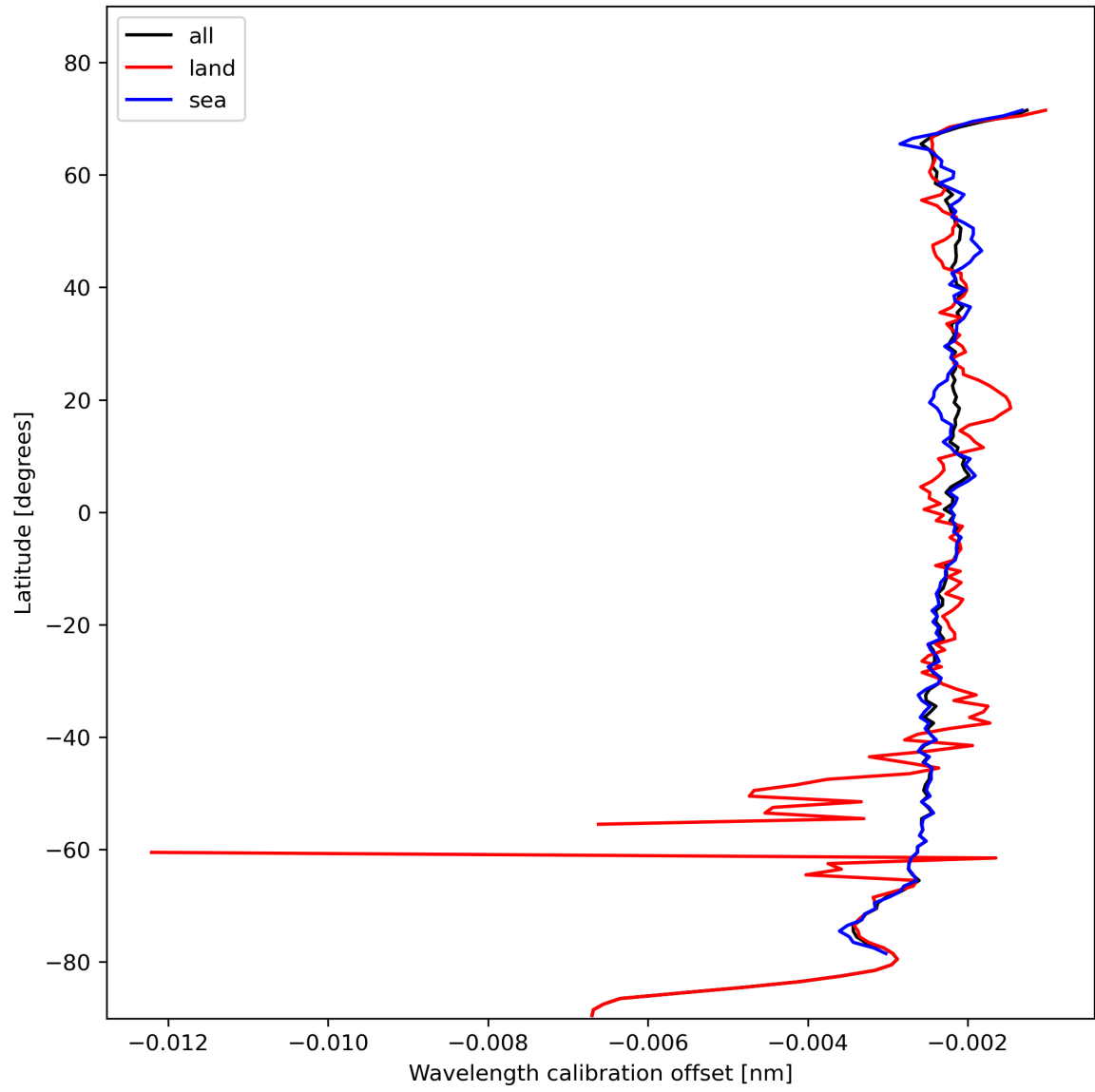
Figure 18: Zonal average of “Wavelength calibration offset” for 2024-02-03 to 2024-02-05.
