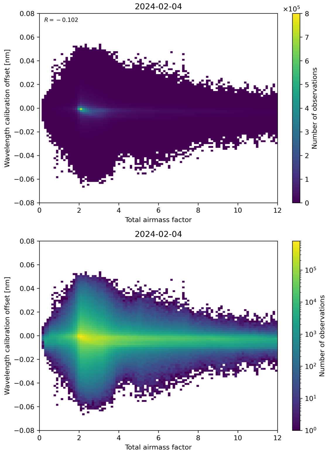
Figure 70: Scatter density plot of “Total airmass factor” against “Wavelength calibration offset” for 2024-02-03 to 2024-02-05.
