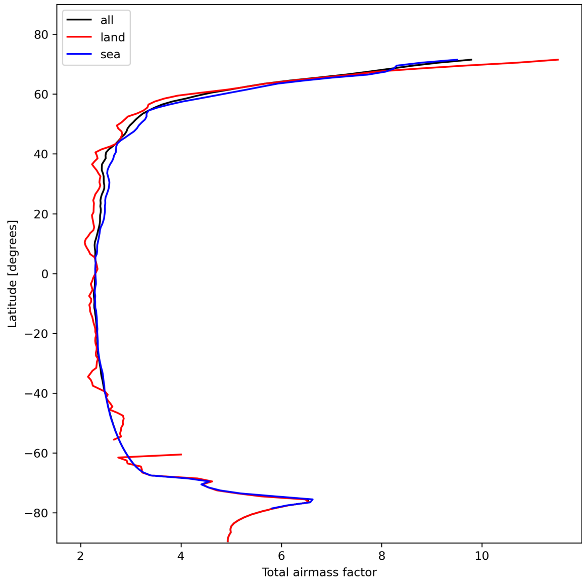
Figure 15: Zonal average of “Total airmass factor” for 2024-02-03 to 2024-02-05.
