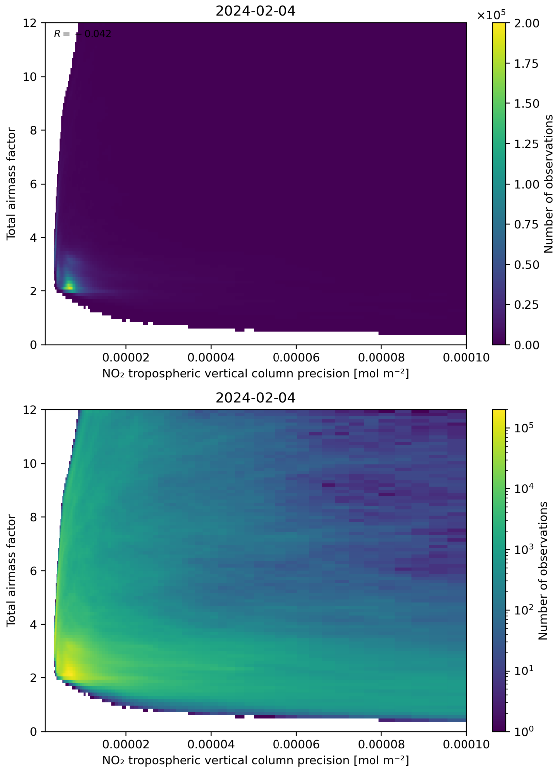
Figure 132: Scatter density plot of “NO 2 tropospheric vertical column precision” against “Total air mass factor” for 2024-02-03 to 2024-02-05.
