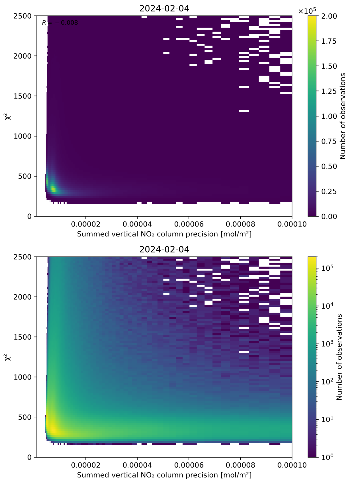
Figure 107: Scatter density plot of “Summed vertical NO 2 column precision” against “ \chi^2 ” for 2024-02-03 to 2024-02-05.
