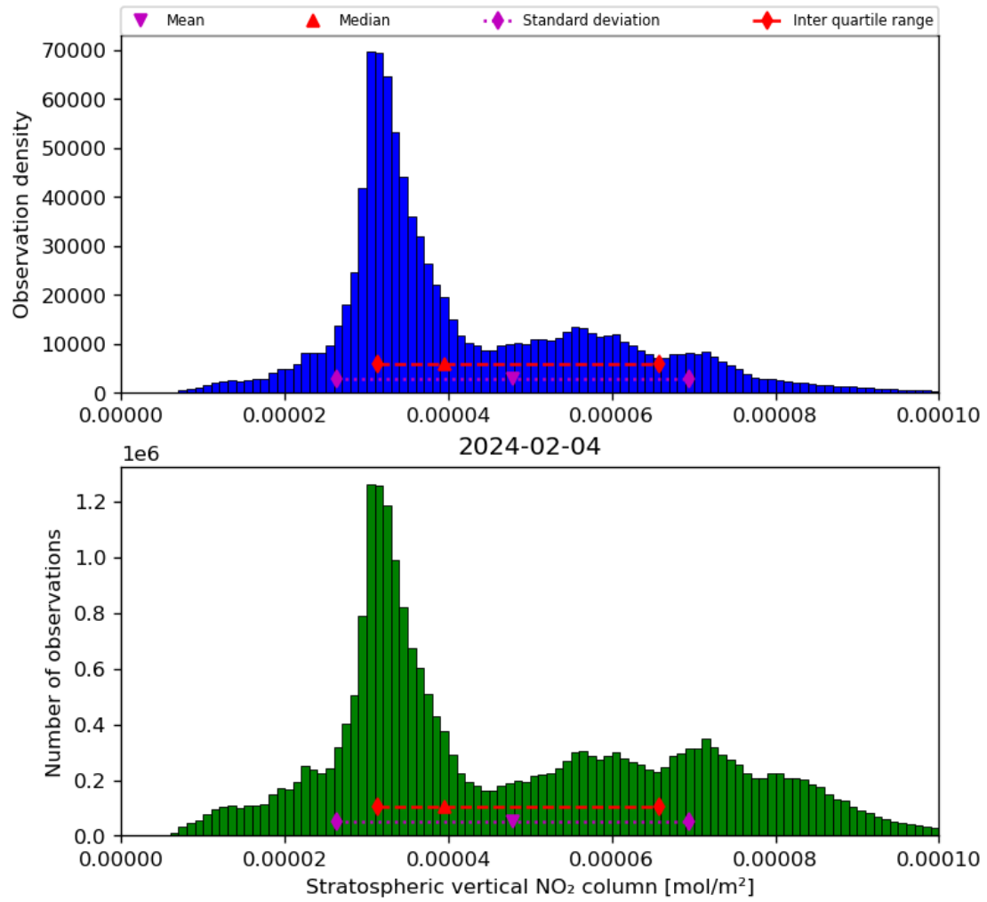
Figure 36: Histogram of “Stratospheric vertical NO 2 column” for 2024-02-03 to 2024-02-05
