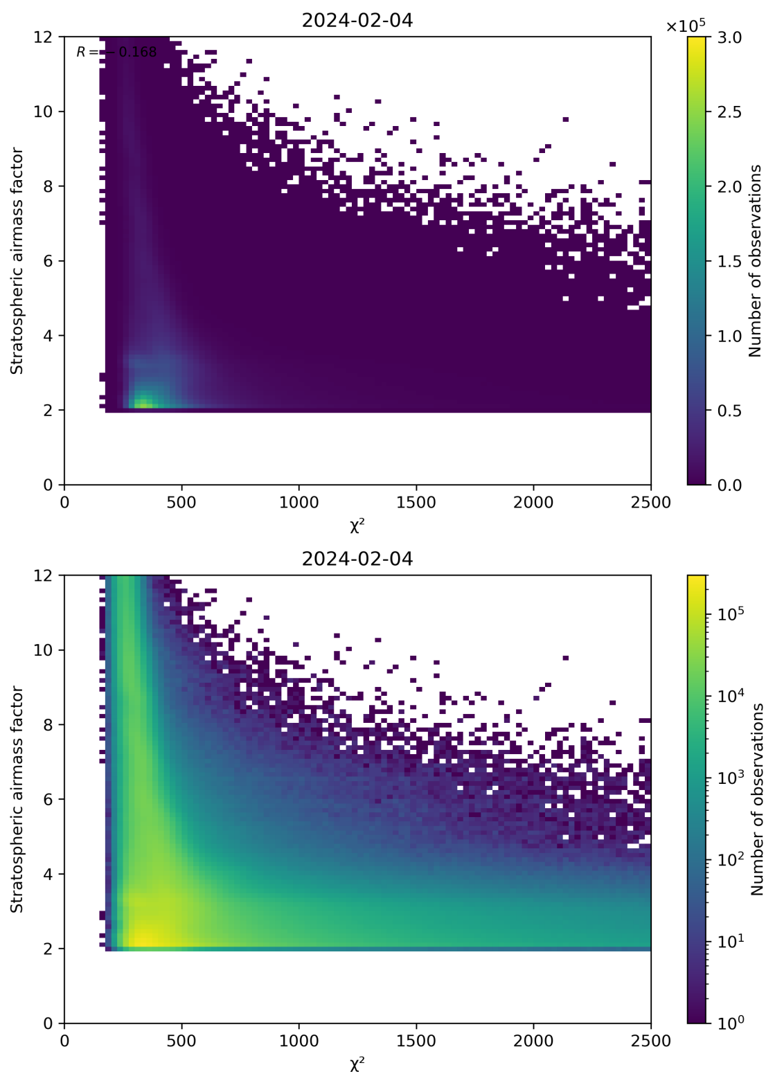
Figure 81: Scatter density plot of “ \chi^2 ” against “Stratospheric airmass factor” for 2024-02-03 to 2024-02-05.
