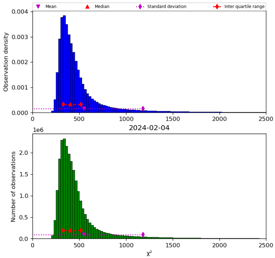
Figure 42: Histogram of “ \chi^2 ” for 2024-02-03 to 2024-02-05
