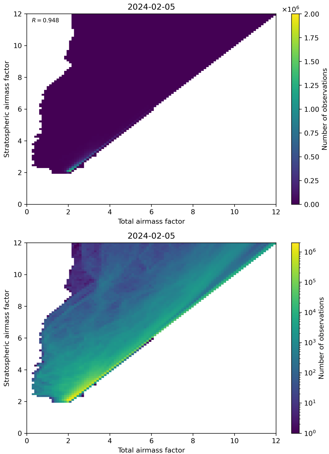
Figure 62: Scatter density plot of “Total airmass factor” against “Stratospheric airmass factor” for 2024-02-04 to 2024-02-06.
