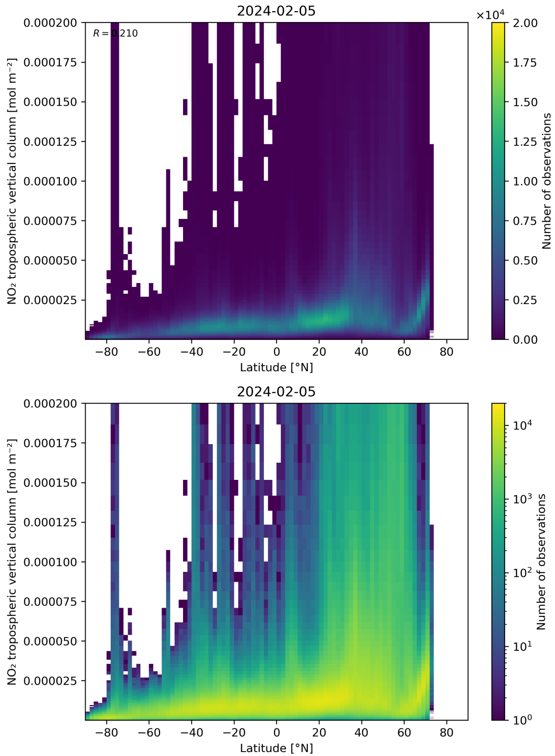
Figure 92: Scatter density plot of “Latitude” against “NO 2 tropospheric vertical column” for 2024-02-04 to 2024-02-06.
