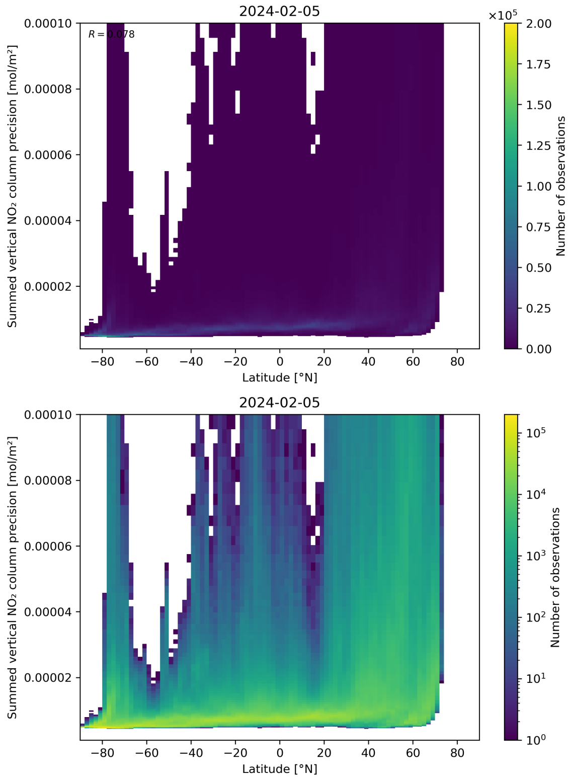
Figure 89: Scatter density plot of “Latitude” against “Summed vertical NO 2 column precision” for 2024-02-04 to 2024-02-06.
