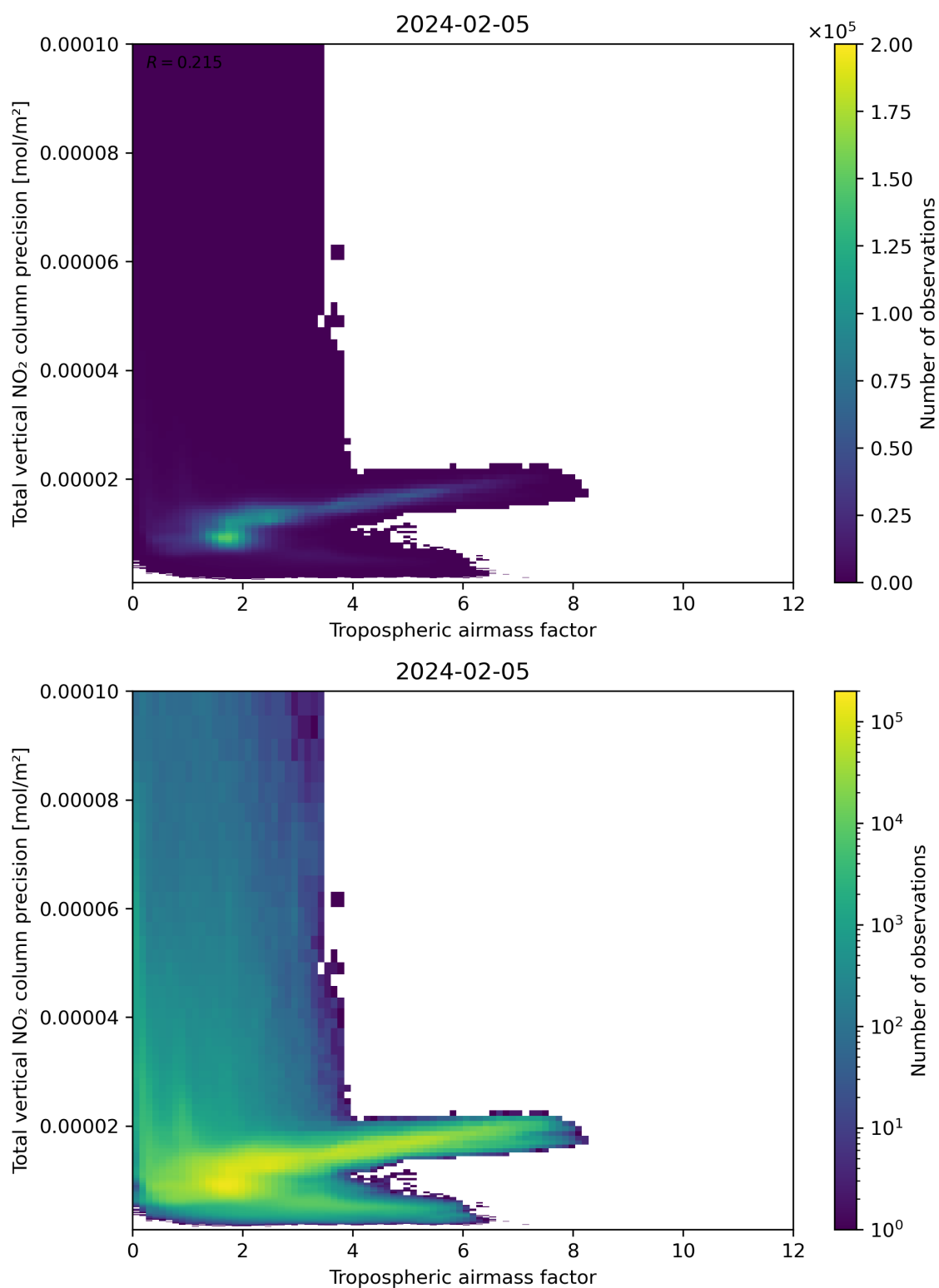
Figure 78: Scatter density plot of “Tropospheric air mass factor” against “Total vertical NO 2 column precision” for 2024-02-04 to 2024-02-06.
