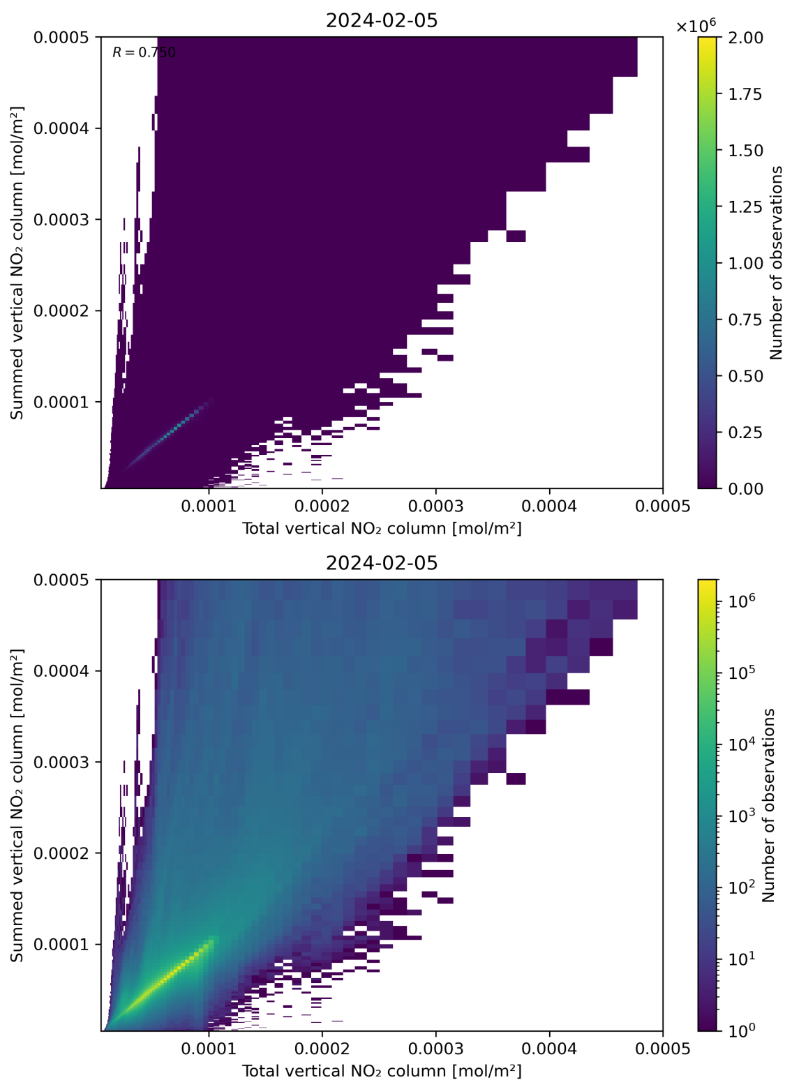
Figure 112: Scatter density plot of “Total vertical NO 2 column” against “Summed vertical NO 2 column” for 2024-02-04 to 2024-02-06.
