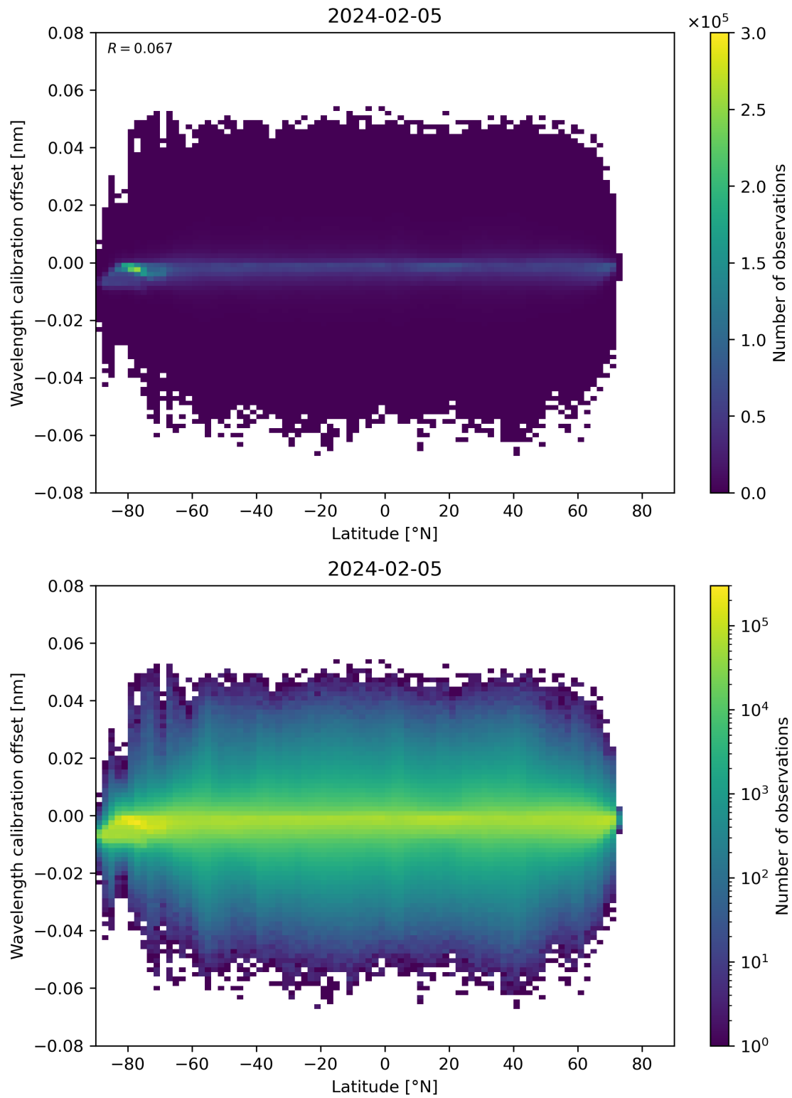
Figure 95: Scatter density plot of “Latitude” against “Wavelength calibration offset” for 2024-02-04 to 2024-02-06.
