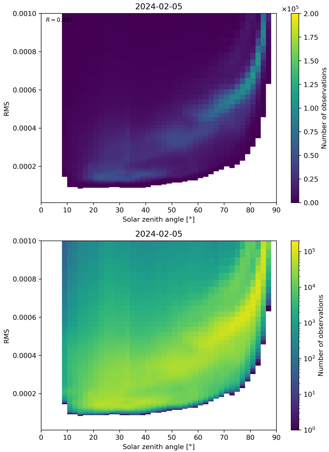
Figure 157: Scatter density plot of “Solar zenith angle” against “RMS” for 2024-02-04 to 2024-02-06.
