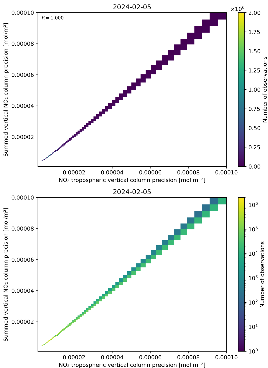
Figure 137: Scatter density plot of “NO 2 tropospheric vertical column precision” against “Summed vertical NO 2 column precision” for 2024-02-04 to 2024-02-06.
