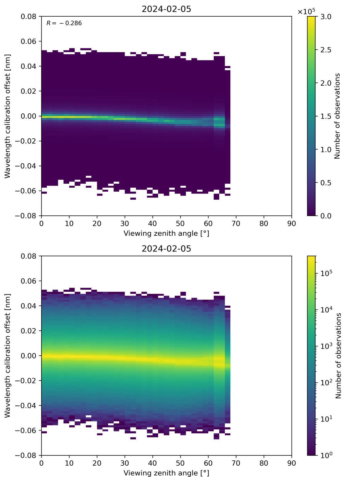
Figure 173: Scatter density plot of “Viewing zenith angle” against “Wavelength calibration offset” for 2024-02-04 to 2024-02-06.
