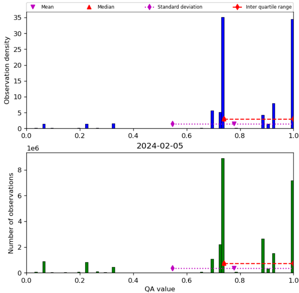
Figure 28: Histogram of “QA value” for 2024-02-04 to 2024-02-06
