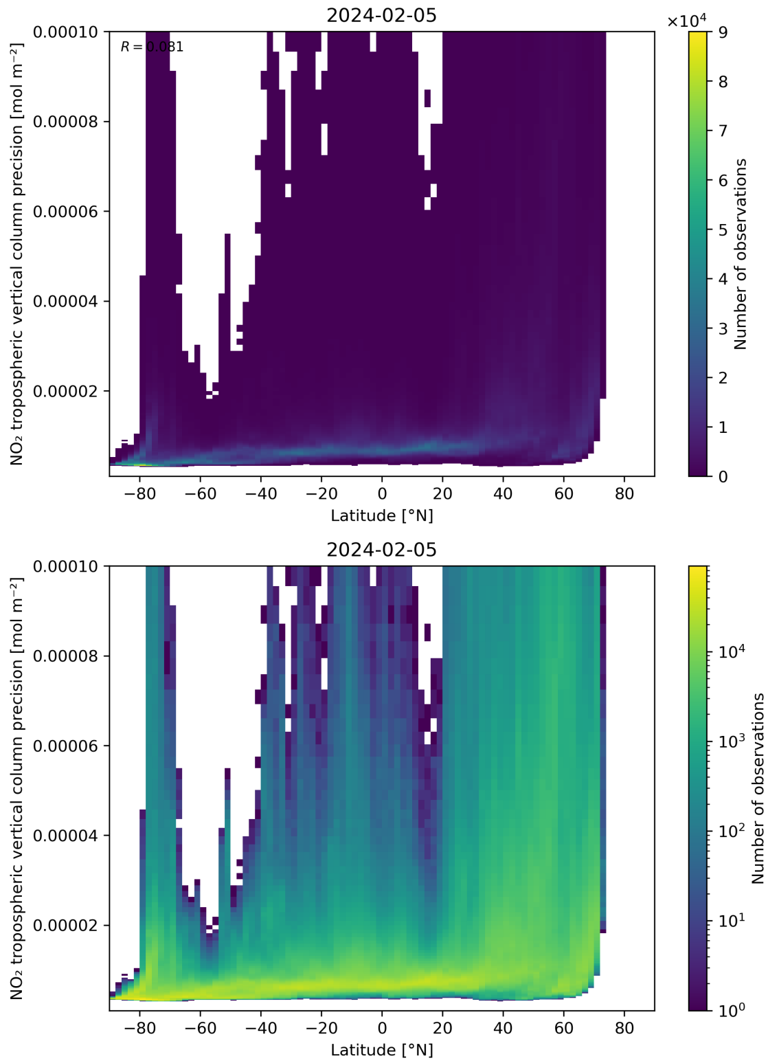
Figure 93: Scatter density plot of “Latitude” against “NO 2 tropospheric vertical column precision” for 2024-02-04 to 2024-02-06.
