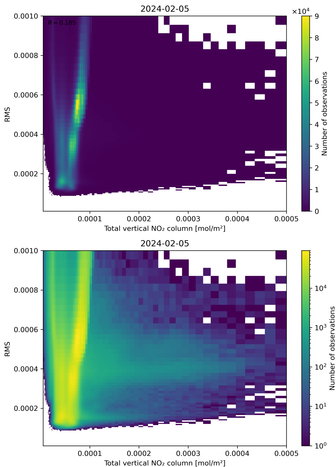
Figure 120: Scatter density plot of “Total vertical NO 2 column” against “RMS” for 2024-02-04 to 2024-02-06.
