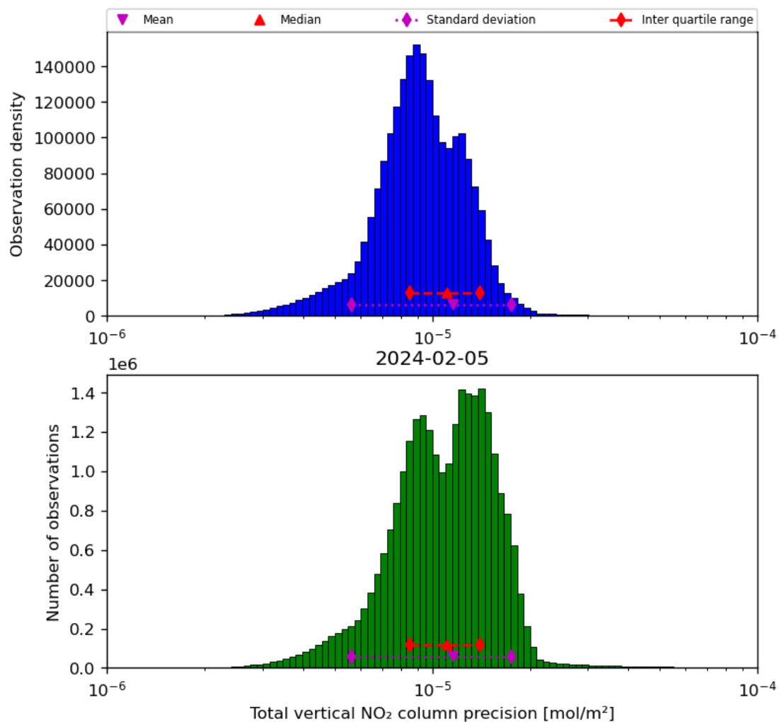
Figure 39: Histogram of “Total vertical NO 2 column precision” for 2024-02-04 to 2024-02-06
