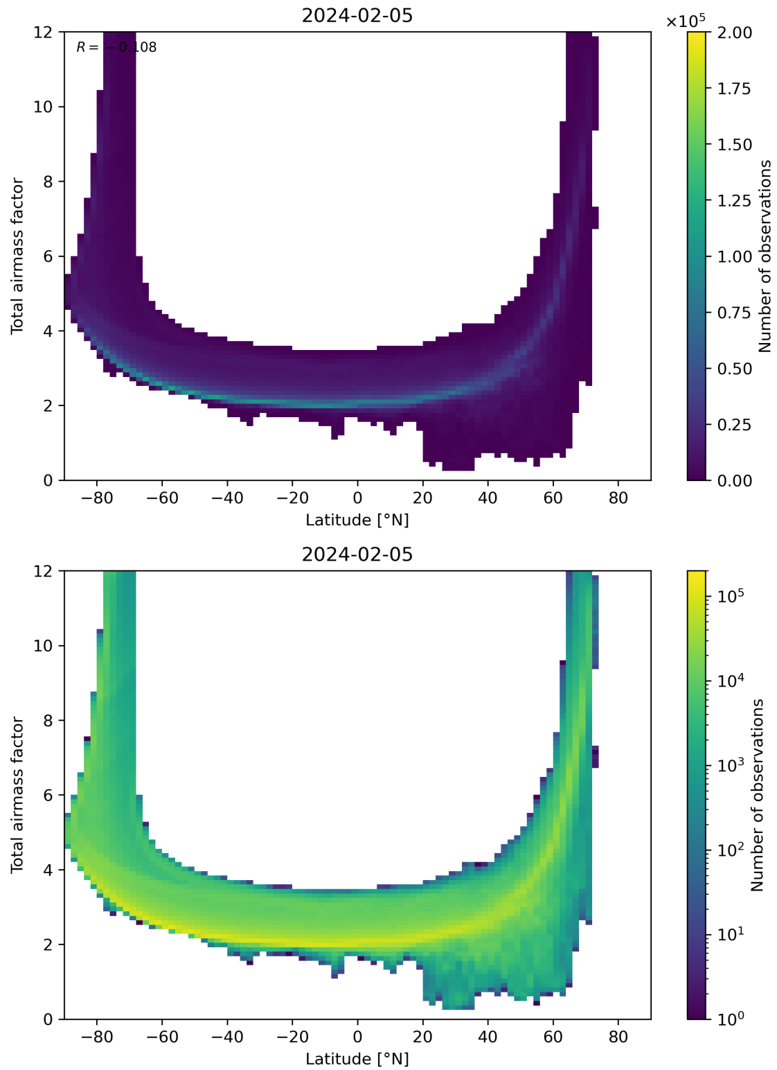
Figure 84: Scatter density plot of “Latitude” against “Total airmass factor” for 2024-02-04 to 2024-02-06.
