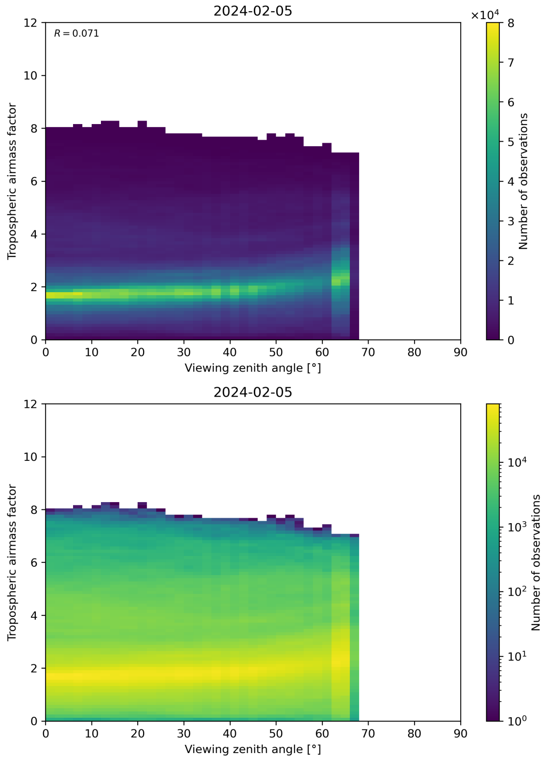
Figure 161: Scatter density plot of “Viewing zenith angle” against “Tropospheric airmass factor” for 2024-02-04 to 2024-02-06.
