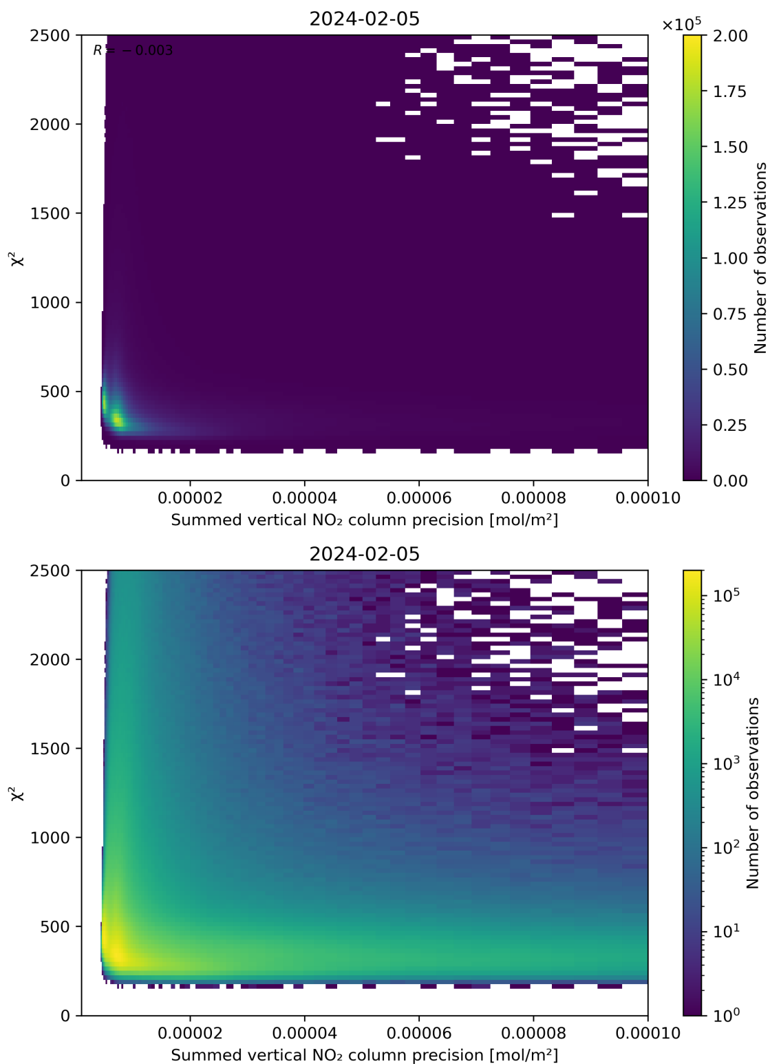
Figure 107: Scatter density plot of “Summed vertical NO 2 column precision” against “ \chi^2 ” for 2024-02-04 to 2024-02-06.
