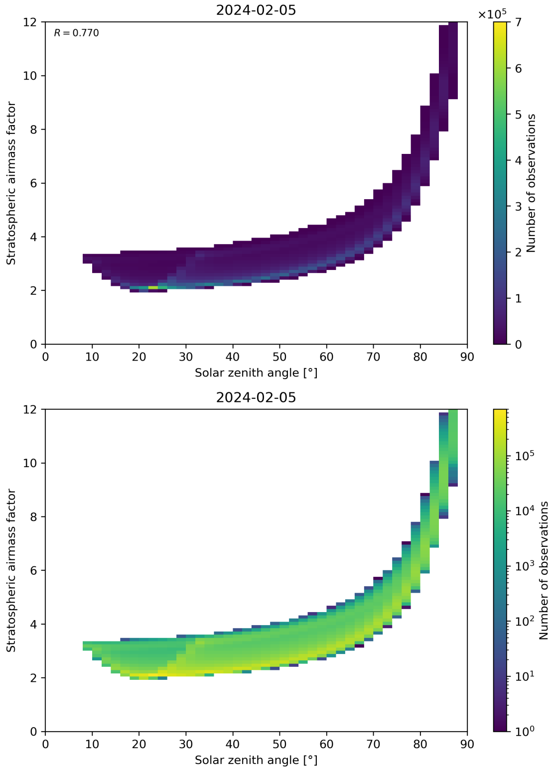
Figure 145: Scatter density plot of “Solar zenith angle” against “Stratospheric airmass factor” for 2024-02-04 to 2024-02-06.
