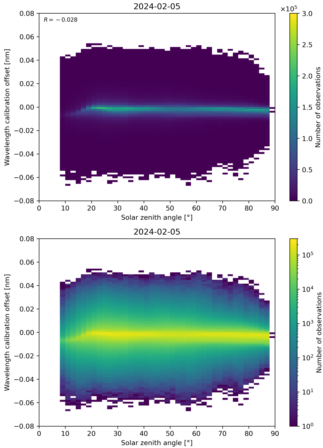
Figure 158: Scatter density plot of “Solar zenith angle” against “Wavelength calibration offset” for 2024-02-04 to 2024-02-06.
