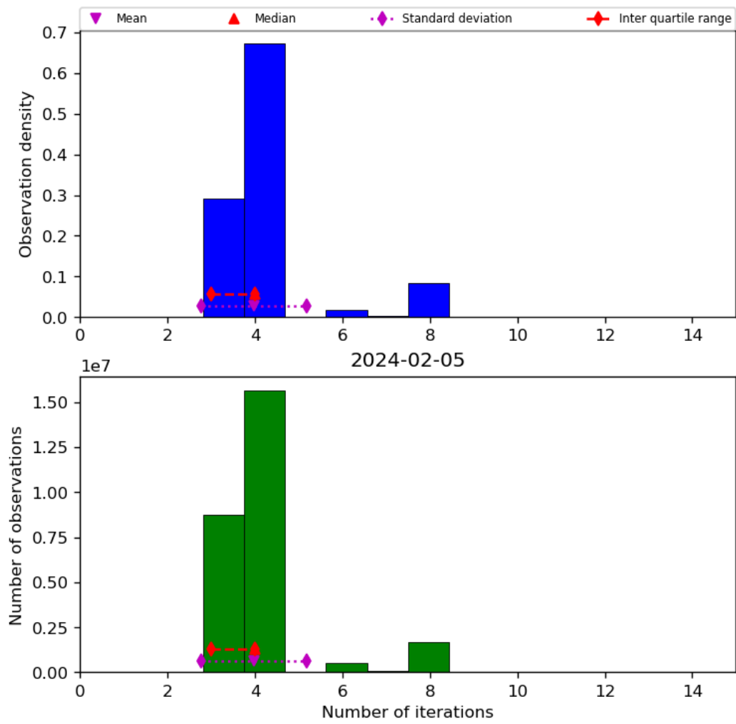
Figure 34: Histogram of “Number of iterations” for 2024-02-04 to 2024-02-06
