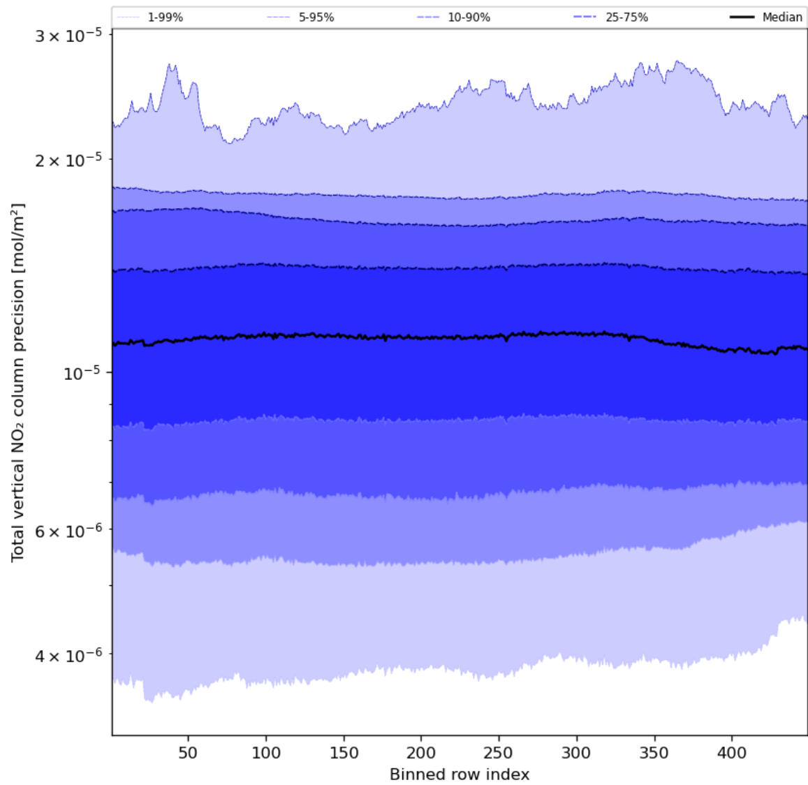
Figure 56: Along track statistics of “Total vertical NO 2 column precision” for 2024-02-04 to 2024-02-06
