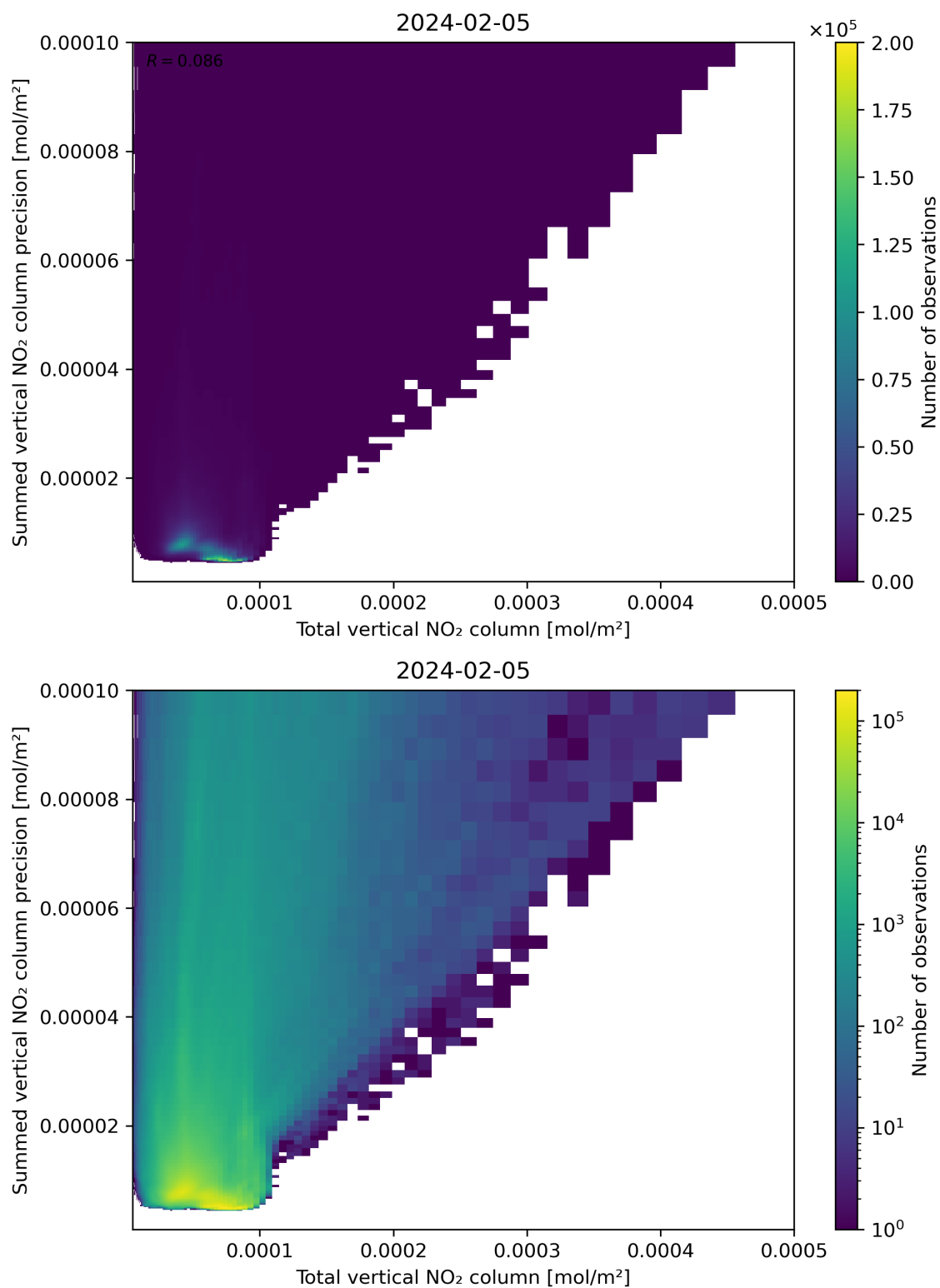
Figure 113: Scatter density plot of “Total vertical NO 2 column” against “Summed vertical NO 2 column precision” for 2024-02-04 to 2024-02-06.
