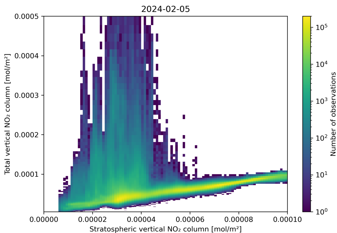
Figure 100: Scatter density plot of “Stratospheric vertical NO 2 column” against “Total vertical NO 2 column” for 2024-02-04 to 2024-02-06.
