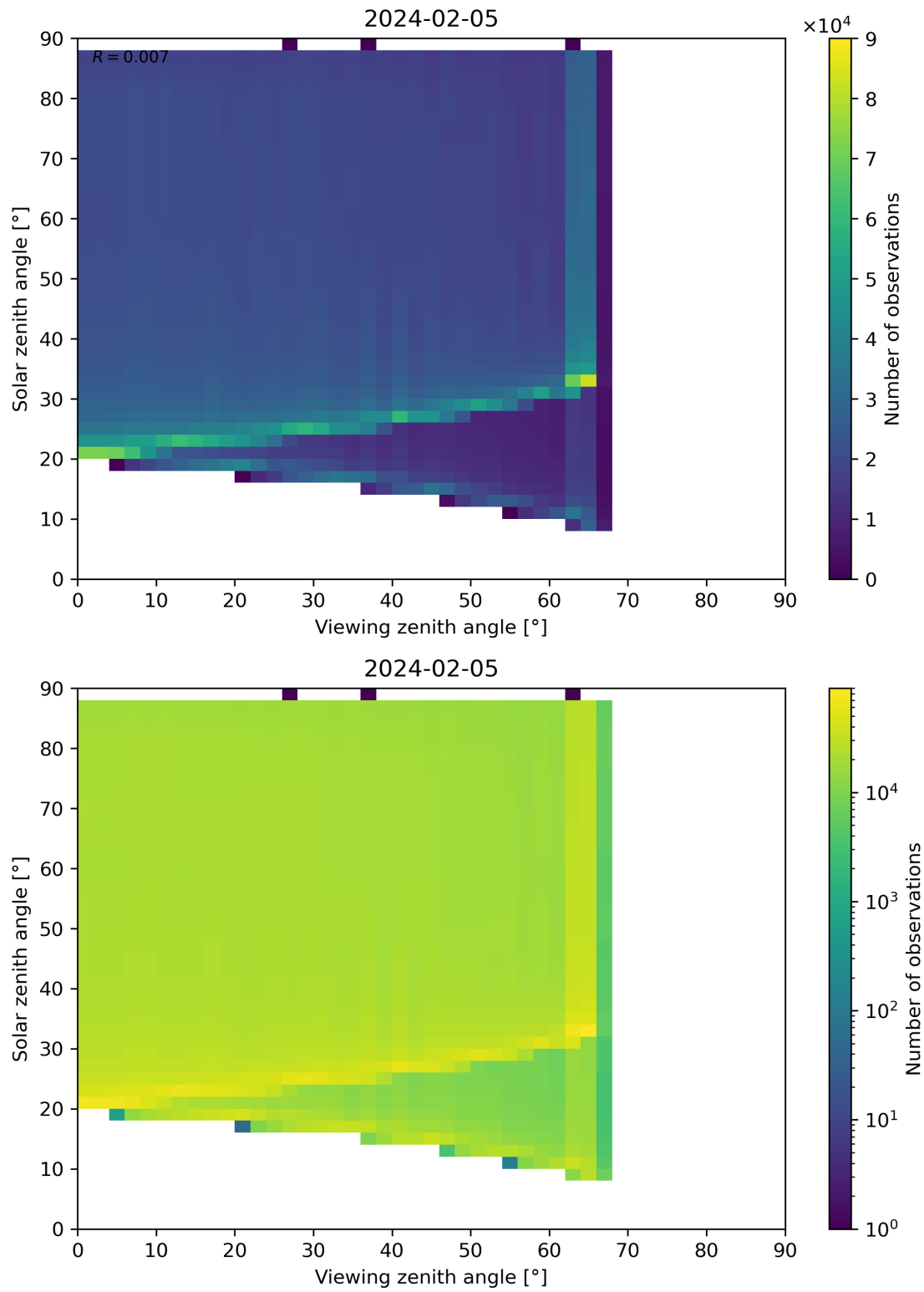
Figure 172: Scatter density plot of “Viewing zenith angle” against “Solar zenith angle” for 2024-02-04 to 2024-02-06.
