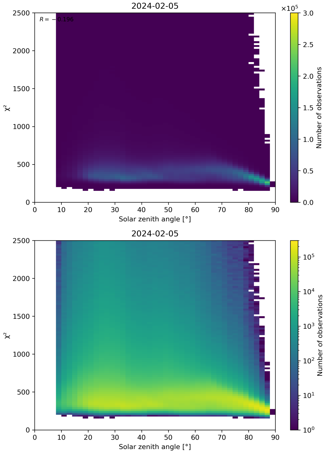
Figure 148: Scatter density plot of “Solar zenith angle” against “ \chi^2 ” for 2024-02-04 to 2024-02-06.
