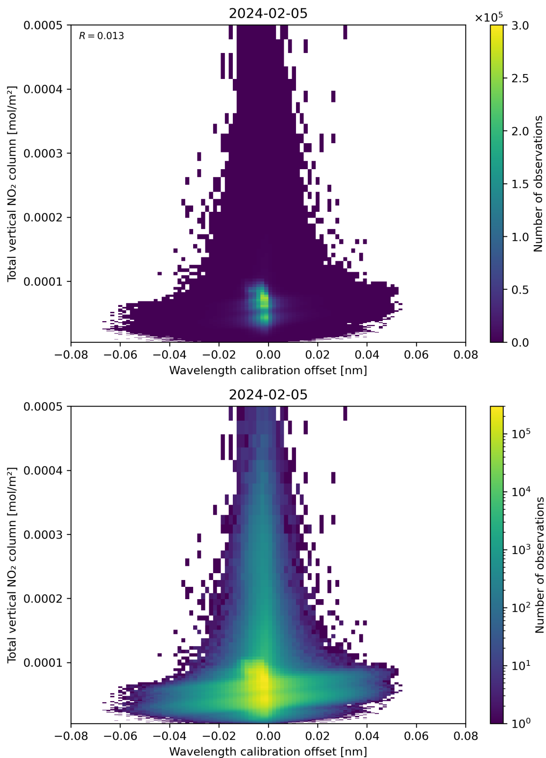
Figure 179: Scatter density plot of “Wavelength calibration offset” against “Total vertical NO 2 column” for 2024-02-04 to 2024-02-06.
