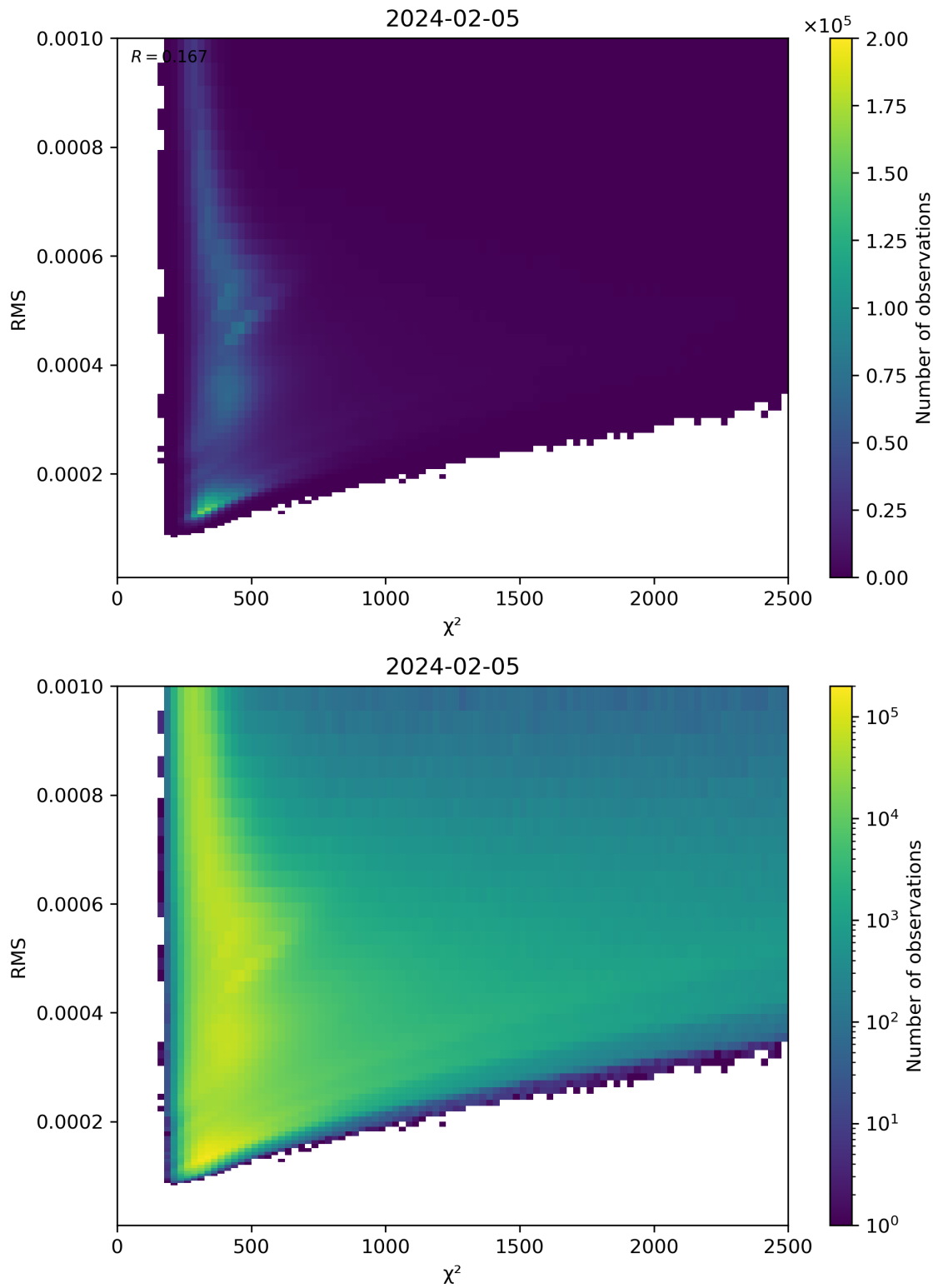
Figure 82: Scatter density plot of “ \chi^2 ” against “RMS” for 2024-02-04 to 2024-02-06.
