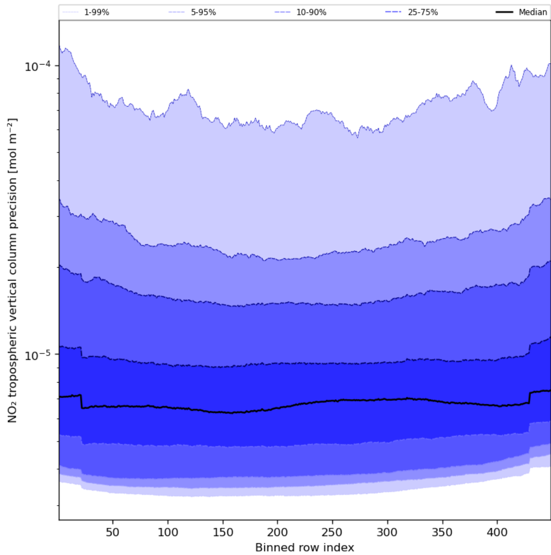
Figure 47: Along track statistics of “NO 2 tropospheric vertical column precision” for 2024-02-04 to 2024-02-06
