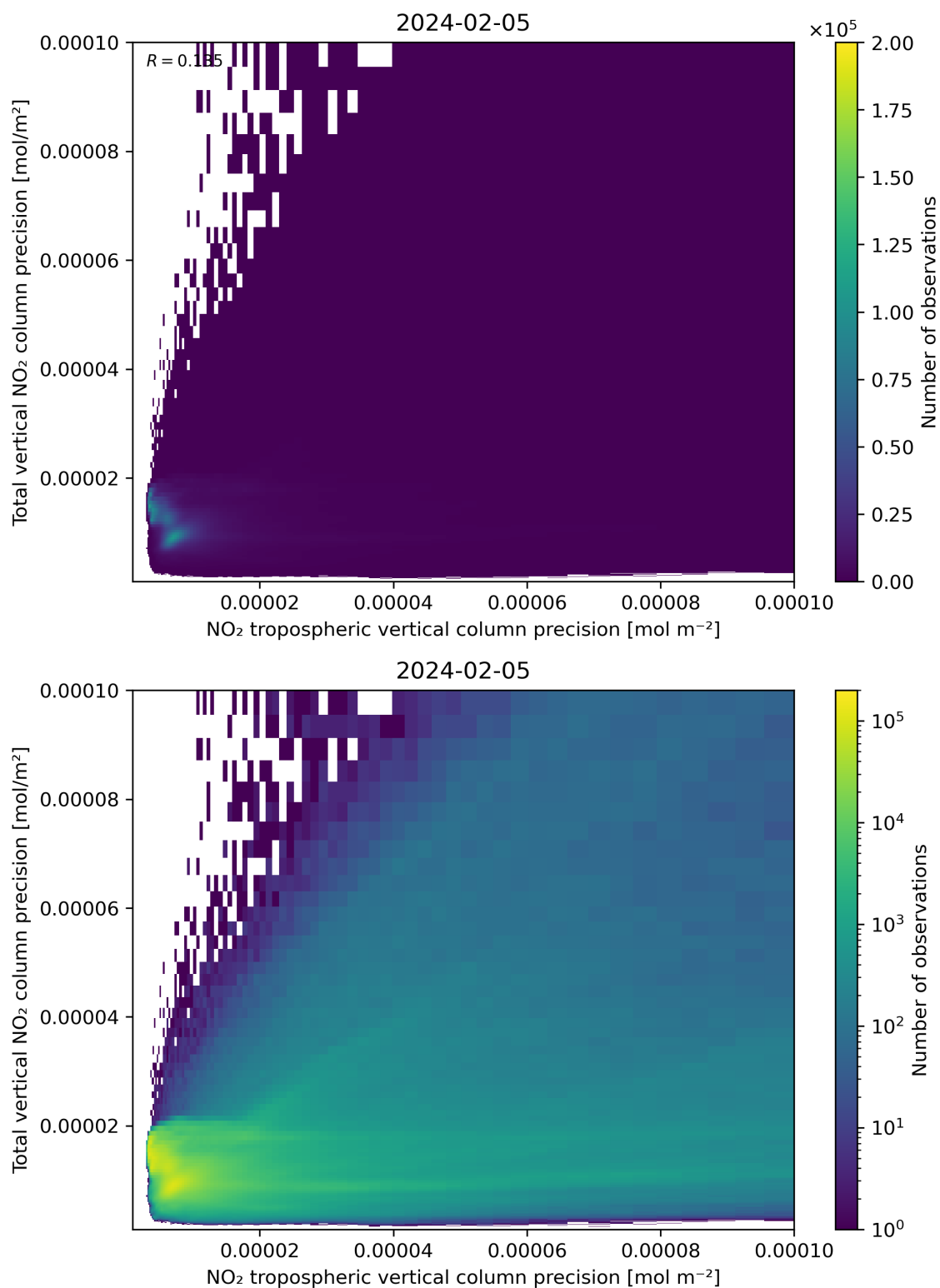
Figure 139: Scatter density plot of “NO 2 tropospheric vertical column precision” against “Total vertical NO 2 column precision” for 2024-02-04 to 2024-02-06.
