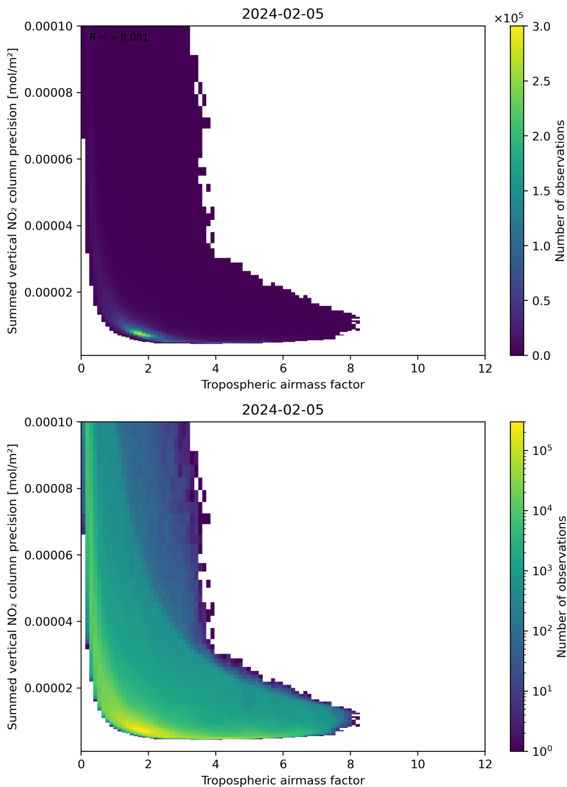
Figure 76: Scatter density plot of “Tropospheric air mass factor” against “Summed vertical NO 2 column precision” for 2024-02-04 to 2024-02-06.
