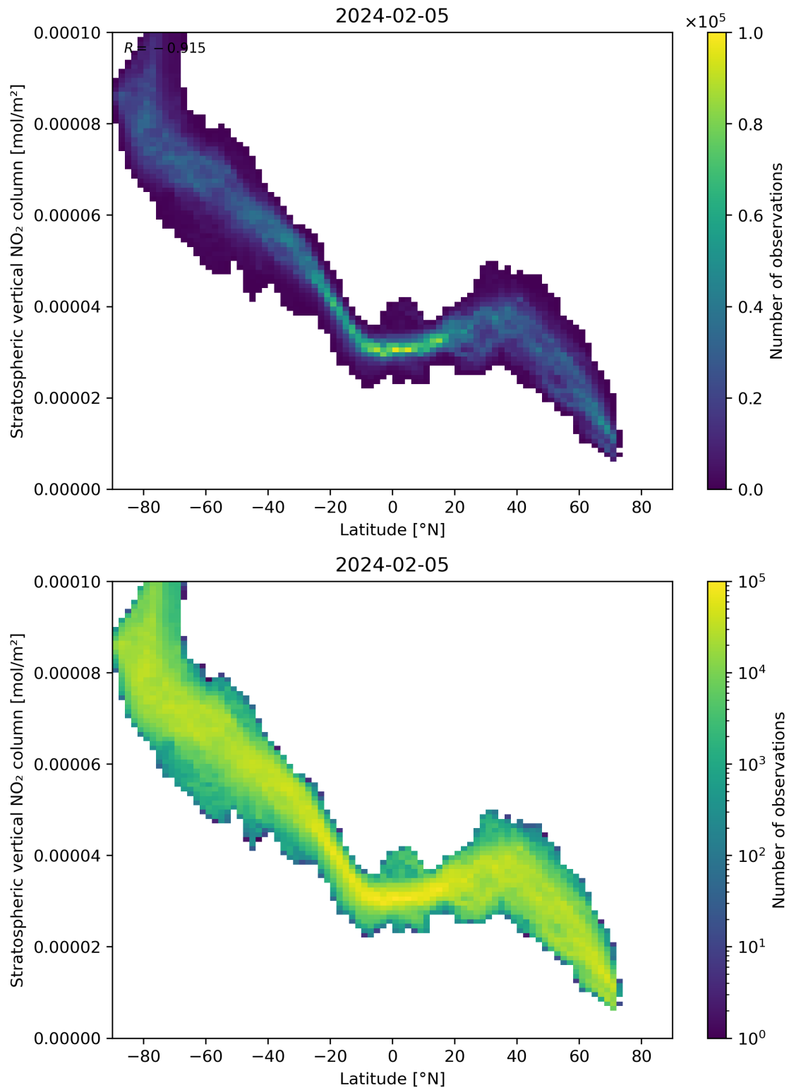
Figure 87: Scatter density plot of “Latitude” against “Stratospheric vertical NO 2 column” for 2024-02-04 to 2024-02-06.
