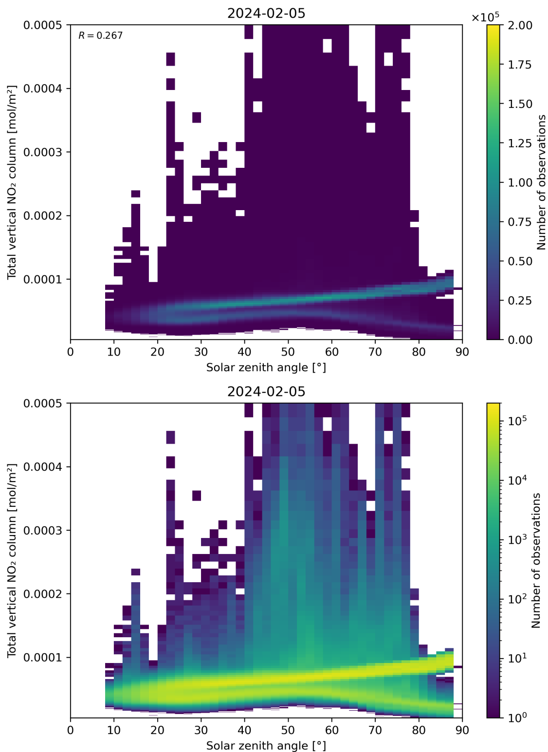
Figure 153: Scatter density plot of “Solar zenith angle” against “Total vertical NO 2 column” for 2024-02-04 to 2024-02-06.
