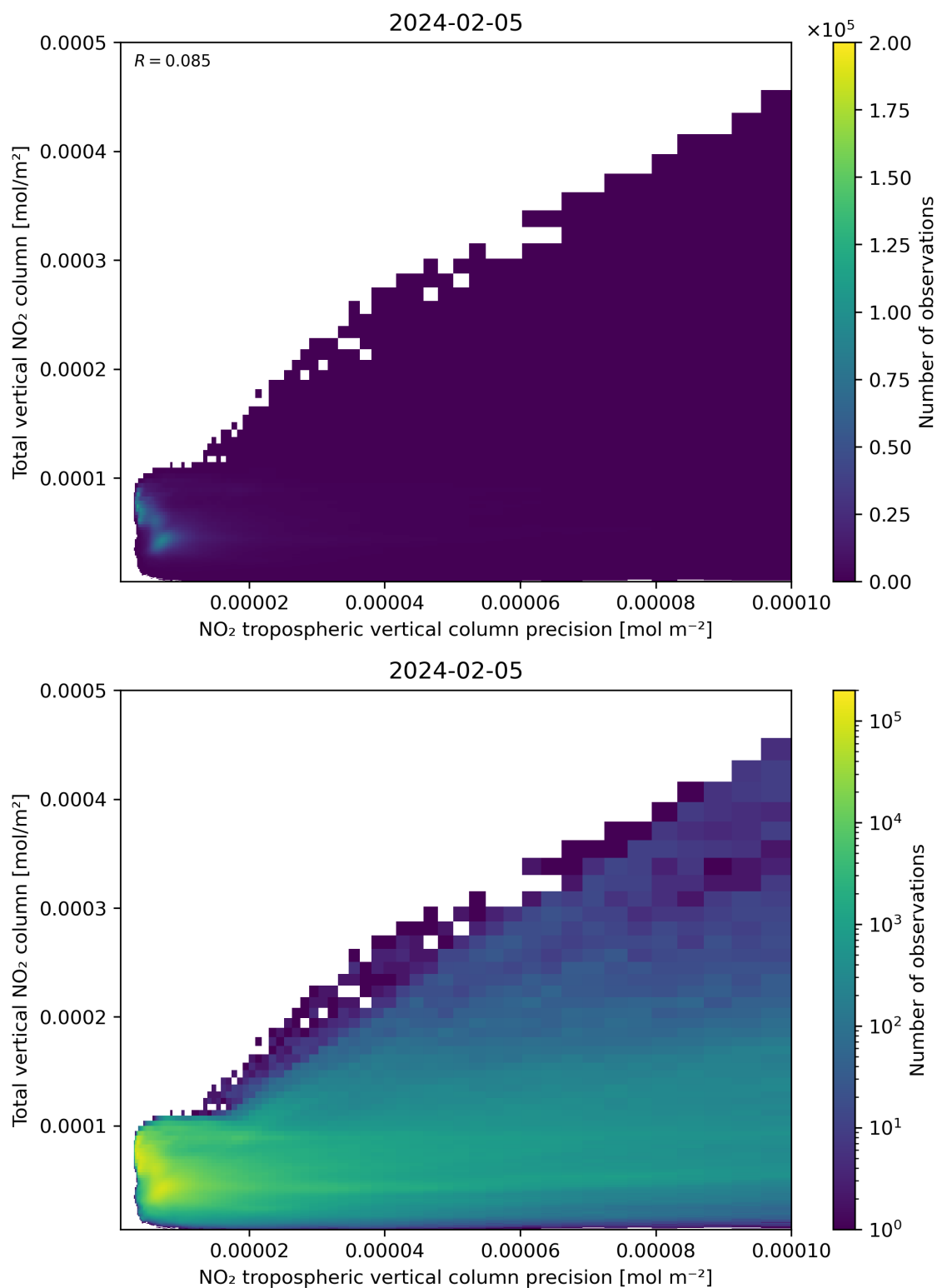
Figure 138: Scatter density plot of “NO 2 tropospheric vertical column precision” against “Total vertical NO 2 column” for 2024-02-04 to 2024-02-06.
