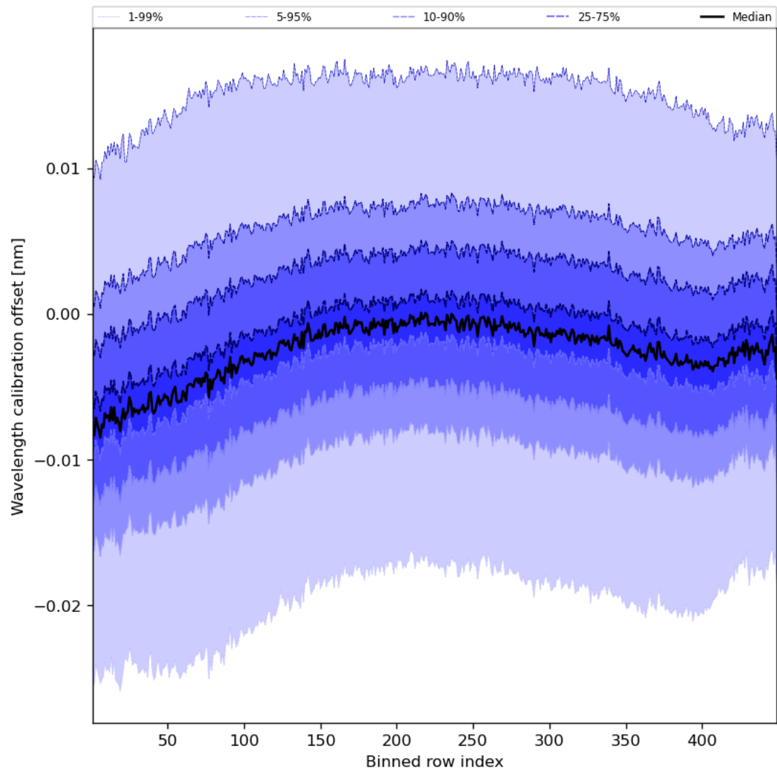
Figure 52: Along track statistics of “Wavelength calibration offset” for 2024-02-04 to 2024-02-06
