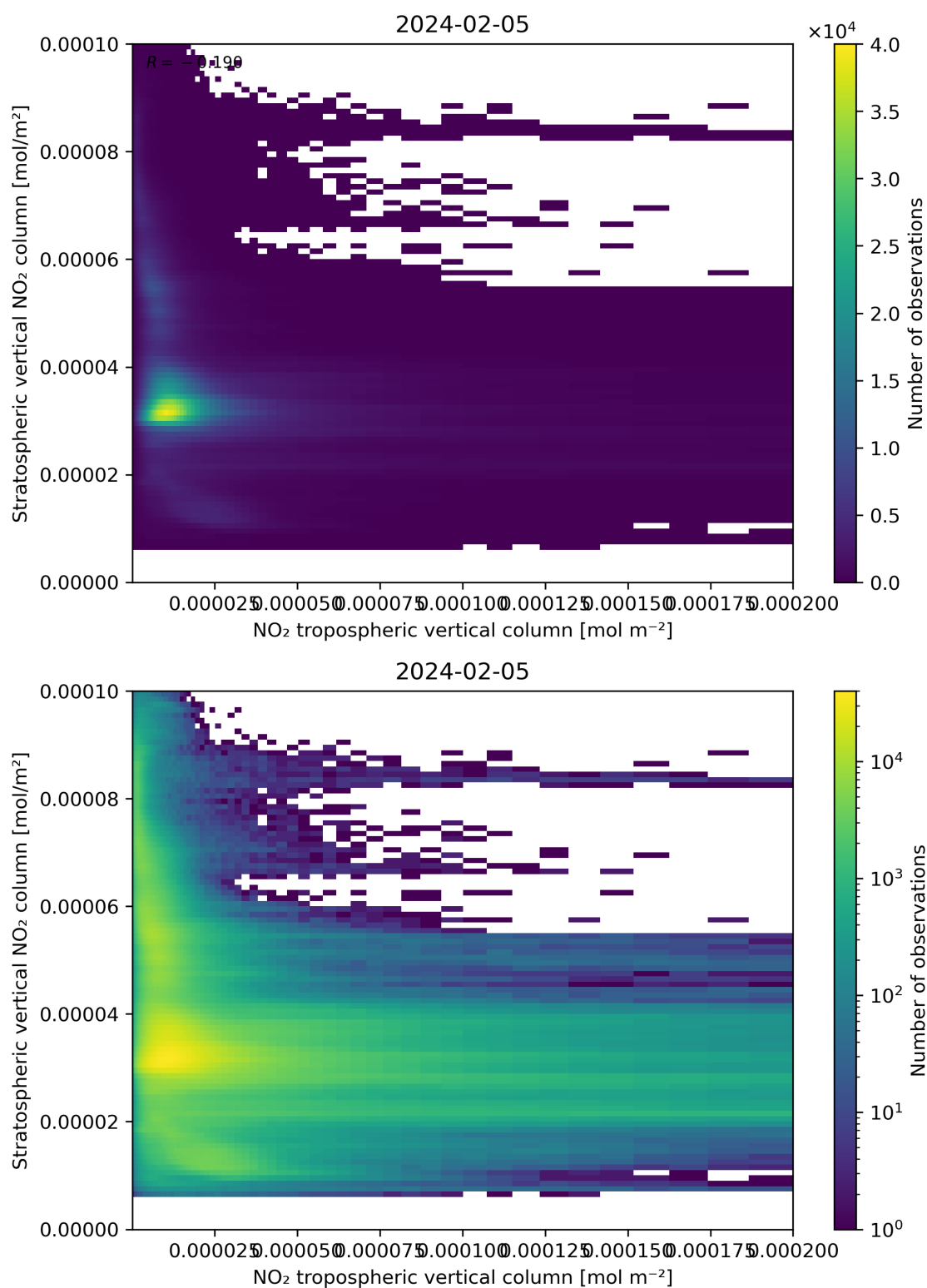
Figure 125: Scatter density plot of “NO 2 tropospheric vertical column” against “Stratospheric vertical NO 2 column” for 2024-02-04 to 2024-02-06.
