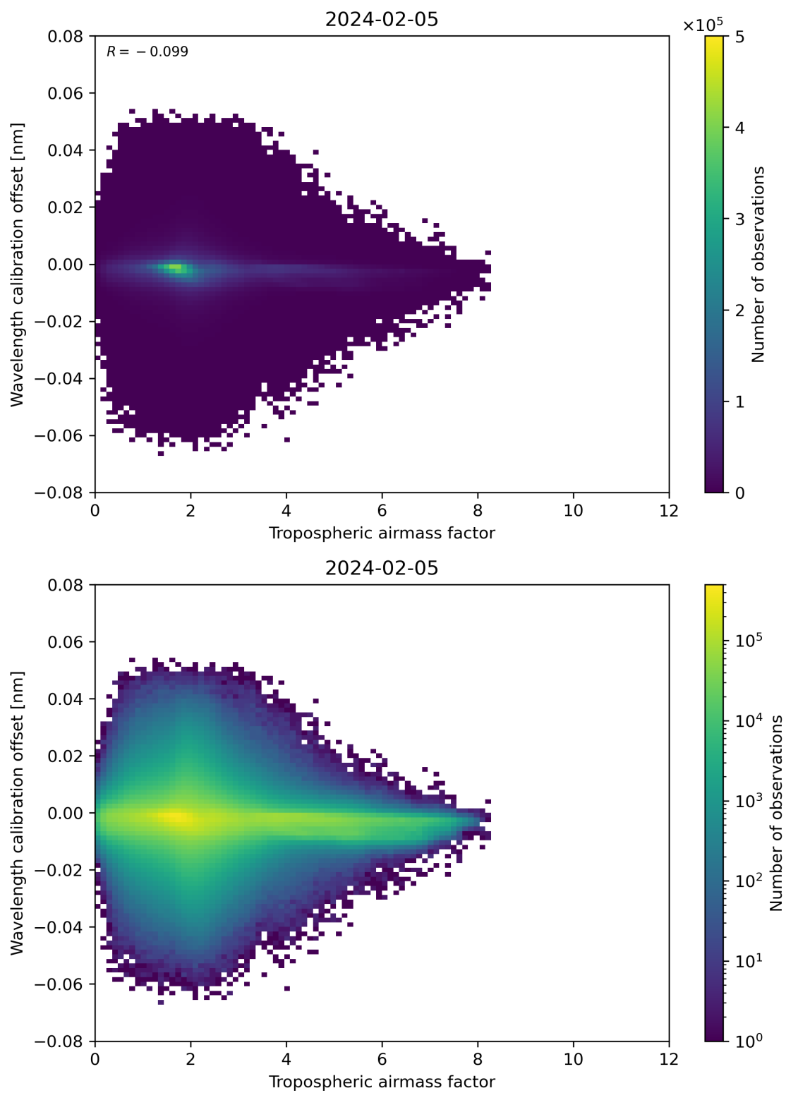
Figure 80: Scatter density plot of “Tropospheric airmass factor” against “Wavelength calibration offset” for 2024-02-04 to 2024-02-06.
