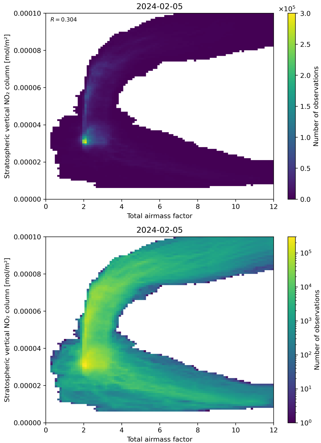
Figure 64: Scatter density plot of “Total airmass factor” against “Stratospheric vertical NO 2 column” for 2024-02-04 to 2024-02-06.
