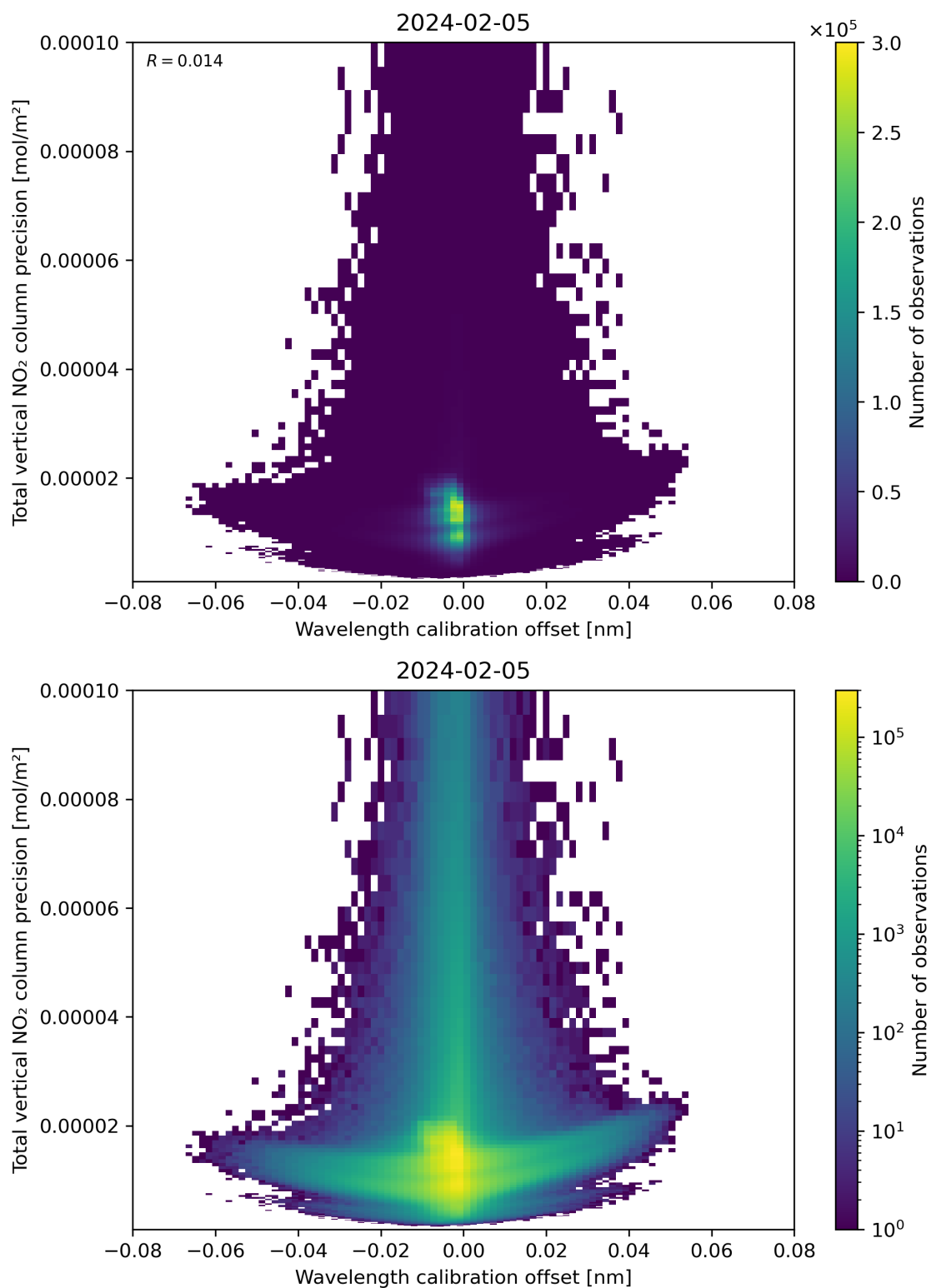
Figure 180: Scatter density plot of “Wavelength calibration offset” against “Total vertical NO 2 column precision” for 2024-02-04 to 2024-02-06.
