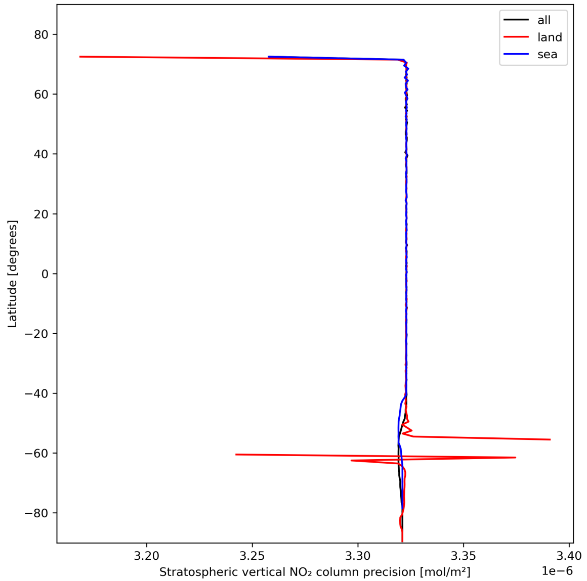
Figure 20: Zonal average of “Stratospheric vertical NO 2 column precision” for 2024-02-04 to 2024-02-06.
