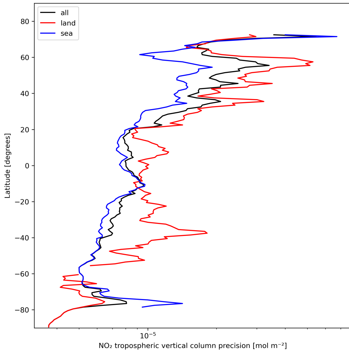
Figure 13: Zonal average of “NO 2 tropospheric vertical column precision” for 2024-02-04 to 2024-02-06.
