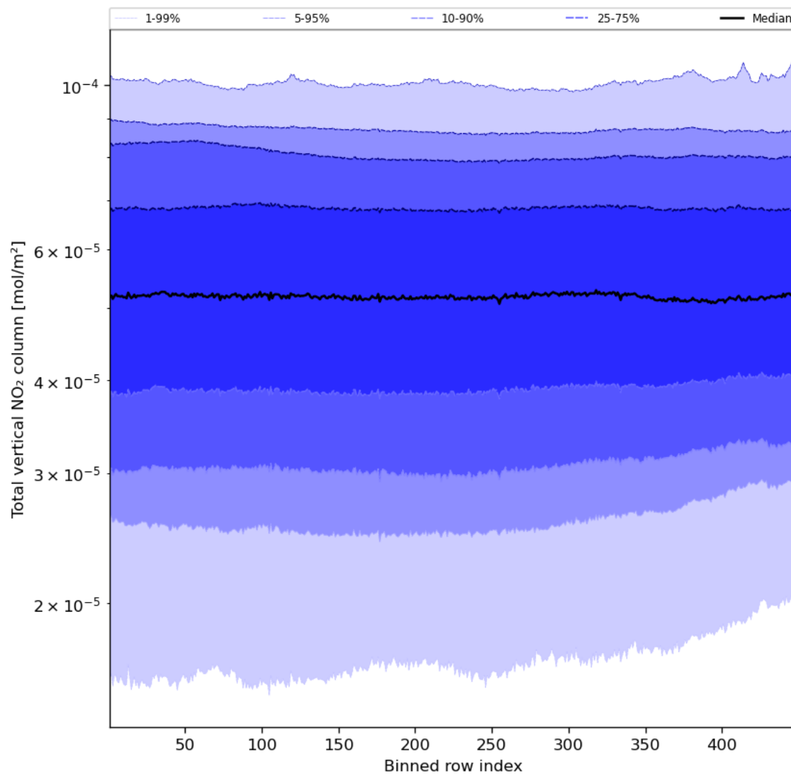
Figure 55: Along track statistics of “Total vertical NO 2 column” for 2024-02-04 to 2024-02-06
