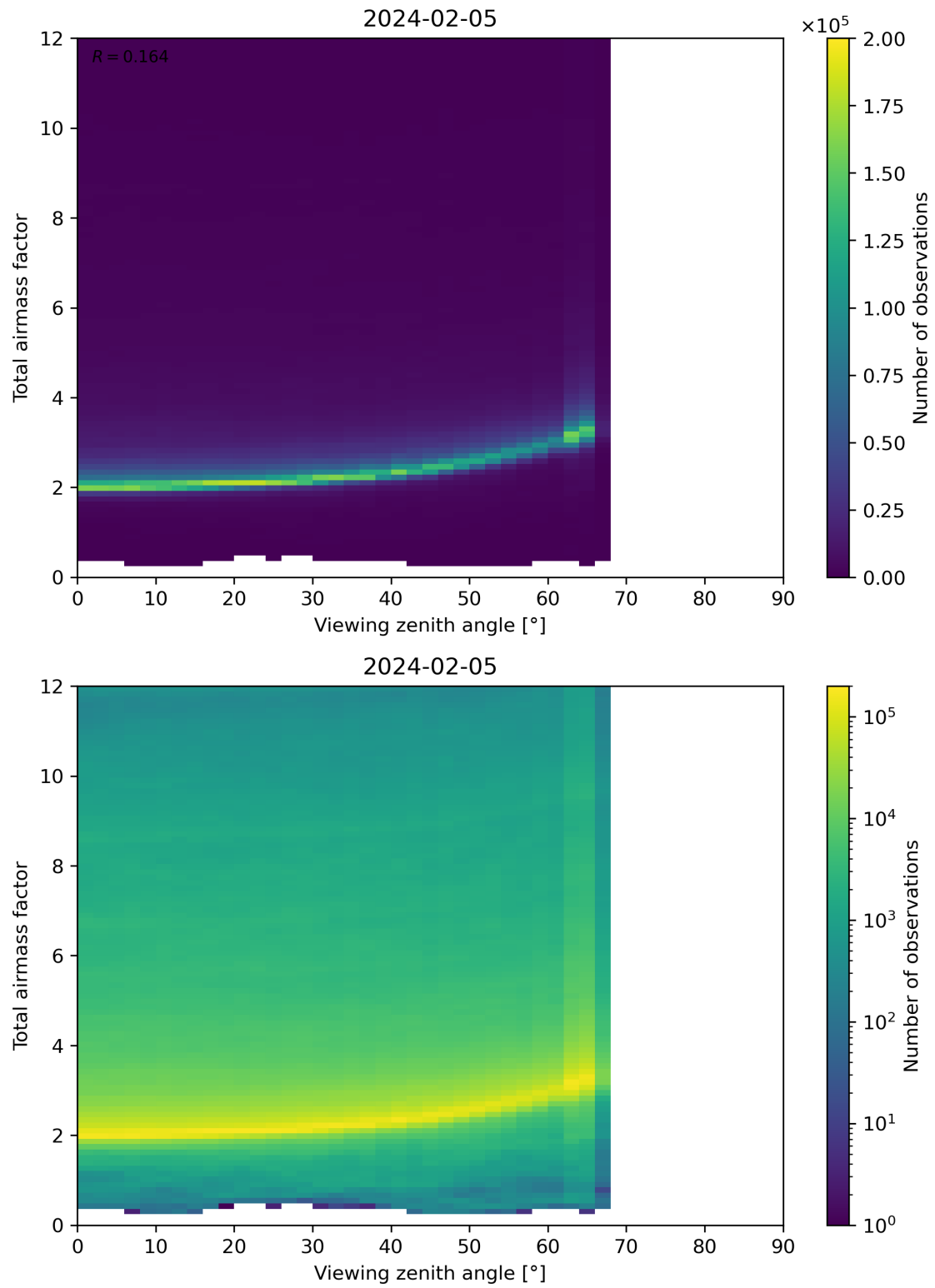
Figure 160: Scatter density plot of “Viewing zenith angle” against “Total airmass factor” for 2024-02-04 to 2024-02-06.
