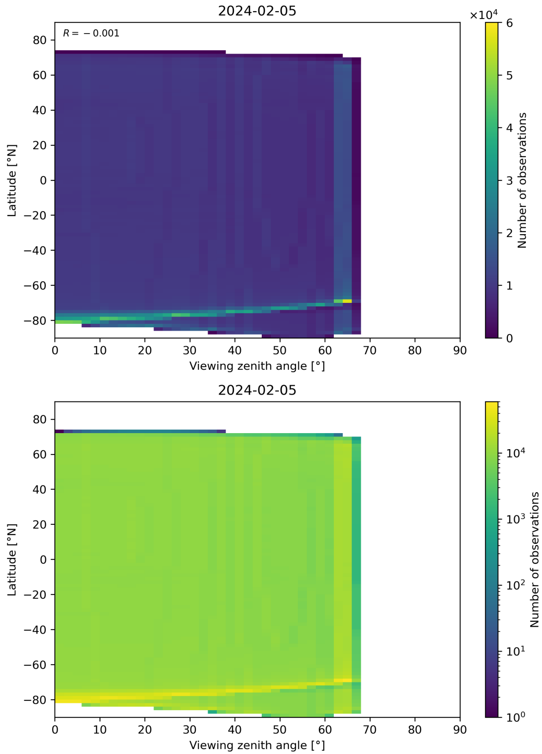
Figure 163: Scatter density plot of “Viewing zenith angle” against “Latitude” for 2024-02-04 to 2024-02-06.
