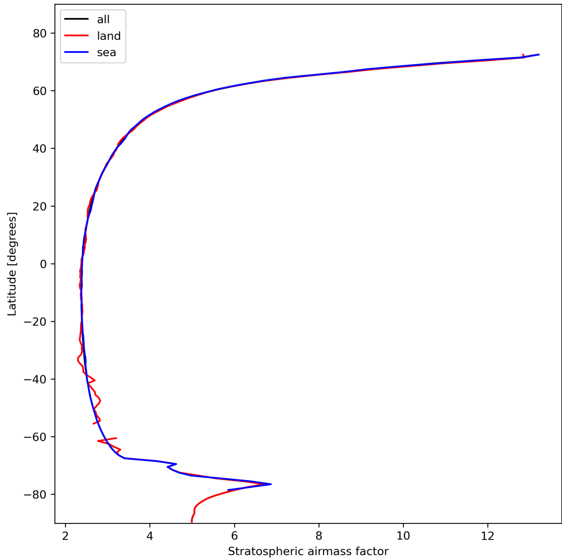
Figure 27: Zonal average of “Stratospheric airmass factor” for 2024-02-04 to 2024-02-06.
