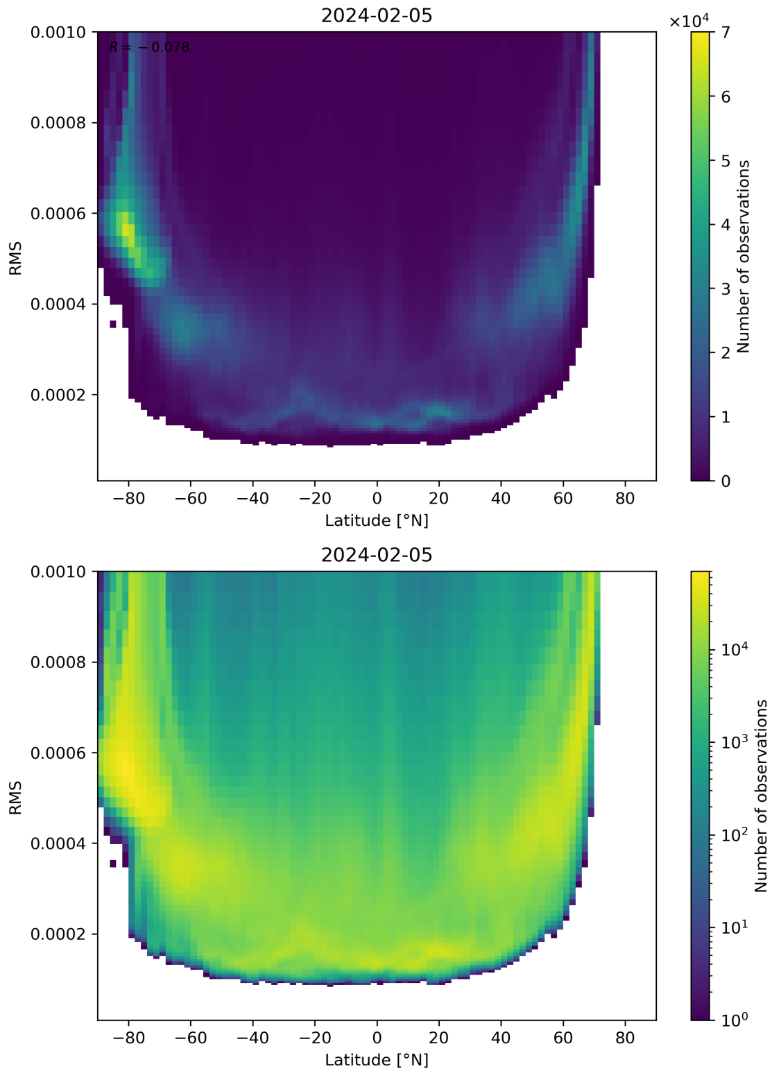
Figure 94: Scatter density plot of “Latitude” against “RMS” for 2024-02-04 to 2024-02-06.
