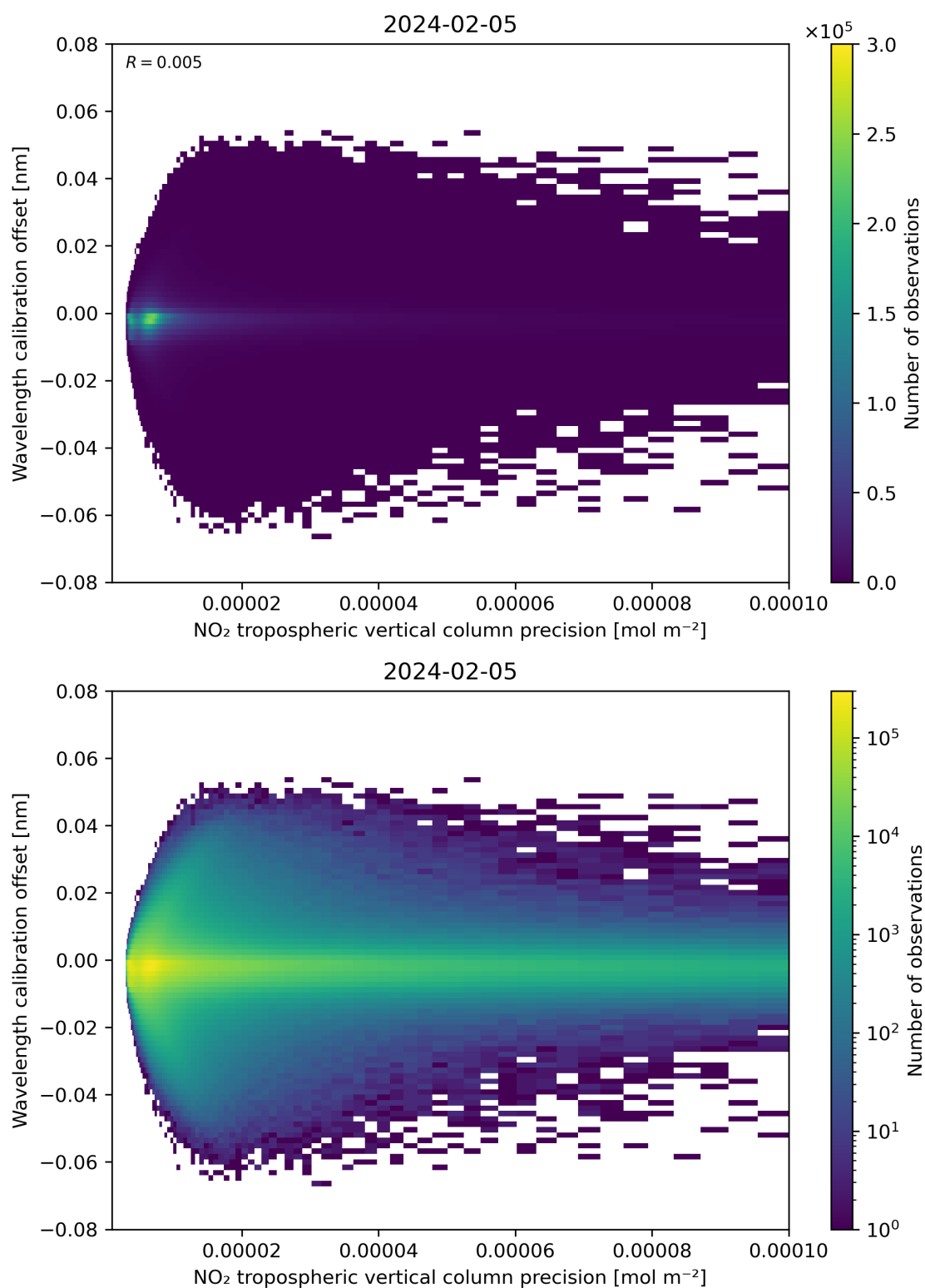
Figure 141: Scatter density plot of “NO 2 tropospheric vertical column precision” against “Wavelength calibration offset” for 2024-02-04 to 2024-02-06.
