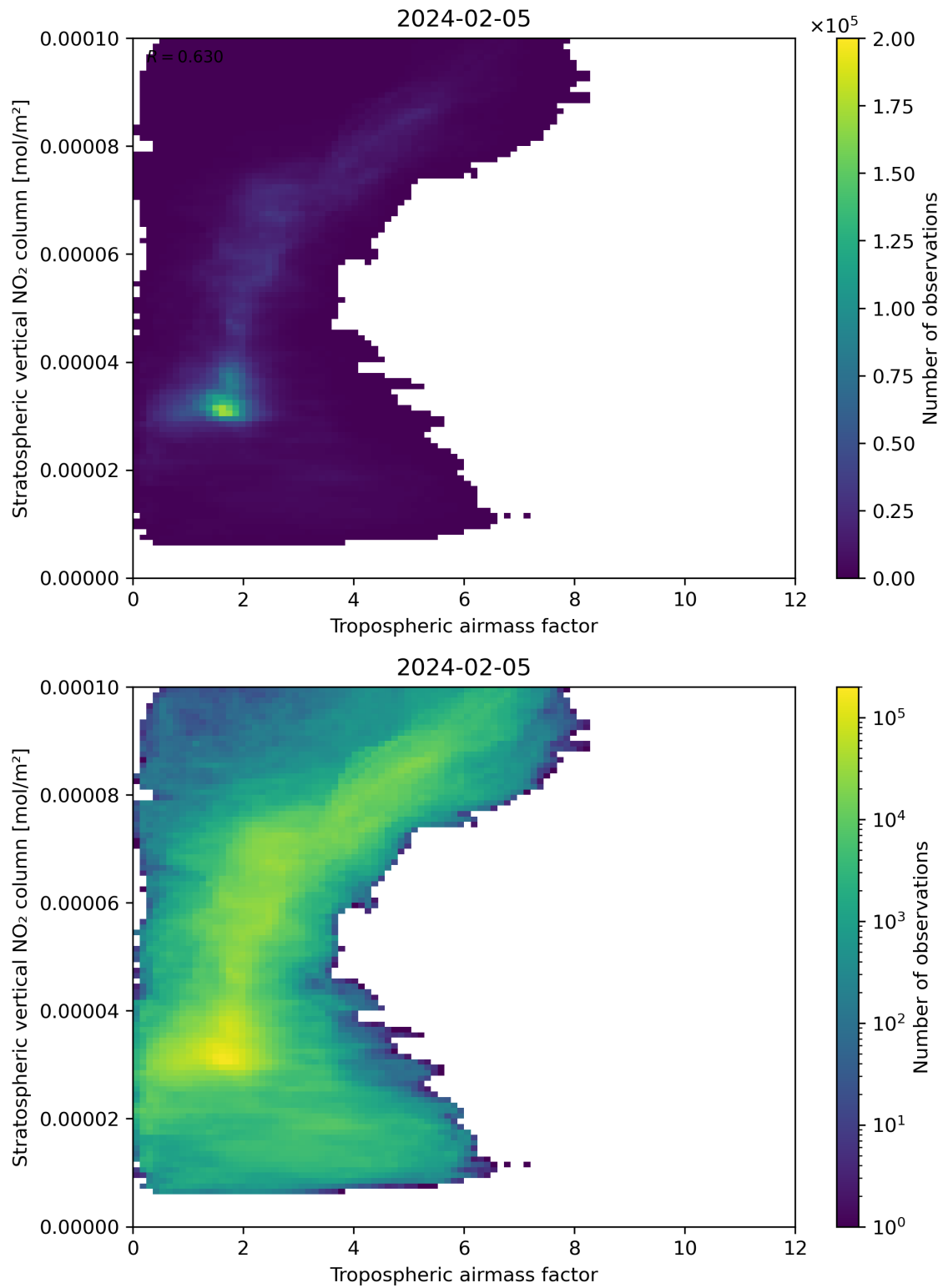
Figure 74: Scatter density plot of “Tropospheric air mass factor” against “Stratospheric vertical NO 2 column” for 2024-02-04 to 2024-02-06.
