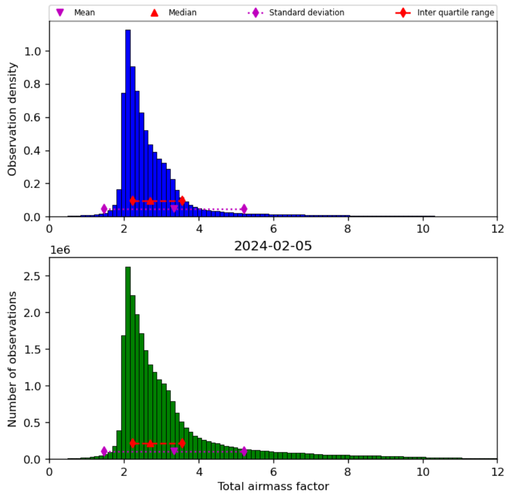
Figure 32: Histogram of “Total airmass factor” for 2024-02-04 to 2024-02-06
