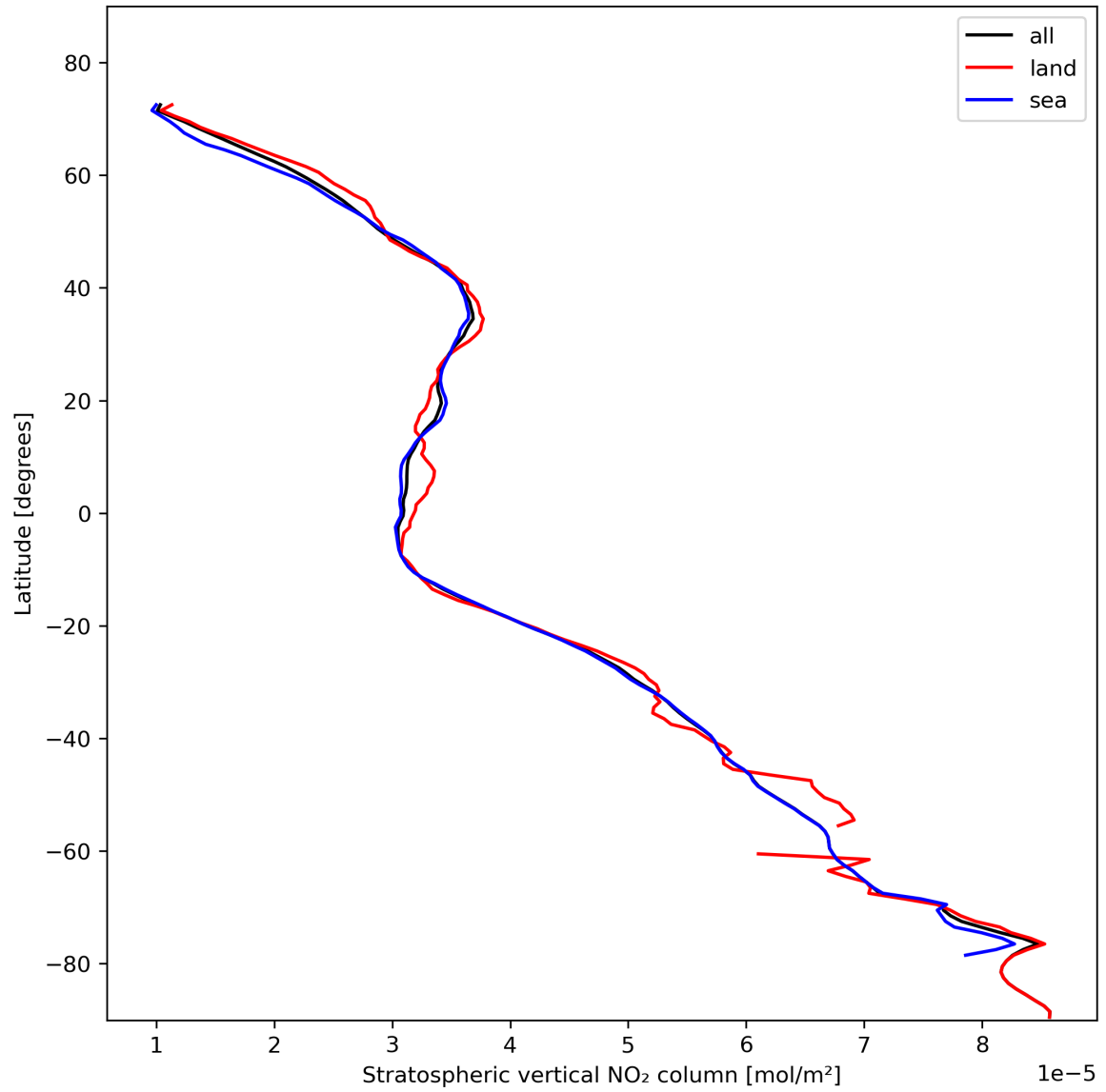
Figure 19: Zonal average of “Stratospheric vertical NO 2 column” for 2024-02-04 to 2024-02-06.
