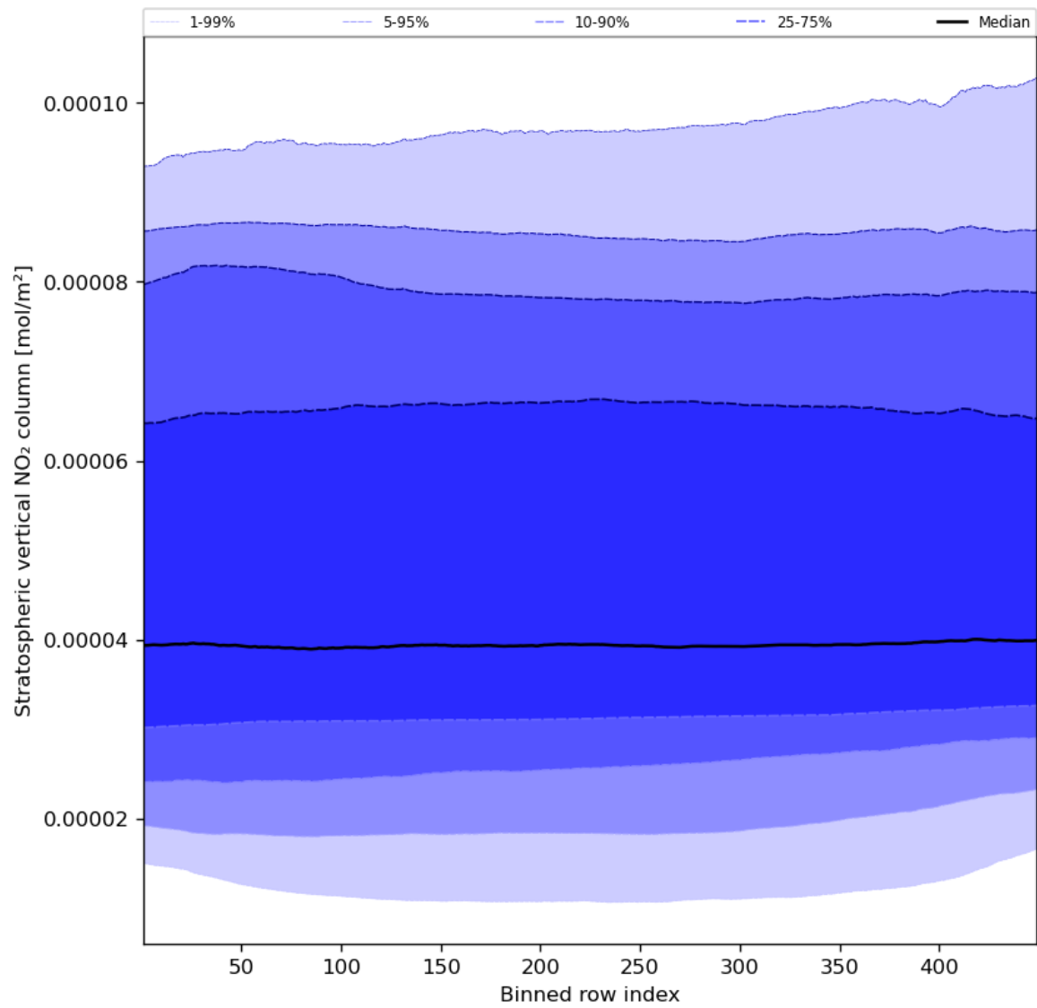
Figure 53: Along track statistics of “Stratospheric vertical NO 2 column” for 2024-02-04 to 2024-02-06
