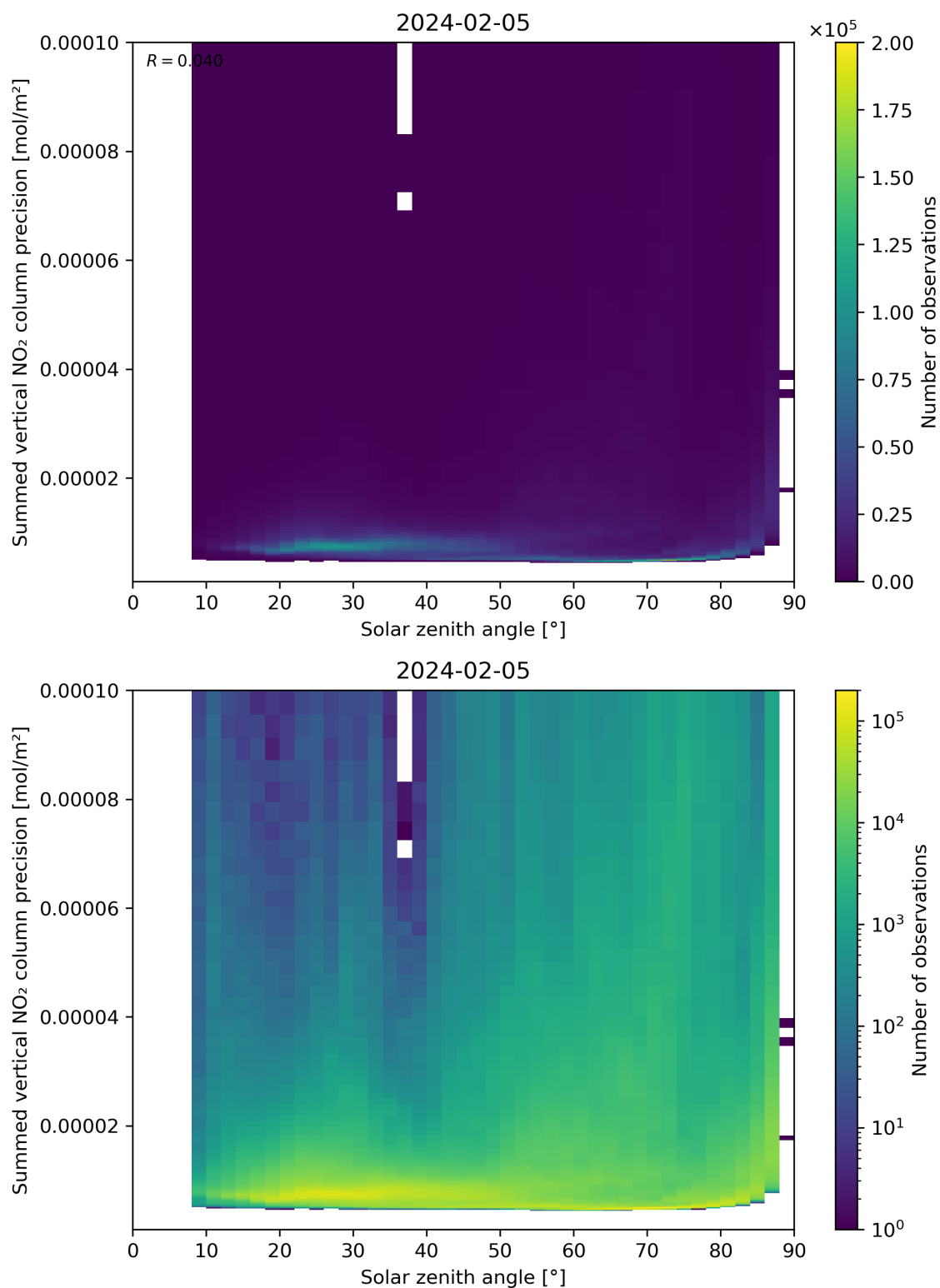
Figure 152: Scatter density plot of “Solar zenith angle” against “Summed vertical NO 2 column precision” for 2024-02-04 to 2024-02-06.
