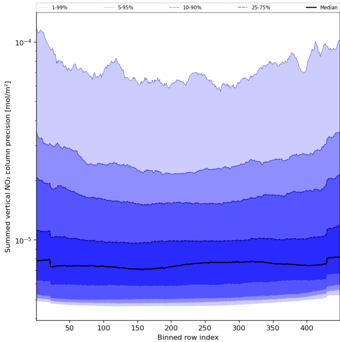
Figure 58: Along track statistics of “Summed vertical NO 2 column precision” for 2024-02-04 to 2024-02-06
