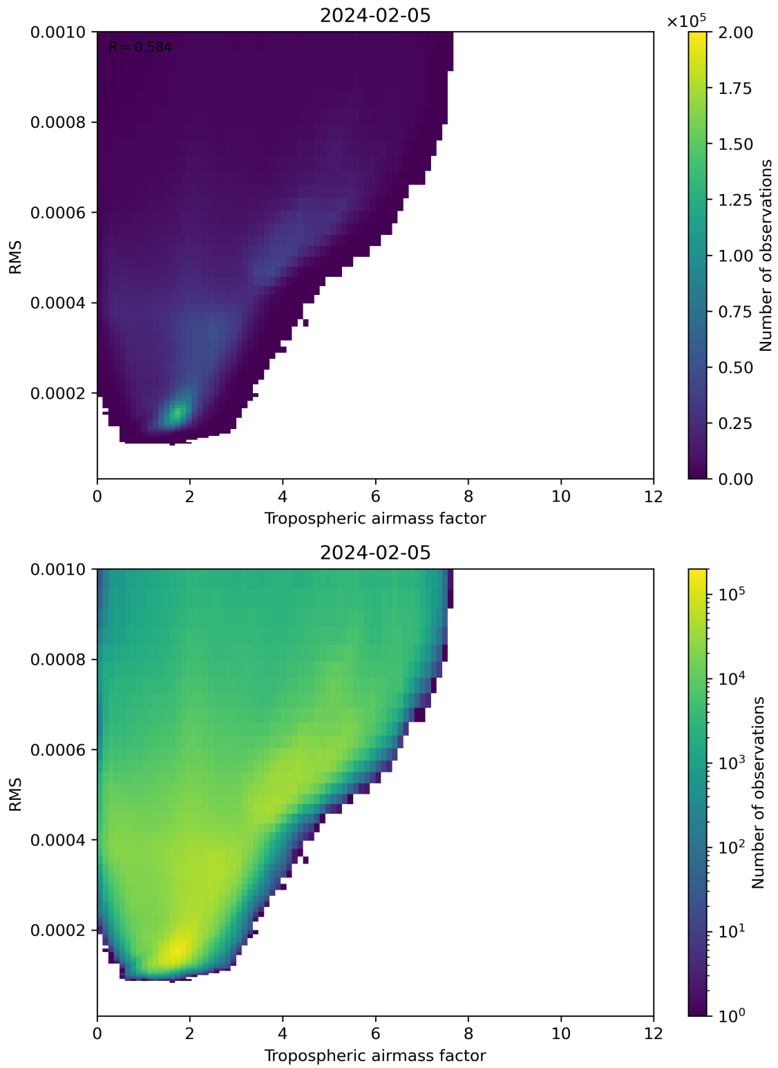
Figure 79: Scatter density plot of “Tropospheric airmass factor” against “RMS” for 2024-02-04 to 2024-02-06.
