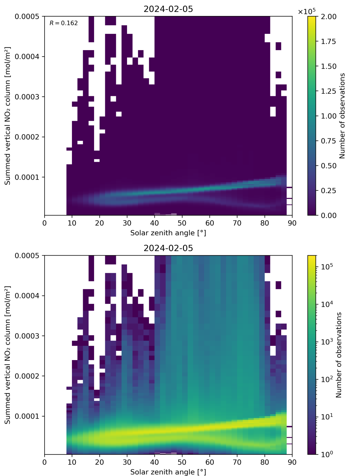
Figure 151: Scatter density plot of “Solar zenith angle” against “Summed vertical NO 2 column” for 2024-02-04 to 2024-02-06.
