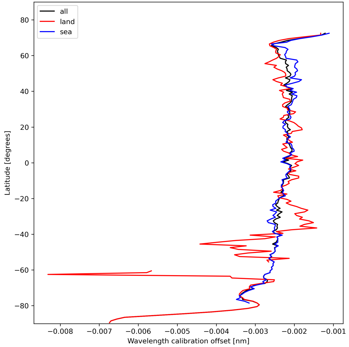
Figure 18: Zonal average of “Wavelength calibration offset” for 2024-02-04 to 2024-02-06.
