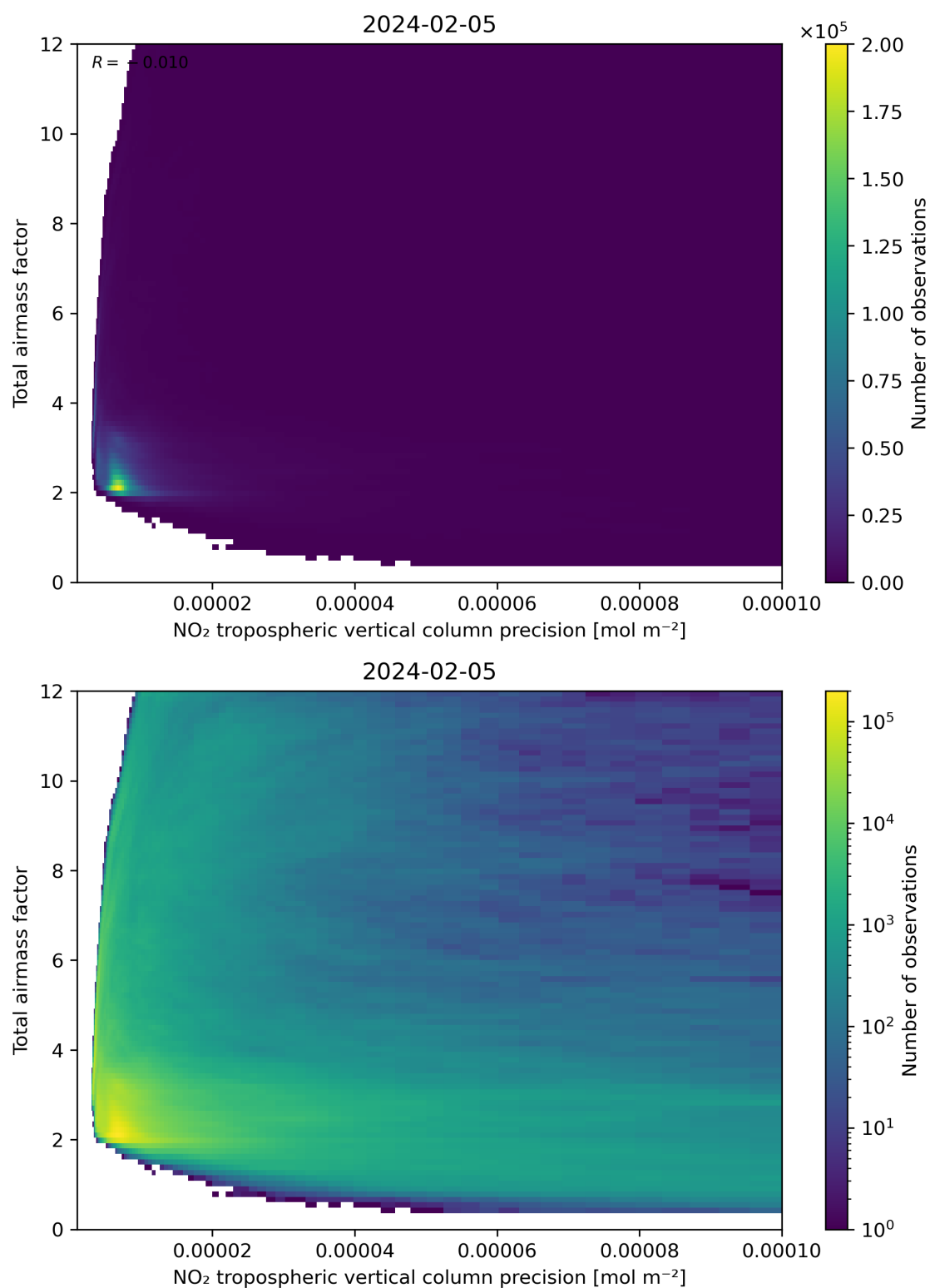
Figure 132: Scatter density plot of “NO 2 tropospheric vertical column precision” against “Total air mass factor” for 2024-02-04 to 2024-02-06.
