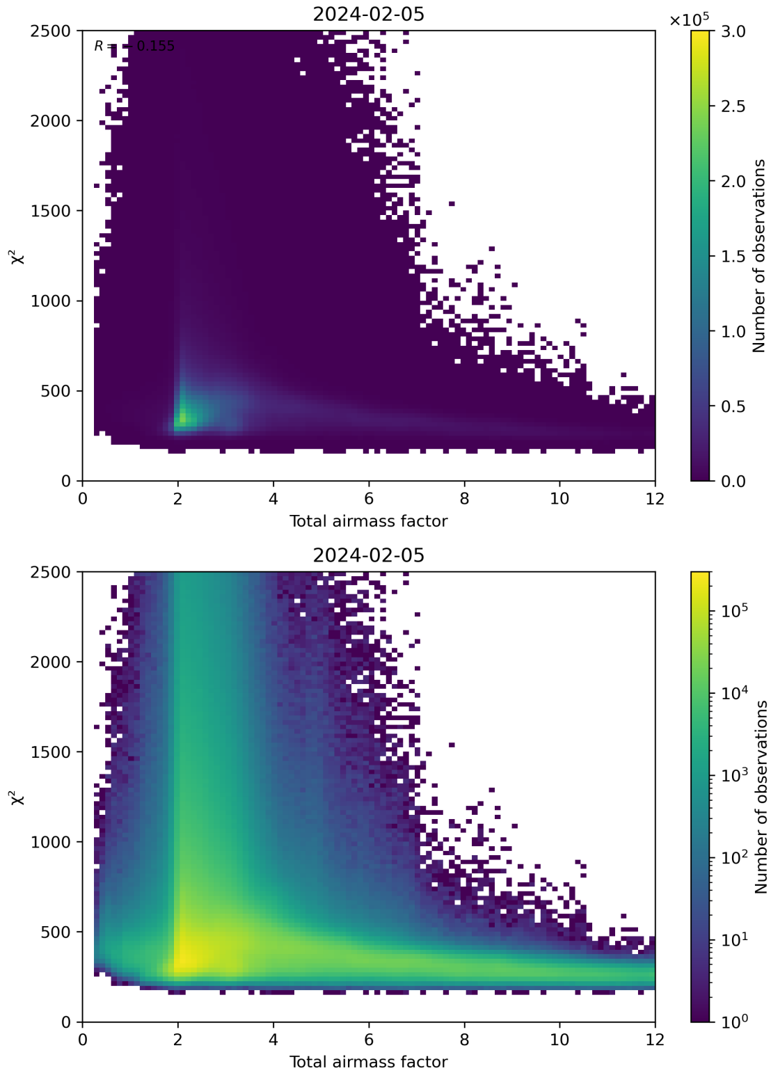
Figure 63: Scatter density plot of “Total airmass factor” against “ \chi^2 ” for 2024-02-04 to 2024-02-06.
