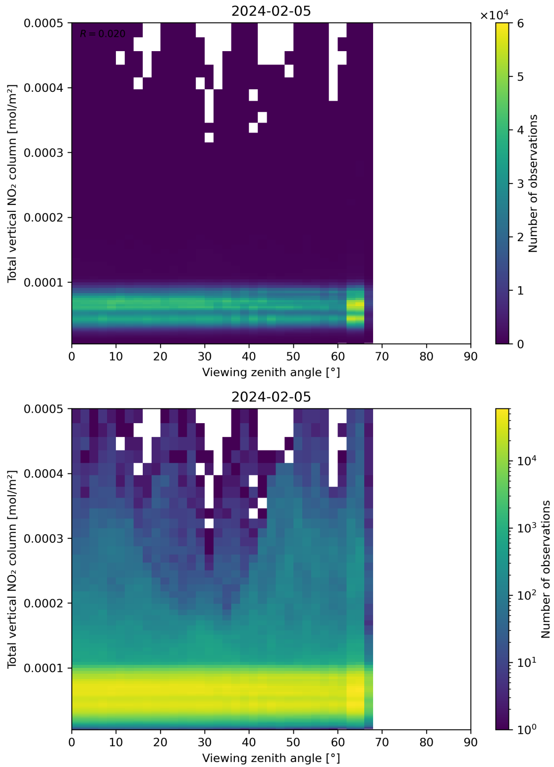
Figure 167: Scatter density plot of “Viewing zenith angle” against “Total vertical NO 2 column” for 2024-02-04 to 2024-02-06.
