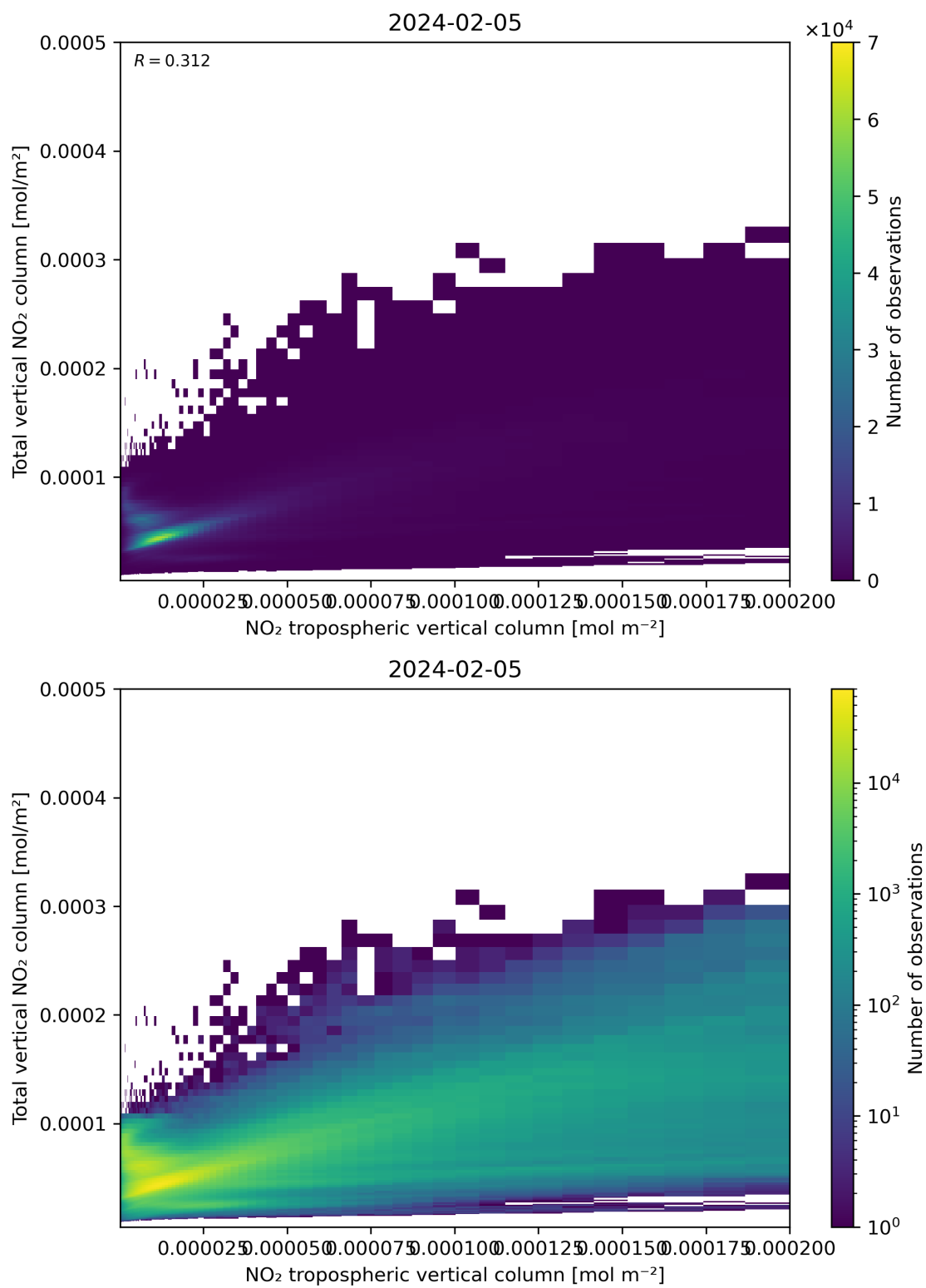
Figure 128: Scatter density plot of “NO 2 tropospheric vertical column” against “Total vertical NO 2 column” for 2024-02-04 to 2024-02-06.
