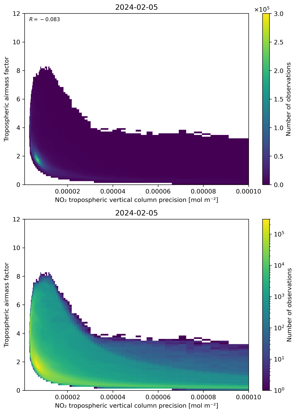
Figure 133: Scatter density plot of “NO 2 tropospheric vertical column precision” against “Tropospheric airmass factor” for 2024-02-04 to 2024-02-06.
