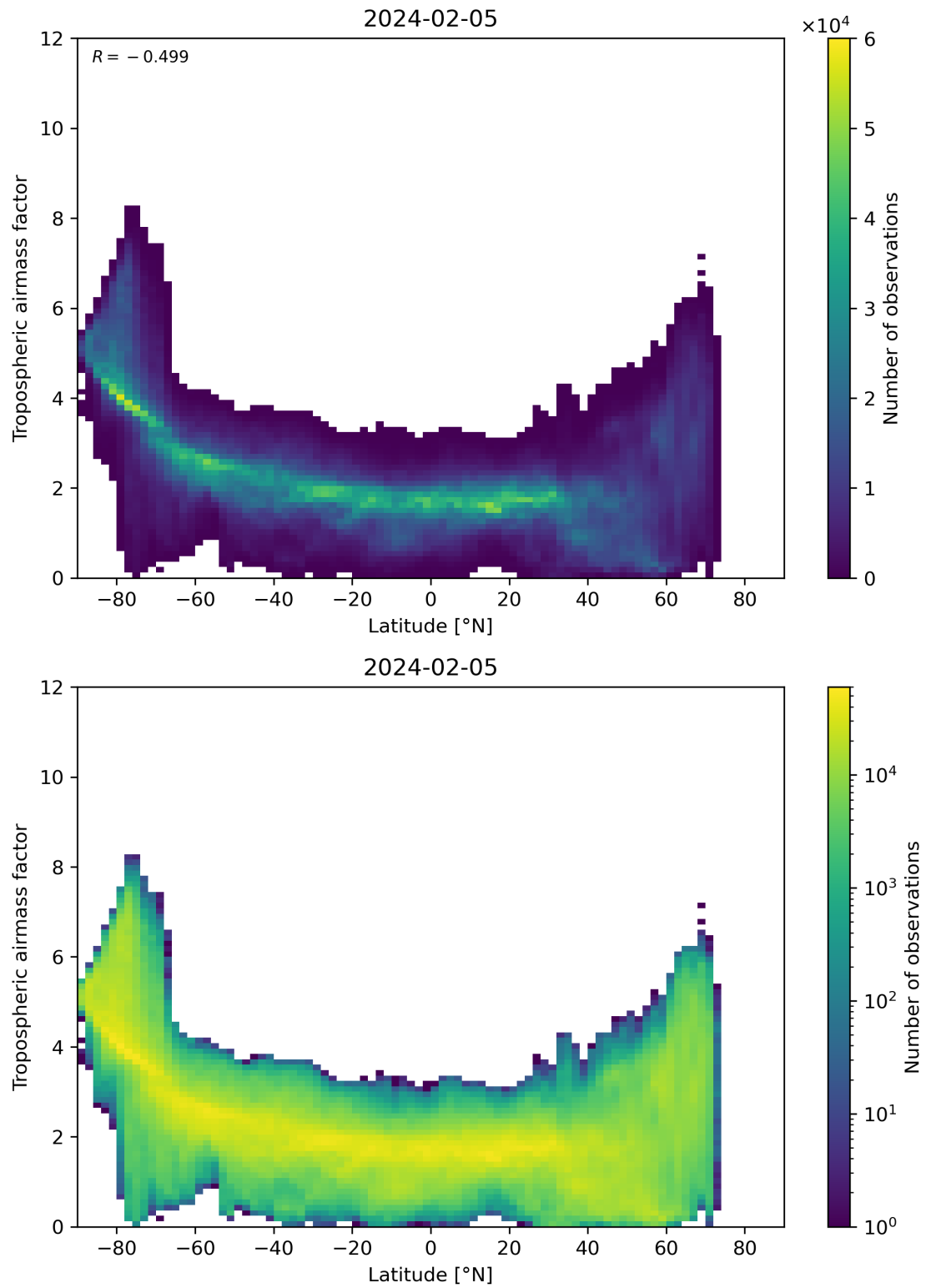
Figure 85: Scatter density plot of “Latitude” against “Tropospheric airmass factor” for 2024-02-04 to 2024-02-06.
