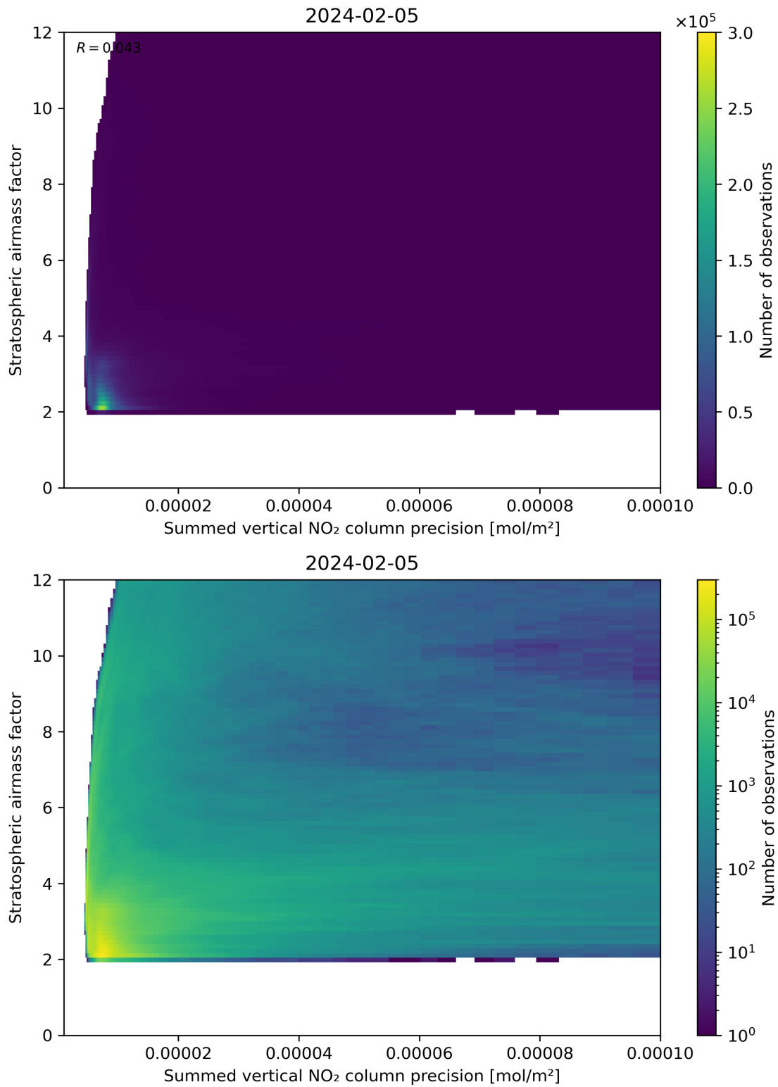
Figure 106: Scatter density plot of “Summed vertical NO 2 column precision” against “Stratospheric airmass factor” for 2024-02-04 to 2024-02-06.
