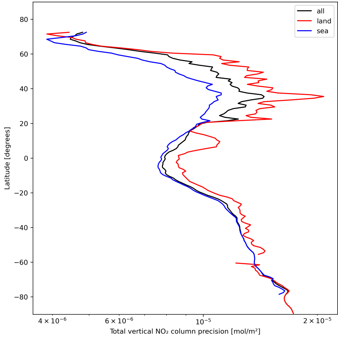
Figure 22: Zonal average of “Total vertical NO 2 column precision” for 2024-02-04 to 2024-02-06.
