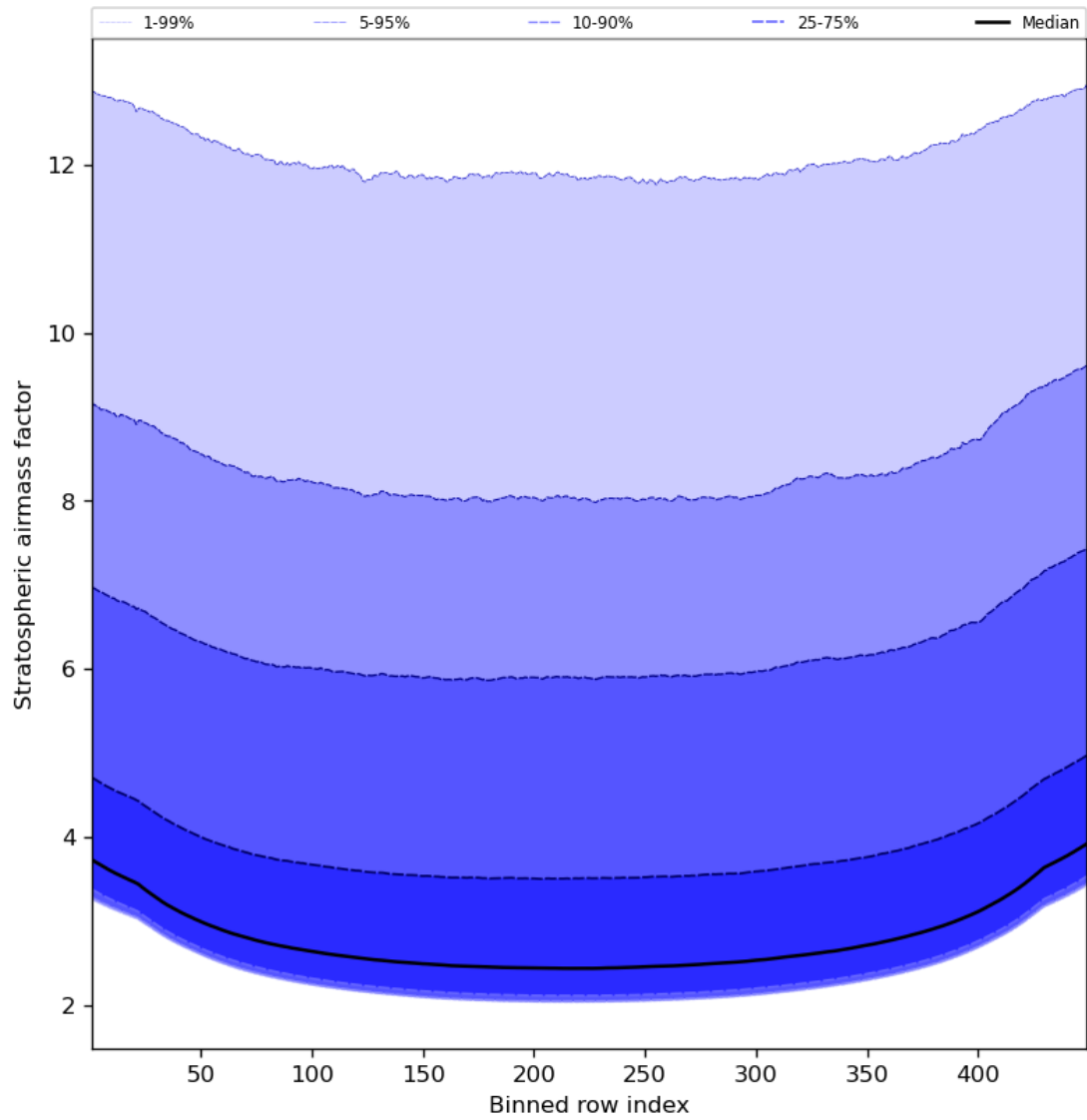
Figure 61: Along track statistics of “Stratospheric airmass factor” for 2024-02-04 to 2024-02-06
