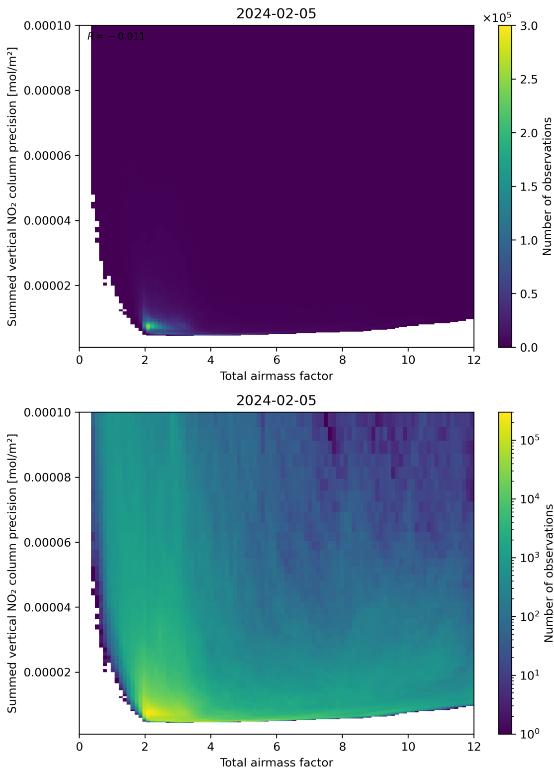
Figure 66: Scatter density plot of “Total airmass factor” against “Summed vertical NO 2 column precision” for 2024-02-04 to 2024-02-06.
