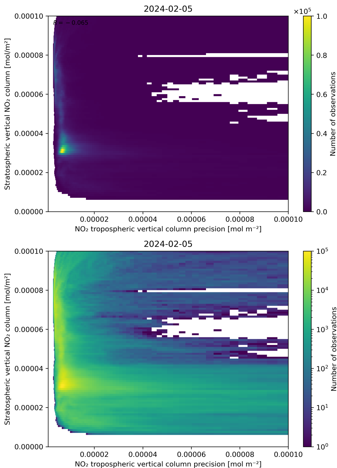
Figure 135: Scatter density plot of “NO 2 tropospheric vertical column precision” against “Stratospheric vertical NO 2 column” for 2024-02-04 to 2024-02-06.
