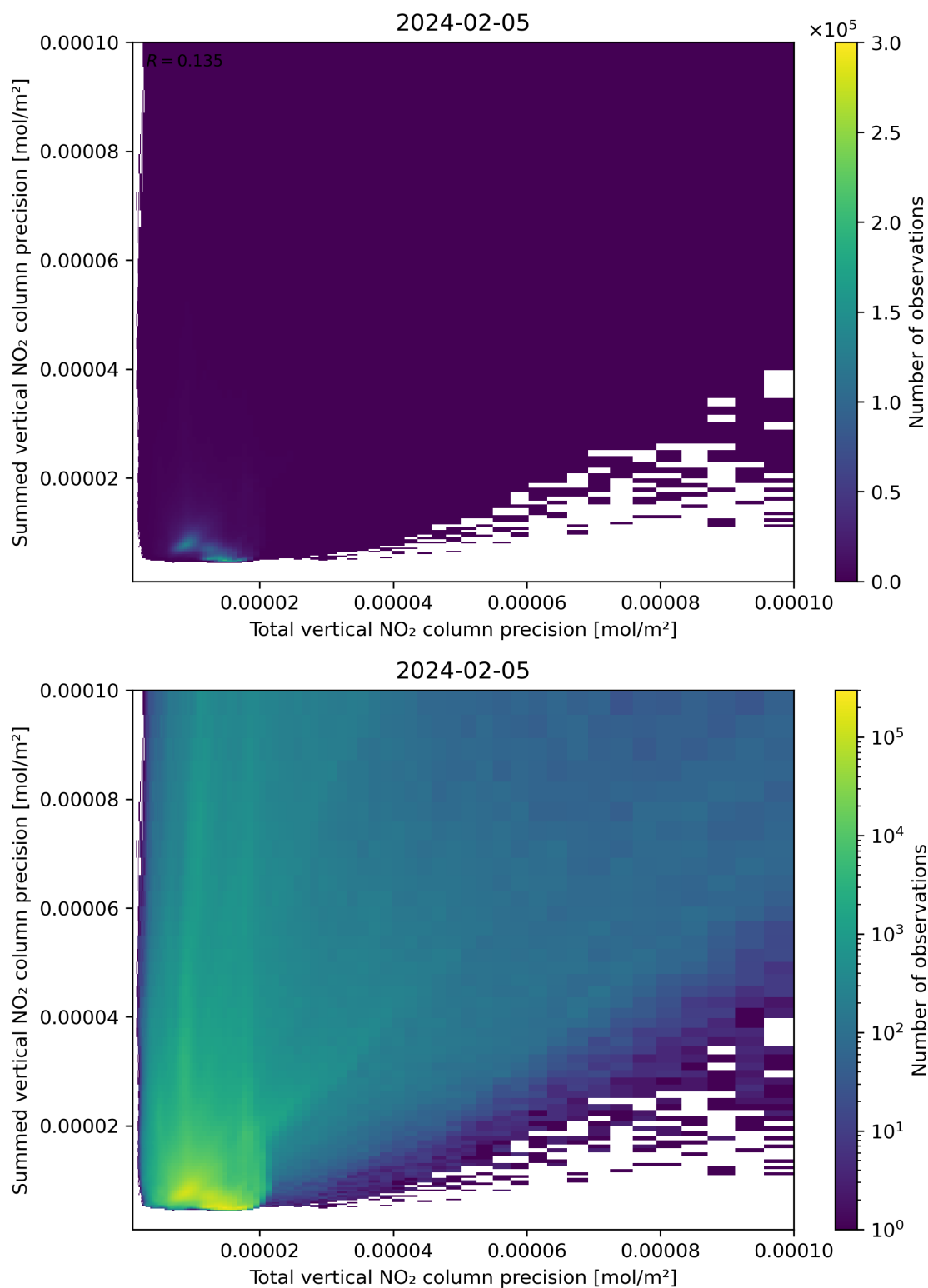
Figure 118: Scatter density plot of “Total vertical NO 2 column precision” against “Summed vertical NO 2 column precision” for 2024-02-04 to 2024-02-06.
