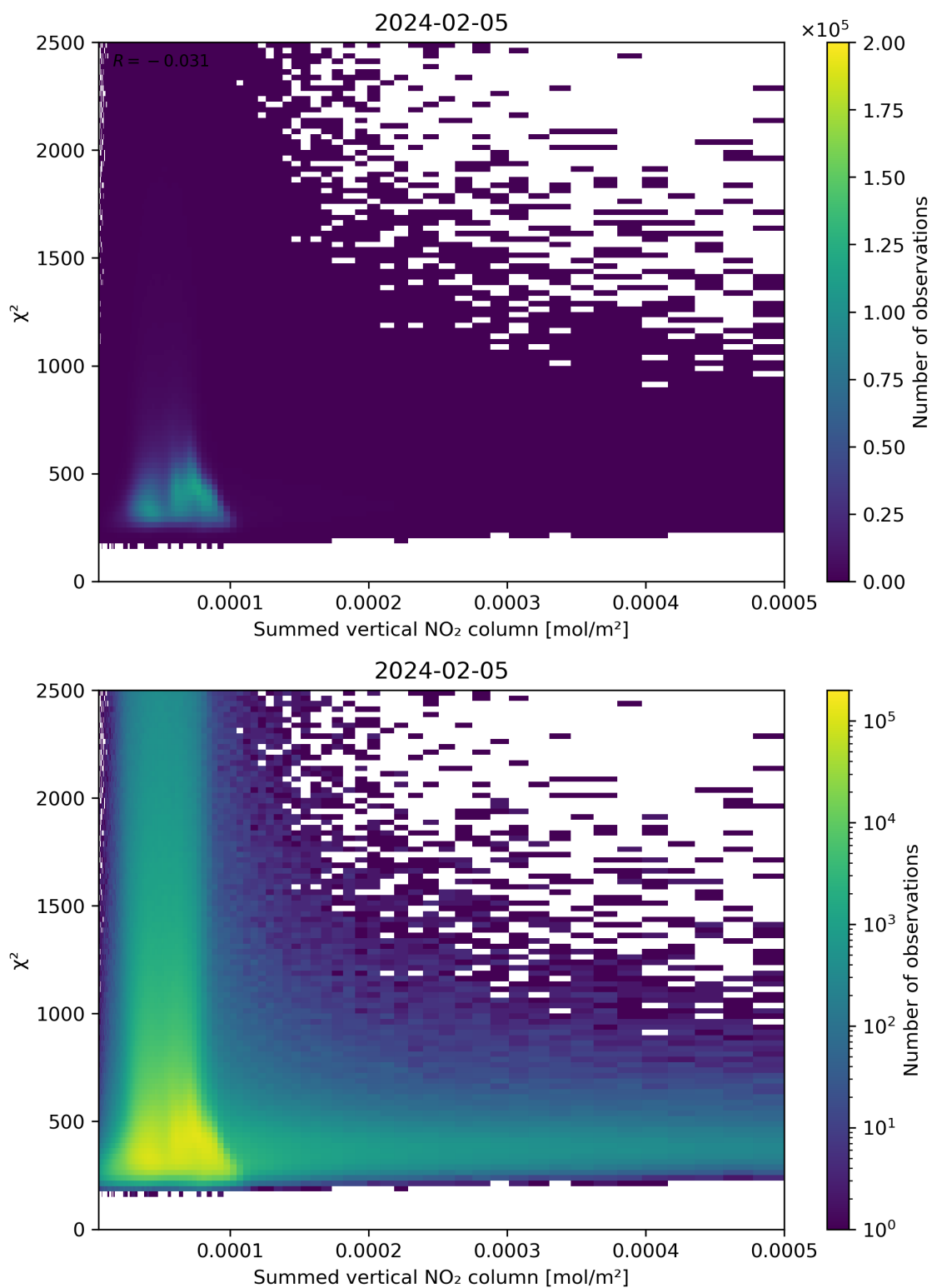
Figure 104: Scatter density plot of “Summed vertical NO 2 column” against “ \chi^2 ” for 2024-02-04 to 2024-02-06.
