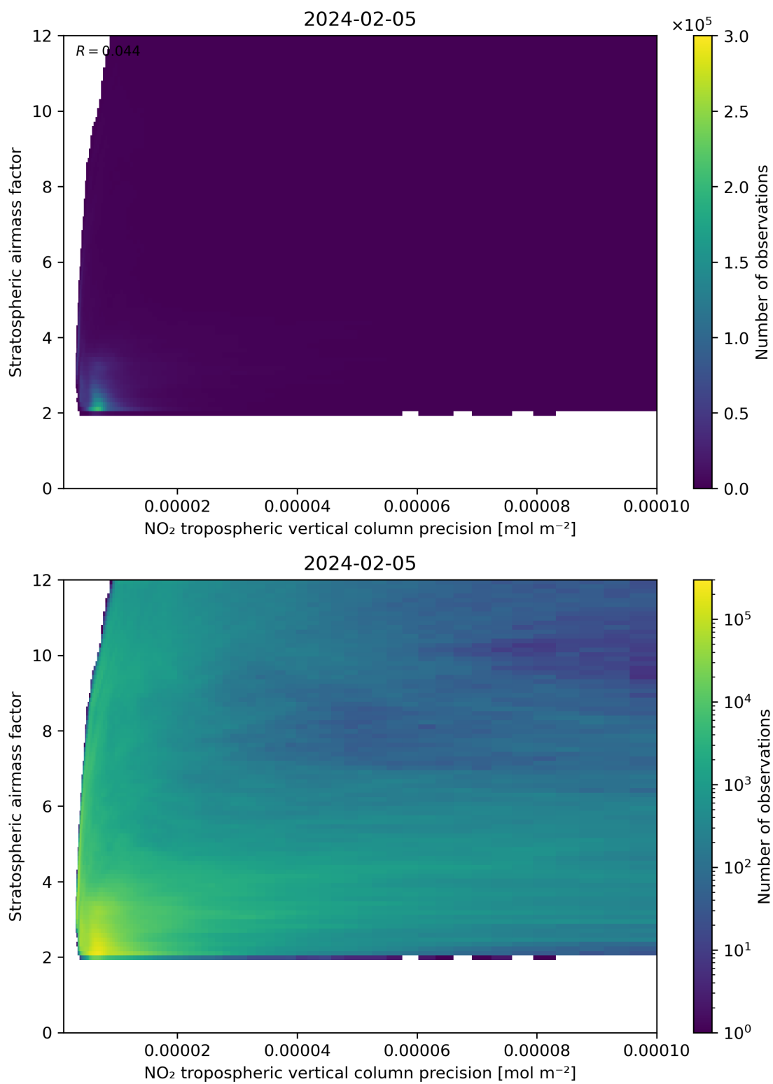
Figure 131: Scatter density plot of “NO 2 tropospheric vertical column precision” against “Stratospheric airmass factor” for 2024-02-04 to 2024-02-06.
