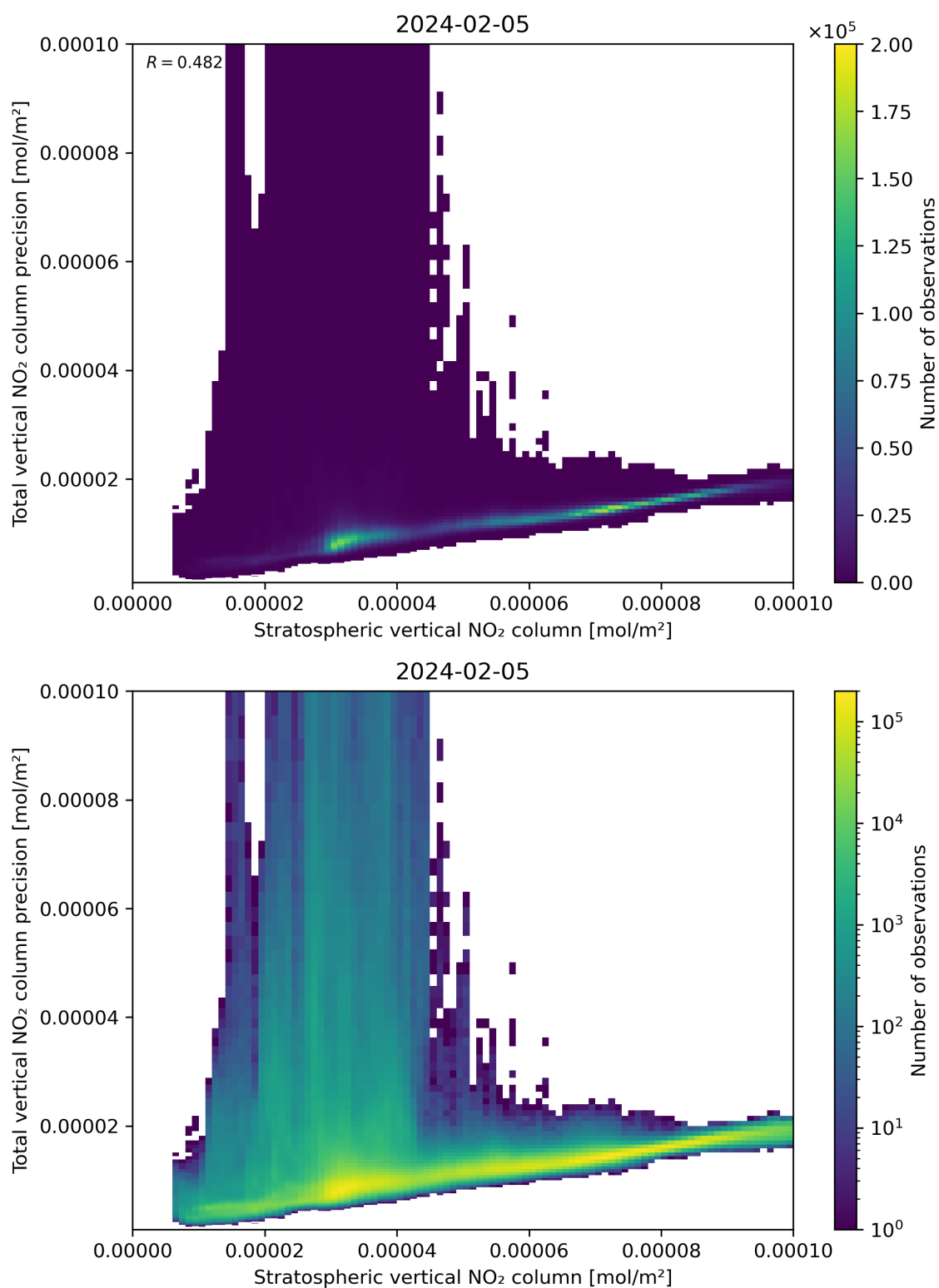
Figure 101: Scatter density plot of “Stratospheric vertical NO 2 column” against “Total vertical NO 2 column precision” for 2024-02-04 to 2024-02-06.
