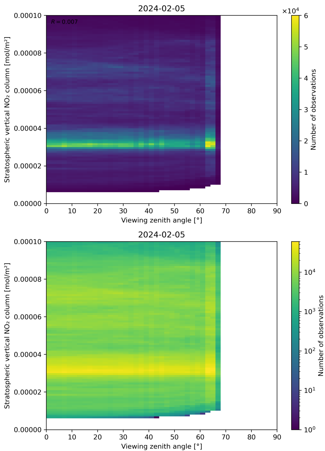
Figure 164: Scatter density plot of “Viewing zenith angle” against “Stratospheric vertical NO 2 column” for 2024-02-04 to 2024-02-06.
