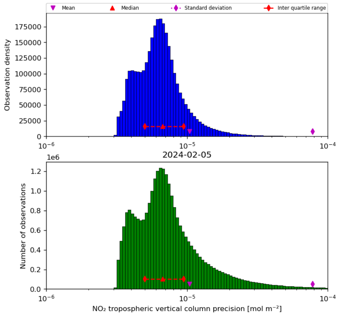
Figure 30: Histogram of “NO 2 tropospheric vertical column precision” for 2024-02-04 to 2024-02-06
