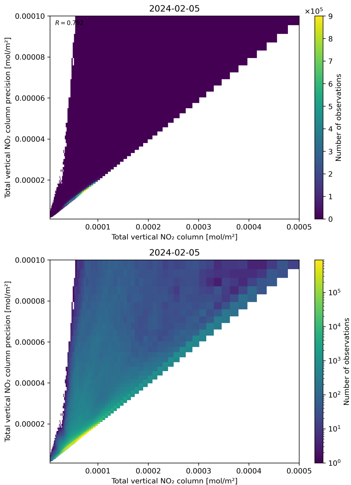
Figure 114: Scatter density plot of “Total vertical NO 2 column” against “Total vertical NO 2 column precision” for 2024-02-04 to 2024-02-06.
