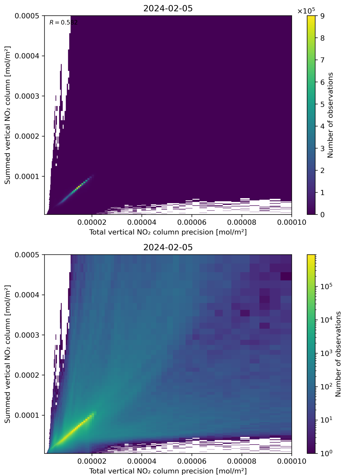
Figure 117: Scatter density plot of “Total vertical NO 2 column precision” against “Summed vertical NO 2 column” for 2024-02-04 to 2024-02-06.
