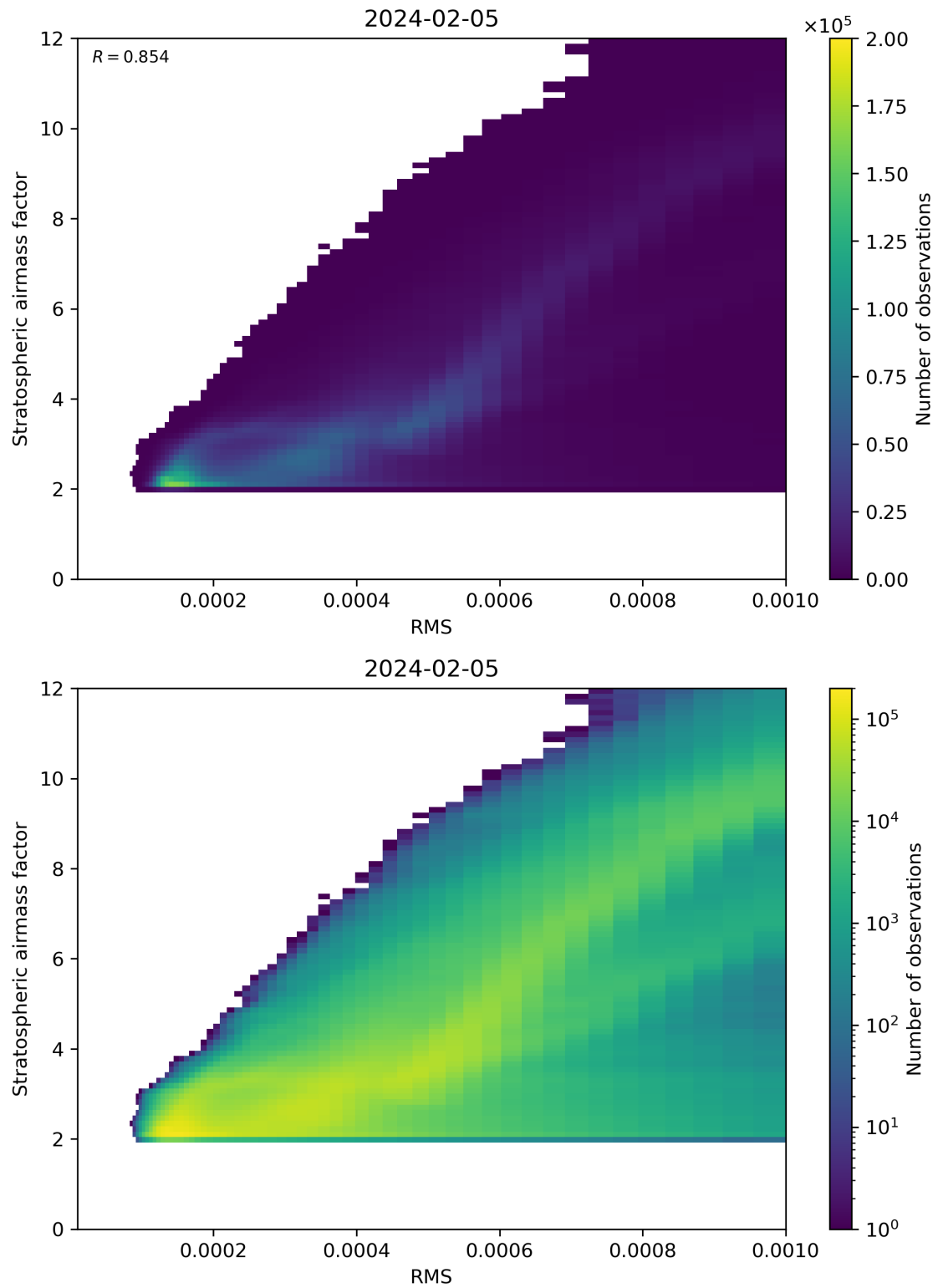
Figure 144: Scatter density plot of “RMS” against “Stratospheric airmass factor” for 2024-02-04 to 2024-02-06.
