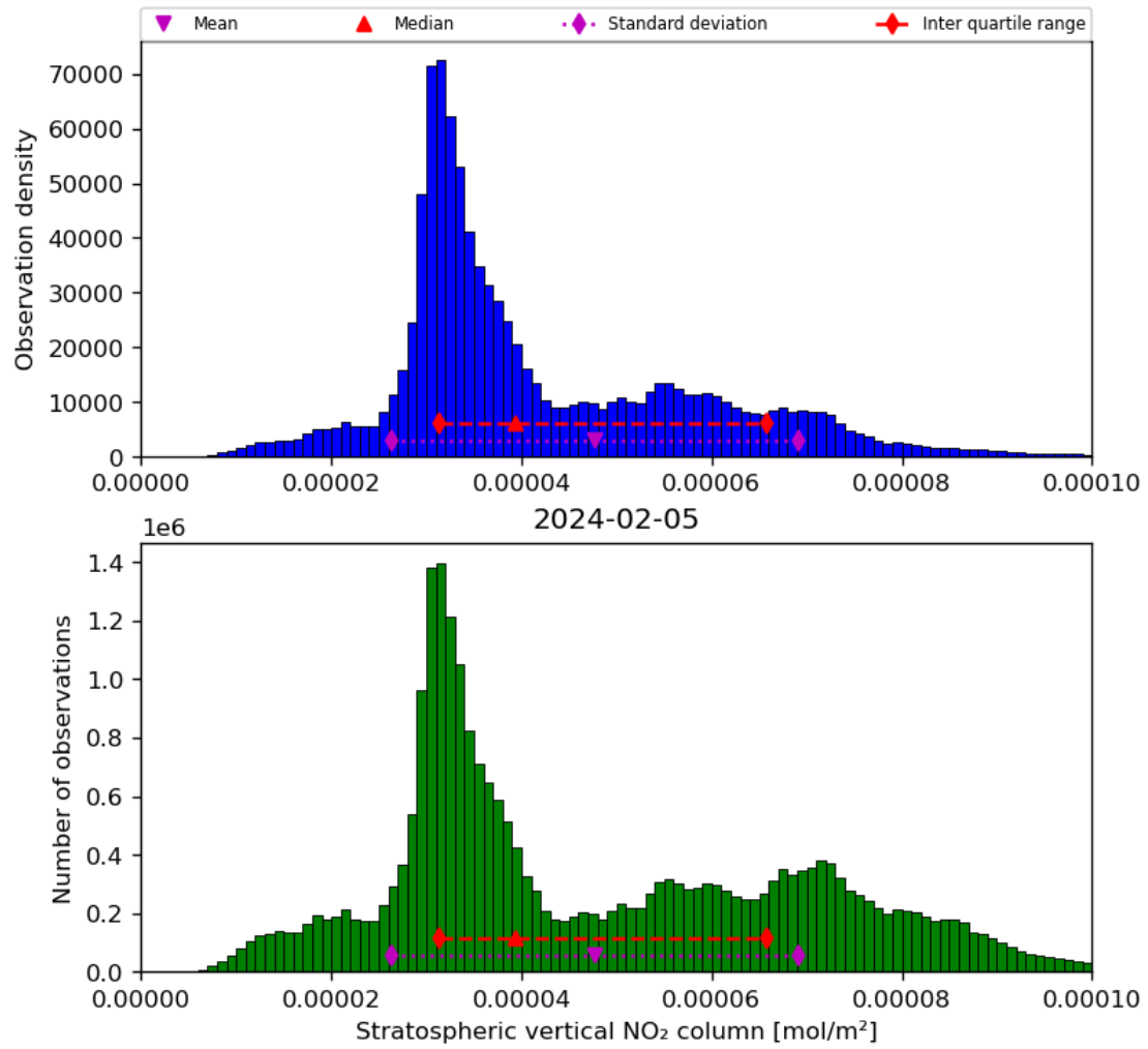
Figure 36: Histogram of “Stratospheric vertical NO 2 column” for 2024-02-04 to 2024-02-06
