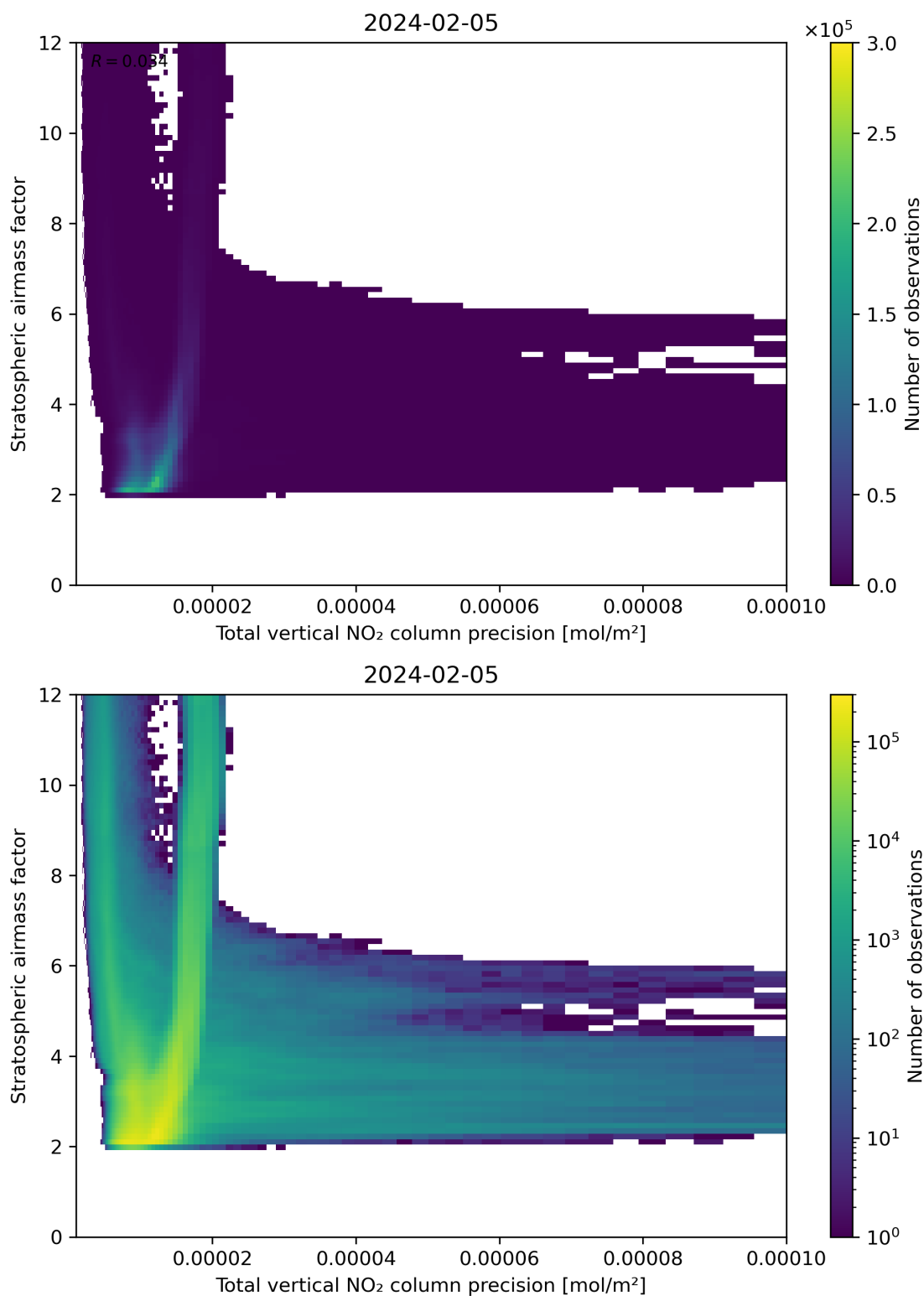
Figure 115: Scatter density plot of “Total vertical NO 2 column precision” against “Stratospheric air mass factor” for 2024-02-04 to 2024-02-06.
