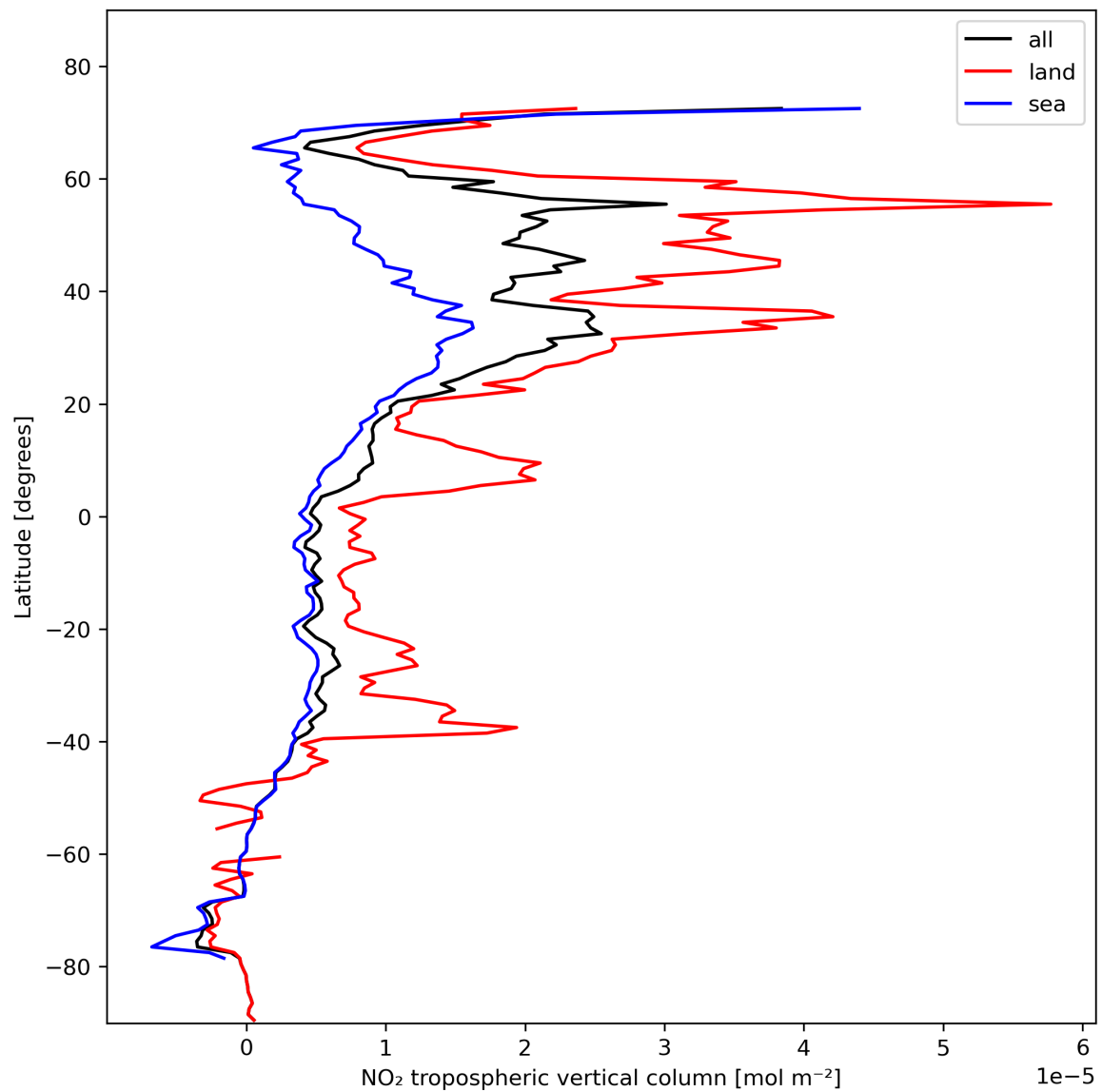
Figure 12: Zonal average of “NO 2 tropospheric vertical column” for 2024-02-04 to 2024-02-06.
