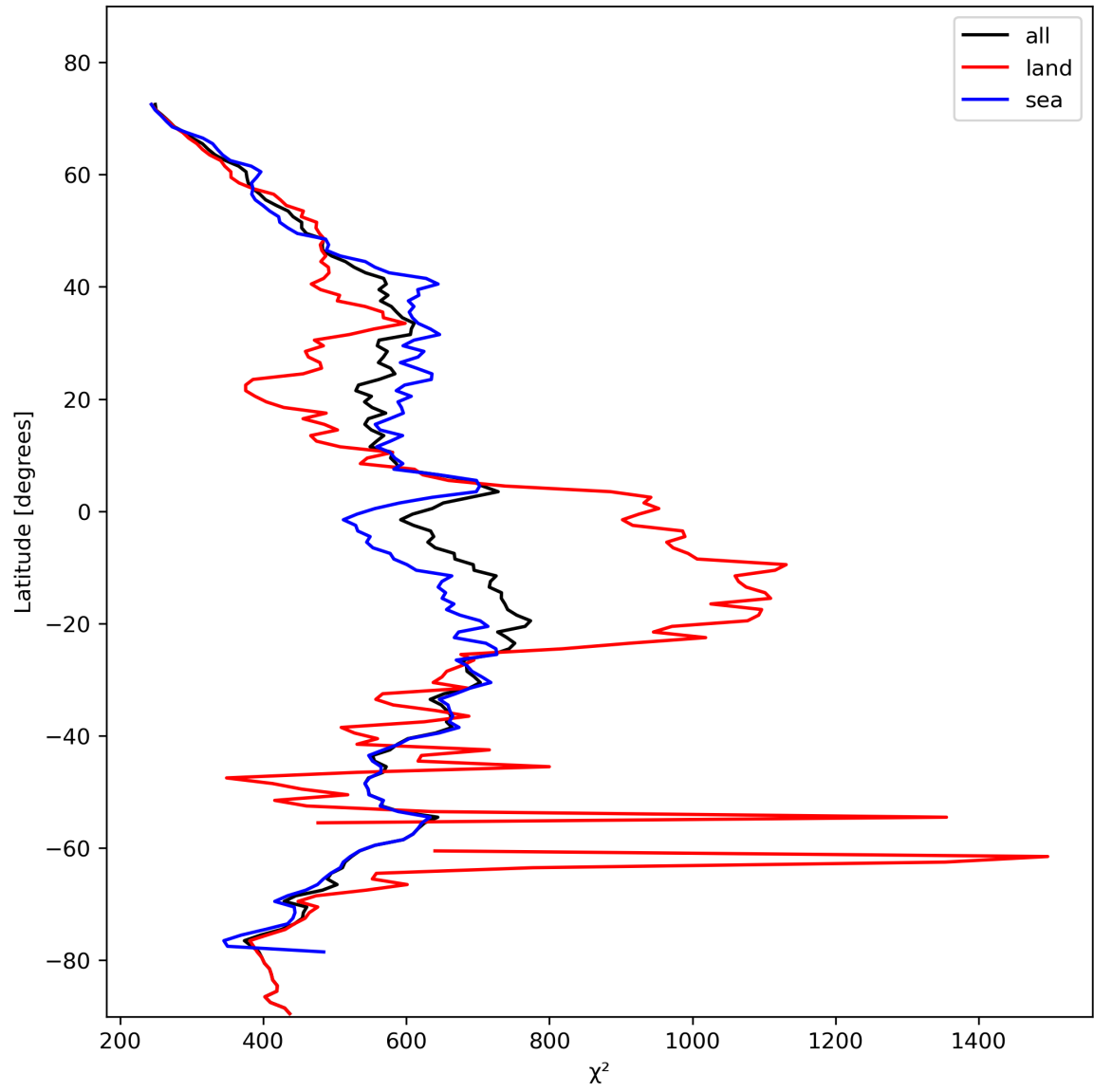
Figure 25: Zonal average of “ \chi^2 ” for 2024-02-04 to 2024-02-06.
