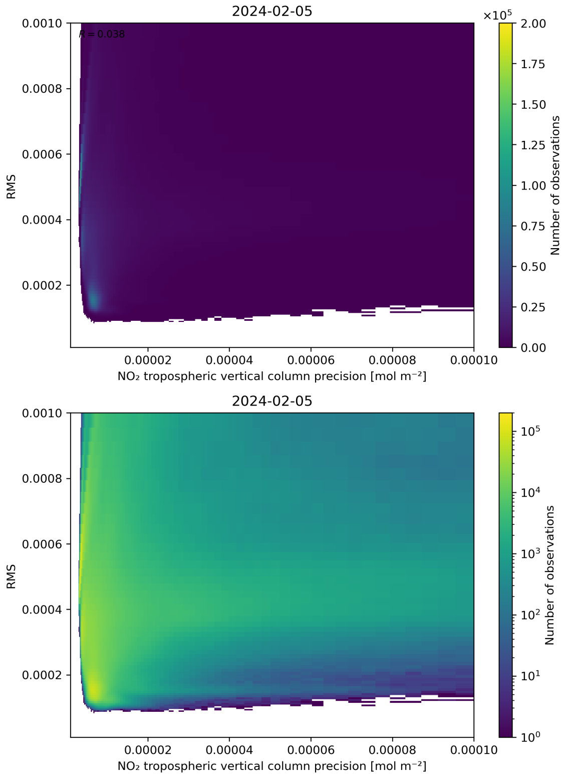
Figure 140: Scatter density plot of “NO 2 tropospheric vertical column precision” against “RMS” for 2024-02-04 to 2024-02-06.
