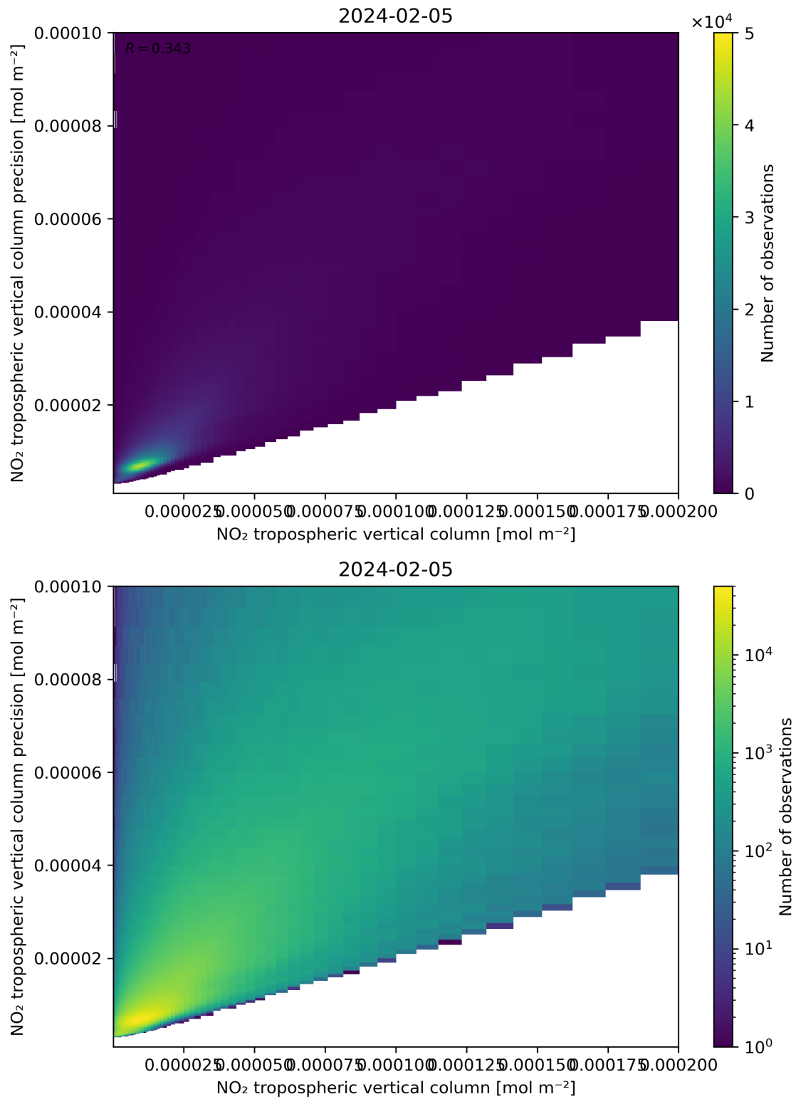
Figure 130: Scatter density plot of “NO 2 tropospheric vertical column” against “NO 2 tropospheric vertical column precision” for 2024-02-04 to 2024-02-06.
