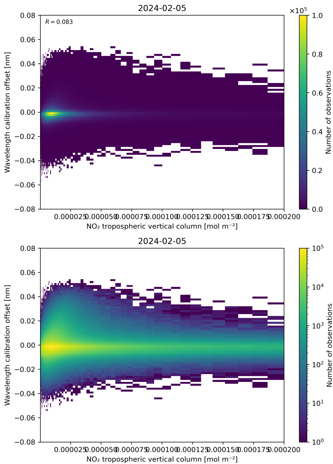
Figure 143: Scatter density plot of “NO 2 tropospheric vertical column” against “Wavelength calibration offset” for 2024-02-04 to 2024-02-06.
