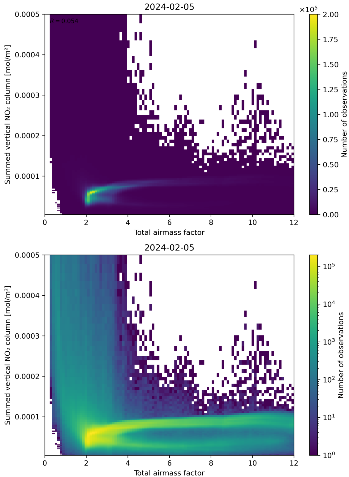
Figure 65: Scatter density plot of “Total airmass factor” against “Summed vertical NO 2 column” for 2024-02-04 to 2024-02-06.
