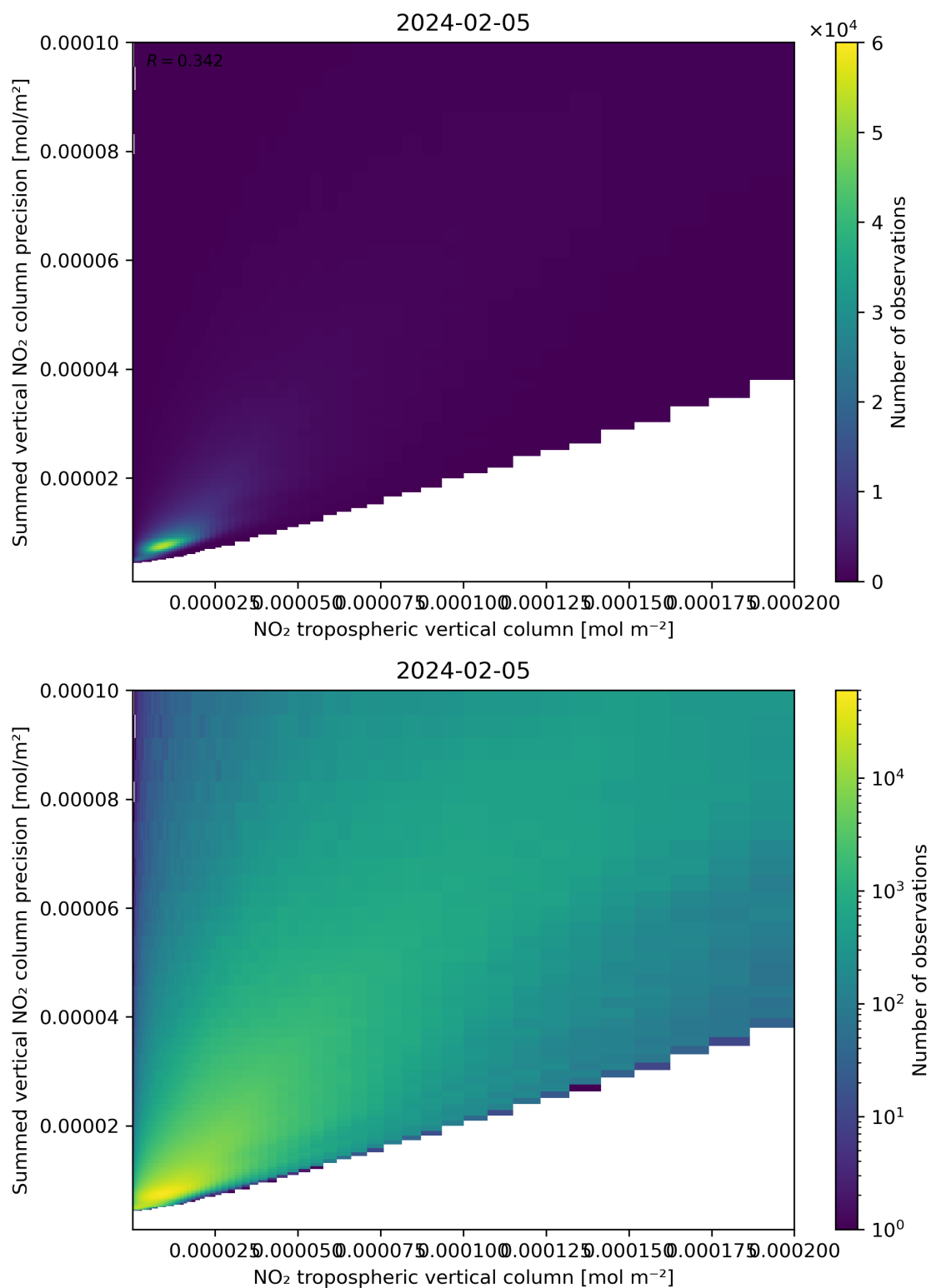
Figure 127: Scatter density plot of “NO 2 tropospheric vertical column” against “Summed vertical NO 2 column precision” for 2024-02-04 to 2024-02-06.
