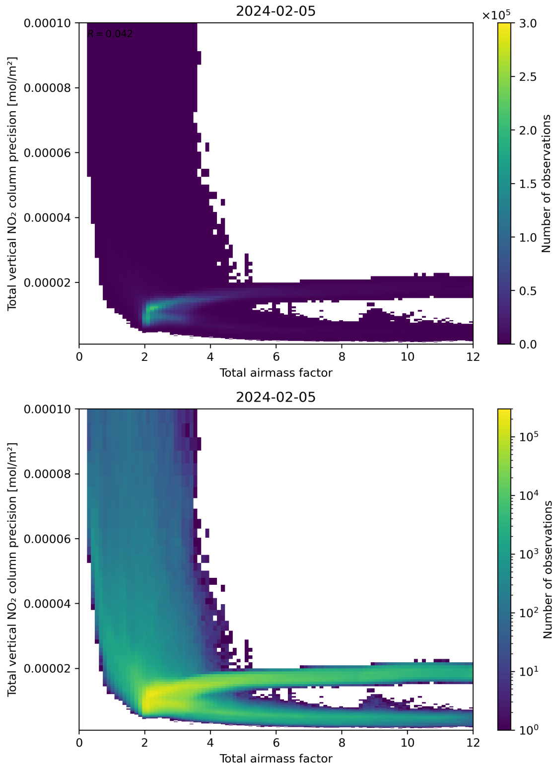
Figure 68: Scatter density plot of “Total airmass factor” against “Total vertical NO 2 column precision” for 2024-02-04 to 2024-02-06.
