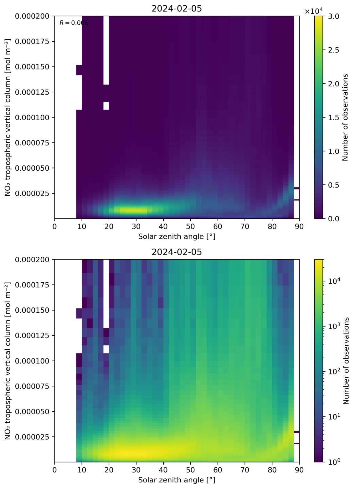
Figure 155: Scatter density plot of “Solar zenith angle” against “NO 2 tropospheric vertical column” for 2024-02-04 to 2024-02-06.
