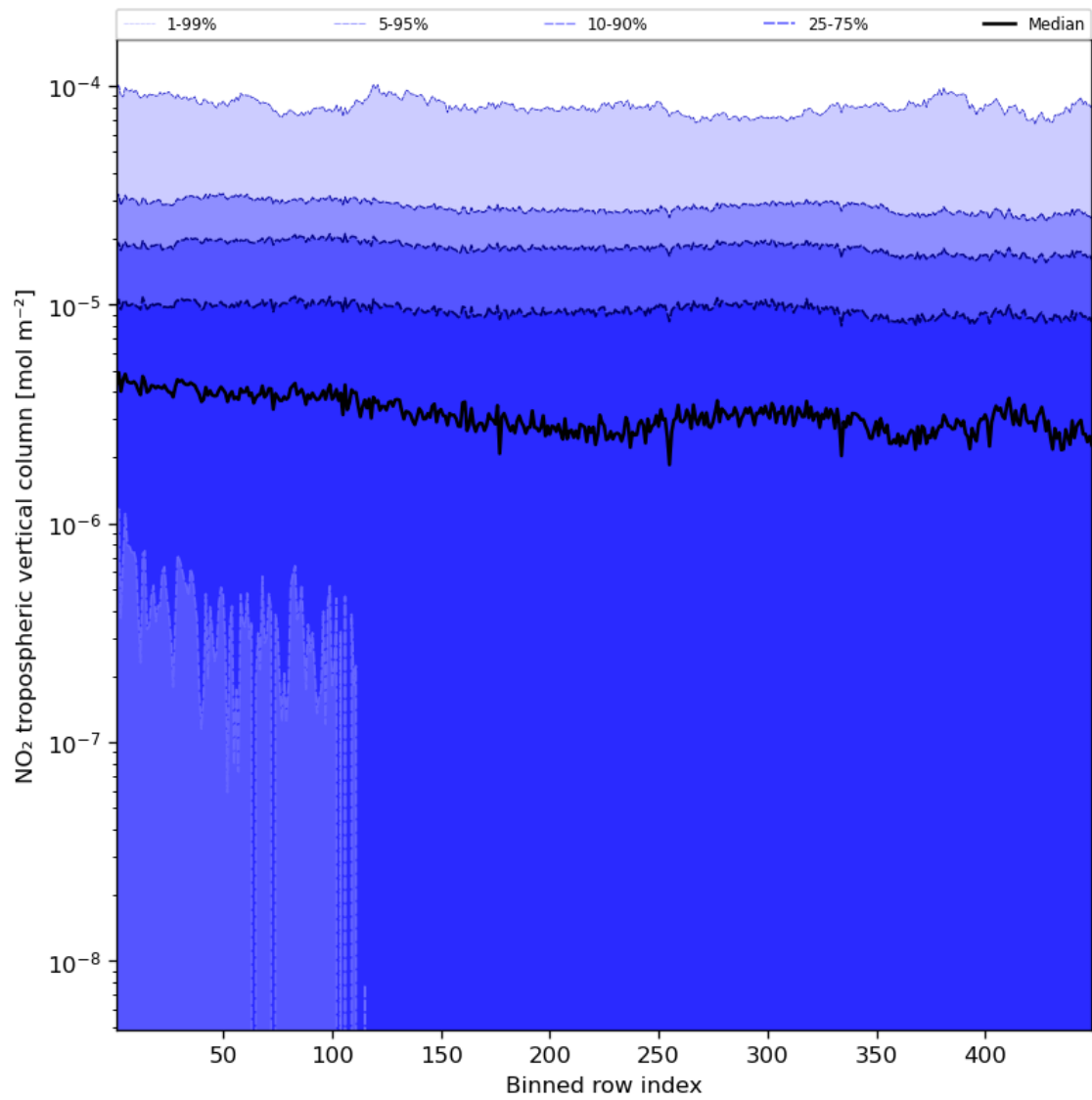
Figure 46: Along track statistics of “NO 2 tropospheric vertical column” for 2024-02-04 to 2024-02-06
