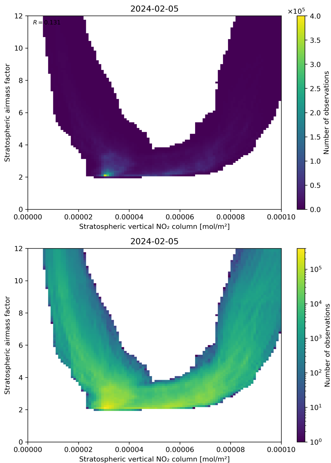
Figure 96: Scatter density plot of “Stratospheric vertical NO 2 column” against “Stratospheric airmass factor” for 2024-02-04 to 2024-02-06.
