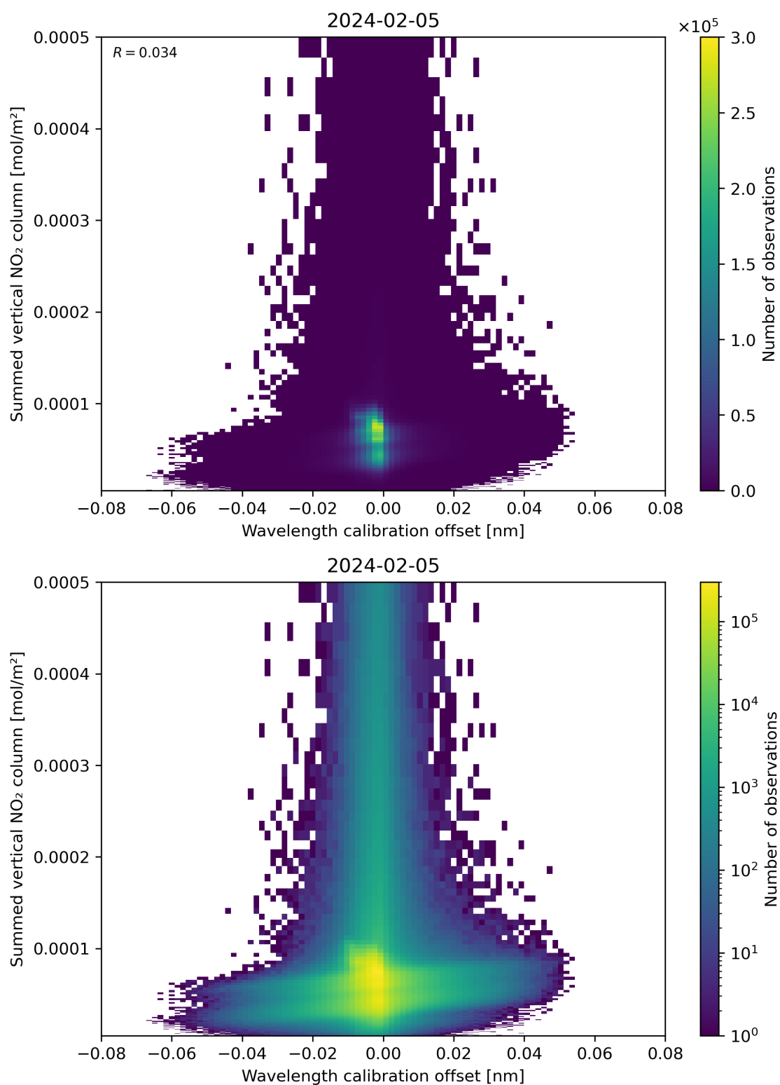
Figure 177: Scatter density plot of “Wavelength calibration offset” against “Summed vertical NO 2 column” for 2024-02-04 to 2024-02-06.
