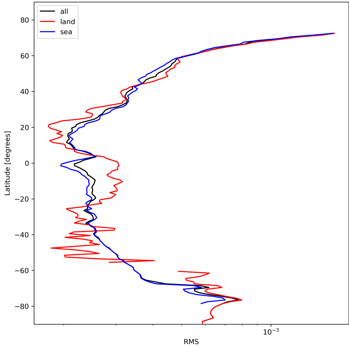
Figure 26: Zonal average of “RMS” for 2024-02-04 to 2024-02-06.
