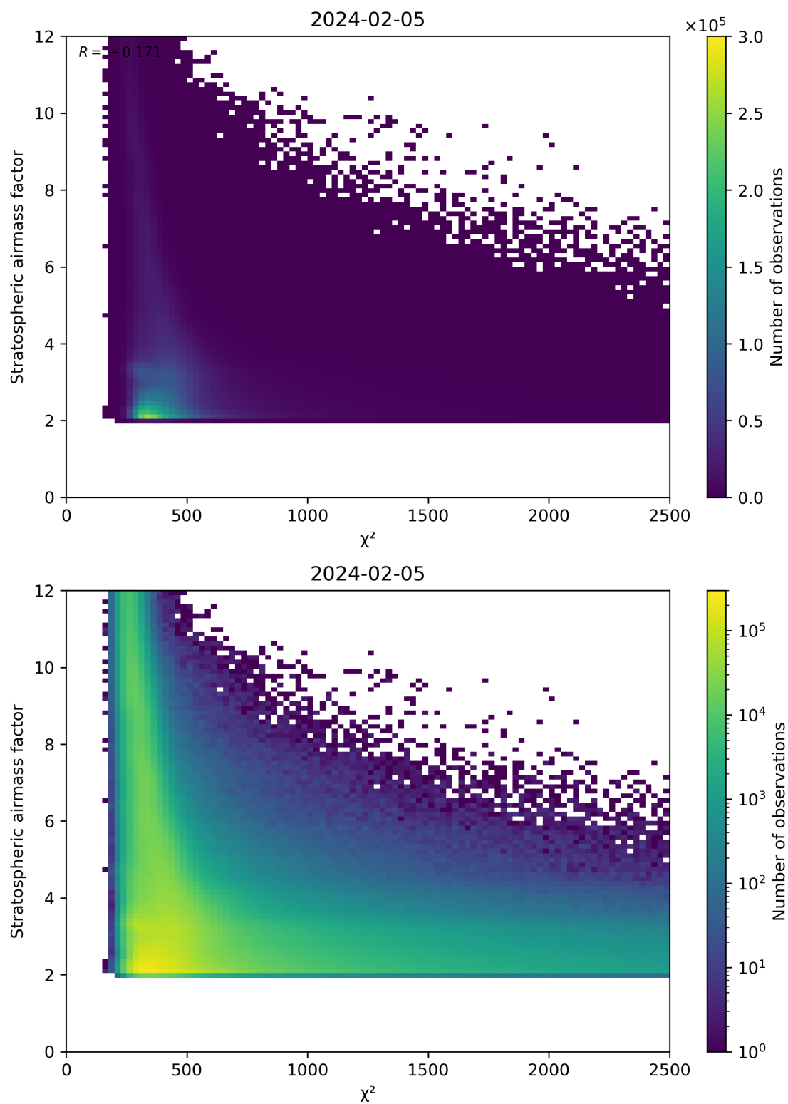
Figure 81: Scatter density plot of “ \chi^2 ” against “Stratospheric airmass factor” for 2024-02-04 to 2024-02-06.
