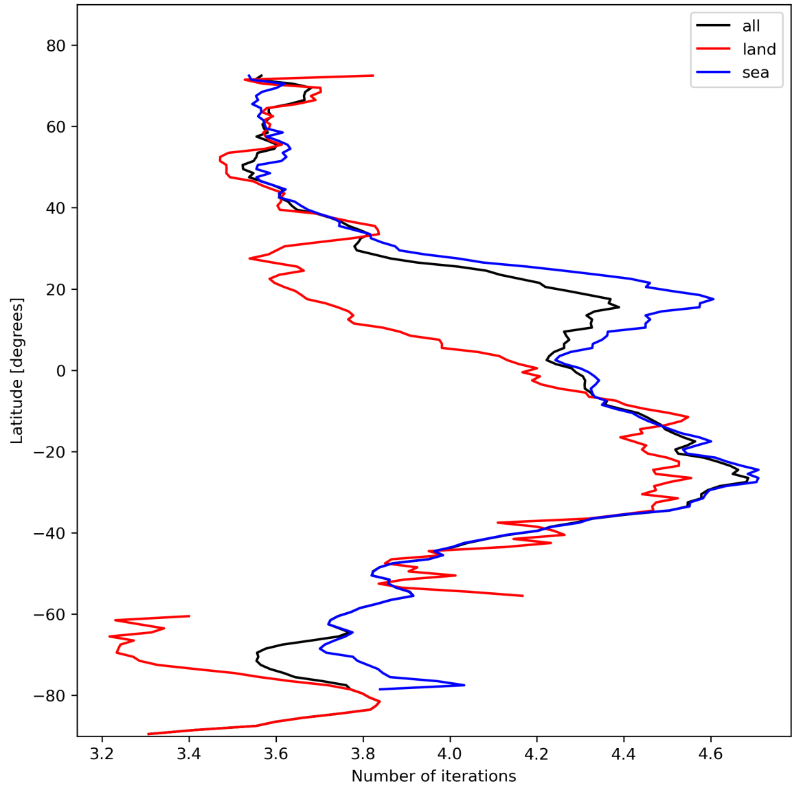
Figure 17: Zonal average of “Number of iterations” for 2024-02-04 to 2024-02-06.
