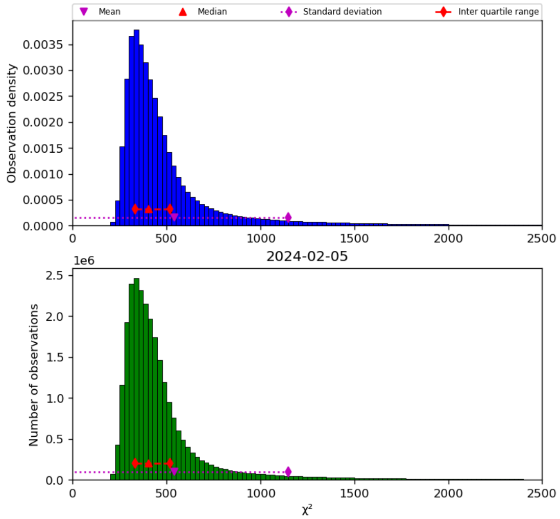
Figure 42: Histogram of “ \chi^2 ” for 2024-02-04 to 2024-02-06
