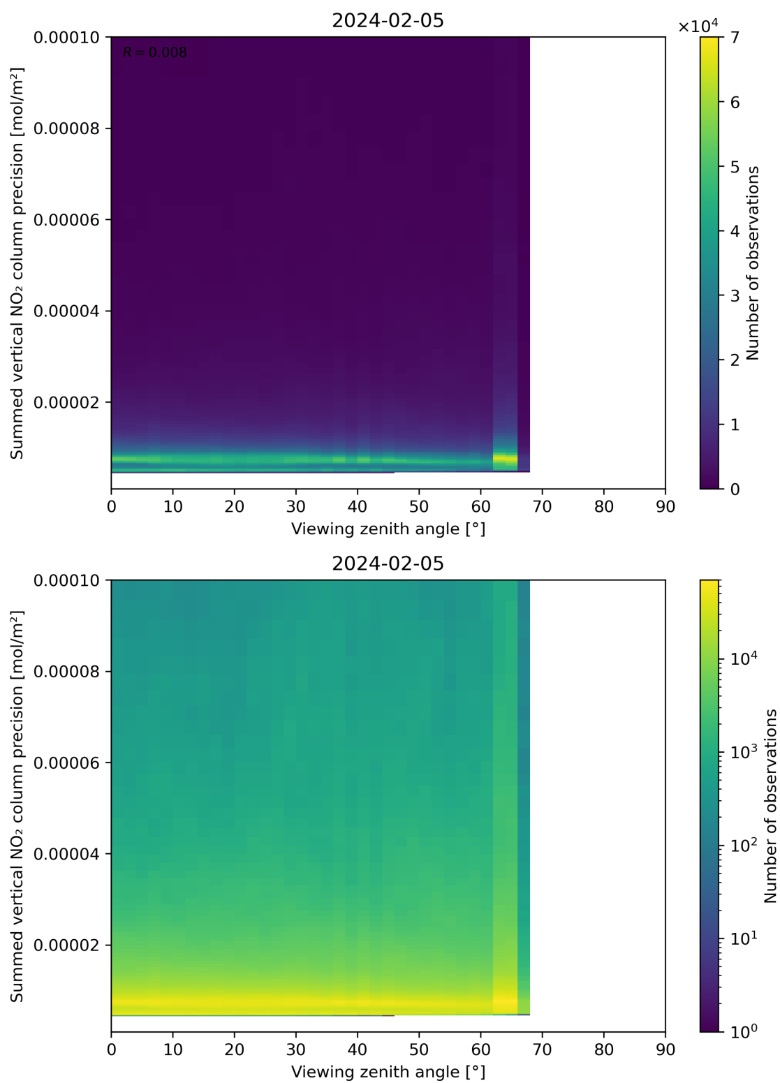
Figure 166: Scatter density plot of “Viewing zenith angle” against “Summed vertical NO 2 column precision” for 2024-02-04 to 2024-02-06.
