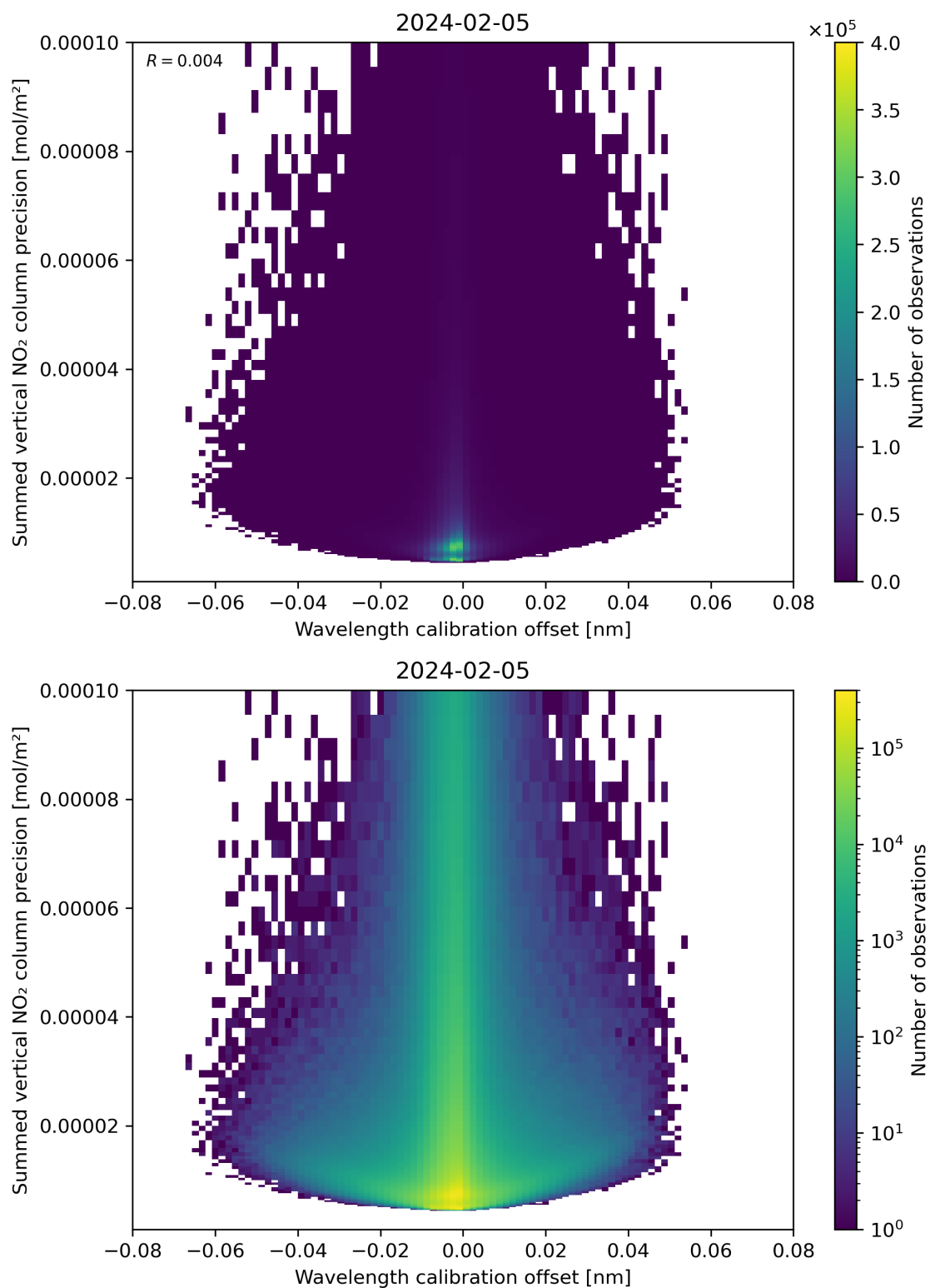
Figure 178: Scatter density plot of “Wavelength calibration offset” against “Summed vertical NO 2 column precision” for 2024-02-04 to 2024-02-06.
