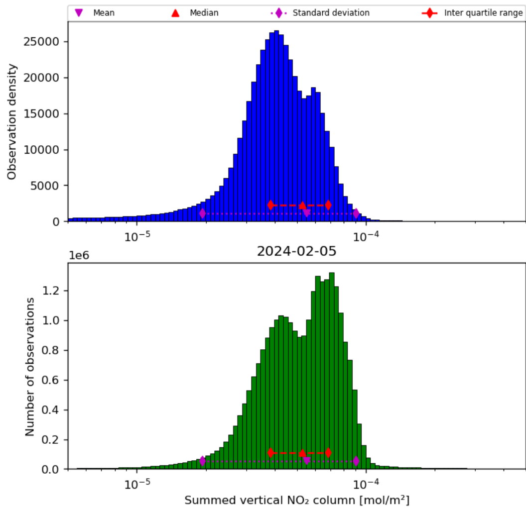
Figure 40: Histogram of “Summed vertical NO 2 column” for 2024-02-04 to 2024-02-06
