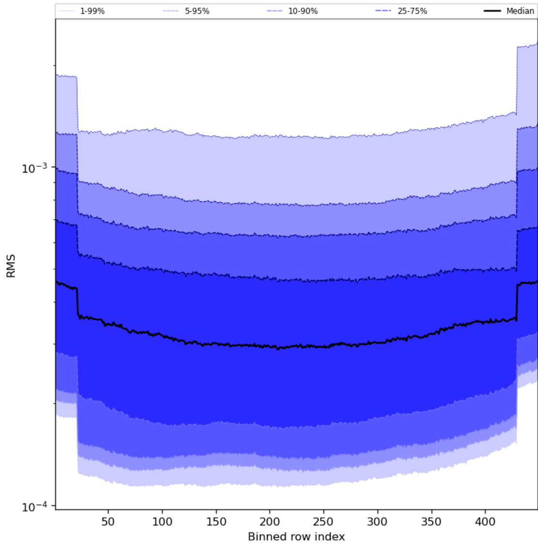
Figure 60: Along track statistics of “RMS” for 2024-02-04 to 2024-02-06
