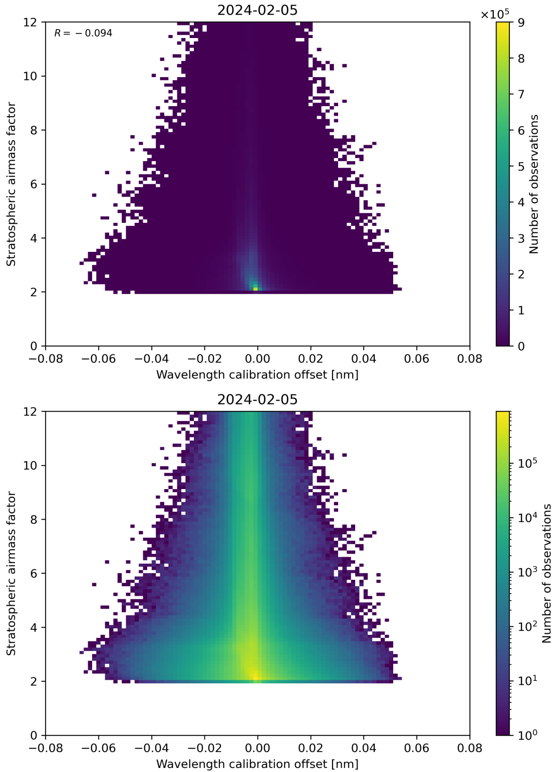
Figure 174: Scatter density plot of “Wavelength calibration offset” against “Stratospheric airmass factor” for 2024-02-04 to 2024-02-06.
