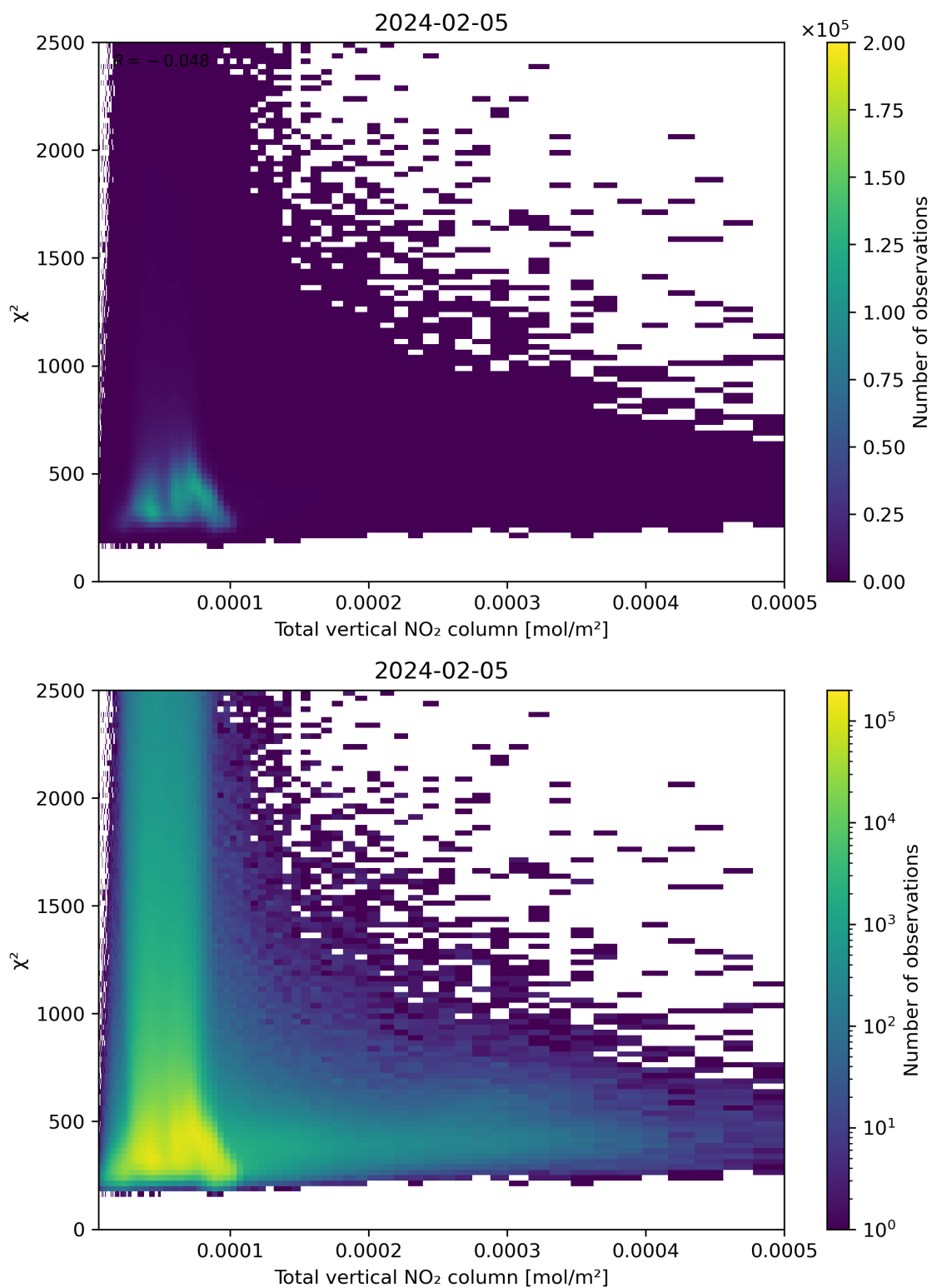
Figure 111: Scatter density plot of “Total vertical NO 2 column” against “ \chi^2 ” for 2024-02-04 to 2024-02-06.
