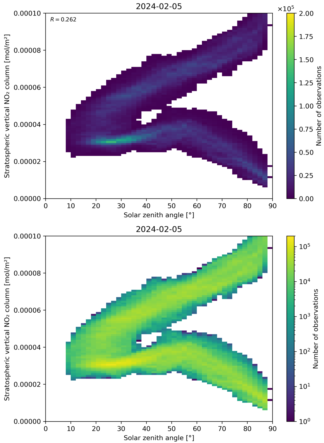
Figure 150: Scatter density plot of “Solar zenith angle” against “Stratospheric vertical NO 2 column” for 2024-02-04 to 2024-02-06.
