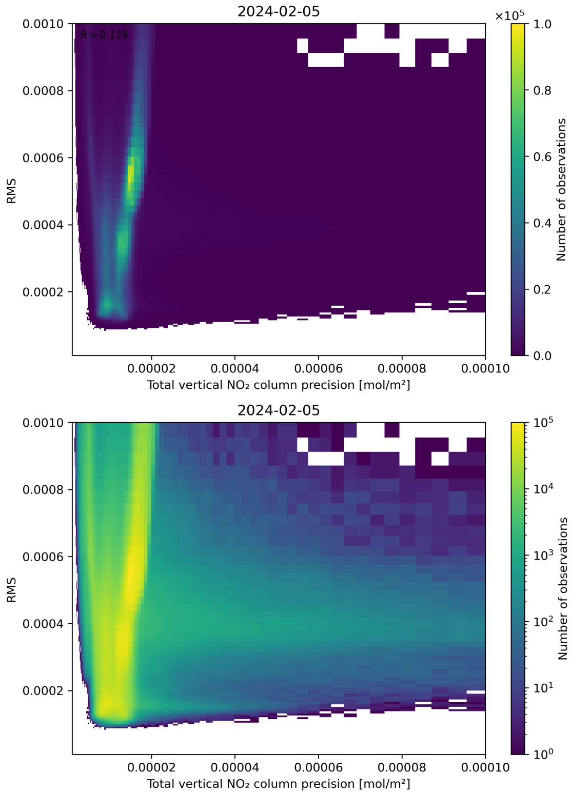
Figure 119: Scatter density plot of “Total vertical NO 2 column precision” against “RMS” for 2024-02-04 to 2024-02-06.
