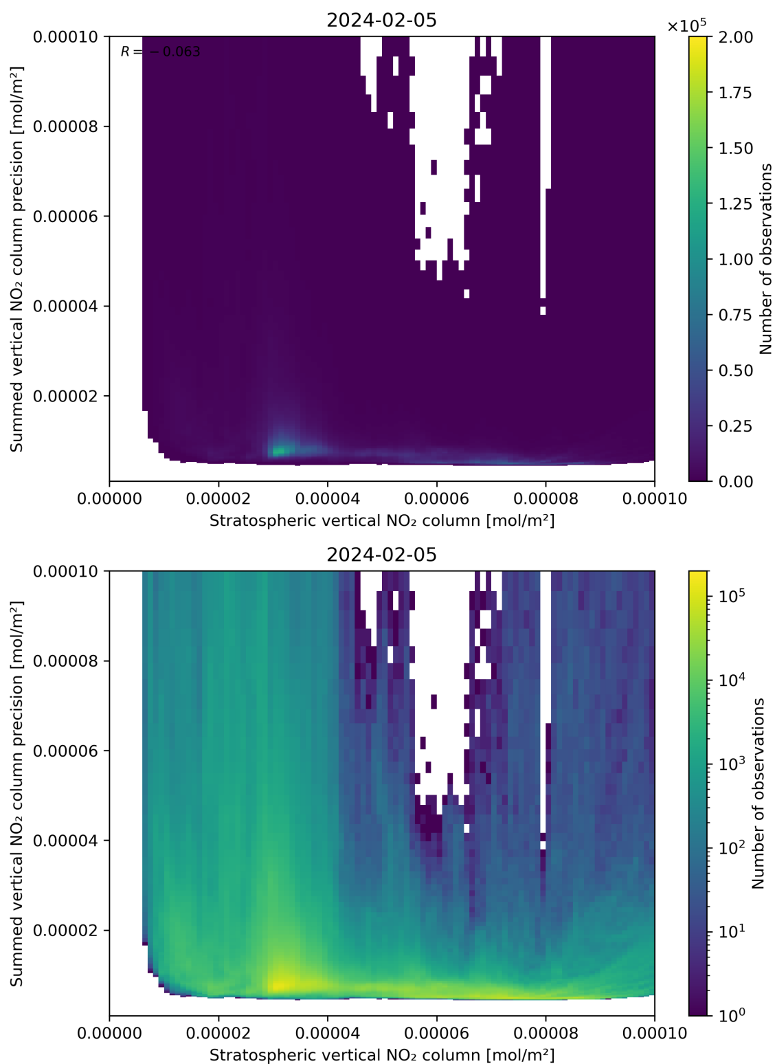
Figure 99: Scatter density plot of “Stratospheric vertical NO 2 column” against “Summed vertical NO 2 column precision” for 2024-02-04 to 2024-02-06.
