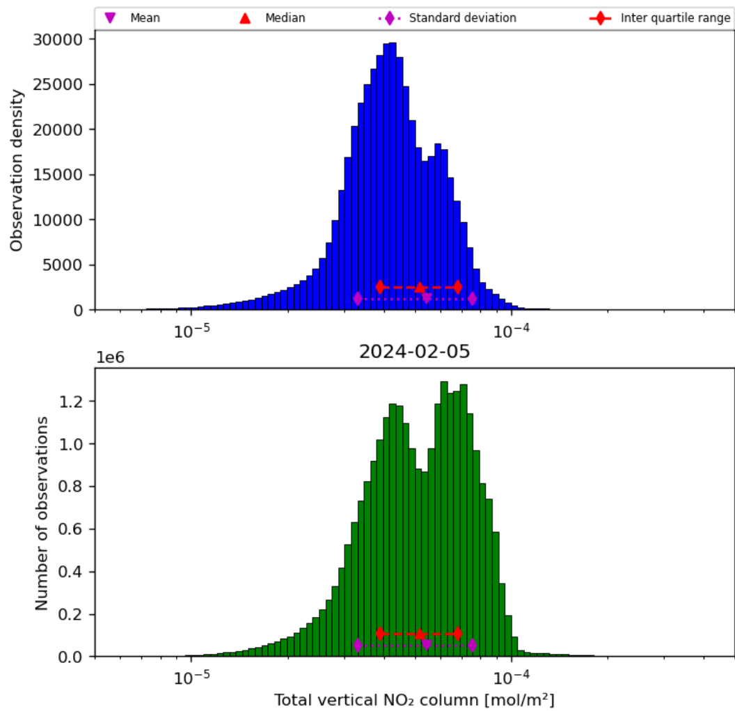
Figure 38: Histogram of “Total vertical NO 2 column” for 2024-02-04 to 2024-02-06
