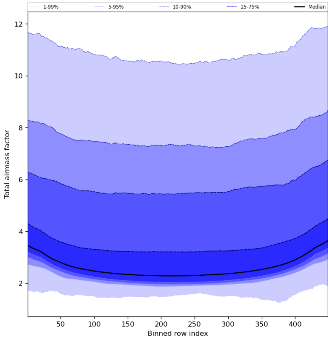
Figure 49: Along track statistics of “Total airmass factor” for 2024-02-04 to 2024-02-06
