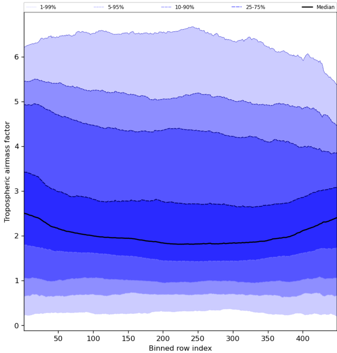
Figure 48: Along track statistics of “Tropospheric air mass factor” for 2024-02-04 to 2024-02-06
