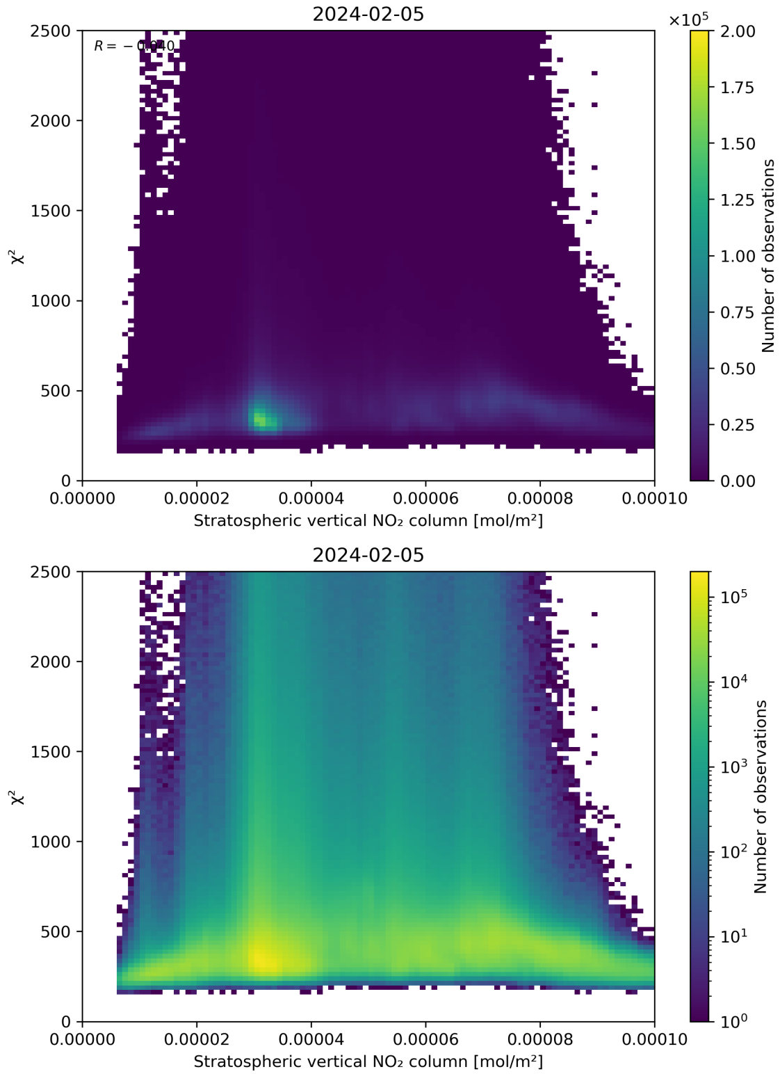
Figure 97: Scatter density plot of “Stratospheric vertical NO 2 column” against “ \chi^2 ” for 2024-02-04 to 2024-02-06.
