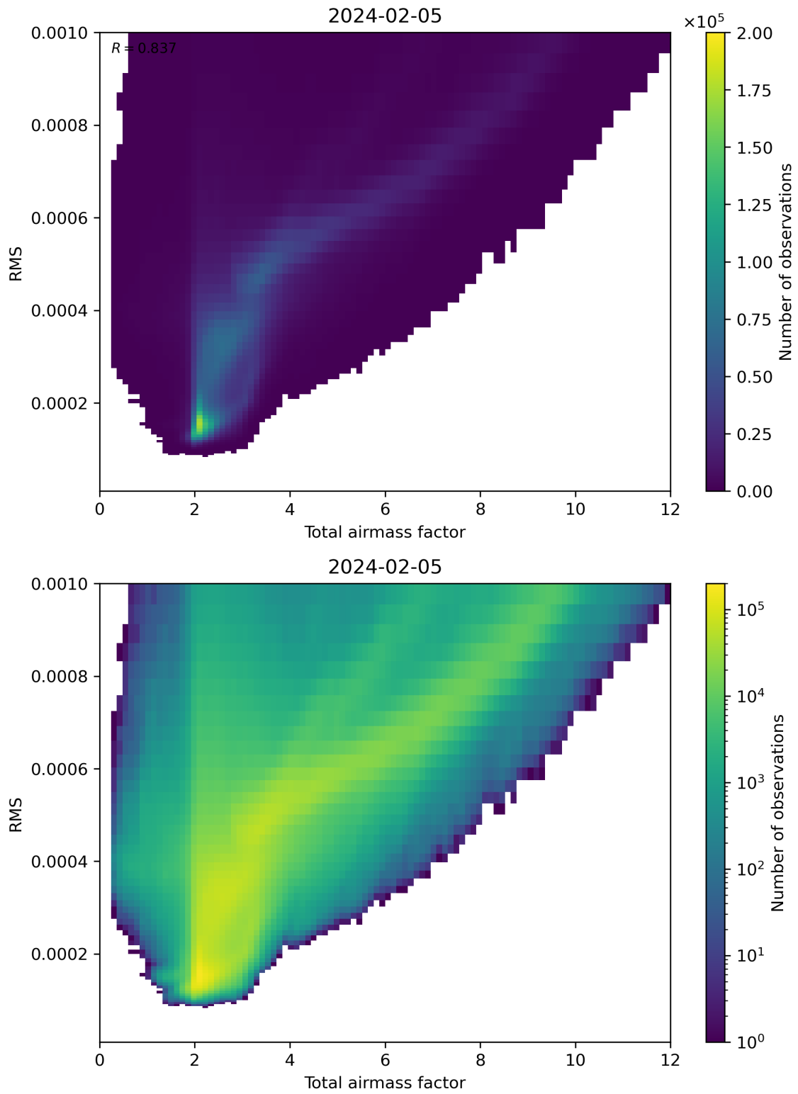
Figure 69: Scatter density plot of “Total airmass factor” against “RMS” for 2024-02-04 to 2024-02-06.
