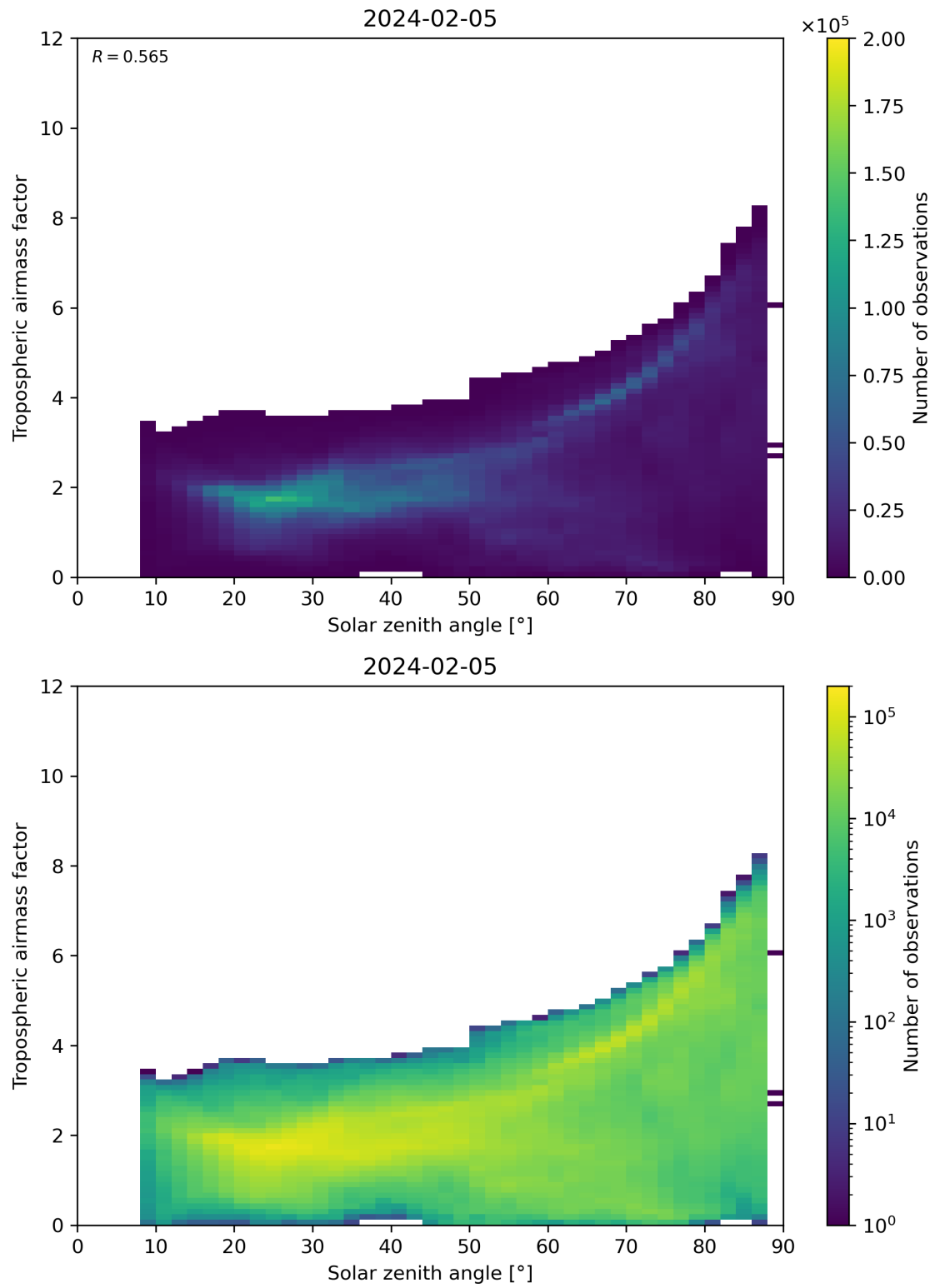
Figure 147: Scatter density plot of “Solar zenith angle” against “Tropospheric airmass factor” for 2024-02-04 to 2024-02-06.
