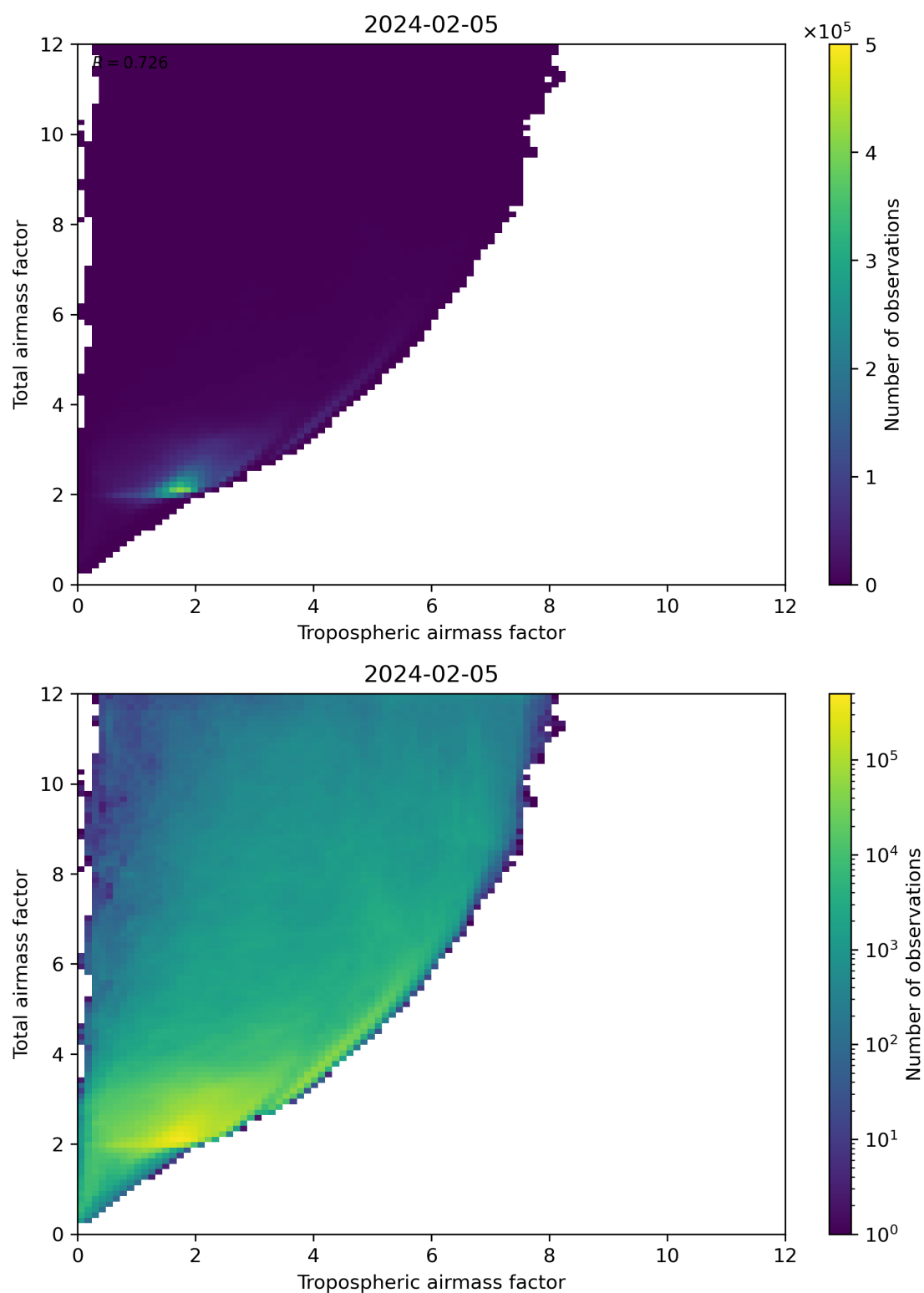
Figure 72: Scatter density plot of “Tropospheric airmass factor” against “Total airmass factor” for 2024-02-04 to 2024-02-06.
