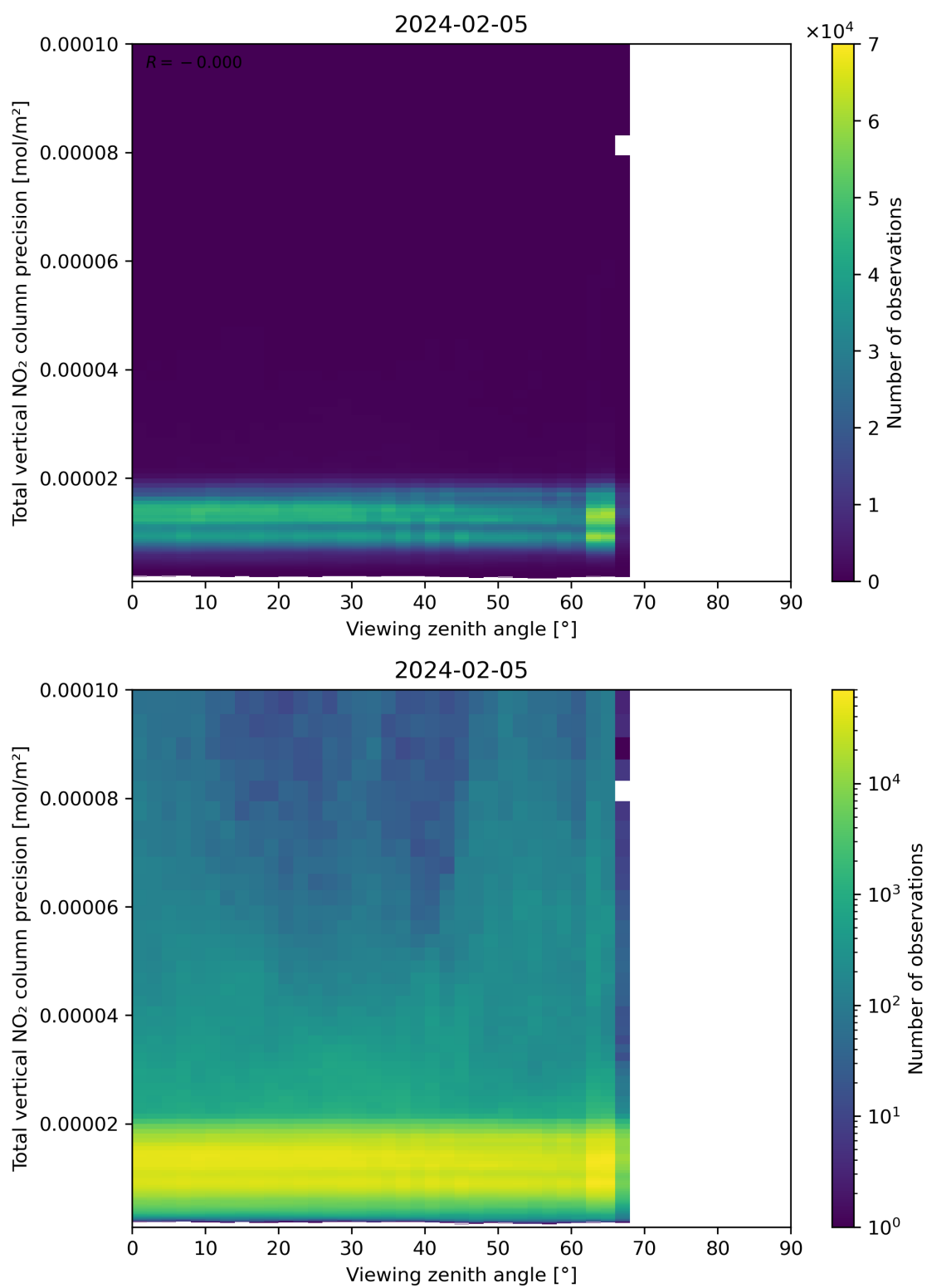
Figure 168: Scatter density plot of “Viewing zenith angle” against “Total vertical NO 2 column precision” for 2024-02-04 to 2024-02-06.
