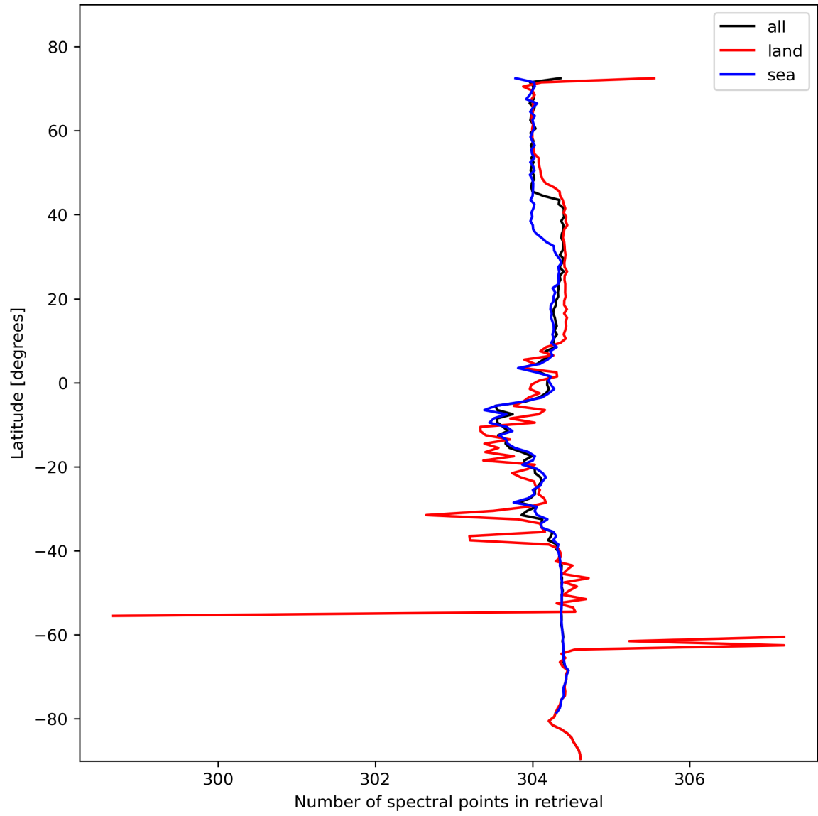
Figure 16: Zonal average of “Number of spectral points in retrieval” for 2024-02-04 to 2024-02-06.
