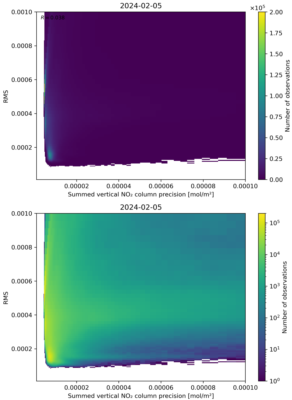
Figure 108: Scatter density plot of “Summed vertical NO 2 column precision” against “RMS” for 2024-02-04 to 2024-02-06.
