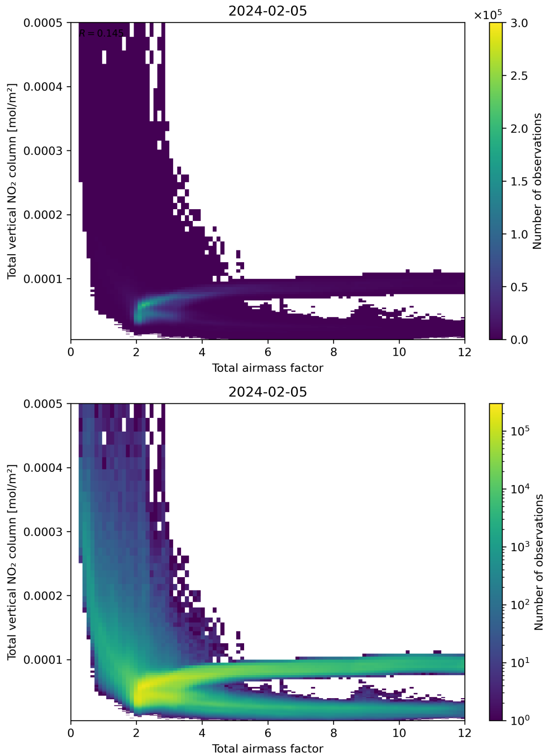
Figure 67: Scatter density plot of “Total airmass factor” against “Total vertical NO 2 column” for 2024-02-04 to 2024-02-06.
