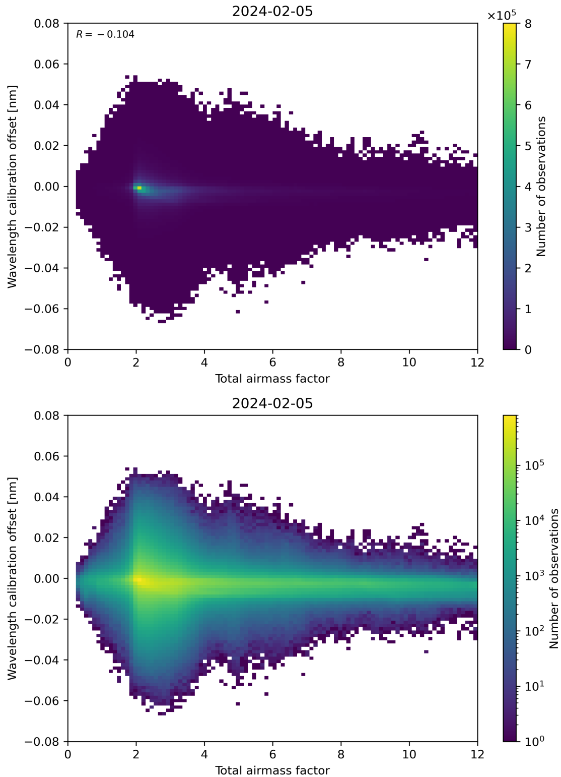
Figure 70: Scatter density plot of “Total airmass factor” against “Wavelength calibration offset” for 2024-02-04 to 2024-02-06.
