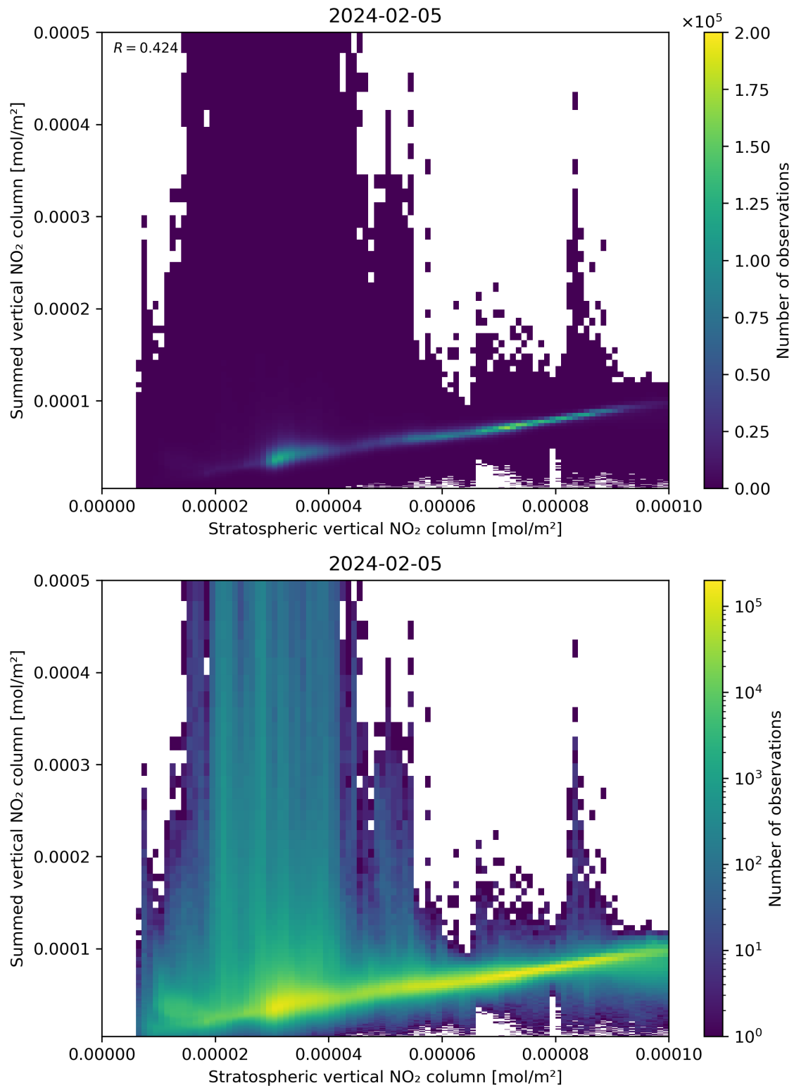
Figure 98: Scatter density plot of “Stratospheric vertical NO 2 column” against “Summed vertical NO 2 column” for 2024-02-04 to 2024-02-06.
