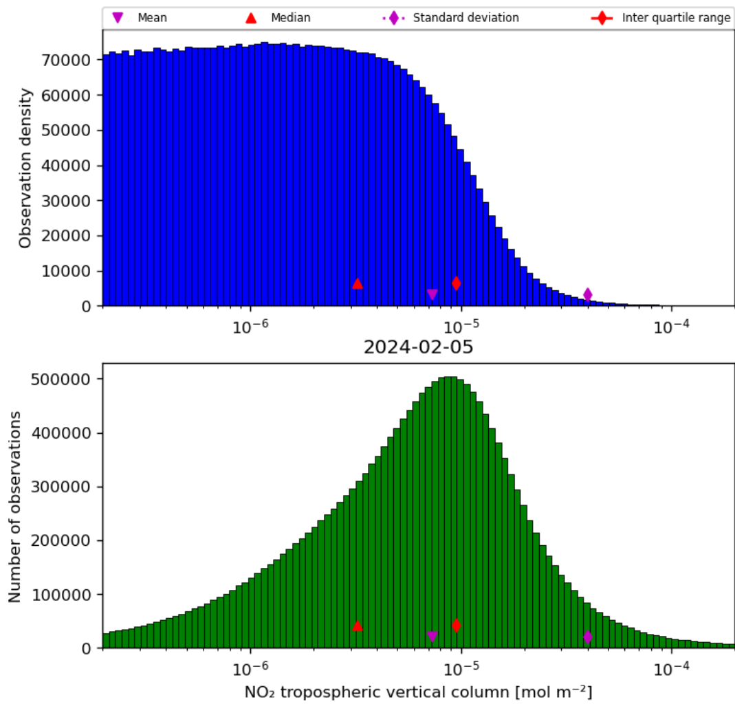
Figure 29: Histogram of “NO 2 tropospheric vertical column” for 2024-02-04 to 2024-02-06
