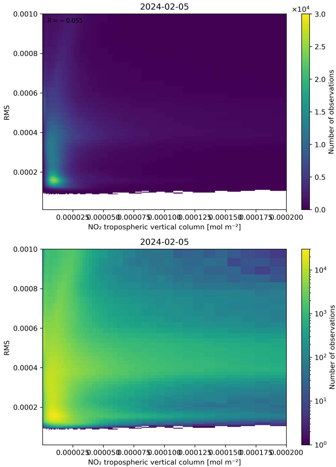
Figure 142: Scatter density plot of “NO 2 tropospheric vertical column” against “RMS” for 2024-02-04 to 2024-02-06.
