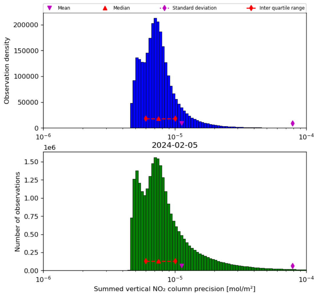
Figure 41: Histogram of "Summed vertical NO 2 column precision" for 2024-02-04 to 2024-02-06
