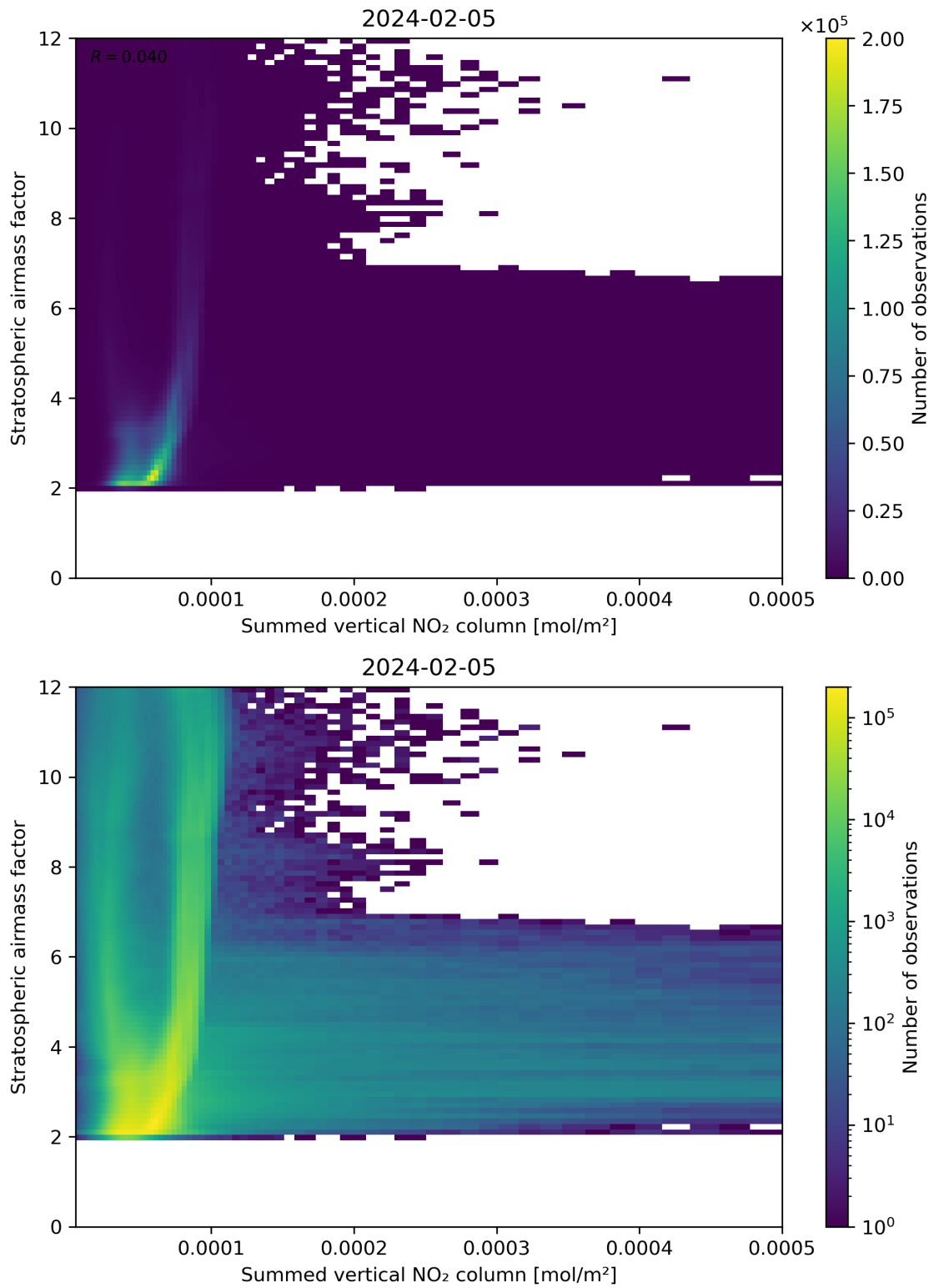
Figure 103: Scatter density plot of “Summed vertical NO 2 column” against “Stratospheric air mass factor” for 2024-02-04 to 2024-02-06.
