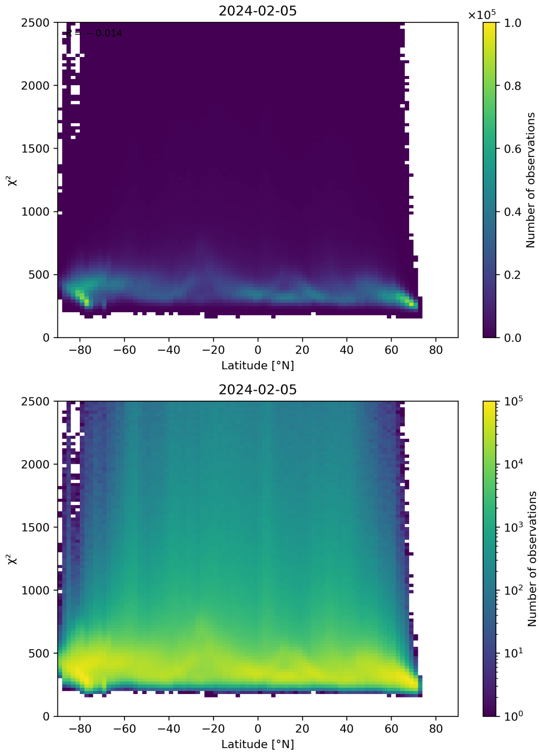
Figure 86: Scatter density plot of “Latitude” against “ \chi^2 ” for 2024-02-04 to 2024-02-06.
