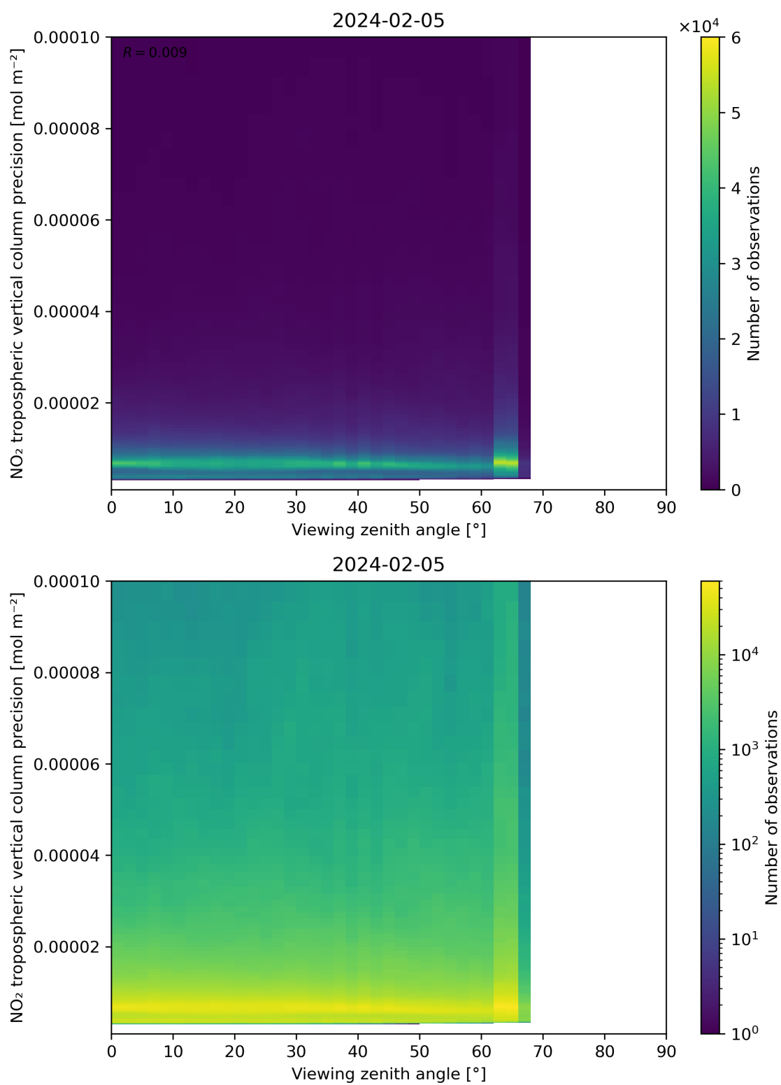
Figure 170: Scatter density plot of “Viewing zenith angle” against “NO 2 tropospheric vertical column precision” for 2024-02-04 to 2024-02-06.
