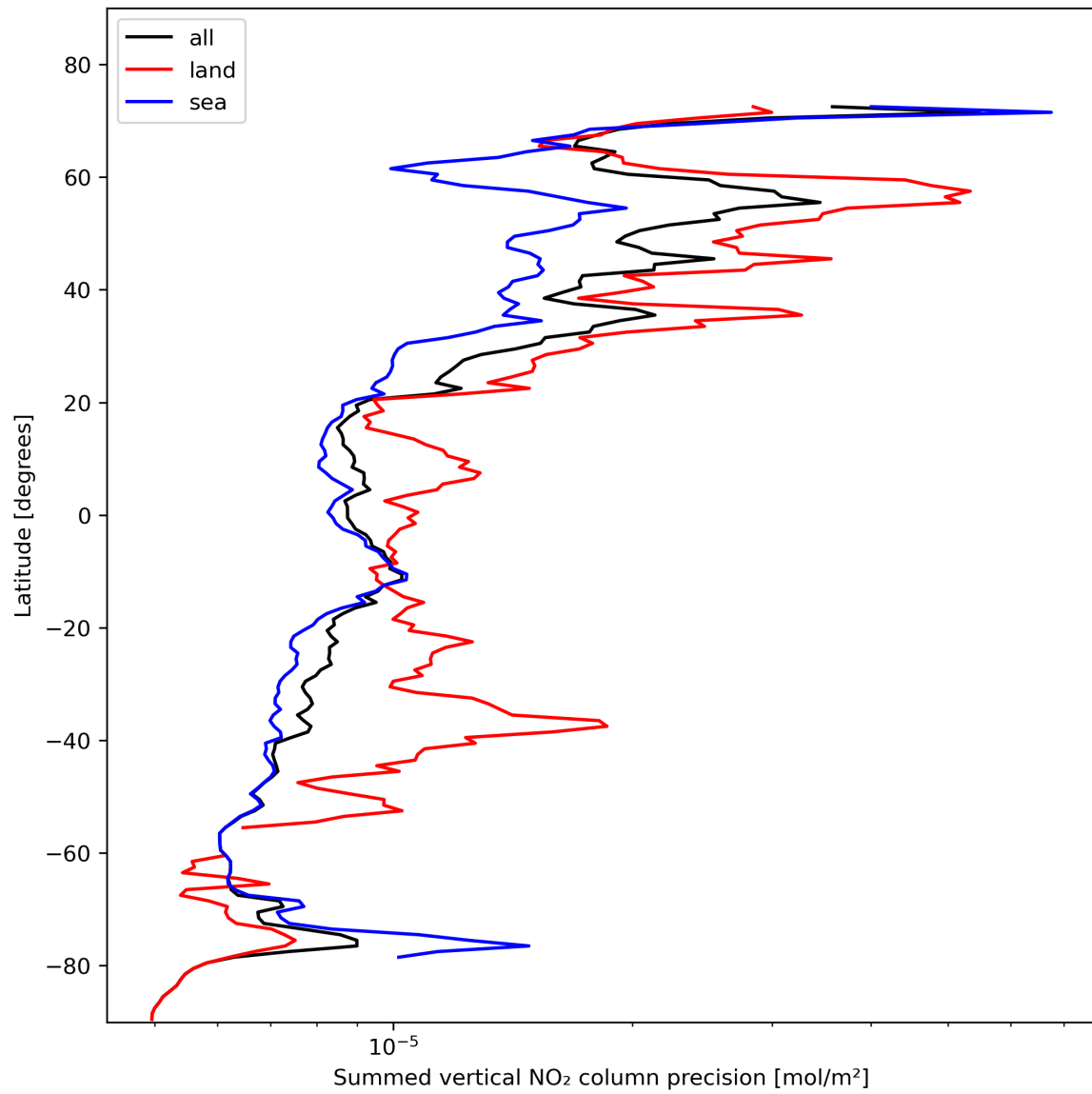
Figure 24: Zonal average of “Summed vertical NO 2 column precision” for 2024-02-04 to 2024-02-06.
