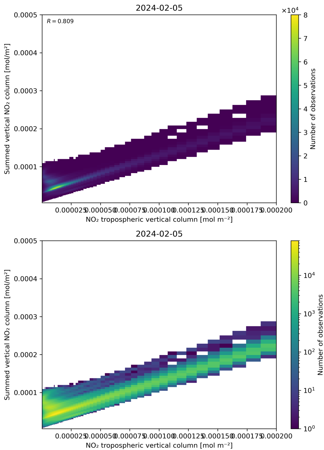
Figure 126: Scatter density plot of “NO 2 tropospheric vertical column” against “Summed vertical NO 2 column” for 2024-02-04 to 2024-02-06.
