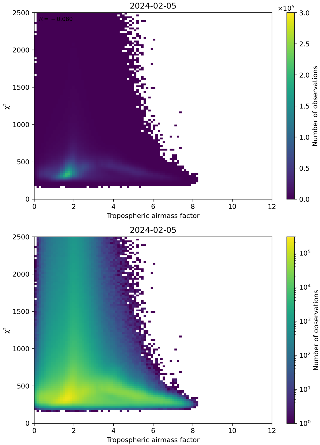
Figure 73: Scatter density plot of “Tropospheric airmass factor” against “ \chi^2 ” for 2024-02-04 to 2024-02-06.
