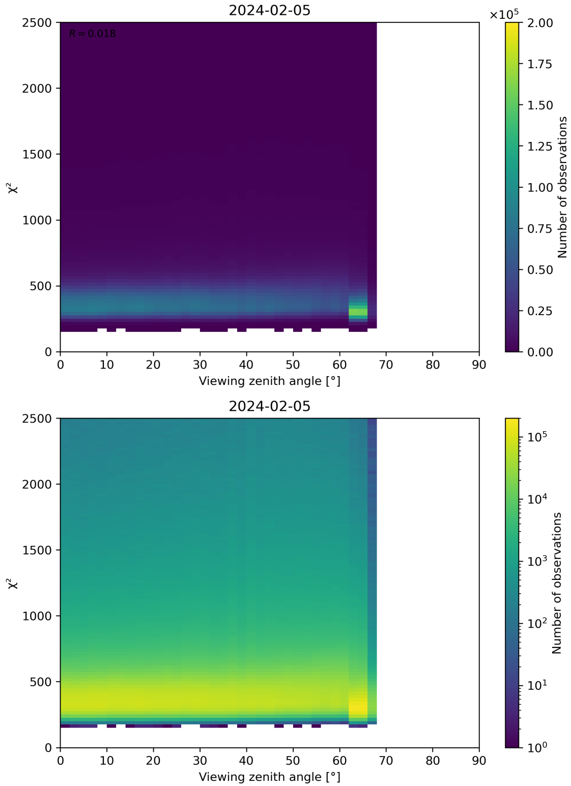
Figure 162: Scatter density plot of “Viewing zenith angle” against “ \chi^2 ” for 2024-02-04 to 2024-02-06.
