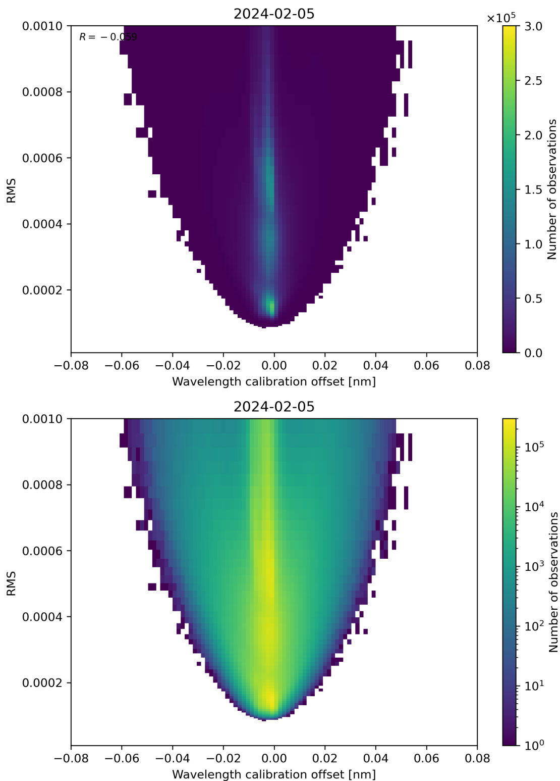
Figure 181: Scatter density plot of “Wavelength calibration offset” against “RMS” for 2024-02-04 to 2024-02-06.
