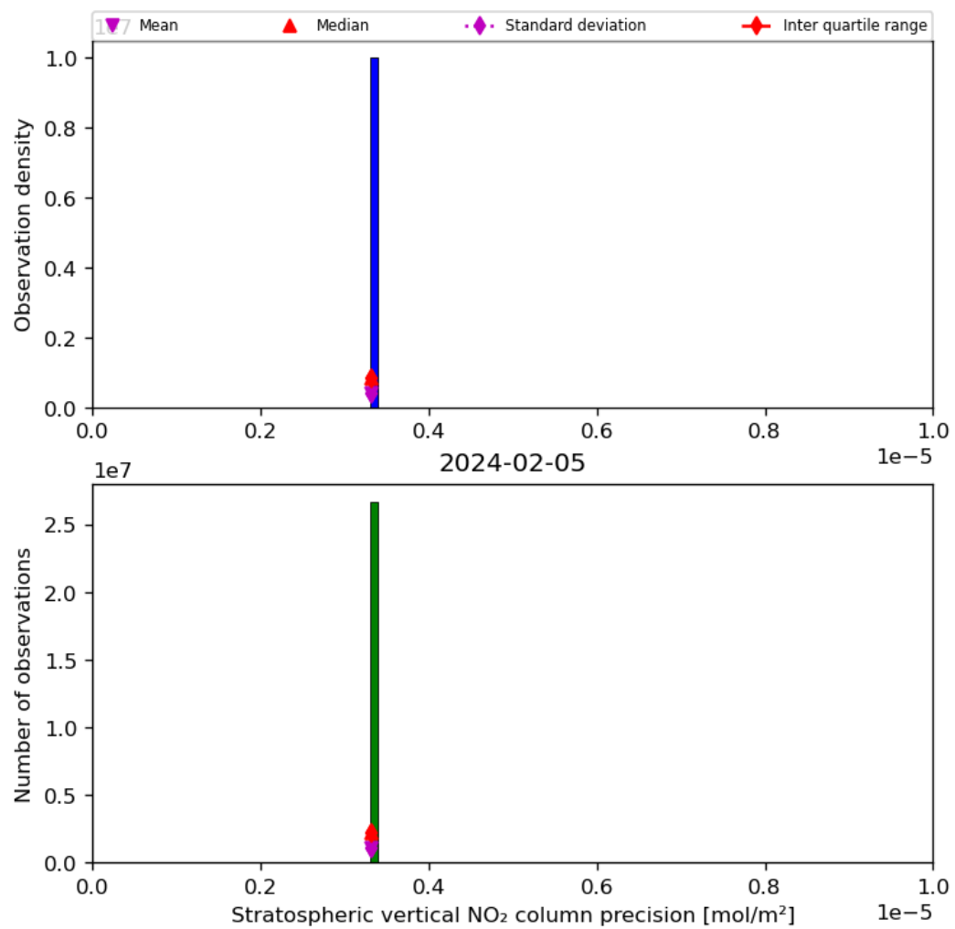
Figure 37: Histogram of “Stratospheric vertical NO 2 column precision” for 2024-02-04 to 2024-02-06
