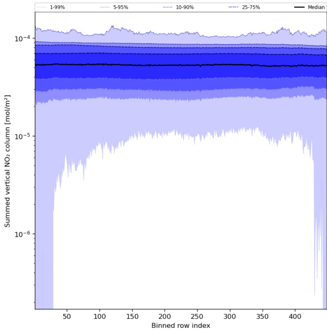
Figure 57: Along track statistics of “Summed vertical NO 2 column” for 2024-02-04 to 2024-02-06
