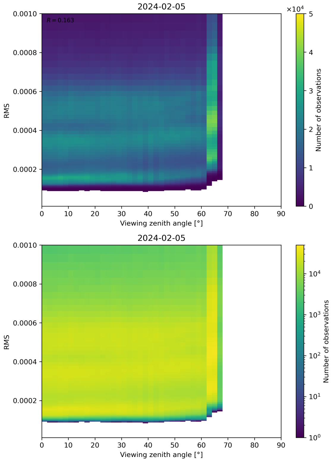
Figure 171: Scatter density plot of “Viewing zenith angle” against “RMS” for 2024-02-04 to 2024-02-06.
