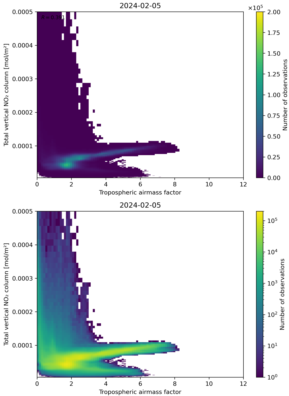
Figure 77: Scatter density plot of “Tropospheric airmass factor” against “Total vertical NO 2 column” for 2024-02-04 to 2024-02-06.
