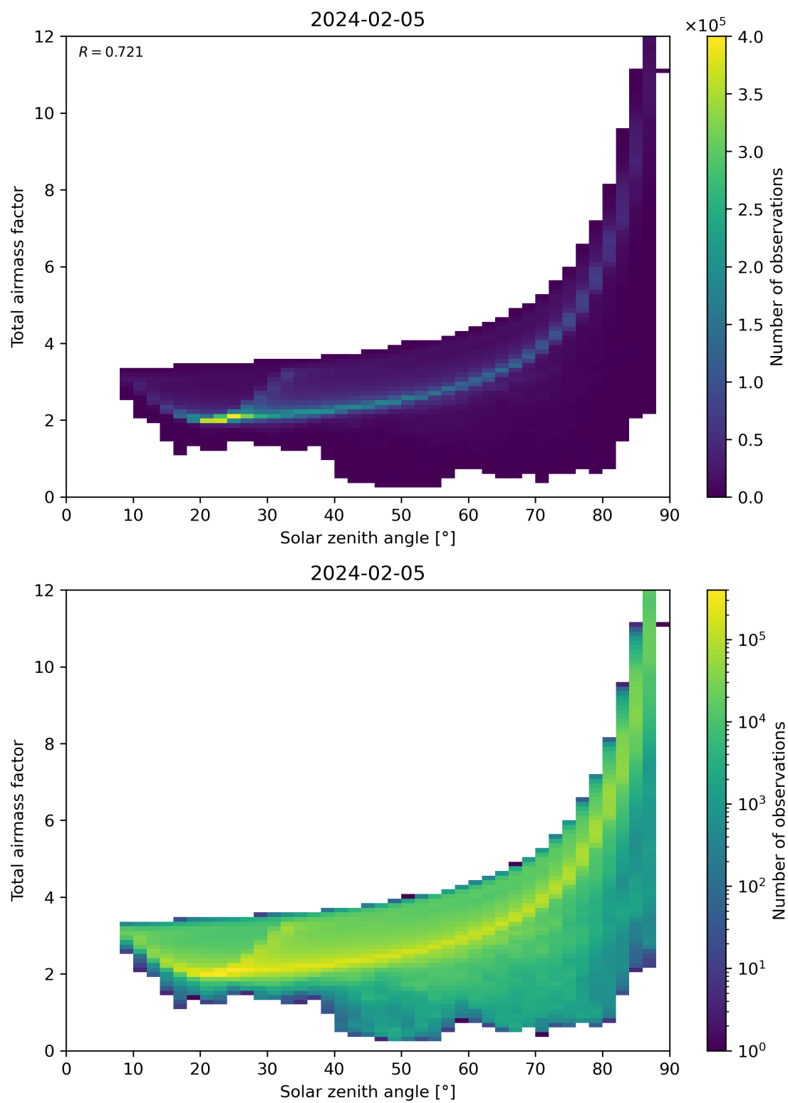
Figure 146: Scatter density plot of “Solar zenith angle” against “Total air mass factor” for 2024-02-04 to 2024-02-06.
