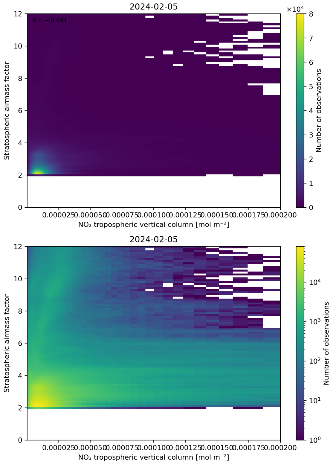
Figure 121: Scatter density plot of “NO 2 tropospheric vertical column” against “Stratospheric airmass factor” for 2024-02-04 to 2024-02-06.
