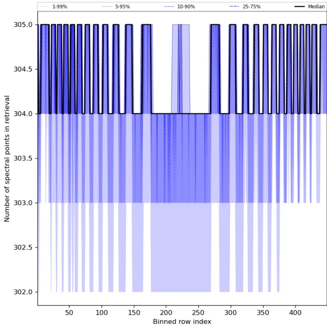
Figure 50: Along track statistics of “Number of spectral points in retrieval” for 2024-02-04 to 2024-02-06
