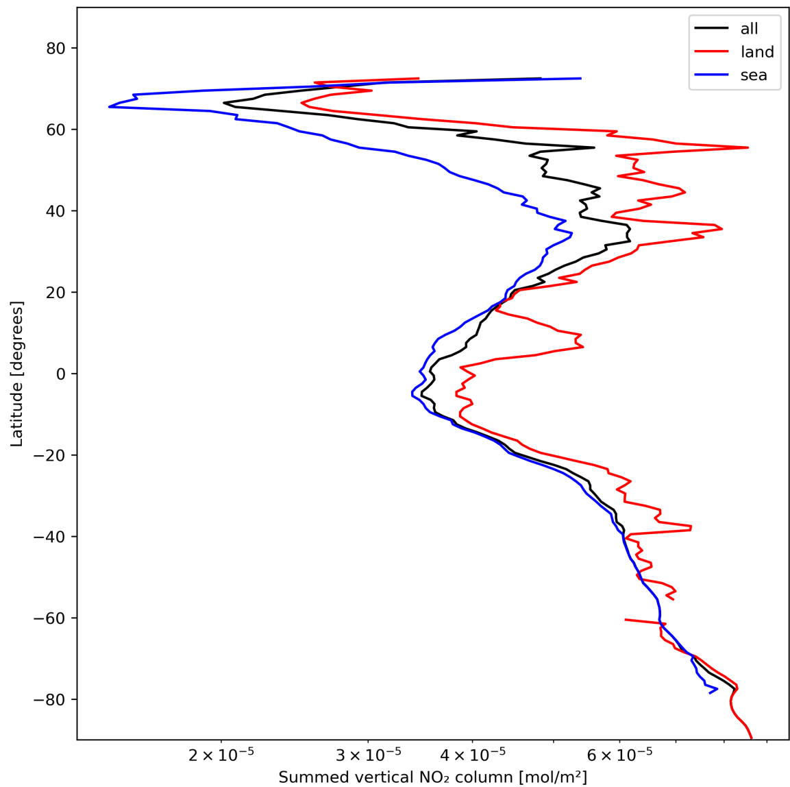
Figure 23: Zonal average of “Summed vertical NO 2 column” for 2024-02-04 to 2024-02-06.
