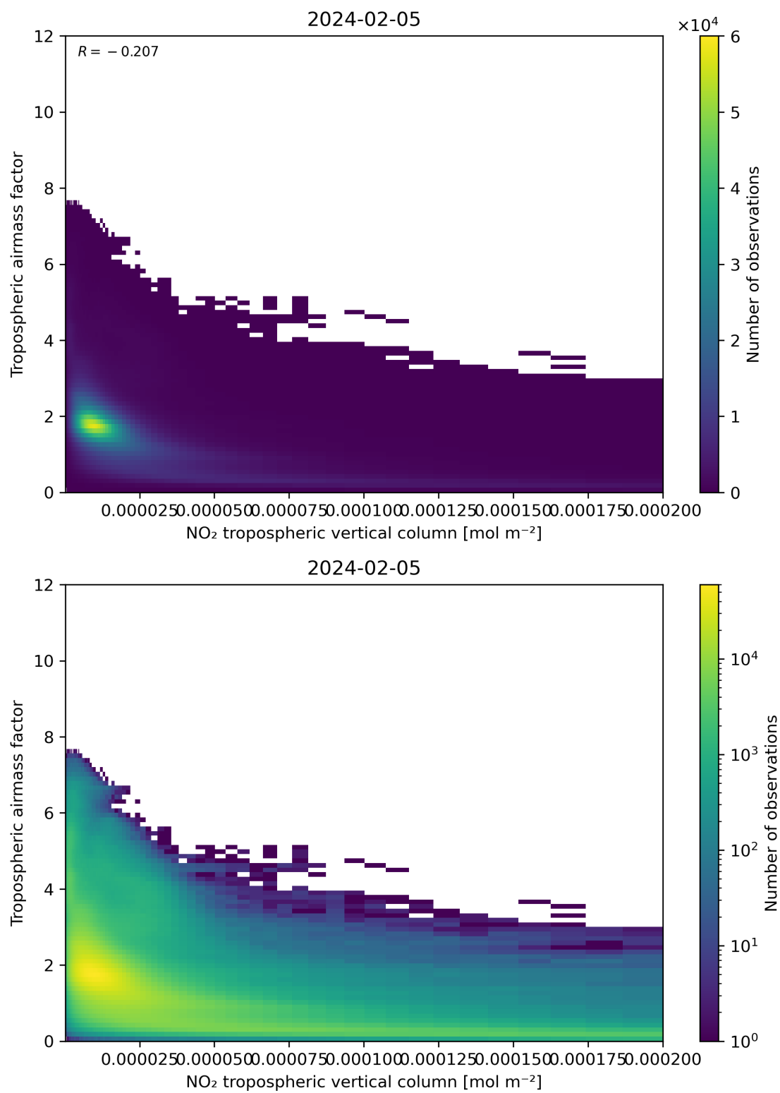
Figure 123: Scatter density plot of “NO 2 tropospheric vertical column” against “Tropospheric air mass factor” for 2024-02-04 to 2024-02-06.
