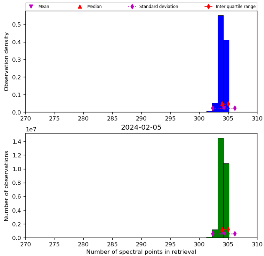
Figure 33: Histogram of “Number of spectral points in retrieval” for 2024-02-04 to 2024-02-06
