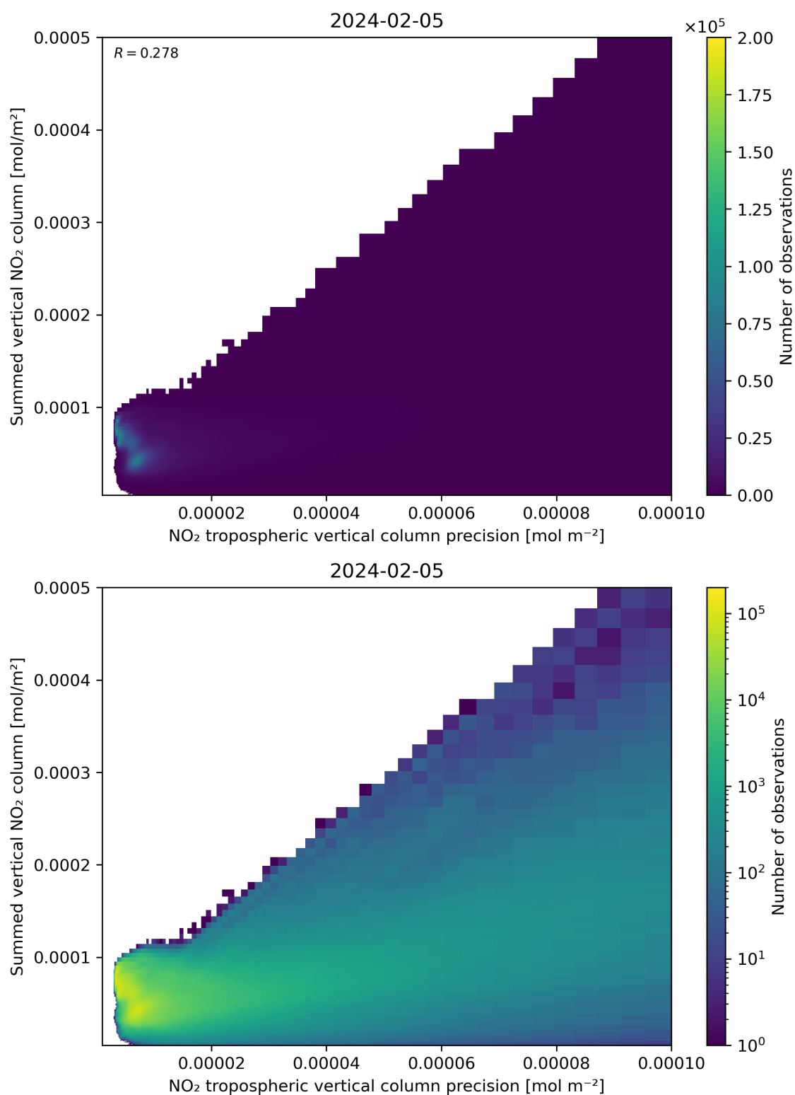
Figure 136: Scatter density plot of “NO 2 tropospheric vertical column precision” against “Summed vertical NO 2 column” for 2024-02-04 to 2024-02-06.
