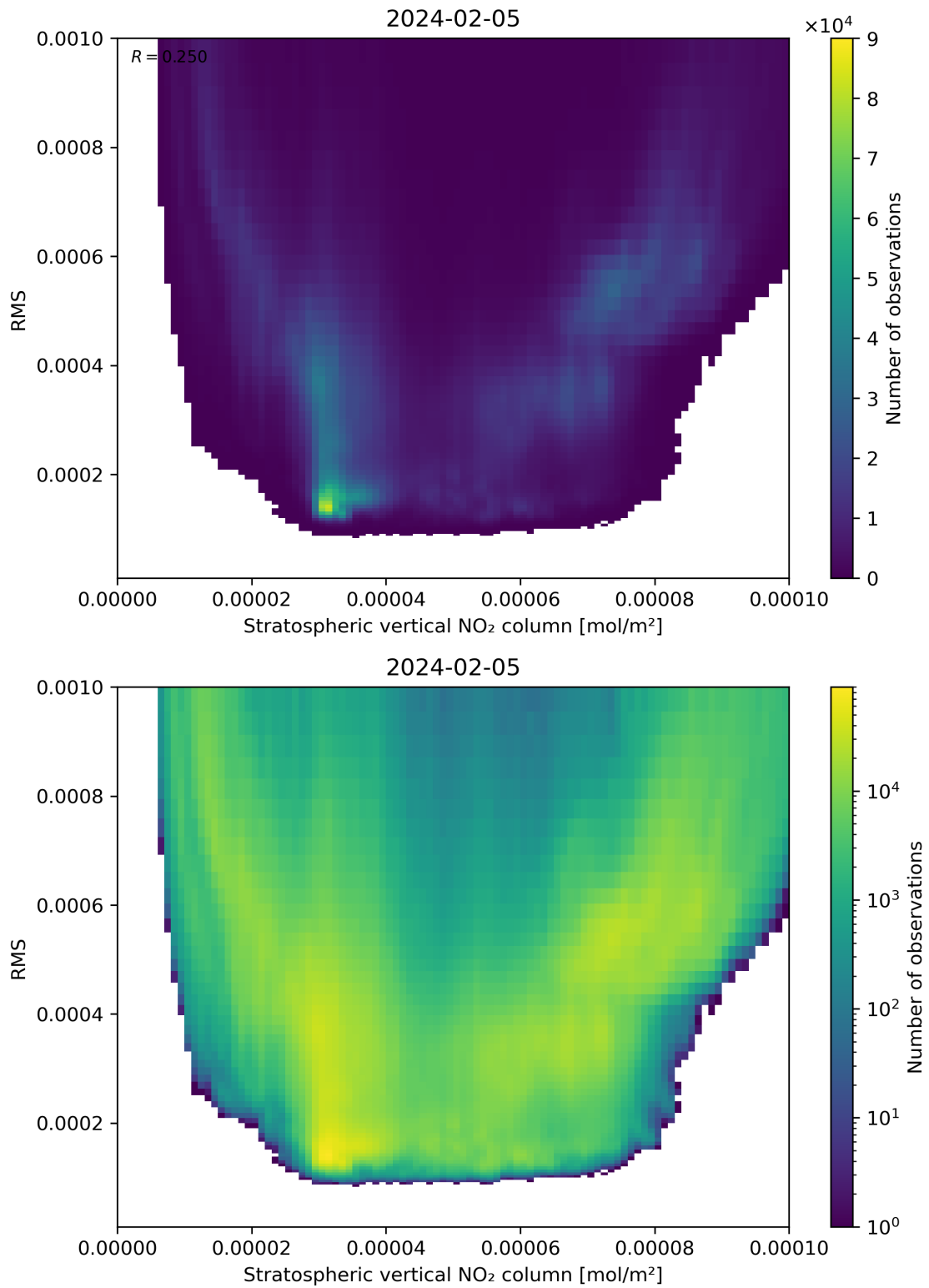
Figure 102: Scatter density plot of “Stratospheric vertical NO 2 column” against “RMS” for 2024-02-04 to 2024-02-06.
