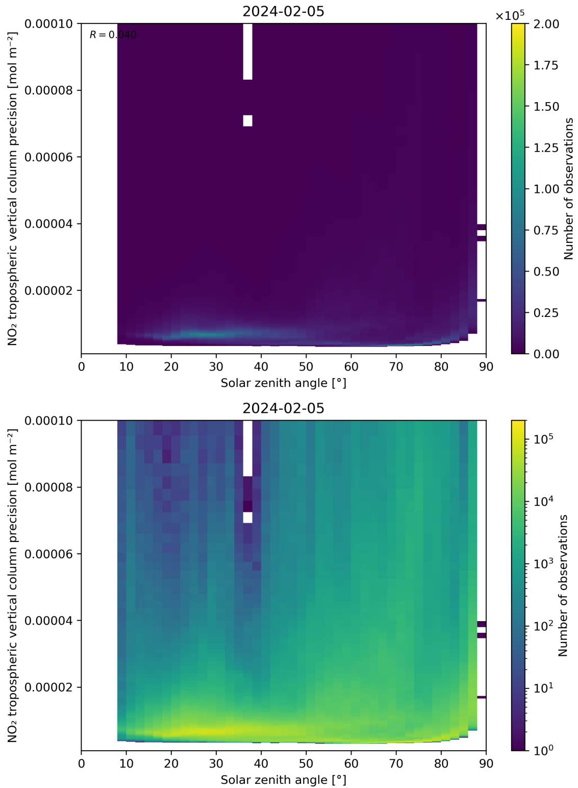
Figure 156: Scatter density plot of “Solar zenith angle” against “NO 2 tropospheric vertical column precision” for 2024-02-04 to 2024-02-06.
