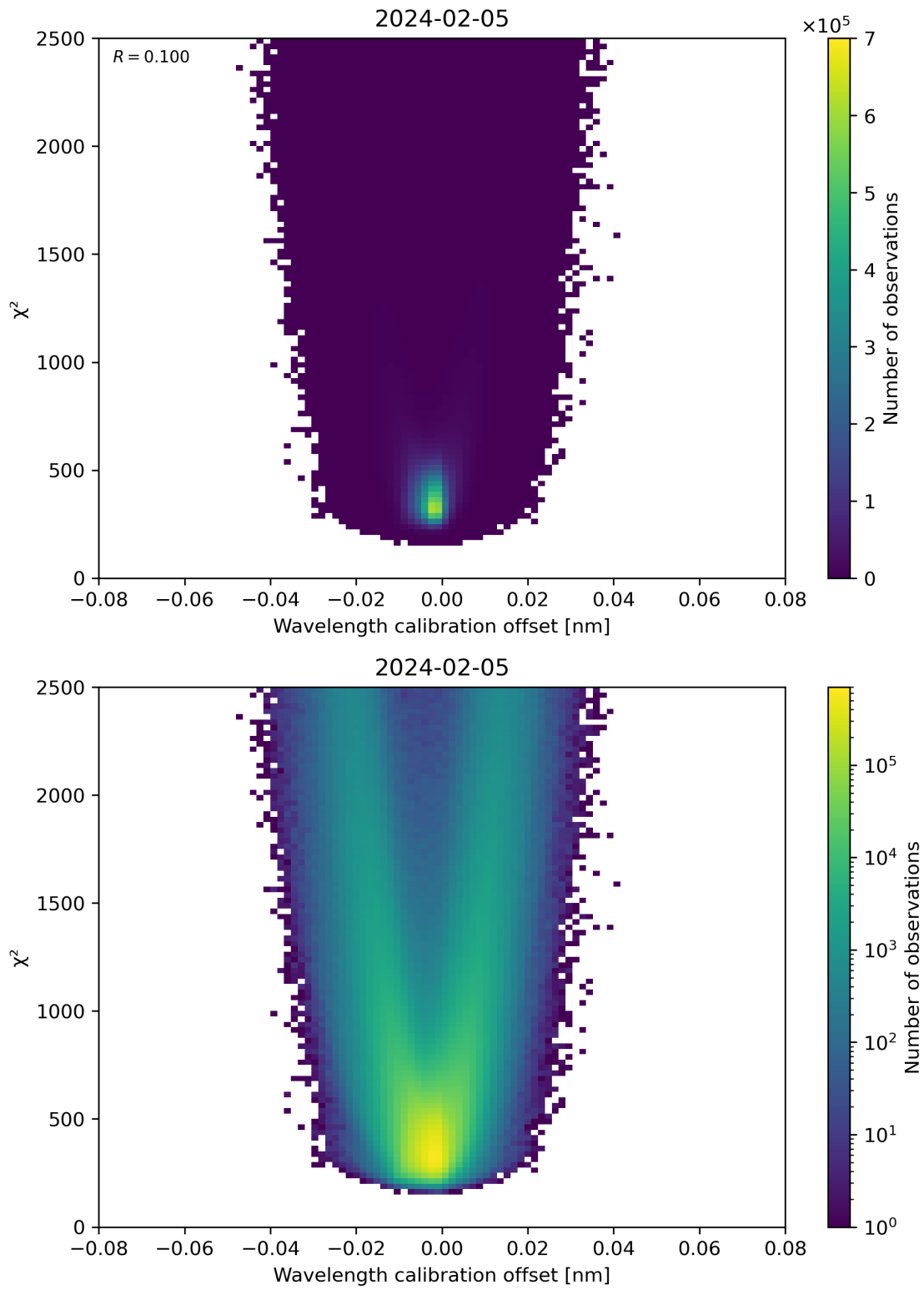
Figure 175: Scatter density plot of “Wavelength calibration offset” against “ \chi^2 ” for 2024-02-04 to 2024-02-06.
