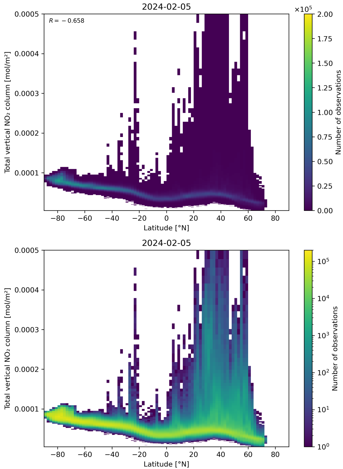
Figure 90: Scatter density plot of “Latitude” against “Total vertical NO 2 column” for 2024-02-04 to 2024-02-06.
