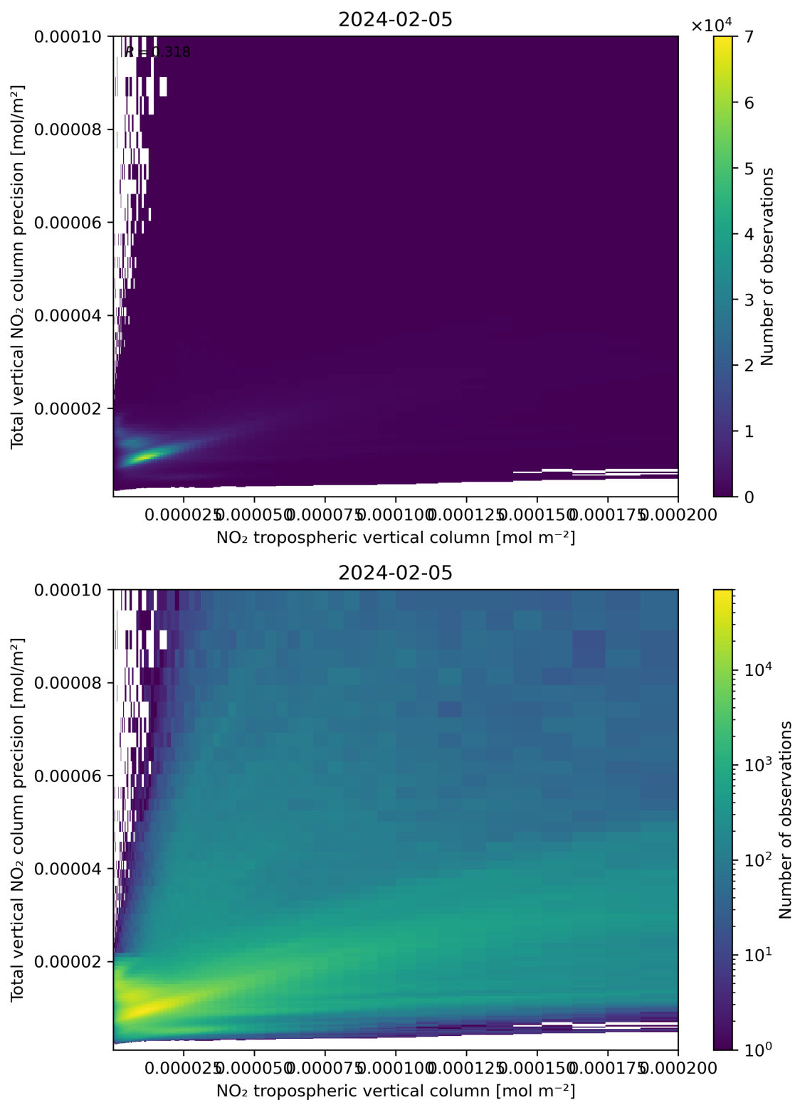
Figure 129: Scatter density plot of “NO 2 tropospheric vertical column” against “Total vertical NO 2 column precision” for 2024-02-04 to 2024-02-06.
