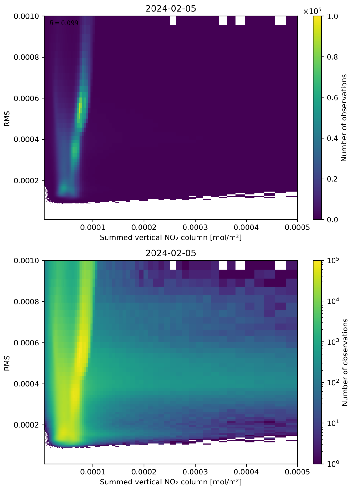
Figure 109: Scatter density plot of “Summed vertical NO 2 column” against “RMS” for 2024-02-04 to 2024-02-06.
