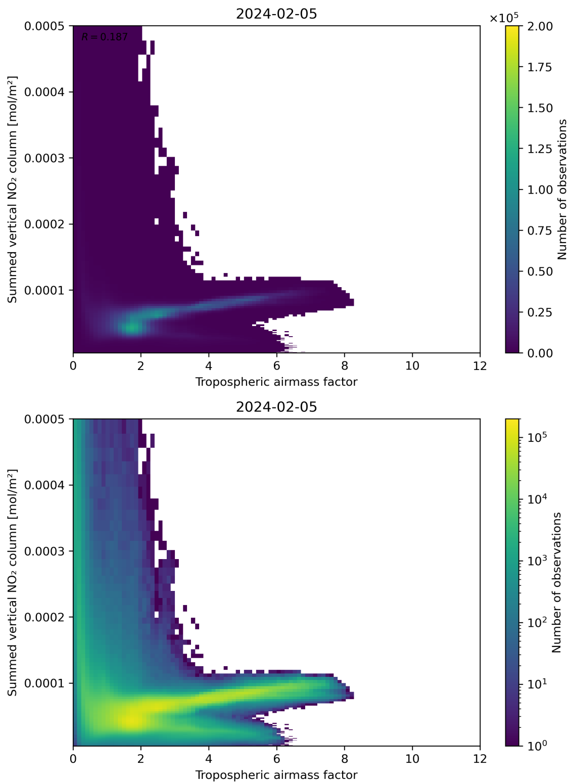
Figure 75: Scatter density plot of “Tropospheric airmass factor” against “Summed vertical NO 2 column” for 2024-02-04 to 2024-02-06.
