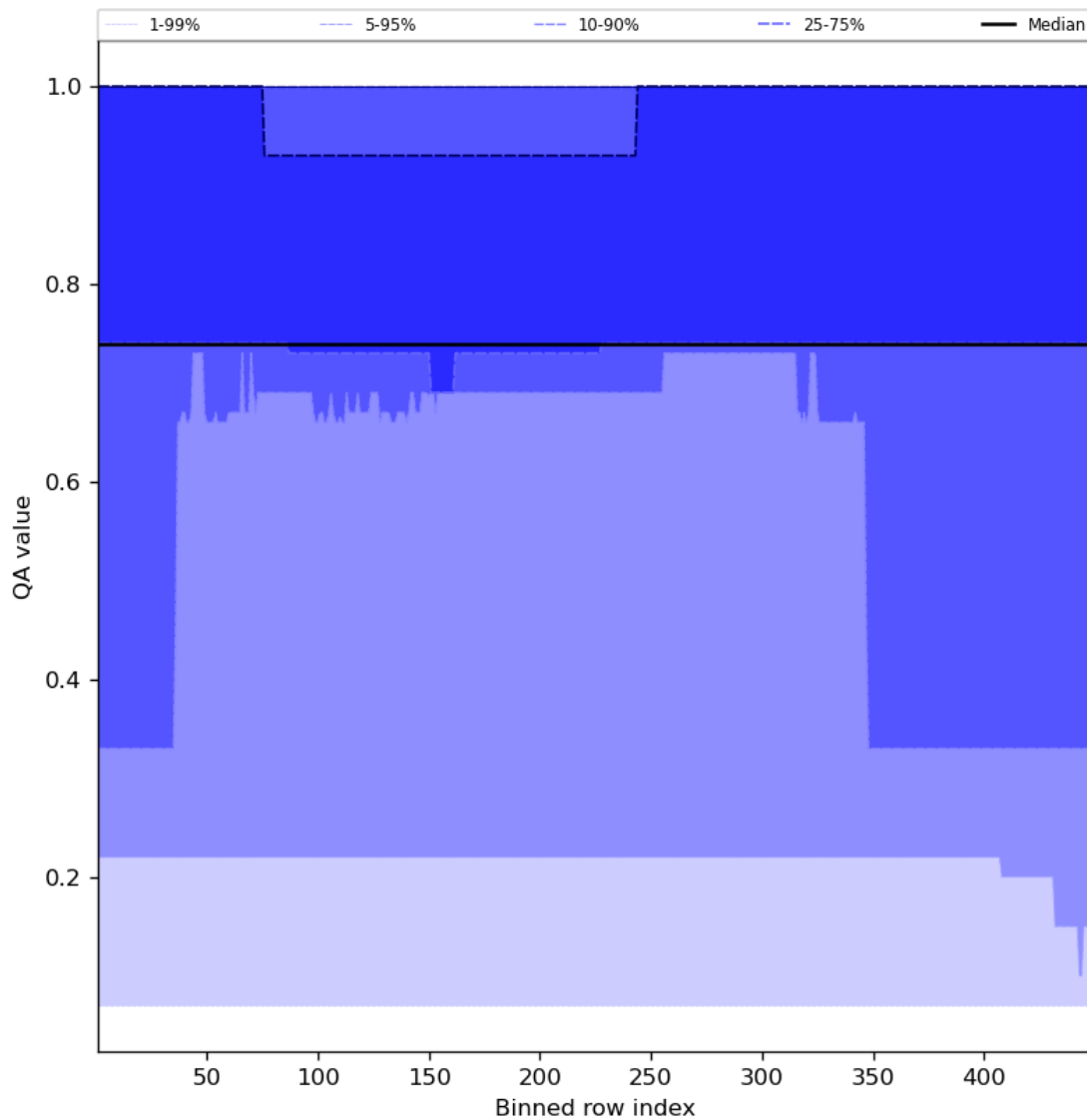
Figure 45: Along track statistics of “QA value” for 2024-02-04 to 2024-02-06
