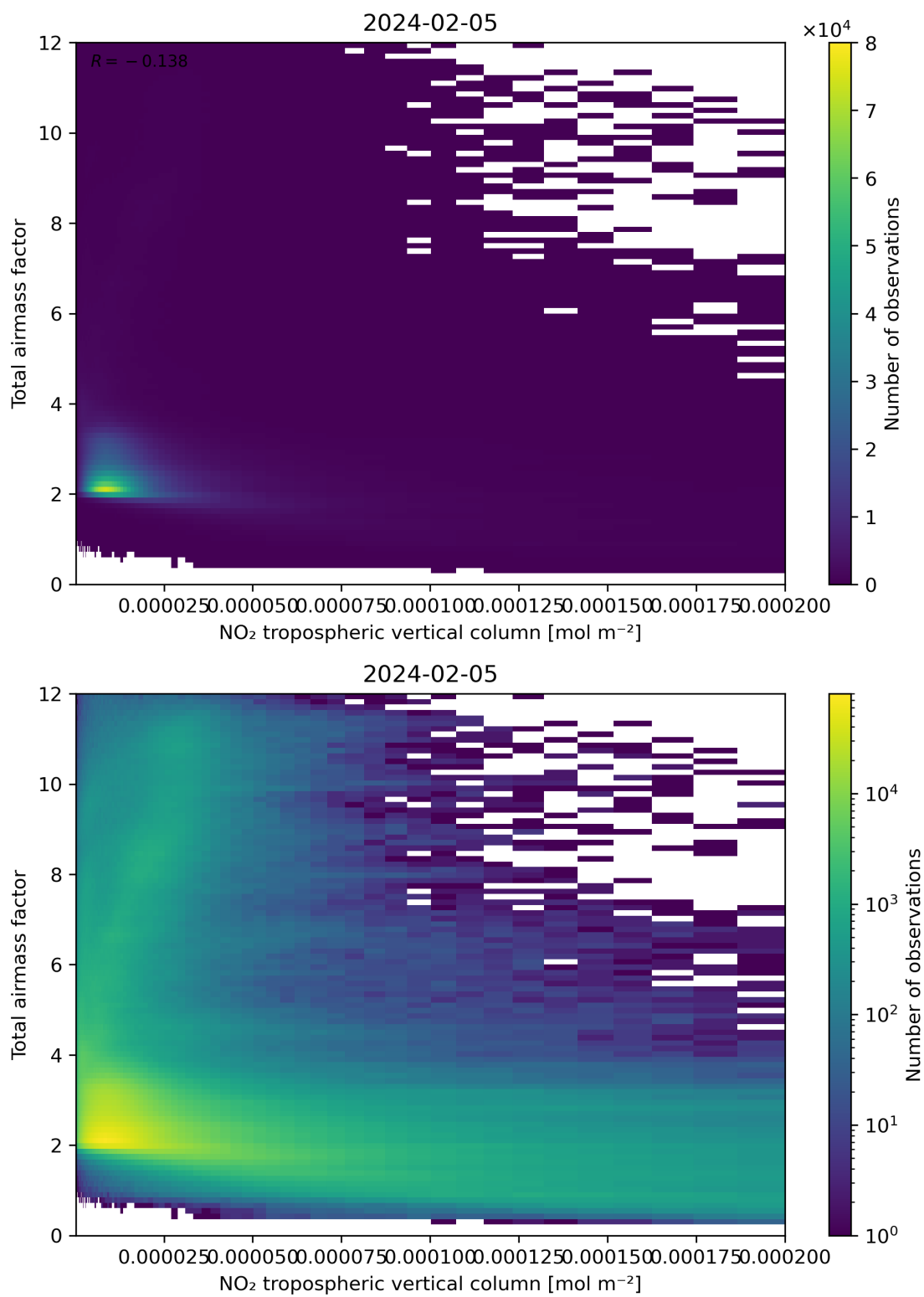
Figure 122: Scatter density plot of “NO 2 tropospheric vertical column” against “Total air mass factor” for 2024-02-04 to 2024-02-06.
