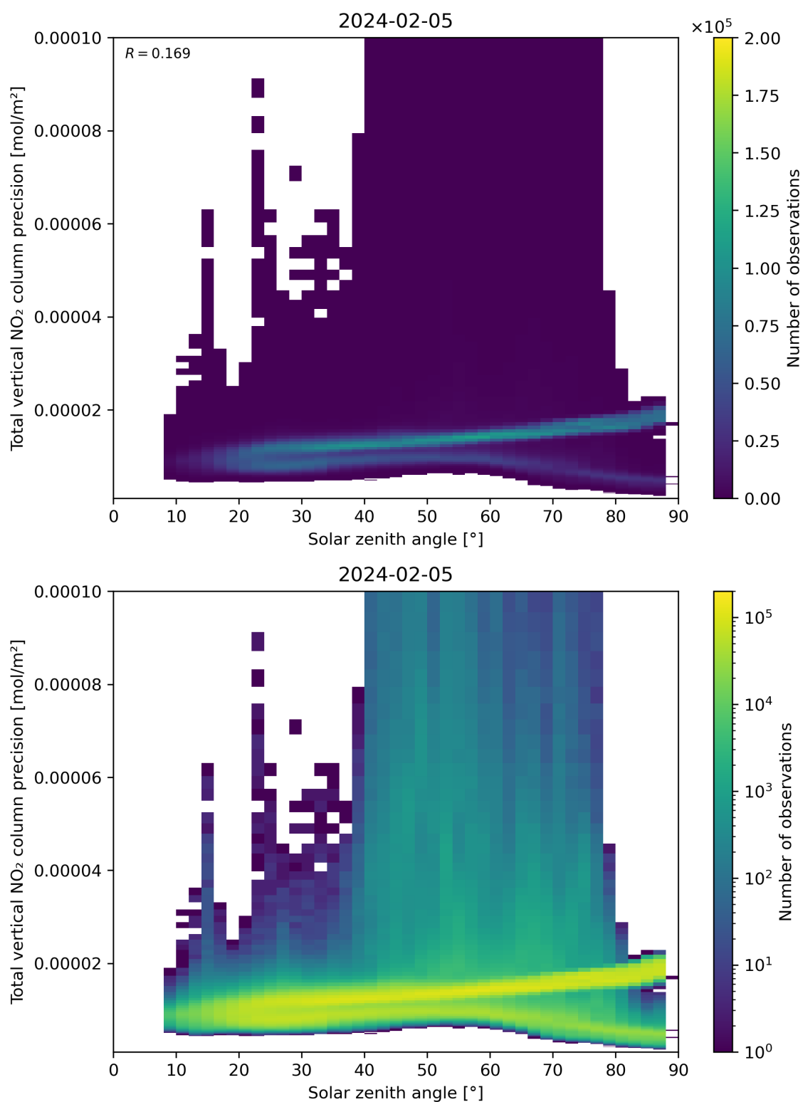
Figure 154: Scatter density plot of “Solar zenith angle” against “Total vertical NO 2 column precision” for 2024-02-04 to 2024-02-06.
