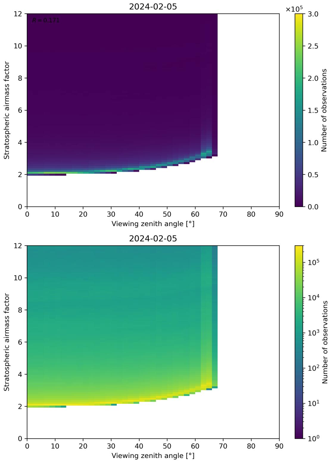
Figure 159: Scatter density plot of “Viewing zenith angle” against “Stratospheric airmass factor” for 2024-02-04 to 2024-02-06.
