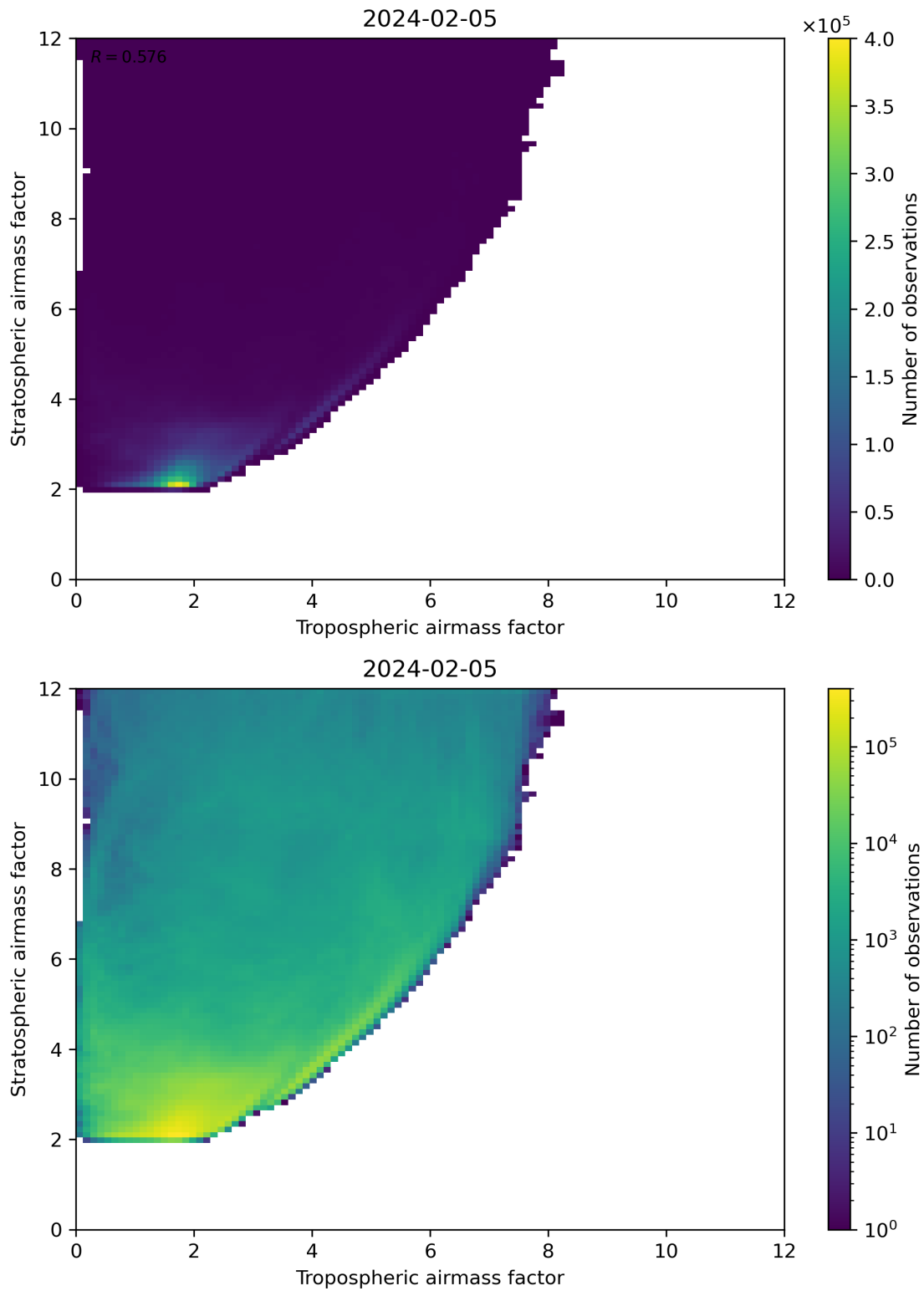
Figure 71: Scatter density plot of “Tropospheric airmass factor” against “Stratospheric airmass factor” for 2024-02-04 to 2024-02-06.
