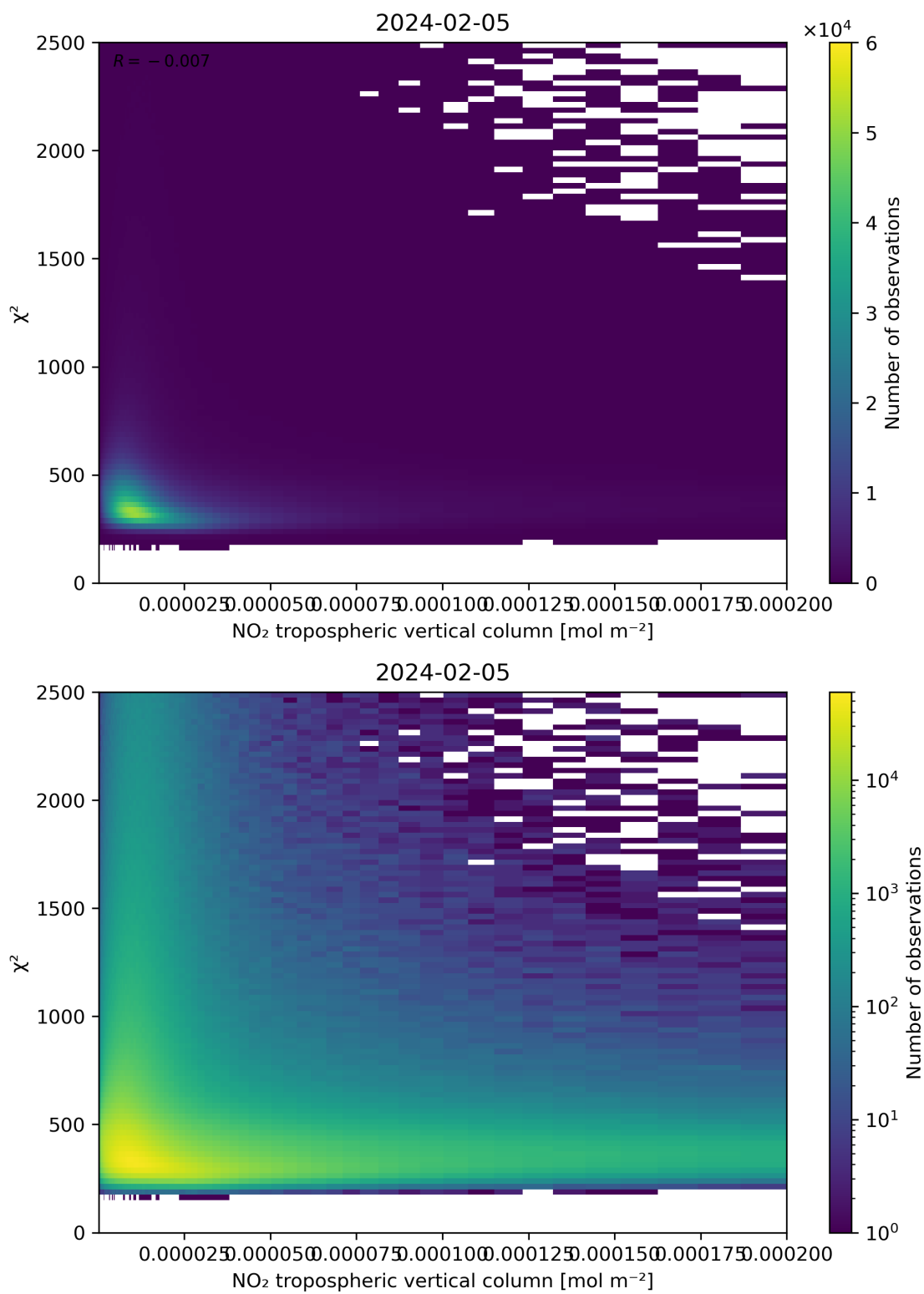
Figure 124: Scatter density plot of “NO 2 tropospheric vertical column” against “ \chi^2 ” for 2024-02-04 to 2024-02-06.
