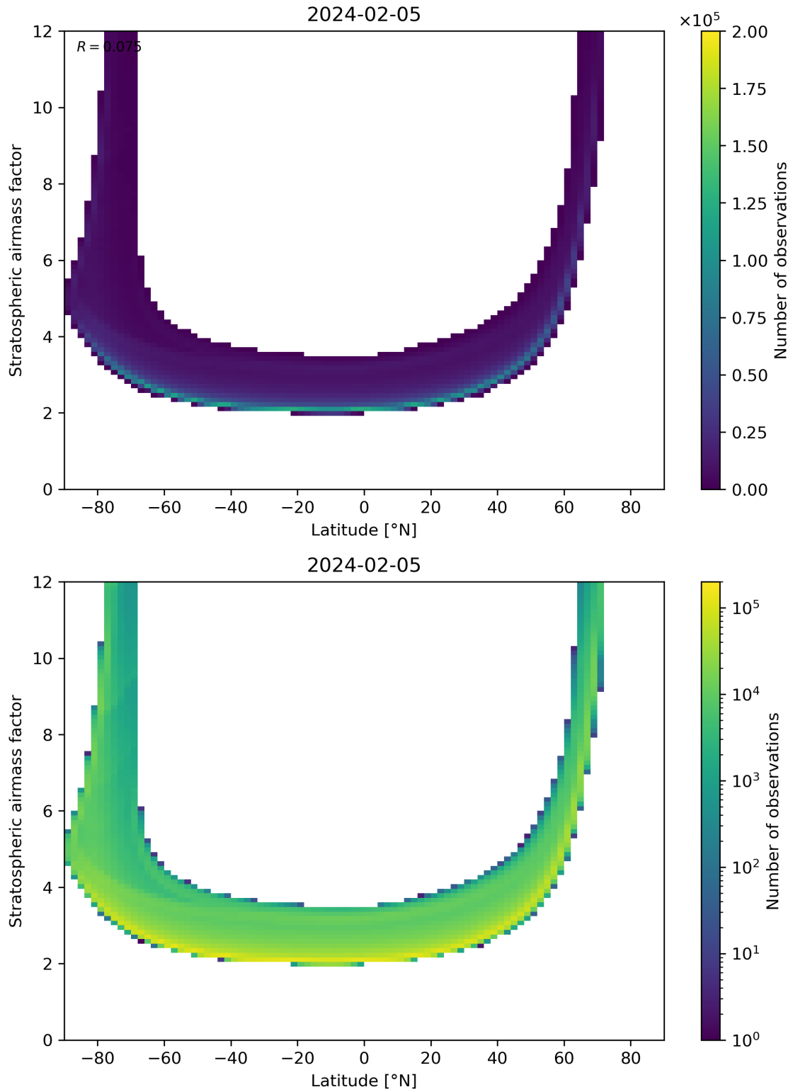
Figure 83: Scatter density plot of “Latitude” against “Stratospheric airmass factor” for 2024-02-04 to 2024-02-06.
