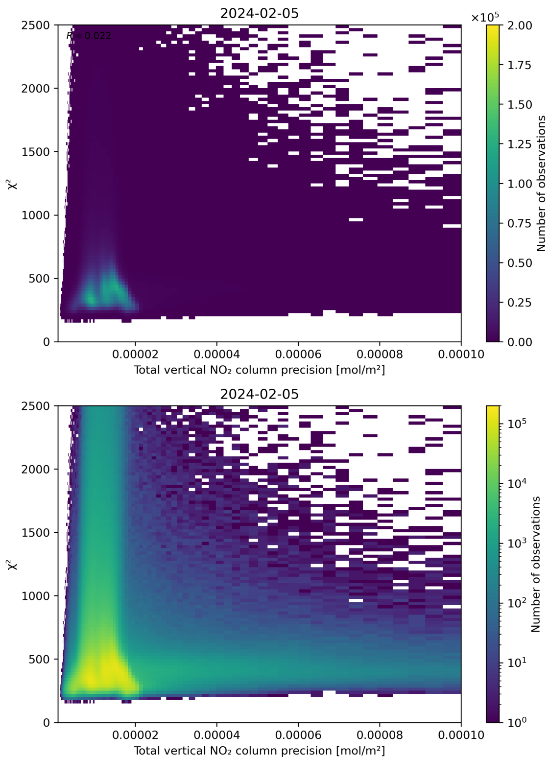
Figure 116: Scatter density plot of “Total vertical NO 2 column precision” against “ \chi^2 ” for 2024-02-04 to 2024-02-06.
