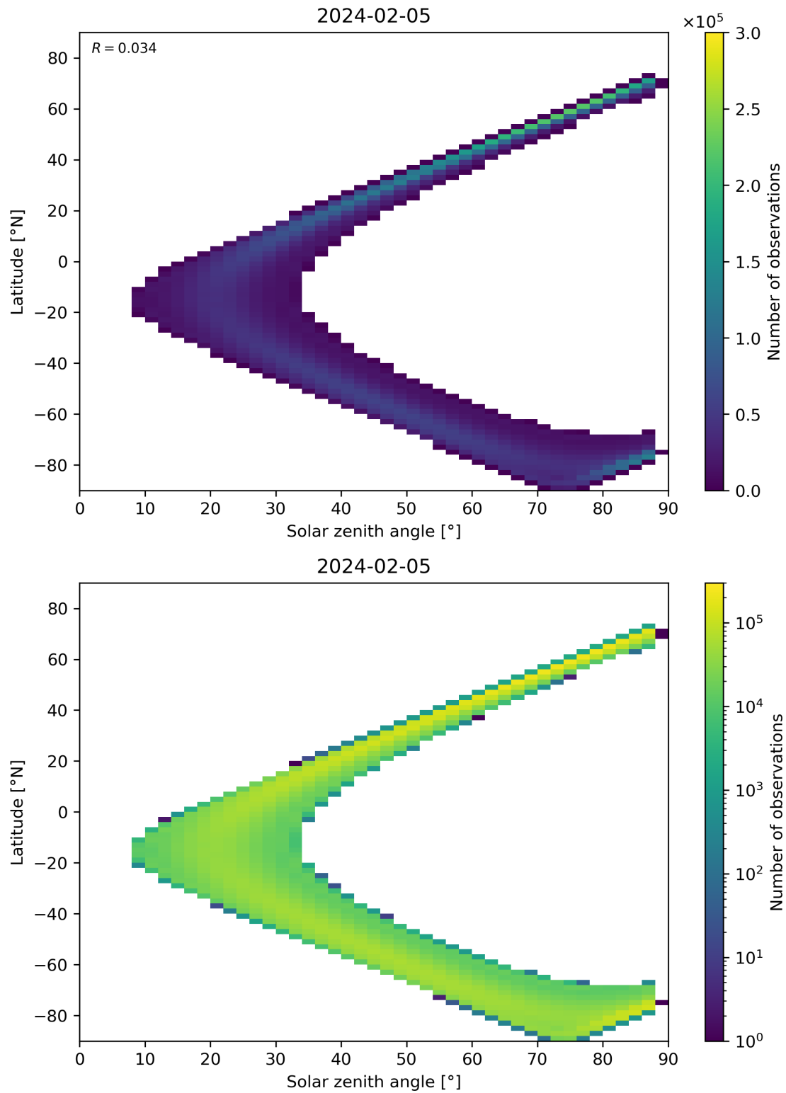
Figure 149: Scatter density plot of “Solar zenith angle” against “Latitude” for 2024-02-04 to 2024-02-06.
