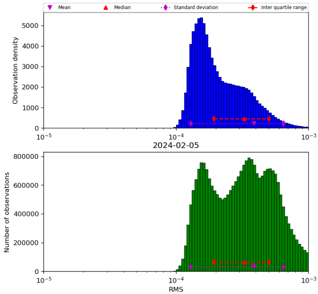
Figure 43: Histogram of “RMS” for 2024-02-04 to 2024-02-06
