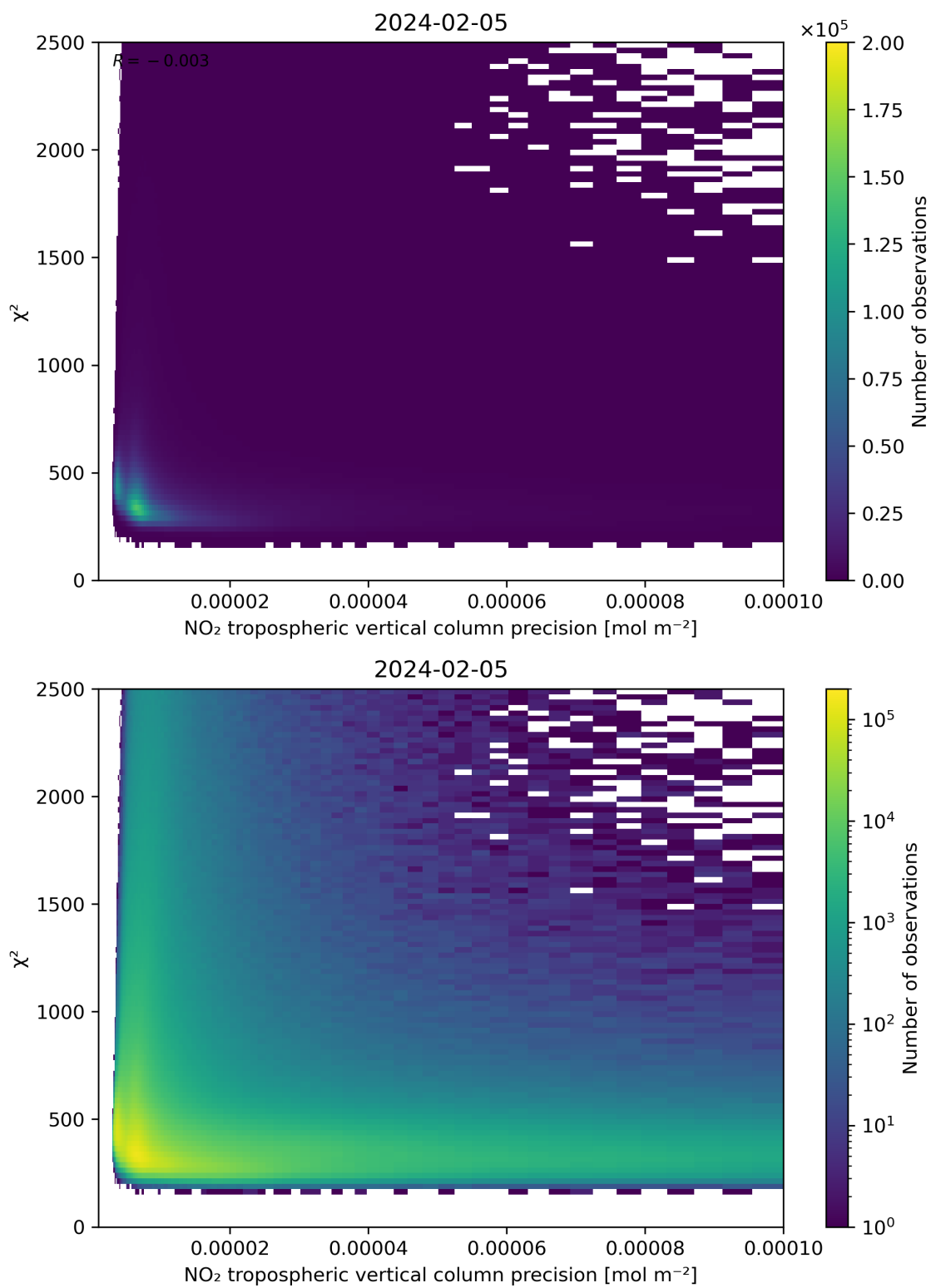
Figure 134: Scatter density plot of “NO 2 tropospheric vertical column precision” against “ \chi^2 ” for 2024-02-04 to 2024-02-06.
