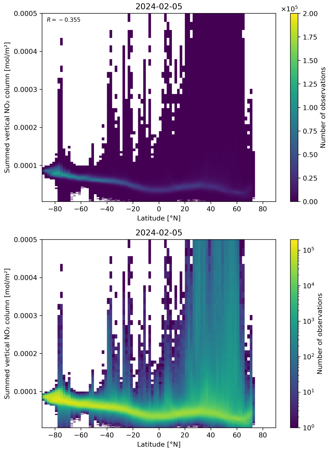
Figure 88: Scatter density plot of “Latitude” against “Summed vertical NO 2 column” for 2024-02-04 to 2024-02-06.
