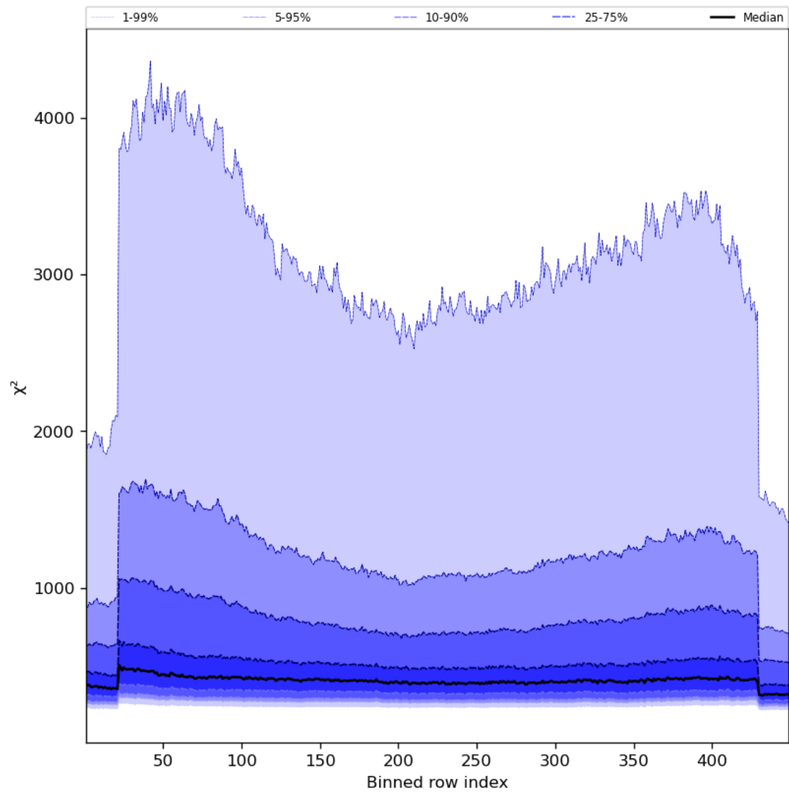
Figure 59: Along track statistics of “ \chi^2 ” for 2024-02-04 to 2024-02-06
