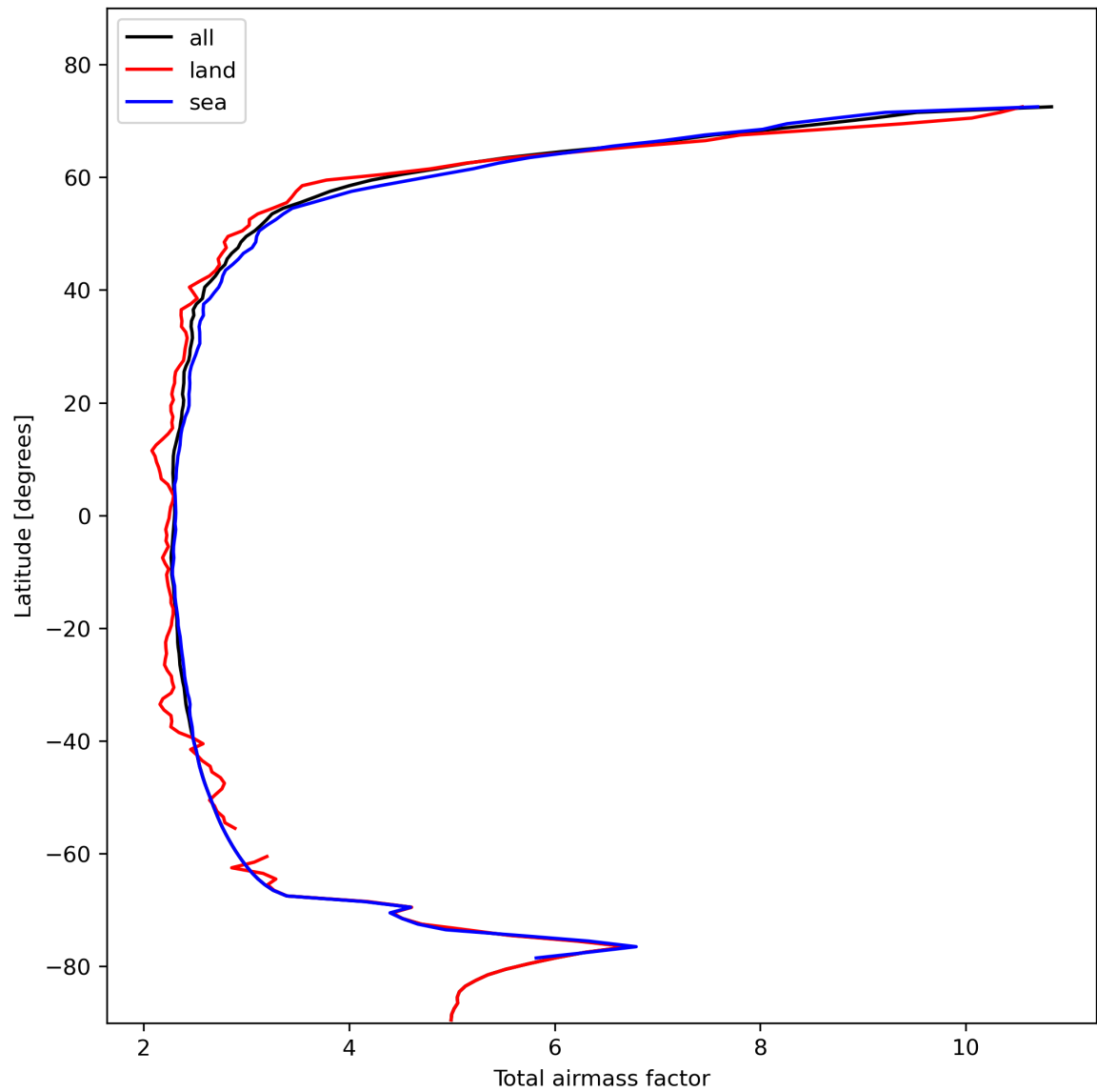
Figure 15: Zonal average of “Total airmass factor” for 2024-02-04 to 2024-02-06.
