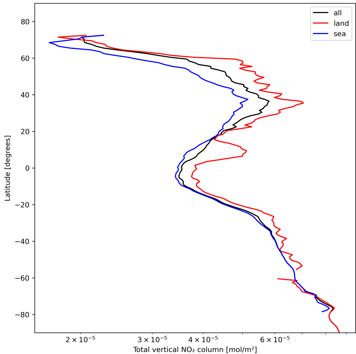
Figure 21: Zonal average of “Total vertical NO 2 column” for 2024-02-04 to 2024-02-06.
