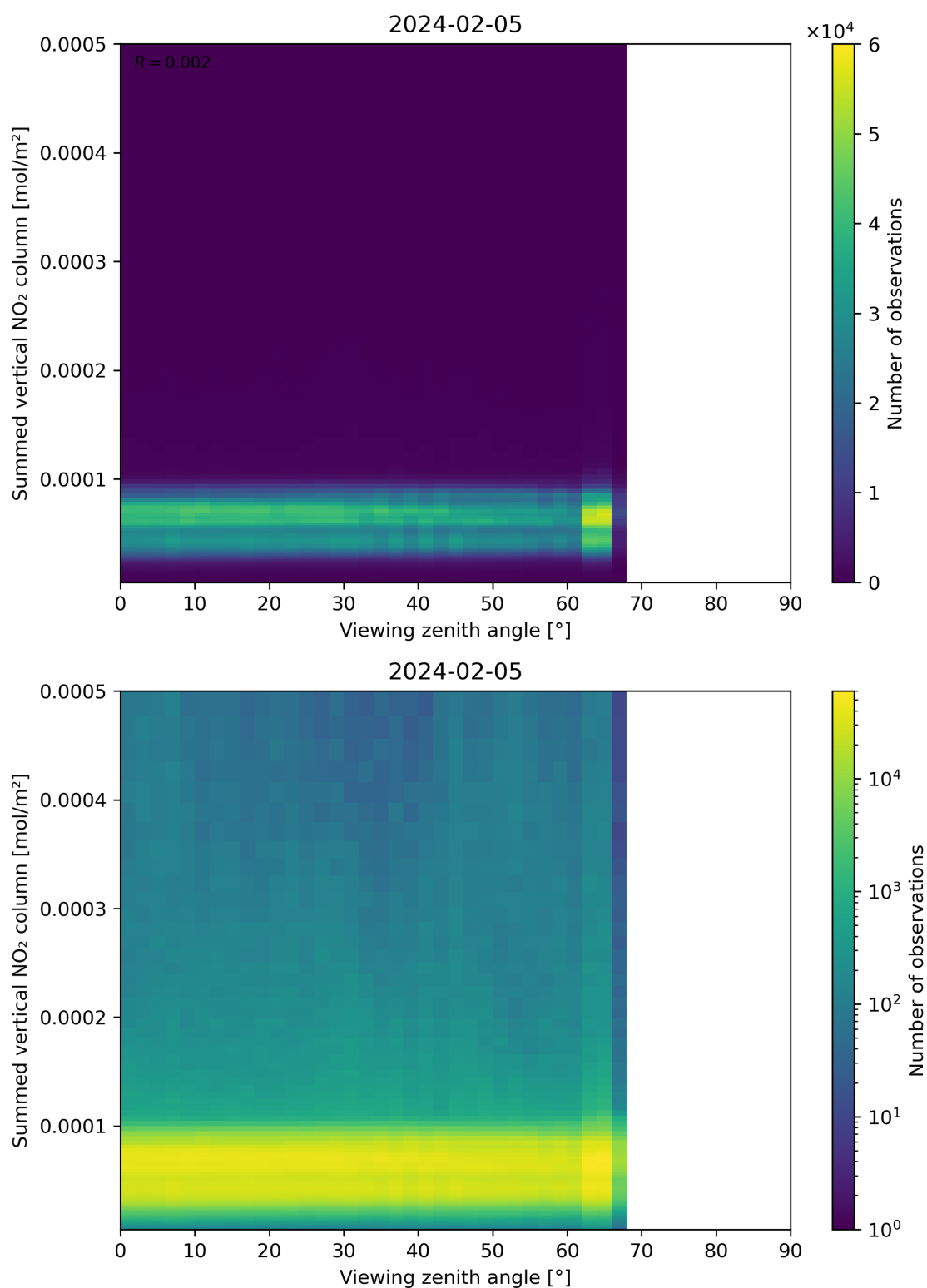
Figure 165: Scatter density plot of “Viewing zenith angle” against “Summed vertical NO 2 column” for 2024-02-04 to 2024-02-06.
