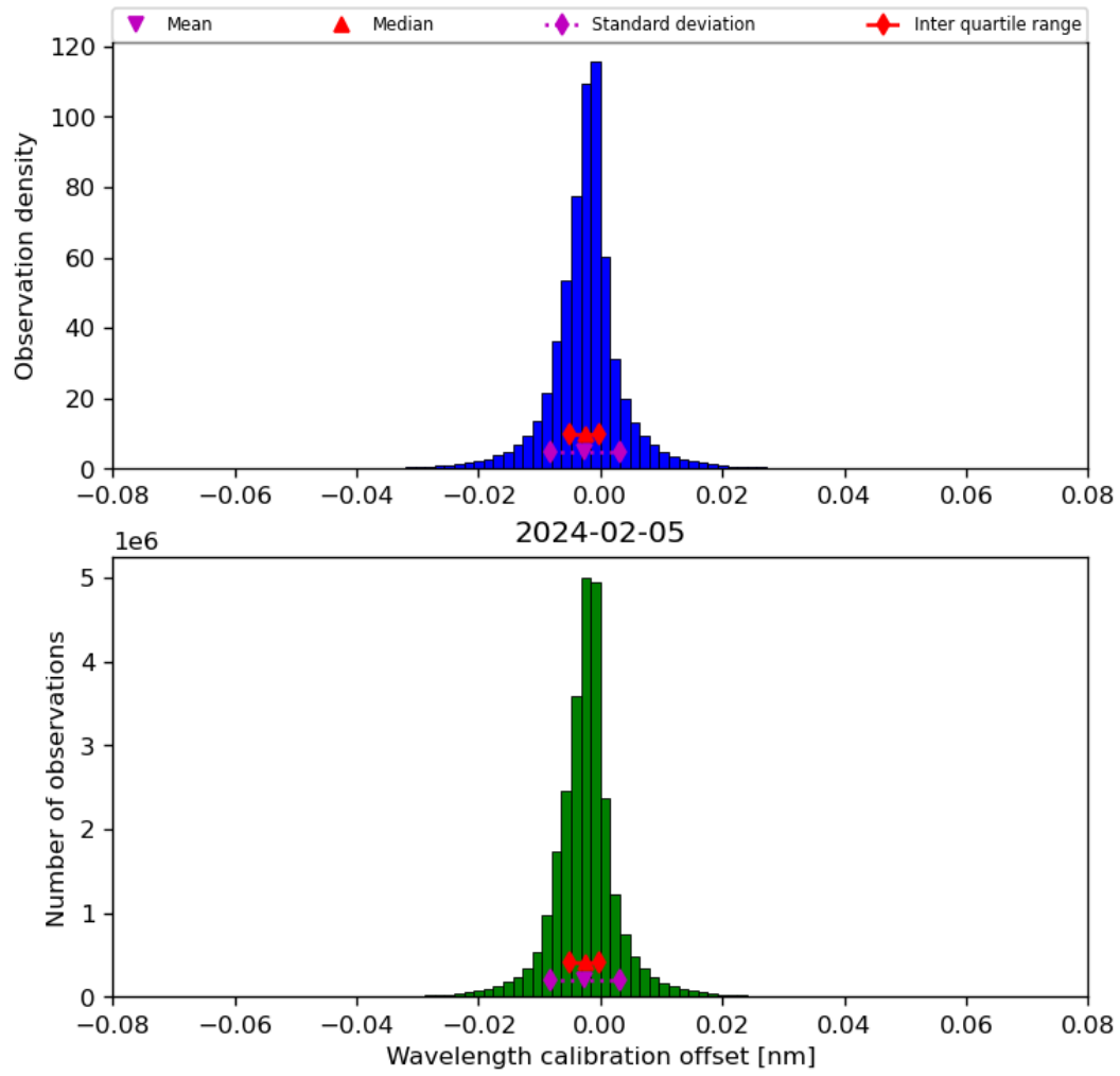
Figure 35: Histogram of “Wavelength calibration offset” for 2024-02-04 to 2024-02-06
