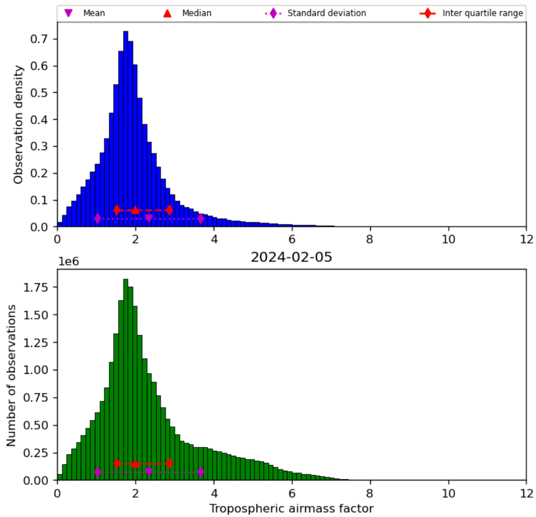
Figure 31: Histogram of “Tropospheric airmass factor” for 2024-02-04 to 2024-02-06
