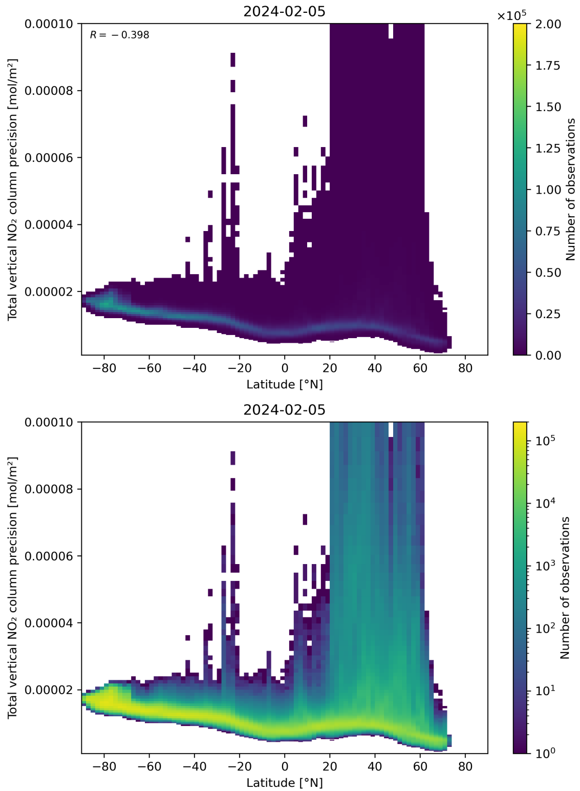
Figure 91: Scatter density plot of “Latitude” against “Total vertical NO 2 column precision” for 2024-02-04 to 2024-02-06.
