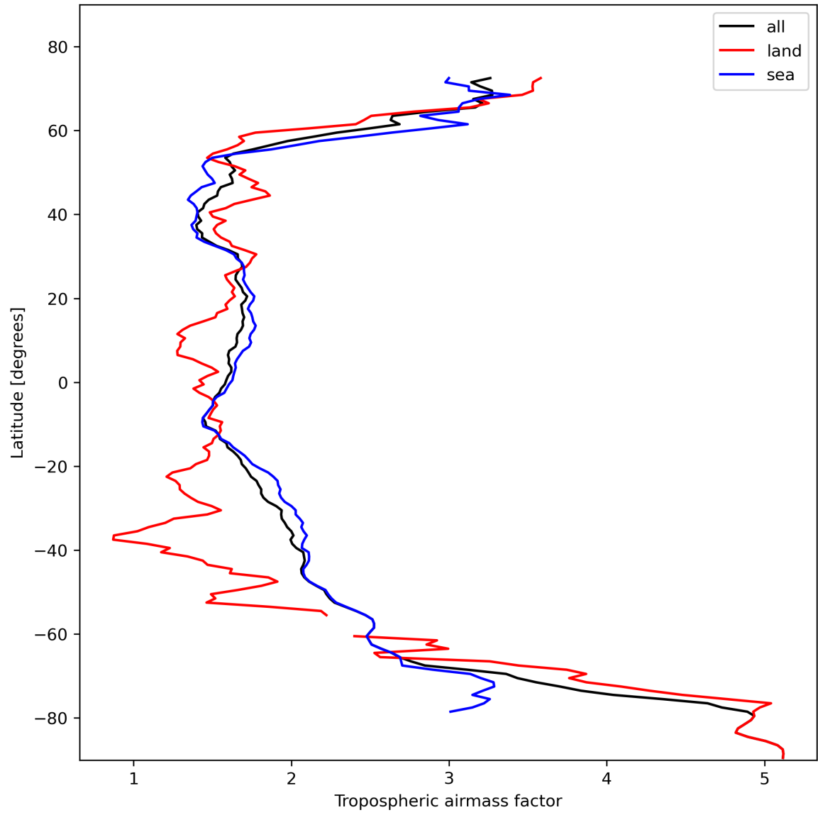
Figure 14: Zonal average of “Tropospheric airmass factor” for 2024-02-04 to 2024-02-06.
