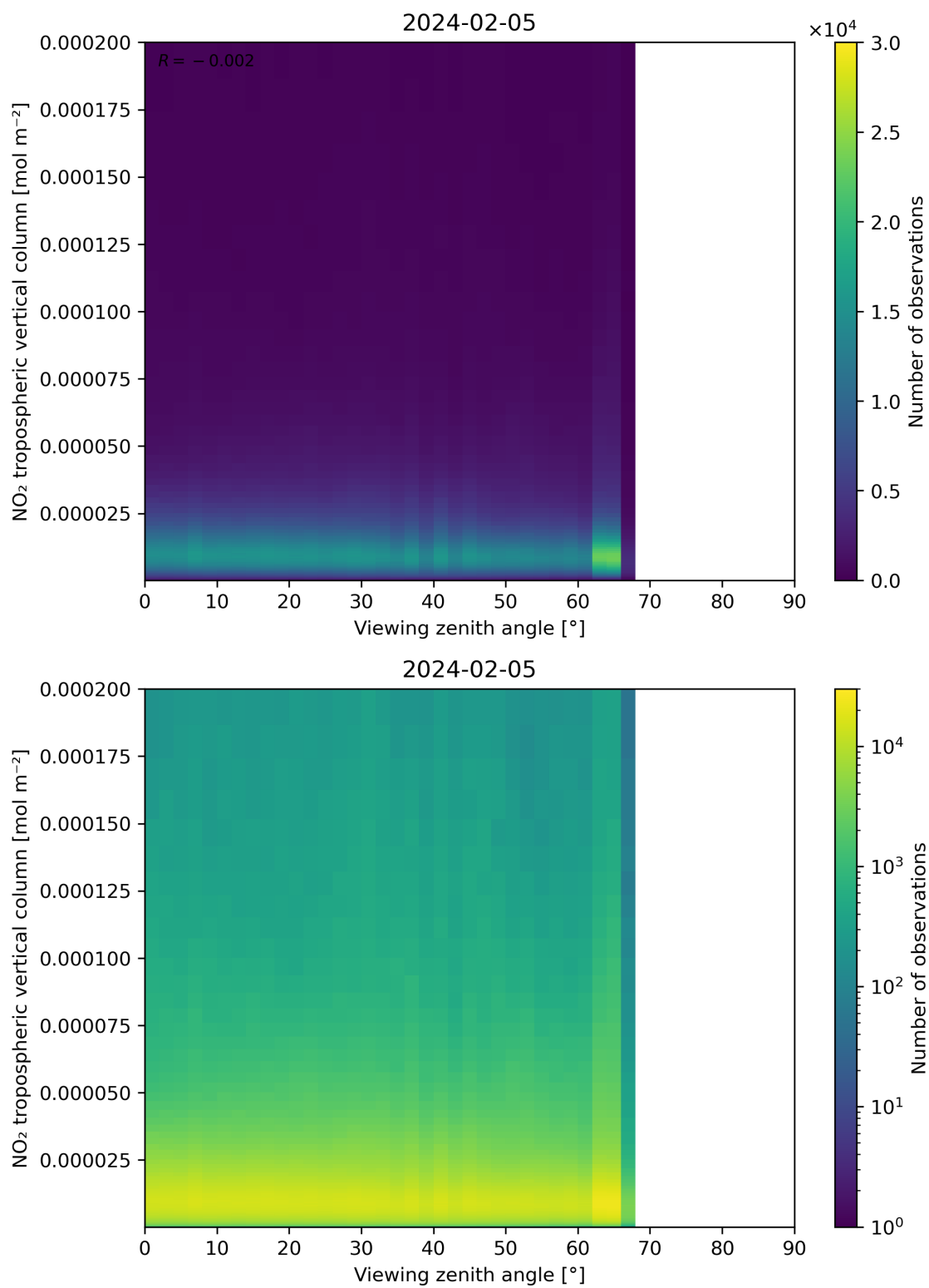
Figure 169: Scatter density plot of “Viewing zenith angle” against “NO 2 tropospheric vertical column” for 2024-02-04 to 2024-02-06.
