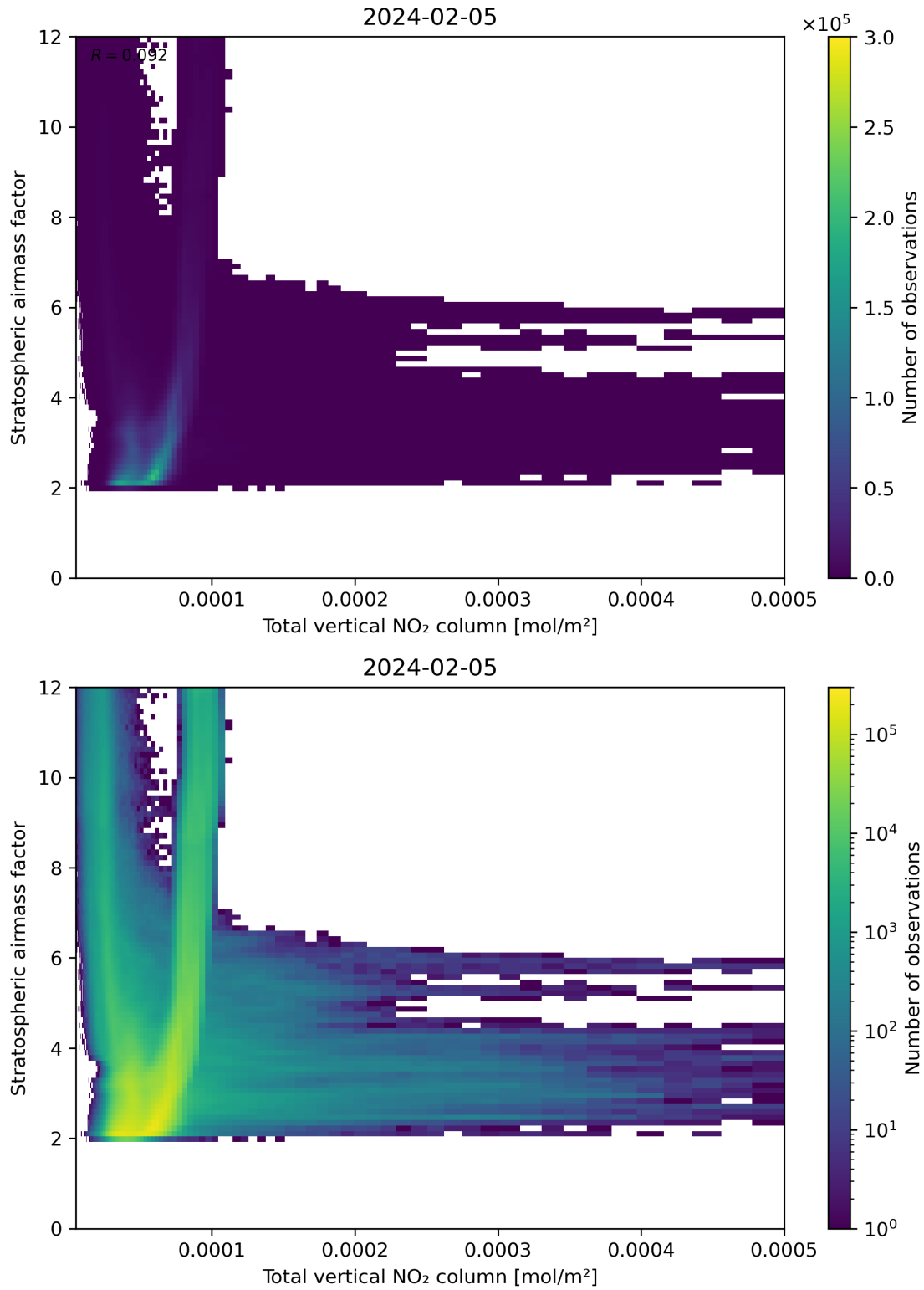
Figure 110: Scatter density plot of “Total vertical NO 2 column” against “Stratospheric airmass factor” for 2024-02-04 to 2024-02-06.
