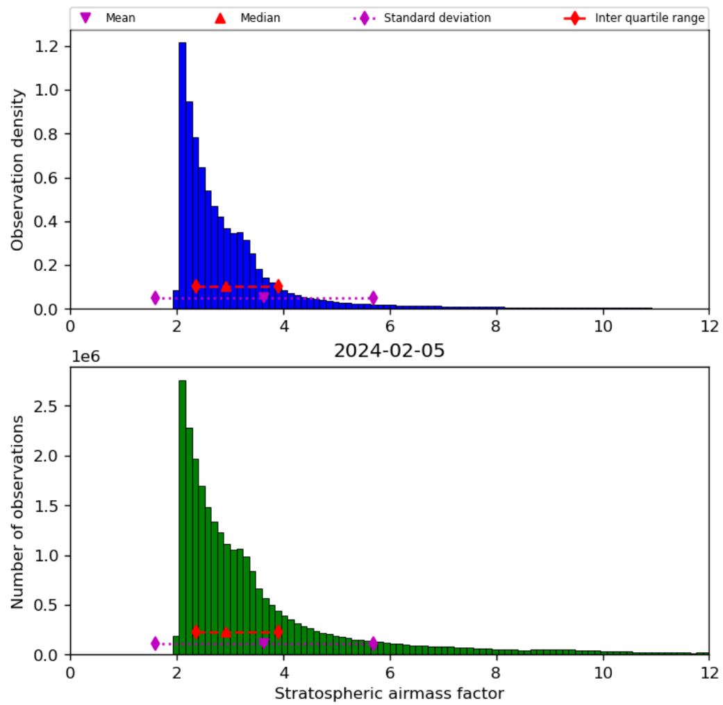
Figure 44: Histogram of “Stratospheric airmass factor” for 2024-02-04 to 2024-02-06
