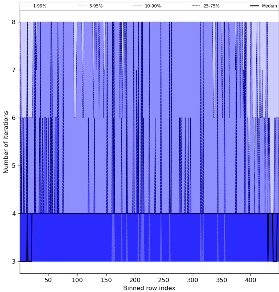
Figure 51: Along track statistics of “Number of iterations” for 2024-02-04 to 2024-02-06
