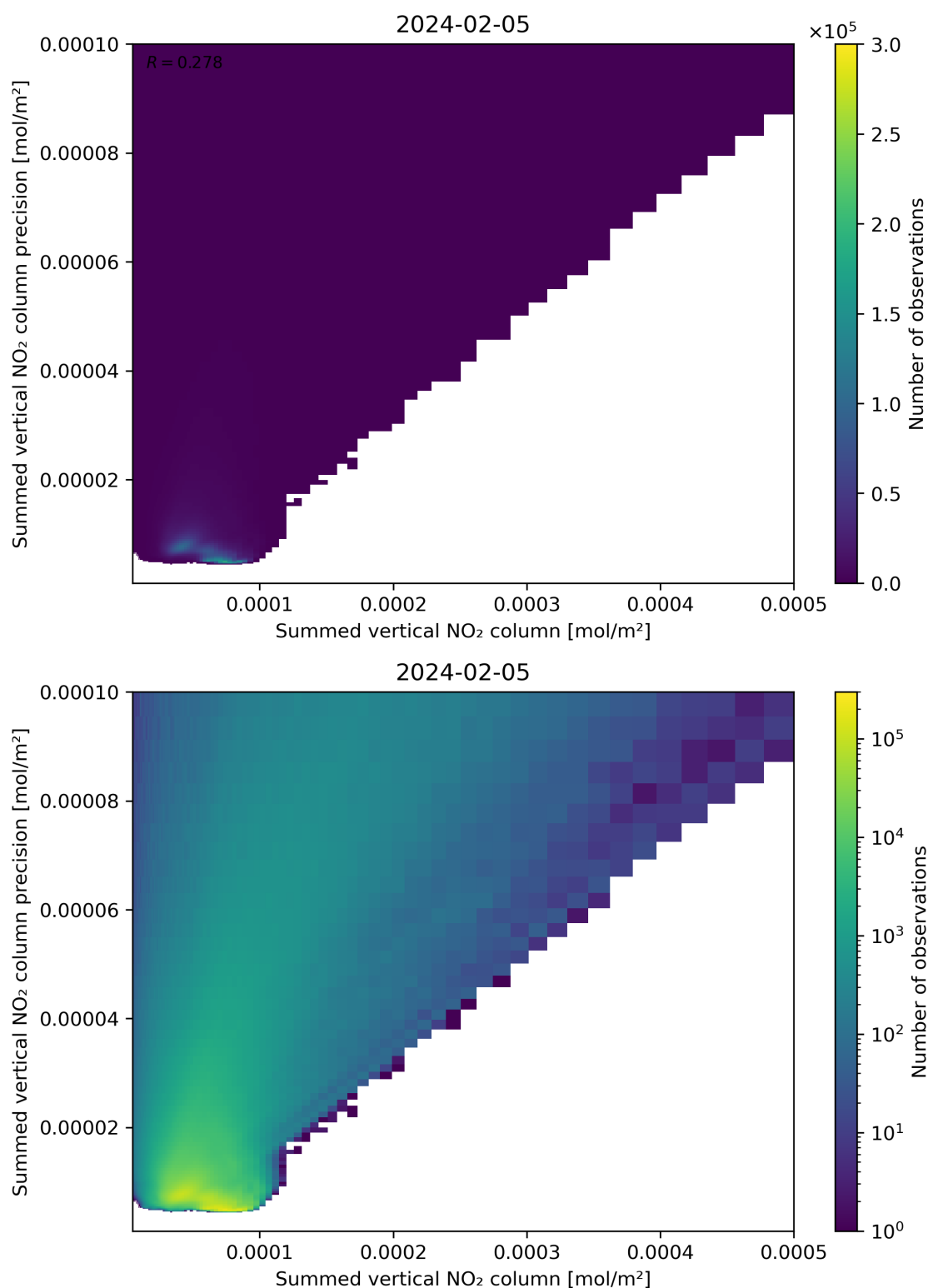
Figure 105: Scatter density plot of “Summed vertical NO 2 column” against “Summed vertical NO 2 column precision” for 2024-02-04 to 2024-02-06.
