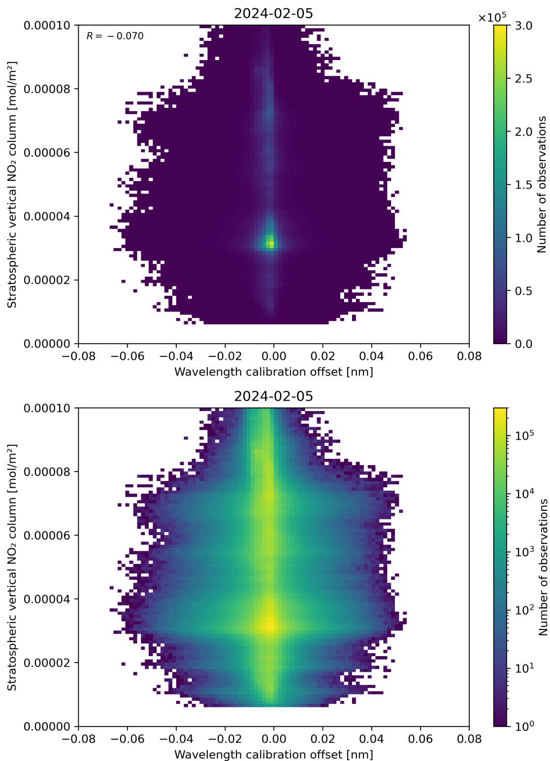
Figure 176: Scatter density plot of “Wavelength calibration offset” against “Stratospheric vertical NO 2 column” for 2024-02-04 to 2024-02-06.
