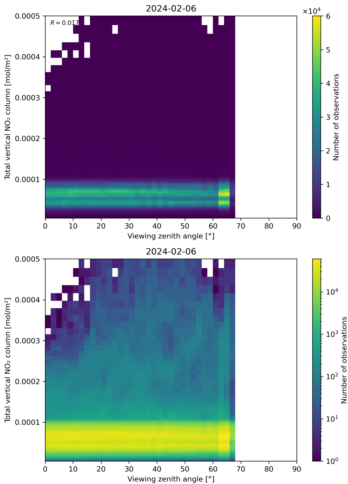
Figure 167: Scatter density plot of “Viewing zenith angle” against “Total vertical NO 2 column” for 2024-02-06 to 2024-02-07.
