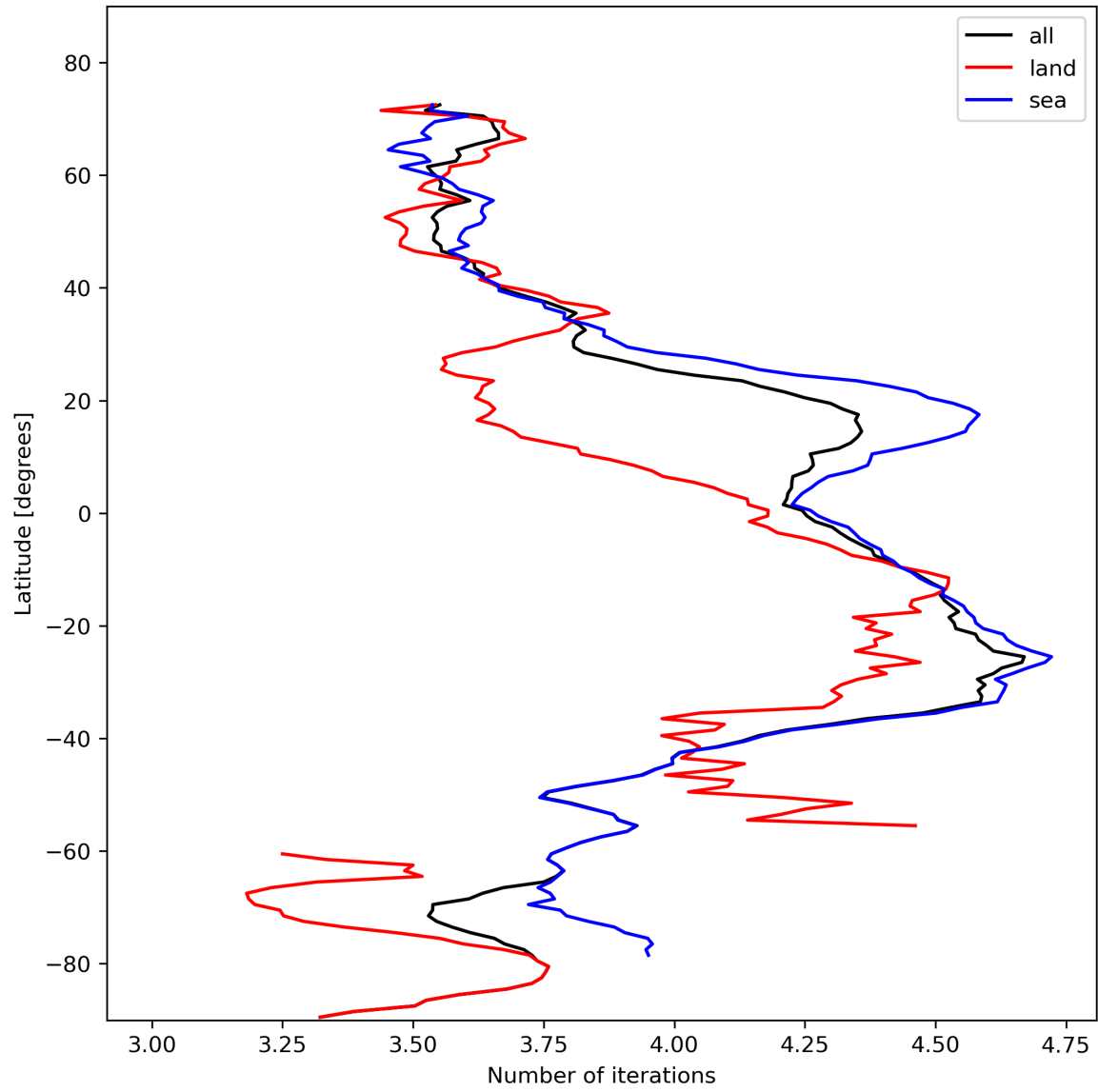
Figure 17: Zonal average of “Number of iterations” for 2024-02-06 to 2024-02-07.
