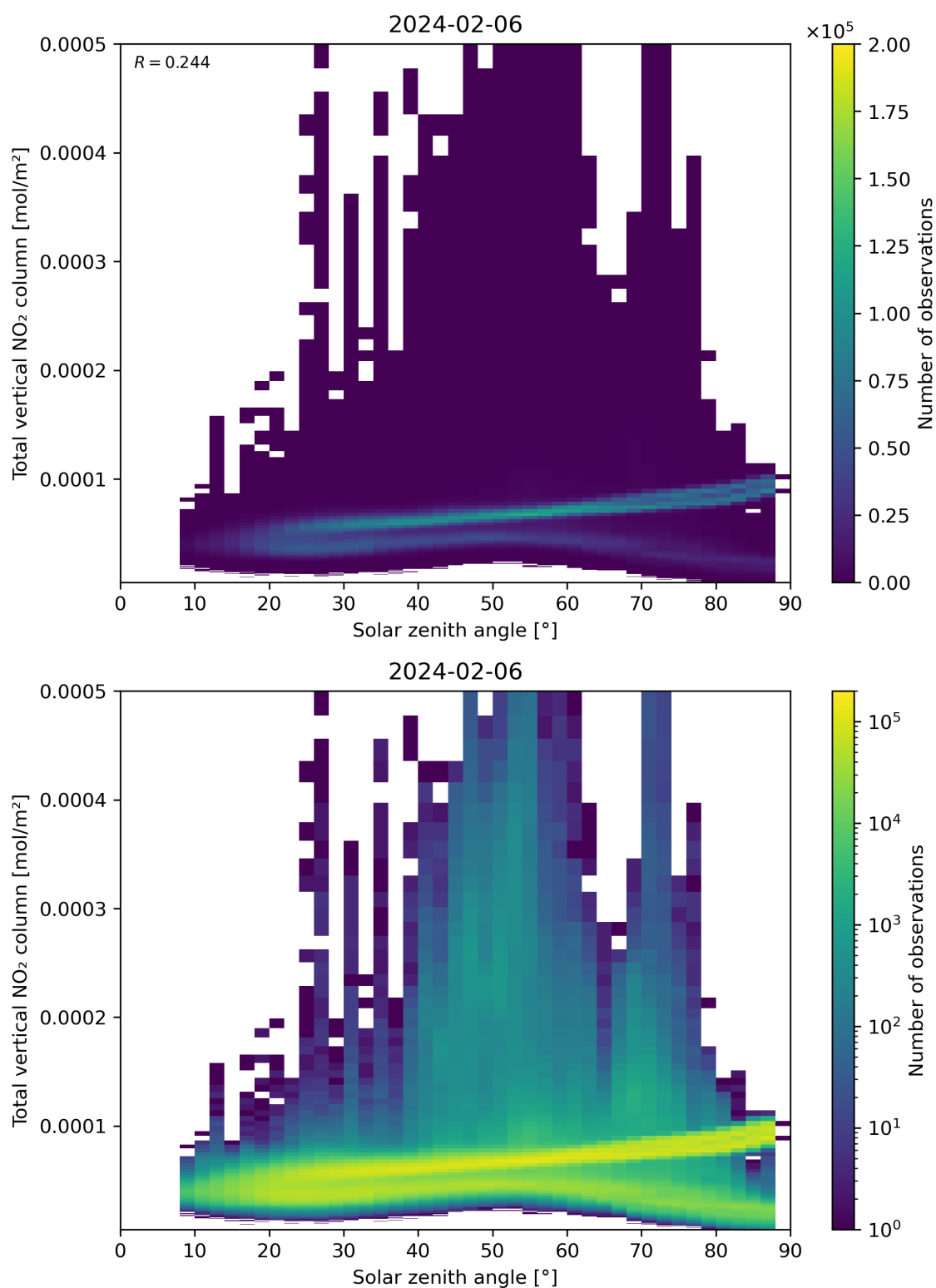
Figure 153: Scatter density plot of “Solar zenith angle” against “Total vertical NO 2 column” for 2024-02-06 to 2024-02-07.
