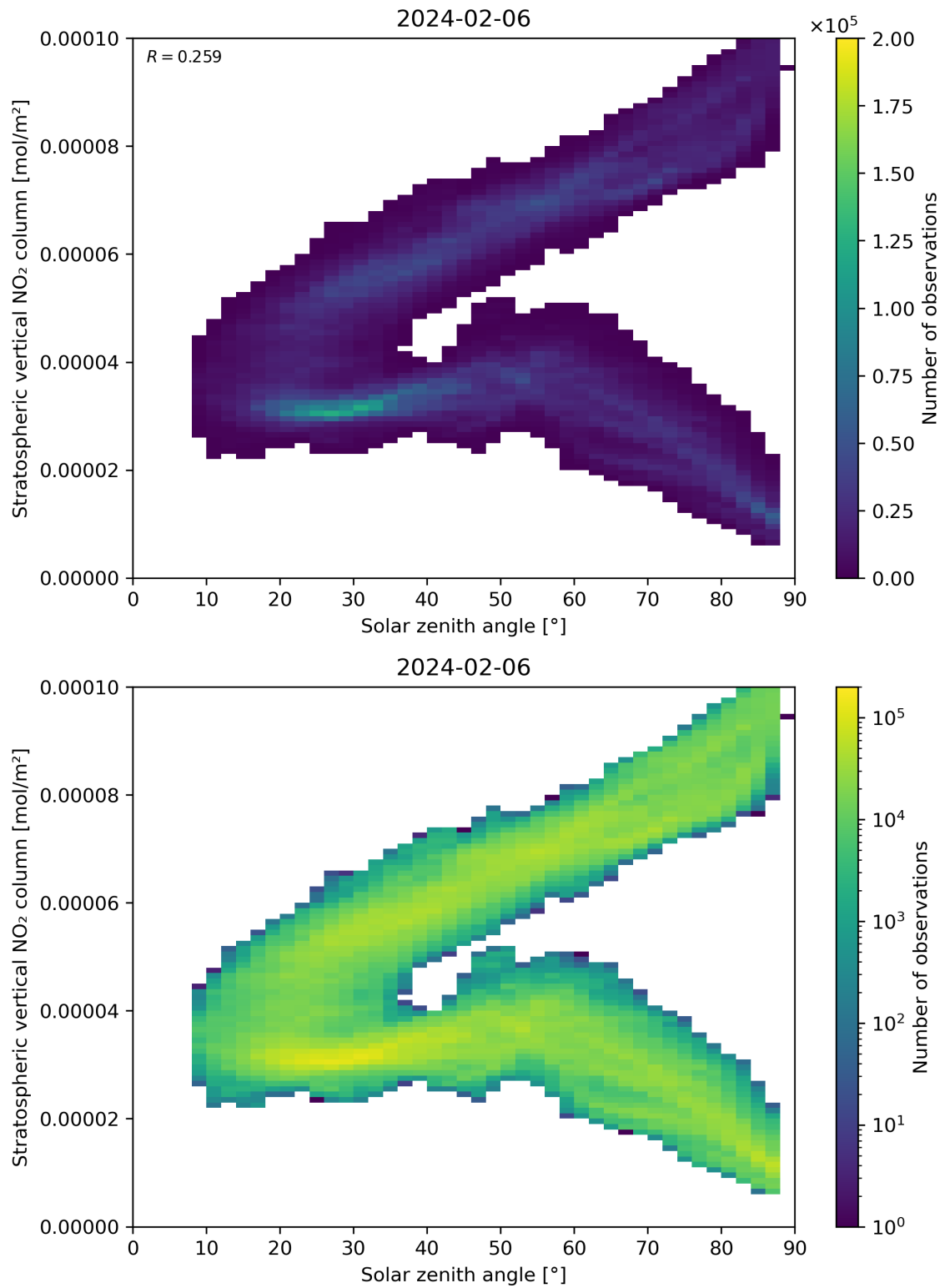
Figure 150: Scatter density plot of “Solar zenith angle” against “Stratospheric vertical NO 2 column” for 2024-02-06 to 2024-02-07.
