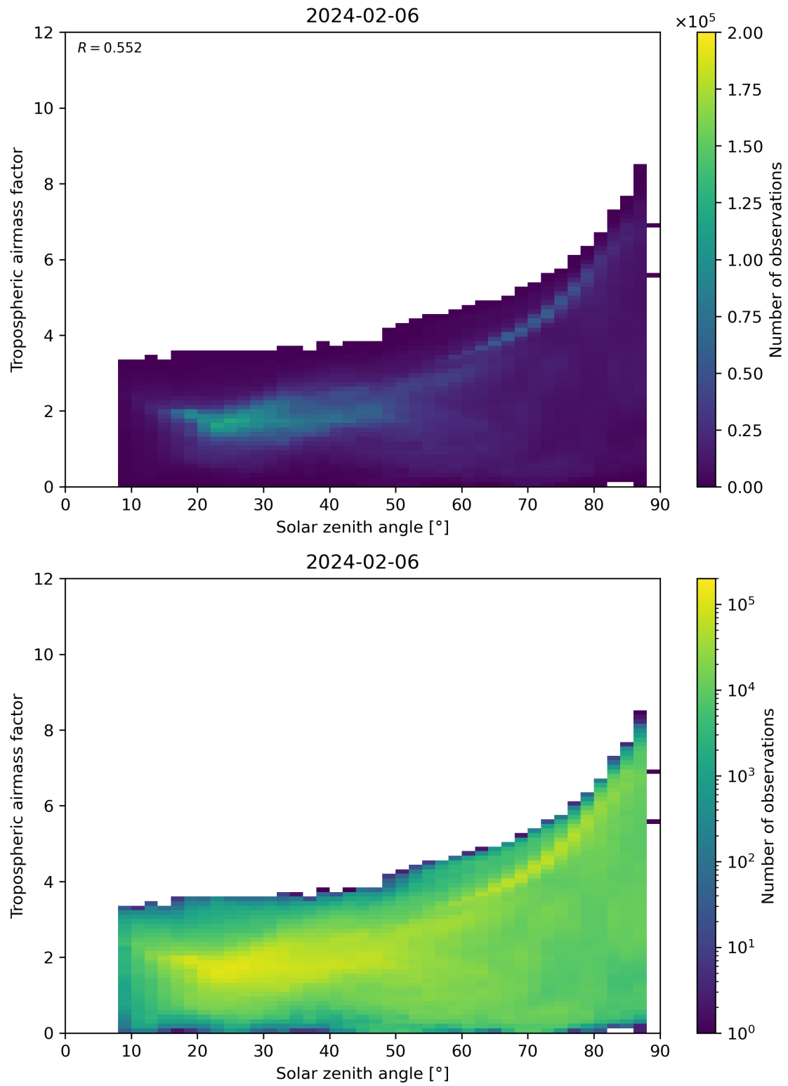
Figure 147: Scatter density plot of “Solar zenith angle” against “Tropospheric airmass factor” for 2024-02-06 to 2024-02-07.
