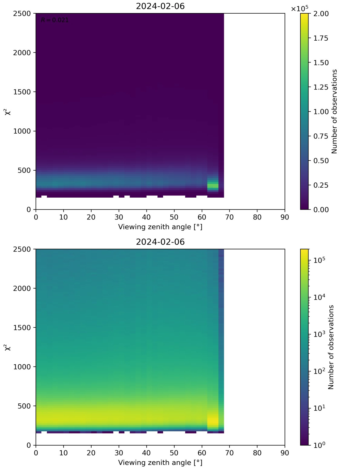
Figure 162: Scatter density plot of “Viewing zenith angle” against “ \chi^2 ” for 2024-02-06 to 2024-02-07.
