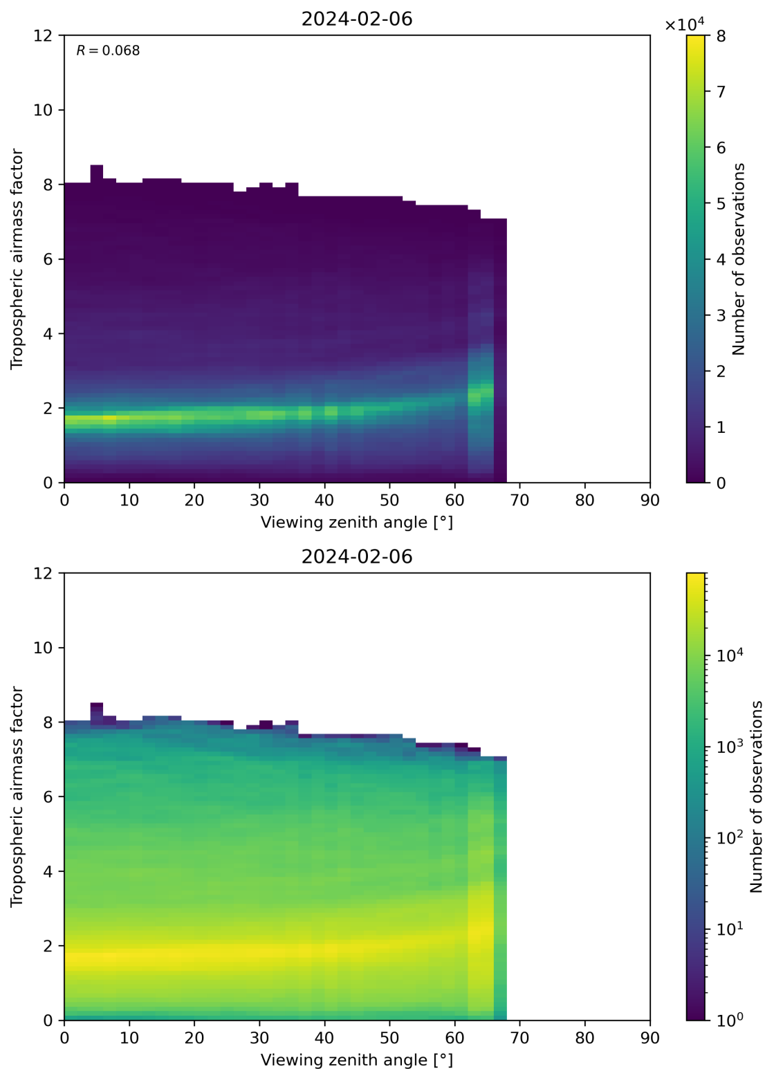
Figure 161: Scatter density plot of “Viewing zenith angle” against “Tropospheric airmass factor” for 2024-02-06 to 2024-02-07.
