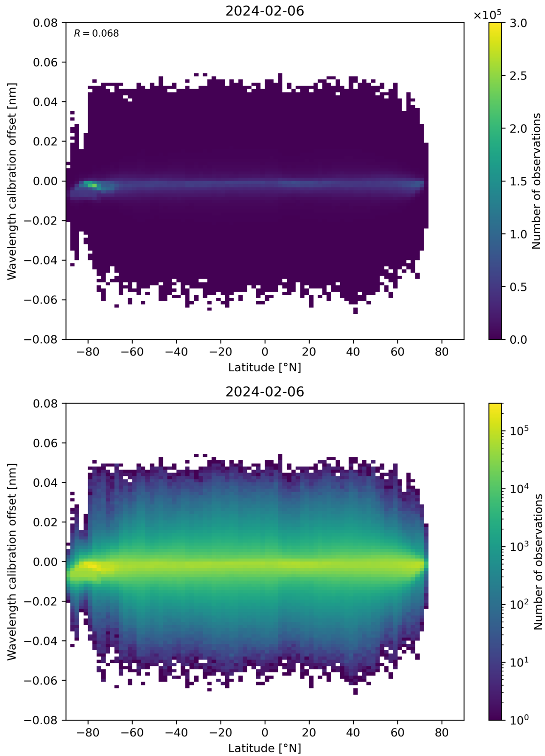
Figure 95: Scatter density plot of “Latitude” against “Wavelength calibration offset” for 2024-02-06 to 2024-02-07.
