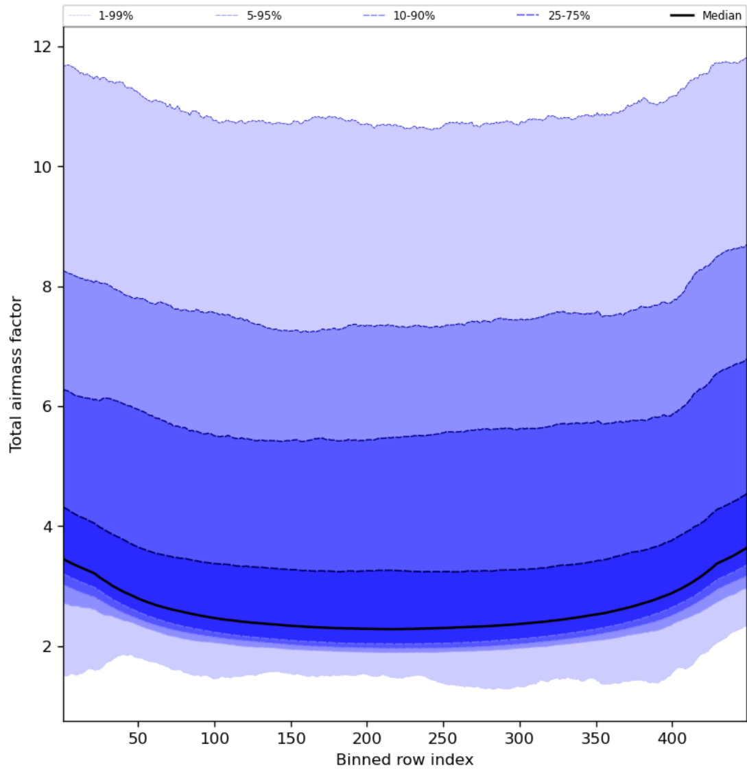
Figure 49: Along track statistics of “Total airmass factor” for 2024-02-06 to 2024-02-07
