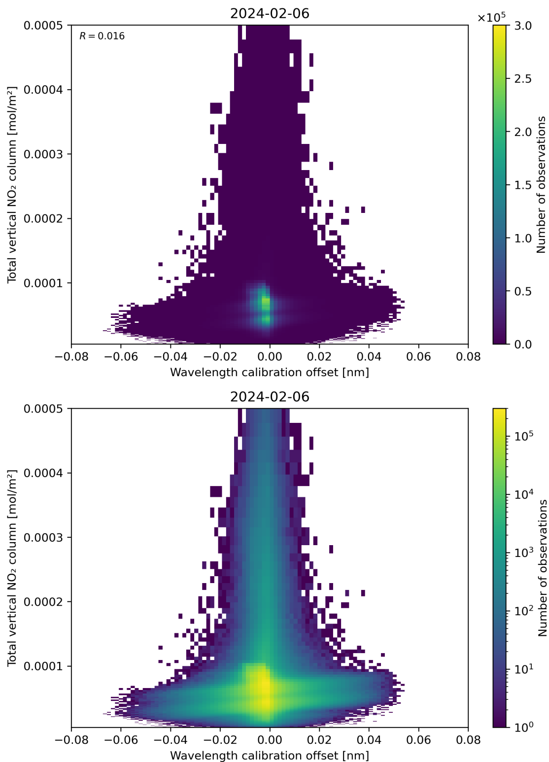
Figure 179: Scatter density plot of “Wavelength calibration offset” against “Total vertical NO 2 column” for 2024-02-06 to 2024-02-07.
