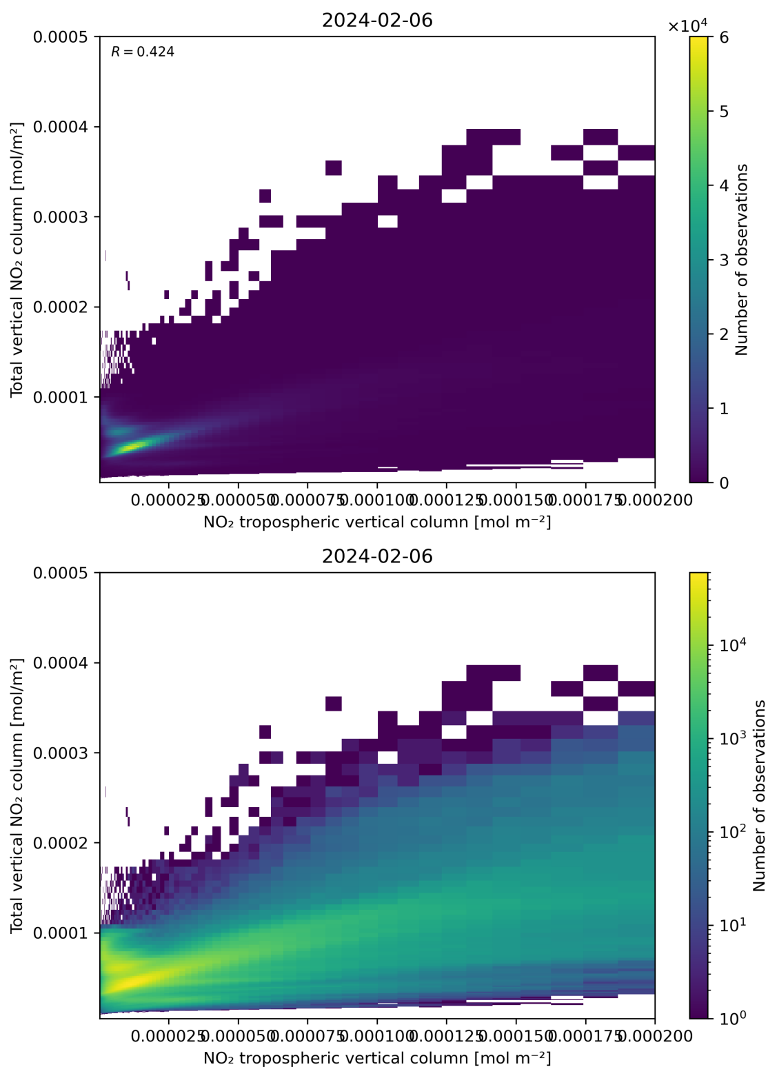
Figure 128: Scatter density plot of “NO 2 tropospheric vertical column” against “Total vertical NO 2 column” for 2024-02-06 to 2024-02-07.
