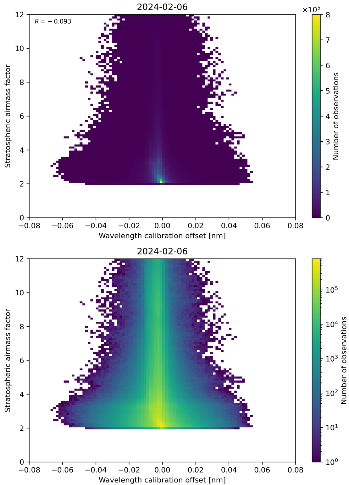
Figure 174: Scatter density plot of “Wavelength calibration offset” against “Stratospheric air mass factor” for 2024-02-06 to 2024-02-07.
