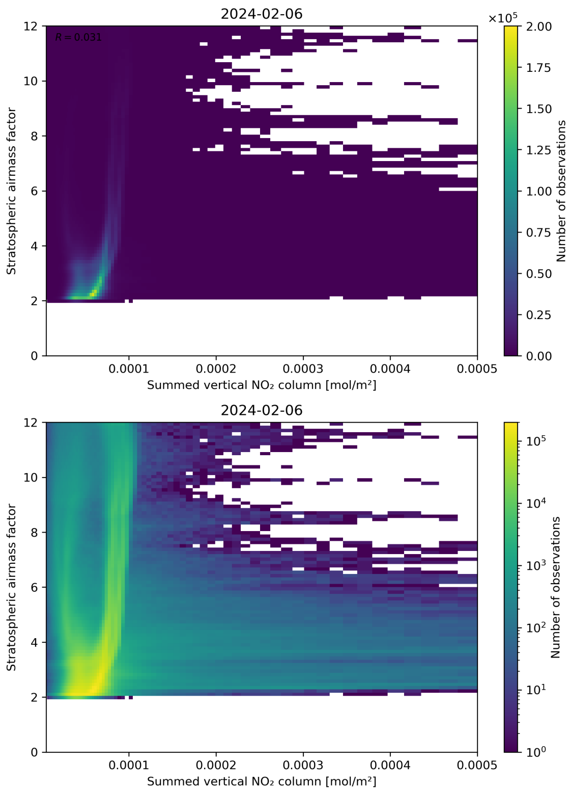
Figure 103: Scatter density plot of “Summed vertical NO 2 column” against “Stratospheric air mass factor” for 2024-02-06 to 2024-02-07.
