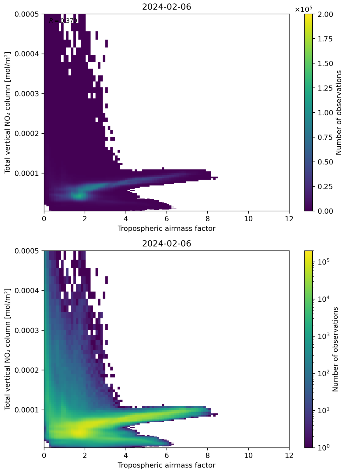
Figure 77: Scatter density plot of “Tropospheric airmass factor” against “Total vertical NO 2 column” for 2024-02-06 to 2024-02-07.
