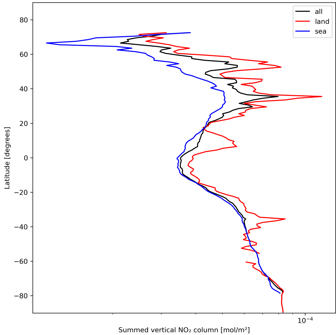
Figure 23: Zonal average of “Summed vertical NO 2 column” for 2024-02-06 to 2024-02-07.
