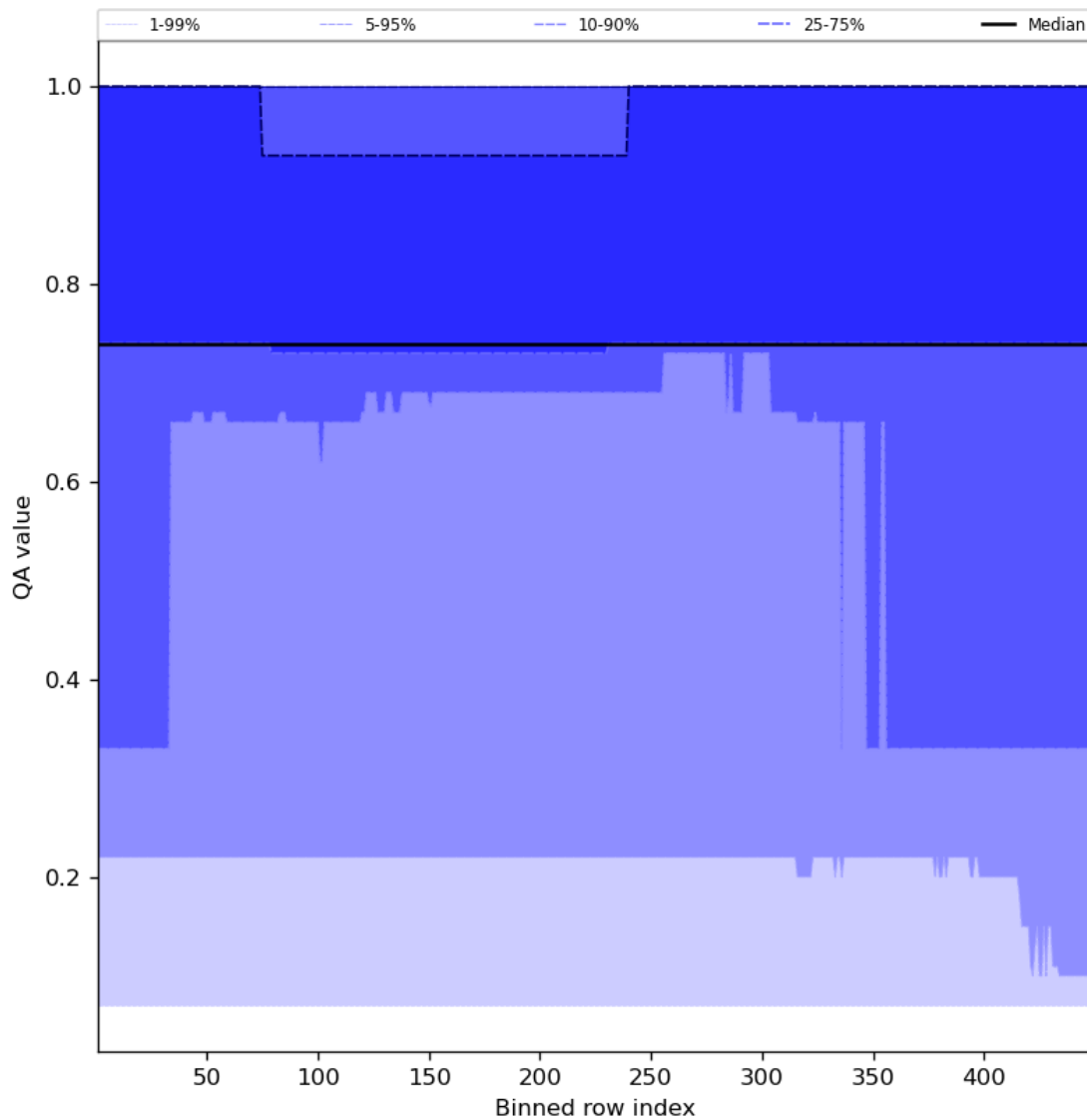
Figure 45: Along track statistics of “QA value” for 2024-02-06 to 2024-02-07
