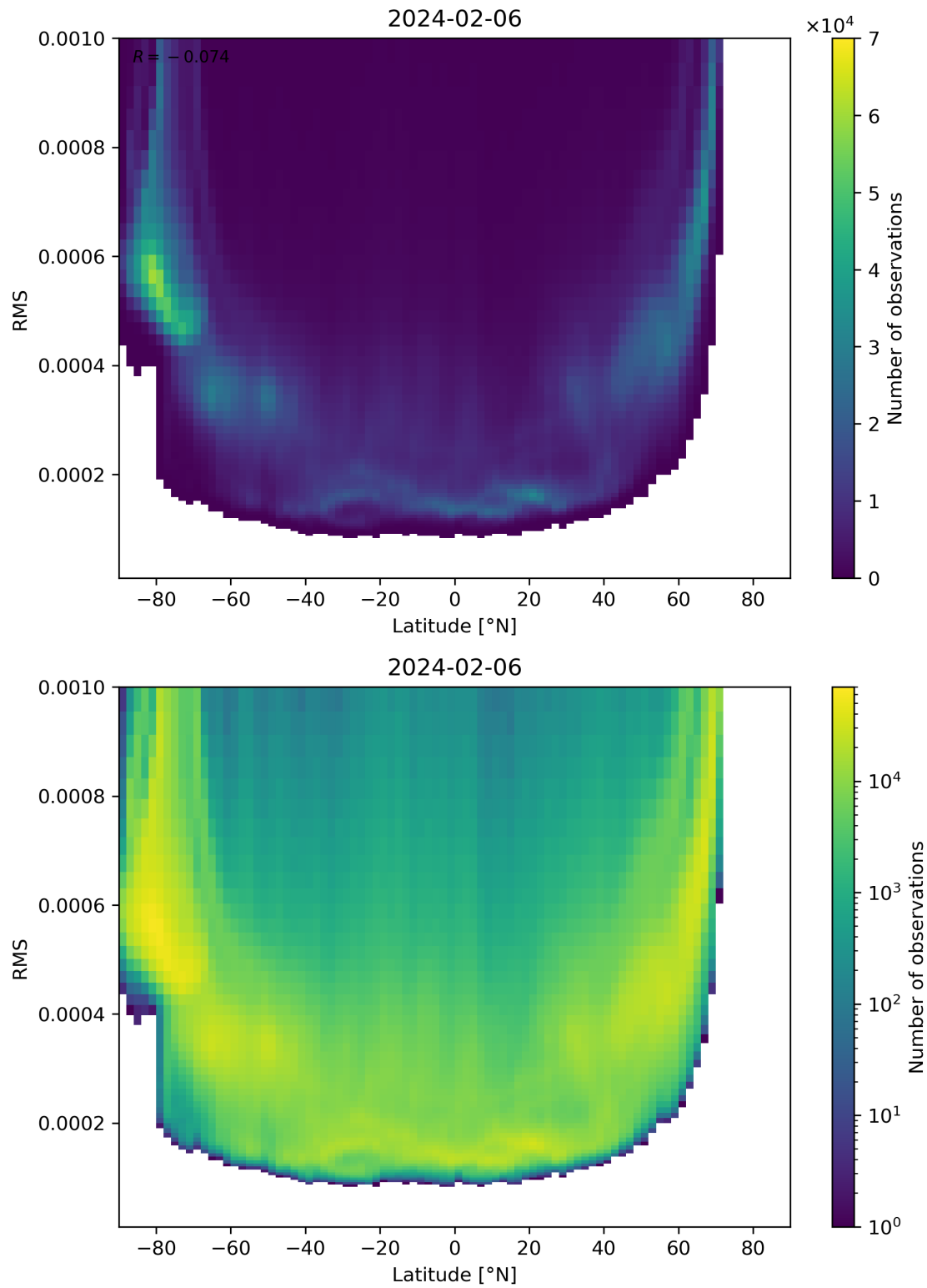
Figure 94: Scatter density plot of “Latitude” against “RMS” for 2024-02-06 to 2024-02-07.
