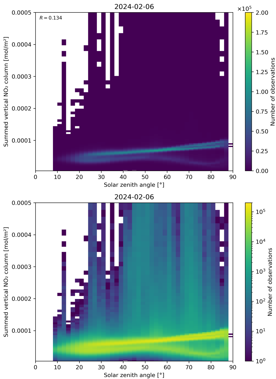
Figure 151: Scatter density plot of “Solar zenith angle” against “Summed vertical NO 2 column” for 2024-02-06 to 2024-02-07.
