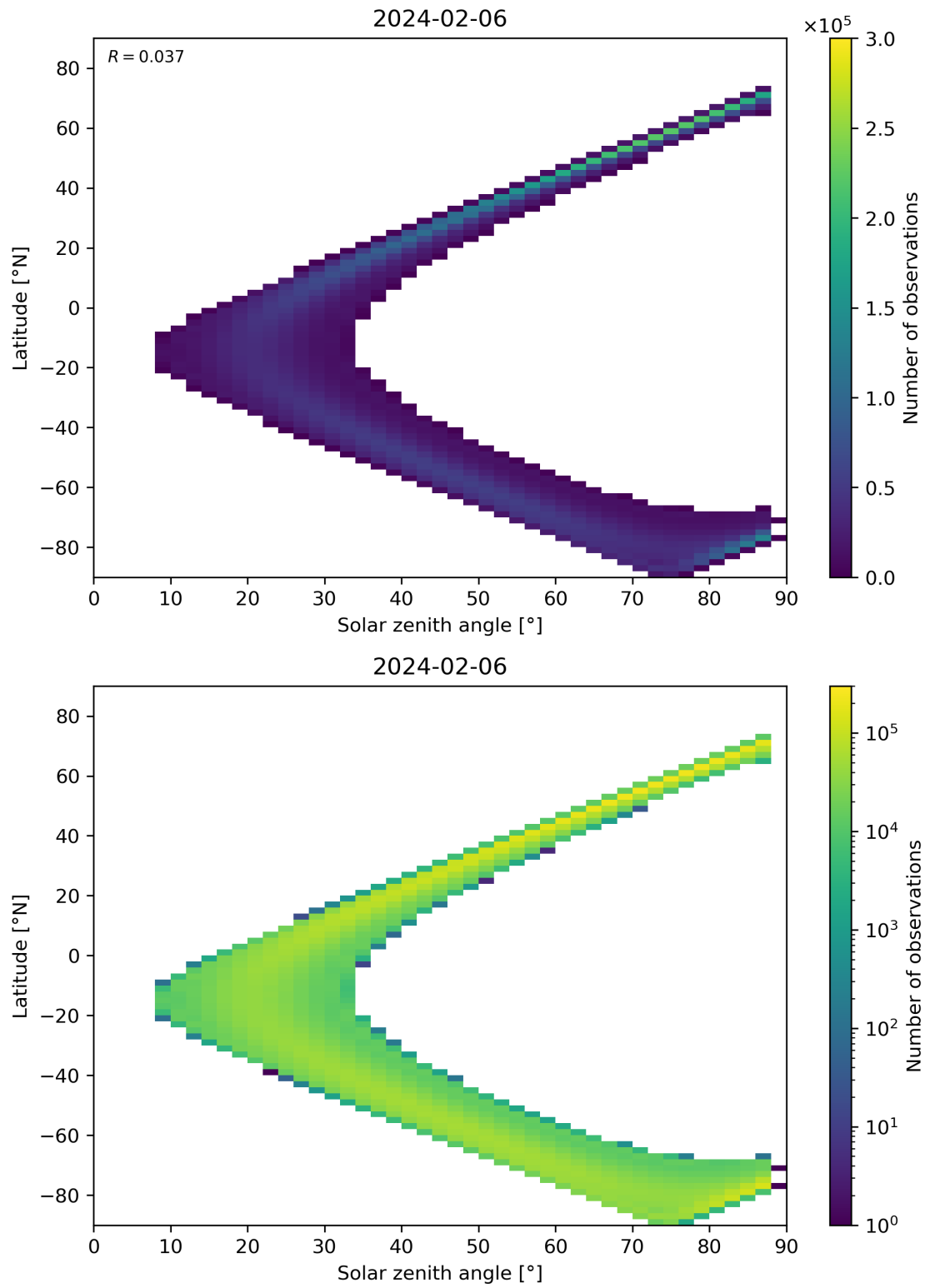
Figure 149: Scatter density plot of “Solar zenith angle” against “Latitude” for 2024-02-06 to 2024-02-07.
