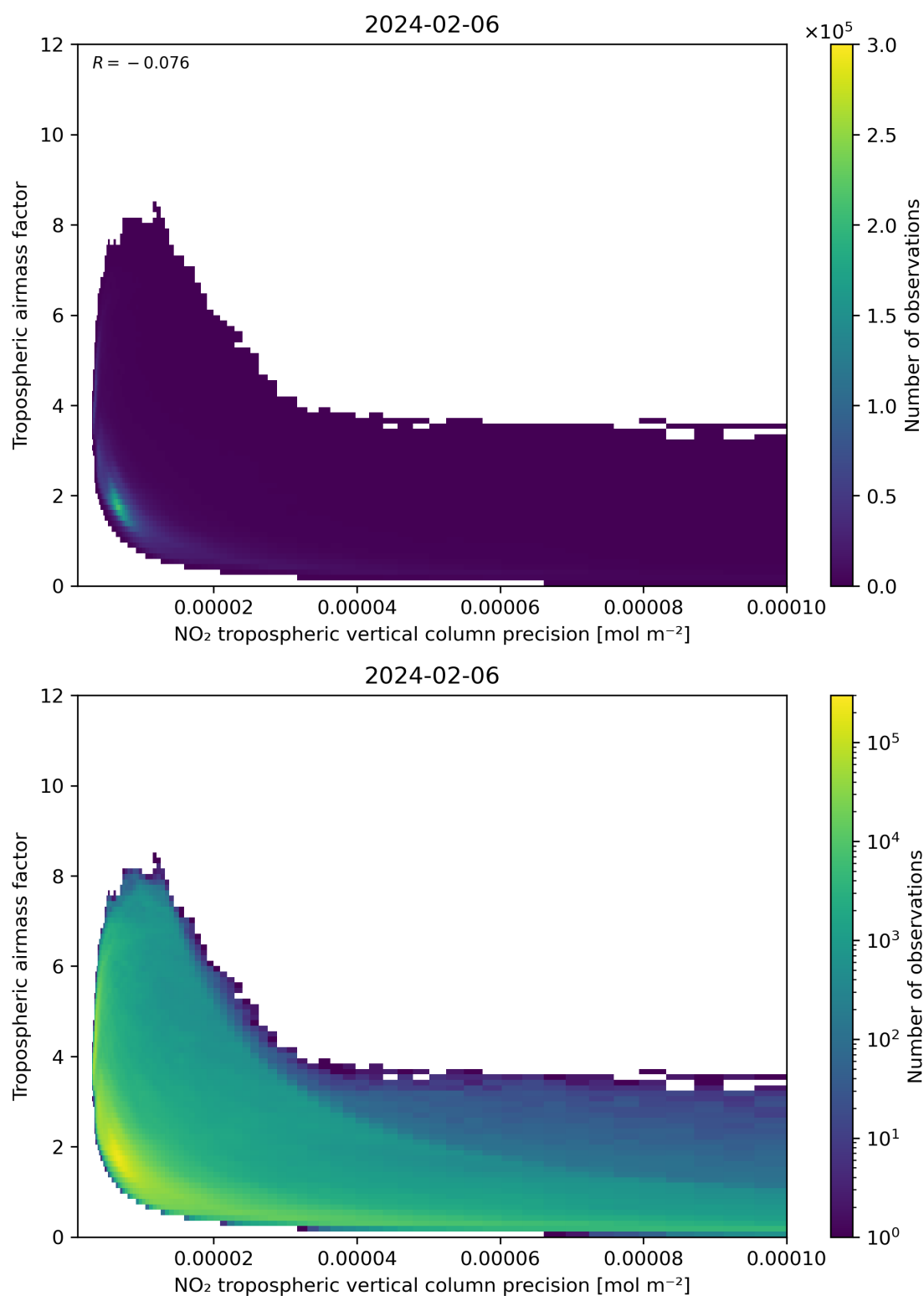
Figure 133: Scatter density plot of “NO 2 tropospheric vertical column precision” against “Tropospheric airmass factor” for 2024-02-06 to 2024-02-07.
