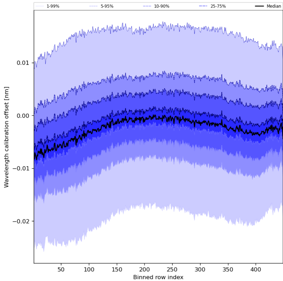
Figure 52: Along track statistics of “Wavelength calibration offset” for 2024-02-06 to 2024-02-07
