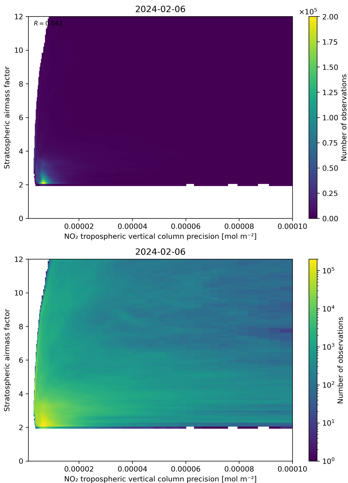
Figure 131: Scatter density plot of “NO 2 tropospheric vertical column precision” against “Stratospheric airmass factor” for 2024-02-06 to 2024-02-07.
