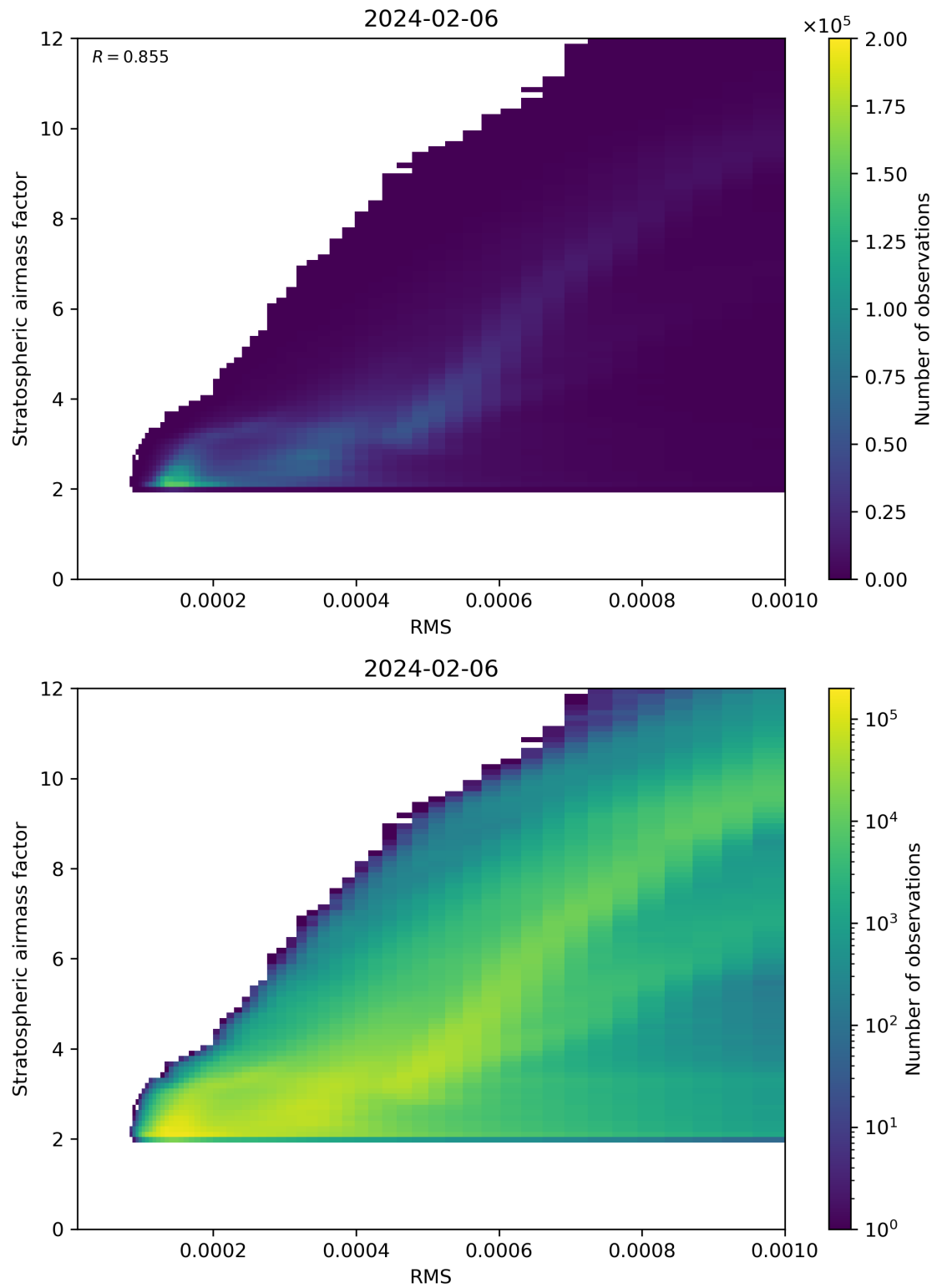
Figure 144: Scatter density plot of “RMS” against “Stratospheric airmass factor” for 2024-02-06 to 2024-02-07.
