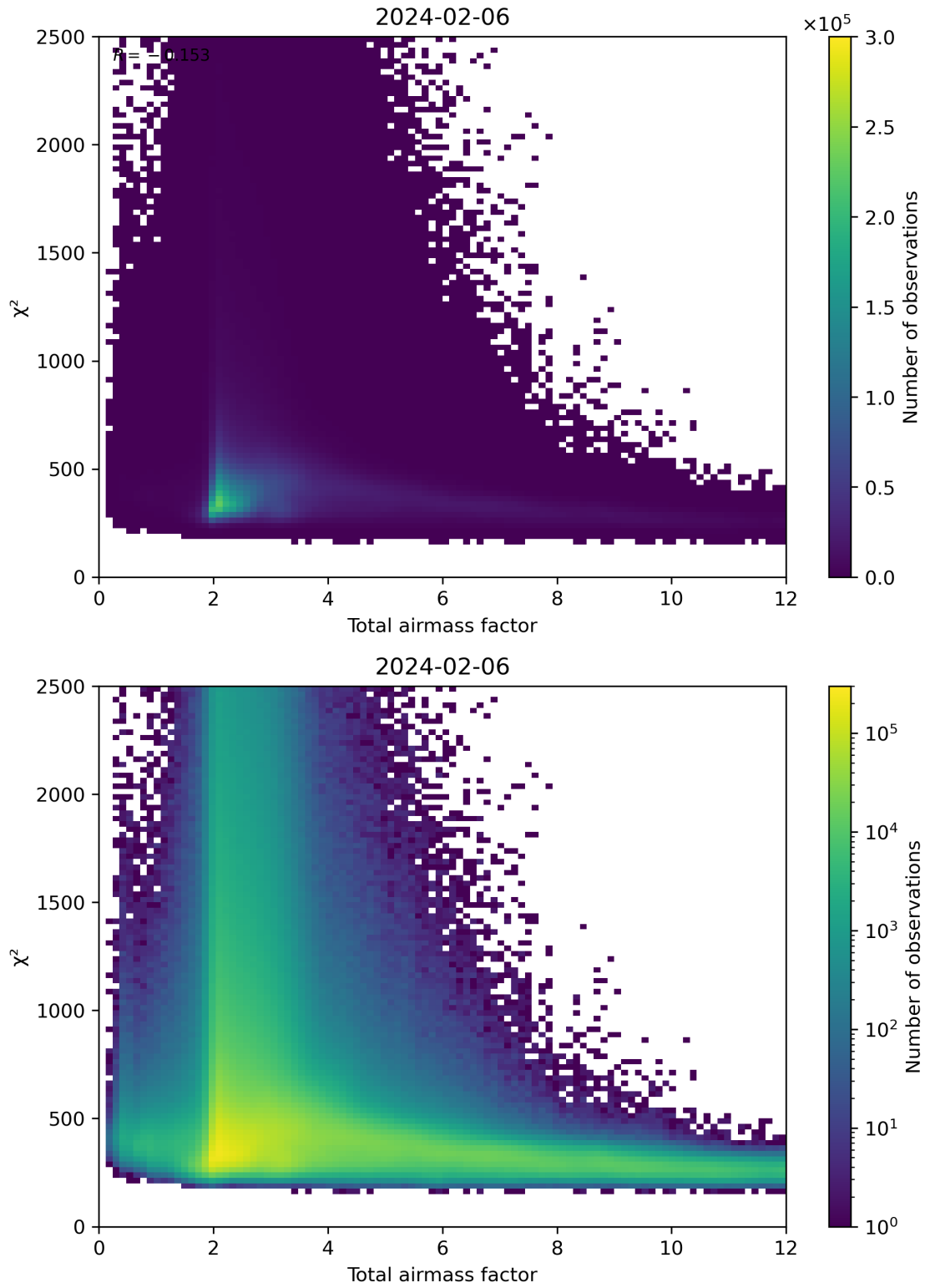
Figure 63: Scatter density plot of “Total airmass factor” against “ \chi^2 ” for 2024-02-06 to 2024-02-07.
