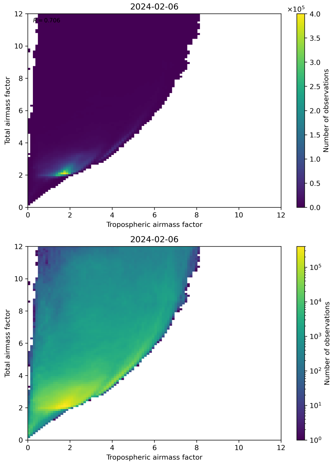
Figure 72: Scatter density plot of “Tropospheric airmass factor” against “Total airmass factor” for 2024-02-06 to 2024-02-07.
