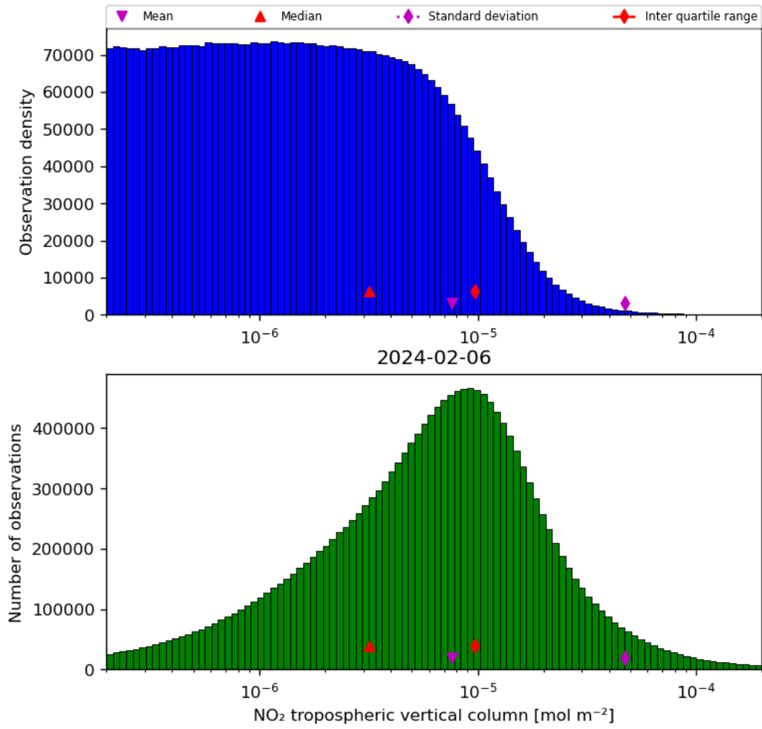
Figure 29: Histogram of "NO 2 tropospheric vertical column" for 2024-02-06 to 2024-02-07
