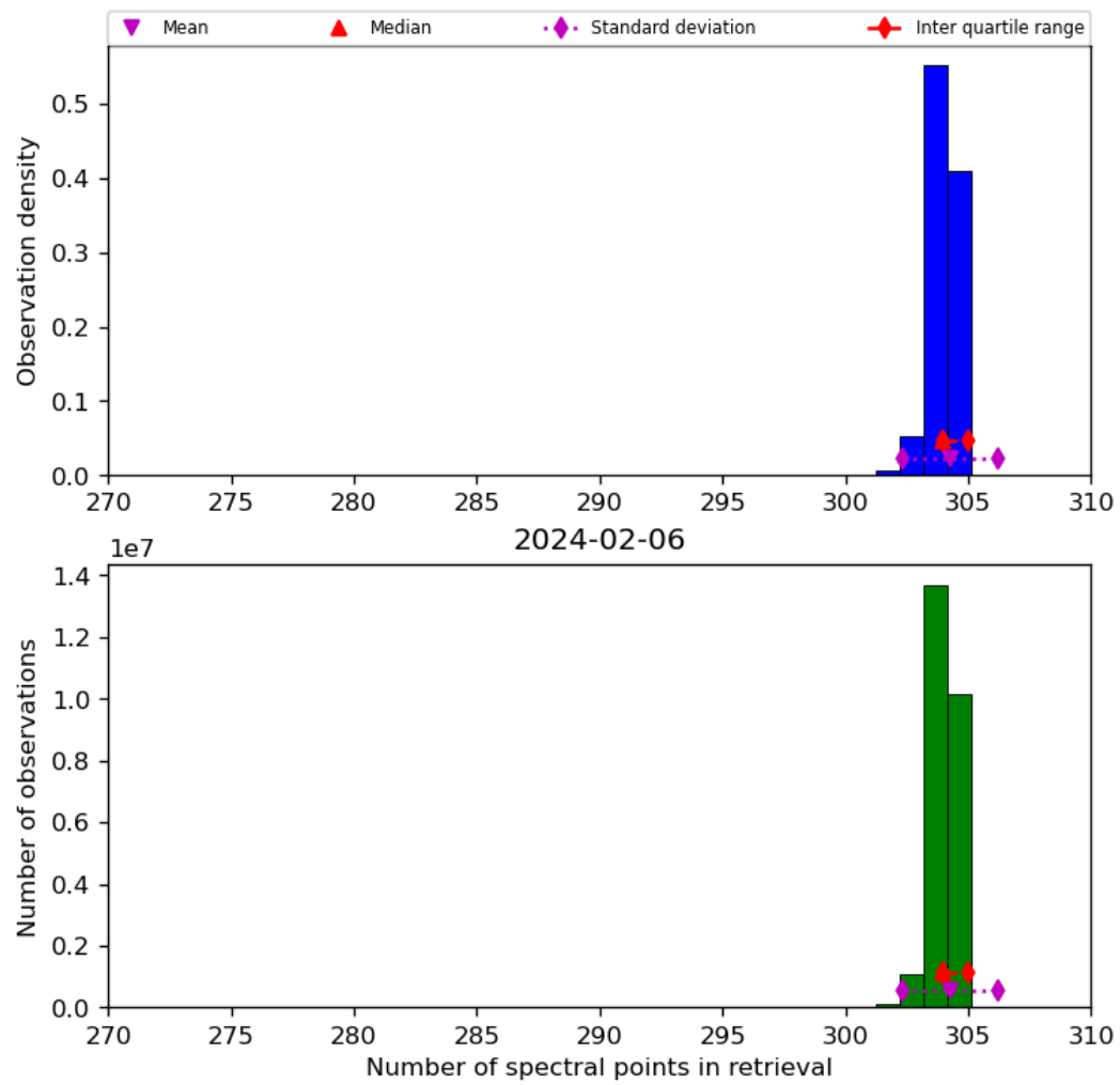
Figure 33: Histogram of “Number of spectral points in retrieval” for 2024-02-06 to 2024-02-07
