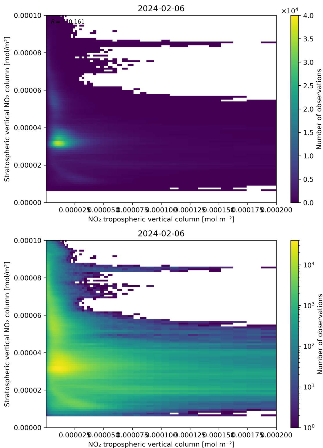
Figure 125: Scatter density plot of “NO 2 tropospheric vertical column” against “Stratospheric vertical NO 2 column” for 2024-02-06 to 2024-02-07.
