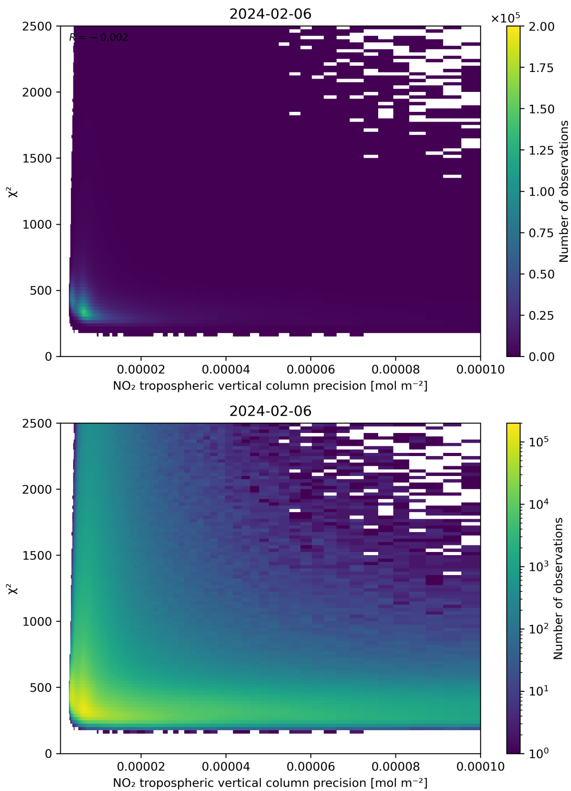
Figure 134: Scatter density plot of “NO 2 tropospheric vertical column precision” against “ \chi^2 ” for 2024-02-06 to 2024-02-07.
