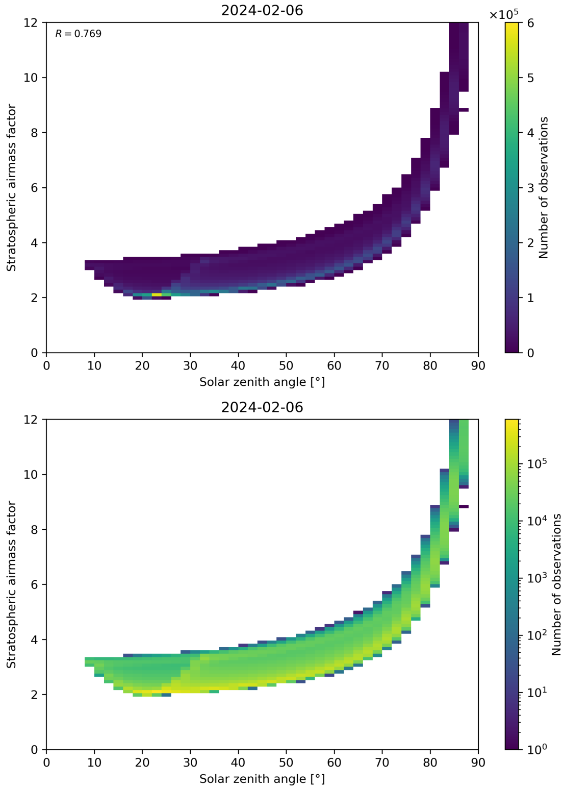
Figure 145: Scatter density plot of “Solar zenith angle” against “Stratospheric airmass factor” for 2024-02-06 to 2024-02-07.
