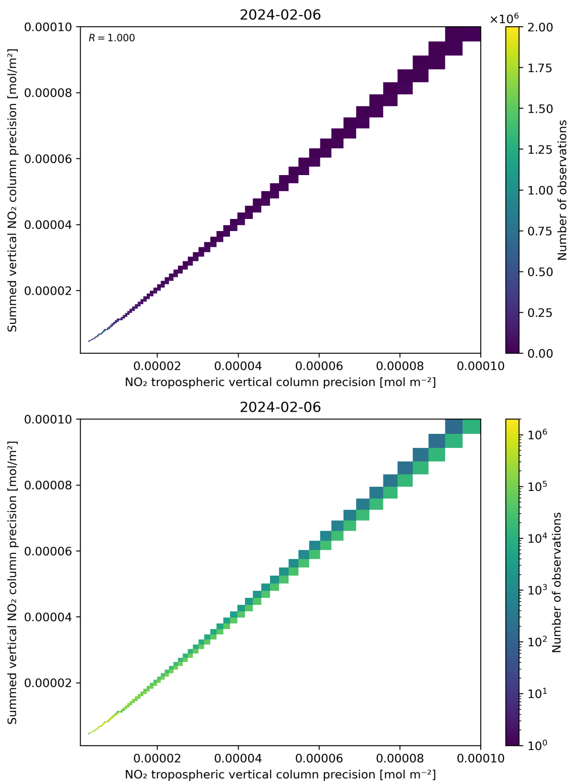
Figure 137: Scatter density plot of “NO 2 tropospheric vertical column precision” against “Summed vertical NO 2 column precision” for 2024-02-06 to 2024-02-07.
