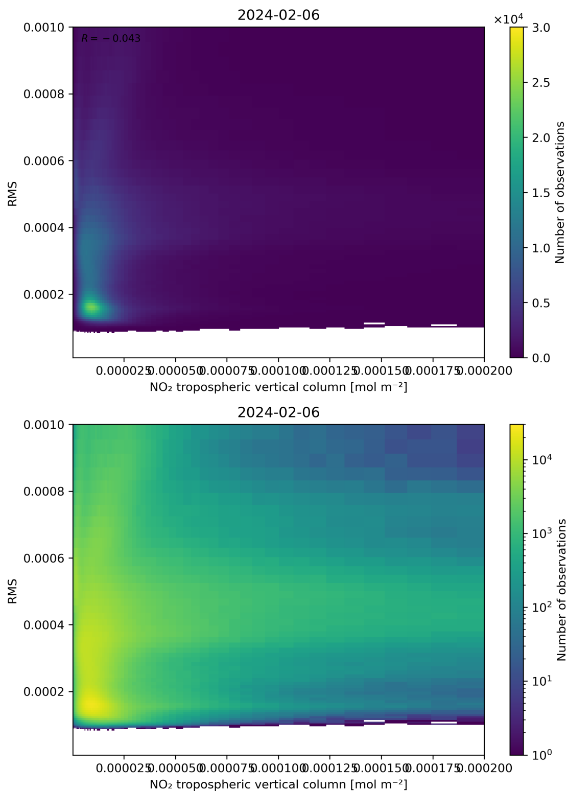
Figure 142: Scatter density plot of “NO 2 tropospheric vertical column” against “RMS” for 2024-02-06 to 2024-02-07.
