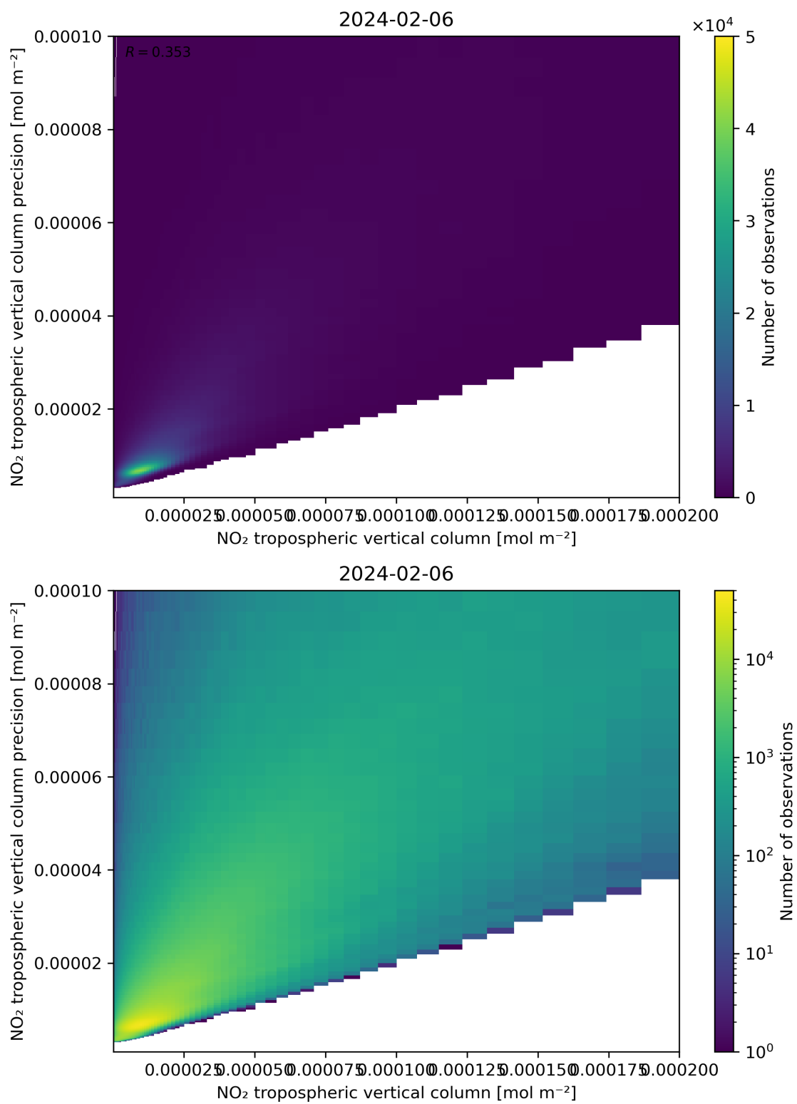
Figure 130: Scatter density plot of “NO 2 tropospheric vertical column” against “NO 2 tropospheric vertical column precision” for 2024-02-06 to 2024-02-07.
