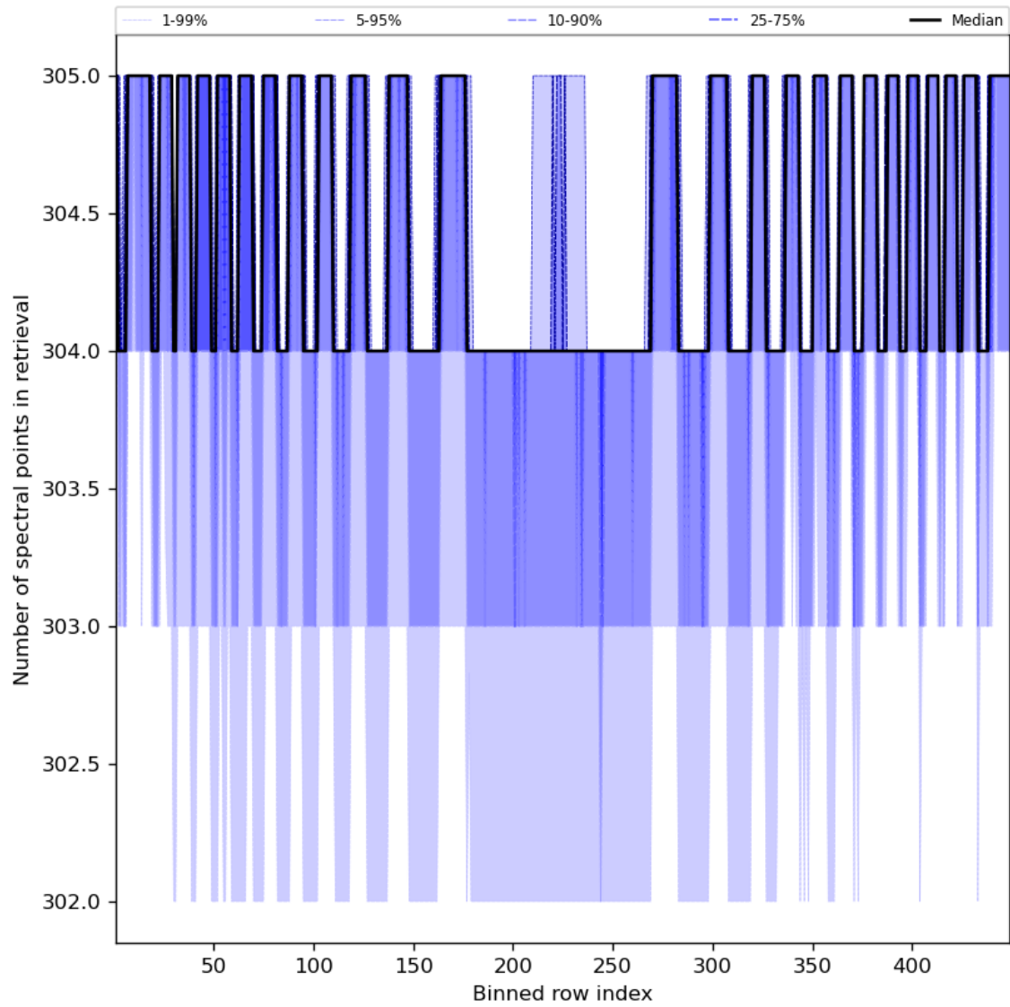
Figure 50: Along track statistics of “Number of spectral points in retrieval” for 2024-02-06 to 2024-02-07
