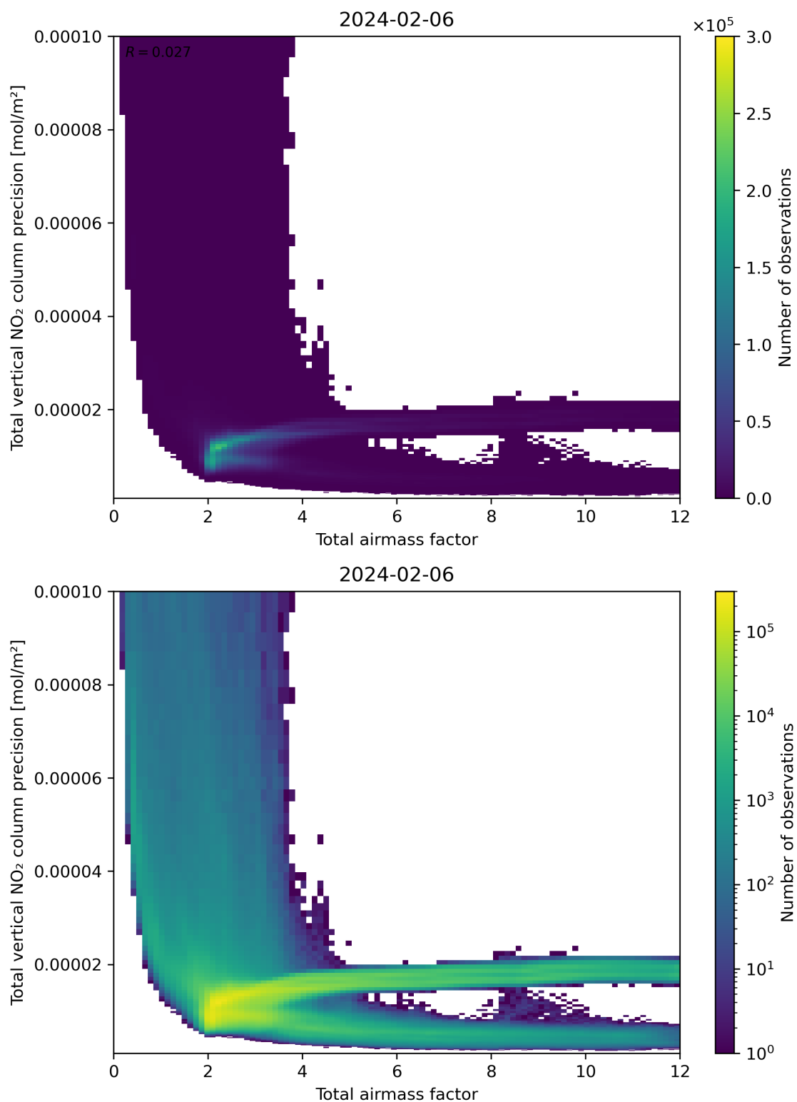
Figure 68: Scatter density plot of “Total airmass factor” against “Total vertical NO 2 column precision” for 2024-02-06 to 2024-02-07.
