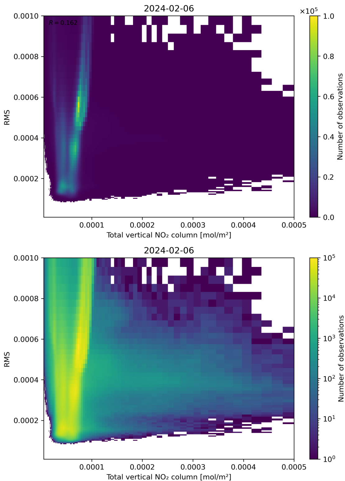
Figure 120: Scatter density plot of “Total vertical NO 2 column” against “RMS” for 2024-02-06 to 2024-02-07.
