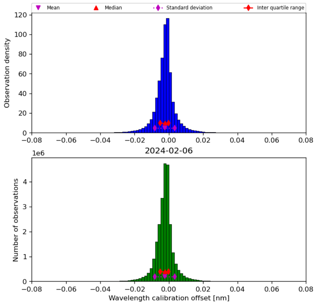
Figure 35: Histogram of “Wavelength calibration offset” for 2024-02-06 to 2024-02-07
