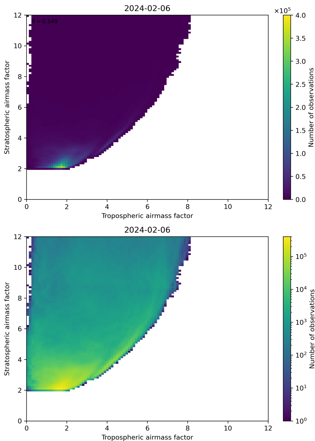
Figure 71: Scatter density plot of “Tropospheric airmass factor” against “Stratospheric airmass factor” for 2024-02-06 to 2024-02-07.
