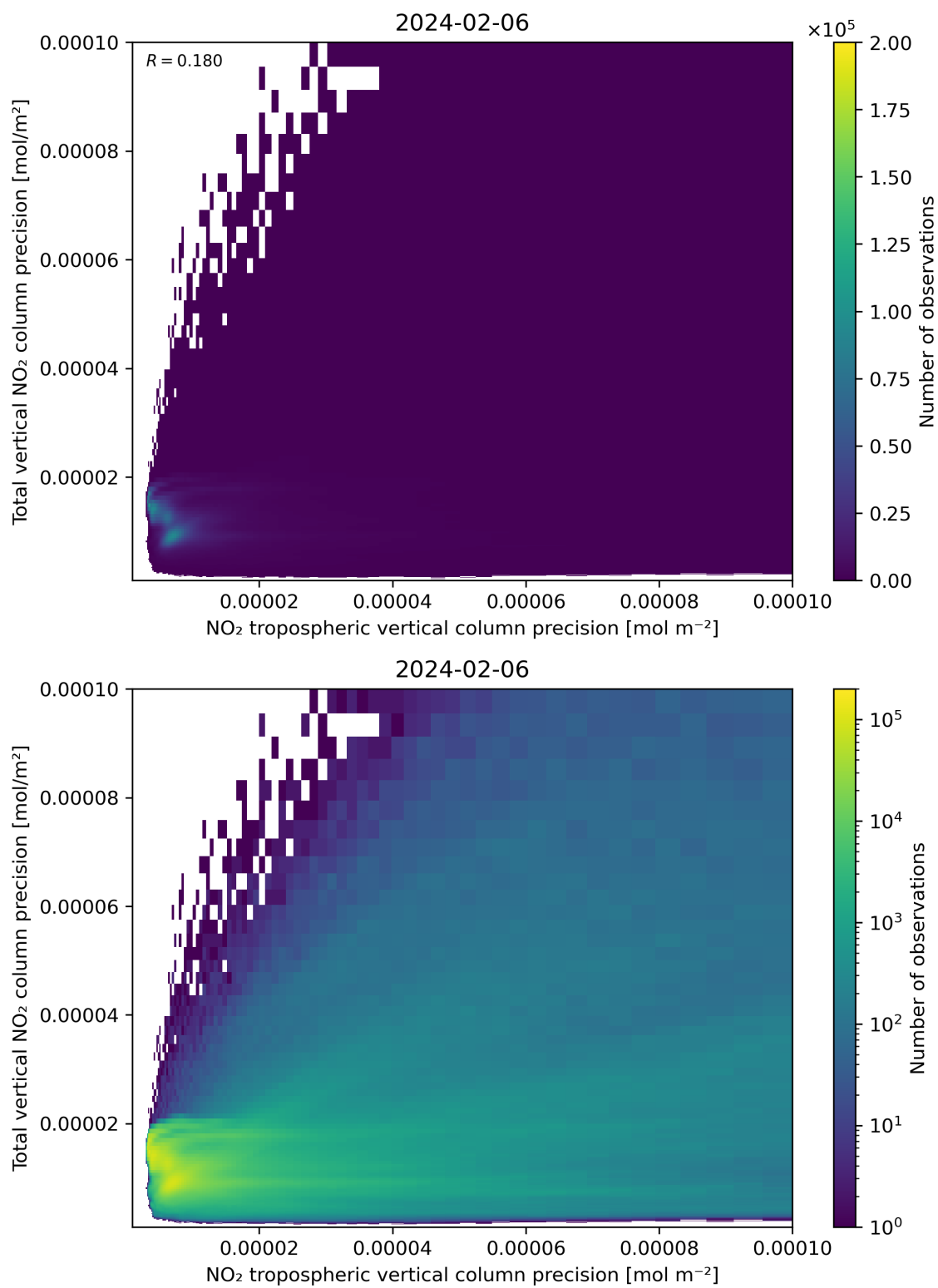
Figure 139: Scatter density plot of “NO 2 tropospheric vertical column precision” against “Total vertical NO 2 column precision” for 2024-02-06 to 2024-02-07.
