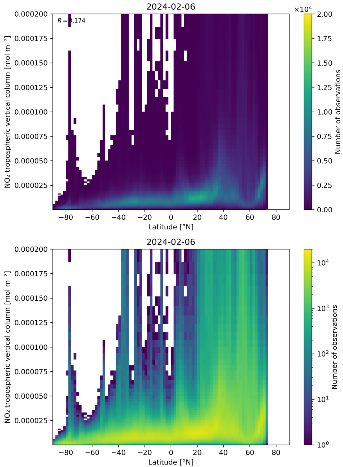
Figure 92: Scatter density plot of “Latitude” against “NO 2 tropospheric vertical column” for 2024-02-06 to 2024-02-07.
