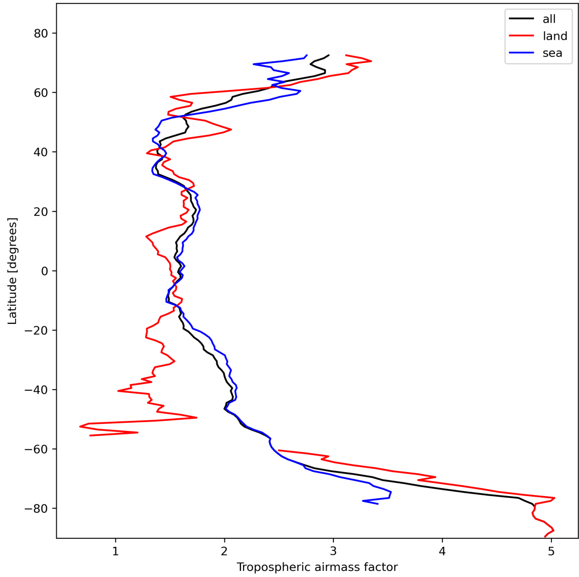
Figure 14: Zonal average of “Tropospheric airmass factor” for 2024-02-06 to 2024-02-07.
