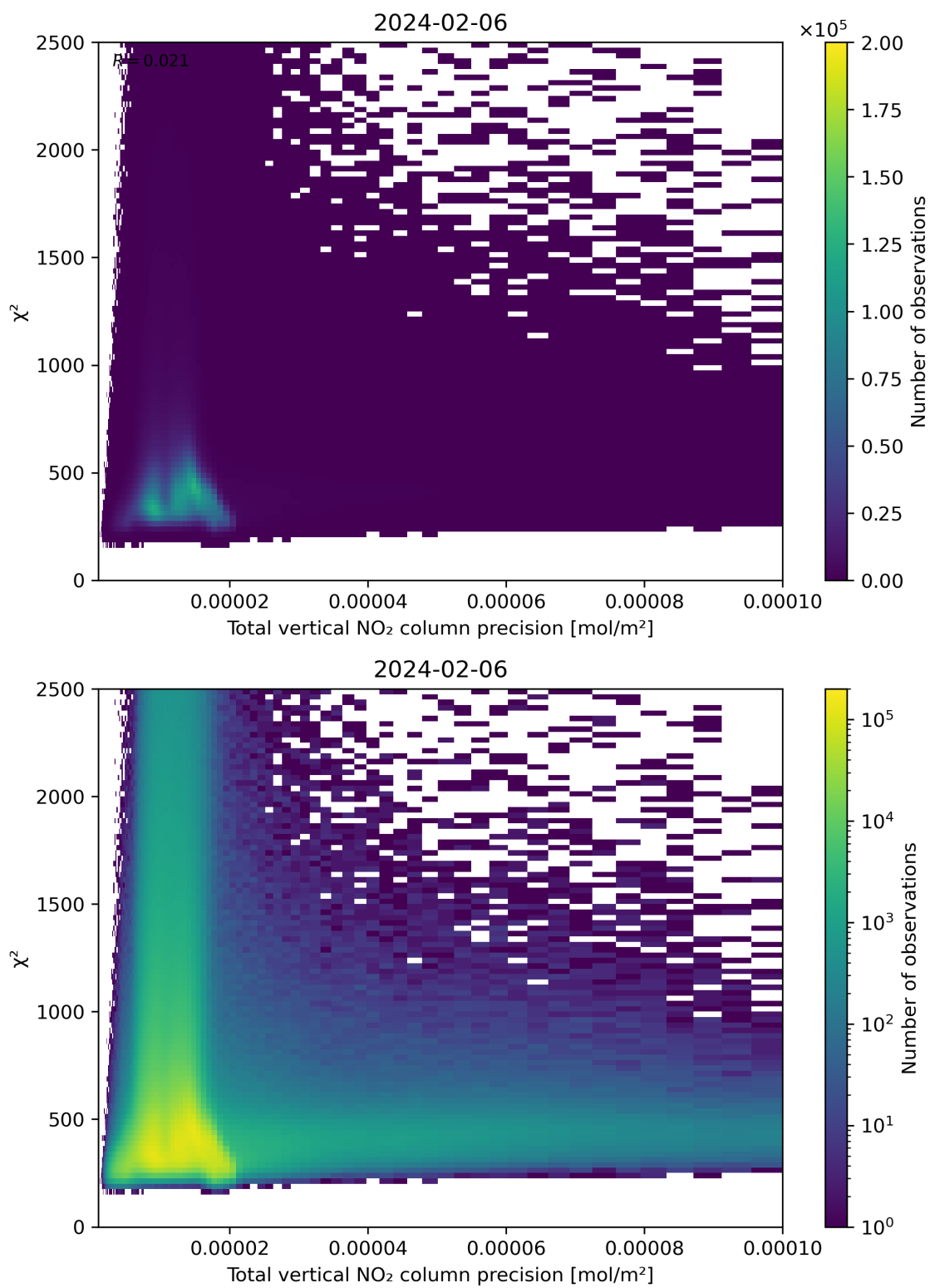
Figure 116: Scatter density plot of “Total vertical NO 2 column precision” against “ \chi^2 ” for 2024-02-06 to 2024-02-07.
