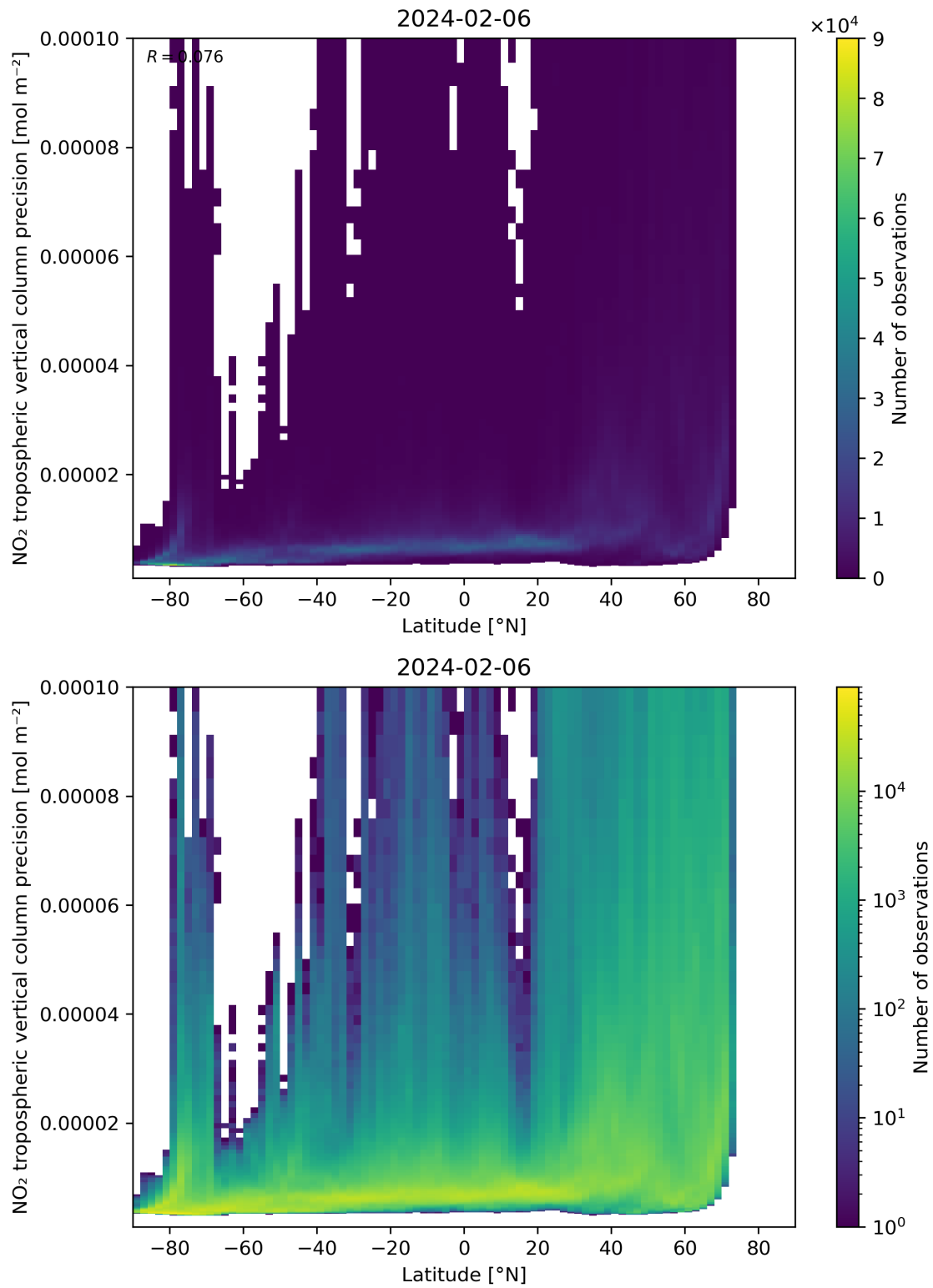
Figure 93: Scatter density plot of “Latitude” against “NO 2 tropospheric vertical column precision” for 2024-02-06 to 2024-02-07.
