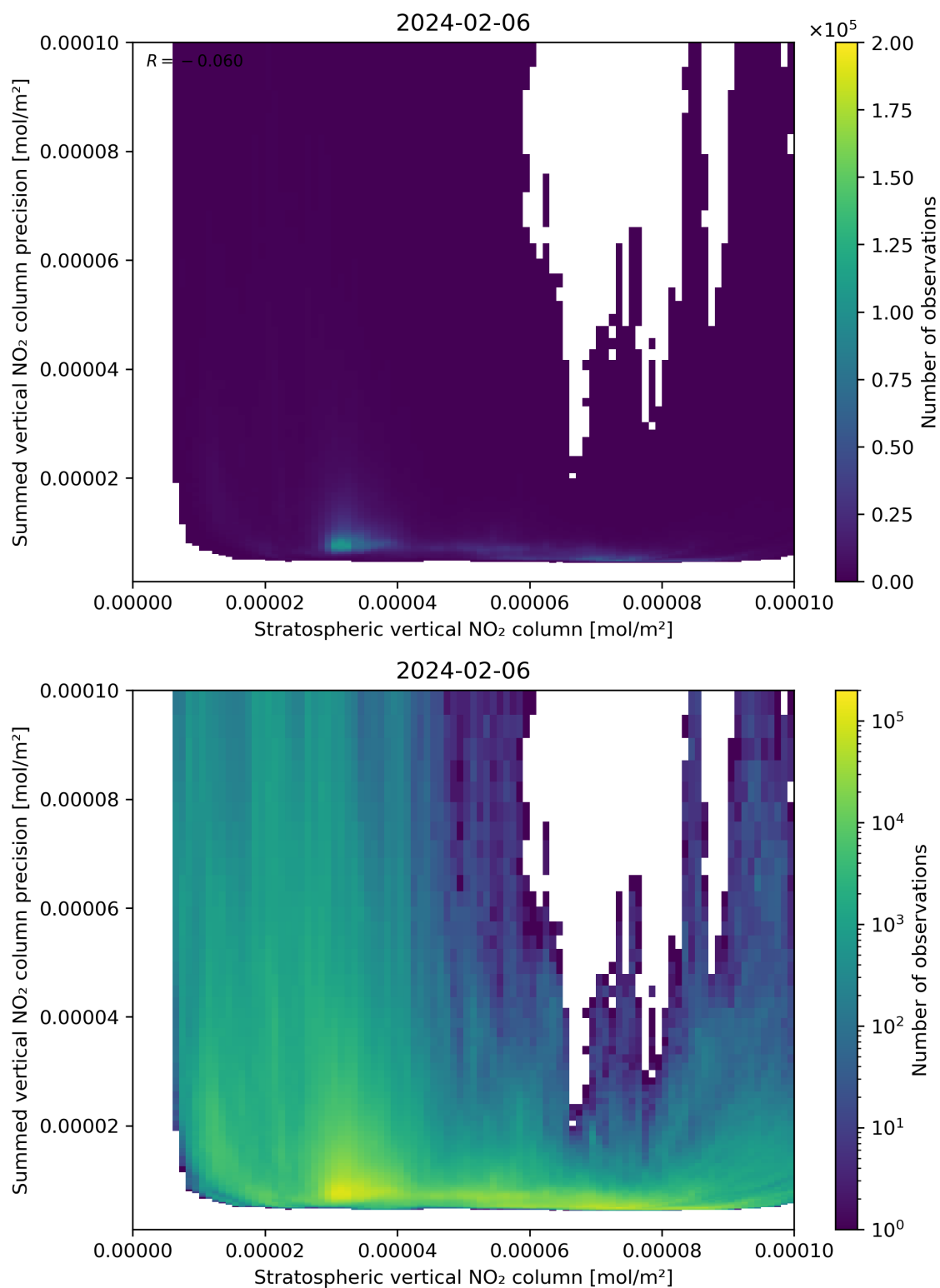
Figure 99: Scatter density plot of “Stratospheric vertical NO 2 column” against “Summed vertical NO 2 column precision” for 2024-02-06 to 2024-02-07.
