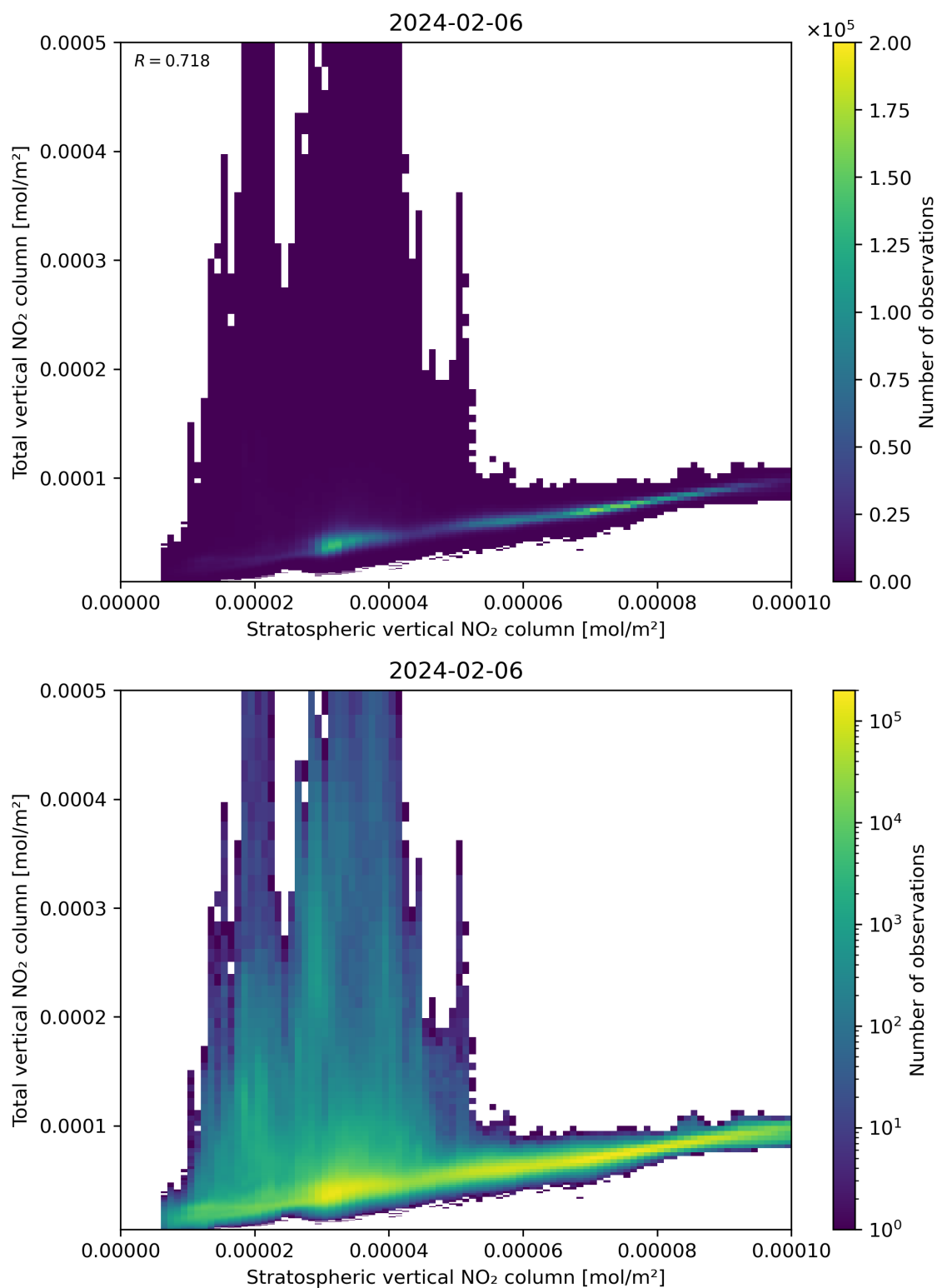
Figure 100: Scatter density plot of “Stratospheric vertical NO 2 column” against “Total vertical NO 2 column” for 2024-02-06 to 2024-02-07.
