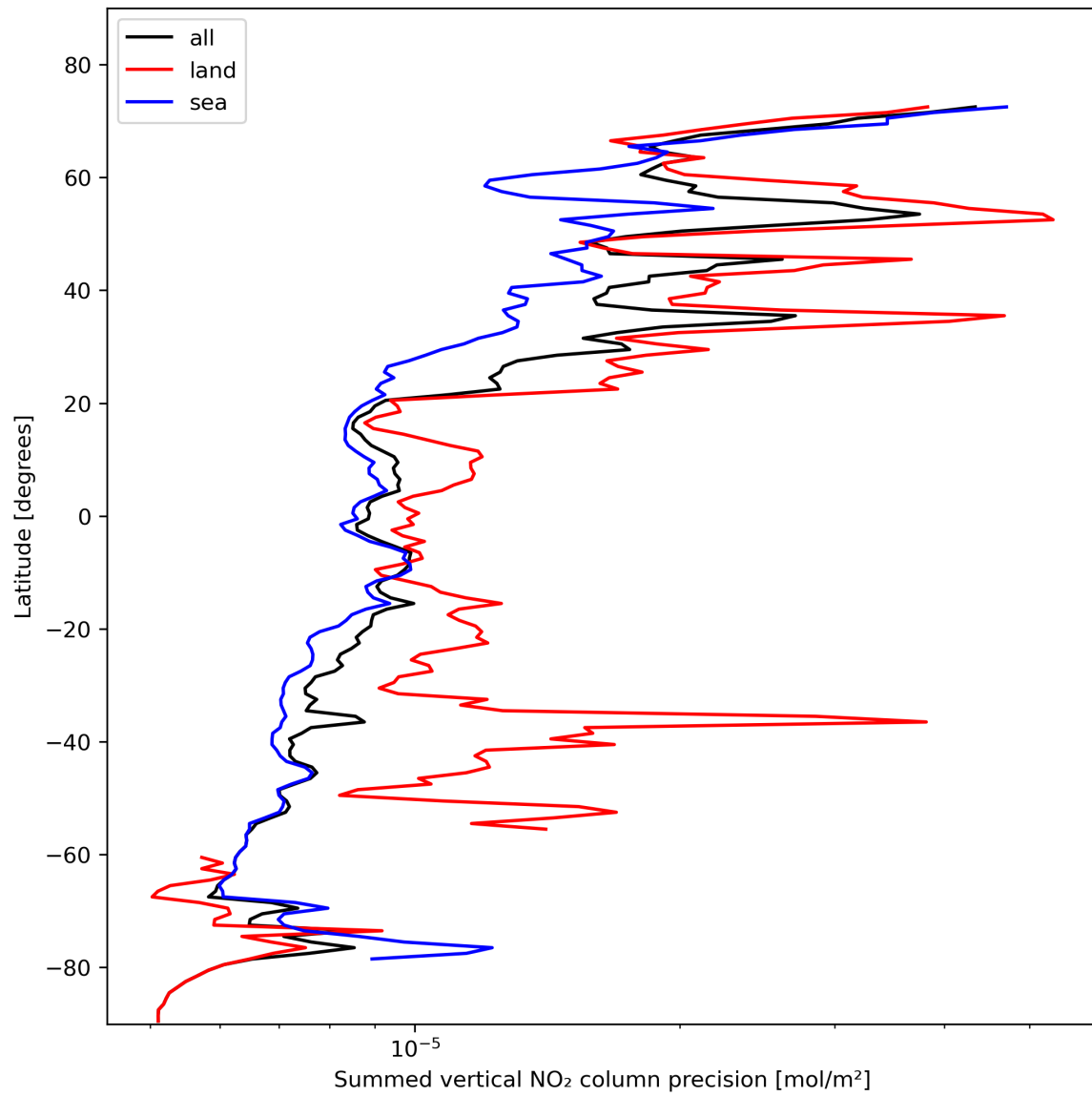
Figure 24: Zonal average of “Summed vertical NO 2 column precision” for 2024-02-06 to 2024-02-07.
