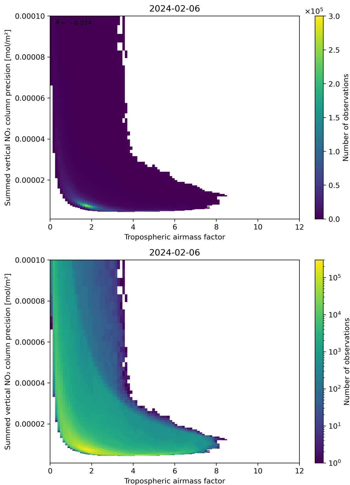
Figure 76: Scatter density plot of “Tropospheric air mass factor” against “Summed vertical NO 2 column precision” for 2024-02-06 to 2024-02-07.
