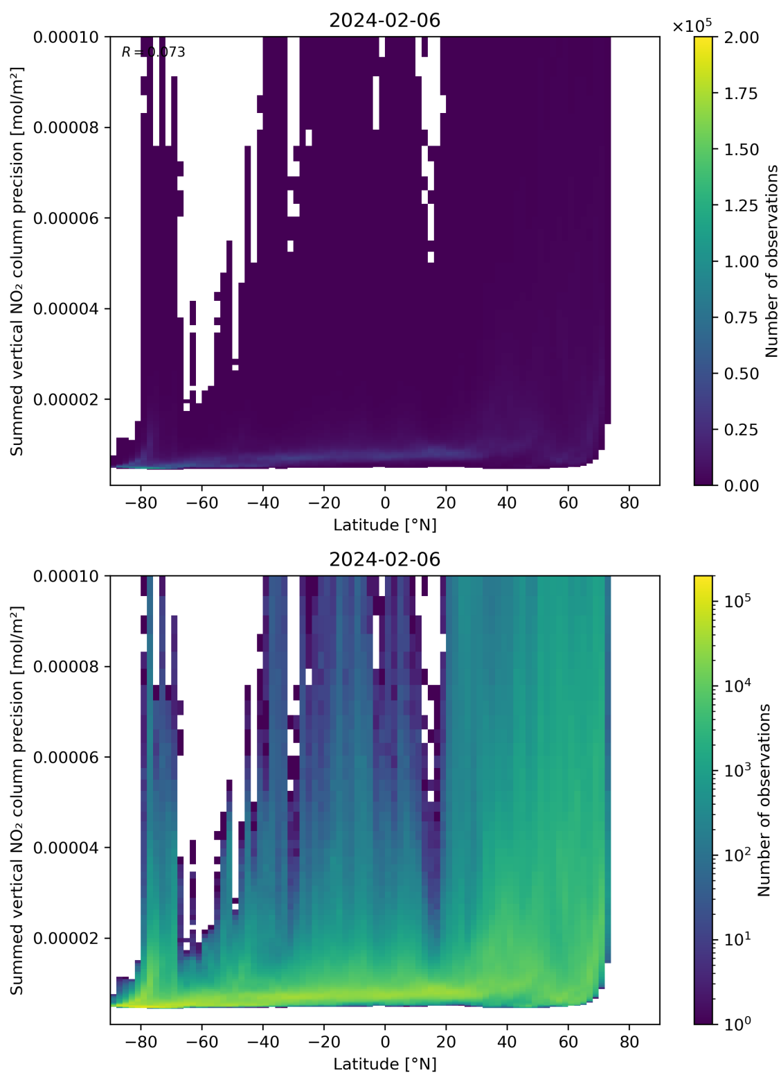
Figure 89: Scatter density plot of “Latitude” against “Summed vertical NO 2 column precision” for 2024-02-06 to 2024-02-07.
