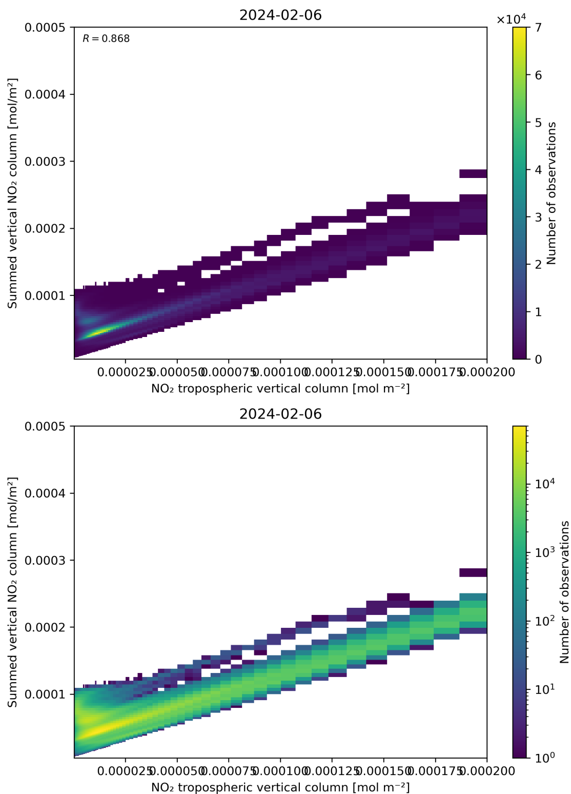
Figure 126: Scatter density plot of “NO 2 tropospheric vertical column” against “Summed vertical NO 2 column” for 2024-02-06 to 2024-02-07.
