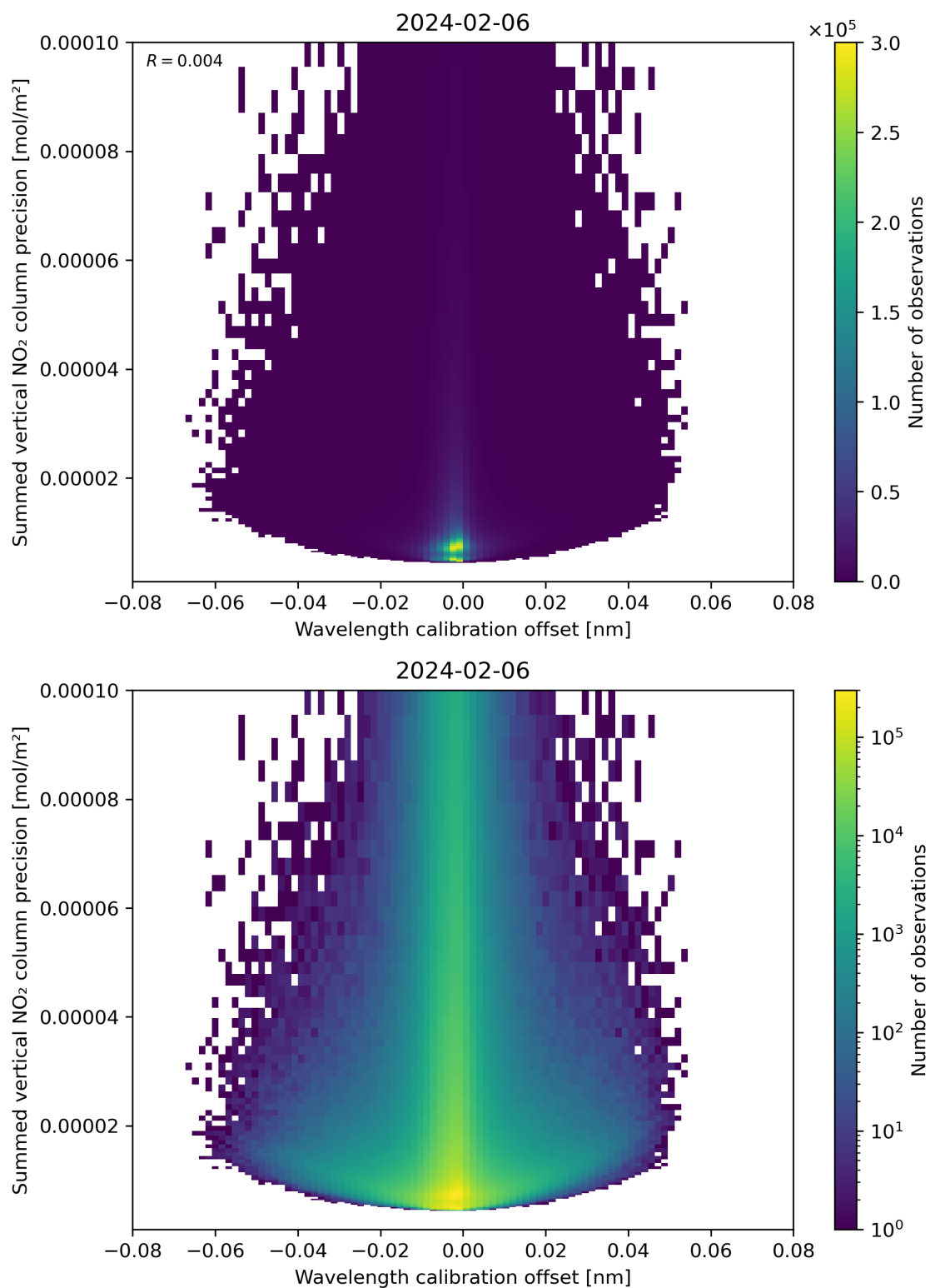
Figure 178: Scatter density plot of “Wavelength calibration offset” against “Summed vertical NO 2 column precision” for 2024-02-06 to 2024-02-07.
