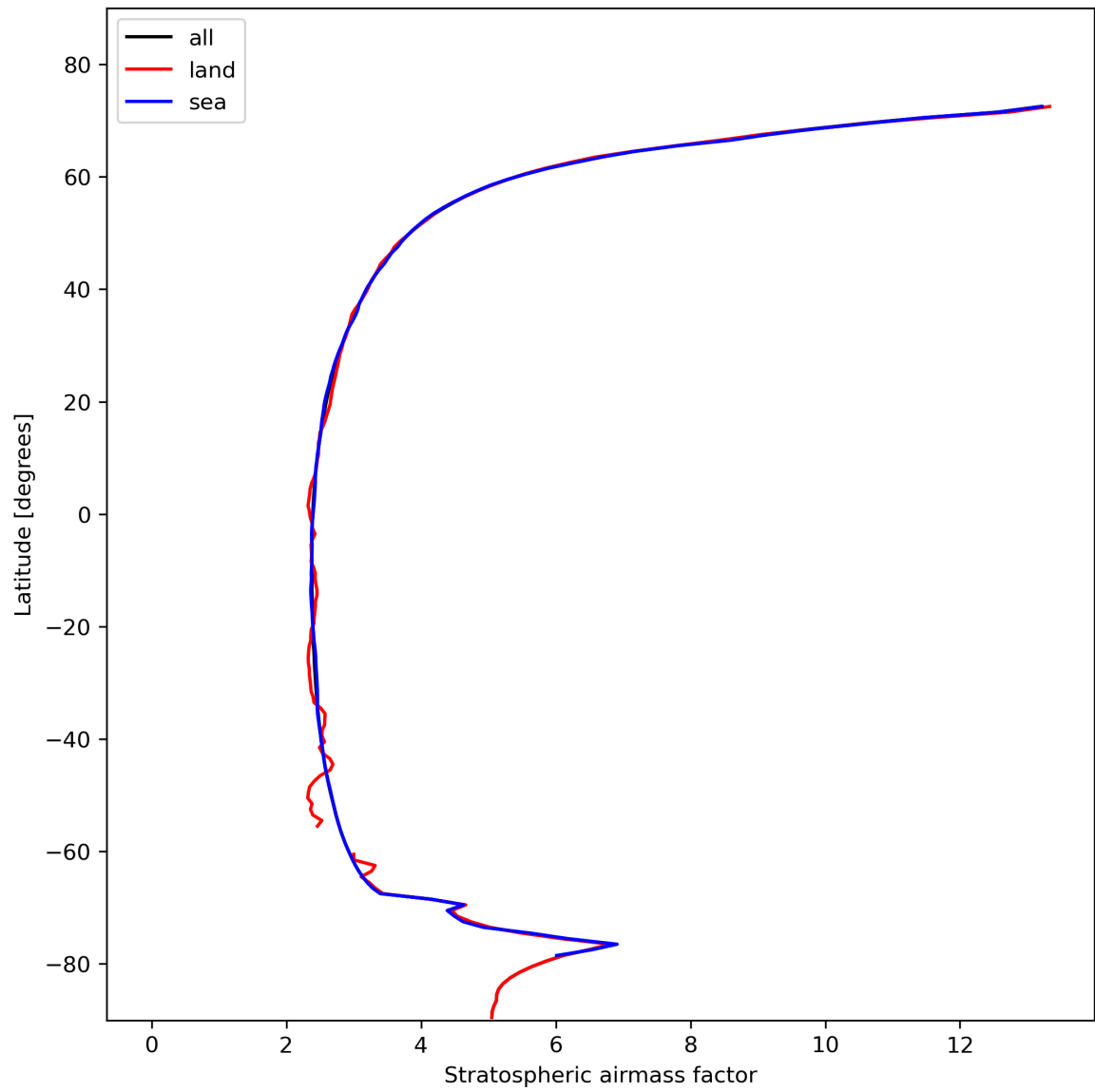
Figure 27: Zonal average of “Stratospheric airmass factor” for 2024-02-06 to 2024-02-07.
