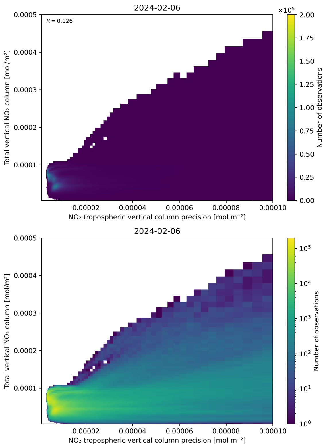
Figure 138: Scatter density plot of “NO 2 tropospheric vertical column precision” against “Total vertical NO 2 column” for 2024-02-06 to 2024-02-07.
