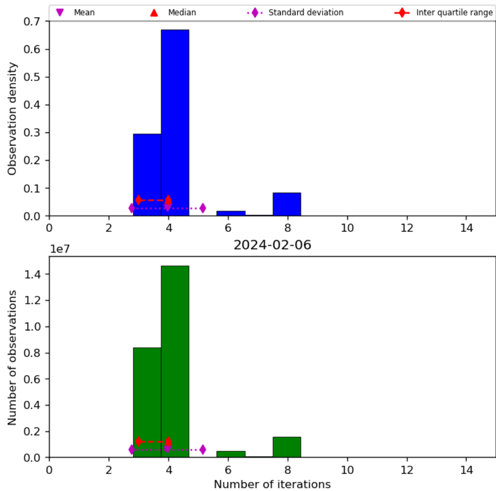
Figure 34: Histogram of “Number of iterations” for 2024-02-06 to 2024-02-07
