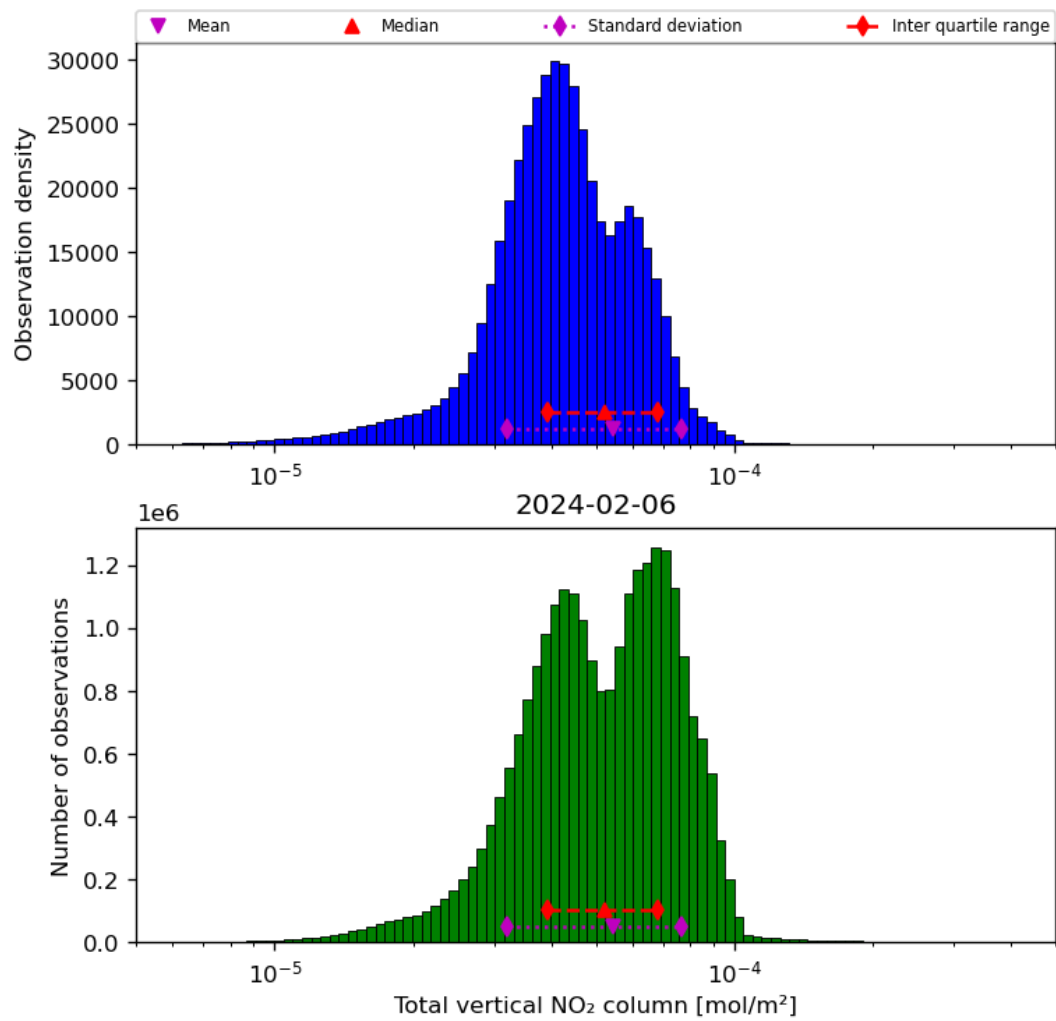
Figure 38: Histogram of “Total vertical NO 2 column” for 2024-02-06 to 2024-02-07
