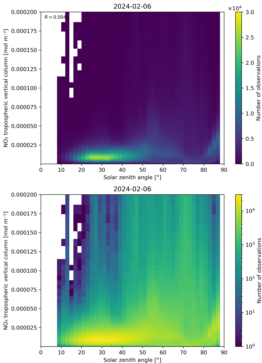
Figure 155: Scatter density plot of “Solar zenith angle” against “NO 2 tropospheric vertical column” for 2024-02-06 to 2024-02-07.
