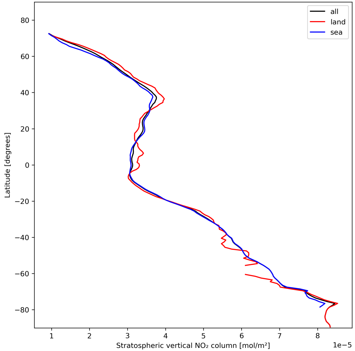
Figure 19: Zonal average of “Stratospheric vertical NO 2 column” for 2024-02-06 to 2024-02-07.
