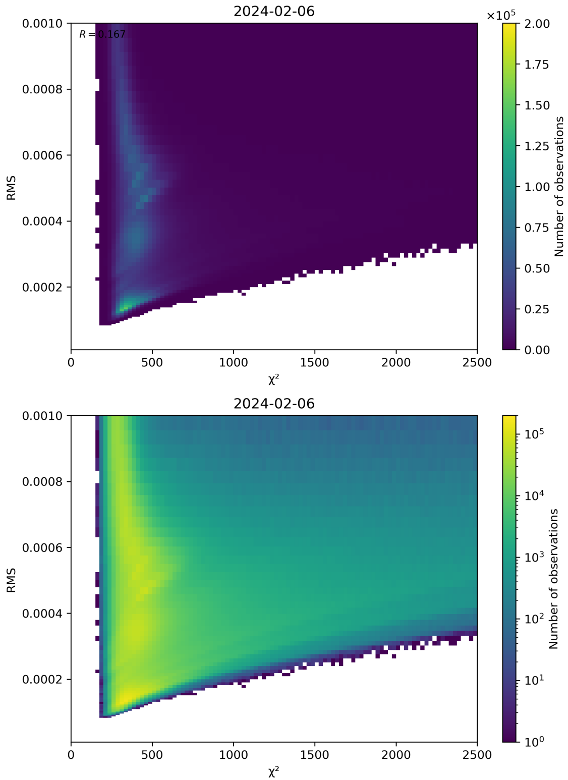
Figure 82: Scatter density plot of “ \chi^2 ” against “RMS” for 2024-02-06 to 2024-02-07.
