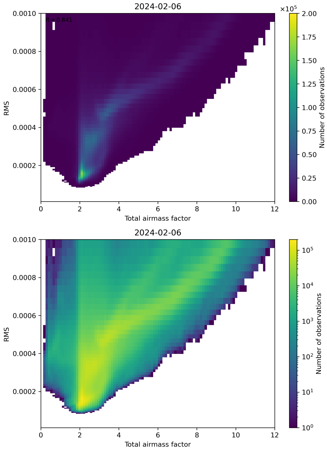
Figure 69: Scatter density plot of “Total airmass factor” against “RMS” for 2024-02-06 to 2024-02-07.
