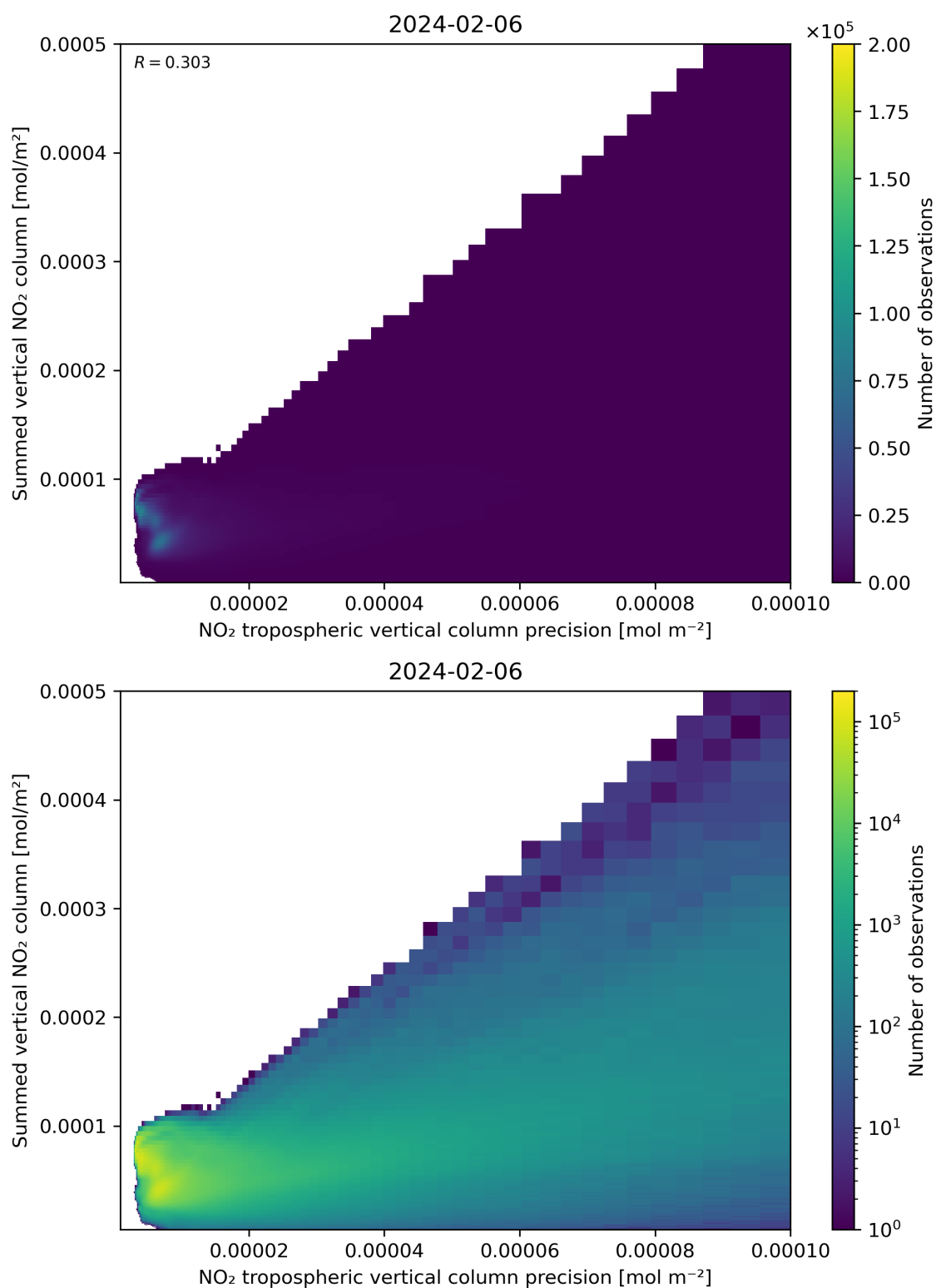
Figure 136: Scatter density plot of “NO 2 tropospheric vertical column precision” against “Summed vertical NO 2 column” for 2024-02-06 to 2024-02-07.
