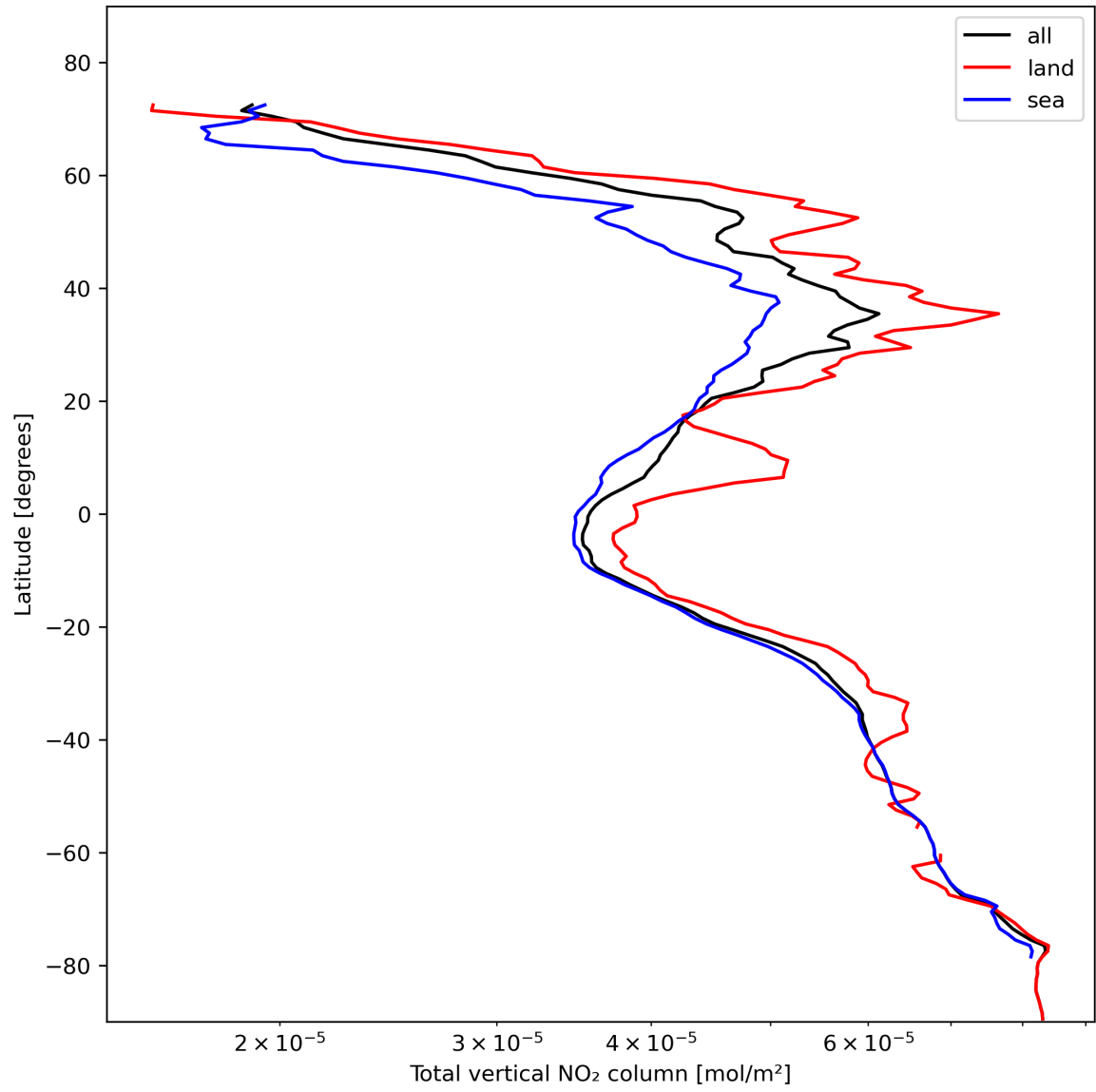
Figure 21: Zonal average of “Total vertical NO 2 column” for 2024-02-06 to 2024-02-07.
