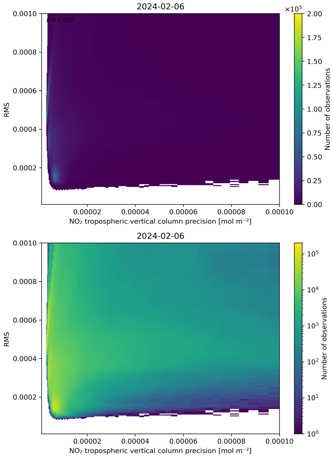
Figure 140: Scatter density plot of “NO 2 tropospheric vertical column precision” against “RMS” for 2024-02-06 to 2024-02-07.
