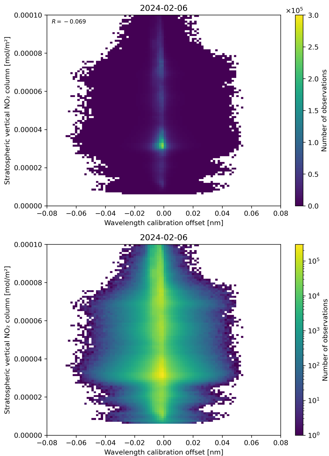
Figure 176: Scatter density plot of “Wavelength calibration offset” against “Stratospheric vertical NO 2 column” for 2024-02-06 to 2024-02-07.
