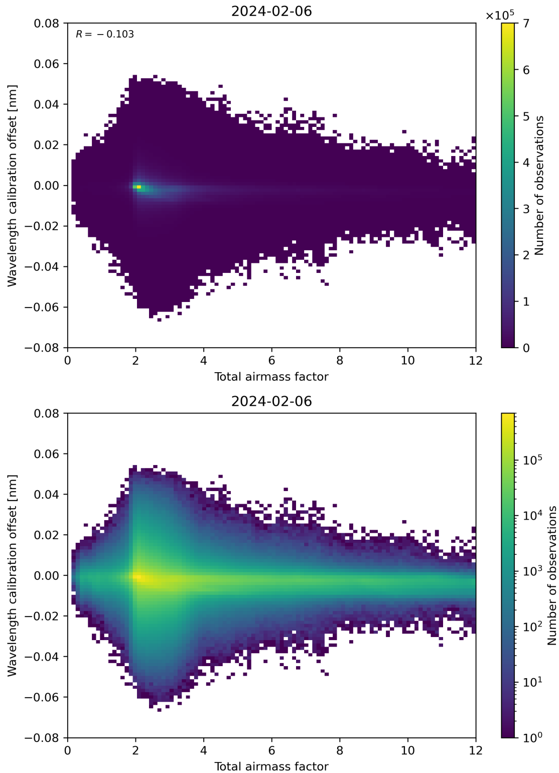
Figure 70: Scatter density plot of “Total airmass factor” against “Wavelength calibration offset” for 2024-02-06 to 2024-02-07.
