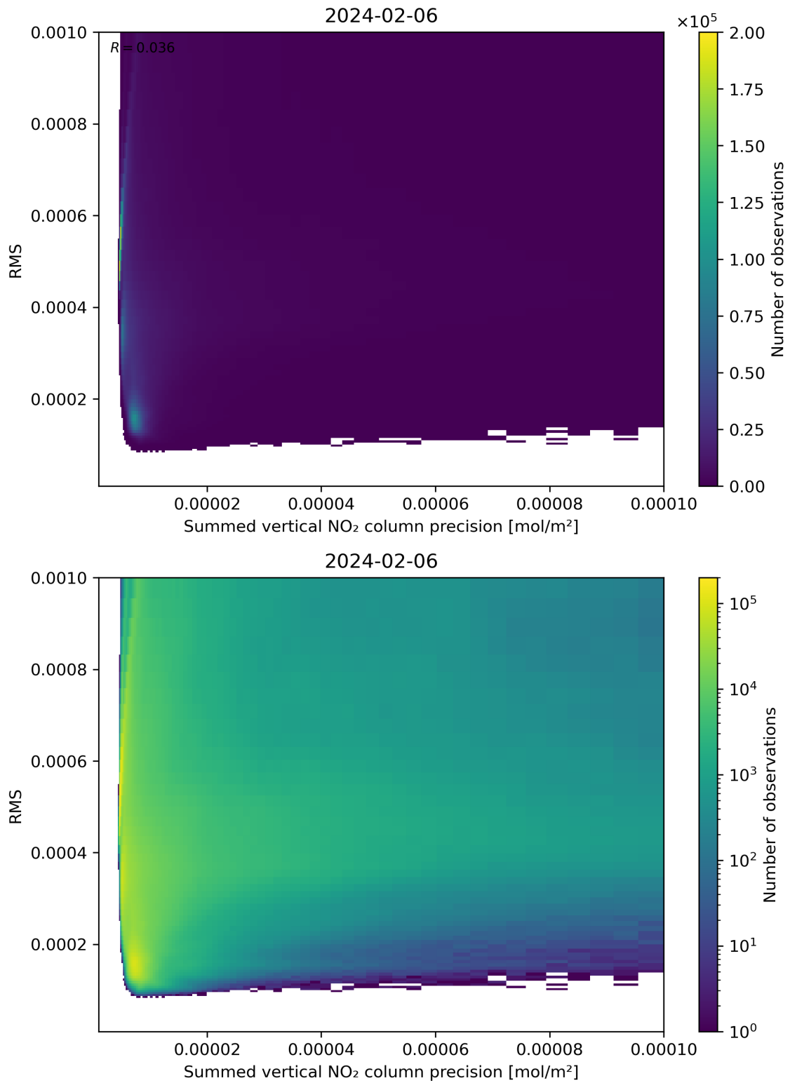
Figure 108: Scatter density plot of “Summed vertical NO 2 column precision” against “RMS” for 2024-02-06 to 2024-02-07.
