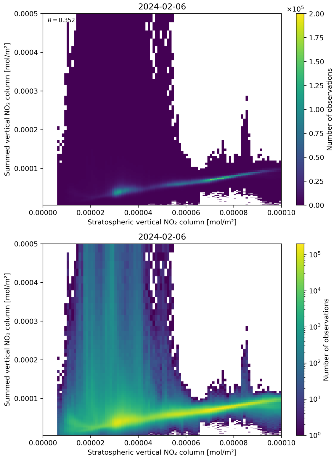
Figure 98: Scatter density plot of “Stratospheric vertical NO 2 column” against “Summed vertical NO 2 column” for 2024-02-06 to 2024-02-07.
