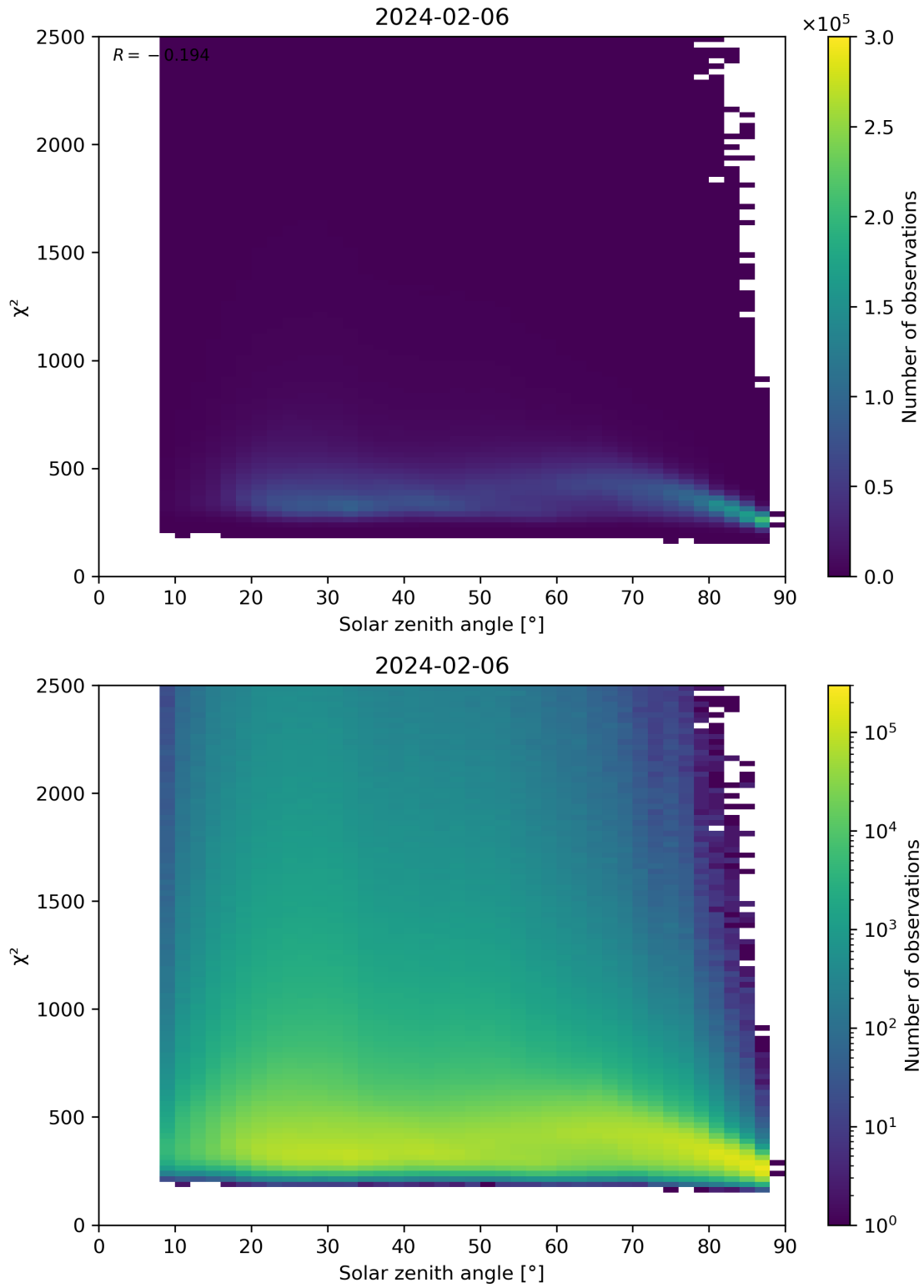
Figure 148: Scatter density plot of “Solar zenith angle” against “ \chi^2 ” for 2024-02-06 to 2024-02-07.
