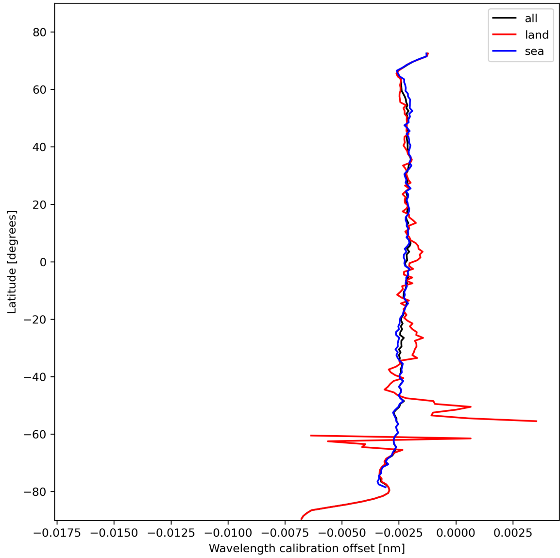
Figure 18: Zonal average of “Wavelength calibration offset” for 2024-02-06 to 2024-02-07.
