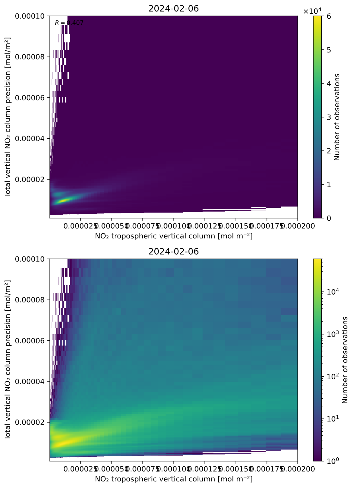
Figure 129: Scatter density plot of “NO 2 tropospheric vertical column” against “Total vertical NO 2 column precision” for 2024-02-06 to 2024-02-07.
