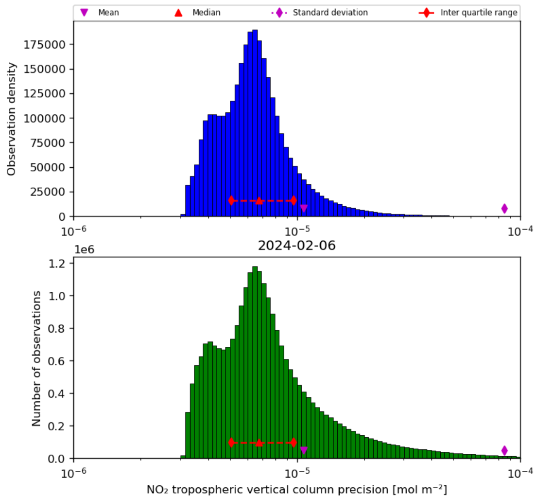
Figure 30: Histogram of “NO 2 tropospheric vertical column precision” for 2024-02-06 to 2024-02-07
