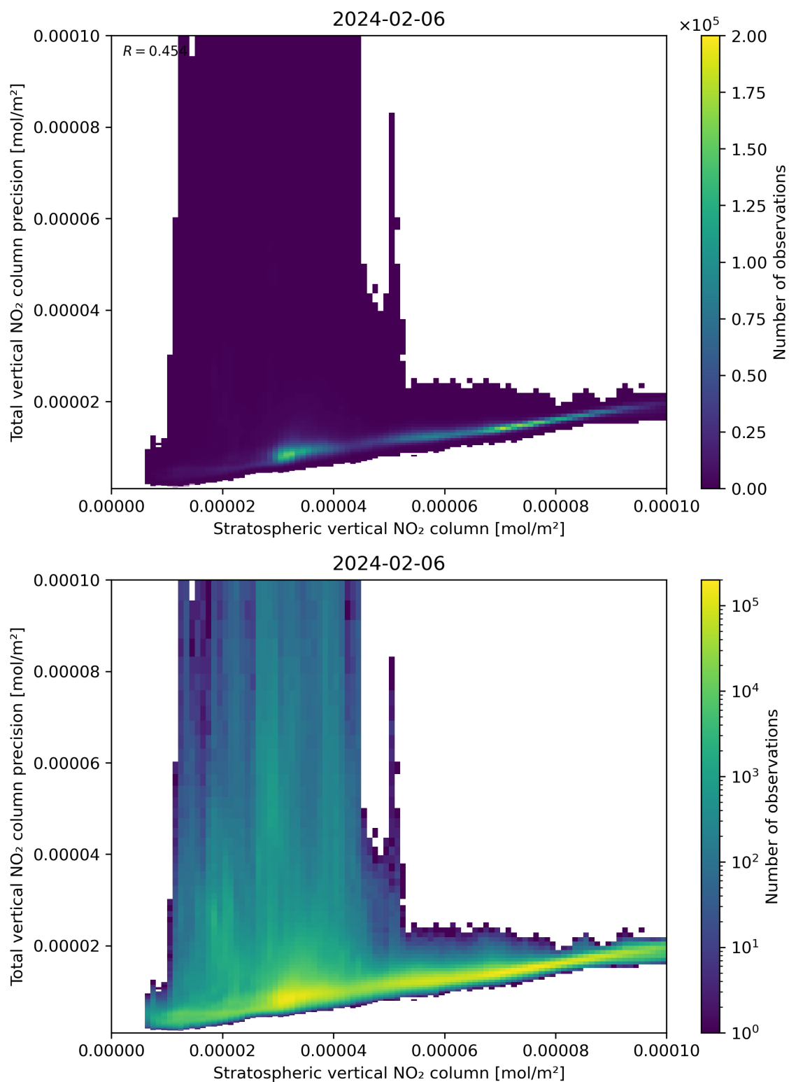
Figure 101: Scatter density plot of “Stratospheric vertical NO 2 column” against “Total vertical NO 2 column precision” for 2024-02-06 to 2024-02-07.
