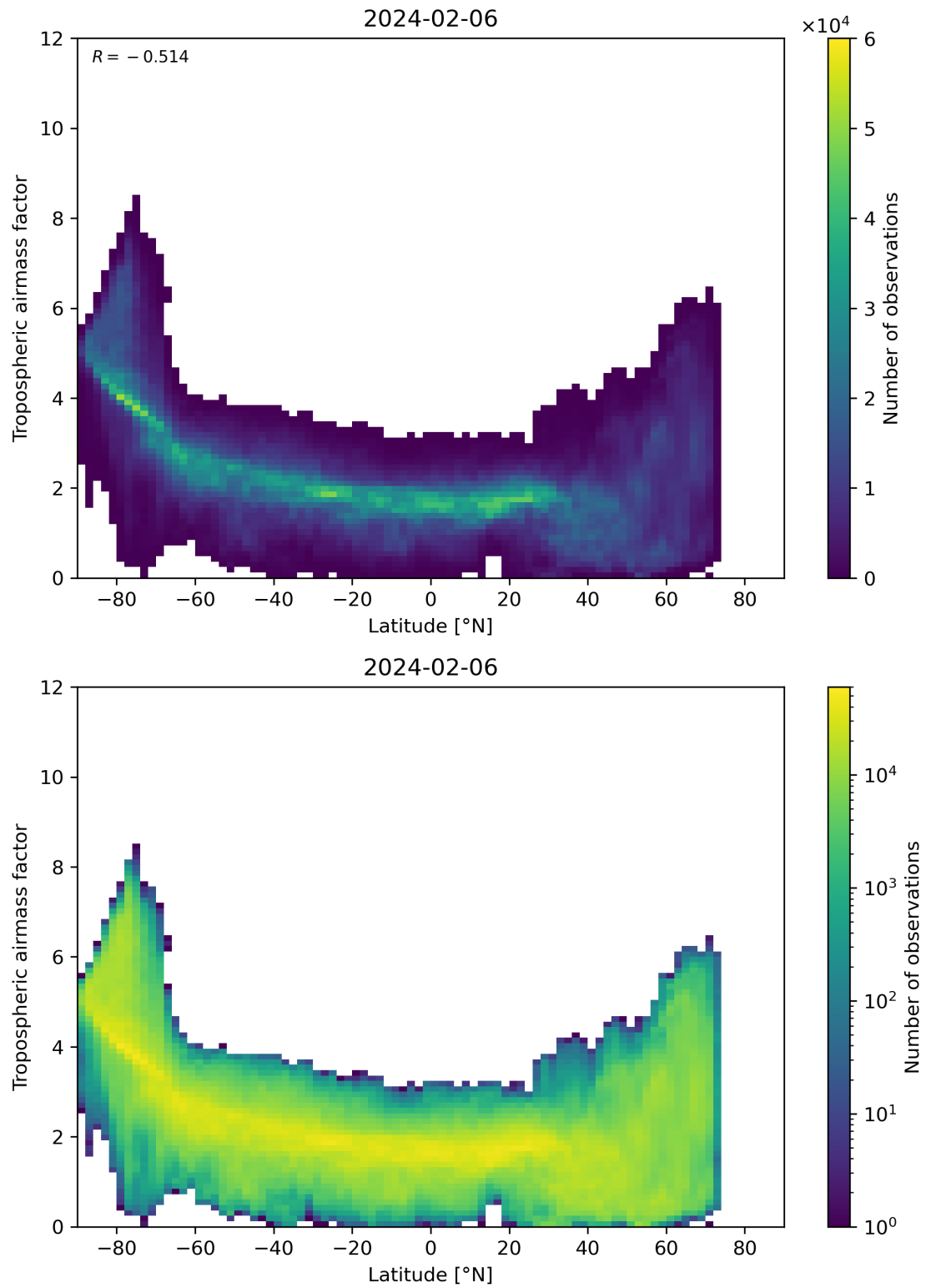
Figure 85: Scatter density plot of “Latitude” against “Tropospheric airmass factor” for 2024-02-06 to 2024-02-07.
