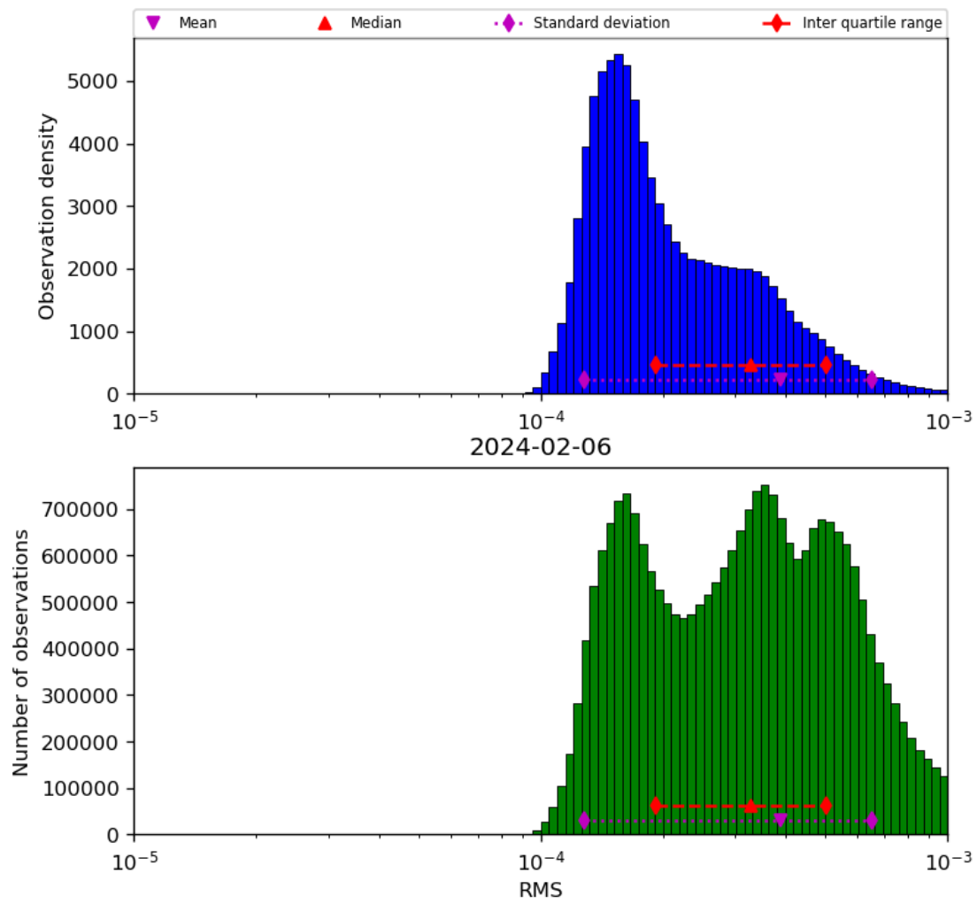
Figure 43: Histogram of “RMS” for 2024-02-06 to 2024-02-07
