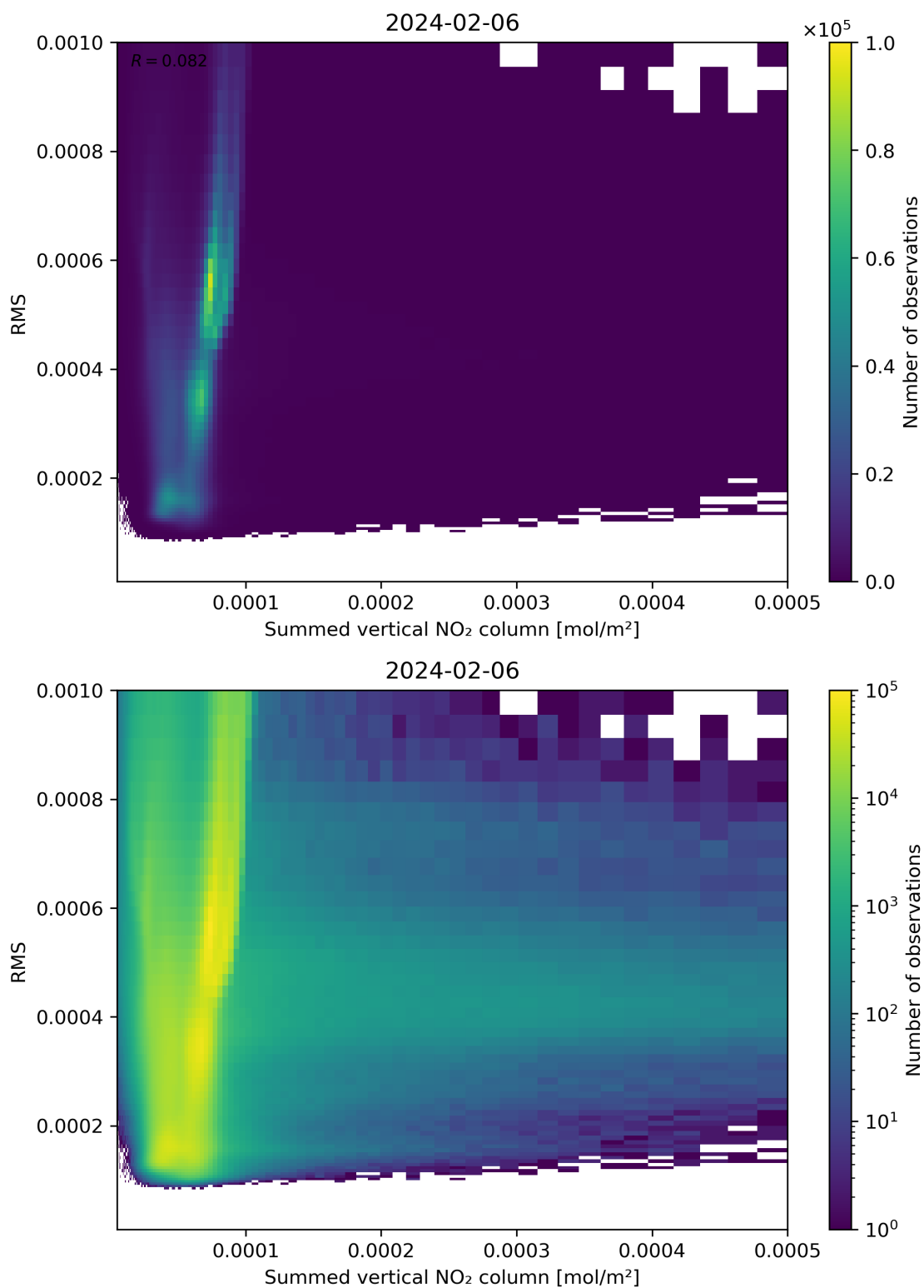
Figure 109: Scatter density plot of “Summed vertical NO 2 column” against “RMS” for 2024-02-06 to 2024-02-07.
