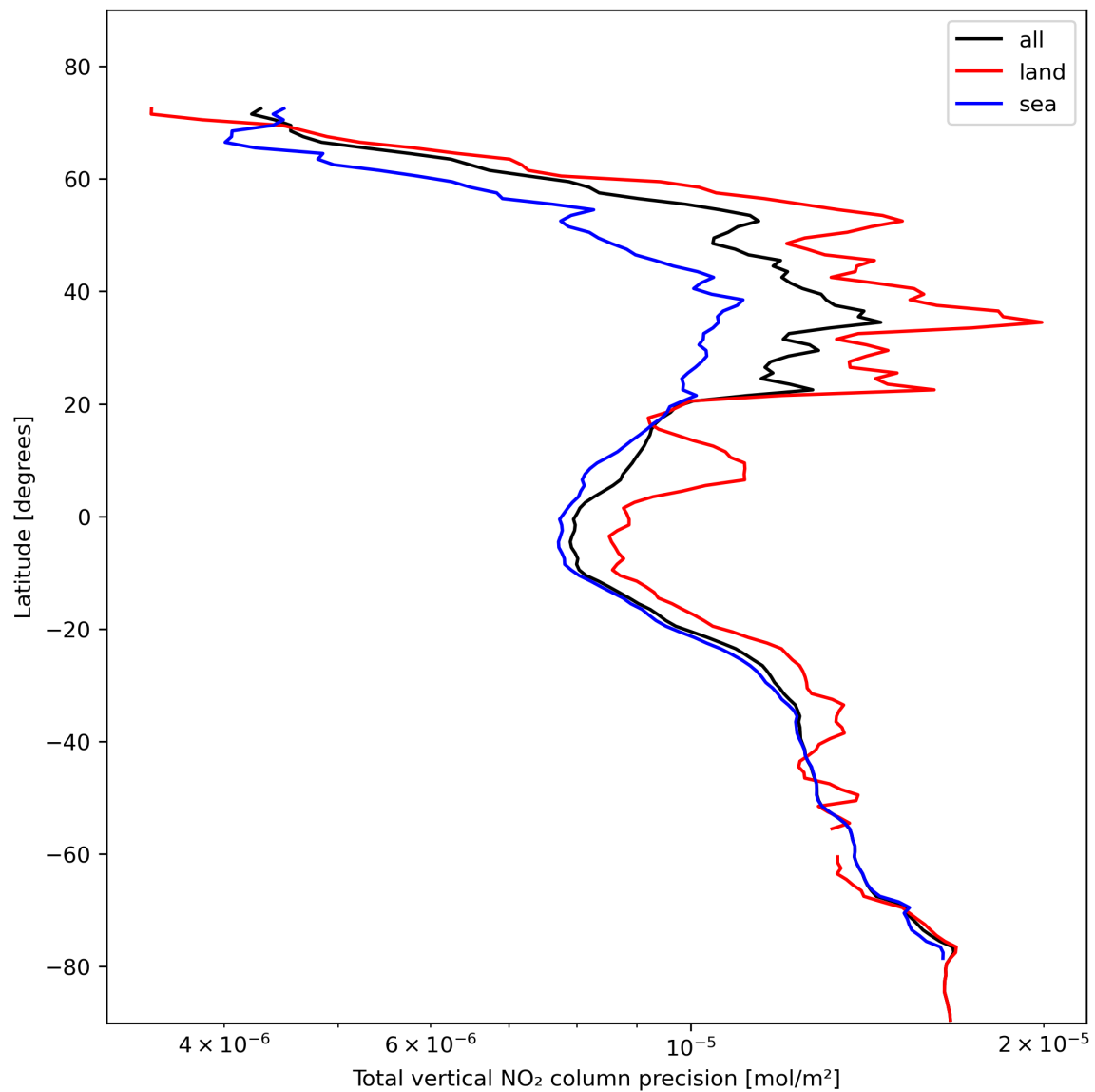
Figure 22: Zonal average of "Total vertical NO 2 column precision" for 2024-02-06 to 2024-02-07.
