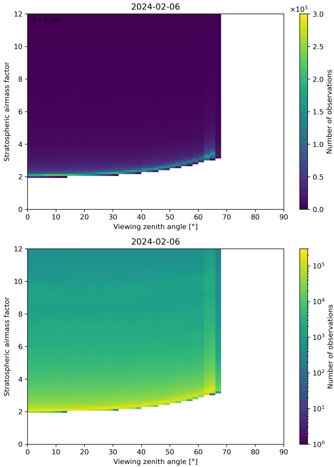
Figure 159: Scatter density plot of “Viewing zenith angle” against “Stratospheric airmass factor” for 2024-02-06 to 2024-02-07.
