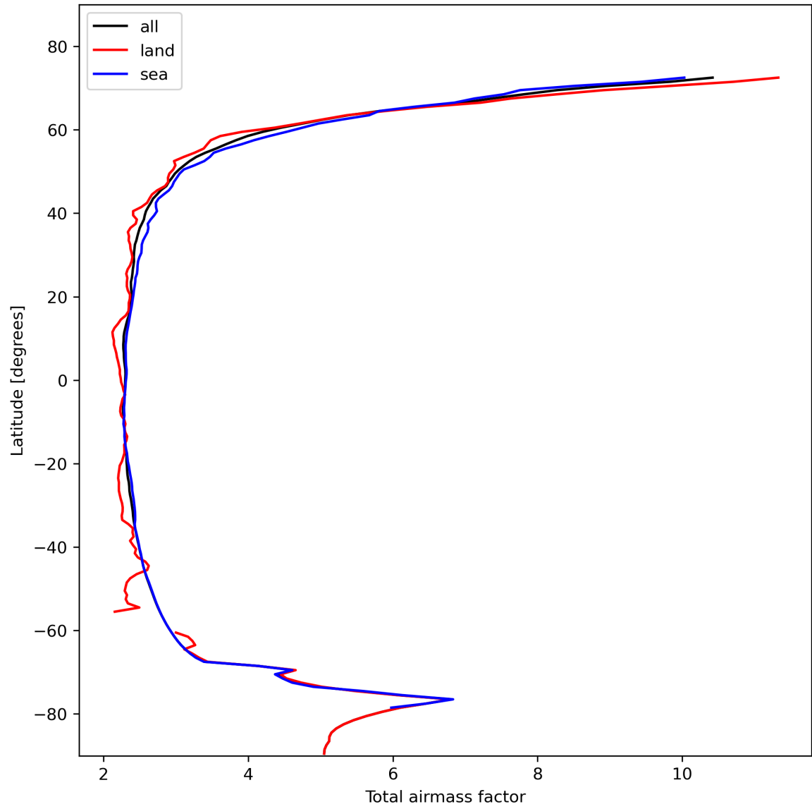
Figure 15: Zonal average of “Total airmass factor” for 2024-02-06 to 2024-02-07.
