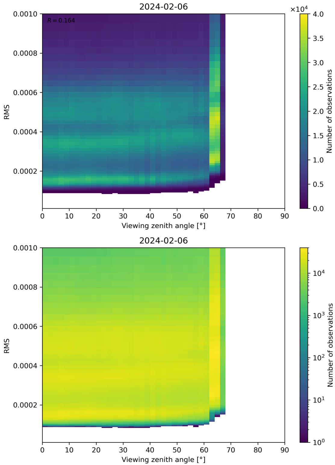
Figure 171: Scatter density plot of “Viewing zenith angle” against “RMS” for 2024-02-06 to 2024-02-07.
