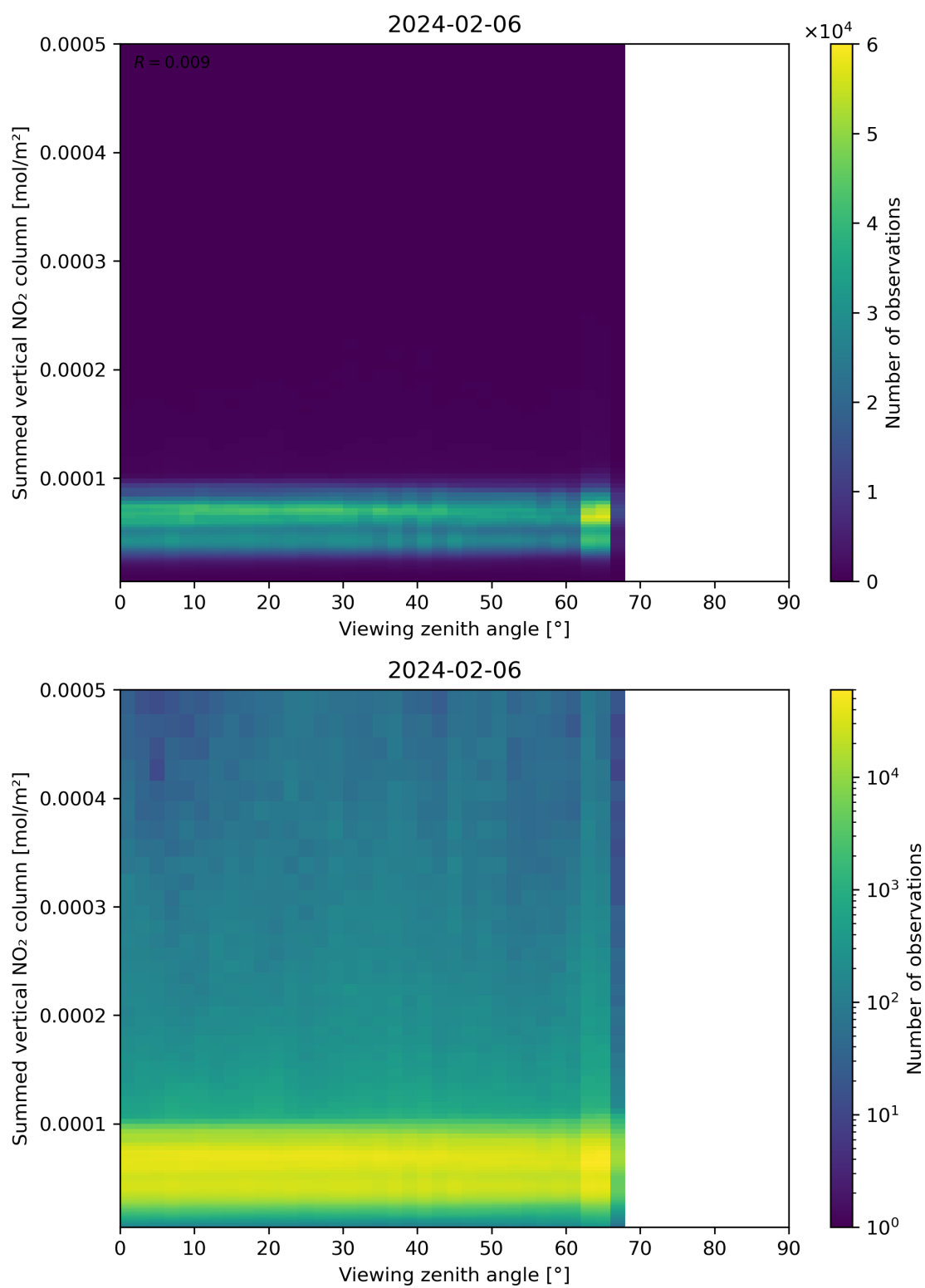
Figure 165: Scatter density plot of “Viewing zenith angle” against “Summed vertical NO 2 column” for 2024-02-06 to 2024-02-07.
