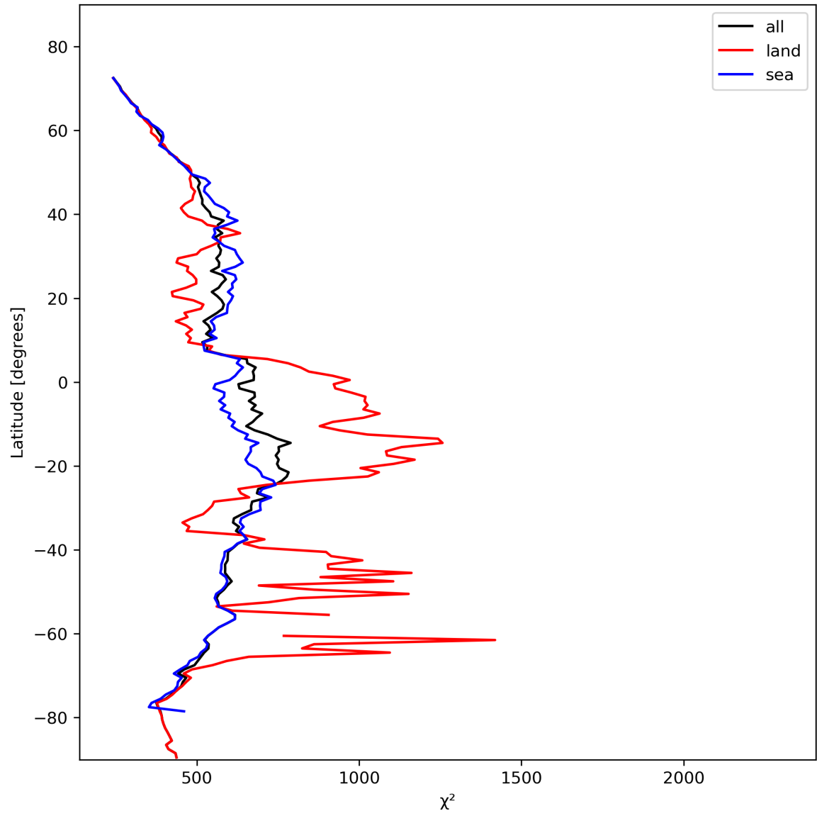
Figure 25: Zonal average of “ \chi^2 ” for 2024-02-06 to 2024-02-07.
