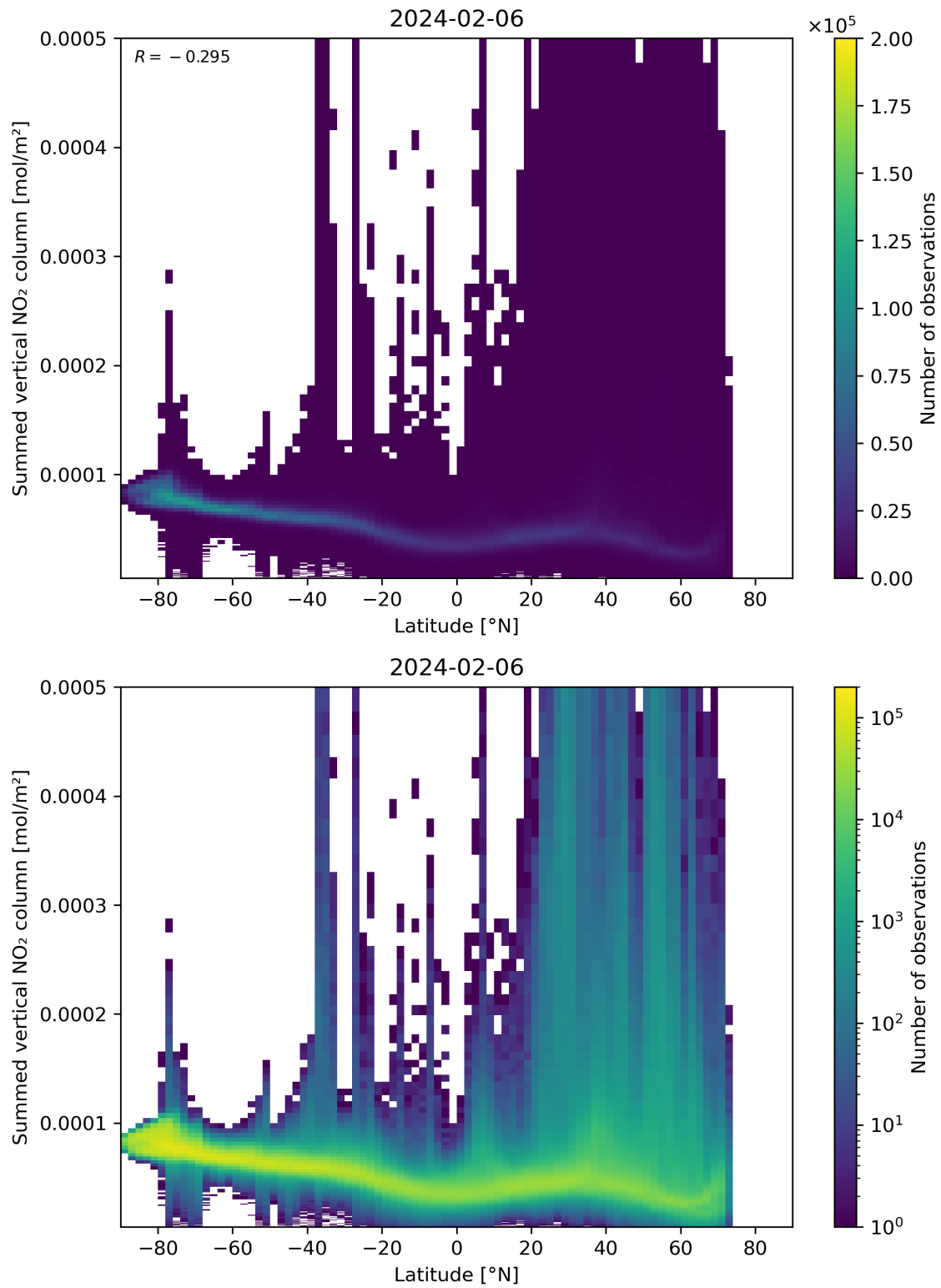
Figure 88: Scatter density plot of “Latitude” against “Summed vertical NO 2 column” for 2024-02-06 to 2024-02-07.
