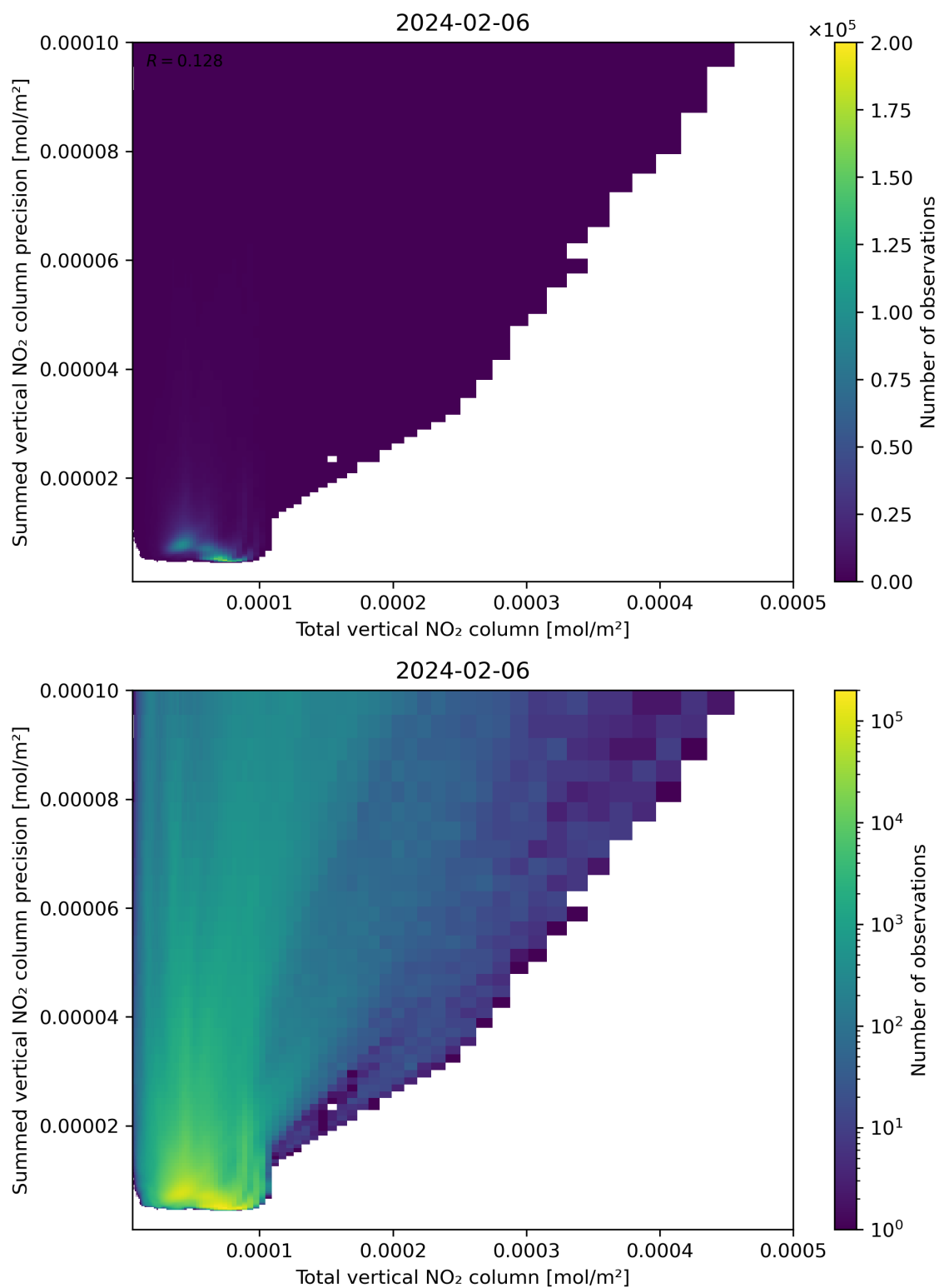
Figure 113: Scatter density plot of “Total vertical NO 2 column” against “Summed vertical NO 2 column precision” for 2024-02-06 to 2024-02-07.
