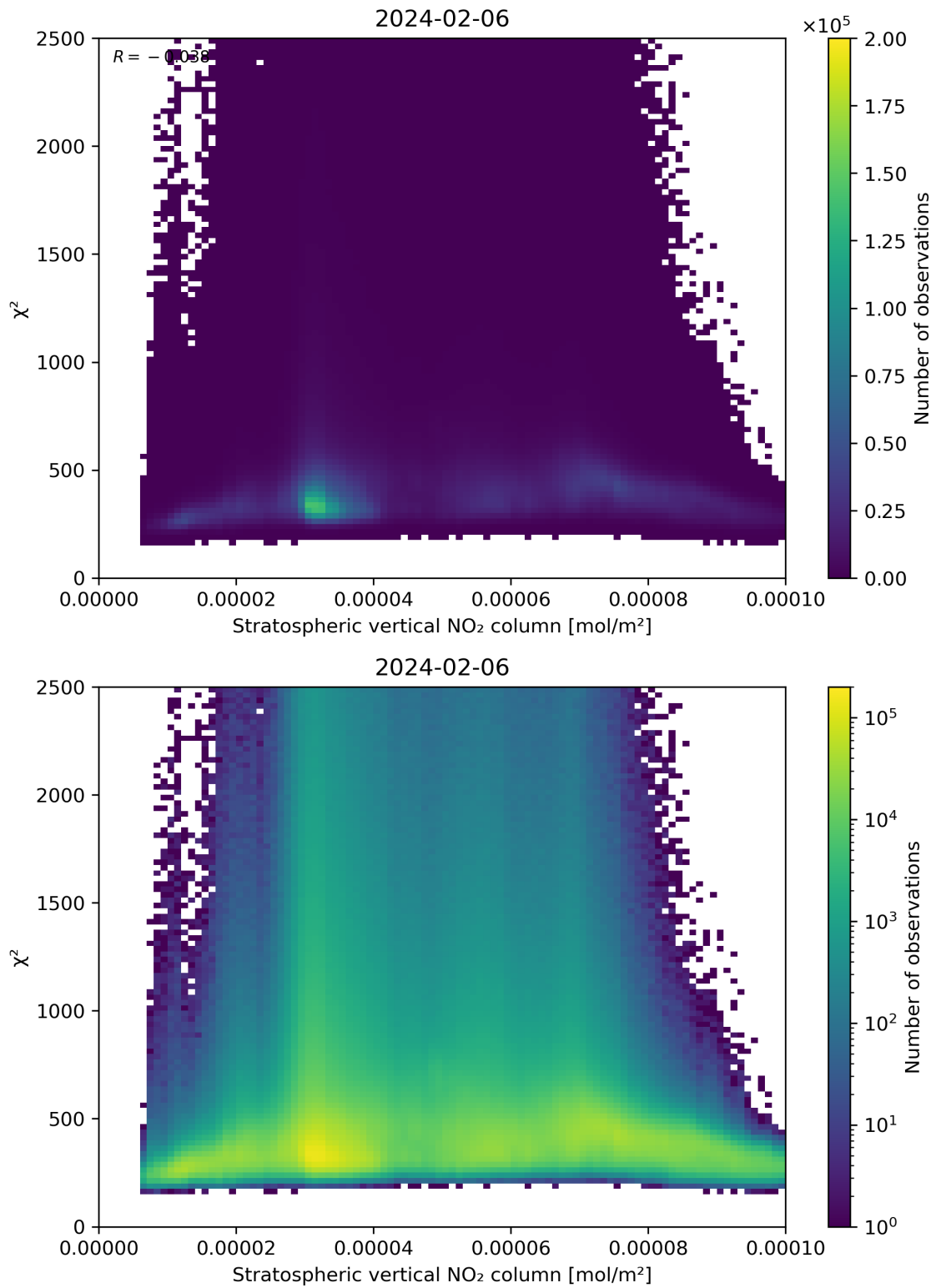
Figure 97: Scatter density plot of “Stratospheric vertical NO 2 column” against “ \chi^2 ” for 2024-02-06 to 2024-02-07.
