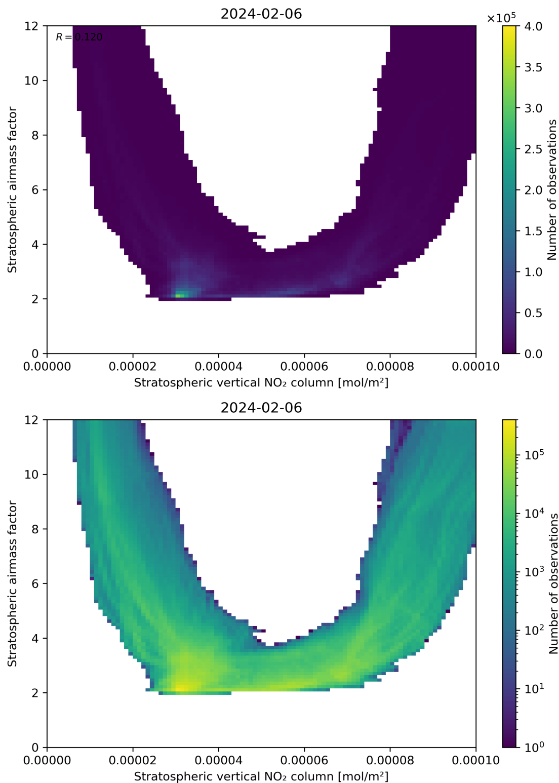
Figure 96: Scatter density plot of “Stratospheric vertical NO 2 column” against “Stratospheric airmass factor” for 2024-02-06 to 2024-02-07.
