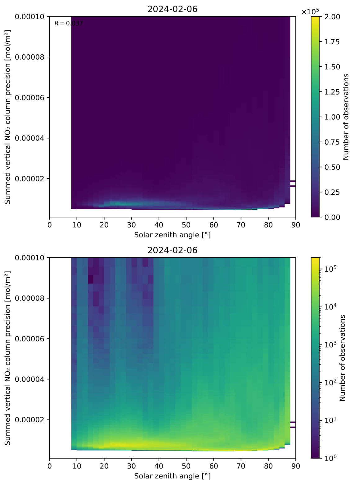
Figure 152: Scatter density plot of “Solar zenith angle” against “Summed vertical NO 2 column precision” for 2024-02-06 to 2024-02-07.
