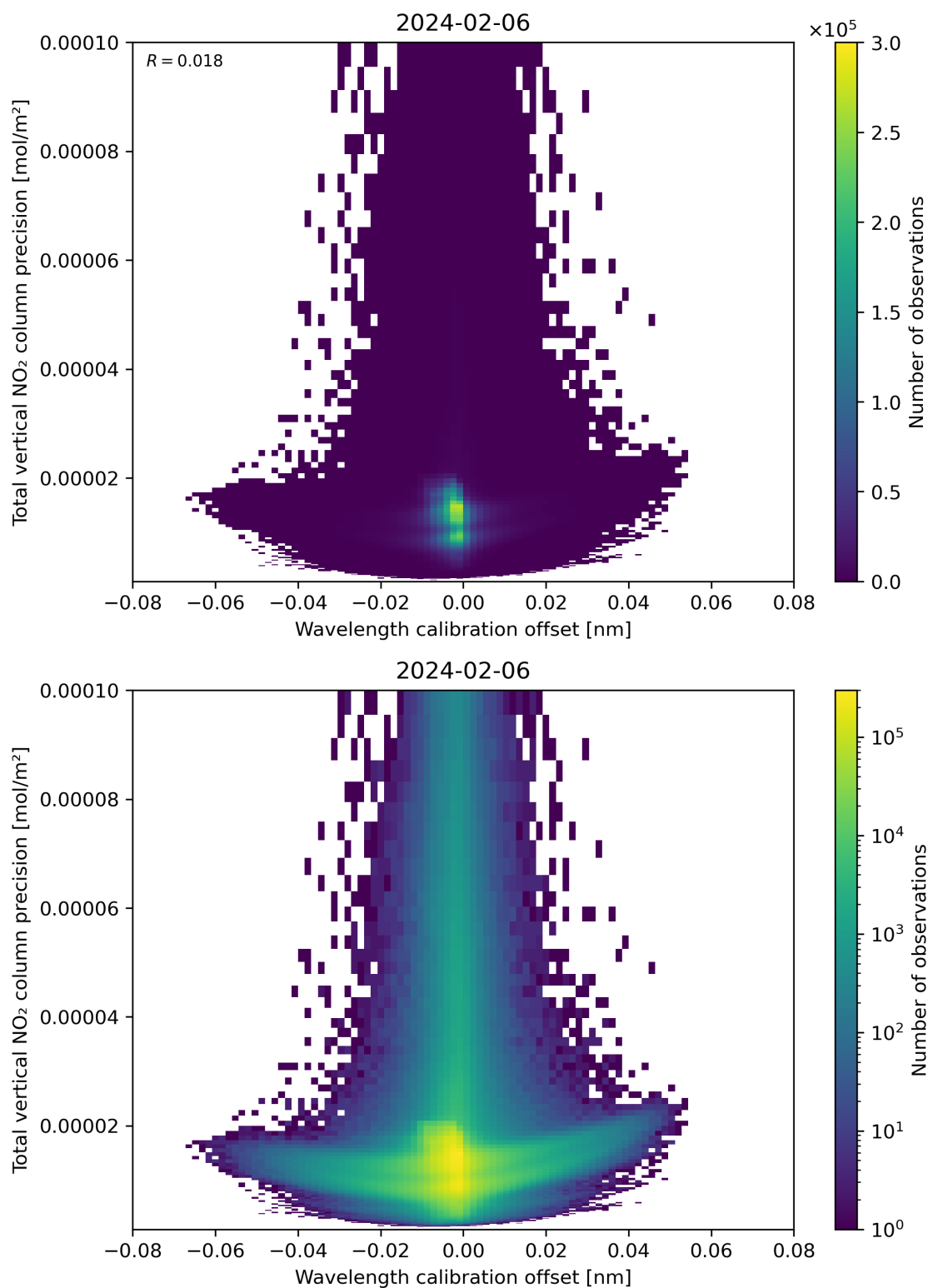
Figure 180: Scatter density plot of “Wavelength calibration offset” against “Total vertical NO 2 column precision” for 2024-02-06 to 2024-02-07.
