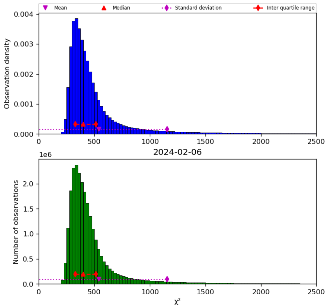
Figure 42: Histogram of “ \chi^2 ” for 2024-02-06 to 2024-02-07
