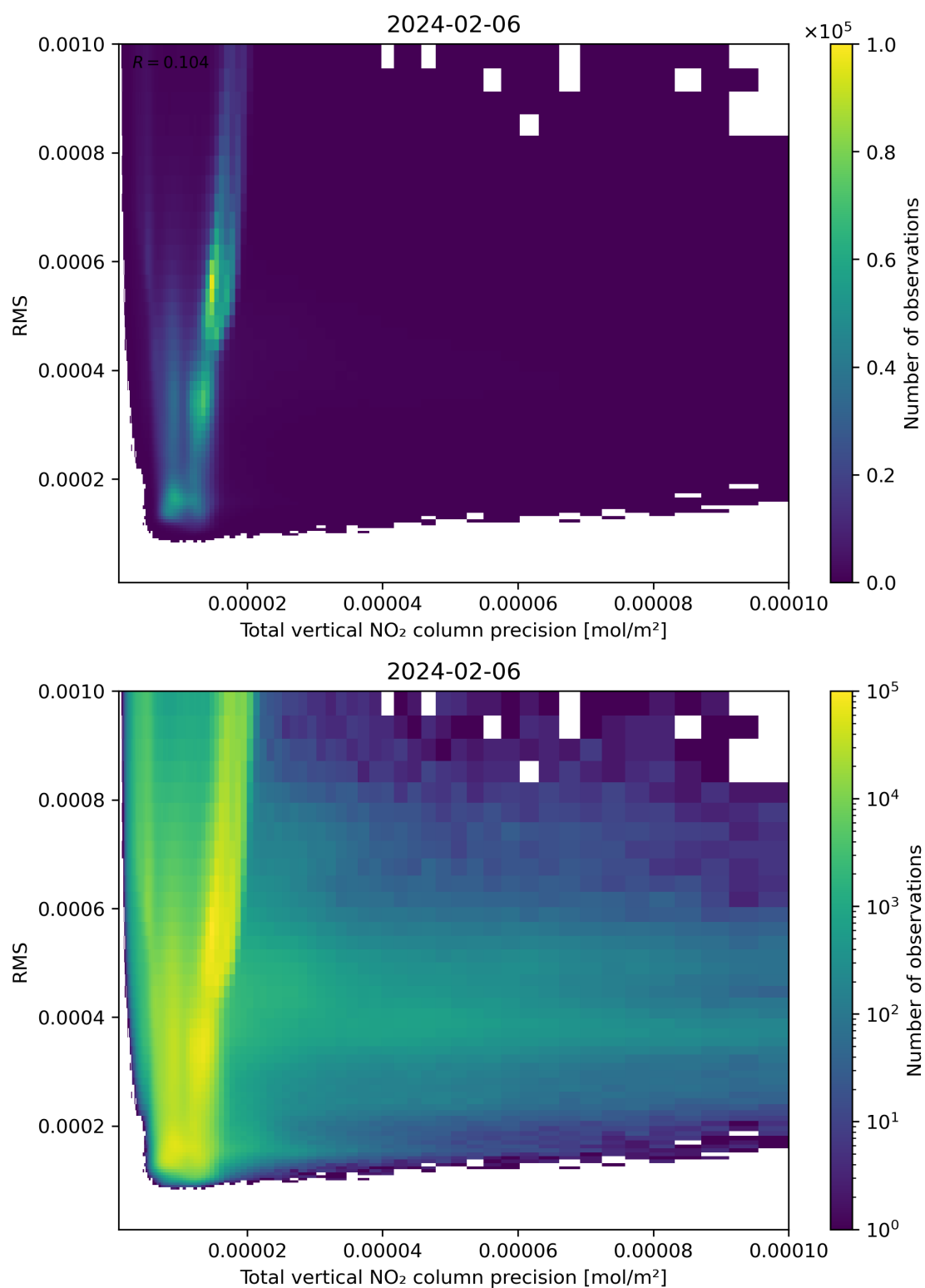
Figure 119: Scatter density plot of “Total vertical NO 2 column precision” against “RMS” for 2024-02-06 to 2024-02-07.
