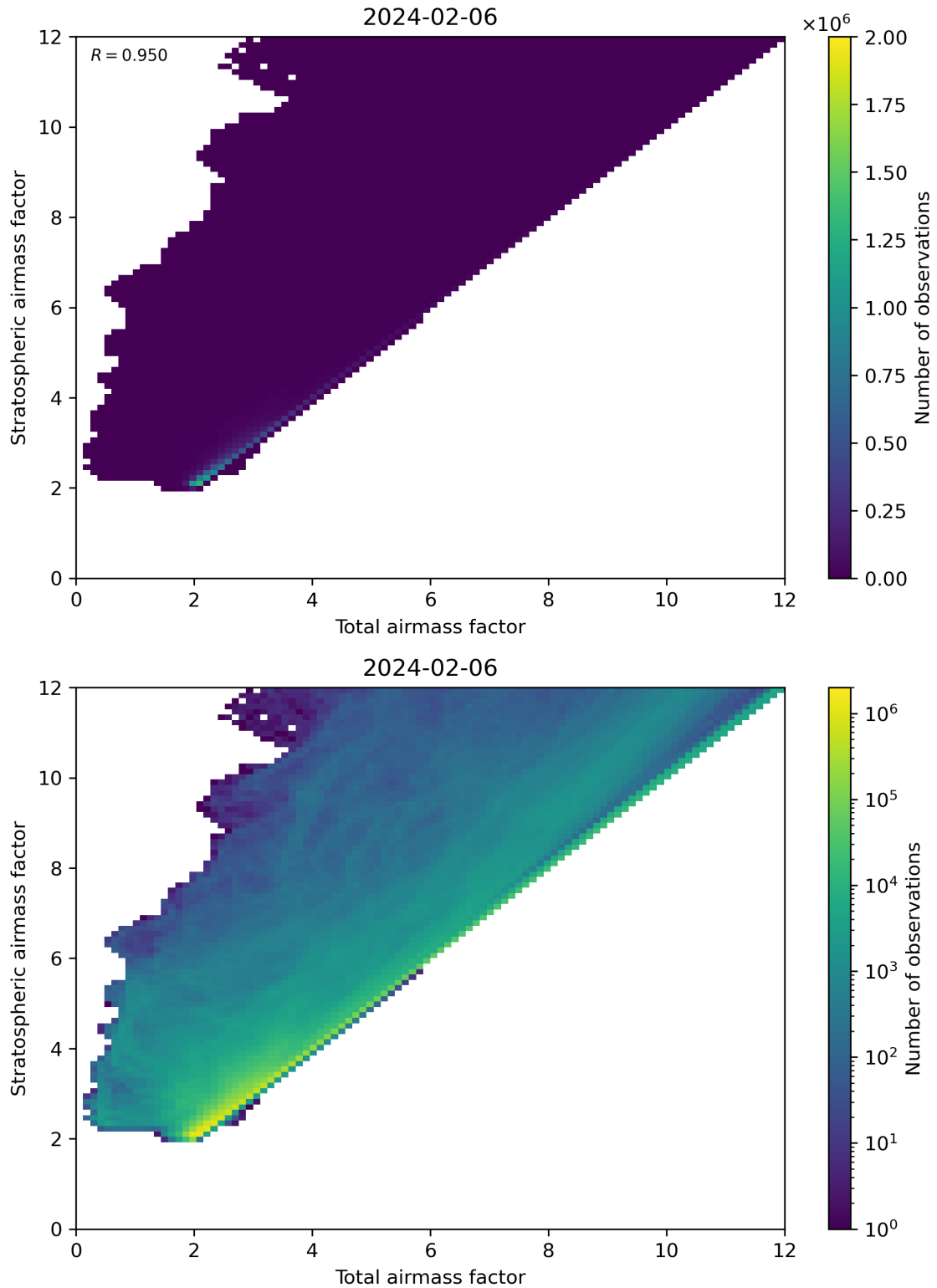
Figure 62: Scatter density plot of “Total airmass factor” against “Stratospheric airmass factor” for 2024-02-06 to 2024-02-07.
