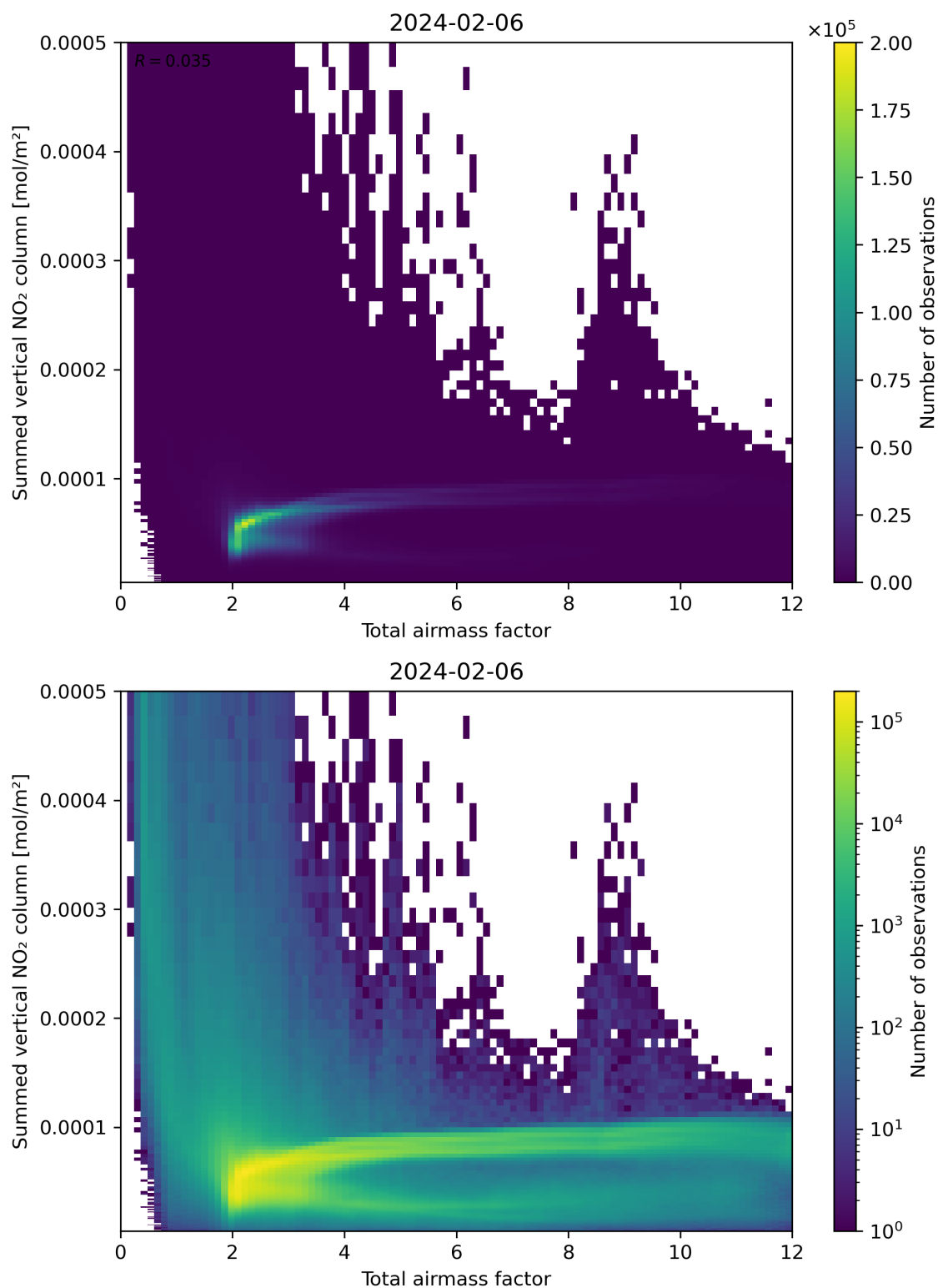
Figure 65: Scatter density plot of “Total airmass factor” against “Summed vertical NO 2 column” for 2024-02-06 to 2024-02-07.
