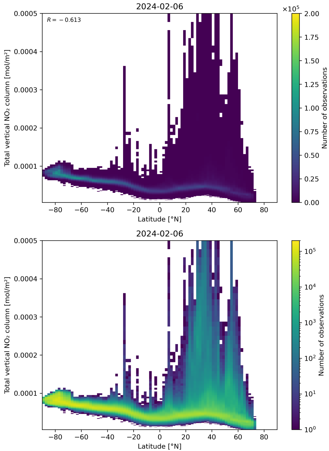
Figure 90: Scatter density plot of “Latitude” against “Total vertical NO 2 column” for 2024-02-06 to 2024-02-07.
