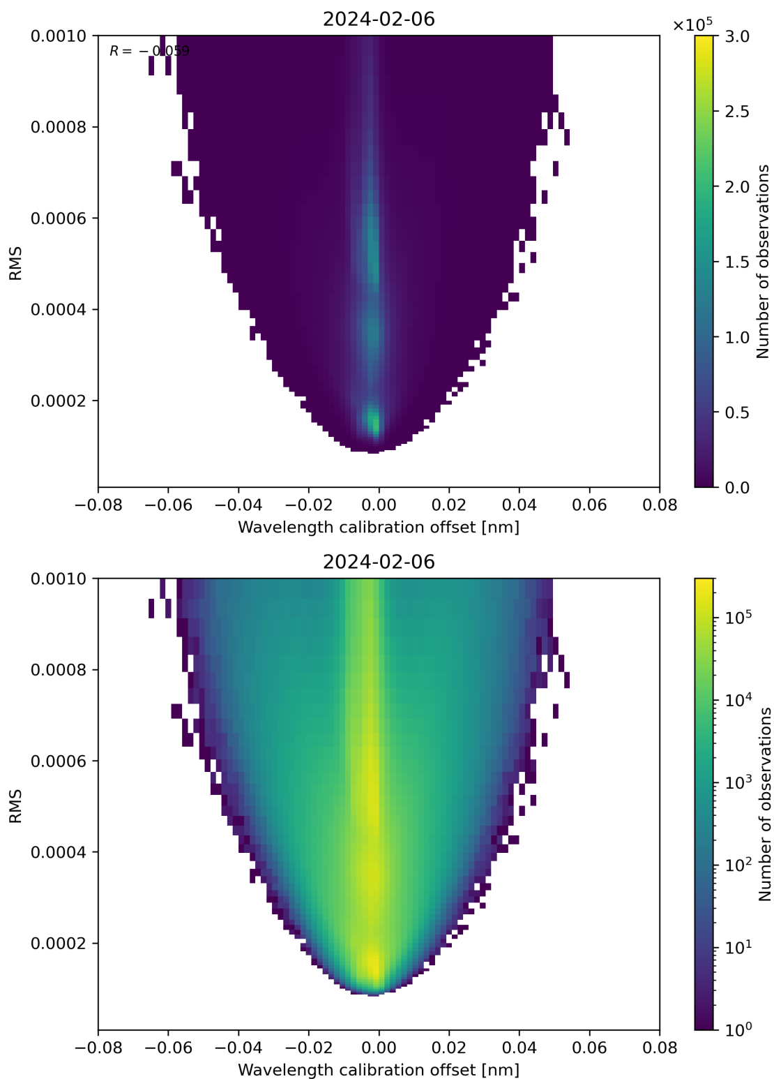
Figure 181: Scatter density plot of “Wavelength calibration offset” against “RMS” for 2024-02-06 to 2024-02-07.
