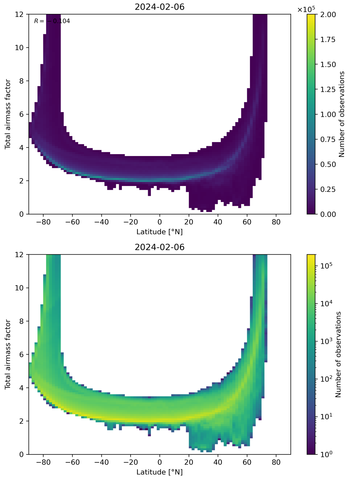
Figure 84: Scatter density plot of “Latitude” against “Total airmass factor” for 2024-02-06 to 2024-02-07.
