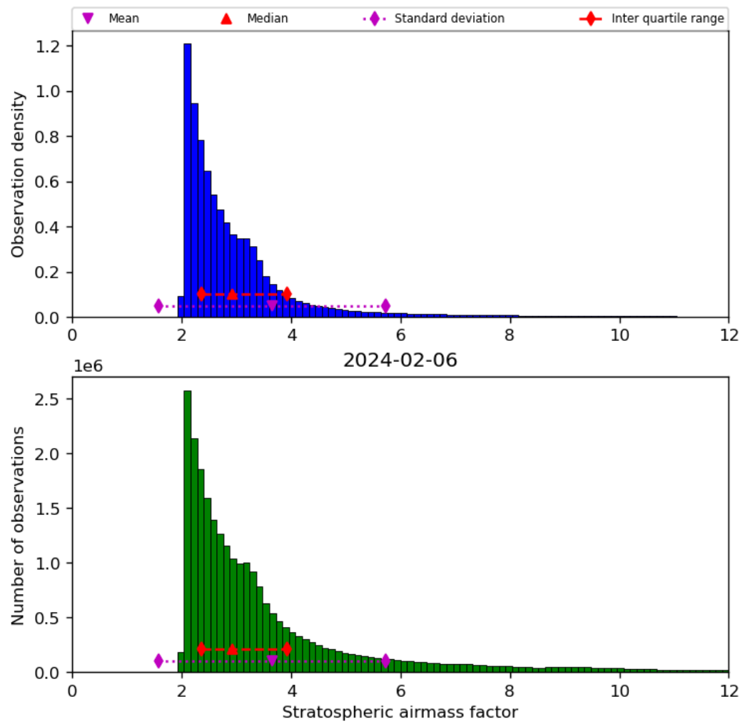
Figure 44: Histogram of “Stratospheric airmass factor” for 2024-02-06 to 2024-02-07
