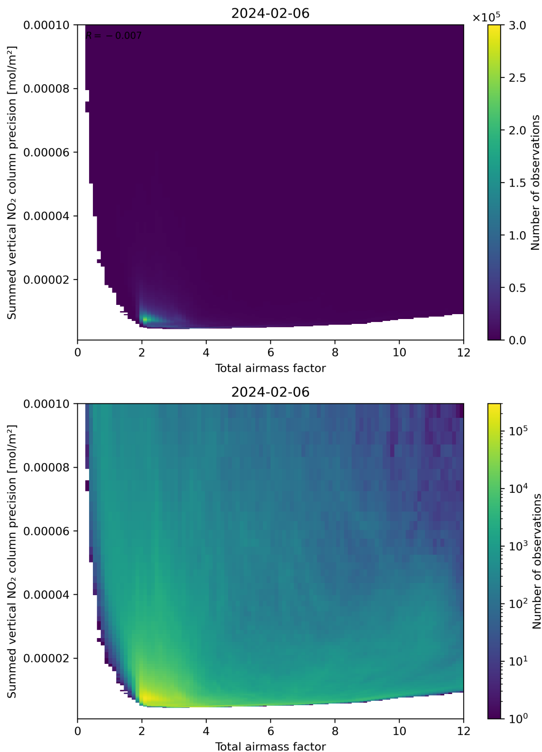
Figure 66: Scatter density plot of “Total airmass factor” against “Summed vertical NO 2 column precision” for 2024-02-06 to 2024-02-07.
