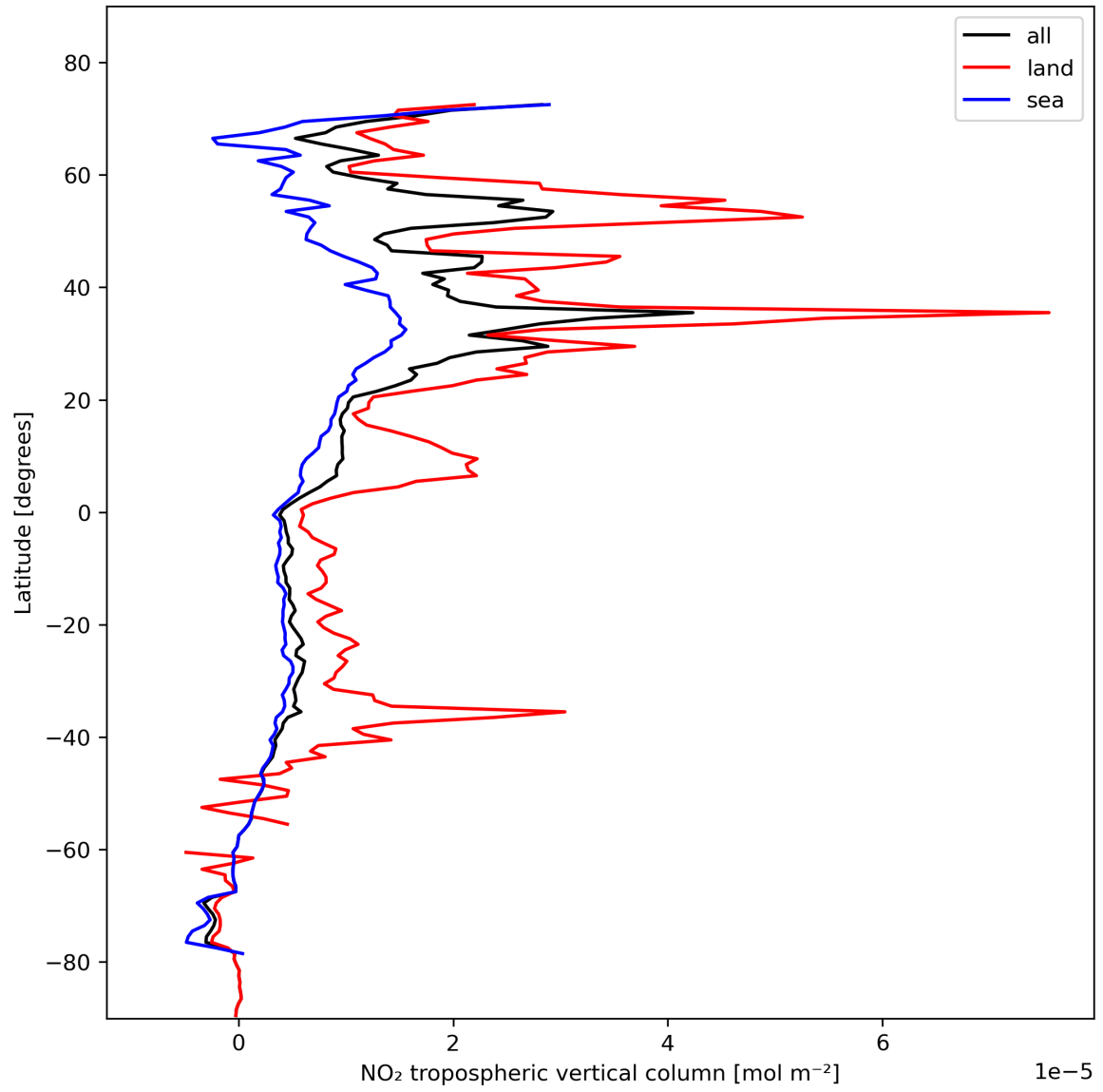
Figure 12: Zonal average of “NO 2 tropospheric vertical column” for 2024-02-06 to 2024-02-07.
