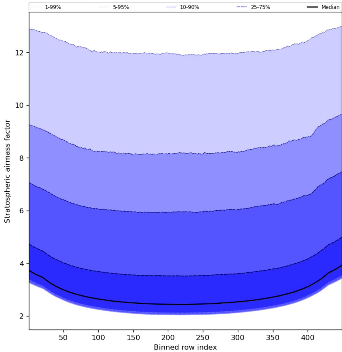
Figure 61: Along track statistics of “Stratospheric air mass factor” for 2024-02-06 to 2024-02-07
