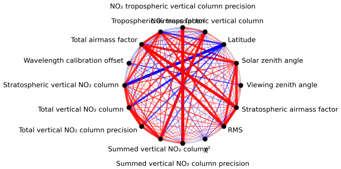
Figure 1: Map of correlation graph for 2024-02-06 to 2024-02-07.
