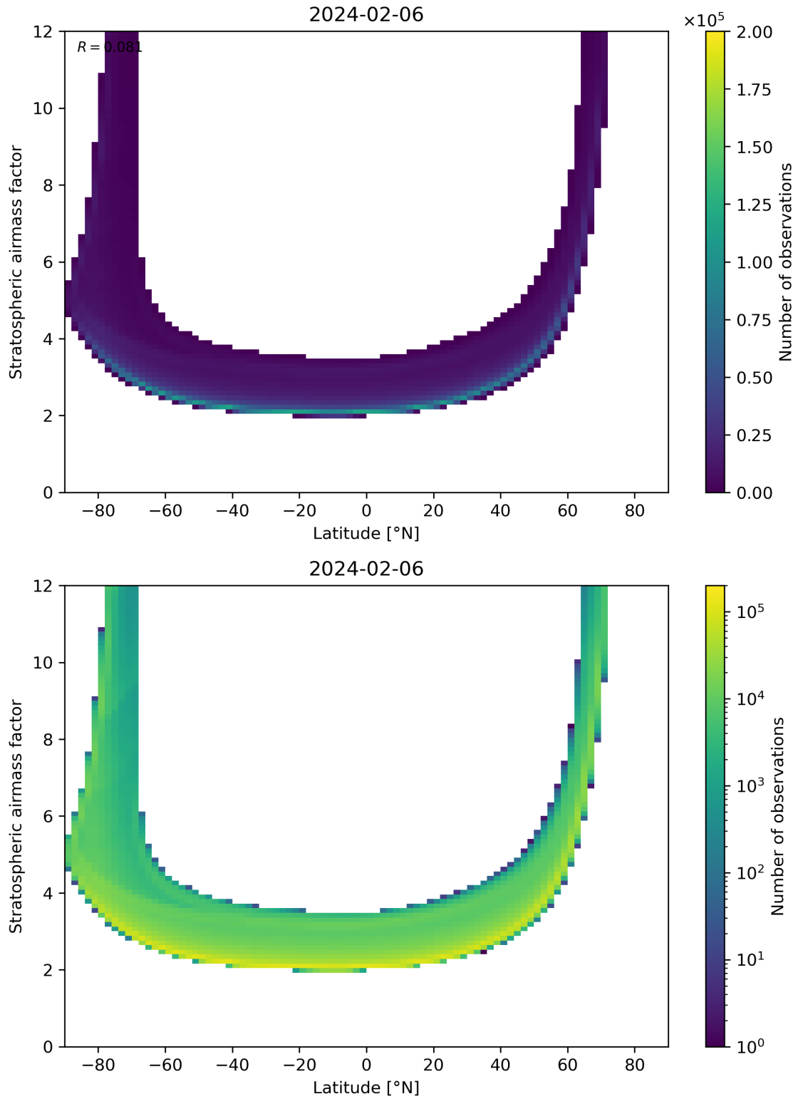
Figure 83: Scatter density plot of “Latitude” against “Stratospheric airmass factor” for 2024-02-06 to 2024-02-07.
