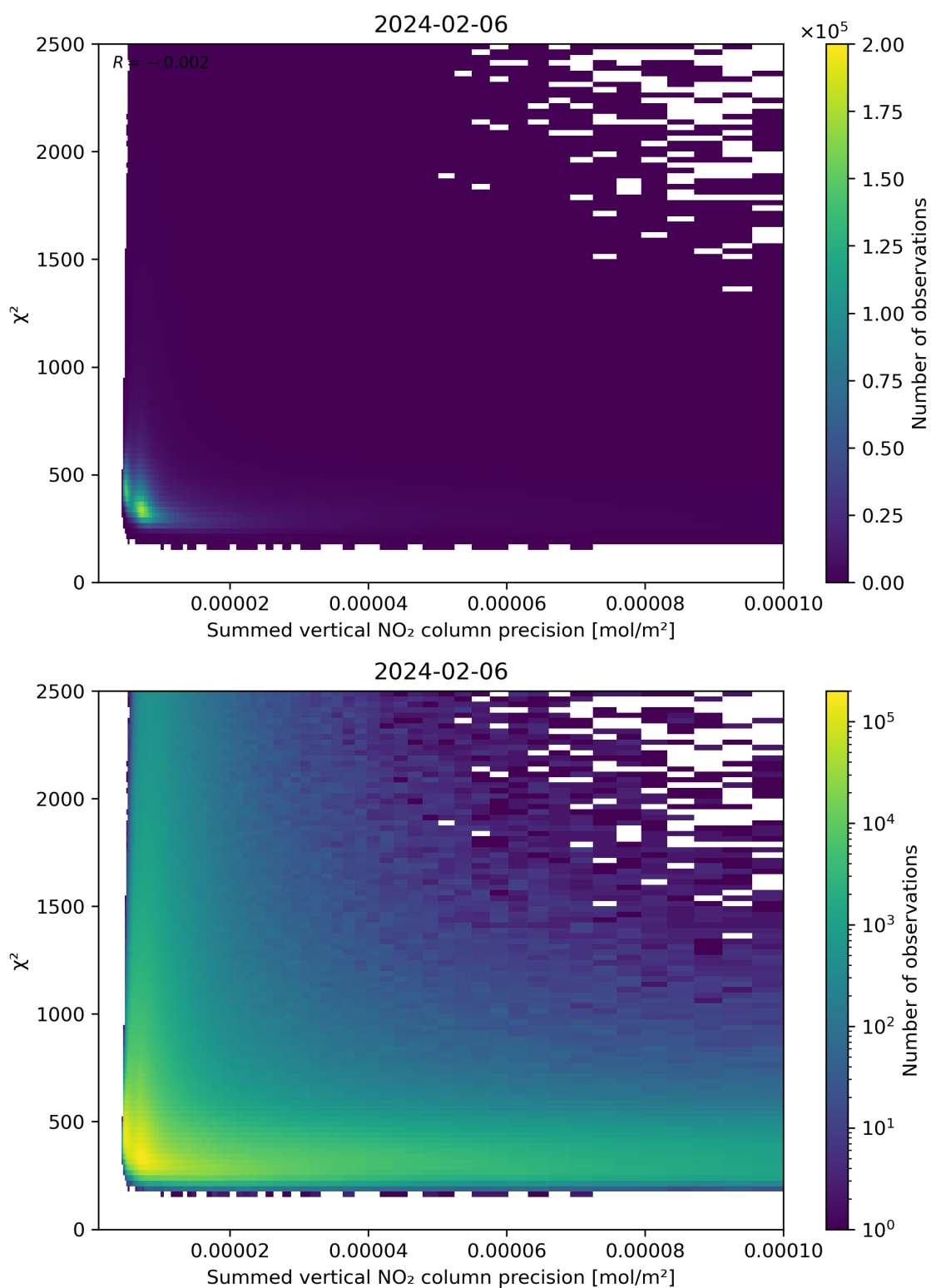
Figure 107: Scatter density plot of “Summed vertical NO 2 column precision” against “ \chi^2 ” for 2024-02-06 to 2024-02-07.
