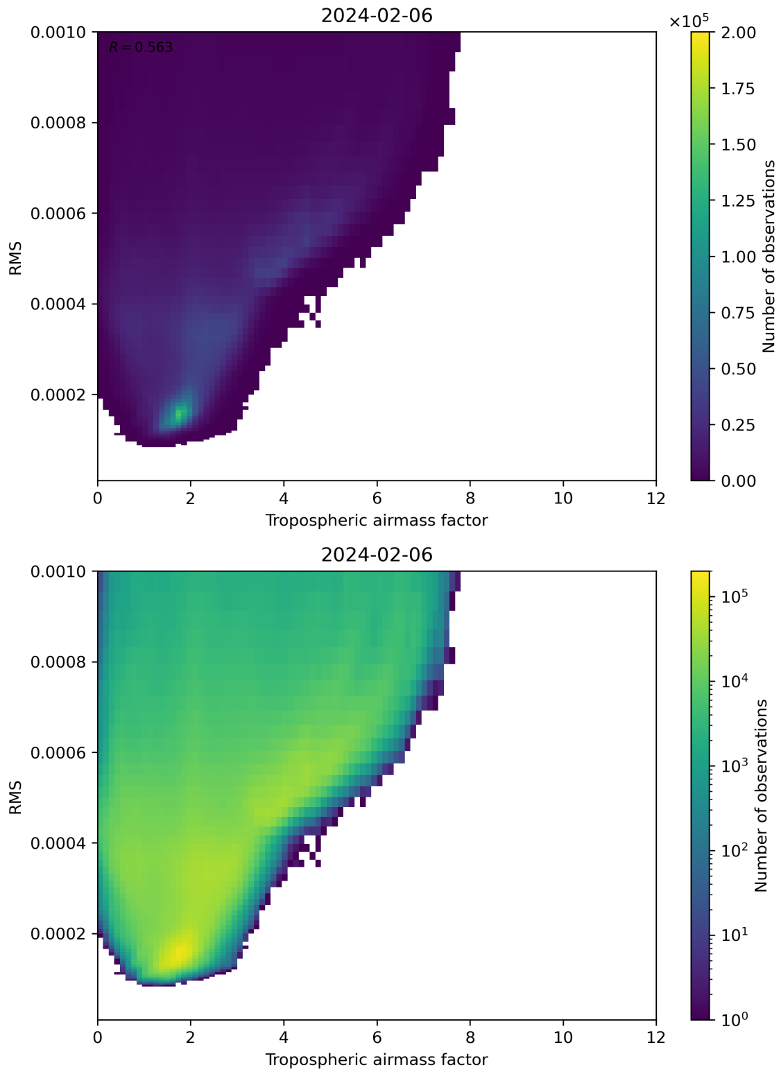
Figure 79: Scatter density plot of “Tropospheric airmass factor” against “RMS” for 2024-02-06 to 2024-02-07.
