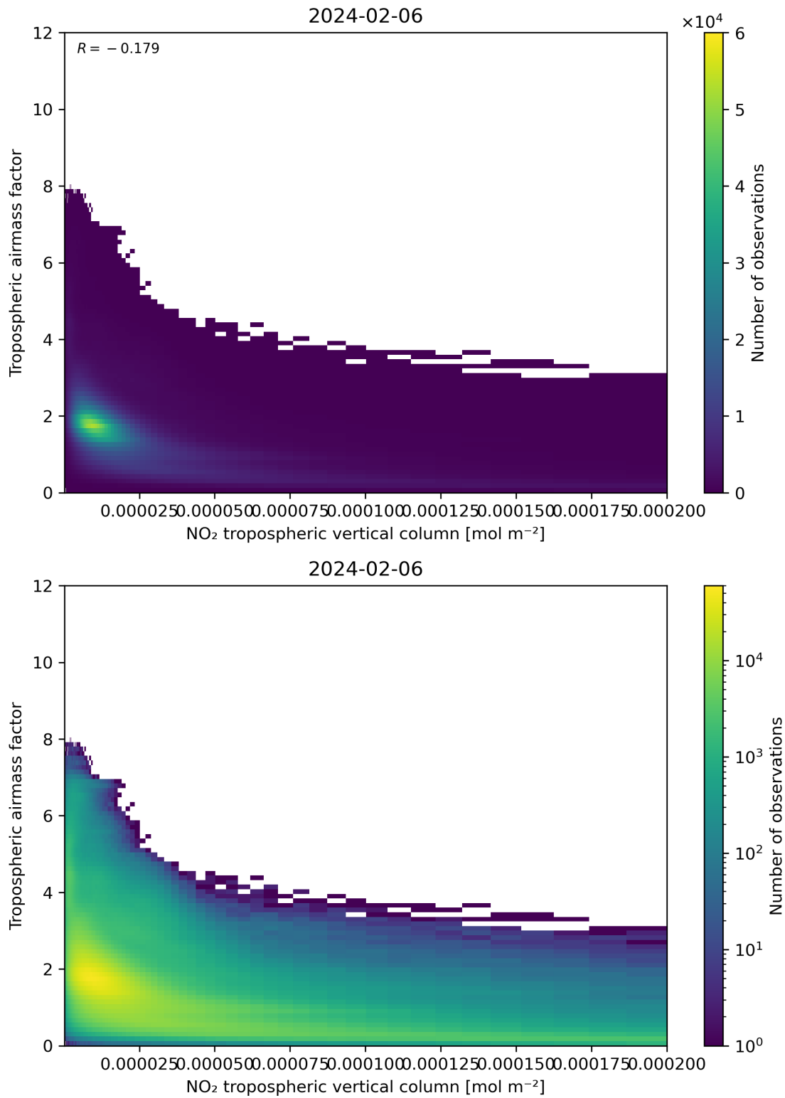
Figure 123: Scatter density plot of “NO 2 tropospheric vertical column” against “Tropospheric air mass factor” for 2024-02-06 to 2024-02-07.
