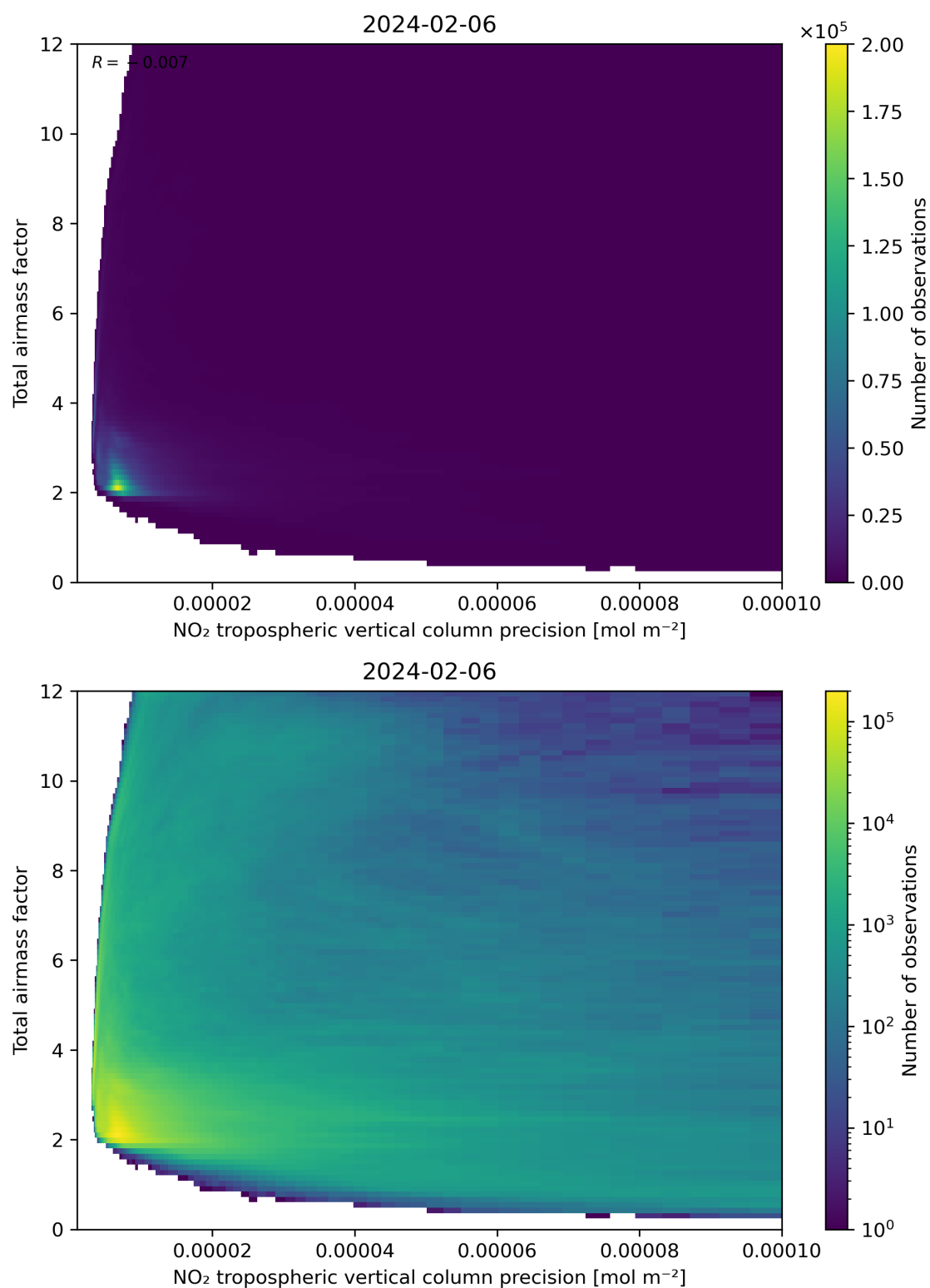
Figure 132: Scatter density plot of “NO 2 tropospheric vertical column precision” against “Total air mass factor” for 2024-02-06 to 2024-02-07.
