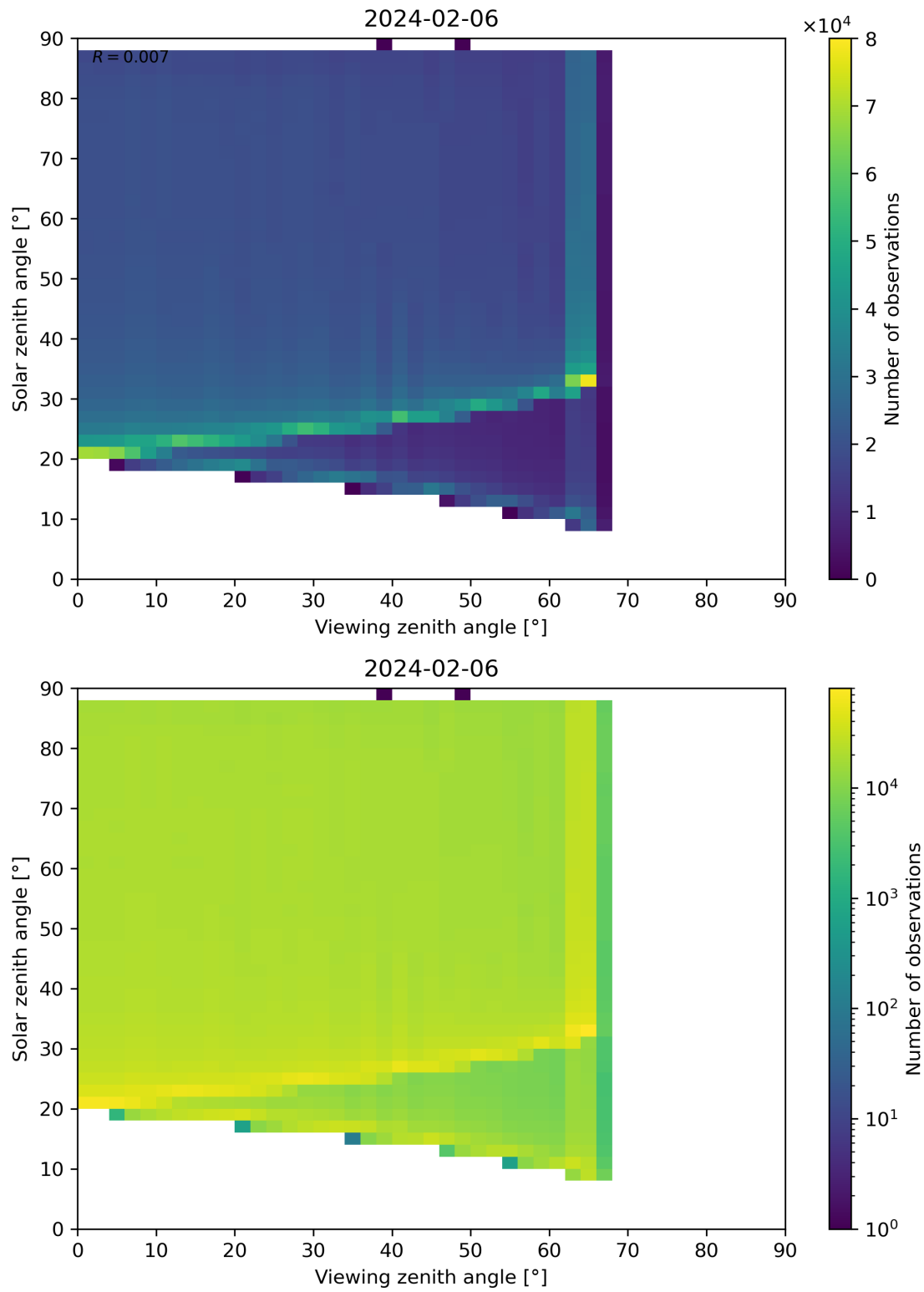
Figure 172: Scatter density plot of “Viewing zenith angle” against “Solar zenith angle” for 2024-02-06 to 2024-02-07.
