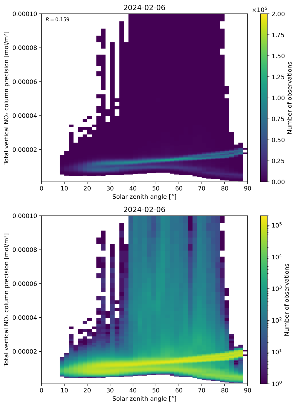
Figure 154: Scatter density plot of “Solar zenith angle” against “Total vertical NO 2 column precision” for 2024-02-06 to 2024-02-07.
