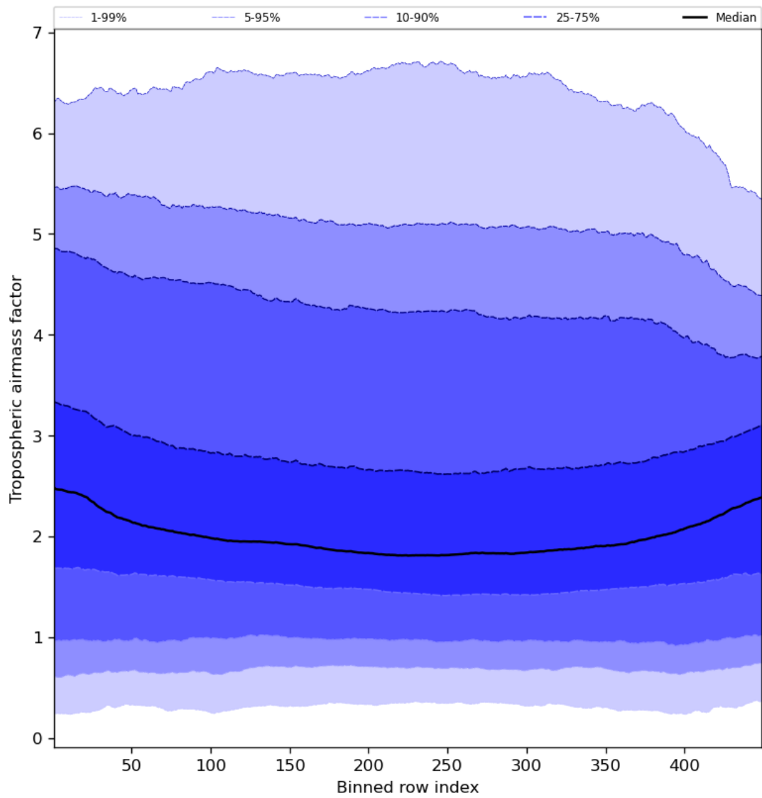
Figure 48: Along track statistics of “Tropospheric air mass factor” for 2024-02-06 to 2024-02-07
