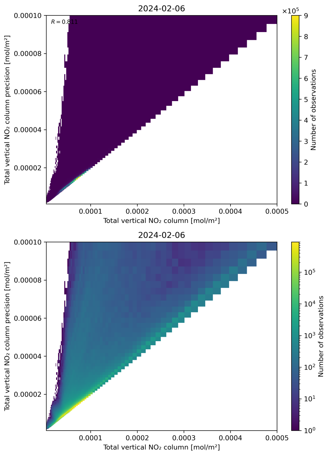
Figure 114: Scatter density plot of “Total vertical NO 2 column” against “Total vertical NO 2 column precision” for 2024-02-06 to 2024-02-07.
