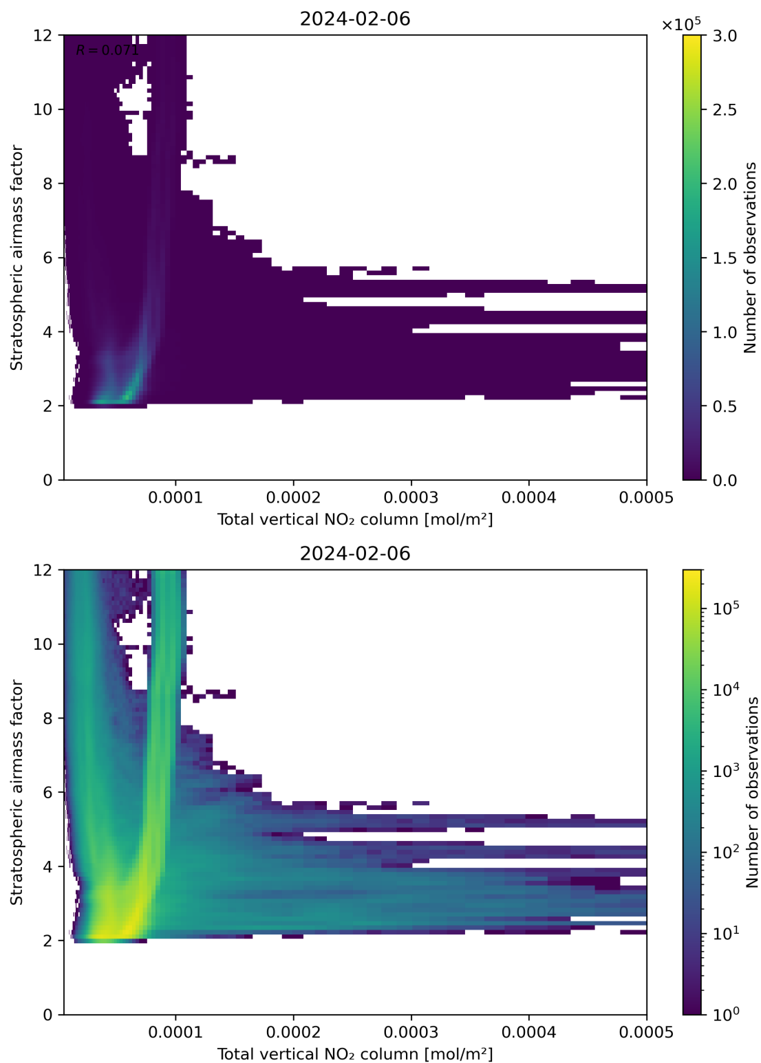
Figure 110: Scatter density plot of “Total vertical NO 2 column” against “Stratospheric airmass factor” for 2024-02-06 to 2024-02-07.
