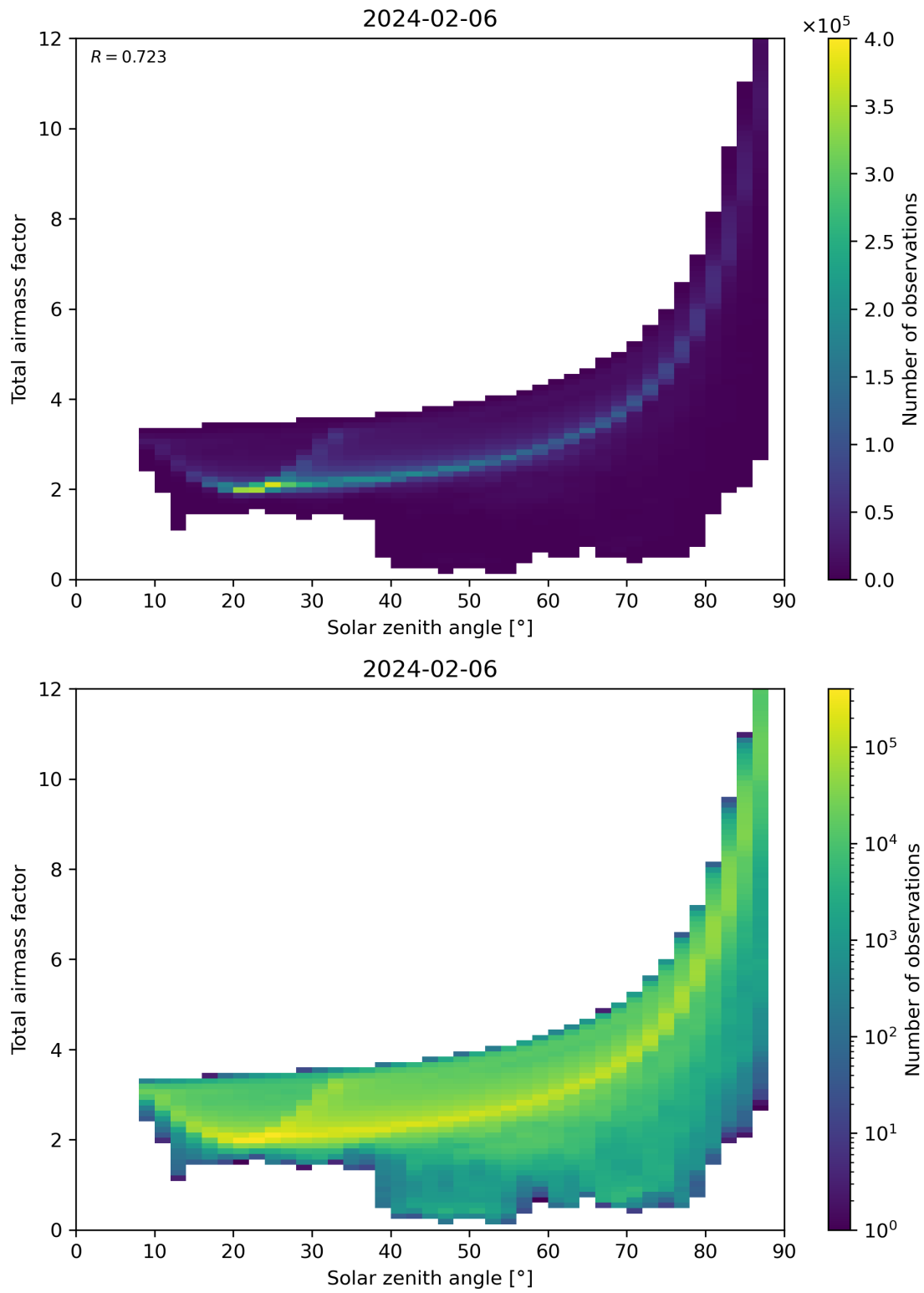
Figure 146: Scatter density plot of “Solar zenith angle” against “Total air mass factor” for 2024-02-06 to 2024-02-07.
