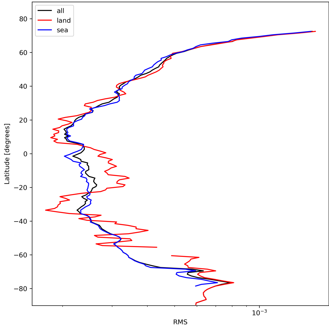
Figure 26: Zonal average of “RMS” for 2024-02-06 to 2024-02-07.
