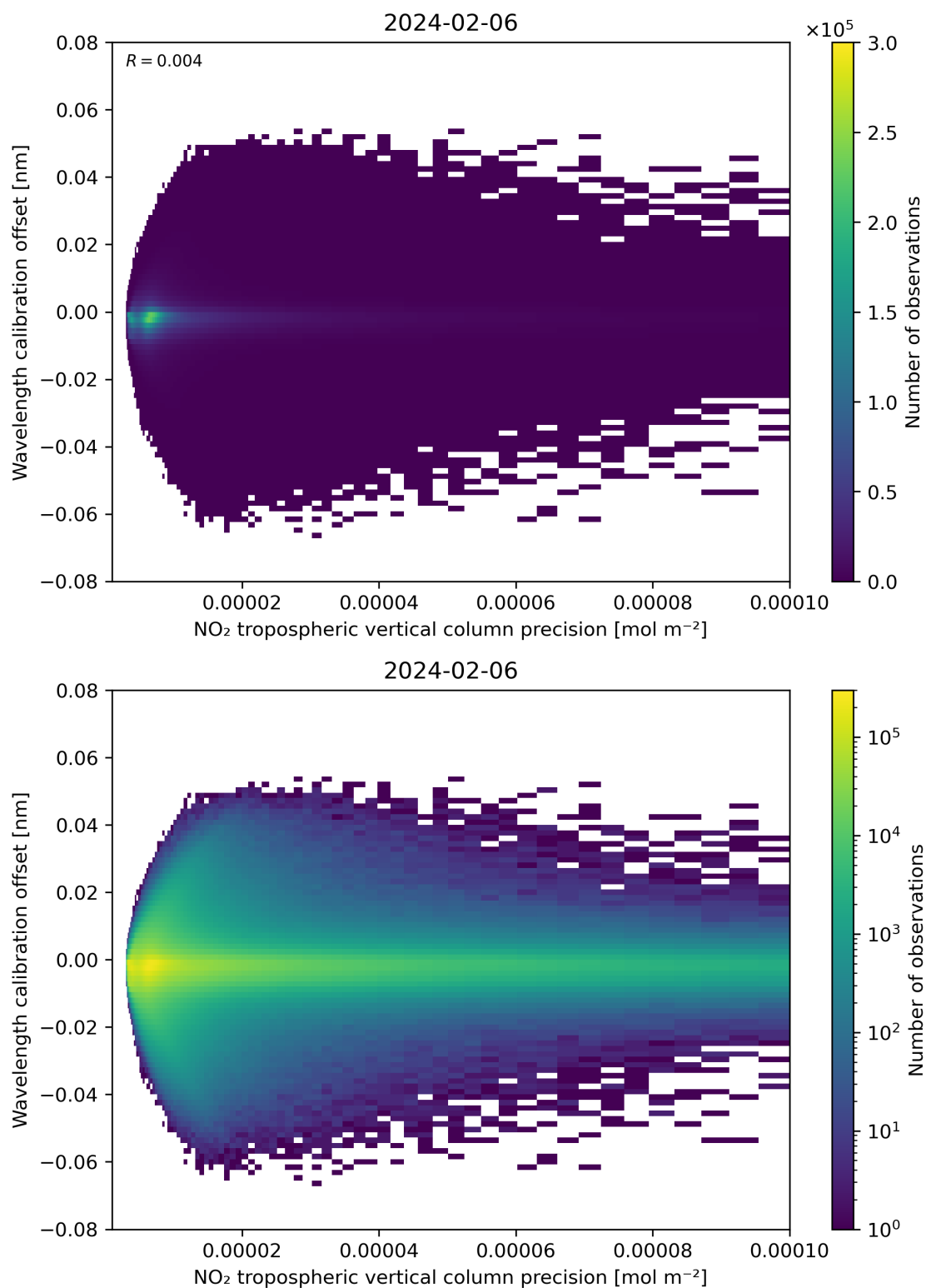
Figure 141: Scatter density plot of “NO 2 tropospheric vertical column precision” against “Wavelength calibration offset” for 2024-02-06 to 2024-02-07.
