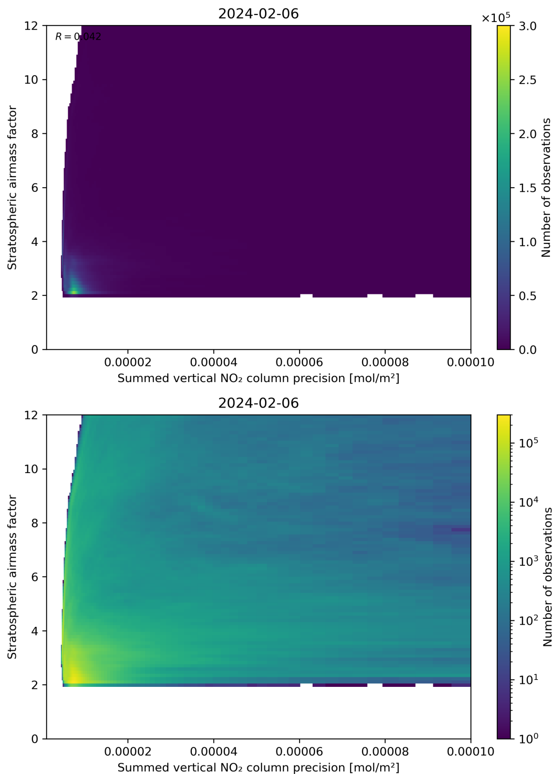
Figure 106: Scatter density plot of “Summed vertical NO 2 column precision” against “Stratospheric airmass factor” for 2024-02-06 to 2024-02-07.
