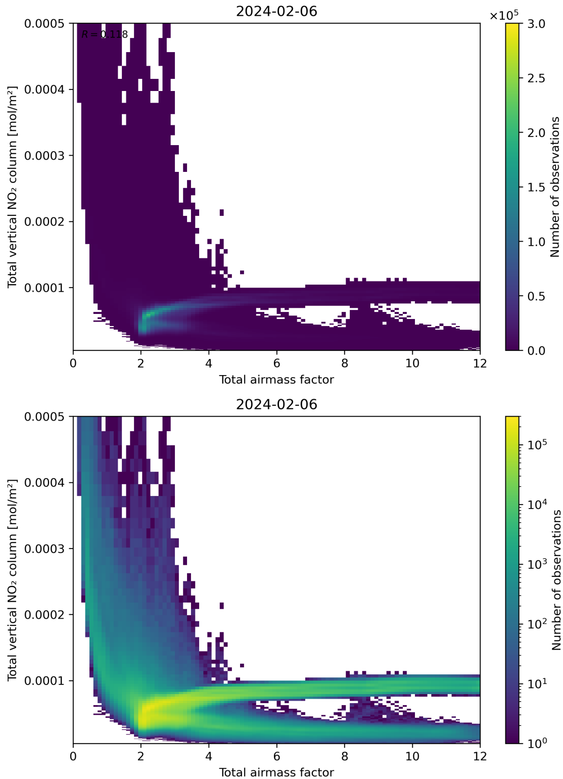
Figure 67: Scatter density plot of “Total airmass factor” against “Total vertical NO 2 column” for 2024-02-06 to 2024-02-07.
