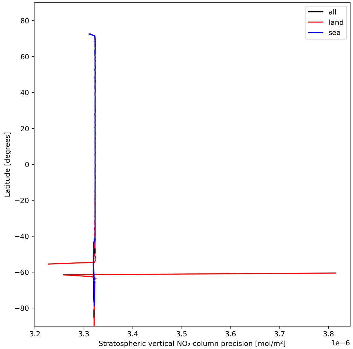
Figure 20: Zonal average of “Stratospheric vertical NO 2 column precision” for 2024-02-06 to 2024-02-07.
