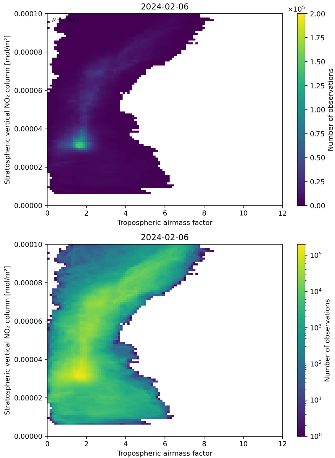
Figure 74: Scatter density plot of “Tropospheric air mass factor” against “Stratospheric vertical NO 2 column” for 2024-02-06 to 2024-02-07.
