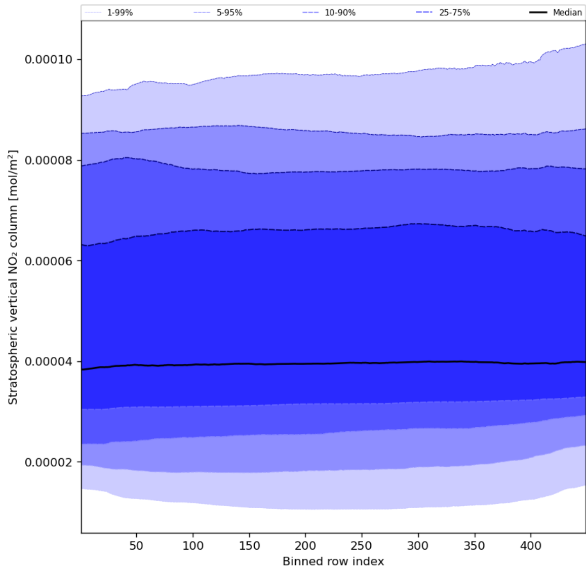
Figure 53: Along track statistics of “Stratospheric vertical NO 2 column” for 2024-02-06 to 2024-02-07
