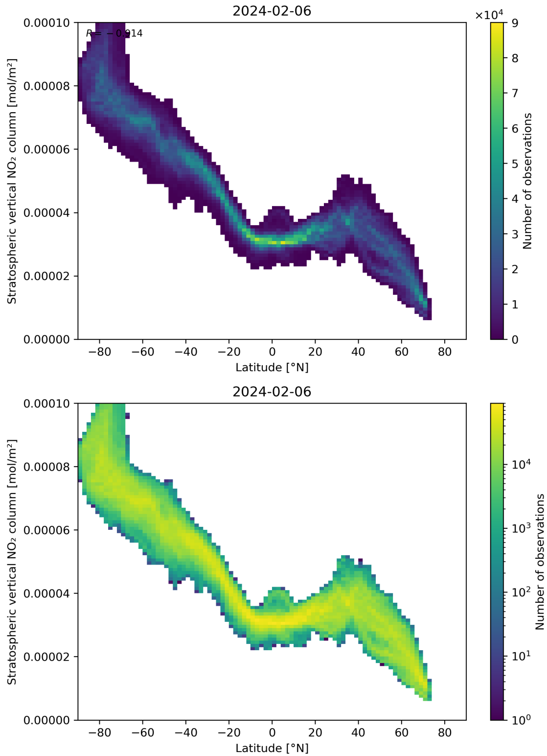
Figure 87: Scatter density plot of “Latitude” against “Stratospheric vertical NO 2 column” for 2024-02-06 to 2024-02-07.
