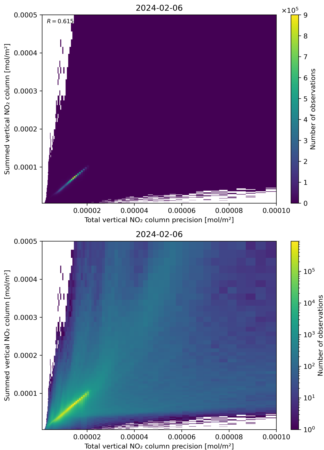
Figure 117: Scatter density plot of “Total vertical NO 2 column precision” against “Summed vertical NO 2 column” for 2024-02-06 to 2024-02-07.
