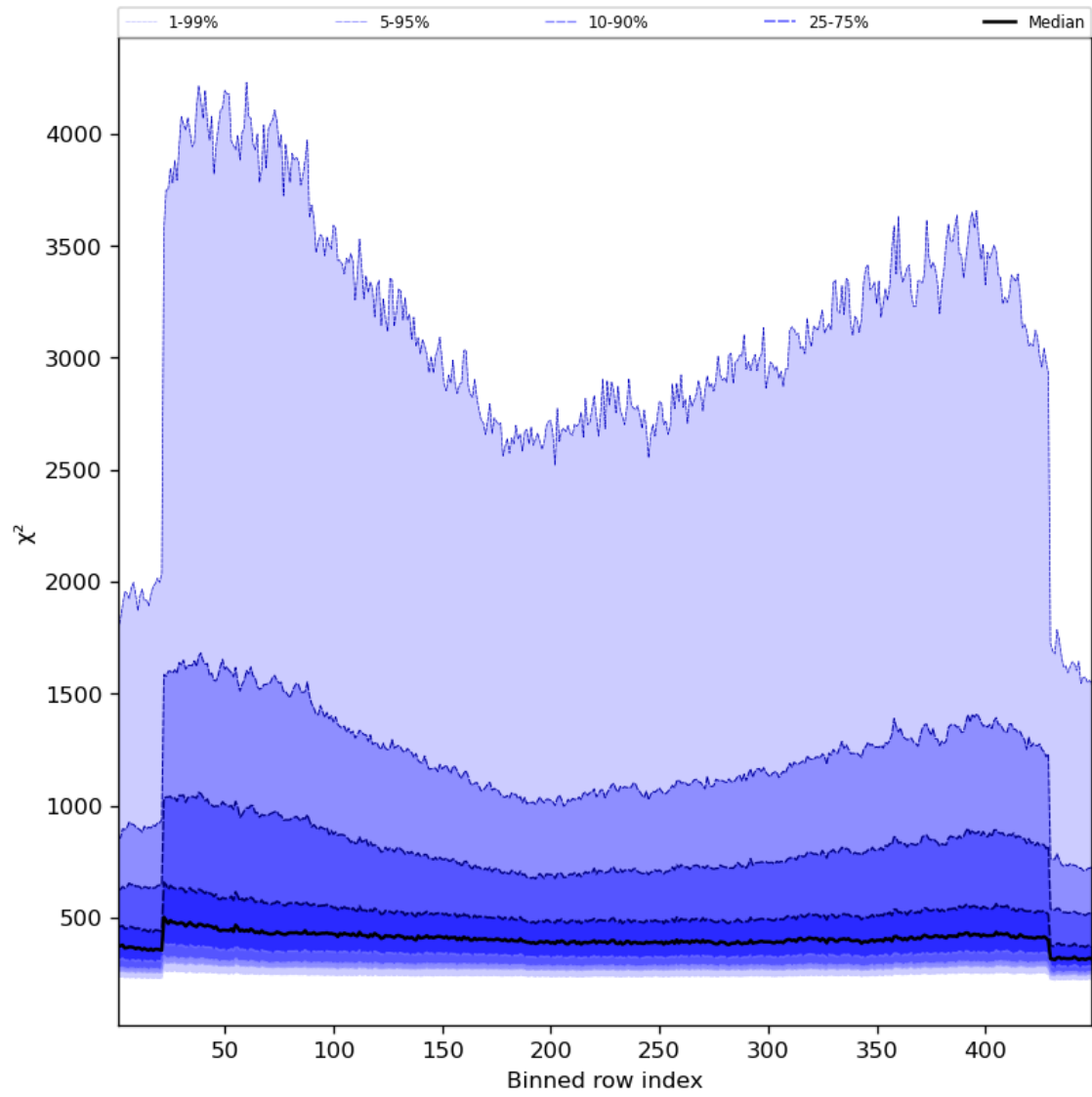
Figure 59: Along track statistics of “ \chi^2 ” for 2024-02-06 to 2024-02-07
