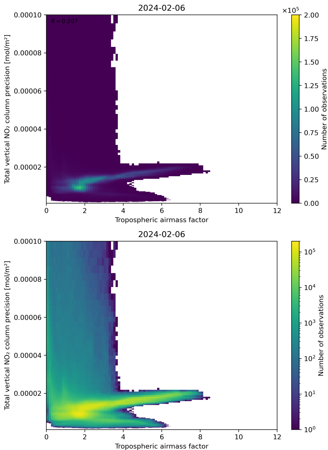
Figure 78: Scatter density plot of “Tropospheric air mass factor” against “Total vertical NO 2 column precision” for 2024-02-06 to 2024-02-07.
