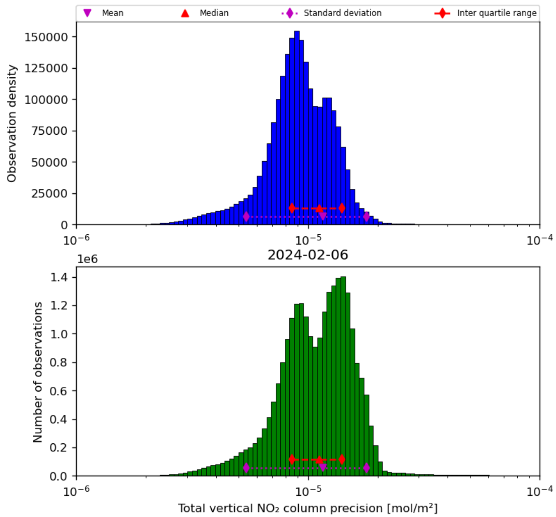
Figure 39: Histogram of “Total vertical NO 2 column precision” for 2024-02-06 to 2024-02-07
