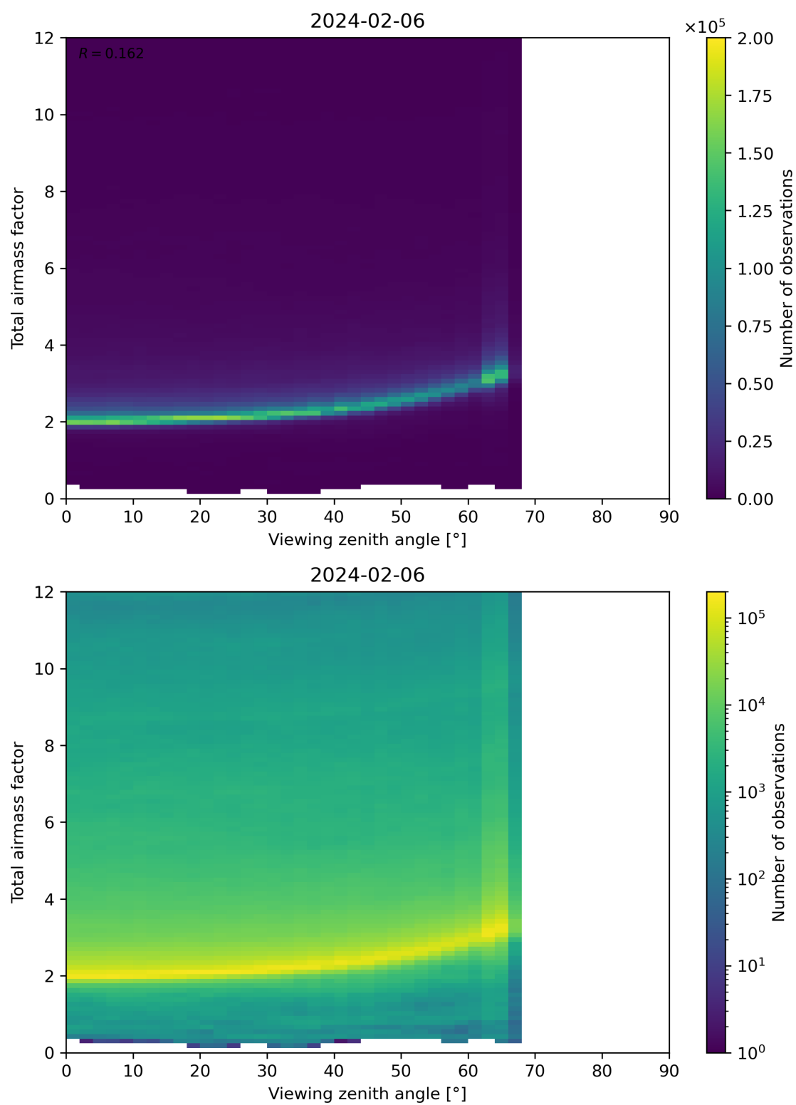
Figure 160: Scatter density plot of “Viewing zenith angle” against “Total airmass factor” for 2024-02-06 to 2024-02-07.
