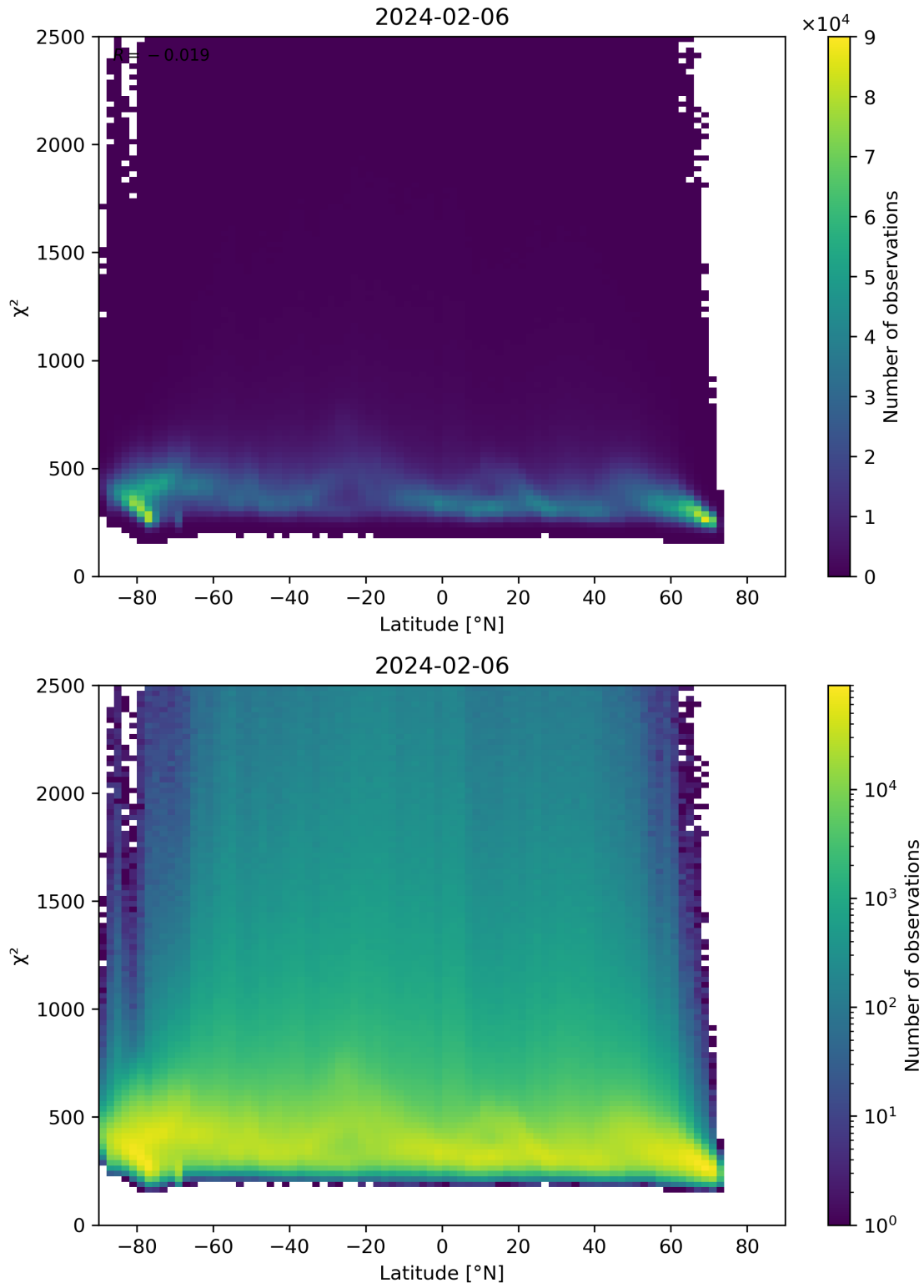
Figure 86: Scatter density plot of “Latitude” against “ \chi^2 ” for 2024-02-06 to 2024-02-07.
