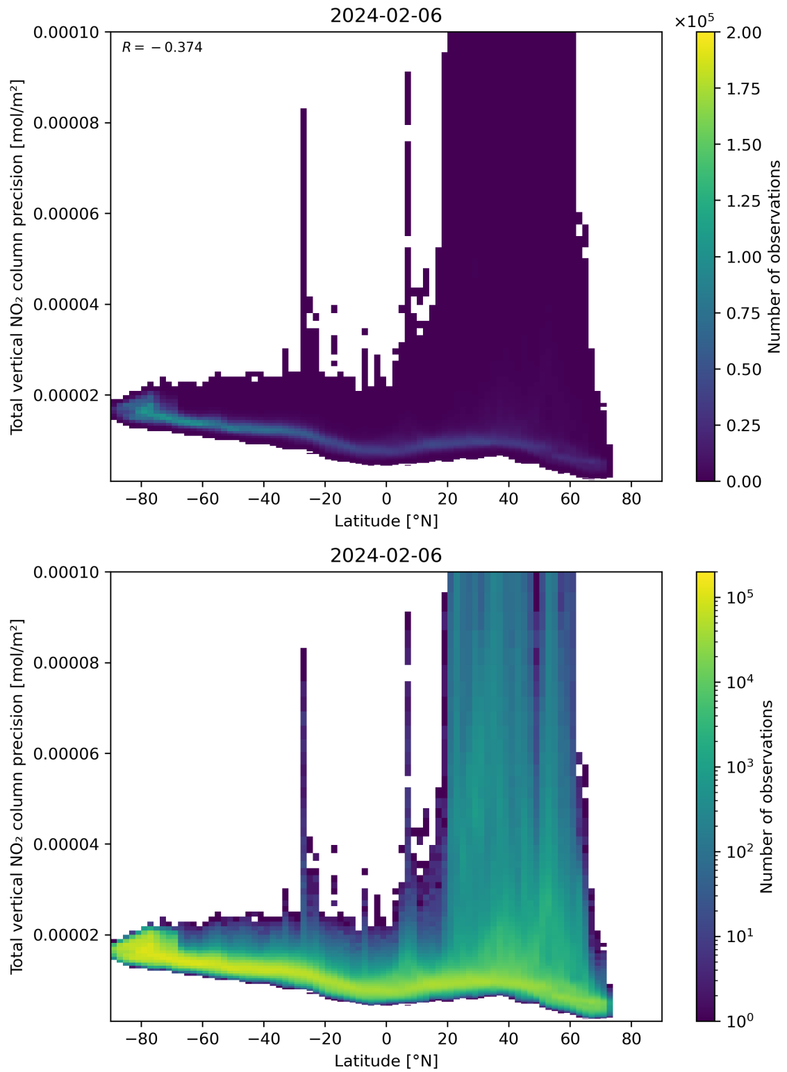
Figure 91: Scatter density plot of “Latitude” against “Total vertical NO 2 column precision” for 2024-02-06 to 2024-02-07.
