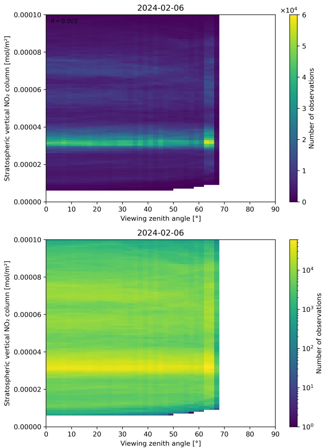
Figure 164: Scatter density plot of “Viewing zenith angle” against “Stratospheric vertical NO 2 column” for 2024-02-06 to 2024-02-07.
