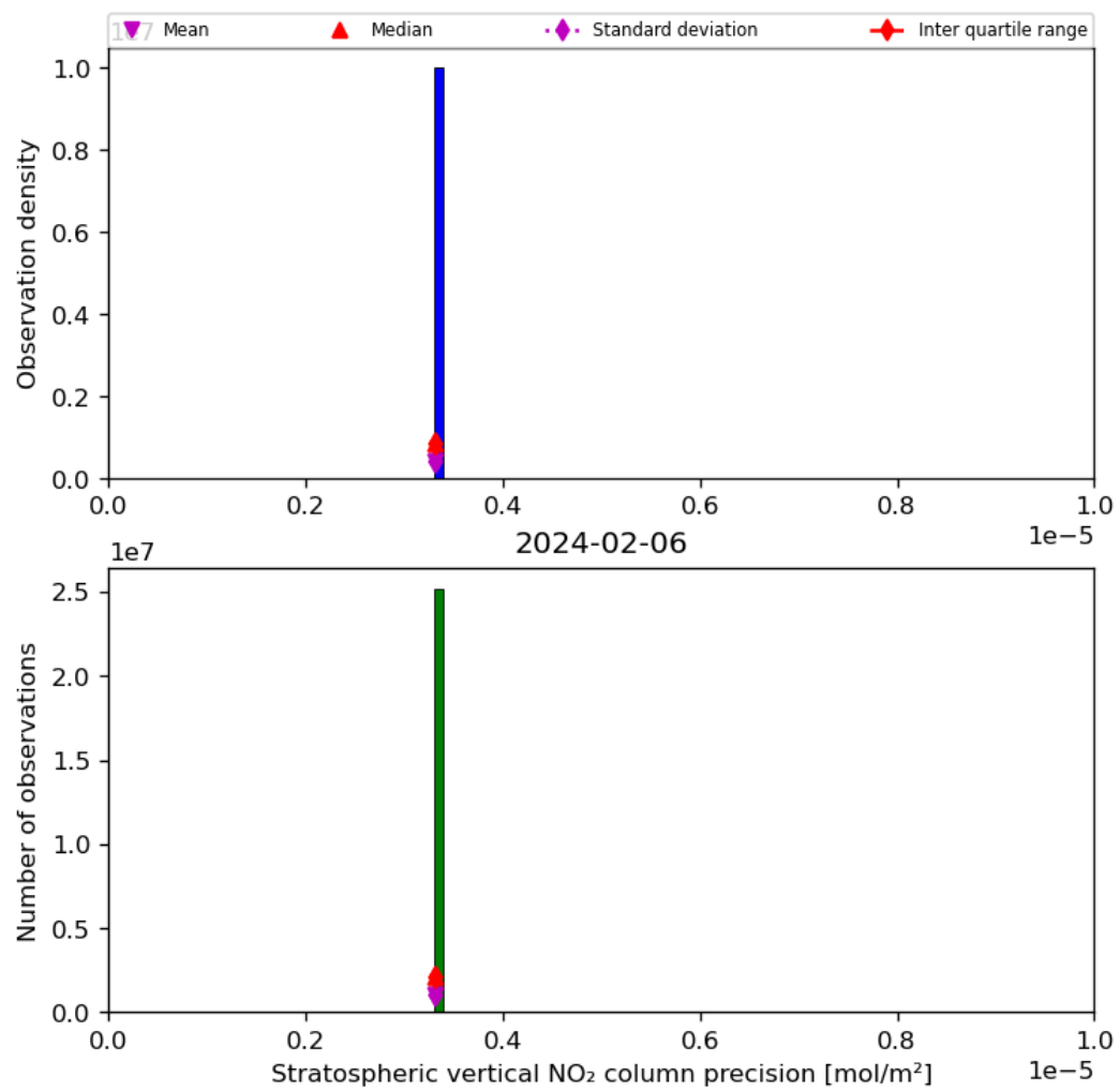
Figure 37: Histogram of “Stratospheric vertical NO 2 column precision” for 2024-02-06 to 2024-02-07
