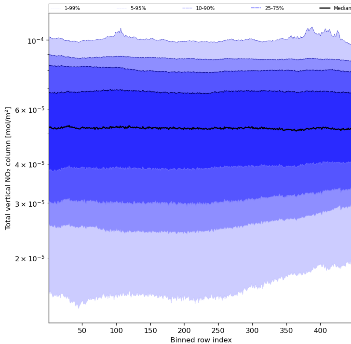
Figure 55: Along track statistics of “Total vertical NO 2 column” for 2024-02-06 to 2024-02-07
