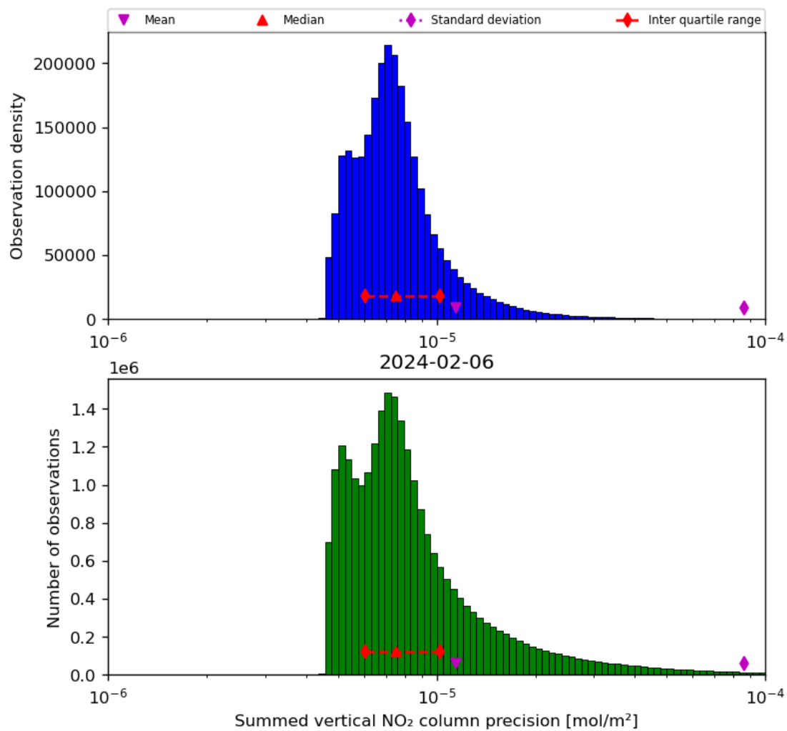
Figure 41: Histogram of “Summed vertical NO 2 column precision” for 2024-02-06 to 2024-02-07
