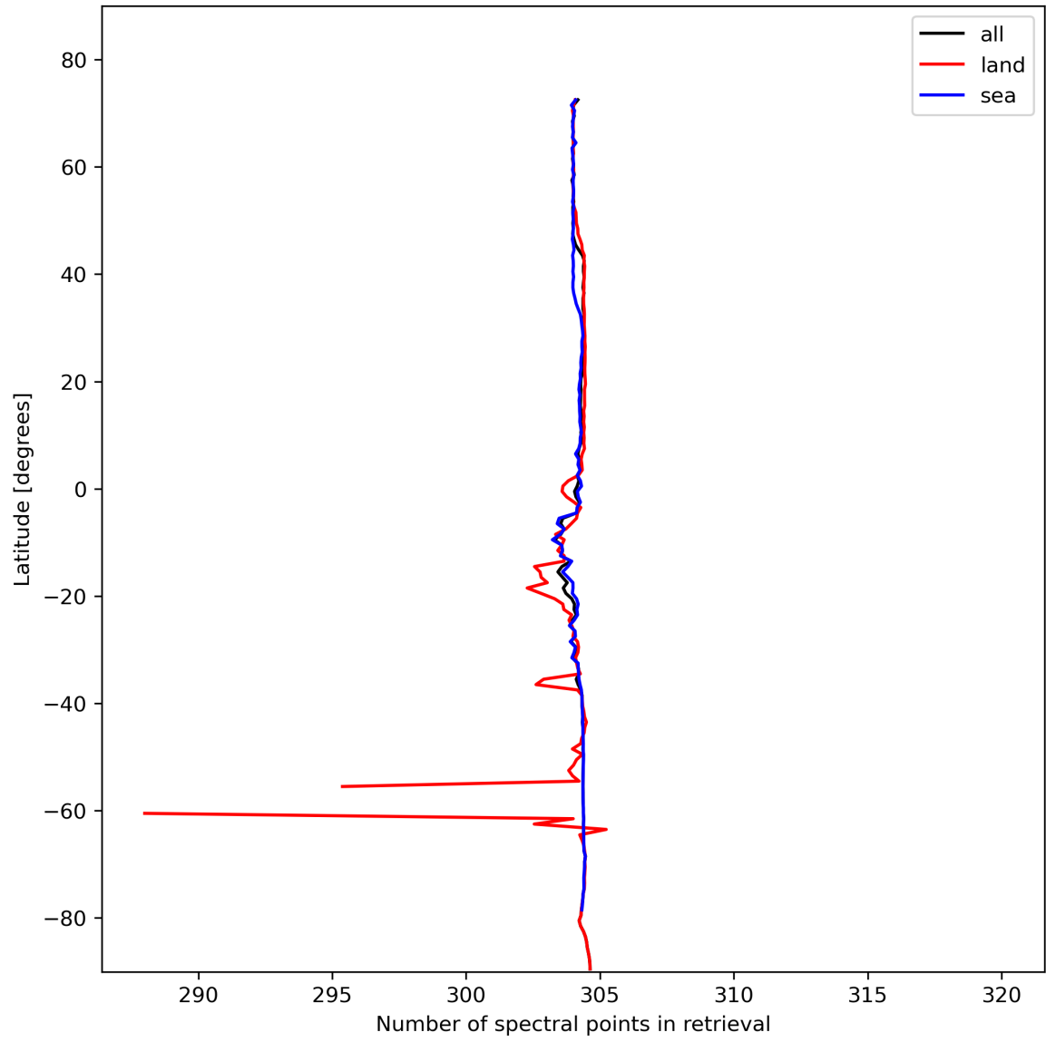
Figure 16: Zonal average of “Number of spectral points in retrieval” for 2024-02-06 to 2024-02-07.
