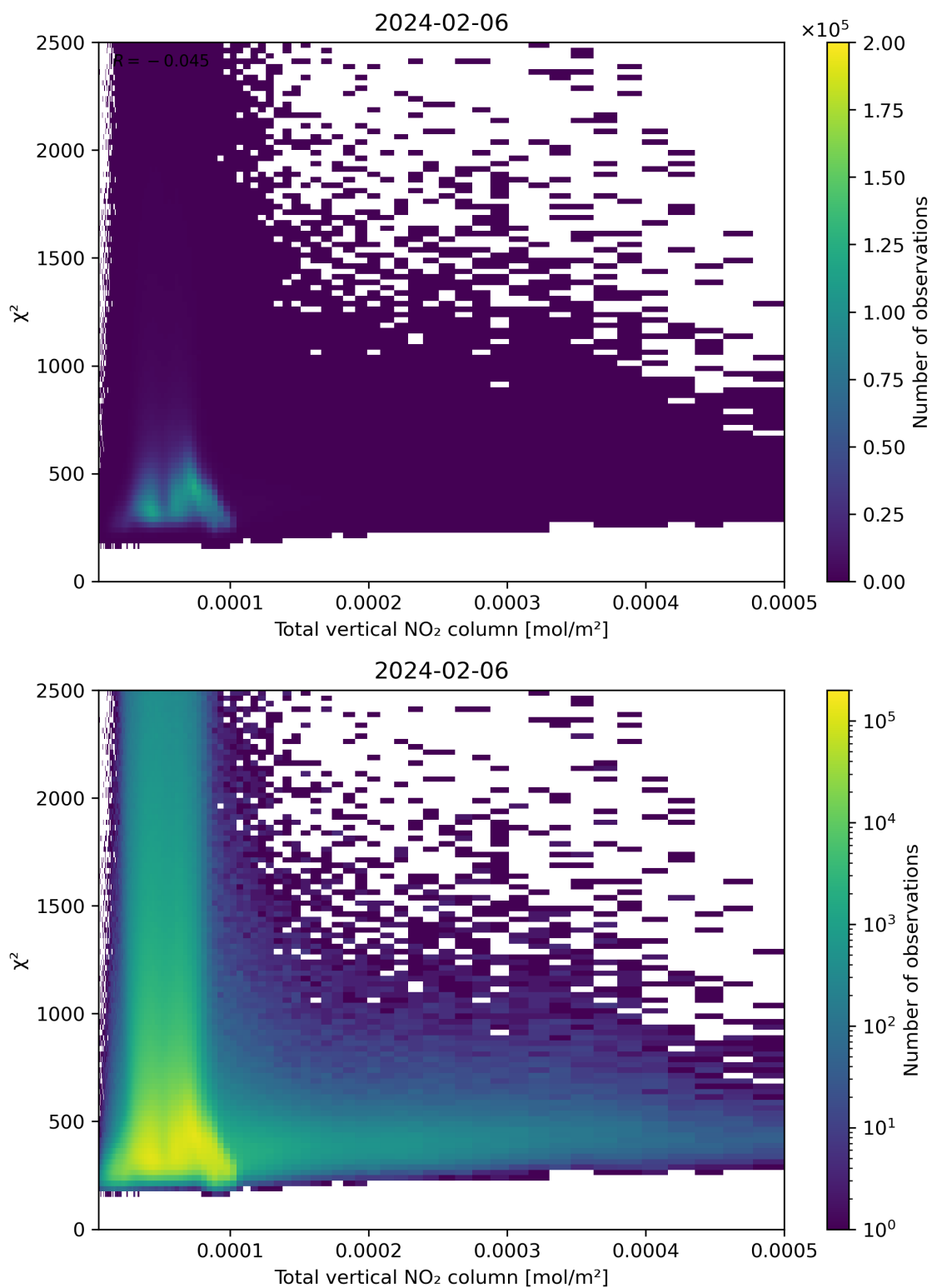
Figure 111: Scatter density plot of “Total vertical NO 2 column” against “ \chi^2 ” for 2024-02-06 to 2024-02-07.
