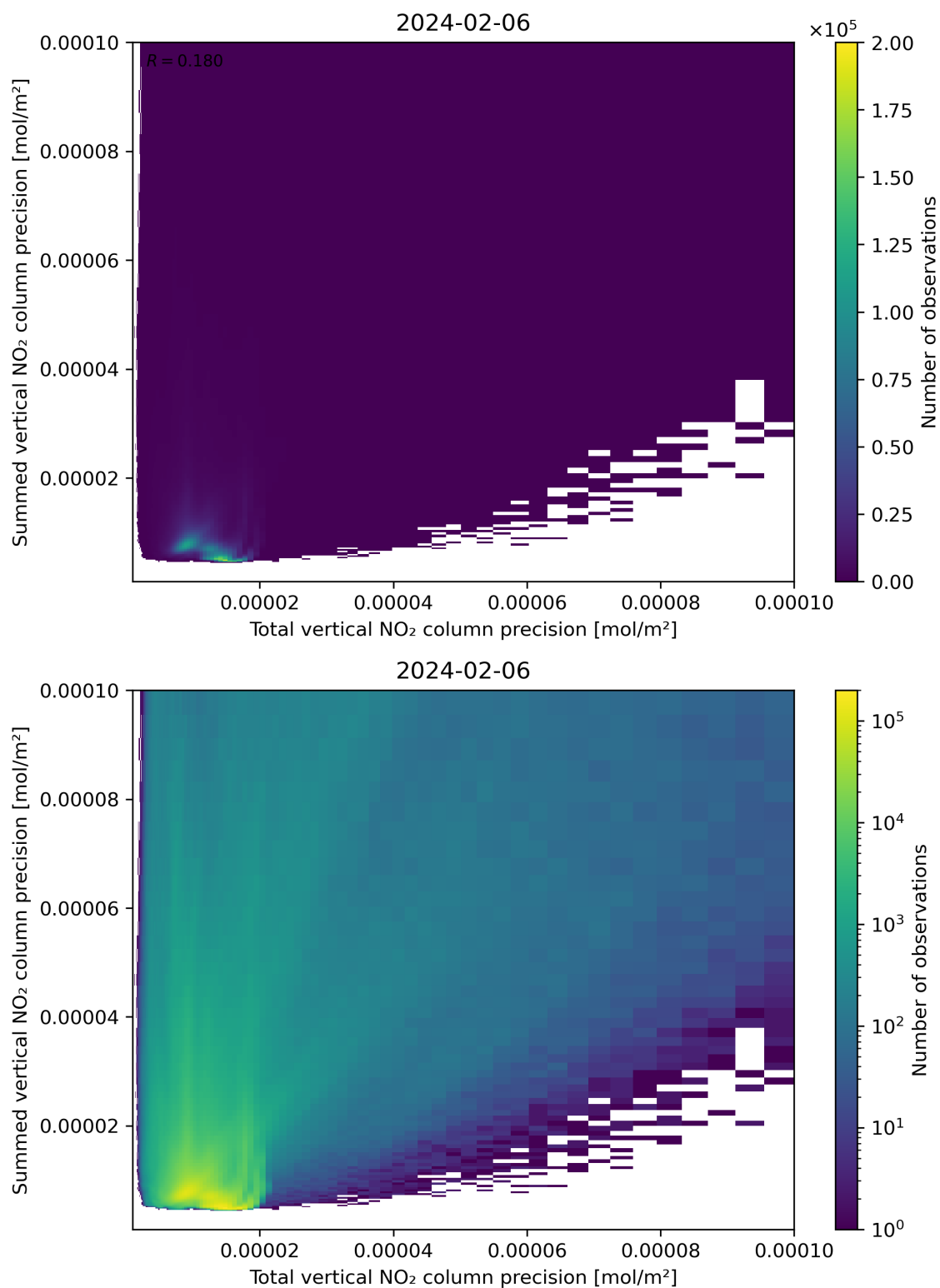
Figure 118: Scatter density plot of “Total vertical NO 2 column precision” against “Summed vertical NO 2 column precision” for 2024-02-06 to 2024-02-07.
