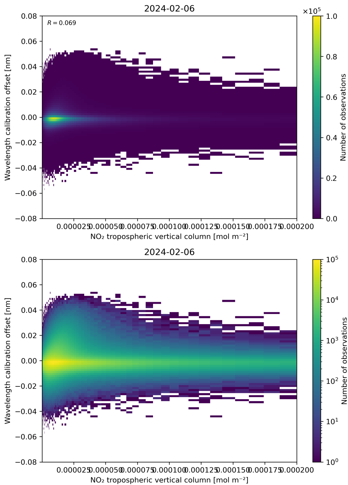
Figure 143: Scatter density plot of “NO 2 tropospheric vertical column” against “Wavelength calibration offset” for 2024-02-06 to 2024-02-07.
