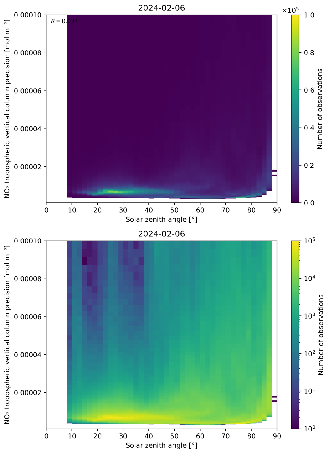
Figure 156: Scatter density plot of “Solar zenith angle” against “NO 2 tropospheric vertical column precision” for 2024-02-06 to 2024-02-07.
