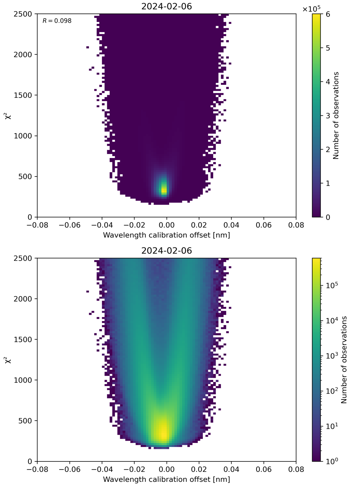
Figure 175: Scatter density plot of “Wavelength calibration offset” against “ \chi^2 ” for 2024-02-06 to 2024-02-07.
