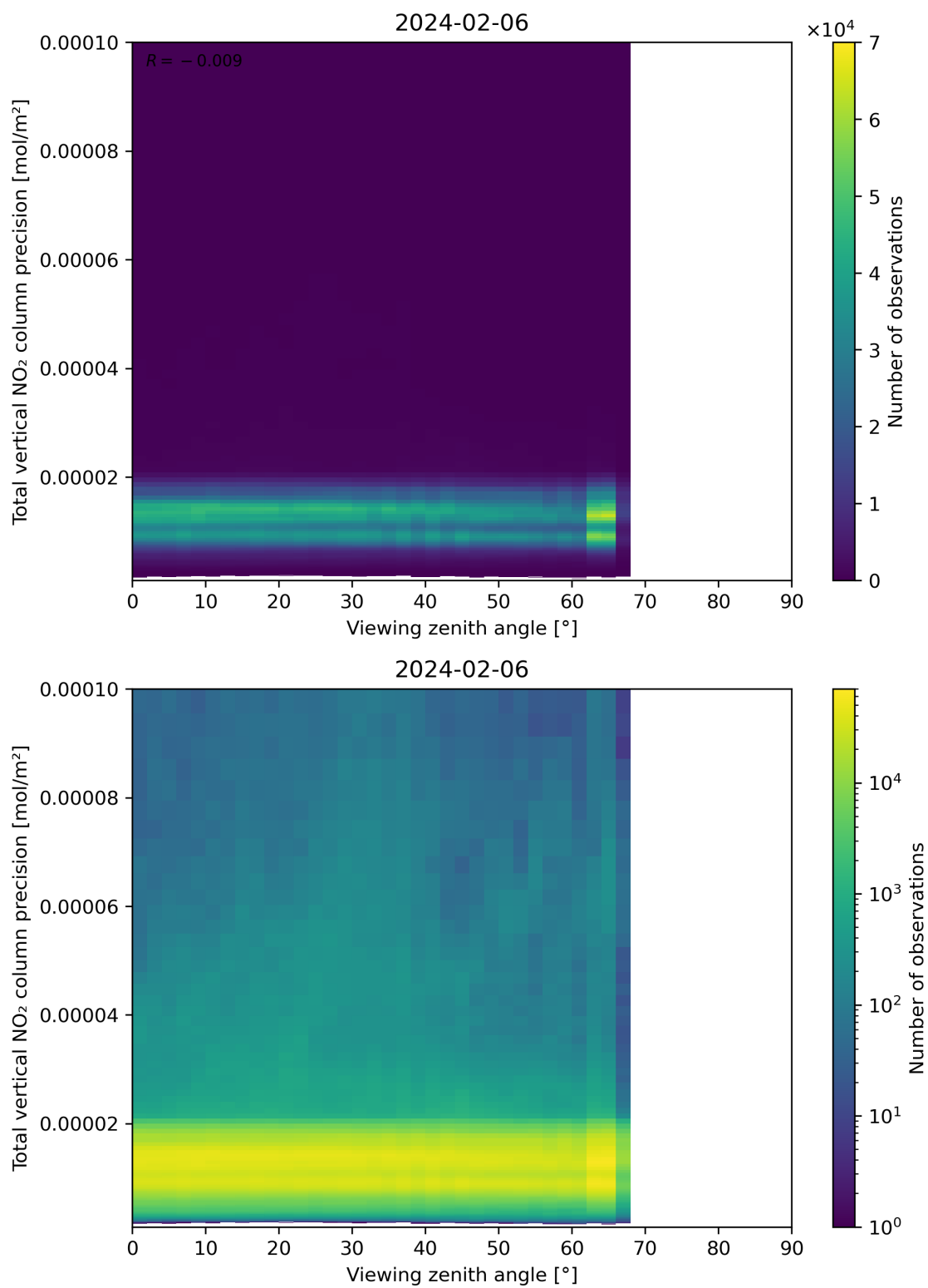
Figure 168: Scatter density plot of “Viewing zenith angle” against “Total vertical NO 2 column precision” for 2024-02-06 to 2024-02-07.
