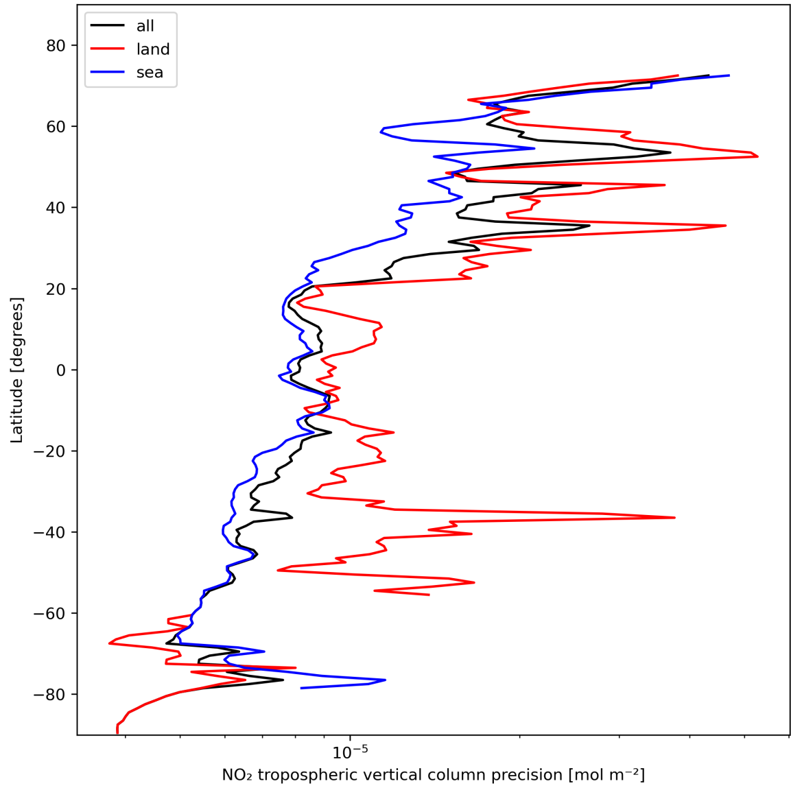
Figure 13: Zonal average of “NO 2 tropospheric vertical column precision” for 2024-02-06 to 2024-02-07.
