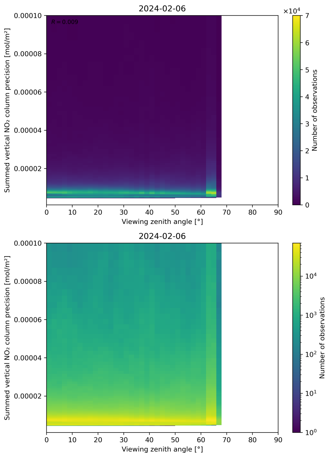
Figure 166: Scatter density plot of “Viewing zenith angle” against “Summed vertical NO 2 column precision” for 2024-02-06 to 2024-02-07.
