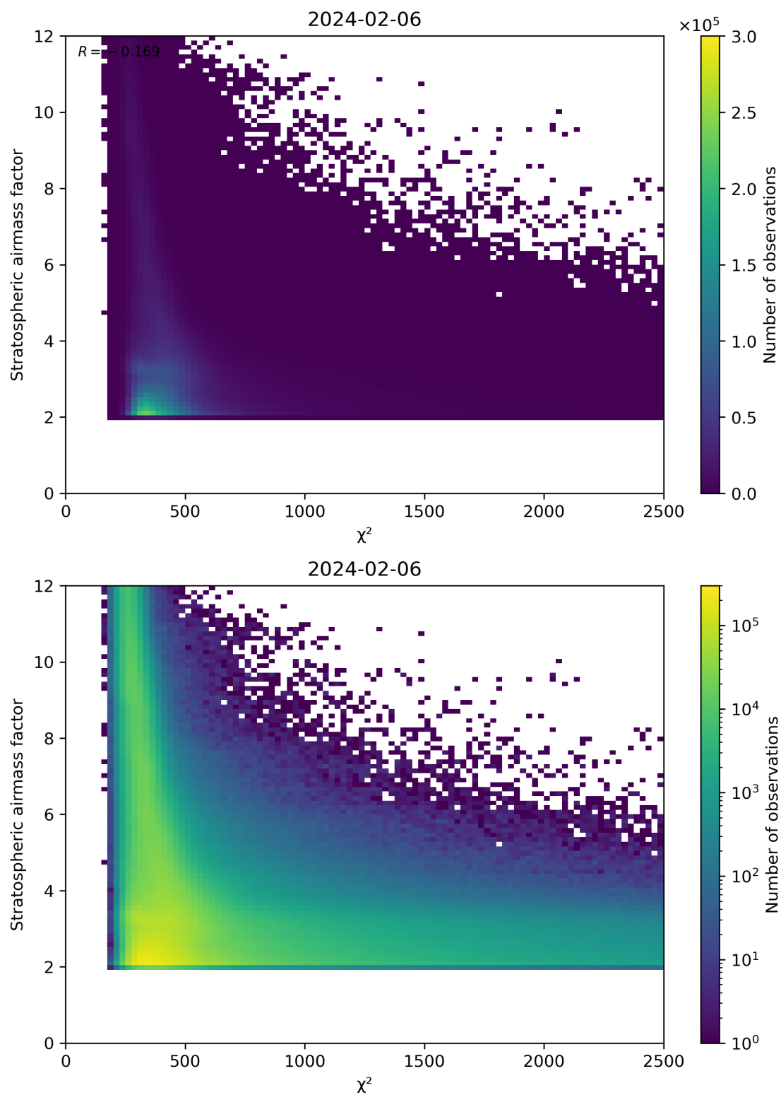
Figure 81: Scatter density plot of “ \chi^2 ” against “Stratospheric airmass factor” for 2024-02-06 to 2024-02-07.
