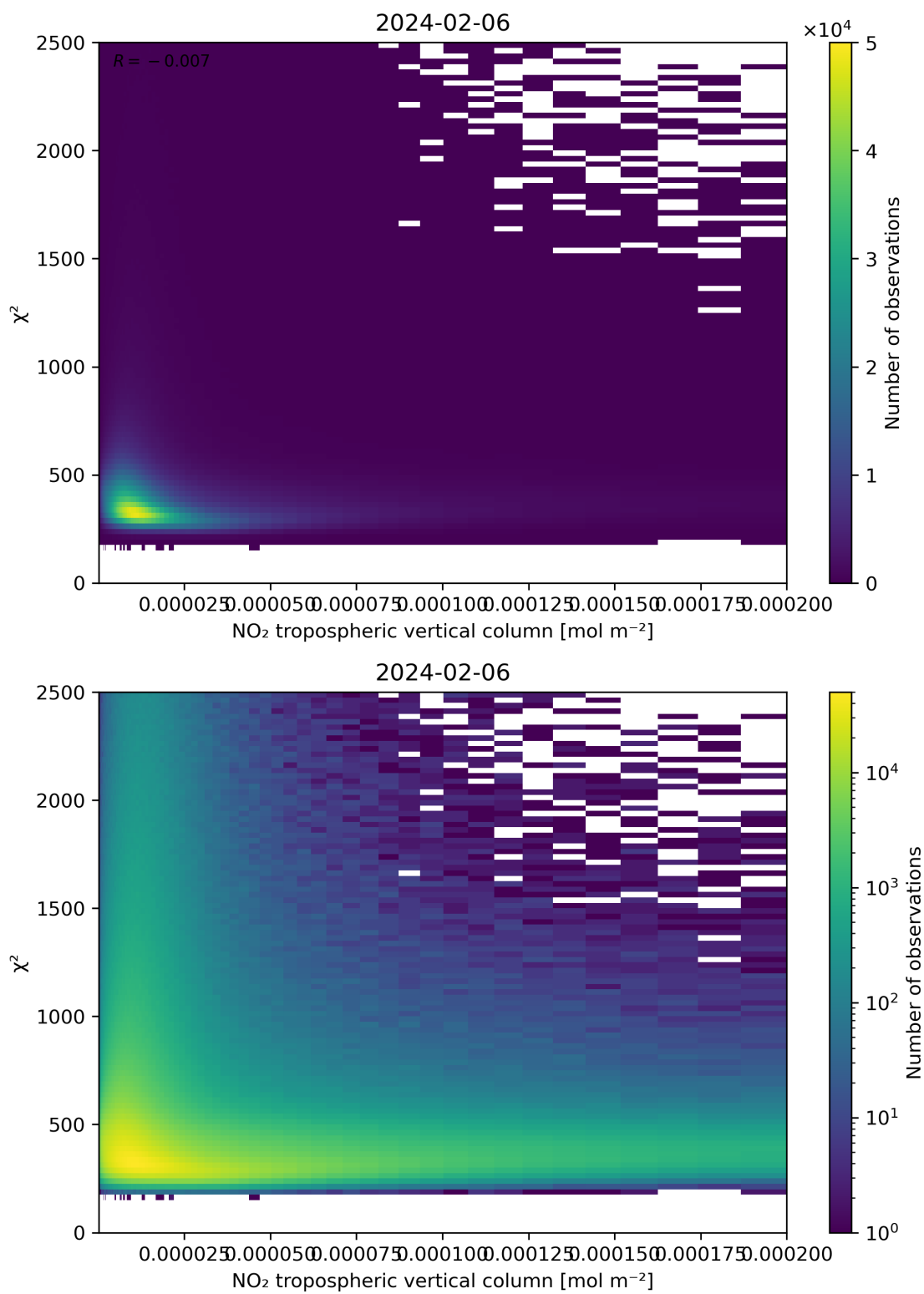
Figure 124: Scatter density plot of “NO 2 tropospheric vertical column” against “ \chi^2 ” for 2024-02-06 to 2024-02-07.
