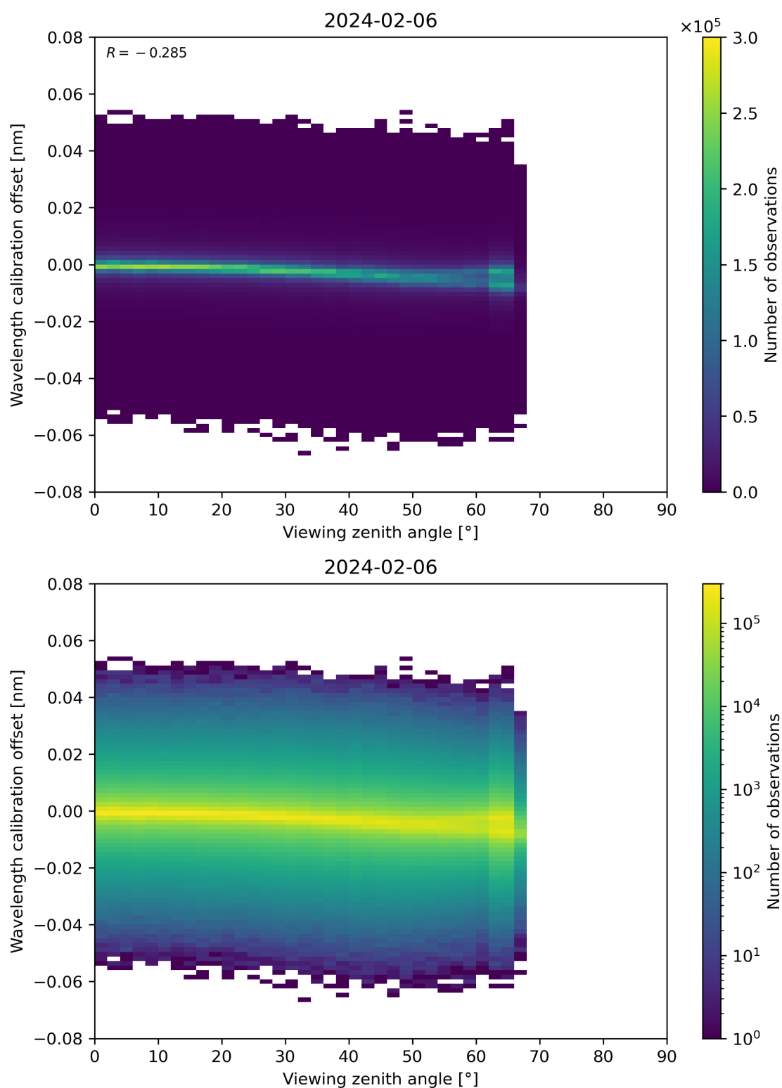
Figure 173: Scatter density plot of “Viewing zenith angle” against “Wavelength calibration offset” for 2024-02-06 to 2024-02-07.
