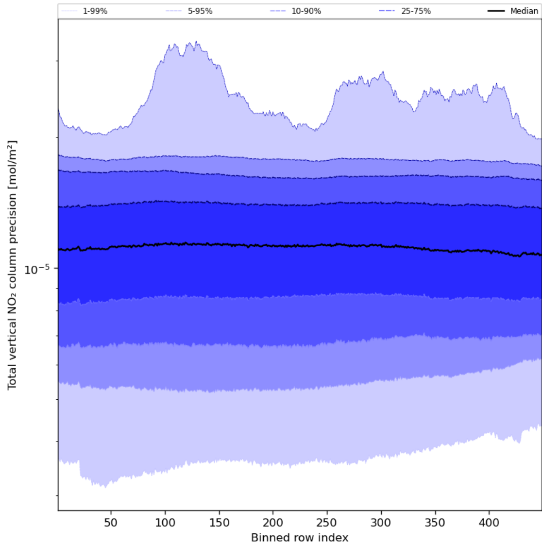
Figure 56: Along track statistics of “Total vertical NO 2 column precision” for 2024-02-06 to 2024-02-07
