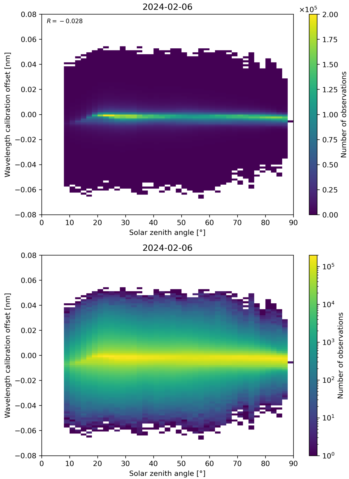
Figure 158: Scatter density plot of “Solar zenith angle” against “Wavelength calibration offset” for 2024-02-06 to 2024-02-07.
