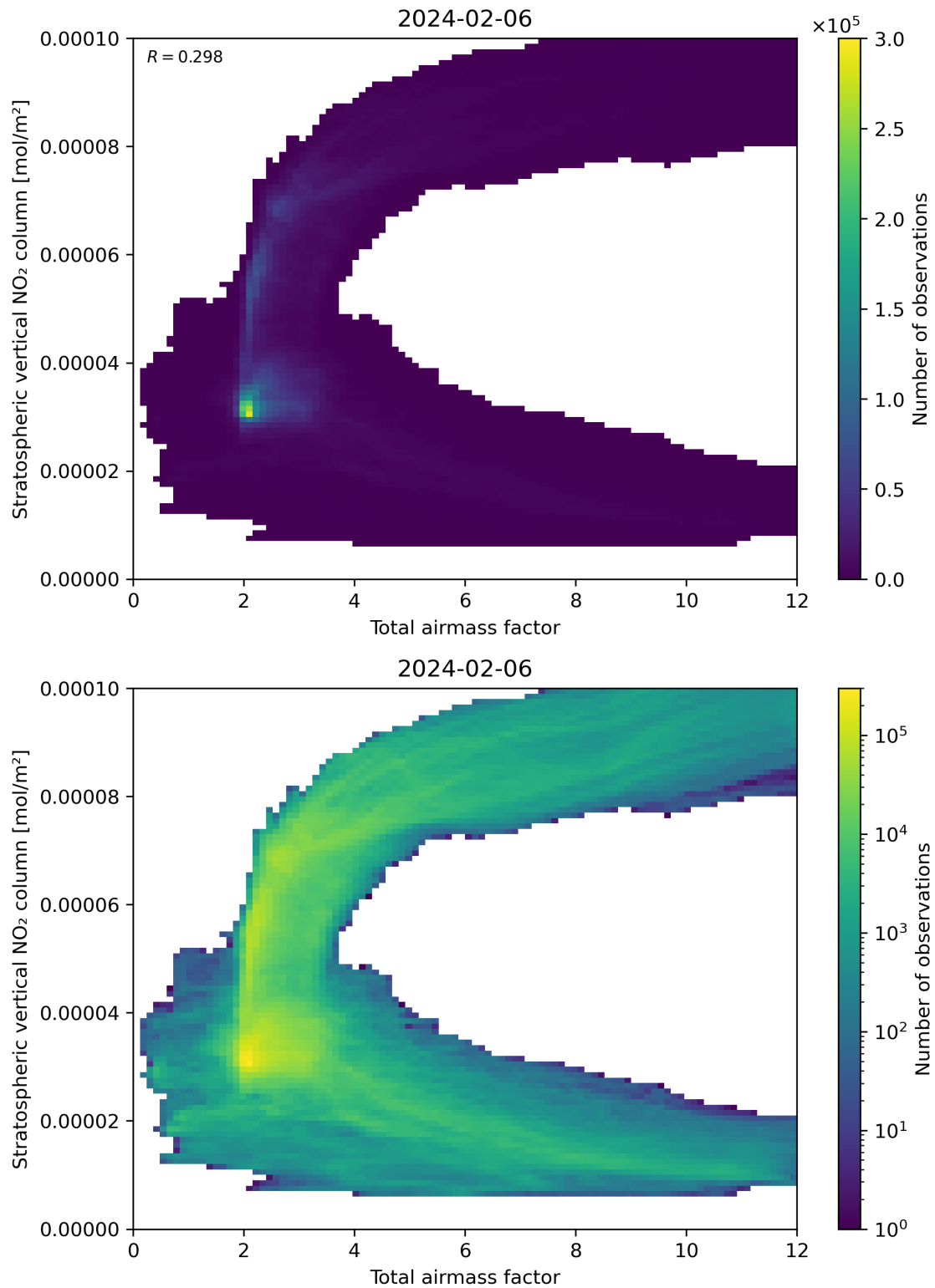
Figure 64: Scatter density plot of “Total airmass factor” against “Stratospheric vertical \text{NO}_2 column” for 2024-02-06 to 2024-02-07.
