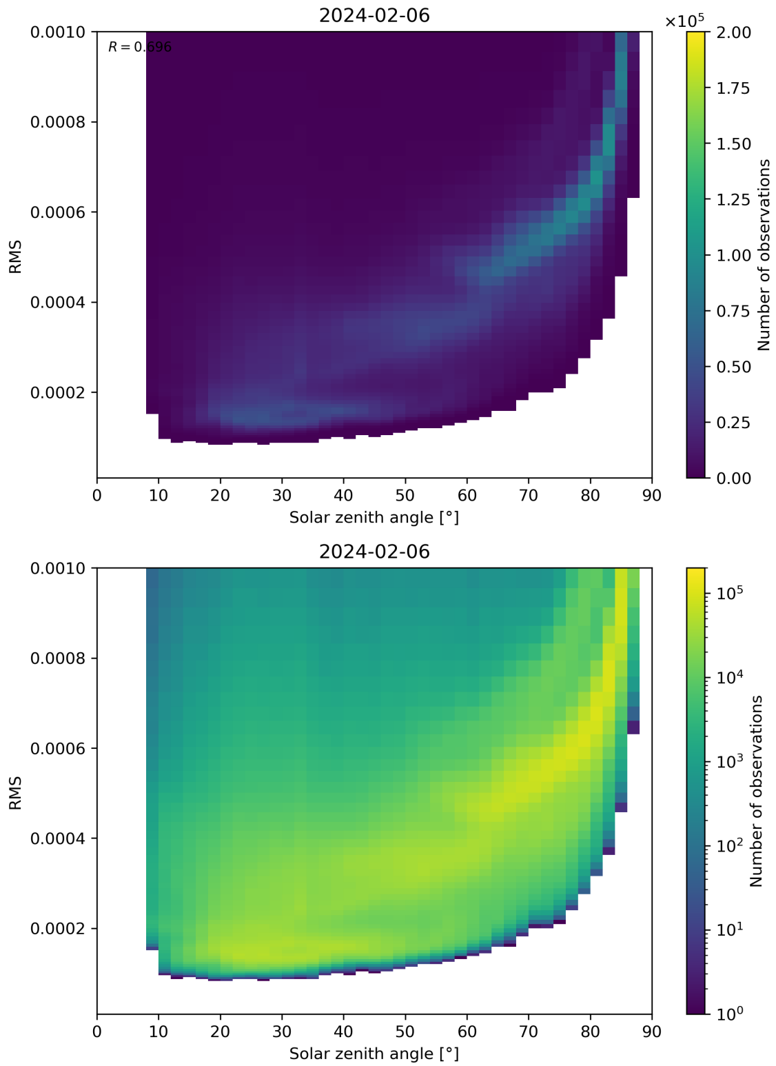
Figure 157: Scatter density plot of “Solar zenith angle” against “RMS” for 2024-02-06 to 2024-02-07.
