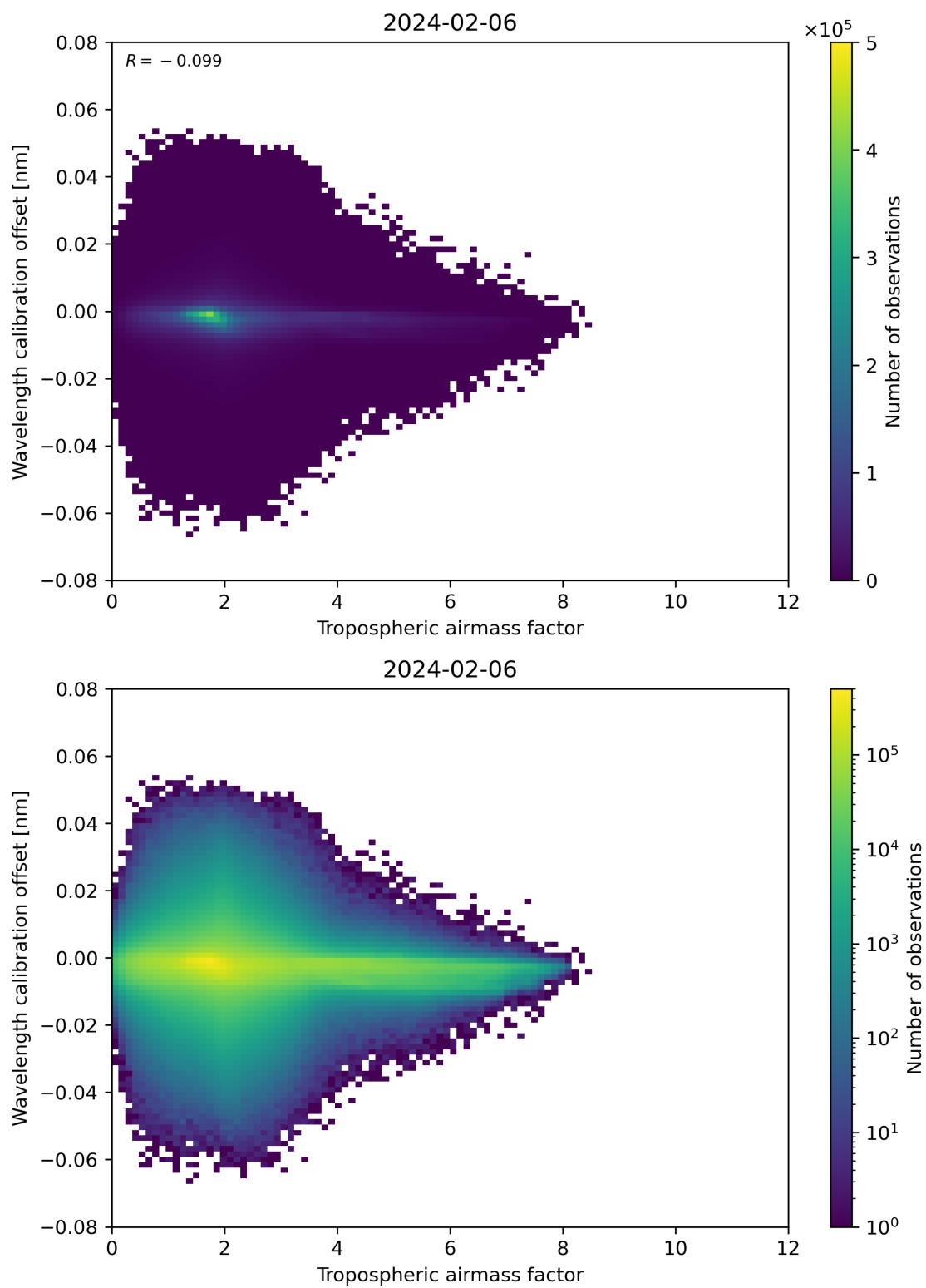
Figure 80: Scatter density plot of “Tropospheric airmass factor” against “Wavelength calibration offset” for 2024-02-06 to 2024-02-07.
