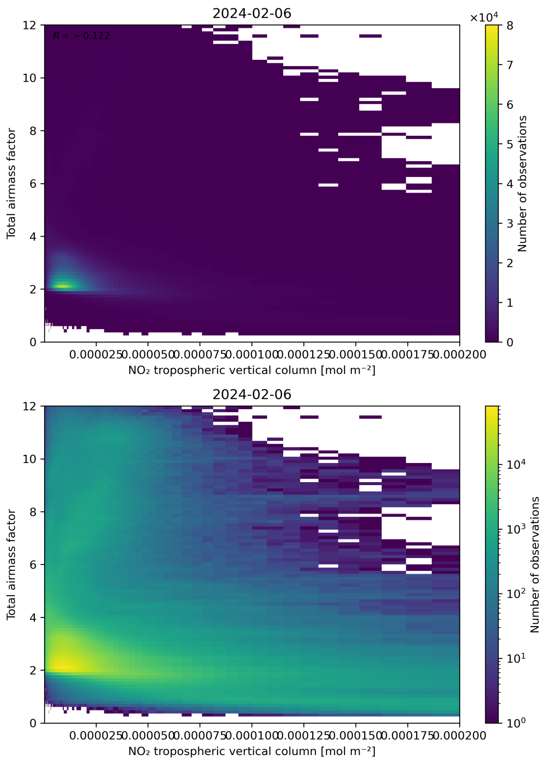
Figure 122: Scatter density plot of “NO 2 tropospheric vertical column” against “Total air mass factor” for 2024-02-06 to 2024-02-07.
