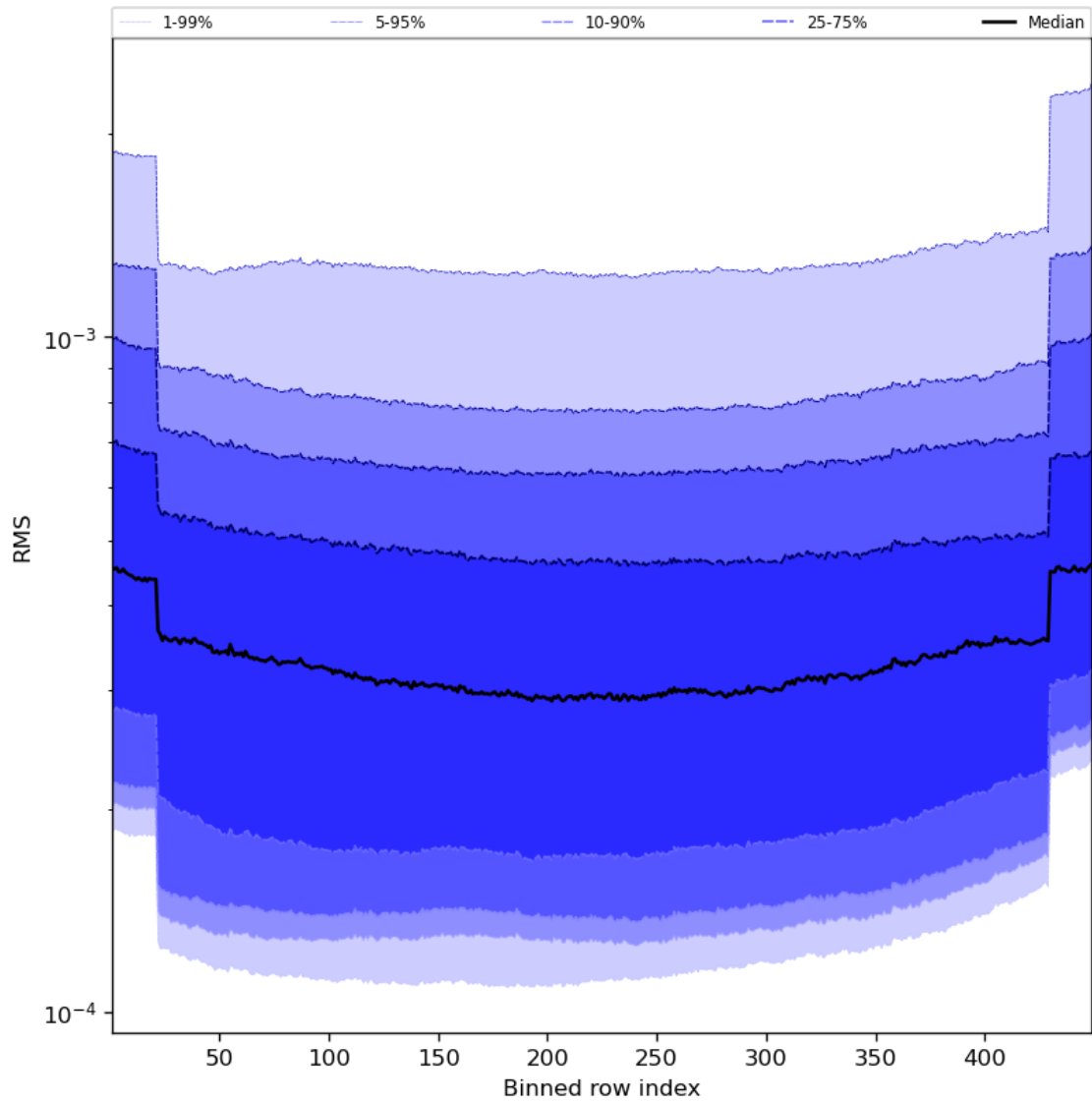
Figure 60: Along track statistics of “RMS” for 2024-02-06 to 2024-02-07
