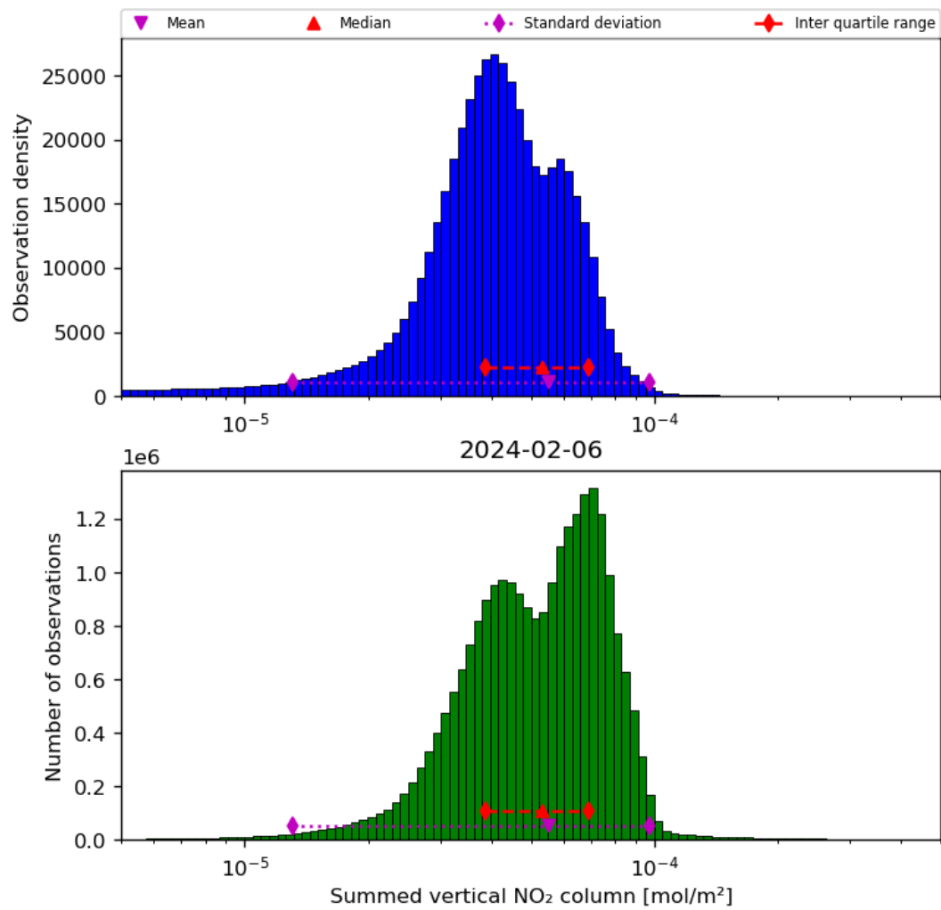
Figure 40: Histogram of “Summed vertical NO 2 column” for 2024-02-06 to 2024-02-07
