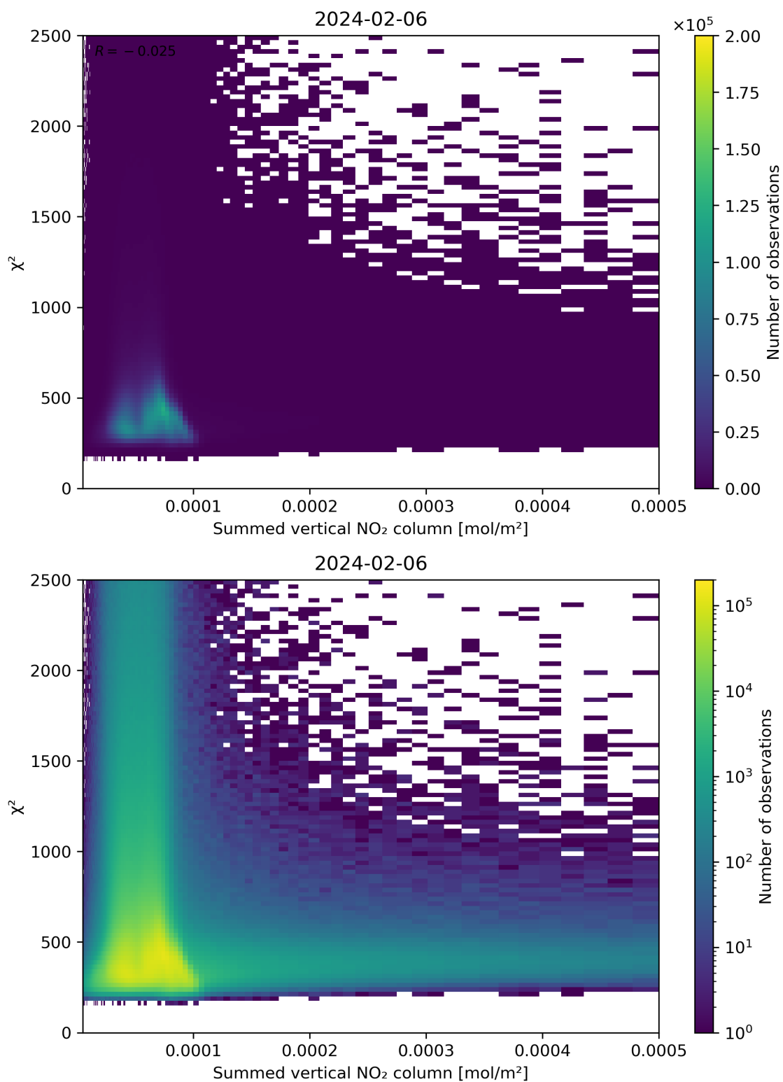
Figure 104: Scatter density plot of “Summed vertical NO 2 column” against “ \chi^2 ” for 2024-02-06 to 2024-02-07.
