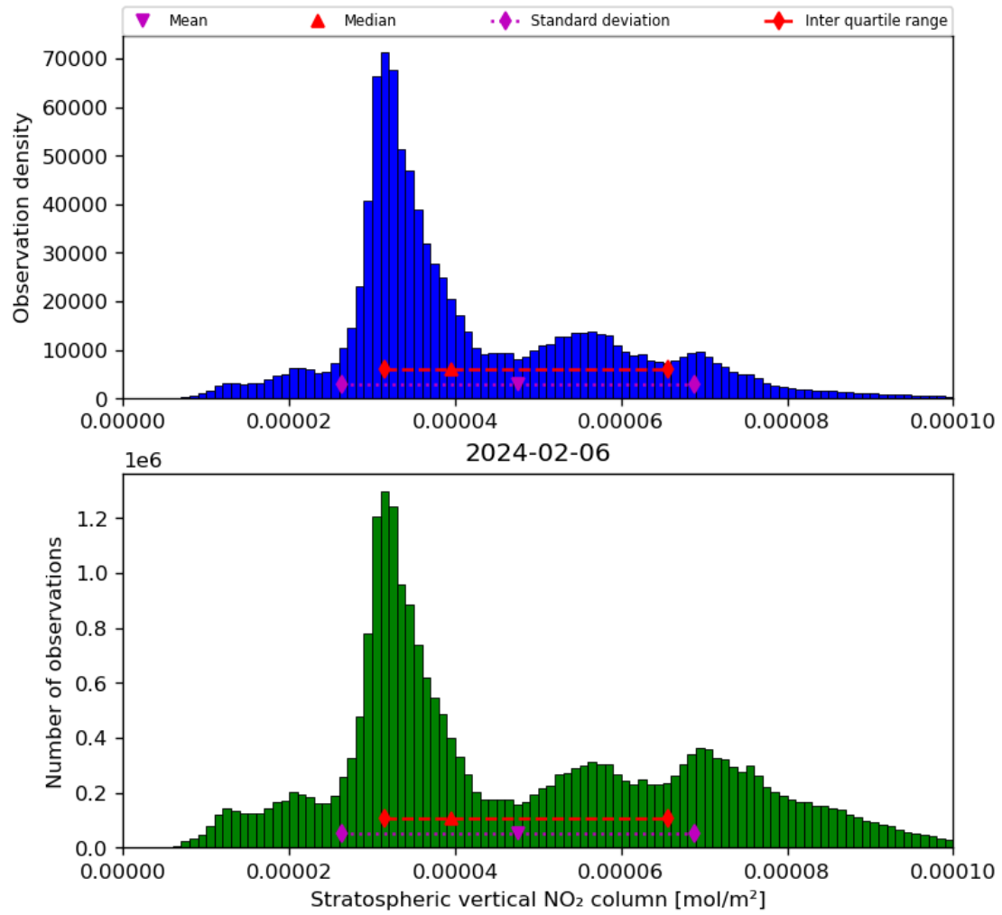
Figure 36: Histogram of “Stratospheric vertical NO 2 column” for 2024-02-06 to 2024-02-07
