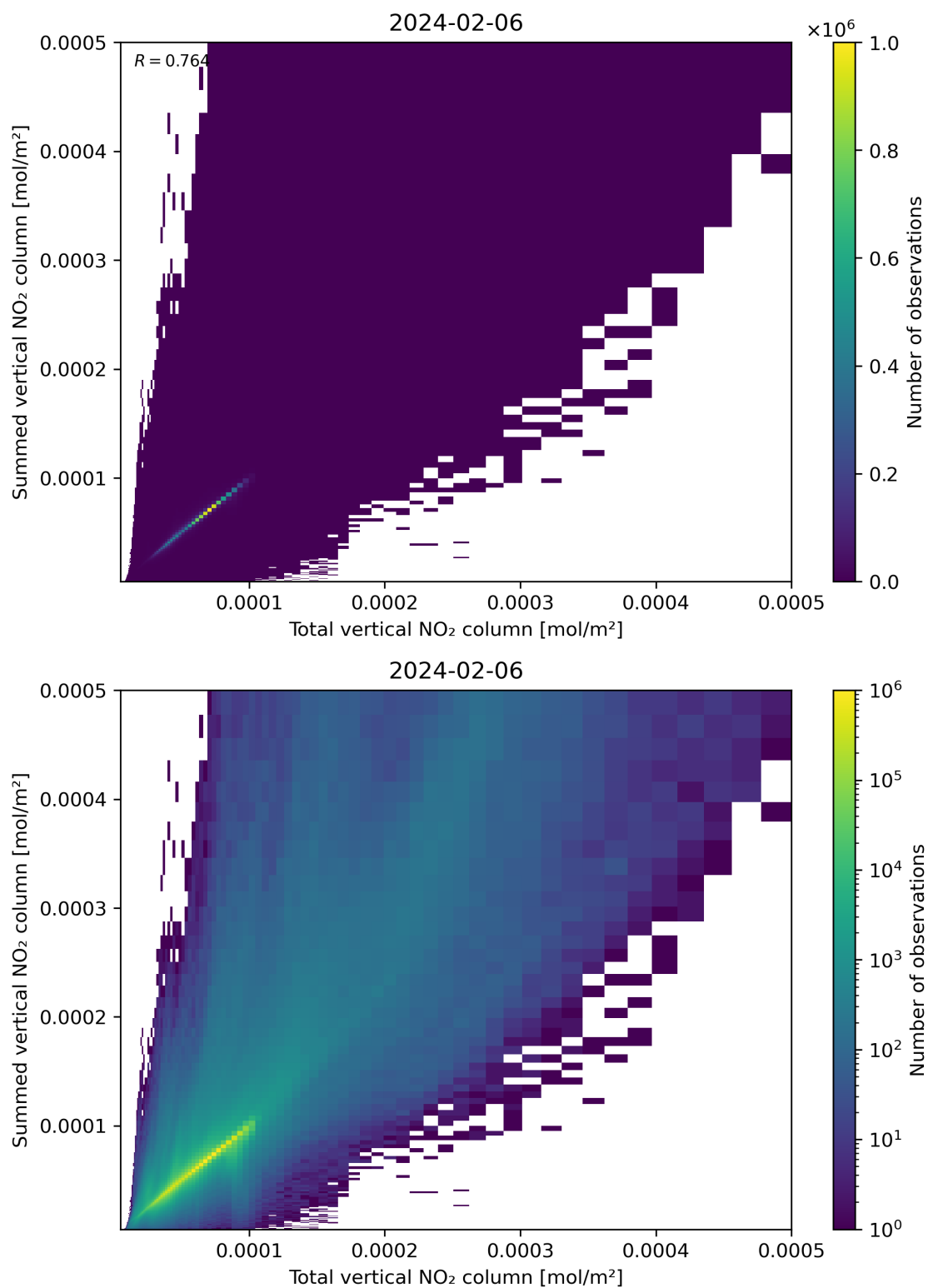
Figure 112: Scatter density plot of “Total vertical NO 2 column” against “Summed vertical NO 2 column” for 2024-02-06 to 2024-02-07.
