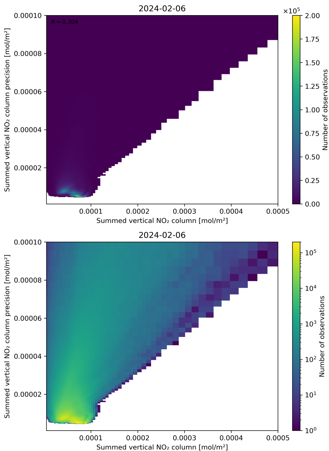
Figure 105: Scatter density plot of “Summed vertical NO 2 column” against “Summed vertical NO 2 column precision” for 2024-02-06 to 2024-02-07.
