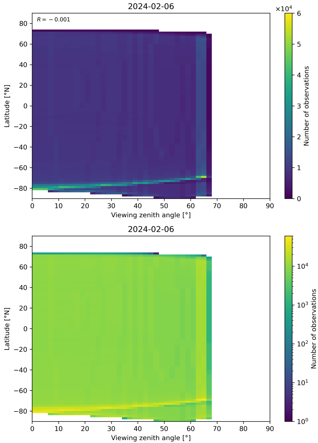
Figure 163: Scatter density plot of “Viewing zenith angle” against “Latitude” for 2024-02-06 to 2024-02-07.
