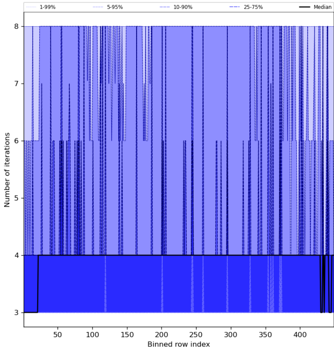
Figure 51: Along track statistics of “Number of iterations” for 2024-02-06 to 2024-02-07
