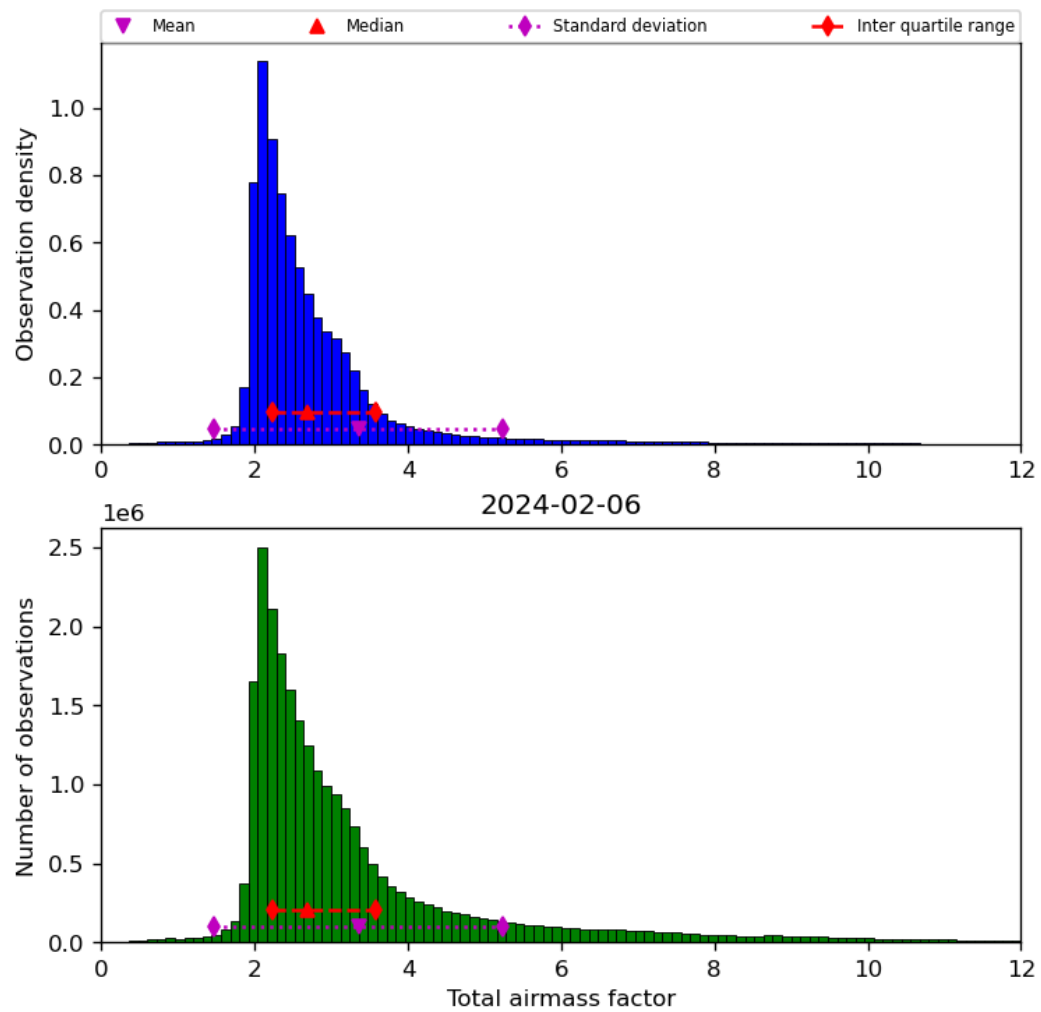
Figure 32: Histogram of “Total airmass factor” for 2024-02-06 to 2024-02-07
