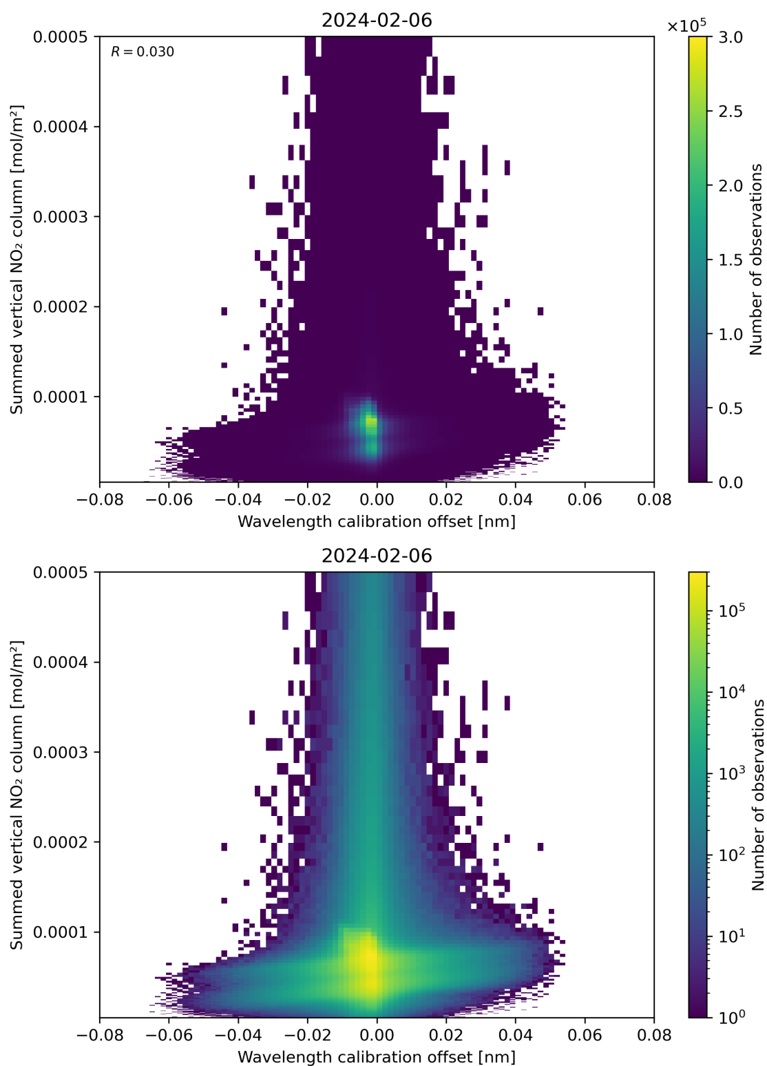
Figure 177: Scatter density plot of “Wavelength calibration offset” against “Summed vertical NO 2 column” for 2024-02-06 to 2024-02-07.
