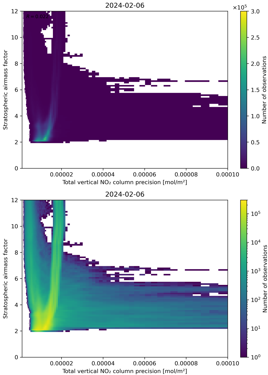
Figure 115: Scatter density plot of “Total vertical NO 2 column precision” against “Stratospheric air mass factor” for 2024-02-06 to 2024-02-07.
