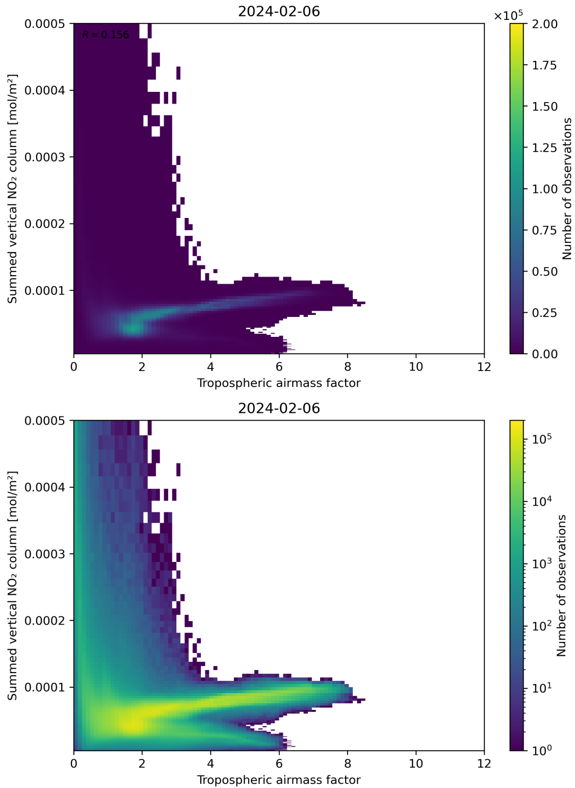
Figure 75: Scatter density plot of “Tropospheric airmass factor” against “Summed vertical NO 2 column” for 2024-02-06 to 2024-02-07.
