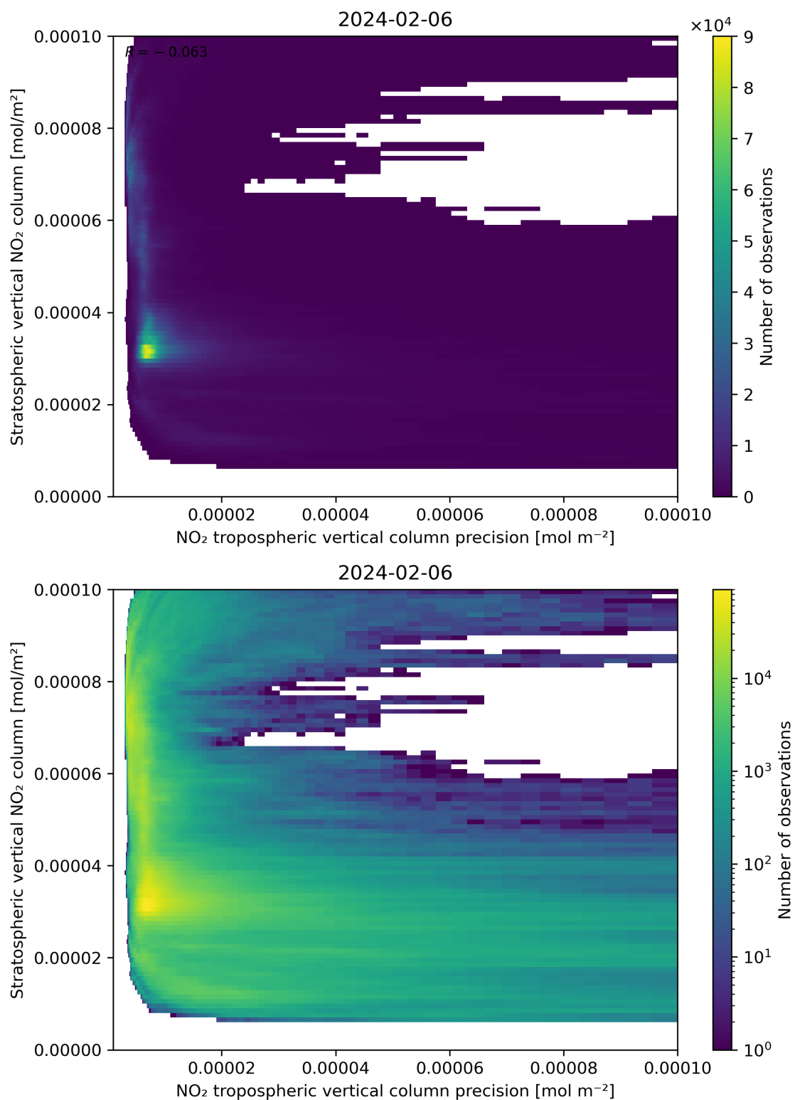
Figure 135: Scatter density plot of “NO 2 tropospheric vertical column precision” against “Stratospheric vertical NO 2 column” for 2024-02-06 to 2024-02-07.
