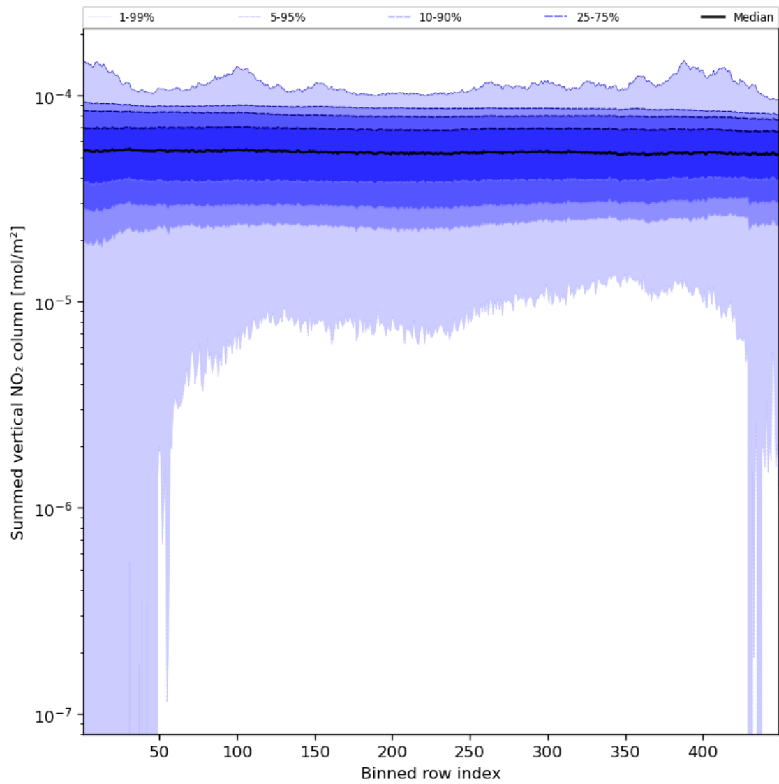
Figure 57: Along track statistics of “Summed vertical NO 2 column” for 2024-02-06 to 2024-02-07
