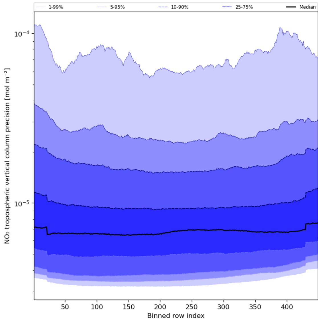
Figure 47: Along track statistics of “NO 2 tropospheric vertical column precision” for 2024-02-06 to 2024-02-07
