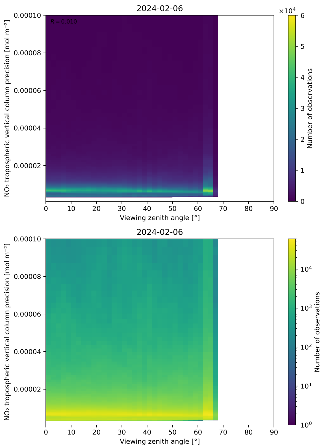
Figure 170: Scatter density plot of “Viewing zenith angle” against “NO 2 tropospheric vertical column precision” for 2024-02-06 to 2024-02-07.
