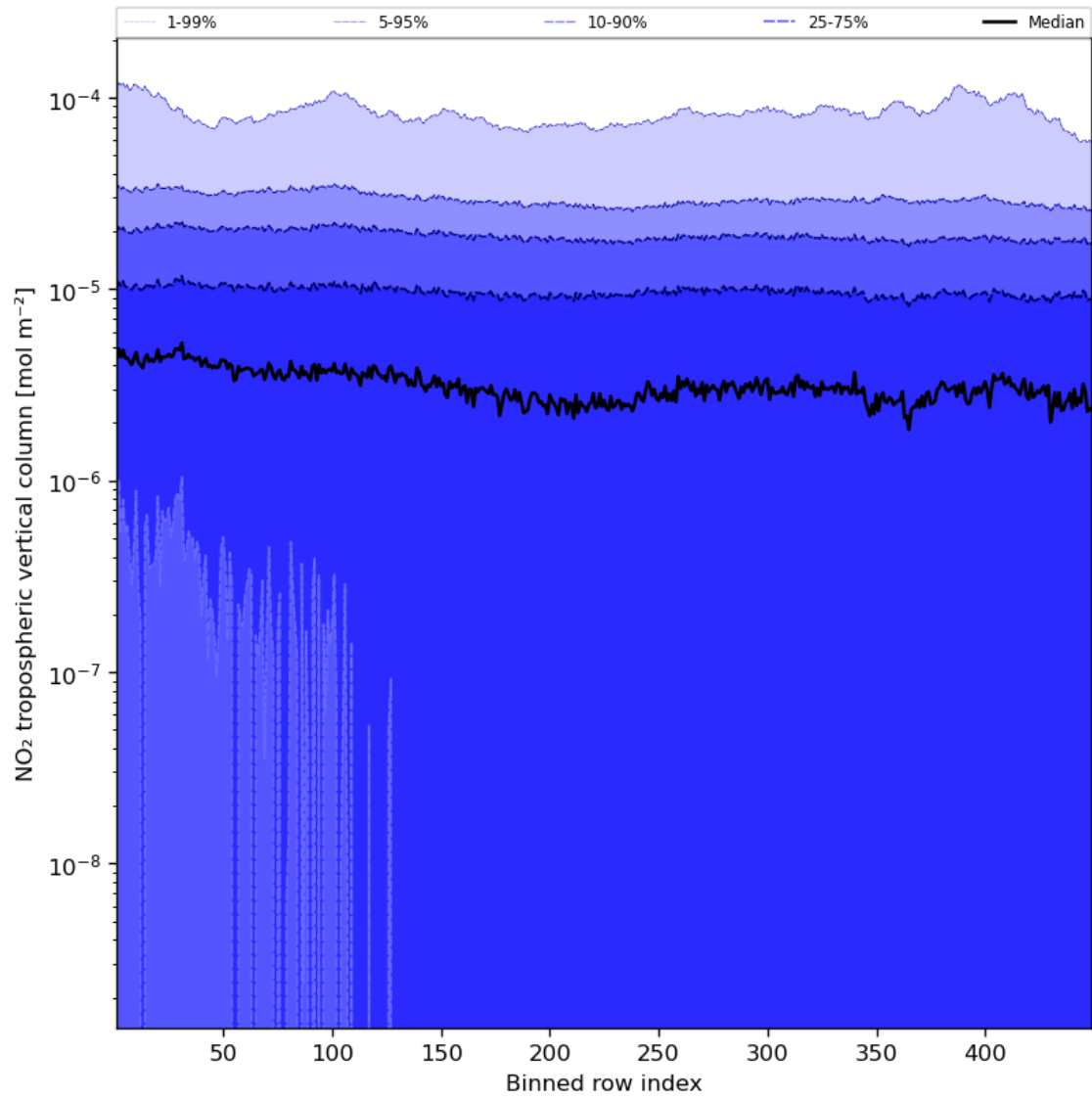
Figure 46: Along track statistics of “NO 2 tropospheric vertical column” for 2024-02-06 to 2024-02-07
