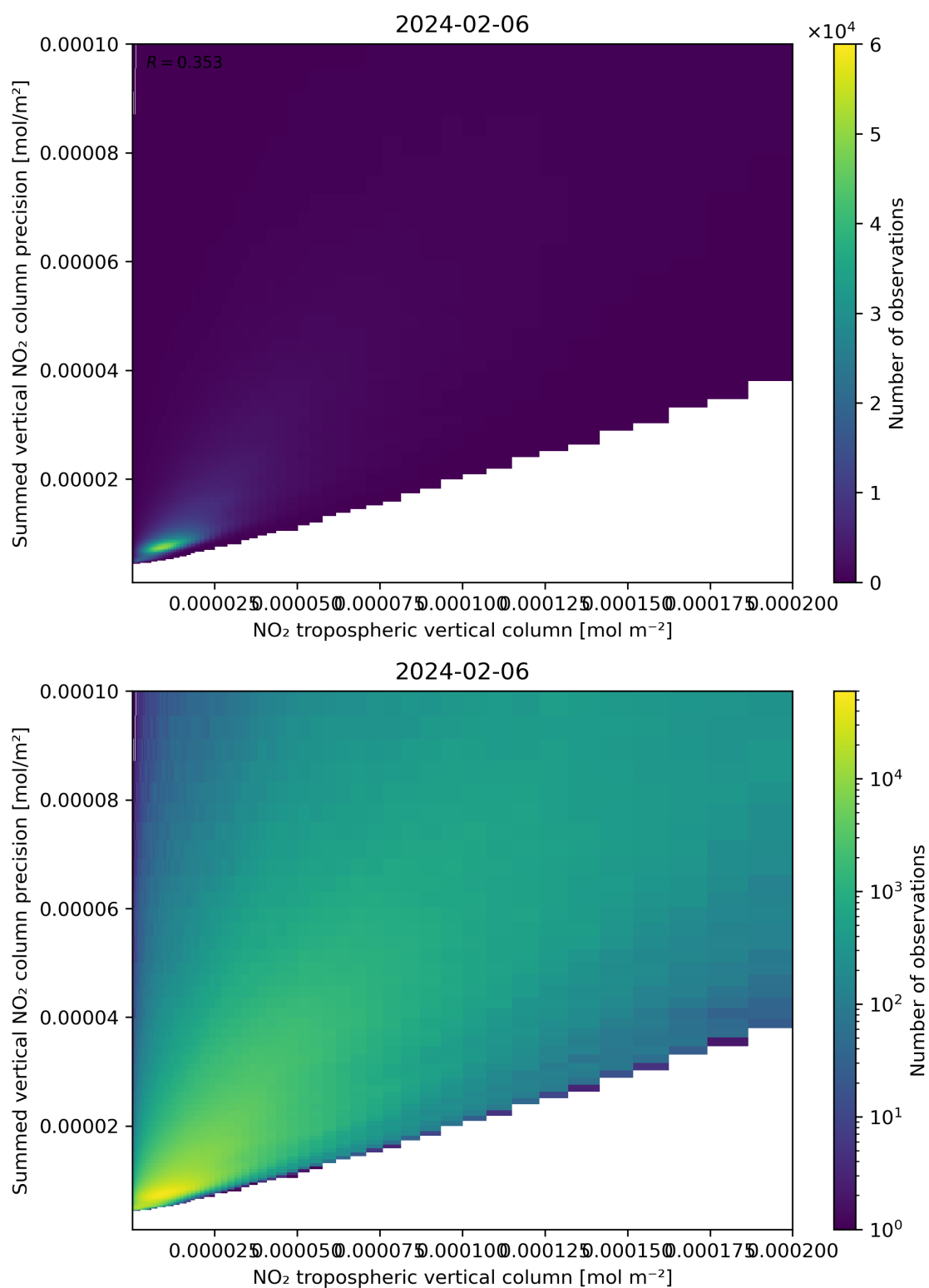
Figure 127: Scatter density plot of “NO 2 tropospheric vertical column” against “Summed vertical NO 2 column precision” for 2024-02-06 to 2024-02-07.
