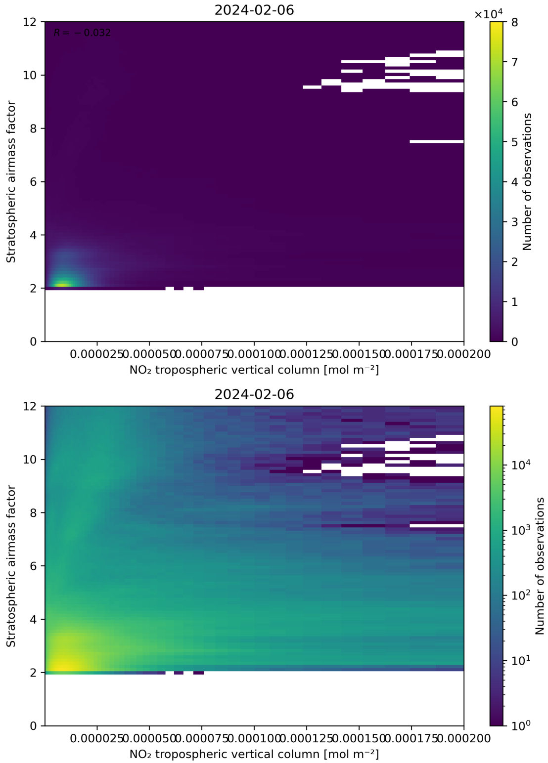
Figure 121: Scatter density plot of “NO 2 tropospheric vertical column” against “Stratospheric airmass factor” for 2024-02-06 to 2024-02-07.
