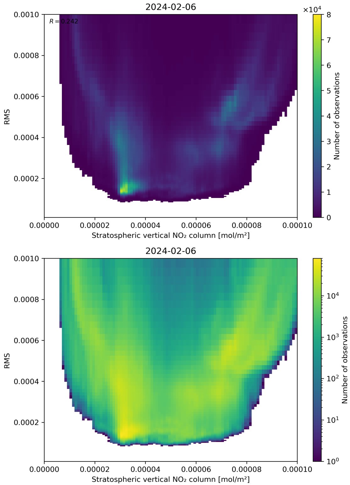
Figure 102: Scatter density plot of “Stratospheric vertical NO 2 column” against “RMS” for 2024-02-06 to 2024-02-07.
