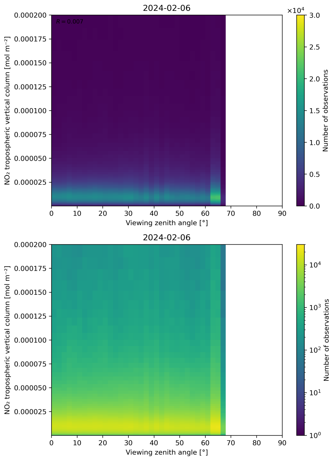
Figure 169: Scatter density plot of “Viewing zenith angle” against “NO 2 tropospheric vertical column” for 2024-02-06 to 2024-02-07.
