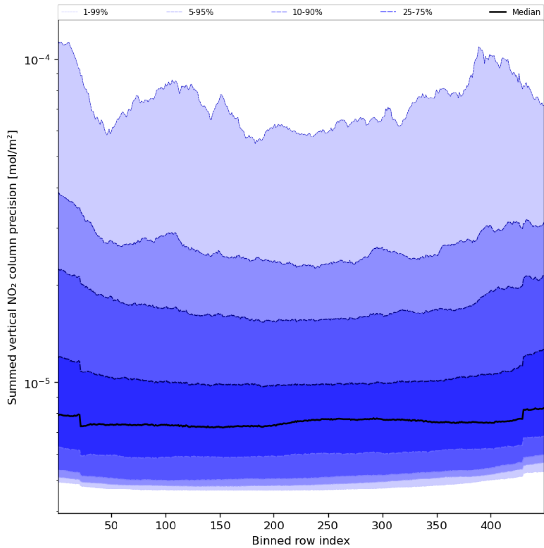
Figure 58: Along track statistics of “Summed vertical NO 2 column precision” for 2024-02-06 to 2024-02-07
