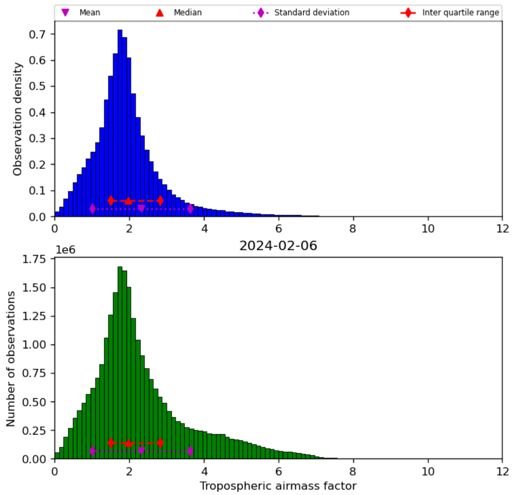
Figure 31: Histogram of “Tropospheric airmass factor” for 2024-02-06 to 2024-02-07
