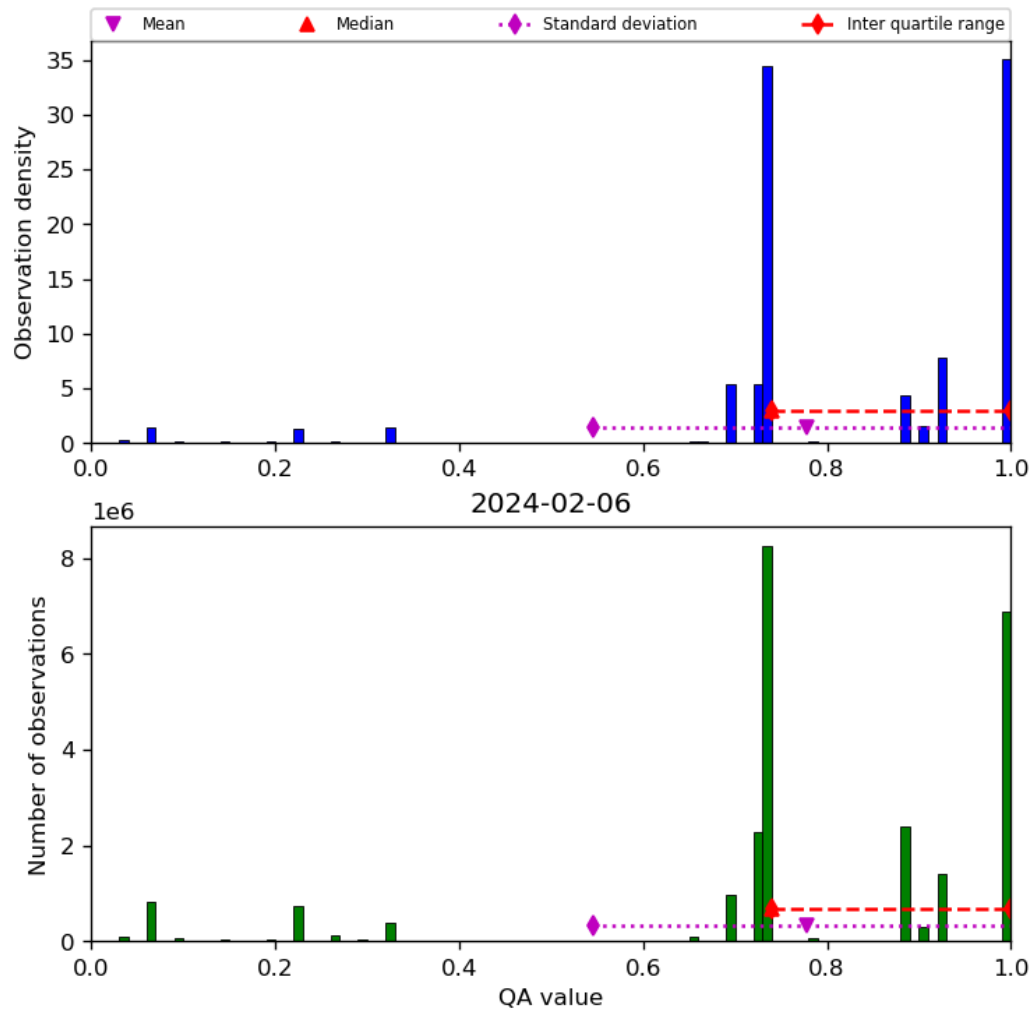
Figure 28: Histogram of “QA value” for 2024-02-06 to 2024-02-07
