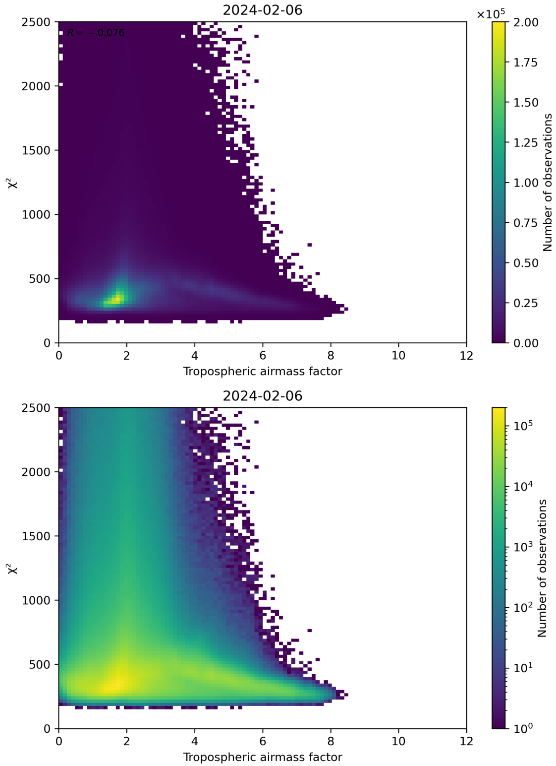
Figure 73: Scatter density plot of “Tropospheric airmass factor” against “ \chi^2 ” for 2024-02-06 to 2024-02-07.
