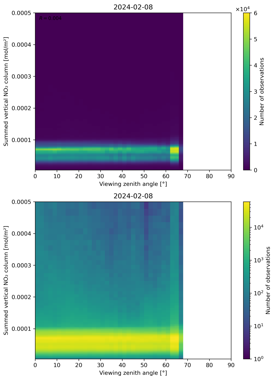
Figure 165: Scatter density plot of “Viewing zenith angle” against “Summed vertical NO 2 column” for 2024-02-07 to 2024-02-09.
