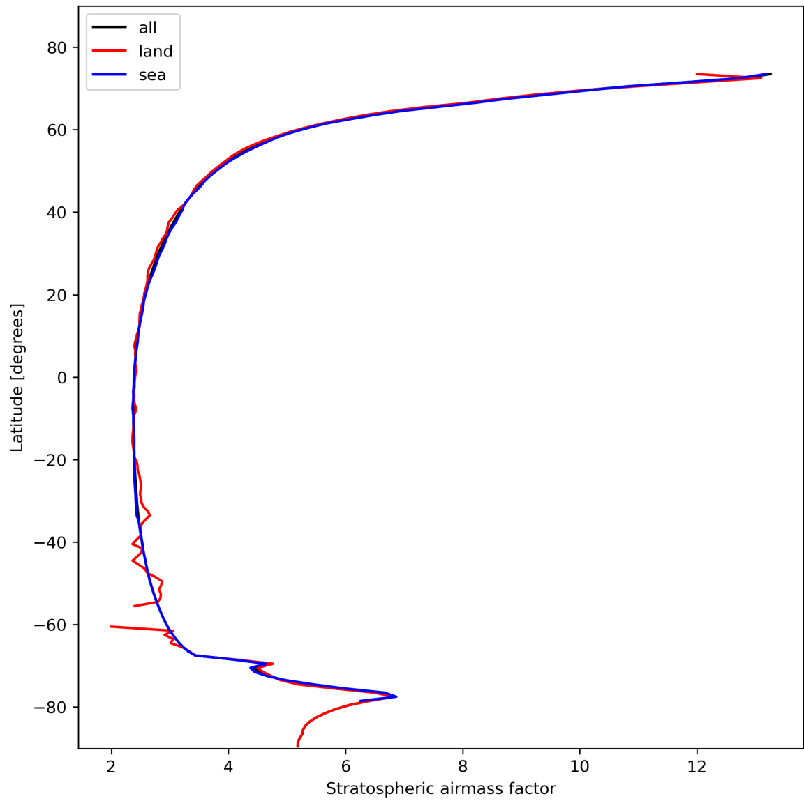
Figure 27: Zonal average of “Stratospheric air mass factor” for 2024-02-07 to 2024-02-09.
