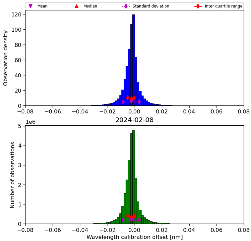
Figure 35: Histogram of “Wavelength calibration offset” for 2024-02-07 to 2024-02-09
