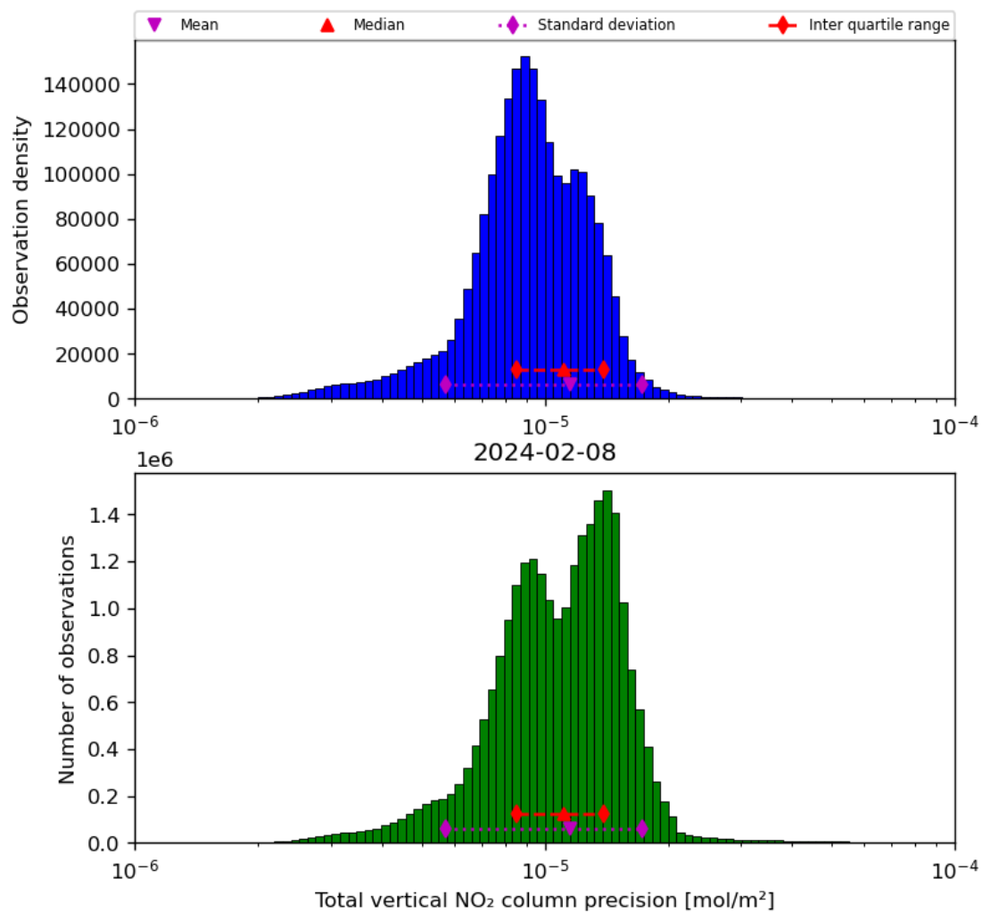
Figure 39: Histogram of “Total vertical NO 2 column precision” for 2024-02-07 to 2024-02-09
