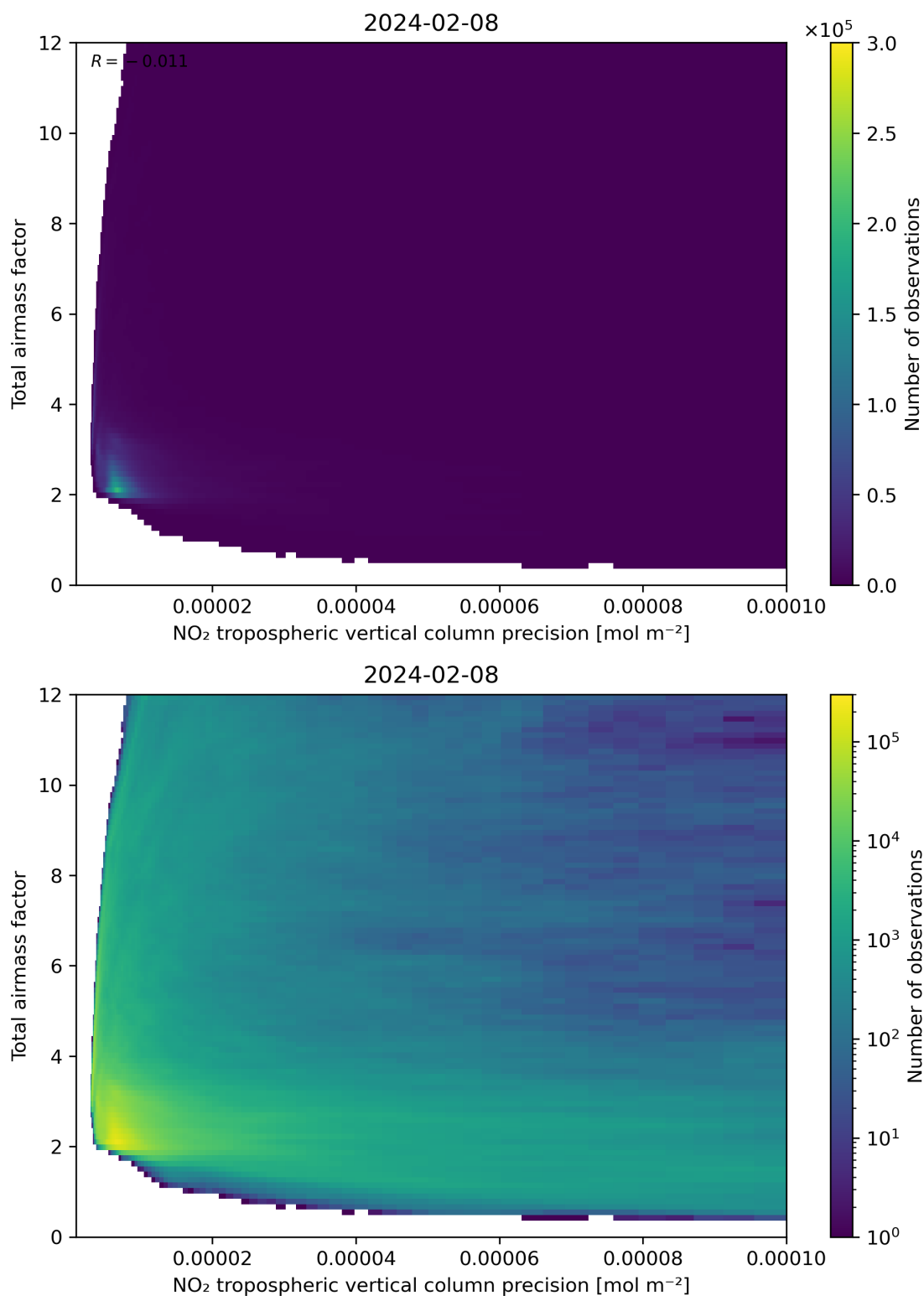
Figure 132: Scatter density plot of “NO 2 tropospheric vertical column precision” against “Total air mass factor” for 2024-02-07 to 2024-02-09.
