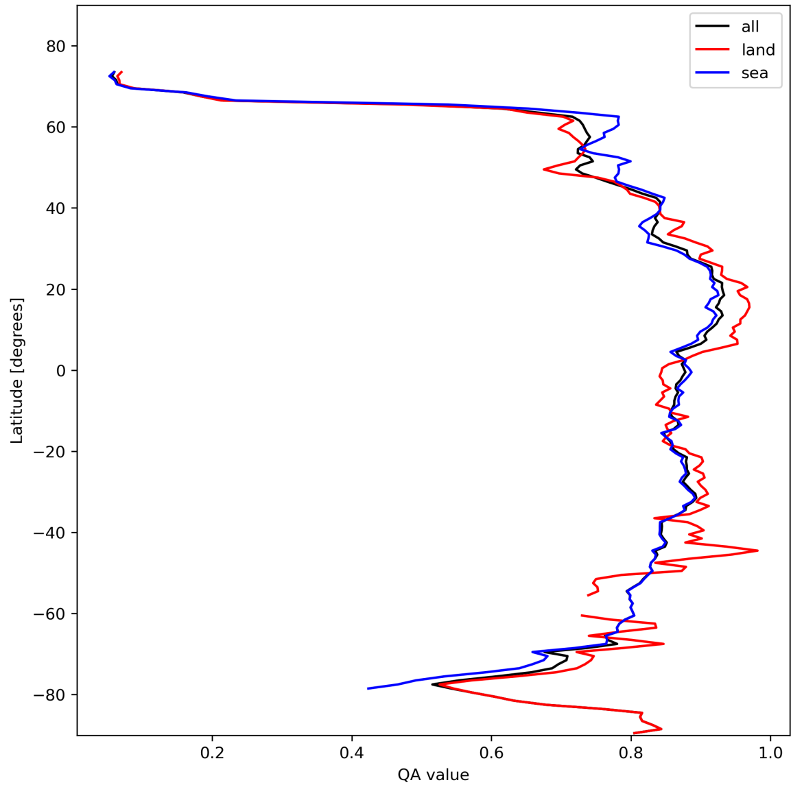
Figure 11: Zonal average of “QA value” for 2024-02-07 to 2024-02-09.
