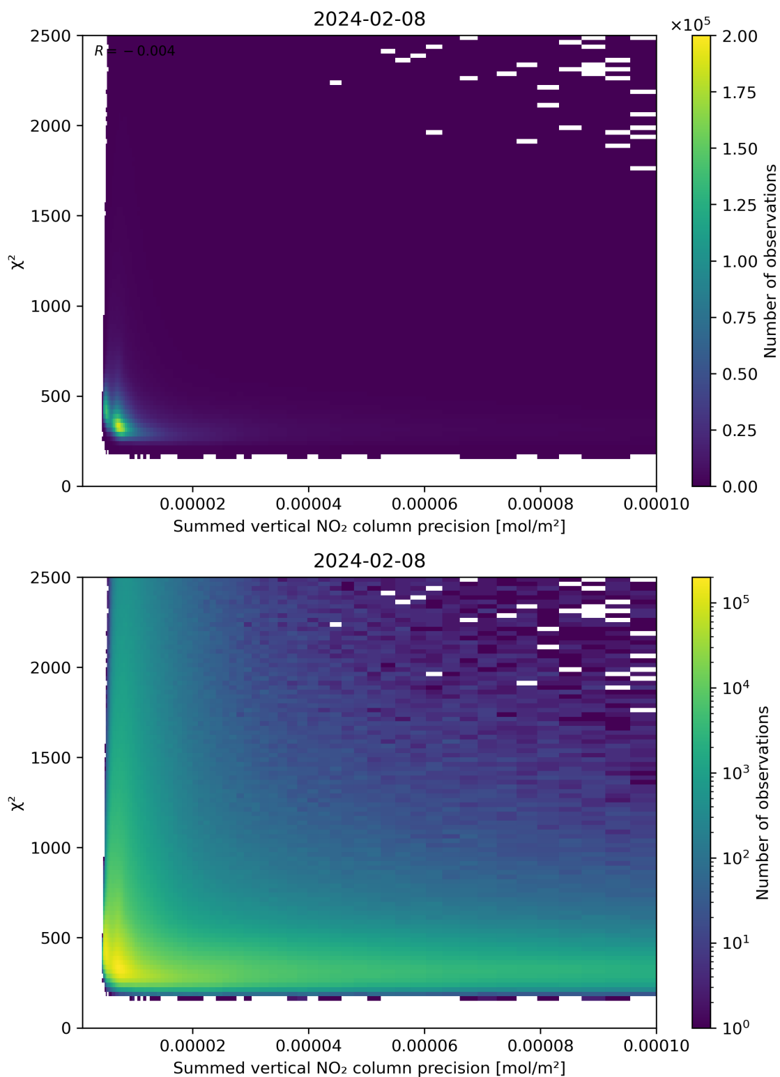
Figure 107: Scatter density plot of “Summed vertical NO 2 column precision” against “ \chi^2 ” for 2024-02-07 to 2024-02-09.
