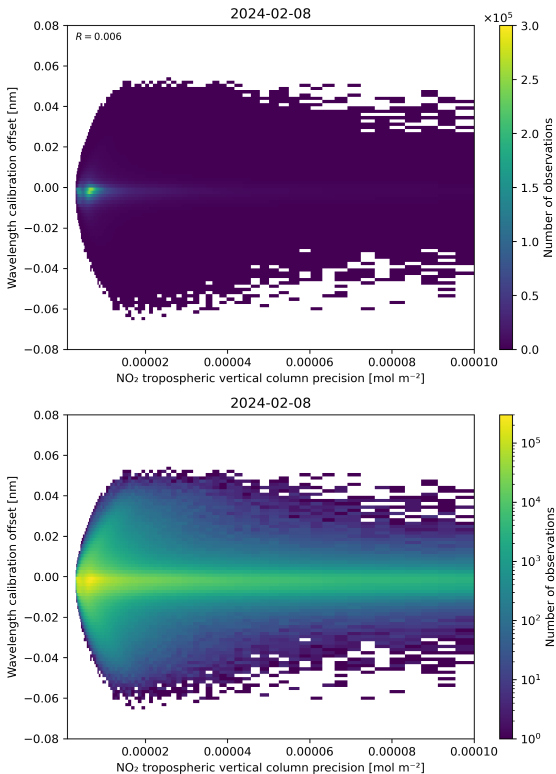
Figure 141: Scatter density plot of “NO 2 tropospheric vertical column precision” against “Wavelength calibration offset” for 2024-02-07 to 2024-02-09.
