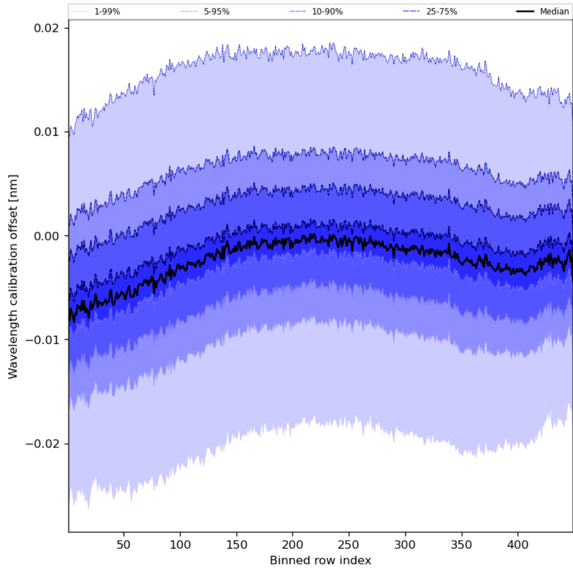
Figure 52: Along track statistics of “Wavelength calibration offset” for 2024-02-07 to 2024-02-09
