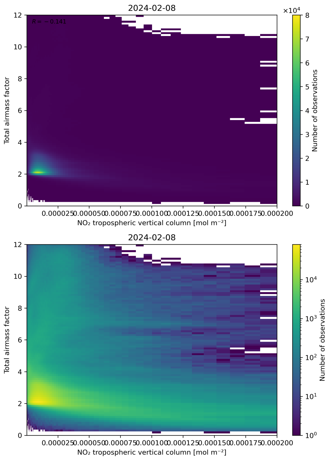
Figure 122: Scatter density plot of “NO 2 tropospheric vertical column” against “Total air mass factor” for 2024-02-07 to 2024-02-09.
