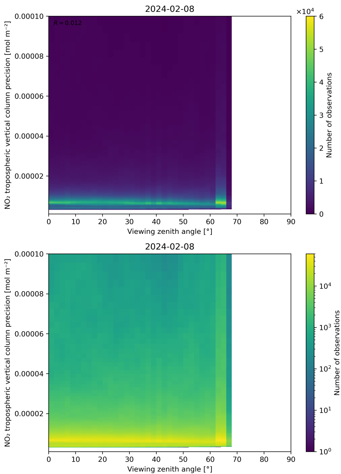
Figure 170: Scatter density plot of “Viewing zenith angle” against “NO 2 tropospheric vertical column precision” for 2024-02-07 to 2024-02-09.
