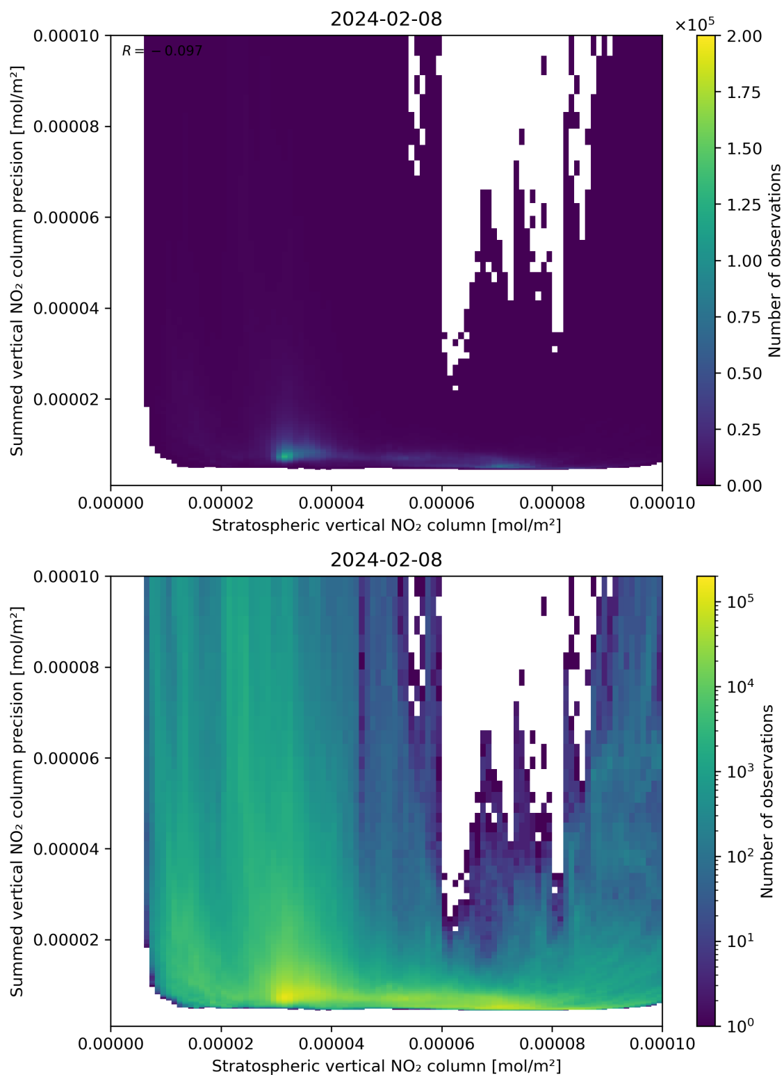
Figure 99: Scatter density plot of “Stratospheric vertical NO 2 column” against “Summed vertical NO 2 column precision” for 2024-02-07 to 2024-02-09.
