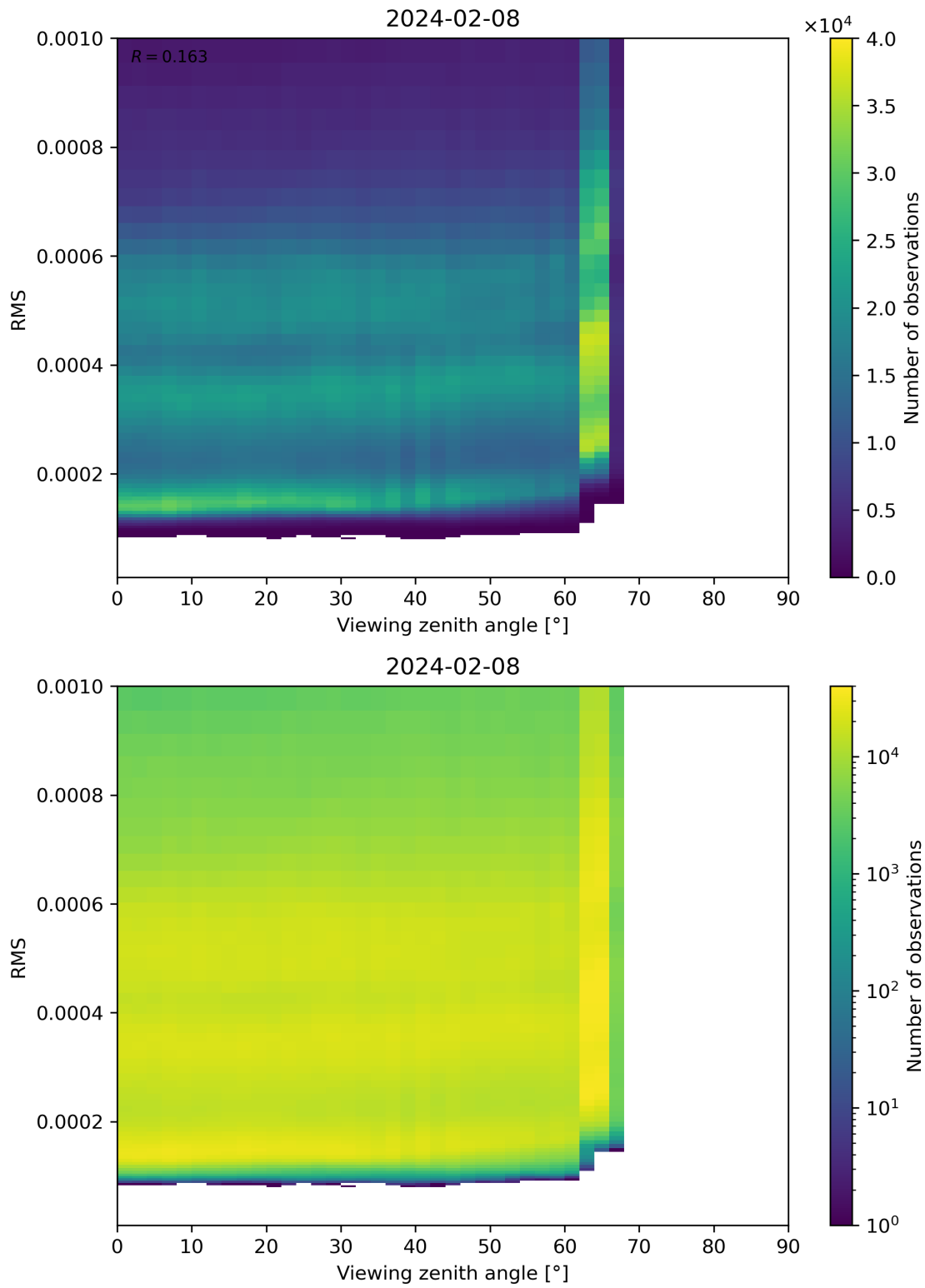
Figure 171: Scatter density plot of “Viewing zenith angle” against “RMS” for 2024-02-07 to 2024-02-09.
