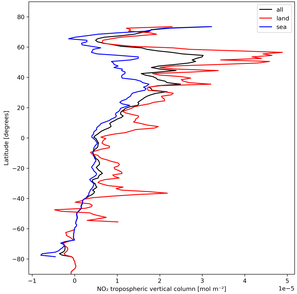
Figure 12: Zonal average of “NO 2 tropospheric vertical column” for 2024-02-07 to 2024-02-09.
