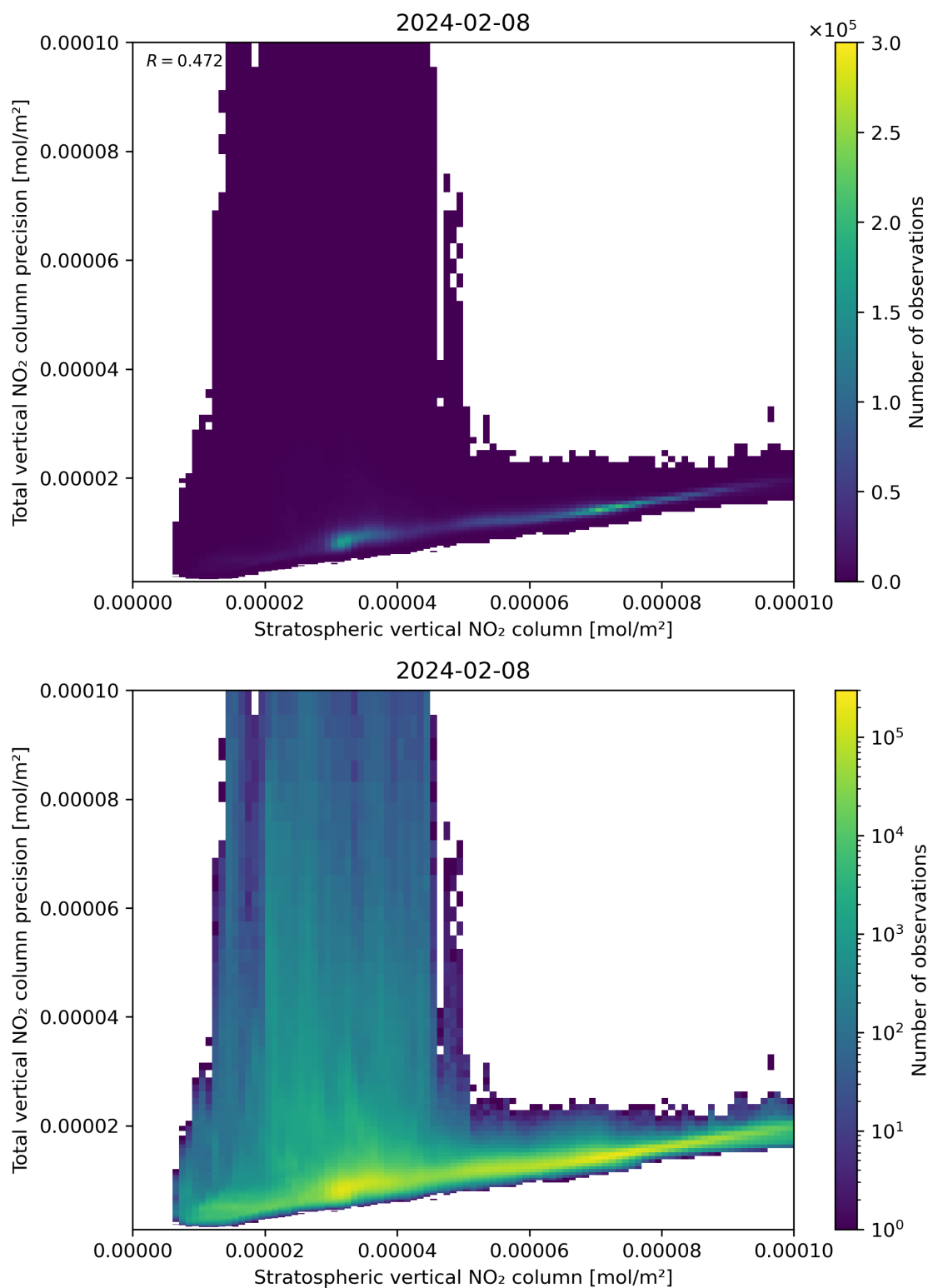
Figure 101: Scatter density plot of “Stratospheric vertical NO 2 column” against “Total vertical NO 2 column precision” for 2024-02-07 to 2024-02-09.
