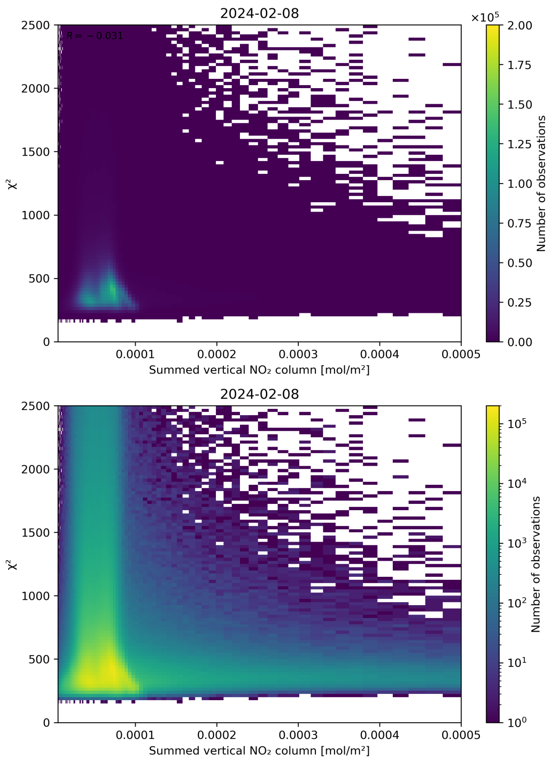
Figure 104: Scatter density plot of “Summed vertical NO 2 column” against “ \chi^2 ” for 2024-02-07 to 2024-02-09.
