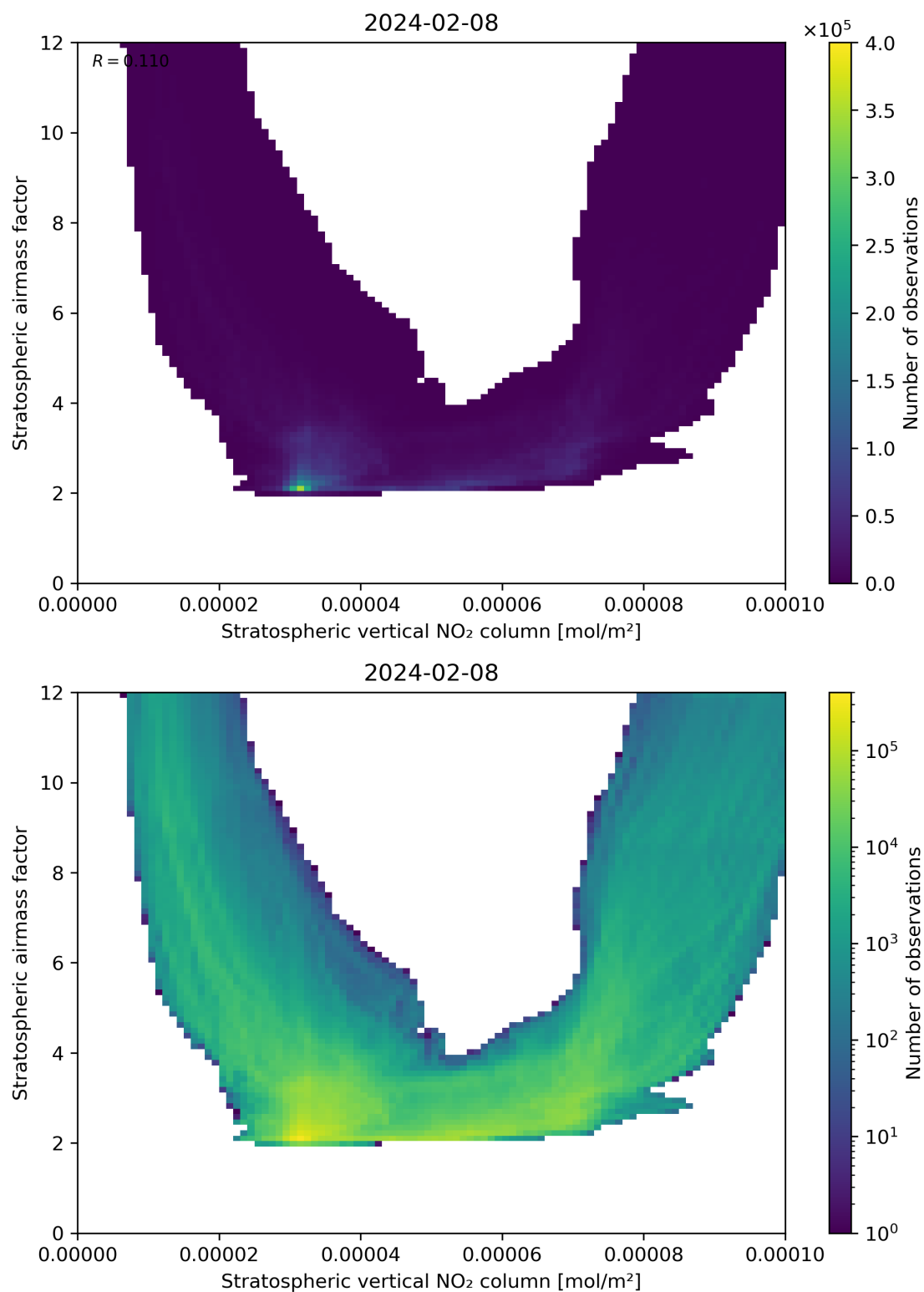
Figure 96: Scatter density plot of “Stratospheric vertical NO 2 column” against “Stratospheric airmass factor” for 2024-02-07 to 2024-02-09.
