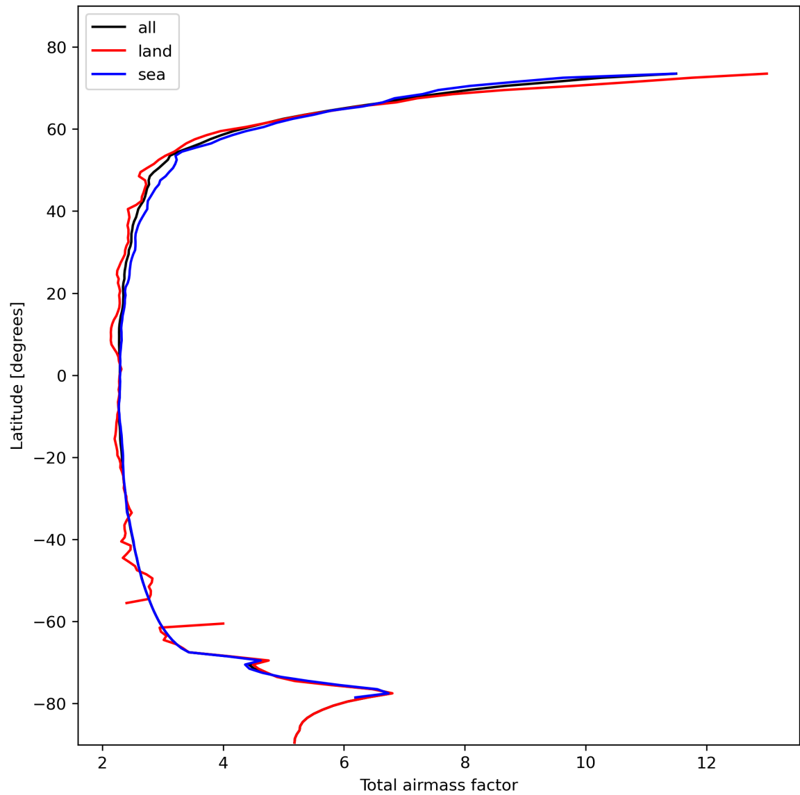
Figure 15: Zonal average of “Total airmass factor” for 2024-02-07 to 2024-02-09.
