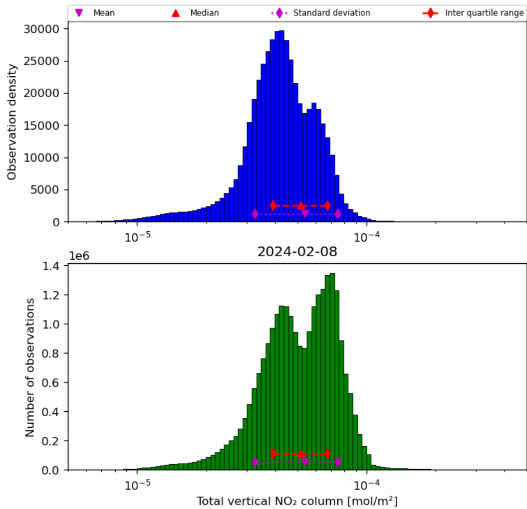
Figure 38: Histogram of “Total vertical NO 2 column” for 2024-02-07 to 2024-02-09
