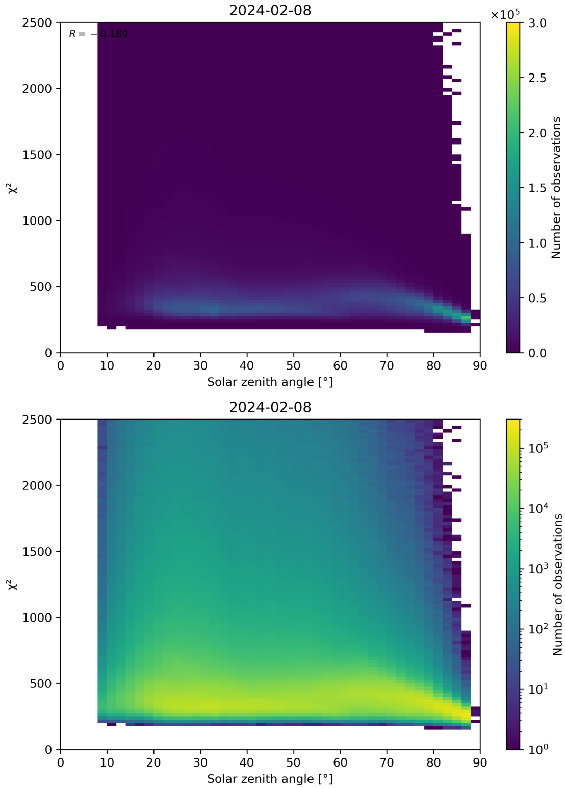
Figure 148: Scatter density plot of “Solar zenith angle” against “ \chi^2 ” for 2024-02-07 to 2024-02-09.
