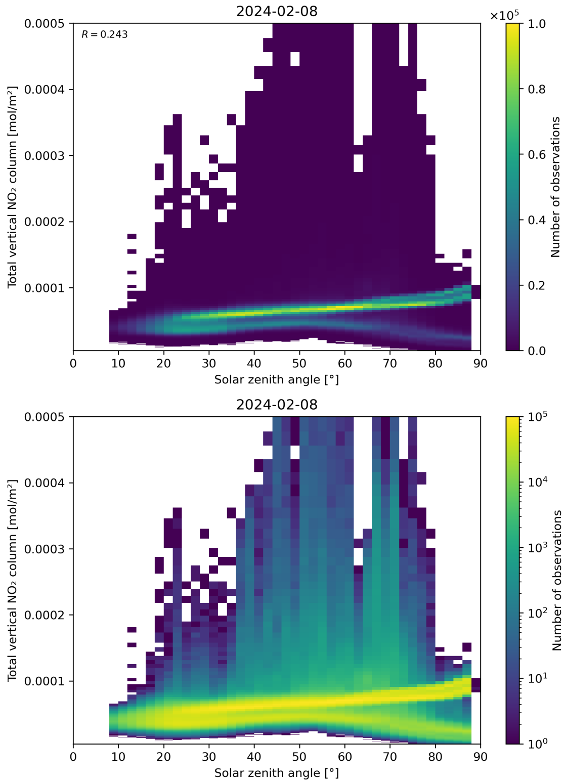
Figure 153: Scatter density plot of “Solar zenith angle” against “Total vertical NO 2 column” for 2024-02-07 to 2024-02-09.
