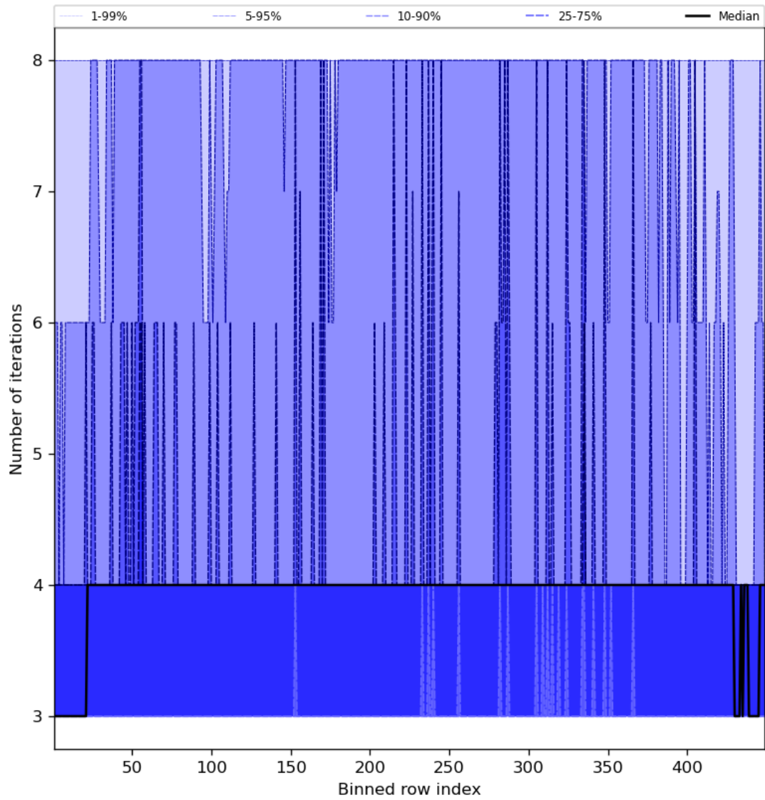
Figure 51: Along track statistics of “Number of iterations” for 2024-02-07 to 2024-02-09
