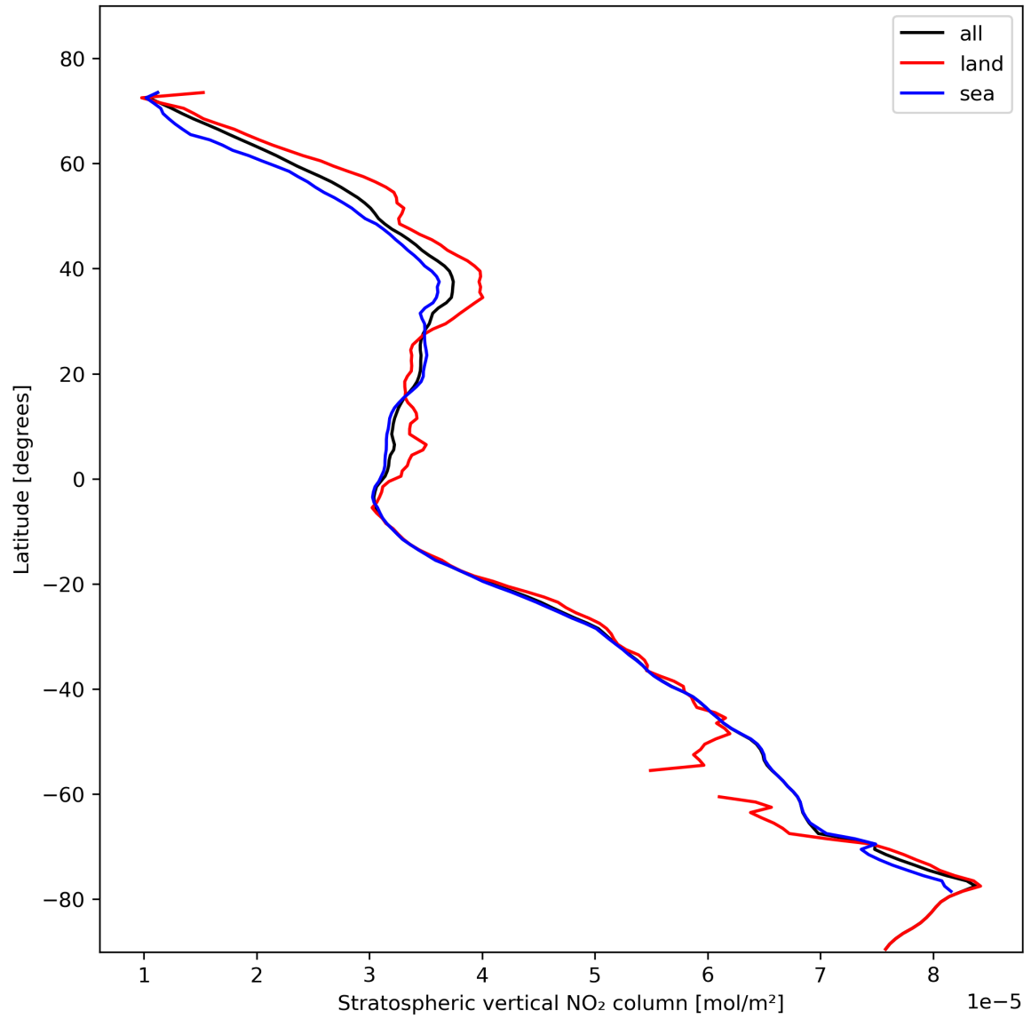
Figure 19: Zonal average of “Stratospheric vertical NO 2 column” for 2024-02-07 to 2024-02-09.
