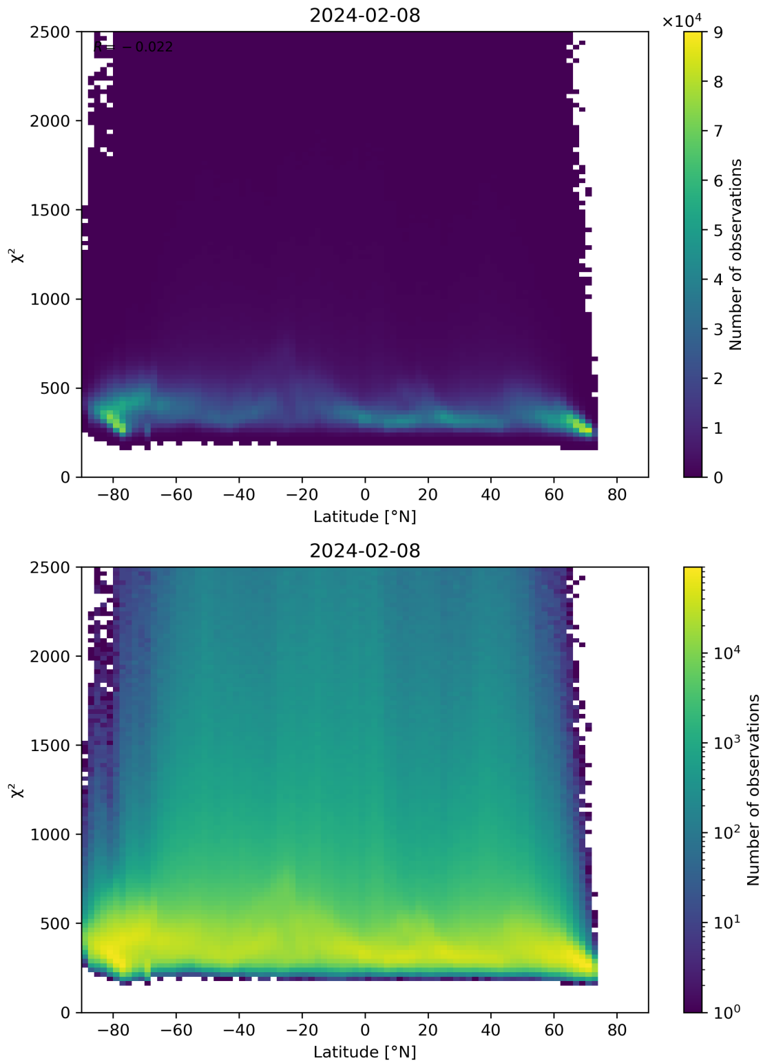
Figure 86: Scatter density plot of “Latitude” against “ \chi^2 ” for 2024-02-07 to 2024-02-09.
