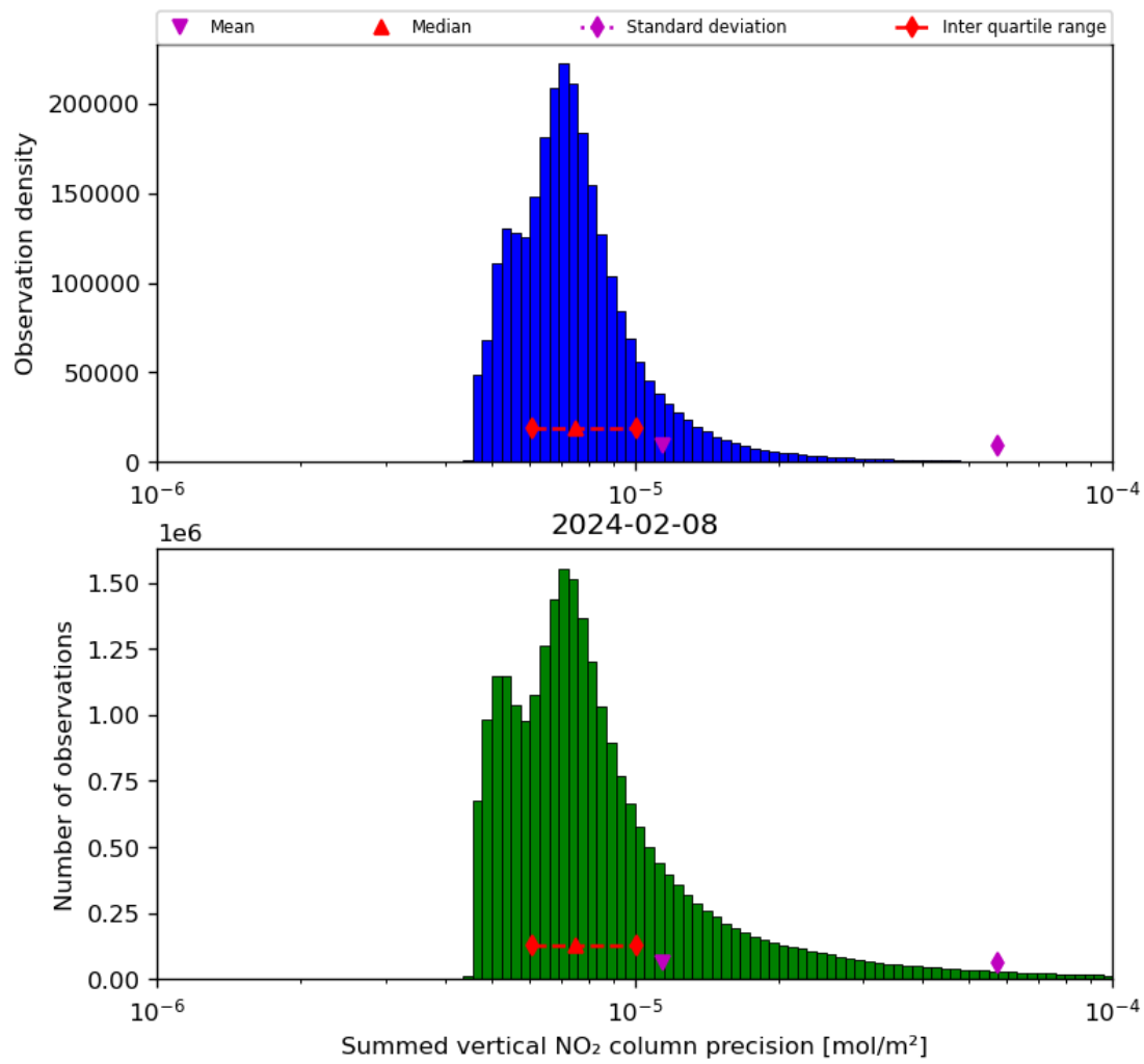
Figure 41: Histogram of "Summed vertical NO 2 column precision" for 2024-02-07 to 2024-02-09
