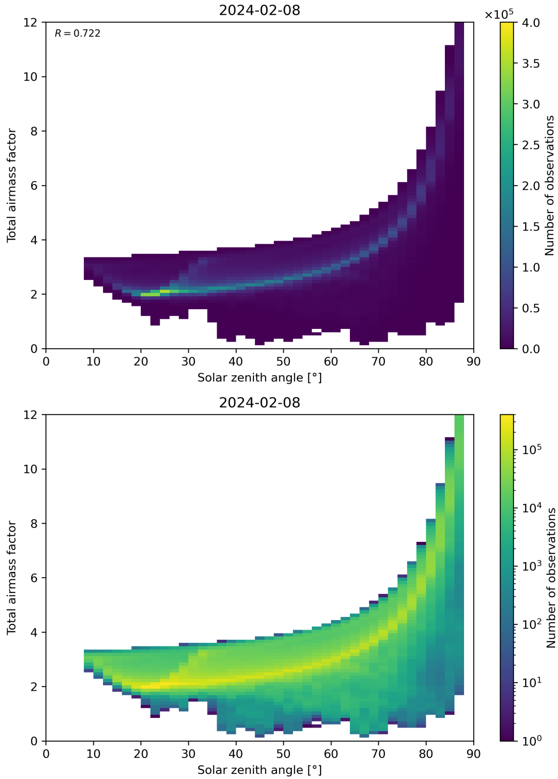
Figure 146: Scatter density plot of “Solar zenith angle” against “Total air mass factor” for 2024-02-07 to 2024-02-09.
