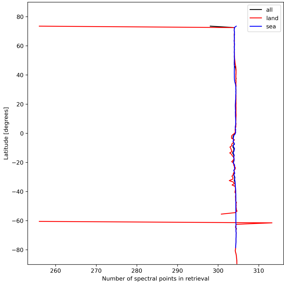
Figure 16: Zonal average of “Number of spectral points in retrieval” for 2024-02-07 to 2024-02-09.
