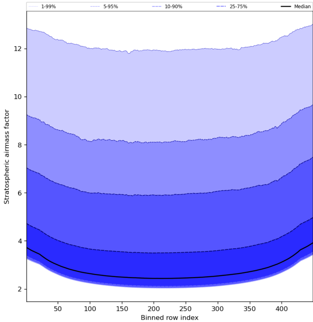
Figure 61: Along track statistics of “Stratospheric air mass factor” for 2024-02-07 to 2024-02-09
