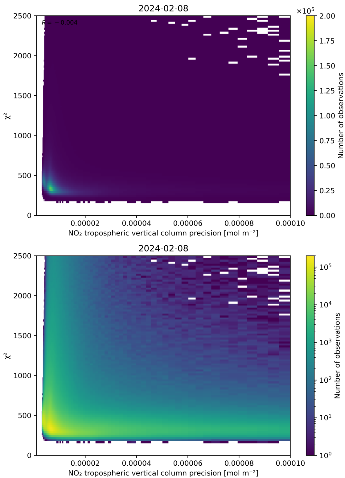
Figure 134: Scatter density plot of “NO 2 tropospheric vertical column precision” against “ \chi^2 ” for 2024-02-07 to 2024-02-09.
