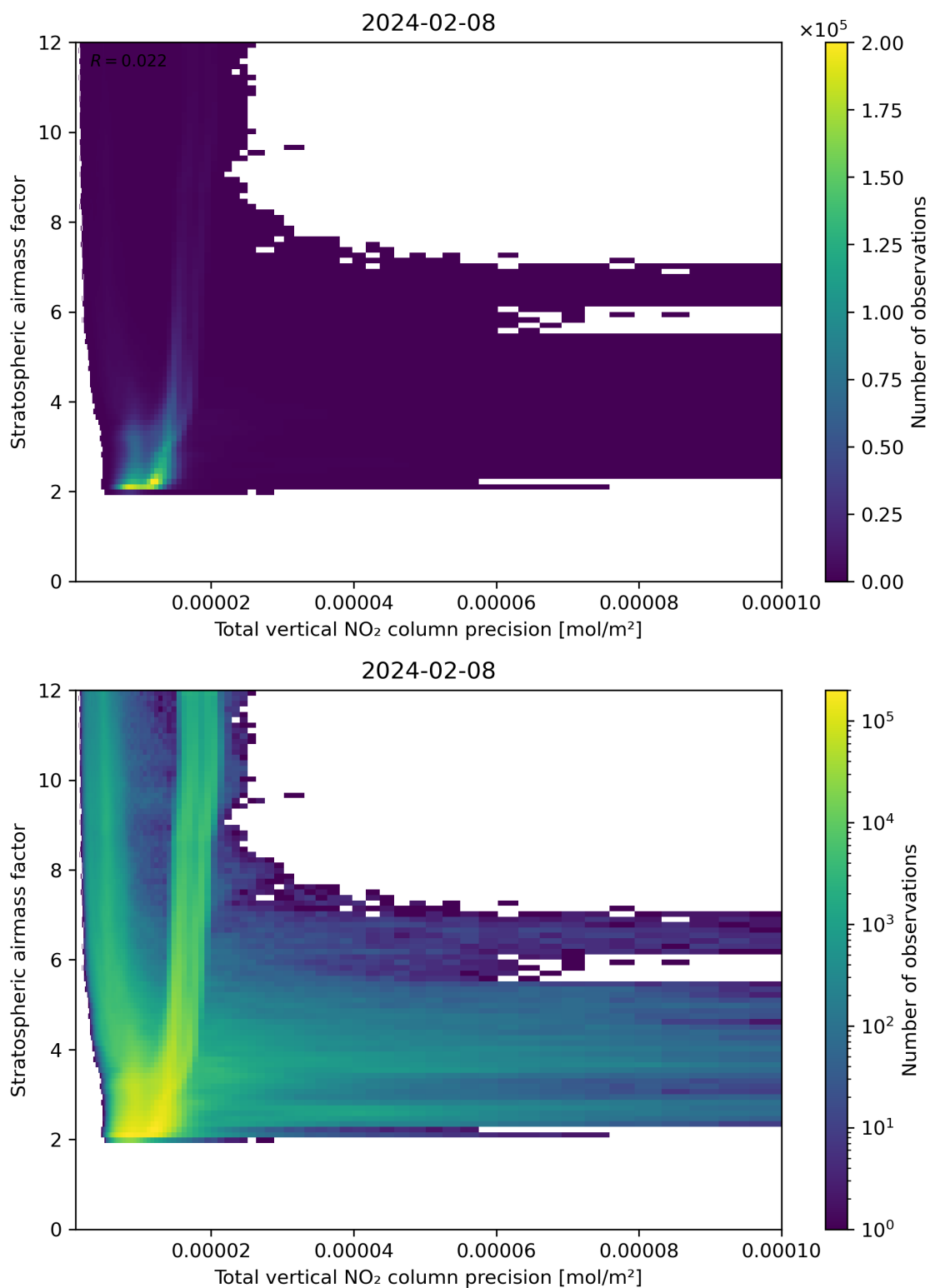
Figure 115: Scatter density plot of “Total vertical NO 2 column precision” against “Stratospheric air mass factor” for 2024-02-07 to 2024-02-09.
