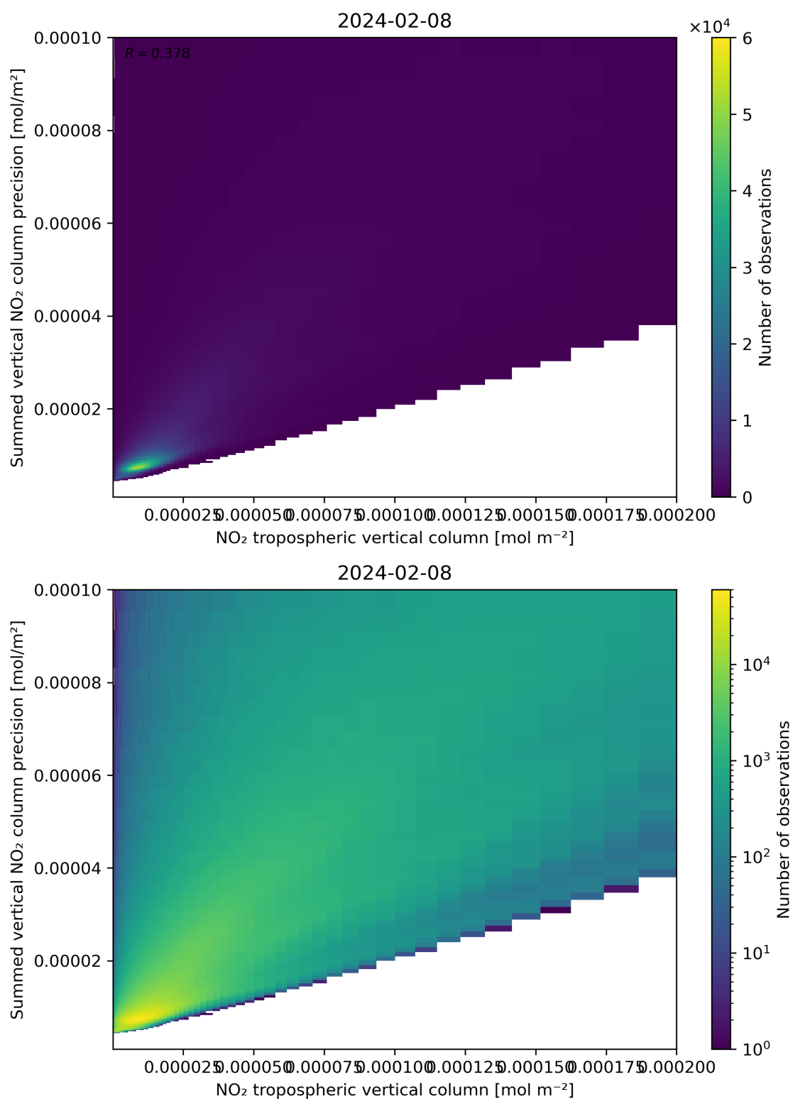
Figure 127: Scatter density plot of “NO 2 tropospheric vertical column” against “Summed vertical NO 2 column precision” for 2024-02-07 to 2024-02-09.
