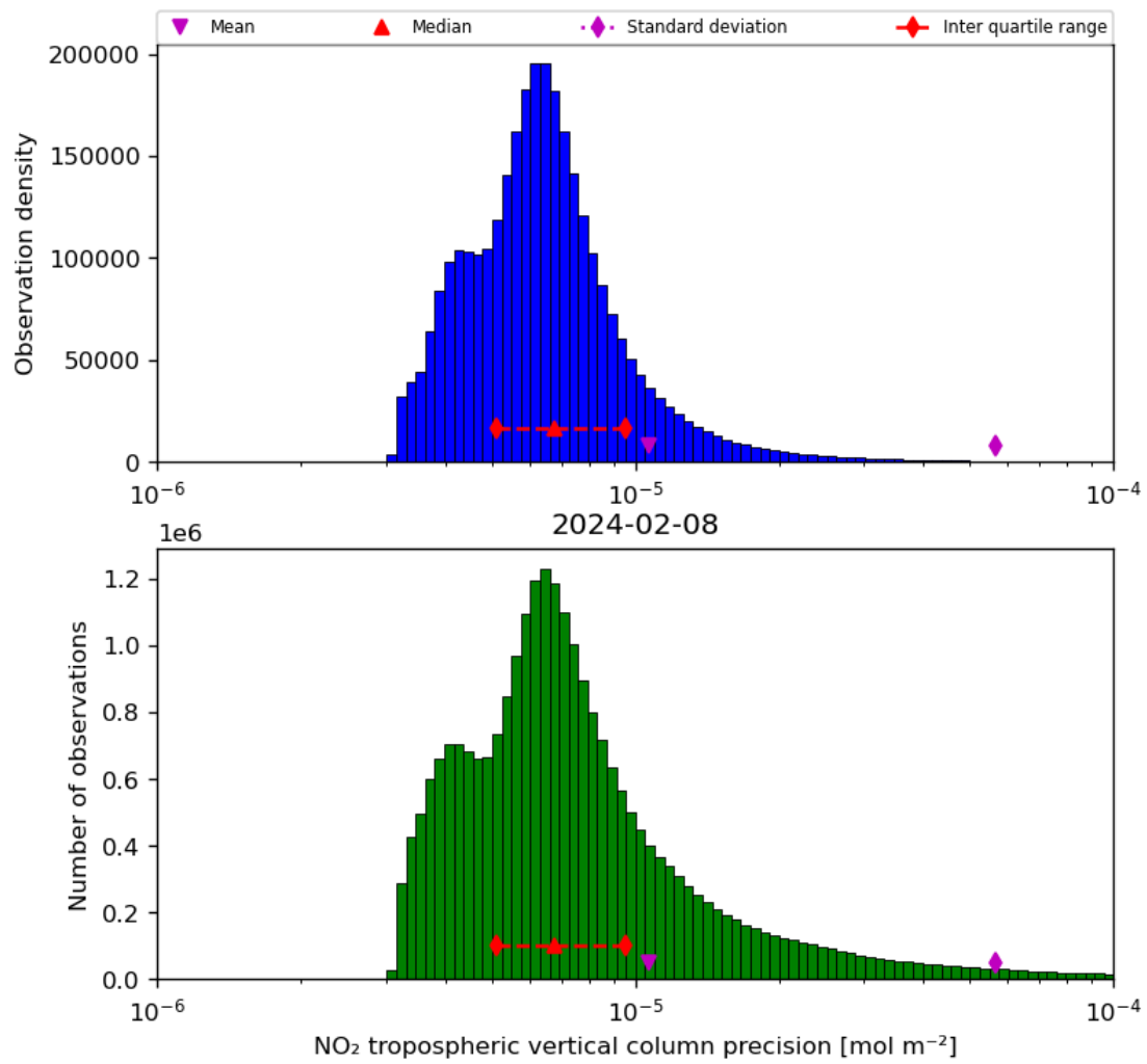
Figure 30: Histogram of “NO 2 tropospheric vertical column precision” for 2024-02-07 to 2024-02-09
