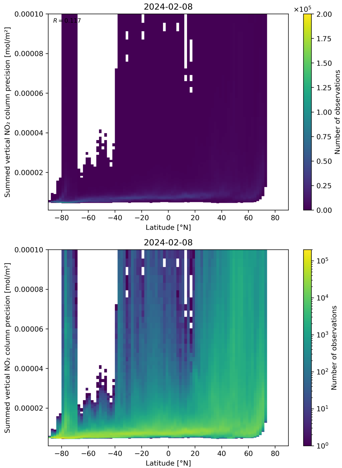
Figure 89: Scatter density plot of “Latitude” against “Summed vertical NO 2 column precision” for 2024-02-07 to 2024-02-09.
