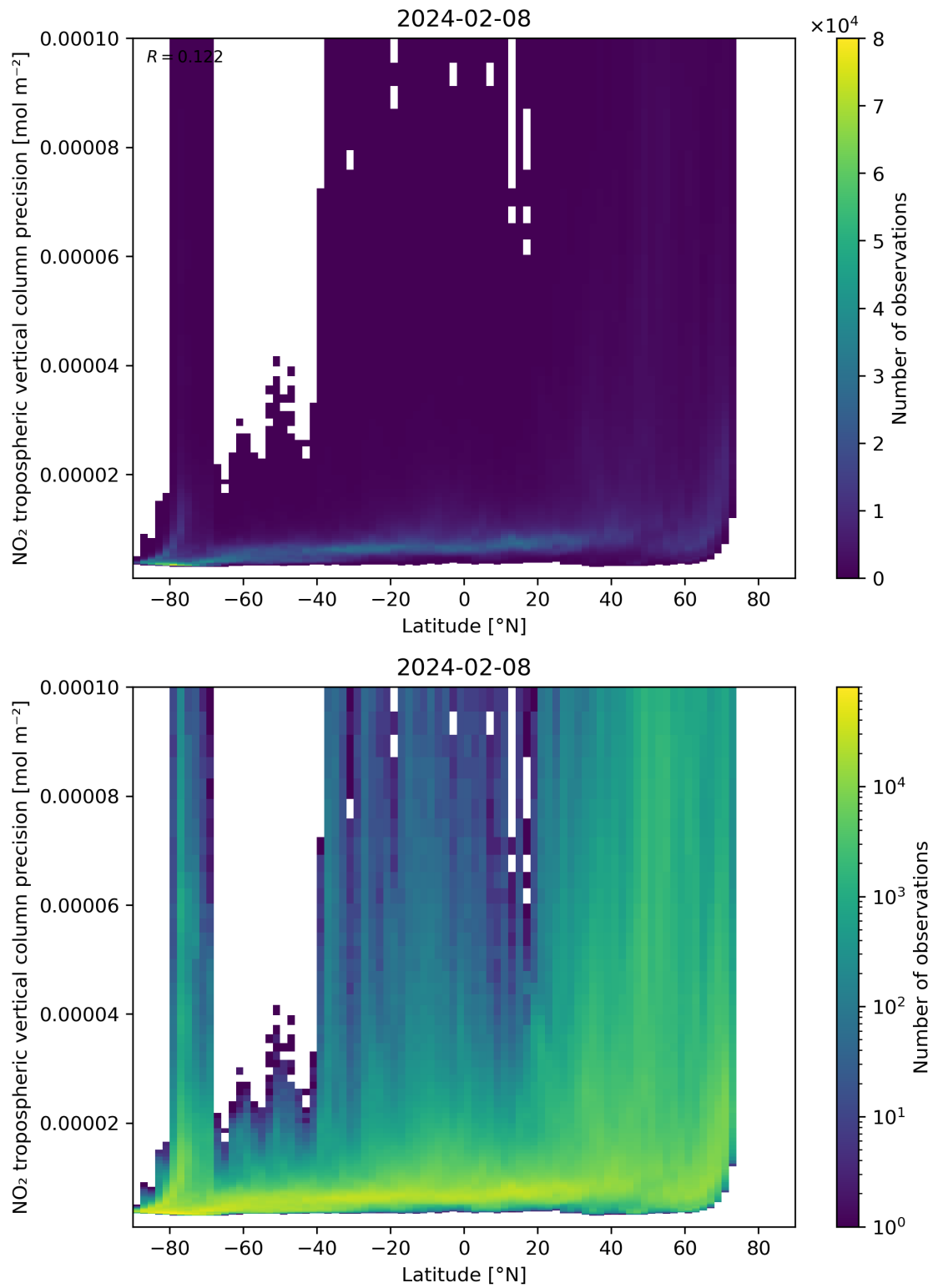
Figure 93: Scatter density plot of “Latitude” against “NO 2 tropospheric vertical column precision” for 2024-02-07 to 2024-02-09.
