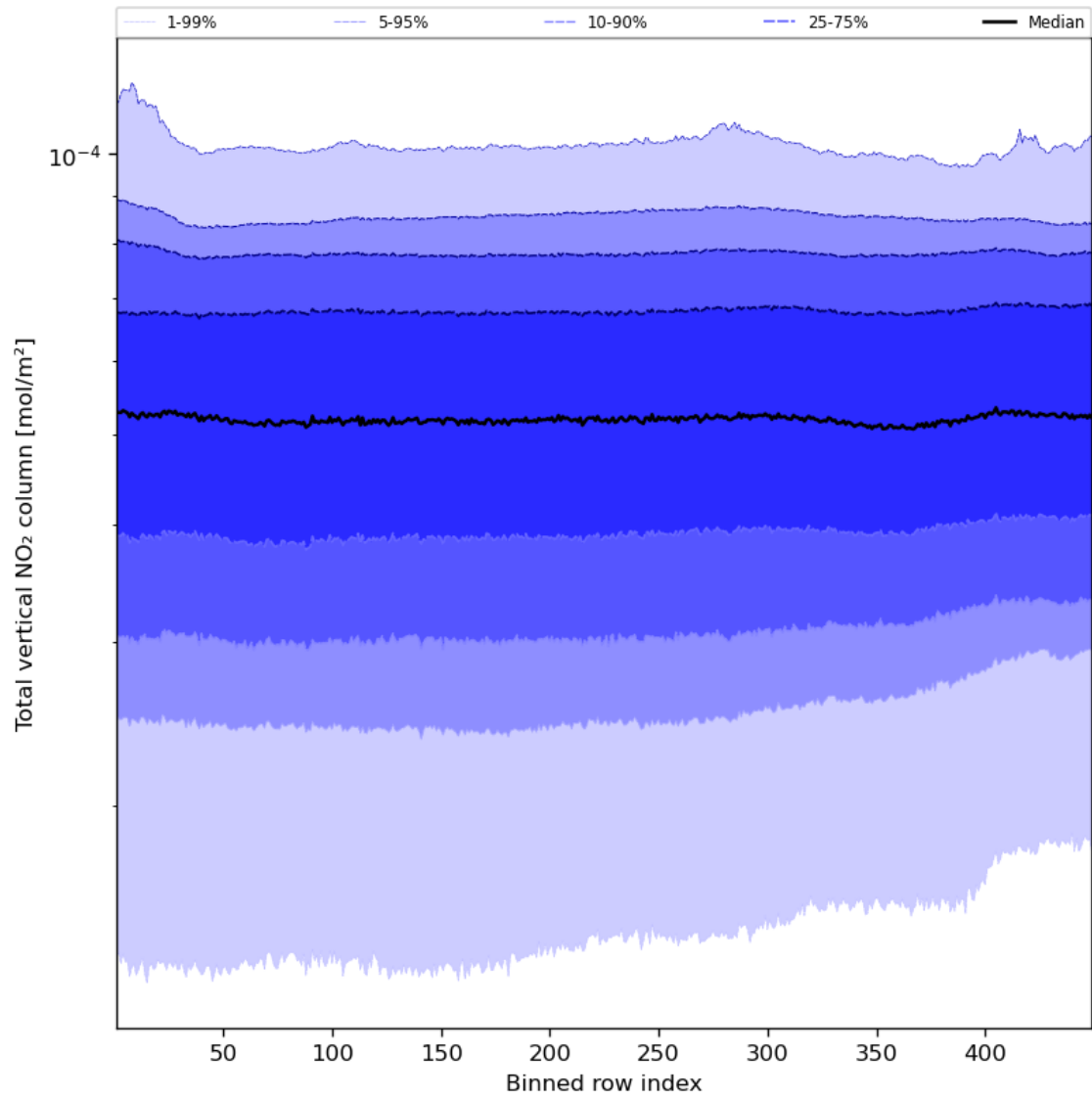
Figure 55: Along track statistics of “Total vertical NO 2 column” for 2024-02-07 to 2024-02-09
