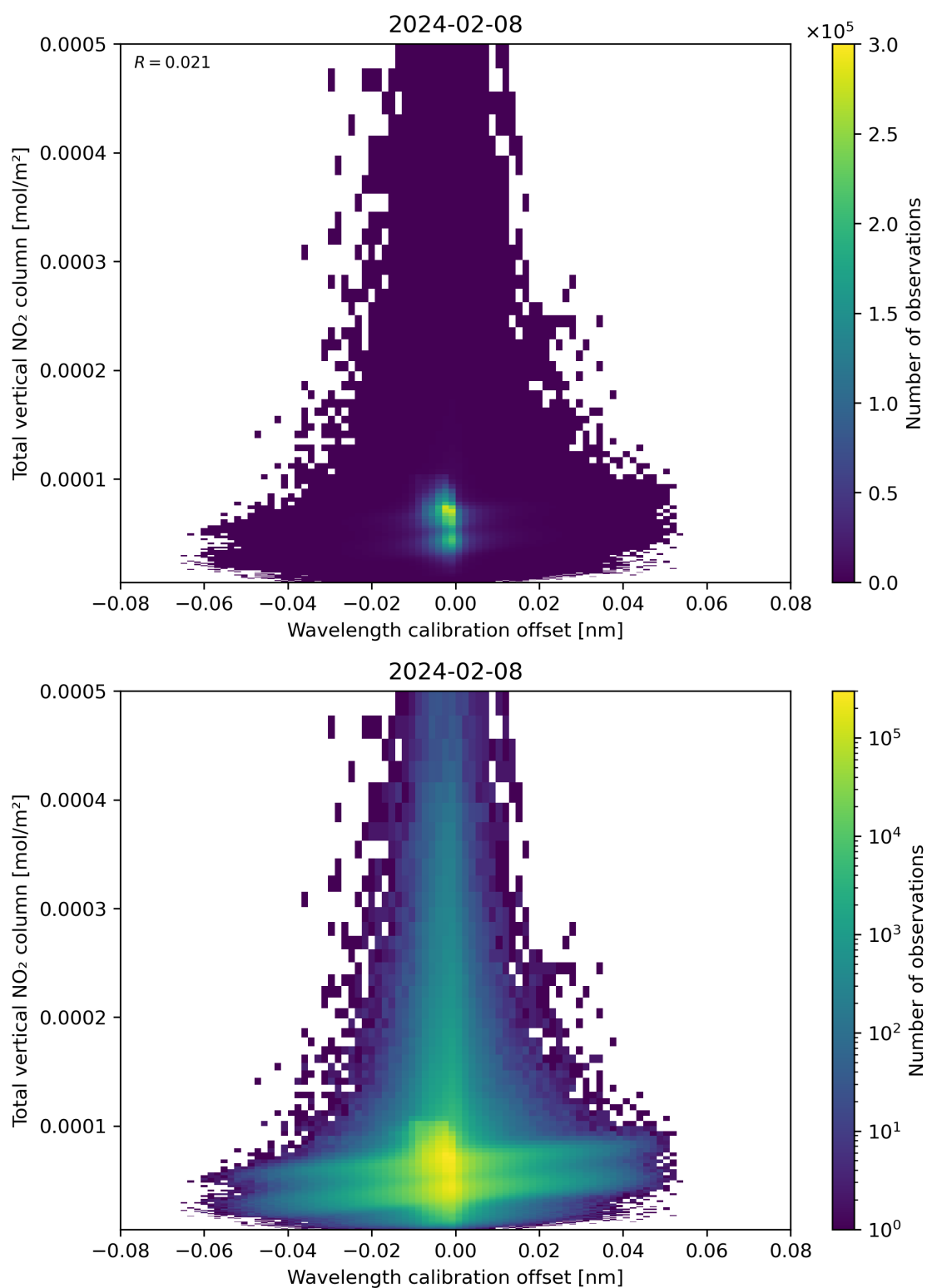
Figure 179: Scatter density plot of “Wavelength calibration offset” against “Total vertical NO 2 column” for 2024-02-07 to 2024-02-09.
