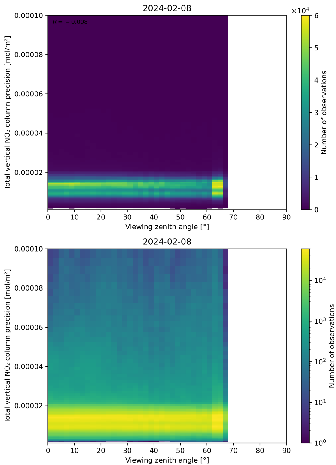
Figure 168: Scatter density plot of “Viewing zenith angle” against “Total vertical NO 2 column precision” for 2024-02-07 to 2024-02-09.
