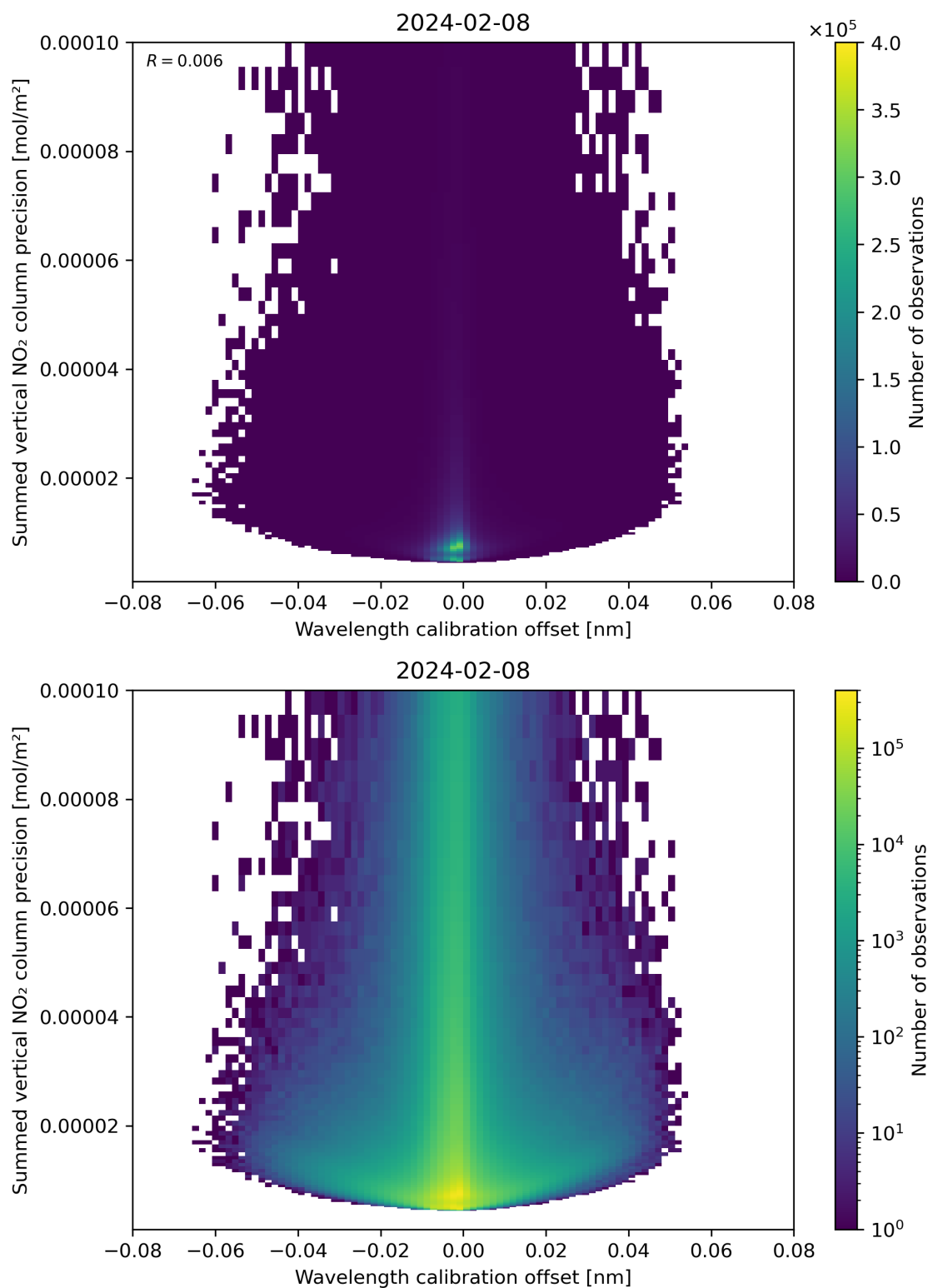
Figure 178: Scatter density plot of “Wavelength calibration offset” against “Summed vertical NO 2 column precision” for 2024-02-07 to 2024-02-09.
