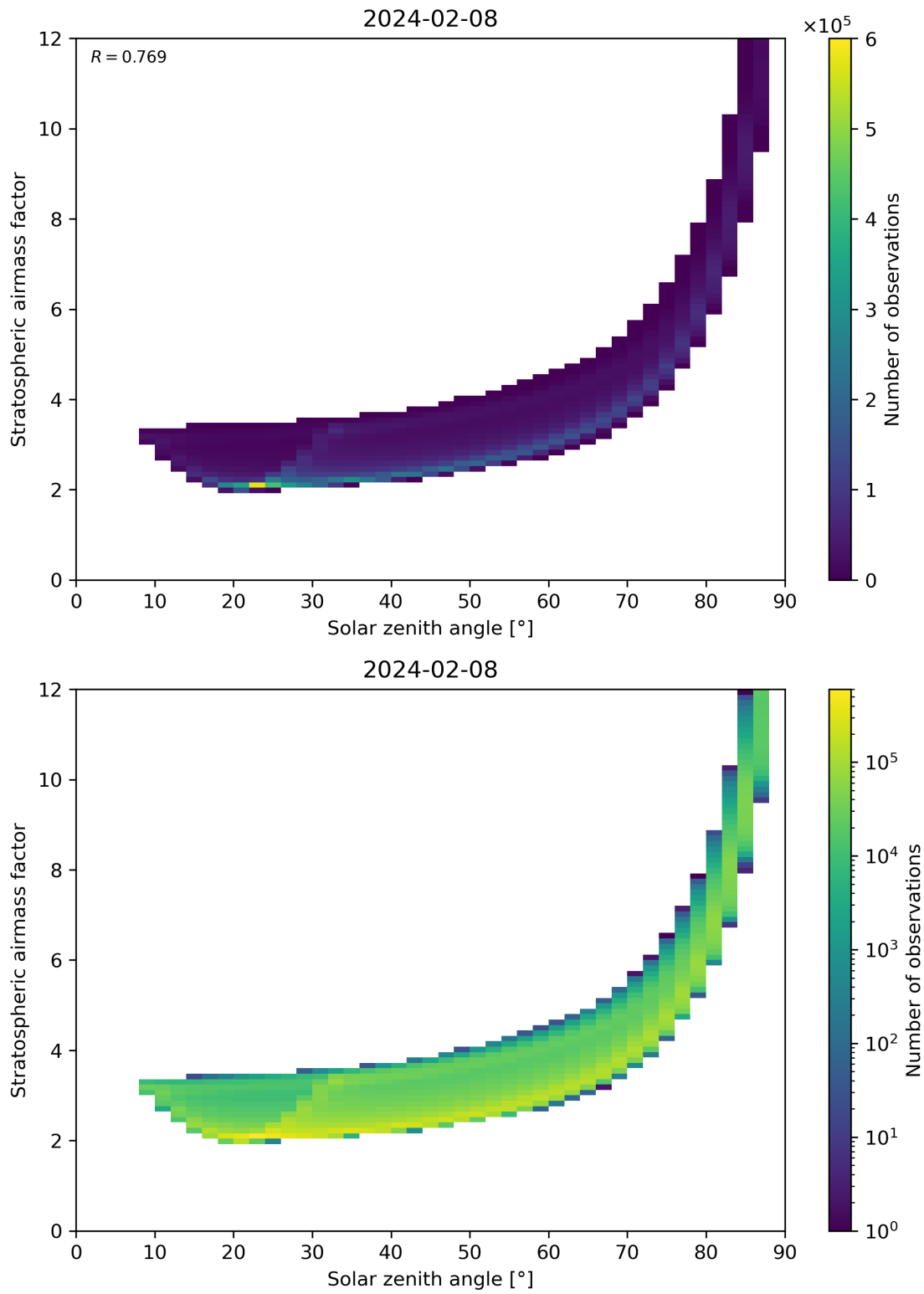
Figure 145: Scatter density plot of “Solar zenith angle” against “Stratospheric airmass factor” for 2024-02-07 to 2024-02-09.
