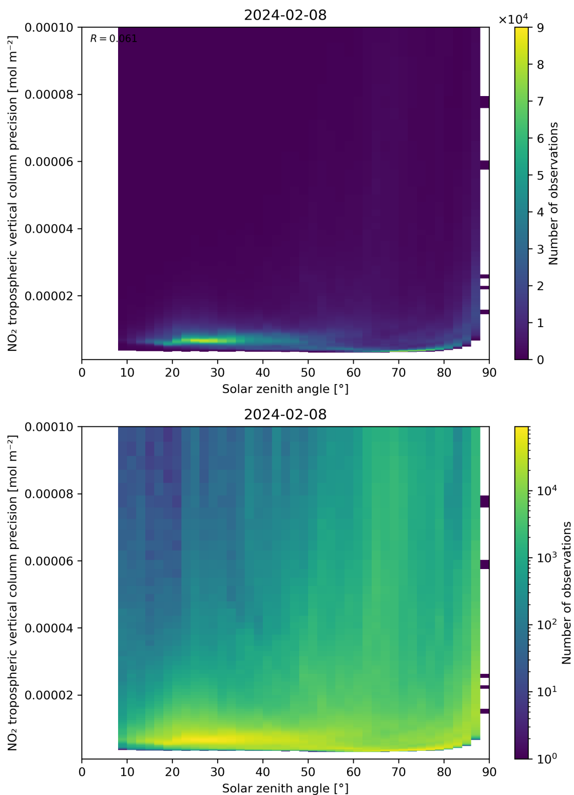
Figure 156: Scatter density plot of “Solar zenith angle” against “NO 2 tropospheric vertical column precision” for 2024-02-07 to 2024-02-09.
