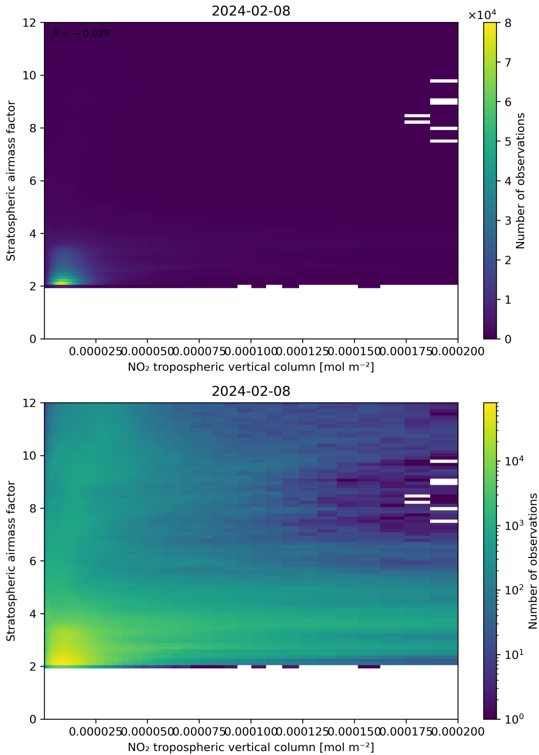
Figure 121: Scatter density plot of “NO 2 tropospheric vertical column” against “Stratospheric airmass factor” for 2024-02-07 to 2024-02-09.
