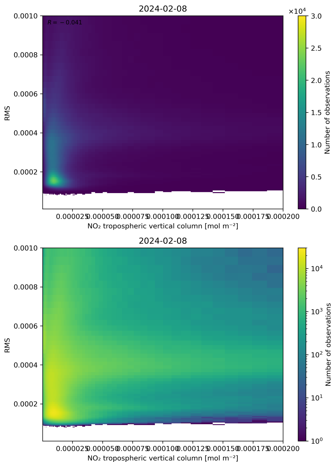
Figure 142: Scatter density plot of “NO 2 tropospheric vertical column” against “RMS” for 2024-02-07 to 2024-02-09.
