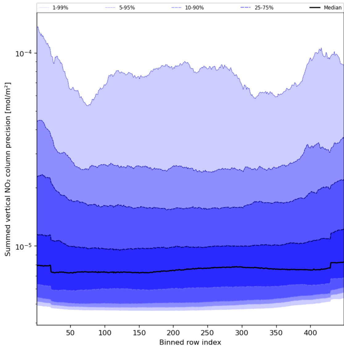
Figure 58: Along track statistics of “Summed vertical NO 2 column precision” for 2024-02-07 to 2024-02-09
