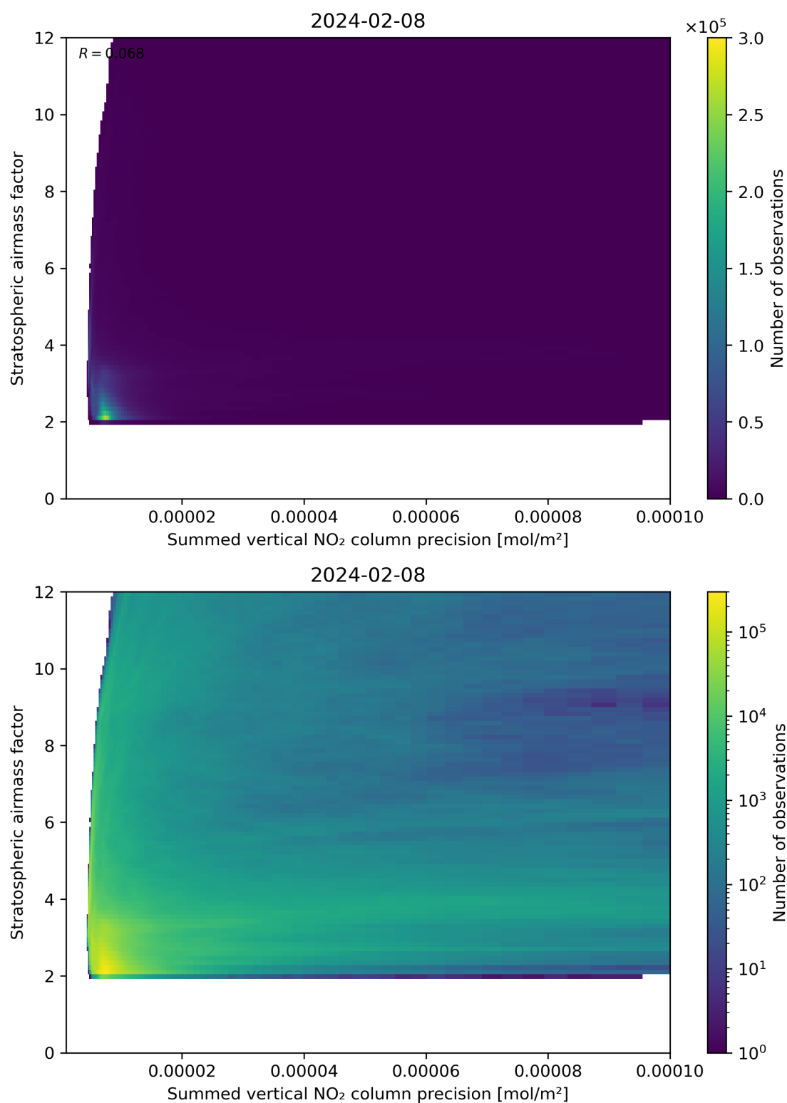
Figure 106: Scatter density plot of “Summed vertical NO 2 column precision” against “Stratospheric airmass factor” for 2024-02-07 to 2024-02-09.
