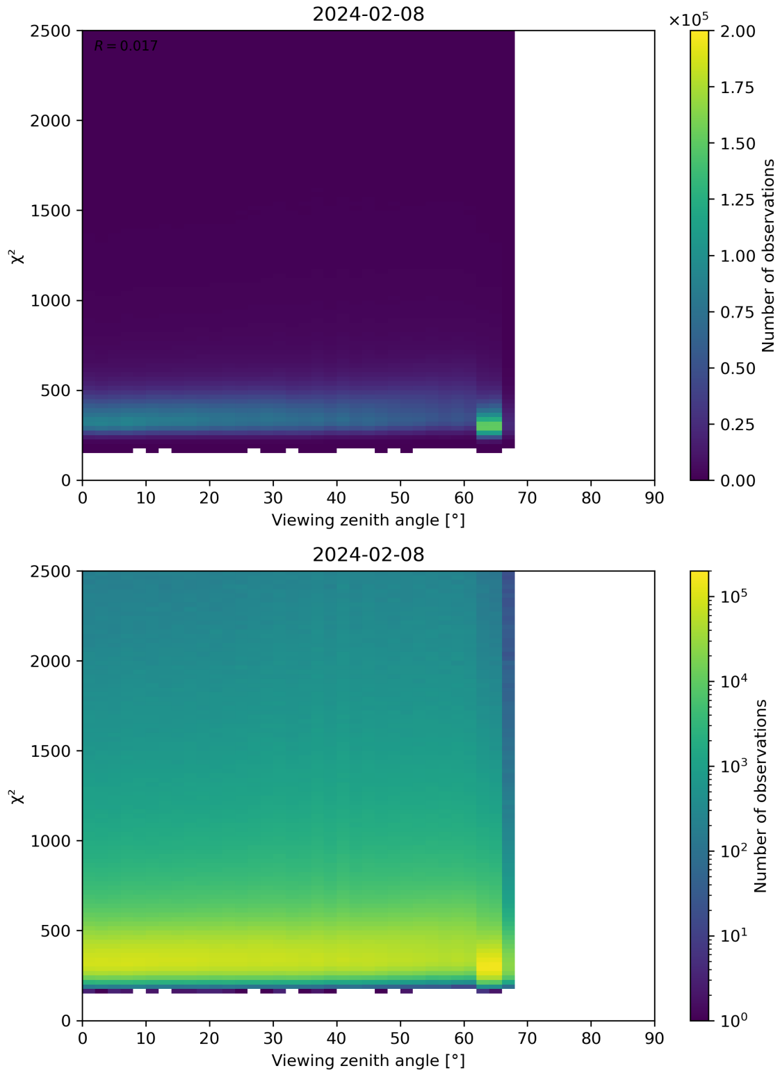
Figure 162: Scatter density plot of “Viewing zenith angle” against “ \chi^2 ” for 2024-02-07 to 2024-02-09.
