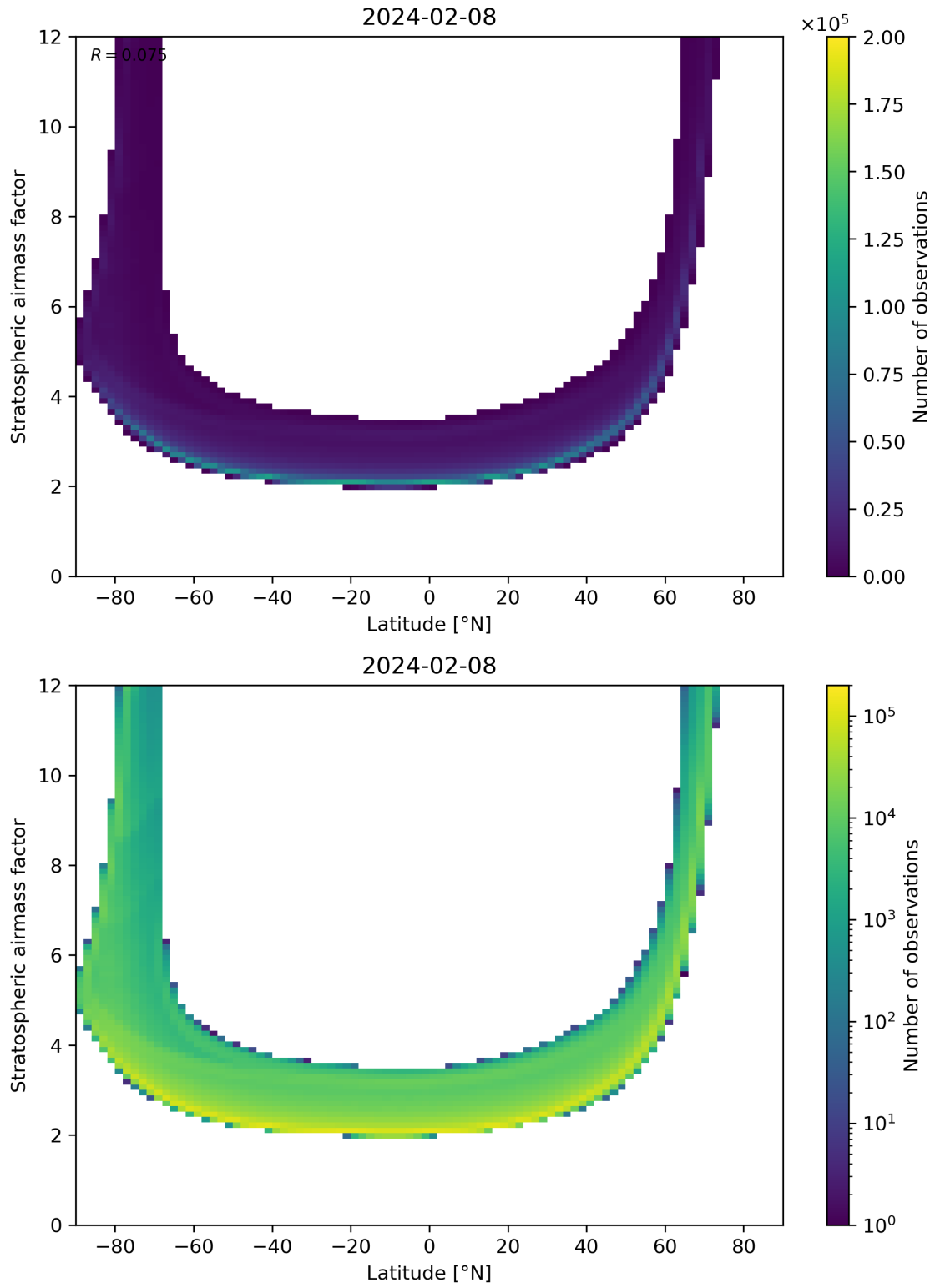
Figure 83: Scatter density plot of “Latitude” against “Stratospheric airmass factor” for 2024-02-07 to 2024-02-09.
