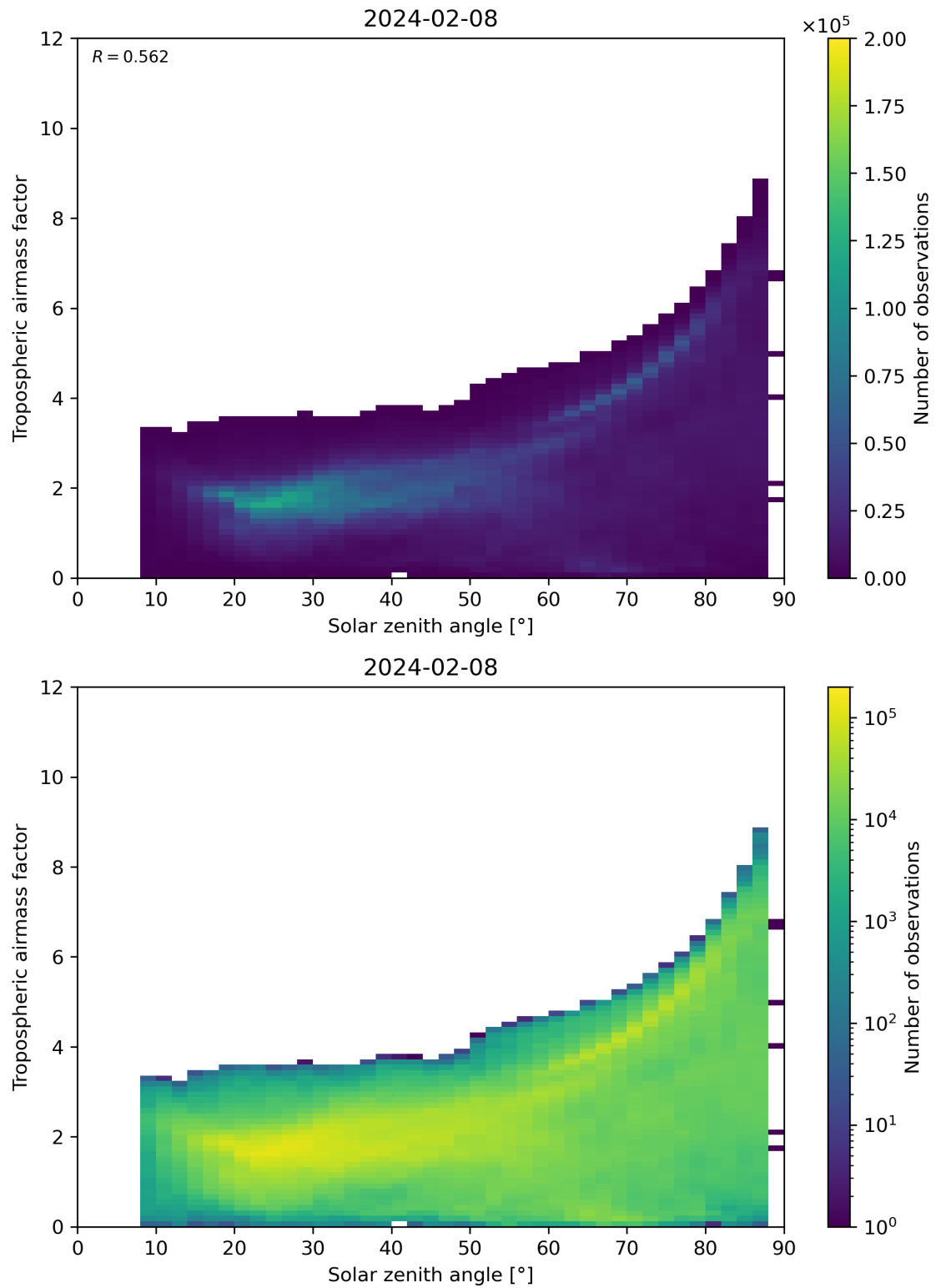
Figure 147: Scatter density plot of “Solar zenith angle” against “Tropospheric airmass factor” for 2024-02-07 to 2024-02-09.
