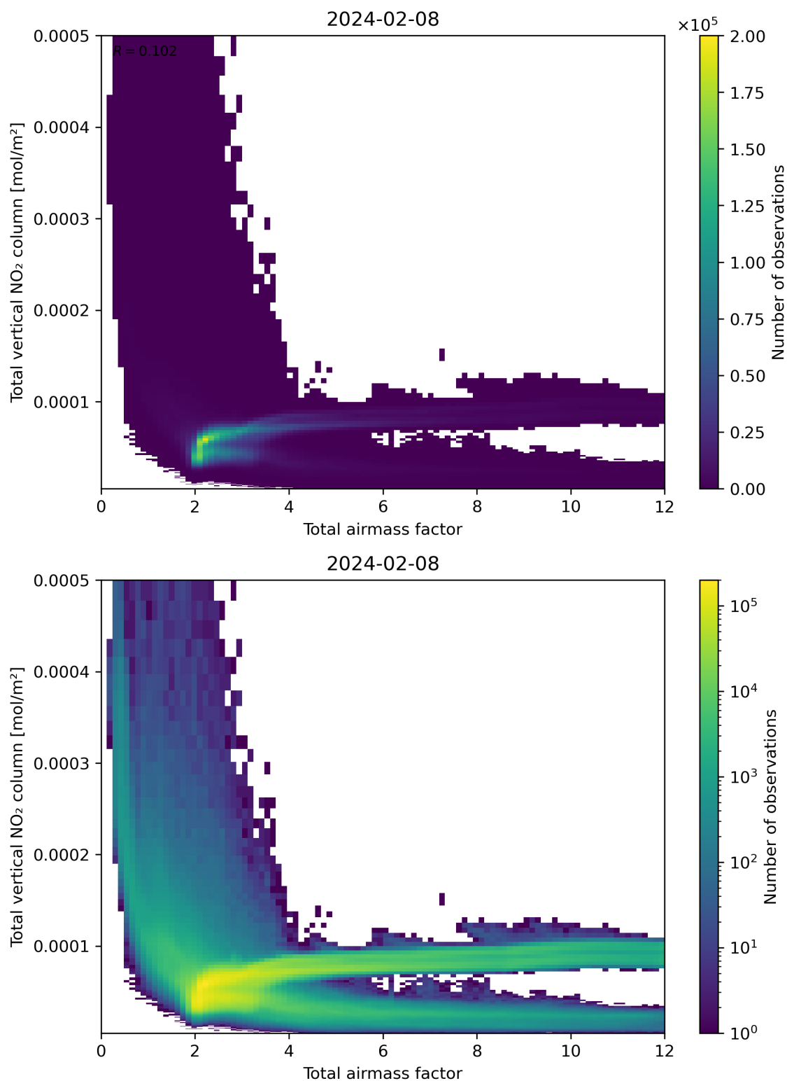
Figure 67: Scatter density plot of “Total airmass factor” against “Total vertical NO 2 column” for 2024-02-07 to 2024-02-09.
