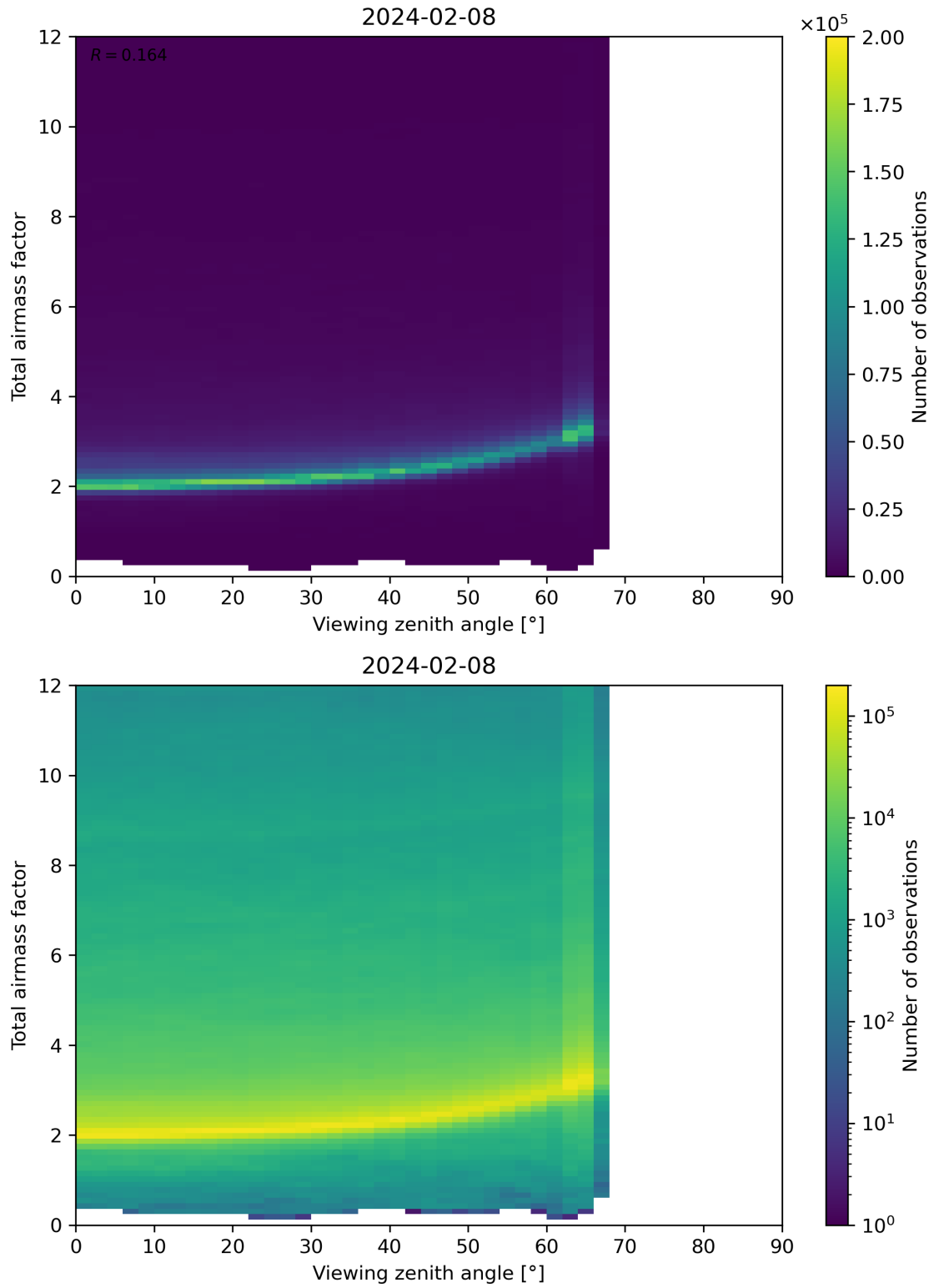
Figure 160: Scatter density plot of “Viewing zenith angle” against “Total airmass factor” for 2024-02-07 to 2024-02-09.
