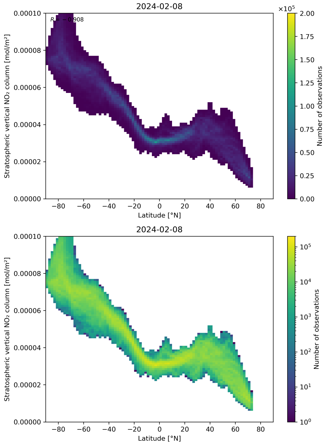
Figure 87: Scatter density plot of “Latitude” against “Stratospheric vertical NO 2 column” for 2024-02-07 to 2024-02-09.
