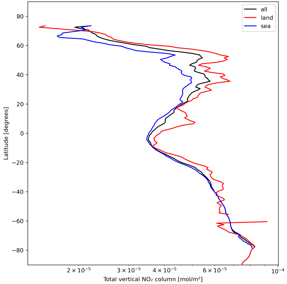
Figure 21: Zonal average of “Total vertical NO 2 column” for 2024-02-07 to 2024-02-09.
