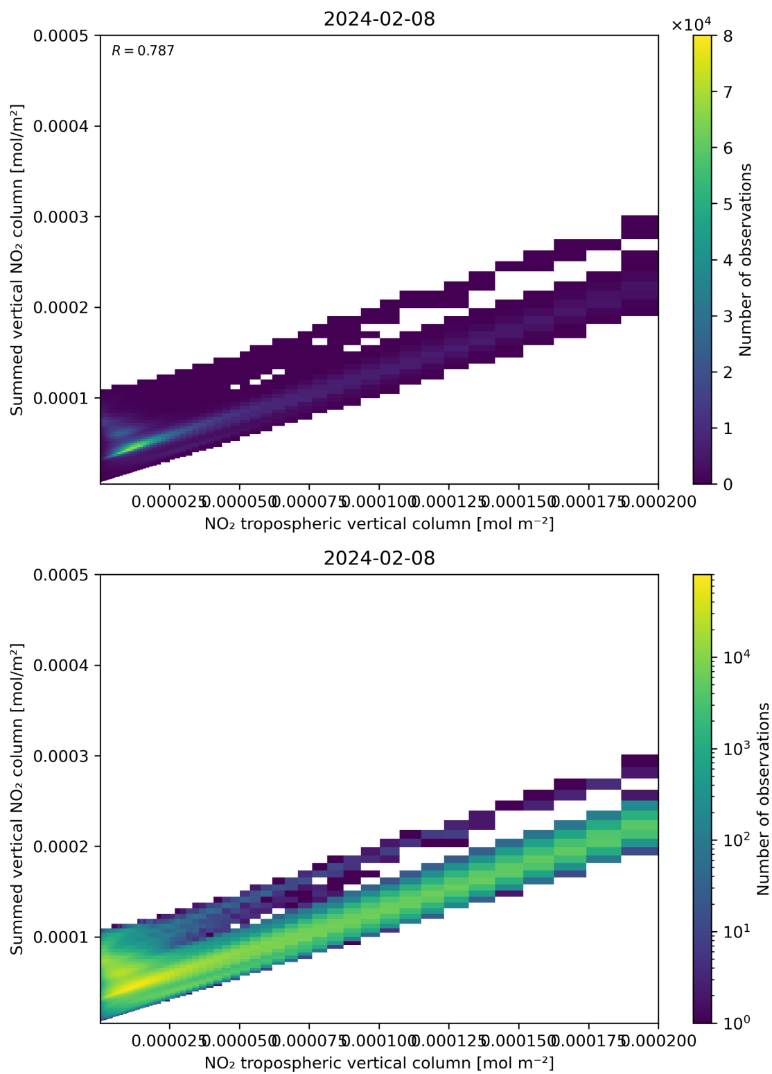
Figure 126: Scatter density plot of “NO 2 tropospheric vertical column” against “Summed vertical NO 2 column” for 2024-02-07 to 2024-02-09.
