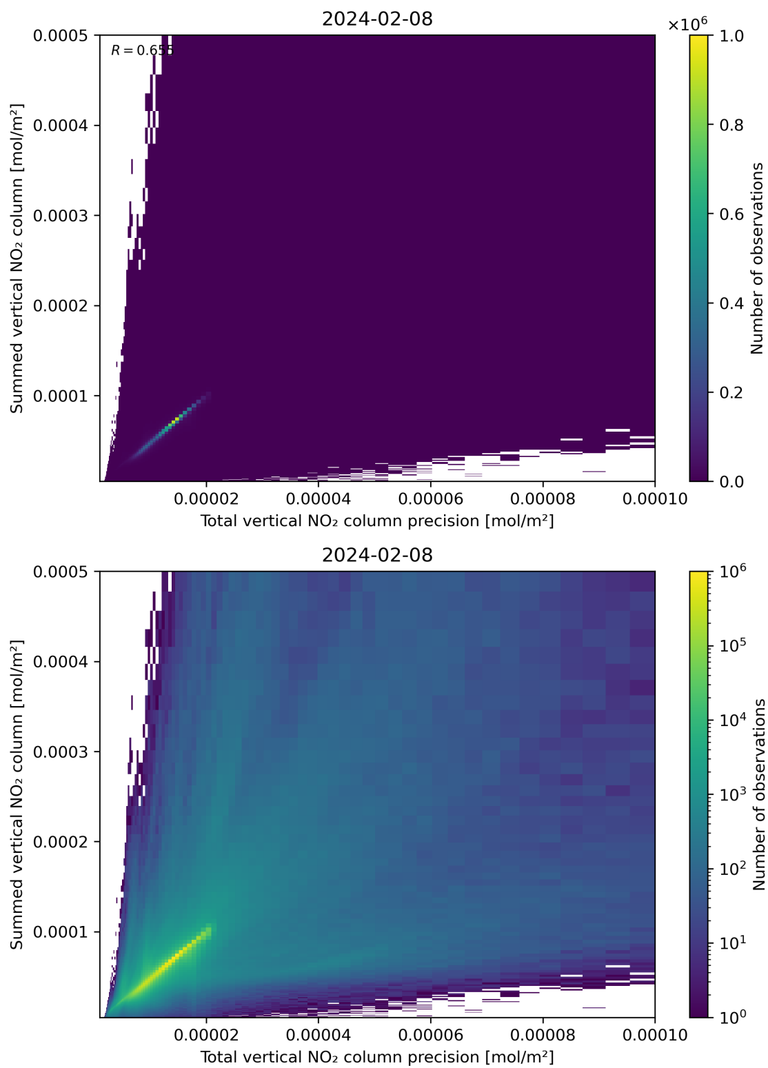
Figure 117: Scatter density plot of “Total vertical NO 2 column precision” against “Summed vertical NO 2 column” for 2024-02-07 to 2024-02-09.
