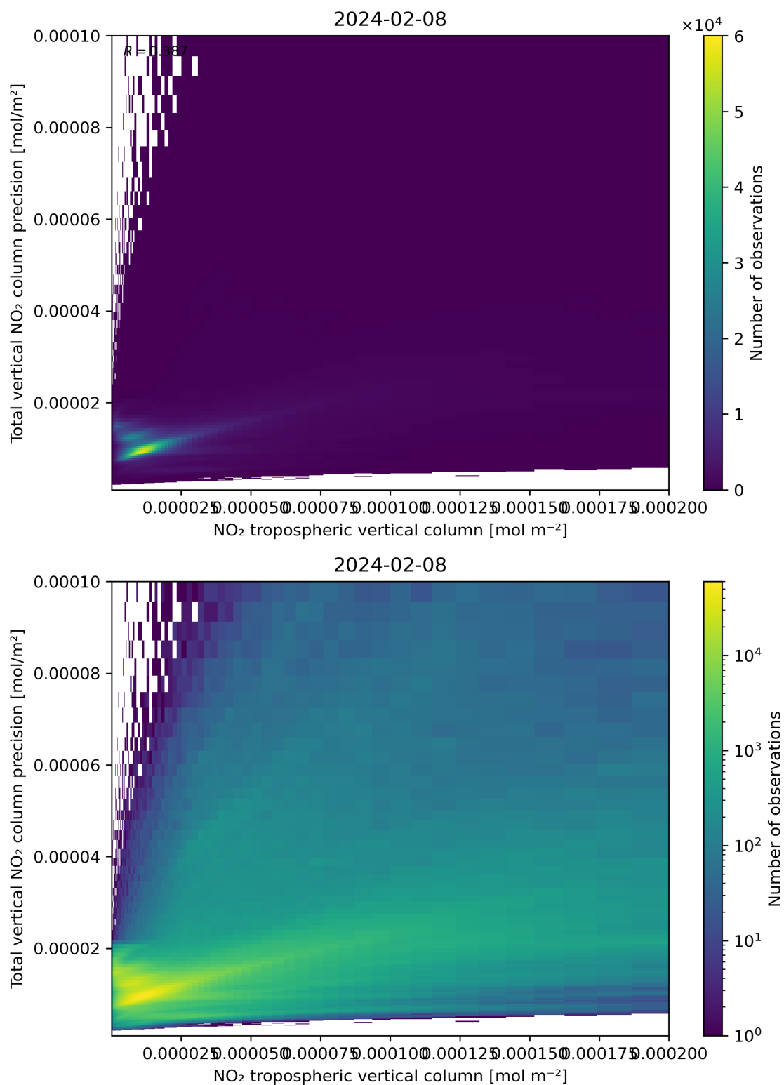
Figure 129: Scatter density plot of “NO 2 tropospheric vertical column” against “Total vertical NO 2 column precision” for 2024-02-07 to 2024-02-09.
