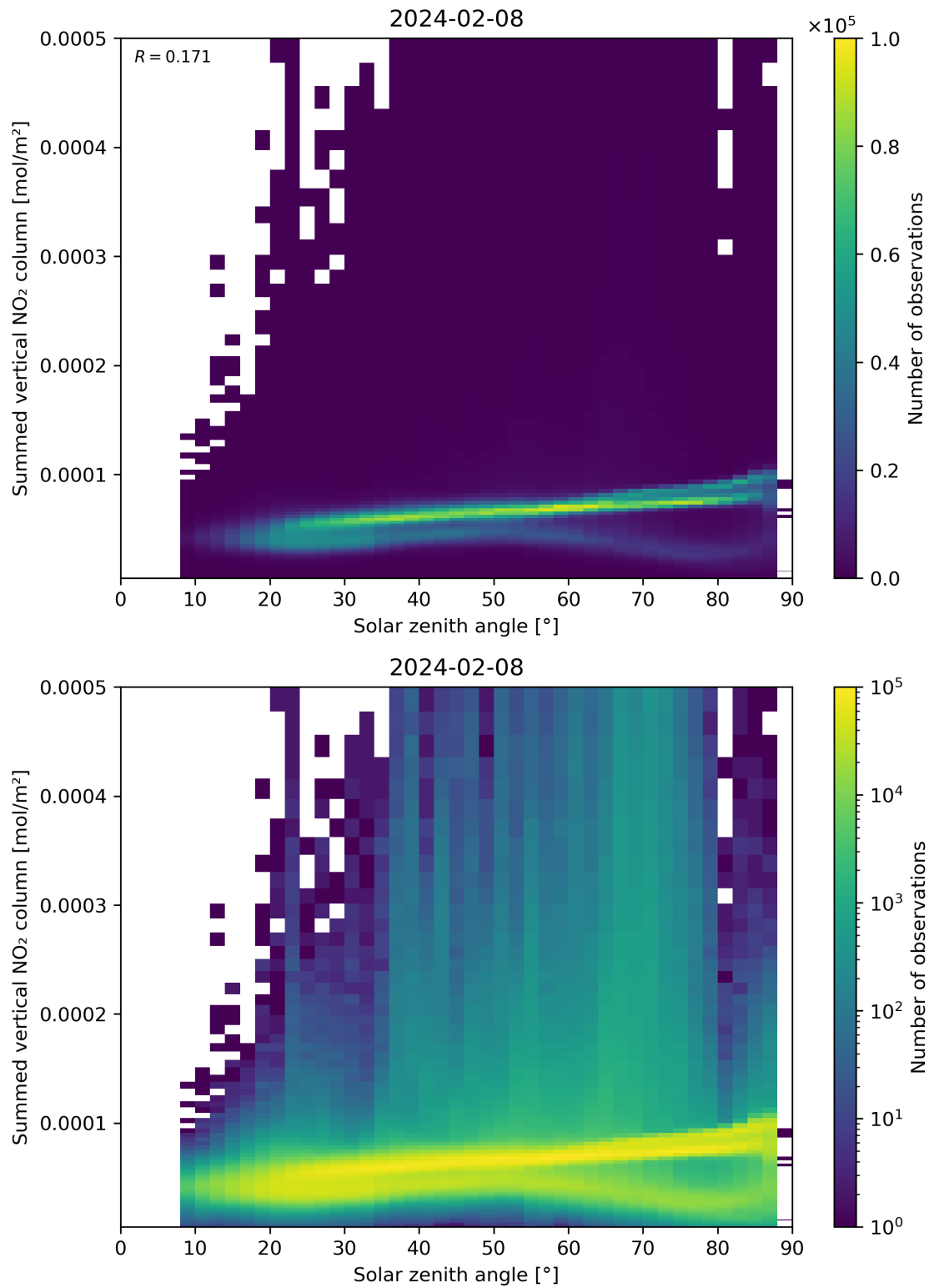
Figure 151: Scatter density plot of “Solar zenith angle” against “Summed vertical NO 2 column” for 2024-02-07 to 2024-02-09.
