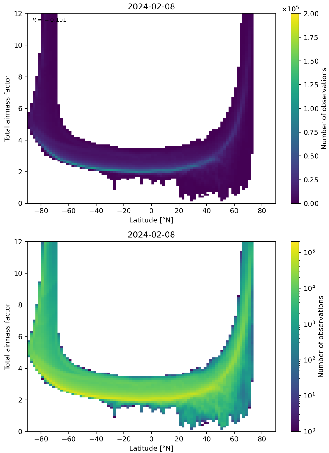
Figure 84: Scatter density plot of “Latitude” against “Total airmass factor” for 2024-02-07 to 2024-02-09.
