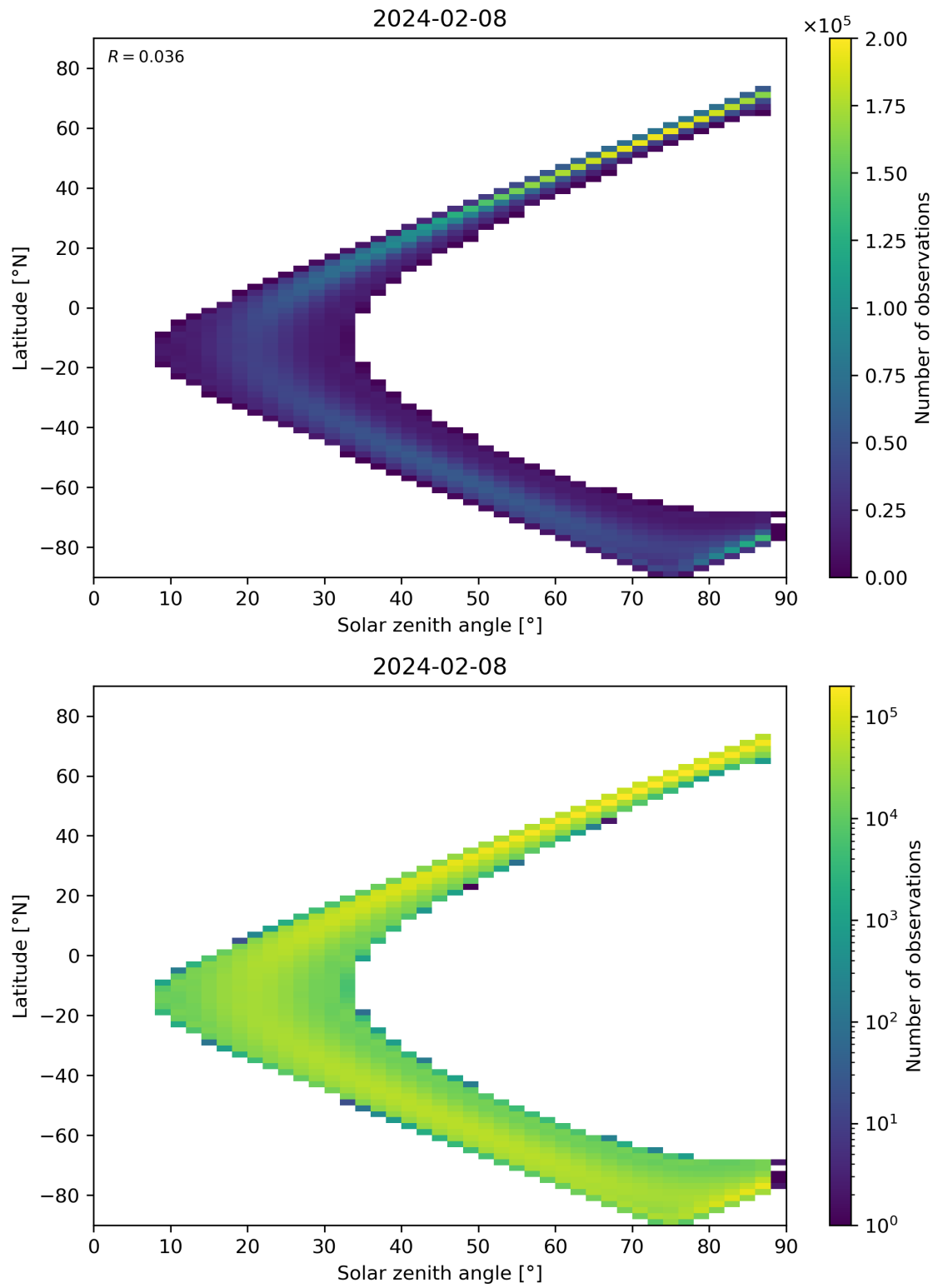
Figure 149: Scatter density plot of “Solar zenith angle” against “Latitude” for 2024-02-07 to 2024-02-09.
