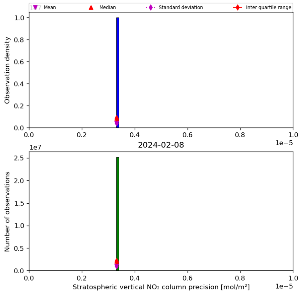
Figure 37: Histogram of “Stratospheric vertical NO 2 column precision” for 2024-02-07 to 2024-02-09
