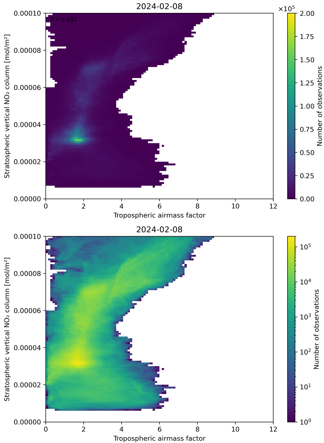
Figure 74: Scatter density plot of “Tropospheric air mass factor” against “Stratospheric vertical NO 2 column” for 2024-02-07 to 2024-02-09.
