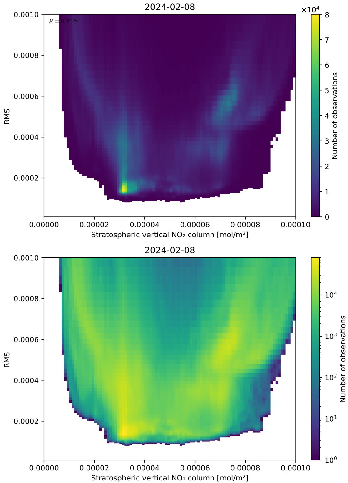
Figure 102: Scatter density plot of “Stratospheric vertical NO 2 column” against “RMS” for 2024-02-07 to 2024-02-09.
