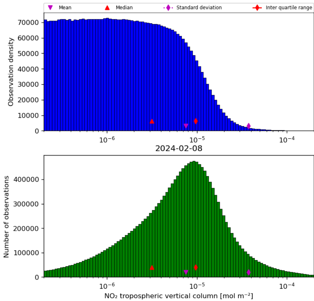
Figure 29: Histogram of “NO 2 tropospheric vertical column” for 2024-02-07 to 2024-02-09
