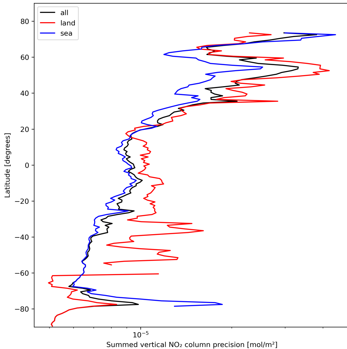
Figure 24: Zonal average of “Summed vertical NO 2 column precision” for 2024-02-07 to 2024-02-09.
