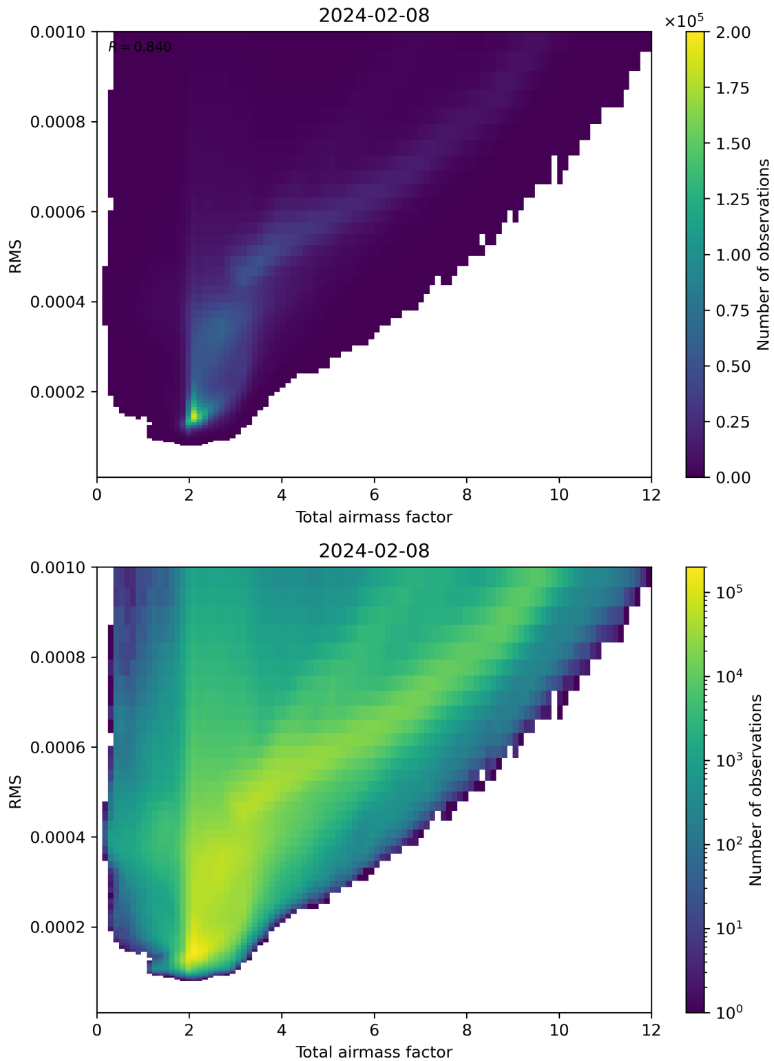
Figure 69: Scatter density plot of “Total airmass factor” against “RMS” for 2024-02-07 to 2024-02-09.
