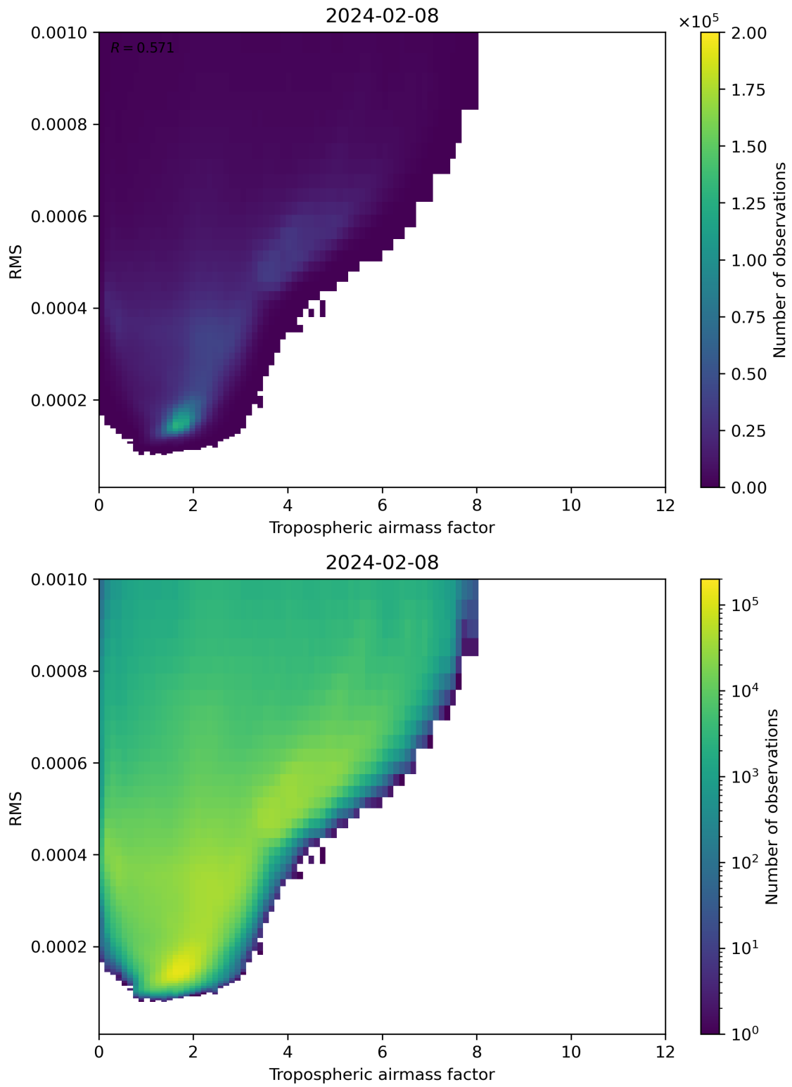
Figure 79: Scatter density plot of “Tropospheric airmass factor” against “RMS” for 2024-02-07 to 2024-02-09.
