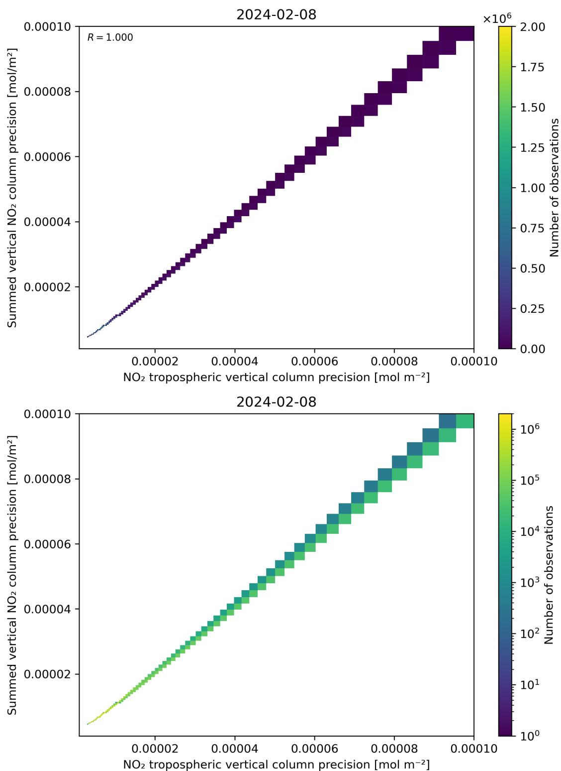
Figure 137: Scatter density plot of “NO 2 tropospheric vertical column precision” against “Summed vertical NO 2 column precision” for 2024-02-07 to 2024-02-09.
