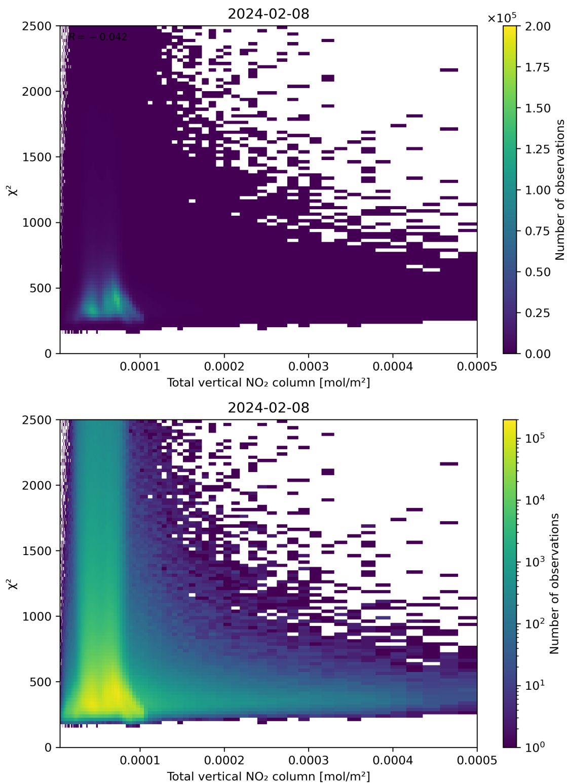
Figure 111: Scatter density plot of “Total vertical NO 2 column” against “ \chi^2 ” for 2024-02-07 to 2024-02-09.
