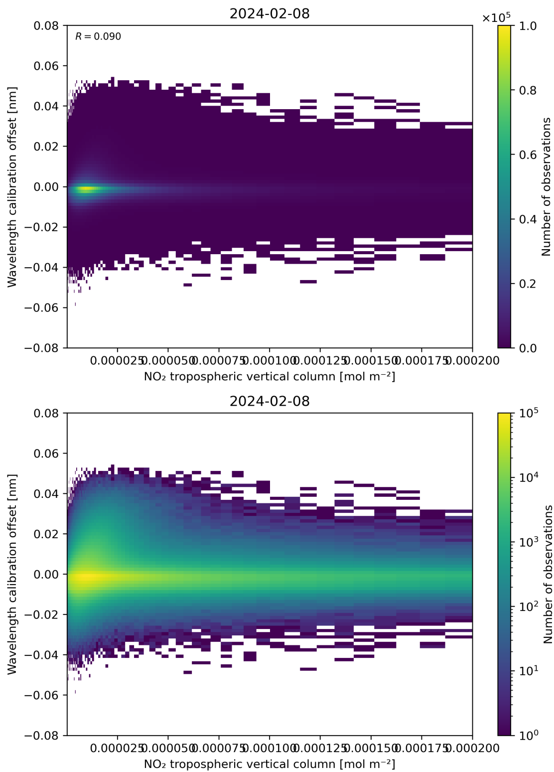
Figure 143: Scatter density plot of “NO 2 tropospheric vertical column” against “Wavelength calibration offset” for 2024-02-07 to 2024-02-09.
