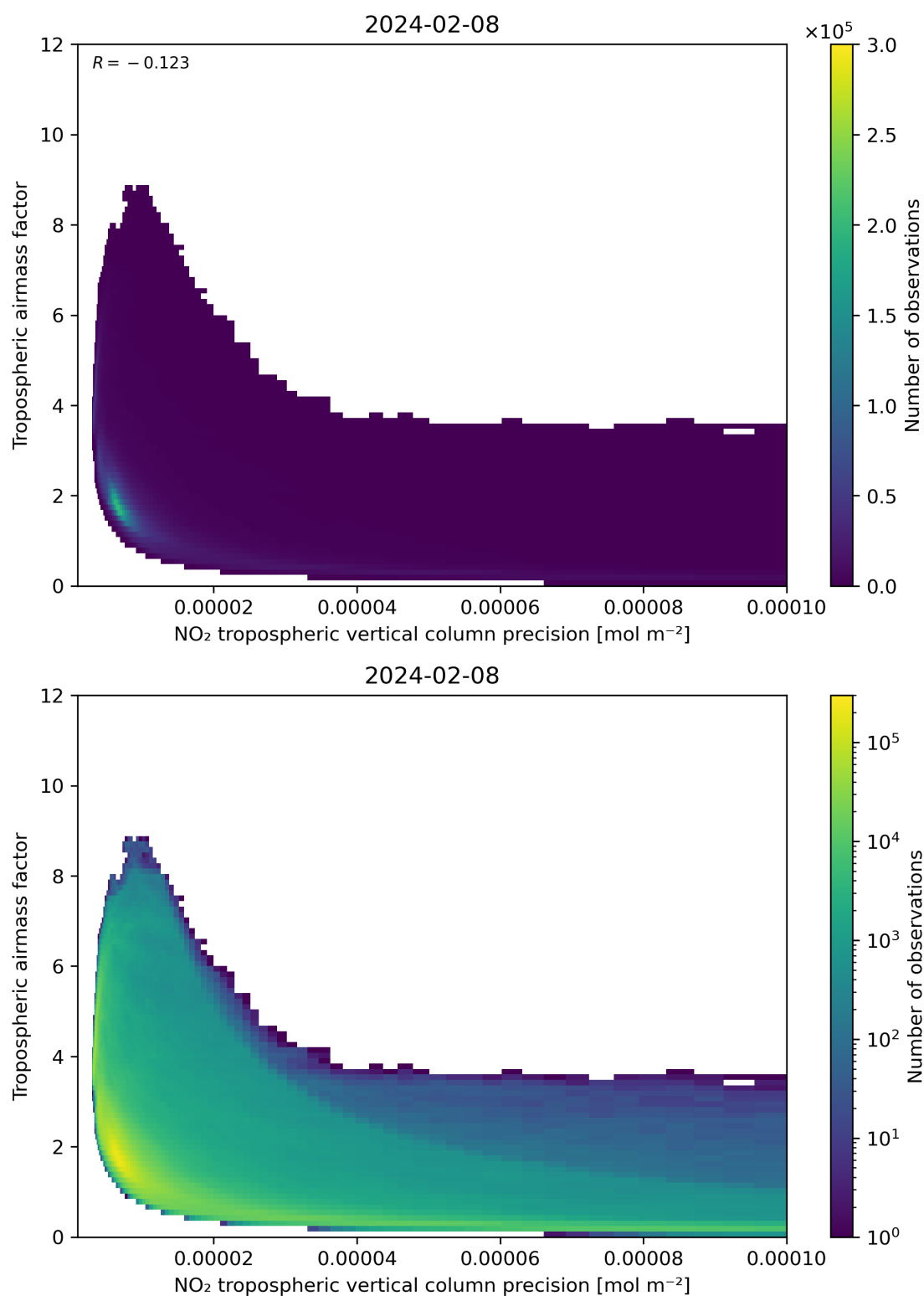
Figure 133: Scatter density plot of “NO 2 tropospheric vertical column precision” against “Tropospheric airmass factor” for 2024-02-07 to 2024-02-09.
