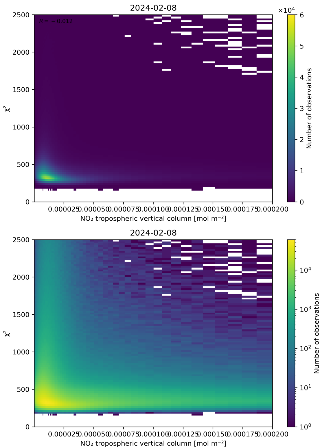
Figure 124: Scatter density plot of “NO 2 tropospheric vertical column” against “ \chi^2 ” for 2024-02-07 to 2024-02-09.
