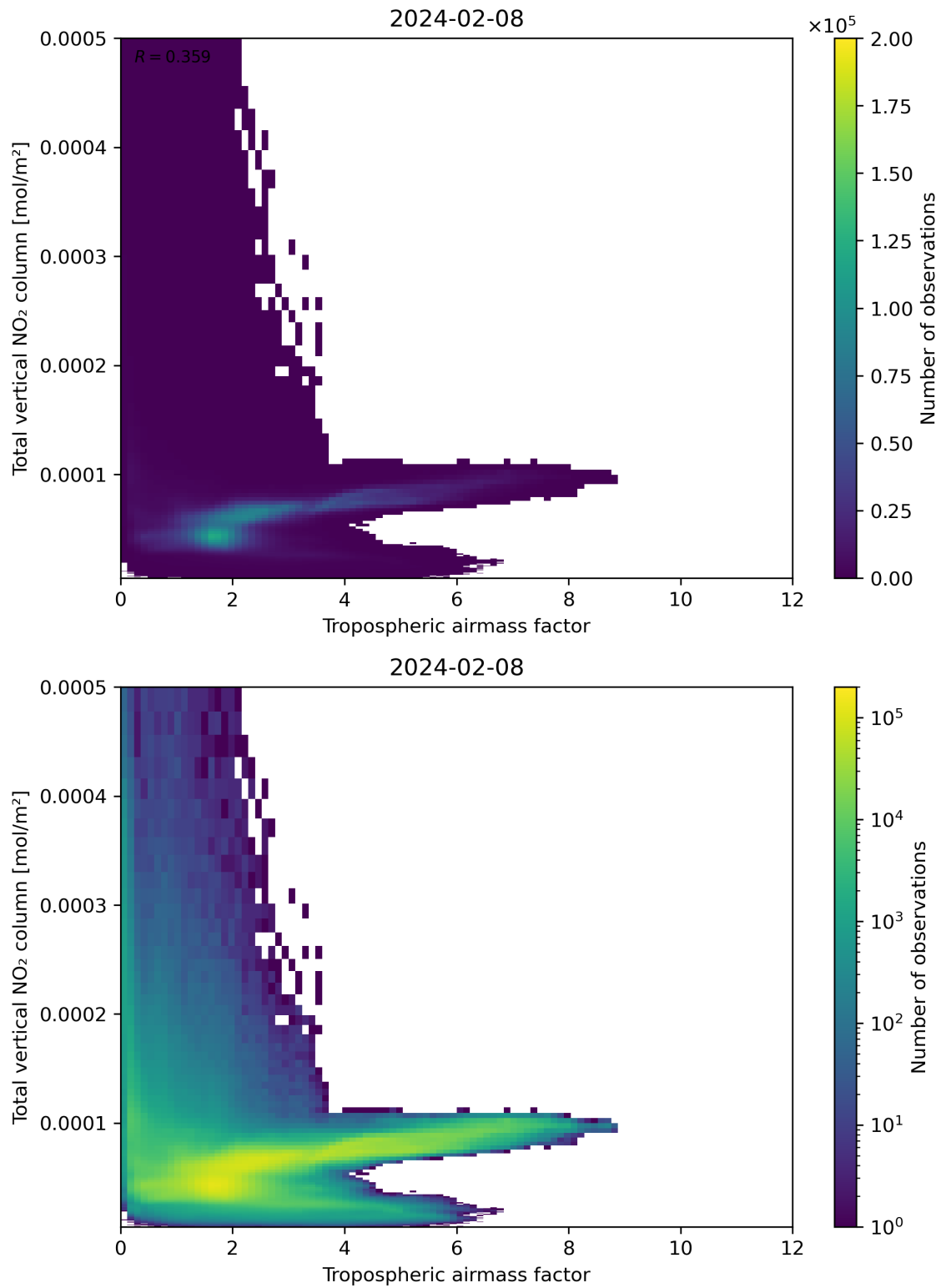
Figure 77: Scatter density plot of “Tropospheric airmass factor” against “Total vertical NO 2 column” for 2024-02-07 to 2024-02-09.
