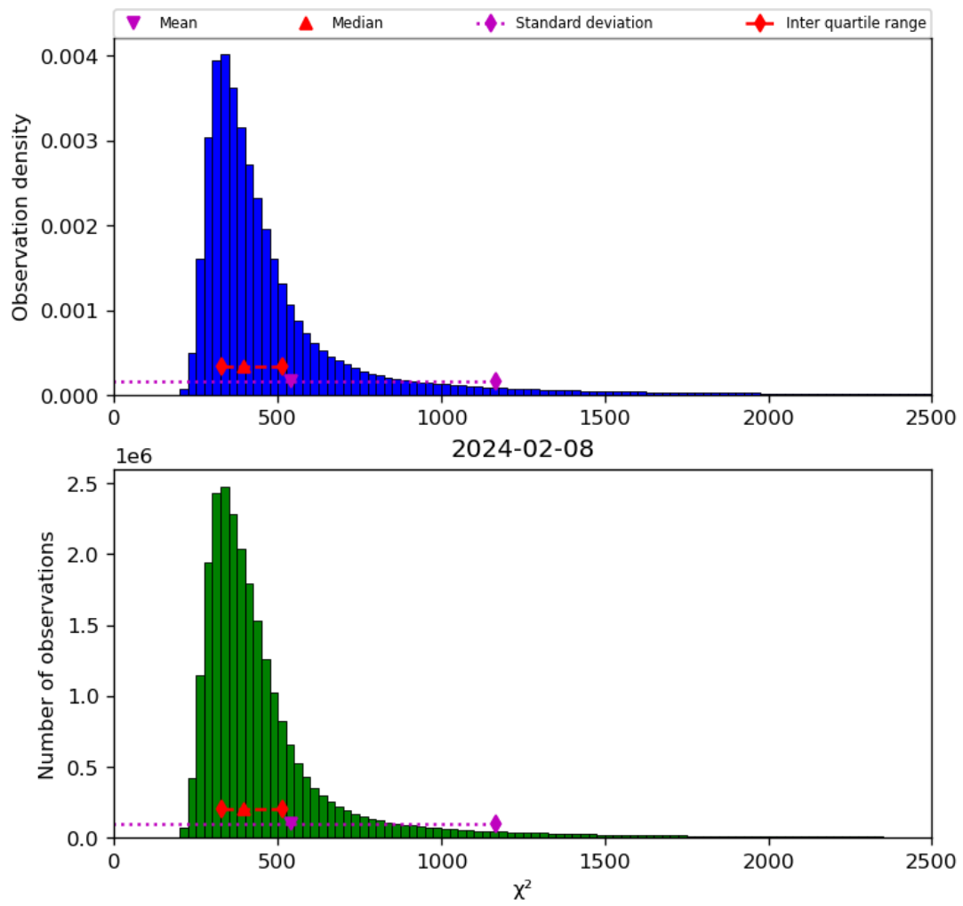
Figure 42: Histogram of " \chi^2 " for 2024-02-07 to 2024-02-09
