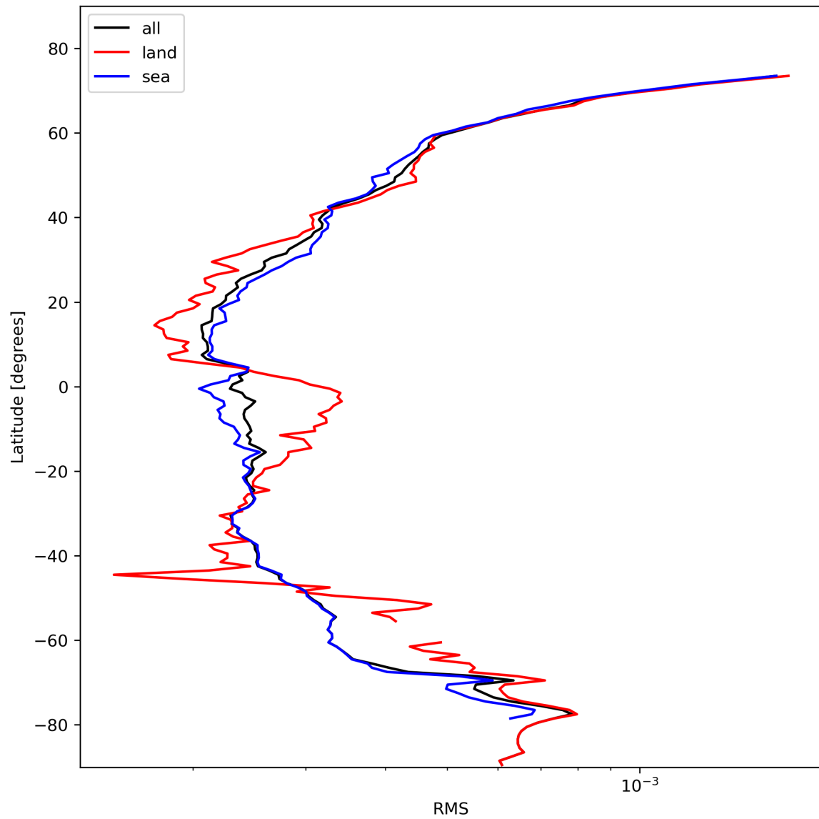
Figure 26: Zonal average of “RMS” for 2024-02-07 to 2024-02-09.
