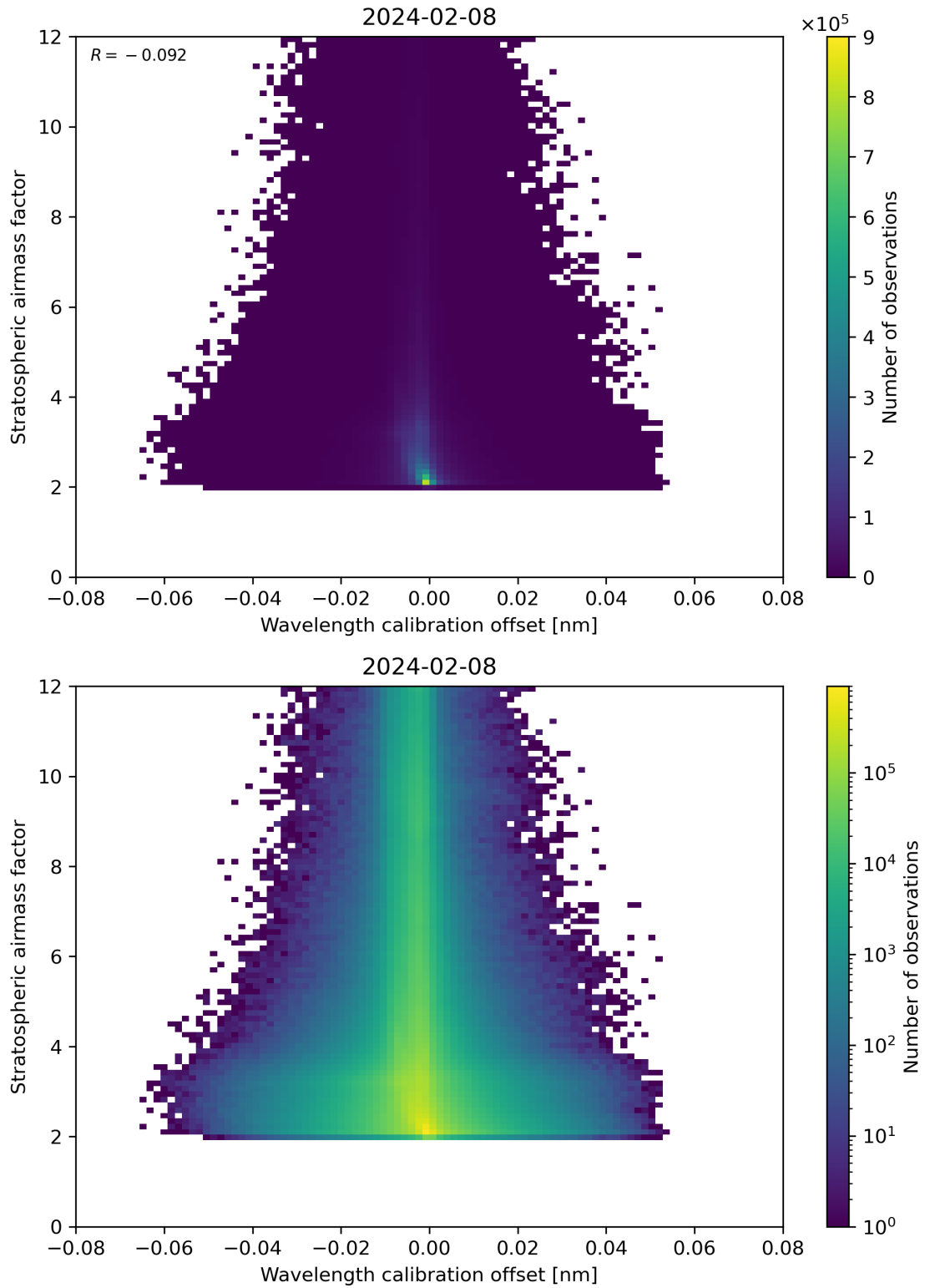
Figure 174: Scatter density plot of “Wavelength calibration offset” against “Stratospheric airmass factor” for 2024-02-07 to 2024-02-09.
