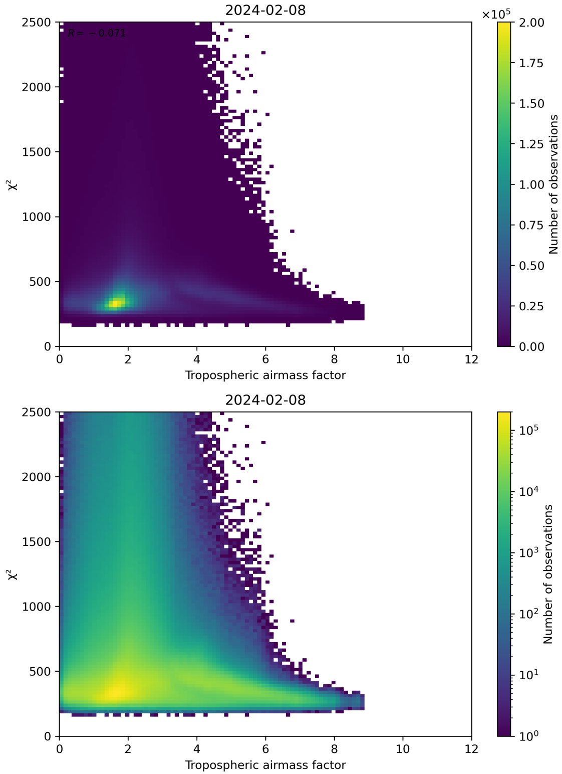
Figure 73: Scatter density plot of “Tropospheric airmass factor” against “ \chi^2 ” for 2024-02-07 to 2024-02-09.
