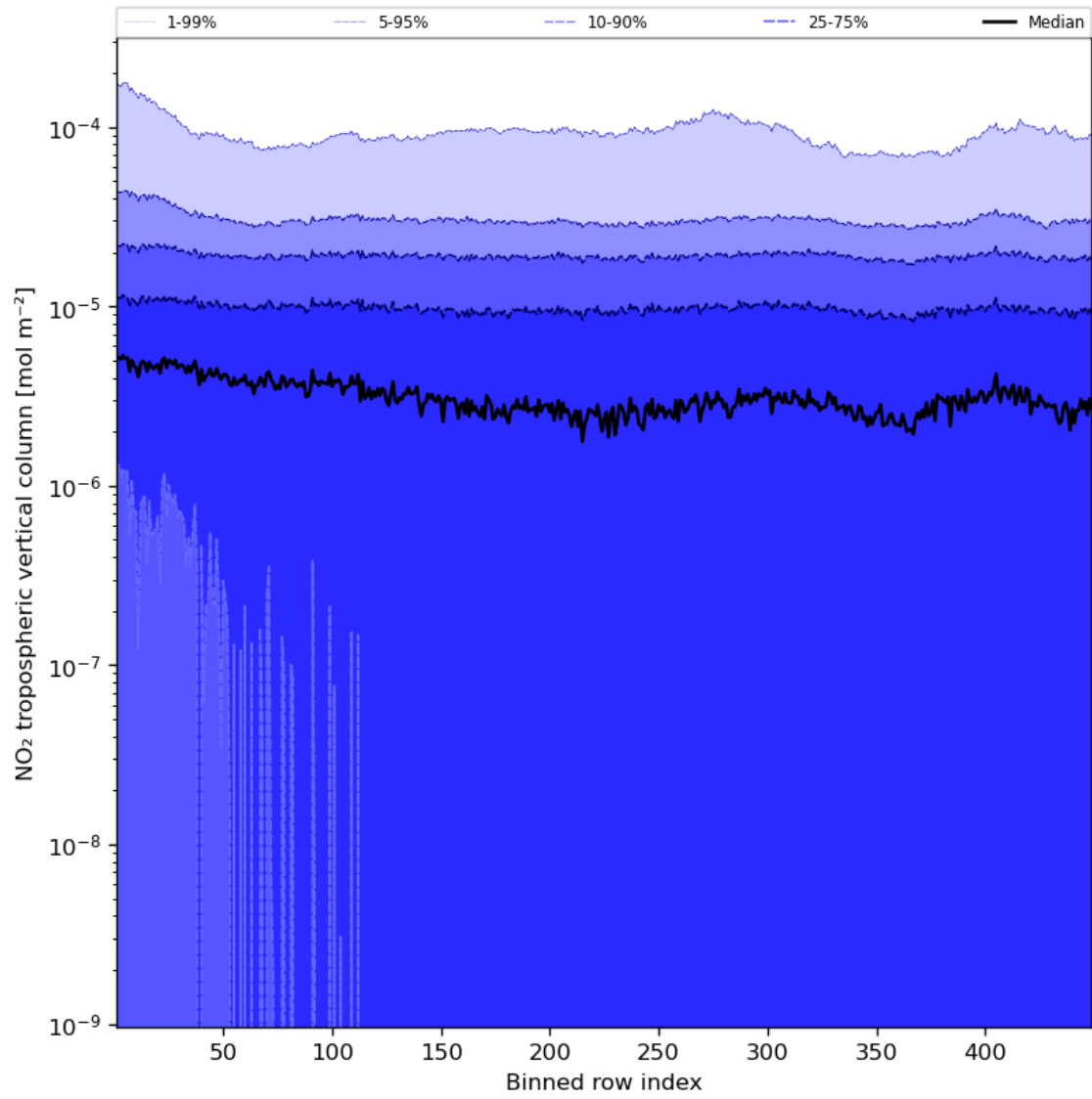
Figure 46: Along track statistics of “NO 2 tropospheric vertical column” for 2024-02-07 to 2024-02-09
