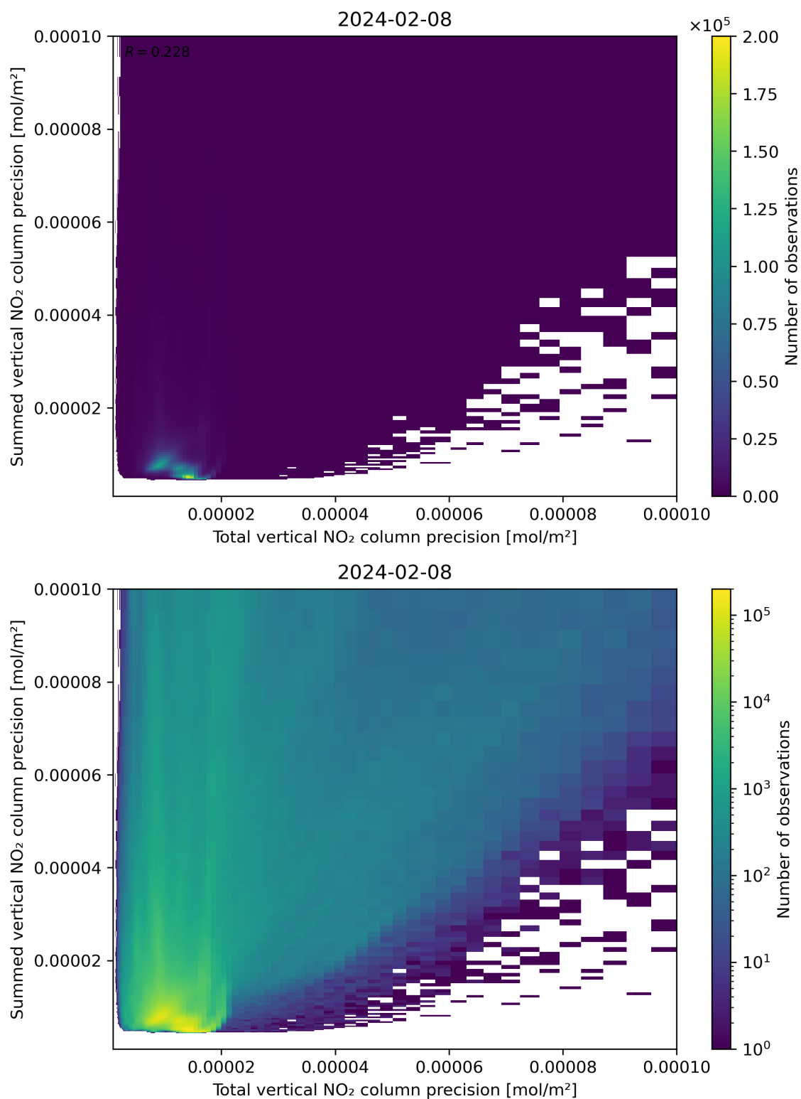
Figure 118: Scatter density plot of “Total vertical NO 2 column precision” against “Summed vertical NO 2 column precision” for 2024-02-07 to 2024-02-09.
