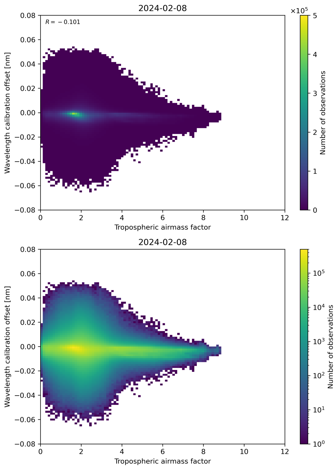
Figure 80: Scatter density plot of “Tropospheric airmass factor” against “Wavelength calibration offset” for 2024-02-07 to 2024-02-09.
