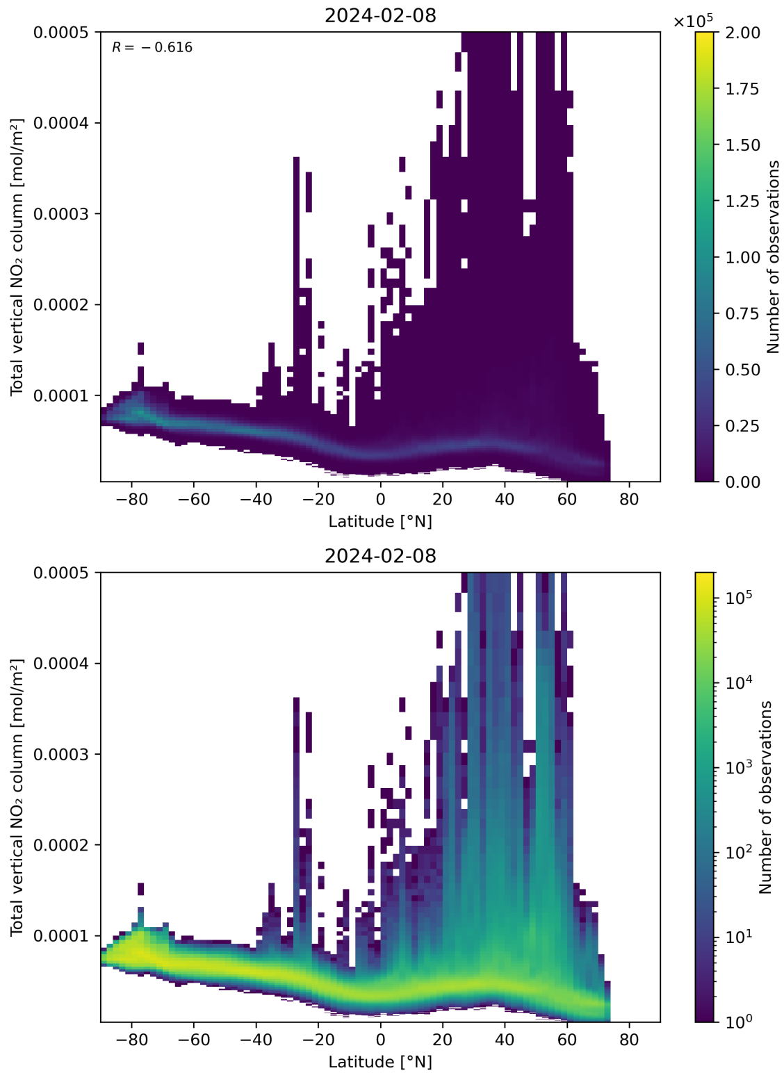
Figure 90: Scatter density plot of “Latitude” against “Total vertical NO 2 column” for 2024-02-07 to 2024-02-09.
