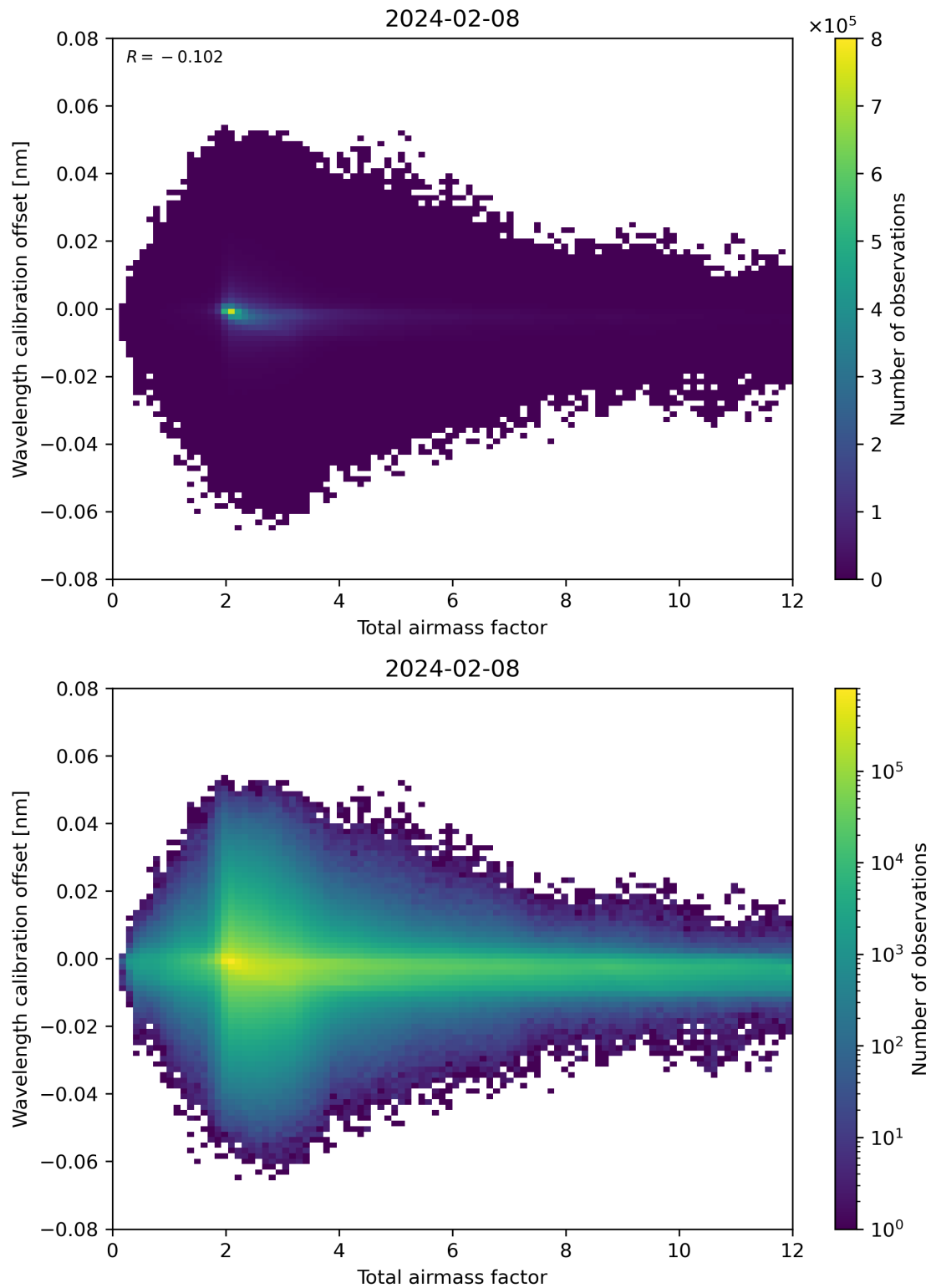
Figure 70: Scatter density plot of “Total airmass factor” against “Wavelength calibration offset” for 2024-02-07 to 2024-02-09.
