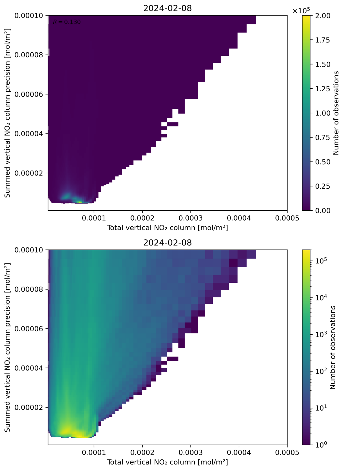
Figure 113: Scatter density plot of “Total vertical NO 2 column” against “Summed vertical NO 2 column precision” for 2024-02-07 to 2024-02-09.
