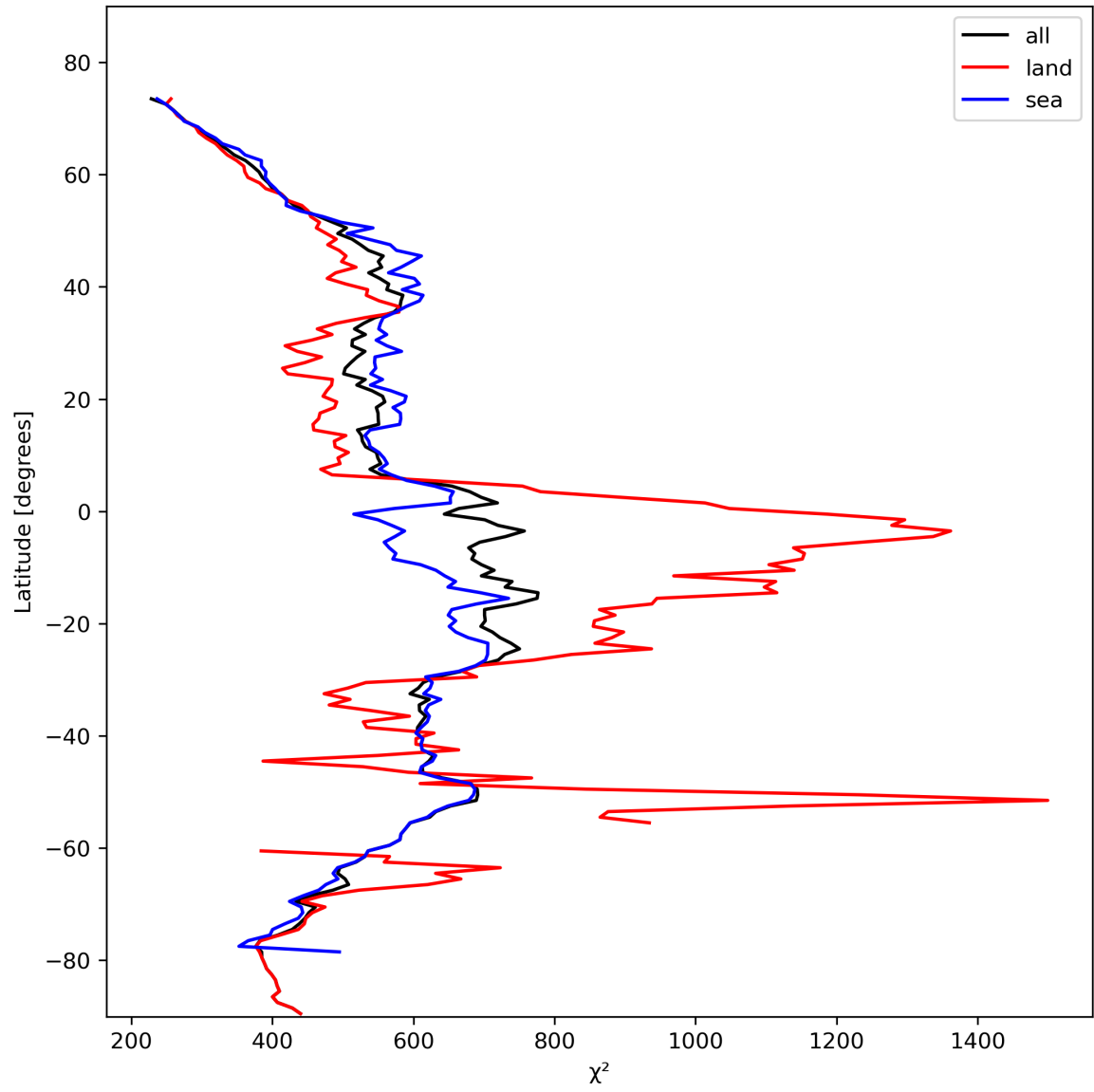
Figure 25: Zonal average of “ \chi^2 ” for 2024-02-07 to 2024-02-09.
