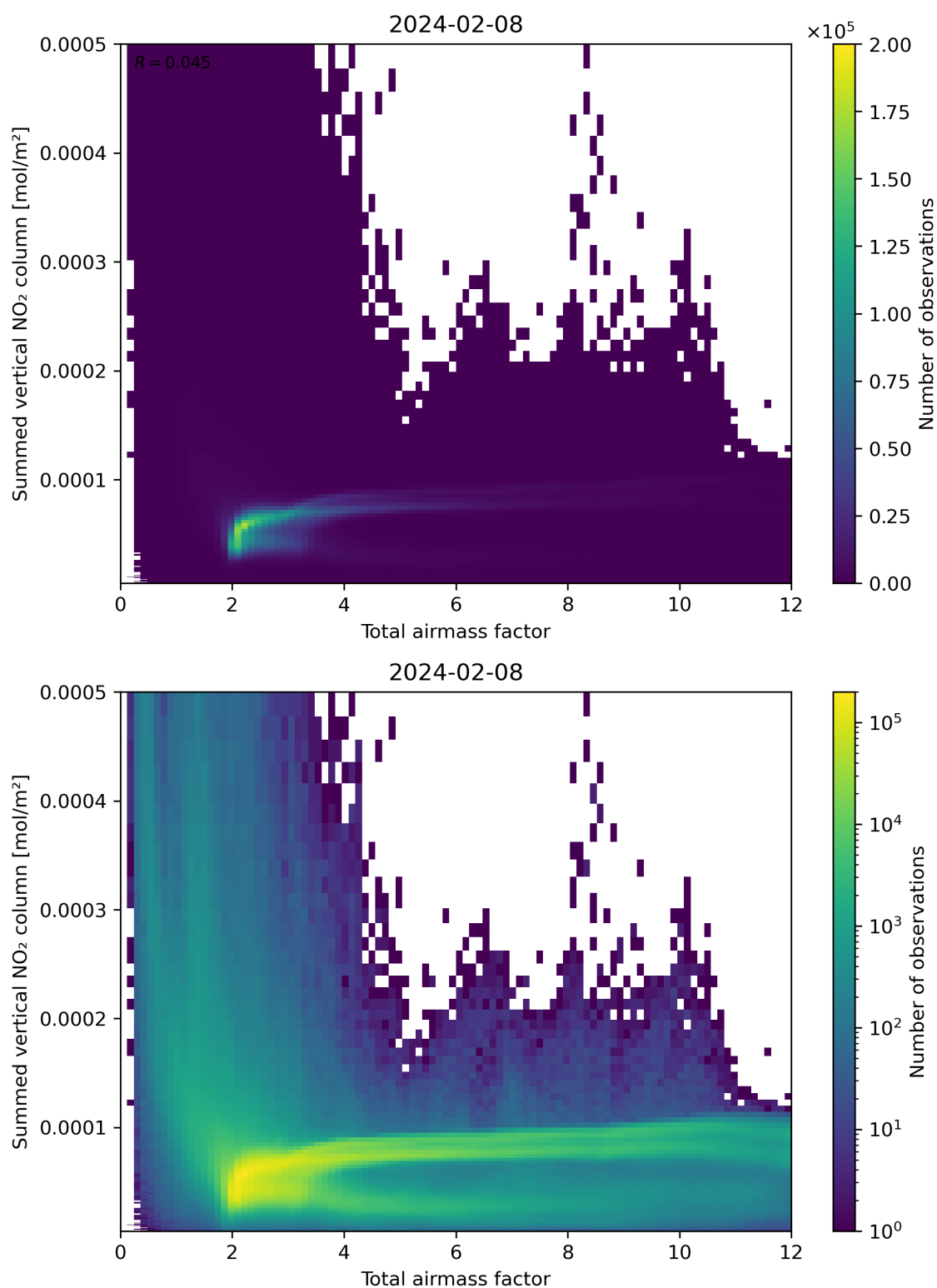
Figure 65: Scatter density plot of “Total airmass factor” against “Summed vertical NO 2 column” for 2024-02-07 to 2024-02-09.
