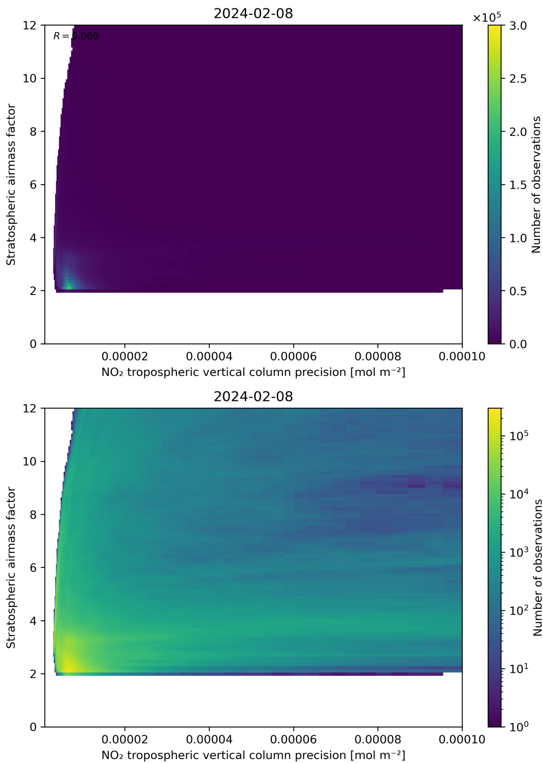
Figure 131: Scatter density plot of “NO 2 tropospheric vertical column precision” against “Stratospheric airmass factor” for 2024-02-07 to 2024-02-09.
