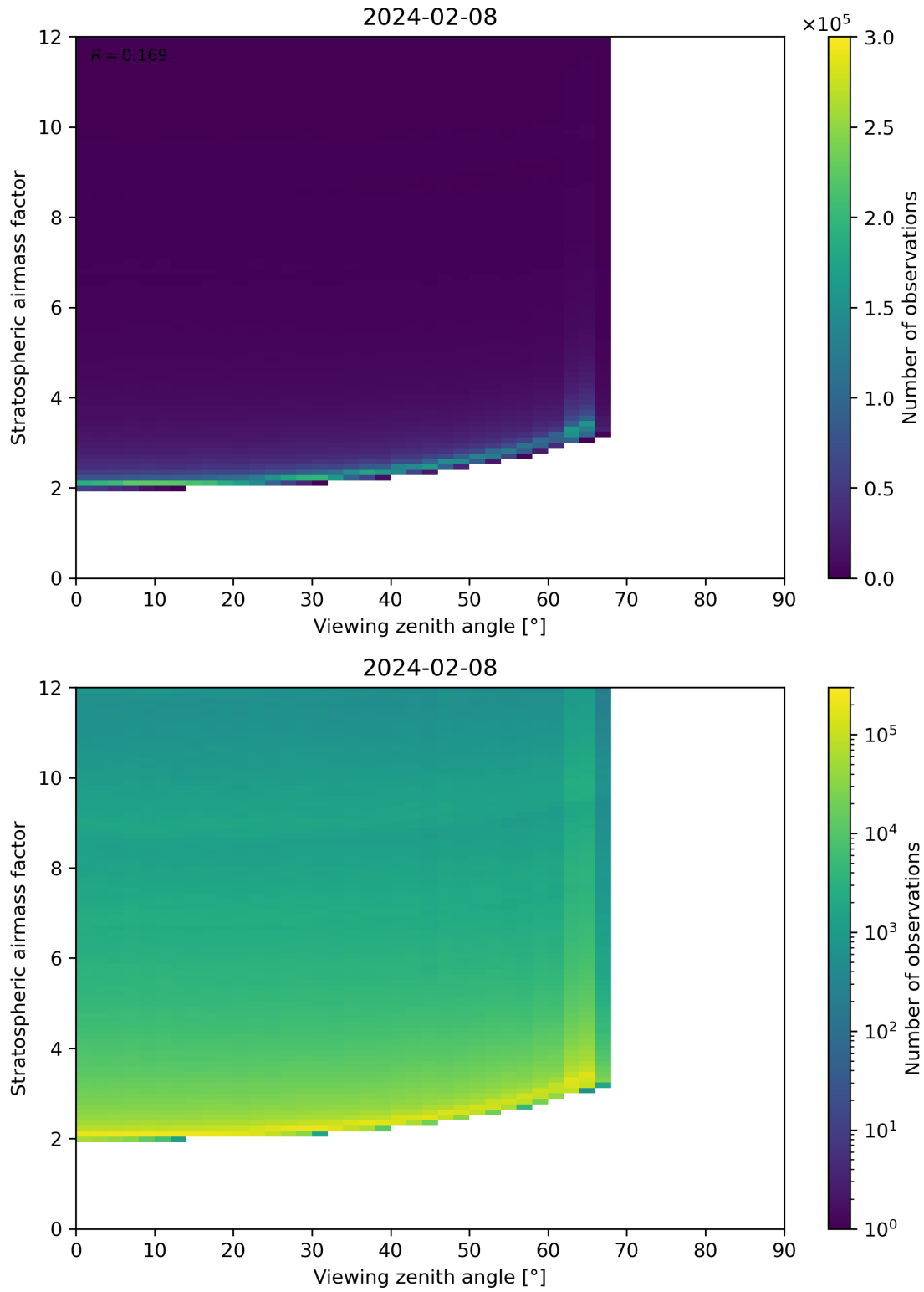
Figure 159: Scatter density plot of “Viewing zenith angle” against “Stratospheric airmass factor” for 2024-02-07 to 2024-02-09.
