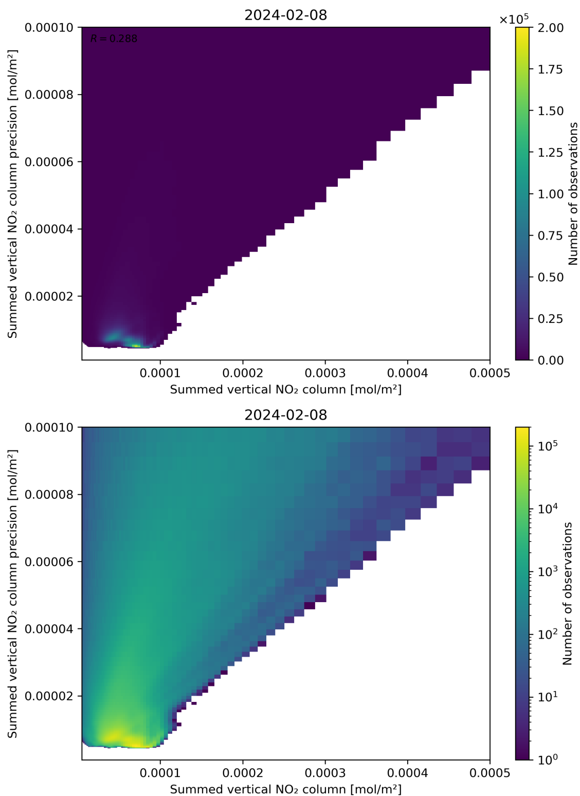
Figure 105: Scatter density plot of “Summed vertical NO 2 column” against “Summed vertical NO 2 column precision” for 2024-02-07 to 2024-02-09.
