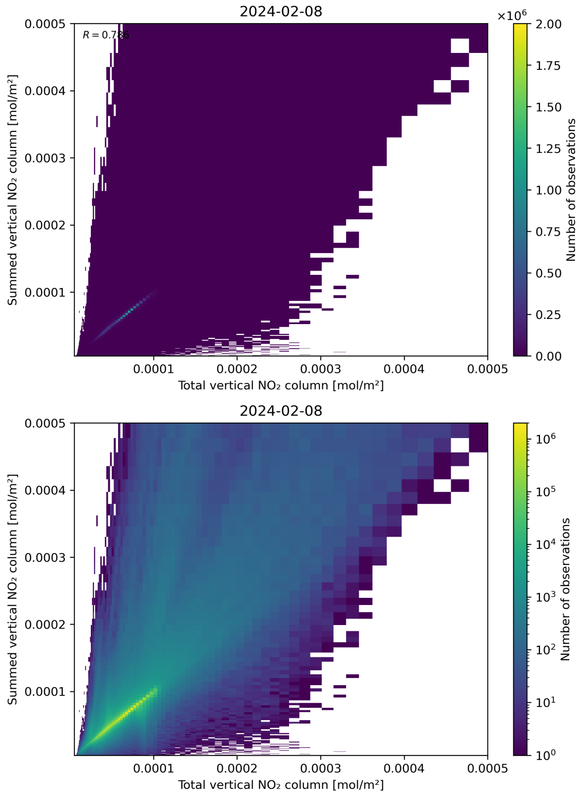
Figure 112: Scatter density plot of “Total vertical NO 2 column” against “Summed vertical NO 2 column” for 2024-02-07 to 2024-02-09.
