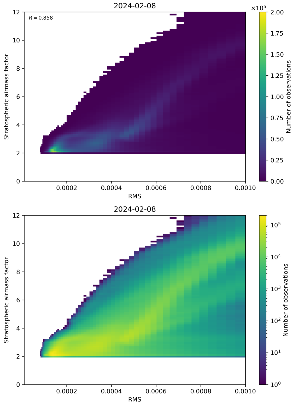
Figure 144: Scatter density plot of “RMS” against “Stratospheric airmass factor” for 2024-02-07 to 2024-02-09.
