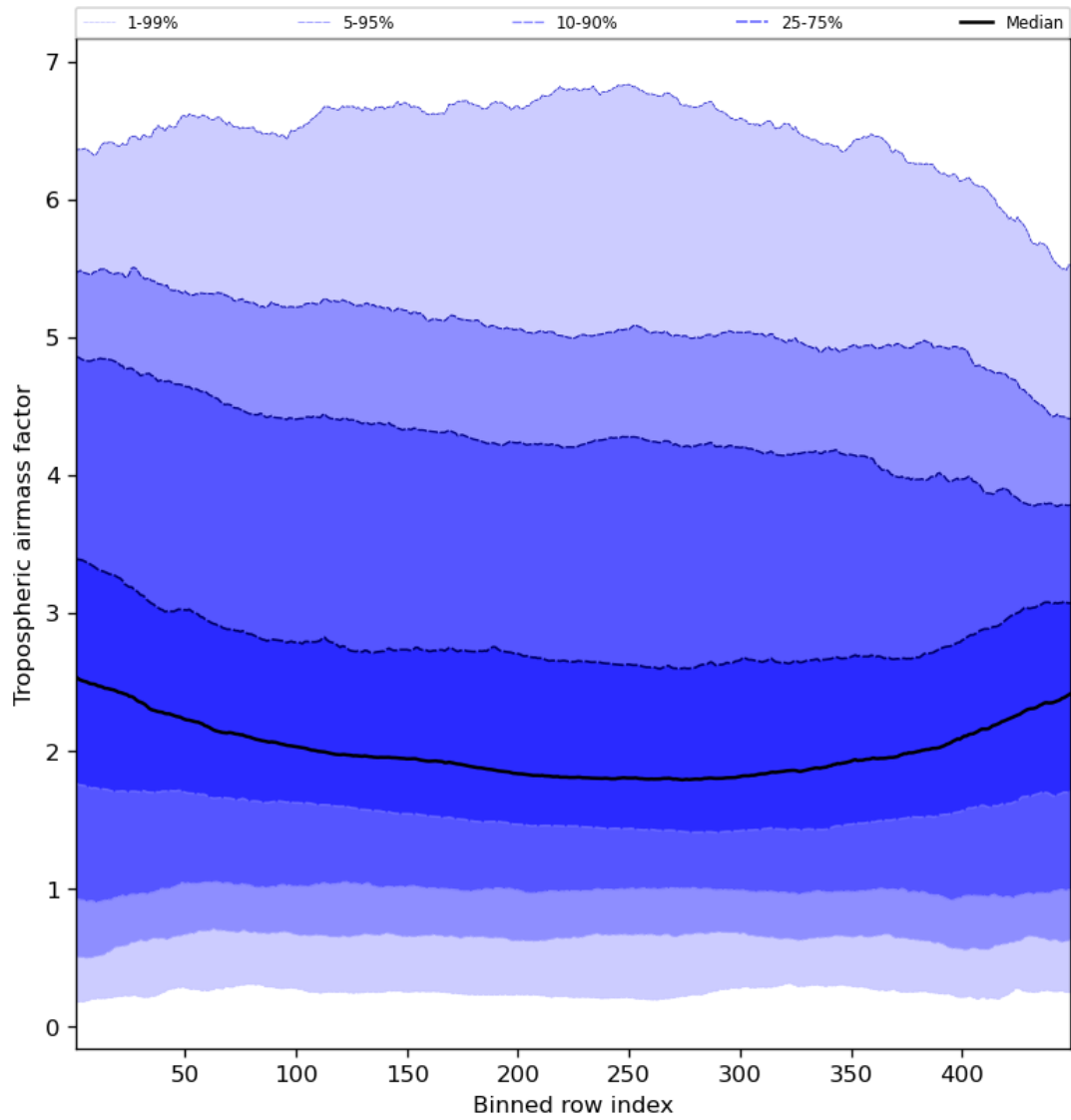
Figure 48: Along track statistics of “Tropospheric air mass factor” for 2024-02-07 to 2024-02-09
