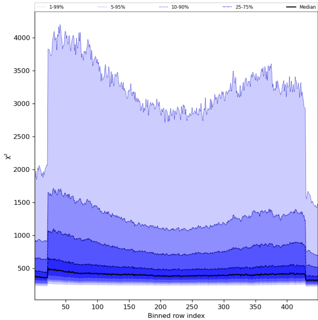
Figure 59: Along track statistics of “ \chi^2 ” for 2024-02-07 to 2024-02-09
