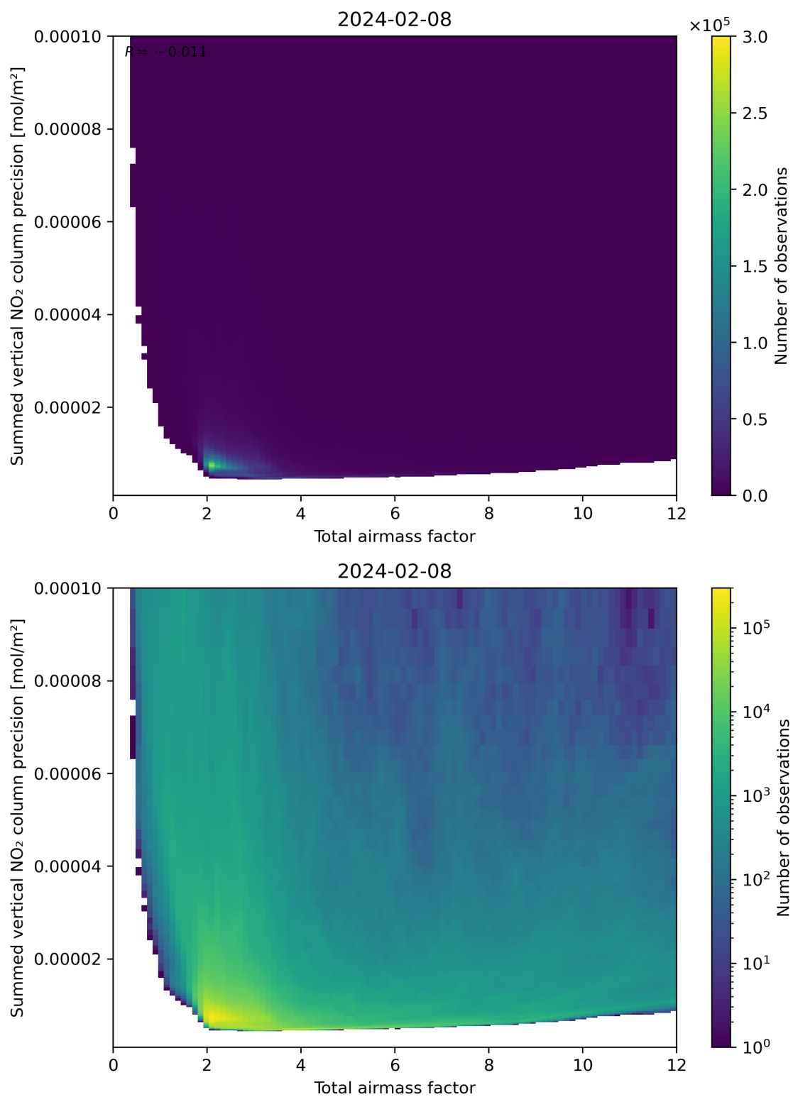
Figure 66: Scatter density plot of “Total airmass factor” against “Summed vertical NO 2 column precision” for 2024-02-07 to 2024-02-09.
