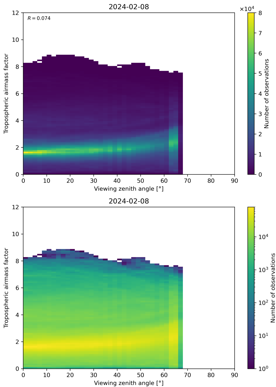
Figure 161: Scatter density plot of “Viewing zenith angle” against “Tropospheric airmass factor” for 2024-02-07 to 2024-02-09.
