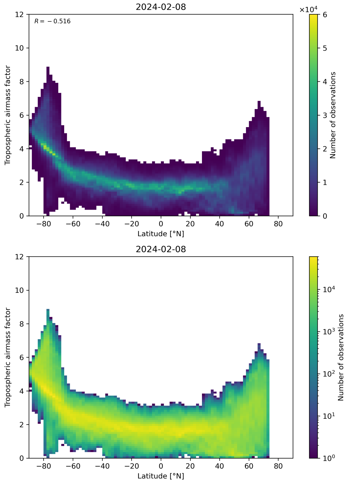
Figure 85: Scatter density plot of “Latitude” against “Tropospheric air mass factor” for 2024-02-07 to 2024-02-09.
