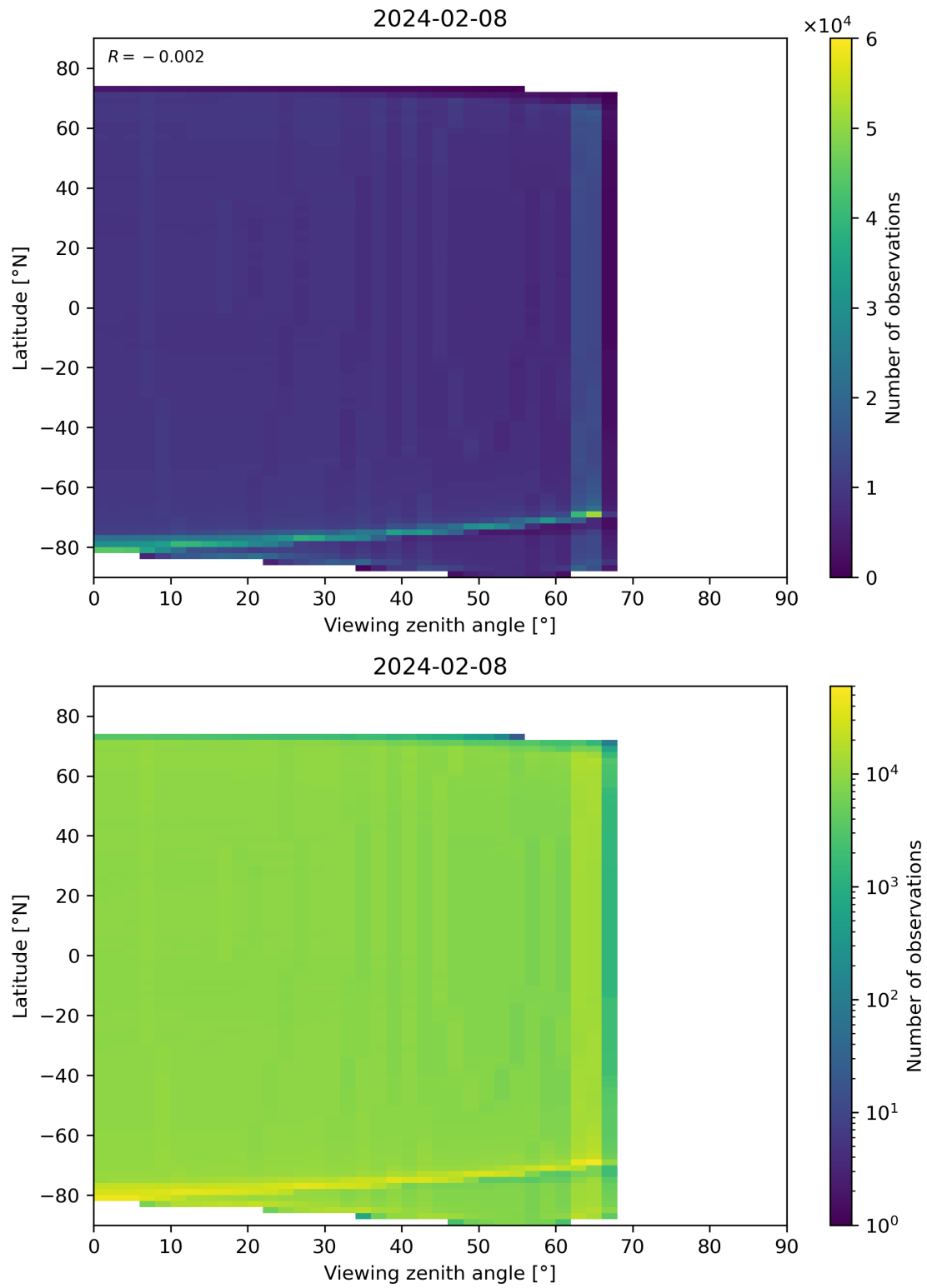
Figure 163: Scatter density plot of “Viewing zenith angle” against “Latitude” for 2024-02-07 to 2024-02-09.
