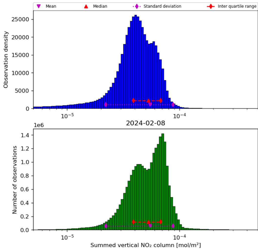
Figure 40: Histogram of “Summed vertical NO 2 column” for 2024-02-07 to 2024-02-09
