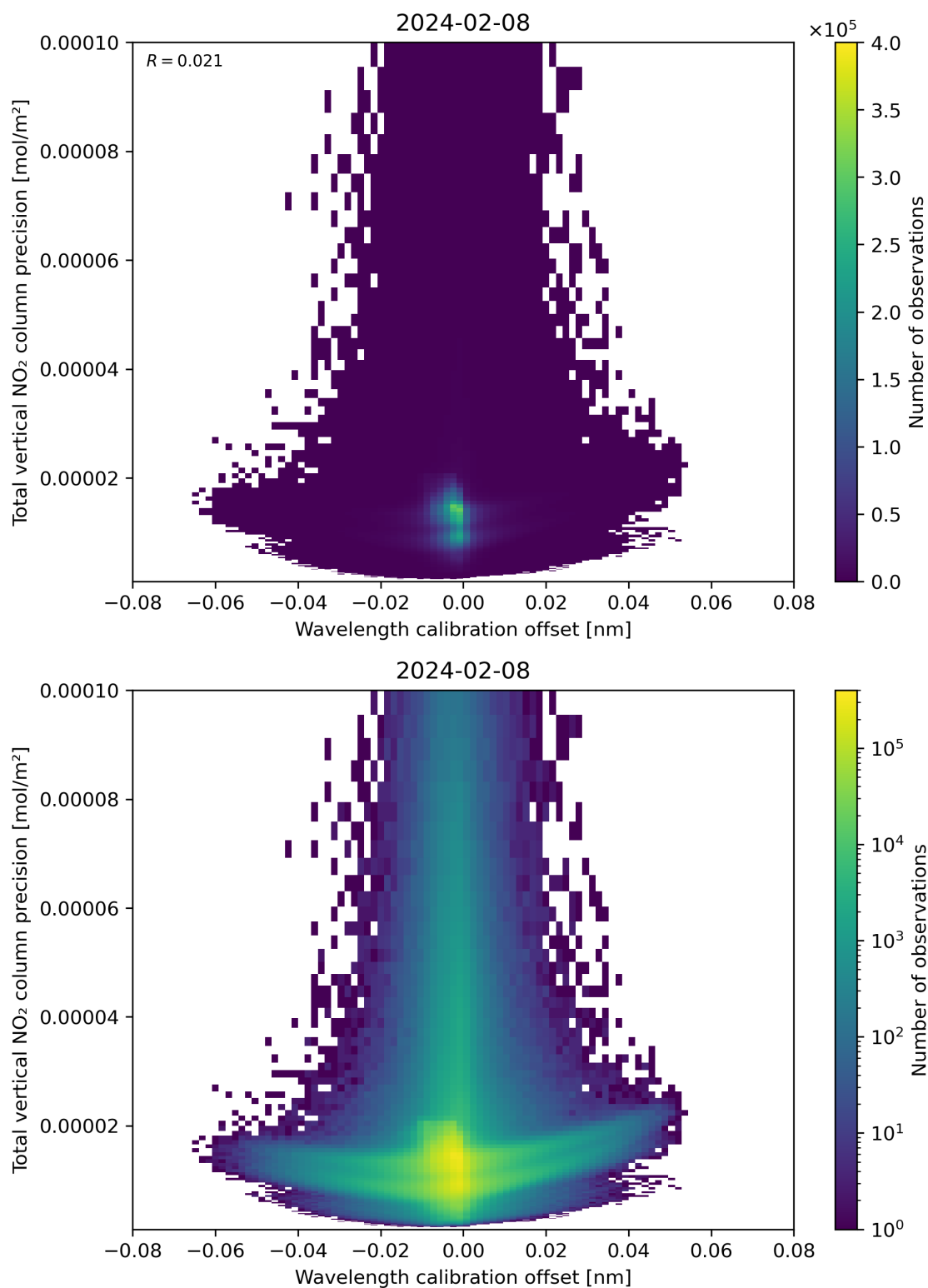
Figure 180: Scatter density plot of “Wavelength calibration offset” against “Total vertical NO 2 column precision” for 2024-02-07 to 2024-02-09.
