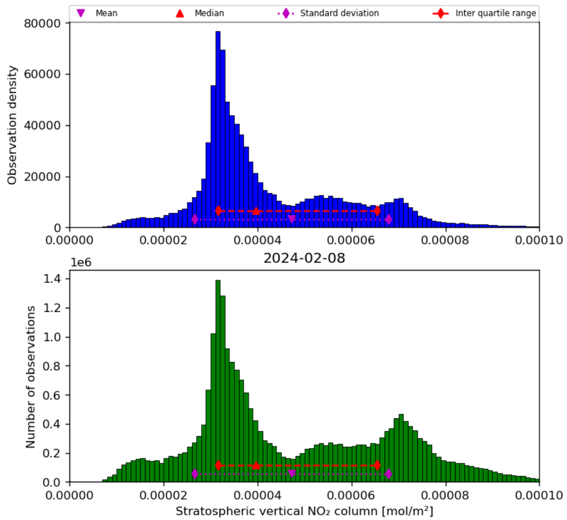
Figure 36: Histogram of “Stratospheric vertical NO 2 column” for 2024-02-07 to 2024-02-09
