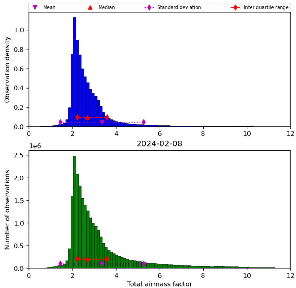
Figure 32: Histogram of “Total airmass factor” for 2024-02-07 to 2024-02-09
