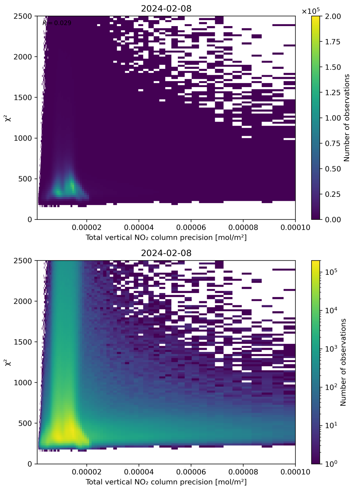
Figure 116: Scatter density plot of “Total vertical NO 2 column precision” against “ \chi^2 ” for 2024-02-07 to 2024-02-09.
