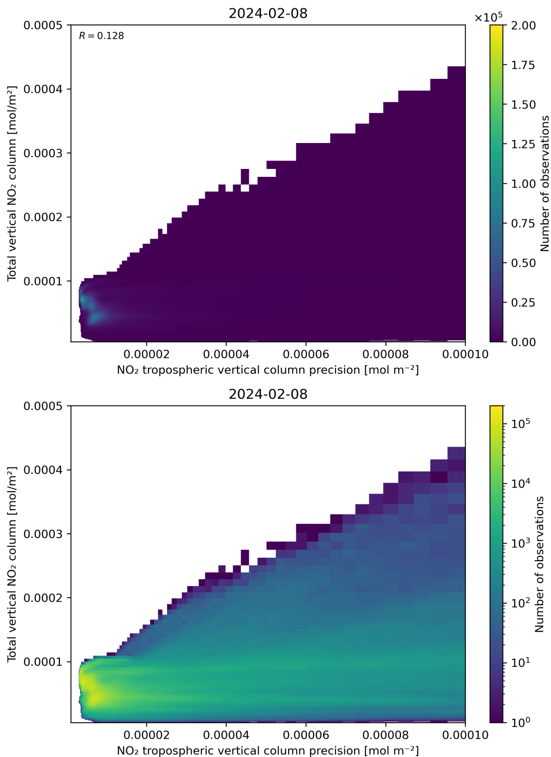
Figure 138: Scatter density plot of “NO 2 tropospheric vertical column precision” against “Total vertical NO 2 column” for 2024-02-07 to 2024-02-09.
