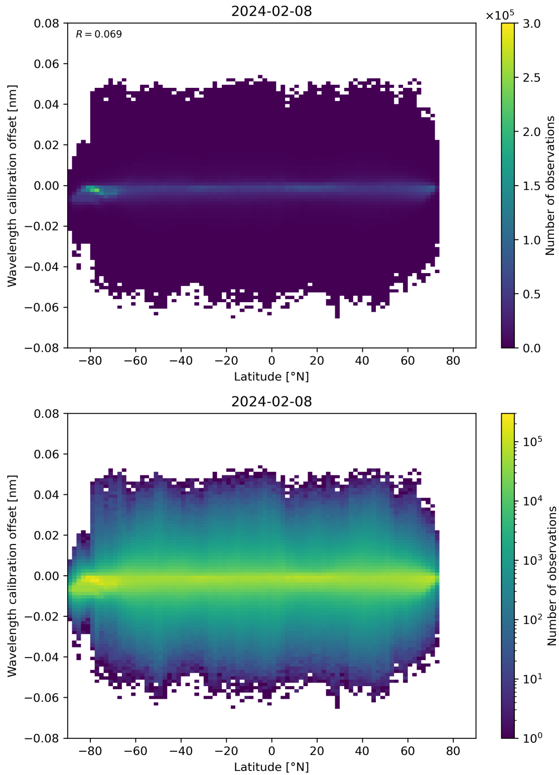
Figure 95: Scatter density plot of “Latitude” against “Wavelength calibration offset” for 2024-02-07 to 2024-02-09.
