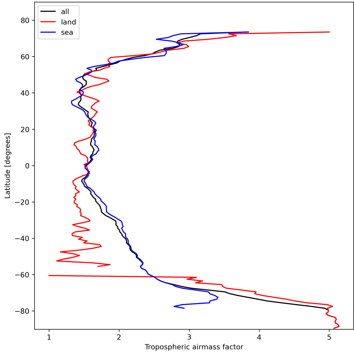
Figure 14: Zonal average of “Tropospheric airmass factor” for 2024-02-07 to 2024-02-09.
