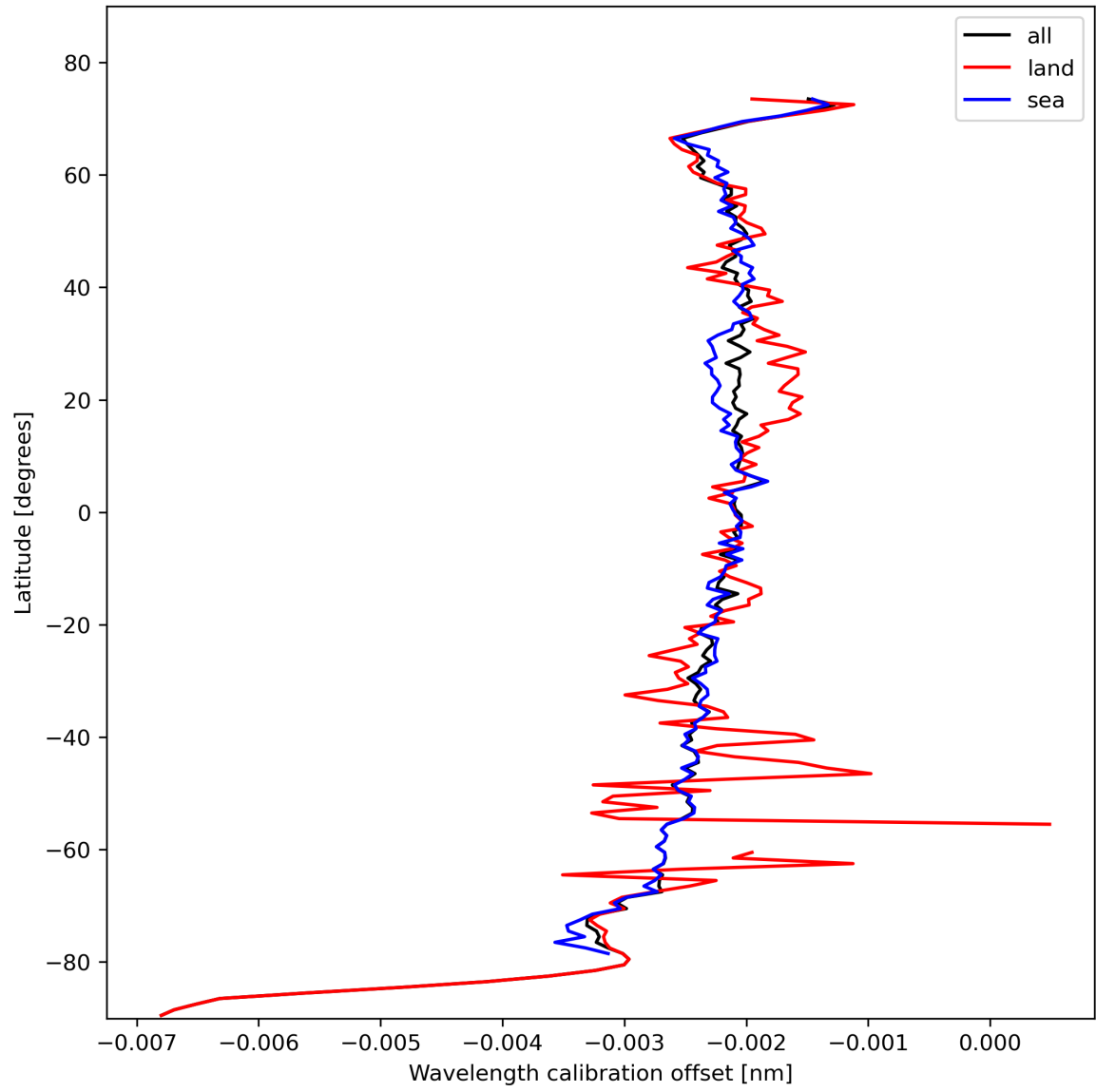
Figure 18: Zonal average of “Wavelength calibration offset” for 2024-02-07 to 2024-02-09.
