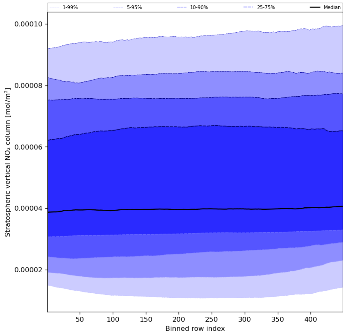
Figure 53: Along track statistics of “Stratospheric vertical NO 2 column” for 2024-02-07 to 2024-02-09
