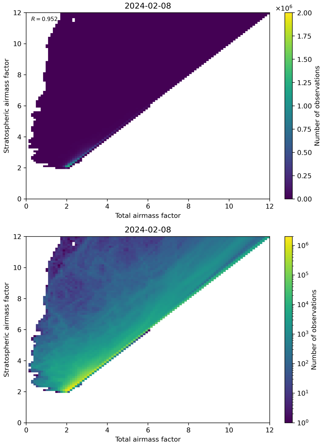
Figure 62: Scatter density plot of “Total airmass factor” against “Stratospheric airmass factor” for 2024-02-07 to 2024-02-09.
