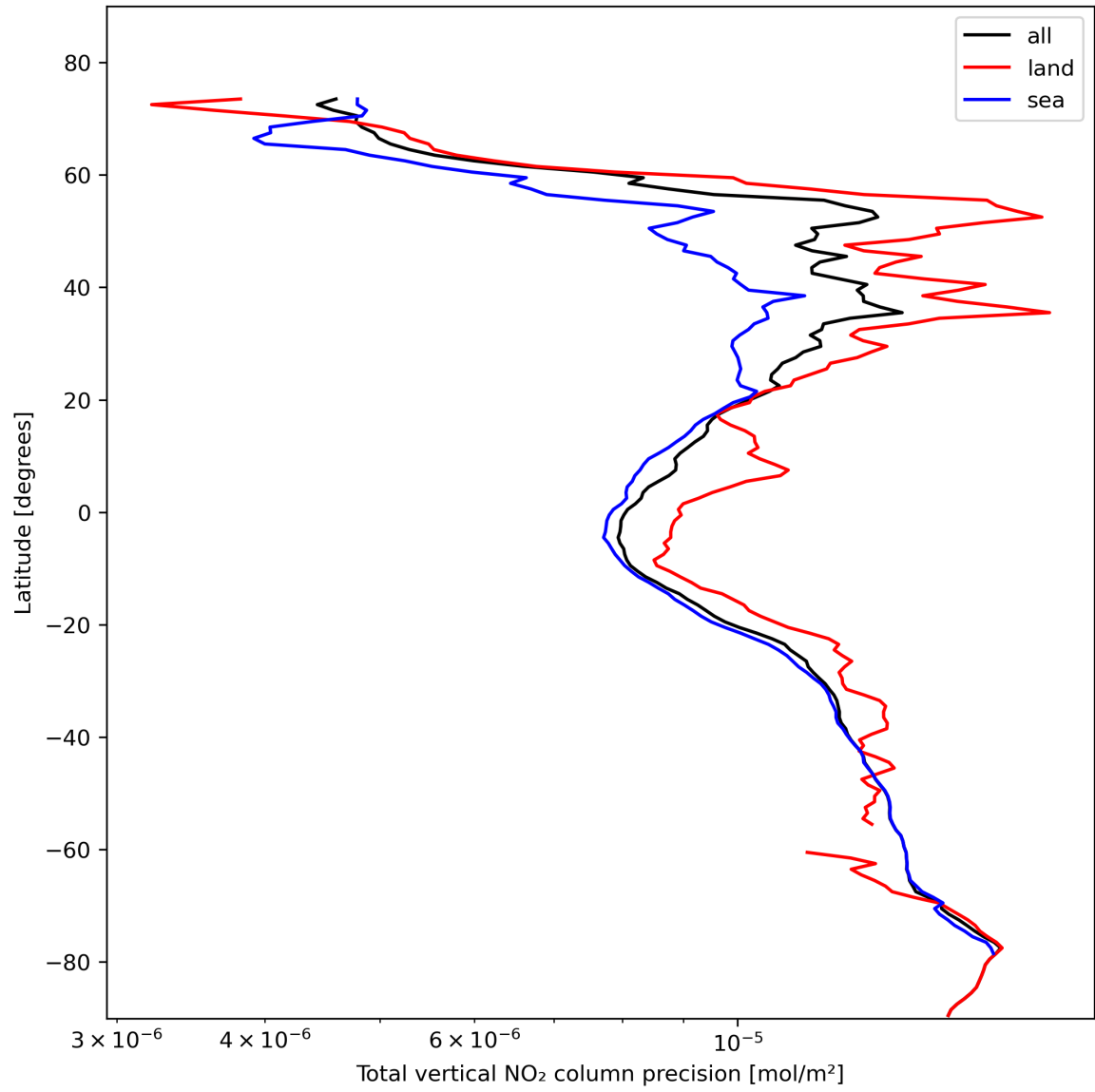
Figure 22: Zonal average of “Total vertical NO 2 column precision” for 2024-02-07 to 2024-02-09.
