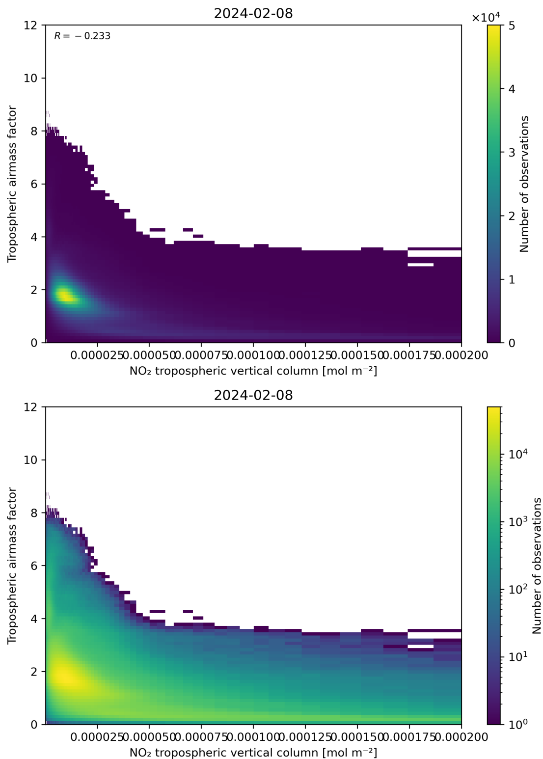
Figure 123: Scatter density plot of “NO 2 tropospheric vertical column” against “Tropospheric airmass factor” for 2024-02-07 to 2024-02-09.
