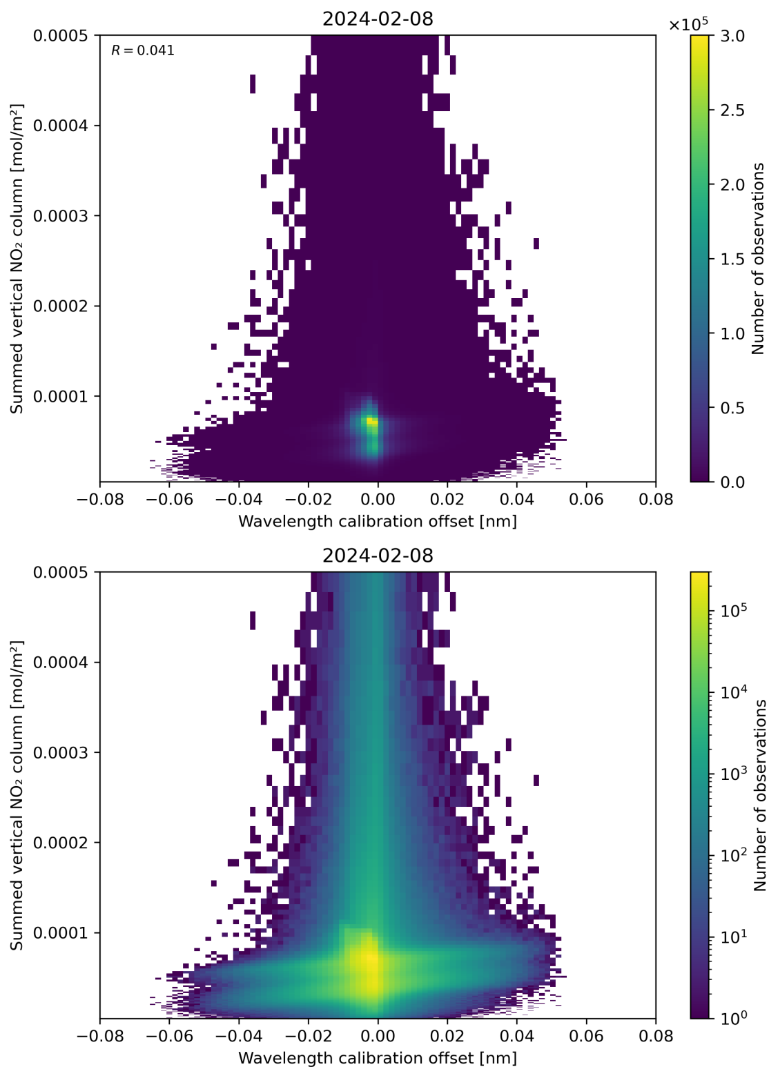
Figure 177: Scatter density plot of “Wavelength calibration offset” against “Summed vertical NO 2 column” for 2024-02-07 to 2024-02-09.
