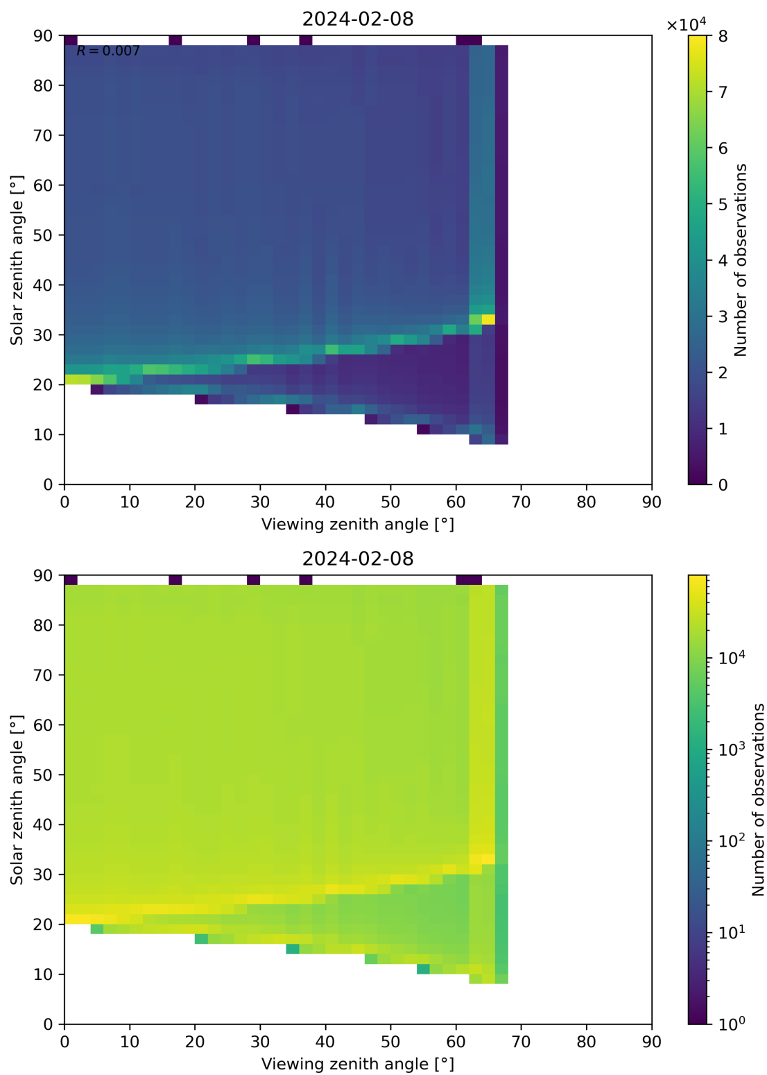
Figure 172: Scatter density plot of “Viewing zenith angle” against “Solar zenith angle” for 2024-02-07 to 2024-02-09.
