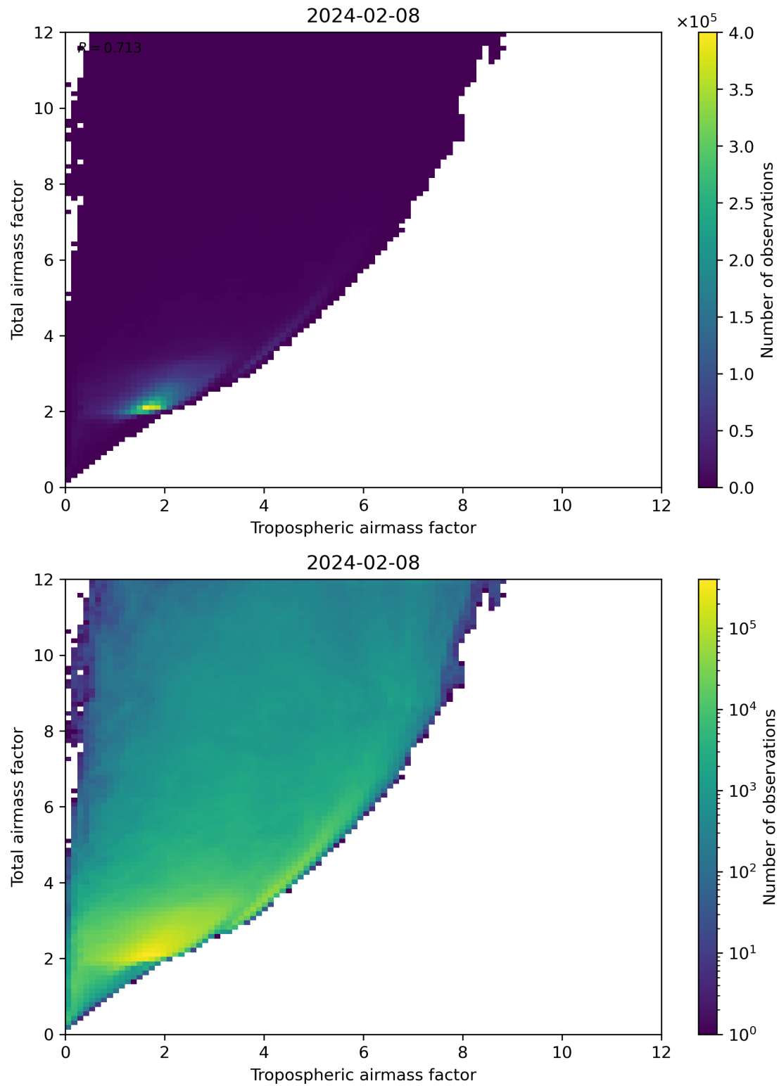
Figure 72: Scatter density plot of “Tropospheric airmass factor” against “Total airmass factor” for 2024-02-07 to 2024-02-09.
