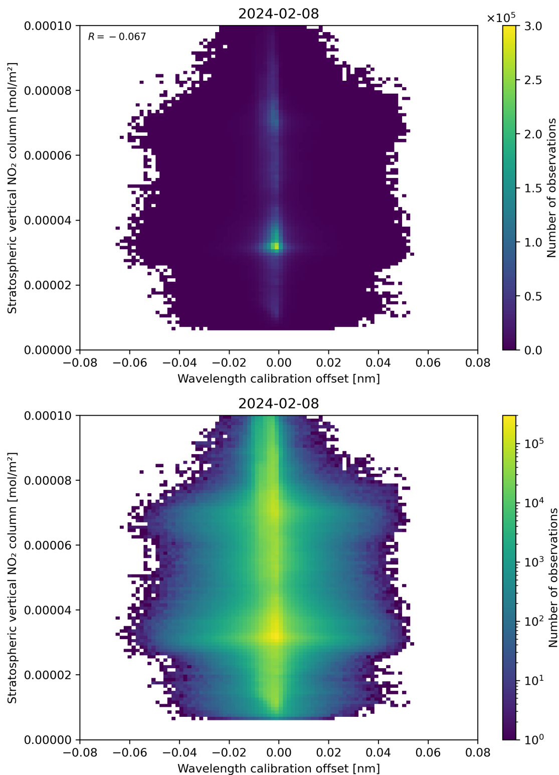
Figure 176: Scatter density plot of “Wavelength calibration offset” against “Stratospheric vertical NO 2 column” for 2024-02-07 to 2024-02-09.
