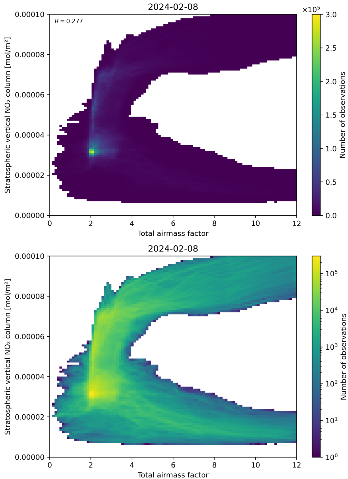
Figure 64: Scatter density plot of “Total airmass factor” against “Stratospheric vertical NO 2 column” for 2024-02-07 to 2024-02-09.
