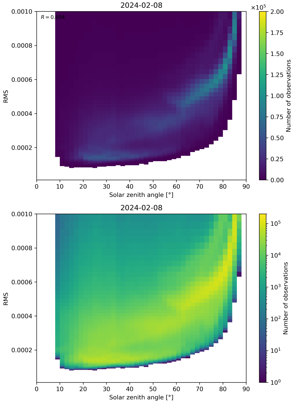
Figure 157: Scatter density plot of “Solar zenith angle” against “RMS” for 2024-02-07 to 2024-02-09.
