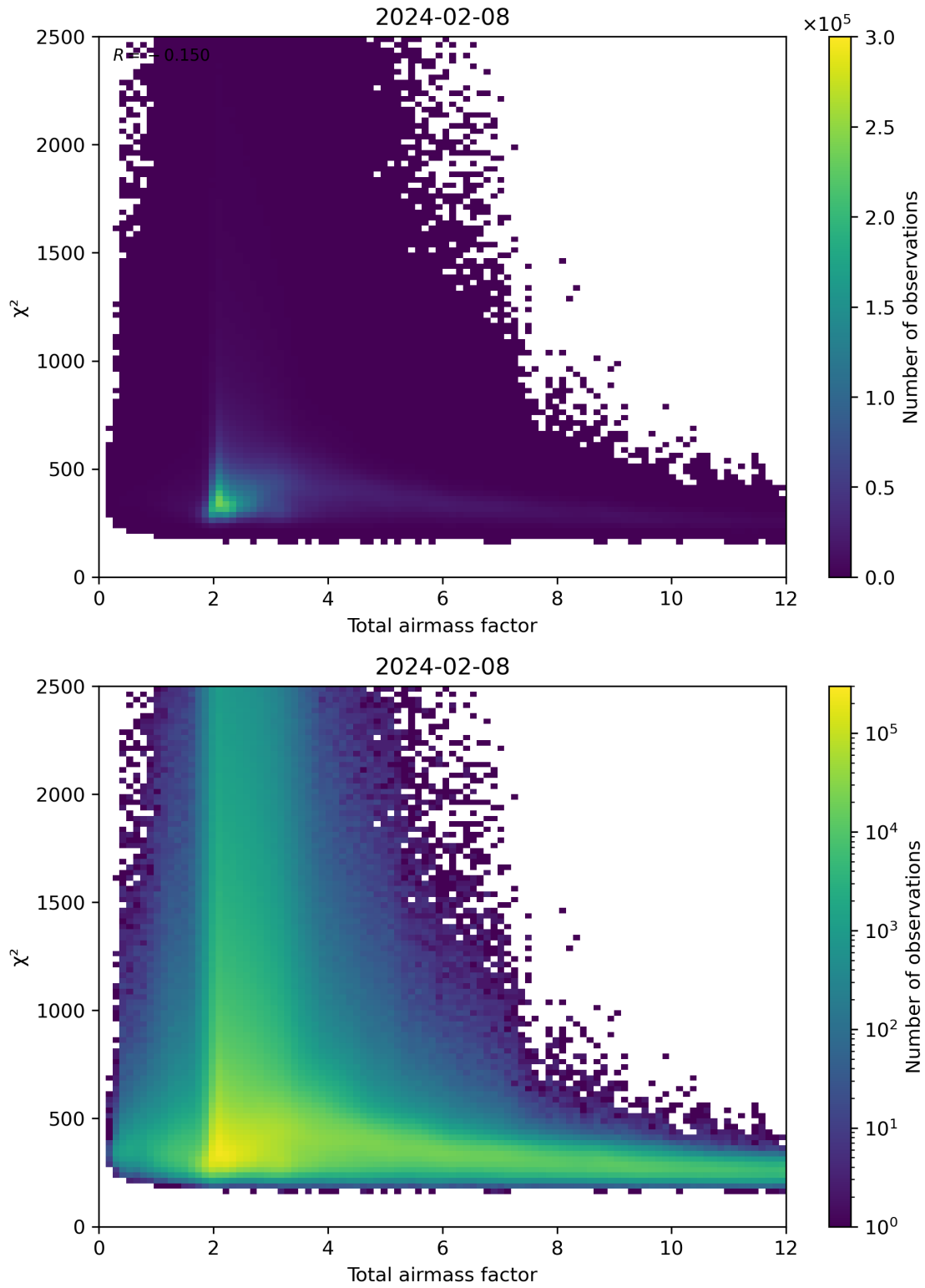
Figure 63: Scatter density plot of “Total airmass factor” against “ \chi^2 ” for 2024-02-07 to 2024-02-09.
