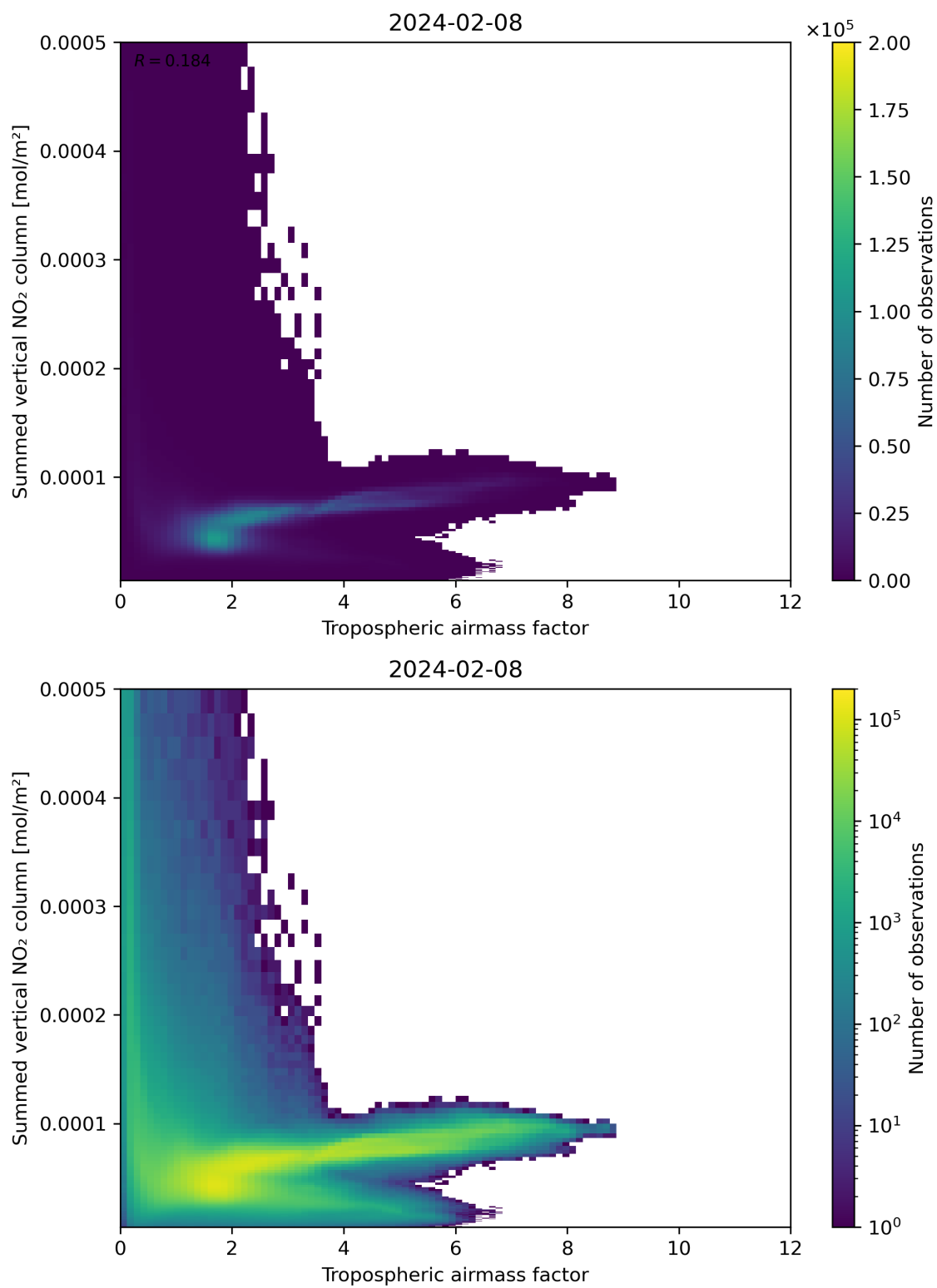
Figure 75: Scatter density plot of “Tropospheric airmass factor” against “Summed vertical NO 2 column” for 2024-02-07 to 2024-02-09.
