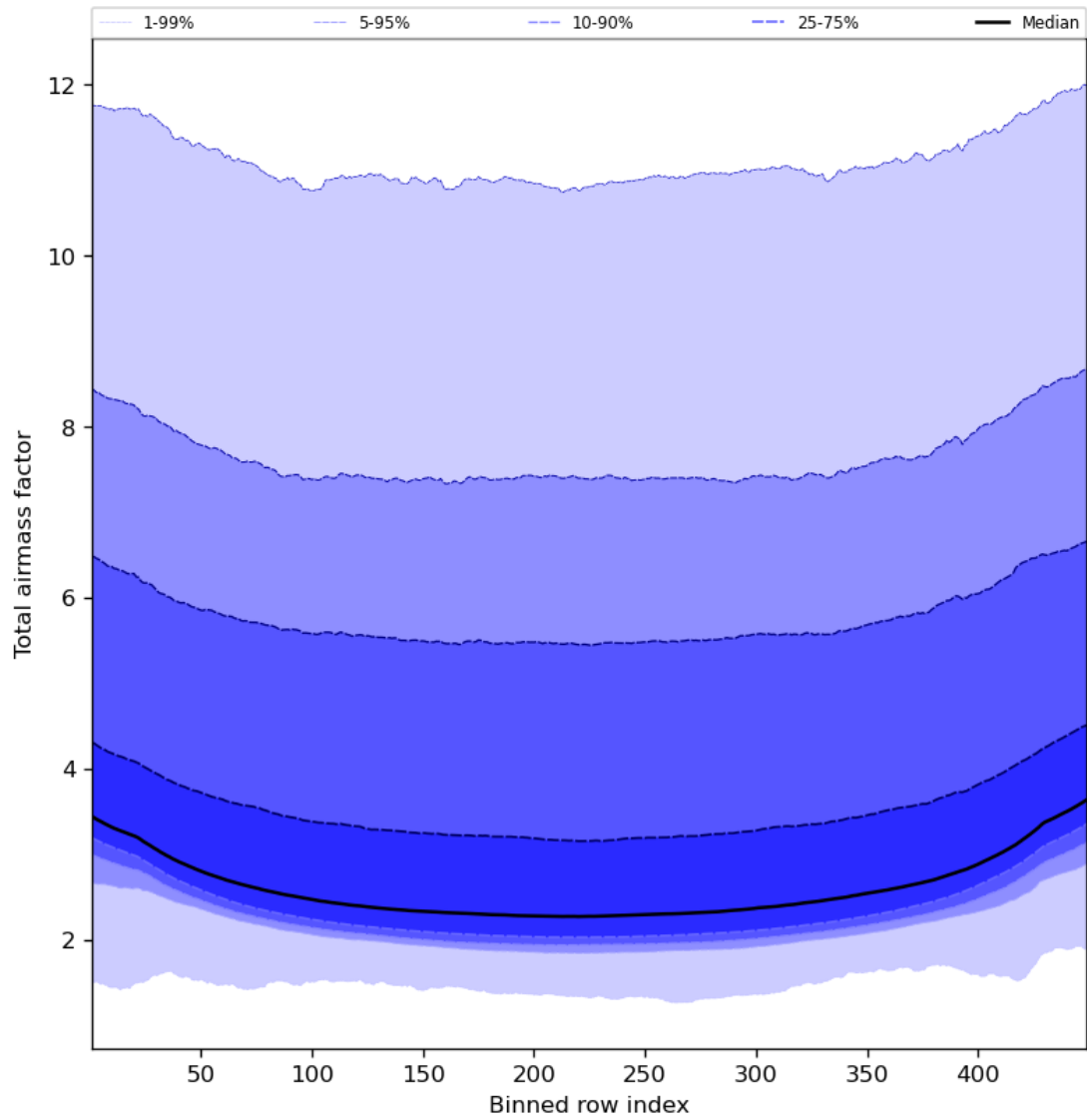
Figure 49: Along track statistics of “Total airmass factor” for 2024-02-07 to 2024-02-09
