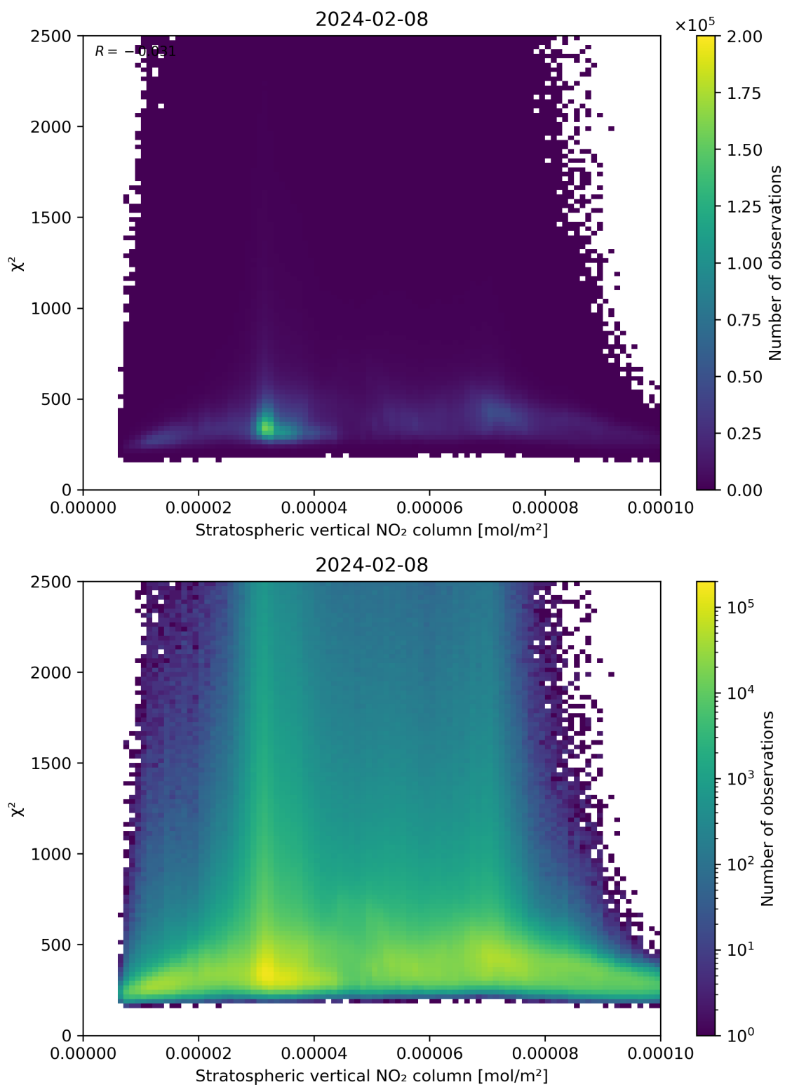
Figure 97: Scatter density plot of “Stratospheric vertical NO 2 column” against “ \chi^2 ” for 2024-02-07 to 2024-02-09.
