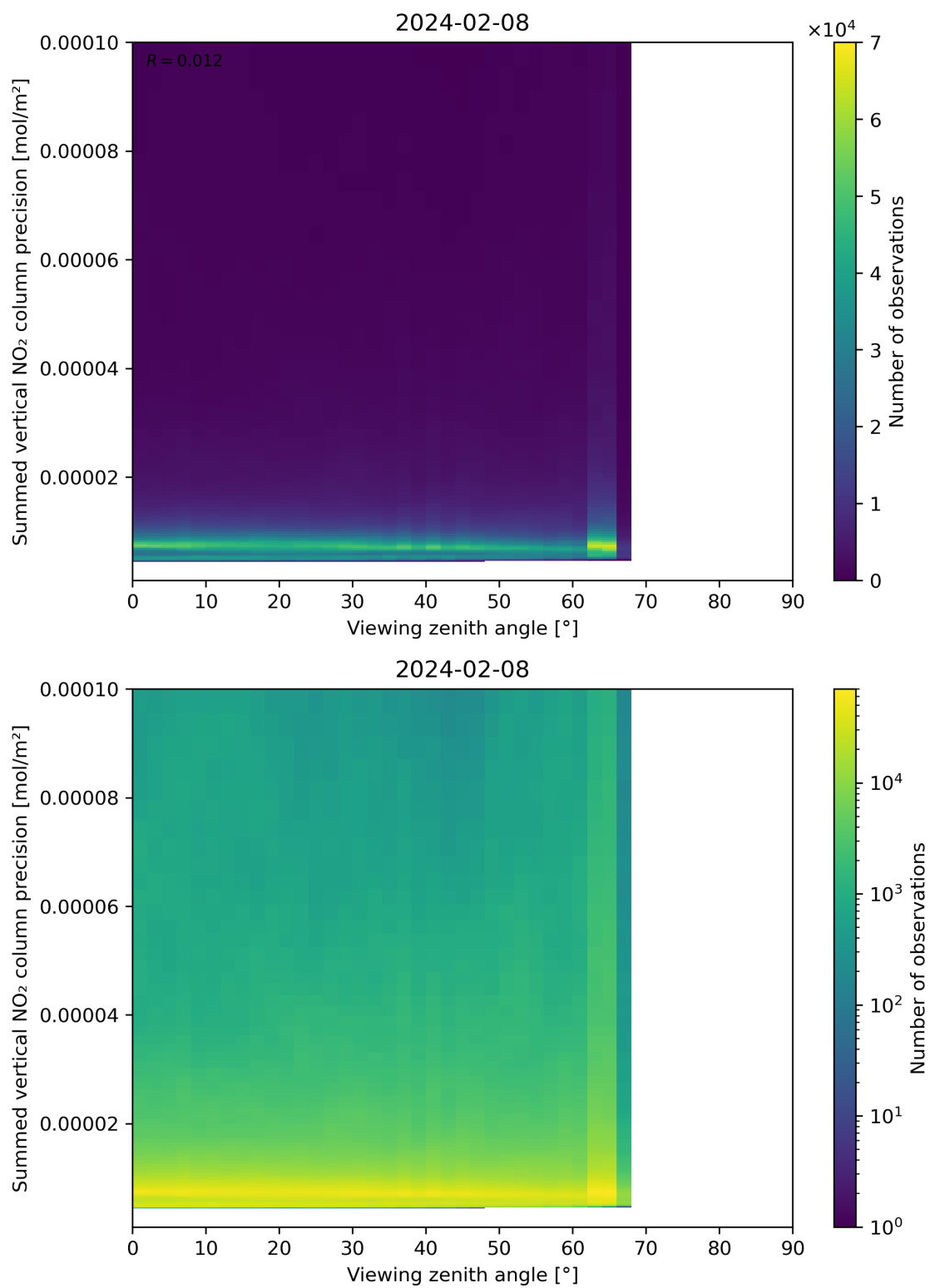
Figure 166: Scatter density plot of “Viewing zenith angle” against “Summed vertical NO 2 column precision” for 2024-02-07 to 2024-02-09.
