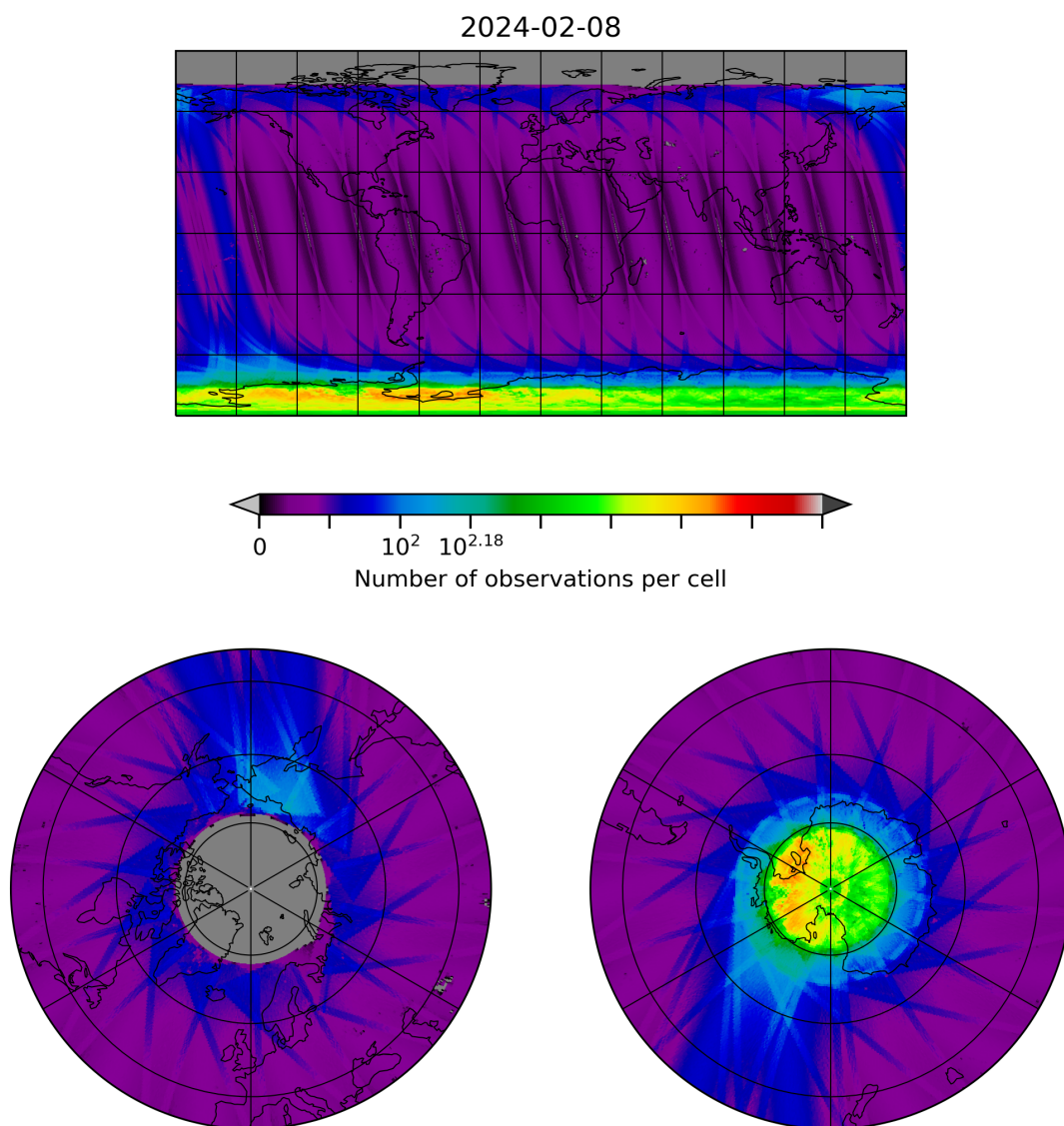
Figure 10: Map of the number of observations for 2024-02-07 to 2024-02-09
