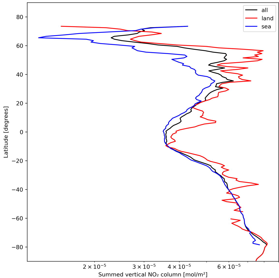
Figure 23: Zonal average of “Summed vertical NO 2 column” for 2024-02-07 to 2024-02-09.
