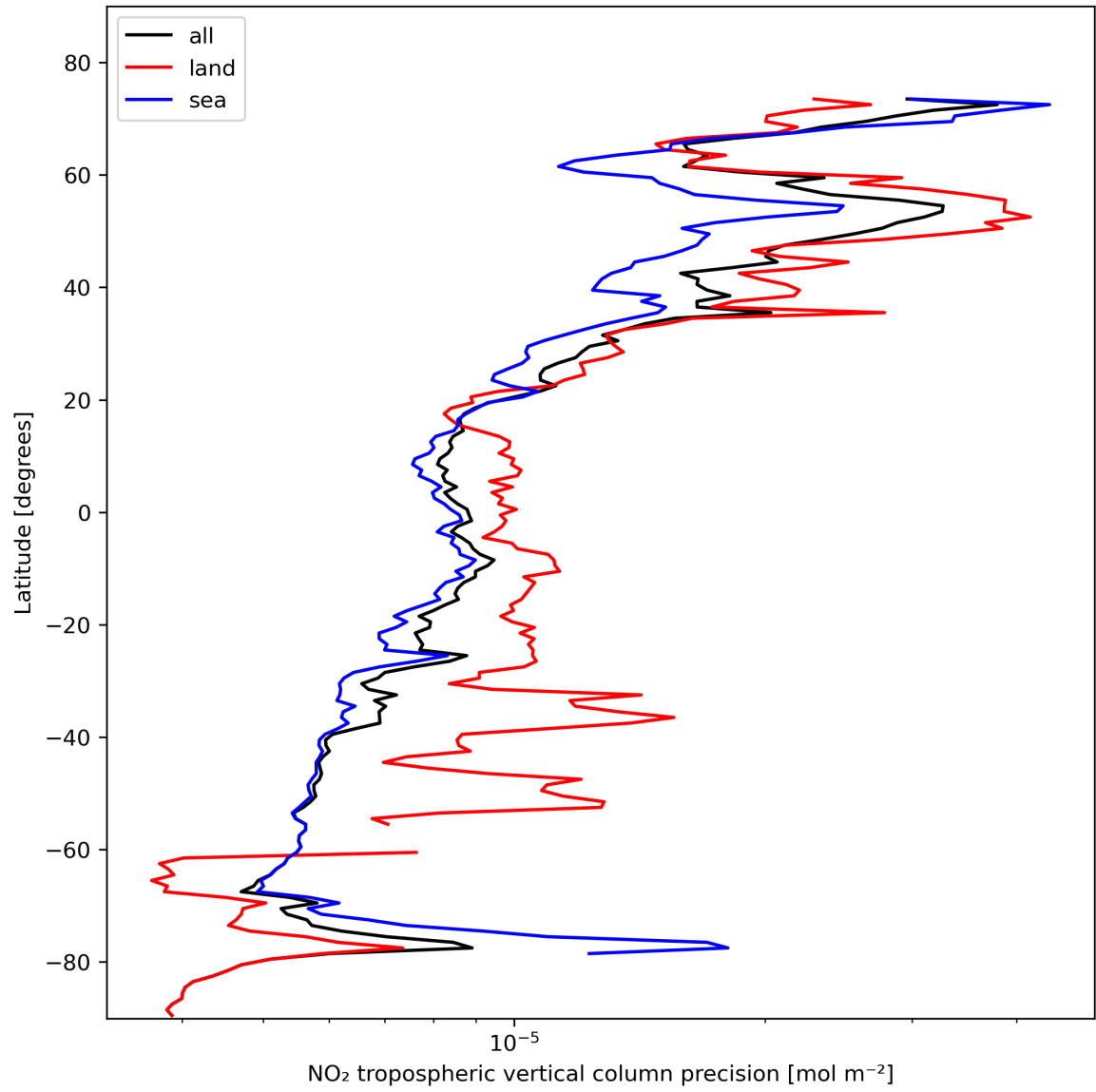
Figure 13: Zonal average of “NO 2 tropospheric vertical column precision” for 2024-02-07 to 2024-02-09.
