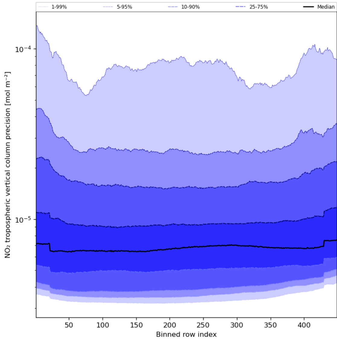
Figure 47: Along track statistics of “NO 2 tropospheric vertical column precision” for 2024-02-07 to 2024-02-09
