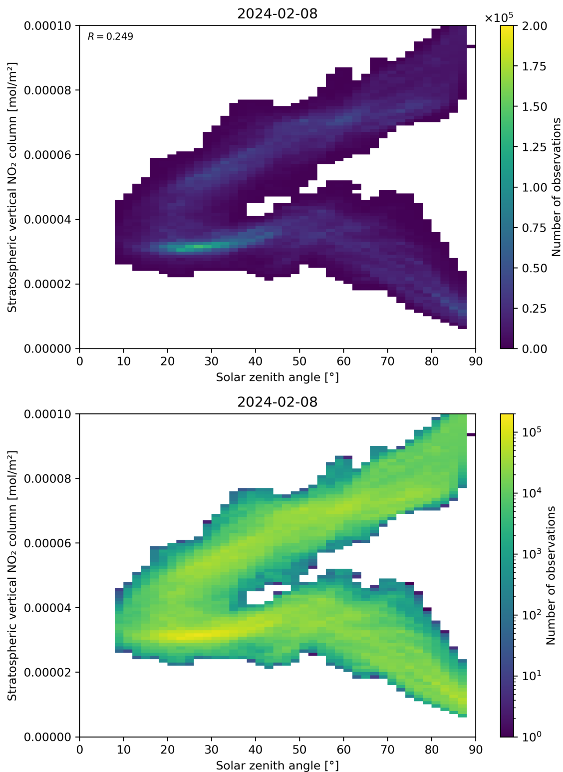
Figure 150: Scatter density plot of “Solar zenith angle” against “Stratospheric vertical NO 2 column” for 2024-02-07 to 2024-02-09.
