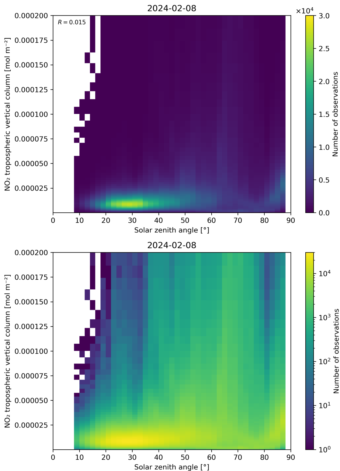
Figure 155: Scatter density plot of “Solar zenith angle” against “NO 2 tropospheric vertical column” for 2024-02-07 to 2024-02-09.
