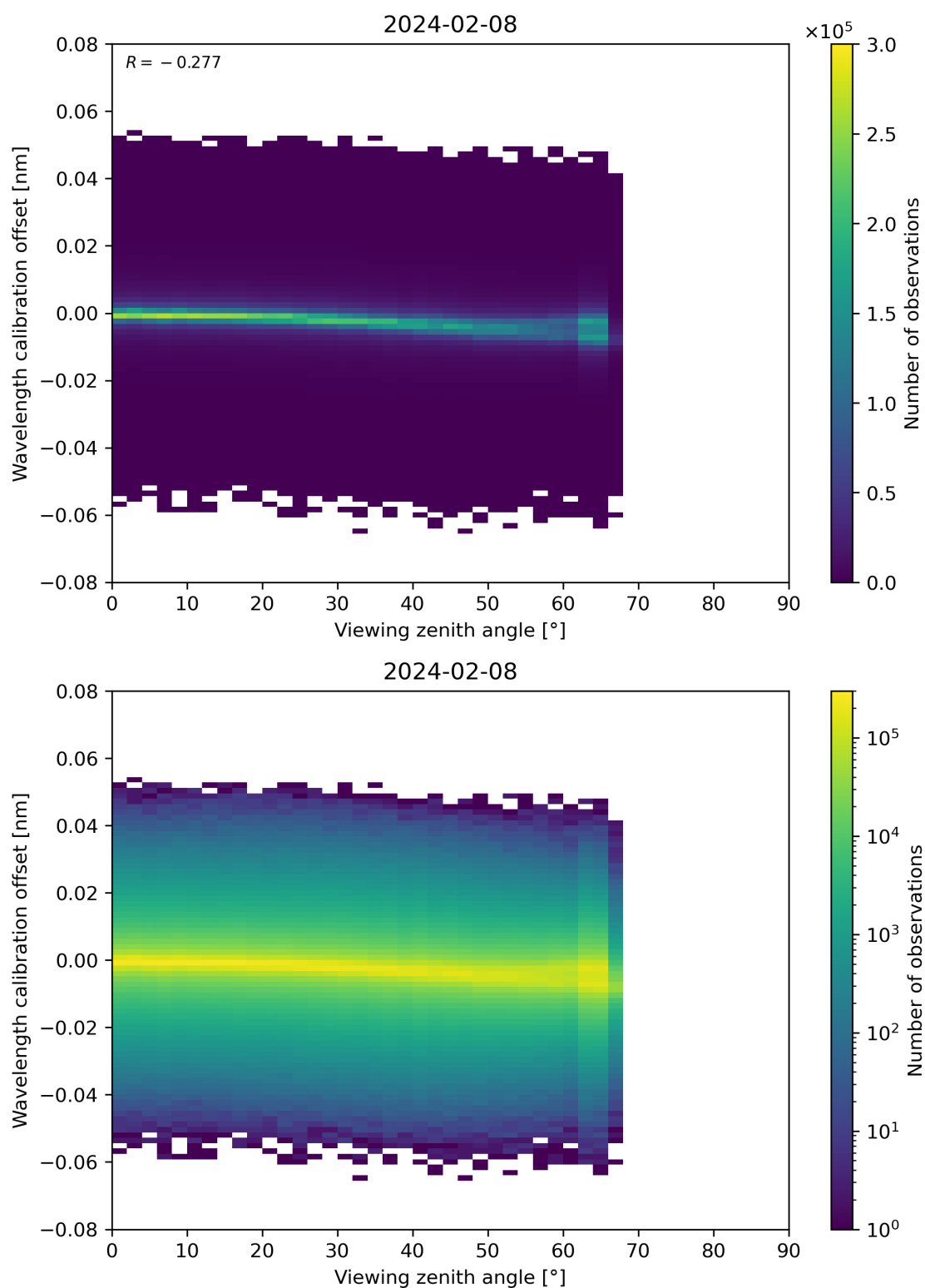
Figure 173: Scatter density plot of “Viewing zenith angle” against “Wavelength calibration offset” for 2024-02-07 to 2024-02-09.
