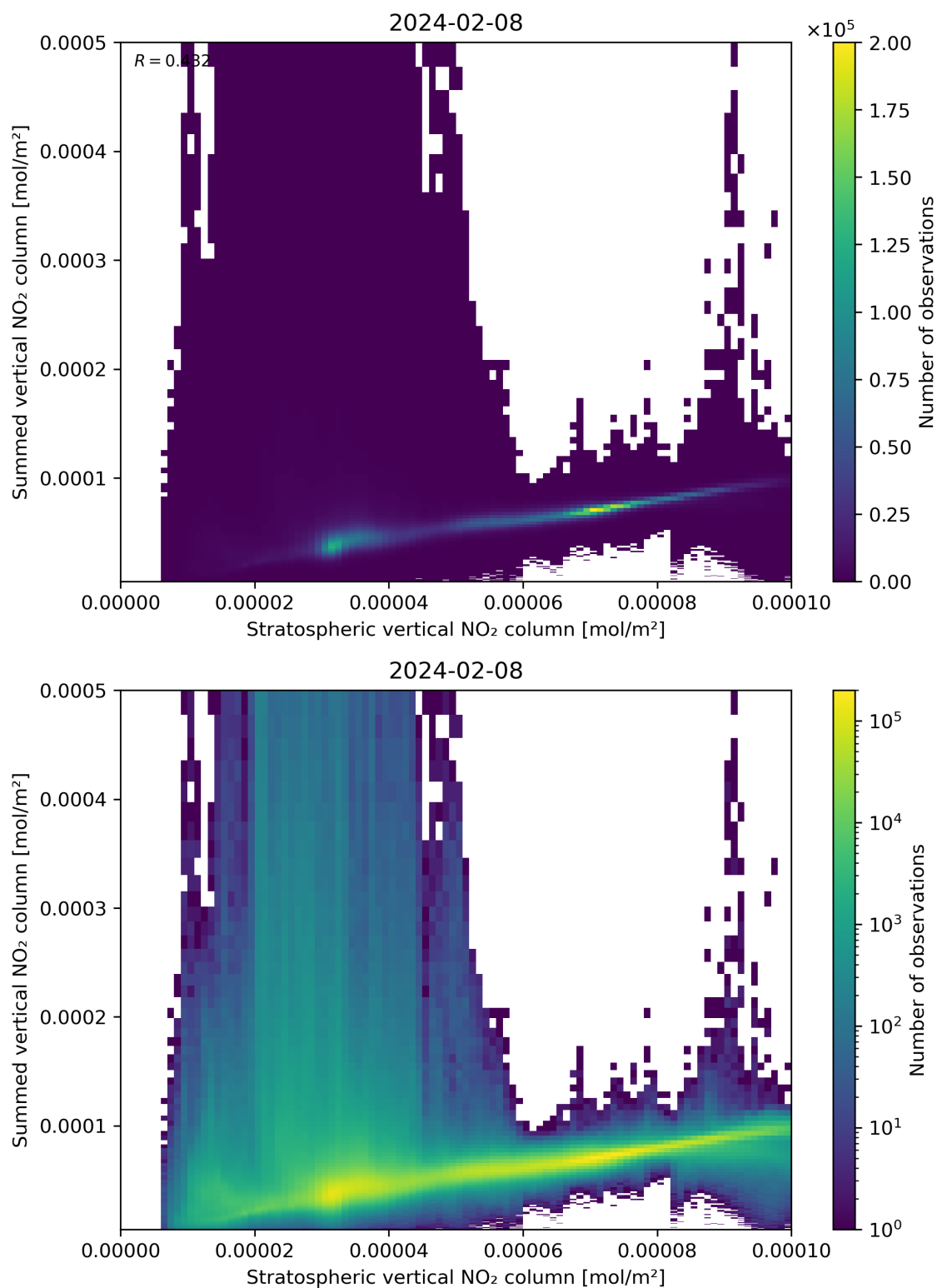
Figure 98: Scatter density plot of “Stratospheric vertical NO 2 column” against “Summed vertical NO 2 column” for 2024-02-07 to 2024-02-09.
