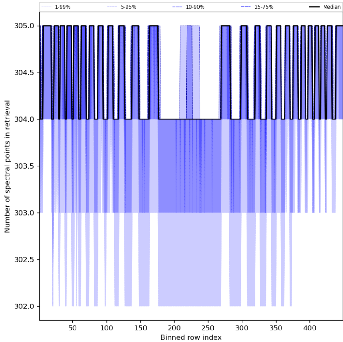
Figure 50: Along track statistics of “Number of spectral points in retrieval” for 2024-02-07 to 2024-02-09
