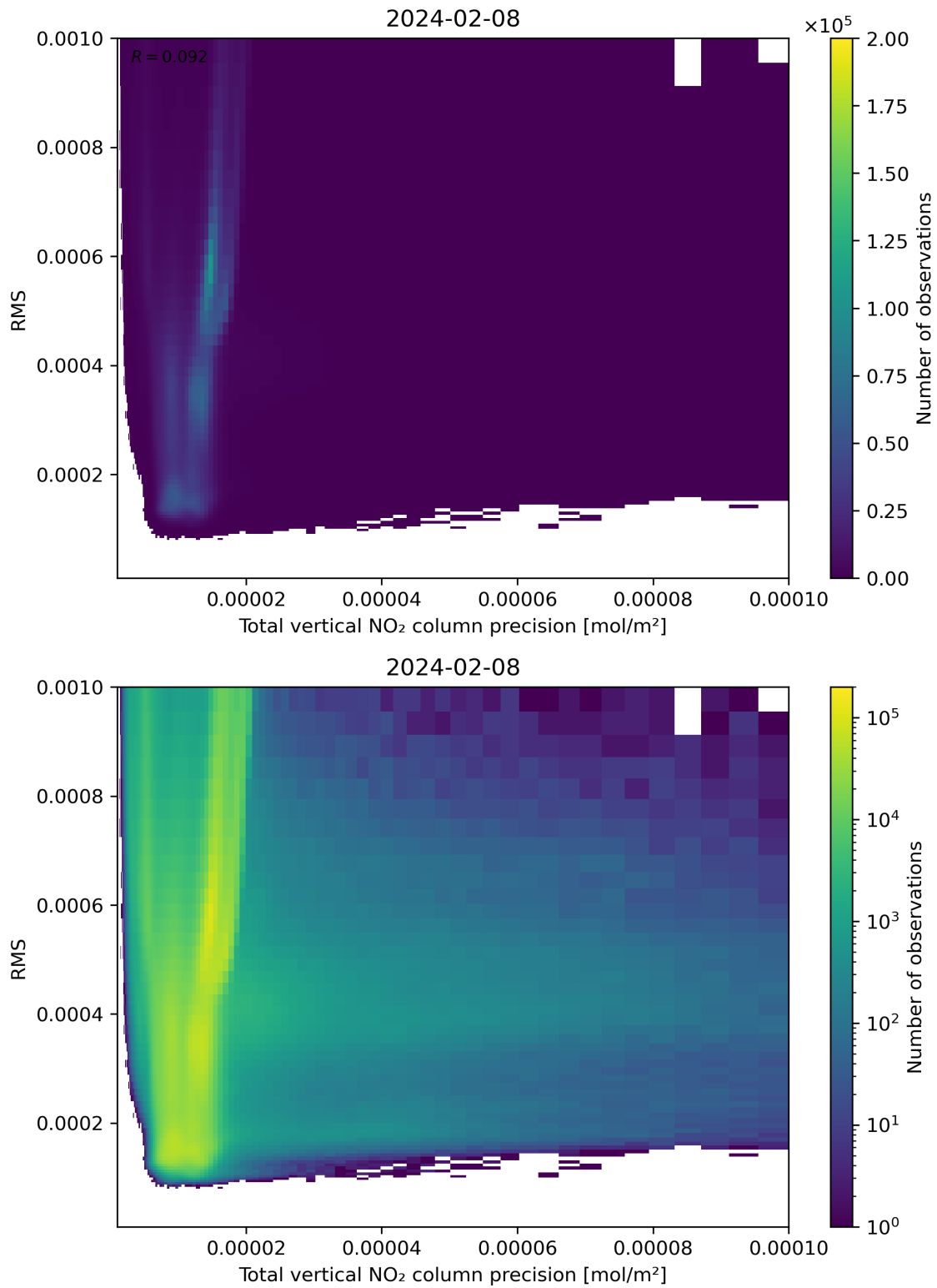
Figure 119: Scatter density plot of “Total vertical NO 2 column precision” against “RMS” for 2024-02-07 to 2024-02-09.
