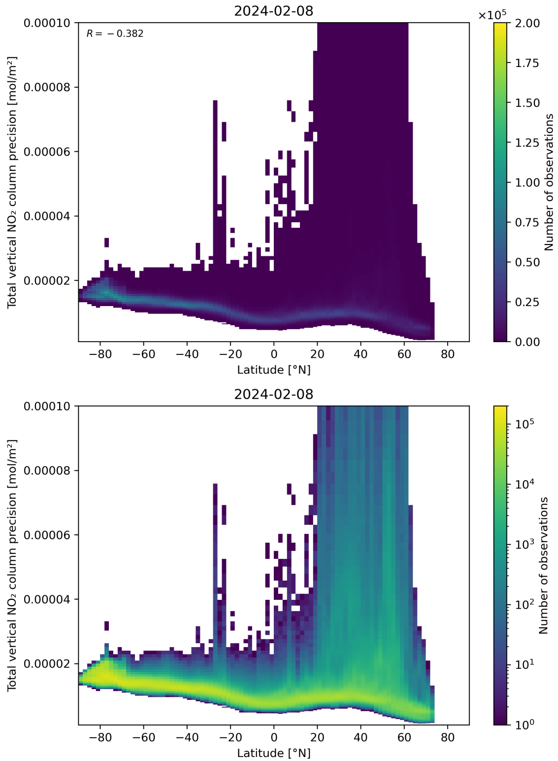
Figure 91: Scatter density plot of “Latitude” against “Total vertical NO 2 column precision” for 2024-02-07 to 2024-02-09.
