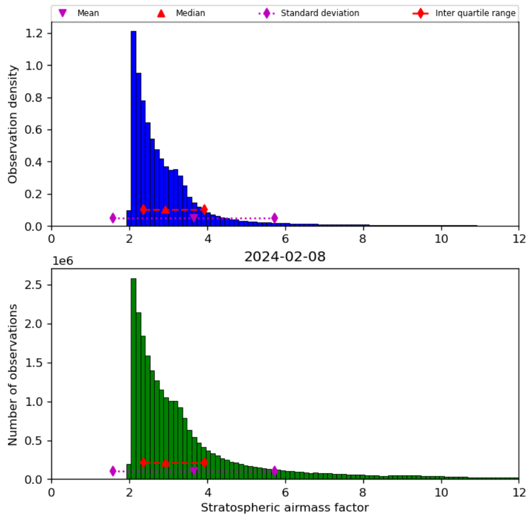
Figure 44: Histogram of “Stratospheric airmass factor” for 2024-02-07 to 2024-02-09
