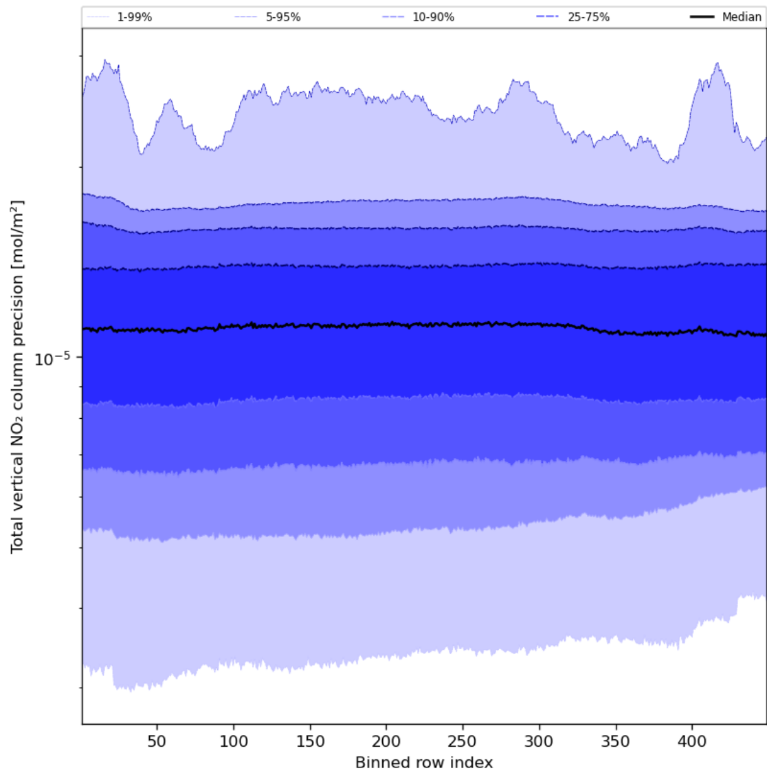
Figure 56: Along track statistics of “Total vertical NO 2 column precision” for 2024-02-07 to 2024-02-09
