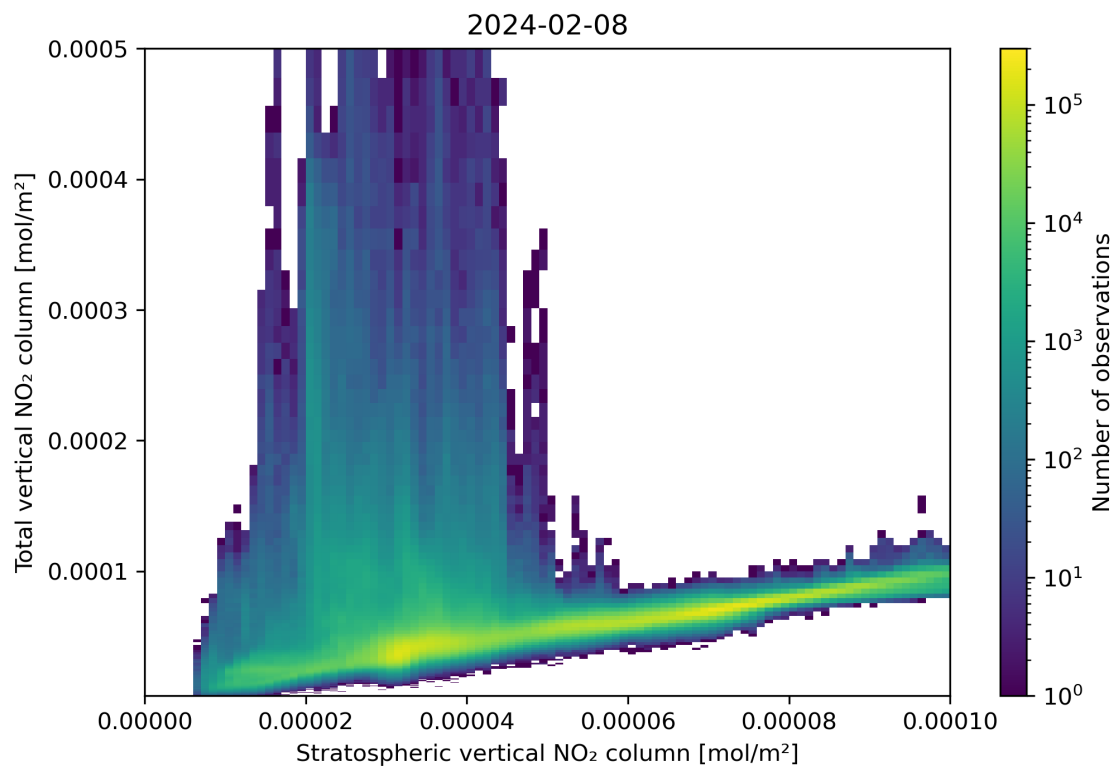
Figure 100: Scatter density plot of “Stratospheric vertical NO 2 column” against “Total vertical NO 2 column” for 2024-02-07 to 2024-02-09.
