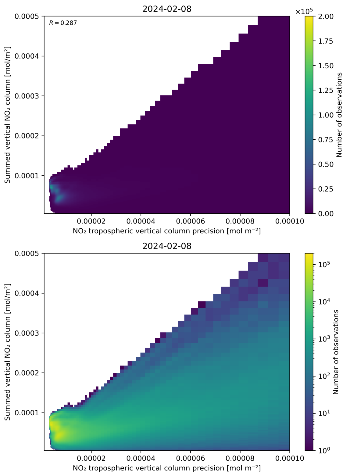
Figure 136: Scatter density plot of “NO 2 tropospheric vertical column precision” against “Summed vertical NO 2 column” for 2024-02-07 to 2024-02-09.
