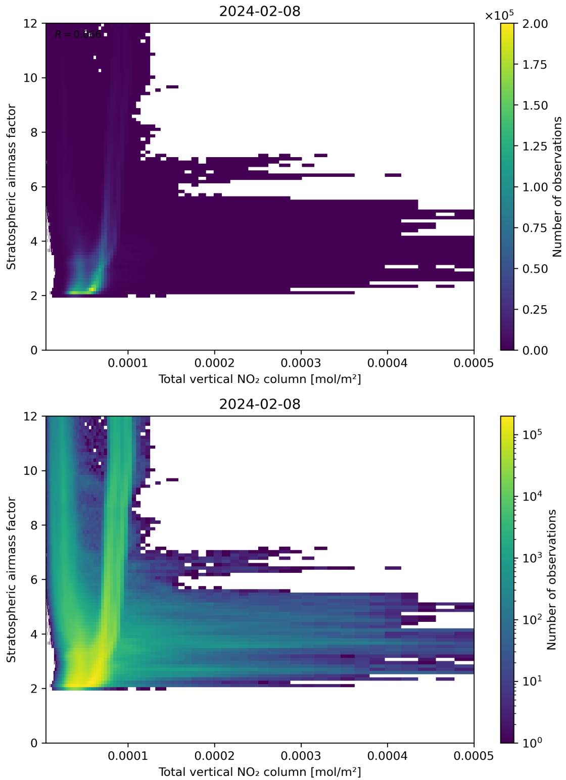
Figure 110: Scatter density plot of “Total vertical NO 2 column” against “Stratospheric airmass factor” for 2024-02-07 to 2024-02-09.
