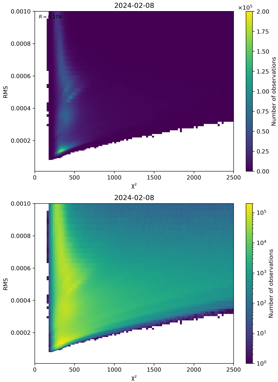
Figure 82: Scatter density plot of “ \chi^2 ” against “RMS” for 2024-02-07 to 2024-02-09.
