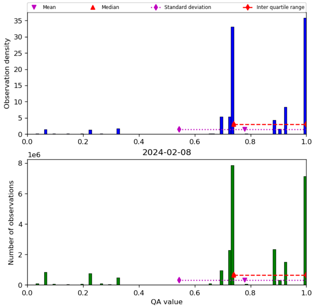
Figure 28: Histogram of “QA value” for 2024-02-07 to 2024-02-09
