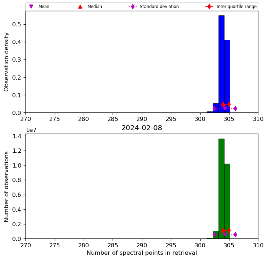
Figure 33: Histogram of “Number of spectral points in retrieval” for 2024-02-07 to 2024-02-09
