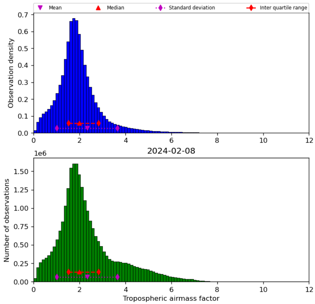
Figure 31: Histogram of “Tropospheric airmass factor” for 2024-02-07 to 2024-02-09
