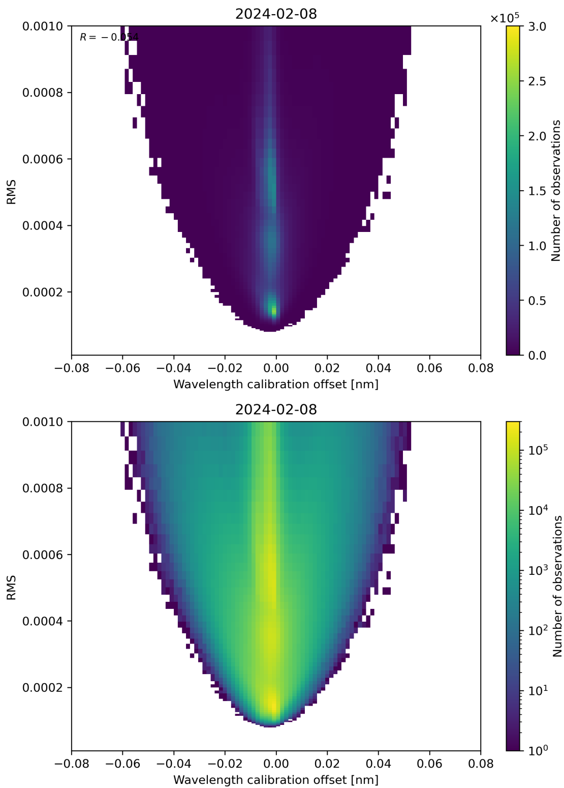
Figure 181: Scatter density plot of “Wavelength calibration offset” against “RMS” for 2024-02-07 to 2024-02-09.
