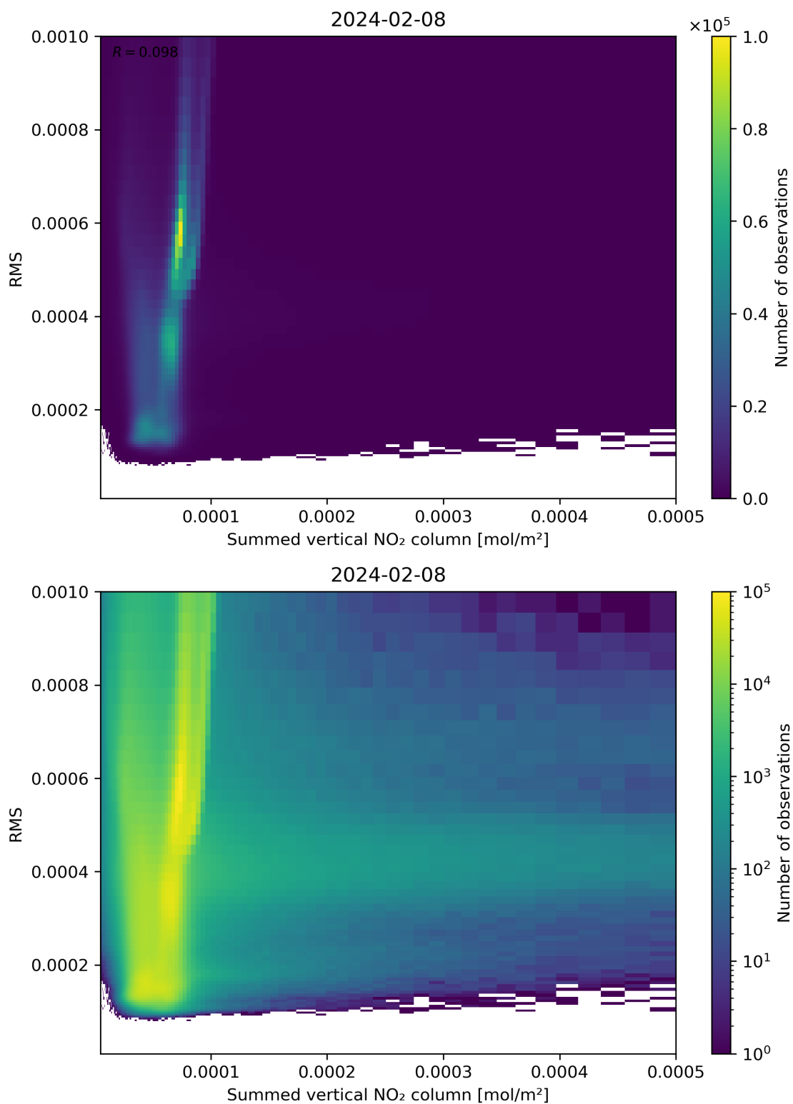
Figure 109: Scatter density plot of “Summed vertical NO 2 column” against “RMS” for 2024-02-07 to 2024-02-09.
