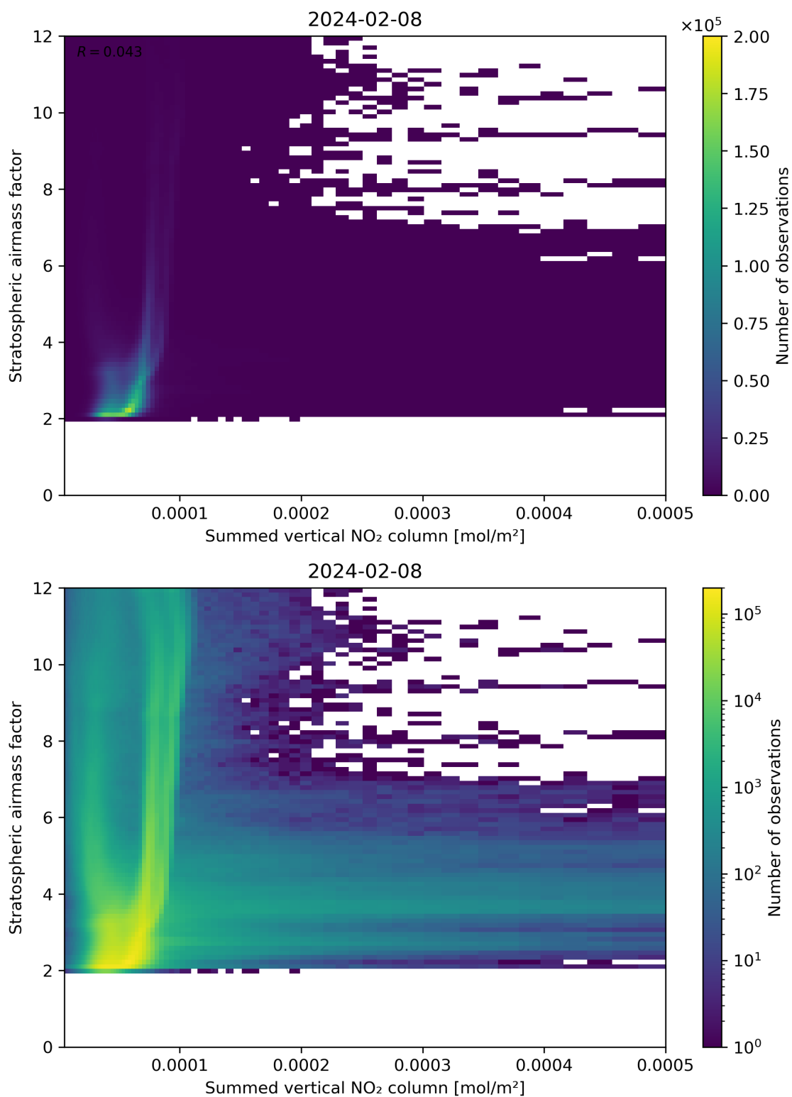
Figure 103: Scatter density plot of “Summed vertical NO 2 column” against “Stratospheric air mass factor” for 2024-02-07 to 2024-02-09.
