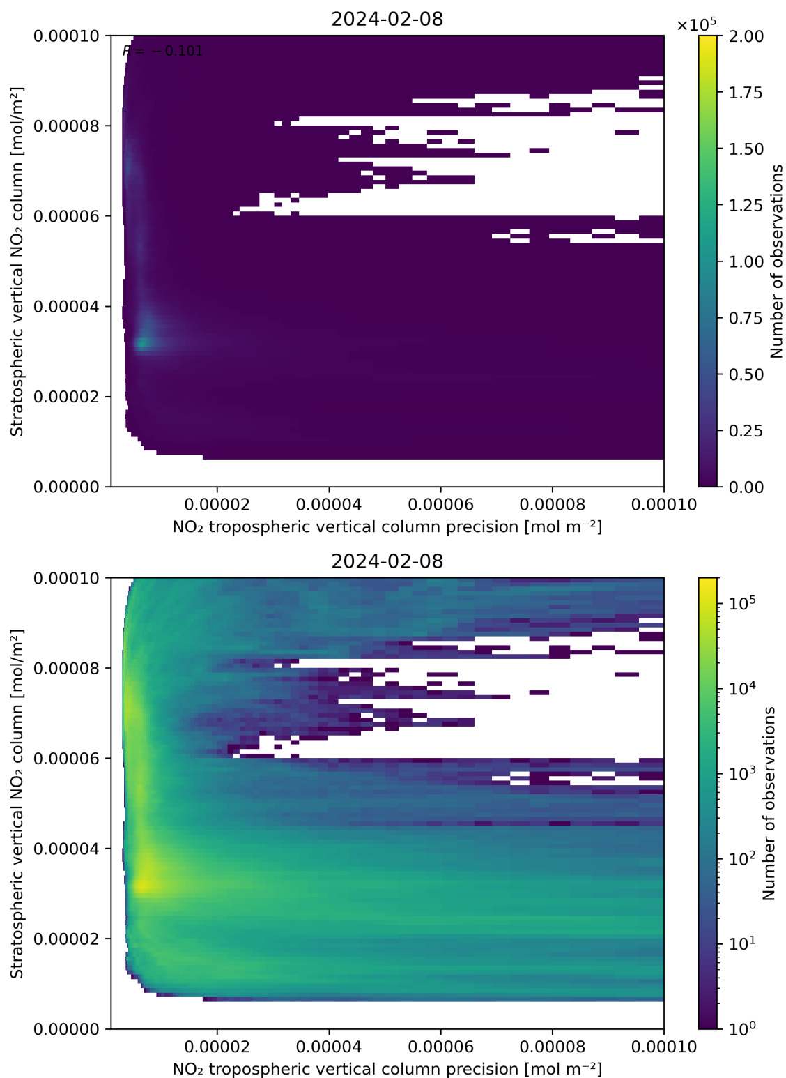
Figure 135: Scatter density plot of “NO 2 tropospheric vertical column precision” against “Stratospheric vertical NO 2 column” for 2024-02-07 to 2024-02-09.
