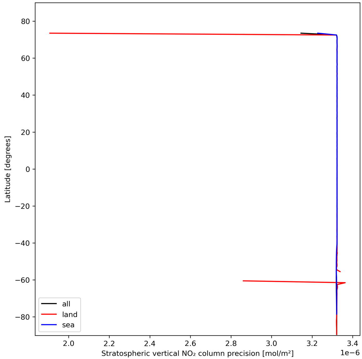
Figure 20: Zonal average of “Stratospheric vertical NO 2 column precision” for 2024-02-07 to 2024-02-09.
