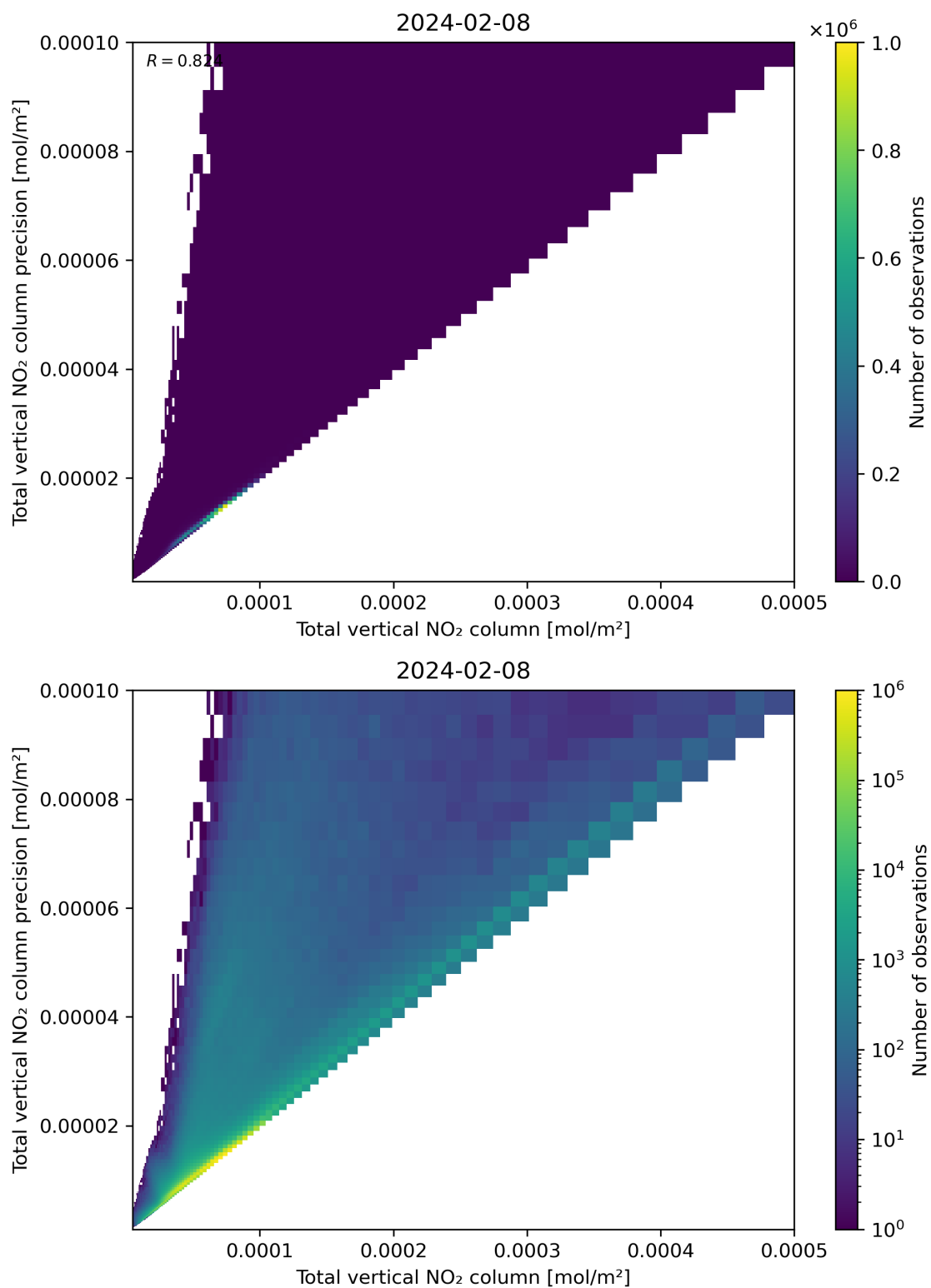
Figure 114: Scatter density plot of “Total vertical NO 2 column” against “Total vertical NO 2 column precision” for 2024-02-07 to 2024-02-09.
