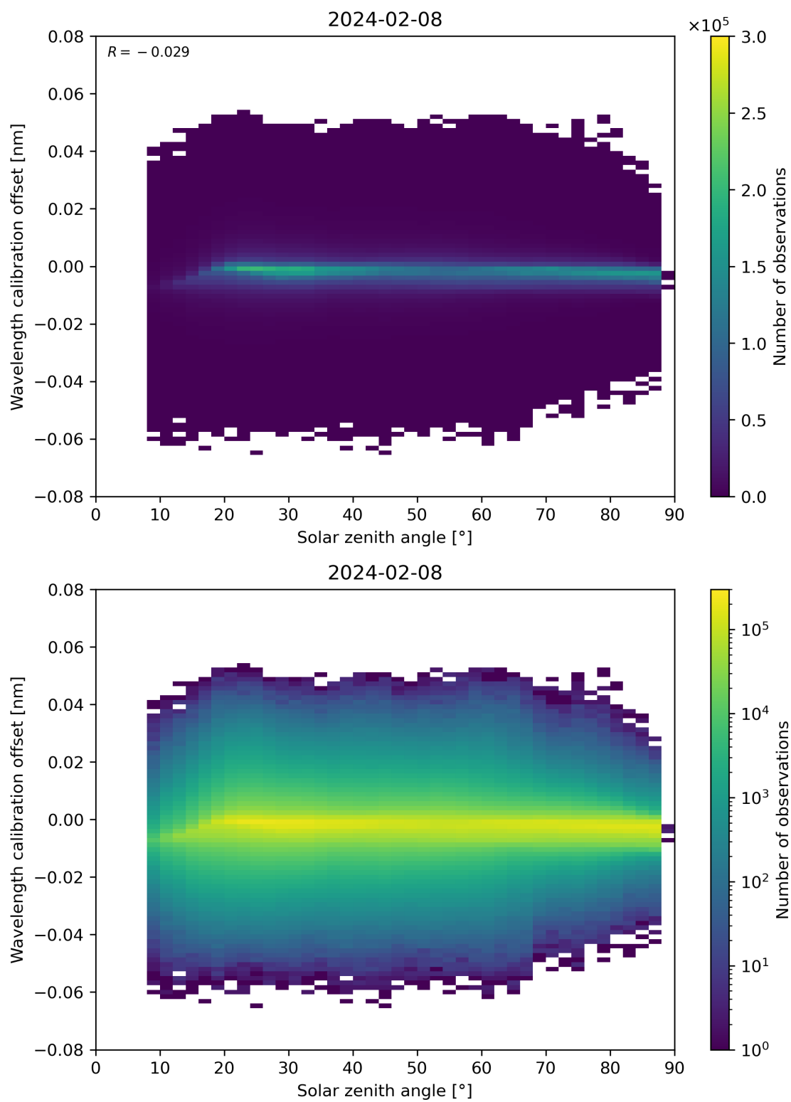
Figure 158: Scatter density plot of “Solar zenith angle” against “Wavelength calibration offset” for 2024-02-07 to 2024-02-09.
