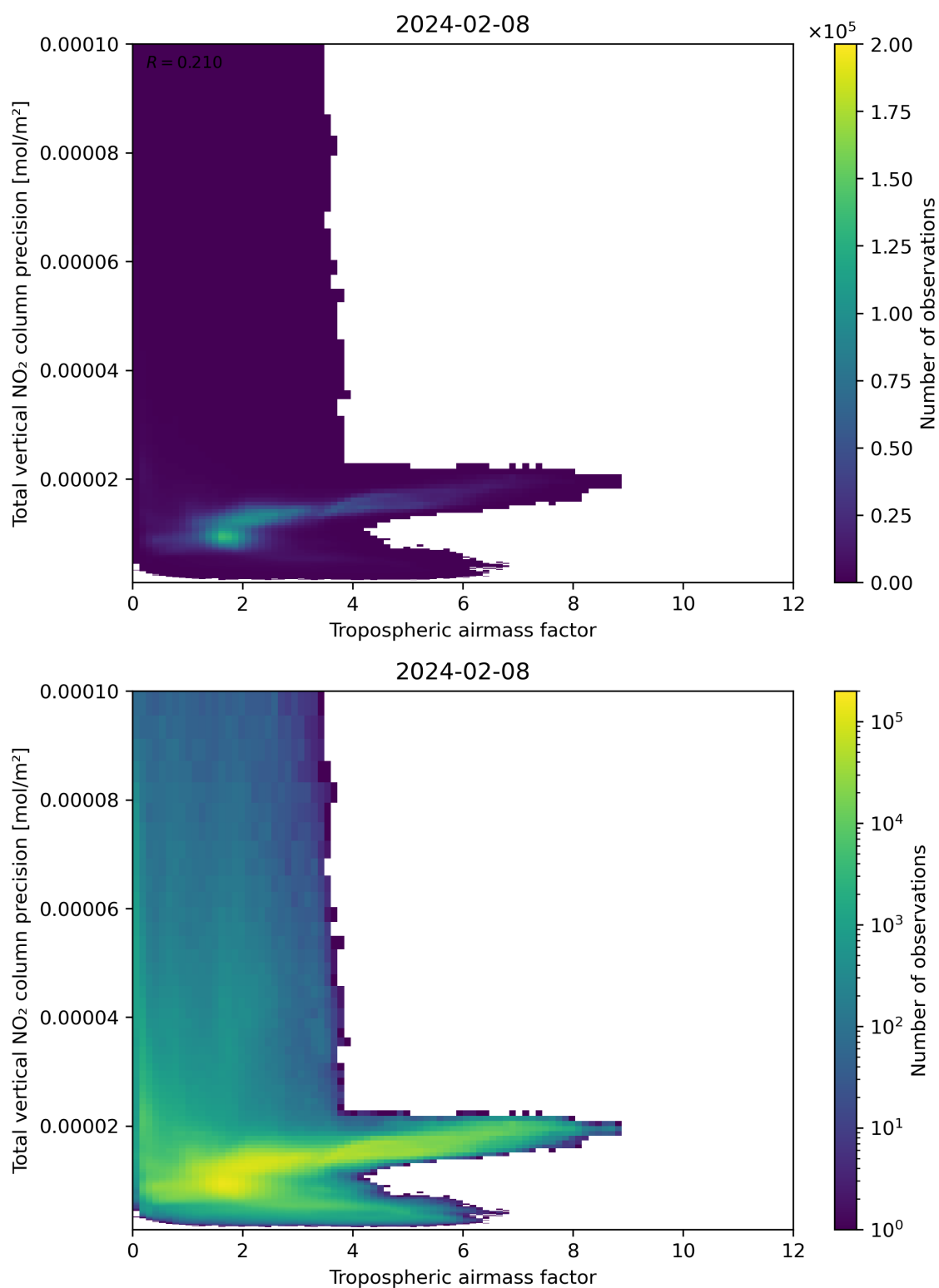
Figure 78: Scatter density plot of “Tropospheric air mass factor” against “Total vertical NO 2 column precision” for 2024-02-07 to 2024-02-09.
