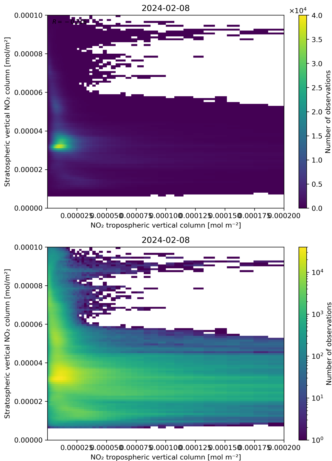
Figure 125: Scatter density plot of “NO 2 tropospheric vertical column” against “Stratospheric vertical NO 2 column” for 2024-02-07 to 2024-02-09.
