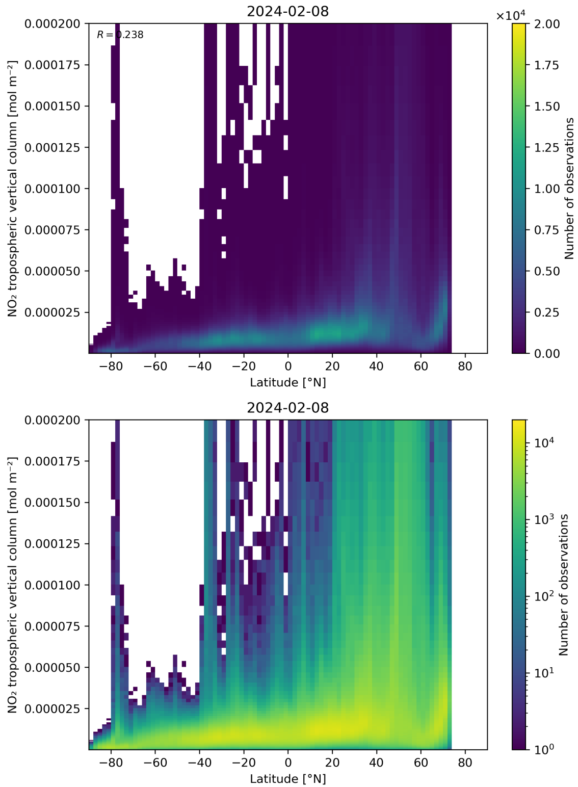
Figure 92: Scatter density plot of “Latitude” against “NO 2 tropospheric vertical column” for 2024-02-07 to 2024-02-09.
