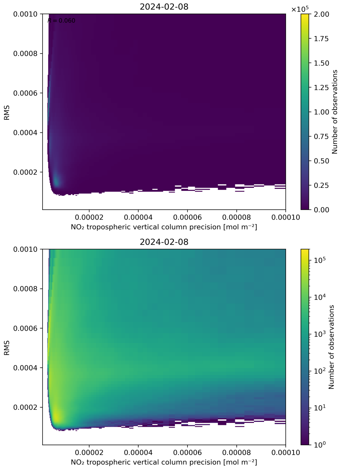
Figure 140: Scatter density plot of “NO 2 tropospheric vertical column precision” against “RMS” for 2024-02-07 to 2024-02-09.
