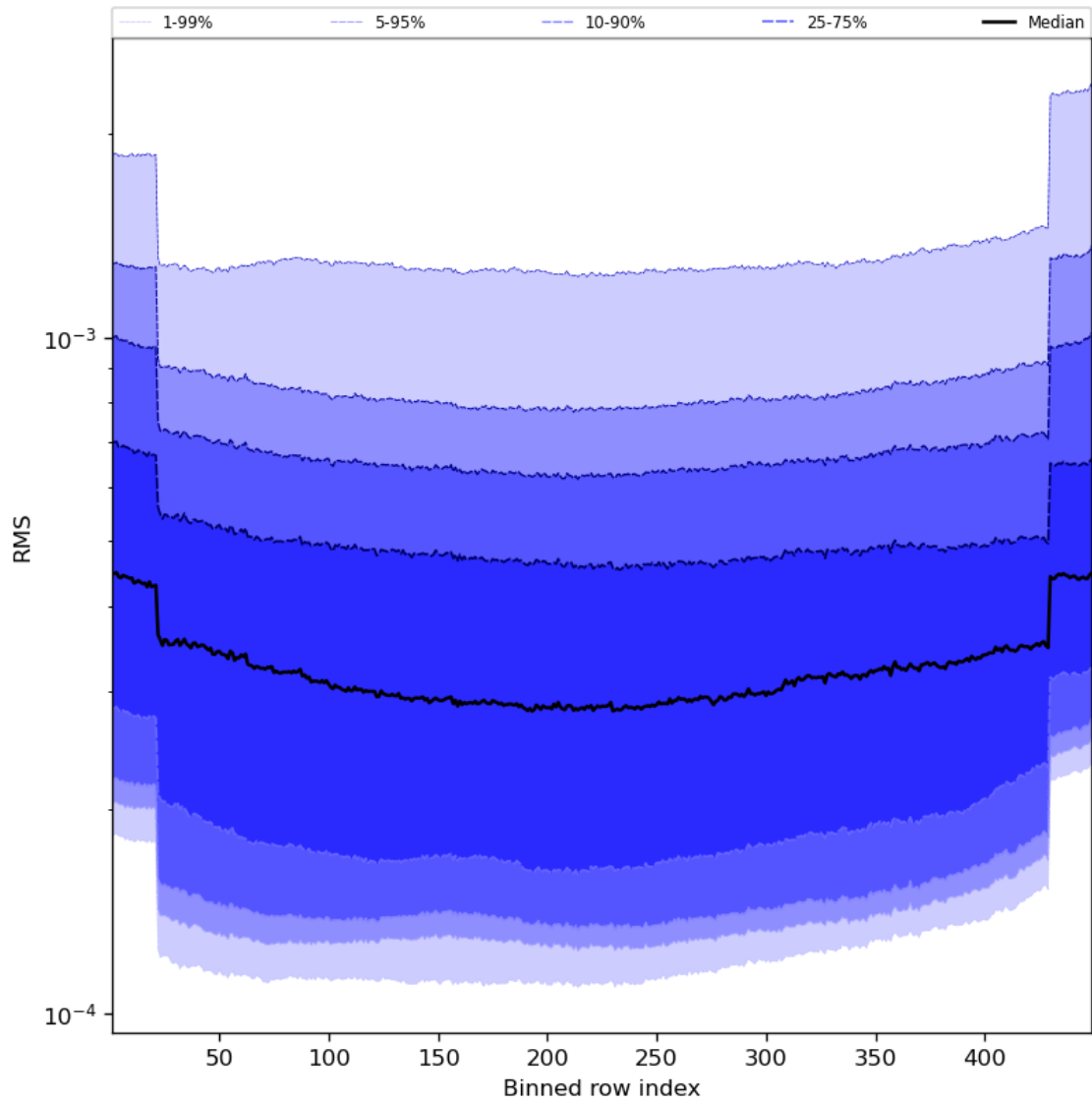
Figure 60: Along track statistics of “RMS” for 2024-02-07 to 2024-02-09
