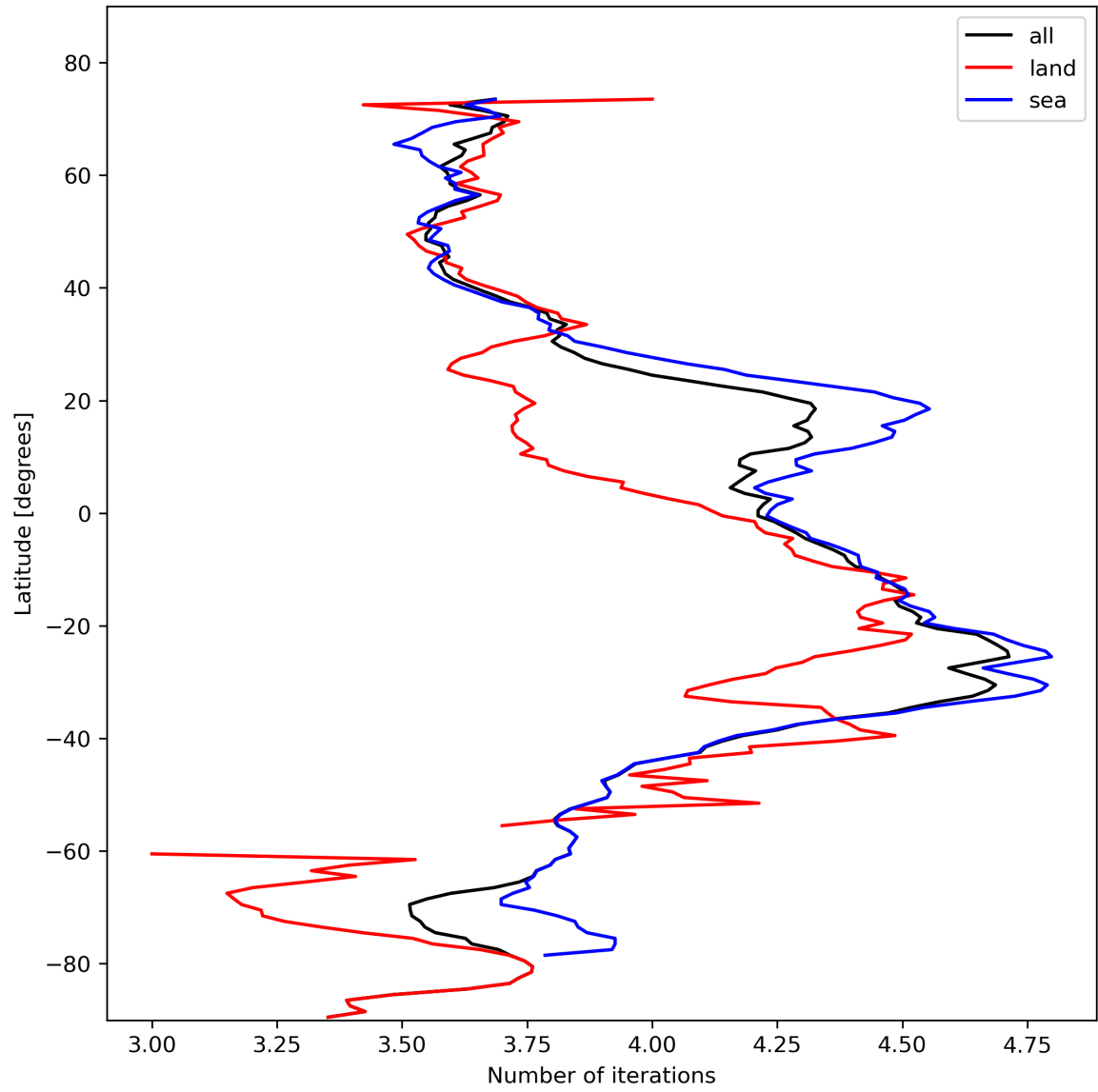
Figure 17: Zonal average of “Number of iterations” for 2024-02-07 to 2024-02-09.
