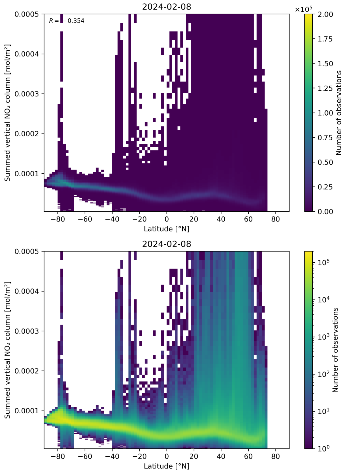
Figure 88: Scatter density plot of “Latitude” against “Summed vertical NO 2 column” for 2024-02-07 to 2024-02-09.
