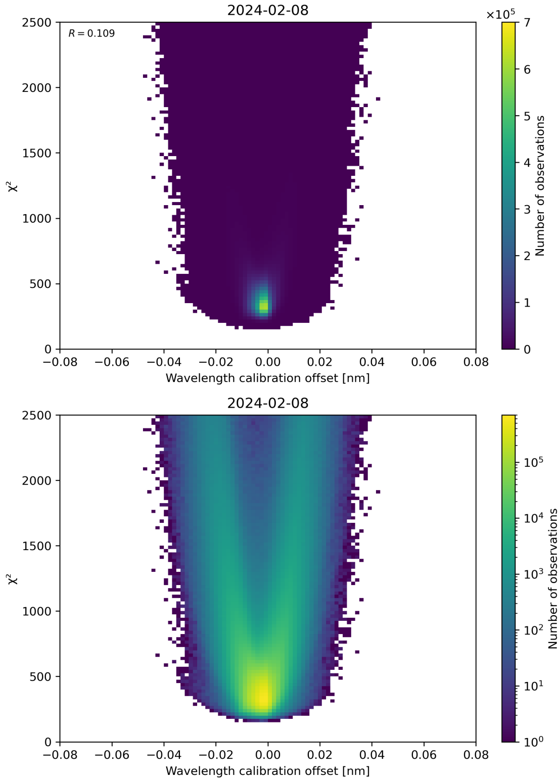
Figure 175: Scatter density plot of “Wavelength calibration offset” against “ \chi^2 ” for 2024-02-07 to 2024-02-09.
