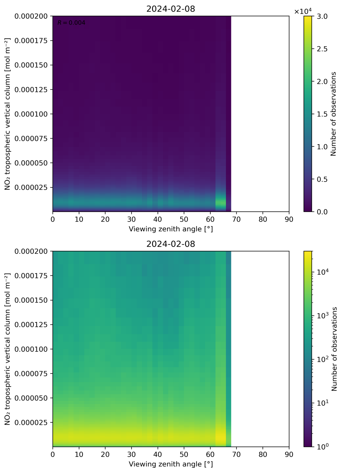
Figure 169: Scatter density plot of “Viewing zenith angle” against “NO 2 tropospheric vertical column” for 2024-02-07 to 2024-02-09.
