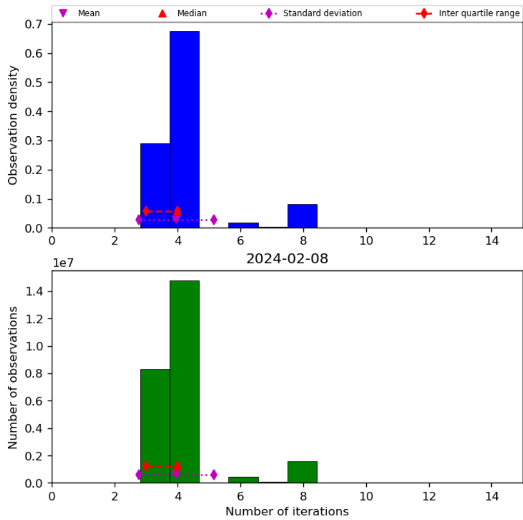
Figure 34: Histogram of “Number of iterations” for 2024-02-07 to 2024-02-09
