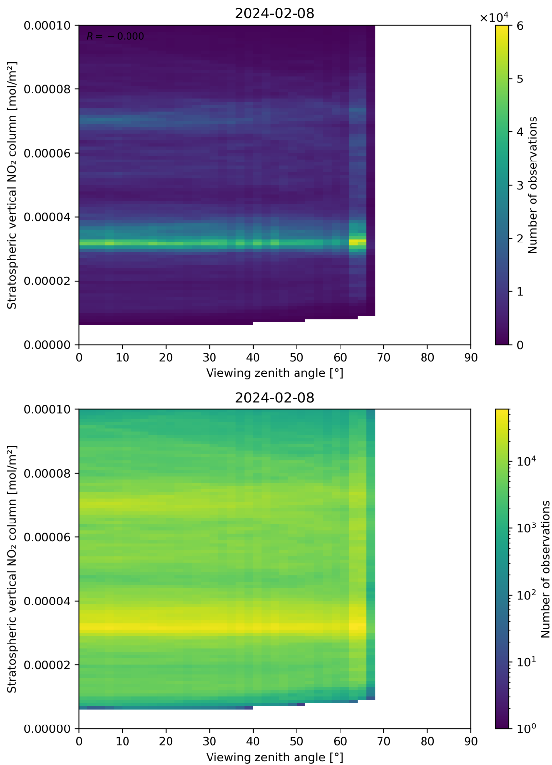
Figure 164: Scatter density plot of “Viewing zenith angle” against “Stratospheric vertical NO 2 column” for 2024-02-07 to 2024-02-09.
