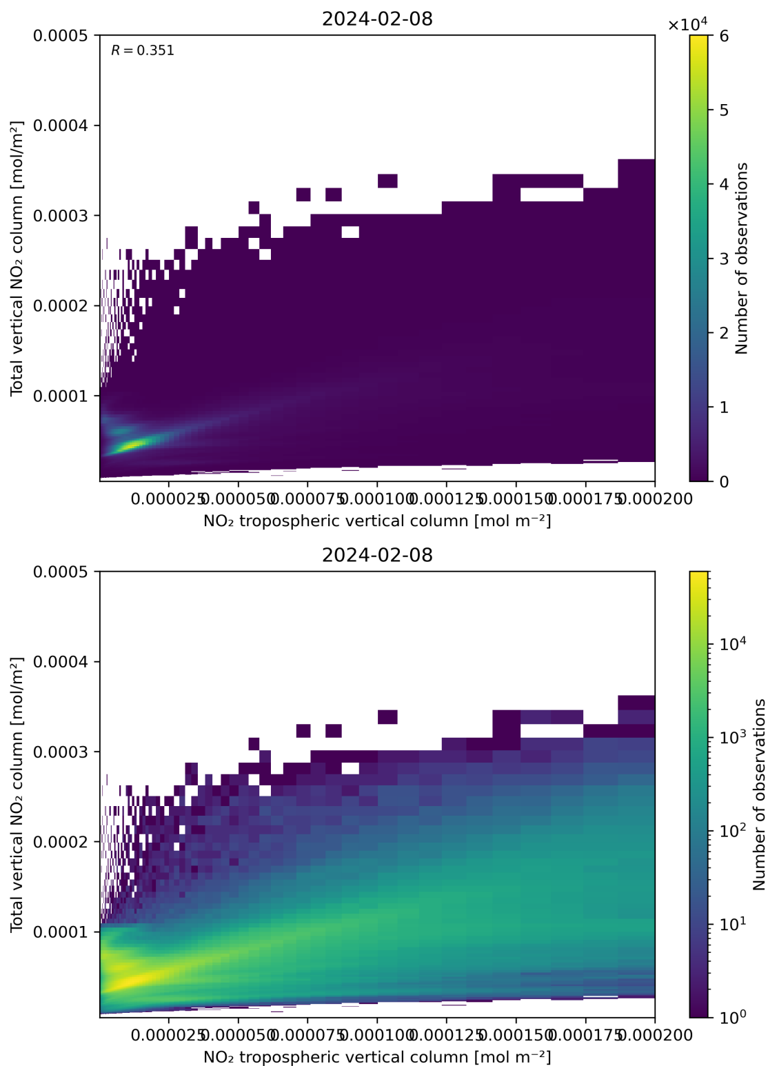
Figure 128: Scatter density plot of “NO 2 tropospheric vertical column” against “Total vertical NO 2 column” for 2024-02-07 to 2024-02-09.
