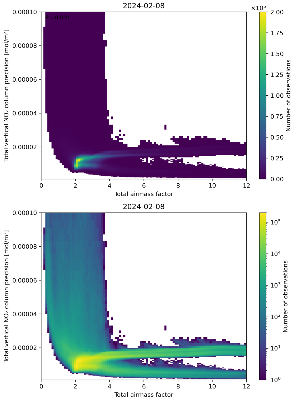
Figure 68: Scatter density plot of “Total airmass factor” against “Total vertical NO 2 column precision” for 2024-02-07 to 2024-02-09.
