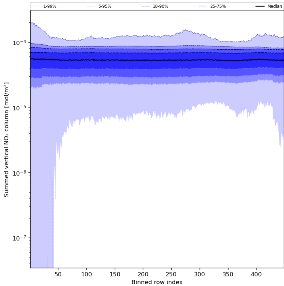
Figure 57: Along track statistics of “Summed vertical NO 2 column” for 2024-02-07 to 2024-02-09
