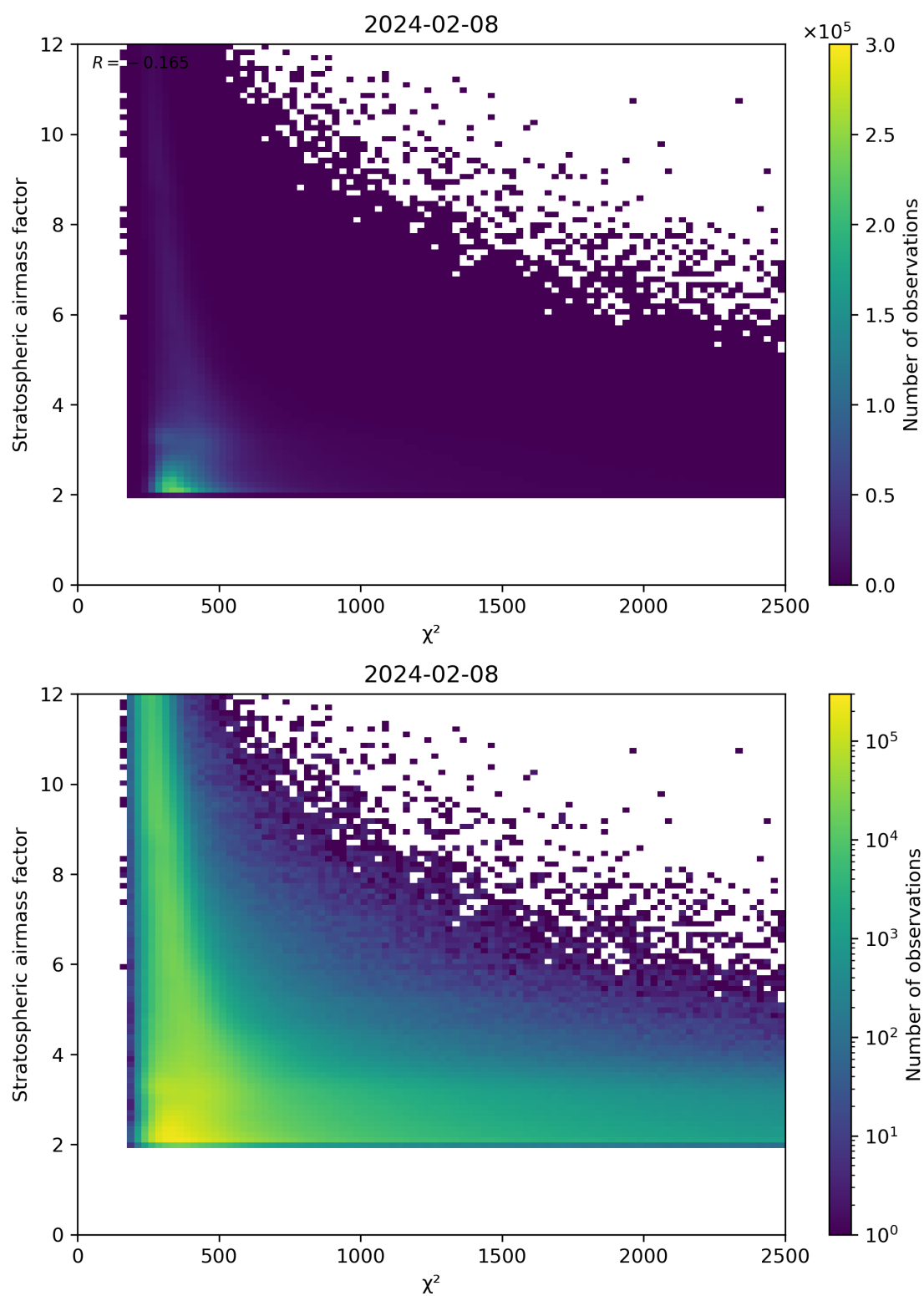
Figure 81: Scatter density plot of “ \chi^2 ” against “Stratospheric airmass factor” for 2024-02-07 to 2024-02-09.
