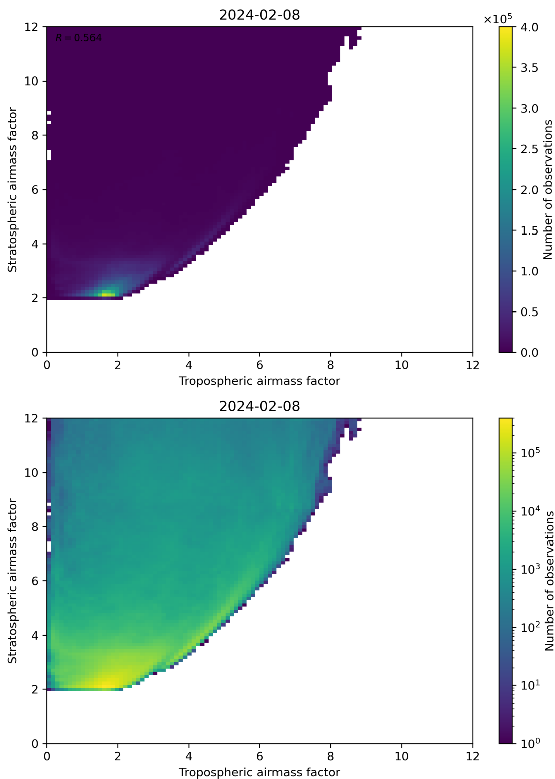
Figure 71: Scatter density plot of “Tropospheric airmass factor” against “Stratospheric airmass factor” for 2024-02-07 to 2024-02-09.
