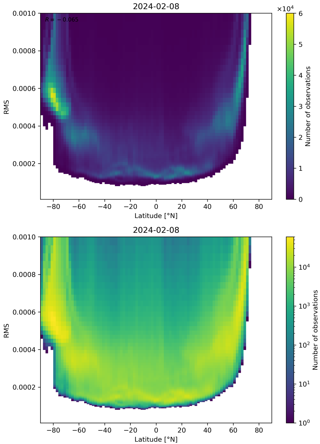
Figure 94: Scatter density plot of “Latitude” against “RMS” for 2024-02-07 to 2024-02-09.
