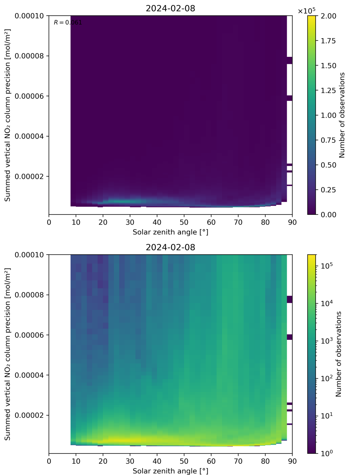
Figure 152: Scatter density plot of “Solar zenith angle” against “Summed vertical NO 2 column precision” for 2024-02-07 to 2024-02-09.
