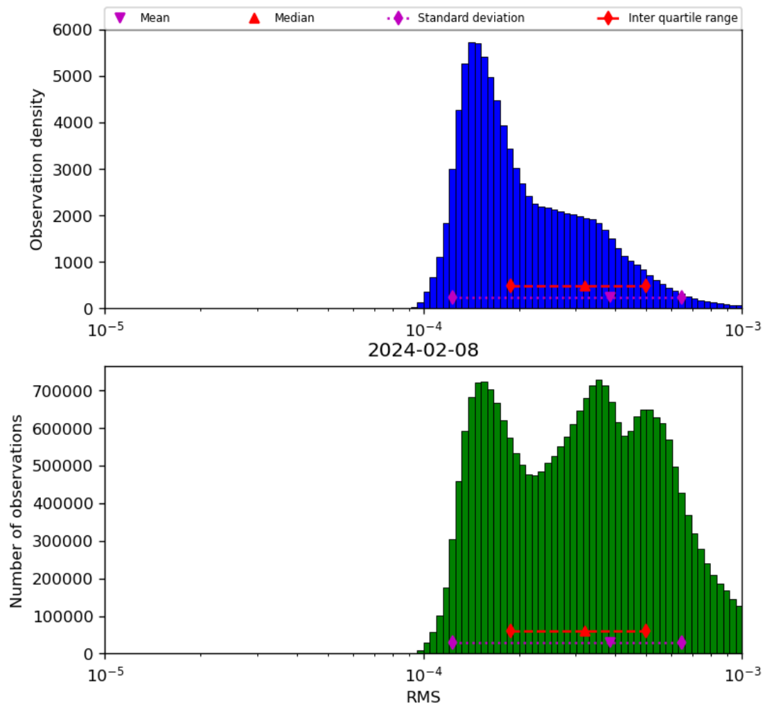
Figure 43: Histogram of “RMS” for 2024-02-07 to 2024-02-09
