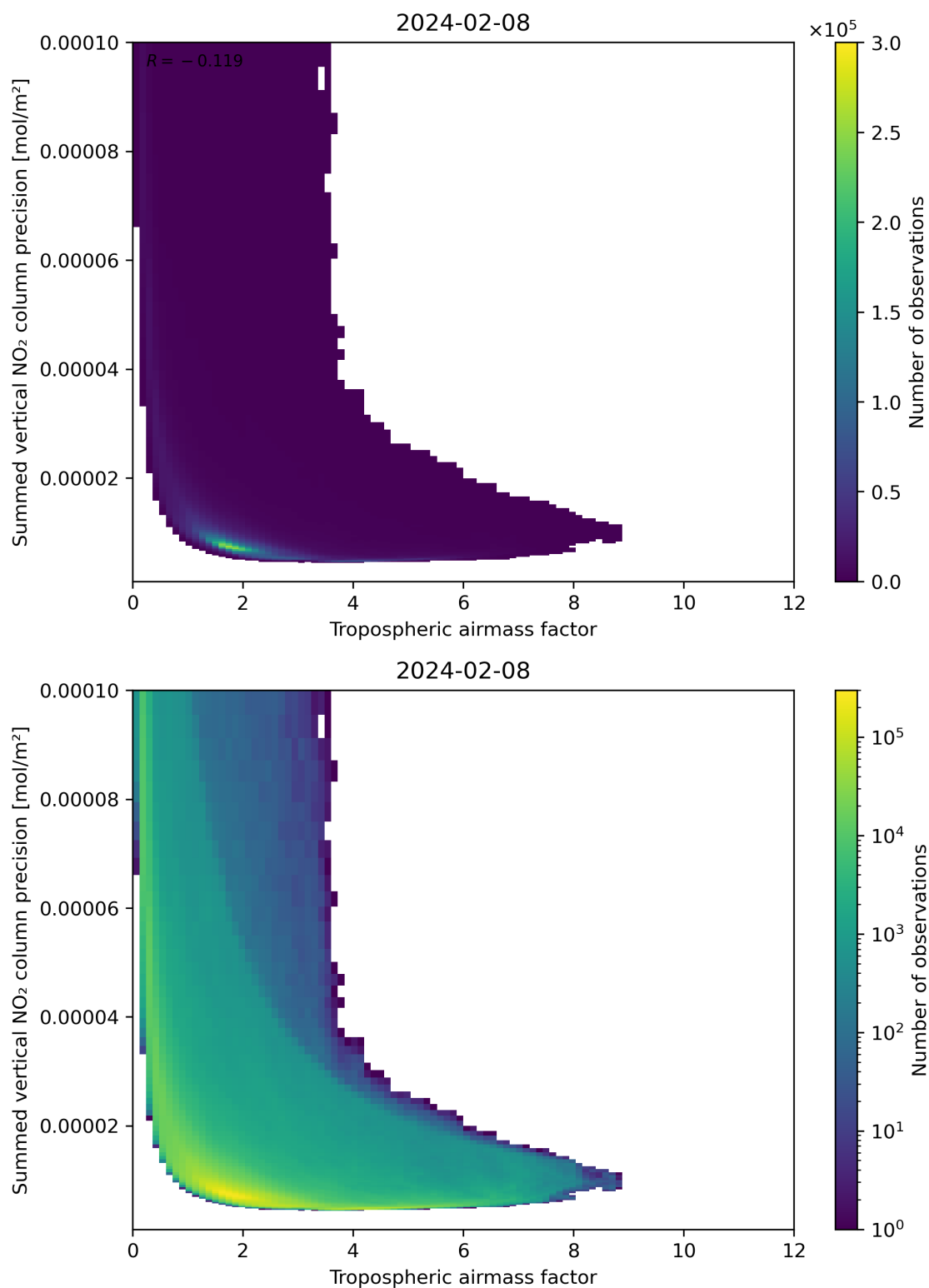
Figure 76: Scatter density plot of “Tropospheric air mass factor” against “Summed vertical NO 2 column precision” for 2024-02-07 to 2024-02-09.
