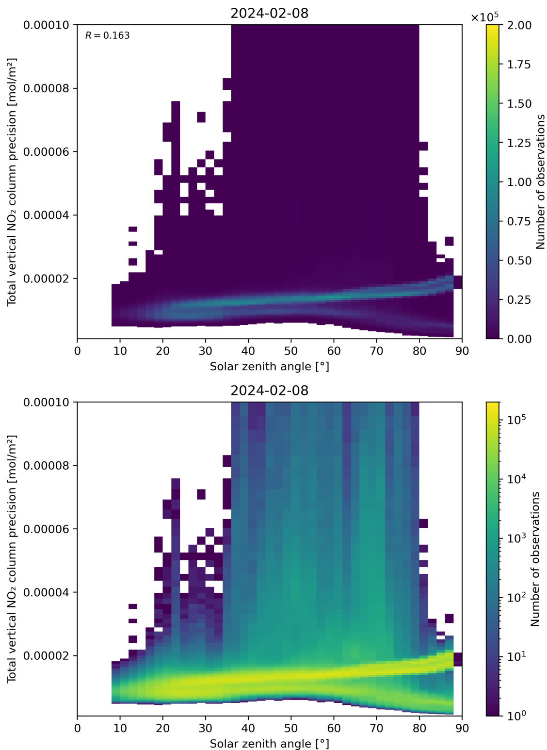
Figure 154: Scatter density plot of “Solar zenith angle” against “Total vertical NO 2 column precision” for 2024-02-07 to 2024-02-09.
