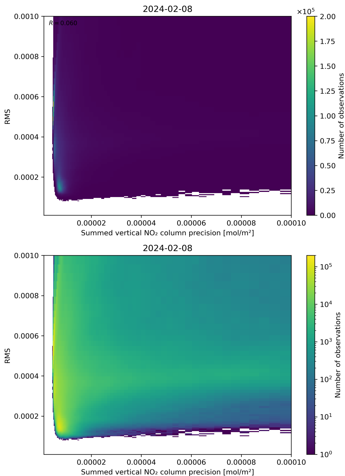
Figure 108: Scatter density plot of “Summed vertical NO 2 column precision” against “RMS” for 2024-02-07 to 2024-02-09.
