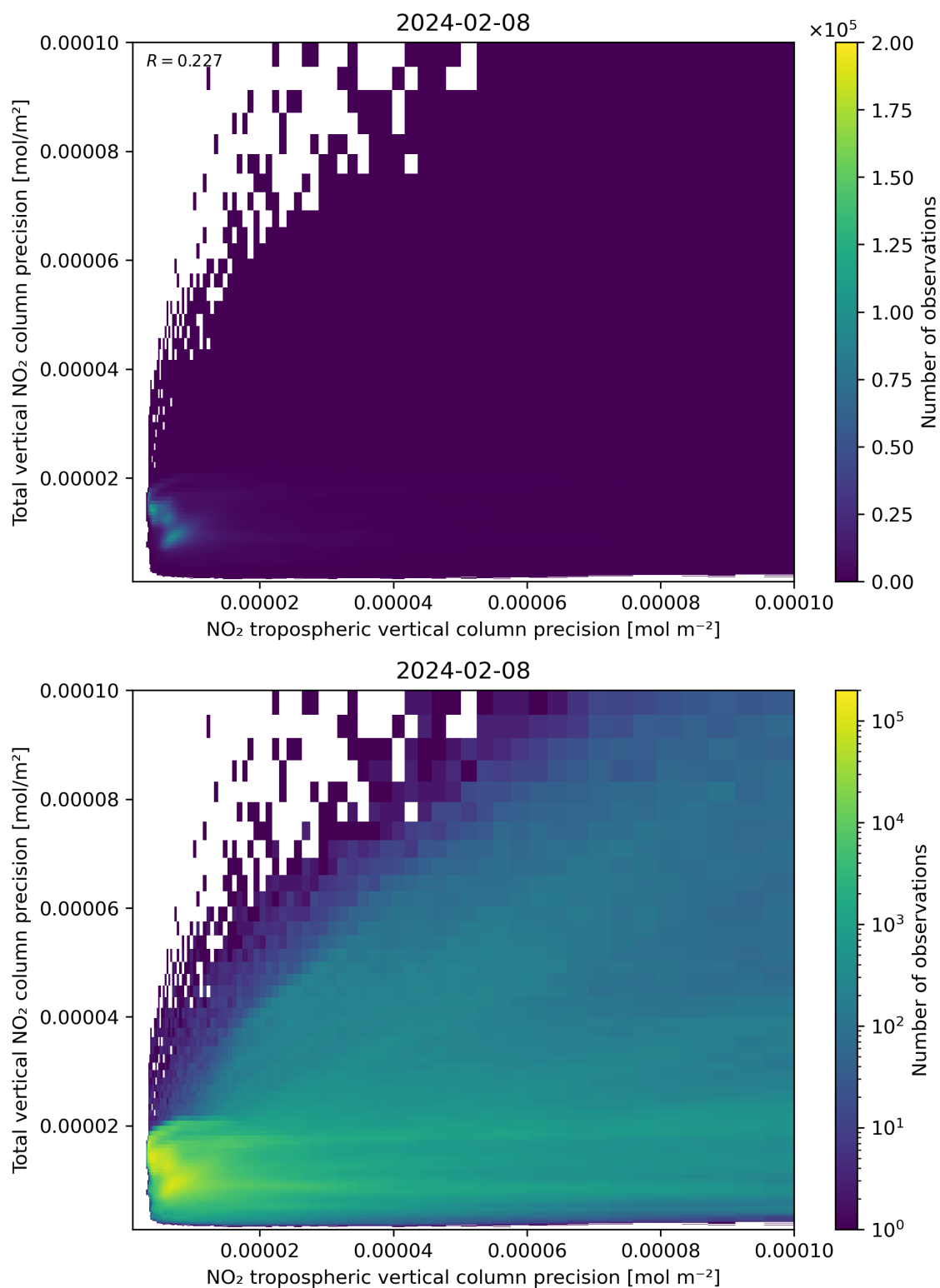
Figure 139: Scatter density plot of “NO 2 tropospheric vertical column precision” against “Total vertical NO 2 column precision” for 2024-02-07 to 2024-02-09.
