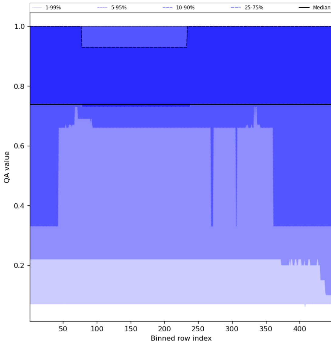
Figure 45: Along track statistics of “QA value” for 2024-02-07 to 2024-02-09
