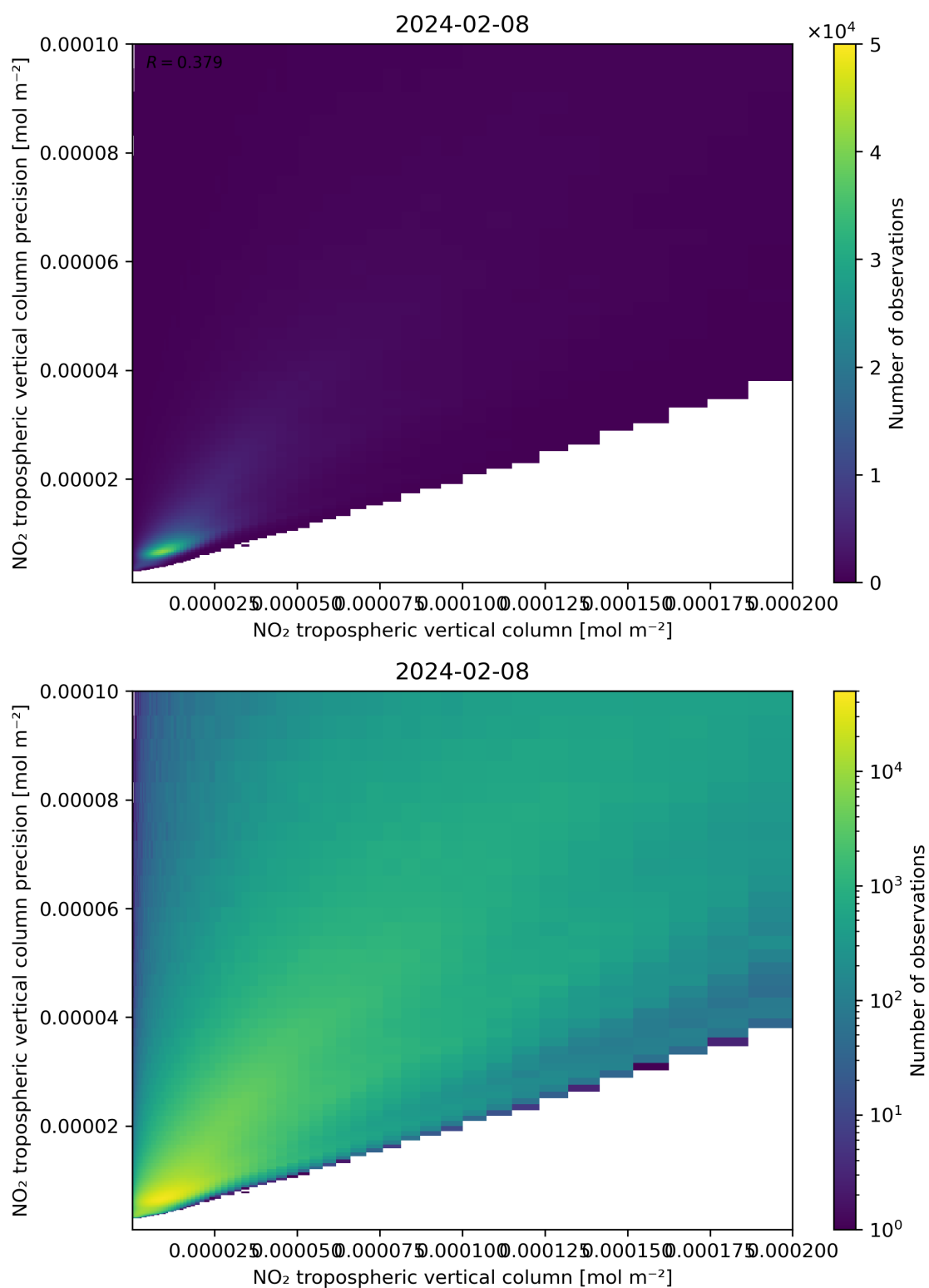
Figure 130: Scatter density plot of “NO 2 tropospheric vertical column” against “NO 2 tropospheric vertical column precision” for 2024-02-07 to 2024-02-09.
