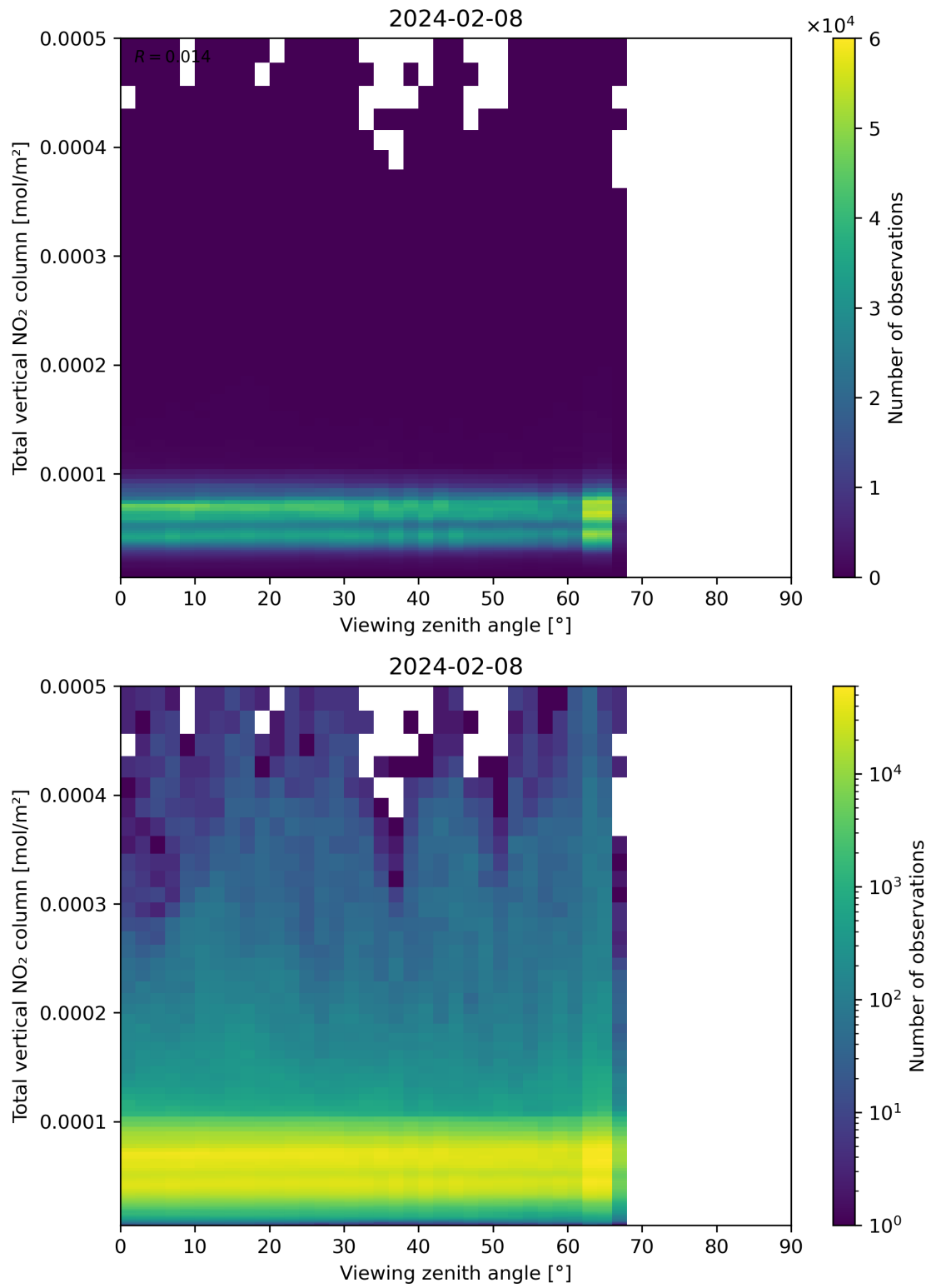
Figure 167: Scatter density plot of “Viewing zenith angle” against “Total vertical NO 2 column” for 2024-02-07 to 2024-02-09.
