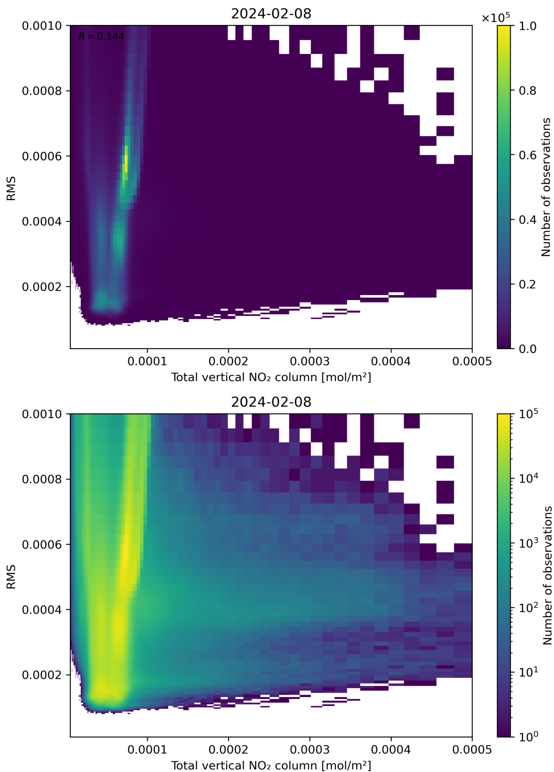
Figure 120: Scatter density plot of “Total vertical NO 2 column” against “RMS” for 2024-02-07 to 2024-02-09.
