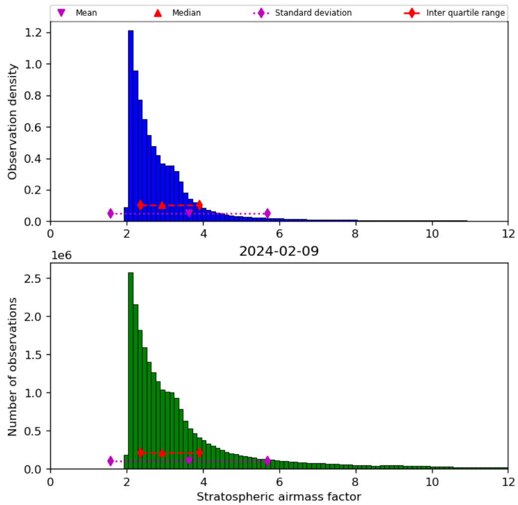
Figure 44: Histogram of “Stratospheric airmass factor” for 2024-02-08 to 2024-02-10
