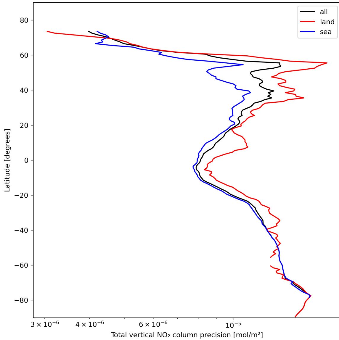
Figure 22: Zonal average of “Total vertical NO 2 column precision” for 2024-02-08 to 2024-02-10.
