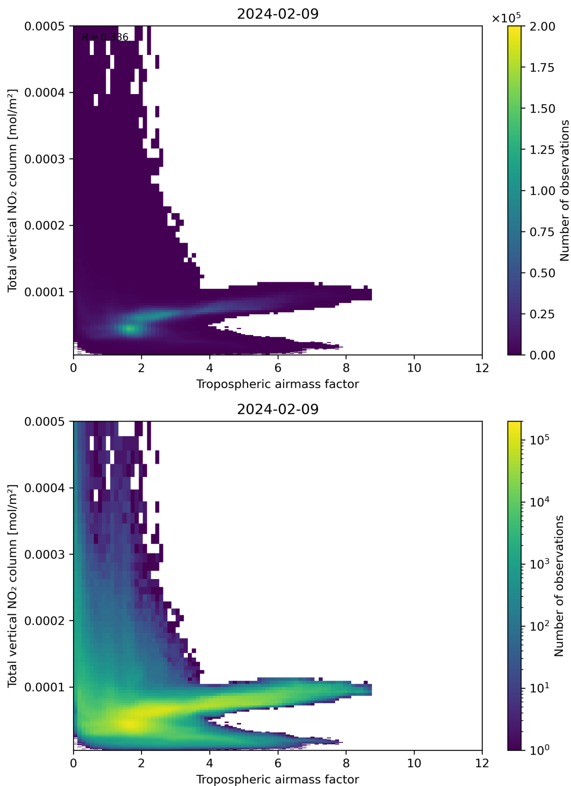
Figure 77: Scatter density plot of “Tropospheric airmass factor” against “Total vertical NO 2 column” for 2024-02-08 to 2024-02-10.
