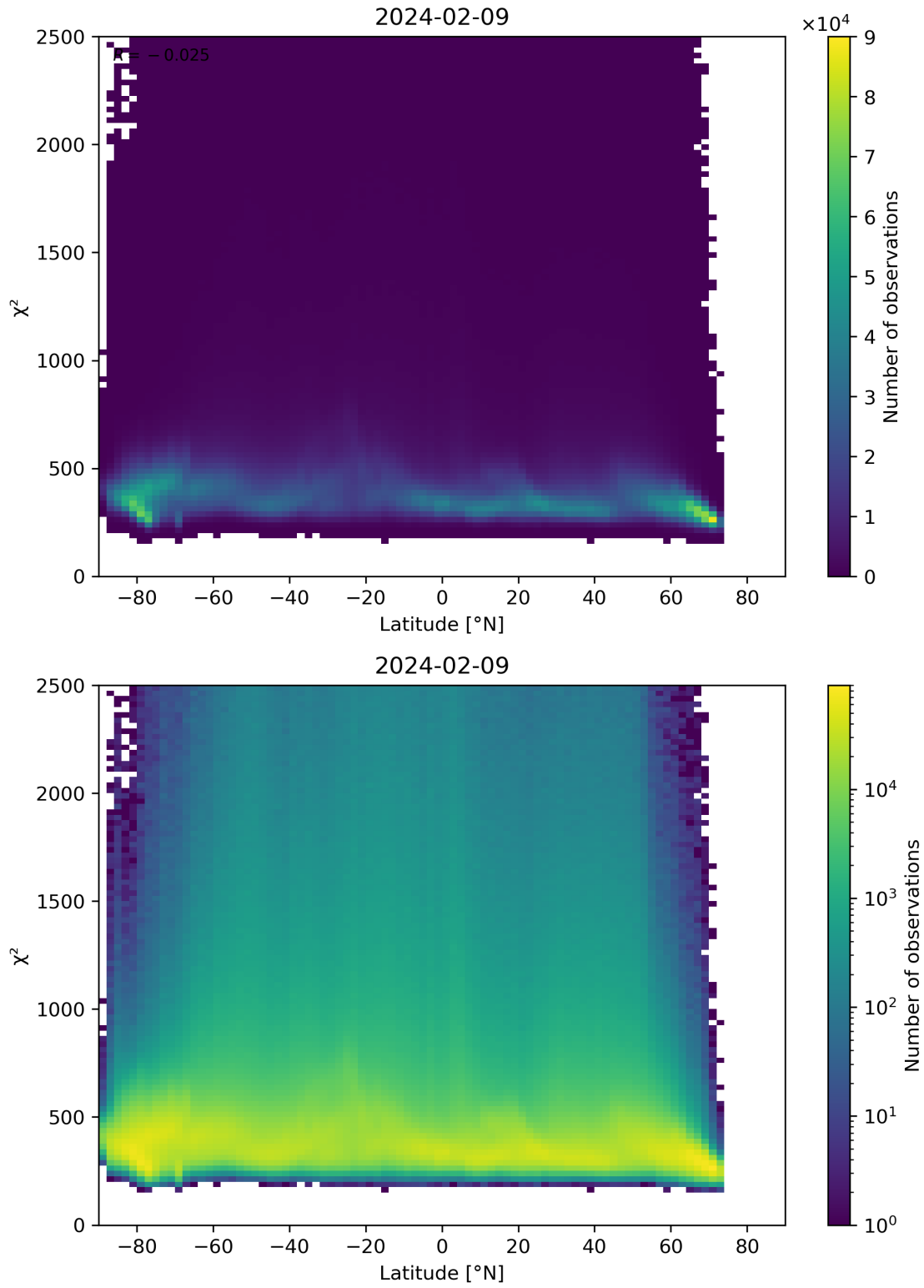
Figure 86: Scatter density plot of “Latitude” against “ \chi^2 ” for 2024-02-08 to 2024-02-10.
