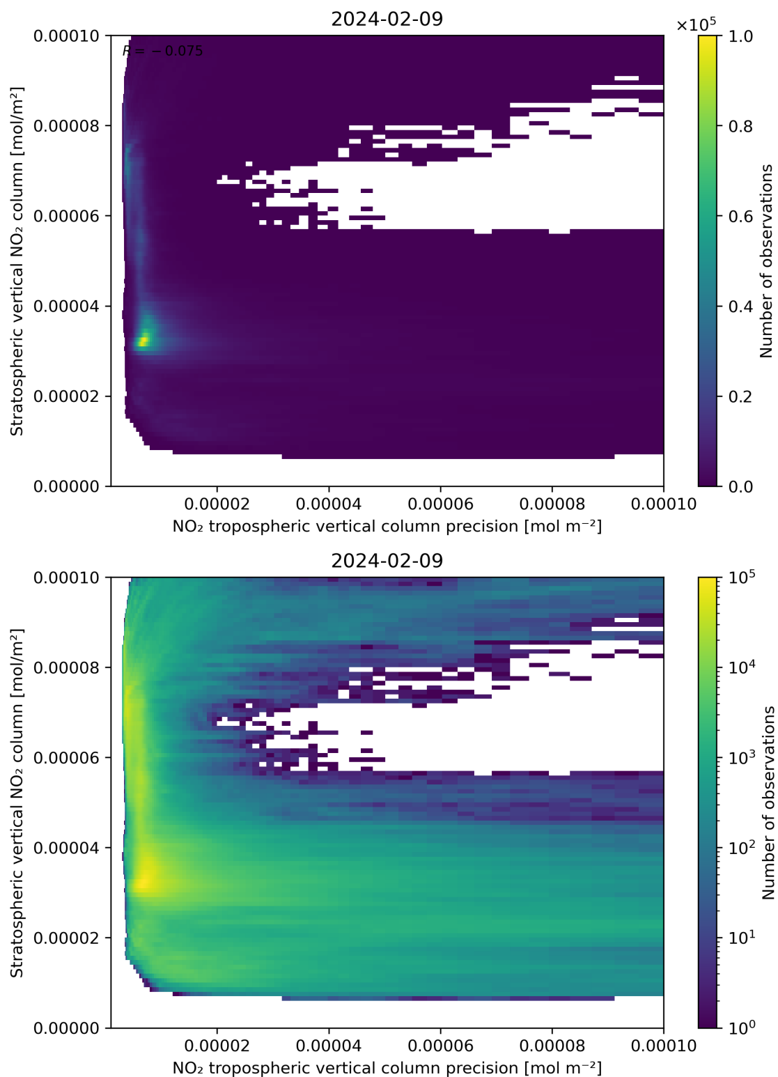
Figure 135: Scatter density plot of “NO 2 tropospheric vertical column precision” against “Stratospheric vertical NO 2 column” for 2024-02-08 to 2024-02-10.
