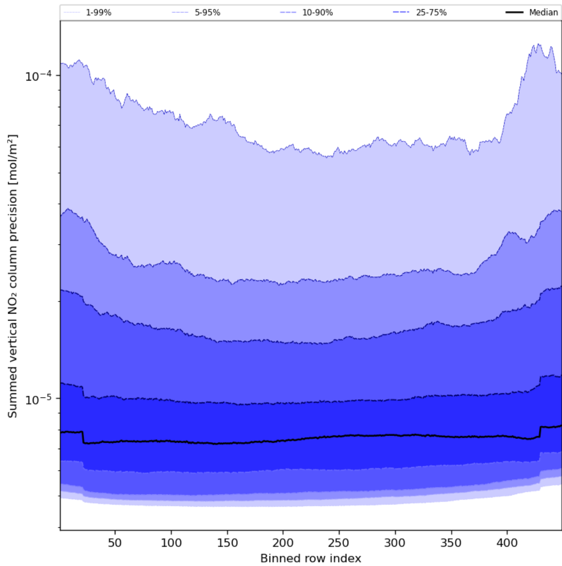
Figure 58: Along track statistics of “Summed vertical NO 2 column precision” for 2024-02-08 to 2024-02-10
