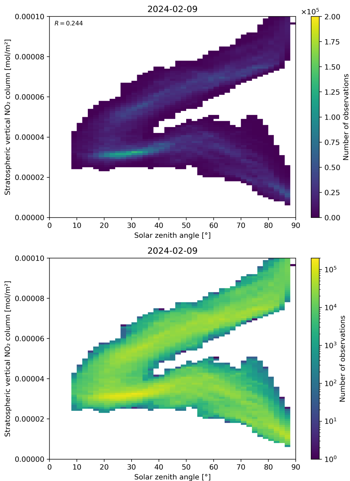
Figure 150: Scatter density plot of “Solar zenith angle” against “Stratospheric vertical NO 2 column” for 2024-02-08 to 2024-02-10.
