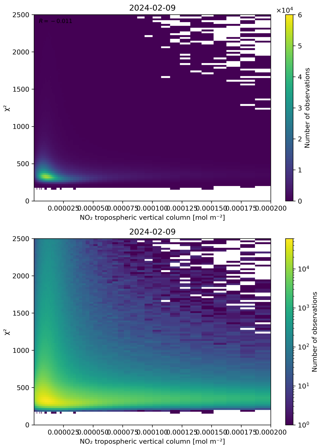
Figure 124: Scatter density plot of “NO 2 tropospheric vertical column” against “ \chi^2 ” for 2024-02-08 to 2024-02-10.
