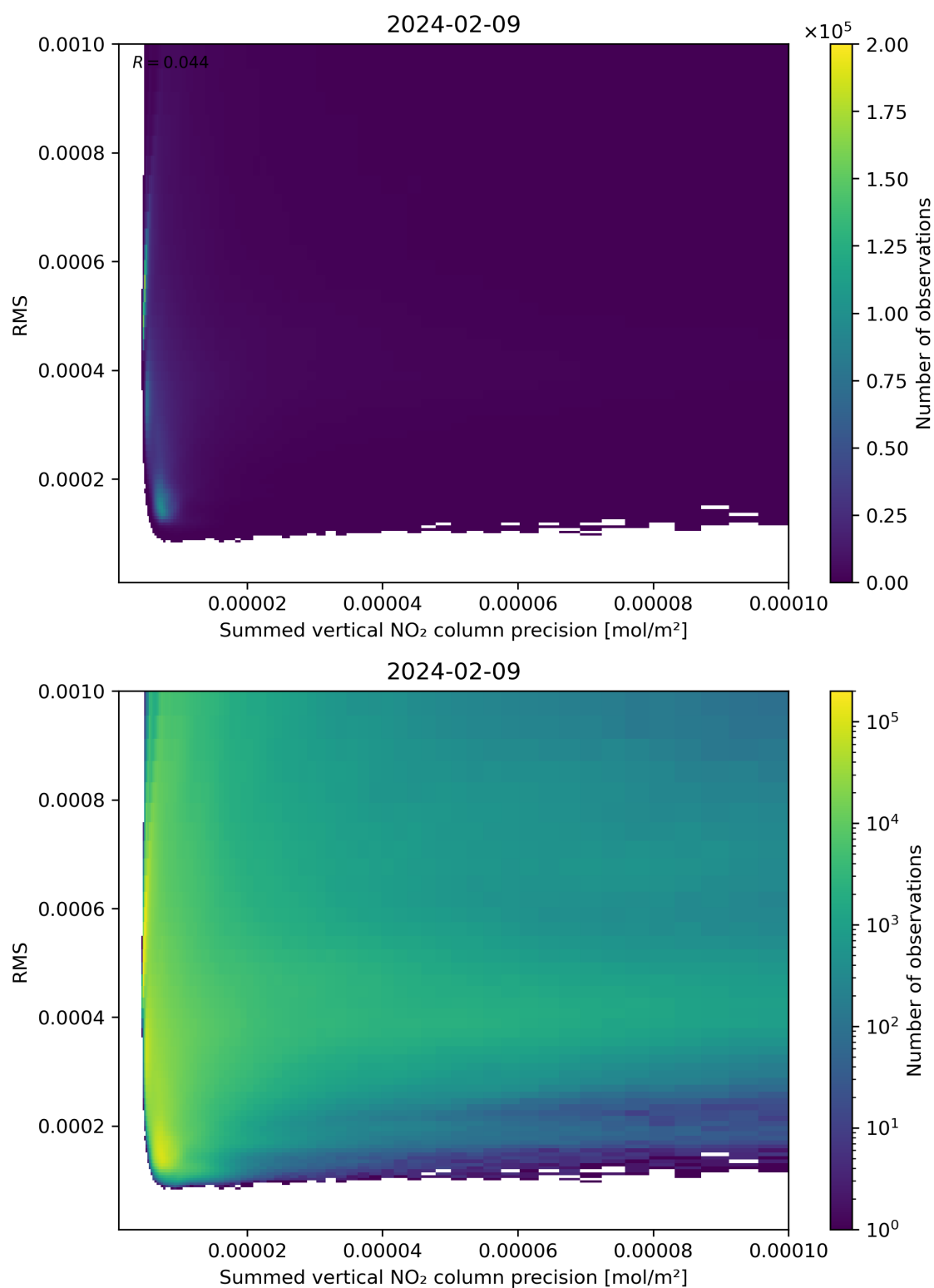
Figure 108: Scatter density plot of “Summed vertical NO 2 column precision” against “RMS” for 2024-02-08 to 2024-02-10.
