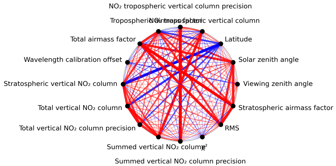
Figure 1: Map of correlation graph for 2024-02-08 to 2024-02-10.
