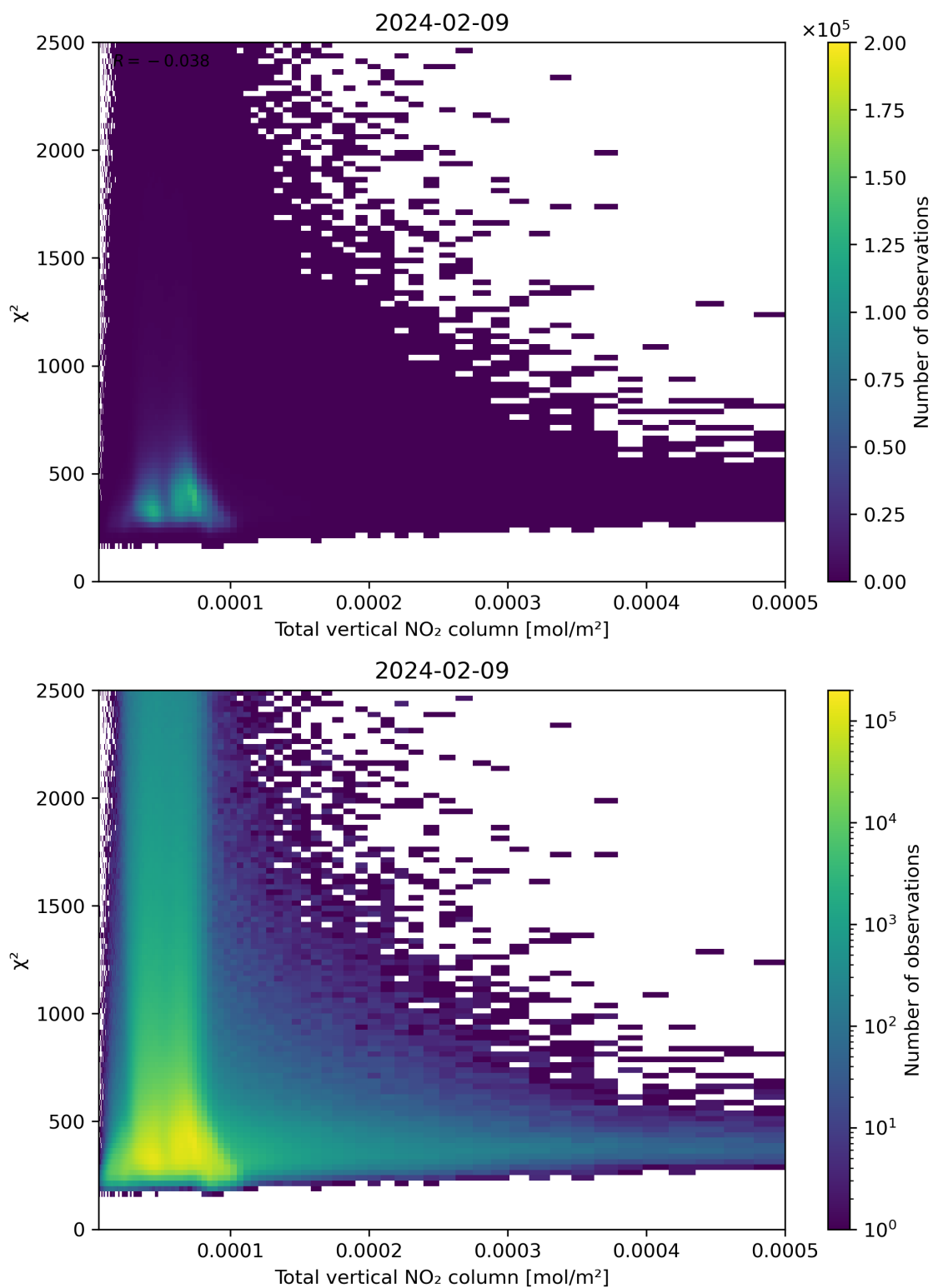
Figure 111: Scatter density plot of “Total vertical NO 2 column” against “ \chi^2 ” for 2024-02-08 to 2024-02-10.
