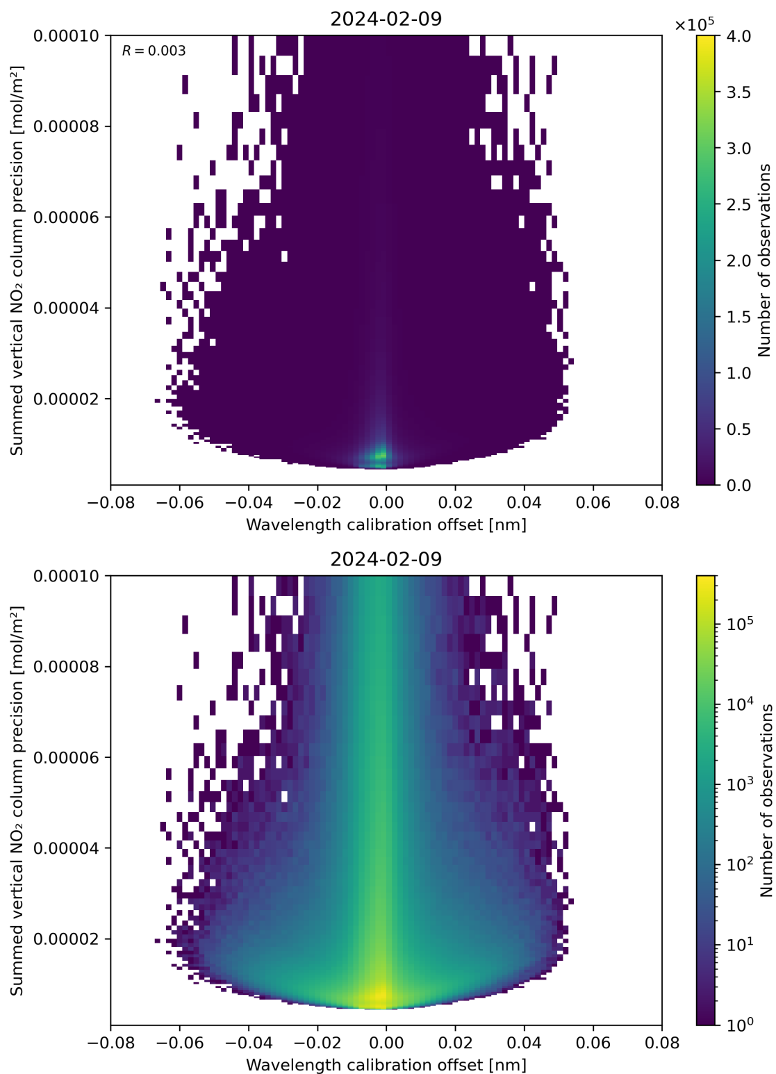
Figure 178: Scatter density plot of “Wavelength calibration offset” against “Summed vertical NO 2 column precision” for 2024-02-08 to 2024-02-10.
