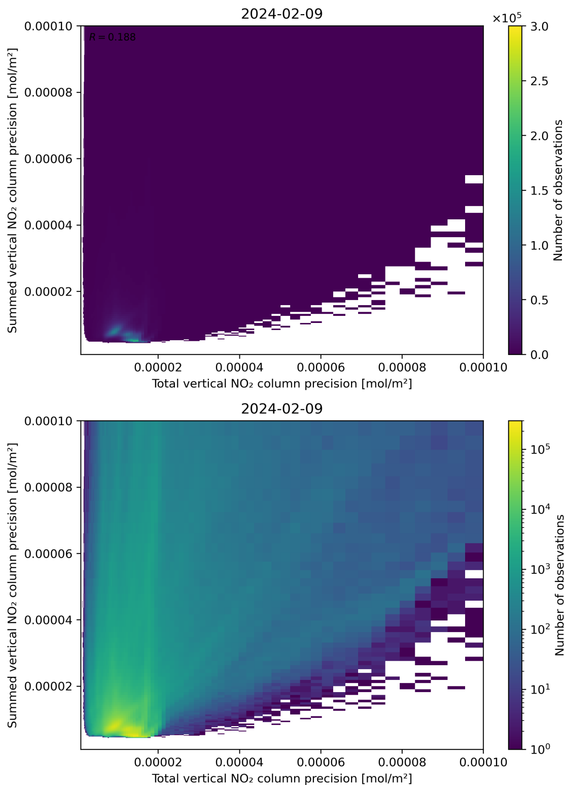
Figure 118: Scatter density plot of “Total vertical NO 2 column precision” against “Summed vertical NO 2 column precision” for 2024-02-08 to 2024-02-10.
