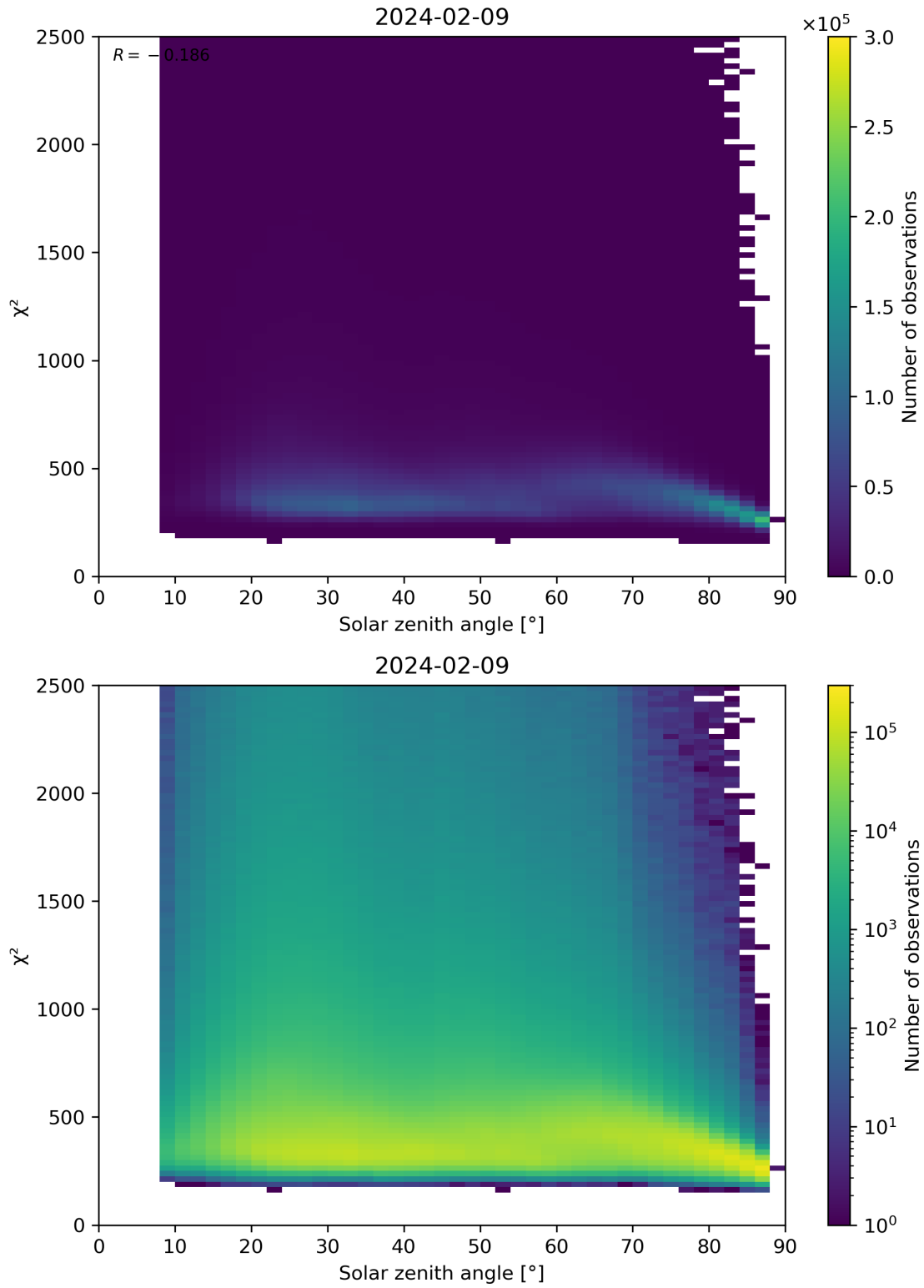
Figure 148: Scatter density plot of “Solar zenith angle” against “ \chi^2 ” for 2024-02-08 to 2024-02-10.
