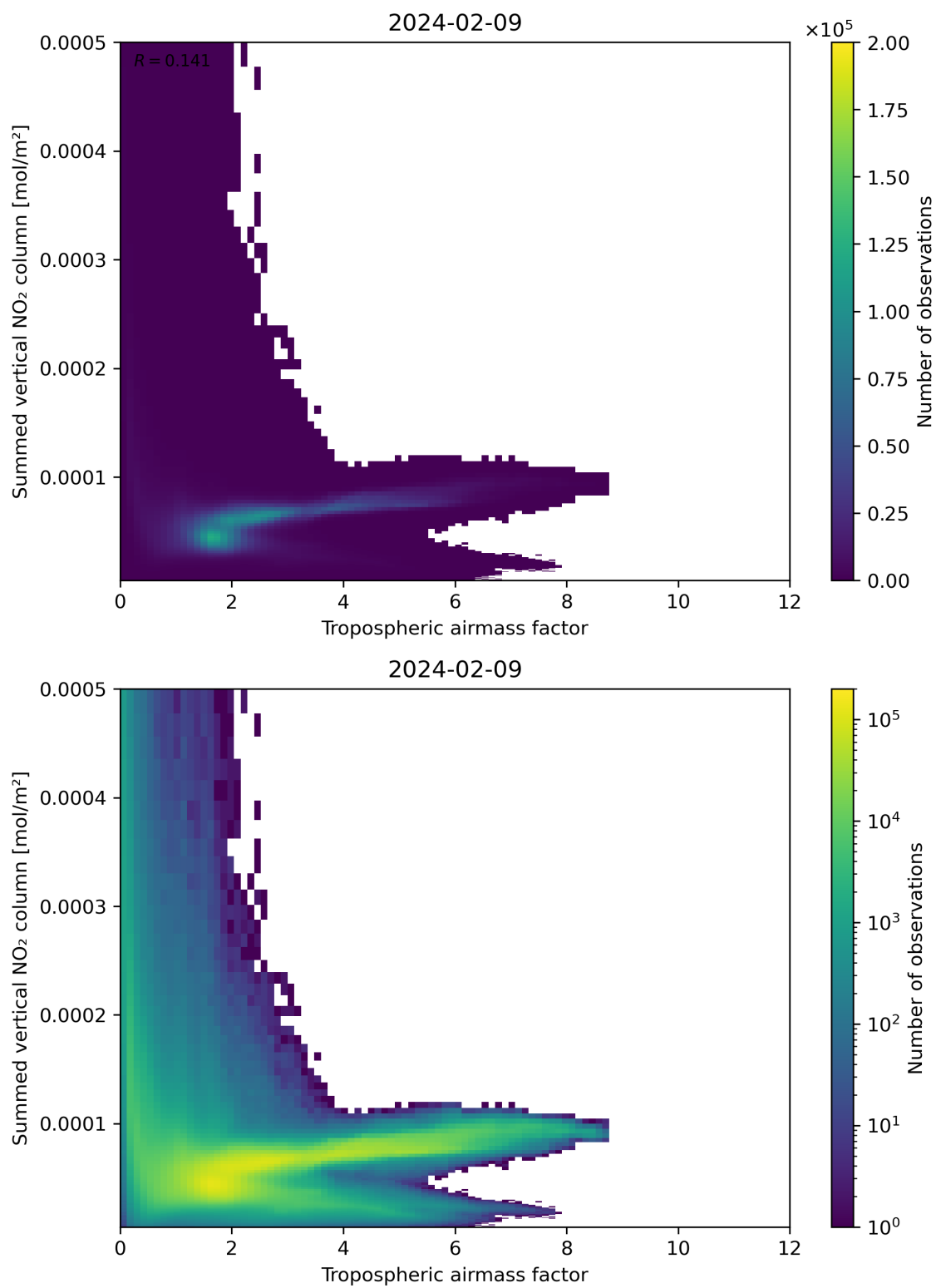
Figure 75: Scatter density plot of “Tropospheric air mass factor” against “Summed vertical NO 2 column” for 2024-02-08 to 2024-02-10.
