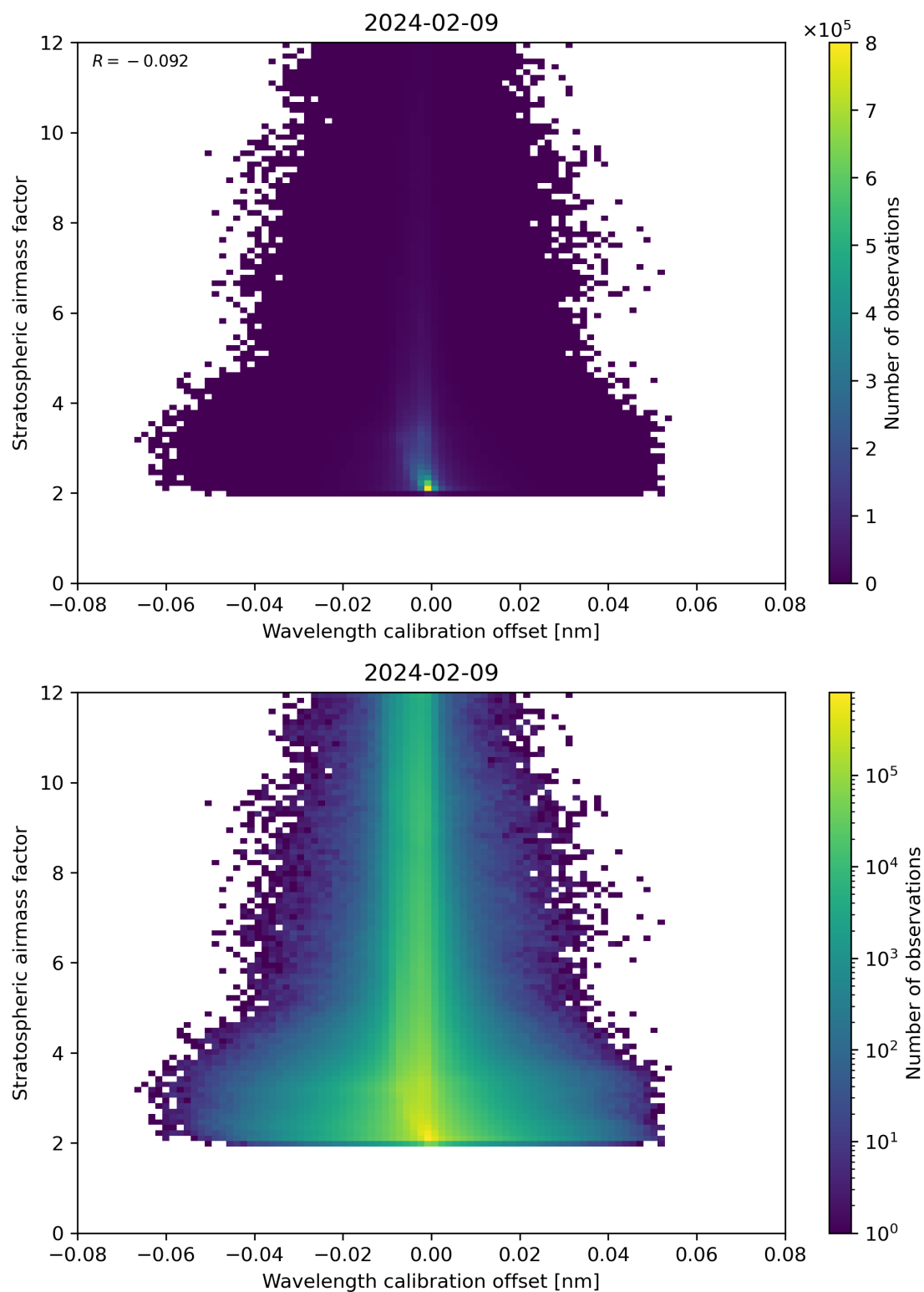
Figure 174: Scatter density plot of “Wavelength calibration offset” against “Stratospheric airmass factor” for 2024-02-08 to 2024-02-10.
