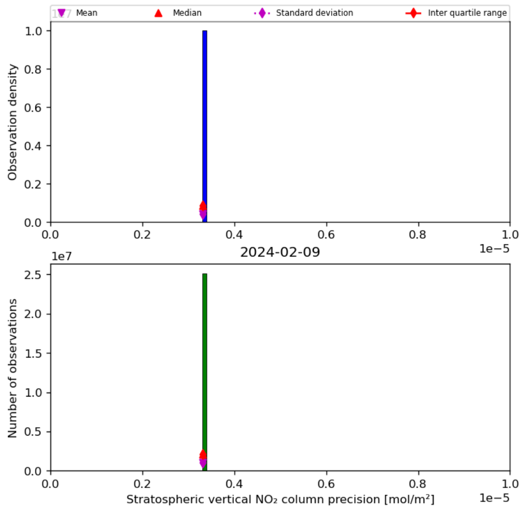
Figure 37: Histogram of “Stratospheric vertical NO 2 column precision” for 2024-02-08 to 2024-02-10
