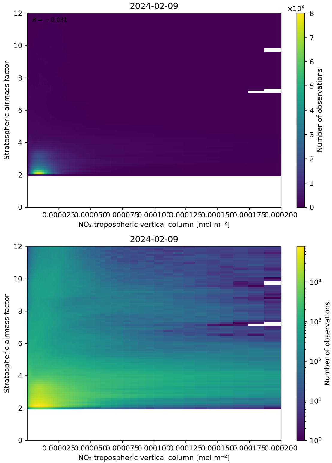
Figure 121: Scatter density plot of “NO 2 tropospheric vertical column” against “Stratospheric airmass factor” for 2024-02-08 to 2024-02-10.
