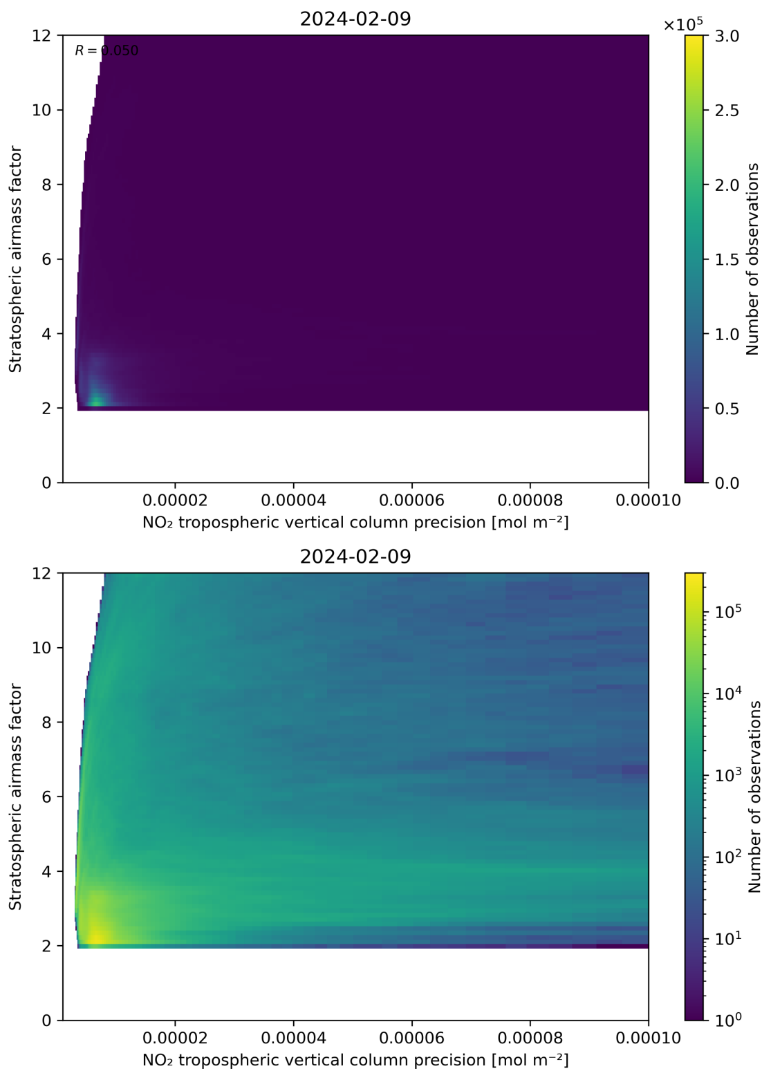
Figure 131: Scatter density plot of “NO 2 tropospheric vertical column precision” against “Stratospheric airmass factor” for 2024-02-08 to 2024-02-10.
