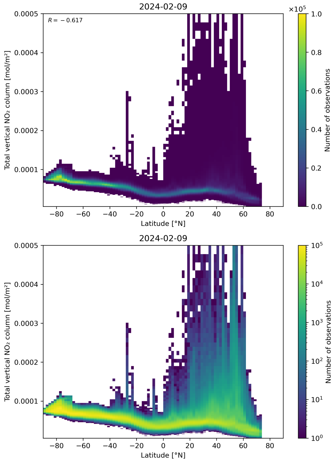
Figure 90: Scatter density plot of “Latitude” against “Total vertical NO 2 column” for 2024-02-08 to 2024-02-10.
