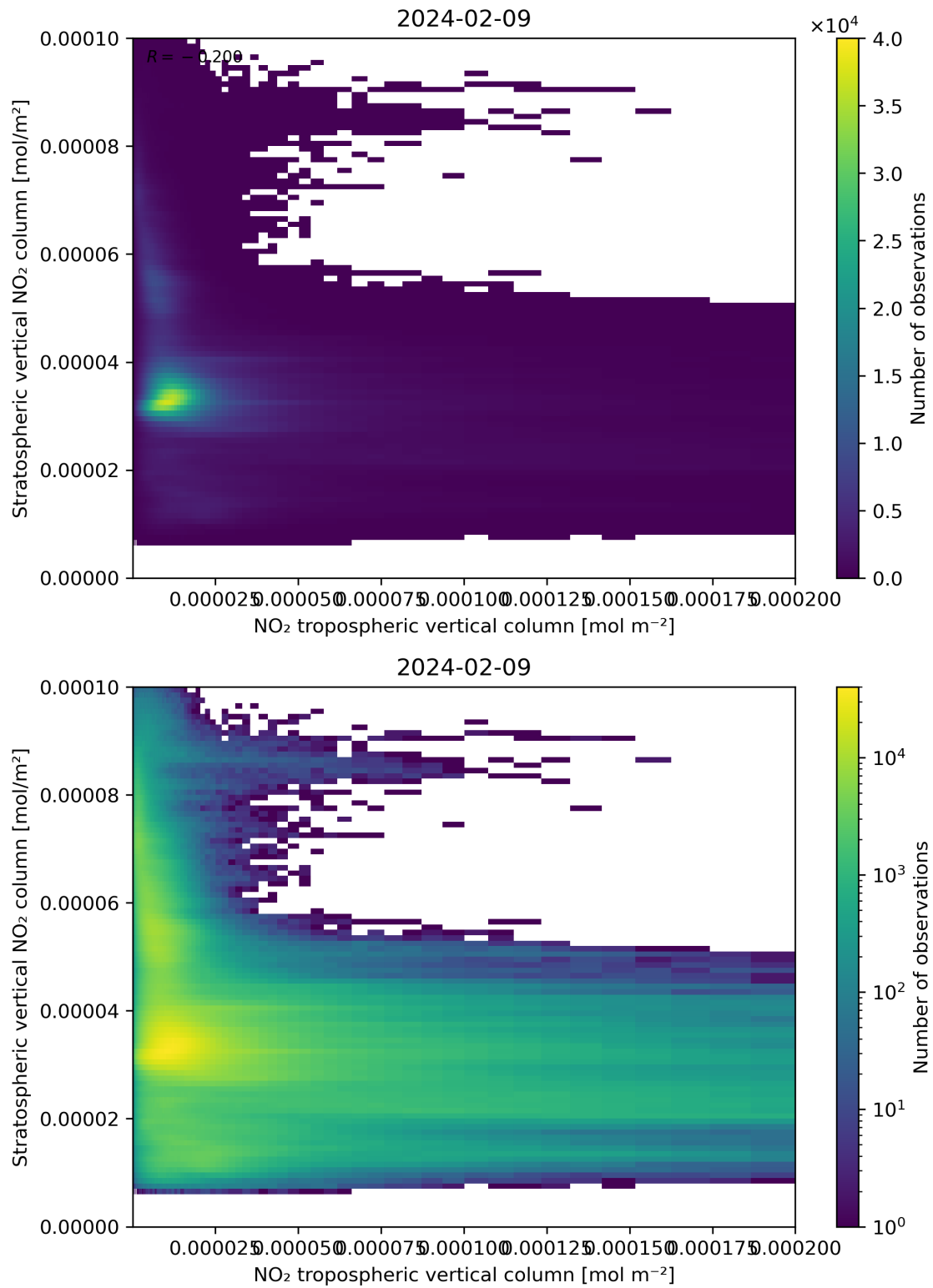
Figure 125: Scatter density plot of “NO 2 tropospheric vertical column” against “Stratospheric vertical NO 2 column” for 2024-02-08 to 2024-02-10.
