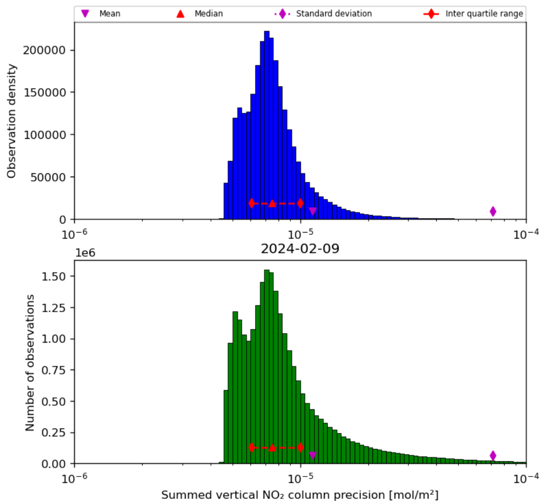
Figure 41: Histogram of "Summed vertical NO 2 column precision" for 2024-02-08 to 2024-02-10
