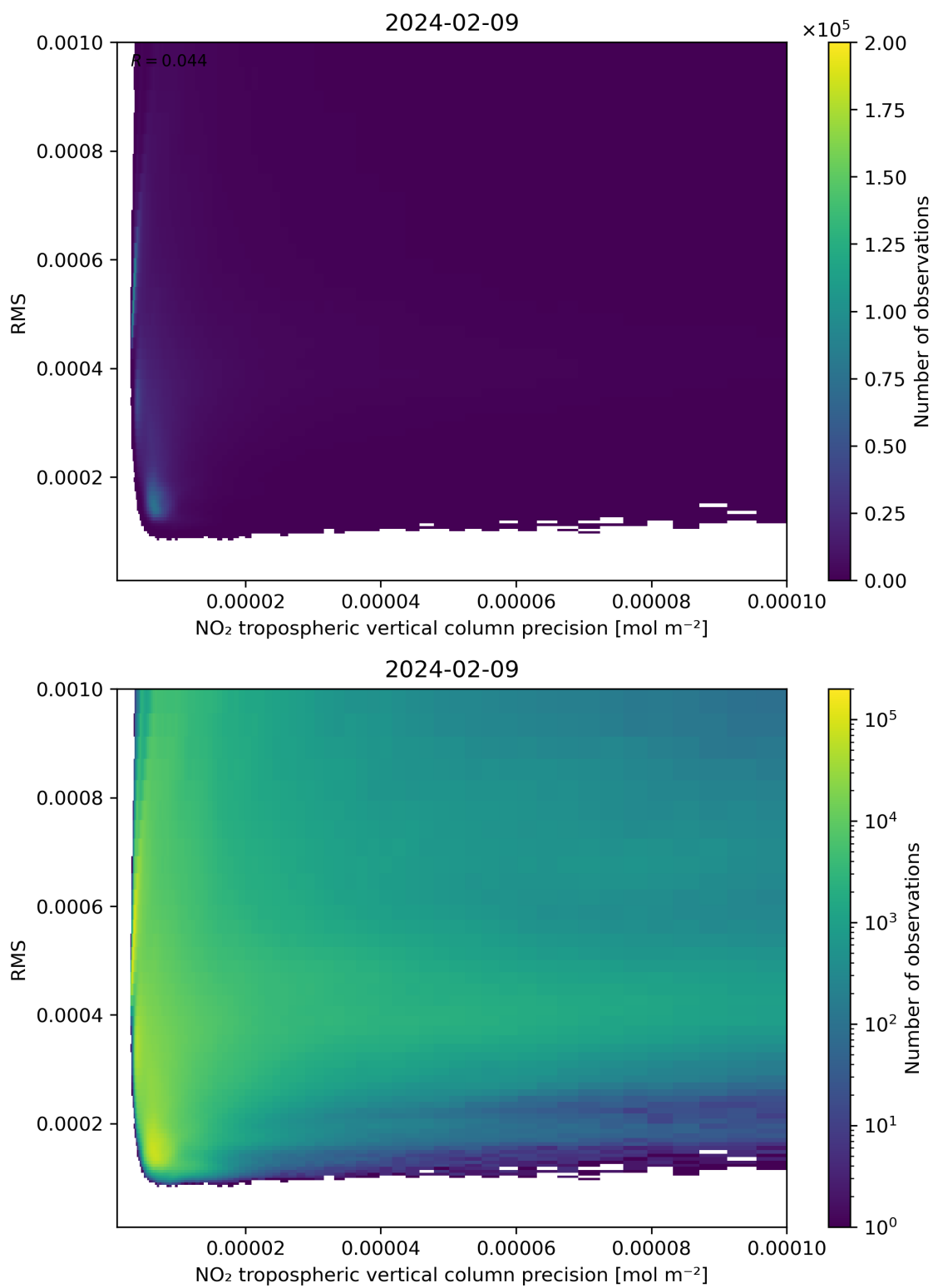
Figure 140: Scatter density plot of “NO 2 tropospheric vertical column precision” against “RMS” for 2024-02-08 to 2024-02-10.
