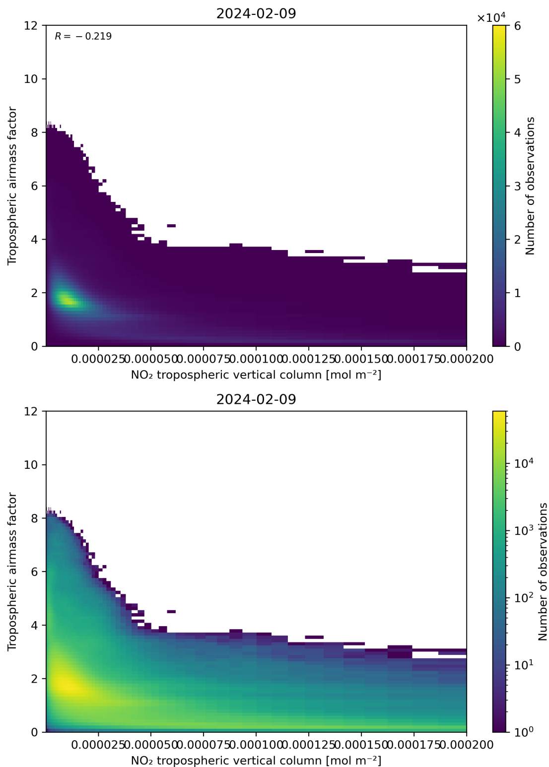
Figure 123: Scatter density plot of “NO 2 tropospheric vertical column” against “Tropospheric airmass factor” for 2024-02-08 to 2024-02-10.
