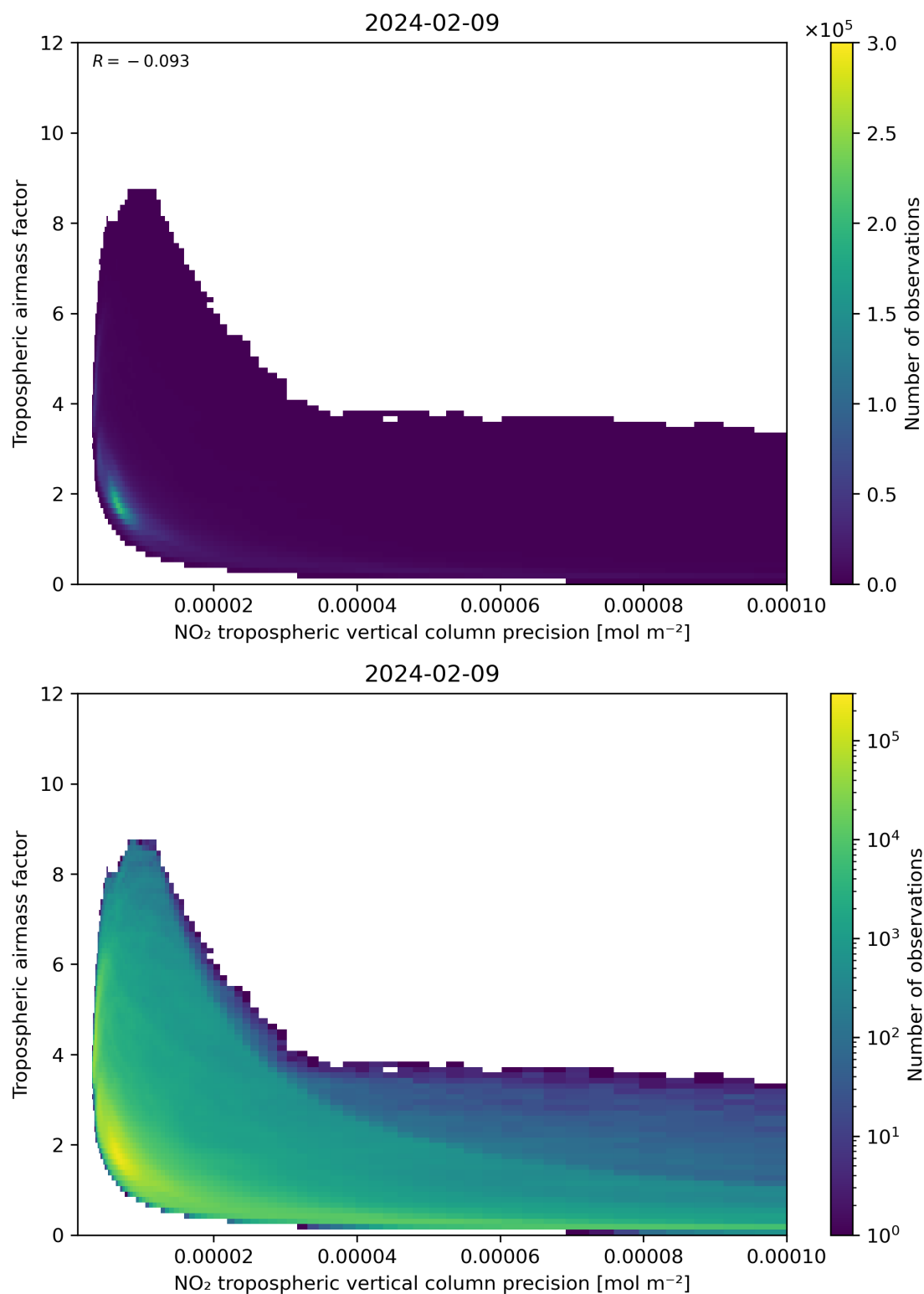
Figure 133: Scatter density plot of “NO 2 tropospheric vertical column precision” against “Tropospheric airmass factor” for 2024-02-08 to 2024-02-10.
