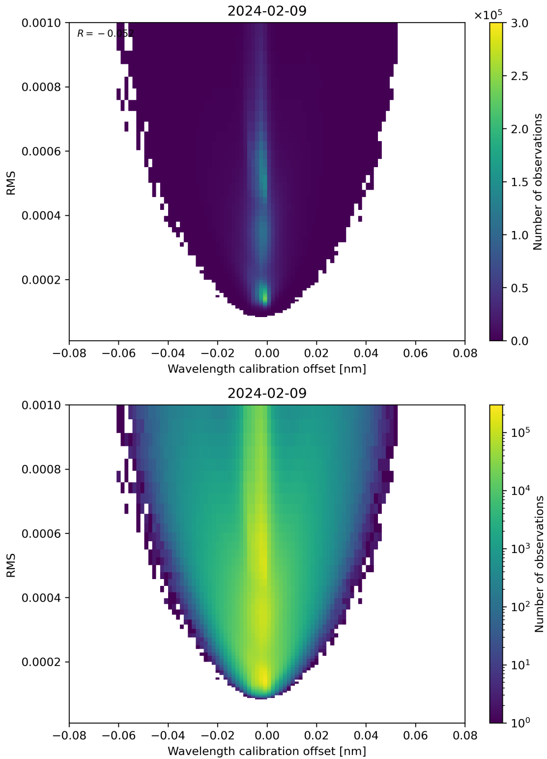
Figure 181: Scatter density plot of “Wavelength calibration offset” against “RMS” for 2024-02-08 to 2024-02-10.
