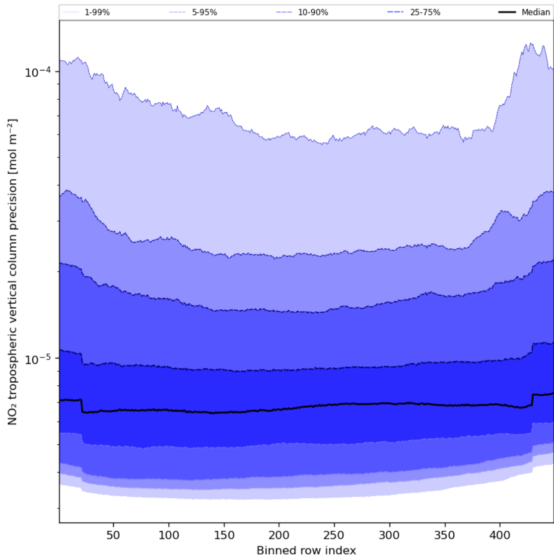
Figure 47: Along track statistics of “NO 2 tropospheric vertical column precision” for 2024-02-08 to 2024-02-10
