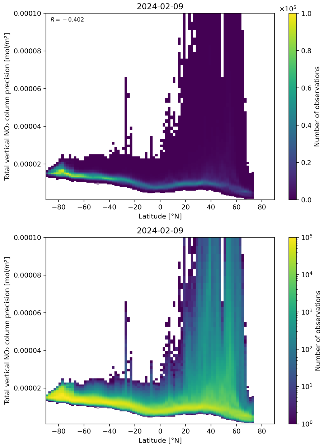
Figure 91: Scatter density plot of “Latitude” against “Total vertical NO 2 column precision” for 2024-02-08 to 2024-02-10.
