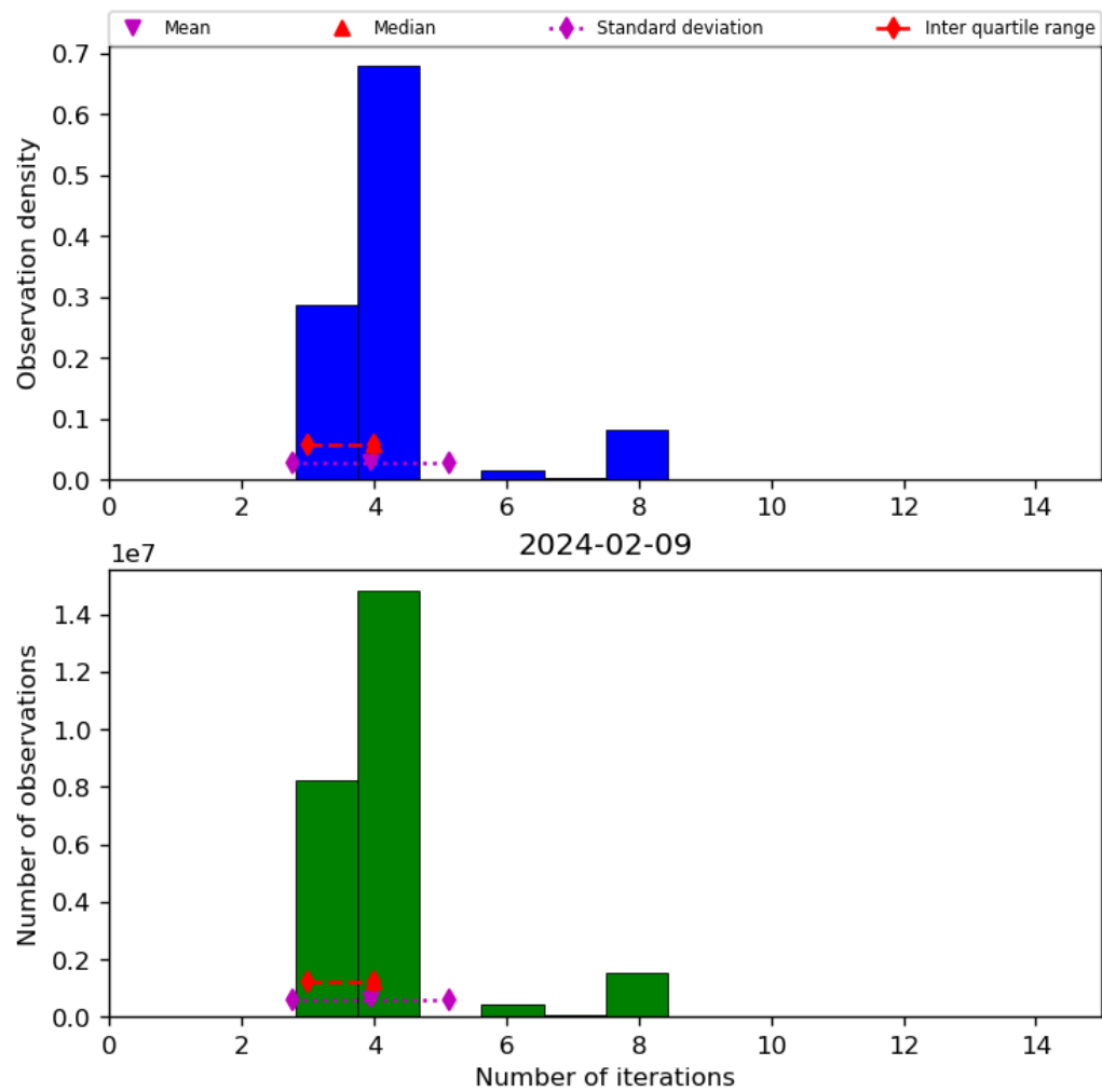
Figure 34: Histogram of “Number of iterations” for 2024-02-08 to 2024-02-10
