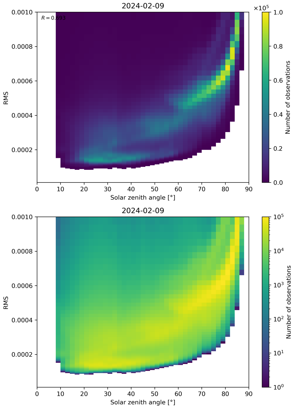
Figure 157: Scatter density plot of “Solar zenith angle” against “RMS” for 2024-02-08 to 2024-02-10.
