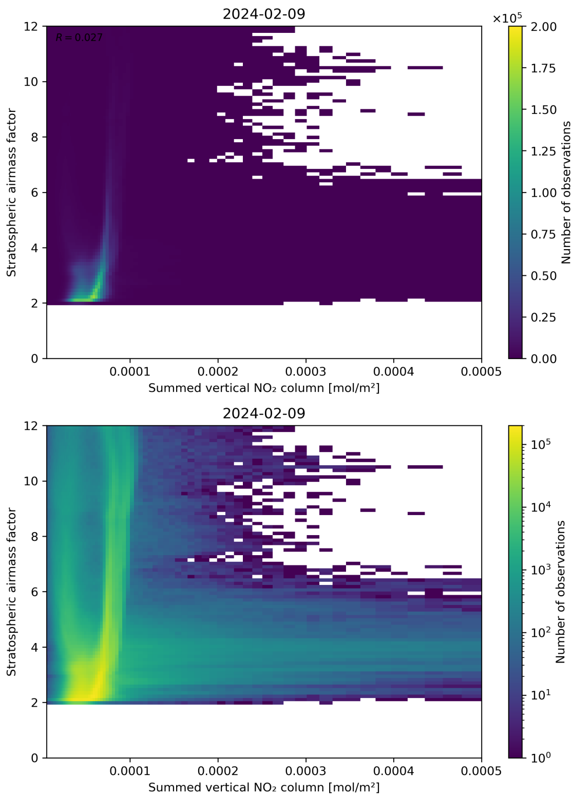
Figure 103: Scatter density plot of “Summed vertical NO 2 column” against “Stratospheric air mass factor” for 2024-02-08 to 2024-02-10.
