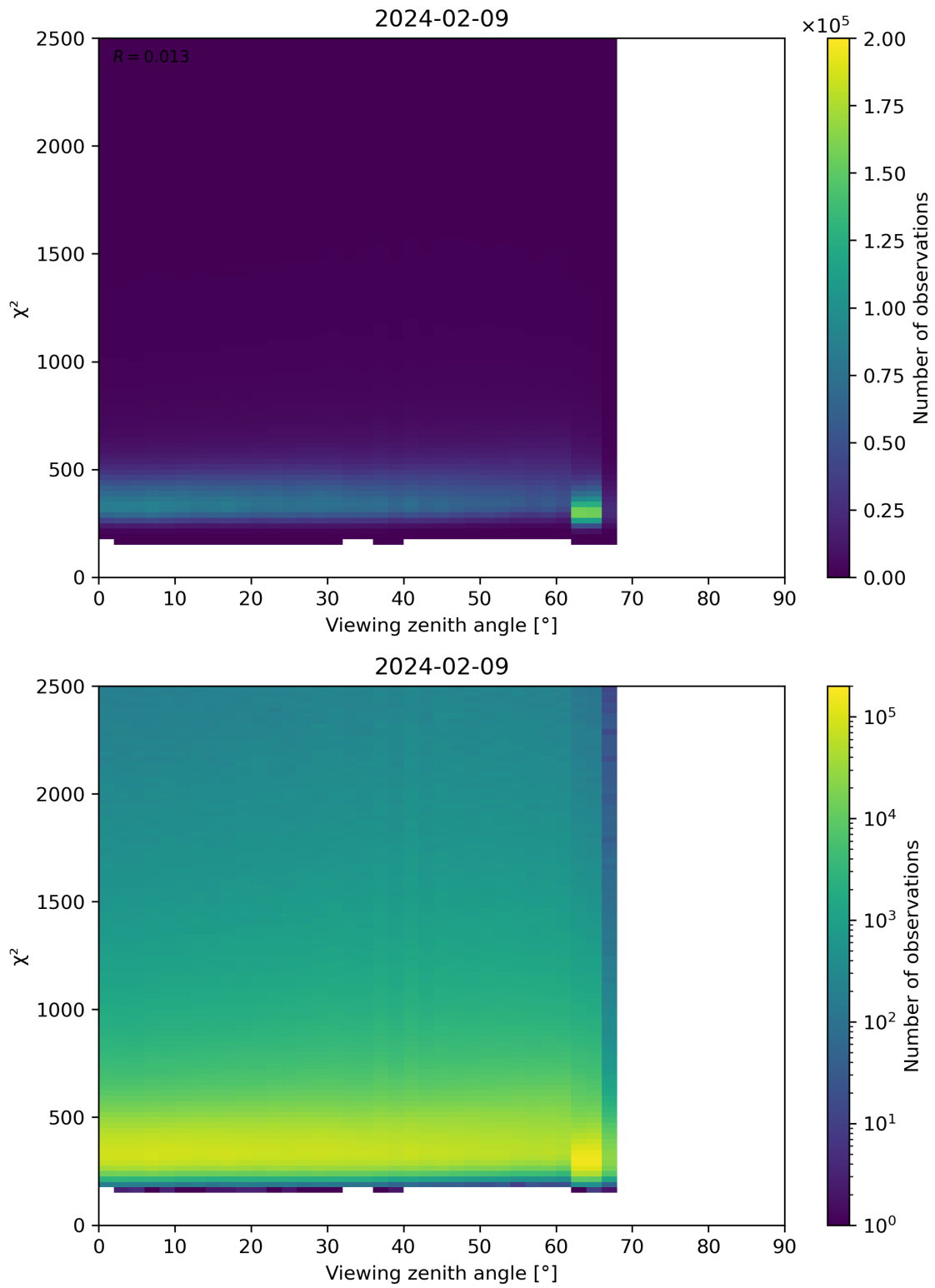
Figure 162: Scatter density plot of “Viewing zenith angle” against “ \chi^2 ” for 2024-02-08 to 2024-02-10.
