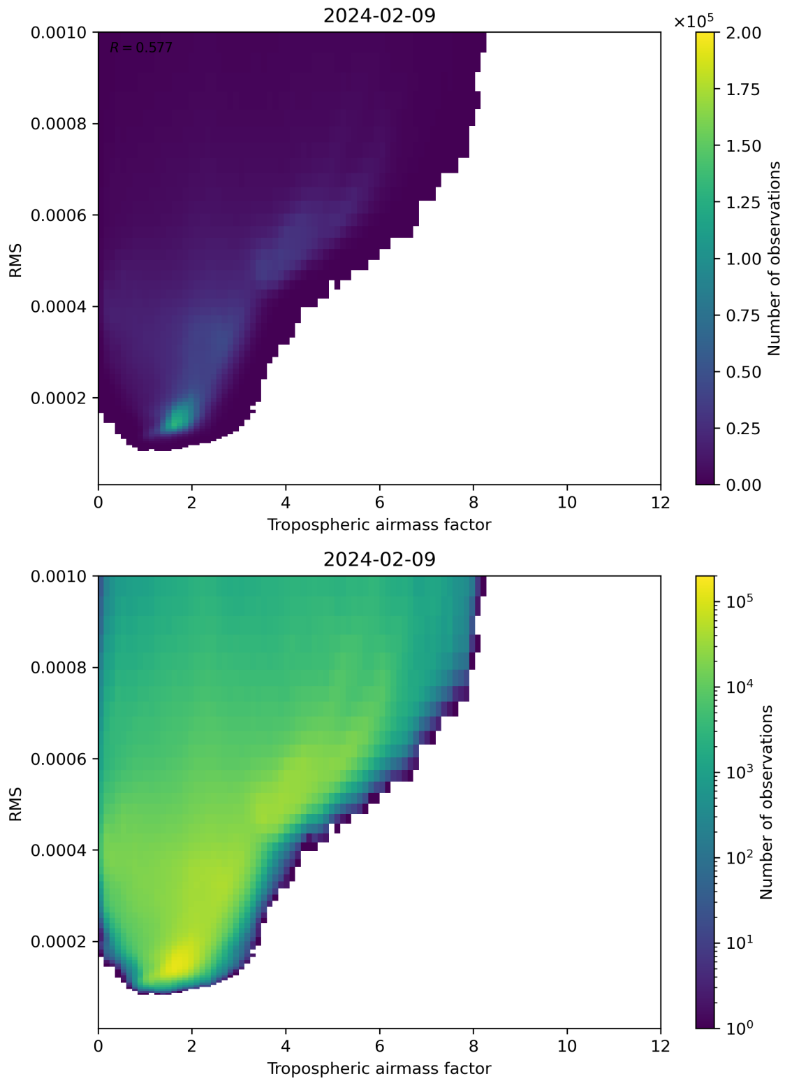
Figure 79: Scatter density plot of “Tropospheric airmass factor” against “RMS” for 2024-02-08 to 2024-02-10.
