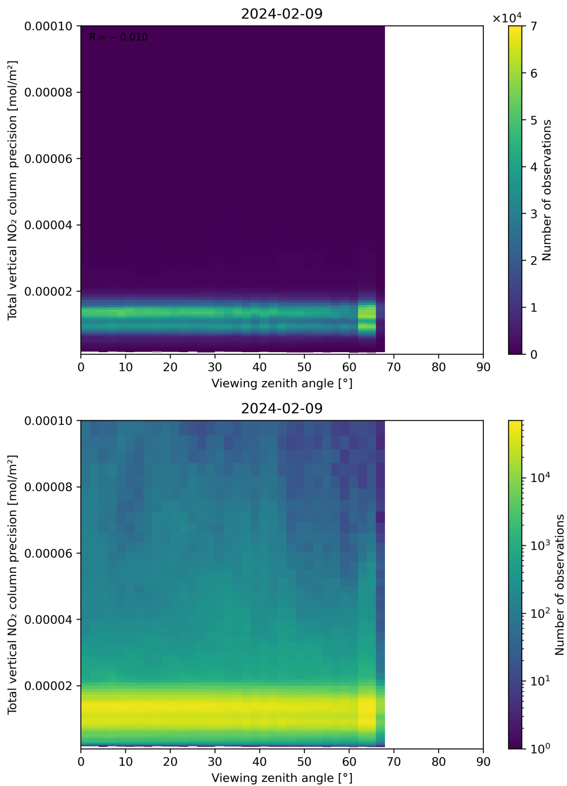
Figure 168: Scatter density plot of “Viewing zenith angle” against “Total vertical NO 2 column precision” for 2024-02-08 to 2024-02-10.
