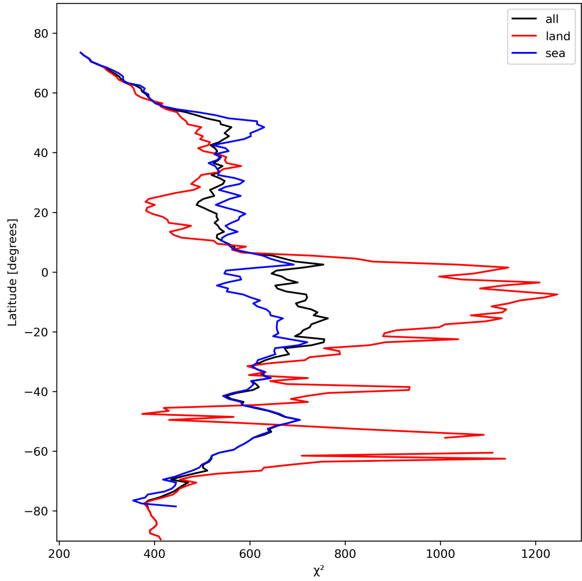
Figure 25: Zonal average of “ \chi^2 ” for 2024-02-08 to 2024-02-10.
