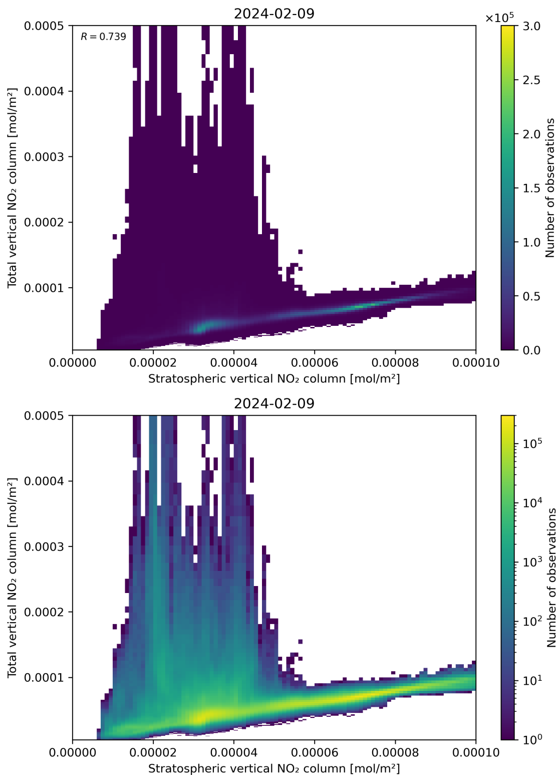
Figure 100: Scatter density plot of “Stratospheric vertical NO 2 column” against “Total vertical NO 2 column” for 2024-02-08 to 2024-02-10.
