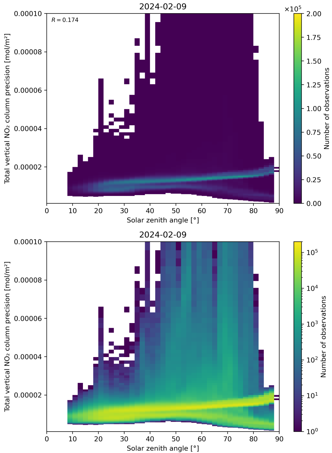
Figure 154: Scatter density plot of “Solar zenith angle” against “Total vertical NO 2 column precision” for 2024-02-08 to 2024-02-10.
