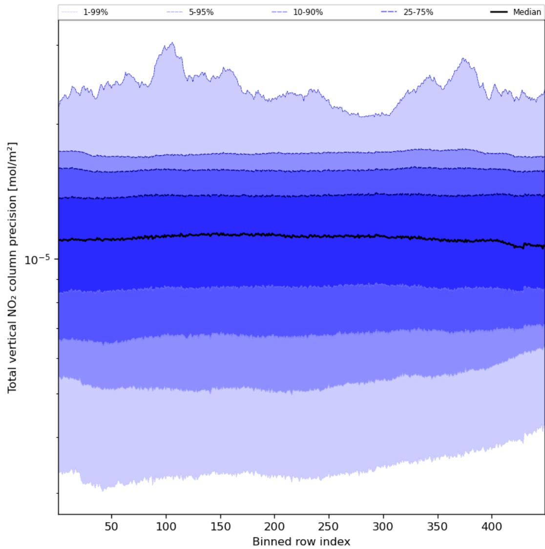
Figure 56: Along track statistics of “Total vertical NO 2 column precision” for 2024-02-08 to 2024-02-10
