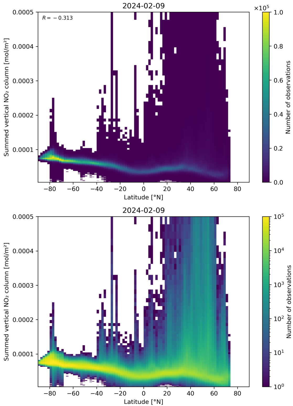
Figure 88: Scatter density plot of “Latitude” against “Summed vertical NO 2 column” for 2024-02-08 to 2024-02-10.
