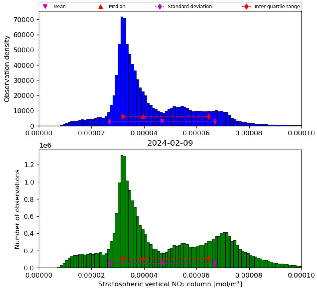
Figure 36: Histogram of “Stratospheric vertical NO 2 column” for 2024-02-08 to 2024-02-10
