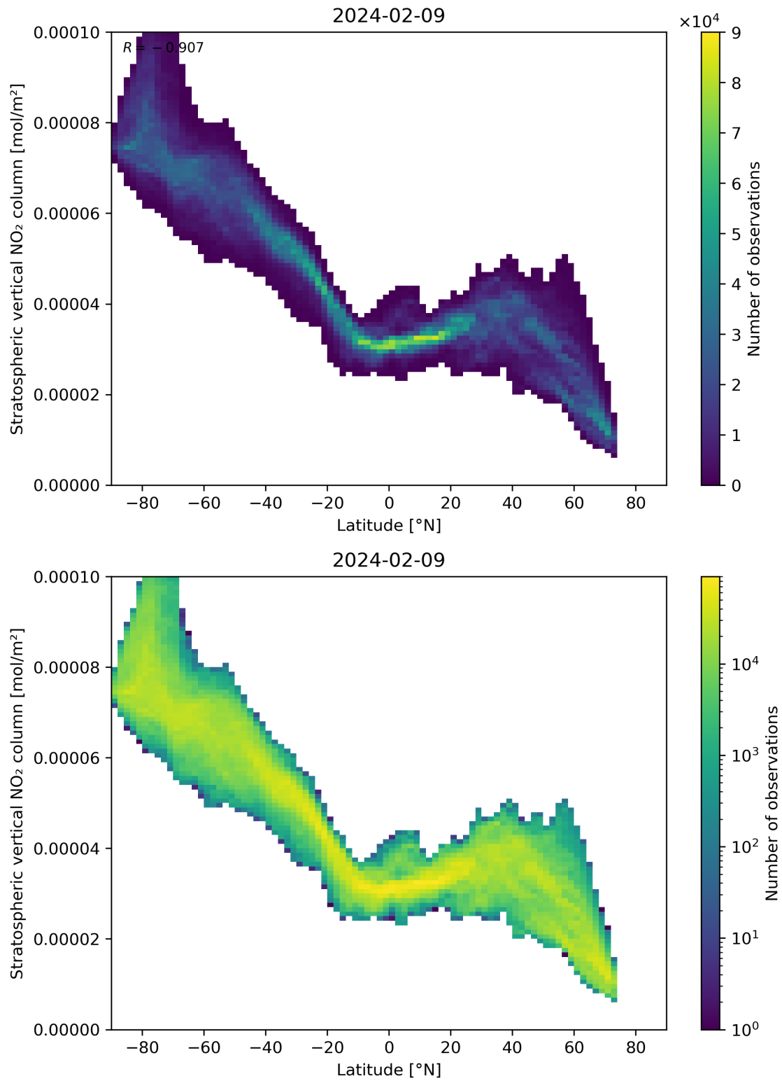
Figure 87: Scatter density plot of “Latitude” against “Stratospheric vertical NO 2 column” for 2024-02-08 to 2024-02-10.
