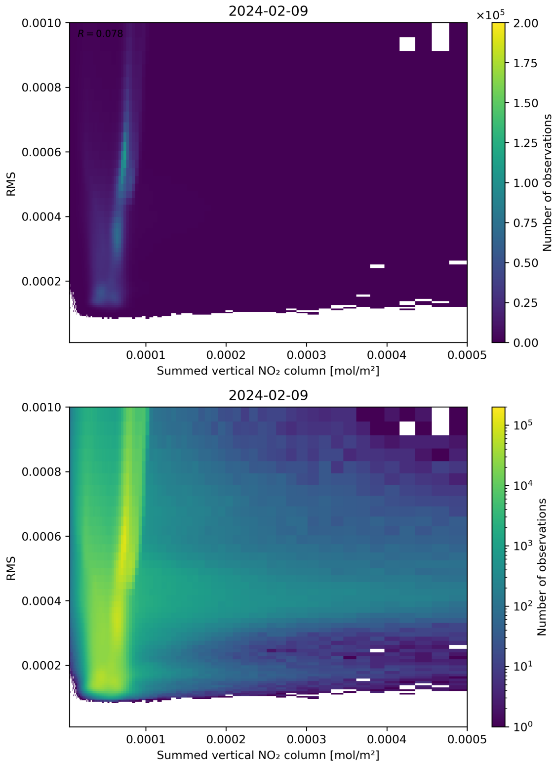
Figure 109: Scatter density plot of “Summed vertical NO 2 column” against “RMS” for 2024-02-08 to 2024-02-10.
