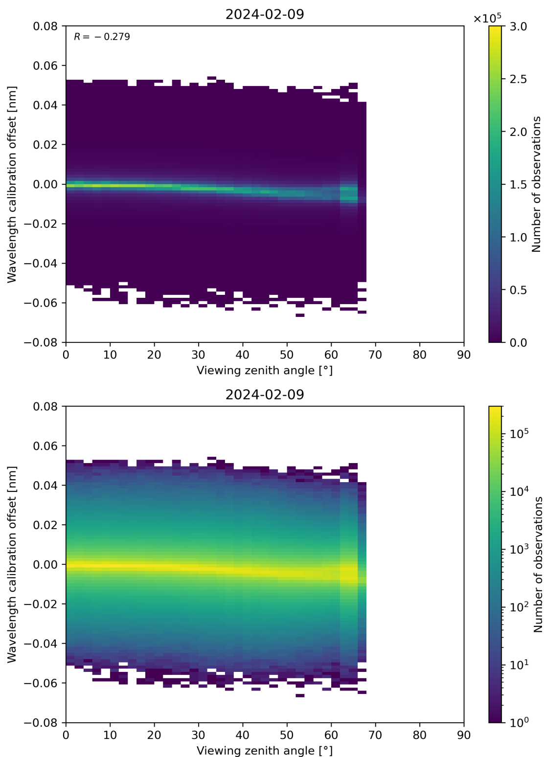
Figure 173: Scatter density plot of “Viewing zenith angle” against “Wavelength calibration offset” for 2024-02-08 to 2024-02-10.
