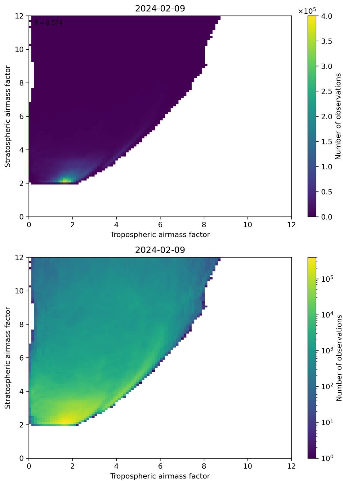
Figure 71: Scatter density plot of “Tropospheric airmass factor” against “Stratospheric airmass factor” for 2024-02-08 to 2024-02-10.
