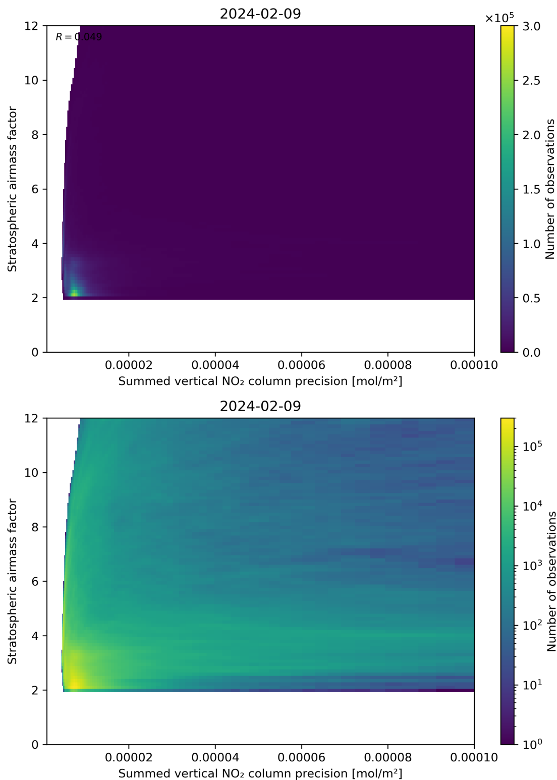
Figure 106: Scatter density plot of “Summed vertical NO 2 column precision” against “Stratospheric airmass factor” for 2024-02-08 to 2024-02-10.
