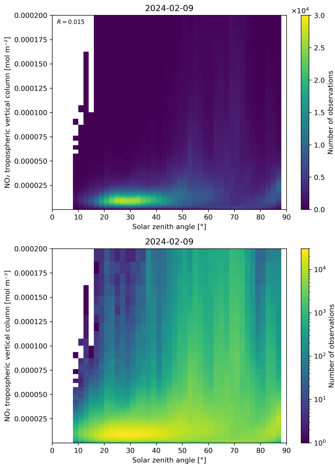
Figure 155: Scatter density plot of “Solar zenith angle” against “NO 2 tropospheric vertical column” for 2024-02-08 to 2024-02-10.
