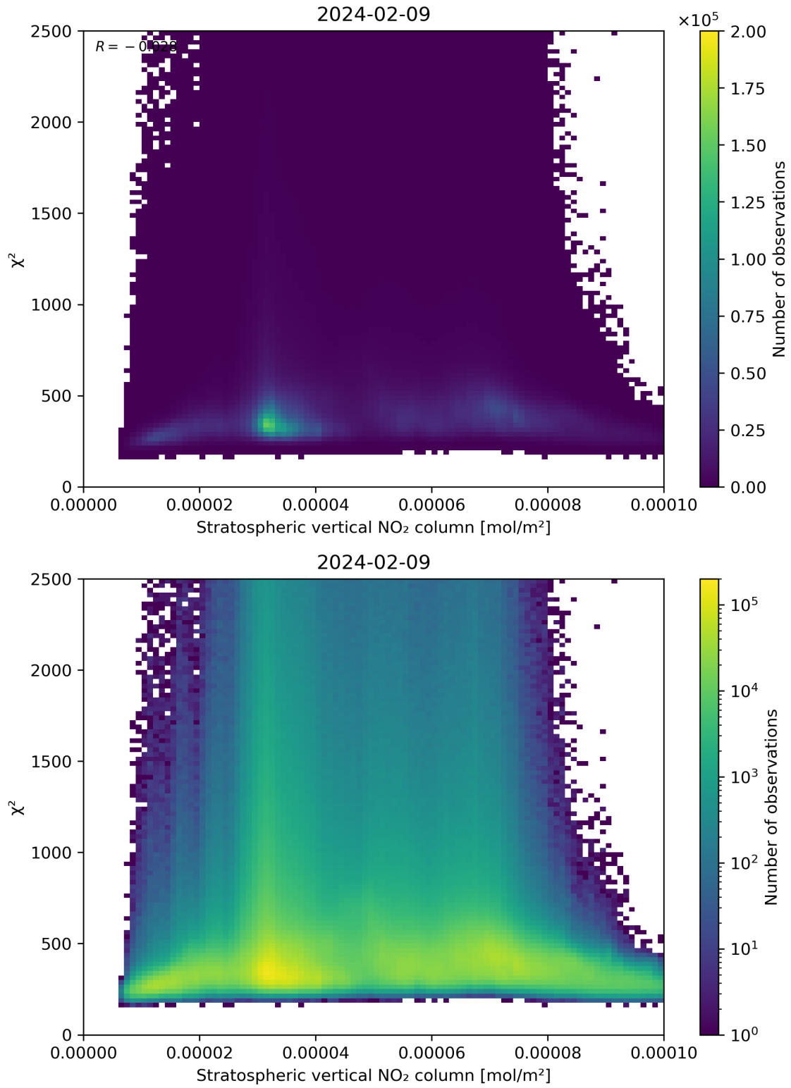
Figure 97: Scatter density plot of “Stratospheric vertical NO 2 column” against “ \chi^2 ” for 2024-02-08 to 2024-02-10.
