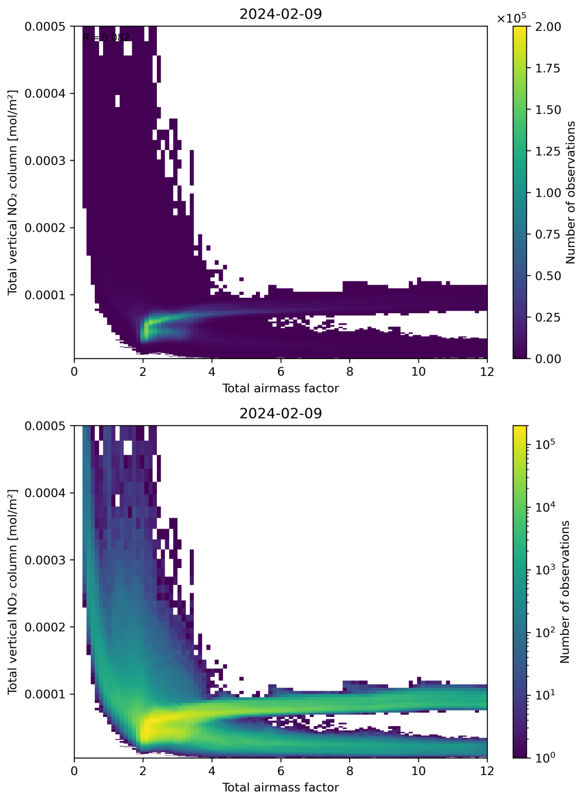
Figure 67: Scatter density plot of “Total airmass factor” against “Total vertical NO 2 column” for 2024-02-08 to 2024-02-10.
