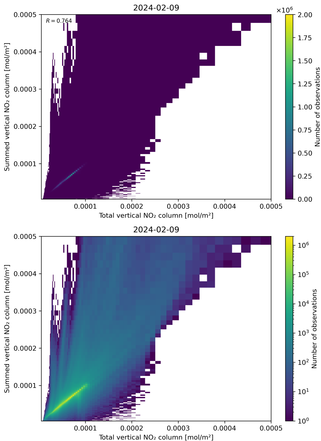
Figure 112: Scatter density plot of “Total vertical NO 2 column” against “Summed vertical NO 2 column” for 2024-02-08 to 2024-02-10.
