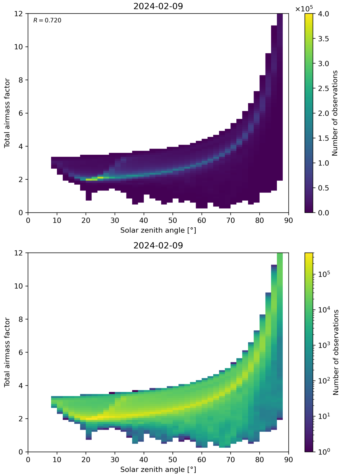
Figure 146: Scatter density plot of “Solar zenith angle” against “Total air mass factor” for 2024-02-08 to 2024-02-10.
