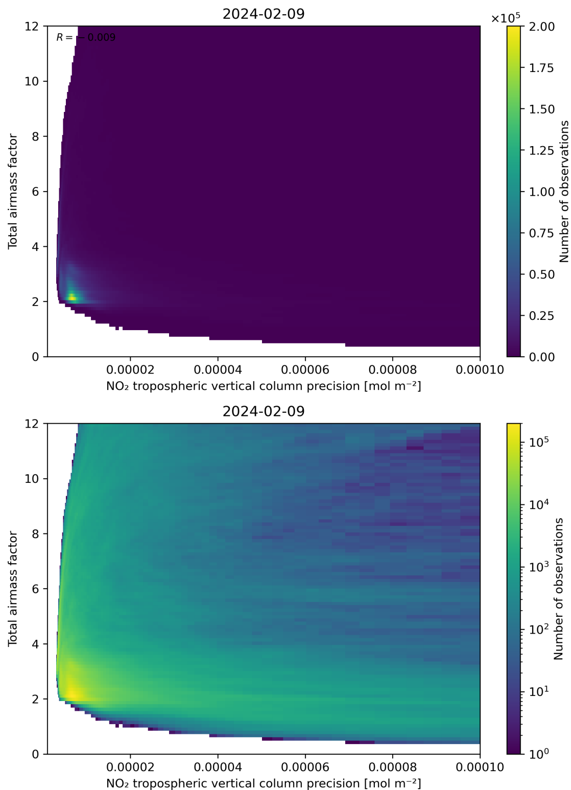
Figure 132: Scatter density plot of “NO 2 tropospheric vertical column precision” against “Total air mass factor” for 2024-02-08 to 2024-02-10.
