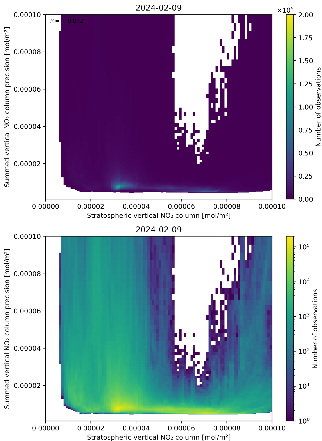
Figure 99: Scatter density plot of “Stratospheric vertical NO 2 column” against “Summed vertical NO 2 column precision” for 2024-02-08 to 2024-02-10.
