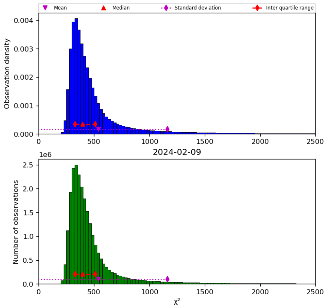
Figure 42: Histogram of " \chi^2 " for 2024-02-08 to 2024-02-10
