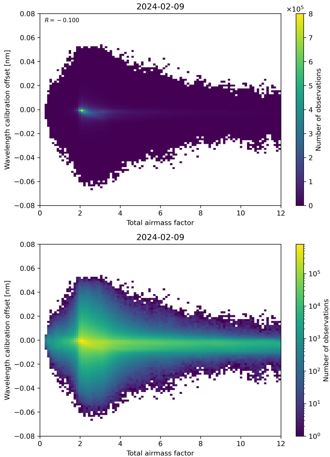
Figure 70: Scatter density plot of “Total airmass factor” against “Wavelength calibration offset” for 2024-02-08 to 2024-02-10.
