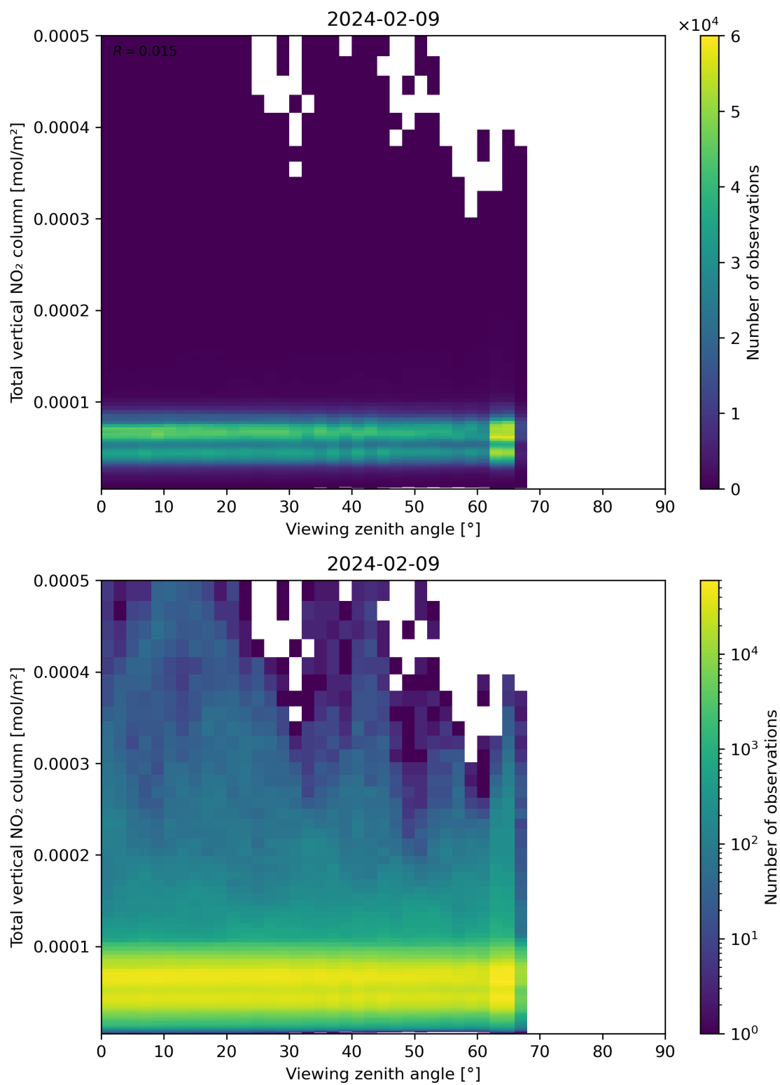
Figure 167: Scatter density plot of “Viewing zenith angle” against “Total vertical NO 2 column” for 2024-02-08 to 2024-02-10.
