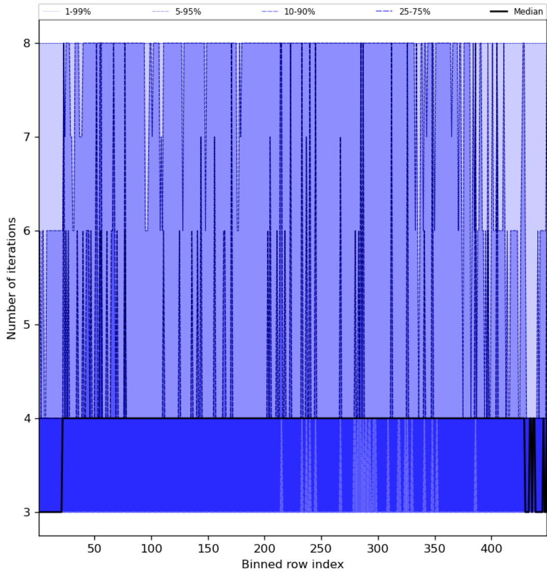
Figure 51: Along track statistics of “Number of iterations” for 2024-02-08 to 2024-02-10
