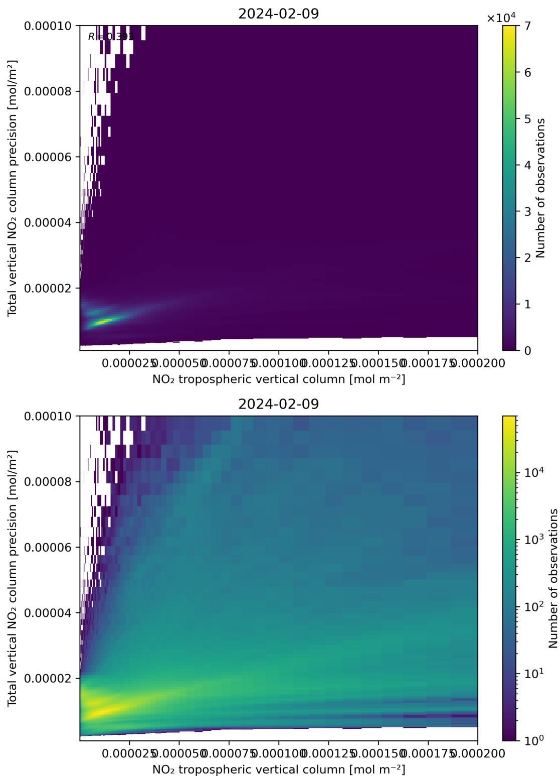
Figure 129: Scatter density plot of “NO 2 tropospheric vertical column” against “Total vertical NO 2 column precision” for 2024-02-08 to 2024-02-10.
