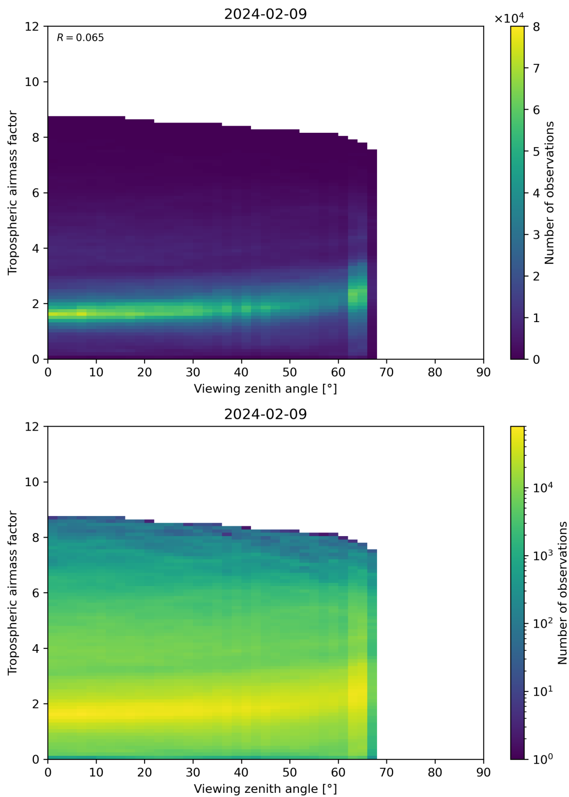
Figure 161: Scatter density plot of “Viewing zenith angle” against “Tropospheric airmass factor” for 2024-02-08 to 2024-02-10.
