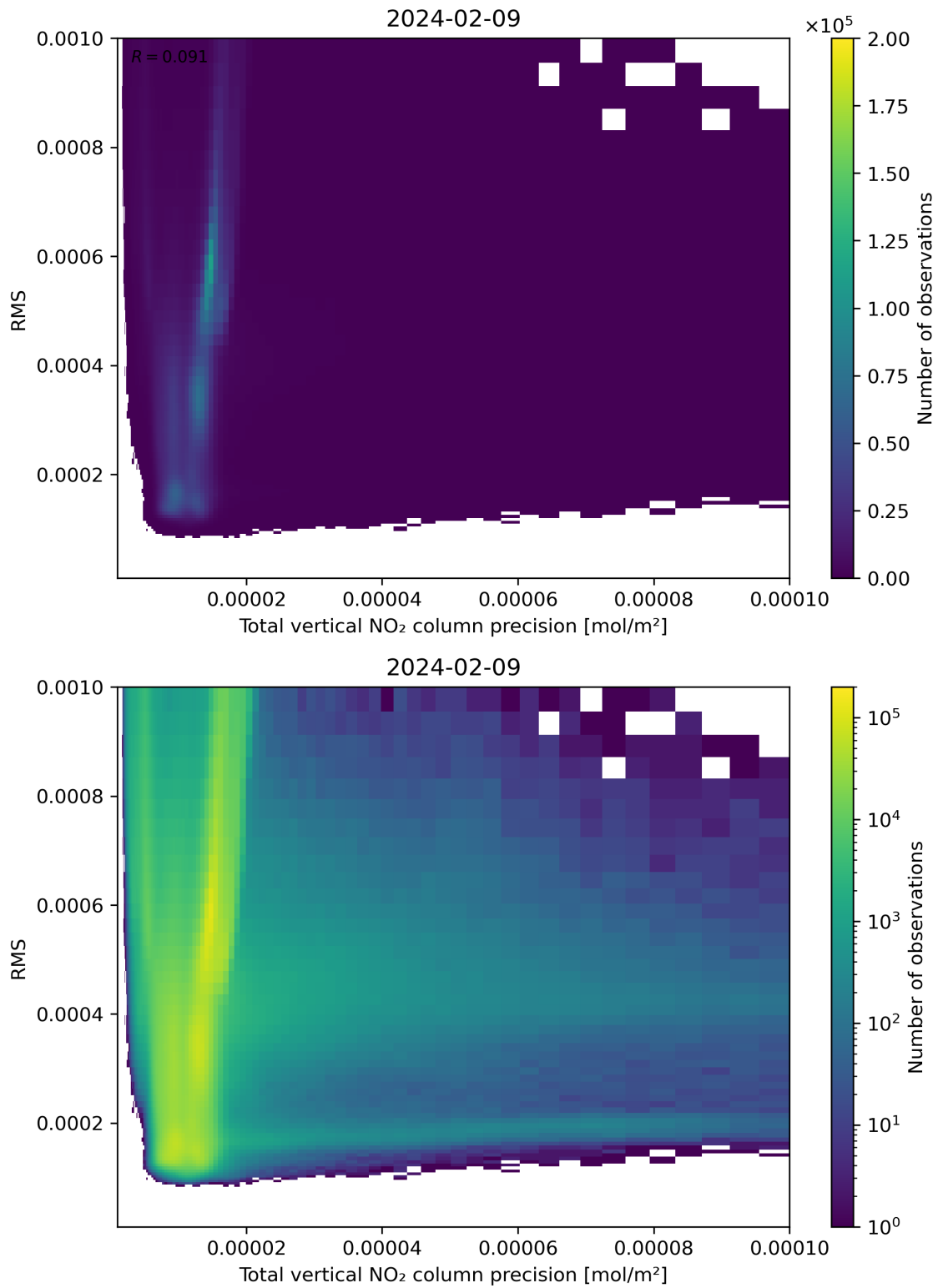
Figure 119: Scatter density plot of “Total vertical NO 2 column precision” against “RMS” for 2024-02-08 to 2024-02-10.
