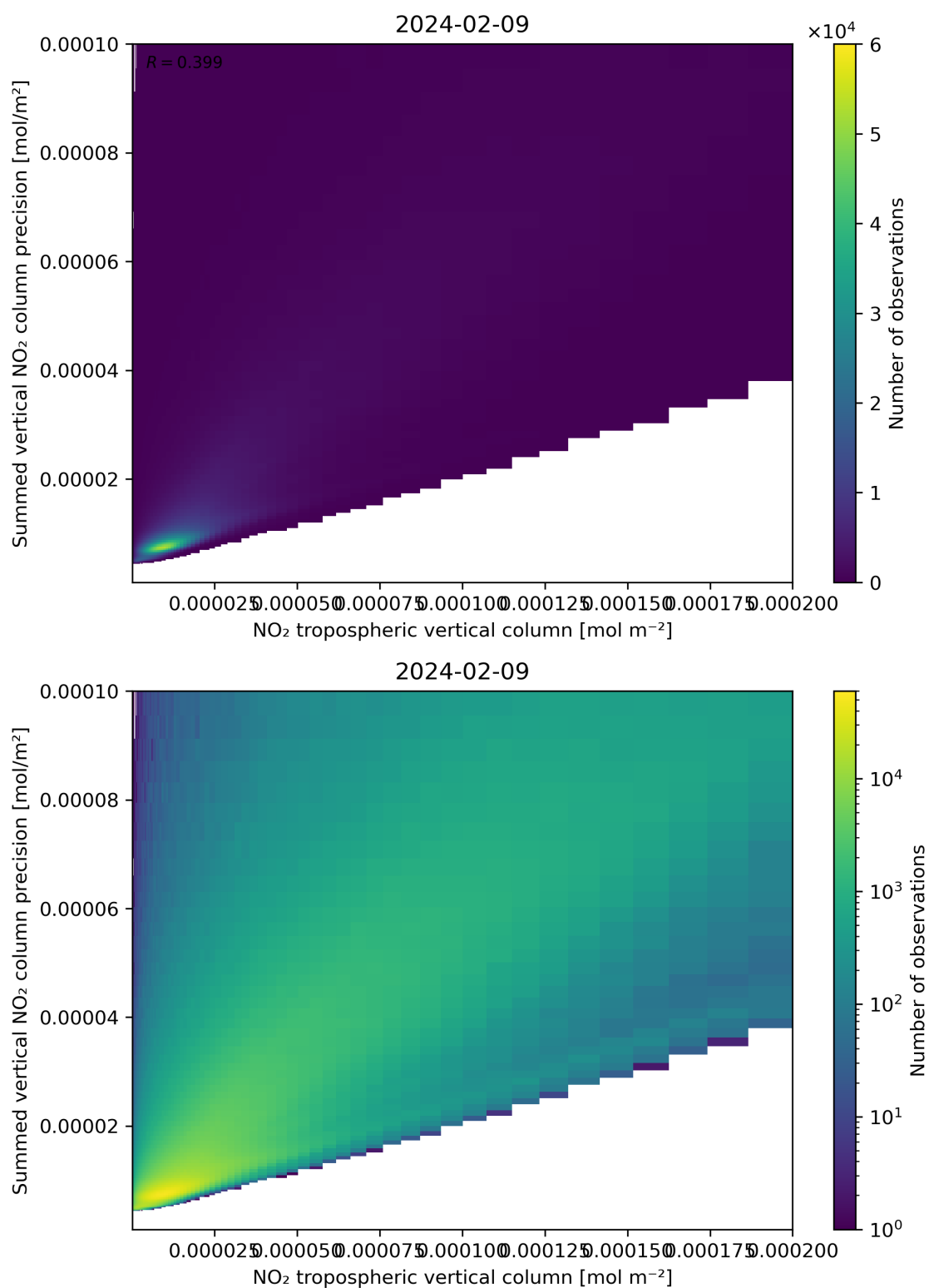
Figure 127: Scatter density plot of “NO 2 tropospheric vertical column” against “Summed vertical NO 2 column precision” for 2024-02-08 to 2024-02-10.
