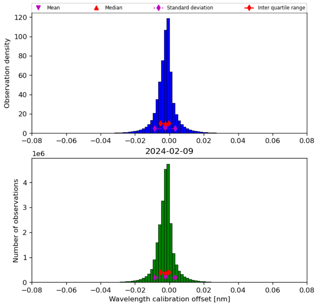
Figure 35: Histogram of “Wavelength calibration offset” for 2024-02-08 to 2024-02-10
