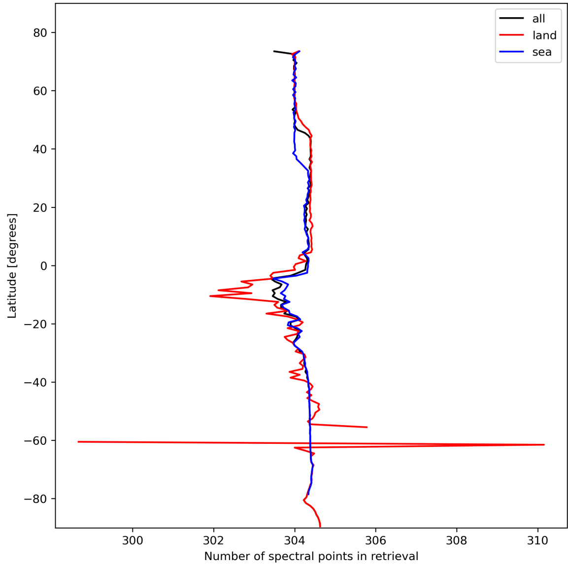
Figure 16: Zonal average of “Number of spectral points in retrieval” for 2024-02-08 to 2024-02-10.
