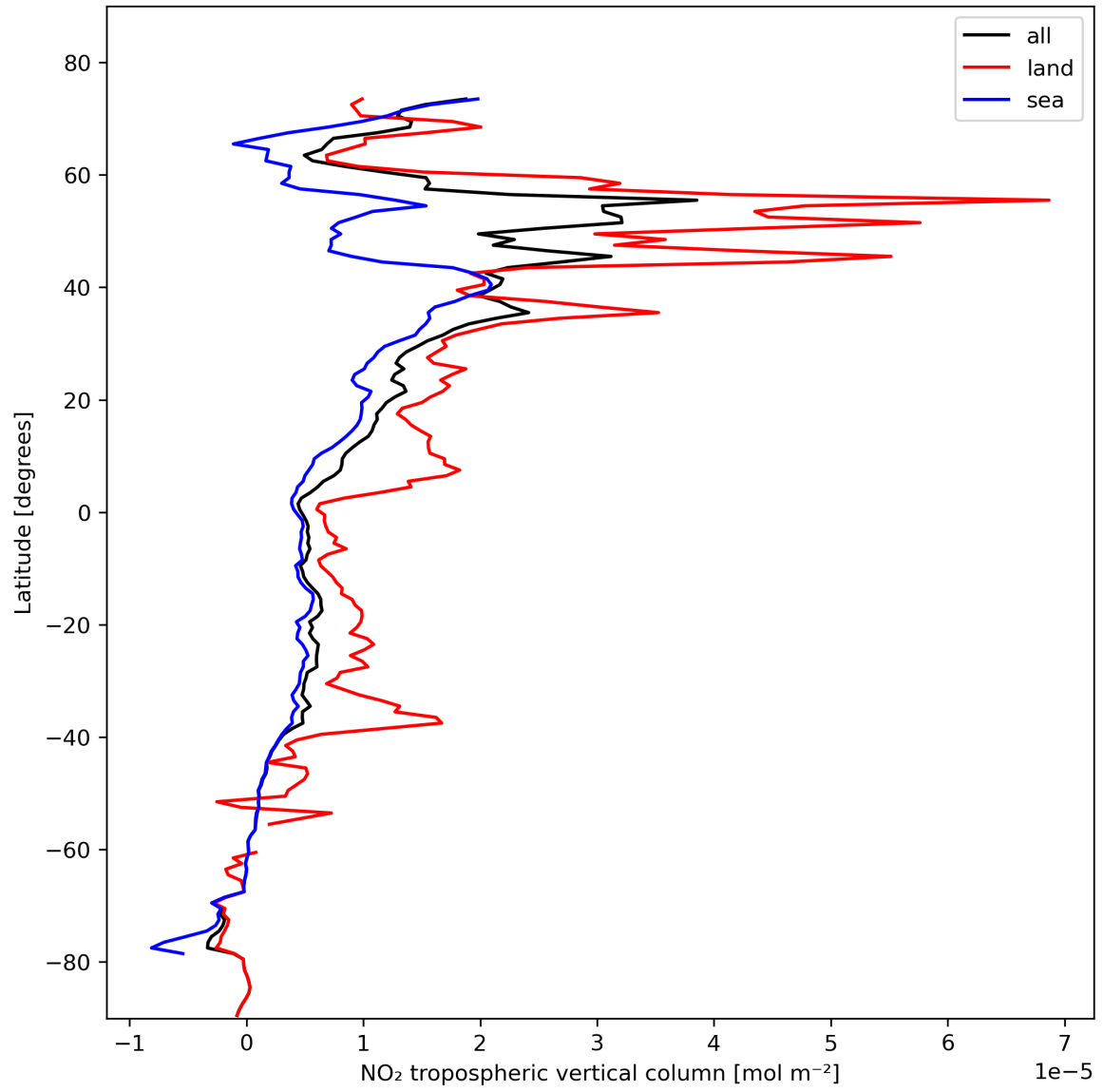
Figure 12: Zonal average of “NO 2 tropospheric vertical column” for 2024-02-08 to 2024-02-10.
