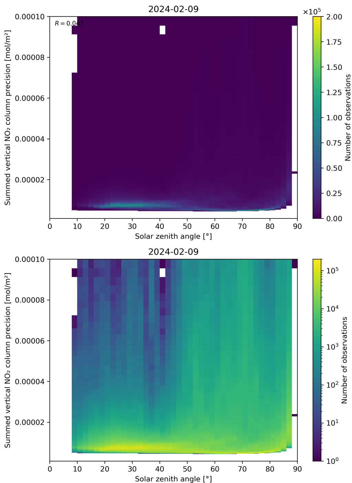
Figure 152: Scatter density plot of “Solar zenith angle” against “Summed vertical NO 2 column precision” for 2024-02-08 to 2024-02-10.
