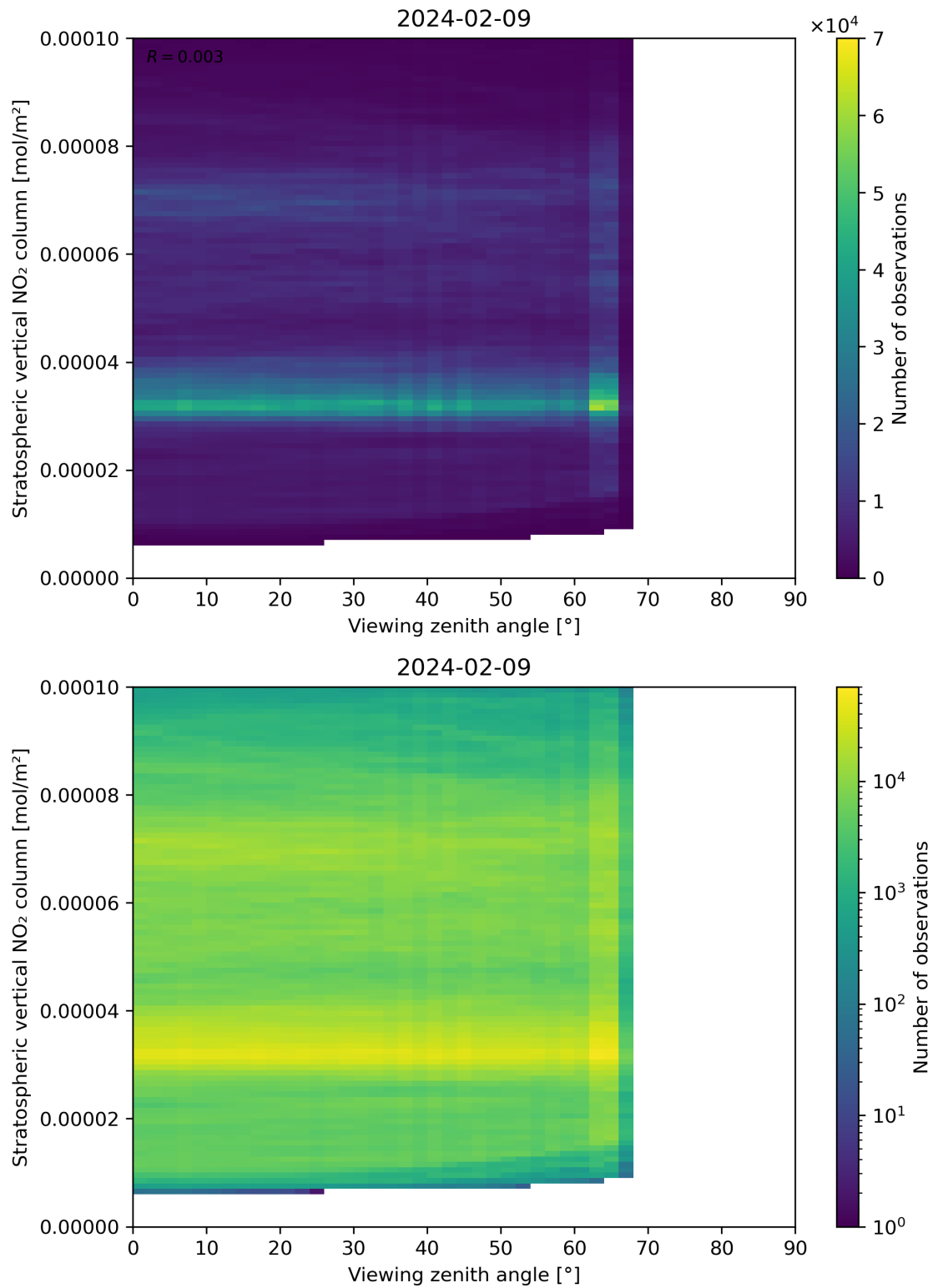
Figure 164: Scatter density plot of “Viewing zenith angle” against “Stratospheric vertical NO 2 column” for 2024-02-08 to 2024-02-10.
