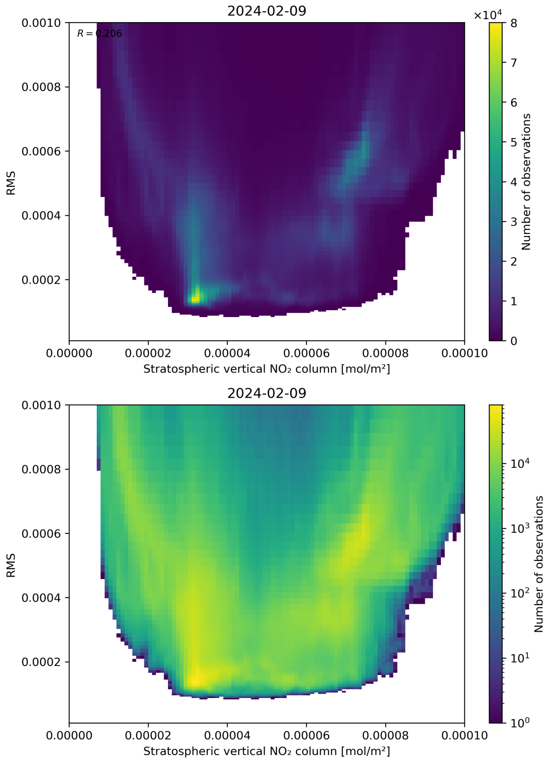
Figure 102: Scatter density plot of “Stratospheric vertical NO 2 column” against “RMS” for 2024-02-08 to 2024-02-10.
