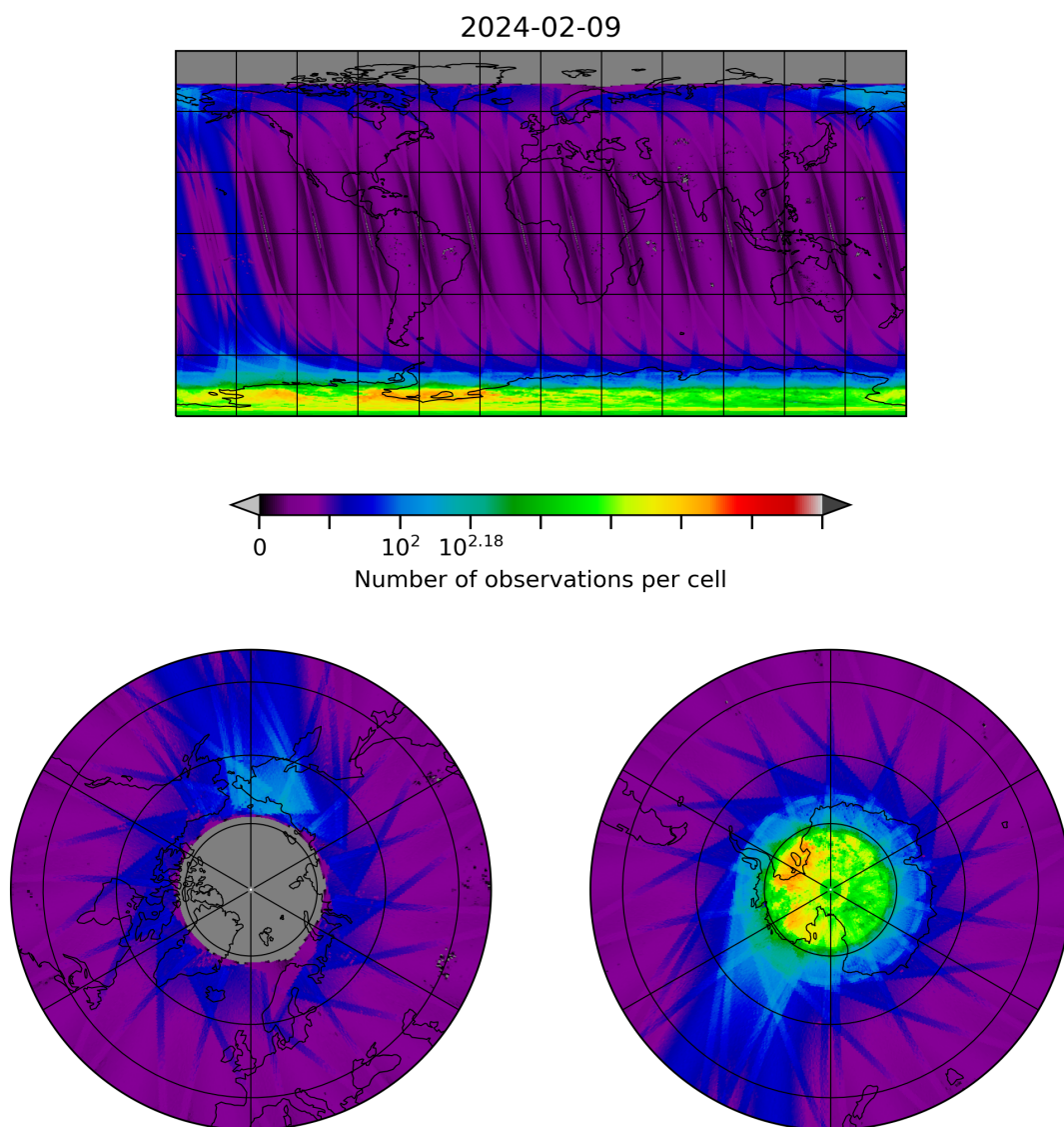
Figure 10: Map of the number of observations for 2024-02-08 to 2024-02-10
