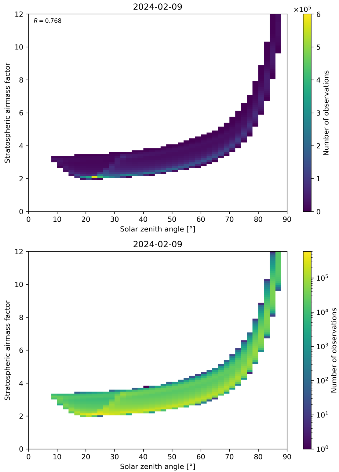
Figure 145: Scatter density plot of “Solar zenith angle” against “Stratospheric airmass factor” for 2024-02-08 to 2024-02-10.
