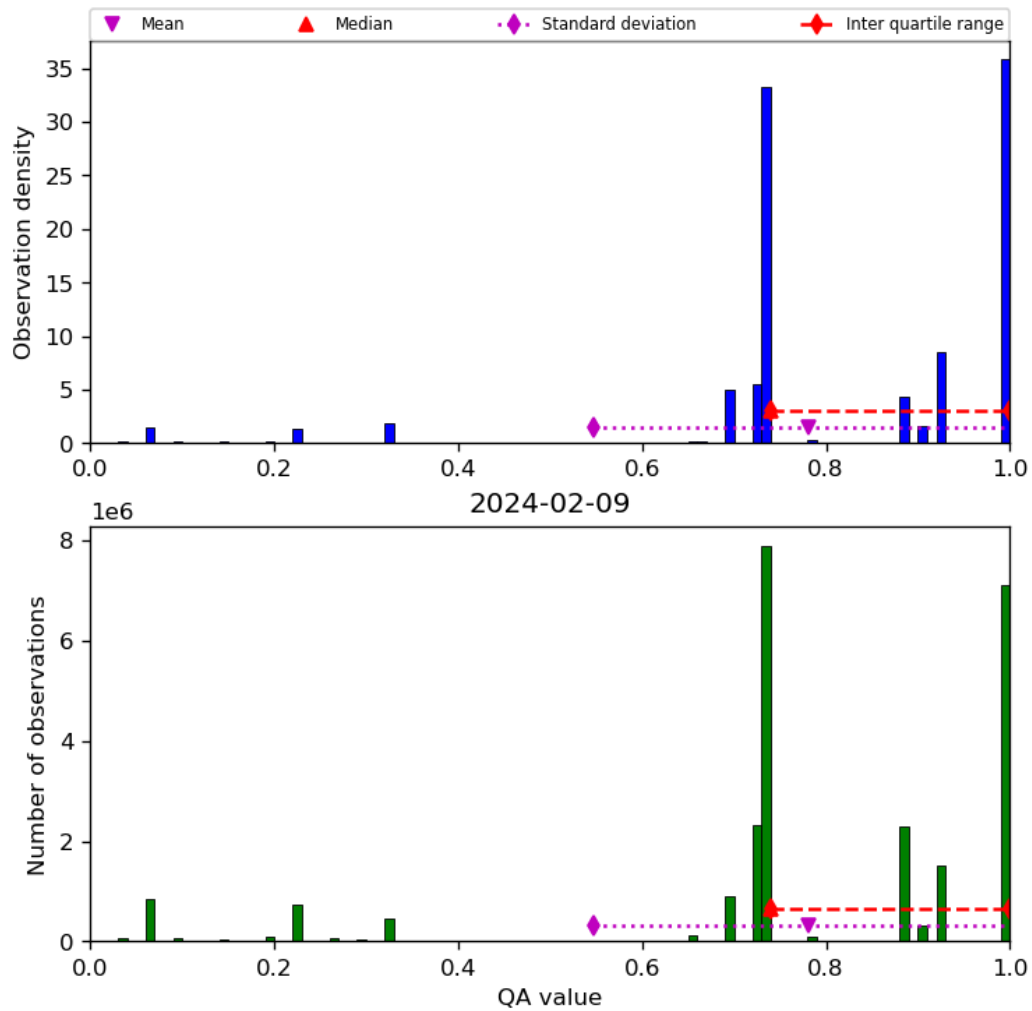
Figure 28: Histogram of “QA value” for 2024-02-08 to 2024-02-10
