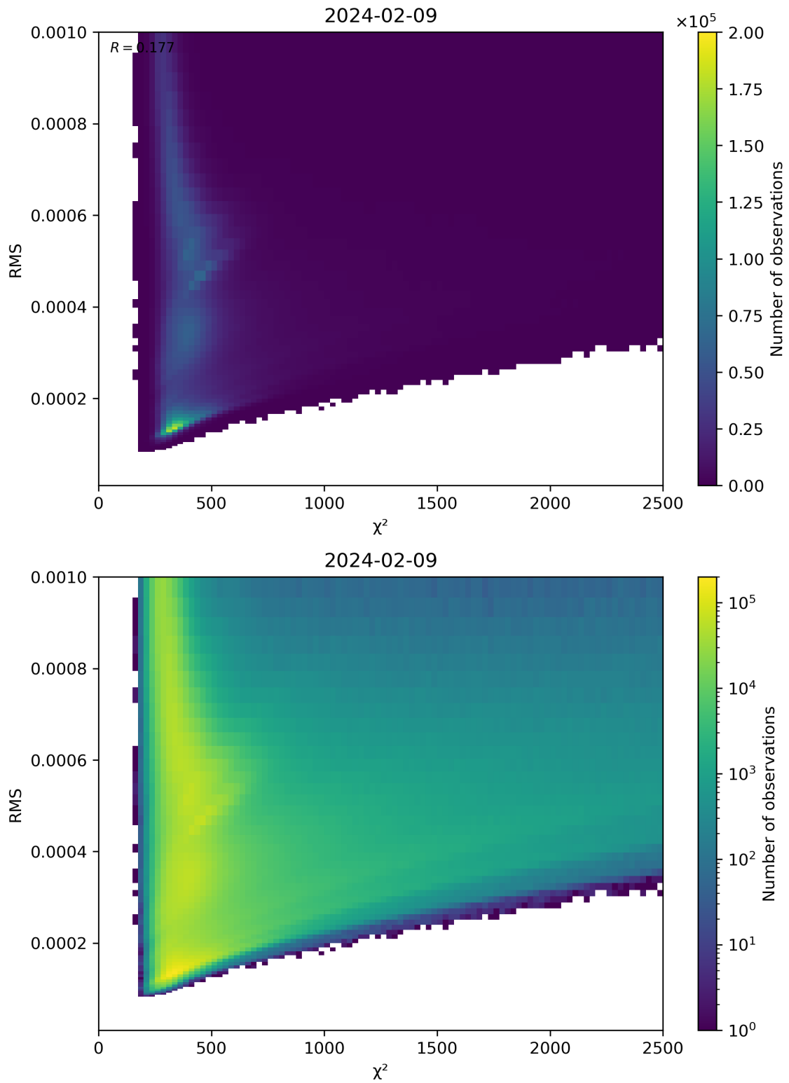
Figure 82: Scatter density plot of “ \chi^2 ” against “RMS” for 2024-02-08 to 2024-02-10.
