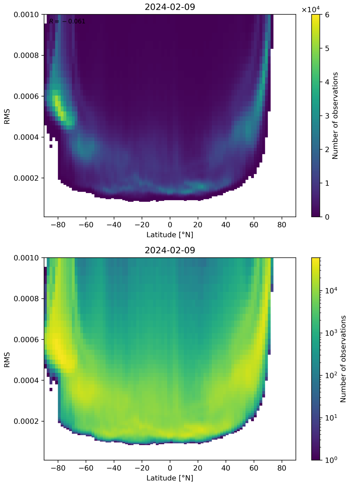
Figure 94: Scatter density plot of “Latitude” against “RMS” for 2024-02-08 to 2024-02-10.
