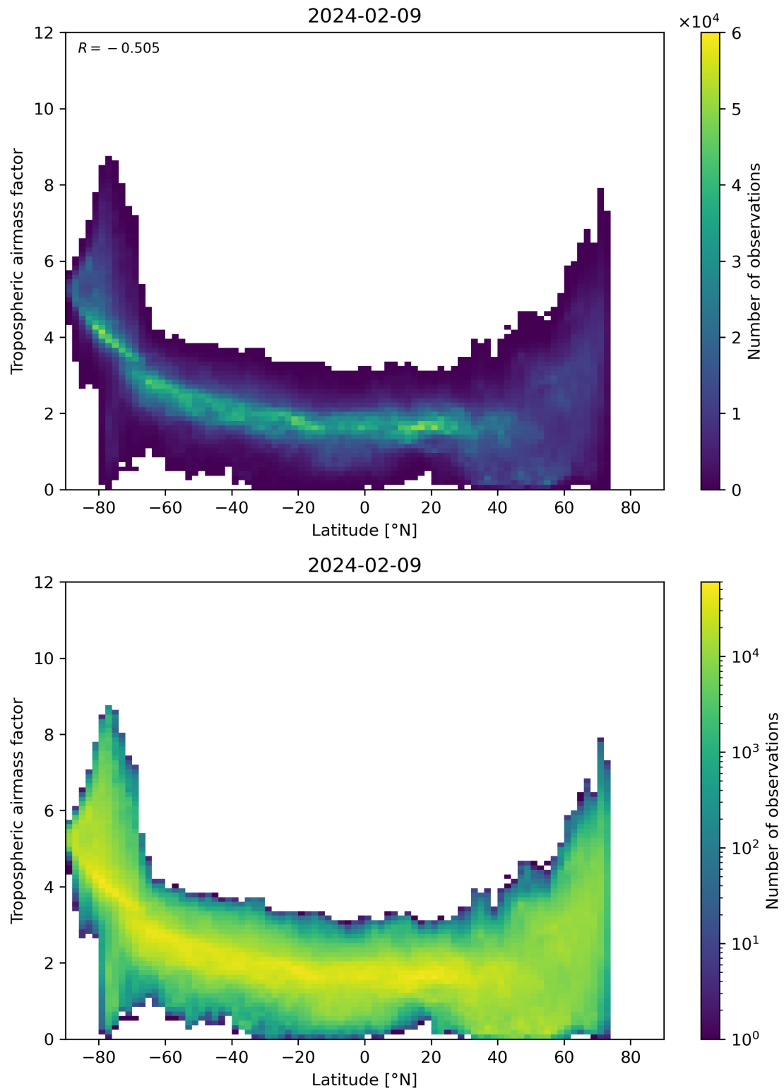
Figure 85: Scatter density plot of “Latitude” against “Tropospheric airmass factor” for 2024-02-08 to 2024-02-10.
