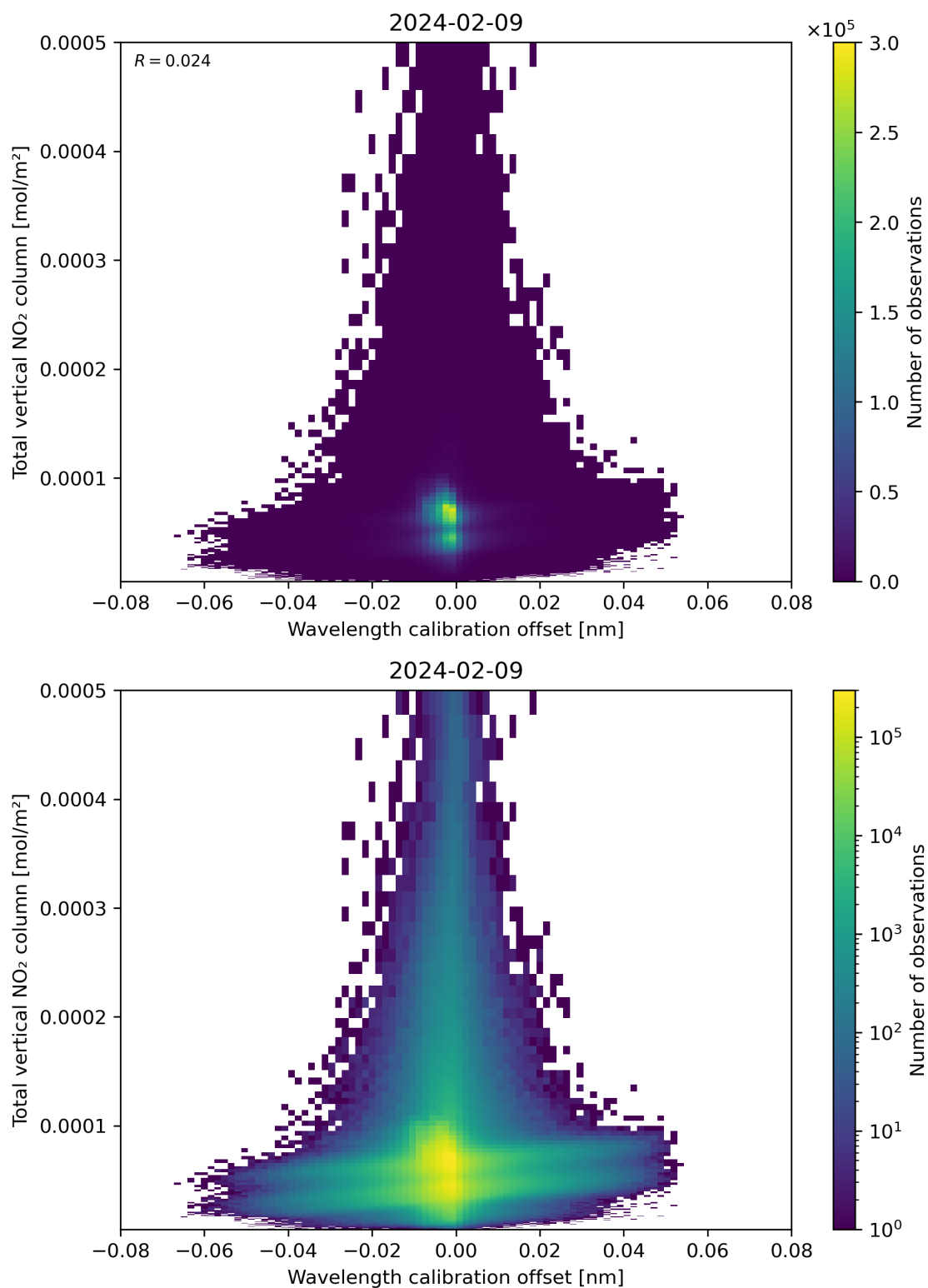
Figure 179: Scatter density plot of “Wavelength calibration offset” against “Total vertical NO 2 column” for 2024-02-08 to 2024-02-10.
