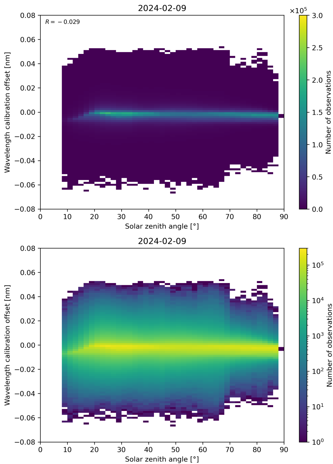
Figure 158: Scatter density plot of “Solar zenith angle” against “Wavelength calibration offset” for 2024-02-08 to 2024-02-10.
