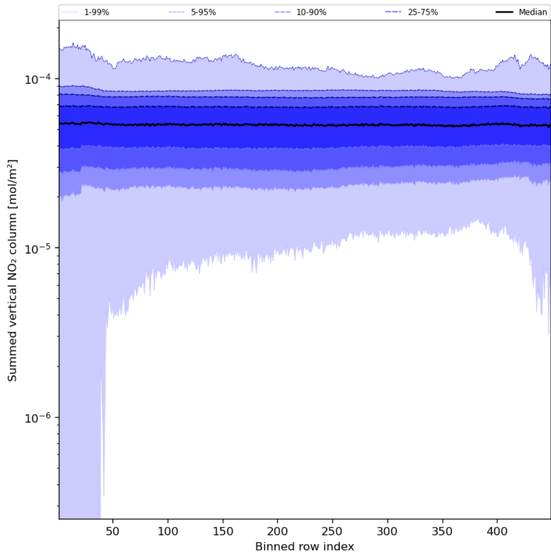
Figure 57: Along track statistics of “Summed vertical NO 2 column” for 2024-02-08 to 2024-02-10
