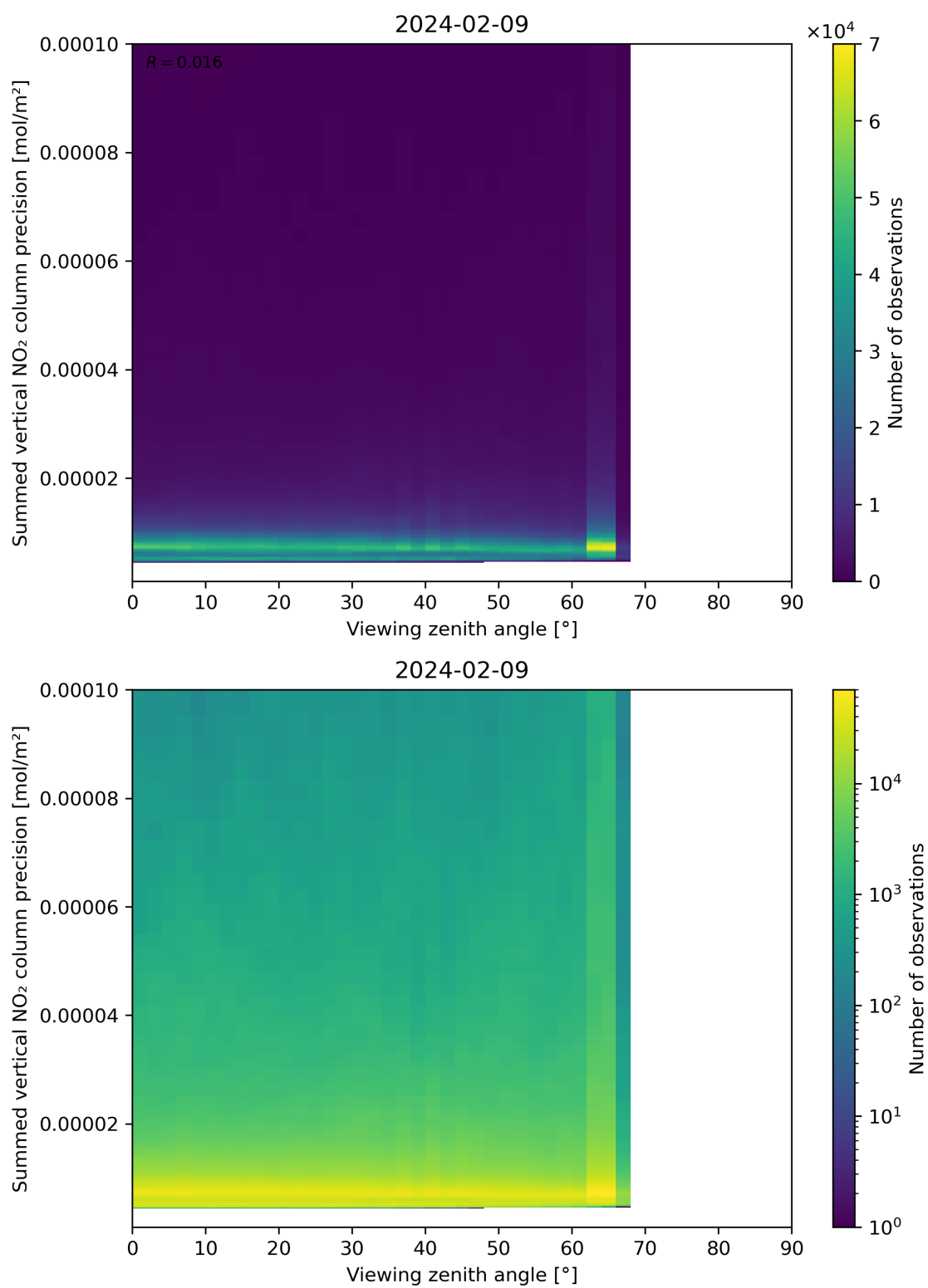
Figure 166: Scatter density plot of “Viewing zenith angle” against “Summed vertical NO 2 column precision” for 2024-02-08 to 2024-02-10.
