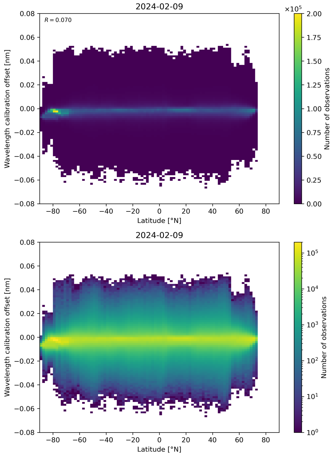
Figure 95: Scatter density plot of “Latitude” against “Wavelength calibration offset” for 2024-02-08 to 2024-02-10.
