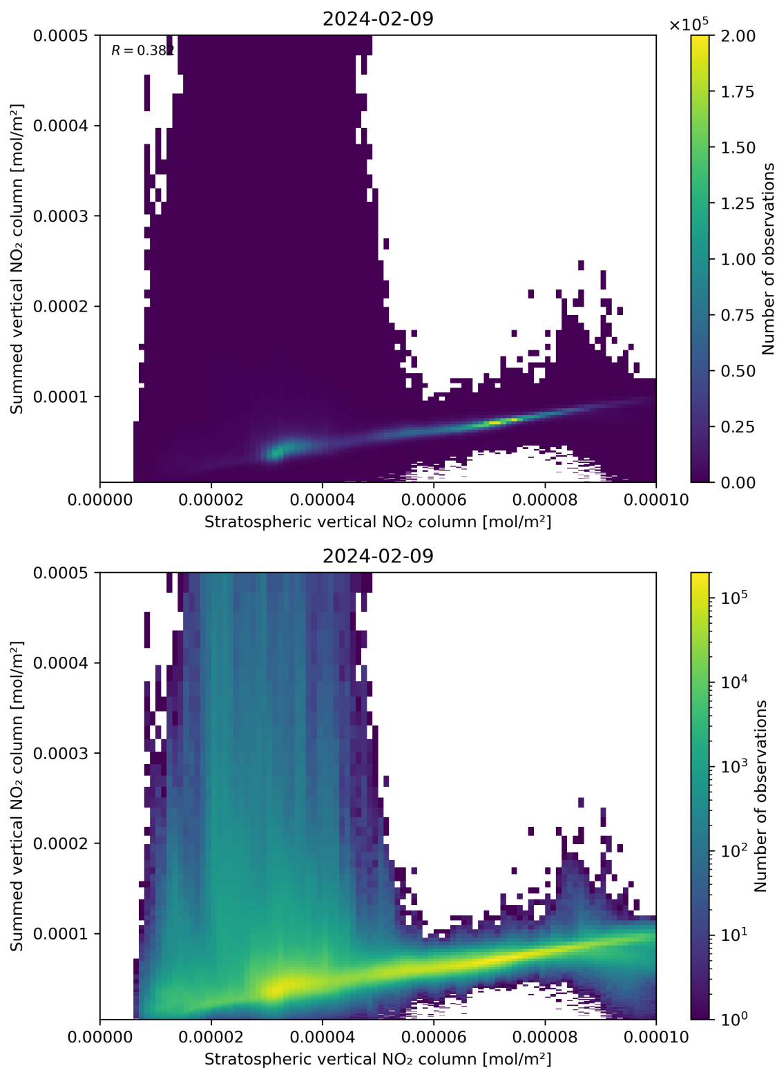
Figure 98: Scatter density plot of “Stratospheric vertical NO 2 column” against “Summed vertical NO 2 column” for 2024-02-08 to 2024-02-10.
