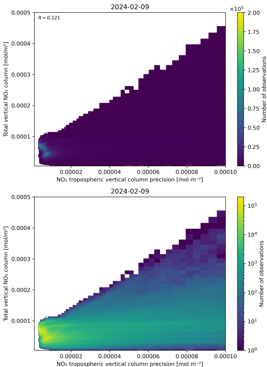
Figure 138: Scatter density plot of “NO 2 tropospheric vertical column precision” against “Total vertical NO 2 column” for 2024-02-08 to 2024-02-10.
