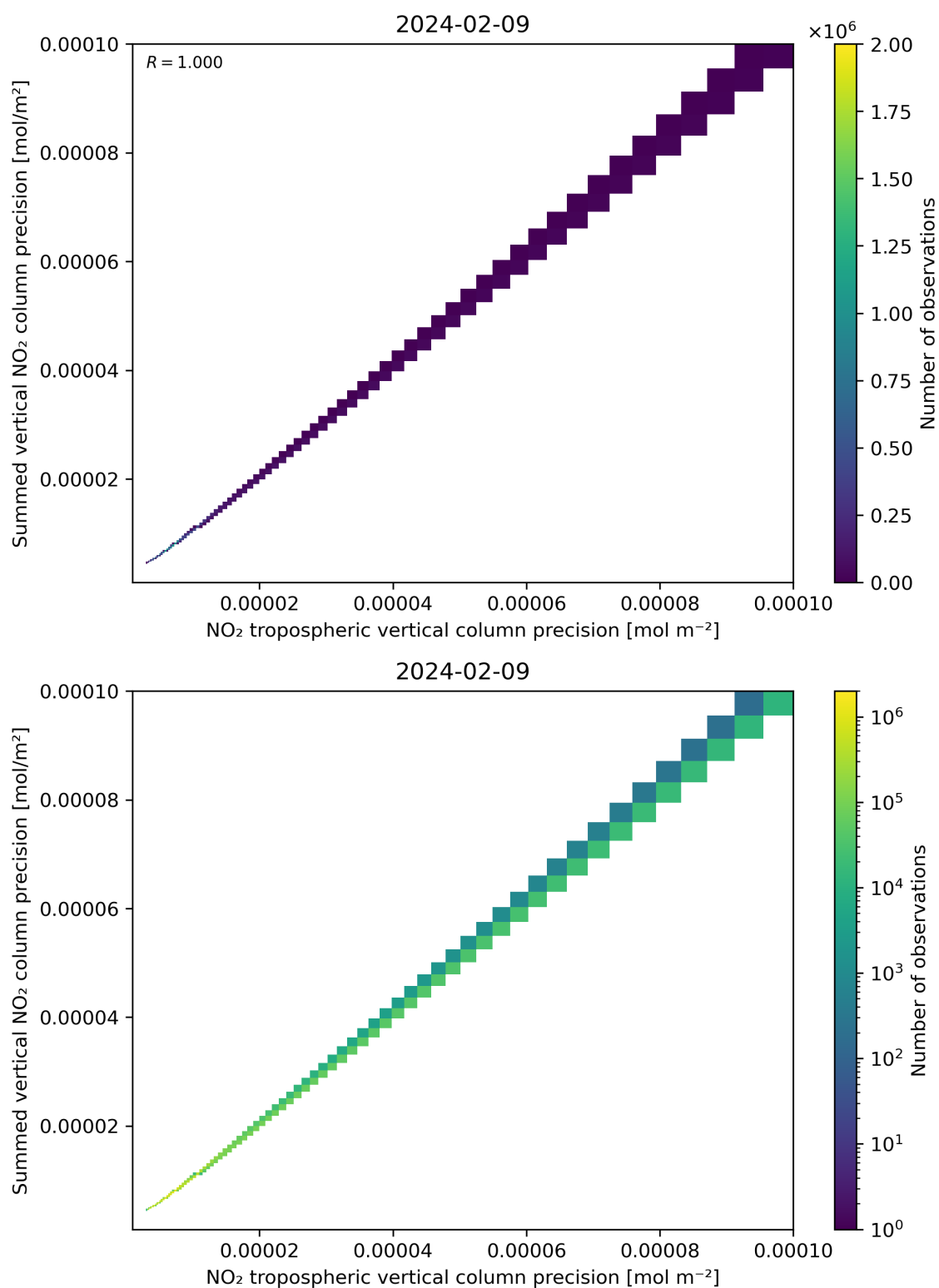
Figure 137: Scatter density plot of “NO 2 tropospheric vertical column precision” against “Summed vertical NO 2 column precision” for 2024-02-08 to 2024-02-10.
