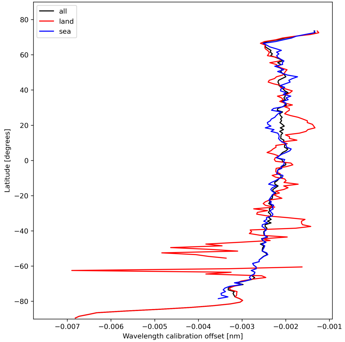
Figure 18: Zonal average of “Wavelength calibration offset” for 2024-02-08 to 2024-02-10.
