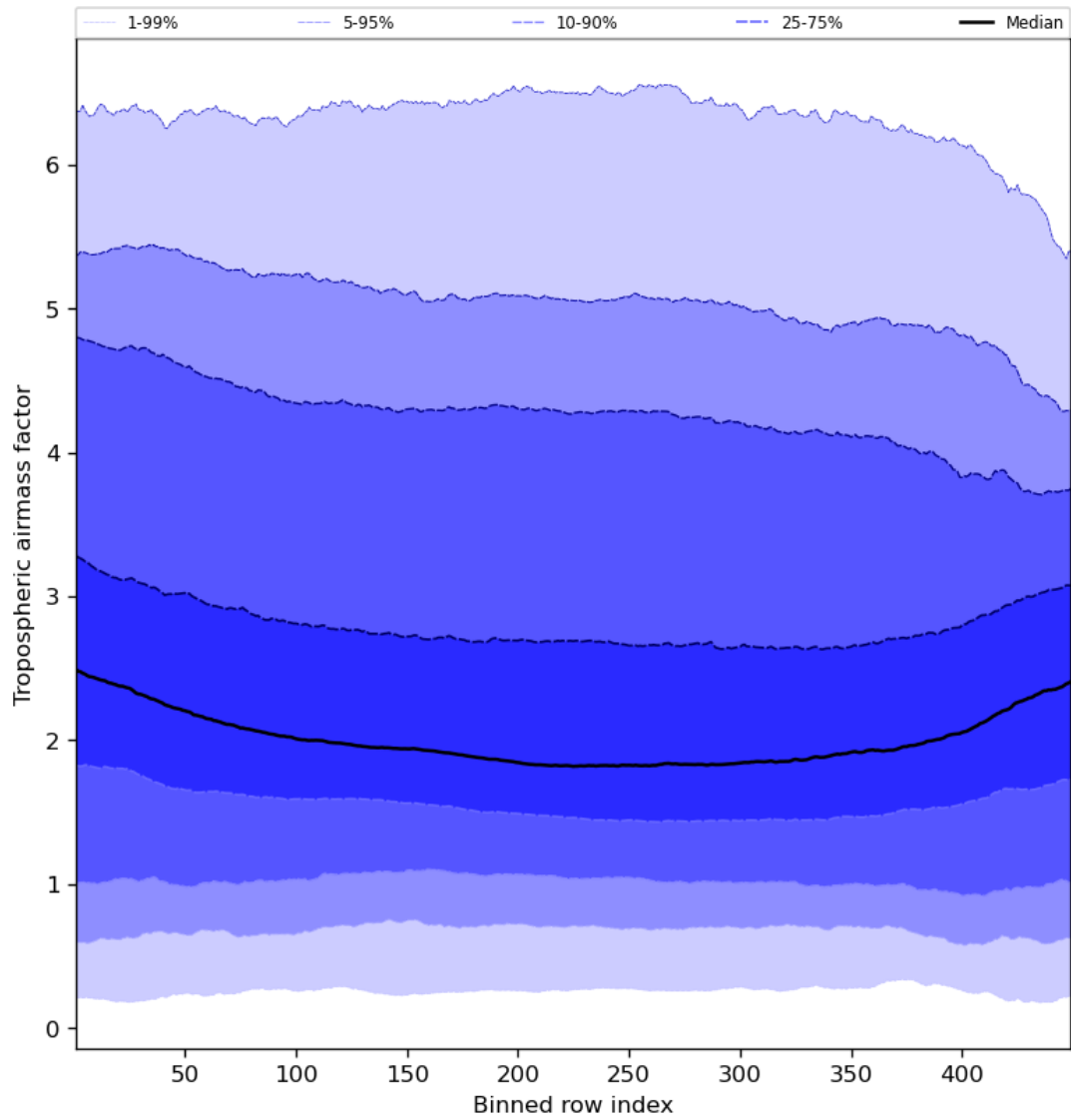
Figure 48: Along track statistics of “Tropospheric airmass factor” for 2024-02-08 to 2024-02-10
