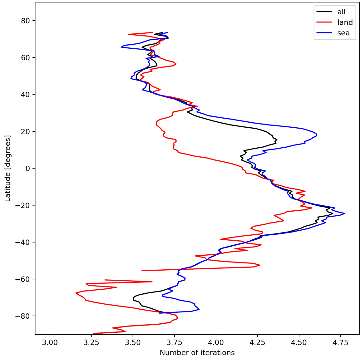
Figure 17: Zonal average of “Number of iterations” for 2024-02-08 to 2024-02-10.
