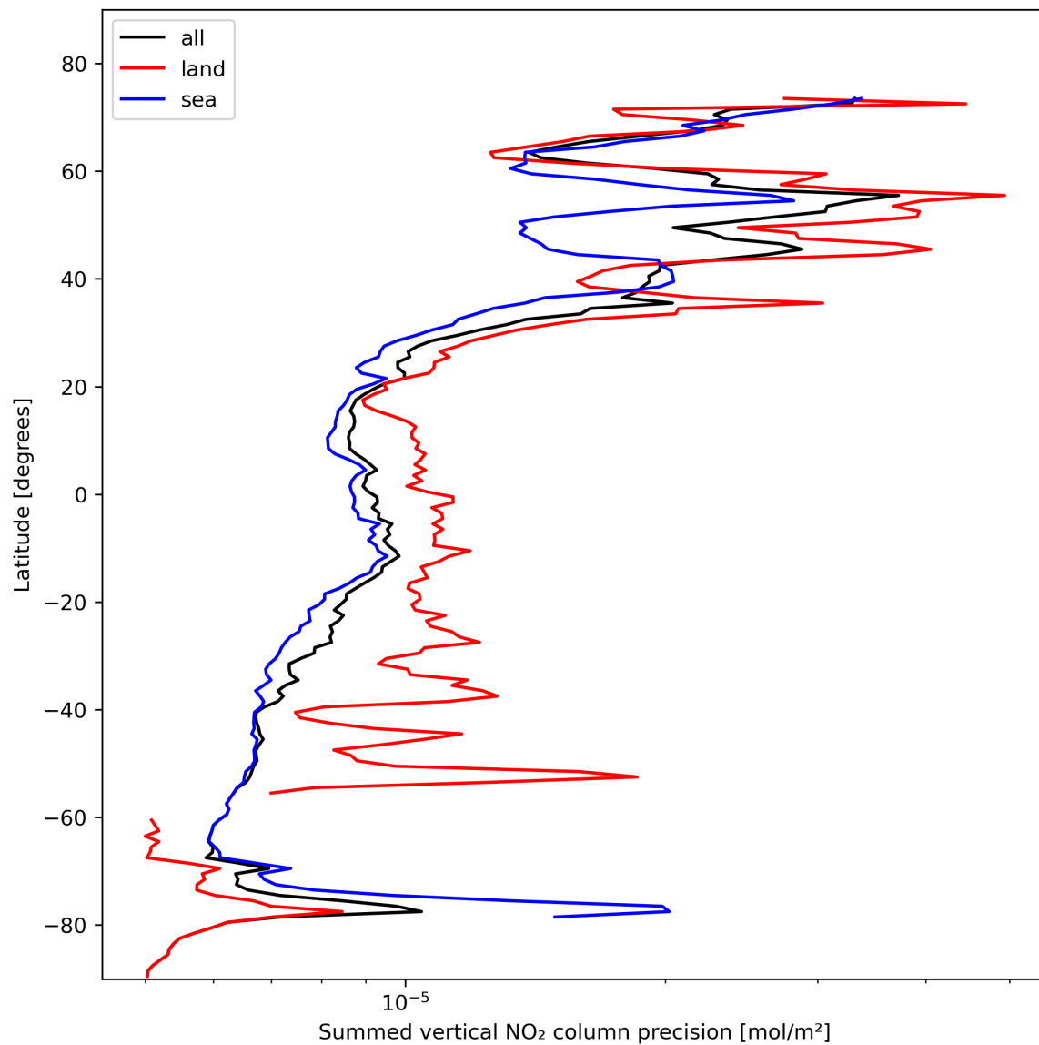
Figure 24: Zonal average of “Summed vertical NO 2 column precision” for 2024-02-08 to 2024-02-10.
