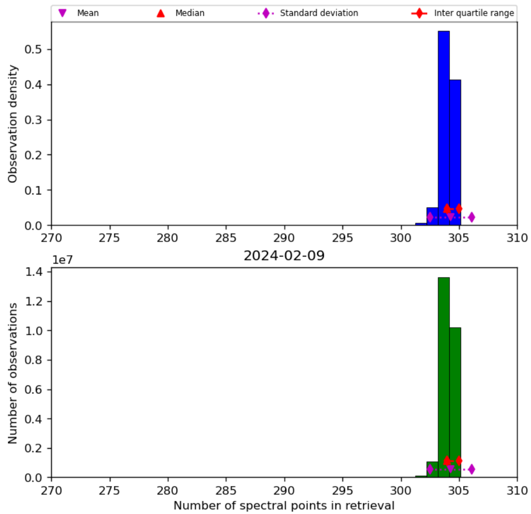
Figure 33: Histogram of “Number of spectral points in retrieval” for 2024-02-08 to 2024-02-10
