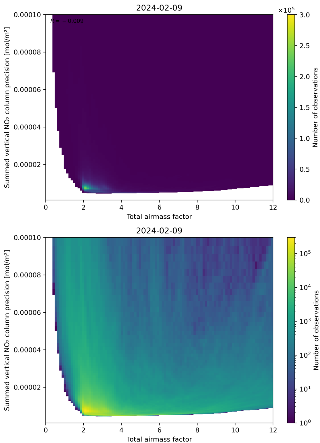
Figure 66: Scatter density plot of “Total airmass factor” against “Summed vertical NO 2 column precision” for 2024-02-08 to 2024-02-10.
