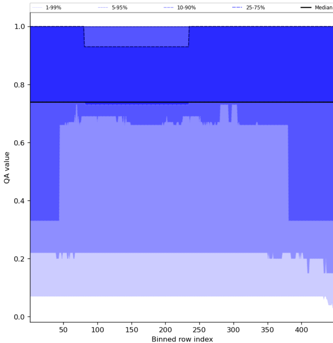
Figure 45: Along track statistics of “QA value” for 2024-02-08 to 2024-02-10
