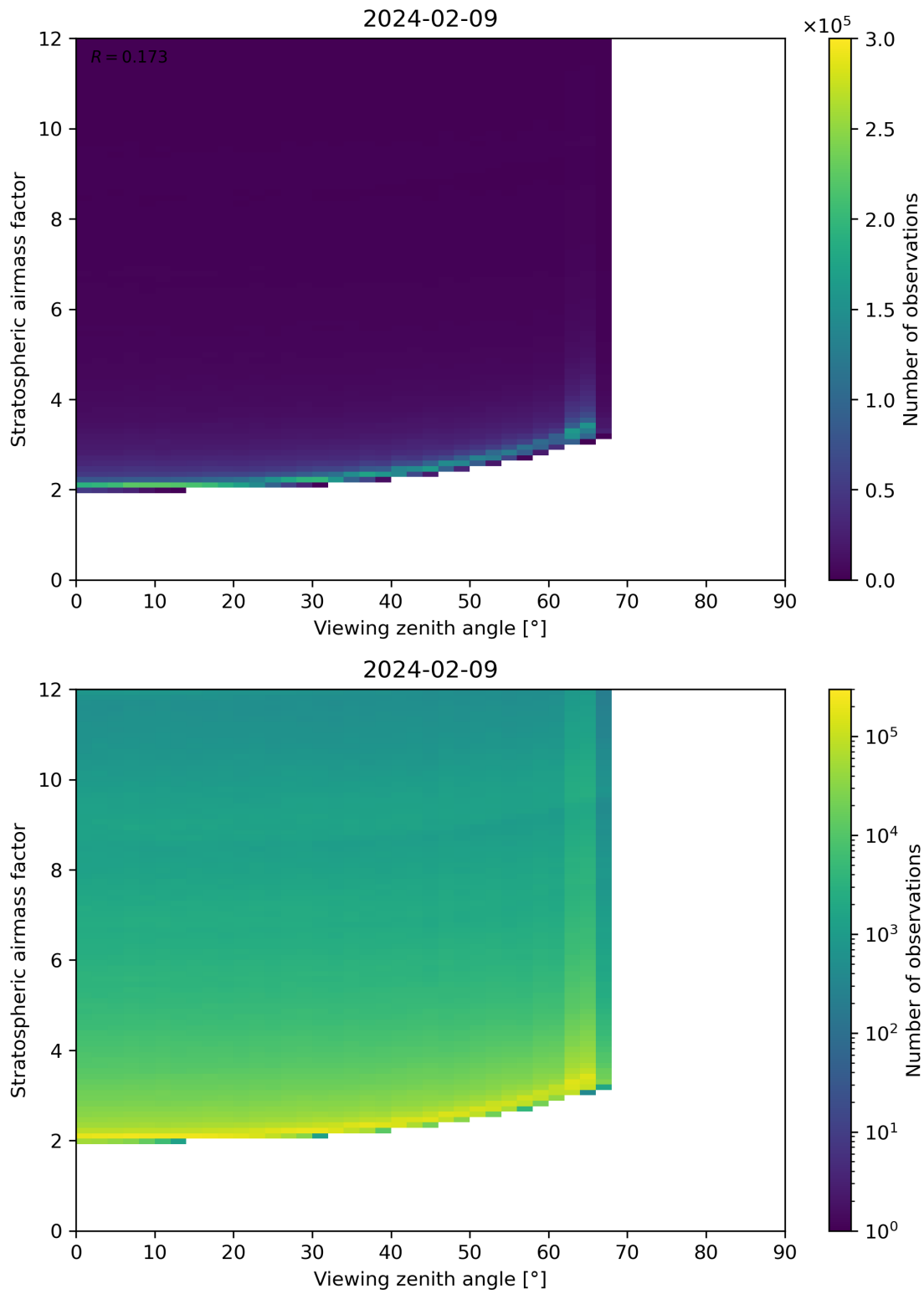
Figure 159: Scatter density plot of “Viewing zenith angle” against “Stratospheric airmass factor” for 2024-02-08 to 2024-02-10.
