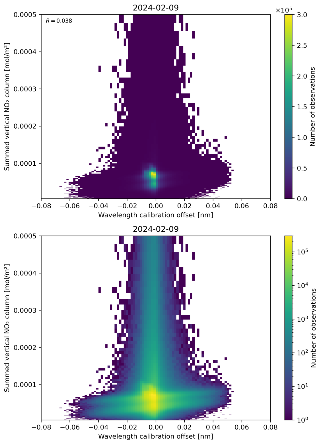
Figure 177: Scatter density plot of “Wavelength calibration offset” against “Summed vertical NO 2 column” for 2024-02-08 to 2024-02-10.
