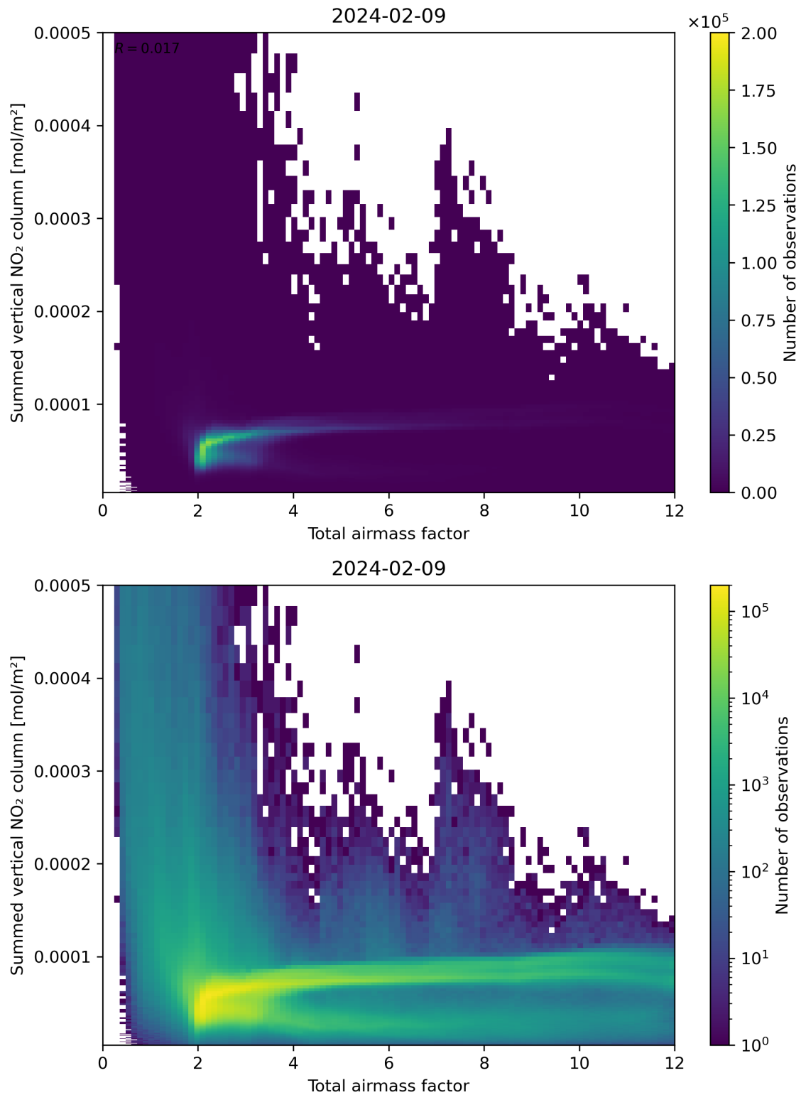
Figure 65: Scatter density plot of “Total airmass factor” against “Summed vertical NO 2 column” for 2024-02-08 to 2024-02-10.
