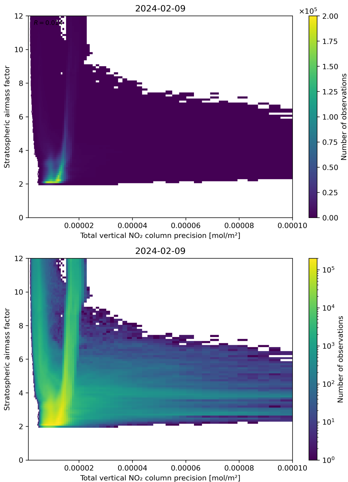
Figure 115: Scatter density plot of “Total vertical NO 2 column precision” against “Stratospheric air mass factor” for 2024-02-08 to 2024-02-10.
