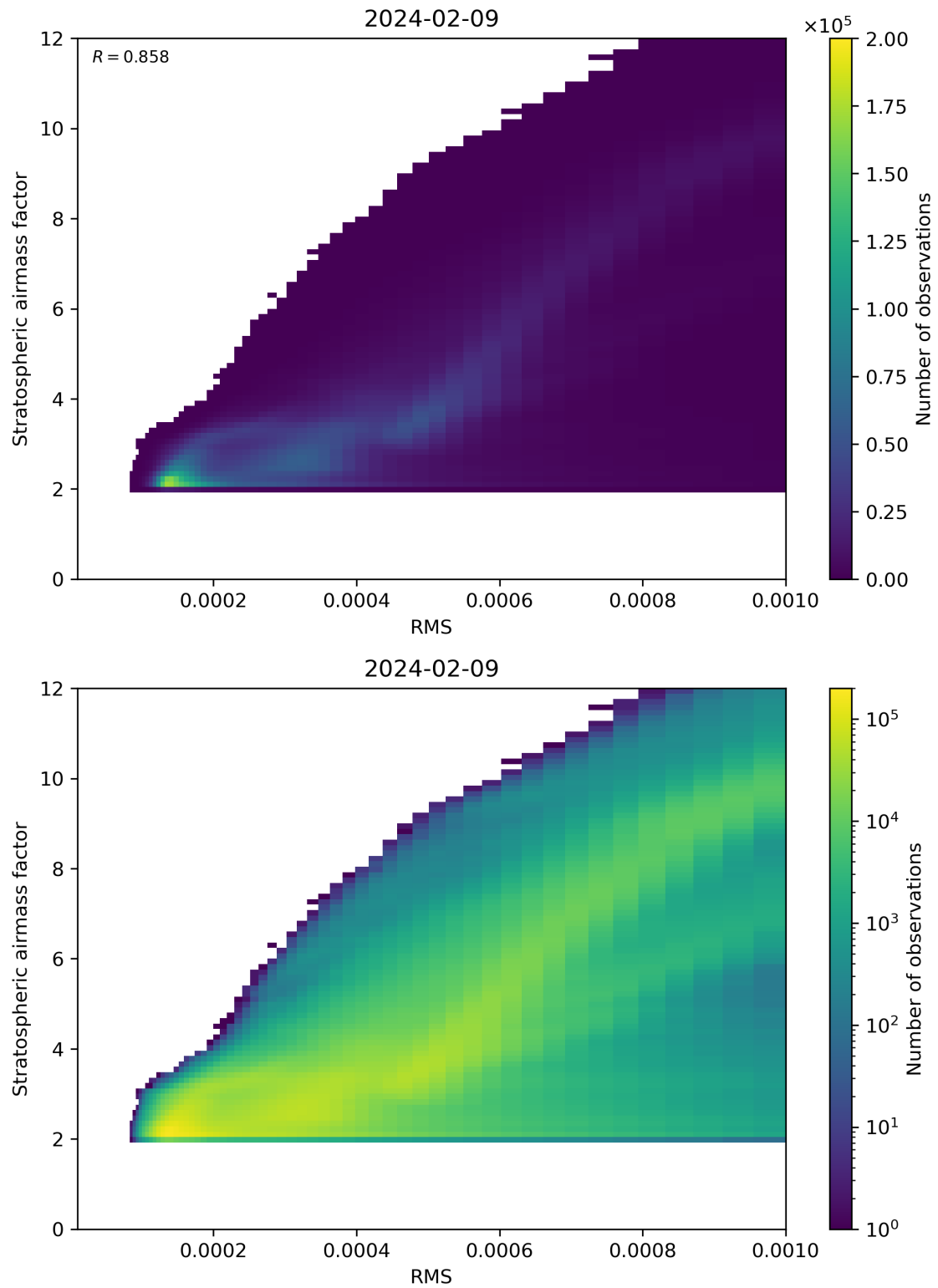
Figure 144: Scatter density plot of “RMS” against “Stratospheric airmass factor” for 2024-02-08 to 2024-02-10.
