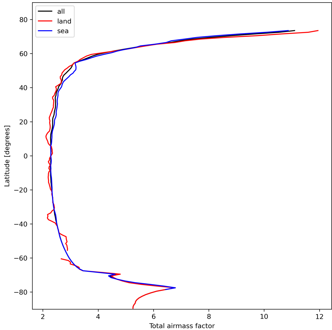
Figure 15: Zonal average of “Total airmass factor” for 2024-02-08 to 2024-02-10.
