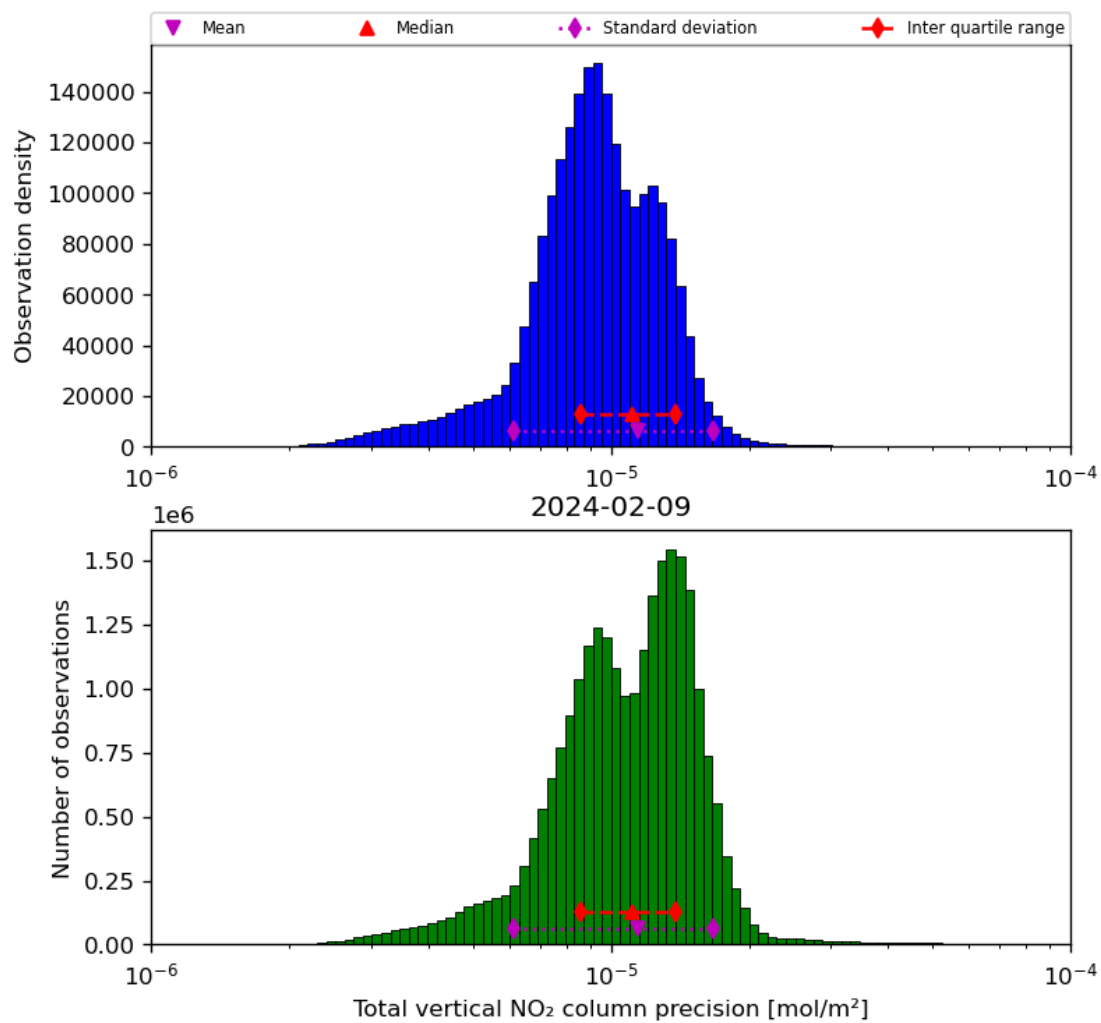
Figure 39: Histogram of “Total vertical NO 2 column precision” for 2024-02-08 to 2024-02-10
