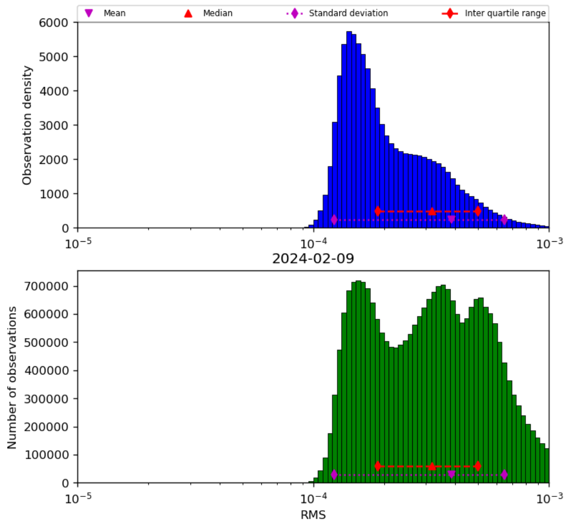
Figure 43: Histogram of “RMS” for 2024-02-08 to 2024-02-10
