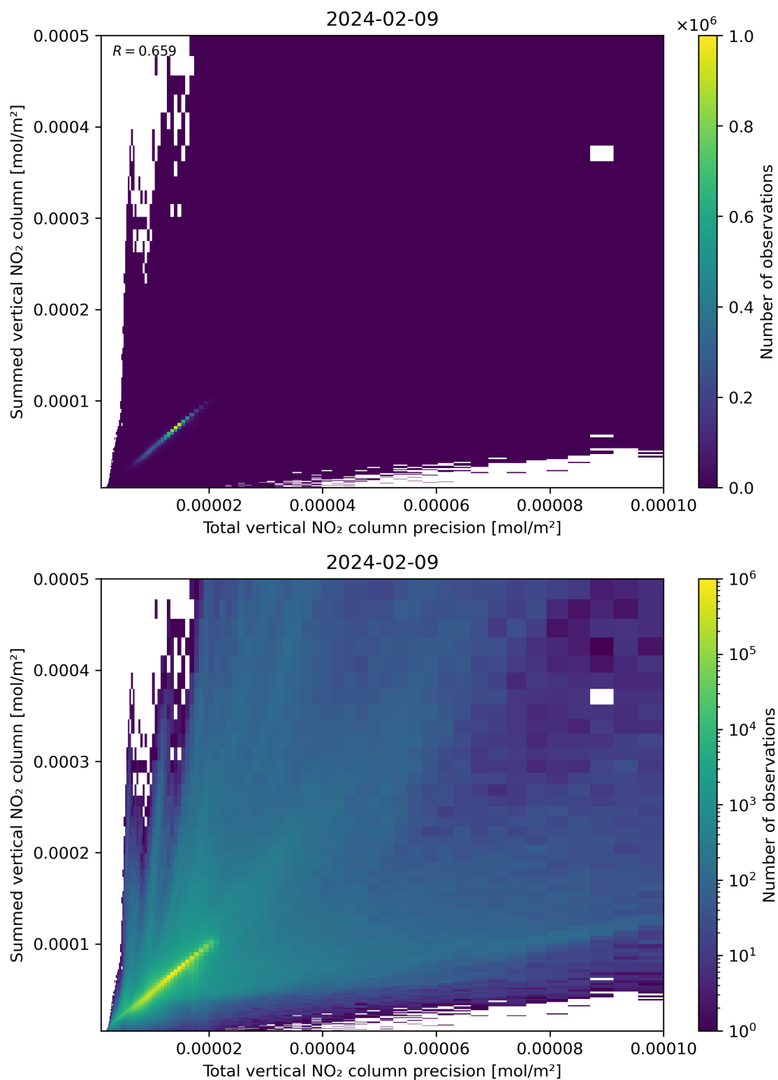
Figure 117: Scatter density plot of “Total vertical NO 2 column precision” against “Summed vertical NO 2 column” for 2024-02-08 to 2024-02-10.
