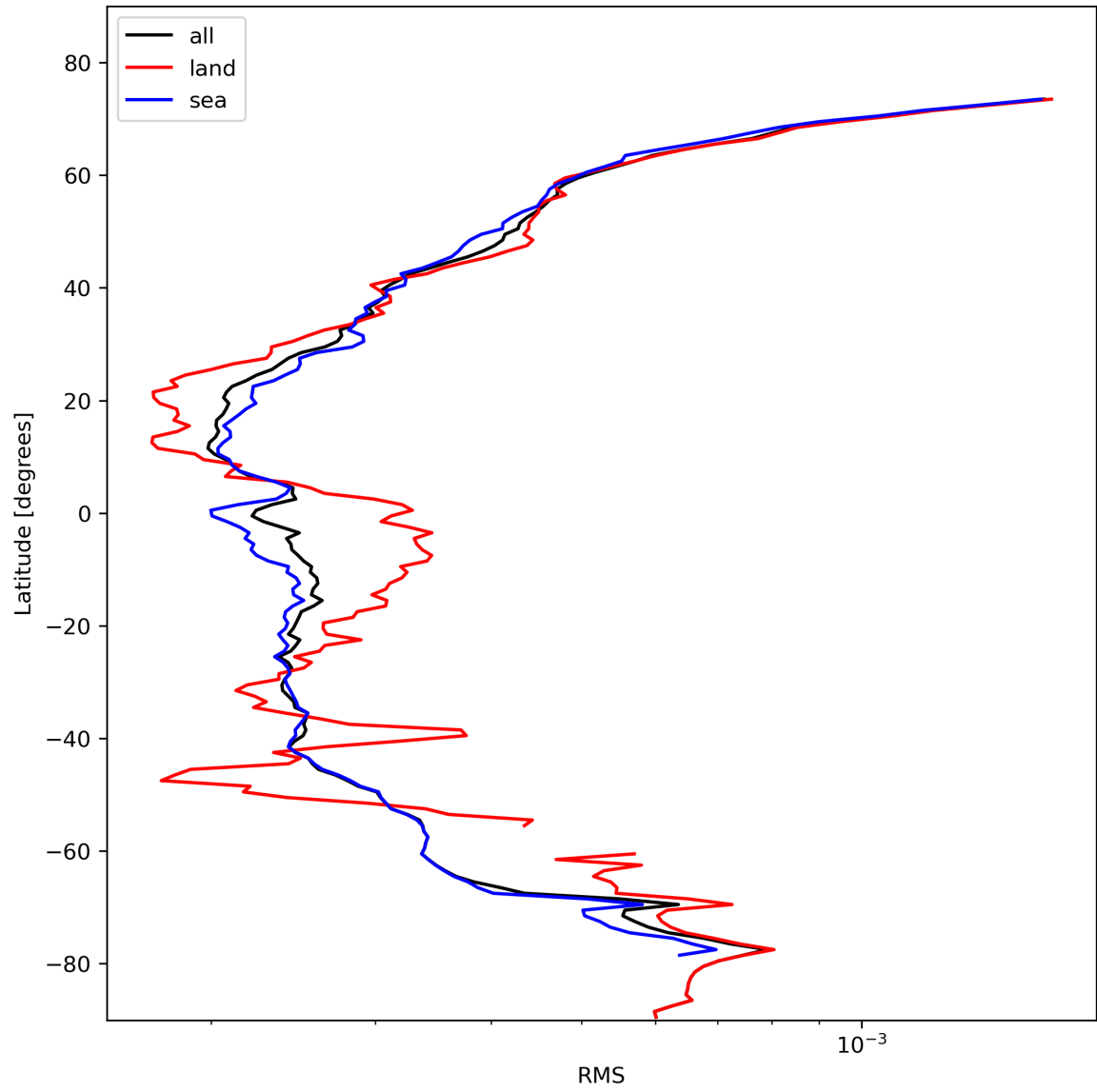
Figure 26: Zonal average of “RMS” for 2024-02-08 to 2024-02-10.
