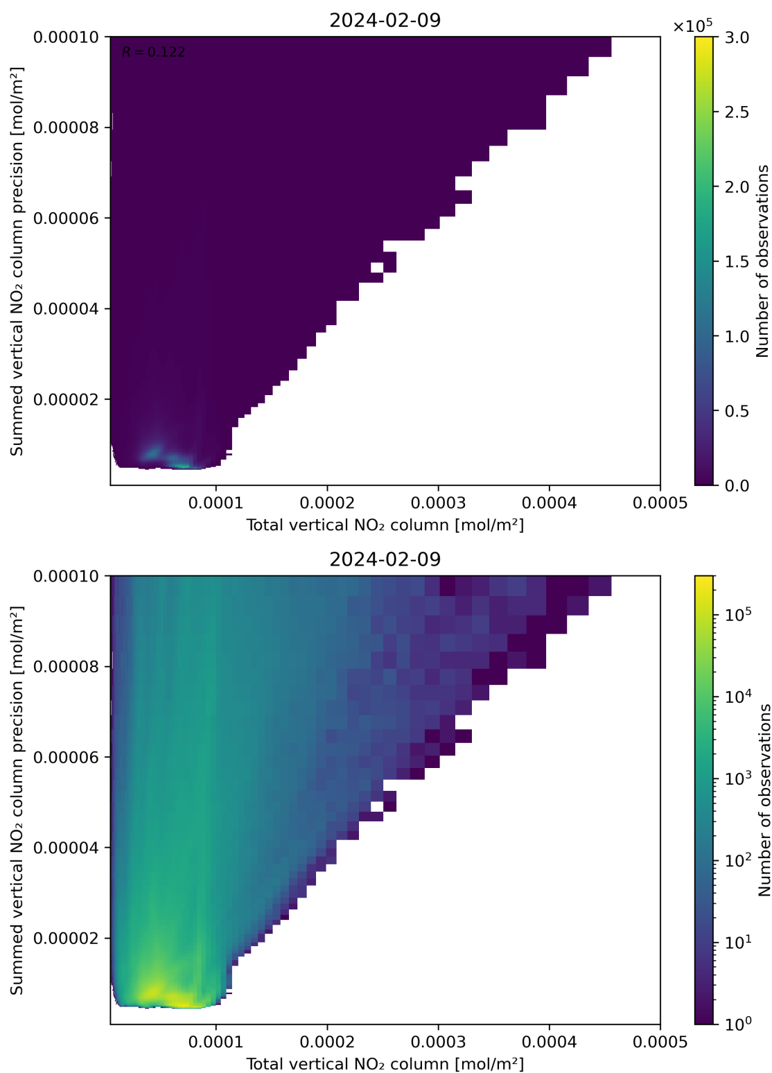
Figure 113: Scatter density plot of “Total vertical NO 2 column” against “Summed vertical NO 2 column precision” for 2024-02-08 to 2024-02-10.
