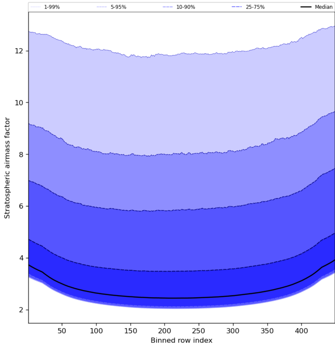
Figure 61: Along track statistics of “Stratospheric airmass factor” for 2024-02-08 to 2024-02-10
