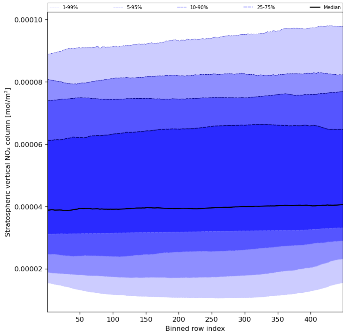
Figure 53: Along track statistics of “Stratospheric vertical NO 2 column” for 2024-02-08 to 2024-02-10
