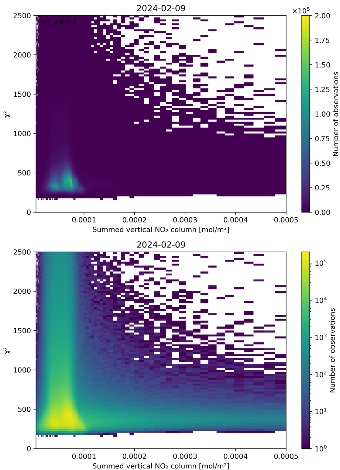
Figure 104: Scatter density plot of “Summed vertical NO 2 column” against “ \chi^2 ” for 2024-02-08 to 2024-02-10.
