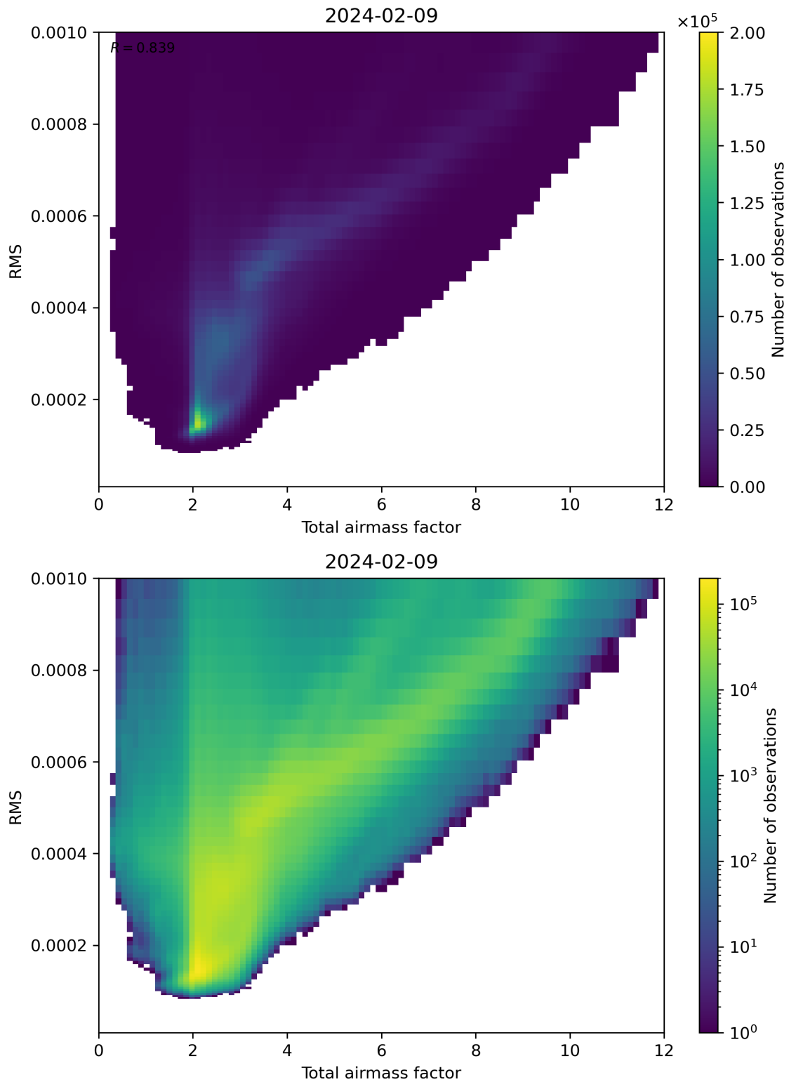
Figure 69: Scatter density plot of “Total airmass factor” against “RMS” for 2024-02-08 to 2024-02-10.
