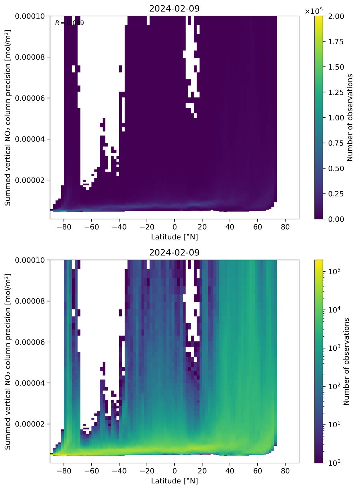
Figure 89: Scatter density plot of “Latitude” against “Summed vertical NO 2 column precision” for 2024-02-08 to 2024-02-10.
