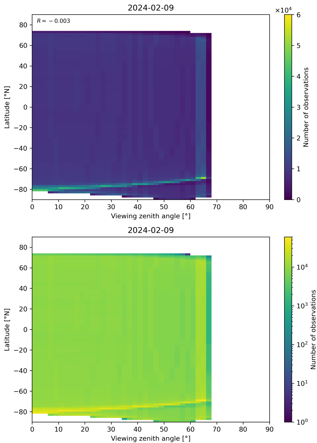
Figure 163: Scatter density plot of “Viewing zenith angle” against “Latitude” for 2024-02-08 to 2024-02-10.
