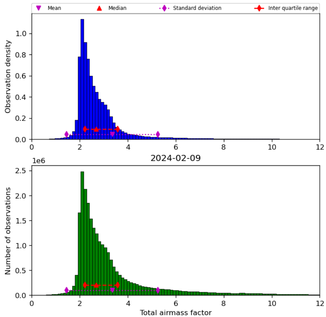
Figure 32: Histogram of “Total airmass factor” for 2024-02-08 to 2024-02-10
