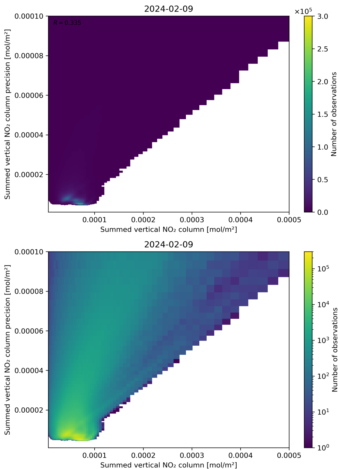
Figure 105: Scatter density plot of “Summed vertical NO 2 column” against “Summed vertical NO 2 column precision” for 2024-02-08 to 2024-02-10.
