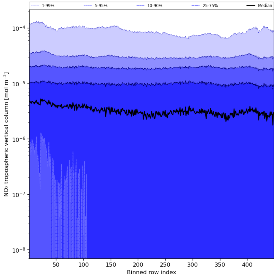
Figure 46: Along track statistics of “NO 2 tropospheric vertical column” for 2024-02-08 to 2024-02-10
