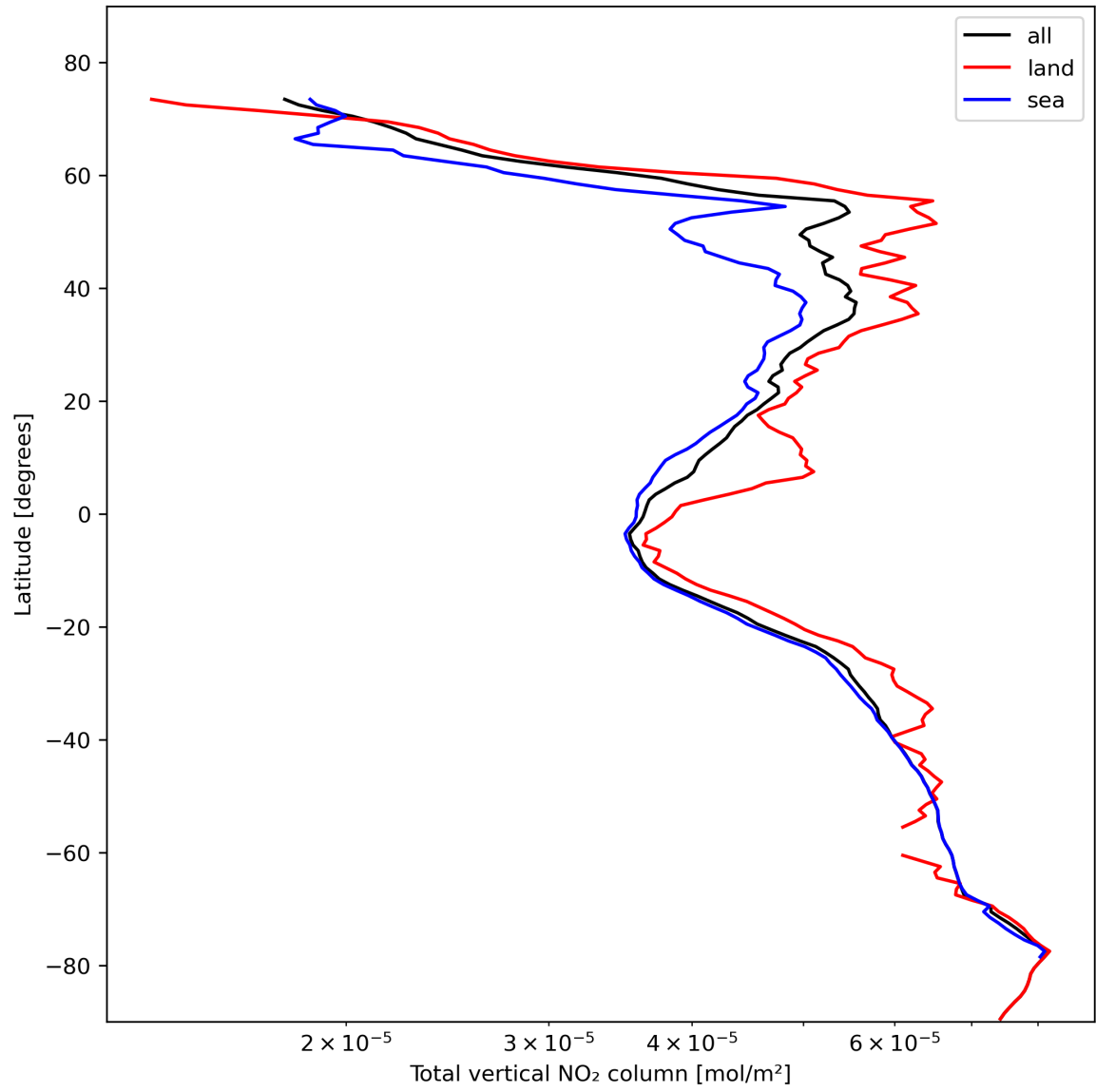
Figure 21: Zonal average of “Total vertical NO 2 column” for 2024-02-08 to 2024-02-10.
