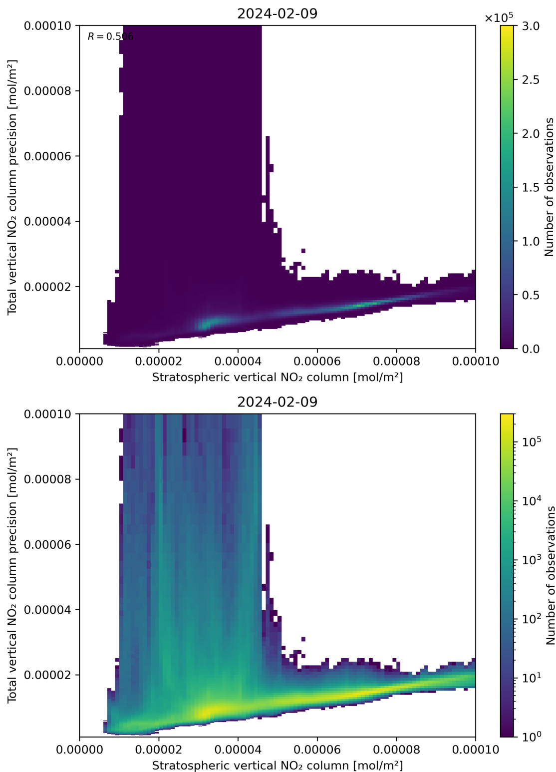
Figure 101: Scatter density plot of “Stratospheric vertical NO 2 column” against “Total vertical NO 2 column precision” for 2024-02-08 to 2024-02-10.
