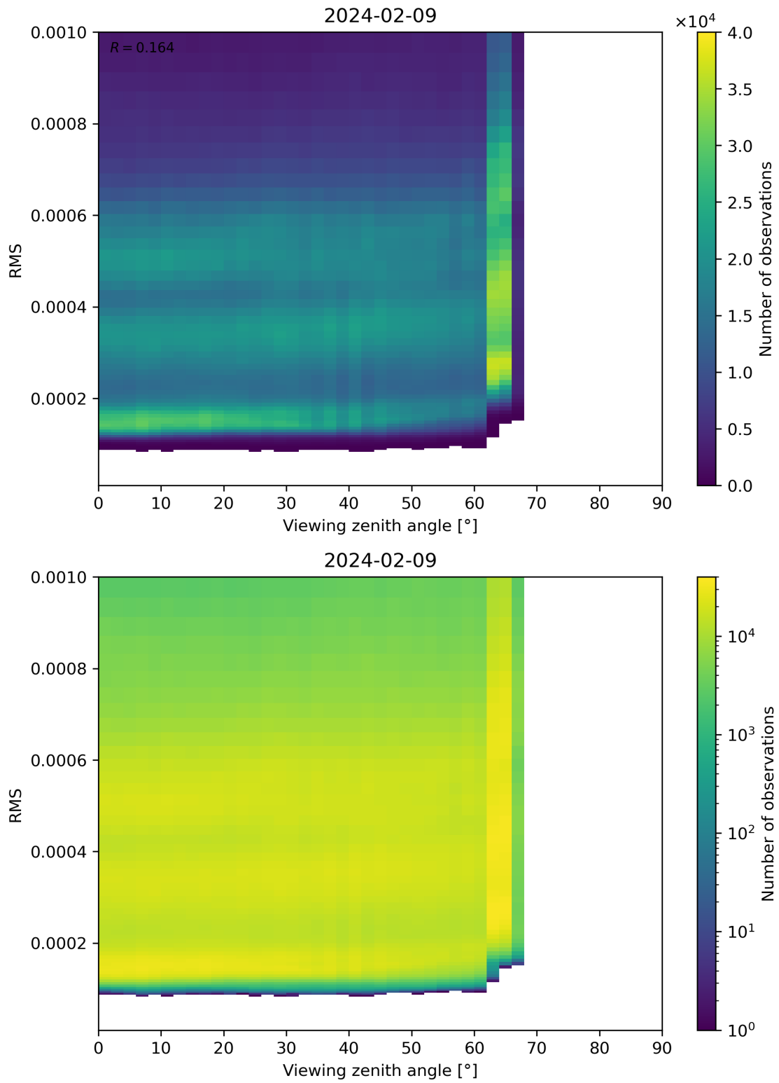
Figure 171: Scatter density plot of “Viewing zenith angle” against “RMS” for 2024-02-08 to 2024-02-10.
