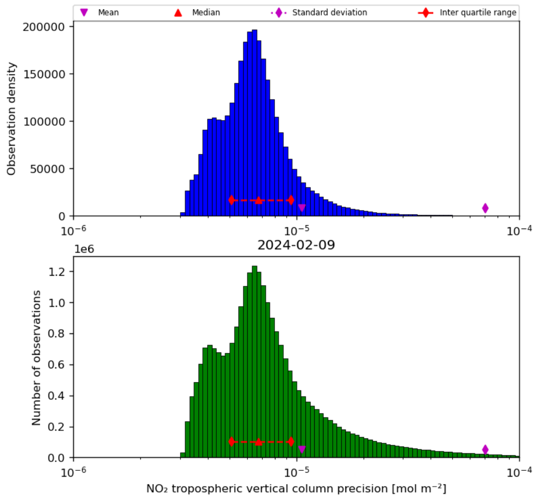
Figure 30: Histogram of “NO 2 tropospheric vertical column precision” for 2024-02-08 to 2024-02-10
