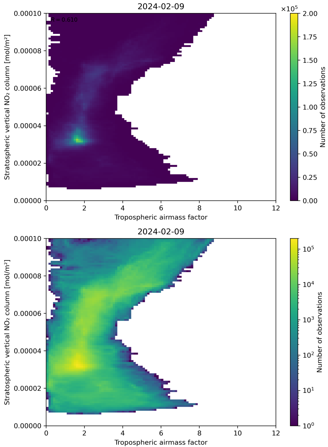
Figure 74: Scatter density plot of “Tropospheric air mass factor” against “Stratospheric vertical NO 2 column” for 2024-02-08 to 2024-02-10.
