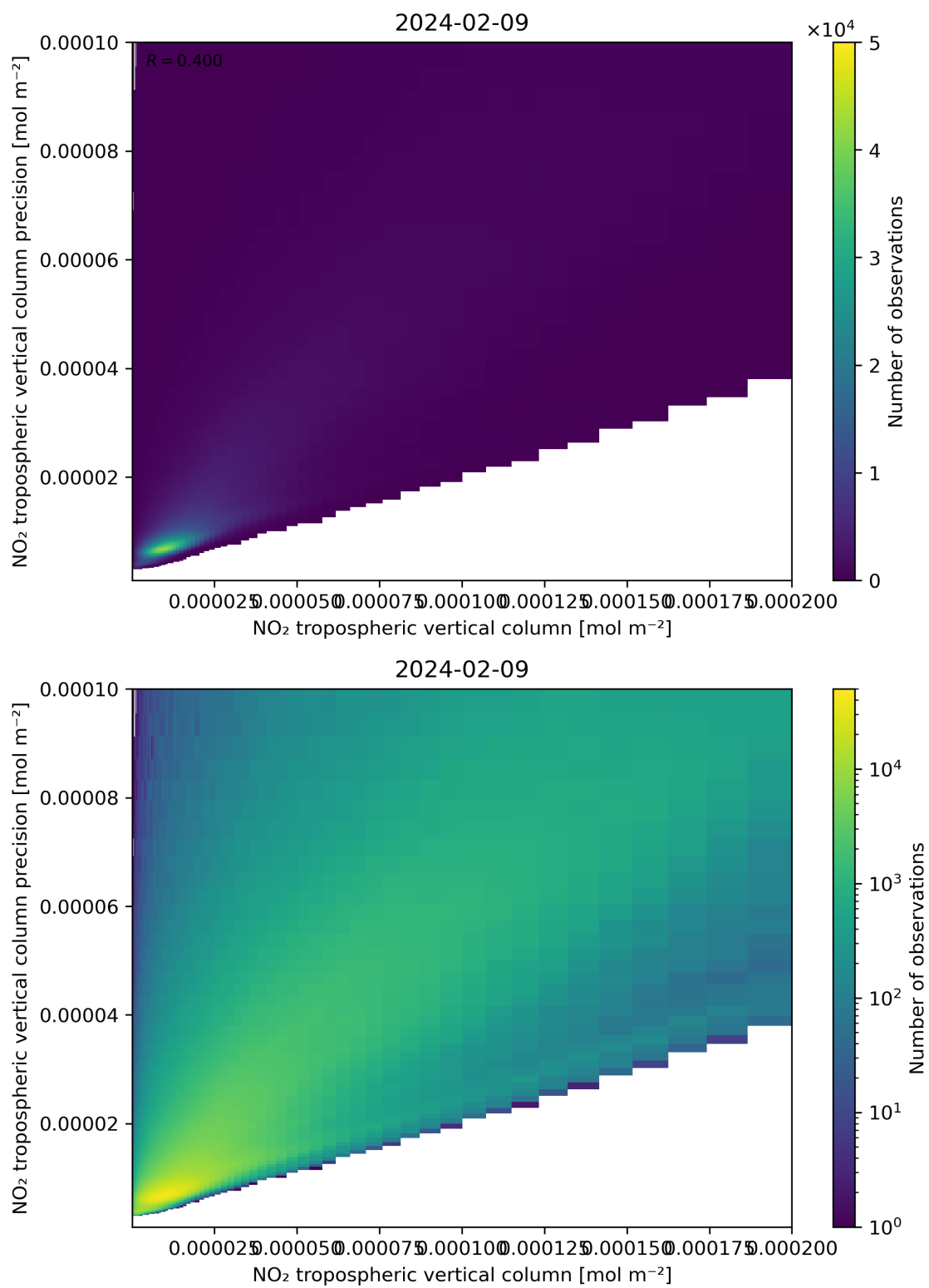
Figure 130: Scatter density plot of “NO 2 tropospheric vertical column” against “NO 2 tropospheric vertical column precision” for 2024-02-08 to 2024-02-10.
