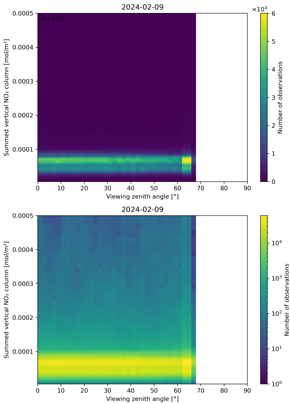
Figure 165: Scatter density plot of “Viewing zenith angle” against “Summed vertical NO 2 column” for 2024-02-08 to 2024-02-10.
