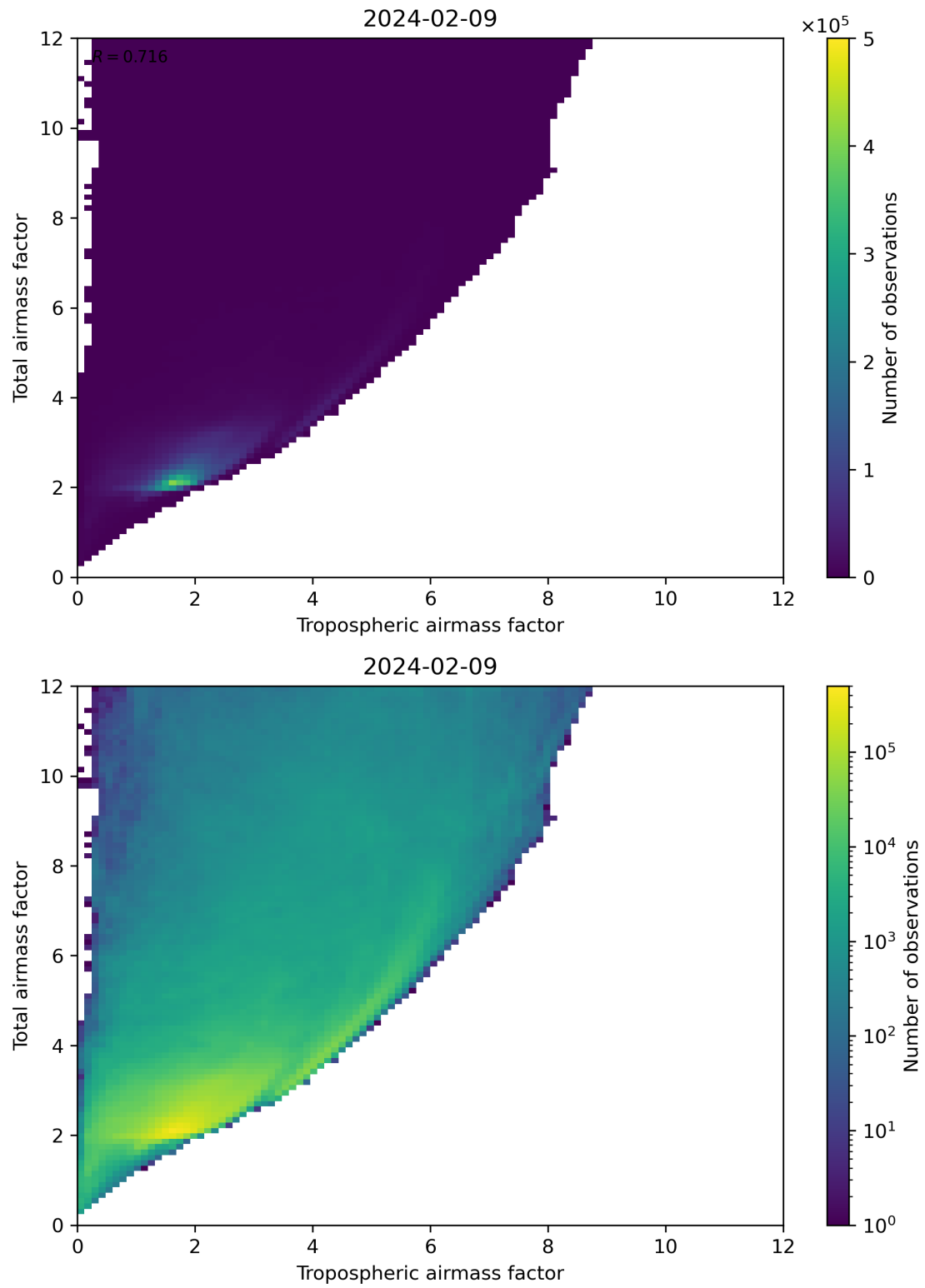
Figure 72: Scatter density plot of “Tropospheric airmass factor” against “Total airmass factor” for 2024-02-08 to 2024-02-10.
