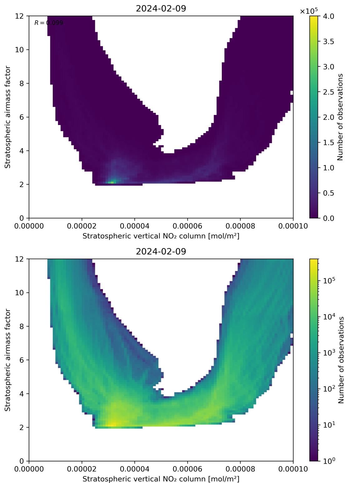
Figure 96: Scatter density plot of “Stratospheric vertical NO 2 column” against “Stratospheric airmass factor” for 2024-02-08 to 2024-02-10.
