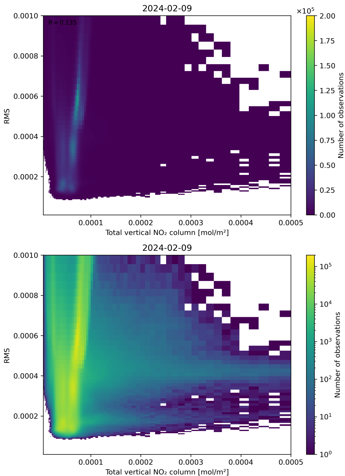
Figure 120: Scatter density plot of “Total vertical NO 2 column” against “RMS” for 2024-02-08 to 2024-02-10.
