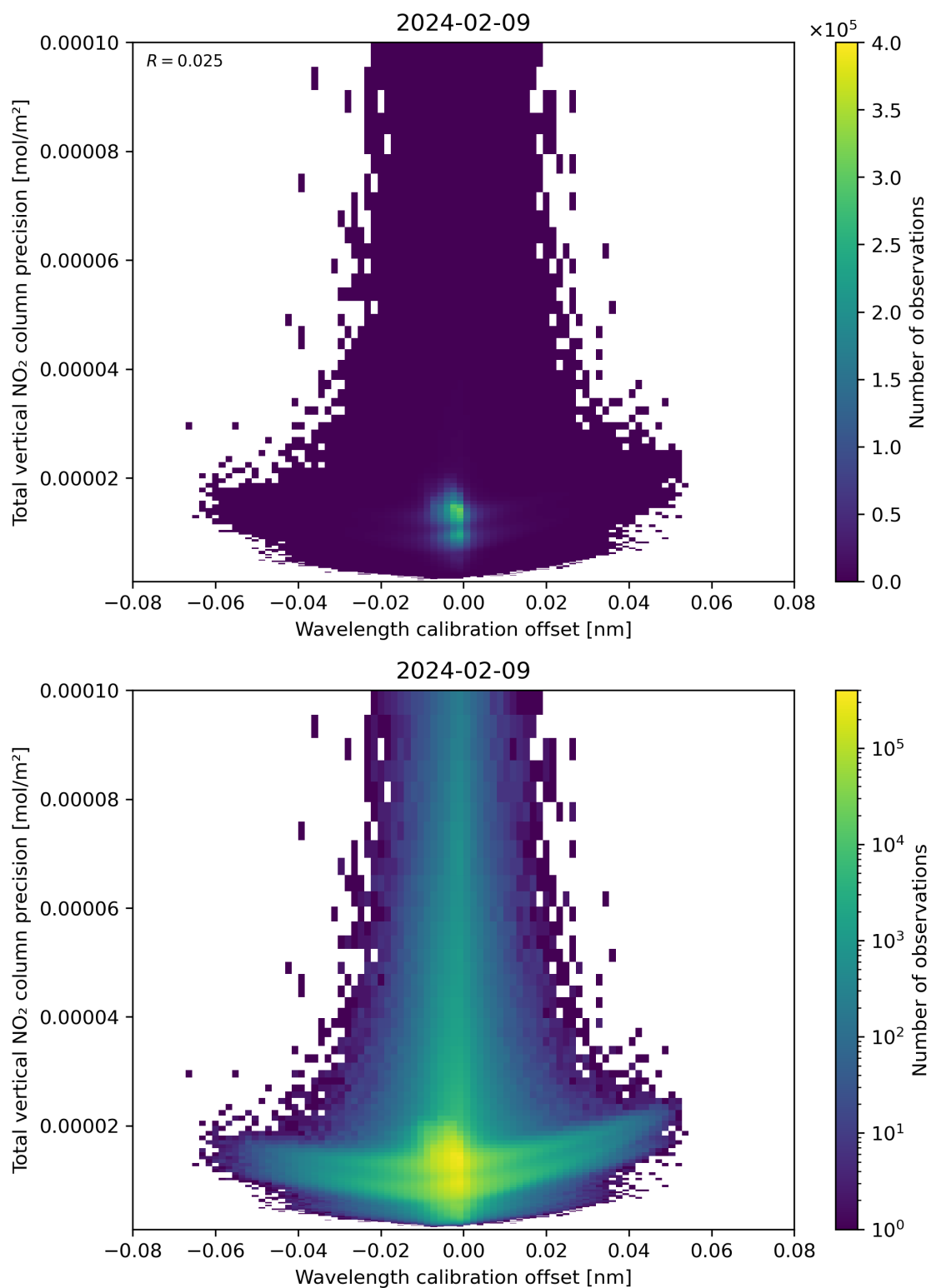
Figure 180: Scatter density plot of “Wavelength calibration offset” against “Total vertical NO 2 column precision” for 2024-02-08 to 2024-02-10.
