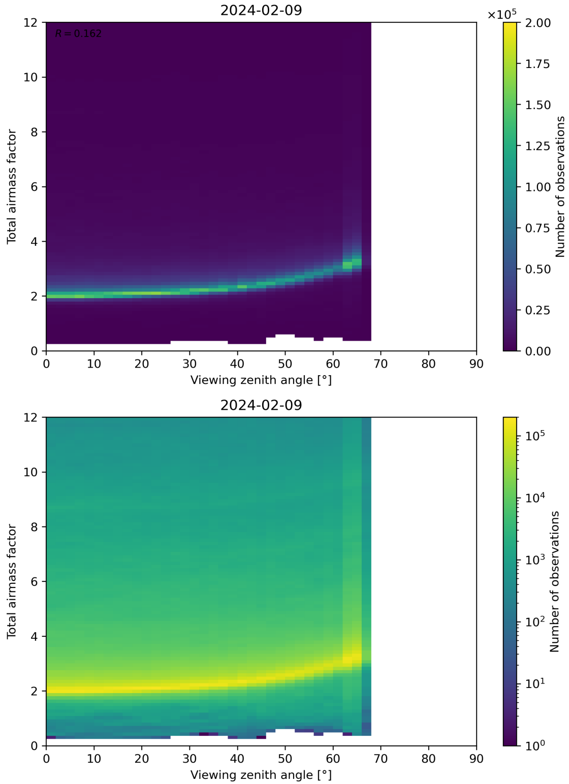
Figure 160: Scatter density plot of “Viewing zenith angle” against “Total airmass factor” for 2024-02-08 to 2024-02-10.
