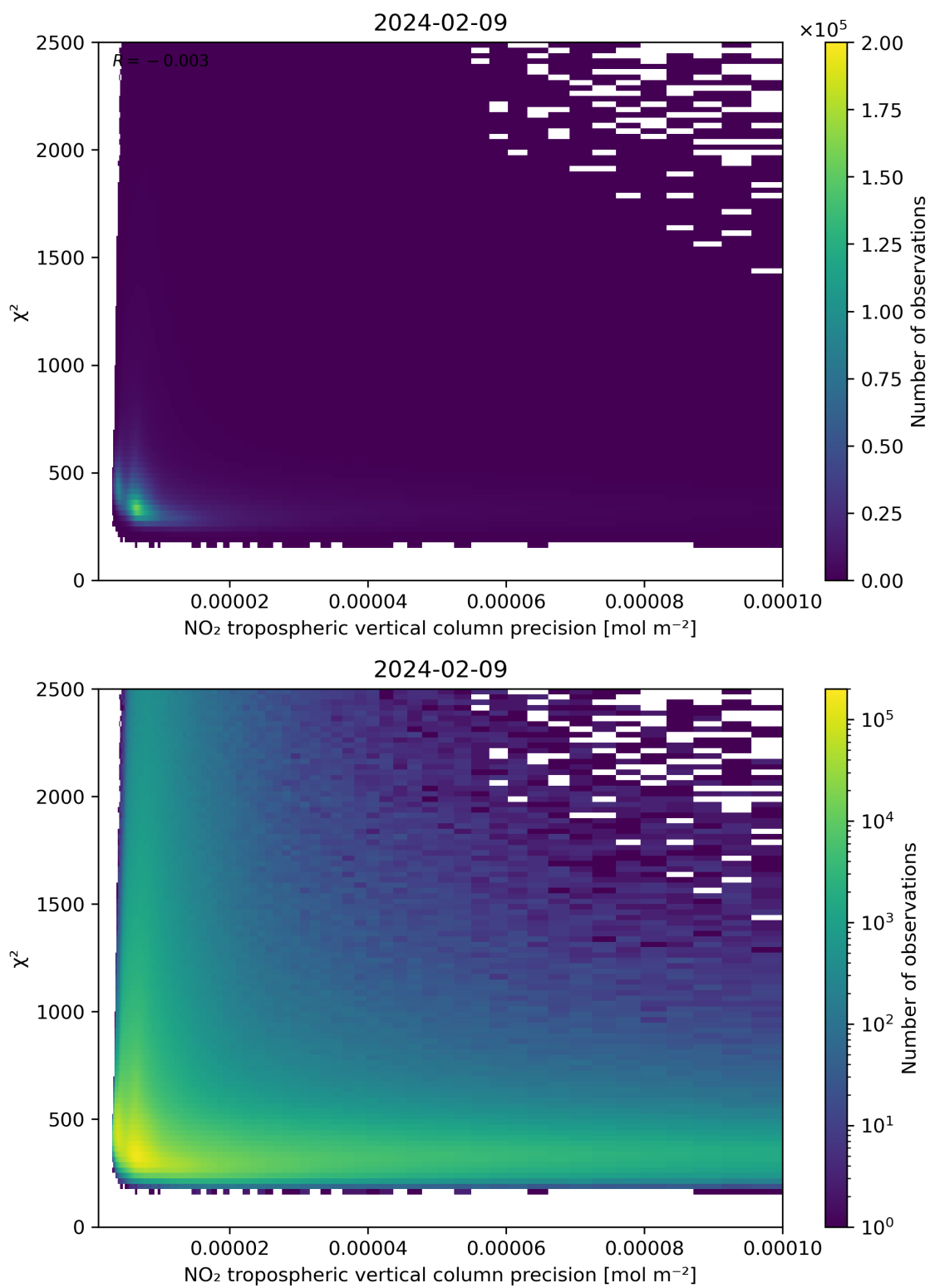
Figure 134: Scatter density plot of “NO 2 tropospheric vertical column precision” against “ \chi^2 ” for 2024-02-08 to 2024-02-10.
