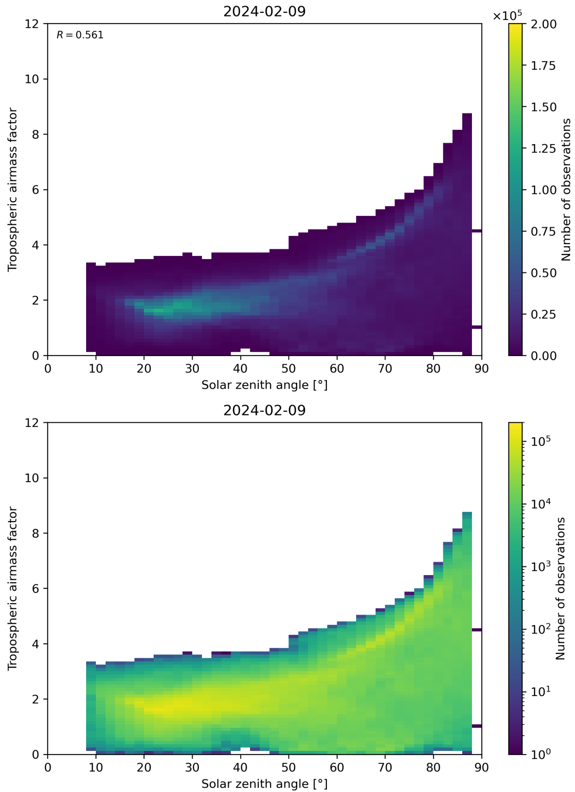
Figure 147: Scatter density plot of “Solar zenith angle” against “Tropospheric airmass factor” for 2024-02-08 to 2024-02-10.
