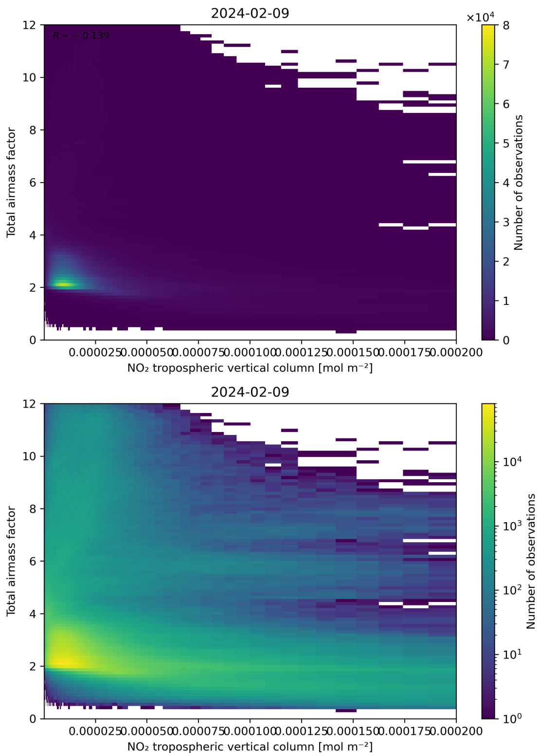
Figure 122: Scatter density plot of “NO 2 tropospheric vertical column” against “Total air mass factor” for 2024-02-08 to 2024-02-10.
