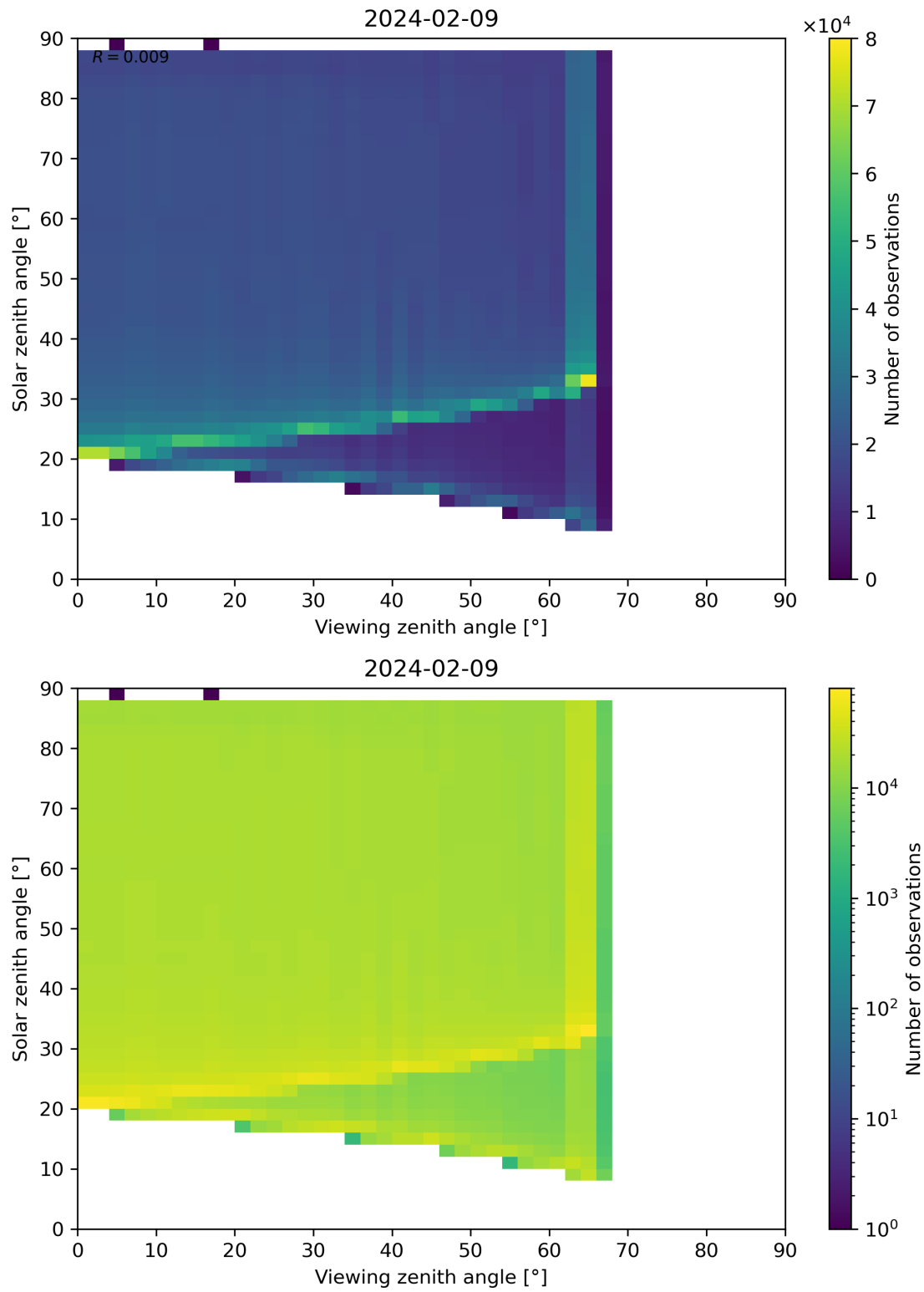
Figure 172: Scatter density plot of “Viewing zenith angle” against “Solar zenith angle” for 2024-02-08 to 2024-02-10.
