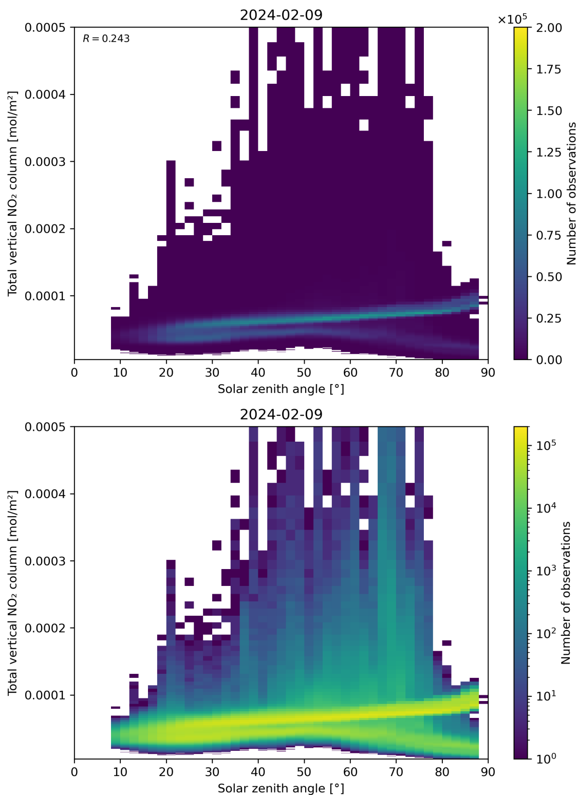
Figure 153: Scatter density plot of “Solar zenith angle” against “Total vertical NO 2 column” for 2024-02-08 to 2024-02-10.
