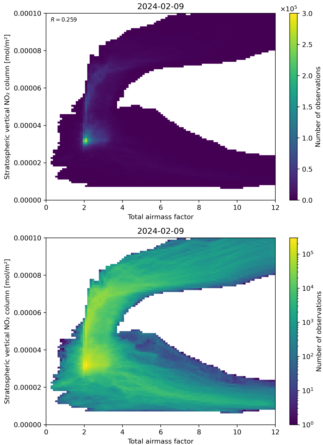
Figure 64: Scatter density plot of “Total airmass factor” against “Stratospheric vertical NO 2 column” for 2024-02-08 to 2024-02-10.
