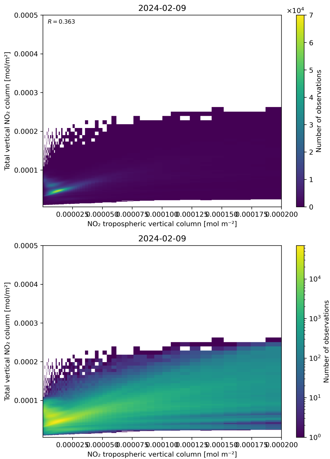
Figure 128: Scatter density plot of “NO 2 tropospheric vertical column” against “Total vertical NO 2 column” for 2024-02-08 to 2024-02-10.
