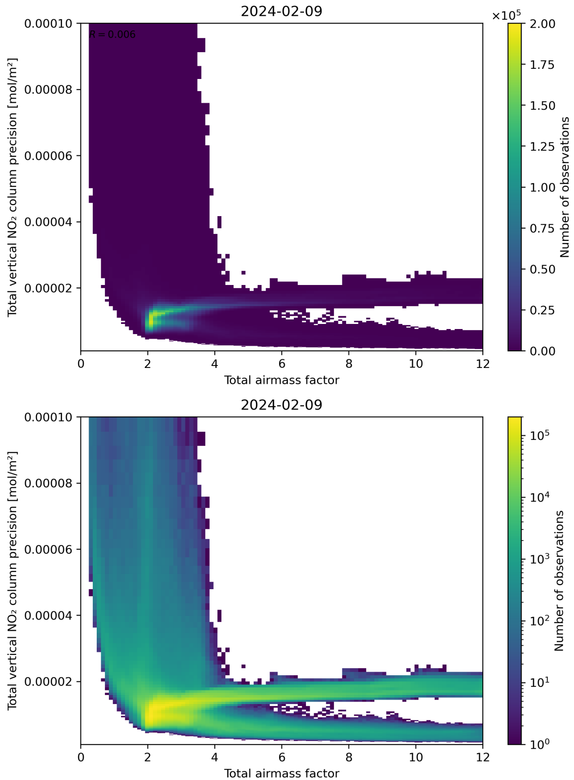
Figure 68: Scatter density plot of “Total airmass factor” against “Total vertical NO 2 column precision” for 2024-02-08 to 2024-02-10.
