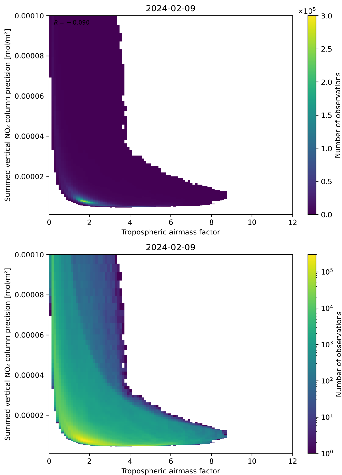
Figure 76: Scatter density plot of “Tropospheric airmass factor” against “Summed vertical NO 2 column precision” for 2024-02-08 to 2024-02-10.
