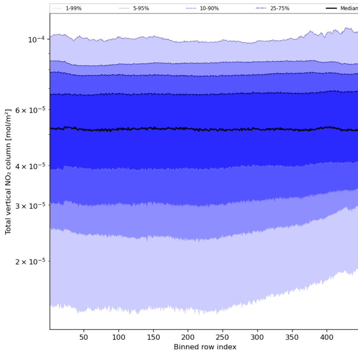
Figure 55: Along track statistics of “Total vertical NO 2 column” for 2024-02-08 to 2024-02-10
