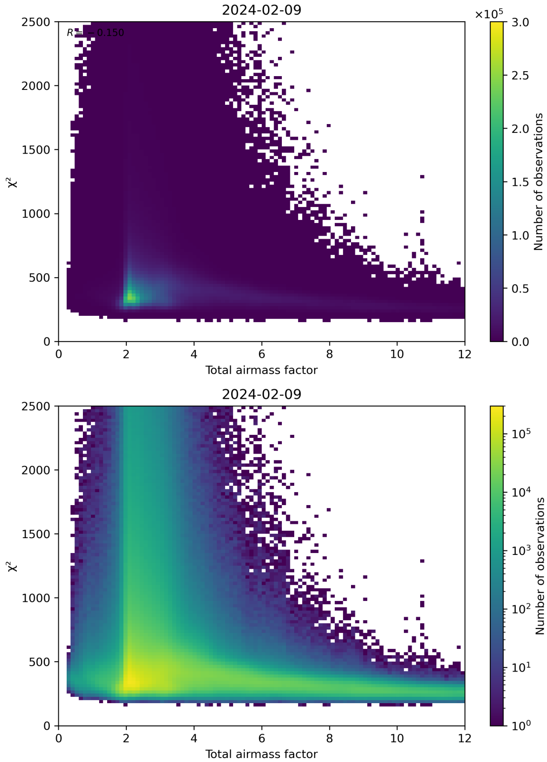
Figure 63: Scatter density plot of “Total airmass factor” against “ \chi^2 ” for 2024-02-08 to 2024-02-10.
