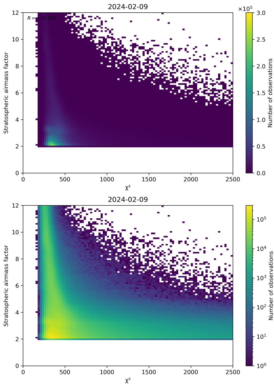
Figure 81: Scatter density plot of “ \chi^2 ” against “Stratospheric airmass factor” for 2024-02-08 to 2024-02-10.
