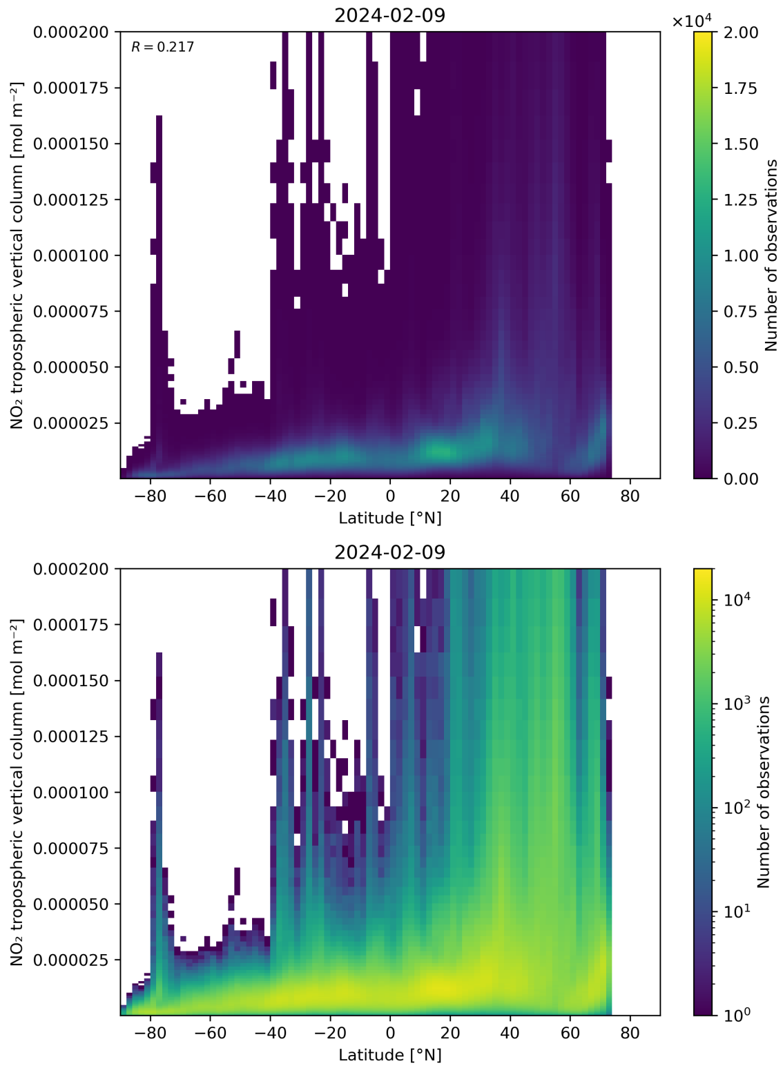
Figure 92: Scatter density plot of “Latitude” against “NO 2 tropospheric vertical column” for 2024-02-08 to 2024-02-10.
