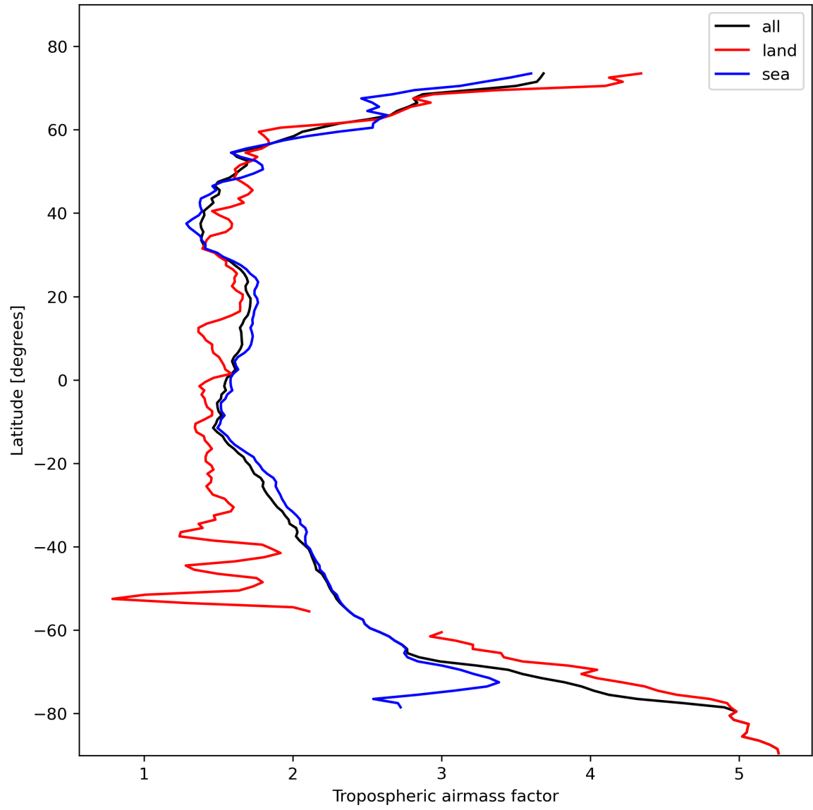
Figure 14: Zonal average of “Tropospheric airmass factor” for 2024-02-08 to 2024-02-10.
