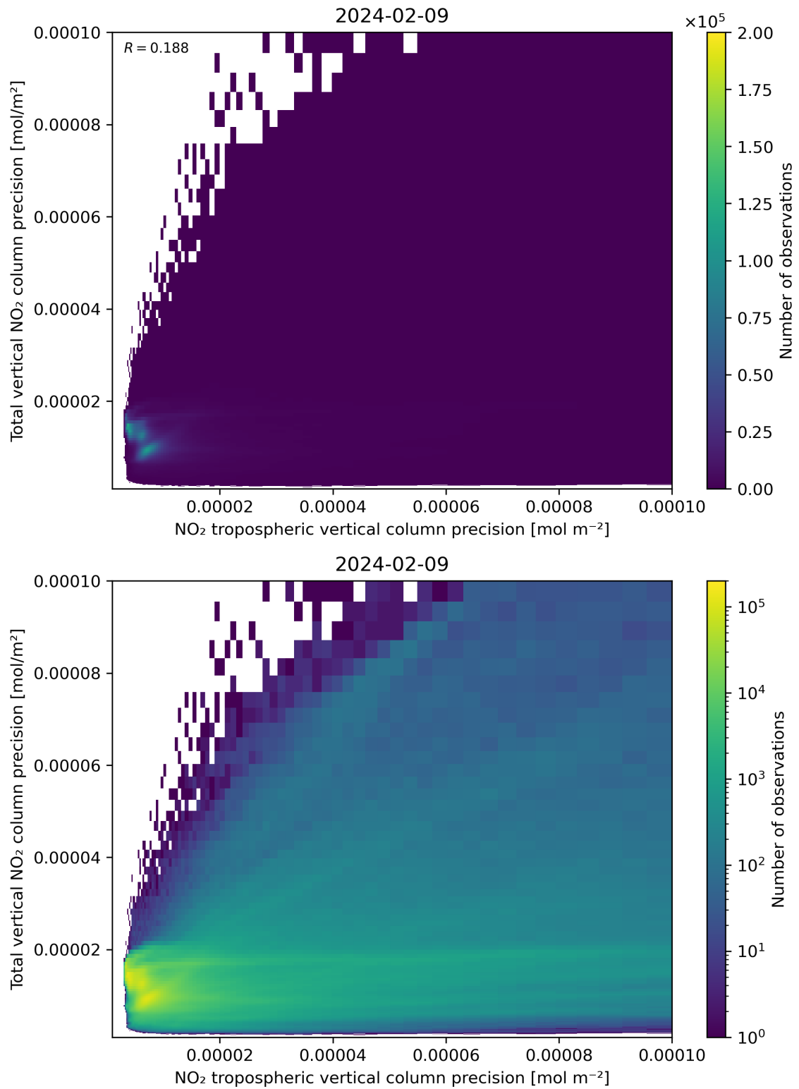
Figure 139: Scatter density plot of “NO 2 tropospheric vertical column precision” against “Total vertical NO 2 column precision” for 2024-02-08 to 2024-02-10.
