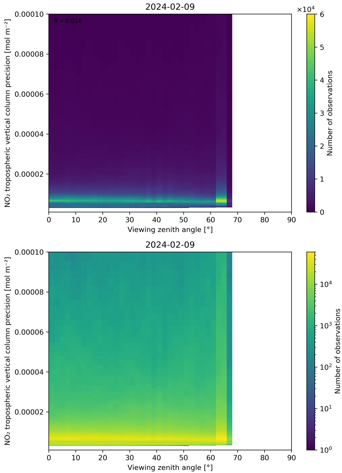
Figure 170: Scatter density plot of “Viewing zenith angle” against “NO 2 tropospheric vertical column precision” for 2024-02-08 to 2024-02-10.
