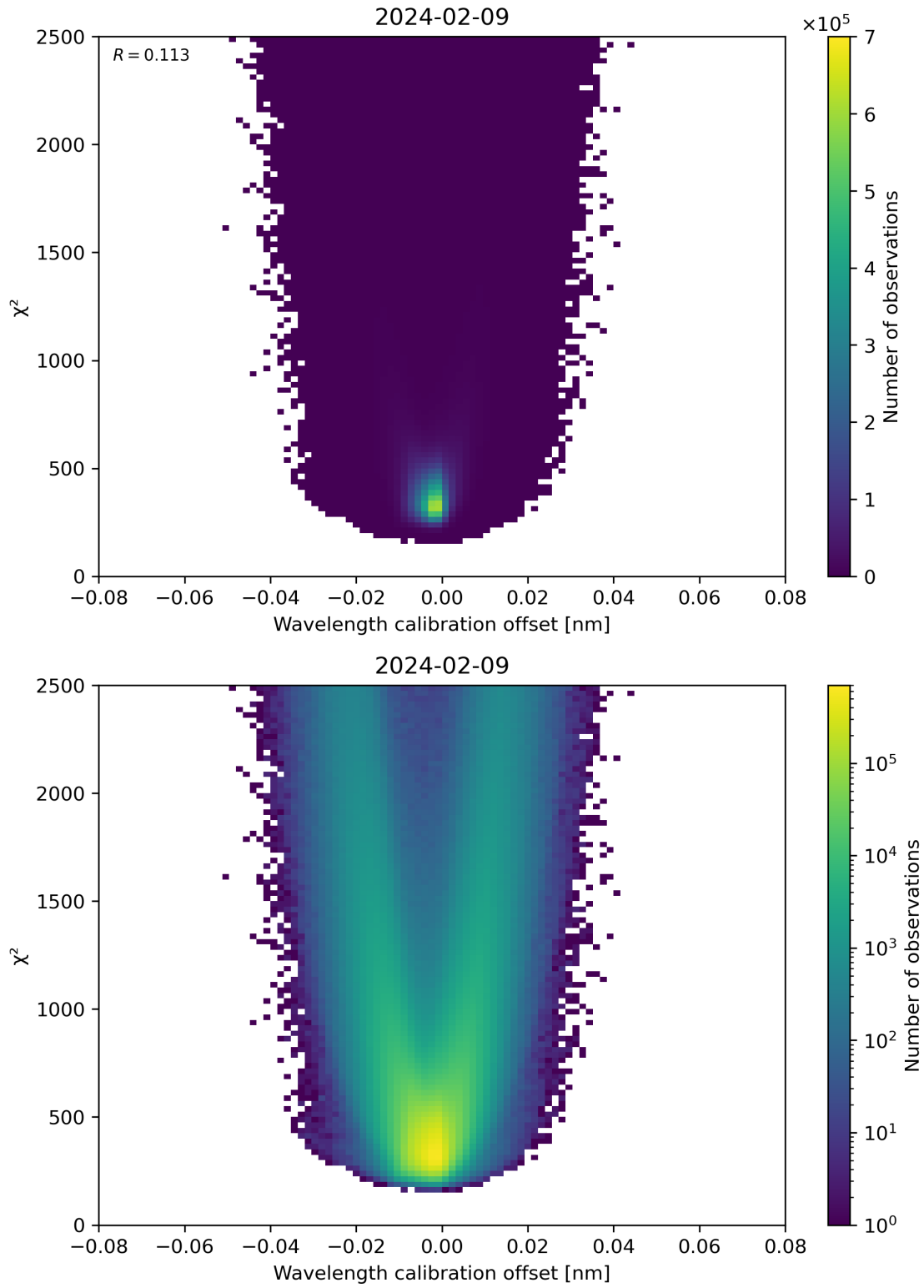
Figure 175: Scatter density plot of “Wavelength calibration offset” against “ \chi^2 ” for 2024-02-08 to 2024-02-10.
