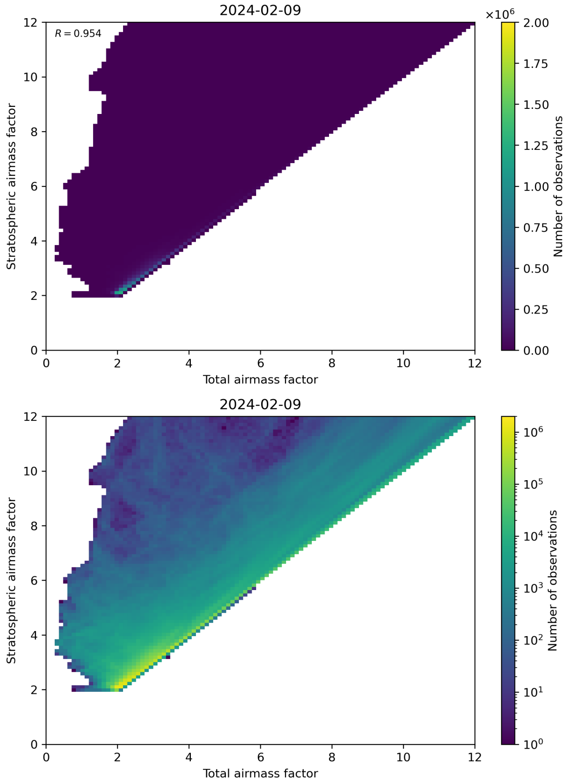
Figure 62: Scatter density plot of “Total airmass factor” against “Stratospheric airmass factor” for 2024-02-08 to 2024-02-10.
