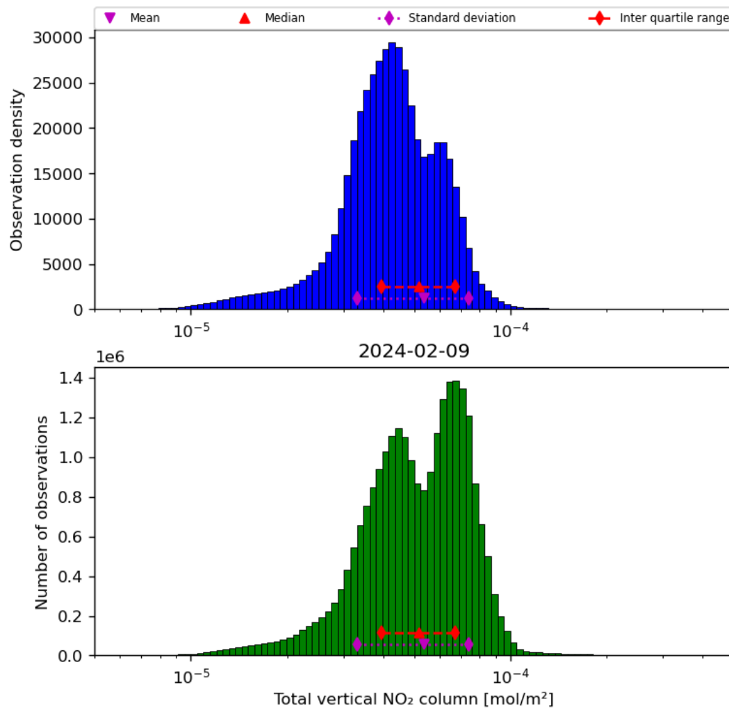
Figure 38: Histogram of “Total vertical NO 2 column” for 2024-02-08 to 2024-02-10
