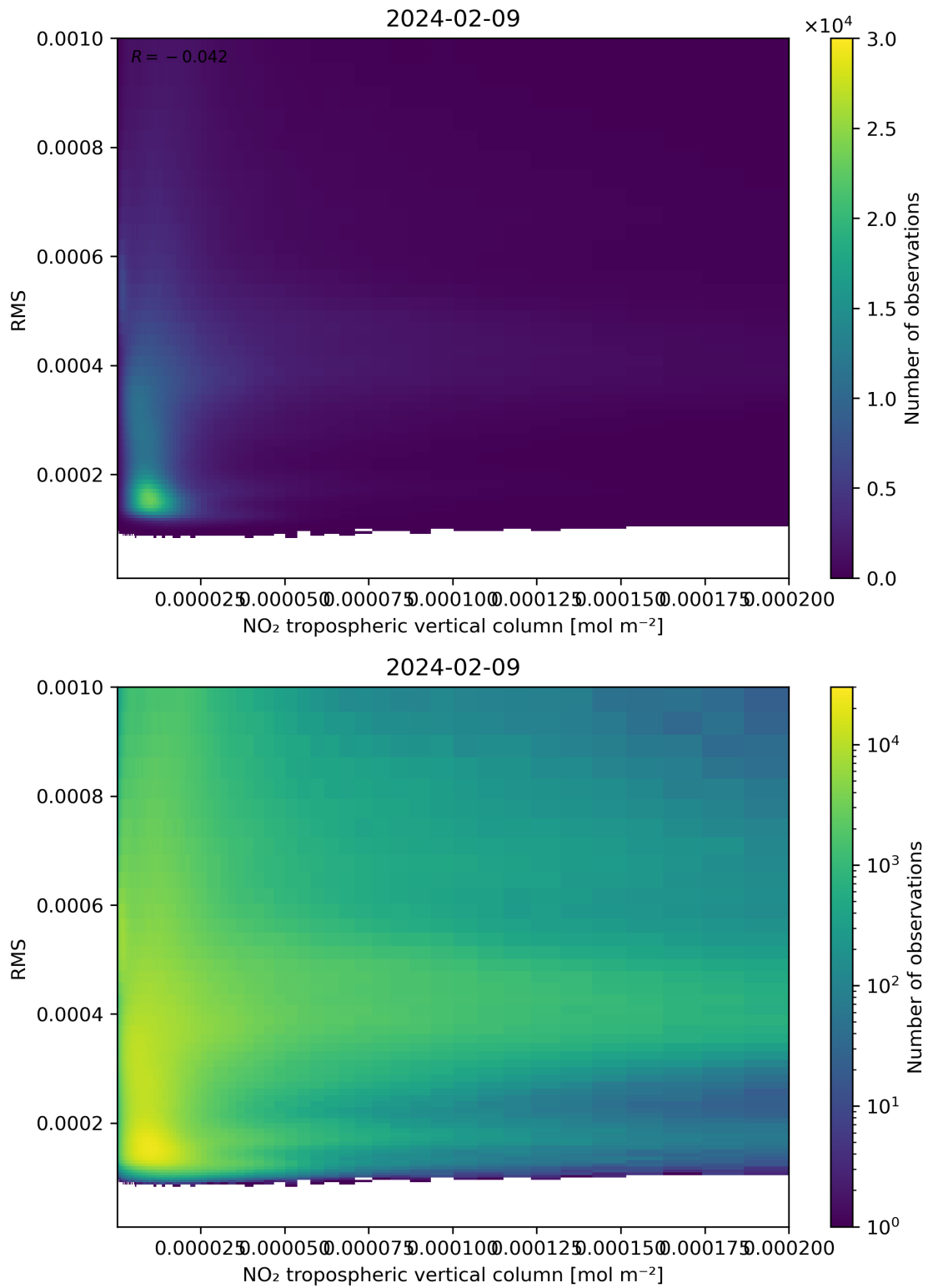
Figure 142: Scatter density plot of “NO 2 tropospheric vertical column” against “RMS” for 2024-02-08 to 2024-02-10.
