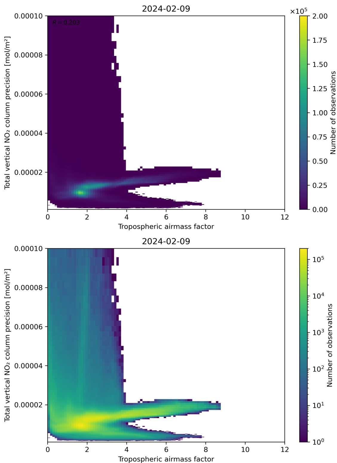
Figure 78: Scatter density plot of “Tropospheric air mass factor” against “Total vertical NO 2 column precision” for 2024-02-08 to 2024-02-10.
