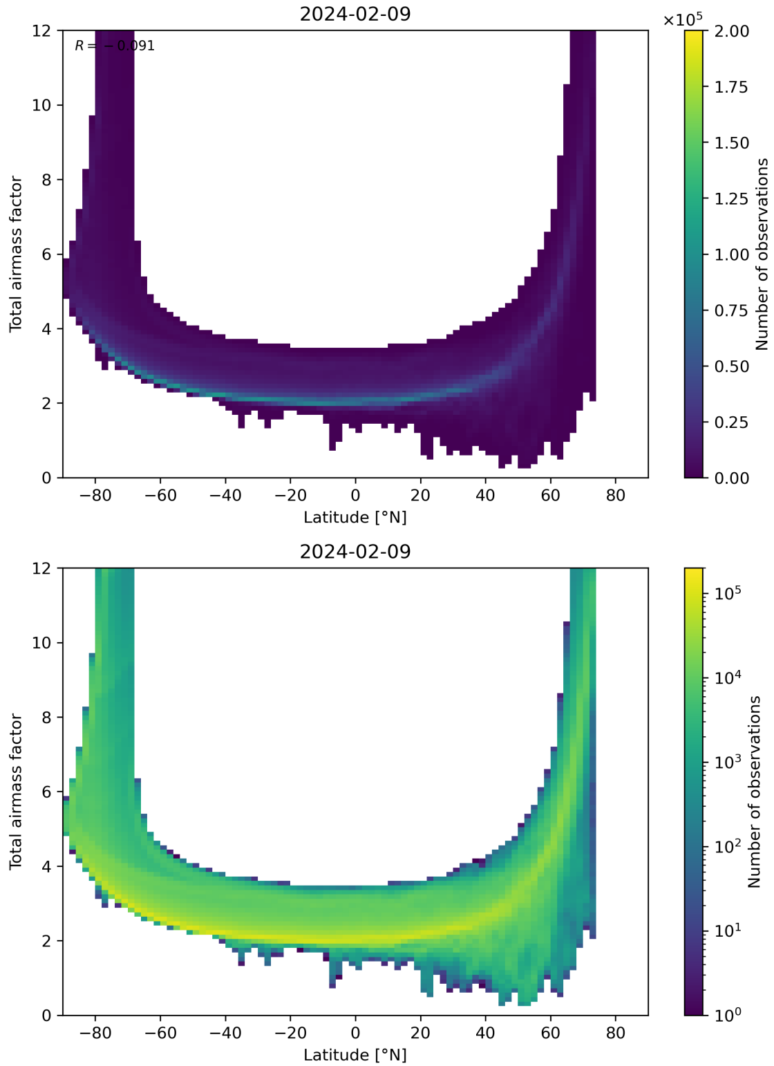
Figure 84: Scatter density plot of “Latitude” against “Total airmass factor” for 2024-02-08 to 2024-02-10.
