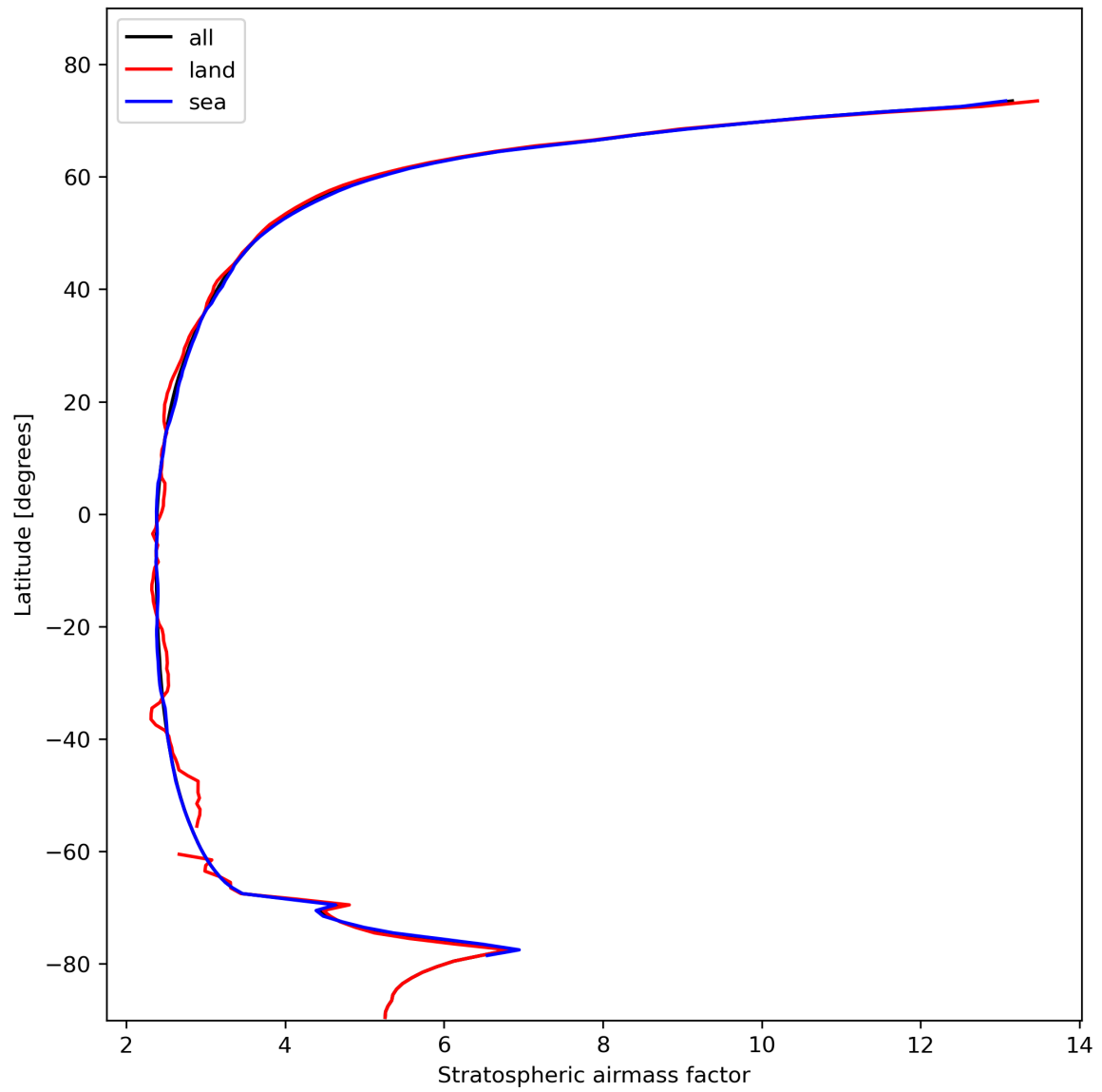
Figure 27: Zonal average of “Stratospheric airmass factor” for 2024-02-08 to 2024-02-10.
