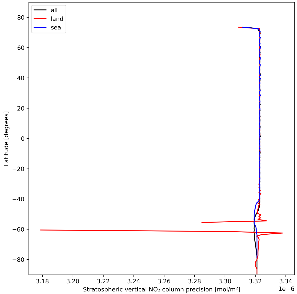
Figure 20: Zonal average of “Stratospheric vertical NO 2 column precision” for 2024-02-08 to 2024-02-10.
