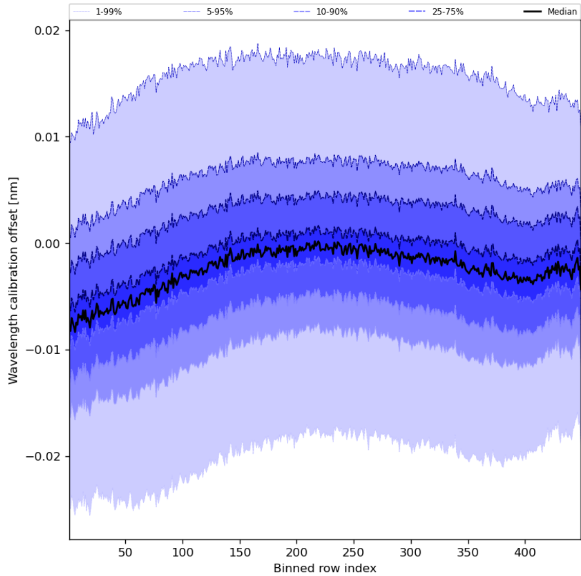
Figure 52: Along track statistics of “Wavelength calibration offset” for 2024-02-08 to 2024-02-10
