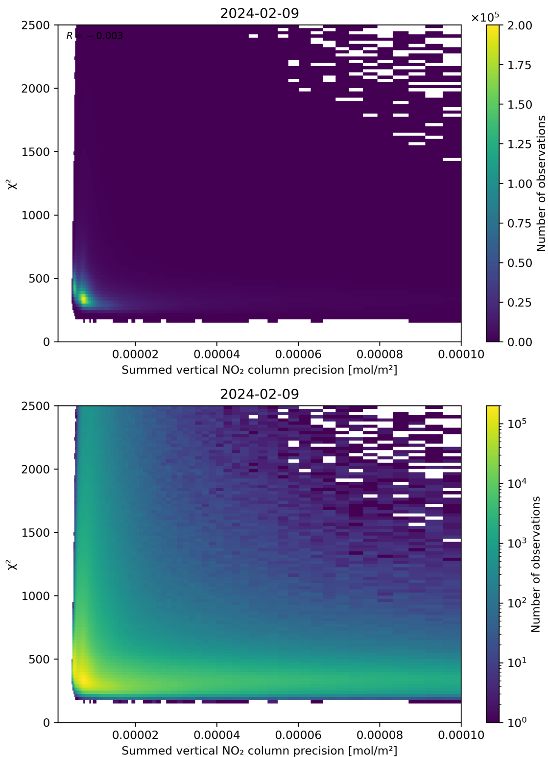
Figure 107: Scatter density plot of “Summed vertical NO 2 column precision” against “ \chi^2 ” for 2024-02-08 to 2024-02-10.
