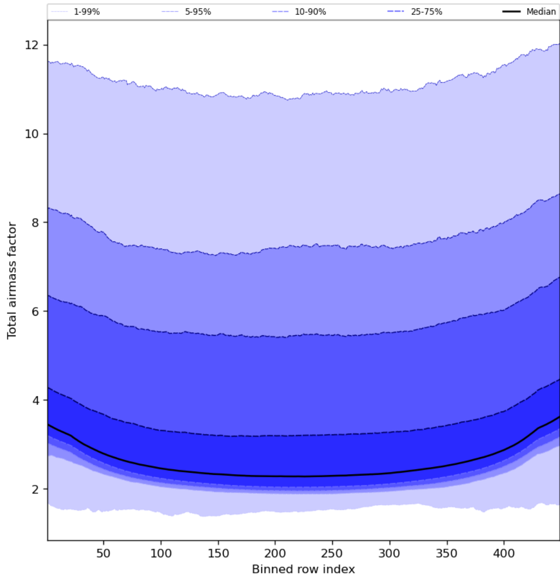
Figure 49: Along track statistics of “Total airmass factor” for 2024-02-08 to 2024-02-10
