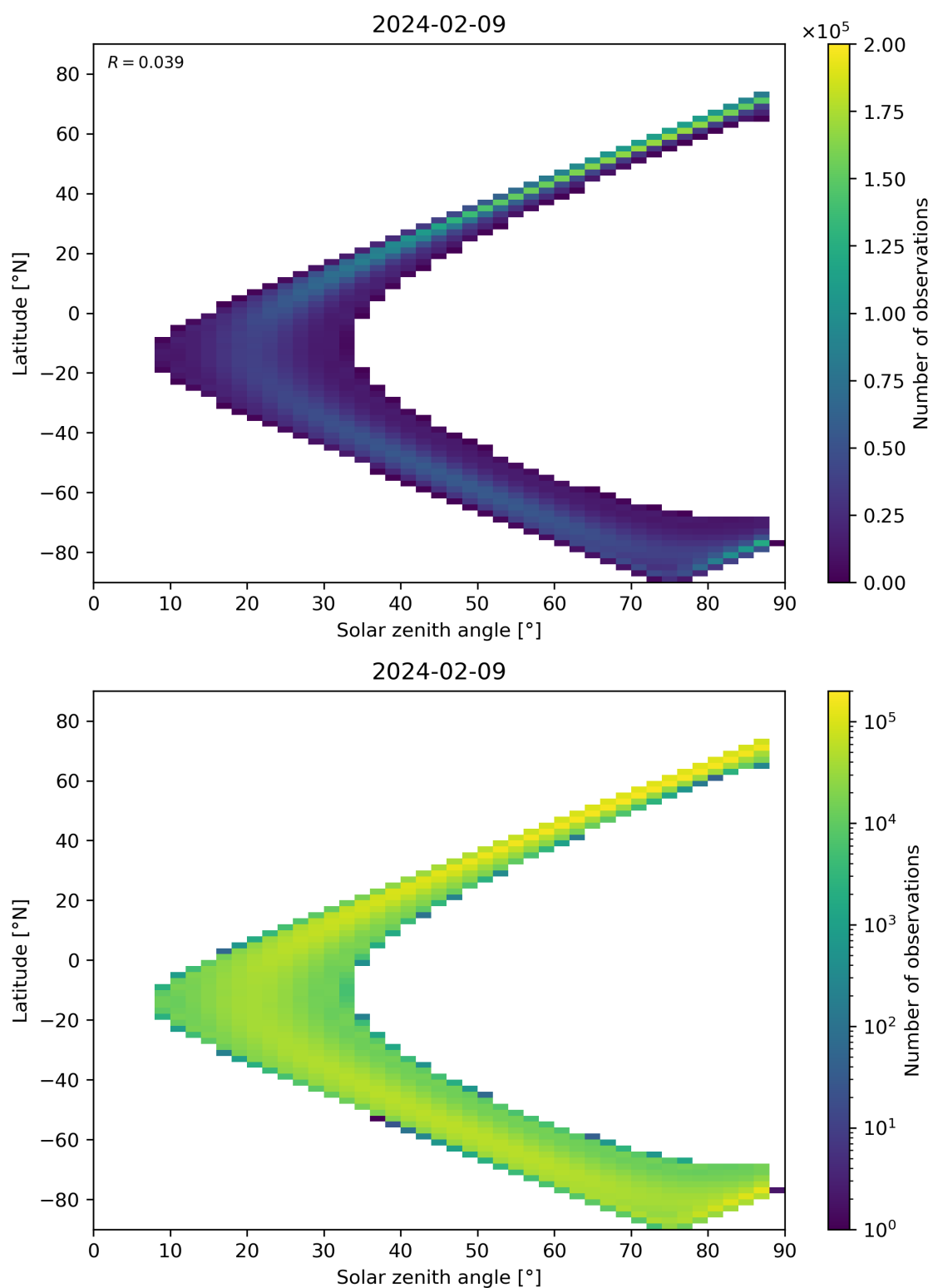
Figure 149: Scatter density plot of “Solar zenith angle” against “Latitude” for 2024-02-08 to 2024-02-10.
