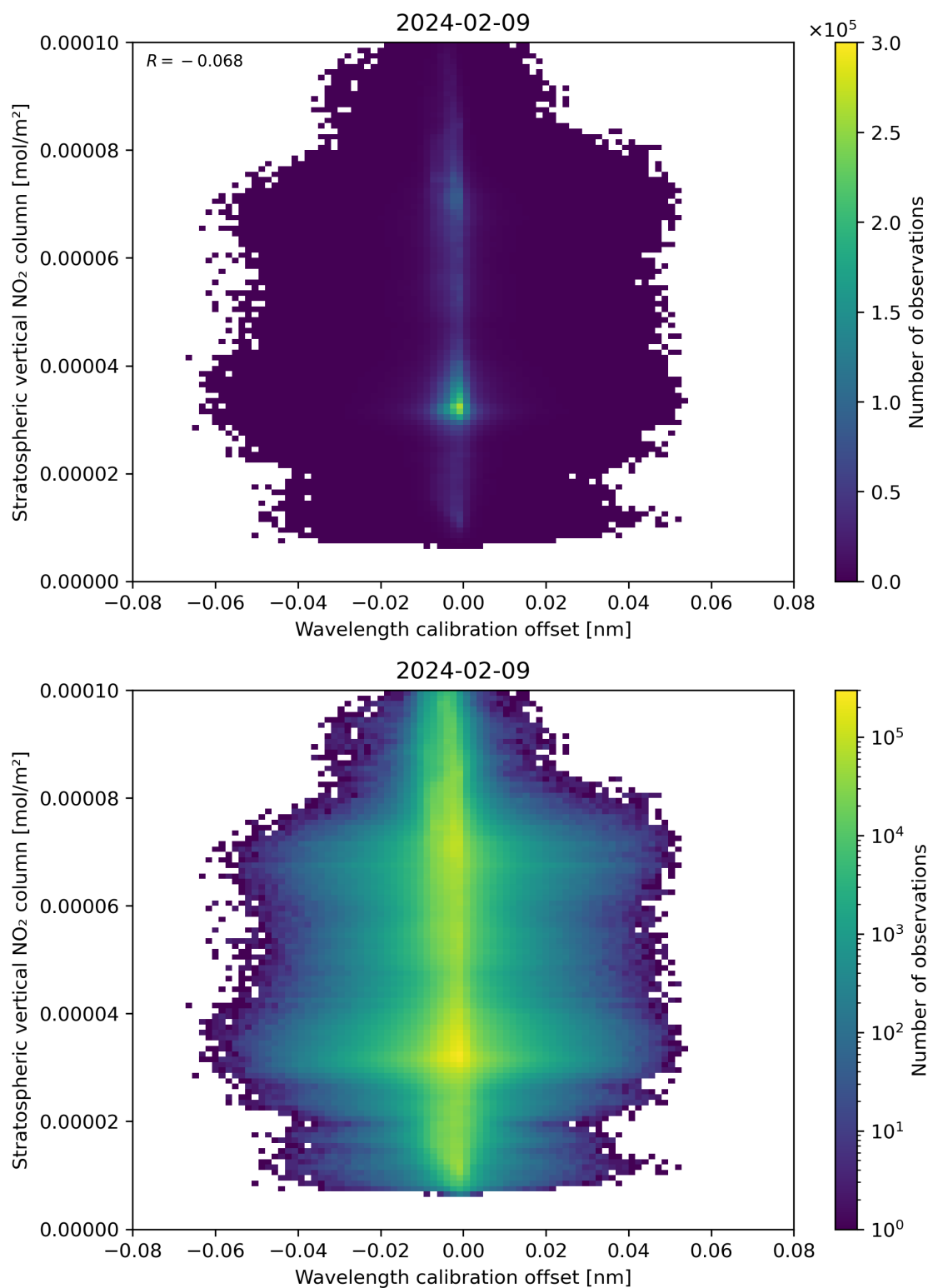
Figure 176: Scatter density plot of “Wavelength calibration offset” against “Stratospheric vertical NO 2 column” for 2024-02-08 to 2024-02-10.
