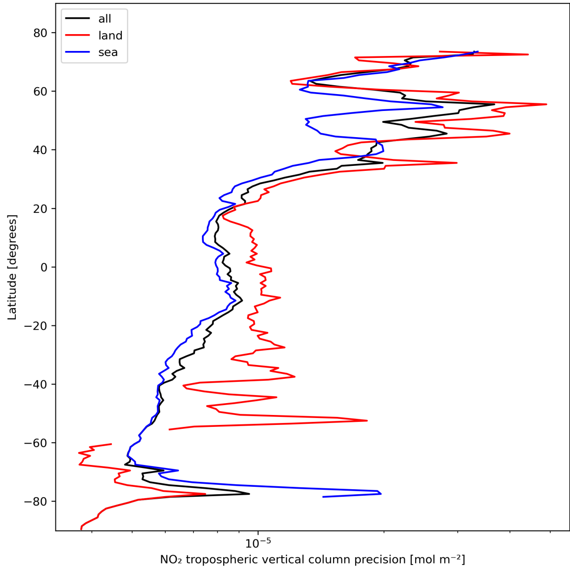
Figure 13: Zonal average of “NO 2 tropospheric vertical column precision” for 2024-02-08 to 2024-02-10.
