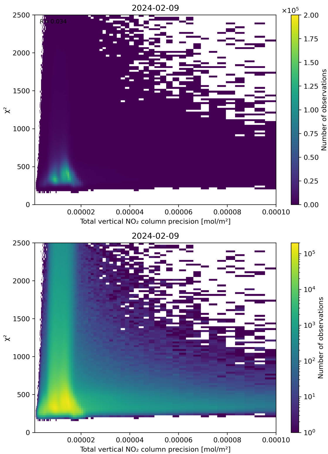
Figure 116: Scatter density plot of “Total vertical NO 2 column precision” against “ \chi^2 ” for 2024-02-08 to 2024-02-10.
