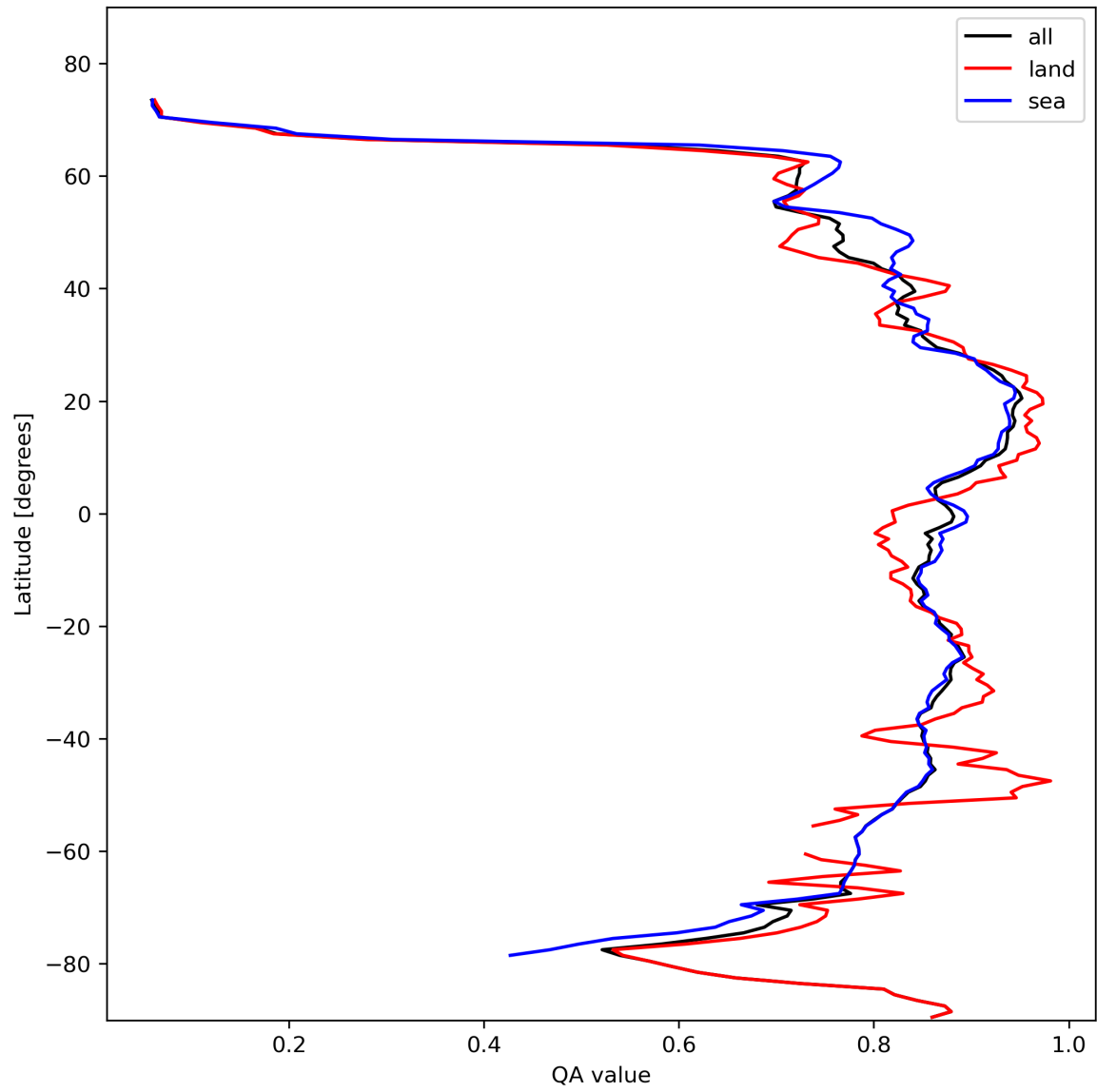
Figure 11: Zonal average of “QA value” for 2024-02-08 to 2024-02-10.
