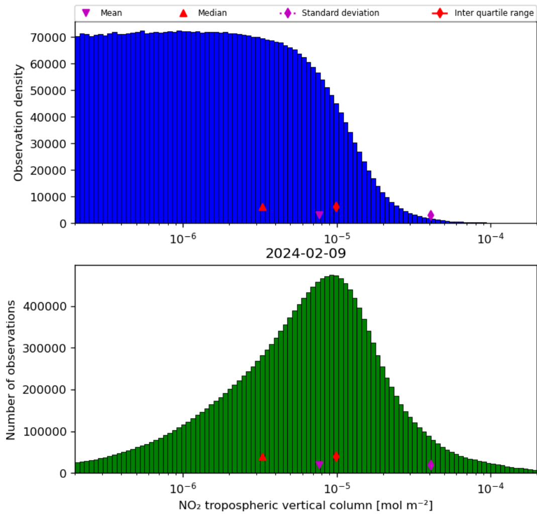
Figure 29: Histogram of “NO 2 tropospheric vertical column” for 2024-02-08 to 2024-02-10
