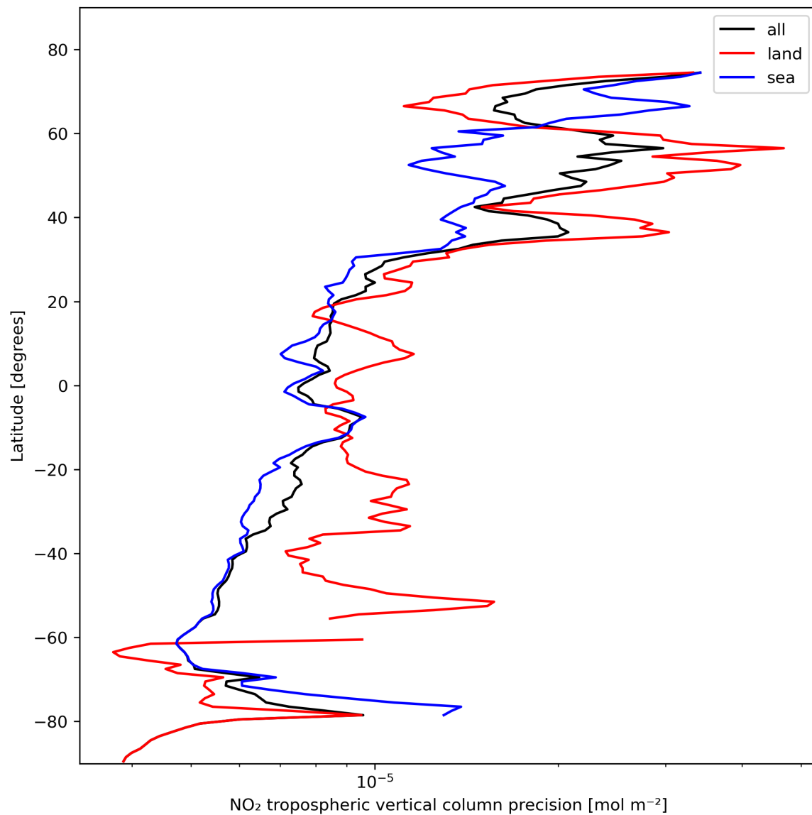
Figure 13: Zonal average of “NO 2 tropospheric vertical column precision” for 2024-02-11 to 2024-02-13.
