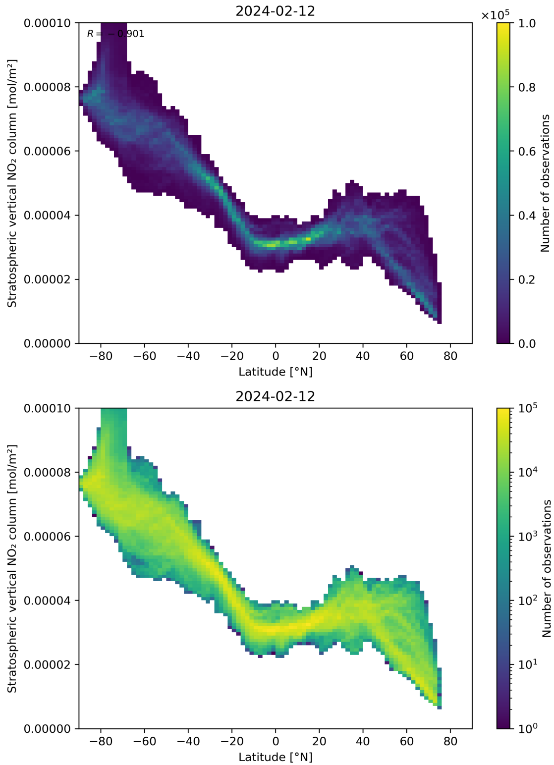
Figure 87: Scatter density plot of “Latitude” against “Stratospheric vertical NO 2 column” for 2024-02-11 to 2024-02-13.
