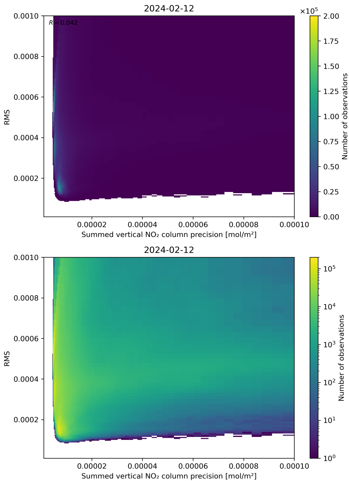
Figure 108: Scatter density plot of “Summed vertical NO 2 column precision” against “RMS” for 2024-02-11 to 2024-02-13.
