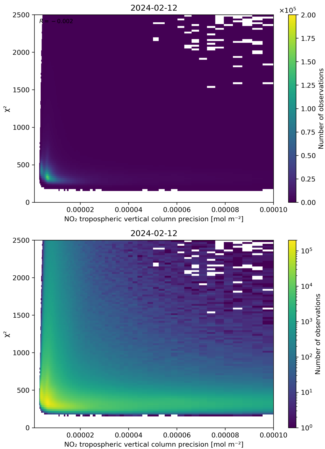
Figure 134: Scatter density plot of “NO 2 tropospheric vertical column precision” against “ \chi^2 ” for 2024-02-11 to 2024-02-13.
