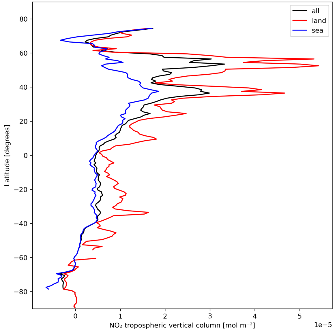
Figure 12: Zonal average of “NO 2 tropospheric vertical column” for 2024-02-11 to 2024-02-13.
