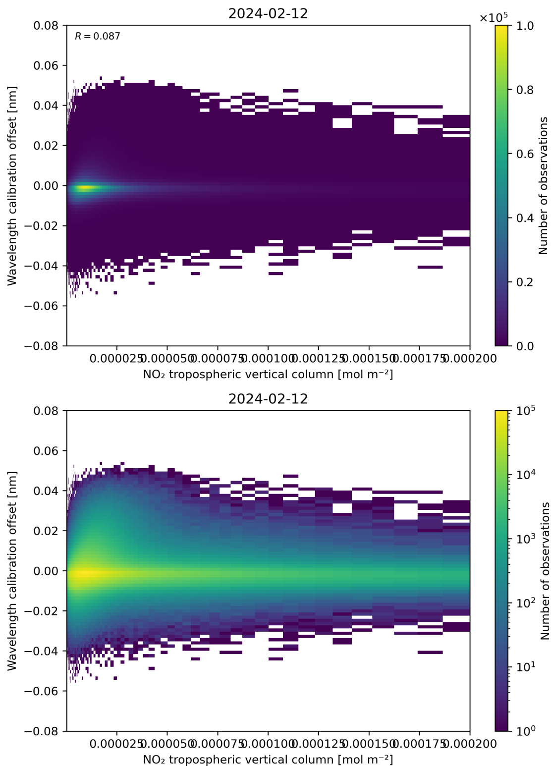
Figure 143: Scatter density plot of “NO 2 tropospheric vertical column” against “Wavelength calibration offset” for 2024-02-11 to 2024-02-13.
