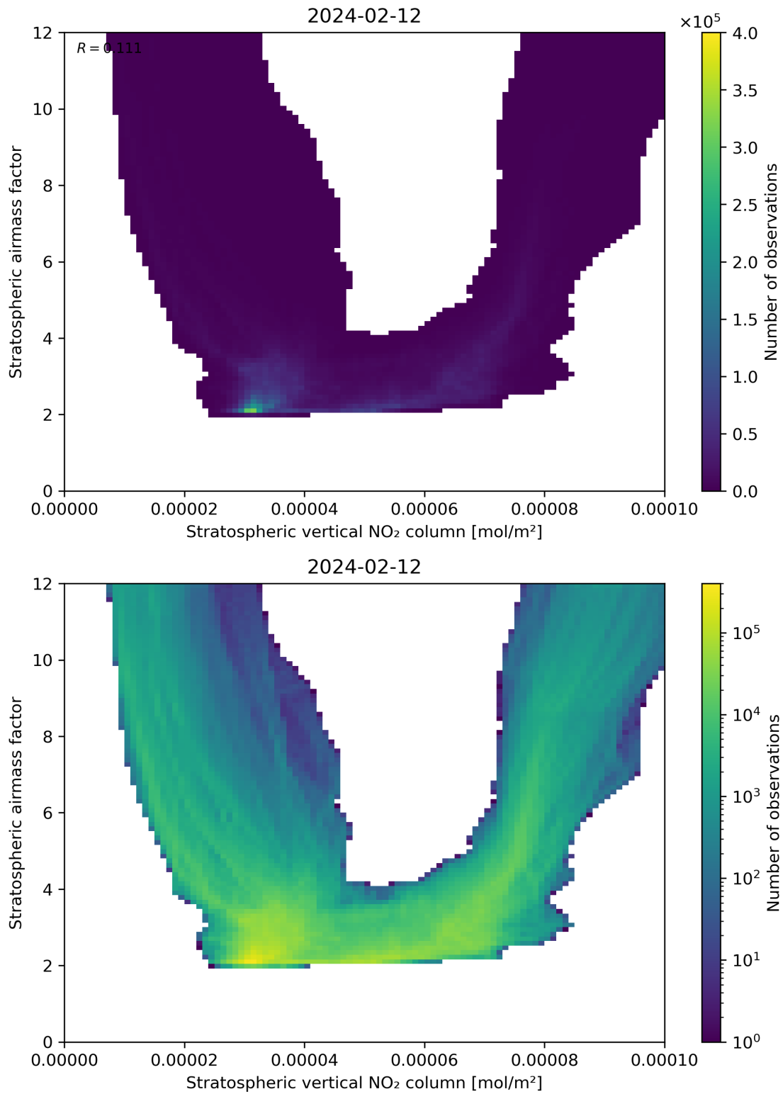
Figure 96: Scatter density plot of “Stratospheric vertical NO 2 column” against “Stratospheric airmass factor” for 2024-02-11 to 2024-02-13.
