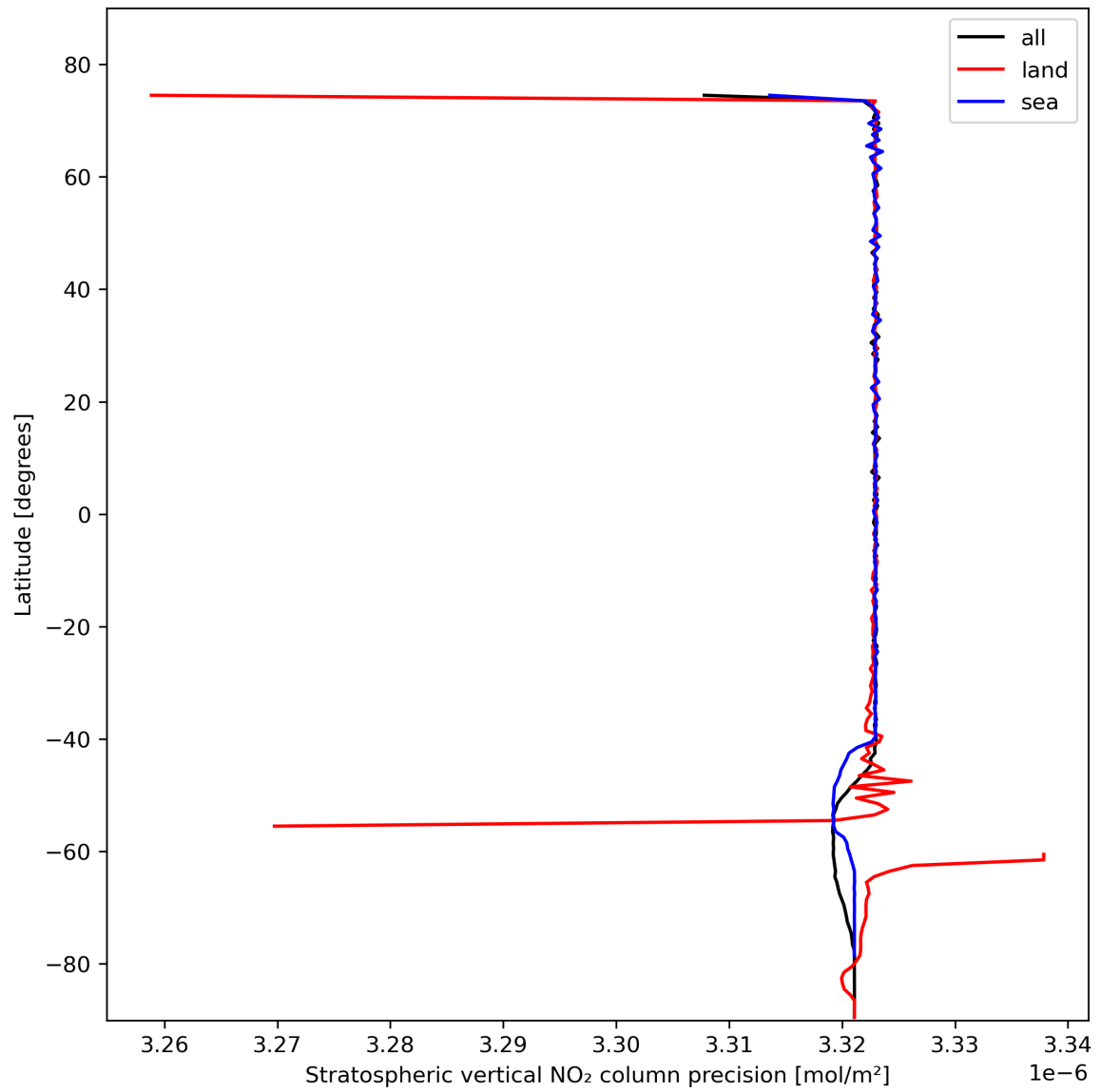
Figure 20: Zonal average of “Stratospheric vertical NO 2 column precision” for 2024-02-11 to 2024-02-13.
