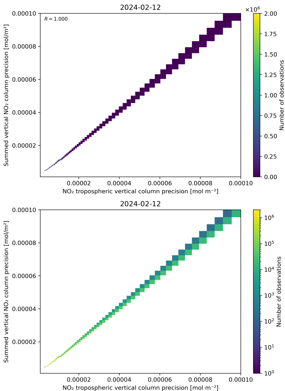
Figure 137: Scatter density plot of “NO 2 tropospheric vertical column precision” against “Summed vertical NO 2 column precision” for 2024-02-11 to 2024-02-13.
