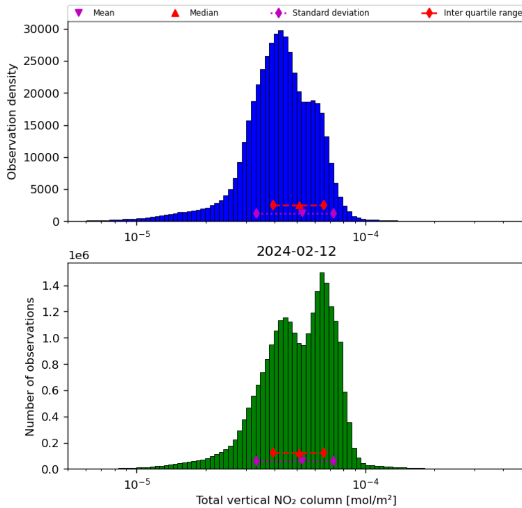
Figure 38: Histogram of “Total vertical NO 2 column” for 2024-02-11 to 2024-02-13
