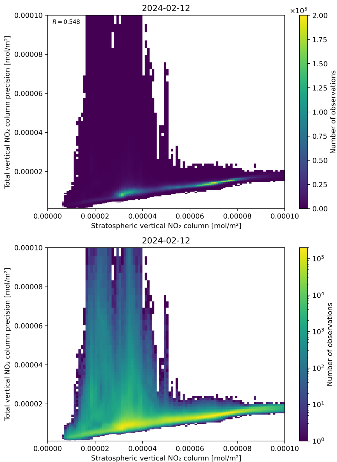
Figure 101: Scatter density plot of “Stratospheric vertical NO 2 column” against “Total vertical NO 2 column precision” for 2024-02-11 to 2024-02-13.
