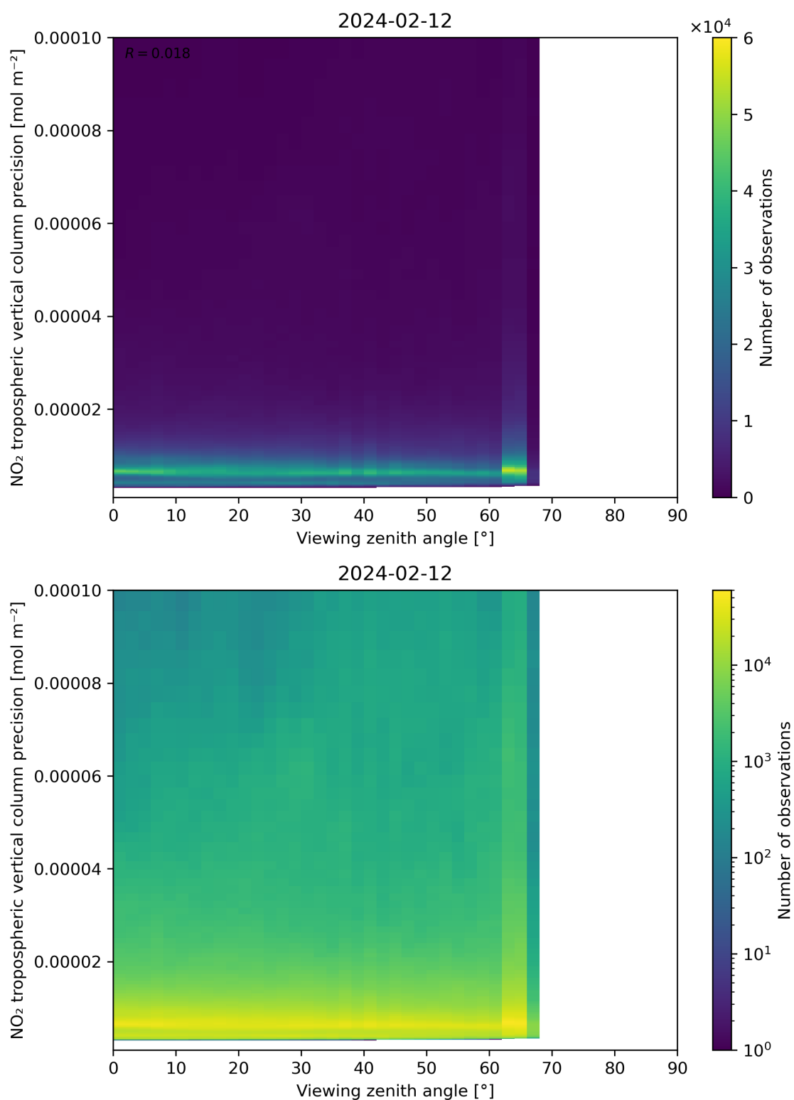
Figure 170: Scatter density plot of “Viewing zenith angle” against “NO 2 tropospheric vertical column precision” for 2024-02-11 to 2024-02-13.
