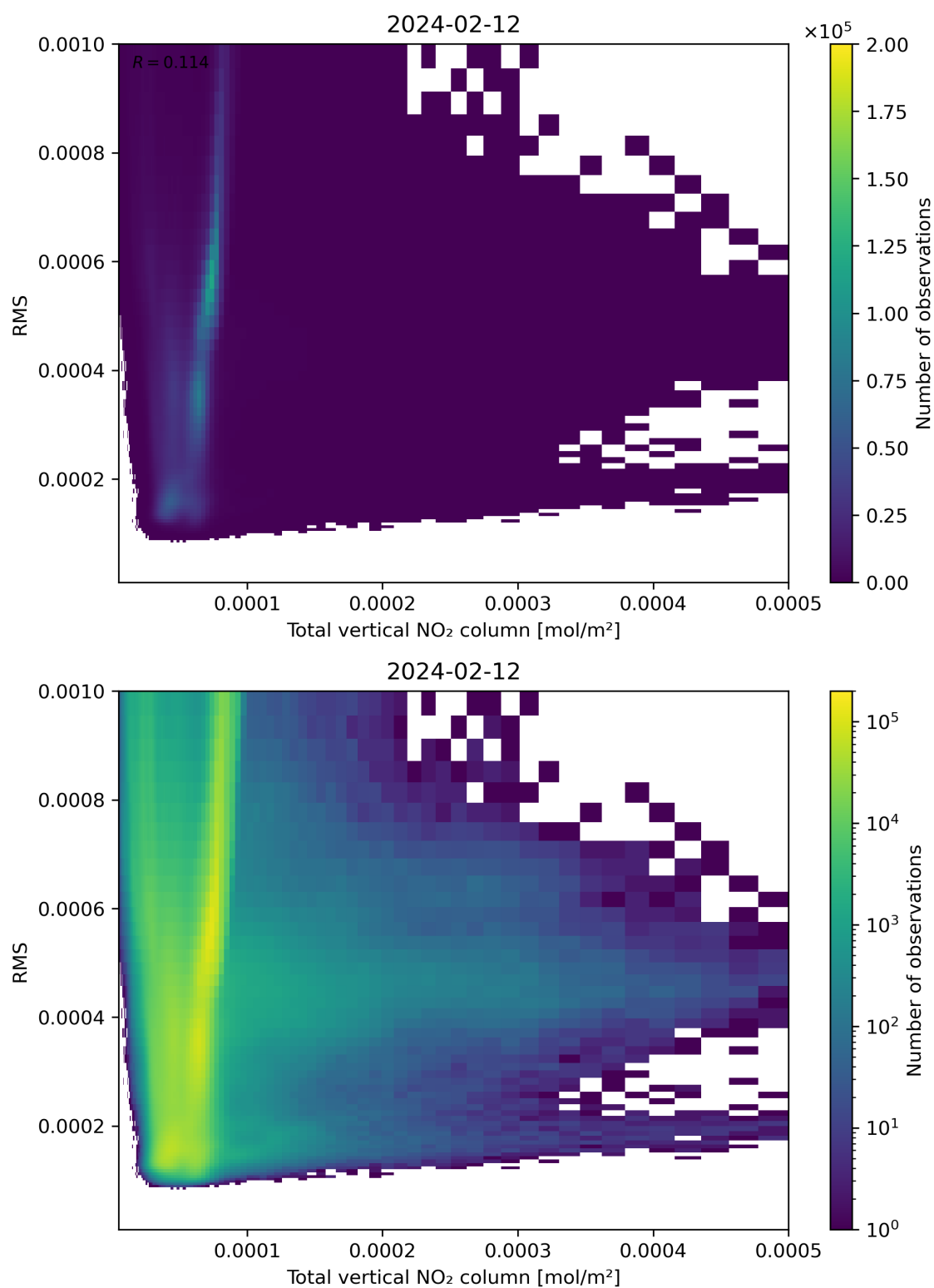
Figure 120: Scatter density plot of “Total vertical NO 2 column” against “RMS” for 2024-02-11 to 2024-02-13.
