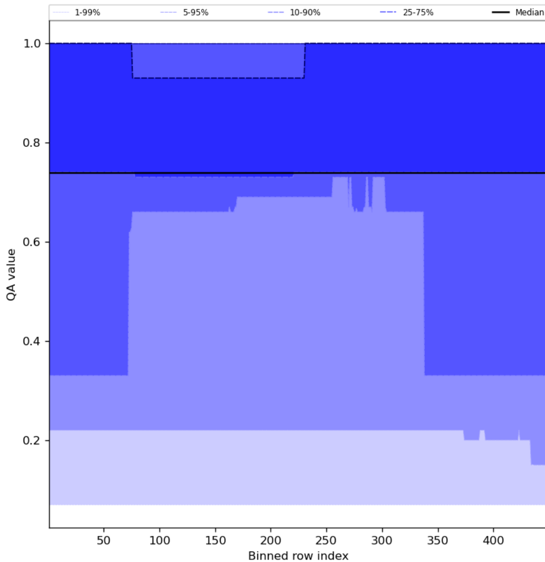
Figure 45: Along track statistics of “QA value” for 2024-02-11 to 2024-02-13
