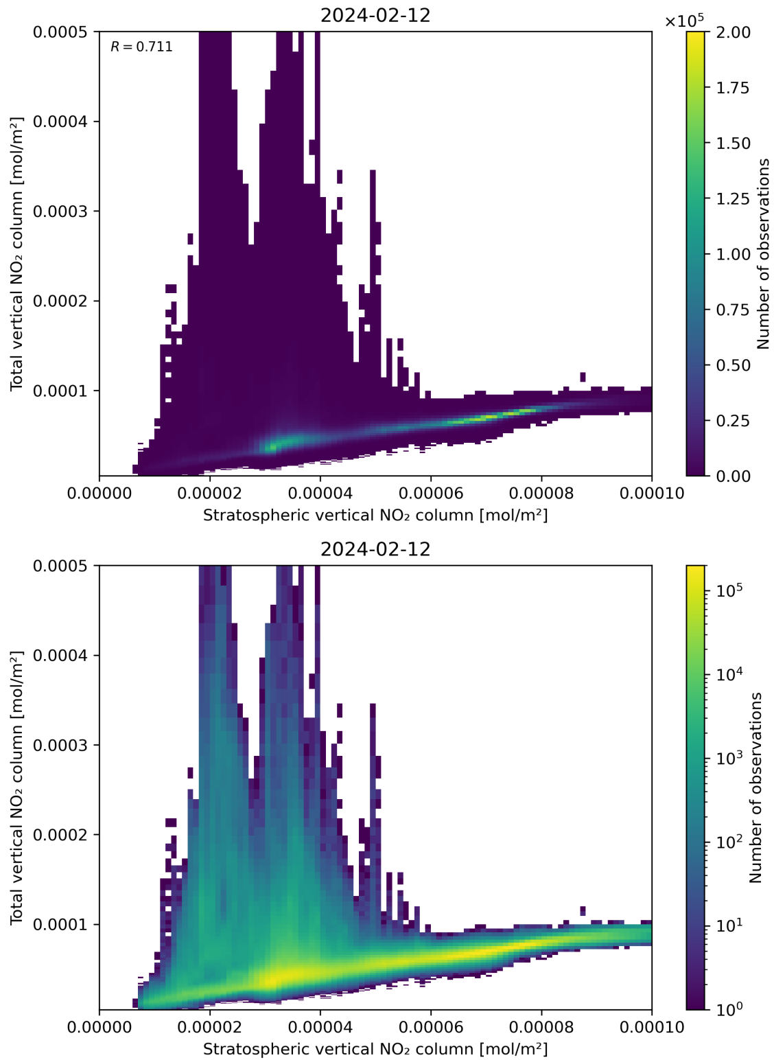
Figure 100: Scatter density plot of “Stratospheric vertical NO 2 column” against “Total vertical NO 2 column” for 2024-02-11 to 2024-02-13.
