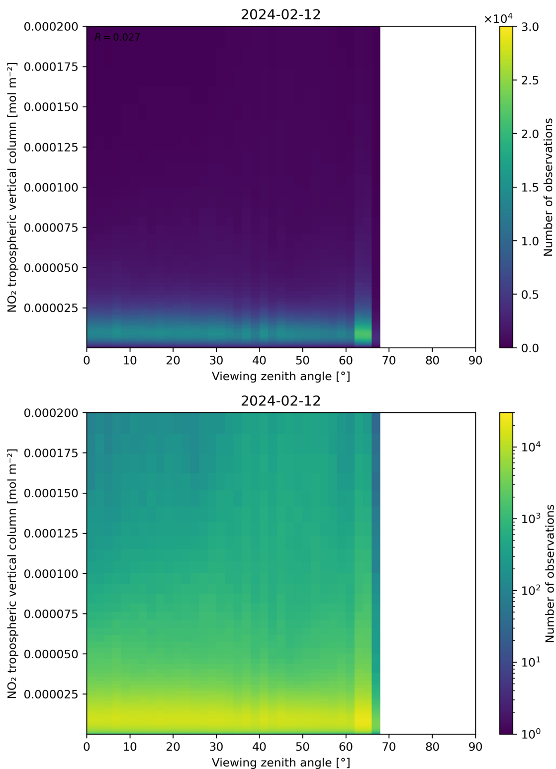
Figure 169: Scatter density plot of “Viewing zenith angle” against “NO 2 tropospheric vertical column” for 2024-02-11 to 2024-02-13.
