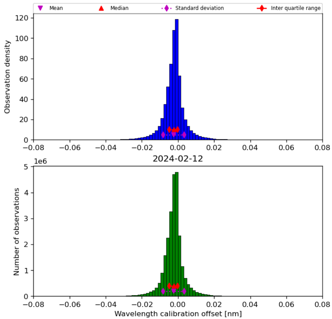
Figure 35: Histogram of “Wavelength calibration offset” for 2024-02-11 to 2024-02-13
