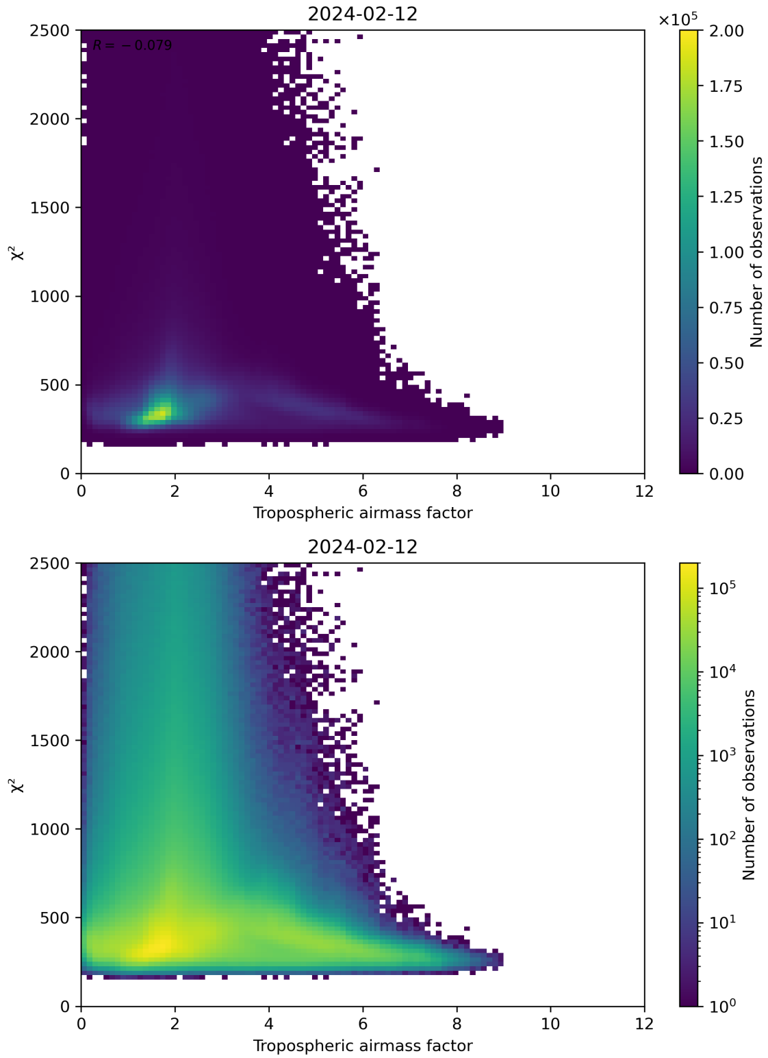
Figure 73: Scatter density plot of “Tropospheric airmass factor” against “ \chi^2 ” for 2024-02-11 to 2024-02-13.
