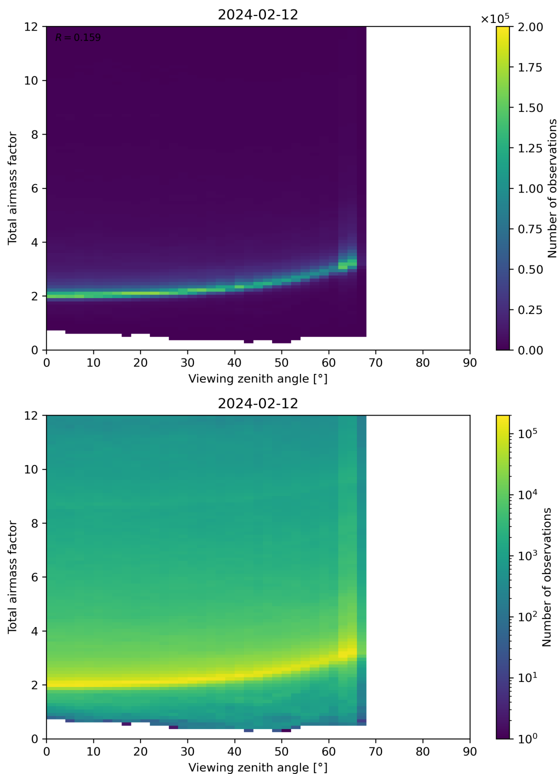
Figure 160: Scatter density plot of “Viewing zenith angle” against “Total airmass factor” for 2024-02-11 to 2024-02-13.
