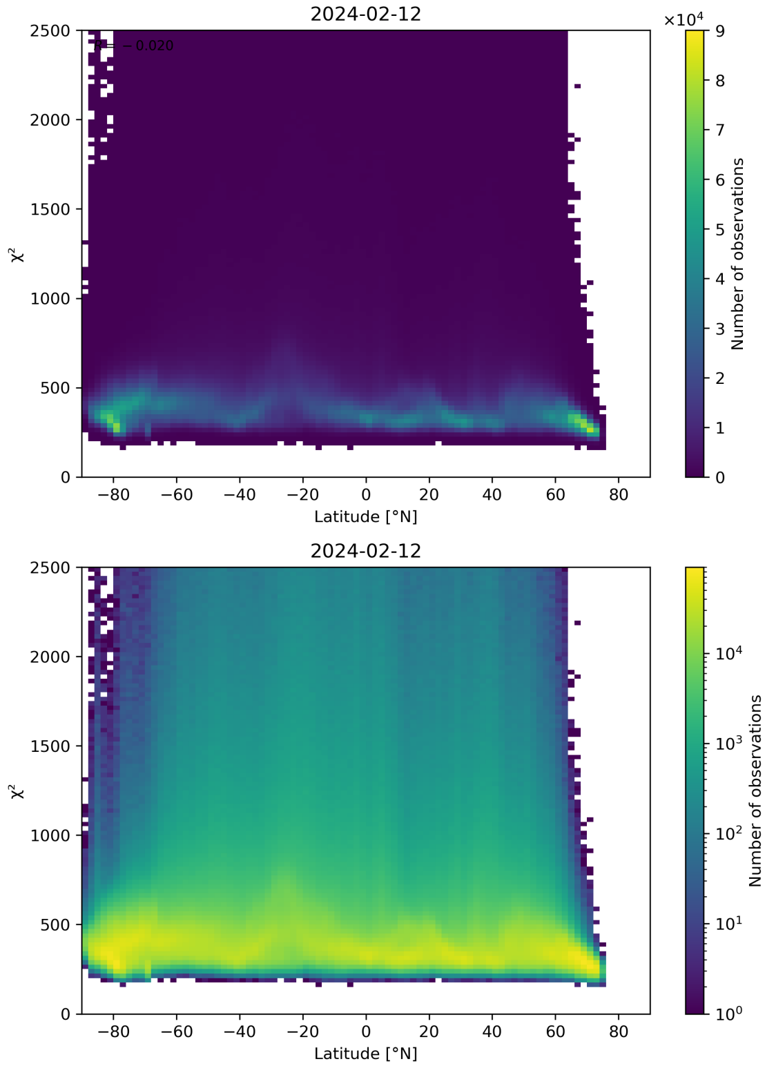
Figure 86: Scatter density plot of “Latitude” against “ \chi^2 ” for 2024-02-11 to 2024-02-13.
