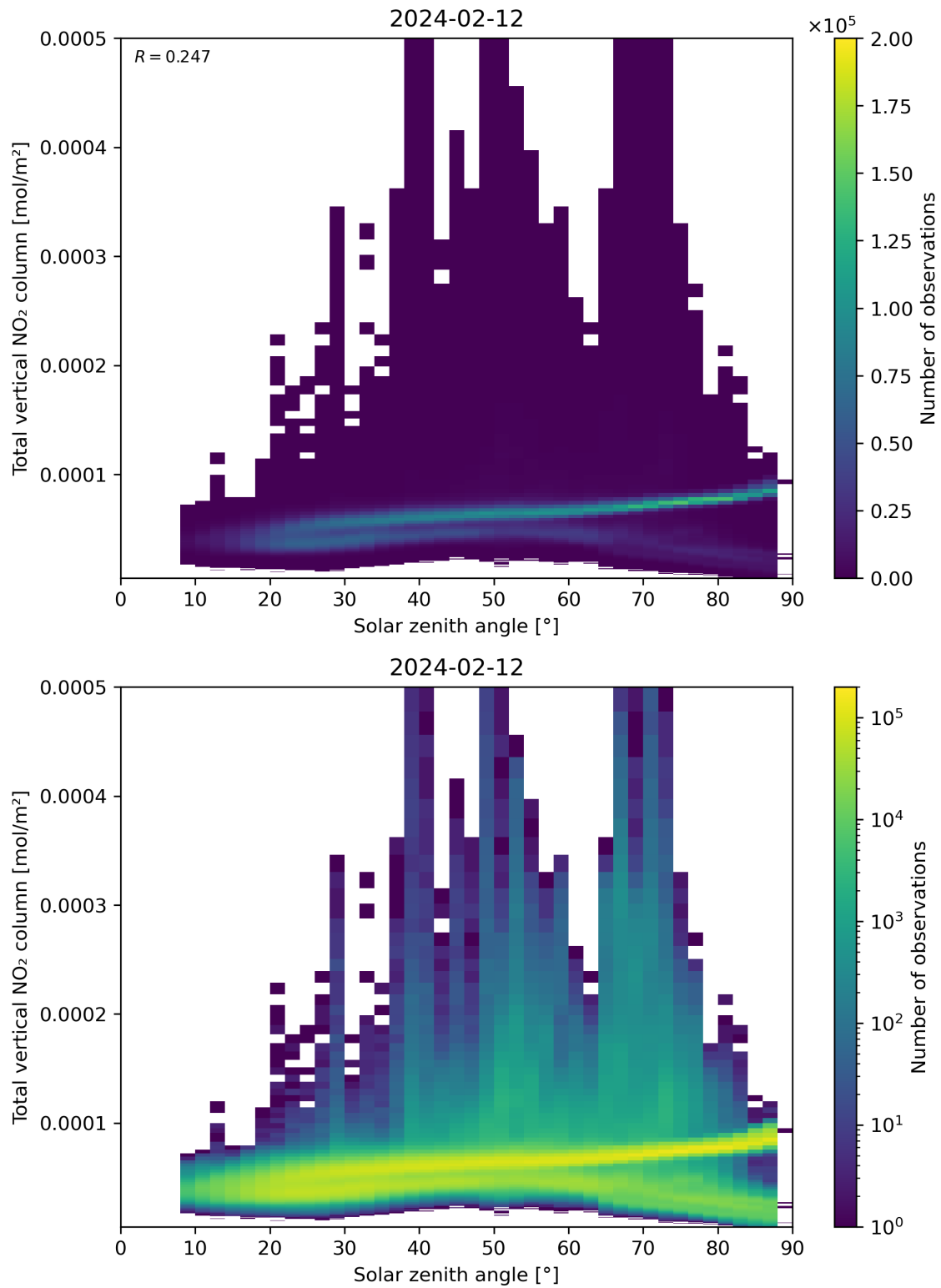
Figure 153: Scatter density plot of “Solar zenith angle” against “Total vertical NO 2 column” for 2024-02-11 to 2024-02-13.
