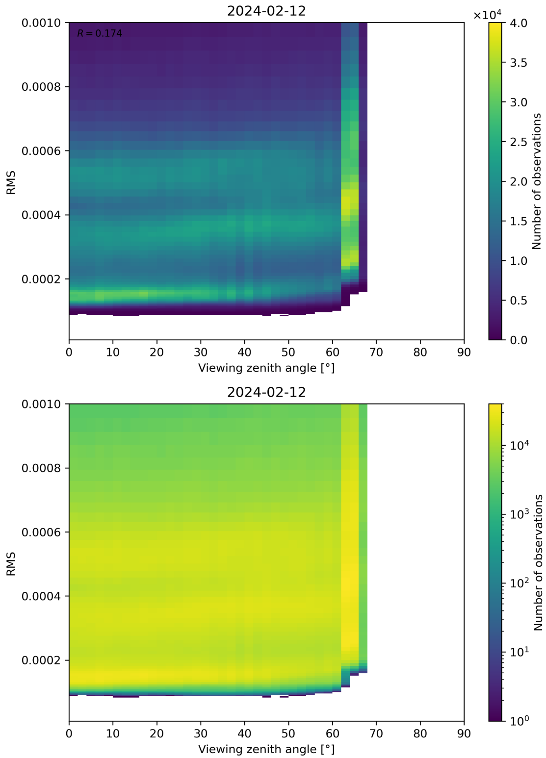
Figure 171: Scatter density plot of “Viewing zenith angle” against “RMS” for 2024-02-11 to 2024-02-13.
