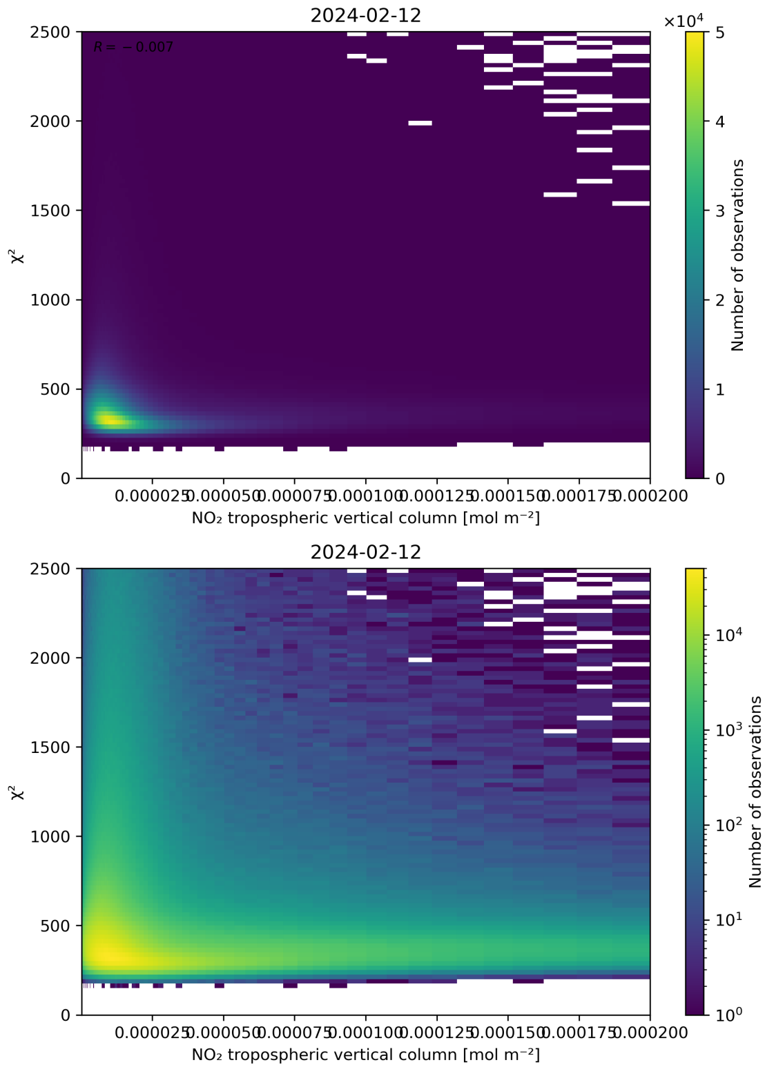
Figure 124: Scatter density plot of “NO 2 tropospheric vertical column” against “ \chi^2 ” for 2024-02-11 to 2024-02-13.
