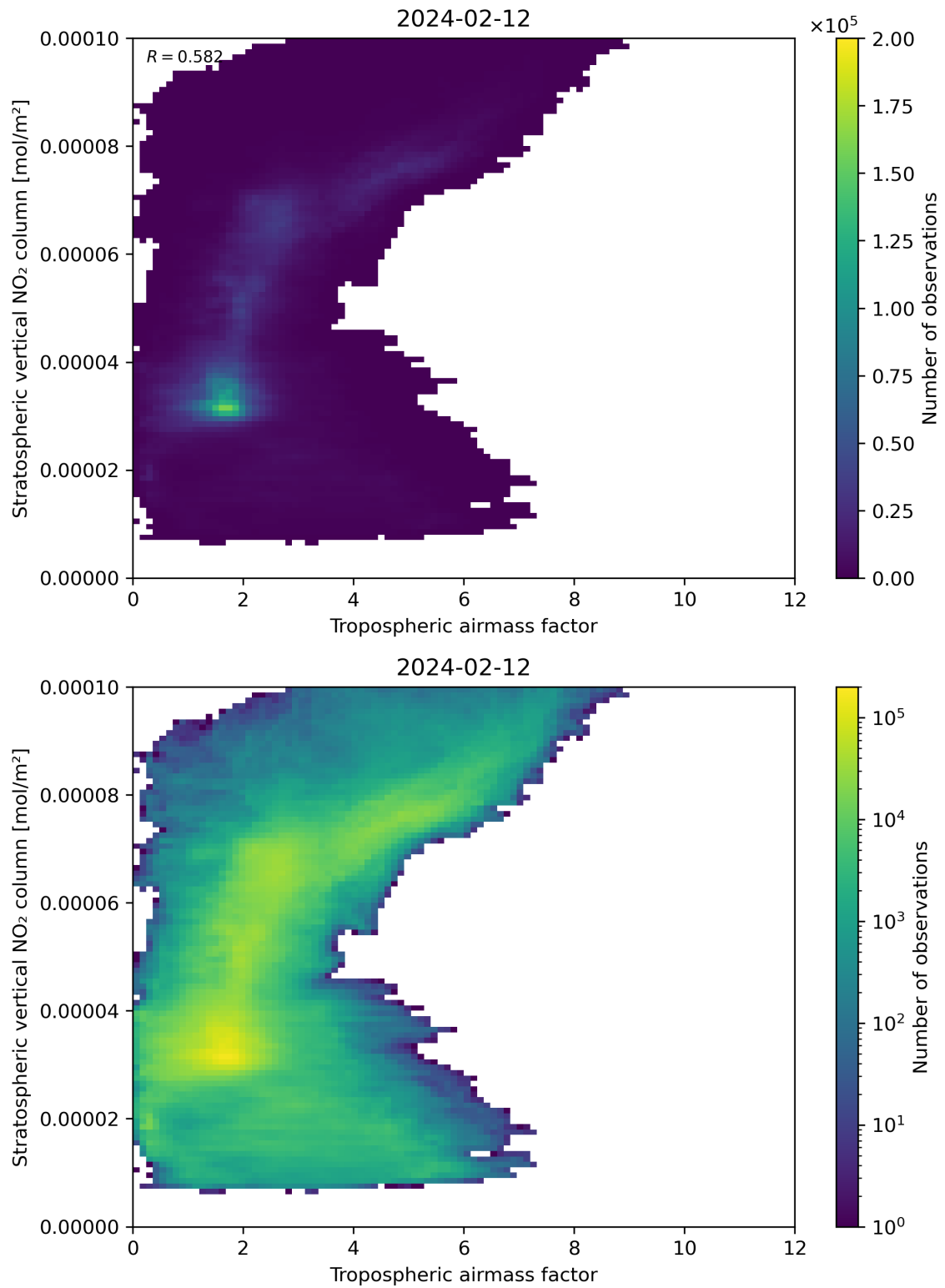
Figure 74: Scatter density plot of “Tropospheric air mass factor” against “Stratospheric vertical NO 2 column” for 2024-02-11 to 2024-02-13.
