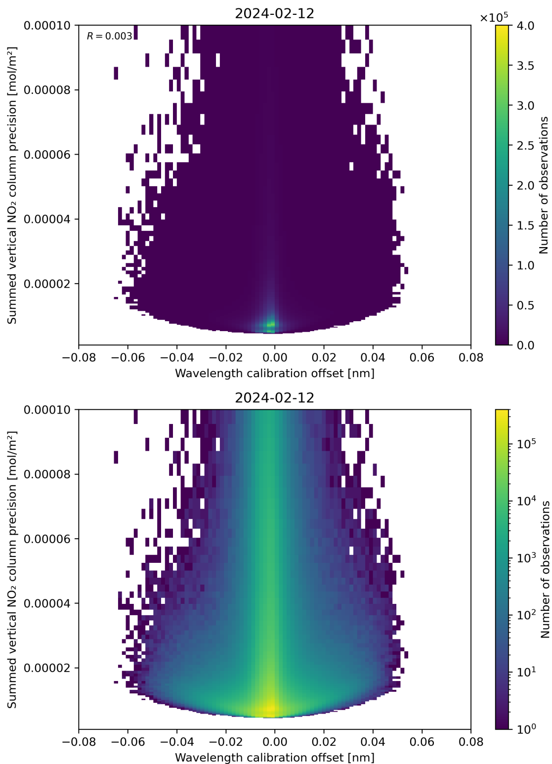
Figure 178: Scatter density plot of “Wavelength calibration offset” against “Summed vertical NO 2 column precision” for 2024-02-11 to 2024-02-13.
