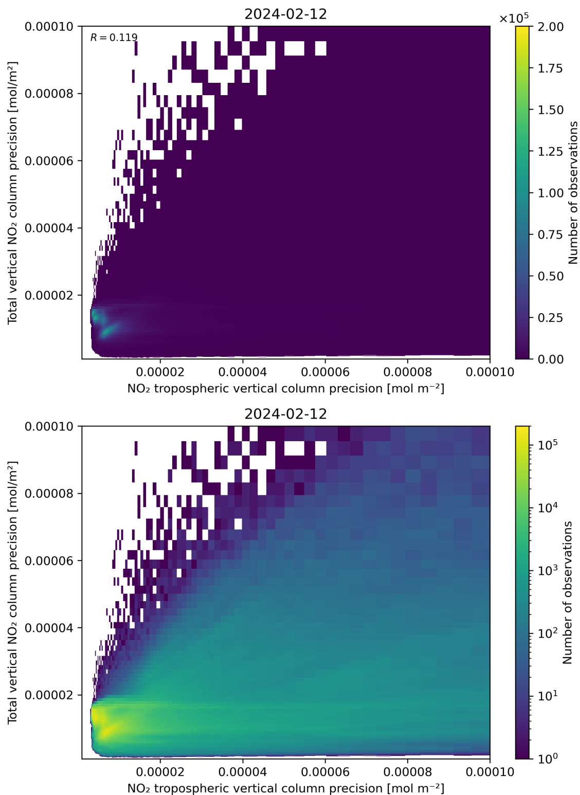
Figure 139: Scatter density plot of “NO 2 tropospheric vertical column precision” against “Total vertical NO 2 column precision” for 2024-02-11 to 2024-02-13.
