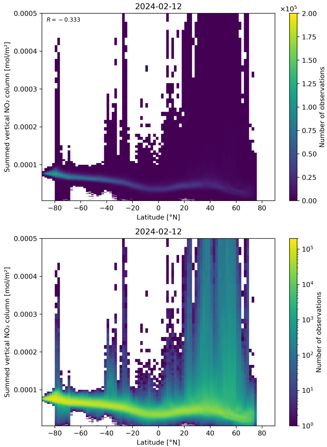
Figure 88: Scatter density plot of “Latitude” against “Summed vertical NO 2 column” for 2024-02-11 to 2024-02-13.
