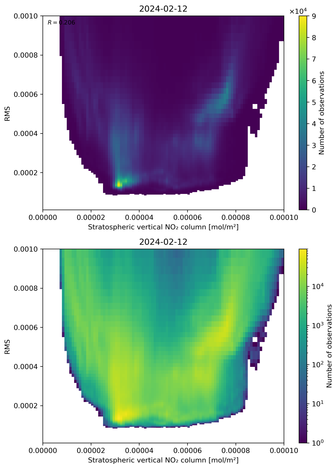
Figure 102: Scatter density plot of “Stratospheric vertical NO 2 column” against “RMS” for 2024-02-11 to 2024-02-13.
