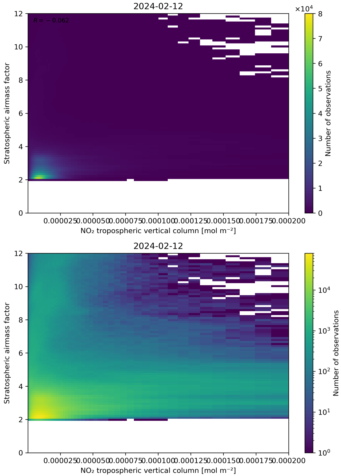
Figure 121: Scatter density plot of “NO 2 tropospheric vertical column” against “Stratospheric air mass factor” for 2024-02-11 to 2024-02-13.
