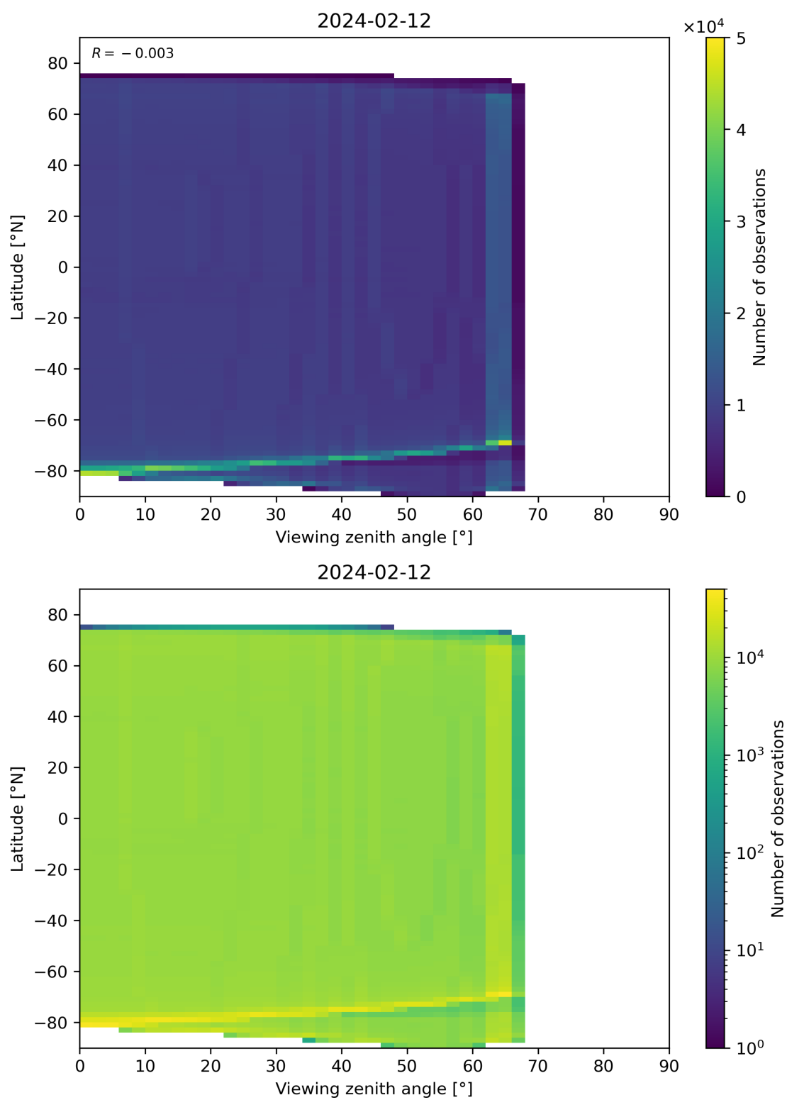
Figure 163: Scatter density plot of “Viewing zenith angle” against “Latitude” for 2024-02-11 to 2024-02-13.
