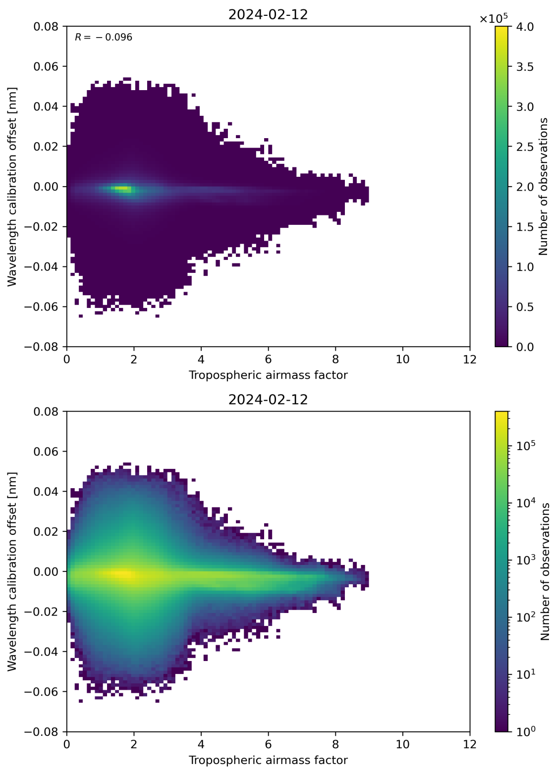
Figure 80: Scatter density plot of “Tropospheric airmass factor” against “Wavelength calibration offset” for 2024-02-11 to 2024-02-13.
