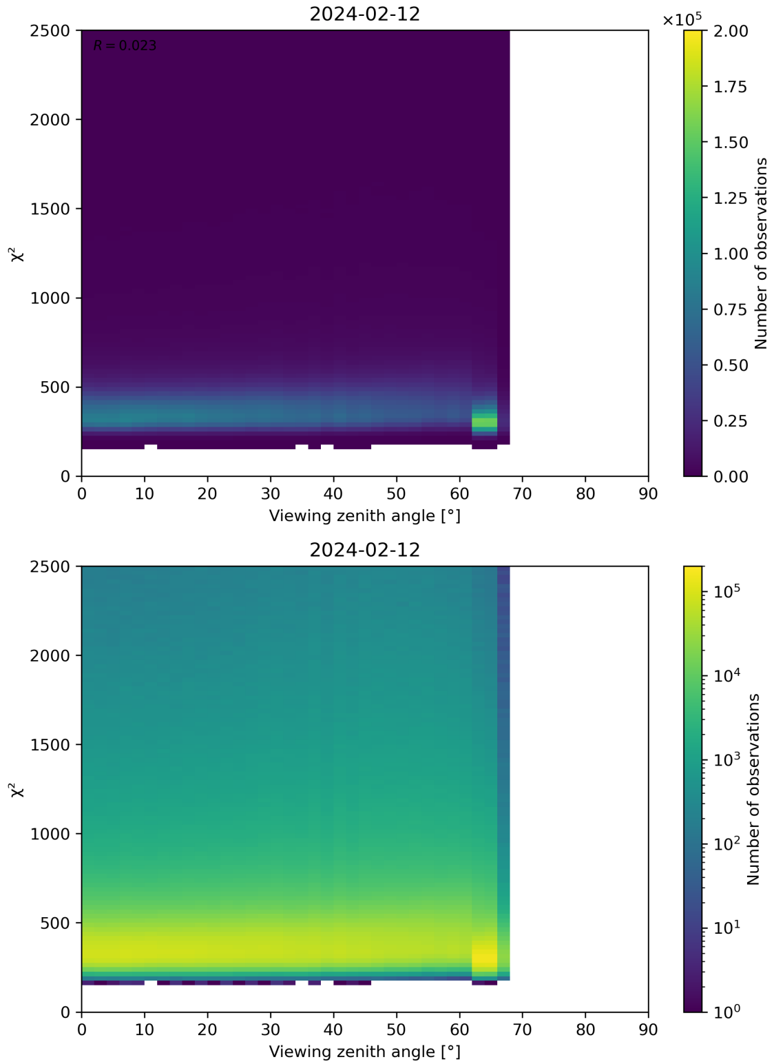
Figure 162: Scatter density plot of “Viewing zenith angle” against “ \chi^2 ” for 2024-02-11 to 2024-02-13.
