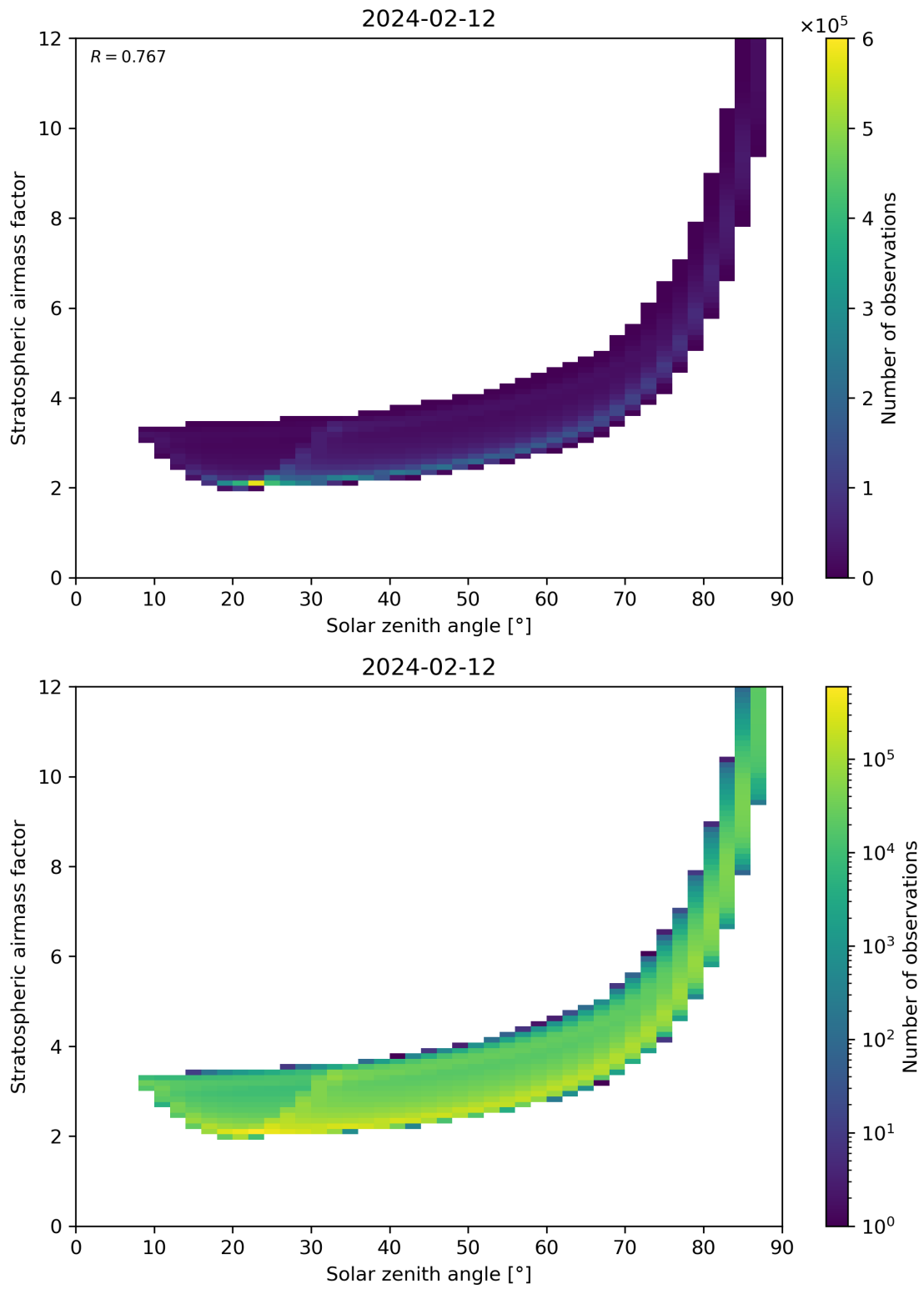
Figure 145: Scatter density plot of “Solar zenith angle” against “Stratospheric airmass factor” for 2024-02-11 to 2024-02-13.
