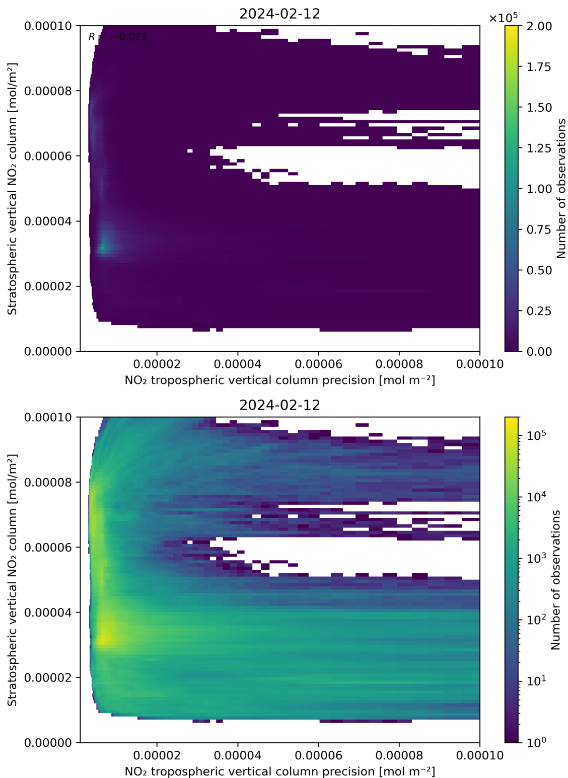
Figure 135: Scatter density plot of “NO 2 tropospheric vertical column precision” against “Stratospheric vertical NO 2 column” for 2024-02-11 to 2024-02-13.
