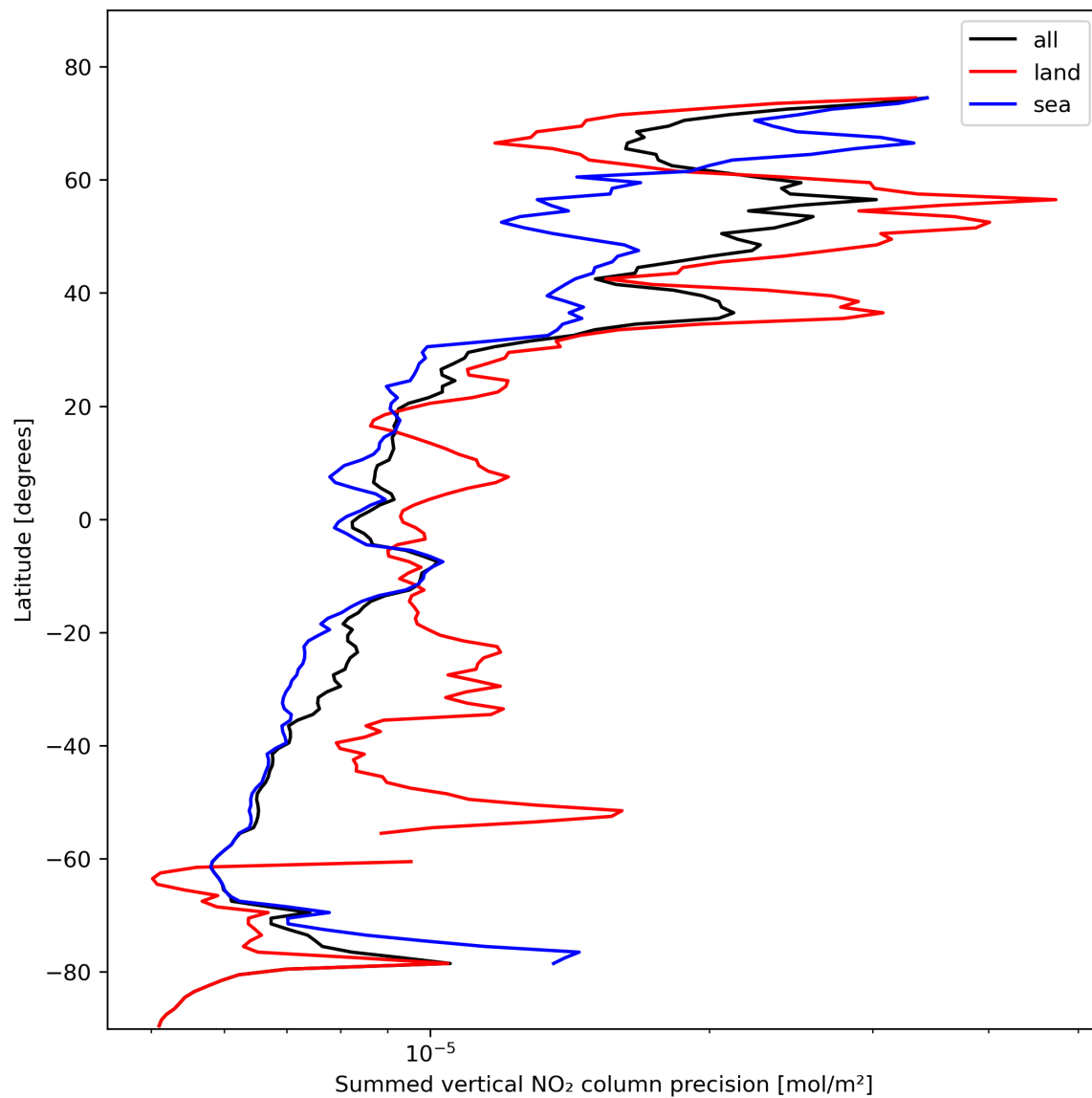
Figure 24: Zonal average of “Summed vertical NO 2 column precision” for 2024-02-11 to 2024-02-13.
