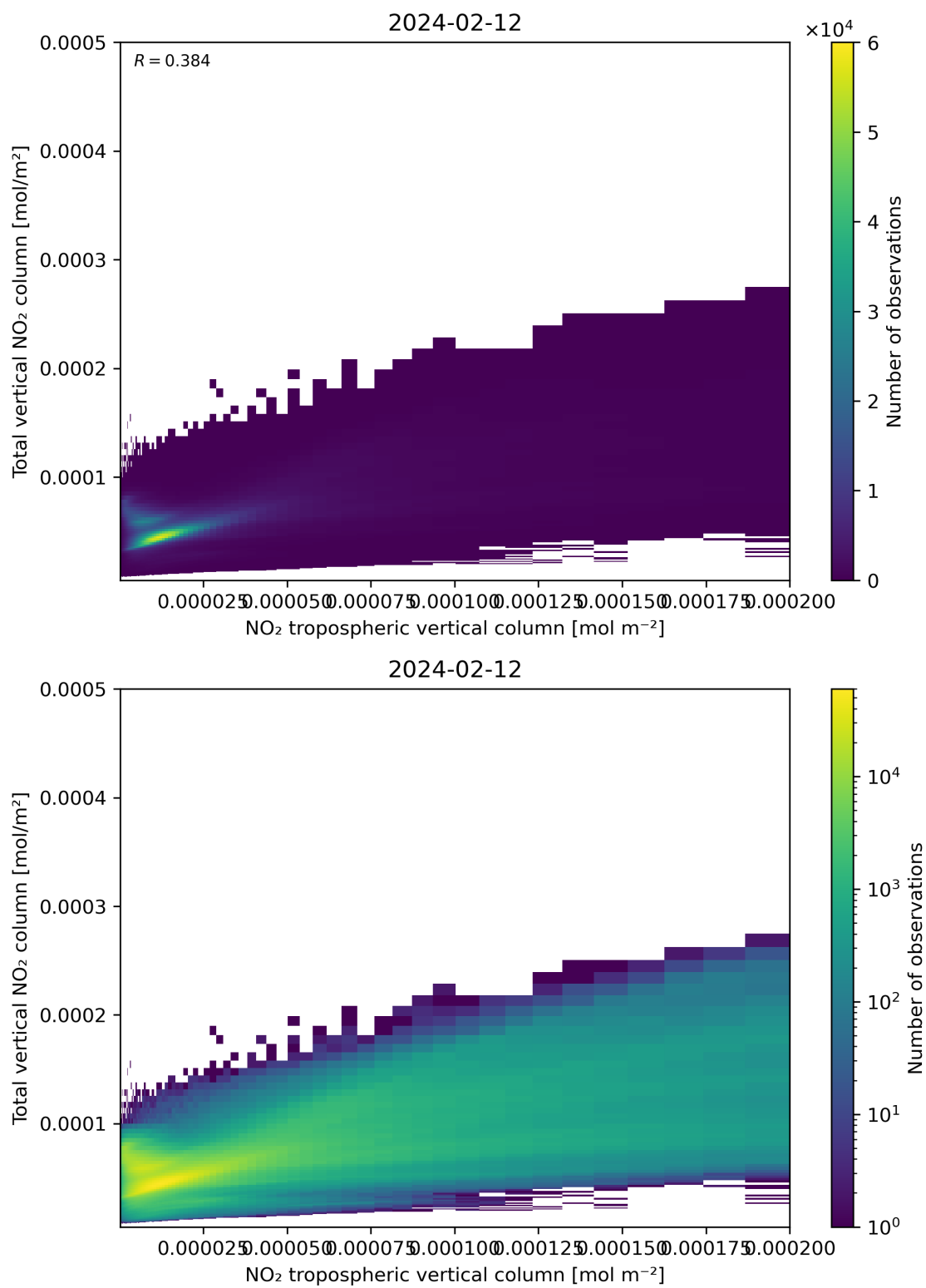
Figure 128: Scatter density plot of “NO 2 tropospheric vertical column” against “Total vertical NO 2 column” for 2024-02-11 to 2024-02-13.
