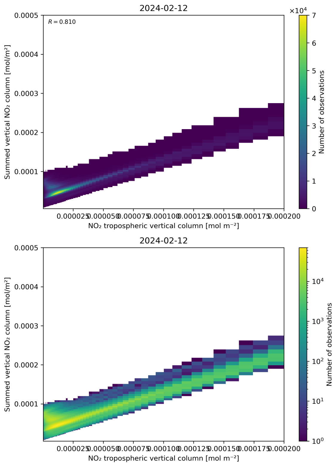
Figure 126: Scatter density plot of “NO 2 tropospheric vertical column” against “Summed vertical NO 2 column” for 2024-02-11 to 2024-02-13.
