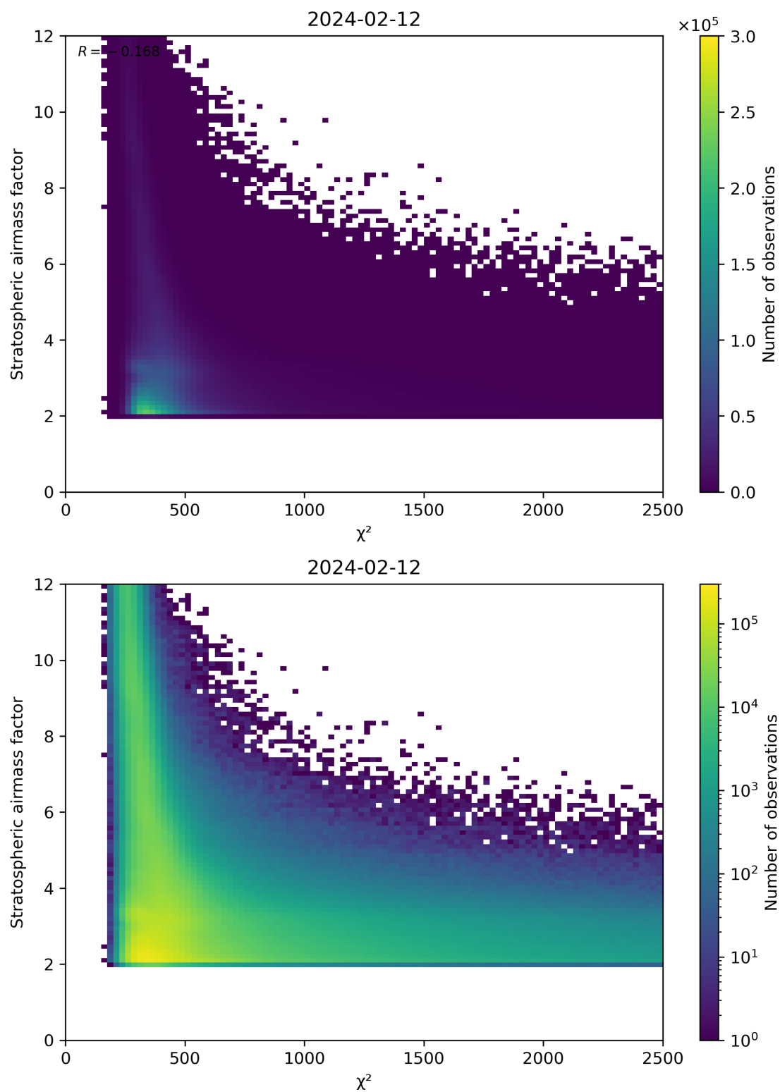
Figure 81: Scatter density plot of “ \chi^2 ” against “Stratospheric airmass factor” for 2024-02-11 to 2024-02-13.
