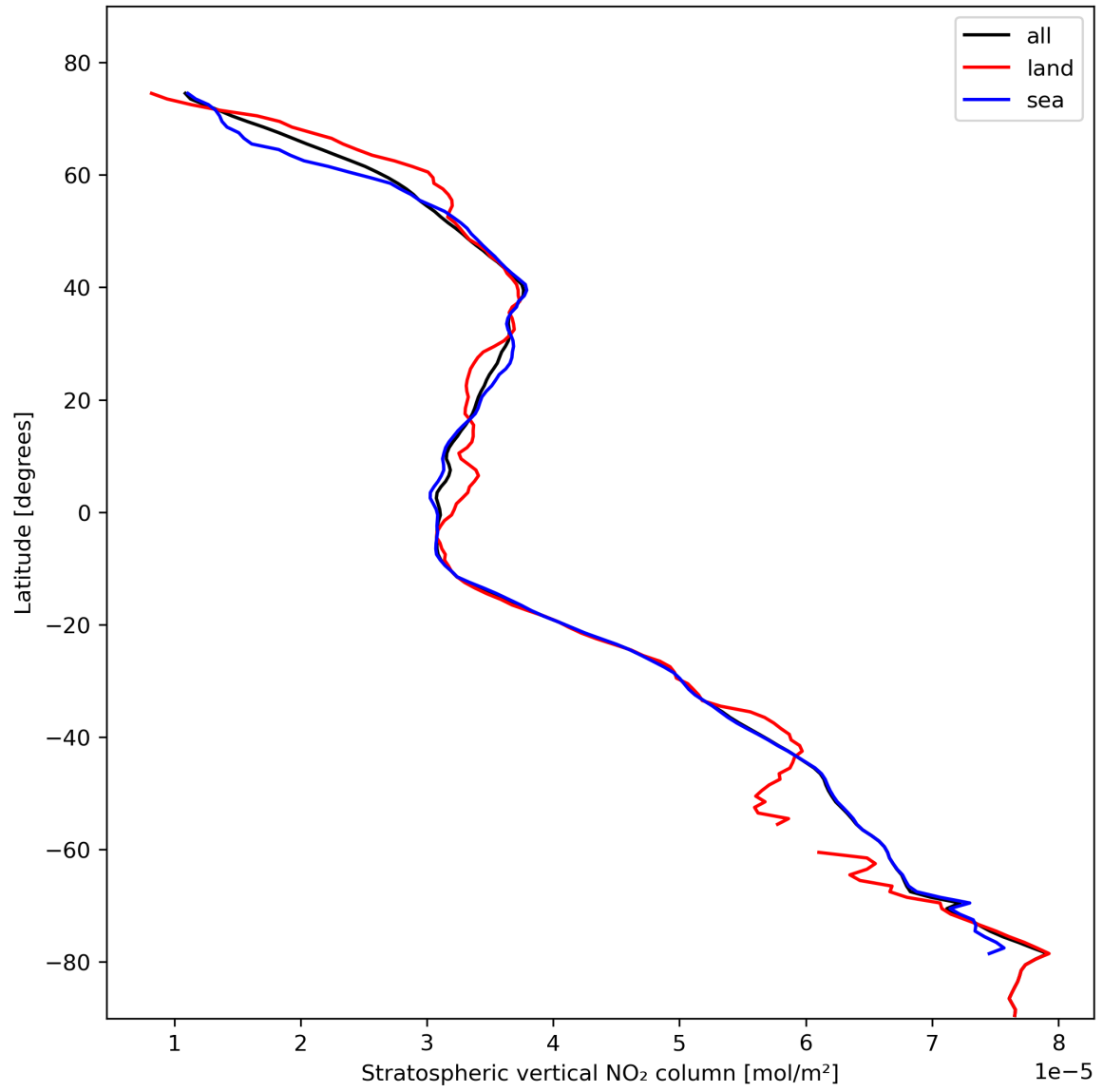
Figure 19: Zonal average of “Stratospheric vertical NO 2 column” for 2024-02-11 to 2024-02-13.
