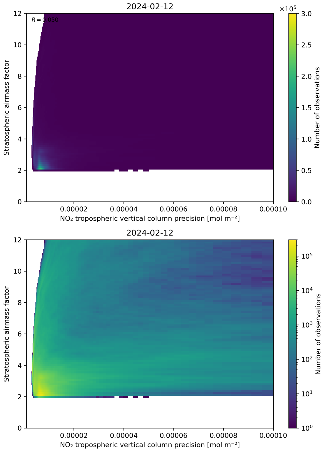
Figure 131: Scatter density plot of “NO 2 tropospheric vertical column precision” against “Stratospheric airmass factor” for 2024-02-11 to 2024-02-13.
