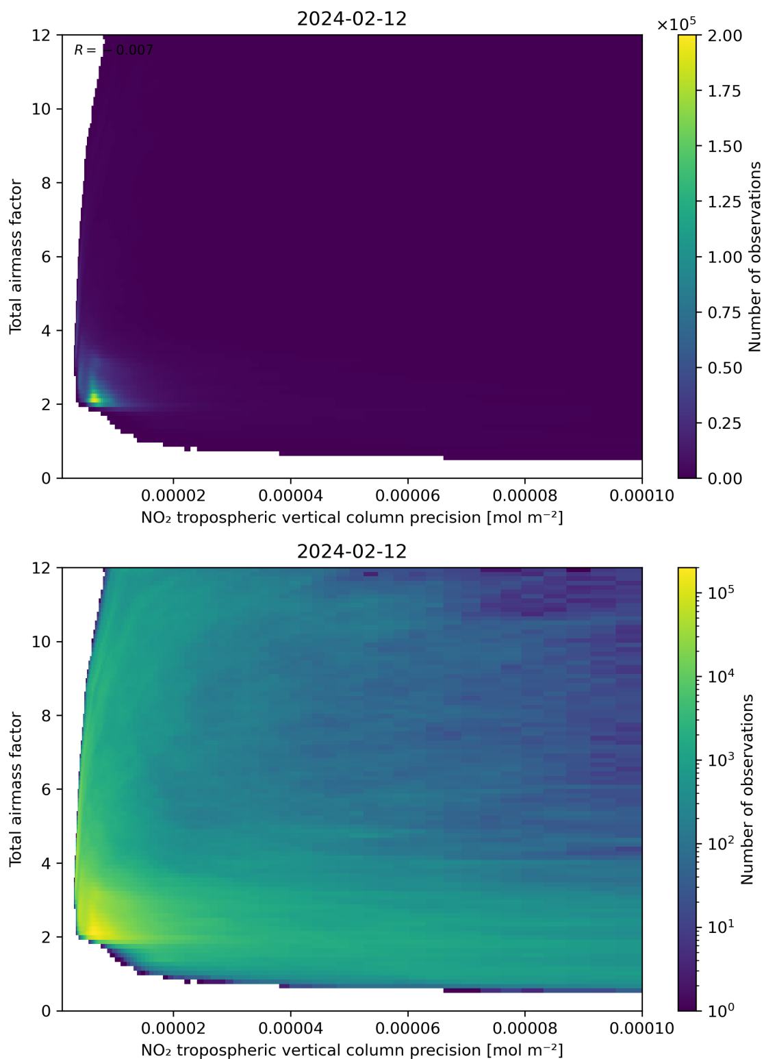
Figure 132: Scatter density plot of “NO 2 tropospheric vertical column precision” against “Total airmass factor” for 2024-02-11 to 2024-02-13.
