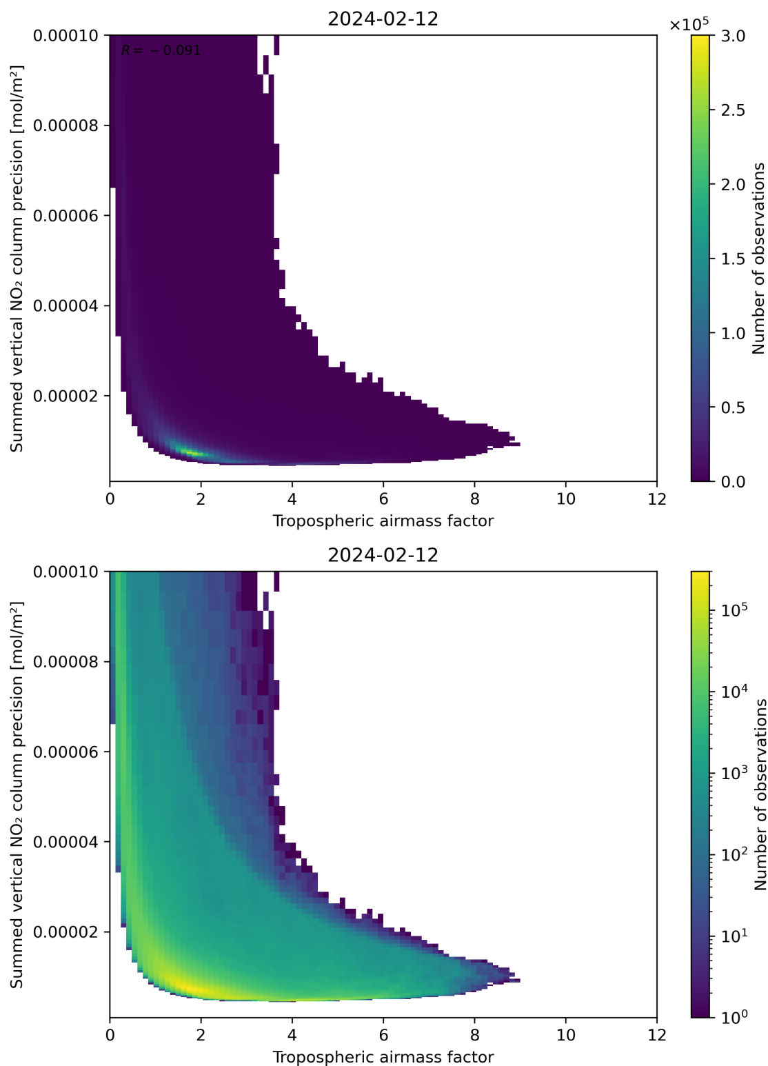
Figure 76: Scatter density plot of “Tropospheric air mass factor” against “Summed vertical NO 2 column precision” for 2024-02-11 to 2024-02-13.
