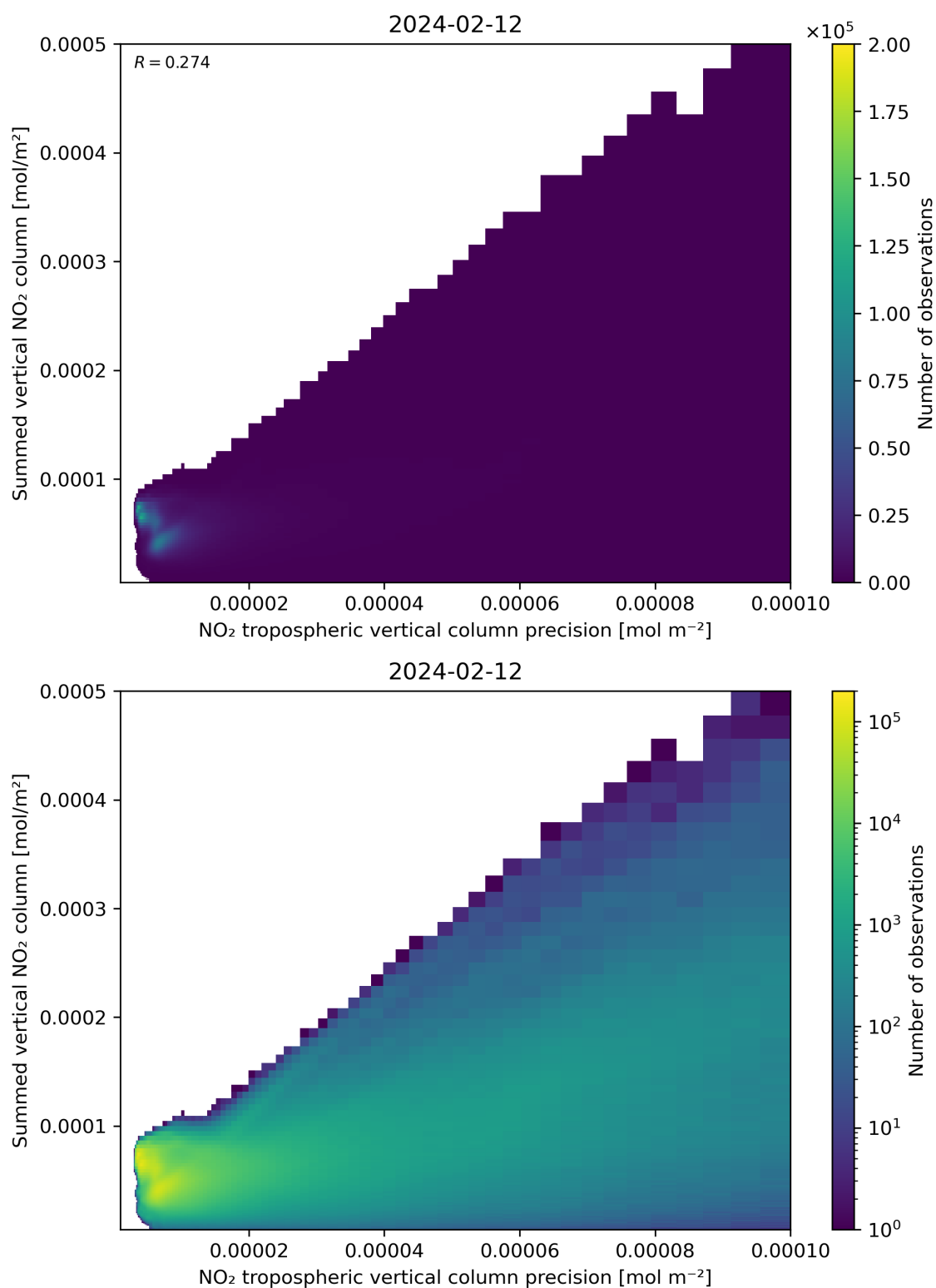
Figure 136: Scatter density plot of “NO 2 tropospheric vertical column precision” against “Summed vertical NO 2 column” for 2024-02-11 to 2024-02-13.
