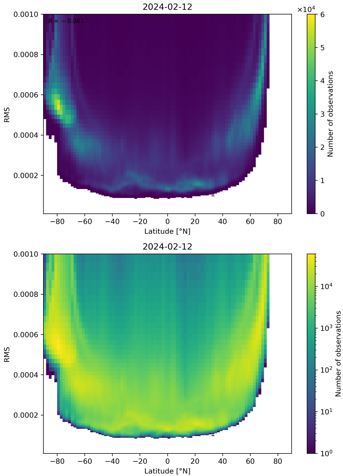
Figure 94: Scatter density plot of “Latitude” against “RMS” for 2024-02-11 to 2024-02-13.
