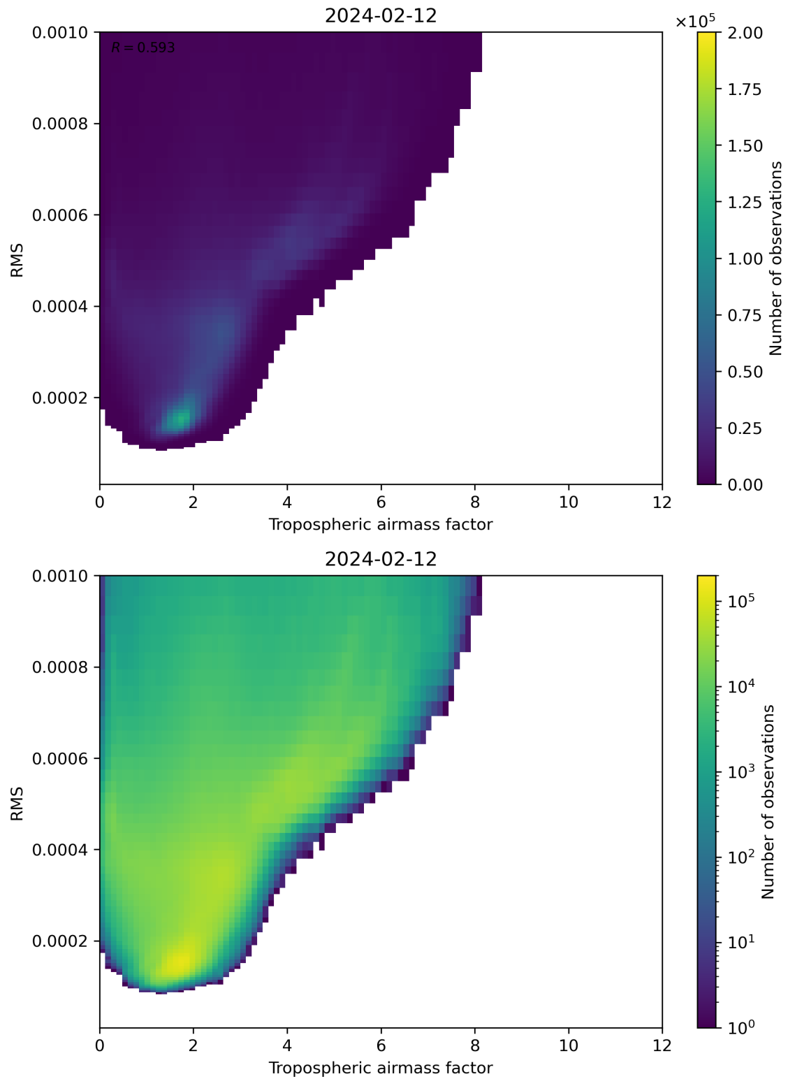
Figure 79: Scatter density plot of “Tropospheric airmass factor” against “RMS” for 2024-02-11 to 2024-02-13.
