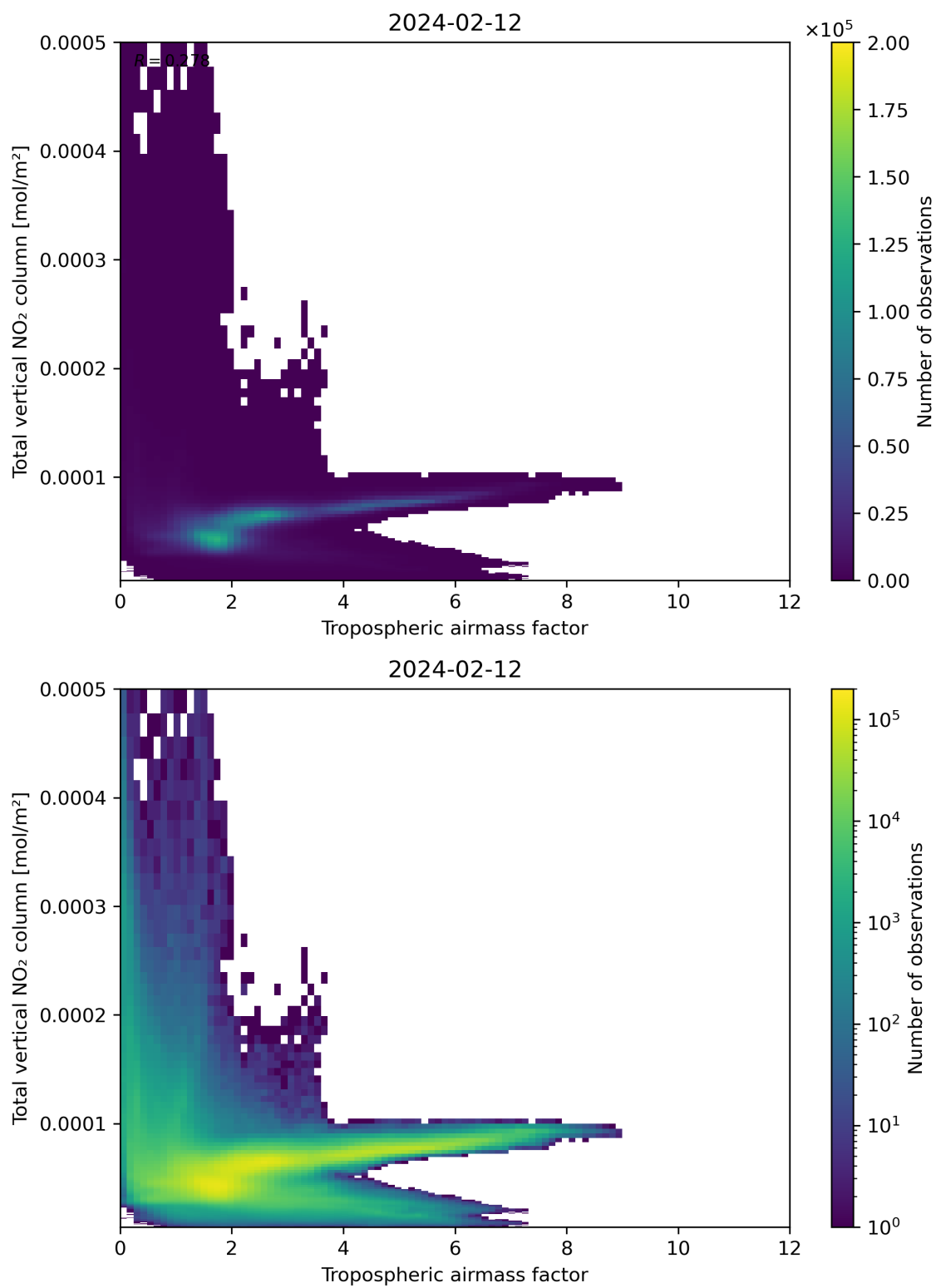
Figure 77: Scatter density plot of “Tropospheric airmass factor” against “Total vertical NO 2 column” for 2024-02-11 to 2024-02-13.
