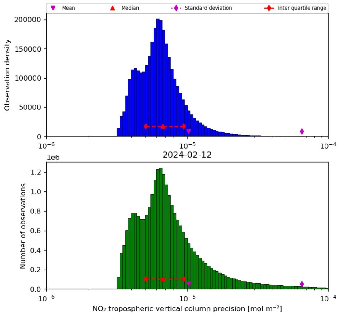
Figure 30: Histogram of “NO 2 tropospheric vertical column precision” for 2024-02-11 to 2024-02-13
