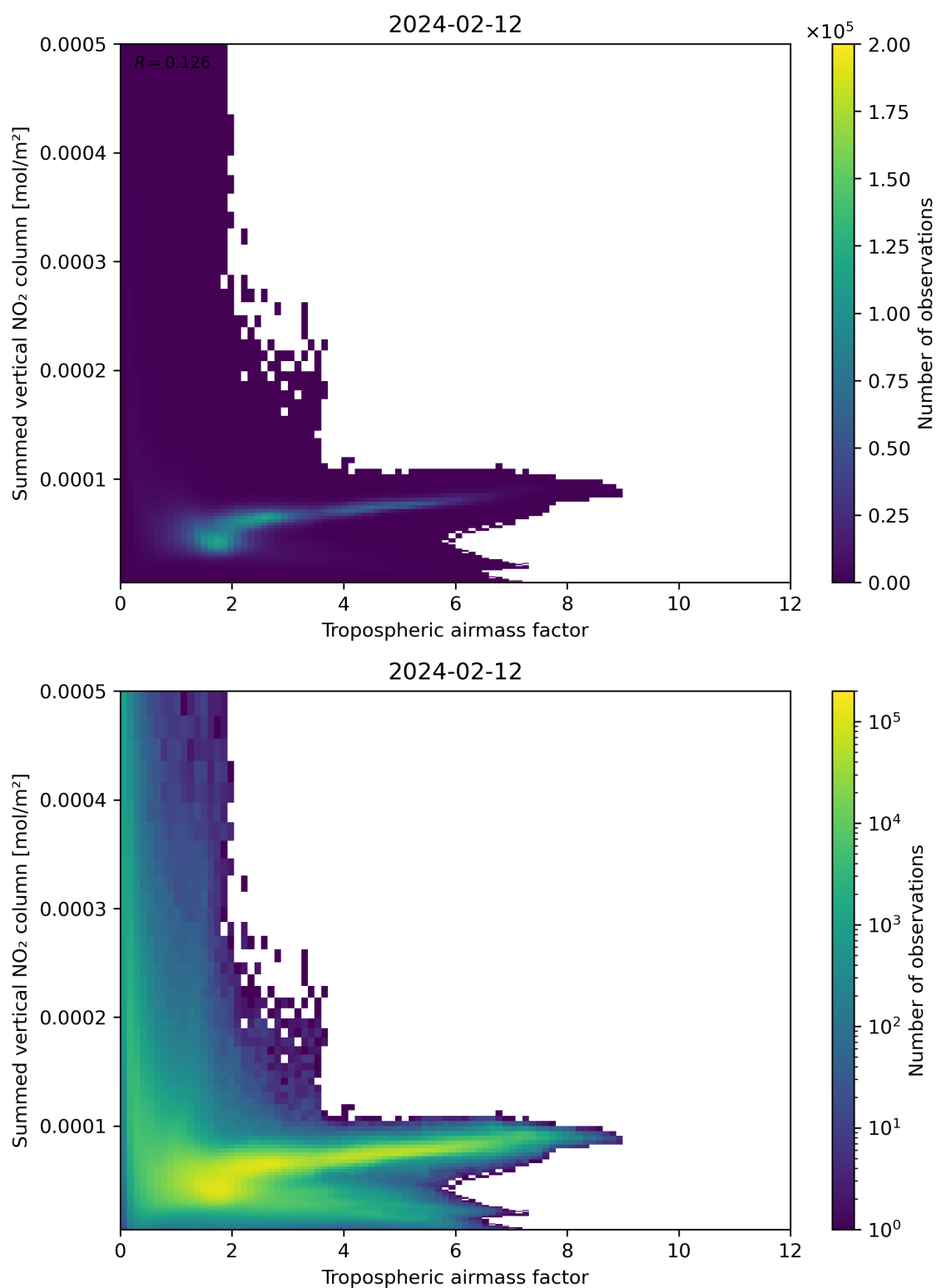
Figure 75: Scatter density plot of “Tropospheric air mass factor” against “Summed vertical NO 2 column” for 2024-02-11 to 2024-02-13.
