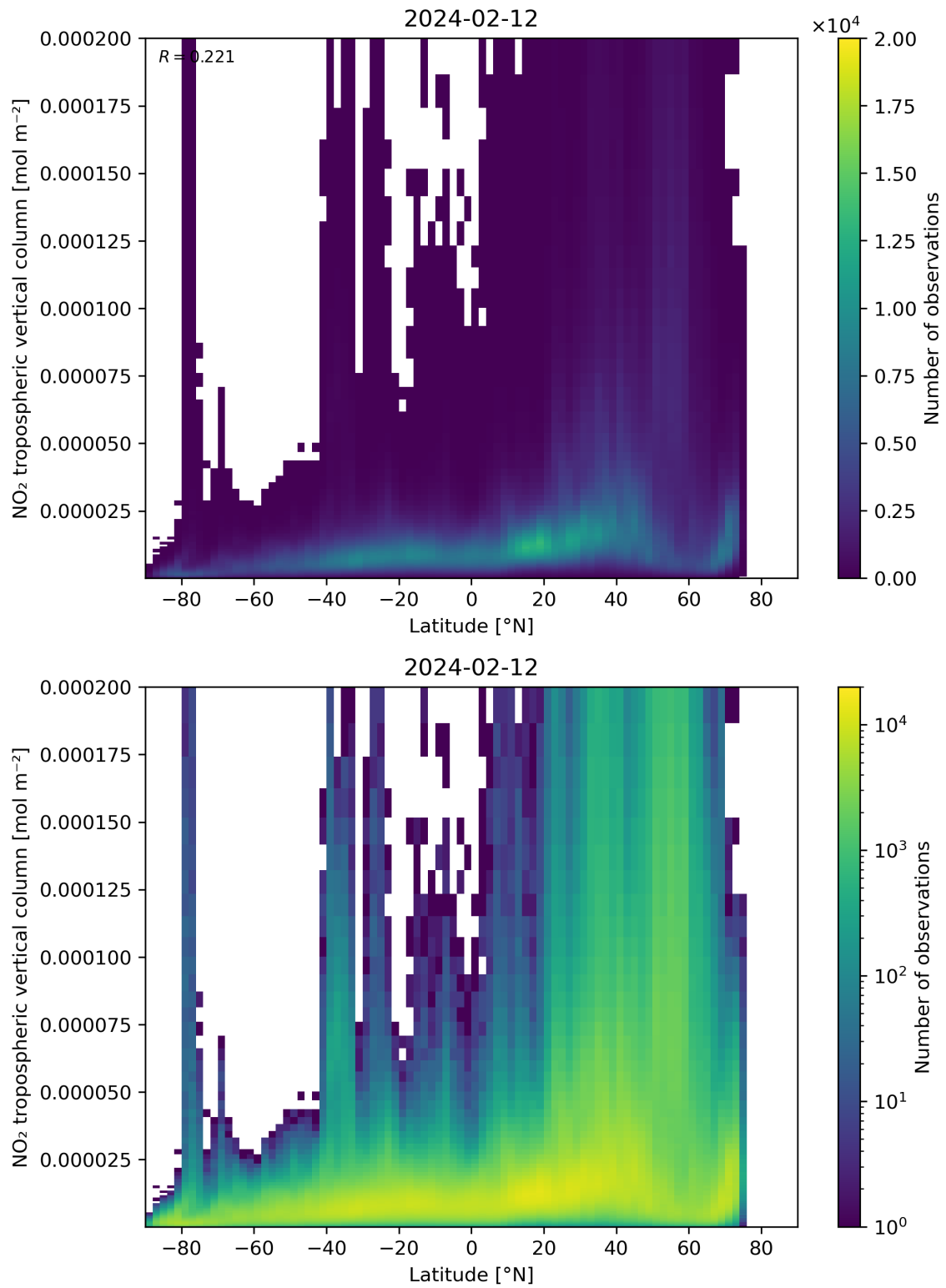
Figure 92: Scatter density plot of “Latitude” against “NO 2 tropospheric vertical column” for 2024-02-11 to 2024-02-13.
