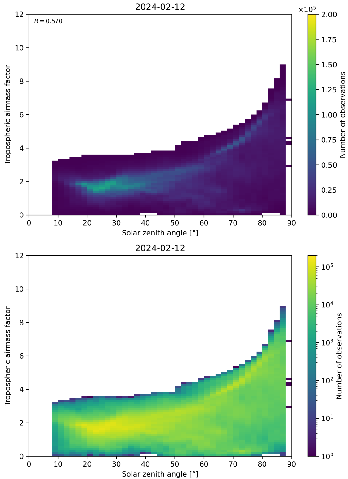
Figure 147: Scatter density plot of “Solar zenith angle” against “Tropospheric airmass factor” for 2024-02-11 to 2024-02-13.
