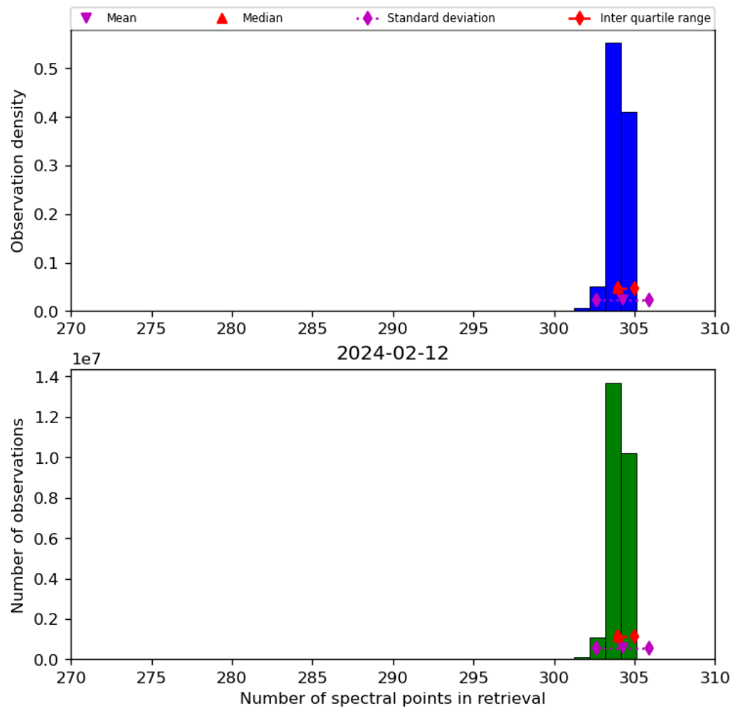
Figure 33: Histogram of “Number of spectral points in retrieval” for 2024-02-11 to 2024-02-13
