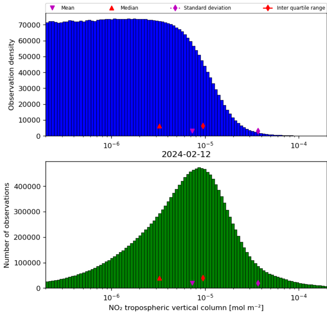
Figure 29: Histogram of “NO 2 tropospheric vertical column” for 2024-02-11 to 2024-02-13
