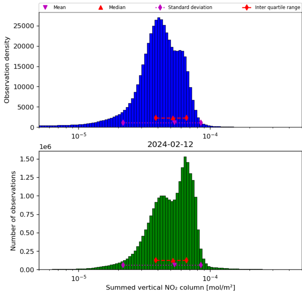
Figure 40: Histogram of “Summed vertical NO 2 column” for 2024-02-11 to 2024-02-13
