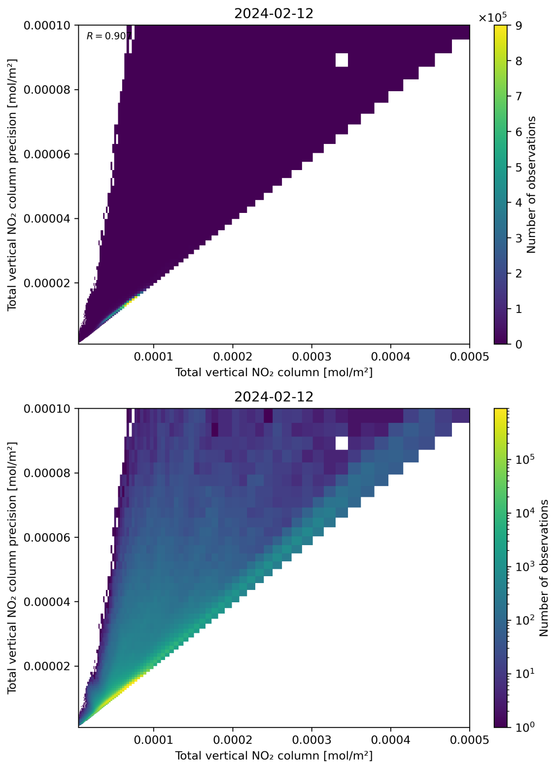
Figure 114: Scatter density plot of “Total vertical NO 2 column” against “Total vertical NO 2 column precision” for 2024-02-11 to 2024-02-13.
