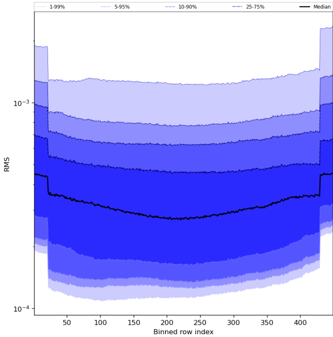
Figure 60: Along track statistics of “RMS” for 2024-02-11 to 2024-02-13
