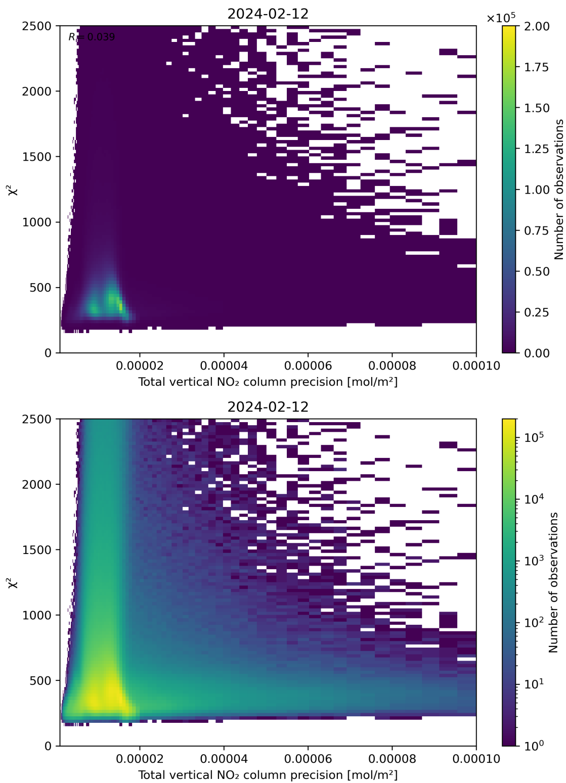
Figure 116: Scatter density plot of “Total vertical NO 2 column precision” against “ \chi^2 ” for 2024-02-11 to 2024-02-13.
