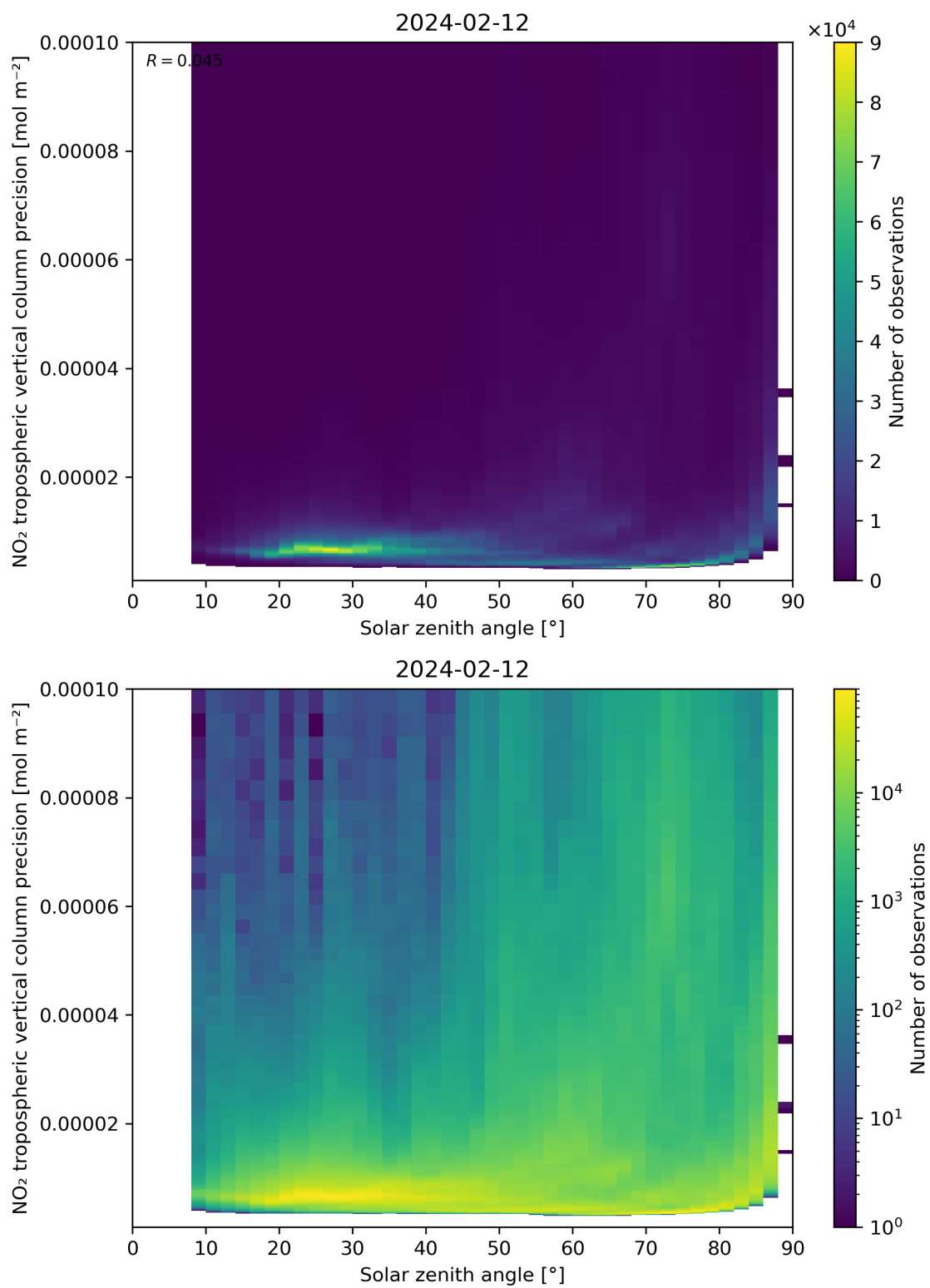
Figure 156: Scatter density plot of “Solar zenith angle” against “NO 2 tropospheric vertical column precision” for 2024-02-11 to 2024-02-13.
