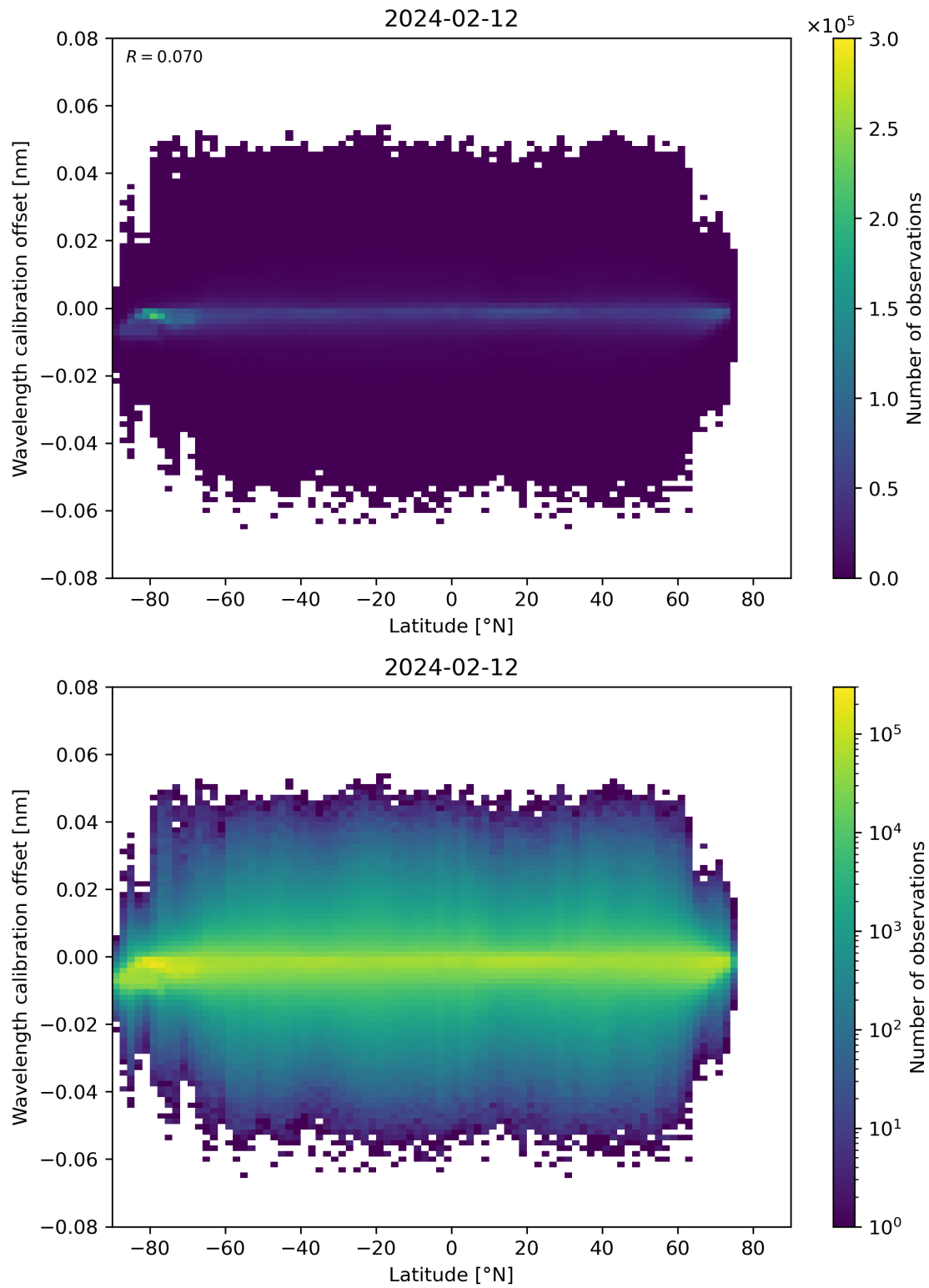
Figure 95: Scatter density plot of “Latitude” against “Wavelength calibration offset” for 2024-02-11 to 2024-02-13.
