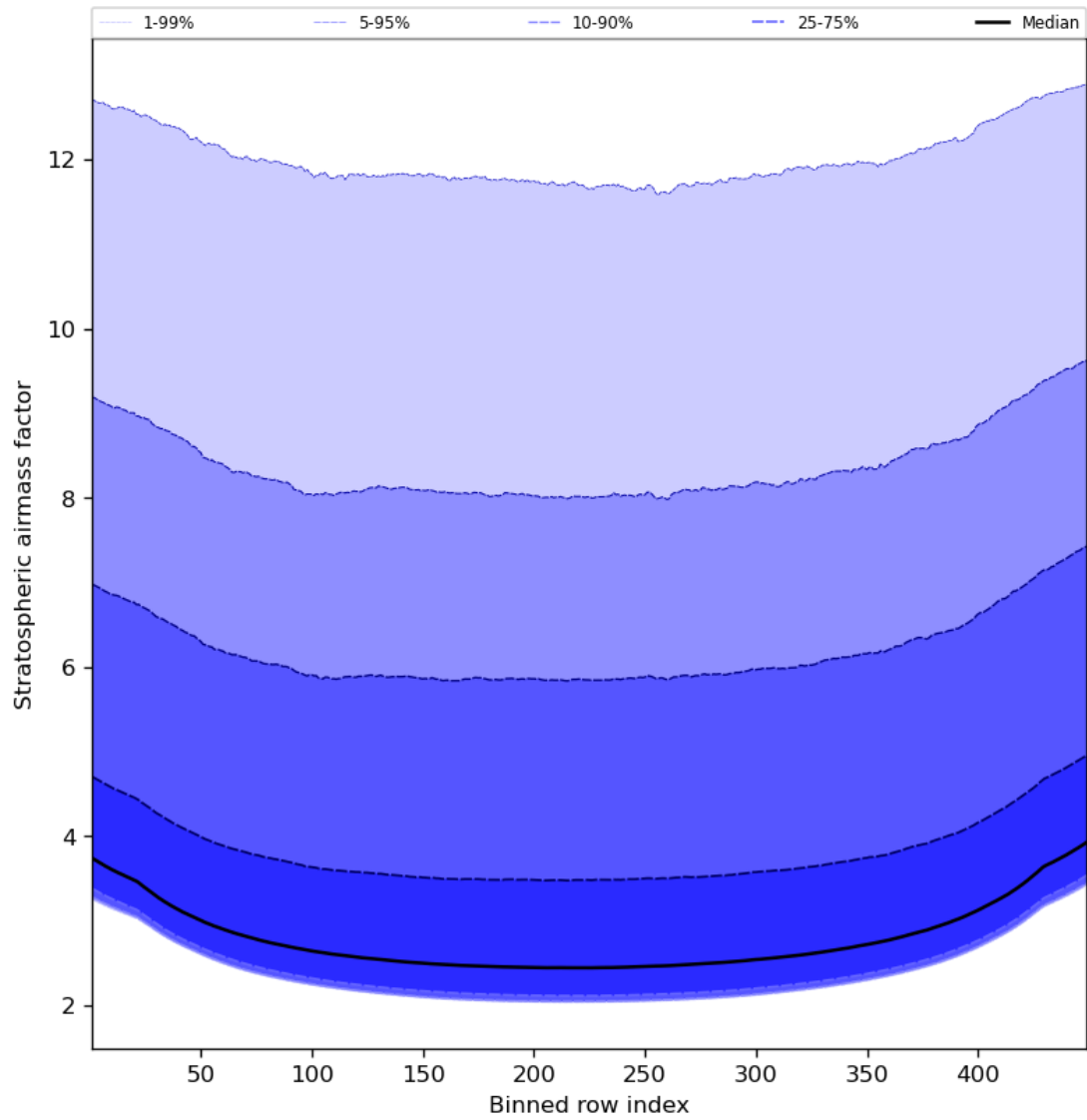
Figure 61: Along track statistics of “Stratospheric airmass factor” for 2024-02-11 to 2024-02-13
