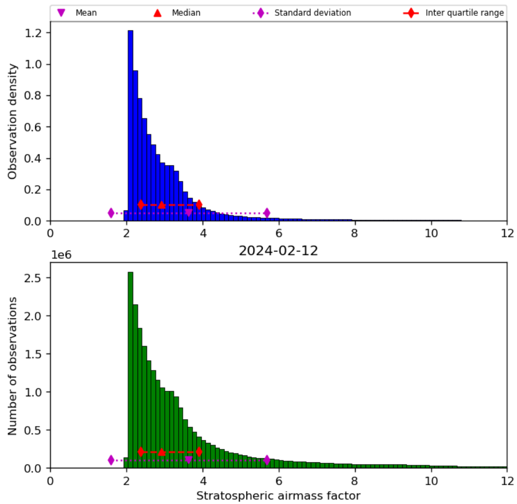
Figure 44: Histogram of “Stratospheric airmass factor” for 2024-02-11 to 2024-02-13
