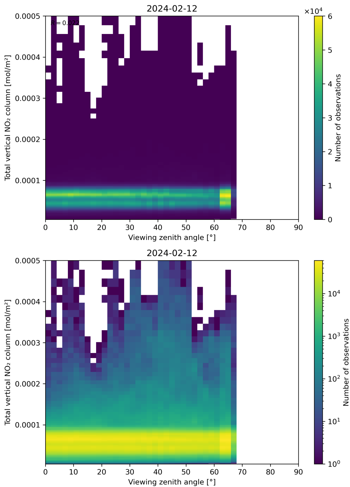
Figure 167: Scatter density plot of “Viewing zenith angle” against “Total vertical NO 2 column” for 2024-02-11 to 2024-02-13.
