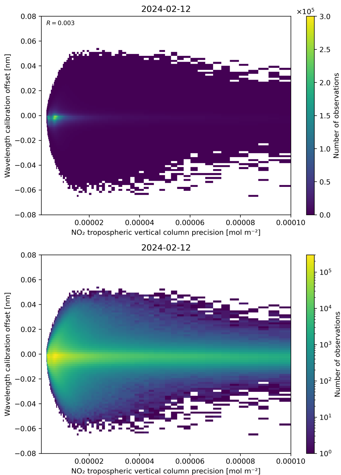
Figure 141: Scatter density plot of “NO 2 tropospheric vertical column precision” against “Wavelength calibration offset” for 2024-02-11 to 2024-02-13.
