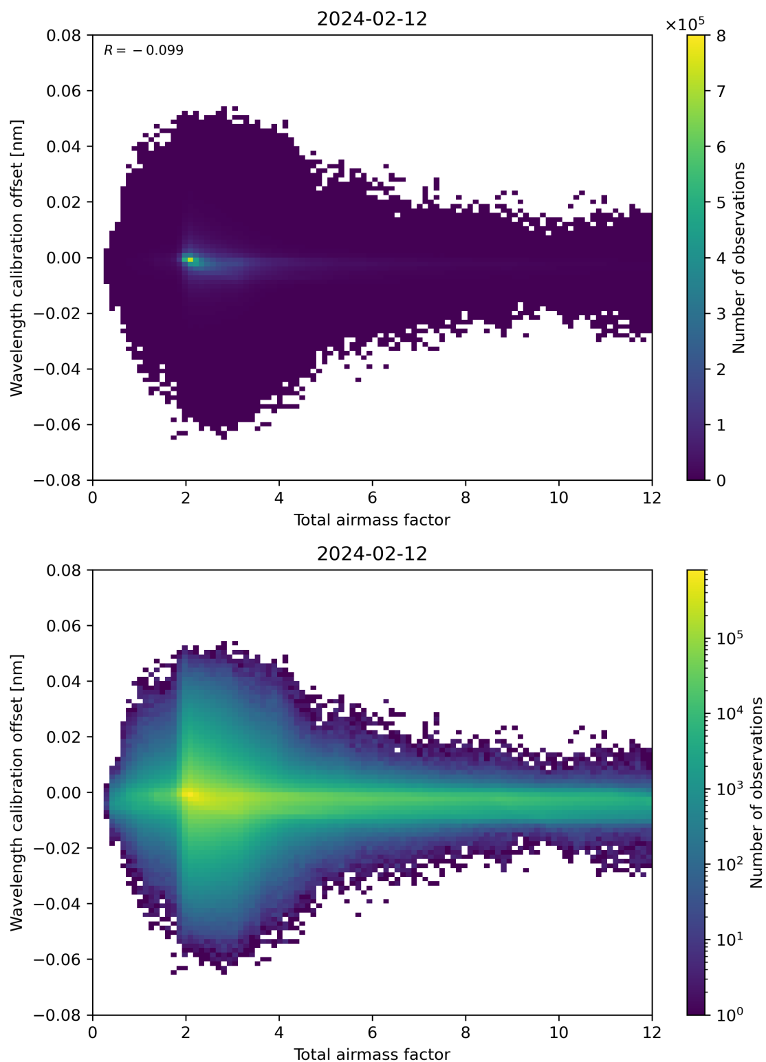
Figure 70: Scatter density plot of “Total airmass factor” against “Wavelength calibration offset” for 2024-02-11 to 2024-02-13.
