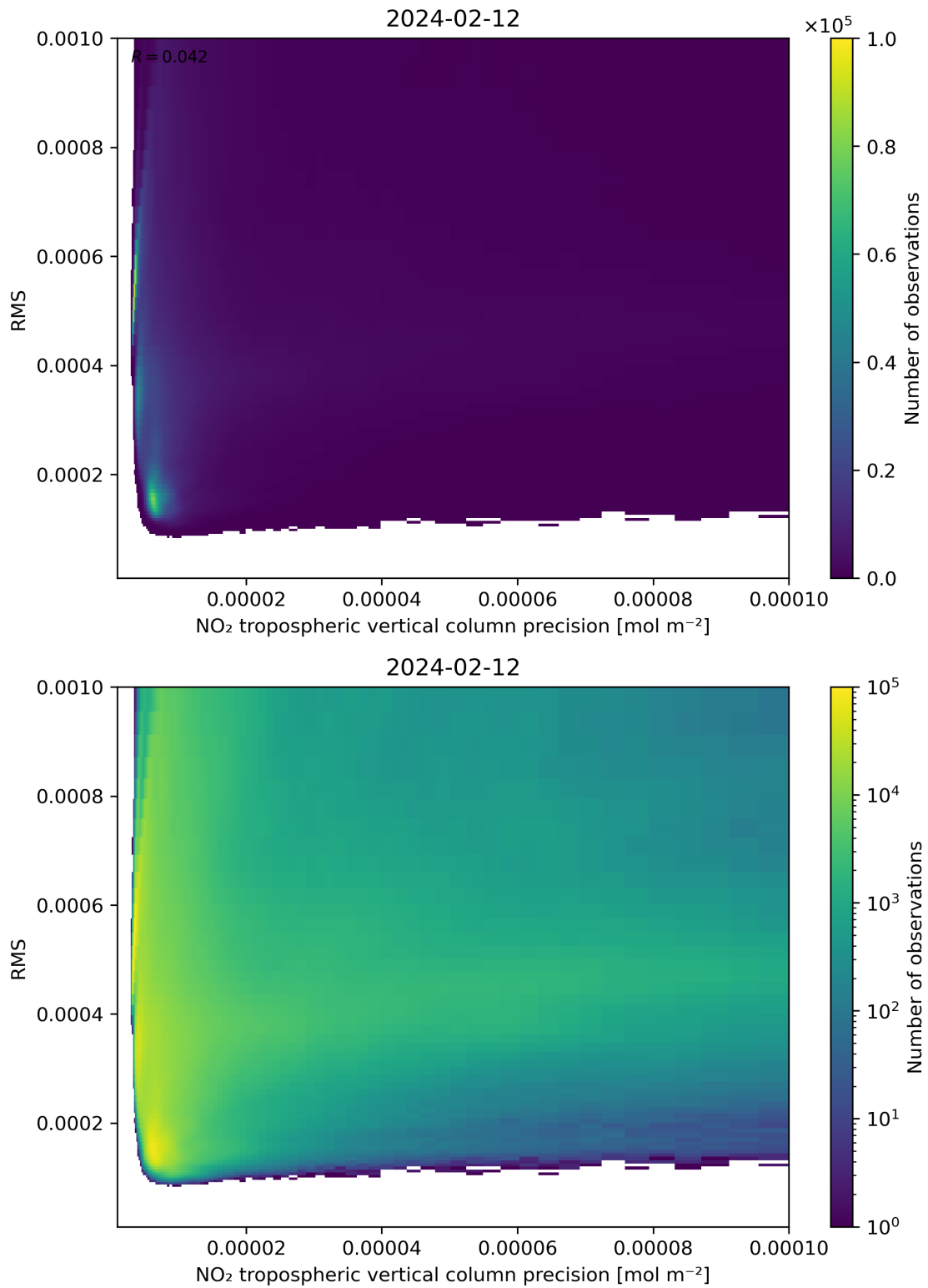
Figure 140: Scatter density plot of “NO 2 tropospheric vertical column precision” against “RMS” for 2024-02-11 to 2024-02-13.
