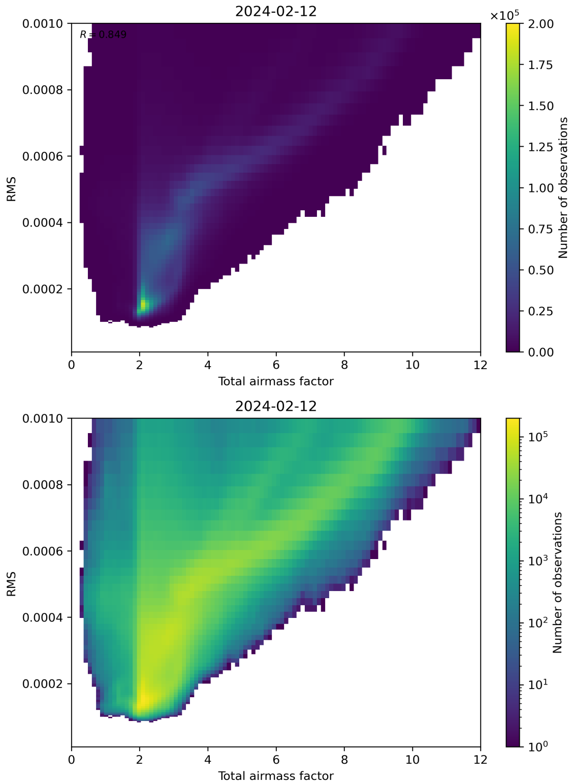
Figure 69: Scatter density plot of “Total airmass factor” against “RMS” for 2024-02-11 to 2024-02-13.
