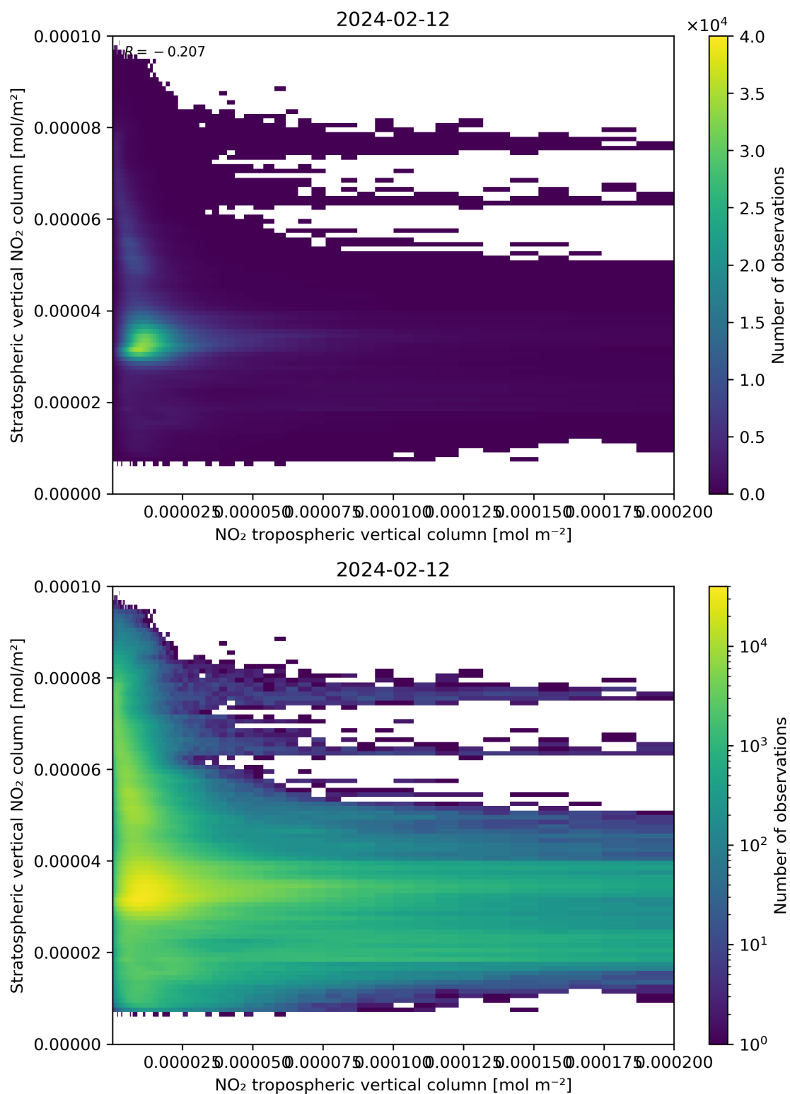
Figure 125: Scatter density plot of “NO 2 tropospheric vertical column” against “Stratospheric vertical NO 2 column” for 2024-02-11 to 2024-02-13.
