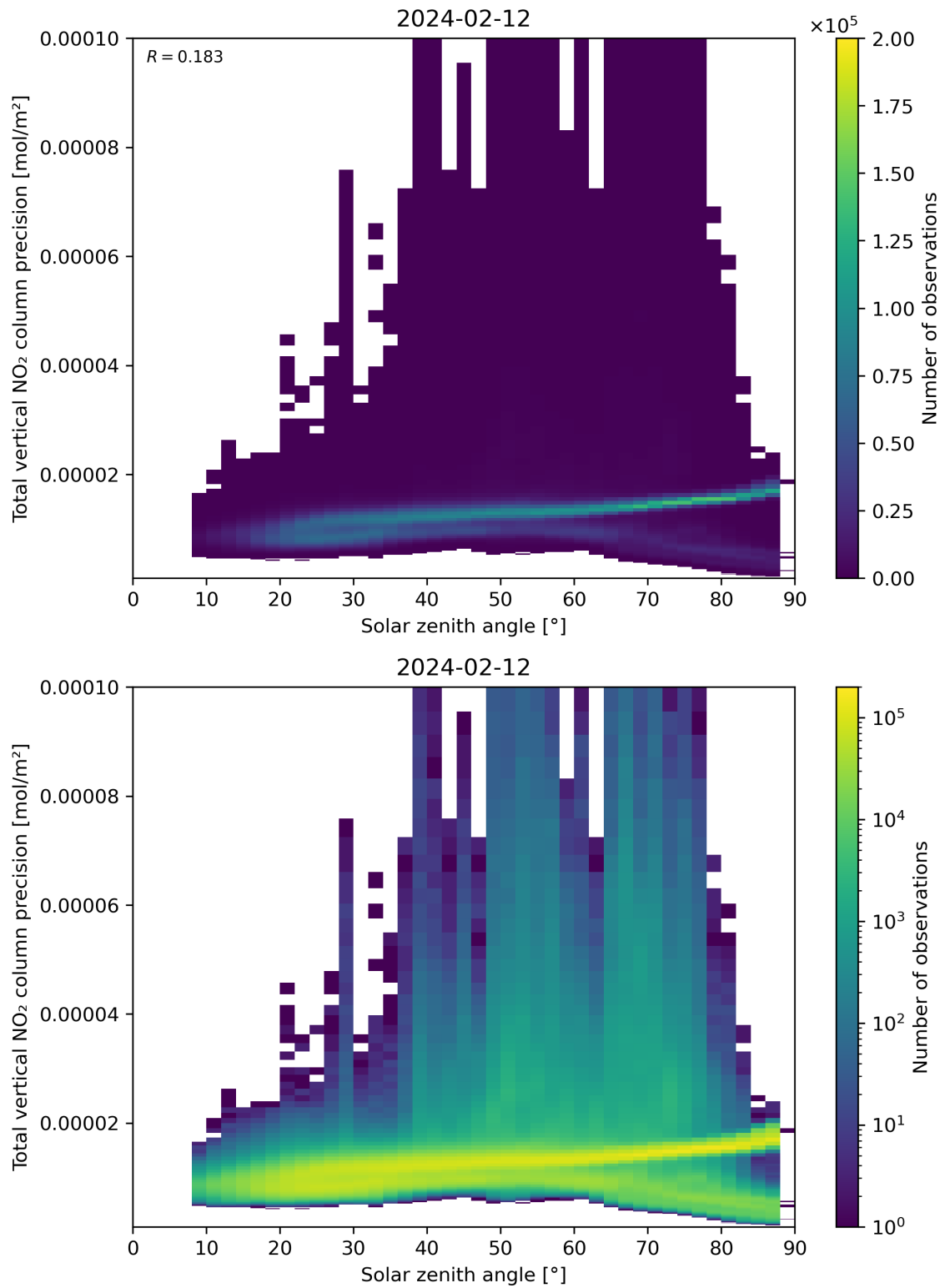
Figure 154: Scatter density plot of “Solar zenith angle” against “Total vertical NO 2 column precision” for 2024-02-11 to 2024-02-13.
