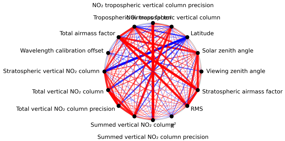
Figure 1: Map of correlation graph for 2024-02-11 to 2024-02-13.
