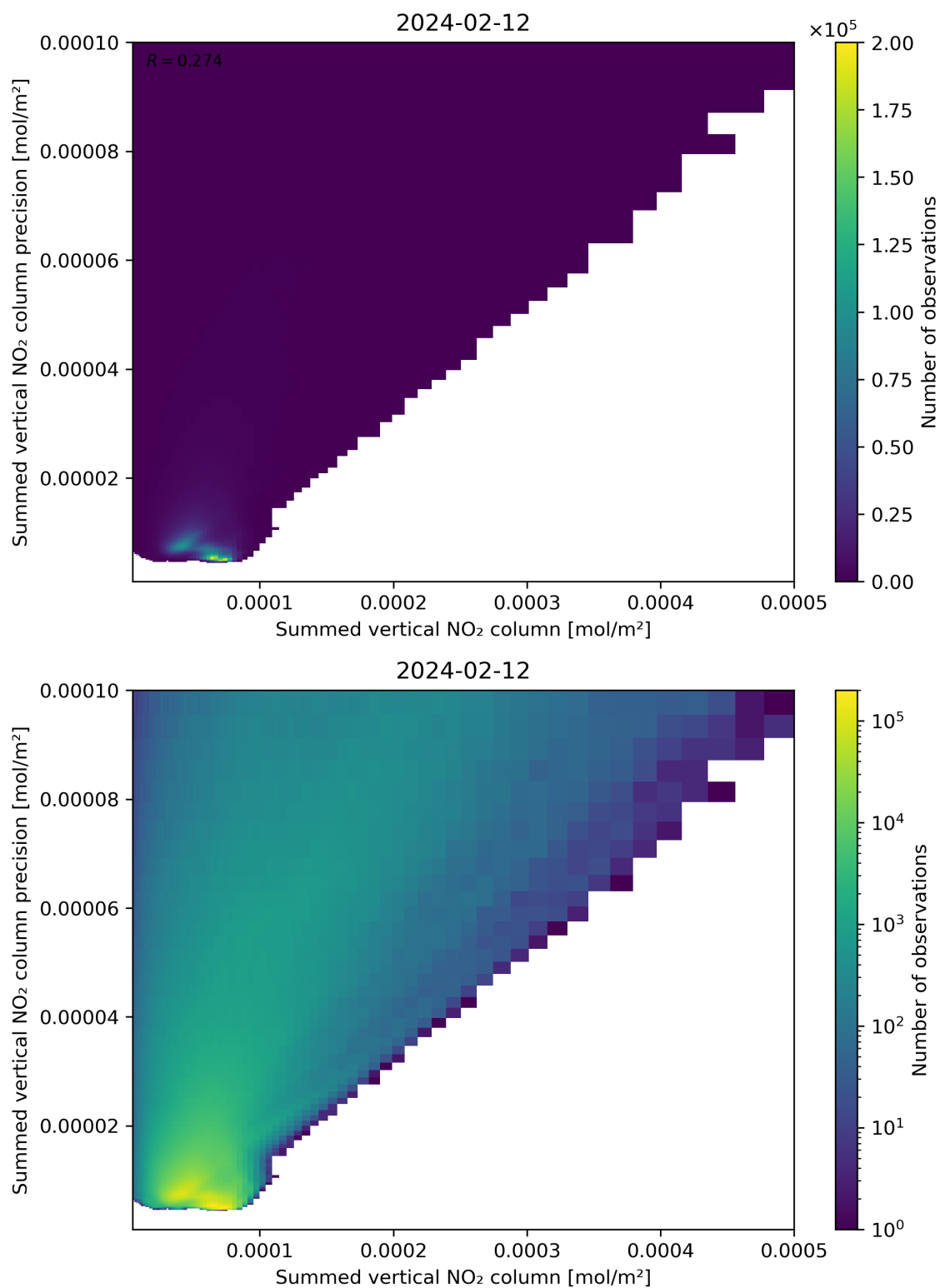
Figure 105: Scatter density plot of “Summed vertical NO 2 column” against “Summed vertical NO 2 column precision” for 2024-02-11 to 2024-02-13.
