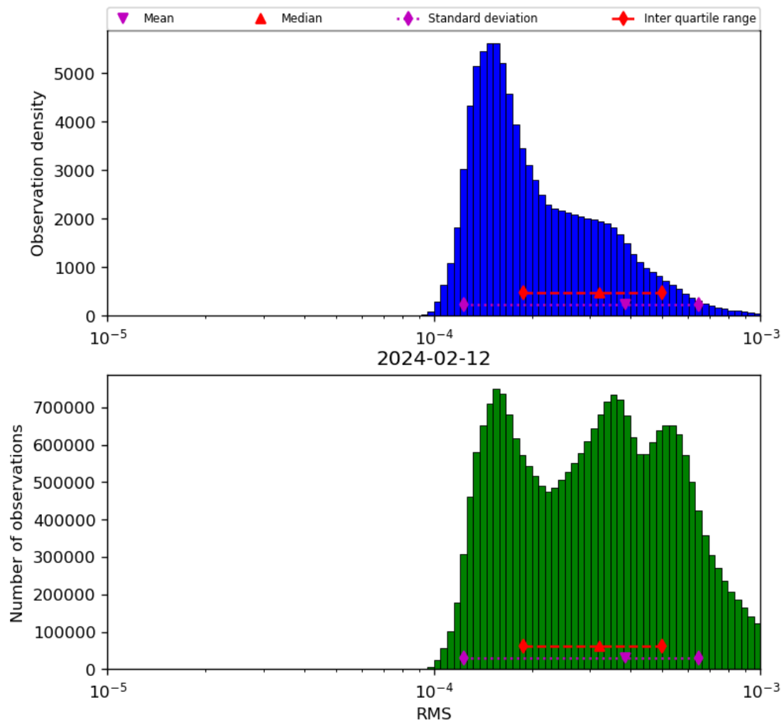
Figure 43: Histogram of “RMS” for 2024-02-11 to 2024-02-13
