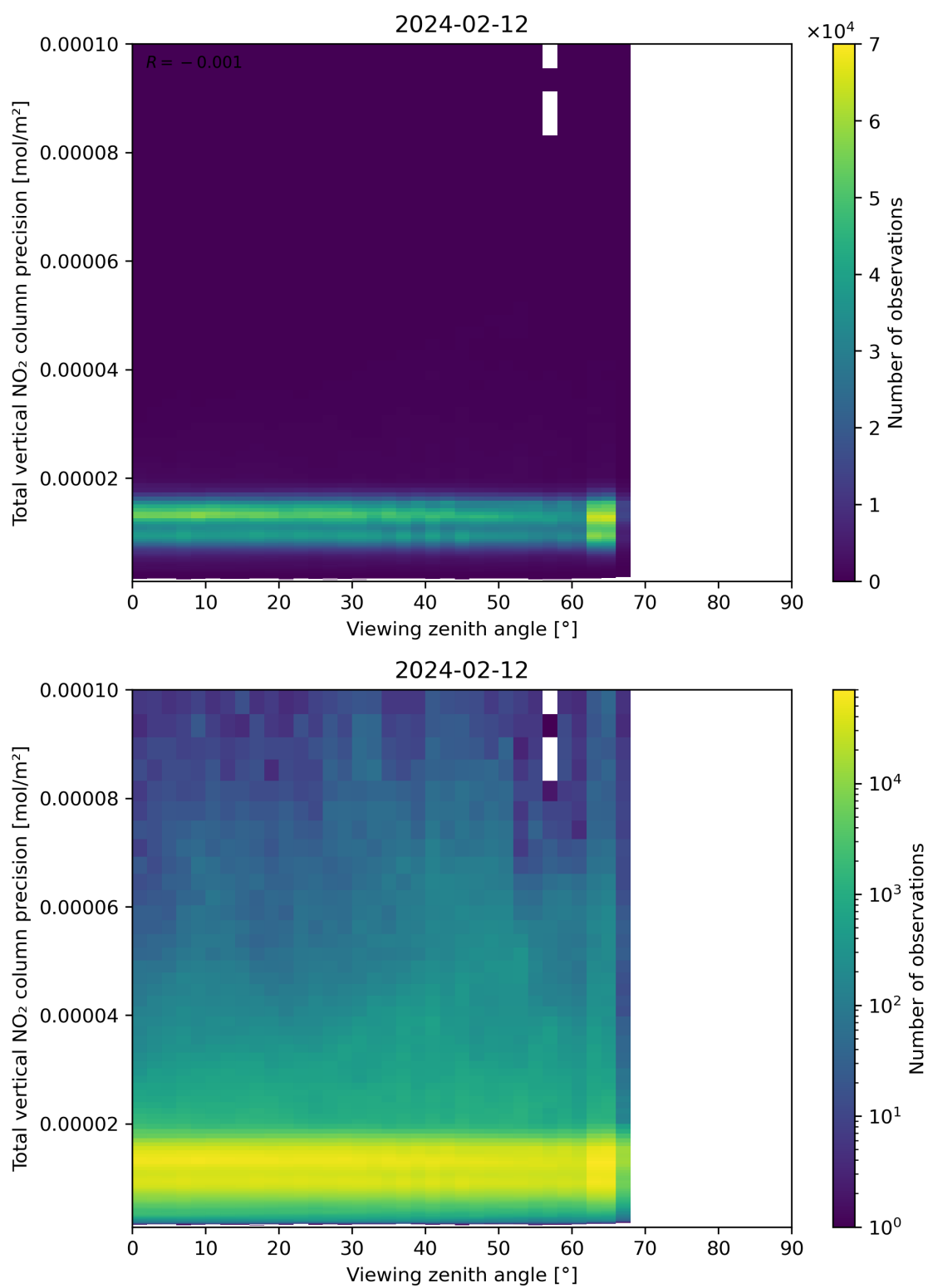
Figure 168: Scatter density plot of “Viewing zenith angle” against “Total vertical NO 2 column precision” for 2024-02-11 to 2024-02-13.
