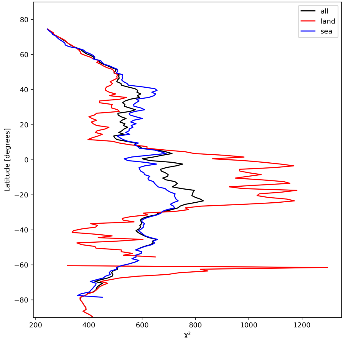
Figure 25: Zonal average of “ \chi^2 ” for 2024-02-11 to 2024-02-13.
