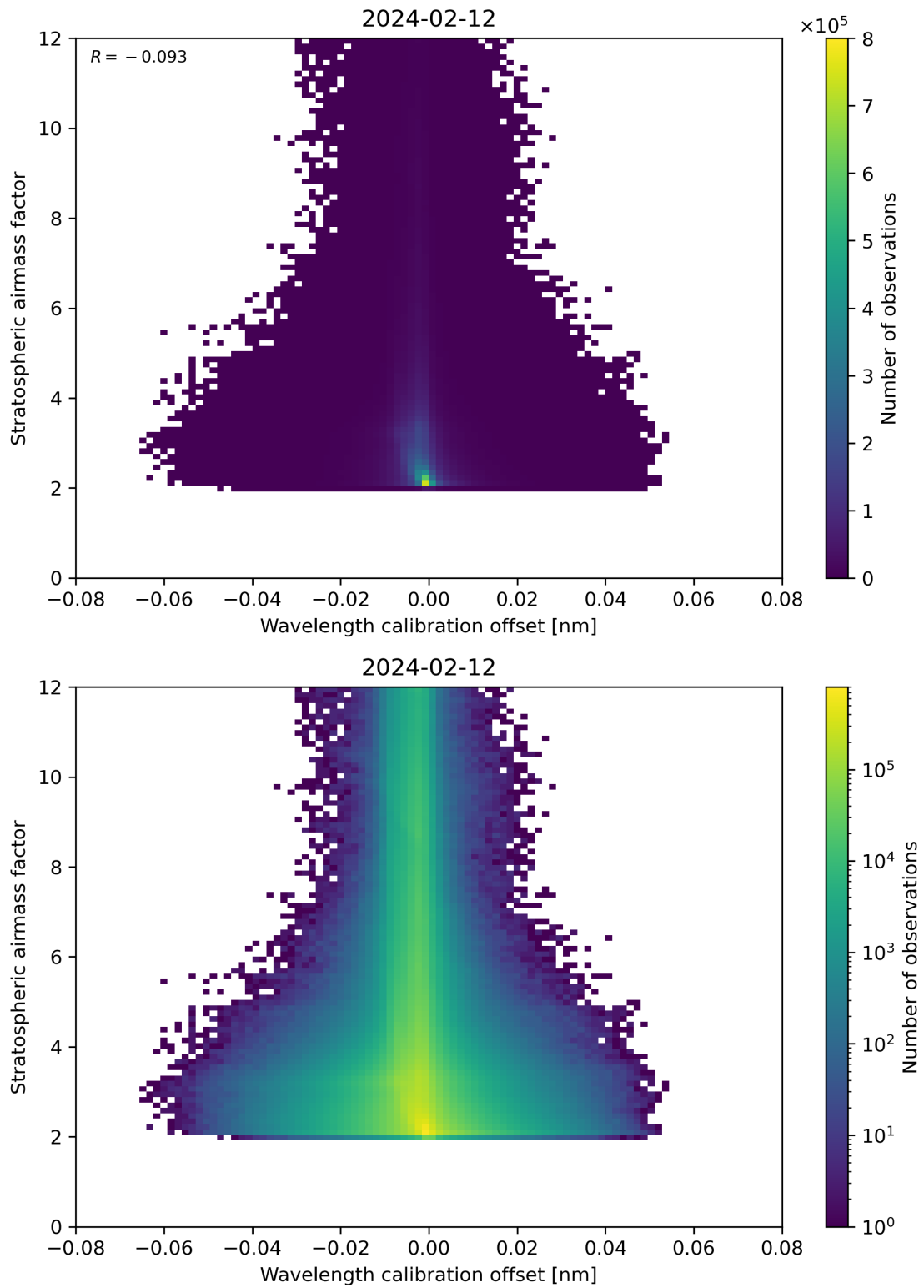
Figure 174: Scatter density plot of “Wavelength calibration offset” against “Stratospheric airmass factor” for 2024-02-11 to 2024-02-13.
