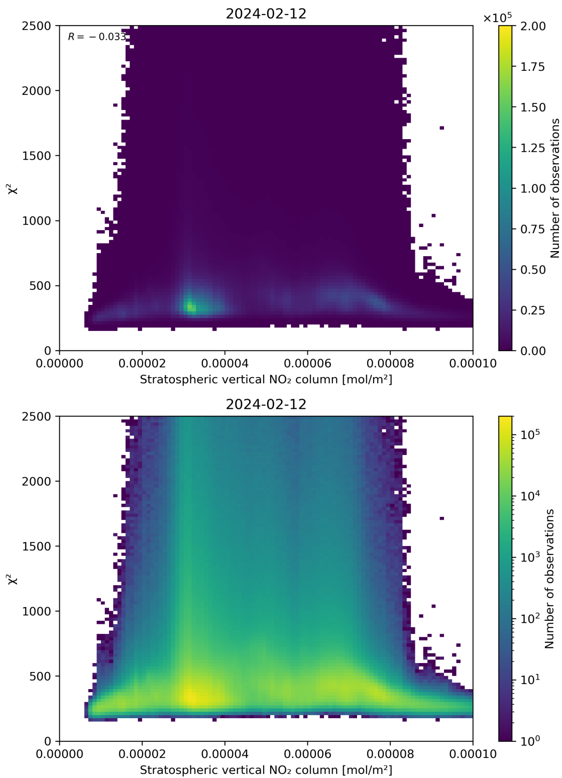
Figure 97: Scatter density plot of “Stratospheric vertical NO 2 column” against “ \chi^2 ” for 2024-02-11 to 2024-02-13.
