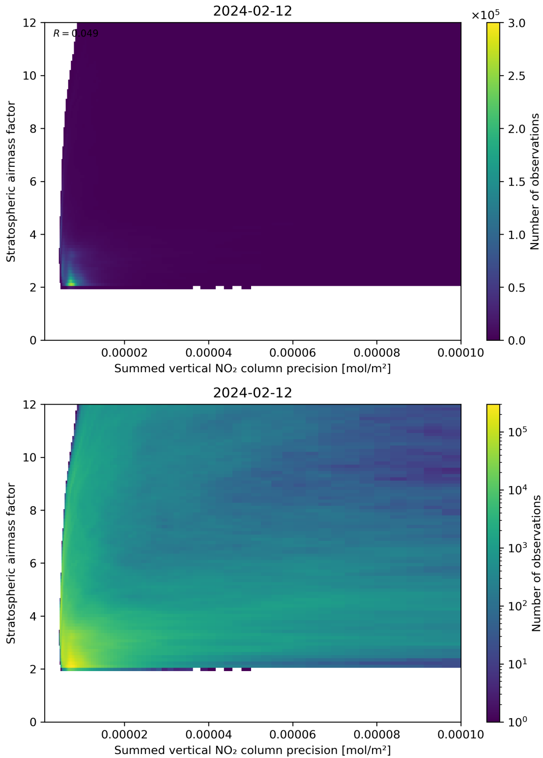
Figure 106: Scatter density plot of “Summed vertical NO 2 column precision” against “Stratospheric airmass factor” for 2024-02-11 to 2024-02-13.
