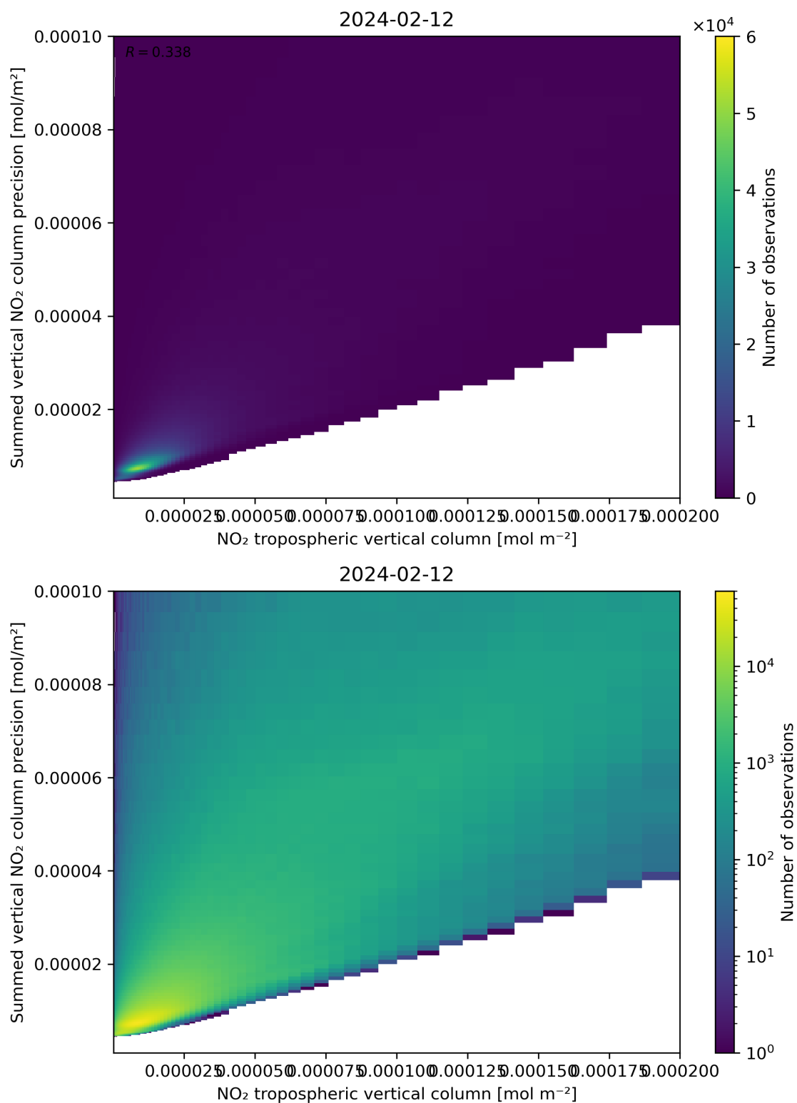
Figure 127: Scatter density plot of “NO 2 tropospheric vertical column” against “Summed vertical NO 2 column precision” for 2024-02-11 to 2024-02-13.
