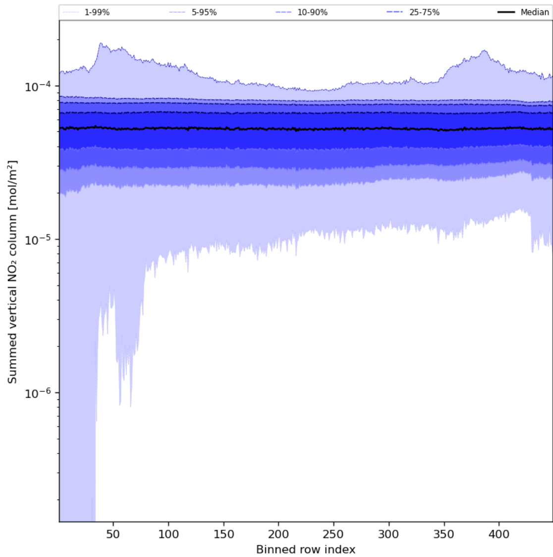
Figure 57: Along track statistics of “Summed vertical NO 2 column” for 2024-02-11 to 2024-02-13
