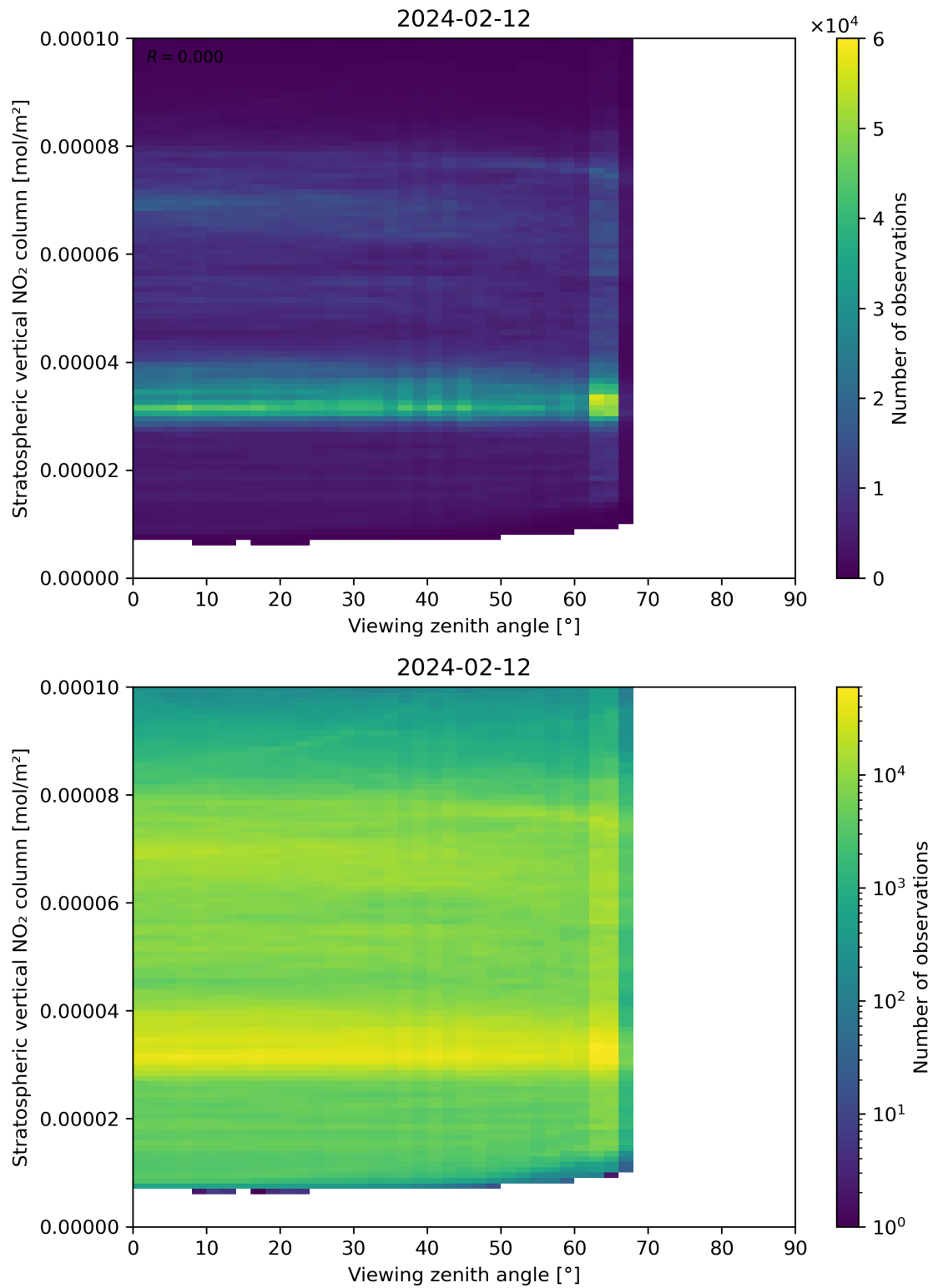
Figure 164: Scatter density plot of “Viewing zenith angle” against “Stratospheric vertical NO 2 column” for 2024-02-11 to 2024-02-13.
