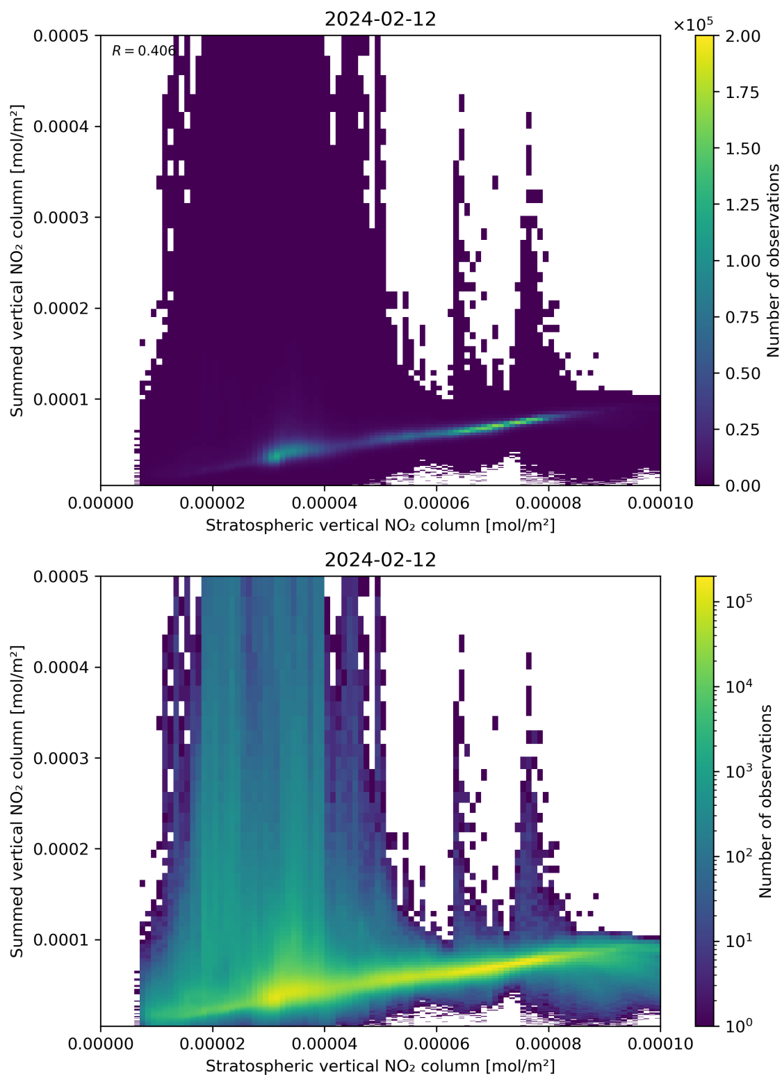
Figure 98: Scatter density plot of “Stratospheric vertical NO 2 column” against “Summed vertical NO 2 column” for 2024-02-11 to 2024-02-13.
