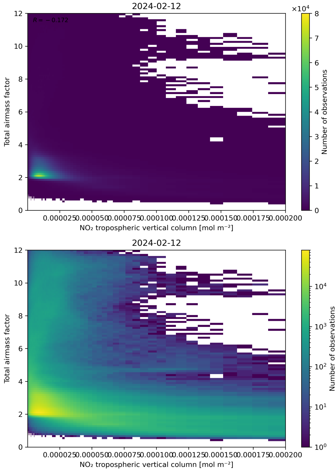
Figure 122: Scatter density plot of “NO 2 tropospheric vertical column” against “Total air mass factor” for 2024-02-11 to 2024-02-13.
