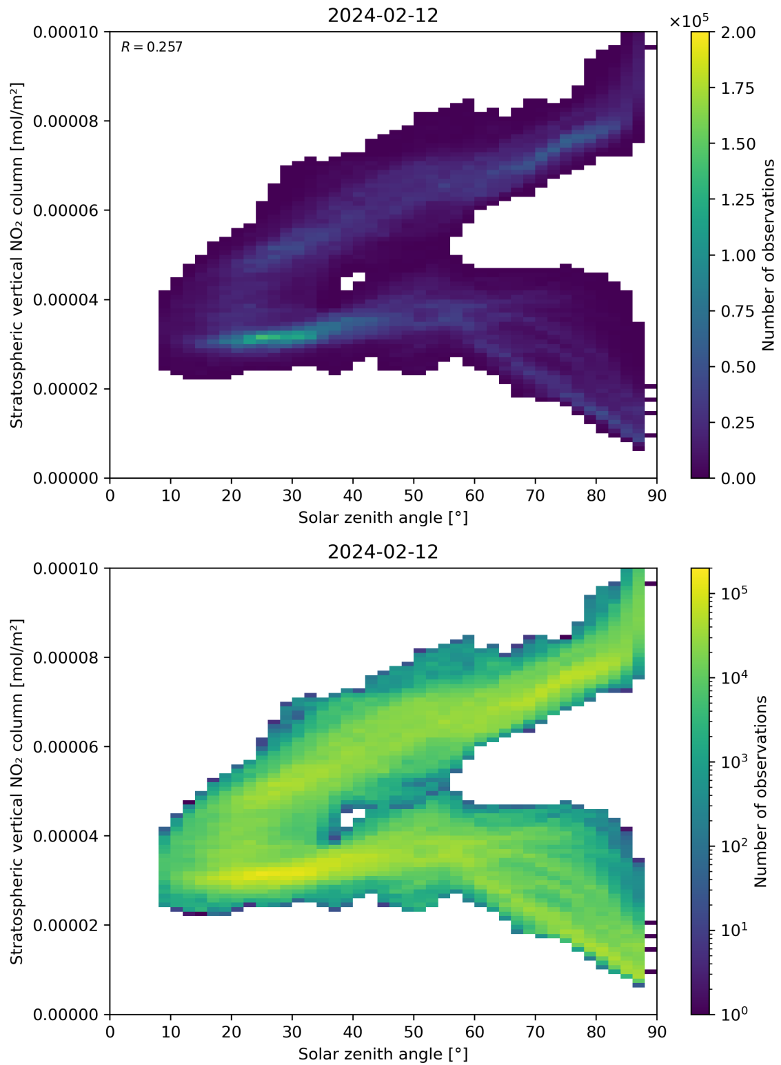
Figure 150: Scatter density plot of “Solar zenith angle” against “Stratospheric vertical NO 2 column” for 2024-02-11 to 2024-02-13.
