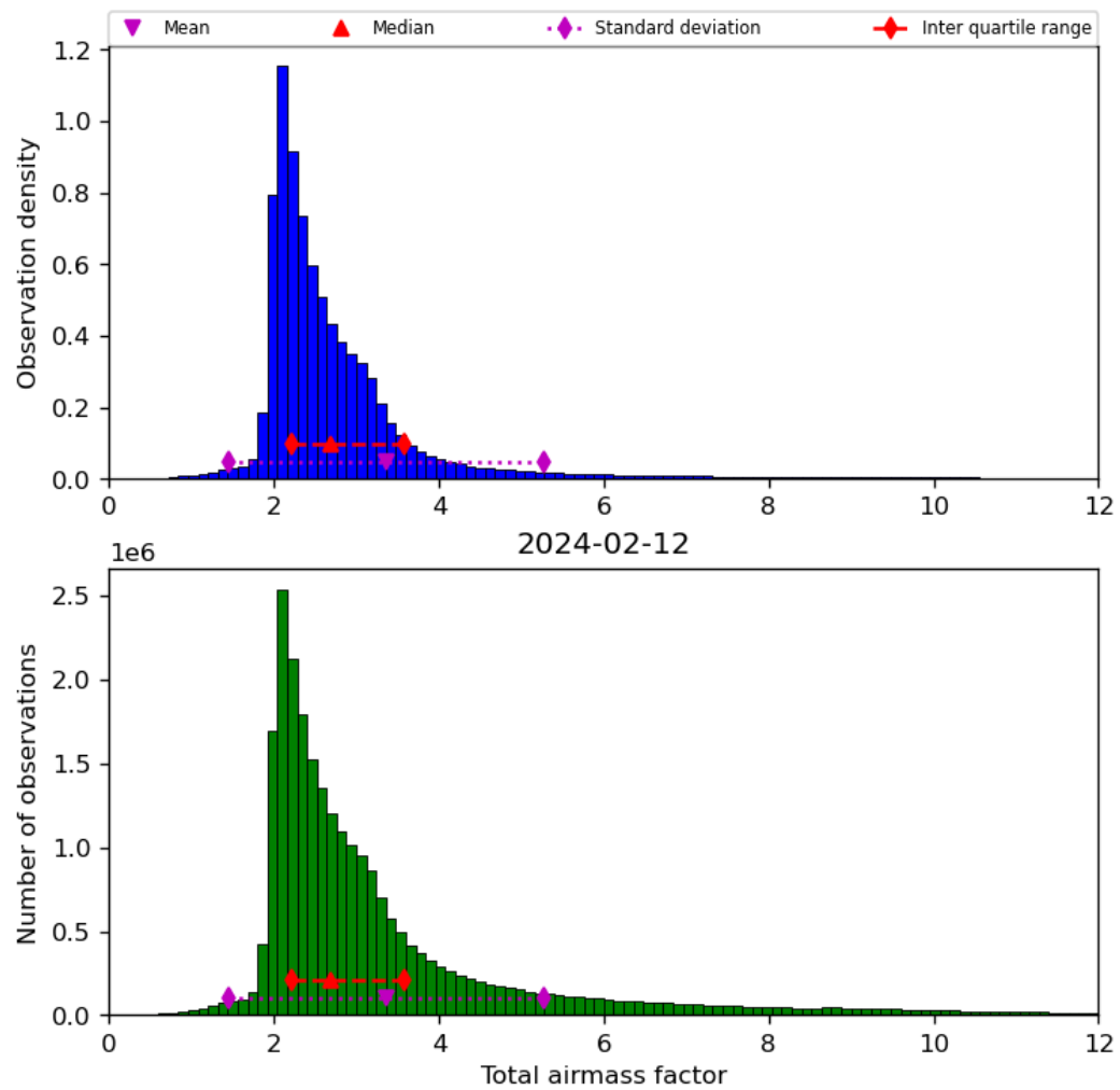
Figure 32: Histogram of “Total airmass factor” for 2024-02-11 to 2024-02-13
