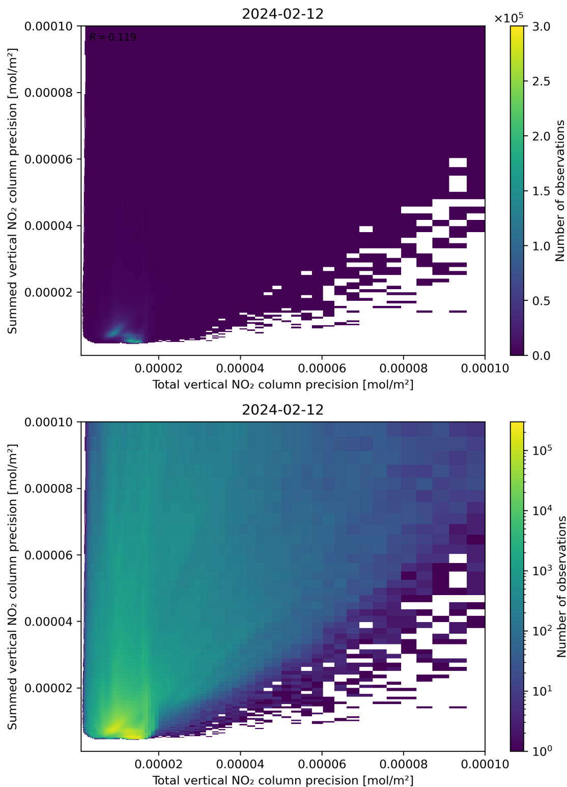
Figure 118: Scatter density plot of “Total vertical NO 2 column precision” against “Summed vertical NO 2 column precision” for 2024-02-11 to 2024-02-13.
