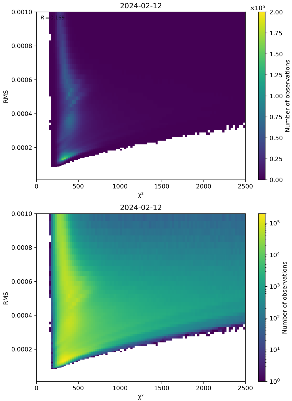
Figure 82: Scatter density plot of “ \chi^2 ” against “RMS” for 2024-02-11 to 2024-02-13.
