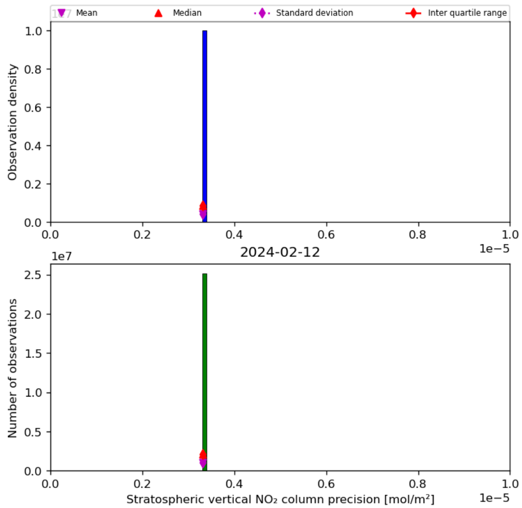
Figure 37: Histogram of “Stratospheric vertical NO 2 column precision” for 2024-02-11 to 2024-02-13
