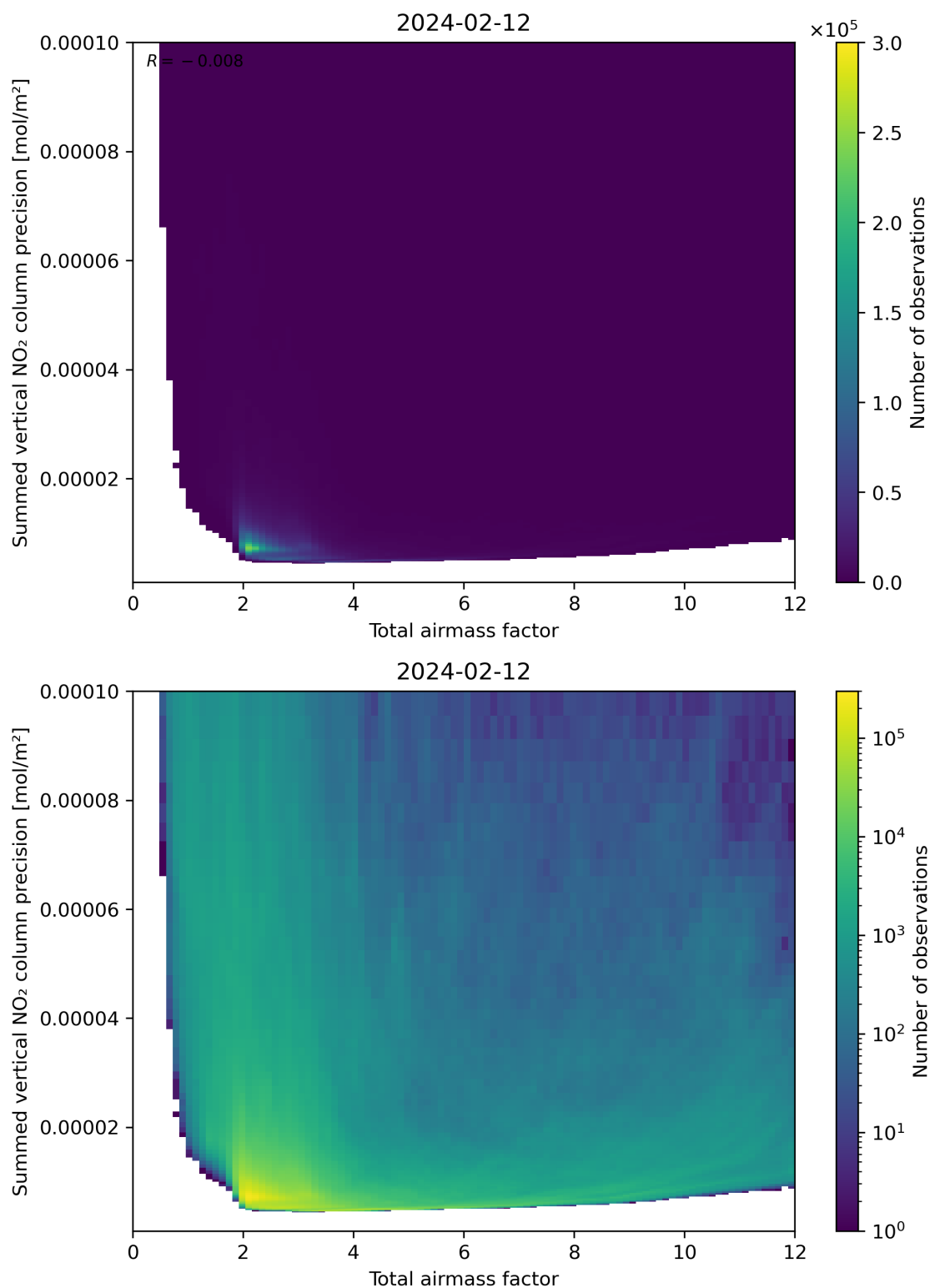
Figure 66: Scatter density plot of “Total airmass factor” against “Summed vertical NO 2 column precision” for 2024-02-11 to 2024-02-13.
