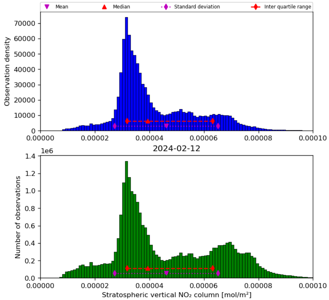
Figure 36: Histogram of “Stratospheric vertical NO 2 column” for 2024-02-11 to 2024-02-13
