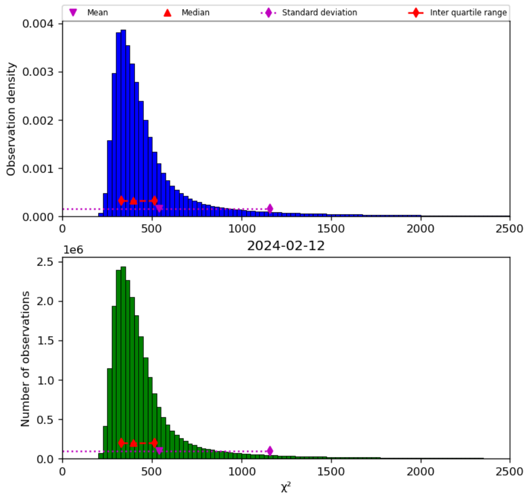
Figure 42: Histogram of “ \chi^2 ” for 2024-02-11 to 2024-02-13
