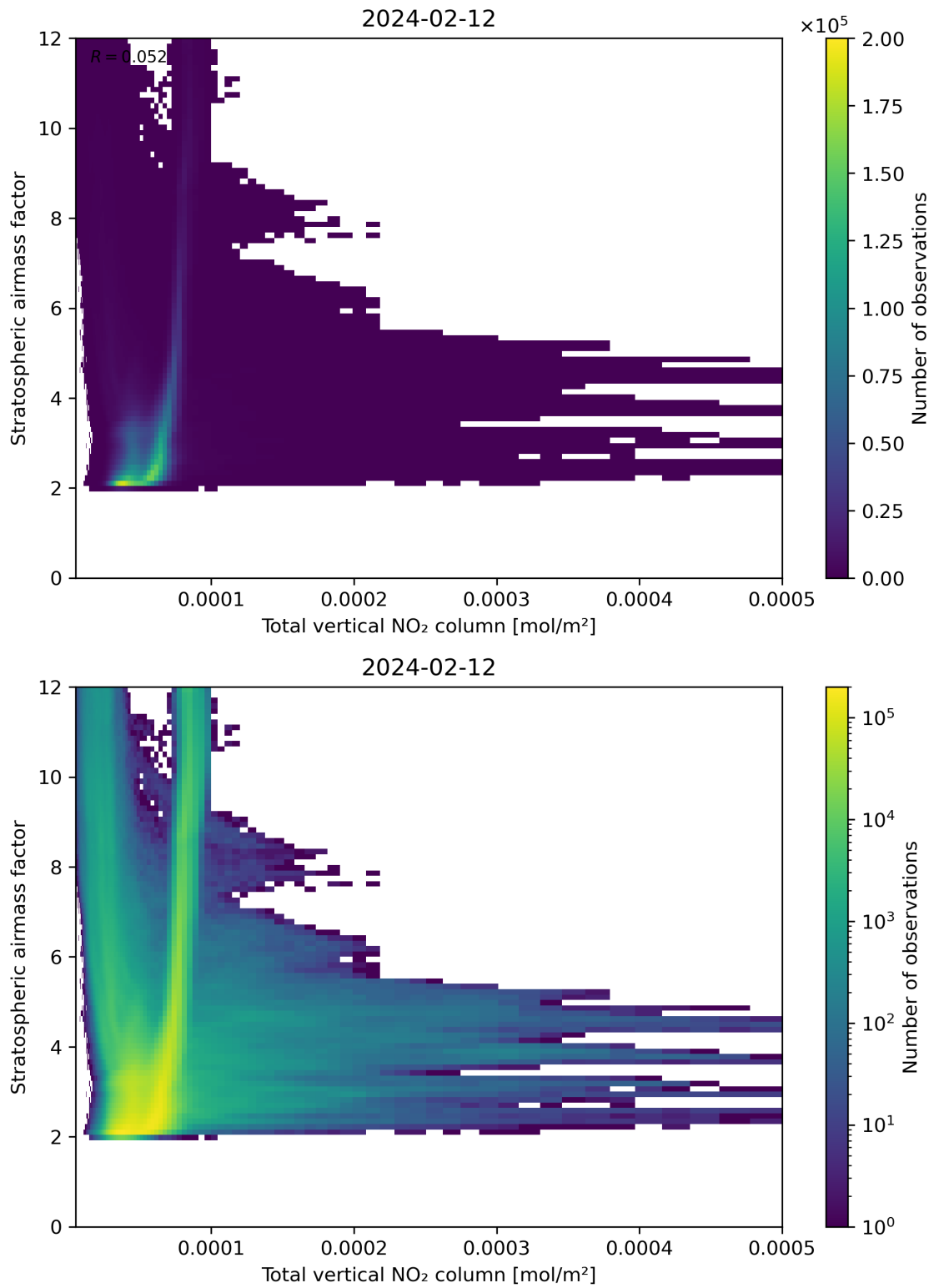
Figure 110: Scatter density plot of “Total vertical NO 2 column” against “Stratospheric airmass factor” for 2024-02-11 to 2024-02-13.
