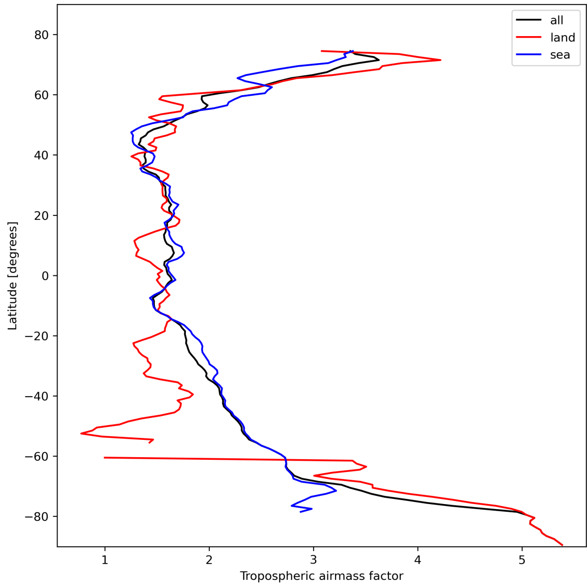
Figure 14: Zonal average of “Tropospheric airmass factor” for 2024-02-11 to 2024-02-13.
