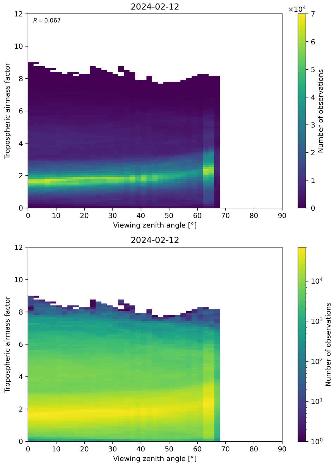
Figure 161: Scatter density plot of “Viewing zenith angle” against “Tropospheric airmass factor” for 2024-02-11 to 2024-02-13.
