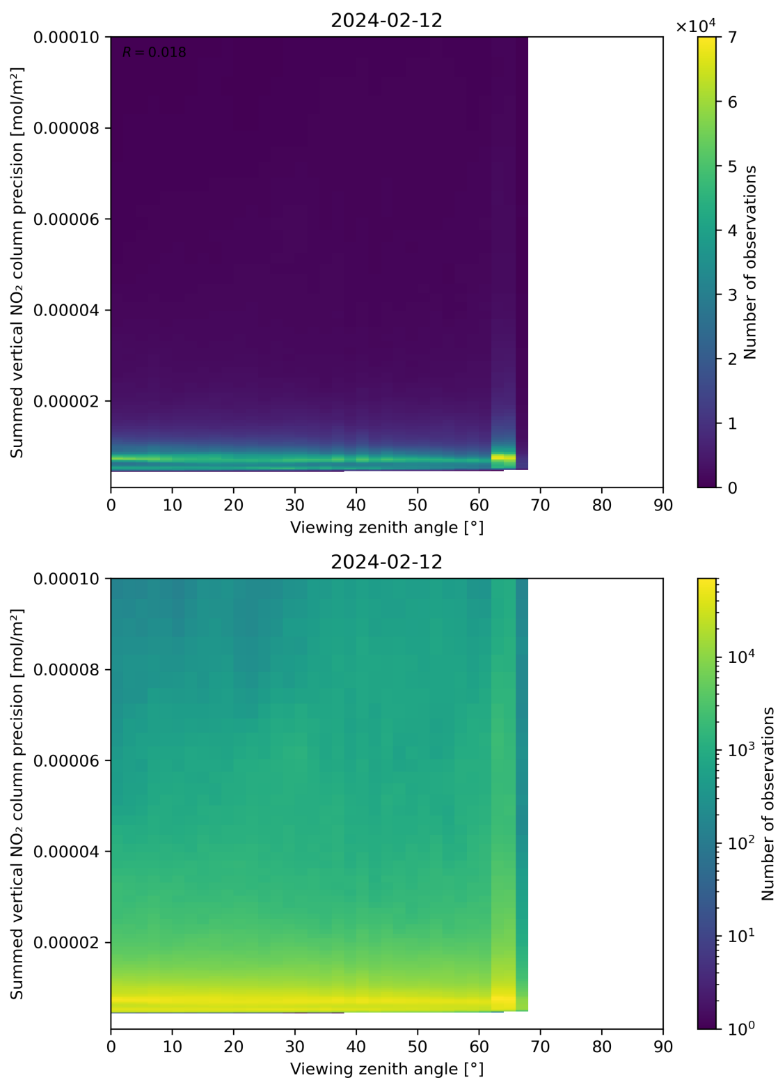
Figure 166: Scatter density plot of “Viewing zenith angle” against “Summed vertical NO 2 column precision” for 2024-02-11 to 2024-02-13.
