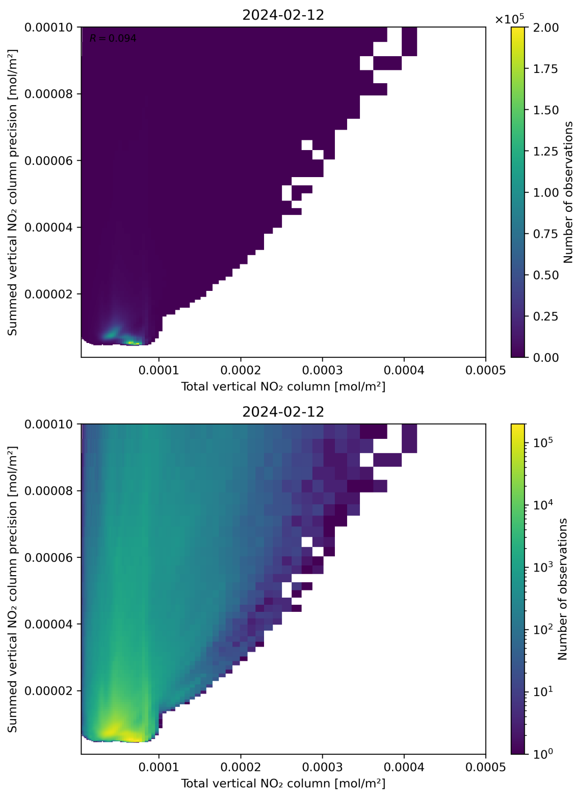
Figure 113: Scatter density plot of “Total vertical NO 2 column” against “Summed vertical NO 2 column precision” for 2024-02-11 to 2024-02-13.
