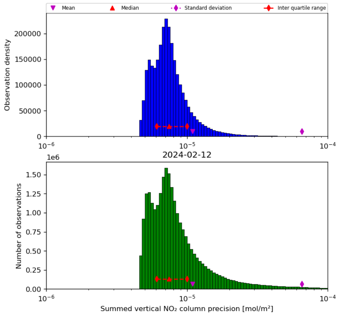
Figure 41: Histogram of “Summed vertical NO 2 column precision” for 2024-02-11 to 2024-02-13
