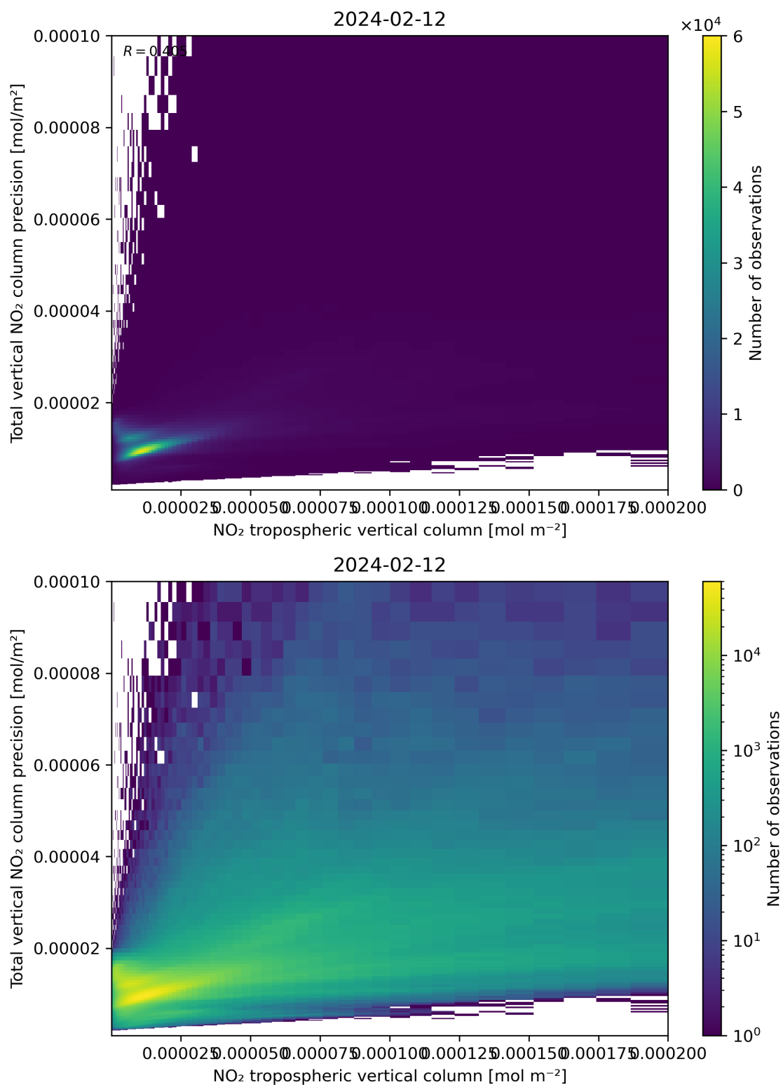
Figure 129: Scatter density plot of “NO 2 tropospheric vertical column” against “Total vertical NO 2 column precision” for 2024-02-11 to 2024-02-13.
