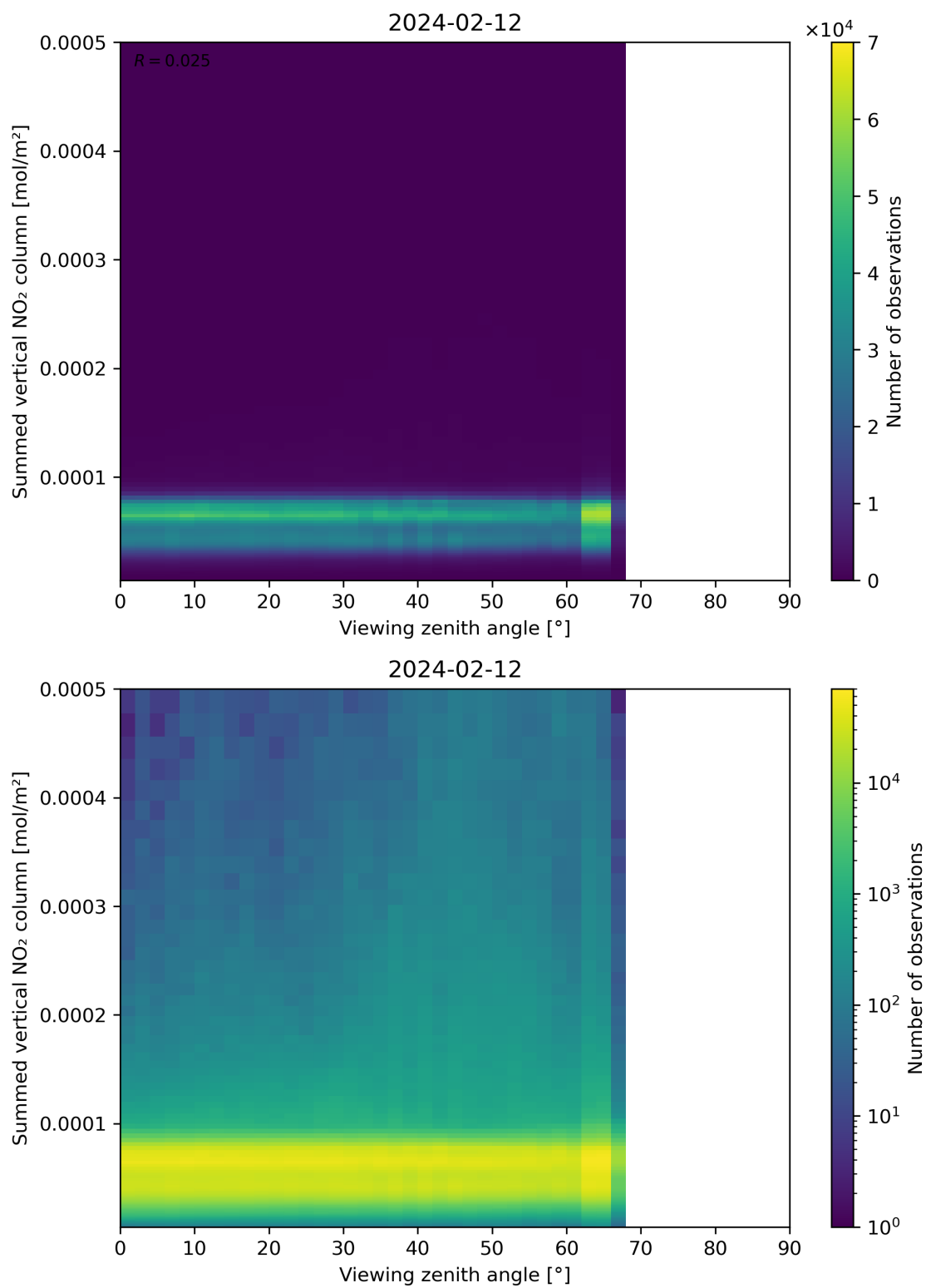
Figure 165: Scatter density plot of “Viewing zenith angle” against “Summed vertical NO 2 column” for 2024-02-11 to 2024-02-13.
