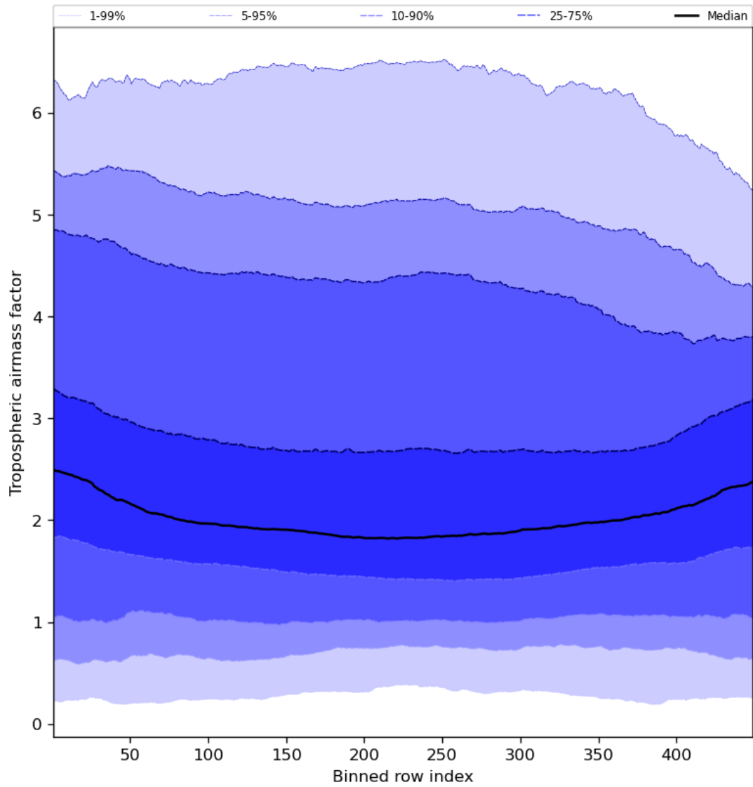
Figure 48: Along track statistics of “Tropospheric airmass factor” for 2024-02-11 to 2024-02-13
