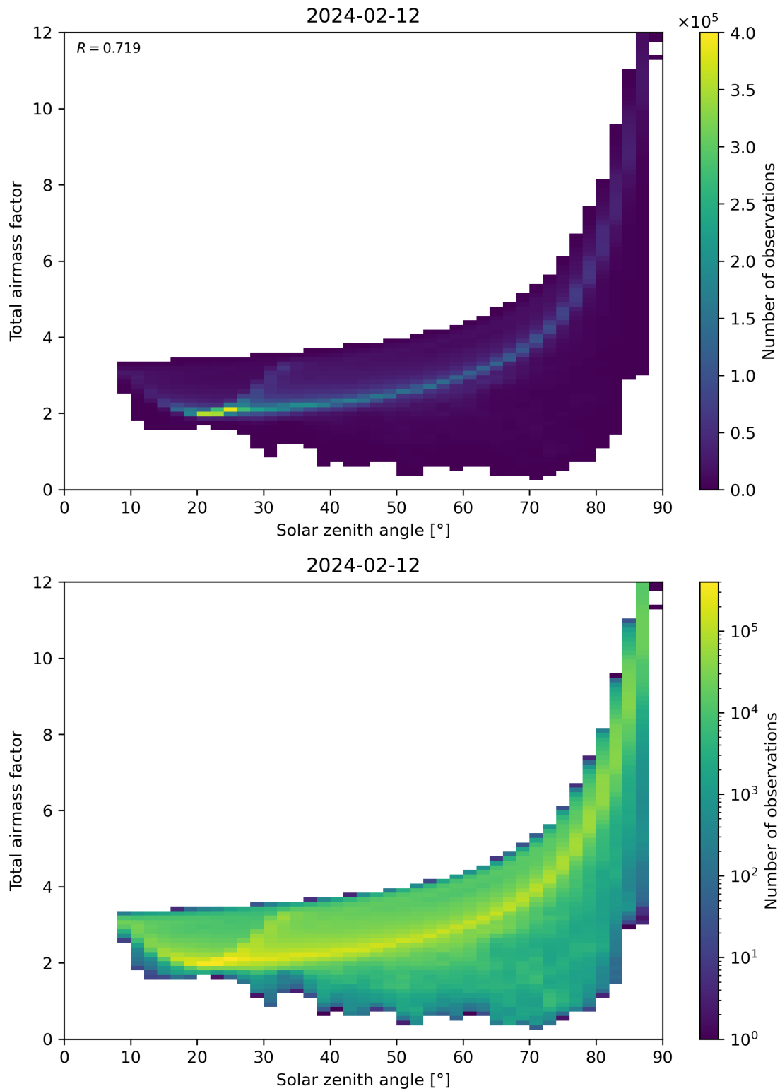
Figure 146: Scatter density plot of “Solar zenith angle” against “Total air mass factor” for 2024-02-11 to 2024-02-13.
