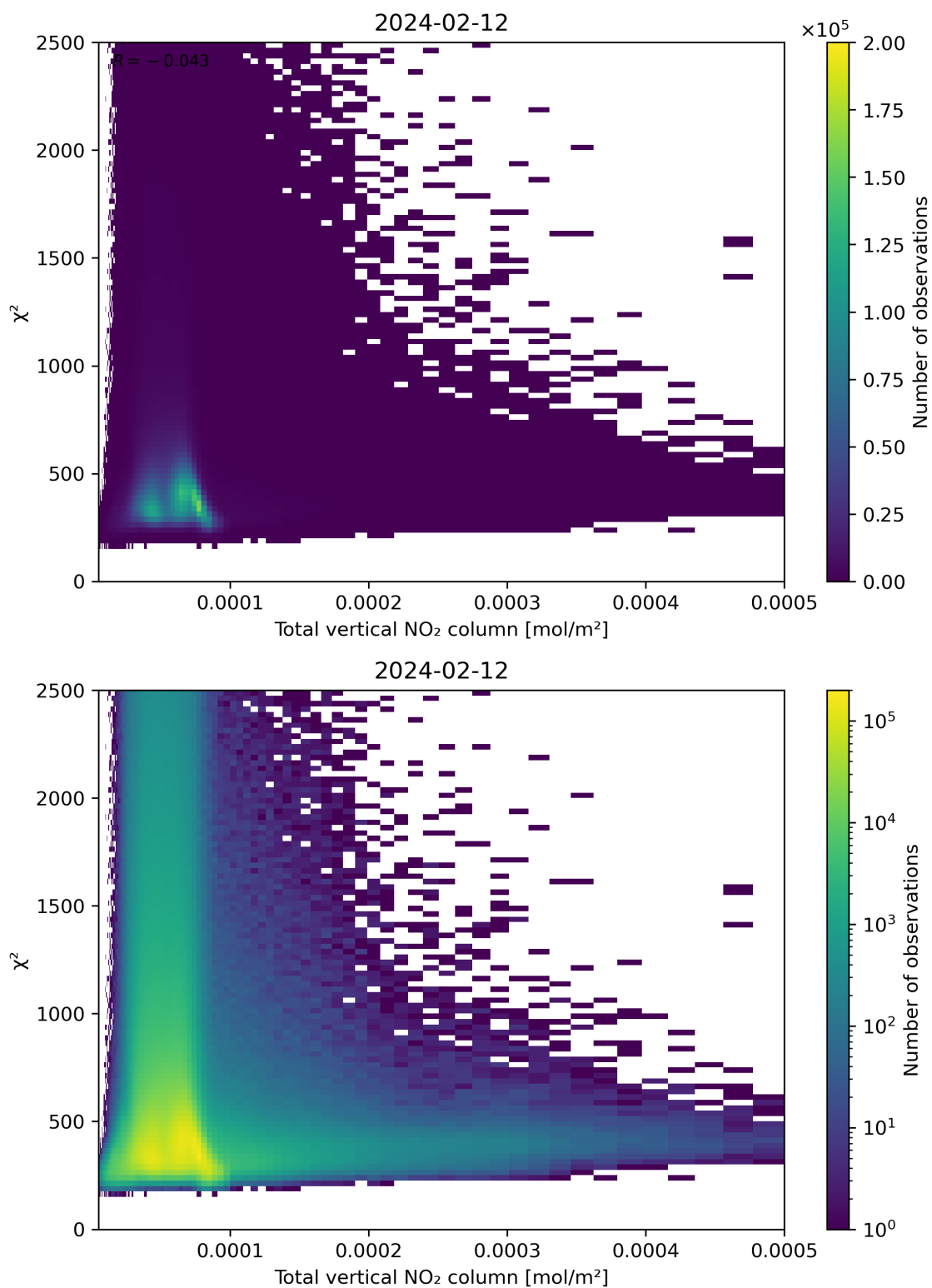
Figure 111: Scatter density plot of “Total vertical NO 2 column” against “ \chi^2 ” for 2024-02-11 to 2024-02-13.
