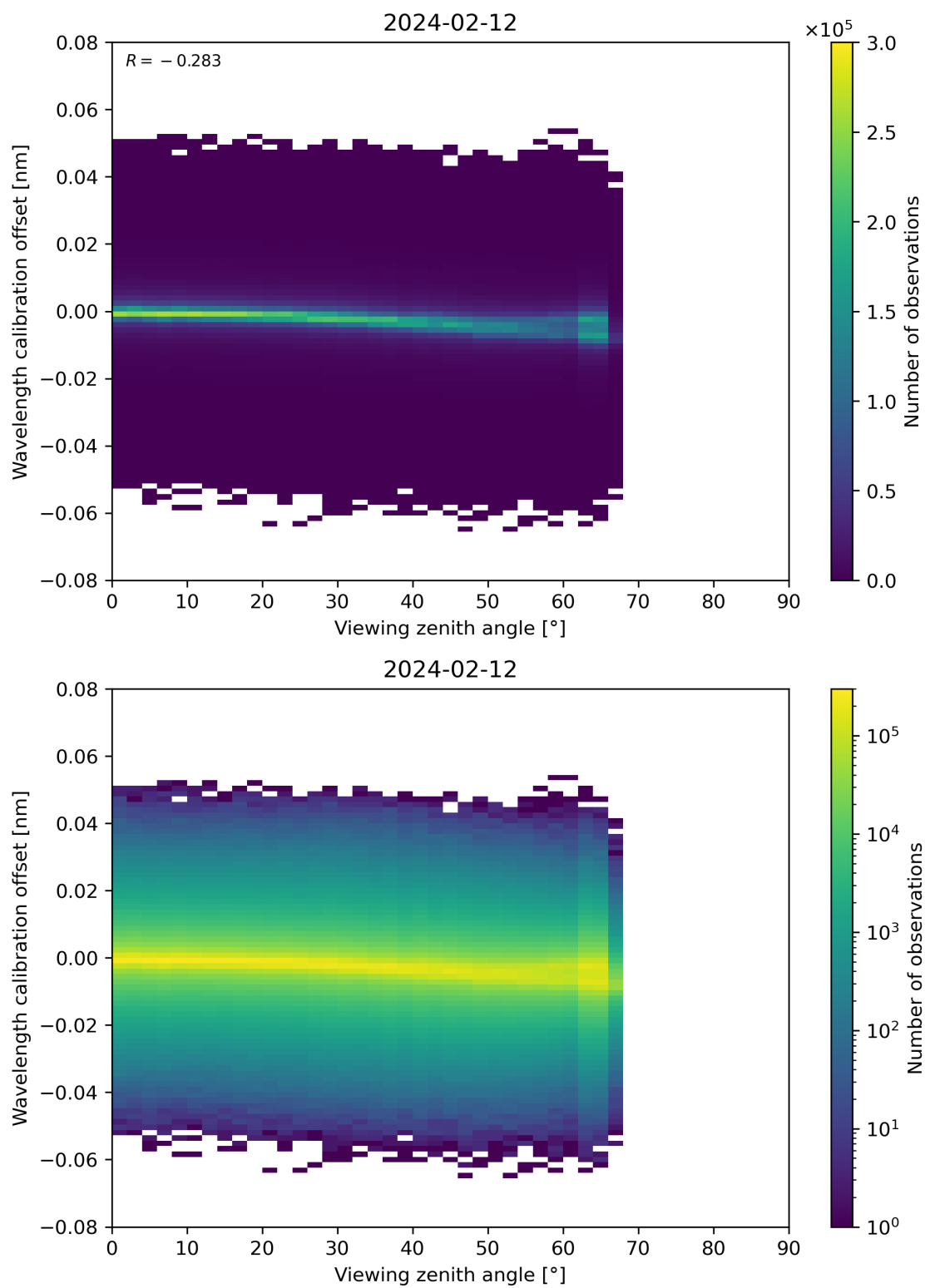
Figure 173: Scatter density plot of “Viewing zenith angle” against “Wavelength calibration offset” for 2024-02-11 to 2024-02-13.
