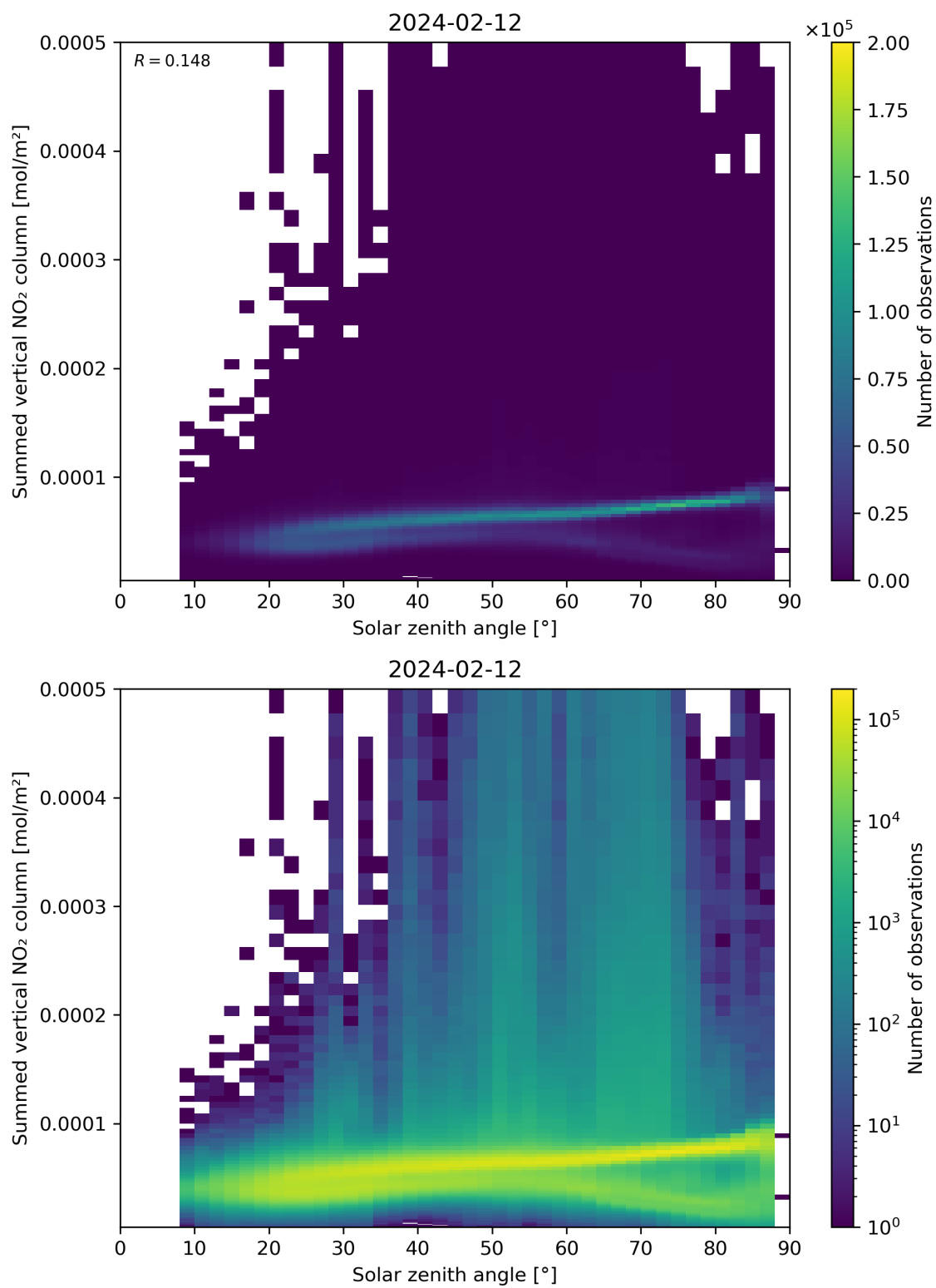
Figure 151: Scatter density plot of “Solar zenith angle” against “Summed vertical NO 2 column” for 2024-02-11 to 2024-02-13.
