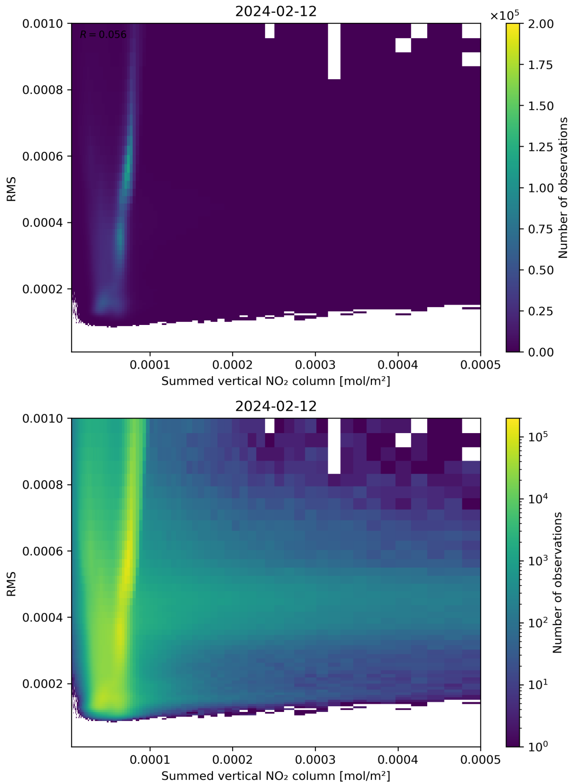
Figure 109: Scatter density plot of “Summed vertical NO 2 column” against “RMS” for 2024-02-11 to 2024-02-13.
