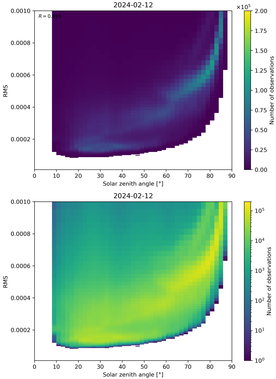
Figure 157: Scatter density plot of “Solar zenith angle” against “RMS” for 2024-02-11 to 2024-02-13.
