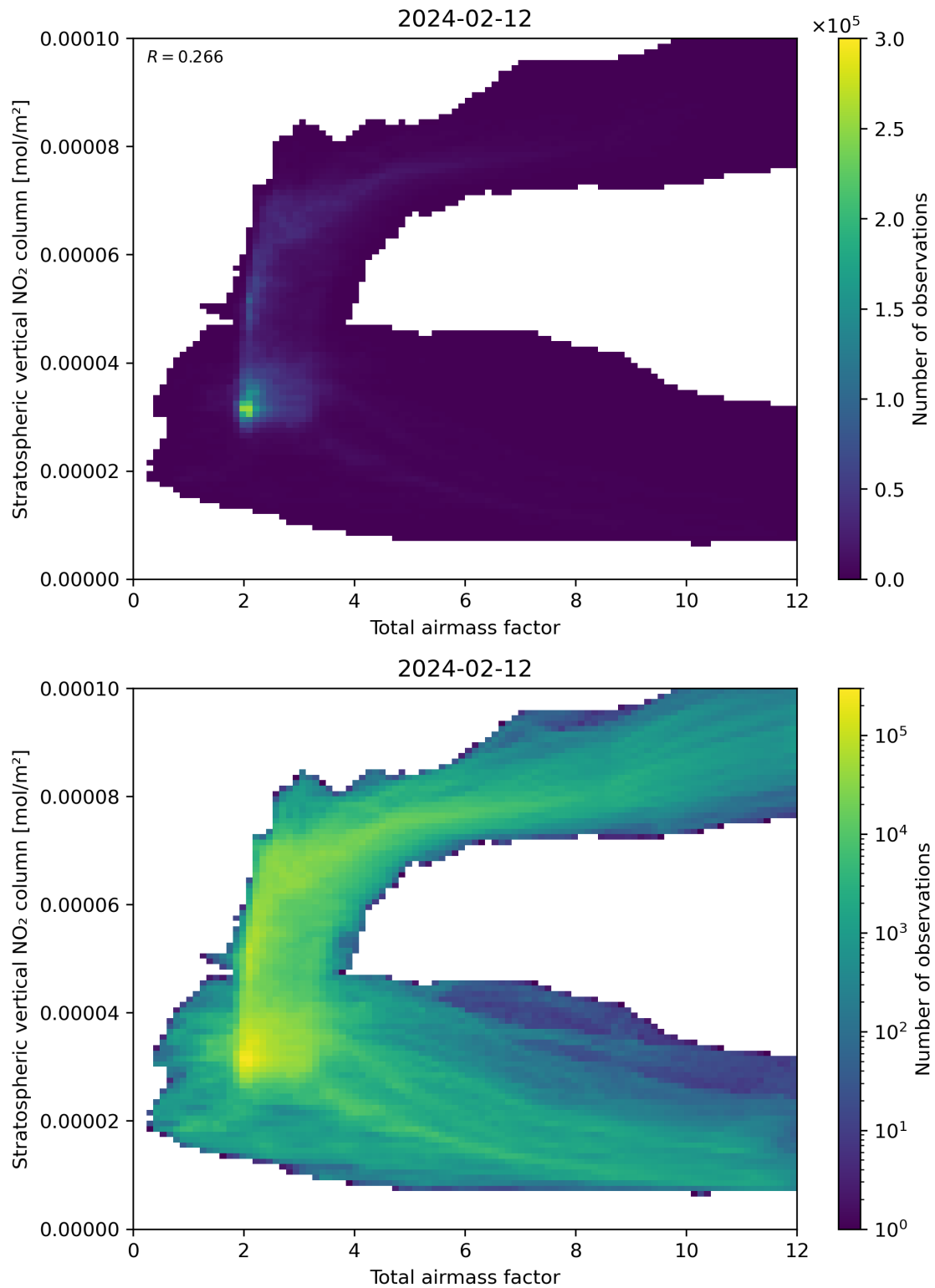
Figure 64: Scatter density plot of “Total airmass factor” against “Stratospheric vertical \text{NO}_2 column” for 2024-02-11 to 2024-02-13.
