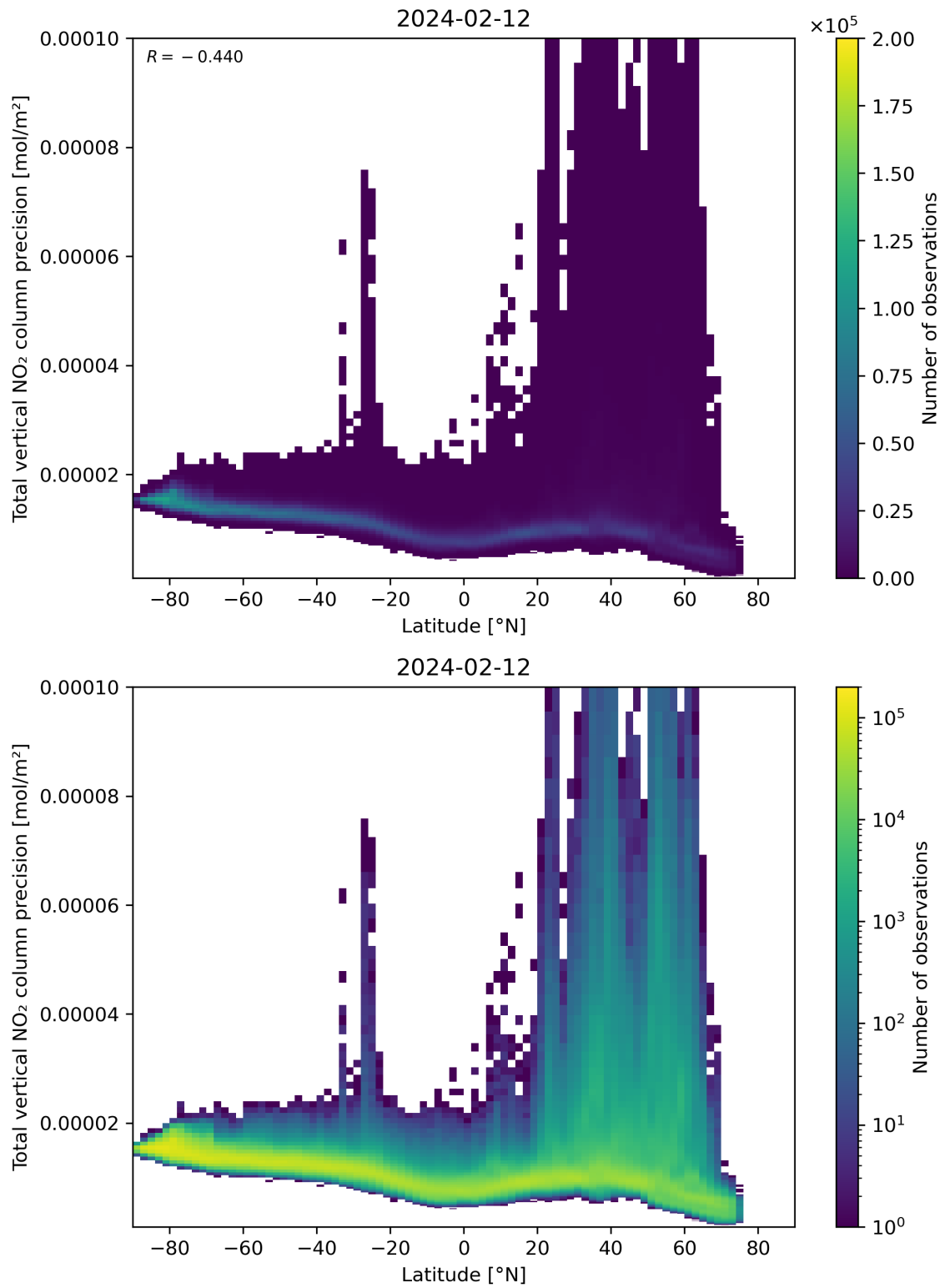
Figure 91: Scatter density plot of “Latitude” against “Total vertical NO 2 column precision” for 2024-02-11 to 2024-02-13.
