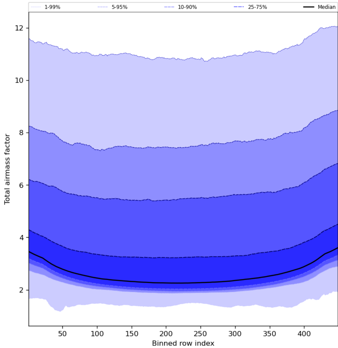
Figure 49: Along track statistics of “Total airmass factor” for 2024-02-11 to 2024-02-13
