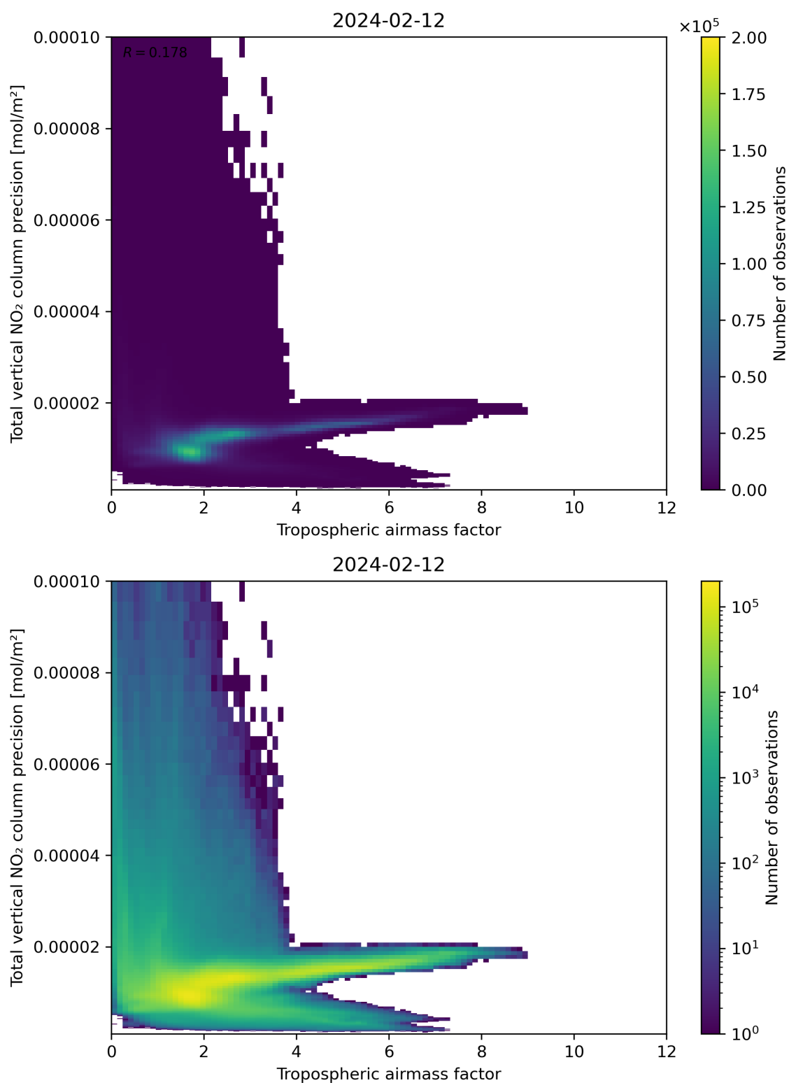
Figure 78: Scatter density plot of “Tropospheric air mass factor” against “Total vertical NO 2 column precision” for 2024-02-11 to 2024-02-13.
