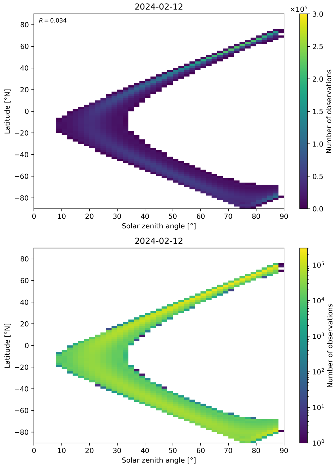
Figure 149: Scatter density plot of “Solar zenith angle” against “Latitude” for 2024-02-11 to 2024-02-13.
