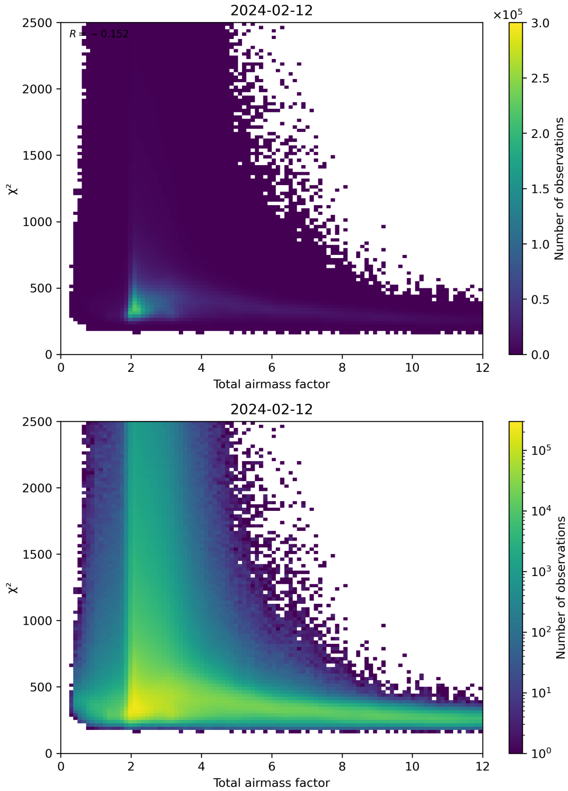
Figure 63: Scatter density plot of “Total airmass factor” against “ \chi^2 ” for 2024-02-11 to 2024-02-13.
