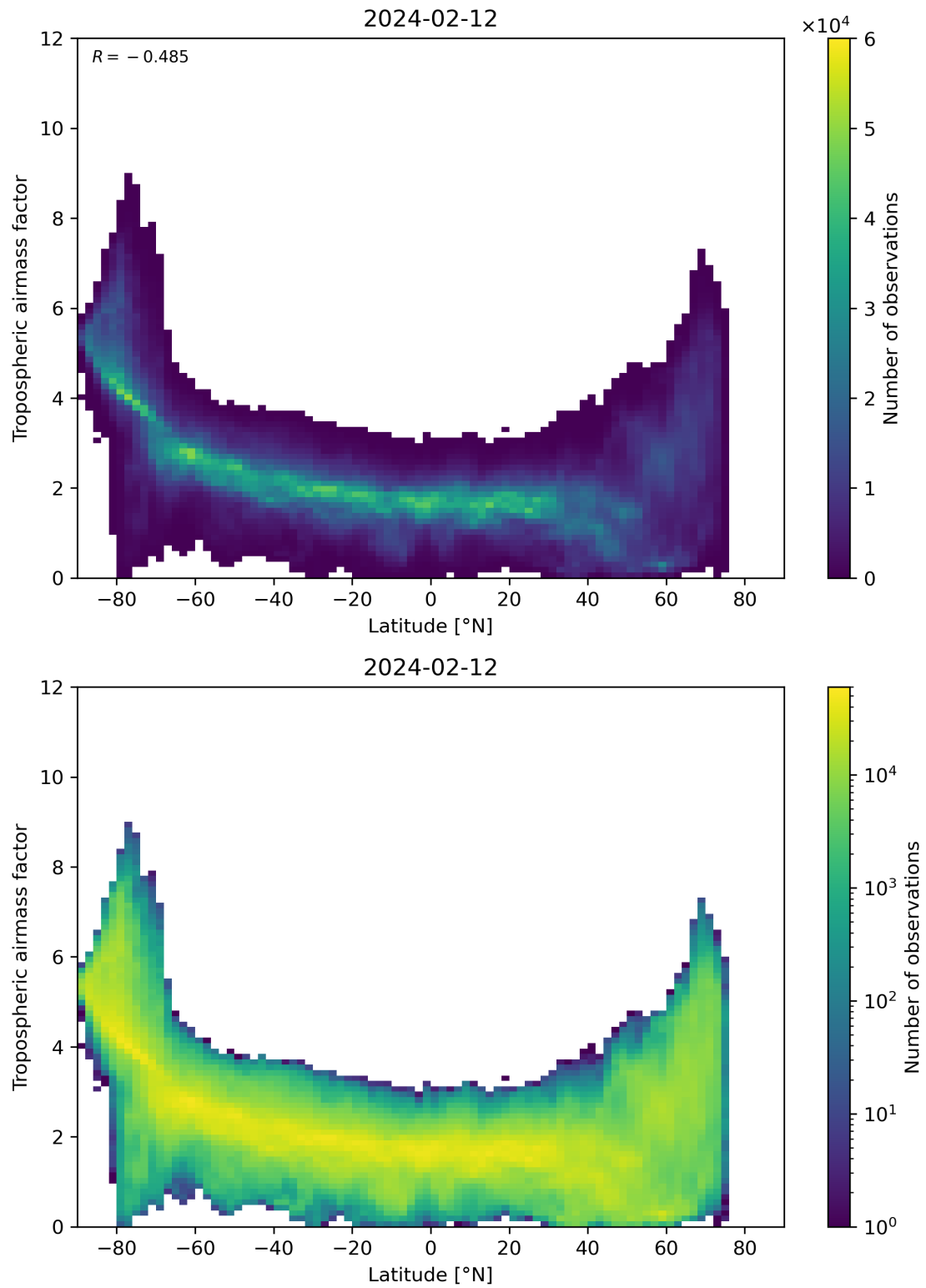
Figure 85: Scatter density plot of “Latitude” against “Tropospheric airmass factor” for 2024-02-11 to 2024-02-13.
