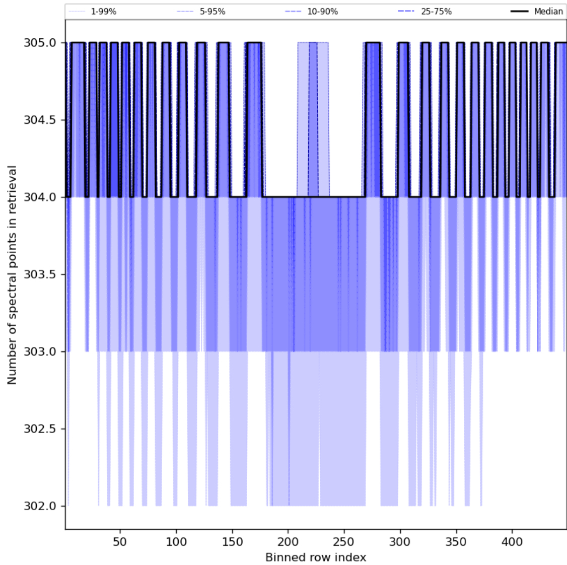
Figure 50: Along track statistics of “Number of spectral points in retrieval” for 2024-02-11 to 2024-02-13
