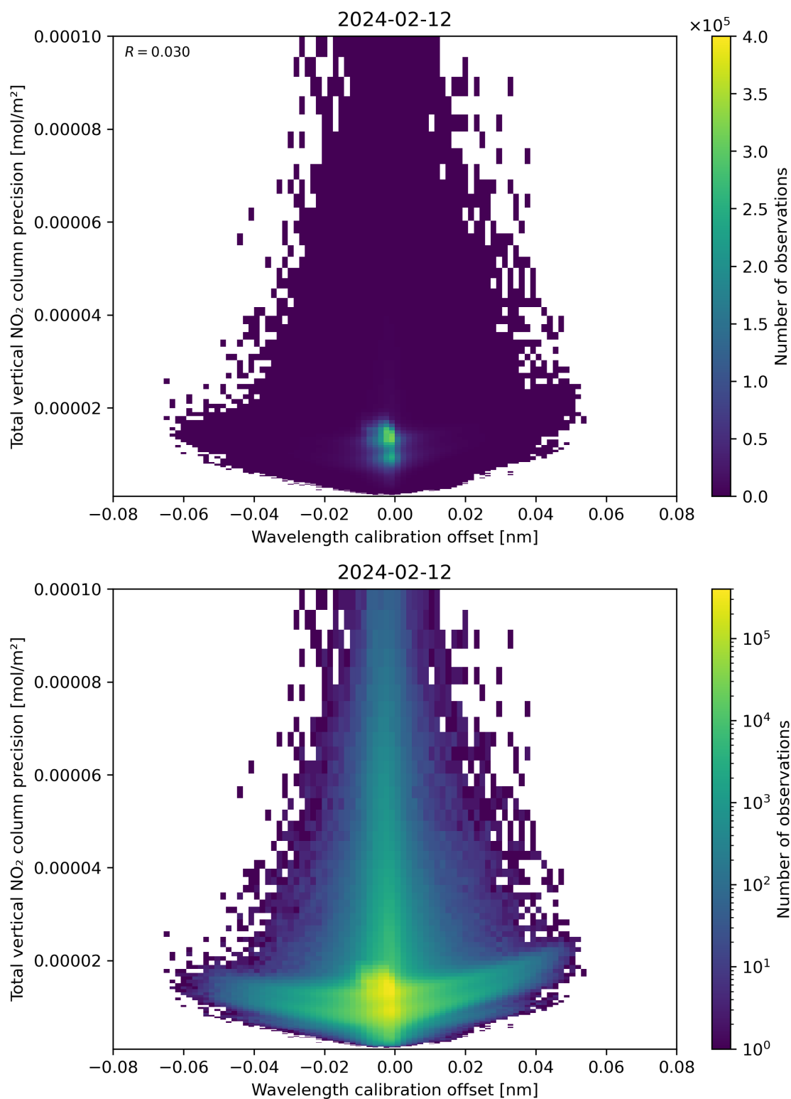
Figure 180: Scatter density plot of “Wavelength calibration offset” against “Total vertical NO 2 column precision” for 2024-02-11 to 2024-02-13.
