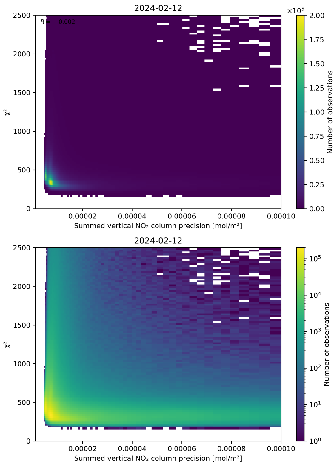
Figure 107: Scatter density plot of “Summed vertical NO 2 column precision” against “ \chi^2 ” for 2024-02-11 to 2024-02-13.
