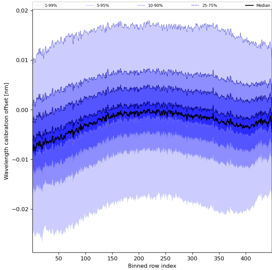
Figure 52: Along track statistics of “Wavelength calibration offset” for 2024-02-11 to 2024-02-13
