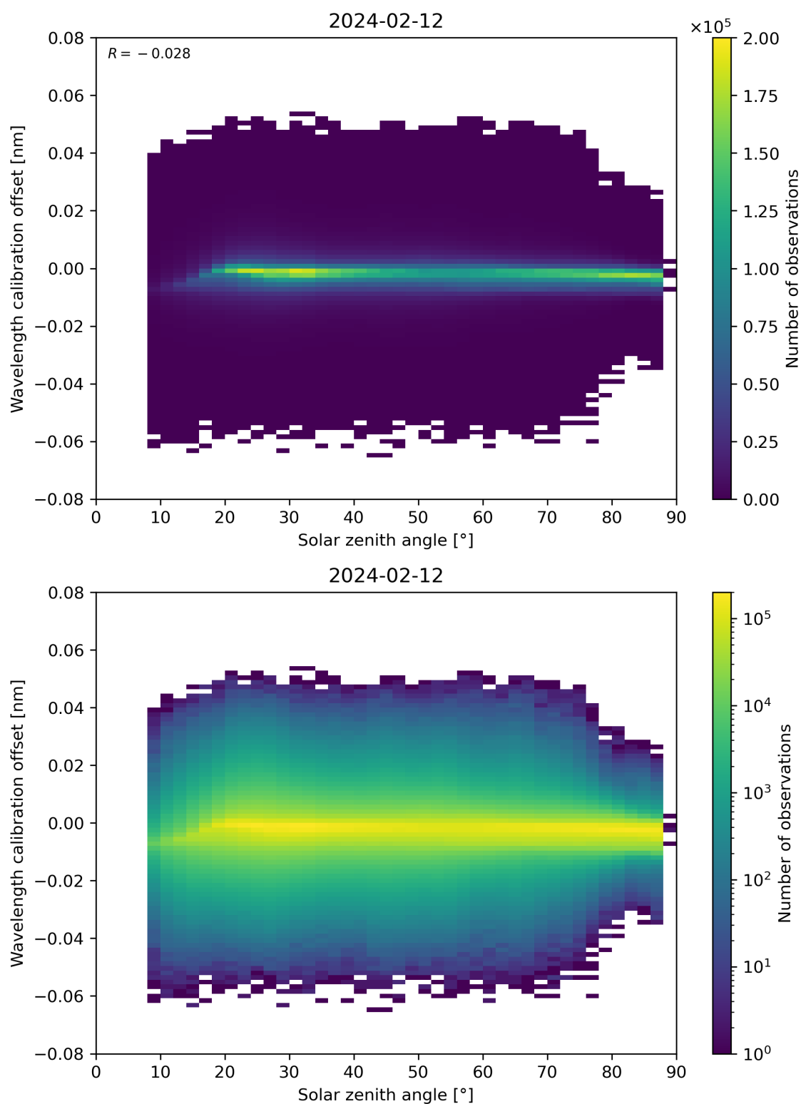
Figure 158: Scatter density plot of “Solar zenith angle” against “Wavelength calibration offset” for 2024-02-11 to 2024-02-13.
