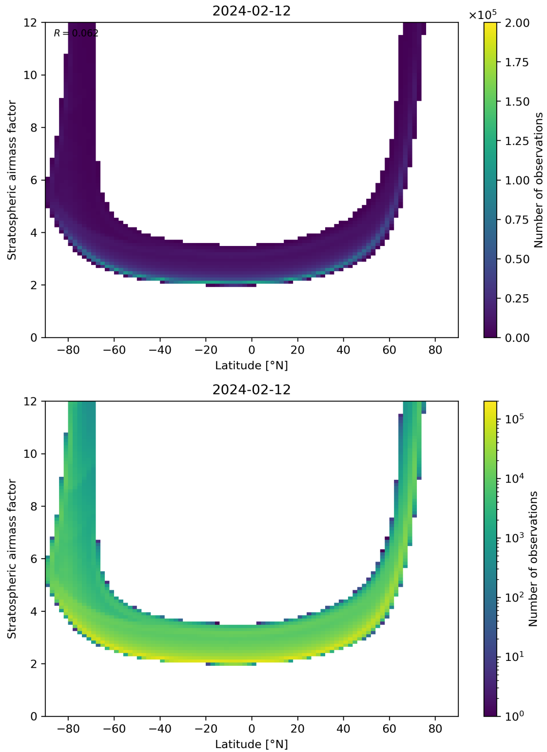
Figure 83: Scatter density plot of “Latitude” against “Stratospheric airmass factor” for 2024-02-11 to 2024-02-13.
