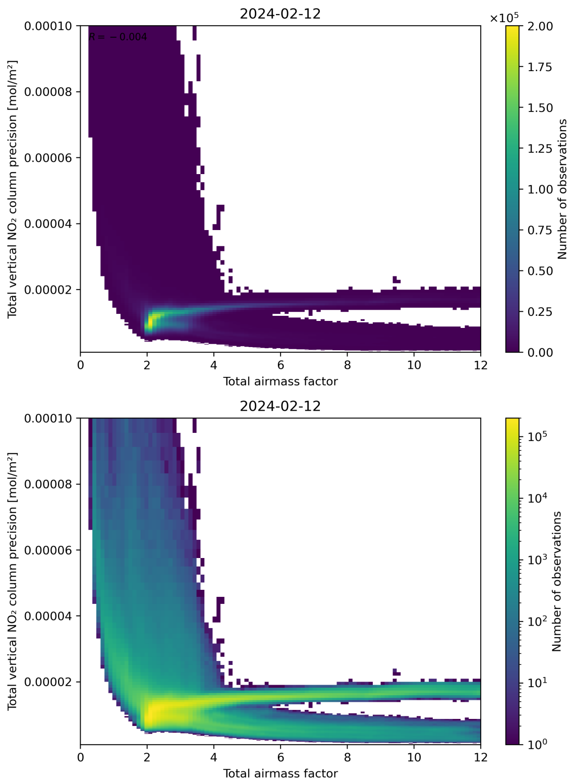
Figure 68: Scatter density plot of “Total airmass factor” against “Total vertical NO 2 column precision” for 2024-02-11 to 2024-02-13.
