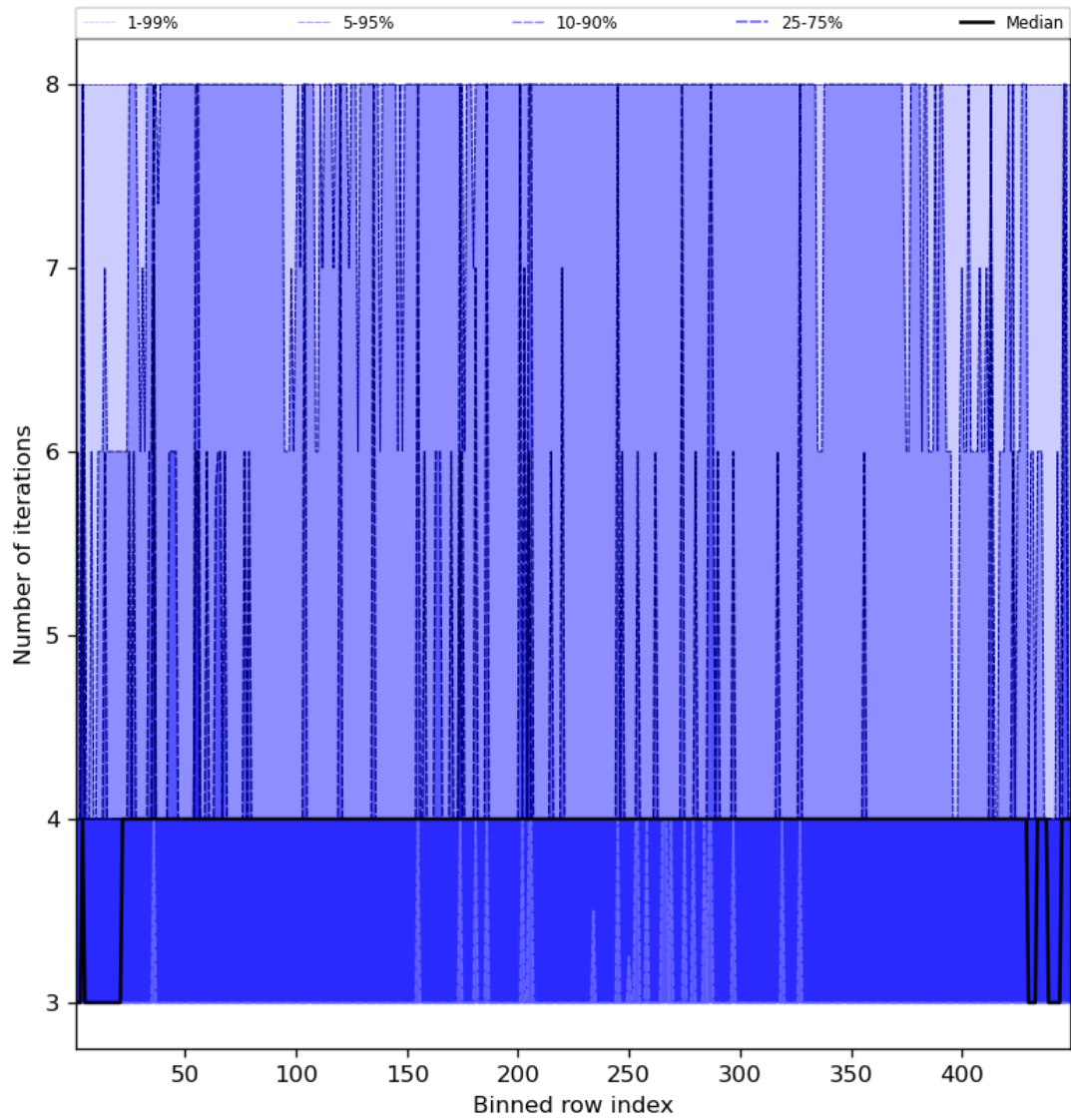
Figure 51: Along track statistics of “Number of iterations” for 2024-02-11 to 2024-02-13
