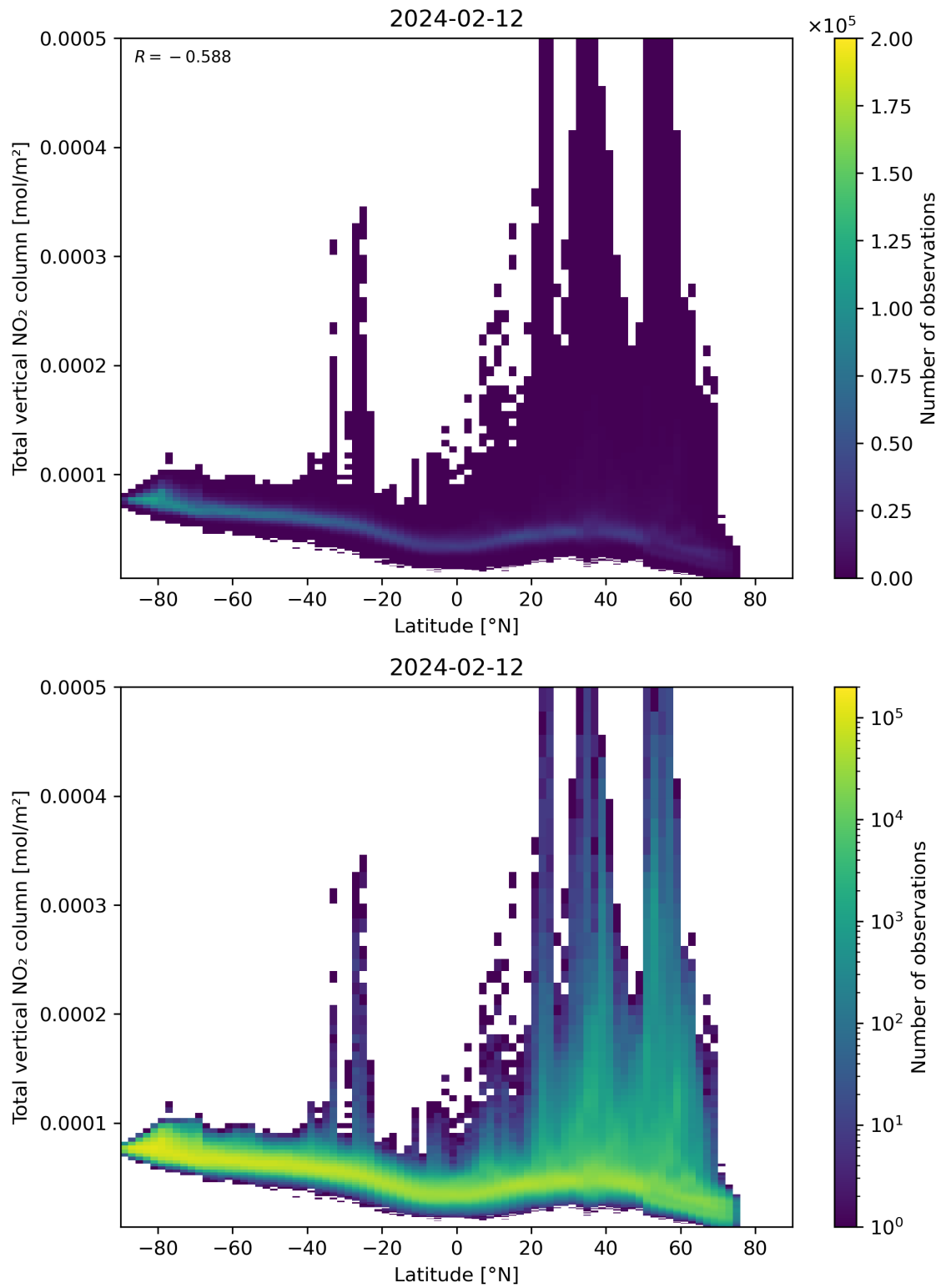
Figure 90: Scatter density plot of “Latitude” against “Total vertical NO 2 column” for 2024-02-11 to 2024-02-13.
