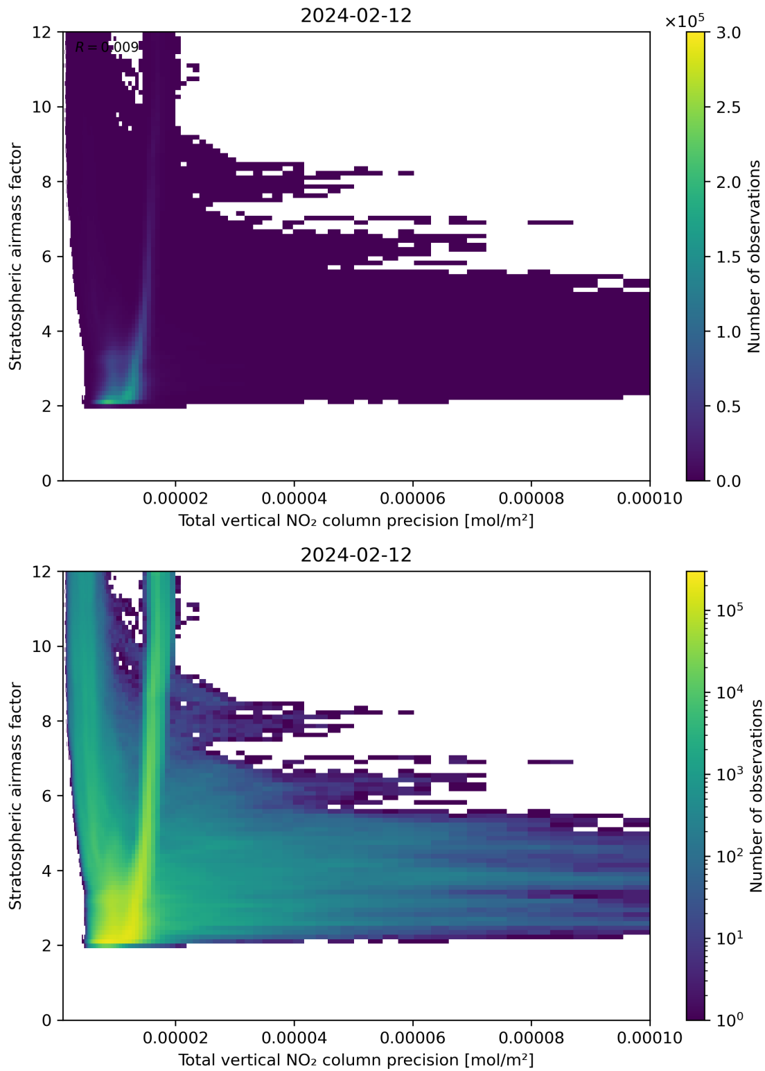
Figure 115: Scatter density plot of “Total vertical NO 2 column precision” against “Stratospheric air mass factor” for 2024-02-11 to 2024-02-13.
