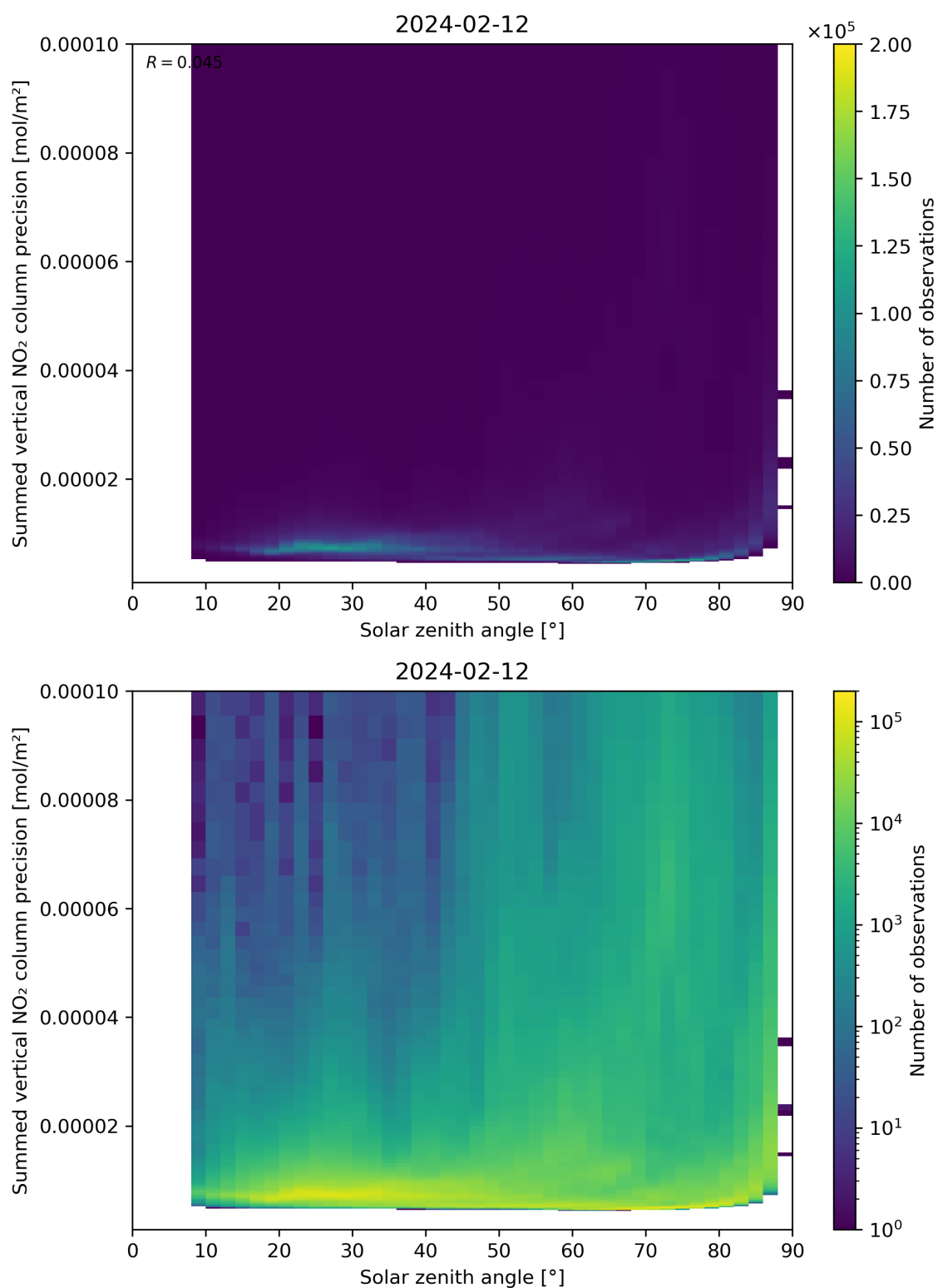
Figure 152: Scatter density plot of “Solar zenith angle” against “Summed vertical NO 2 column precision” for 2024-02-11 to 2024-02-13.
