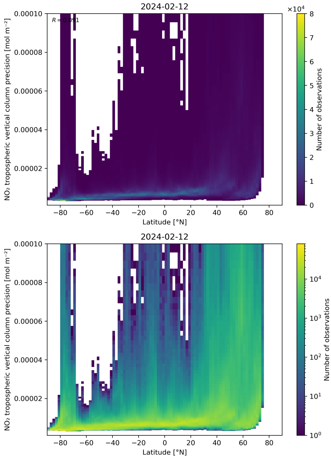
Figure 93: Scatter density plot of “Latitude” against “NO 2 tropospheric vertical column precision” for 2024-02-11 to 2024-02-13.
