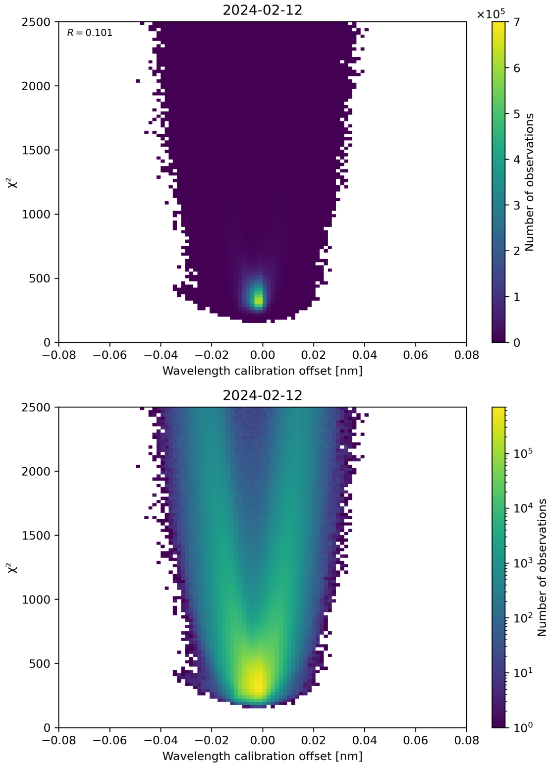
Figure 175: Scatter density plot of “Wavelength calibration offset” against “ \chi^2 ” for 2024-02-11 to 2024-02-13.
