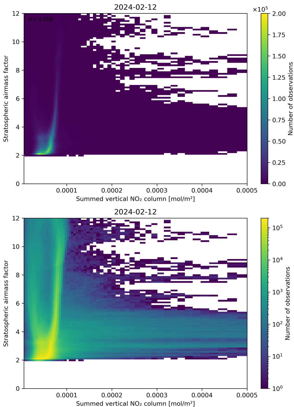
Figure 103: Scatter density plot of “Summed vertical NO 2 column” against “Stratospheric airmass factor” for 2024-02-11 to 2024-02-13.
