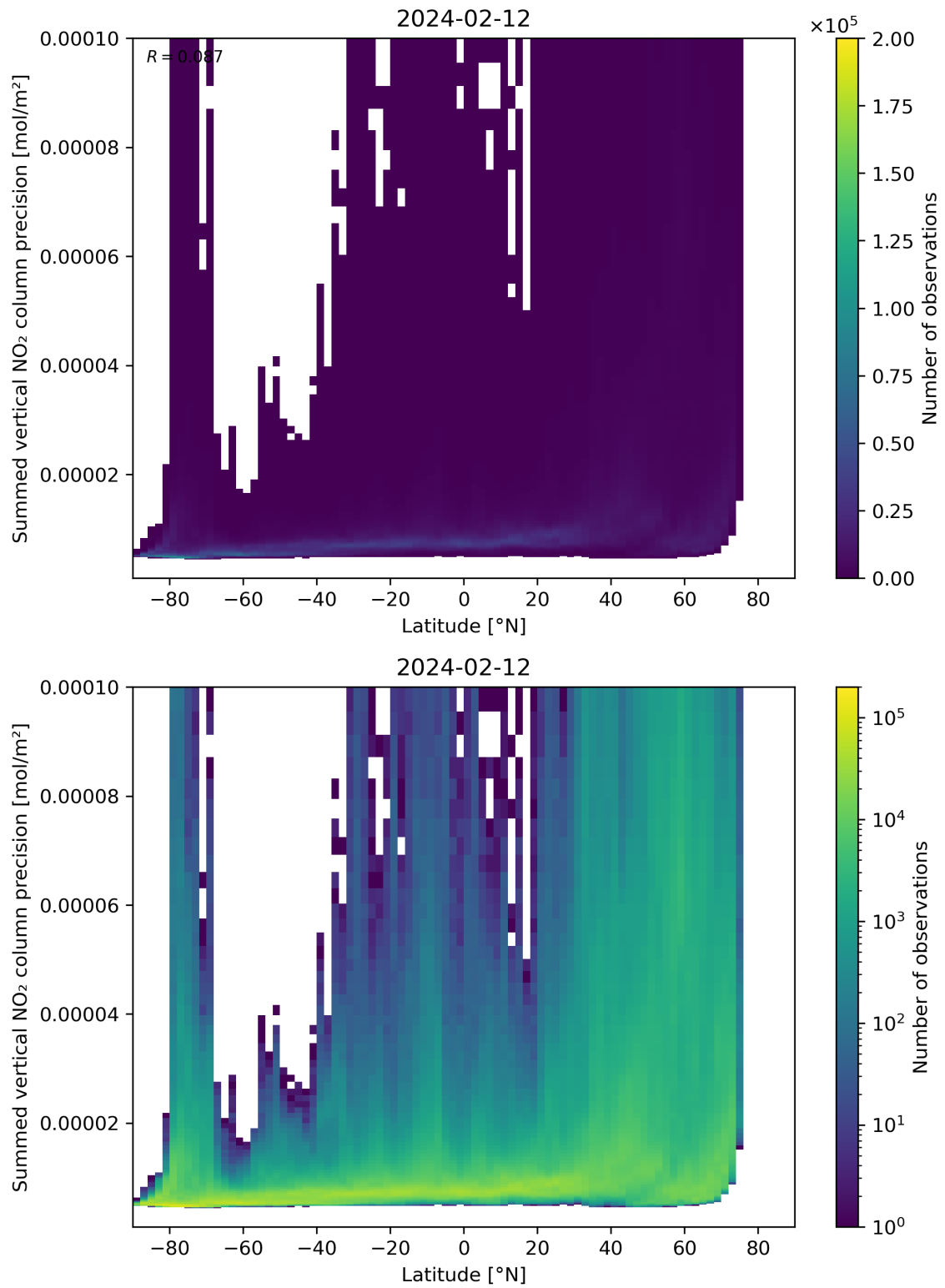
Figure 89: Scatter density plot of “Latitude” against “Summed vertical NO 2 column precision” for 2024-02-11 to 2024-02-13.
