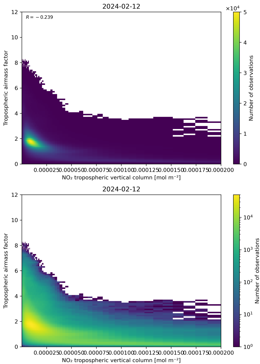
Figure 123: Scatter density plot of “NO 2 tropospheric vertical column” against “Tropospheric air mass factor” for 2024-02-11 to 2024-02-13.
