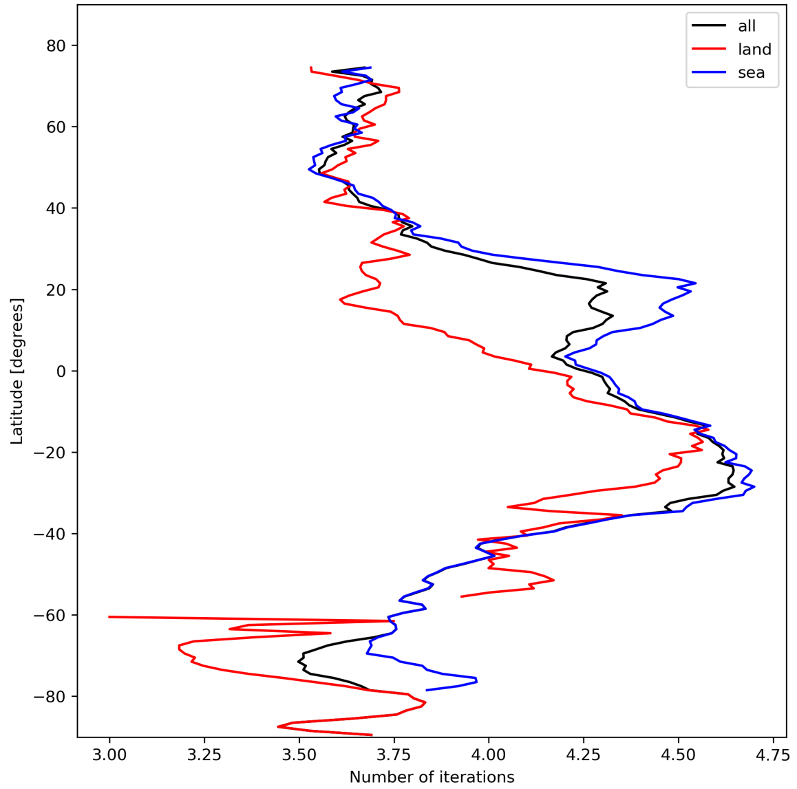
Figure 17: Zonal average of “Number of iterations” for 2024-02-11 to 2024-02-13.
