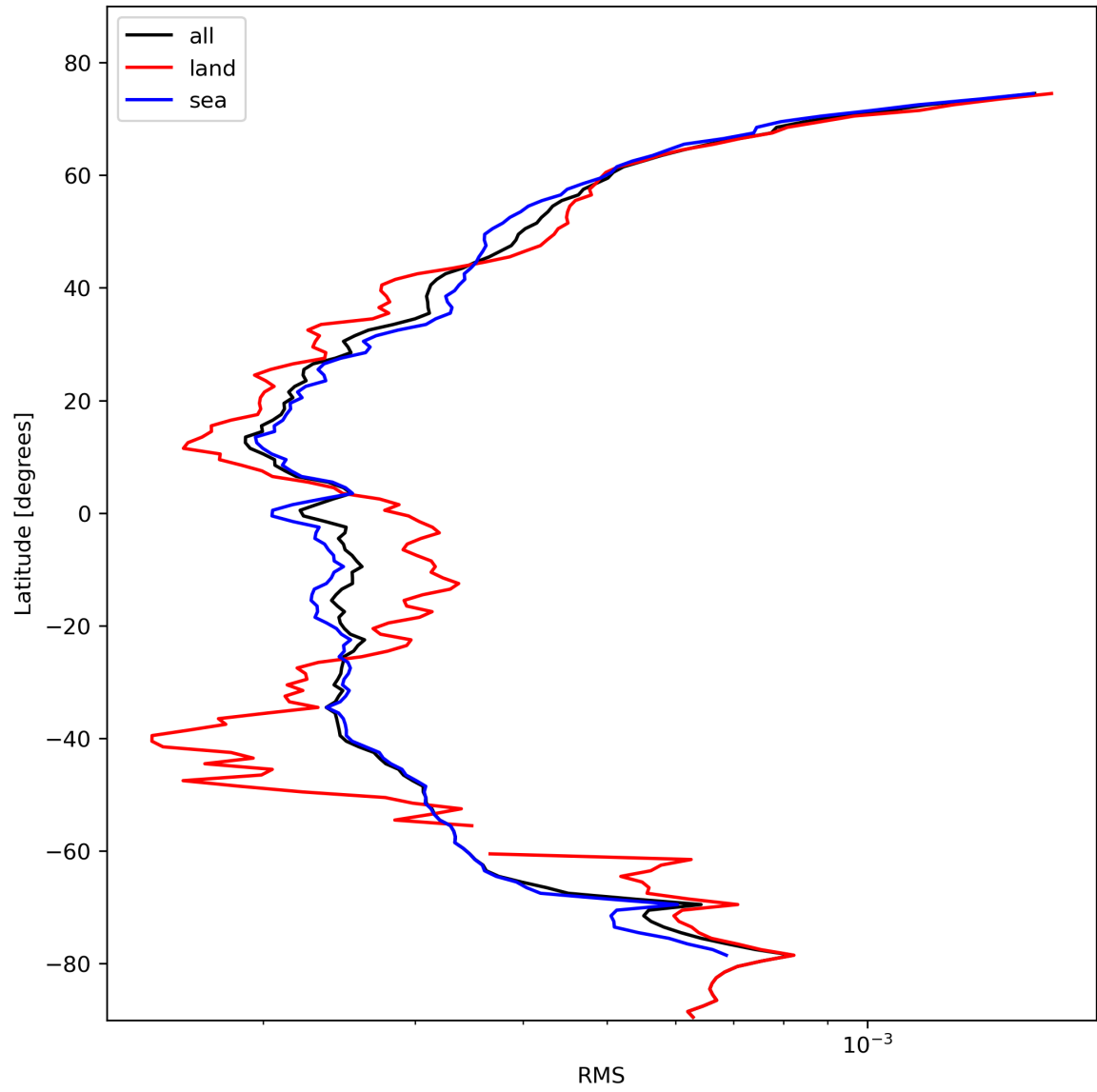
Figure 26: Zonal average of “RMS” for 2024-02-11 to 2024-02-13.
