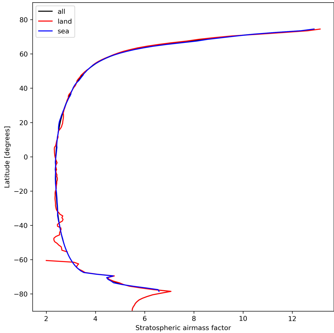
Figure 27: Zonal average of “Stratospheric airmass factor” for 2024-02-11 to 2024-02-13.
