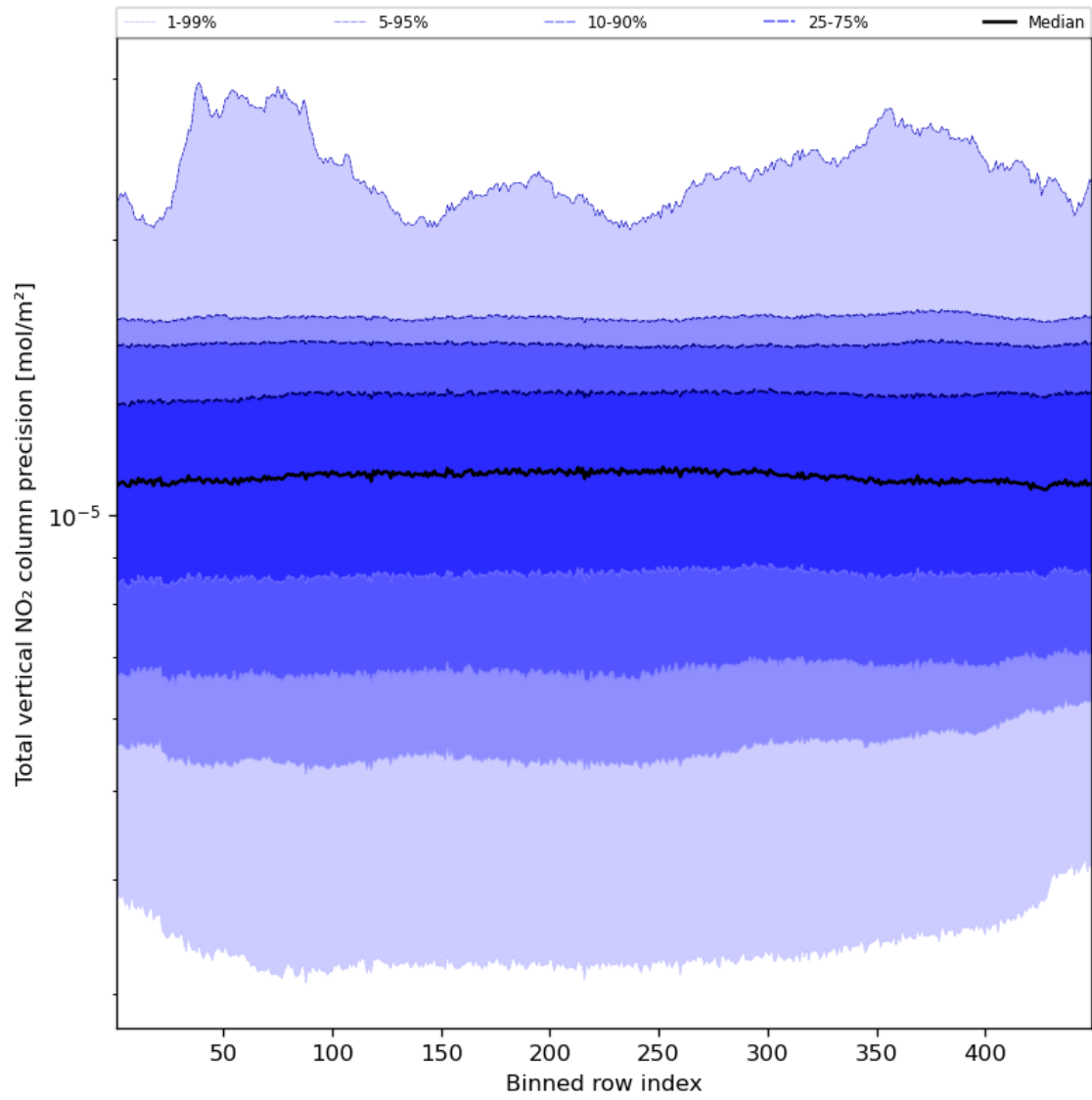
Figure 56: Along track statistics of “Total vertical NO 2 column precision” for 2024-02-11 to 2024-02-13
