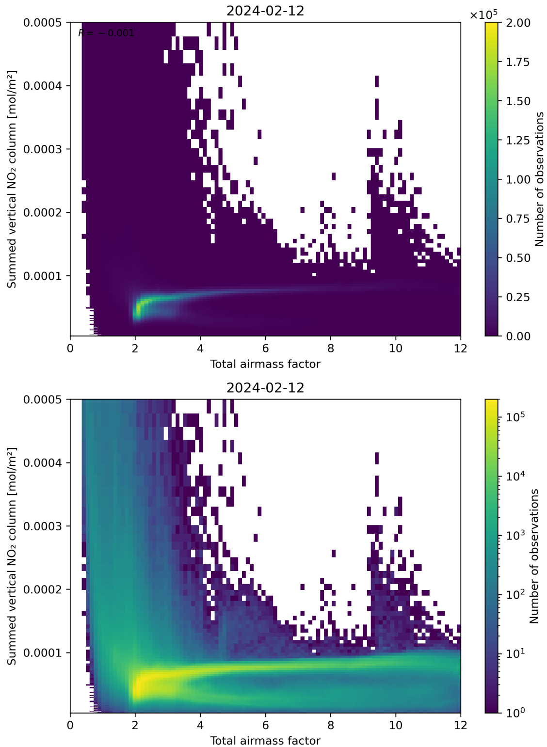
Figure 65: Scatter density plot of “Total airmass factor” against “Summed vertical NO 2 column” for 2024-02-11 to 2024-02-13.
