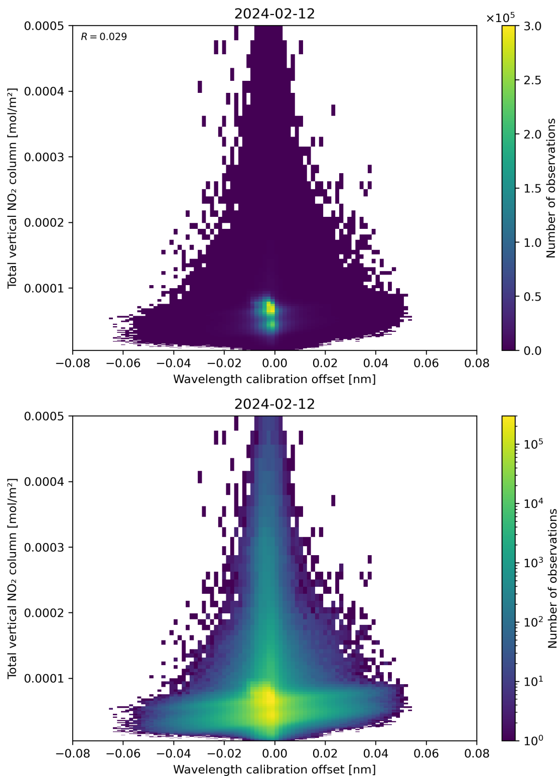
Figure 179: Scatter density plot of “Wavelength calibration offset” against “Total vertical NO 2 column” for 2024-02-11 to 2024-02-13.
