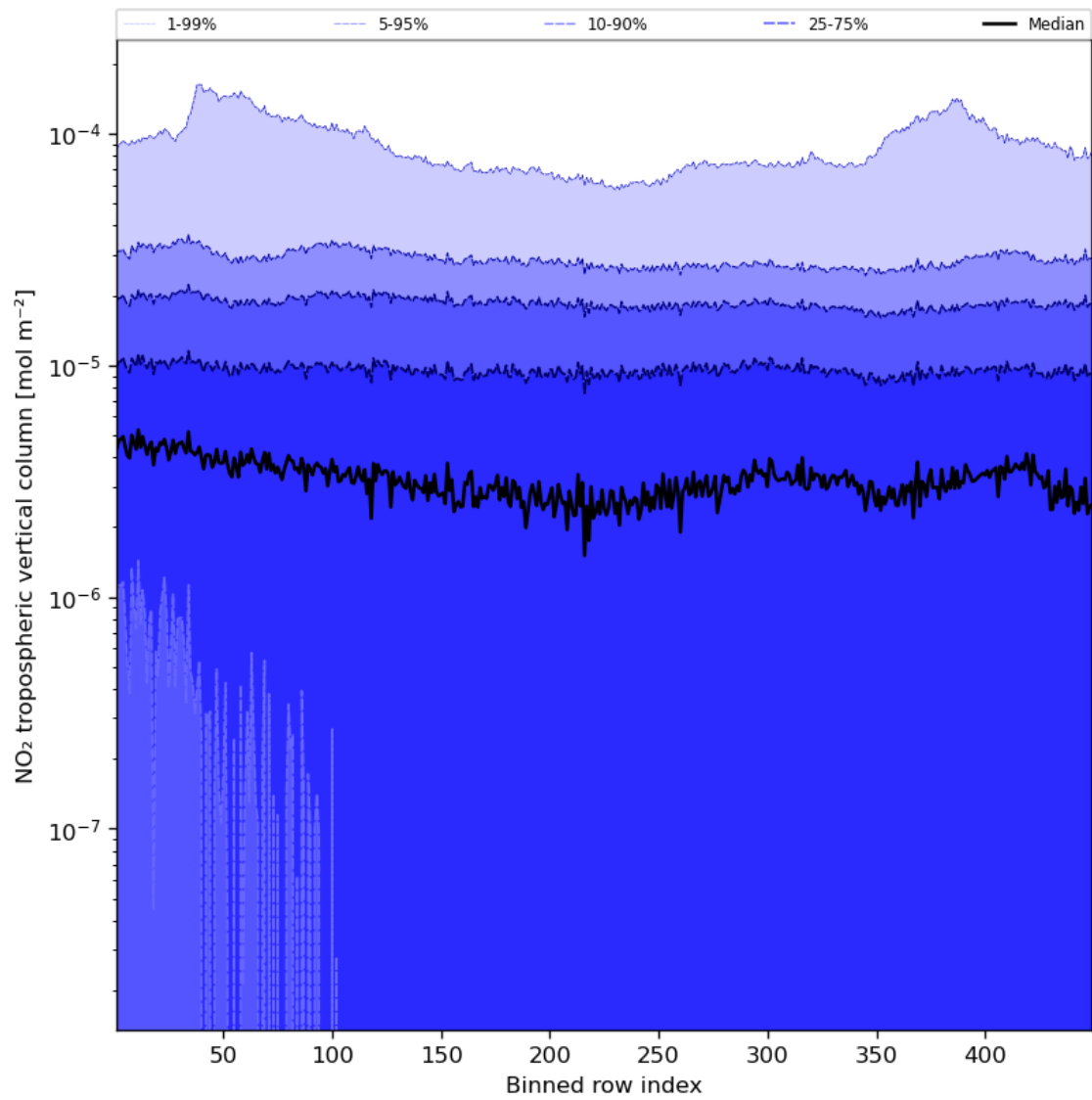
Figure 46: Along track statistics of “NO 2 tropospheric vertical column” for 2024-02-11 to 2024-02-13
