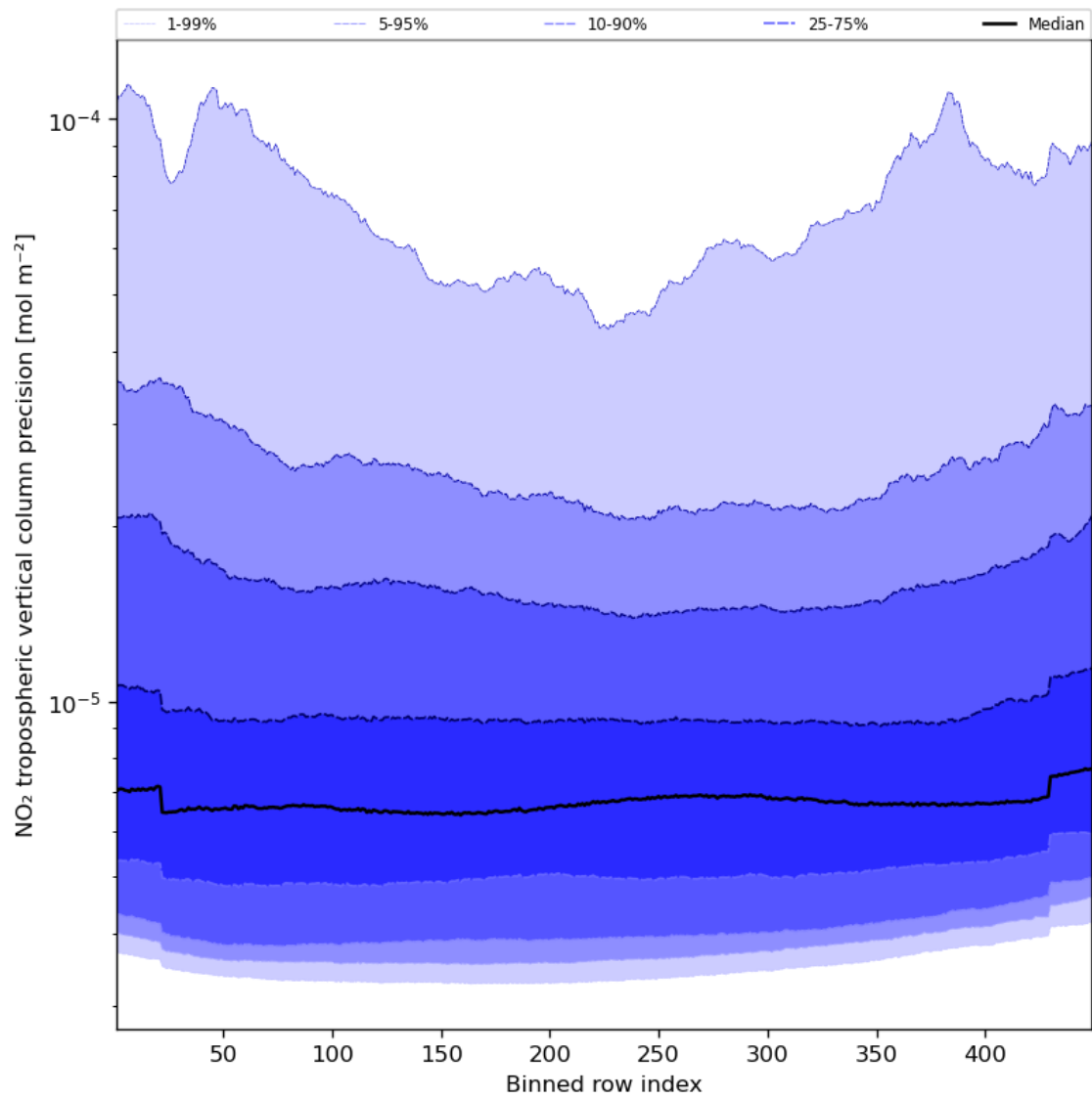
Figure 47: Along track statistics of “NO 2 tropospheric vertical column precision” for 2024-02-11 to 2024-02-13
