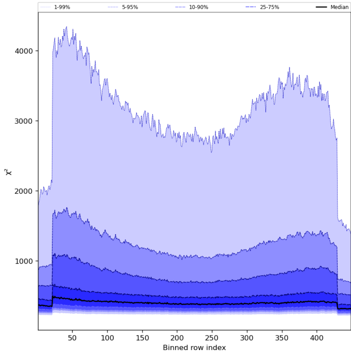
Figure 59: Along track statistics of “ \chi^2 ” for 2024-02-11 to 2024-02-13
