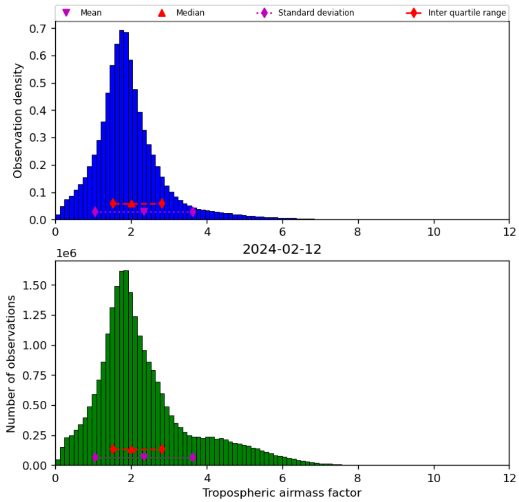
Figure 31: Histogram of “Tropospheric airmass factor” for 2024-02-11 to 2024-02-13
