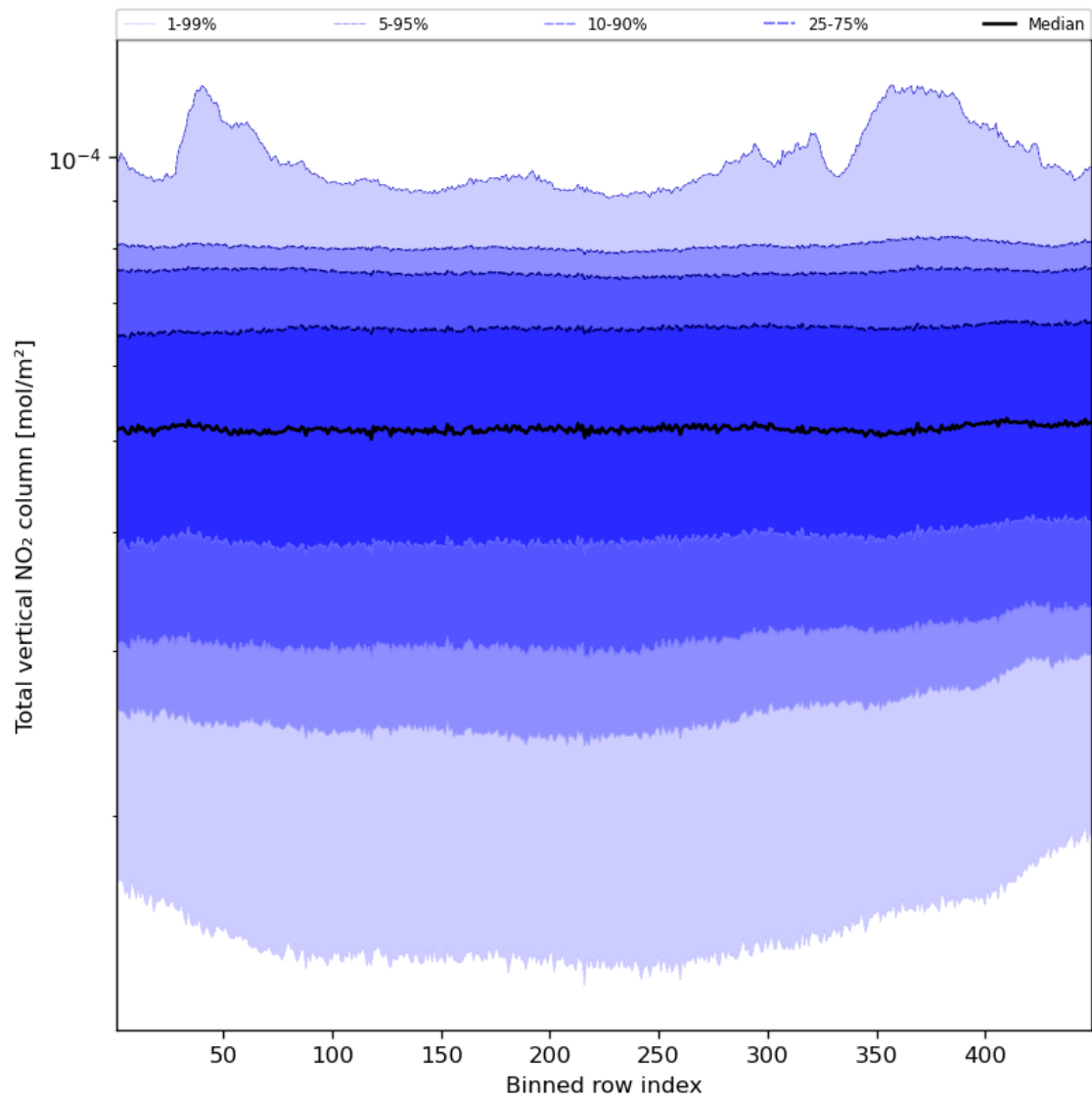
Figure 55: Along track statistics of “Total vertical NO 2 column” for 2024-02-11 to 2024-02-13
