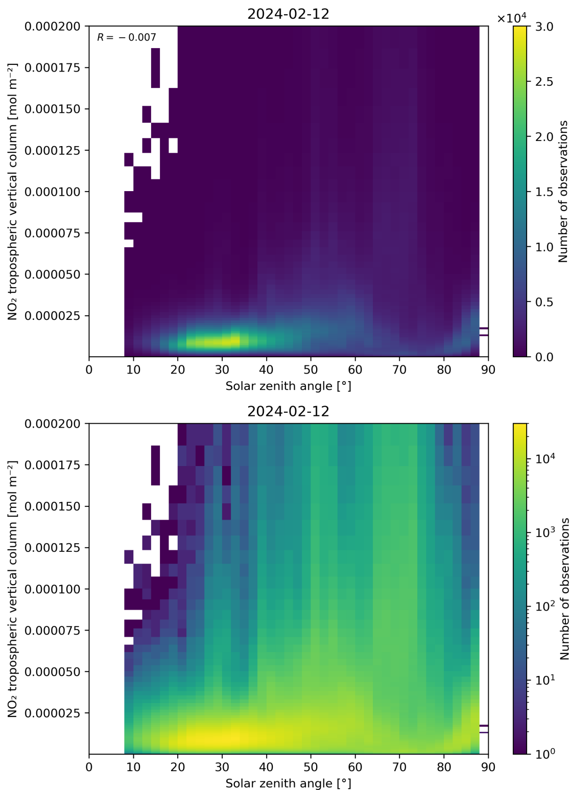
Figure 155: Scatter density plot of “Solar zenith angle” against “NO 2 tropospheric vertical column” for 2024-02-11 to 2024-02-13.
