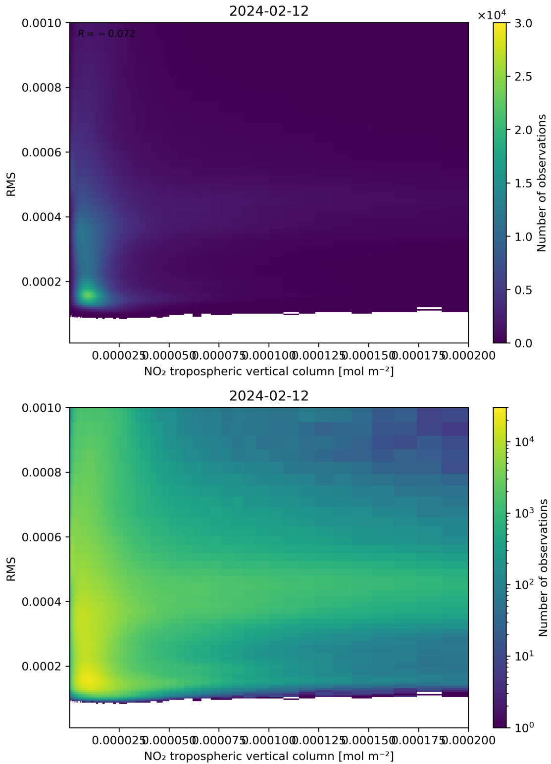
Figure 142: Scatter density plot of “NO 2 tropospheric vertical column” against “RMS” for 2024-02-11 to 2024-02-13.
