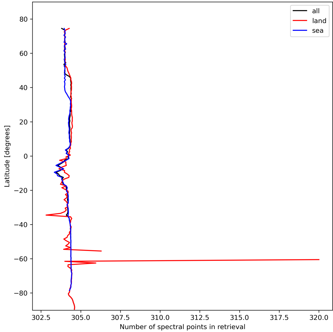
Figure 16: Zonal average of “Number of spectral points in retrieval” for 2024-02-11 to 2024-02-13.
