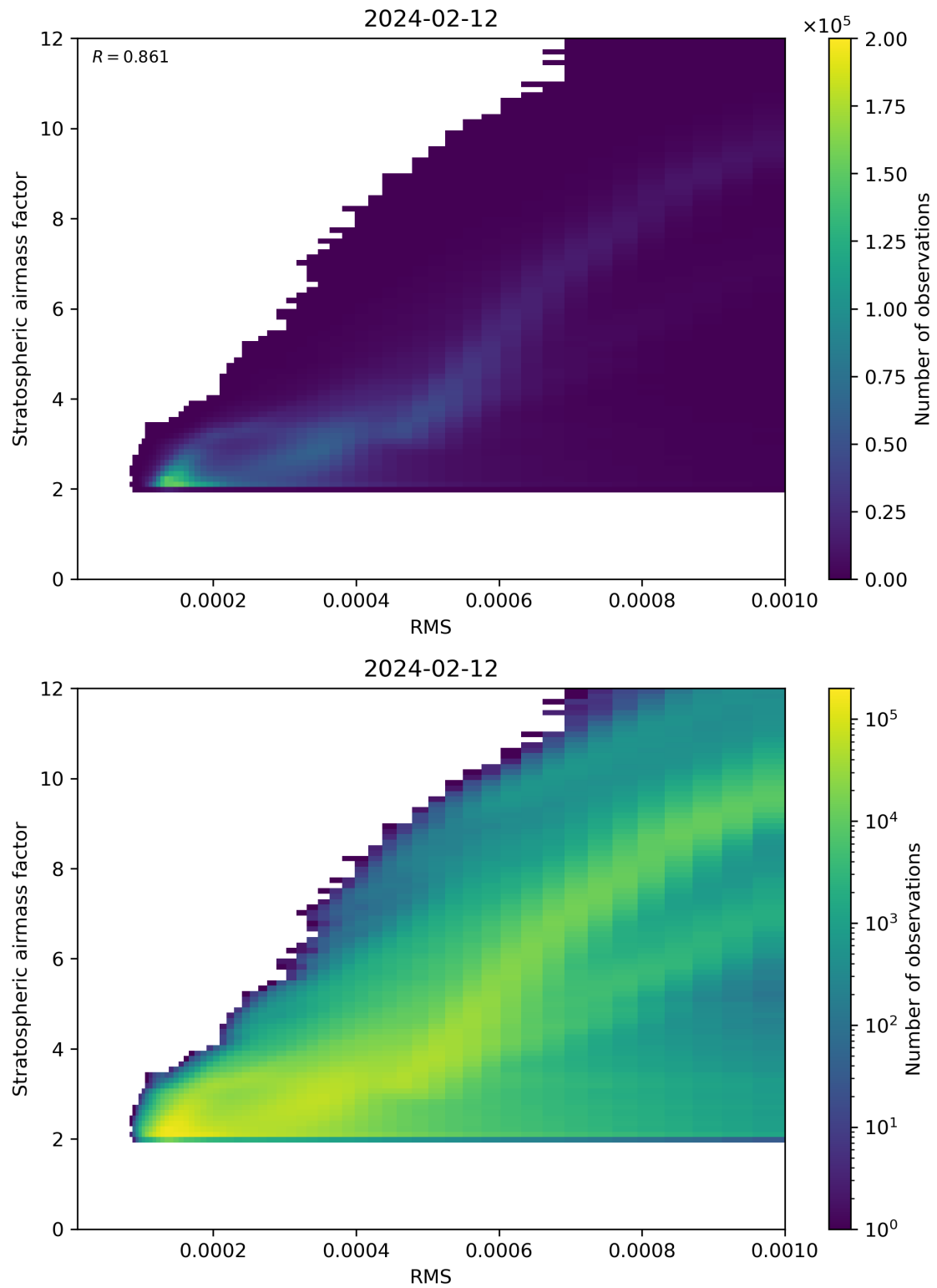
Figure 144: Scatter density plot of “RMS” against “Stratospheric airmass factor” for 2024-02-11 to 2024-02-13.
