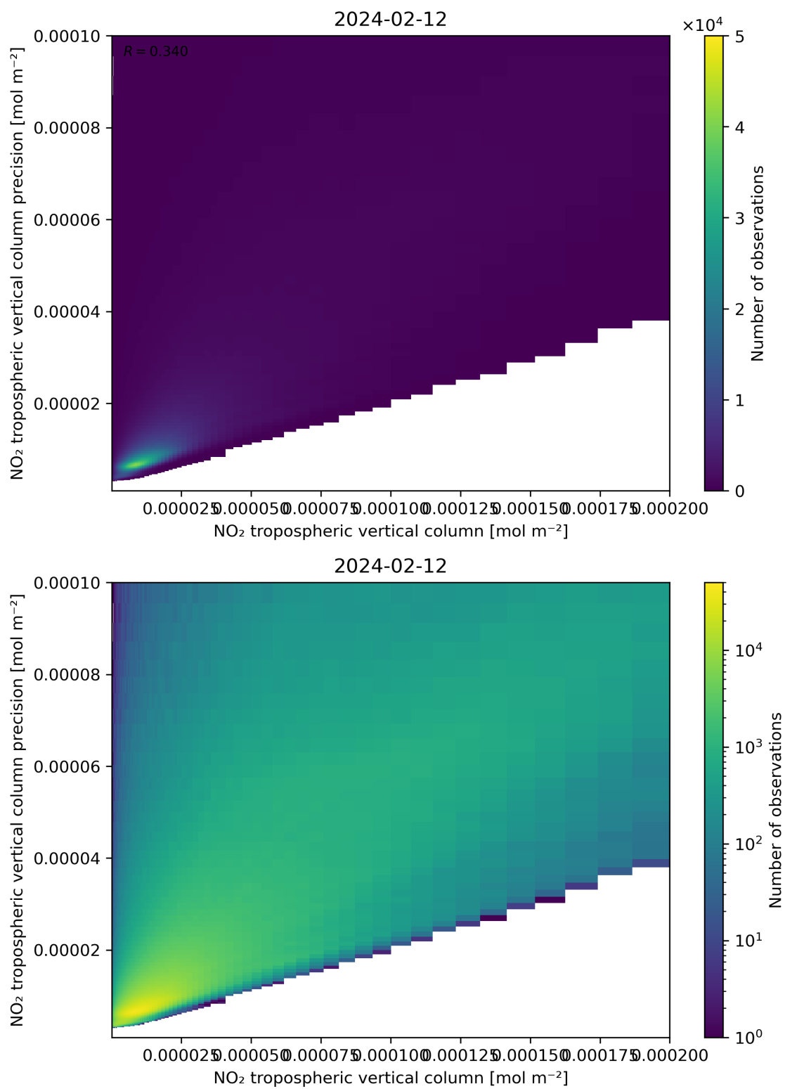
Figure 130: Scatter density plot of “NO 2 tropospheric vertical column” against “NO 2 tropospheric vertical column precision” for 2024-02-11 to 2024-02-13.
