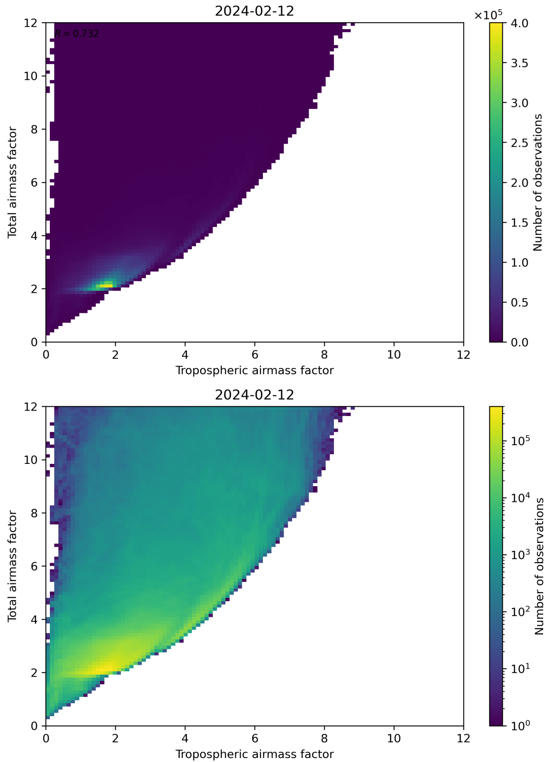
Figure 72: Scatter density plot of “Tropospheric airmass factor” against “Total airmass factor” for 2024-02-11 to 2024-02-13.
