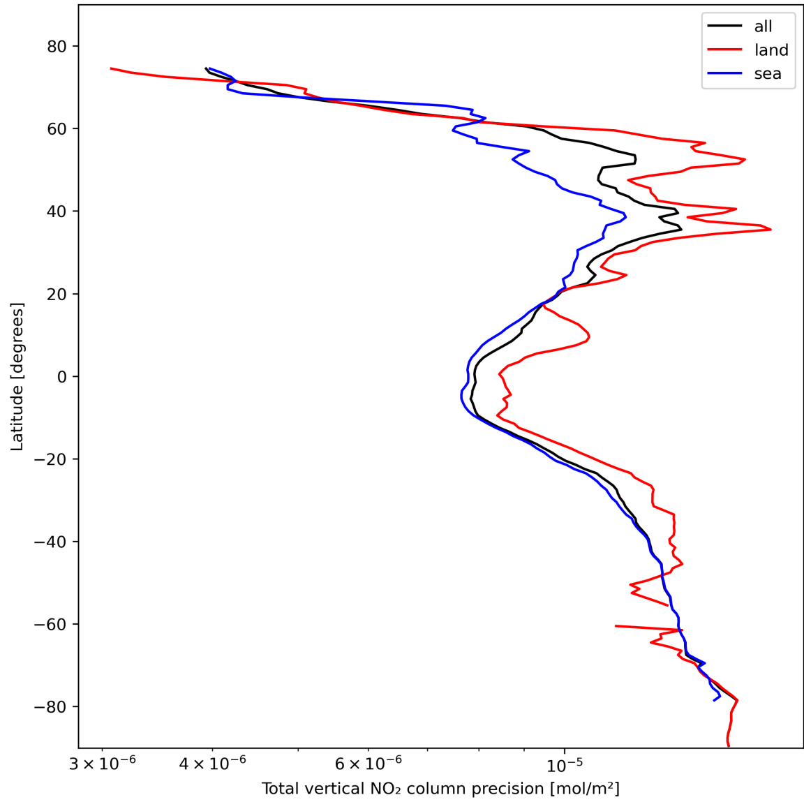
Figure 22: Zonal average of “Total vertical NO 2 column precision” for 2024-02-11 to 2024-02-13.
