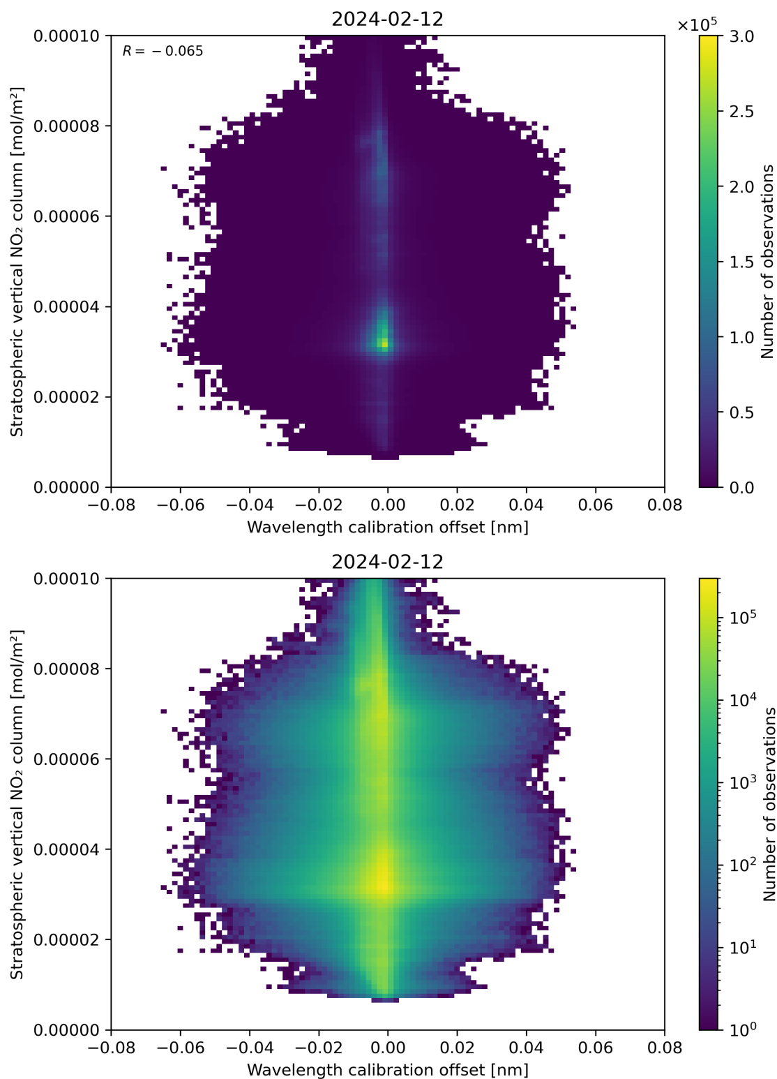
Figure 176: Scatter density plot of “Wavelength calibration offset” against “Stratospheric vertical NO 2 column” for 2024-02-11 to 2024-02-13.
