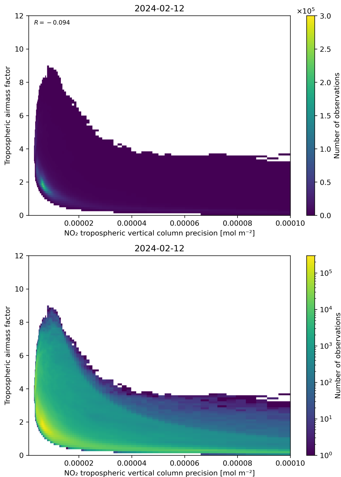
Figure 133: Scatter density plot of “NO 2 tropospheric vertical column precision” against “Tropospheric airmass factor” for 2024-02-11 to 2024-02-13.
