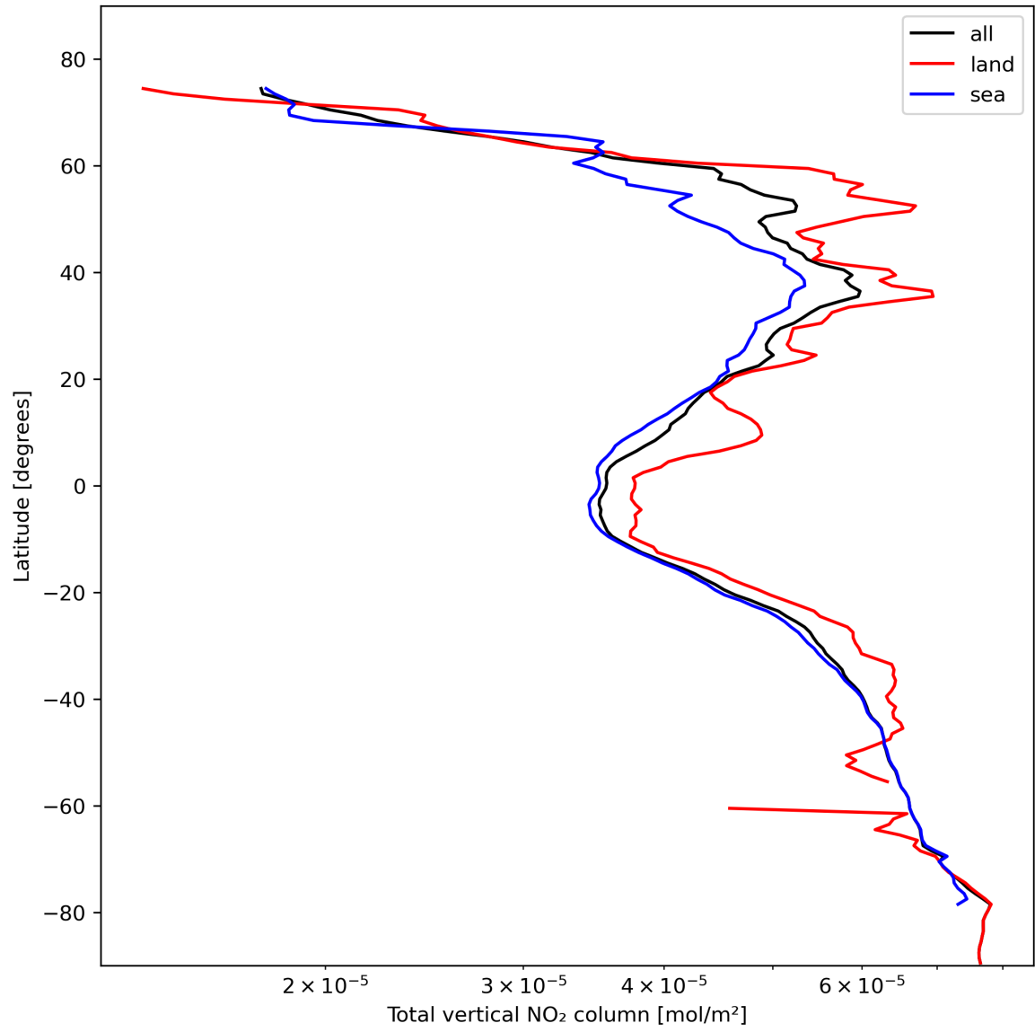
Figure 21: Zonal average of “Total vertical NO 2 column” for 2024-02-11 to 2024-02-13.
