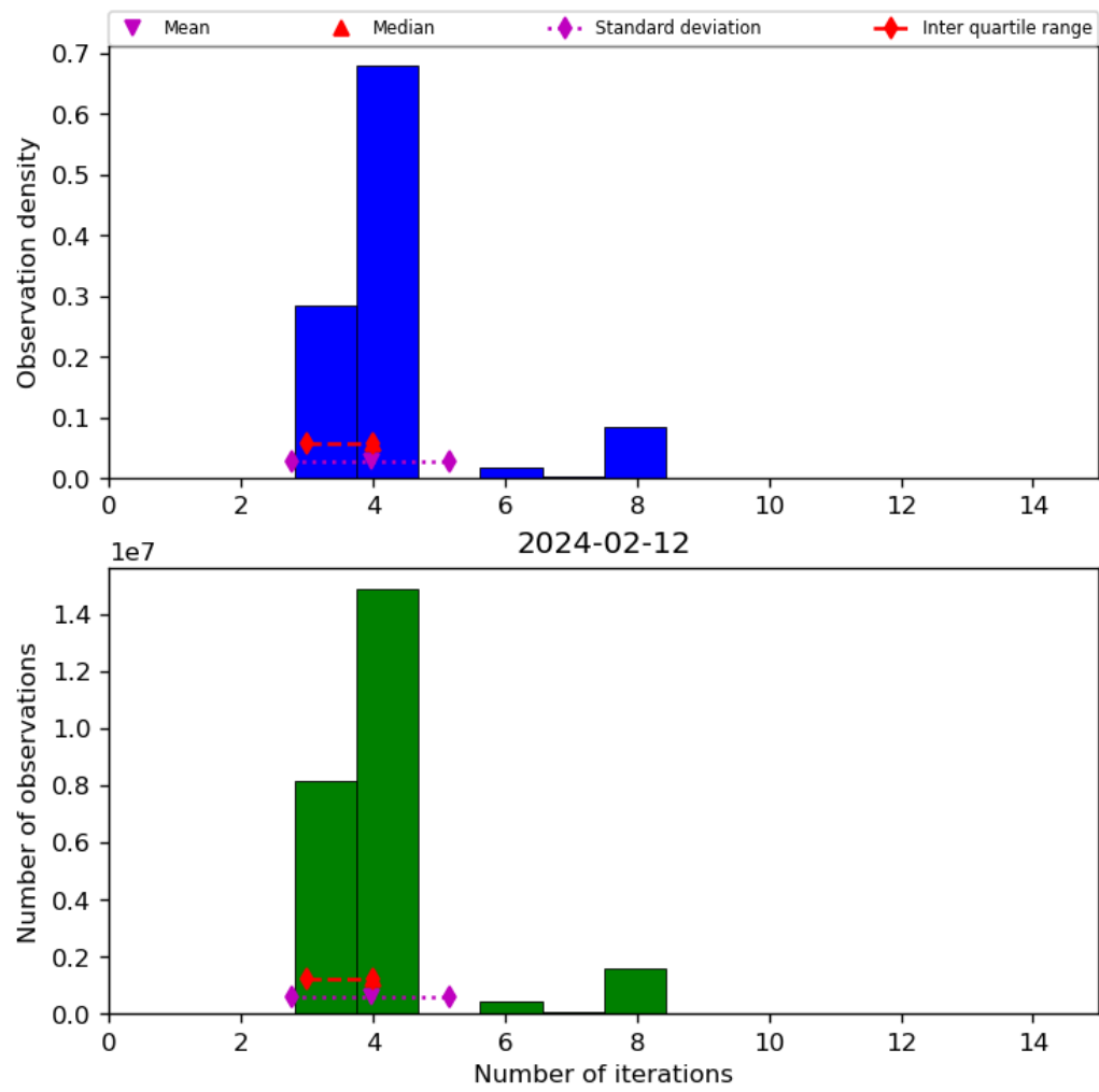
Figure 34: Histogram of “Number of iterations” for 2024-02-11 to 2024-02-13
