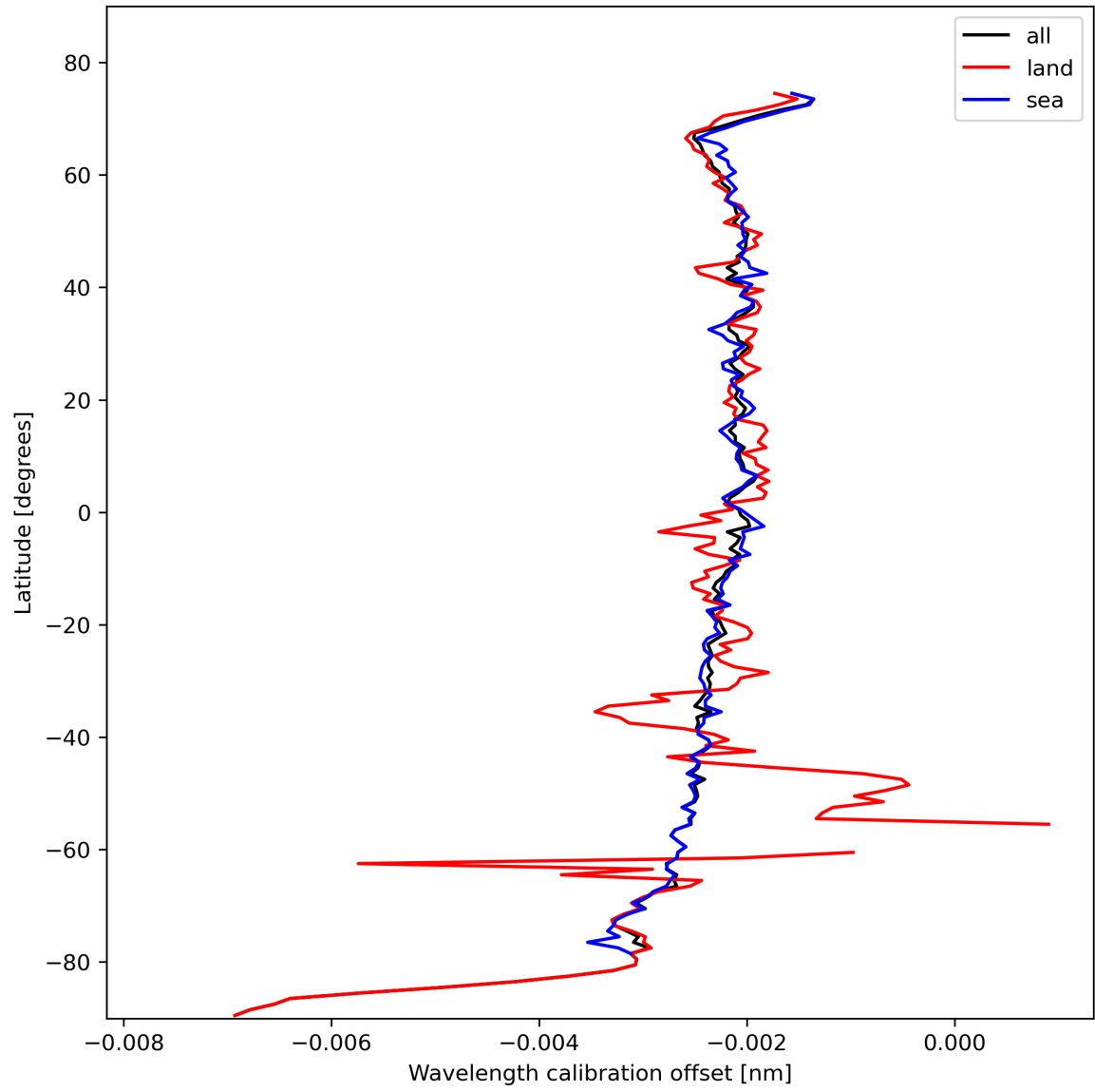
Figure 18: Zonal average of “Wavelength calibration offset” for 2024-02-11 to 2024-02-13.
