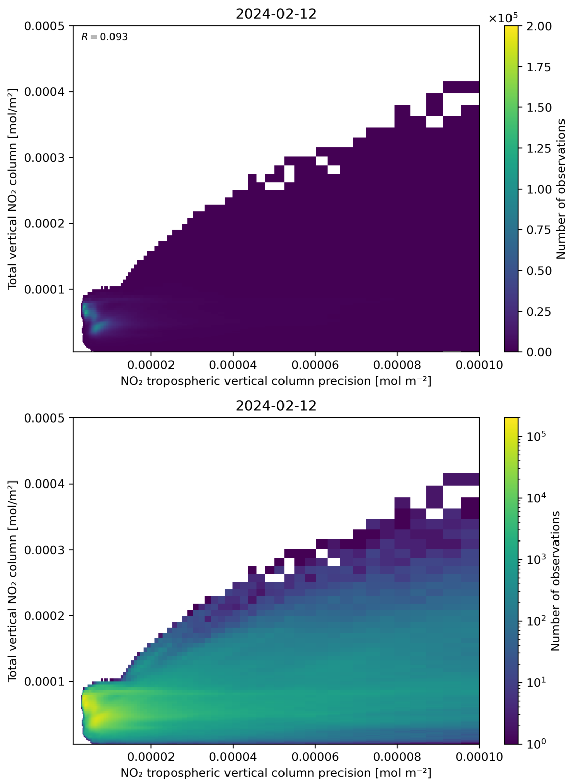
Figure 138: Scatter density plot of “NO 2 tropospheric vertical column precision” against “Total vertical NO 2 column” for 2024-02-11 to 2024-02-13.
