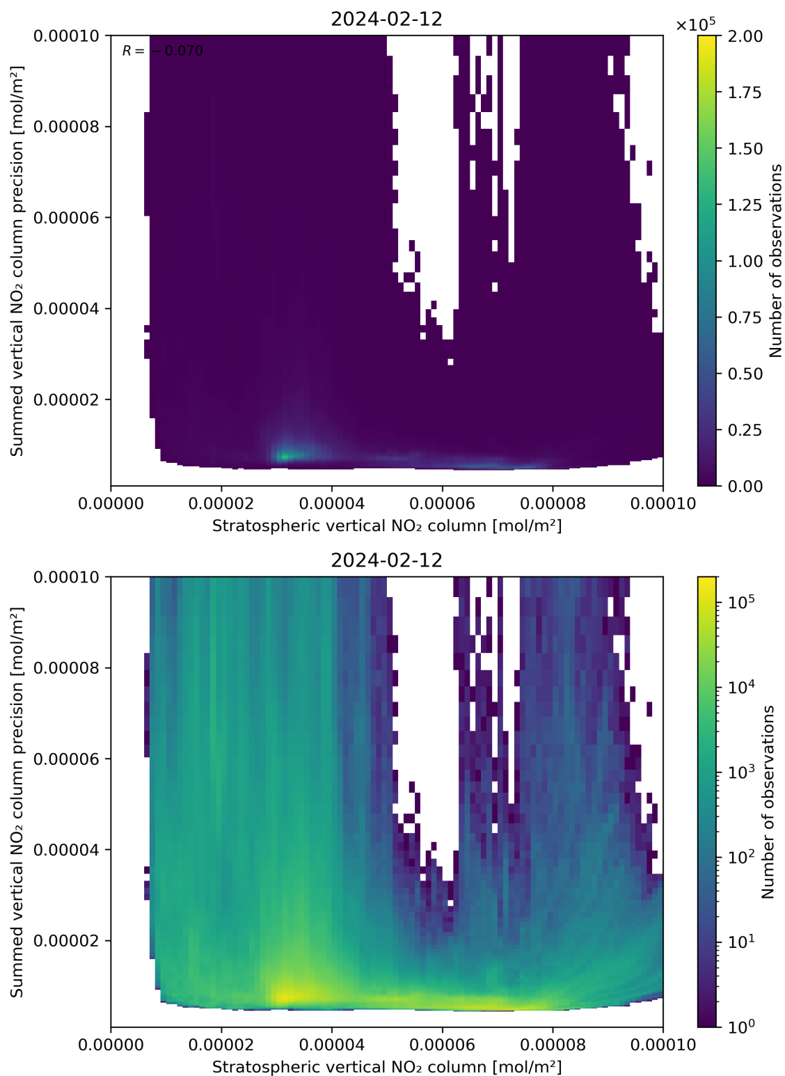
Figure 99: Scatter density plot of “Stratospheric vertical NO 2 column” against “Summed vertical NO 2 column precision” for 2024-02-11 to 2024-02-13.
