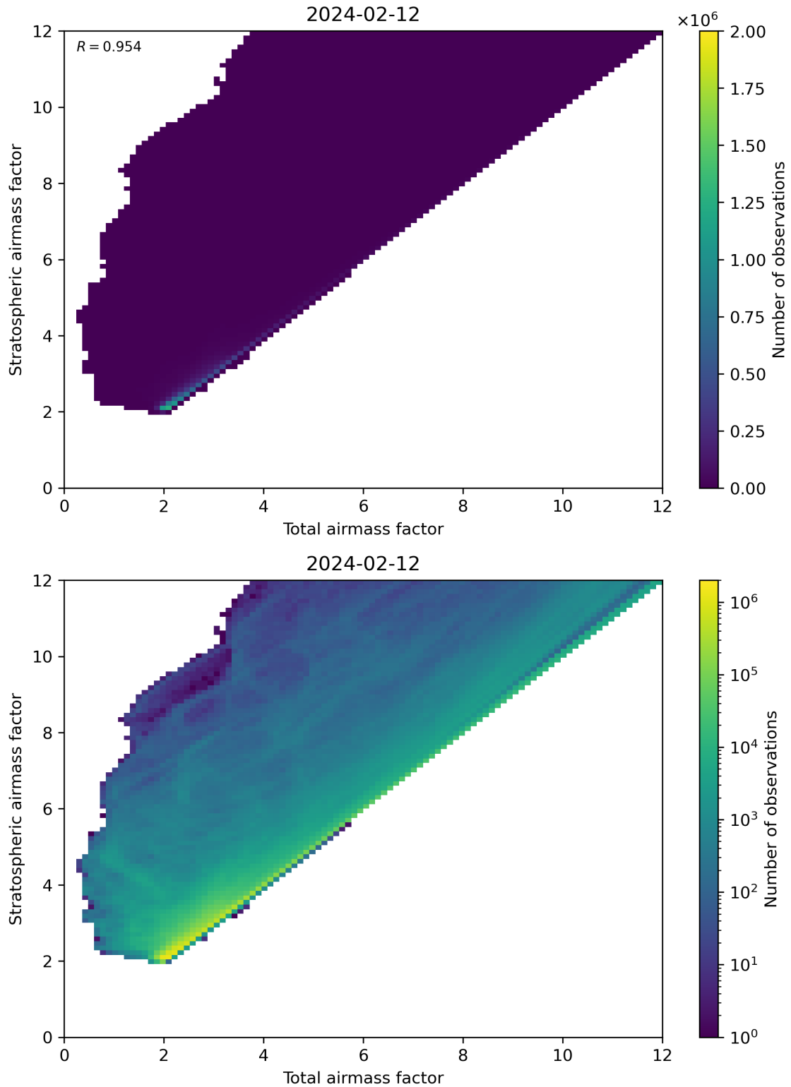
Figure 62: Scatter density plot of “Total airmass factor” against “Stratospheric airmass factor” for 2024-02-11 to 2024-02-13.
