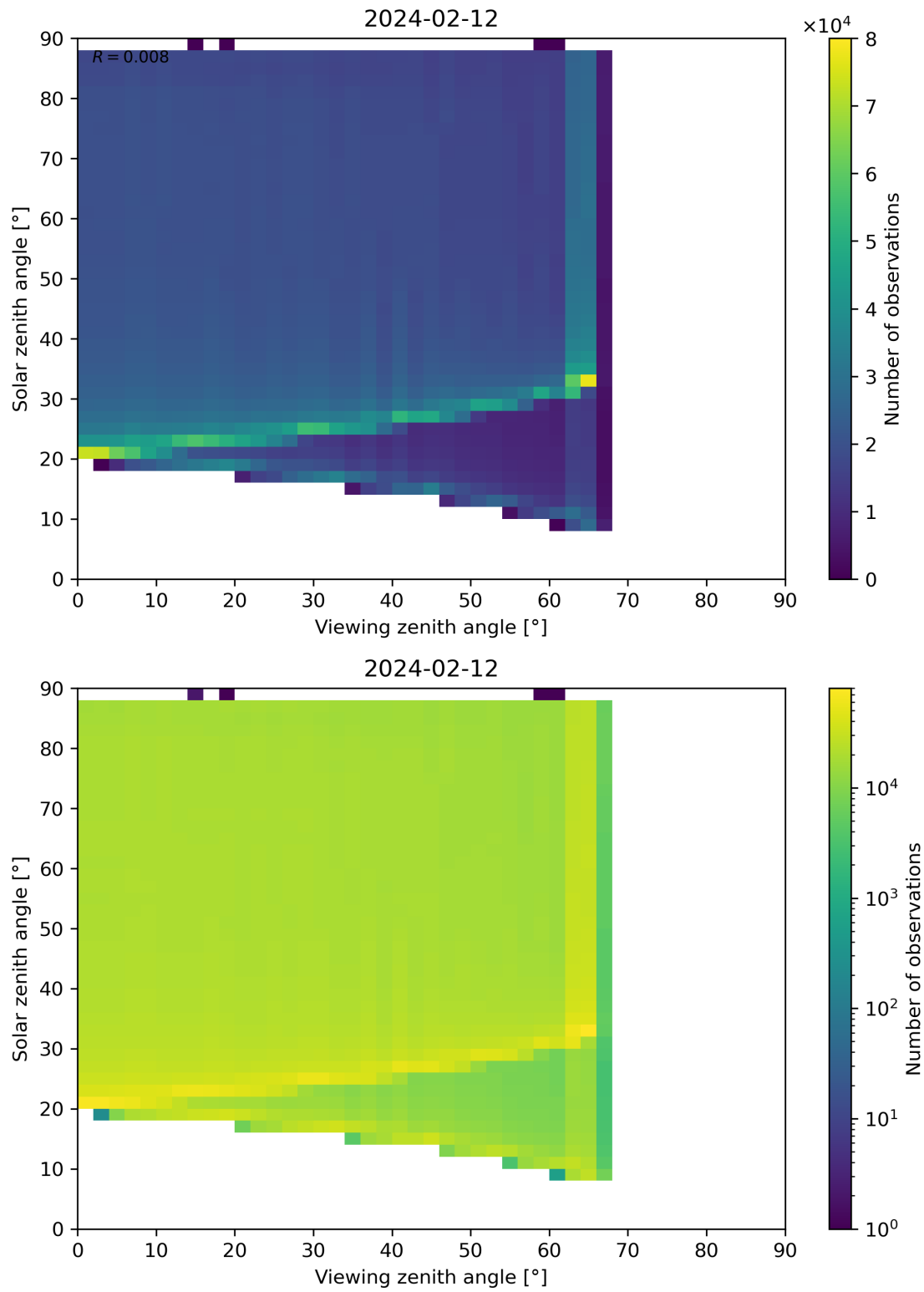
Figure 172: Scatter density plot of “Viewing zenith angle” against “Solar zenith angle” for 2024-02-11 to 2024-02-13.
