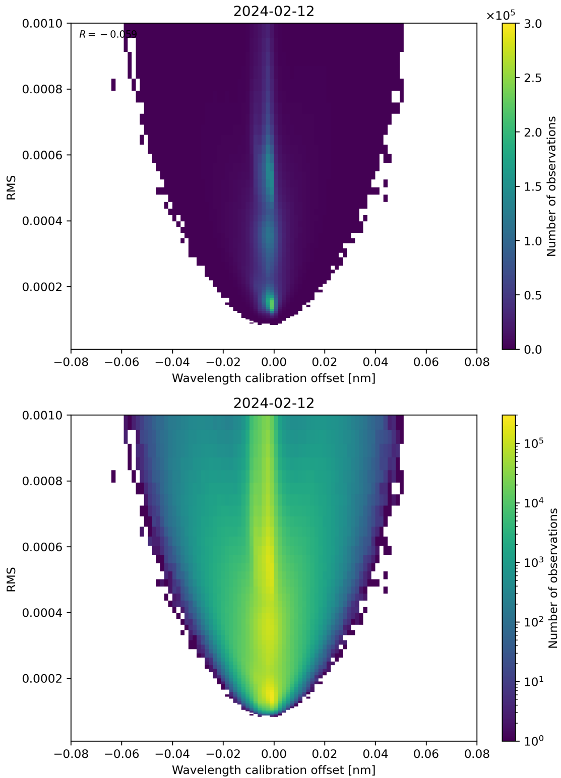
Figure 181: Scatter density plot of “Wavelength calibration offset” against “RMS” for 2024-02-11 to 2024-02-13.
