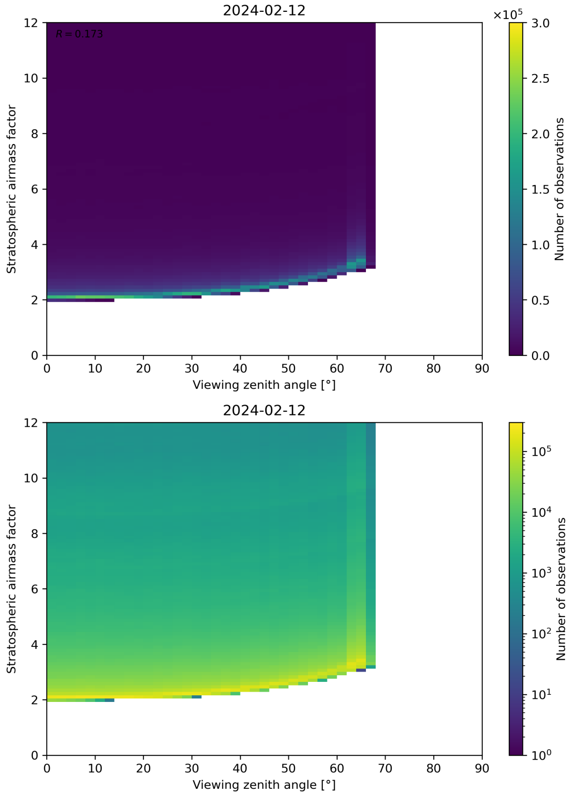
Figure 159: Scatter density plot of “Viewing zenith angle” against “Stratospheric airmass factor” for 2024-02-11 to 2024-02-13.
