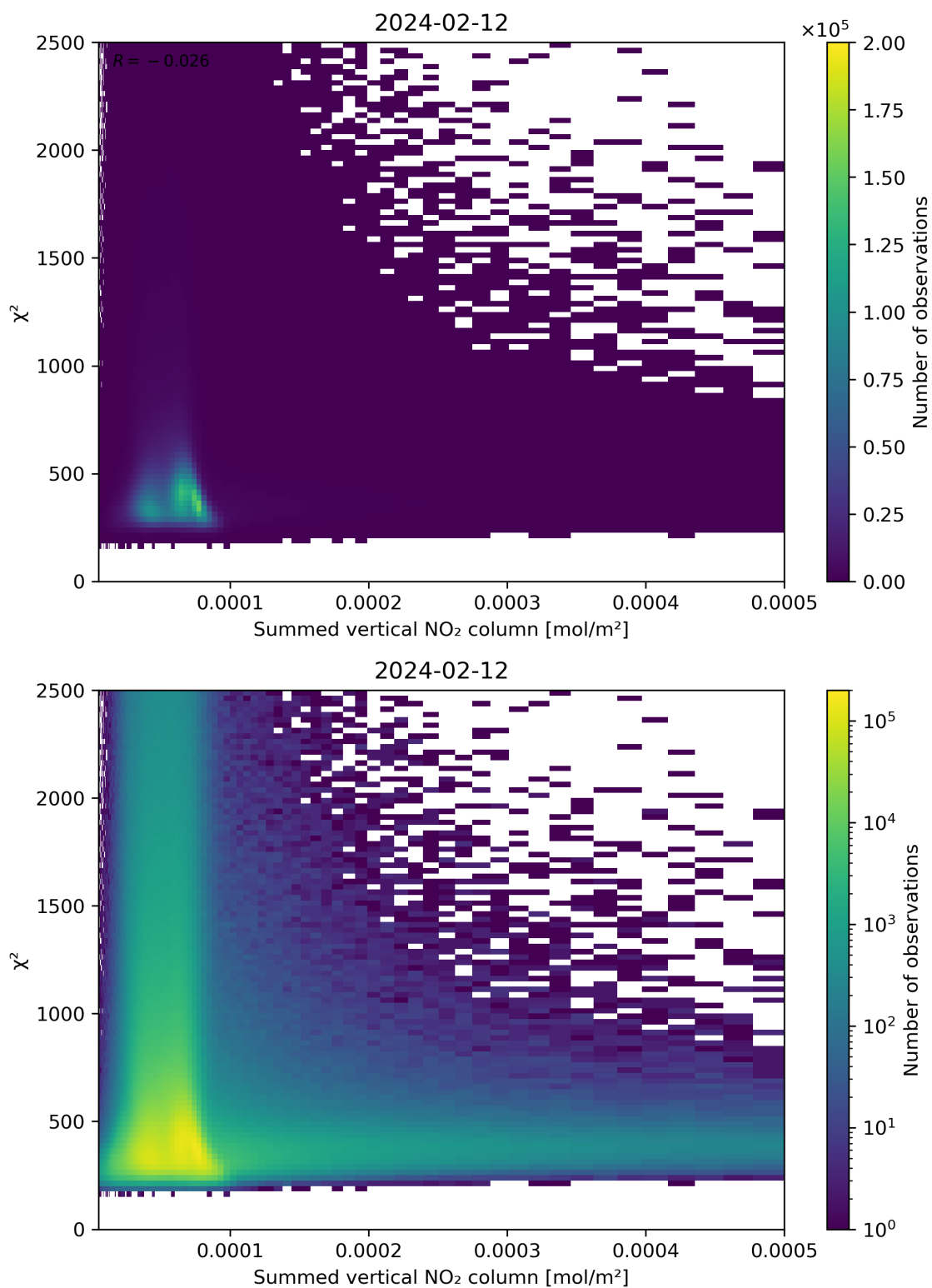
Figure 104: Scatter density plot of “Summed vertical NO 2 column” against “ \chi^2 ” for 2024-02-11 to 2024-02-13.
