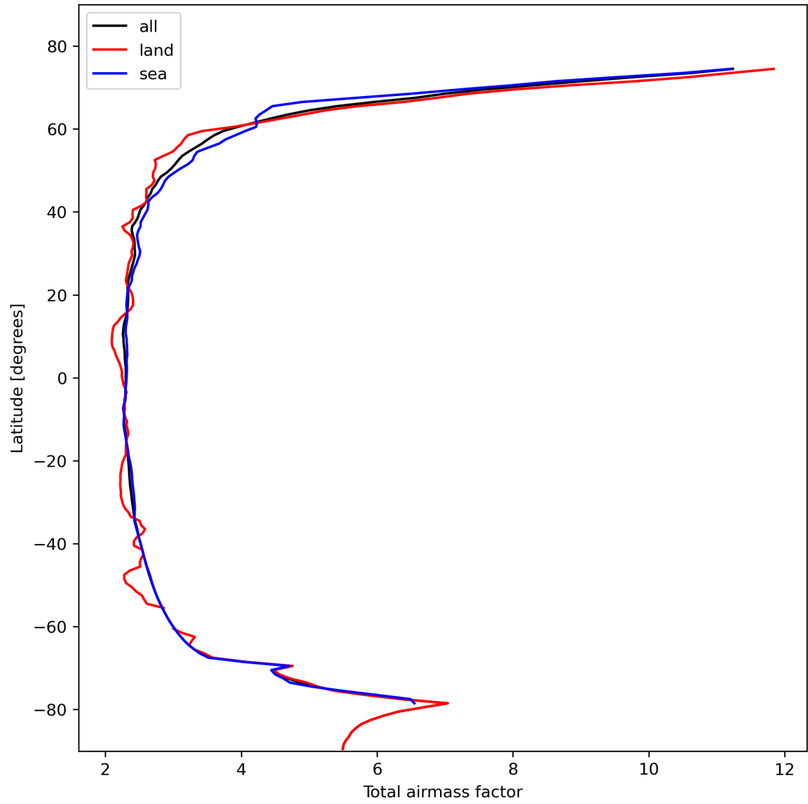
Figure 15: Zonal average of “Total airmass factor” for 2024-02-11 to 2024-02-13.
