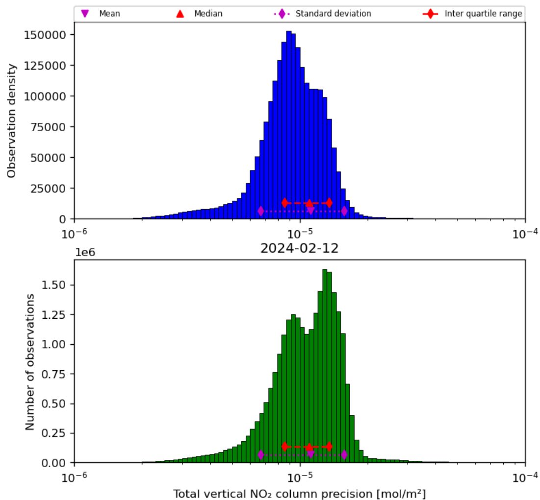
Figure 39: Histogram of “Total vertical NO 2 column precision” for 2024-02-11 to 2024-02-13
