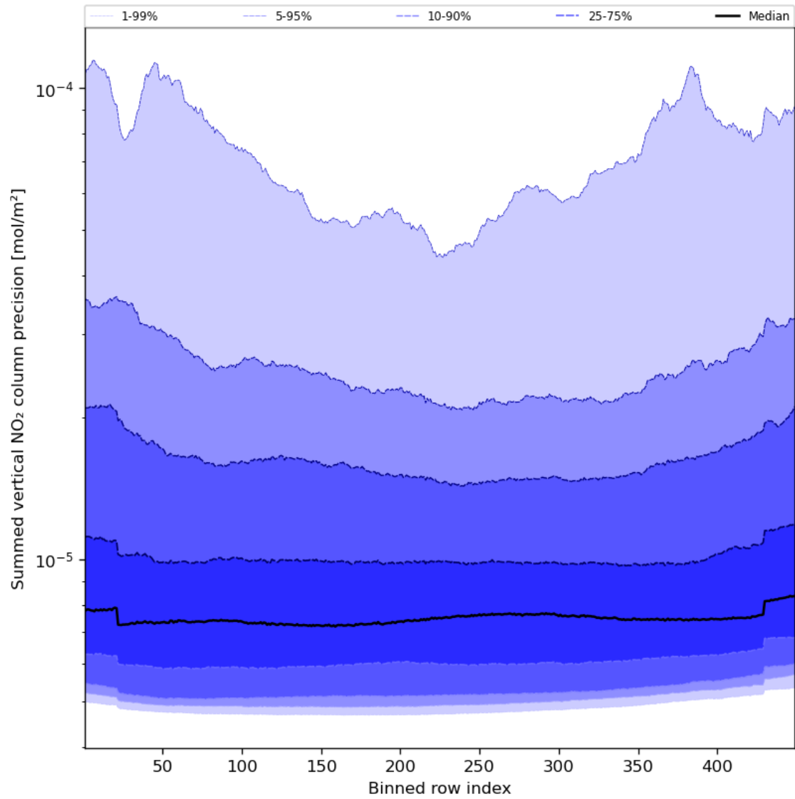
Figure 58: Along track statistics of “Summed vertical NO 2 column precision” for 2024-02-11 to 2024-02-13
