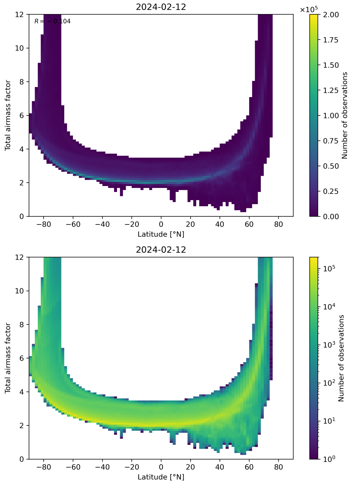
Figure 84: Scatter density plot of “Latitude” against “Total airmass factor” for 2024-02-11 to 2024-02-13.
