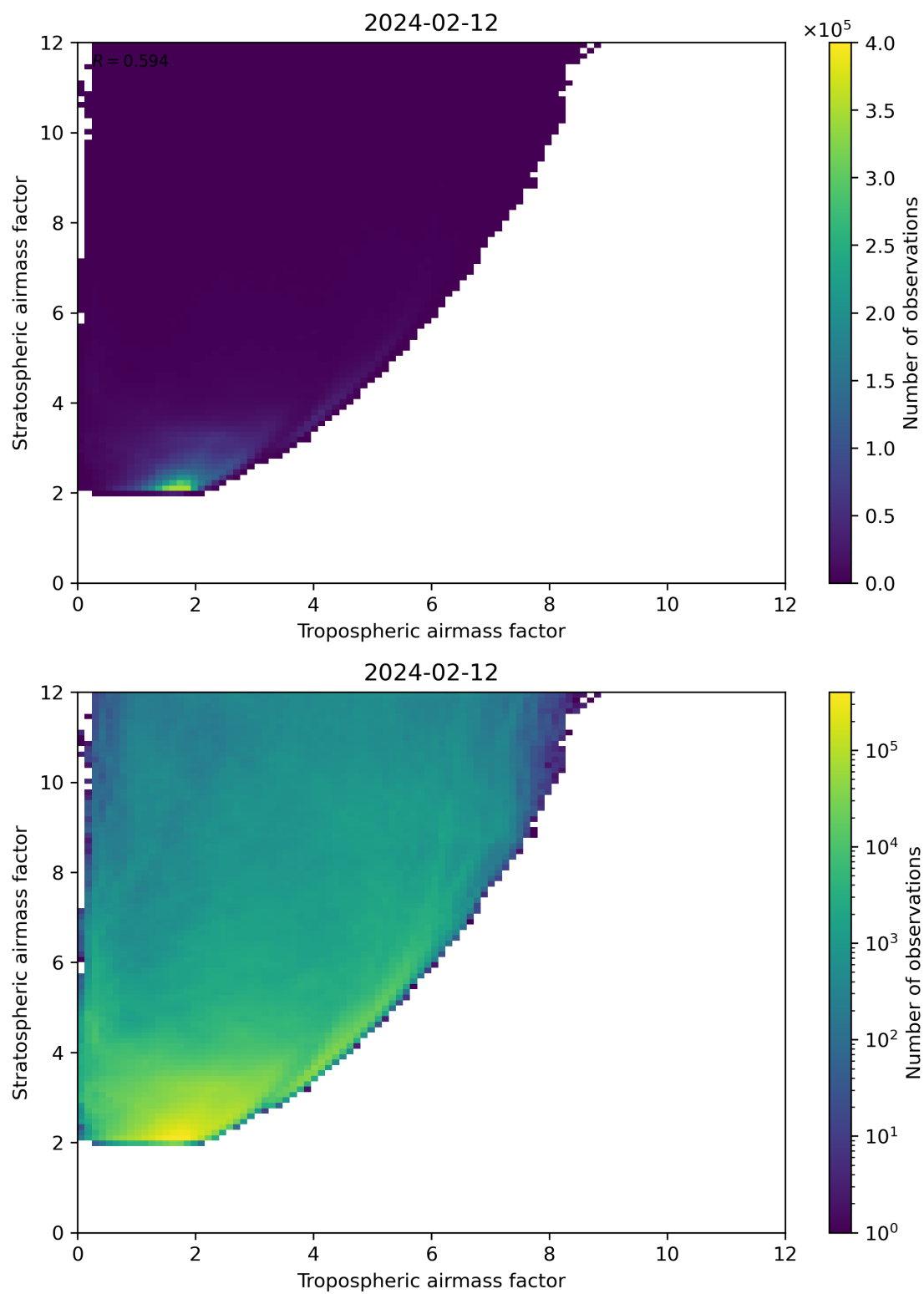
Figure 71: Scatter density plot of “Tropospheric airmass factor” against “Stratospheric airmass factor” for 2024-02-11 to 2024-02-13.
