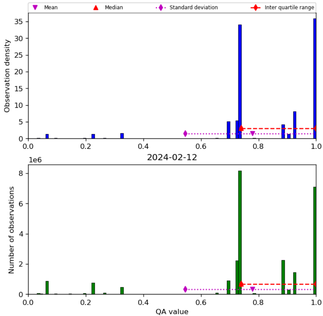
Figure 28: Histogram of “QA value” for 2024-02-11 to 2024-02-13
