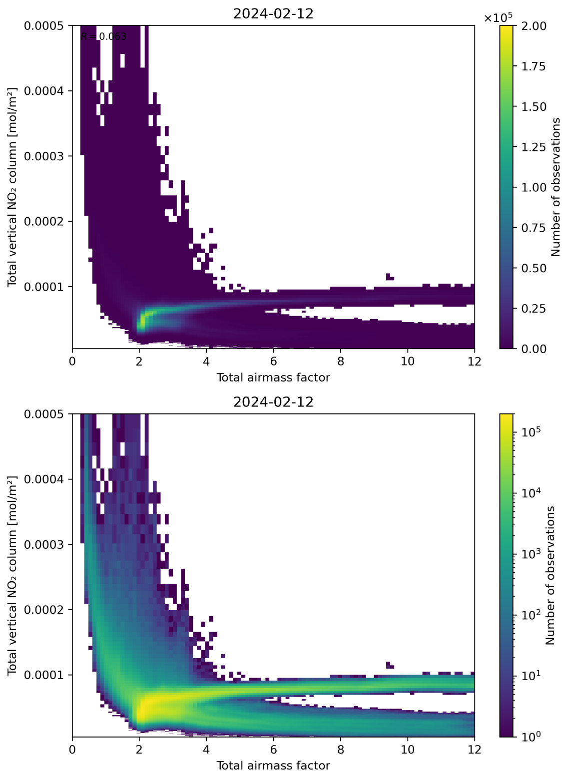
Figure 67: Scatter density plot of “Total airmass factor” against “Total vertical NO 2 column” for 2024-02-11 to 2024-02-13.
