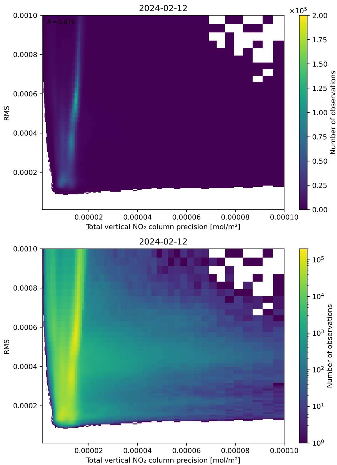
Figure 119: Scatter density plot of “Total vertical NO 2 column precision” against “RMS” for 2024-02-11 to 2024-02-13.
