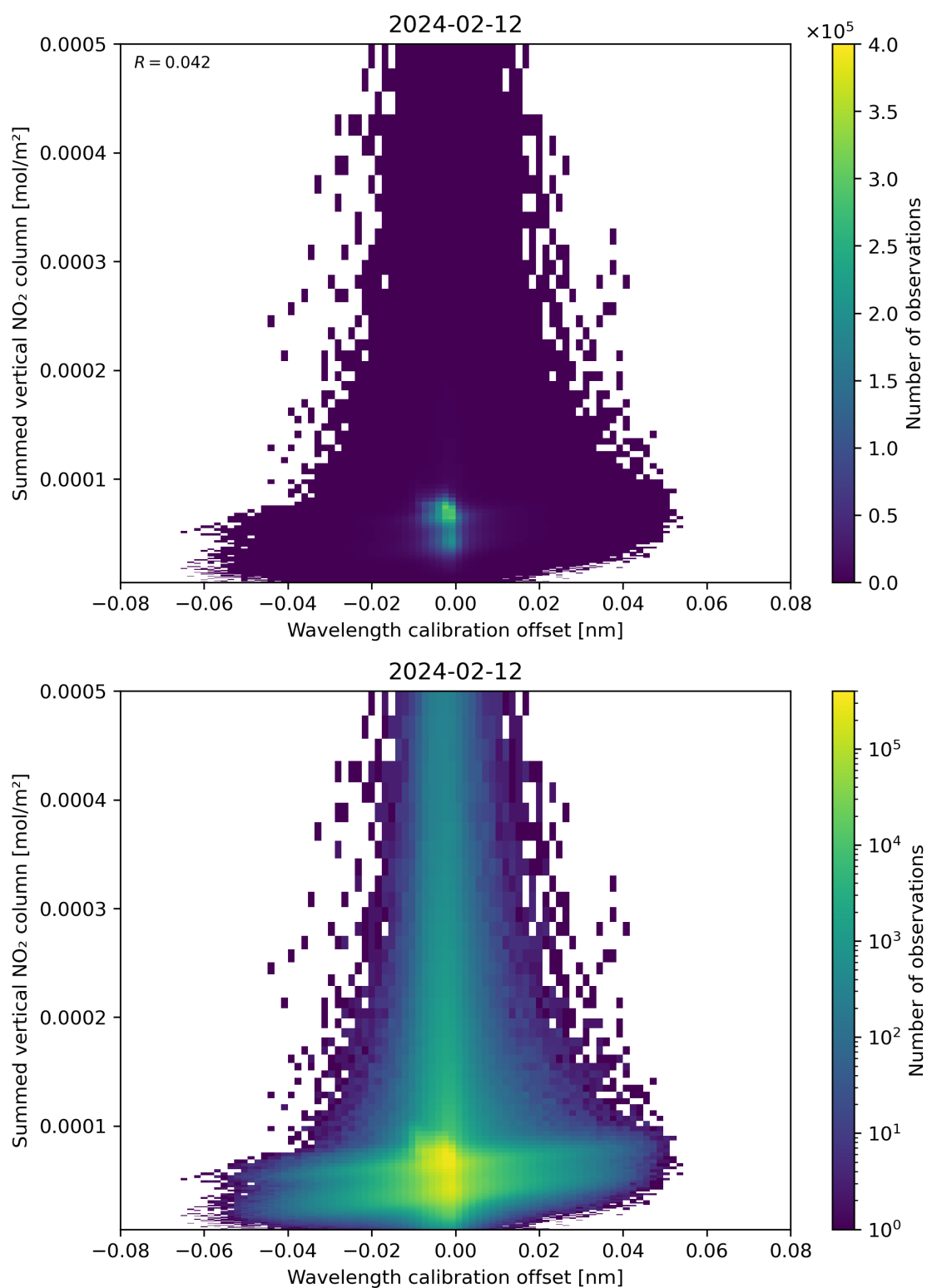
Figure 177: Scatter density plot of “Wavelength calibration offset” against “Summed vertical NO 2 column” for 2024-02-11 to 2024-02-13.
