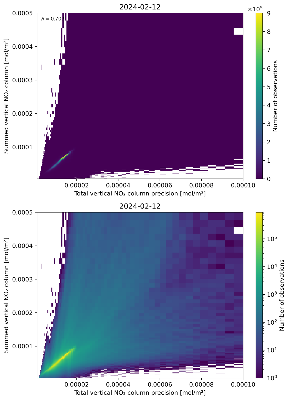
Figure 117: Scatter density plot of “Total vertical NO 2 column precision” against “Summed vertical NO 2 column” for 2024-02-11 to 2024-02-13.
