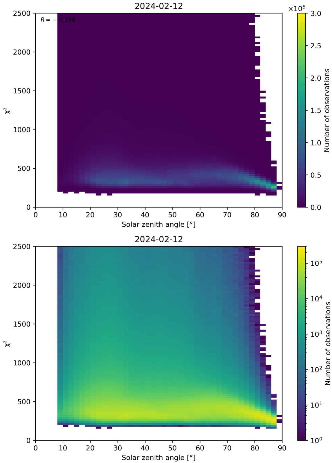
Figure 148: Scatter density plot of “Solar zenith angle” against “ \chi^2 ” for 2024-02-11 to 2024-02-13.
