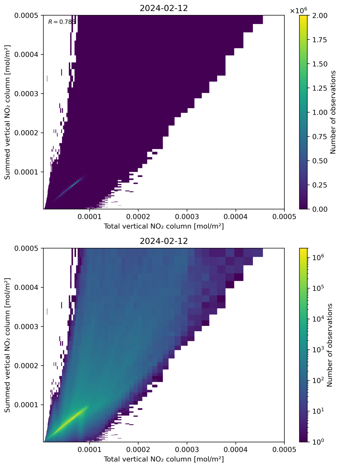
Figure 112: Scatter density plot of “Total vertical NO 2 column” against “Summed vertical NO 2 column” for 2024-02-11 to 2024-02-13.
