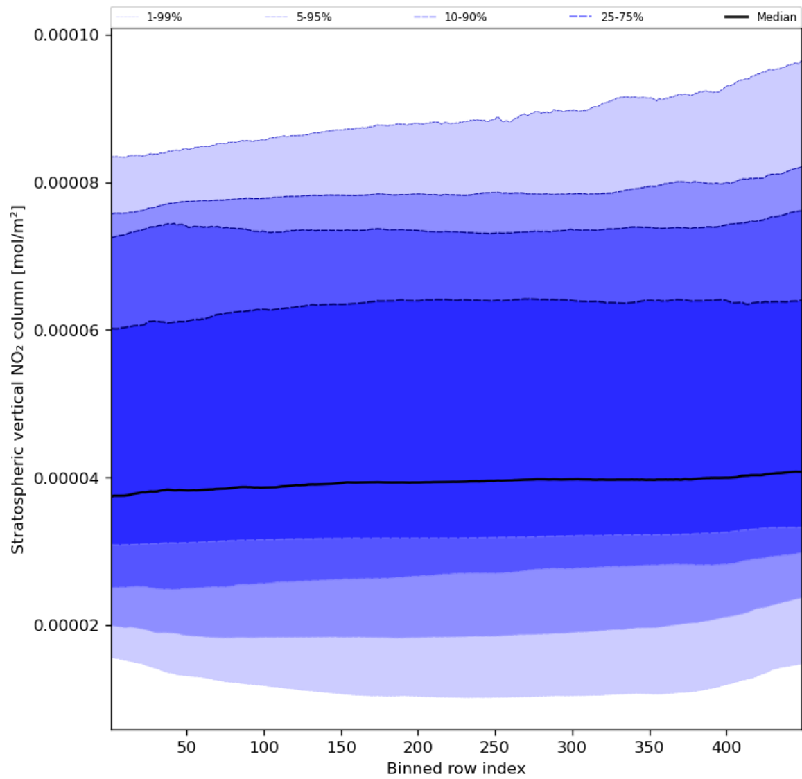
Figure 53: Along track statistics of “Stratospheric vertical NO 2 column” for 2024-02-11 to 2024-02-13
