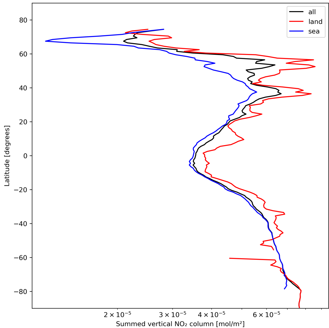
Figure 23: Zonal average of “Summed vertical NO 2 column” for 2024-02-11 to 2024-02-13.
