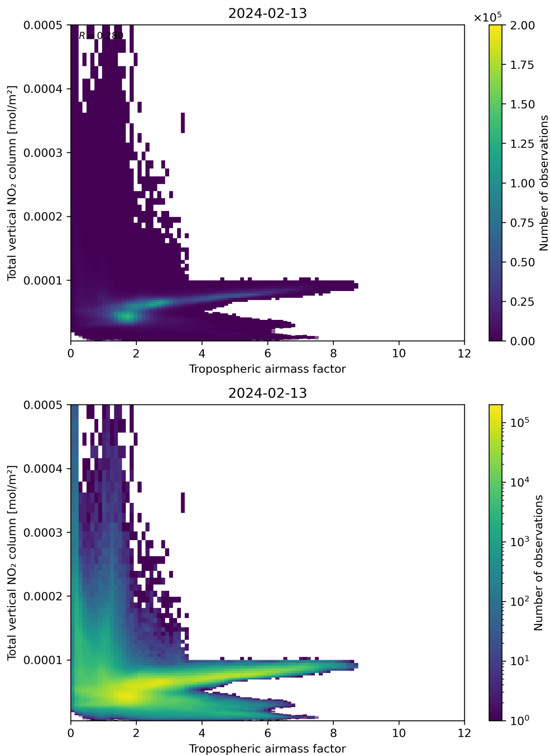
Figure 77: Scatter density plot of “Tropospheric airmass factor” against “Total vertical NO 2 column” for 2024-02-12 to 2024-02-14.
