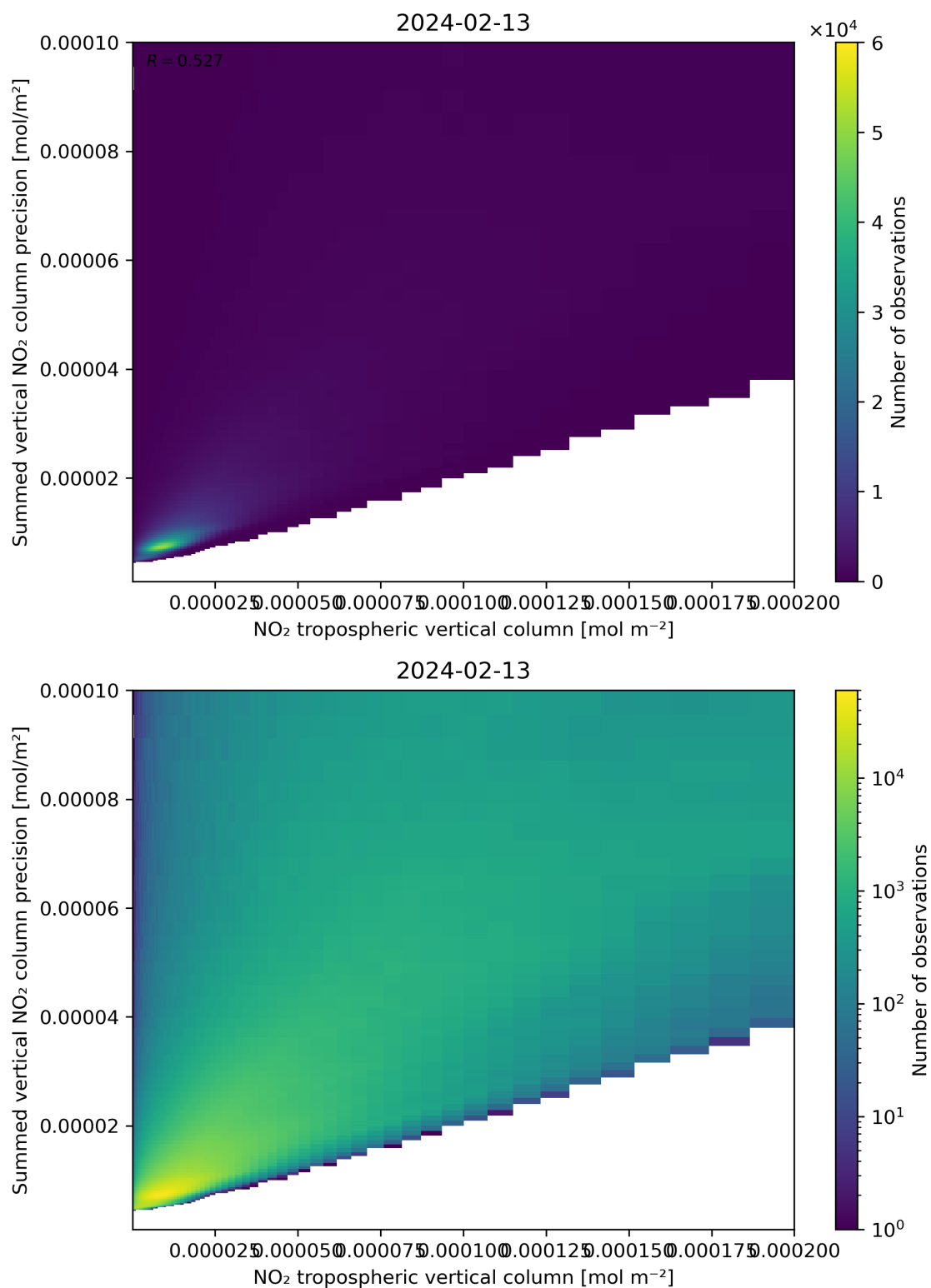
Figure 127: Scatter density plot of “NO 2 tropospheric vertical column” against “Summed vertical NO 2 column precision” for 2024-02-12 to 2024-02-14.
