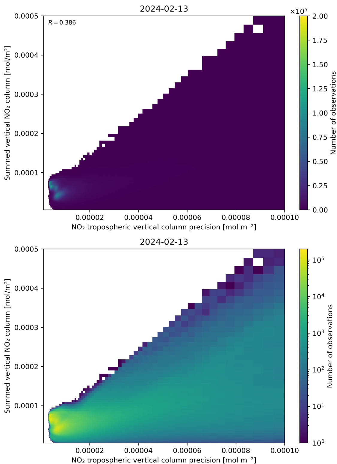
Figure 136: Scatter density plot of “NO 2 tropospheric vertical column precision” against “Summed vertical NO 2 column” for 2024-02-12 to 2024-02-14.
