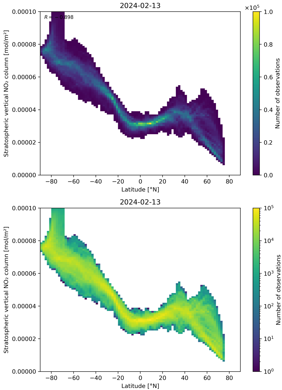
Figure 87: Scatter density plot of “Latitude” against “Stratospheric vertical NO 2 column” for 2024-02-12 to 2024-02-14.
