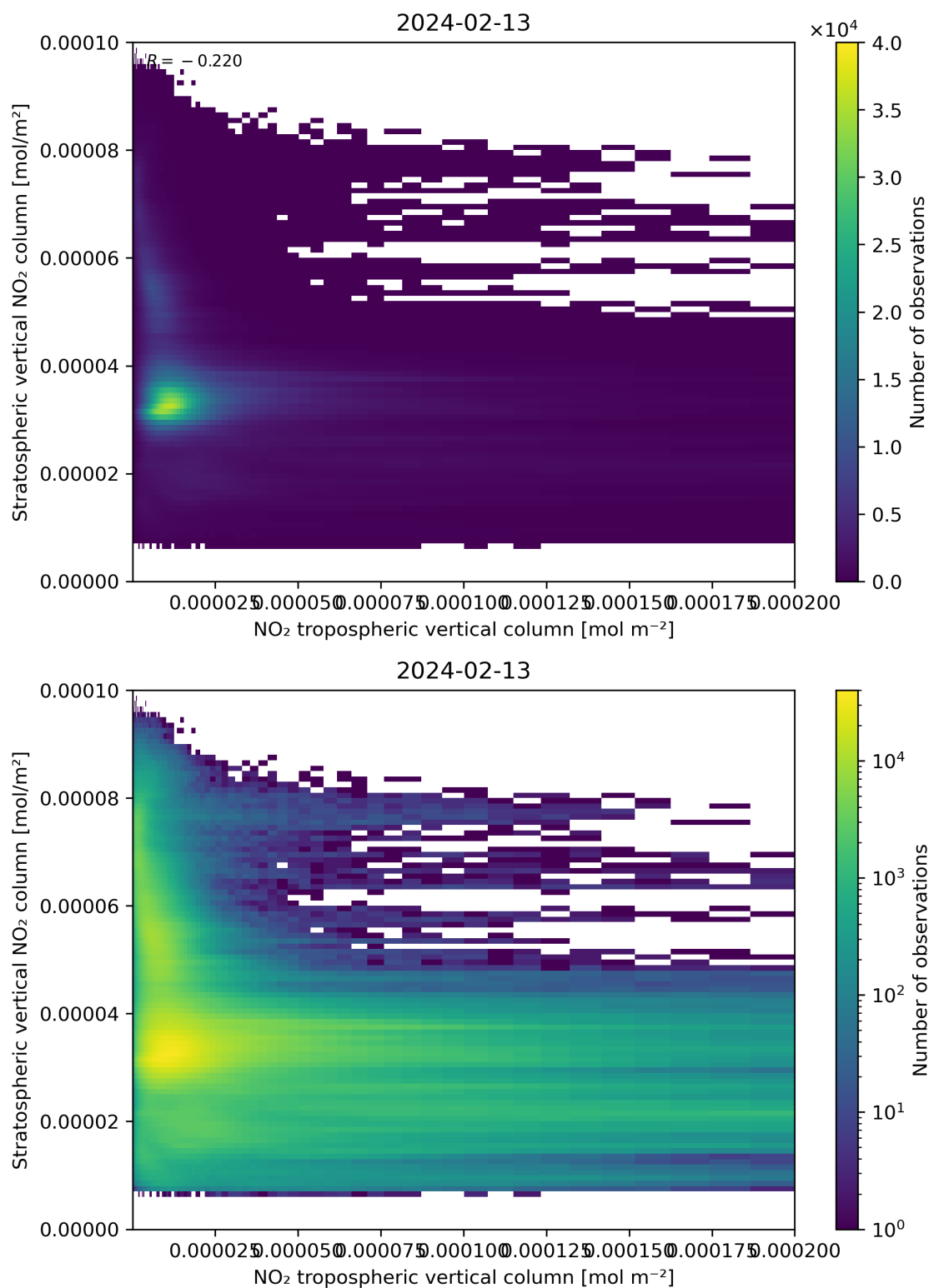
Figure 125: Scatter density plot of “NO 2 tropospheric vertical column” against “Stratospheric vertical NO 2 column” for 2024-02-12 to 2024-02-14.
