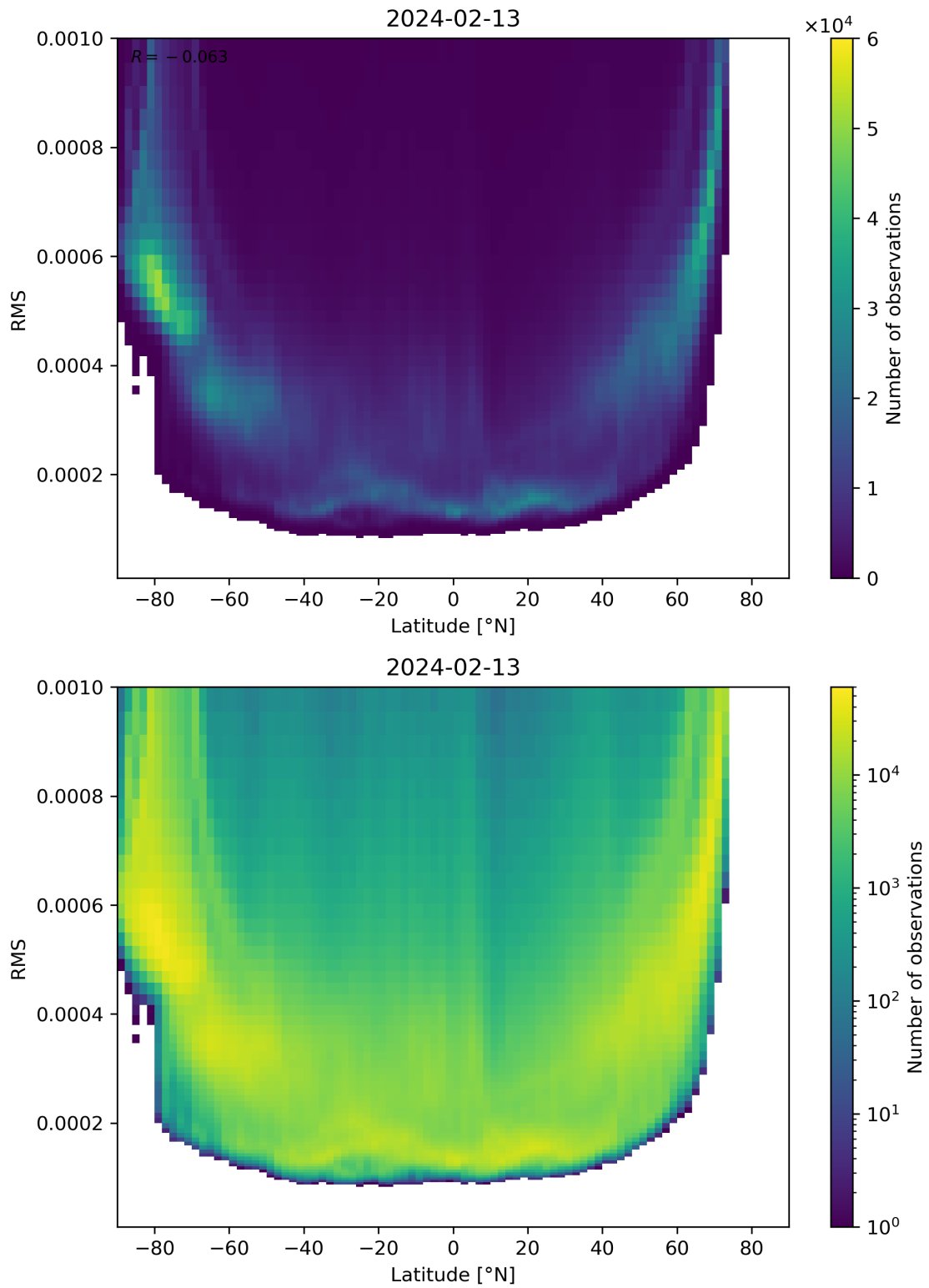
Figure 94: Scatter density plot of “Latitude” against “RMS” for 2024-02-12 to 2024-02-14.
