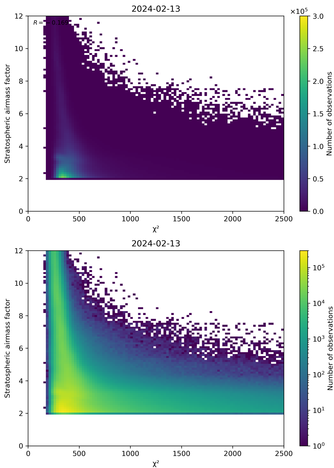
Figure 81: Scatter density plot of “ \chi^2 ” against “Stratospheric airmass factor” for 2024-02-12 to 2024-02-14.
