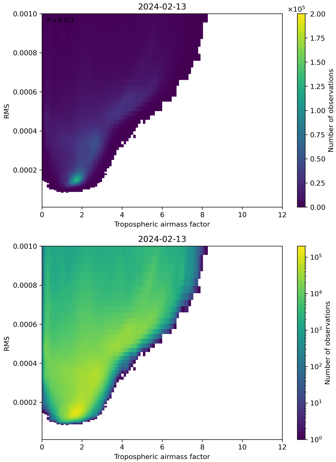
Figure 79: Scatter density plot of “Tropospheric airmass factor” against “RMS” for 2024-02-12 to 2024-02-14.
