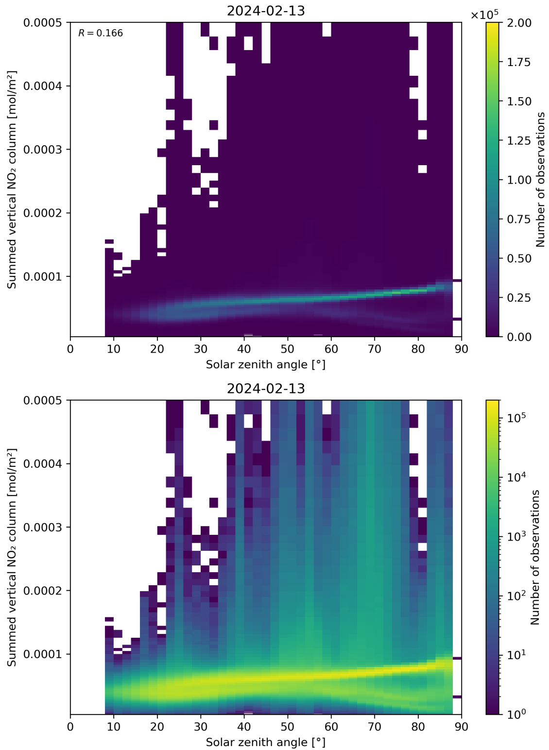
Figure 151: Scatter density plot of “Solar zenith angle” against “Summed vertical NO 2 column” for 2024-02-12 to 2024-02-14.
