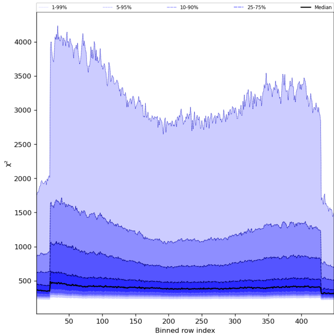
Figure 59: Along track statistics of “ \chi^2 ” for 2024-02-12 to 2024-02-14
