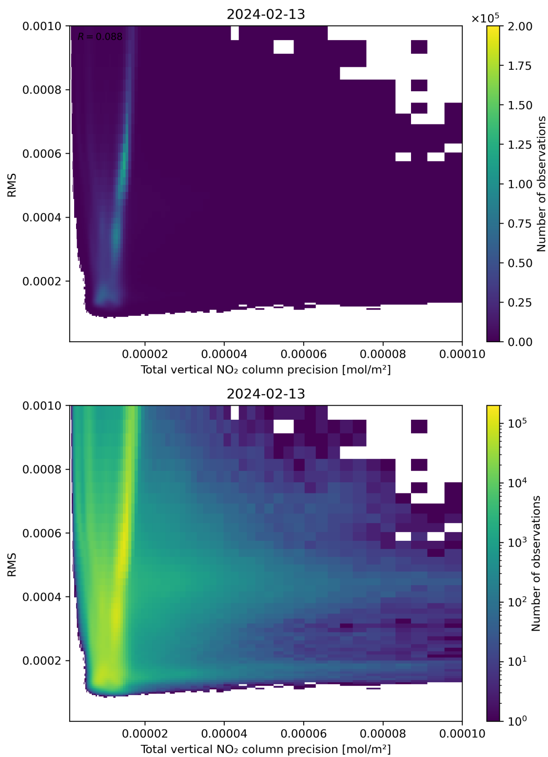
Figure 119: Scatter density plot of “Total vertical NO 2 column precision” against “RMS” for 2024-02-12 to 2024-02-14.
