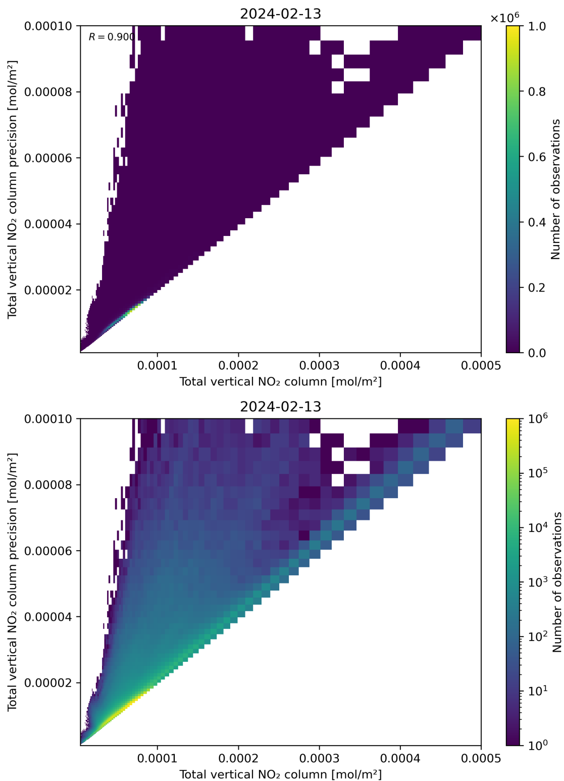
Figure 114: Scatter density plot of “Total vertical NO 2 column” against “Total vertical NO 2 column precision” for 2024-02-12 to 2024-02-14.
