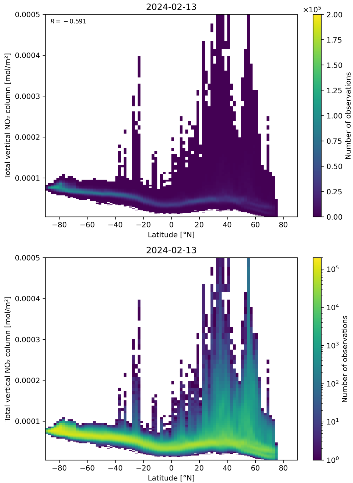
Figure 90: Scatter density plot of “Latitude” against “Total vertical NO 2 column” for 2024-02-12 to 2024-02-14.
