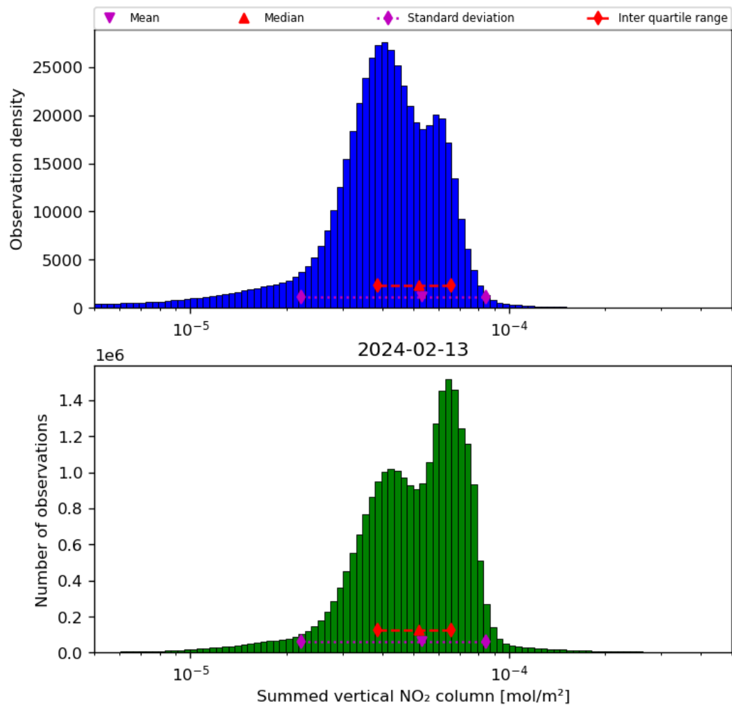
Figure 40: Histogram of “Summed vertical NO 2 column” for 2024-02-12 to 2024-02-14
