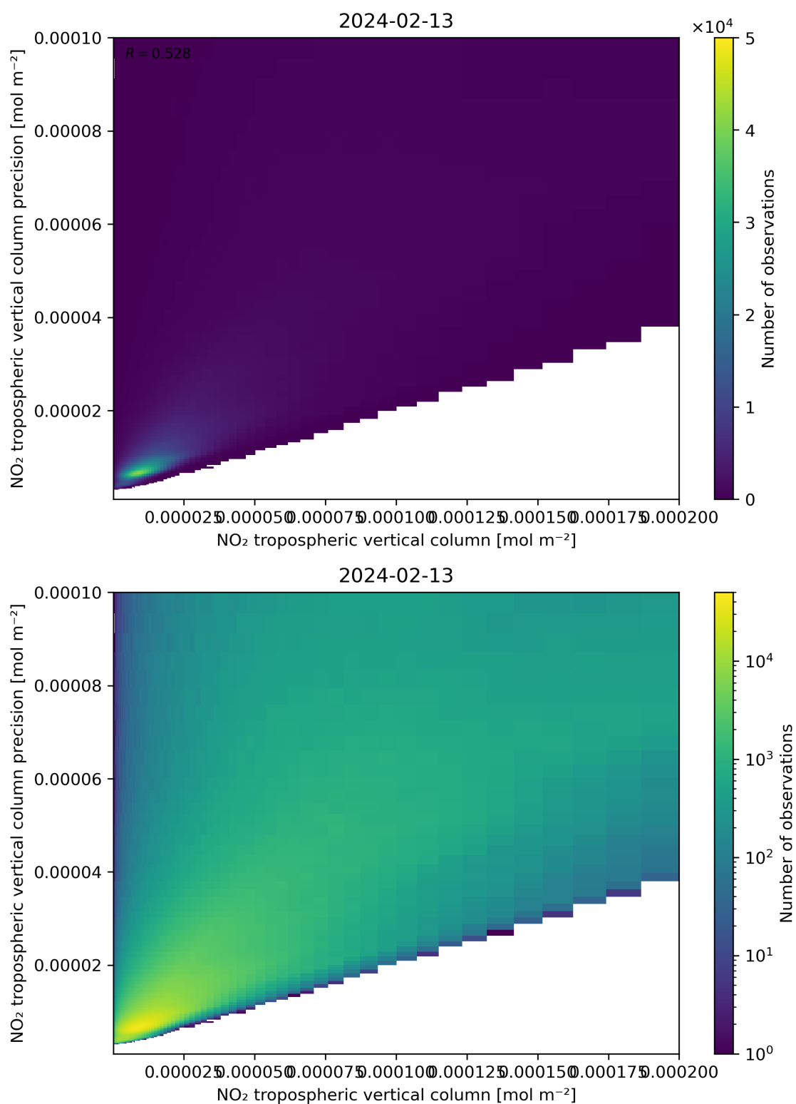
Figure 130: Scatter density plot of “NO 2 tropospheric vertical column” against “NO 2 tropospheric vertical column precision” for 2024-02-12 to 2024-02-14.
