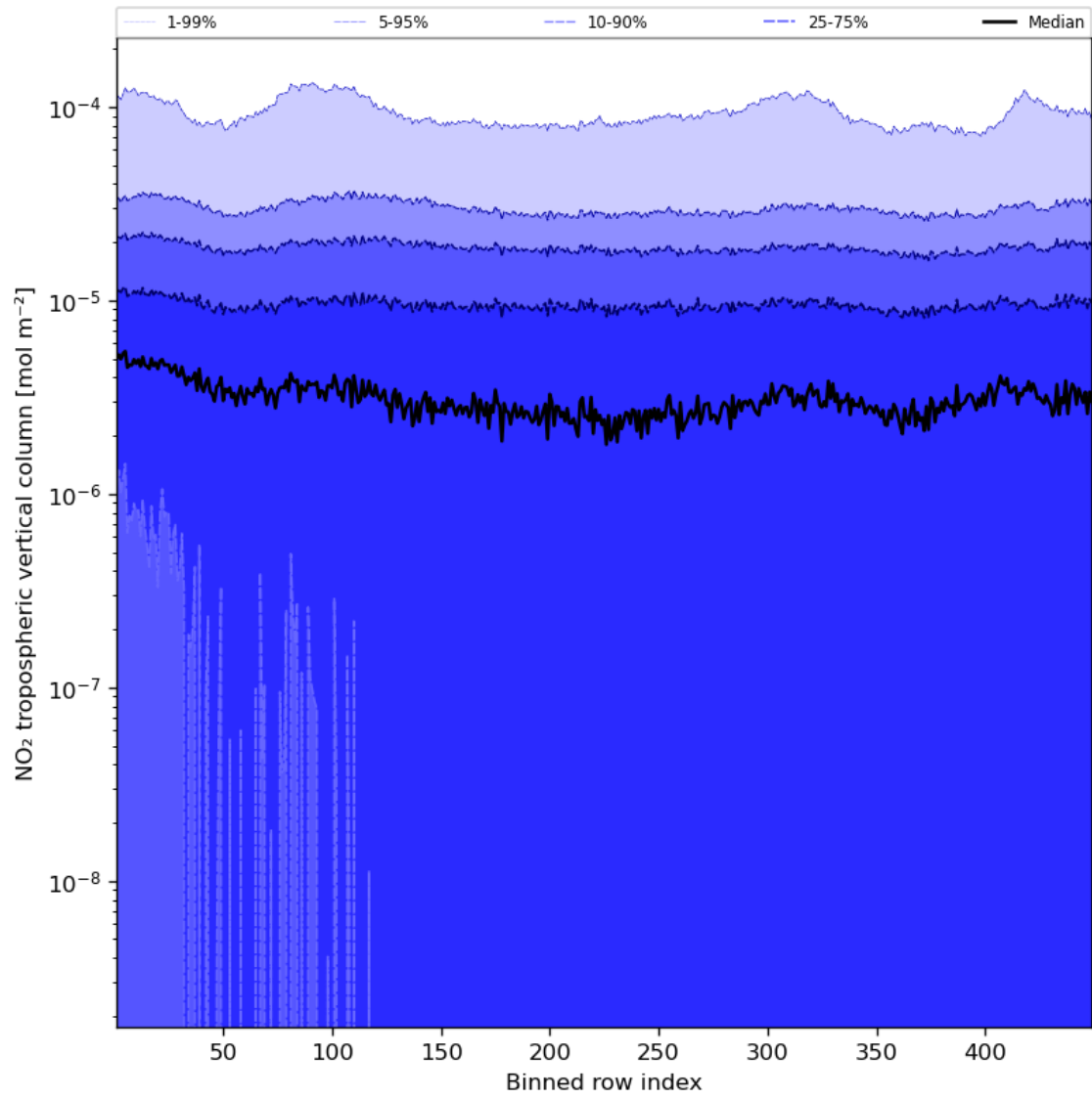
Figure 46: Along track statistics of “NO 2 tropospheric vertical column” for 2024-02-12 to 2024-02-14
