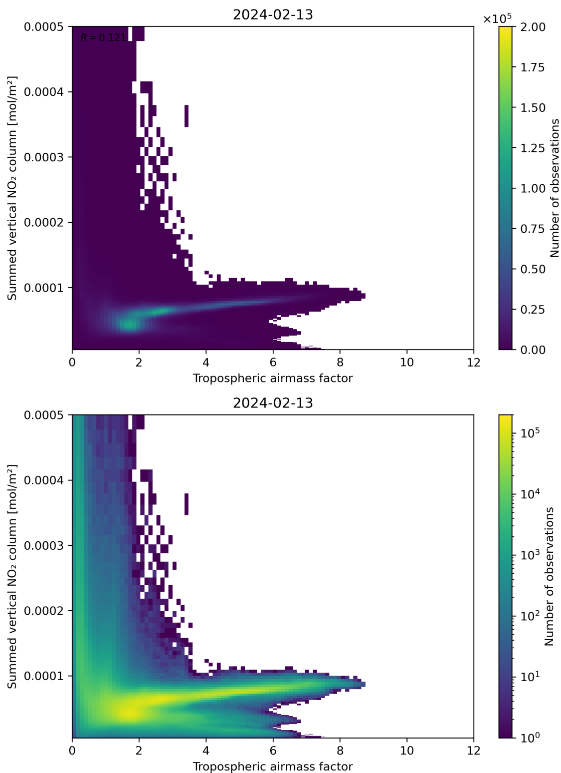
Figure 75: Scatter density plot of “Tropospheric airmass factor” against “Summed vertical NO 2 column” for 2024-02-12 to 2024-02-14.
