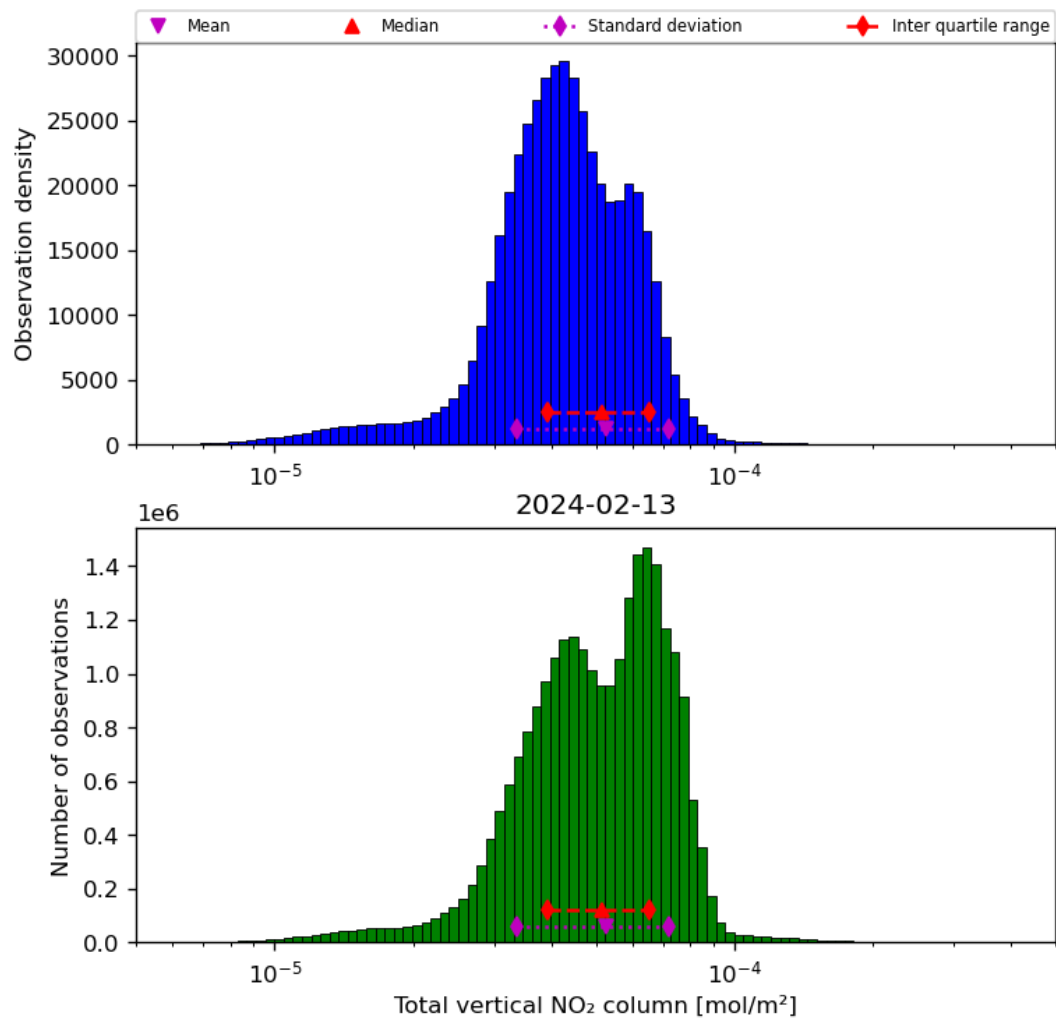
Figure 38: Histogram of “Total vertical NO 2 column” for 2024-02-12 to 2024-02-14
