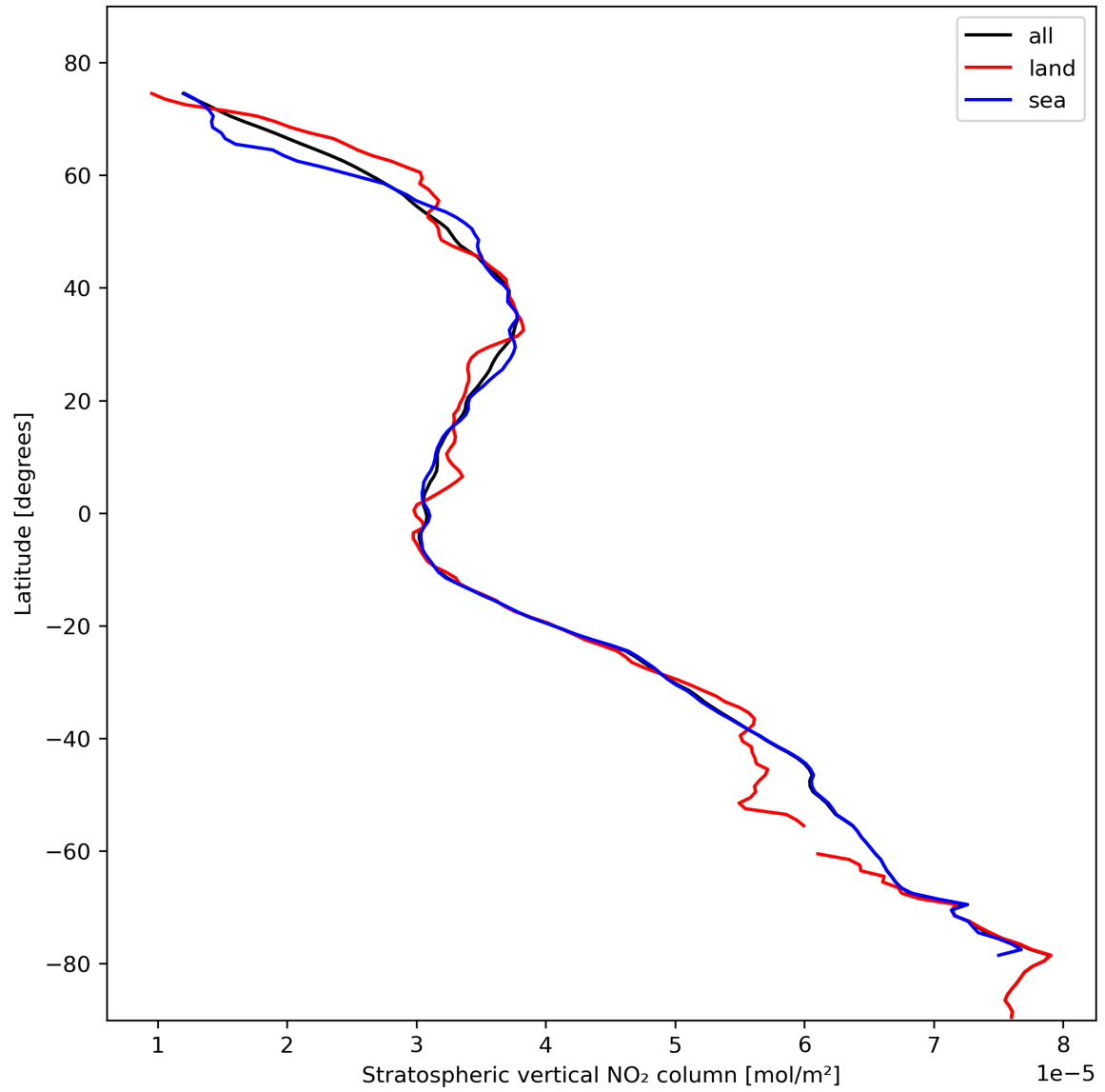
Figure 19: Zonal average of “Stratospheric vertical NO 2 column” for 2024-02-12 to 2024-02-14.
