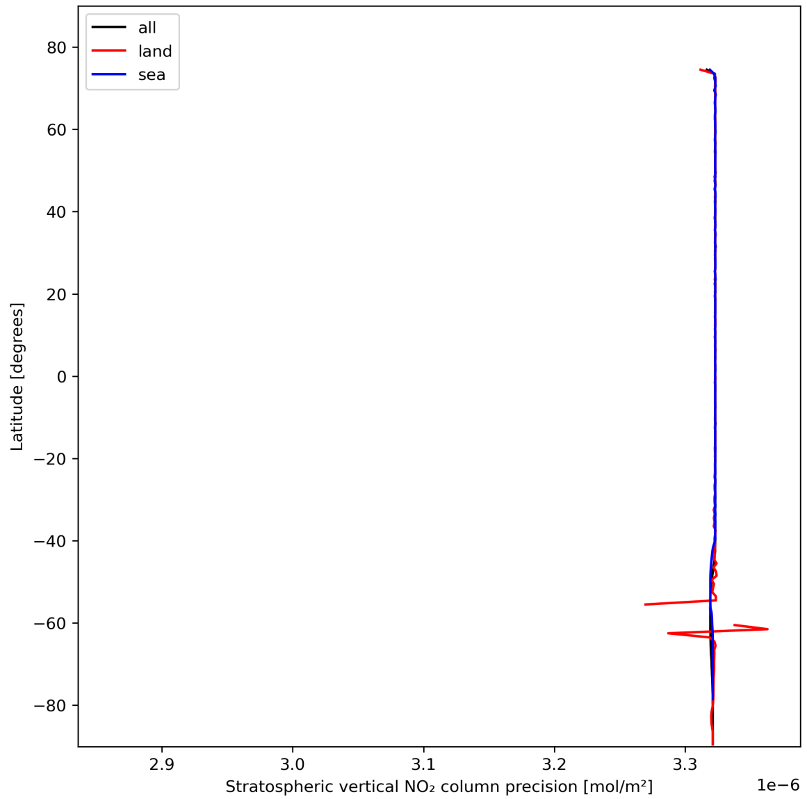
Figure 20: Zonal average of “Stratospheric vertical NO 2 column precision” for 2024-02-12 to 2024-02-14.
