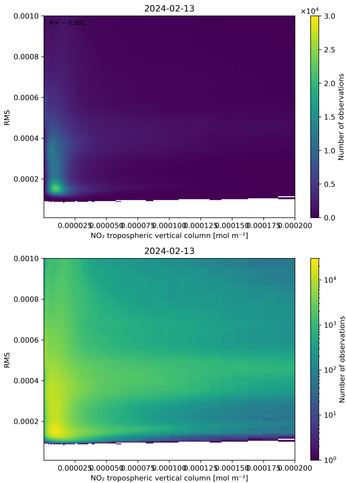
Figure 142: Scatter density plot of “NO 2 tropospheric vertical column” against “RMS” for 2024-02-12 to 2024-02-14.
