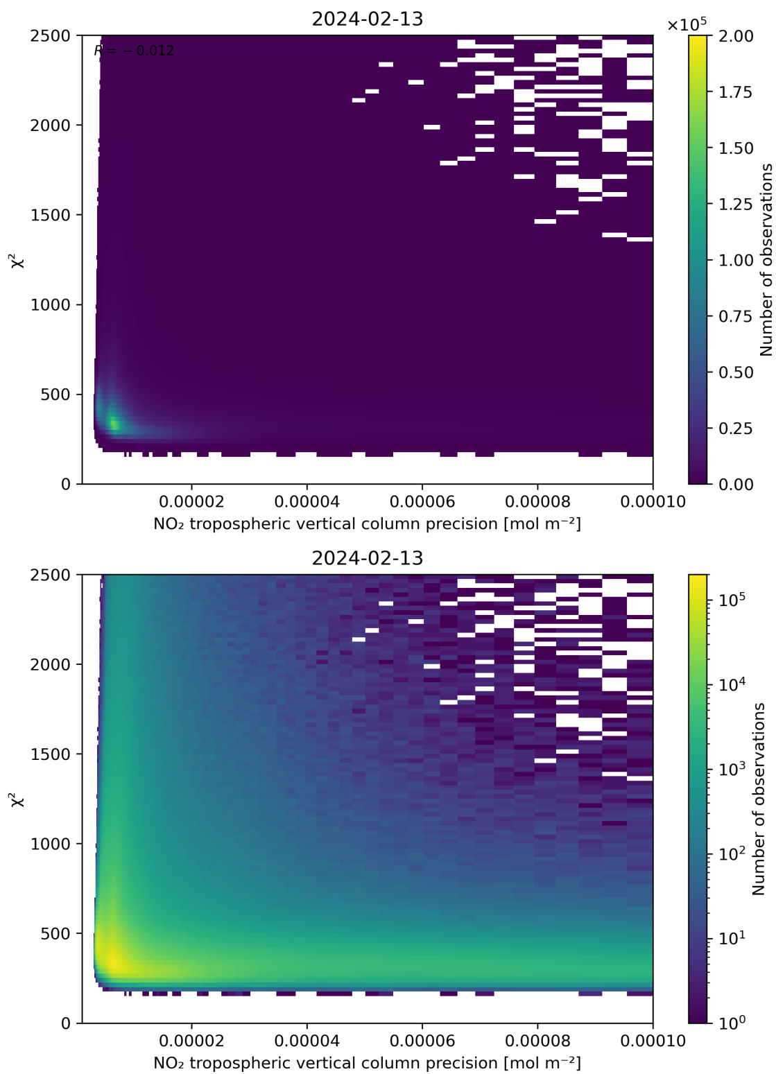
Figure 134: Scatter density plot of “NO 2 tropospheric vertical column precision” against “ \chi^2 ” for 2024-02-12 to 2024-02-14.
