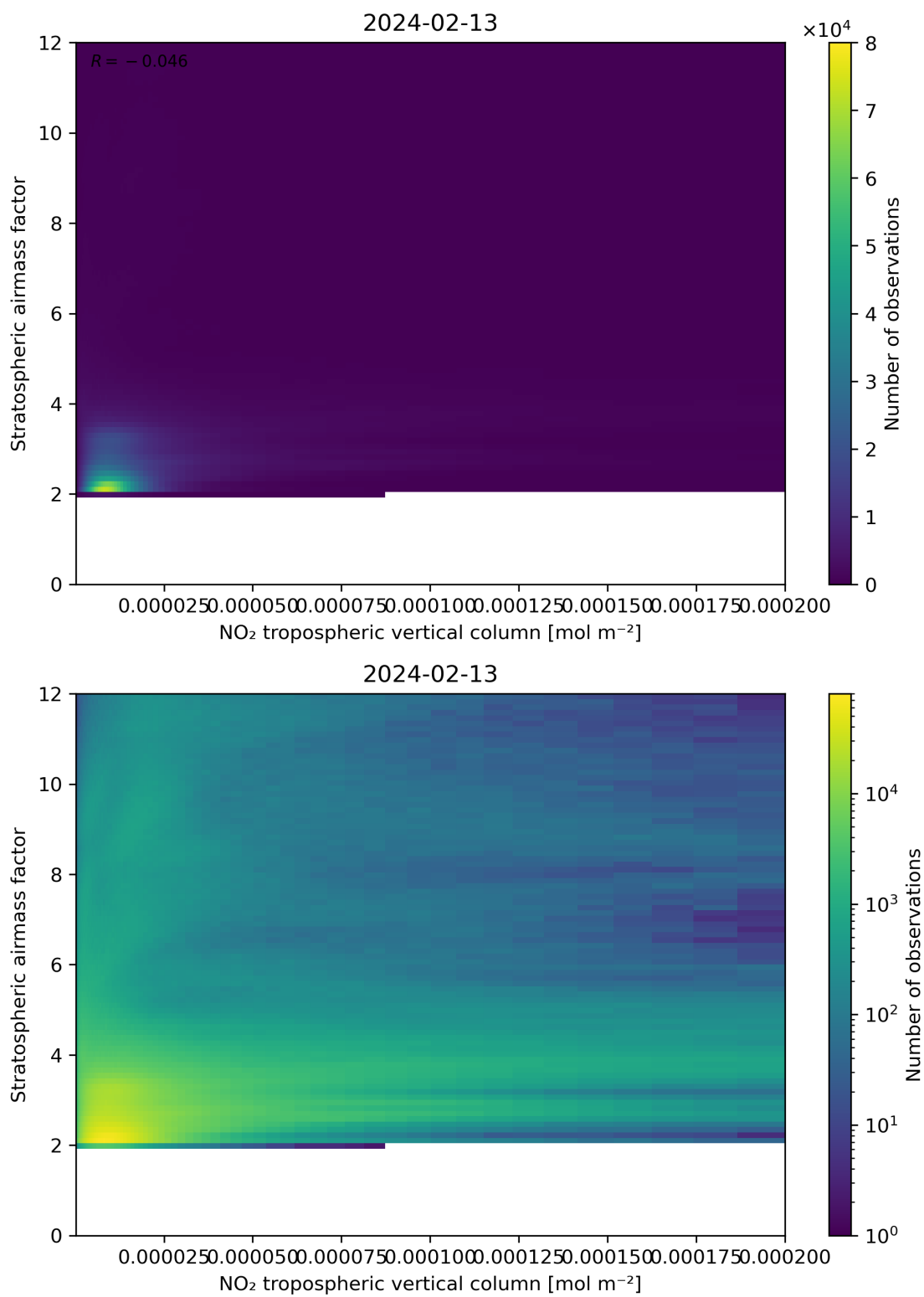
Figure 121: Scatter density plot of “NO 2 tropospheric vertical column” against “Stratospheric airmass factor” for 2024-02-12 to 2024-02-14.
