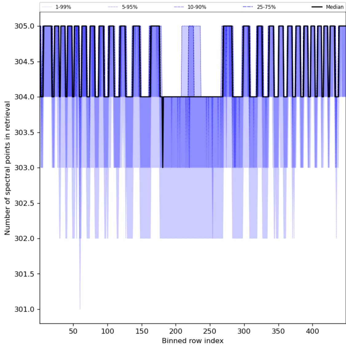
Figure 50: Along track statistics of “Number of spectral points in retrieval” for 2024-02-12 to 2024-02-14
