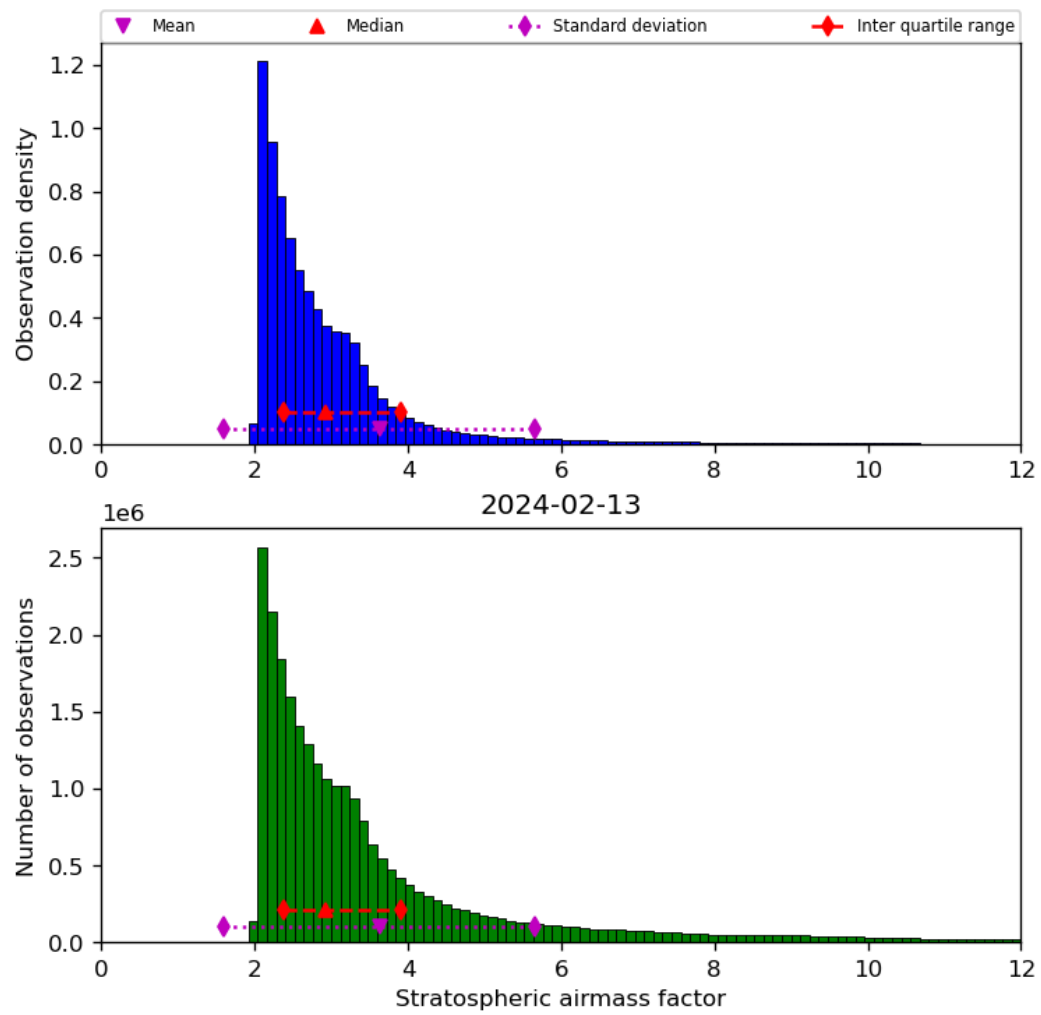
Figure 44: Histogram of “Stratospheric airmass factor” for 2024-02-12 to 2024-02-14
