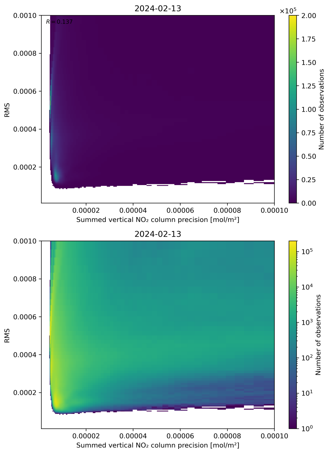
Figure 108: Scatter density plot of “Summed vertical NO 2 column precision” against “RMS” for 2024-02-12 to 2024-02-14.
