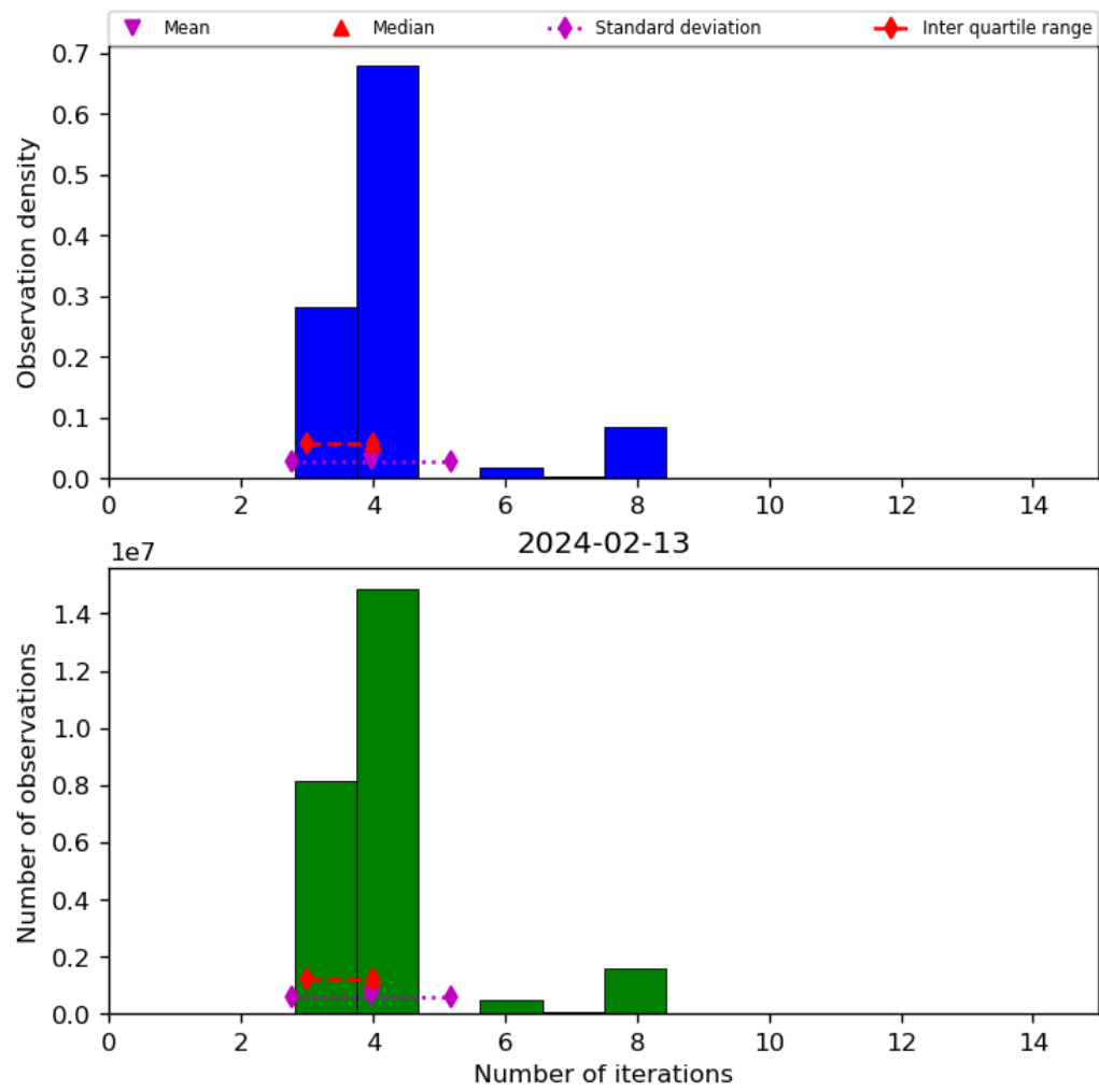
Figure 34: Histogram of “Number of iterations” for 2024-02-12 to 2024-02-14
