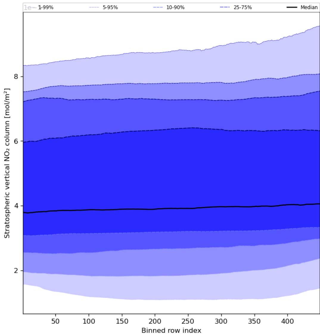
Figure 53: Along track statistics of “Stratospheric vertical NO 2 column” for 2024-02-12 to 2024-02-14
