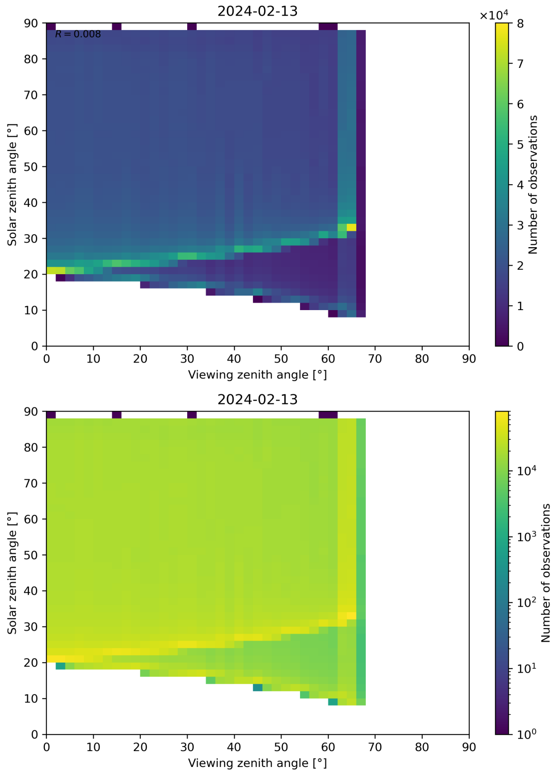
Figure 172: Scatter density plot of “Viewing zenith angle” against “Solar zenith angle” for 2024-02-12 to 2024-02-14.
