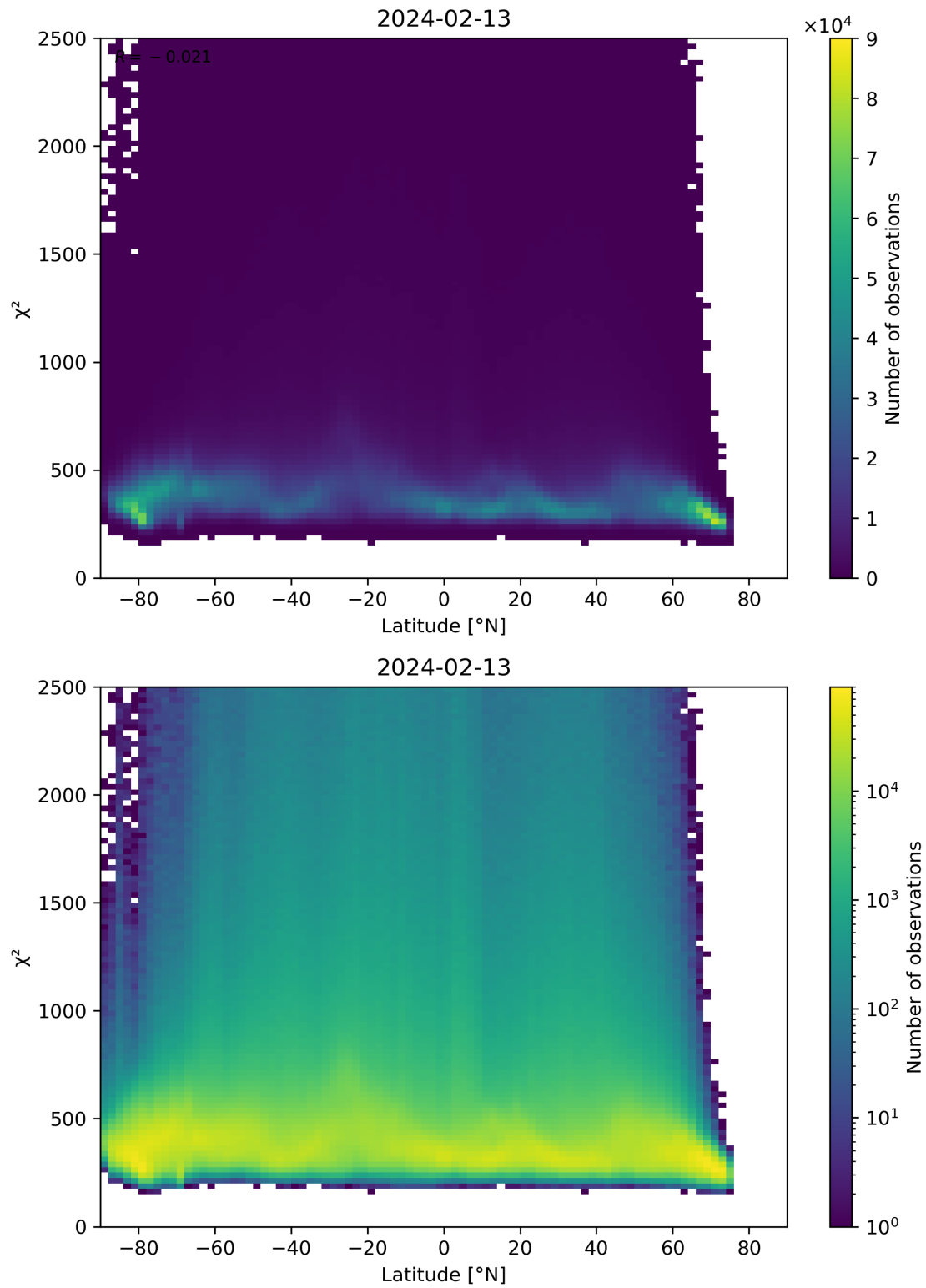
Figure 86: Scatter density plot of “Latitude” against “ \chi^2 ” for 2024-02-12 to 2024-02-14.
