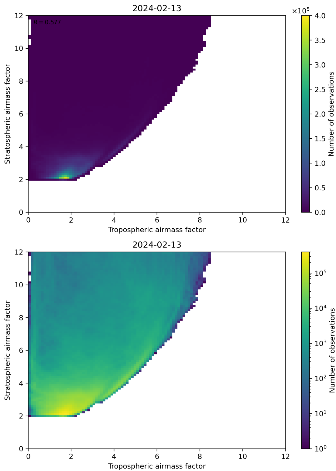
Figure 71: Scatter density plot of “Tropospheric airmass factor” against “Stratospheric airmass factor” for 2024-02-12 to 2024-02-14.
