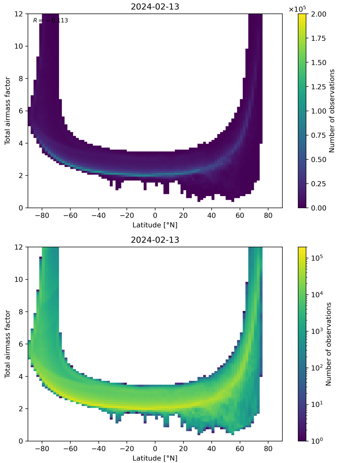
Figure 84: Scatter density plot of “Latitude” against “Total airmass factor” for 2024-02-12 to 2024-02-14.
