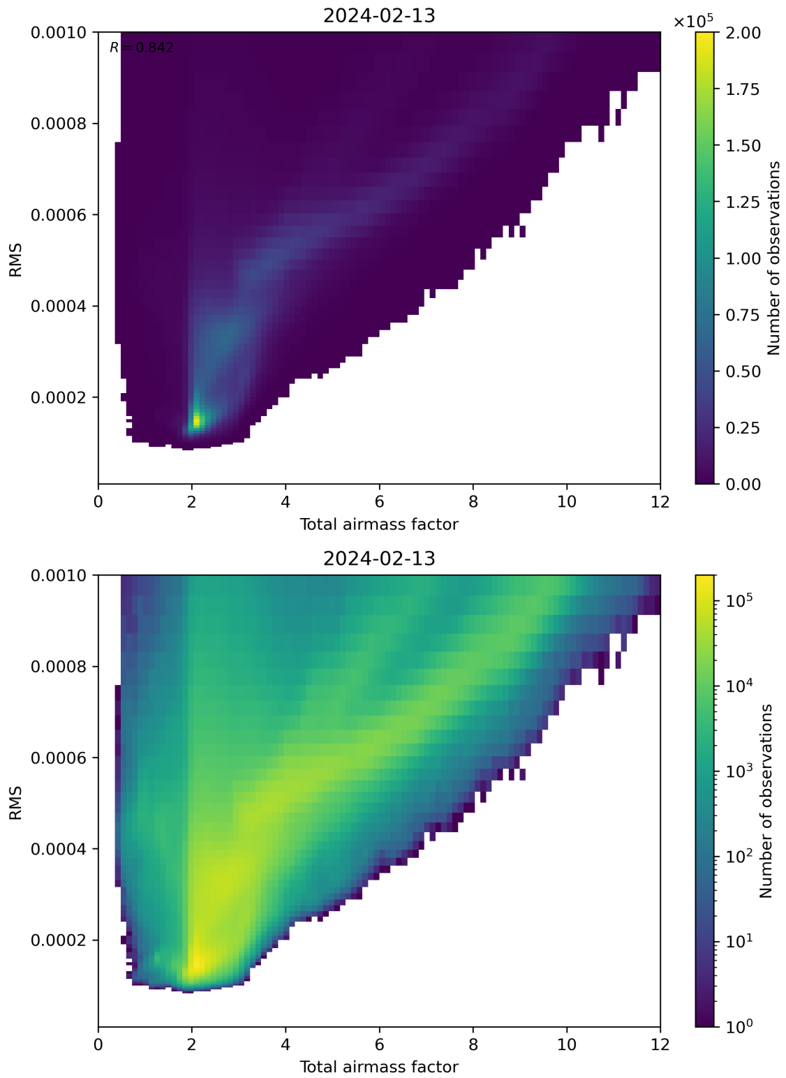
Figure 69: Scatter density plot of “Total airmass factor” against “RMS” for 2024-02-12 to 2024-02-14.
