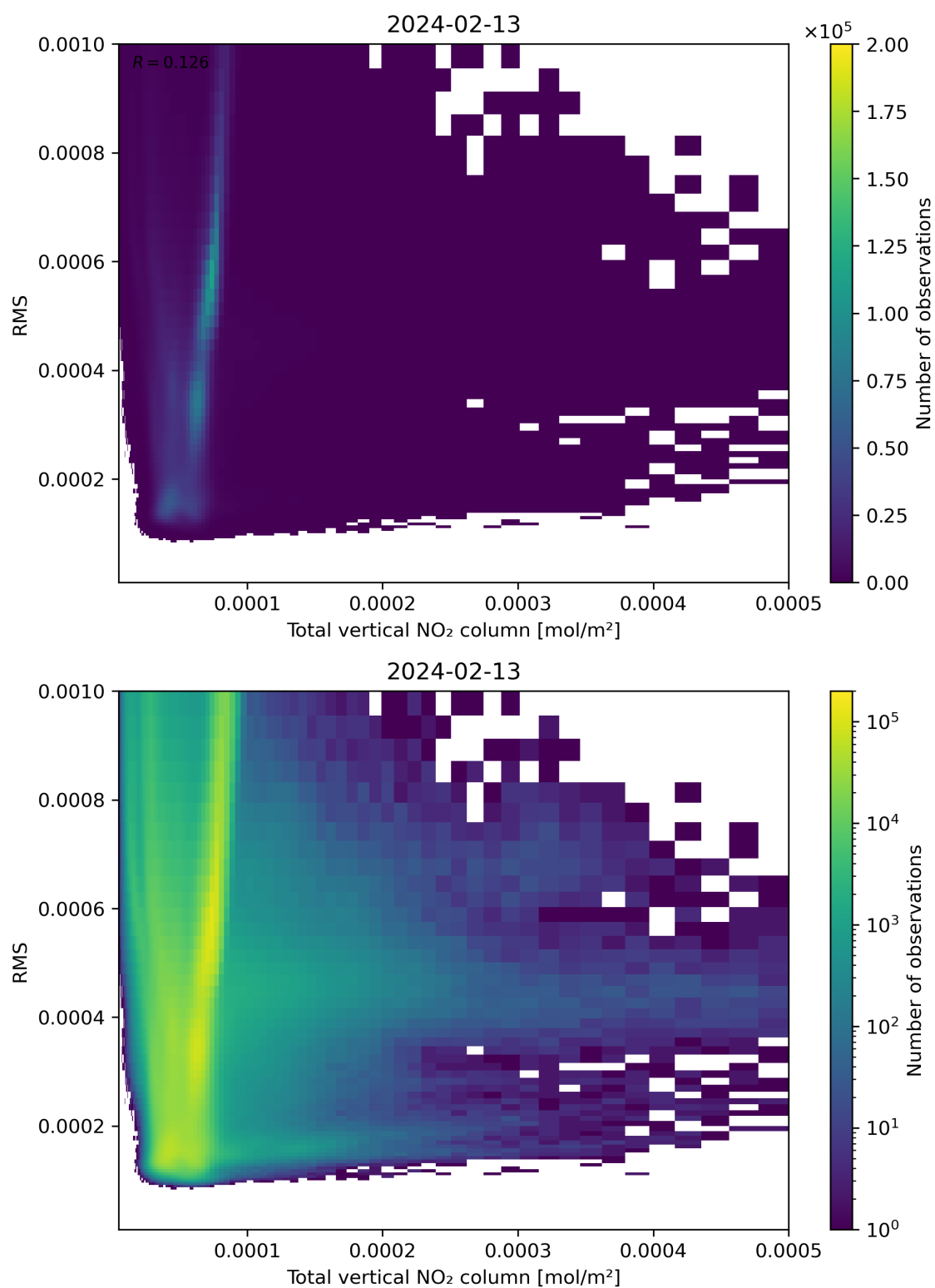
Figure 120: Scatter density plot of “Total vertical NO 2 column” against “RMS” for 2024-02-12 to 2024-02-14.
