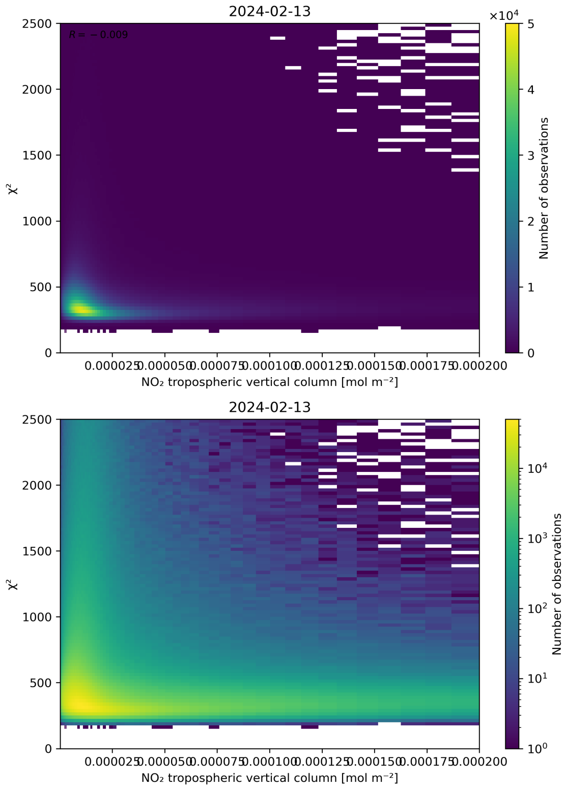
Figure 124: Scatter density plot of “NO 2 tropospheric vertical column” against “ \chi^2 ” for 2024-02-12 to 2024-02-14.
