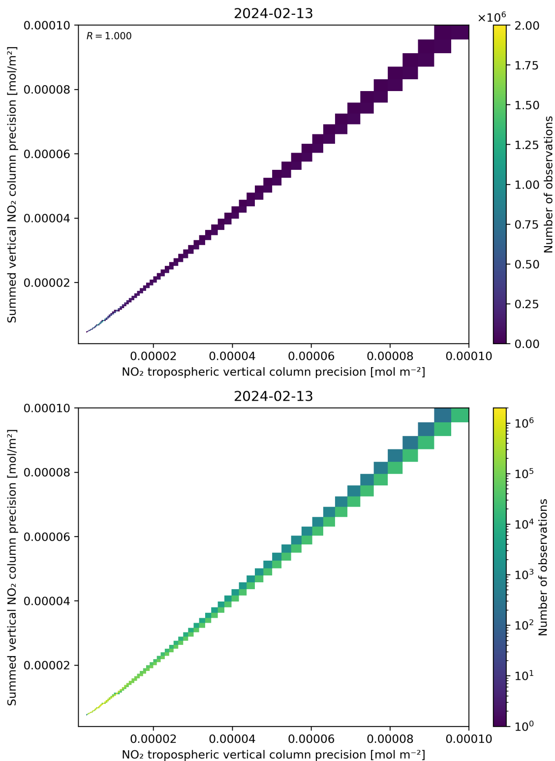
Figure 137: Scatter density plot of “NO 2 tropospheric vertical column precision” against “Summed vertical NO 2 column precision” for 2024-02-12 to 2024-02-14.
