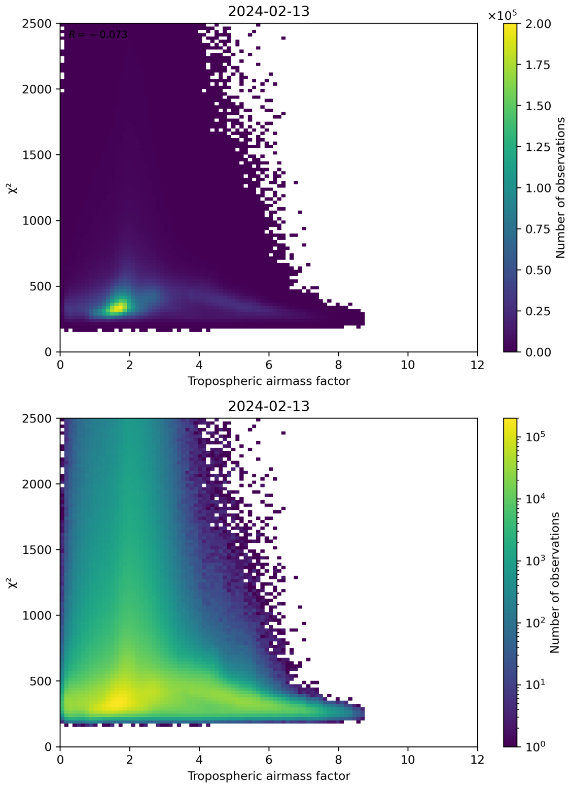
Figure 73: Scatter density plot of “Tropospheric airmass factor” against “ \chi^2 ” for 2024-02-12 to 2024-02-14.
