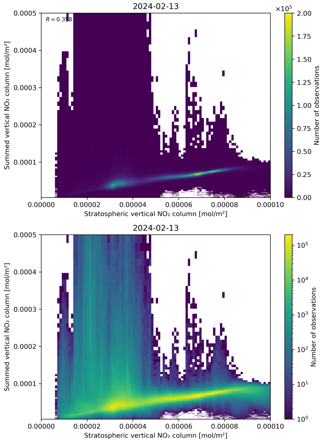
Figure 98: Scatter density plot of “Stratospheric vertical NO 2 column” against “Summed vertical NO 2 column” for 2024-02-12 to 2024-02-14.
