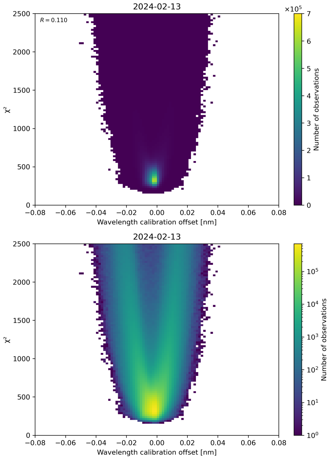
Figure 175: Scatter density plot of “Wavelength calibration offset” against “ \chi^2 ” for 2024-02-12 to 2024-02-14.
