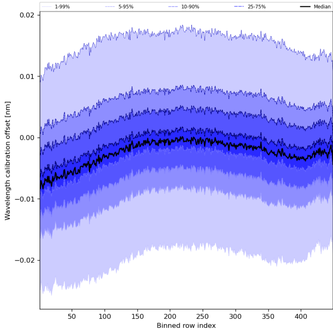
Figure 52: Along track statistics of “Wavelength calibration offset” for 2024-02-12 to 2024-02-14
