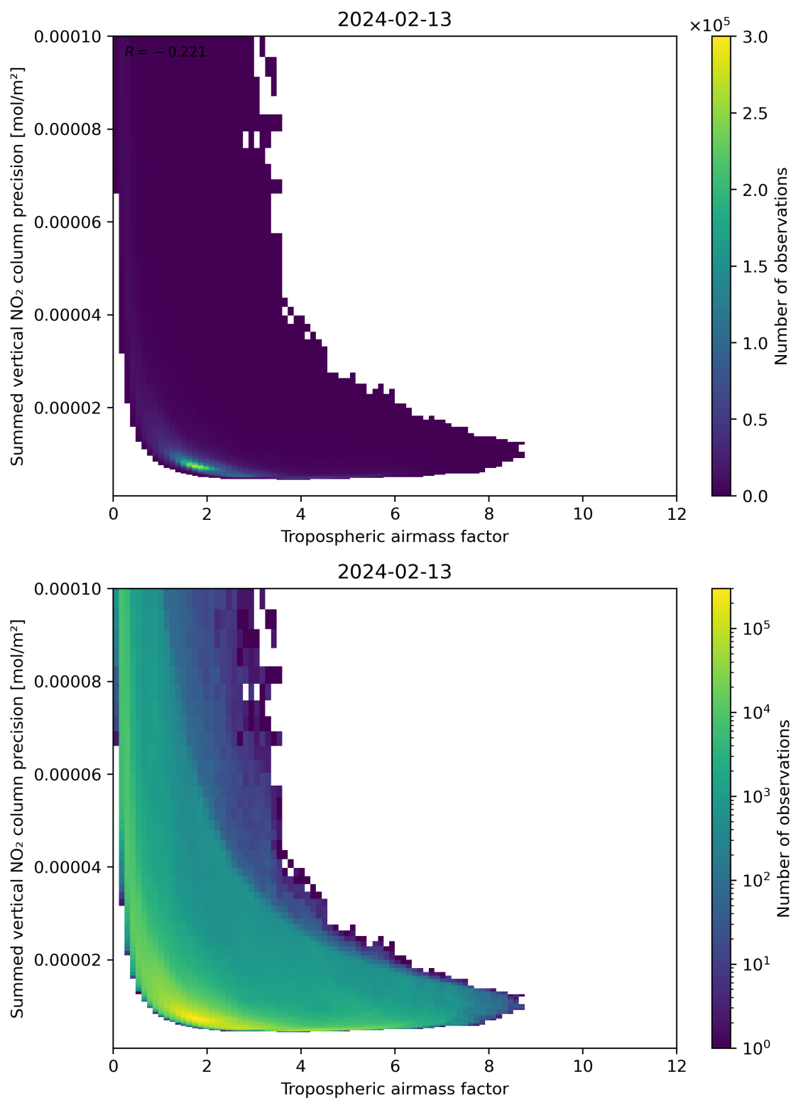
Figure 76: Scatter density plot of “Tropospheric air mass factor” against “Summed vertical NO 2 column precision” for 2024-02-12 to 2024-02-14.
