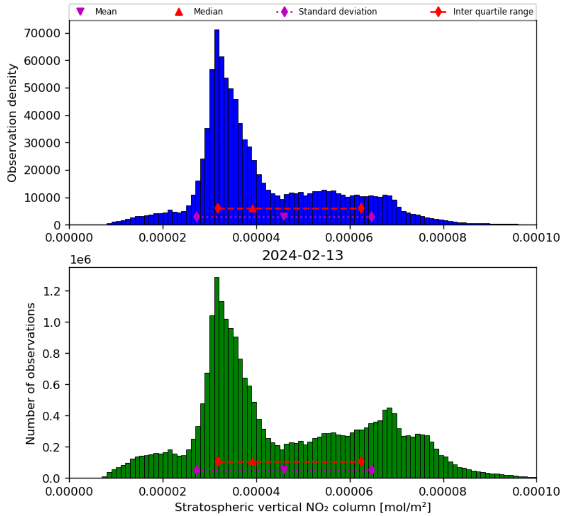
Figure 36: Histogram of “Stratospheric vertical NO 2 column” for 2024-02-12 to 2024-02-14
