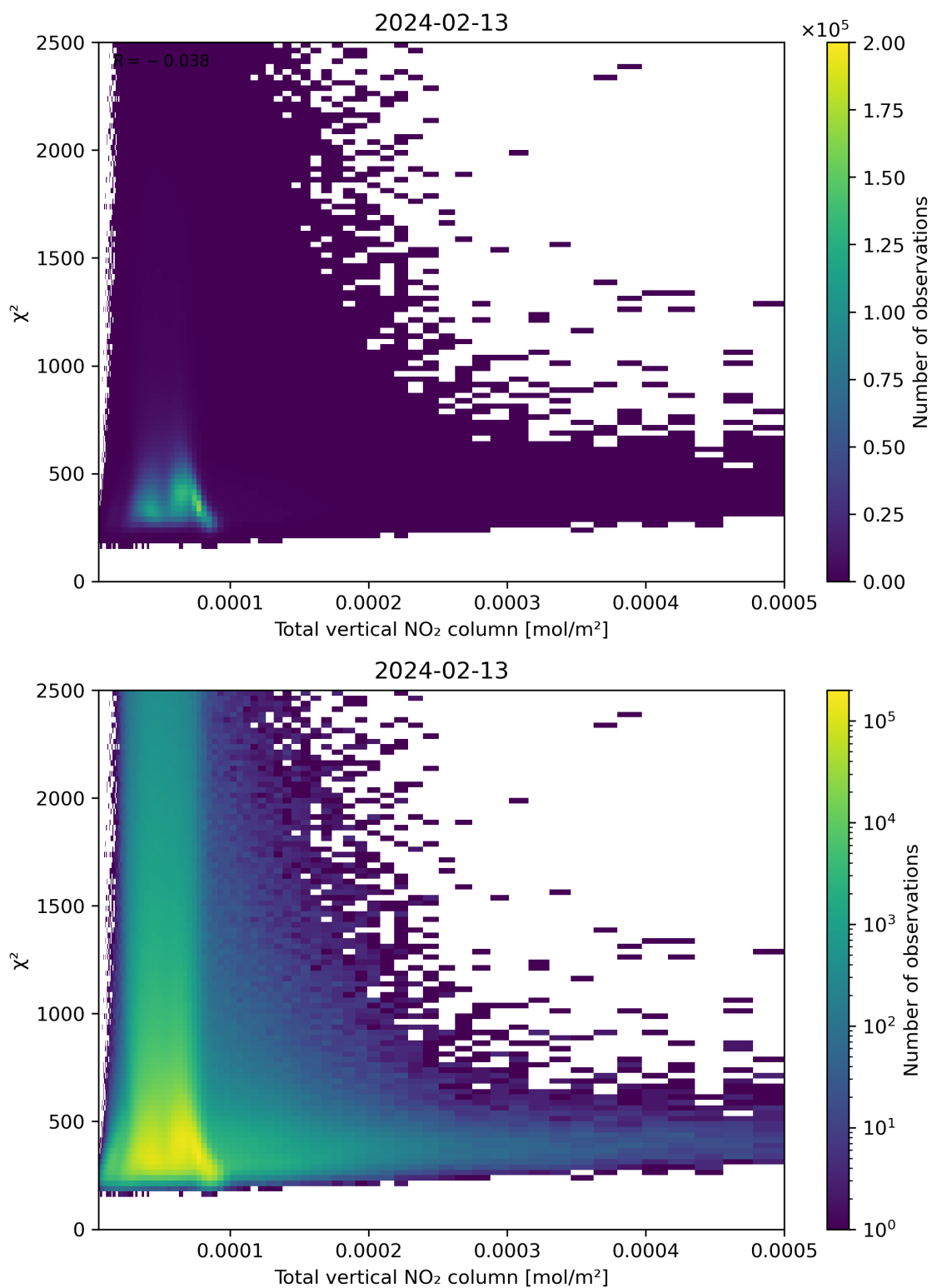
Figure 111: Scatter density plot of “Total vertical NO 2 column” against “ \chi^2 ” for 2024-02-12 to 2024-02-14.
