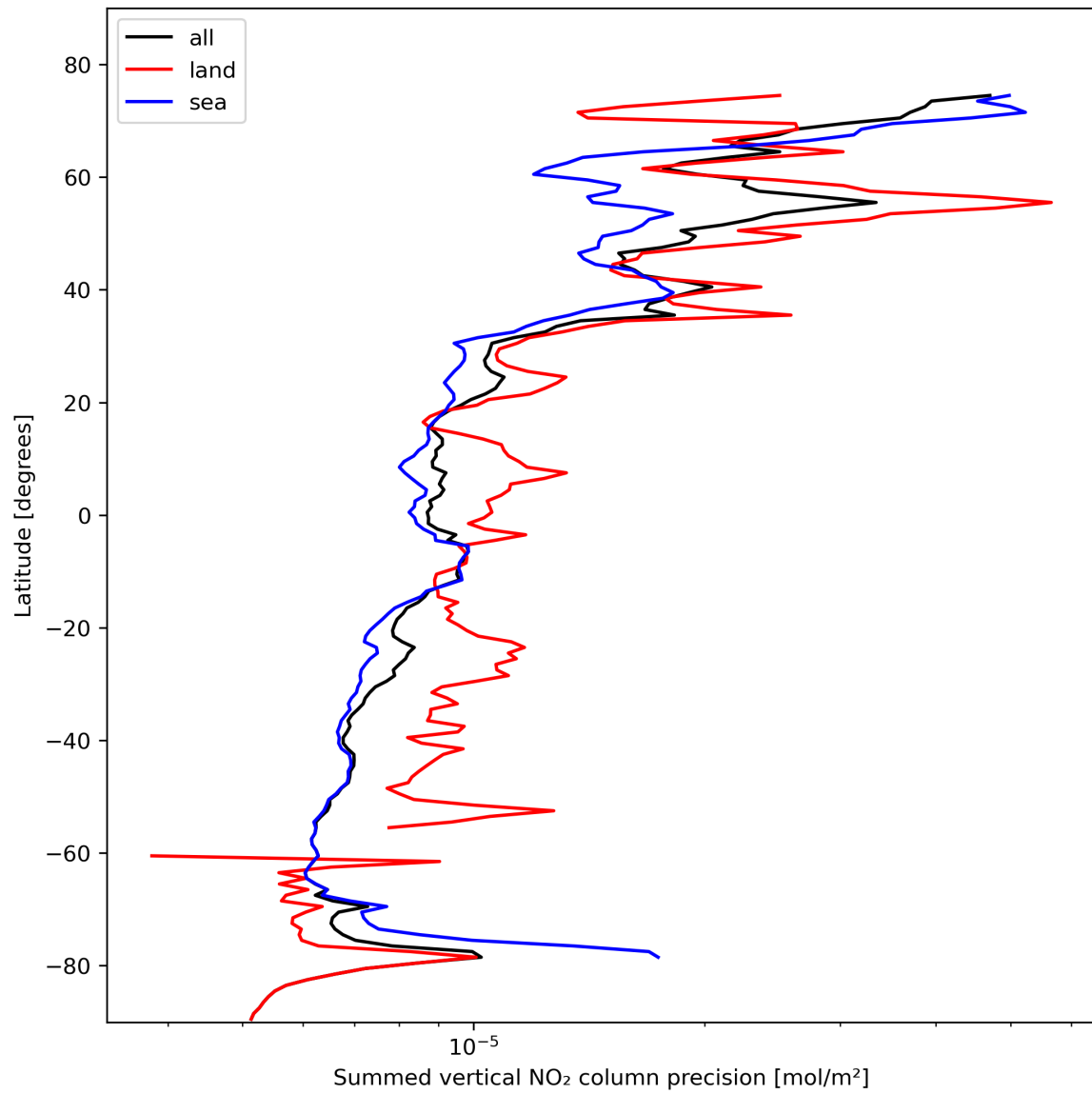
Figure 24: Zonal average of “Summed vertical NO 2 column precision” for 2024-02-12 to 2024-02-14.
