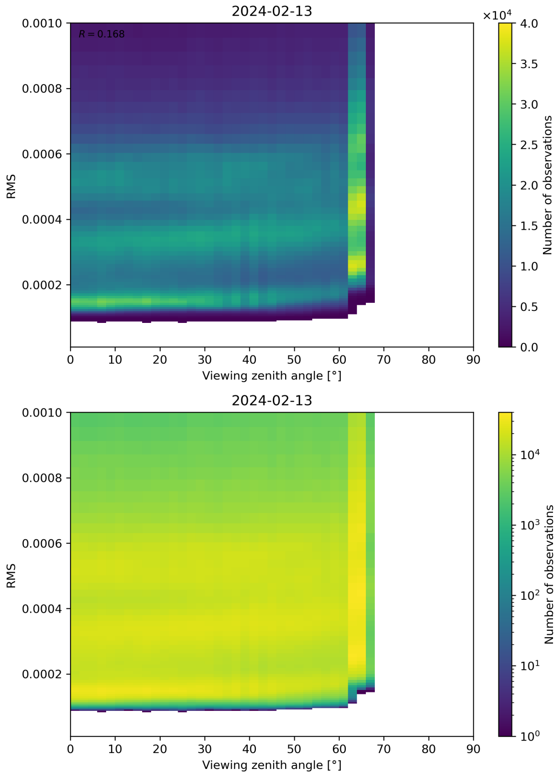
Figure 171: Scatter density plot of “Viewing zenith angle” against “RMS” for 2024-02-12 to 2024-02-14.
