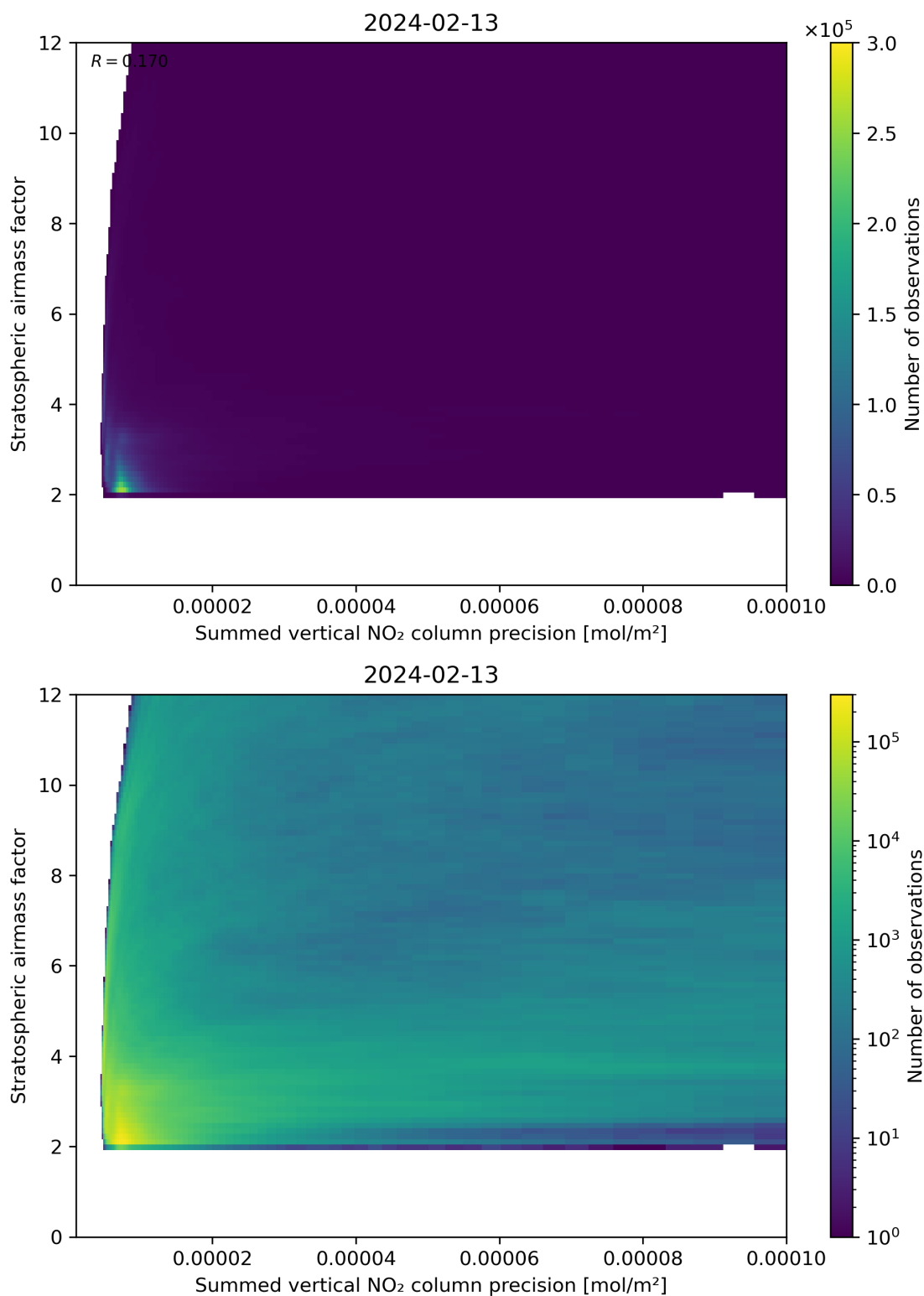
Figure 106: Scatter density plot of “Summed vertical NO 2 column precision” against “Stratospheric airmass factor” for 2024-02-12 to 2024-02-14.
