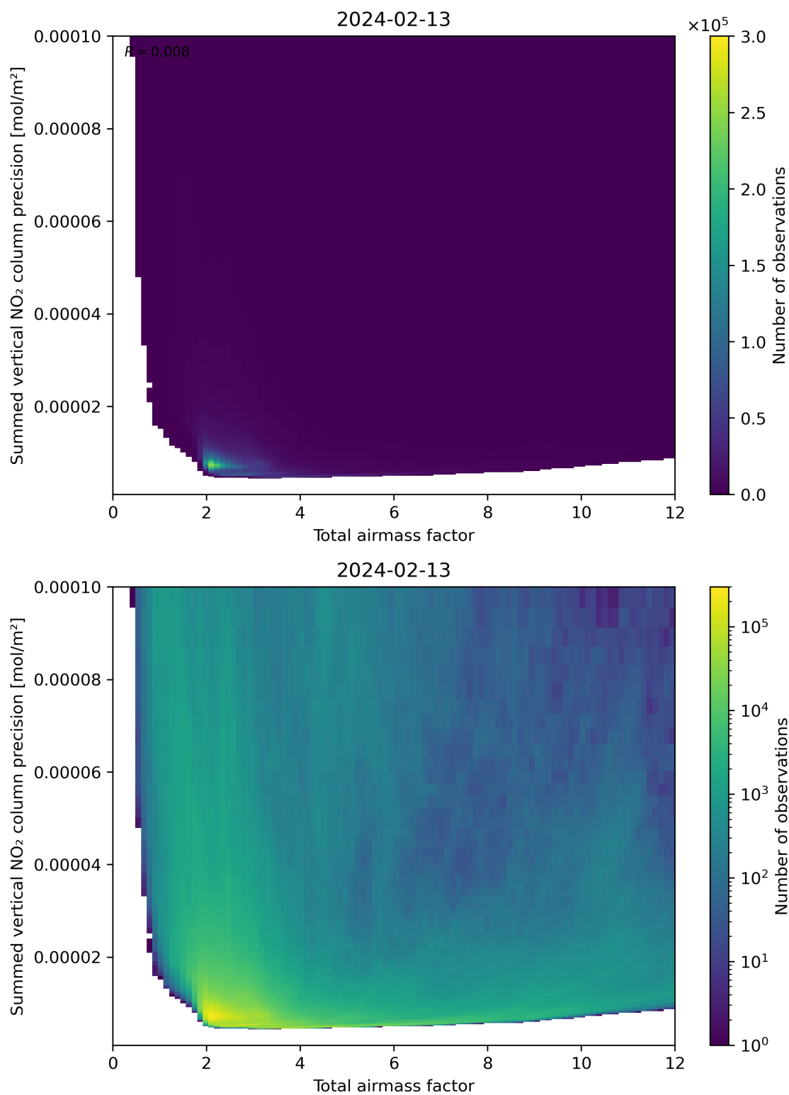
Figure 66: Scatter density plot of “Total airmass factor” against “Summed vertical NO 2 column precision” for 2024-02-12 to 2024-02-14.
