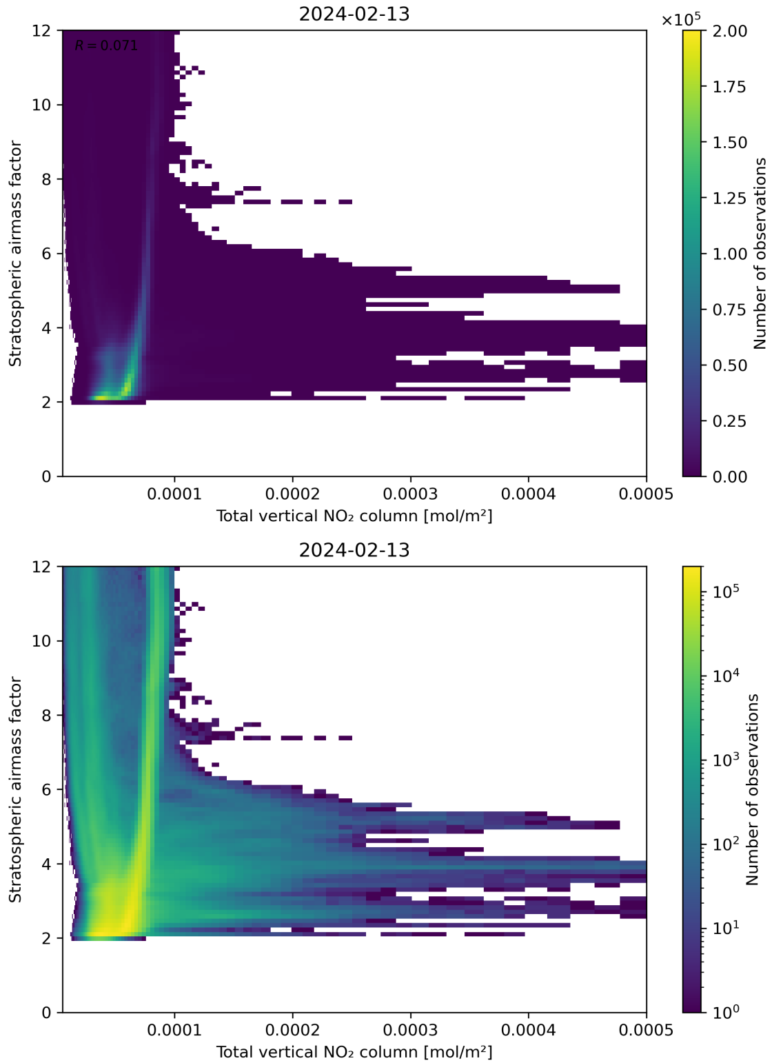
Figure 110: Scatter density plot of “Total vertical NO 2 column” against “Stratospheric airmass factor” for 2024-02-12 to 2024-02-14.
