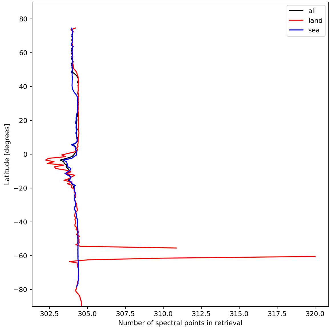
Figure 16: Zonal average of “Number of spectral points in retrieval” for 2024-02-12 to 2024-02-14.
