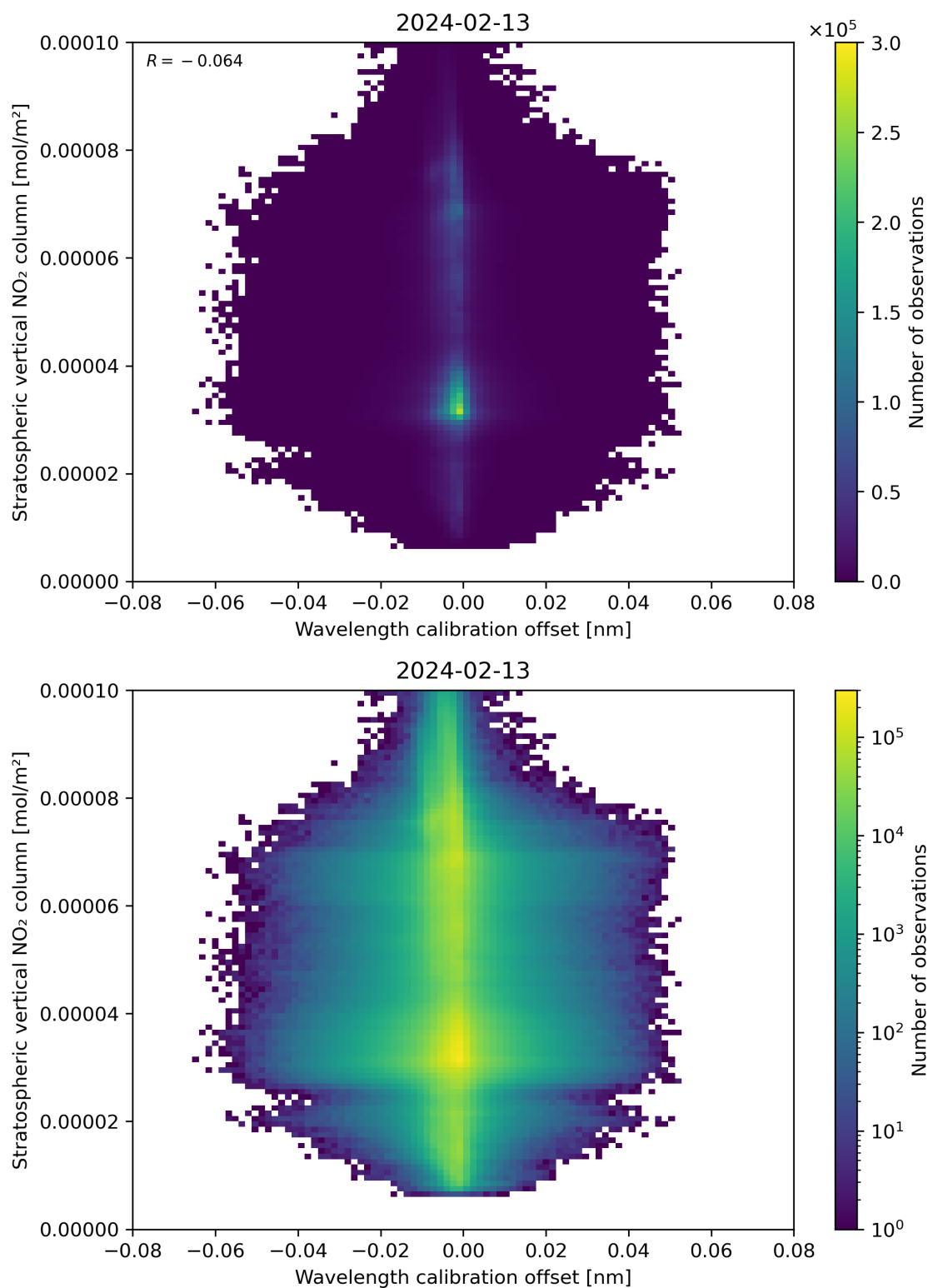
Figure 176: Scatter density plot of “Wavelength calibration offset” against “Stratospheric vertical NO 2 column” for 2024-02-12 to 2024-02-14.
