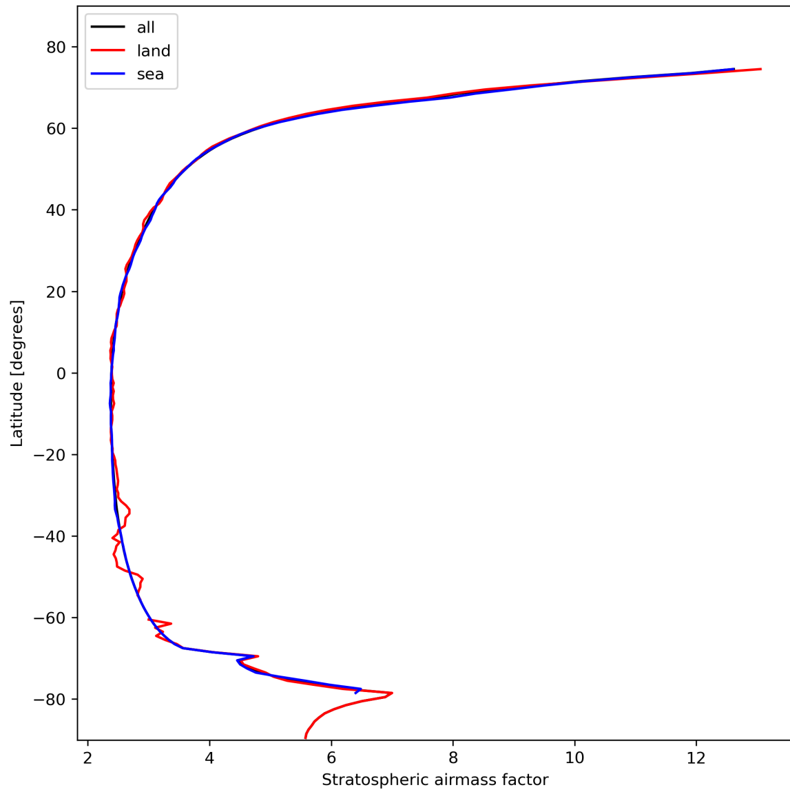
Figure 27: Zonal average of “Stratospheric airmass factor” for 2024-02-12 to 2024-02-14.
