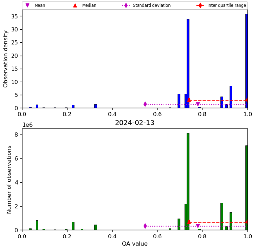
Figure 28: Histogram of “QA value” for 2024-02-12 to 2024-02-14
