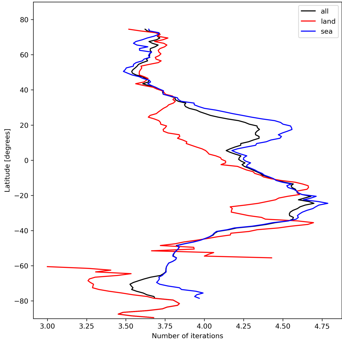
Figure 17: Zonal average of “Number of iterations” for 2024-02-12 to 2024-02-14.
