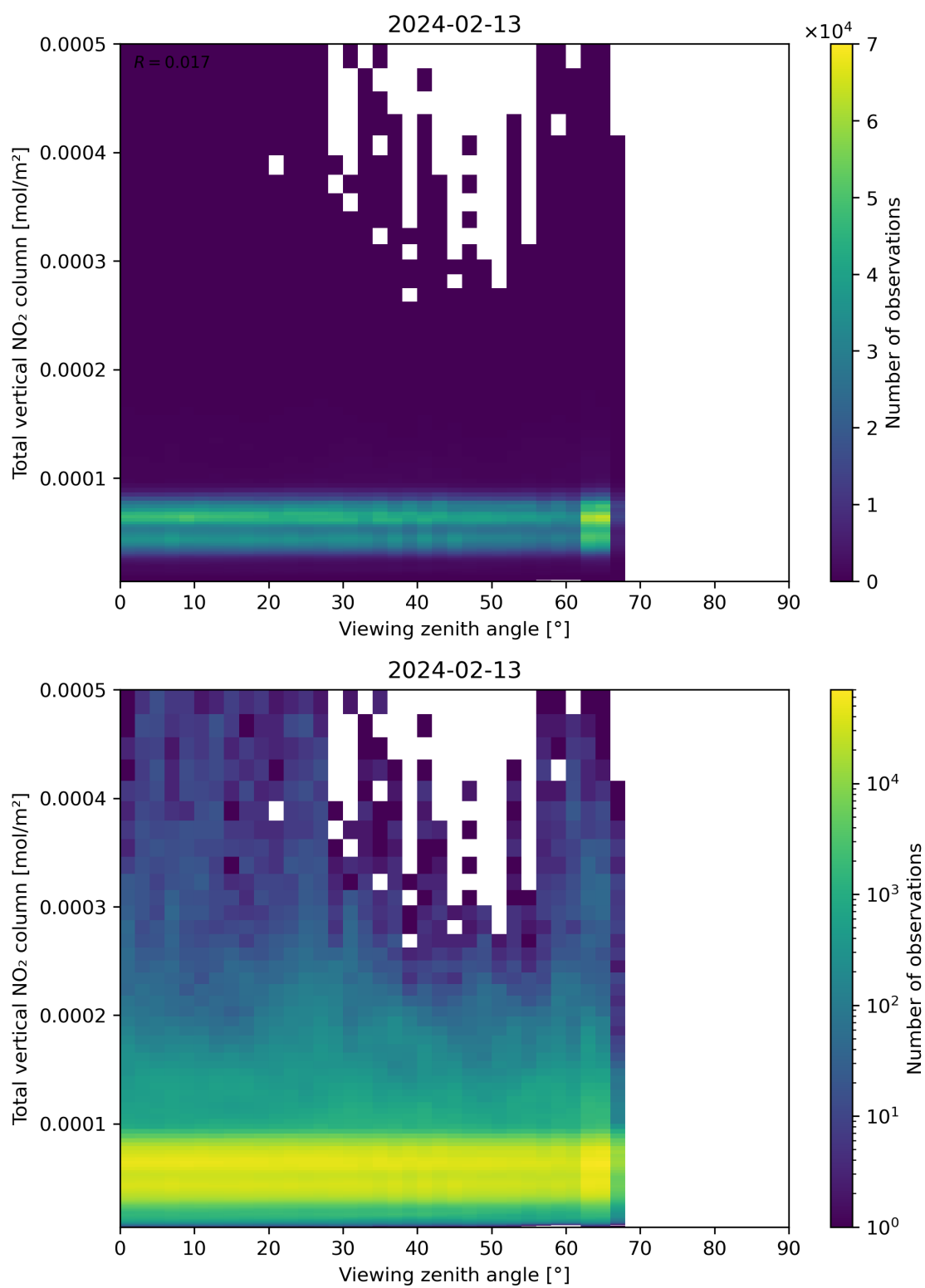
Figure 167: Scatter density plot of “Viewing zenith angle” against “Total vertical NO 2 column” for 2024-02-12 to 2024-02-14.
