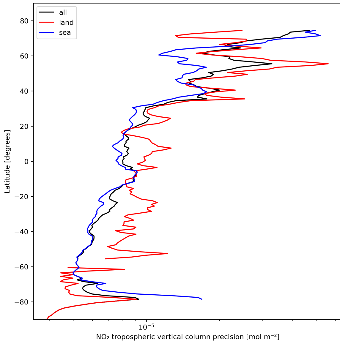
Figure 13: Zonal average of “NO 2 tropospheric vertical column precision” for 2024-02-12 to 2024-02-14.
