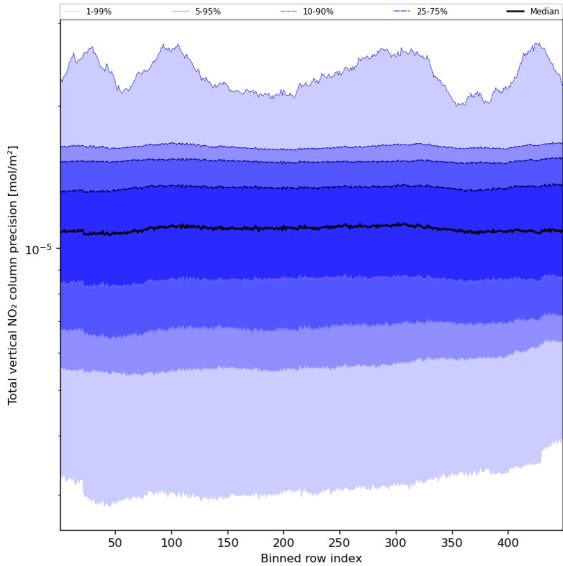
Figure 56: Along track statistics of “Total vertical NO 2 column precision” for 2024-02-12 to 2024-02-14
