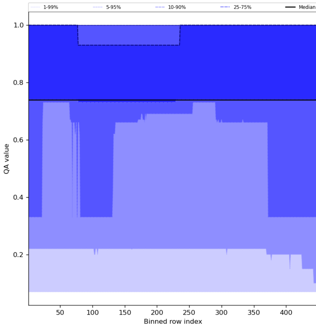
Figure 45: Along track statistics of “QA value” for 2024-02-12 to 2024-02-14
