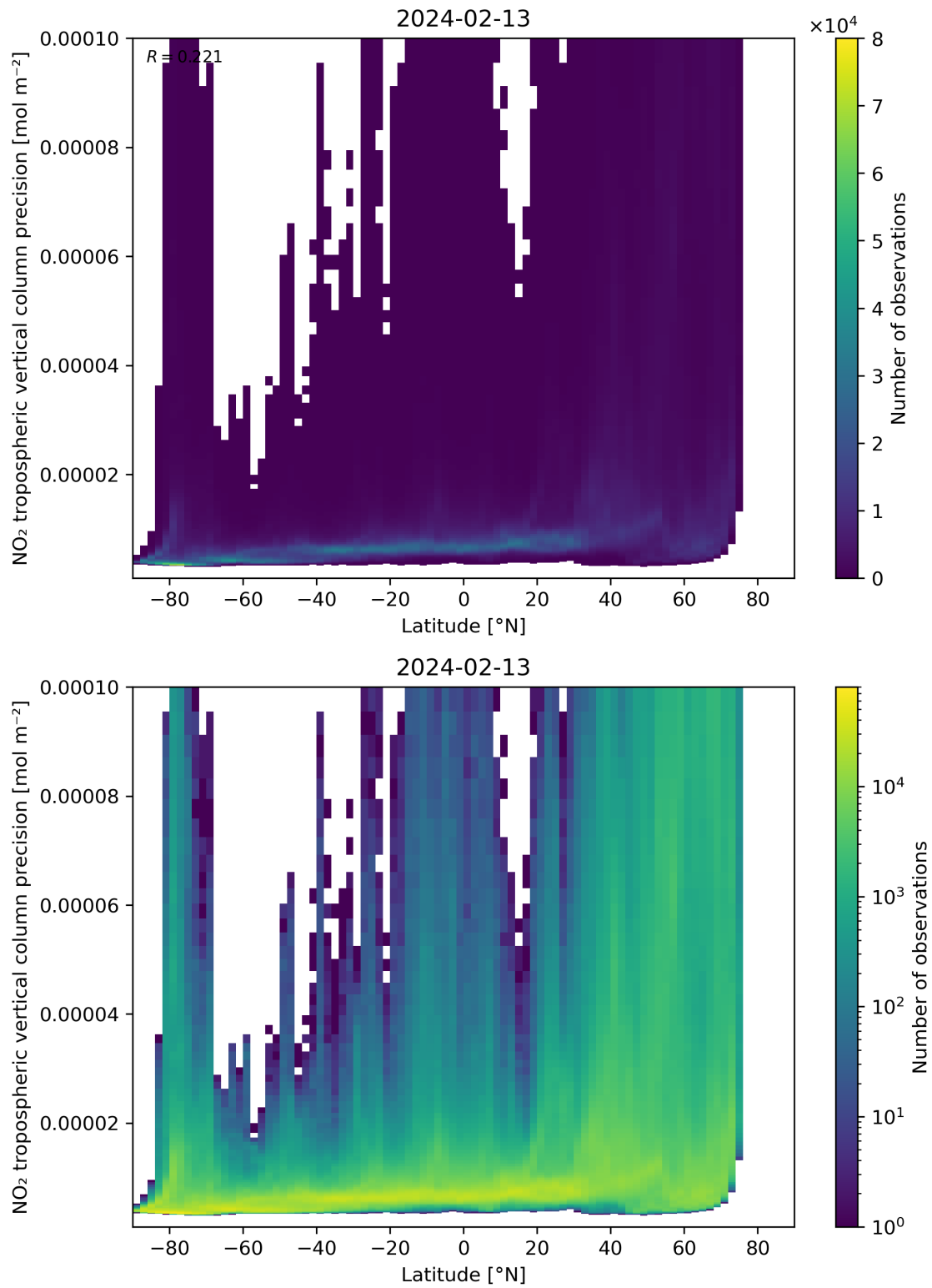
Figure 93: Scatter density plot of “Latitude” against “NO 2 tropospheric vertical column precision” for 2024-02-12 to 2024-02-14.
