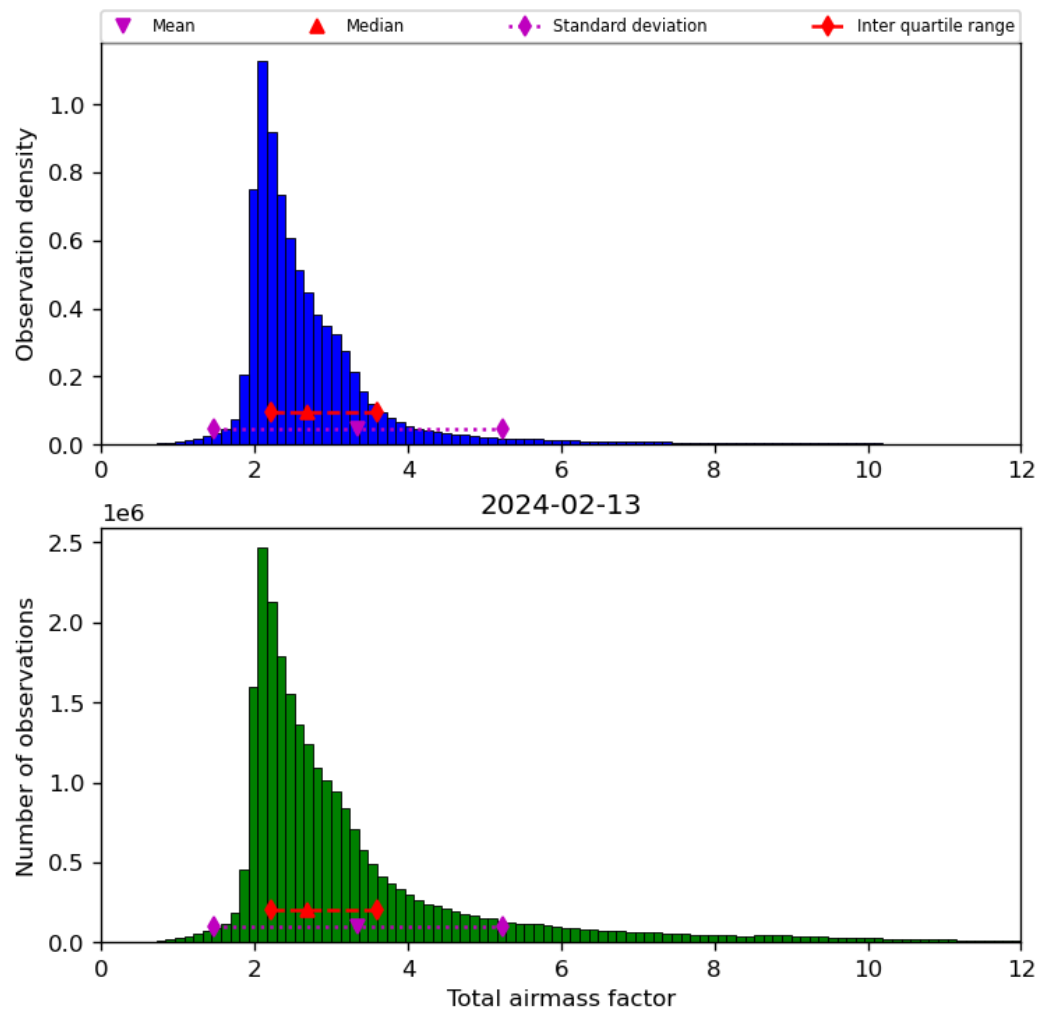
Figure 32: Histogram of “Total airmass factor” for 2024-02-12 to 2024-02-14
