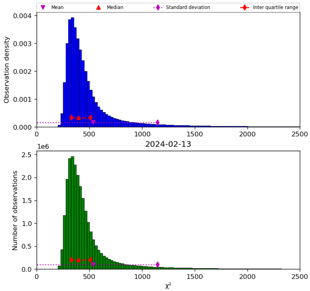
Figure 42: Histogram of “ \chi^2 ” for 2024-02-12 to 2024-02-14
