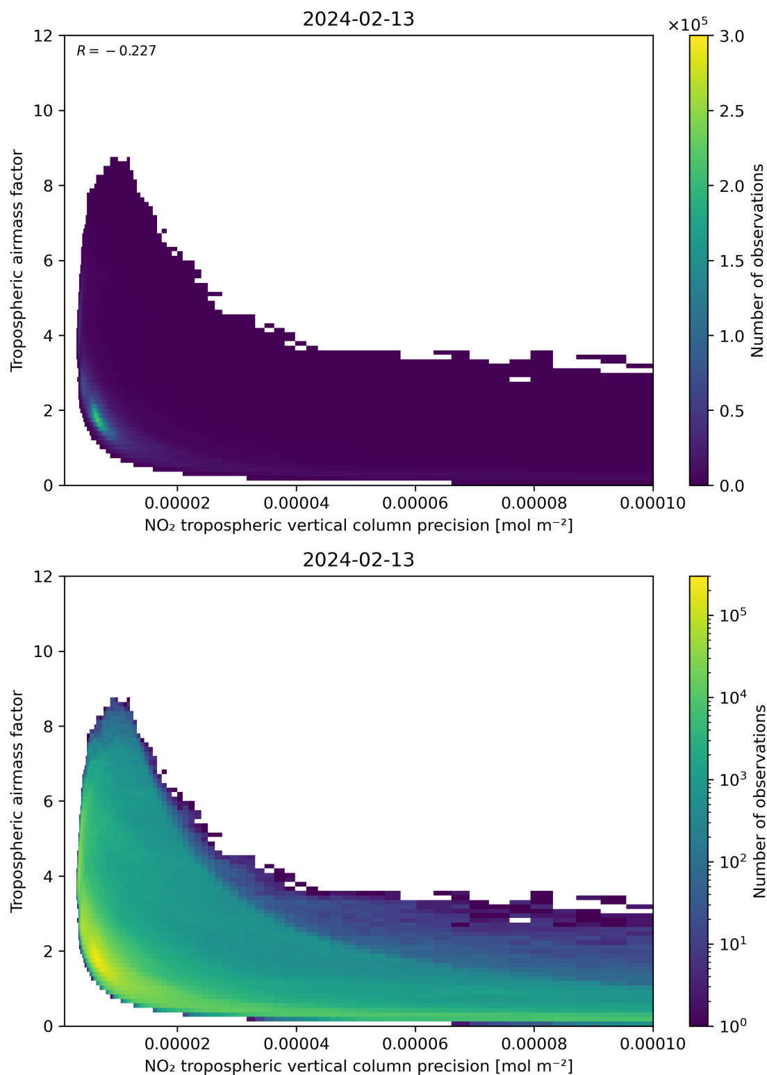
Figure 133: Scatter density plot of “NO 2 tropospheric vertical column precision” against “Tropospheric airmass factor” for 2024-02-12 to 2024-02-14.
