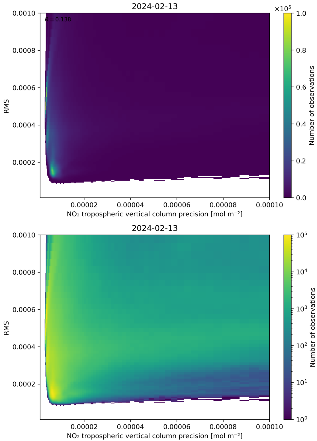
Figure 140: Scatter density plot of “NO 2 tropospheric vertical column precision” against “RMS” for 2024-02-12 to 2024-02-14.
