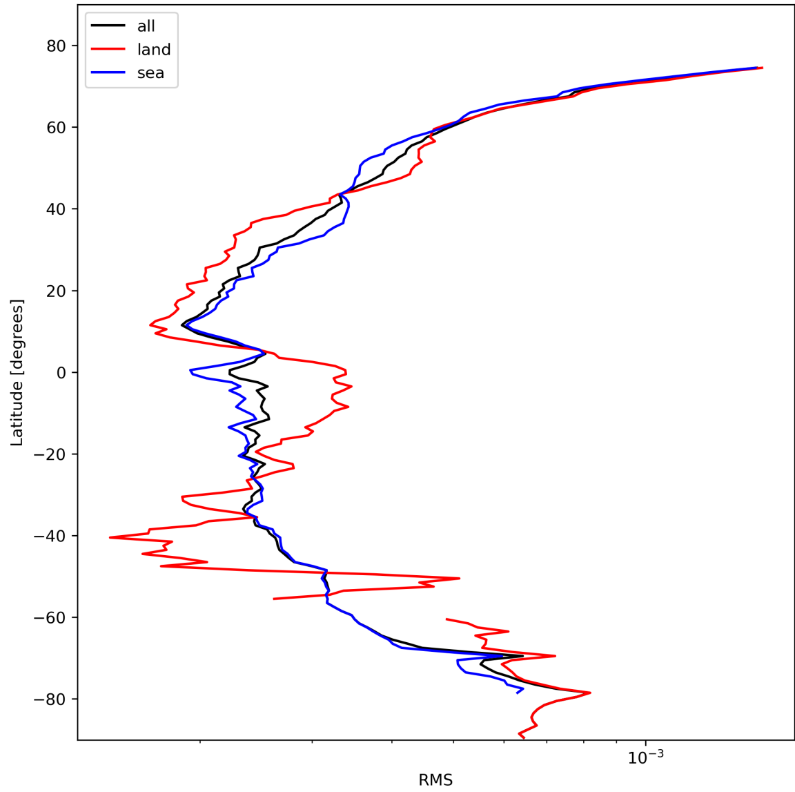
Figure 26: Zonal average of “RMS” for 2024-02-12 to 2024-02-14.
