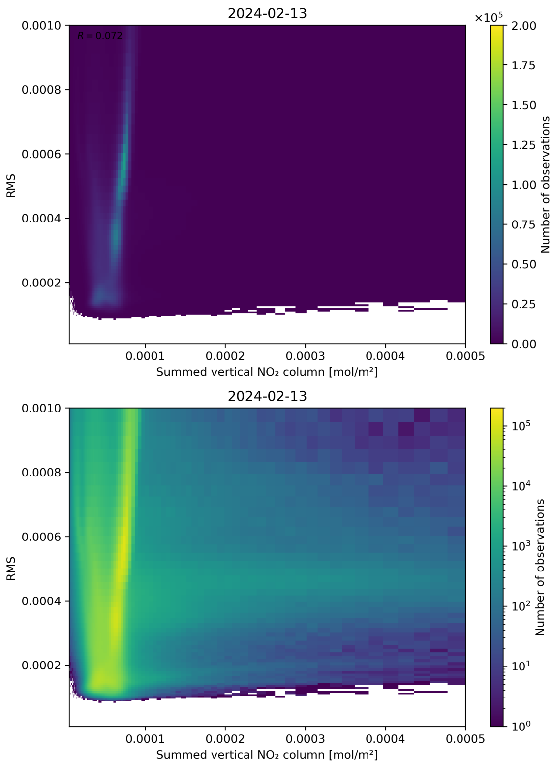
Figure 109: Scatter density plot of “Summed vertical NO 2 column” against “RMS” for 2024-02-12 to 2024-02-14.
