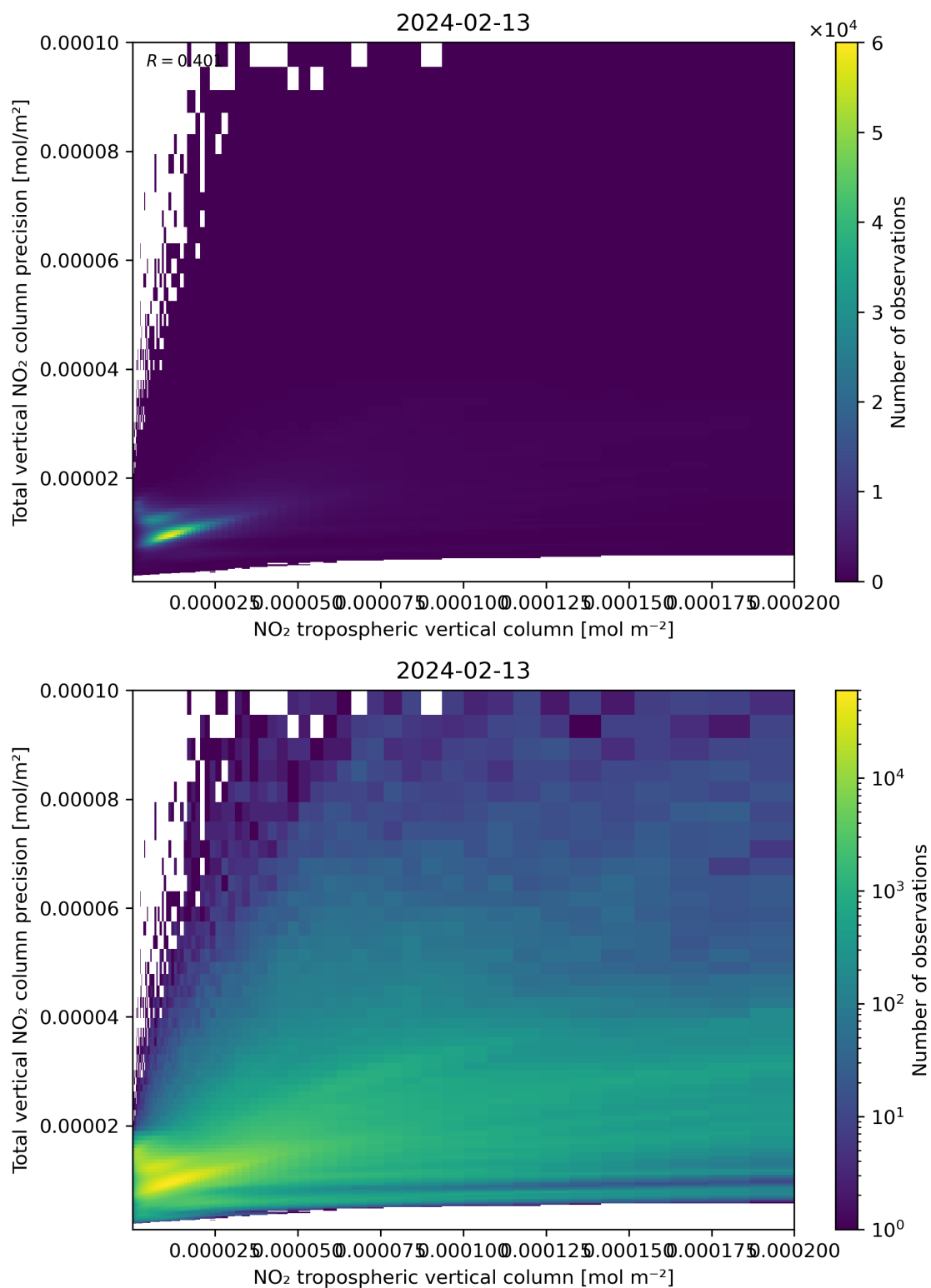
Figure 129: Scatter density plot of “NO 2 tropospheric vertical column” against “Total vertical NO 2 column precision” for 2024-02-12 to 2024-02-14.
