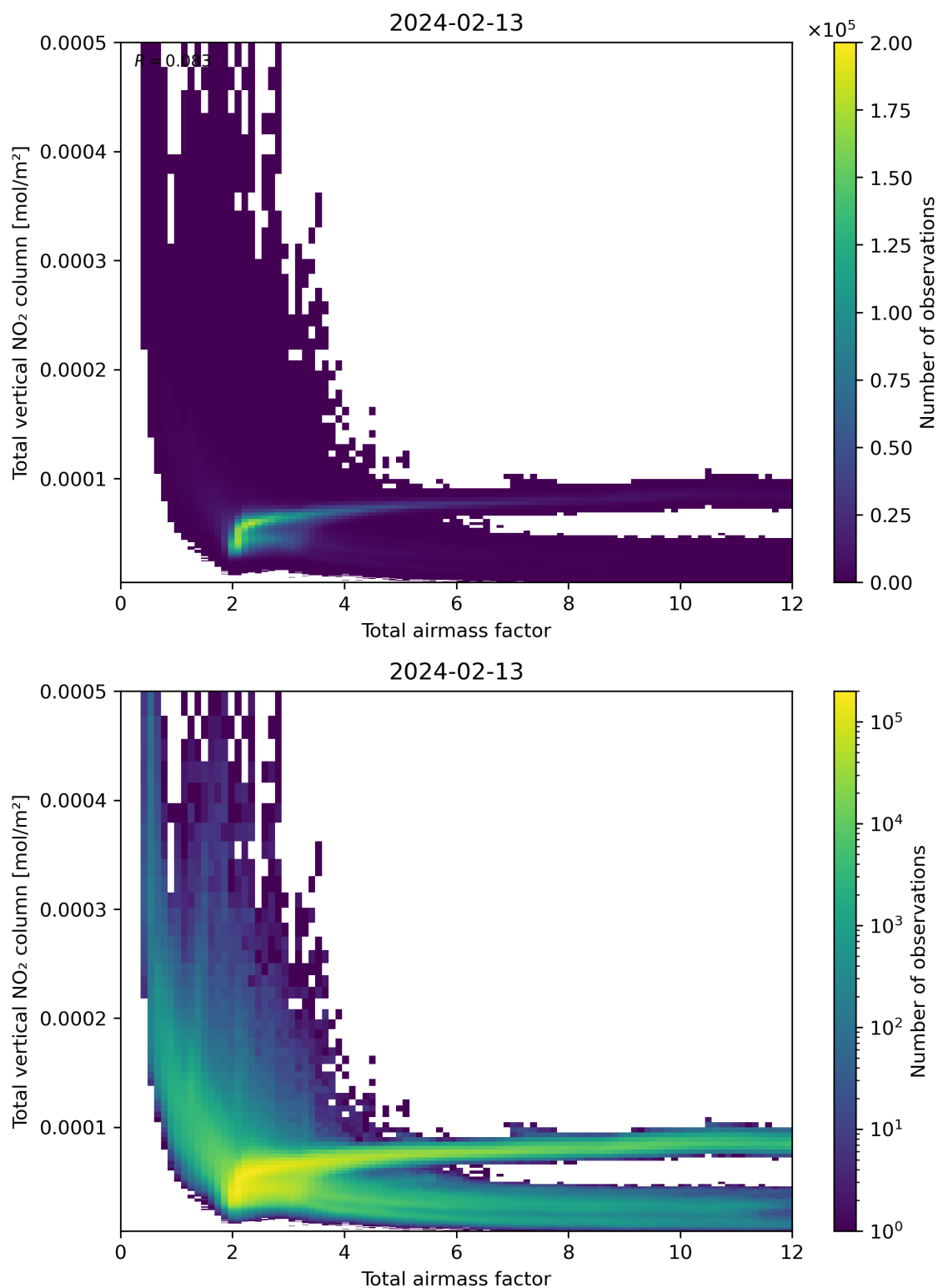
Figure 67: Scatter density plot of “Total airmass factor” against “Total vertical NO 2 column” for 2024-02-12 to 2024-02-14.
