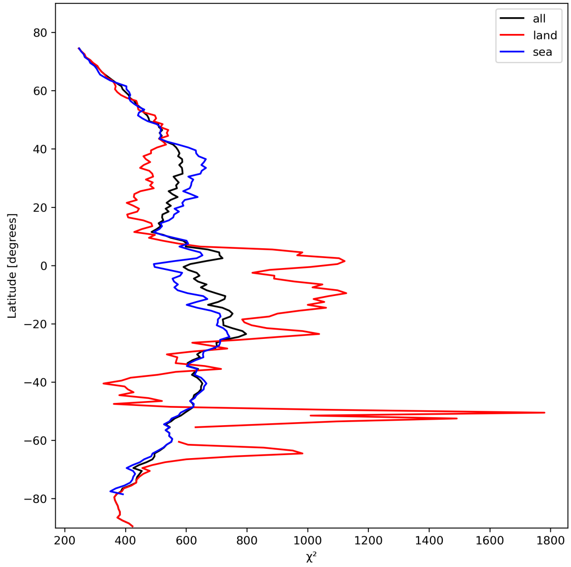
Figure 25: Zonal average of “ \chi^2 ” for 2024-02-12 to 2024-02-14.
