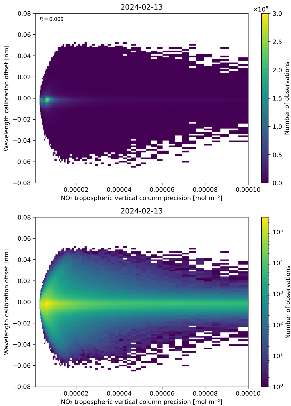
Figure 141: Scatter density plot of “NO 2 tropospheric vertical column precision” against “Wavelength calibration offset” for 2024-02-12 to 2024-02-14.
