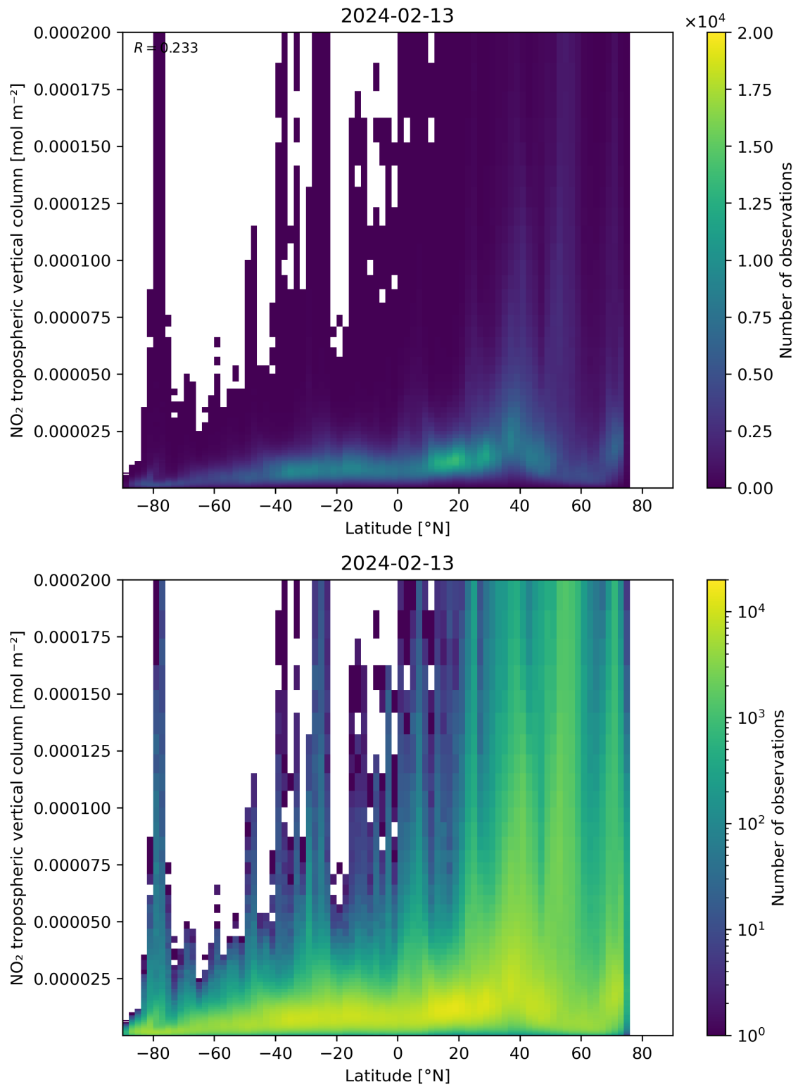
Figure 92: Scatter density plot of “Latitude” against “NO 2 tropospheric vertical column” for 2024-02-12 to 2024-02-14.
