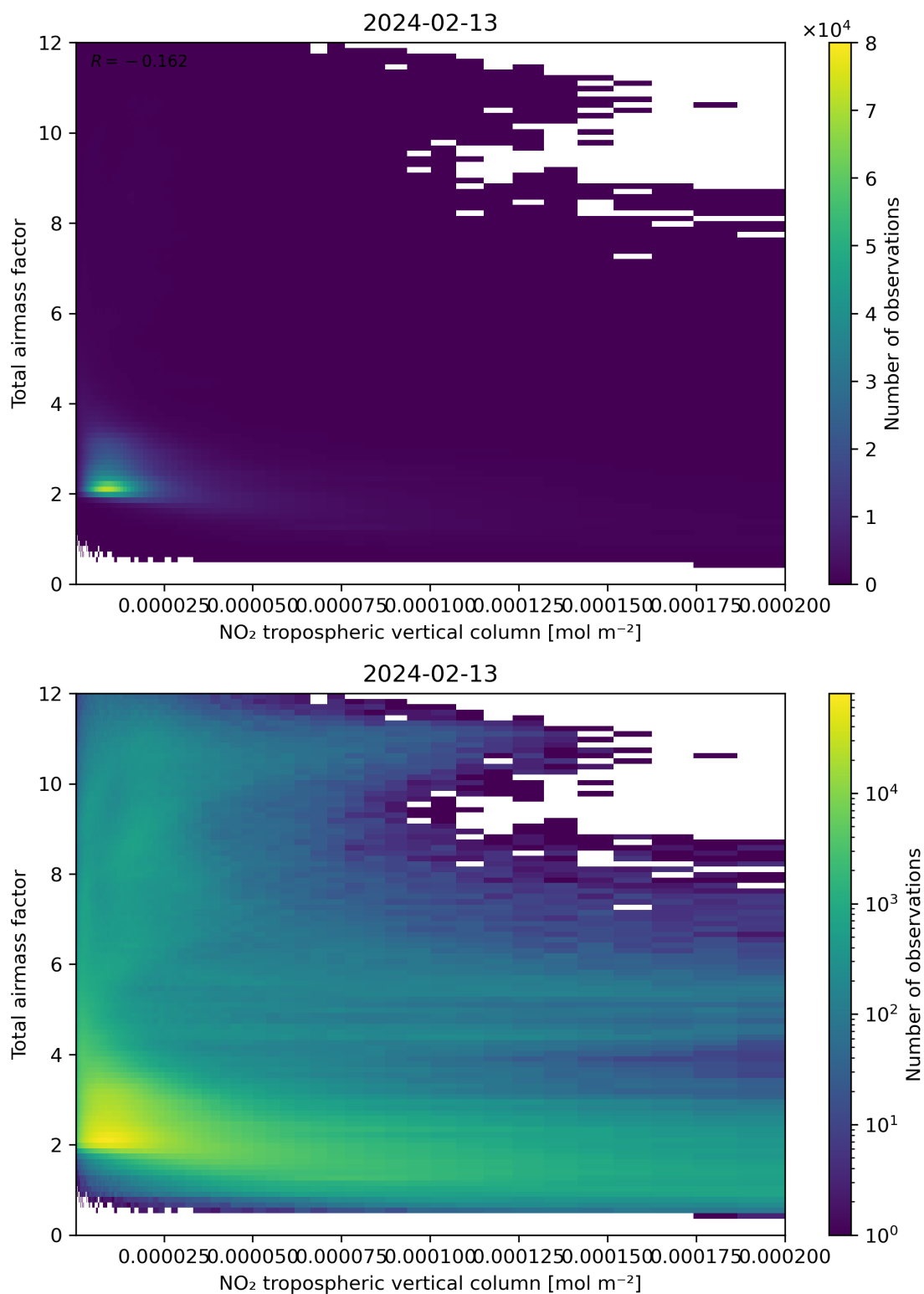
Figure 122: Scatter density plot of “NO 2 tropospheric vertical column” against “Total air mass factor” for 2024-02-12 to 2024-02-14.
