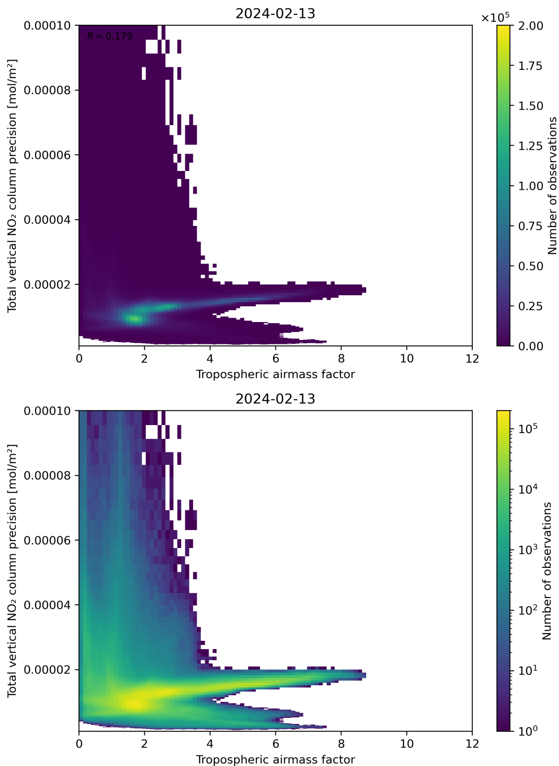
Figure 78: Scatter density plot of “Tropospheric air mass factor” against “Total vertical NO 2 column precision” for 2024-02-12 to 2024-02-14.
