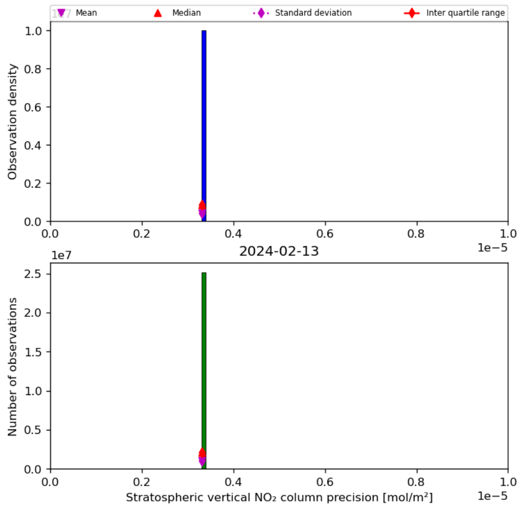
Figure 37: Histogram of “Stratospheric vertical NO 2 column precision” for 2024-02-12 to 2024-02-14
