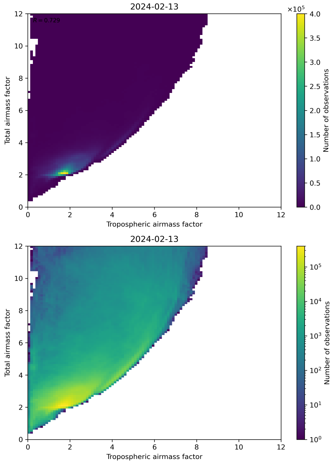
Figure 72: Scatter density plot of “Tropospheric airmass factor” against “Total airmass factor” for 2024-02-12 to 2024-02-14.
