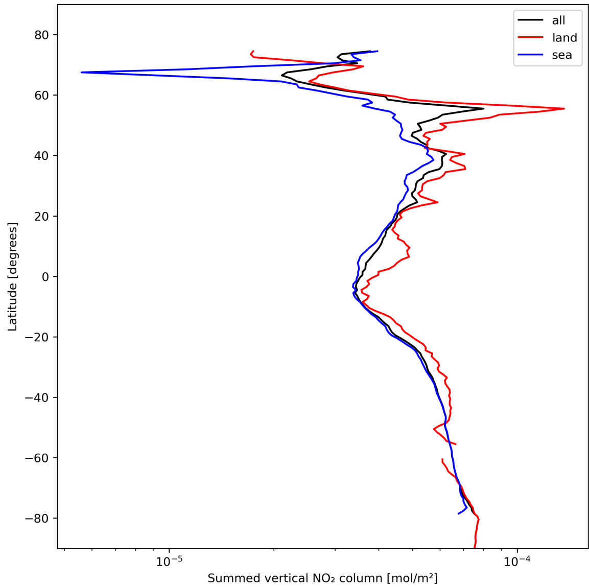
Figure 23: Zonal average of “Summed vertical NO 2 column” for 2024-02-12 to 2024-02-14.
