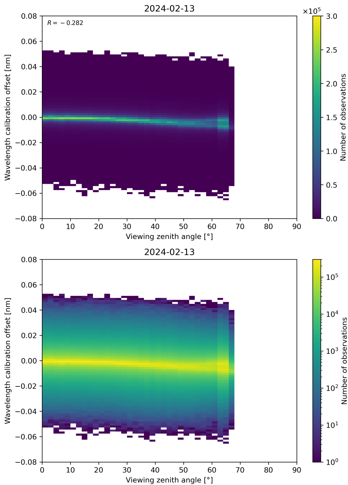
Figure 173: Scatter density plot of “Viewing zenith angle” against “Wavelength calibration offset” for 2024-02-12 to 2024-02-14.
