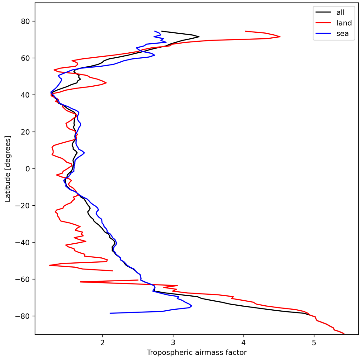
Figure 14: Zonal average of “Tropospheric airmass factor” for 2024-02-12 to 2024-02-14.
