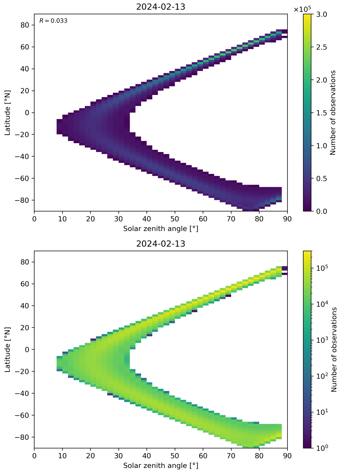
Figure 149: Scatter density plot of “Solar zenith angle” against “Latitude” for 2024-02-12 to 2024-02-14.
