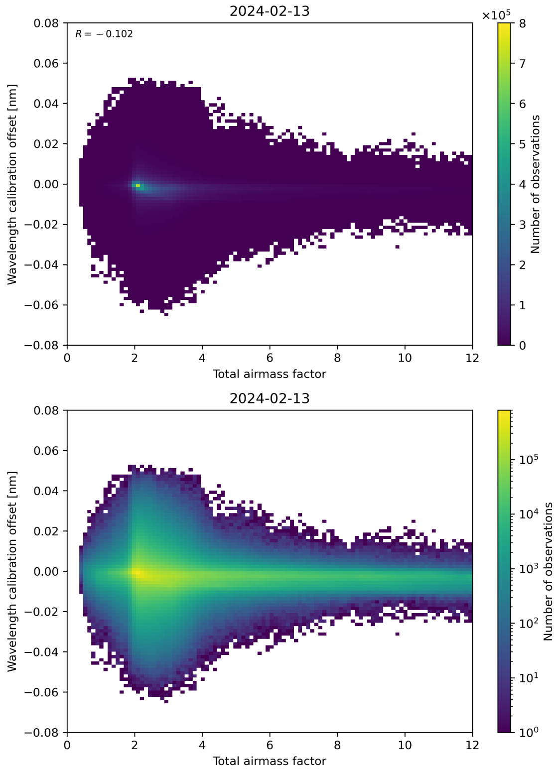
Figure 70: Scatter density plot of “Total airmass factor” against “Wavelength calibration offset” for 2024-02-12 to 2024-02-14.
