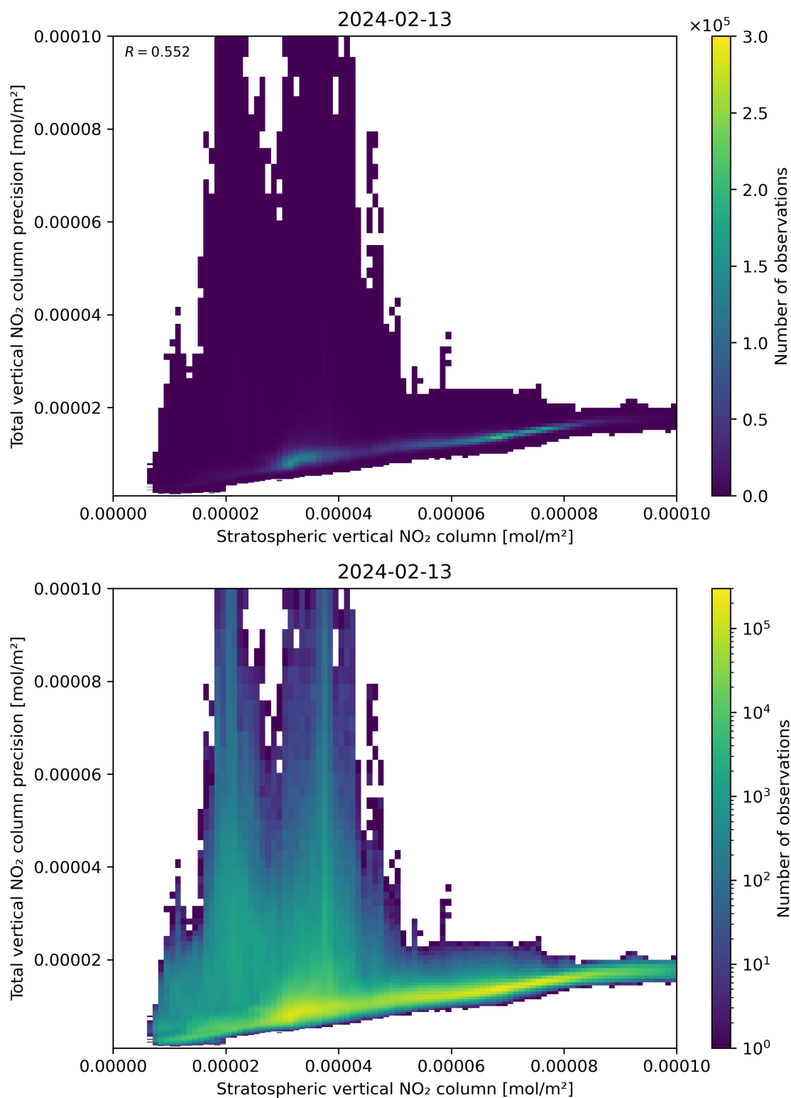
Figure 101: Scatter density plot of “Stratospheric vertical NO 2 column” against “Total vertical NO 2 column precision” for 2024-02-12 to 2024-02-14.
