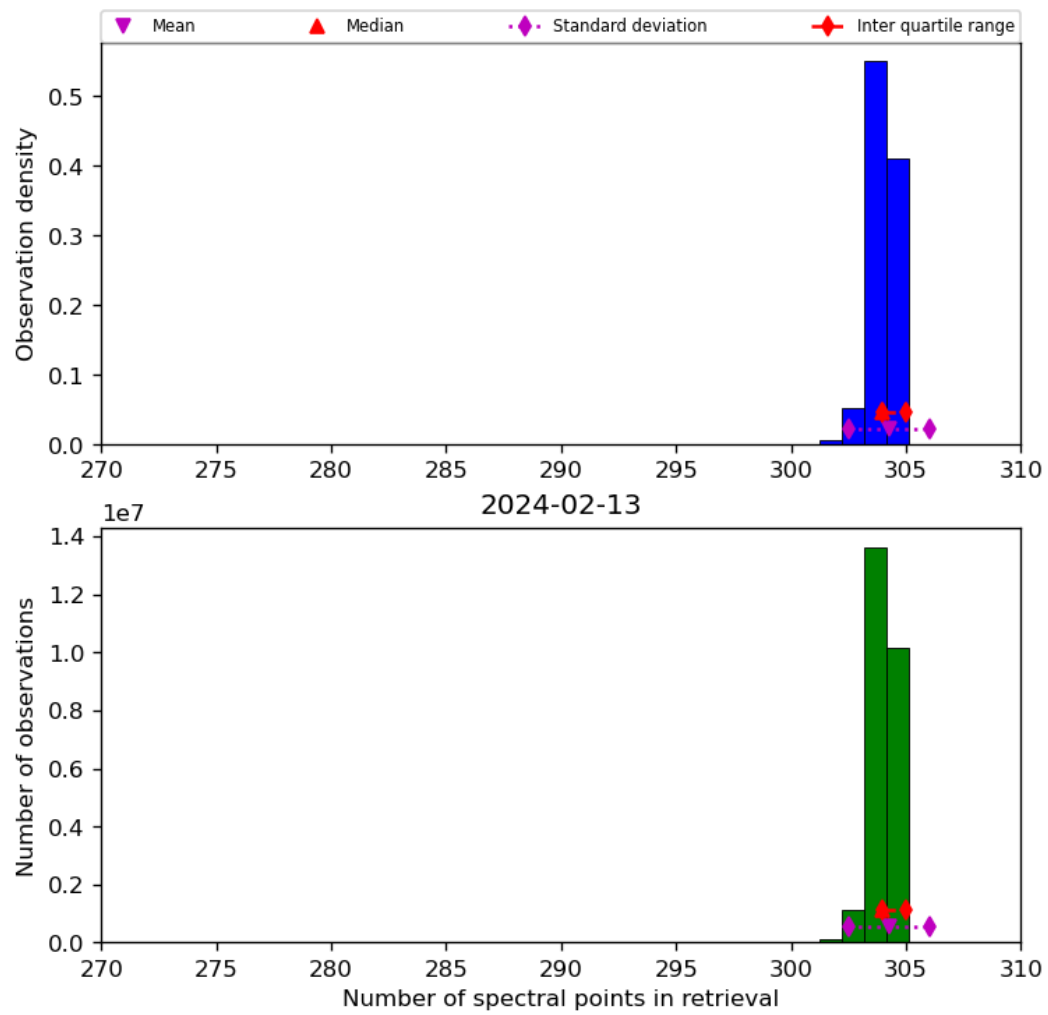
Figure 33: Histogram of “Number of spectral points in retrieval” for 2024-02-12 to 2024-02-14
