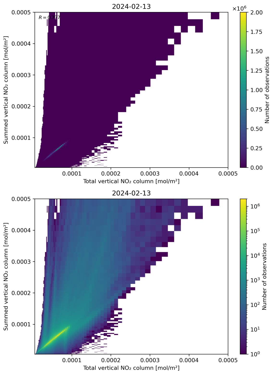
Figure 112: Scatter density plot of “Total vertical NO 2 column” against “Summed vertical NO 2 column” for 2024-02-12 to 2024-02-14.
