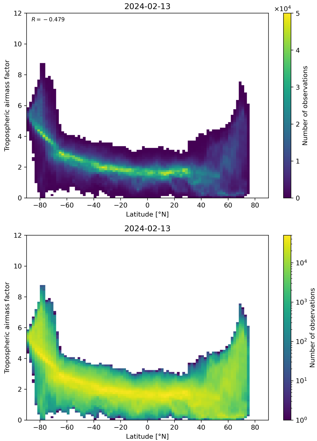
Figure 85: Scatter density plot of “Latitude” against “Tropospheric airmass factor” for 2024-02-12 to 2024-02-14.
