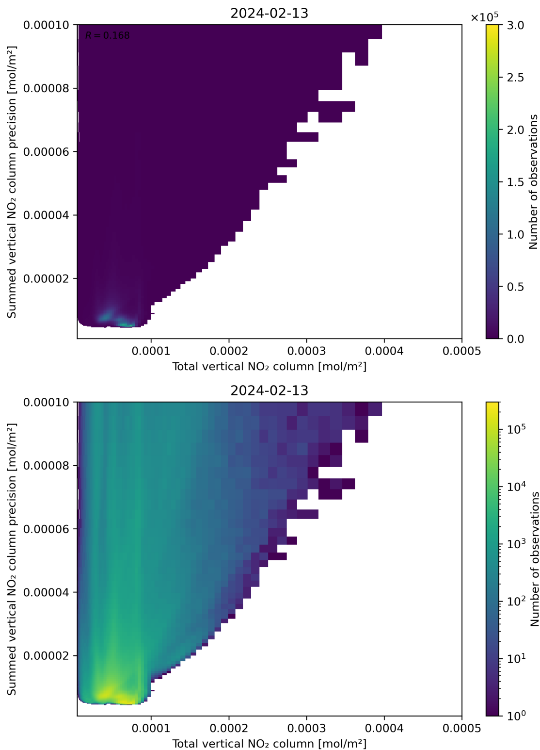
Figure 113: Scatter density plot of “Total vertical NO 2 column” against “Summed vertical NO 2 column precision” for 2024-02-12 to 2024-02-14.
