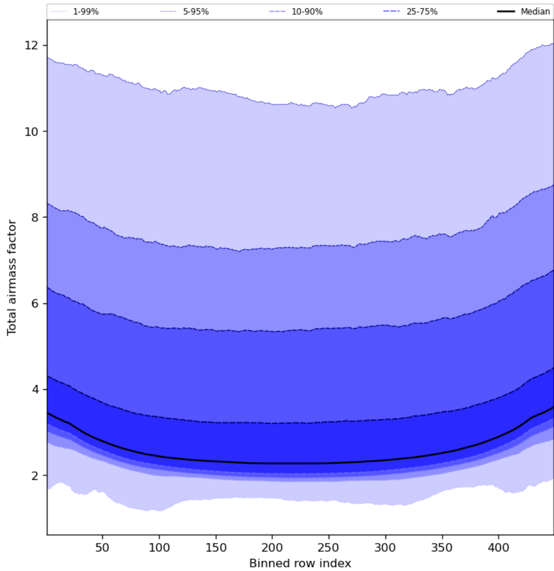
Figure 49: Along track statistics of “Total airmass factor” for 2024-02-12 to 2024-02-14
