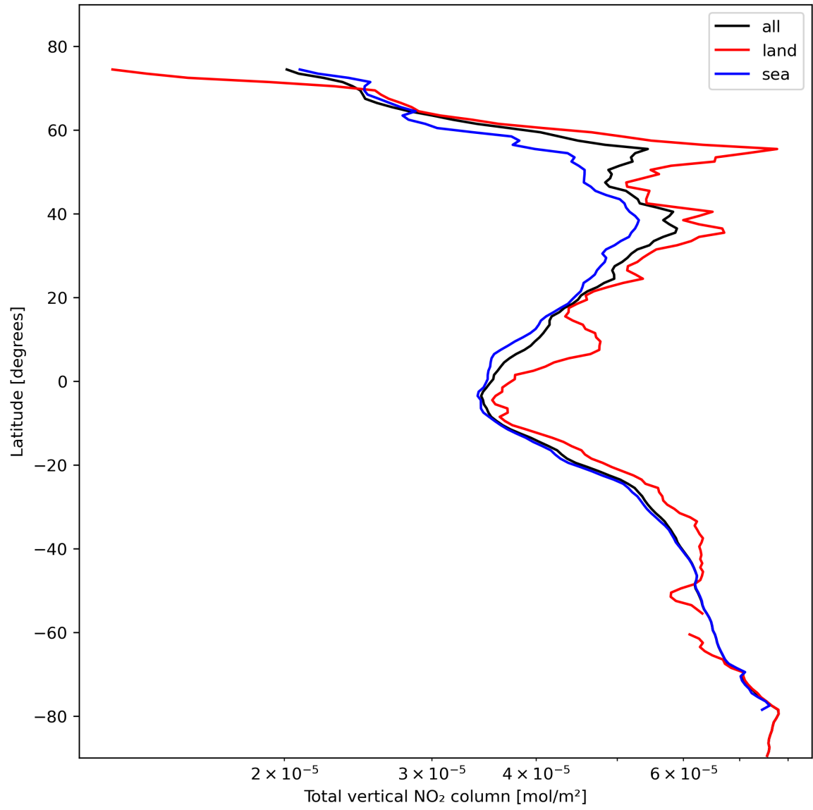
Figure 21: Zonal average of “Total vertical NO 2 column” for 2024-02-12 to 2024-02-14.
