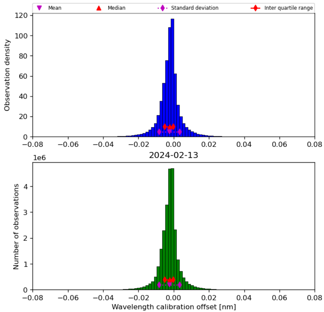
Figure 35: Histogram of “Wavelength calibration offset” for 2024-02-12 to 2024-02-14
