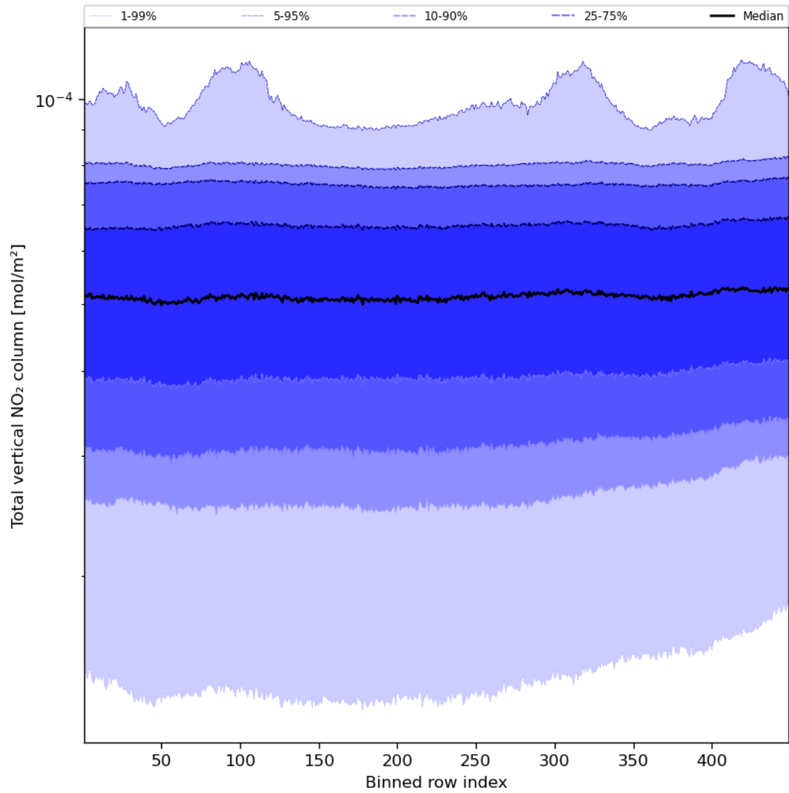
Figure 55: Along track statistics of “Total vertical NO 2 column” for 2024-02-12 to 2024-02-14
