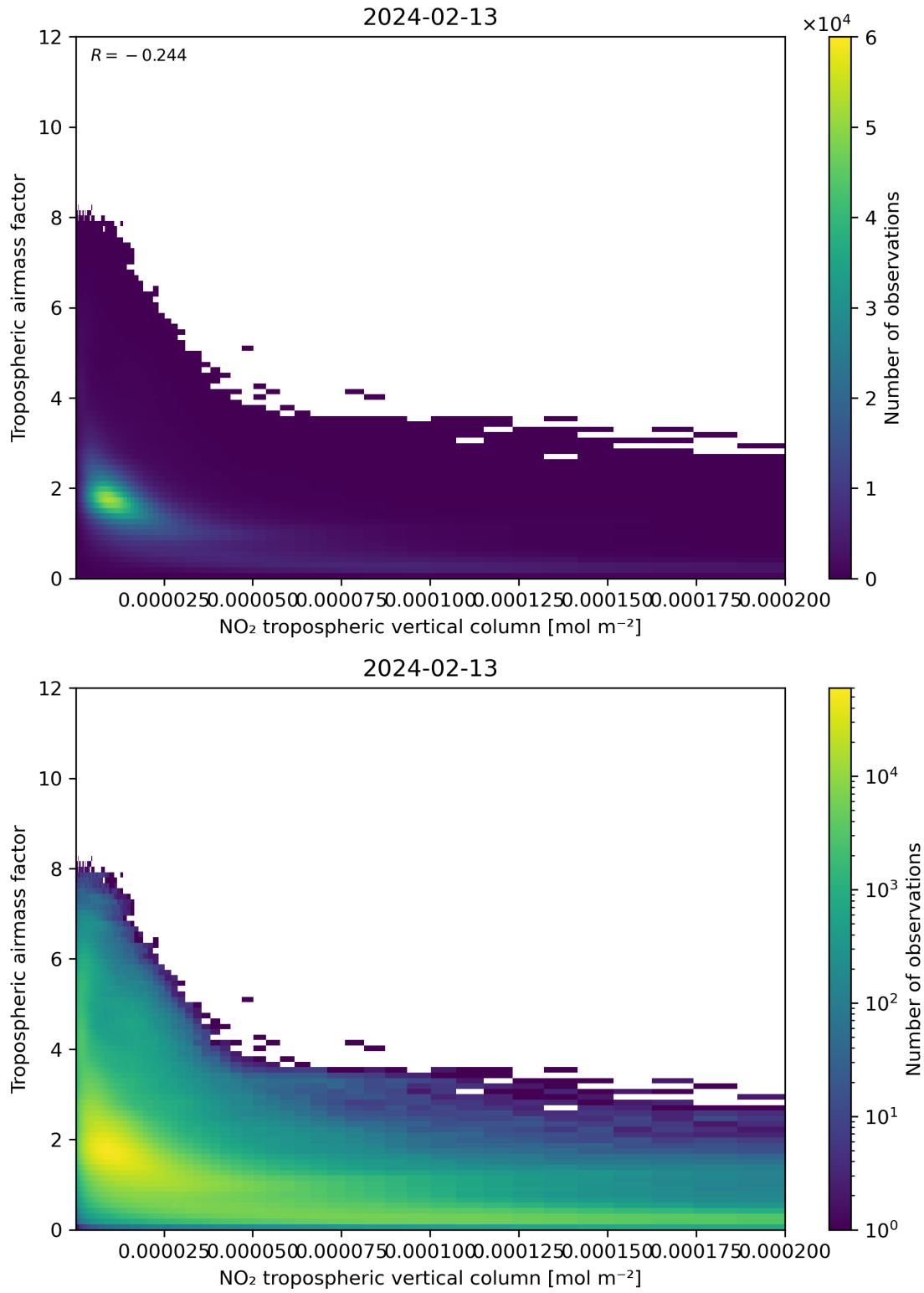
Figure 123: Scatter density plot of “NO 2 tropospheric vertical column” against “Tropospheric air mass factor” for 2024-02-12 to 2024-02-14.
