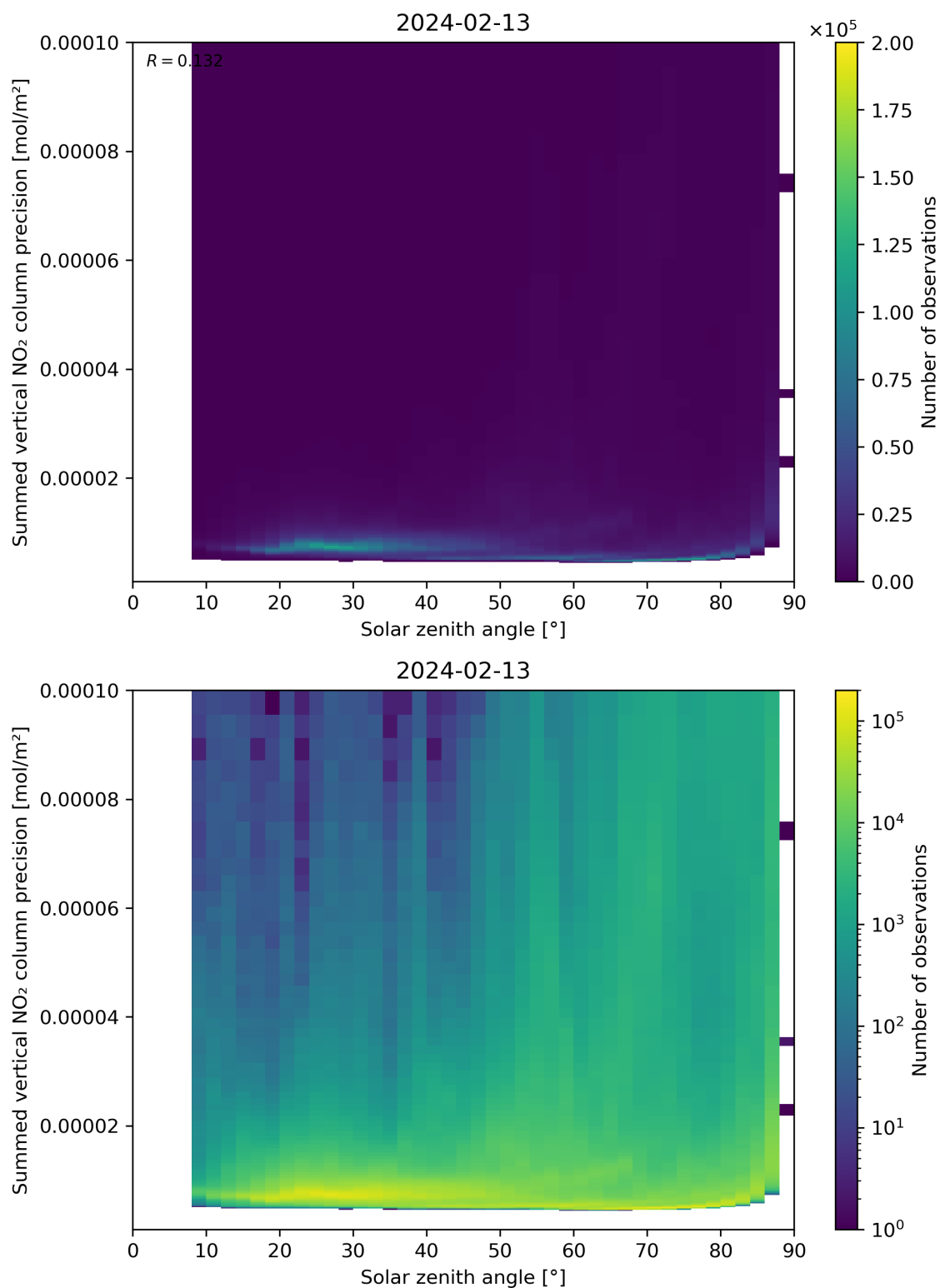
Figure 152: Scatter density plot of “Solar zenith angle” against “Summed vertical NO 2 column precision” for 2024-02-12 to 2024-02-14.
