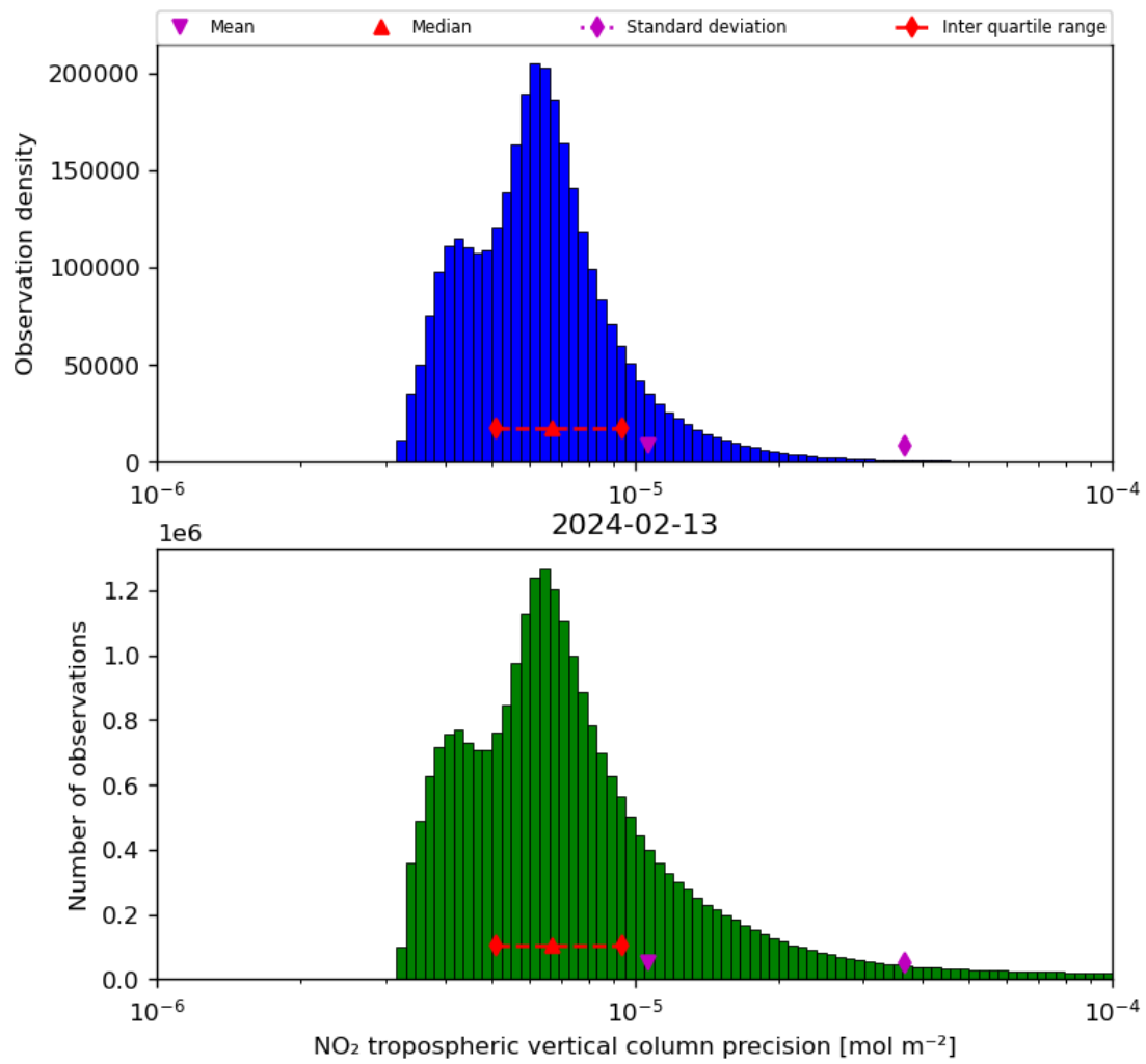
Figure 30: Histogram of “NO 2 tropospheric vertical column precision” for 2024-02-12 to 2024-02-14
