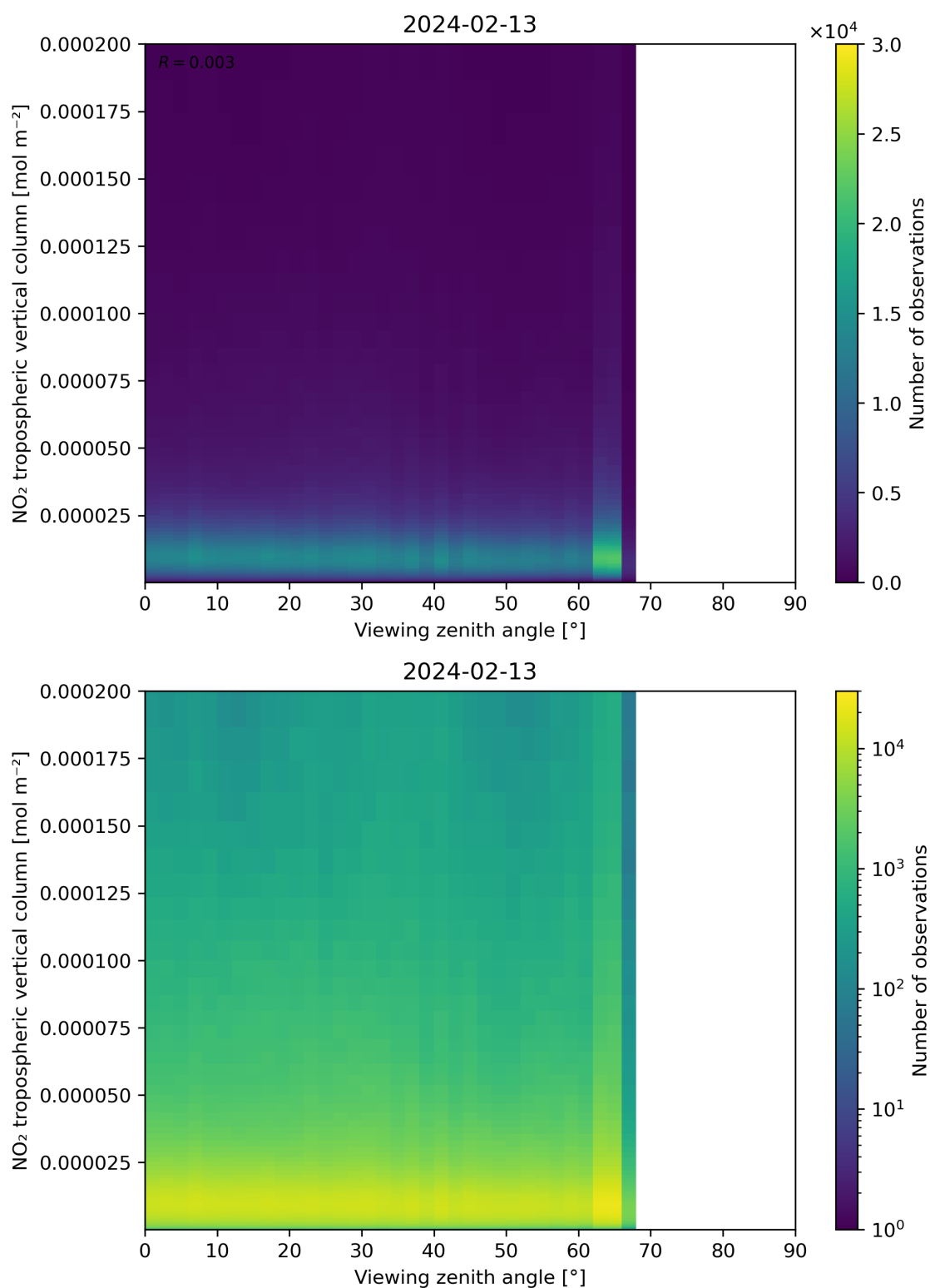
Figure 169: Scatter density plot of “Viewing zenith angle” against “NO 2 tropospheric vertical column” for 2024-02-12 to 2024-02-14.
