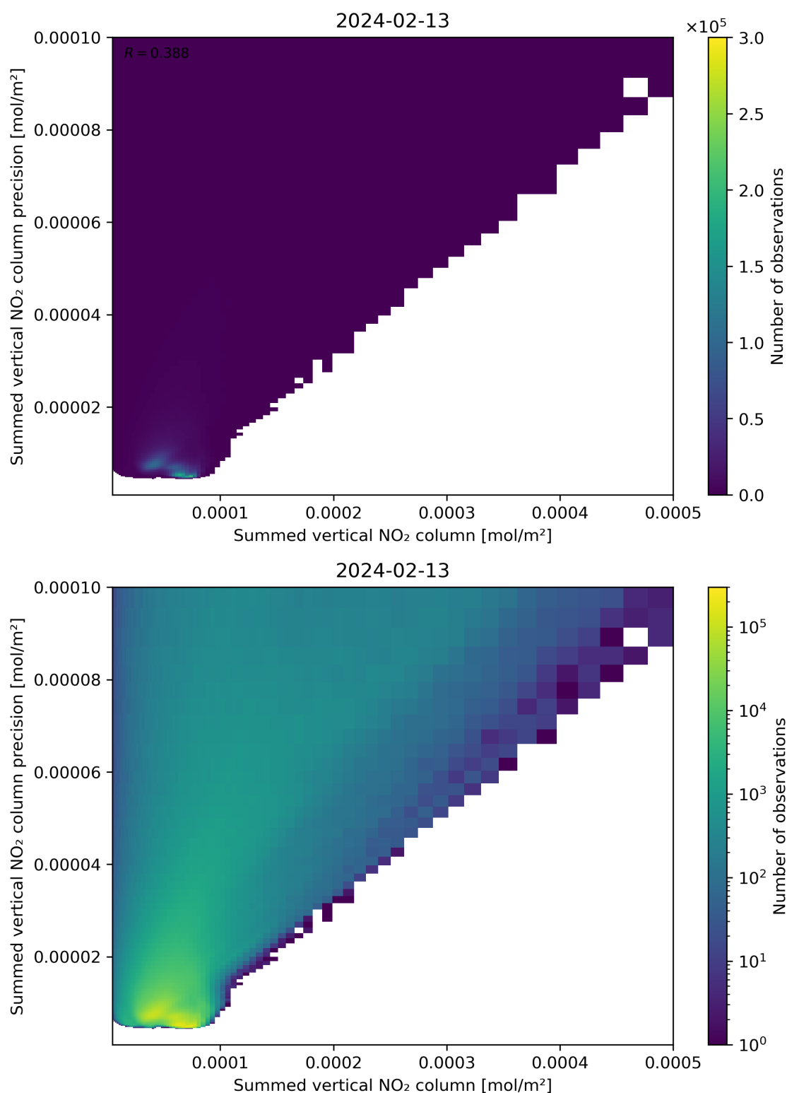
Figure 105: Scatter density plot of “Summed vertical NO 2 column” against “Summed vertical NO 2 column precision” for 2024-02-12 to 2024-02-14.
