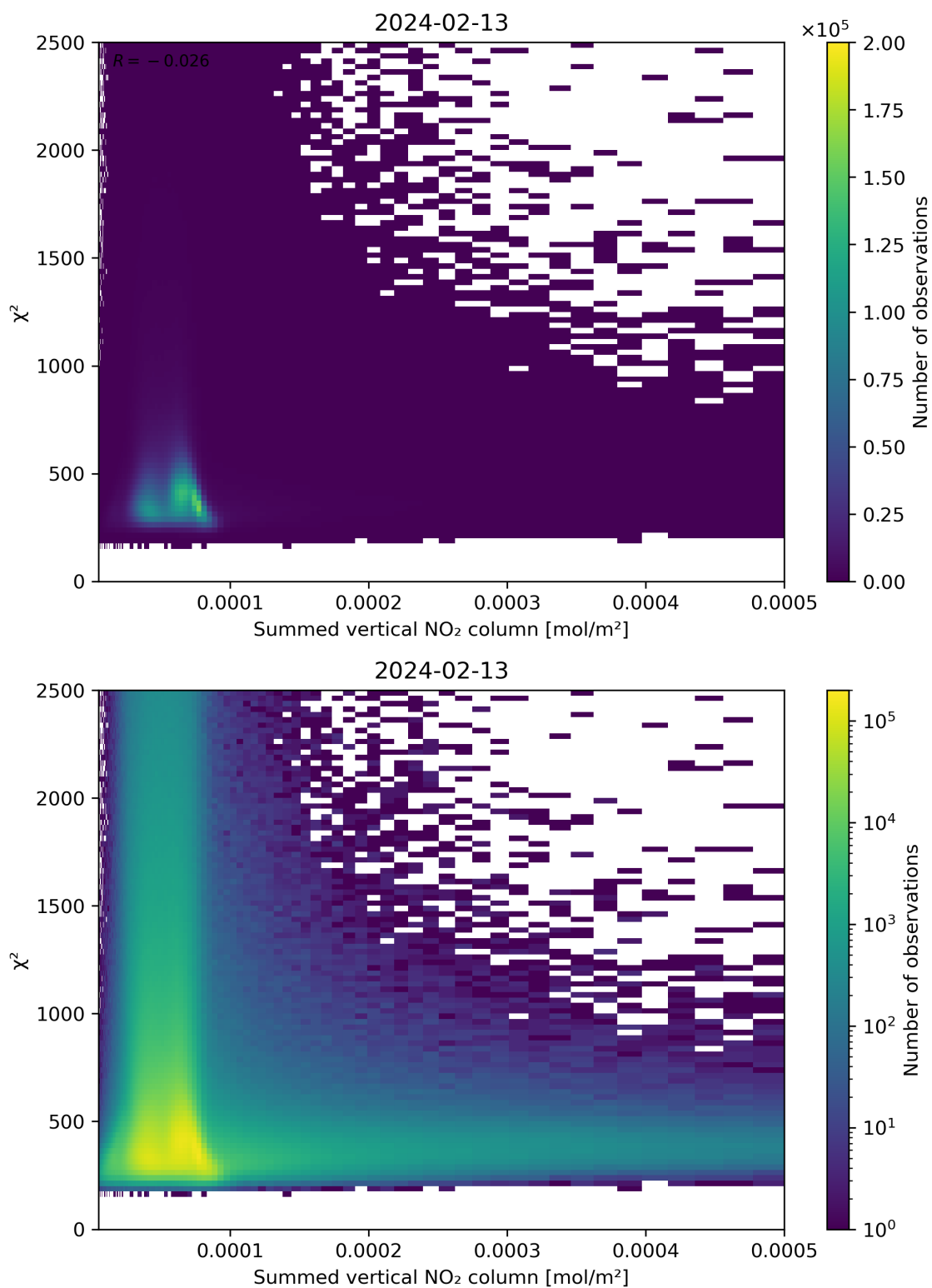
Figure 104: Scatter density plot of “Summed vertical NO 2 column” against “ \chi^2 ” for 2024-02-12 to 2024-02-14.
