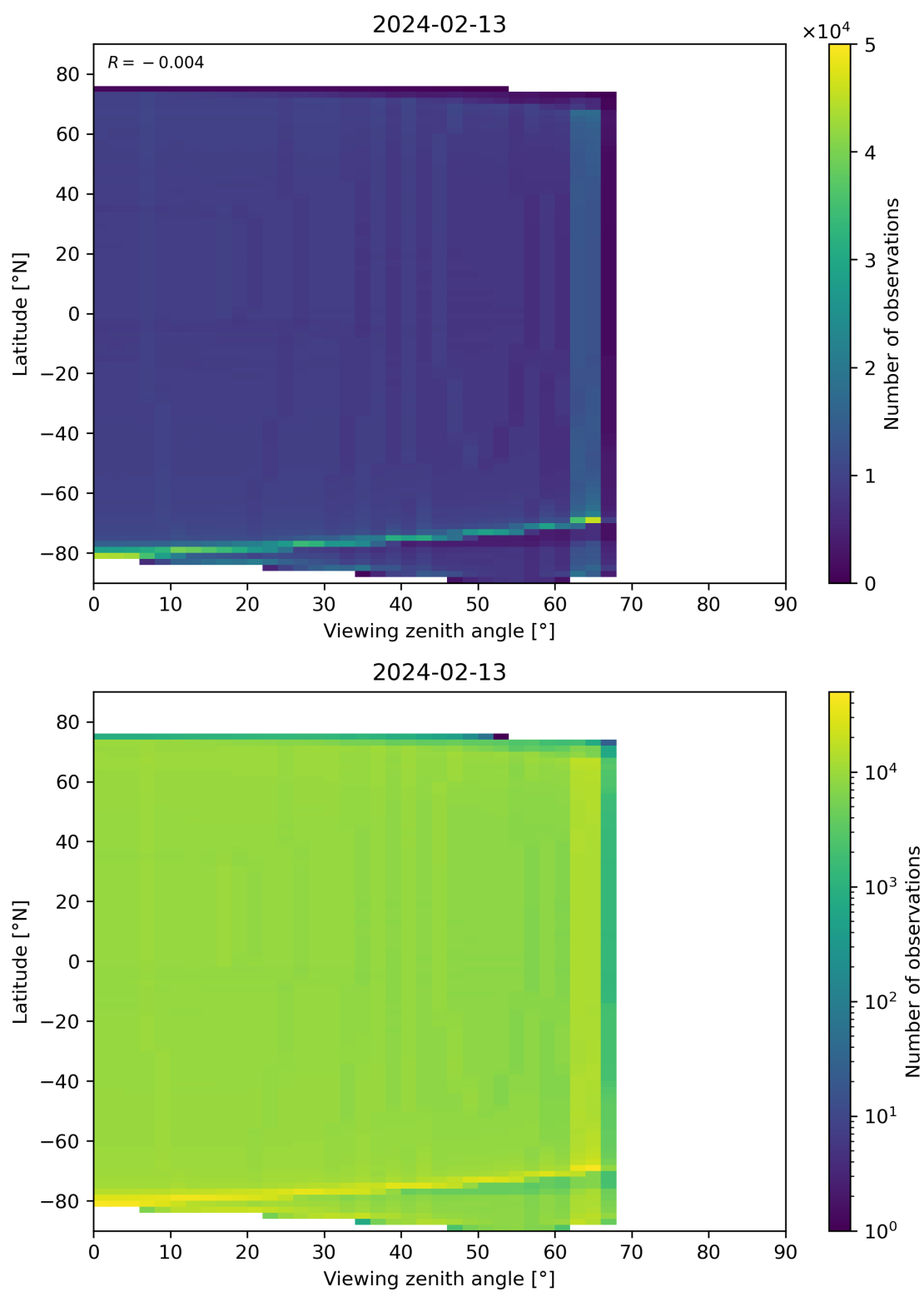
Figure 163: Scatter density plot of “Viewing zenith angle” against “Latitude” for 2024-02-12 to 2024-02-14.
