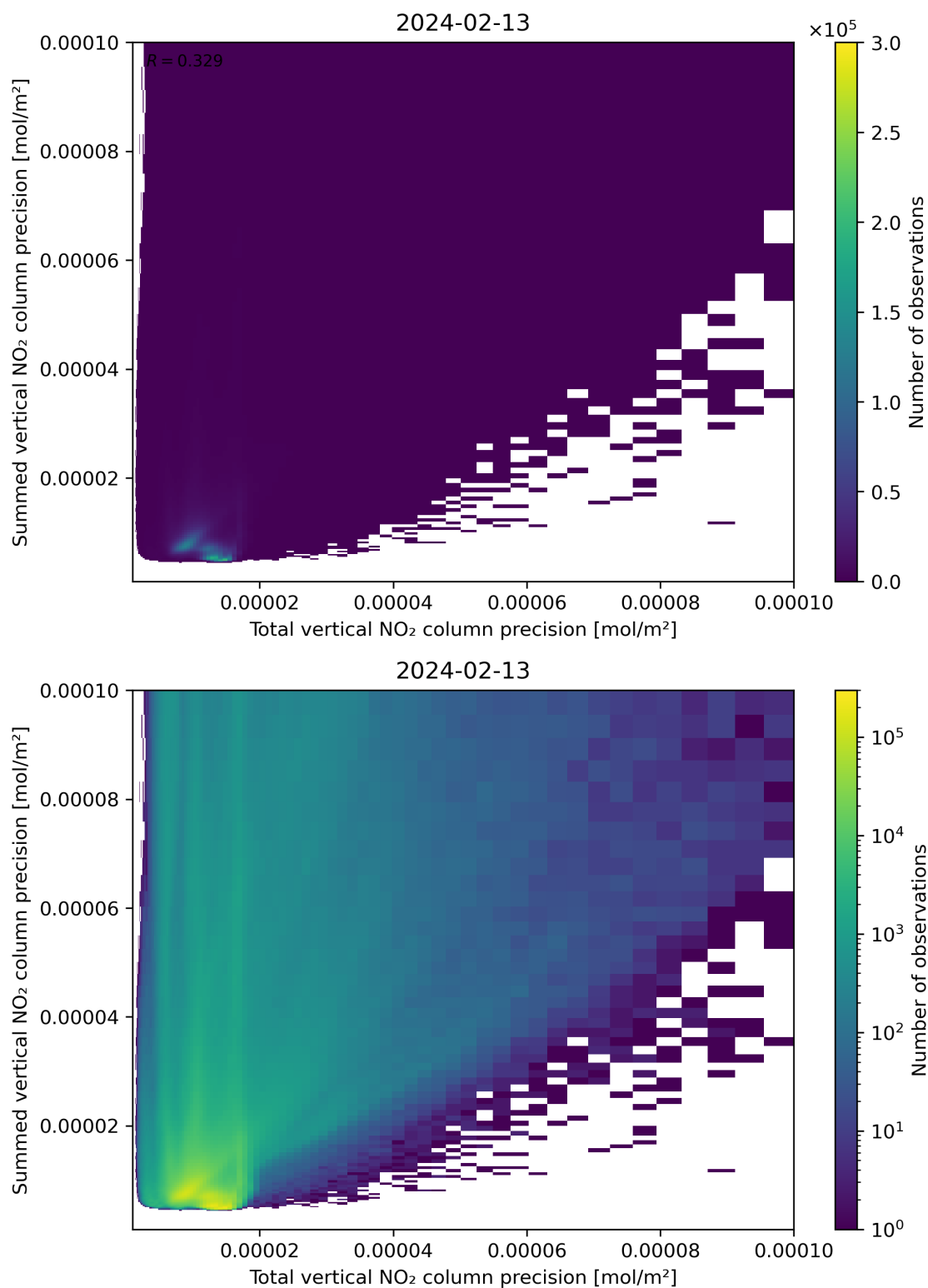
Figure 118: Scatter density plot of “Total vertical NO 2 column precision” against “Summed vertical NO 2 column precision” for 2024-02-12 to 2024-02-14.
