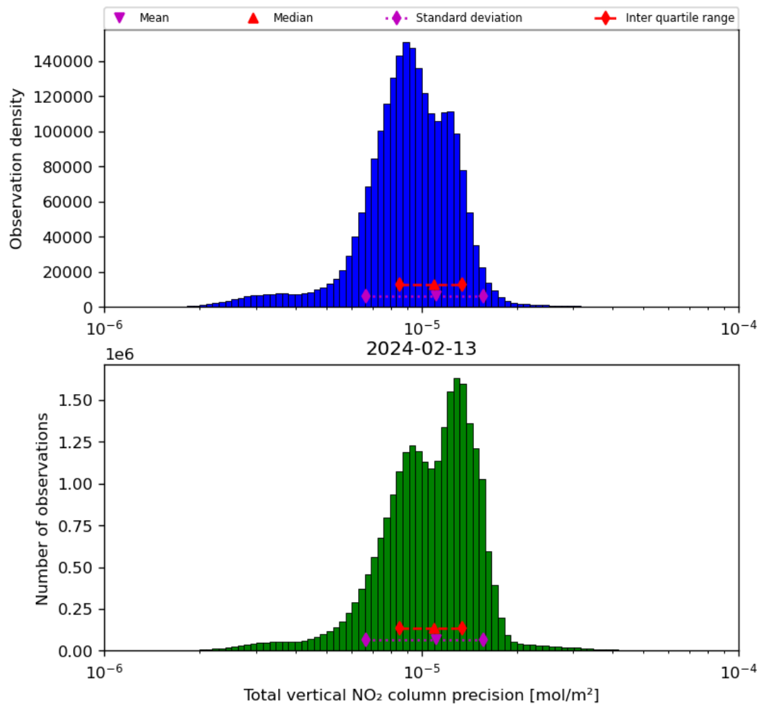
Figure 39: Histogram of “Total vertical NO 2 column precision” for 2024-02-12 to 2024-02-14
