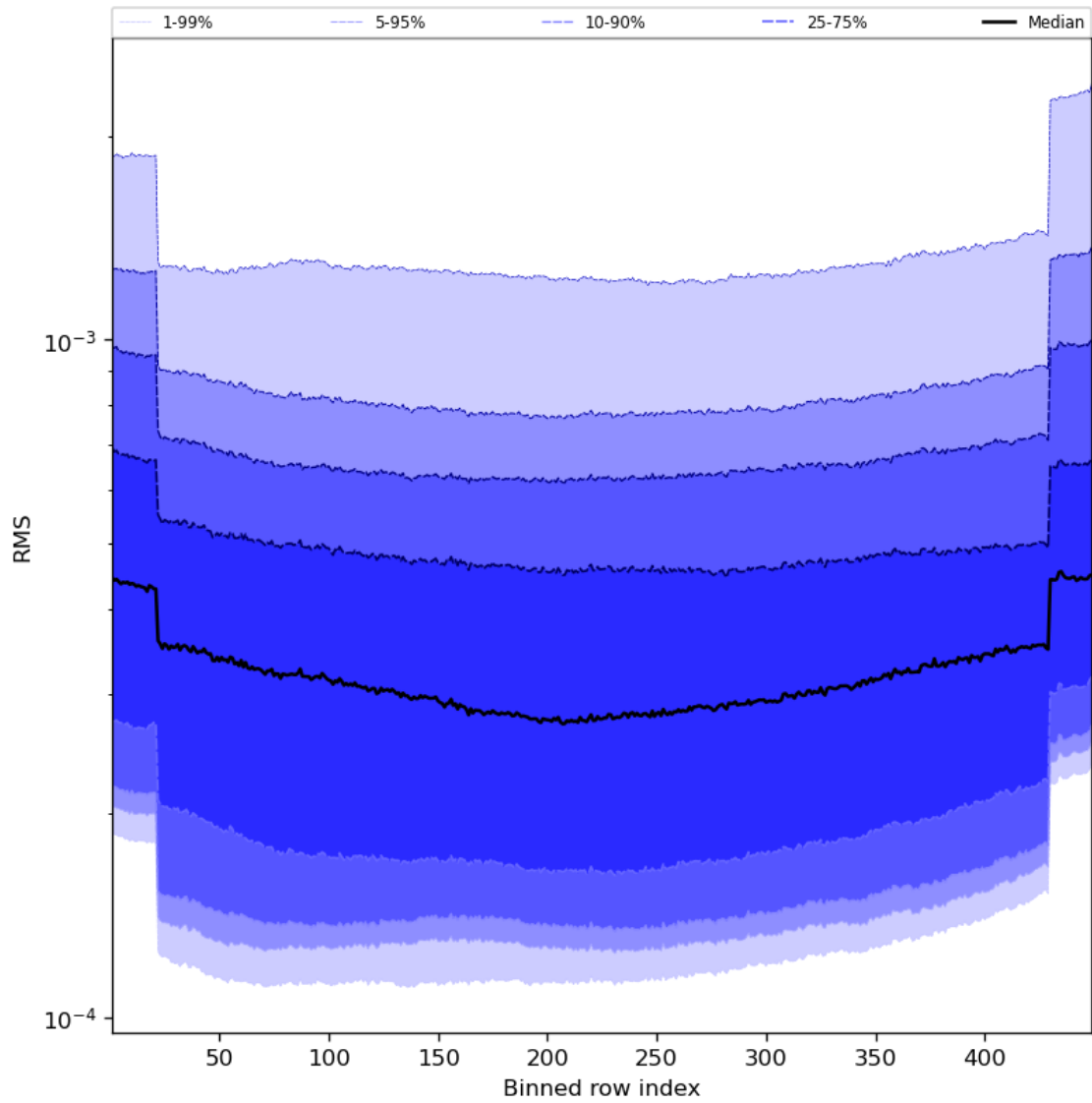
Figure 60: Along track statistics of “RMS” for 2024-02-12 to 2024-02-14
