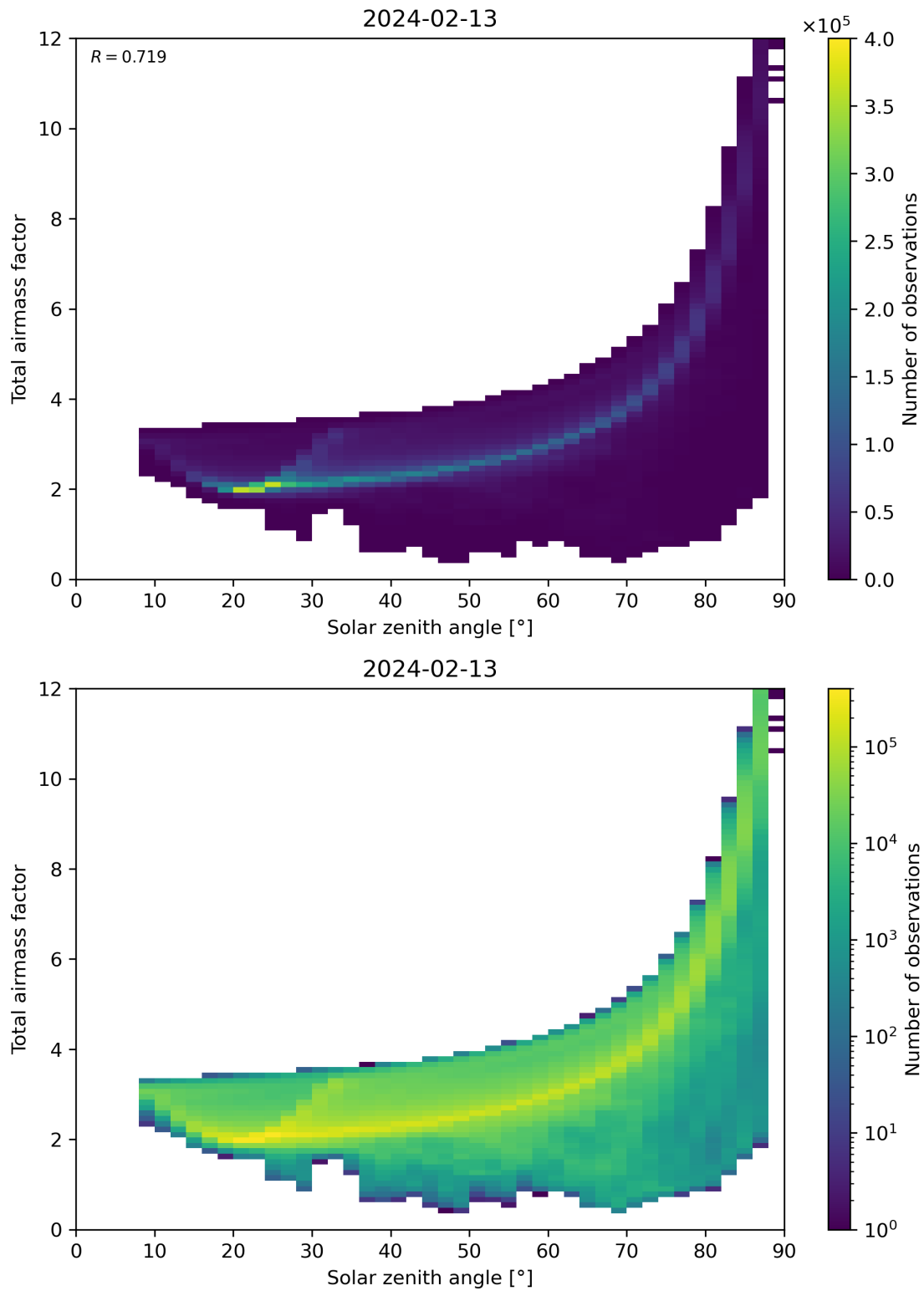
Figure 146: Scatter density plot of “Solar zenith angle” against “Total air mass factor” for 2024-02-12 to 2024-02-14.
