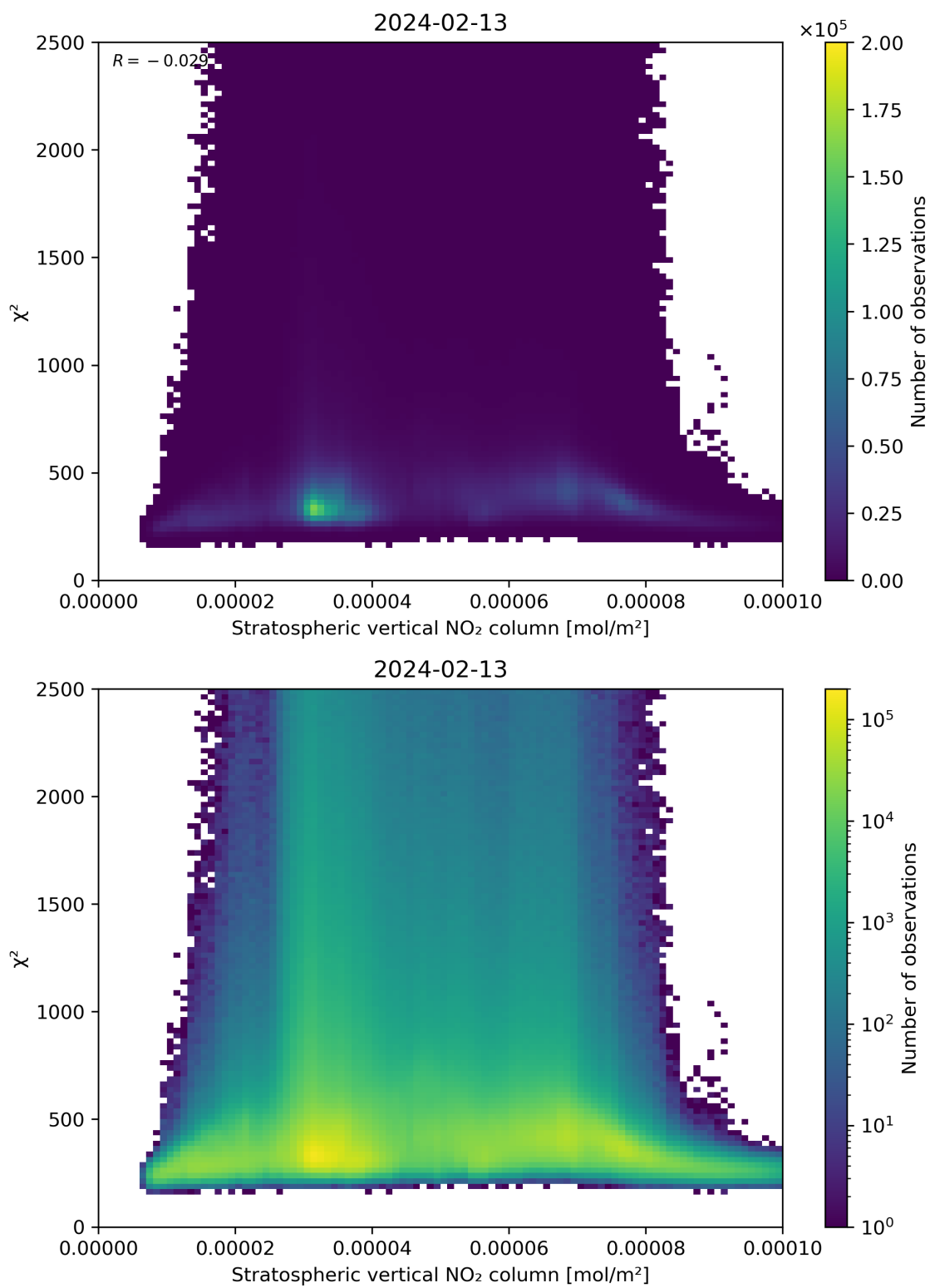
Figure 97: Scatter density plot of “Stratospheric vertical NO 2 column” against “ \chi^2 ” for 2024-02-12 to 2024-02-14.
