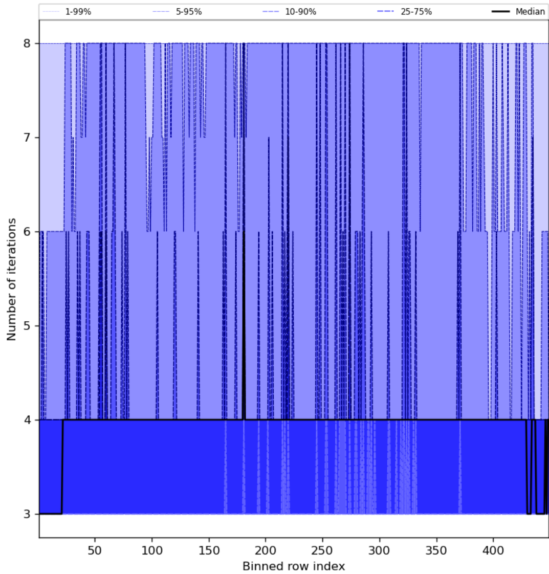
Figure 51: Along track statistics of “Number of iterations” for 2024-02-12 to 2024-02-14
