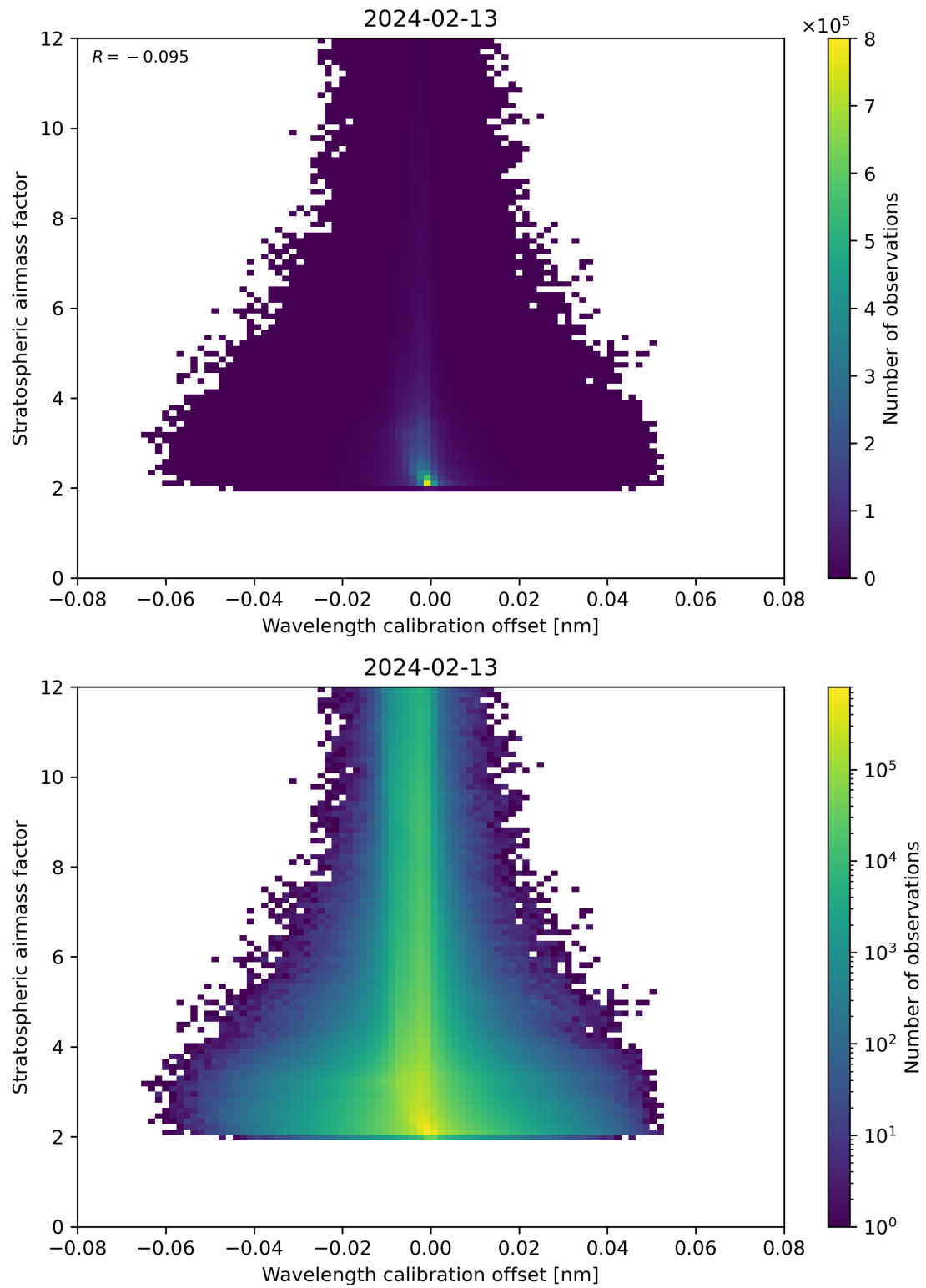
Figure 174: Scatter density plot of “Wavelength calibration offset” against “Stratospheric airmass factor” for 2024-02-12 to 2024-02-14.
