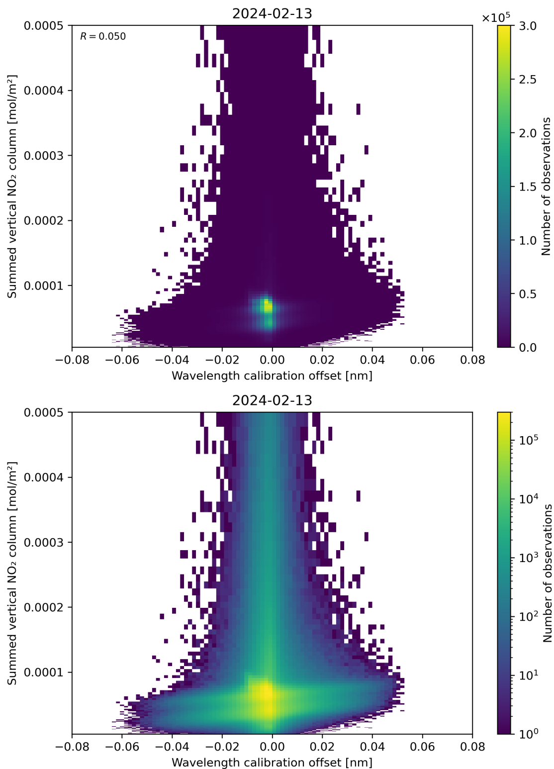
Figure 177: Scatter density plot of “Wavelength calibration offset” against “Summed vertical NO 2 column” for 2024-02-12 to 2024-02-14.
