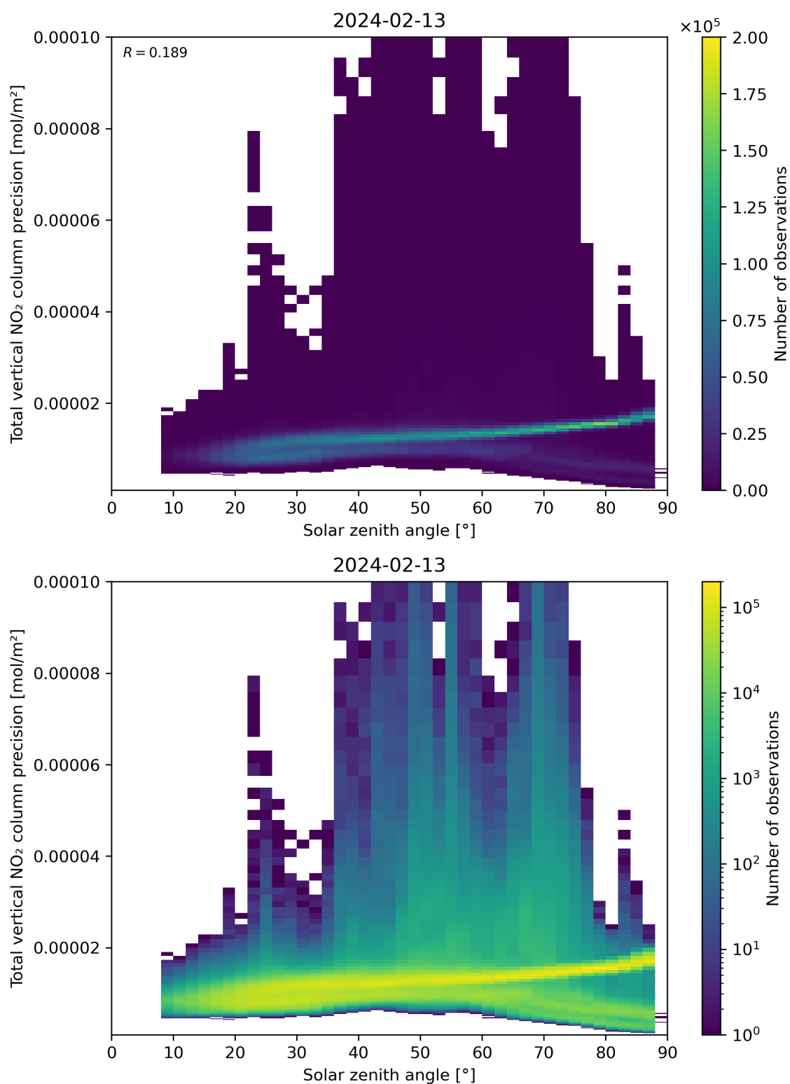
Figure 154: Scatter density plot of “Solar zenith angle” against “Total vertical NO 2 column precision” for 2024-02-12 to 2024-02-14.
