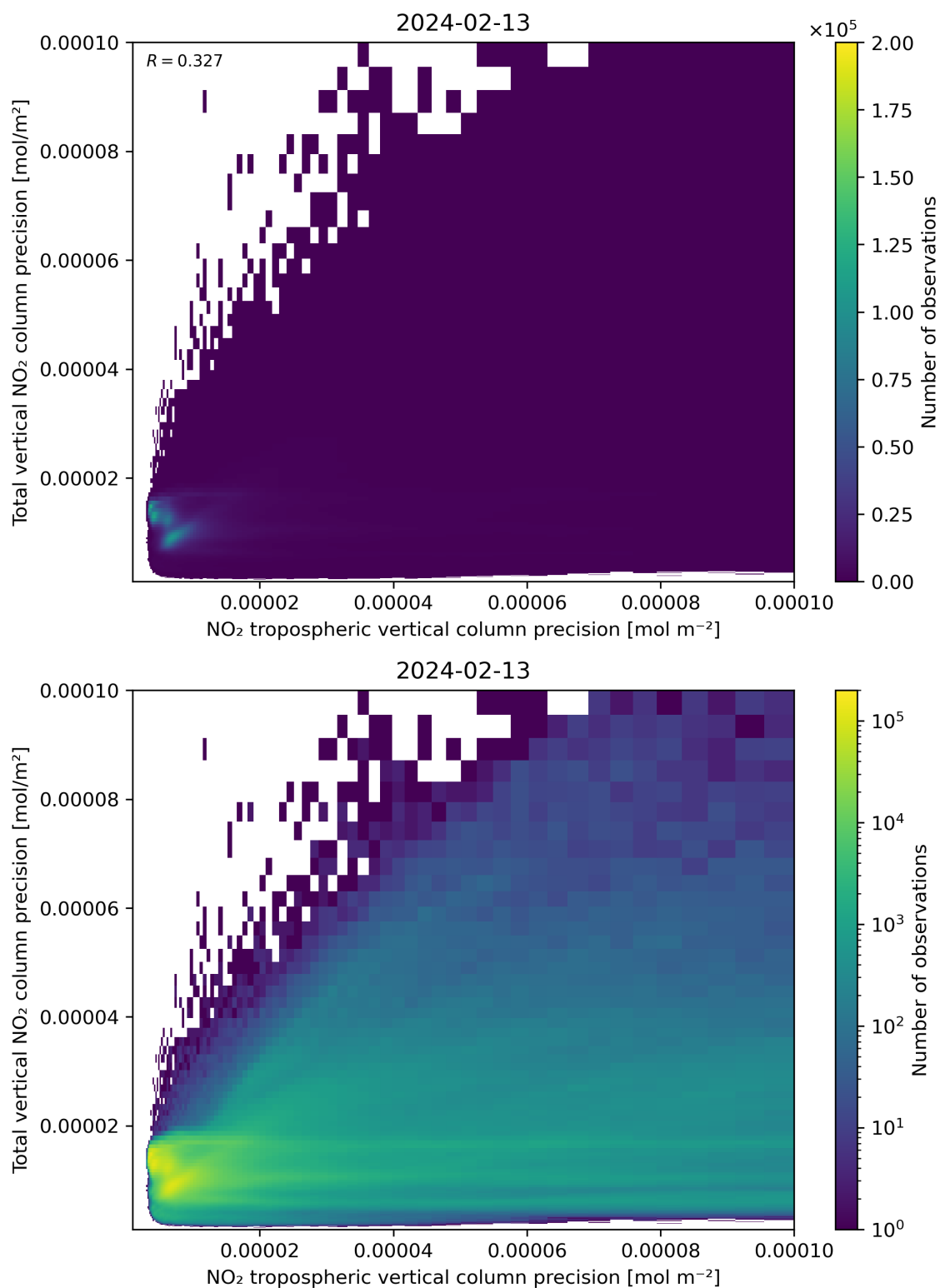
Figure 139: Scatter density plot of “NO 2 tropospheric vertical column precision” against “Total vertical NO 2 column precision” for 2024-02-12 to 2024-02-14.
