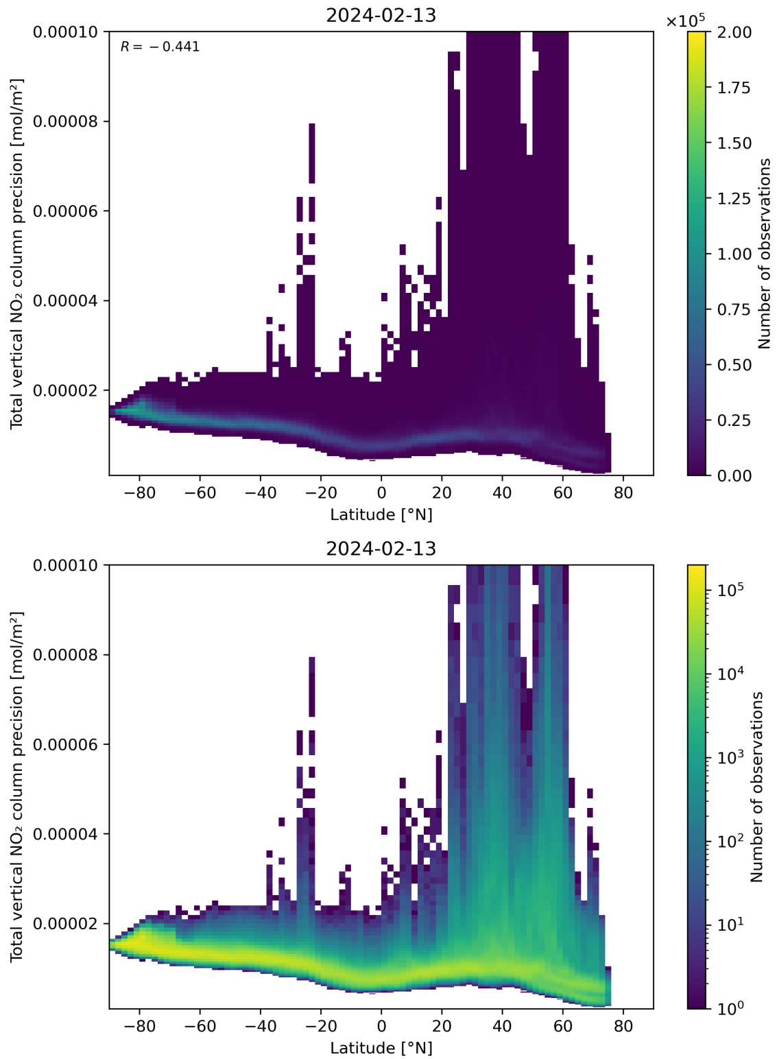
Figure 91: Scatter density plot of “Latitude” against “Total vertical NO 2 column precision” for 2024-02-12 to 2024-02-14.
