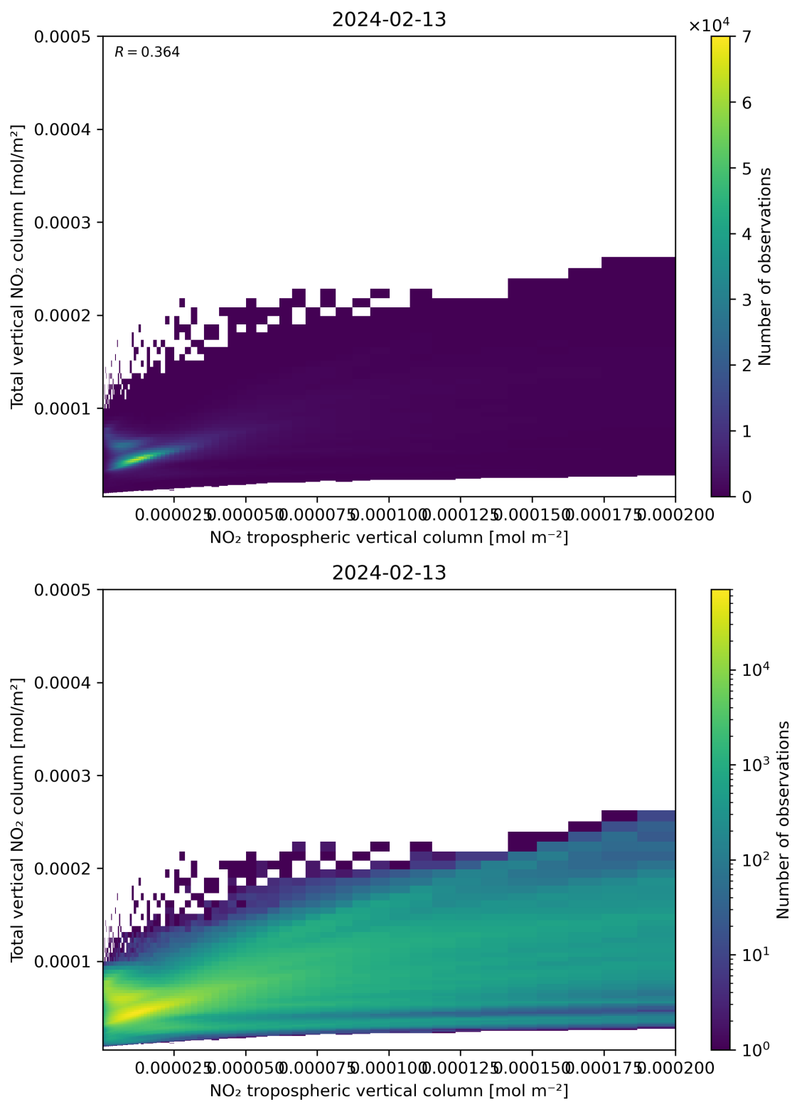
Figure 128: Scatter density plot of “NO 2 tropospheric vertical column” against “Total vertical NO 2 column” for 2024-02-12 to 2024-02-14.
