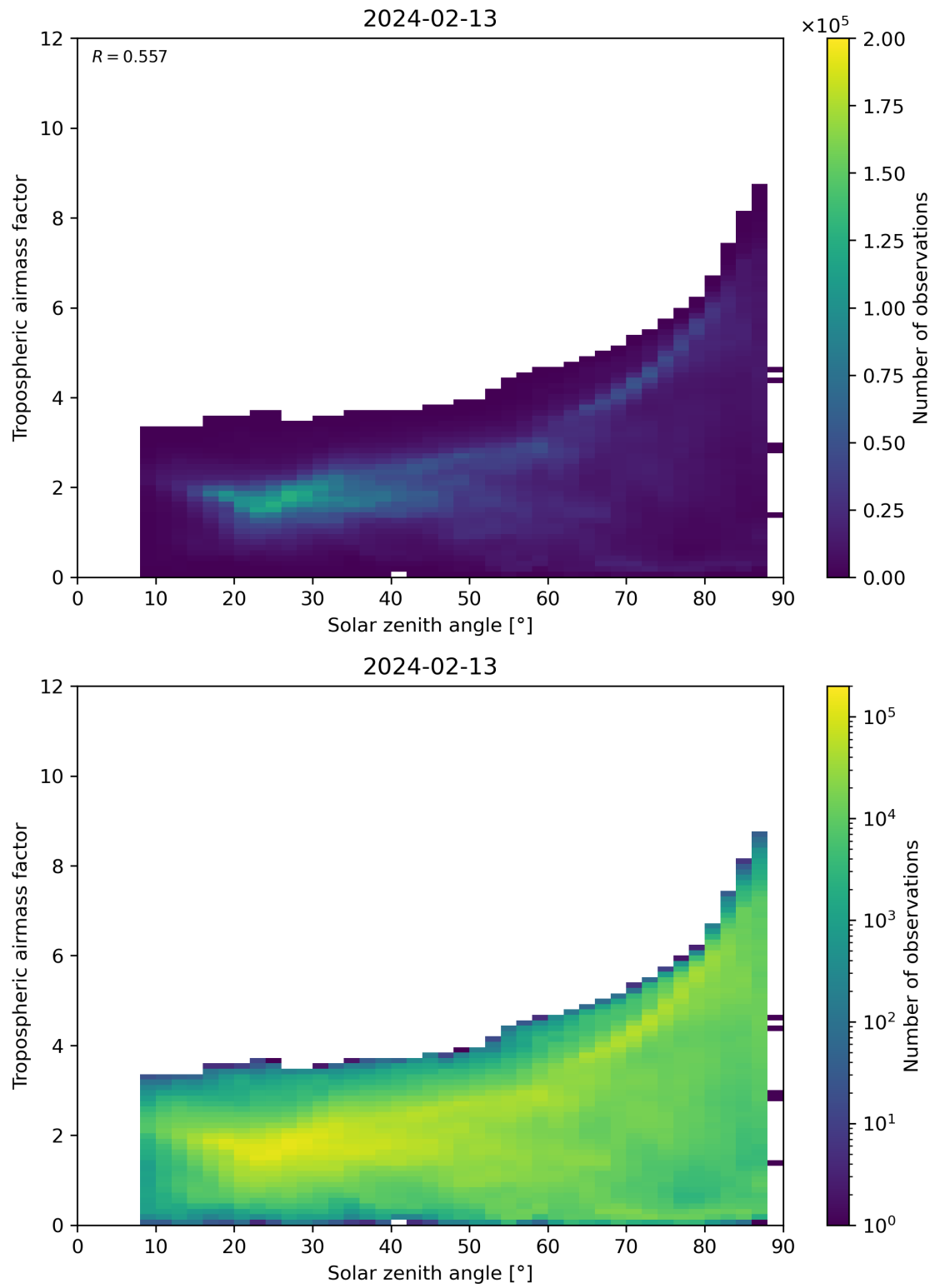
Figure 147: Scatter density plot of “Solar zenith angle” against “Tropospheric airmass factor” for 2024-02-12 to 2024-02-14.
