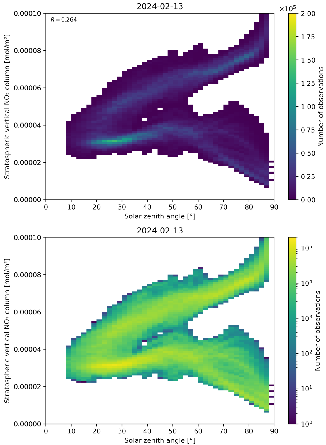
Figure 150: Scatter density plot of “Solar zenith angle” against “Stratospheric vertical NO 2 column” for 2024-02-12 to 2024-02-14.
