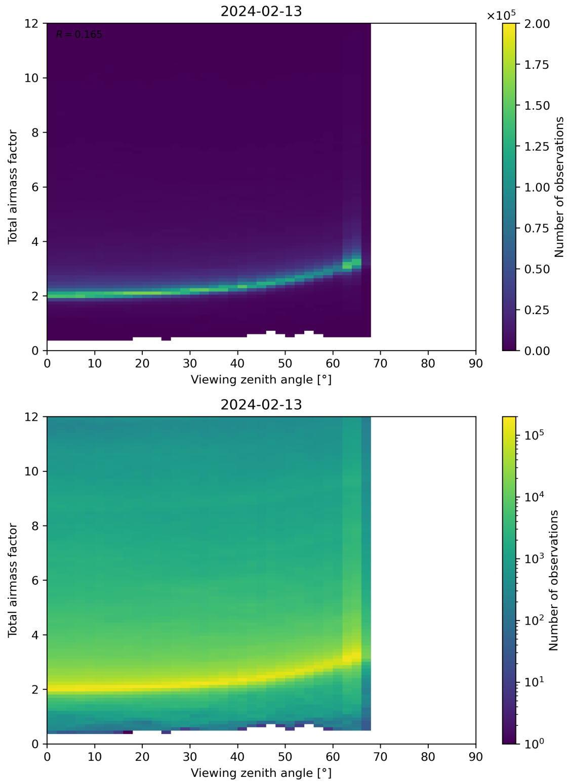
Figure 160: Scatter density plot of “Viewing zenith angle” against “Total airmass factor” for 2024-02-12 to 2024-02-14.
