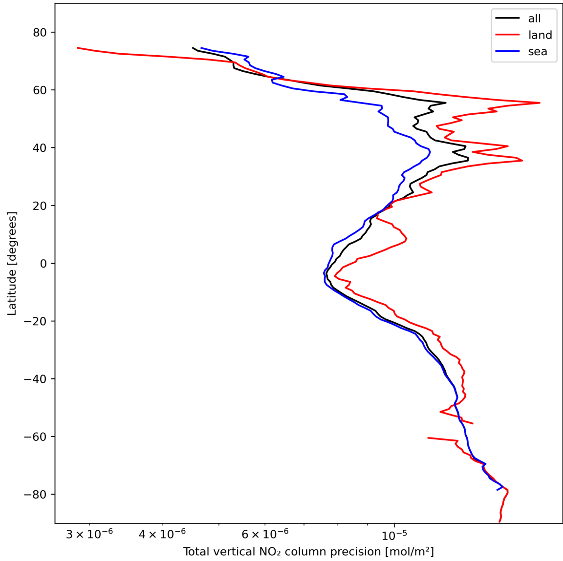
Figure 22: Zonal average of “Total vertical NO 2 column precision” for 2024-02-12 to 2024-02-14.
