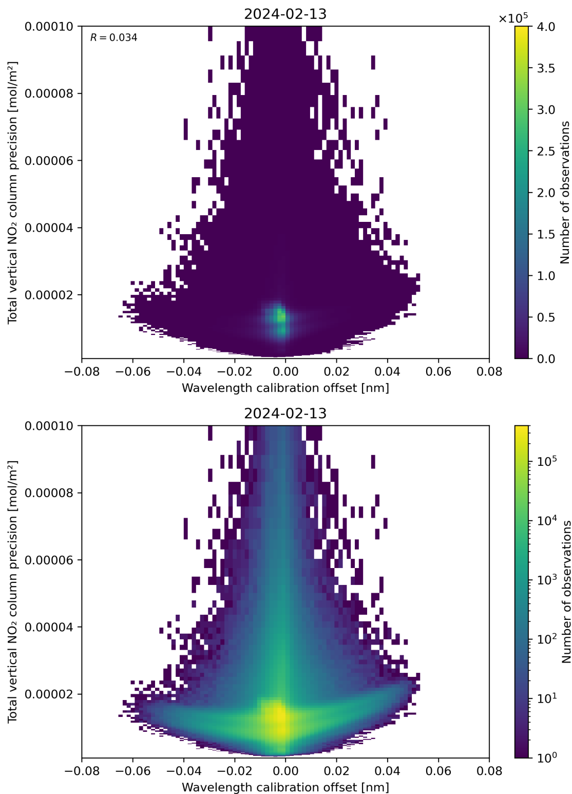
Figure 180: Scatter density plot of “Wavelength calibration offset” against “Total vertical NO 2 column precision” for 2024-02-12 to 2024-02-14.
