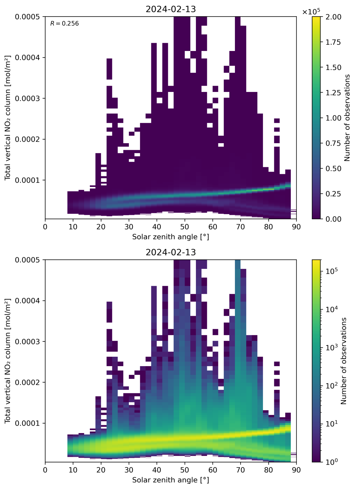
Figure 153: Scatter density plot of “Solar zenith angle” against “Total vertical NO 2 column” for 2024-02-12 to 2024-02-14.
