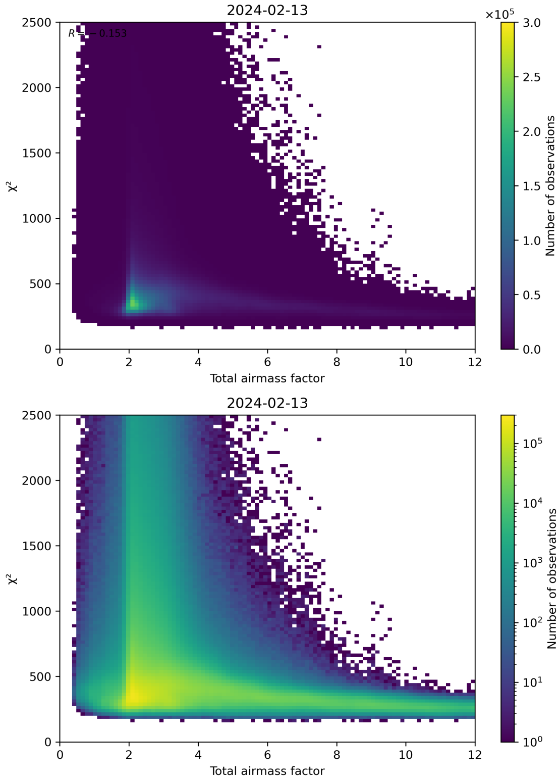
Figure 63: Scatter density plot of “Total airmass factor” against “ \chi^2 ” for 2024-02-12 to 2024-02-14.
