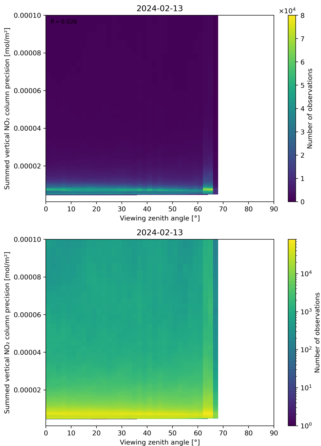
Figure 166: Scatter density plot of “Viewing zenith angle” against “Summed vertical NO 2 column precision” for 2024-02-12 to 2024-02-14.
