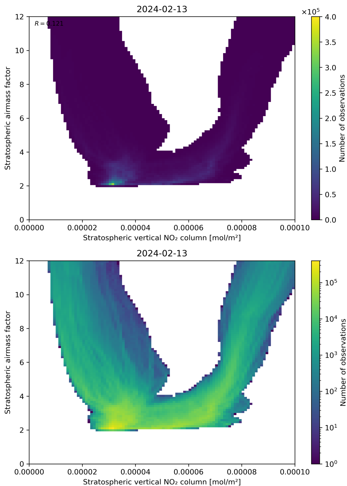
Figure 96: Scatter density plot of “Stratospheric vertical NO 2 column” against “Stratospheric airmass factor” for 2024-02-12 to 2024-02-14.
