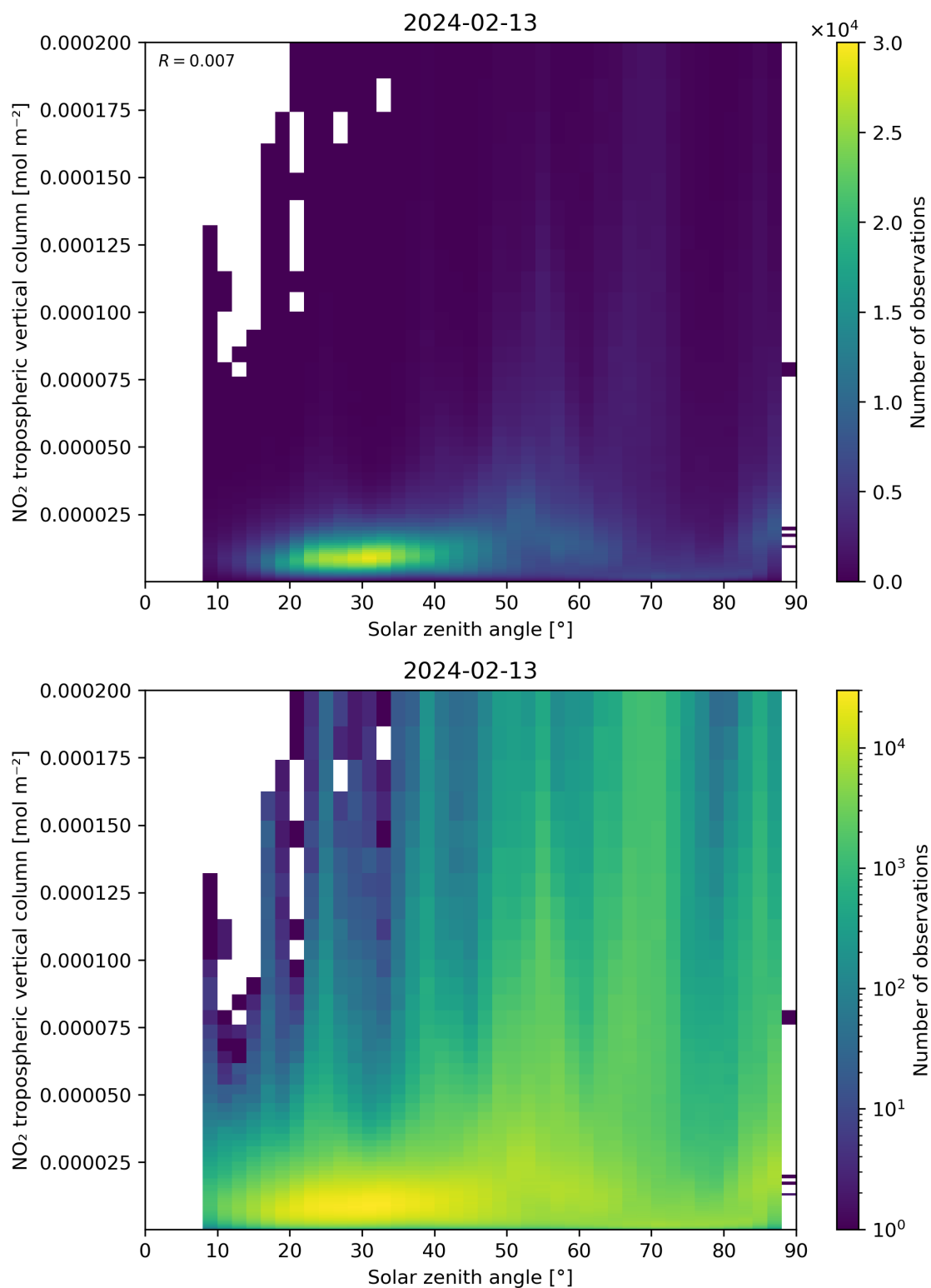
Figure 155: Scatter density plot of “Solar zenith angle” against “NO 2 tropospheric vertical column” for 2024-02-12 to 2024-02-14.
