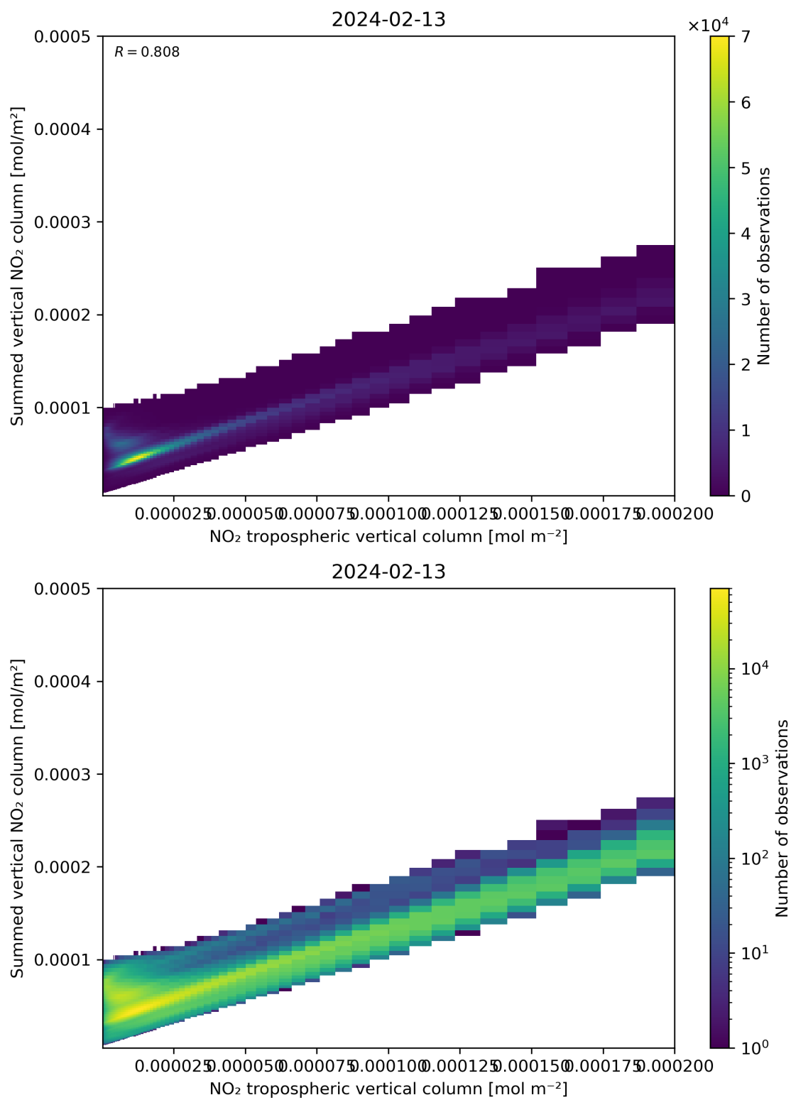
Figure 126: Scatter density plot of “NO 2 tropospheric vertical column” against “Summed vertical NO 2 column” for 2024-02-12 to 2024-02-14.
