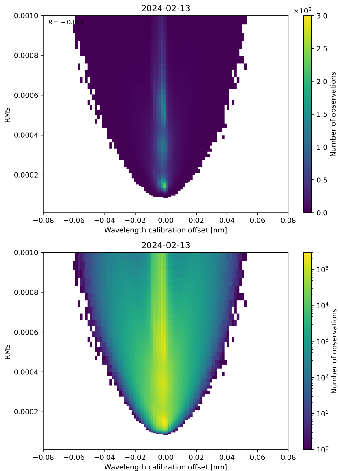
Figure 181: Scatter density plot of “Wavelength calibration offset” against “RMS” for 2024-02-12 to 2024-02-14.
