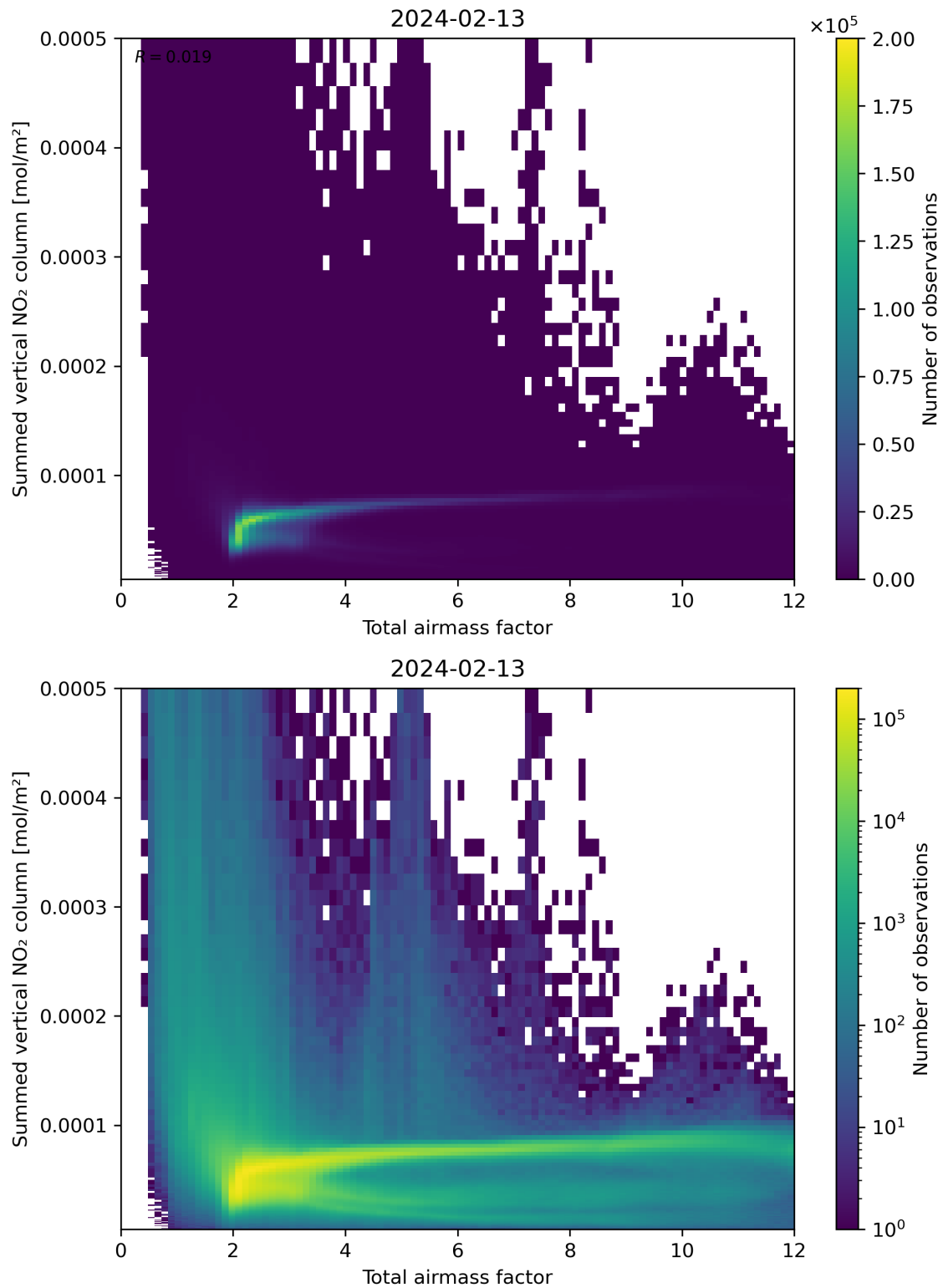
Figure 65: Scatter density plot of “Total airmass factor” against “Summed vertical NO 2 column” for 2024-02-12 to 2024-02-14.
