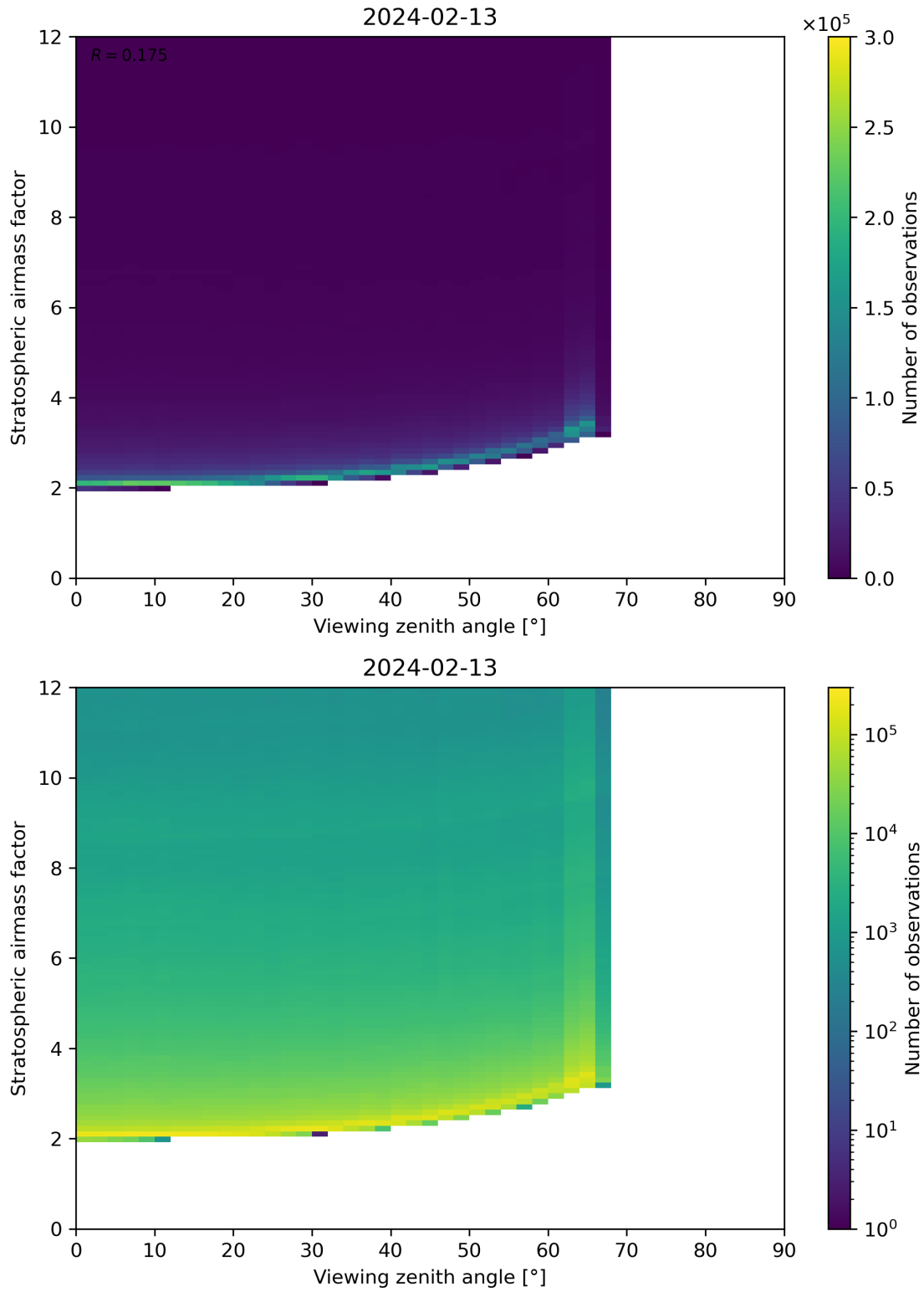
Figure 159: Scatter density plot of “Viewing zenith angle” against “Stratospheric airmass factor” for 2024-02-12 to 2024-02-14.
