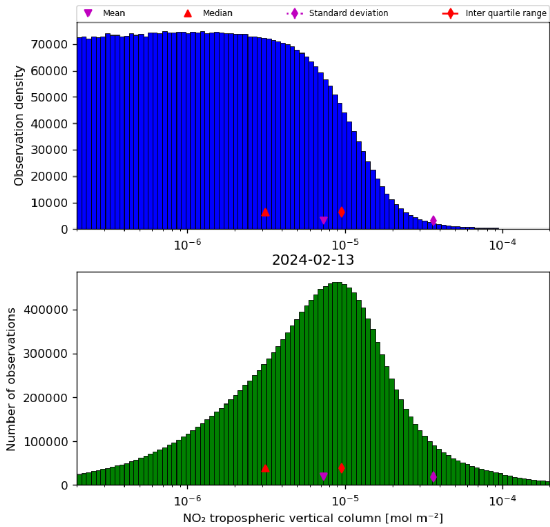
Figure 29: Histogram of “NO 2 tropospheric vertical column” for 2024-02-12 to 2024-02-14
