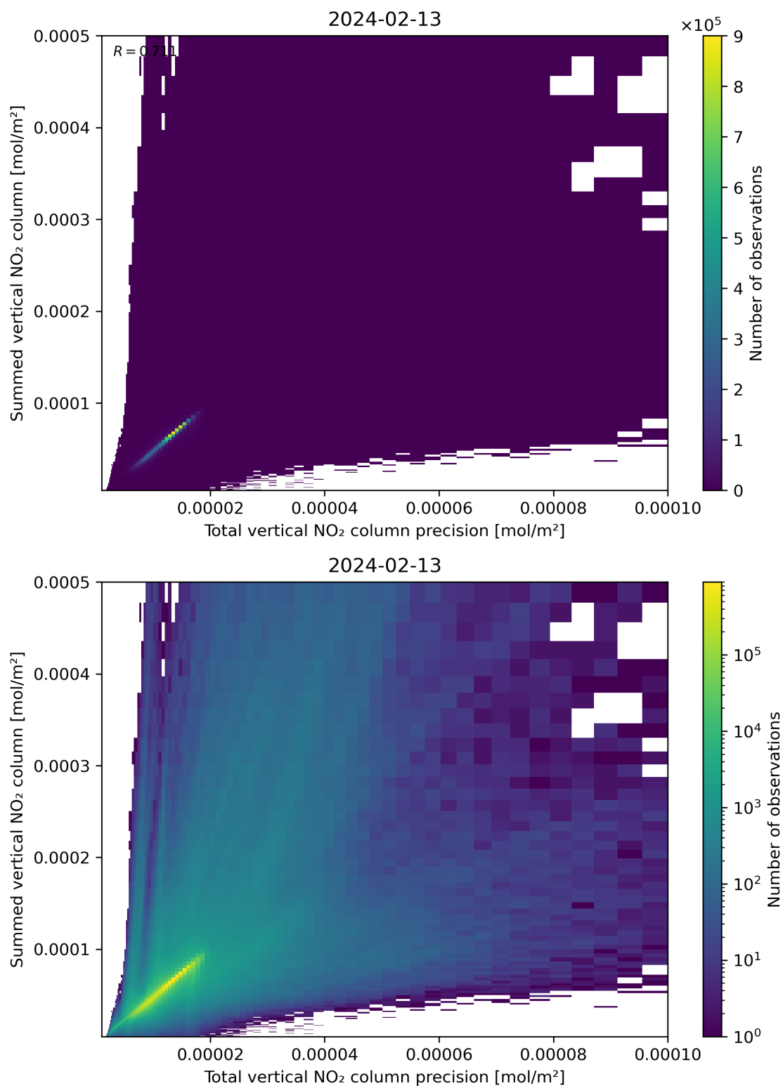
Figure 117: Scatter density plot of “Total vertical NO 2 column precision” against “Summed vertical NO 2 column” for 2024-02-12 to 2024-02-14.
