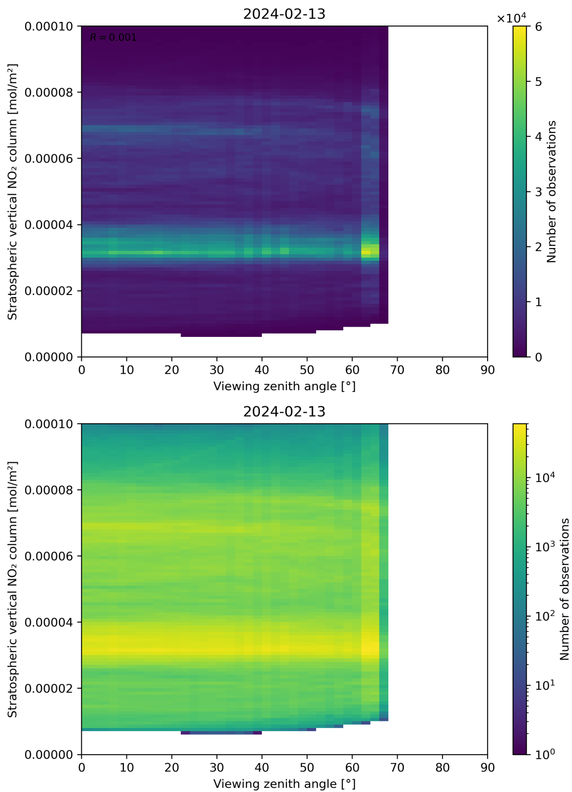
Figure 164: Scatter density plot of “Viewing zenith angle” against “Stratospheric vertical NO 2 column” for 2024-02-12 to 2024-02-14.
