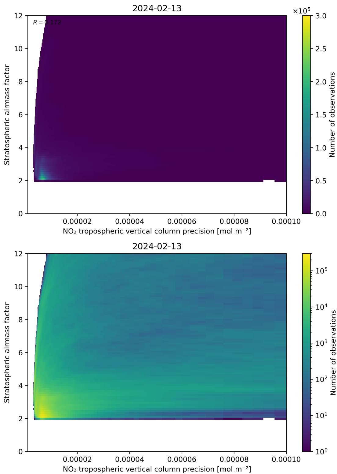
Figure 131: Scatter density plot of “NO 2 tropospheric vertical column precision” against “Stratospheric airmass factor” for 2024-02-12 to 2024-02-14.
