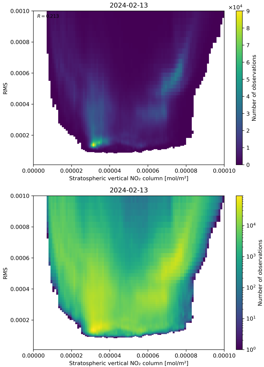
Figure 102: Scatter density plot of “Stratospheric vertical NO 2 column” against “RMS” for 2024-02-12 to 2024-02-14.
