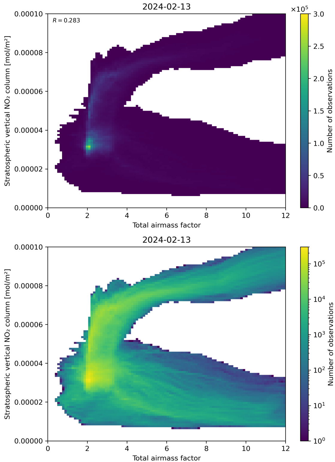
Figure 64: Scatter density plot of “Total airmass factor” against “Stratospheric vertical NO 2 column” for 2024-02-12 to 2024-02-14.
