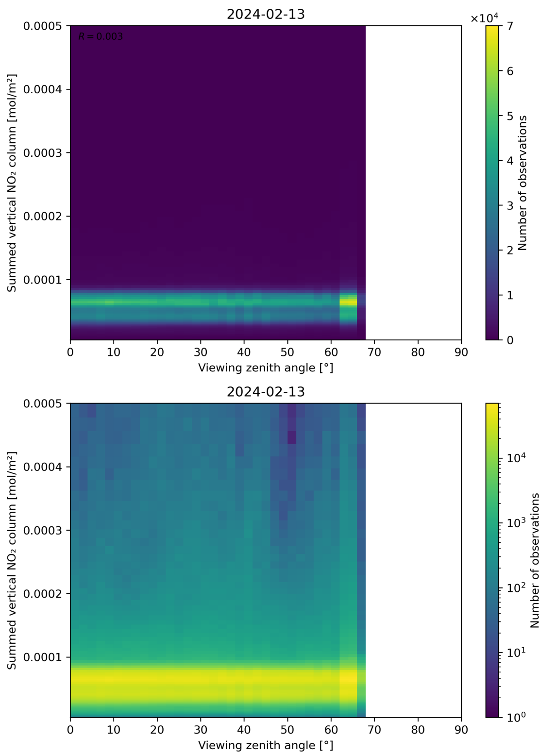
Figure 165: Scatter density plot of “Viewing zenith angle” against “Summed vertical NO 2 column” for 2024-02-12 to 2024-02-14.
