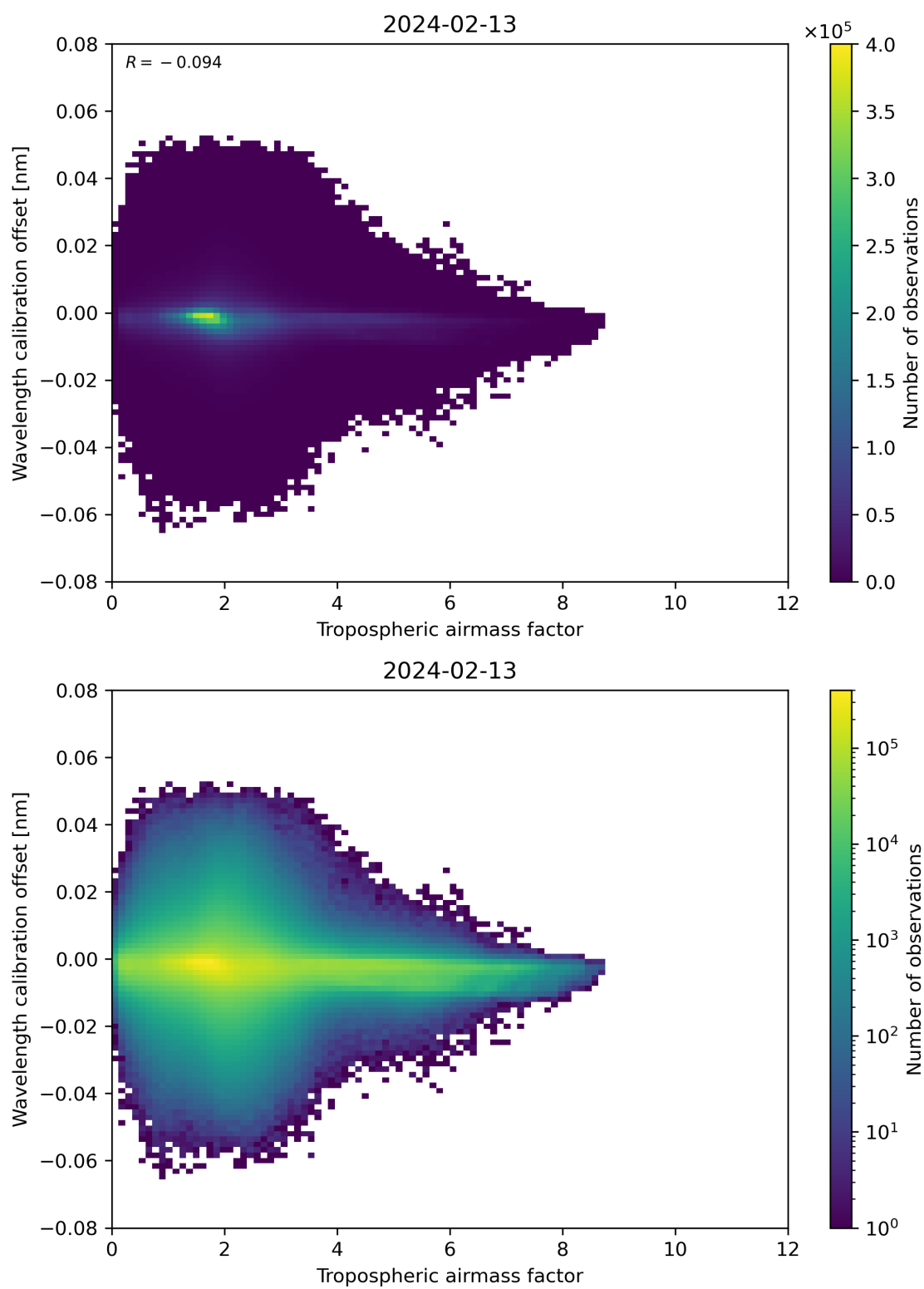
Figure 80: Scatter density plot of “Tropospheric airmass factor” against “Wavelength calibration offset” for 2024-02-12 to 2024-02-14.
