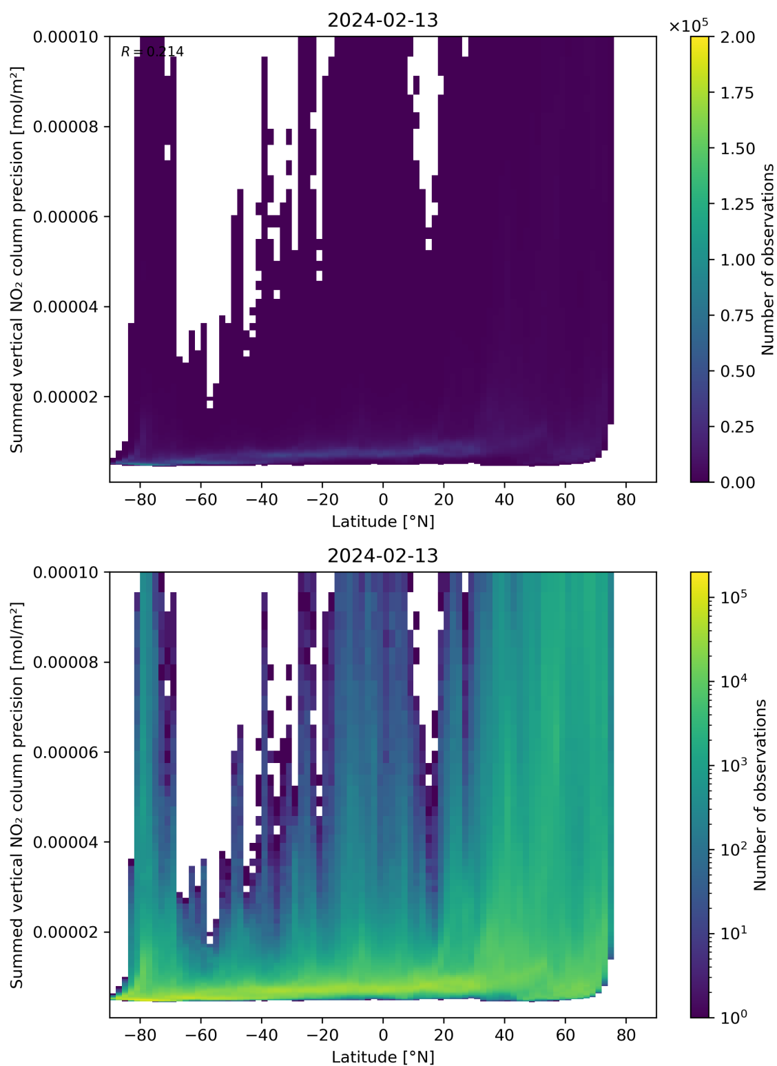
Figure 89: Scatter density plot of “Latitude” against “Summed vertical NO 2 column precision” for 2024-02-12 to 2024-02-14.
