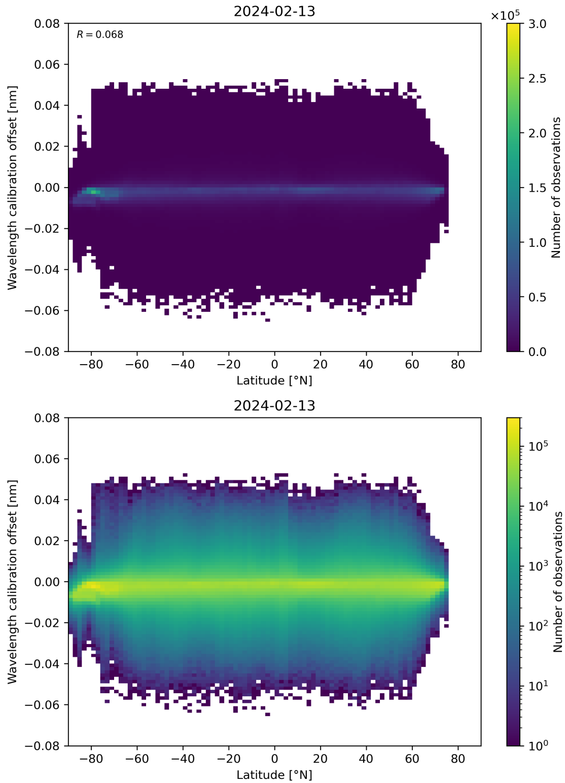
Figure 95: Scatter density plot of “Latitude” against “Wavelength calibration offset” for 2024-02-12 to 2024-02-14.
