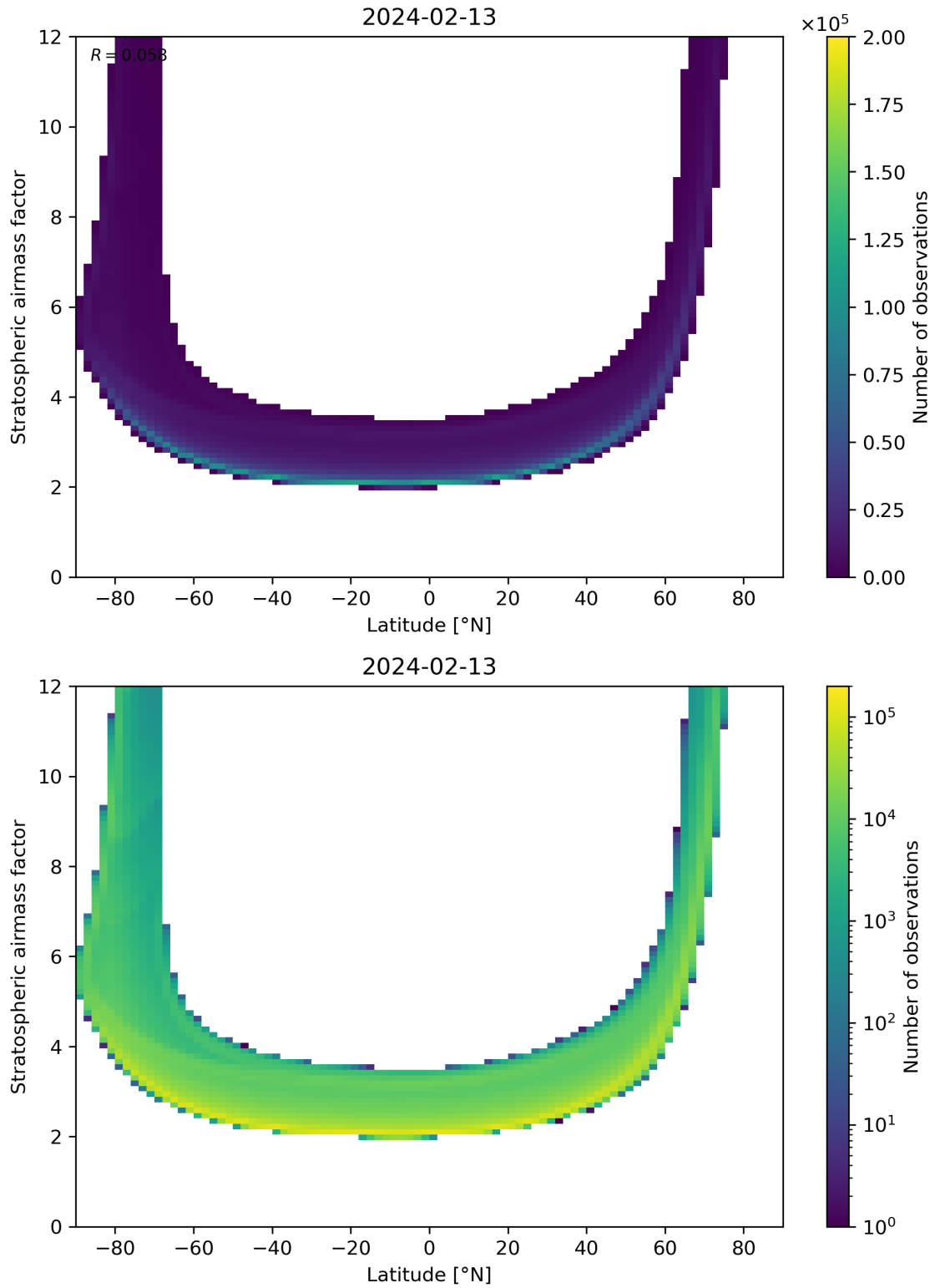
Figure 83: Scatter density plot of “Latitude” against “Stratospheric airmass factor” for 2024-02-12 to 2024-02-14.
