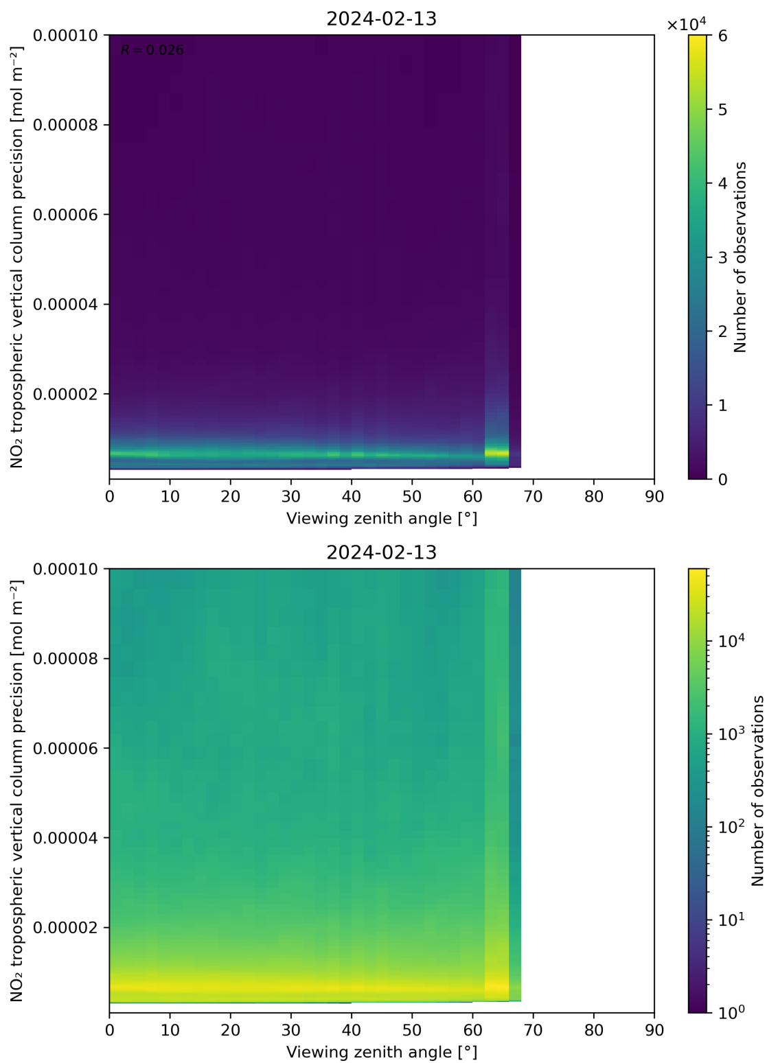
Figure 170: Scatter density plot of “Viewing zenith angle” against “NO 2 tropospheric vertical column precision” for 2024-02-12 to 2024-02-14.
