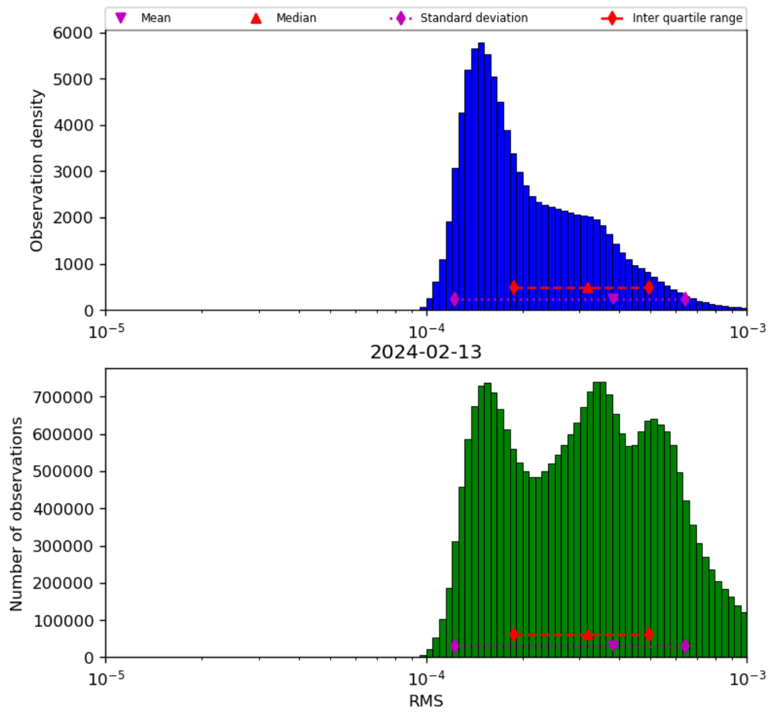
Figure 43: Histogram of “RMS” for 2024-02-12 to 2024-02-14
