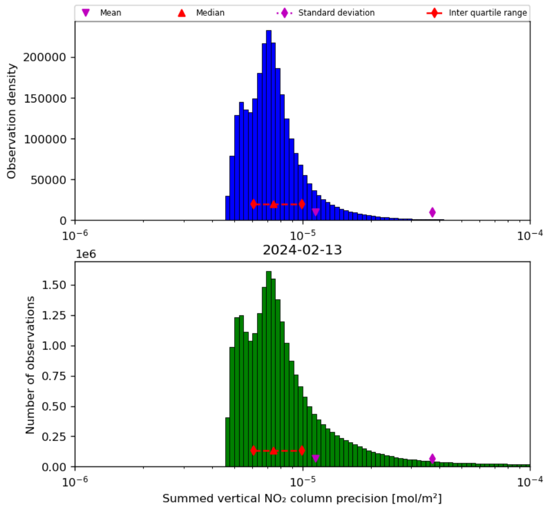
Figure 41: Histogram of “Summed vertical NO 2 column precision” for 2024-02-12 to 2024-02-14
