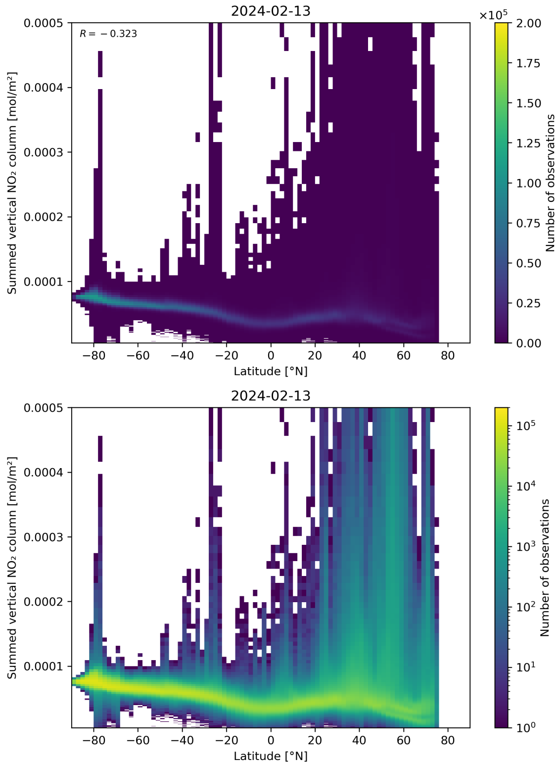
Figure 88: Scatter density plot of “Latitude” against “Summed vertical NO 2 column” for 2024-02-12 to 2024-02-14.
