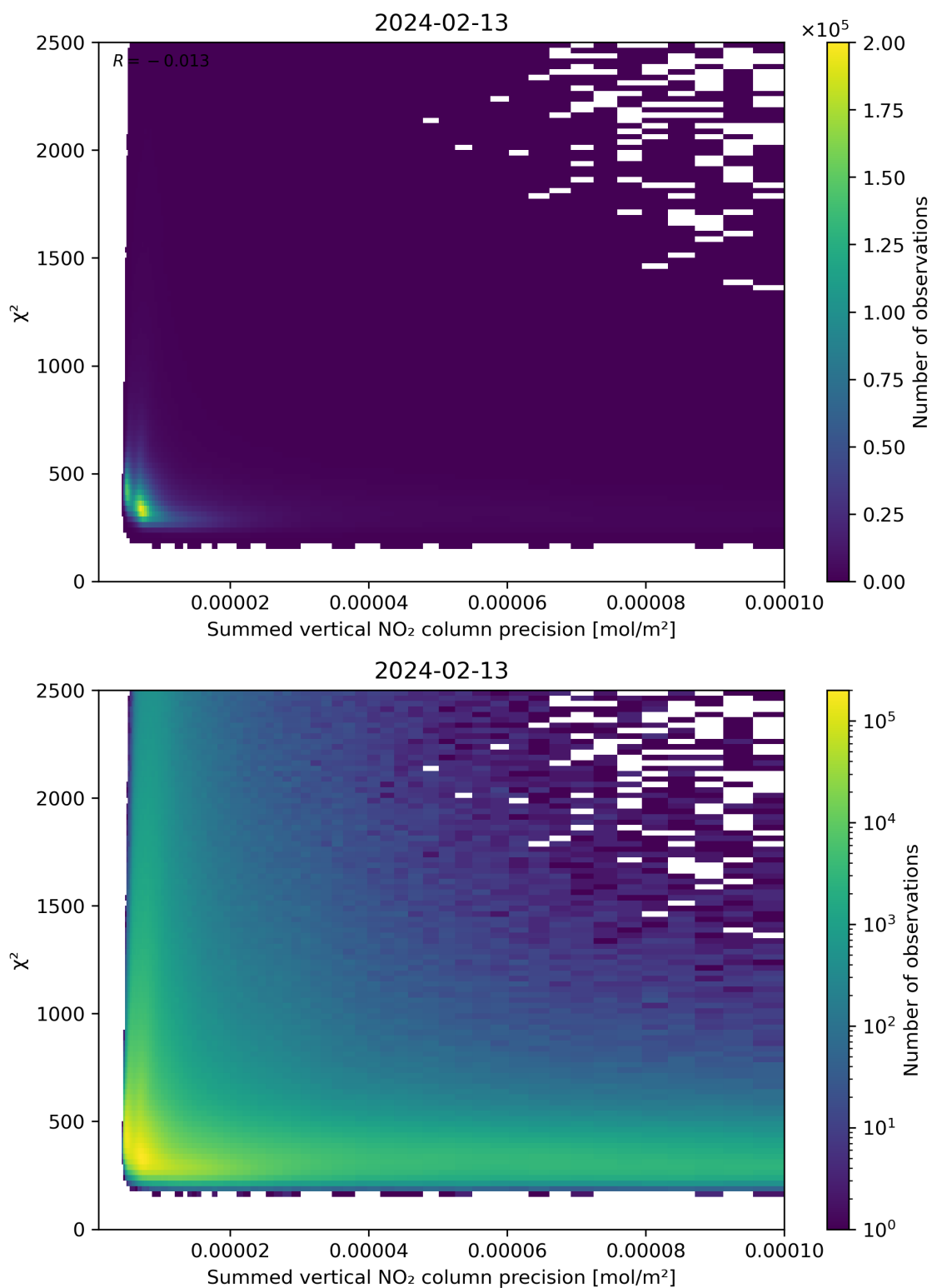
Figure 107: Scatter density plot of “Summed vertical NO 2 column precision” against “ \chi^2 ” for 2024-02-12 to 2024-02-14.
