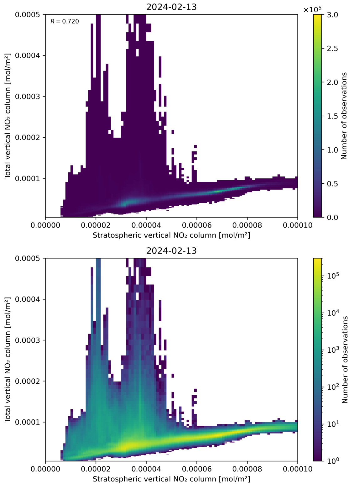
Figure 100: Scatter density plot of “Stratospheric vertical NO 2 column” against “Total vertical NO 2 column” for 2024-02-12 to 2024-02-14.
