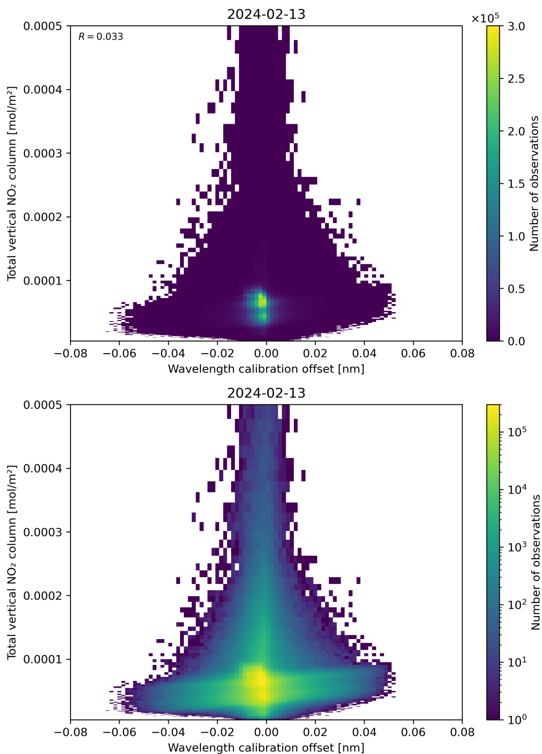
Figure 179: Scatter density plot of “Wavelength calibration offset” against “Total vertical NO 2 column” for 2024-02-12 to 2024-02-14.
