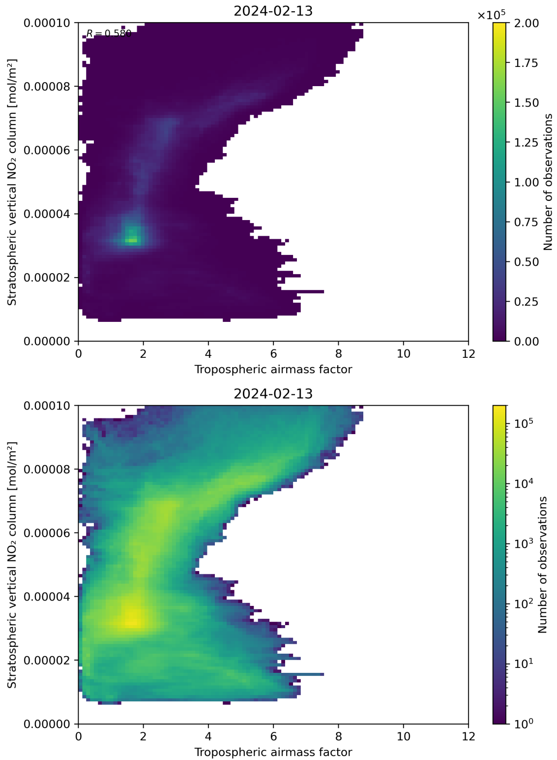
Figure 74: Scatter density plot of “Tropospheric air mass factor” against “Stratospheric vertical NO 2 column” for 2024-02-12 to 2024-02-14.
