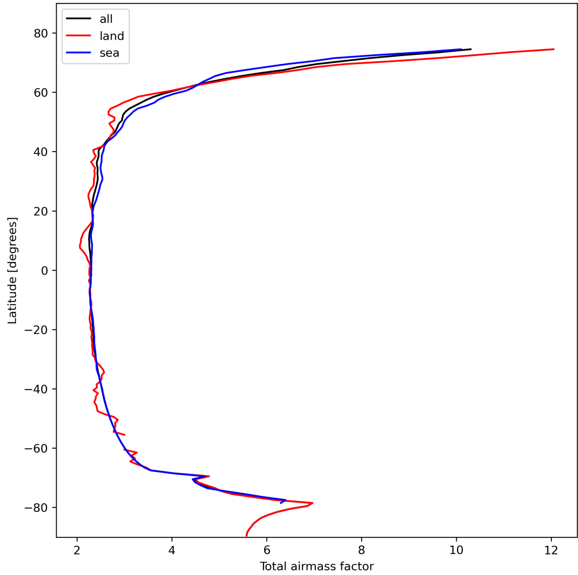
Figure 15: Zonal average of “Total airmass factor” for 2024-02-12 to 2024-02-14.
