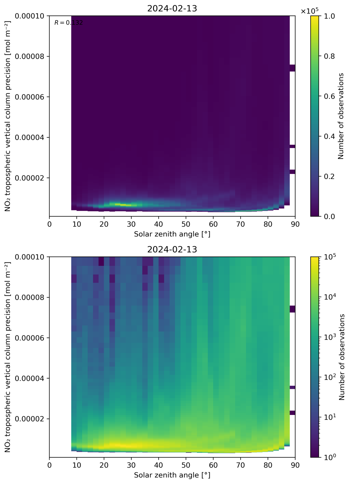
Figure 156: Scatter density plot of “Solar zenith angle” against “NO 2 tropospheric vertical column precision” for 2024-02-12 to 2024-02-14.
