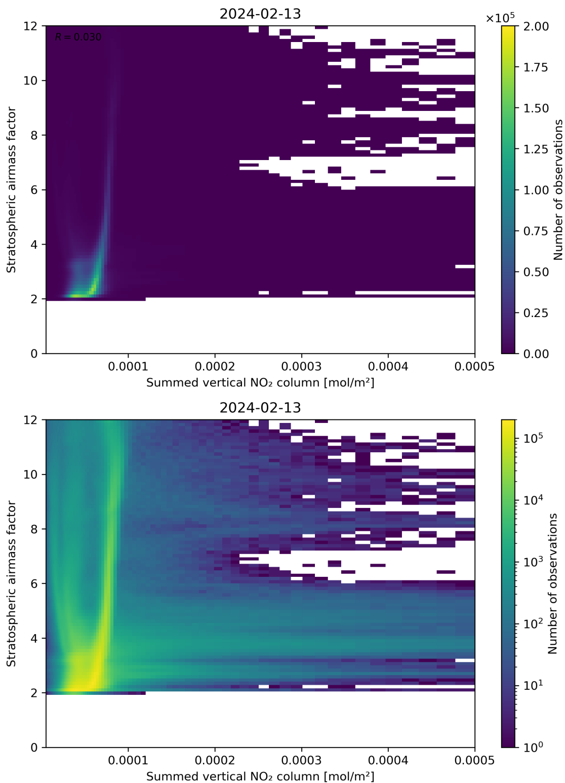
Figure 103: Scatter density plot of “Summed vertical NO 2 column” against “Stratospheric airmass factor” for 2024-02-12 to 2024-02-14.
