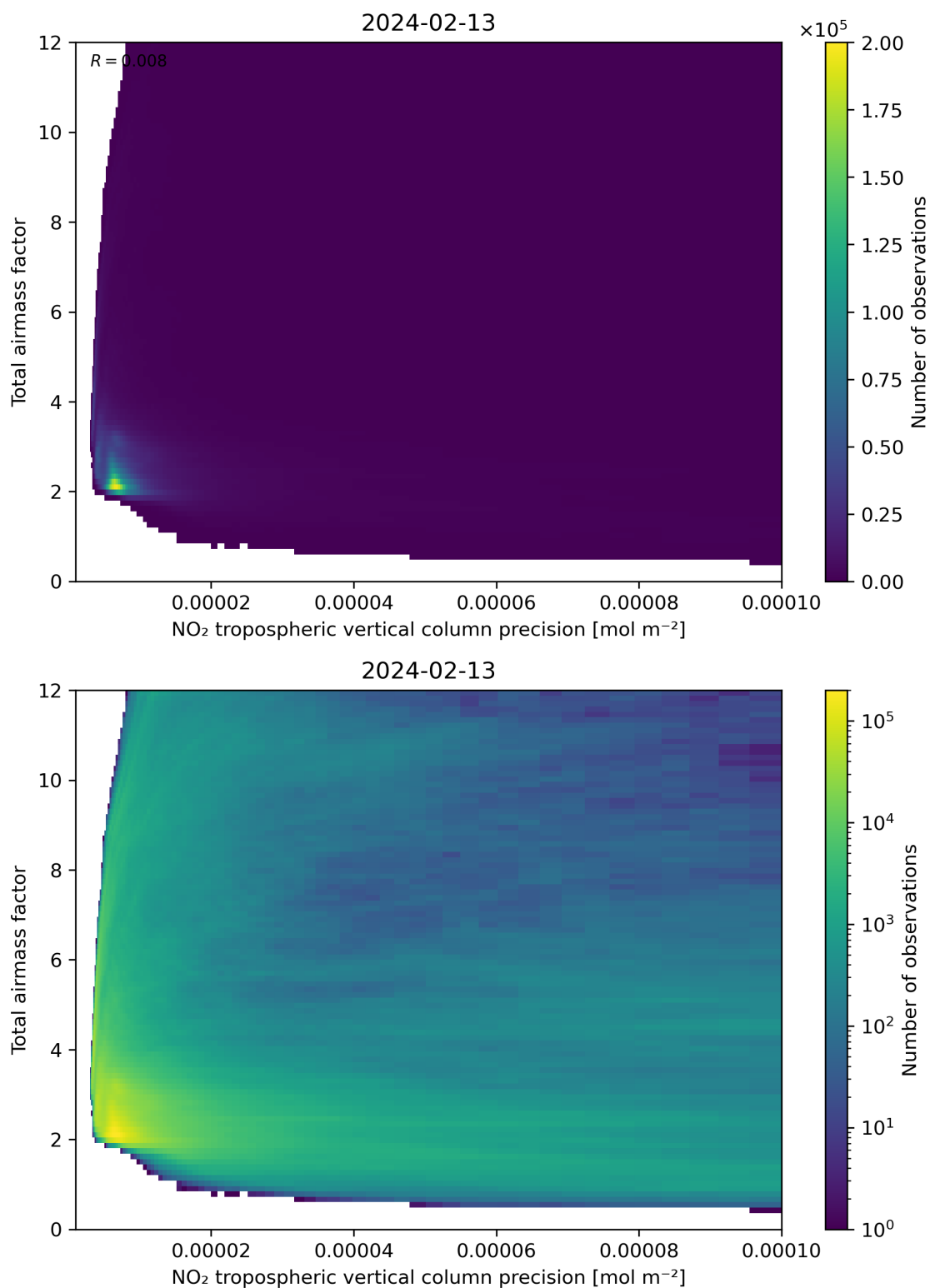
Figure 132: Scatter density plot of “NO 2 tropospheric vertical column precision” against “Total air mass factor” for 2024-02-12 to 2024-02-14.
