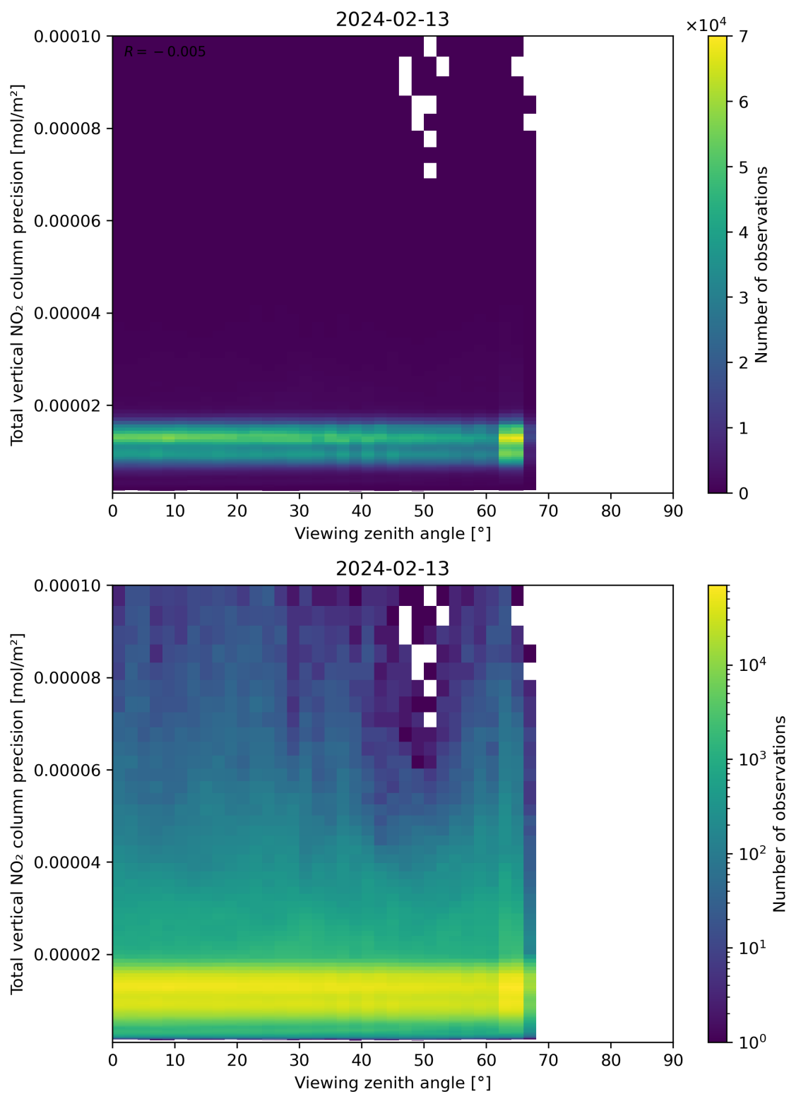
Figure 168: Scatter density plot of “Viewing zenith angle” against “Total vertical NO 2 column precision” for 2024-02-12 to 2024-02-14.
