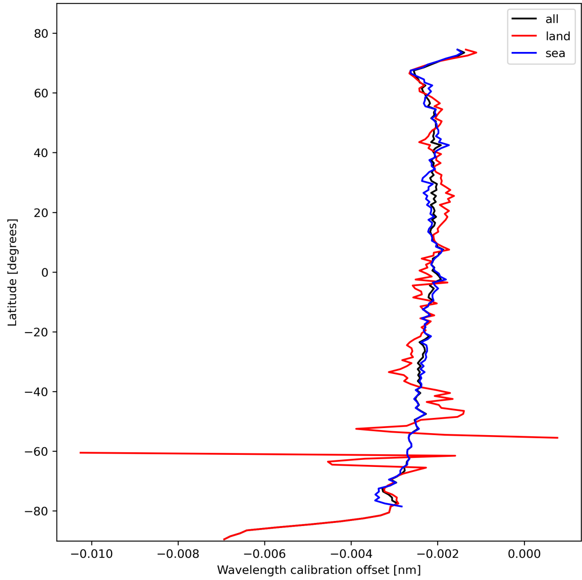
Figure 18: Zonal average of “Wavelength calibration offset” for 2024-02-12 to 2024-02-14.
