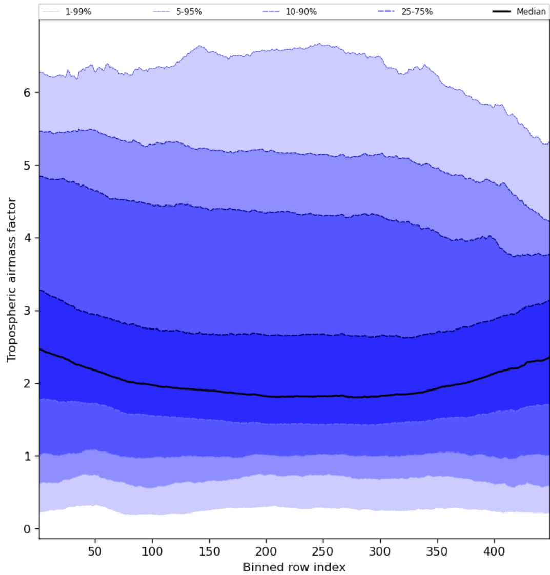
Figure 48: Along track statistics of “Tropospheric airmass factor” for 2024-02-12 to 2024-02-14
