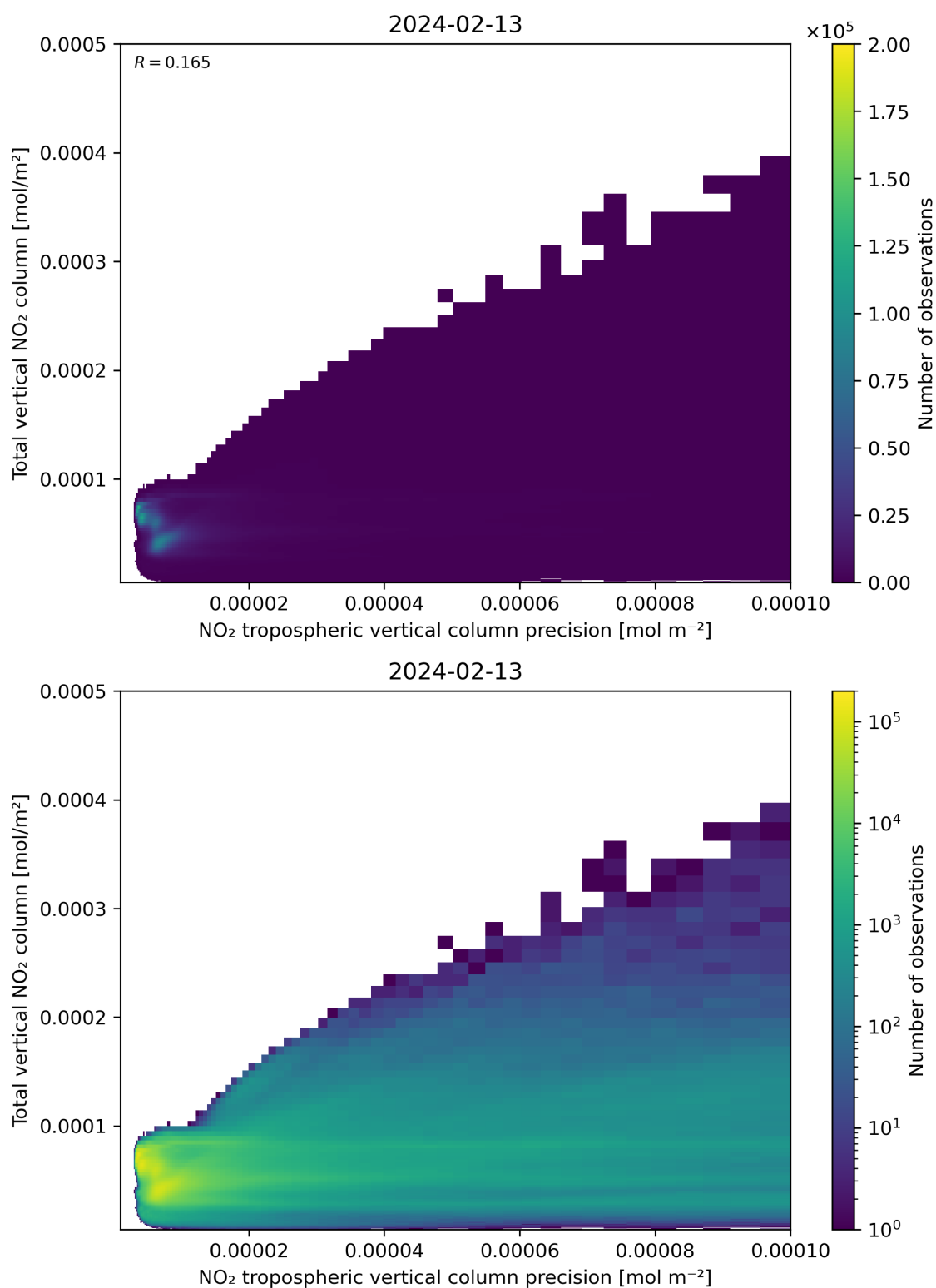
Figure 138: Scatter density plot of “NO 2 tropospheric vertical column precision” against “Total vertical NO 2 column” for 2024-02-12 to 2024-02-14.
