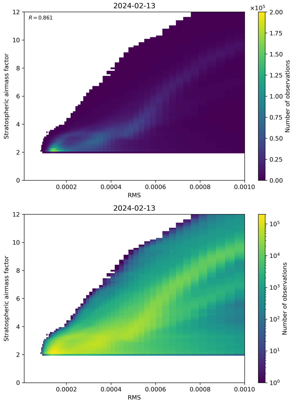
Figure 144: Scatter density plot of “RMS” against “Stratospheric airmass factor” for 2024-02-12 to 2024-02-14.
