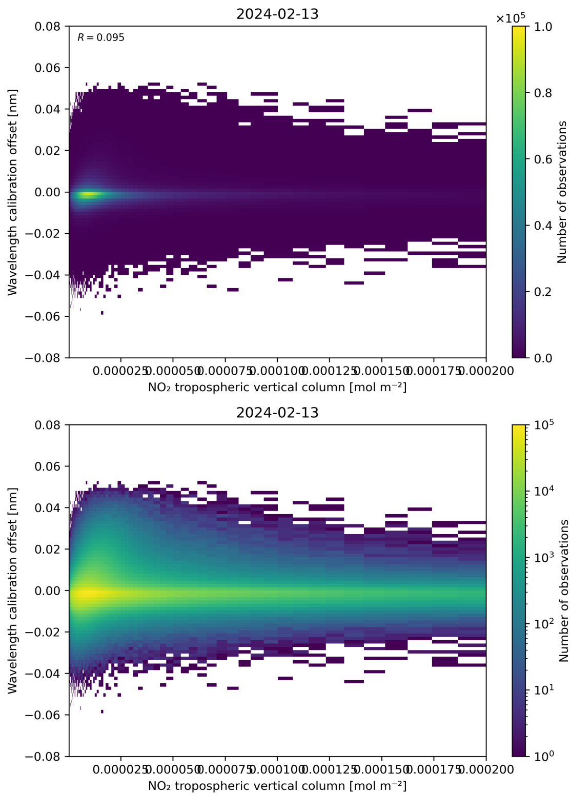
Figure 143: Scatter density plot of “NO 2 tropospheric vertical column” against “Wavelength calibration offset” for 2024-02-12 to 2024-02-14.
