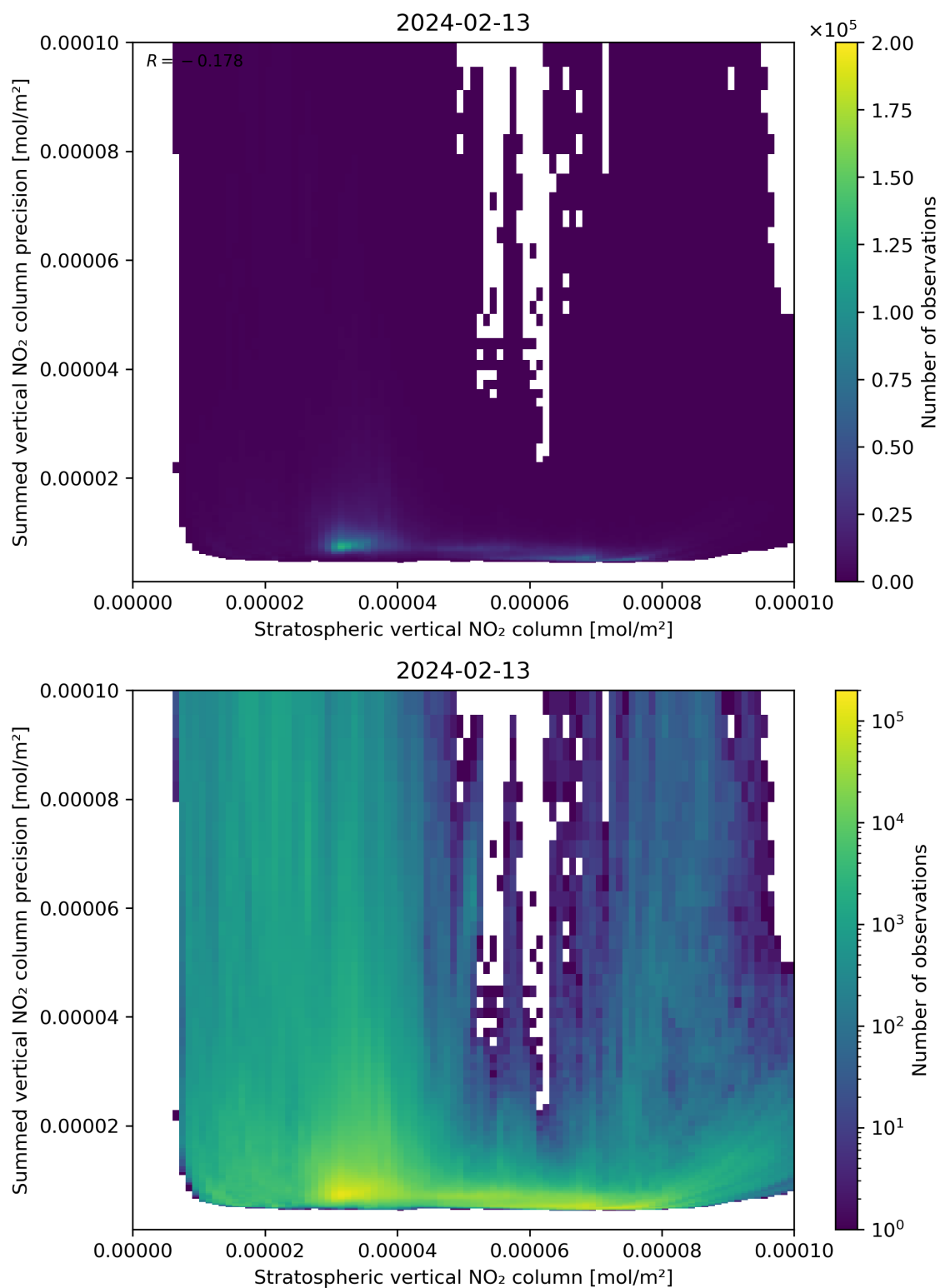
Figure 99: Scatter density plot of “Stratospheric vertical NO 2 column” against “Summed vertical NO 2 column precision” for 2024-02-12 to 2024-02-14.
