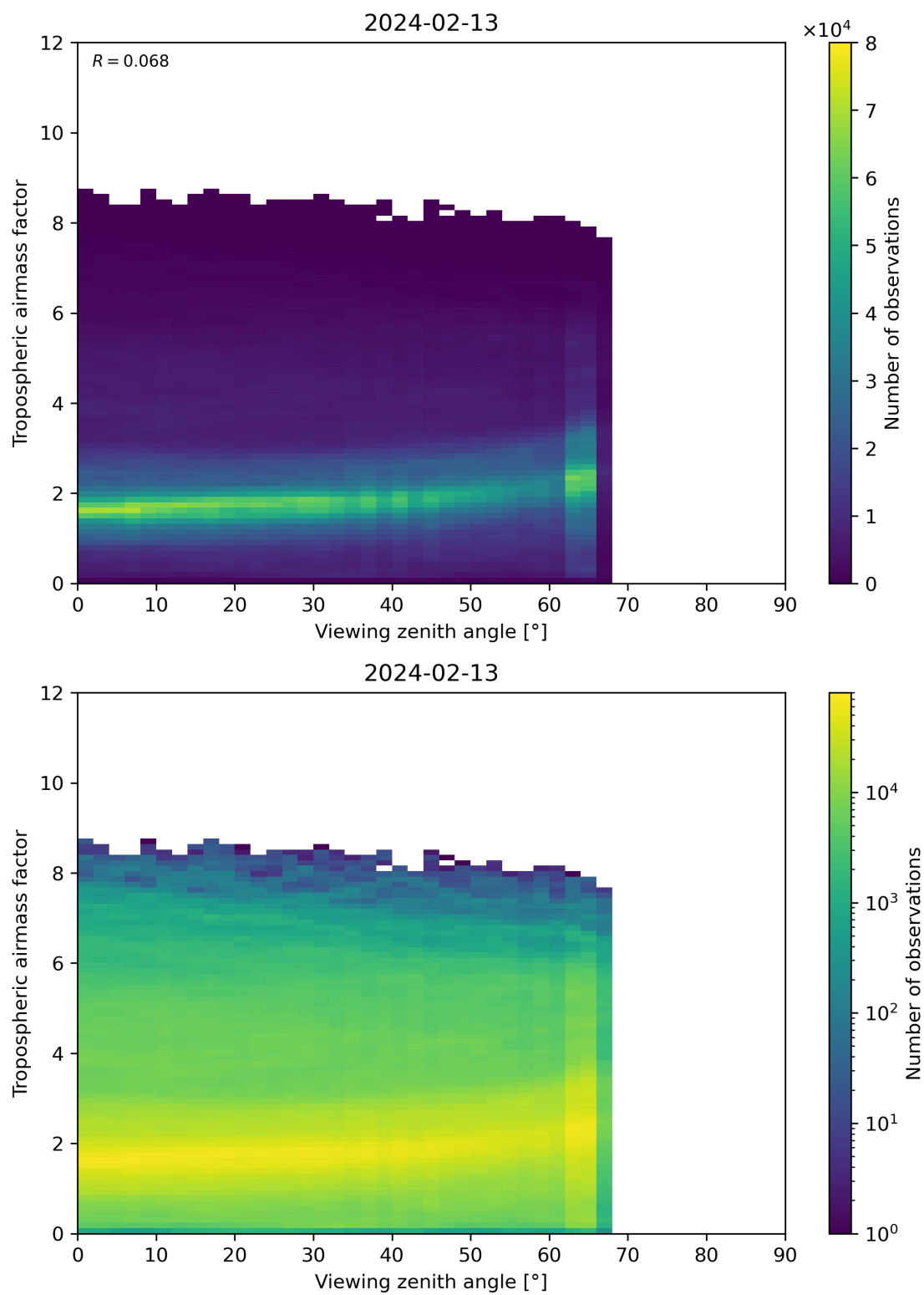
Figure 161: Scatter density plot of “Viewing zenith angle” against “Tropospheric airmass factor” for 2024-02-12 to 2024-02-14.
