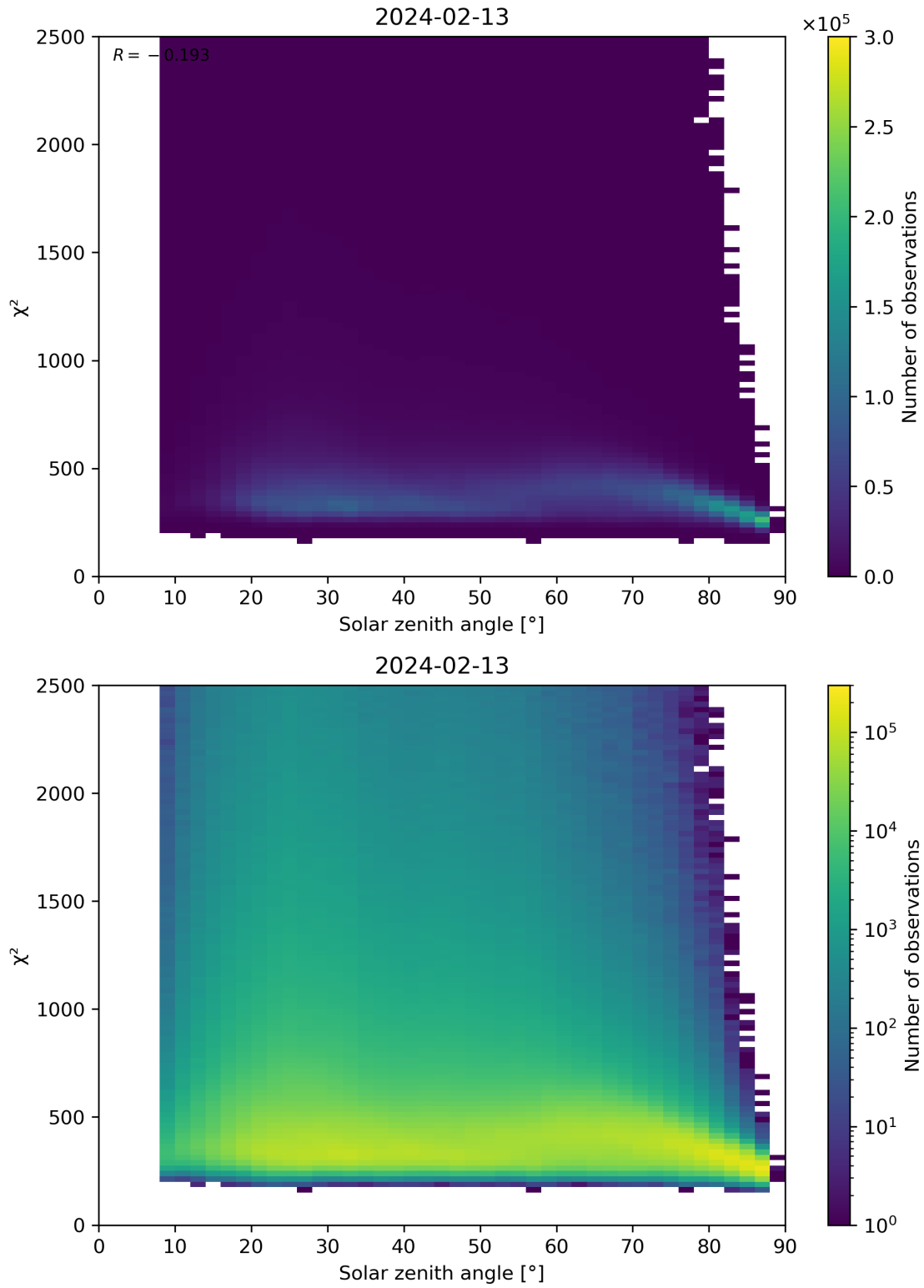
Figure 148: Scatter density plot of “Solar zenith angle” against “ \chi^2 ” for 2024-02-12 to 2024-02-14.
