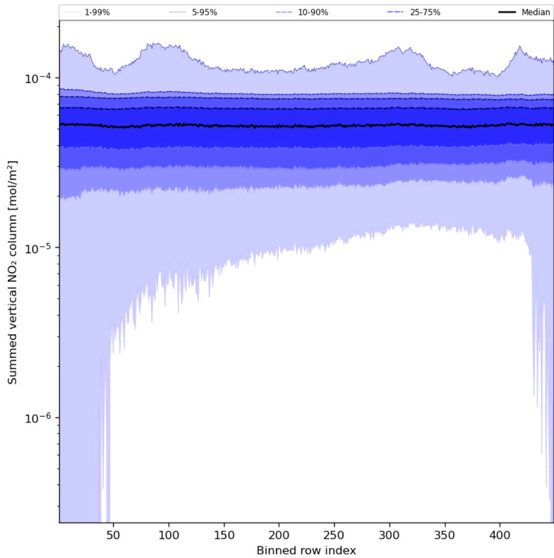
Figure 57: Along track statistics of “Summed vertical NO 2 column” for 2024-02-12 to 2024-02-14
