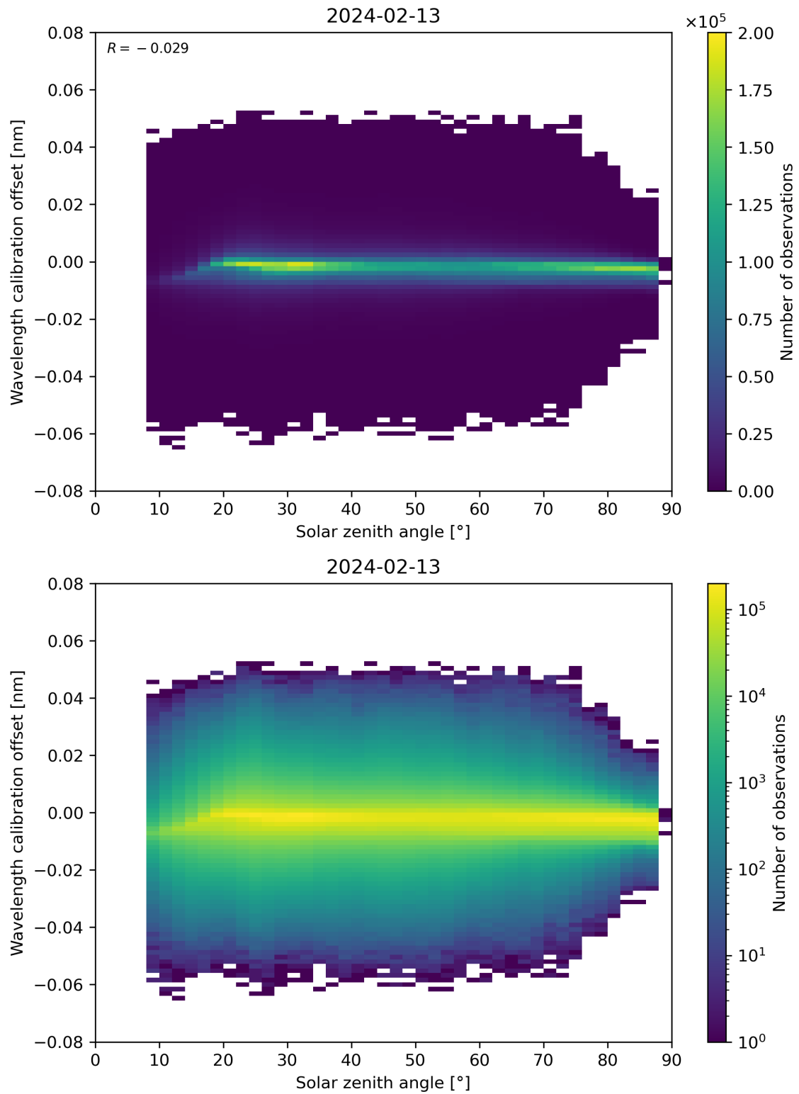
Figure 158: Scatter density plot of “Solar zenith angle” against “Wavelength calibration offset” for 2024-02-12 to 2024-02-14.
