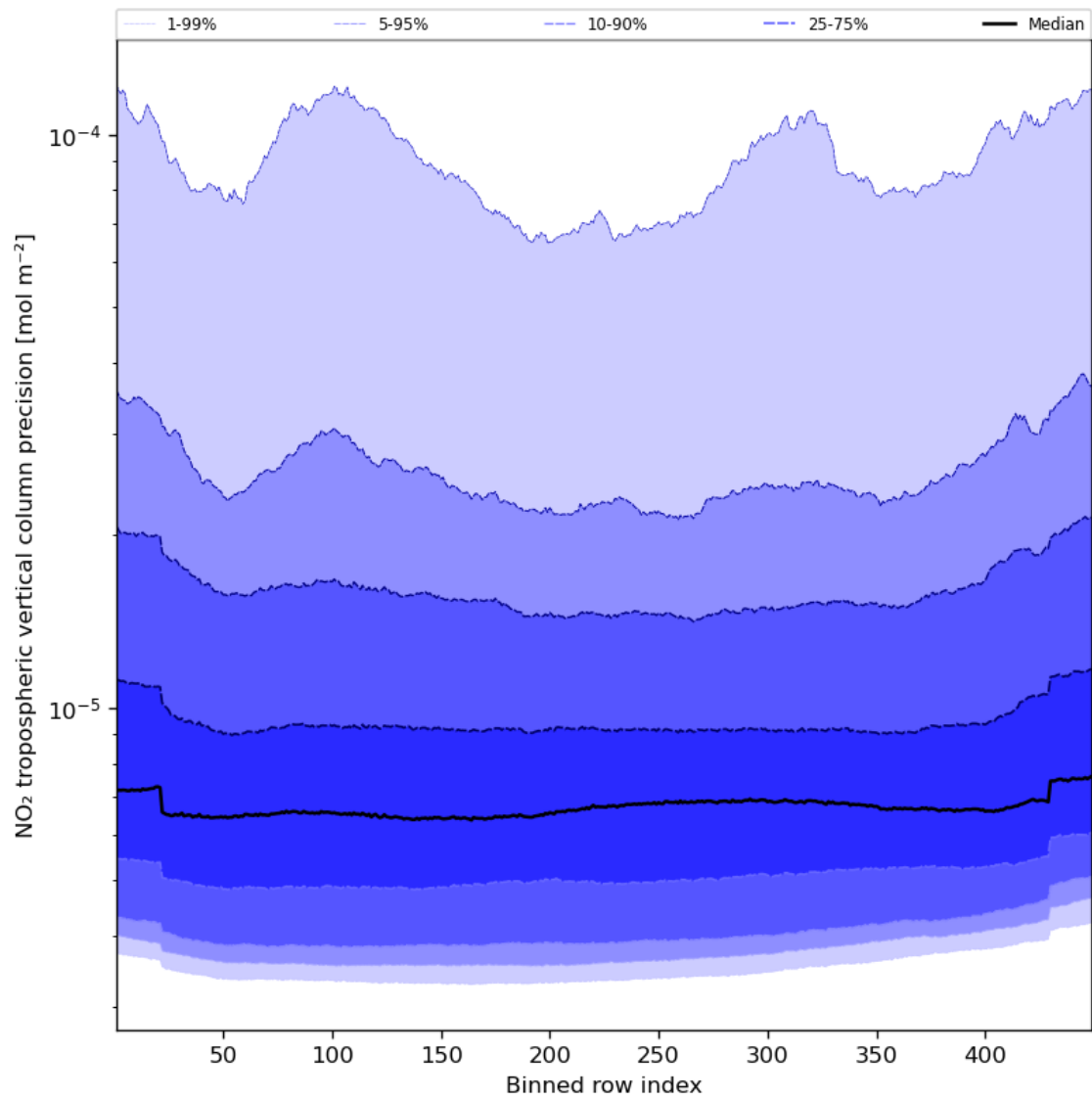
Figure 47: Along track statistics of “NO 2 tropospheric vertical column precision” for 2024-02-12 to 2024-02-14
