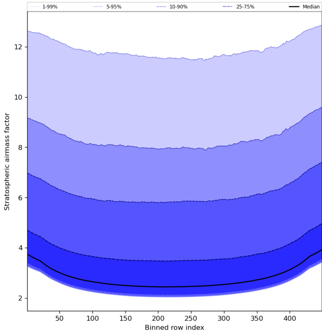
Figure 61: Along track statistics of “Stratospheric airmass factor” for 2024-02-12 to 2024-02-14
