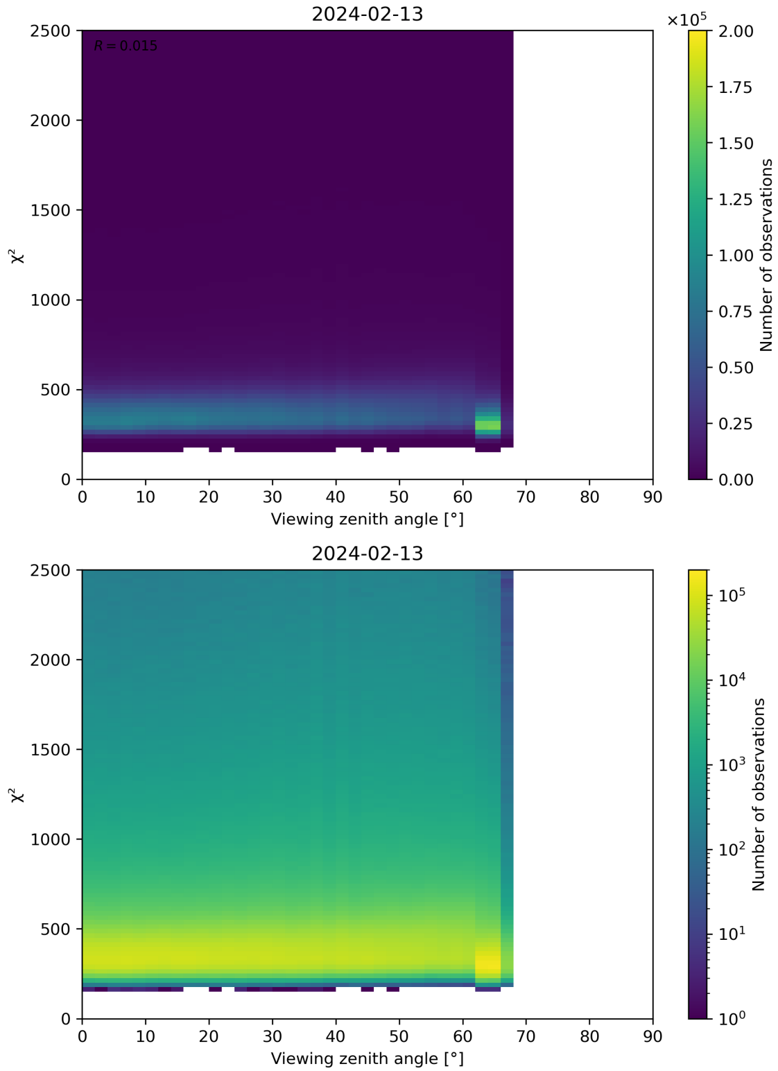
Figure 162: Scatter density plot of “Viewing zenith angle” against “ \chi^2 ” for 2024-02-12 to 2024-02-14.
