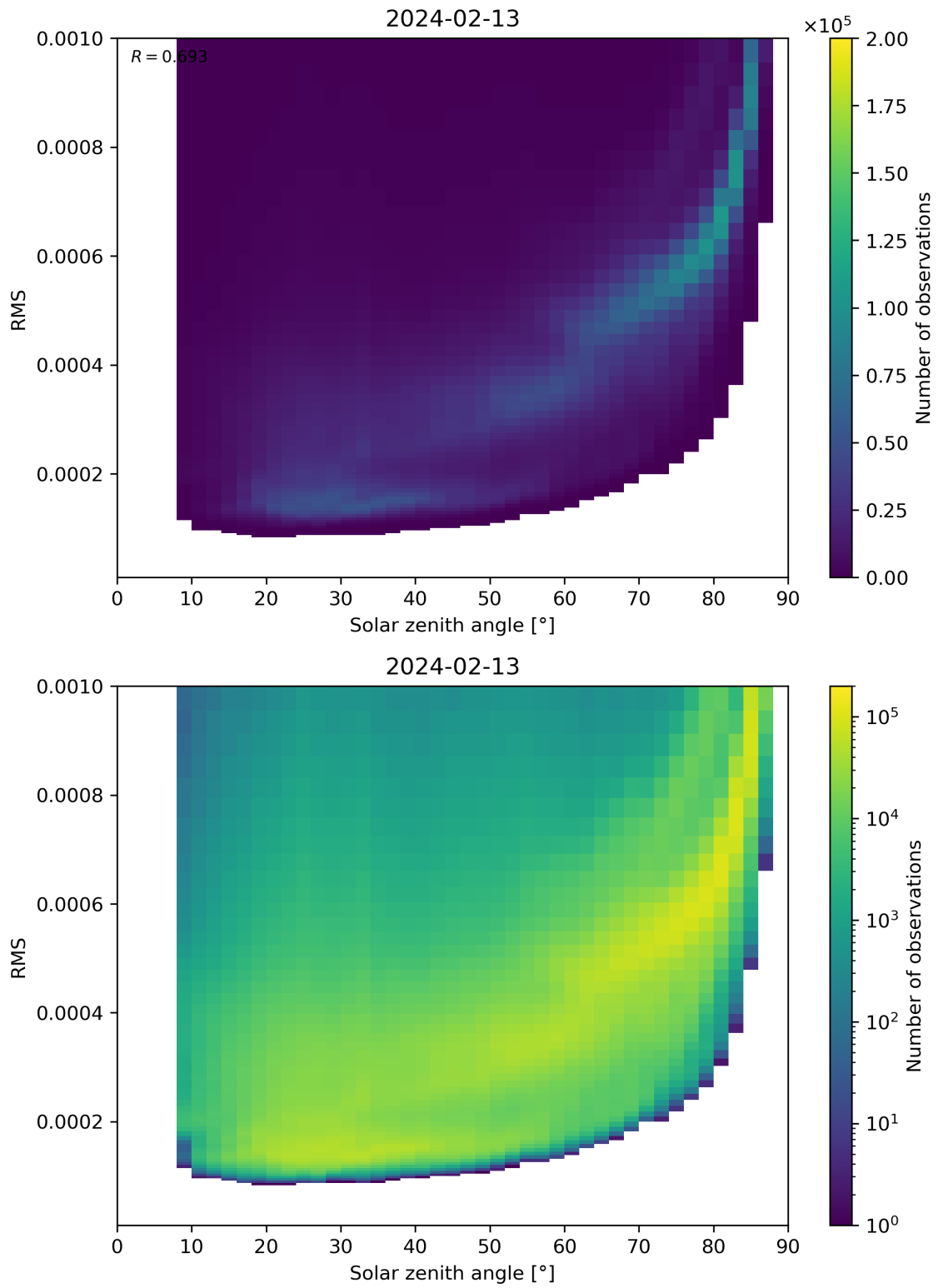
Figure 157: Scatter density plot of “Solar zenith angle” against “RMS” for 2024-02-12 to 2024-02-14.
