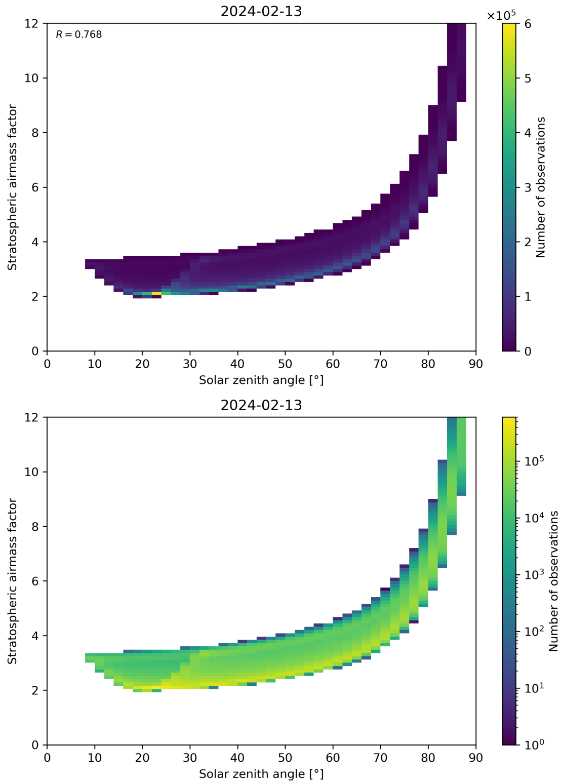
Figure 145: Scatter density plot of “Solar zenith angle” against “Stratospheric airmass factor” for 2024-02-12 to 2024-02-14.
