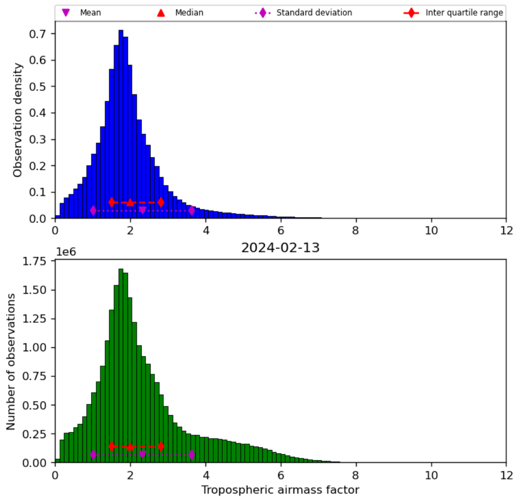
Figure 31: Histogram of “Tropospheric airmass factor” for 2024-02-12 to 2024-02-14
