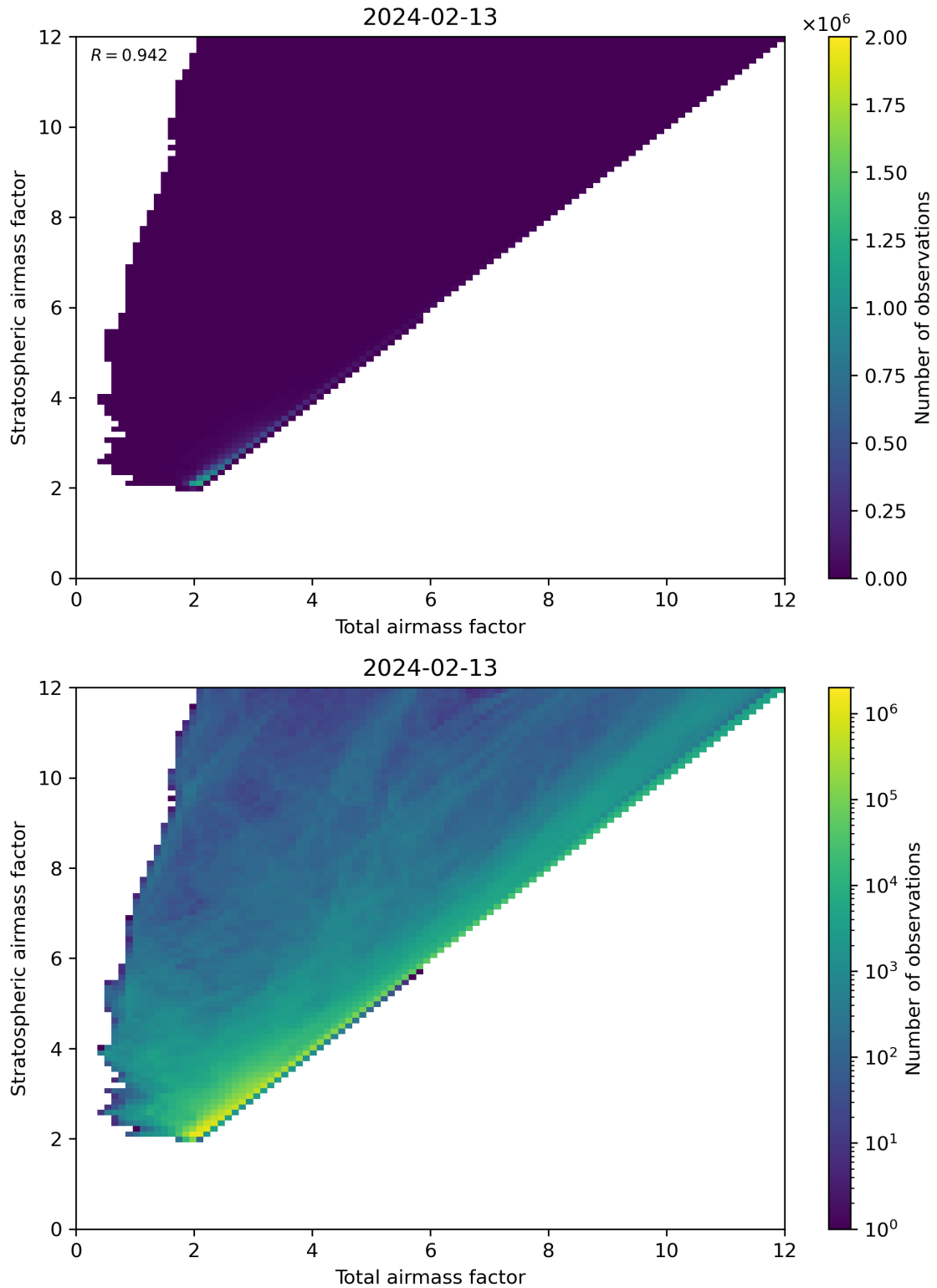
Figure 62: Scatter density plot of “Total airmass factor” against “Stratospheric airmass factor” for 2024-02-12 to 2024-02-14.
