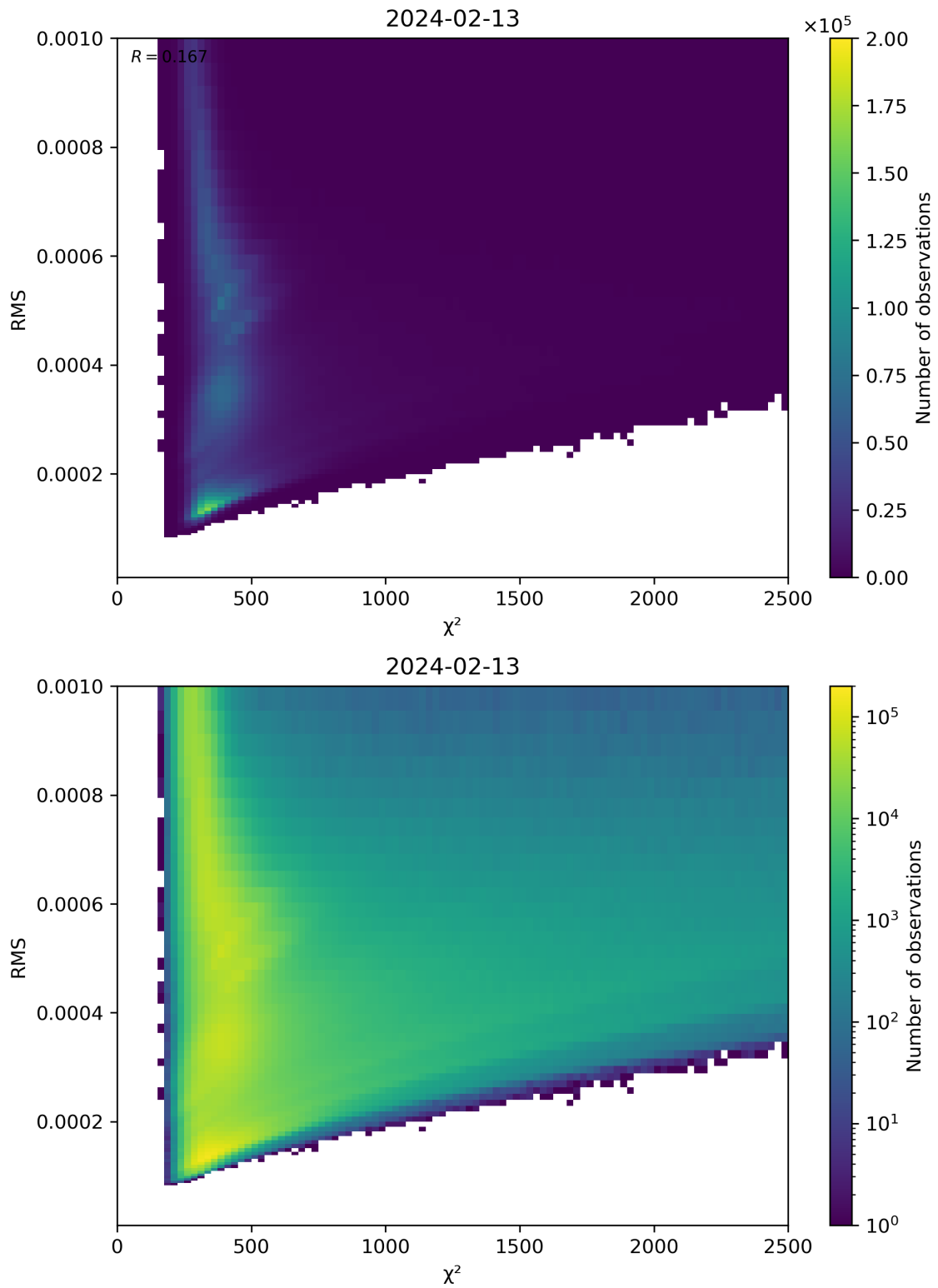
Figure 82: Scatter density plot of “ \chi^2 ” against “RMS” for 2024-02-12 to 2024-02-14.
