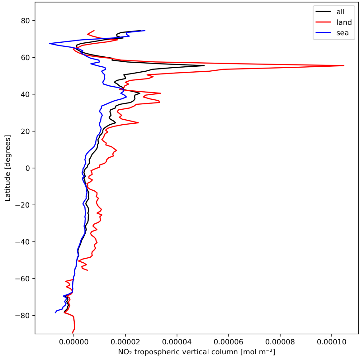
Figure 12: Zonal average of “NO 2 tropospheric vertical column” for 2024-02-12 to 2024-02-14.
