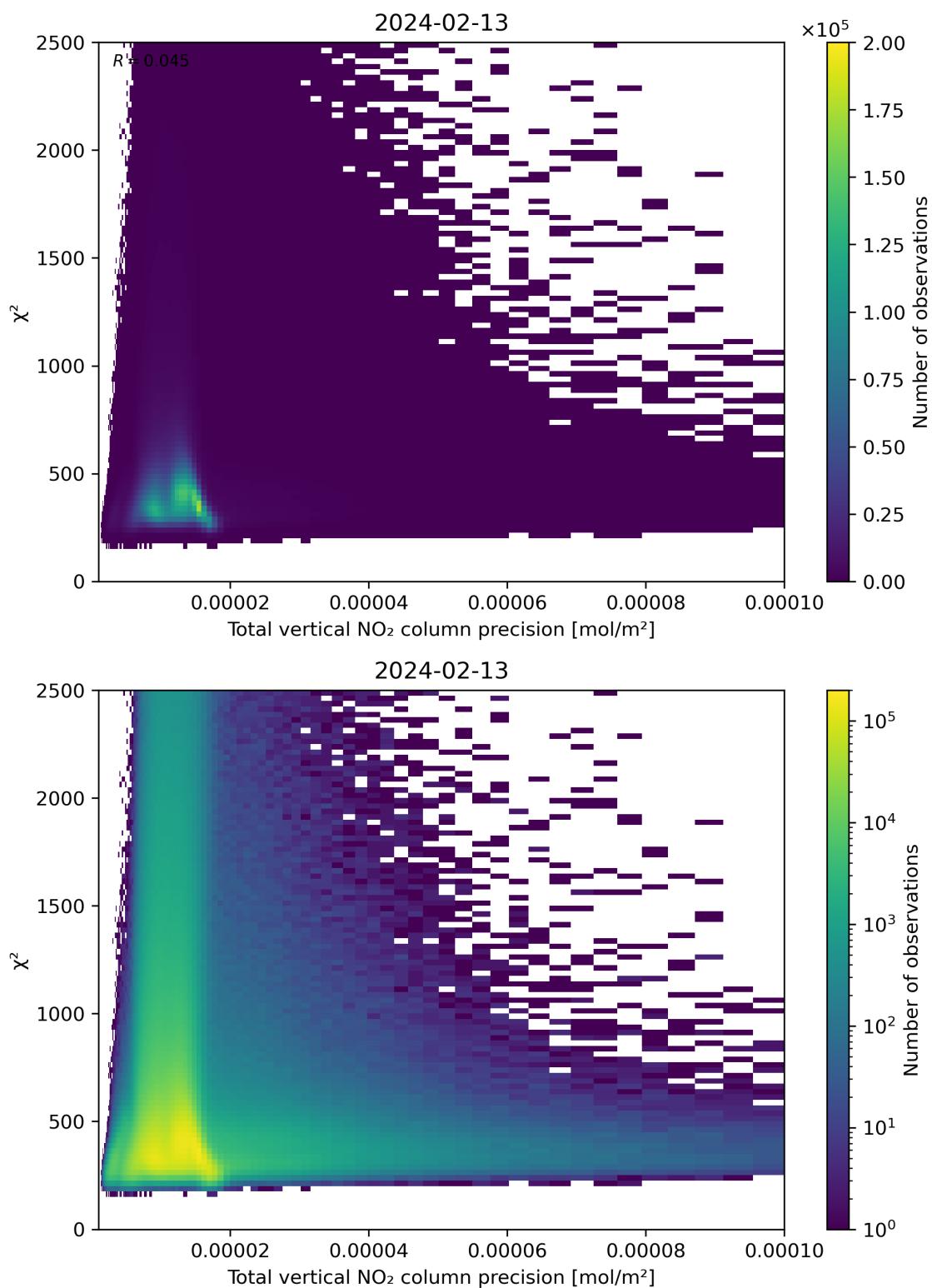
Figure 116: Scatter density plot of “Total vertical NO 2 column precision” against “ \chi^2 ” for 2024-02-12 to 2024-02-14.
