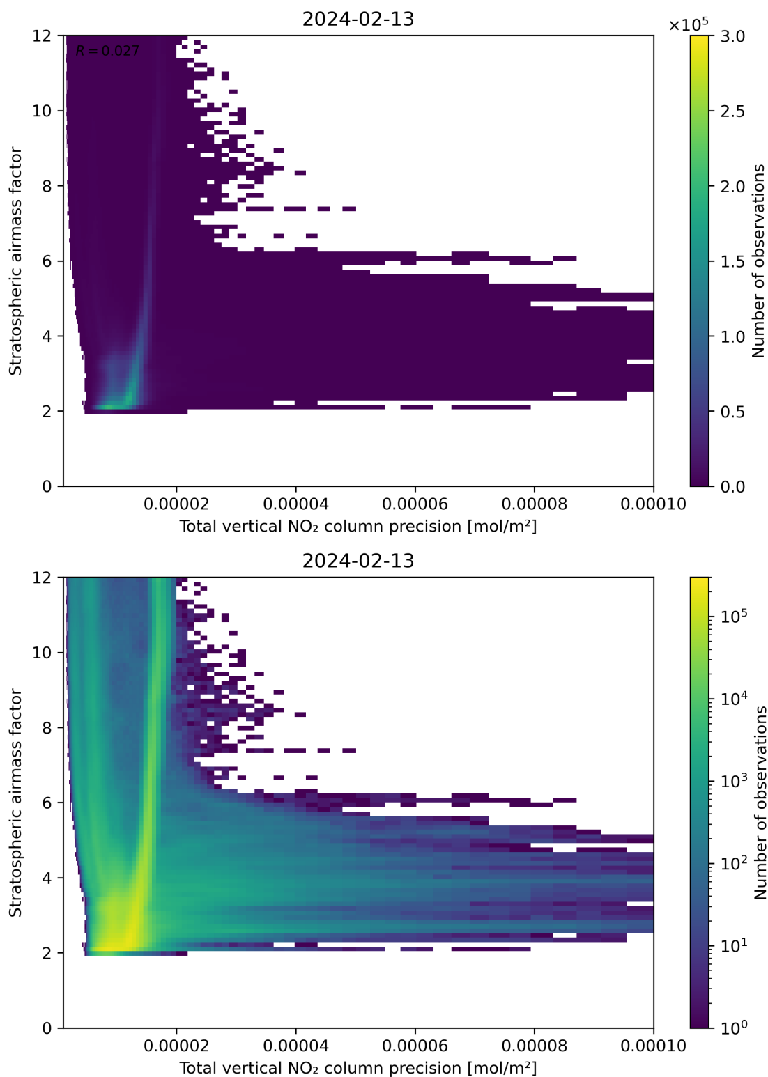
Figure 115: Scatter density plot of “Total vertical NO 2 column precision” against “Stratospheric air mass factor” for 2024-02-12 to 2024-02-14.
