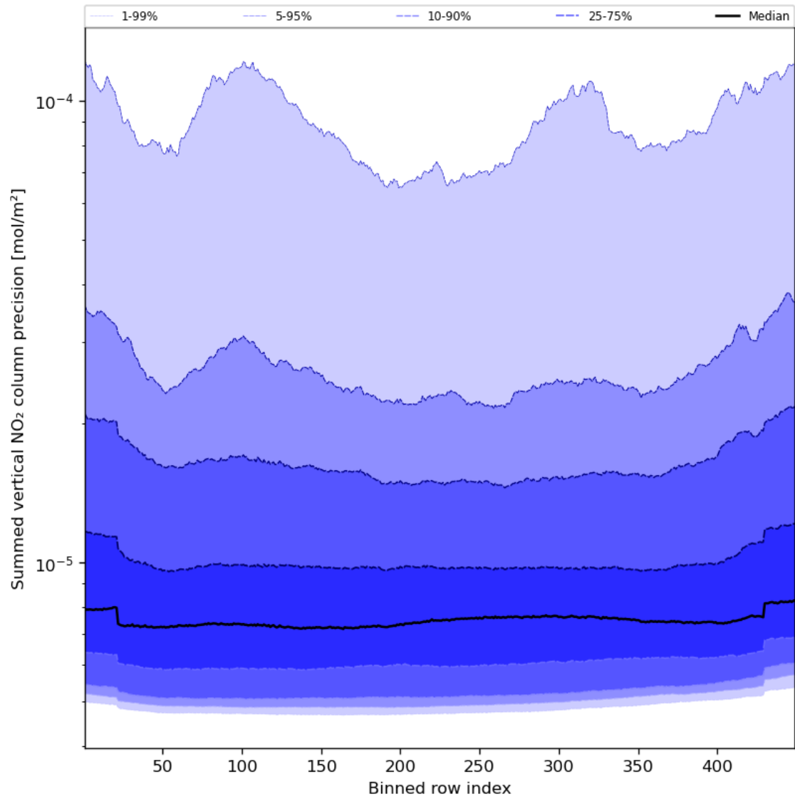
Figure 58: Along track statistics of “Summed vertical NO 2 column precision” for 2024-02-12 to 2024-02-14
