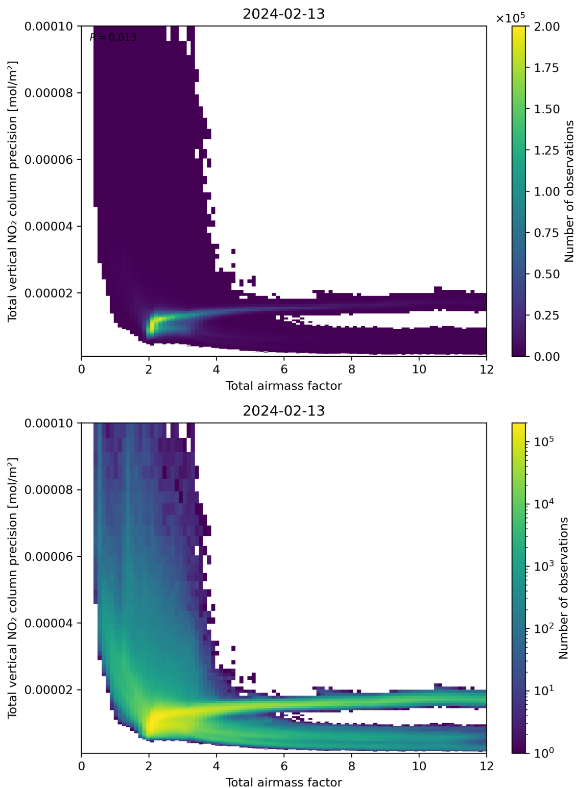
Figure 68: Scatter density plot of “Total airmass factor” against “Total vertical NO 2 column precision” for 2024-02-12 to 2024-02-14.
