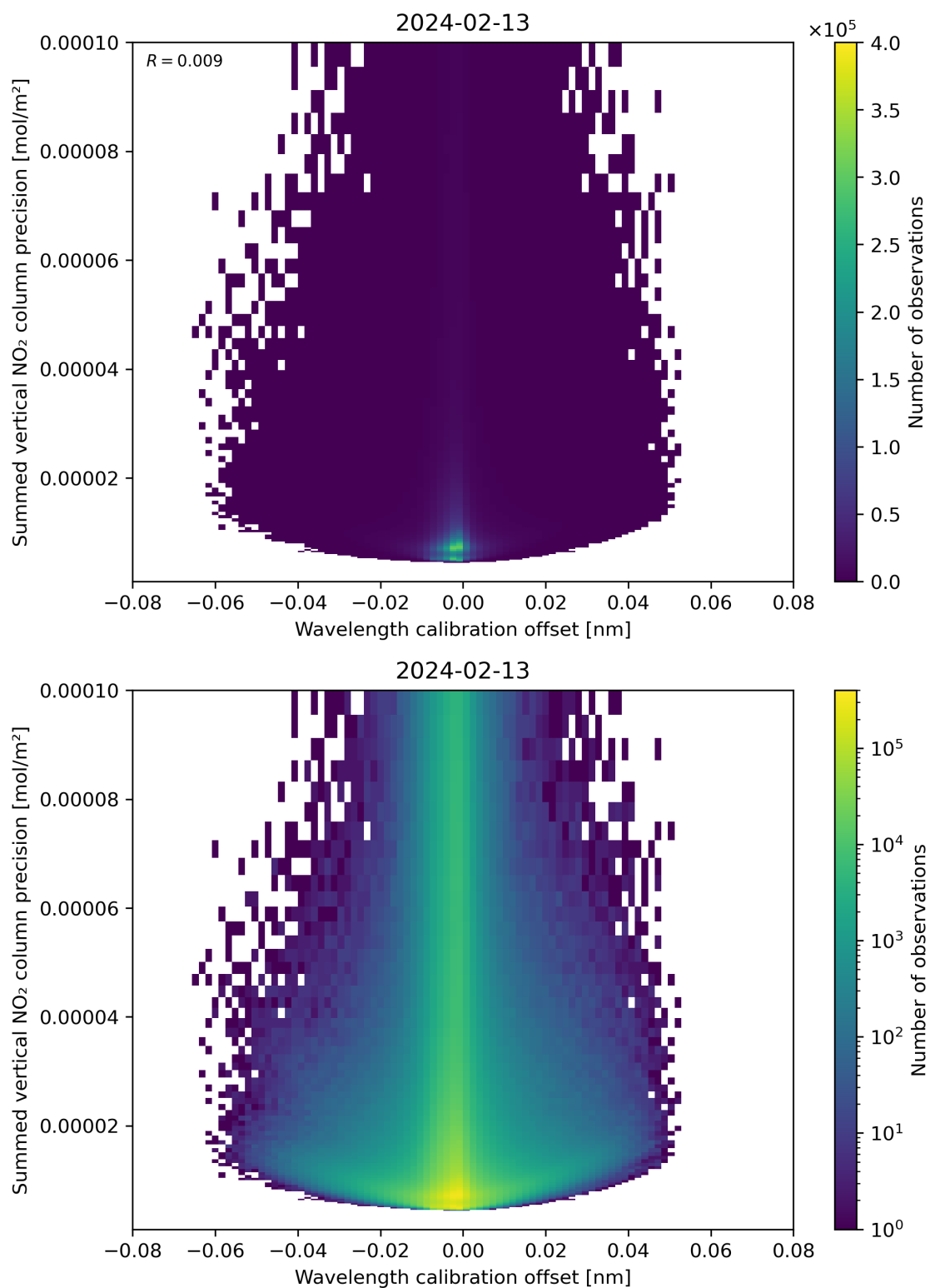
Figure 178: Scatter density plot of “Wavelength calibration offset” against “Summed vertical NO 2 column precision” for 2024-02-12 to 2024-02-14.
