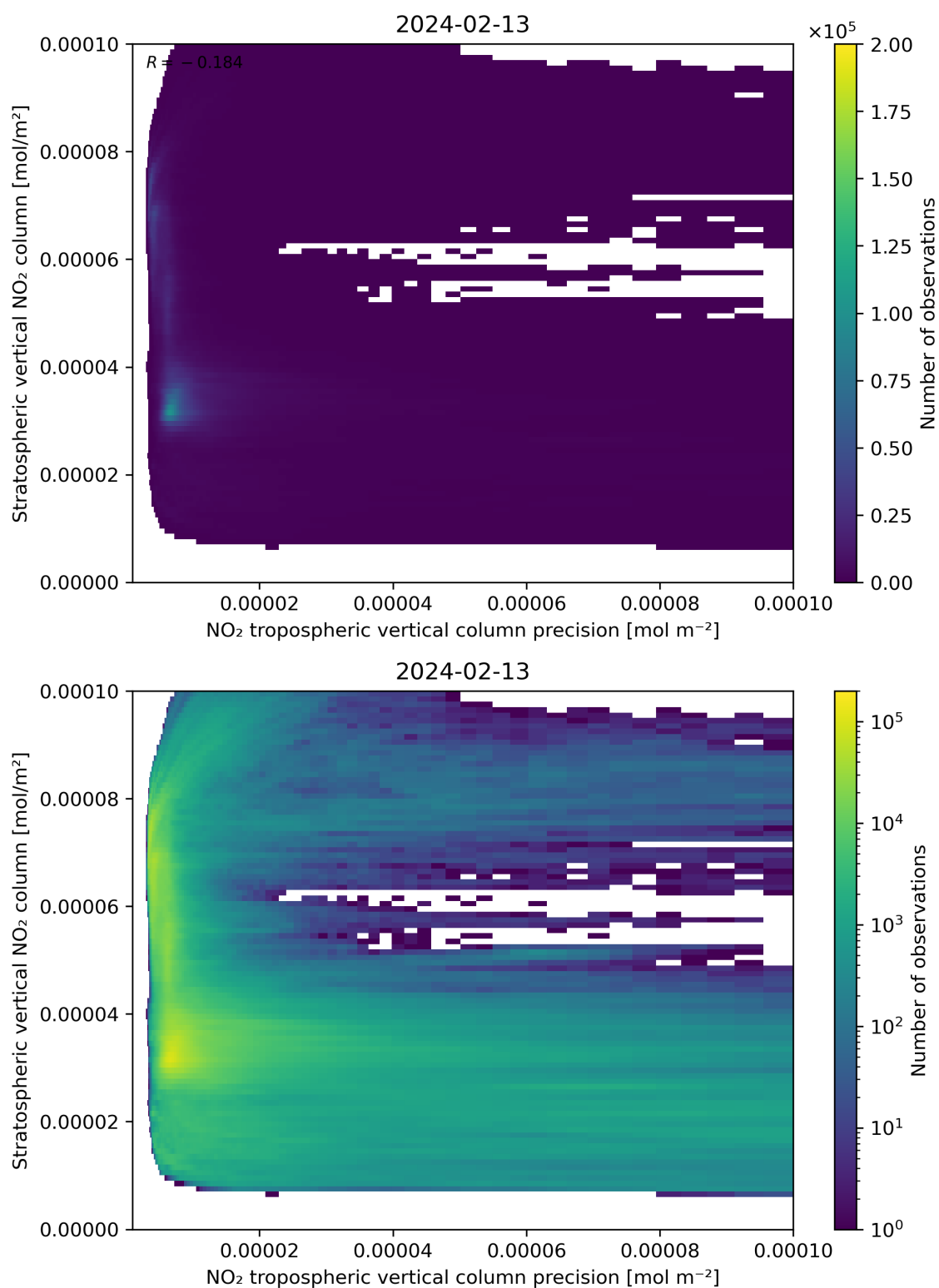
Figure 135: Scatter density plot of “NO 2 tropospheric vertical column precision” against “Stratospheric vertical NO 2 column” for 2024-02-12 to 2024-02-14.
