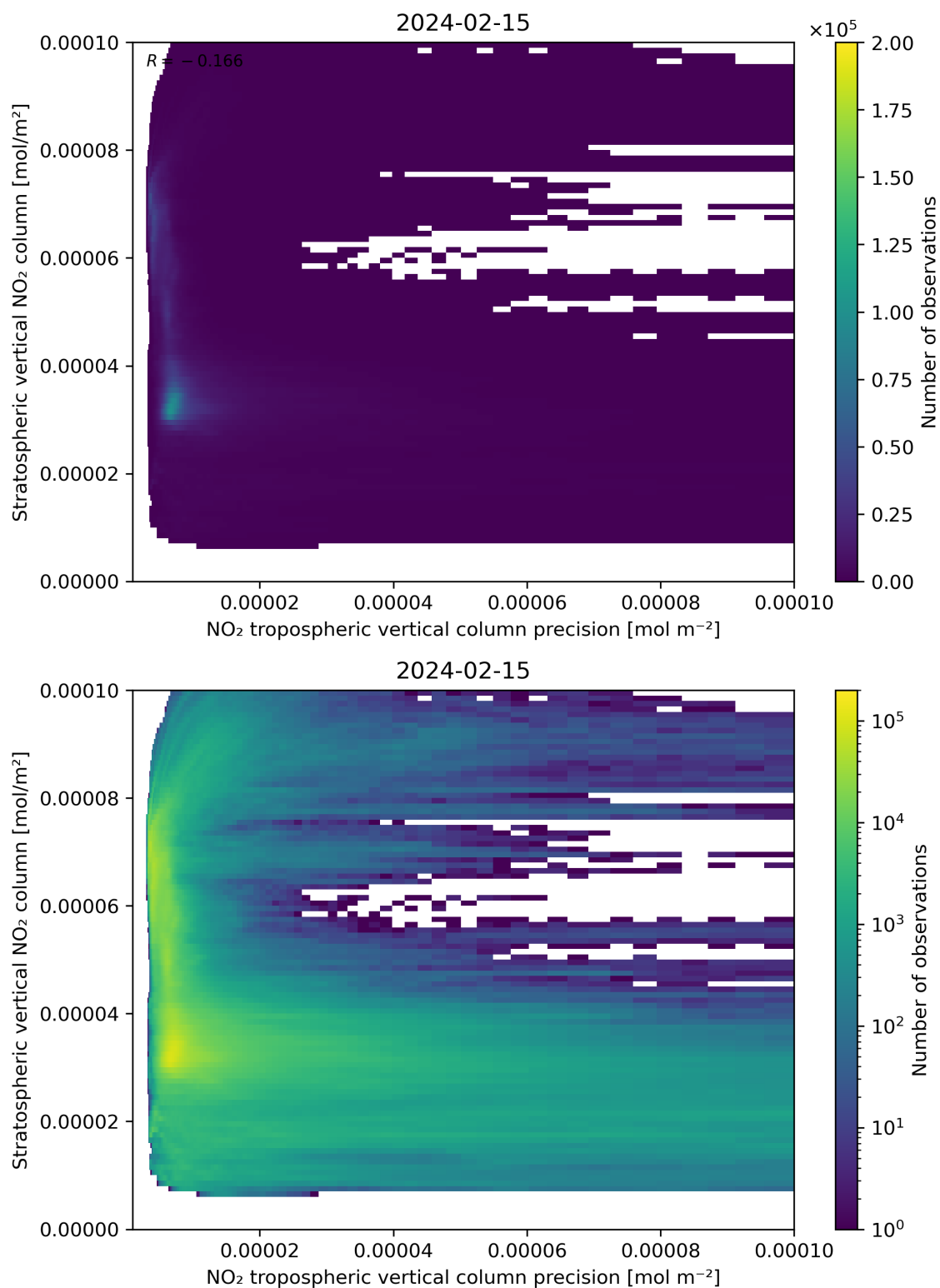
Figure 135: Scatter density plot of “NO 2 tropospheric vertical column precision” against “Stratospheric vertical NO 2 column” for 2024-02-14 to 2024-02-16.
