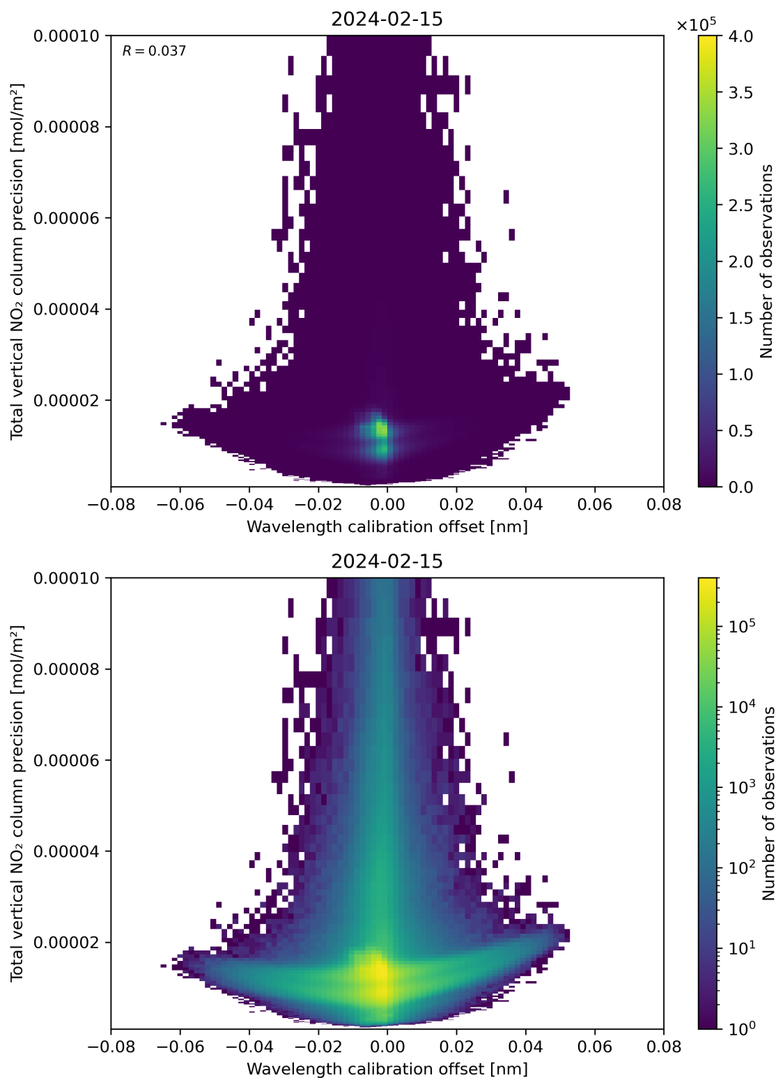
Figure 180: Scatter density plot of “Wavelength calibration offset” against “Total vertical NO 2 column precision” for 2024-02-14 to 2024-02-16.
