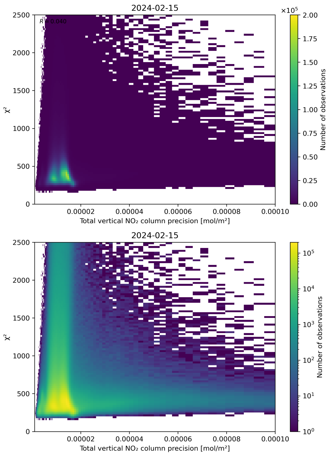
Figure 116: Scatter density plot of “Total vertical NO 2 column precision” against “ \chi^2 ” for 2024-02-14 to 2024-02-16.
