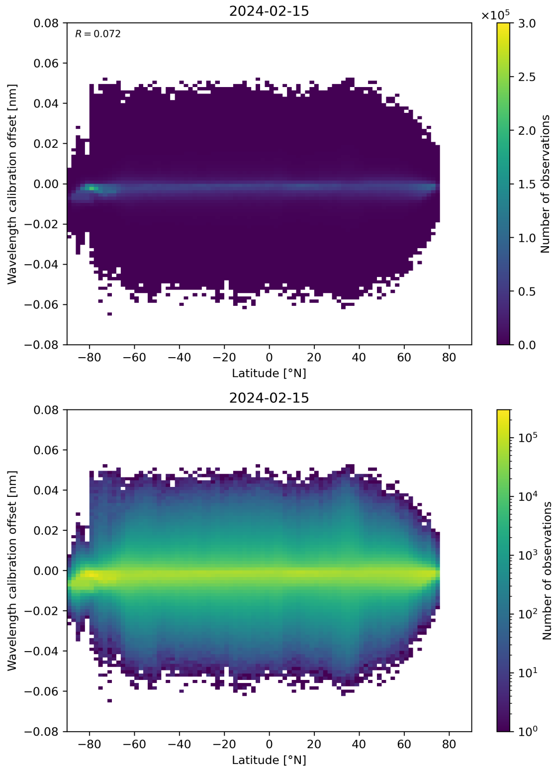
Figure 95: Scatter density plot of “Latitude” against “Wavelength calibration offset” for 2024-02-14 to 2024-02-16.
