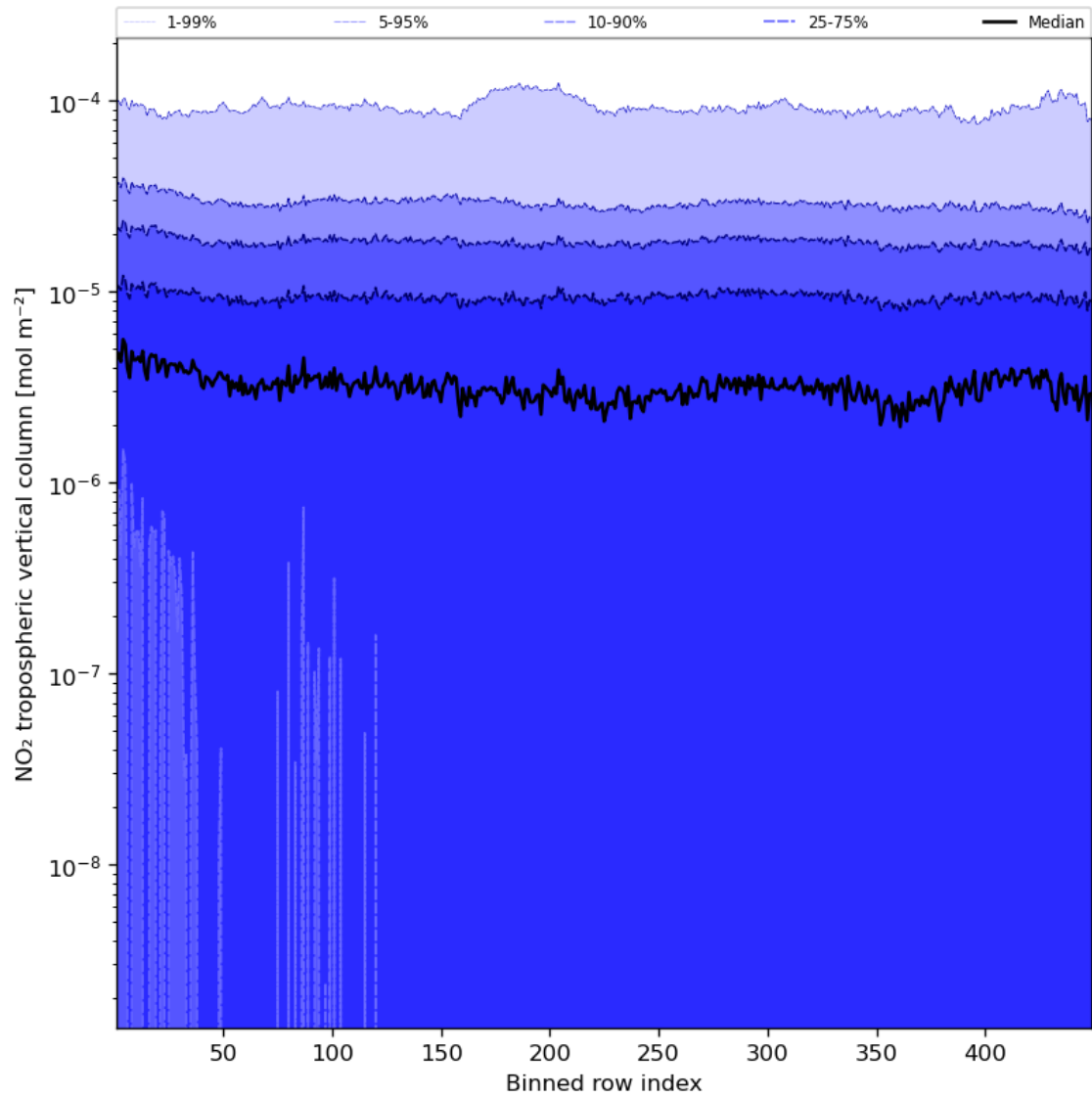
Figure 46: Along track statistics of “NO 2 tropospheric vertical column” for 2024-02-14 to 2024-02-16
