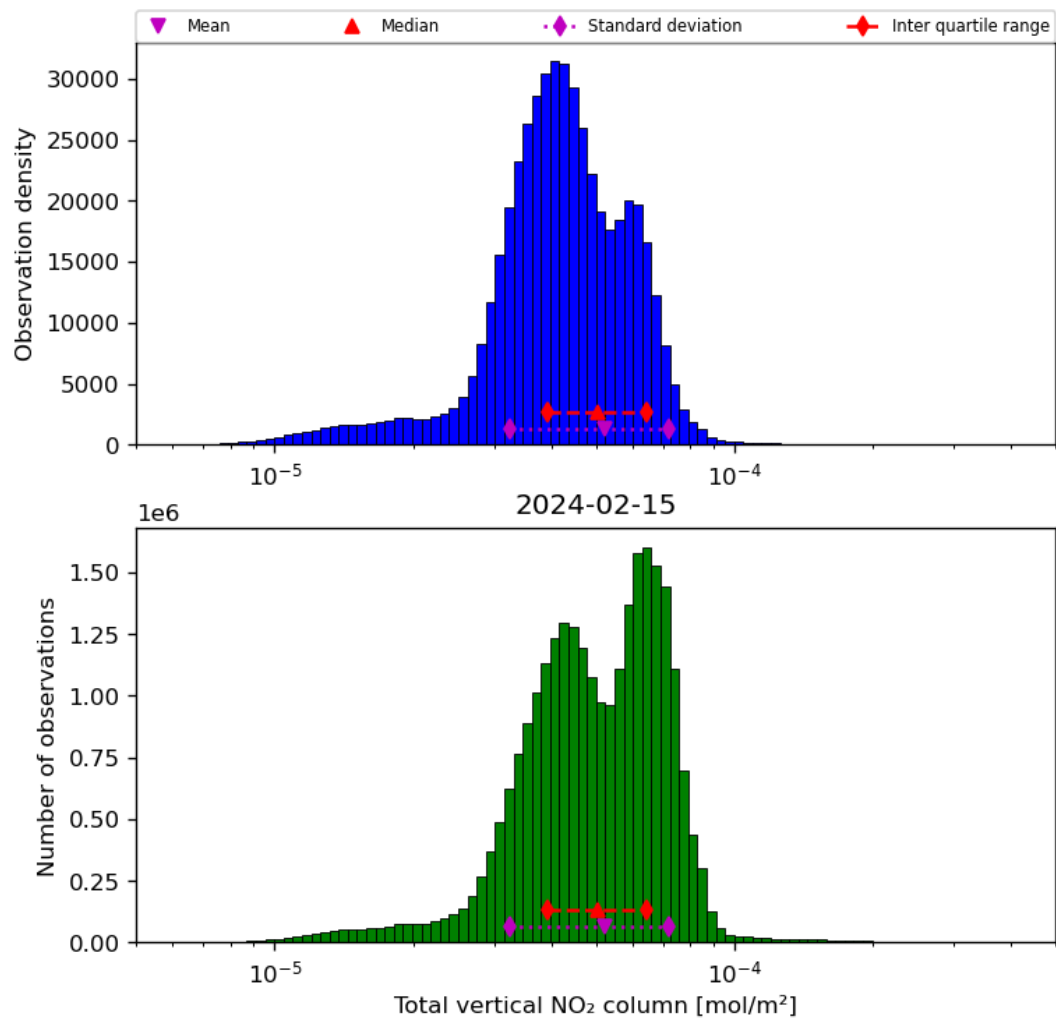
Figure 38: Histogram of “Total vertical NO 2 column” for 2024-02-14 to 2024-02-16
