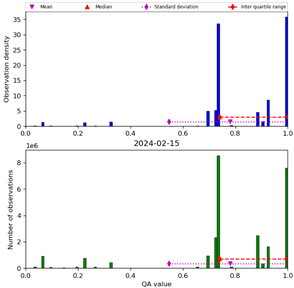
Figure 28: Histogram of “QA value” for 2024-02-14 to 2024-02-16
