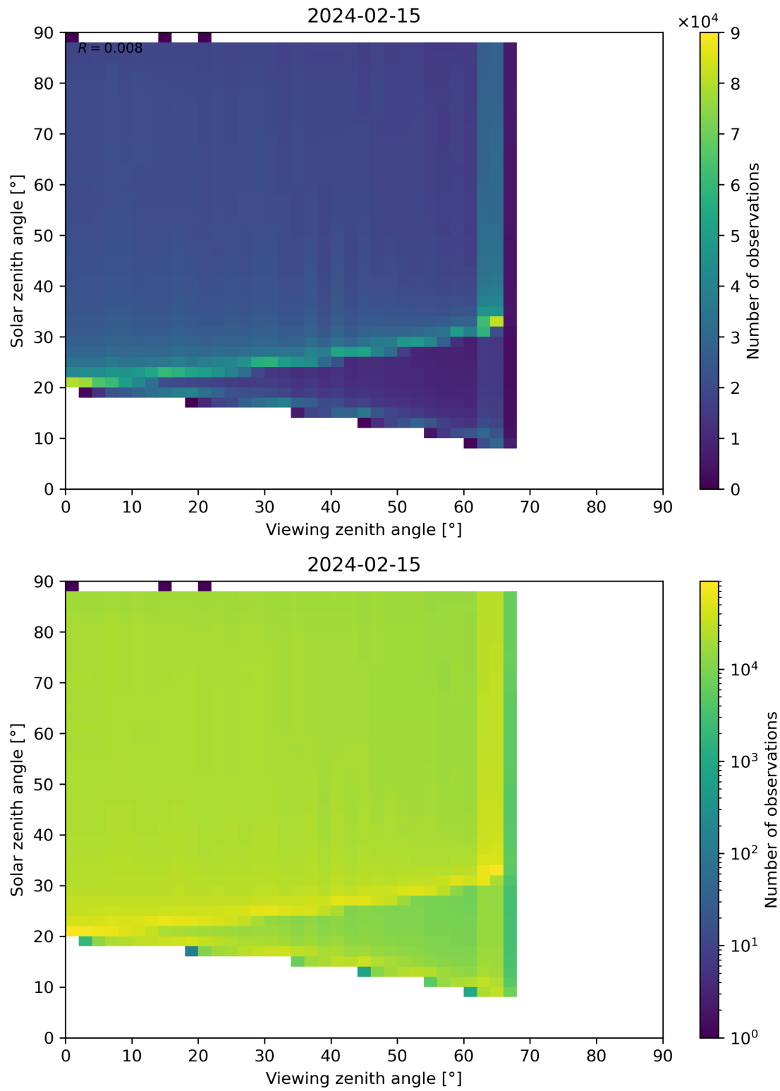
Figure 172: Scatter density plot of “Viewing zenith angle” against “Solar zenith angle” for 2024-02-14 to 2024-02-16.
