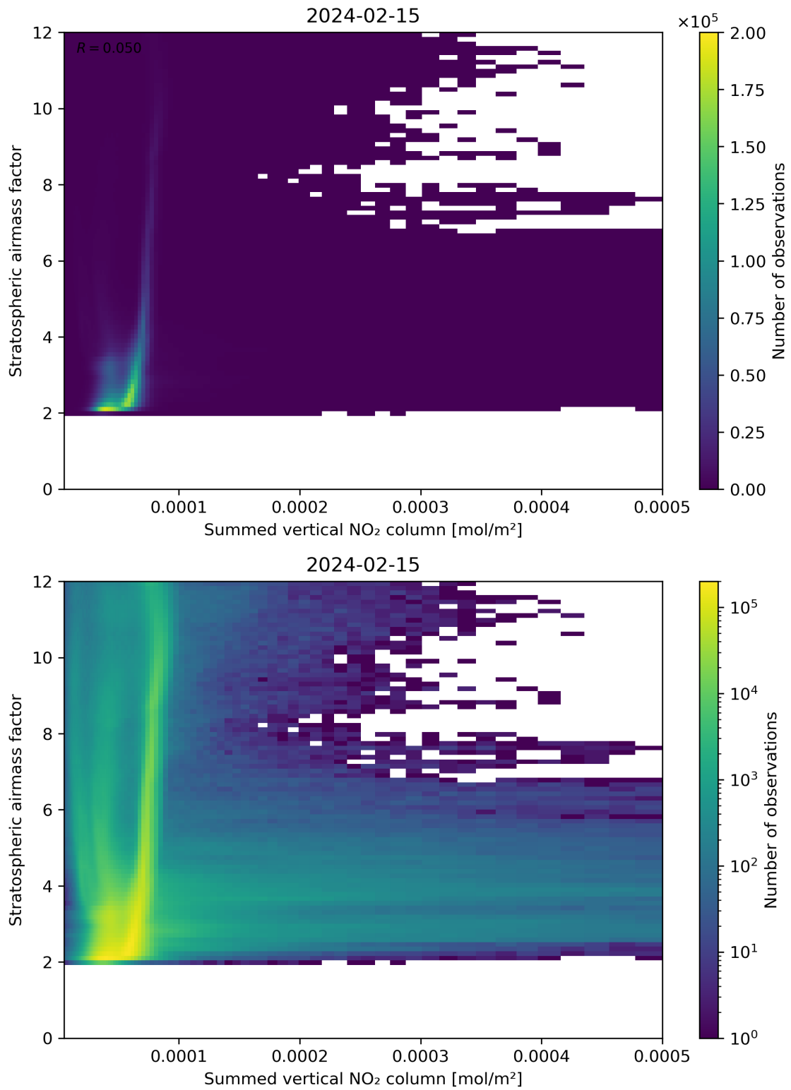
Figure 103: Scatter density plot of “Summed vertical NO 2 column” against “Stratospheric airmass factor” for 2024-02-14 to 2024-02-16.
