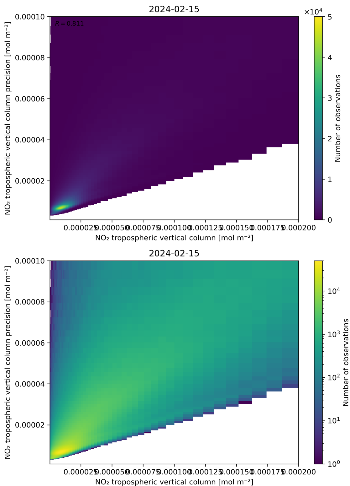
Figure 130: Scatter density plot of “NO 2 tropospheric vertical column” against “NO 2 tropospheric vertical column precision” for 2024-02-14 to 2024-02-16.
