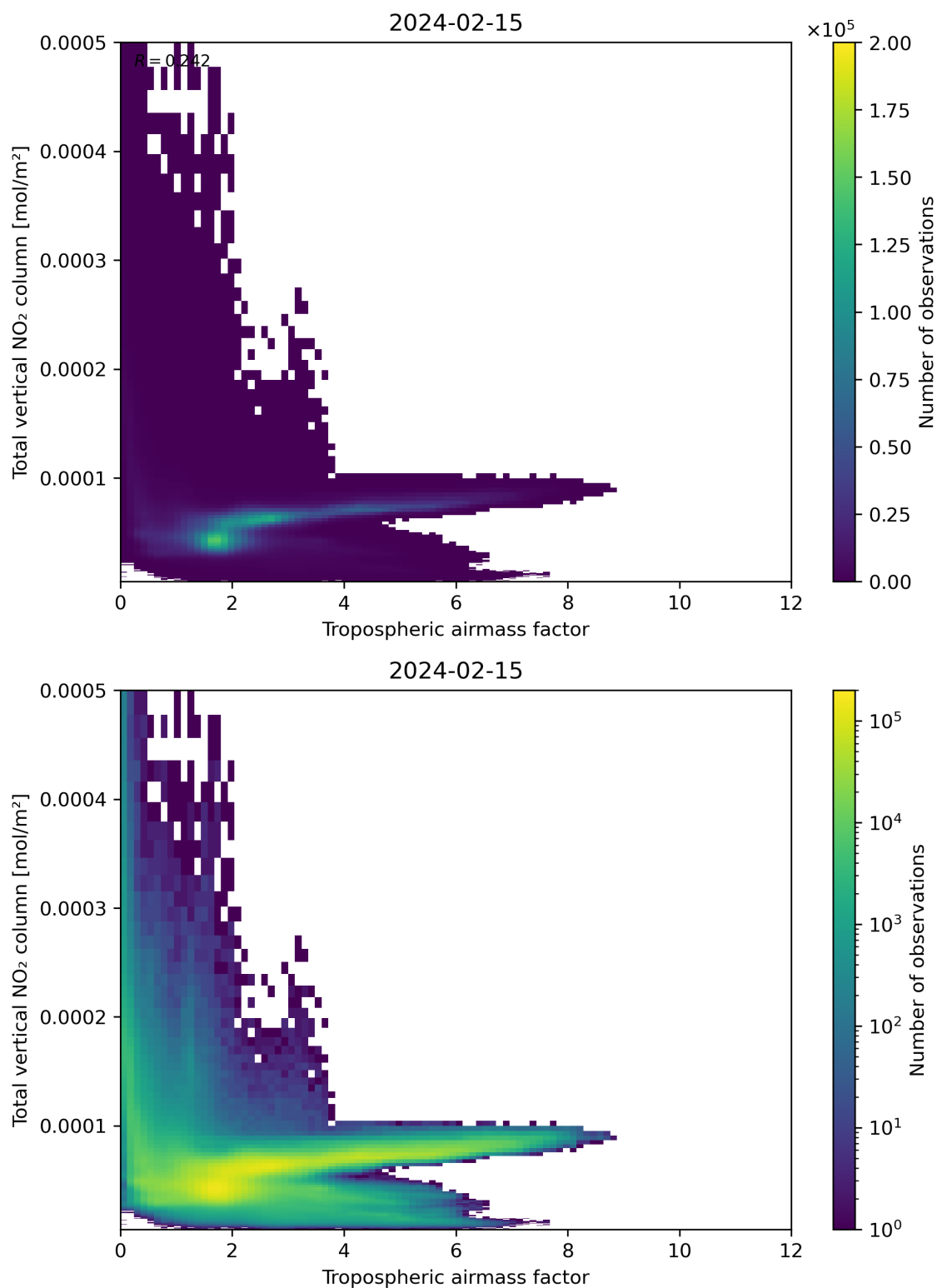
Figure 77: Scatter density plot of “Tropospheric airmass factor” against “Total vertical NO 2 column” for 2024-02-14 to 2024-02-16.
