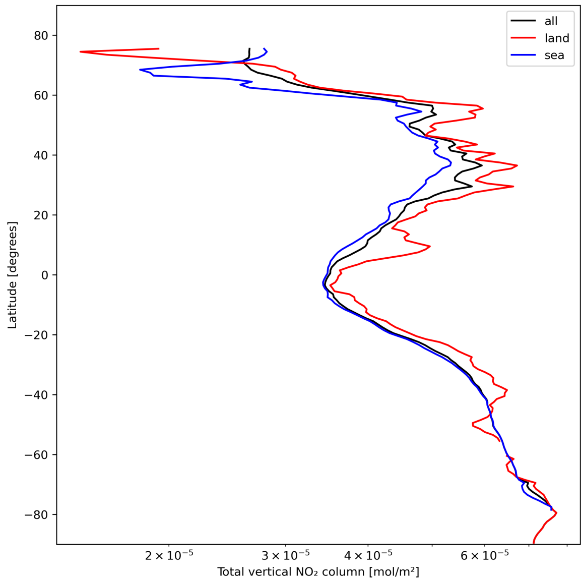
Figure 21: Zonal average of “Total vertical NO 2 column” for 2024-02-14 to 2024-02-16.
