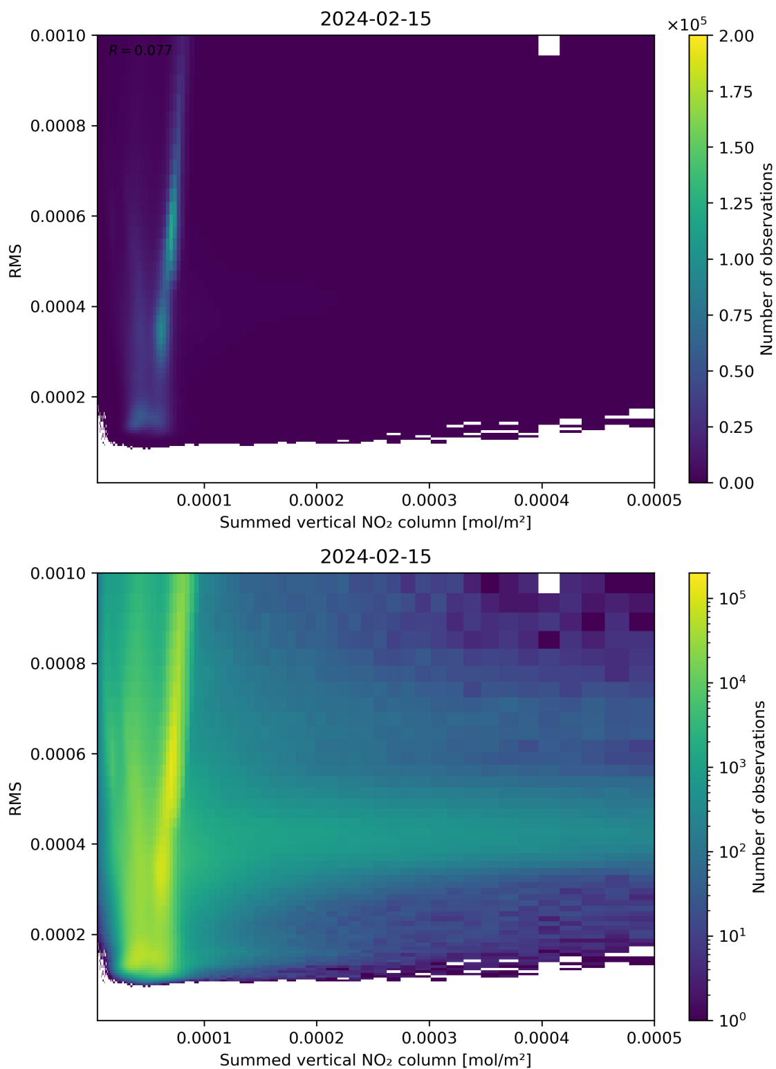
Figure 109: Scatter density plot of “Summed vertical NO 2 column” against “RMS” for 2024-02-14 to 2024-02-16.
