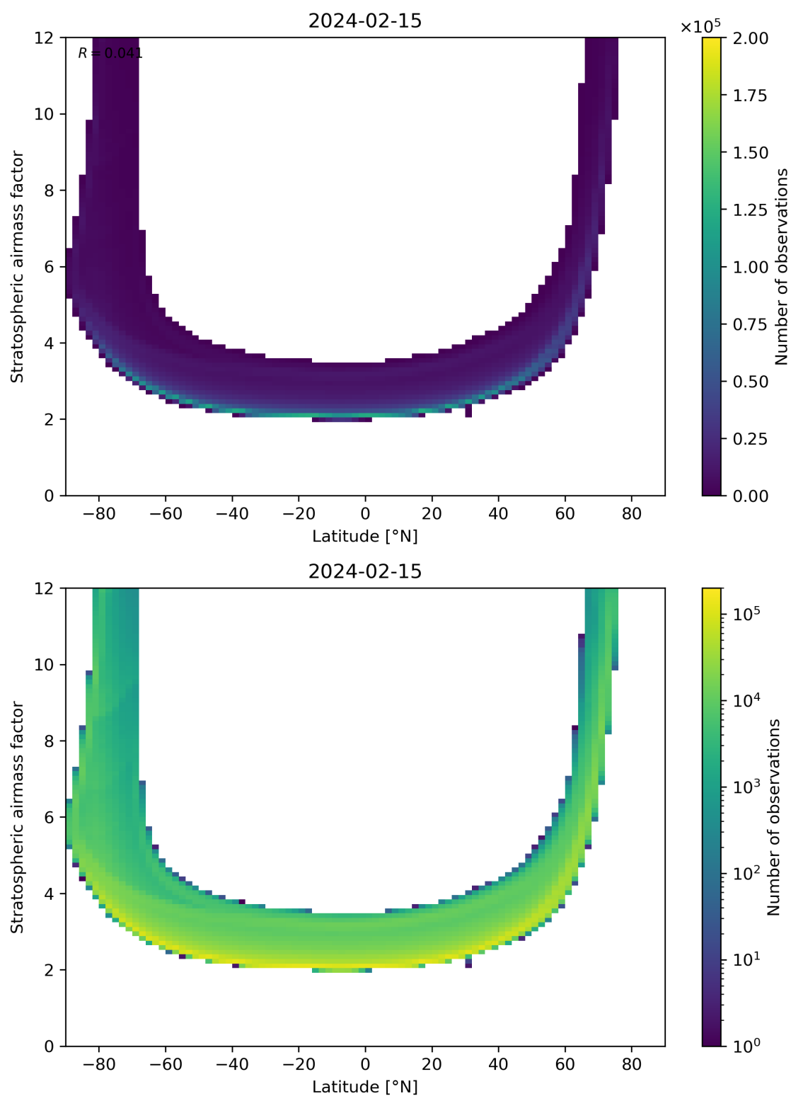
Figure 83: Scatter density plot of “Latitude” against “Stratospheric airmass factor” for 2024-02-14 to 2024-02-16.
