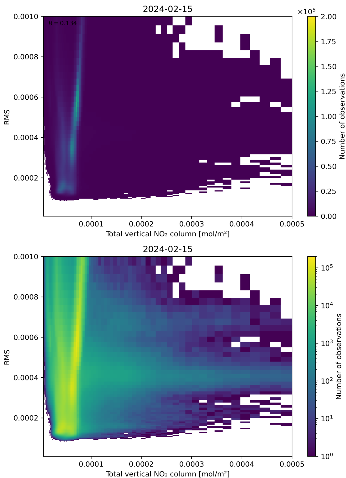
Figure 120: Scatter density plot of “Total vertical NO 2 column” against “RMS” for 2024-02-14 to 2024-02-16.
