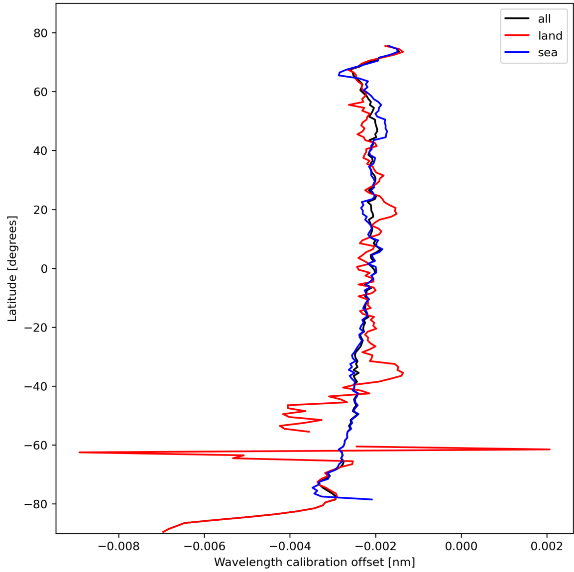
Figure 18: Zonal average of “Wavelength calibration offset” for 2024-02-14 to 2024-02-16.
