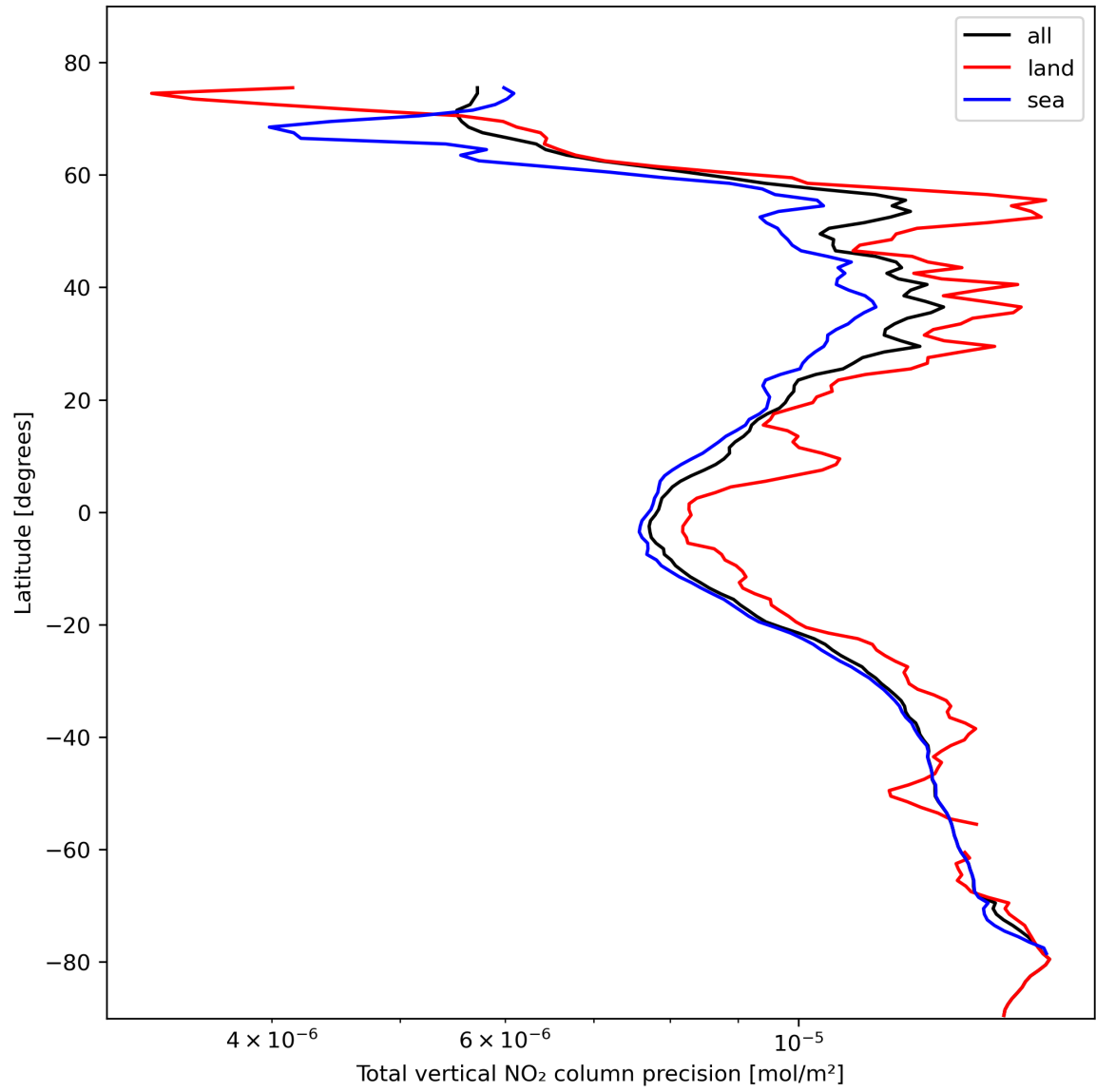
Figure 22: Zonal average of “Total vertical NO 2 column precision” for 2024-02-14 to 2024-02-16.
