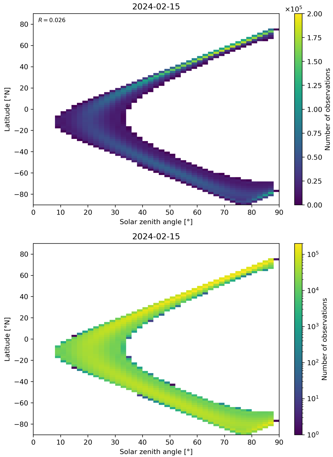
Figure 149: Scatter density plot of “Solar zenith angle” against “Latitude” for 2024-02-14 to 2024-02-16.
