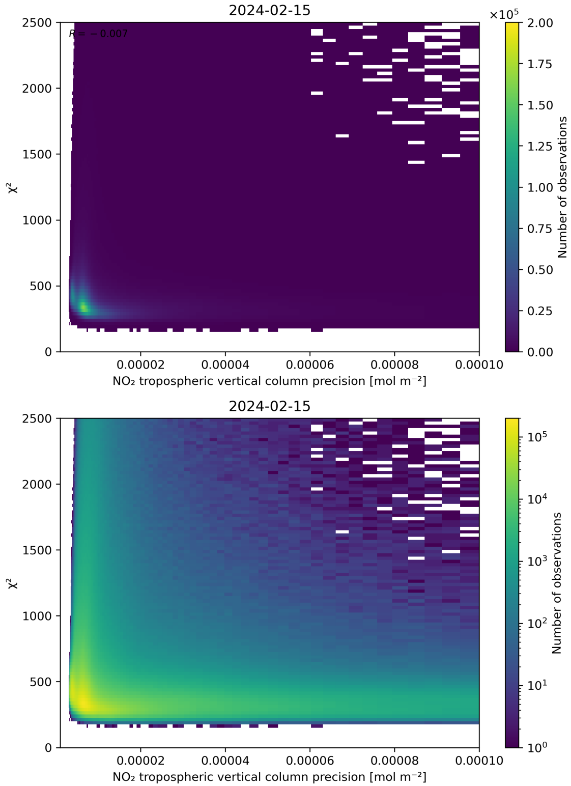
Figure 134: Scatter density plot of “NO 2 tropospheric vertical column precision” against “ \chi^2 ” for 2024-02-14 to 2024-02-16.
