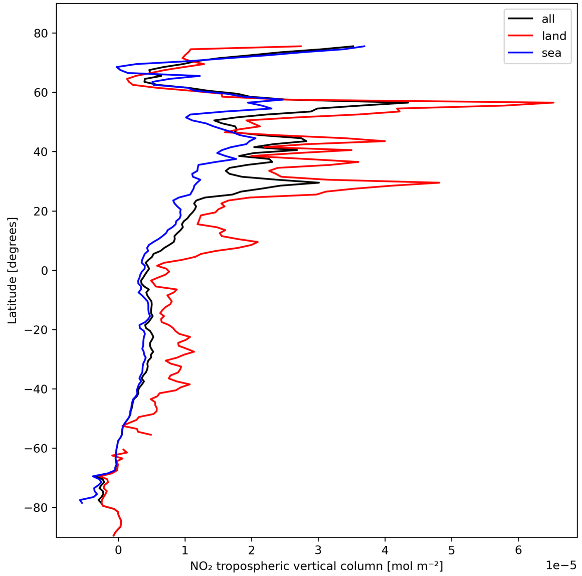
Figure 12: Zonal average of “NO 2 tropospheric vertical column” for 2024-02-14 to 2024-02-16.
