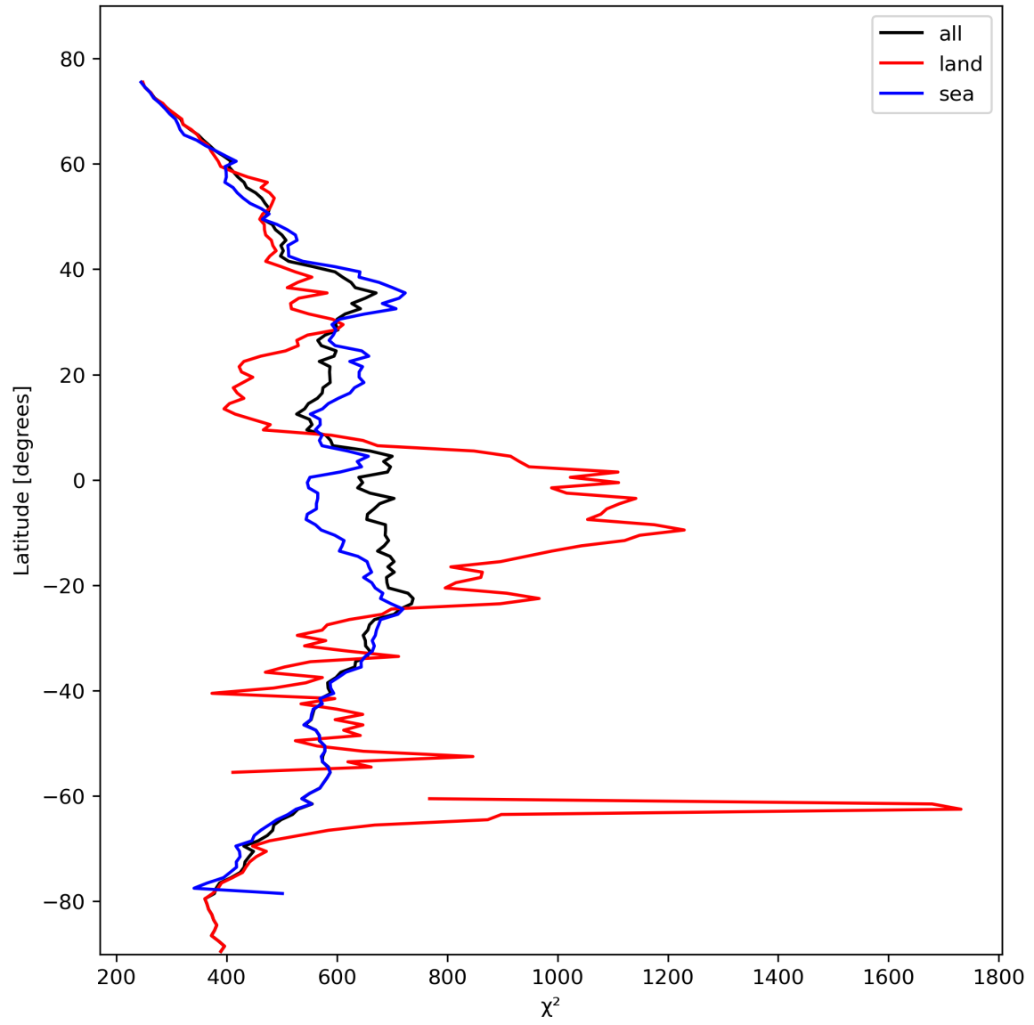
Figure 25: Zonal average of “ \chi^2 ” for 2024-02-14 to 2024-02-16.
