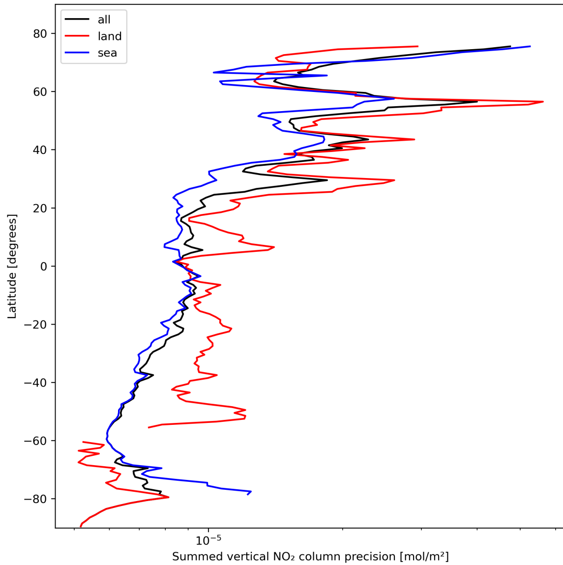
Figure 24: Zonal average of “Summed vertical NO 2 column precision” for 2024-02-14 to 2024-02-16.
