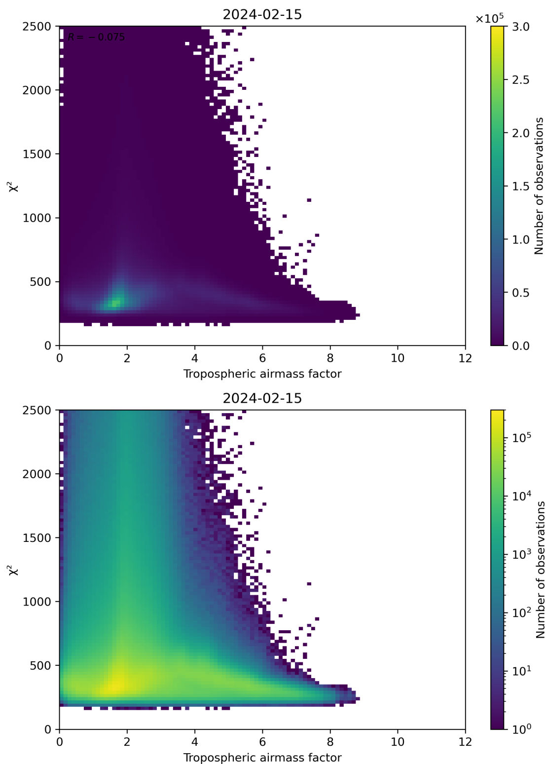
Figure 73: Scatter density plot of “Tropospheric airmass factor” against “ \chi^2 ” for 2024-02-14 to 2024-02-16.
