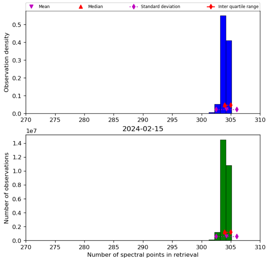
Figure 33: Histogram of “Number of spectral points in retrieval” for 2024-02-14 to 2024-02-16
