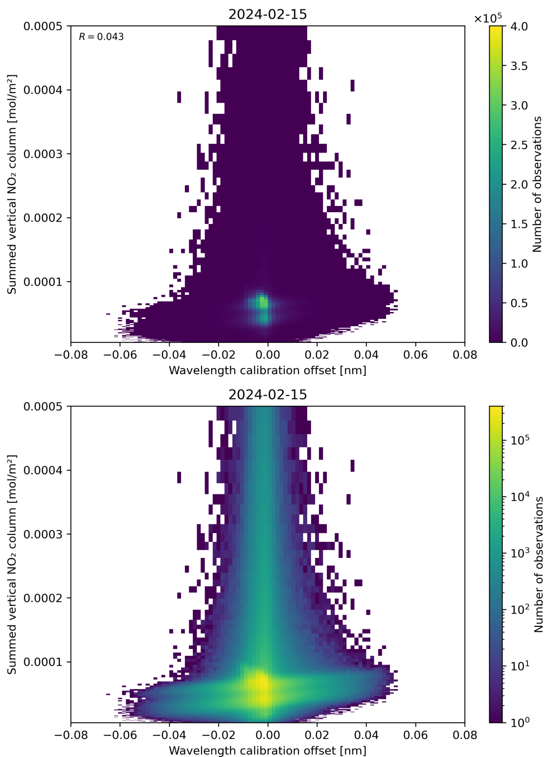
Figure 177: Scatter density plot of “Wavelength calibration offset” against “Summed vertical NO 2 column” for 2024-02-14 to 2024-02-16.
