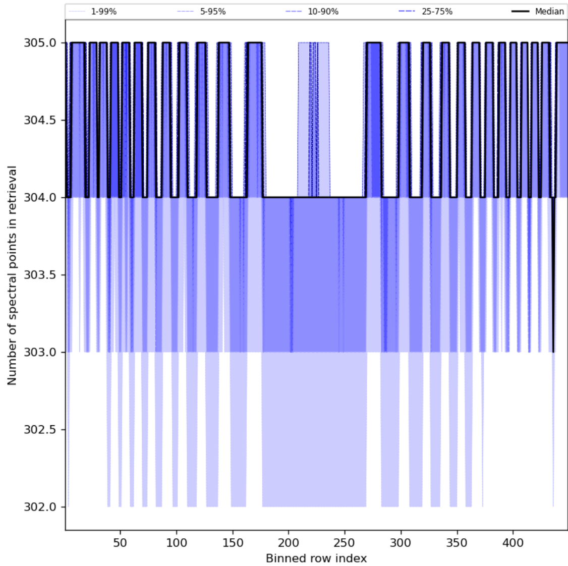
Figure 50: Along track statistics of “Number of spectral points in retrieval” for 2024-02-14 to 2024-02-16
