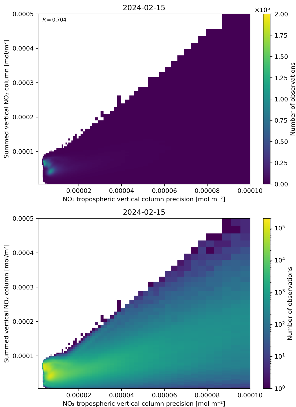
Figure 136: Scatter density plot of “NO 2 tropospheric vertical column precision” against “Summed vertical NO 2 column” for 2024-02-14 to 2024-02-16.
