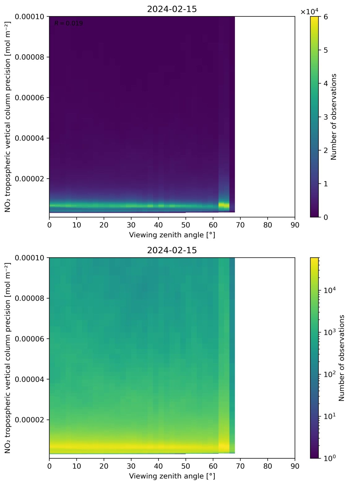
Figure 170: Scatter density plot of “Viewing zenith angle” against “NO 2 tropospheric vertical column precision” for 2024-02-14 to 2024-02-16.
