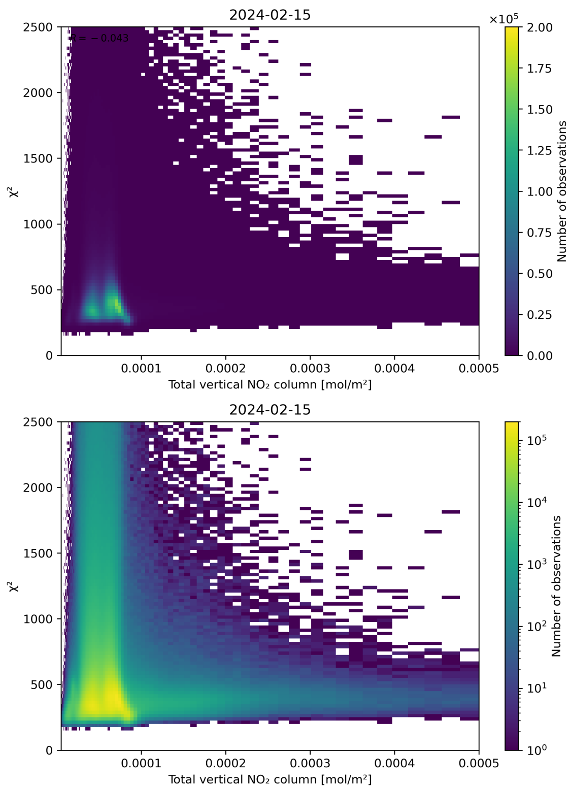
Figure 111: Scatter density plot of “Total vertical NO 2 column” against “ \chi^2 ” for 2024-02-14 to 2024-02-16.
