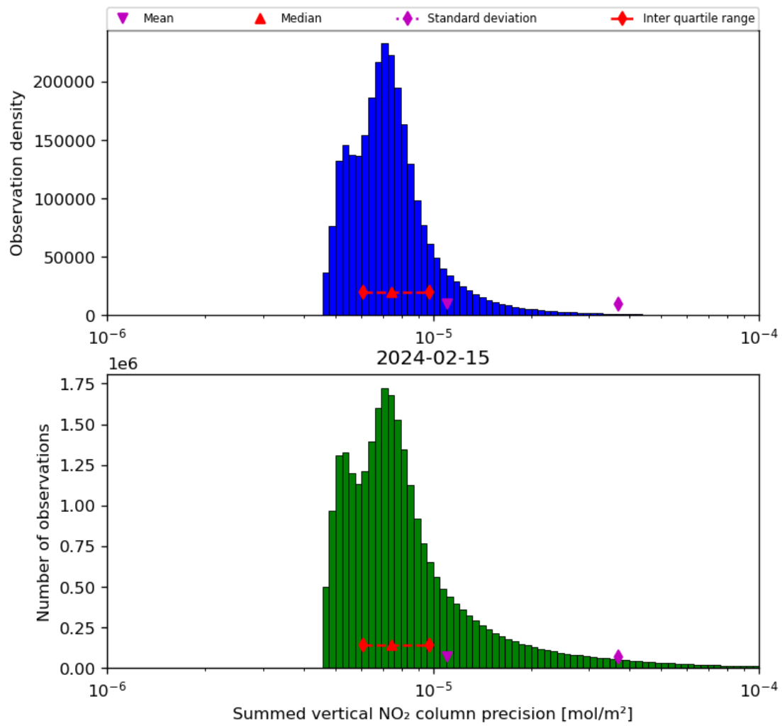
Figure 41: Histogram of “Summed vertical NO 2 column precision” for 2024-02-14 to 2024-02-16
