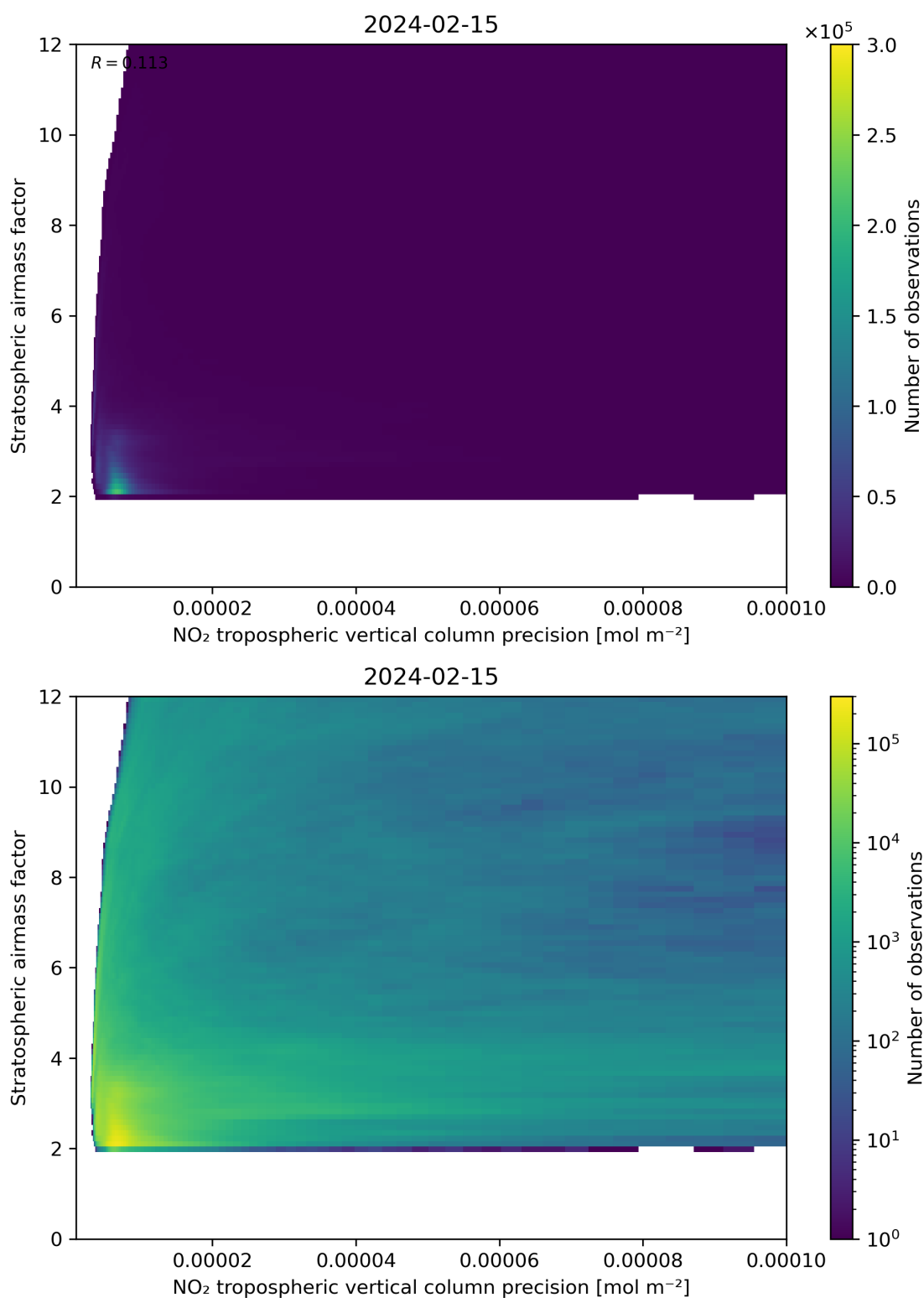
Figure 131: Scatter density plot of “NO 2 tropospheric vertical column precision” against “Stratospheric airmass factor” for 2024-02-14 to 2024-02-16.
