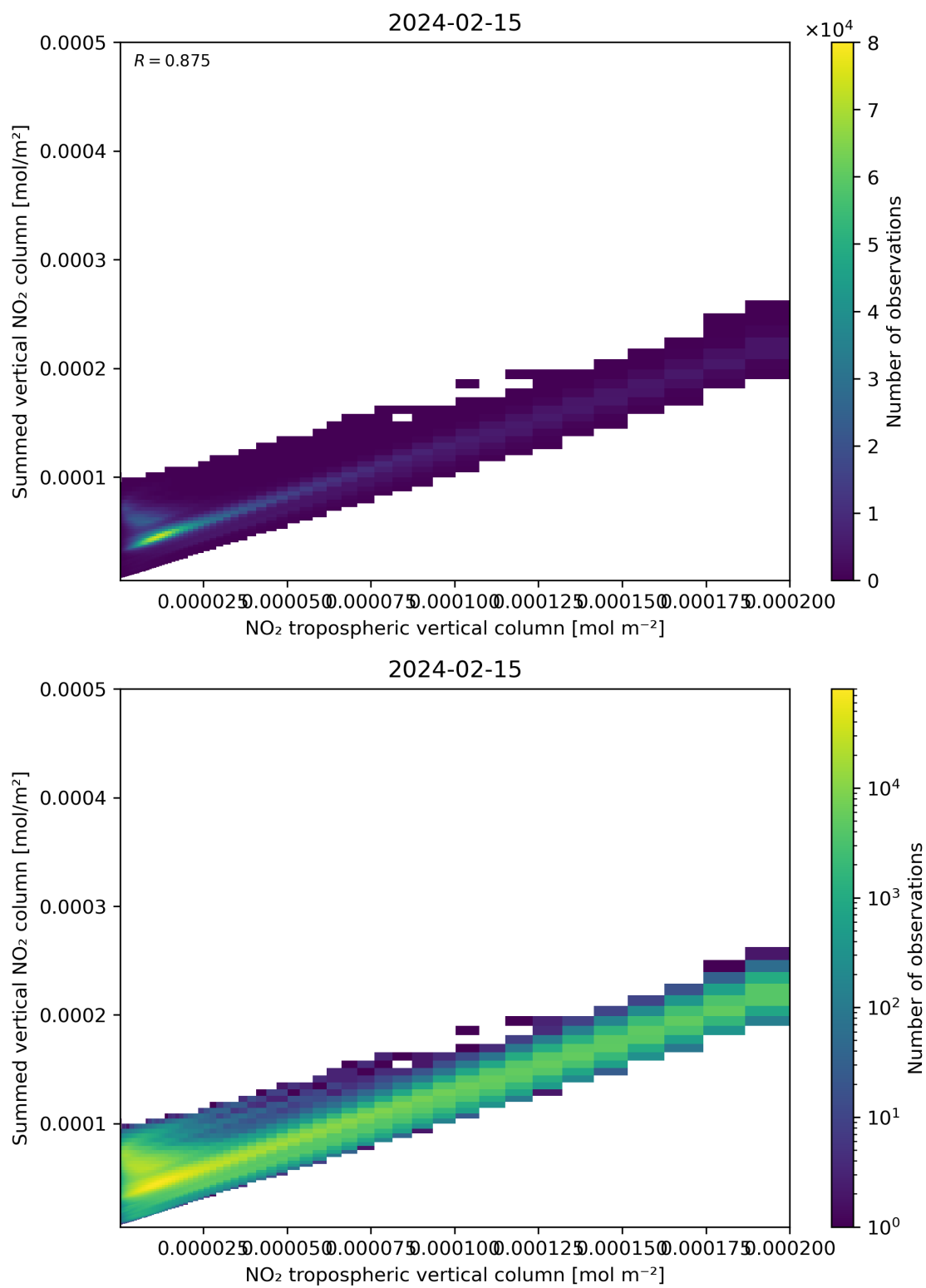
Figure 126: Scatter density plot of “NO 2 tropospheric vertical column” against “Summed vertical NO 2 column” for 2024-02-14 to 2024-02-16.
