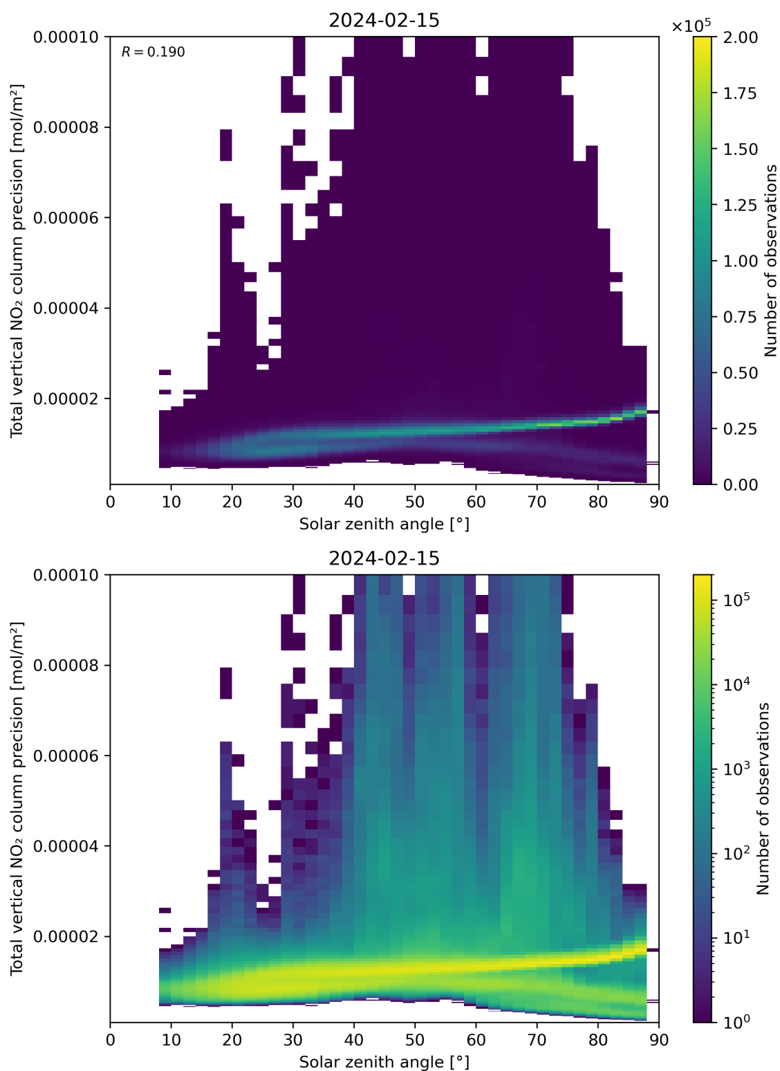
Figure 154: Scatter density plot of “Solar zenith angle” against “Total vertical NO 2 column precision” for 2024-02-14 to 2024-02-16.
