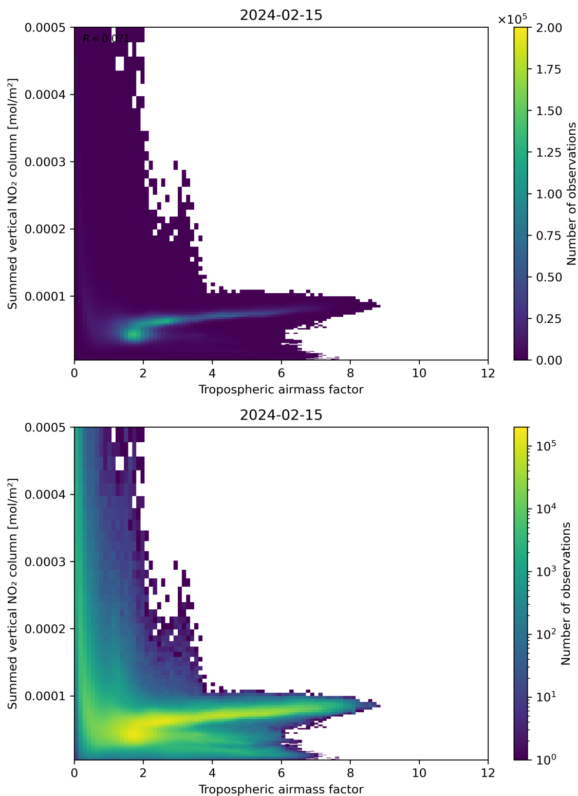
Figure 75: Scatter density plot of “Tropospheric airmass factor” against “Summed vertical NO 2 column” for 2024-02-14 to 2024-02-16.
