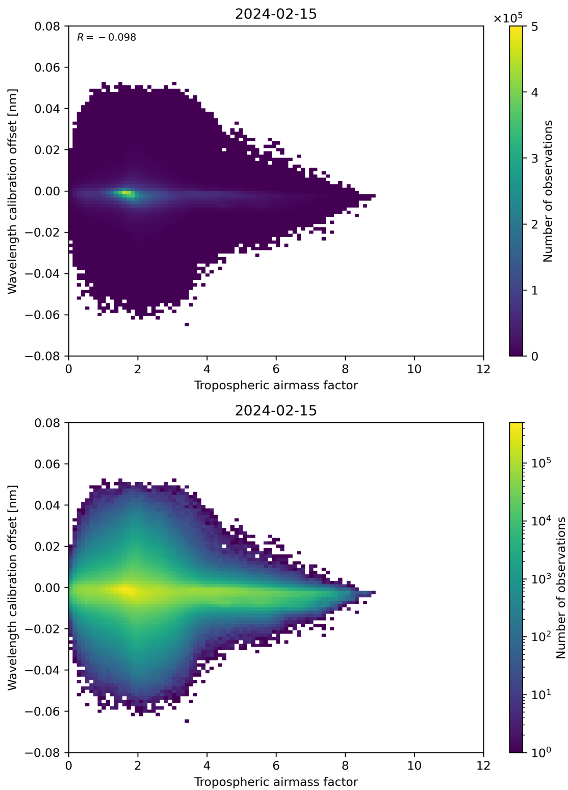
Figure 80: Scatter density plot of “Tropospheric air mass factor” against “Wavelength calibration offset” for 2024-02-14 to 2024-02-16.
