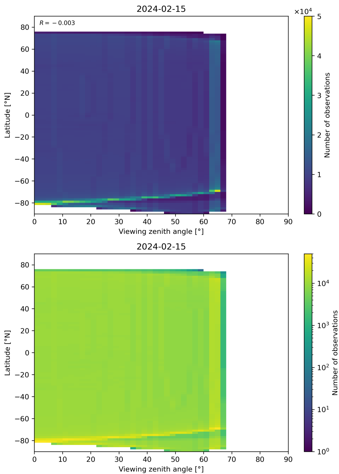
Figure 163: Scatter density plot of “Viewing zenith angle” against “Latitude” for 2024-02-14 to 2024-02-16.
