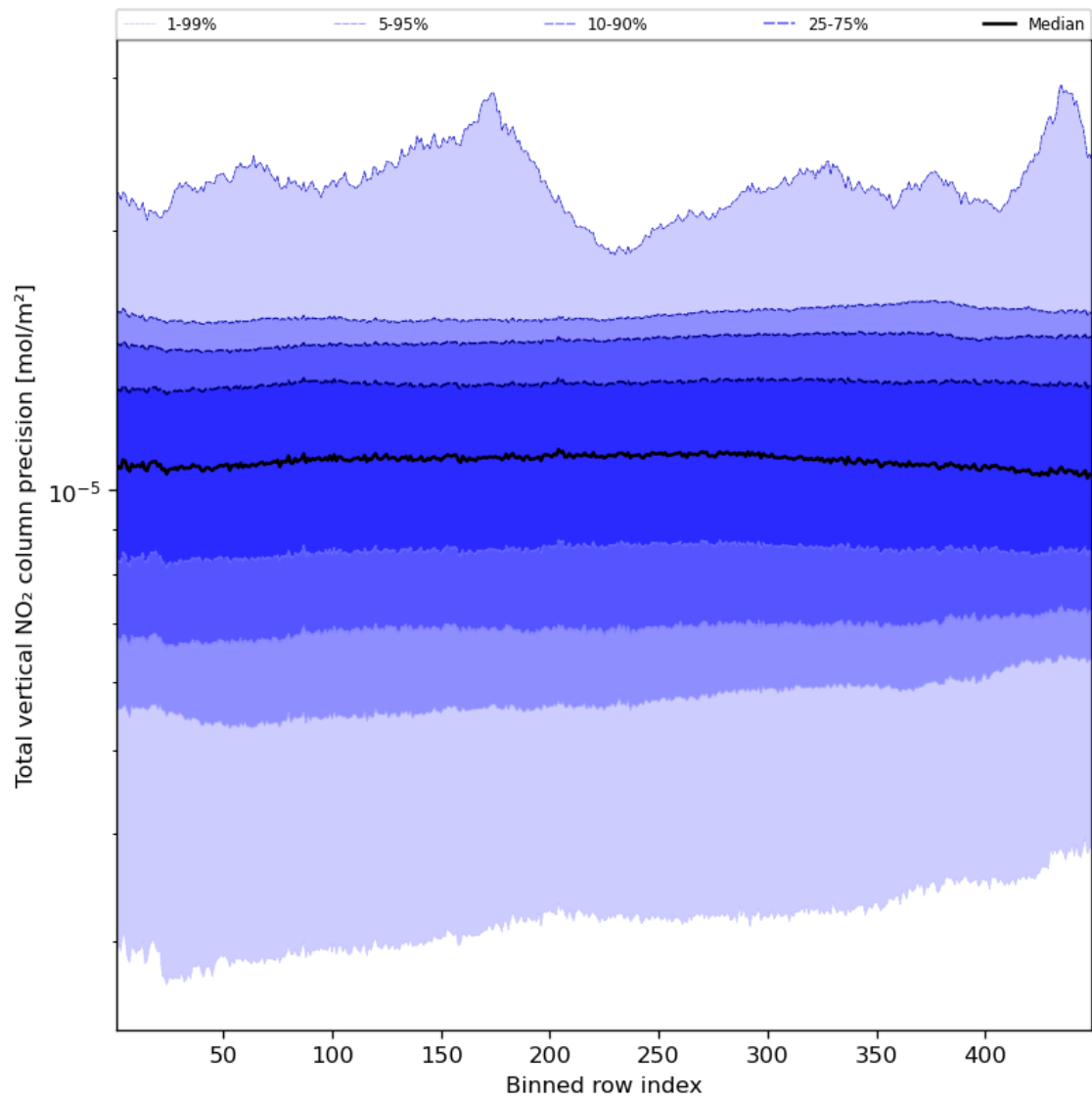
Figure 56: Along track statistics of “Total vertical NO 2 column precision” for 2024-02-14 to 2024-02-16
