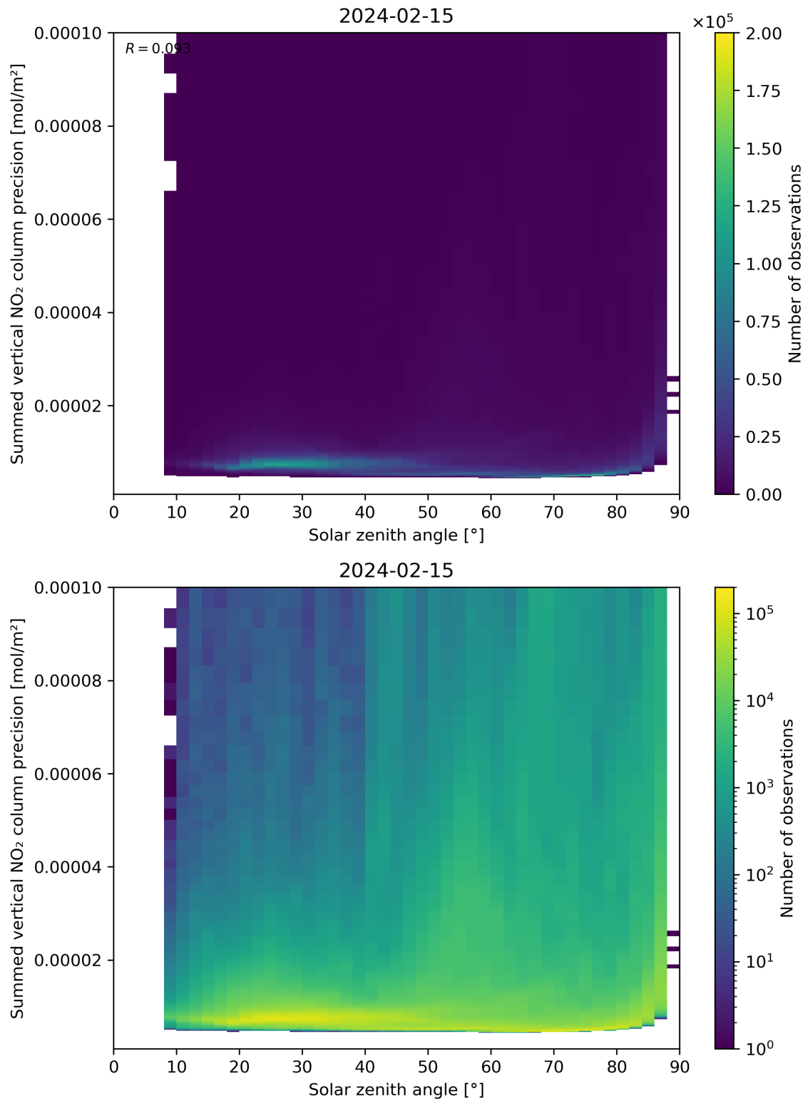
Figure 152: Scatter density plot of “Solar zenith angle” against “Summed vertical NO 2 column precision” for 2024-02-14 to 2024-02-16.
