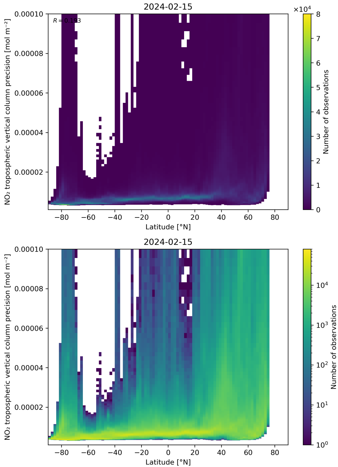
Figure 93: Scatter density plot of “Latitude” against “NO 2 tropospheric vertical column precision” for 2024-02-14 to 2024-02-16.
