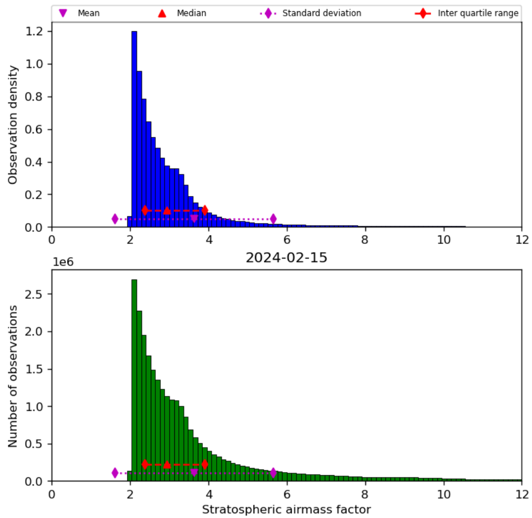
Figure 44: Histogram of “Stratospheric airmass factor” for 2024-02-14 to 2024-02-16
