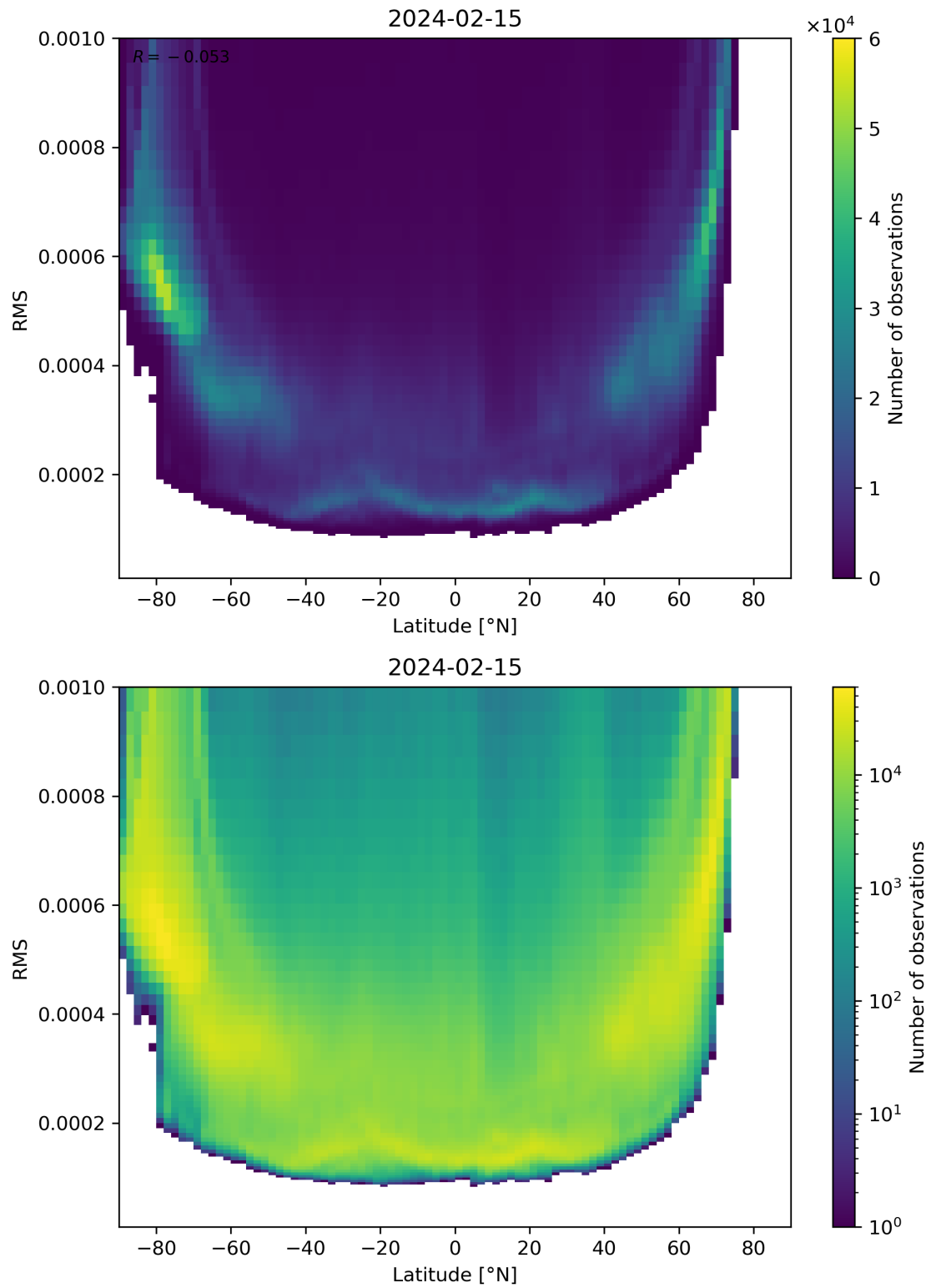
Figure 94: Scatter density plot of “Latitude” against “RMS” for 2024-02-14 to 2024-02-16.
