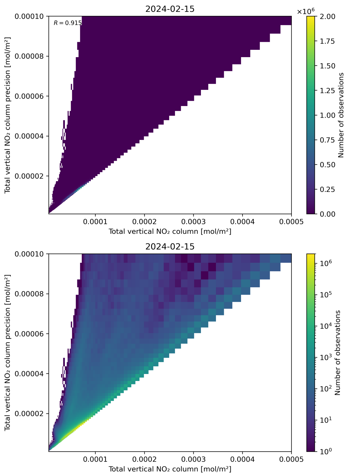
Figure 114: Scatter density plot of “Total vertical NO 2 column” against “Total vertical NO 2 column precision” for 2024-02-14 to 2024-02-16.
