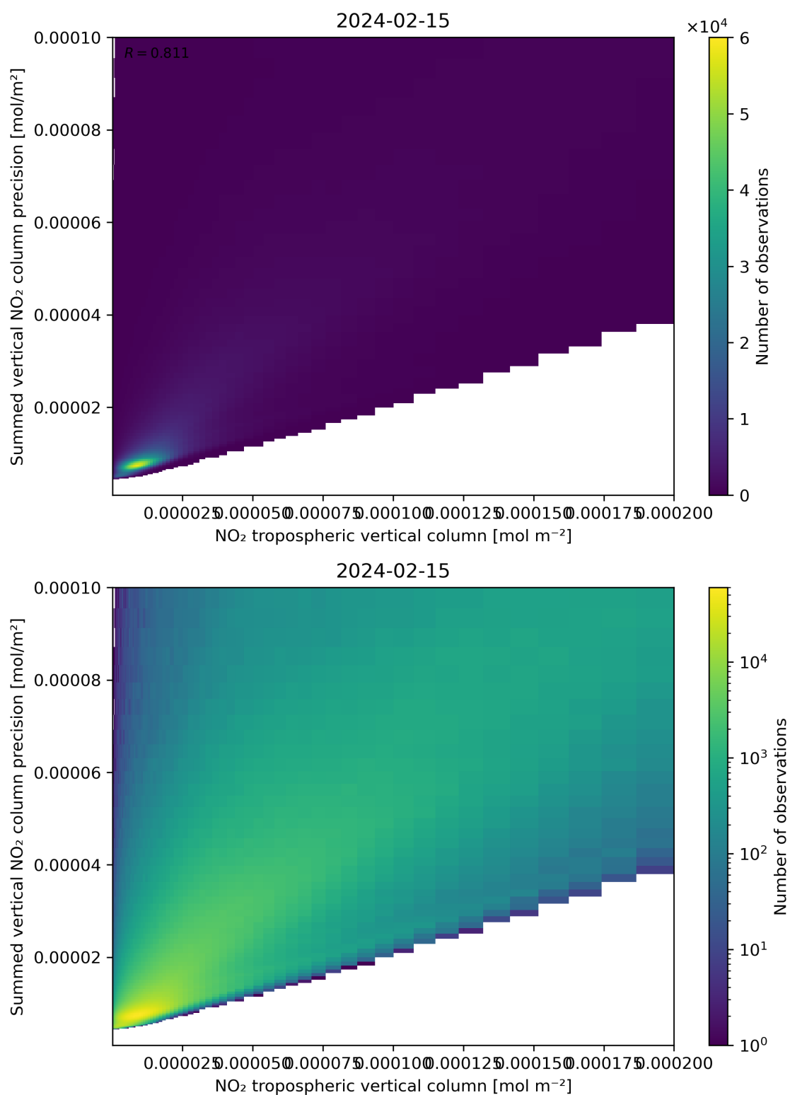
Figure 127: Scatter density plot of “NO 2 tropospheric vertical column” against “Summed vertical NO 2 column precision” for 2024-02-14 to 2024-02-16.
