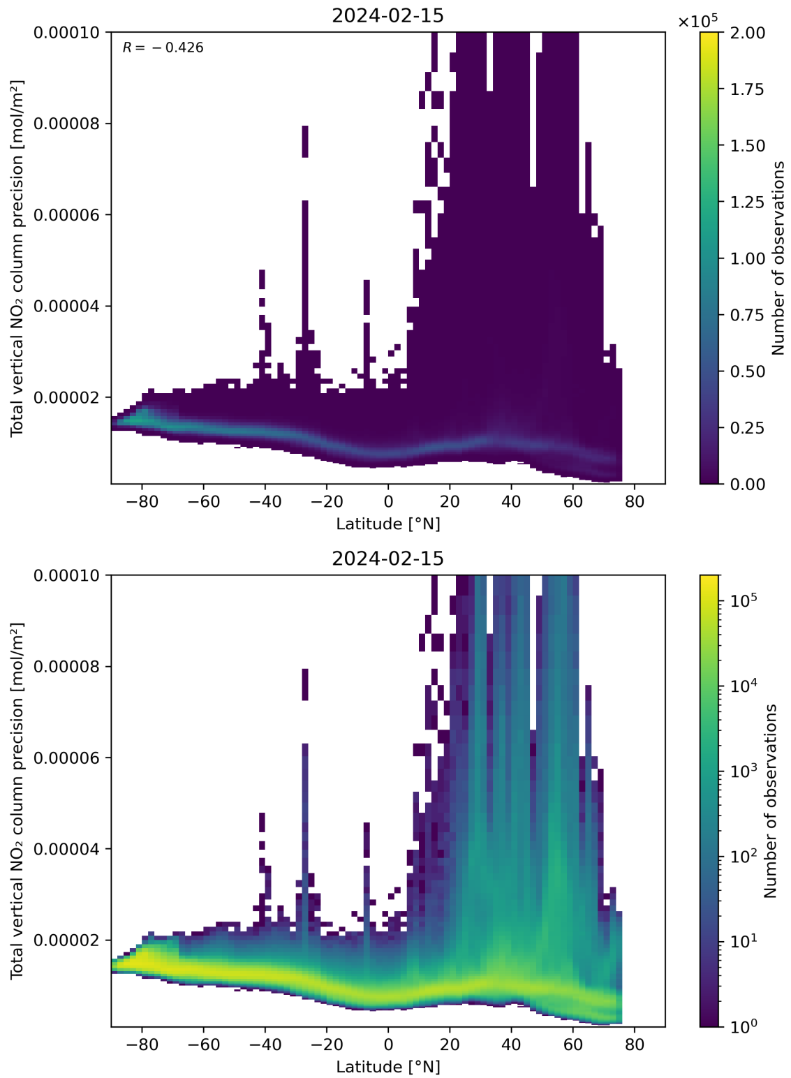
Figure 91: Scatter density plot of “Latitude” against “Total vertical NO 2 column precision” for 2024-02-14 to 2024-02-16.
