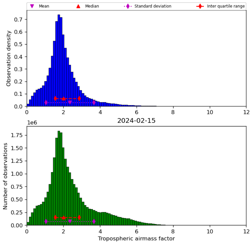
Figure 31: Histogram of “Tropospheric airmass factor” for 2024-02-14 to 2024-02-16
