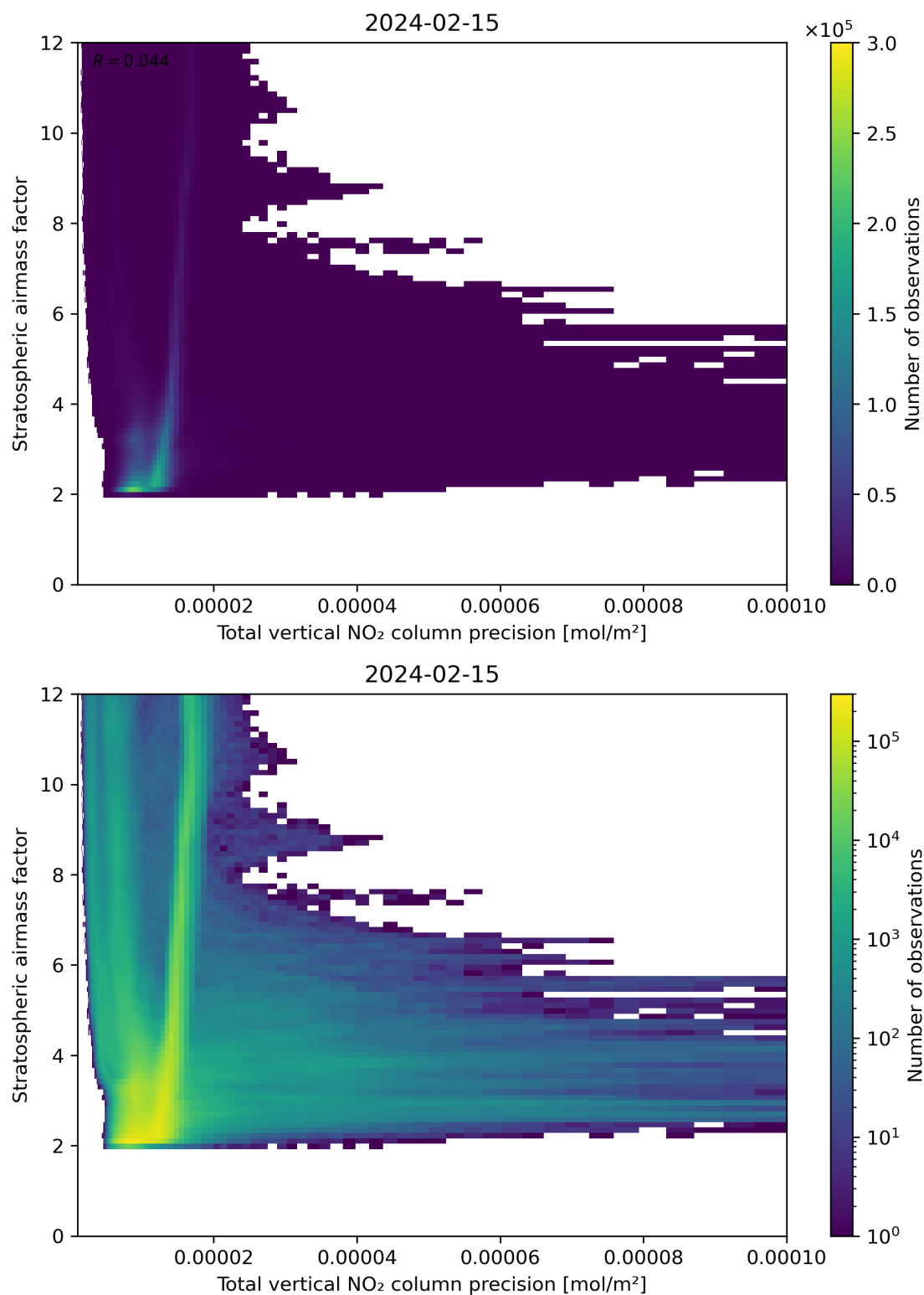
Figure 115: Scatter density plot of “Total vertical NO 2 column precision” against “Stratospheric air mass factor” for 2024-02-14 to 2024-02-16.
