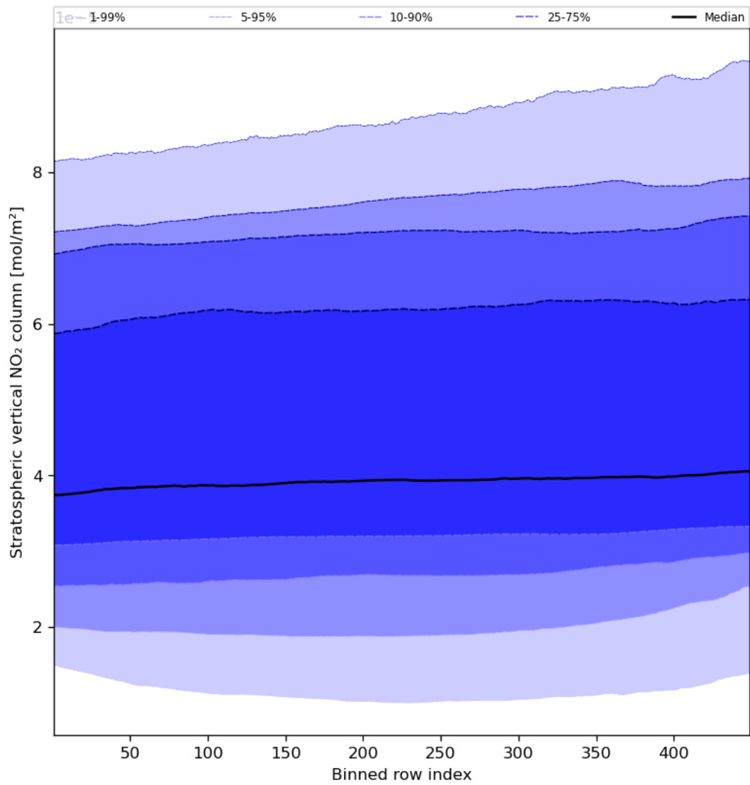
Figure 53: Along track statistics of “Stratospheric vertical NO 2 column” for 2024-02-14 to 2024-02-16
