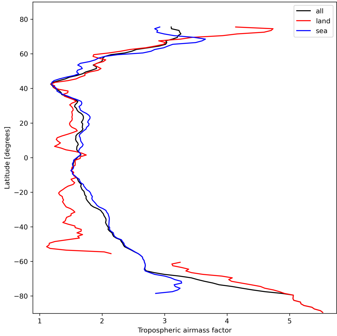
Figure 14: Zonal average of “Tropospheric airmass factor” for 2024-02-14 to 2024-02-16.
