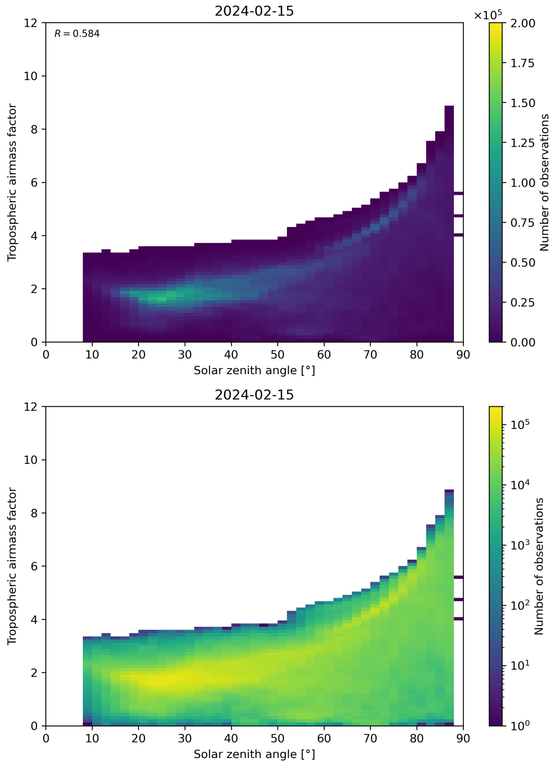
Figure 147: Scatter density plot of “Solar zenith angle” against “Tropospheric airmass factor” for 2024-02-14 to 2024-02-16.
