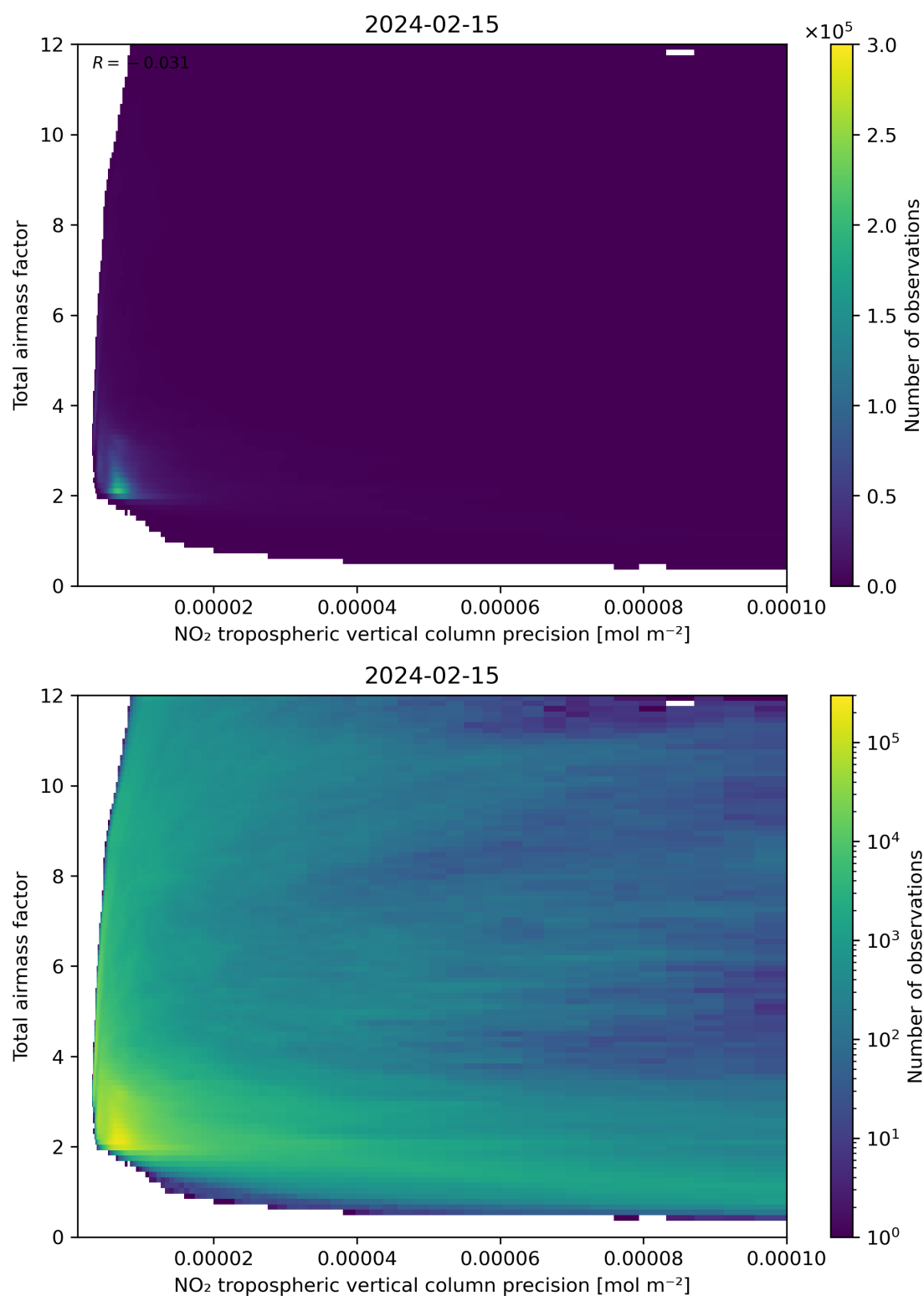
Figure 132: Scatter density plot of “NO 2 tropospheric vertical column precision” against “Total airmass factor” for 2024-02-14 to 2024-02-16.
