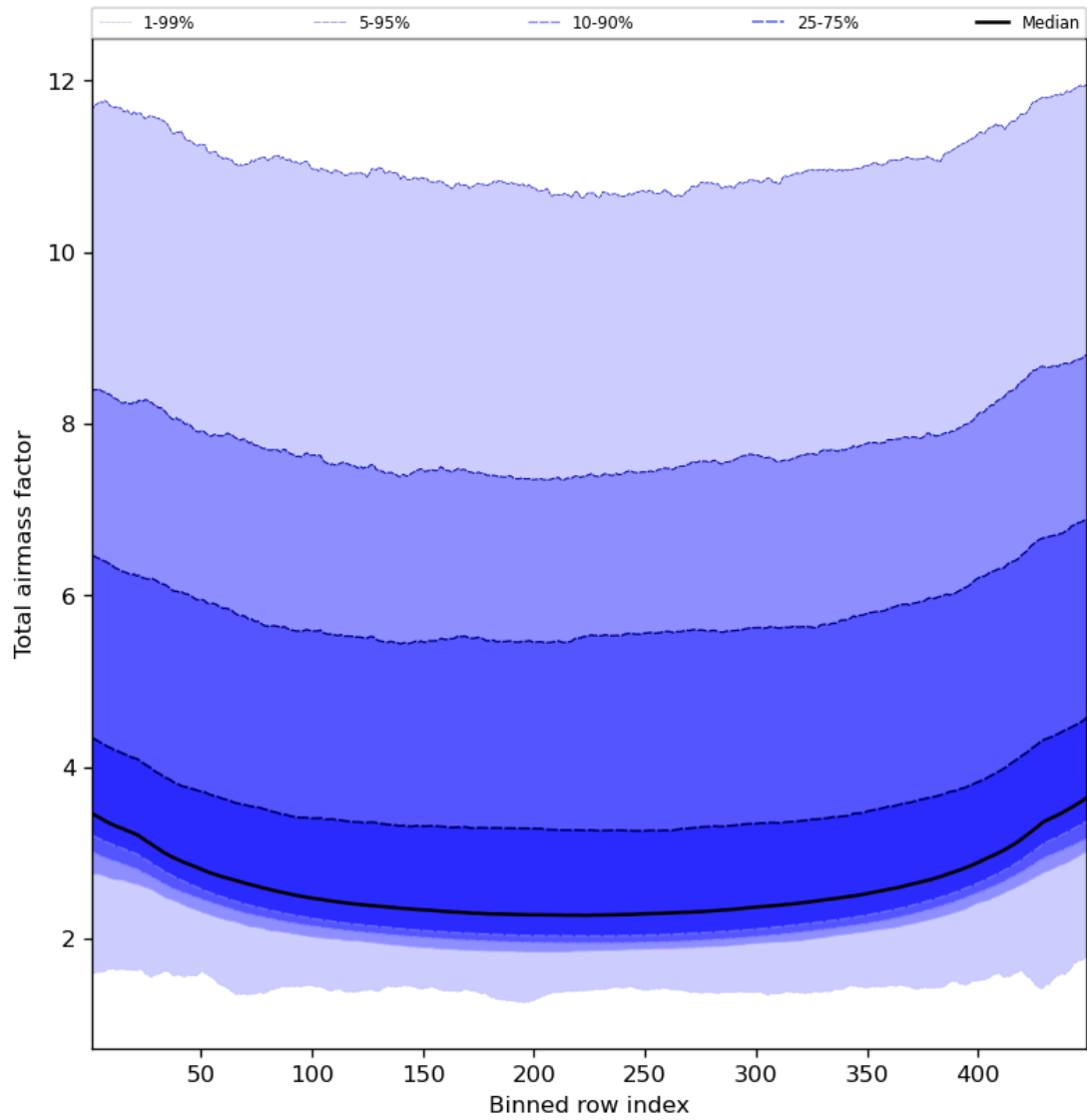
Figure 49: Along track statistics of “Total airmass factor” for 2024-02-14 to 2024-02-16
