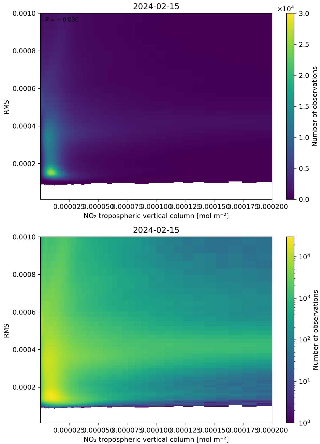
Figure 142: Scatter density plot of “NO 2 tropospheric vertical column” against “RMS” for 2024-02-14 to 2024-02-16.
