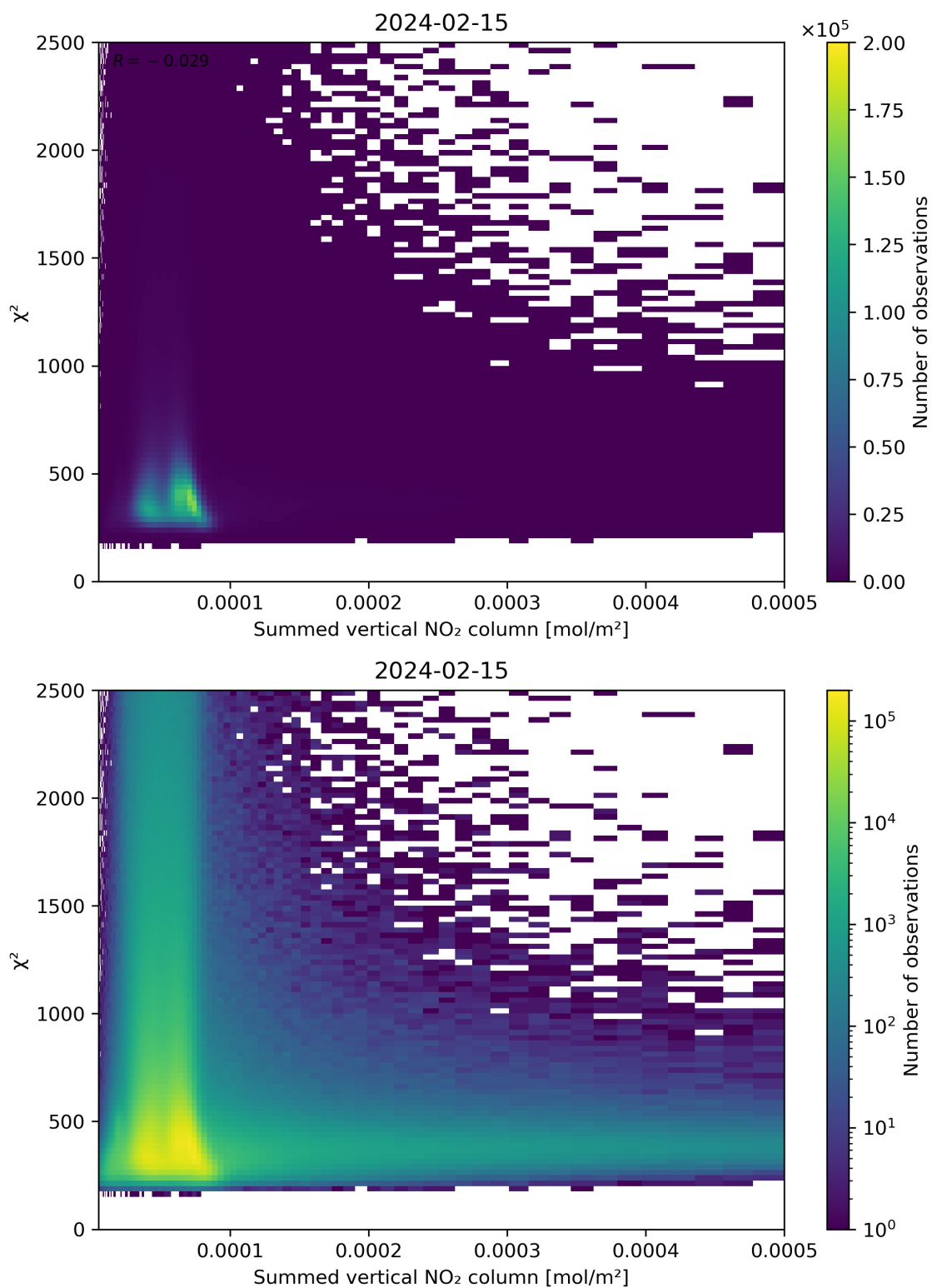
Figure 104: Scatter density plot of “Summed vertical NO 2 column” against “ \chi^2 ” for 2024-02-14 to 2024-02-16.
