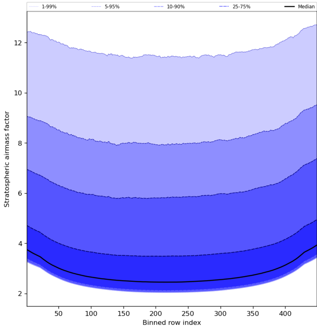
Figure 61: Along track statistics of “Stratospheric airmass factor” for 2024-02-14 to 2024-02-16
