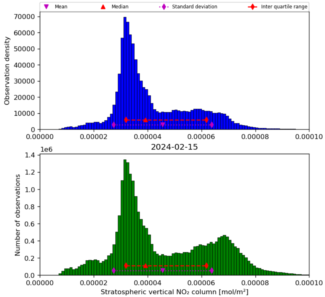
Figure 36: Histogram of “Stratospheric vertical NO 2 column” for 2024-02-14 to 2024-02-16
