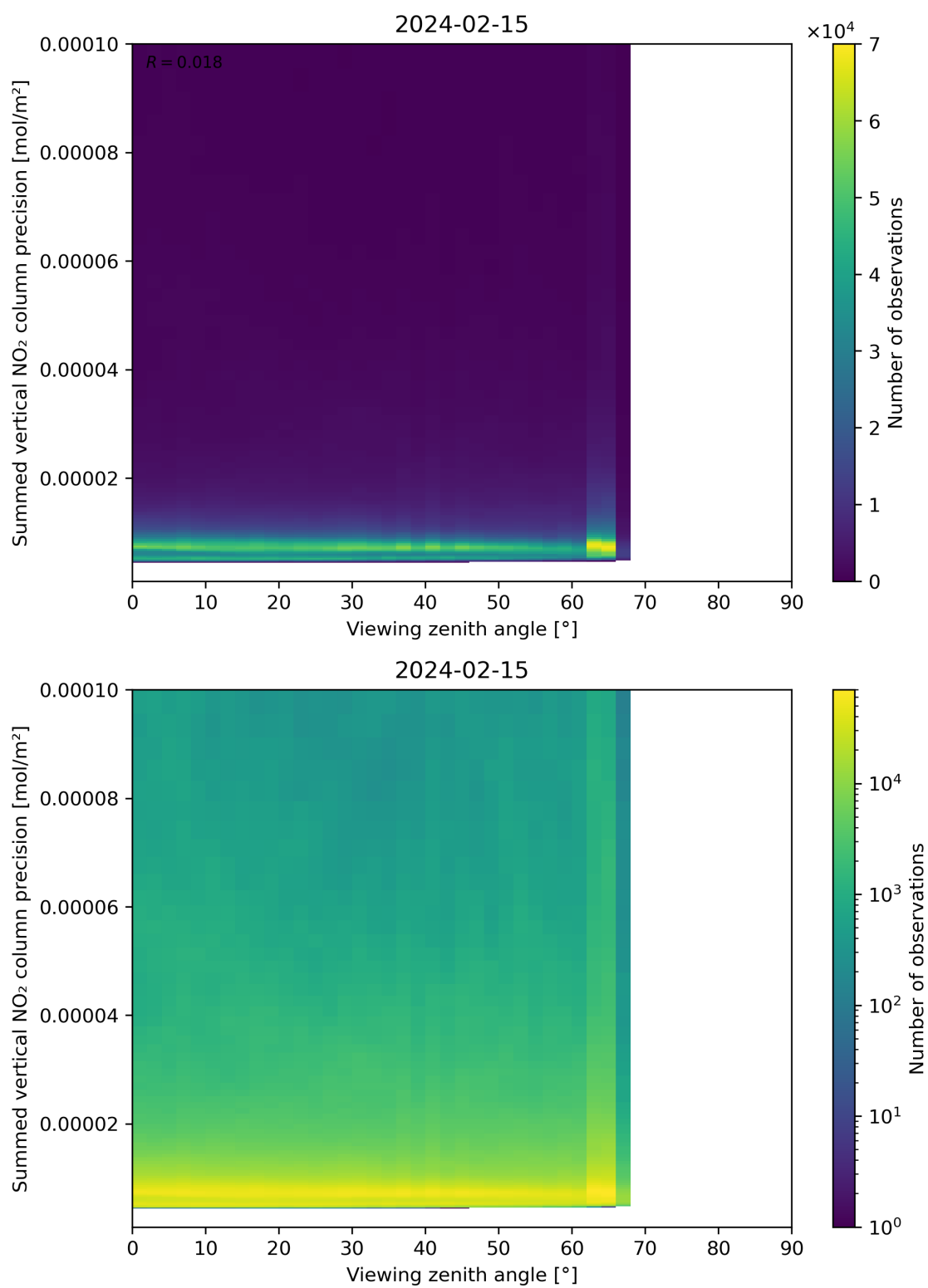
Figure 166: Scatter density plot of “Viewing zenith angle” against “Summed vertical NO 2 column precision” for 2024-02-14 to 2024-02-16.
