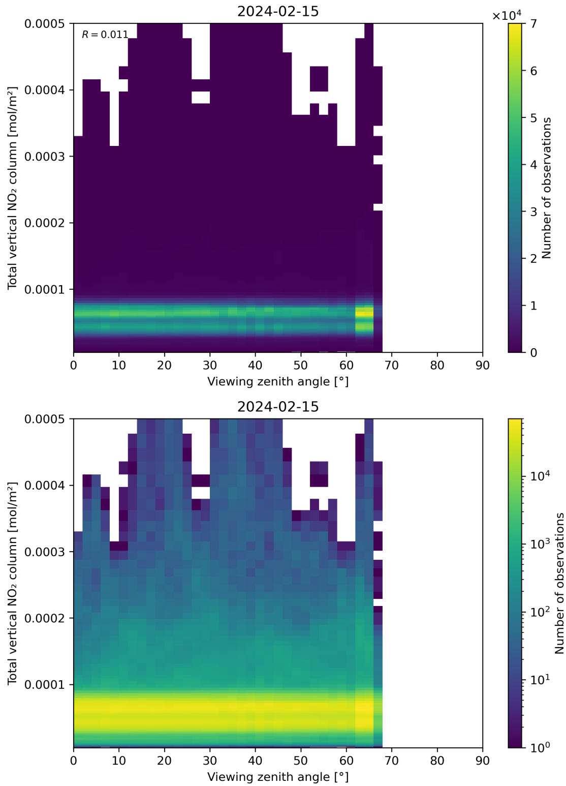
Figure 167: Scatter density plot of “Viewing zenith angle” against “Total vertical NO 2 column” for 2024-02-14 to 2024-02-16.
