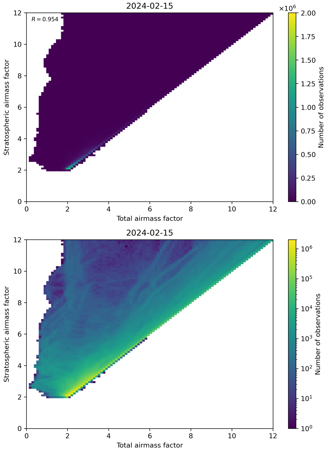
Figure 62: Scatter density plot of “Total airmass factor” against “Stratospheric airmass factor” for 2024-02-14 to 2024-02-16.
