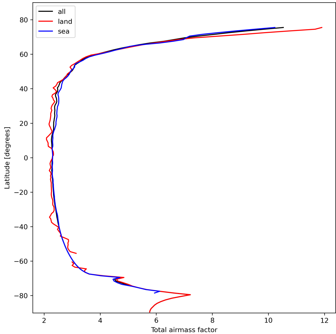
Figure 15: Zonal average of “Total airmass factor” for 2024-02-14 to 2024-02-16.
