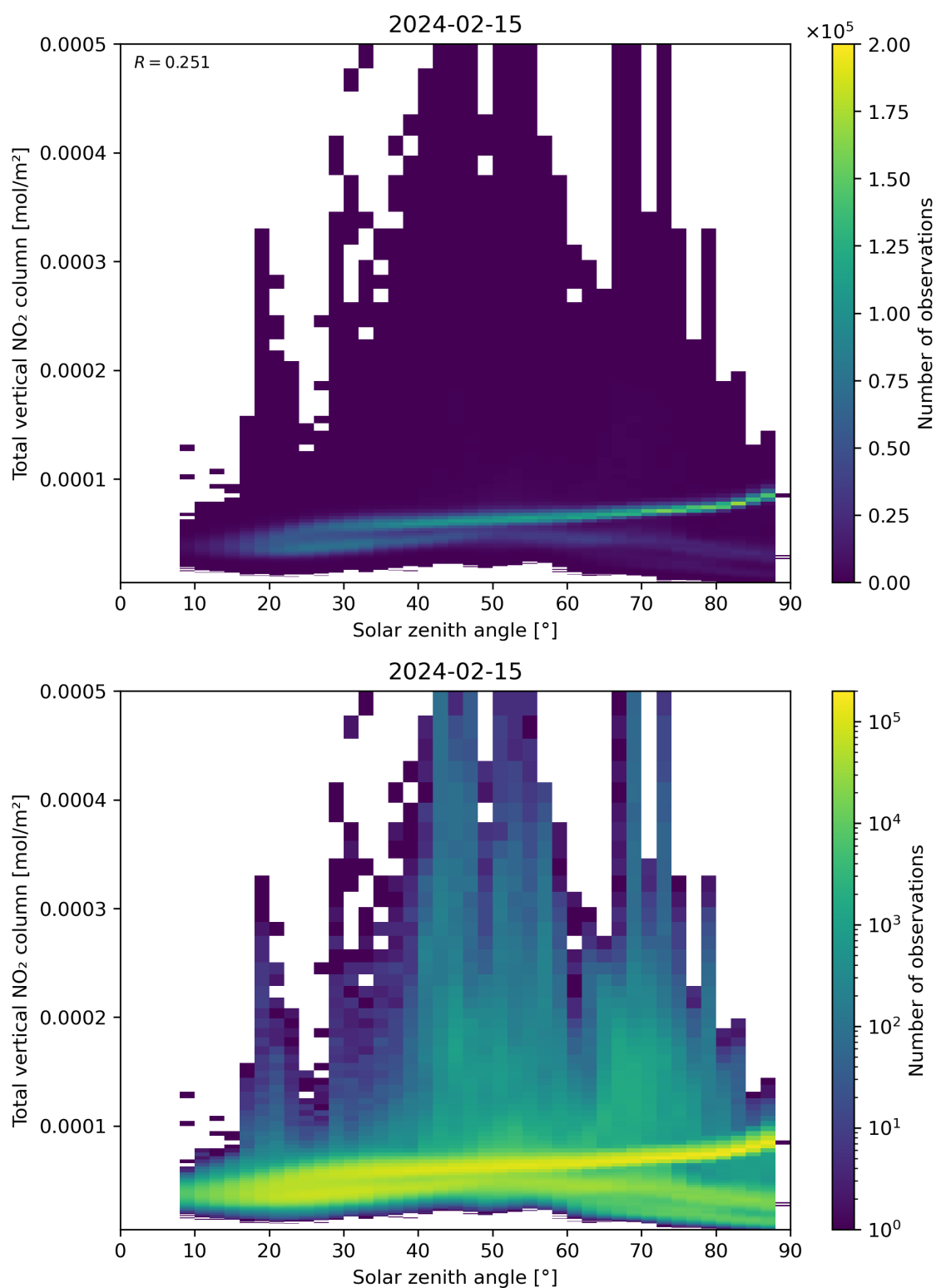
Figure 153: Scatter density plot of “Solar zenith angle” against “Total vertical NO 2 column” for 2024-02-14 to 2024-02-16.
