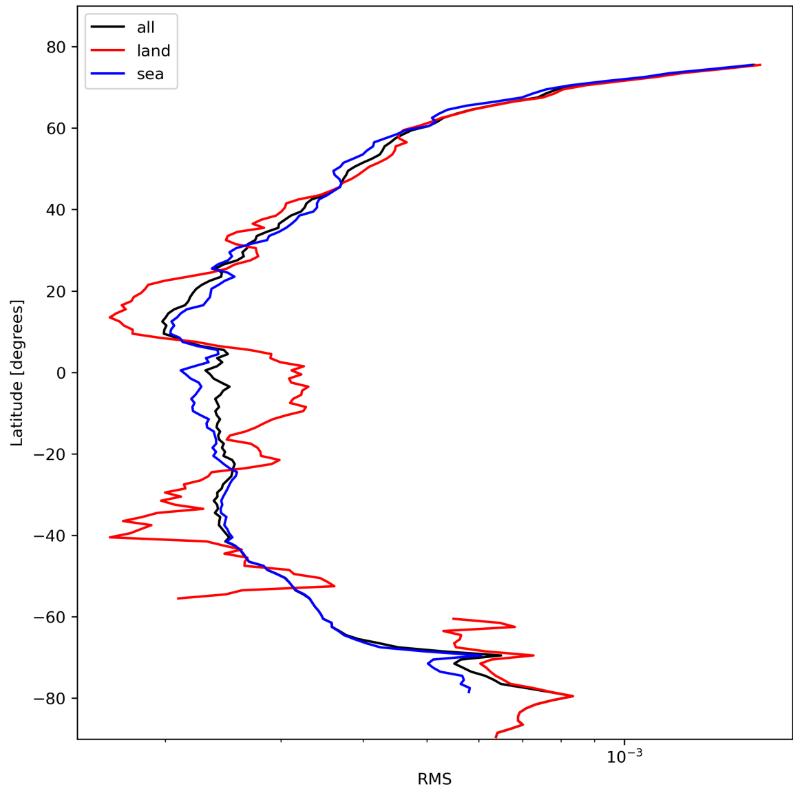
Figure 26: Zonal average of “RMS” for 2024-02-14 to 2024-02-16.
