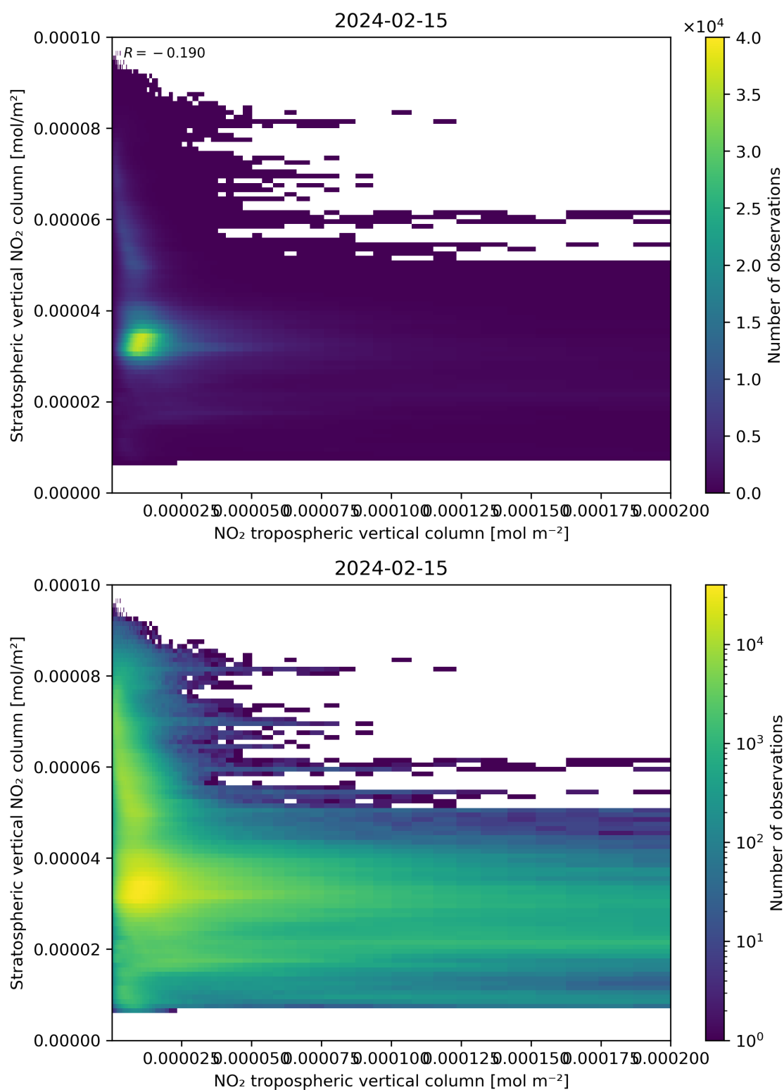
Figure 125: Scatter density plot of “NO 2 tropospheric vertical column” against “Stratospheric vertical NO 2 column” for 2024-02-14 to 2024-02-16.
