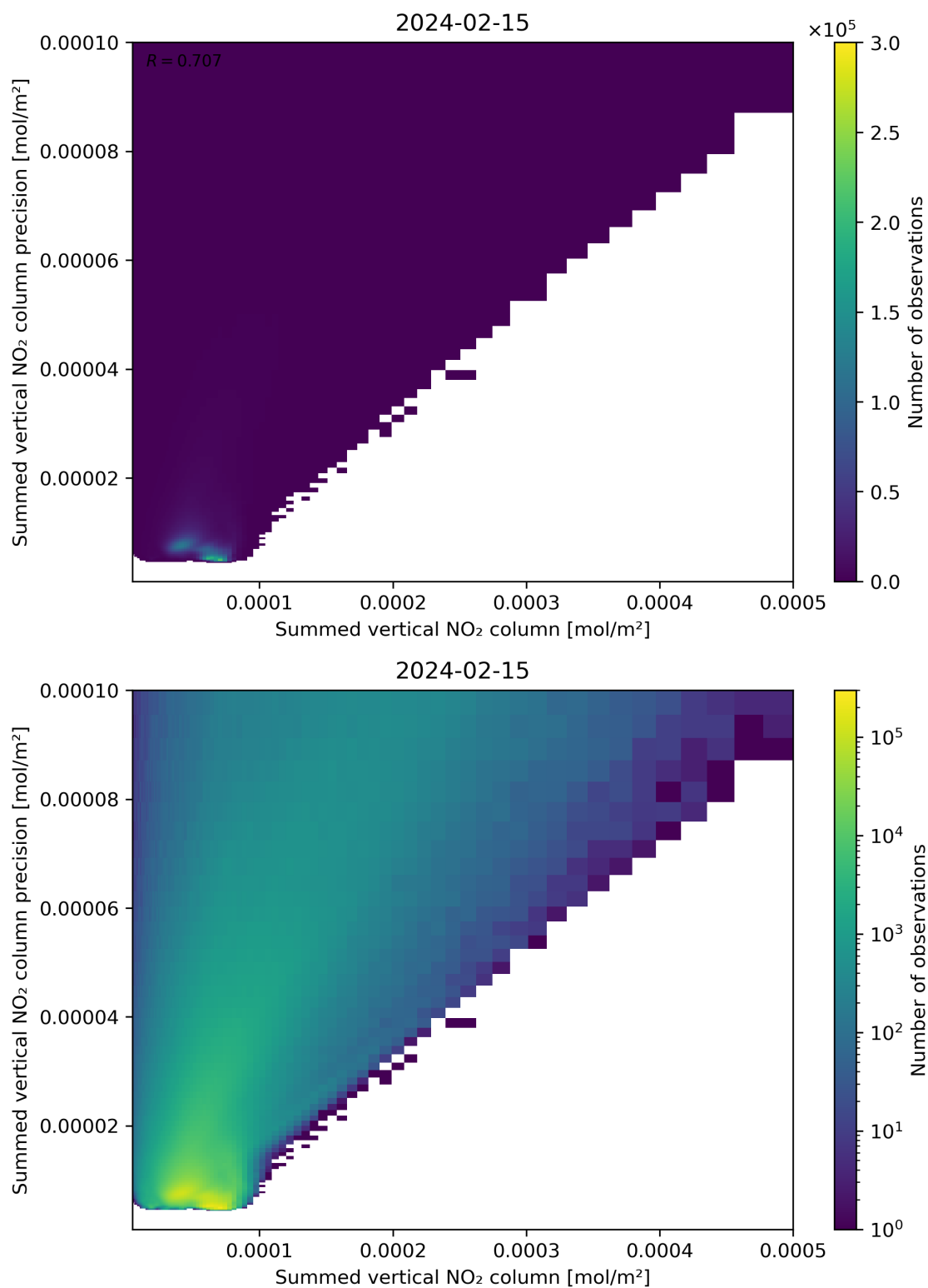
Figure 105: Scatter density plot of “Summed vertical NO 2 column” against “Summed vertical NO 2 column precision” for 2024-02-14 to 2024-02-16.
