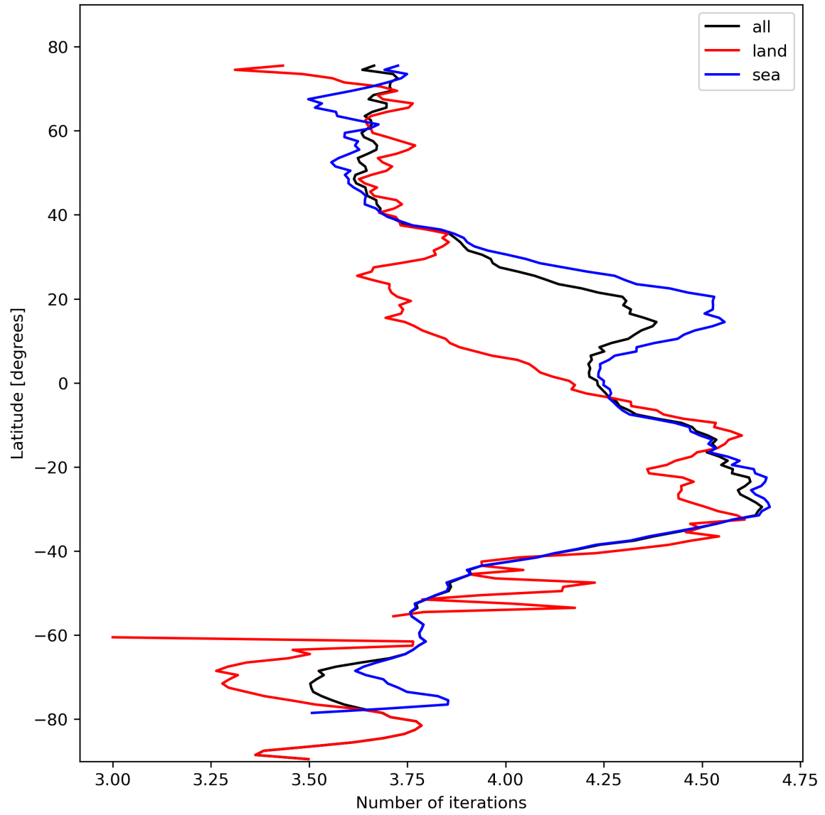
Figure 17: Zonal average of “Number of iterations” for 2024-02-14 to 2024-02-16.
