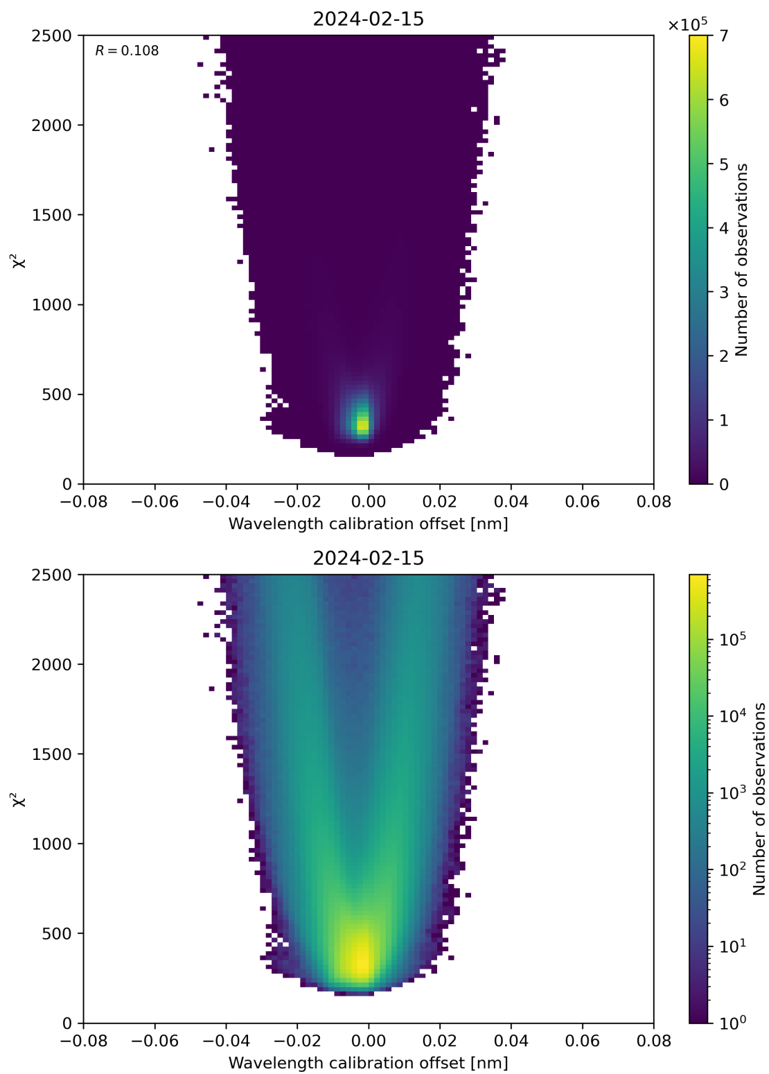
Figure 175: Scatter density plot of “Wavelength calibration offset” against “ \chi^2 ” for 2024-02-14 to 2024-02-16.
