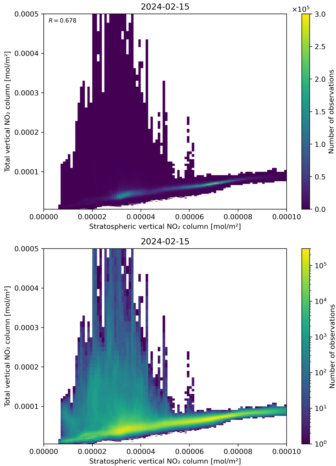
Figure 100: Scatter density plot of “Stratospheric vertical NO 2 column” against “Total vertical NO 2 column” for 2024-02-14 to 2024-02-16.
