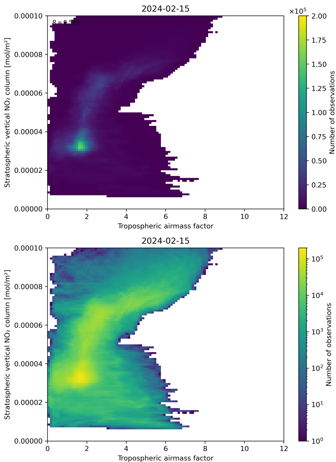
Figure 74: Scatter density plot of “Tropospheric air mass factor” against “Stratospheric vertical NO 2 column” for 2024-02-14 to 2024-02-16.
