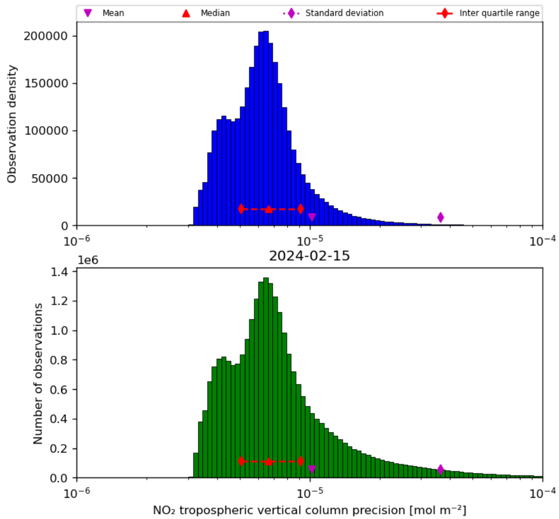
Figure 30: Histogram of “NO 2 tropospheric vertical column precision” for 2024-02-14 to 2024-02-16
