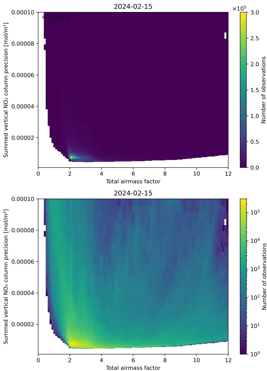
Figure 66: Scatter density plot of “Total airmass factor” against “Summed vertical NO 2 column precision” for 2024-02-14 to 2024-02-16.
