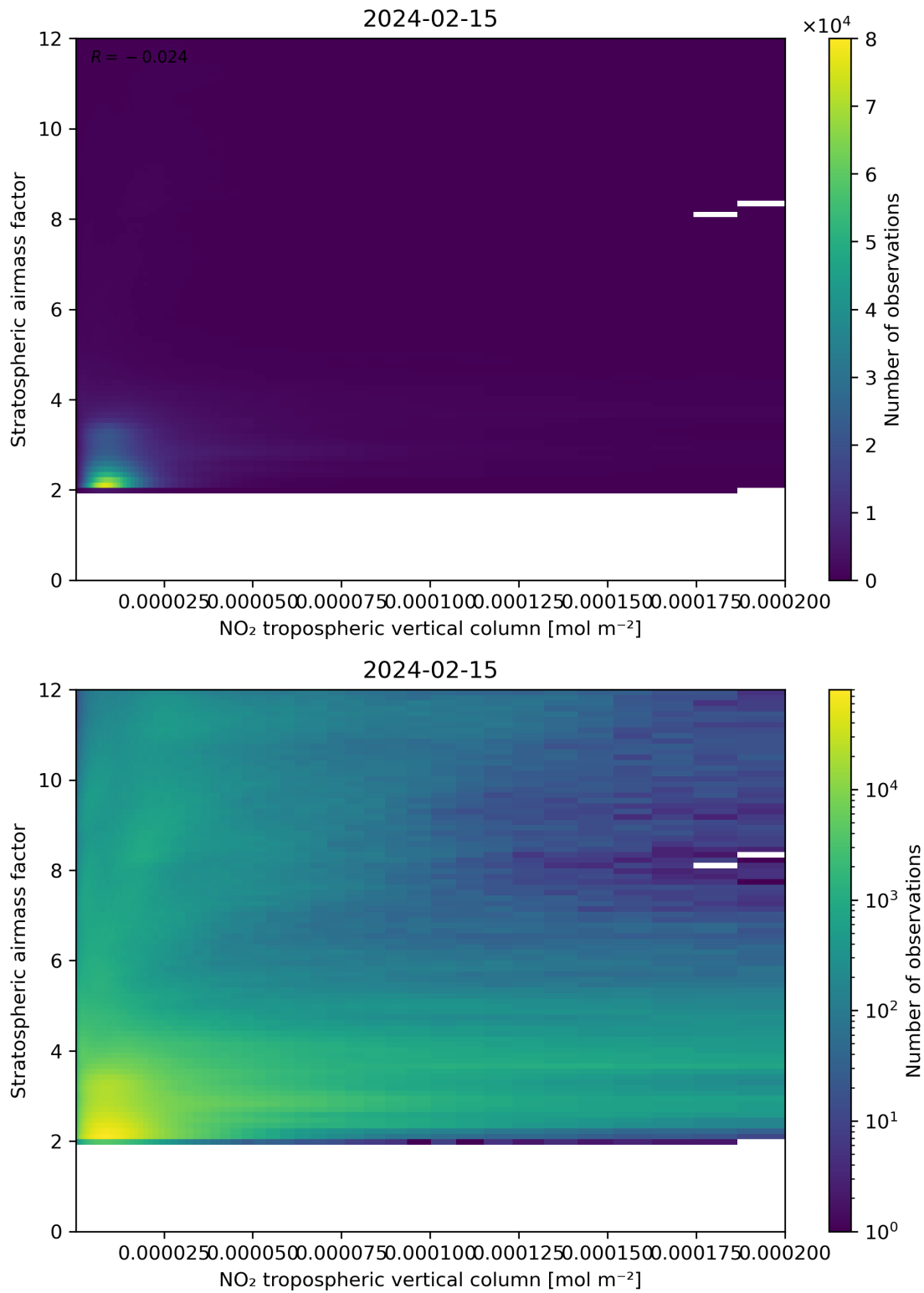
Figure 121: Scatter density plot of “NO 2 tropospheric vertical column” against “Stratospheric air mass factor” for 2024-02-14 to 2024-02-16.
