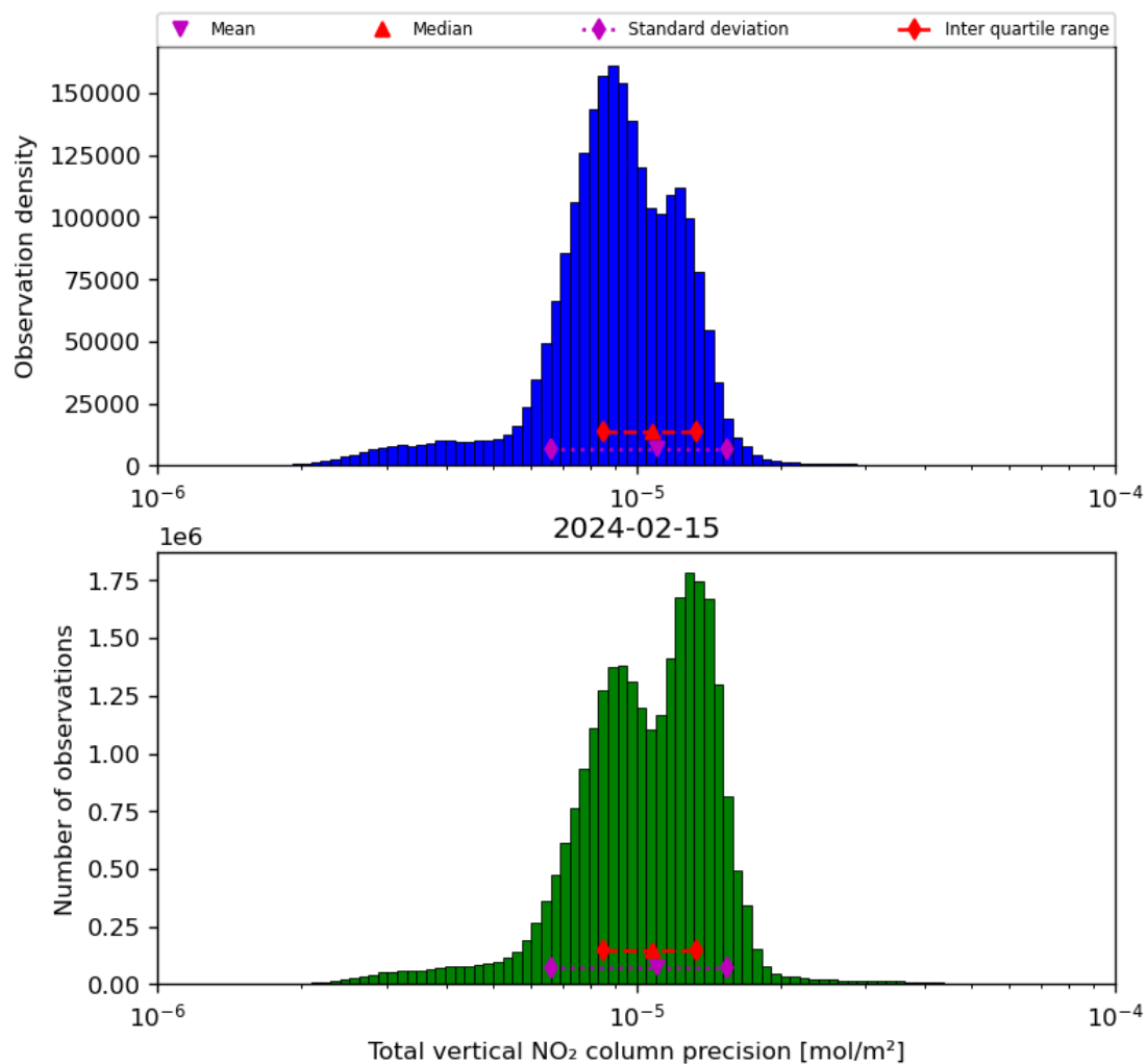
Figure 39: Histogram of “Total vertical NO 2 column precision” for 2024-02-14 to 2024-02-16
