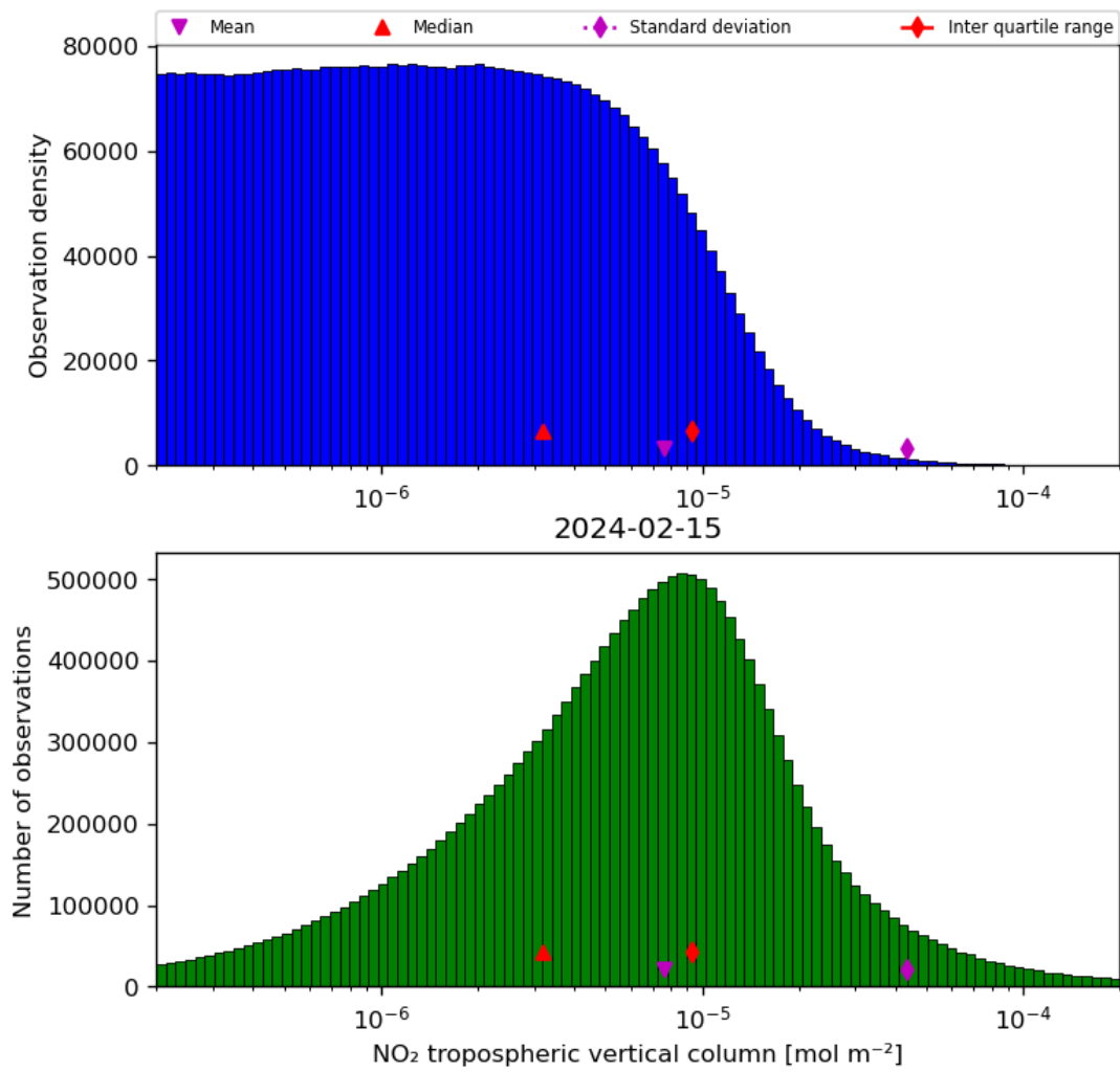
Figure 29: Histogram of “NO 2 tropospheric vertical column” for 2024-02-14 to 2024-02-16
