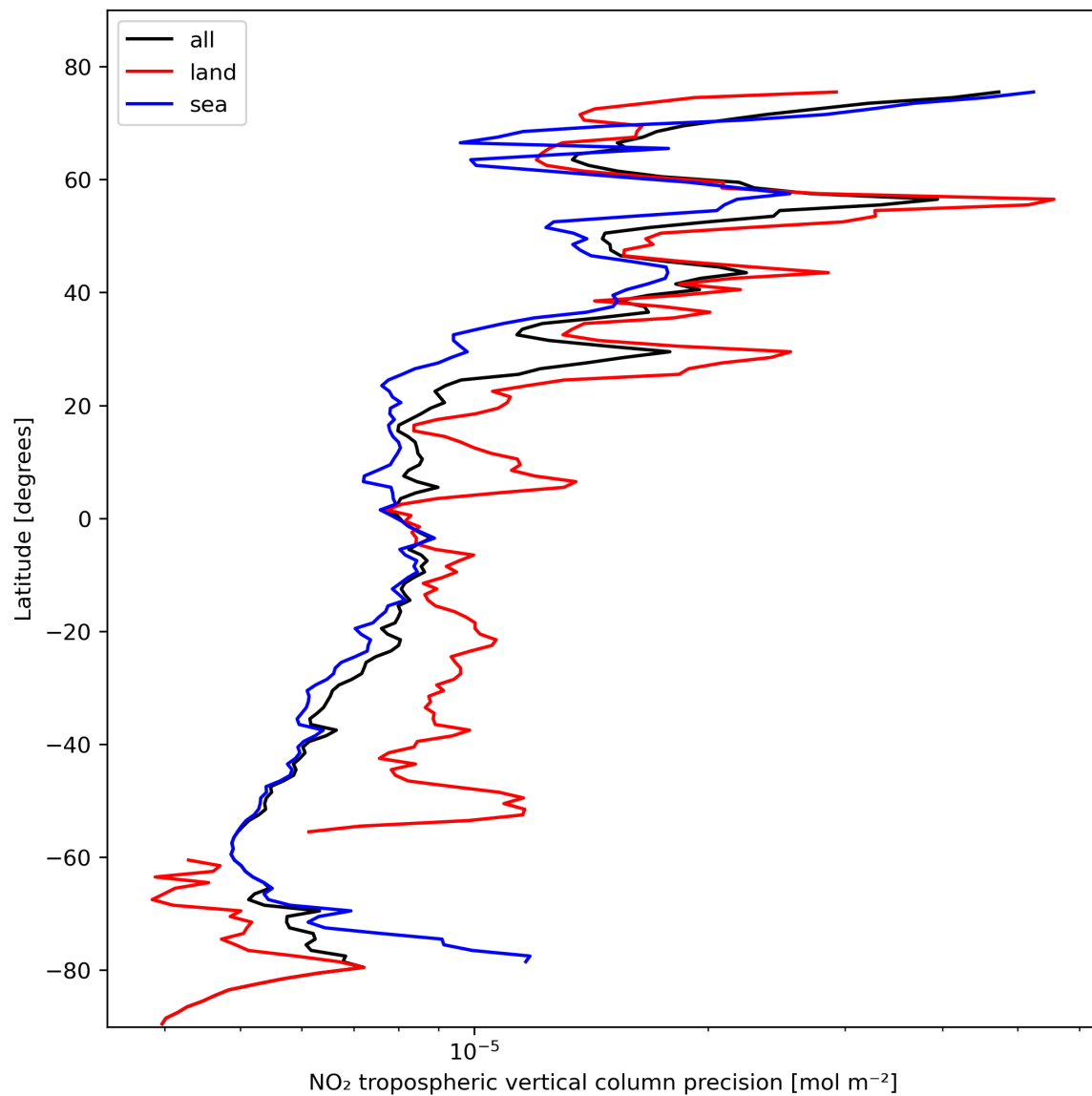
Figure 13: Zonal average of “NO 2 tropospheric vertical column precision” for 2024-02-14 to 2024-02-16.
