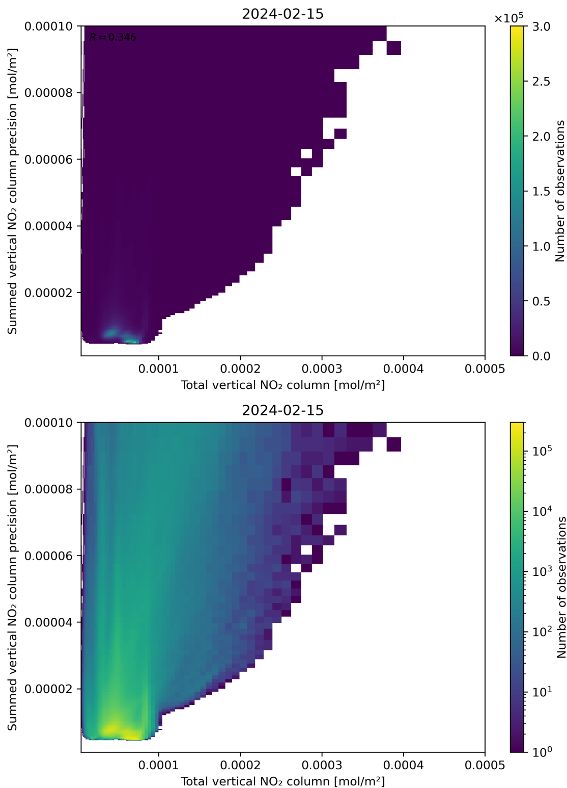
Figure 113: Scatter density plot of “Total vertical NO 2 column” against “Summed vertical NO 2 column precision” for 2024-02-14 to 2024-02-16.
