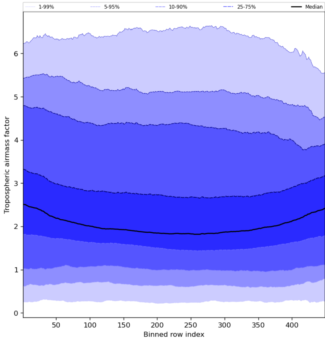
Figure 48: Along track statistics of “Tropospheric airmass factor” for 2024-02-14 to 2024-02-16
