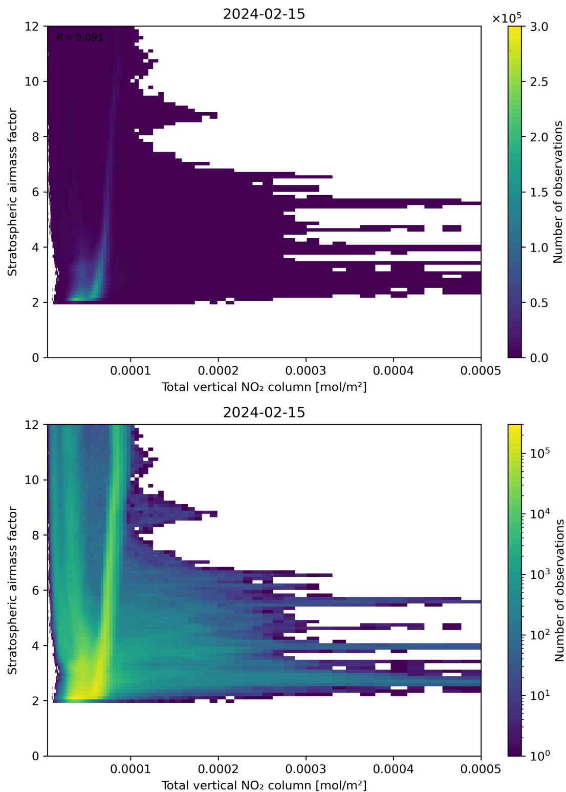
Figure 110: Scatter density plot of “Total vertical NO 2 column” against “Stratospheric air mass factor” for 2024-02-14 to 2024-02-16.
