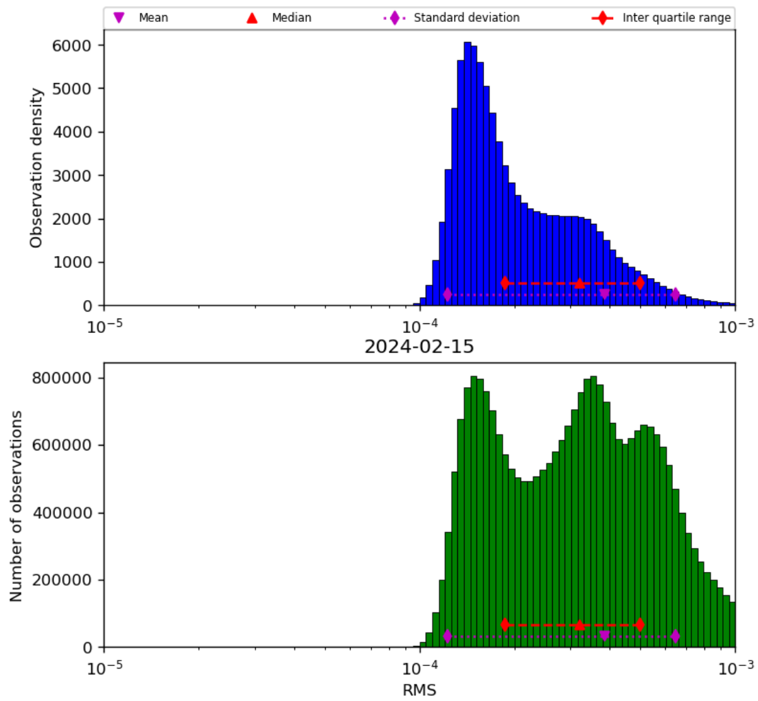
Figure 43: Histogram of “RMS” for 2024-02-14 to 2024-02-16
