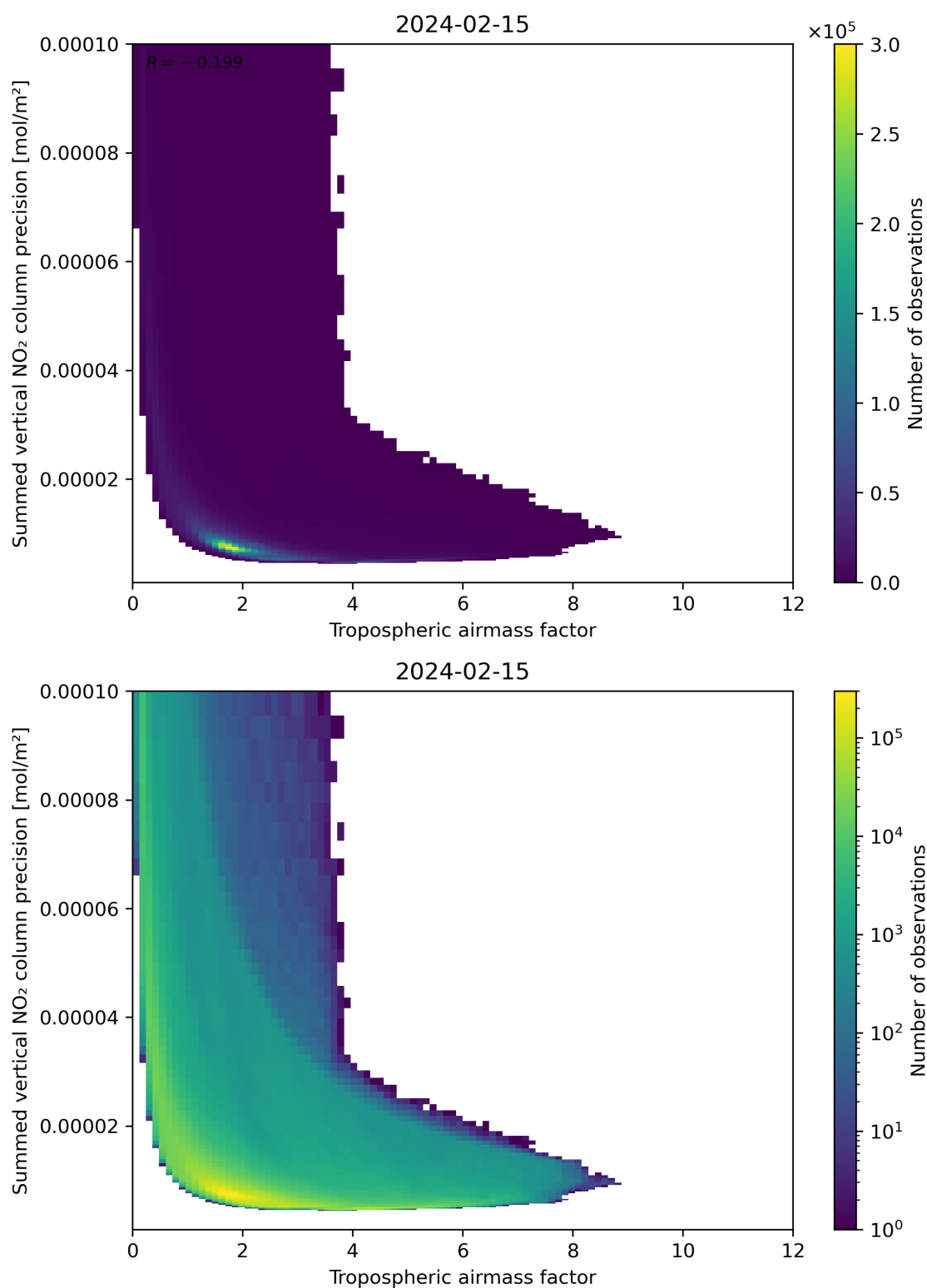
Figure 76: Scatter density plot of “Tropospheric air mass factor” against “Summed vertical NO 2 column precision” for 2024-02-14 to 2024-02-16.
