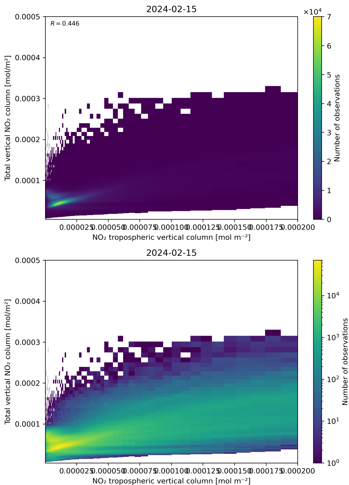
Figure 128: Scatter density plot of “NO 2 tropospheric vertical column” against “Total vertical NO 2 column” for 2024-02-14 to 2024-02-16.
