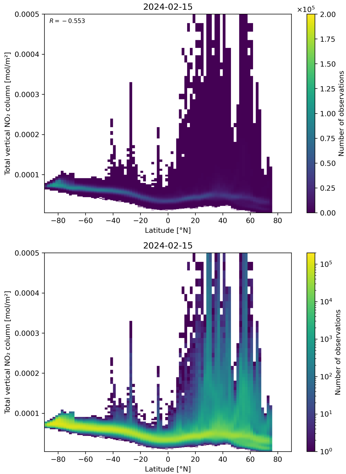
Figure 90: Scatter density plot of “Latitude” against “Total vertical NO 2 column” for 2024-02-14 to 2024-02-16.
