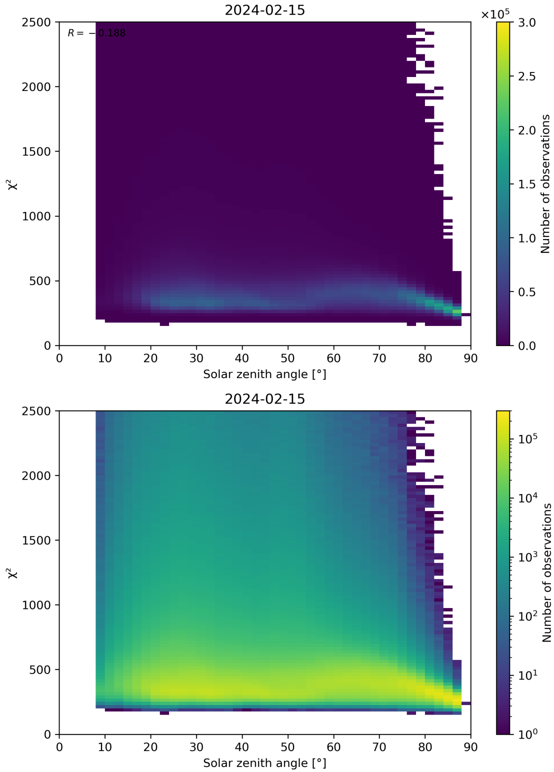
Figure 148: Scatter density plot of “Solar zenith angle” against “ \chi^2 ” for 2024-02-14 to 2024-02-16.
