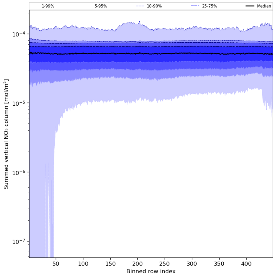
Figure 57: Along track statistics of “Summed vertical NO 2 column” for 2024-02-14 to 2024-02-16
