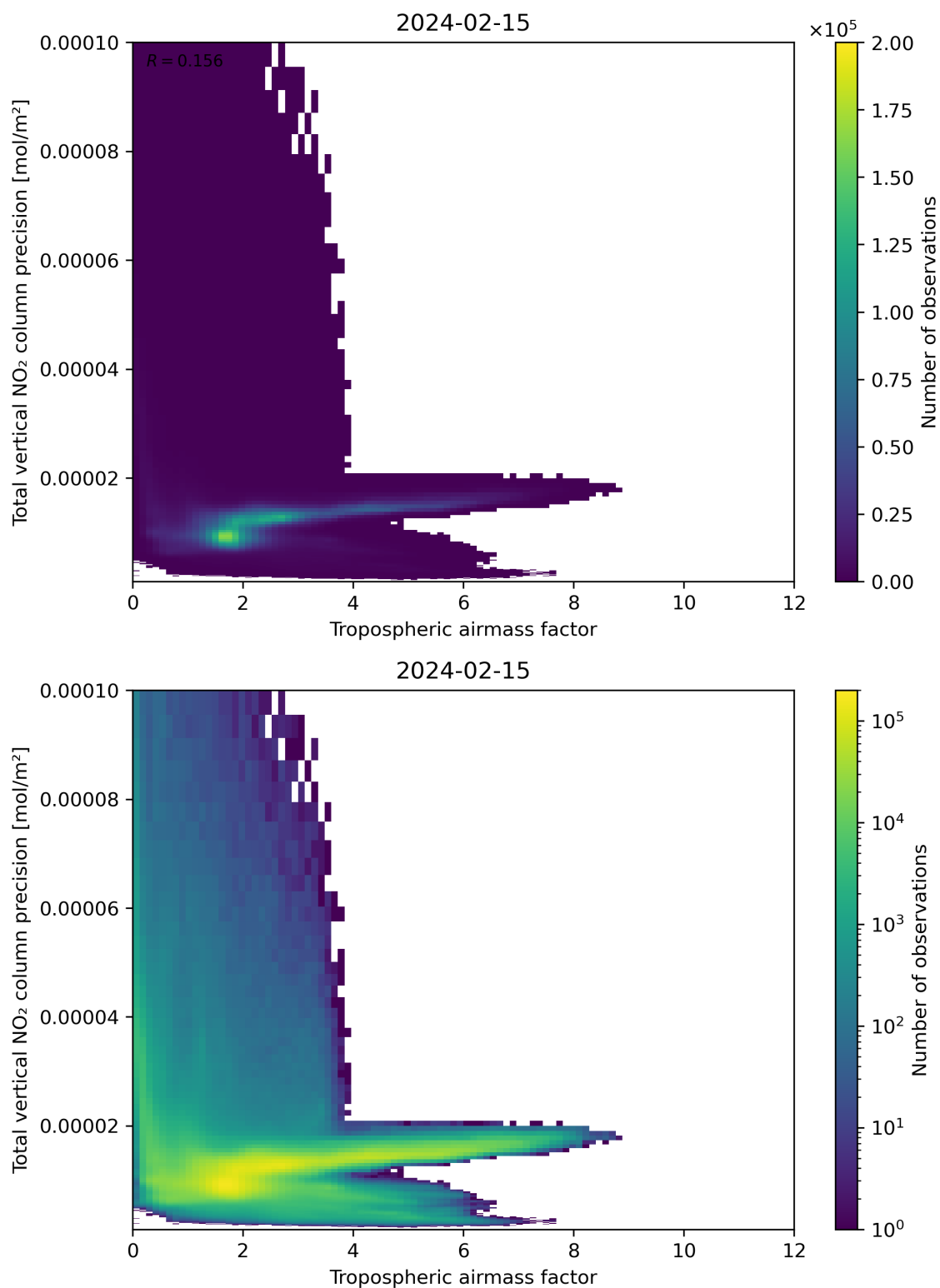
Figure 78: Scatter density plot of “Tropospheric air mass factor” against “Total vertical NO 2 column precision” for 2024-02-14 to 2024-02-16.
