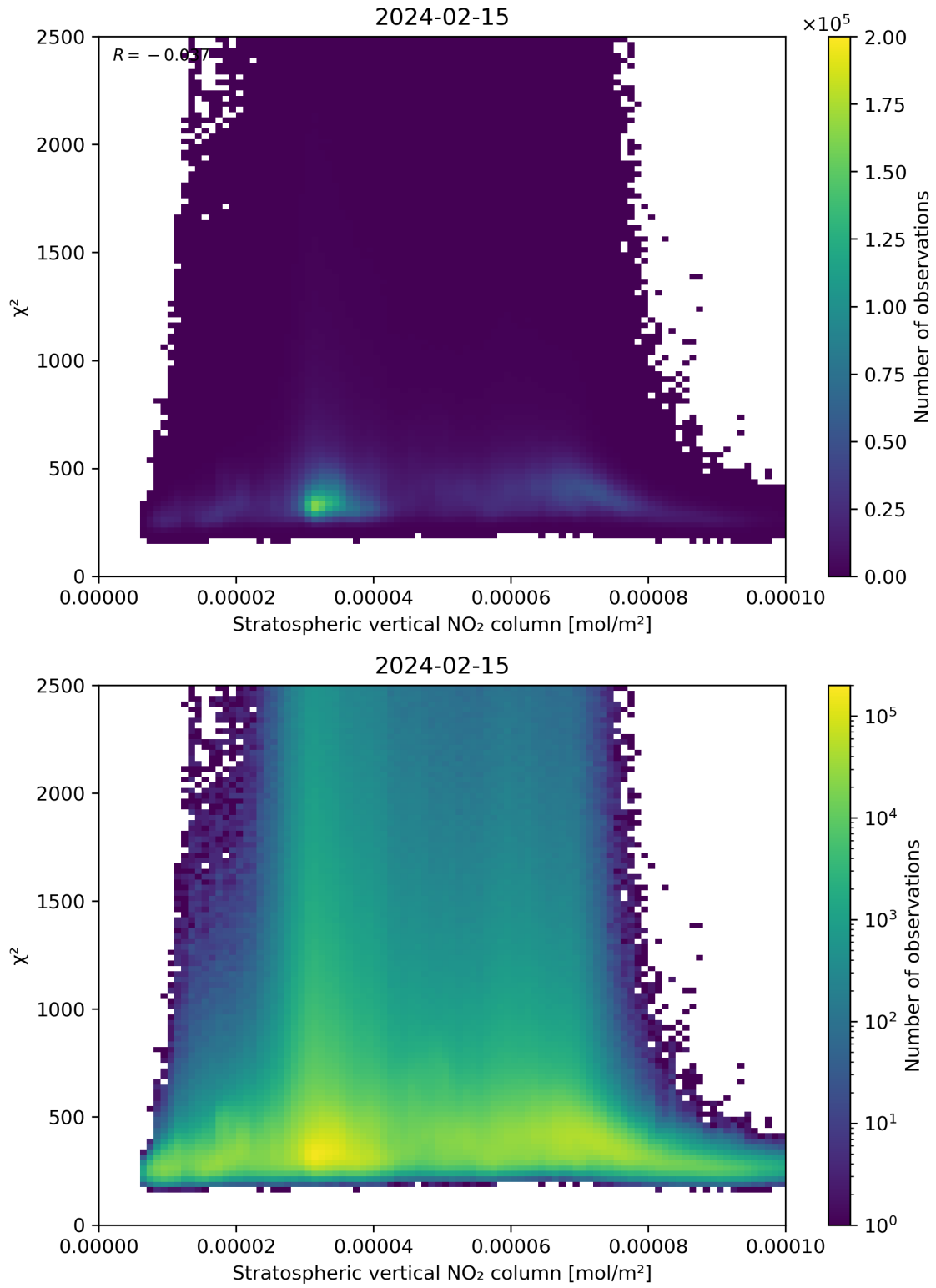
Figure 97: Scatter density plot of “Stratospheric vertical NO 2 column” against “ \chi^2 ” for 2024-02-14 to 2024-02-16.
