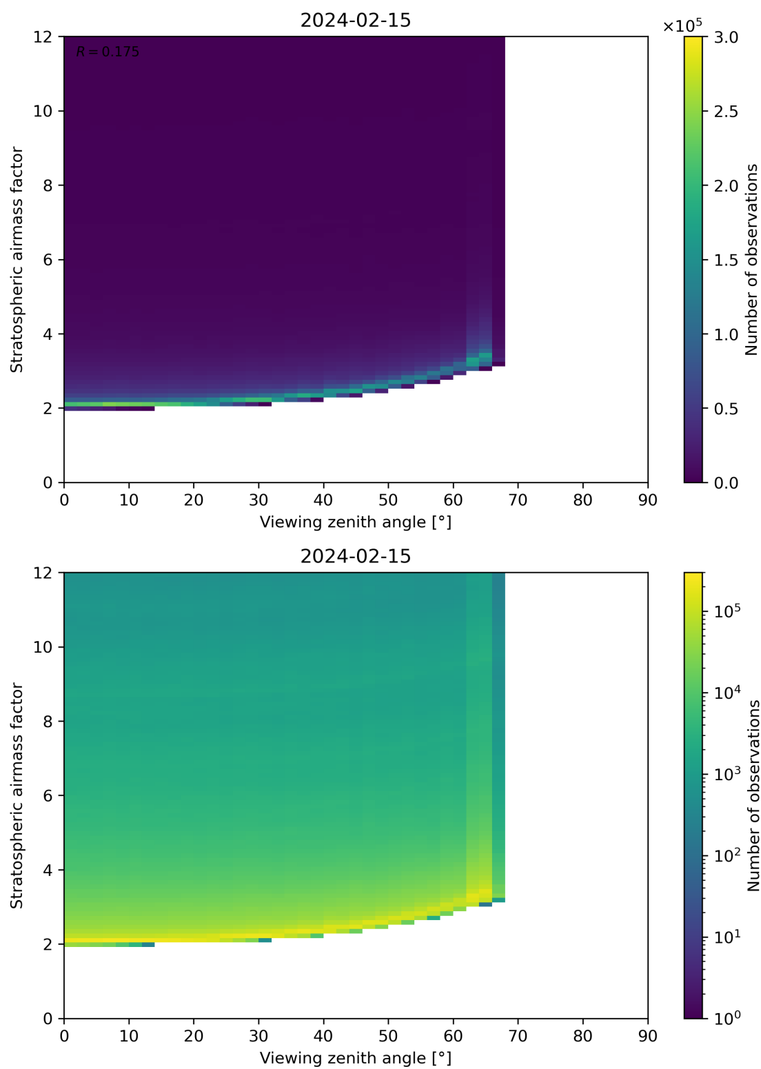
Figure 159: Scatter density plot of “Viewing zenith angle” against “Stratospheric airmass factor” for 2024-02-14 to 2024-02-16.
