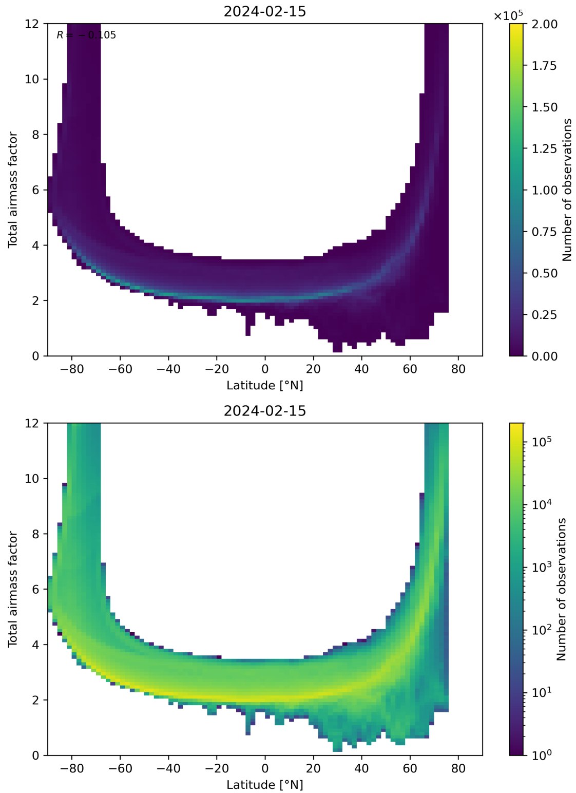
Figure 84: Scatter density plot of “Latitude” against “Total airmass factor” for 2024-02-14 to 2024-02-16.
