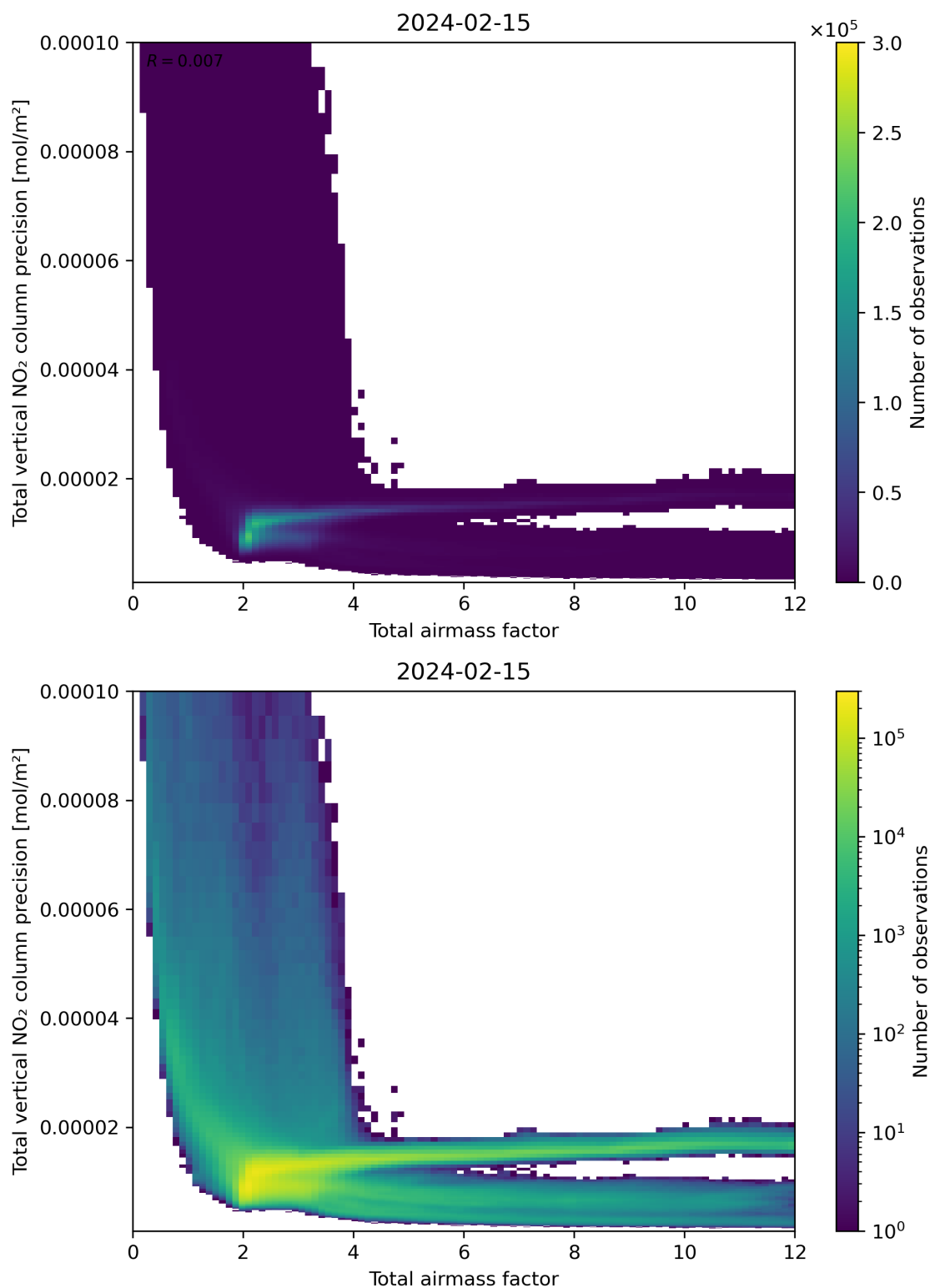
Figure 68: Scatter density plot of “Total airmass factor” against “Total vertical NO 2 column precision” for 2024-02-14 to 2024-02-16.
