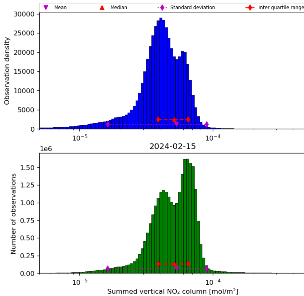
Figure 40: Histogram of “Summed vertical NO 2 column” for 2024-02-14 to 2024-02-16
