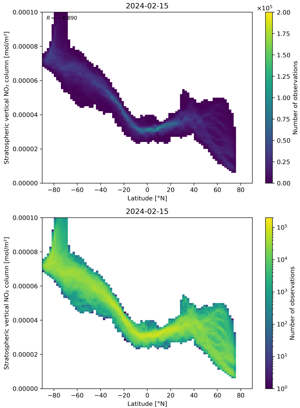
Figure 87: Scatter density plot of “Latitude” against “Stratospheric vertical NO 2 column” for 2024-02-14 to 2024-02-16.
