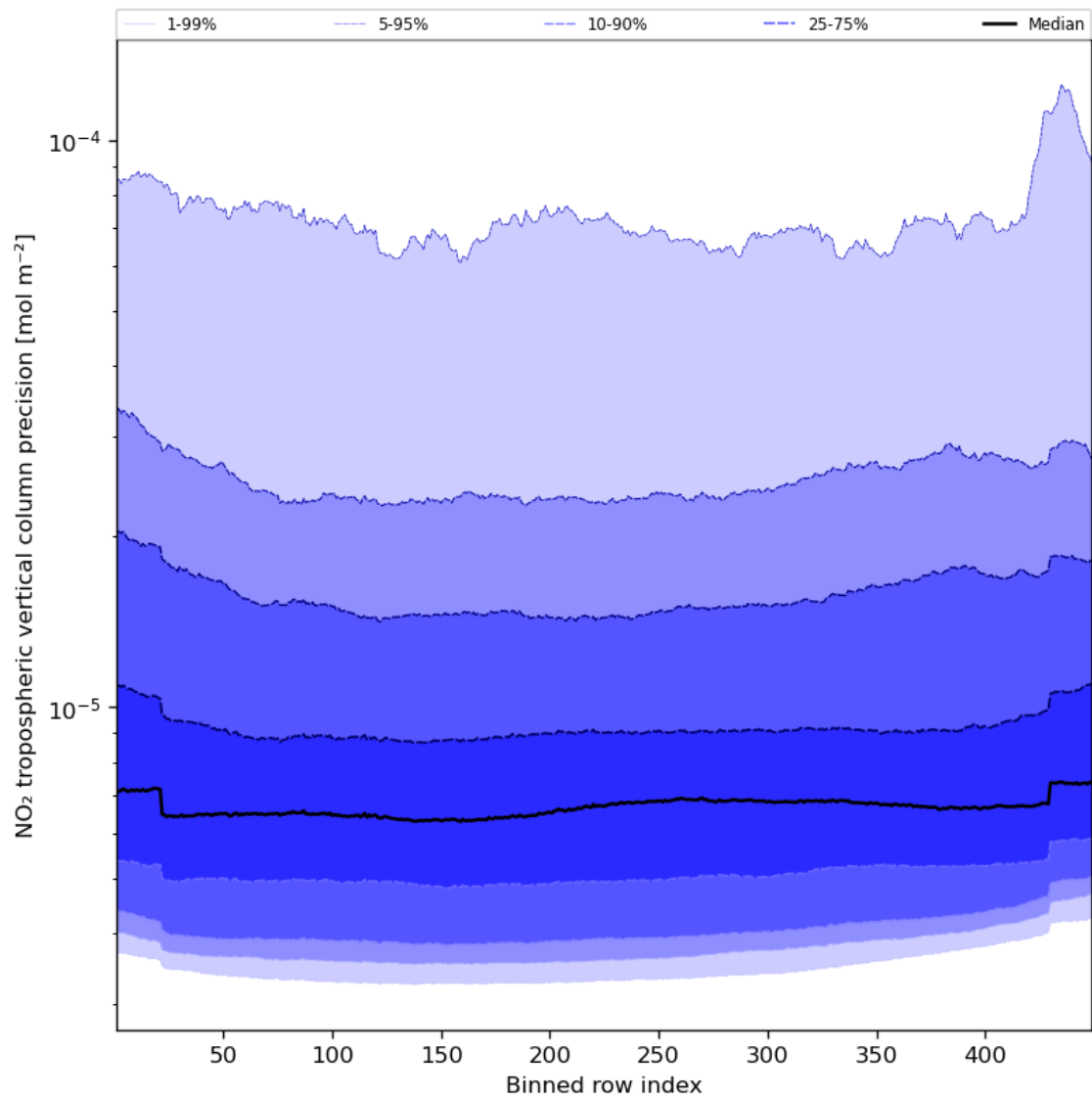
Figure 47: Along track statistics of “NO 2 tropospheric vertical column precision” for 2024-02-14 to 2024-02-16
