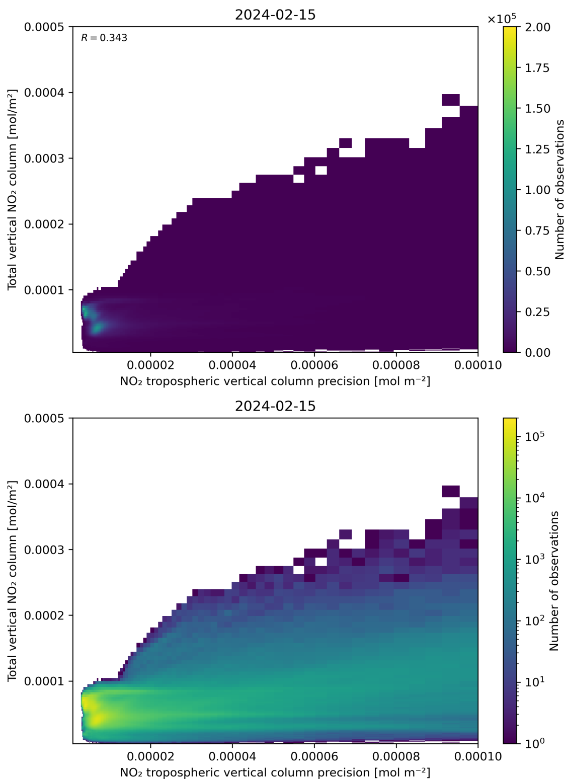
Figure 138: Scatter density plot of “NO 2 tropospheric vertical column precision” against “Total vertical NO 2 column” for 2024-02-14 to 2024-02-16.
