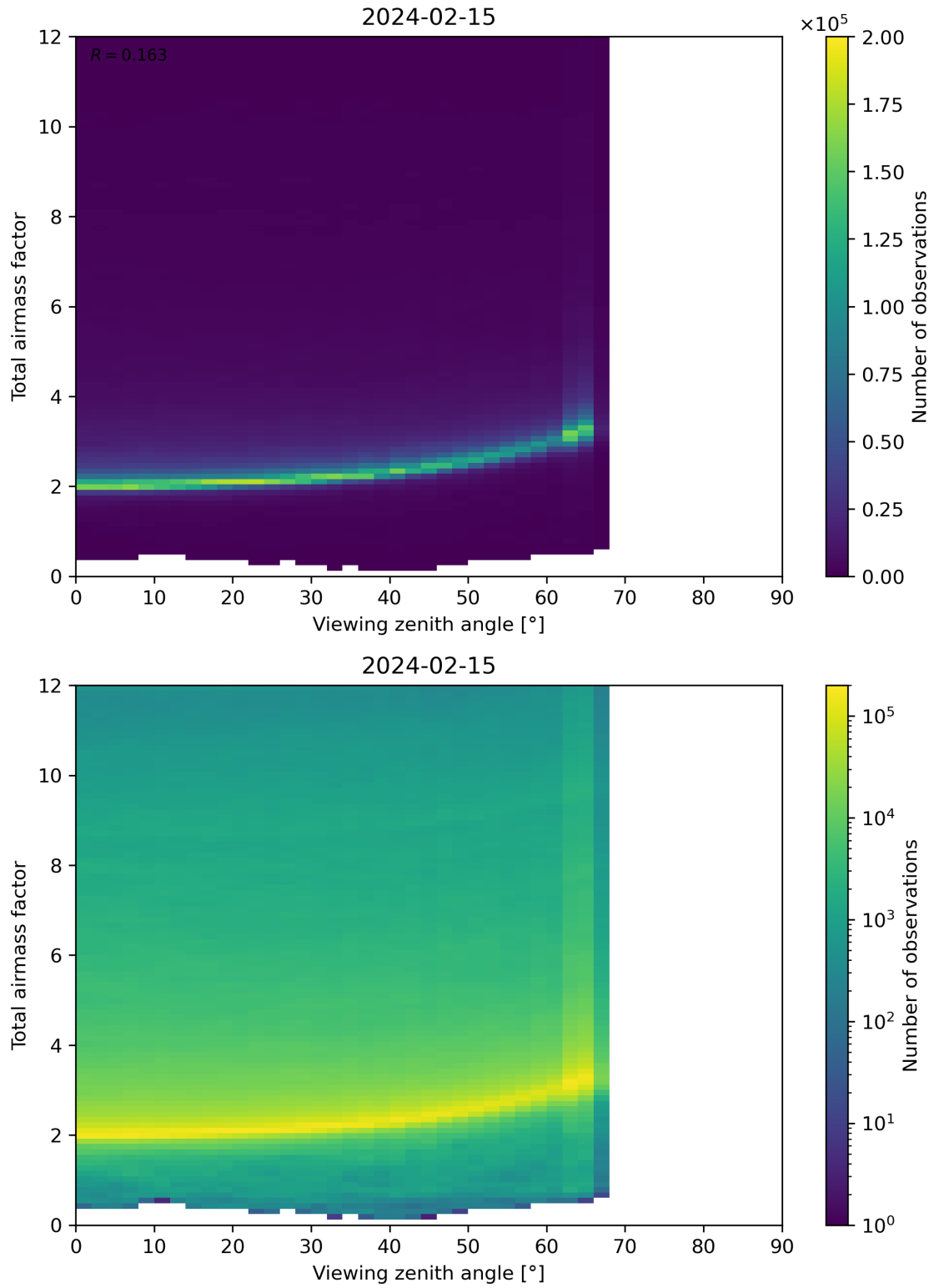
Figure 160: Scatter density plot of “Viewing zenith angle” against “Total airmass factor” for 2024-02-14 to 2024-02-16.
