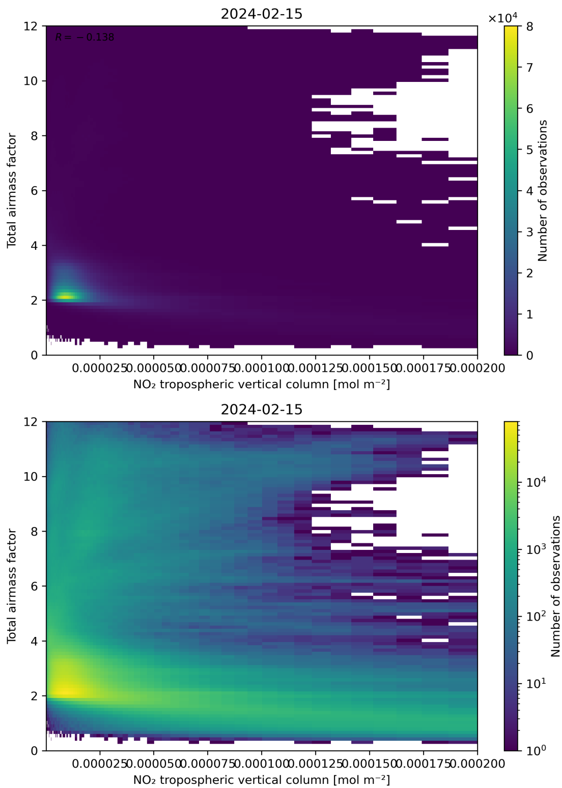
Figure 122: Scatter density plot of “NO 2 tropospheric vertical column” against “Total air mass factor” for 2024-02-14 to 2024-02-16.
