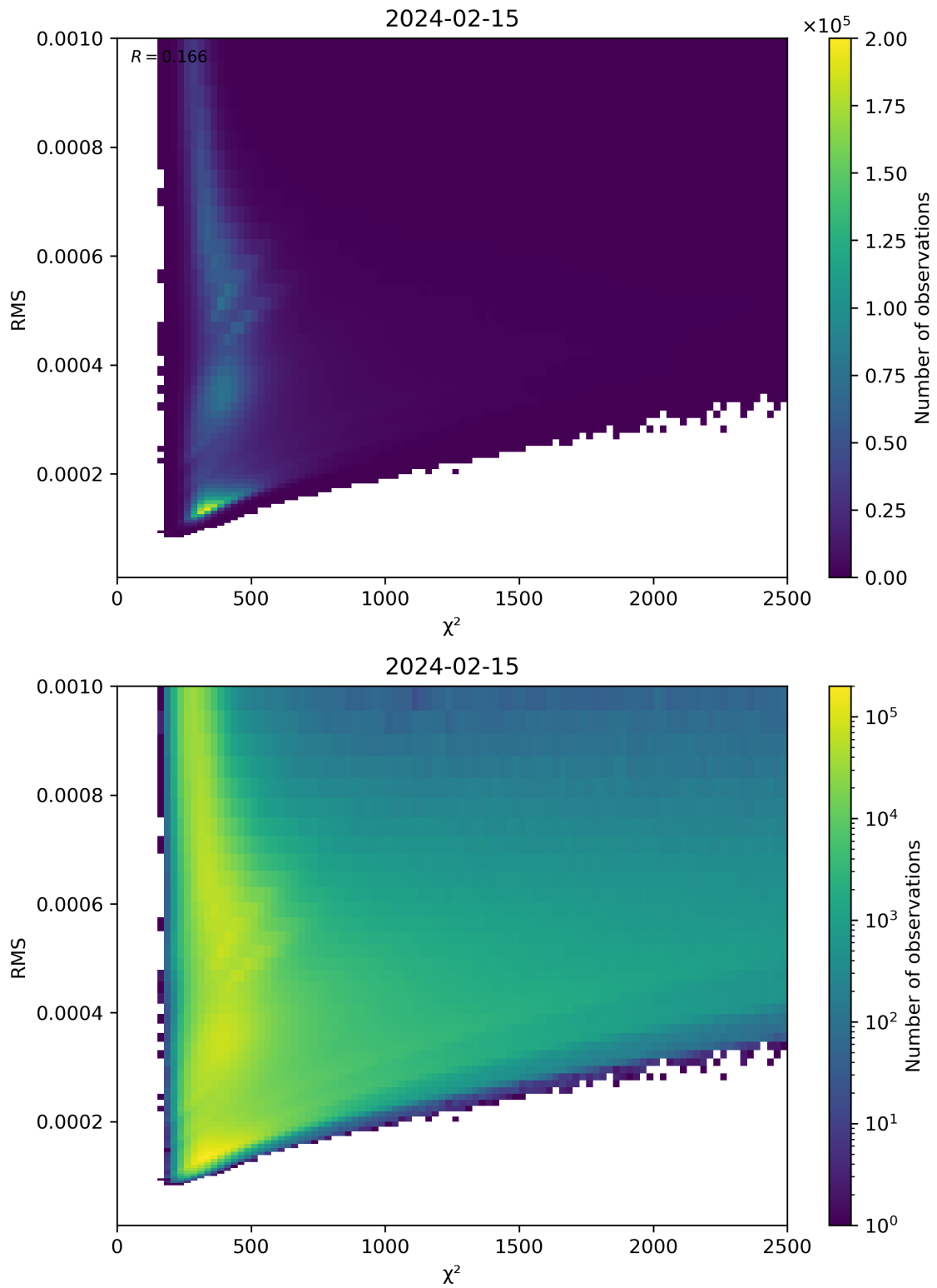
Figure 82: Scatter density plot of “ \chi^2 ” against “RMS” for 2024-02-14 to 2024-02-16.
