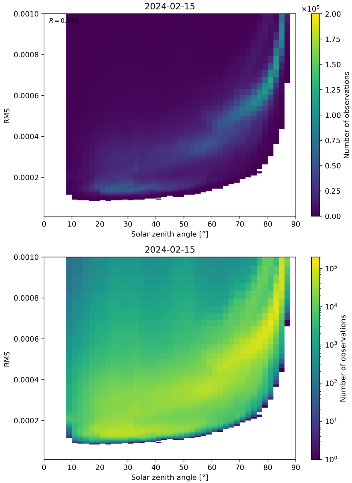
Figure 157: Scatter density plot of “Solar zenith angle” against “RMS” for 2024-02-14 to 2024-02-16.
