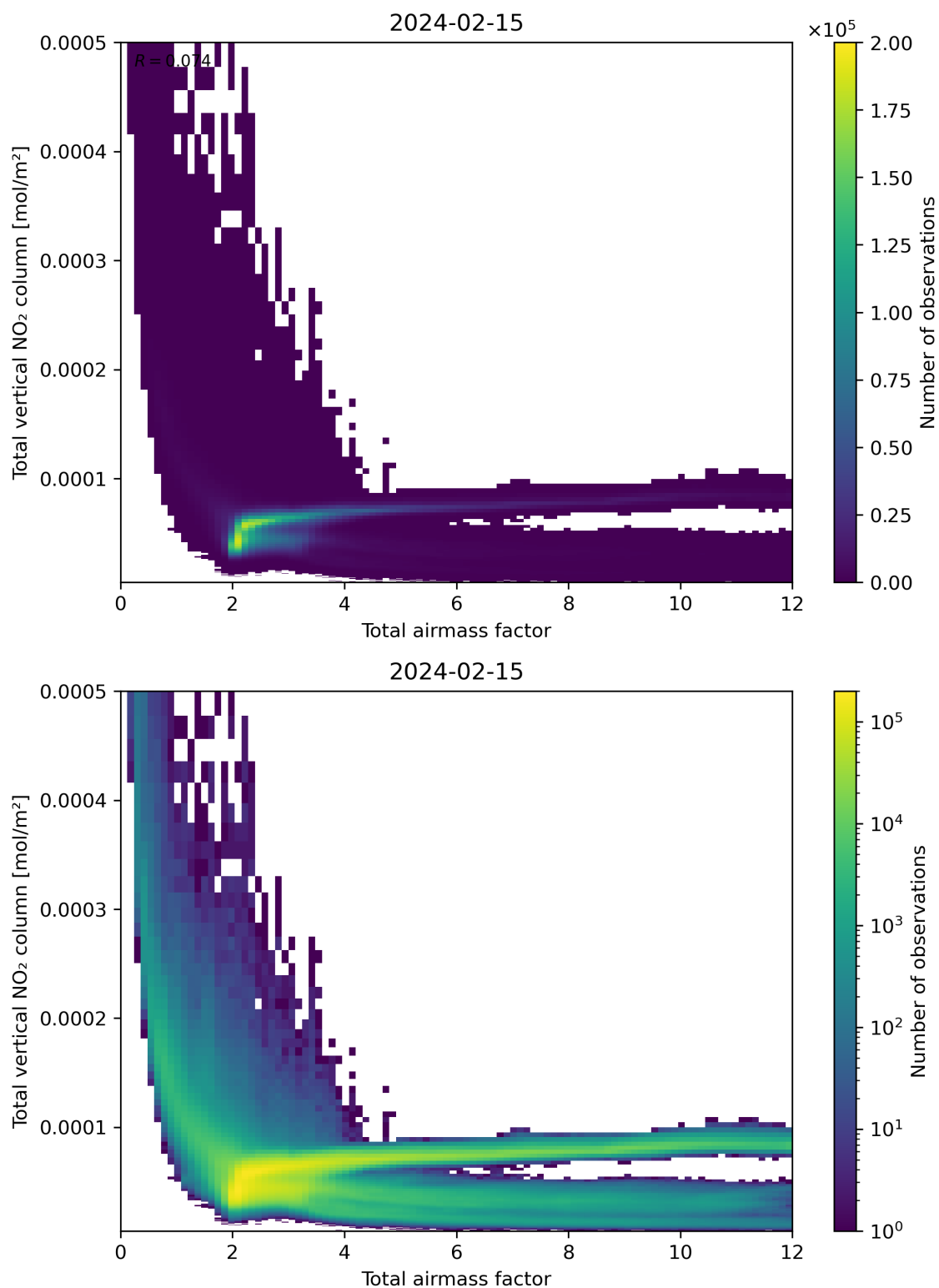
Figure 67: Scatter density plot of “Total airmass factor” against “Total vertical NO 2 column” for 2024-02-14 to 2024-02-16.
