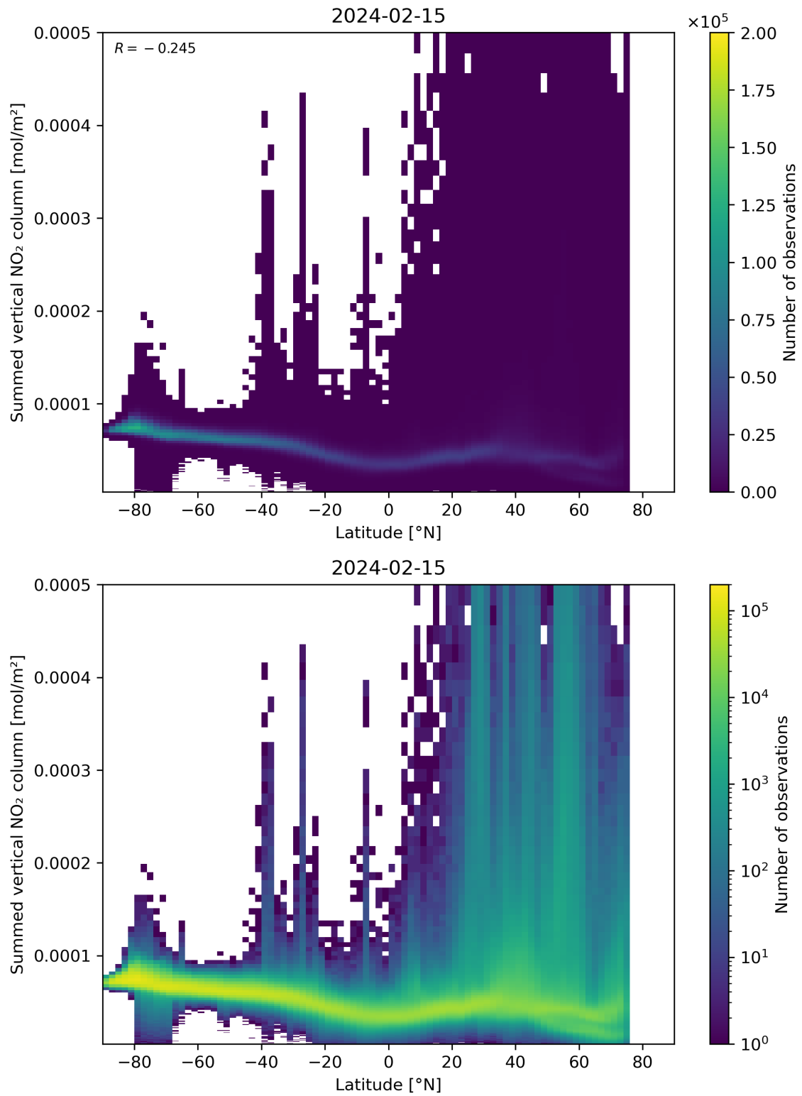
Figure 88: Scatter density plot of “Latitude” against “Summed vertical NO 2 column” for 2024-02-14 to 2024-02-16.
