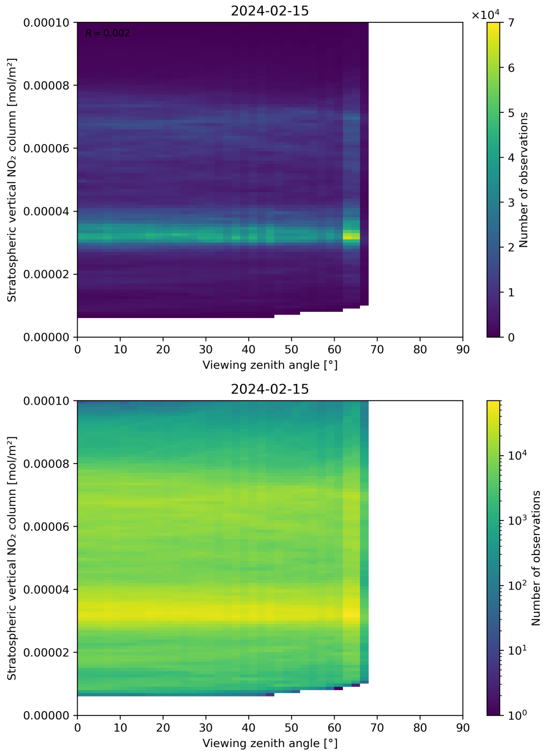
Figure 164: Scatter density plot of “Viewing zenith angle” against “Stratospheric vertical NO 2 column” for 2024-02-14 to 2024-02-16.
