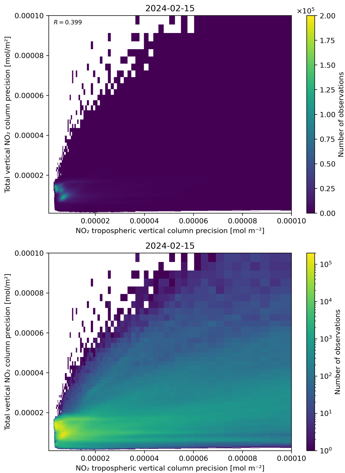
Figure 139: Scatter density plot of “NO 2 tropospheric vertical column precision” against “Total vertical NO 2 column precision” for 2024-02-14 to 2024-02-16.
