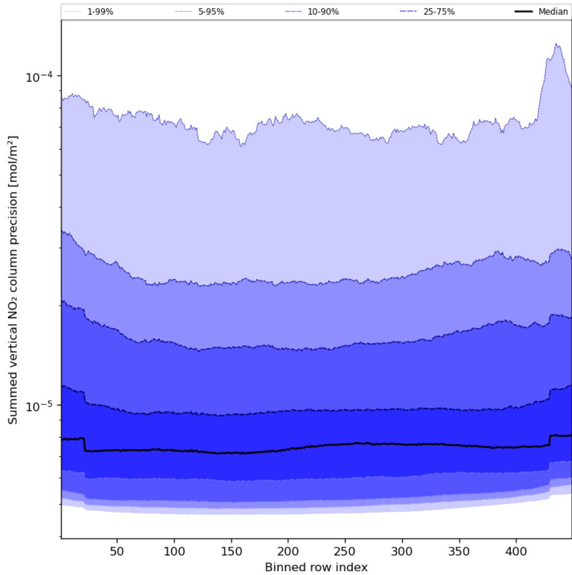
Figure 58: Along track statistics of “Summed vertical NO 2 column precision” for 2024-02-14 to 2024-02-16
