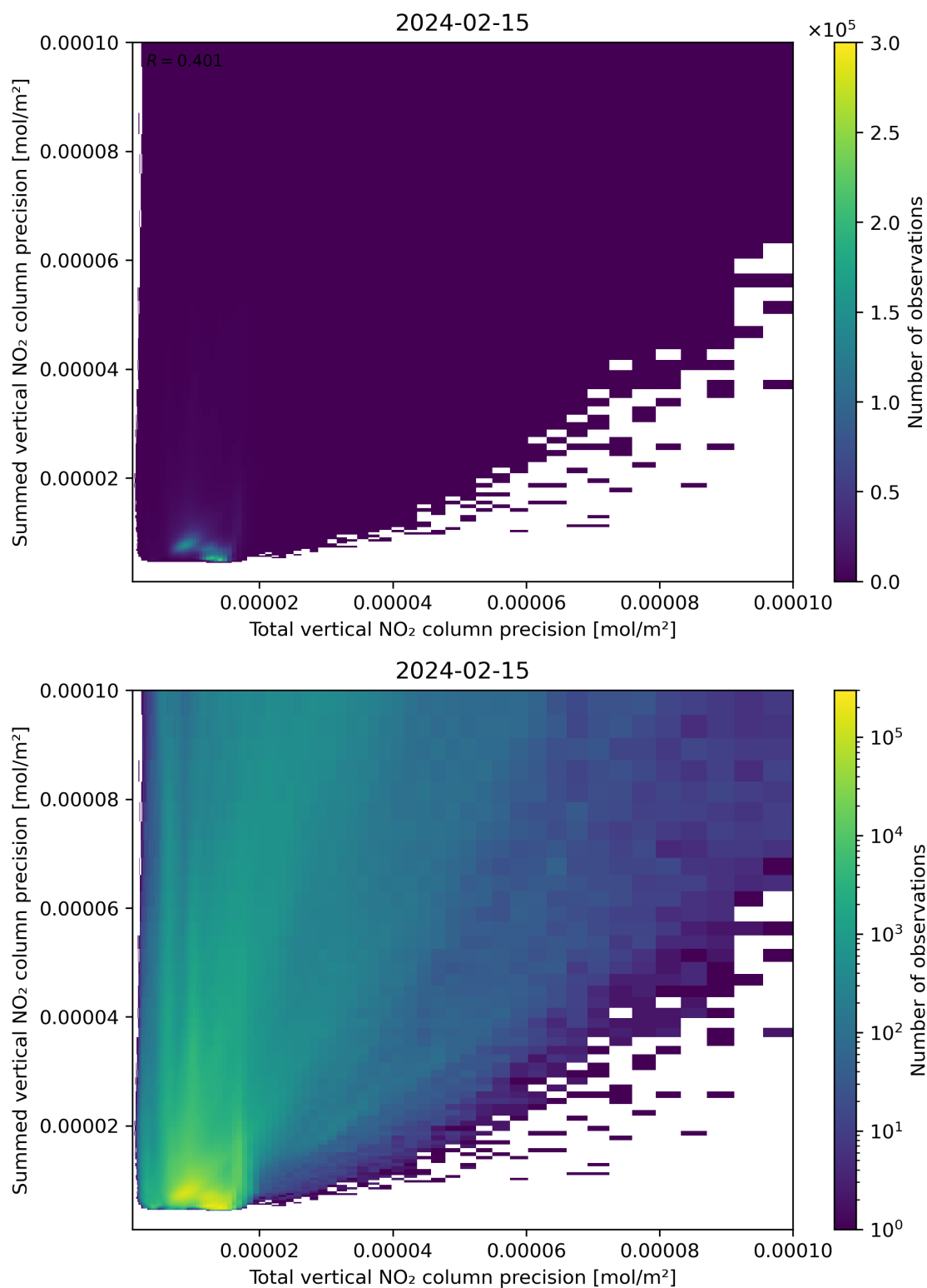
Figure 118: Scatter density plot of “Total vertical NO 2 column precision” against “Summed vertical NO 2 column precision” for 2024-02-14 to 2024-02-16.
