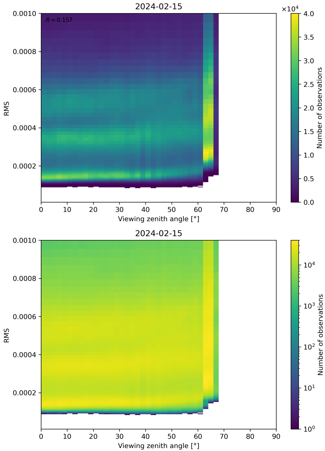
Figure 171: Scatter density plot of “Viewing zenith angle” against “RMS” for 2024-02-14 to 2024-02-16.
