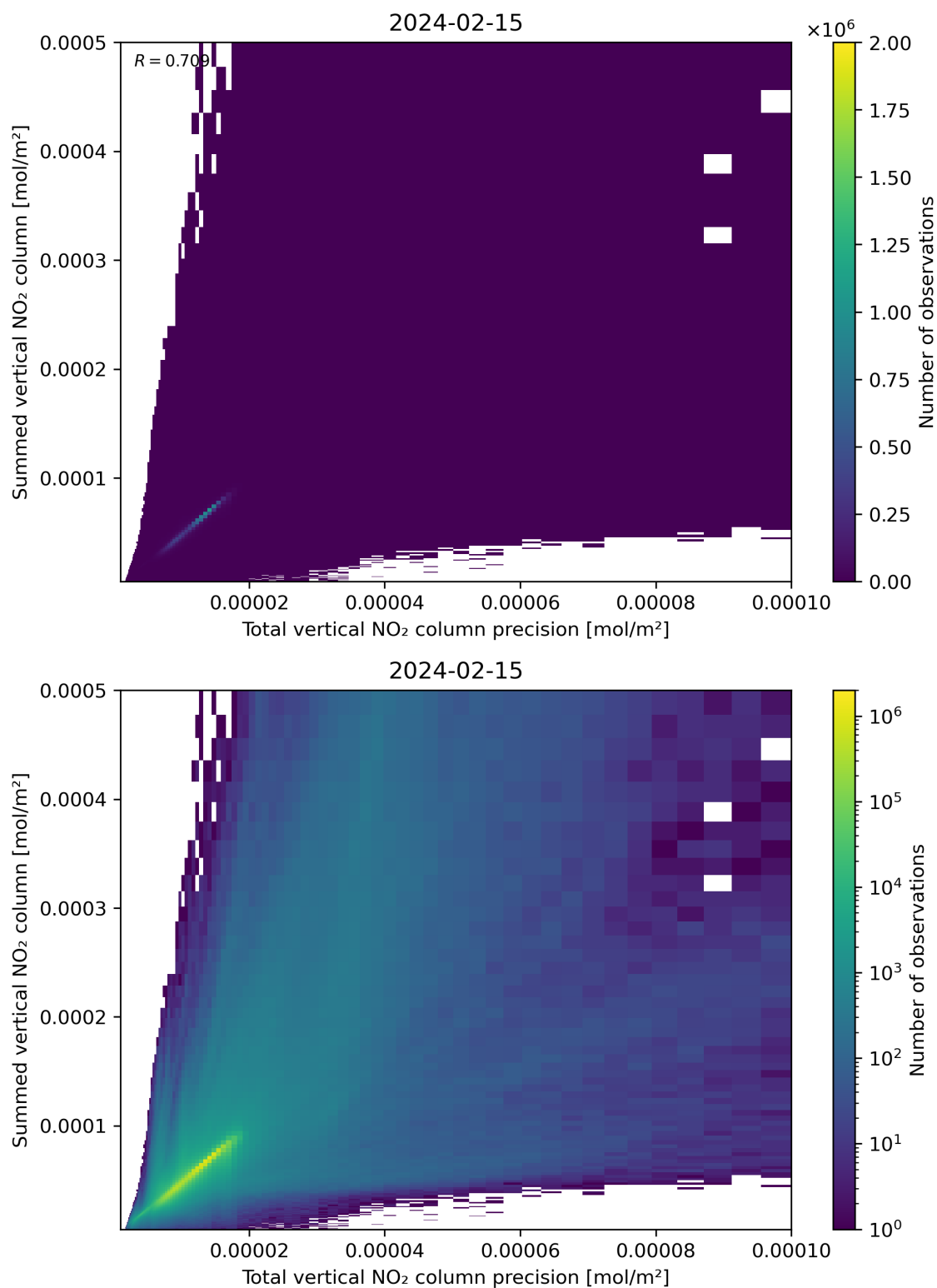
Figure 117: Scatter density plot of “Total vertical NO 2 column precision” against “Summed vertical NO 2 column” for 2024-02-14 to 2024-02-16.
