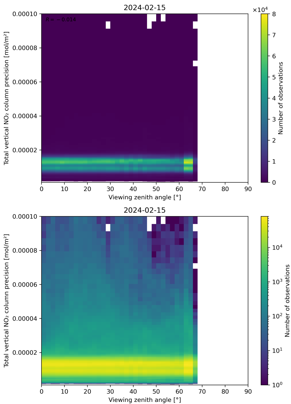
Figure 168: Scatter density plot of “Viewing zenith angle” against “Total vertical NO 2 column precision” for 2024-02-14 to 2024-02-16.
