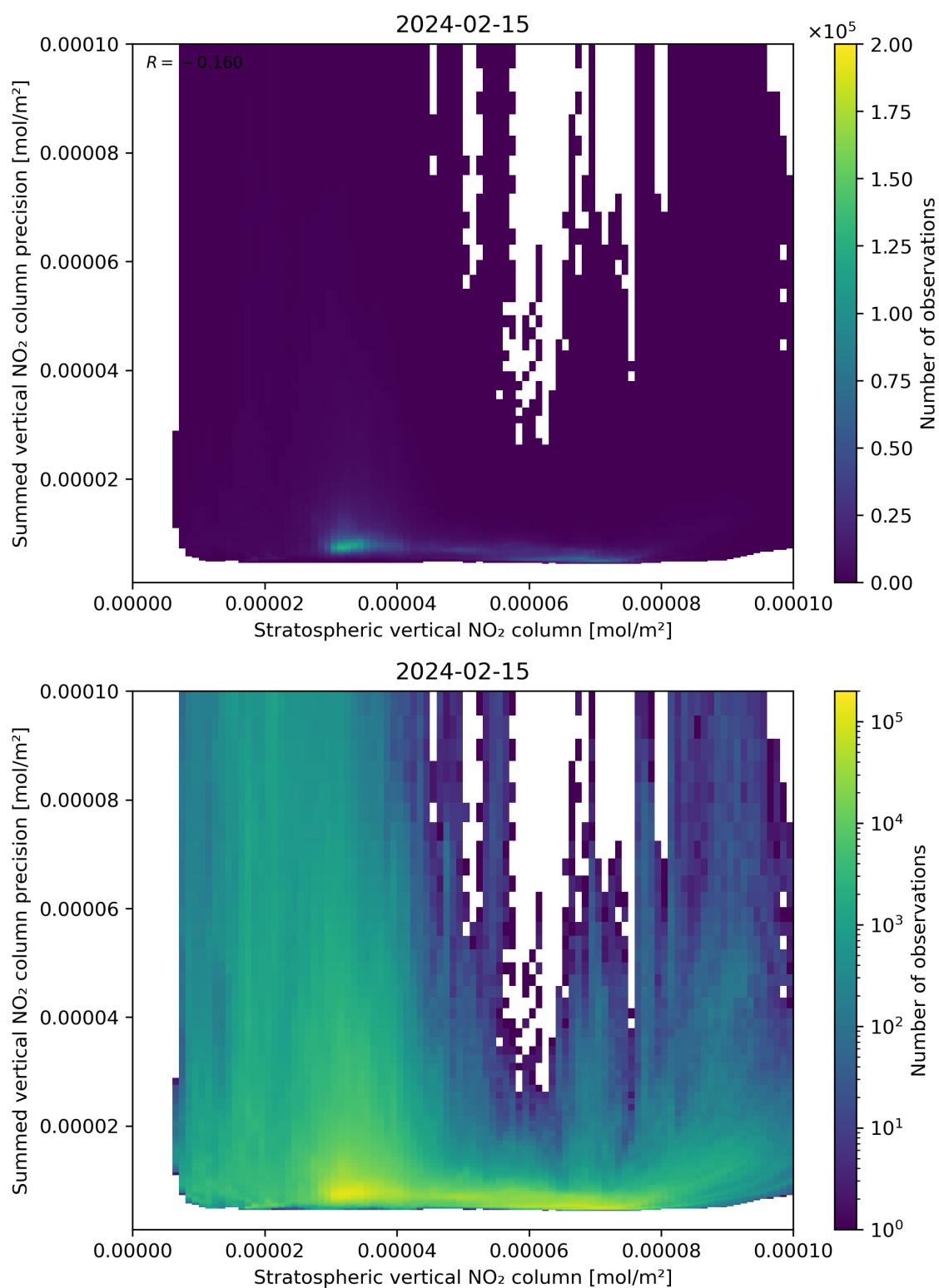
Figure 99: Scatter density plot of “Stratospheric vertical NO 2 column” against “Summed vertical NO 2 column precision” for 2024-02-14 to 2024-02-16.
