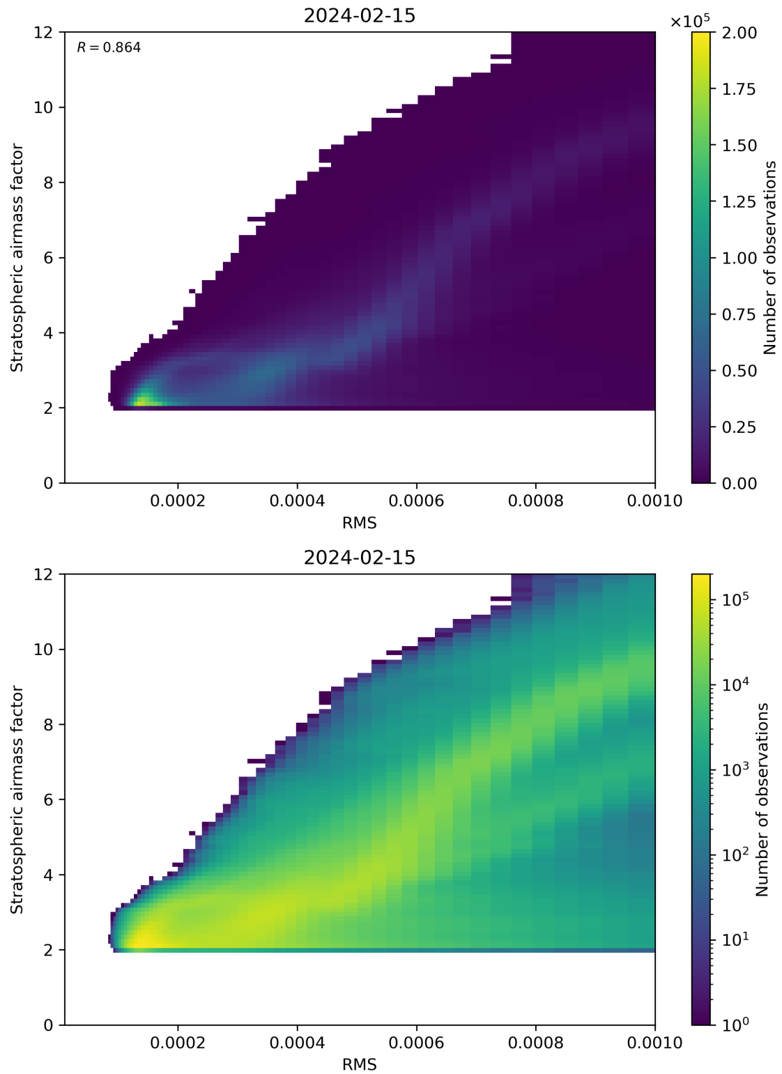
Figure 144: Scatter density plot of “RMS” against “Stratospheric airmass factor” for 2024-02-14 to 2024-02-16.
