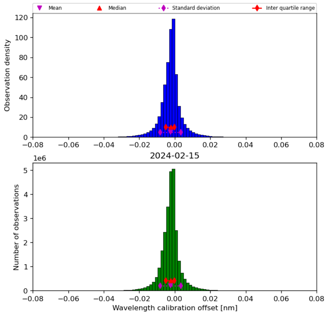
Figure 35: Histogram of “Wavelength calibration offset” for 2024-02-14 to 2024-02-16
