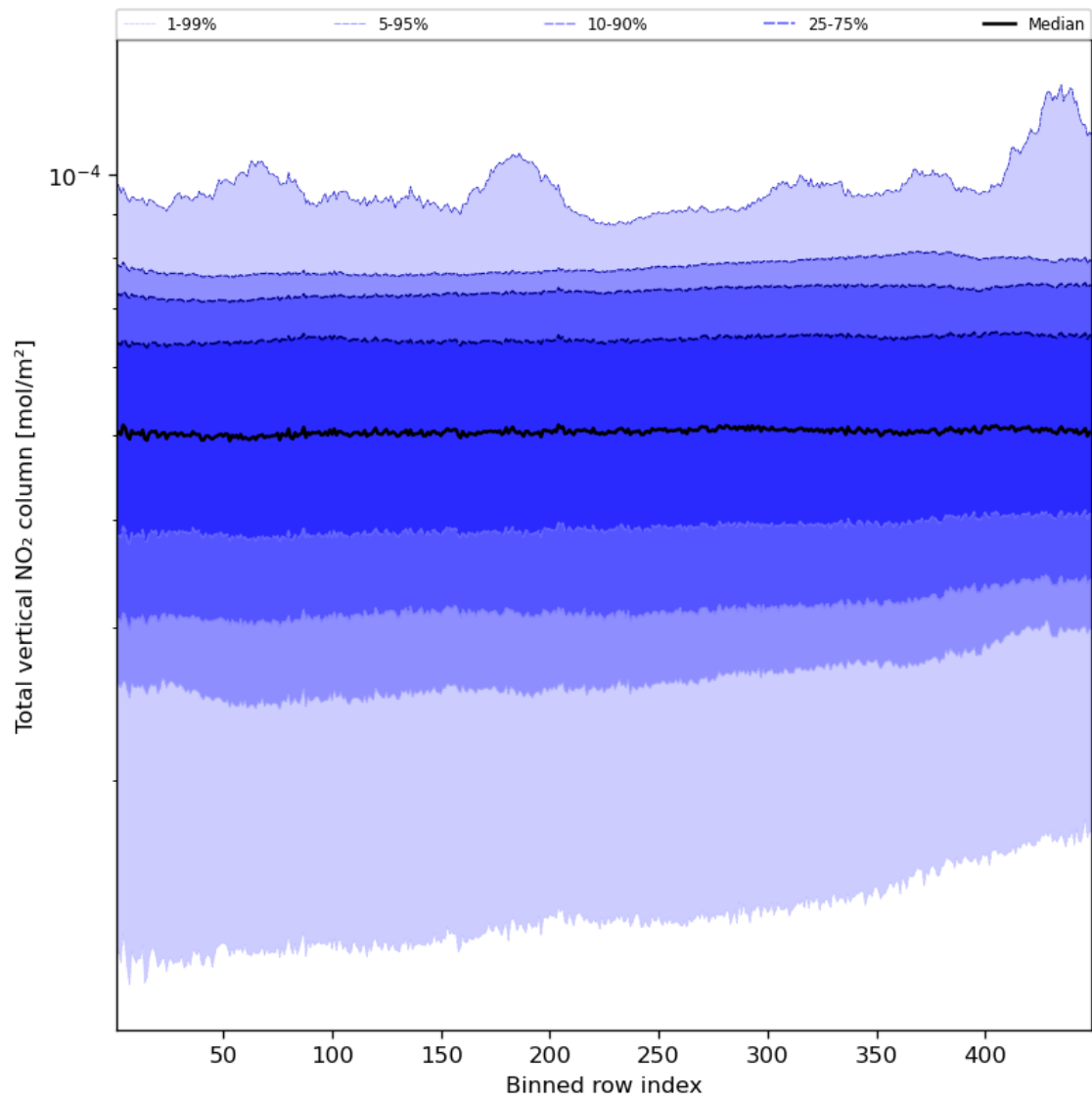
Figure 55: Along track statistics of “Total vertical NO 2 column” for 2024-02-14 to 2024-02-16
