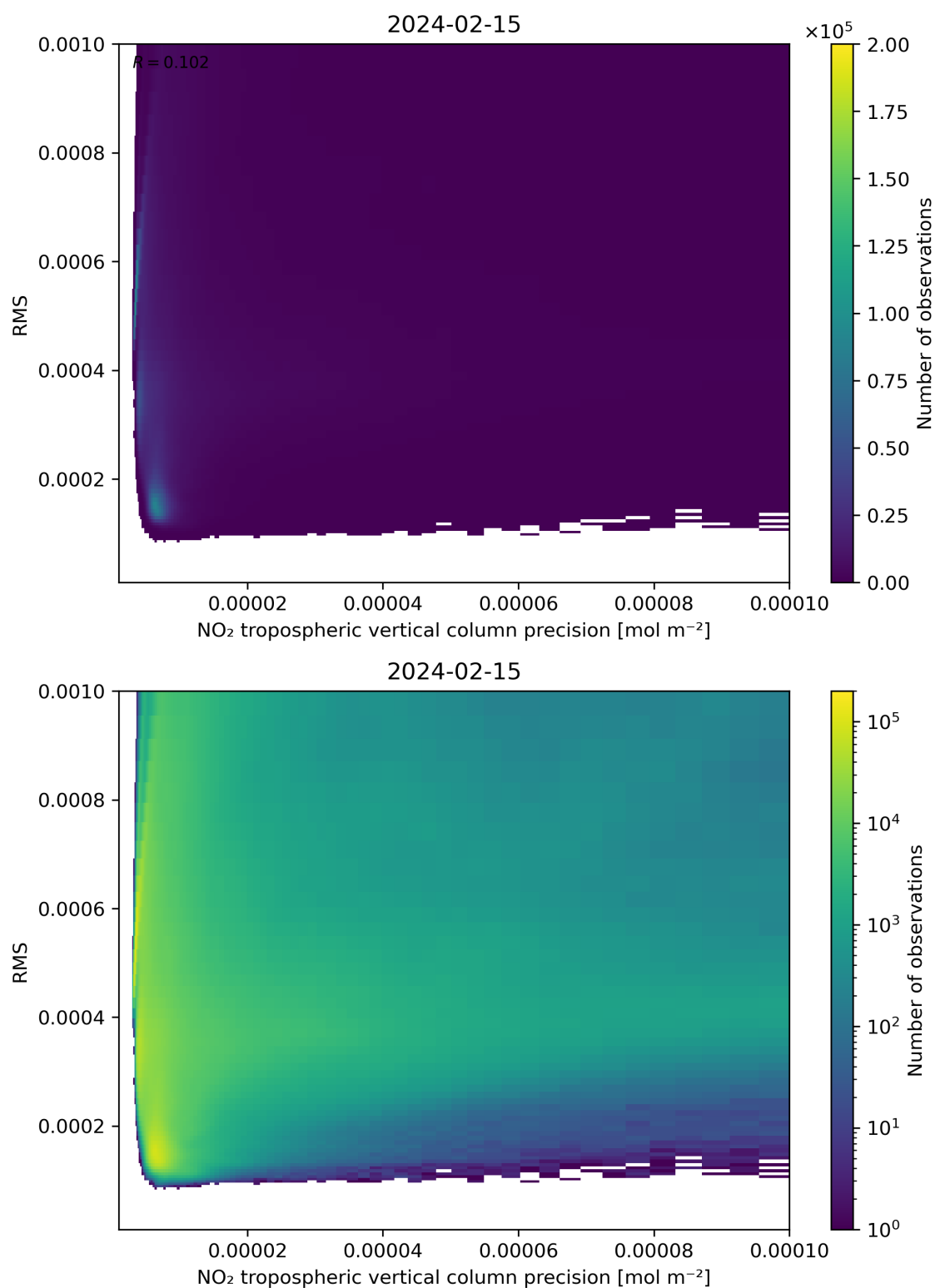
Figure 140: Scatter density plot of “NO 2 tropospheric vertical column precision” against “RMS” for 2024-02-14 to 2024-02-16.
