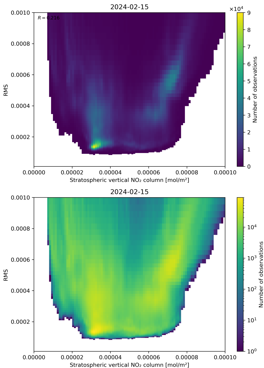
Figure 102: Scatter density plot of “Stratospheric vertical NO 2 column” against “RMS” for 2024-02-14 to 2024-02-16.
