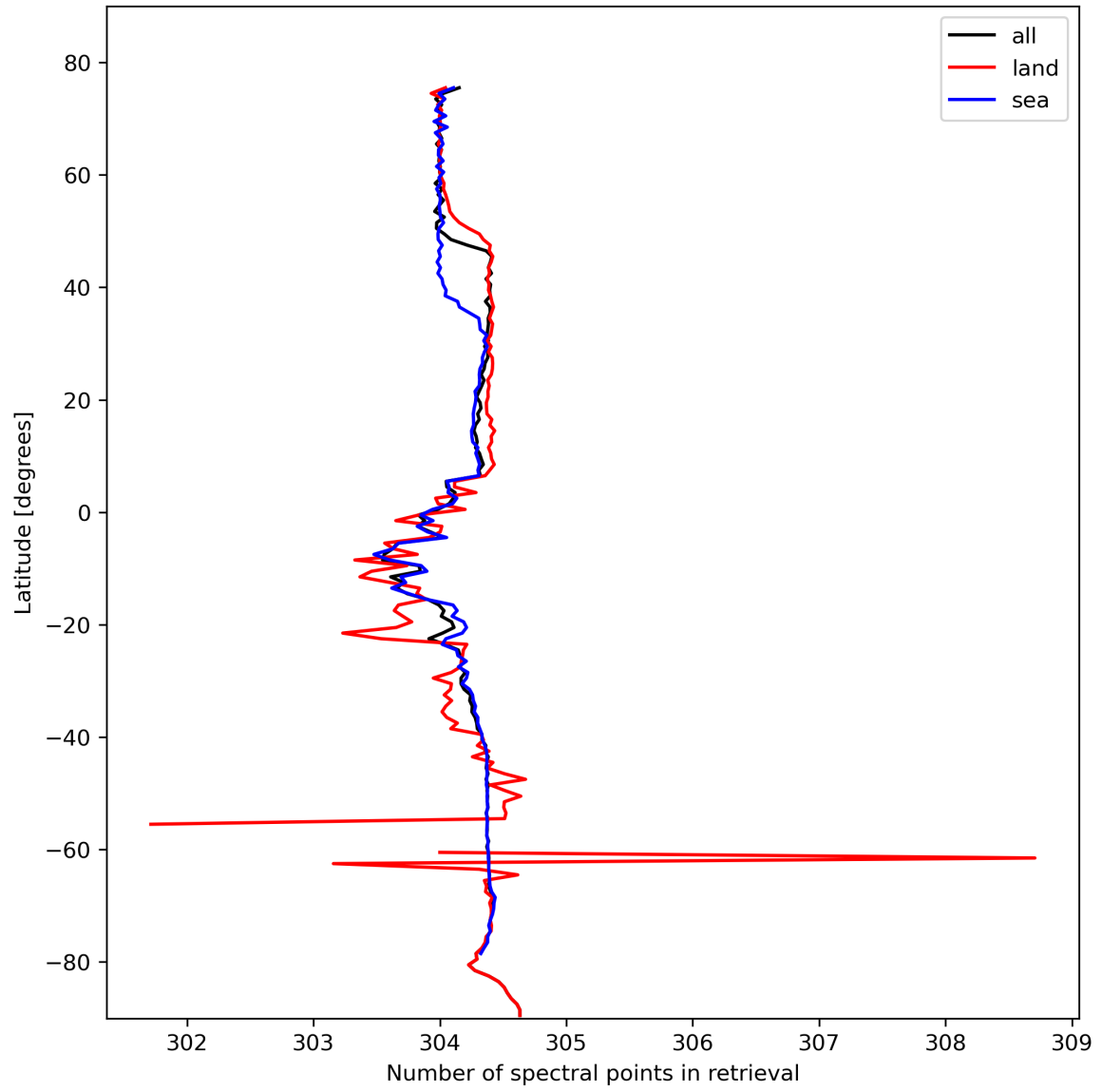
Figure 16: Zonal average of “Number of spectral points in retrieval” for 2024-02-14 to 2024-02-16.
