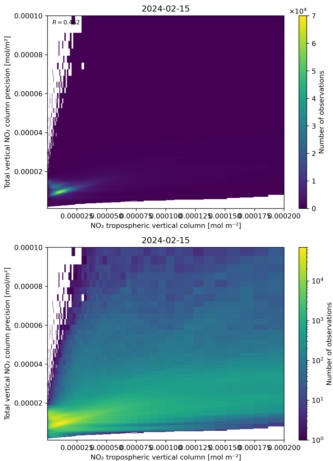
Figure 129: Scatter density plot of “NO 2 tropospheric vertical column” against “Total vertical NO 2 column precision” for 2024-02-14 to 2024-02-16.
