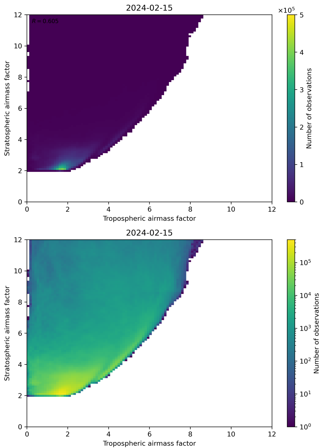
Figure 71: Scatter density plot of “Tropospheric airmass factor” against “Stratospheric airmass factor” for 2024-02-14 to 2024-02-16.
