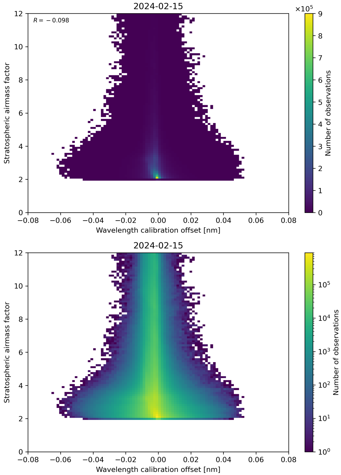
Figure 174: Scatter density plot of “Wavelength calibration offset” against “Stratospheric airmass factor” for 2024-02-14 to 2024-02-16.
