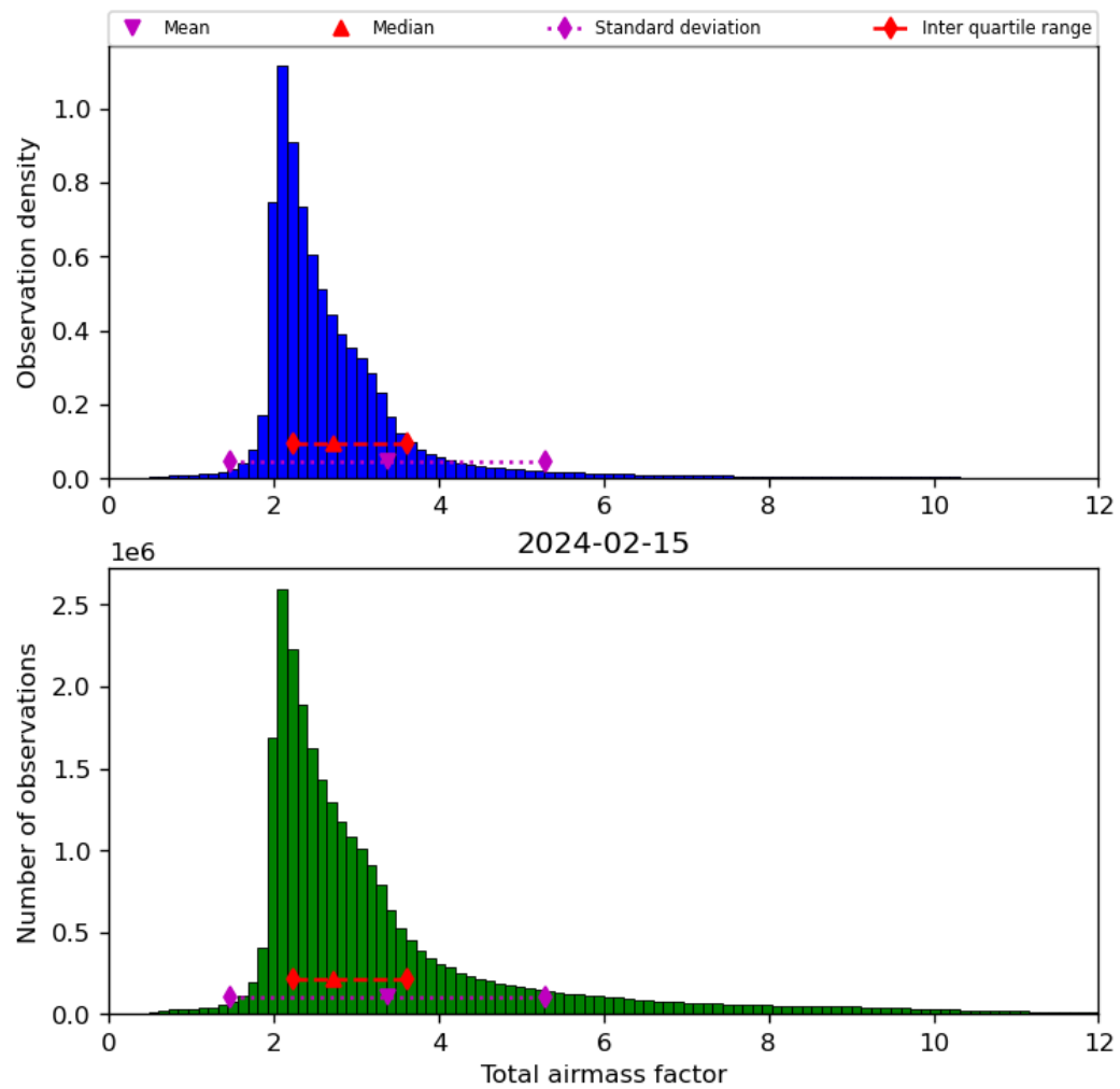
Figure 32: Histogram of “Total airmass factor” for 2024-02-14 to 2024-02-16
