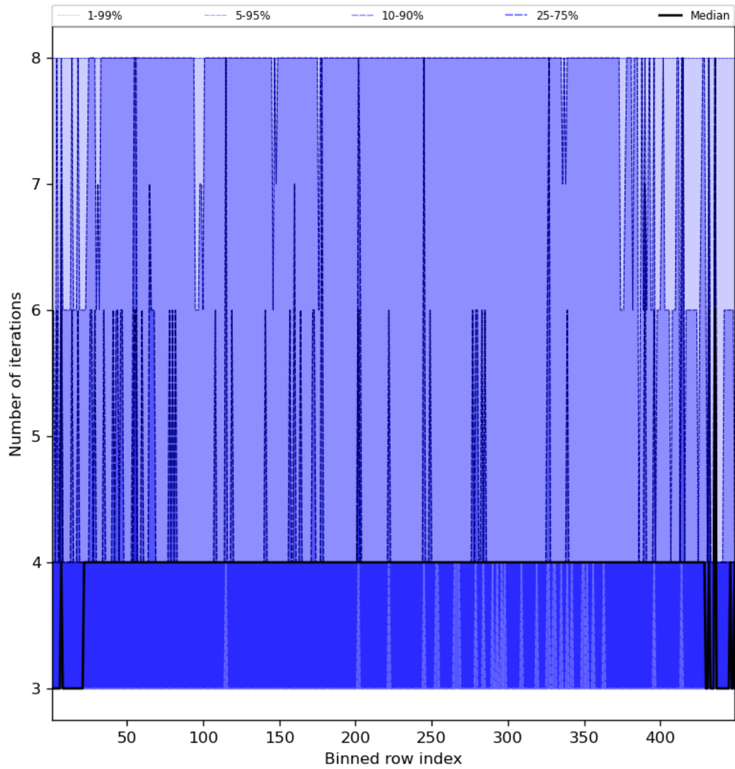
Figure 51: Along track statistics of “Number of iterations” for 2024-02-14 to 2024-02-16
