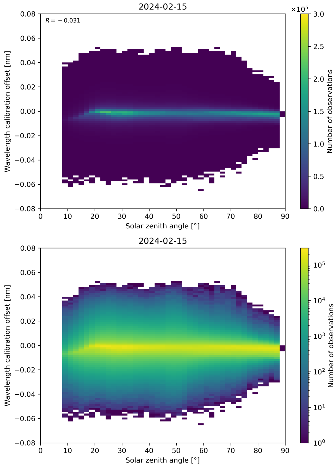
Figure 158: Scatter density plot of “Solar zenith angle” against “Wavelength calibration offset” for 2024-02-14 to 2024-02-16.
