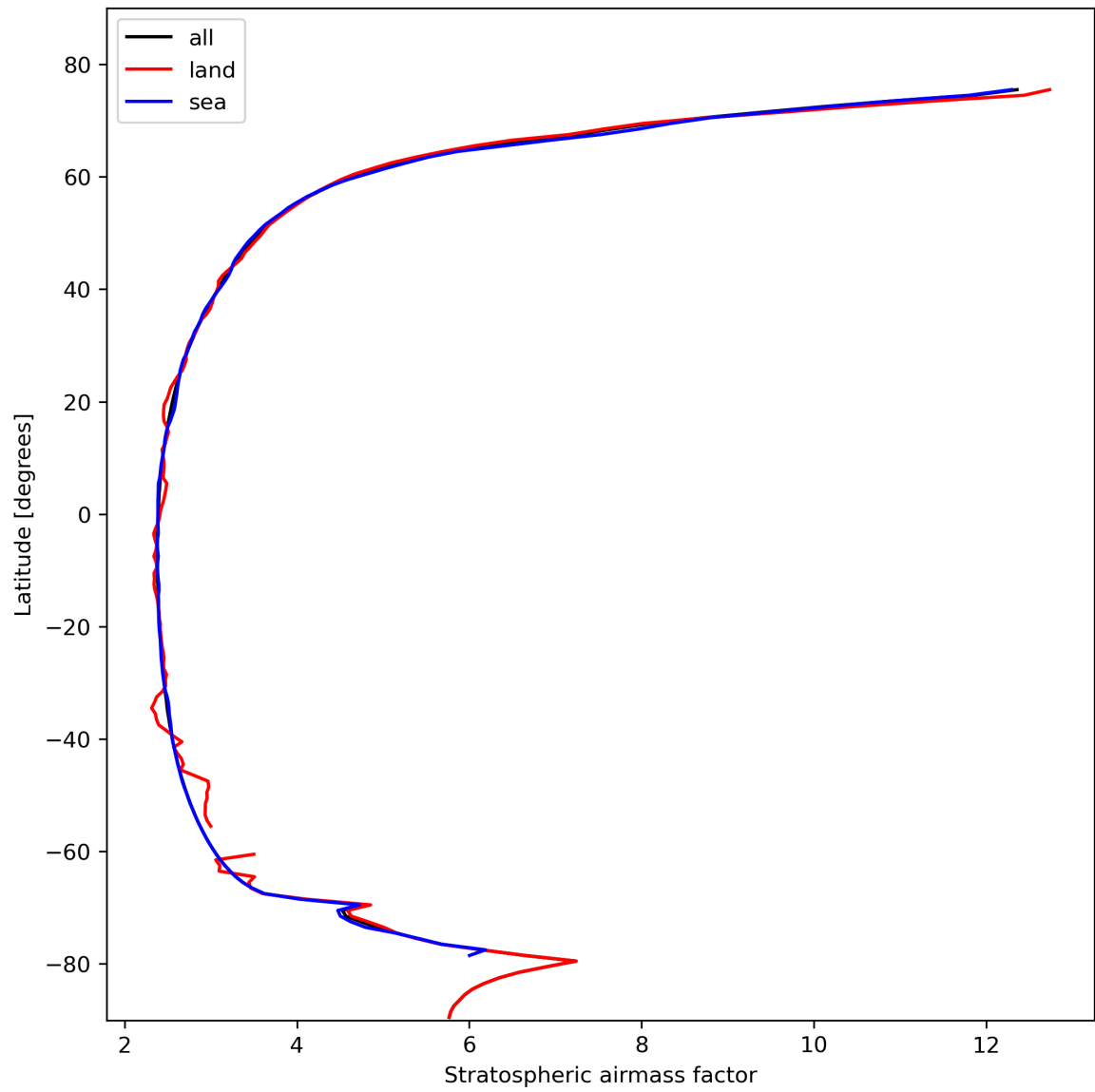
Figure 27: Zonal average of “Stratospheric airmass factor” for 2024-02-14 to 2024-02-16.
