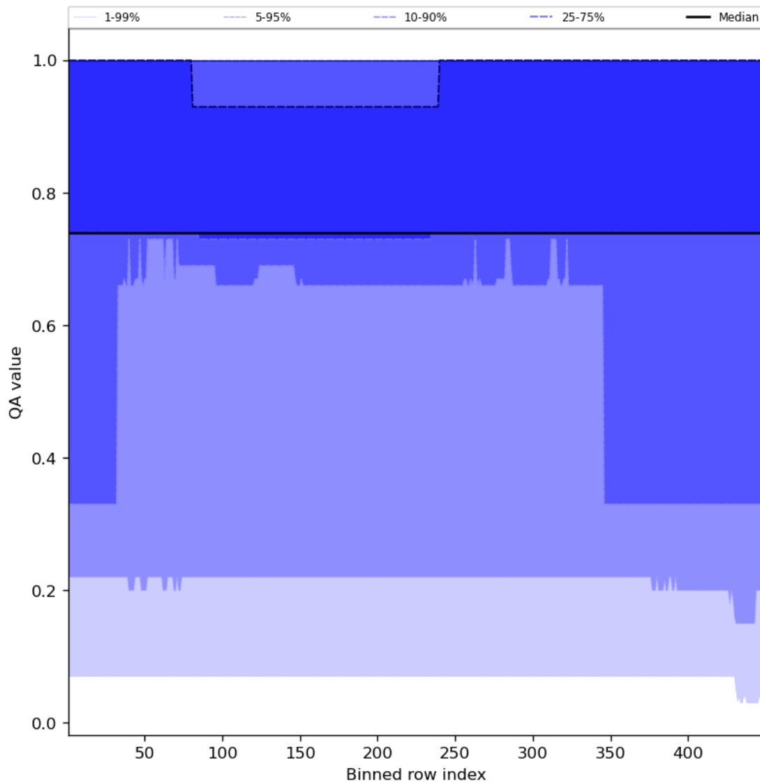
Figure 45: Along track statistics of “QA value” for 2024-02-14 to 2024-02-16
