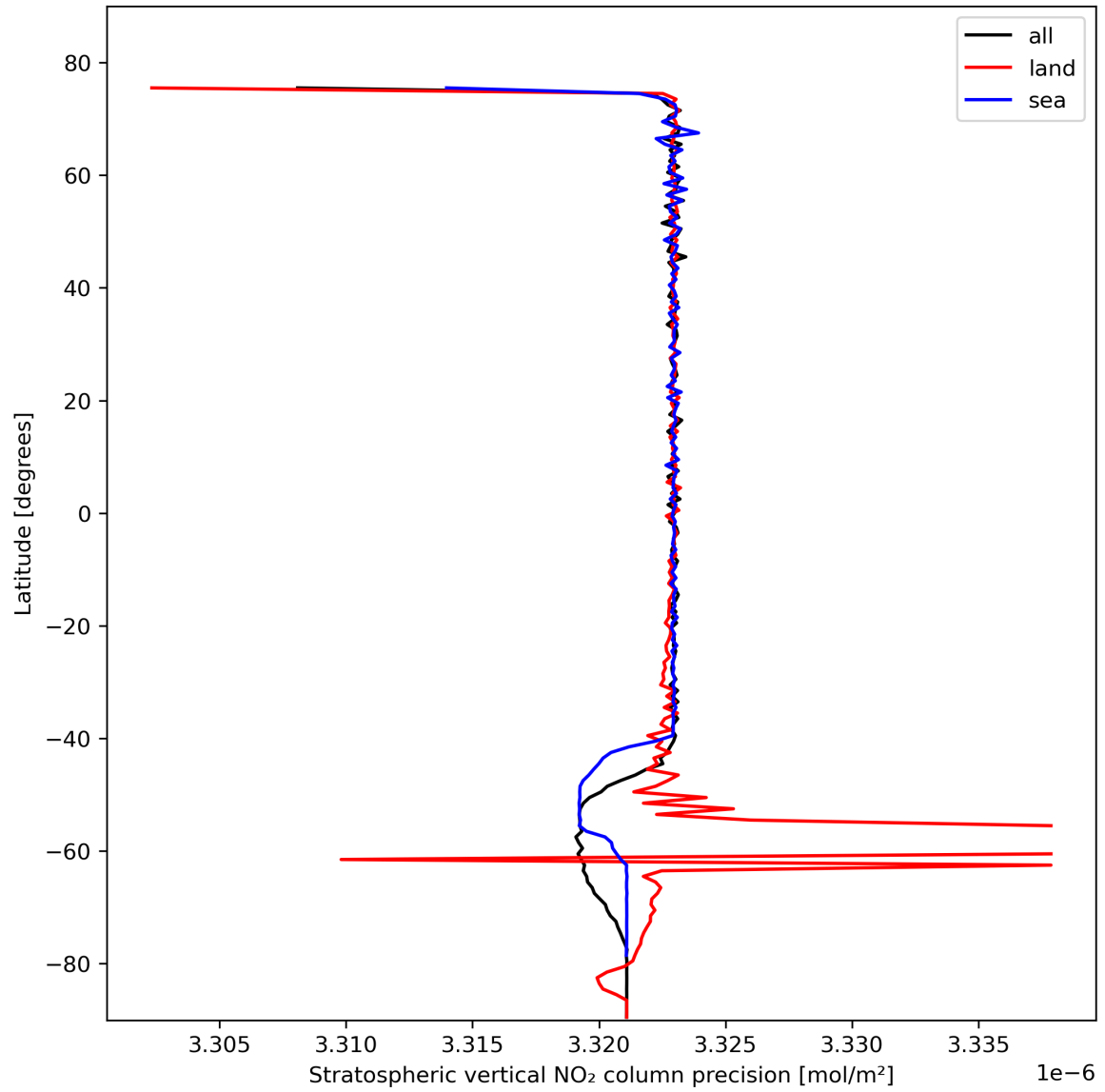
Figure 20: Zonal average of “Stratospheric vertical NO 2 column precision” for 2024-02-14 to 2024-02-16.
