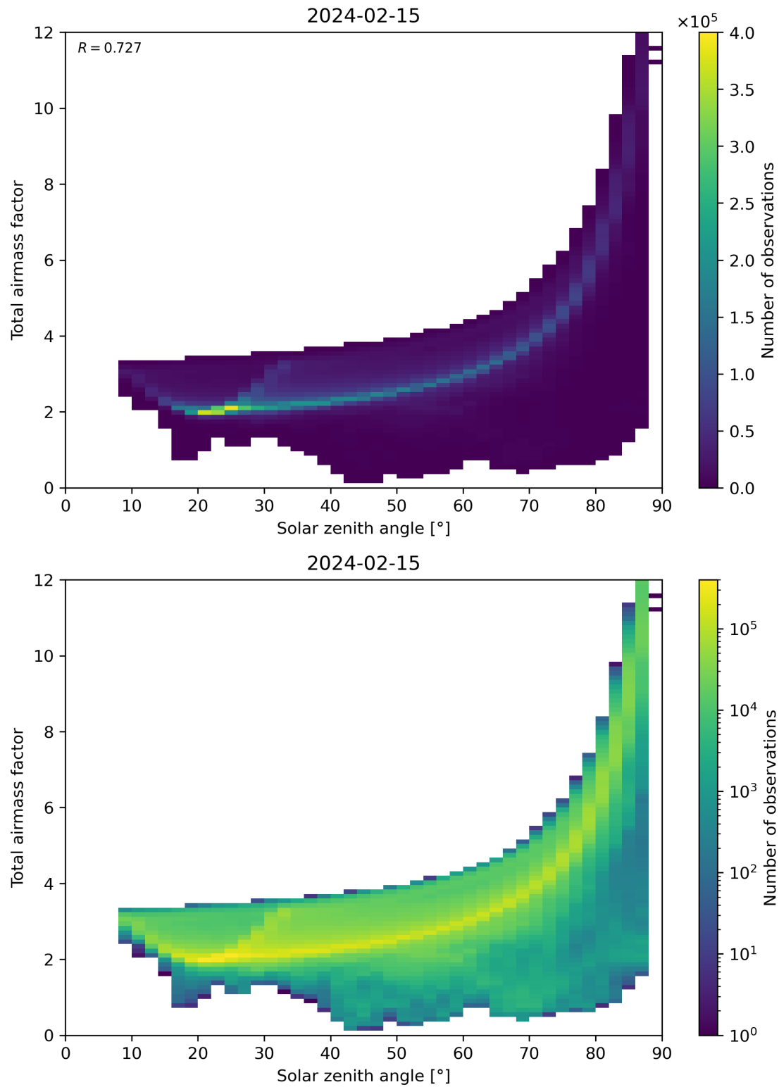
Figure 146: Scatter density plot of “Solar zenith angle” against “Total air mass factor” for 2024-02-14 to 2024-02-16.
