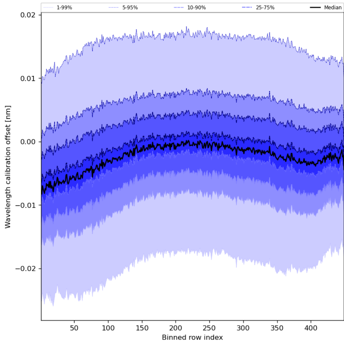
Figure 52: Along track statistics of “Wavelength calibration offset” for 2024-02-14 to 2024-02-16
