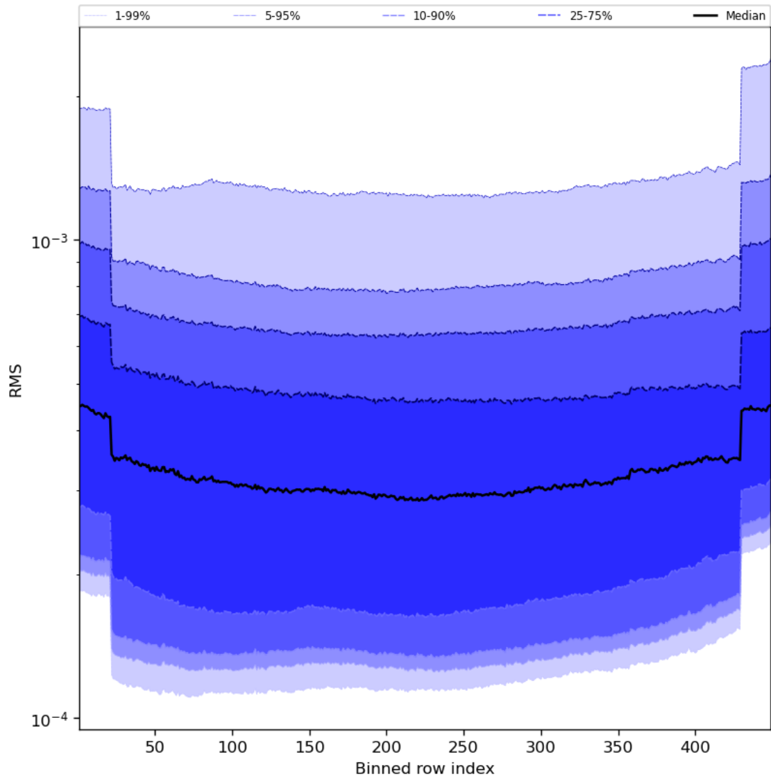
Figure 60: Along track statistics of “RMS” for 2024-02-14 to 2024-02-16
