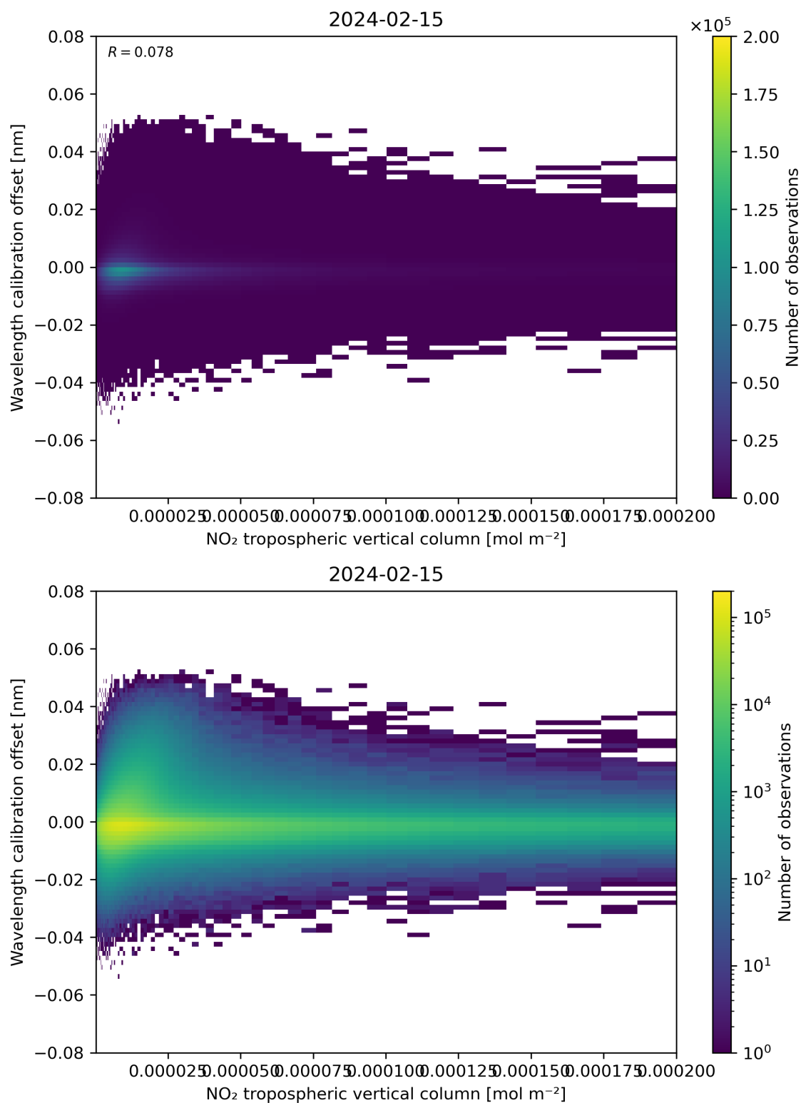
Figure 143: Scatter density plot of “NO 2 tropospheric vertical column” against “Wavelength calibration offset” for 2024-02-14 to 2024-02-16.
