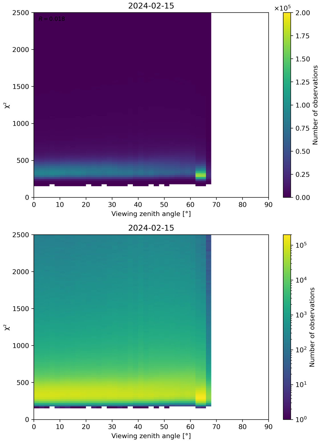
Figure 162: Scatter density plot of “Viewing zenith angle” against “ \chi^2 ” for 2024-02-14 to 2024-02-16.
