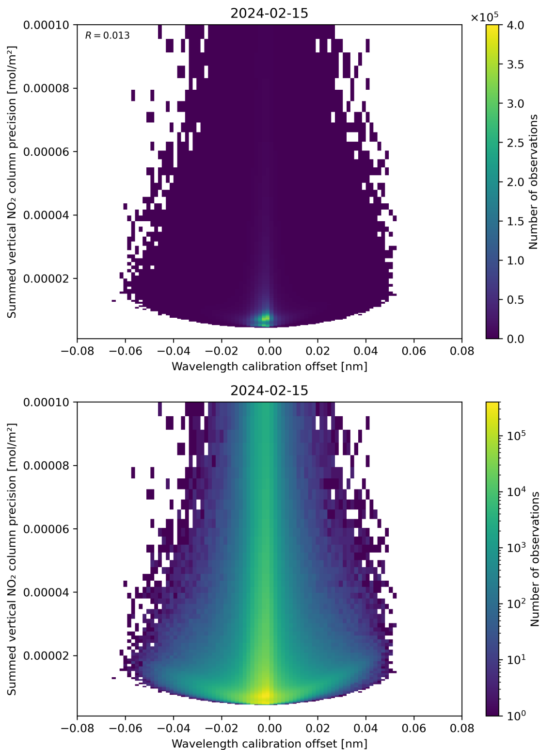
Figure 178: Scatter density plot of “Wavelength calibration offset” against “Summed vertical NO 2 column precision” for 2024-02-14 to 2024-02-16.
