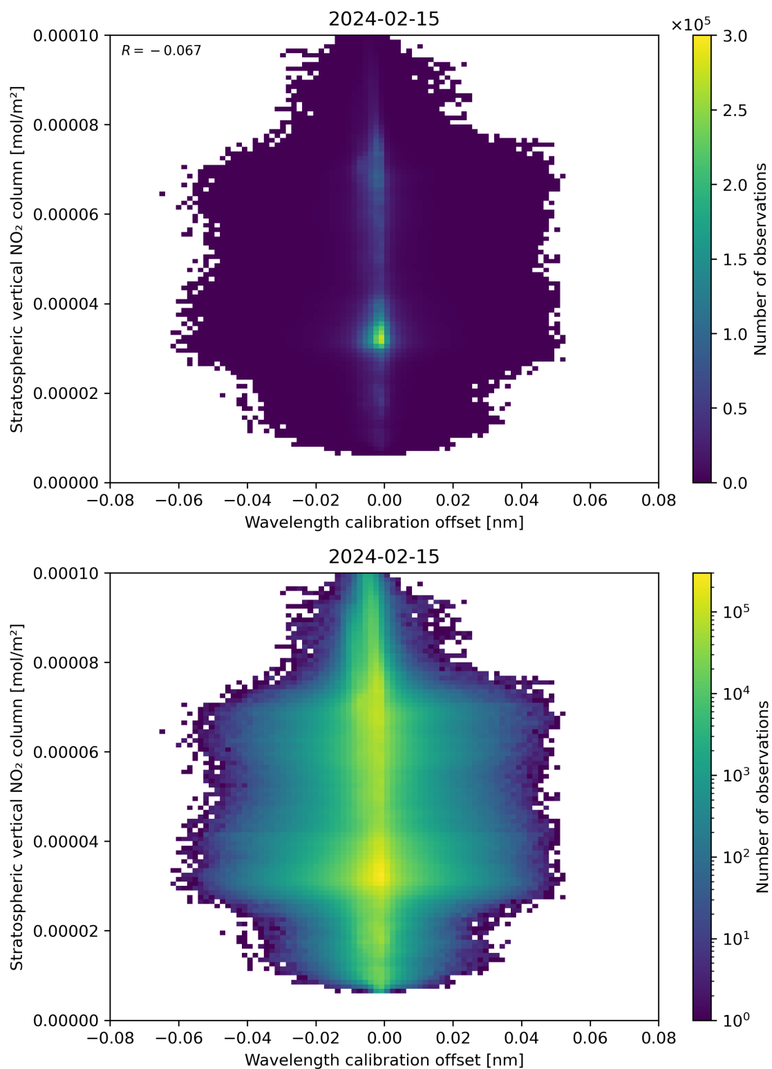
Figure 176: Scatter density plot of “Wavelength calibration offset” against “Stratospheric vertical NO 2 column” for 2024-02-14 to 2024-02-16.
