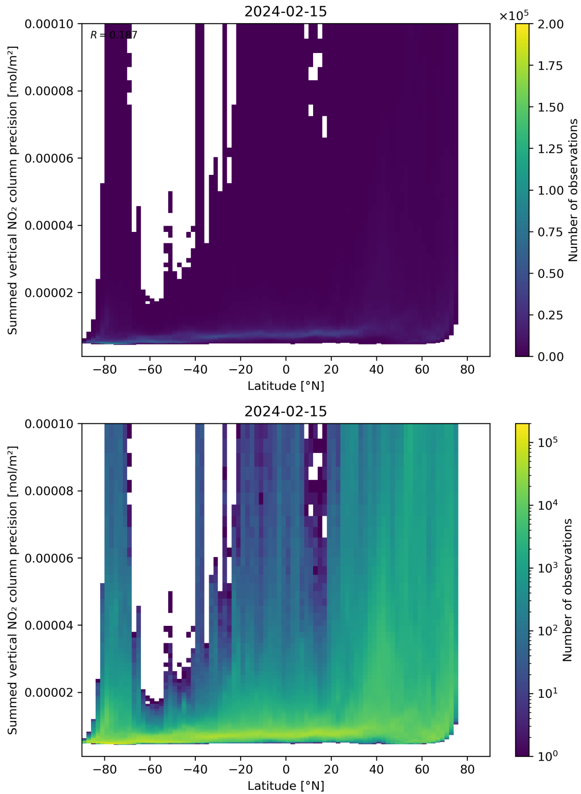
Figure 89: Scatter density plot of “Latitude” against “Summed vertical NO 2 column precision” for 2024-02-14 to 2024-02-16.
