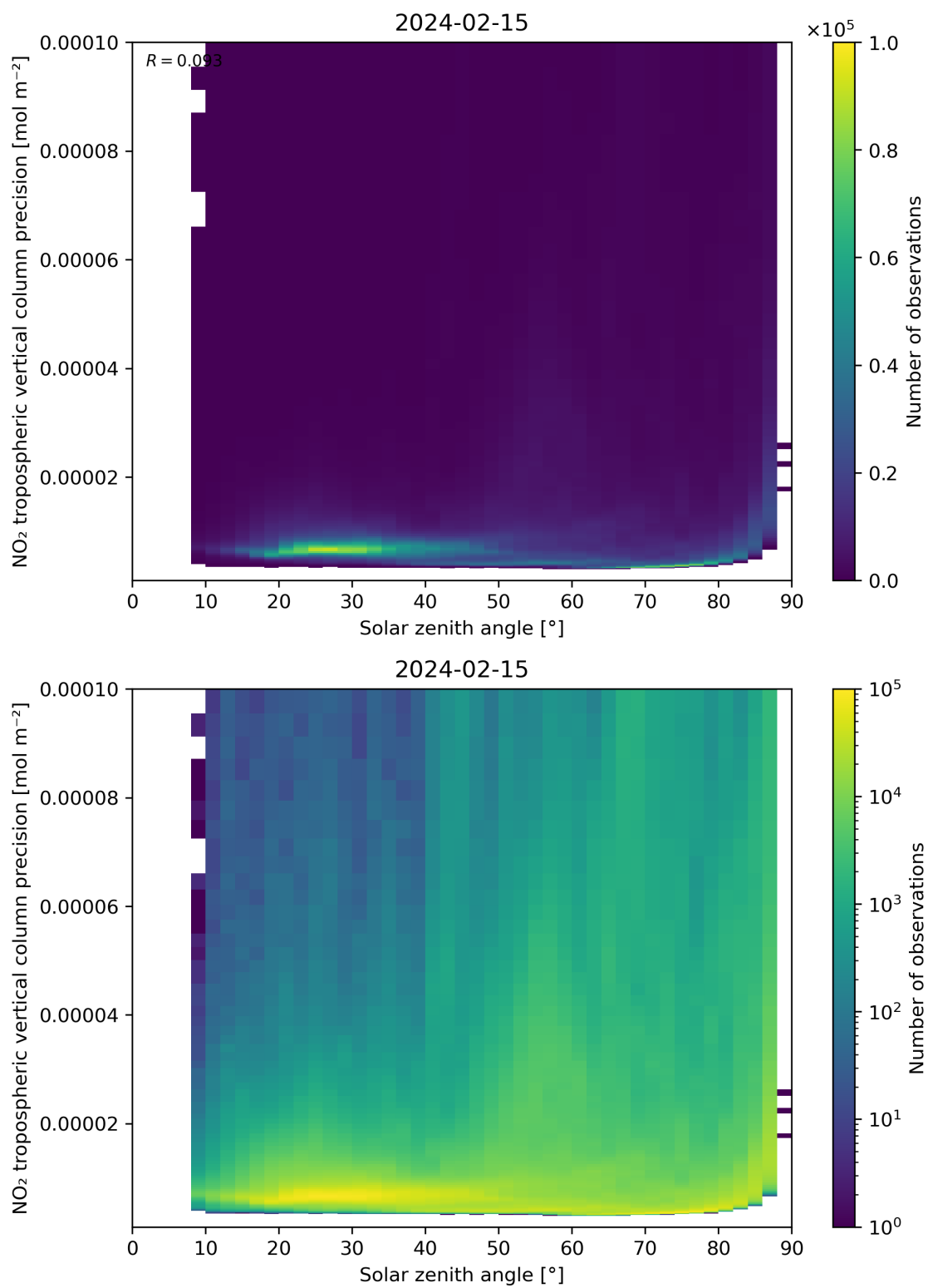
Figure 156: Scatter density plot of “Solar zenith angle” against “NO 2 tropospheric vertical column precision” for 2024-02-14 to 2024-02-16.
