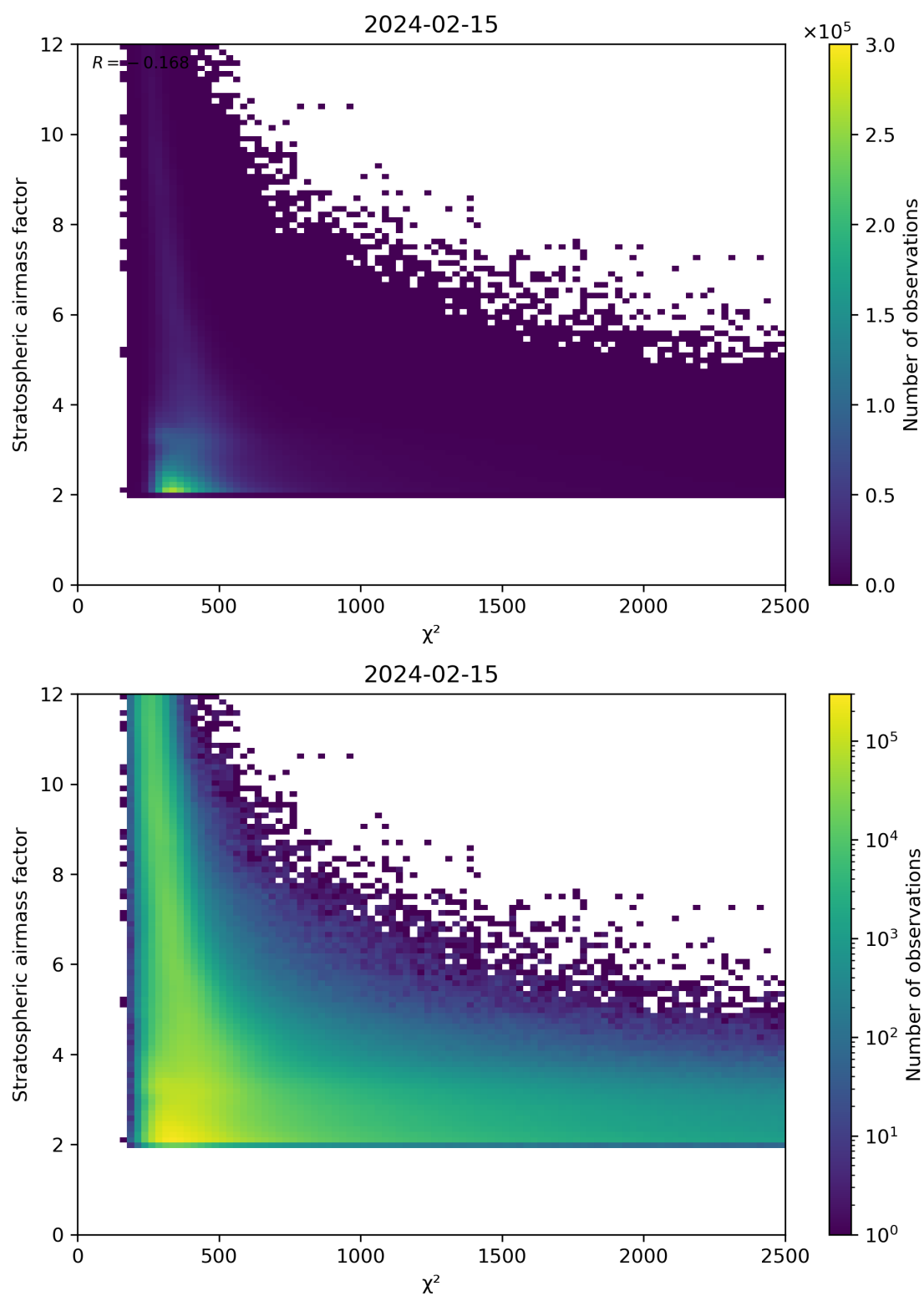
Figure 81: Scatter density plot of “ \chi^2 ” against “Stratospheric airmass factor” for 2024-02-14 to 2024-02-16.
