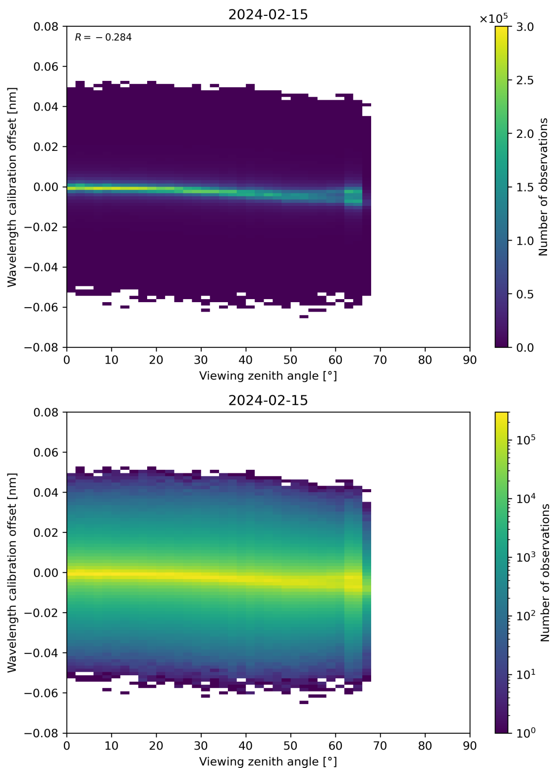
Figure 173: Scatter density plot of “Viewing zenith angle” against “Wavelength calibration offset” for 2024-02-14 to 2024-02-16.
