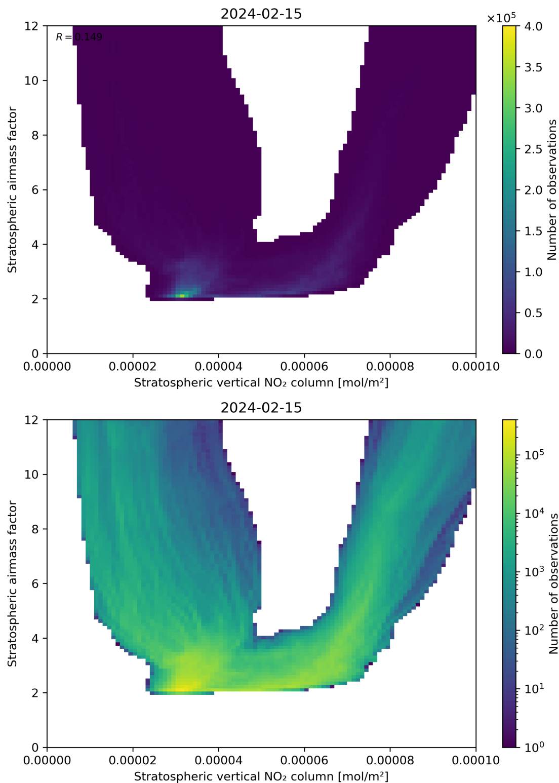
Figure 96: Scatter density plot of “Stratospheric vertical NO 2 column” against “Stratospheric airmass factor” for 2024-02-14 to 2024-02-16.
