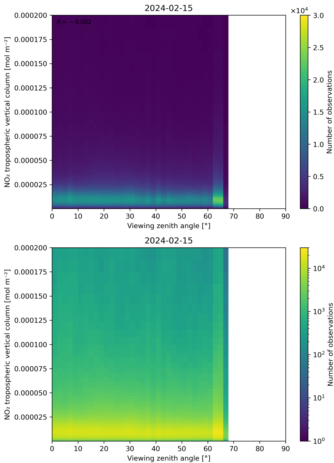
Figure 169: Scatter density plot of “Viewing zenith angle” against “NO 2 tropospheric vertical column” for 2024-02-14 to 2024-02-16.
