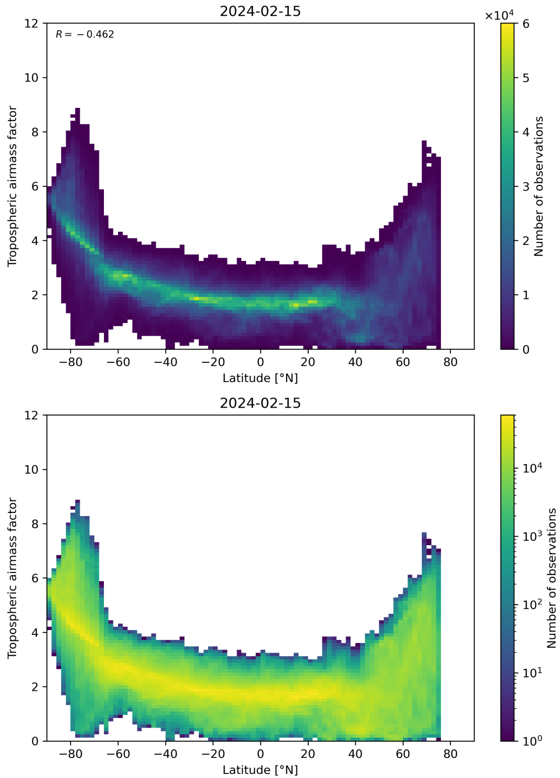
Figure 85: Scatter density plot of “Latitude” against “Tropospheric airmass factor” for 2024-02-14 to 2024-02-16.
