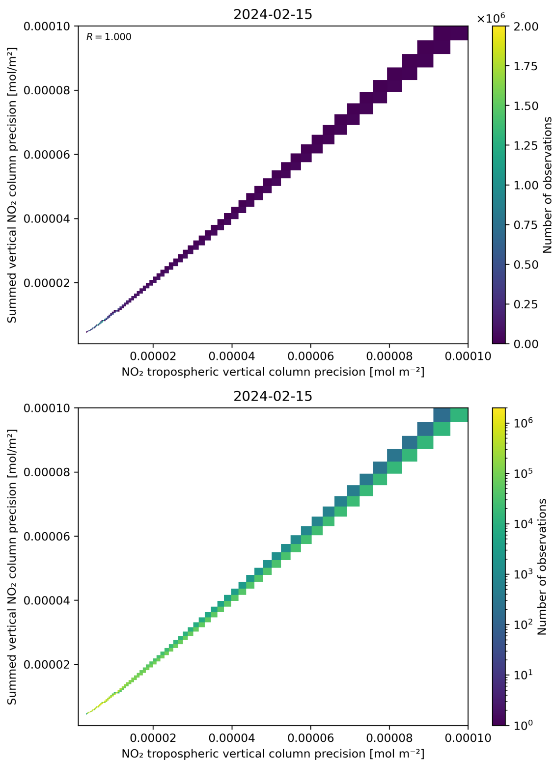
Figure 137: Scatter density plot of “NO 2 tropospheric vertical column precision” against “Summed vertical NO 2 column precision” for 2024-02-14 to 2024-02-16.
