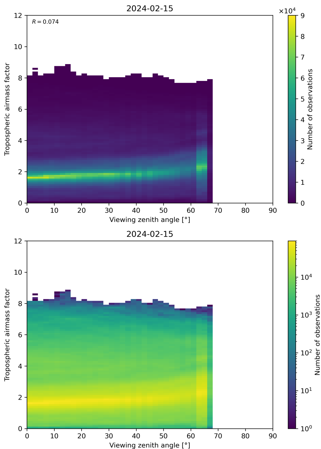
Figure 161: Scatter density plot of “Viewing zenith angle” against “Tropospheric airmass factor” for 2024-02-14 to 2024-02-16.
