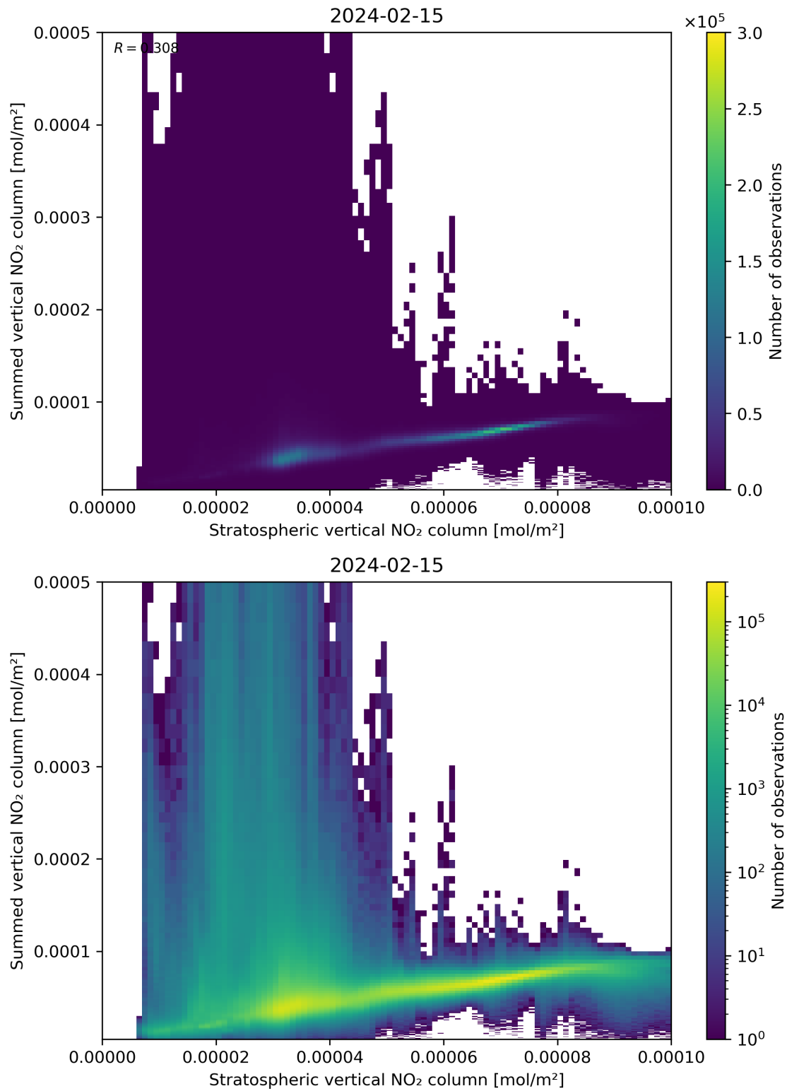
Figure 98: Scatter density plot of “Stratospheric vertical NO 2 column” against “Summed vertical NO 2 column” for 2024-02-14 to 2024-02-16.
