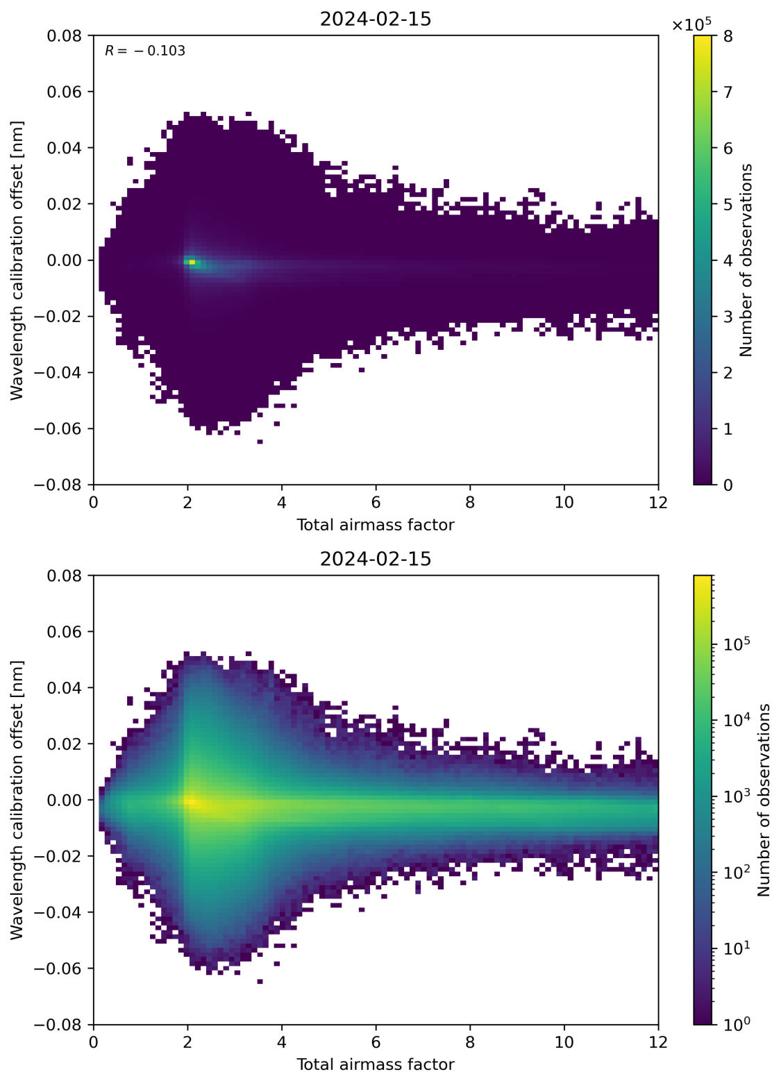
Figure 70: Scatter density plot of “Total airmass factor” against “Wavelength calibration offset” for 2024-02-14 to 2024-02-16.
