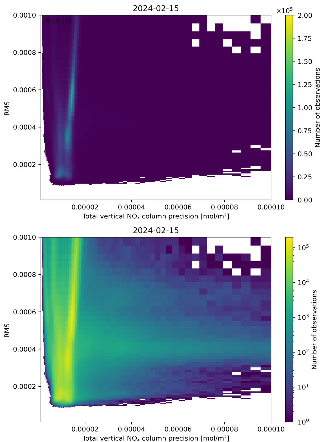
Figure 119: Scatter density plot of “Total vertical NO 2 column precision” against “RMS” for 2024-02-14 to 2024-02-16.
