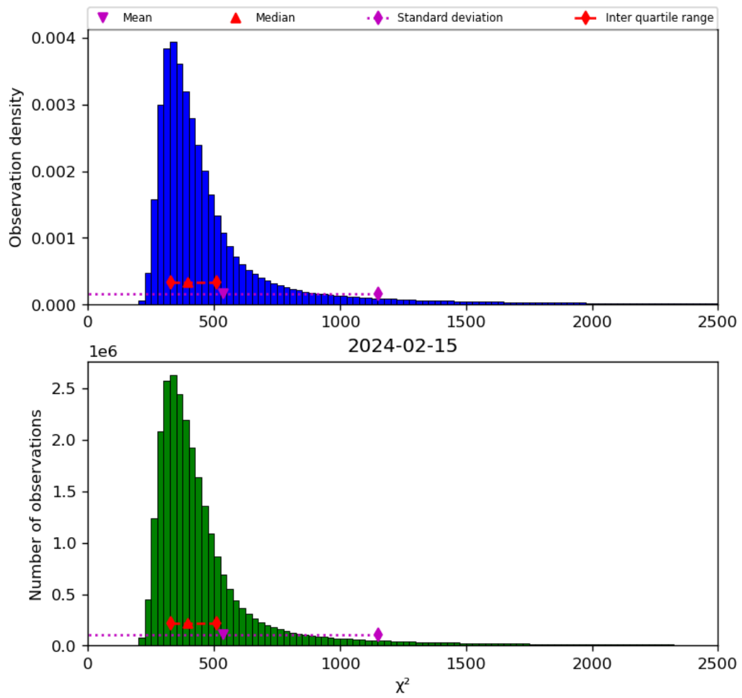
Figure 42: Histogram of “ \chi^2 ” for 2024-02-14 to 2024-02-16
