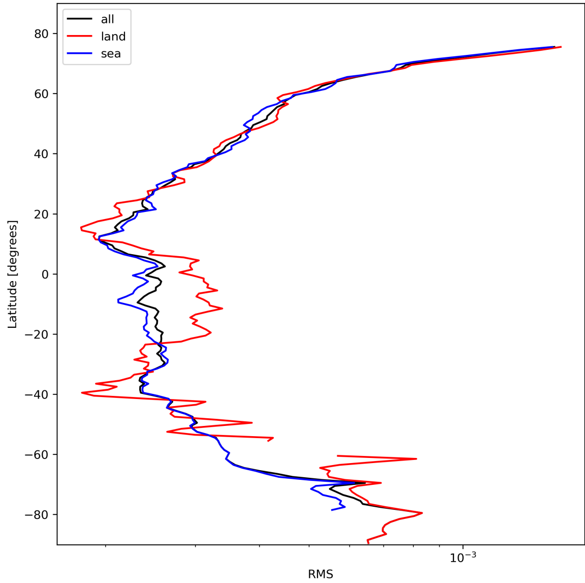
Figure 26: Zonal average of “RMS” for 2024-02-16 to 2024-02-17.
