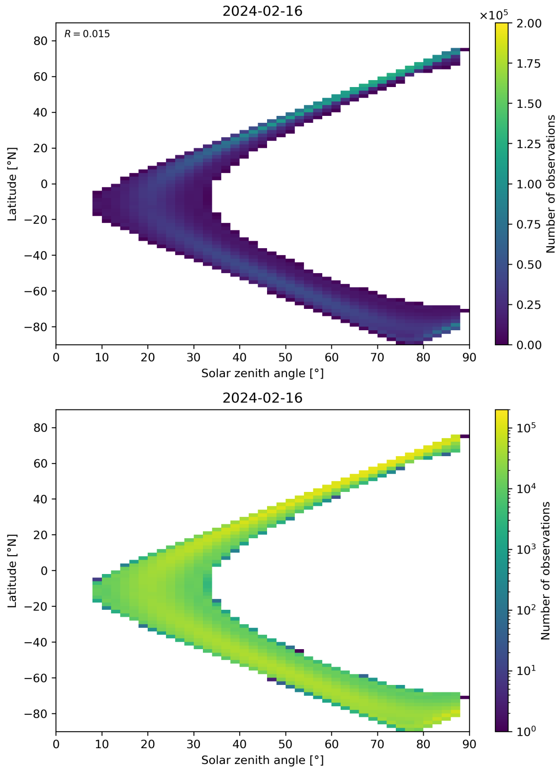
Figure 149: Scatter density plot of “Solar zenith angle” against “Latitude” for 2024-02-16 to 2024-02-17.
