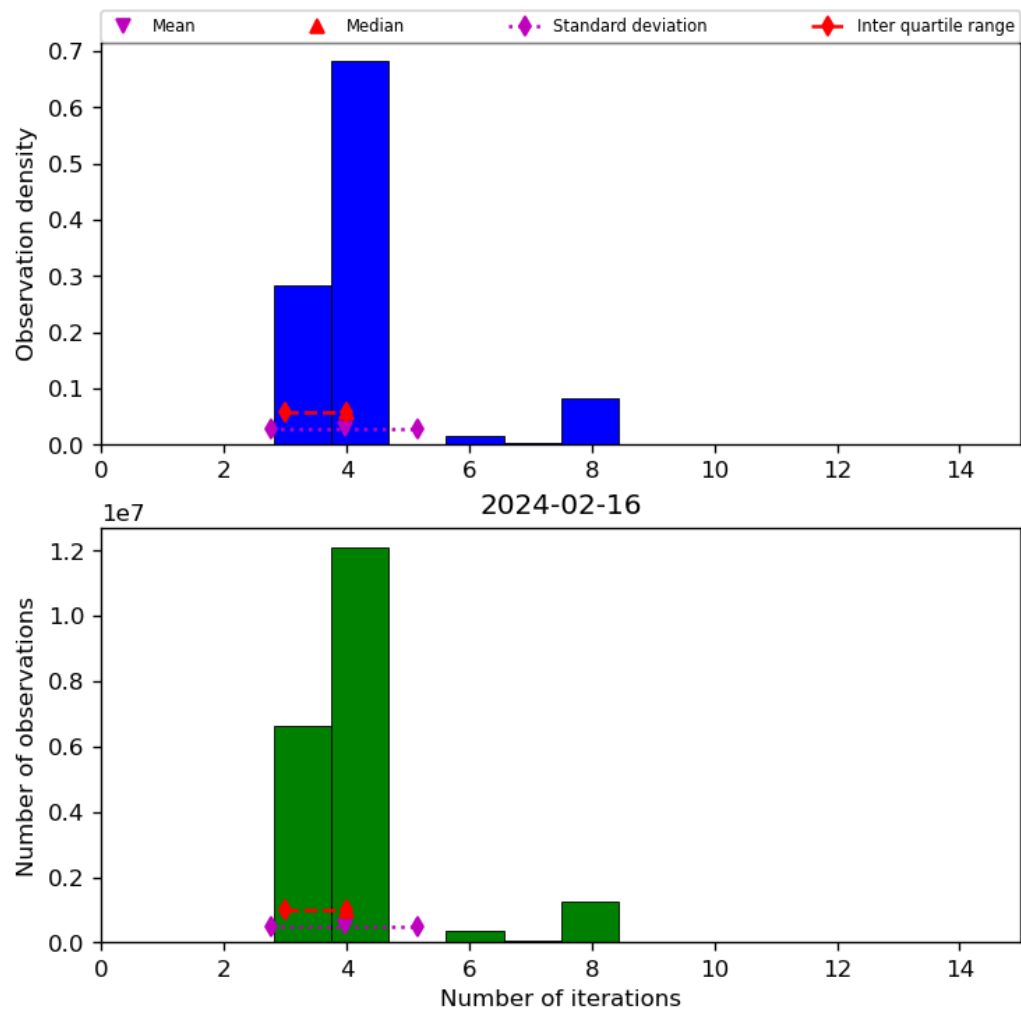
Figure 34: Histogram of “Number of iterations” for 2024-02-16 to 2024-02-17
