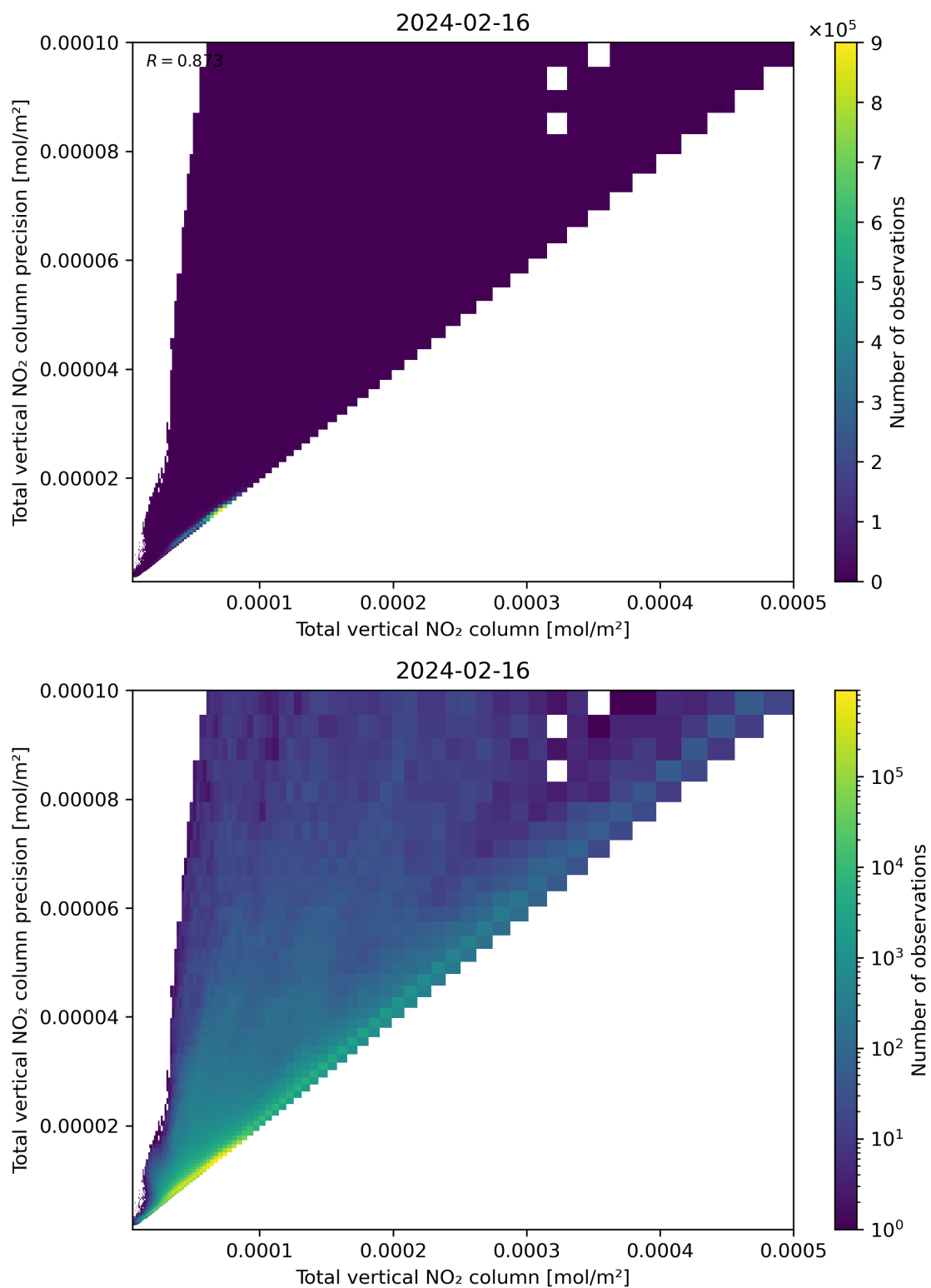
Figure 114: Scatter density plot of “Total vertical NO 2 column” against “Total vertical NO 2 column precision” for 2024-02-16 to 2024-02-17.
