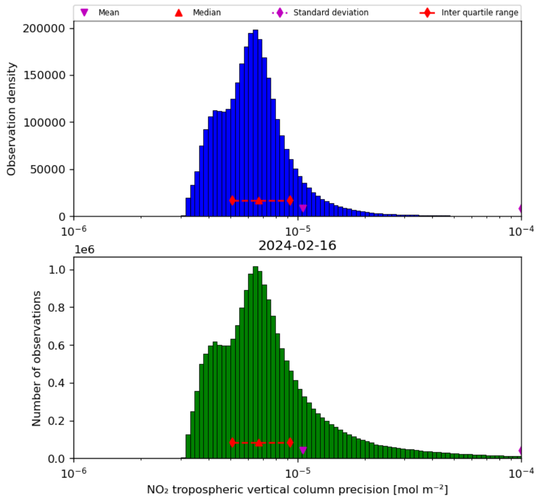
Figure 30: Histogram of “NO 2 tropospheric vertical column precision” for 2024-02-16 to 2024-02-17
