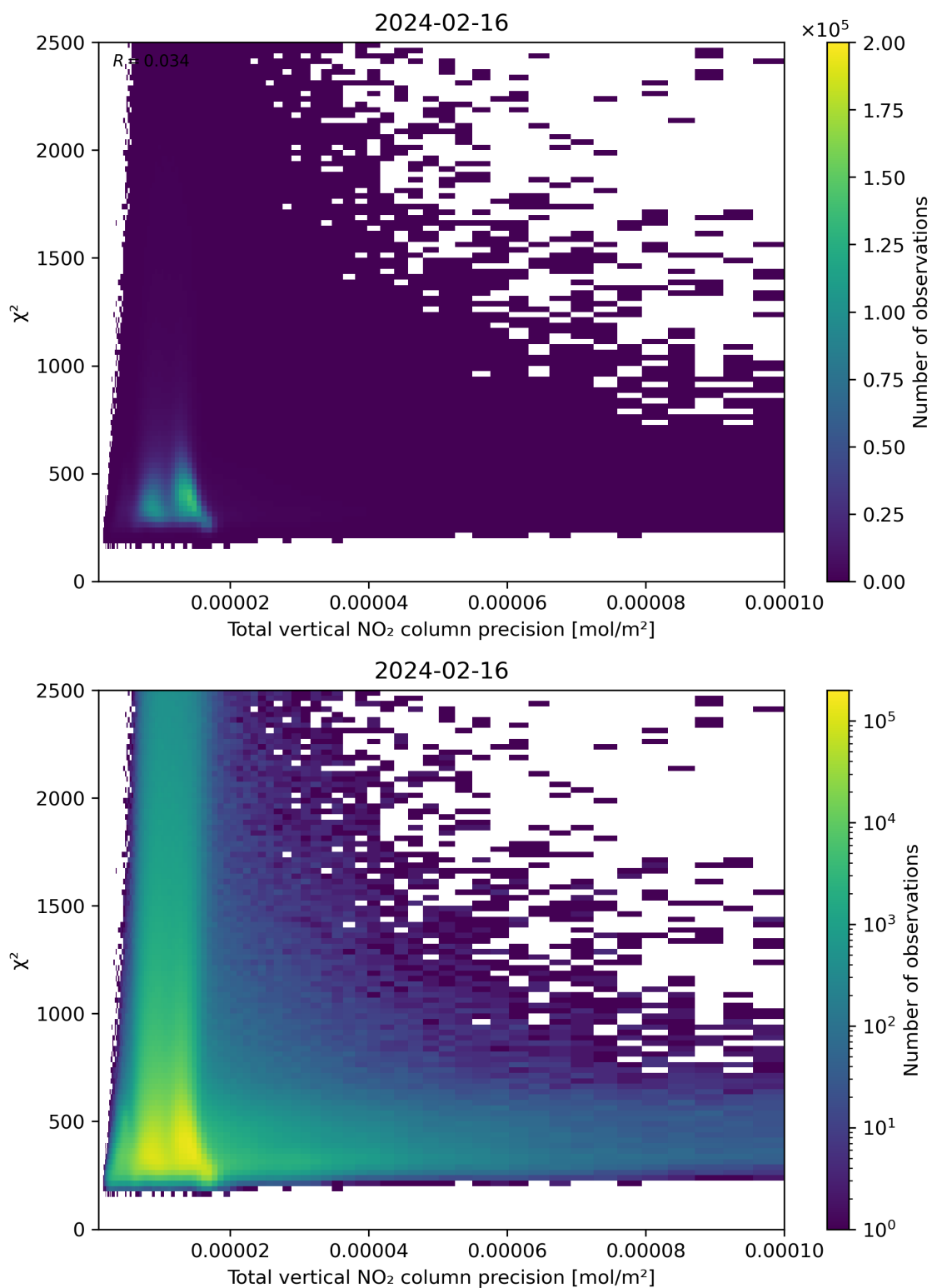
Figure 116: Scatter density plot of “Total vertical NO 2 column precision” against “ \chi^2 ” for 2024-02-16 to 2024-02-17.
