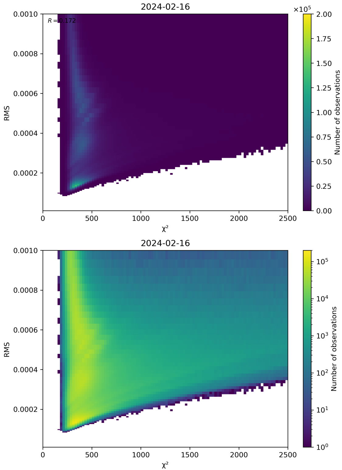
Figure 82: Scatter density plot of “ \chi^2 ” against “RMS” for 2024-02-16 to 2024-02-17.
