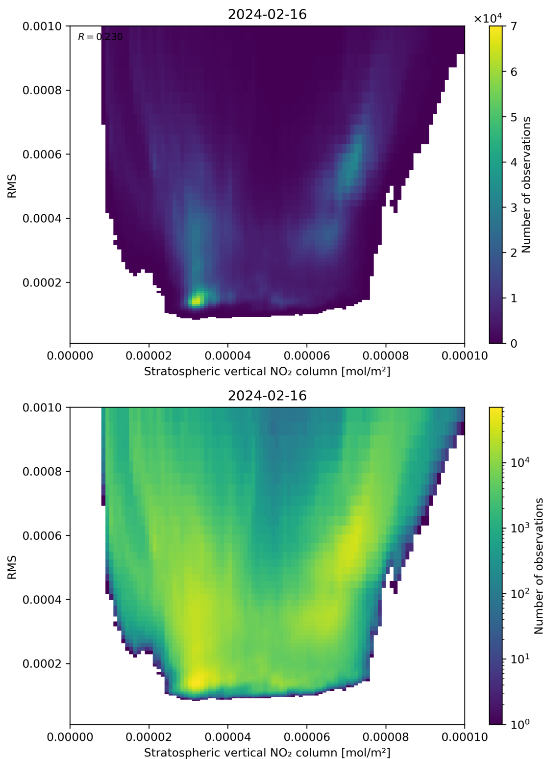
Figure 102: Scatter density plot of “Stratospheric vertical NO 2 column” against “RMS” for 2024-02-16 to 2024-02-17.
