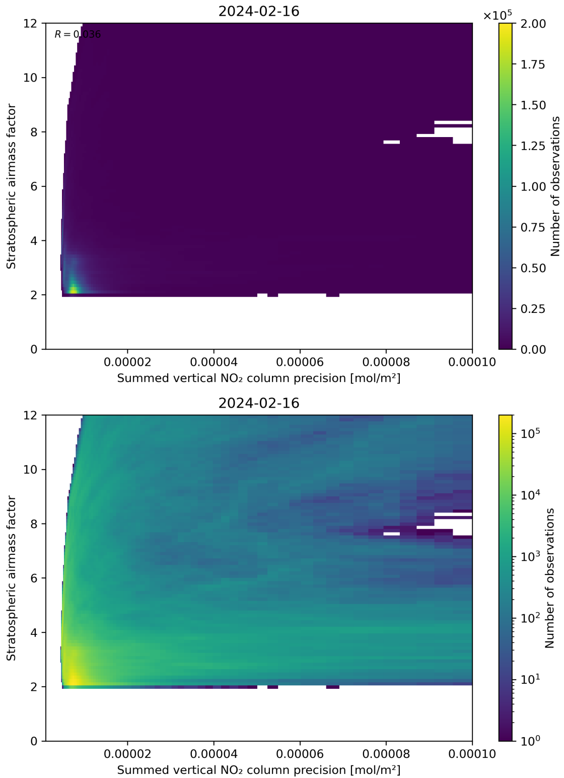
Figure 106: Scatter density plot of “Summed vertical NO 2 column precision” against “Stratospheric airmass factor” for 2024-02-16 to 2024-02-17.
