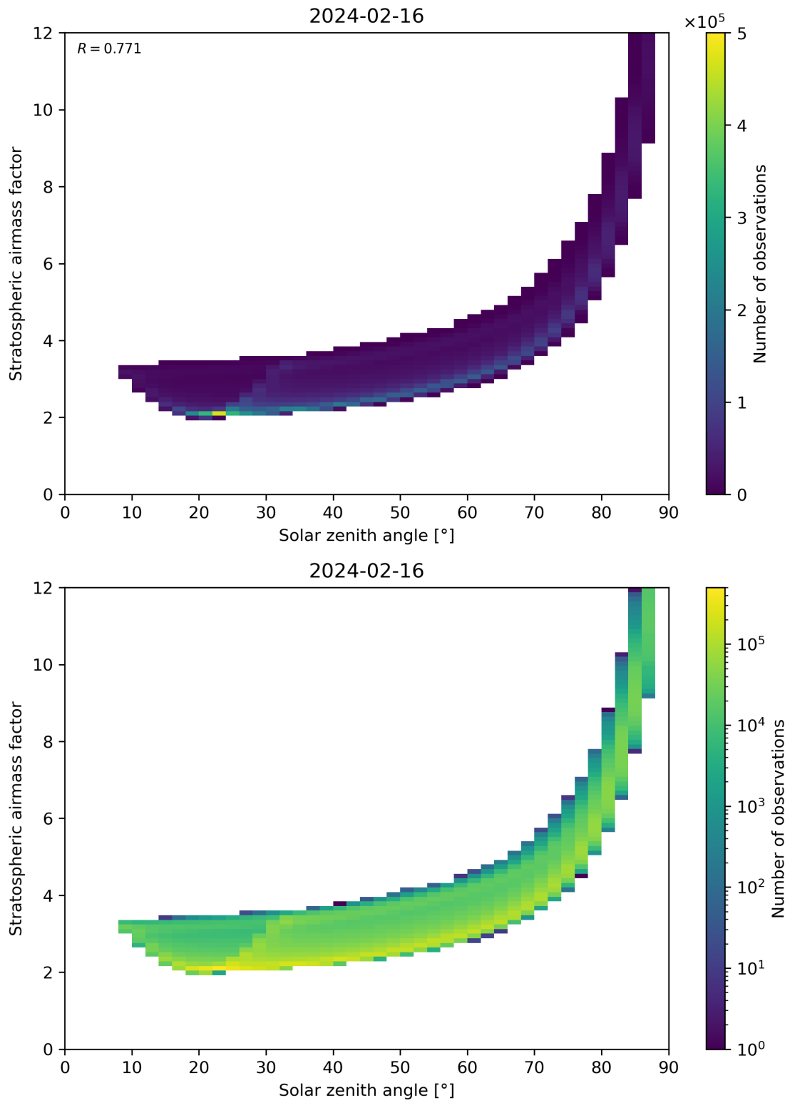
Figure 145: Scatter density plot of “Solar zenith angle” against “Stratospheric airmass factor” for 2024-02-16 to 2024-02-17.
