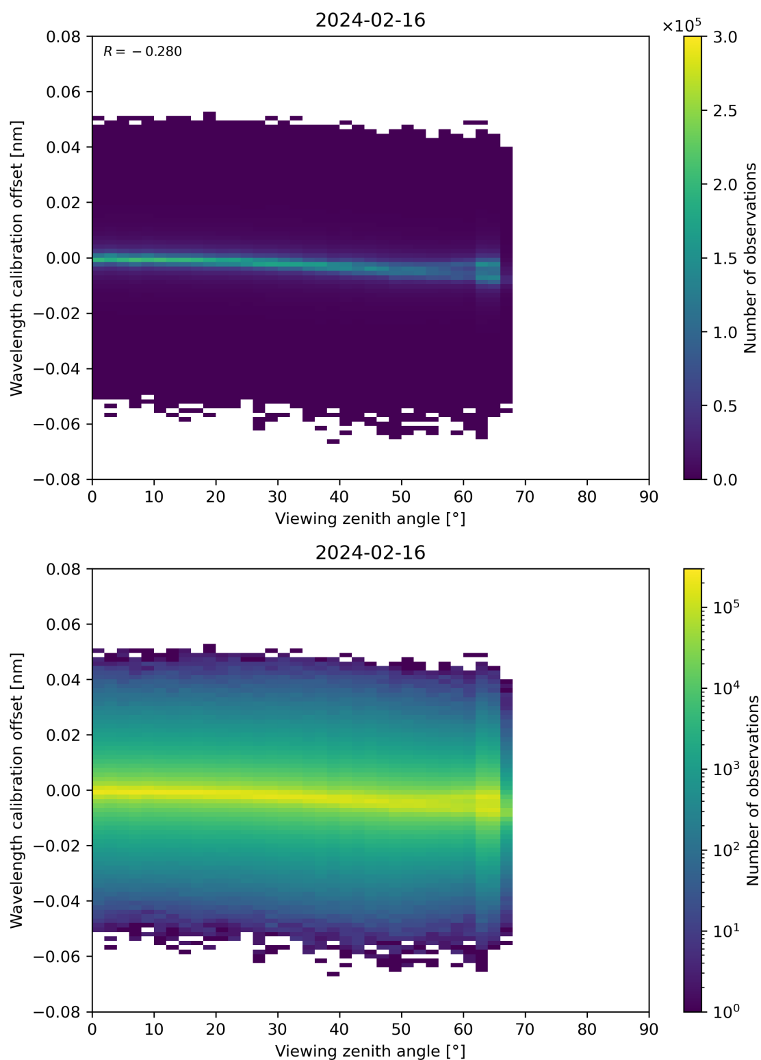
Figure 173: Scatter density plot of “Viewing zenith angle” against “Wavelength calibration offset” for 2024-02-16 to 2024-02-17.
