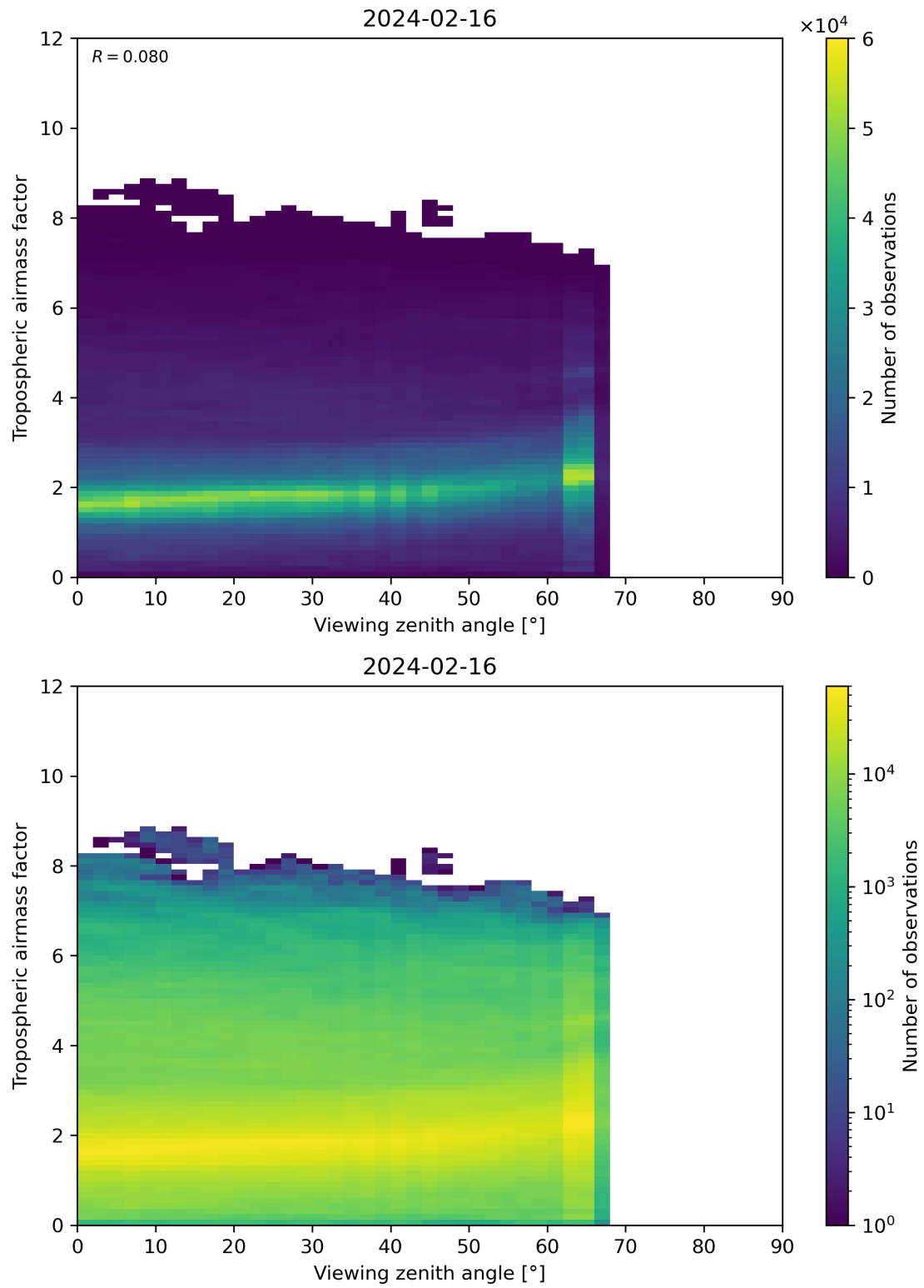
Figure 161: Scatter density plot of “Viewing zenith angle” against “Tropospheric airmass factor” for 2024-02-16 to 2024-02-17.
