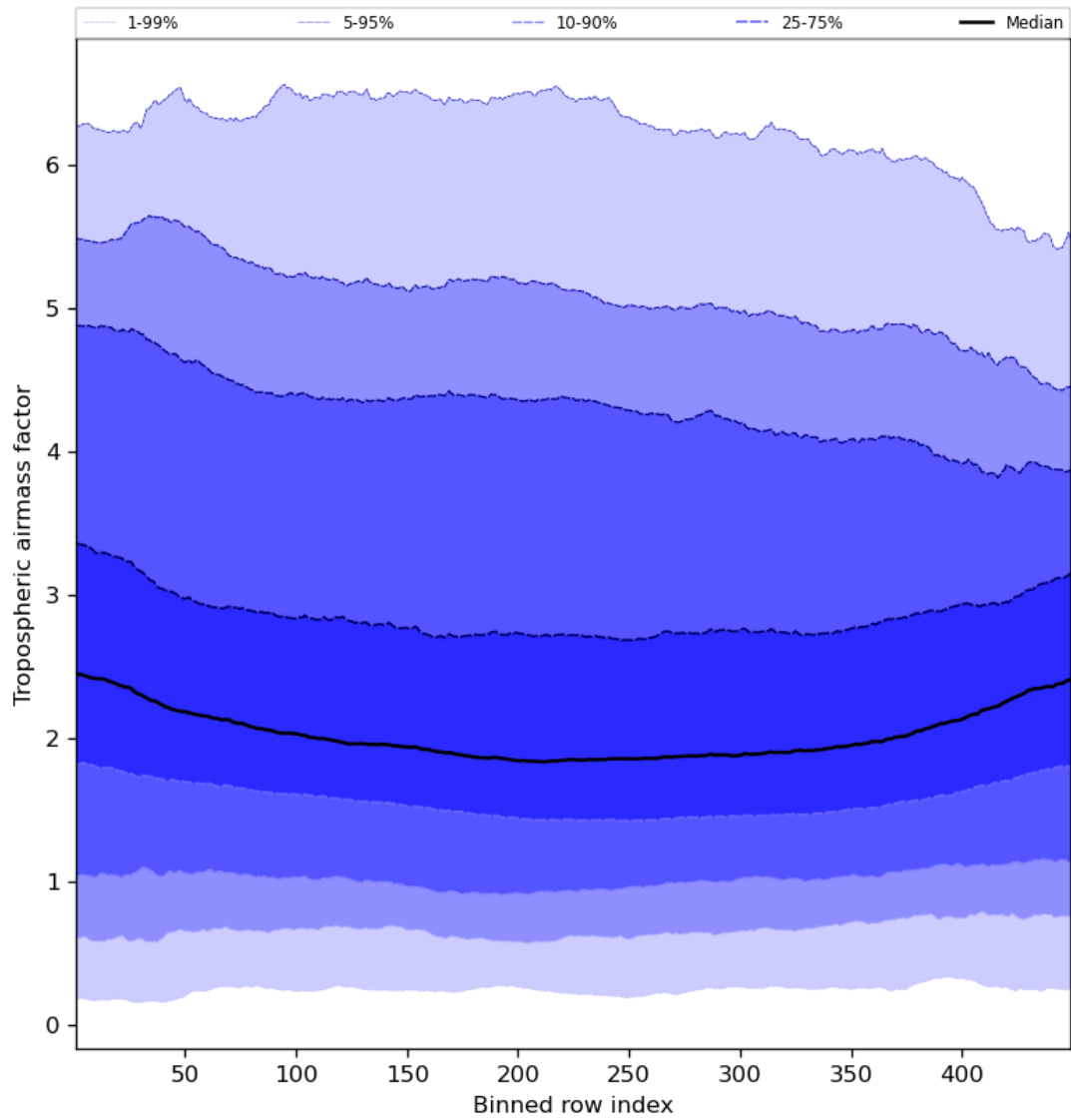
Figure 48: Along track statistics of “Tropospheric airmass factor” for 2024-02-16 to 2024-02-17
