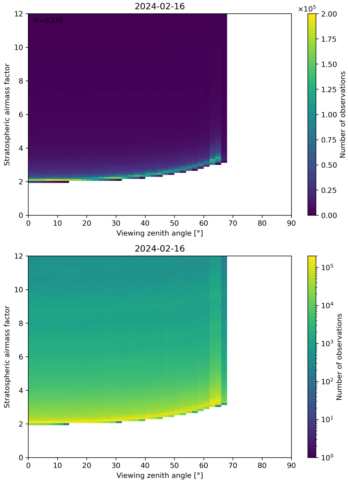
Figure 159: Scatter density plot of “Viewing zenith angle” against “Stratospheric airmass factor” for 2024-02-16 to 2024-02-17.
