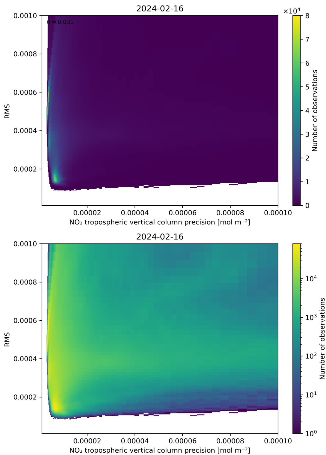
Figure 140: Scatter density plot of “NO 2 tropospheric vertical column precision” against “RMS” for 2024-02-16 to 2024-02-17.
