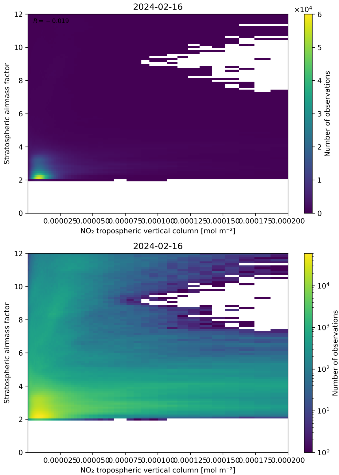
Figure 121: Scatter density plot of “NO 2 tropospheric vertical column” against “Stratospheric airmass factor” for 2024-02-16 to 2024-02-17.
