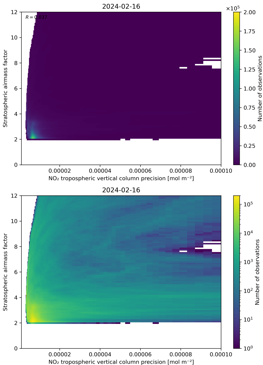
Figure 131: Scatter density plot of “NO 2 tropospheric vertical column precision” against “Stratospheric airmass factor” for 2024-02-16 to 2024-02-17.
