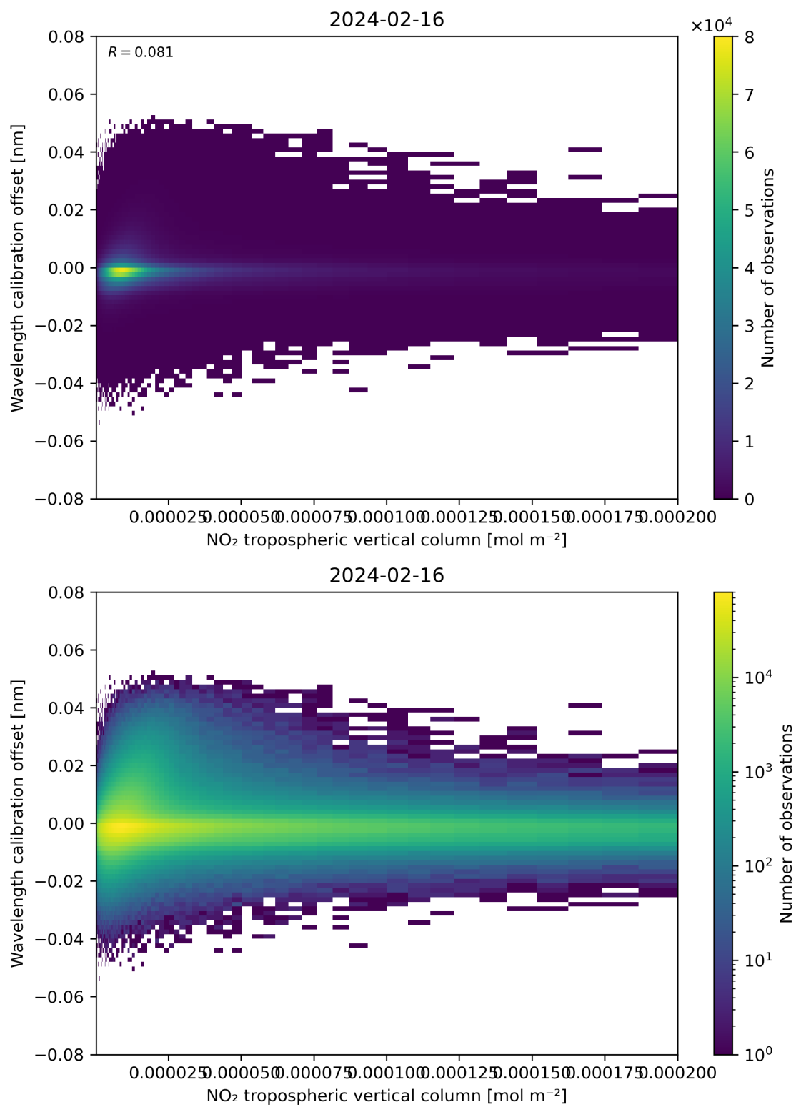
Figure 143: Scatter density plot of “NO 2 tropospheric vertical column” against “Wavelength calibration offset” for 2024-02-16 to 2024-02-17.
