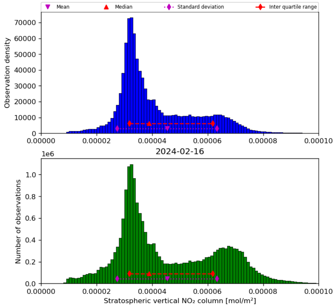
Figure 36: Histogram of “Stratospheric vertical NO 2 column” for 2024-02-16 to 2024-02-17
