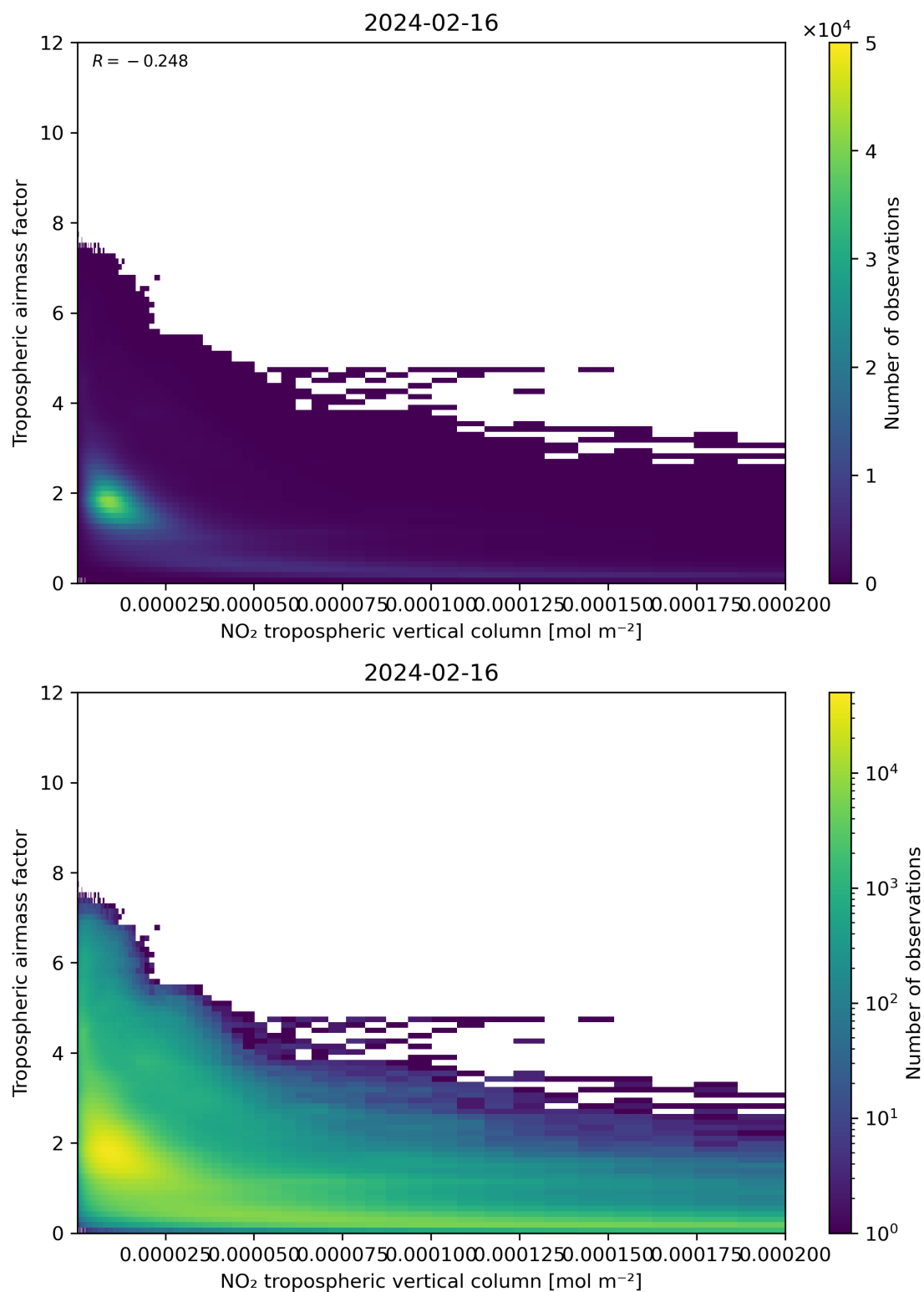
Figure 123: Scatter density plot of “NO 2 tropospheric vertical column” against “Tropospheric airmass factor” for 2024-02-16 to 2024-02-17.
