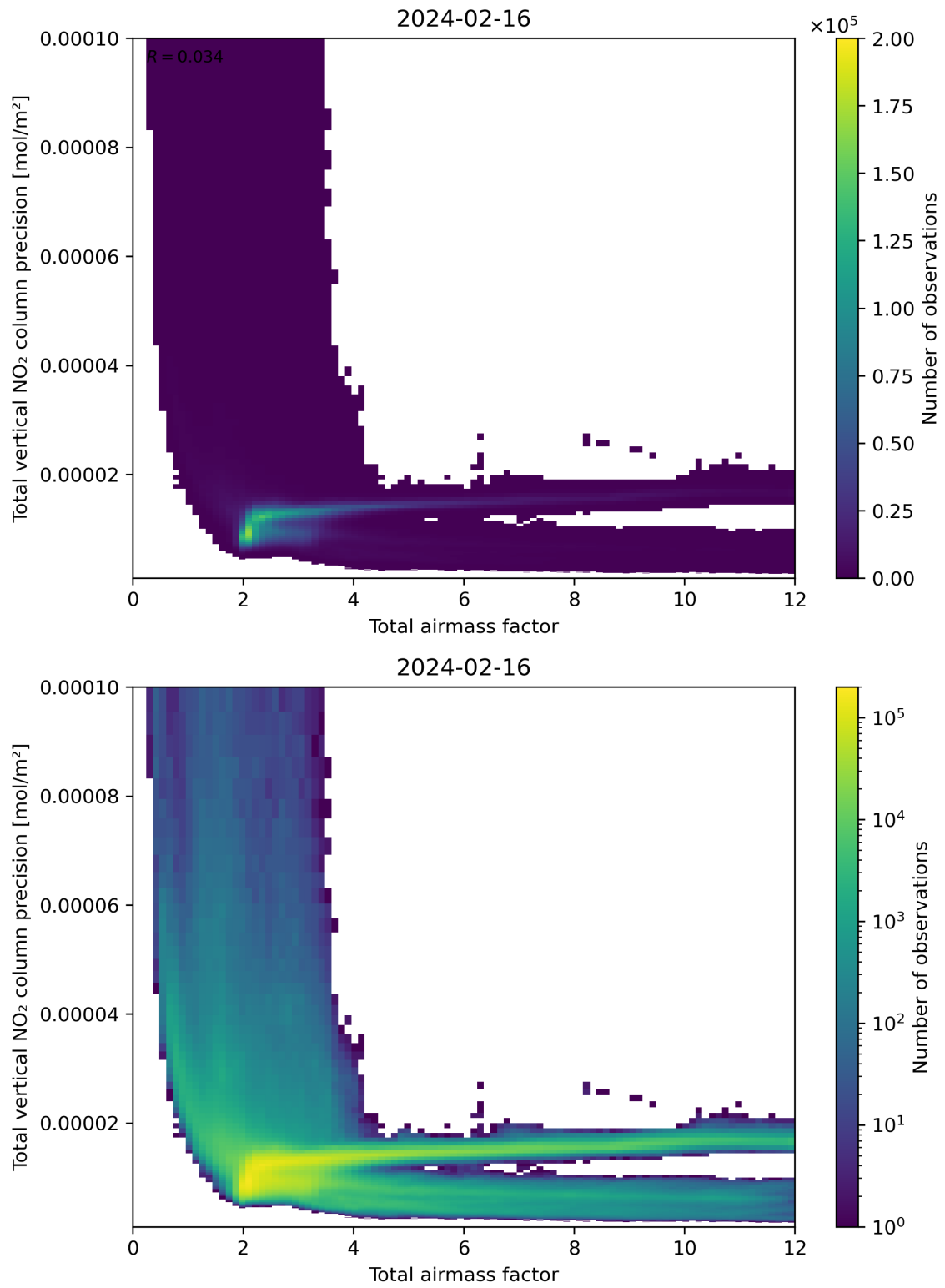
Figure 68: Scatter density plot of “Total airmass factor” against “Total vertical NO 2 column precision” for 2024-02-16 to 2024-02-17.
