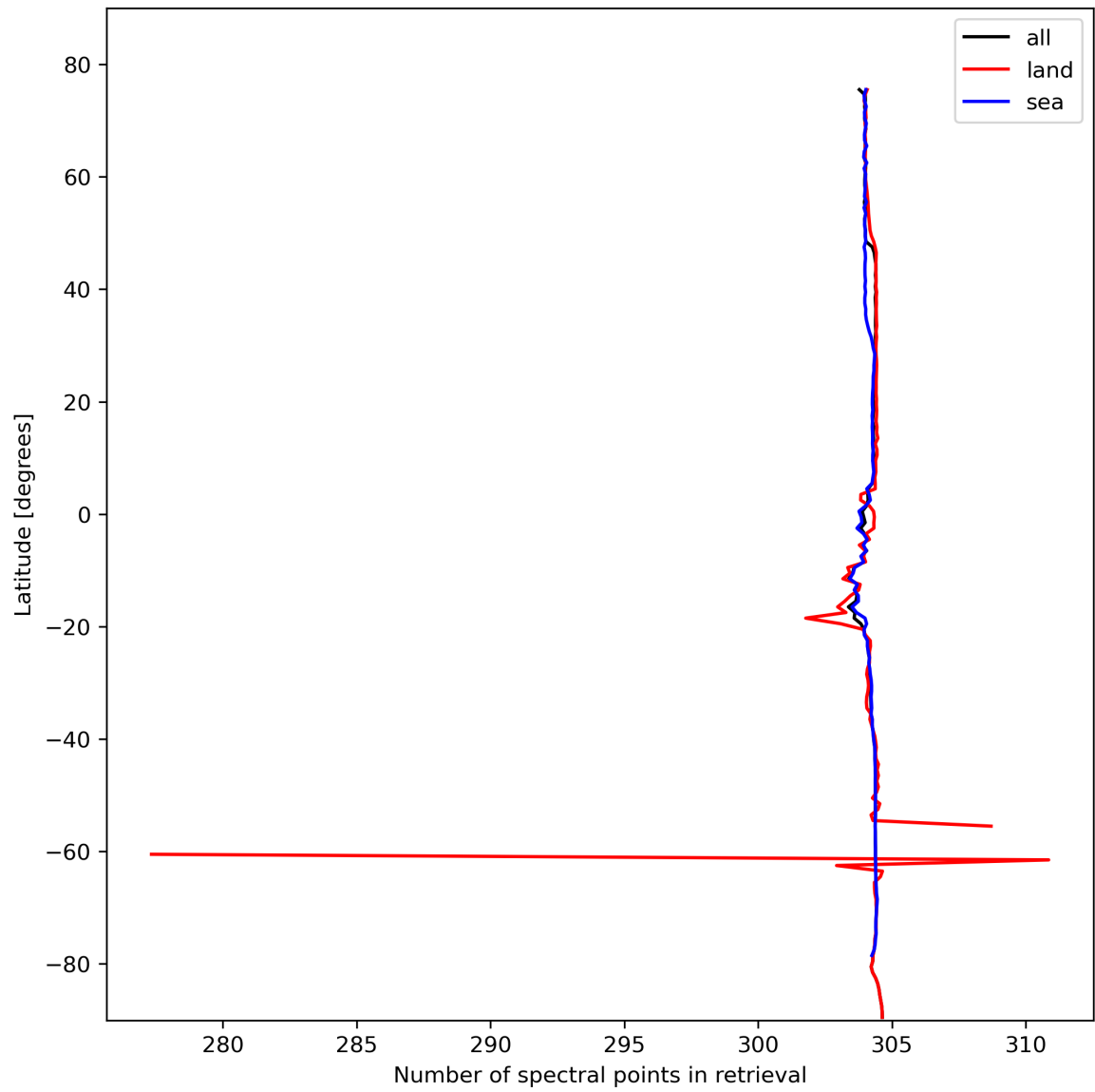
Figure 16: Zonal average of “Number of spectral points in retrieval” for 2024-02-16 to 2024-02-17.
