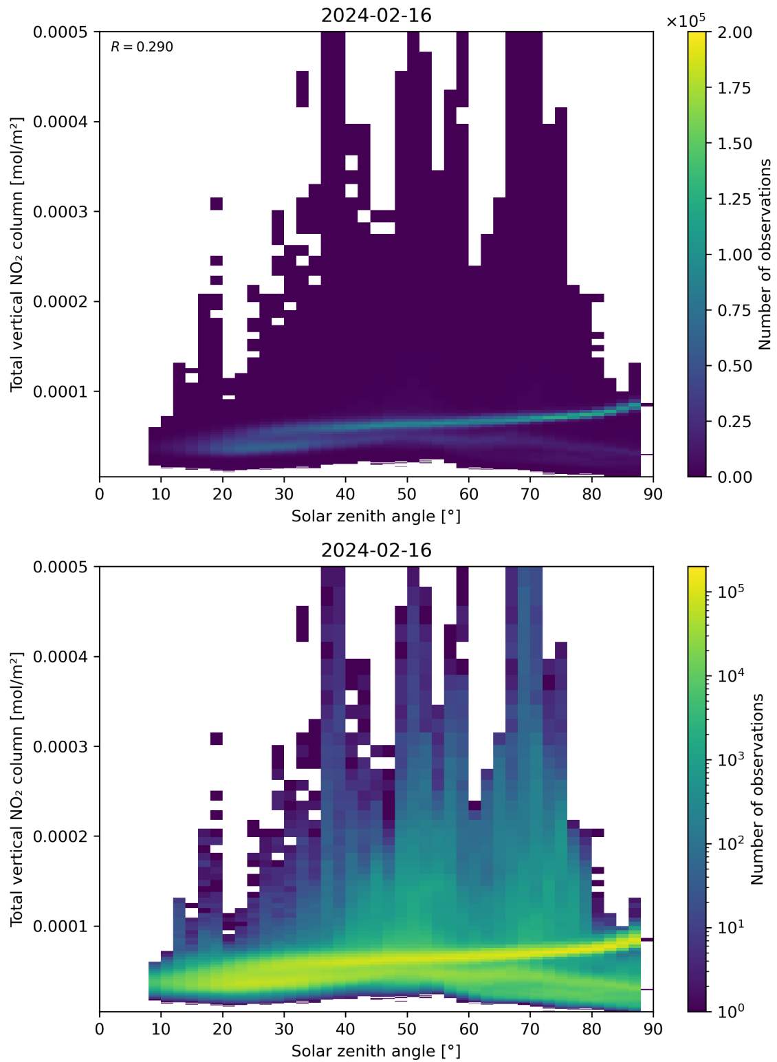
Figure 153: Scatter density plot of “Solar zenith angle” against “Total vertical NO 2 column” for 2024-02-16 to 2024-02-17.
