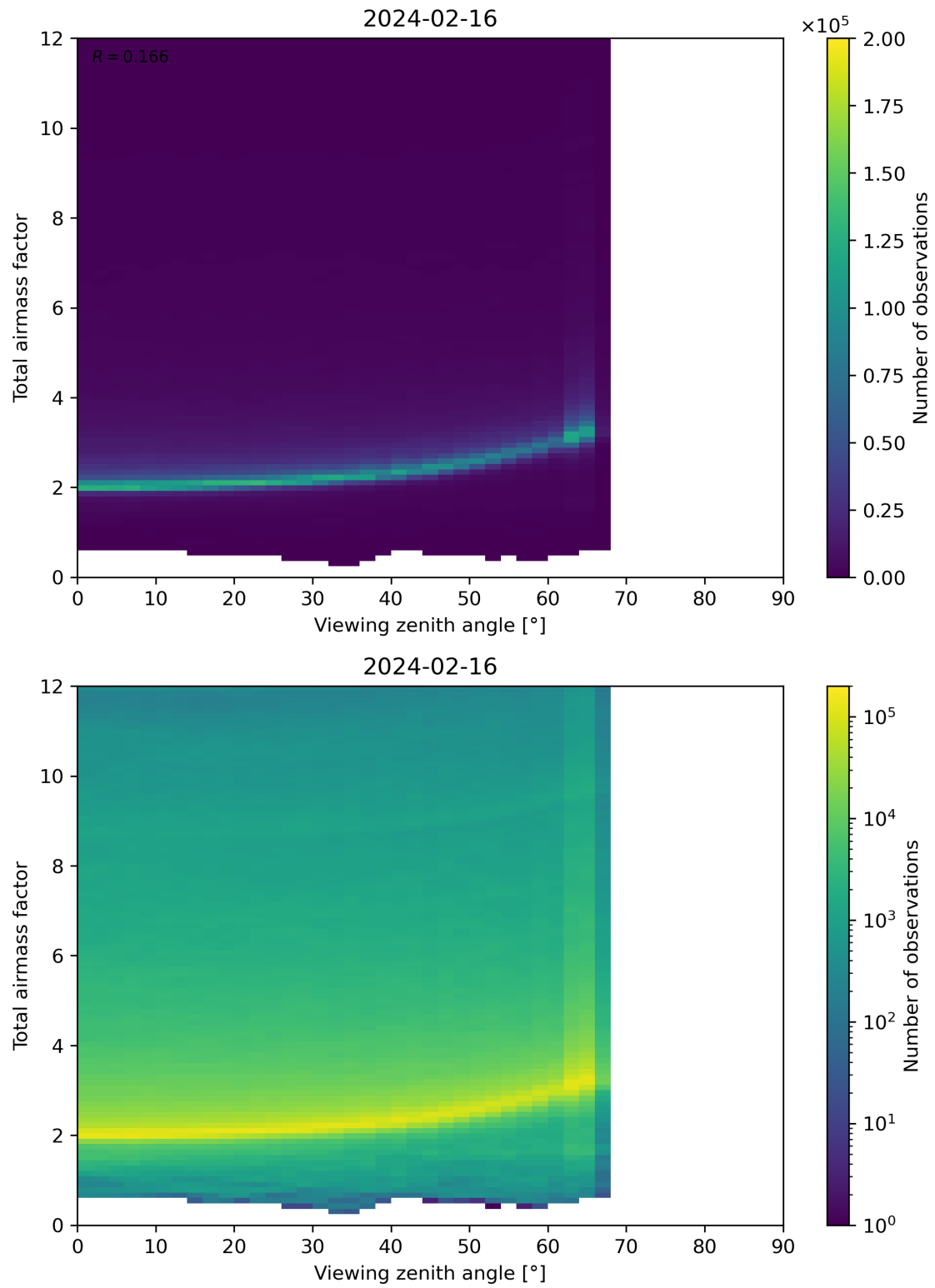
Figure 160: Scatter density plot of “Viewing zenith angle” against “Total airmass factor” for 2024-02-16 to 2024-02-17.
