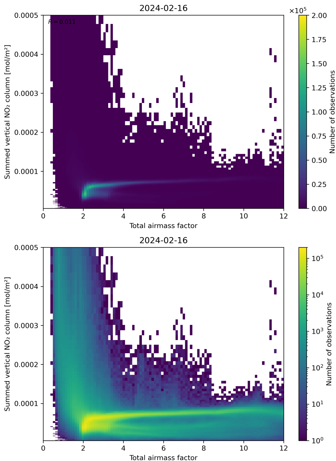
Figure 65: Scatter density plot of “Total airmass factor” against “Summed vertical NO 2 column” for 2024-02-16 to 2024-02-17.
