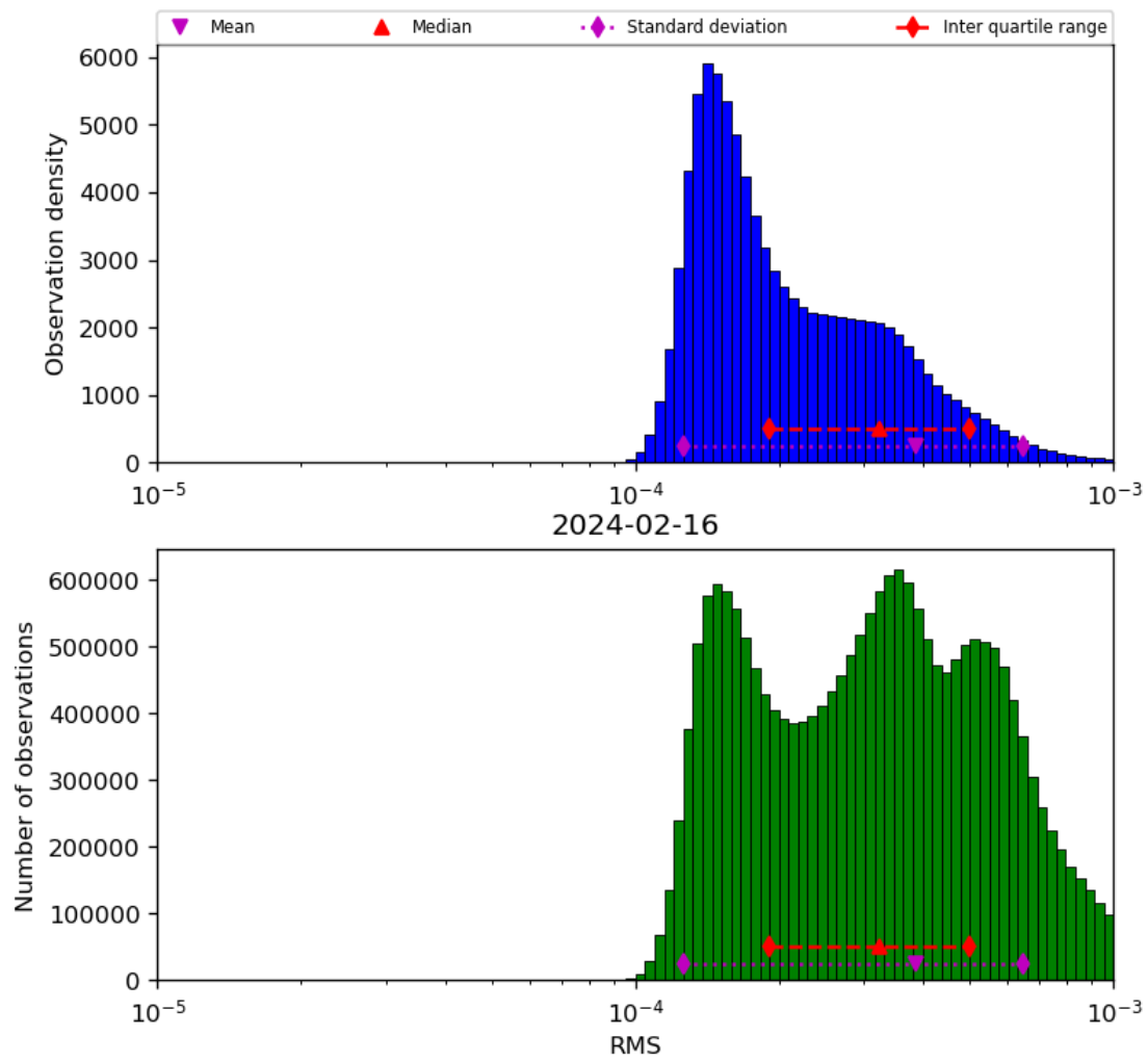
Figure 43: Histogram of “RMS” for 2024-02-16 to 2024-02-17
