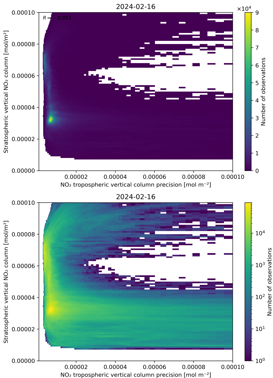
Figure 135: Scatter density plot of “NO 2 tropospheric vertical column precision” against “Stratospheric vertical NO 2 column” for 2024-02-16 to 2024-02-17.
