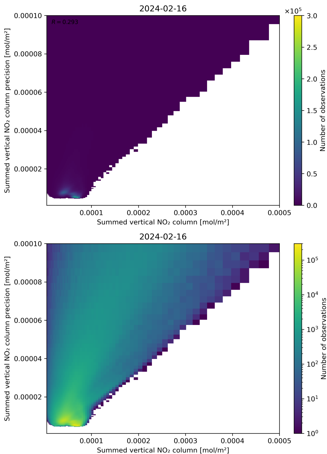
Figure 105: Scatter density plot of “Summed vertical NO 2 column” against “Summed vertical NO 2 column precision” for 2024-02-16 to 2024-02-17.
