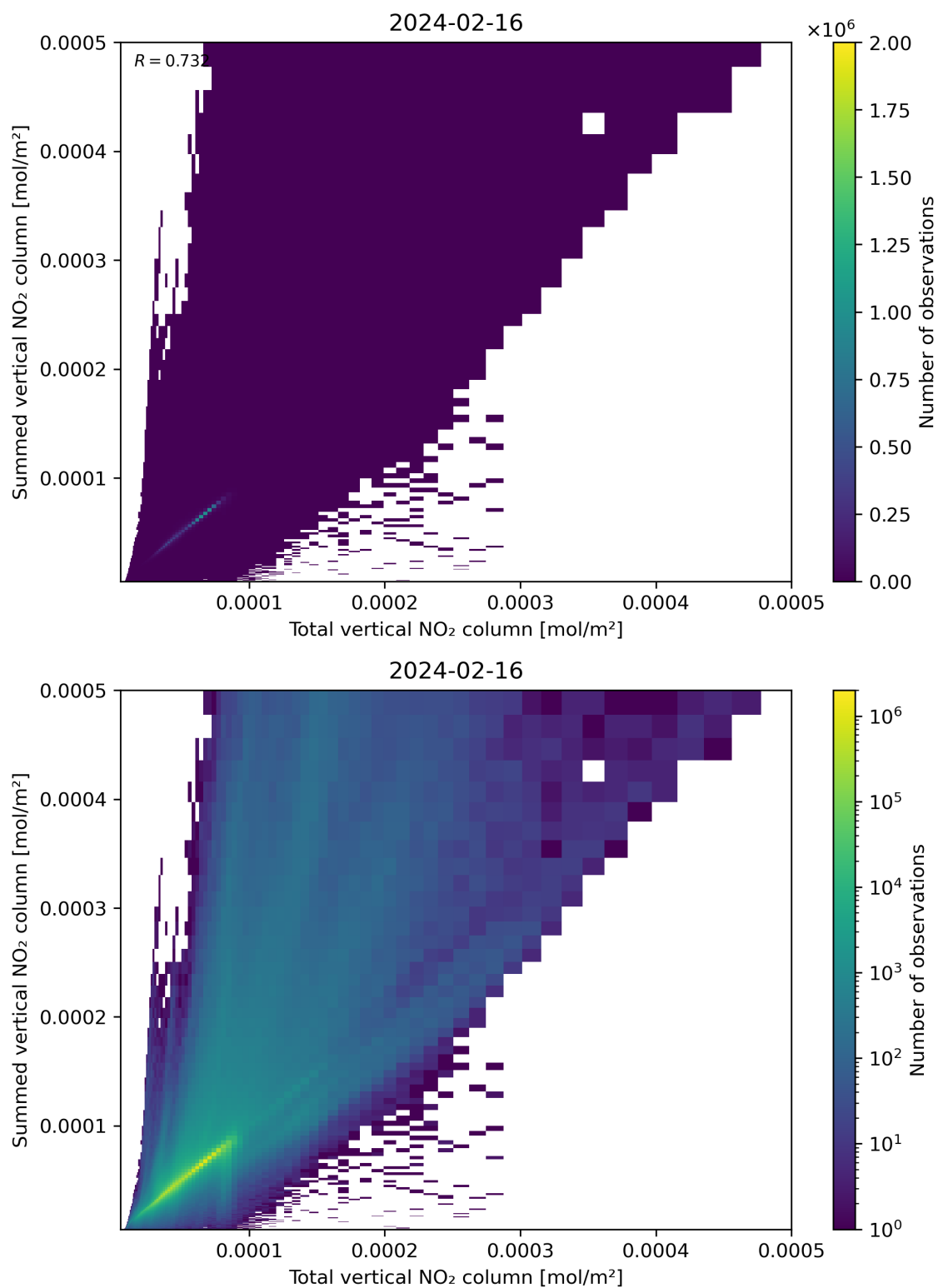
Figure 112: Scatter density plot of “Total vertical NO 2 column” against “Summed vertical NO 2 column” for 2024-02-16 to 2024-02-17.
