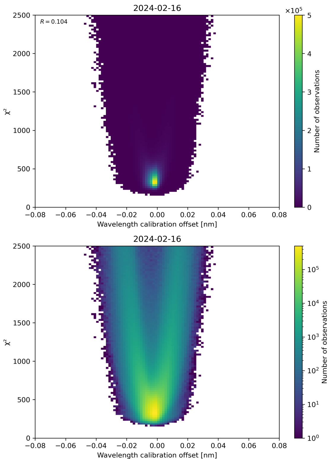
Figure 175: Scatter density plot of “Wavelength calibration offset” against “ \chi^2 ” for 2024-02-16 to 2024-02-17.
