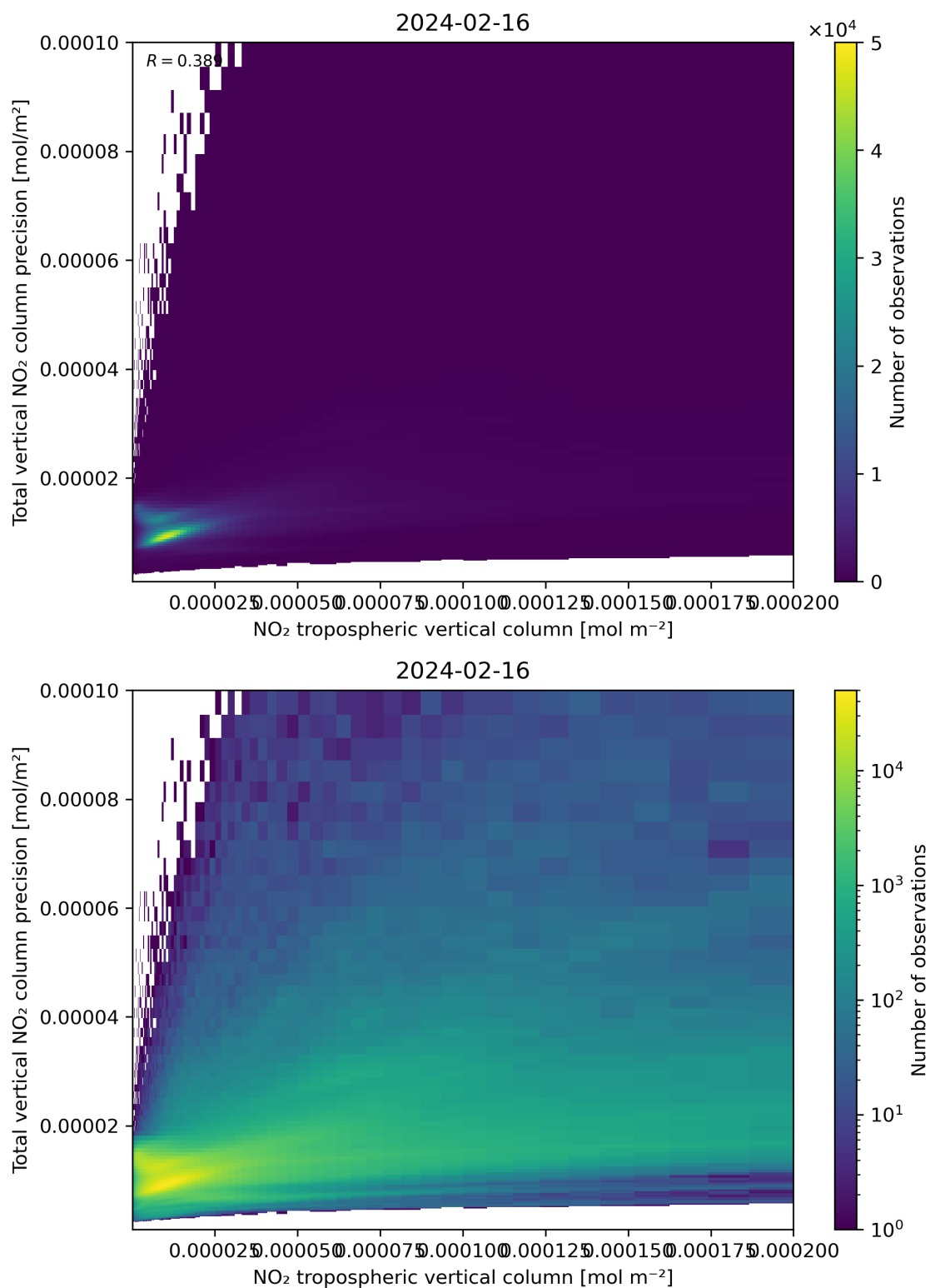
Figure 129: Scatter density plot of “NO 2 tropospheric vertical column” against “Total vertical NO 2 column precision” for 2024-02-16 to 2024-02-17.
