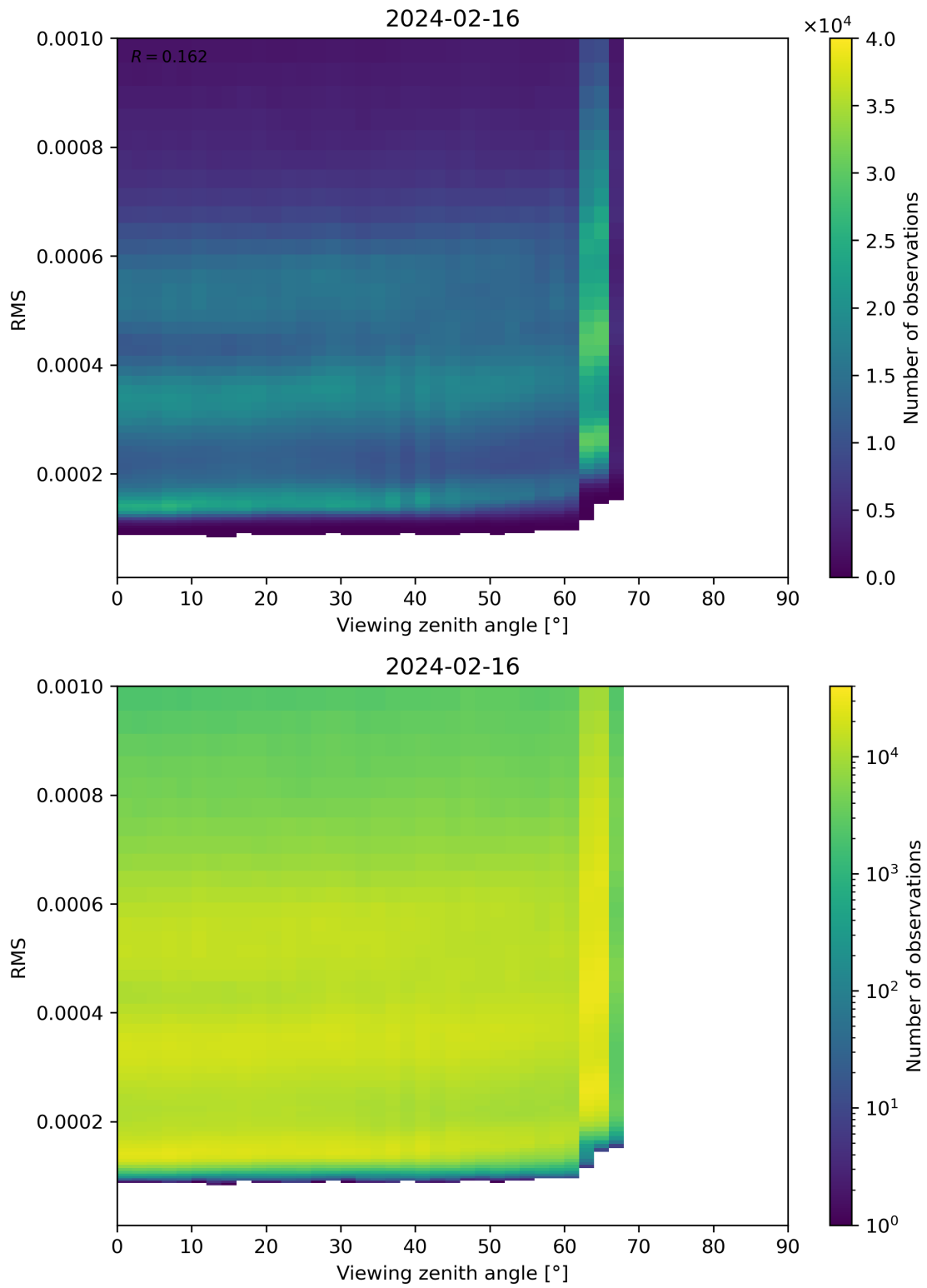
Figure 171: Scatter density plot of “Viewing zenith angle” against “RMS” for 2024-02-16 to 2024-02-17.
