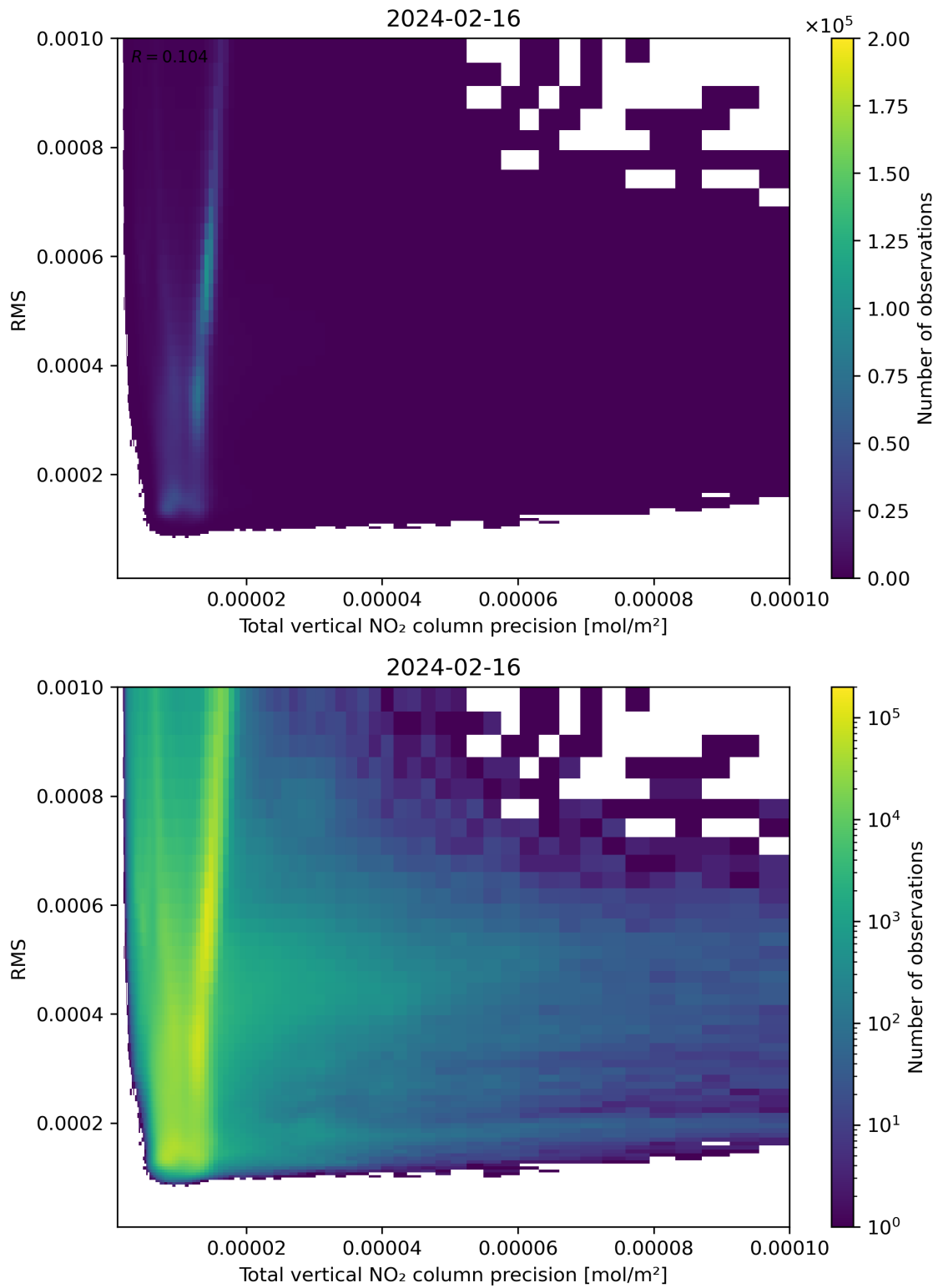
Figure 119: Scatter density plot of “Total vertical NO 2 column precision” against “RMS” for 2024-02-16 to 2024-02-17.
