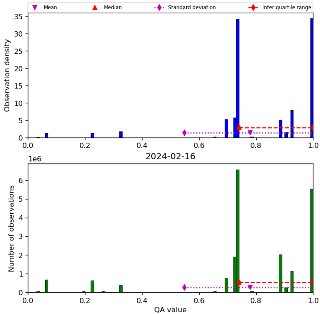
Figure 28: Histogram of “QA value” for 2024-02-16 to 2024-02-17
