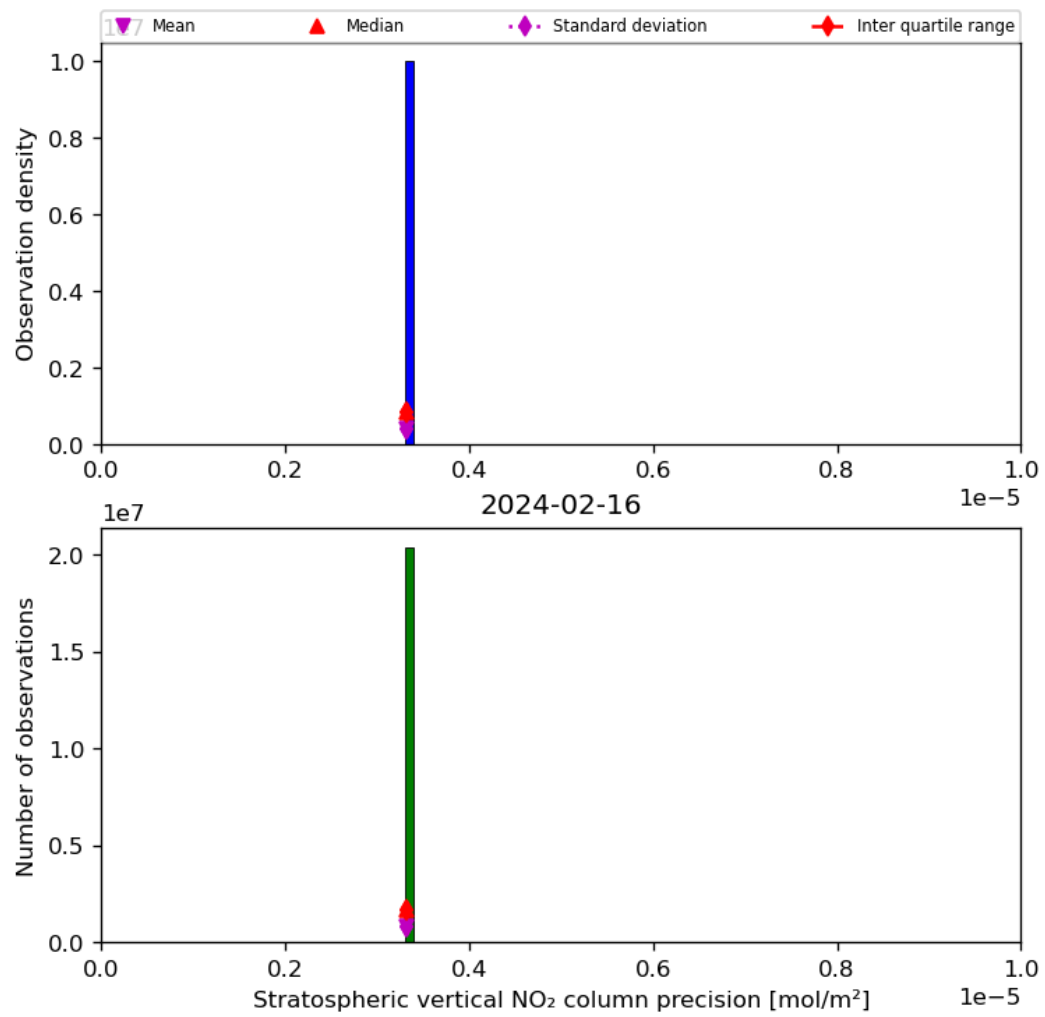
Figure 37: Histogram of “Stratospheric vertical NO 2 column precision” for 2024-02-16 to 2024-02-17
