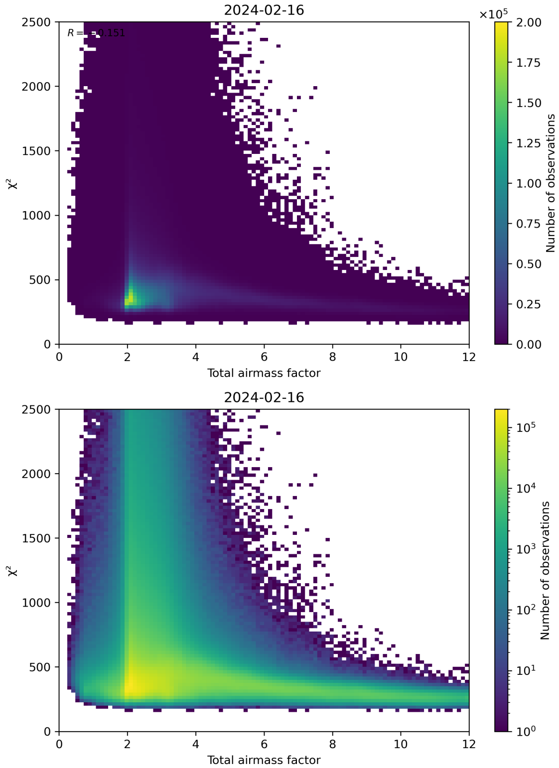
Figure 63: Scatter density plot of “Total airmass factor” against “ \chi^2 ” for 2024-02-16 to 2024-02-17.
