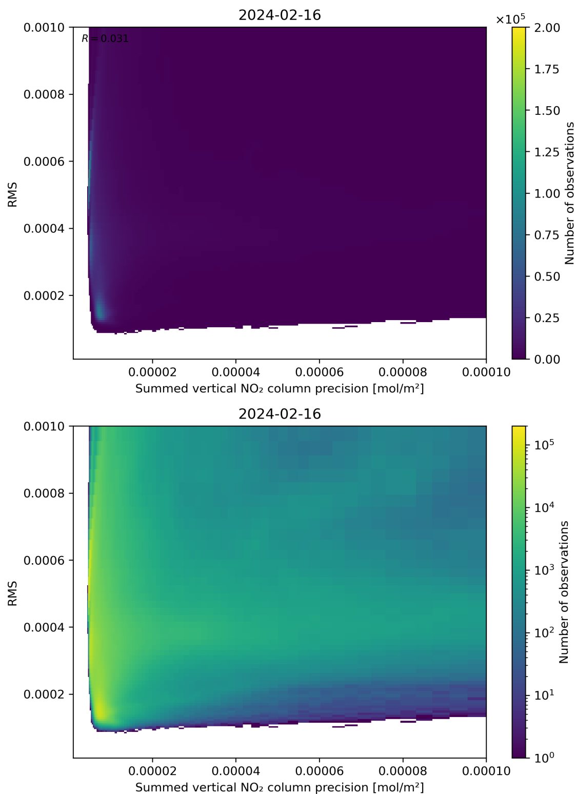
Figure 108: Scatter density plot of “Summed vertical NO 2 column precision” against “RMS” for 2024-02-16 to 2024-02-17.
