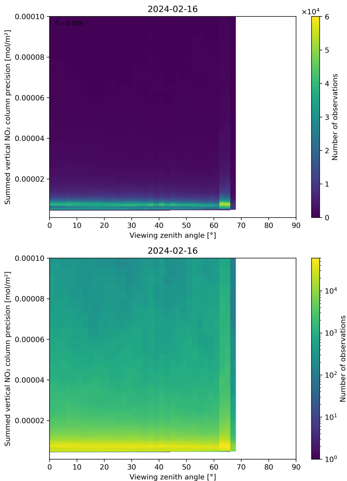
Figure 166: Scatter density plot of “Viewing zenith angle” against “Summed vertical NO 2 column precision” for 2024-02-16 to 2024-02-17.
