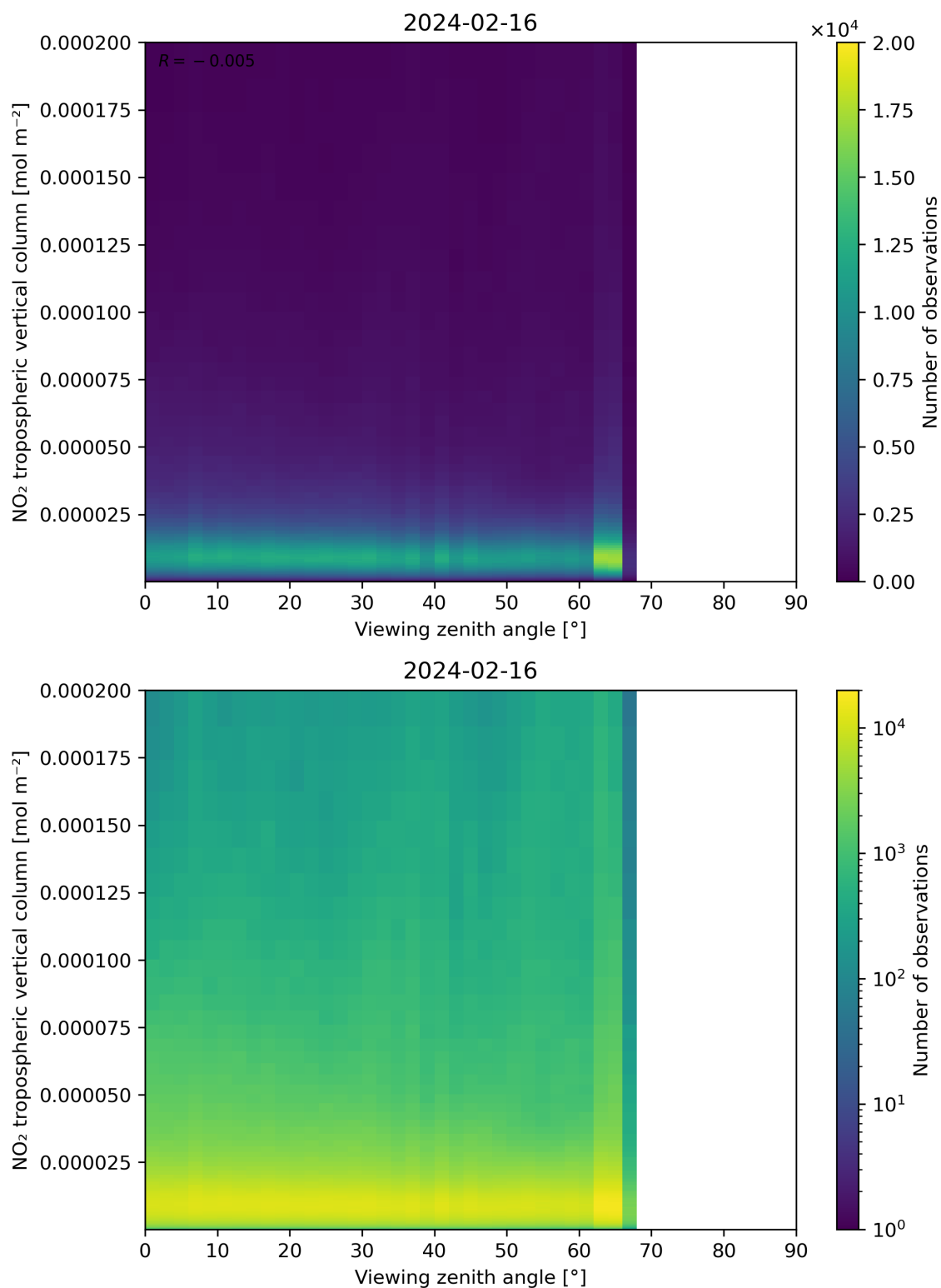
Figure 169: Scatter density plot of “Viewing zenith angle” against “NO 2 tropospheric vertical column” for 2024-02-16 to 2024-02-17.
