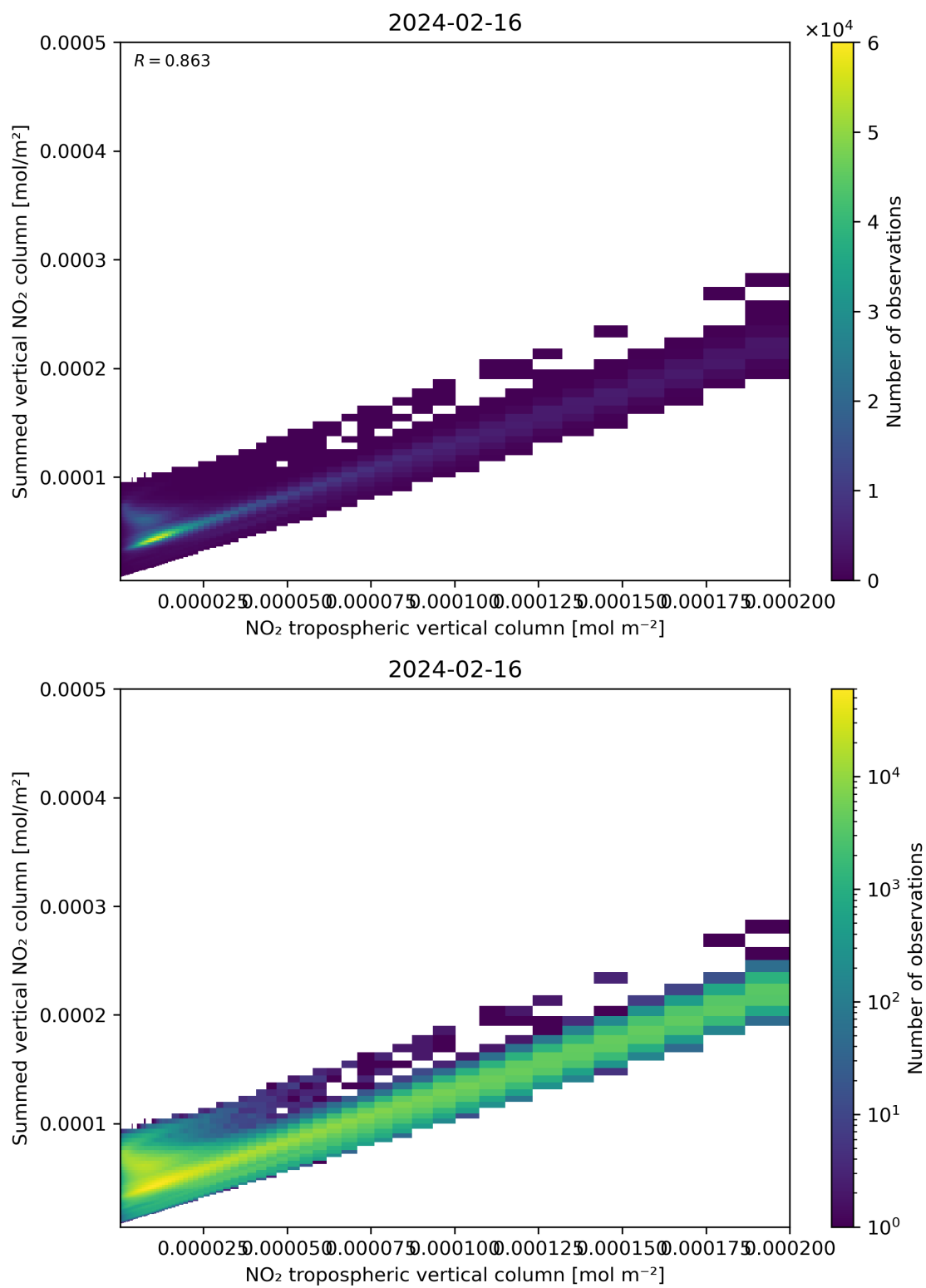
Figure 126: Scatter density plot of “NO 2 tropospheric vertical column” against “Summed vertical NO 2 column” for 2024-02-16 to 2024-02-17.
