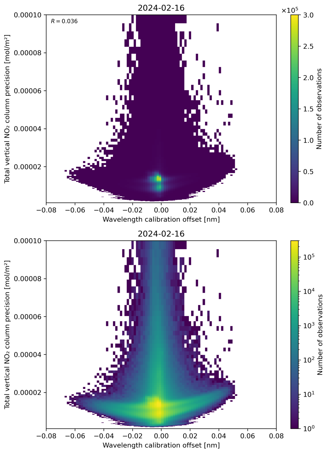
Figure 180: Scatter density plot of “Wavelength calibration offset” against “Total vertical NO 2 column precision” for 2024-02-16 to 2024-02-17.
