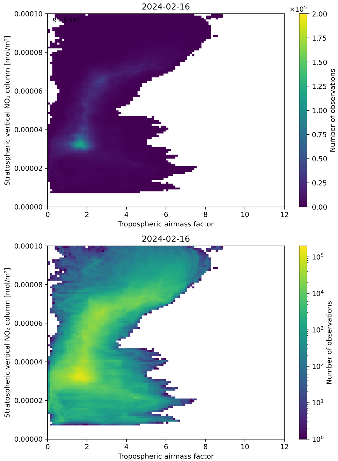
Figure 74: Scatter density plot of “Tropospheric air mass factor” against “Stratospheric vertical NO 2 column” for 2024-02-16 to 2024-02-17.
