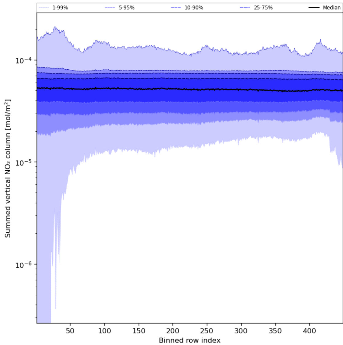
Figure 57: Along track statistics of “Summed vertical NO 2 column” for 2024-02-16 to 2024-02-17
