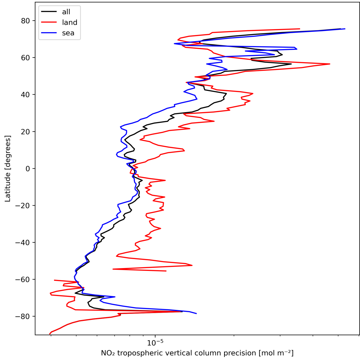
Figure 13: Zonal average of “NO 2 tropospheric vertical column precision” for 2024-02-16 to 2024-02-17.
