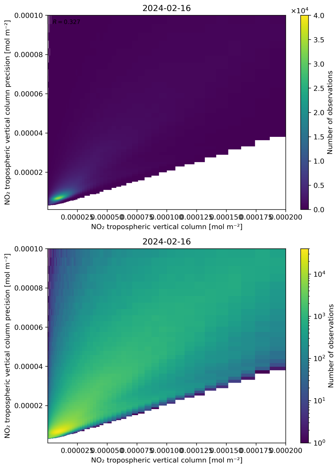
Figure 130: Scatter density plot of “NO 2 tropospheric vertical column” against “NO 2 tropospheric vertical column precision” for 2024-02-16 to 2024-02-17.
