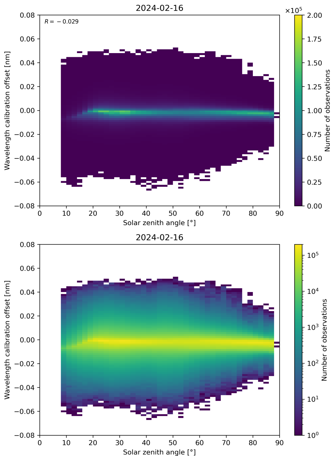
Figure 158: Scatter density plot of “Solar zenith angle” against “Wavelength calibration offset” for 2024-02-16 to 2024-02-17.
