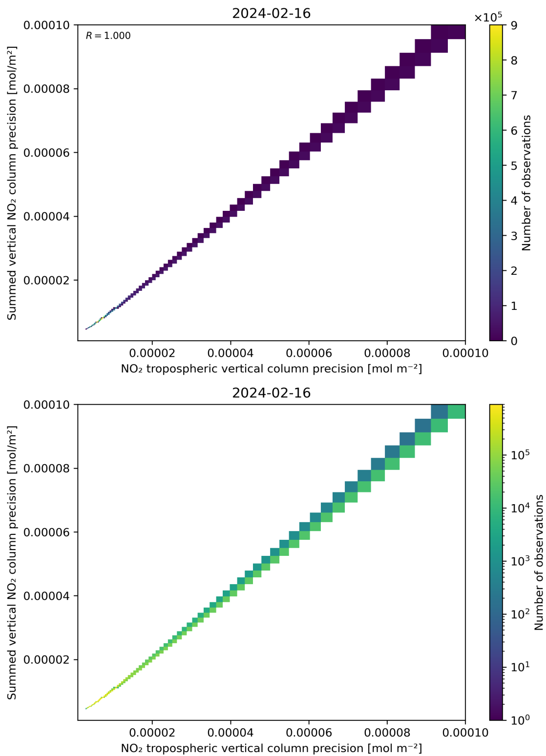
Figure 137: Scatter density plot of “NO 2 tropospheric vertical column precision” against “Summed vertical NO 2 column precision” for 2024-02-16 to 2024-02-17.
