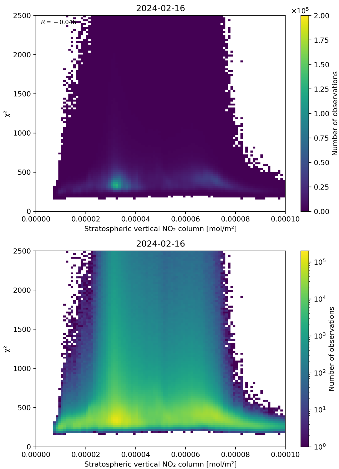
Figure 97: Scatter density plot of “Stratospheric vertical NO 2 column” against “ \chi^2 ” for 2024-02-16 to 2024-02-17.
