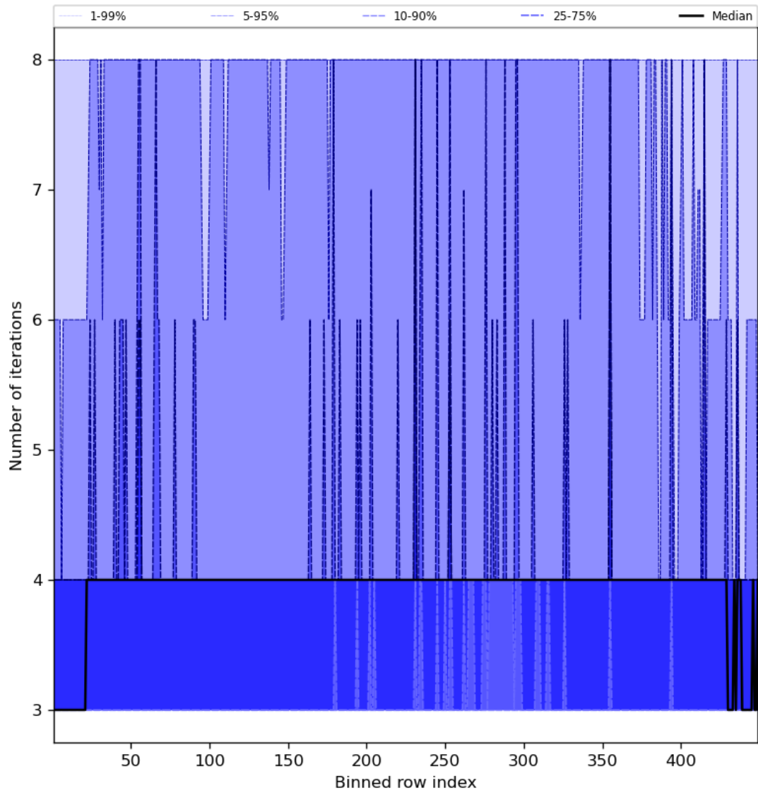
Figure 51: Along track statistics of “Number of iterations” for 2024-02-16 to 2024-02-17
