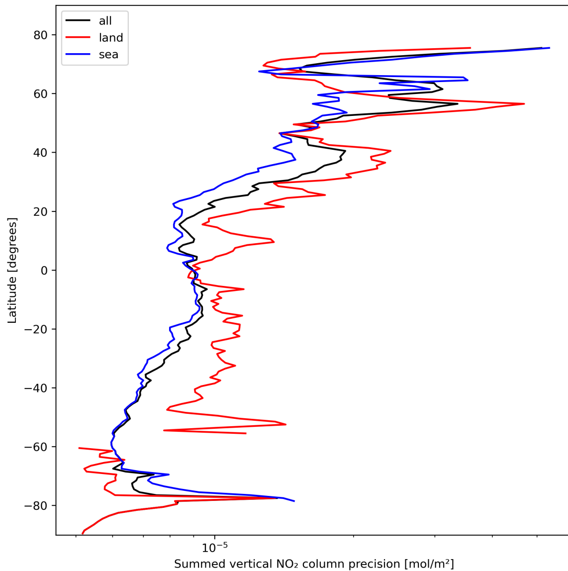
Figure 24: Zonal average of “Summed vertical NO 2 column precision” for 2024-02-16 to 2024-02-17.
