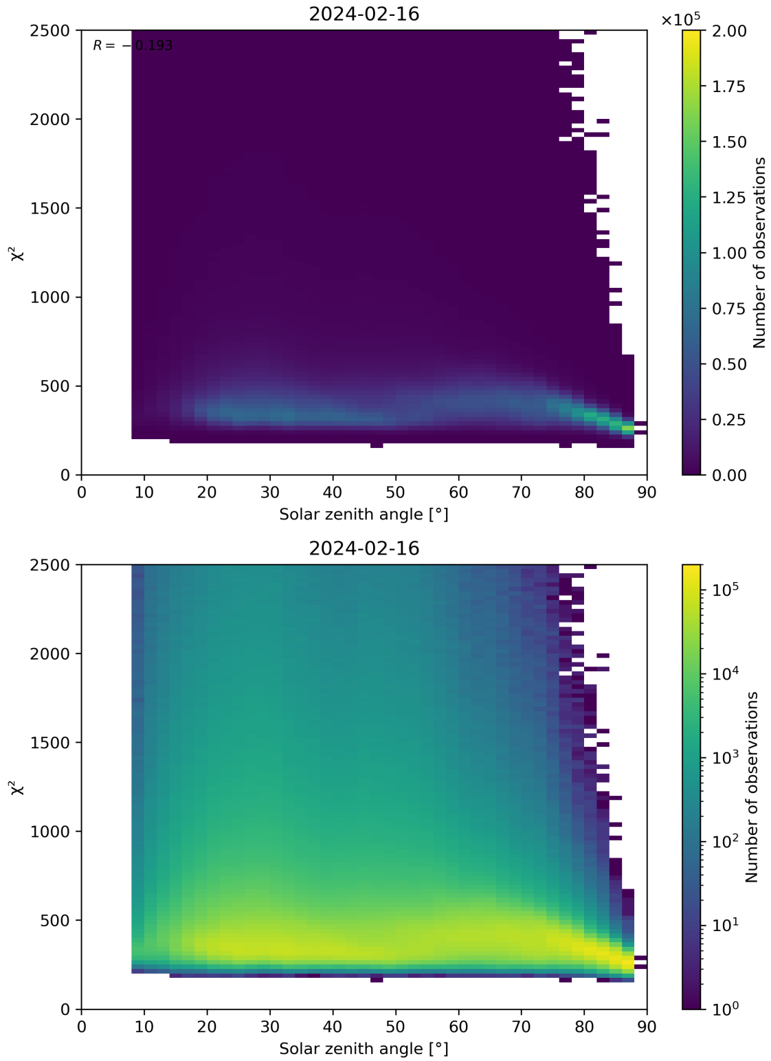
Figure 148: Scatter density plot of “Solar zenith angle” against “ \chi^2 ” for 2024-02-16 to 2024-02-17.
