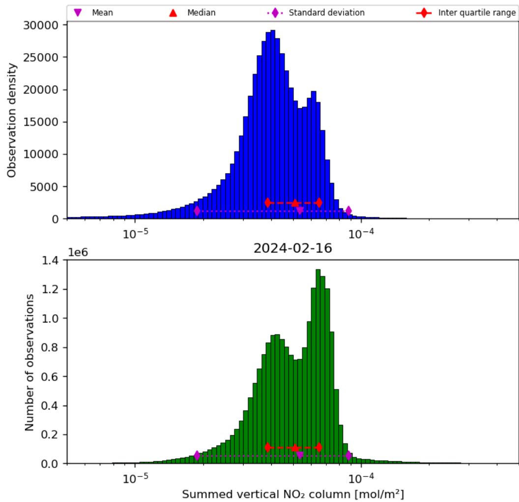
Figure 40: Histogram of “Summed vertical NO 2 column” for 2024-02-16 to 2024-02-17
