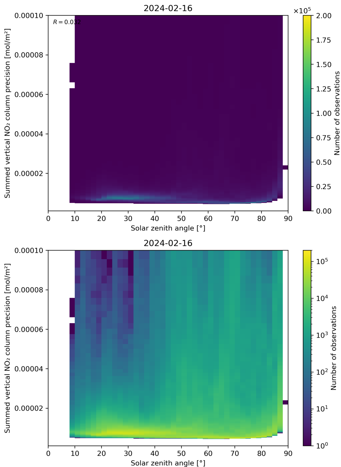
Figure 152: Scatter density plot of “Solar zenith angle” against “Summed vertical NO 2 column precision” for 2024-02-16 to 2024-02-17.
