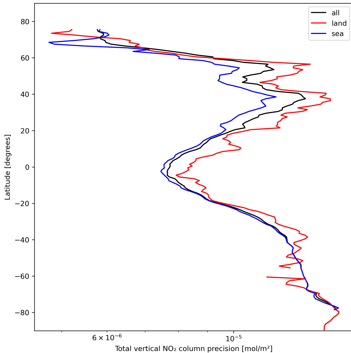
Figure 22: Zonal average of "Total vertical NO 2 column precision" for 2024-02-16 to 2024-02-17.
