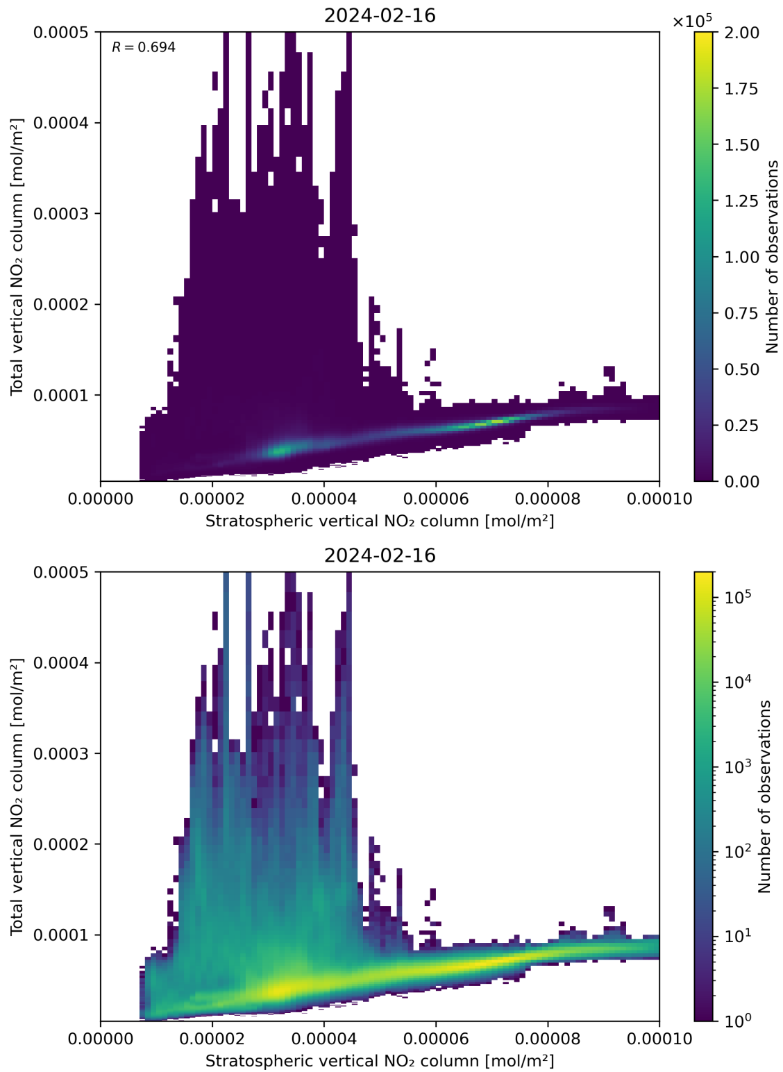
Figure 100: Scatter density plot of “Stratospheric vertical NO 2 column” against “Total vertical NO 2 column” for 2024-02-16 to 2024-02-17.
