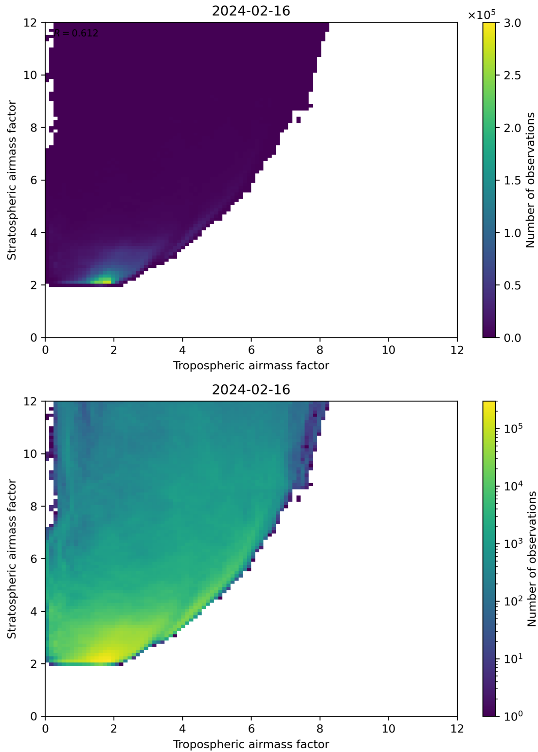
Figure 71: Scatter density plot of “Tropospheric airmass factor” against “Stratospheric airmass factor” for 2024-02-16 to 2024-02-17.
