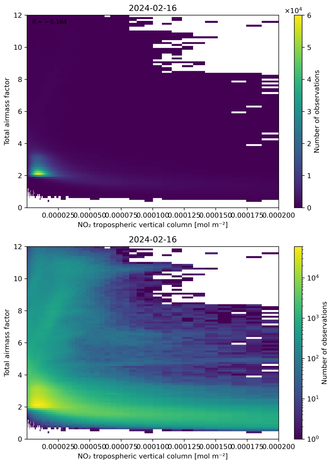
Figure 122: Scatter density plot of “NO 2 tropospheric vertical column” against “Total air mass factor” for 2024-02-16 to 2024-02-17.
