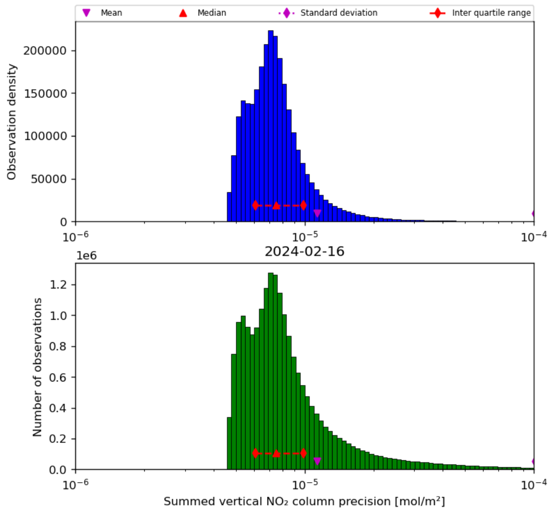
Figure 41: Histogram of “Summed vertical NO 2 column precision” for 2024-02-16 to 2024-02-17
