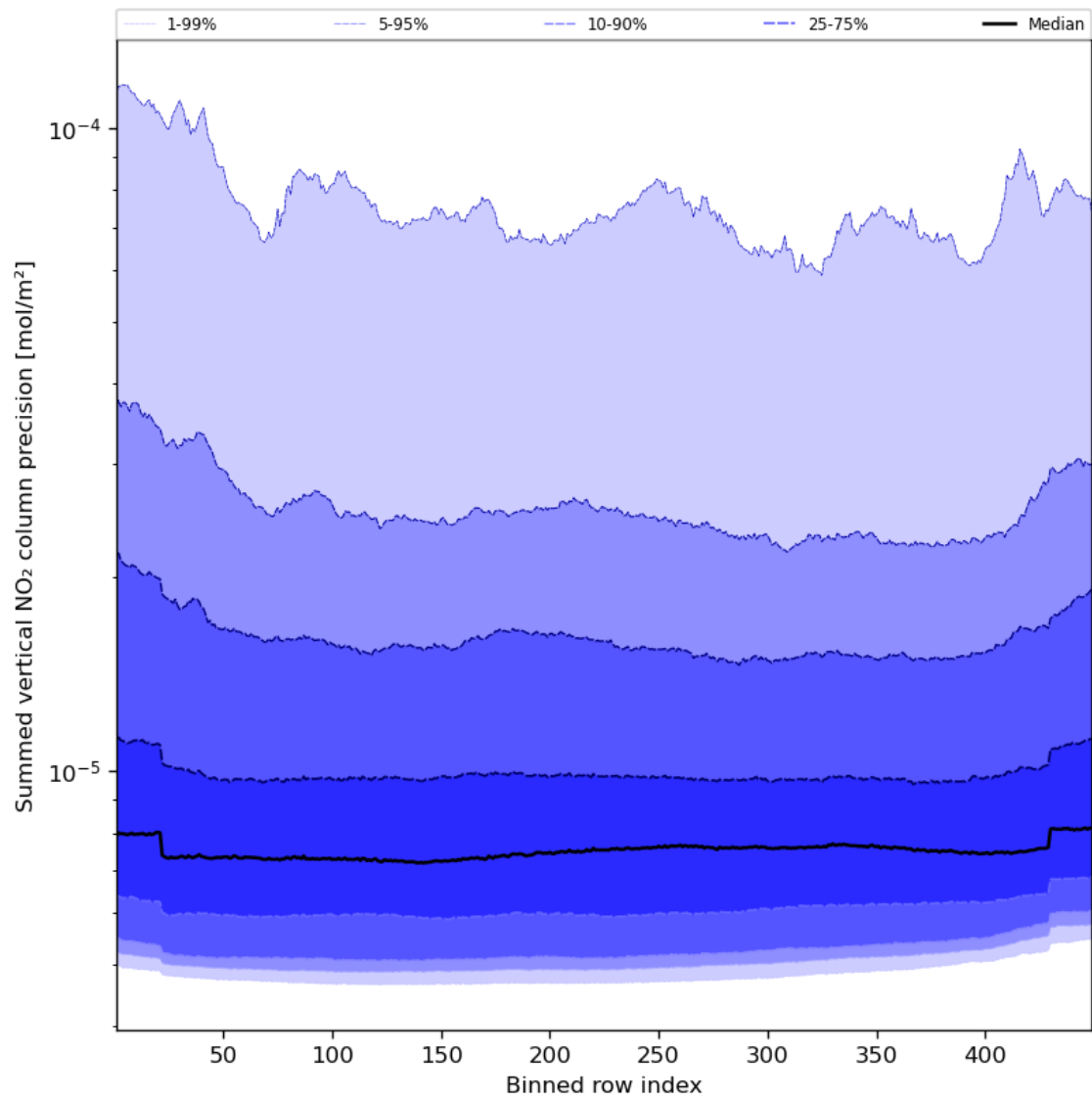
Figure 58: Along track statistics of “Summed vertical NO 2 column precision” for 2024-02-16 to 2024-02-17
