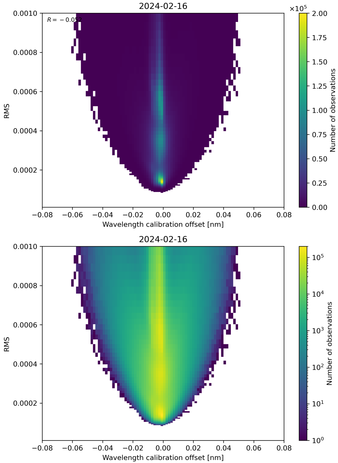
Figure 181: Scatter density plot of “Wavelength calibration offset” against “RMS” for 2024-02-16 to 2024-02-17.
