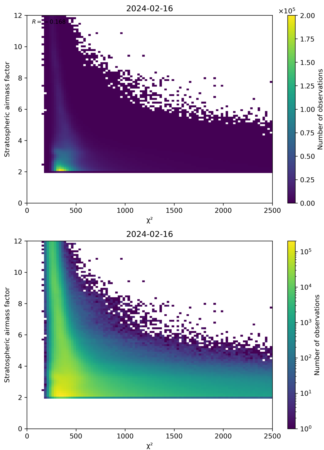
Figure 81: Scatter density plot of “ \chi^2 ” against “Stratospheric airmass factor” for 2024-02-16 to 2024-02-17.
