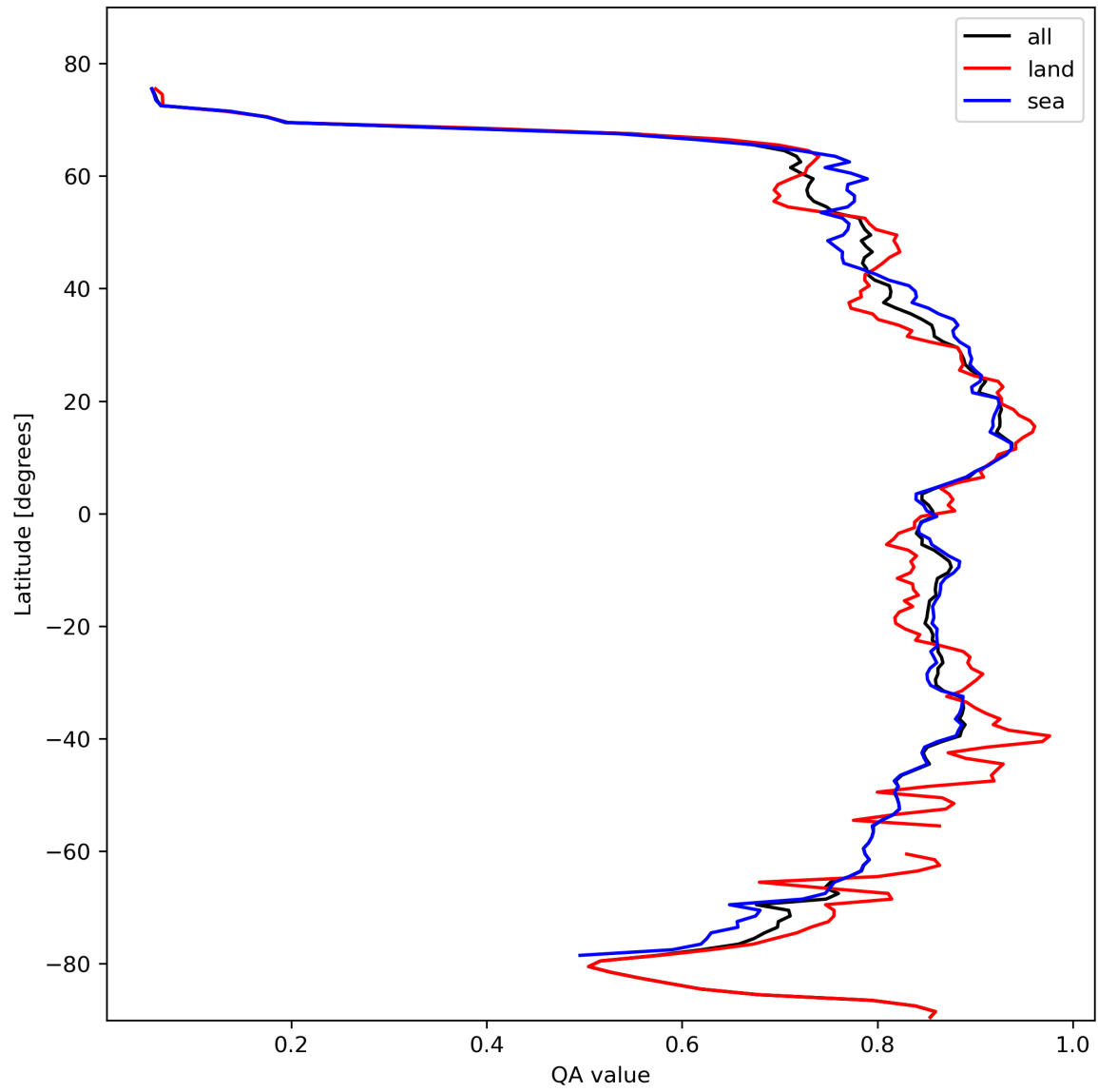
Figure 11: Zonal average of “QA value” for 2024-02-16 to 2024-02-17.
