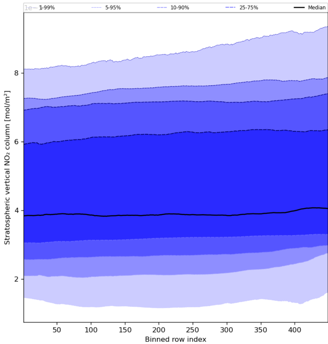
Figure 53: Along track statistics of “Stratospheric vertical NO 2 column” for 2024-02-16 to 2024-02-17
