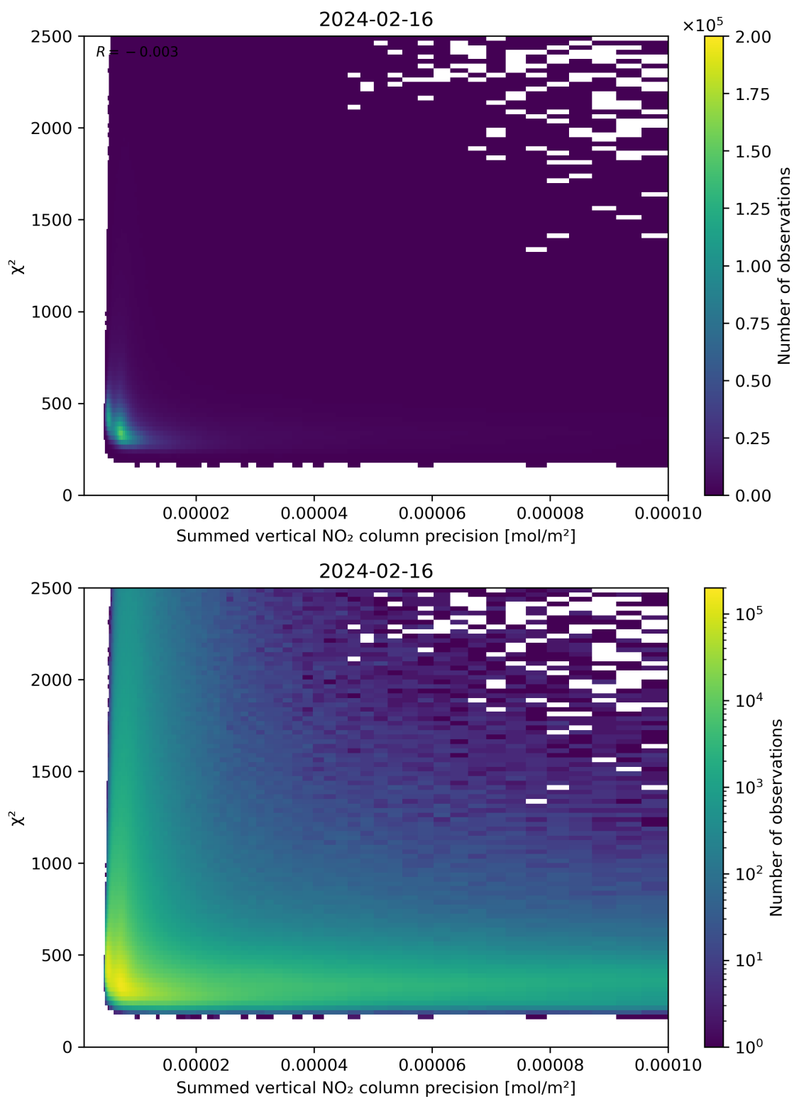
Figure 107: Scatter density plot of “Summed vertical NO 2 column precision” against “ \chi^2 ” for 2024-02-16 to 2024-02-17.
