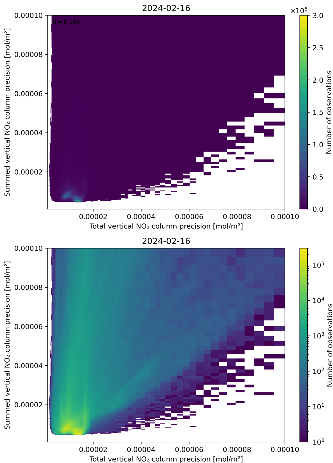
Figure 118: Scatter density plot of “Total vertical NO 2 column precision” against “Summed vertical NO 2 column precision” for 2024-02-16 to 2024-02-17.
