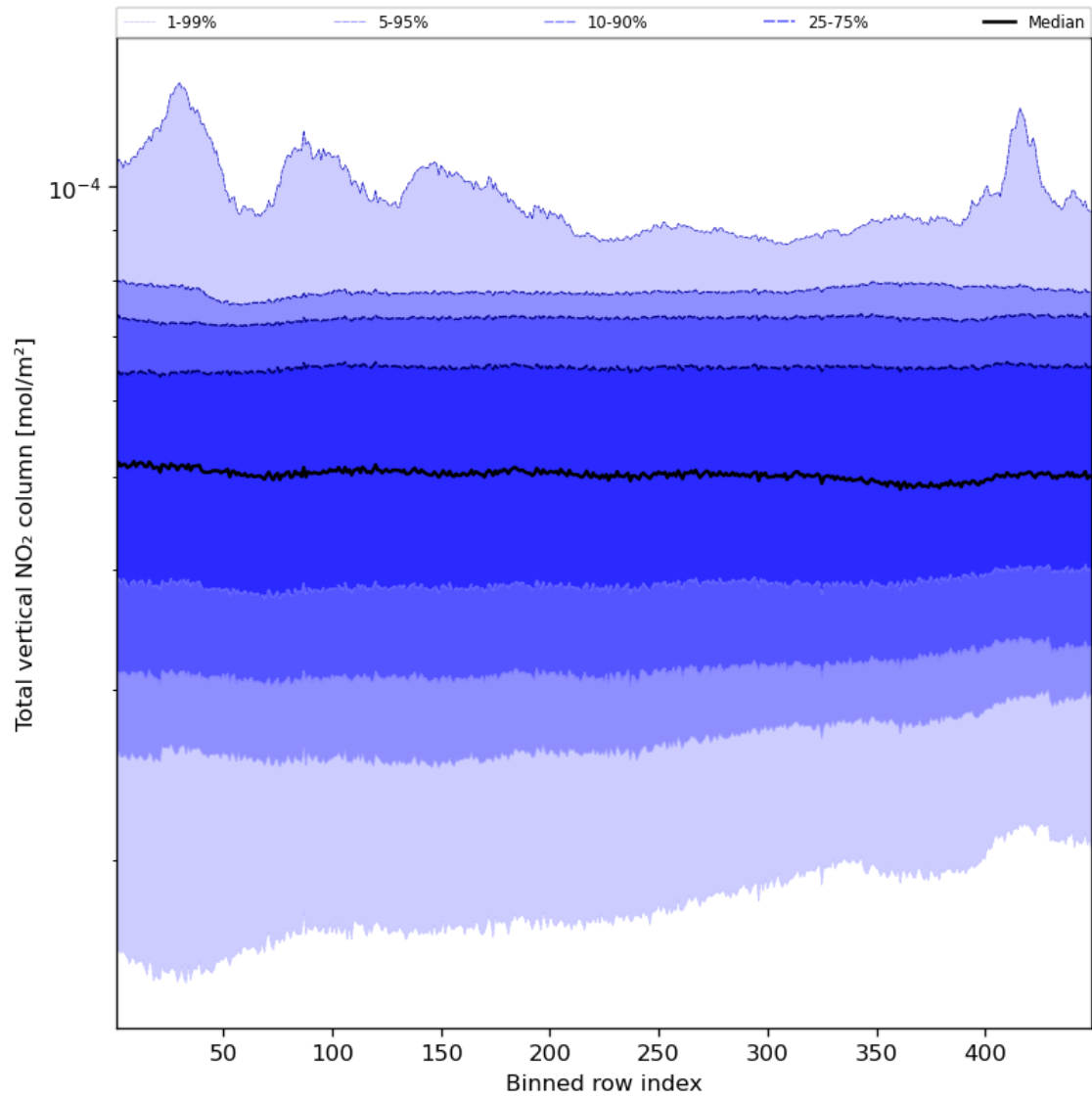
Figure 55: Along track statistics of “Total vertical NO 2 column” for 2024-02-16 to 2024-02-17
