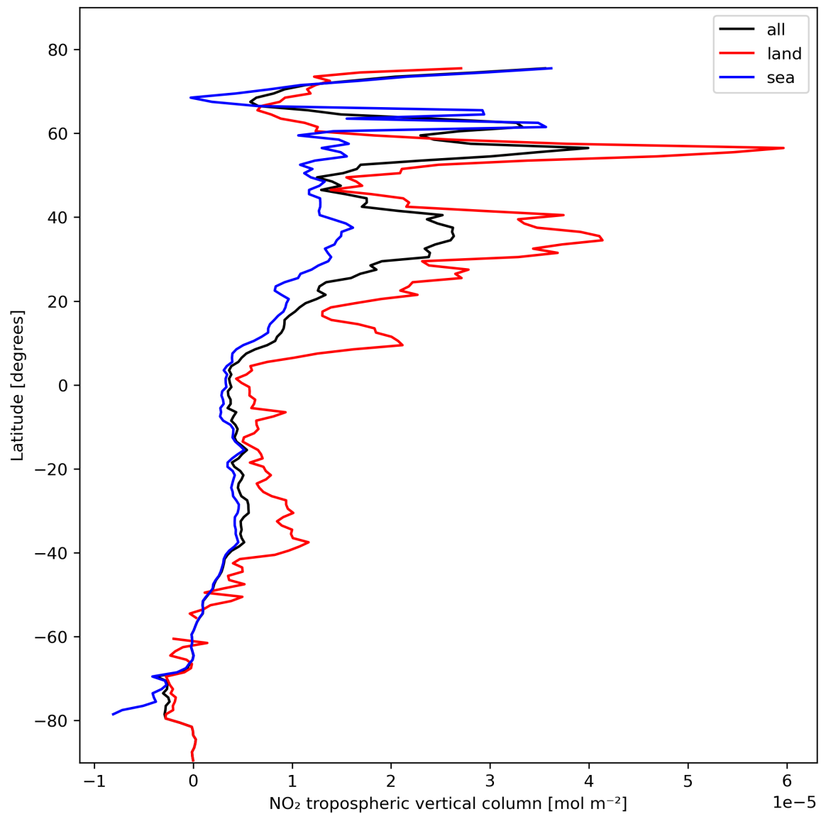
Figure 12: Zonal average of “NO 2 tropospheric vertical column” for 2024-02-16 to 2024-02-17.
