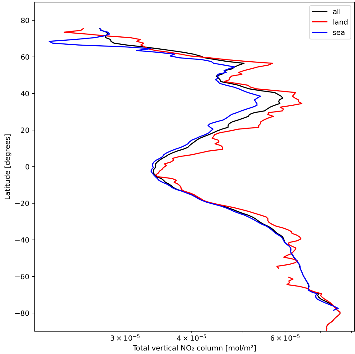
Figure 21: Zonal average of “Total vertical NO 2 column” for 2024-02-16 to 2024-02-17.
