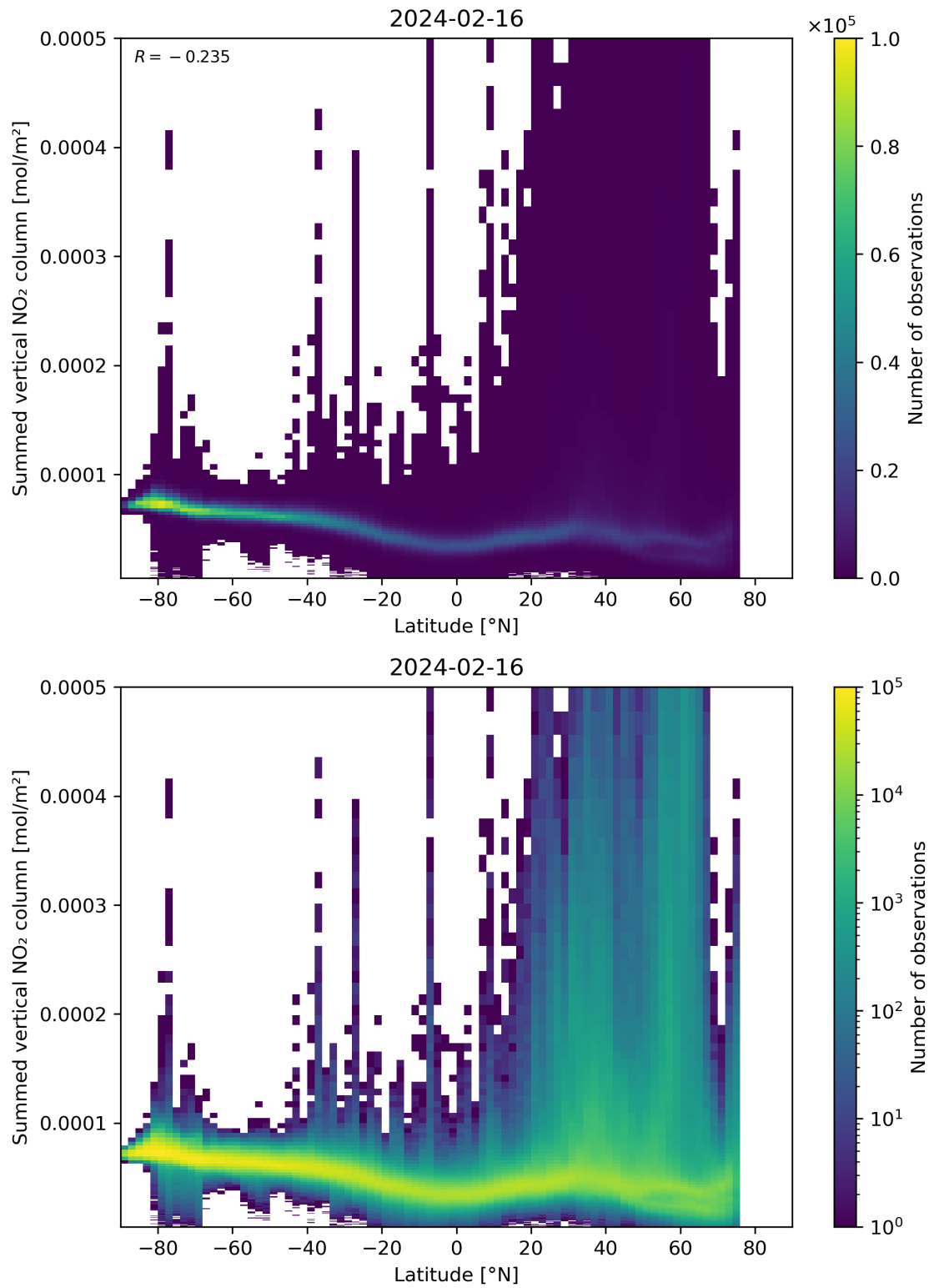
Figure 88: Scatter density plot of “Latitude” against “Summed vertical NO 2 column” for 2024-02-16 to 2024-02-17.
