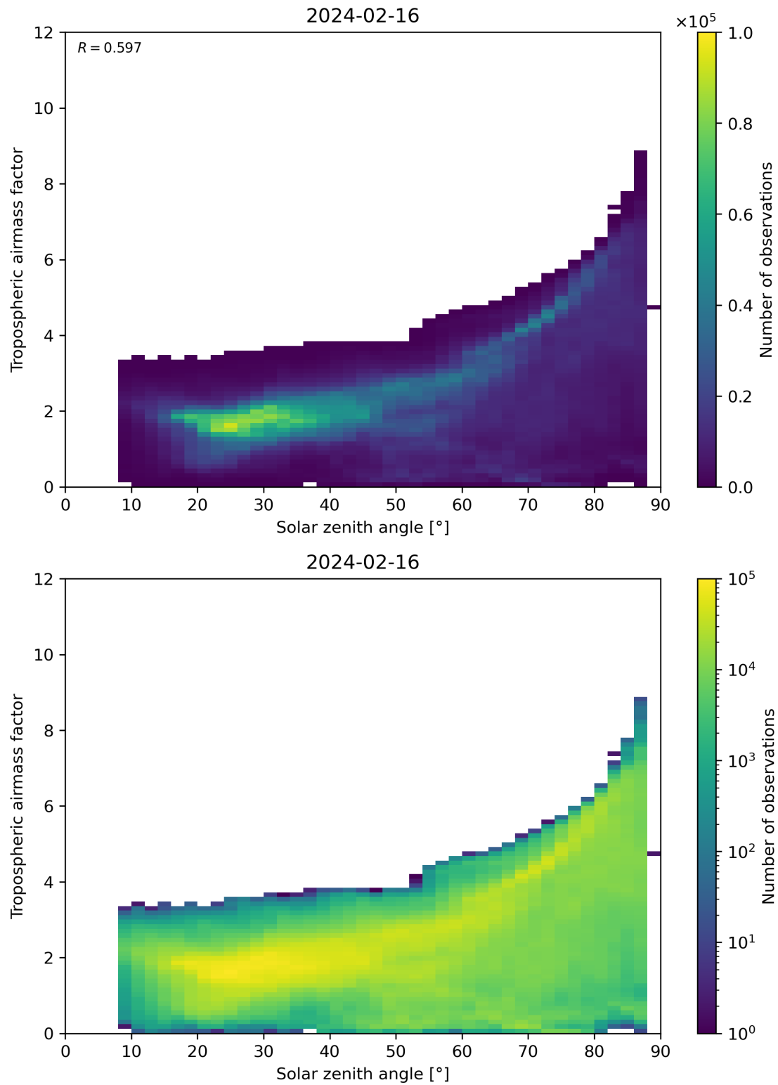
Figure 147: Scatter density plot of “Solar zenith angle” against “Tropospheric airmass factor” for 2024-02-16 to 2024-02-17.
