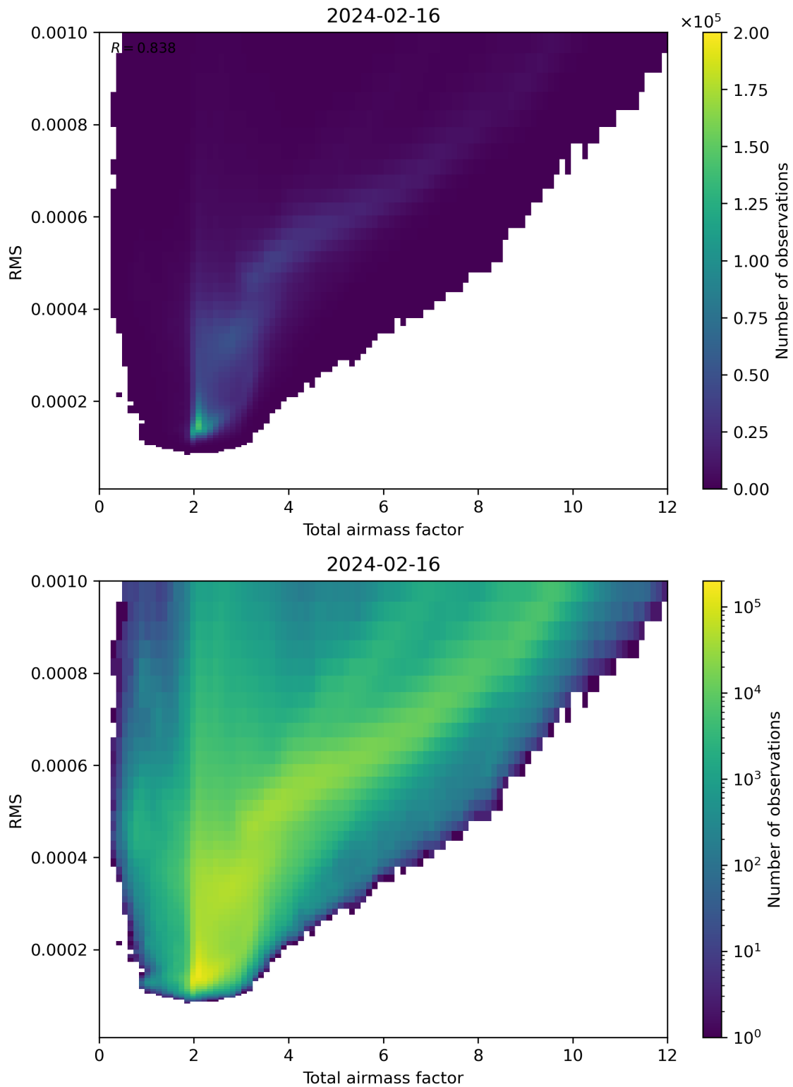
Figure 69: Scatter density plot of “Total airmass factor” against “RMS” for 2024-02-16 to 2024-02-17.
