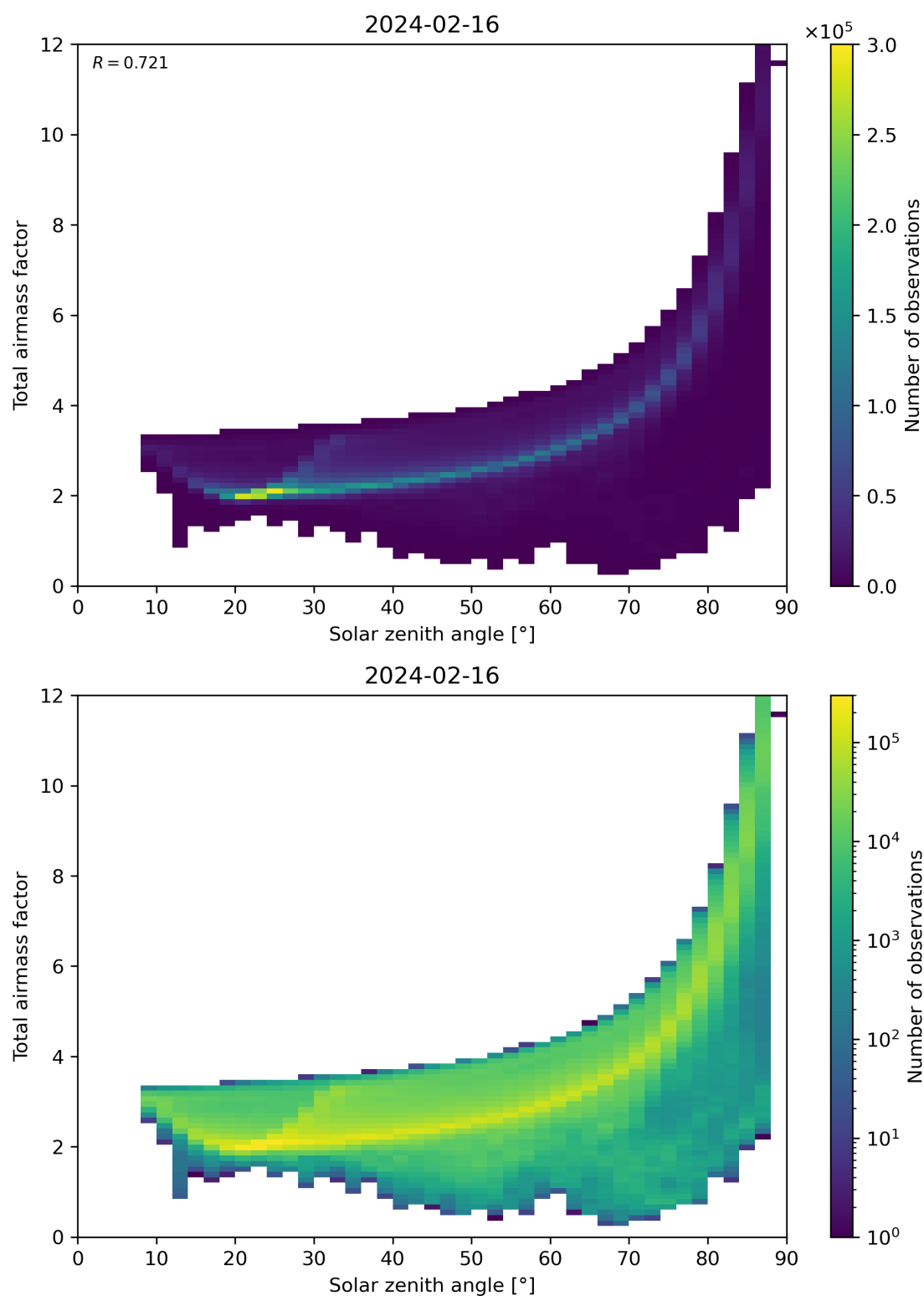
Figure 146: Scatter density plot of “Solar zenith angle” against “Total air mass factor” for 2024-02-16 to 2024-02-17.
