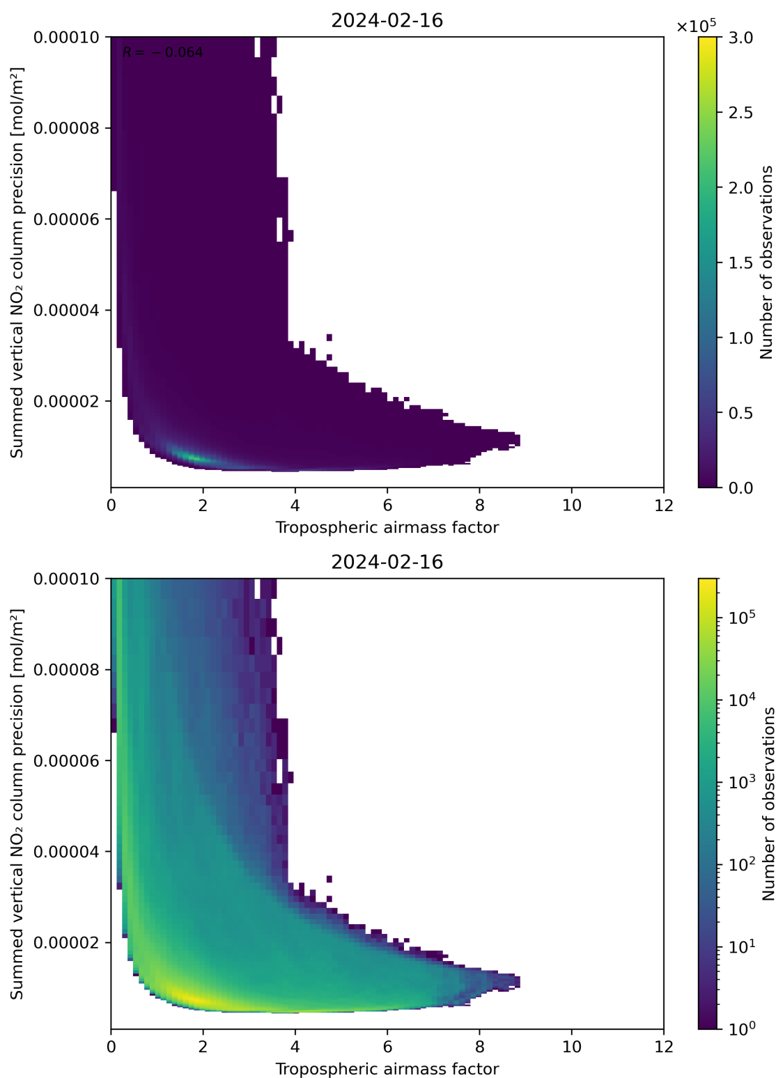
Figure 76: Scatter density plot of “Tropospheric air mass factor” against “Summed vertical NO 2 column precision” for 2024-02-16 to 2024-02-17.
