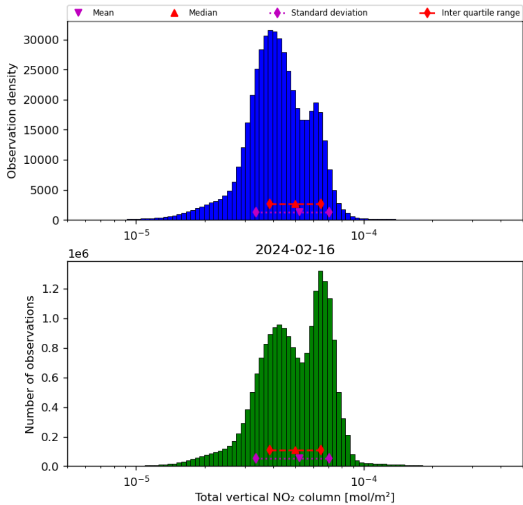
Figure 38: Histogram of “Total vertical NO 2 column” for 2024-02-16 to 2024-02-17
