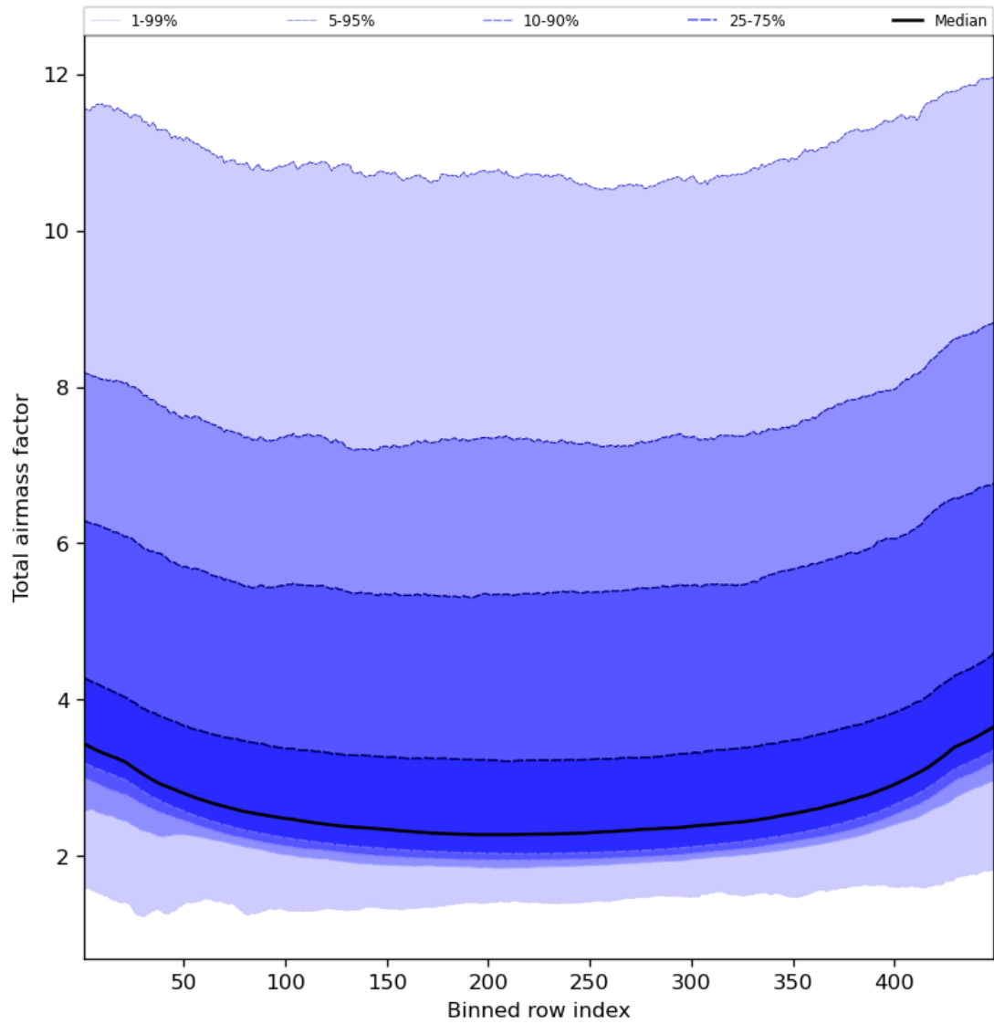
Figure 49: Along track statistics of “Total airmass factor” for 2024-02-16 to 2024-02-17
