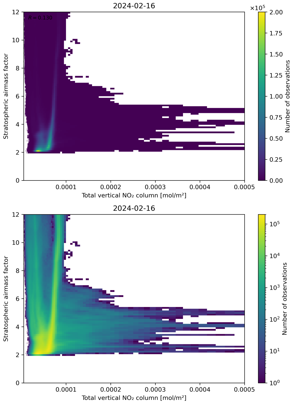
Figure 110: Scatter density plot of “Total vertical NO 2 column” against “Stratospheric airmass factor” for 2024-02-16 to 2024-02-17.
