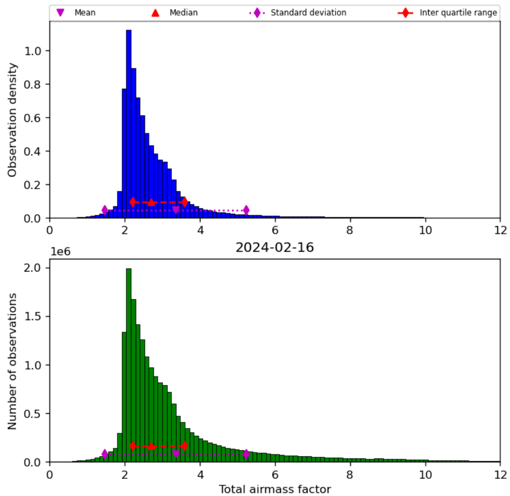
Figure 32: Histogram of “Total airmass factor” for 2024-02-16 to 2024-02-17
