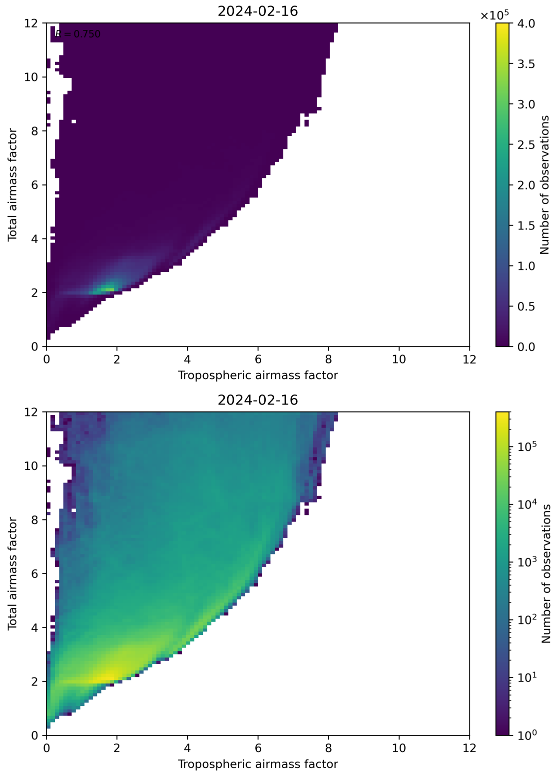
Figure 72: Scatter density plot of “Tropospheric airmass factor” against “Total airmass factor” for 2024-02-16 to 2024-02-17.
