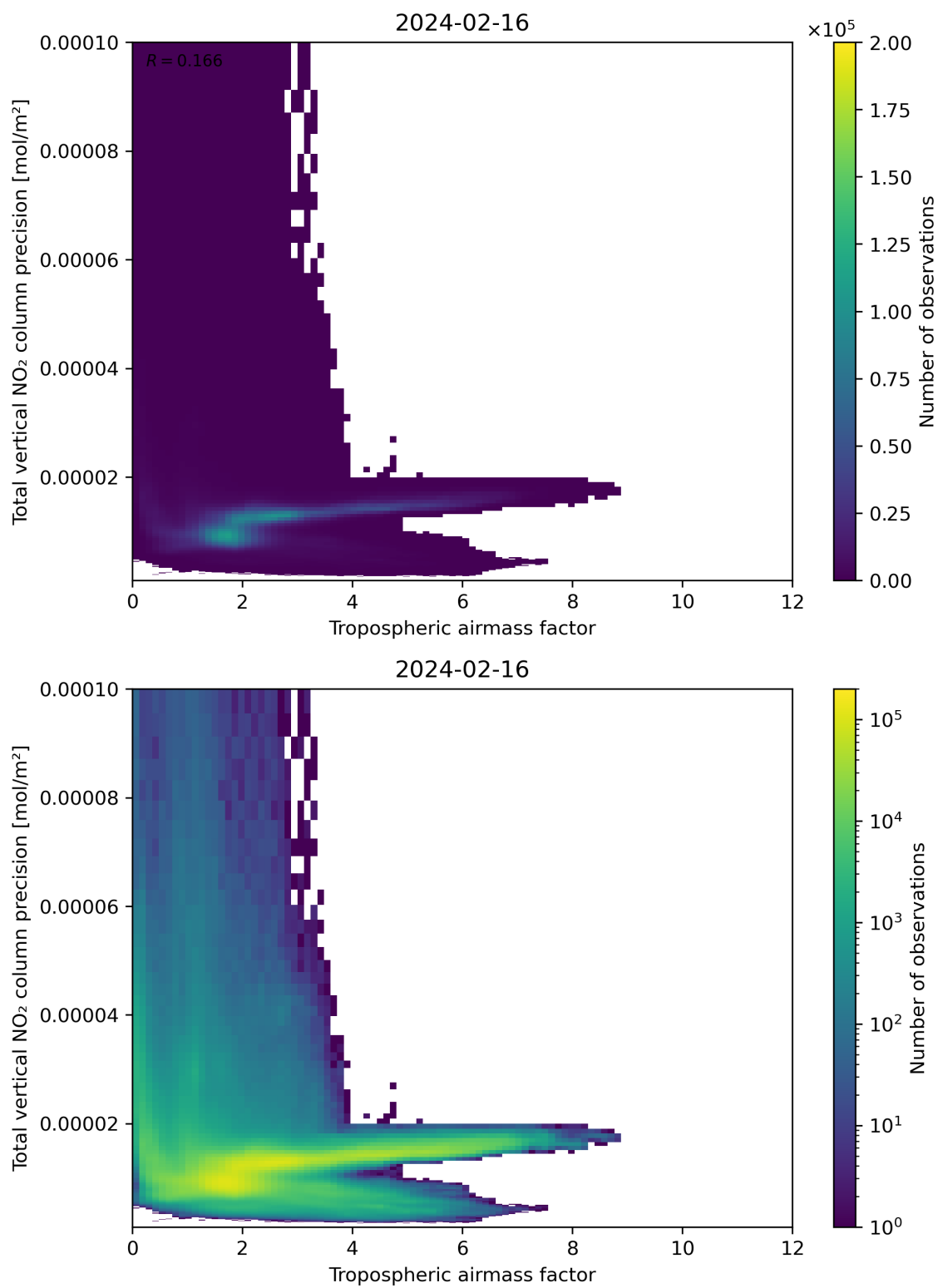
Figure 78: Scatter density plot of “Tropospheric air mass factor” against “Total vertical NO 2 column precision” for 2024-02-16 to 2024-02-17.
