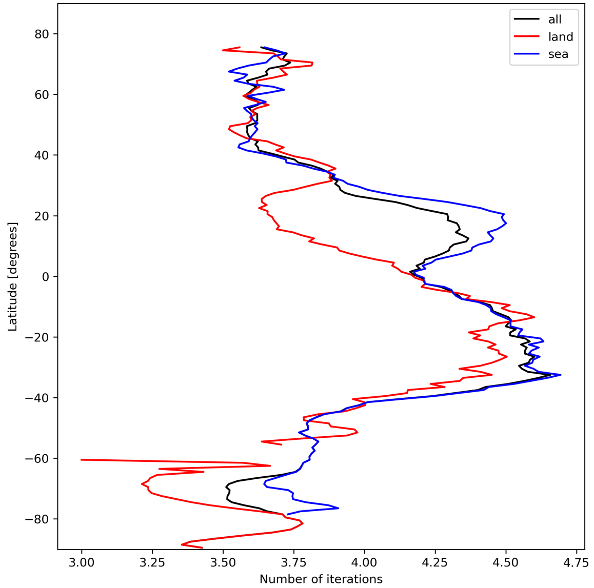
Figure 17: Zonal average of “Number of iterations” for 2024-02-16 to 2024-02-17.
