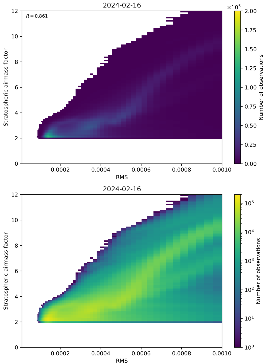
Figure 144: Scatter density plot of “RMS” against “Stratospheric airmass factor” for 2024-02-16 to 2024-02-17.
