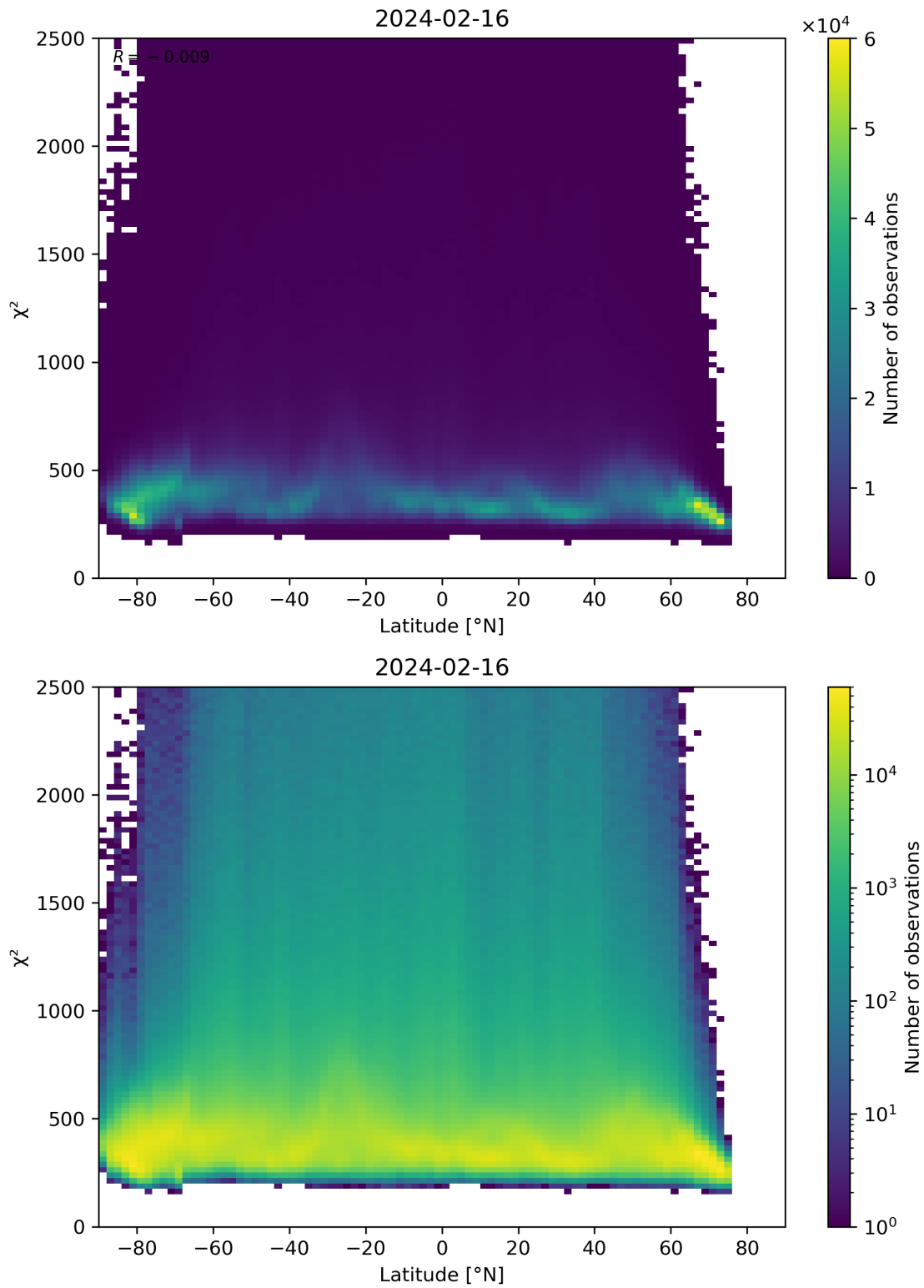
Figure 86: Scatter density plot of “Latitude” against “ \chi^2 ” for 2024-02-16 to 2024-02-17.
