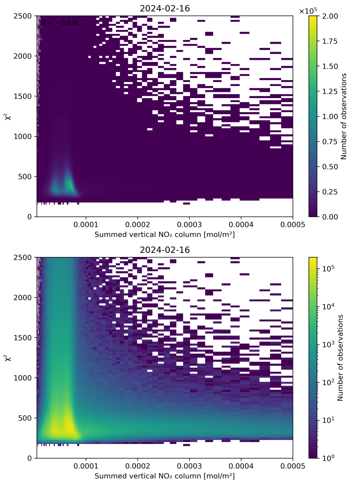
Figure 104: Scatter density plot of “Summed vertical NO 2 column” against “ \chi^2 ” for 2024-02-16 to 2024-02-17.
