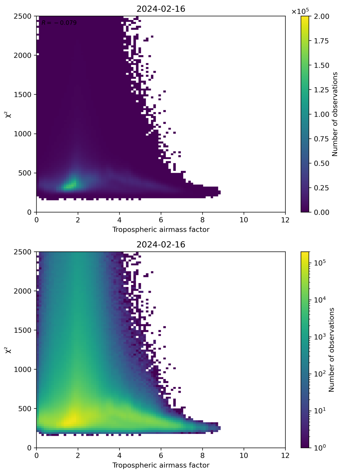
Figure 73: Scatter density plot of “Tropospheric airmass factor” against “ \chi^2 ” for 2024-02-16 to 2024-02-17.
