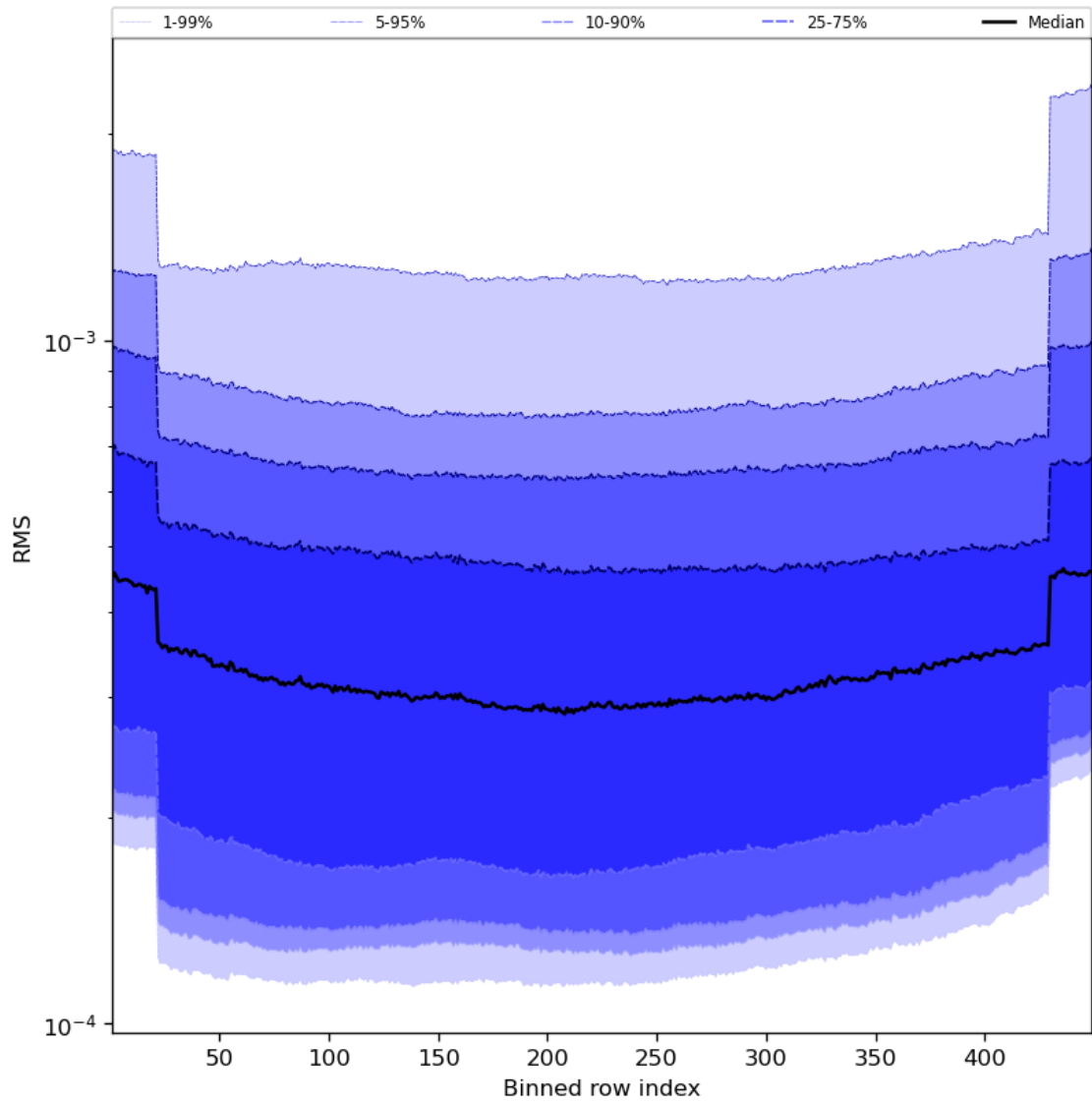
Figure 60: Along track statistics of “RMS” for 2024-02-16 to 2024-02-17
