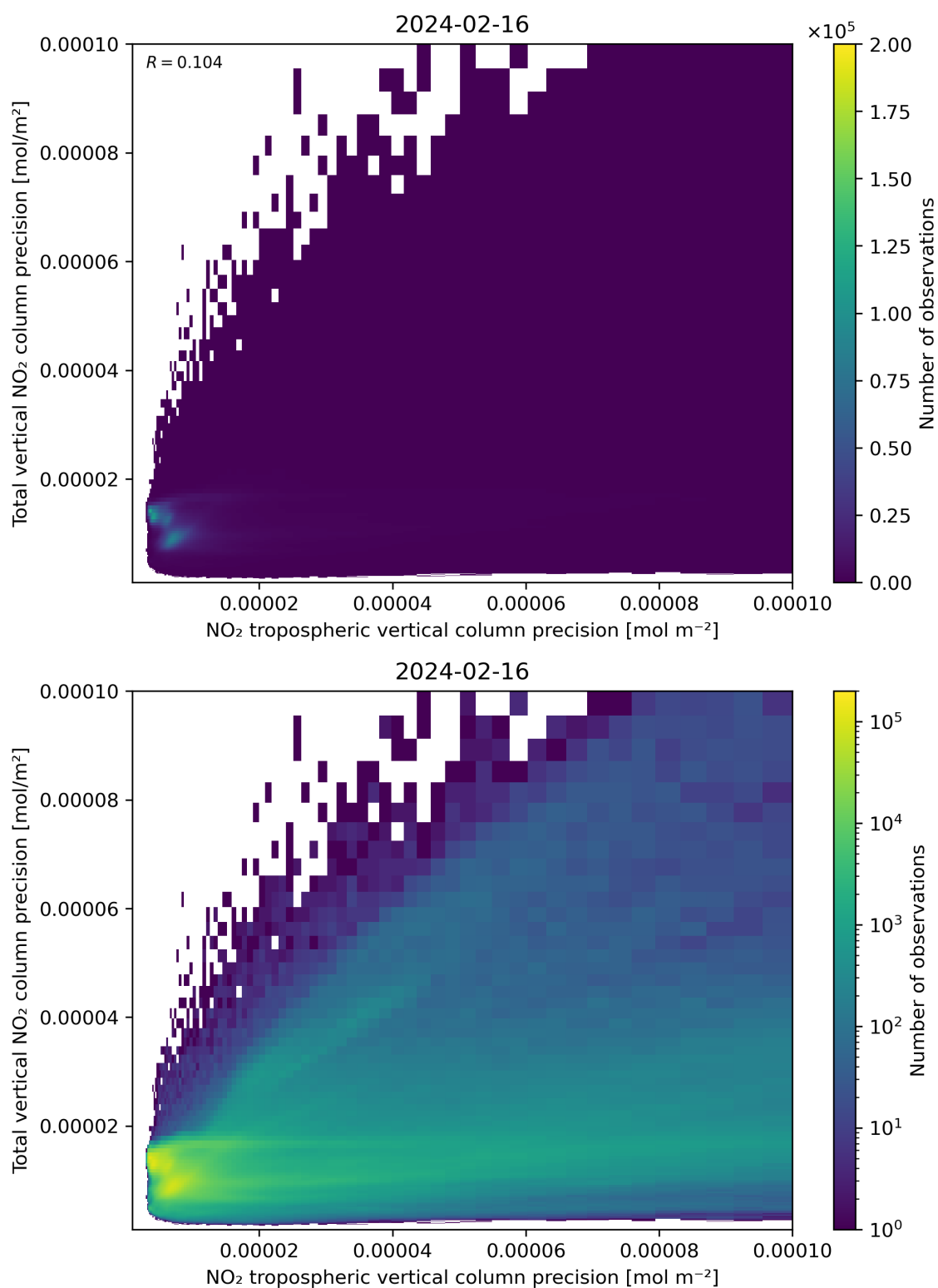
Figure 139: Scatter density plot of “NO 2 tropospheric vertical column precision” against “Total vertical NO 2 column precision” for 2024-02-16 to 2024-02-17.
