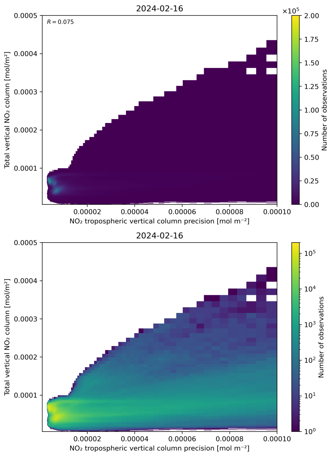
Figure 138: Scatter density plot of “NO 2 tropospheric vertical column precision” against “Total vertical NO 2 column” for 2024-02-16 to 2024-02-17.
