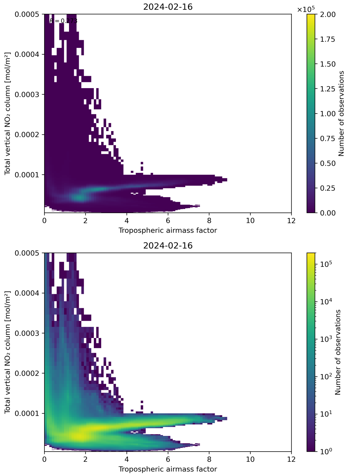
Figure 77: Scatter density plot of “Tropospheric airmass factor” against “Total vertical NO 2 column” for 2024-02-16 to 2024-02-17.
