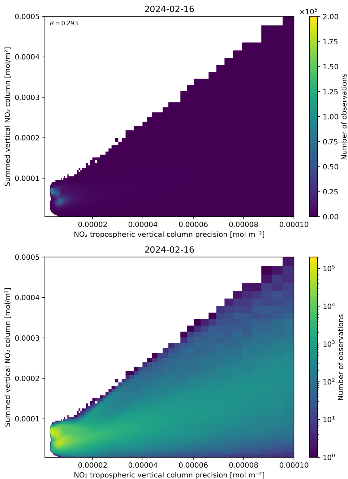
Figure 136: Scatter density plot of “NO 2 tropospheric vertical column precision” against “Summed vertical NO 2 column” for 2024-02-16 to 2024-02-17.
