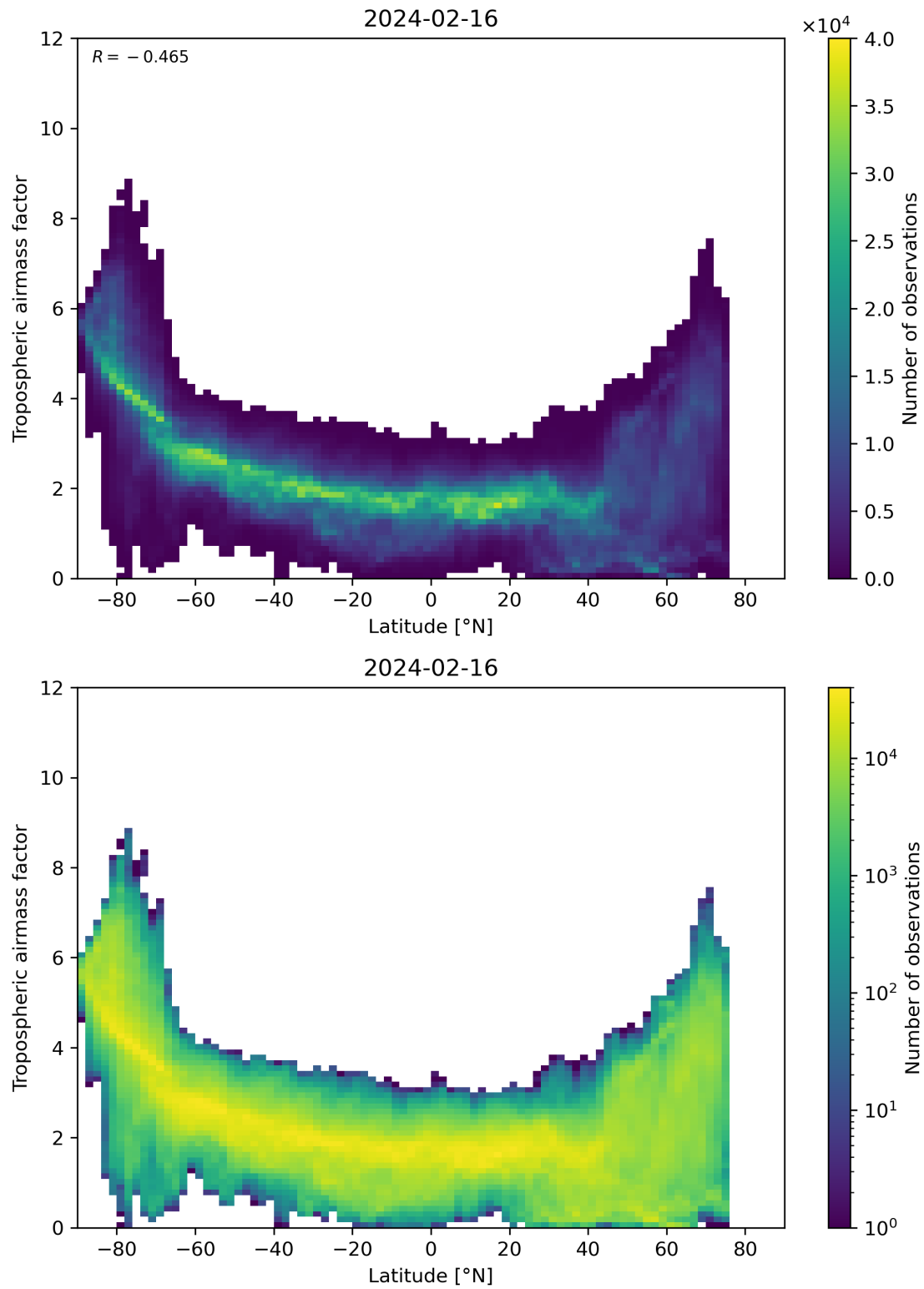
Figure 85: Scatter density plot of “Latitude” against “Tropospheric airmass factor” for 2024-02-16 to 2024-02-17.
