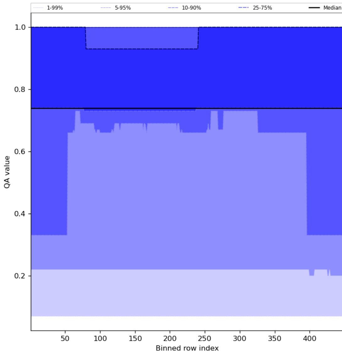
Figure 45: Along track statistics of “QA value” for 2024-02-16 to 2024-02-17
