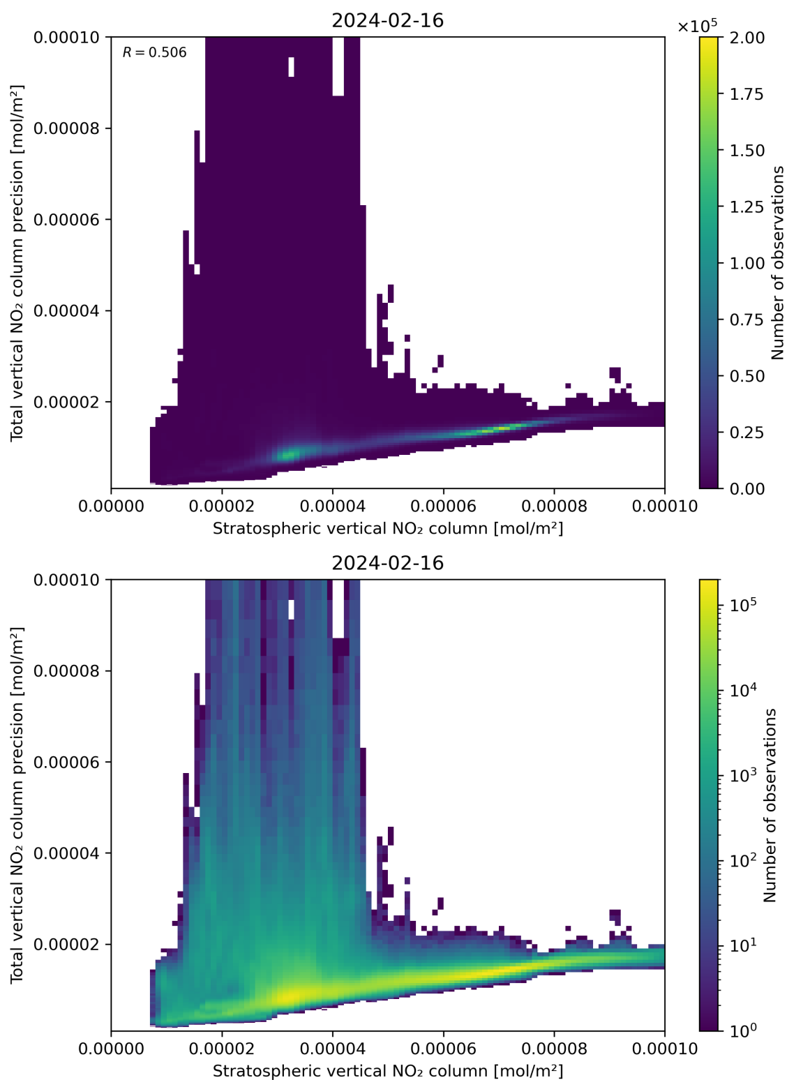
Figure 101: Scatter density plot of “Stratospheric vertical NO 2 column” against “Total vertical NO 2 column precision” for 2024-02-16 to 2024-02-17.
