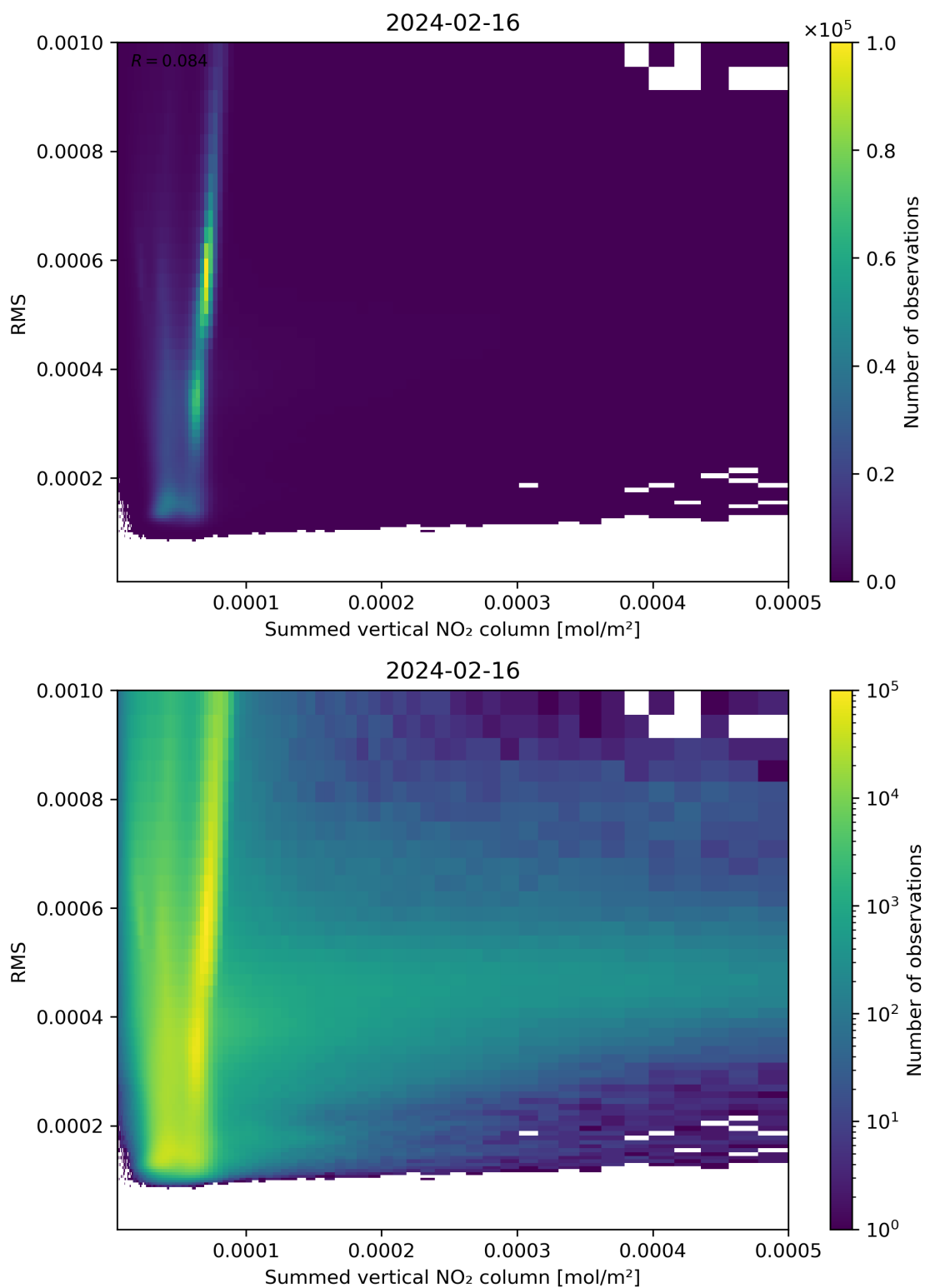
Figure 109: Scatter density plot of “Summed vertical NO 2 column” against “RMS” for 2024-02-16 to 2024-02-17.
