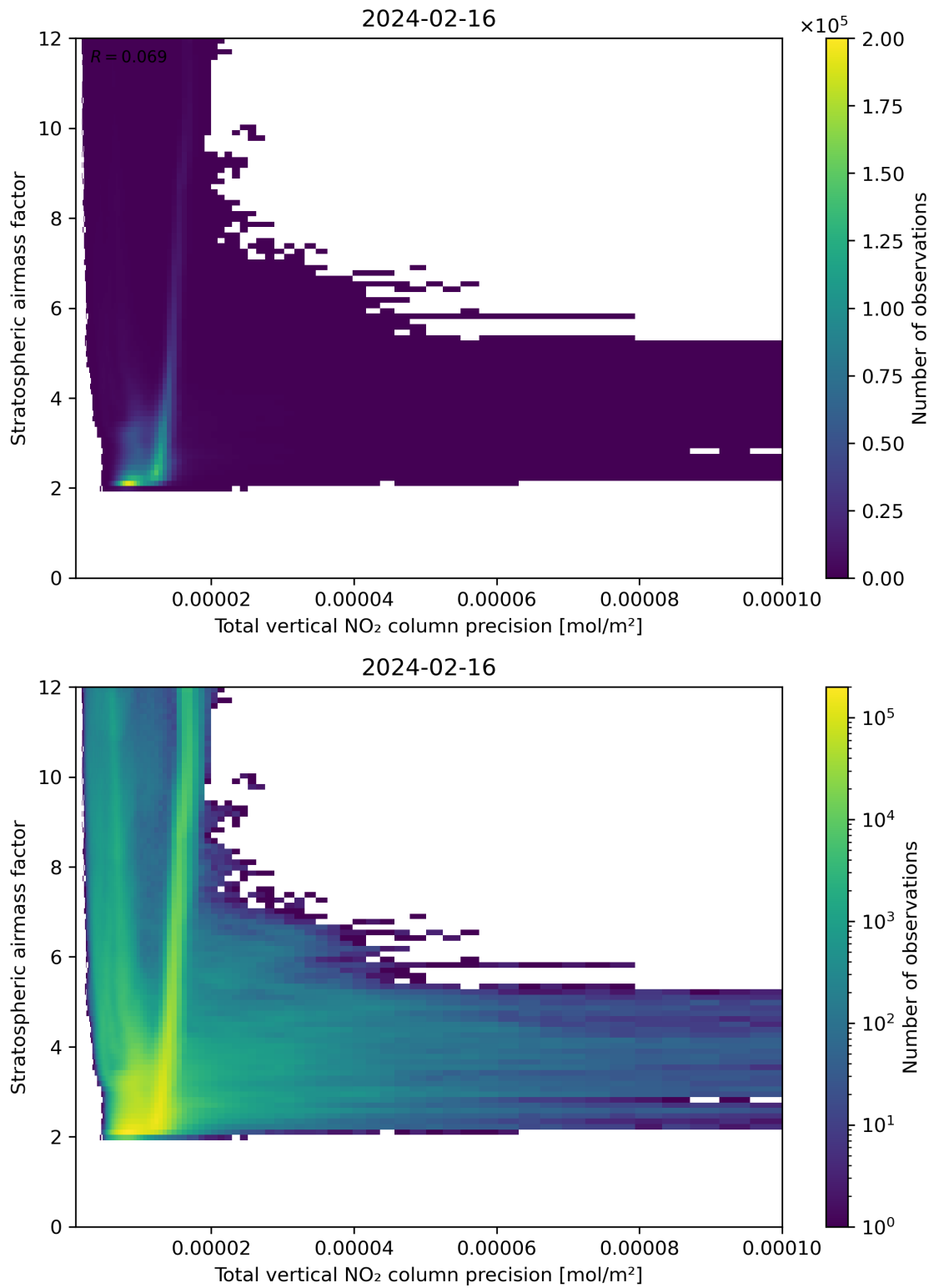
Figure 115: Scatter density plot of “Total vertical NO 2 column precision” against “Stratospheric air mass factor” for 2024-02-16 to 2024-02-17.
