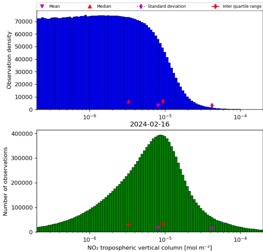
Figure 29: Histogram of “NO 2 tropospheric vertical column” for 2024-02-16 to 2024-02-17
