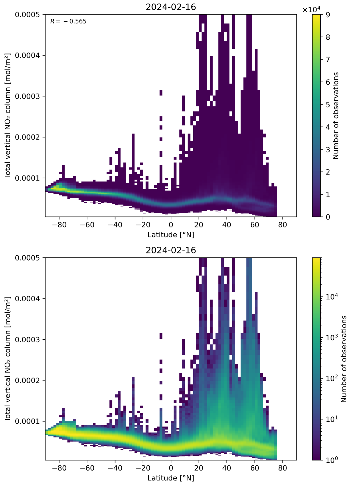
Figure 90: Scatter density plot of “Latitude” against “Total vertical NO 2 column” for 2024-02-16 to 2024-02-17.
