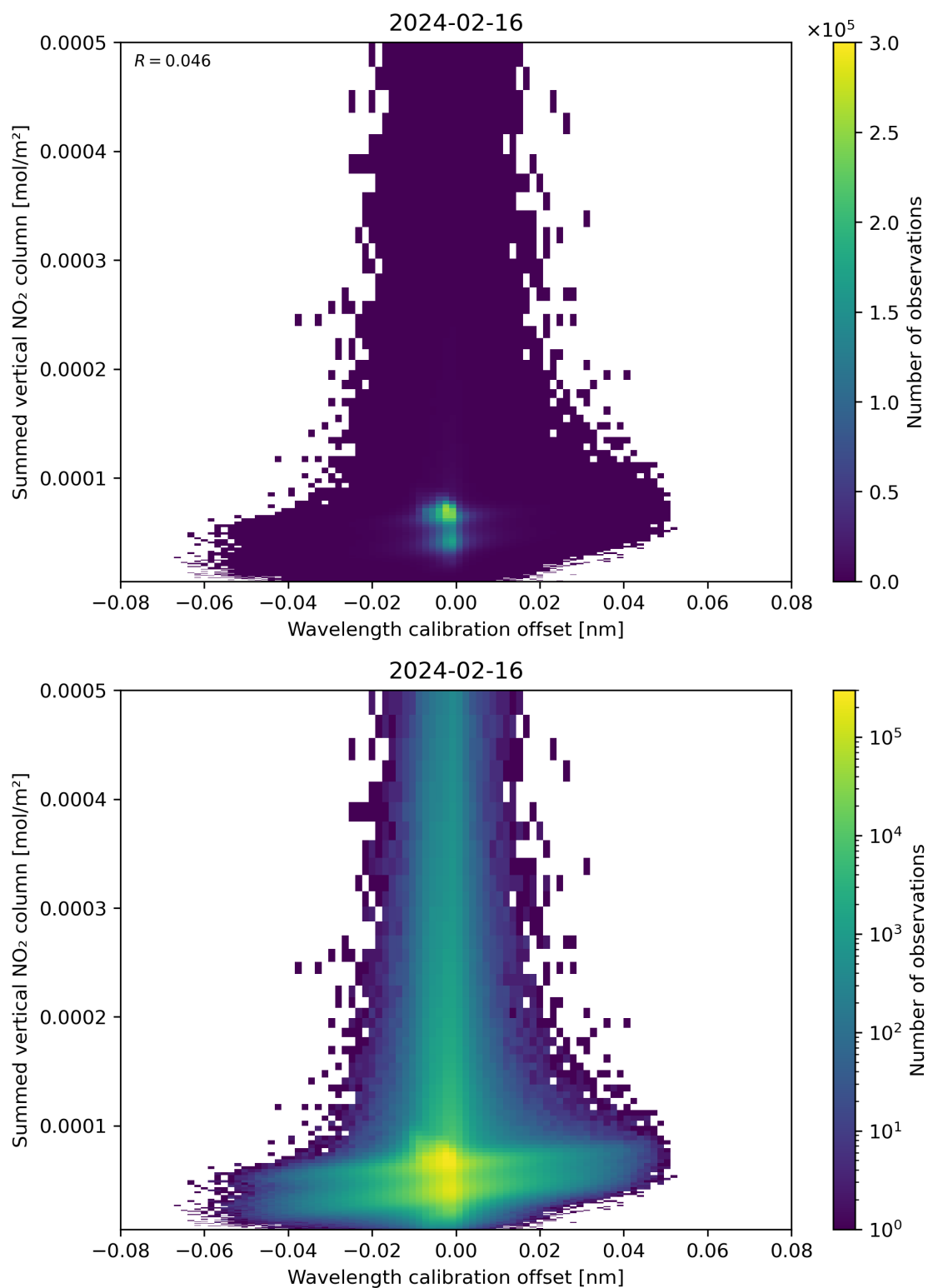
Figure 177: Scatter density plot of “Wavelength calibration offset” against “Summed vertical NO 2 column” for 2024-02-16 to 2024-02-17.
