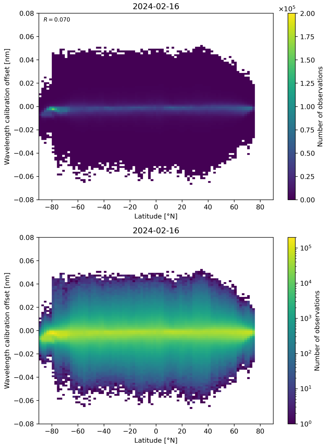
Figure 95: Scatter density plot of “Latitude” against “Wavelength calibration offset” for 2024-02-16 to 2024-02-17.
