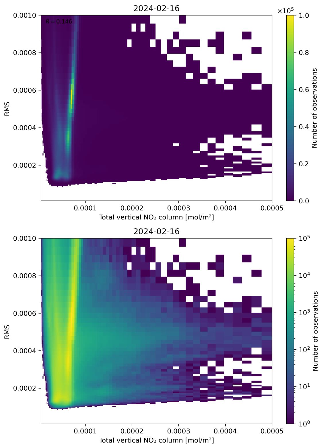
Figure 120: Scatter density plot of “Total vertical NO 2 column” against “RMS” for 2024-02-16 to 2024-02-17.
