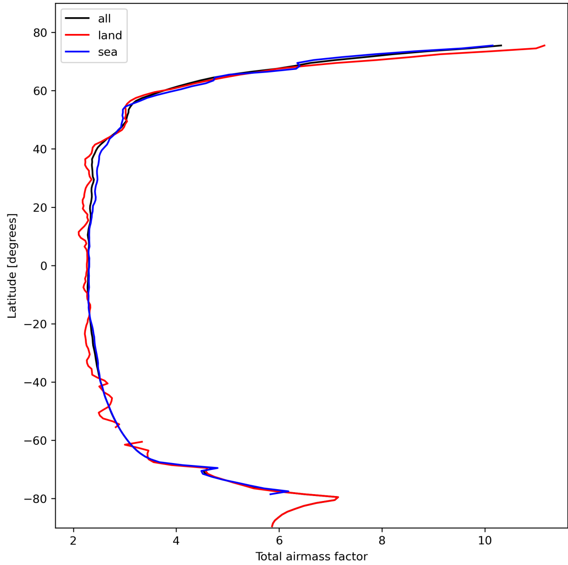
Figure 15: Zonal average of “Total airmass factor” for 2024-02-16 to 2024-02-17.
