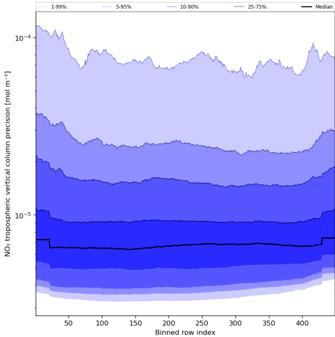
Figure 47: Along track statistics of “NO 2 tropospheric vertical column precision” for 2024-02-16 to 2024-02-17
