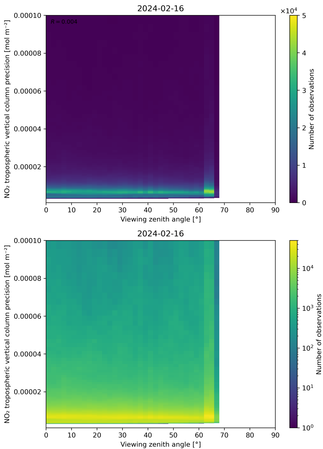
Figure 170: Scatter density plot of “Viewing zenith angle” against “NO 2 tropospheric vertical column precision” for 2024-02-16 to 2024-02-17.
