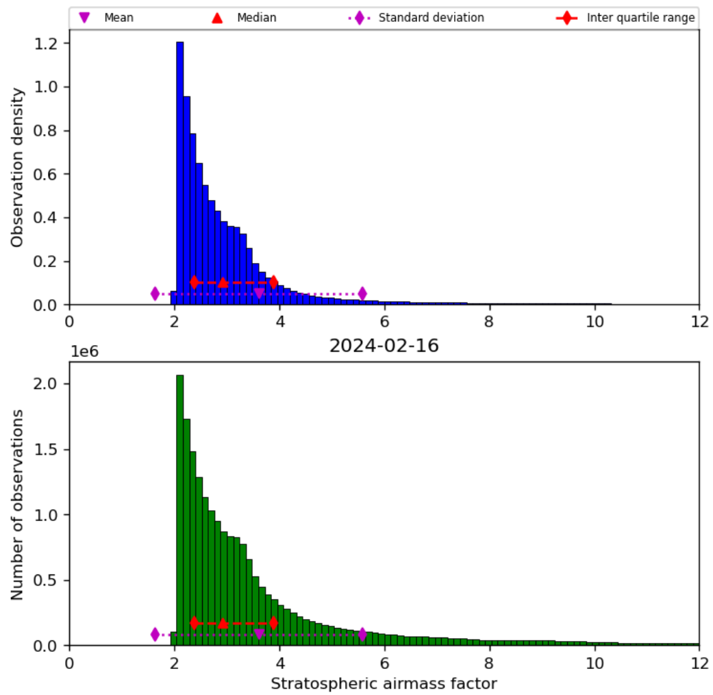
Figure 44: Histogram of “Stratospheric airmass factor” for 2024-02-16 to 2024-02-17
