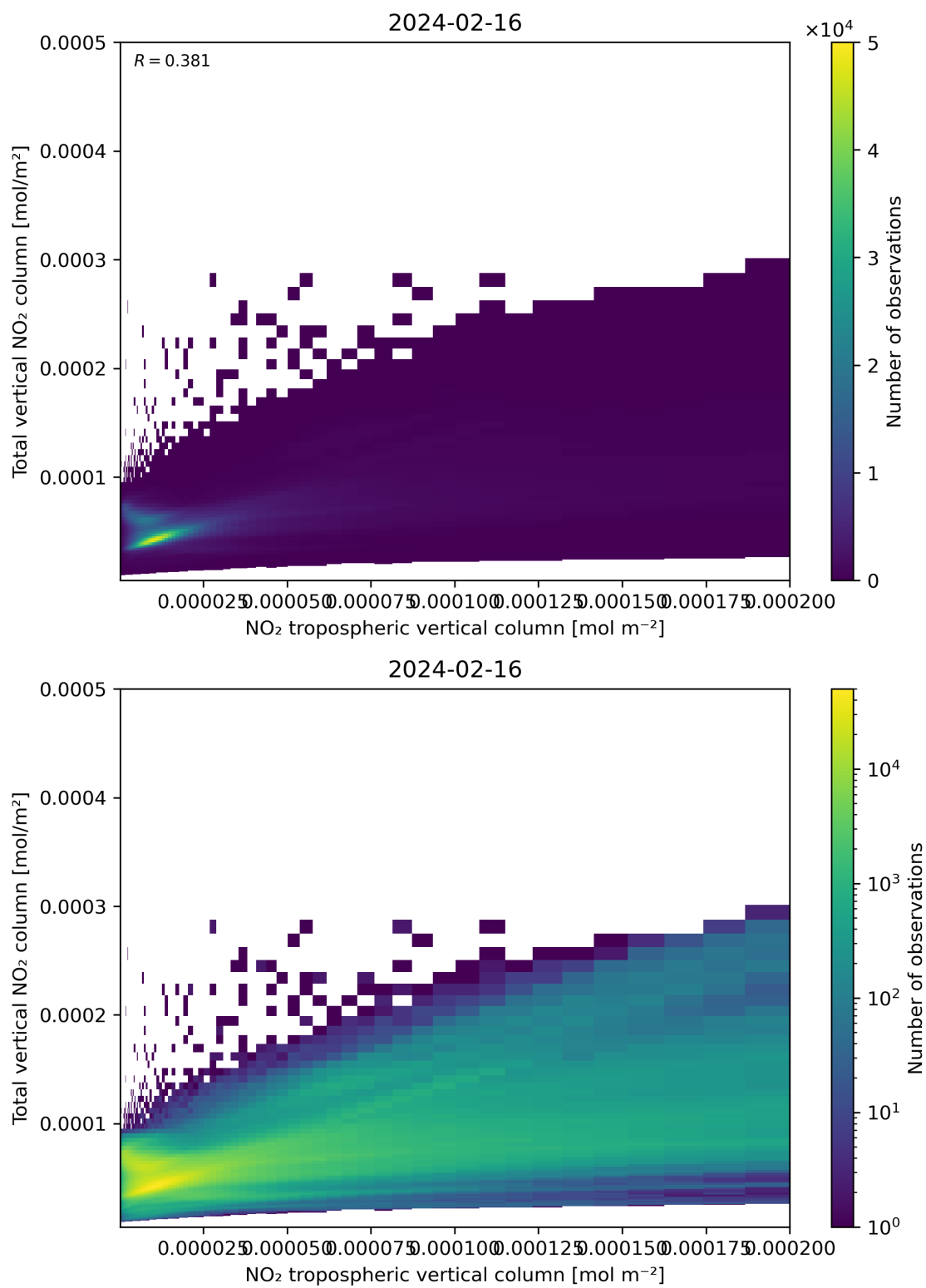
Figure 128: Scatter density plot of “NO 2 tropospheric vertical column” against “Total vertical NO 2 column” for 2024-02-16 to 2024-02-17.
