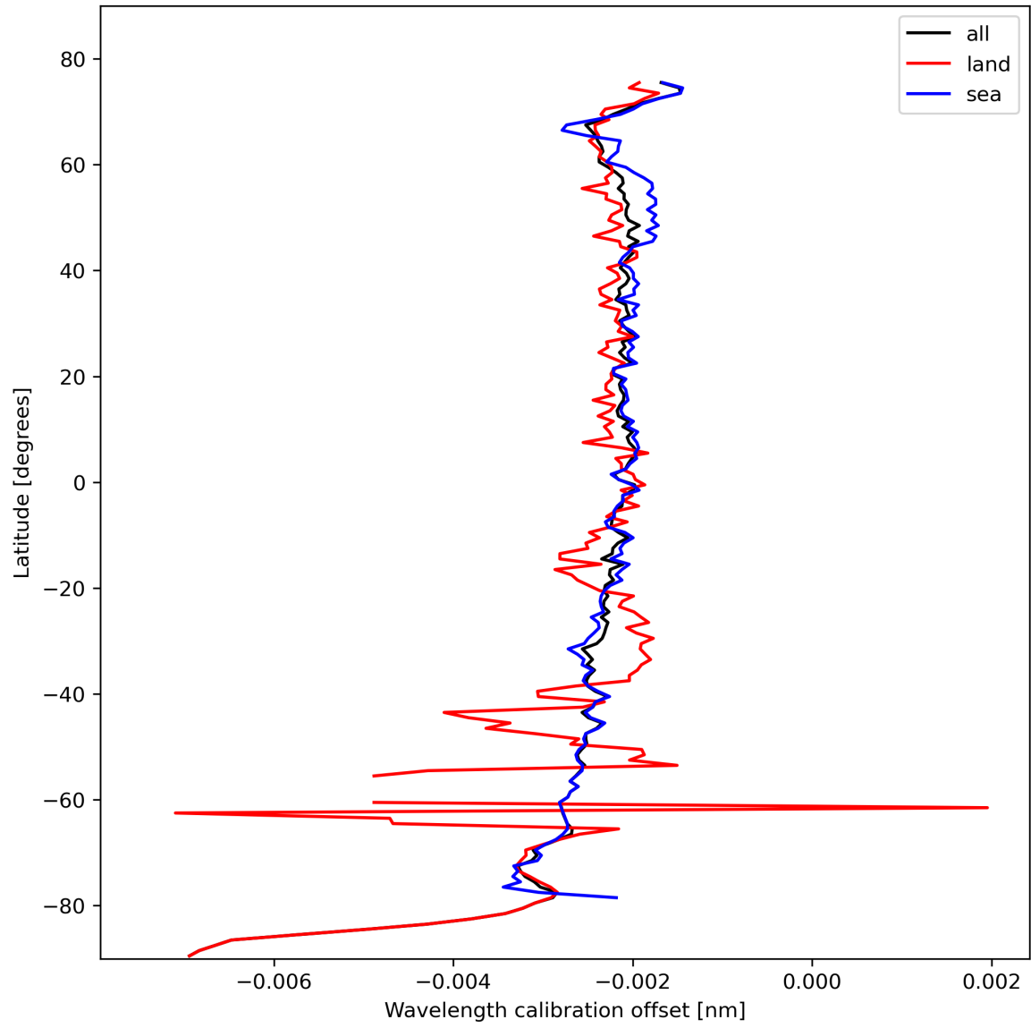
Figure 18: Zonal average of “Wavelength calibration offset” for 2024-02-16 to 2024-02-17.
