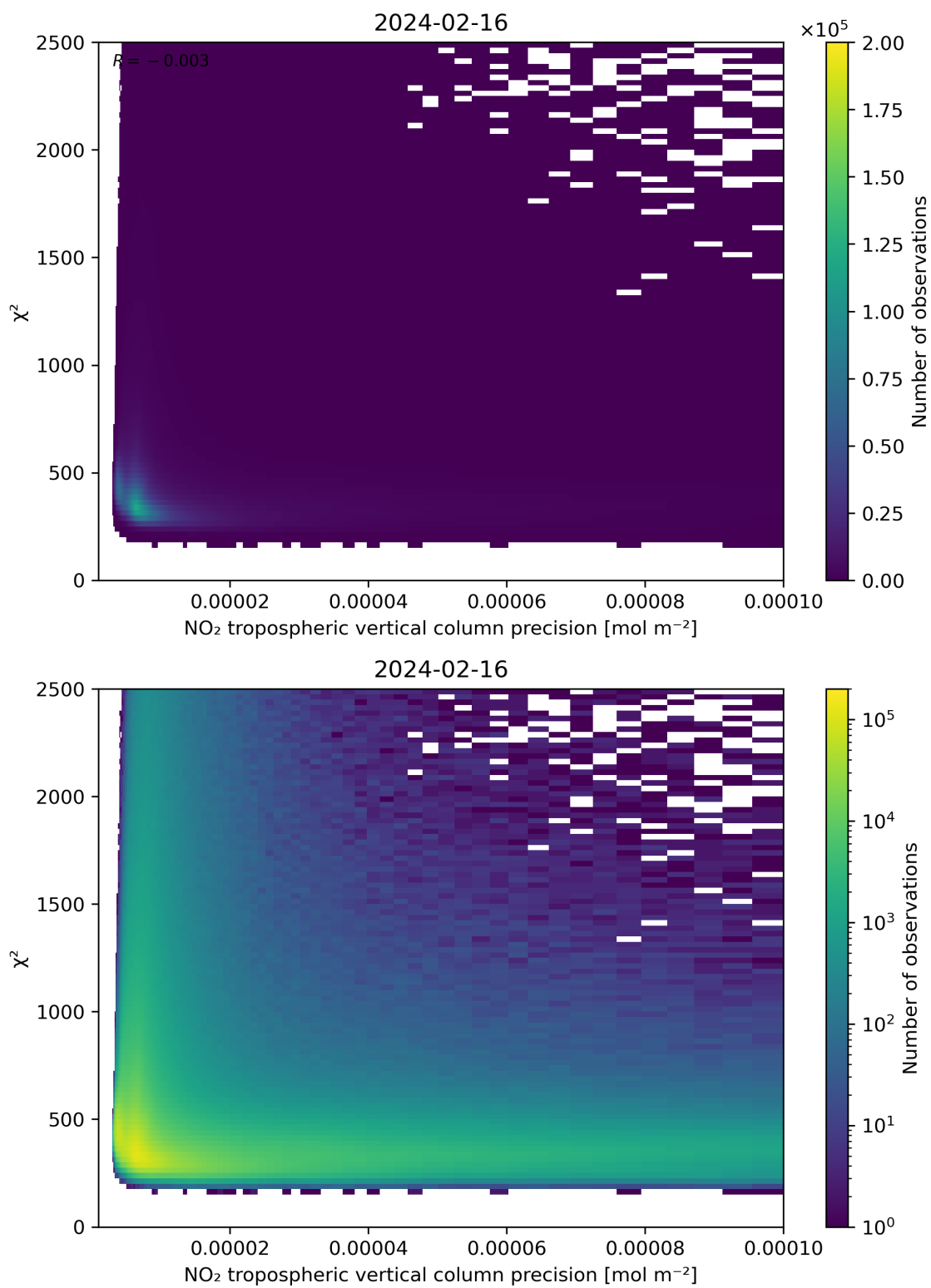
Figure 134: Scatter density plot of “NO 2 tropospheric vertical column precision” against “ \chi^2 ” for 2024-02-16 to 2024-02-17.
