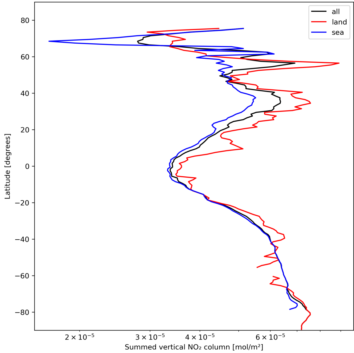
Figure 23: Zonal average of “Summed vertical NO 2 column” for 2024-02-16 to 2024-02-17.
