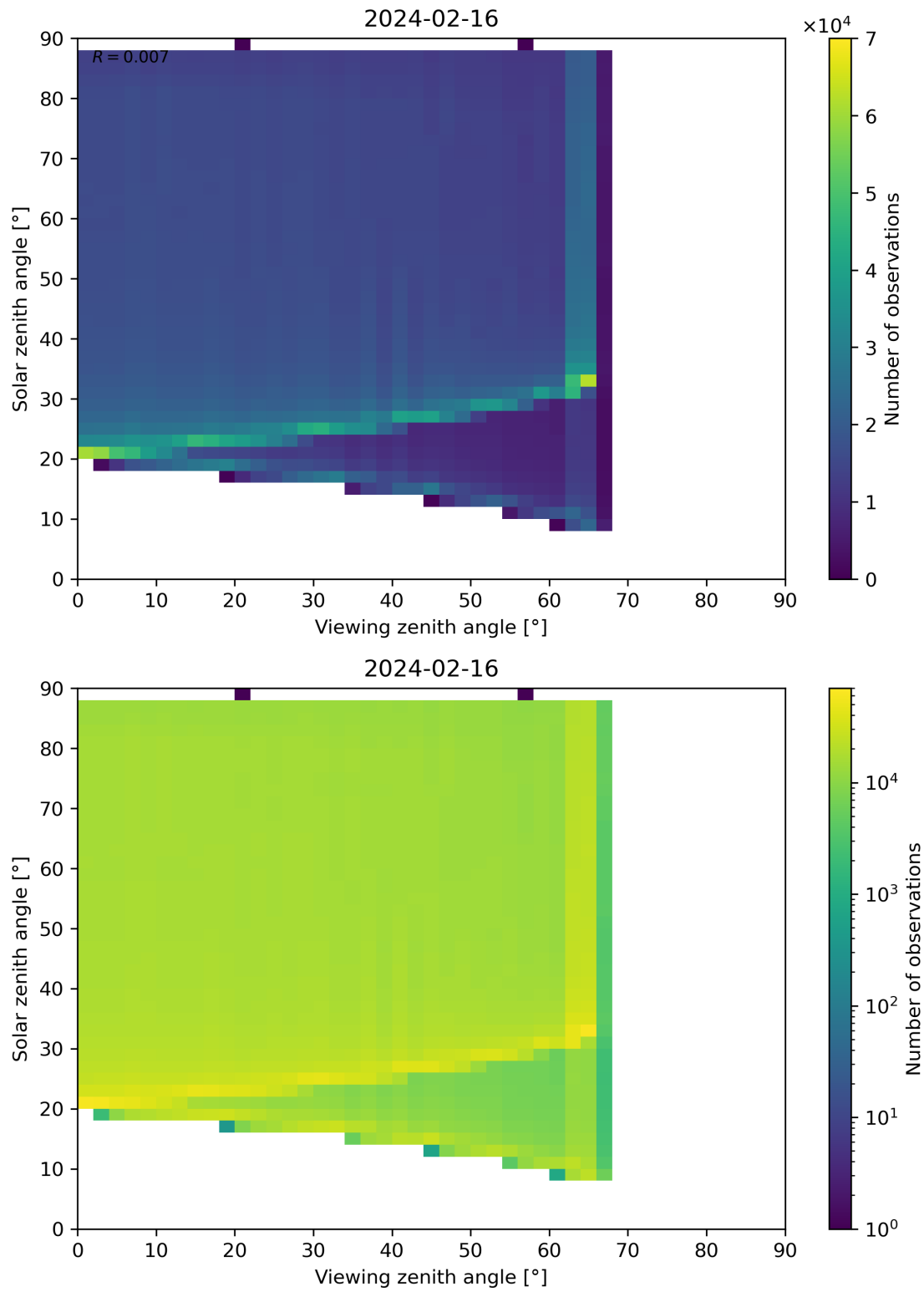
Figure 172: Scatter density plot of “Viewing zenith angle” against “Solar zenith angle” for 2024-02-16 to 2024-02-17.
