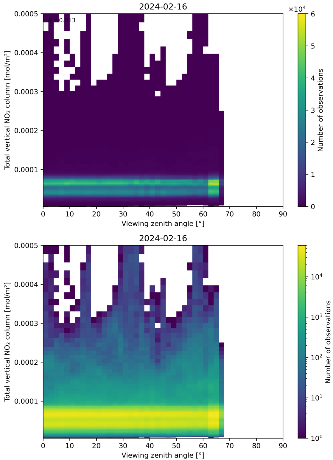
Figure 167: Scatter density plot of “Viewing zenith angle” against “Total vertical NO 2 column” for 2024-02-16 to 2024-02-17.
