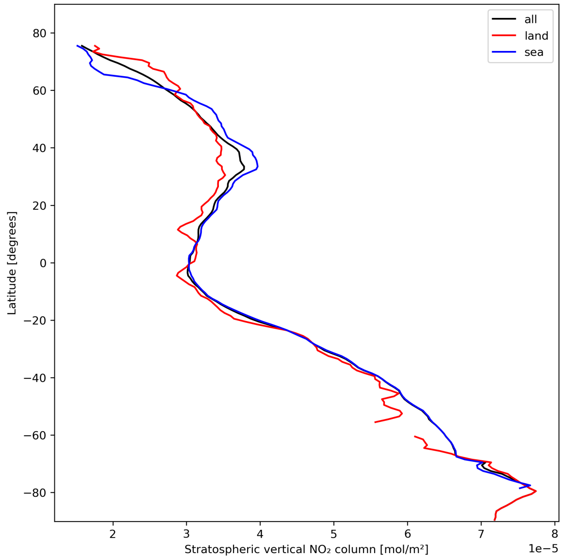
Figure 19: Zonal average of “Stratospheric vertical NO 2 column” for 2024-02-16 to 2024-02-17.
