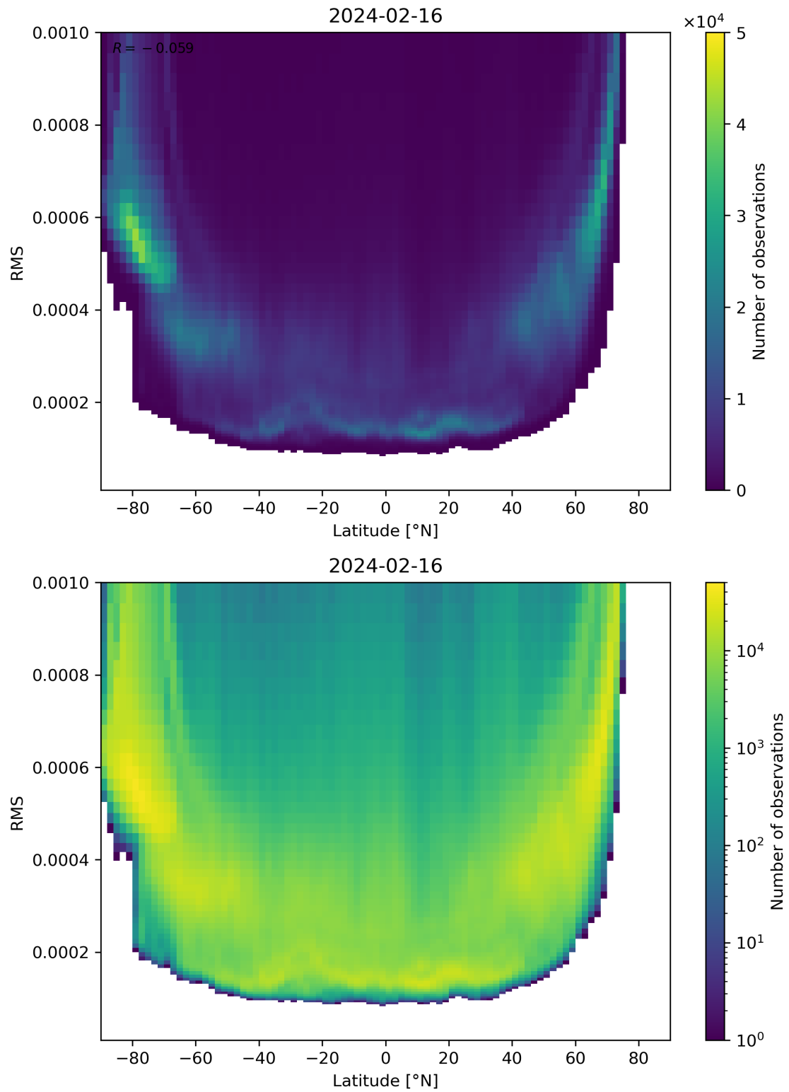
Figure 94: Scatter density plot of “Latitude” against “RMS” for 2024-02-16 to 2024-02-17.
