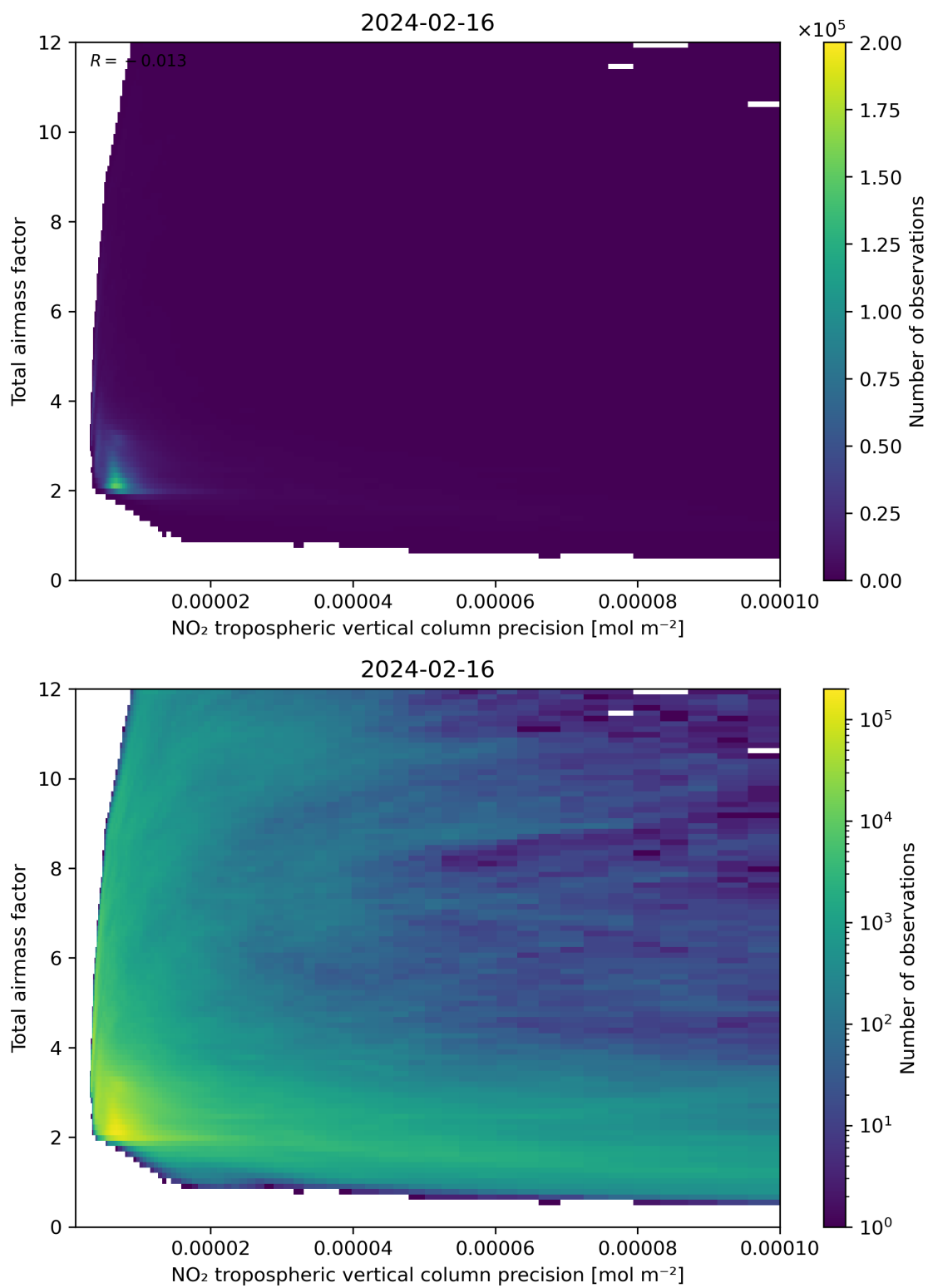
Figure 132: Scatter density plot of “NO 2 tropospheric vertical column precision” against “Total airmass factor” for 2024-02-16 to 2024-02-17.
