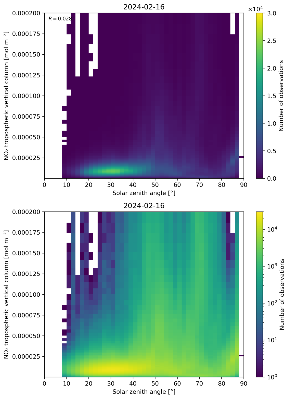
Figure 155: Scatter density plot of “Solar zenith angle” against “NO 2 tropospheric vertical column” for 2024-02-16 to 2024-02-17.
