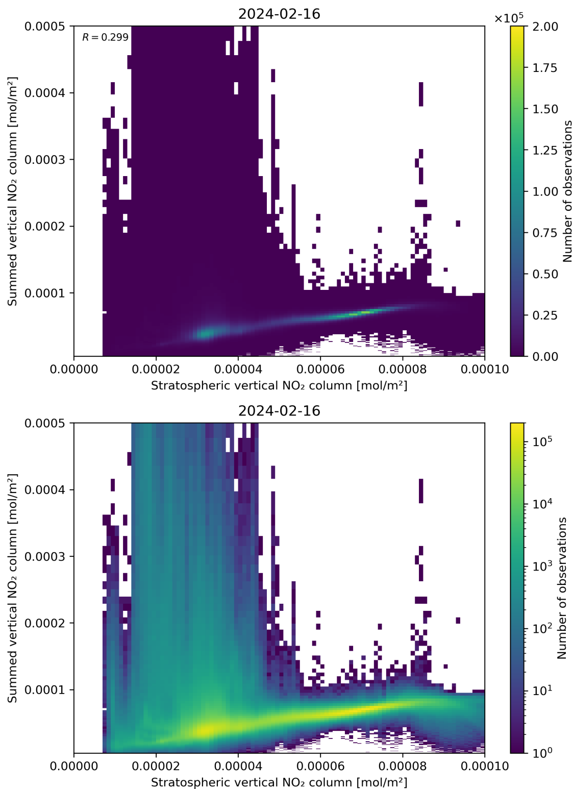
Figure 98: Scatter density plot of “Stratospheric vertical NO 2 column” against “Summed vertical NO 2 column” for 2024-02-16 to 2024-02-17.
