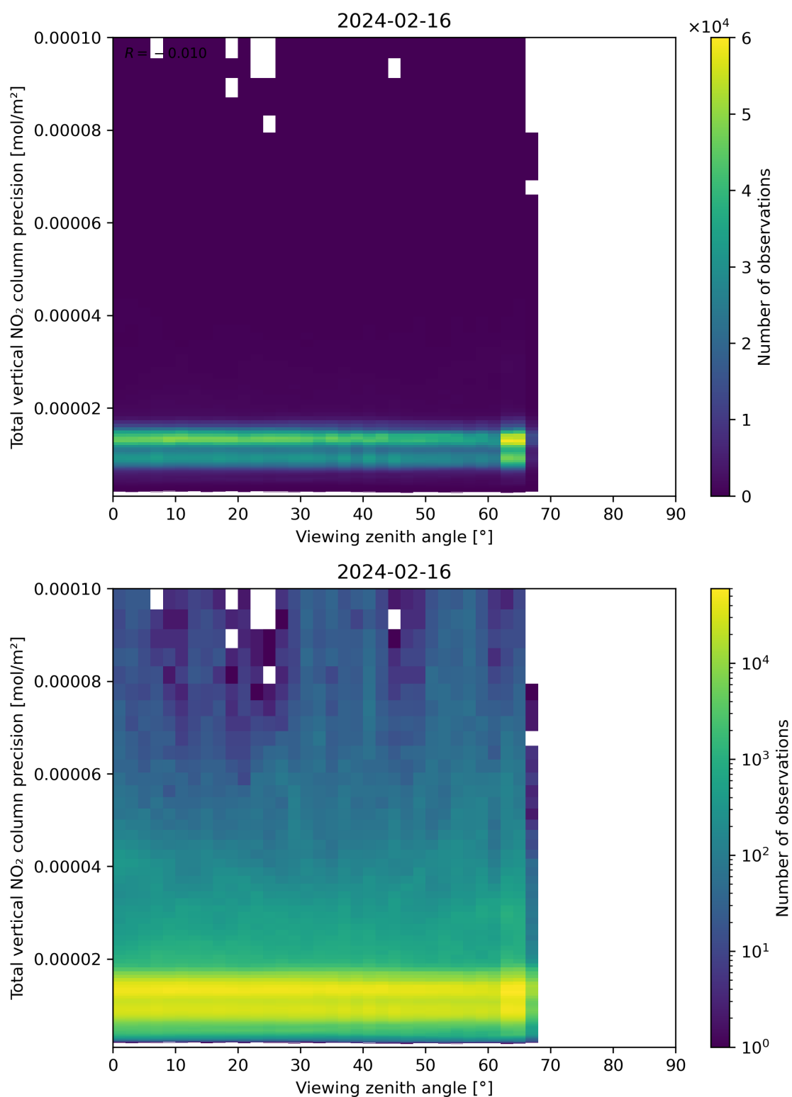
Figure 168: Scatter density plot of “Viewing zenith angle” against “Total vertical NO 2 column precision” for 2024-02-16 to 2024-02-17.
