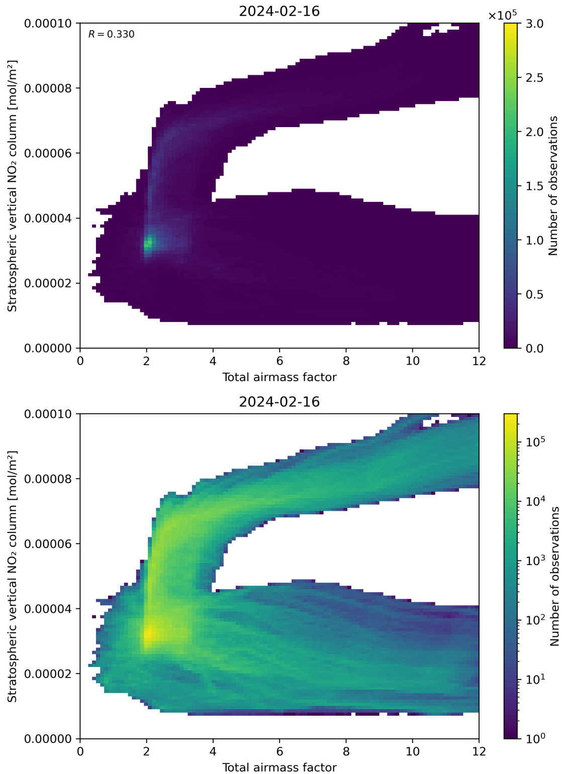
Figure 64: Scatter density plot of “Total airmass factor” against “Stratospheric vertical \text{NO}_2 column” for 2024-02-16 to 2024-02-17.
