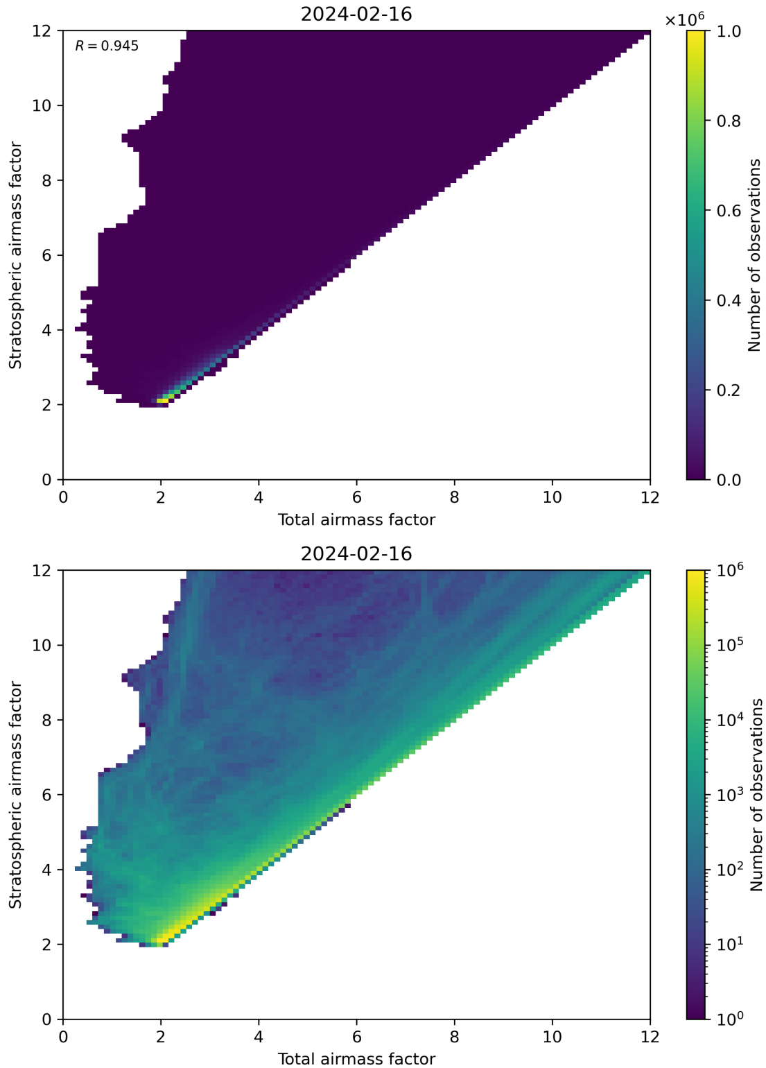
Figure 62: Scatter density plot of “Total airmass factor” against “Stratospheric airmass factor” for 2024-02-16 to 2024-02-17.
