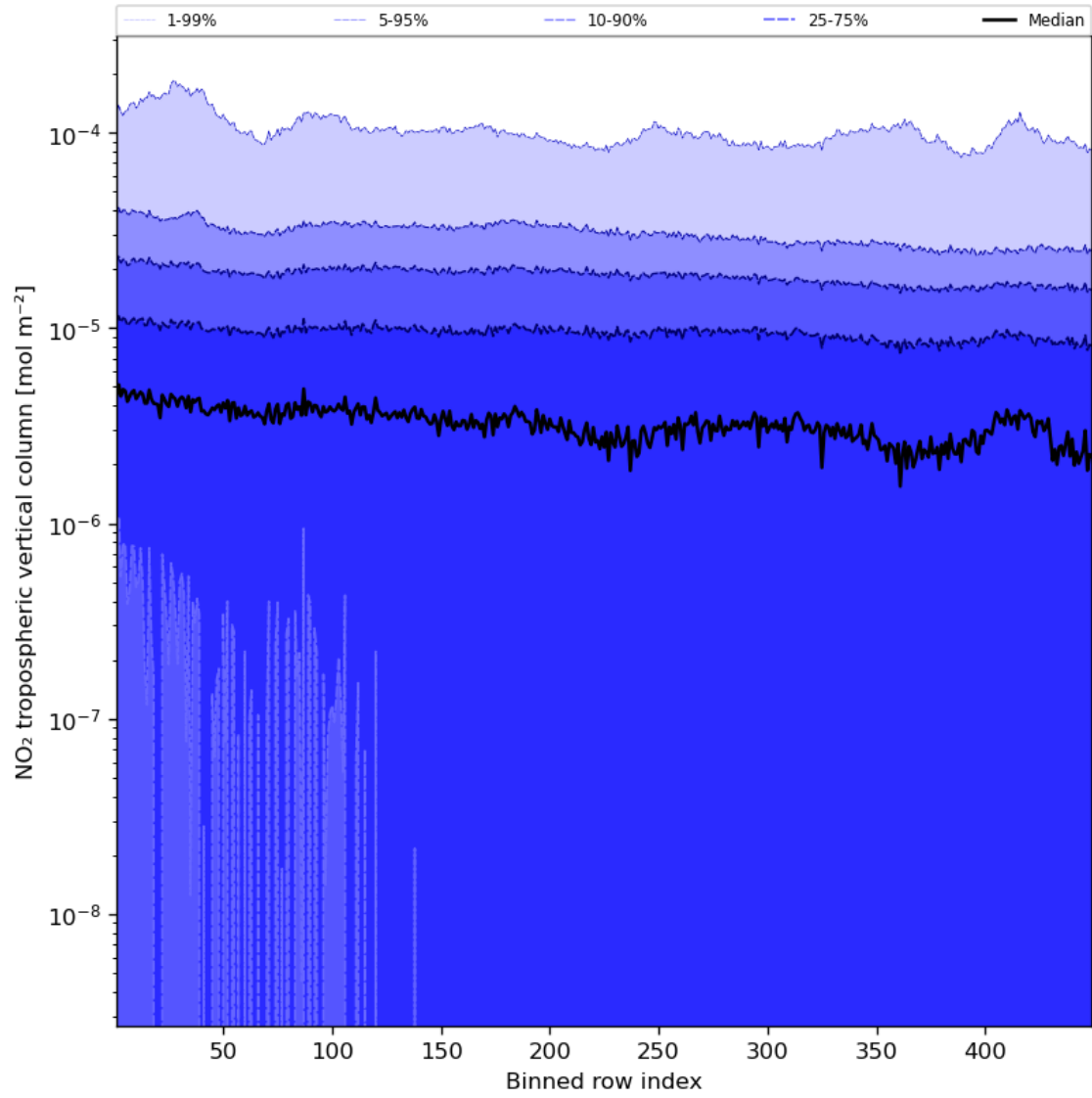
Figure 46: Along track statistics of “NO 2 tropospheric vertical column” for 2024-02-16 to 2024-02-17
