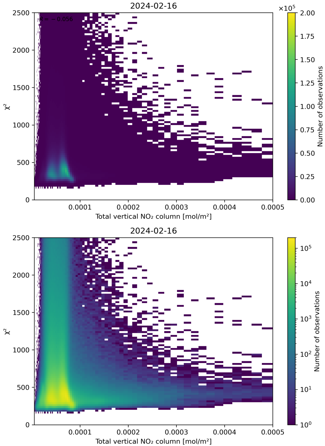
Figure 111: Scatter density plot of “Total vertical NO 2 column” against “ \chi^2 ” for 2024-02-16 to 2024-02-17.
