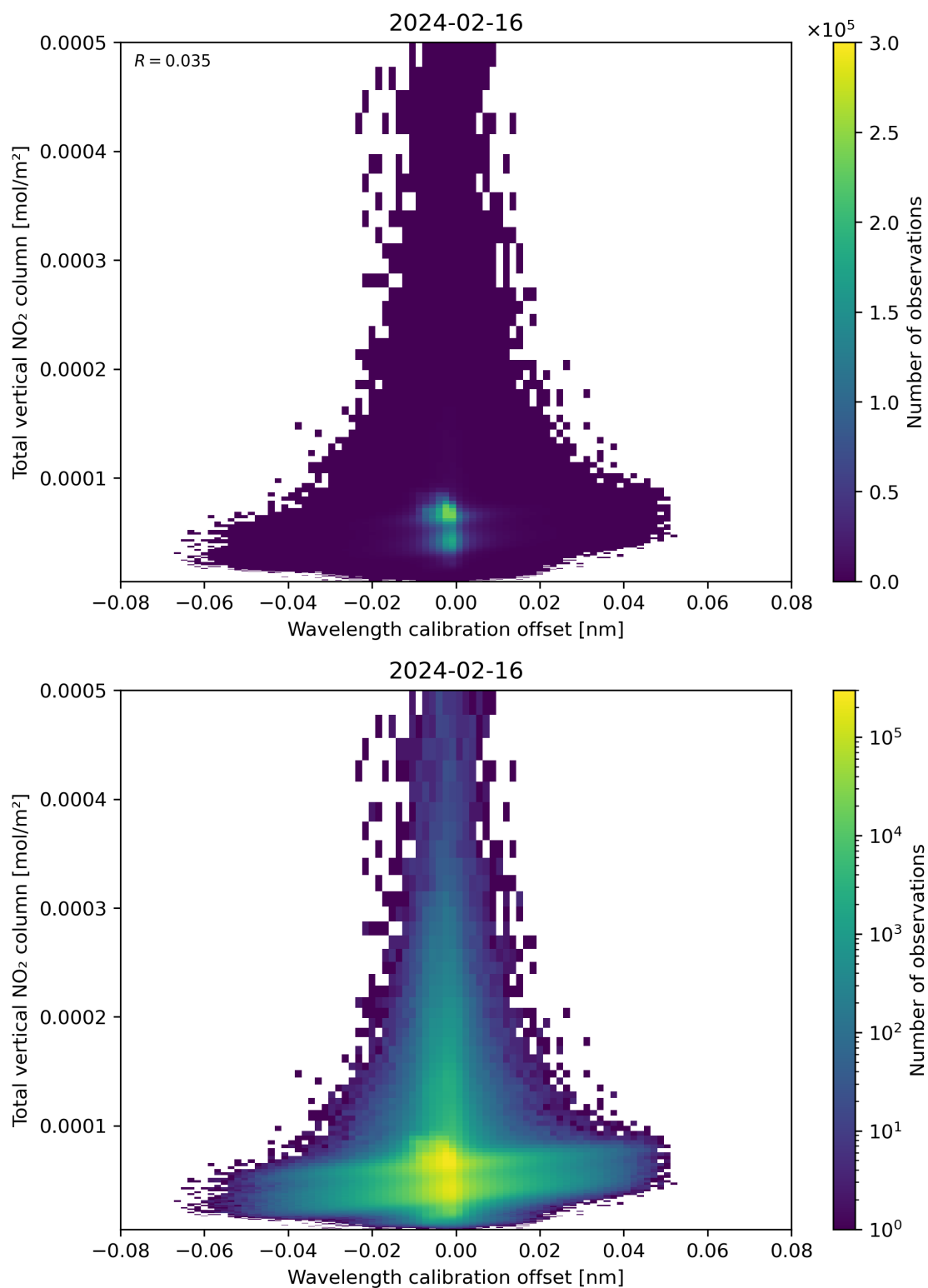
Figure 179: Scatter density plot of “Wavelength calibration offset” against “Total vertical NO 2 column” for 2024-02-16 to 2024-02-17.
