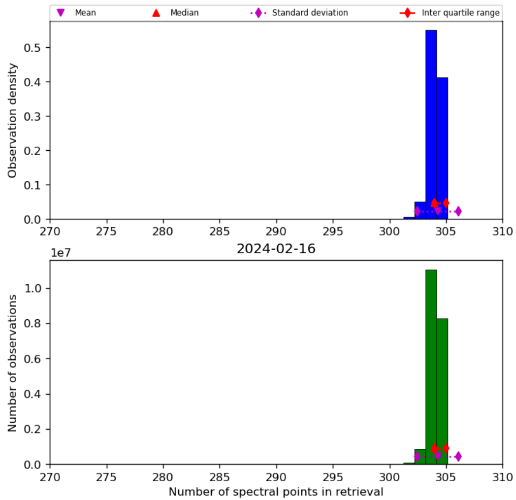
Figure 33: Histogram of “Number of spectral points in retrieval” for 2024-02-16 to 2024-02-17
