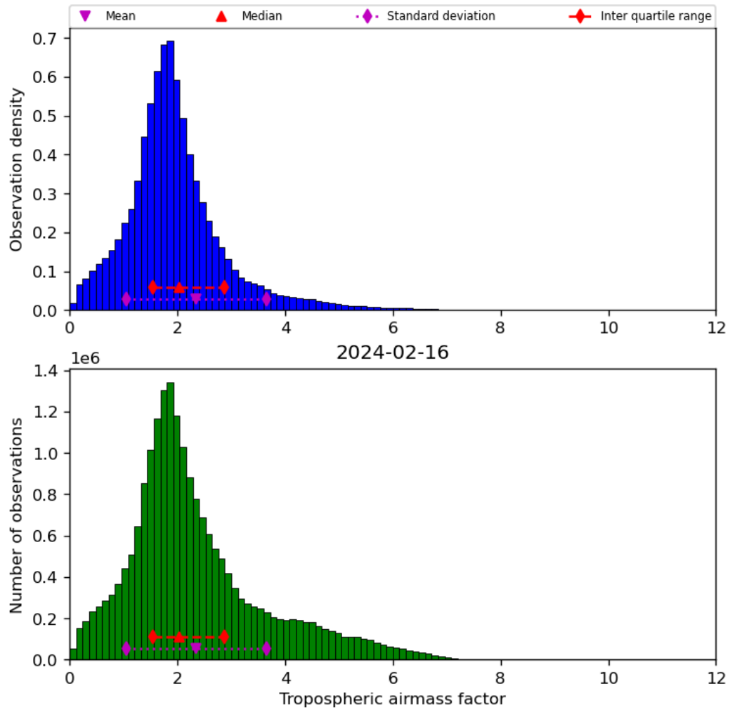
Figure 31: Histogram of “Tropospheric airmass factor” for 2024-02-16 to 2024-02-17
