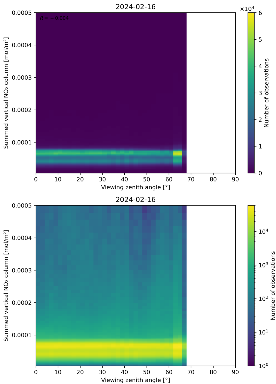
Figure 165: Scatter density plot of “Viewing zenith angle” against “Summed vertical NO 2 column” for 2024-02-16 to 2024-02-17.
