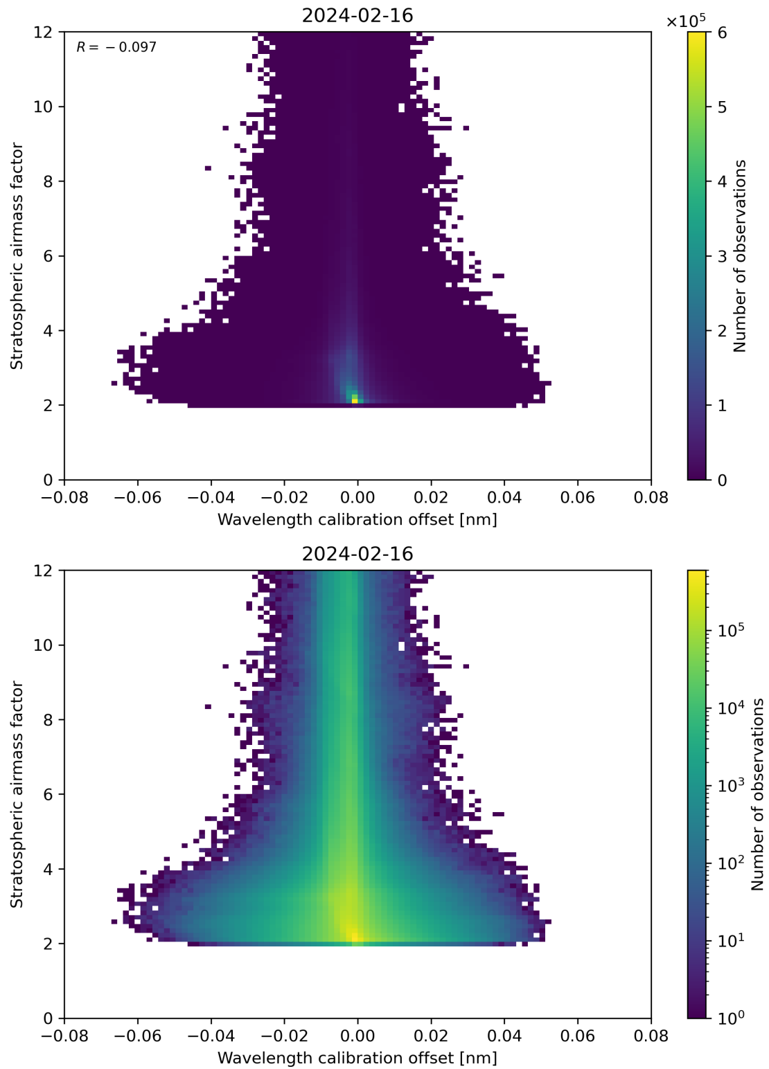
Figure 174: Scatter density plot of “Wavelength calibration offset” against “Stratospheric airmass factor” for 2024-02-16 to 2024-02-17.
