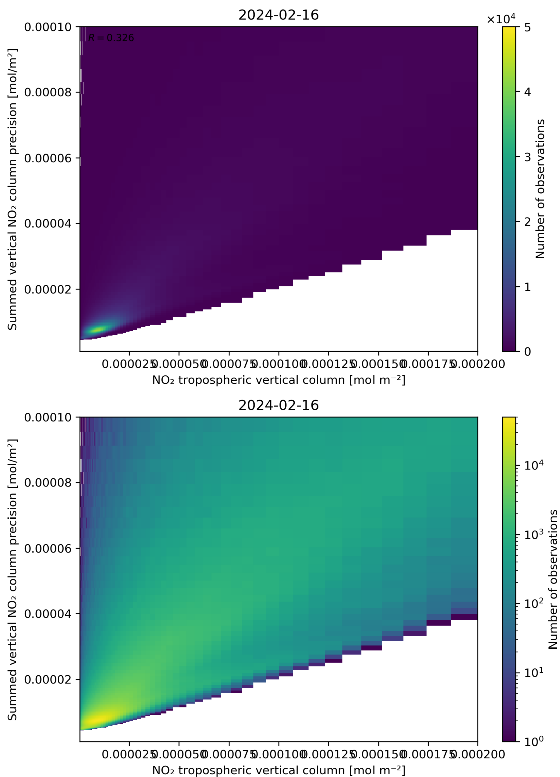
Figure 127: Scatter density plot of “NO 2 tropospheric vertical column” against “Summed vertical NO 2 column precision” for 2024-02-16 to 2024-02-17.
