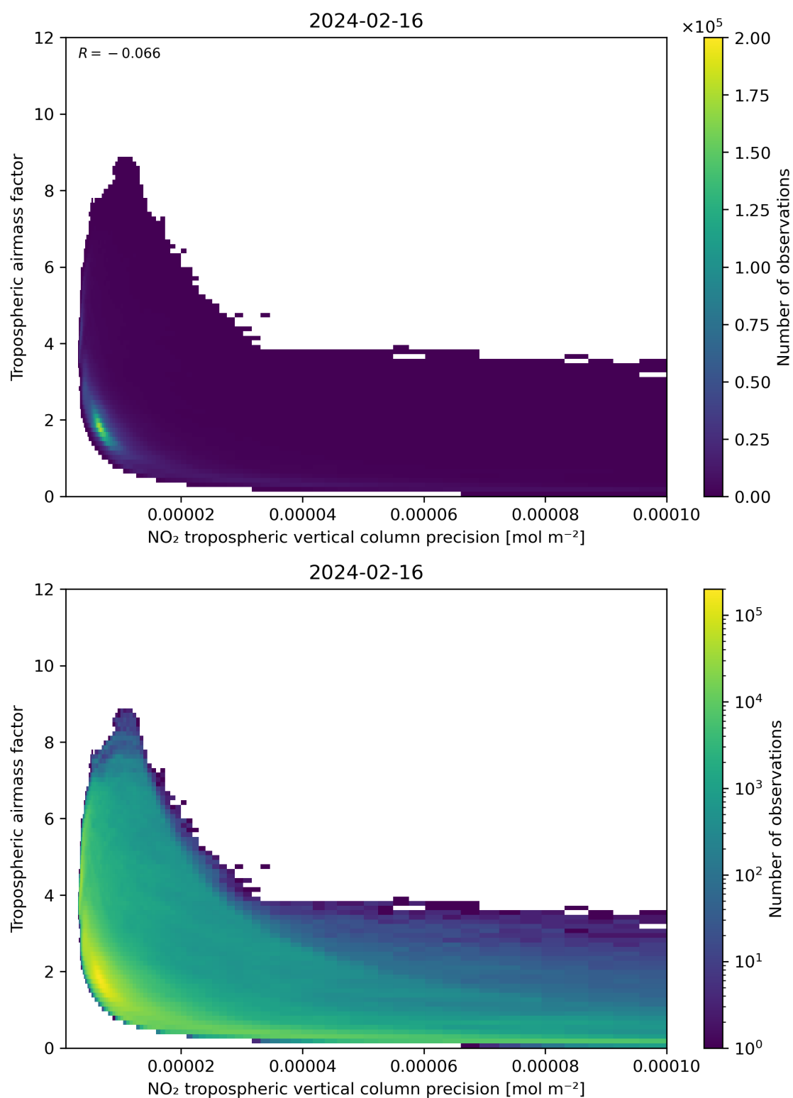
Figure 133: Scatter density plot of “NO 2 tropospheric vertical column precision” against “Tropospheric airmass factor” for 2024-02-16 to 2024-02-17.
