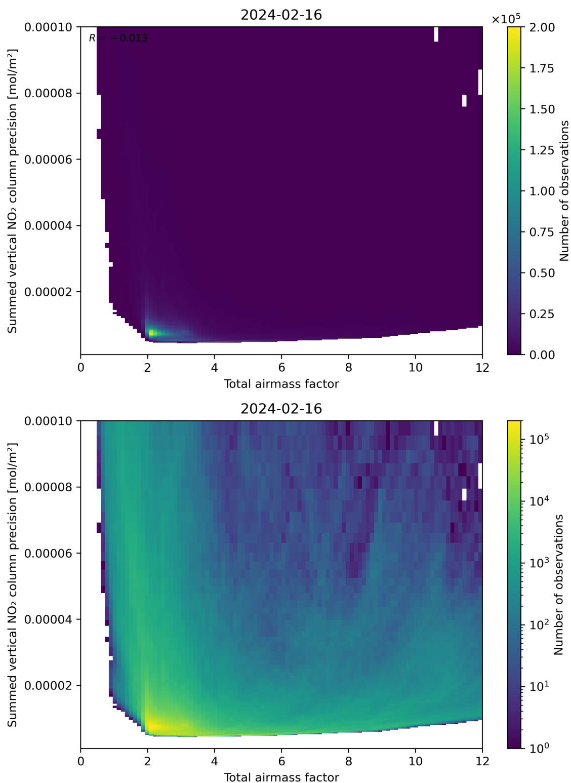
Figure 66: Scatter density plot of “Total airmass factor” against “Summed vertical NO 2 column precision” for 2024-02-16 to 2024-02-17.
