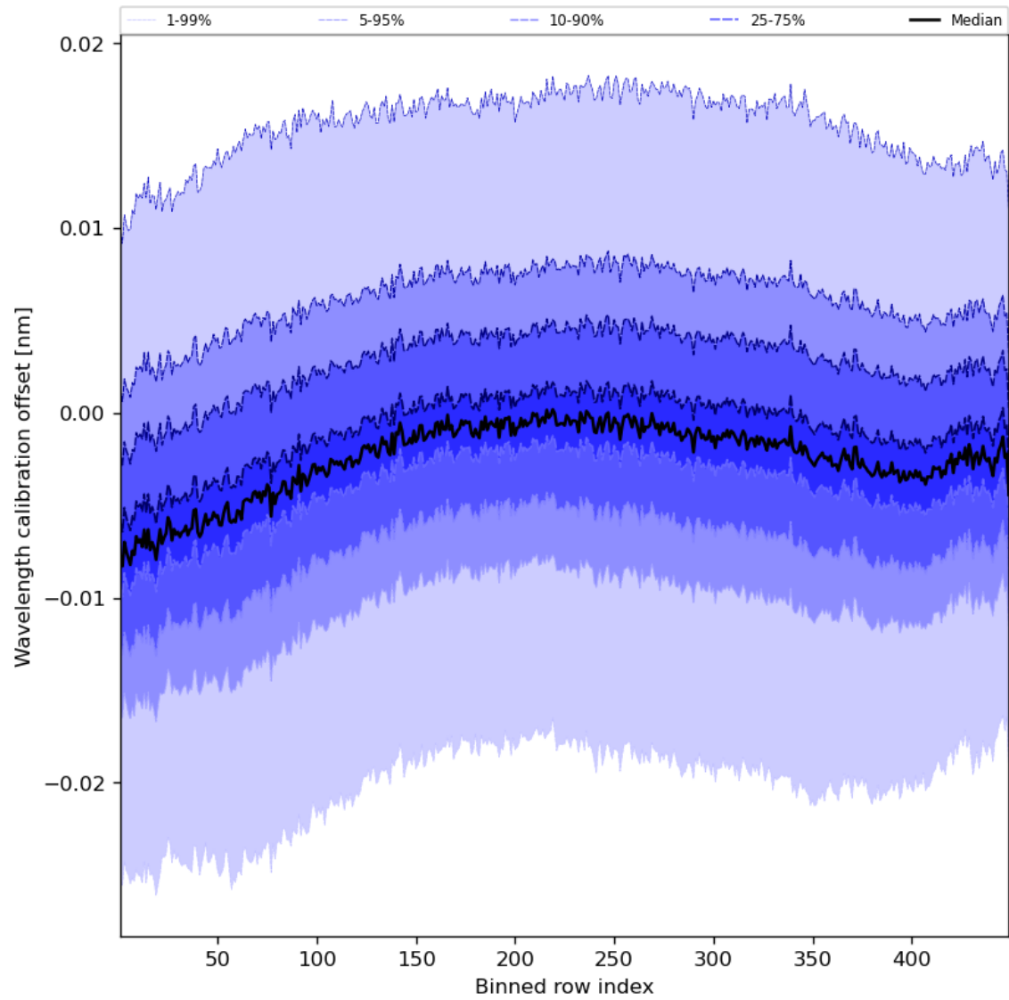
Figure 52: Along track statistics of “Wavelength calibration offset” for 2024-02-16 to 2024-02-17
