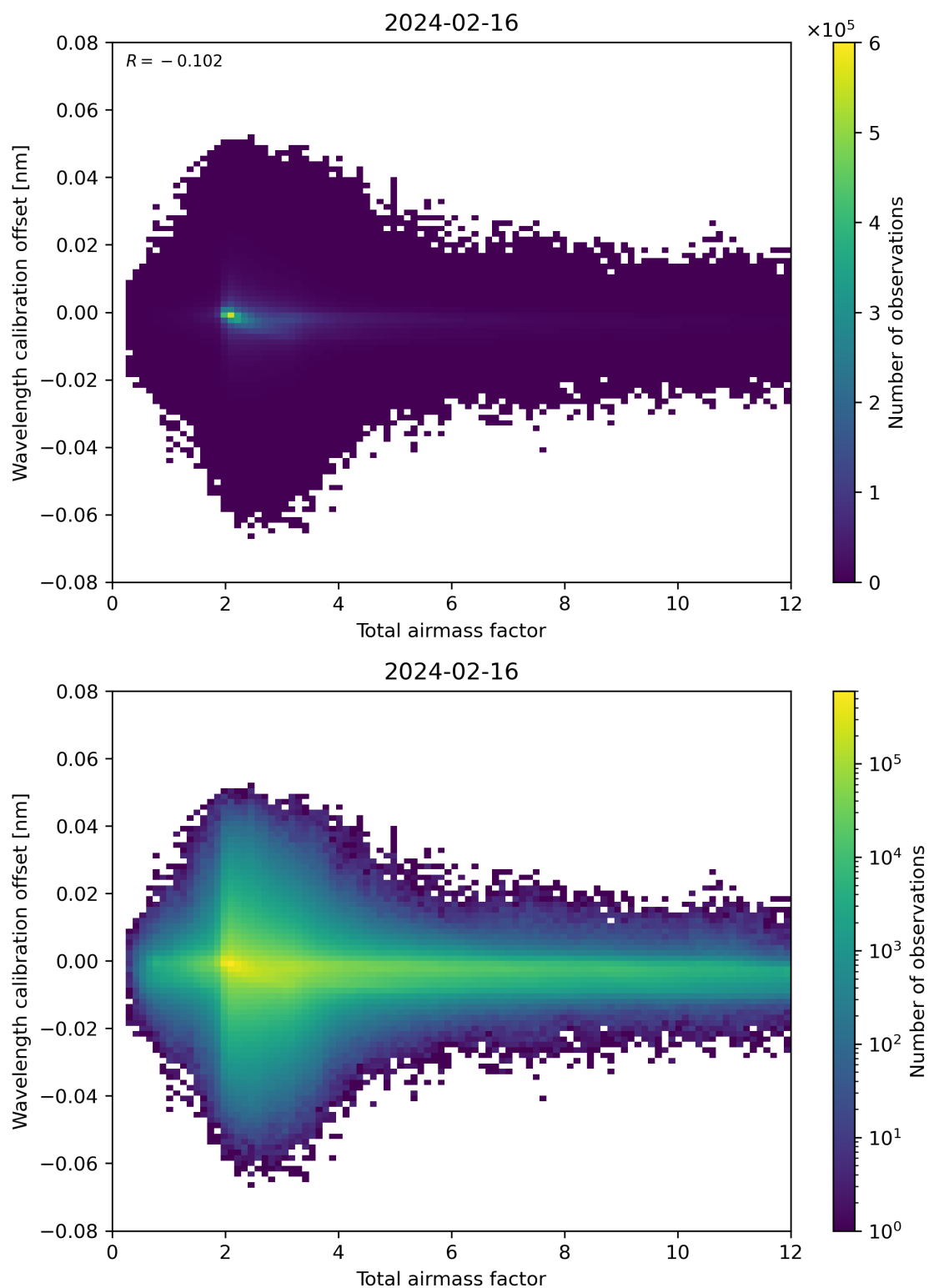
Figure 70: Scatter density plot of “Total airmass factor” against “Wavelength calibration offset” for 2024-02-16 to 2024-02-17.
