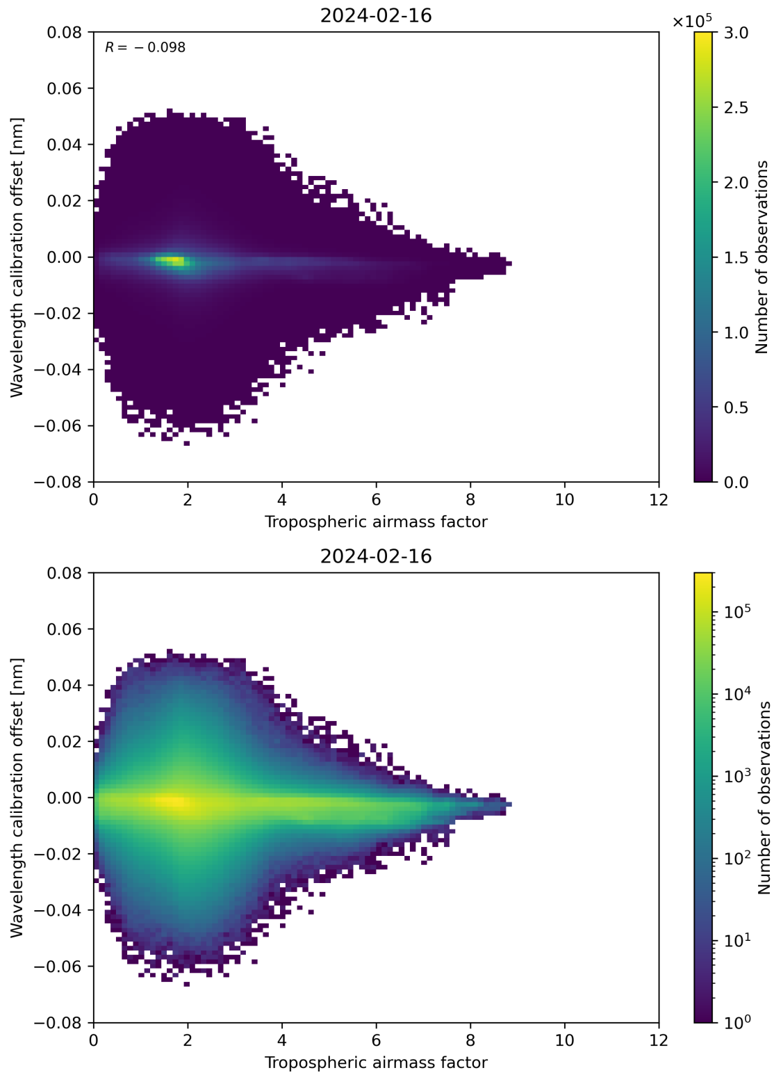
Figure 80: Scatter density plot of “Tropospheric airmass factor” against “Wavelength calibration offset” for 2024-02-16 to 2024-02-17.
