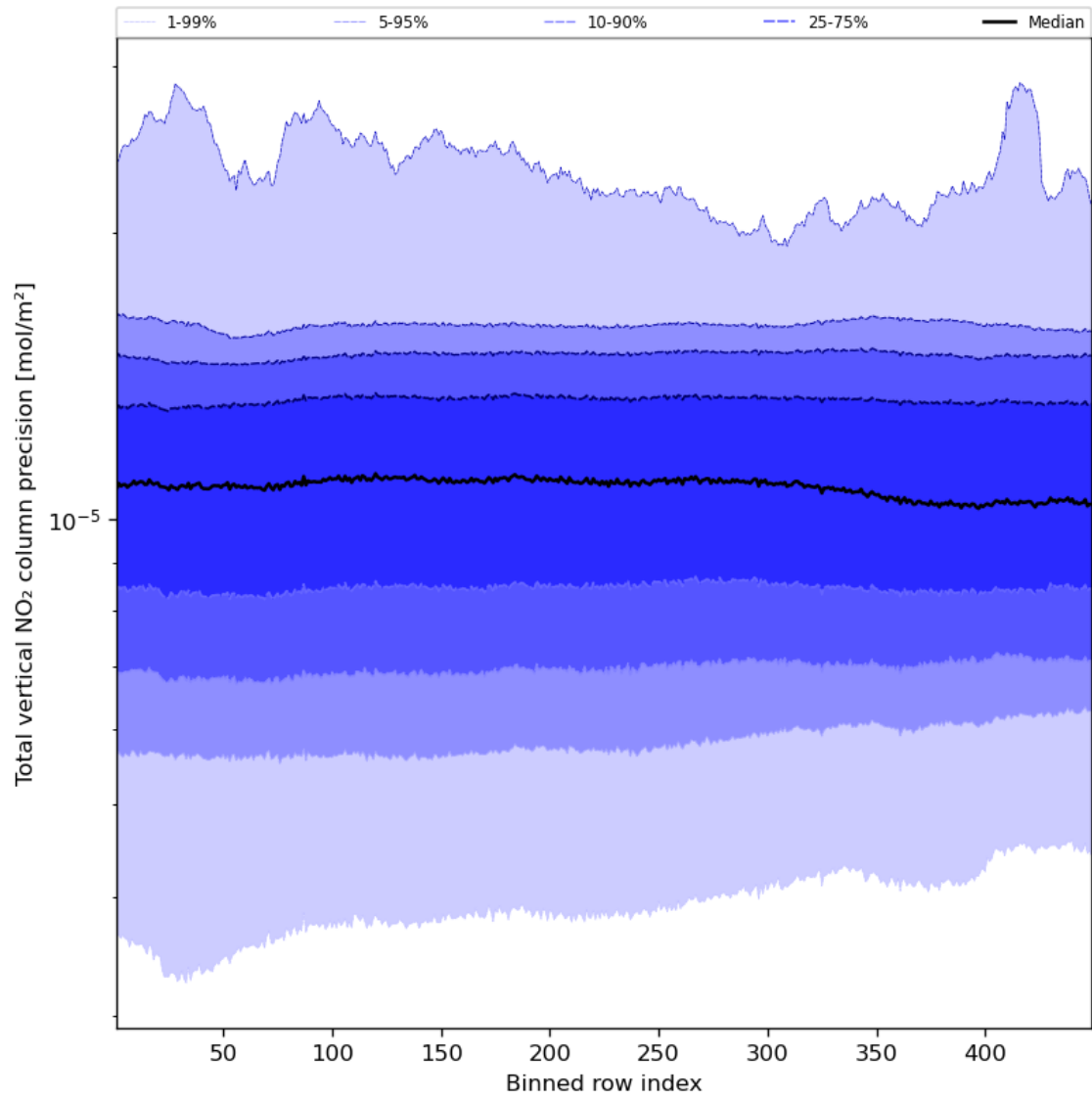
Figure 56: Along track statistics of “Total vertical NO 2 column precision” for 2024-02-16 to 2024-02-17
