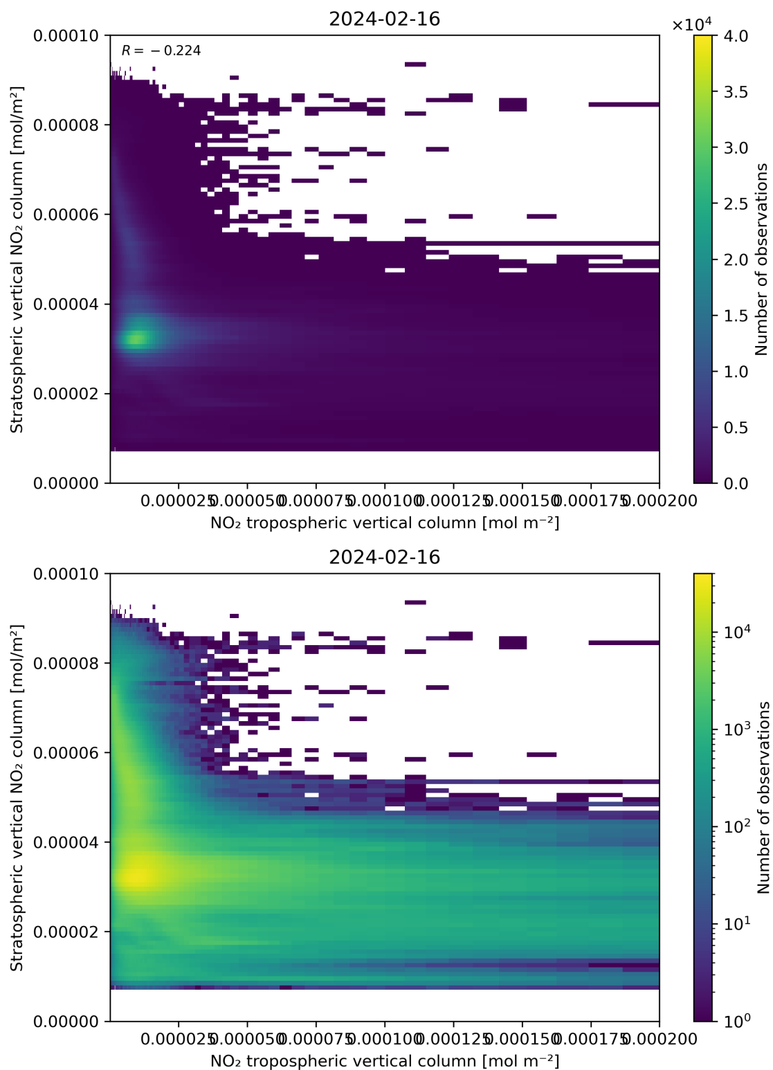
Figure 125: Scatter density plot of “NO 2 tropospheric vertical column” against “Stratospheric vertical NO 2 column” for 2024-02-16 to 2024-02-17.
