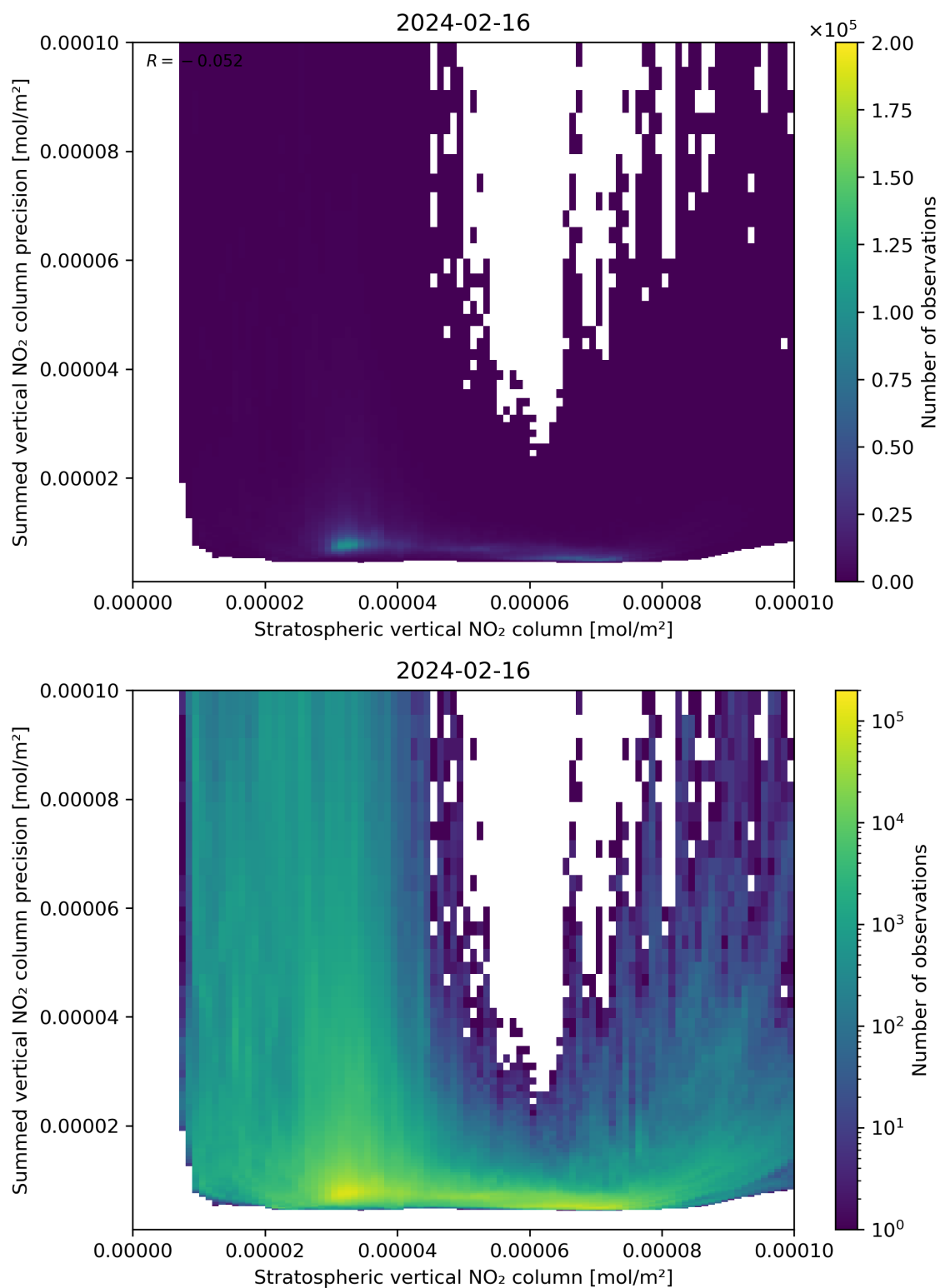
Figure 99: Scatter density plot of “Stratospheric vertical NO 2 column” against “Summed vertical NO 2 column precision” for 2024-02-16 to 2024-02-17.
