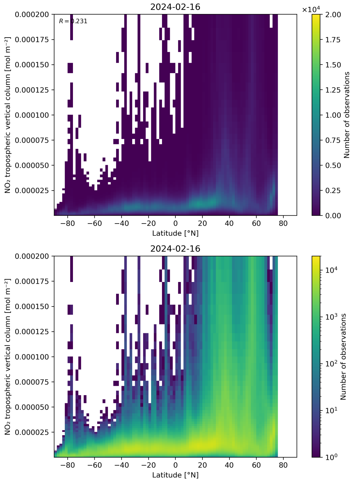
Figure 92: Scatter density plot of “Latitude” against “NO 2 tropospheric vertical column” for 2024-02-16 to 2024-02-17.
