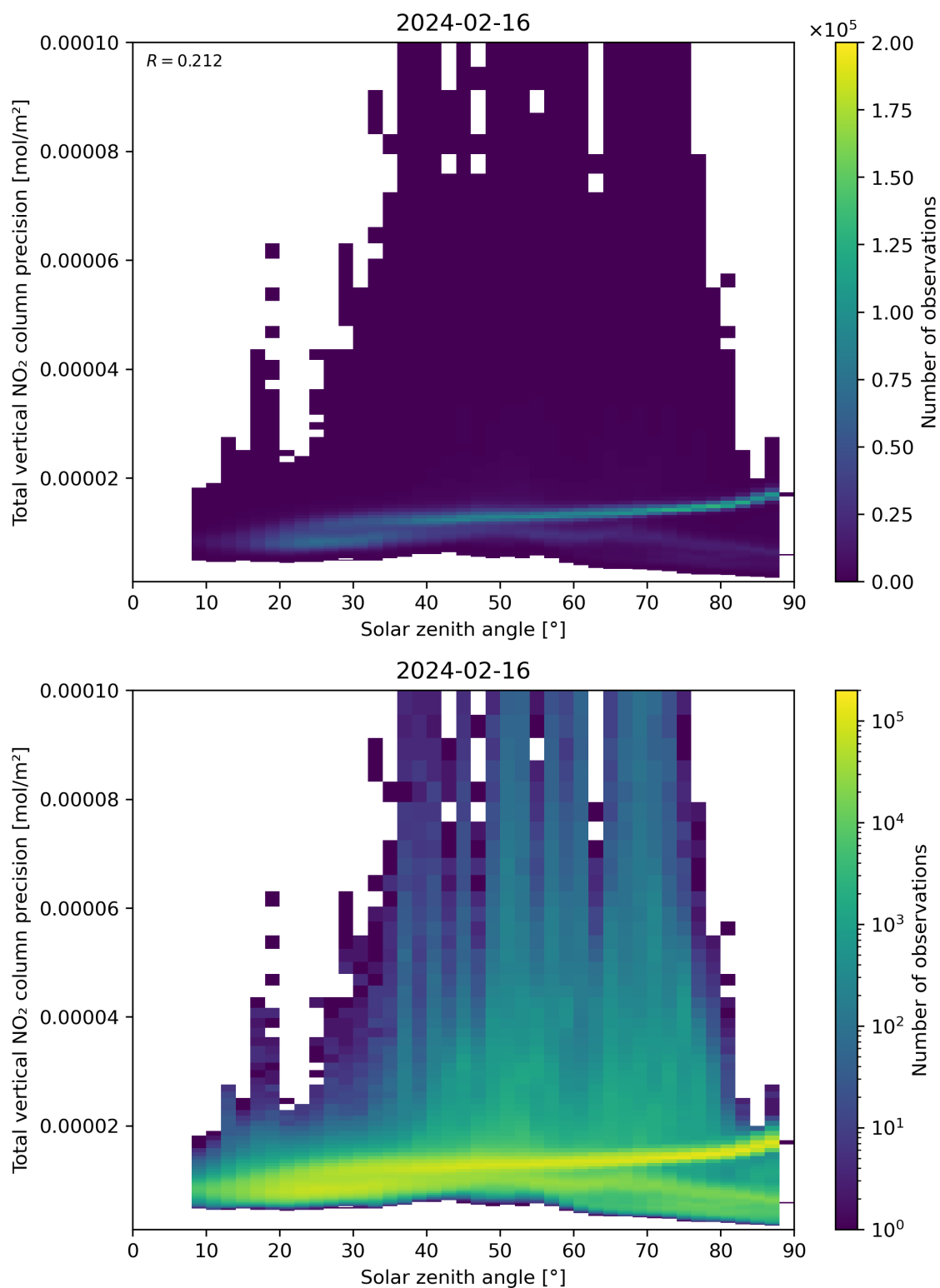
Figure 154: Scatter density plot of “Solar zenith angle” against “Total vertical NO 2 column precision” for 2024-02-16 to 2024-02-17.
