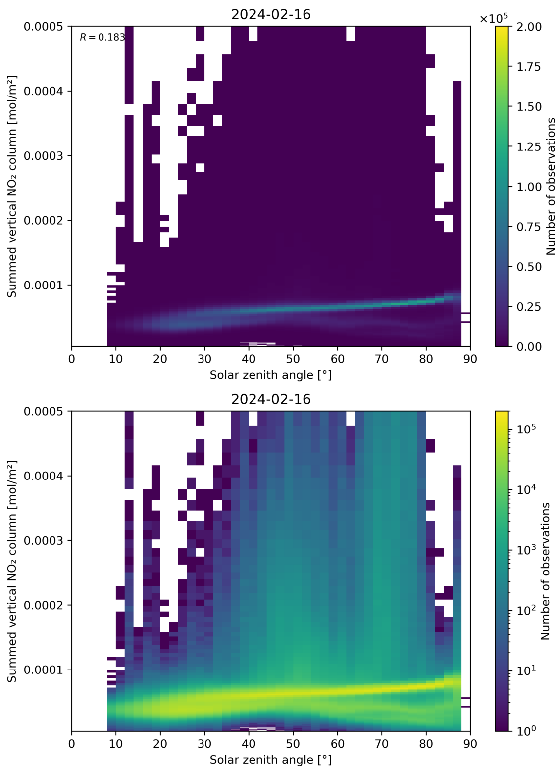
Figure 151: Scatter density plot of “Solar zenith angle” against “Summed vertical NO 2 column” for 2024-02-16 to 2024-02-17.
