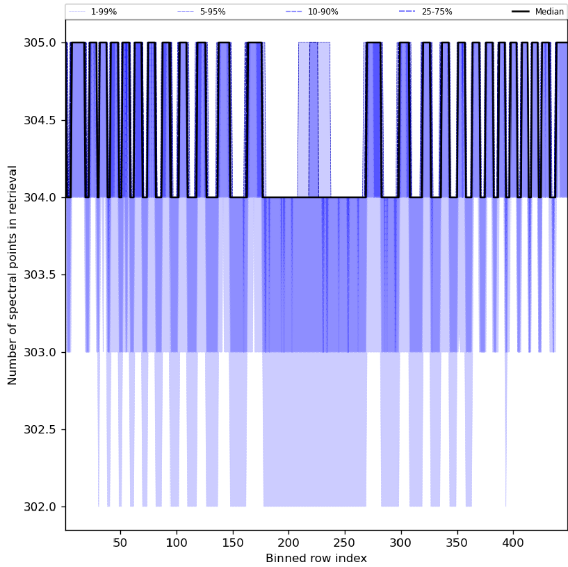
Figure 50: Along track statistics of “Number of spectral points in retrieval” for 2024-02-16 to 2024-02-17
