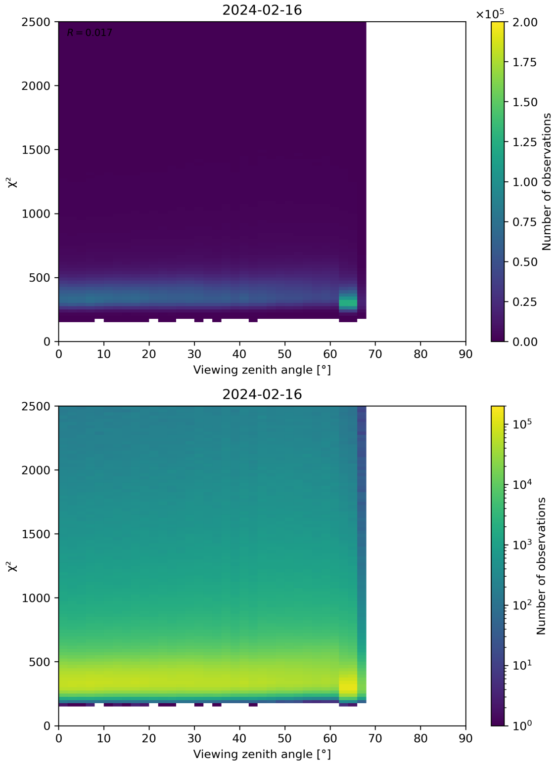
Figure 162: Scatter density plot of “Viewing zenith angle” against “ \chi^2 ” for 2024-02-16 to 2024-02-17.
