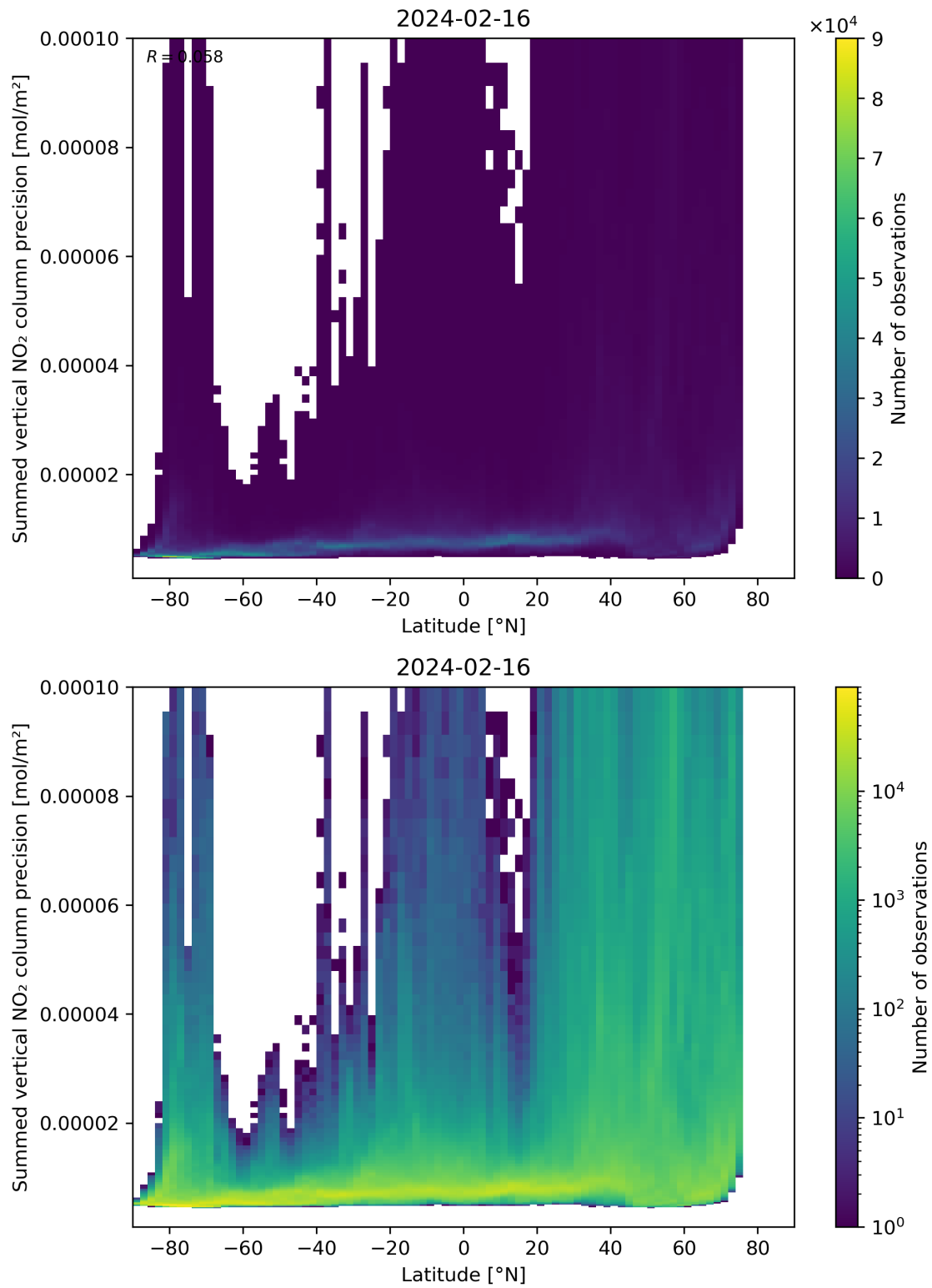
Figure 89: Scatter density plot of “Latitude” against “Summed vertical NO 2 column precision” for 2024-02-16 to 2024-02-17.
