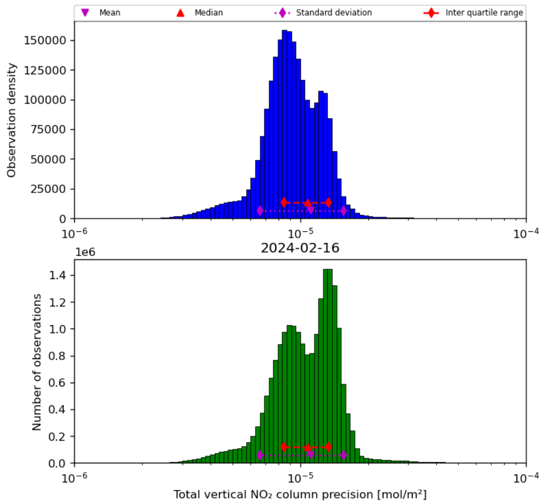
Figure 39: Histogram of “Total vertical NO 2 column precision” for 2024-02-16 to 2024-02-17
