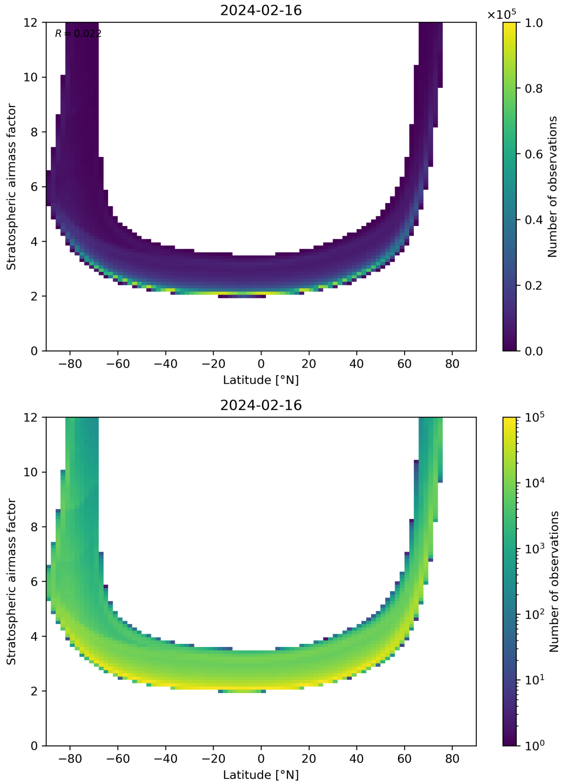
Figure 83: Scatter density plot of “Latitude” against “Stratospheric air mass factor” for 2024-02-16 to 2024-02-17.
