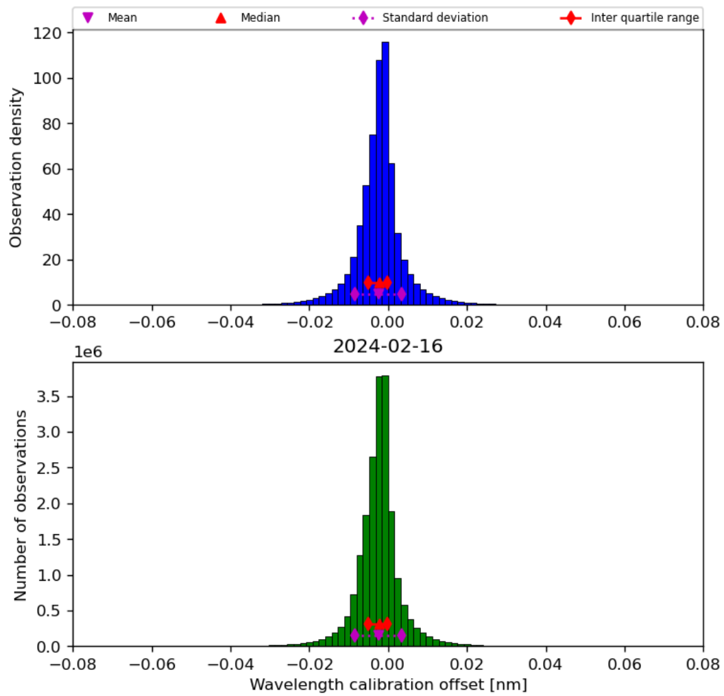
Figure 35: Histogram of “Wavelength calibration offset” for 2024-02-16 to 2024-02-17
