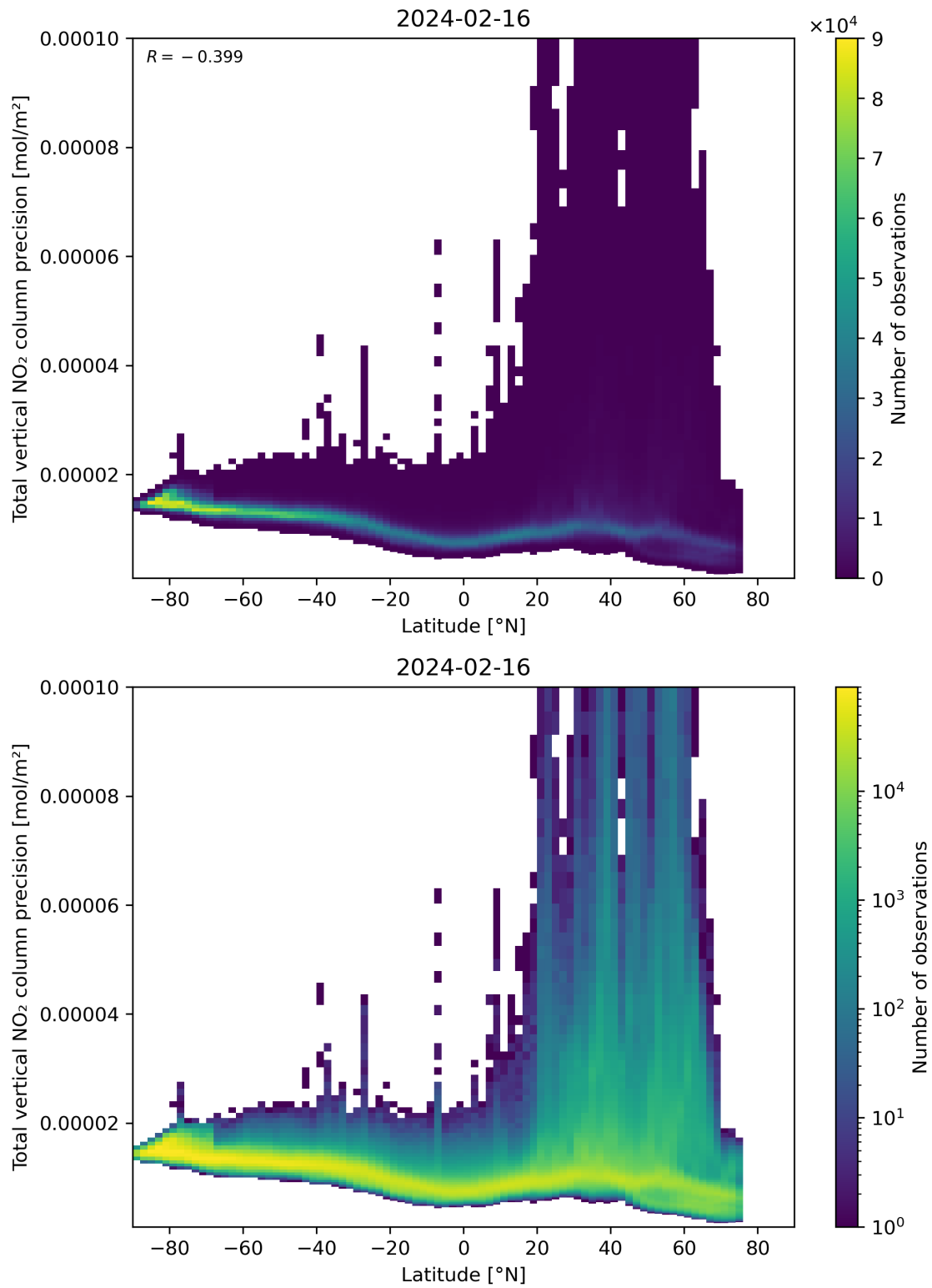
Figure 91: Scatter density plot of “Latitude” against “Total vertical NO 2 column precision” for 2024-02-16 to 2024-02-17.
