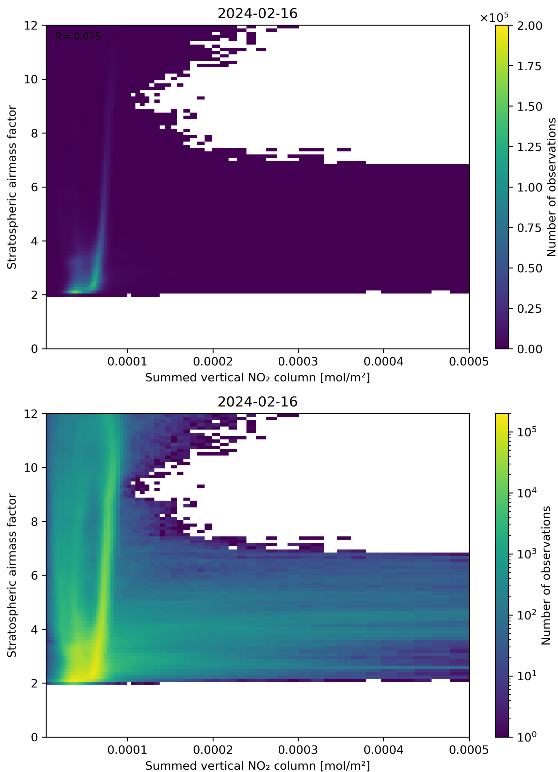
Figure 103: Scatter density plot of “Summed vertical NO 2 column” against “Stratospheric airmass factor” for 2024-02-16 to 2024-02-17.
