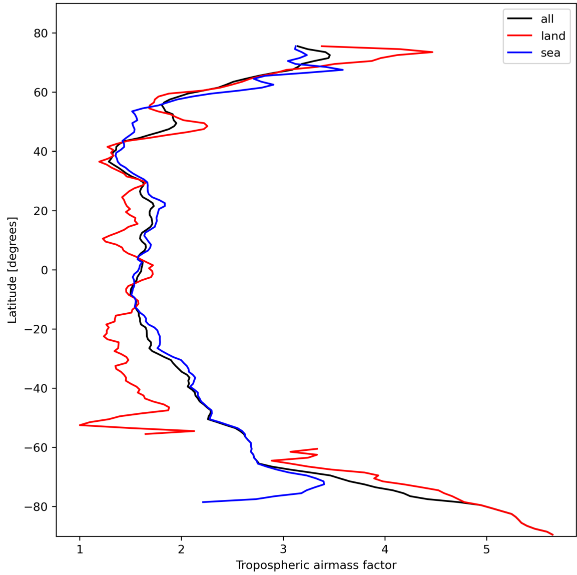
Figure 14: Zonal average of “Tropospheric airmass factor” for 2024-02-16 to 2024-02-17.
