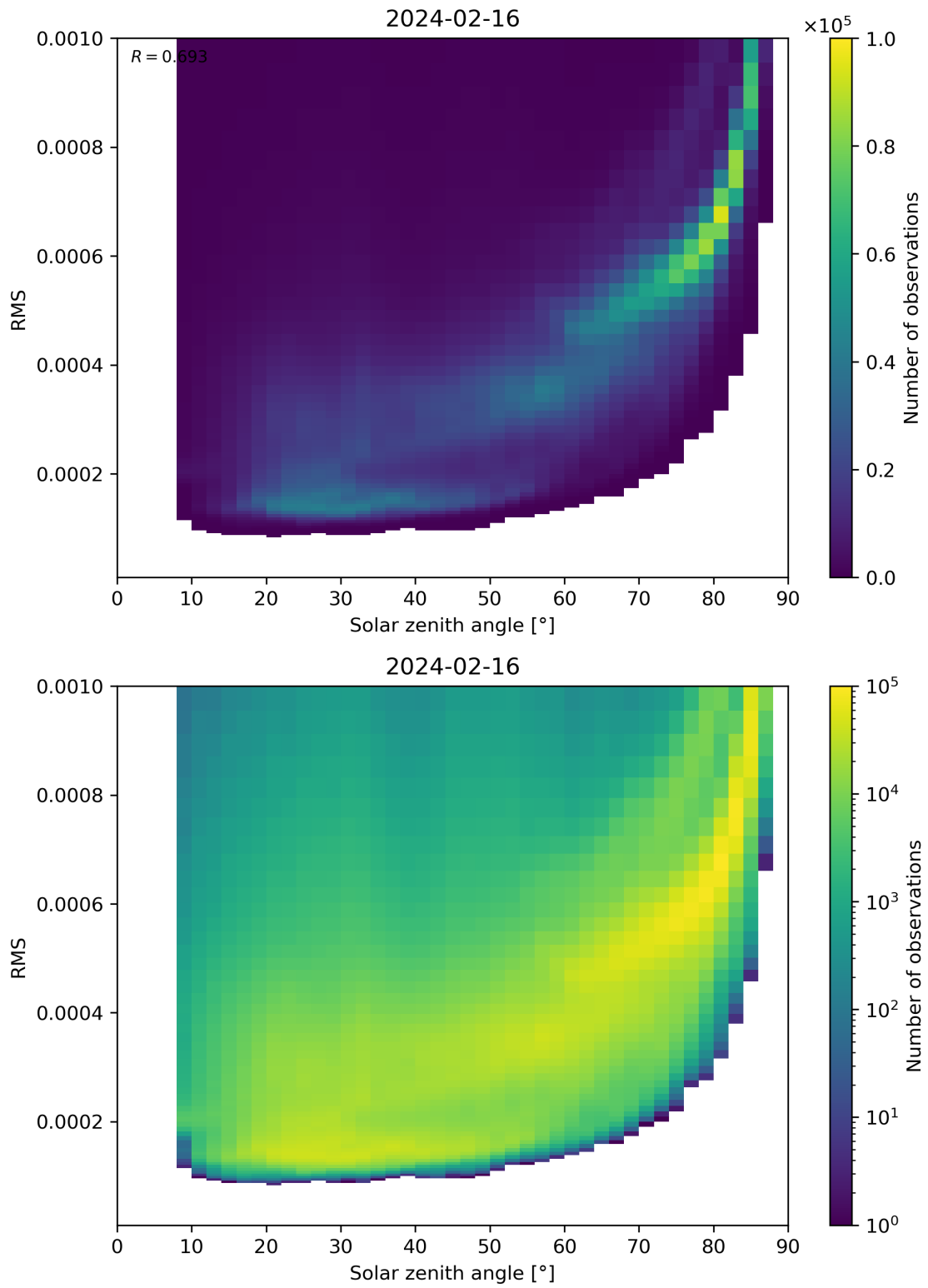
Figure 157: Scatter density plot of “Solar zenith angle” against “RMS” for 2024-02-16 to 2024-02-17.
