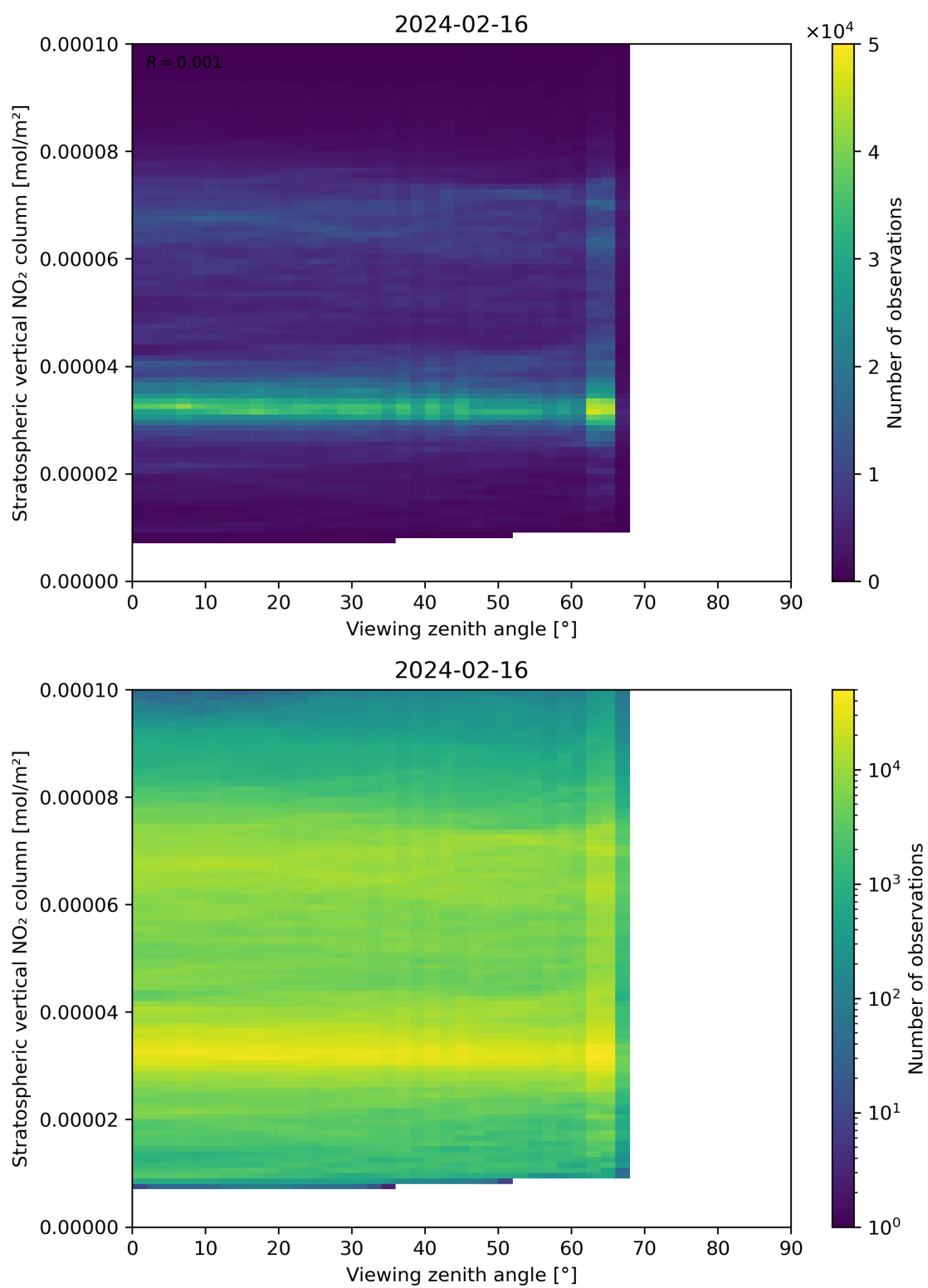
Figure 164: Scatter density plot of “Viewing zenith angle” against “Stratospheric vertical NO 2 column” for 2024-02-16 to 2024-02-17.
