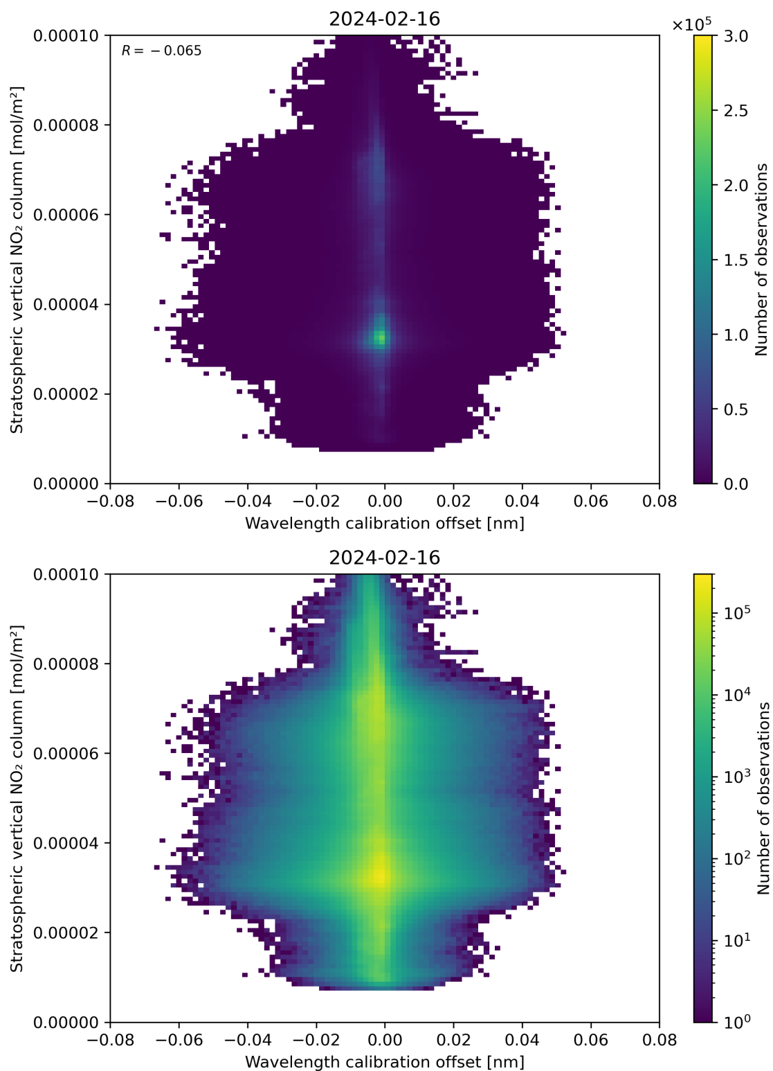
Figure 176: Scatter density plot of “Wavelength calibration offset” against “Stratospheric vertical NO 2 column” for 2024-02-16 to 2024-02-17.
