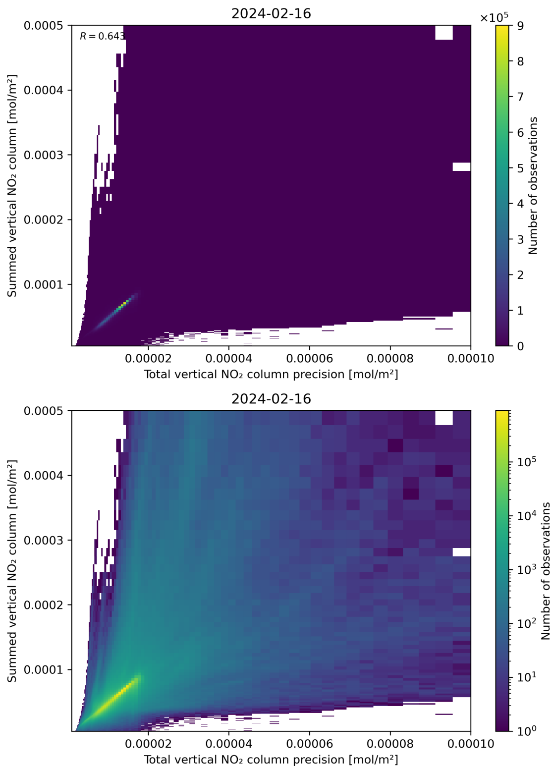
Figure 117: Scatter density plot of “Total vertical NO 2 column precision” against “Summed vertical NO 2 column” for 2024-02-16 to 2024-02-17.
