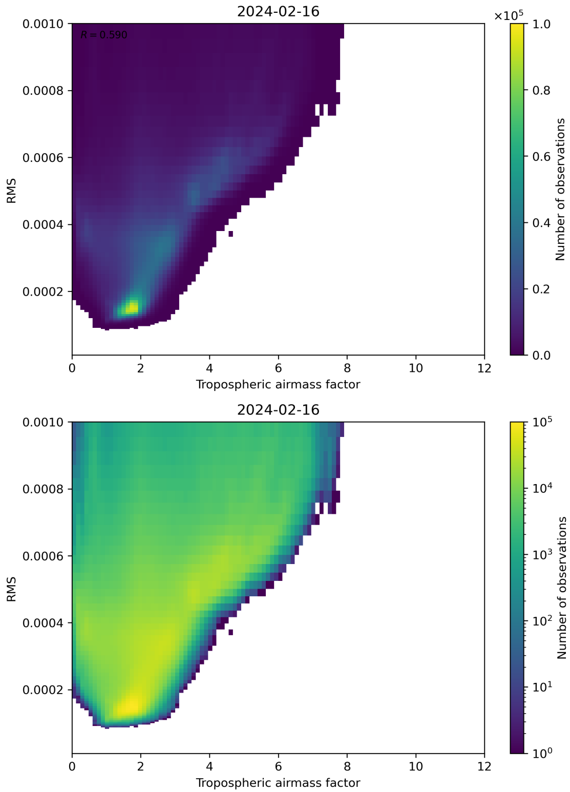
Figure 79: Scatter density plot of “Tropospheric airmass factor” against “RMS” for 2024-02-16 to 2024-02-17.
