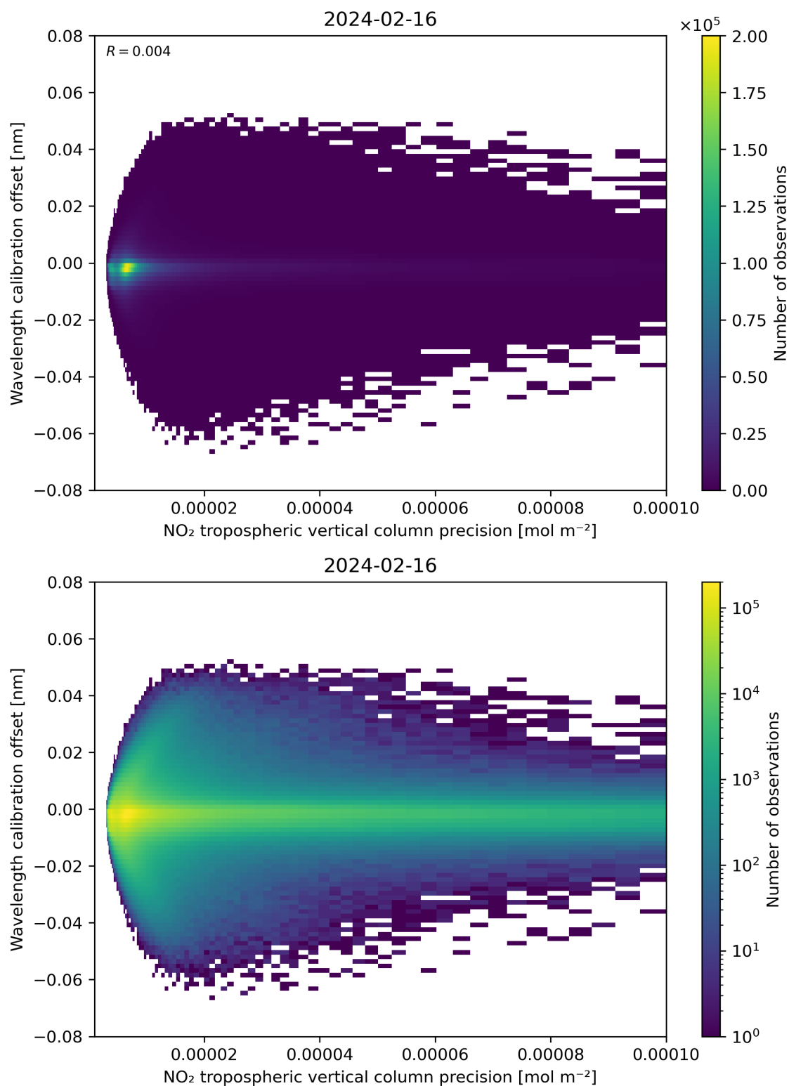
Figure 141: Scatter density plot of “NO 2 tropospheric vertical column precision” against “Wavelength calibration offset” for 2024-02-16 to 2024-02-17.
