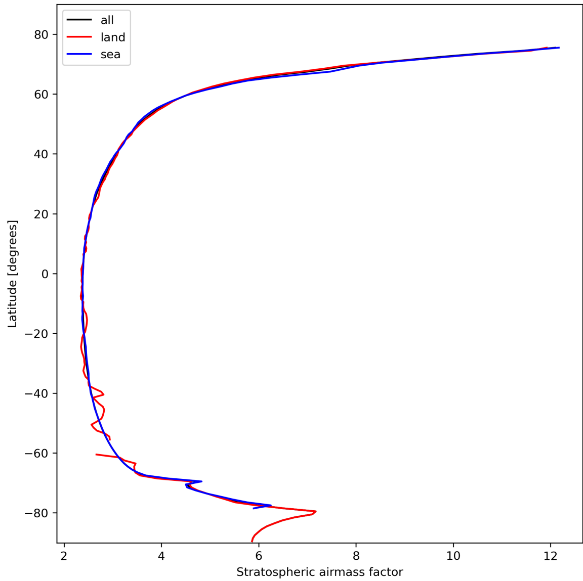
Figure 27: Zonal average of “Stratospheric air mass factor” for 2024-02-16 to 2024-02-17.
