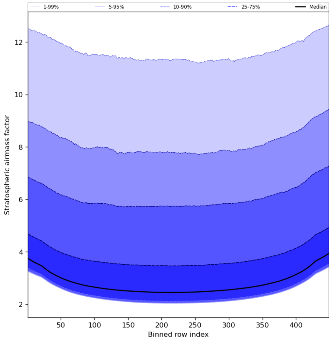
Figure 61: Along track statistics of “Stratospheric airmass factor” for 2024-02-16 to 2024-02-17
