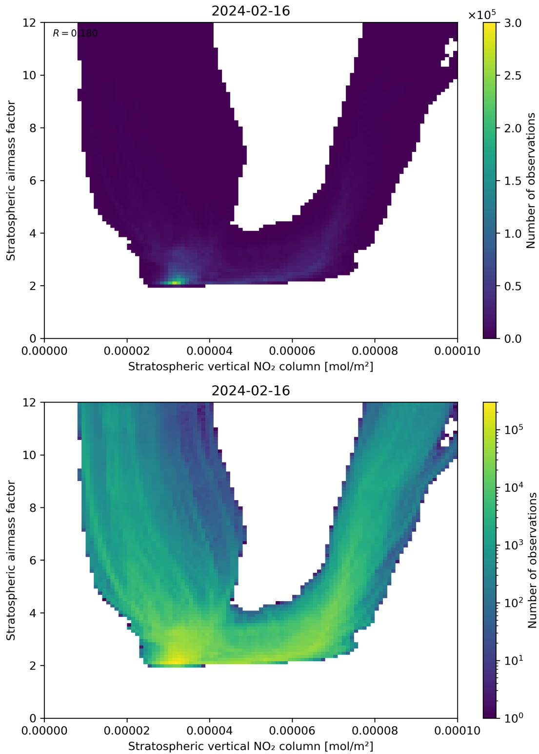
Figure 96: Scatter density plot of “Stratospheric vertical NO 2 column” against “Stratospheric airmass factor” for 2024-02-16 to 2024-02-17.
