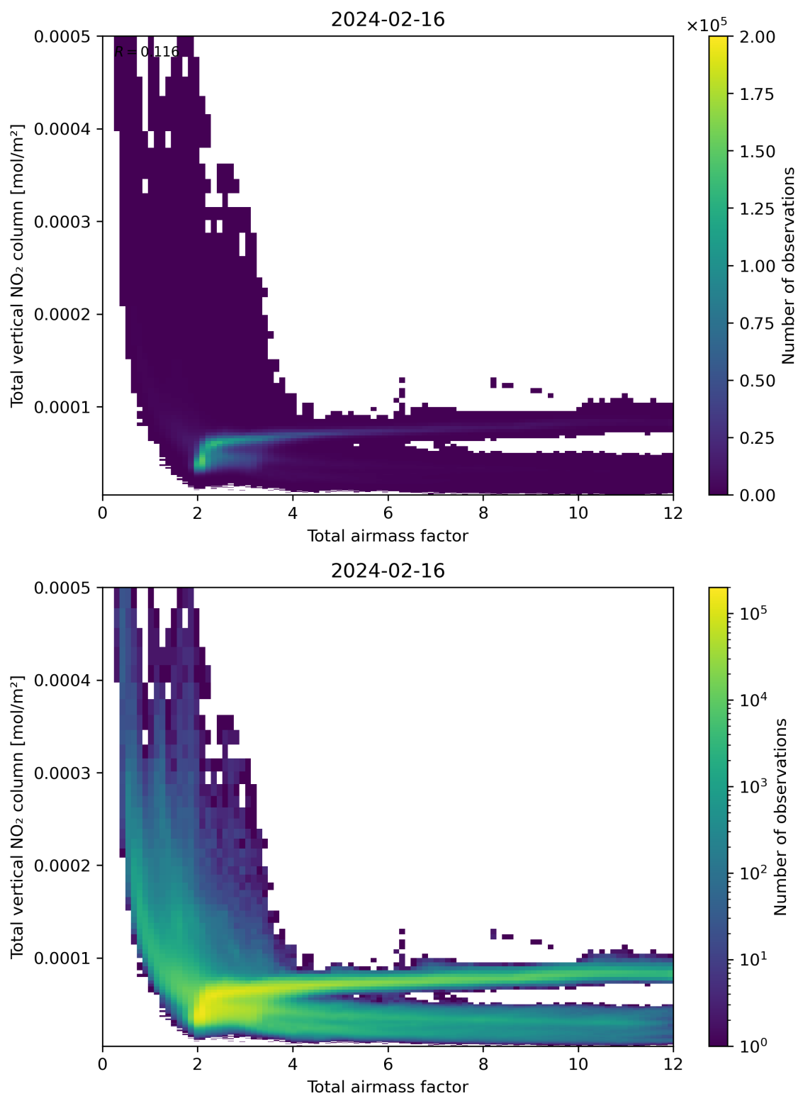
Figure 67: Scatter density plot of “Total airmass factor” against “Total vertical NO 2 column” for 2024-02-16 to 2024-02-17.
