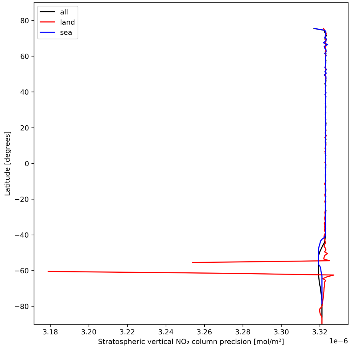
Figure 20: Zonal average of “Stratospheric vertical NO 2 column precision” for 2024-02-16 to 2024-02-17.
