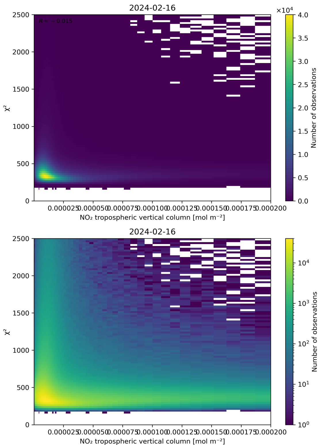
Figure 124: Scatter density plot of “NO 2 tropospheric vertical column” against “ \chi^2 ” for 2024-02-16 to 2024-02-17.
