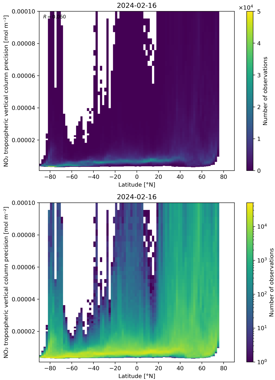
Figure 93: Scatter density plot of “Latitude” against “NO 2 tropospheric vertical column precision” for 2024-02-16 to 2024-02-17.
