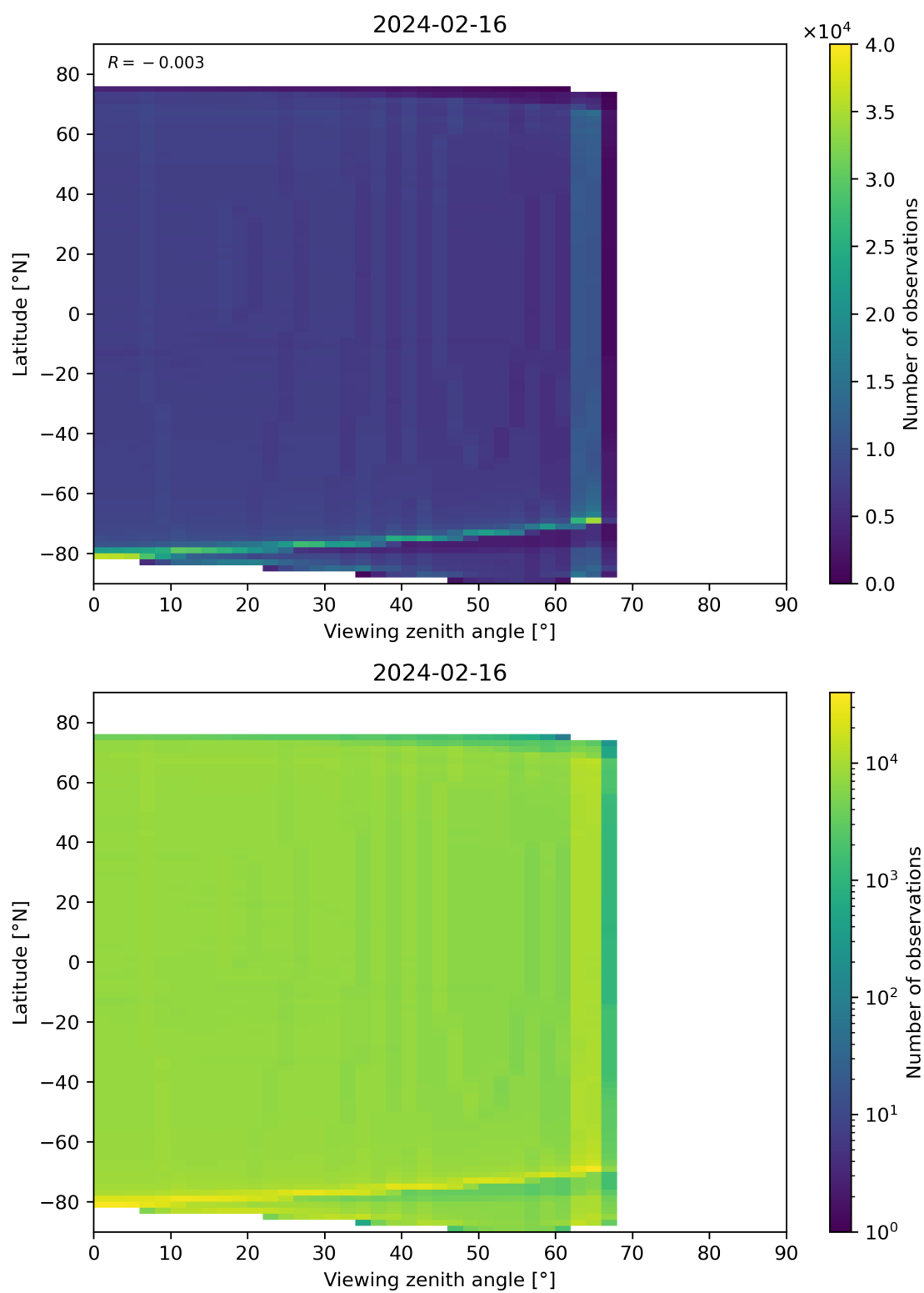
Figure 163: Scatter density plot of “Viewing zenith angle” against “Latitude” for 2024-02-16 to 2024-02-17.
