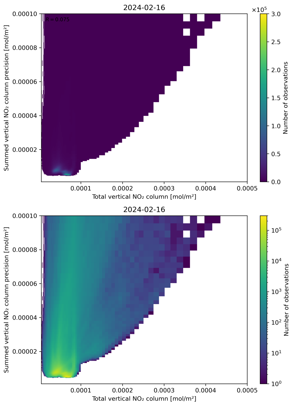
Figure 113: Scatter density plot of “Total vertical NO 2 column” against “Summed vertical NO 2 column precision” for 2024-02-16 to 2024-02-17.
