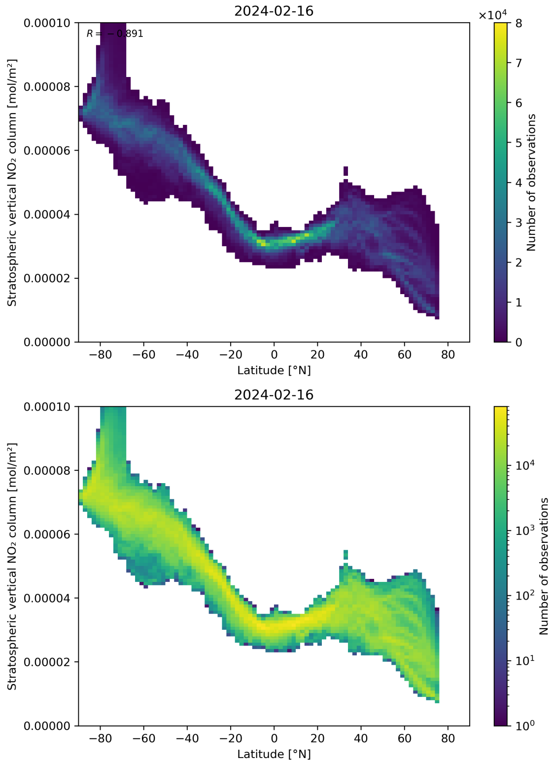
Figure 87: Scatter density plot of “Latitude” against “Stratospheric vertical NO 2 column” for 2024-02-16 to 2024-02-17.
