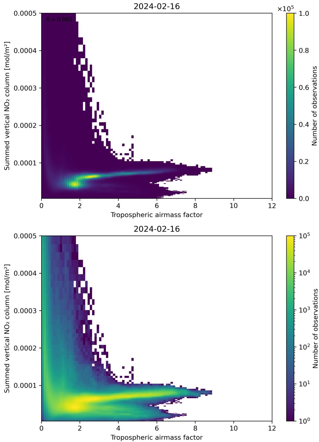
Figure 75: Scatter density plot of “Tropospheric airmass factor” against “Summed vertical NO 2 column” for 2024-02-16 to 2024-02-17.
