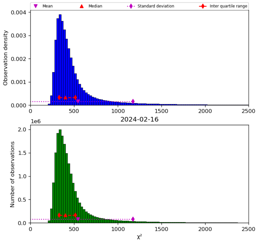
Figure 42: Histogram of “ \chi^2 ” for 2024-02-16 to 2024-02-17
