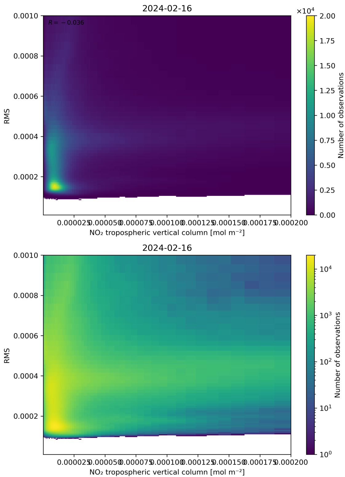
Figure 142: Scatter density plot of “NO 2 tropospheric vertical column” against “RMS” for 2024-02-16 to 2024-02-17.
