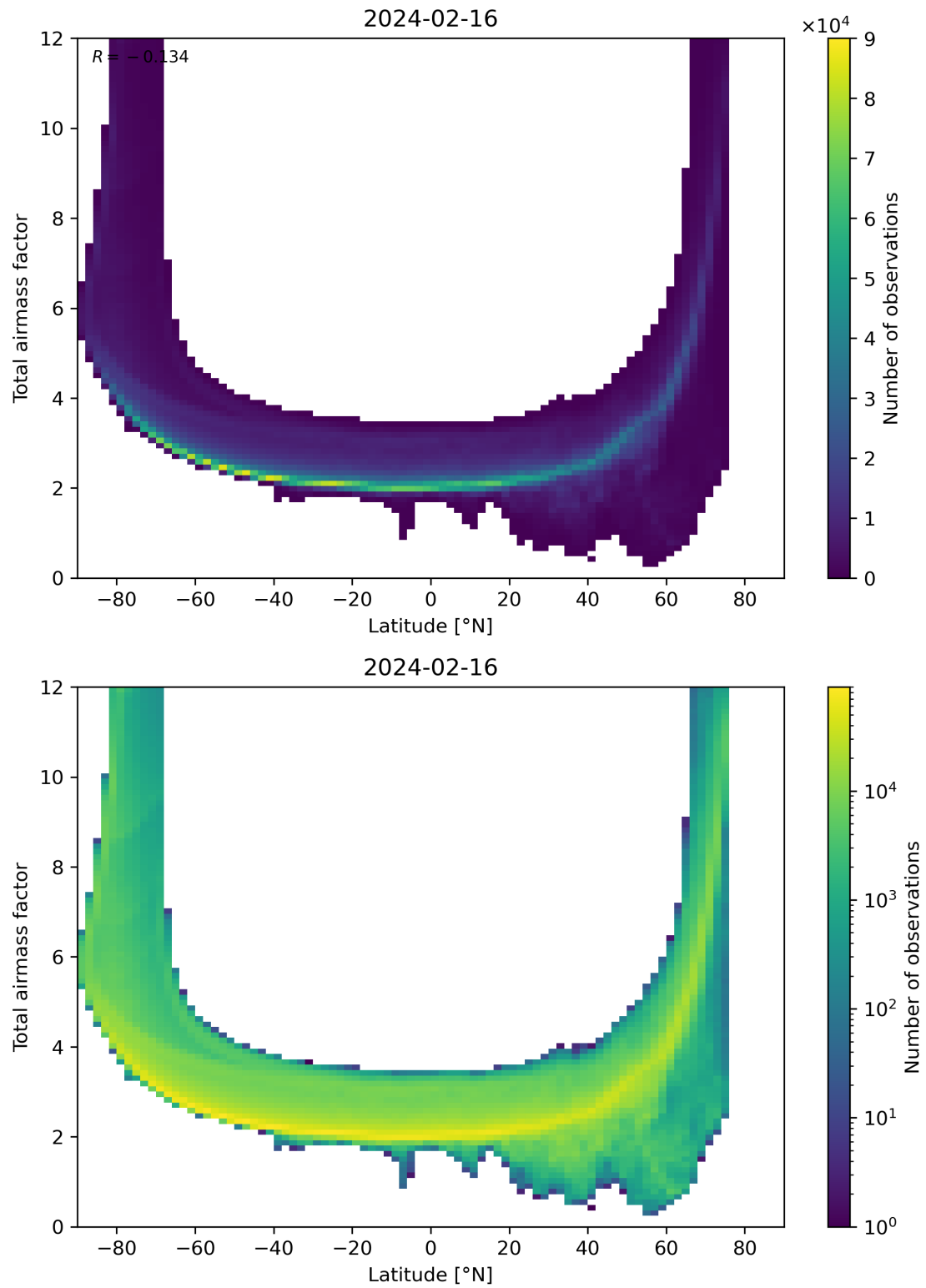
Figure 84: Scatter density plot of “Latitude” against “Total airmass factor” for 2024-02-16 to 2024-02-17.
