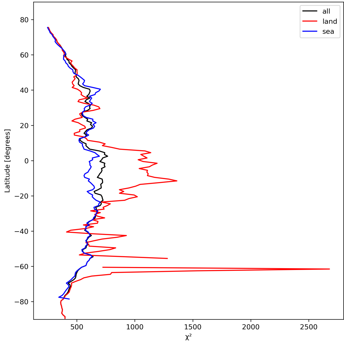
Figure 25: Zonal average of “ \chi^2 ” for 2024-02-16 to 2024-02-17.
