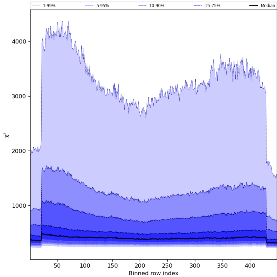
Figure 59: Along track statistics of “ \chi^2 ” for 2024-02-16 to 2024-02-17
