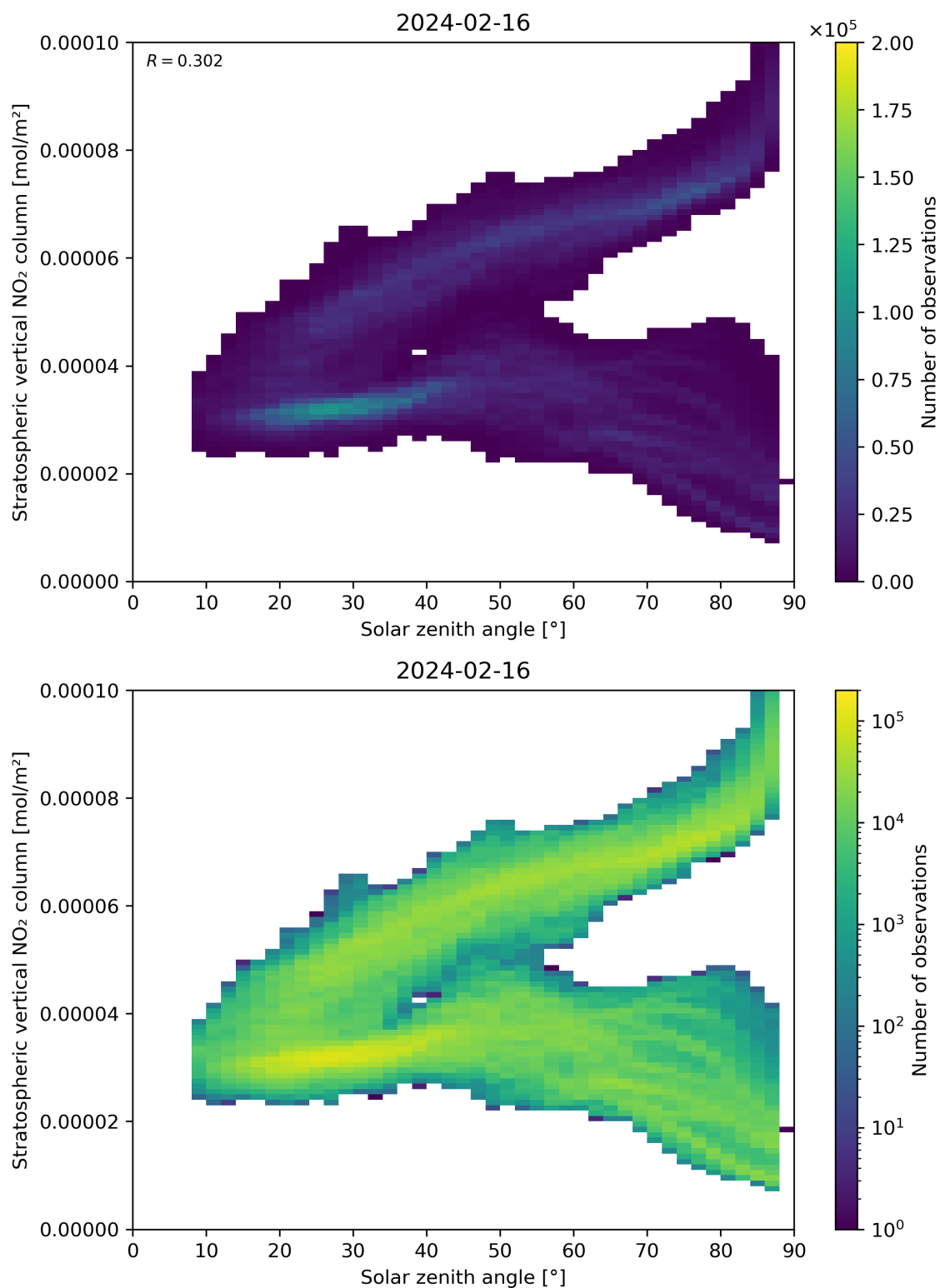
Figure 150: Scatter density plot of “Solar zenith angle” against “Stratospheric vertical NO 2 column” for 2024-02-16 to 2024-02-17.
