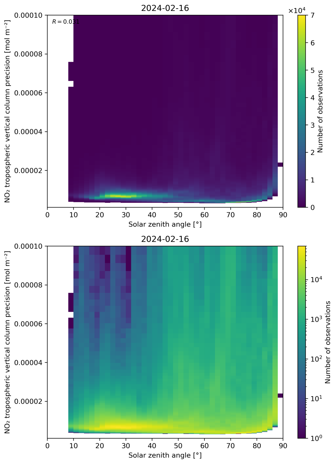
Figure 156: Scatter density plot of “Solar zenith angle” against “NO 2 tropospheric vertical column precision” for 2024-02-16 to 2024-02-17.
