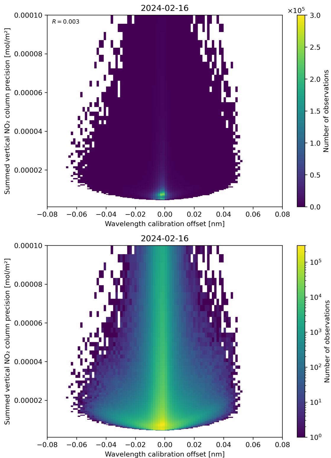
Figure 178: Scatter density plot of “Wavelength calibration offset” against “Summed vertical NO 2 column precision” for 2024-02-16 to 2024-02-17.
