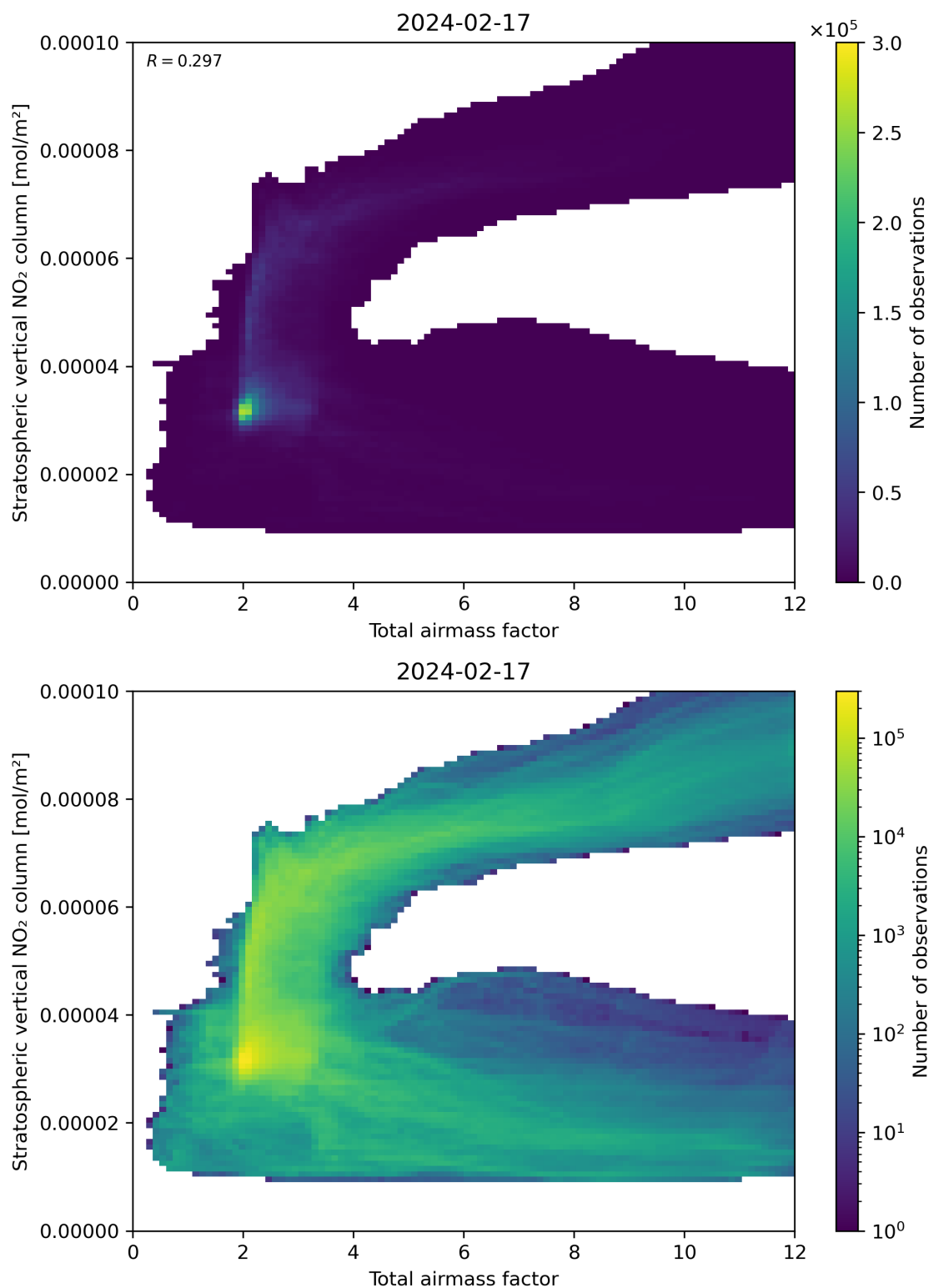
Figure 64: Scatter density plot of “Total airmass factor” against “Stratospheric vertical \text{NO}_2 column” for 2024-02-17 to 2024-02-18.
