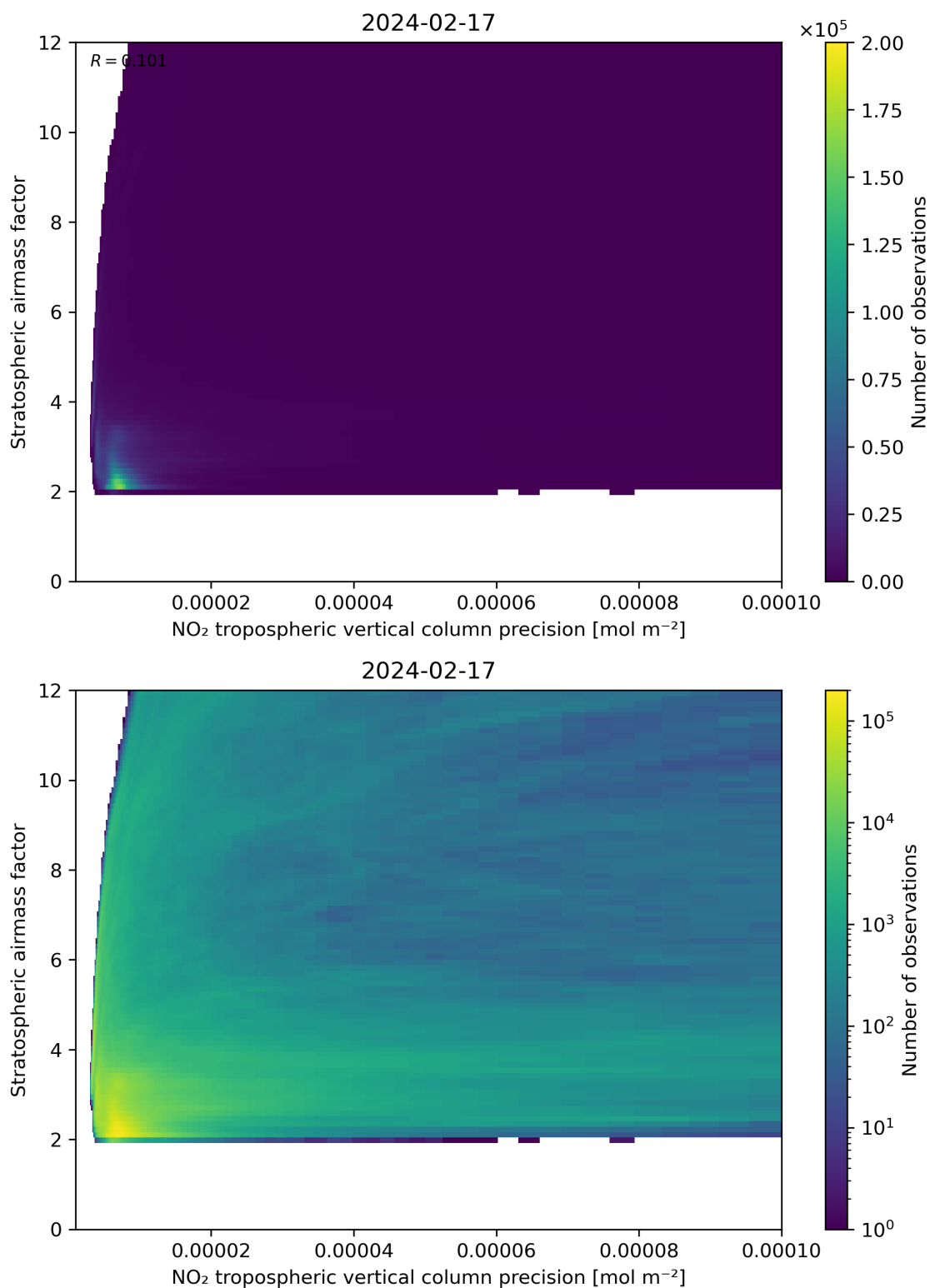
Figure 131: Scatter density plot of “NO 2 tropospheric vertical column precision” against “Stratospheric airmass factor” for 2024-02-17 to 2024-02-18.
