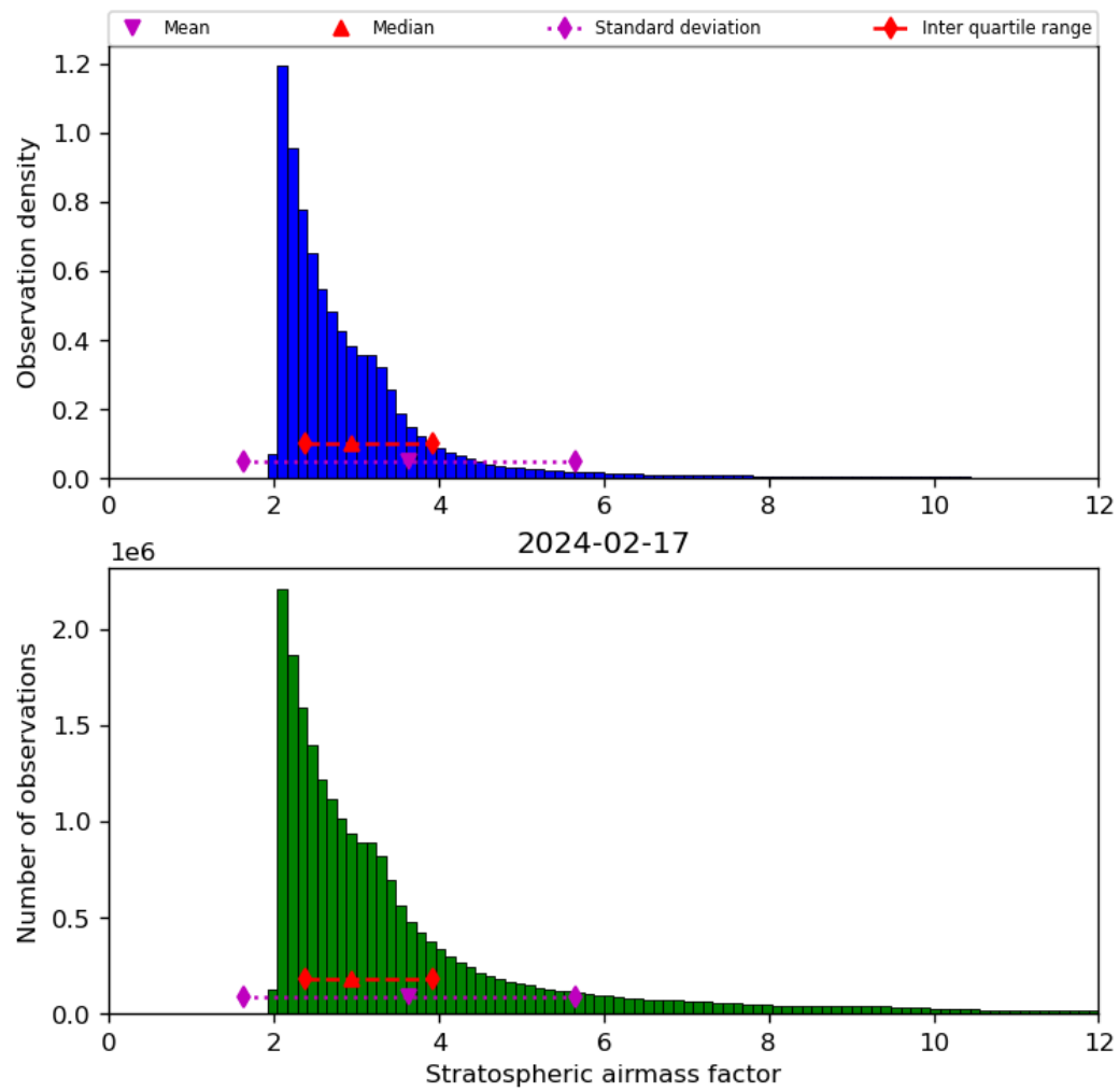
Figure 44: Histogram of “Stratospheric airmass factor” for 2024-02-17 to 2024-02-18
