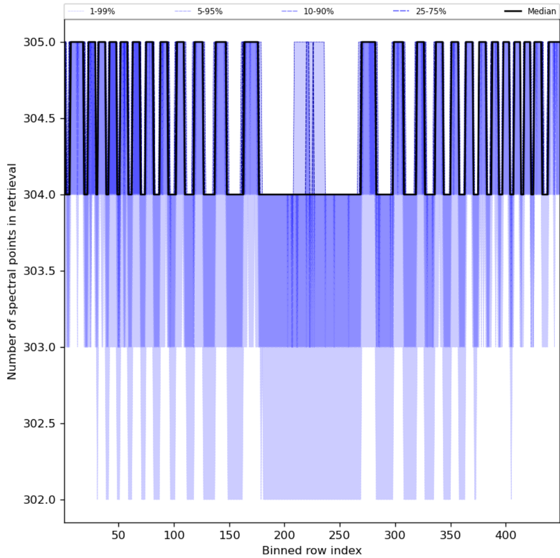
Figure 50: Along track statistics of “Number of spectral points in retrieval” for 2024-02-17 to 2024-02-18
