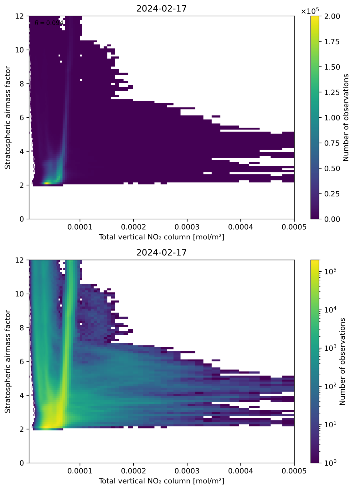
Figure 110: Scatter density plot of “Total vertical NO 2 column” against “Stratospheric air mass factor” for 2024-02-17 to 2024-02-18.
