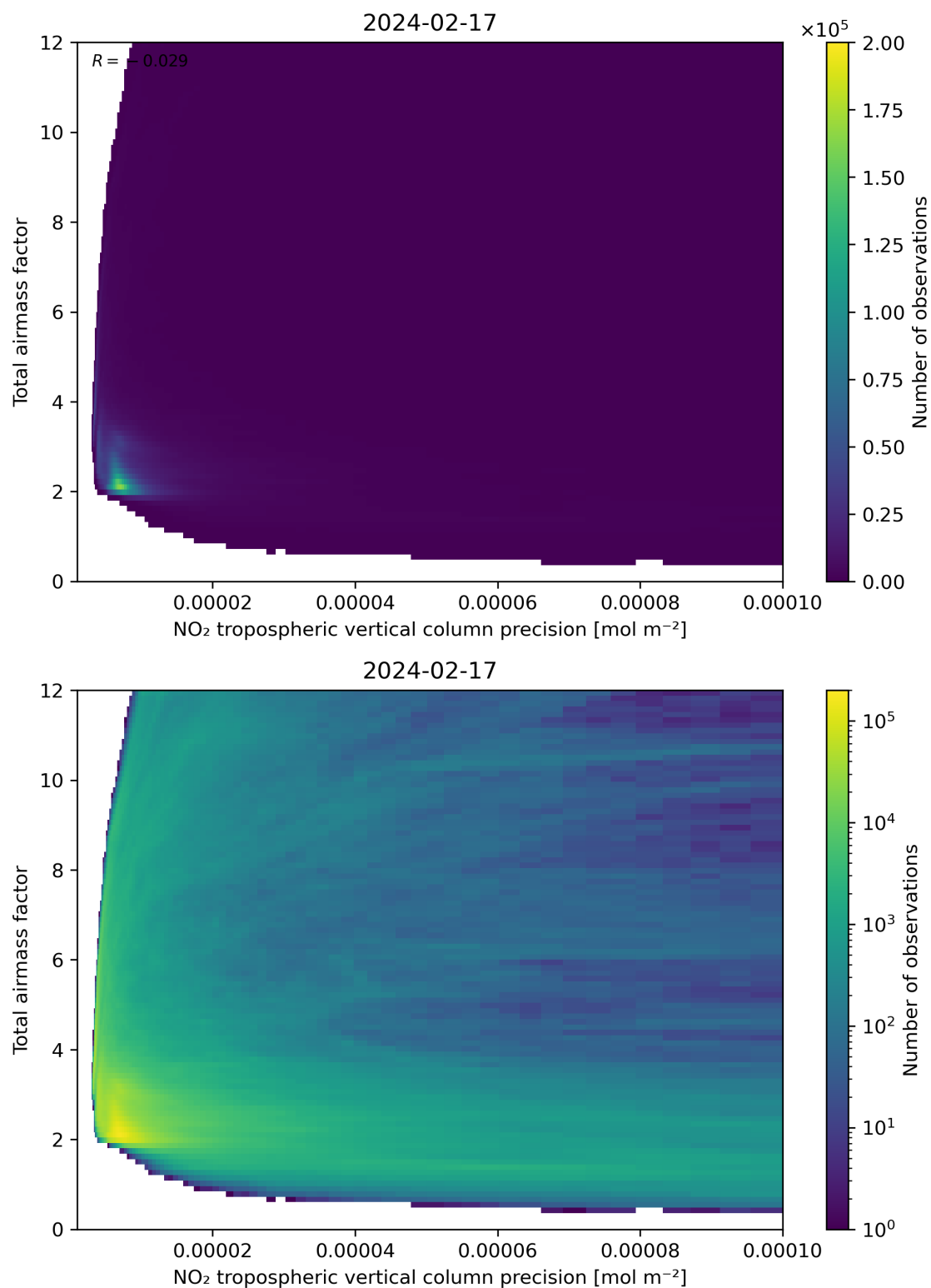
Figure 132: Scatter density plot of “NO 2 tropospheric vertical column precision” against “Total air mass factor” for 2024-02-17 to 2024-02-18.
