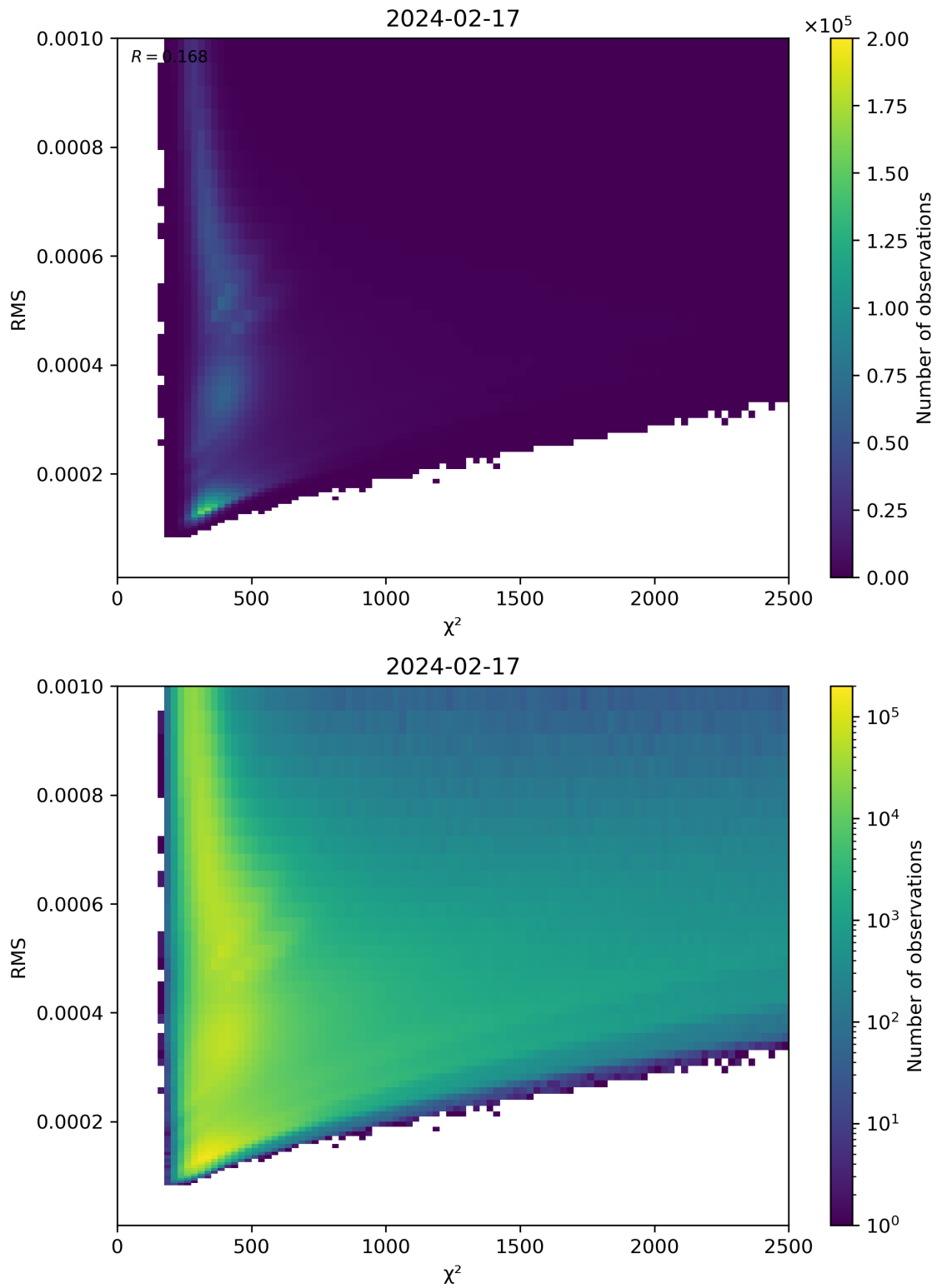
Figure 82: Scatter density plot of “ \chi^2 ” against “RMS” for 2024-02-17 to 2024-02-18.
