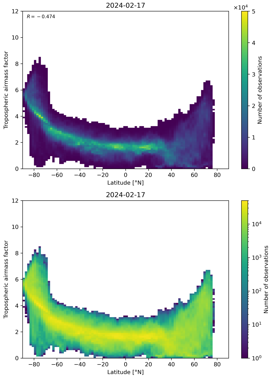
Figure 85: Scatter density plot of “Latitude” against “Tropospheric airmass factor” for 2024-02-17 to 2024-02-18.
