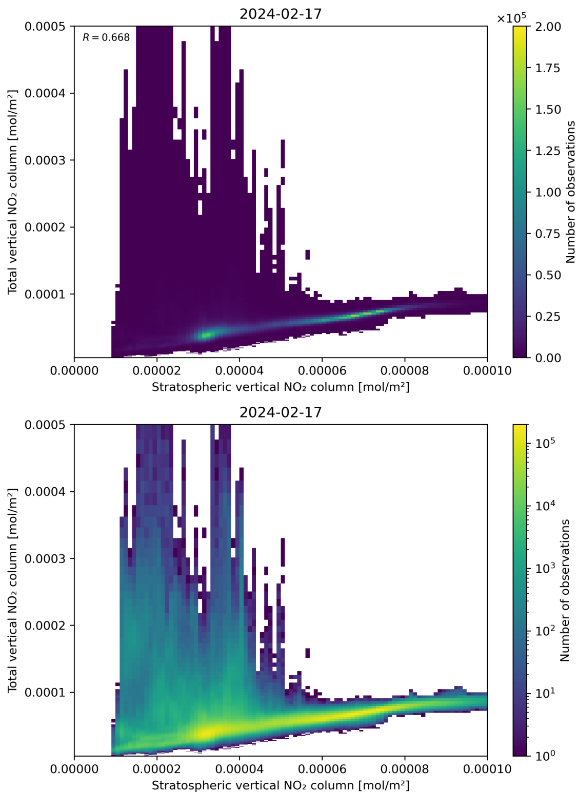
Figure 100: Scatter density plot of “Stratospheric vertical NO 2 column” against “Total vertical NO 2 column” for 2024-02-17 to 2024-02-18.
