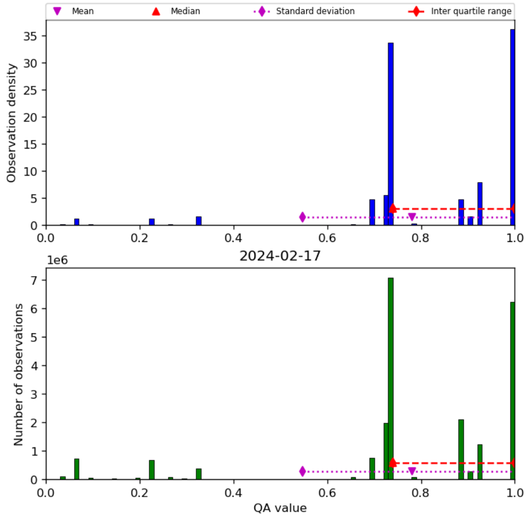
Figure 28: Histogram of “QA value” for 2024-02-17 to 2024-02-18
