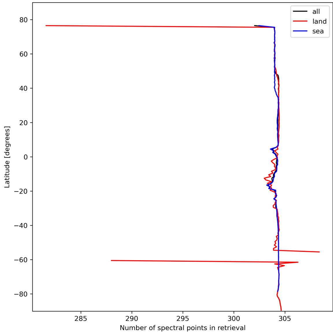
Figure 16: Zonal average of “Number of spectral points in retrieval” for 2024-02-17 to 2024-02-18.
