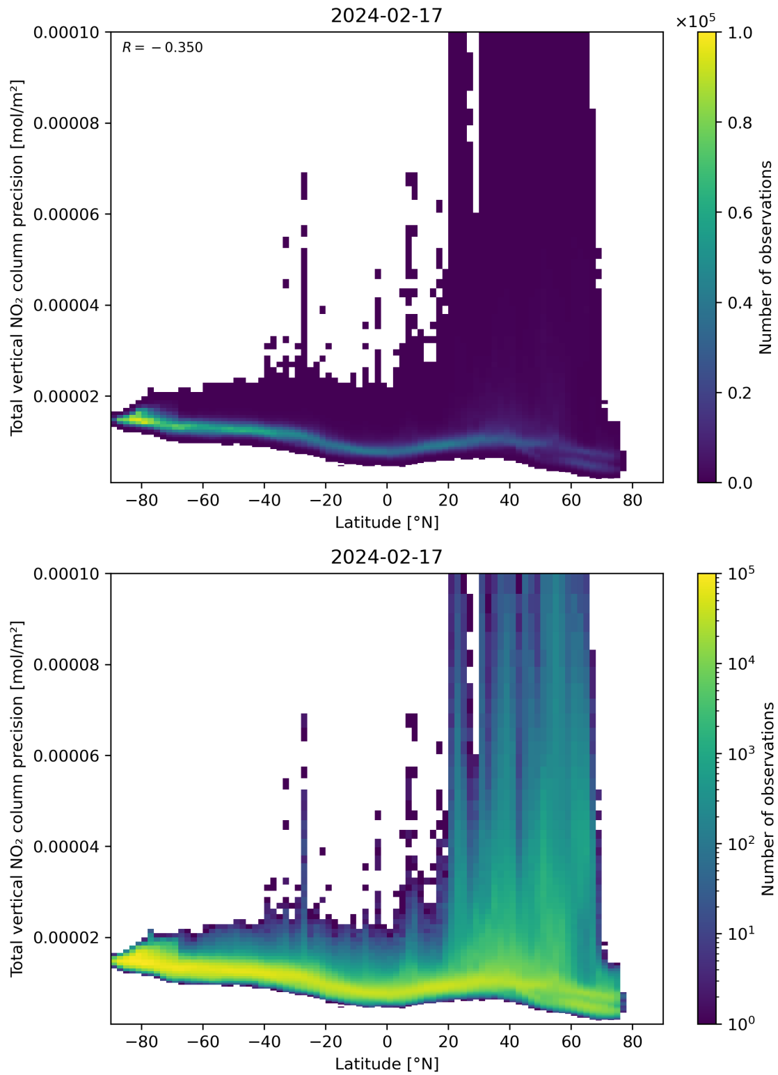
Figure 91: Scatter density plot of “Latitude” against “Total vertical NO 2 column precision” for 2024-02-17 to 2024-02-18.
