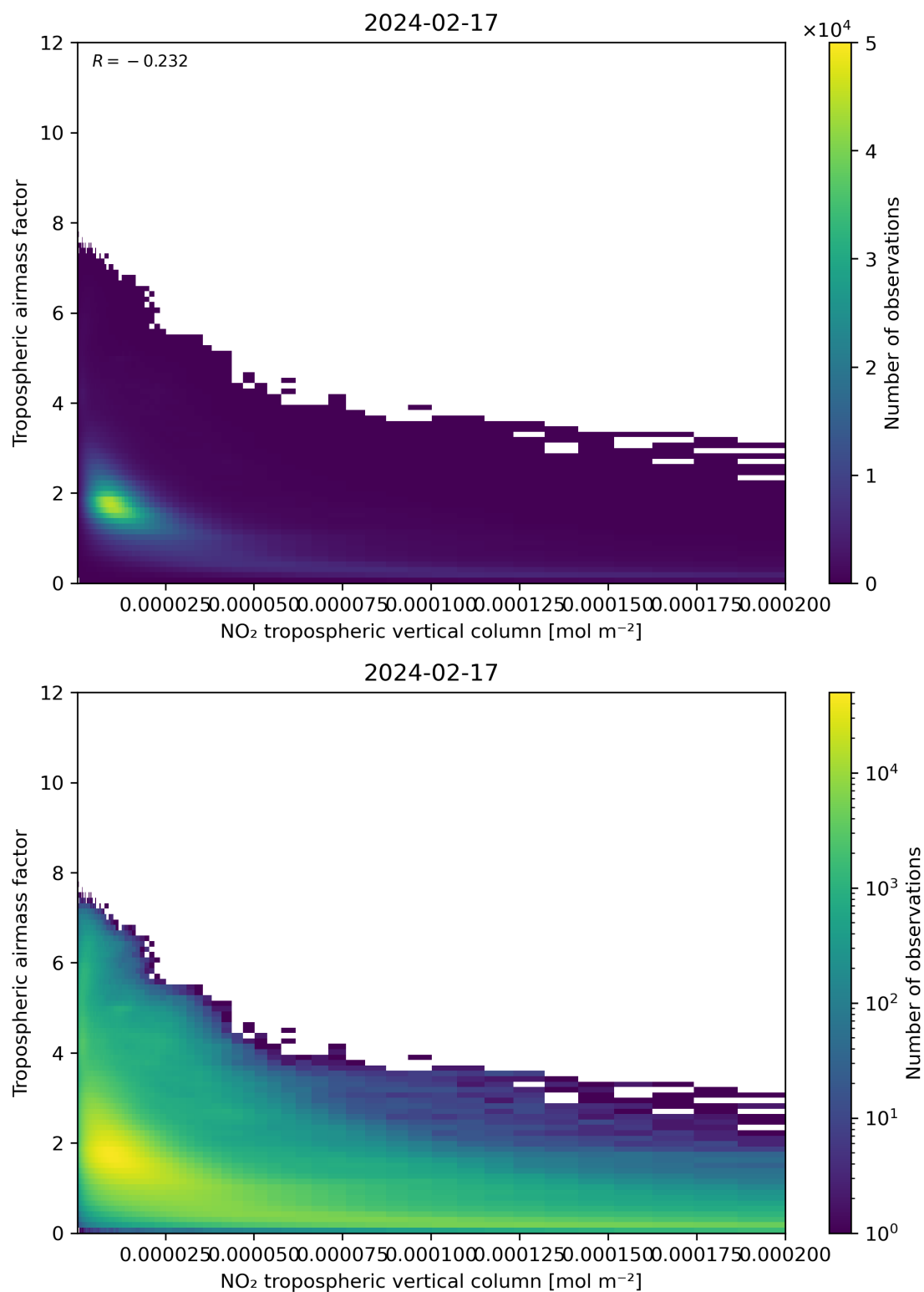
Figure 123: Scatter density plot of “NO 2 tropospheric vertical column” against “Tropospheric air mass factor” for 2024-02-17 to 2024-02-18.
