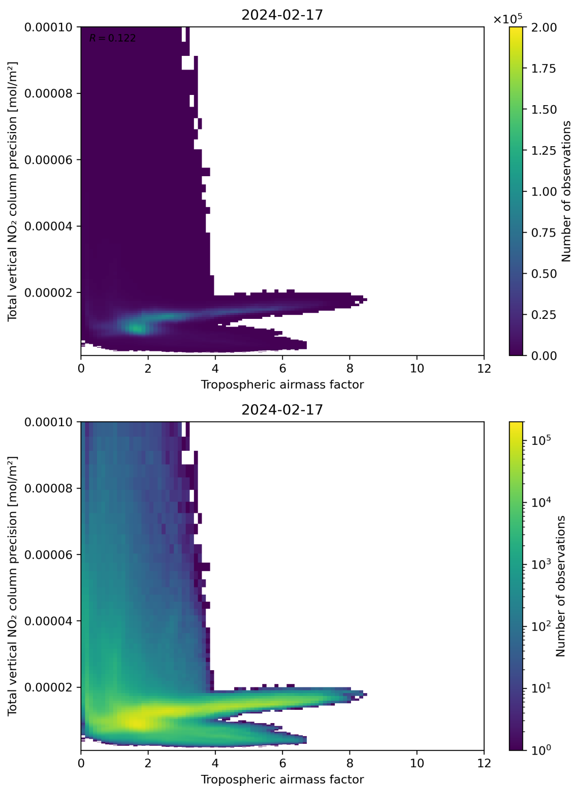
Figure 78: Scatter density plot of “Tropospheric air mass factor” against “Total vertical NO 2 column precision” for 2024-02-17 to 2024-02-18.
