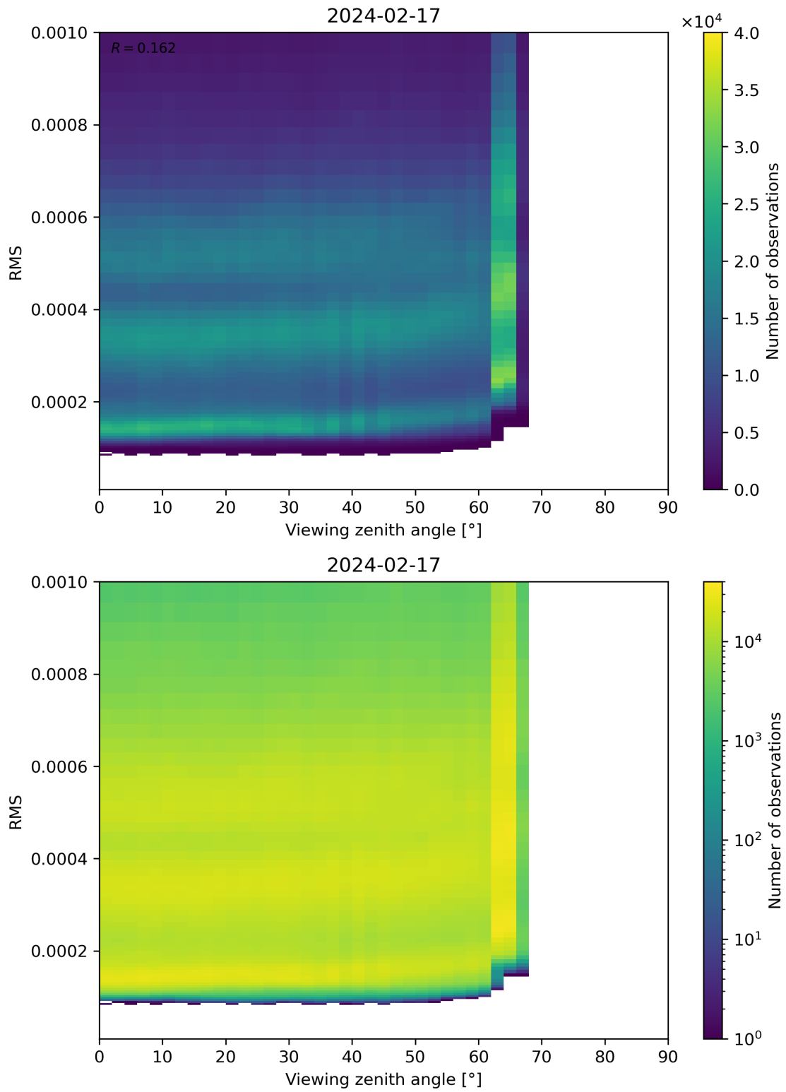
Figure 171: Scatter density plot of “Viewing zenith angle” against “RMS” for 2024-02-17 to 2024-02-18.
