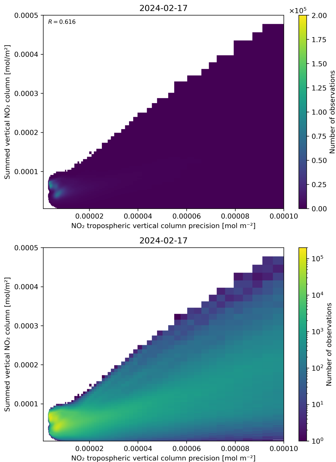
Figure 136: Scatter density plot of “NO 2 tropospheric vertical column precision” against “Summed vertical NO 2 column” for 2024-02-17 to 2024-02-18.
