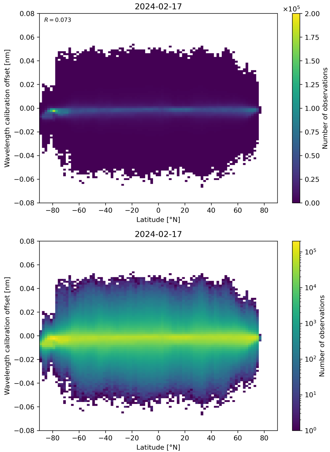
Figure 95: Scatter density plot of “Latitude” against “Wavelength calibration offset” for 2024-02-17 to 2024-02-18.
