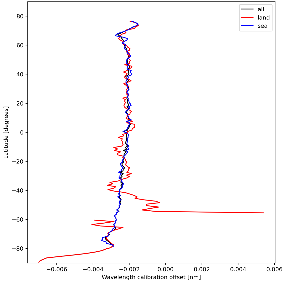
Figure 18: Zonal average of “Wavelength calibration offset” for 2024-02-17 to 2024-02-18.
