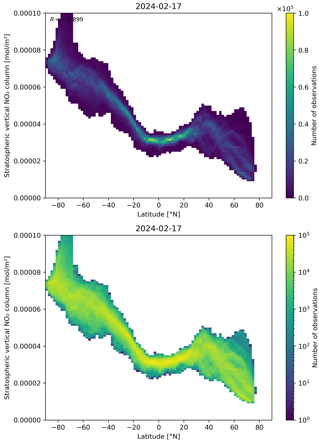
Figure 87: Scatter density plot of “Latitude” against “Stratospheric vertical NO 2 column” for 2024-02-17 to 2024-02-18.
