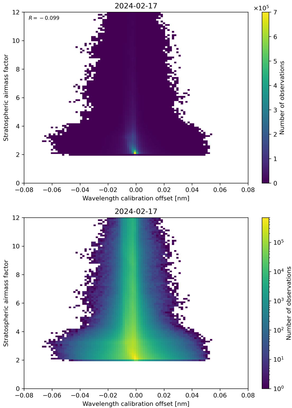
Figure 174: Scatter density plot of “Wavelength calibration offset” against “Stratospheric airmass factor” for 2024-02-17 to 2024-02-18.
