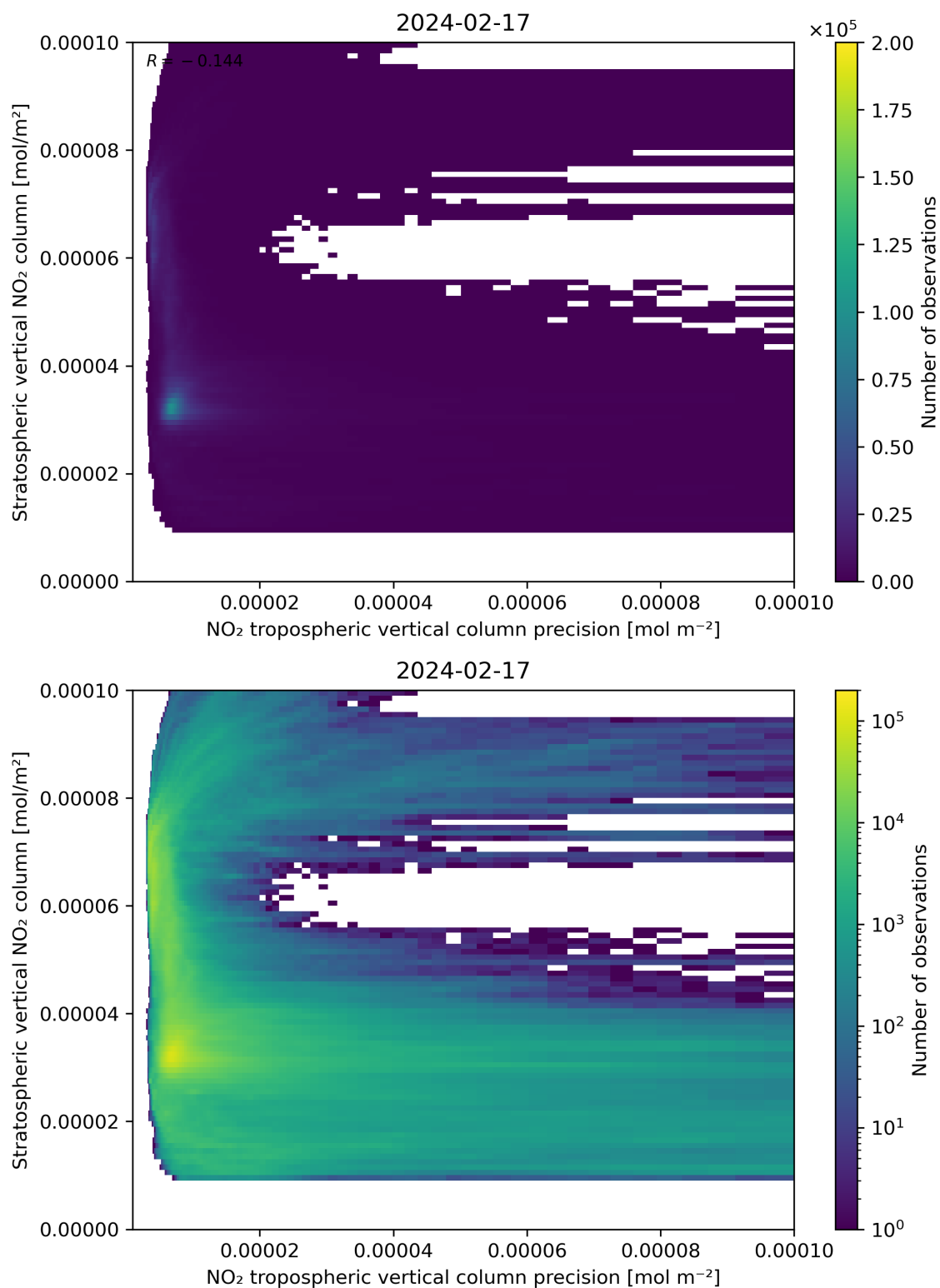
Figure 135: Scatter density plot of “NO 2 tropospheric vertical column precision” against “Stratospheric vertical NO 2 column” for 2024-02-17 to 2024-02-18.
