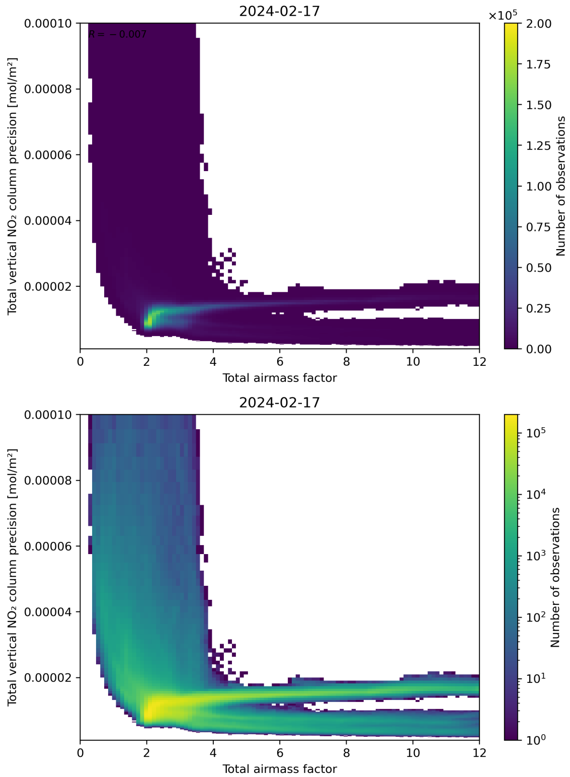
Figure 68: Scatter density plot of “Total airmass factor” against “Total vertical NO 2 column precision” for 2024-02-17 to 2024-02-18.
