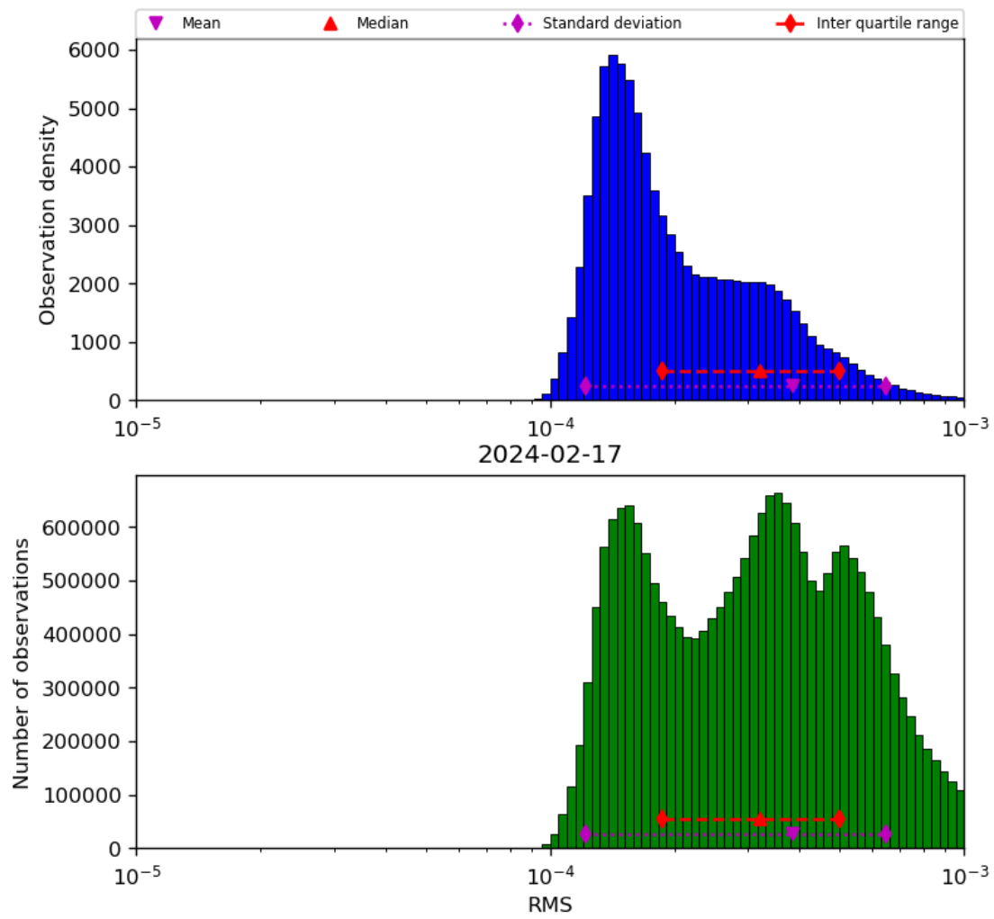
Figure 43: Histogram of “RMS” for 2024-02-17 to 2024-02-18
