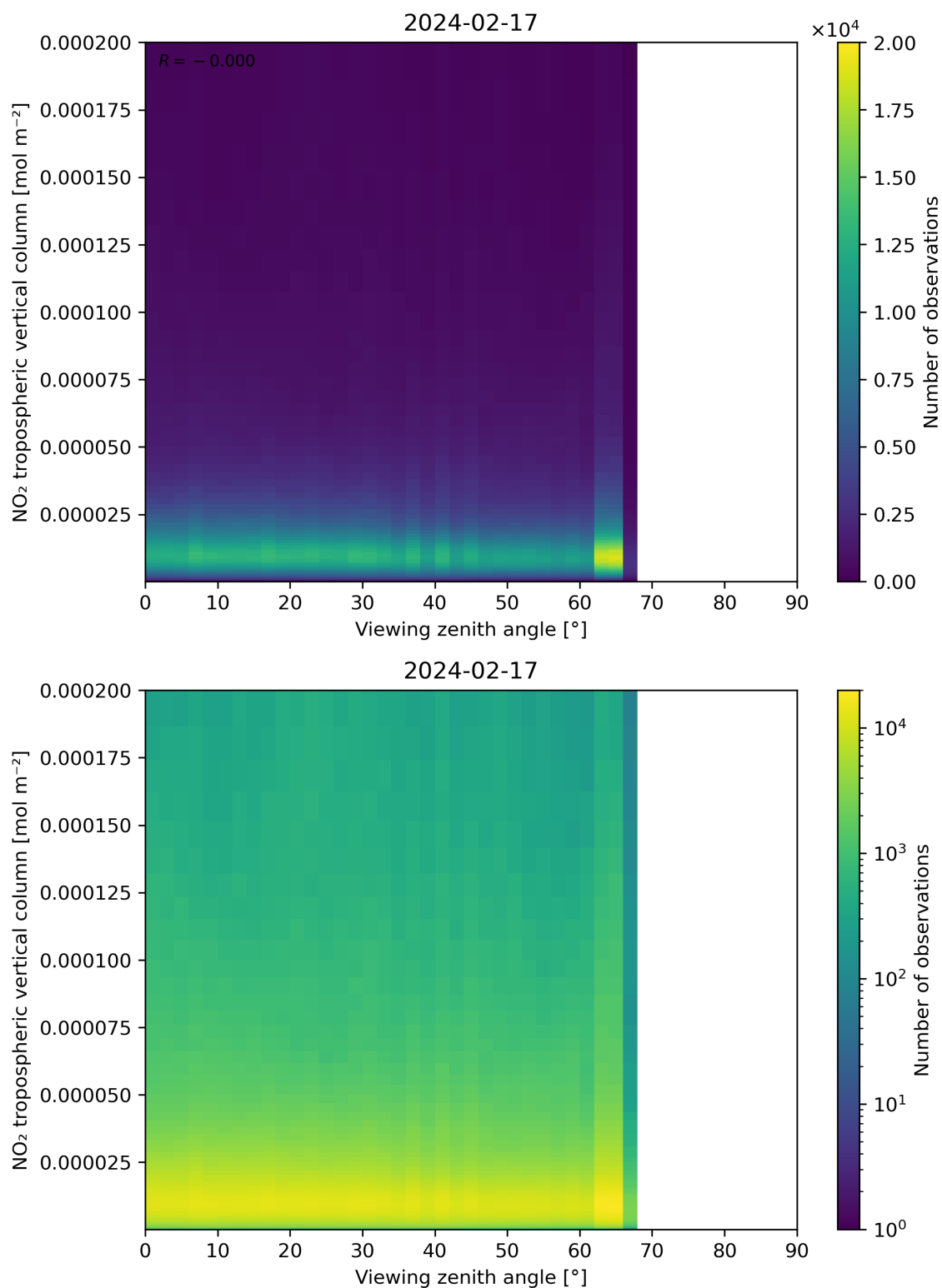
Figure 169: Scatter density plot of “Viewing zenith angle” against “NO 2 tropospheric vertical column” for 2024-02-17 to 2024-02-18.
