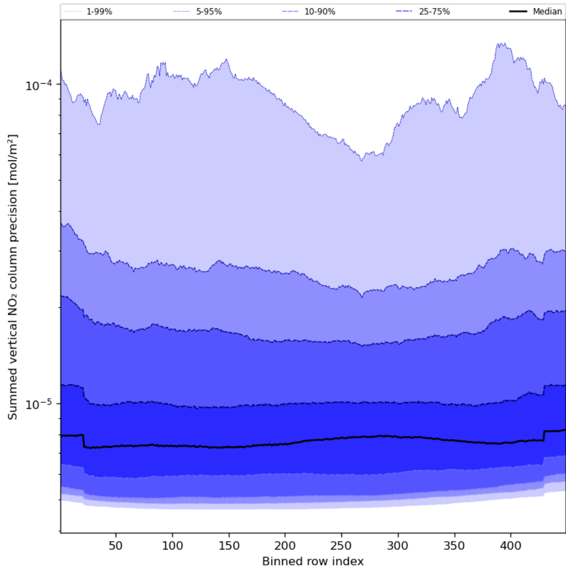
Figure 58: Along track statistics of “Summed vertical NO 2 column precision” for 2024-02-17 to 2024-02-18
