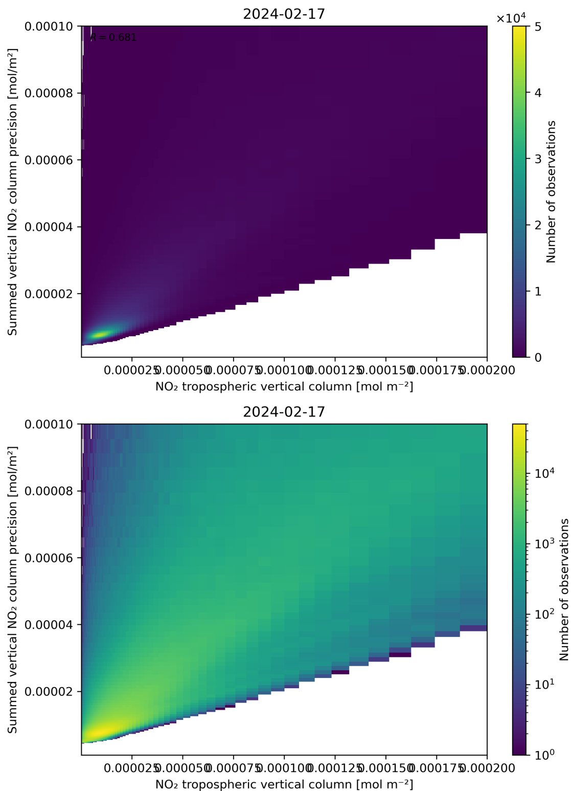
Figure 127: Scatter density plot of “NO 2 tropospheric vertical column” against “Summed vertical NO 2 column precision” for 2024-02-17 to 2024-02-18.
