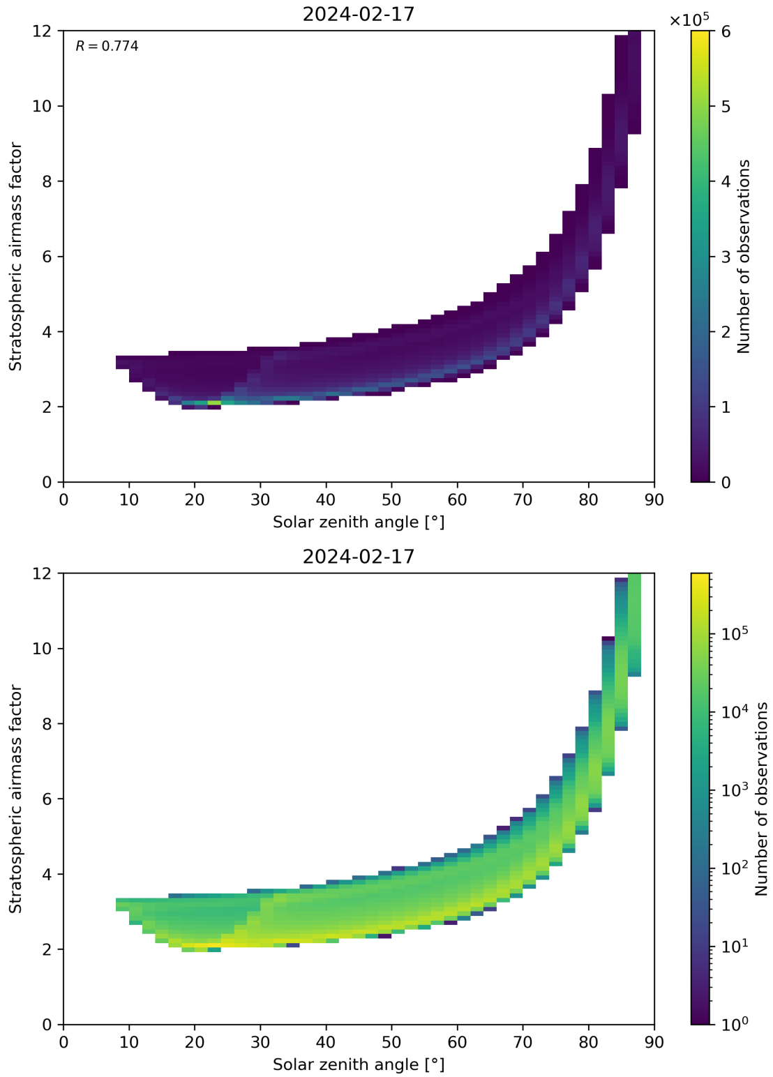
Figure 145: Scatter density plot of “Solar zenith angle” against “Stratospheric airmass factor” for 2024-02-17 to 2024-02-18.
