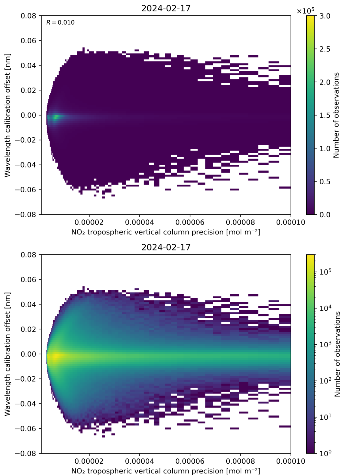
Figure 141: Scatter density plot of “NO 2 tropospheric vertical column precision” against “Wavelength calibration offset” for 2024-02-17 to 2024-02-18.
