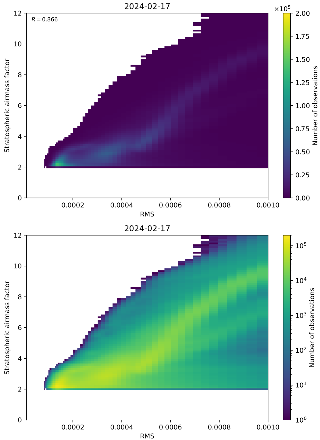
Figure 144: Scatter density plot of “RMS” against “Stratospheric airmass factor” for 2024-02-17 to 2024-02-18.
