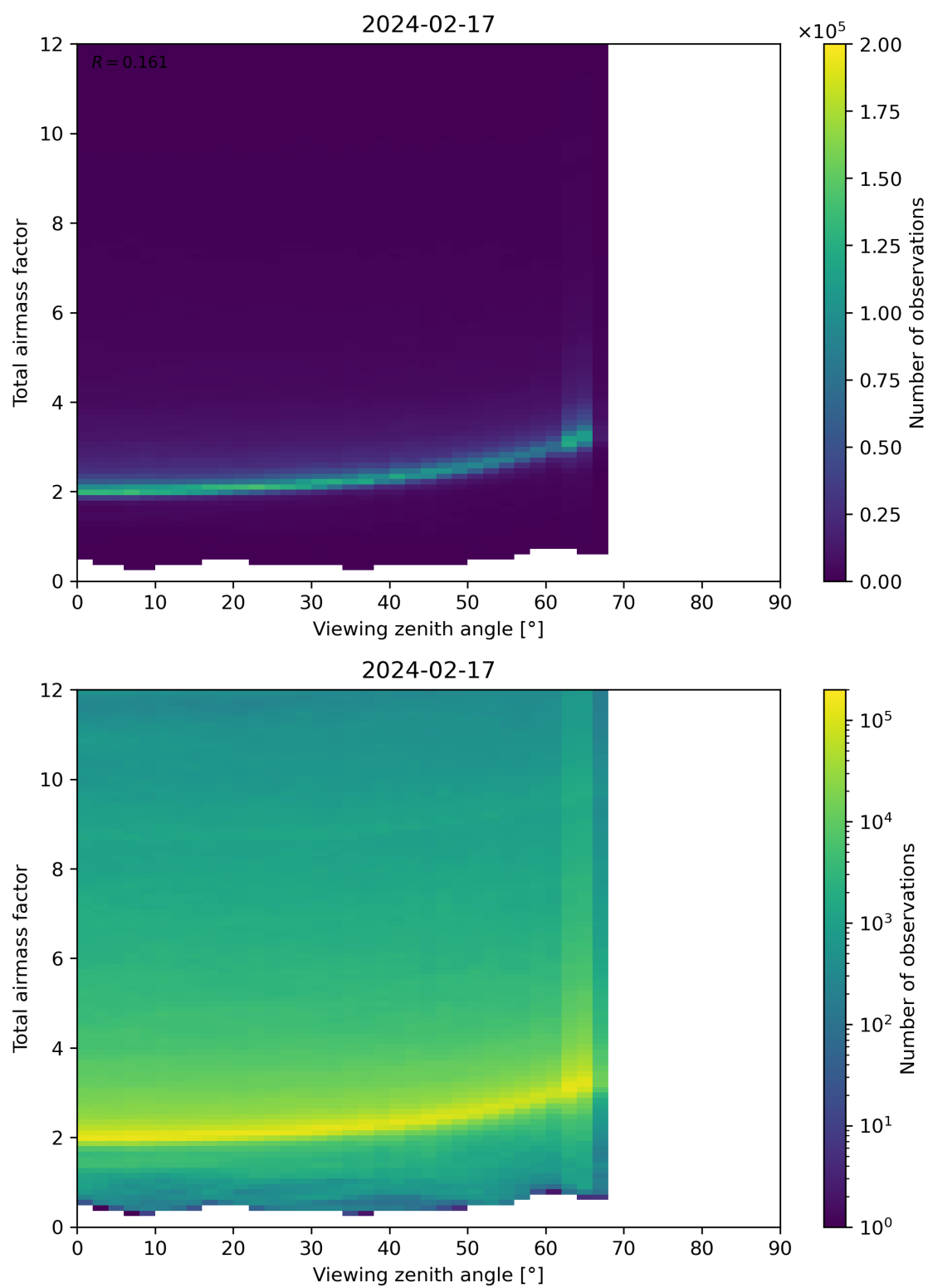
Figure 160: Scatter density plot of “Viewing zenith angle” against “Total airmass factor” for 2024-02-17 to 2024-02-18.
