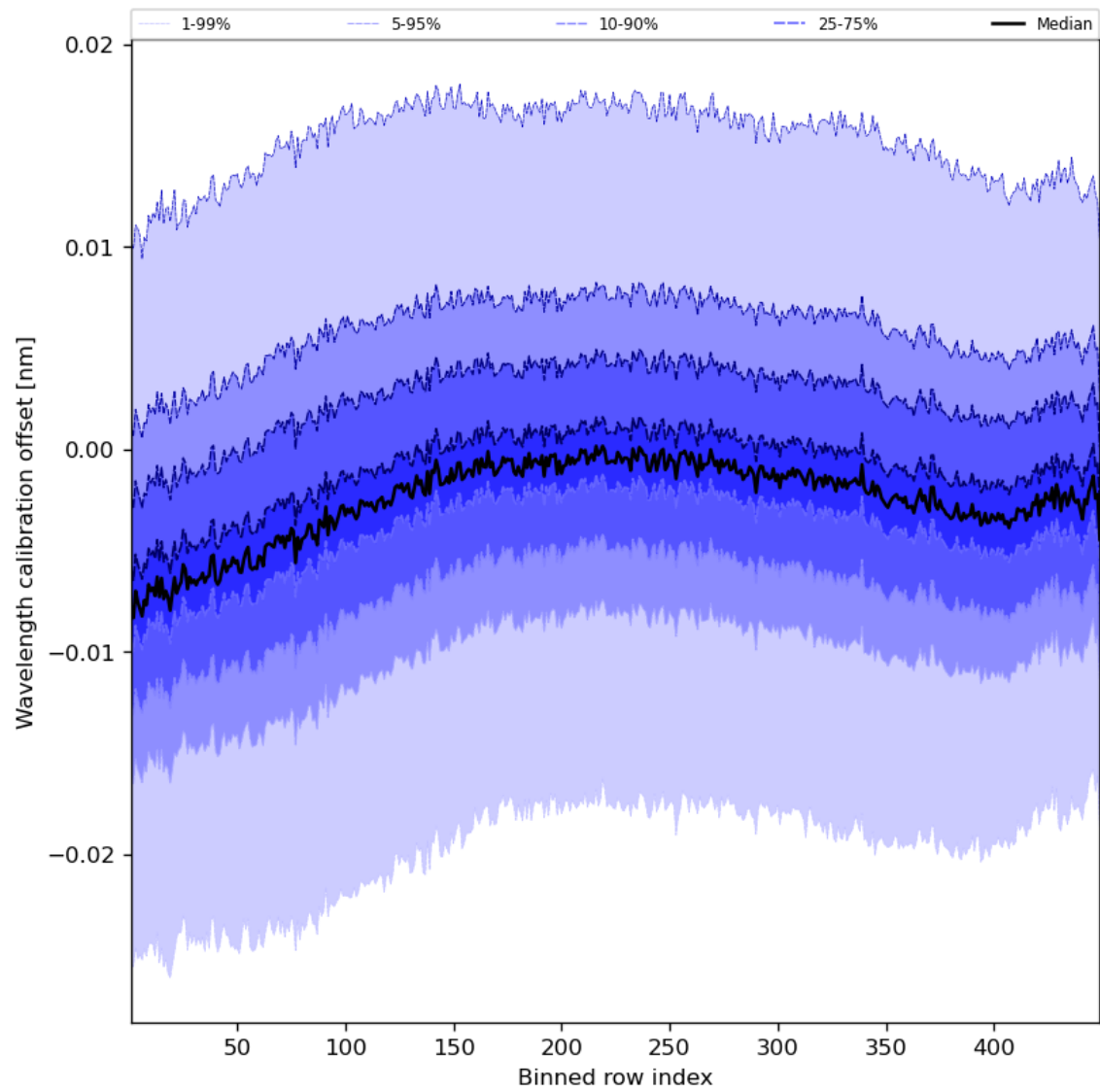
Figure 52: Along track statistics of “Wavelength calibration offset” for 2024-02-17 to 2024-02-18
