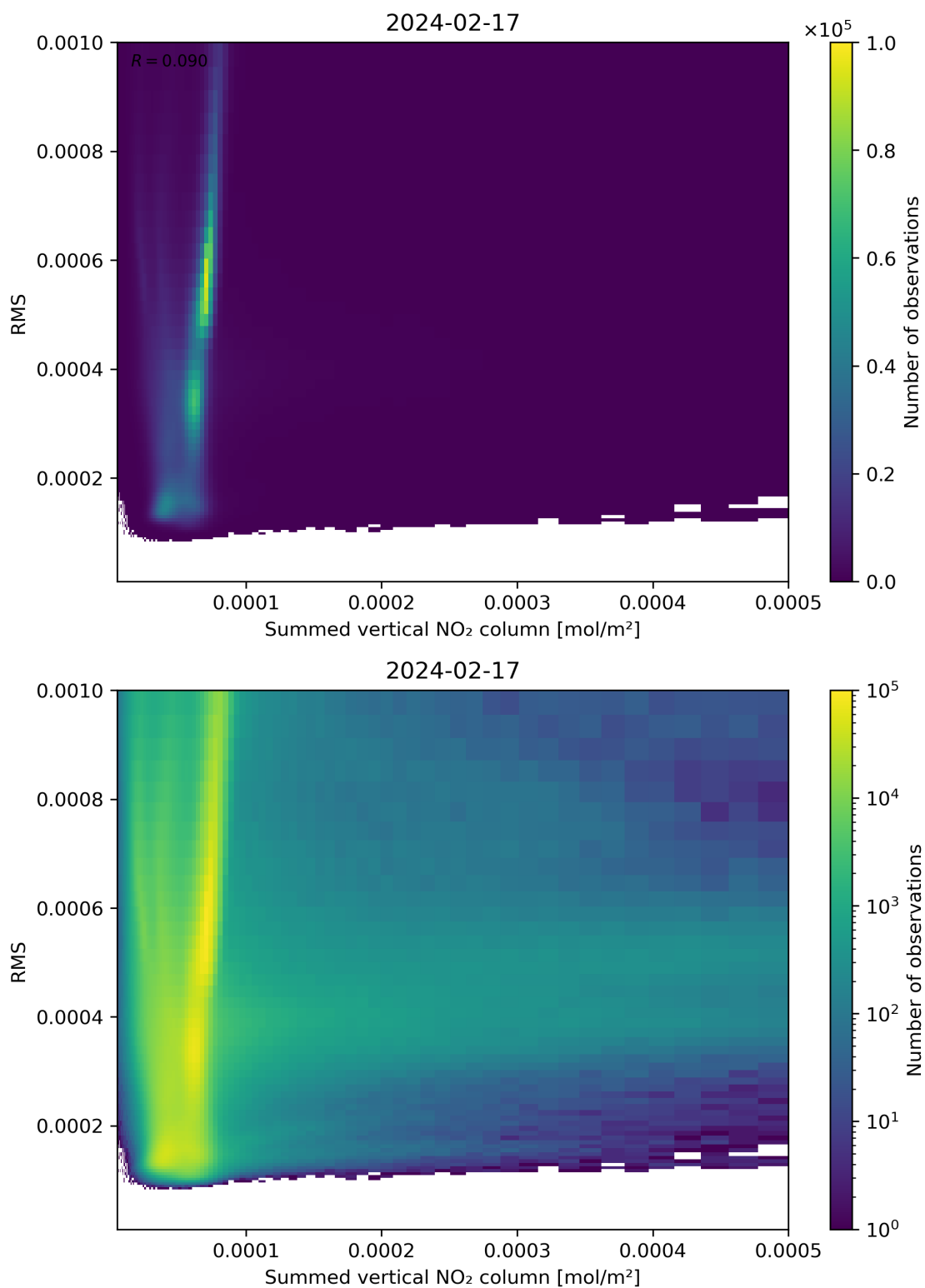
Figure 109: Scatter density plot of “Summed vertical NO 2 column” against “RMS” for 2024-02-17 to 2024-02-18.
