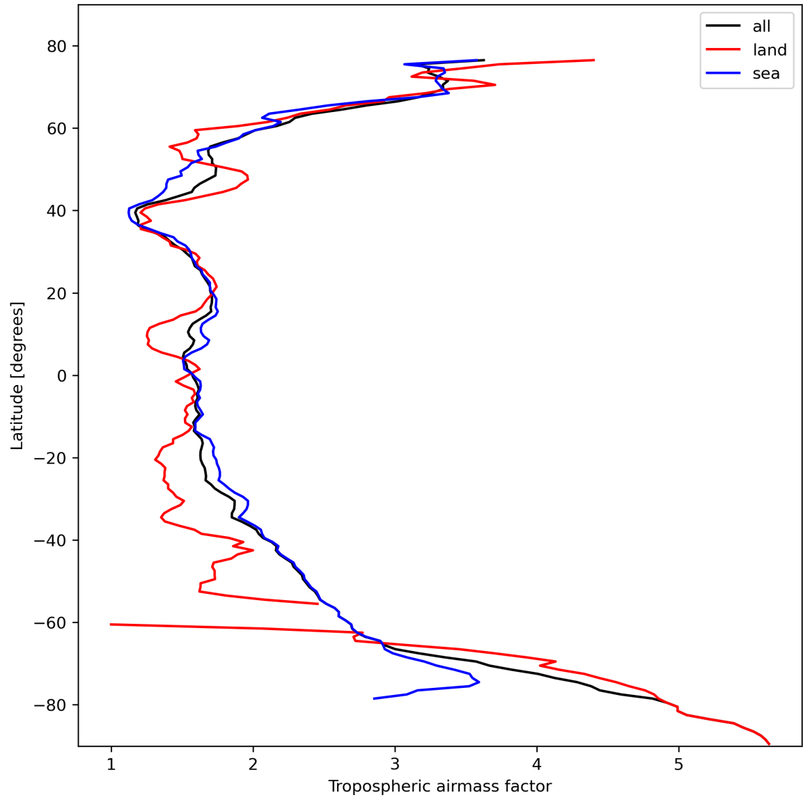
Figure 14: Zonal average of “Tropospheric airmass factor” for 2024-02-17 to 2024-02-18.
