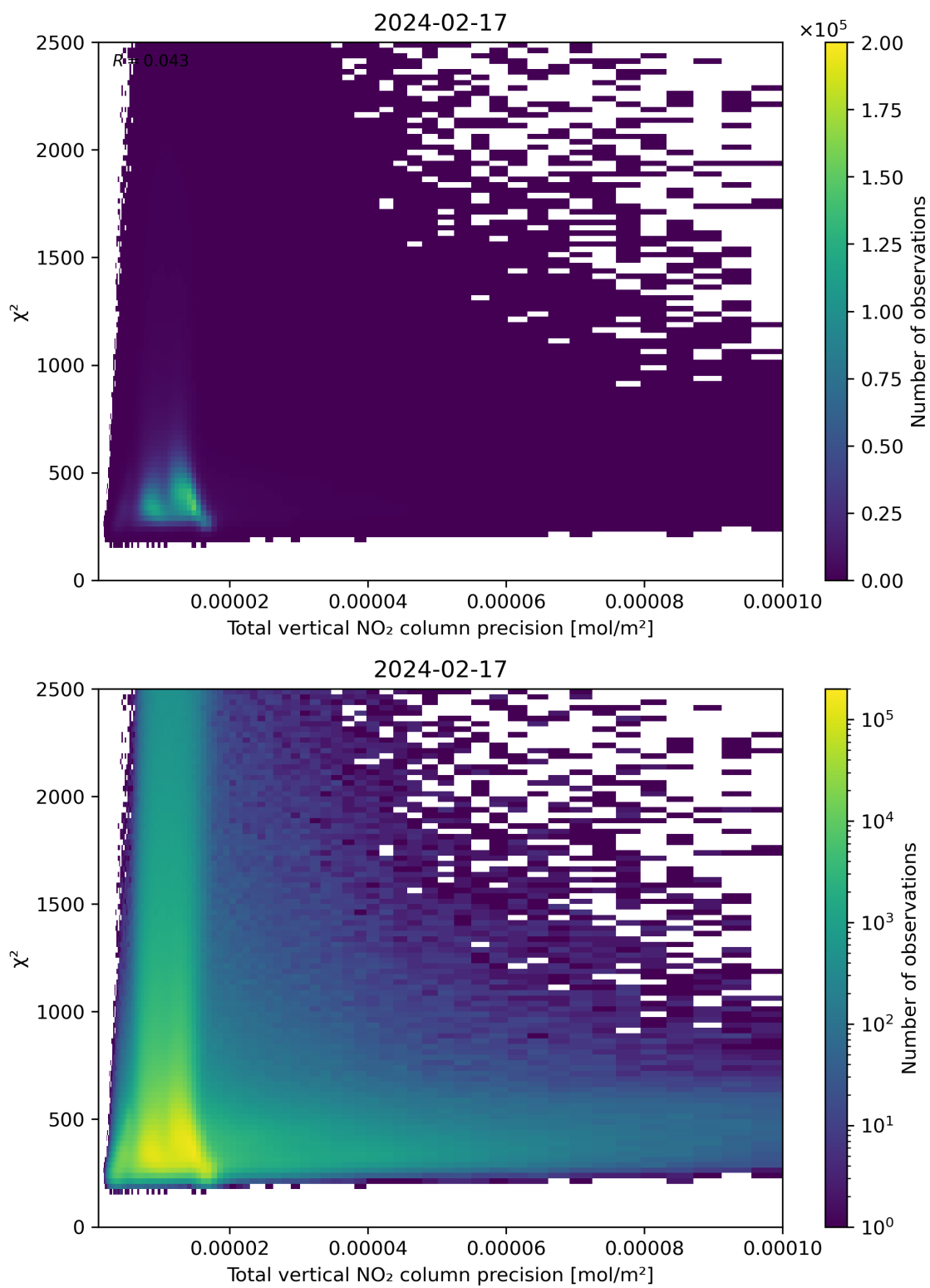
Figure 116: Scatter density plot of “Total vertical NO 2 column precision” against “ \chi^2 ” for 2024-02-17 to 2024-02-18.
