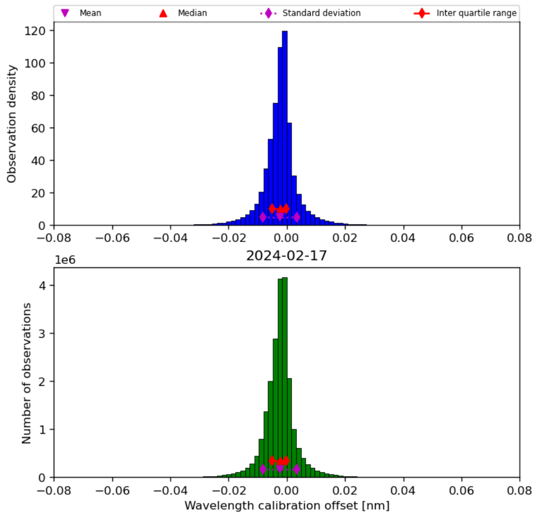
Figure 35: Histogram of “Wavelength calibration offset” for 2024-02-17 to 2024-02-18
