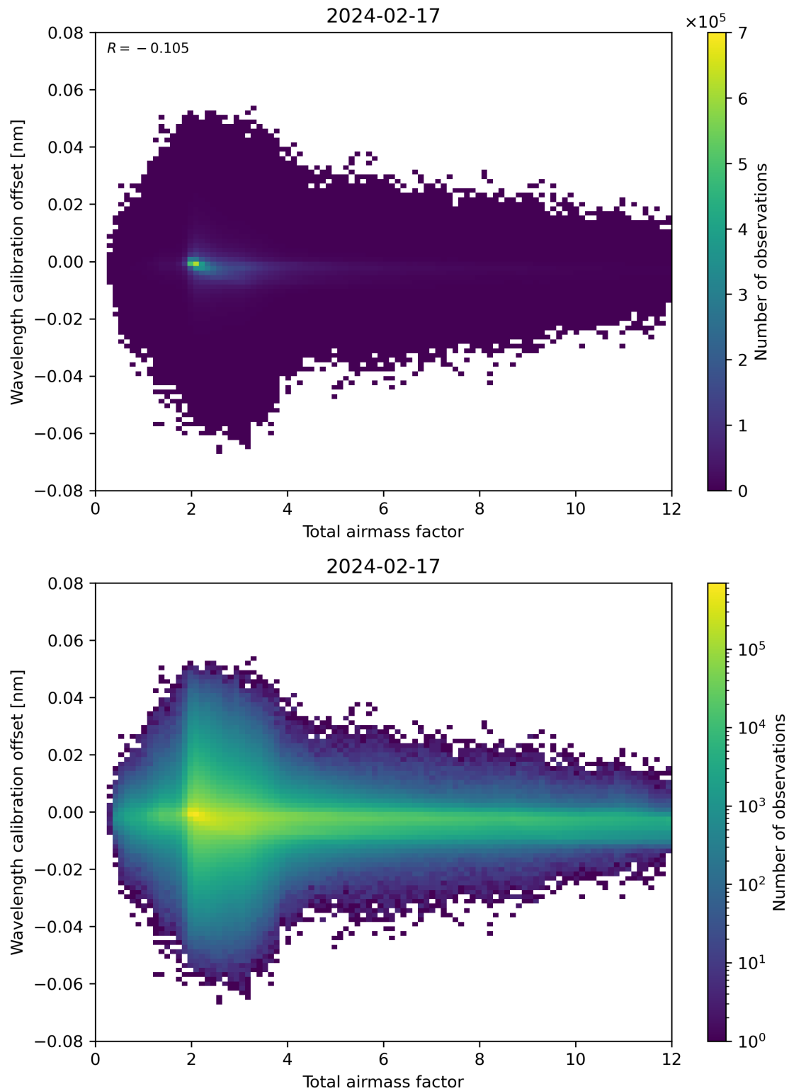
Figure 70: Scatter density plot of “Total airmass factor” against “Wavelength calibration offset” for 2024-02-17 to 2024-02-18.
