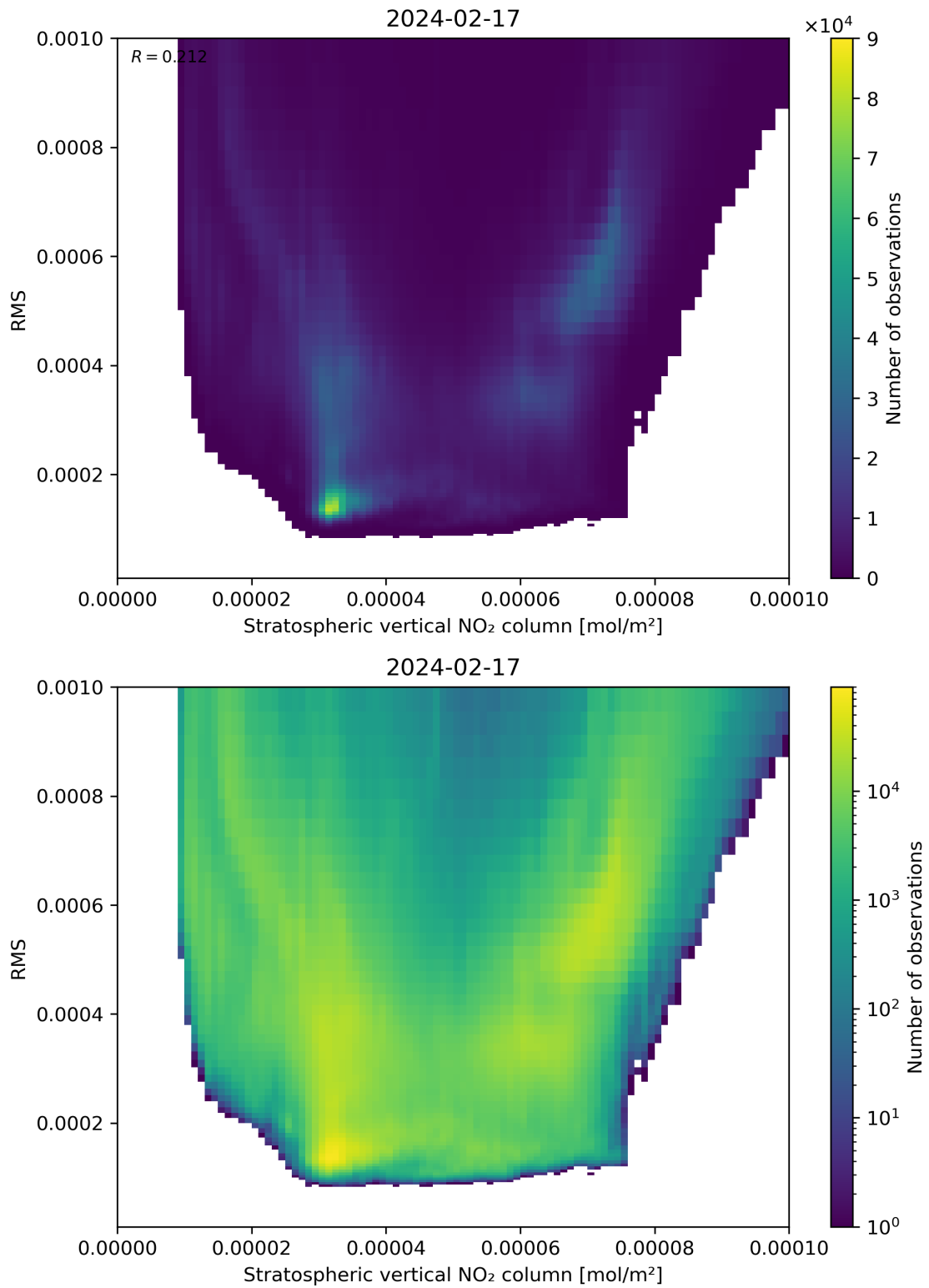
Figure 102: Scatter density plot of “Stratospheric vertical NO 2 column” against “RMS” for 2024-02-17 to 2024-02-18.
