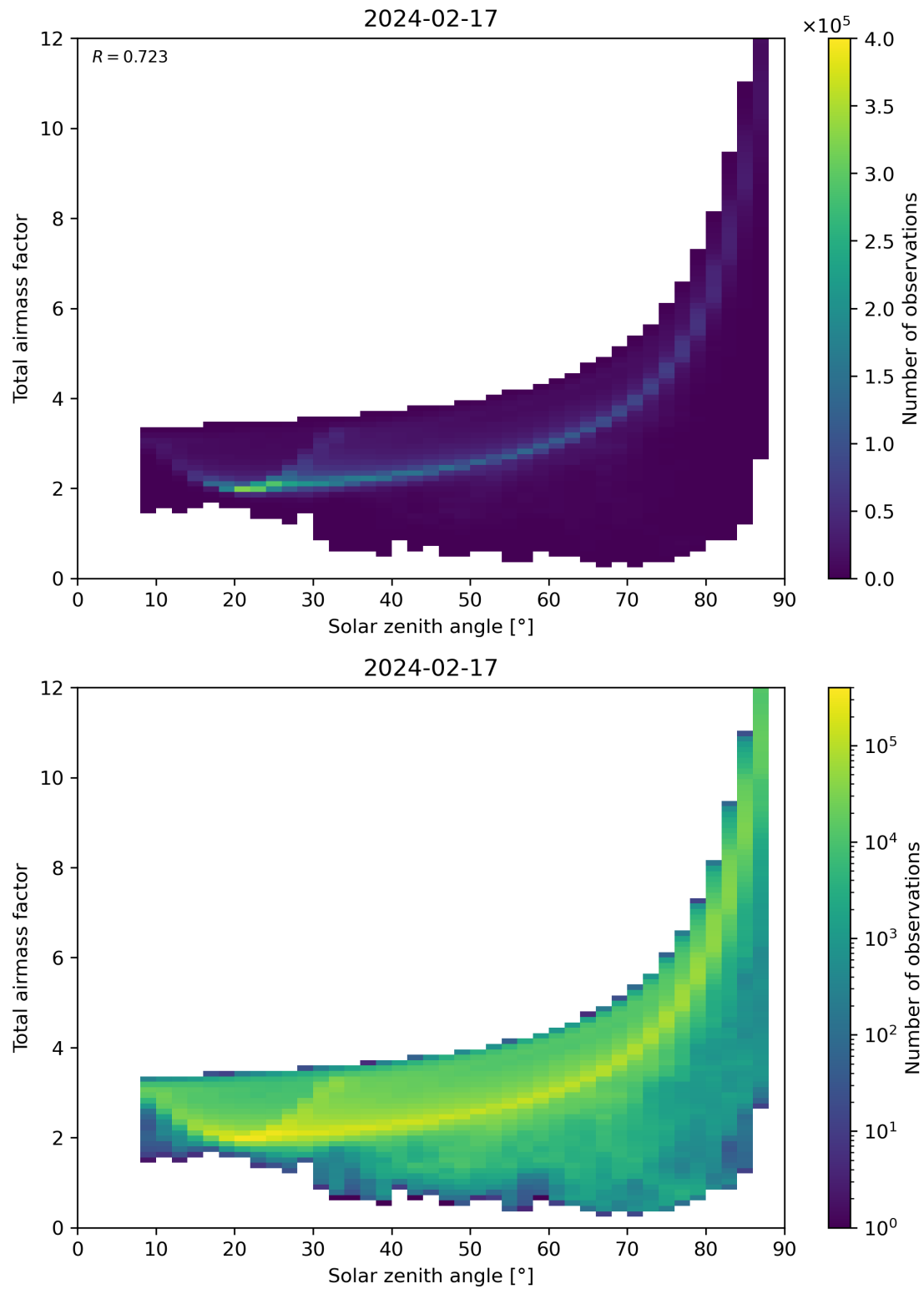
Figure 146: Scatter density plot of “Solar zenith angle” against “Total air mass factor” for 2024-02-17 to 2024-02-18.
