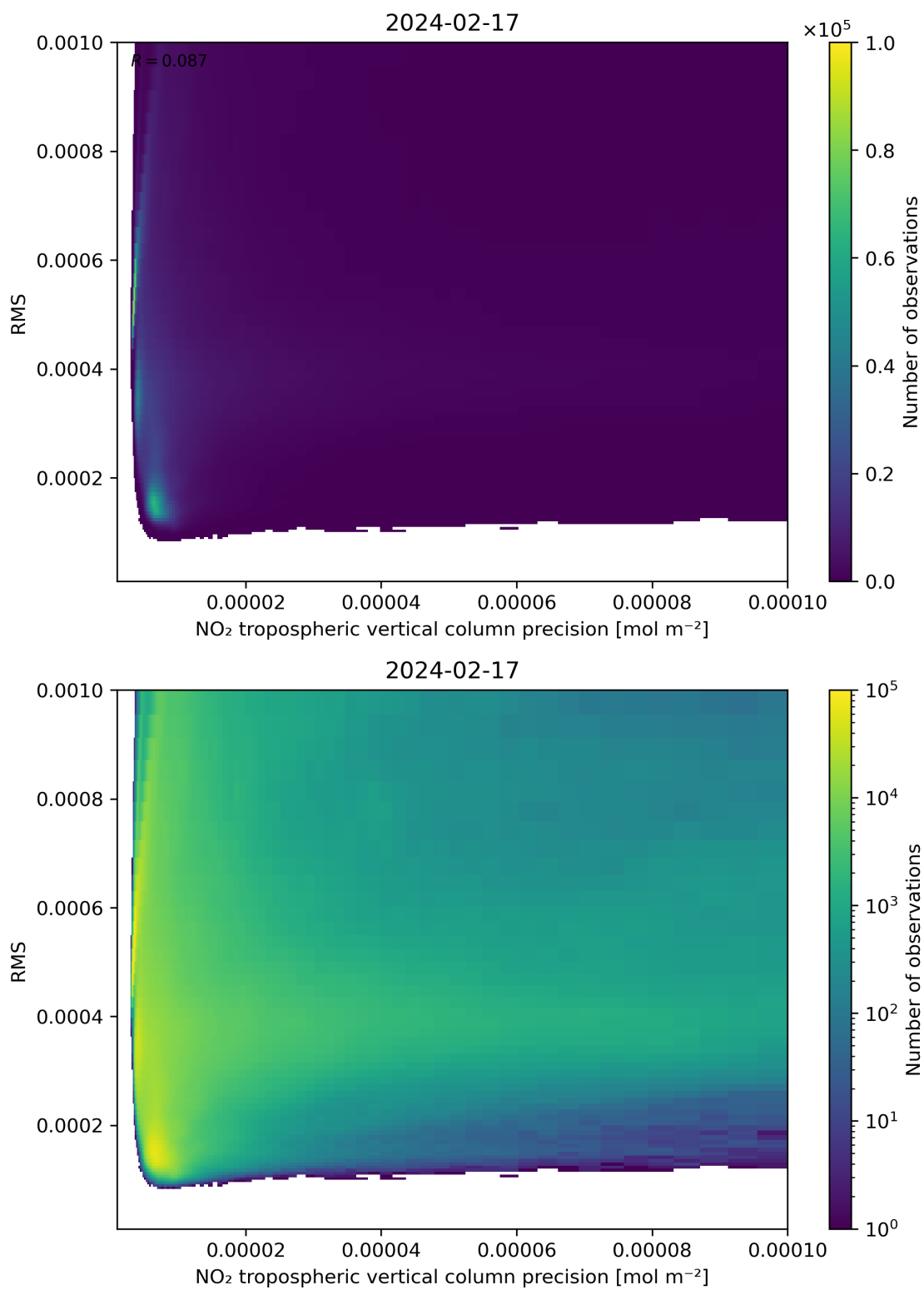
Figure 140: Scatter density plot of “NO 2 tropospheric vertical column precision” against “RMS” for 2024-02-17 to 2024-02-18.
