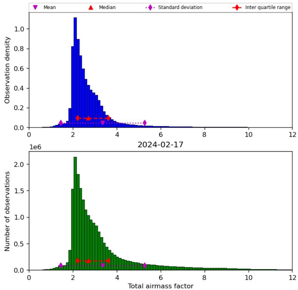
Figure 32: Histogram of “Total airmass factor” for 2024-02-17 to 2024-02-18
