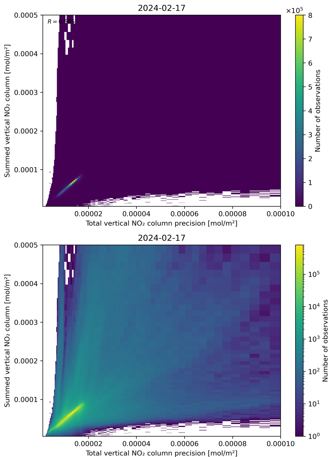
Figure 117: Scatter density plot of “Total vertical NO 2 column precision” against “Summed vertical NO 2 column” for 2024-02-17 to 2024-02-18.
