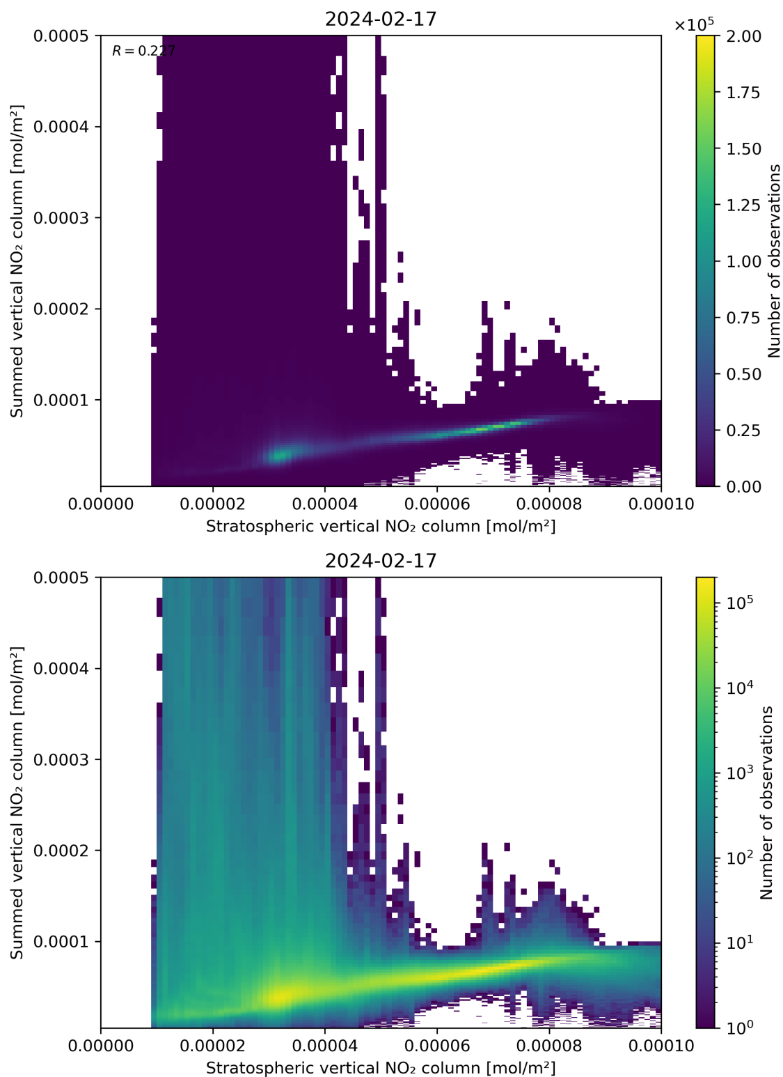
Figure 98: Scatter density plot of “Stratospheric vertical NO 2 column” against “Summed vertical NO 2 column” for 2024-02-17 to 2024-02-18.
