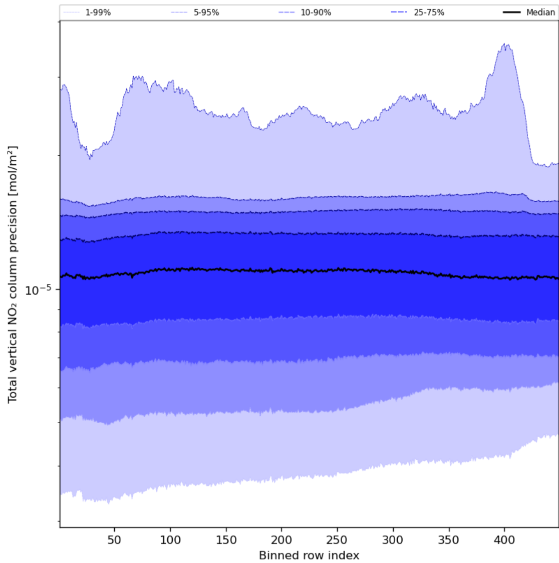
Figure 56: Along track statistics of “Total vertical NO 2 column precision” for 2024-02-17 to 2024-02-18
