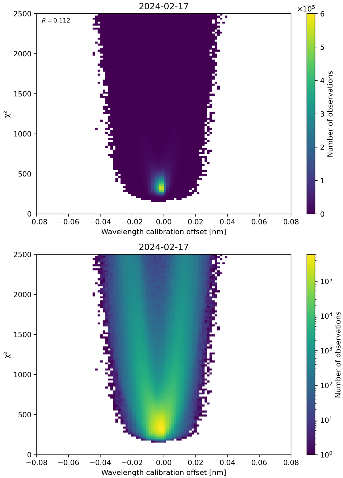
Figure 175: Scatter density plot of “Wavelength calibration offset” against “ \chi^2 ” for 2024-02-17 to 2024-02-18.
