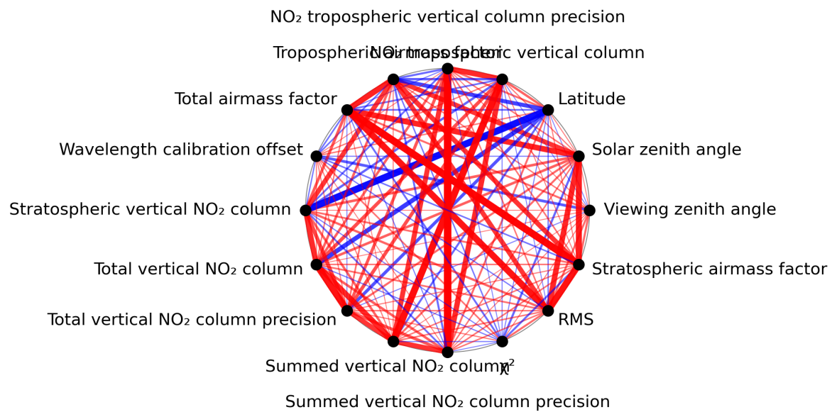
Figure 1: Map of correlation graph for 2024-02-17 to 2024-02-18.
