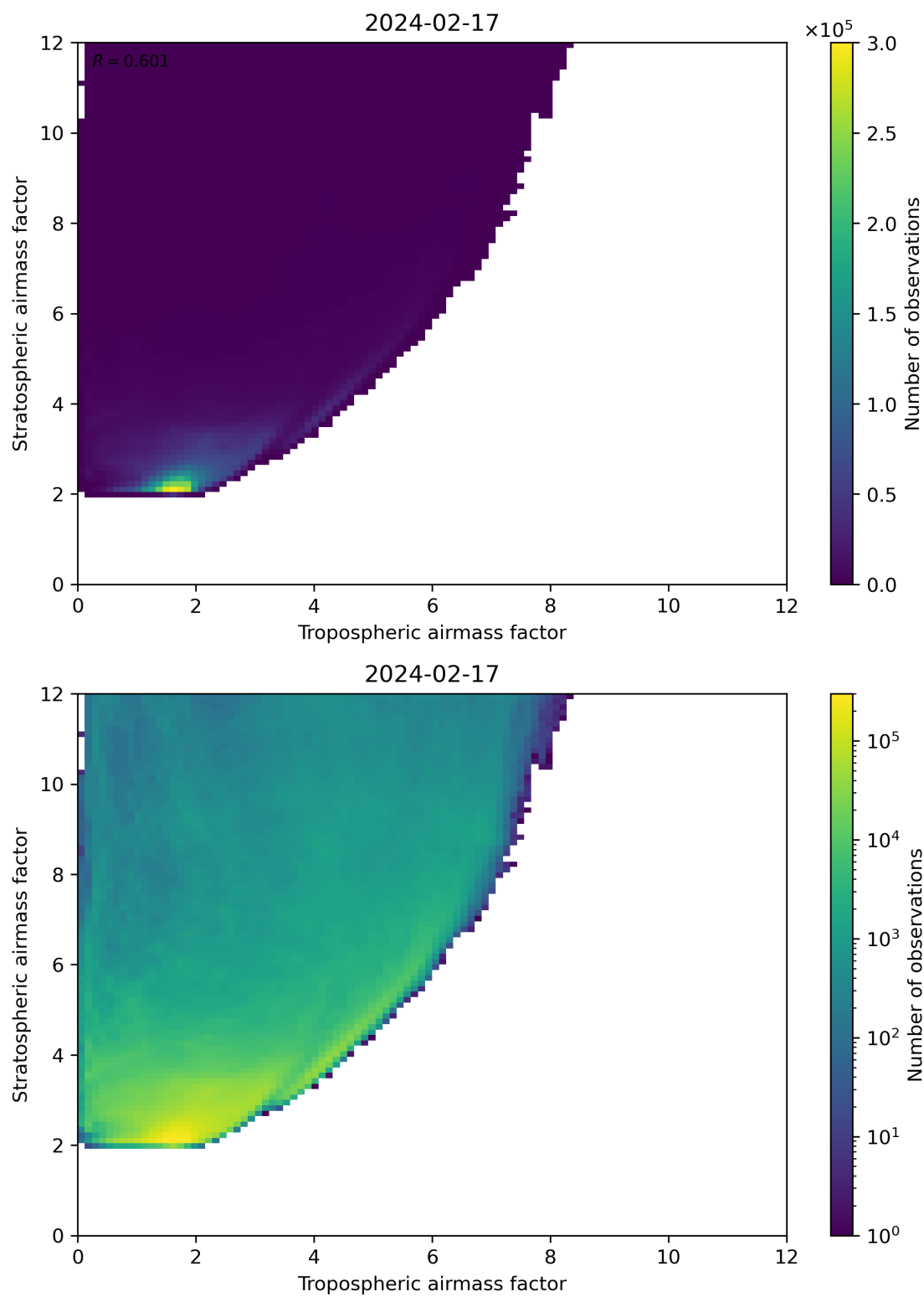
Figure 71: Scatter density plot of “Tropospheric airmass factor” against “Stratospheric airmass factor” for 2024-02-17 to 2024-02-18.
