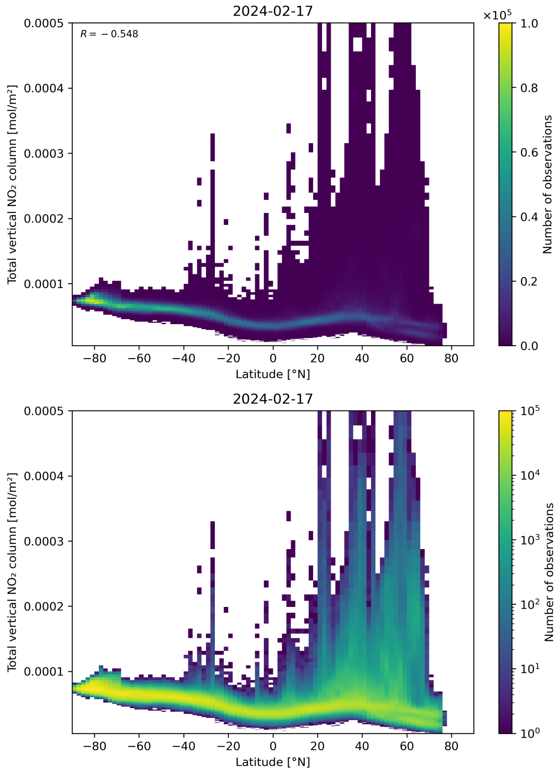
Figure 90: Scatter density plot of “Latitude” against “Total vertical NO 2 column” for 2024-02-17 to 2024-02-18.
