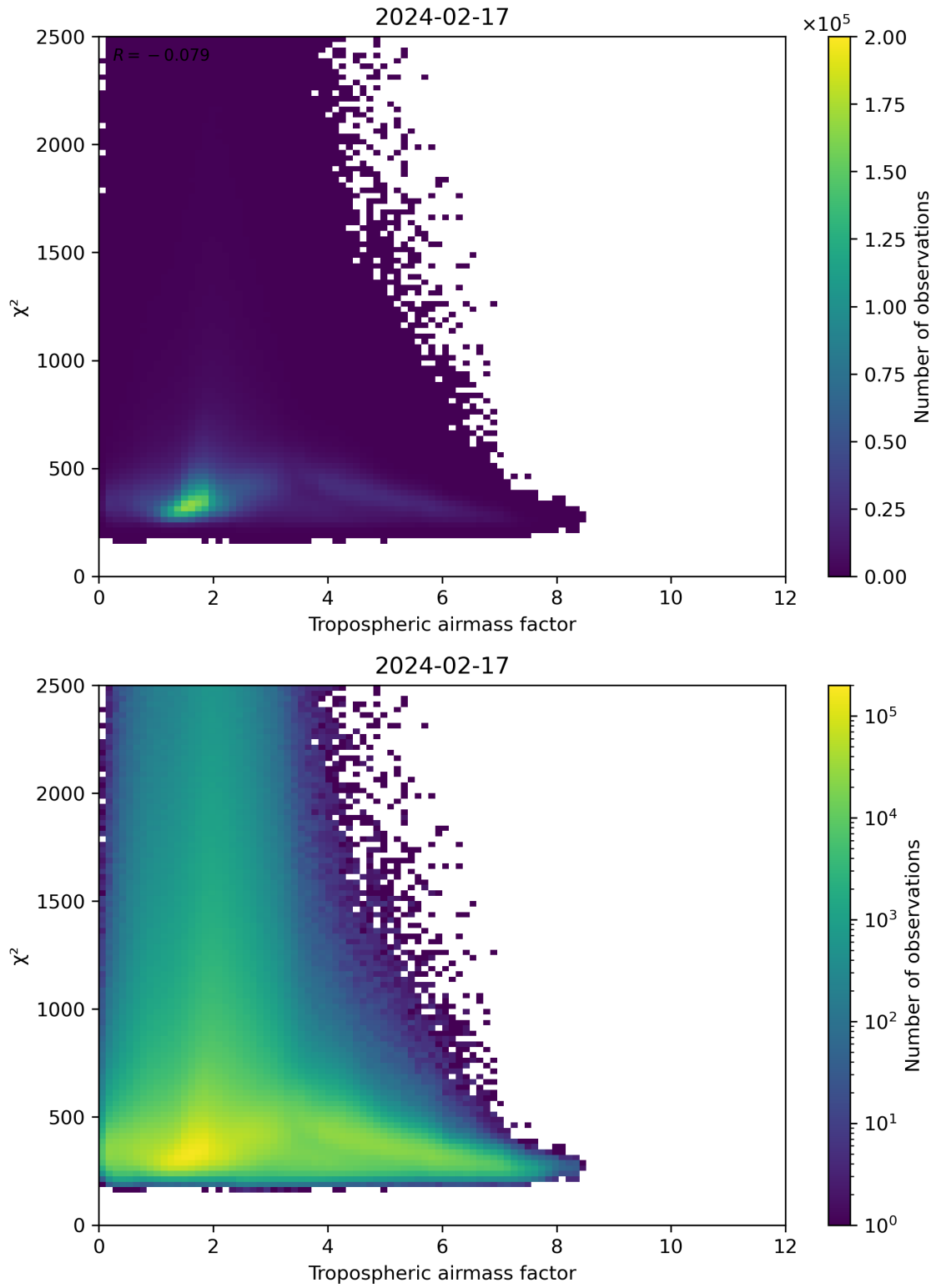
Figure 73: Scatter density plot of “Tropospheric airmass factor” against “ \chi^2 ” for 2024-02-17 to 2024-02-18.
