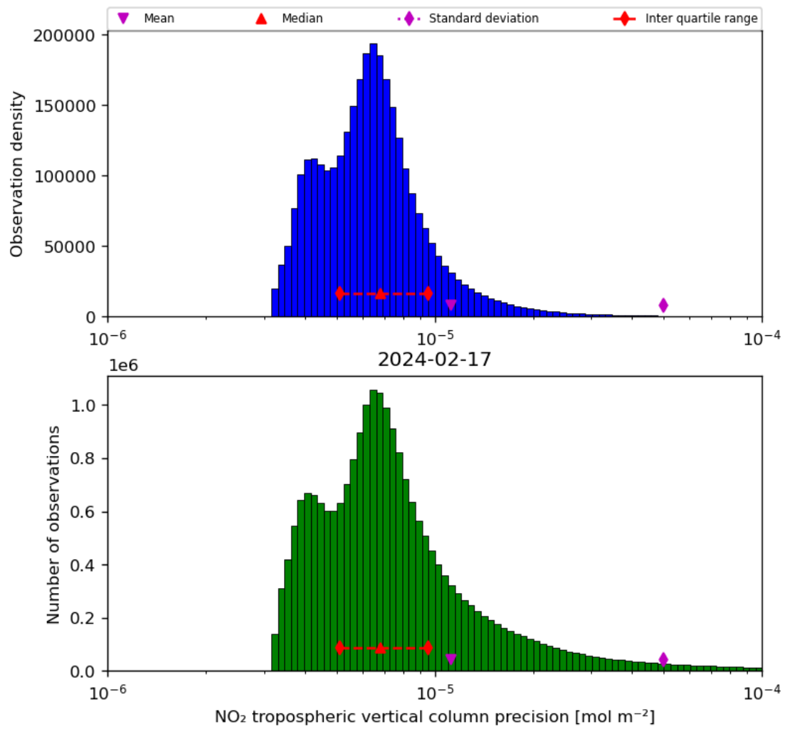
Figure 30: Histogram of “NO 2 tropospheric vertical column precision” for 2024-02-17 to 2024-02-18
