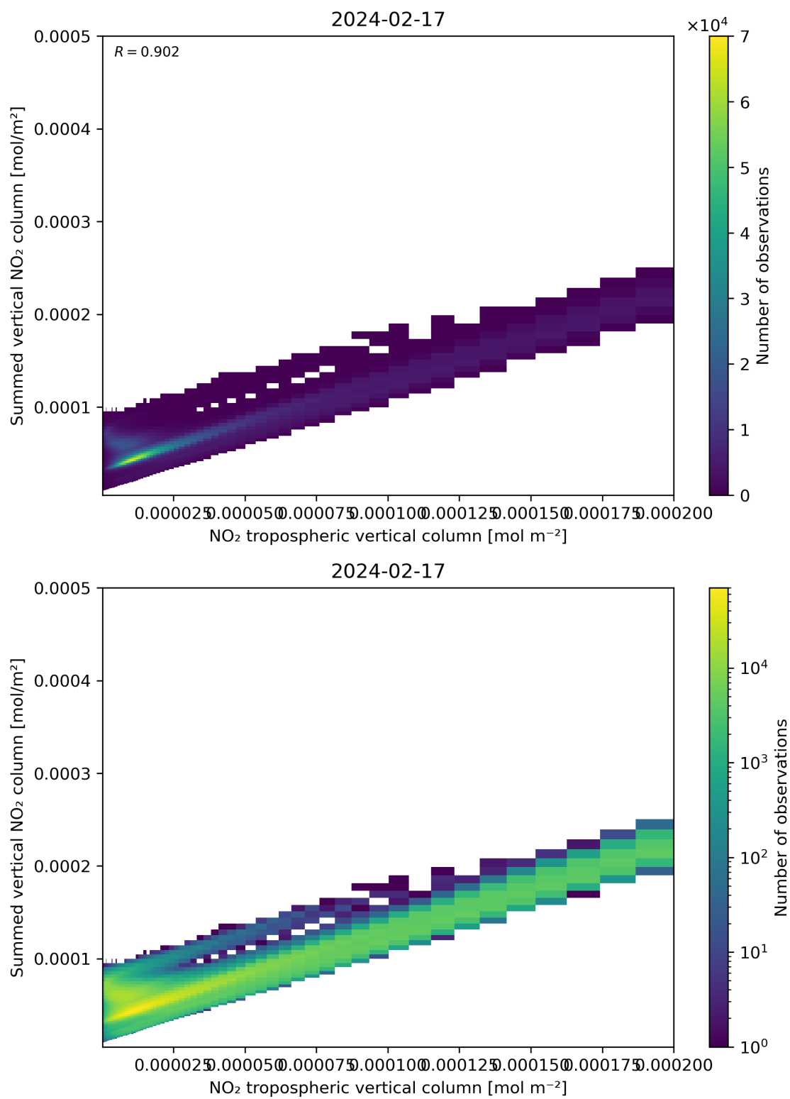
Figure 126: Scatter density plot of “NO 2 tropospheric vertical column” against “Summed vertical NO 2 column” for 2024-02-17 to 2024-02-18.
