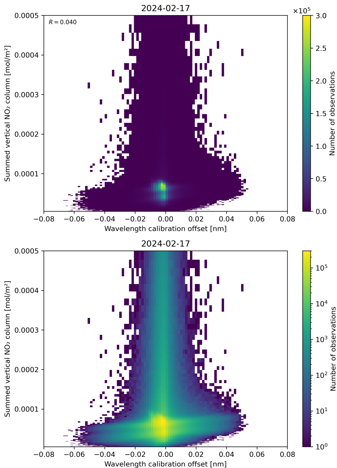
Figure 177: Scatter density plot of “Wavelength calibration offset” against “Summed vertical NO 2 column” for 2024-02-17 to 2024-02-18.
