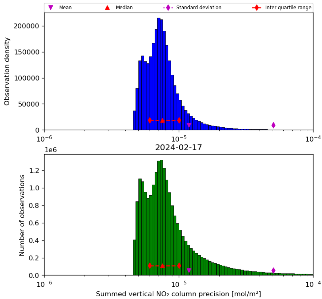
Figure 41: Histogram of “Summed vertical NO 2 column precision” for 2024-02-17 to 2024-02-18
