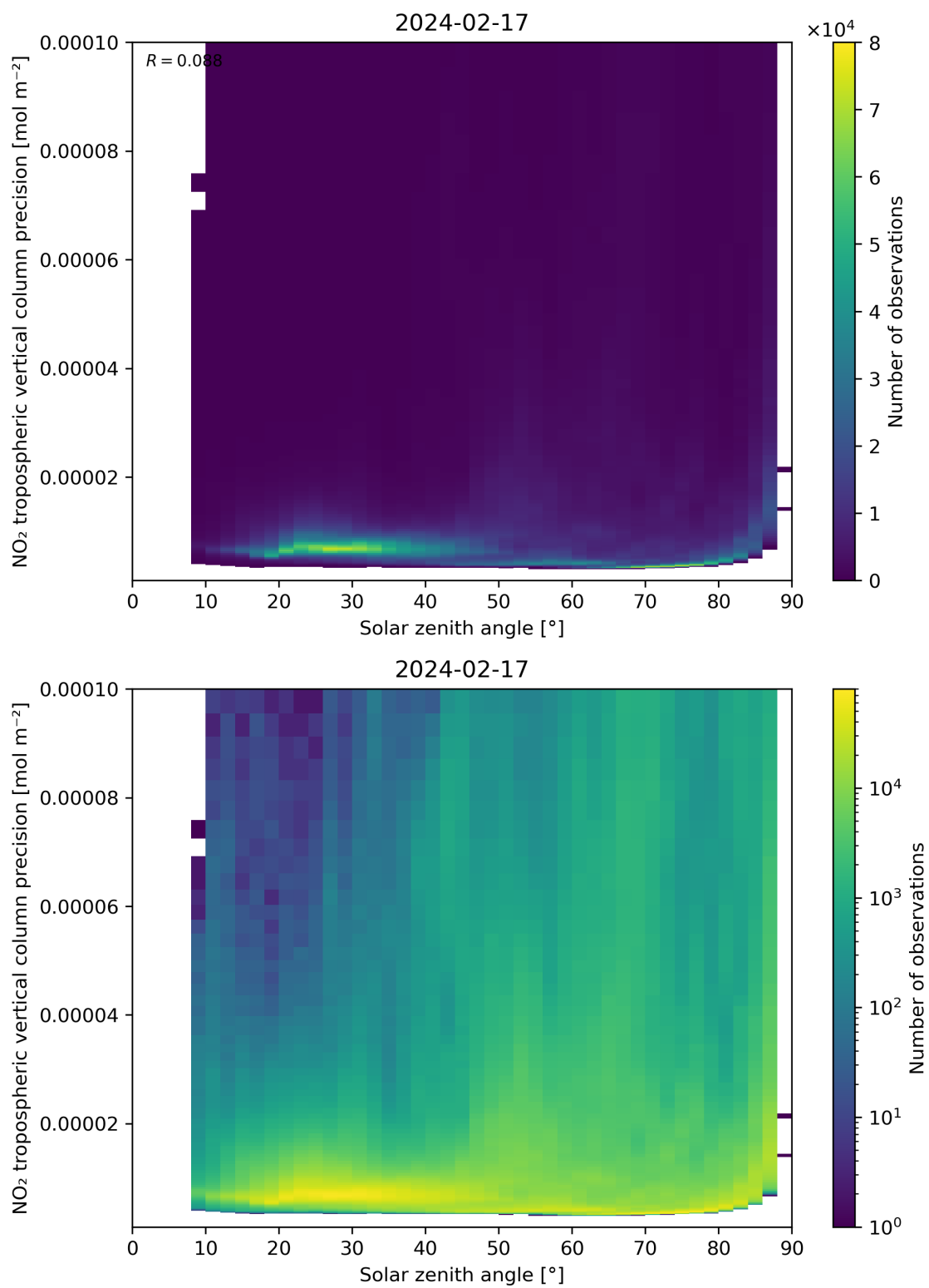
Figure 156: Scatter density plot of “Solar zenith angle” against “NO 2 tropospheric vertical column precision” for 2024-02-17 to 2024-02-18.
