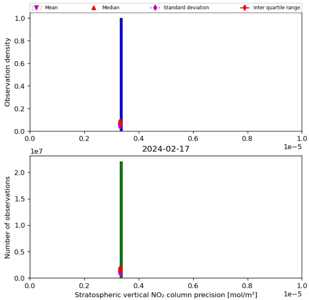
Figure 37: Histogram of “Stratospheric vertical NO 2 column precision” for 2024-02-17 to 2024-02-18
