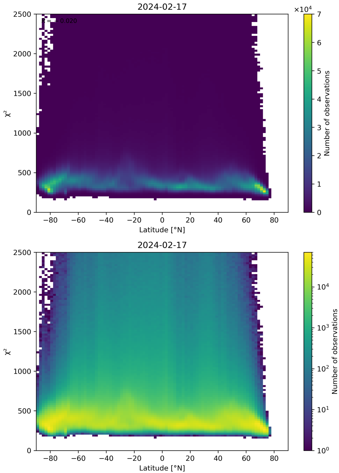
Figure 86: Scatter density plot of “Latitude” against “ \chi^2 ” for 2024-02-17 to 2024-02-18.
