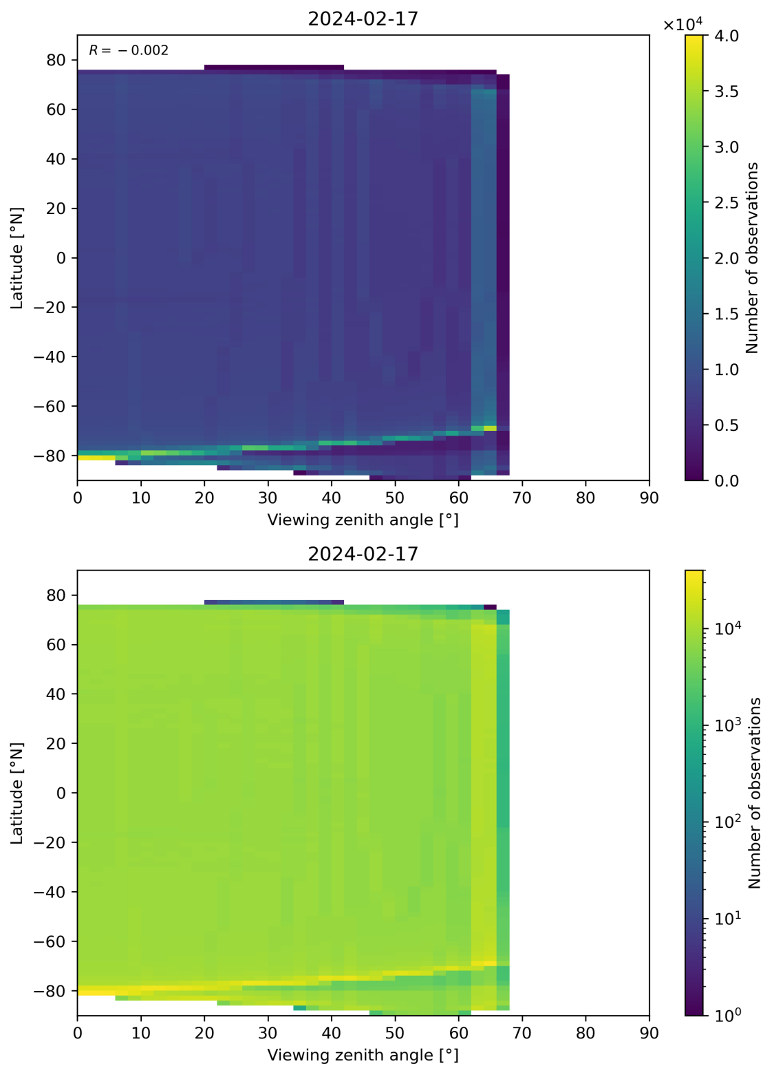
Figure 163: Scatter density plot of “Viewing zenith angle” against “Latitude” for 2024-02-17 to 2024-02-18.
