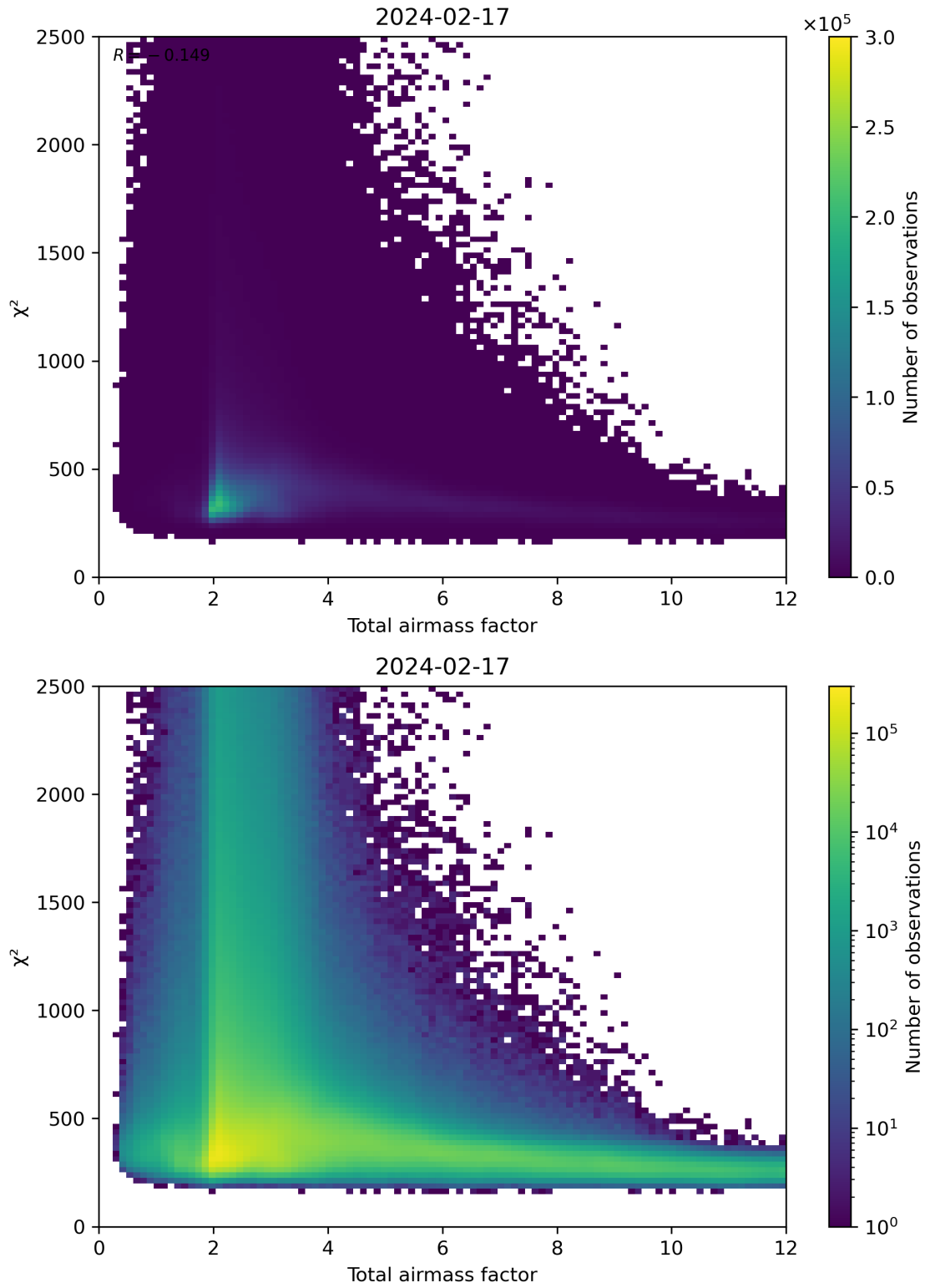
Figure 63: Scatter density plot of “Total airmass factor” against “ \chi^2 ” for 2024-02-17 to 2024-02-18.
