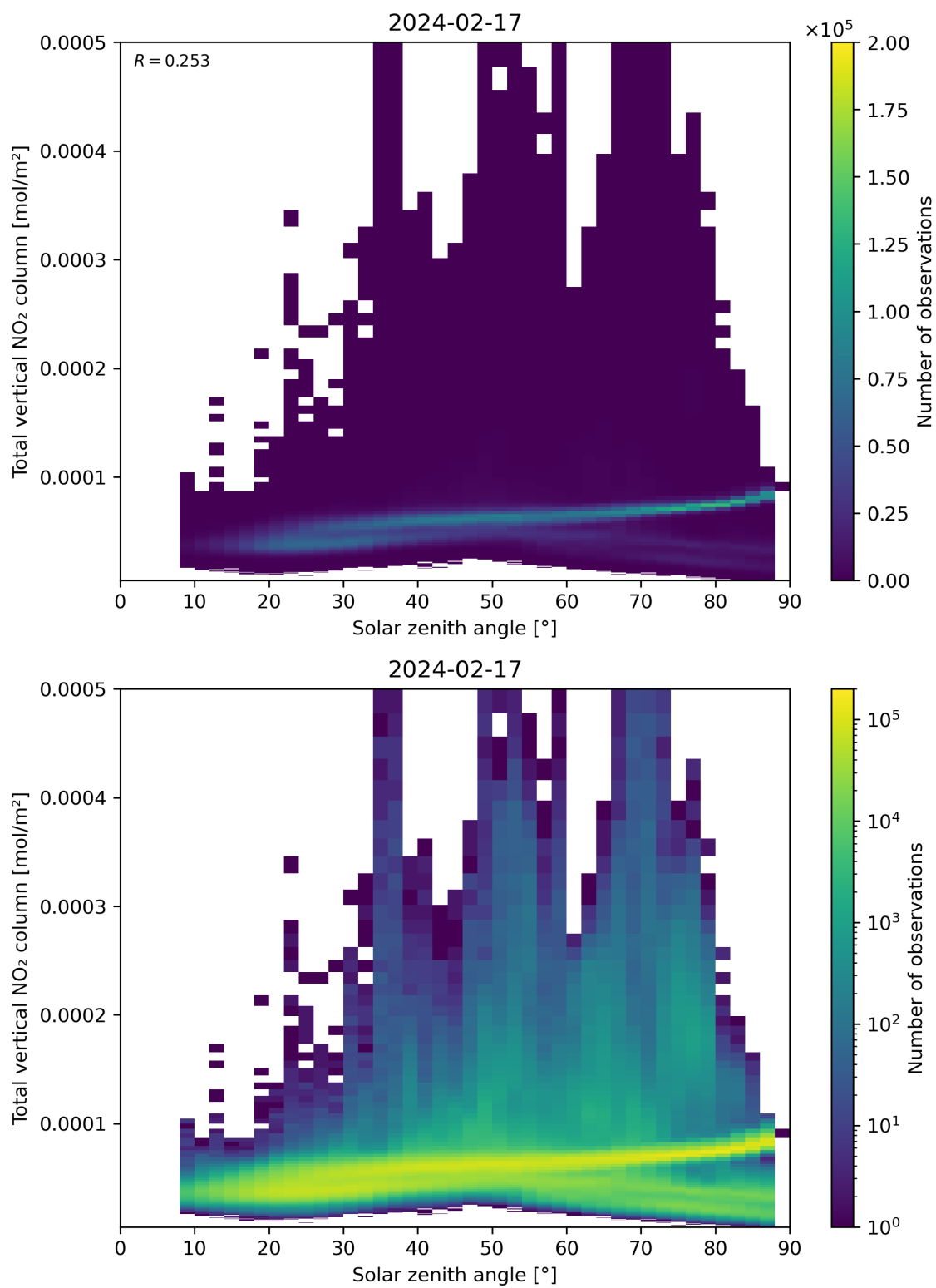
Figure 153: Scatter density plot of “Solar zenith angle” against “Total vertical NO 2 column” for 2024-02-17 to 2024-02-18.
