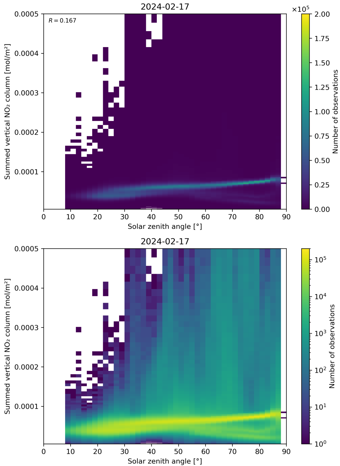
Figure 151: Scatter density plot of “Solar zenith angle” against “Summed vertical NO 2 column” for 2024-02-17 to 2024-02-18.
