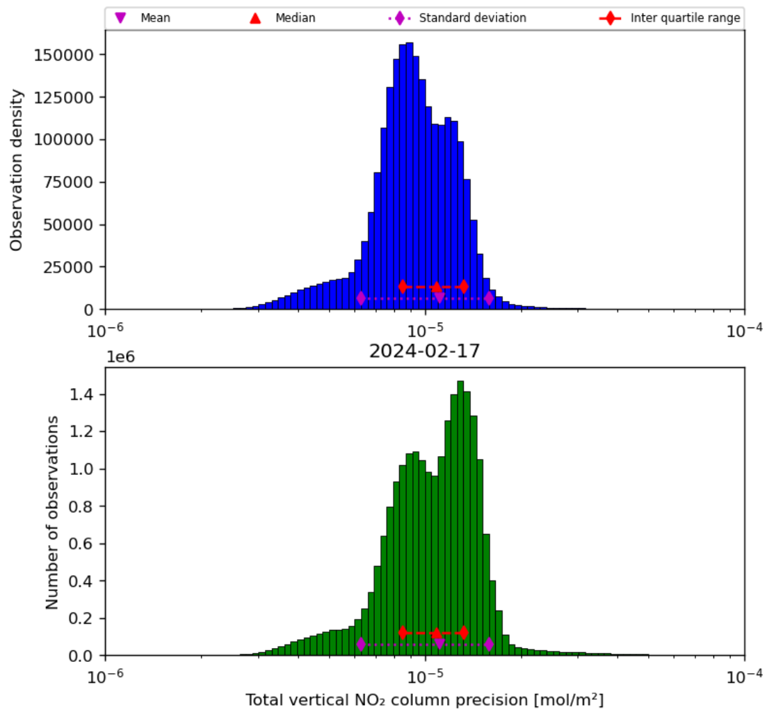
Figure 39: Histogram of “Total vertical NO 2 column precision” for 2024-02-17 to 2024-02-18
