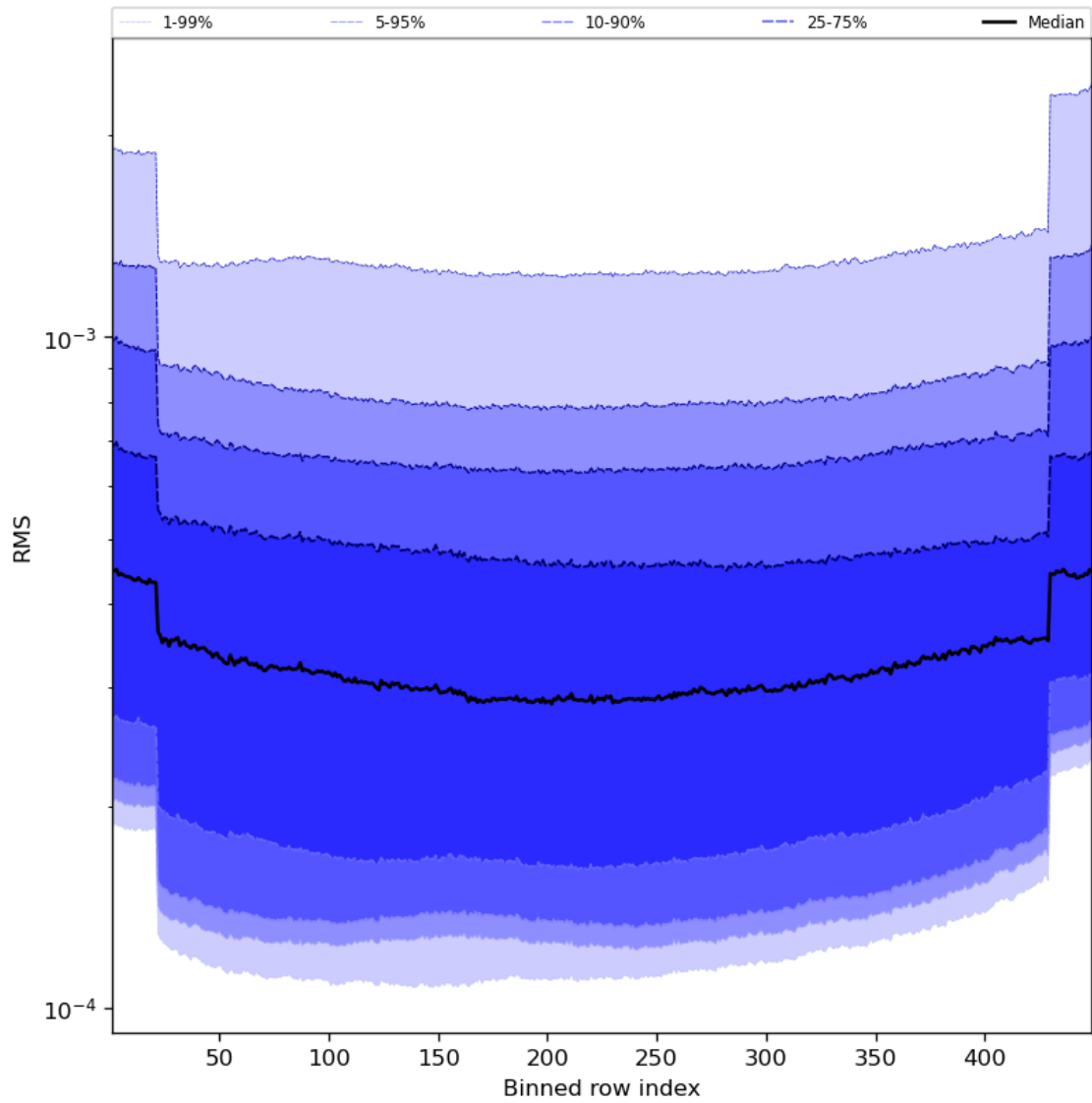
Figure 60: Along track statistics of “RMS” for 2024-02-17 to 2024-02-18
