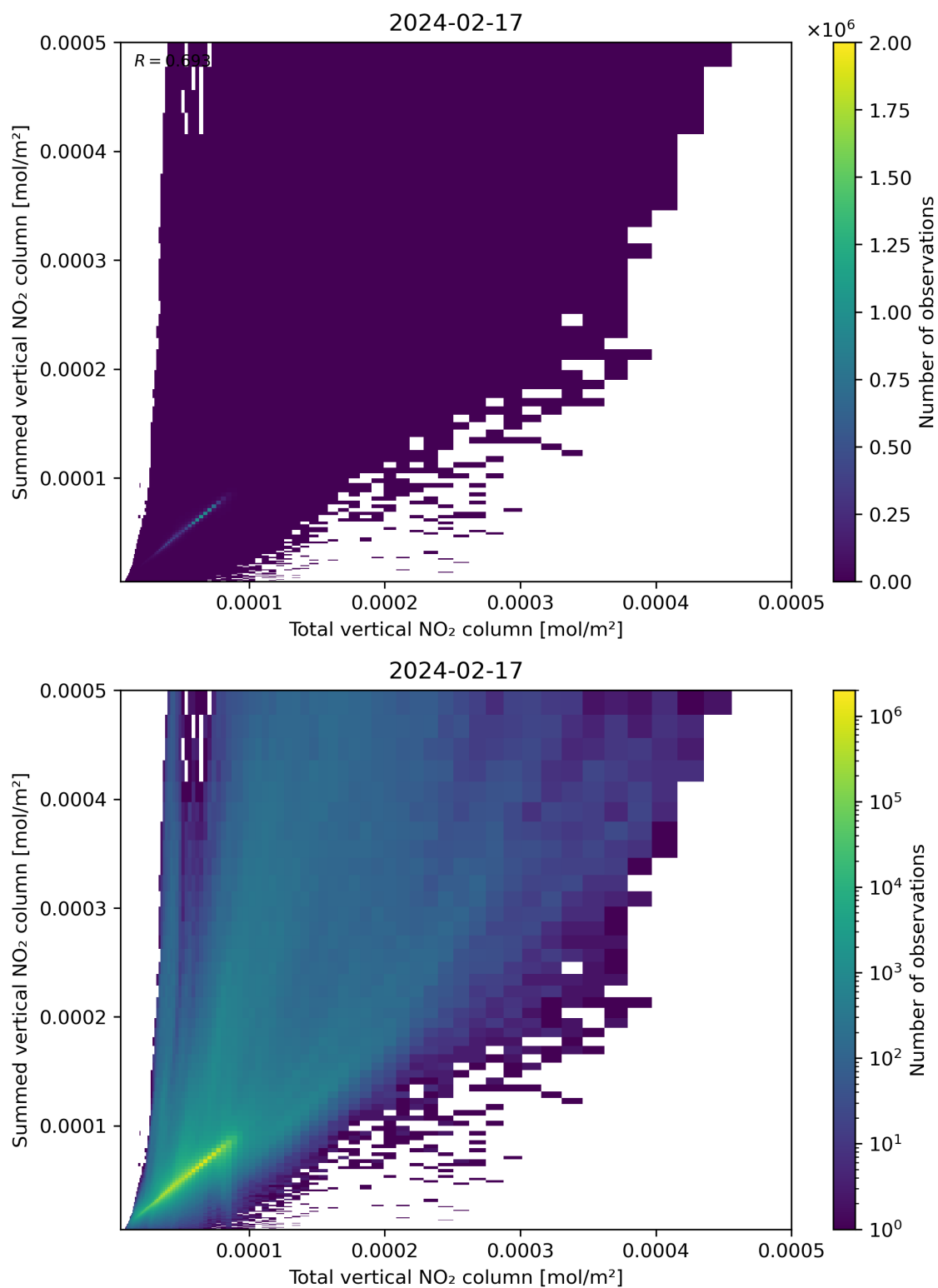
Figure 112: Scatter density plot of “Total vertical NO 2 column” against “Summed vertical NO 2 column” for 2024-02-17 to 2024-02-18.
