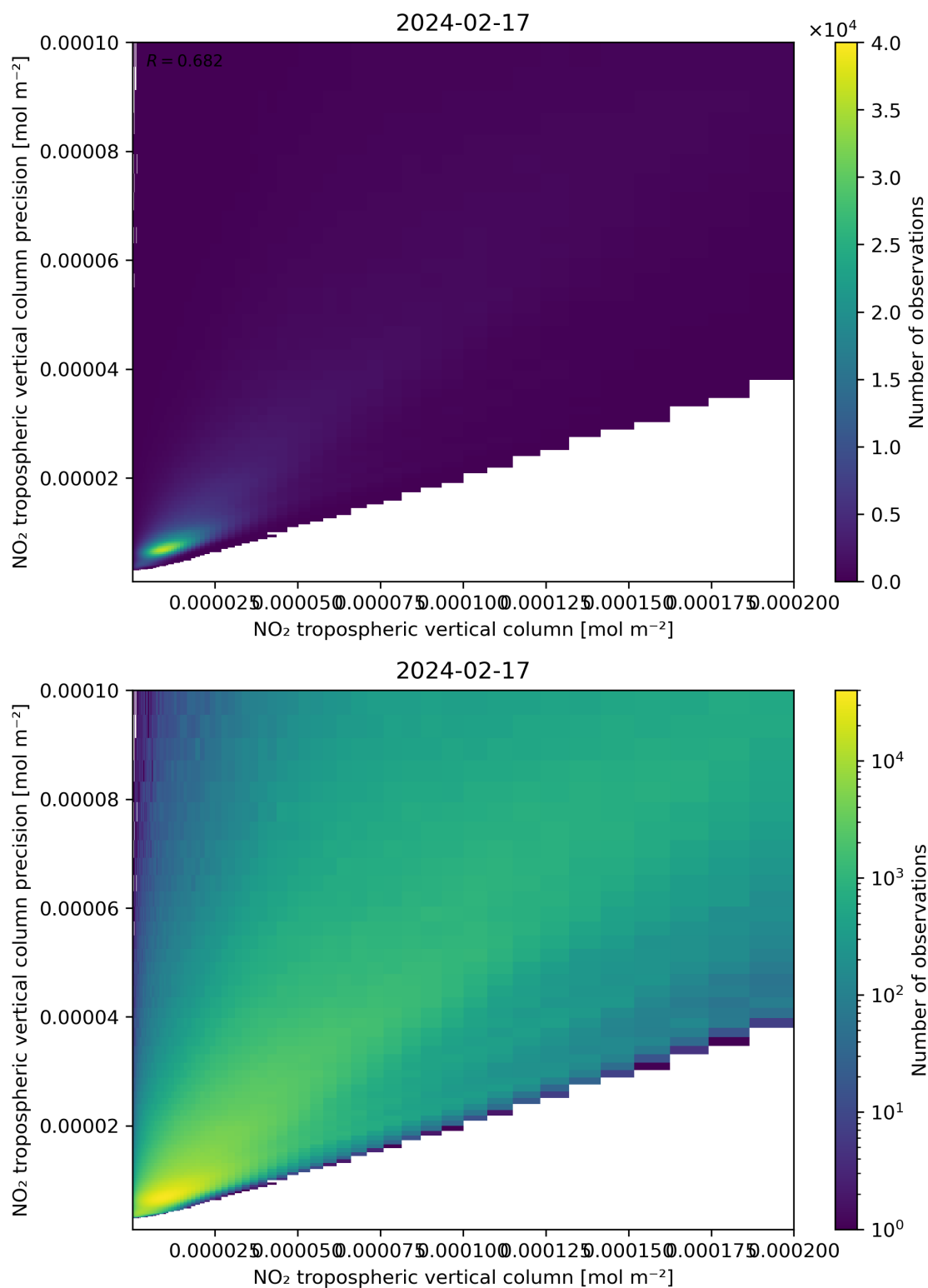
Figure 130: Scatter density plot of “NO 2 tropospheric vertical column” against “NO 2 tropospheric vertical column precision” for 2024-02-17 to 2024-02-18.
