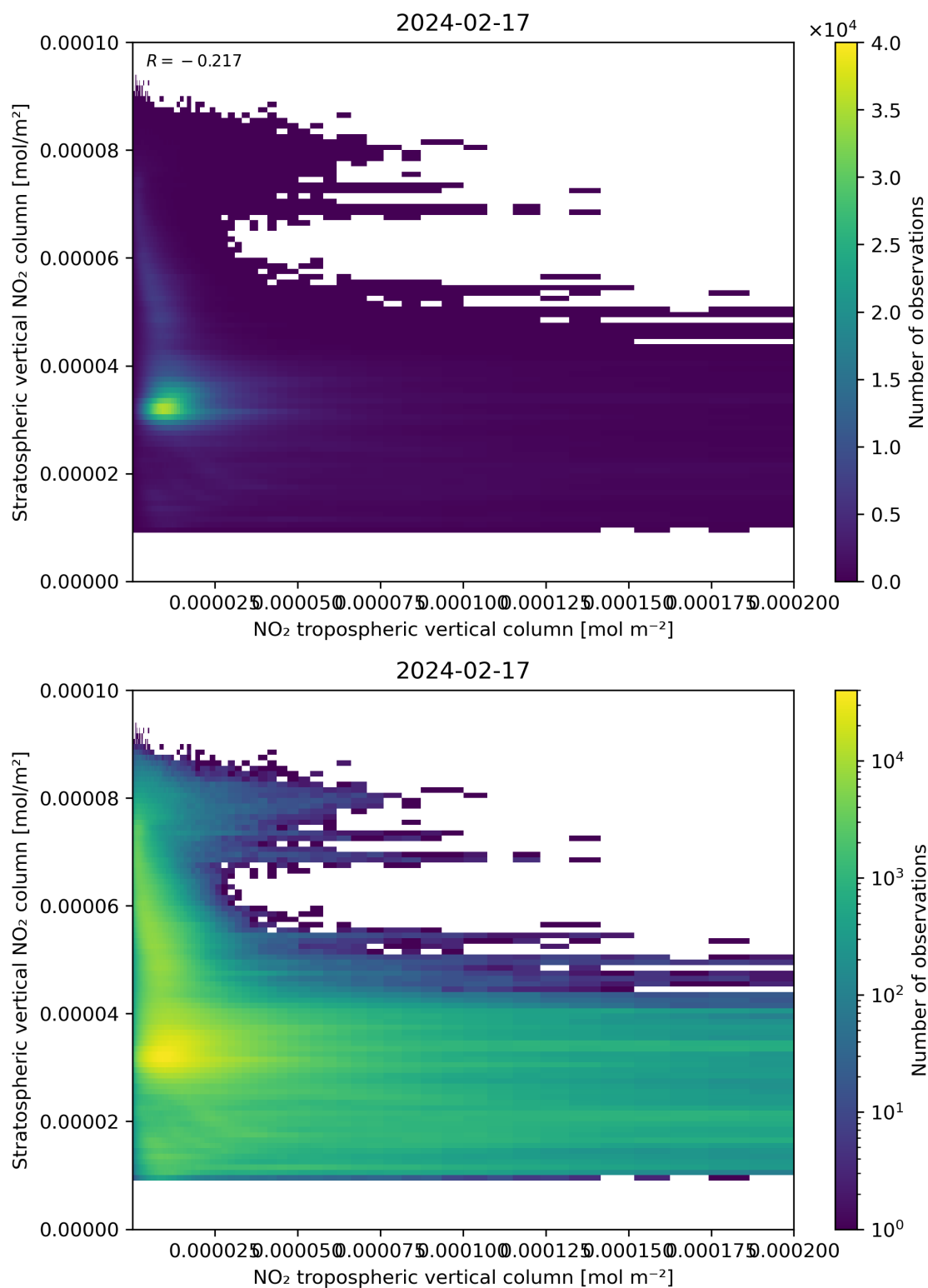
Figure 125: Scatter density plot of “NO 2 tropospheric vertical column” against “Stratospheric vertical NO 2 column” for 2024-02-17 to 2024-02-18.
