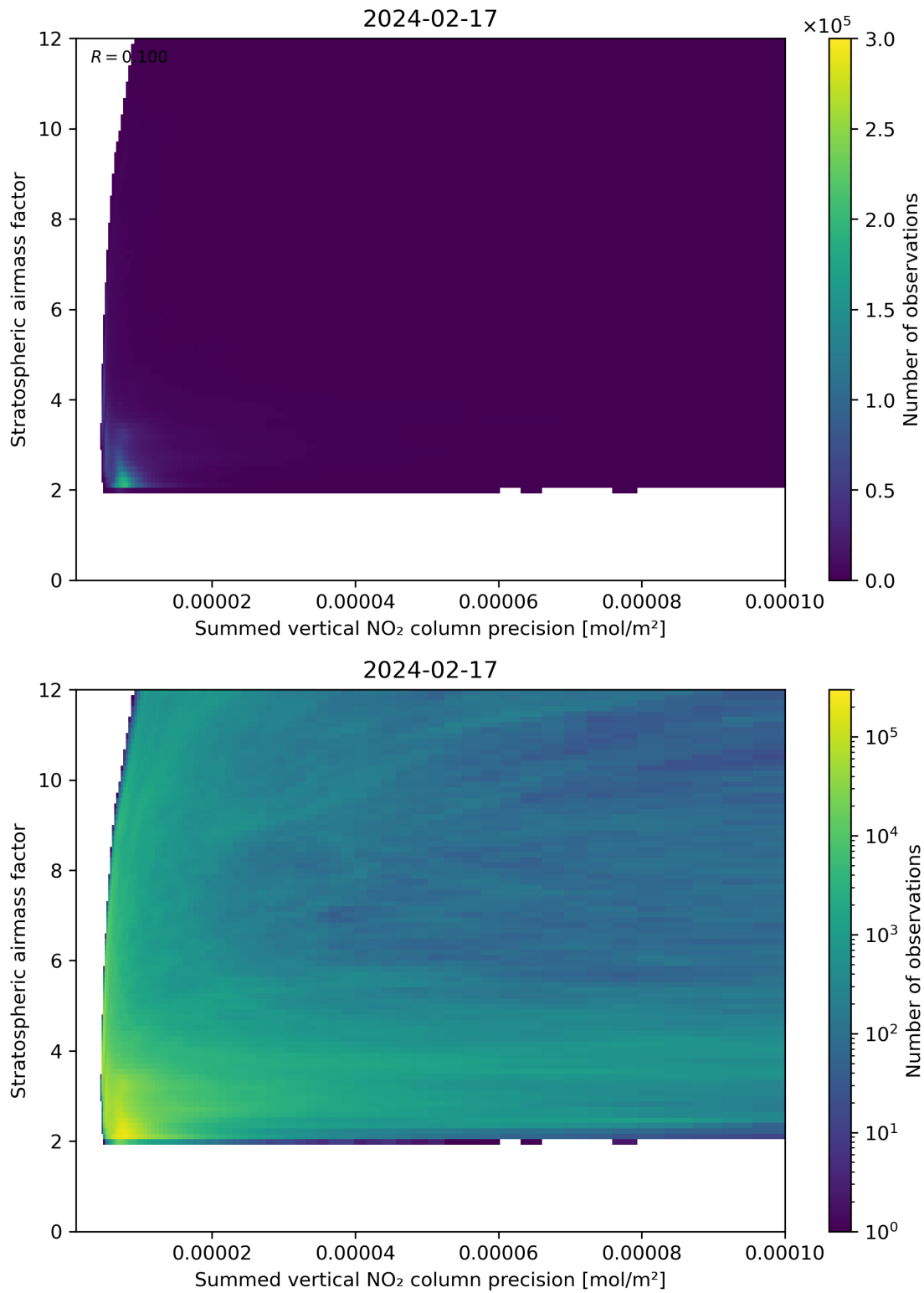
Figure 106: Scatter density plot of “Summed vertical NO 2 column precision” against “Stratospheric airmass factor” for 2024-02-17 to 2024-02-18.
