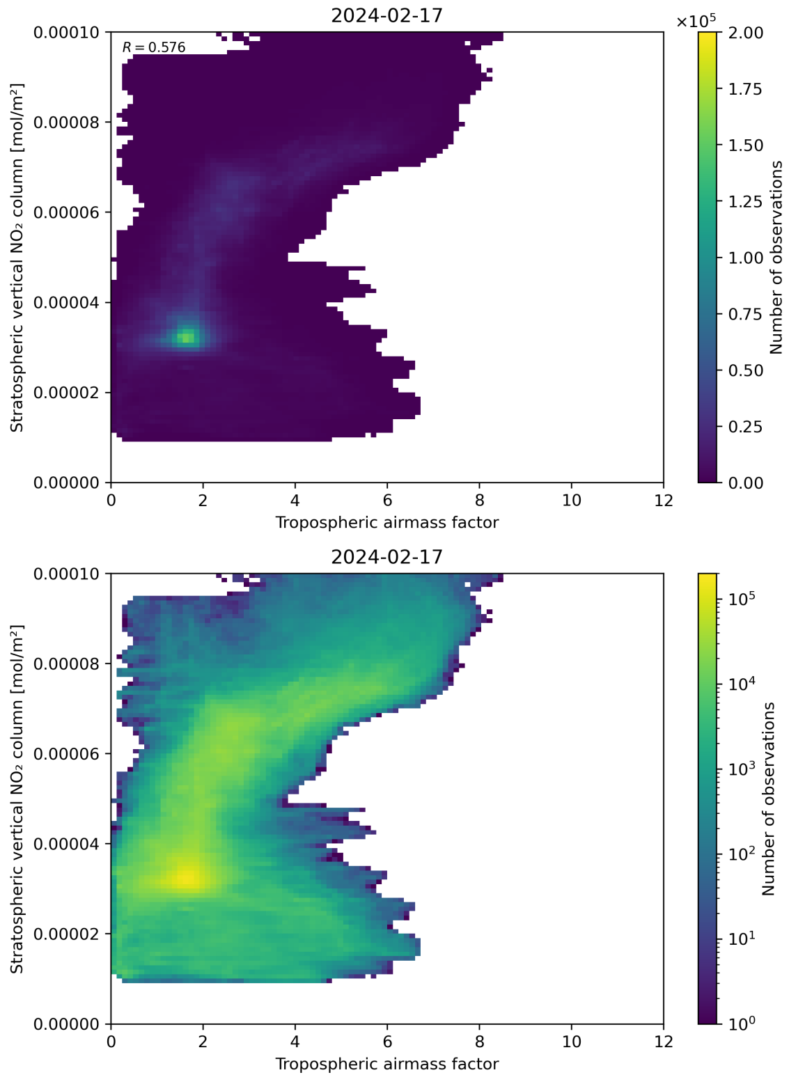
Figure 74: Scatter density plot of “Tropospheric air mass factor” against “Stratospheric vertical NO 2 column” for 2024-02-17 to 2024-02-18.
