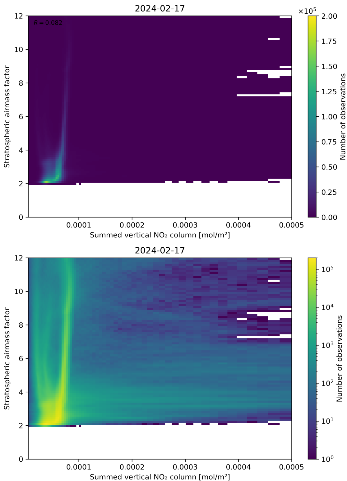
Figure 103: Scatter density plot of “Summed vertical NO 2 column” against “Stratospheric air mass factor” for 2024-02-17 to 2024-02-18.
