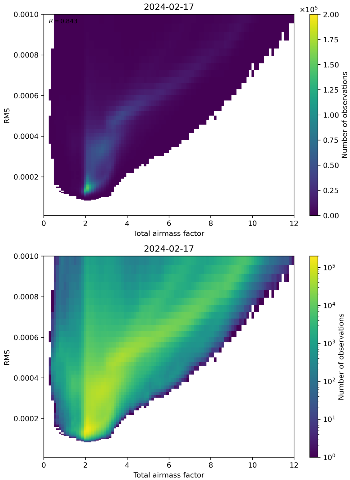
Figure 69: Scatter density plot of “Total airmass factor” against “RMS” for 2024-02-17 to 2024-02-18.
