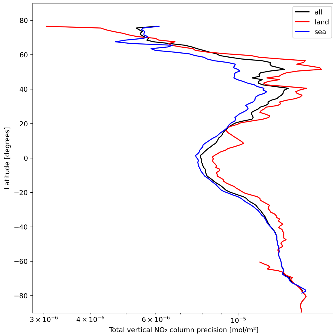
Figure 22: Zonal average of “Total vertical NO 2 column precision” for 2024-02-17 to 2024-02-18.
