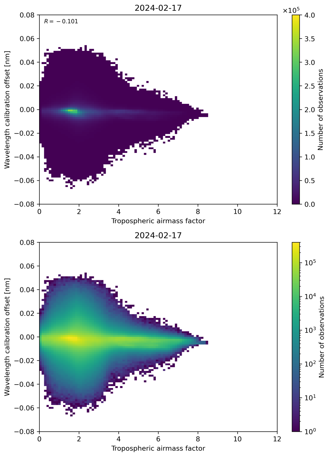
Figure 80: Scatter density plot of “Tropospheric airmass factor” against “Wavelength calibration offset” for 2024-02-17 to 2024-02-18.
