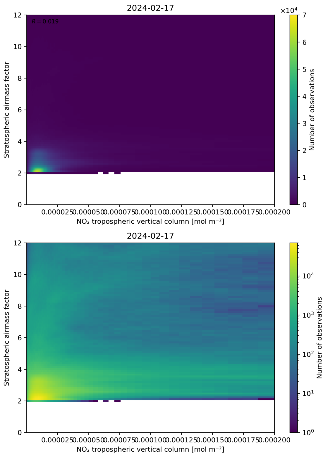
Figure 121: Scatter density plot of “NO 2 tropospheric vertical column” against “Stratospheric airmass factor” for 2024-02-17 to 2024-02-18.
