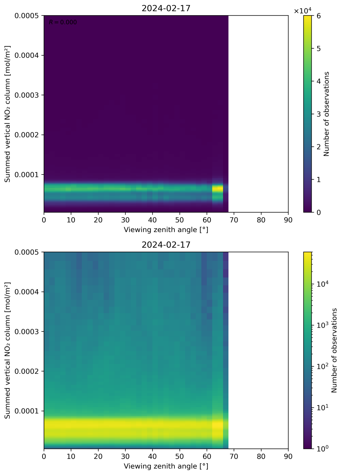
Figure 165: Scatter density plot of “Viewing zenith angle” against “Summed vertical NO 2 column” for 2024-02-17 to 2024-02-18.
