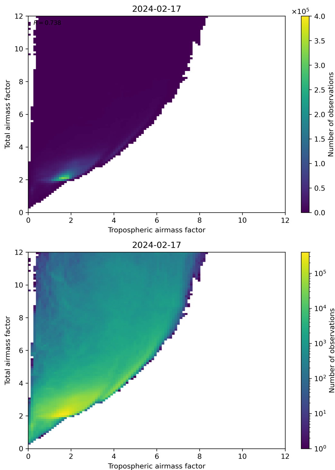
Figure 72: Scatter density plot of “Tropospheric airmass factor” against “Total airmass factor” for 2024-02-17 to 2024-02-18.
