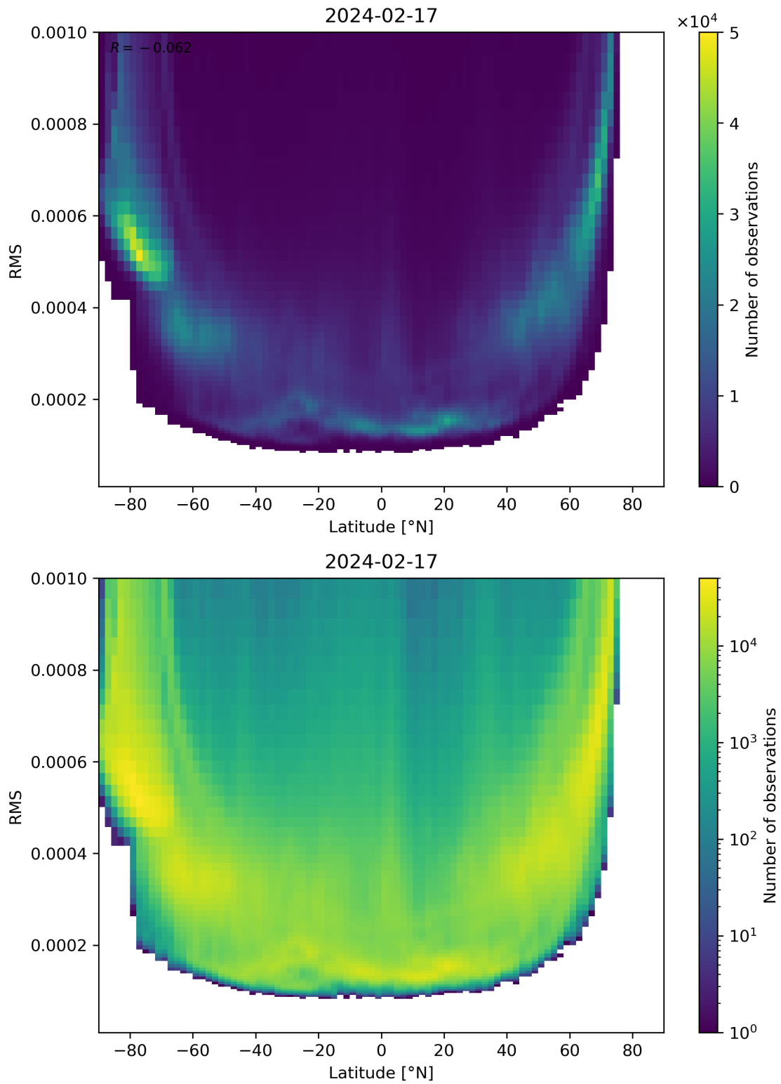
Figure 94: Scatter density plot of “Latitude” against “RMS” for 2024-02-17 to 2024-02-18.
