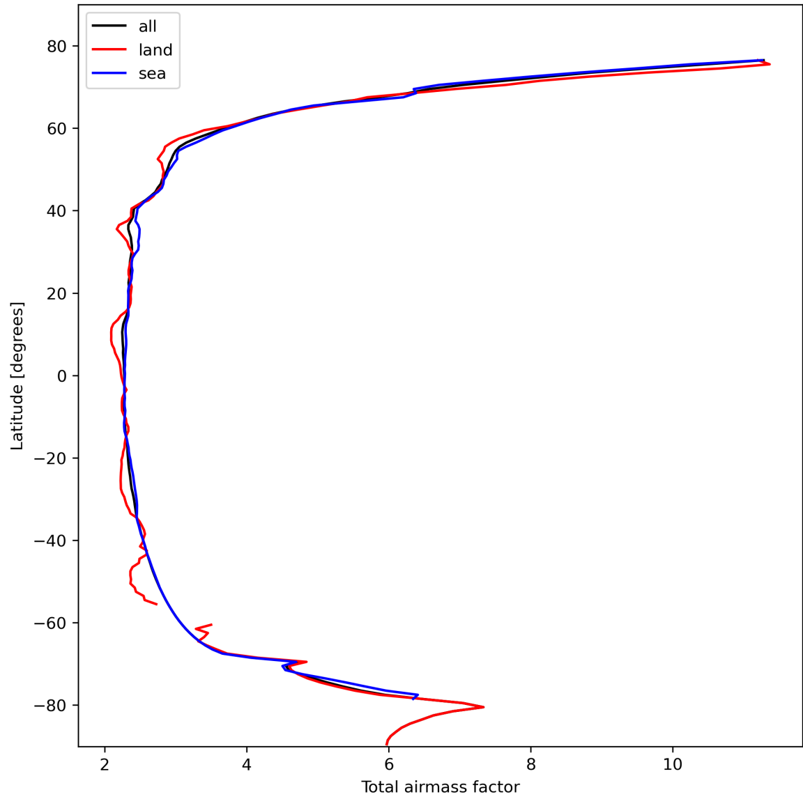
Figure 15: Zonal average of “Total airmass factor” for 2024-02-17 to 2024-02-18.
