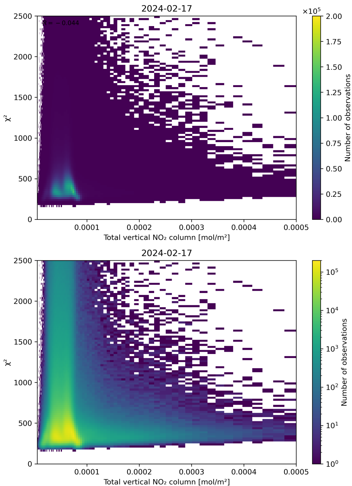
Figure 111: Scatter density plot of “Total vertical NO 2 column” against “ \chi^2 ” for 2024-02-17 to 2024-02-18.
