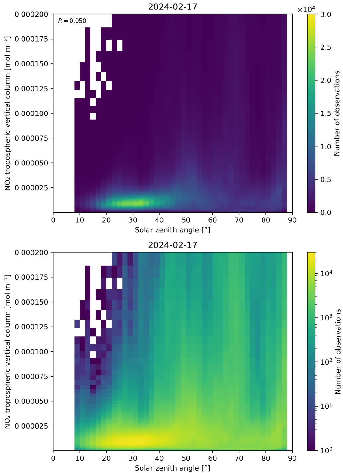
Figure 155: Scatter density plot of “Solar zenith angle” against “NO 2 tropospheric vertical column” for 2024-02-17 to 2024-02-18.
