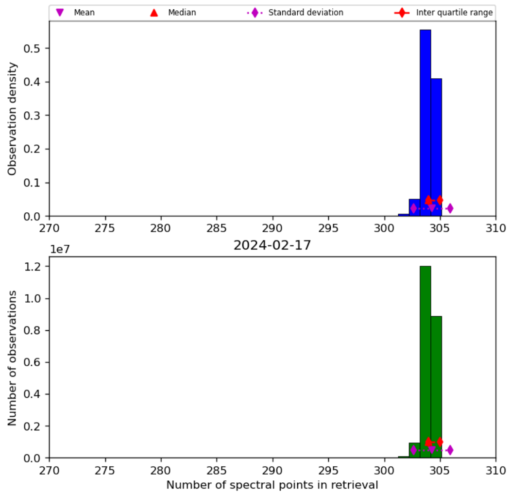
Figure 33: Histogram of “Number of spectral points in retrieval” for 2024-02-17 to 2024-02-18
