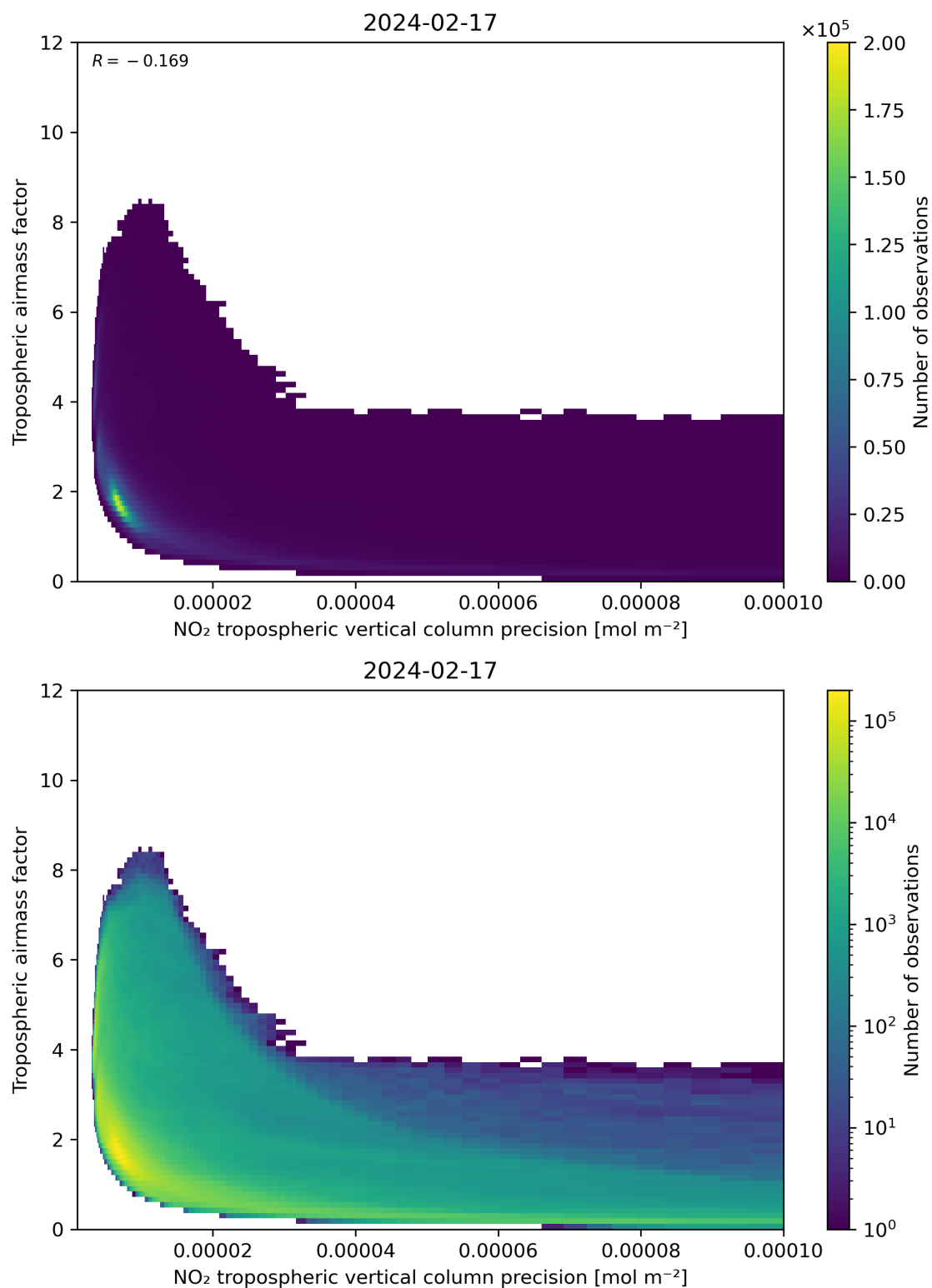
Figure 133: Scatter density plot of “NO 2 tropospheric vertical column precision” against “Tropospheric airmass factor” for 2024-02-17 to 2024-02-18.
