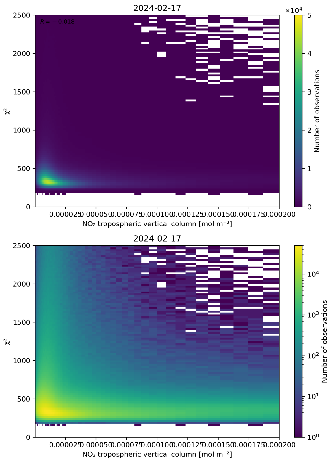
Figure 124: Scatter density plot of “NO 2 tropospheric vertical column” against “ \chi^2 ” for 2024-02-17 to 2024-02-18.
