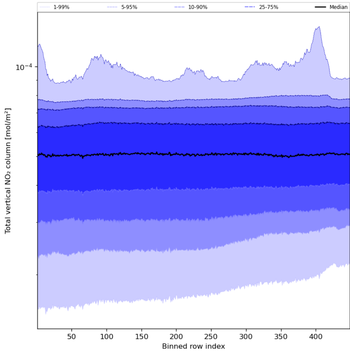
Figure 55: Along track statistics of “Total vertical NO 2 column” for 2024-02-17 to 2024-02-18
