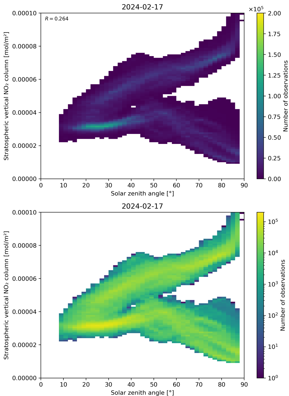
Figure 150: Scatter density plot of “Solar zenith angle” against “Stratospheric vertical NO 2 column” for 2024-02-17 to 2024-02-18.
