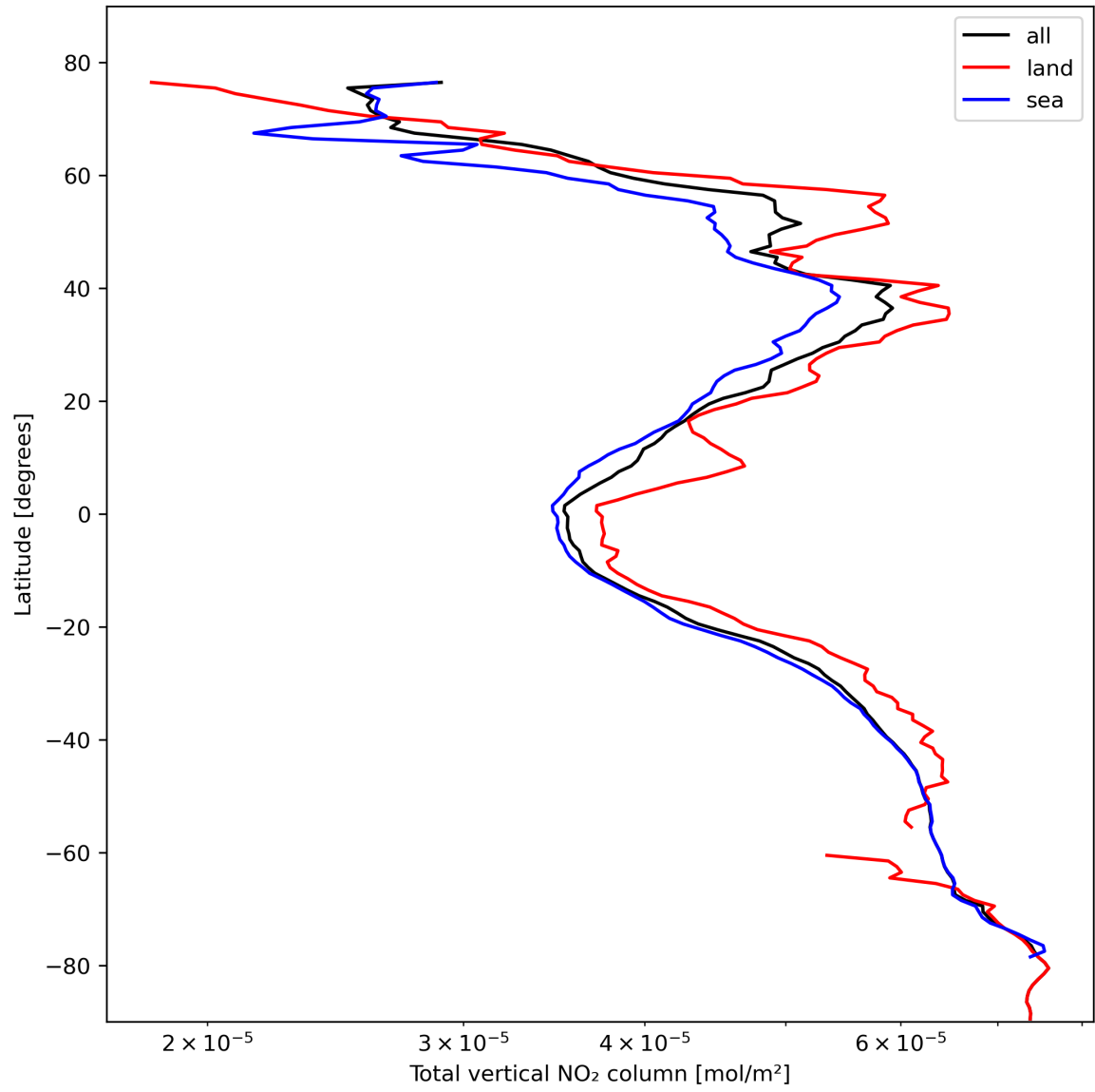
Figure 21: Zonal average of “Total vertical NO 2 column” for 2024-02-17 to 2024-02-18.
