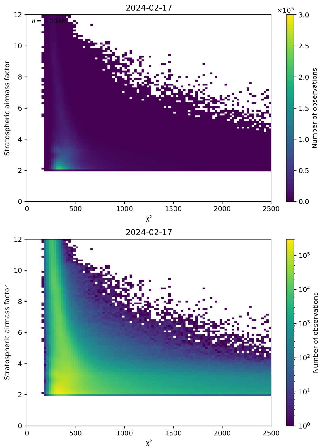
Figure 81: Scatter density plot of “ \chi^2 ” against “Stratospheric airmass factor” for 2024-02-17 to 2024-02-18.
