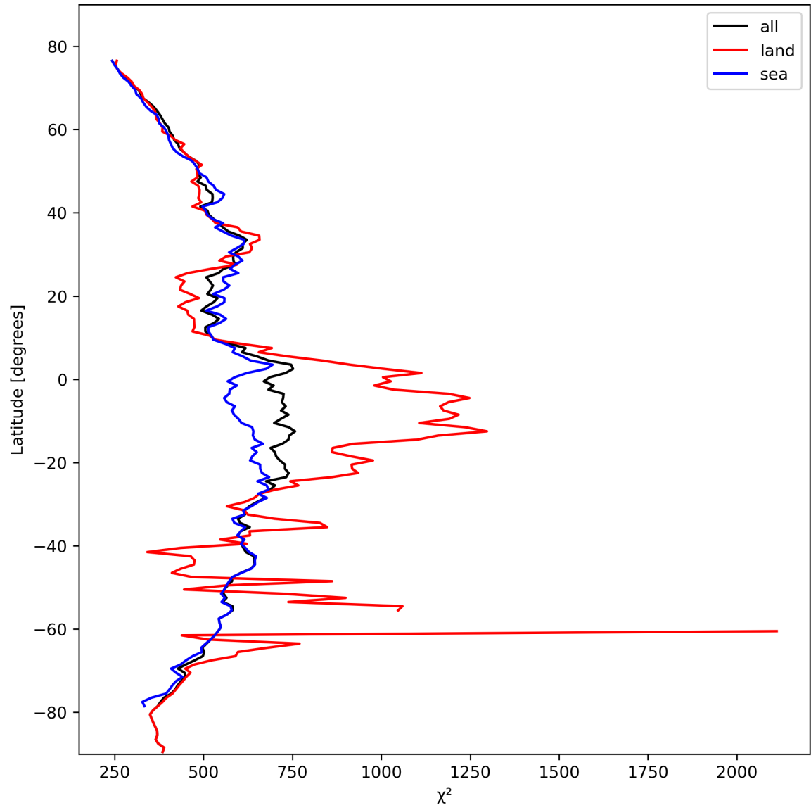
Figure 25: Zonal average of “ \chi^2 ” for 2024-02-17 to 2024-02-18.
