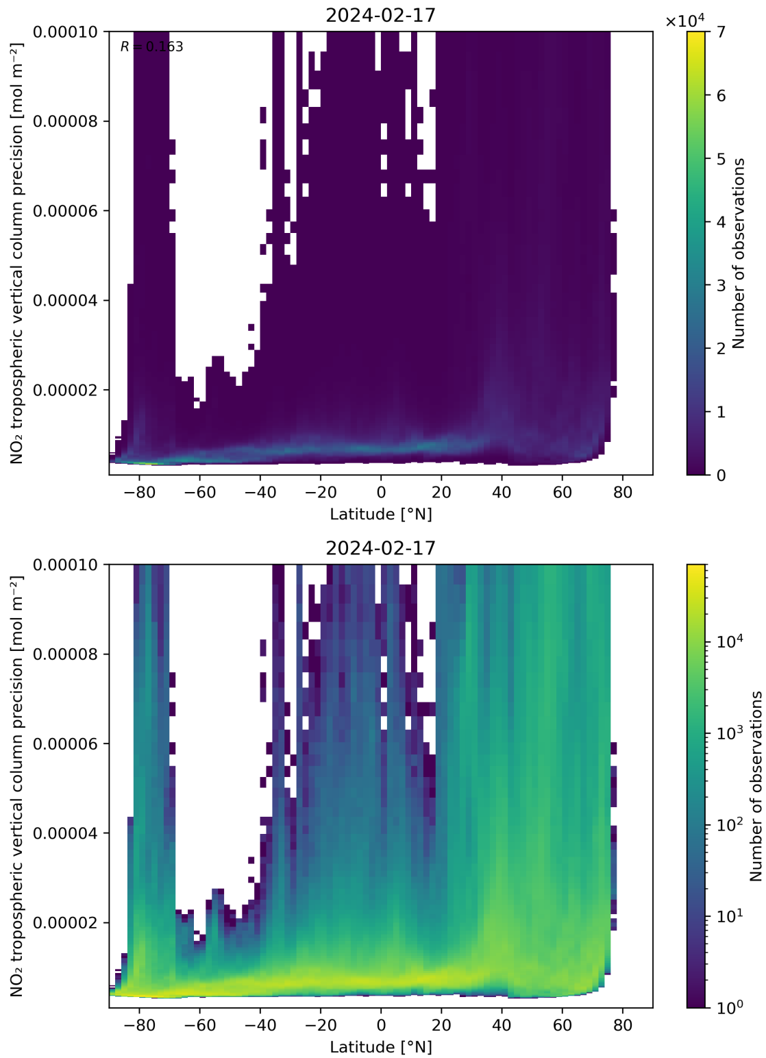
Figure 93: Scatter density plot of “Latitude” against “NO 2 tropospheric vertical column precision” for 2024-02-17 to 2024-02-18.
