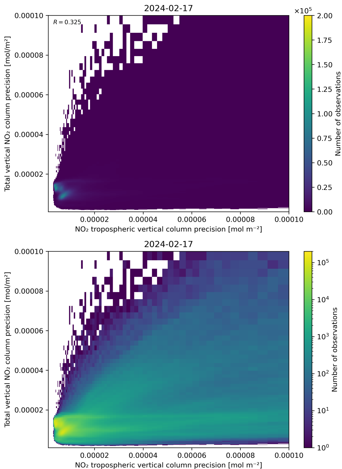
Figure 139: Scatter density plot of “NO 2 tropospheric vertical column precision” against “Total vertical NO 2 column precision” for 2024-02-17 to 2024-02-18.
