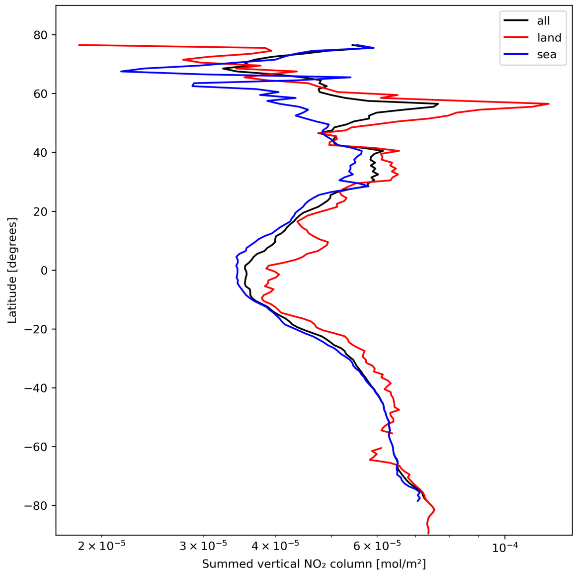
Figure 23: Zonal average of “Summed vertical NO 2 column” for 2024-02-17 to 2024-02-18.
