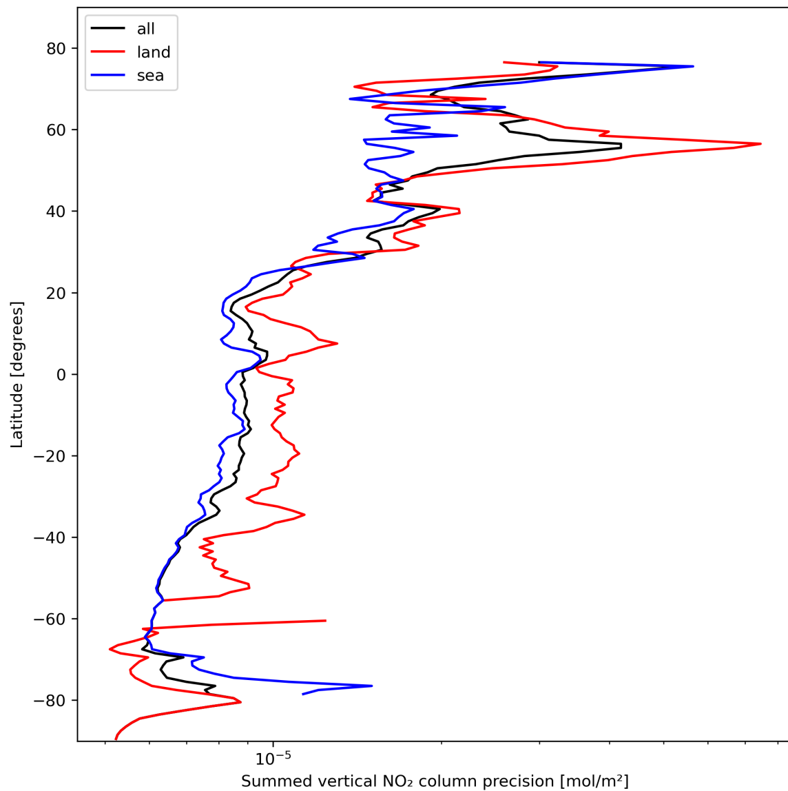
Figure 24: Zonal average of “Summed vertical NO 2 column precision” for 2024-02-17 to 2024-02-18.
