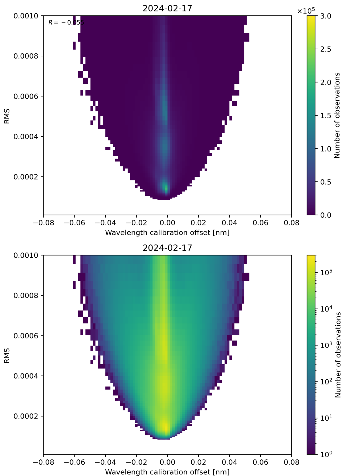
Figure 181: Scatter density plot of “Wavelength calibration offset” against “RMS” for 2024-02-17 to 2024-02-18.
