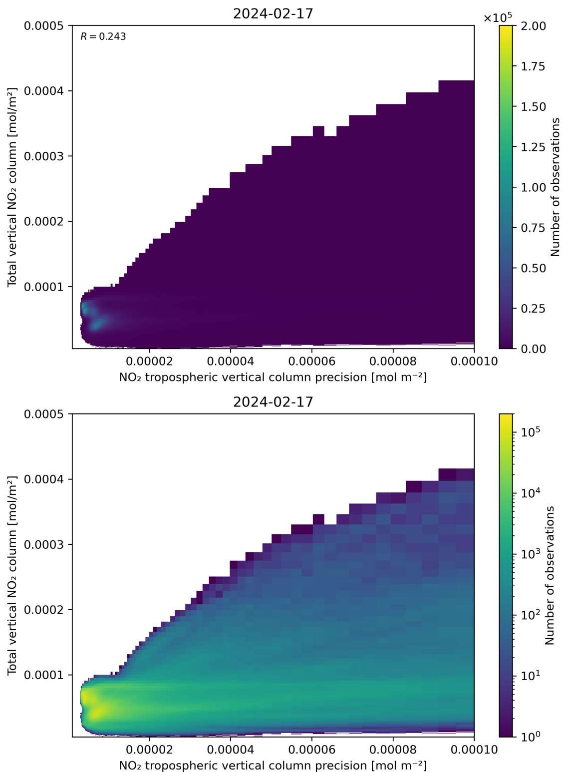
Figure 138: Scatter density plot of “NO 2 tropospheric vertical column precision” against “Total vertical NO 2 column” for 2024-02-17 to 2024-02-18.
