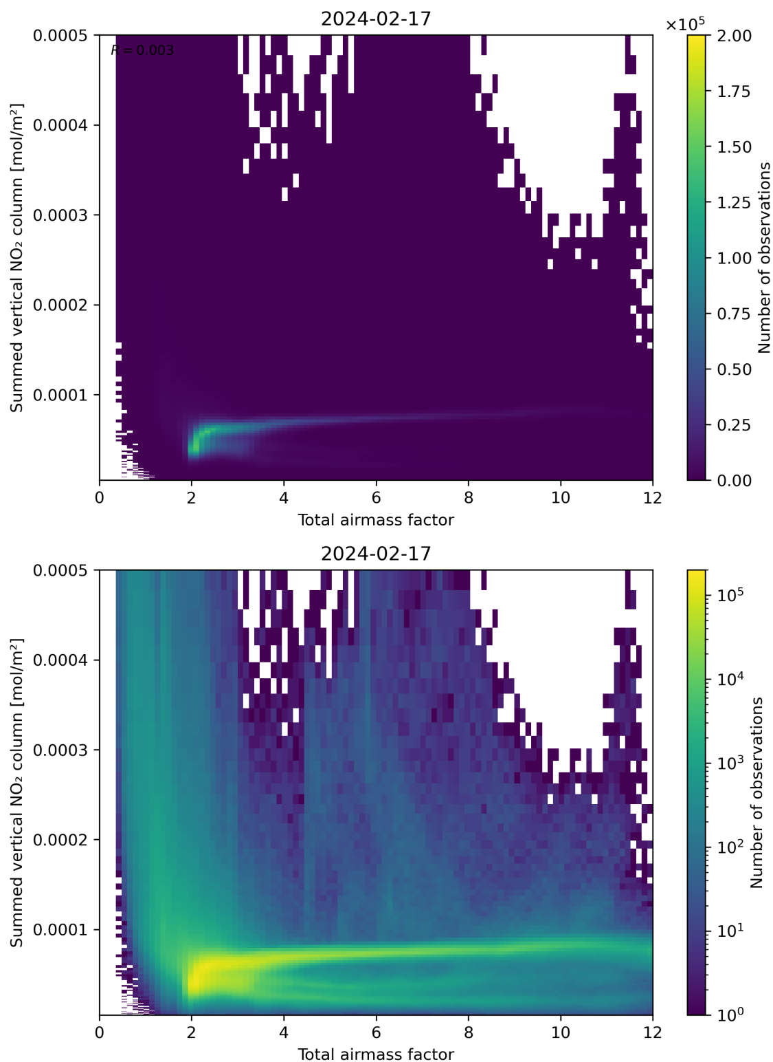
Figure 65: Scatter density plot of “Total airmass factor” against “Summed vertical NO 2 column” for 2024-02-17 to 2024-02-18.
