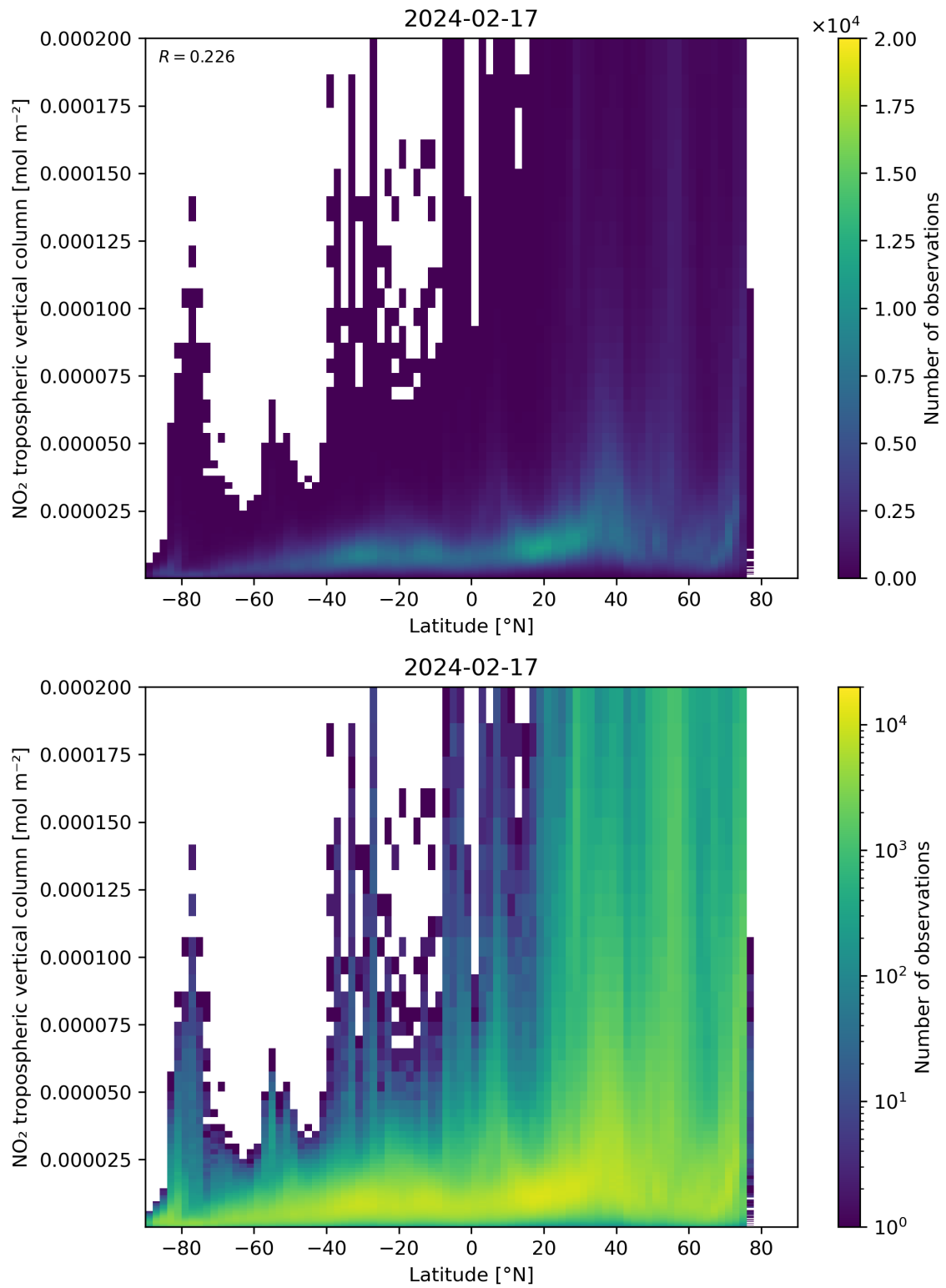
Figure 92: Scatter density plot of “Latitude” against “NO 2 tropospheric vertical column” for 2024-02-17 to 2024-02-18.
