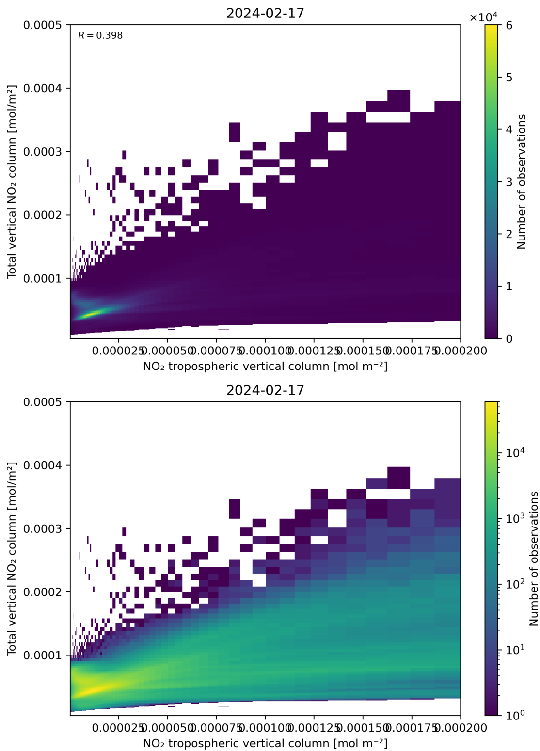
Figure 128: Scatter density plot of “NO 2 tropospheric vertical column” against “Total vertical NO 2 column” for 2024-02-17 to 2024-02-18.
