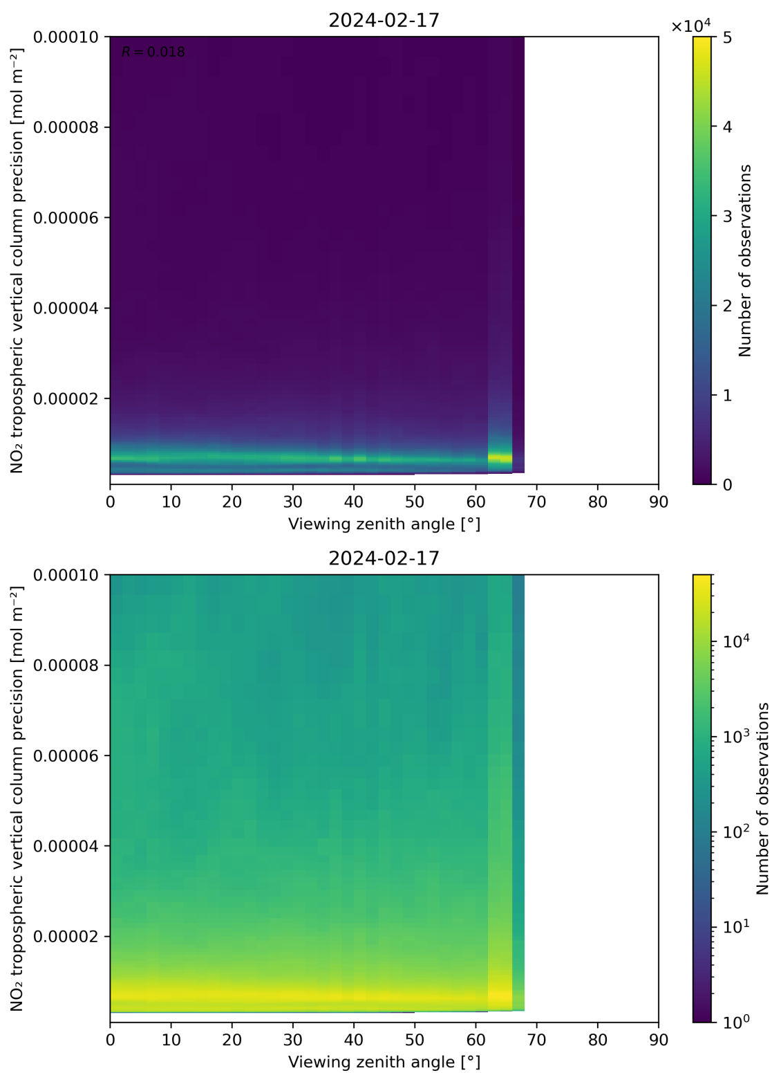
Figure 170: Scatter density plot of “Viewing zenith angle” against “NO 2 tropospheric vertical column precision” for 2024-02-17 to 2024-02-18.
