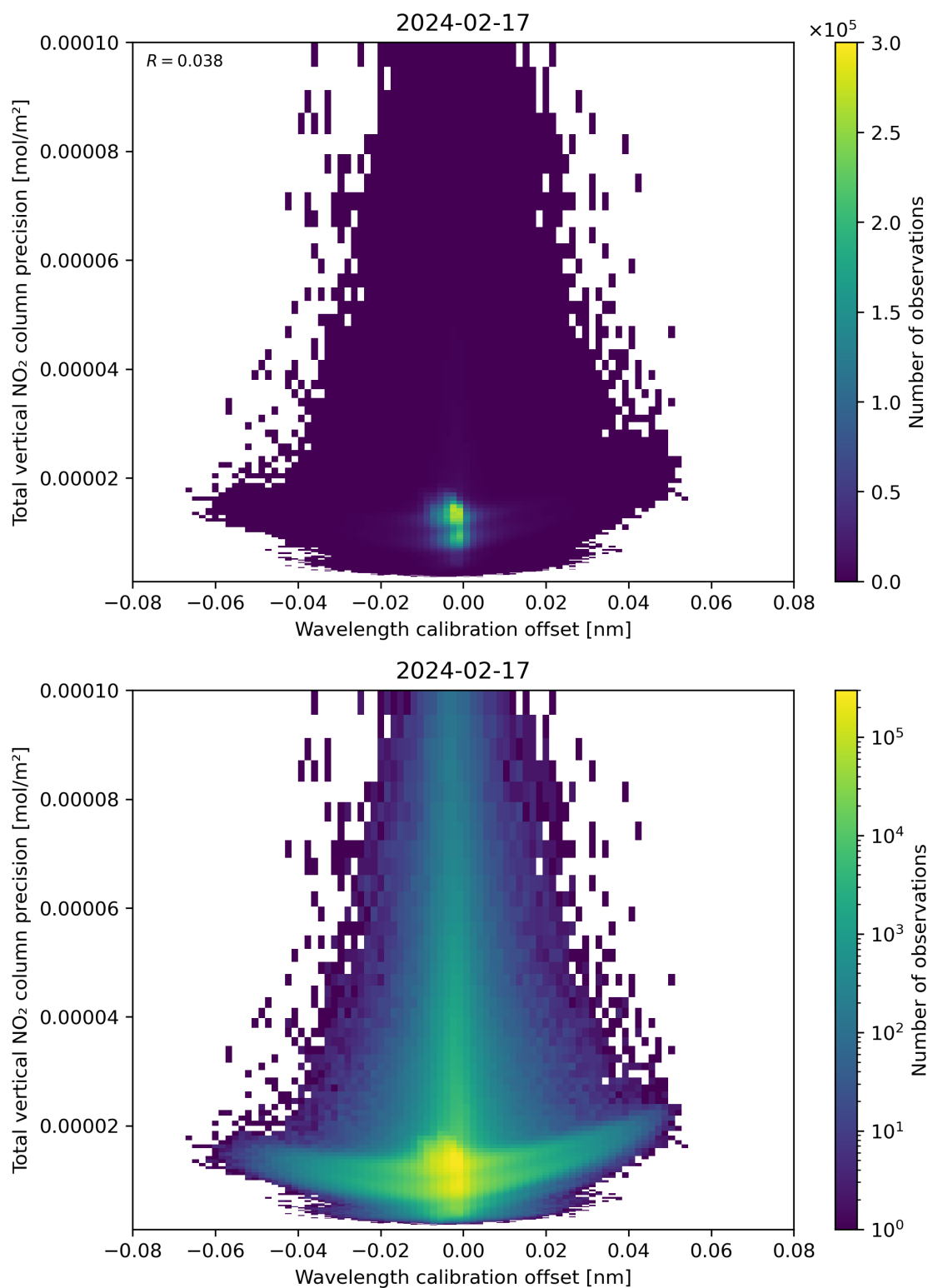
Figure 180: Scatter density plot of “Wavelength calibration offset” against “Total vertical NO 2 column precision” for 2024-02-17 to 2024-02-18.
