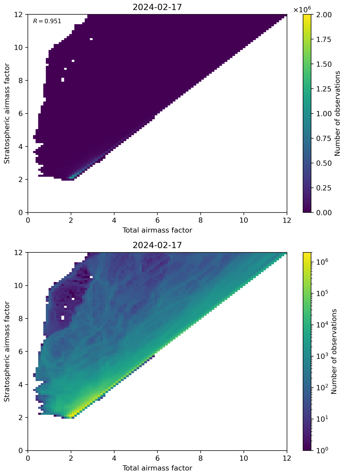
Figure 62: Scatter density plot of “Total airmass factor” against “Stratospheric airmass factor” for 2024-02-17 to 2024-02-18.
