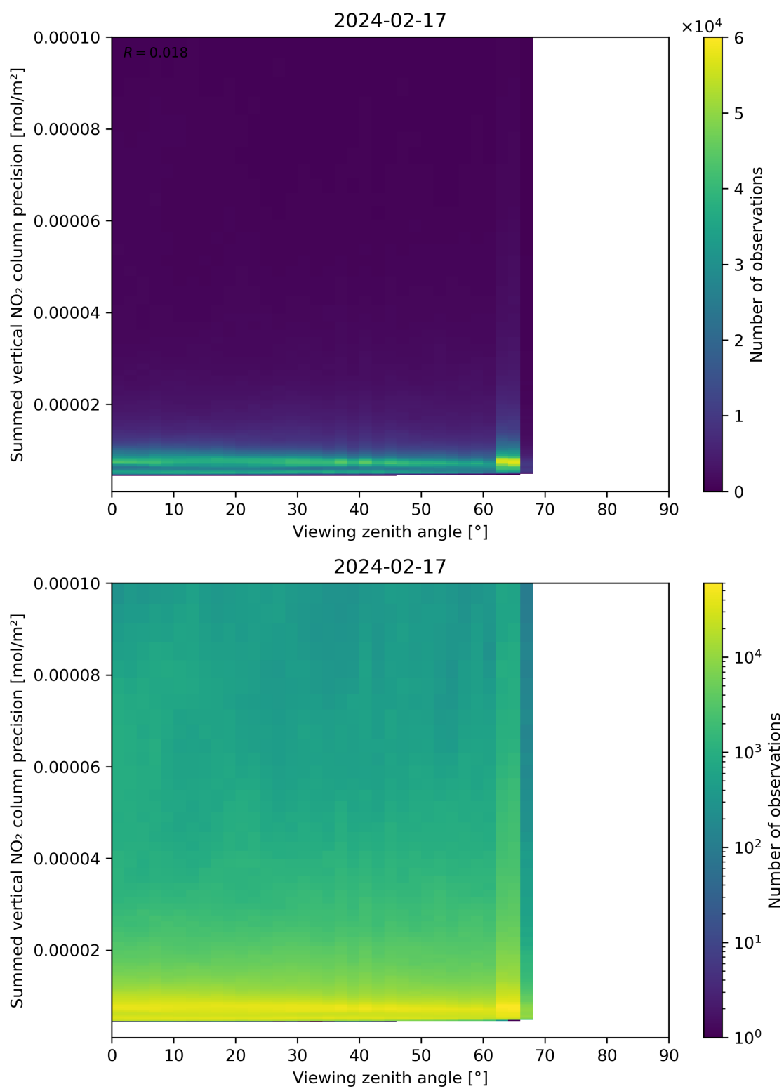
Figure 166: Scatter density plot of “Viewing zenith angle” against “Summed vertical NO 2 column precision” for 2024-02-17 to 2024-02-18.
