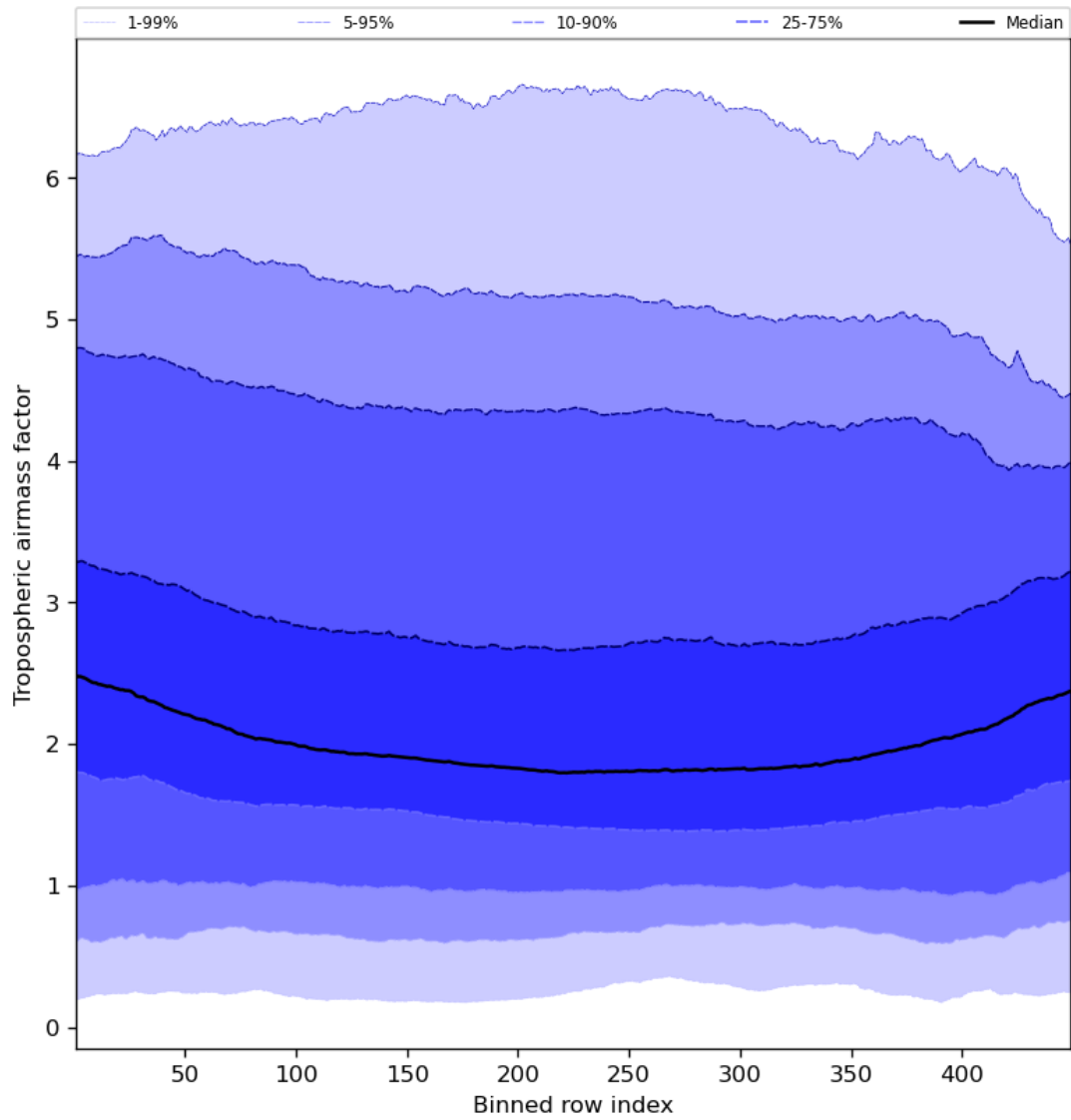
Figure 48: Along track statistics of “Tropospheric airmass factor” for 2024-02-17 to 2024-02-18
