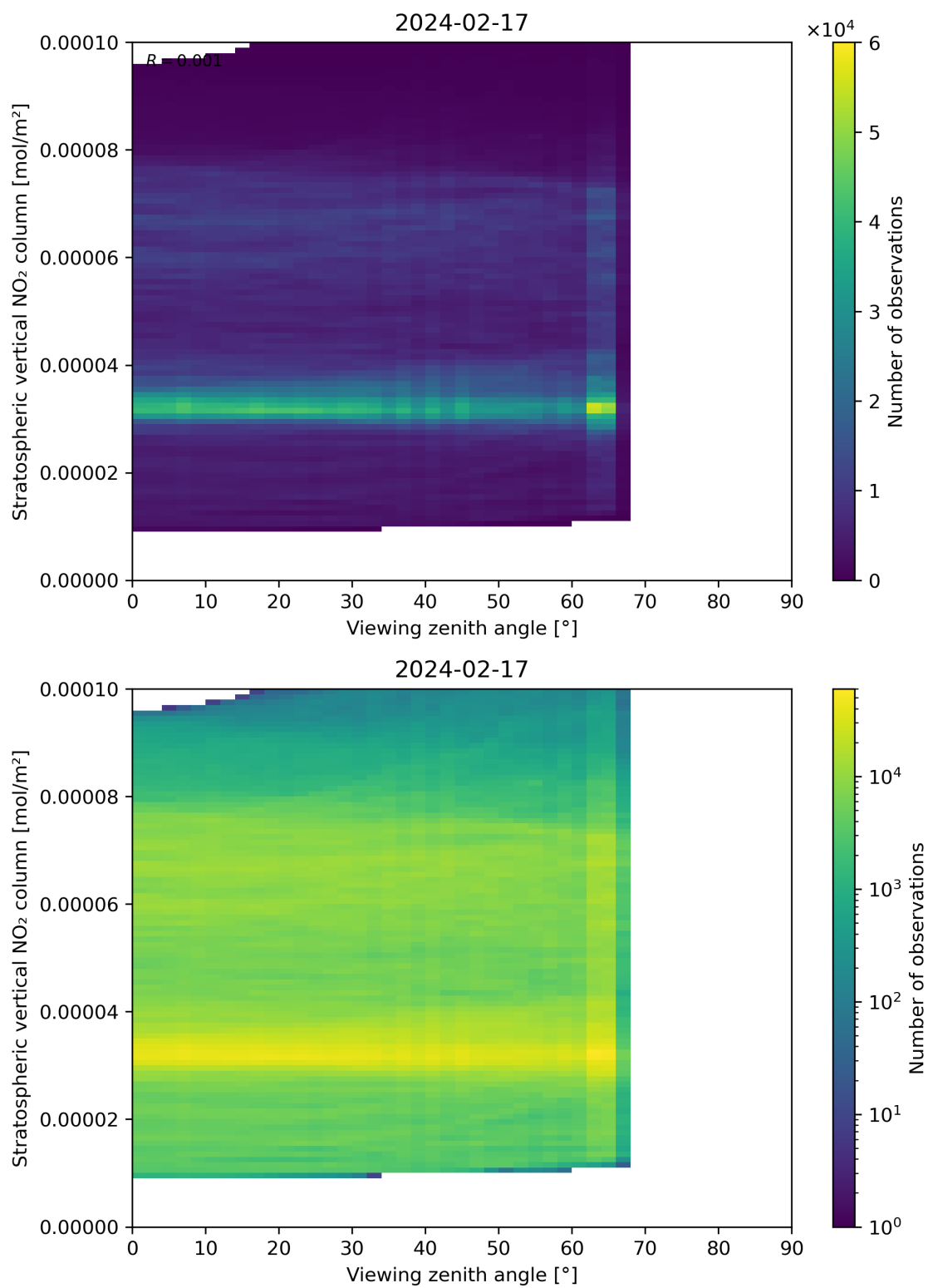
Figure 164: Scatter density plot of “Viewing zenith angle” against “Stratospheric vertical NO 2 column” for 2024-02-17 to 2024-02-18.
