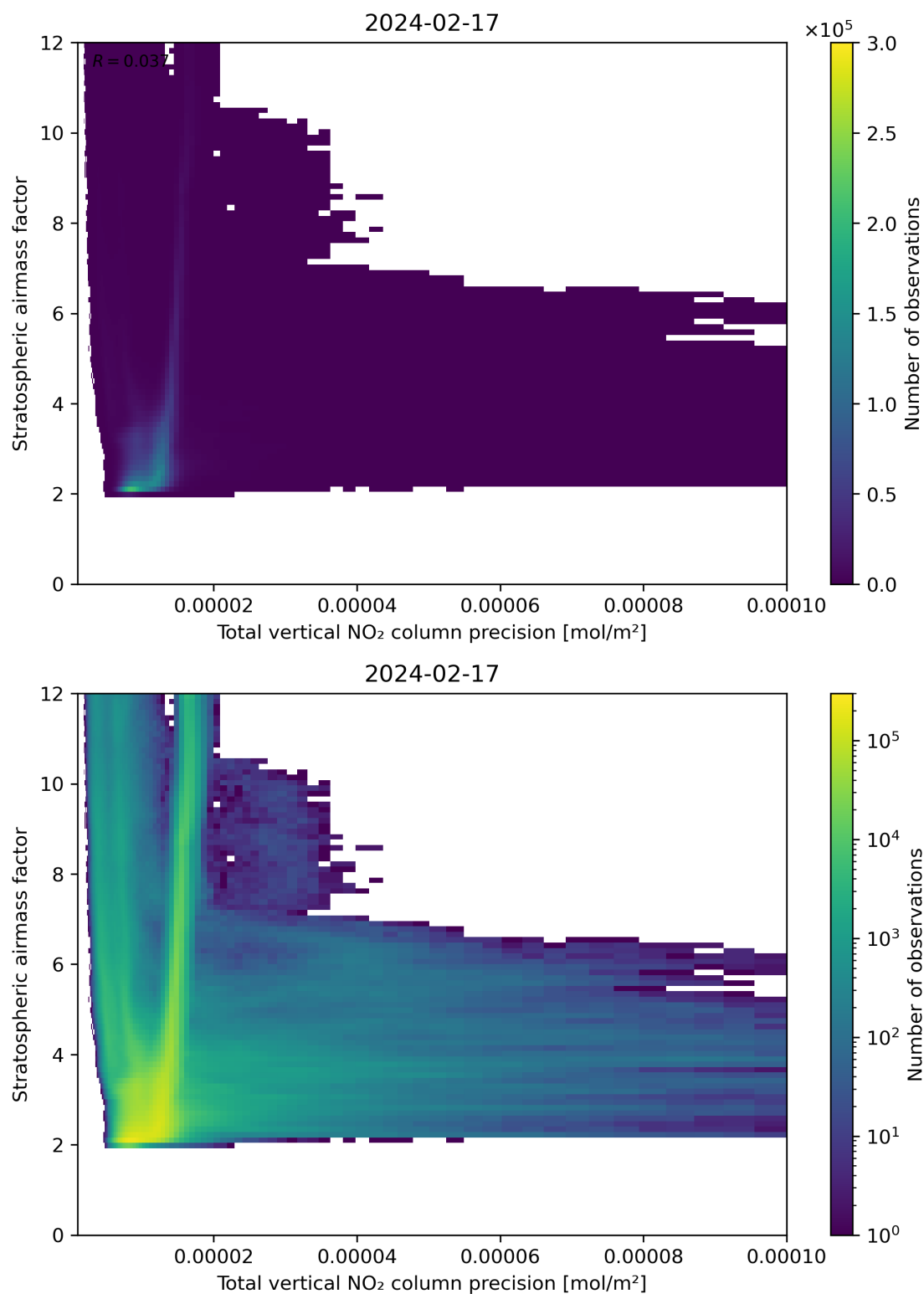
Figure 115: Scatter density plot of “Total vertical NO 2 column precision” against “Stratospheric air mass factor” for 2024-02-17 to 2024-02-18.
