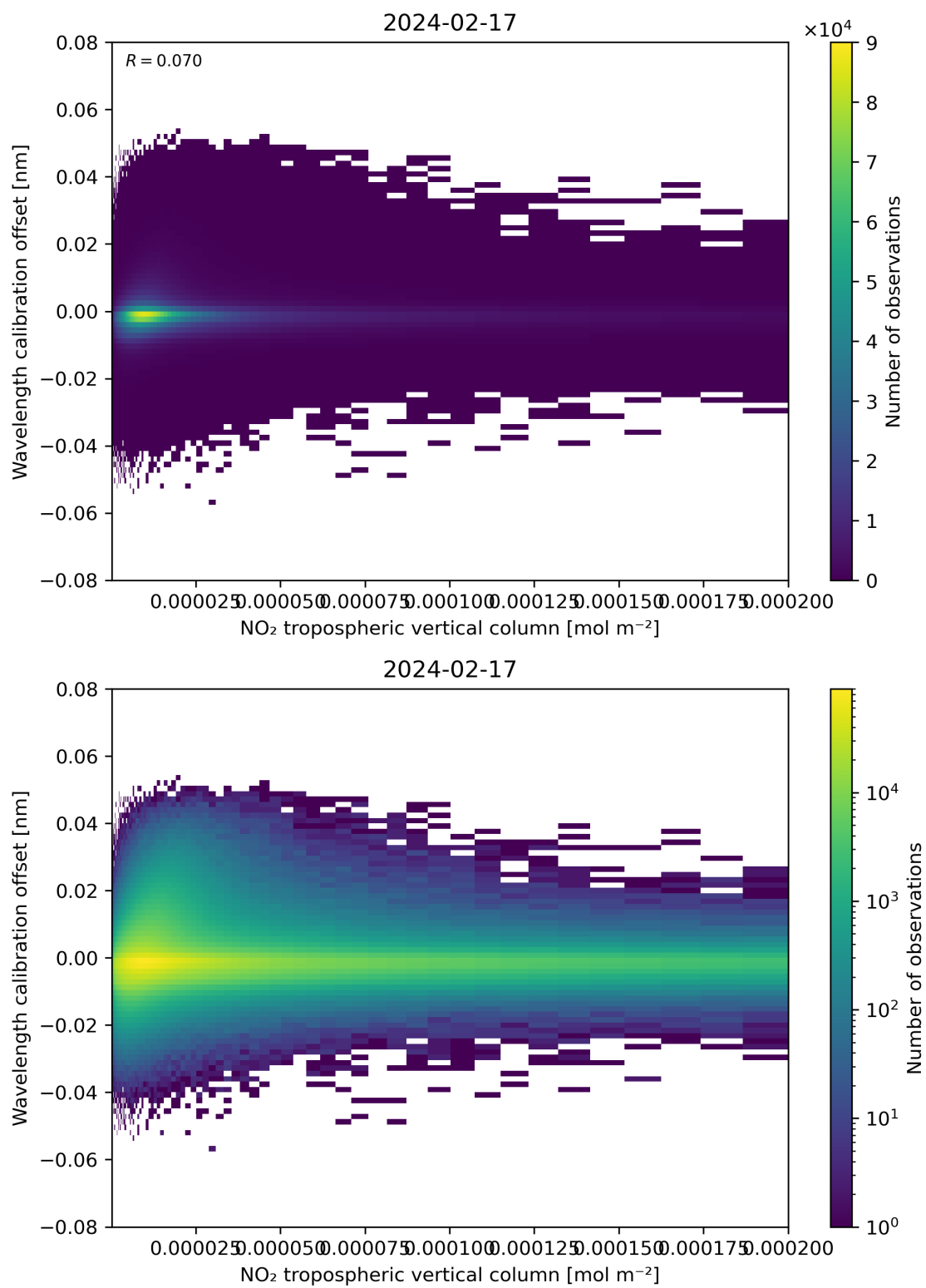
Figure 143: Scatter density plot of “NO 2 tropospheric vertical column” against “Wavelength calibration offset” for 2024-02-17 to 2024-02-18.
