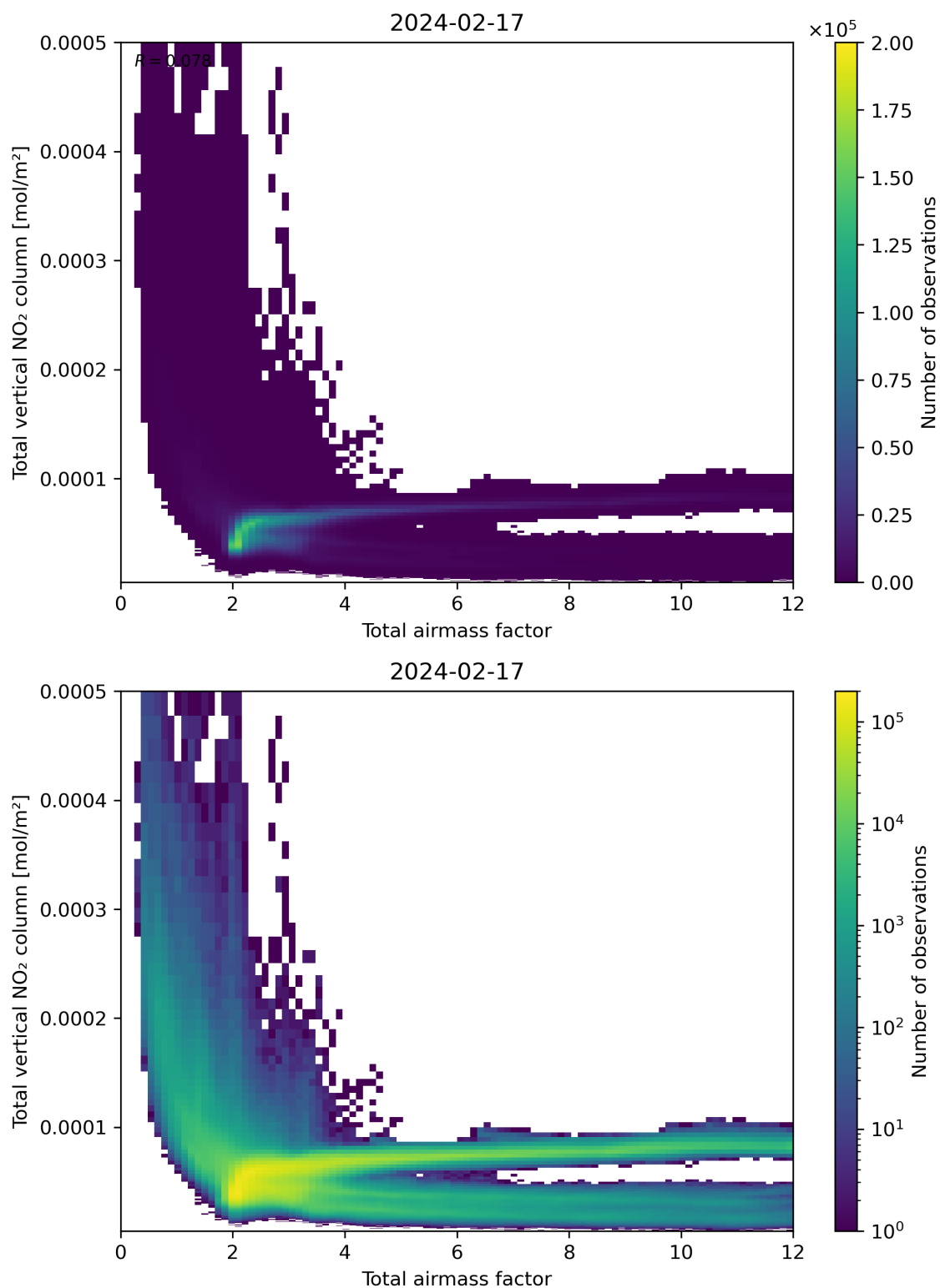
Figure 67: Scatter density plot of “Total airmass factor” against “Total vertical NO 2 column” for 2024-02-17 to 2024-02-18.
