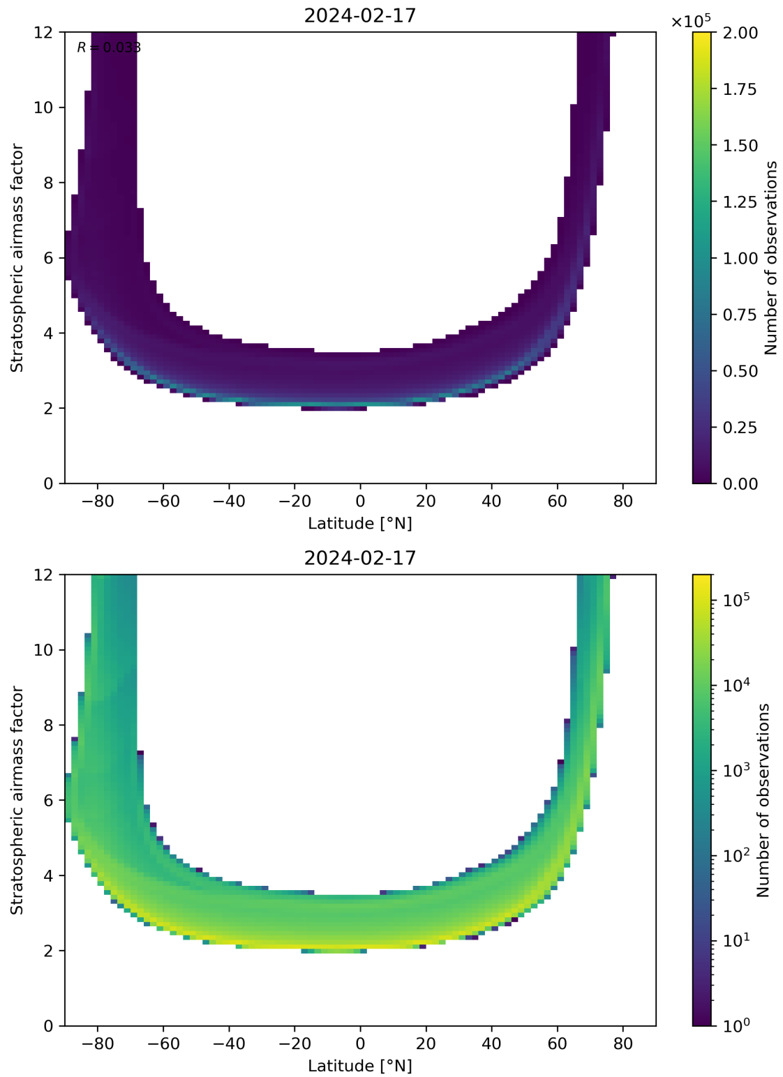
Figure 83: Scatter density plot of “Latitude” against “Stratospheric air mass factor” for 2024-02-17 to 2024-02-18.
