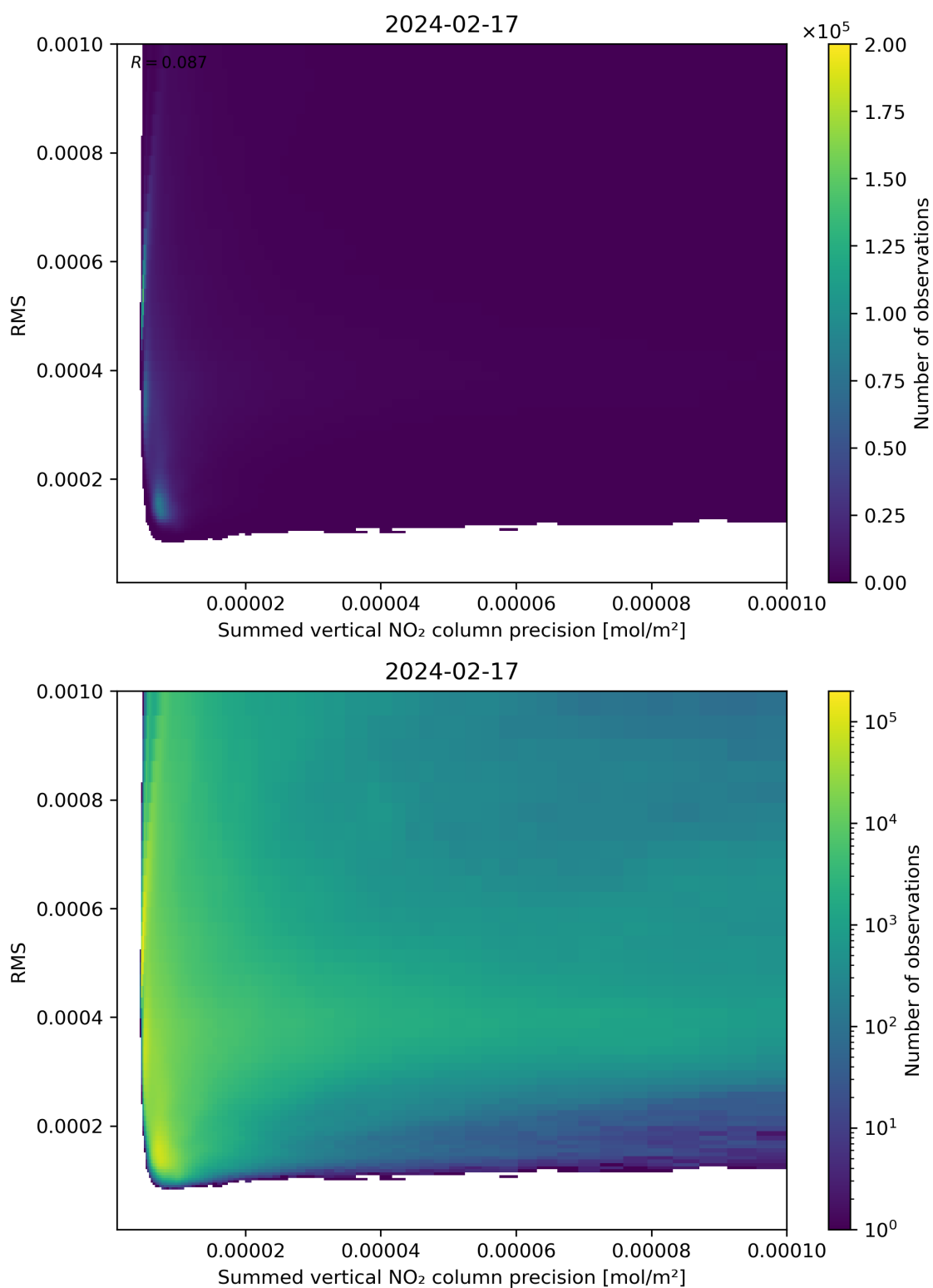
Figure 108: Scatter density plot of “Summed vertical NO 2 column precision” against “RMS” for 2024-02-17 to 2024-02-18.
