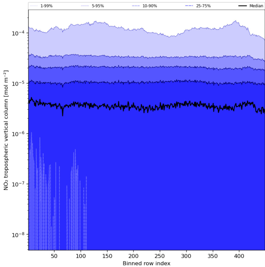
Figure 46: Along track statistics of “NO 2 tropospheric vertical column” for 2024-02-17 to 2024-02-18
