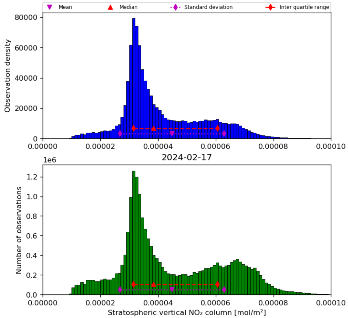
Figure 36: Histogram of “Stratospheric vertical NO 2 column” for 2024-02-17 to 2024-02-18
