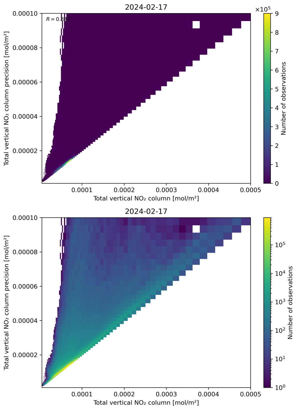
Figure 114: Scatter density plot of “Total vertical NO 2 column” against “Total vertical NO 2 column precision” for 2024-02-17 to 2024-02-18.
