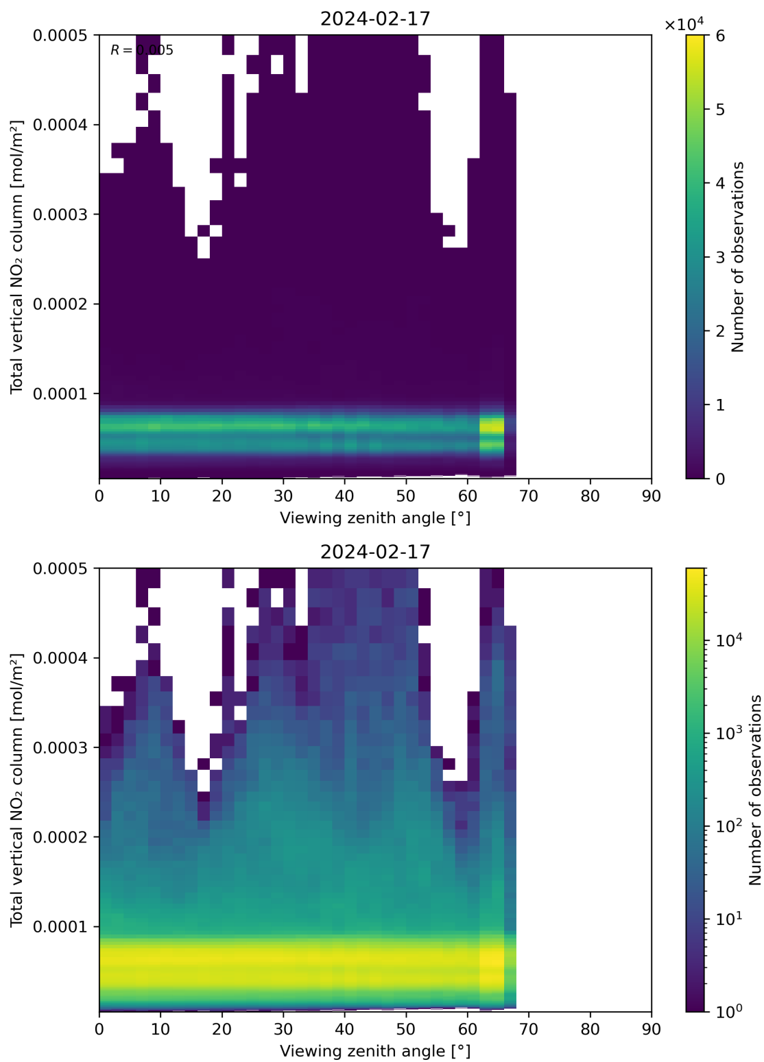
Figure 167: Scatter density plot of “Viewing zenith angle” against “Total vertical NO 2 column” for 2024-02-17 to 2024-02-18.
