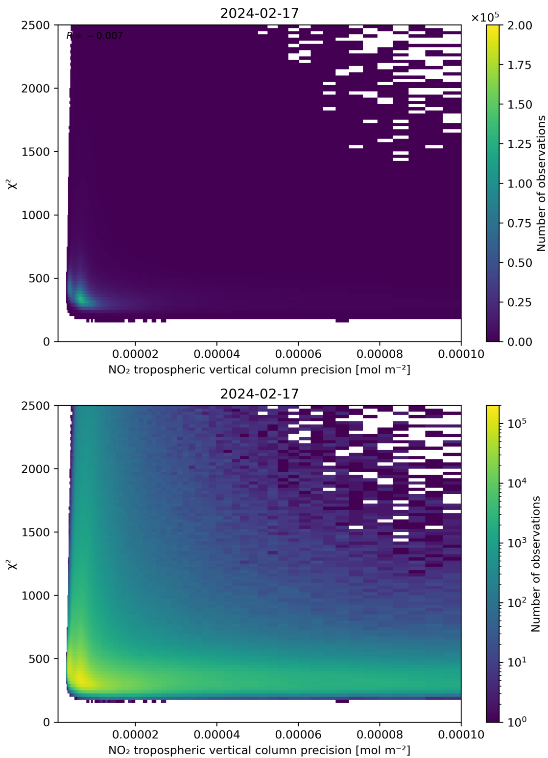
Figure 134: Scatter density plot of “NO 2 tropospheric vertical column precision” against “ \chi^2 ” for 2024-02-17 to 2024-02-18.
