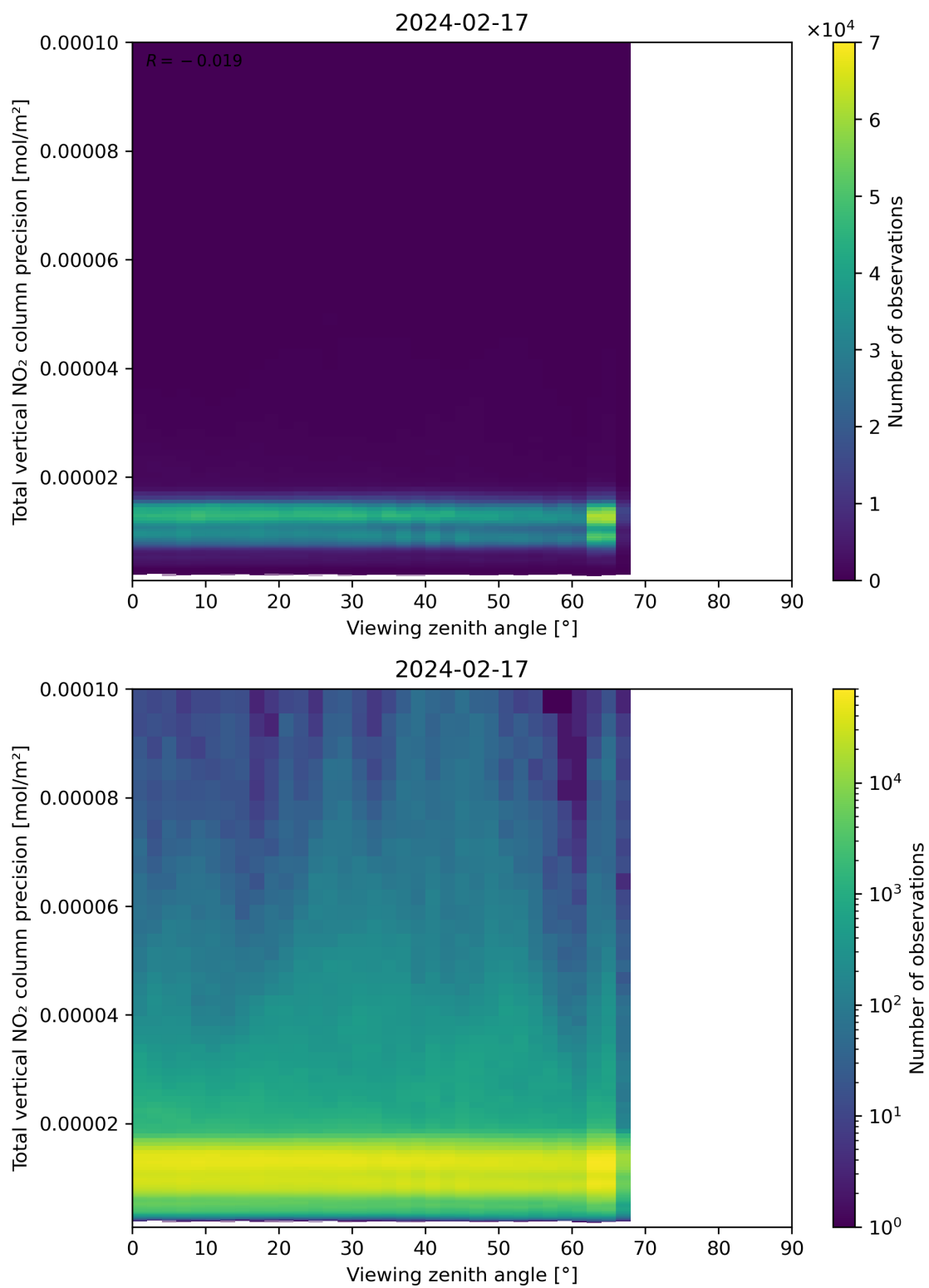
Figure 168: Scatter density plot of “Viewing zenith angle” against “Total vertical NO 2 column precision” for 2024-02-17 to 2024-02-18.
