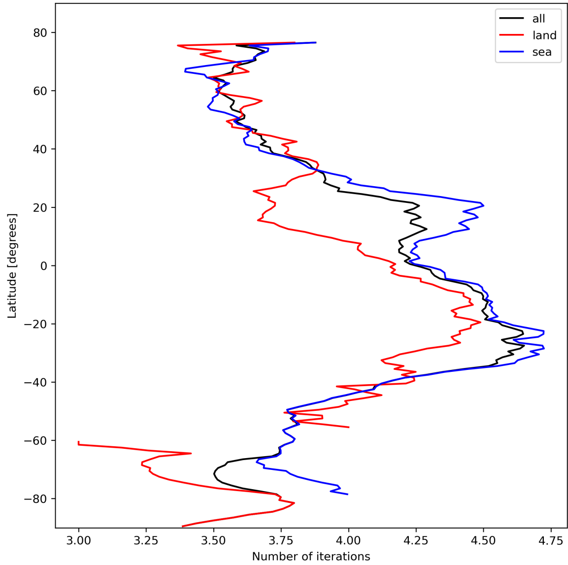
Figure 17: Zonal average of “Number of iterations” for 2024-02-17 to 2024-02-18.
