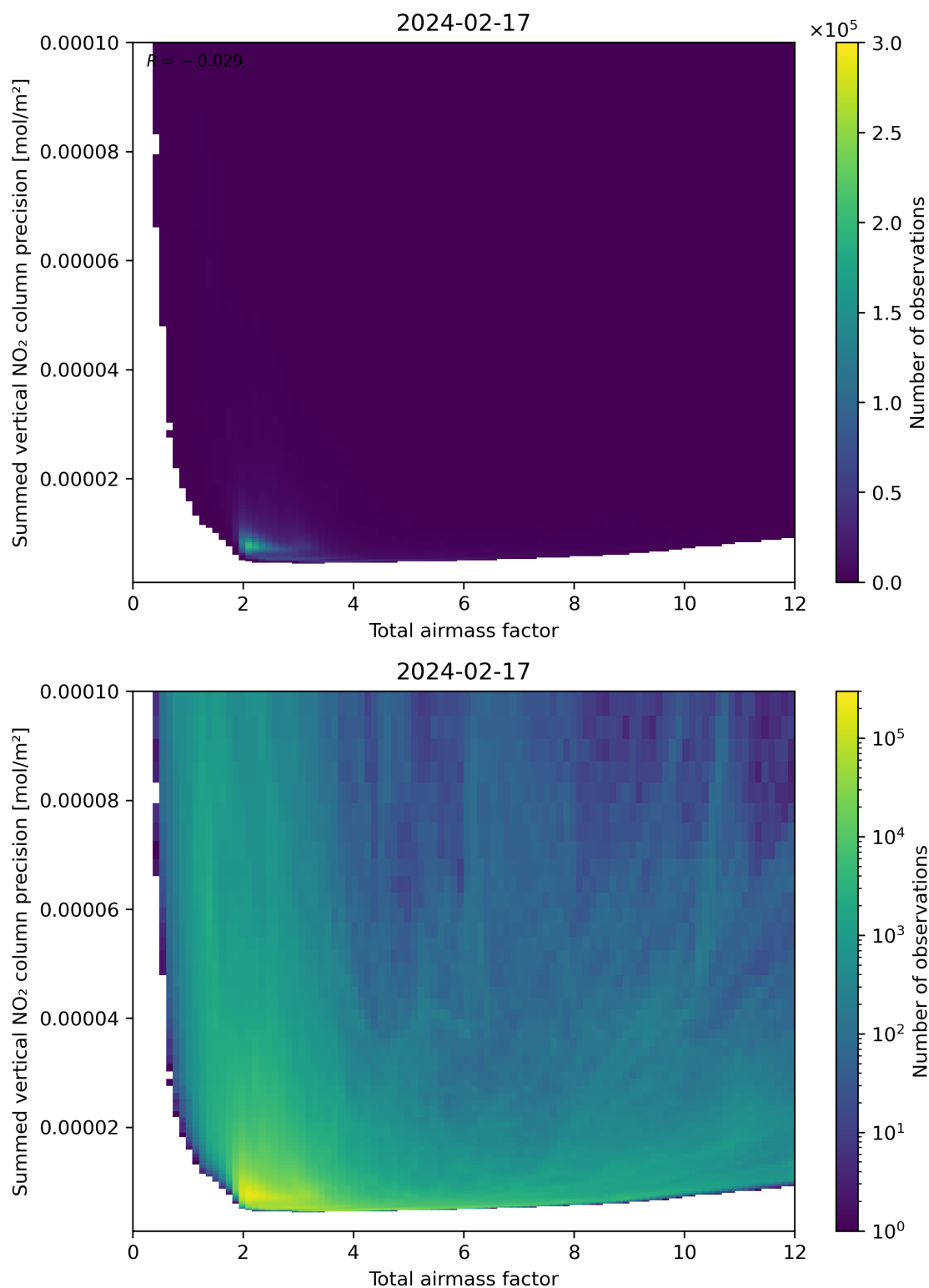
Figure 66: Scatter density plot of “Total airmass factor” against “Summed vertical NO 2 column precision” for 2024-02-17 to 2024-02-18.
