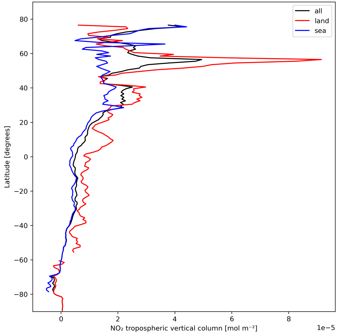
Figure 12: Zonal average of “NO 2 tropospheric vertical column” for 2024-02-17 to 2024-02-18.
