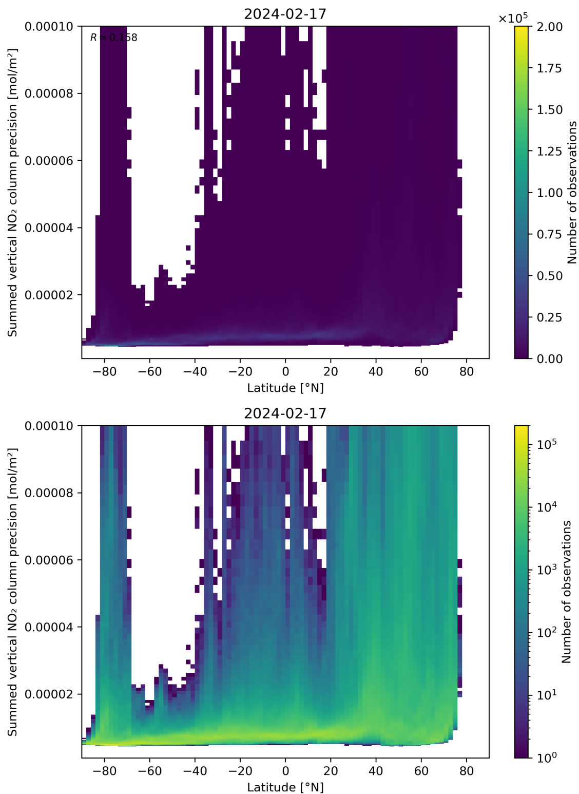
Figure 89: Scatter density plot of “Latitude” against “Summed vertical NO 2 column precision” for 2024-02-17 to 2024-02-18.
