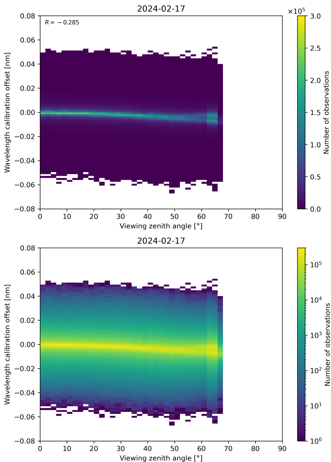
Figure 173: Scatter density plot of “Viewing zenith angle” against “Wavelength calibration offset” for 2024-02-17 to 2024-02-18.
