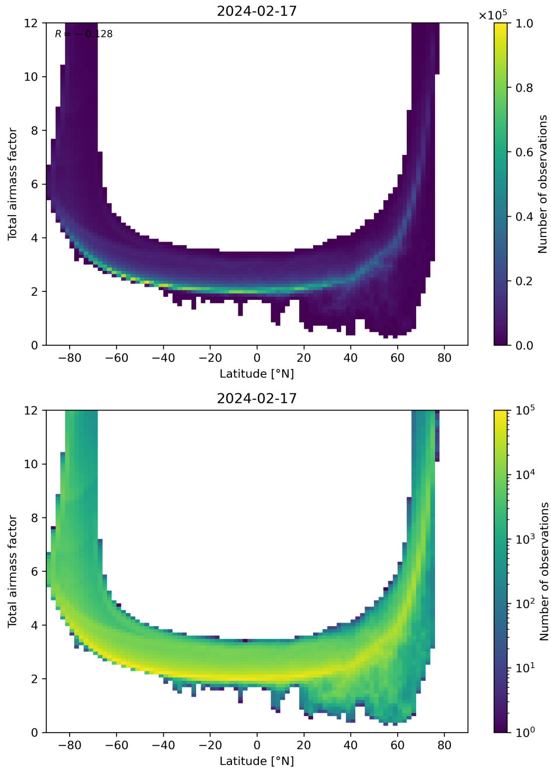
Figure 84: Scatter density plot of “Latitude” against “Total airmass factor” for 2024-02-17 to 2024-02-18.
