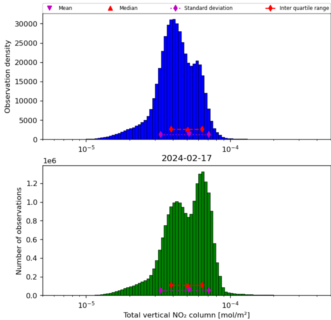
Figure 38: Histogram of “Total vertical NO 2 column” for 2024-02-17 to 2024-02-18
