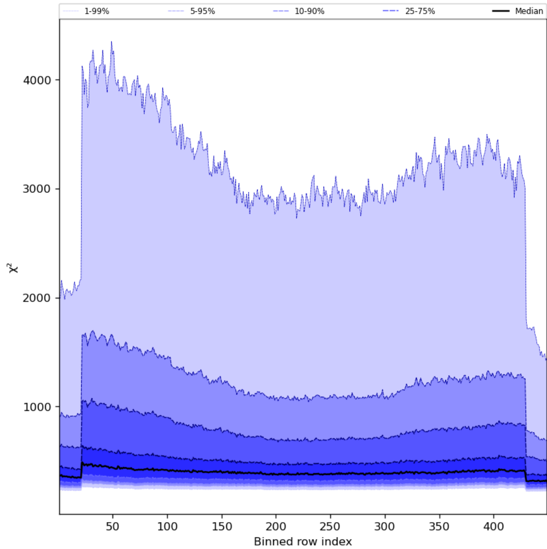
Figure 59: Along track statistics of “ \chi^2 ” for 2024-02-17 to 2024-02-18
