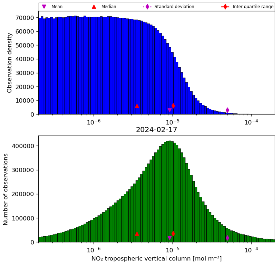
Figure 29: Histogram of “NO 2 tropospheric vertical column” for 2024-02-17 to 2024-02-18
