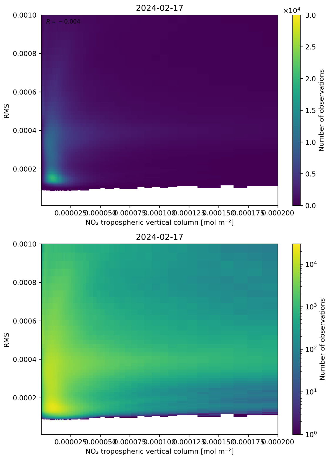
Figure 142: Scatter density plot of “NO 2 tropospheric vertical column” against “RMS” for 2024-02-17 to 2024-02-18.
