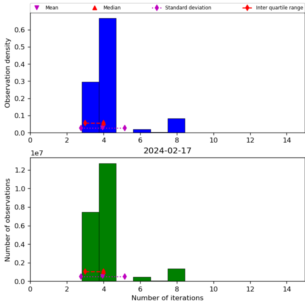
Figure 34: Histogram of “Number of iterations” for 2024-02-17 to 2024-02-18
