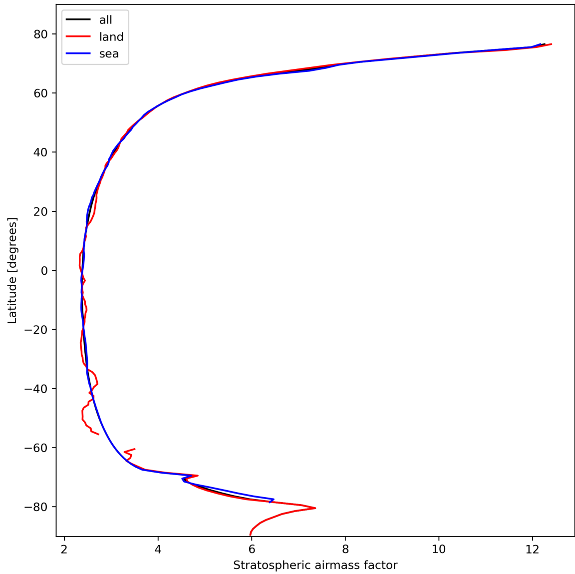
Figure 27: Zonal average of “Stratospheric air mass factor” for 2024-02-17 to 2024-02-18.
