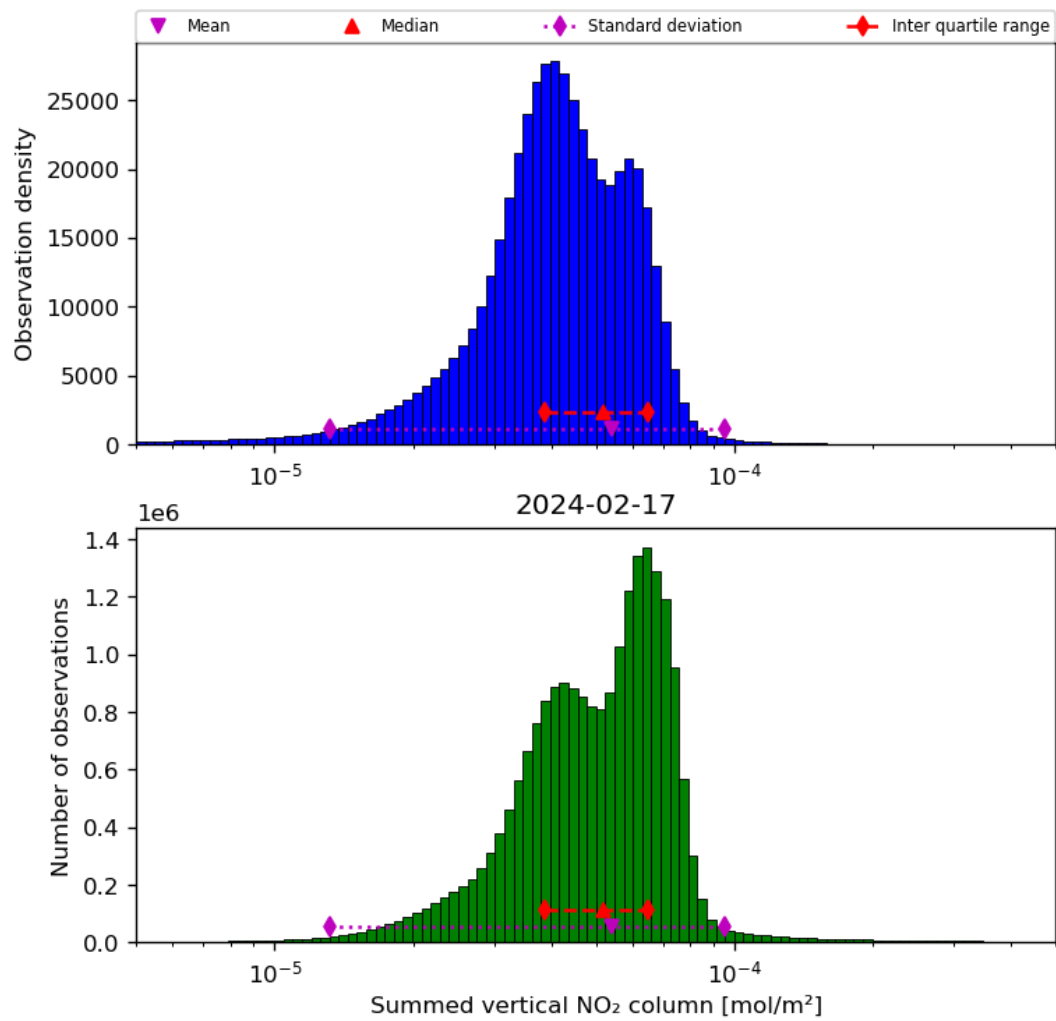
Figure 40: Histogram of “Summed vertical NO 2 column” for 2024-02-17 to 2024-02-18
