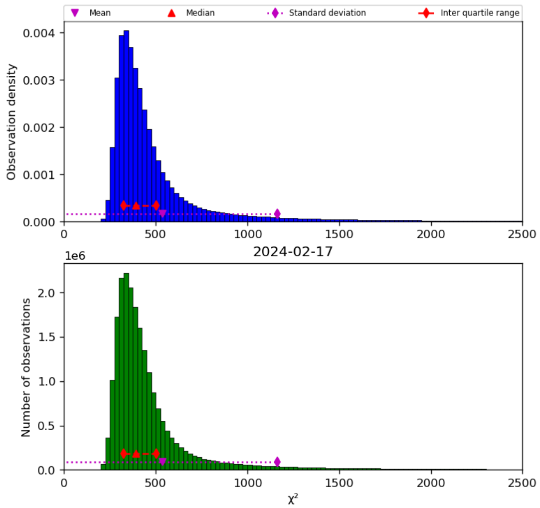
Figure 42: Histogram of “ \chi^2 ” for 2024-02-17 to 2024-02-18
