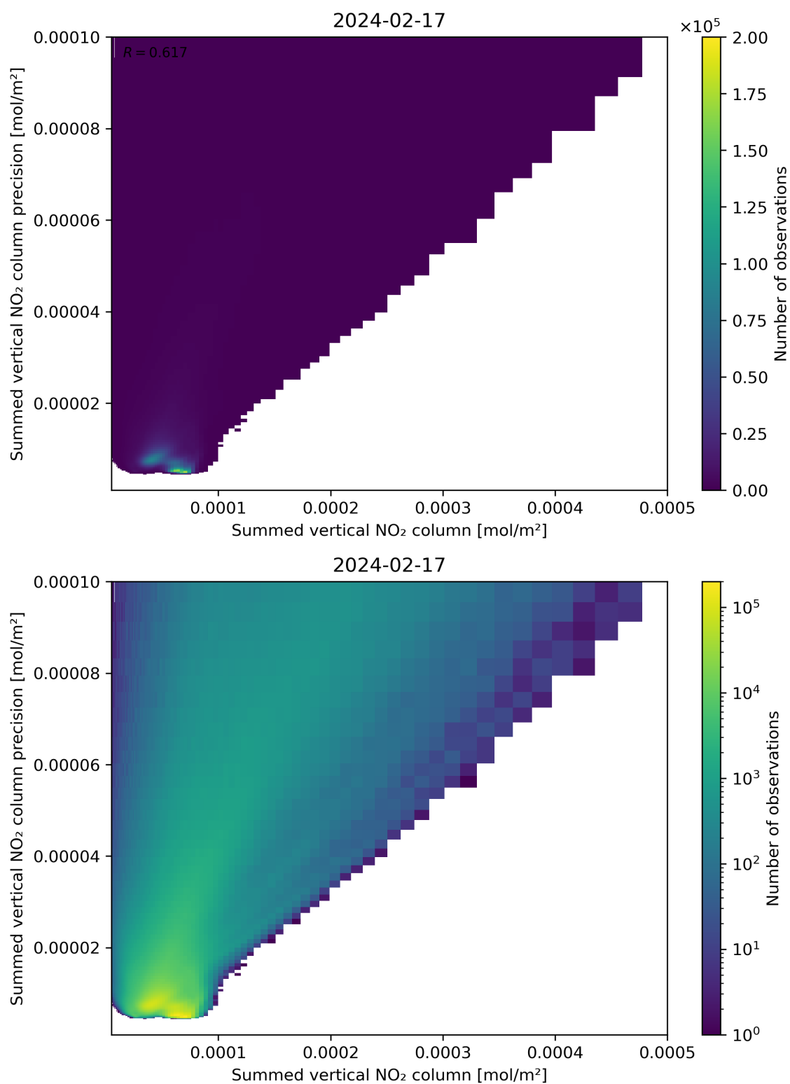
Figure 105: Scatter density plot of “Summed vertical NO 2 column” against “Summed vertical NO 2 column precision” for 2024-02-17 to 2024-02-18.
