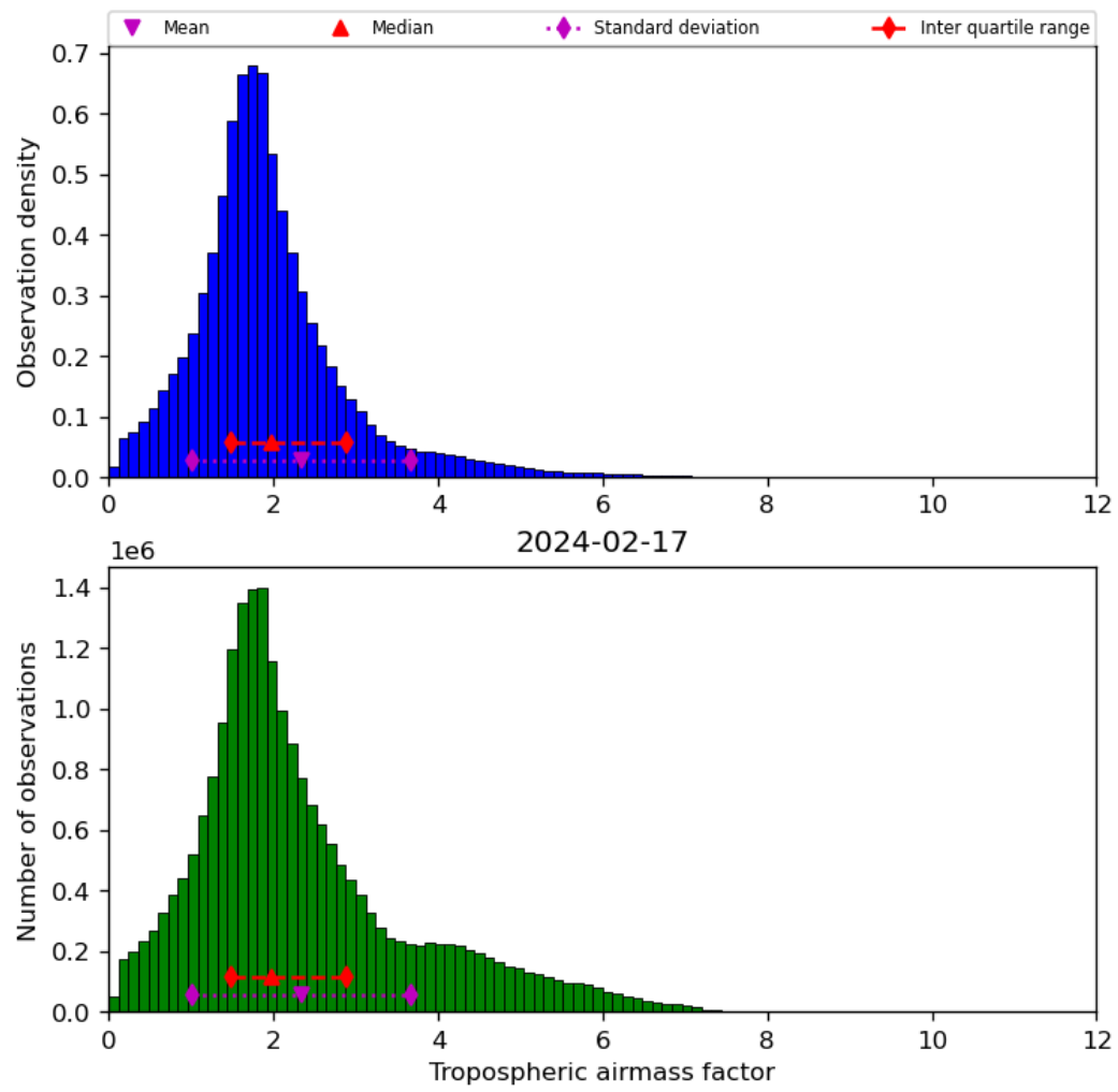
Figure 31: Histogram of “Tropospheric airmass factor” for 2024-02-17 to 2024-02-18
