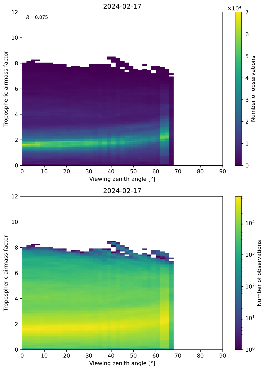
Figure 161: Scatter density plot of “Viewing zenith angle” against “Tropospheric airmass factor” for 2024-02-17 to 2024-02-18.
