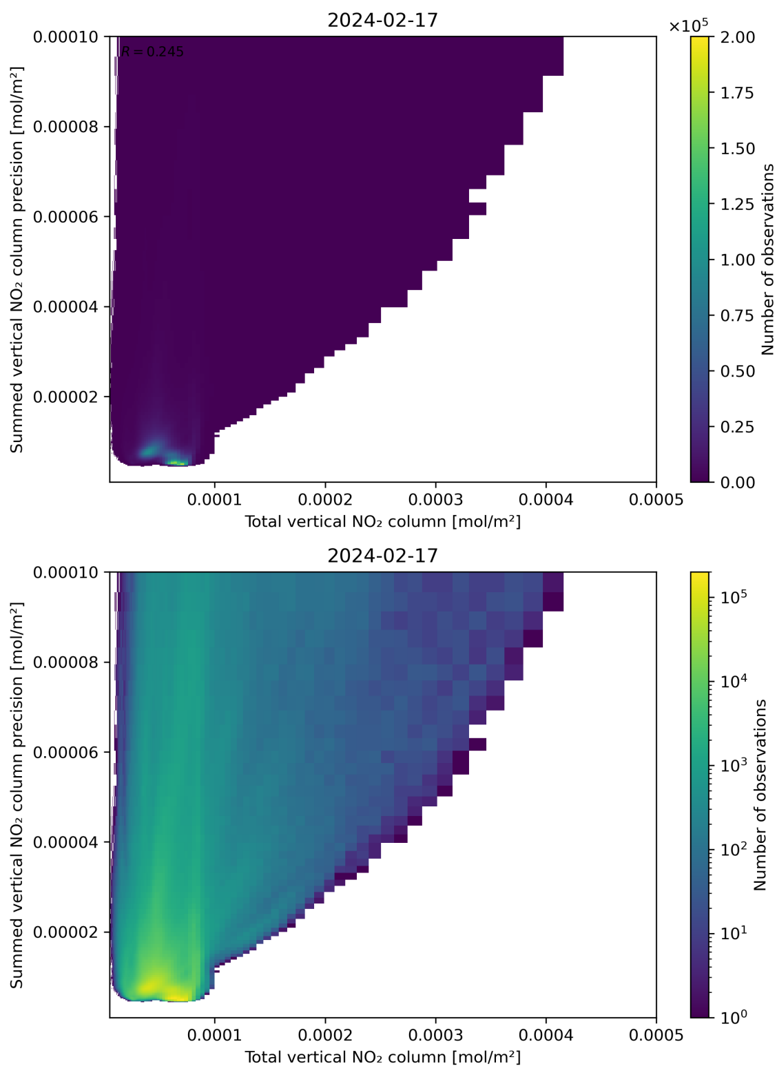
Figure 113: Scatter density plot of “Total vertical NO 2 column” against “Summed vertical NO 2 column precision” for 2024-02-17 to 2024-02-18.
