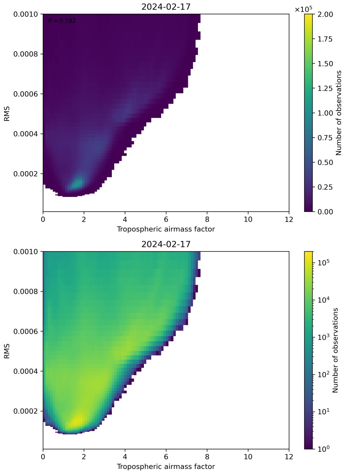
Figure 79: Scatter density plot of “Tropospheric airmass factor” against “RMS” for 2024-02-17 to 2024-02-18.
