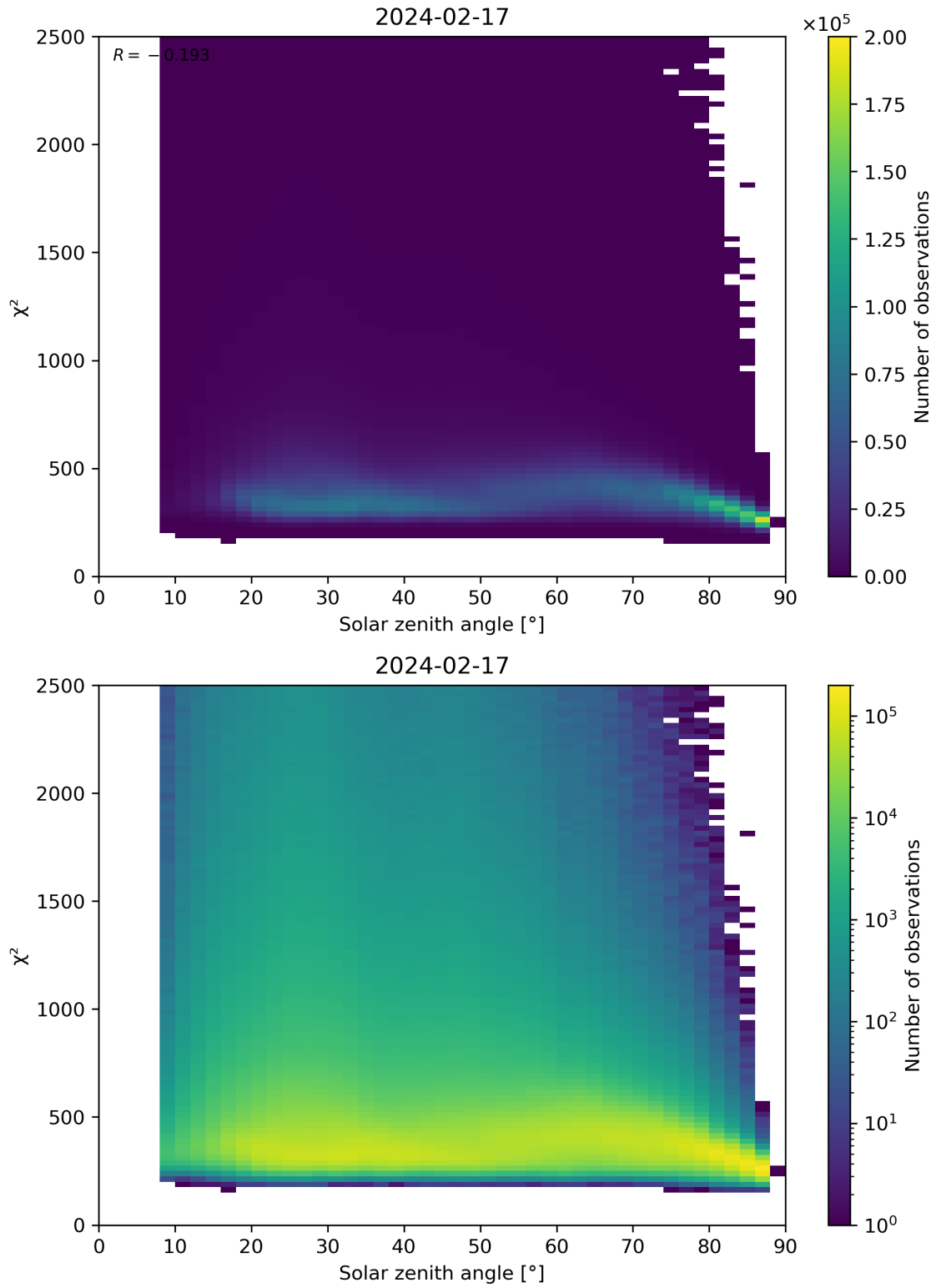
Figure 148: Scatter density plot of “Solar zenith angle” against “ \chi^2 ” for 2024-02-17 to 2024-02-18.
