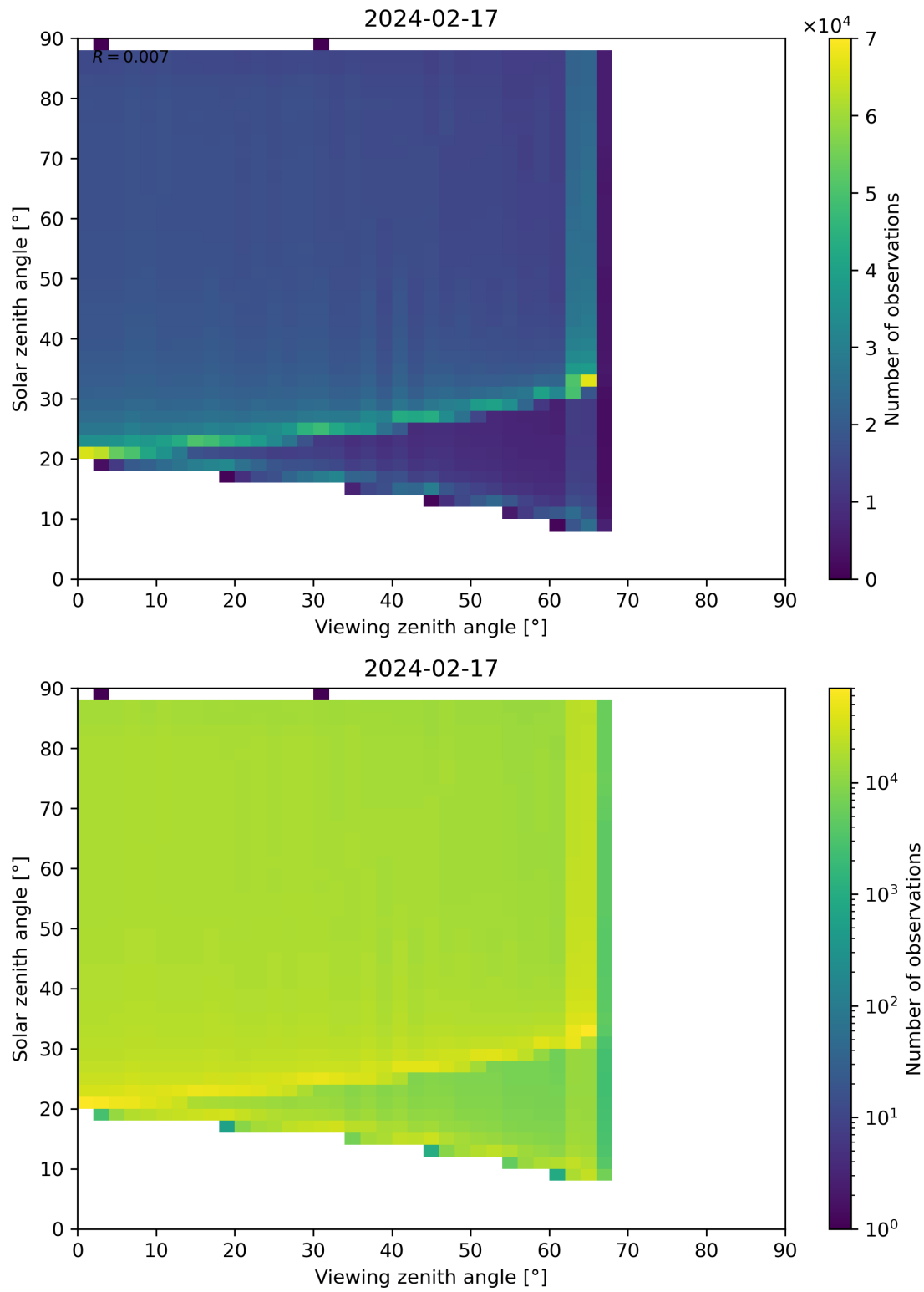
Figure 172: Scatter density plot of “Viewing zenith angle” against “Solar zenith angle” for 2024-02-17 to 2024-02-18.
