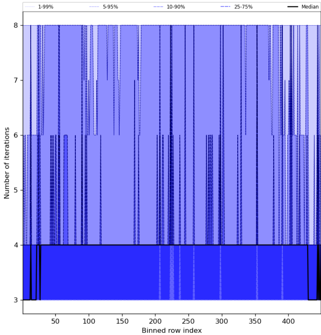
Figure 51: Along track statistics of “Number of iterations” for 2024-02-17 to 2024-02-18
