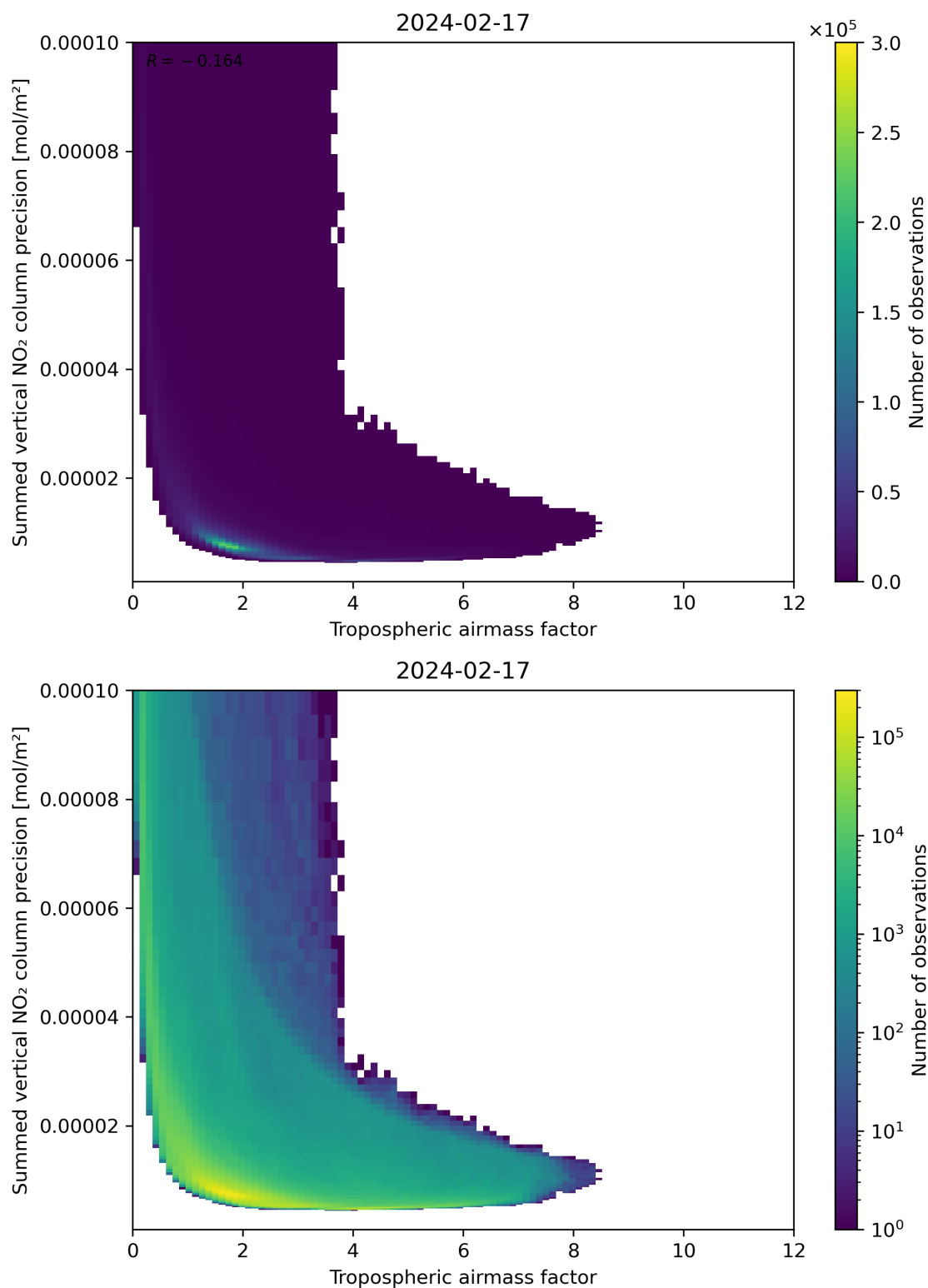
Figure 76: Scatter density plot of “Tropospheric air mass factor” against “Summed vertical NO 2 column precision” for 2024-02-17 to 2024-02-18.
