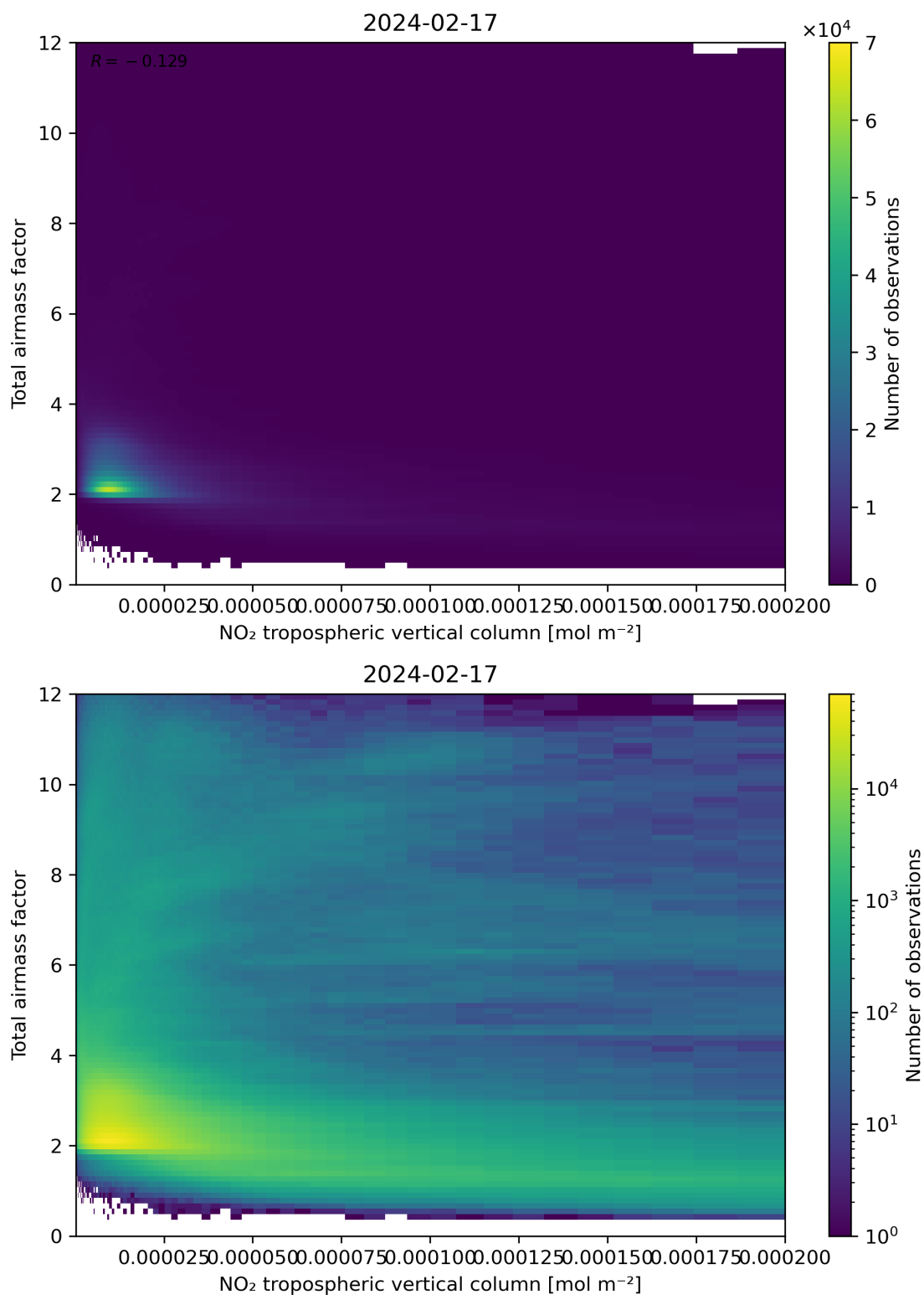
Figure 122: Scatter density plot of “NO 2 tropospheric vertical column” against “Total air mass factor” for 2024-02-17 to 2024-02-18.
