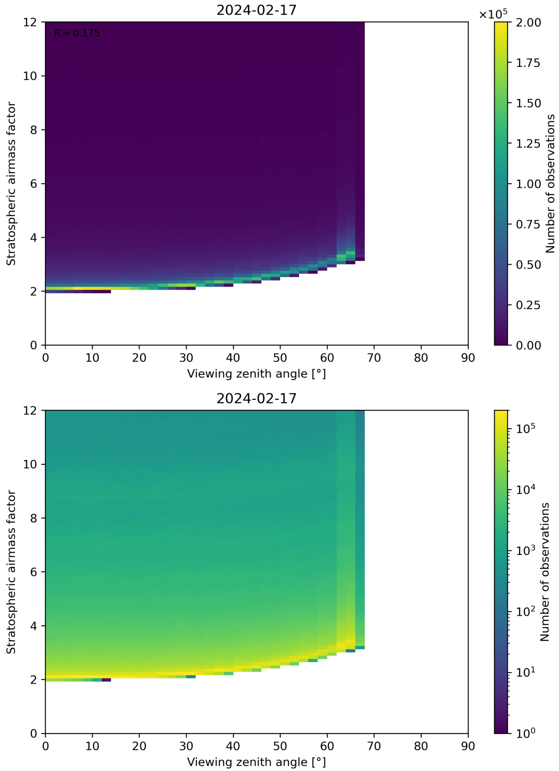
Figure 159: Scatter density plot of “Viewing zenith angle” against “Stratospheric airmass factor” for 2024-02-17 to 2024-02-18.
