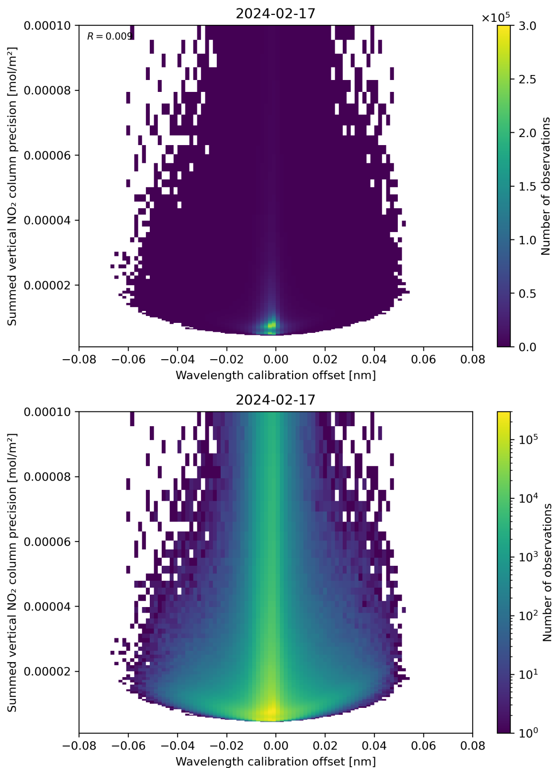
Figure 178: Scatter density plot of “Wavelength calibration offset” against “Summed vertical NO 2 column precision” for 2024-02-17 to 2024-02-18.
