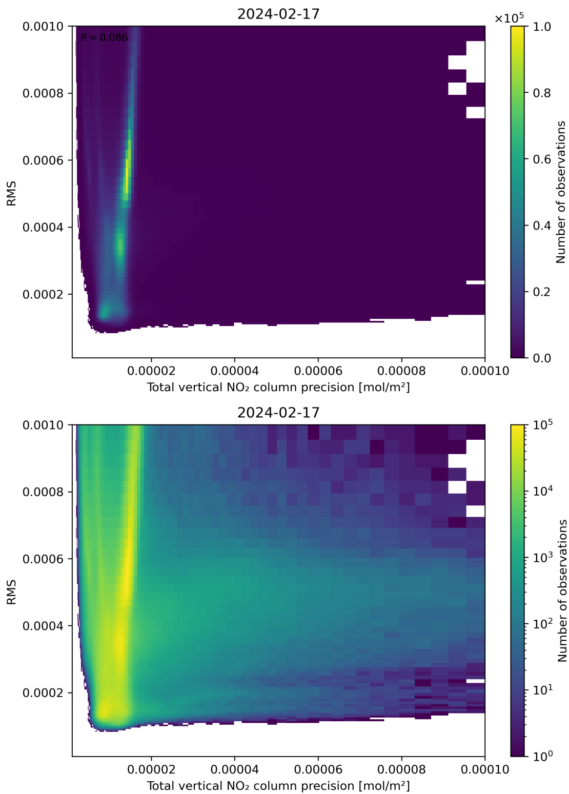
Figure 119: Scatter density plot of “Total vertical NO 2 column precision” against “RMS” for 2024-02-17 to 2024-02-18.
