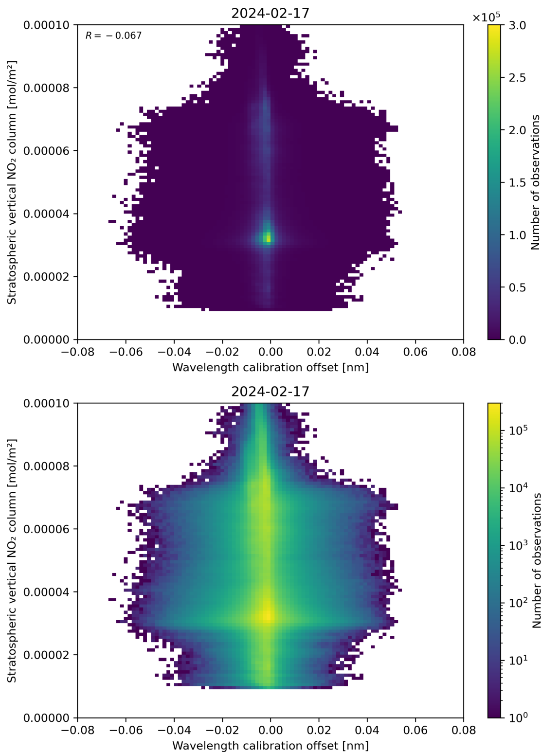
Figure 176: Scatter density plot of “Wavelength calibration offset” against “Stratospheric vertical NO 2 column” for 2024-02-17 to 2024-02-18.
