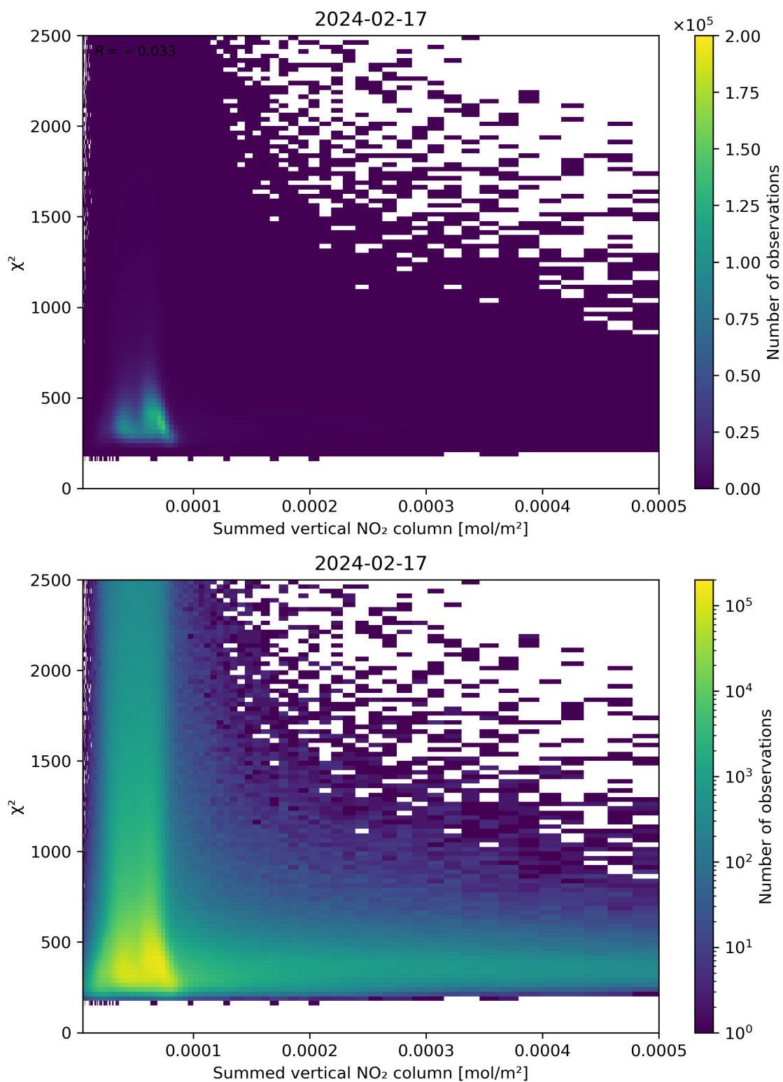
Figure 104: Scatter density plot of “Summed vertical NO 2 column” against “ \chi^2 ” for 2024-02-17 to 2024-02-18.
