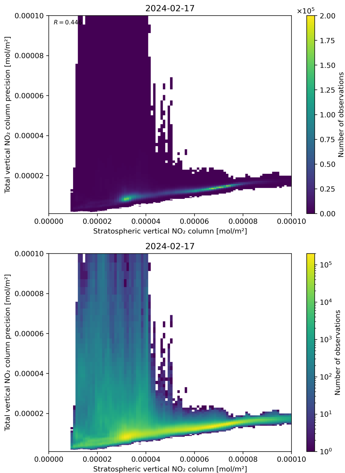
Figure 101: Scatter density plot of “Stratospheric vertical NO 2 column” against “Total vertical NO 2 column precision” for 2024-02-17 to 2024-02-18.
