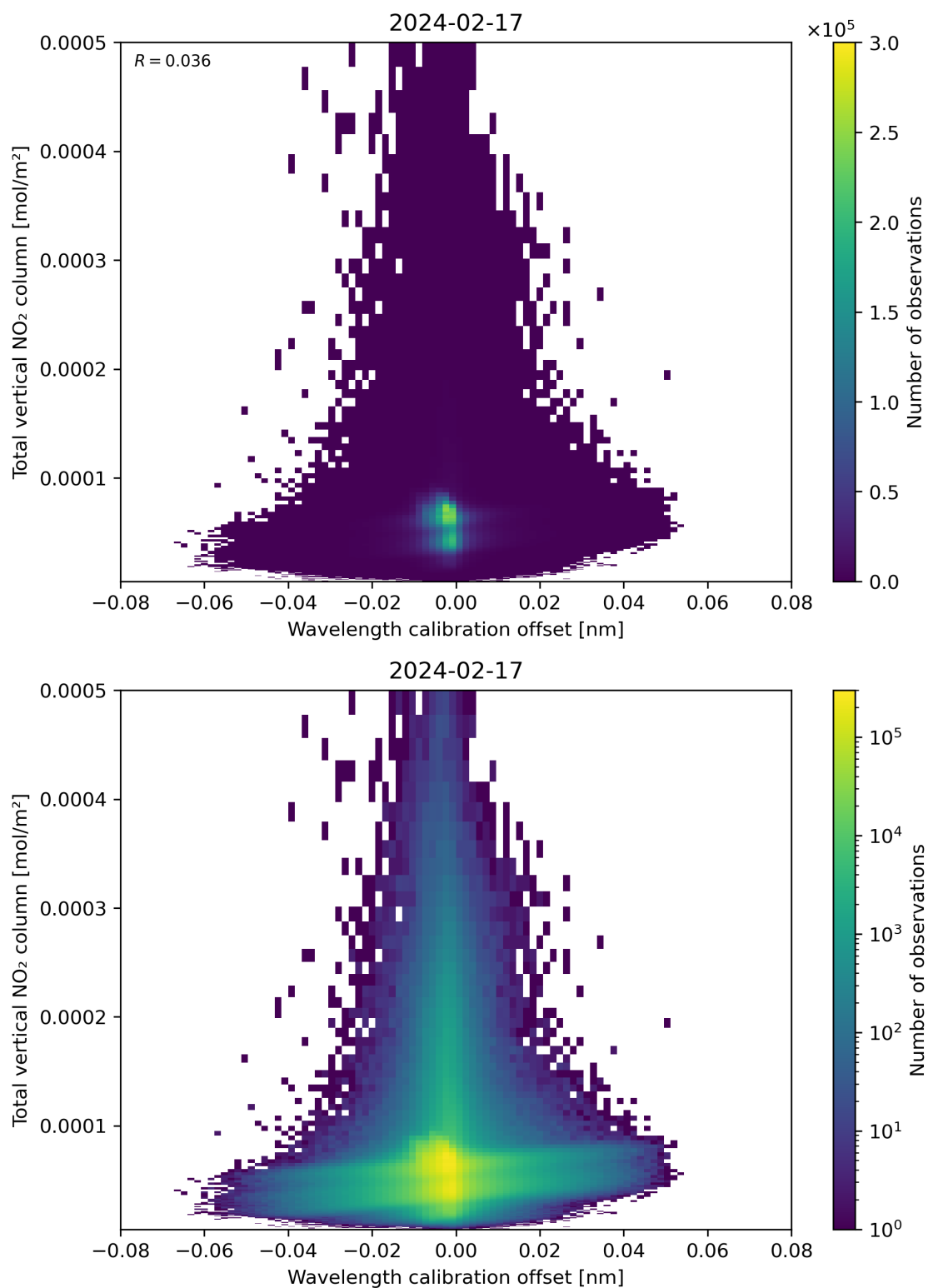
Figure 179: Scatter density plot of “Wavelength calibration offset” against “Total vertical NO 2 column” for 2024-02-17 to 2024-02-18.
