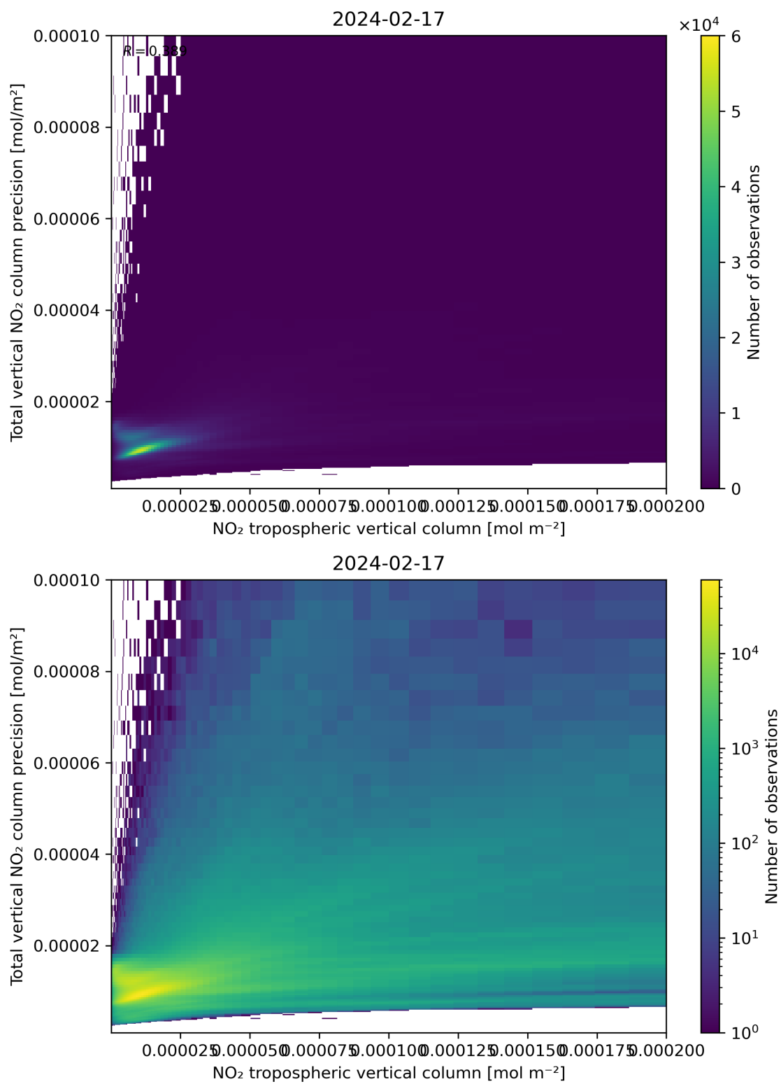
Figure 129: Scatter density plot of “NO 2 tropospheric vertical column” against “Total vertical NO 2 column precision” for 2024-02-17 to 2024-02-18.
