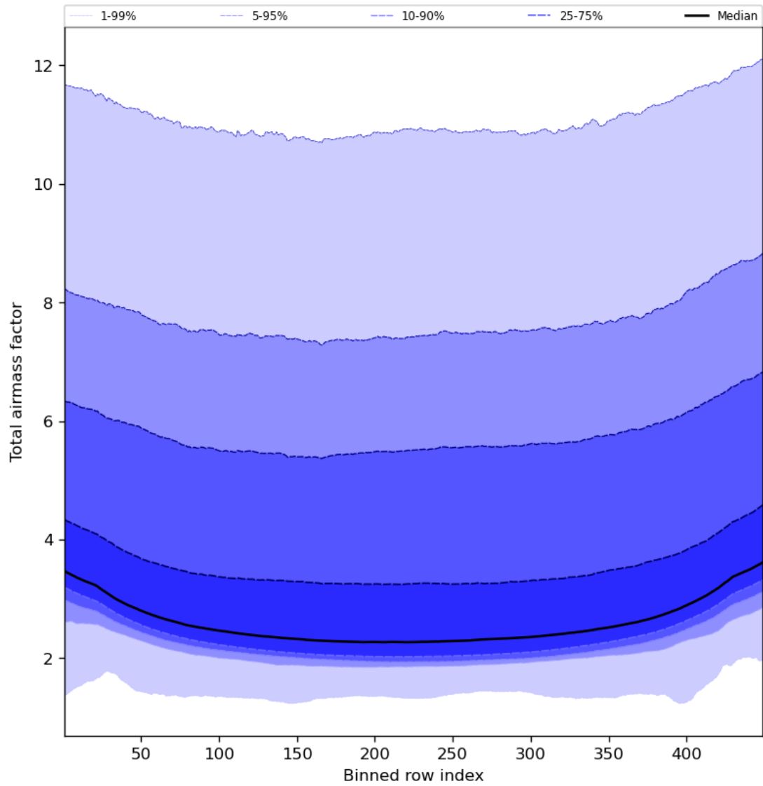
Figure 49: Along track statistics of “Total airmass factor” for 2024-02-17 to 2024-02-18
