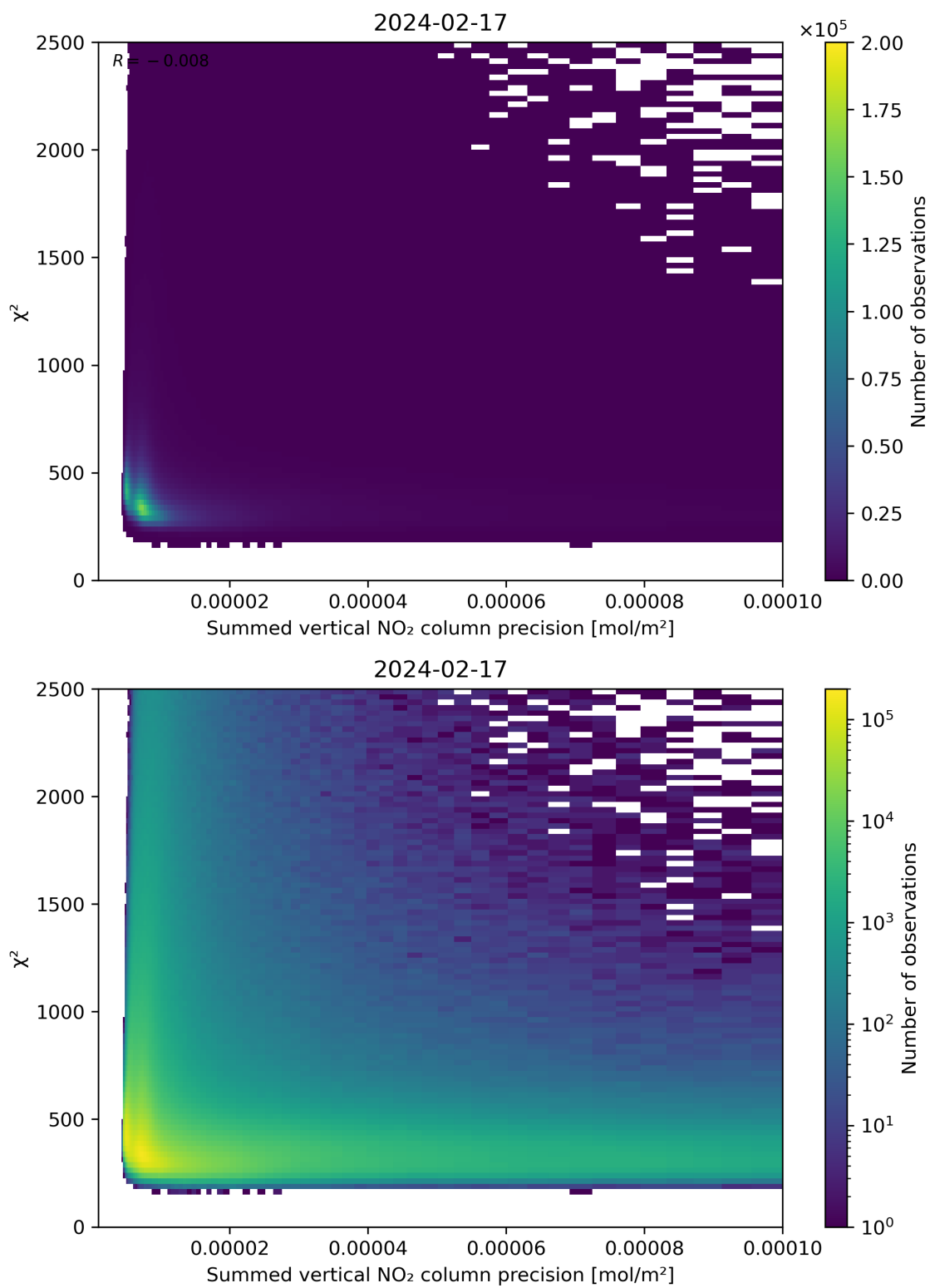
Figure 107: Scatter density plot of “Summed vertical NO 2 column precision” against “ \chi^2 ” for 2024-02-17 to 2024-02-18.
