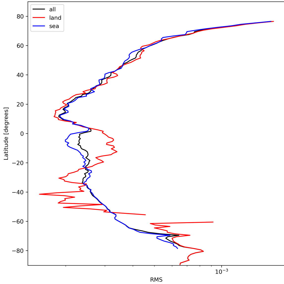
Figure 26: Zonal average of “RMS” for 2024-02-17 to 2024-02-18.
