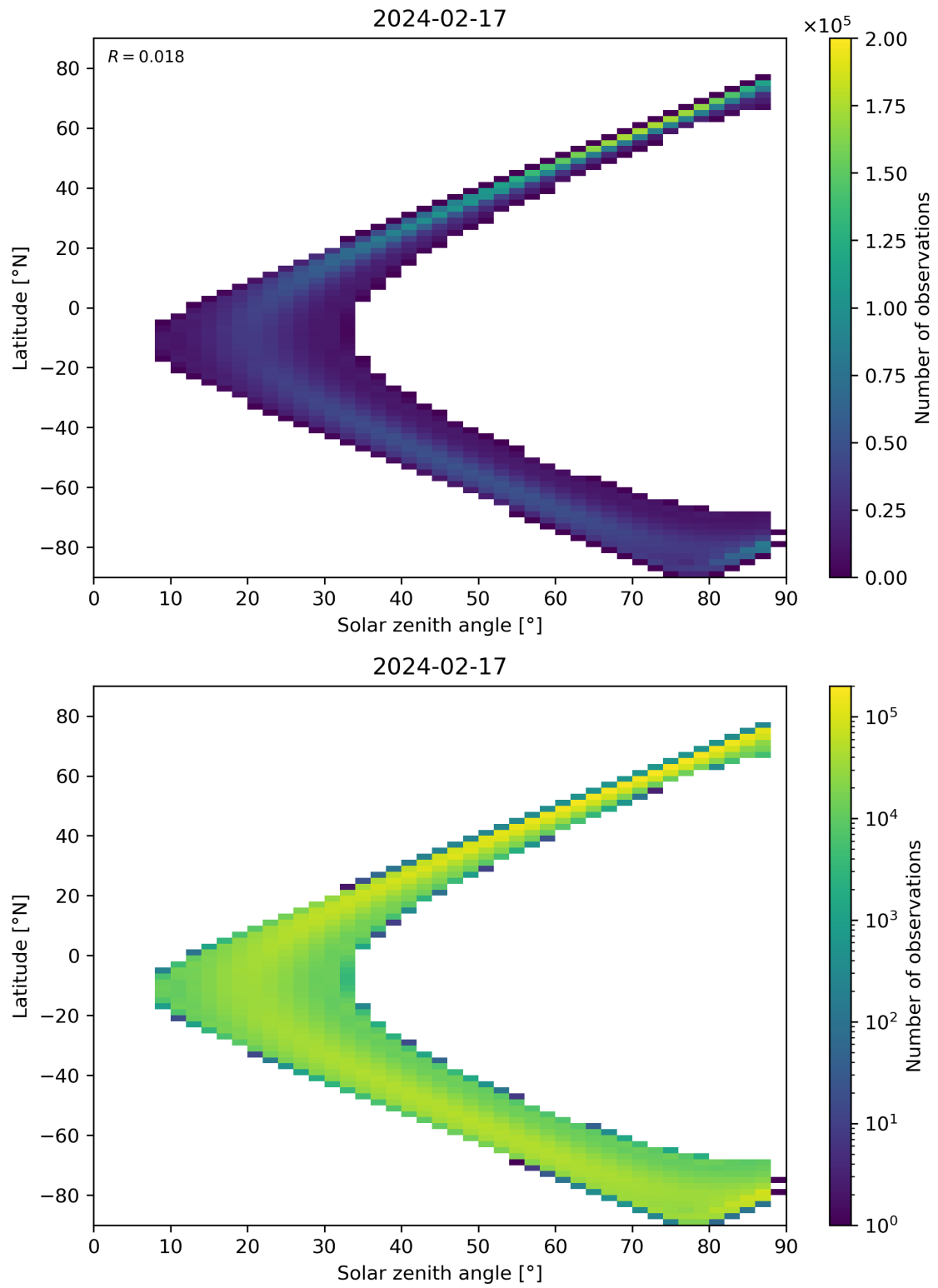
Figure 149: Scatter density plot of “Solar zenith angle” against “Latitude” for 2024-02-17 to 2024-02-18.
