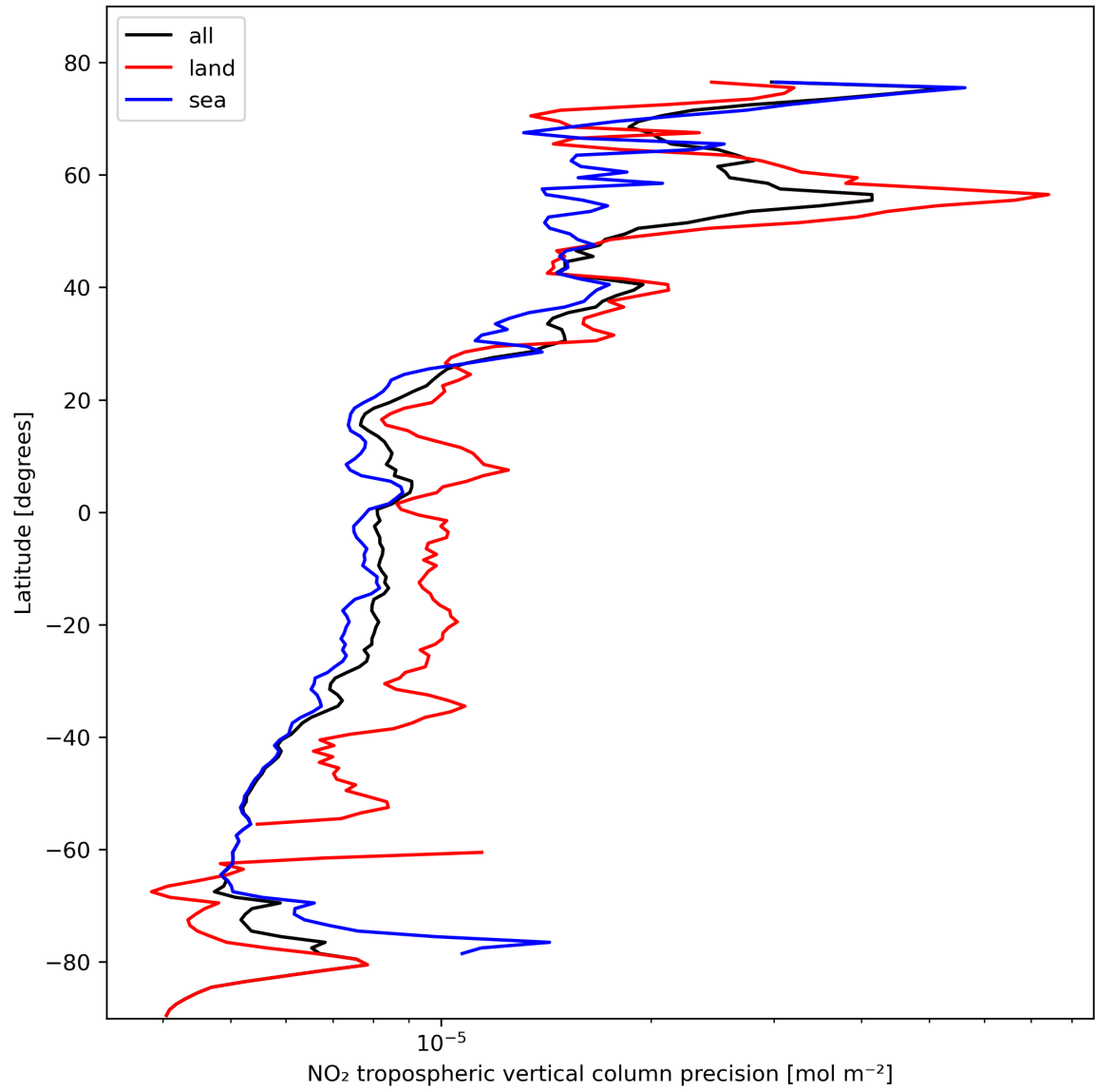
Figure 13: Zonal average of “NO 2 tropospheric vertical column precision” for 2024-02-17 to 2024-02-18.
