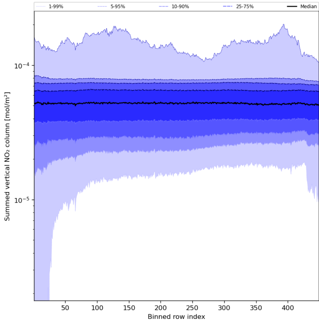
Figure 57: Along track statistics of “Summed vertical NO 2 column” for 2024-02-17 to 2024-02-18
