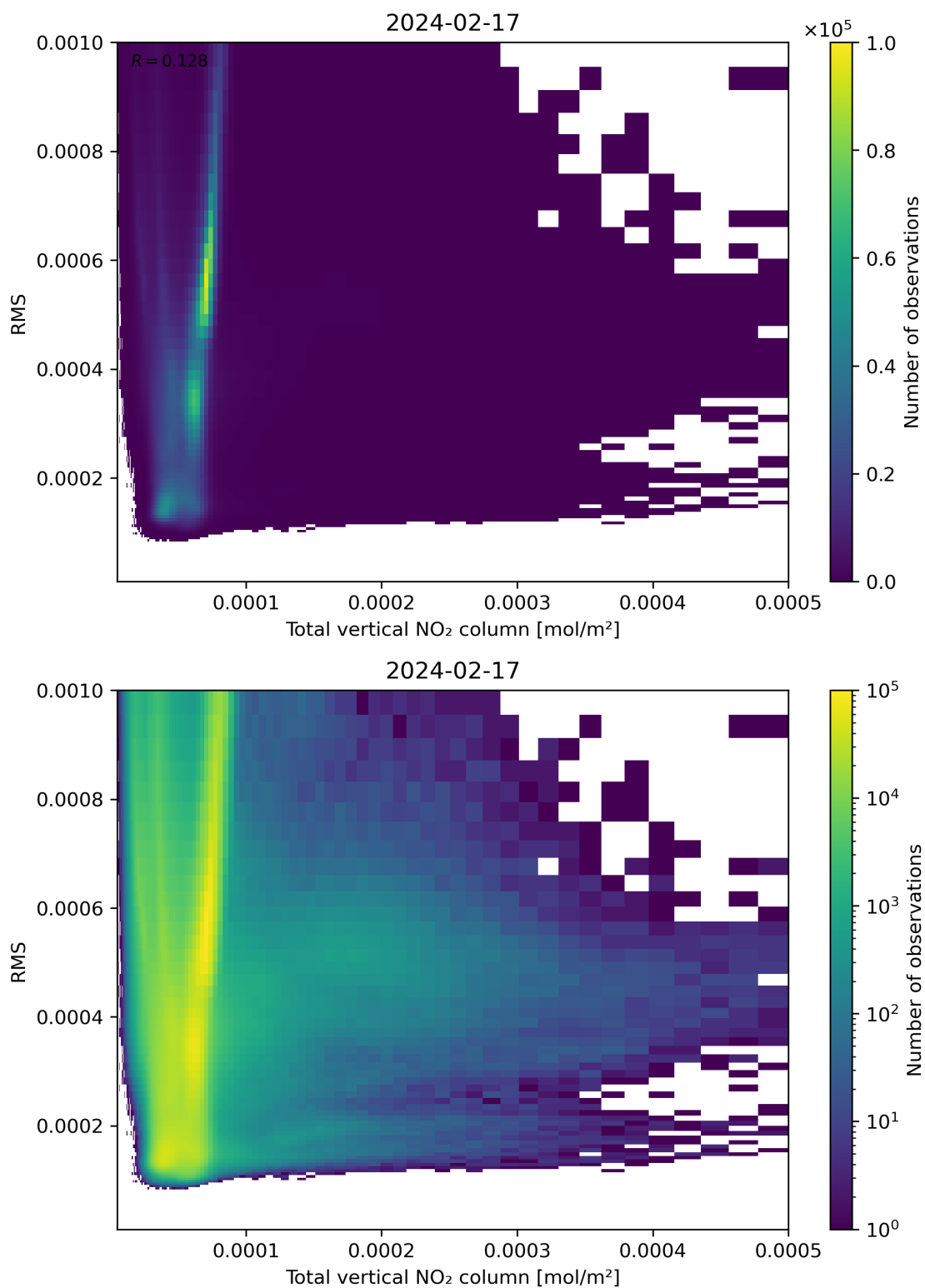
Figure 120: Scatter density plot of “Total vertical NO 2 column” against “RMS” for 2024-02-17 to 2024-02-18.
