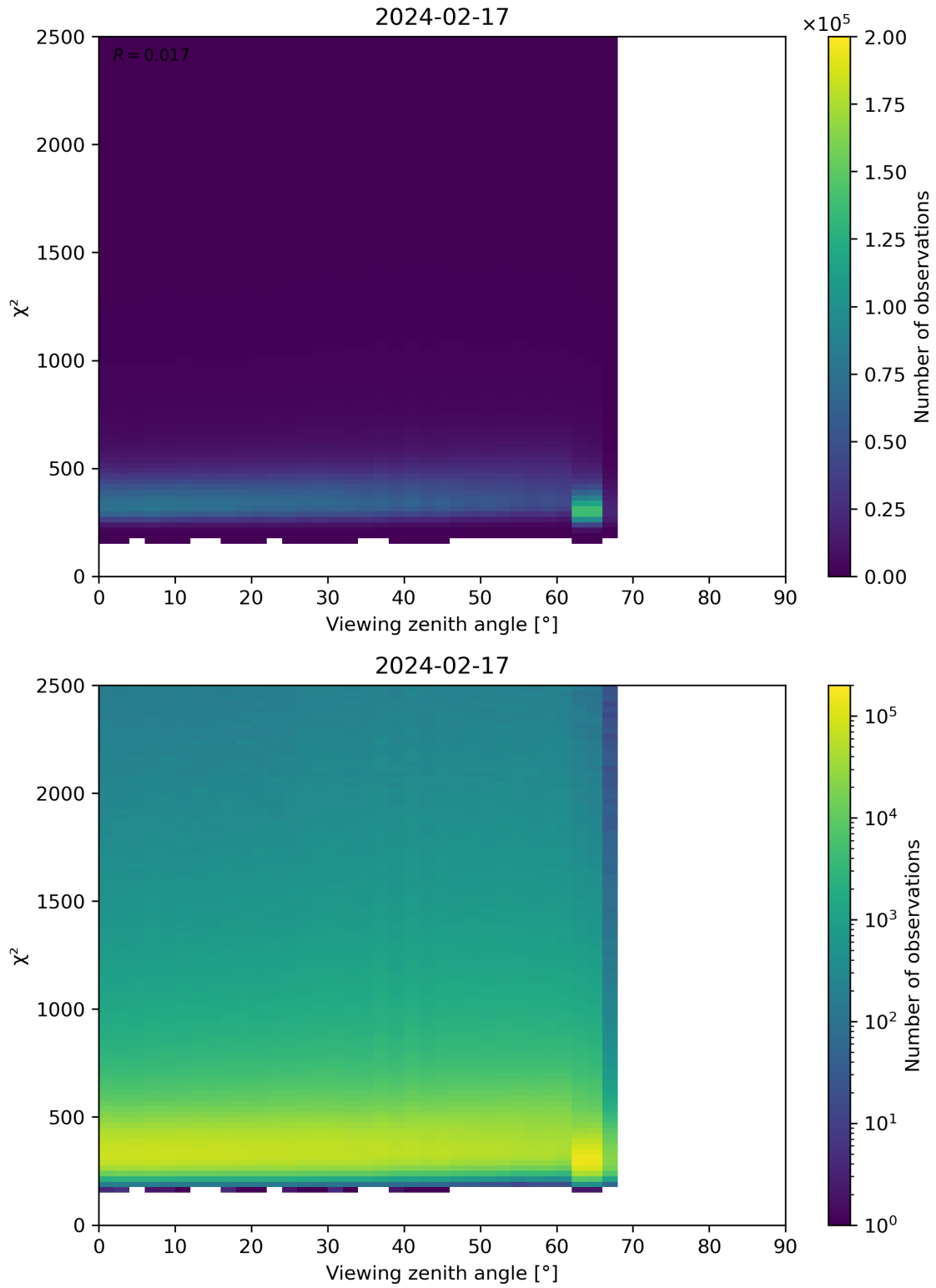
Figure 162: Scatter density plot of “Viewing zenith angle” against “ \chi^2 ” for 2024-02-17 to 2024-02-18.
