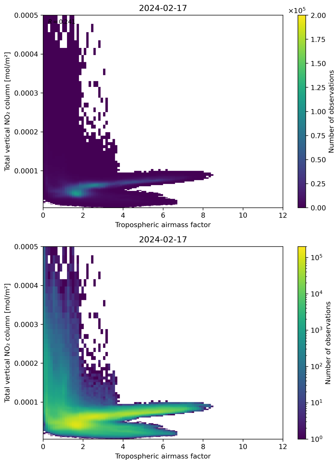
Figure 77: Scatter density plot of “Tropospheric airmass factor” against “Total vertical \text{NO}_2 column” for 2024-02-17 to 2024-02-18.
