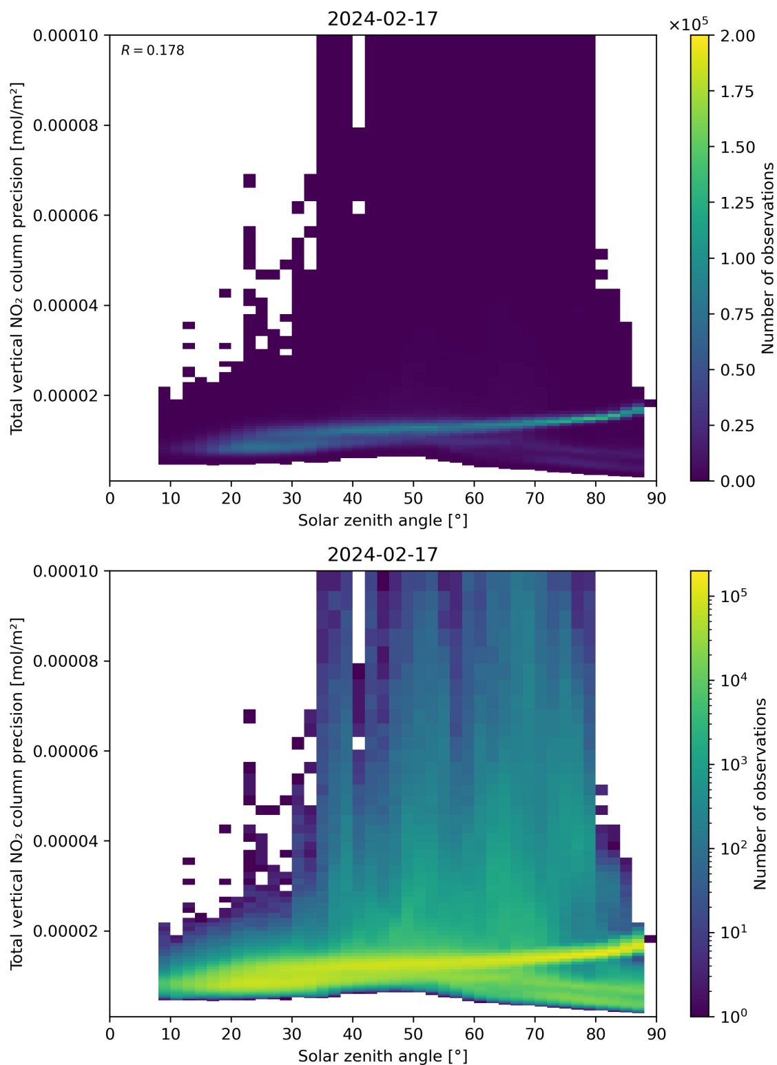
Figure 154: Scatter density plot of “Solar zenith angle” against “Total vertical NO 2 column precision” for 2024-02-17 to 2024-02-18.
