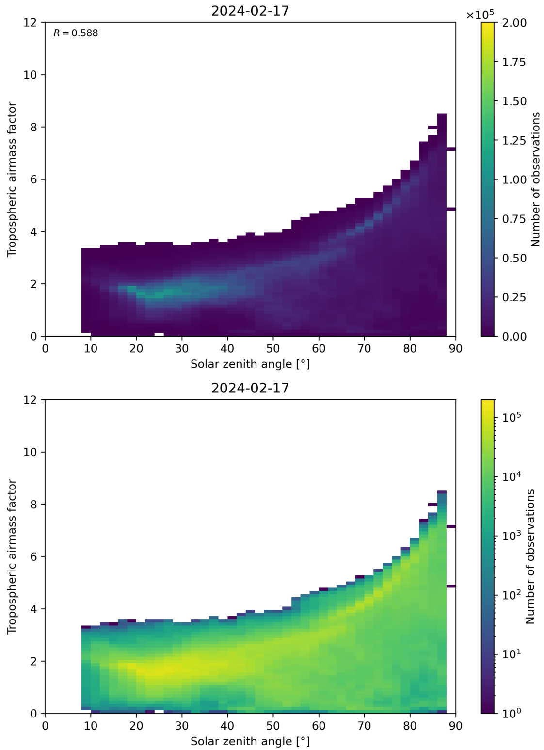
Figure 147: Scatter density plot of “Solar zenith angle” against “Tropospheric airmass factor” for 2024-02-17 to 2024-02-18.
