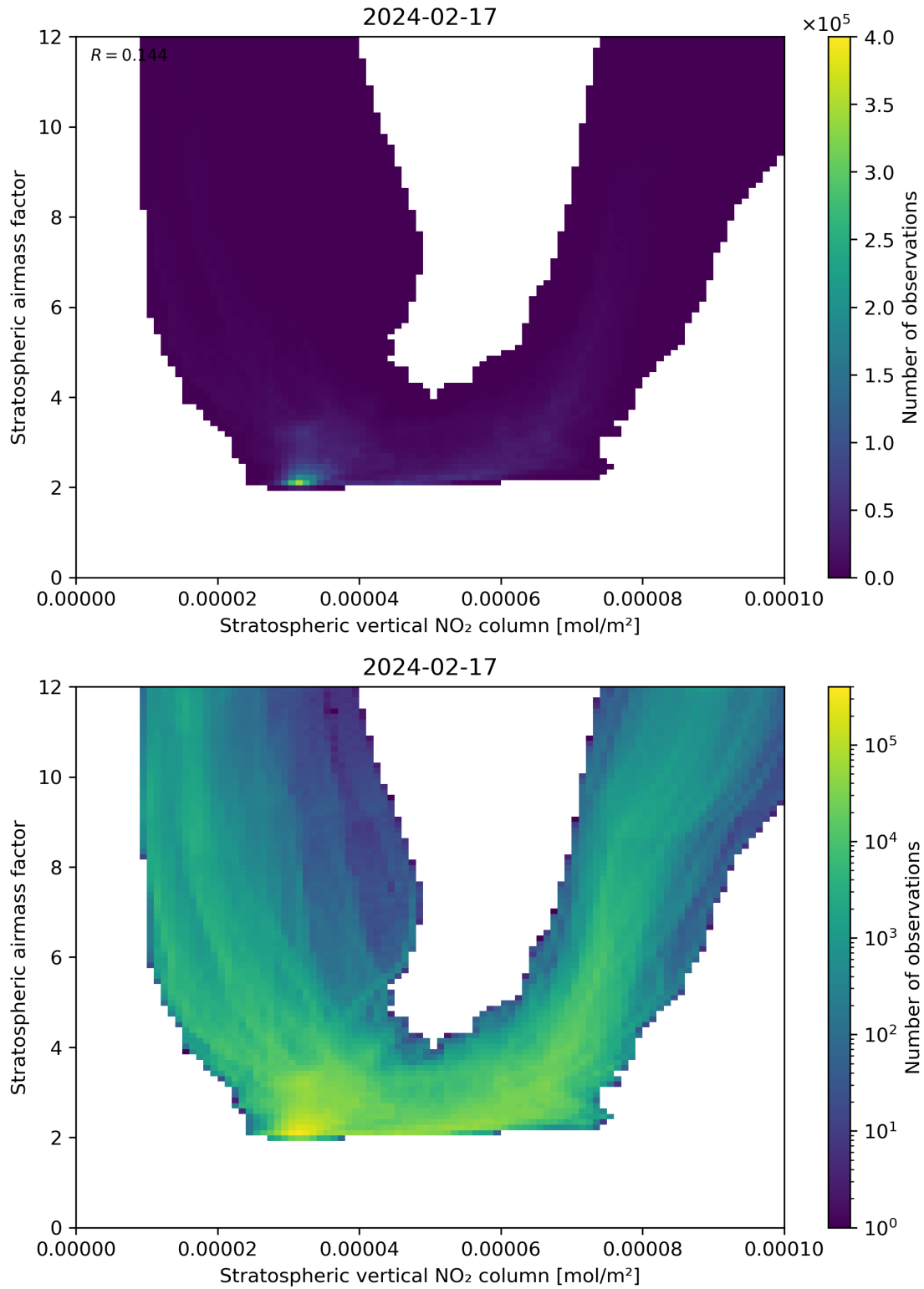
Figure 96: Scatter density plot of “Stratospheric vertical NO 2 column” against “Stratospheric airmass factor” for 2024-02-17 to 2024-02-18.
