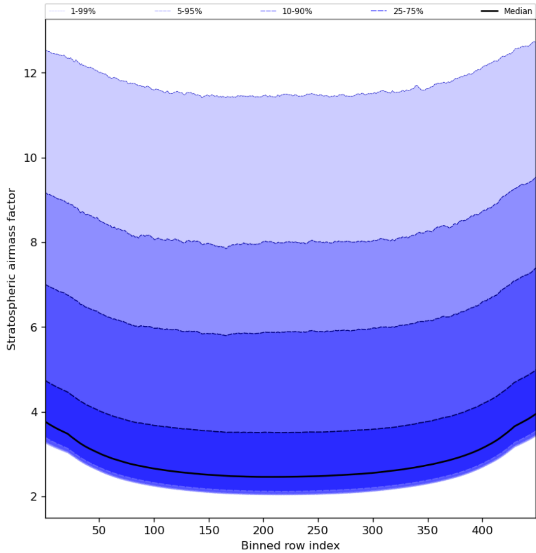
Figure 61: Along track statistics of “Stratospheric airmass factor” for 2024-02-17 to 2024-02-18
