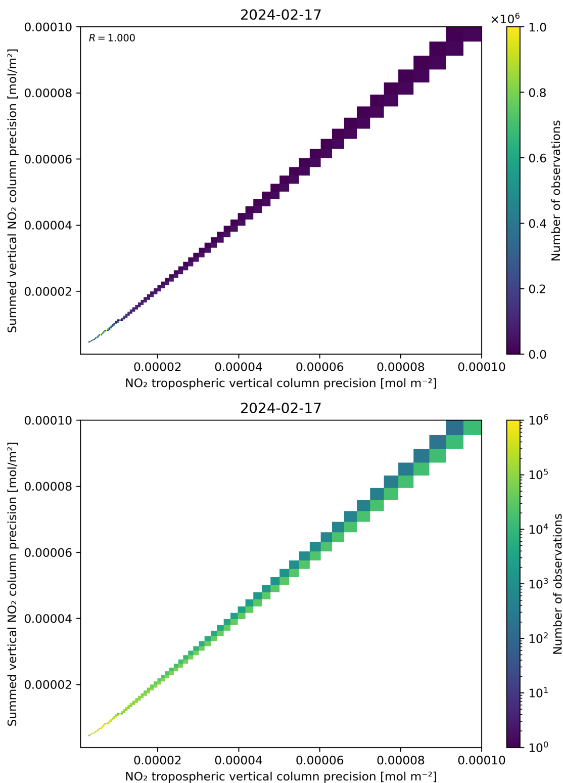
Figure 137: Scatter density plot of “NO 2 tropospheric vertical column precision” against “Summed vertical NO 2 column precision” for 2024-02-17 to 2024-02-18.
