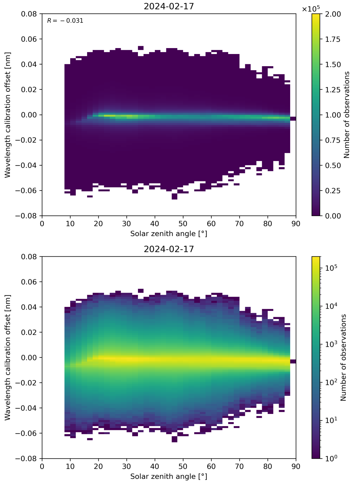
Figure 158: Scatter density plot of “Solar zenith angle” against “Wavelength calibration offset” for 2024-02-17 to 2024-02-18.
