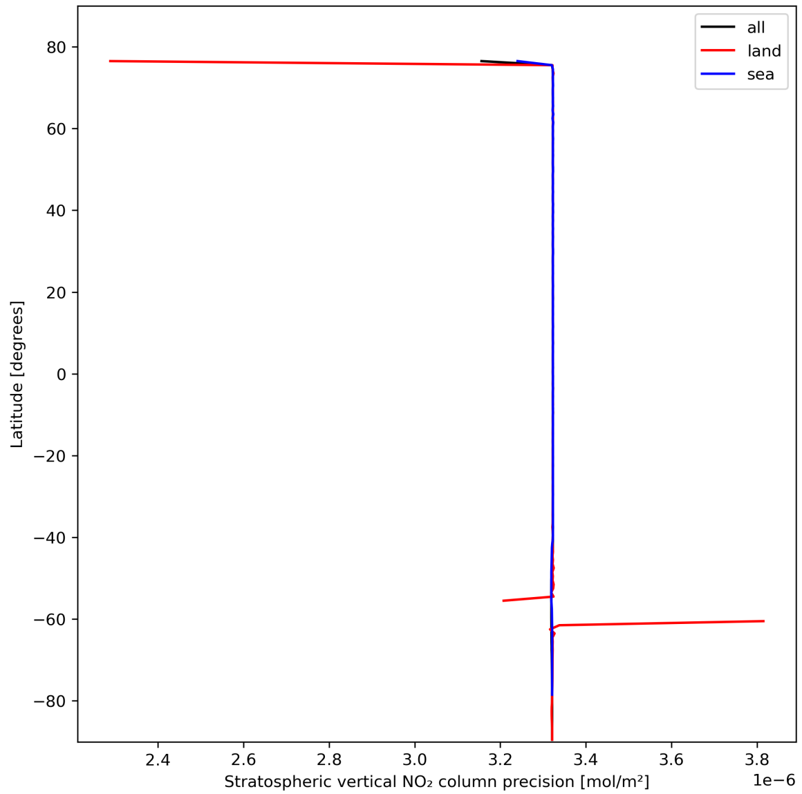
Figure 20: Zonal average of “Stratospheric vertical NO 2 column precision” for 2024-02-17 to 2024-02-18.
