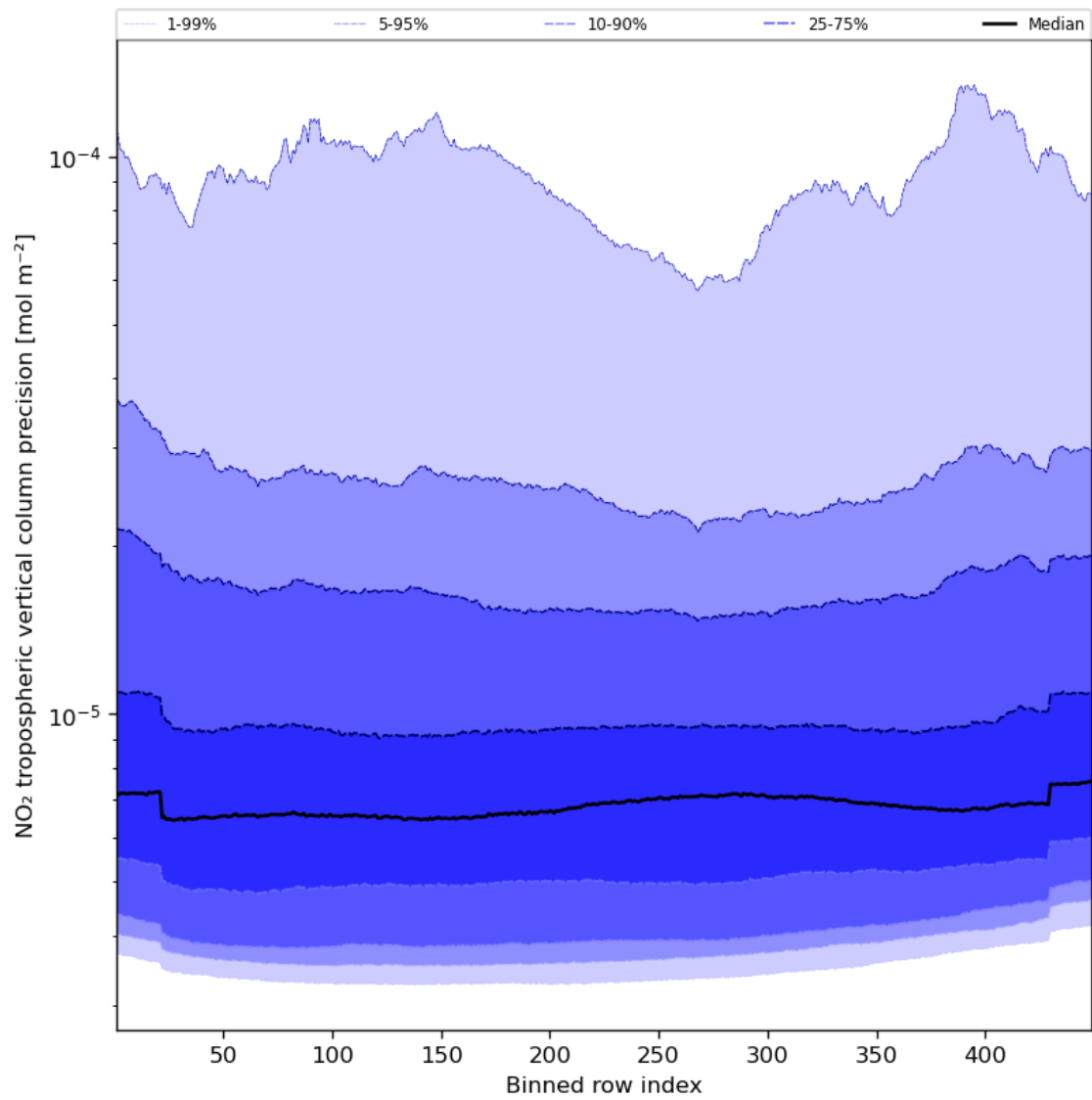
Figure 47: Along track statistics of “NO 2 tropospheric vertical column precision” for 2024-02-17 to 2024-02-18
