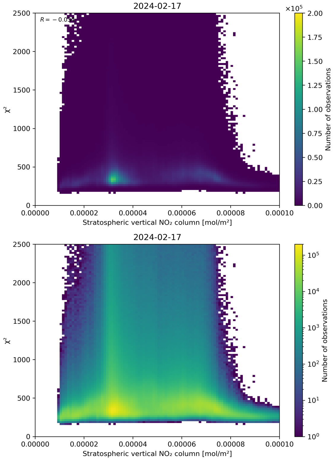
Figure 97: Scatter density plot of “Stratospheric vertical NO 2 column” against “ \chi^2 ” for 2024-02-17 to 2024-02-18.
