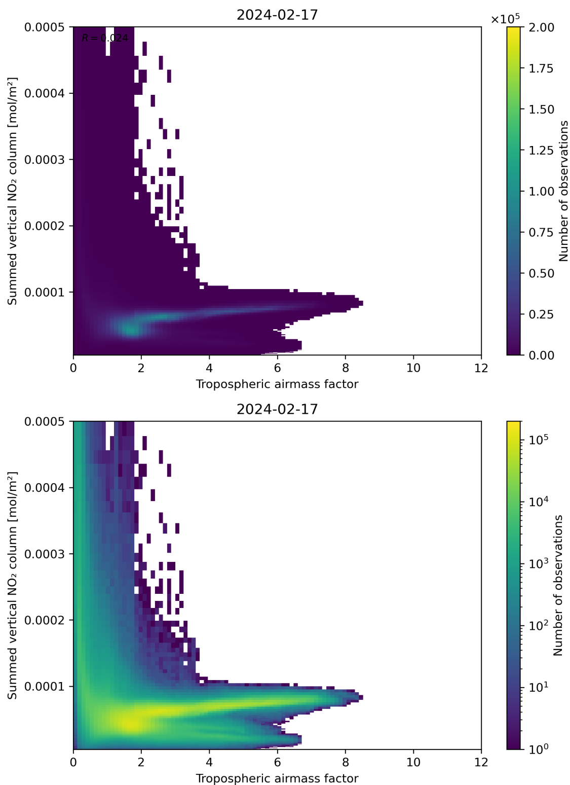
Figure 75: Scatter density plot of “Tropospheric airmass factor” against “Summed vertical NO 2 column” for 2024-02-17 to 2024-02-18.
