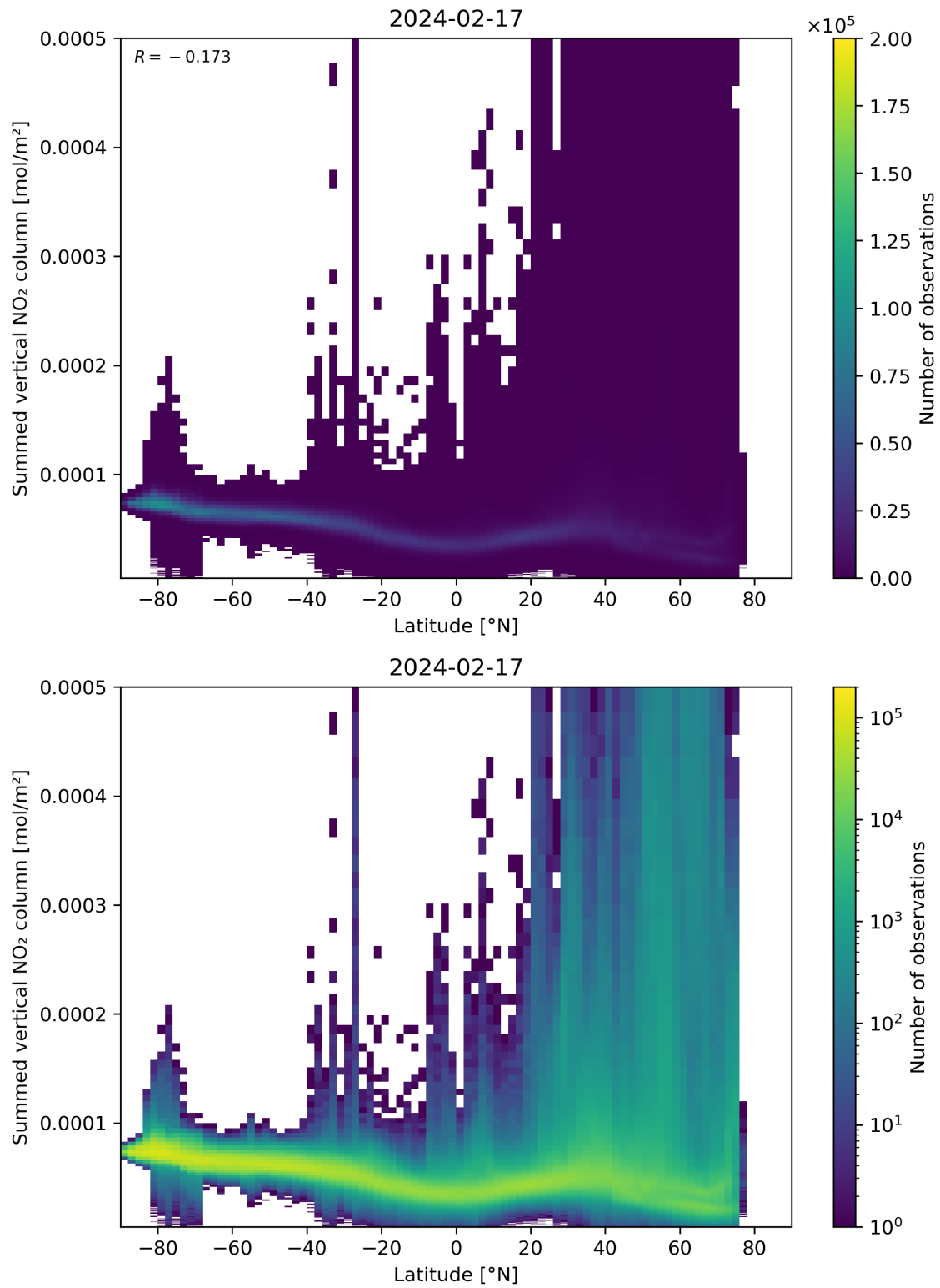
Figure 88: Scatter density plot of “Latitude” against “Summed vertical NO 2 column” for 2024-02-17 to 2024-02-18.
