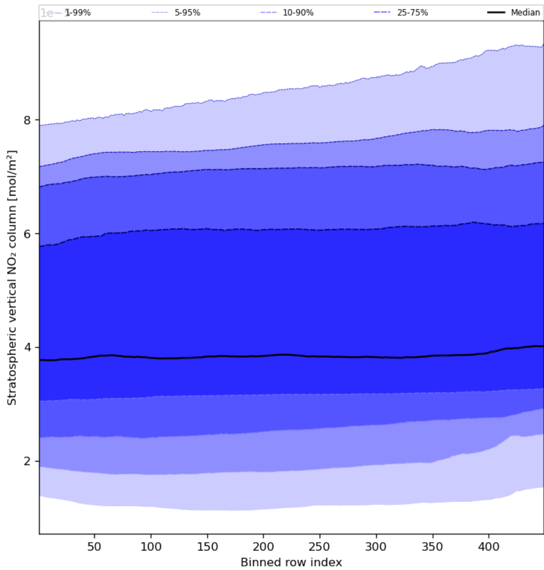
Figure 53: Along track statistics of “Stratospheric vertical NO 2 column” for 2024-02-17 to 2024-02-18
