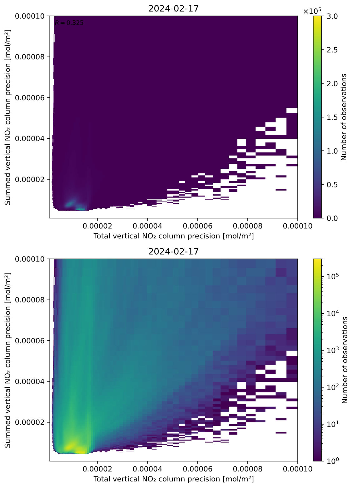
Figure 118: Scatter density plot of “Total vertical NO 2 column precision” against “Summed vertical NO 2 column precision” for 2024-02-17 to 2024-02-18.
