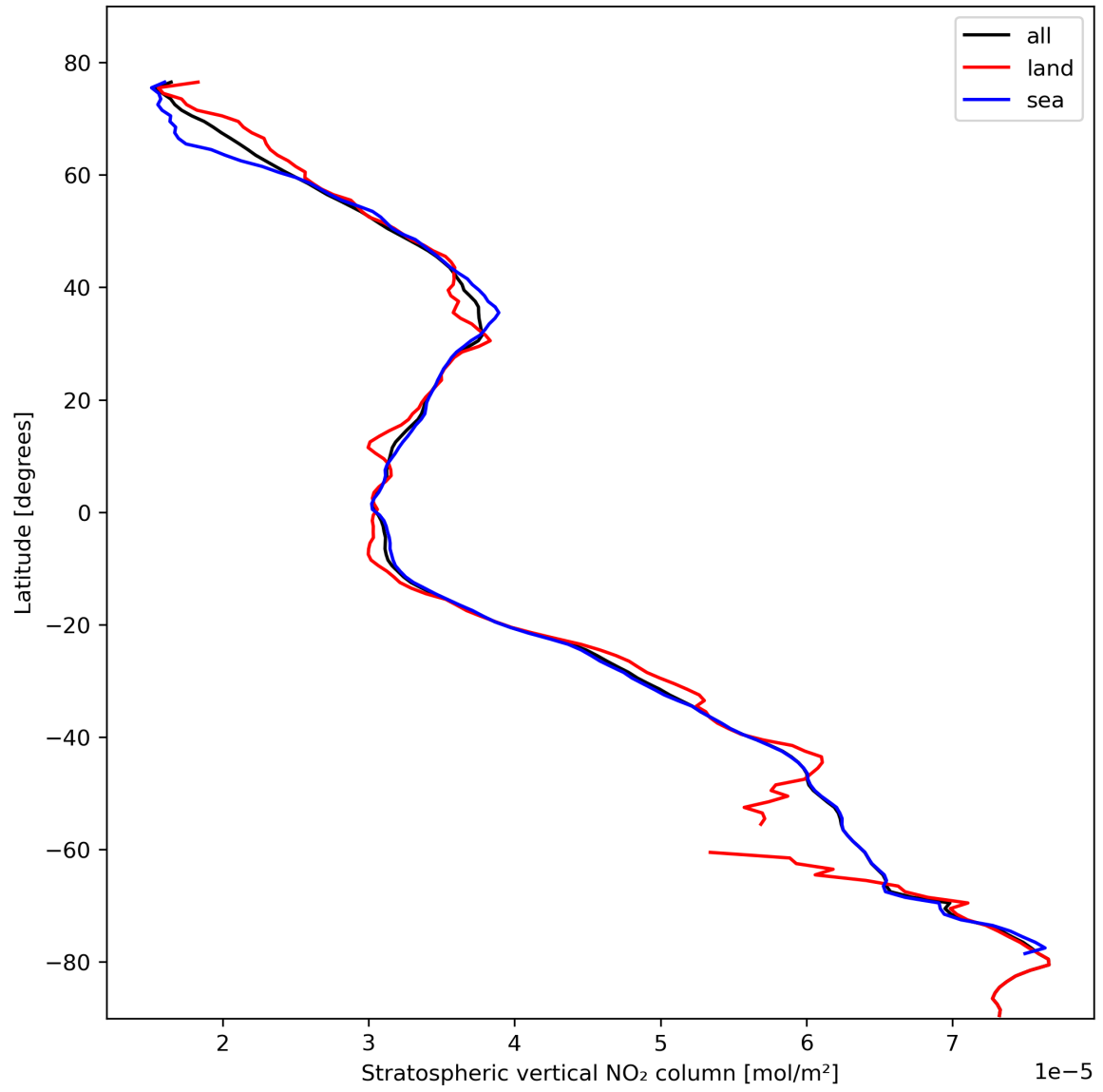
Figure 19: Zonal average of “Stratospheric vertical NO 2 column” for 2024-02-17 to 2024-02-18.
