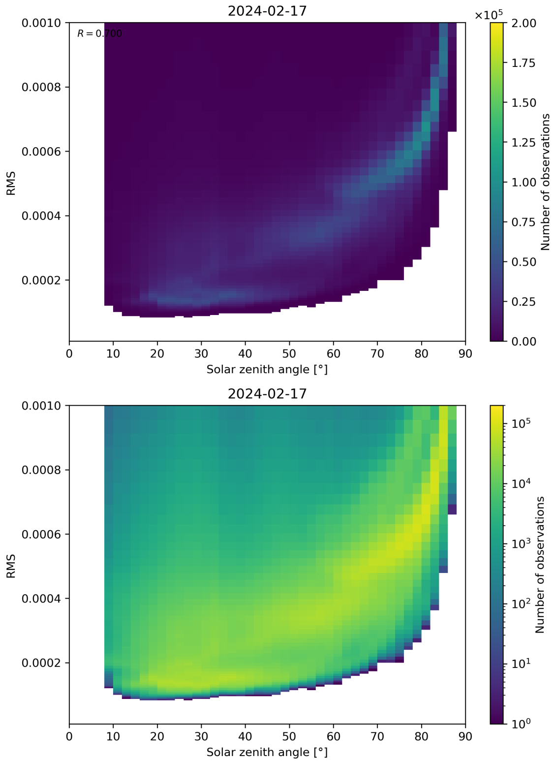
Figure 157: Scatter density plot of “Solar zenith angle” against “RMS” for 2024-02-17 to 2024-02-18.
