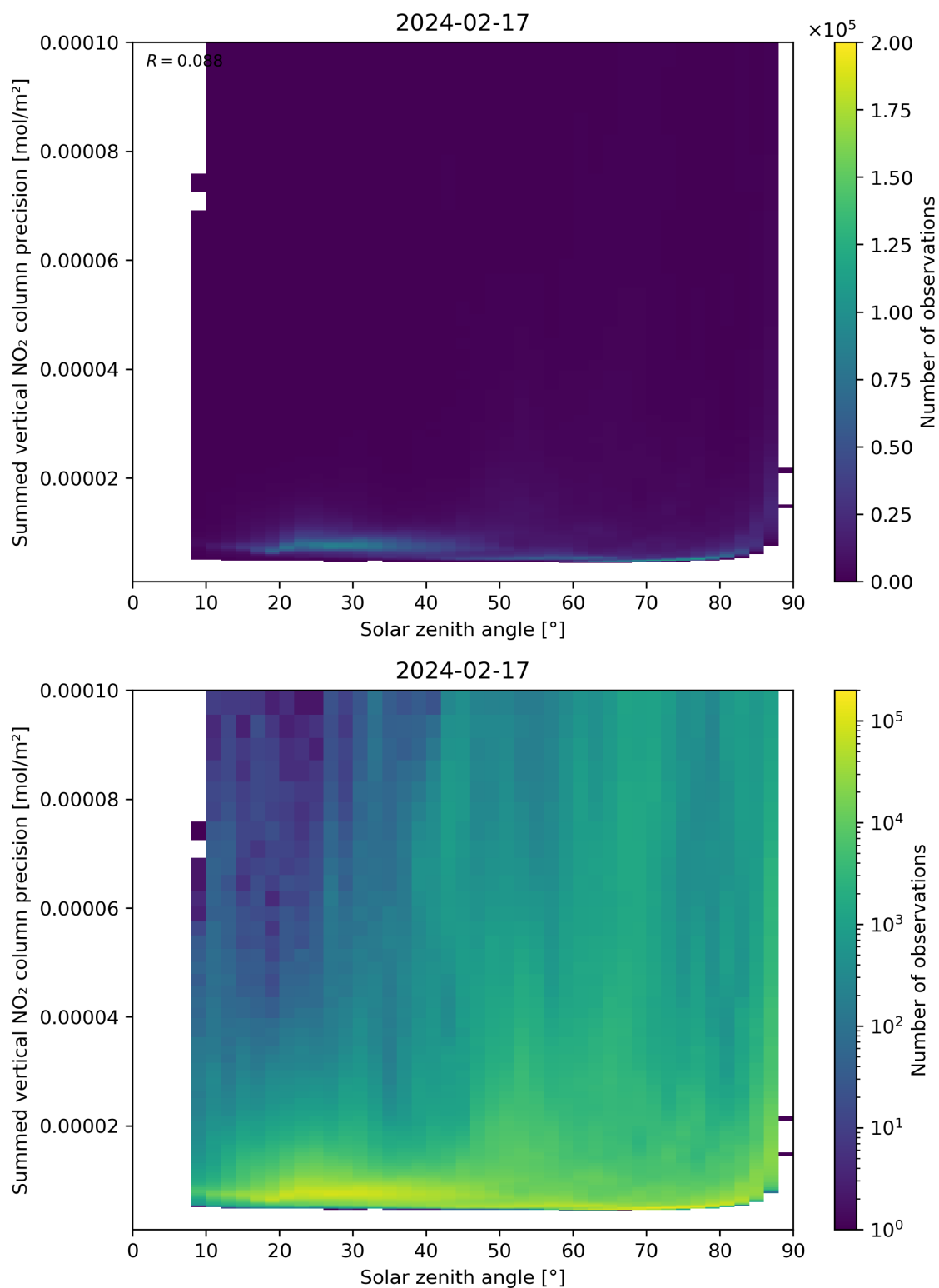
Figure 152: Scatter density plot of “Solar zenith angle” against “Summed vertical NO 2 column precision” for 2024-02-17 to 2024-02-18.
