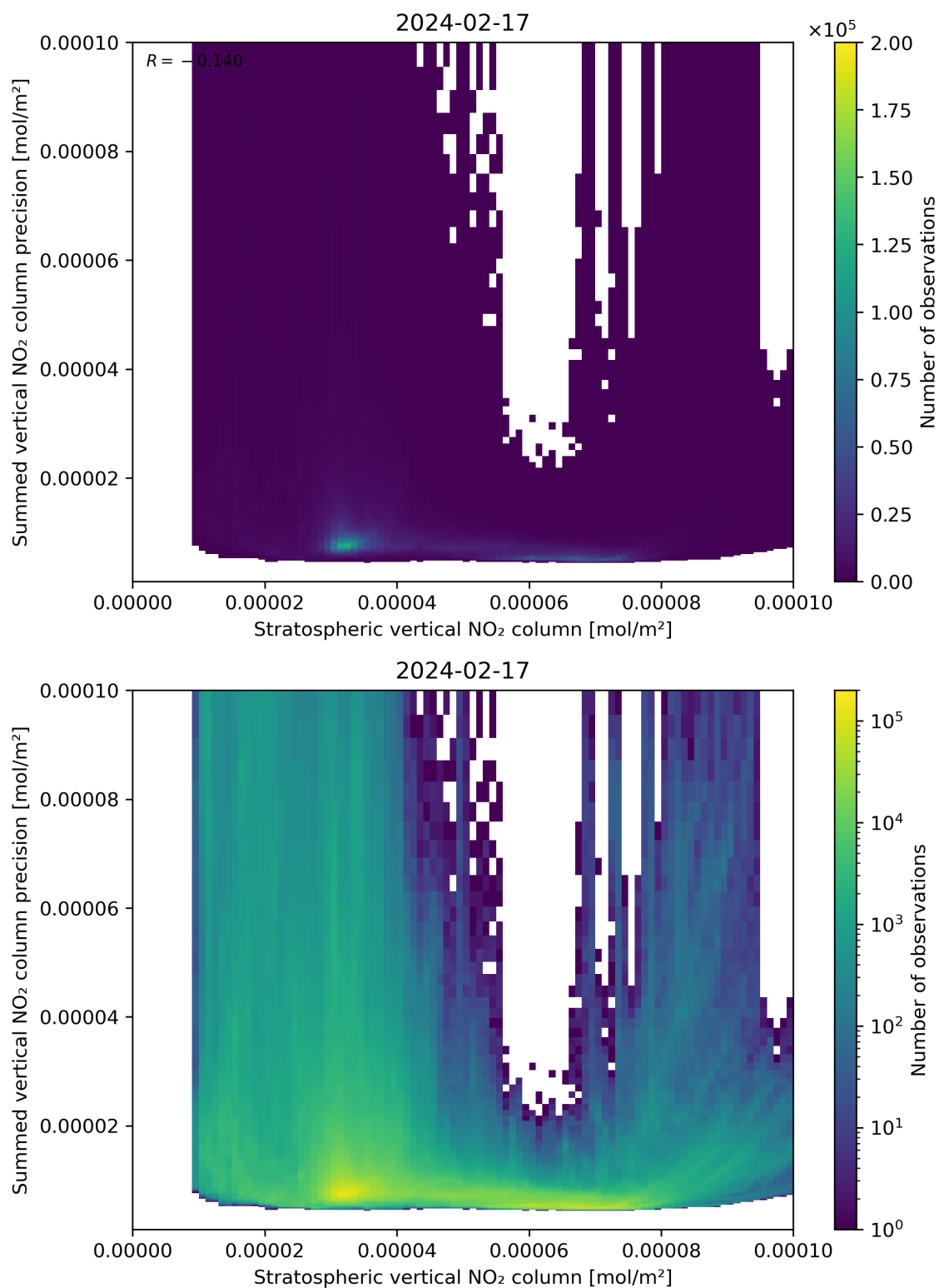
Figure 99: Scatter density plot of “Stratospheric vertical NO 2 column” against “Summed vertical NO 2 column precision” for 2024-02-17 to 2024-02-18.
