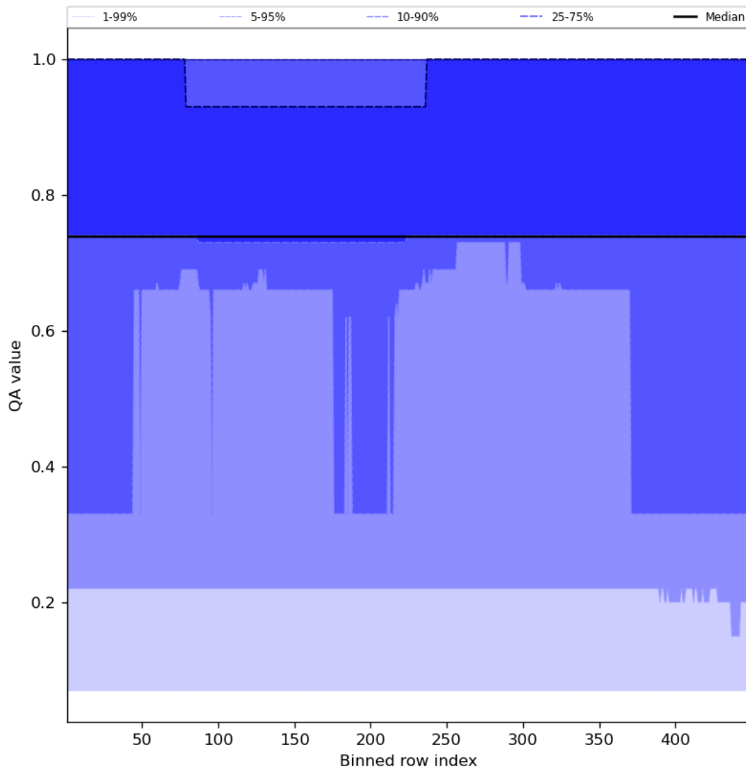
Figure 45: Along track statistics of “QA value” for 2024-02-17 to 2024-02-18
