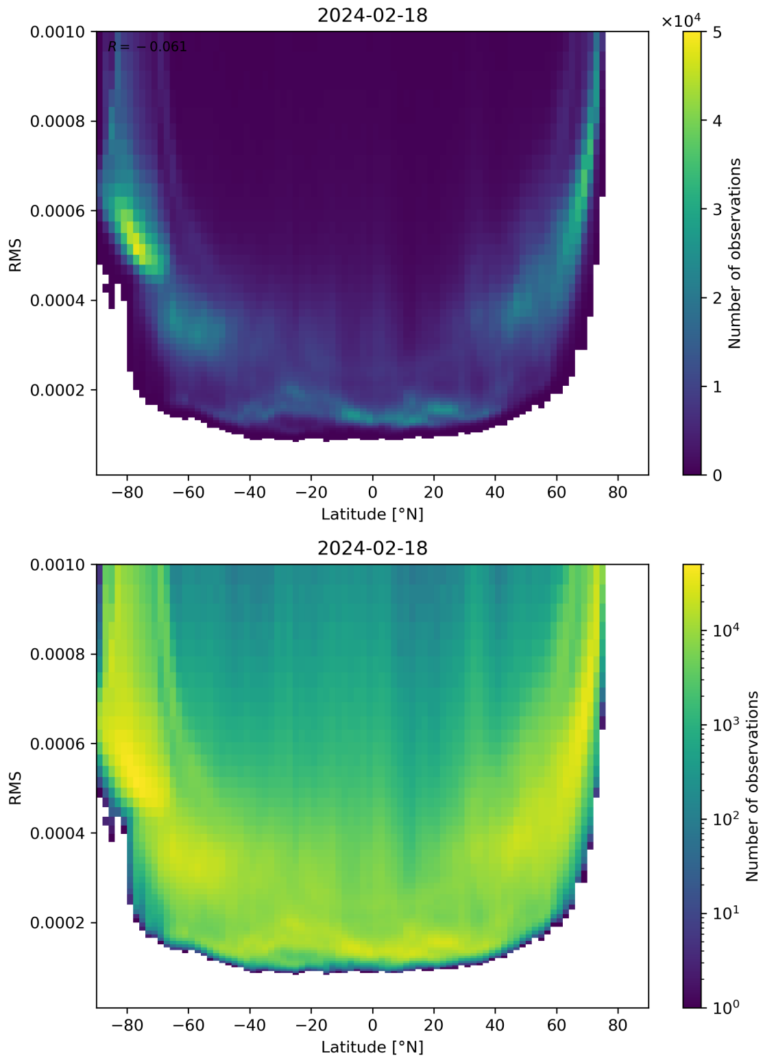
Figure 94: Scatter density plot of “Latitude” against “RMS” for 2024-02-17 to 2024-02-19.
