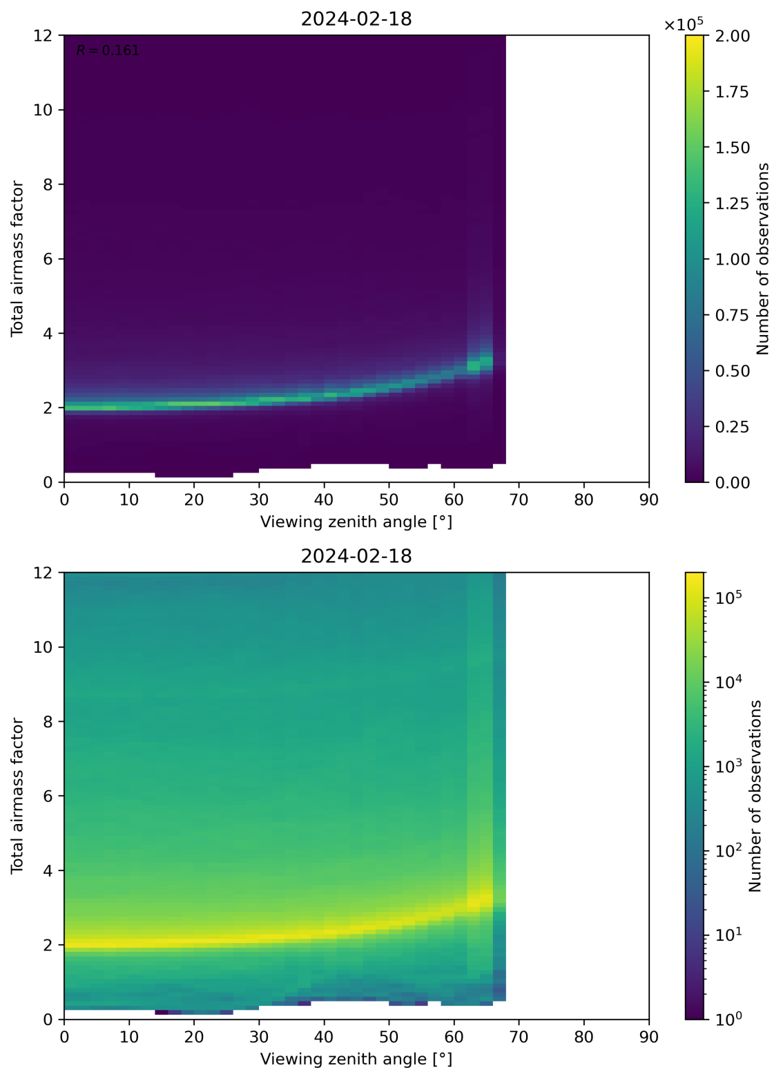
Figure 160: Scatter density plot of “Viewing zenith angle” against “Total airmass factor” for 2024-02-17 to 2024-02-19.
