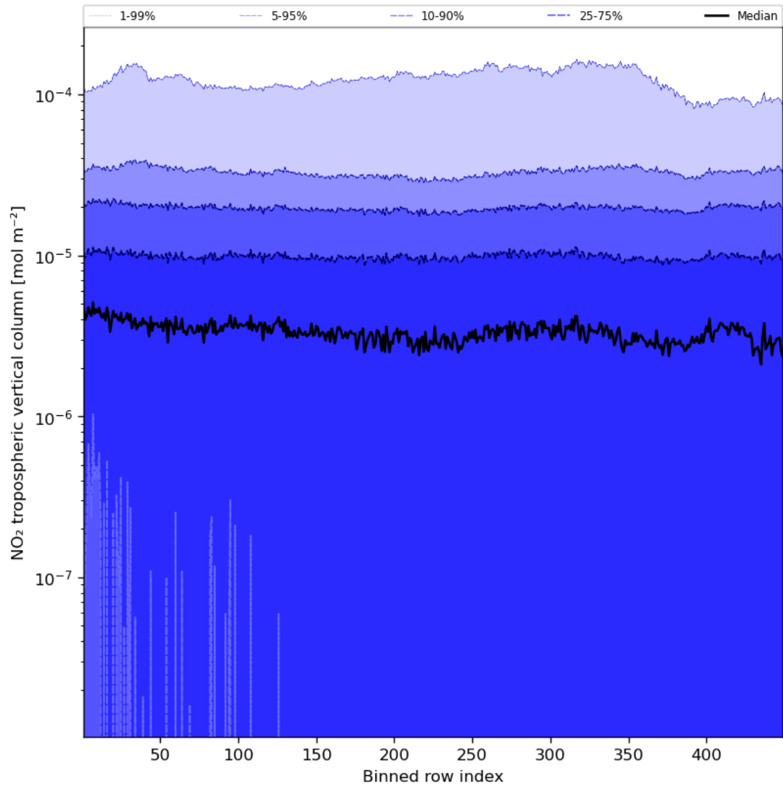
Figure 46: Along track statistics of “NO 2 tropospheric vertical column” for 2024-02-17 to 2024-02-19
