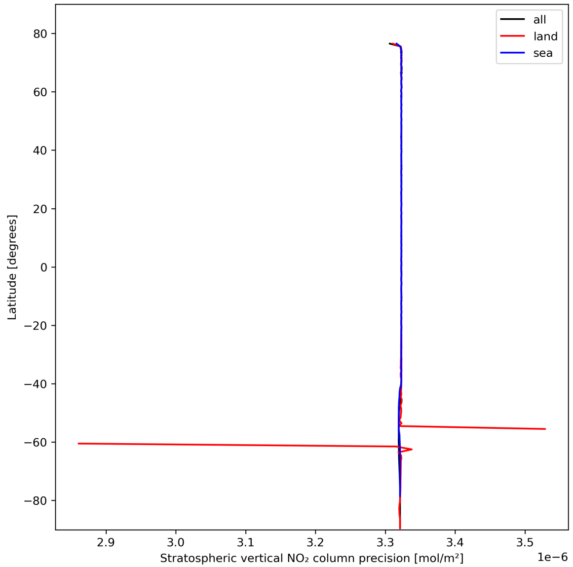
Figure 20: Zonal average of “Stratospheric vertical NO 2 column precision” for 2024-02-17 to 2024-02-19.
