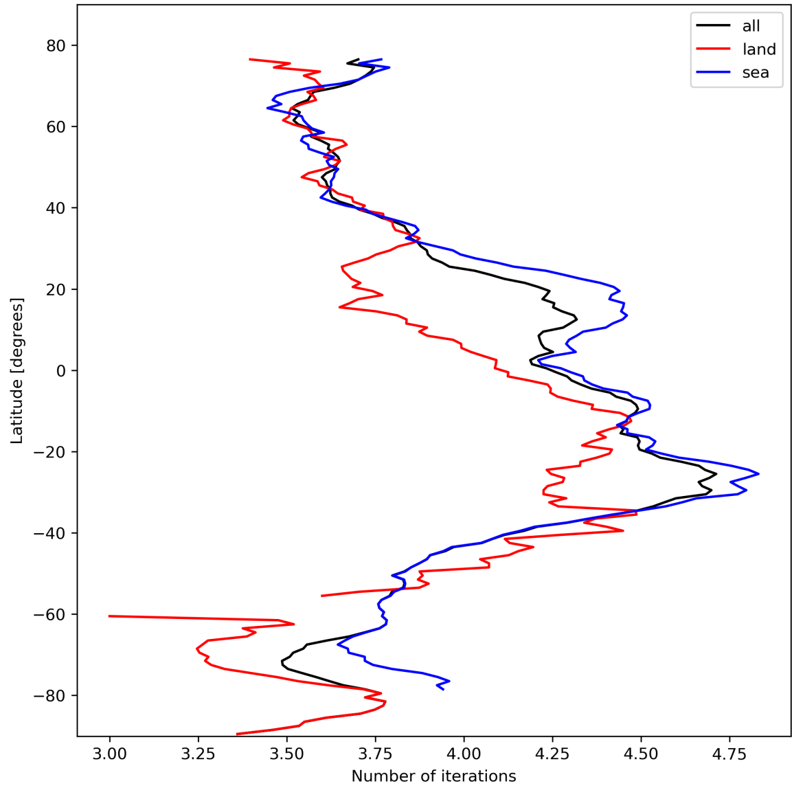
Figure 17: Zonal average of “Number of iterations” for 2024-02-17 to 2024-02-19.
