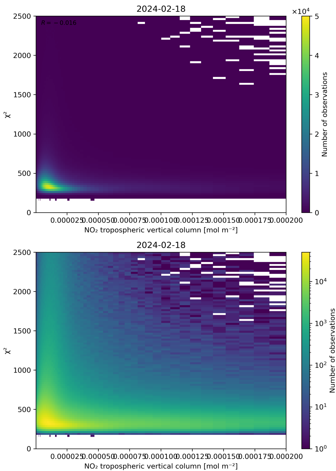
Figure 124: Scatter density plot of “NO 2 tropospheric vertical column” against “ \chi^2 ” for 2024-02-17 to 2024-02-19.
