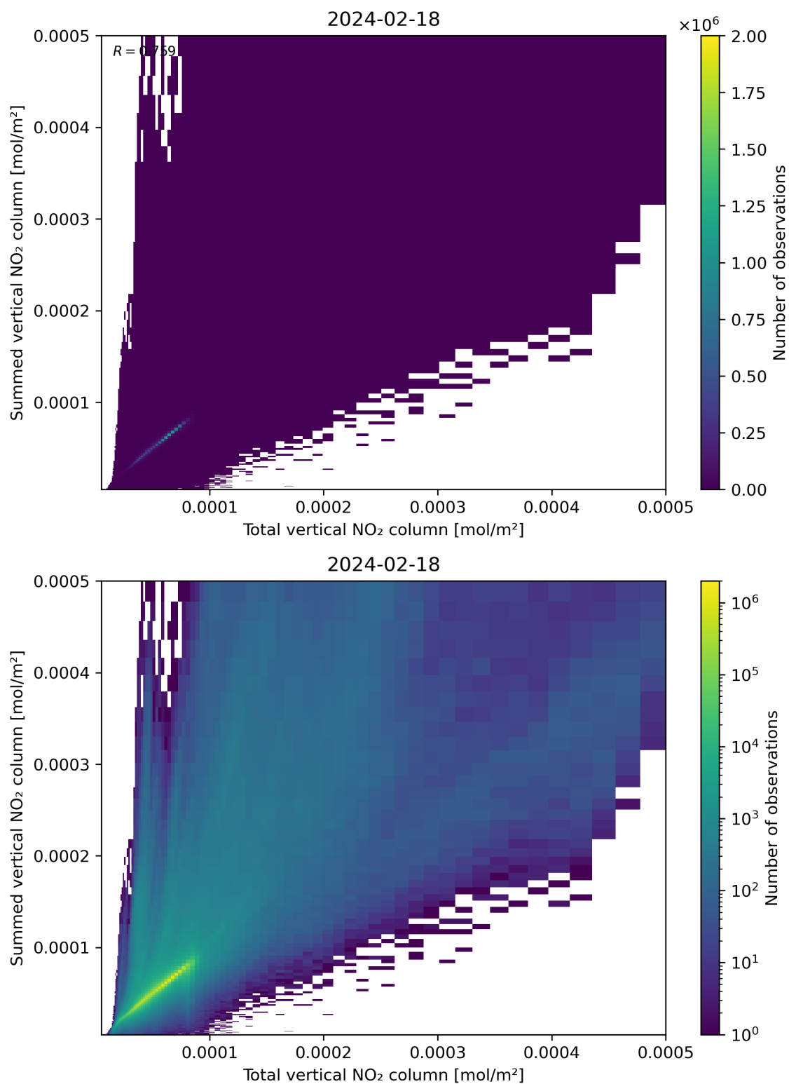
Figure 112: Scatter density plot of “Total vertical NO 2 column” against “Summed vertical NO 2 column” for 2024-02-17 to 2024-02-19.
