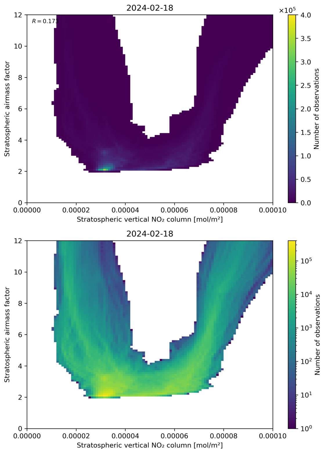
Figure 96: Scatter density plot of “Stratospheric vertical NO 2 column” against “Stratospheric airmass factor” for 2024-02-17 to 2024-02-19.
