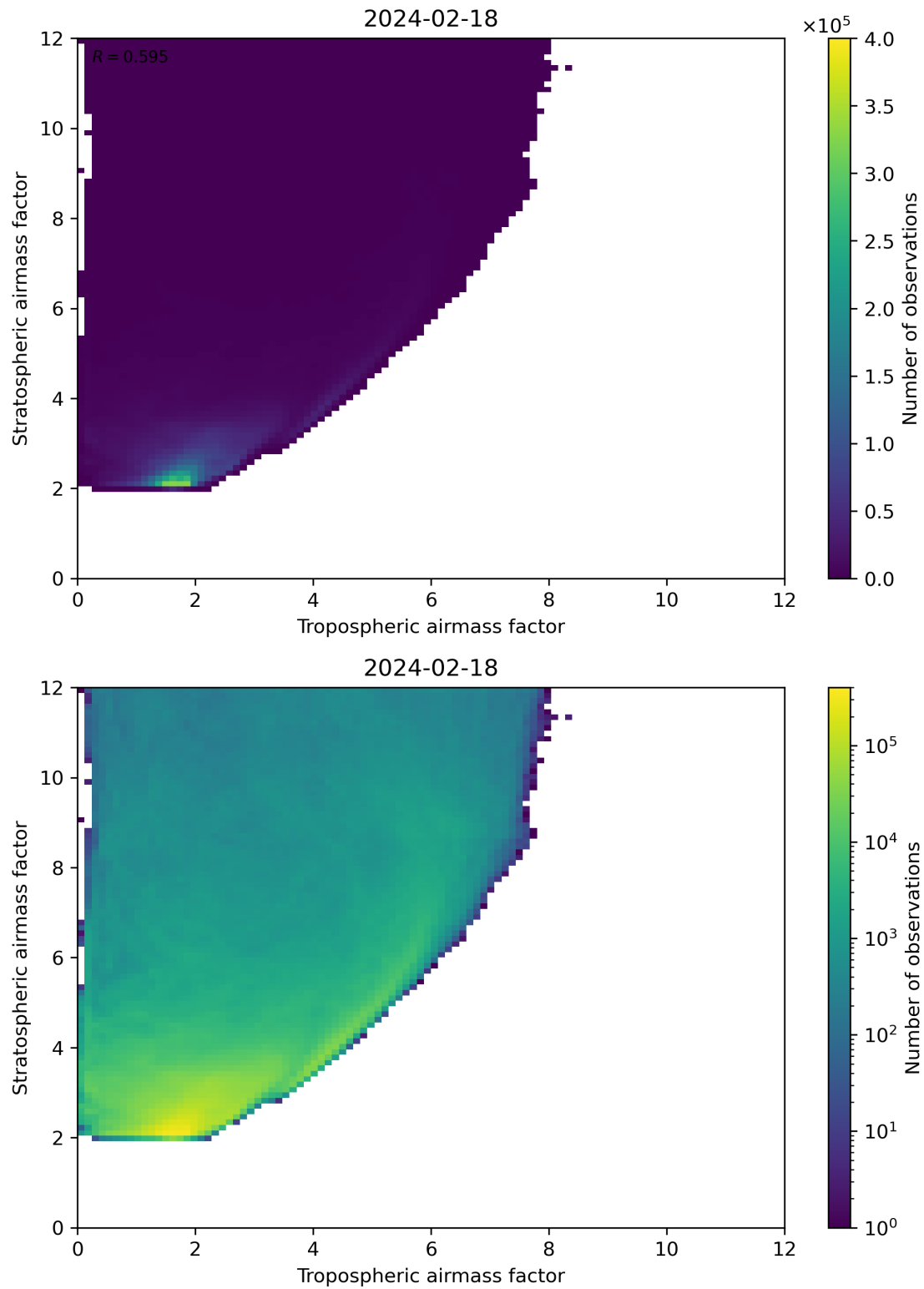
Figure 71: Scatter density plot of “Tropospheric airmass factor” against “Stratospheric airmass factor” for 2024-02-17 to 2024-02-19.
