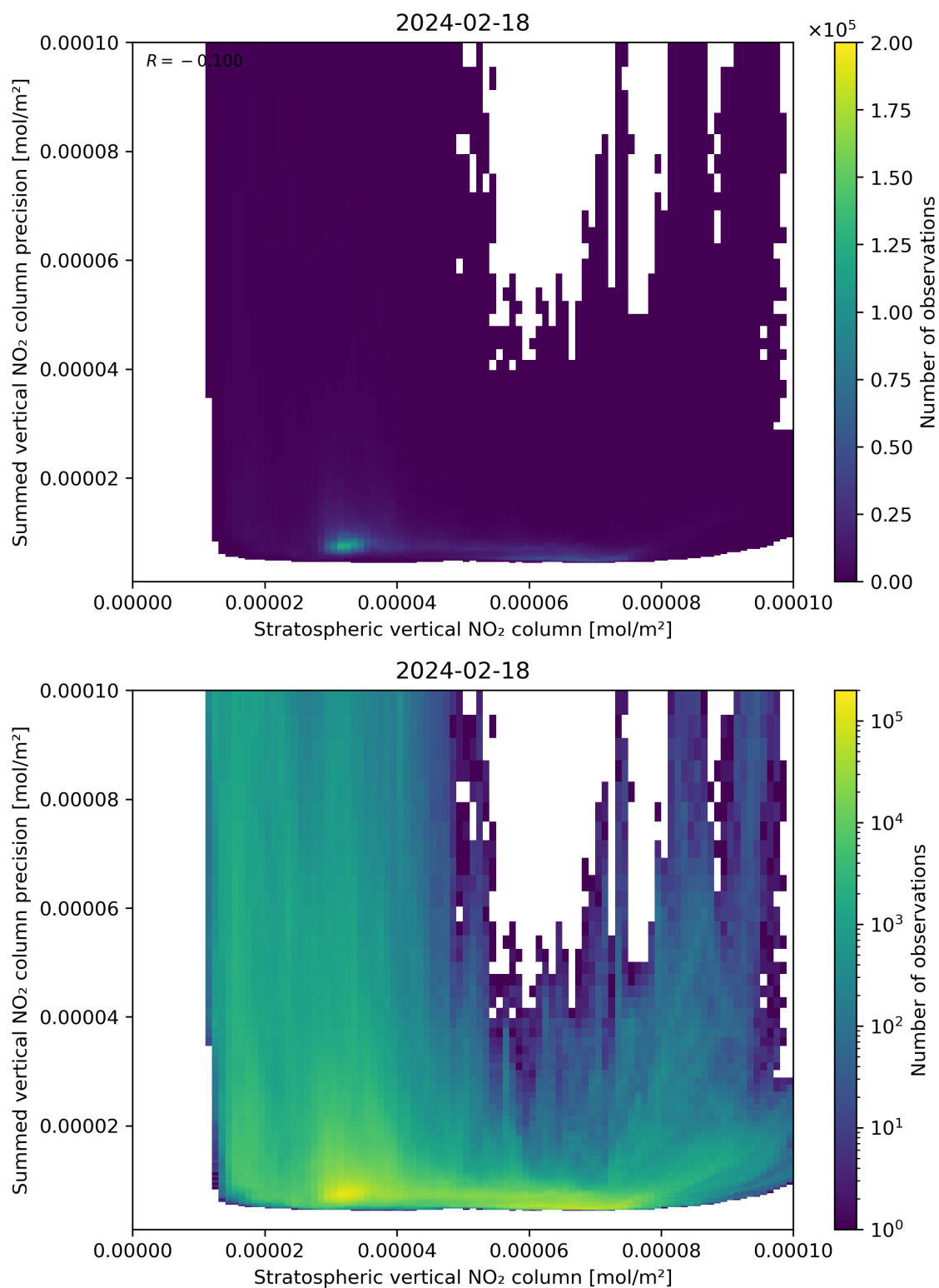
Figure 99: Scatter density plot of “Stratospheric vertical NO 2 column” against “Summed vertical NO 2 column precision” for 2024-02-17 to 2024-02-19.
