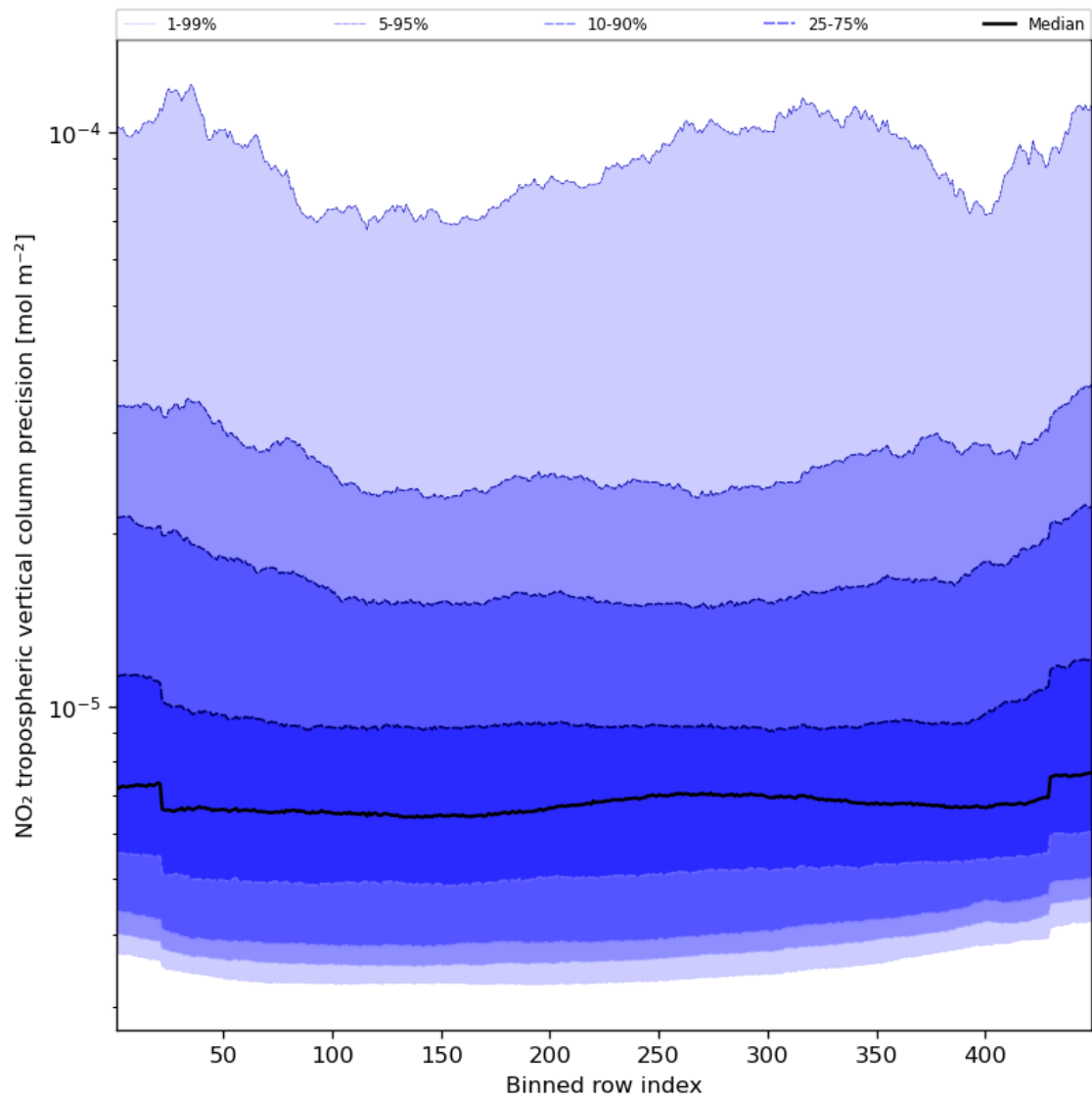
Figure 47: Along track statistics of “NO 2 tropospheric vertical column precision” for 2024-02-17 to 2024-02-19
