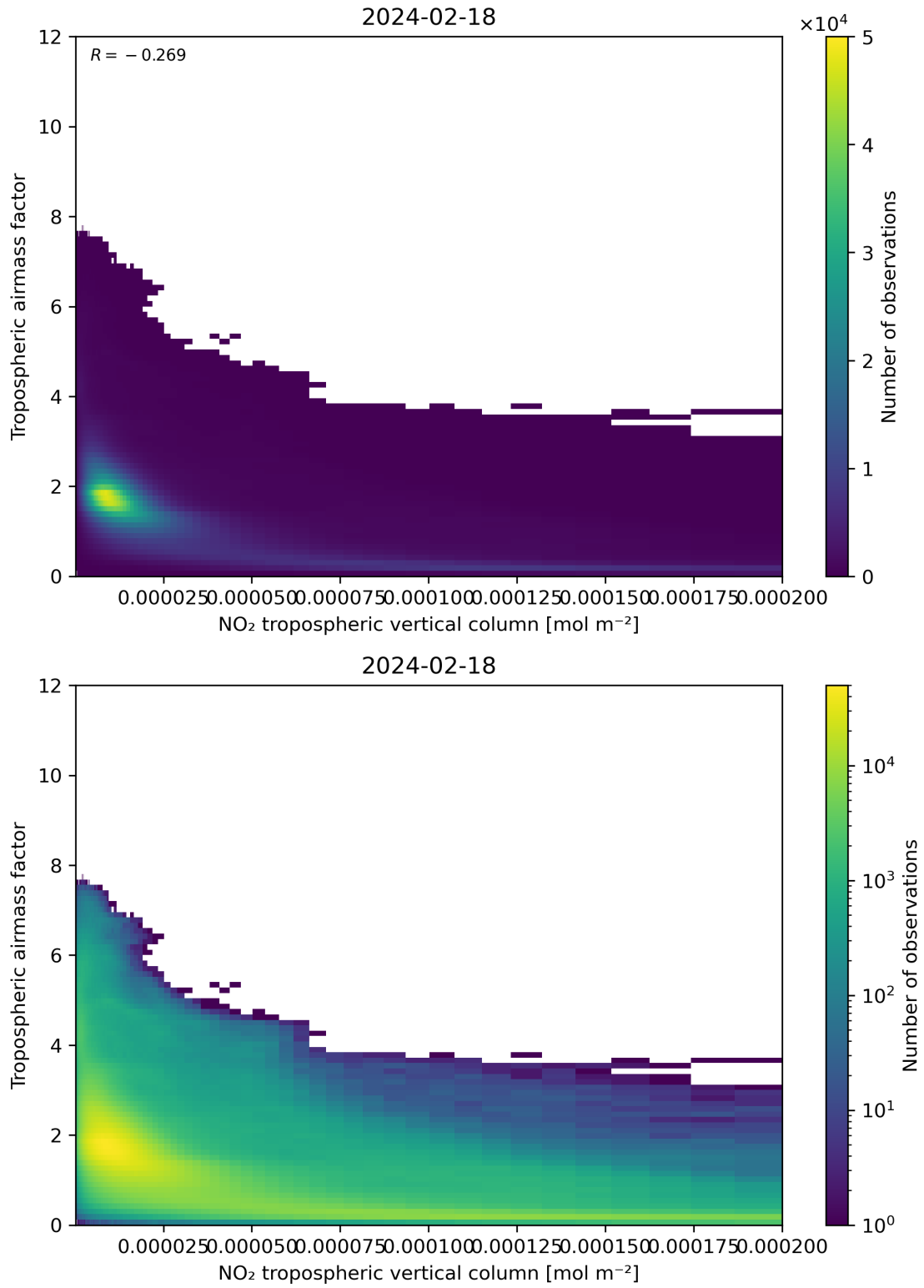
Figure 123: Scatter density plot of “NO 2 tropospheric vertical column” against “Tropospheric air mass factor” for 2024-02-17 to 2024-02-19.
