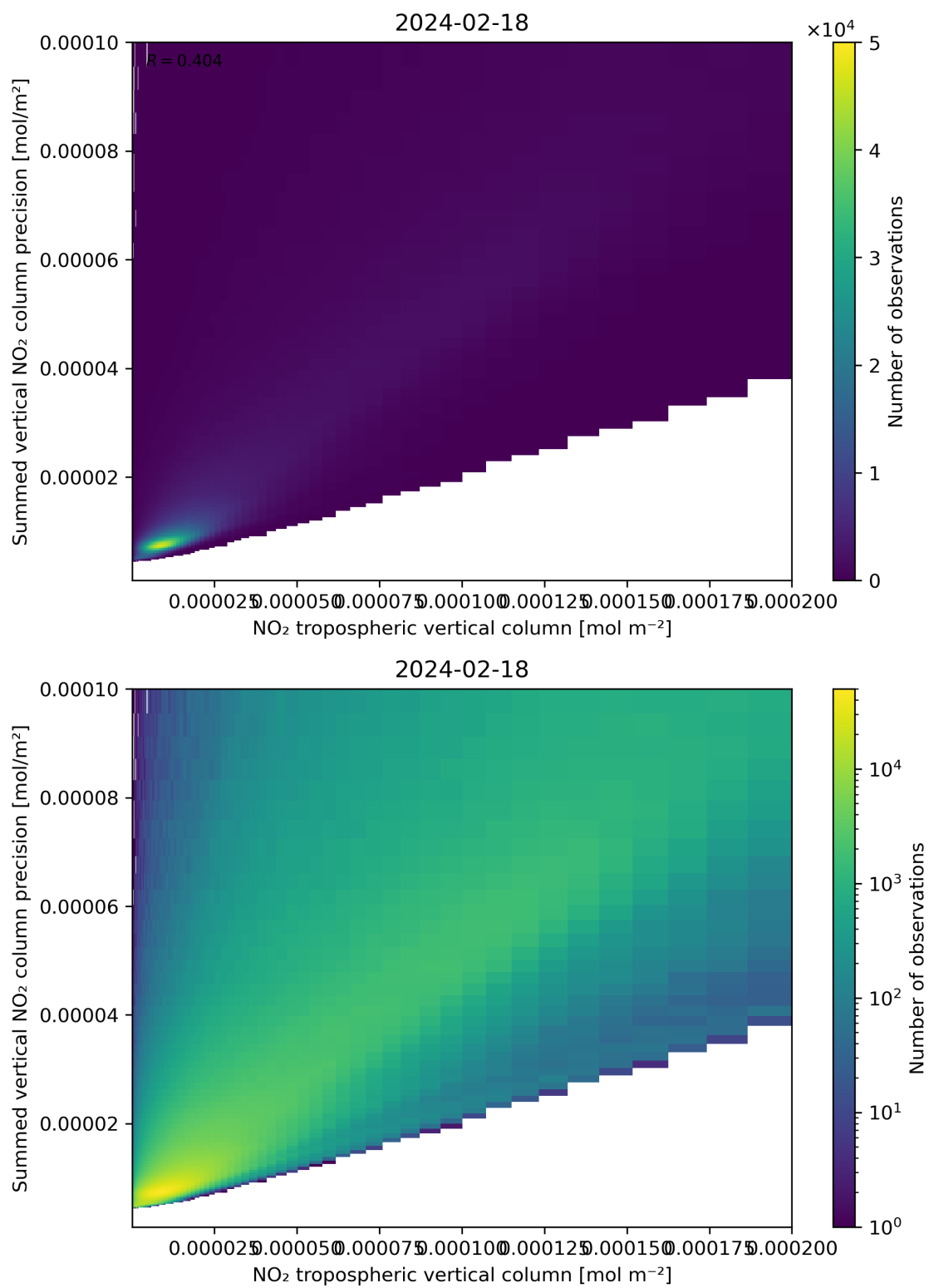
Figure 127: Scatter density plot of “NO 2 tropospheric vertical column” against “Summed vertical NO 2 column precision” for 2024-02-17 to 2024-02-19.
