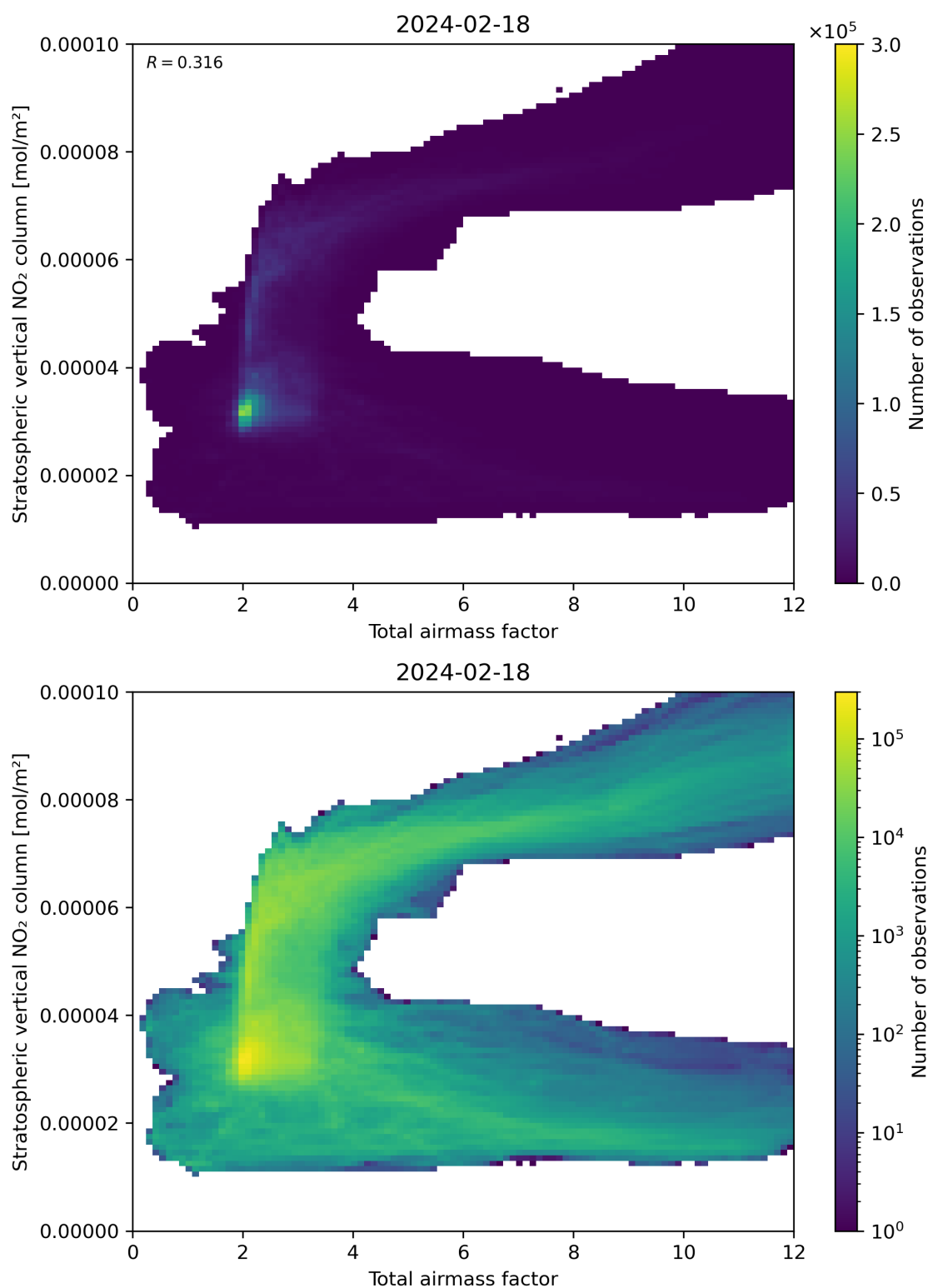
Figure 64: Scatter density plot of “Total airmass factor” against “Stratospheric vertical \text{NO}_2 column” for 2024-02-17 to 2024-02-19.
