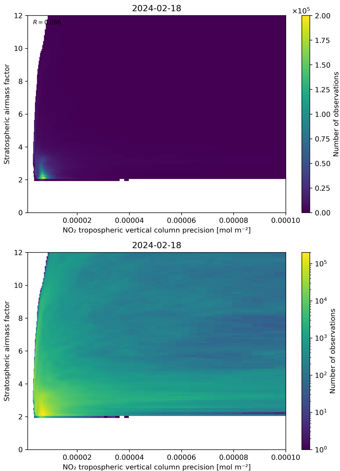
Figure 131: Scatter density plot of “NO 2 tropospheric vertical column precision” against “Stratospheric airmass factor” for 2024-02-17 to 2024-02-19.
