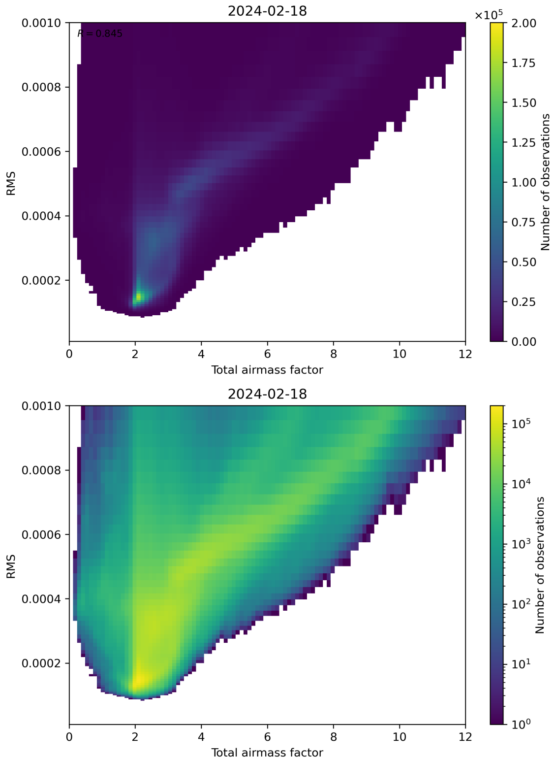
Figure 69: Scatter density plot of “Total airmass factor” against “RMS” for 2024-02-17 to 2024-02-19.
