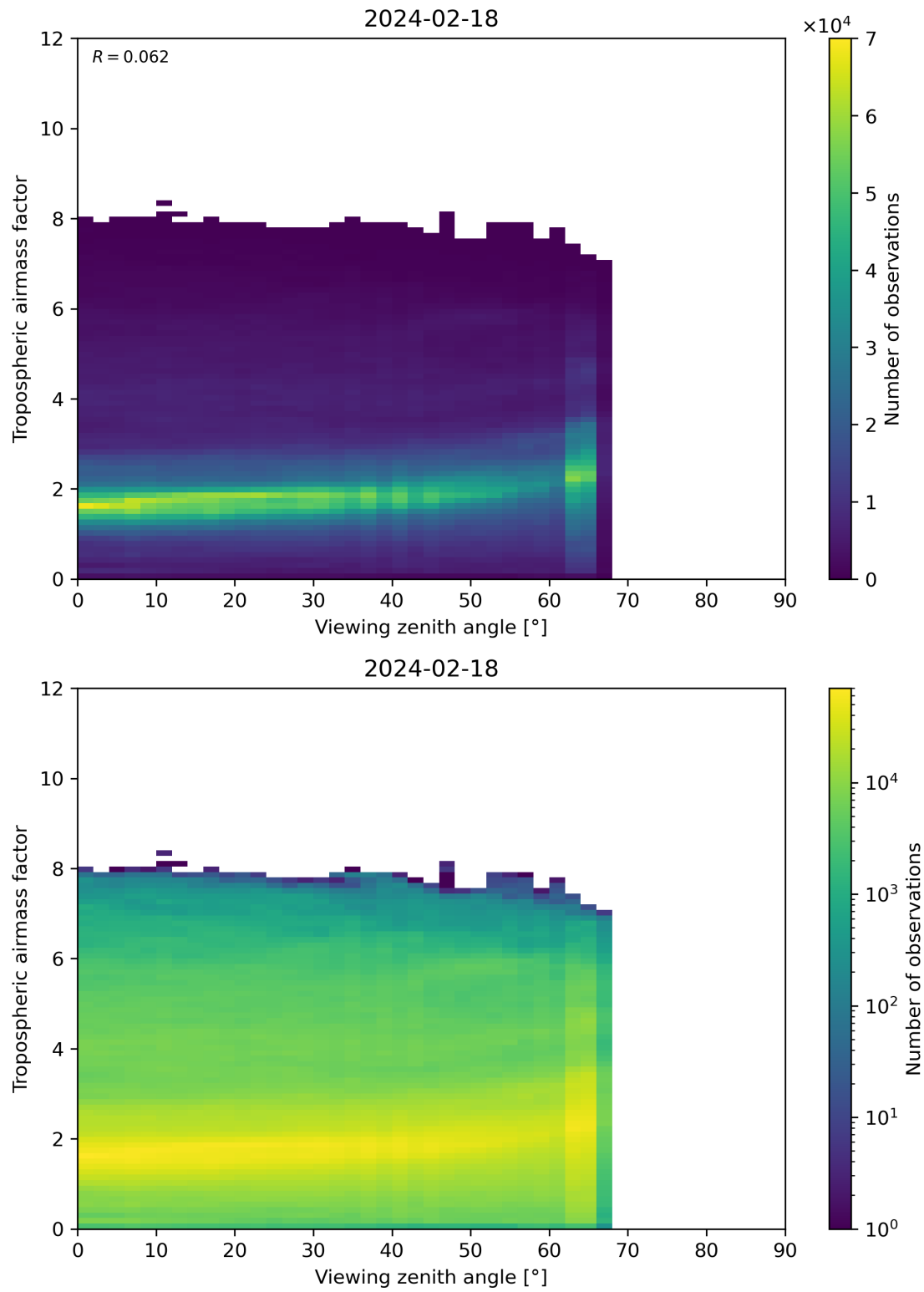
Figure 161: Scatter density plot of “Viewing zenith angle” against “Tropospheric airmass factor” for 2024-02-17 to 2024-02-19.
