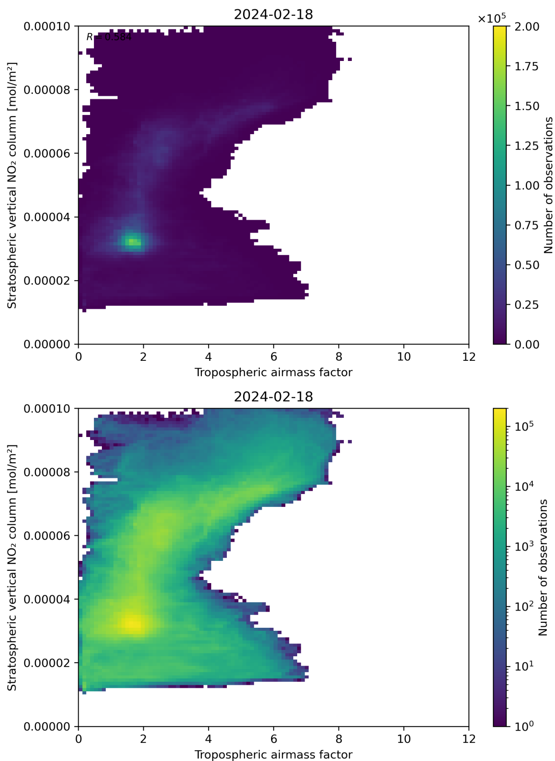
Figure 74: Scatter density plot of “Tropospheric air mass factor” against “Stratospheric vertical NO 2 column” for 2024-02-17 to 2024-02-19.
