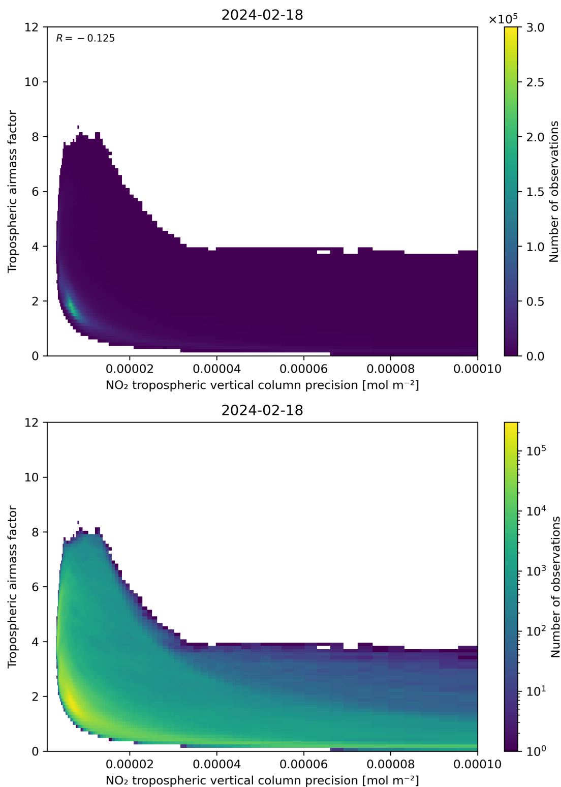
Figure 133: Scatter density plot of “NO 2 tropospheric vertical column precision” against “Tropospheric airmass factor” for 2024-02-17 to 2024-02-19.
