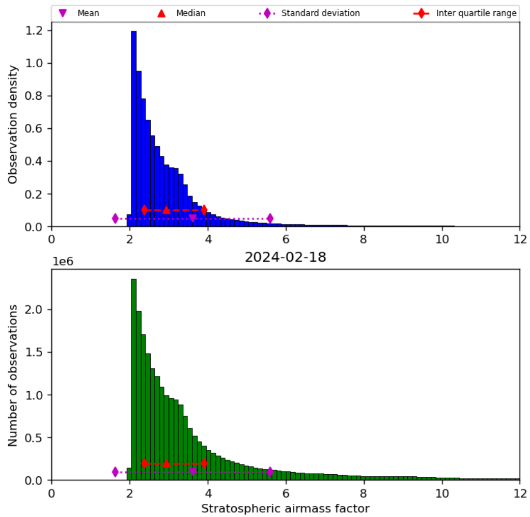
Figure 44: Histogram of “Stratospheric airmass factor” for 2024-02-17 to 2024-02-19
