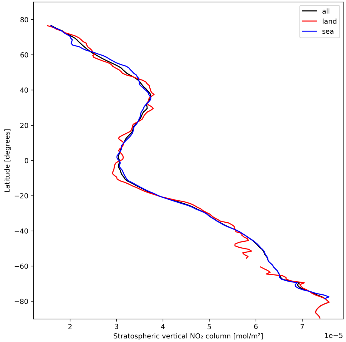
Figure 19: Zonal average of “Stratospheric vertical NO 2 column” for 2024-02-17 to 2024-02-19.
