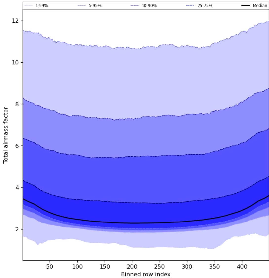
Figure 49: Along track statistics of “Total airmass factor” for 2024-02-17 to 2024-02-19
