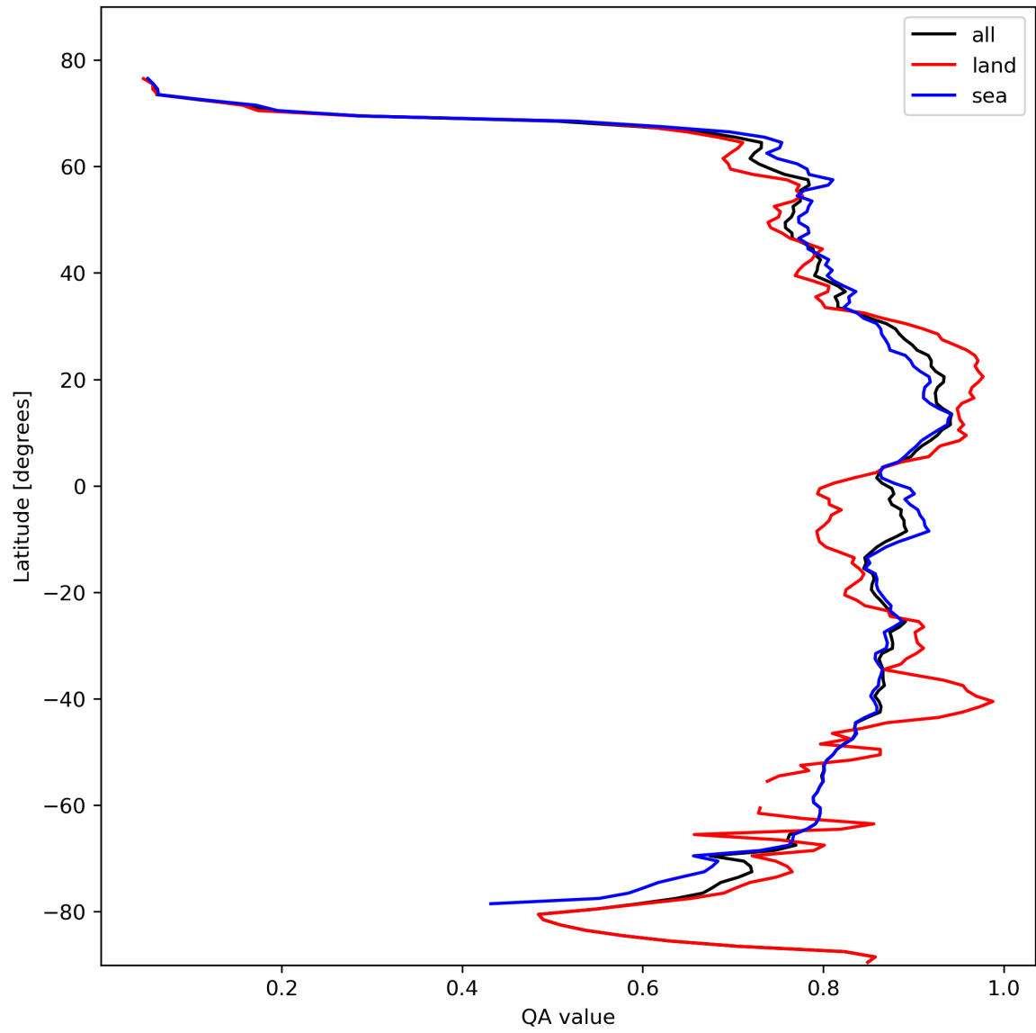
Figure 11: Zonal average of “QA value” for 2024-02-17 to 2024-02-19.
