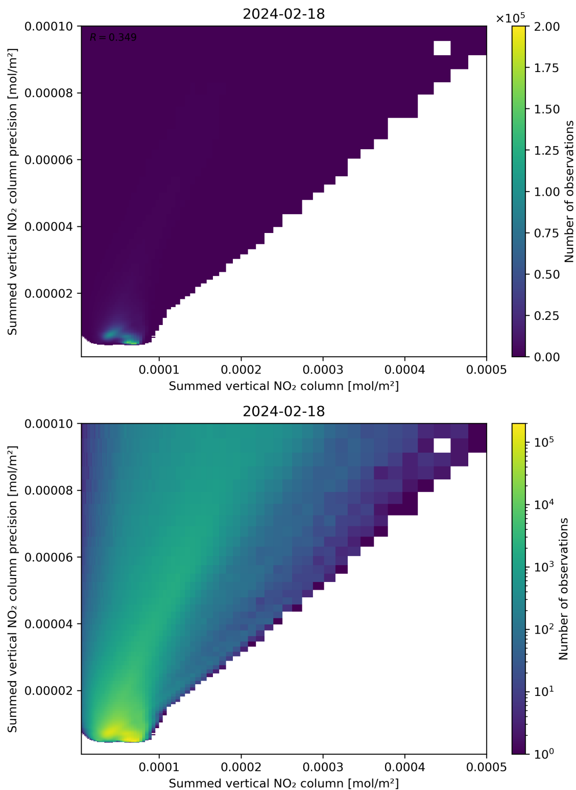
Figure 105: Scatter density plot of “Summed vertical NO 2 column” against “Summed vertical NO 2 column precision” for 2024-02-17 to 2024-02-19.
