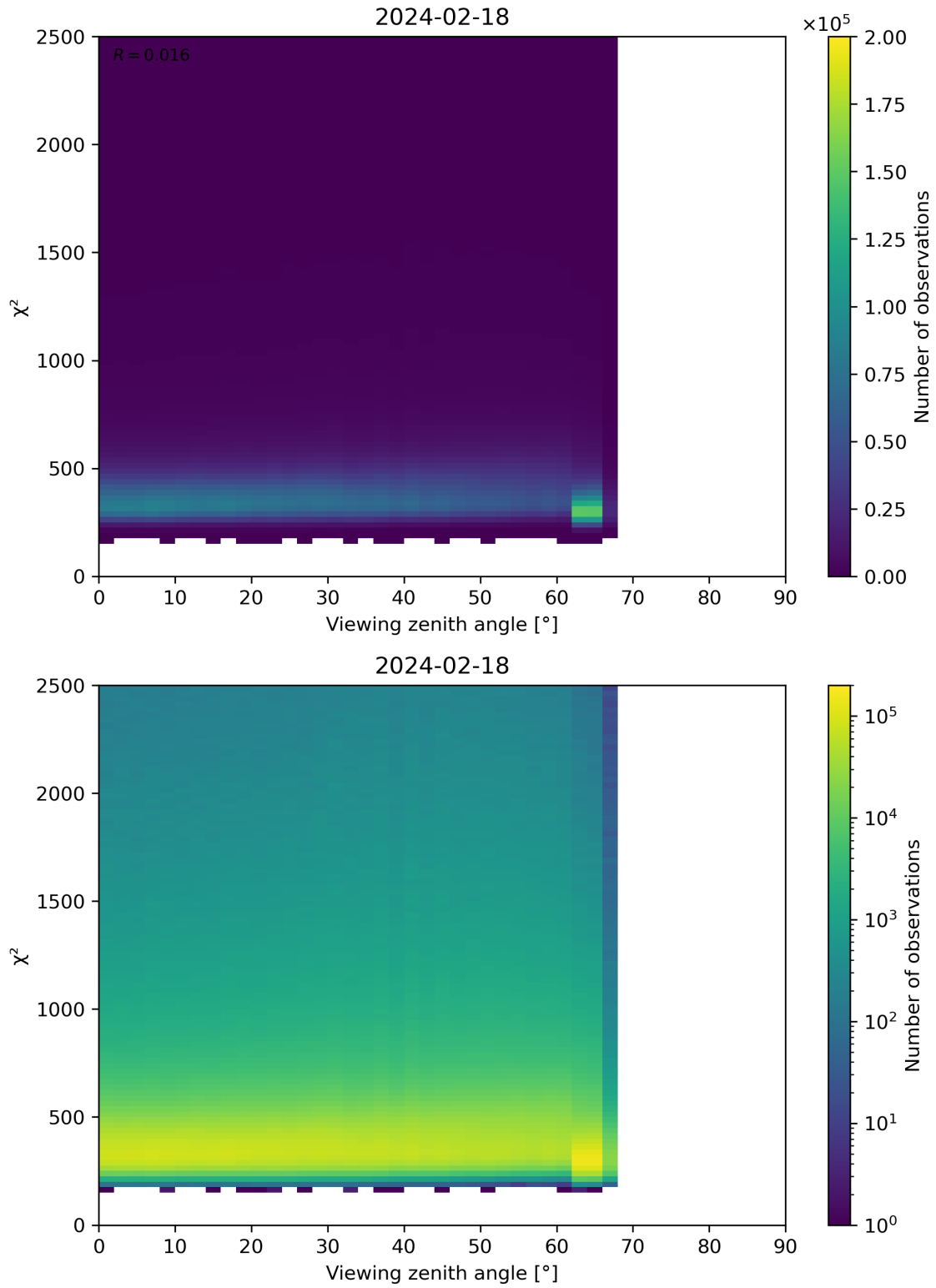
Figure 162: Scatter density plot of “Viewing zenith angle” against “ \chi^2 ” for 2024-02-17 to 2024-02-19.
