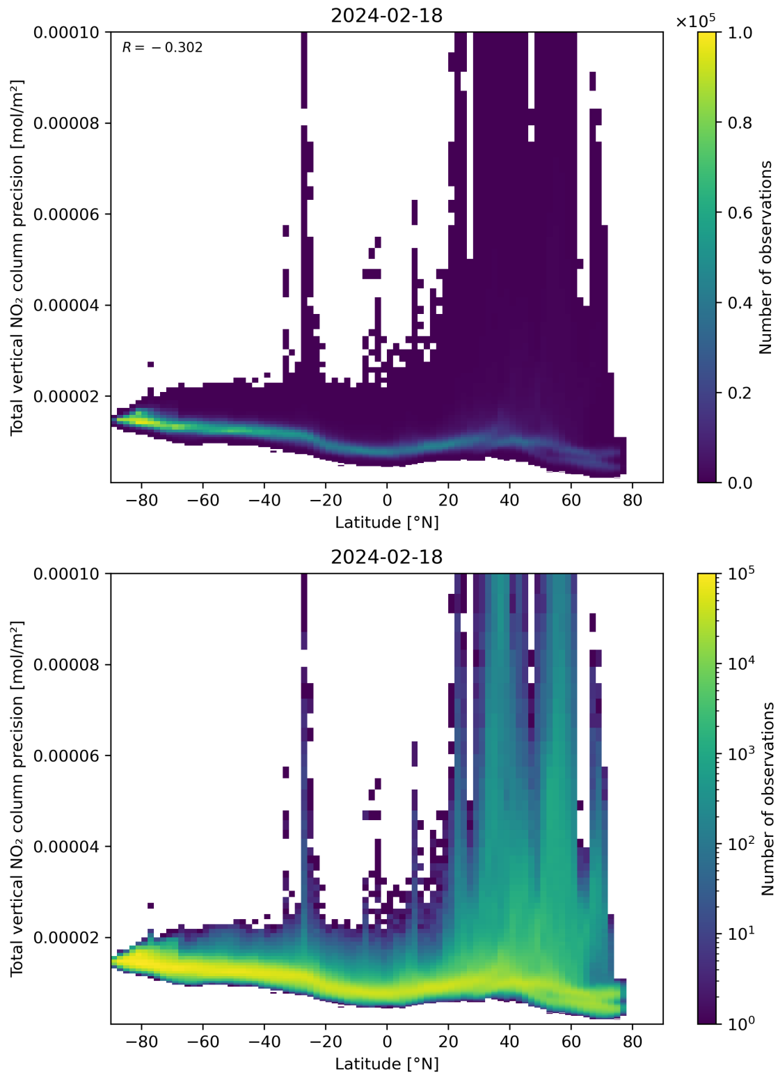
Figure 91: Scatter density plot of “Latitude” against “Total vertical NO 2 column precision” for 2024-02-17 to 2024-02-19.
