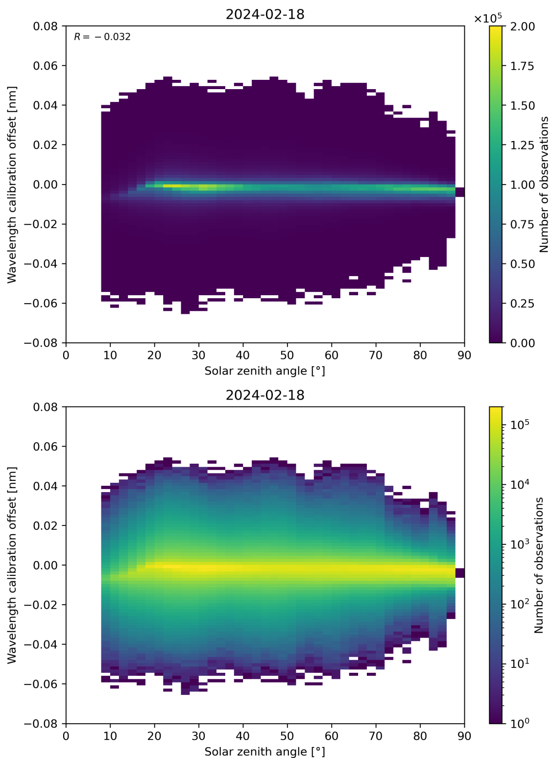
Figure 158: Scatter density plot of “Solar zenith angle” against “Wavelength calibration offset” for 2024-02-17 to 2024-02-19.
