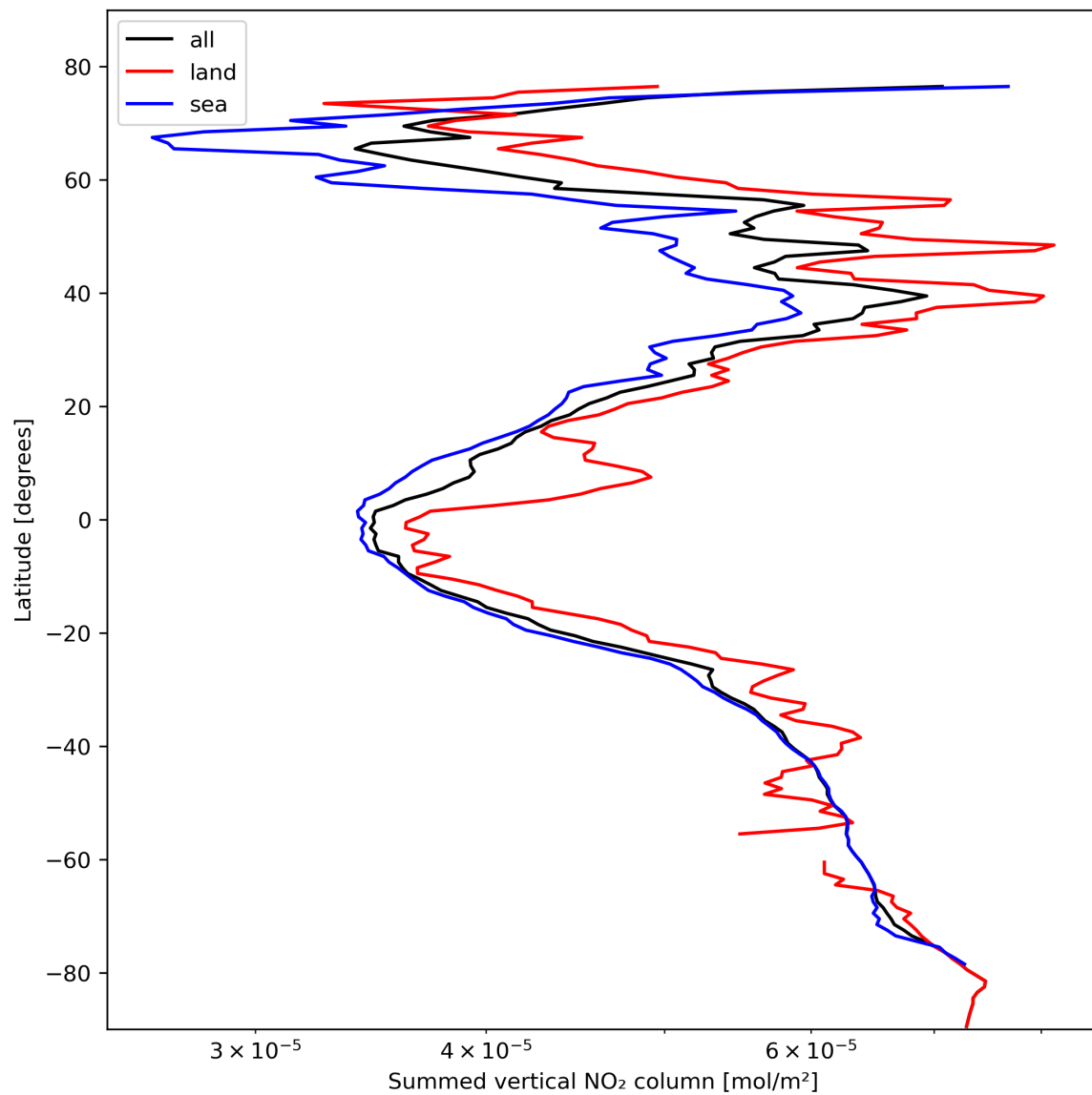
Figure 23: Zonal average of “Summed vertical NO 2 column” for 2024-02-17 to 2024-02-19.
