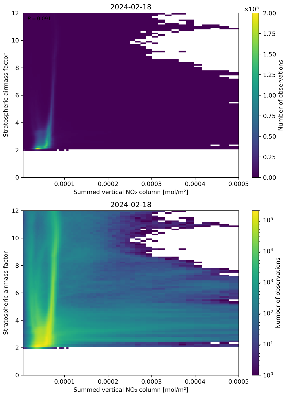
Figure 103: Scatter density plot of “Summed vertical NO 2 column” against “Stratospheric air mass factor” for 2024-02-17 to 2024-02-19.
