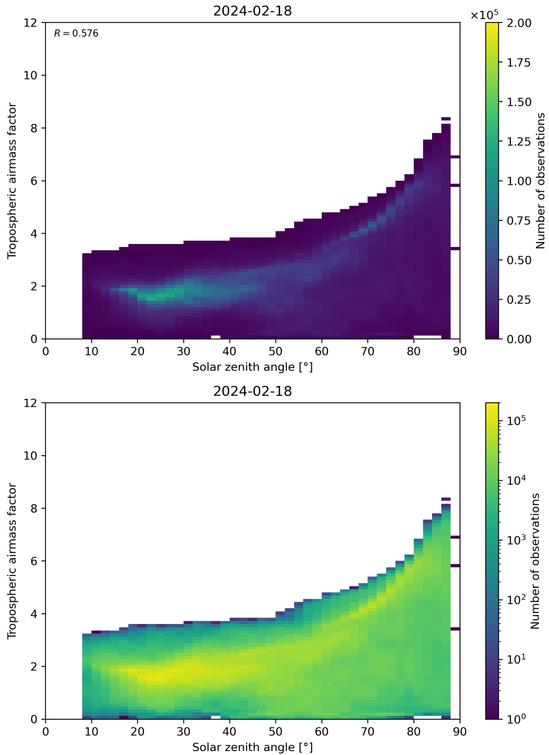
Figure 147: Scatter density plot of “Solar zenith angle” against “Tropospheric airmass factor” for 2024-02-17 to 2024-02-19.
