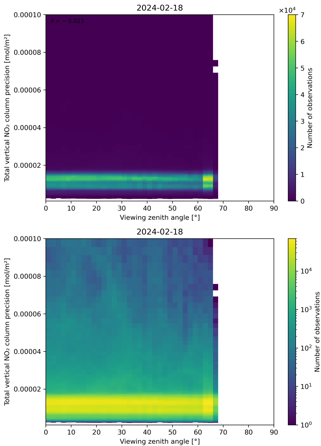
Figure 168: Scatter density plot of “Viewing zenith angle” against “Total vertical NO 2 column precision” for 2024-02-17 to 2024-02-19.
