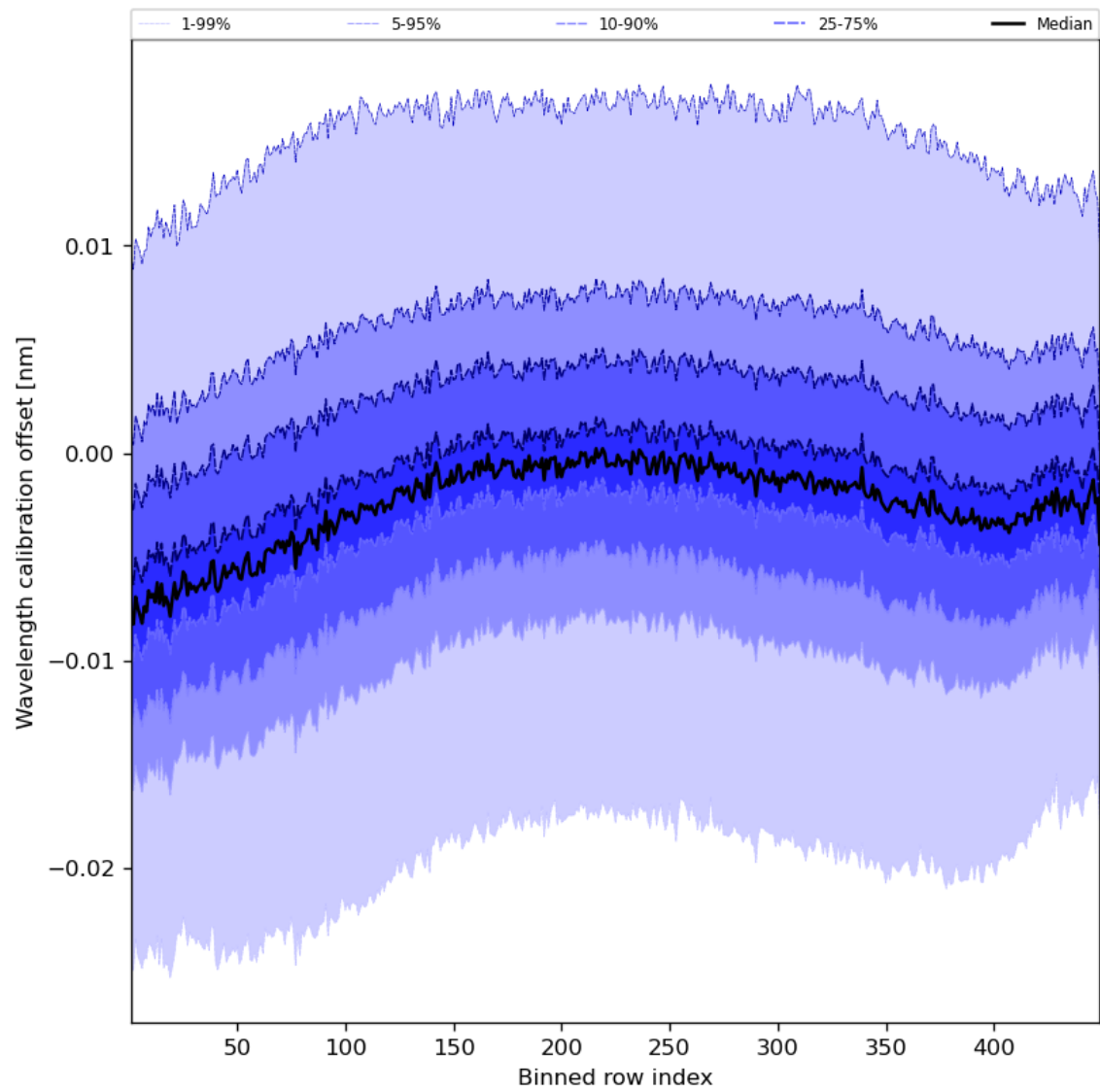
Figure 52: Along track statistics of “Wavelength calibration offset” for 2024-02-17 to 2024-02-19
