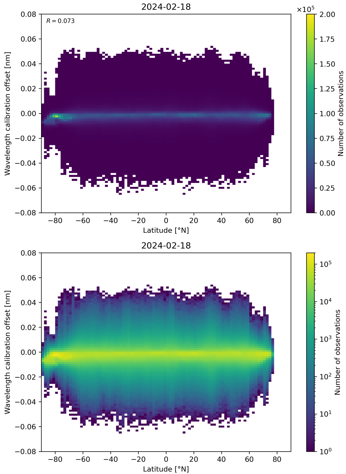
Figure 95: Scatter density plot of “Latitude” against “Wavelength calibration offset” for 2024-02-17 to 2024-02-19.
