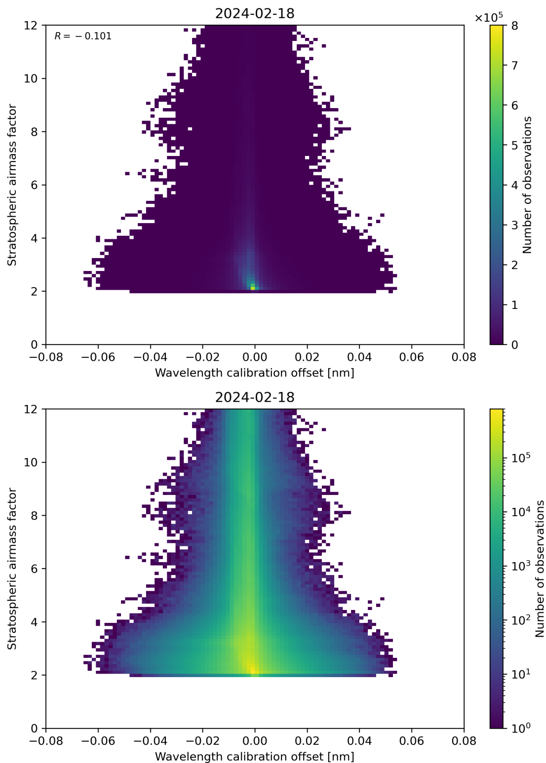
Figure 174: Scatter density plot of “Wavelength calibration offset” against “Stratospheric airmass factor” for 2024-02-17 to 2024-02-19.
