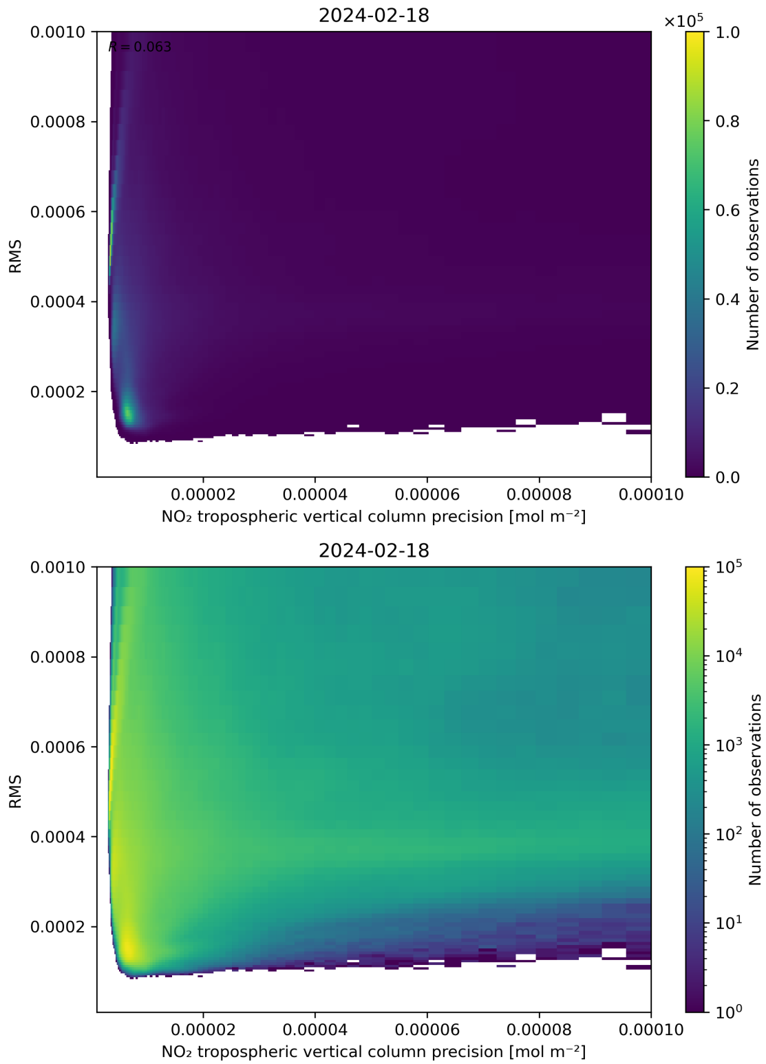
Figure 140: Scatter density plot of “NO 2 tropospheric vertical column precision” against “RMS” for 2024-02-17 to 2024-02-19.
