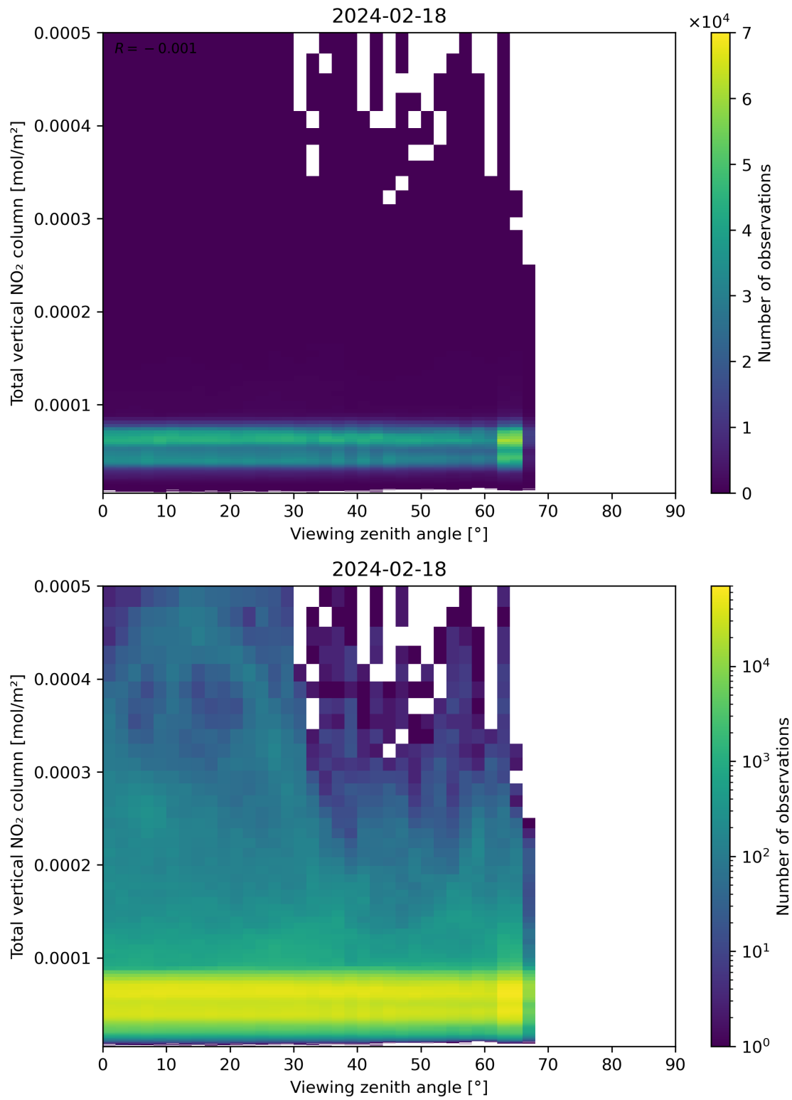
Figure 167: Scatter density plot of “Viewing zenith angle” against “Total vertical NO 2 column” for 2024-02-17 to 2024-02-19.
