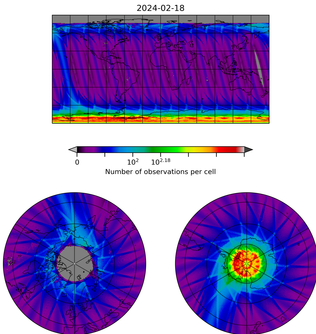
Figure 10: Map of the number of observations for 2024-02-17 to 2024-02-19
