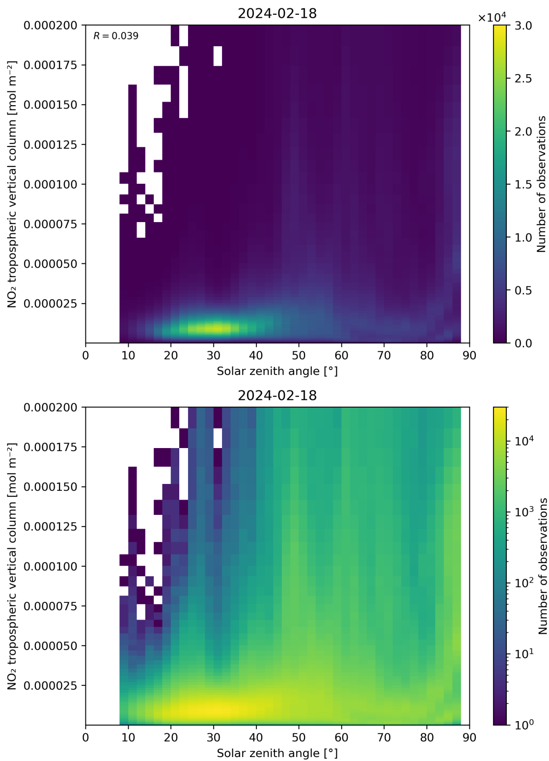
Figure 155: Scatter density plot of “Solar zenith angle” against “NO 2 tropospheric vertical column” for 2024-02-17 to 2024-02-19.
