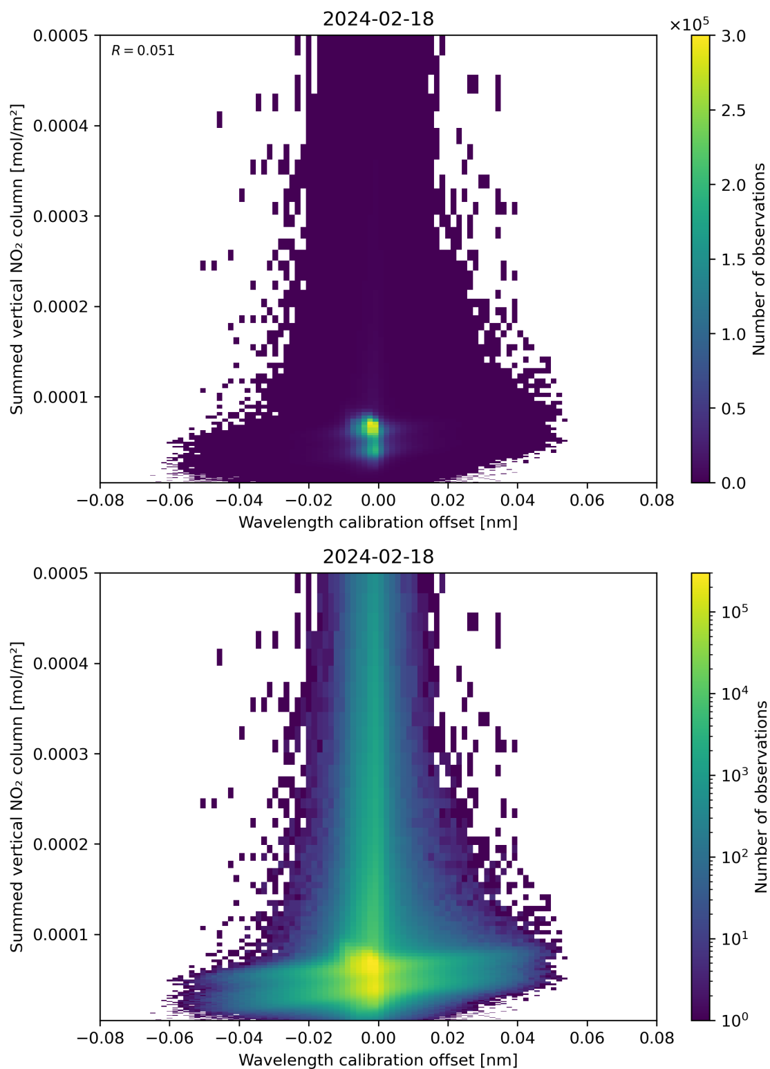
Figure 177: Scatter density plot of “Wavelength calibration offset” against “Summed vertical NO 2 column” for 2024-02-17 to 2024-02-19.
