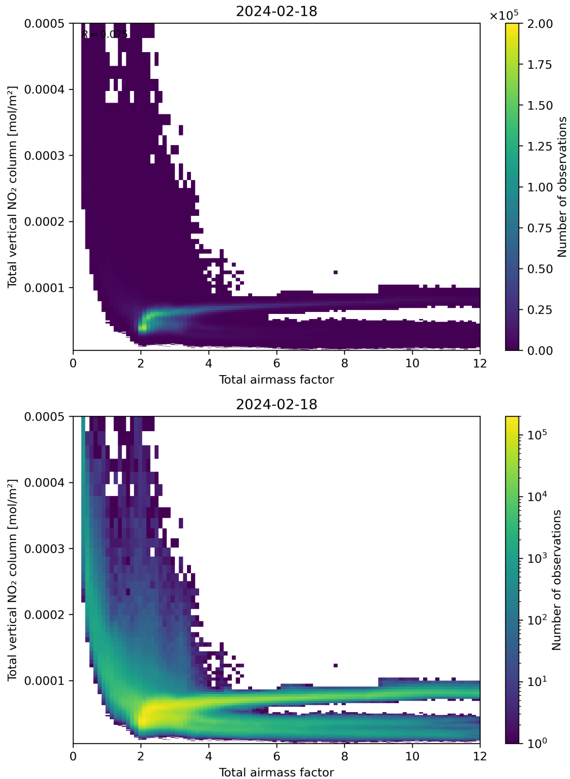
Figure 67: Scatter density plot of “Total airmass factor” against “Total vertical NO 2 column” for 2024-02-17 to 2024-02-19.
