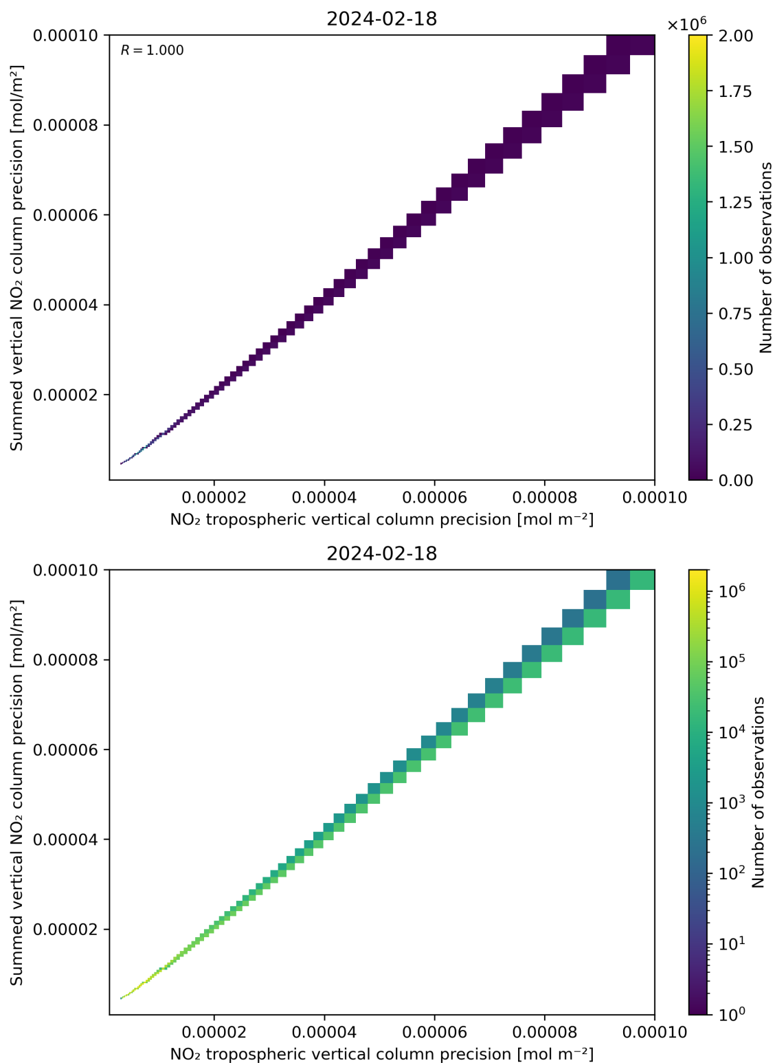
Figure 137: Scatter density plot of “NO 2 tropospheric vertical column precision” against “Summed vertical NO 2 column precision” for 2024-02-17 to 2024-02-19.
