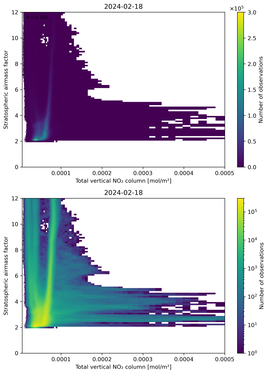
Figure 110: Scatter density plot of “Total vertical NO 2 column” against “Stratospheric airmass factor” for 2024-02-17 to 2024-02-19.
