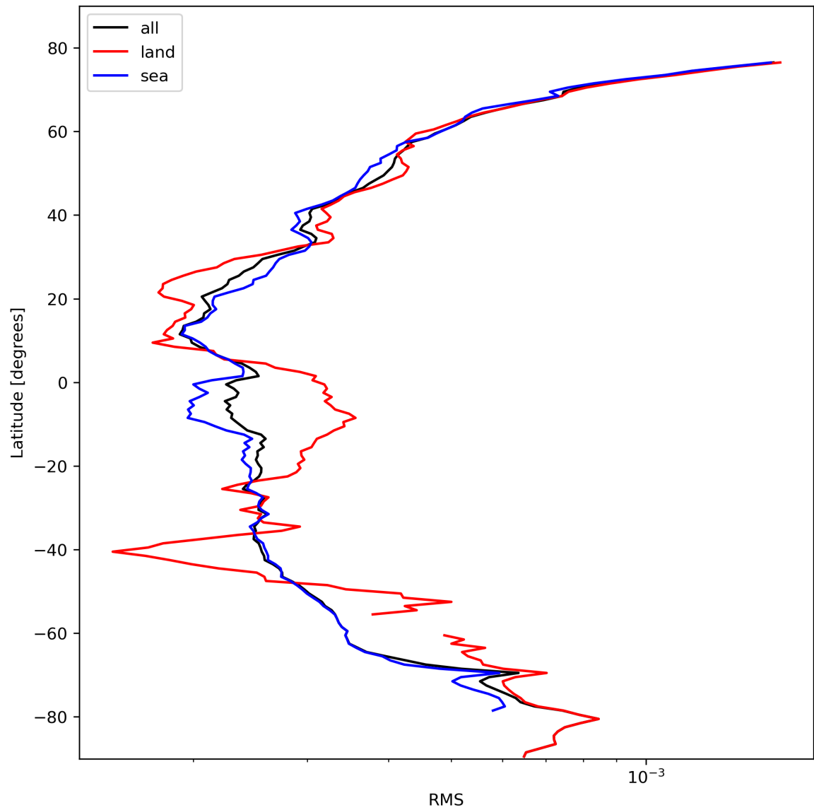
Figure 26: Zonal average of “RMS” for 2024-02-17 to 2024-02-19.
