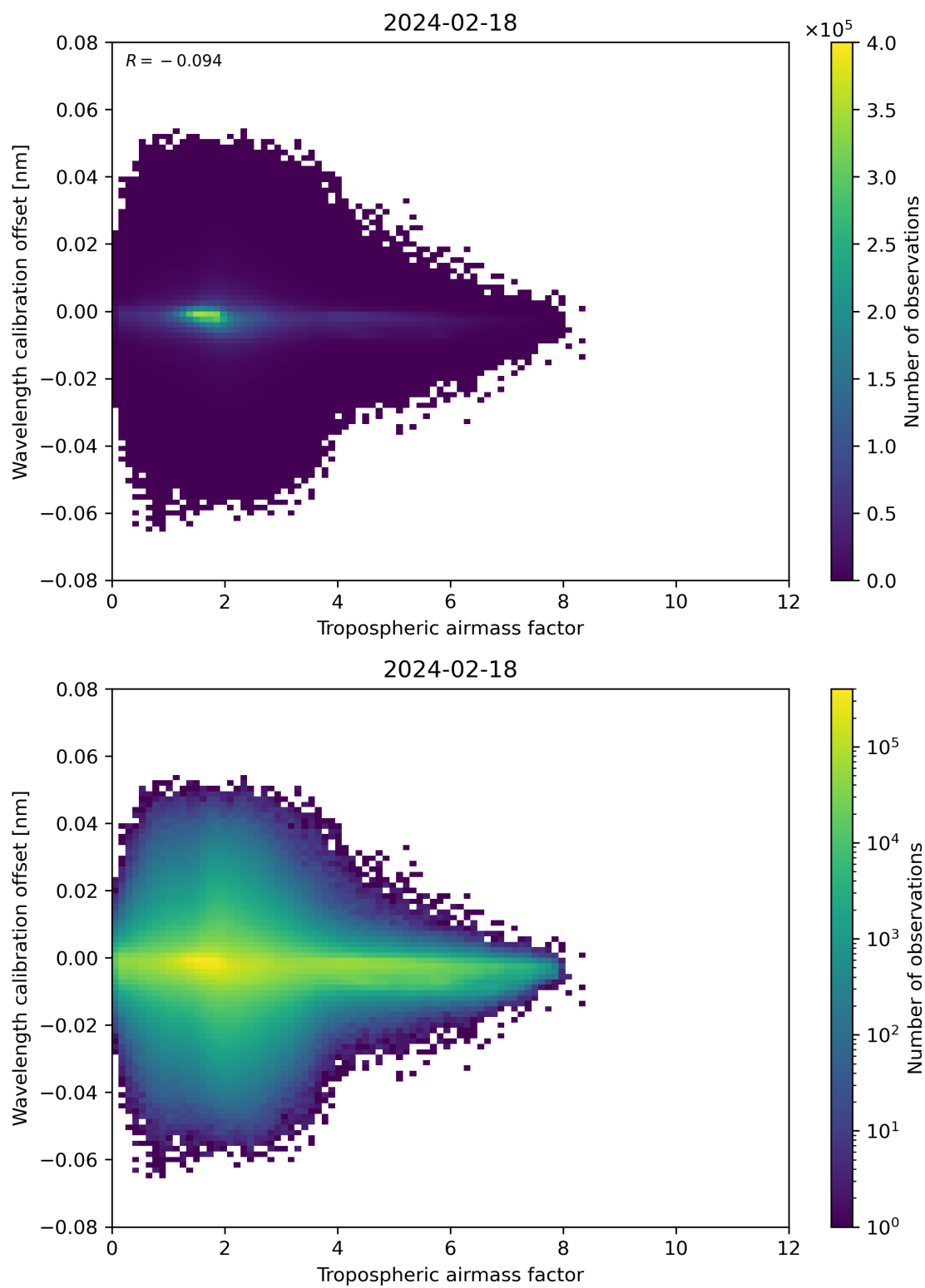
Figure 80: Scatter density plot of “Tropospheric airmass factor” against “Wavelength calibration offset” for 2024-02-17 to 2024-02-19.
