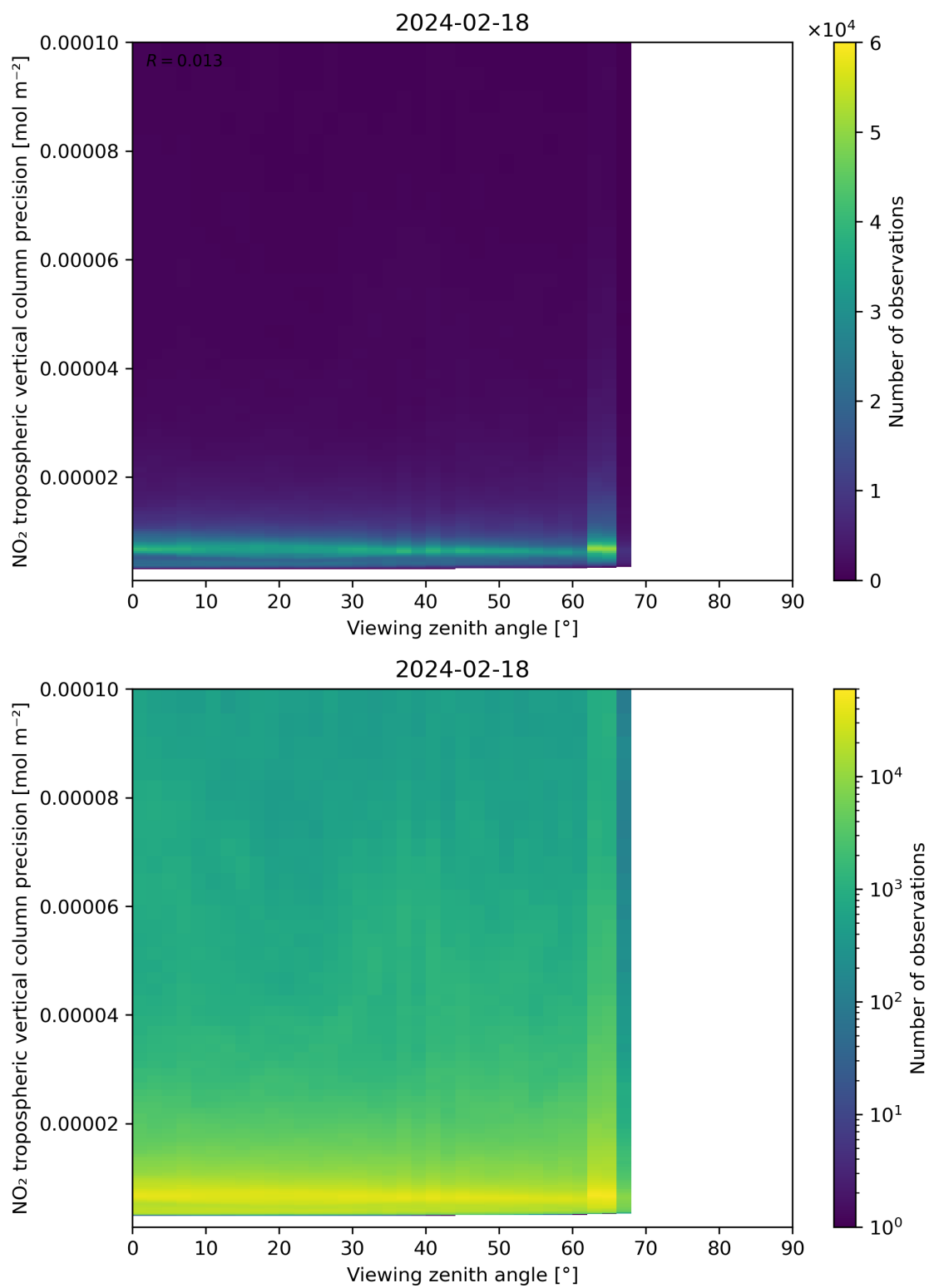
Figure 170: Scatter density plot of “Viewing zenith angle” against “NO 2 tropospheric vertical column precision” for 2024-02-17 to 2024-02-19.
