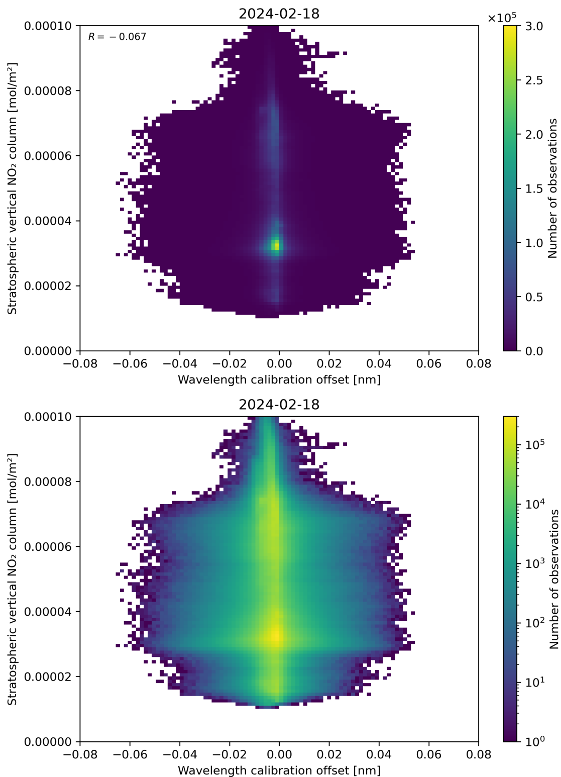
Figure 176: Scatter density plot of “Wavelength calibration offset” against “Stratospheric vertical NO 2 column” for 2024-02-17 to 2024-02-19.
