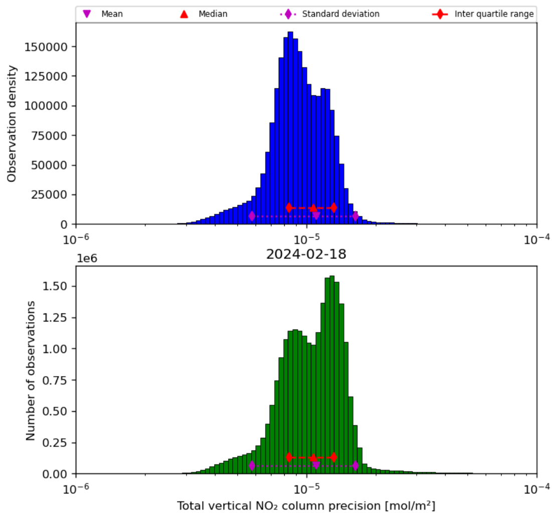
Figure 39: Histogram of “Total vertical NO 2 column precision” for 2024-02-17 to 2024-02-19
