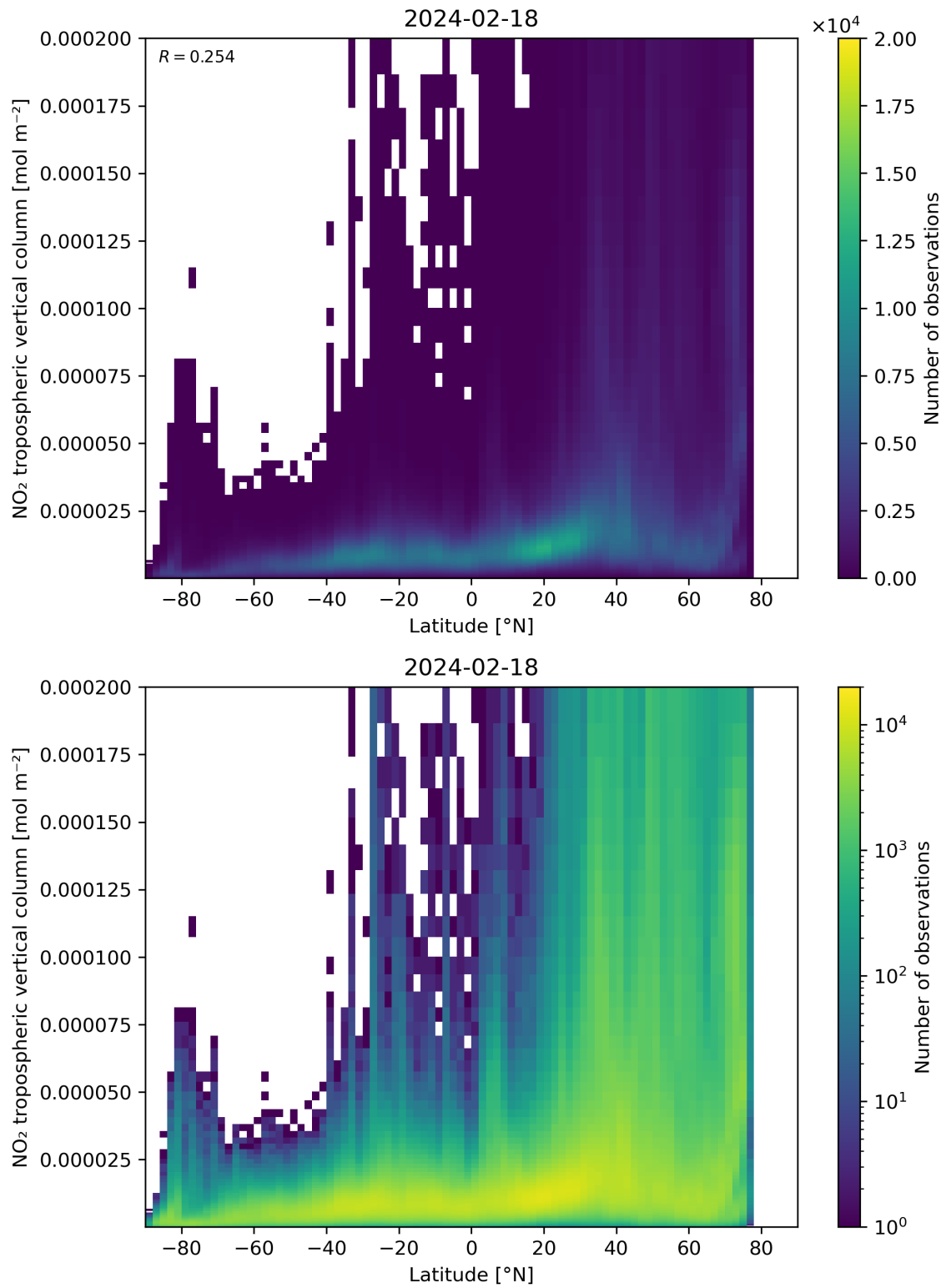
Figure 92: Scatter density plot of “Latitude” against “NO 2 tropospheric vertical column” for 2024-02-17 to 2024-02-19.
