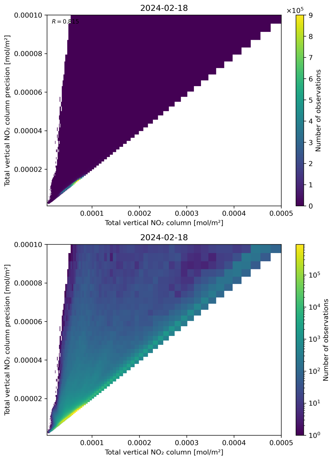
Figure 114: Scatter density plot of “Total vertical NO 2 column” against “Total vertical NO 2 column precision” for 2024-02-17 to 2024-02-19.
