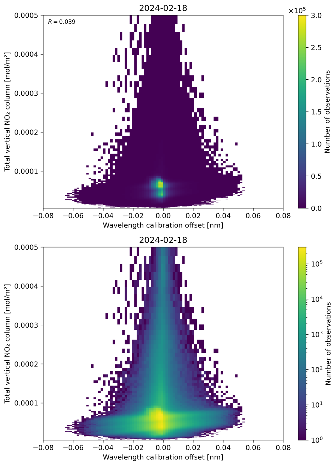
Figure 179: Scatter density plot of “Wavelength calibration offset” against “Total vertical NO 2 column” for 2024-02-17 to 2024-02-19.
