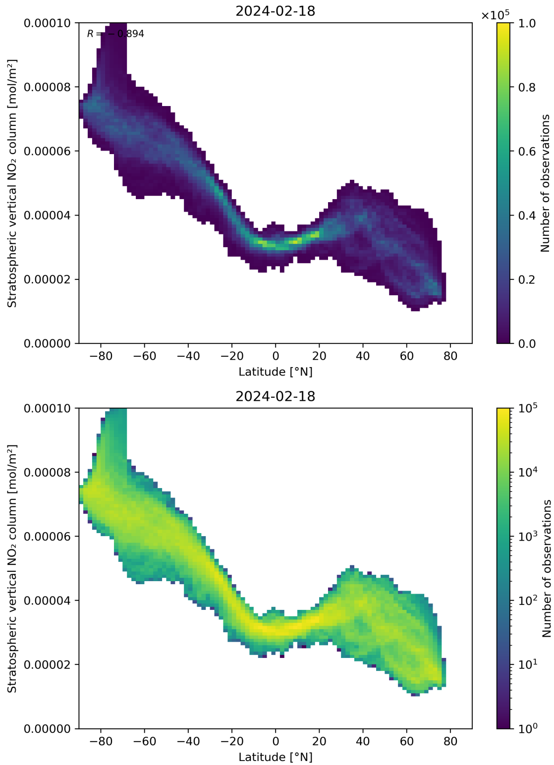
Figure 87: Scatter density plot of “Latitude” against “Stratospheric vertical NO 2 column” for 2024-02-17 to 2024-02-19.
