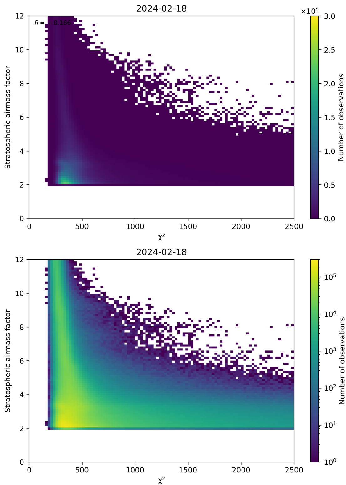
Figure 81: Scatter density plot of “ \chi^2 ” against “Stratospheric airmass factor” for 2024-02-17 to 2024-02-19.
