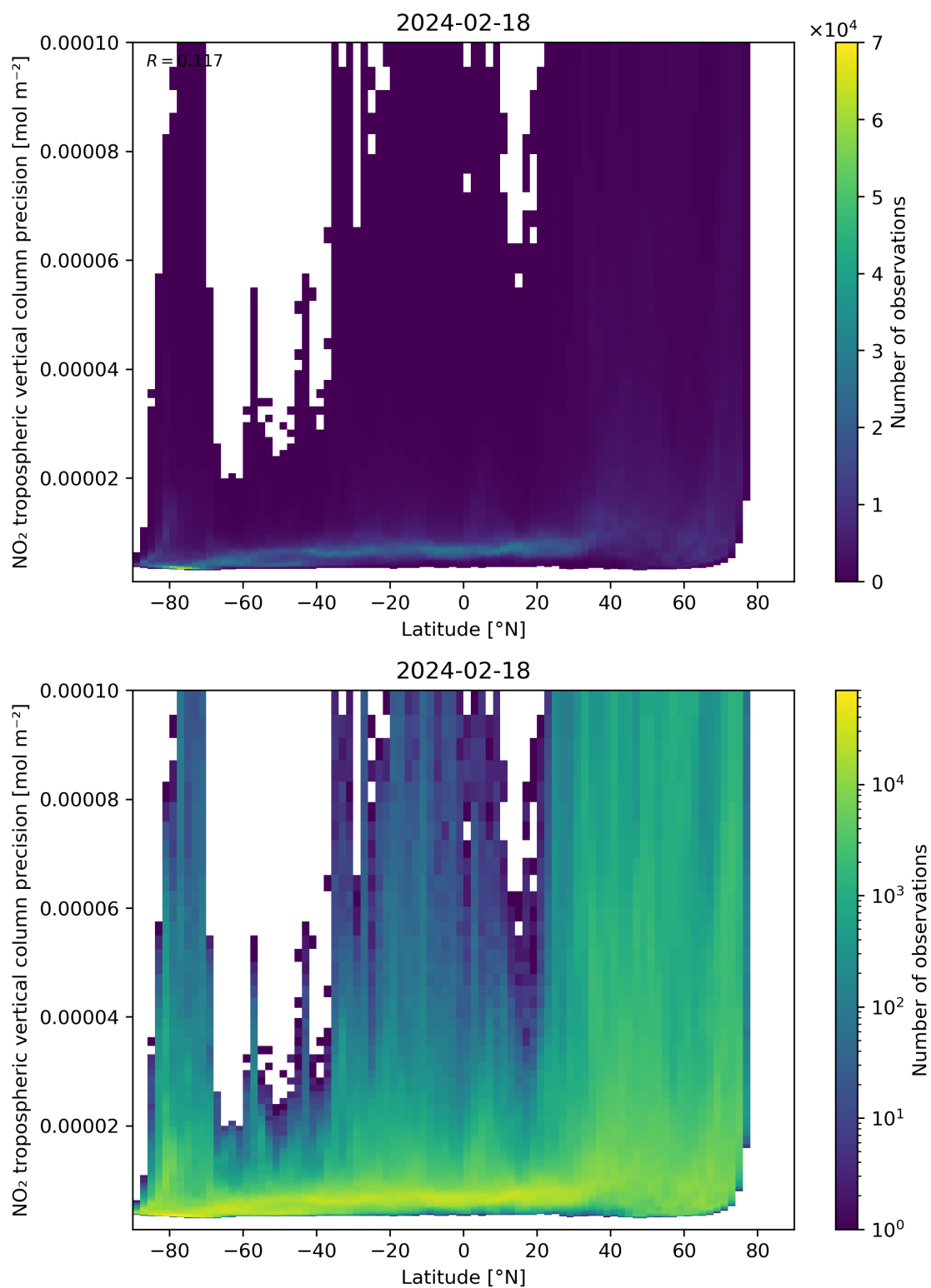
Figure 93: Scatter density plot of “Latitude” against “NO 2 tropospheric vertical column precision” for 2024-02-17 to 2024-02-19.
