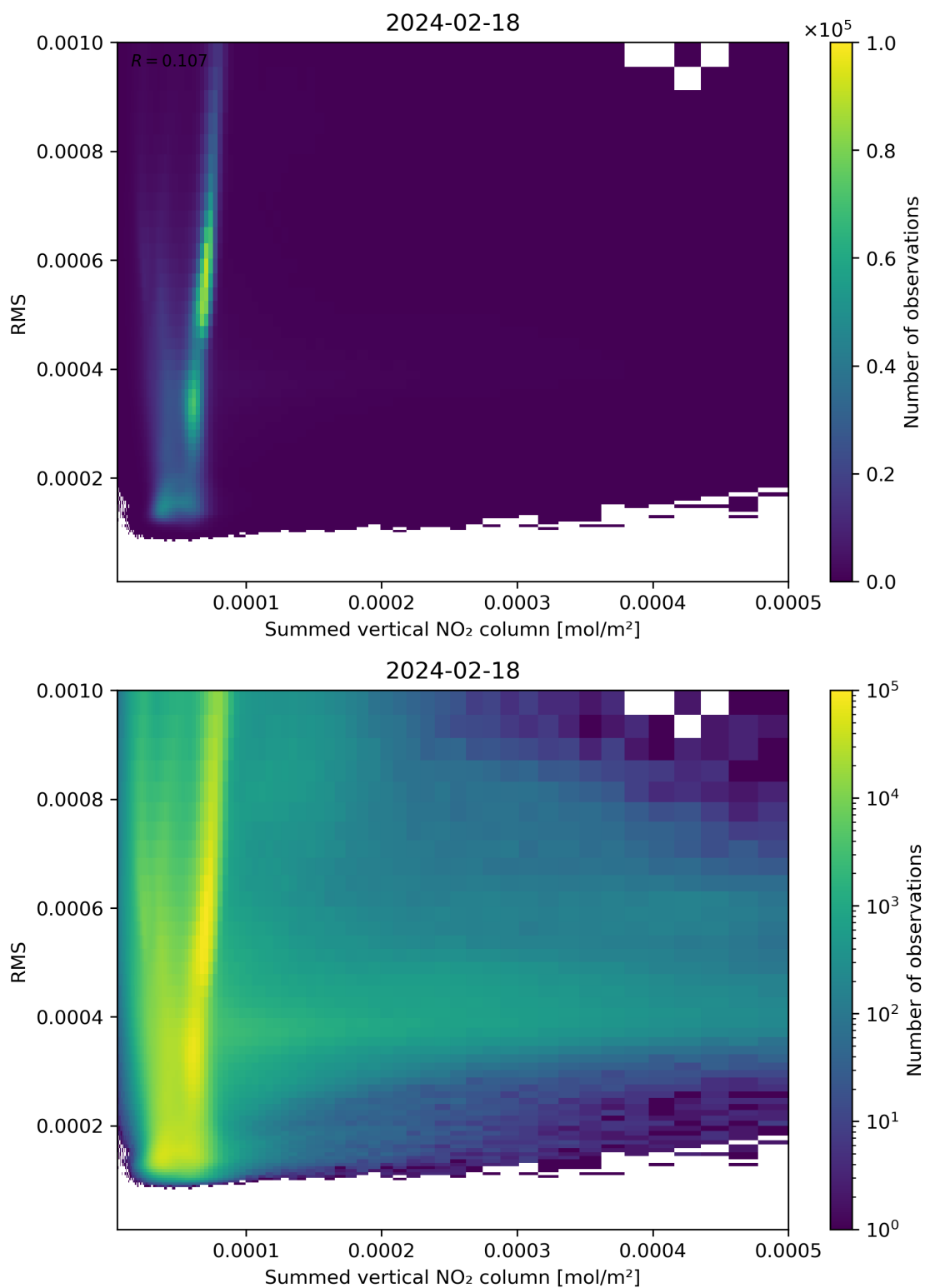
Figure 109: Scatter density plot of “Summed vertical NO 2 column” against “RMS” for 2024-02-17 to 2024-02-19.
