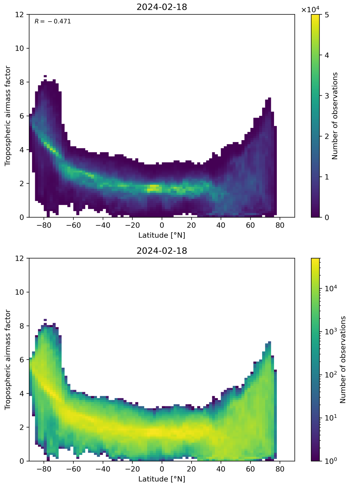
Figure 85: Scatter density plot of “Latitude” against “Tropospheric airmass factor” for 2024-02-17 to 2024-02-19.
