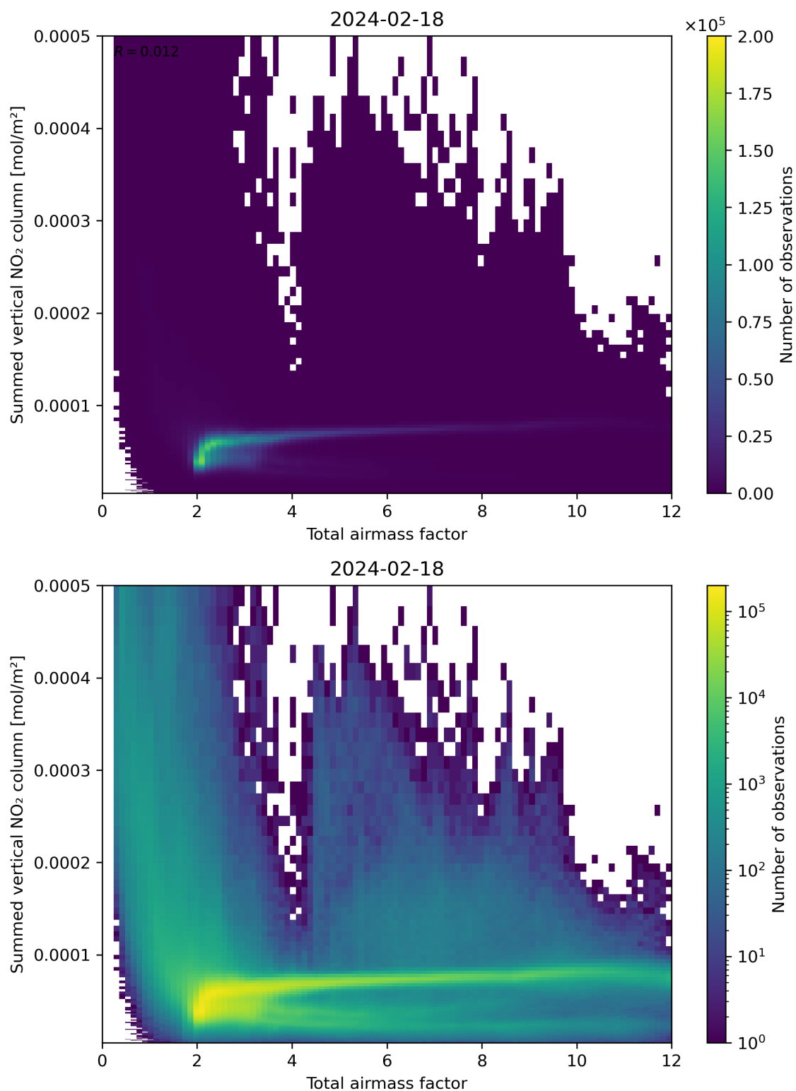
Figure 65: Scatter density plot of “Total airmass factor” against “Summed vertical NO 2 column” for 2024-02-17 to 2024-02-19.
