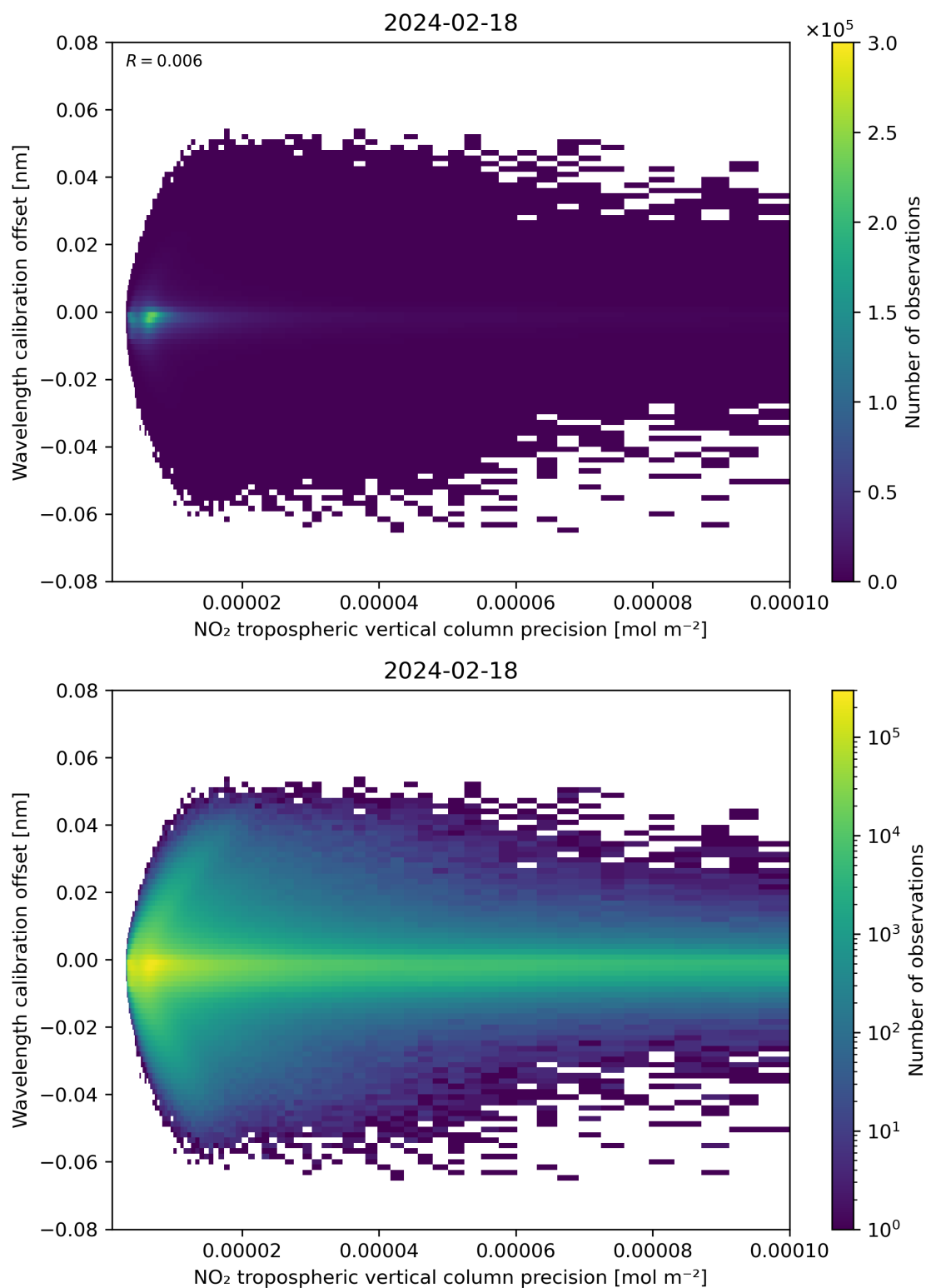
Figure 141: Scatter density plot of “NO 2 tropospheric vertical column precision” against “Wavelength calibration offset” for 2024-02-17 to 2024-02-19.
