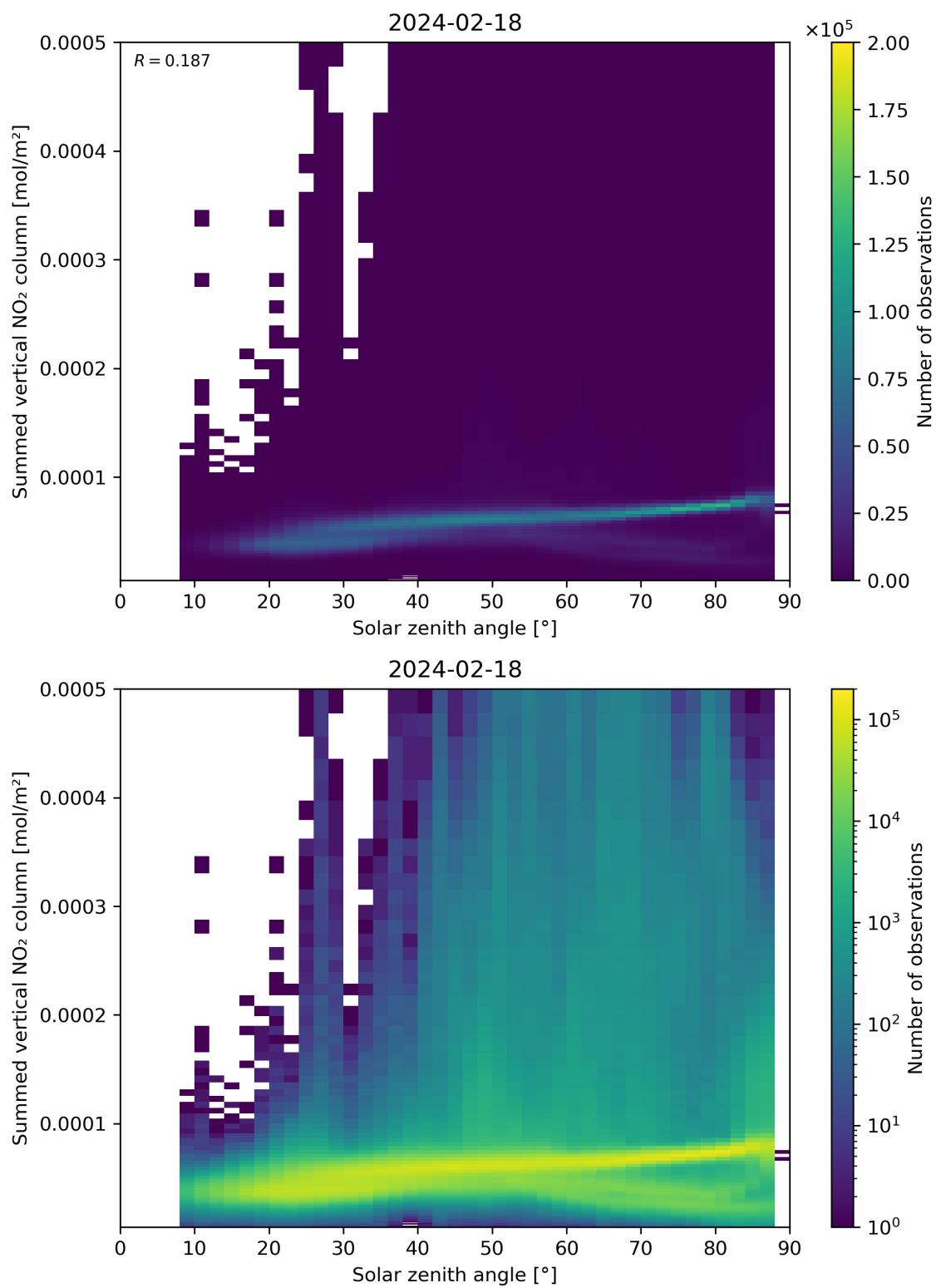
Figure 151: Scatter density plot of “Solar zenith angle” against “Summed vertical NO 2 column” for 2024-02-17 to 2024-02-19.
