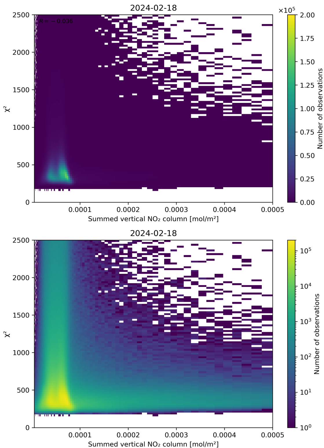
Figure 104: Scatter density plot of “Summed vertical NO 2 column” against “ \chi^2 ” for 2024-02-17 to 2024-02-19.
