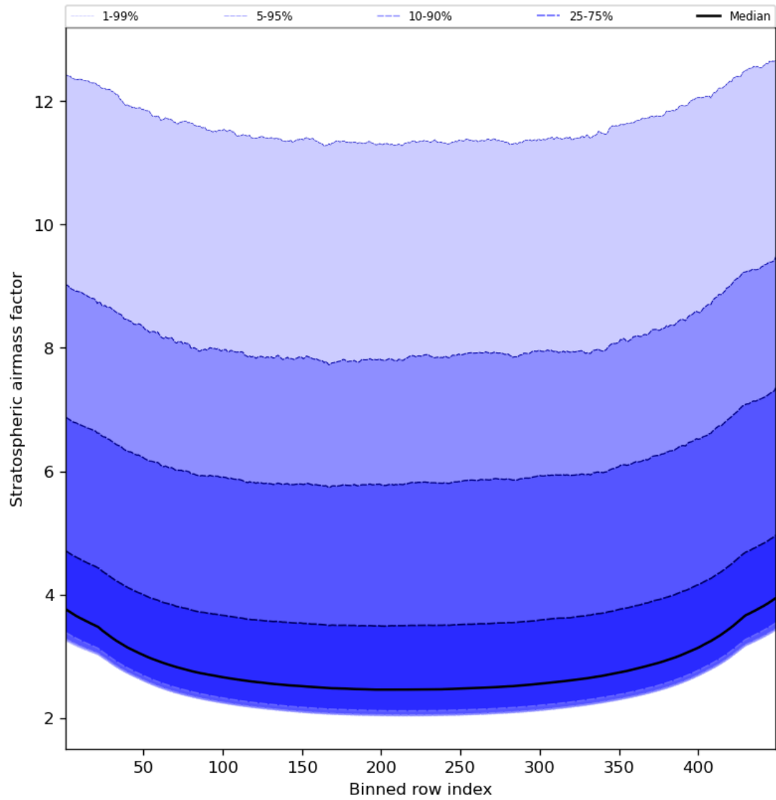
Figure 61: Along track statistics of “Stratospheric airmass factor” for 2024-02-17 to 2024-02-19
