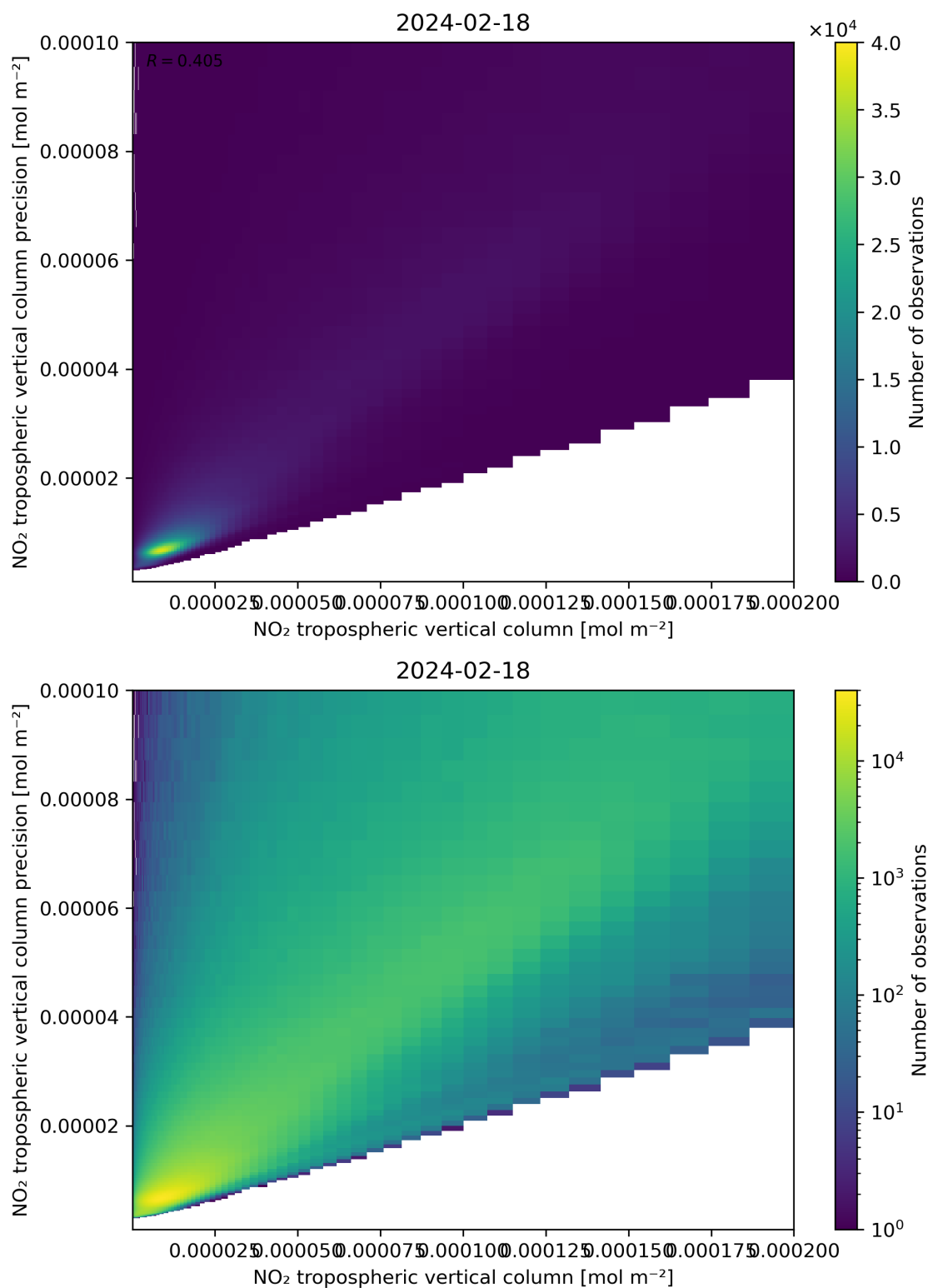
Figure 130: Scatter density plot of “NO 2 tropospheric vertical column” against “NO 2 tropospheric vertical column precision” for 2024-02-17 to 2024-02-19.
