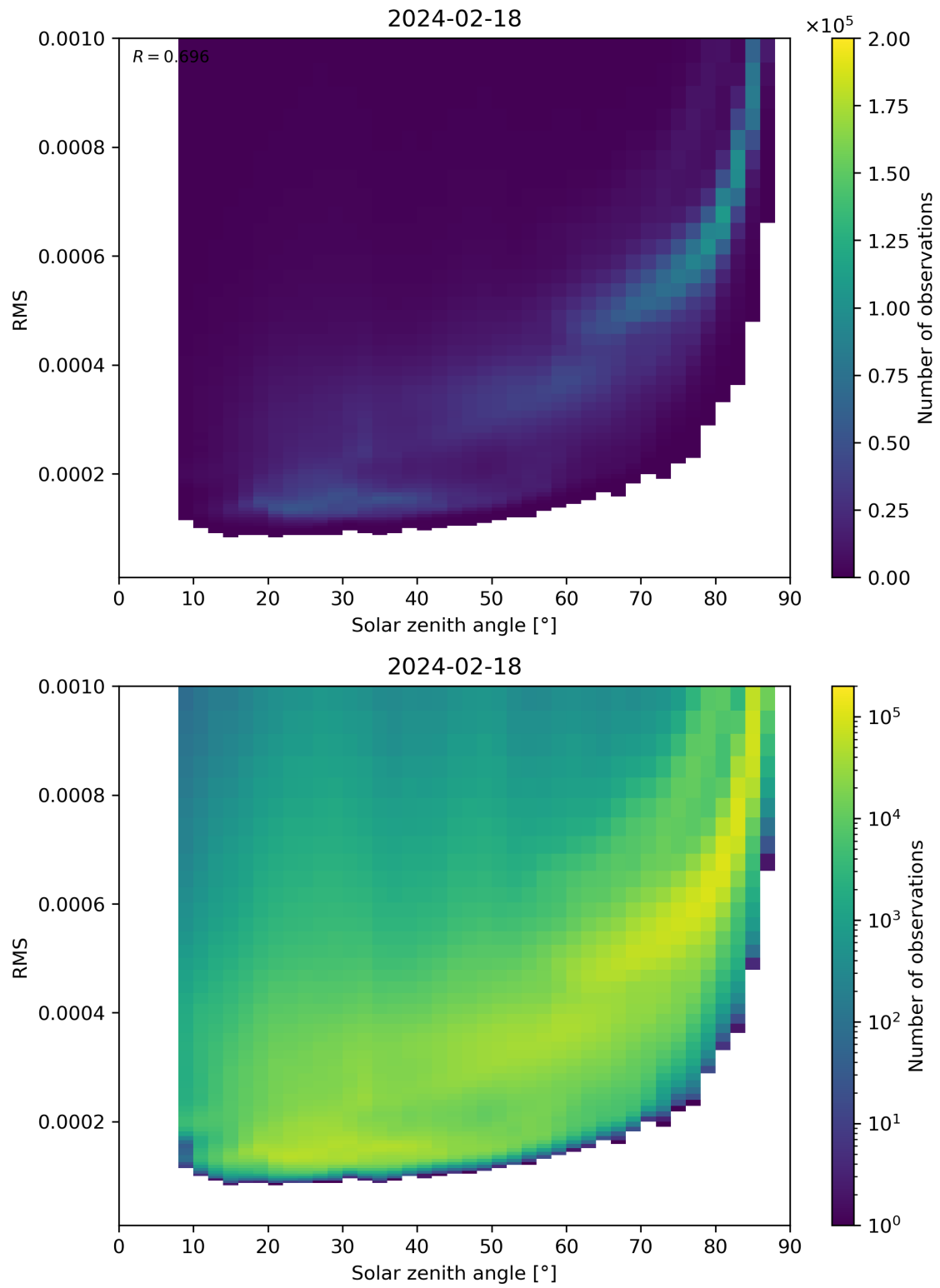
Figure 157: Scatter density plot of “Solar zenith angle” against “RMS” for 2024-02-17 to 2024-02-19.
