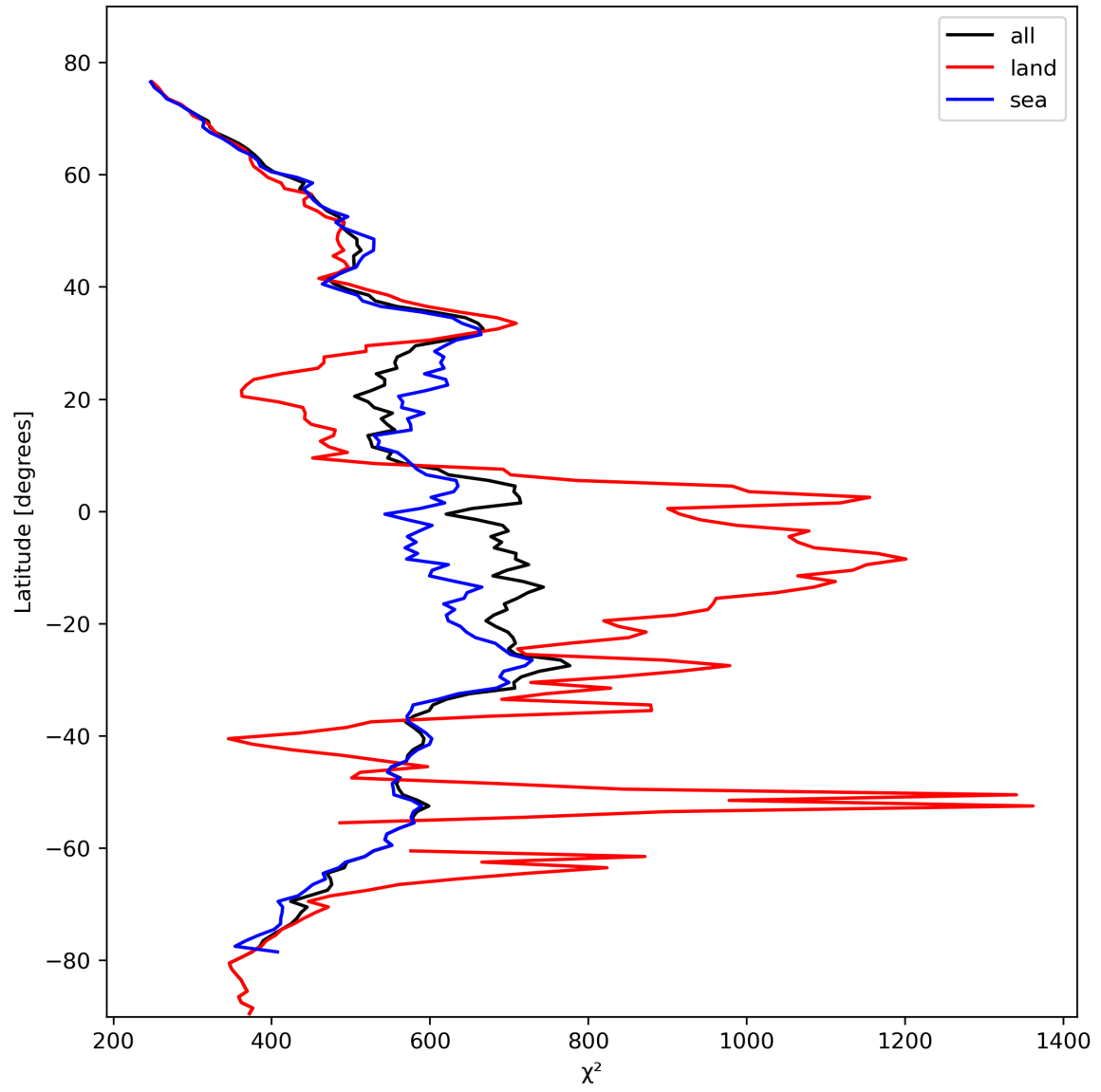
Figure 25: Zonal average of “ \chi^2 ” for 2024-02-17 to 2024-02-19.
