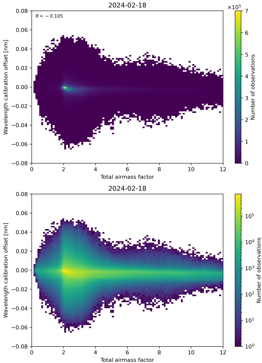
Figure 70: Scatter density plot of “Total airmass factor” against “Wavelength calibration offset” for 2024-02-17 to 2024-02-19.
