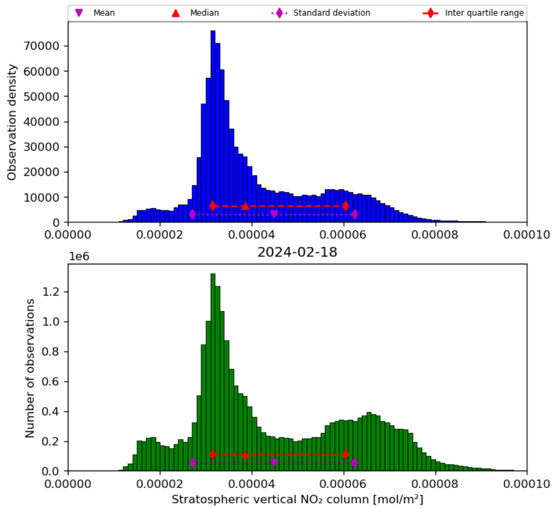
Figure 36: Histogram of “Stratospheric vertical NO 2 column” for 2024-02-17 to 2024-02-19
