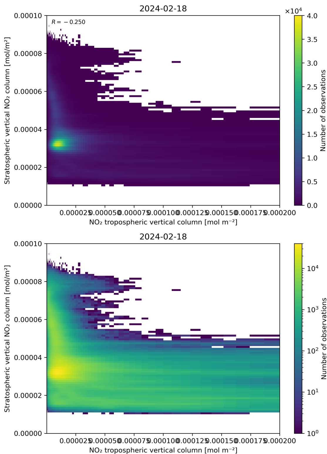
Figure 125: Scatter density plot of “NO 2 tropospheric vertical column” against “Stratospheric vertical NO 2 column” for 2024-02-17 to 2024-02-19.
