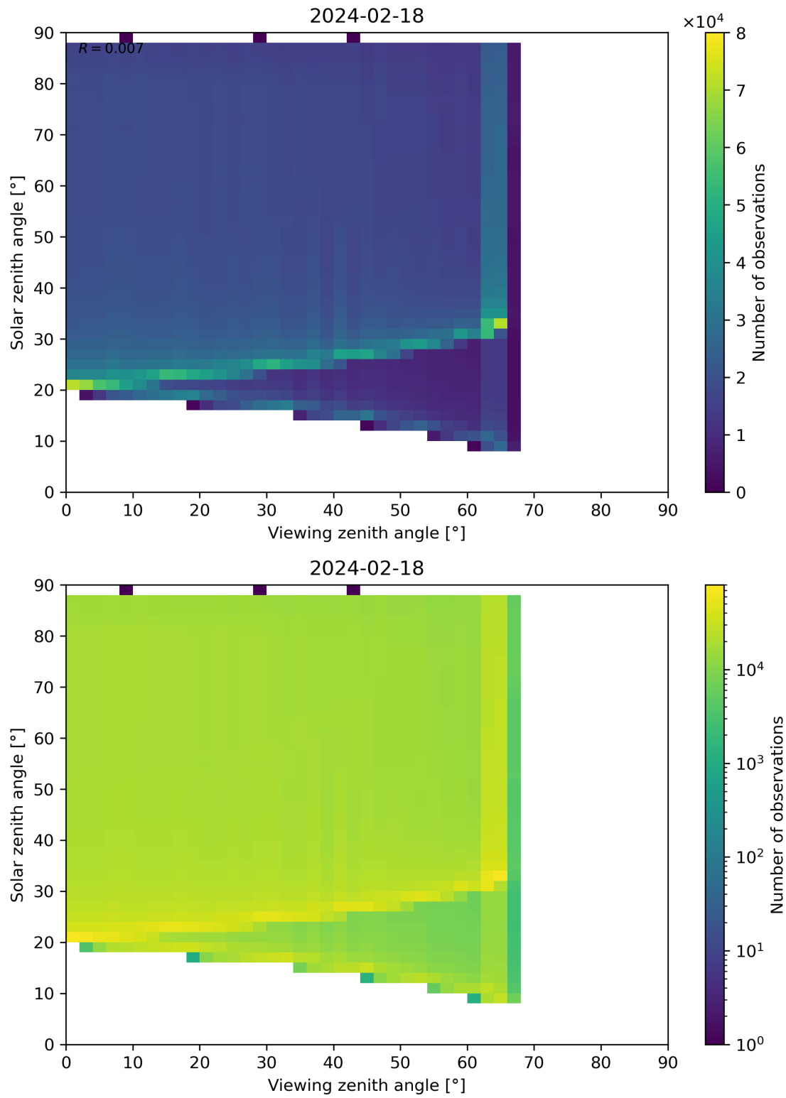
Figure 172: Scatter density plot of “Viewing zenith angle” against “Solar zenith angle” for 2024-02-17 to 2024-02-19.
