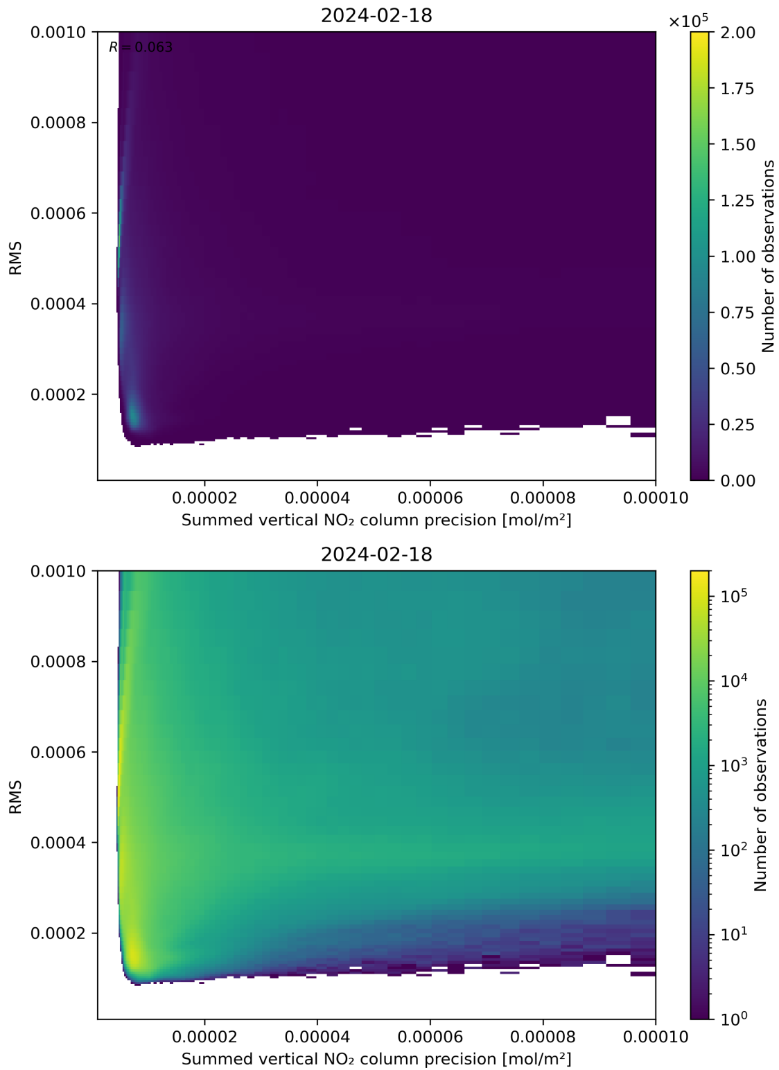
Figure 108: Scatter density plot of “Summed vertical NO 2 column precision” against “RMS” for 2024-02-17 to 2024-02-19.
