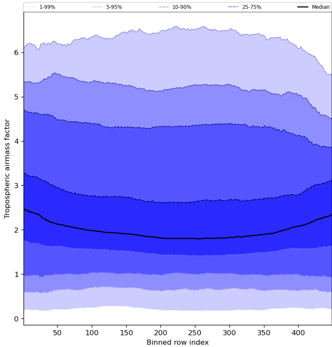
Figure 48: Along track statistics of “Tropospheric air mass factor” for 2024-02-17 to 2024-02-19
