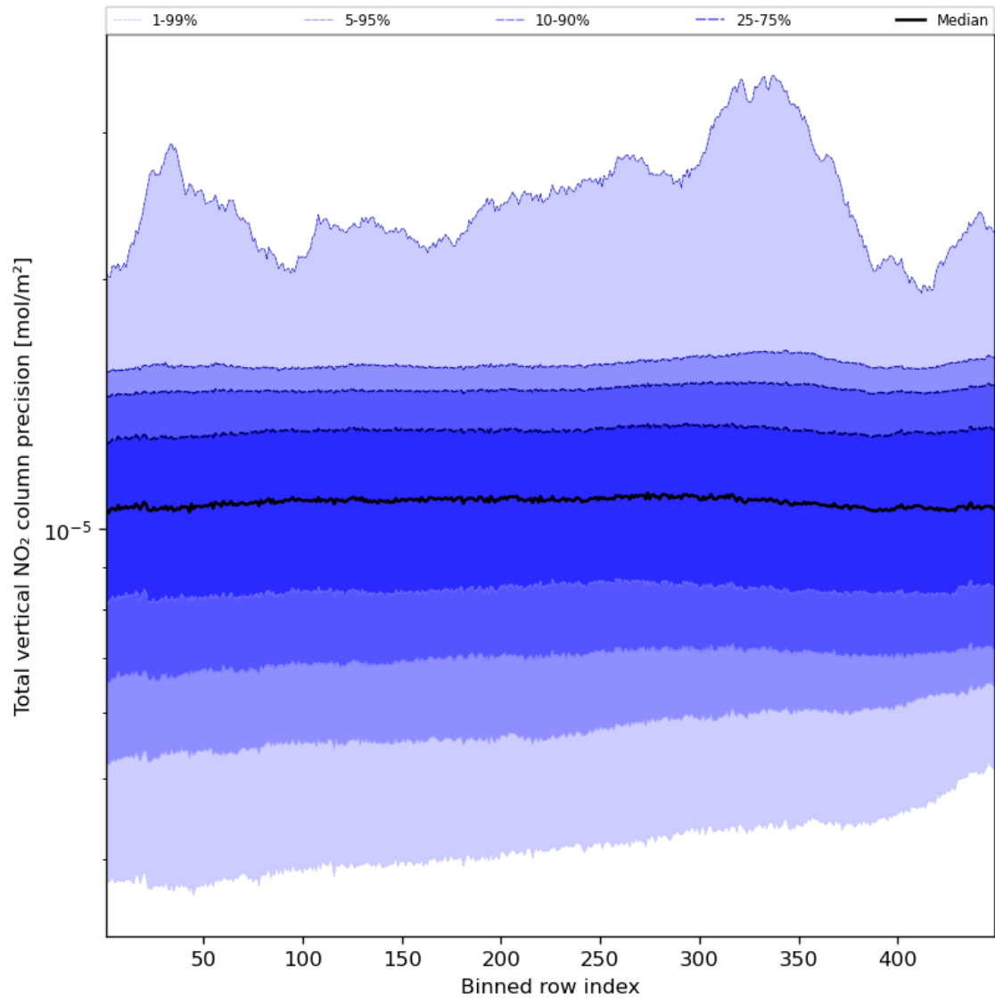
Figure 56: Along track statistics of “Total vertical NO 2 column precision” for 2024-02-17 to 2024-02-19
