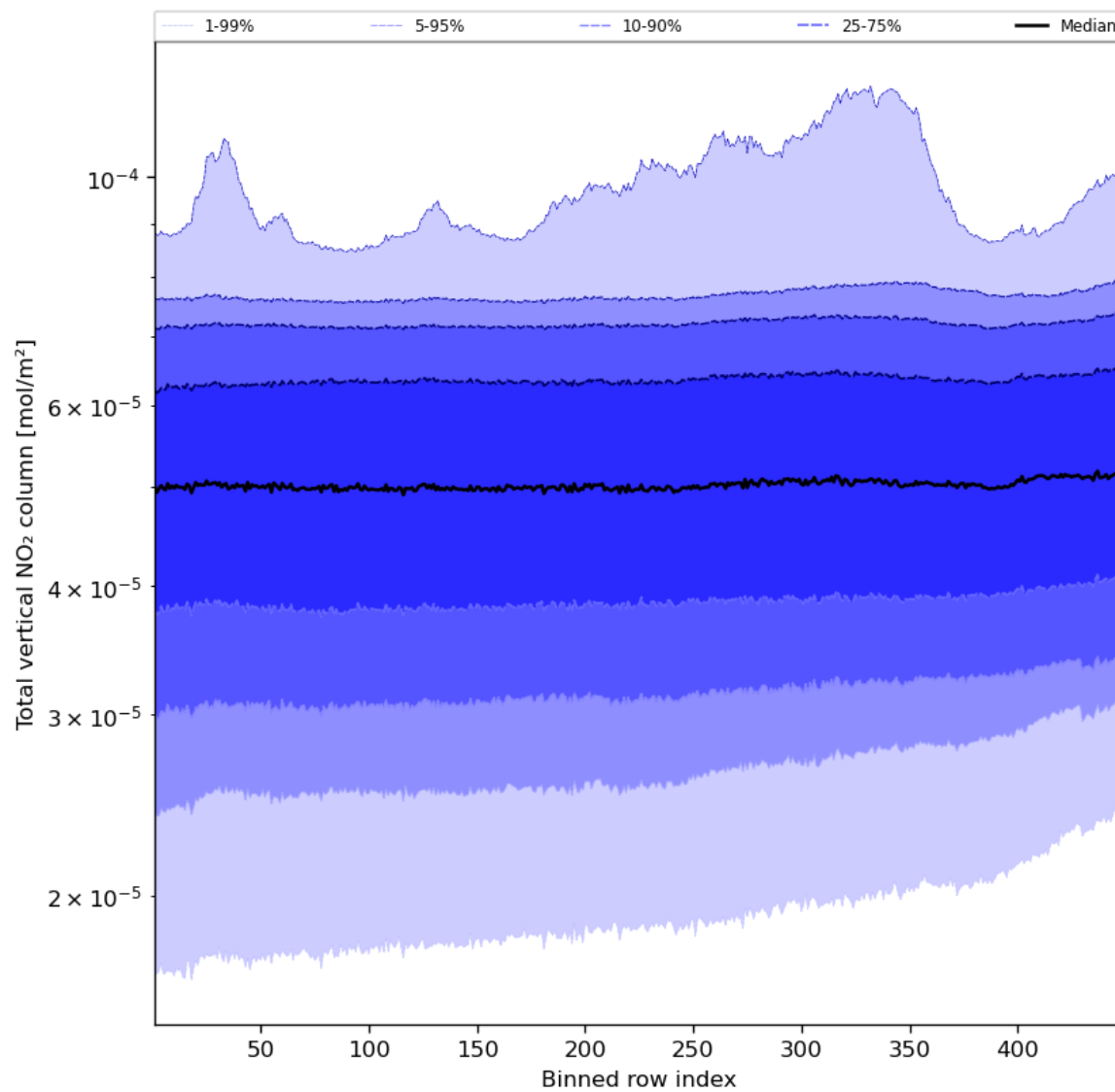
Figure 55: Along track statistics of “Total vertical NO 2 column” for 2024-02-17 to 2024-02-19
