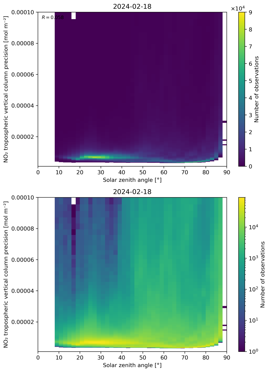
Figure 156: Scatter density plot of “Solar zenith angle” against “NO 2 tropospheric vertical column precision” for 2024-02-17 to 2024-02-19.
