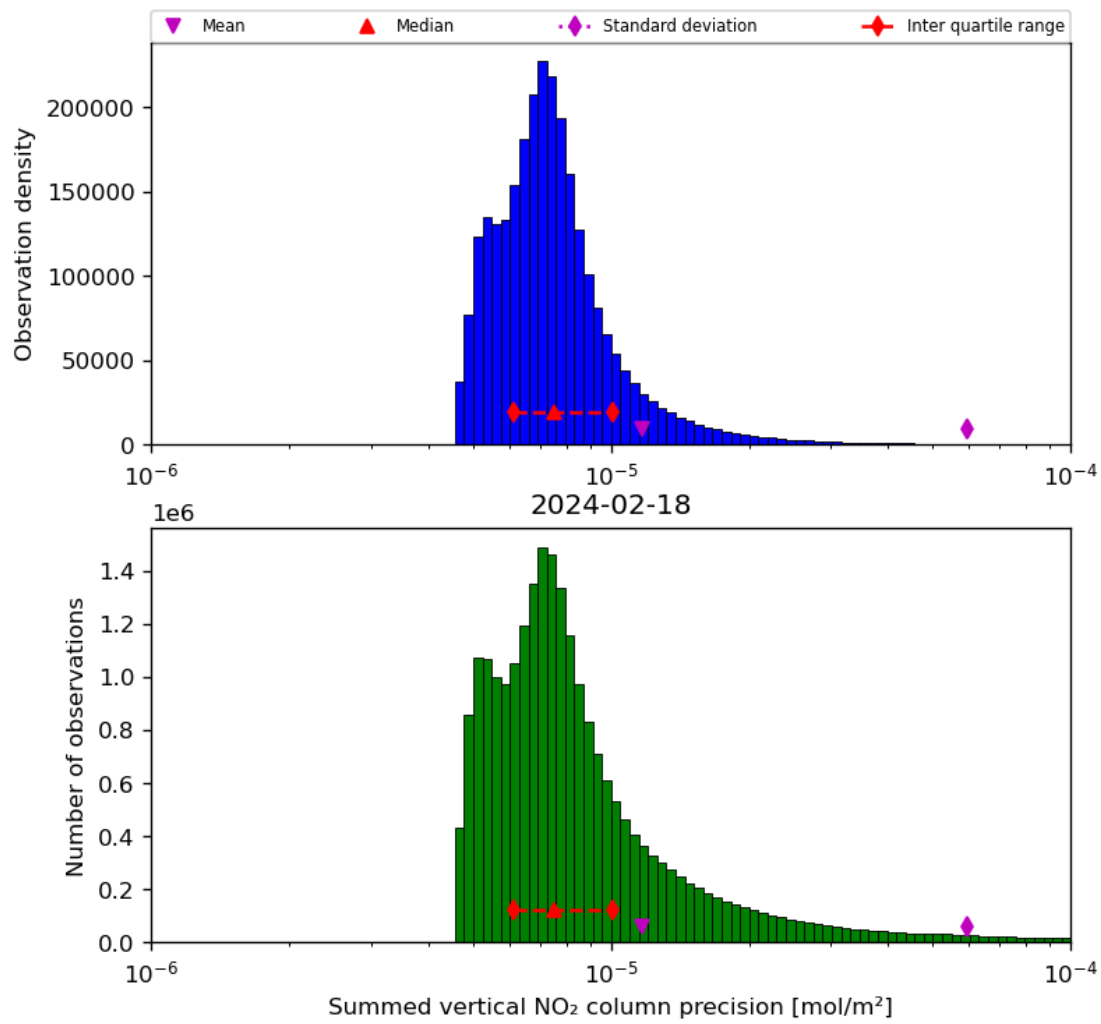
Figure 41: Histogram of "Summed vertical NO 2 column precision" for 2024-02-17 to 2024-02-19
