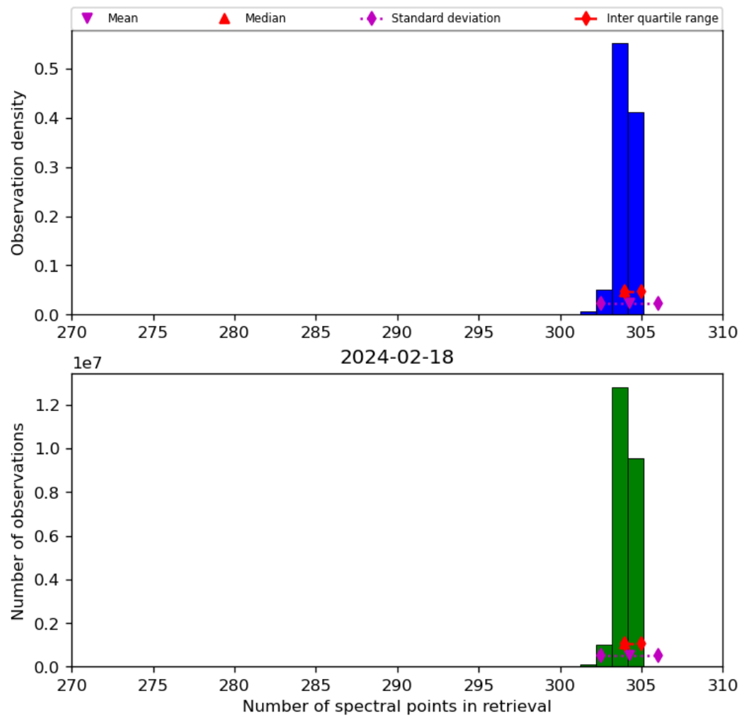
Figure 33: Histogram of “Number of spectral points in retrieval” for 2024-02-17 to 2024-02-19
