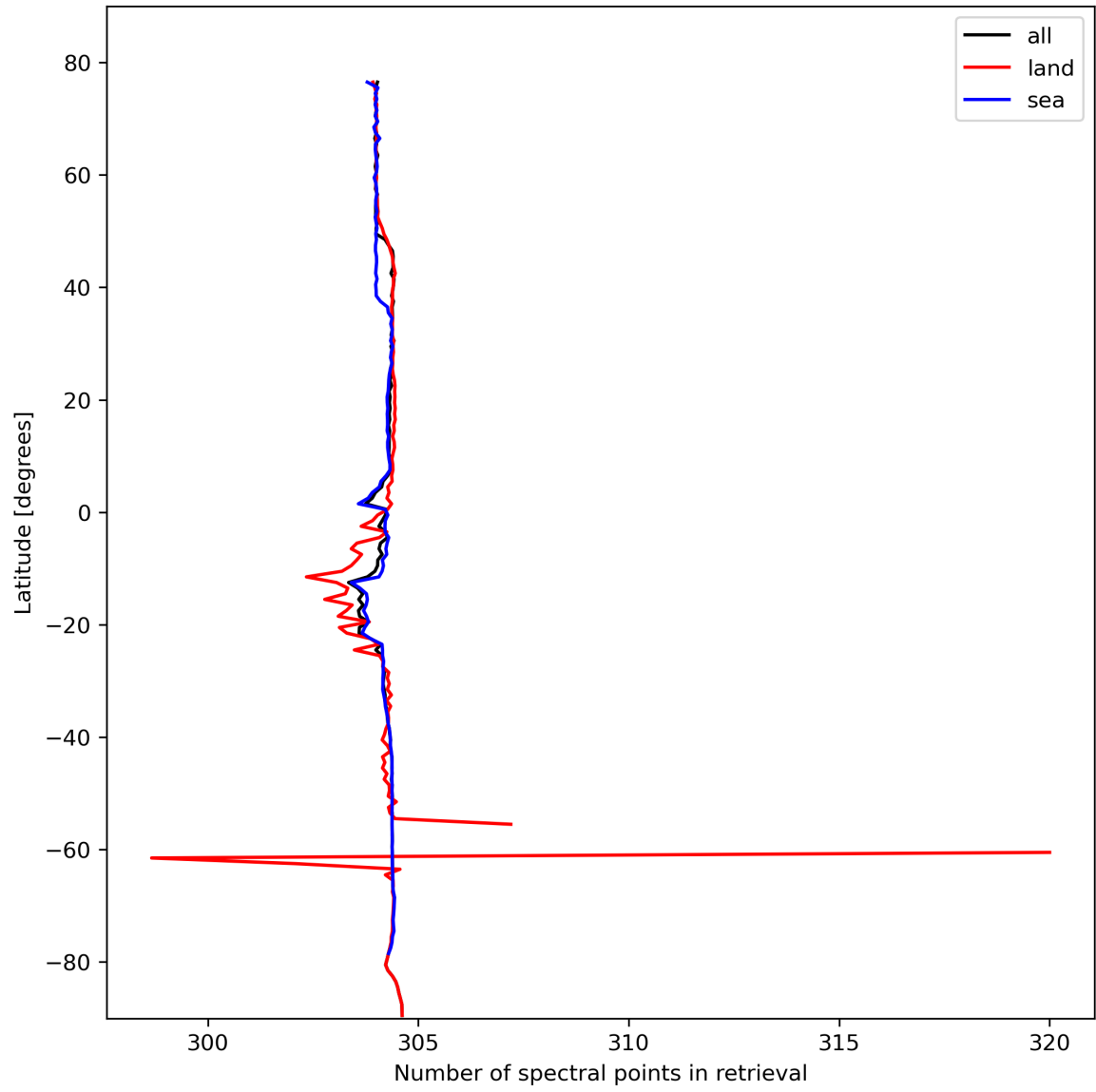
Figure 16: Zonal average of “Number of spectral points in retrieval” for 2024-02-17 to 2024-02-19.
