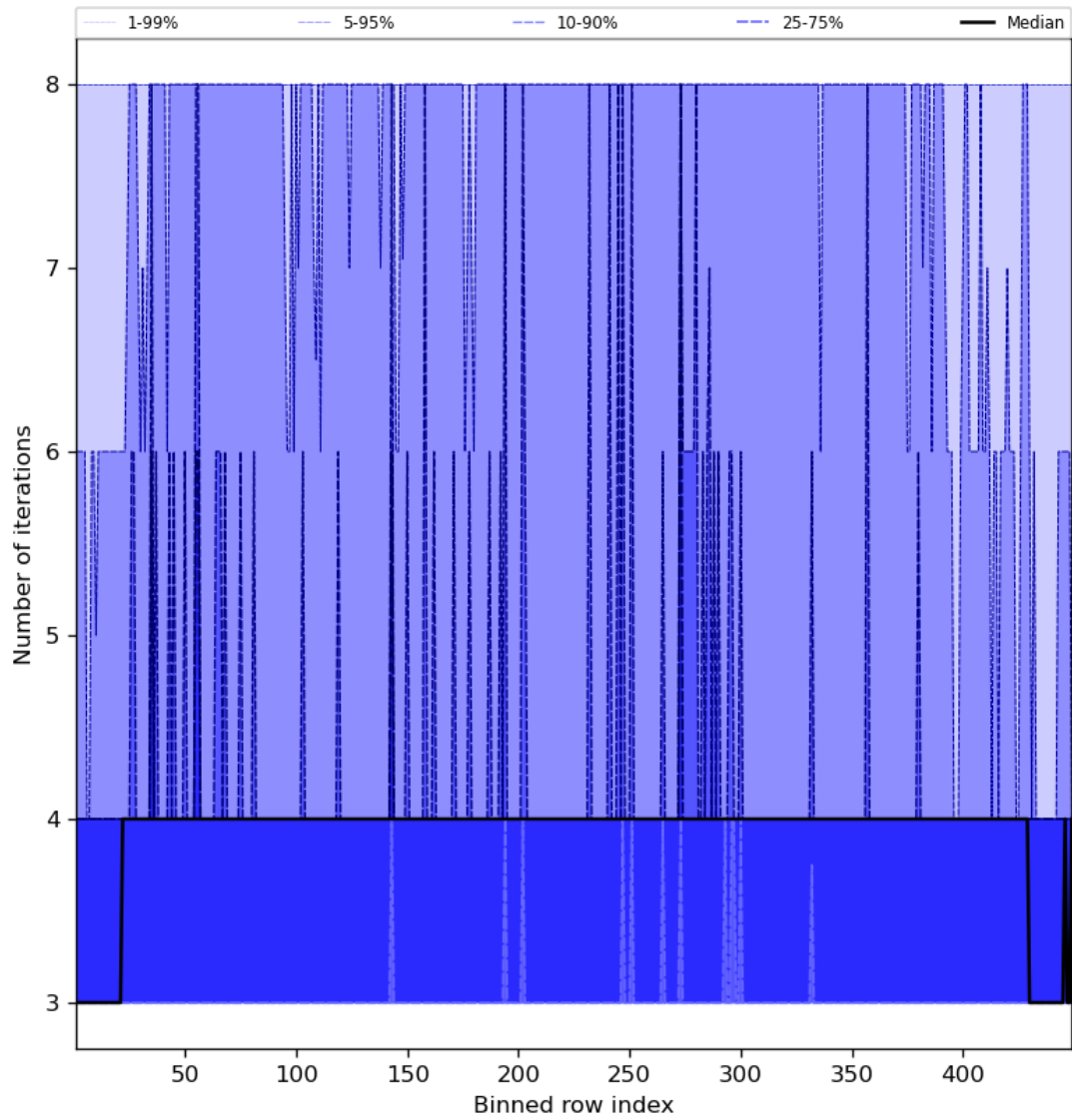
Figure 51: Along track statistics of “Number of iterations” for 2024-02-17 to 2024-02-19
