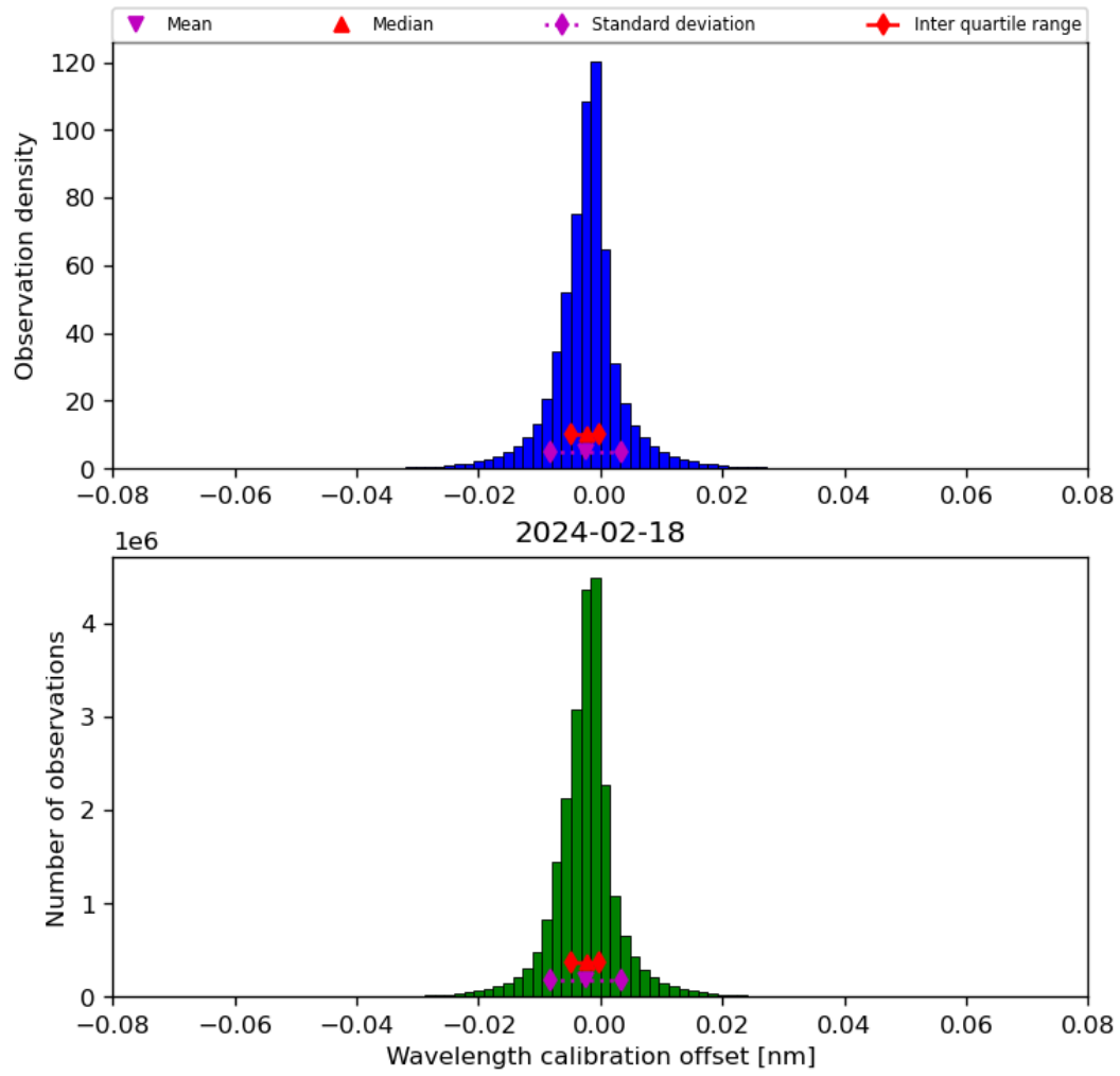
Figure 35: Histogram of “Wavelength calibration offset” for 2024-02-17 to 2024-02-19
