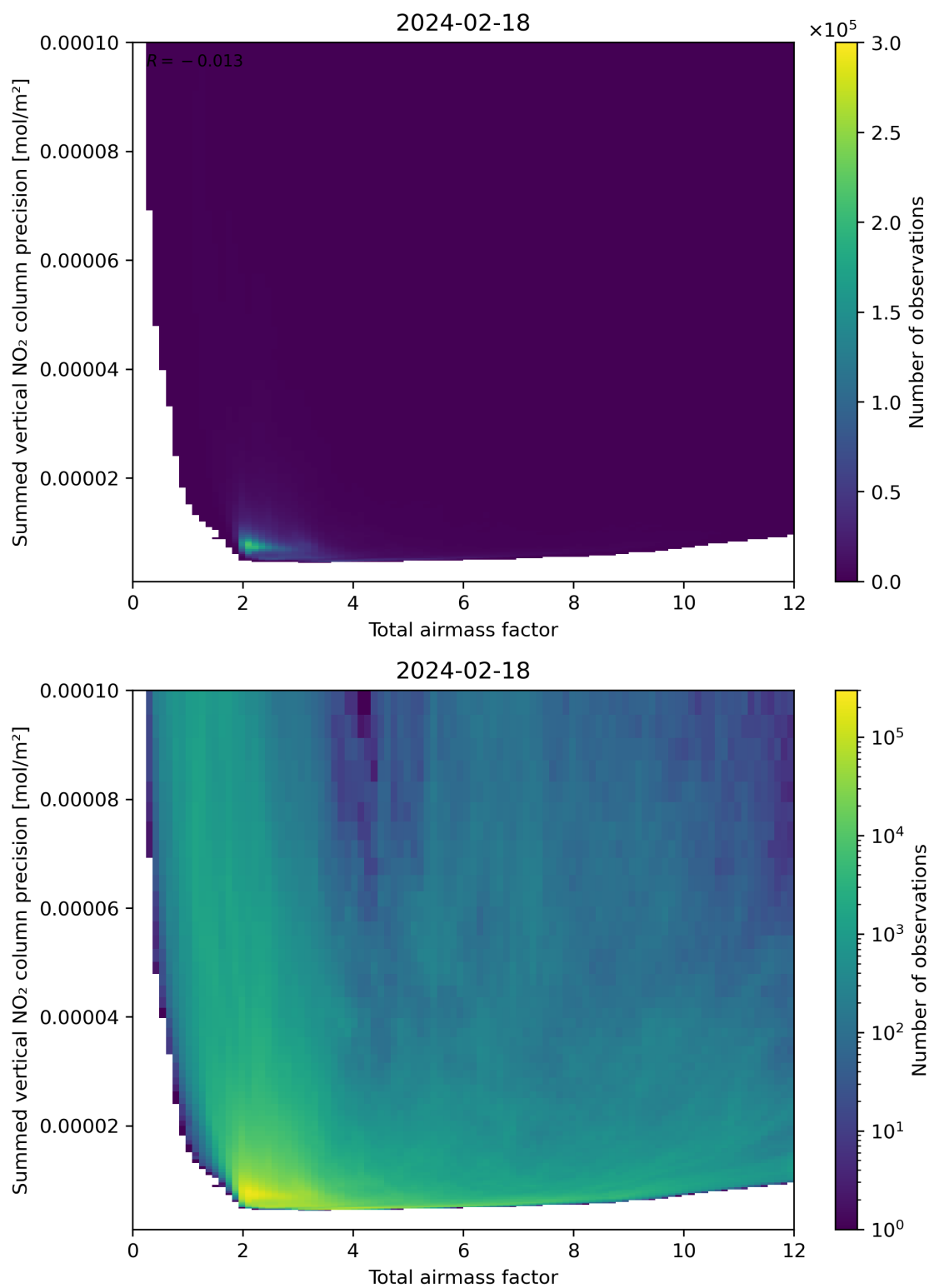
Figure 66: Scatter density plot of “Total airmass factor” against “Summed vertical NO 2 column precision” for 2024-02-17 to 2024-02-19.
