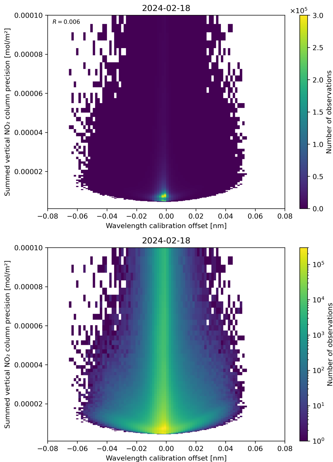
Figure 178: Scatter density plot of “Wavelength calibration offset” against “Summed vertical NO 2 column precision” for 2024-02-17 to 2024-02-19.
