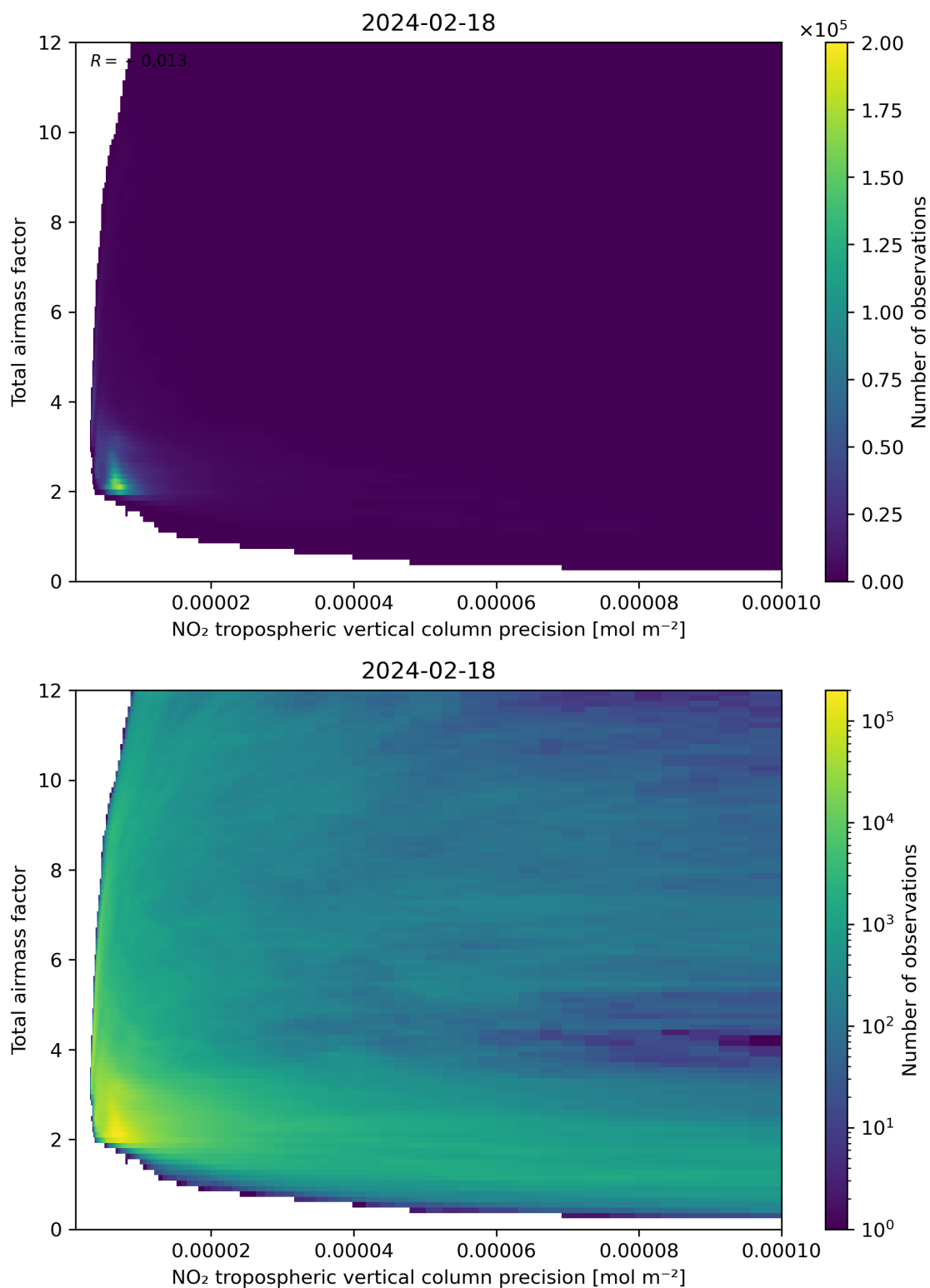
Figure 132: Scatter density plot of “NO 2 tropospheric vertical column precision” against “Total air mass factor” for 2024-02-17 to 2024-02-19.
