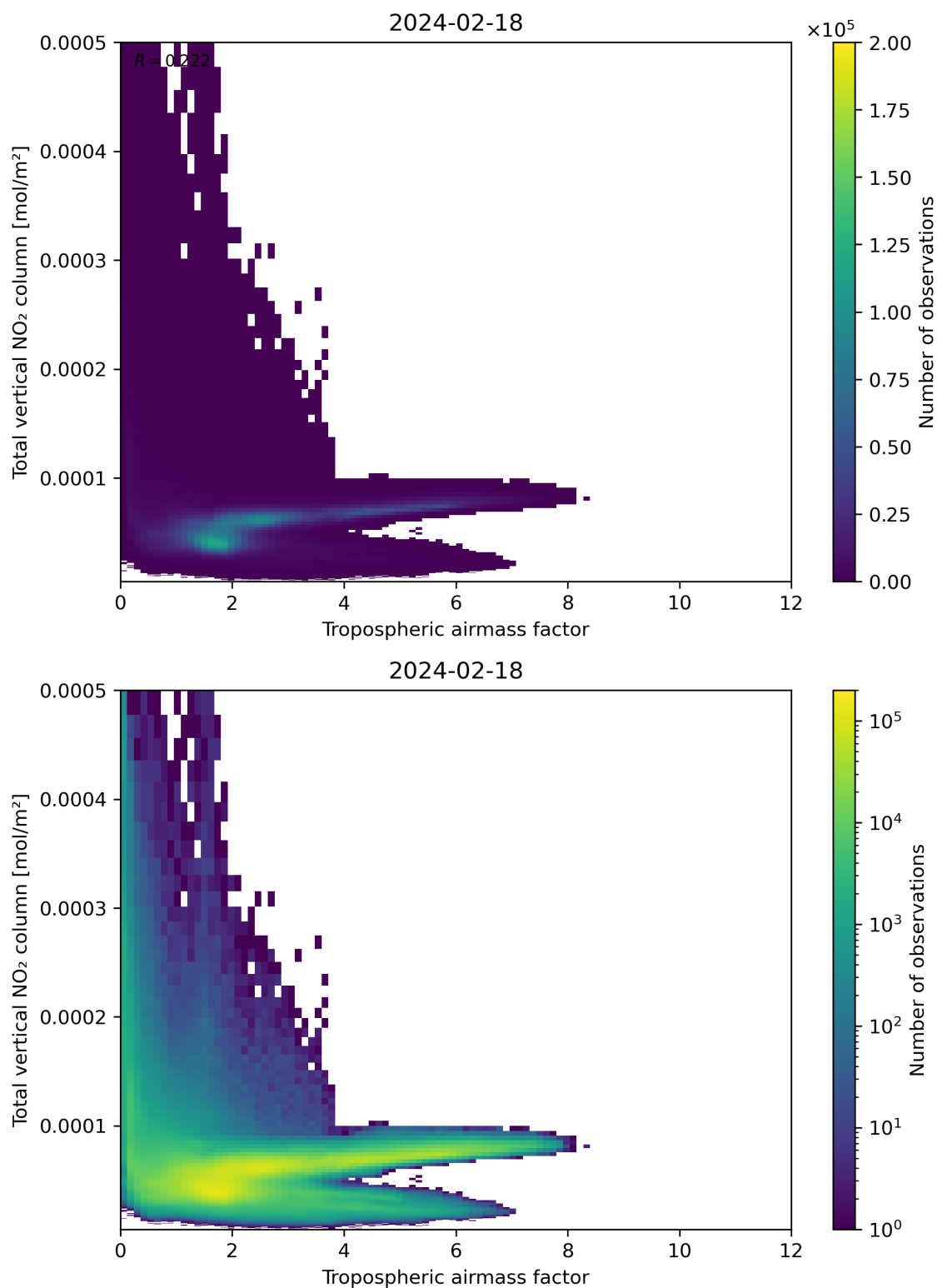
Figure 77: Scatter density plot of “Tropospheric airmass factor” against “Total vertical NO 2 column” for 2024-02-17 to 2024-02-19.
