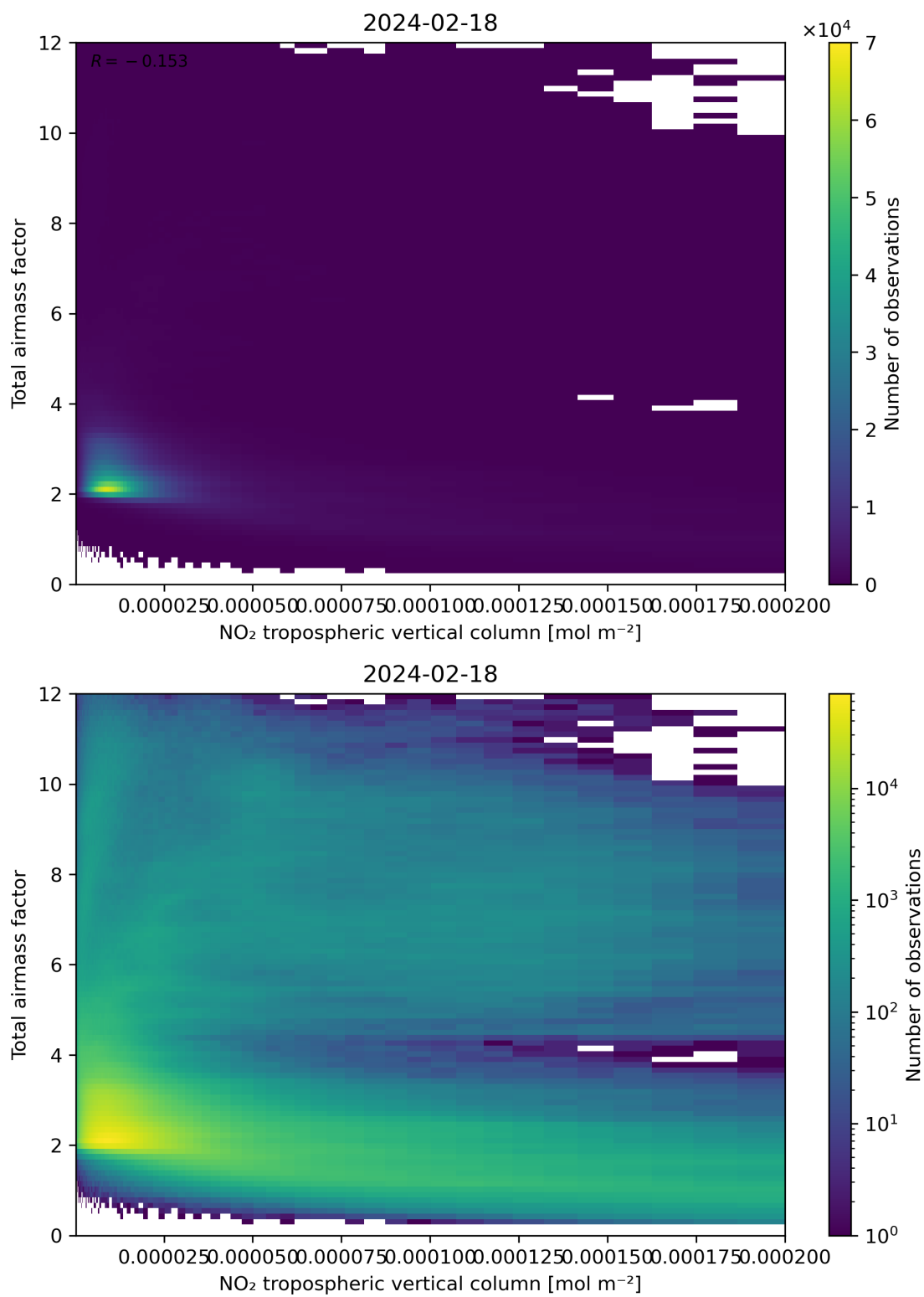
Figure 122: Scatter density plot of “NO 2 tropospheric vertical column” against “Total air mass factor” for 2024-02-17 to 2024-02-19.
