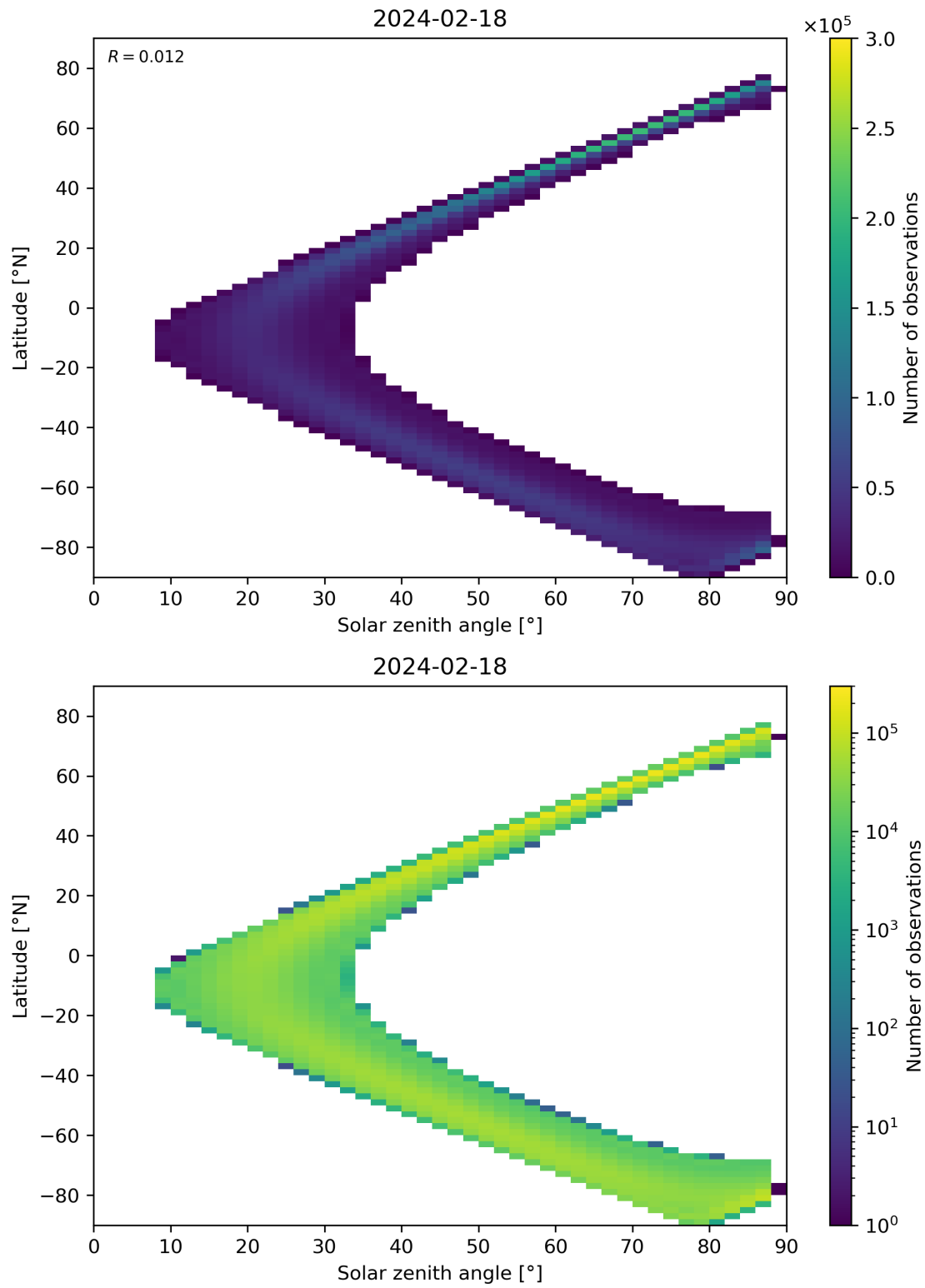
Figure 149: Scatter density plot of “Solar zenith angle” against “Latitude” for 2024-02-17 to 2024-02-19.
