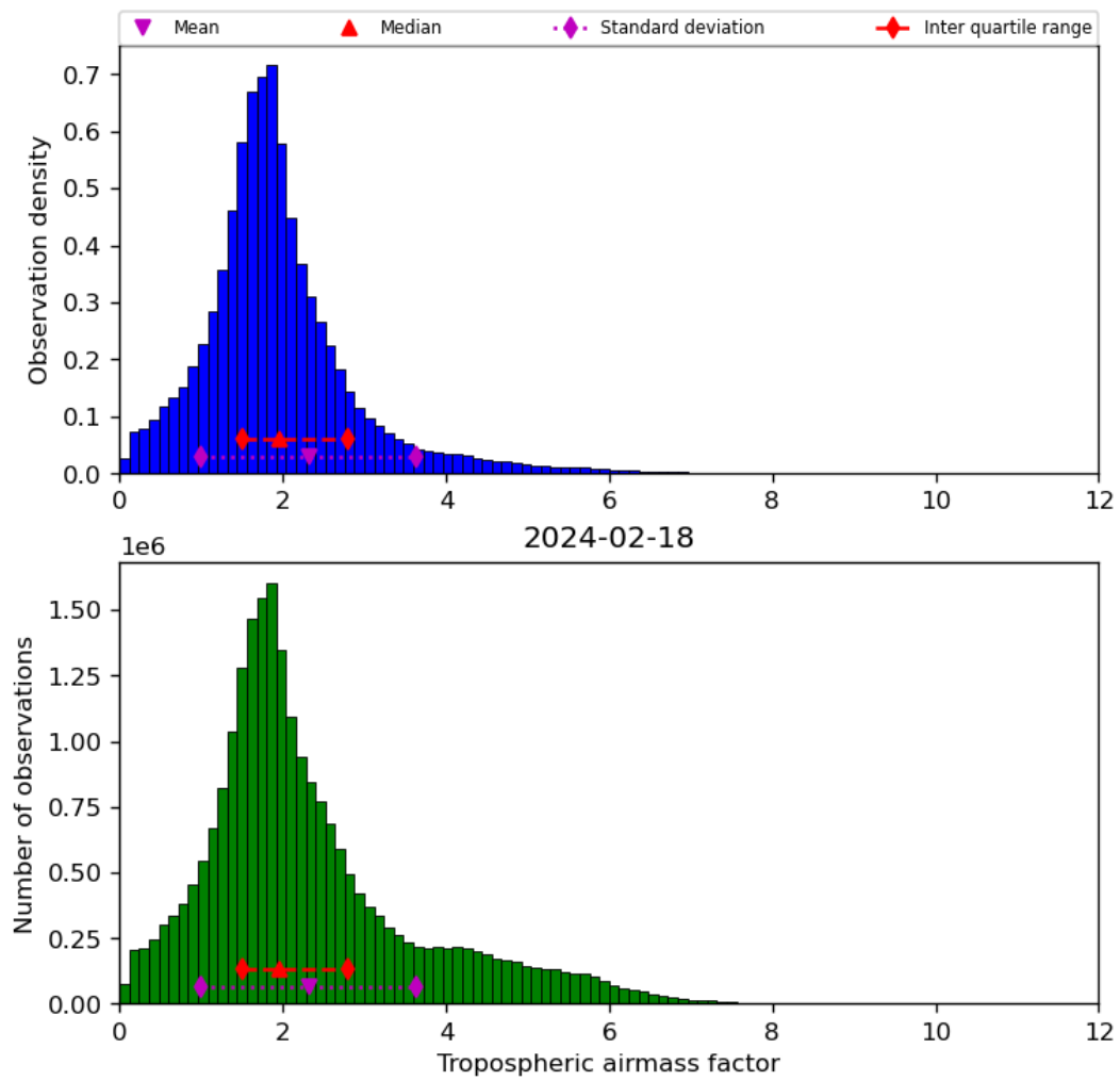
Figure 31: Histogram of “Tropospheric airmass factor” for 2024-02-17 to 2024-02-19
