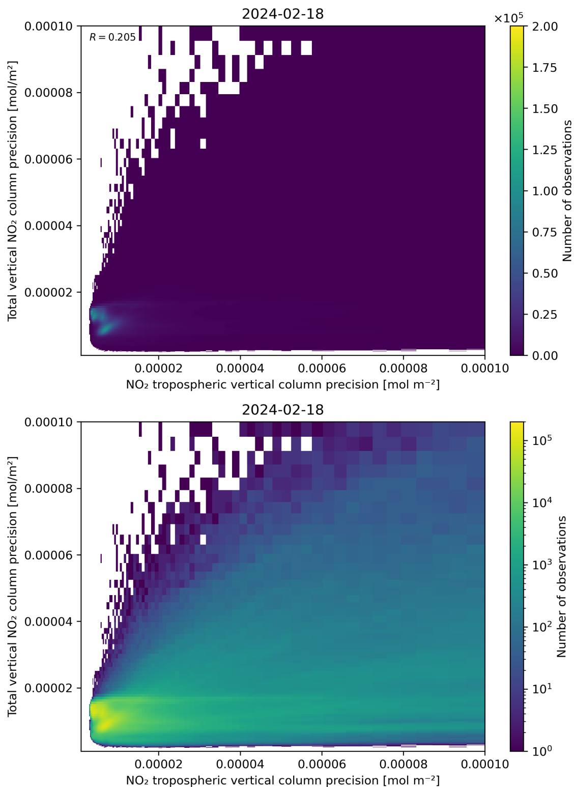
Figure 139: Scatter density plot of “NO 2 tropospheric vertical column precision” against “Total vertical NO 2 column precision” for 2024-02-17 to 2024-02-19.
