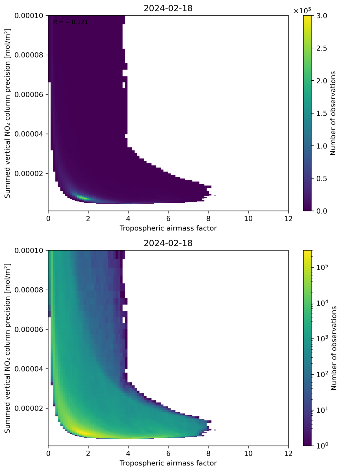
Figure 76: Scatter density plot of “Tropospheric air mass factor” against “Summed vertical NO 2 column precision” for 2024-02-17 to 2024-02-19.
