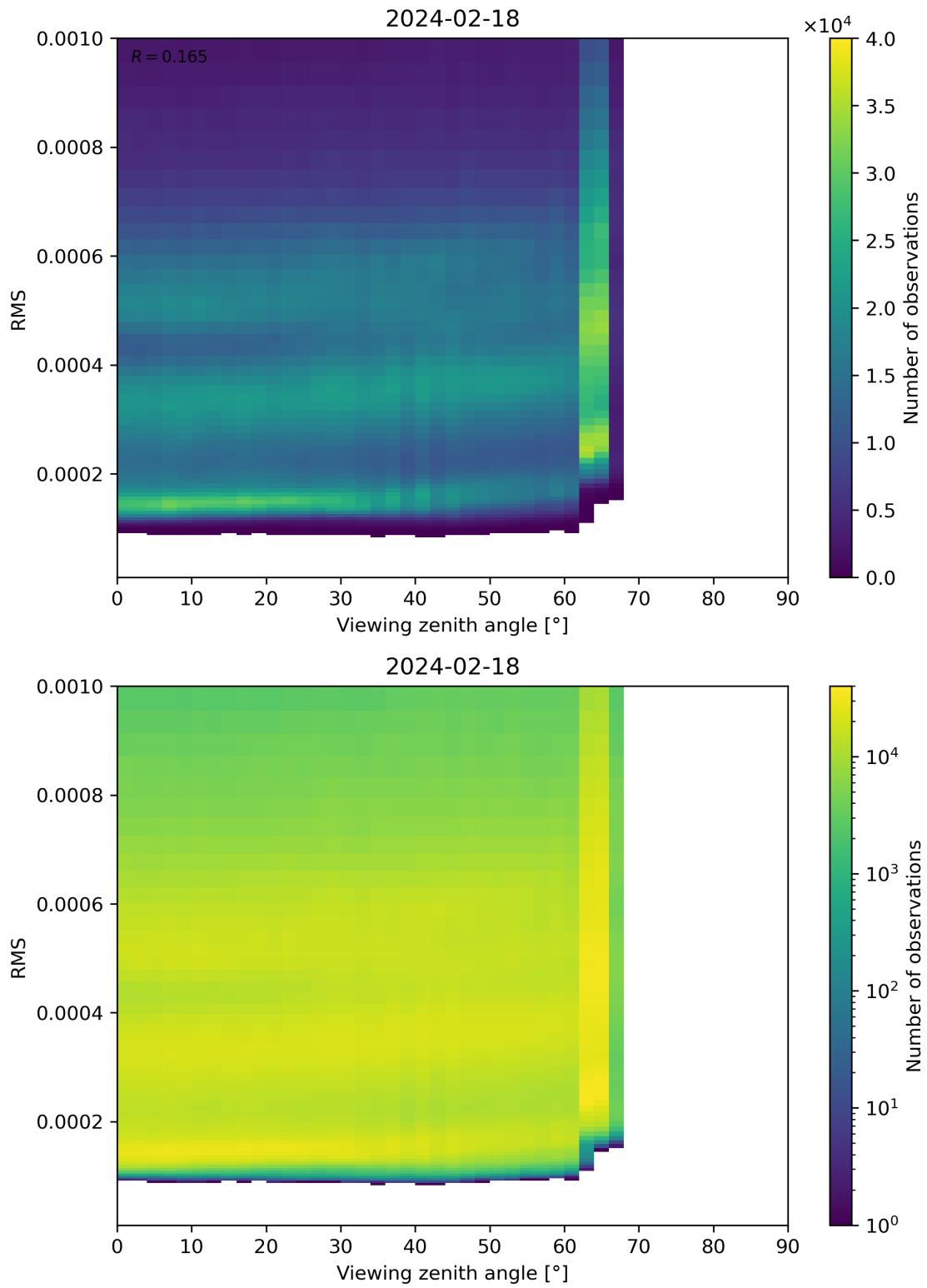
Figure 171: Scatter density plot of “Viewing zenith angle” against “RMS” for 2024-02-17 to 2024-02-19.
