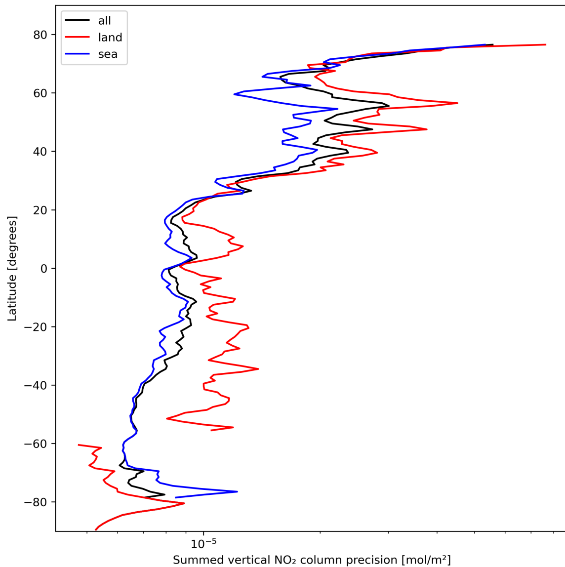
Figure 24: Zonal average of “Summed vertical NO 2 column precision” for 2024-02-17 to 2024-02-19.
