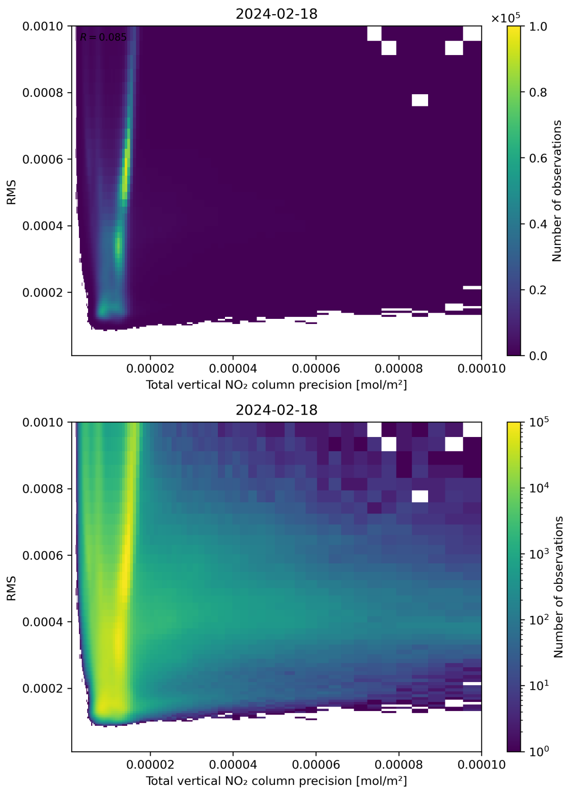
Figure 119: Scatter density plot of “Total vertical NO 2 column precision” against “RMS” for 2024-02-17 to 2024-02-19.
