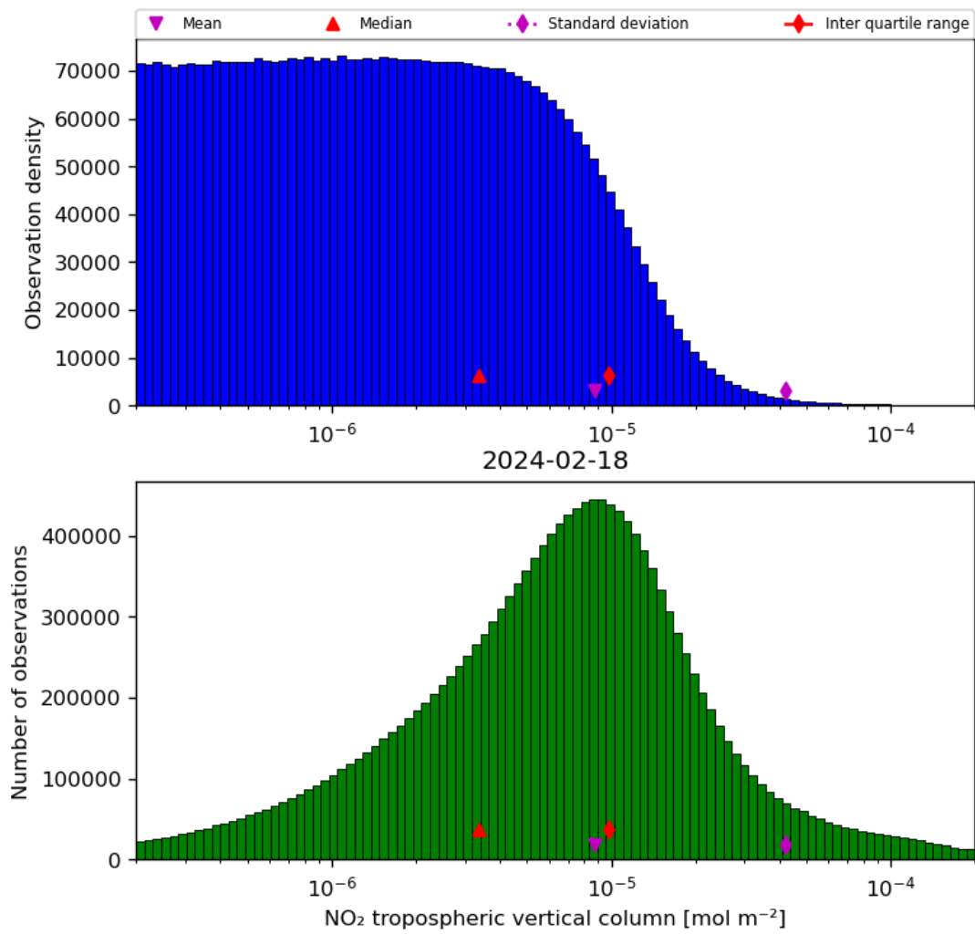
Figure 29: Histogram of “NO 2 tropospheric vertical column” for 2024-02-17 to 2024-02-19
