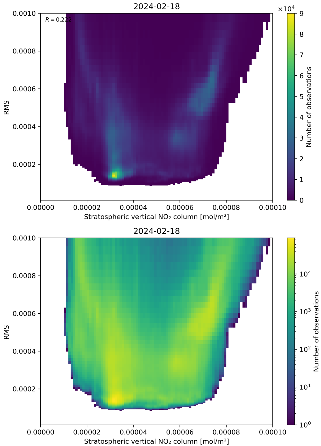
Figure 102: Scatter density plot of “Stratospheric vertical NO 2 column” against “RMS” for 2024-02-17 to 2024-02-19.
