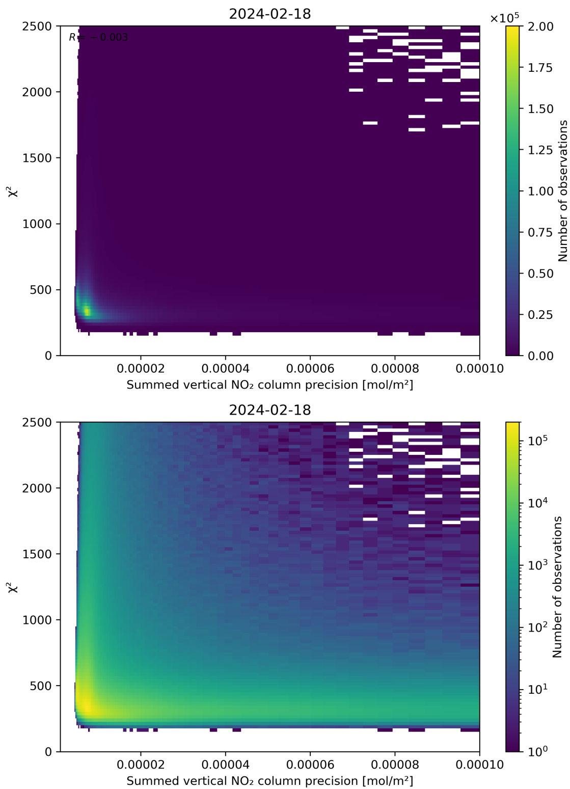
Figure 107: Scatter density plot of “Summed vertical NO 2 column precision” against “ \chi^2 ” for 2024-02-17 to 2024-02-19.
