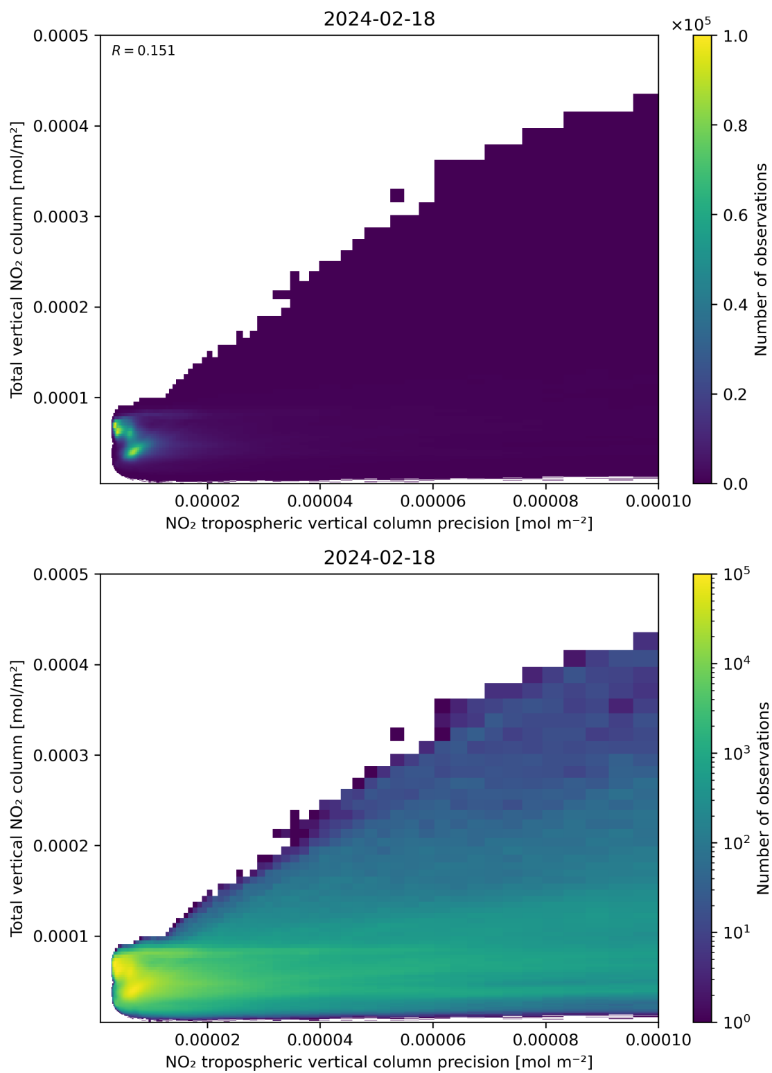
Figure 138: Scatter density plot of “NO 2 tropospheric vertical column precision” against “Total vertical NO 2 column” for 2024-02-17 to 2024-02-19.
