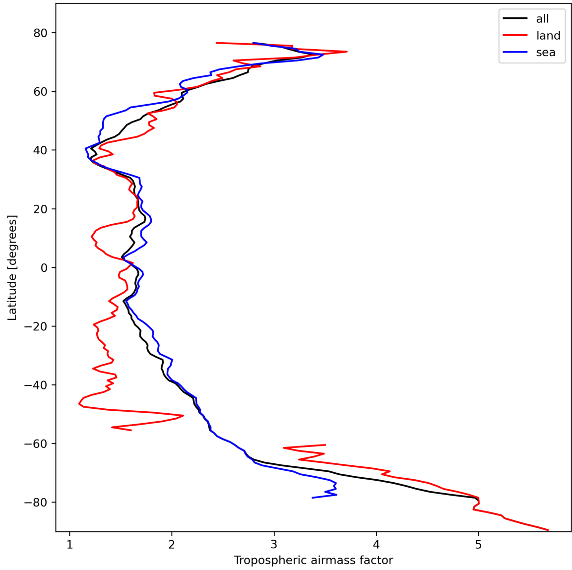
Figure 14: Zonal average of “Tropospheric airmass factor” for 2024-02-17 to 2024-02-19.
