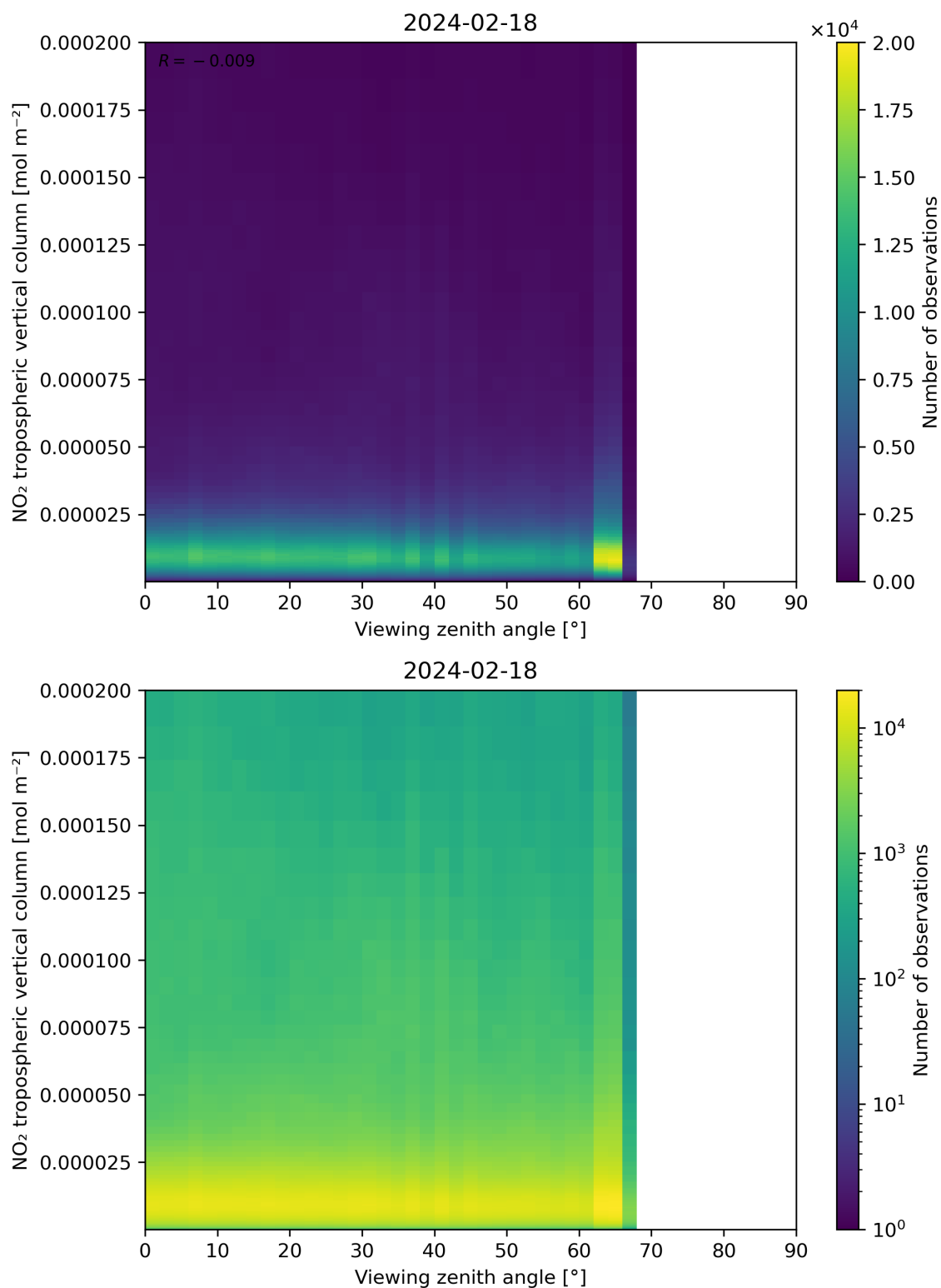
Figure 169: Scatter density plot of “Viewing zenith angle” against “NO 2 tropospheric vertical column” for 2024-02-17 to 2024-02-19.
