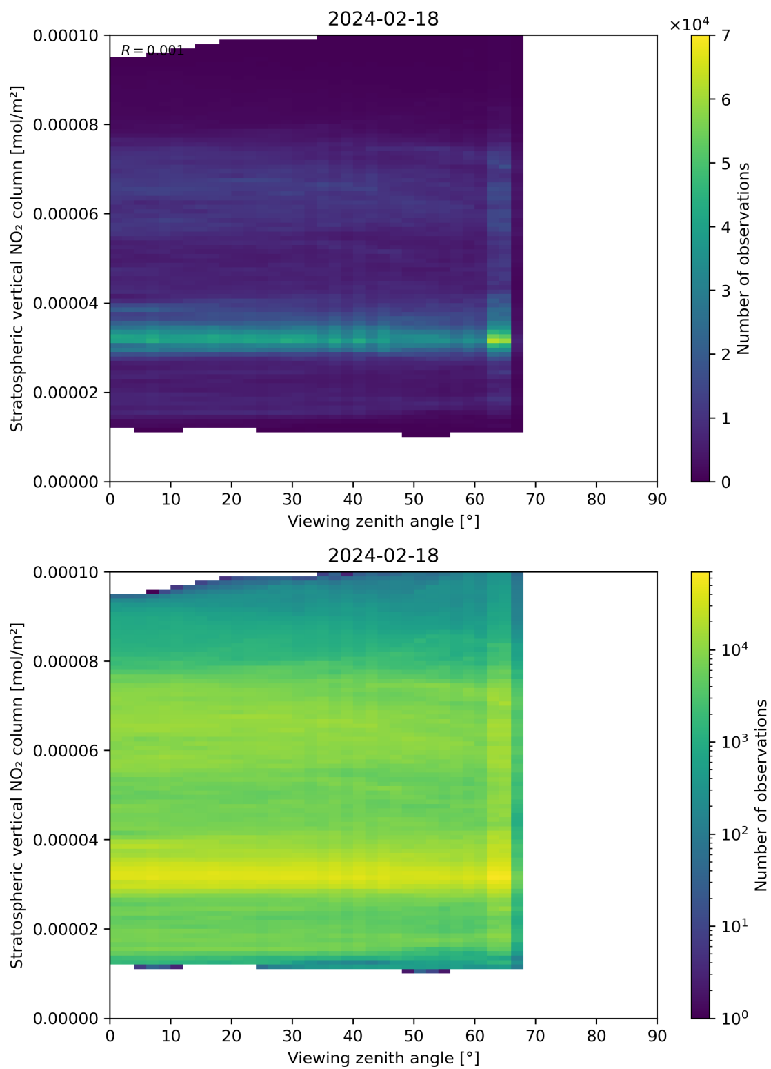
Figure 164: Scatter density plot of “Viewing zenith angle” against “Stratospheric vertical NO 2 column” for 2024-02-17 to 2024-02-19.
