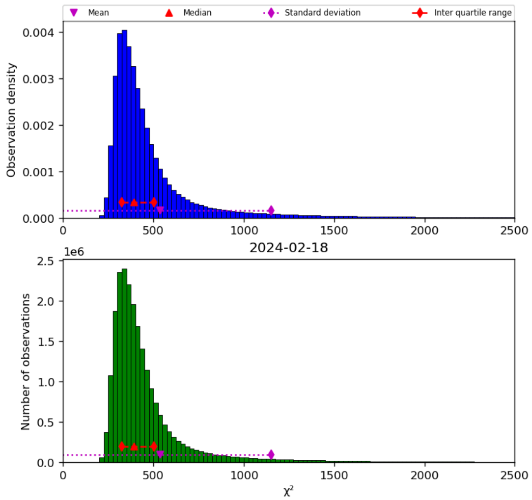
Figure 42: Histogram of “ \chi^2 ” for 2024-02-17 to 2024-02-19
