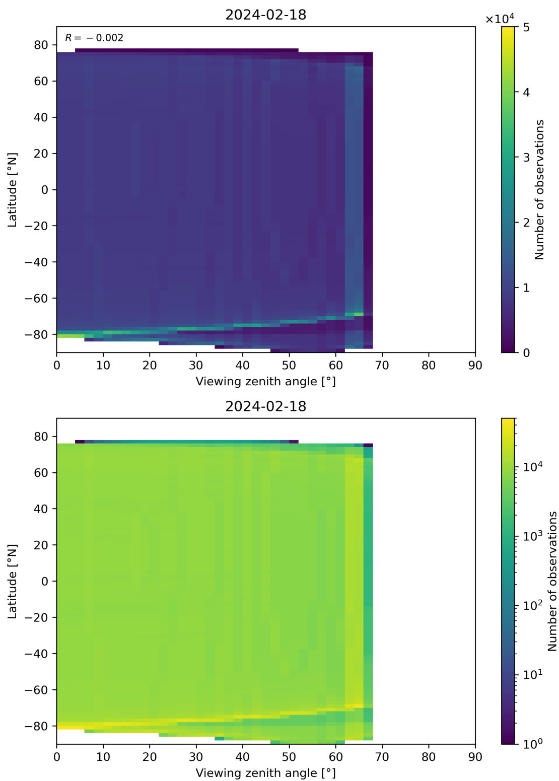
Figure 163: Scatter density plot of “Viewing zenith angle” against “Latitude” for 2024-02-17 to 2024-02-19.
