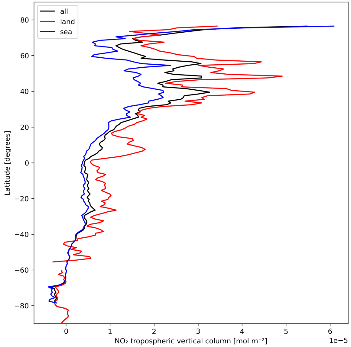
Figure 12: Zonal average of “NO 2 tropospheric vertical column” for 2024-02-17 to 2024-02-19.
