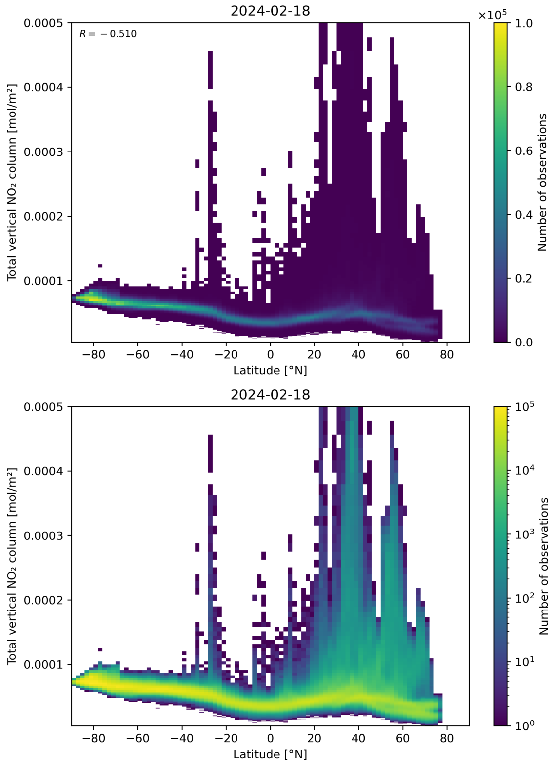
Figure 90: Scatter density plot of “Latitude” against “Total vertical NO 2 column” for 2024-02-17 to 2024-02-19.
