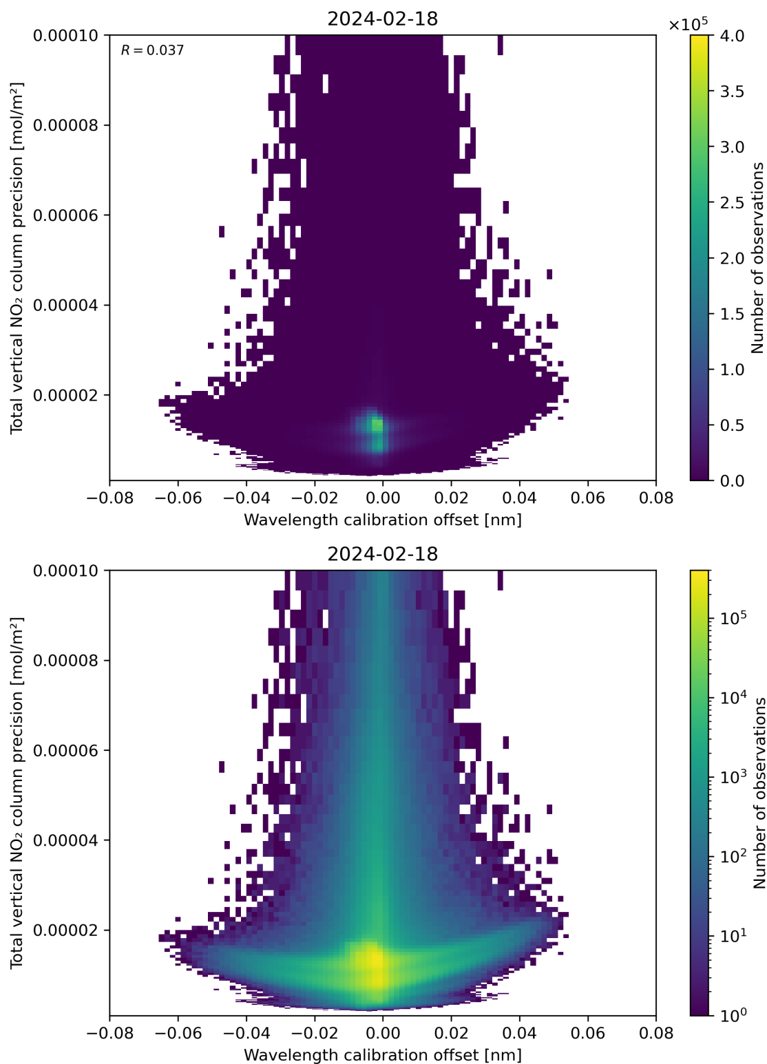
Figure 180: Scatter density plot of “Wavelength calibration offset” against “Total vertical NO 2 column precision” for 2024-02-17 to 2024-02-19.
