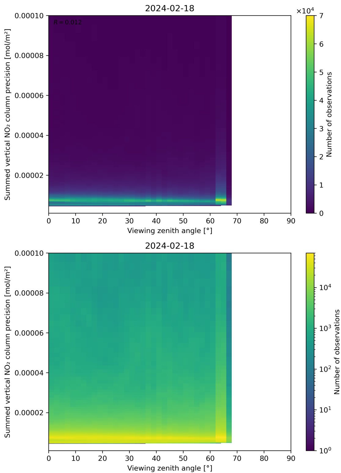
Figure 166: Scatter density plot of “Viewing zenith angle” against “Summed vertical NO 2 column precision” for 2024-02-17 to 2024-02-19.
