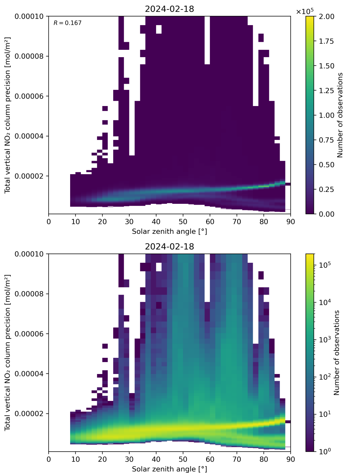
Figure 154: Scatter density plot of “Solar zenith angle” against “Total vertical NO 2 column precision” for 2024-02-17 to 2024-02-19.
