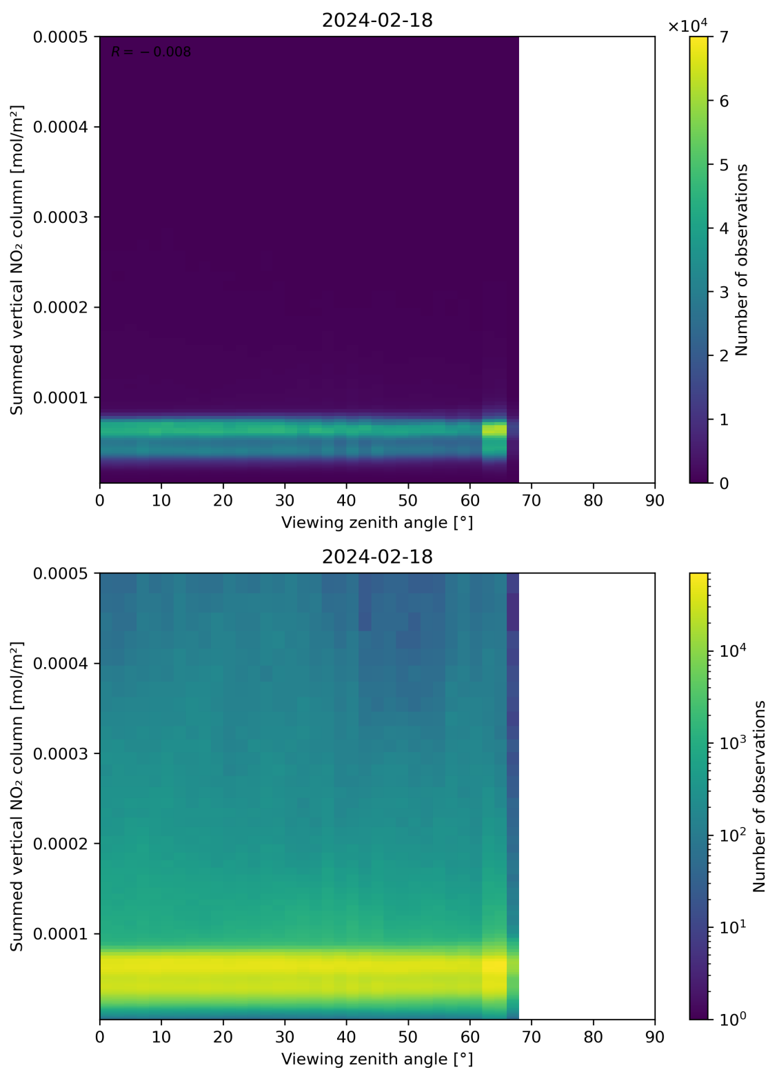
Figure 165: Scatter density plot of “Viewing zenith angle” against “Summed vertical NO 2 column” for 2024-02-17 to 2024-02-19.
