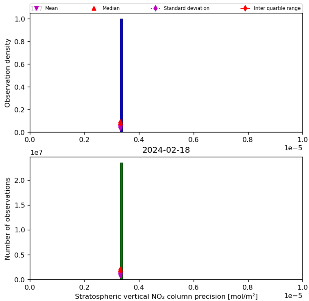
Figure 37: Histogram of “Stratospheric vertical NO 2 column precision” for 2024-02-17 to 2024-02-19
