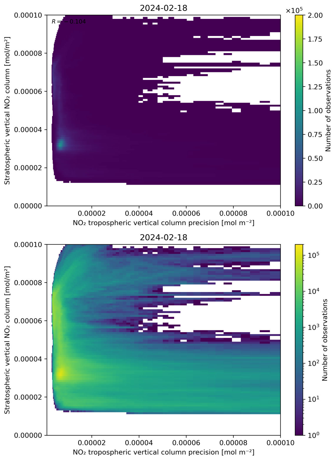
Figure 135: Scatter density plot of “NO 2 tropospheric vertical column precision” against “Stratospheric vertical NO 2 column” for 2024-02-17 to 2024-02-19.
