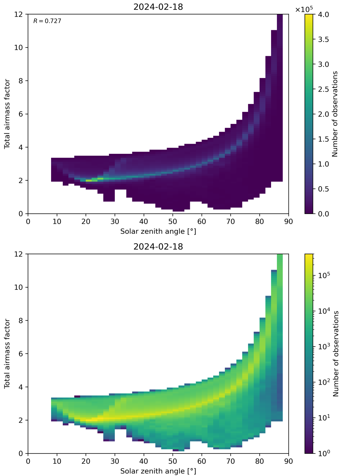
Figure 146: Scatter density plot of “Solar zenith angle” against “Total air mass factor” for 2024-02-17 to 2024-02-19.
