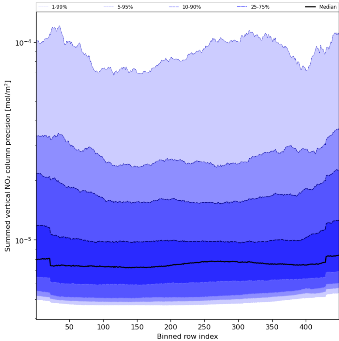
Figure 58: Along track statistics of “Summed vertical NO 2 column precision” for 2024-02-17 to 2024-02-19
