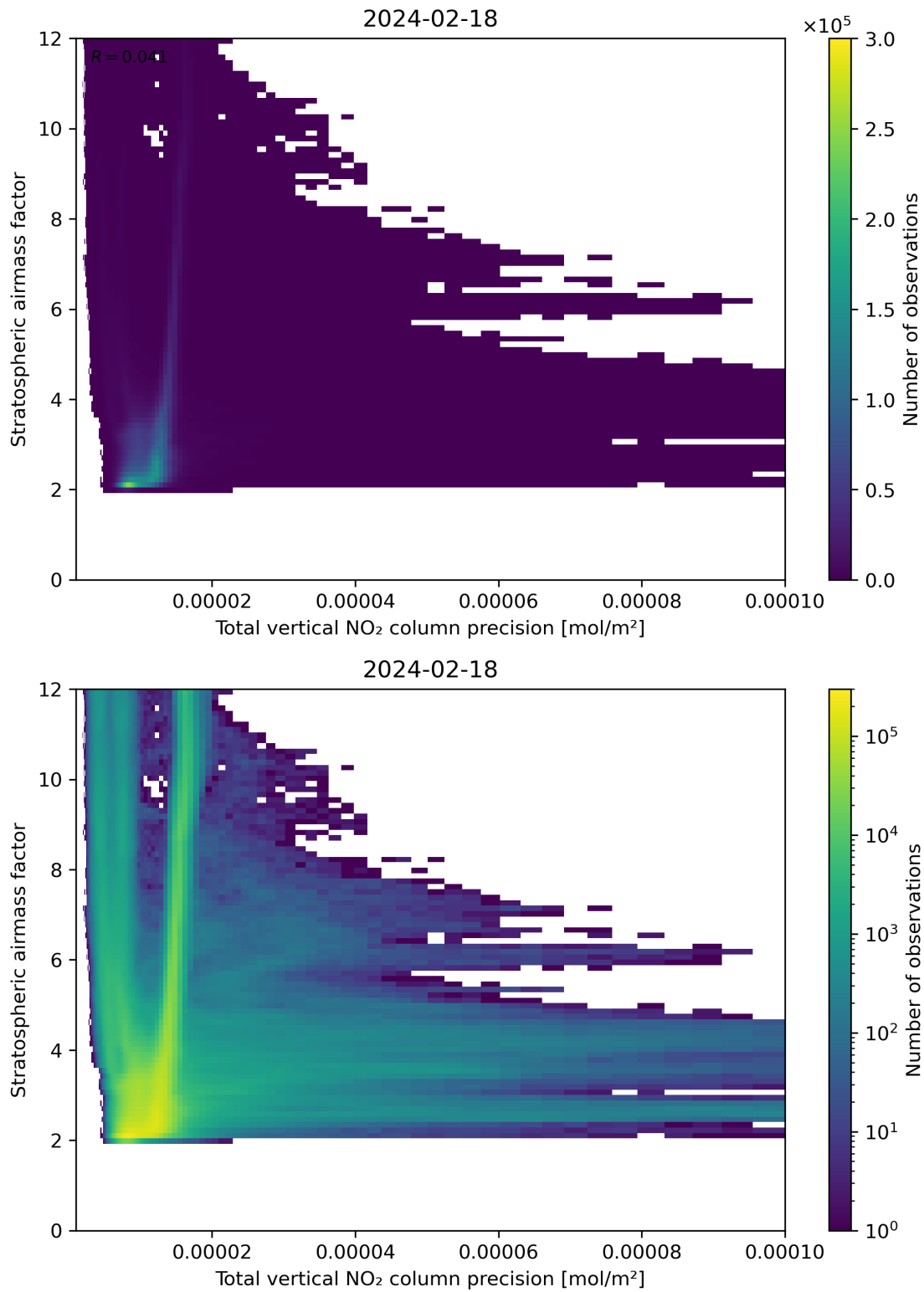
Figure 115: Scatter density plot of “Total vertical NO 2 column precision” against “Stratospheric air mass factor” for 2024-02-17 to 2024-02-19.
