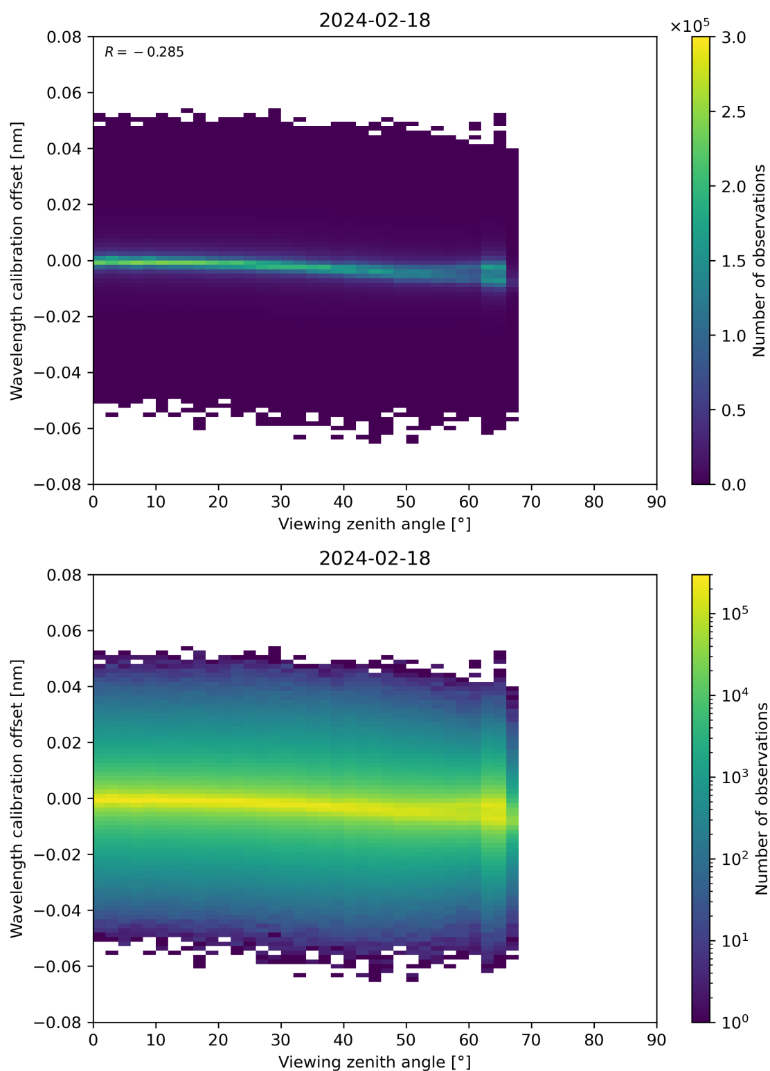
Figure 173: Scatter density plot of “Viewing zenith angle” against “Wavelength calibration offset” for 2024-02-17 to 2024-02-19.
