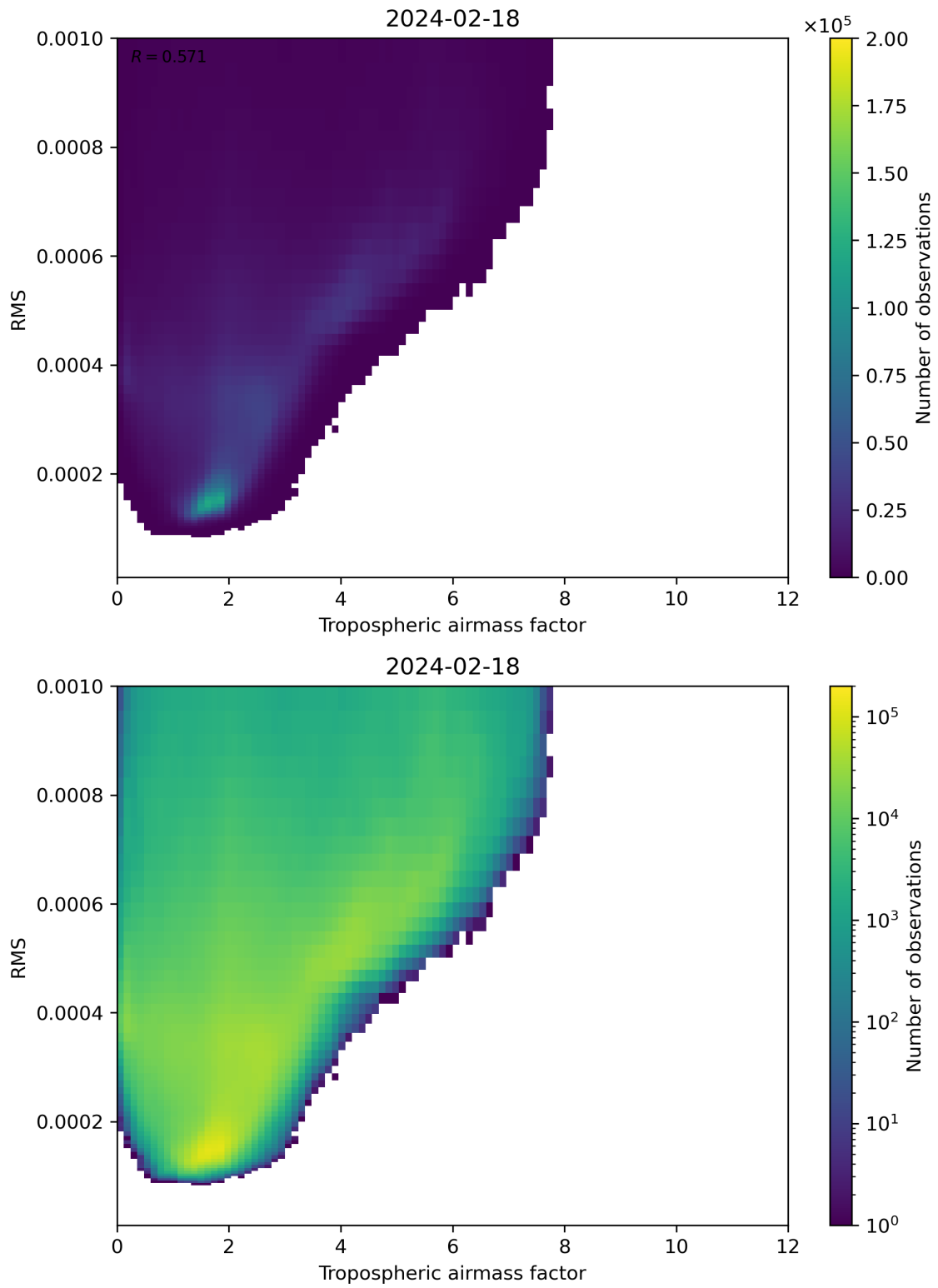
Figure 79: Scatter density plot of “Tropospheric airmass factor” against “RMS” for 2024-02-17 to 2024-02-19.
