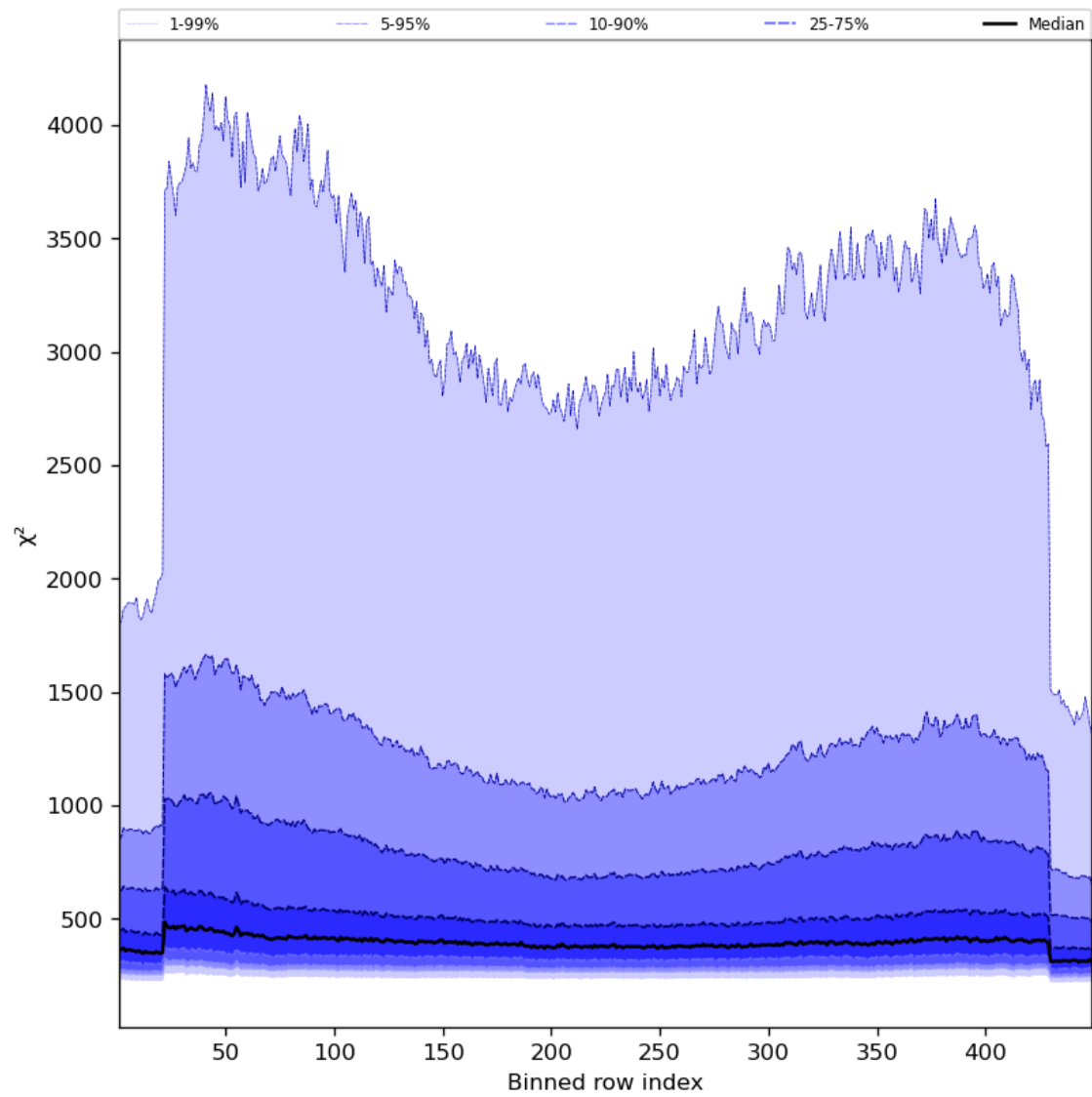
Figure 59: Along track statistics of “ \chi^2 ” for 2024-02-17 to 2024-02-19
