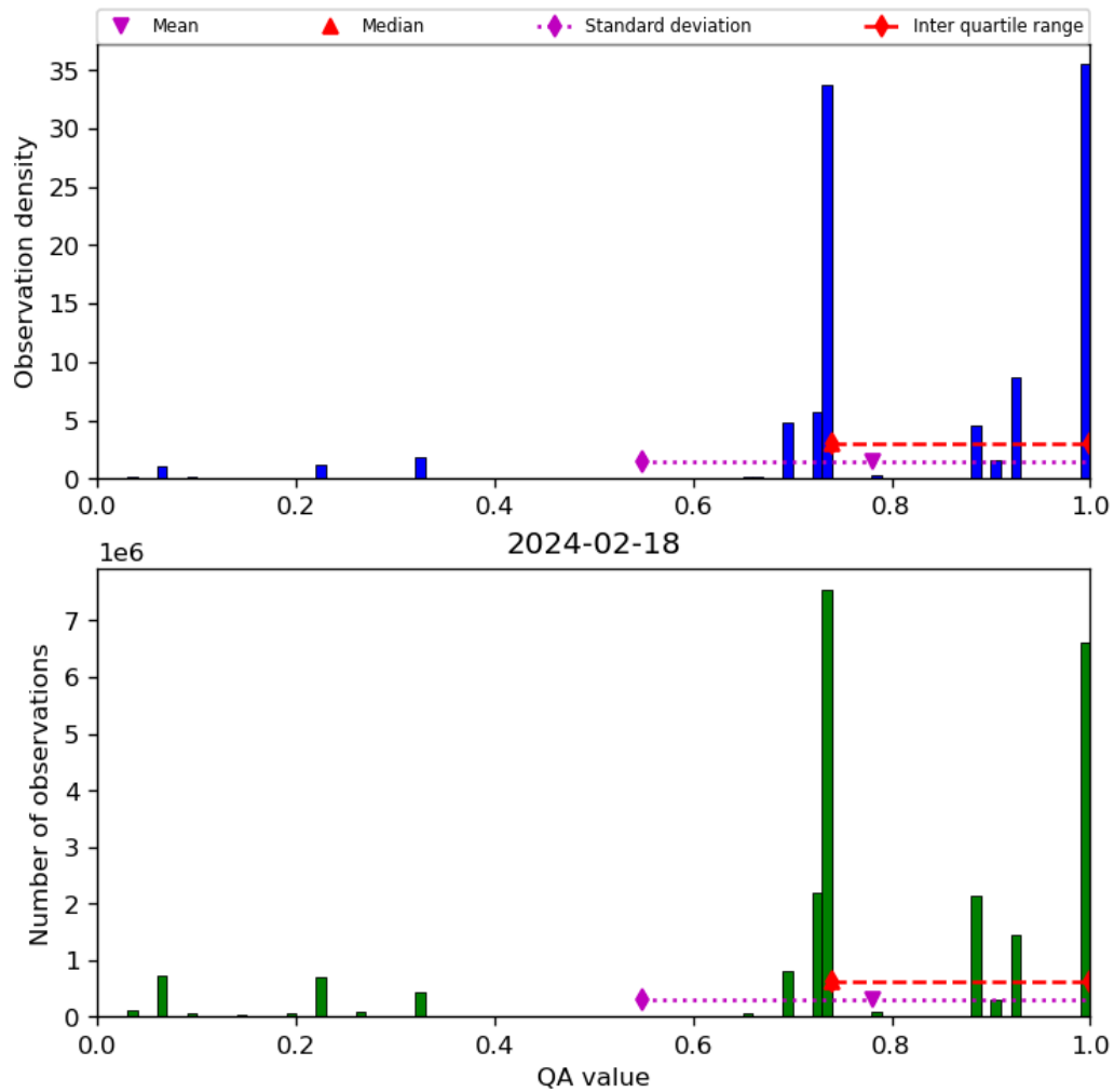
Figure 28: Histogram of “QA value” for 2024-02-17 to 2024-02-19
