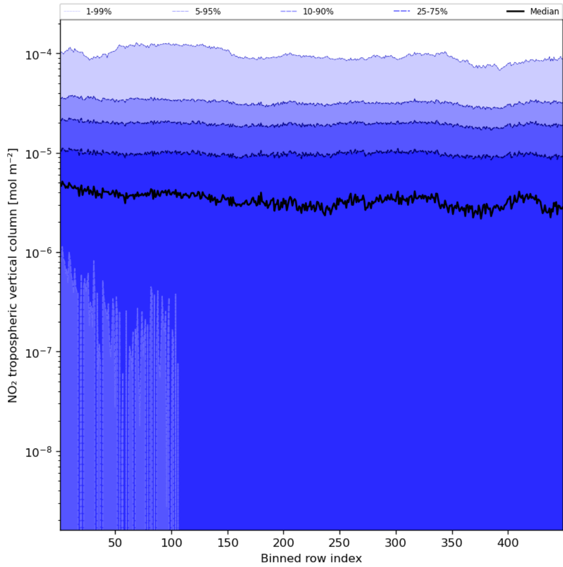
Figure 46: Along track statistics of “NO 2 tropospheric vertical column” for 2024-02-18 to 2024-02-20
