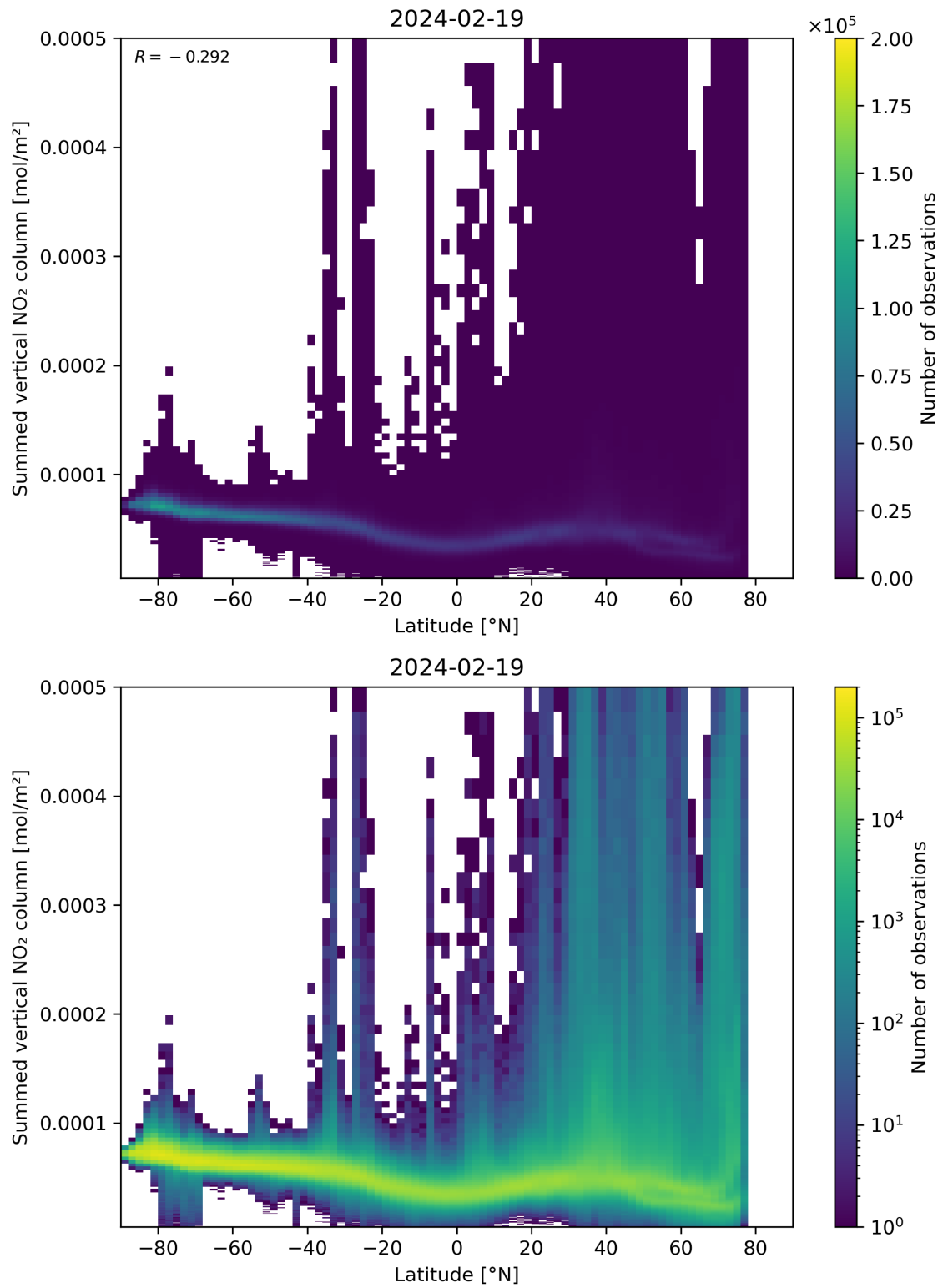
Figure 88: Scatter density plot of “Latitude” against “Summed vertical NO 2 column” for 2024-02-18 to 2024-02-20.
