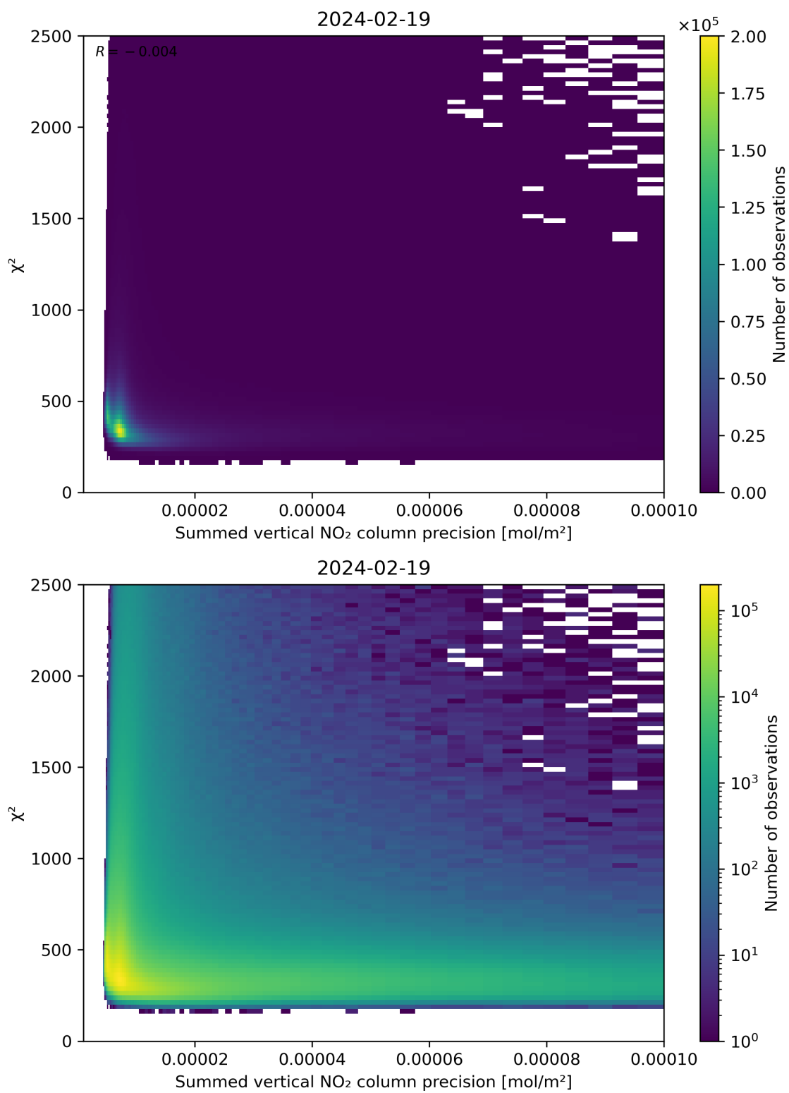
Figure 107: Scatter density plot of “Summed vertical NO 2 column precision” against “ \chi^2 ” for 2024-02-18 to 2024-02-20.
