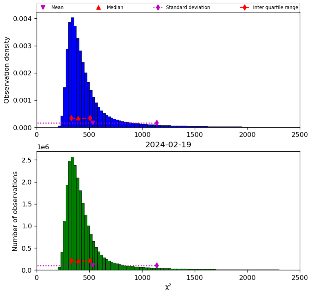
Figure 42: Histogram of “ \chi^2 ” for 2024-02-18 to 2024-02-20
