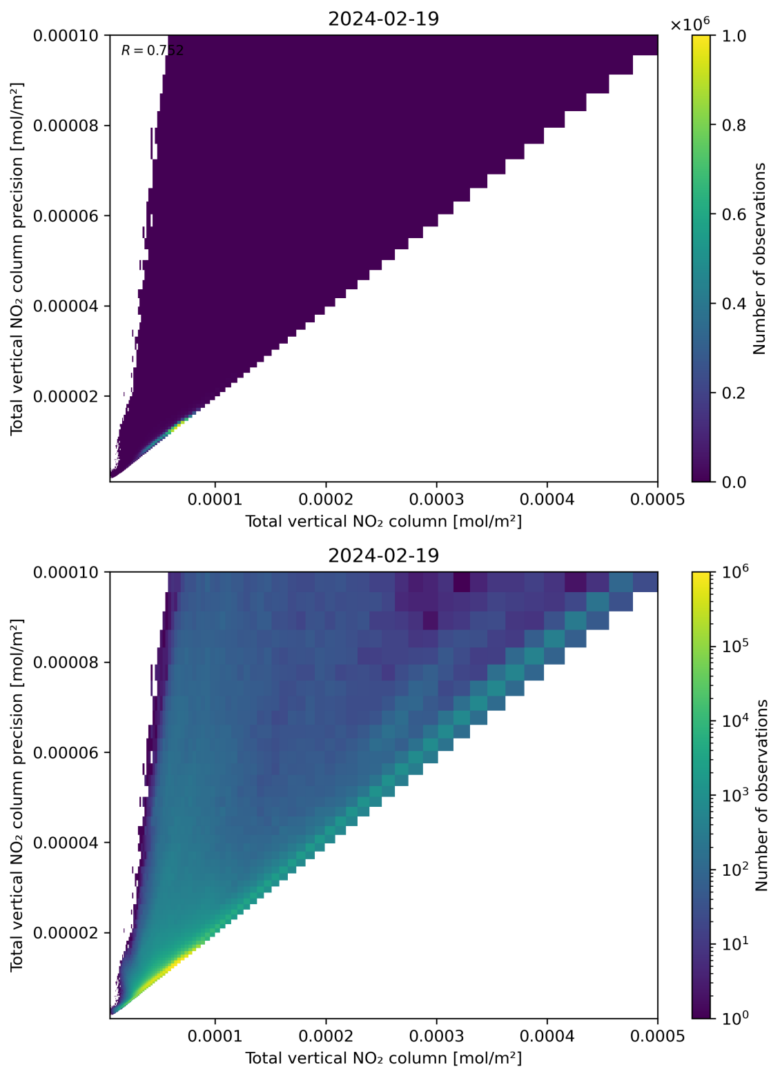
Figure 114: Scatter density plot of “Total vertical NO 2 column” against “Total vertical NO 2 column precision” for 2024-02-18 to 2024-02-20.
