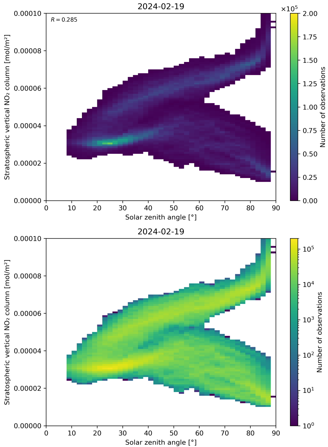
Figure 150: Scatter density plot of “Solar zenith angle” against “Stratospheric vertical NO 2 column” for 2024-02-18 to 2024-02-20.
