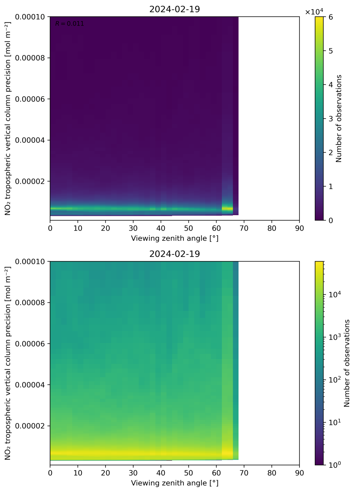
Figure 170: Scatter density plot of “Viewing zenith angle” against “NO 2 tropospheric vertical column precision” for 2024-02-18 to 2024-02-20.
