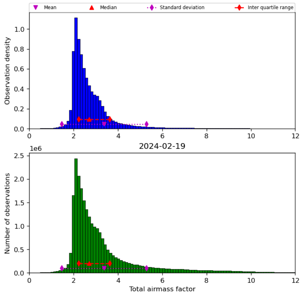
Figure 32: Histogram of “Total airmass factor” for 2024-02-18 to 2024-02-20
