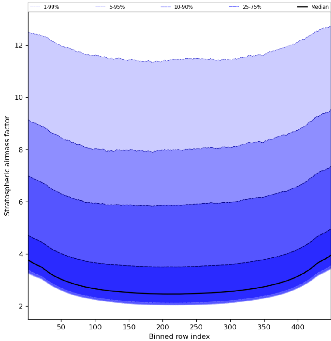
Figure 61: Along track statistics of “Stratospheric airmass factor” for 2024-02-18 to 2024-02-20
