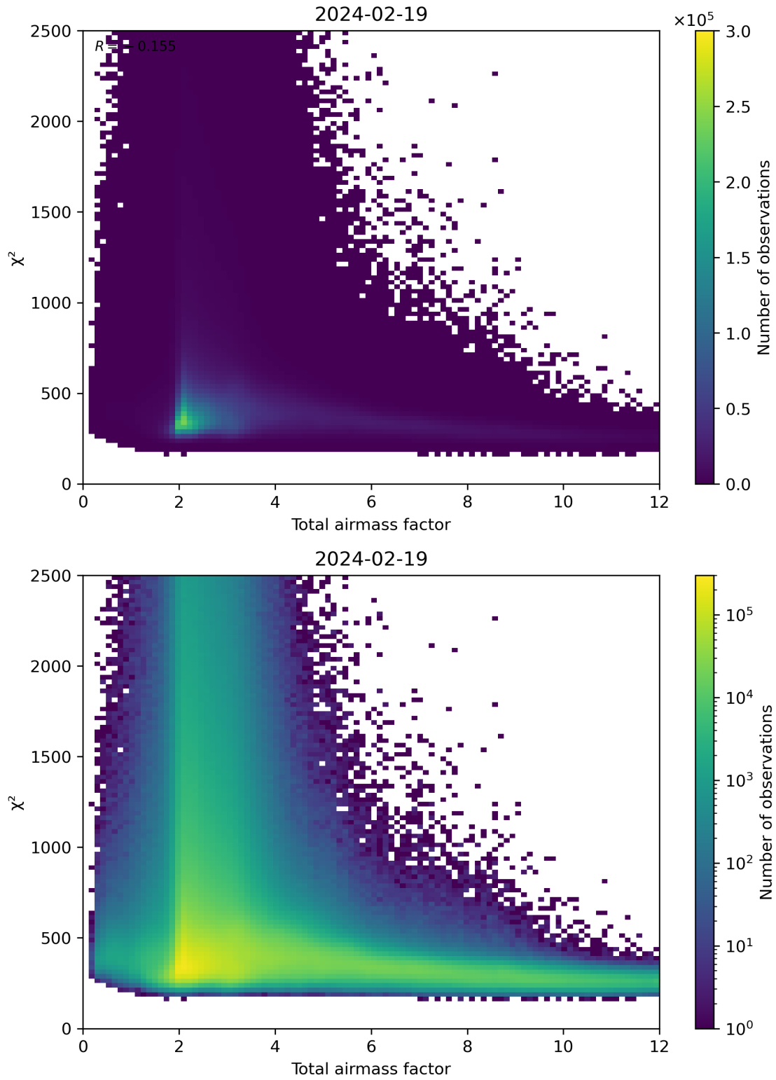
Figure 63: Scatter density plot of “Total airmass factor” against “ \chi^2 ” for 2024-02-18 to 2024-02-20.
