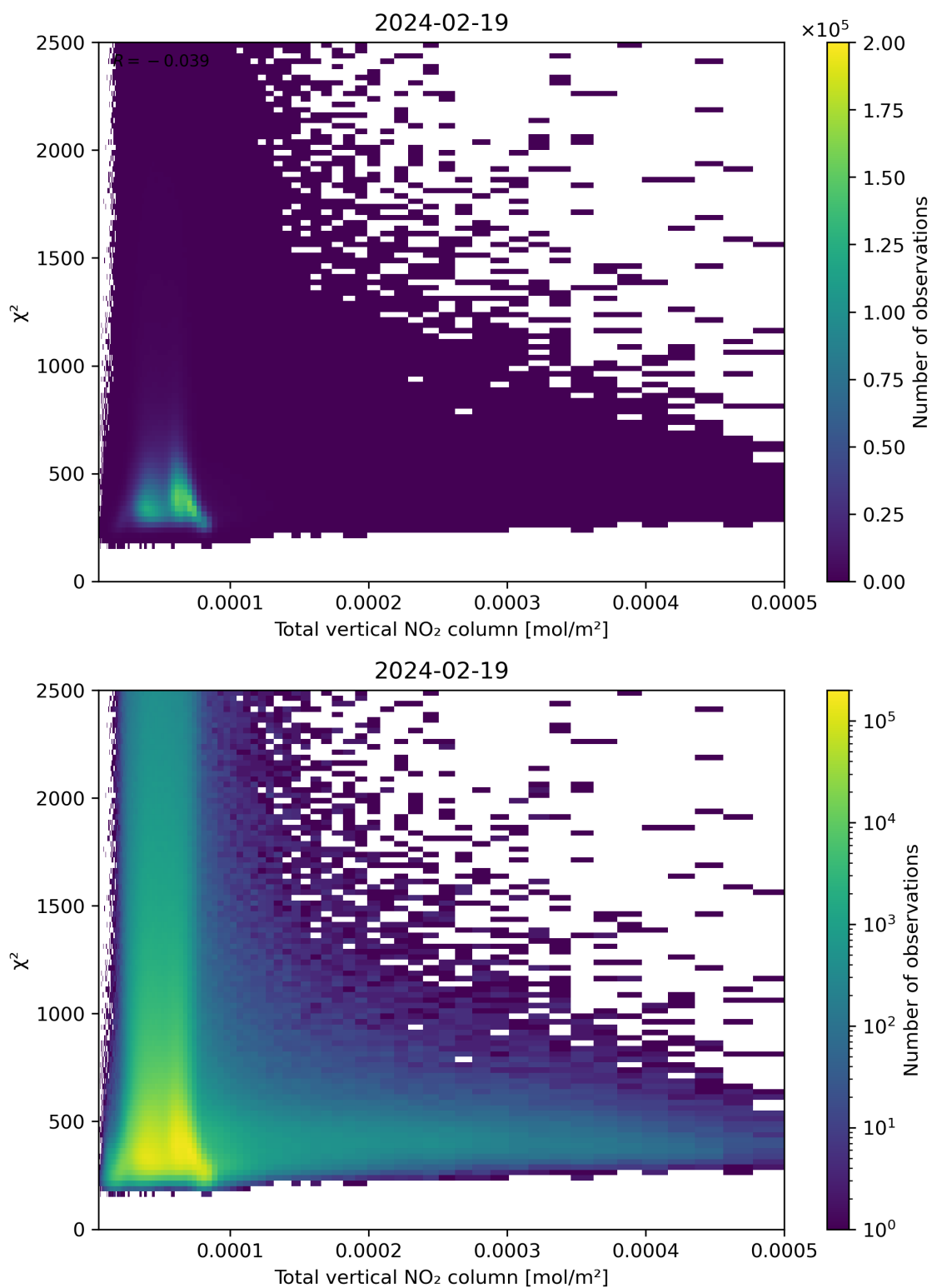
Figure 111: Scatter density plot of “Total vertical NO 2 column” against “ \chi^2 ” for 2024-02-18 to 2024-02-20.
