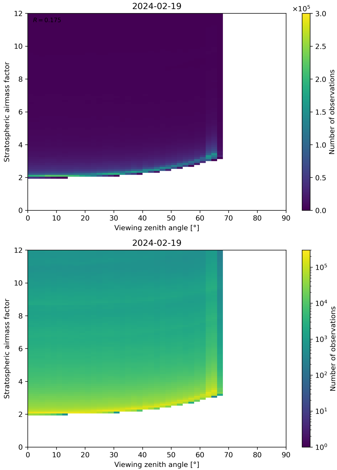
Figure 159: Scatter density plot of “Viewing zenith angle” against “Stratospheric airmass factor” for 2024-02-18 to 2024-02-20.
