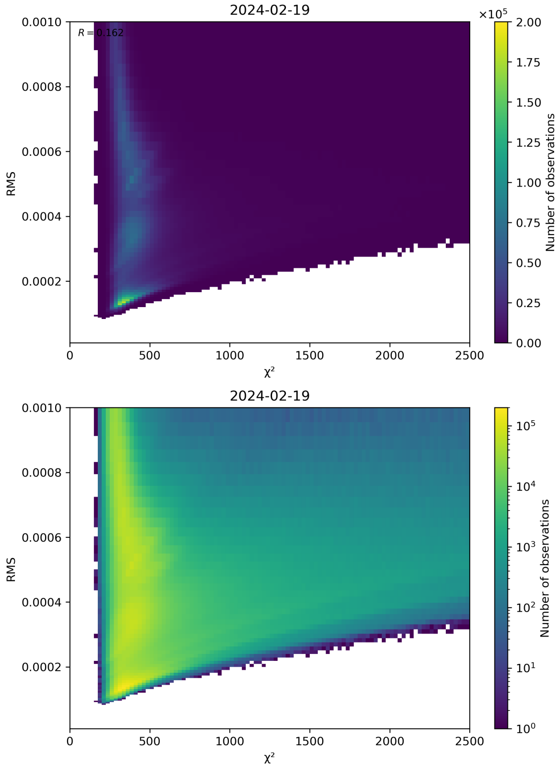
Figure 82: Scatter density plot of “ \chi^2 ” against “RMS” for 2024-02-18 to 2024-02-20.
