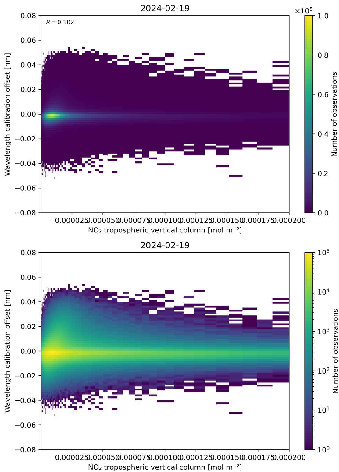
Figure 143: Scatter density plot of “NO 2 tropospheric vertical column” against “Wavelength calibration offset” for 2024-02-18 to 2024-02-20.
