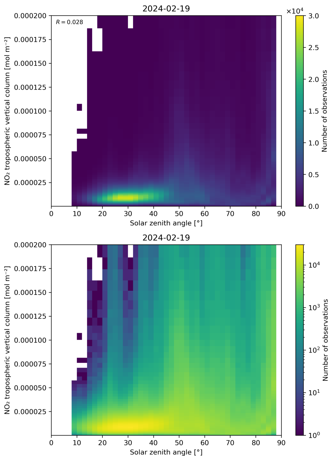
Figure 155: Scatter density plot of “Solar zenith angle” against “NO 2 tropospheric vertical column” for 2024-02-18 to 2024-02-20.
