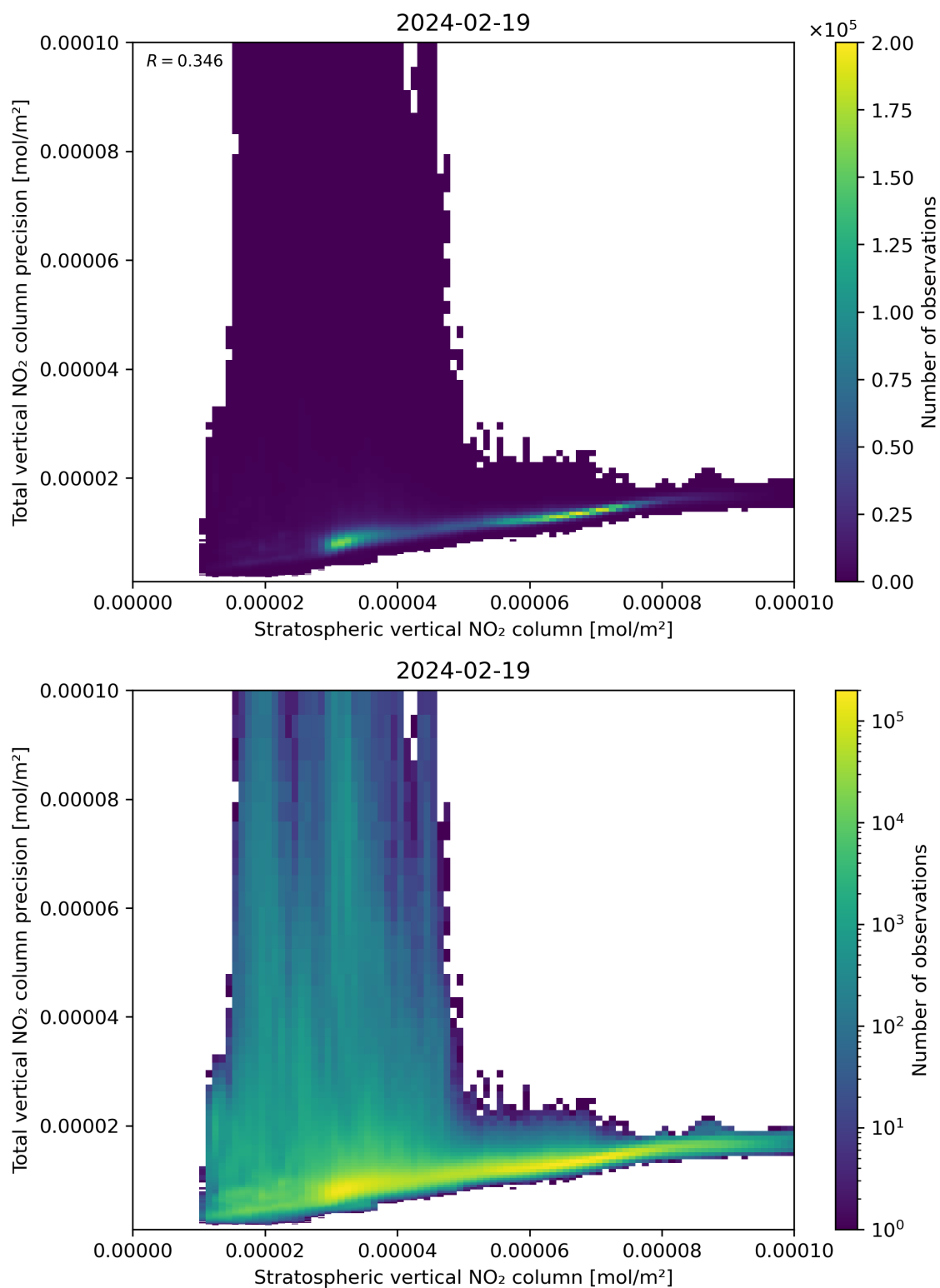
Figure 101: Scatter density plot of “Stratospheric vertical NO 2 column” against “Total vertical NO 2 column precision” for 2024-02-18 to 2024-02-20.
