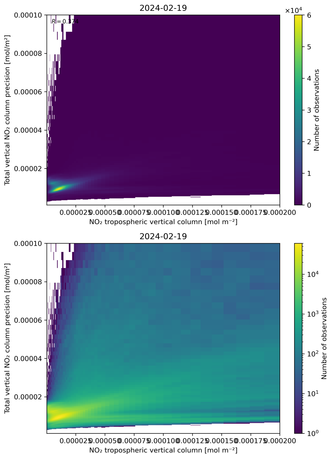
Figure 129: Scatter density plot of “NO 2 tropospheric vertical column” against “Total vertical NO 2 column precision” for 2024-02-18 to 2024-02-20.
