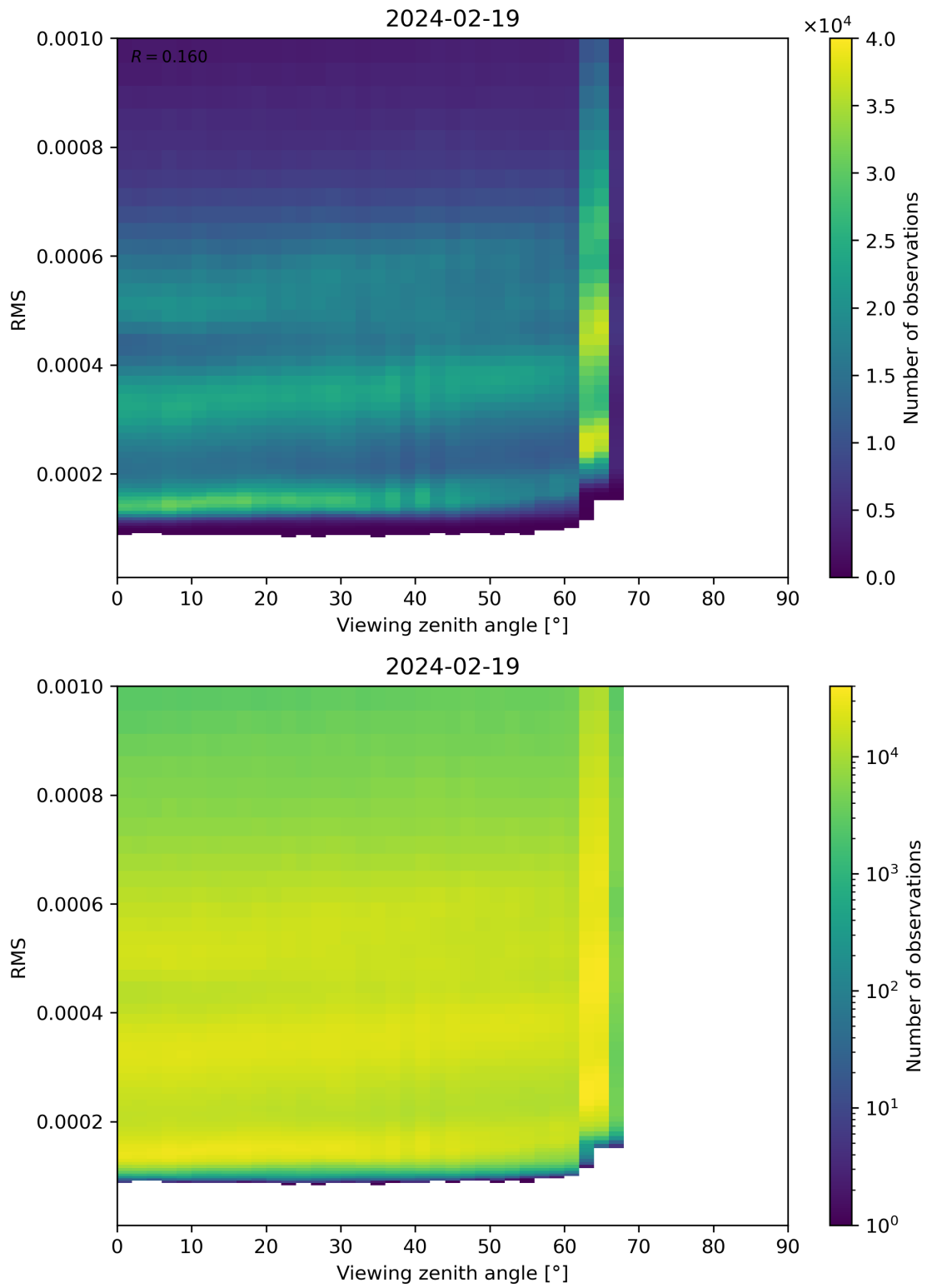
Figure 171: Scatter density plot of “Viewing zenith angle” against “RMS” for 2024-02-18 to 2024-02-20.
