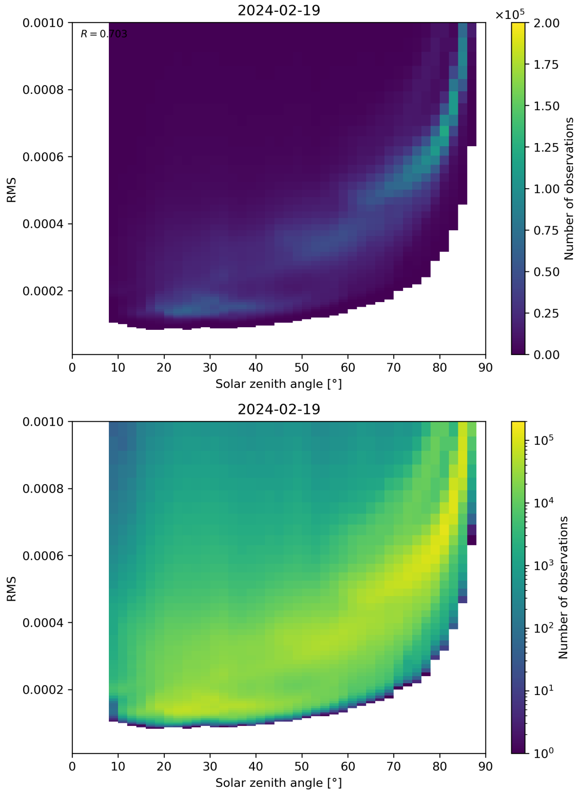
Figure 157: Scatter density plot of “Solar zenith angle” against “RMS” for 2024-02-18 to 2024-02-20.
