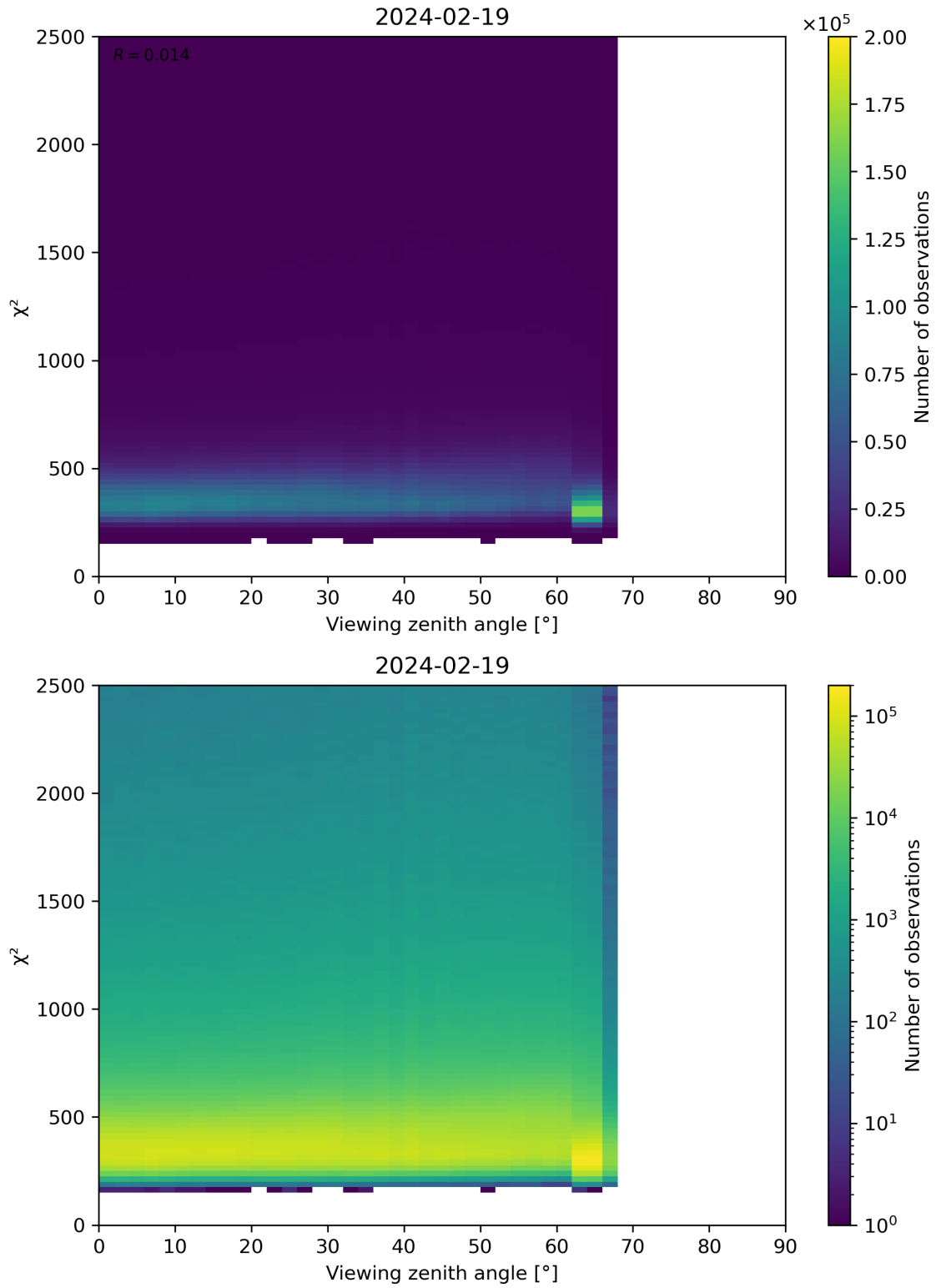
Figure 162: Scatter density plot of “Viewing zenith angle” against “ \chi^2 ” for 2024-02-18 to 2024-02-20.
