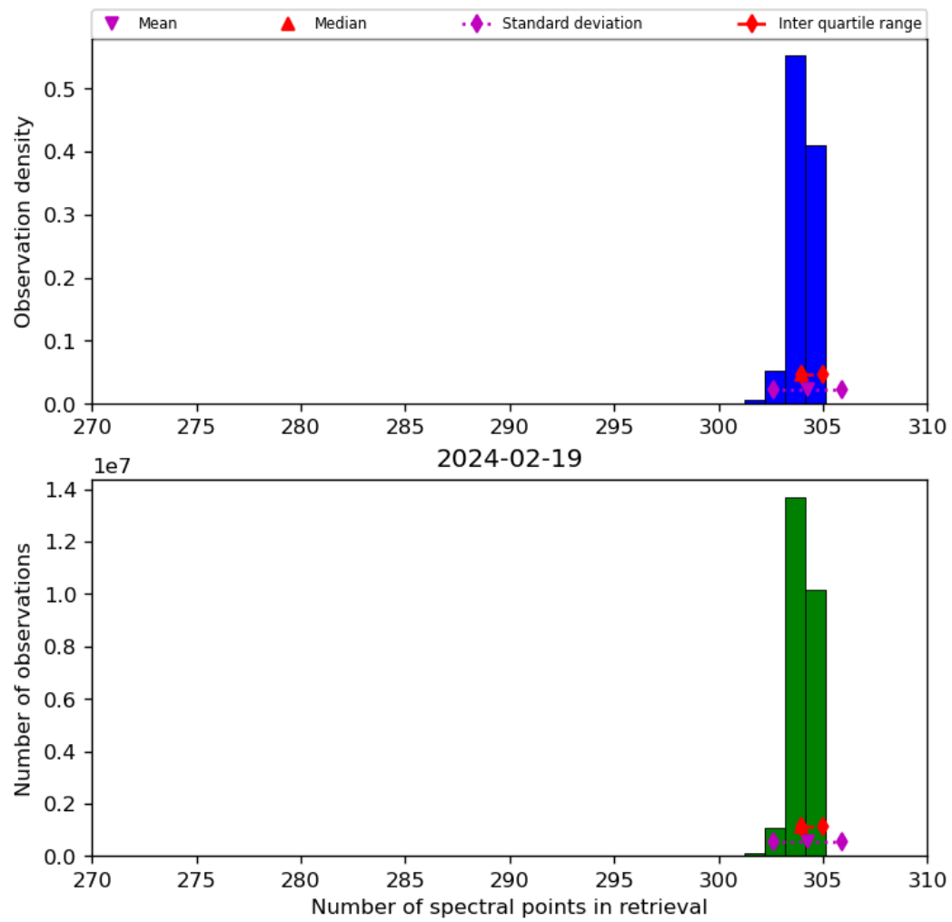
Figure 33: Histogram of “Number of spectral points in retrieval” for 2024-02-18 to 2024-02-20
