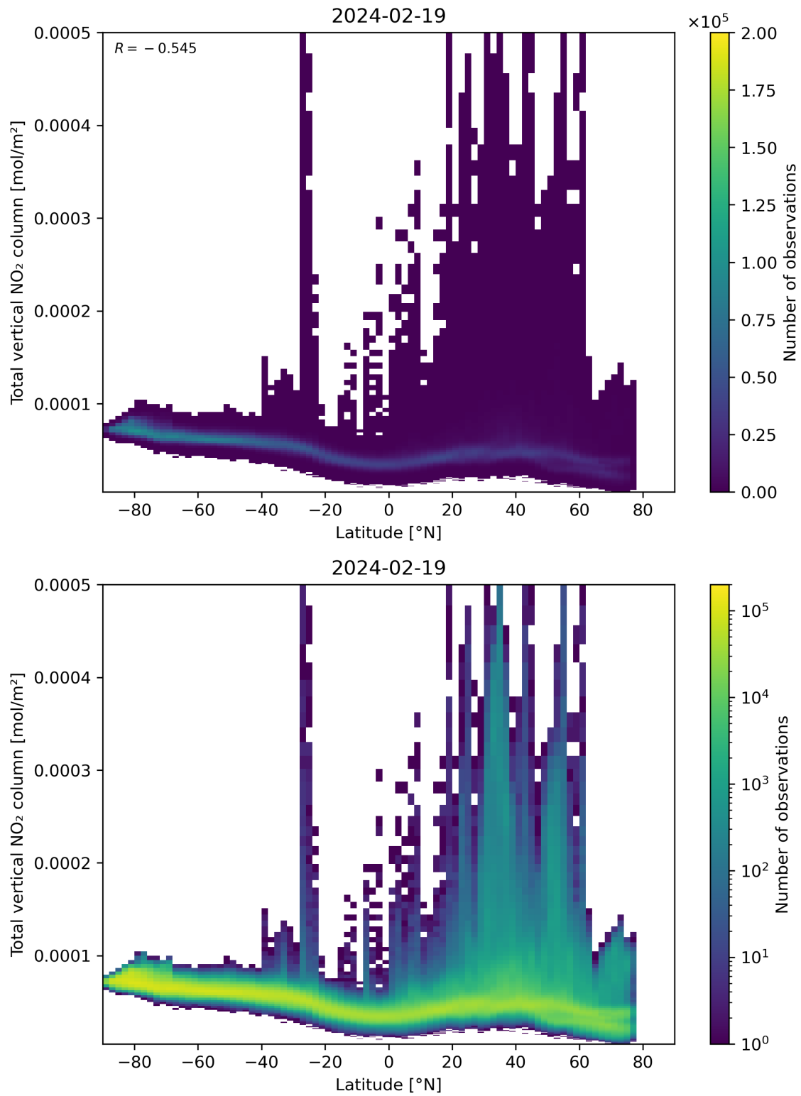
Figure 90: Scatter density plot of “Latitude” against “Total vertical NO 2 column” for 2024-02-18 to 2024-02-20.
