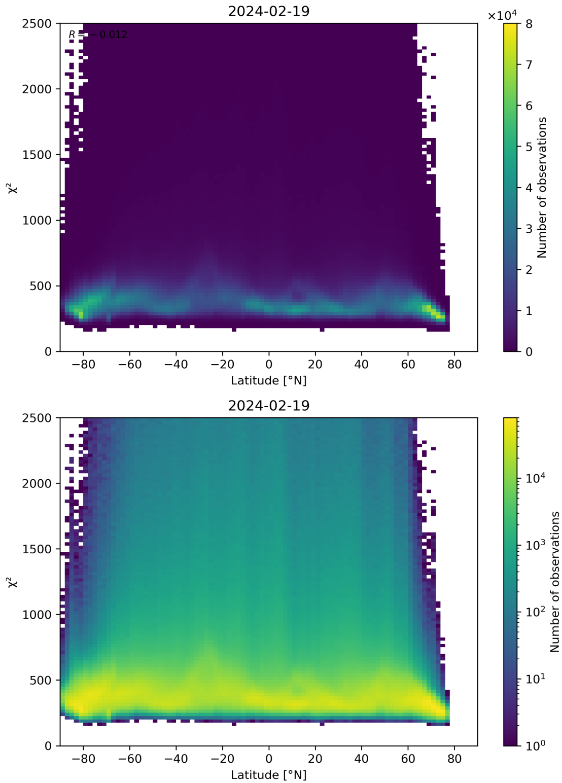
Figure 86: Scatter density plot of “Latitude” against “ \chi^2 ” for 2024-02-18 to 2024-02-20.
