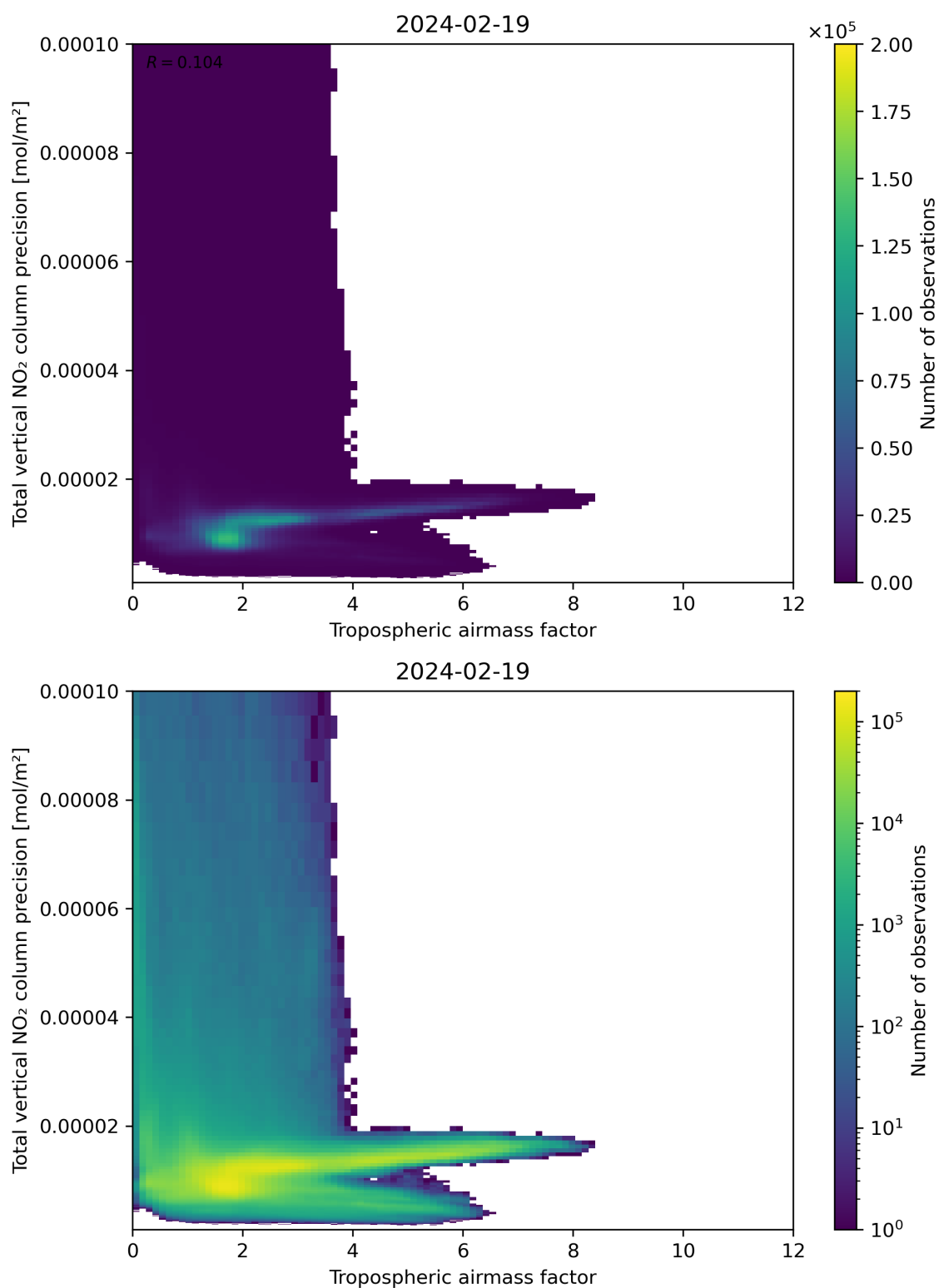
Figure 78: Scatter density plot of “Tropospheric air mass factor” against “Total vertical NO 2 column precision” for 2024-02-18 to 2024-02-20.
