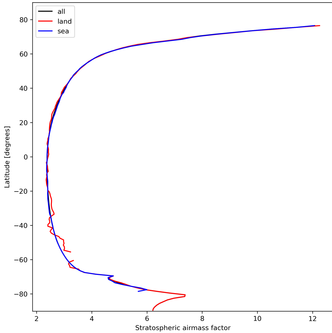
Figure 27: Zonal average of “Stratospheric airmass factor” for 2024-02-18 to 2024-02-20.
