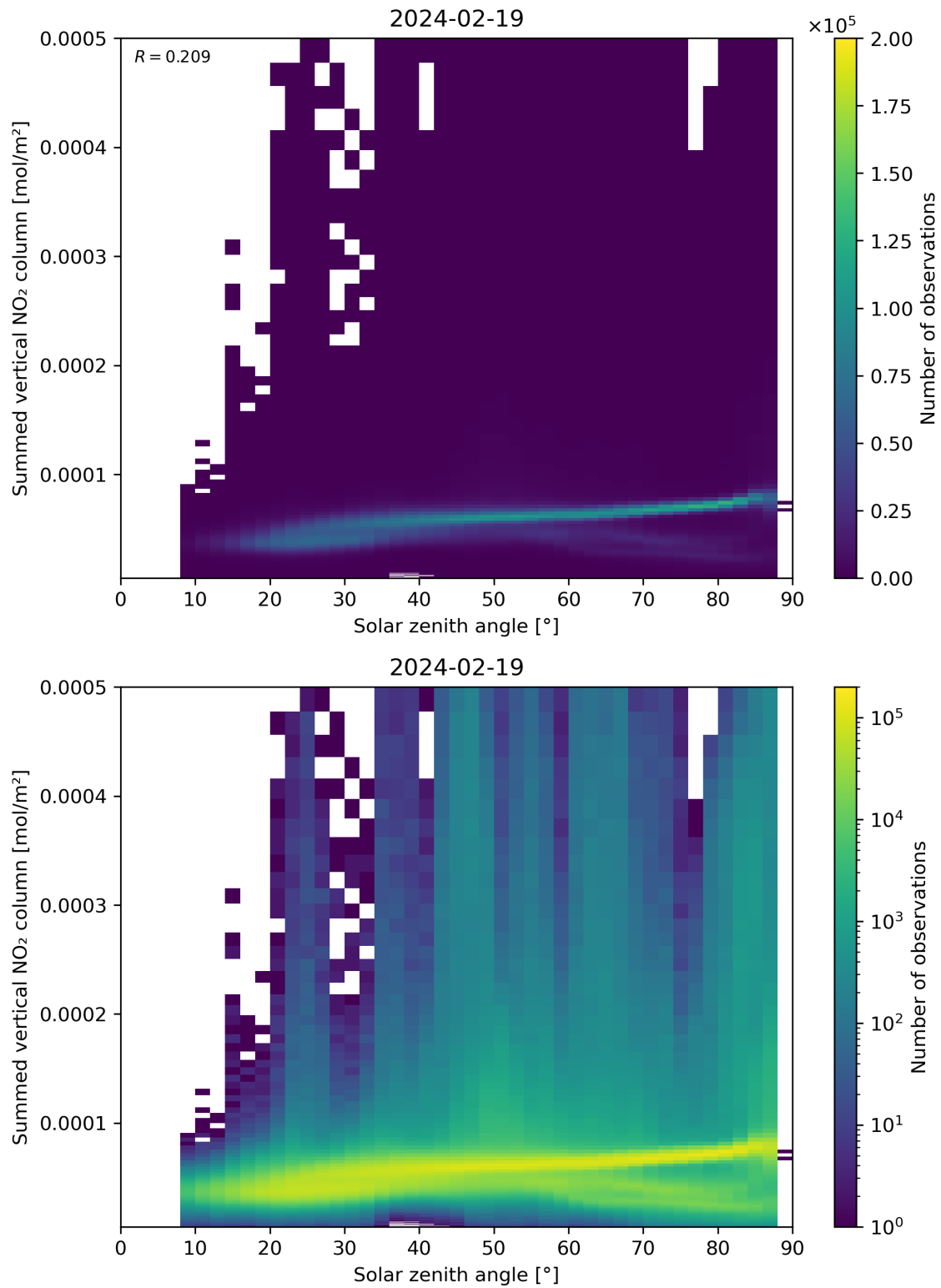
Figure 151: Scatter density plot of “Solar zenith angle” against “Summed vertical NO 2 column” for 2024-02-18 to 2024-02-20.
