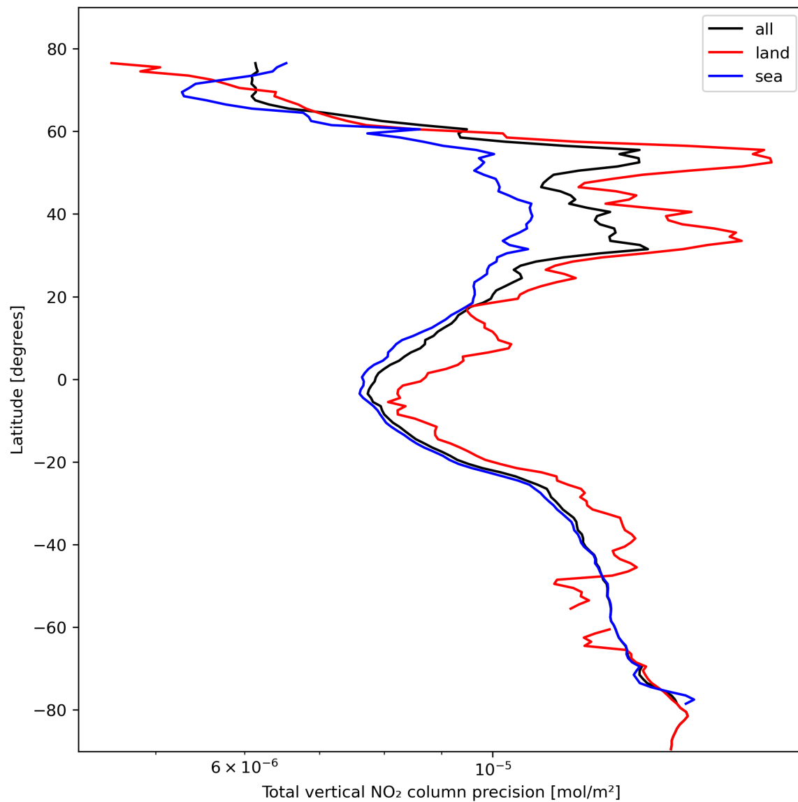
Figure 22: Zonal average of “Total vertical NO 2 column precision” for 2024-02-18 to 2024-02-20.
