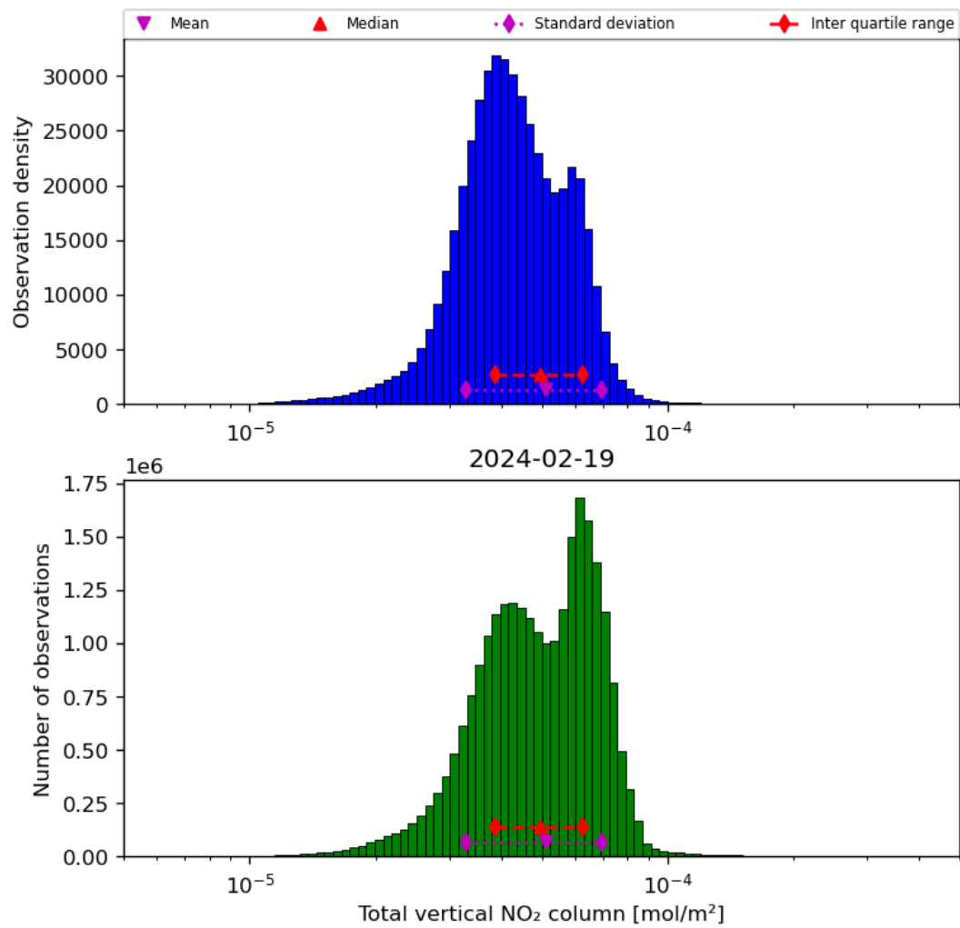
Figure 38: Histogram of “Total vertical NO 2 column” for 2024-02-18 to 2024-02-20
