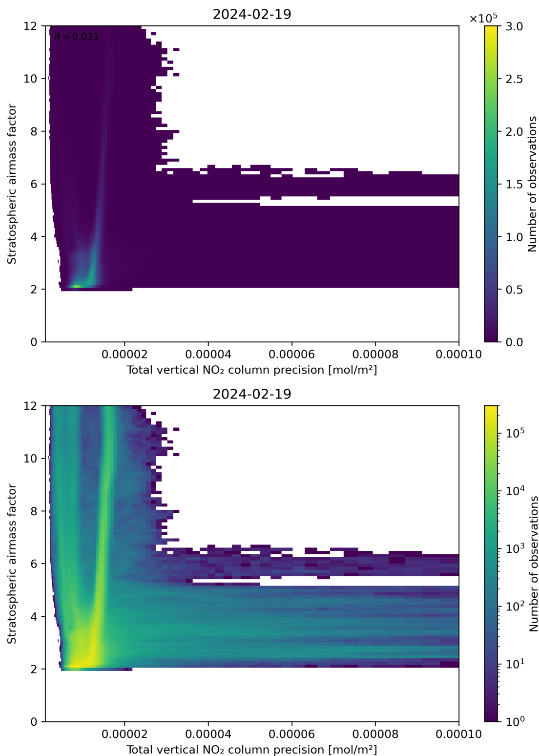
Figure 115: Scatter density plot of “Total vertical NO 2 column precision” against “Stratospheric air mass factor” for 2024-02-18 to 2024-02-20.
