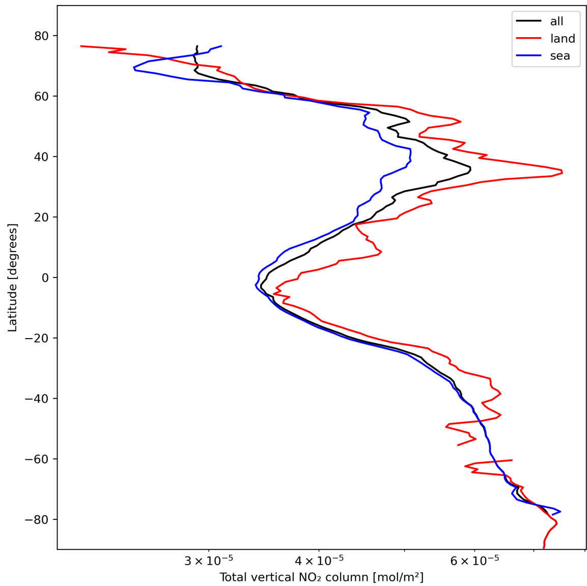
Figure 21: Zonal average of “Total vertical NO 2 column” for 2024-02-18 to 2024-02-20.
