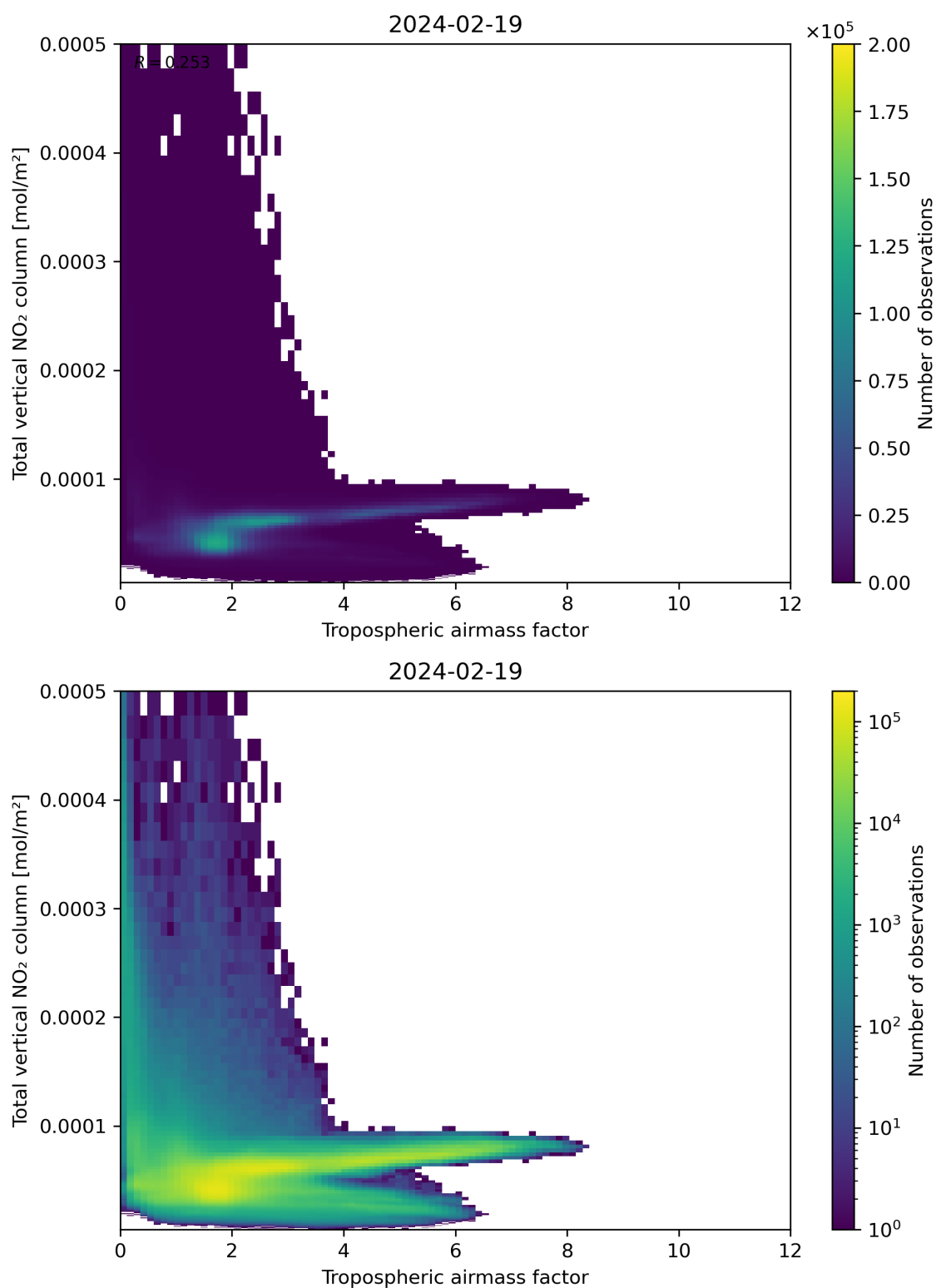
Figure 77: Scatter density plot of “Tropospheric airmass factor” against “Total vertical NO 2 column” for 2024-02-18 to 2024-02-20.
