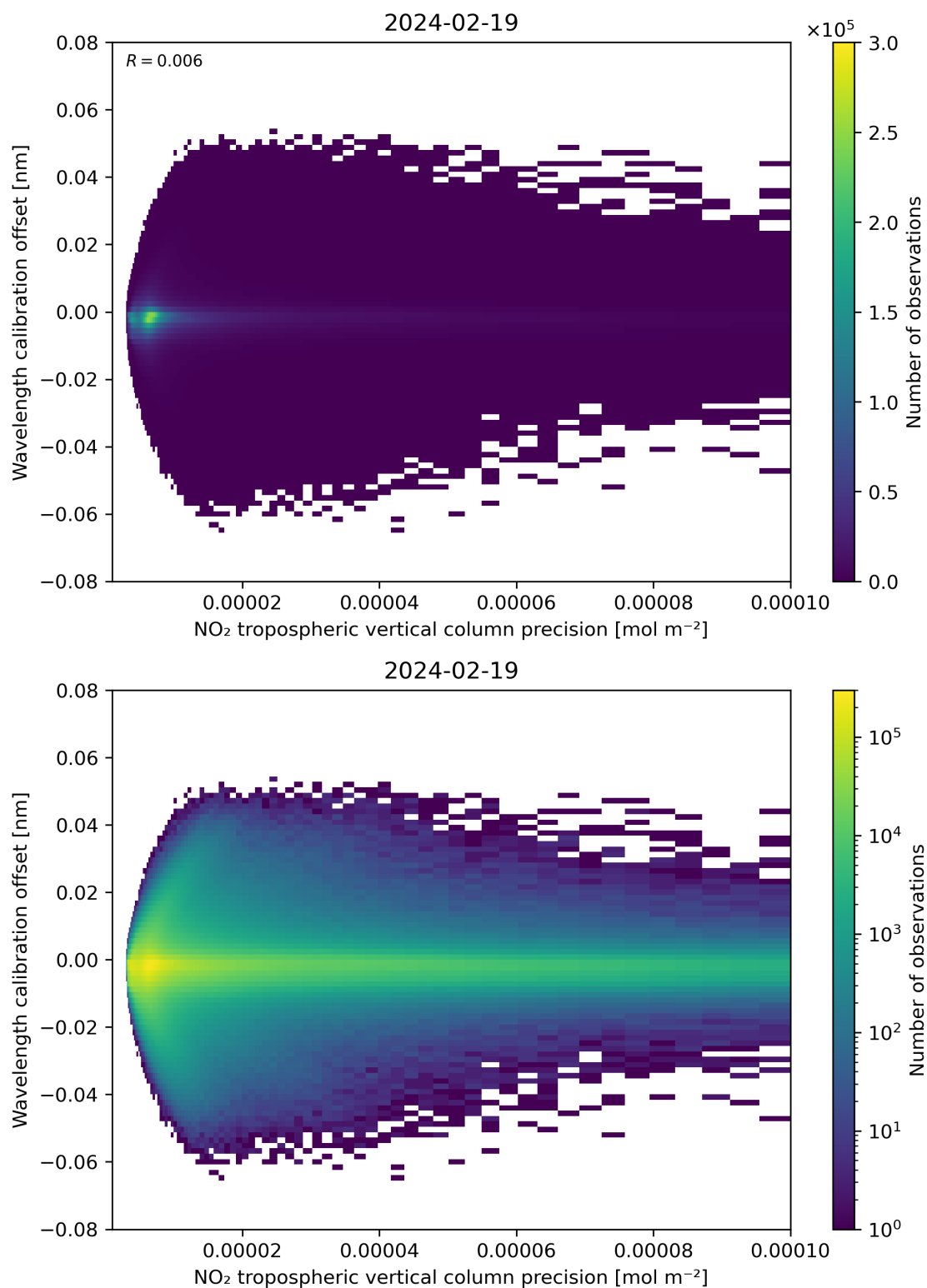
Figure 141: Scatter density plot of “NO 2 tropospheric vertical column precision” against “Wavelength calibration offset” for 2024-02-18 to 2024-02-20.
