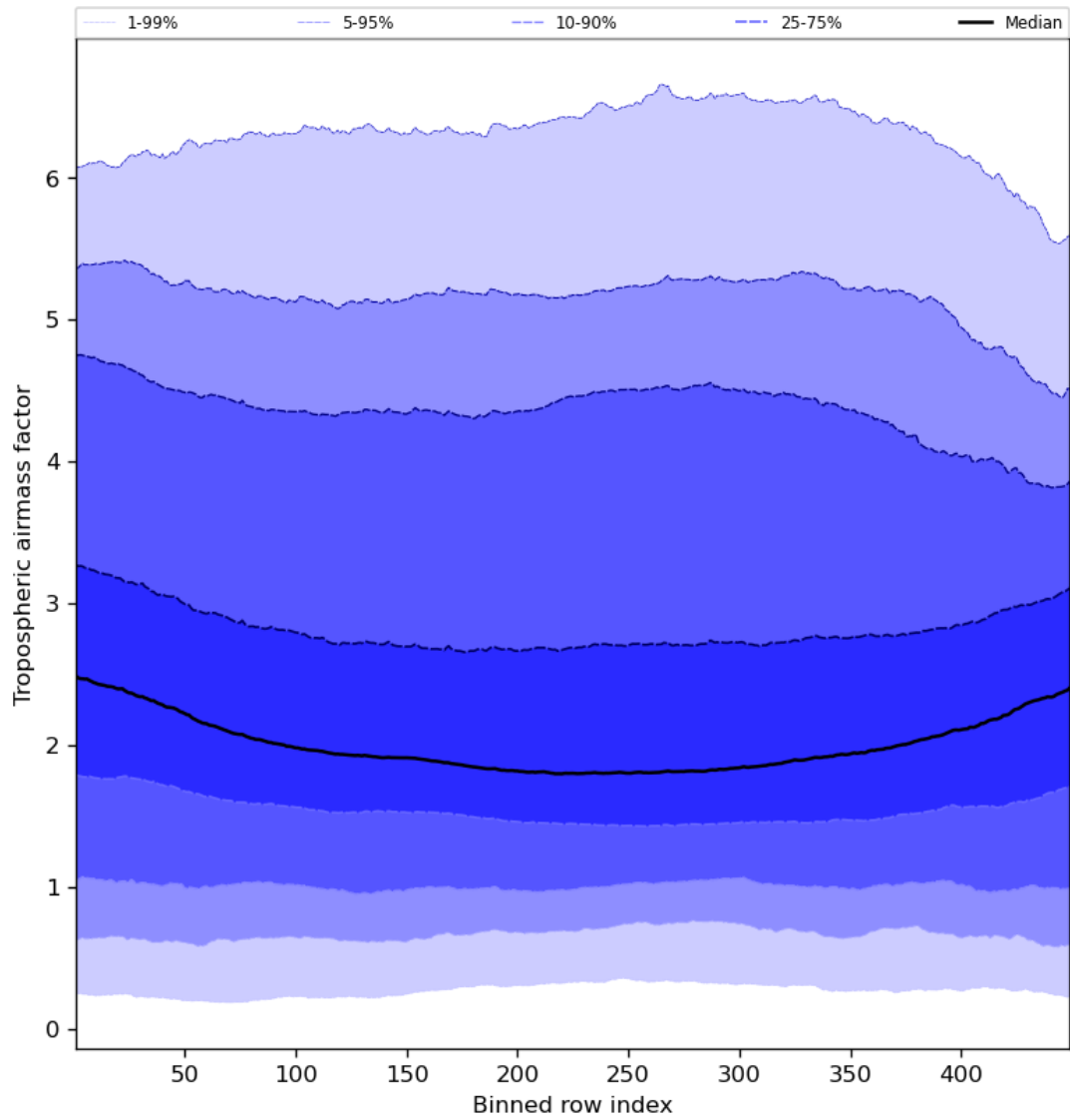
Figure 48: Along track statistics of “Tropospheric air mass factor” for 2024-02-18 to 2024-02-20
