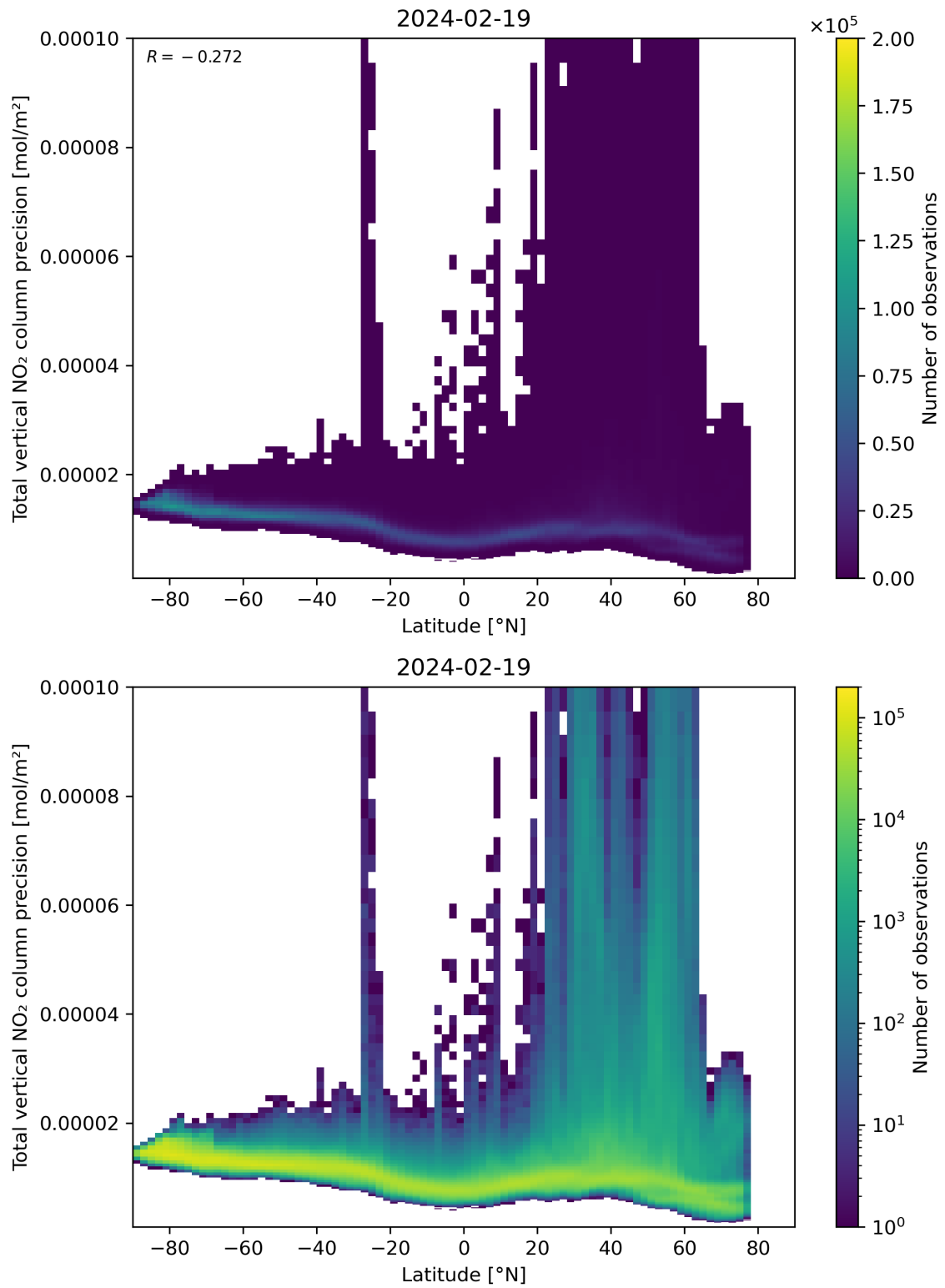
Figure 91: Scatter density plot of “Latitude” against “Total vertical NO 2 column precision” for 2024-02-18 to 2024-02-20.
