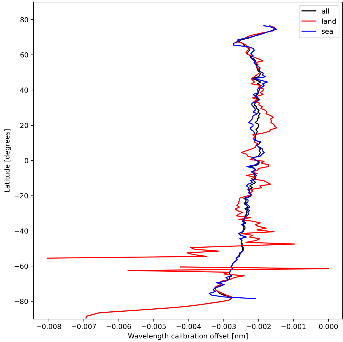
Figure 18: Zonal average of “Wavelength calibration offset” for 2024-02-18 to 2024-02-20.
