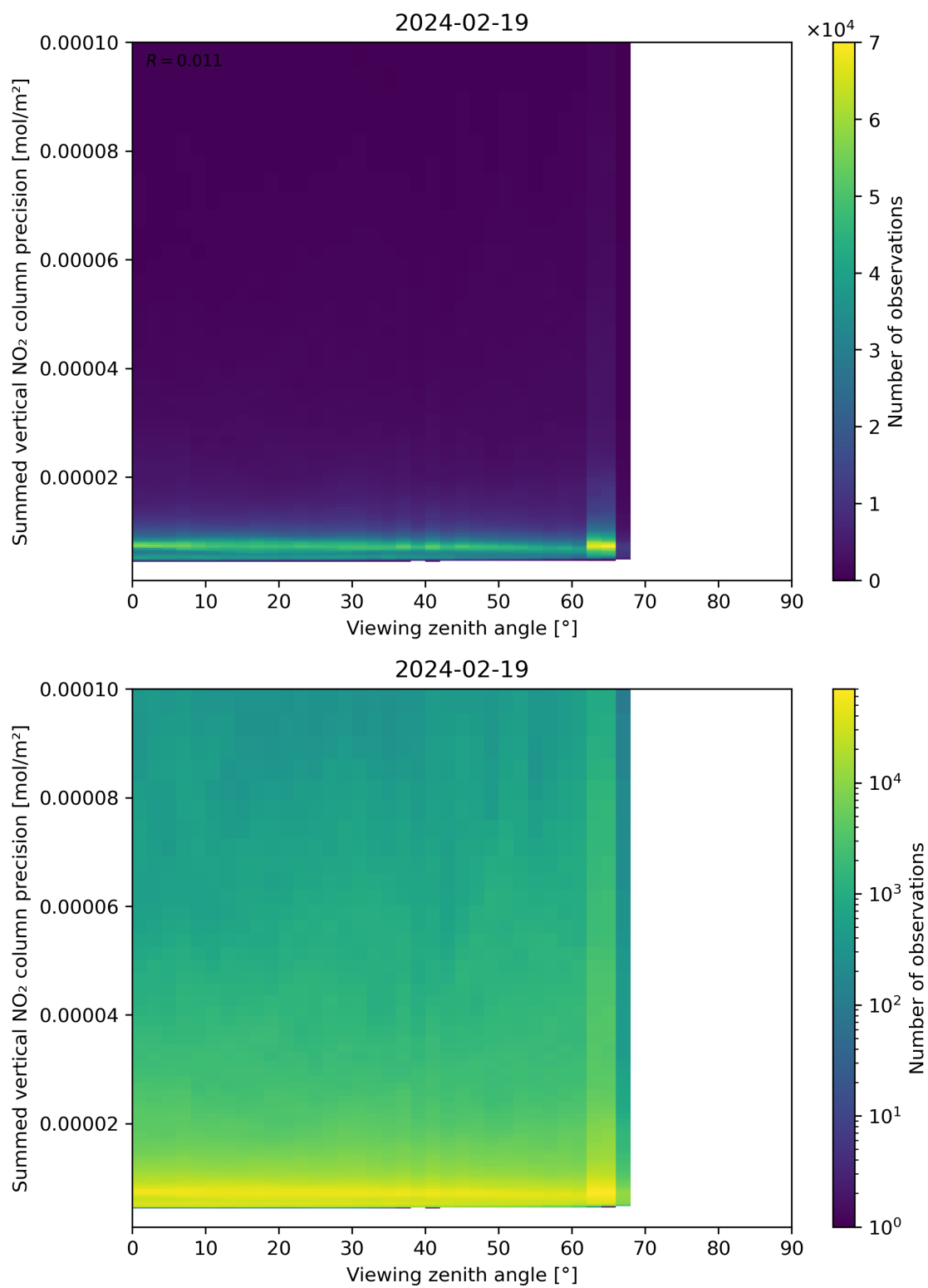
Figure 166: Scatter density plot of “Viewing zenith angle” against “Summed vertical NO 2 column precision” for 2024-02-18 to 2024-02-20.
