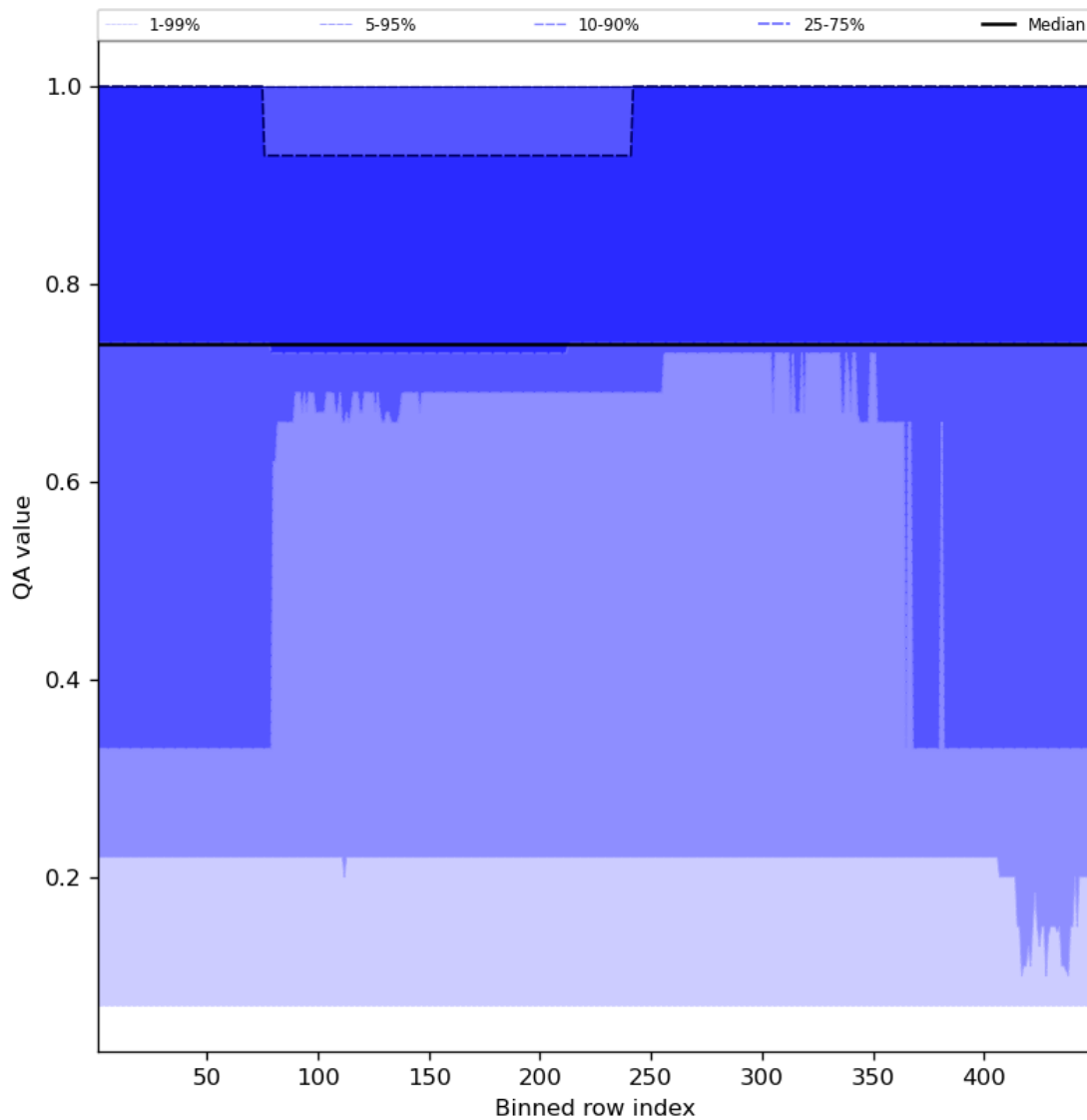
Figure 45: Along track statistics of “QA value” for 2024-02-18 to 2024-02-20
