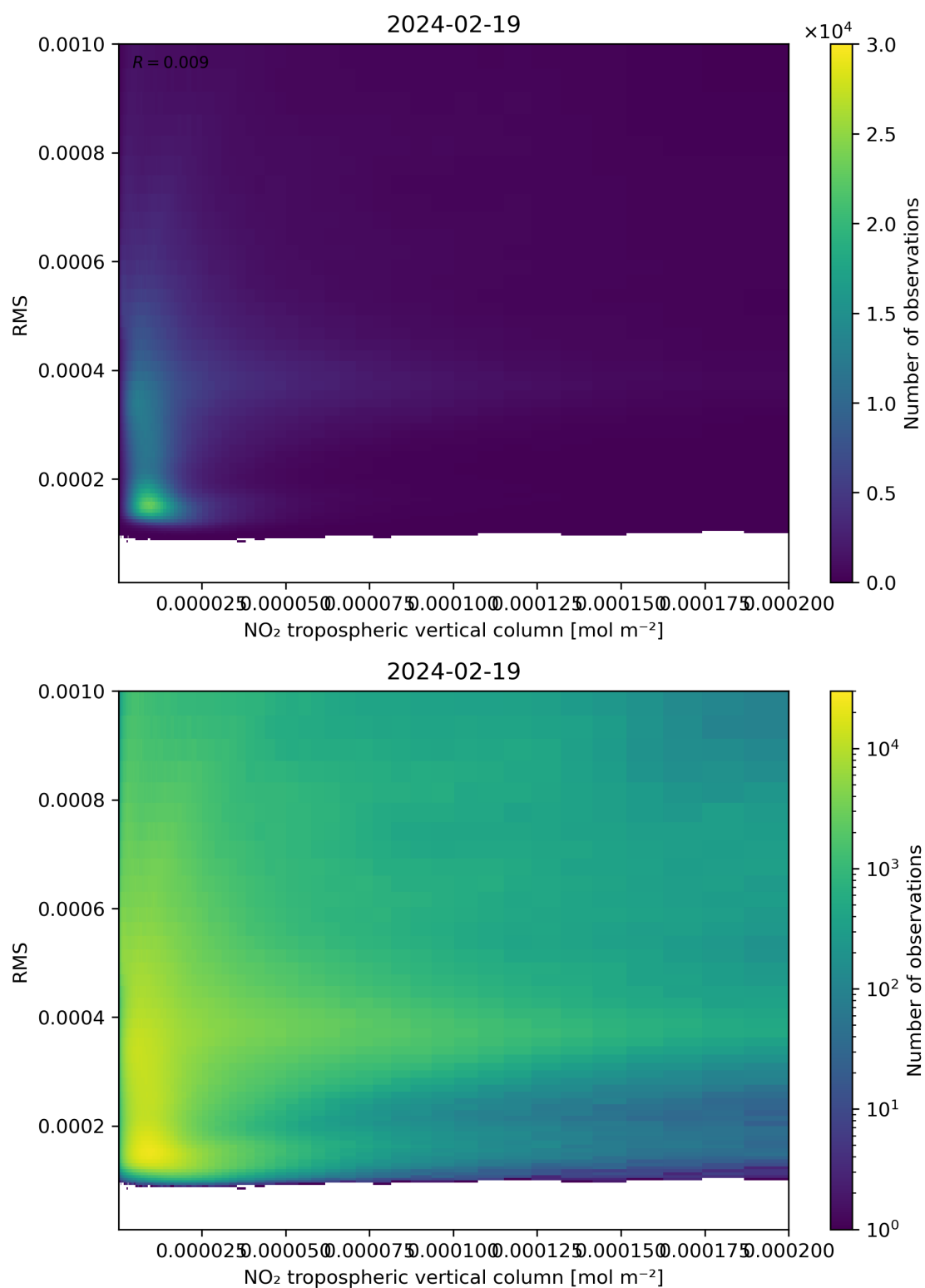
Figure 142: Scatter density plot of “NO 2 tropospheric vertical column” against “RMS” for 2024-02-18 to 2024-02-20.
