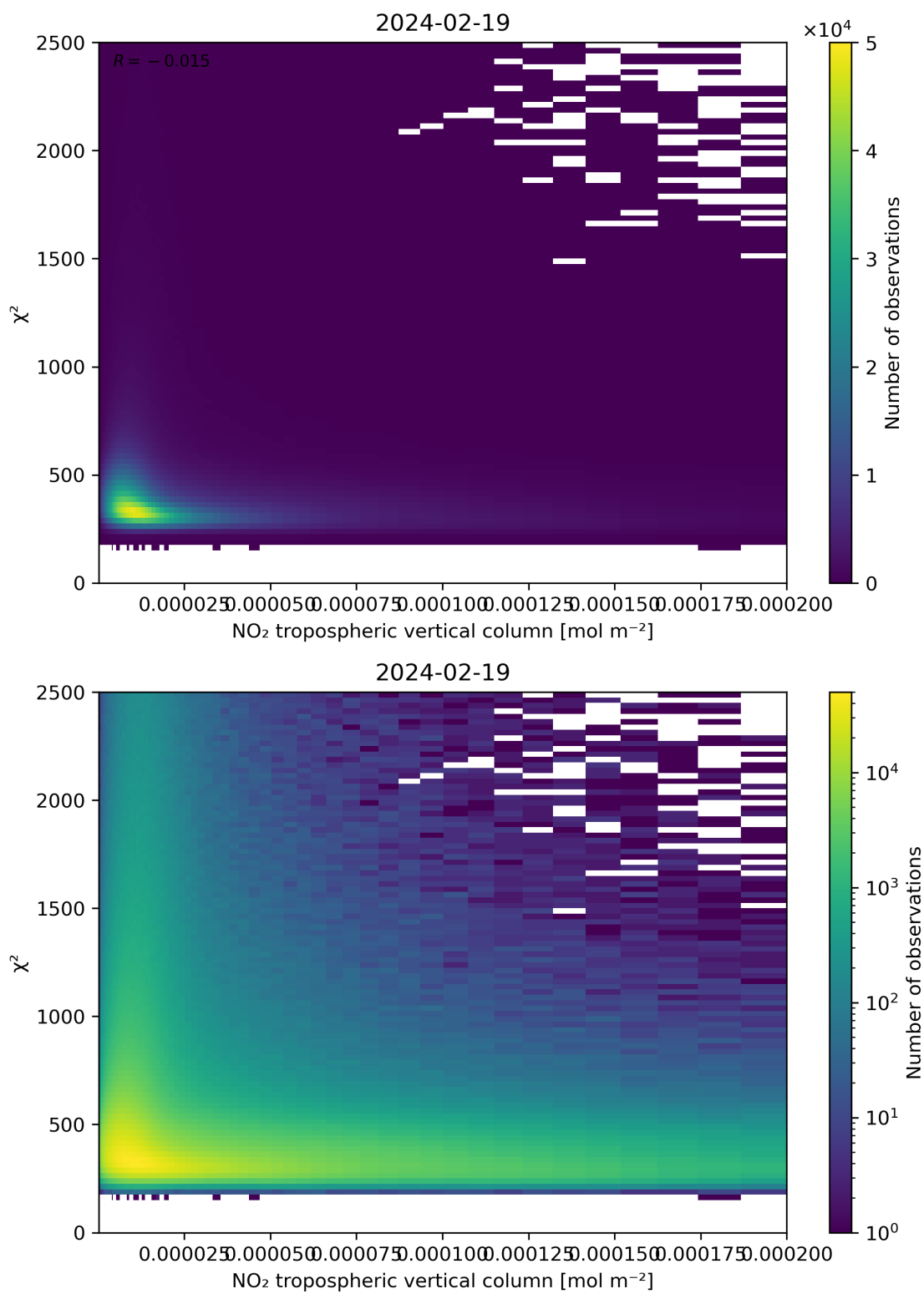
Figure 124: Scatter density plot of “NO 2 tropospheric vertical column” against “ \chi^2 ” for 2024-02-18 to 2024-02-20.
