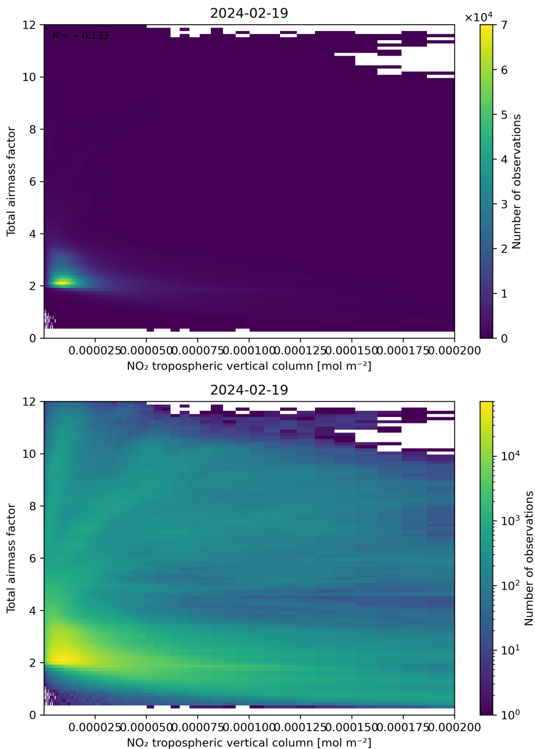
Figure 122: Scatter density plot of “NO 2 tropospheric vertical column” against “Total air mass factor” for 2024-02-18 to 2024-02-20.
