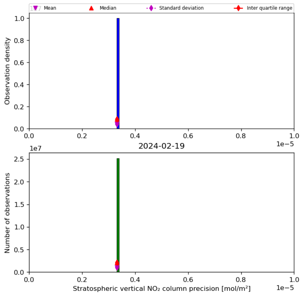
Figure 37: Histogram of “Stratospheric vertical NO 2 column precision” for 2024-02-18 to 2024-02-20
