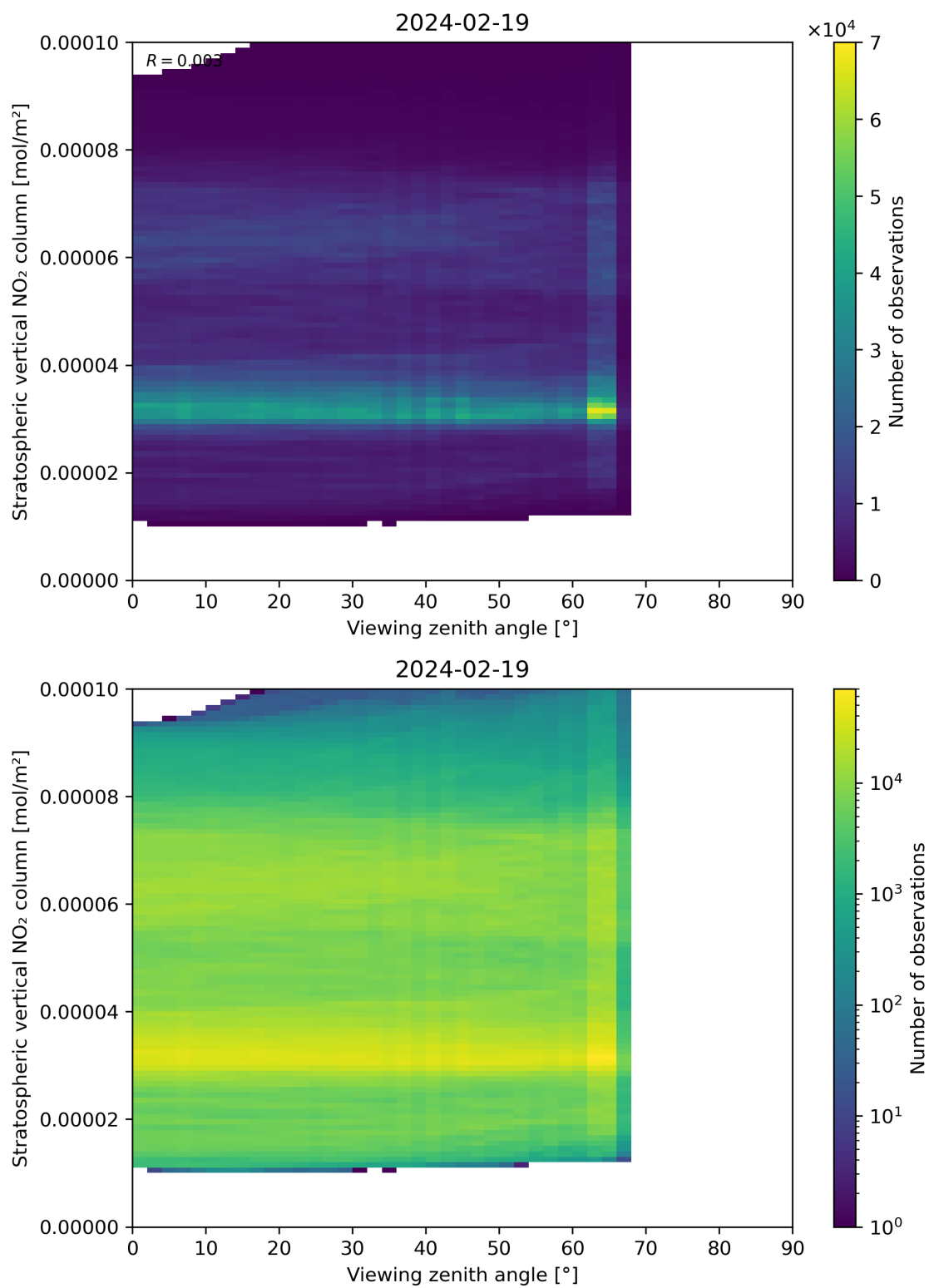
Figure 164: Scatter density plot of “Viewing zenith angle” against “Stratospheric vertical NO 2 column” for 2024-02-18 to 2024-02-20.
