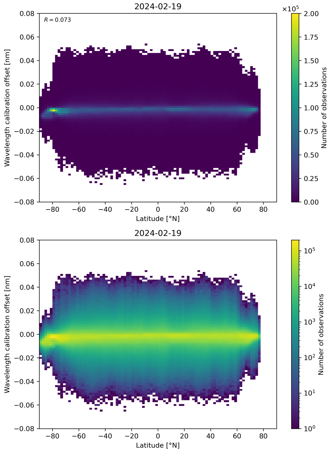
Figure 95: Scatter density plot of “Latitude” against “Wavelength calibration offset” for 2024-02-18 to 2024-02-20.
