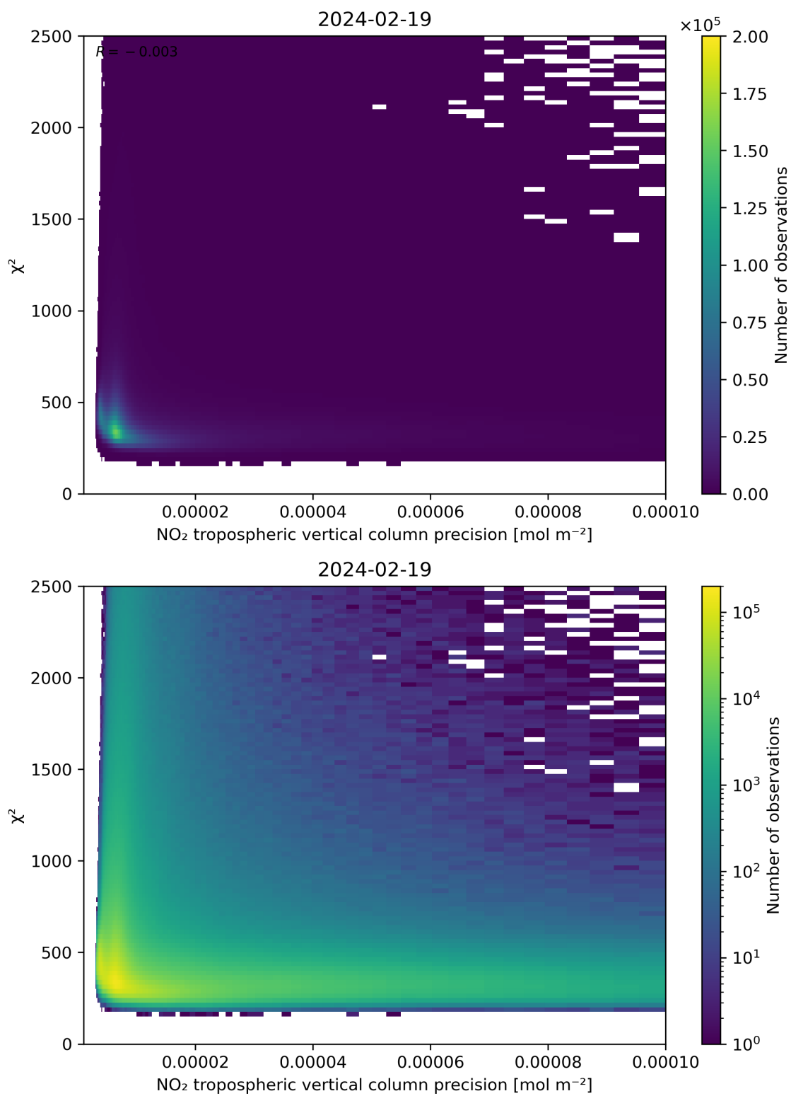
Figure 134: Scatter density plot of “NO 2 tropospheric vertical column precision” against “ \chi^2 ” for 2024-02-18 to 2024-02-20.
