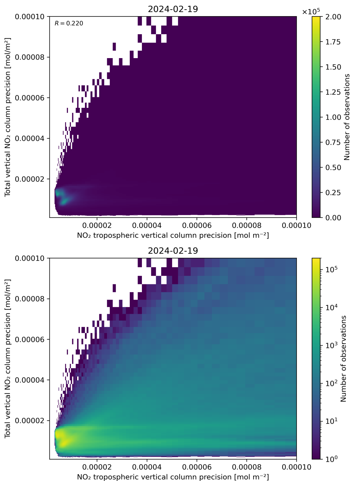
Figure 139: Scatter density plot of “NO 2 tropospheric vertical column precision” against “Total vertical NO 2 column precision” for 2024-02-18 to 2024-02-20.
