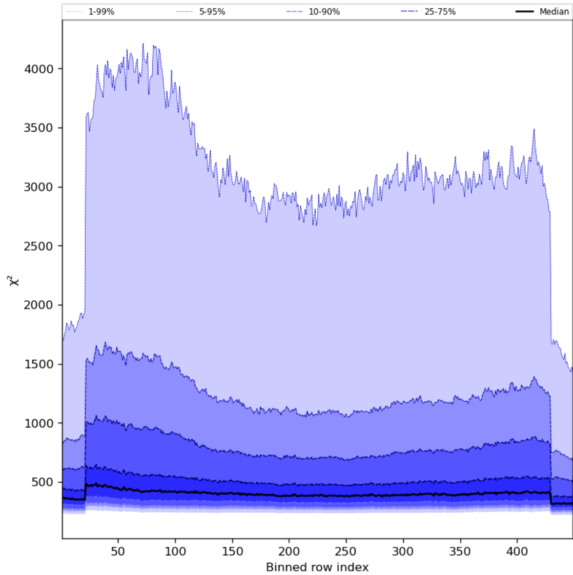
Figure 59: Along track statistics of “ \chi^2 ” for 2024-02-18 to 2024-02-20
