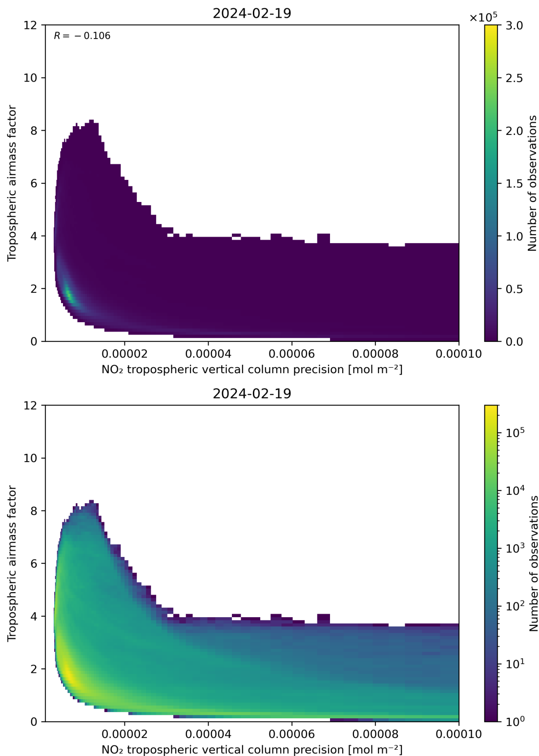
Figure 133: Scatter density plot of “NO 2 tropospheric vertical column precision” against “Tropospheric airmass factor” for 2024-02-18 to 2024-02-20.
