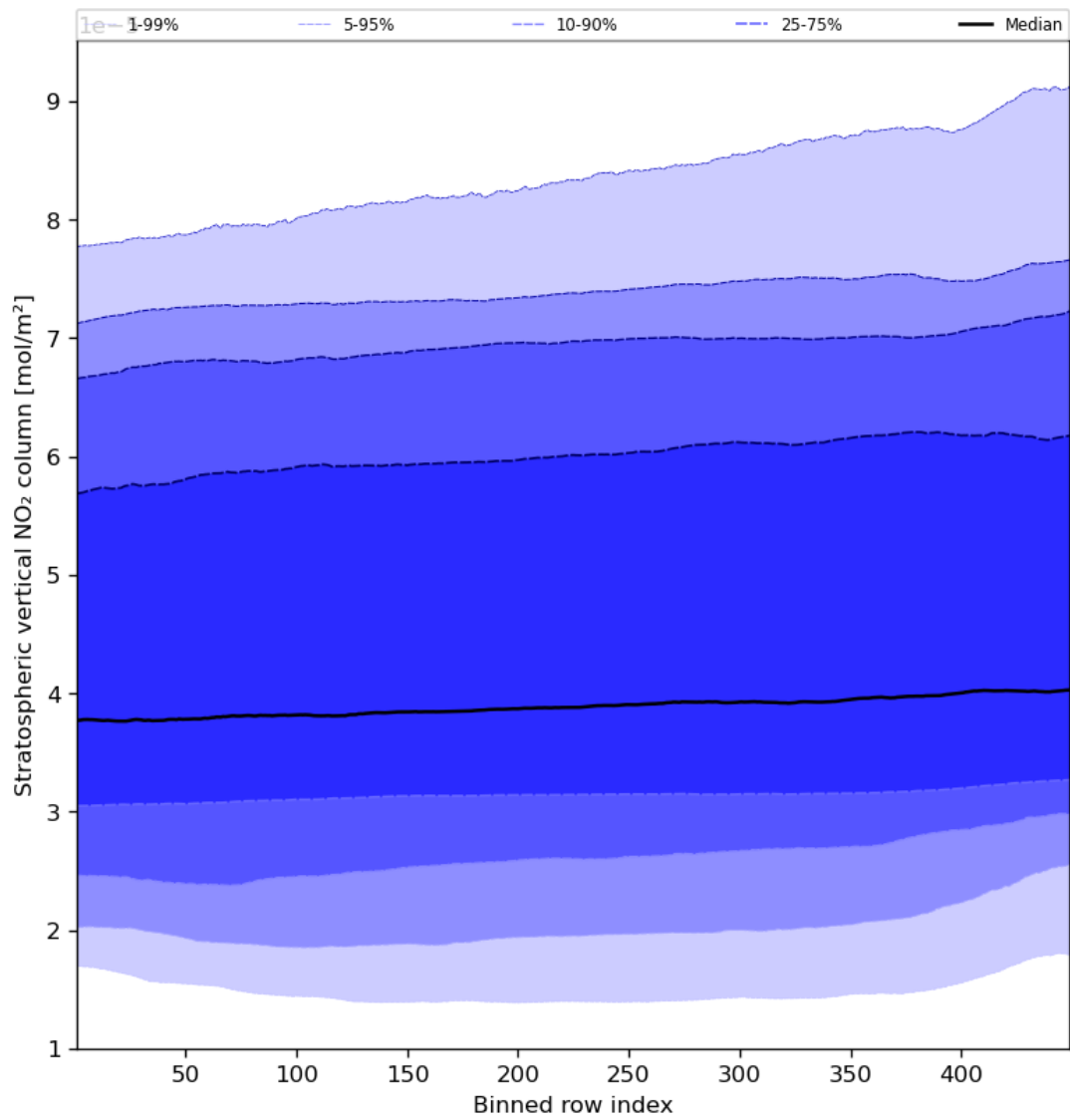
Figure 53: Along track statistics of “Stratospheric vertical NO 2 column” for 2024-02-18 to 2024-02-20
