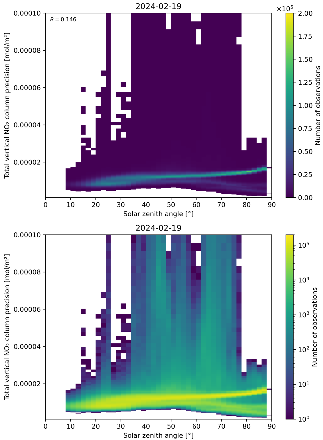
Figure 154: Scatter density plot of “Solar zenith angle” against “Total vertical NO 2 column precision” for 2024-02-18 to 2024-02-20.
