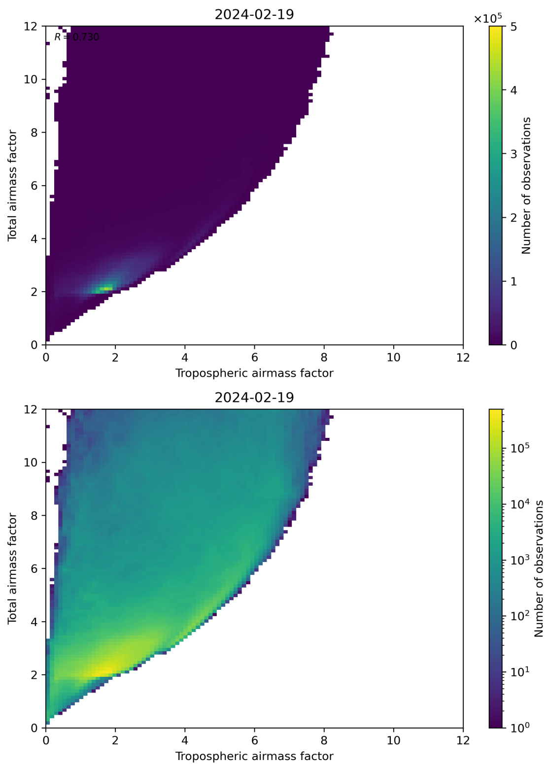
Figure 72: Scatter density plot of “Tropospheric airmass factor” against “Total airmass factor” for 2024-02-18 to 2024-02-20.
