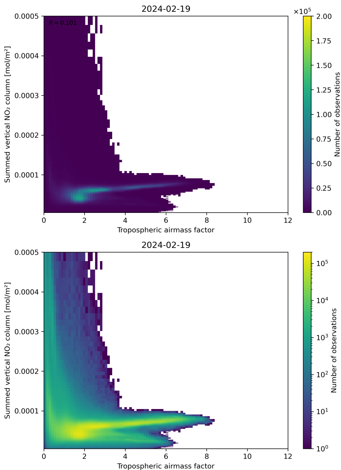
Figure 75: Scatter density plot of “Tropospheric air mass factor” against “Summed vertical NO 2 column” for 2024-02-18 to 2024-02-20.
