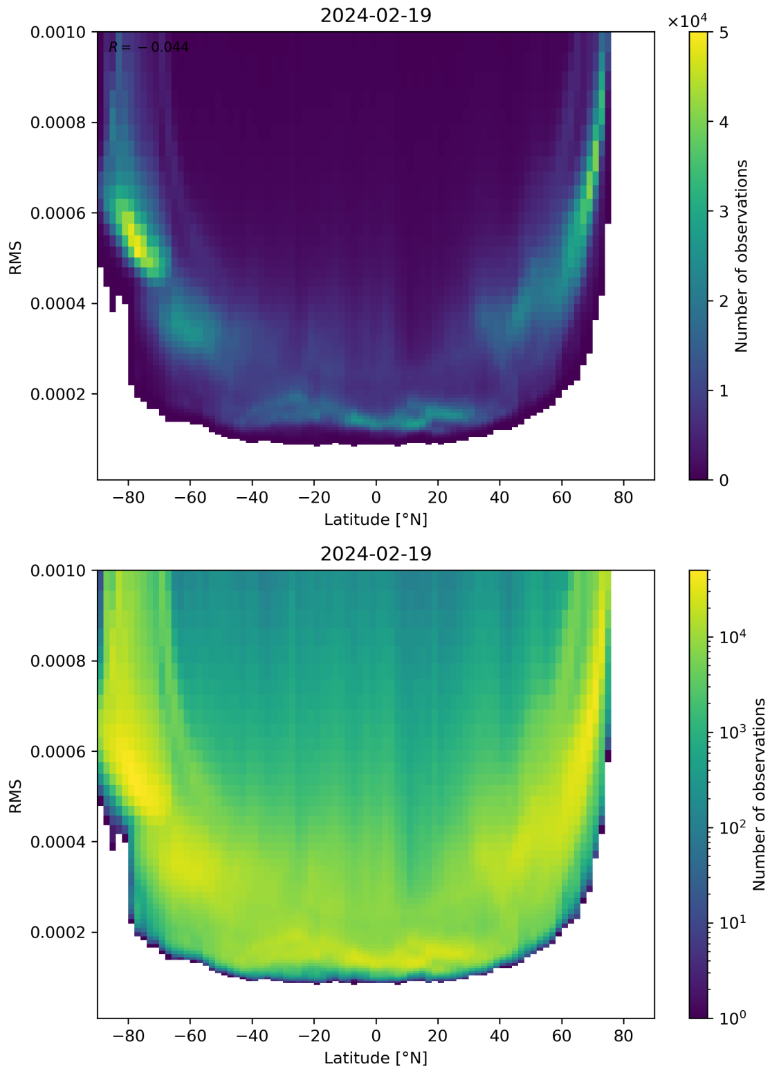
Figure 94: Scatter density plot of “Latitude” against “RMS” for 2024-02-18 to 2024-02-20.
