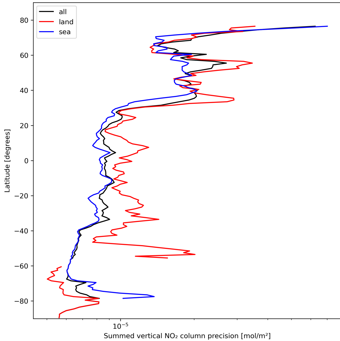
Figure 24: Zonal average of “Summed vertical NO 2 column precision” for 2024-02-18 to 2024-02-20.
