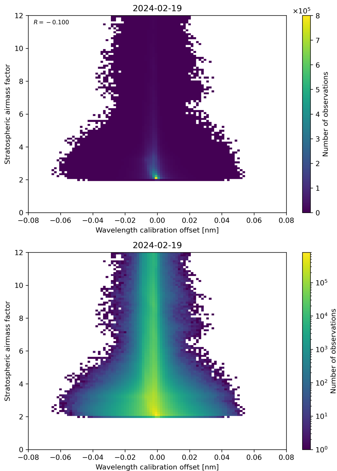
Figure 174: Scatter density plot of “Wavelength calibration offset” against “Stratospheric airmass factor” for 2024-02-18 to 2024-02-20.
