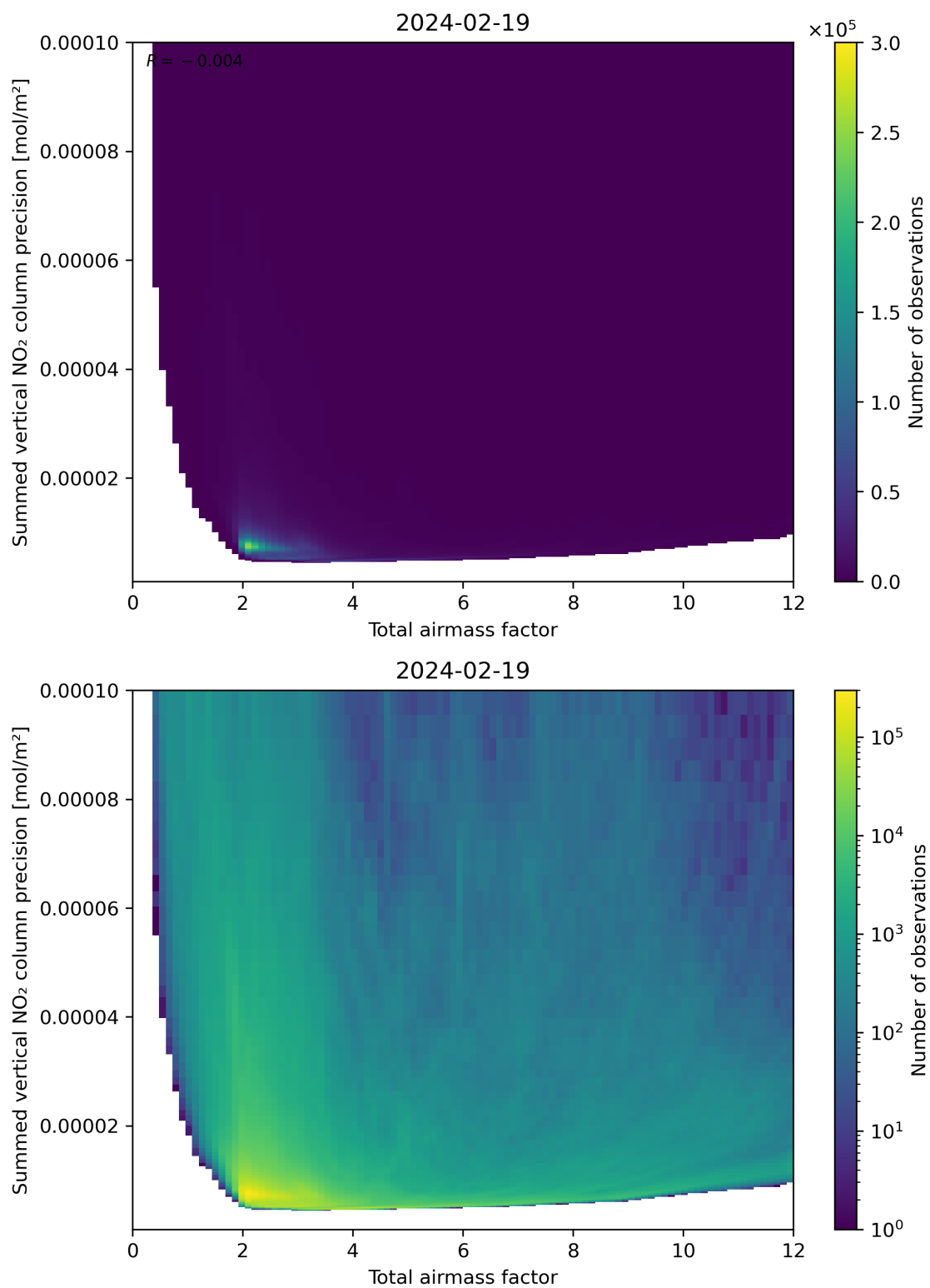
Figure 66: Scatter density plot of “Total airmass factor” against “Summed vertical NO 2 column precision” for 2024-02-18 to 2024-02-20.
