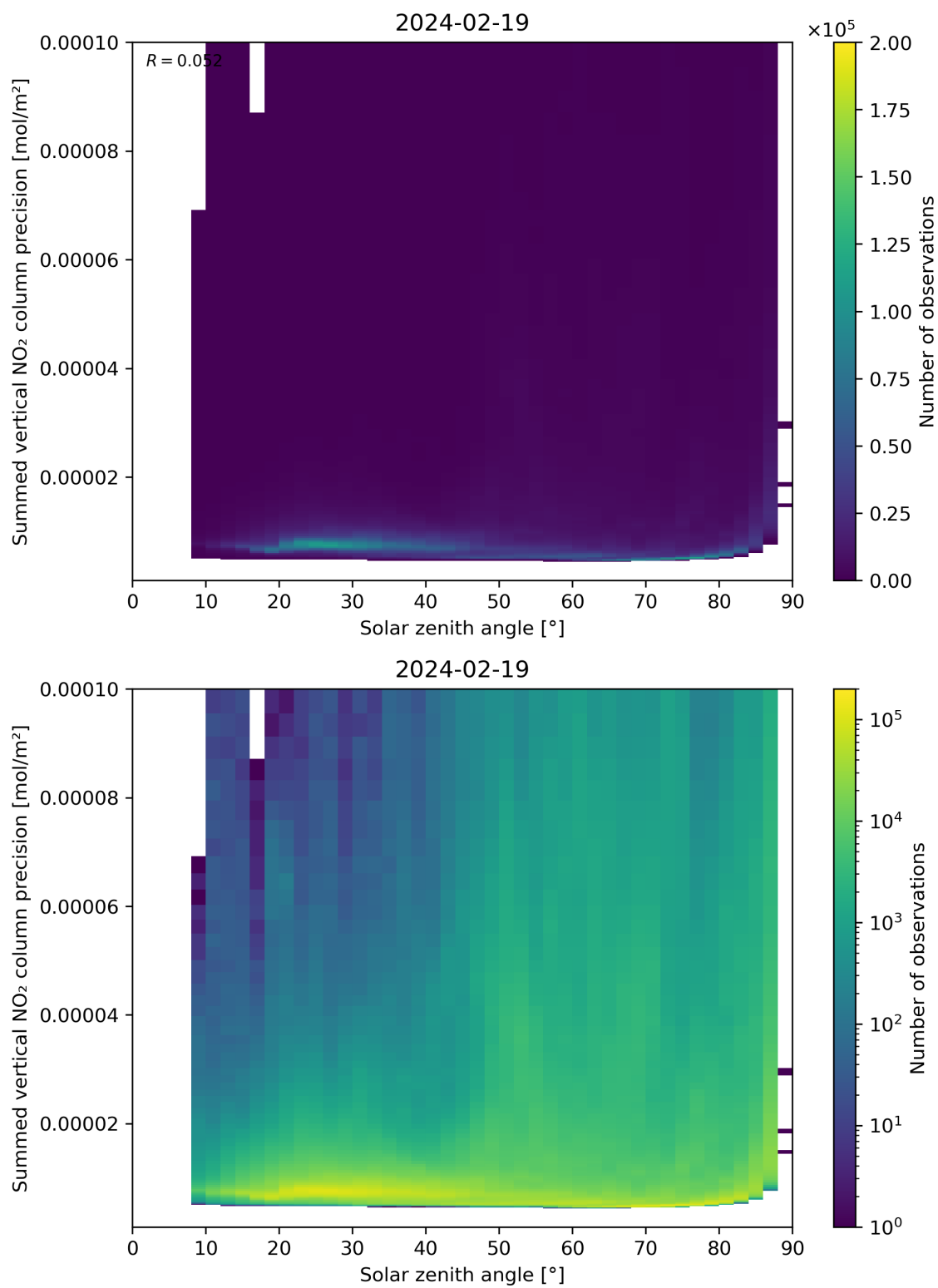
Figure 152: Scatter density plot of “Solar zenith angle” against “Summed vertical NO 2 column precision” for 2024-02-18 to 2024-02-20.
