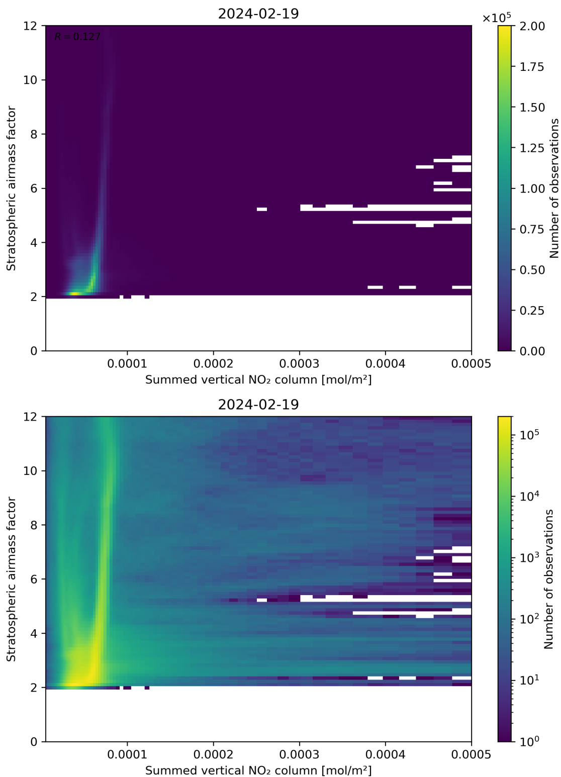
Figure 103: Scatter density plot of “Summed vertical NO 2 column” against “Stratospheric air mass factor” for 2024-02-18 to 2024-02-20.
