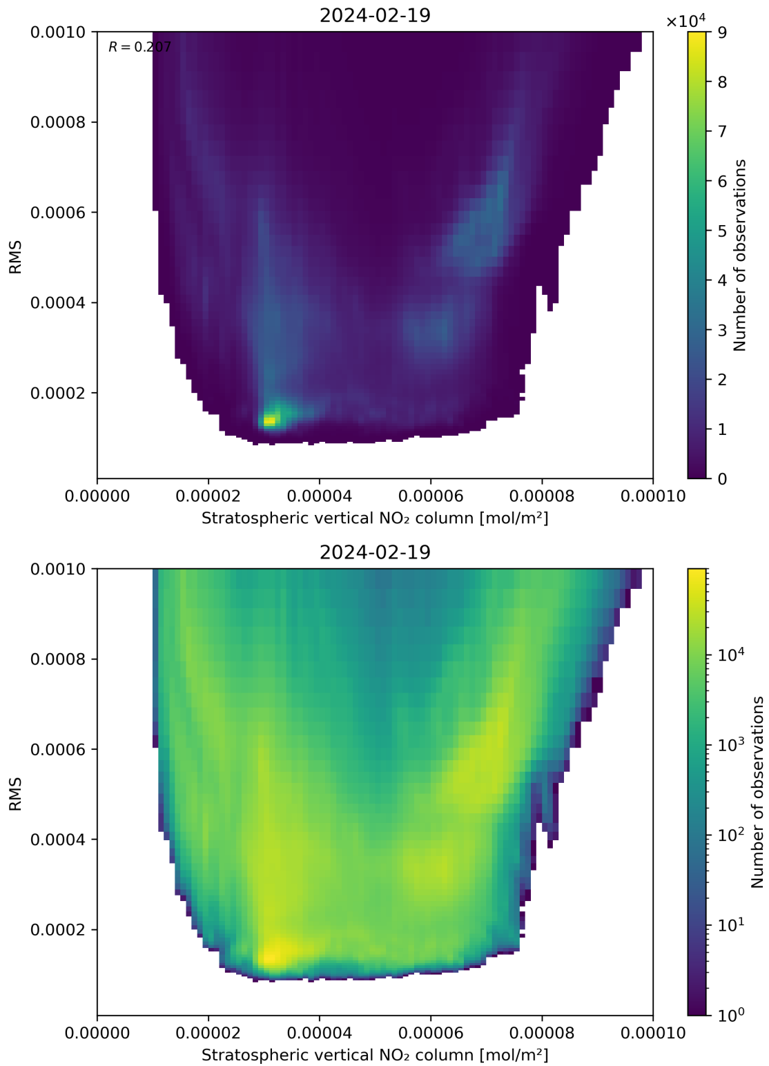
Figure 102: Scatter density plot of “Stratospheric vertical NO 2 column” against “RMS” for 2024-02-18 to 2024-02-20.
