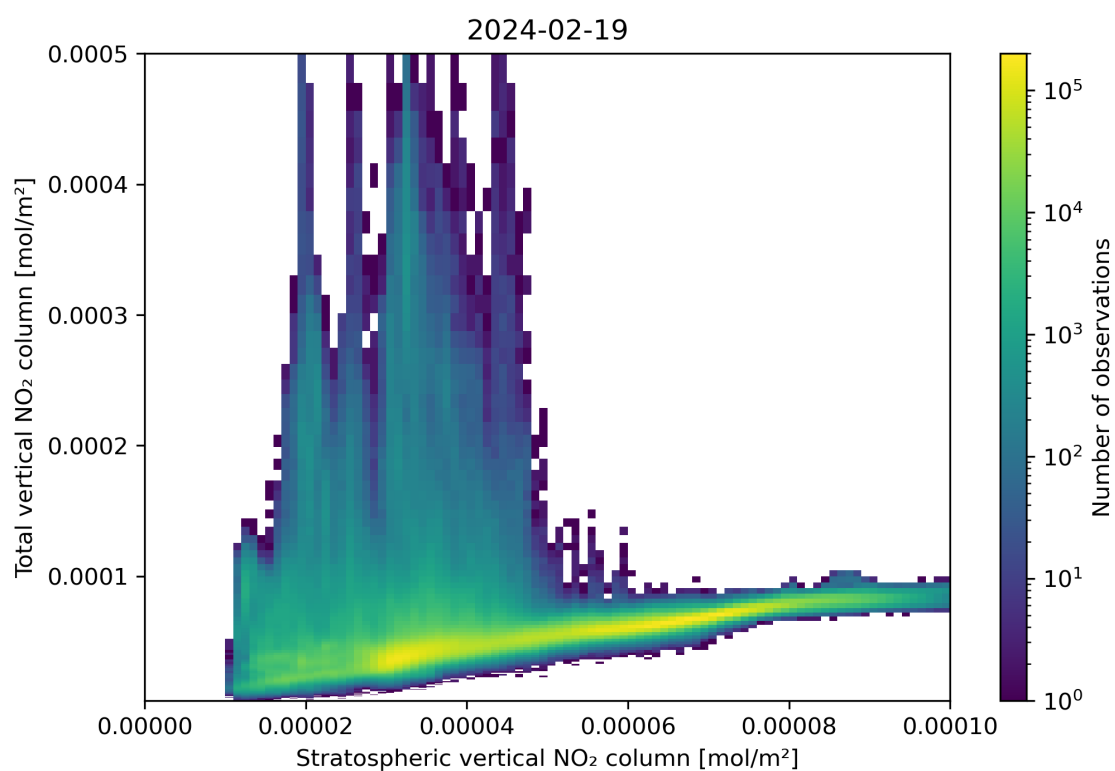
Figure 100: Scatter density plot of “Stratospheric vertical NO 2 column” against “Total vertical NO 2 column” for 2024-02-18 to 2024-02-20.
