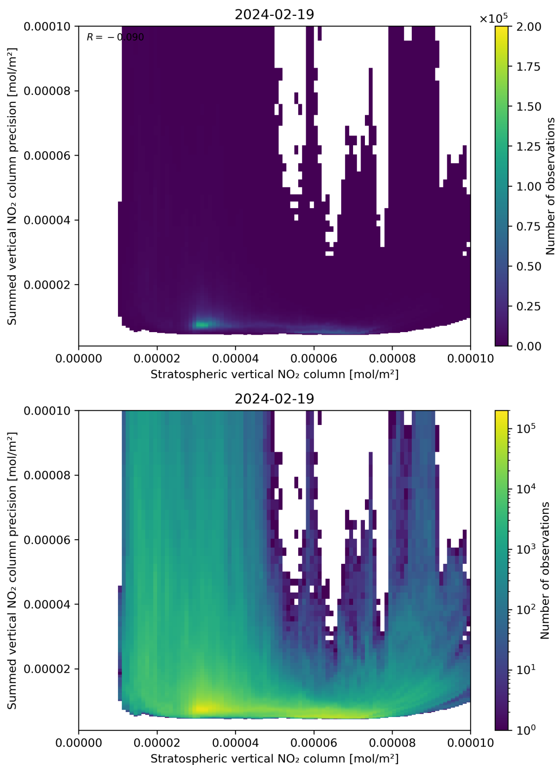
Figure 99: Scatter density plot of “Stratospheric vertical NO 2 column” against “Summed vertical NO 2 column precision” for 2024-02-18 to 2024-02-20.
