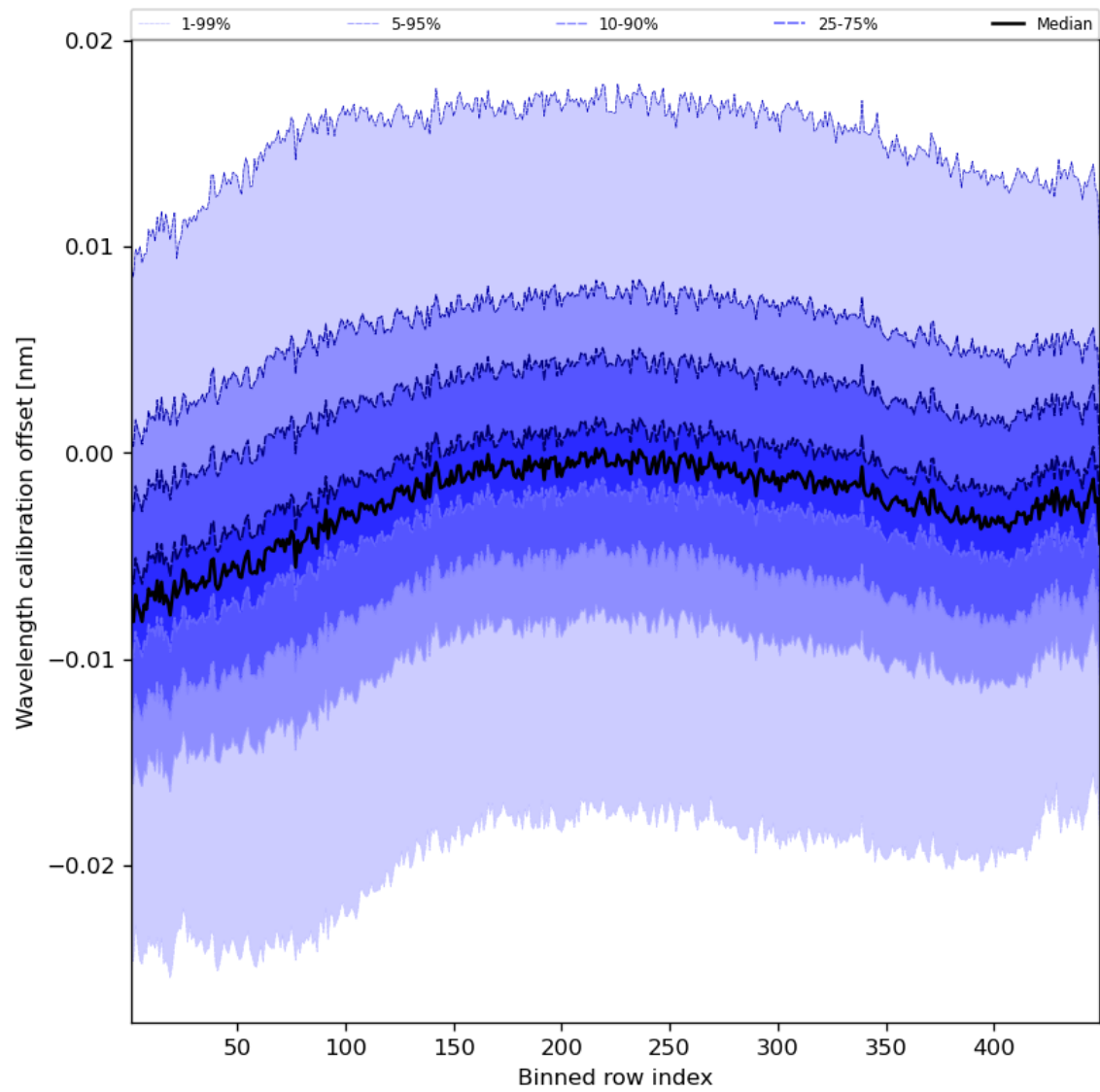
Figure 52: Along track statistics of “Wavelength calibration offset” for 2024-02-18 to 2024-02-20
