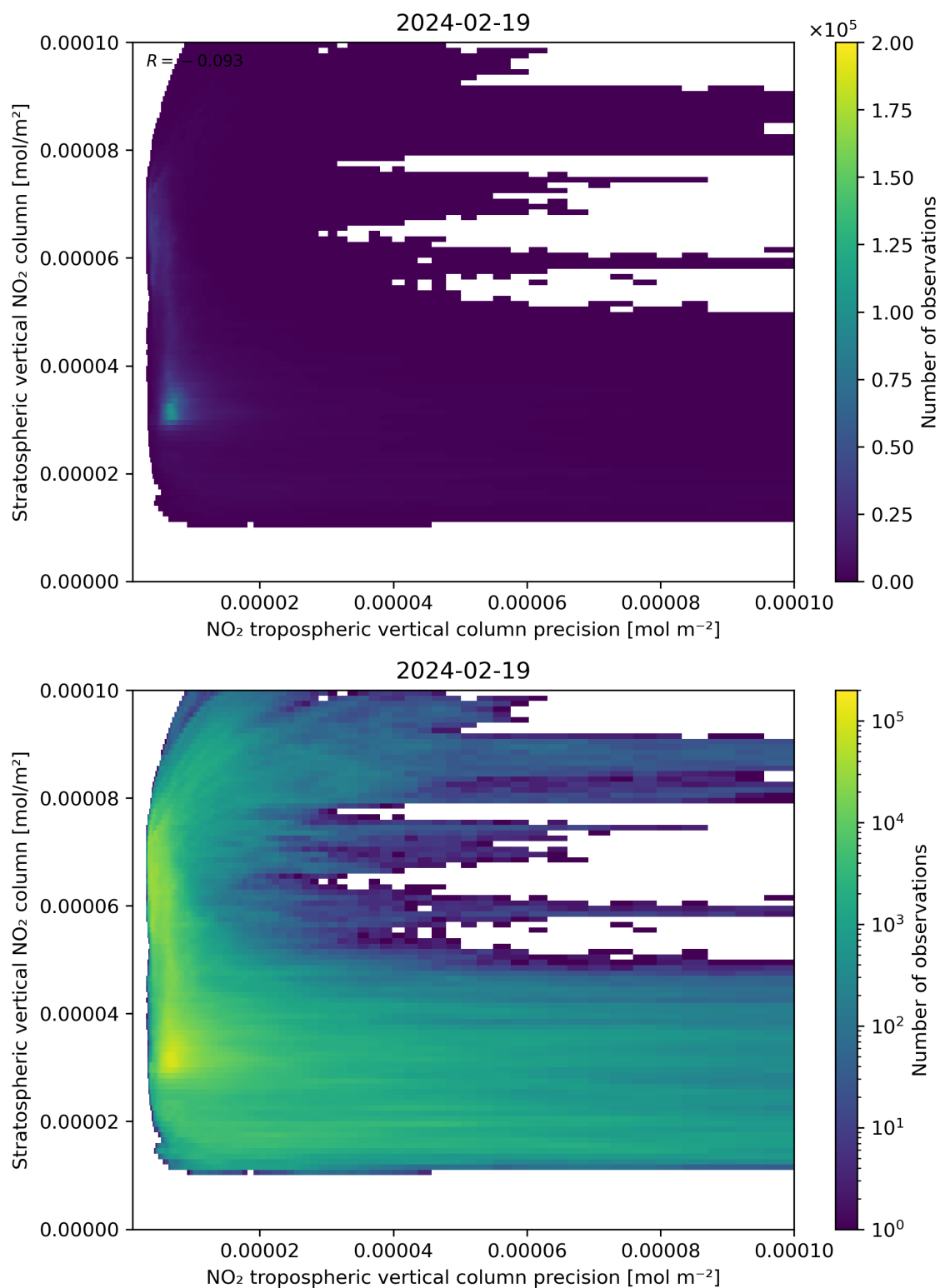
Figure 135: Scatter density plot of “NO 2 tropospheric vertical column precision” against “Stratospheric vertical NO 2 column” for 2024-02-18 to 2024-02-20.
