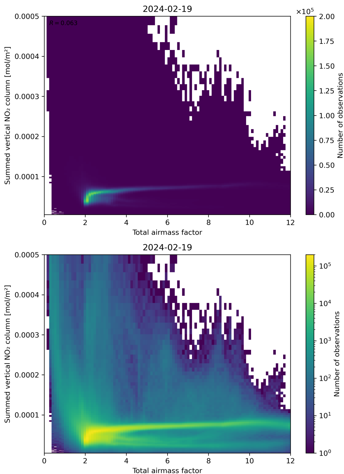
Figure 65: Scatter density plot of “Total airmass factor” against “Summed vertical NO 2 column” for 2024-02-18 to 2024-02-20.
