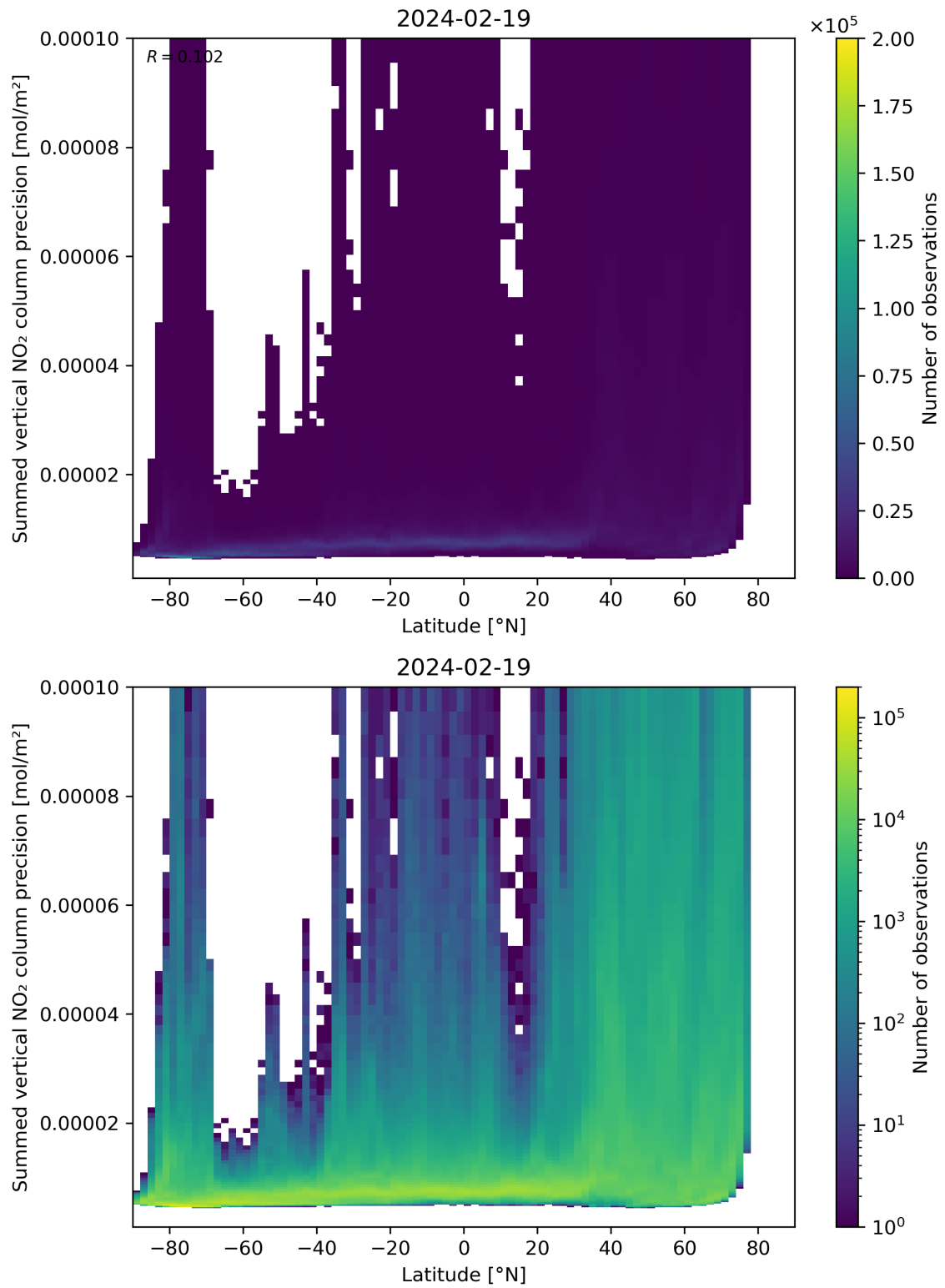
Figure 89: Scatter density plot of “Latitude” against “Summed vertical NO 2 column precision” for 2024-02-18 to 2024-02-20.
