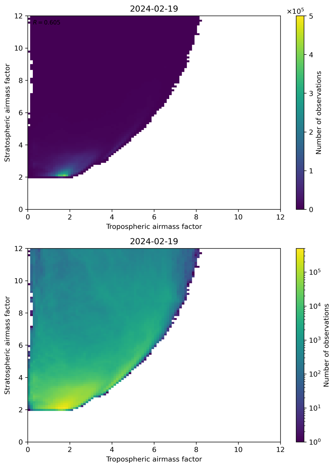
Figure 71: Scatter density plot of “Tropospheric airmass factor” against “Stratospheric airmass factor” for 2024-02-18 to 2024-02-20.
