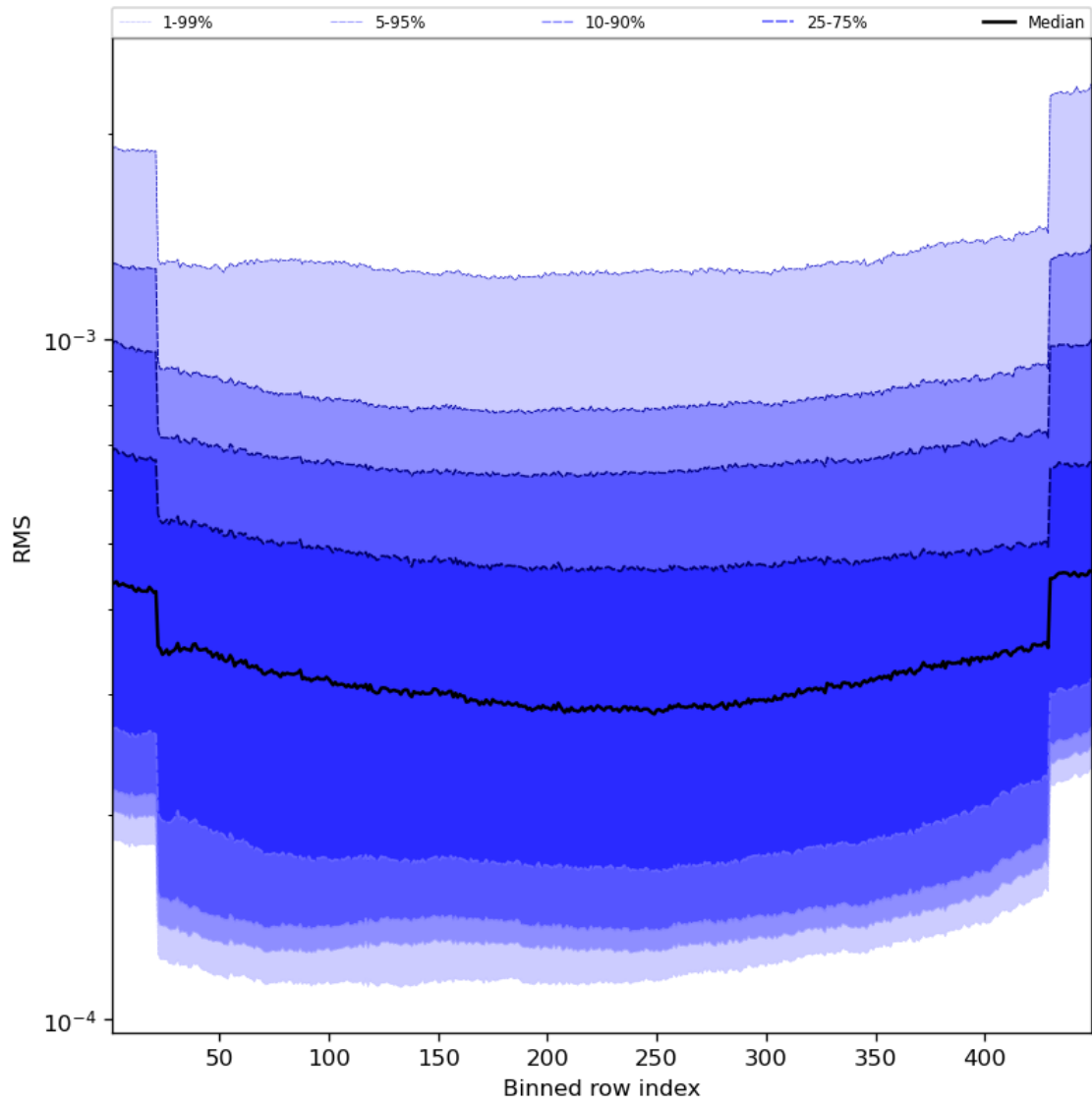
Figure 60: Along track statistics of “RMS” for 2024-02-18 to 2024-02-20
