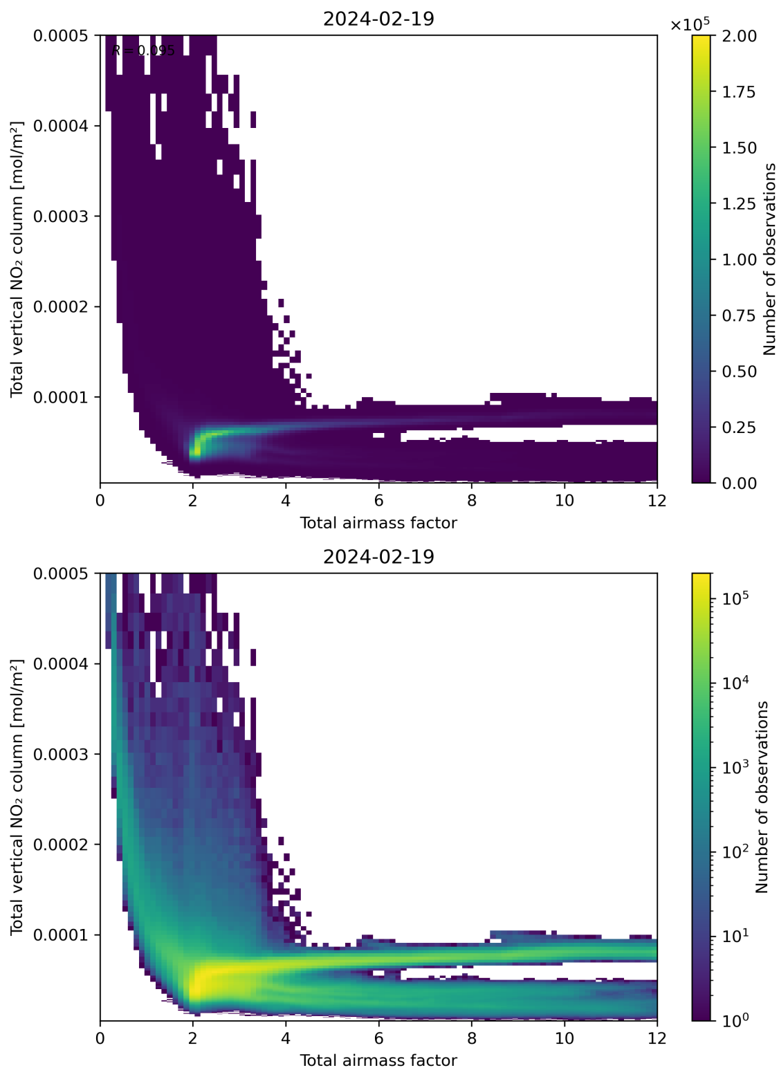
Figure 67: Scatter density plot of “Total airmass factor” against “Total vertical NO 2 column” for 2024-02-18 to 2024-02-20.
