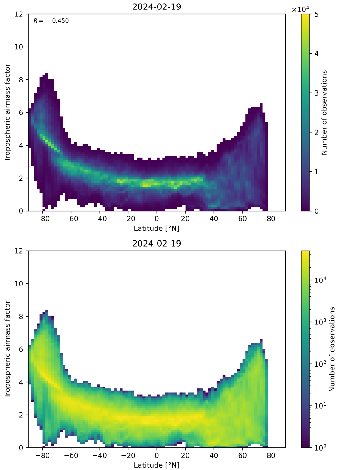
Figure 85: Scatter density plot of “Latitude” against “Tropospheric airmass factor” for 2024-02-18 to 2024-02-20.
