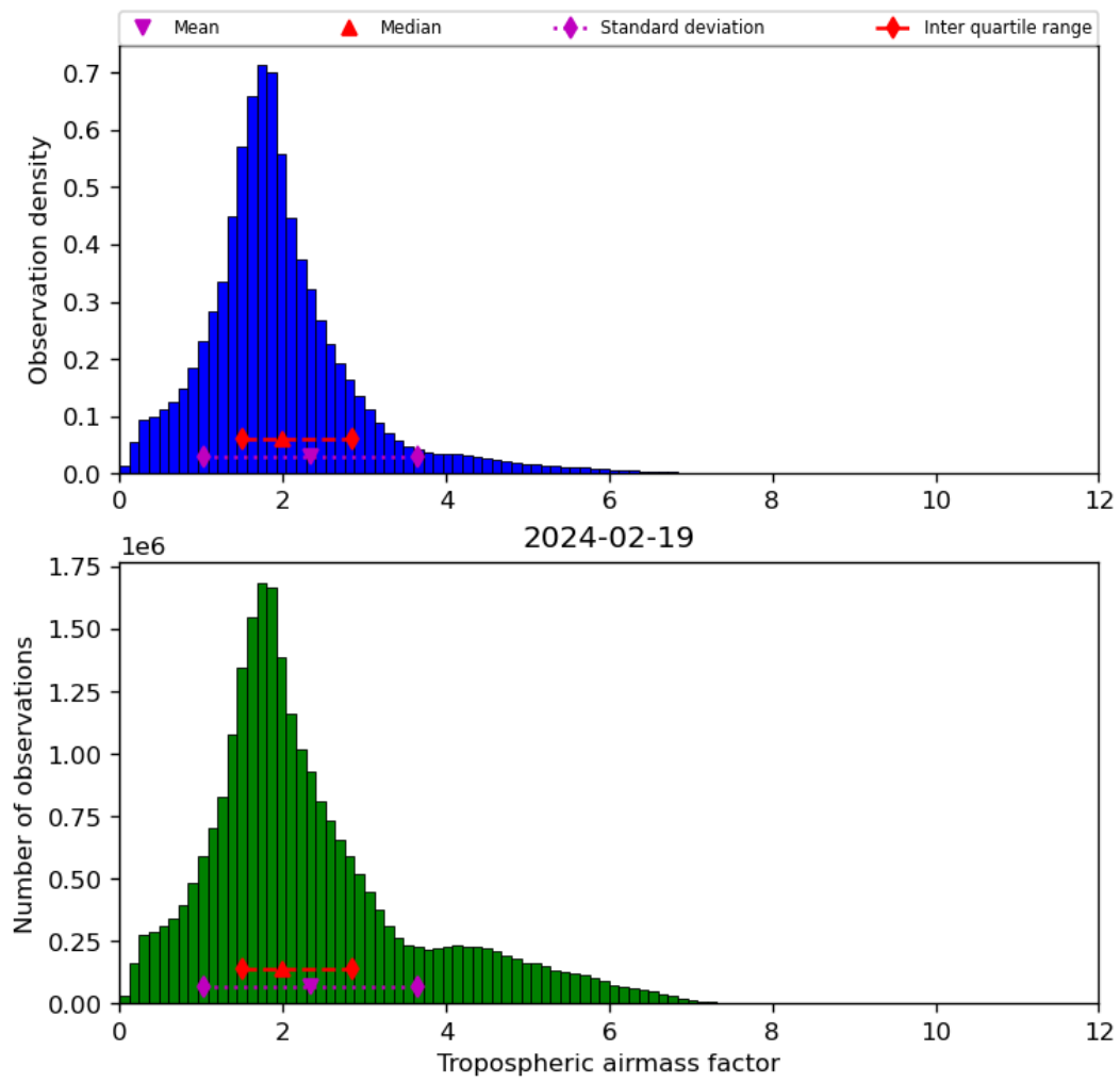
Figure 31: Histogram of “Tropospheric airmass factor” for 2024-02-18 to 2024-02-20
