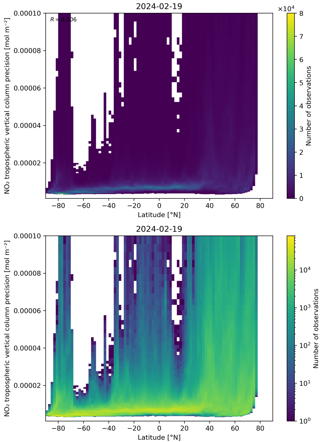
Figure 93: Scatter density plot of “Latitude” against “NO 2 tropospheric vertical column precision” for 2024-02-18 to 2024-02-20.
