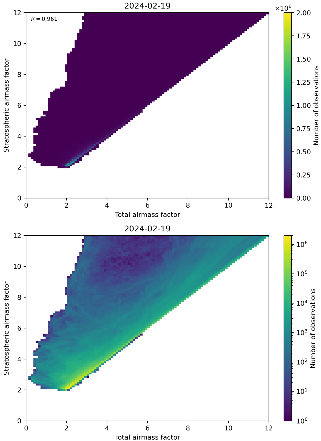
Figure 62: Scatter density plot of “Total airmass factor” against “Stratospheric airmass factor” for 2024-02-18 to 2024-02-20.
