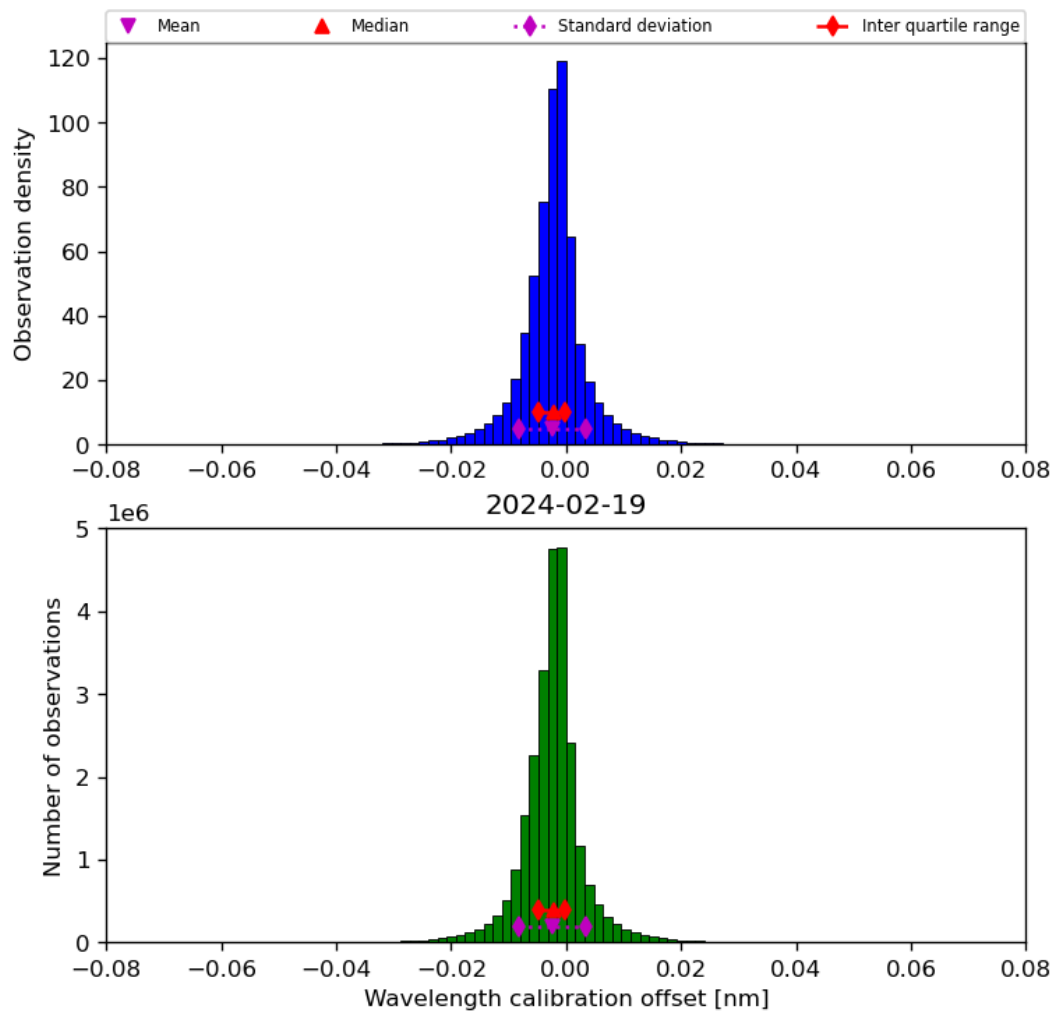
Figure 35: Histogram of “Wavelength calibration offset” for 2024-02-18 to 2024-02-20
