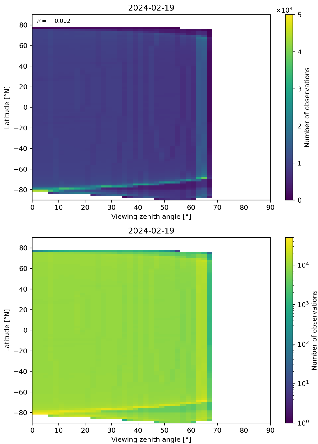
Figure 163: Scatter density plot of “Viewing zenith angle” against “Latitude” for 2024-02-18 to 2024-02-20.
