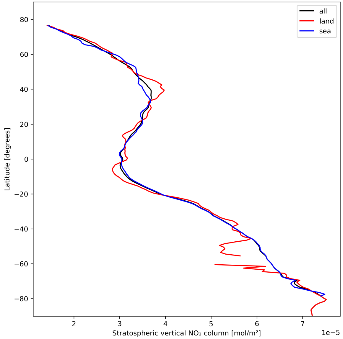
Figure 19: Zonal average of “Stratospheric vertical NO 2 column” for 2024-02-18 to 2024-02-20.
