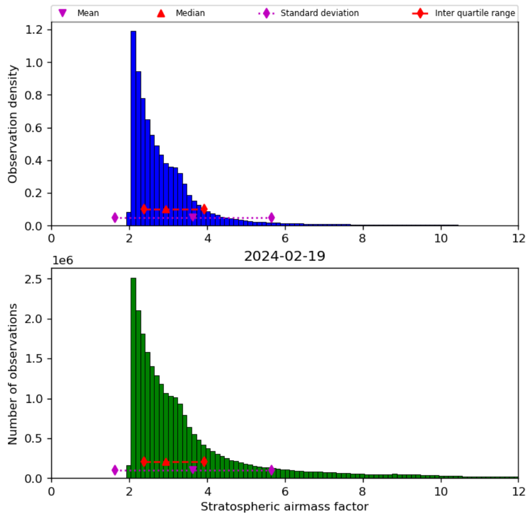
Figure 44: Histogram of “Stratospheric airmass factor” for 2024-02-18 to 2024-02-20
