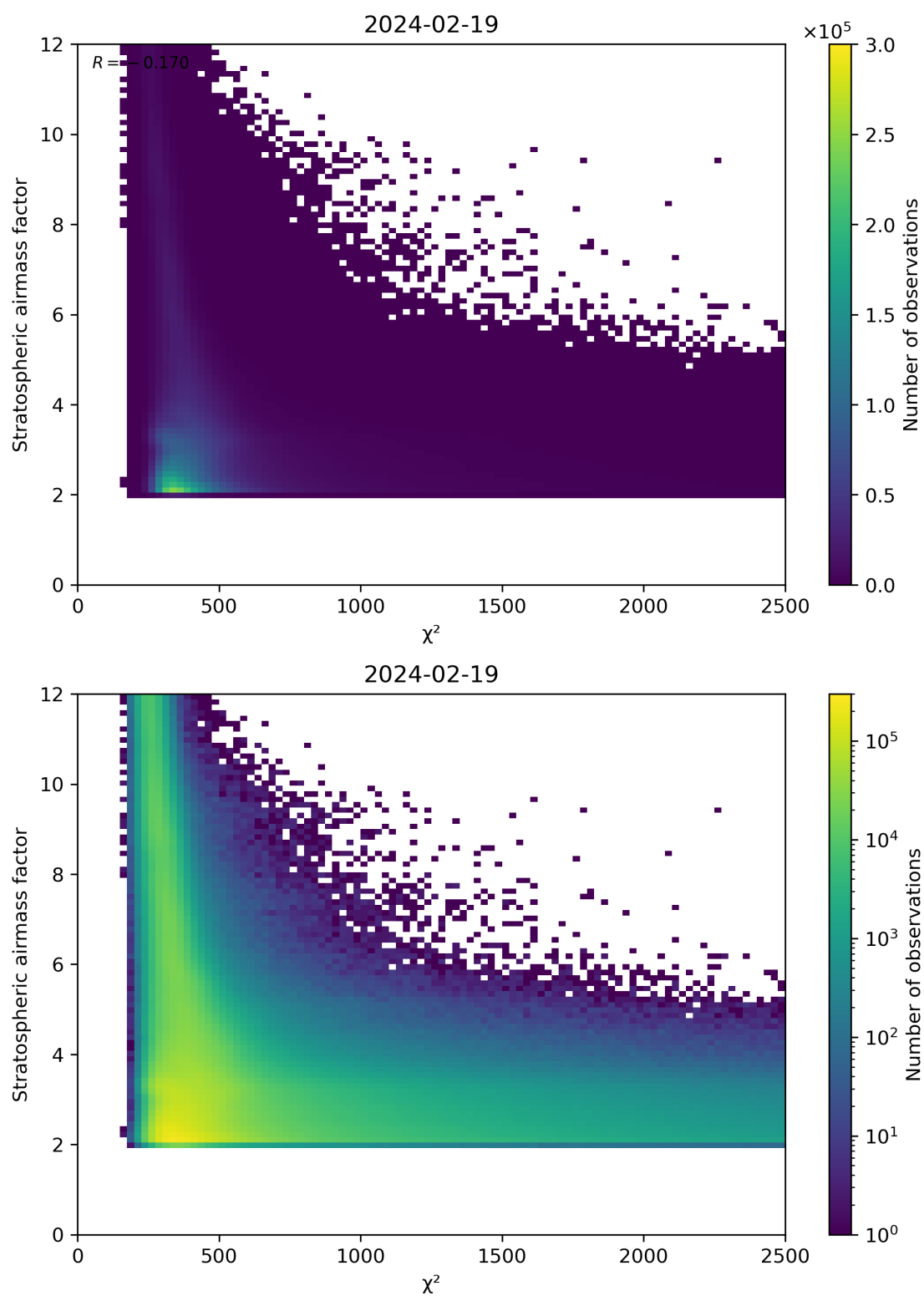
Figure 81: Scatter density plot of “ \chi^2 ” against “Stratospheric airmass factor” for 2024-02-18 to 2024-02-20.
