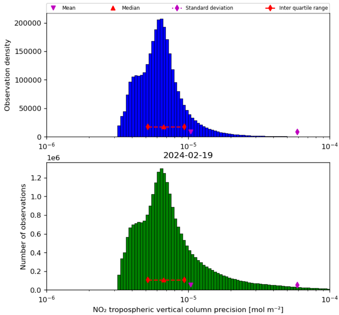
Figure 30: Histogram of “NO 2 tropospheric vertical column precision” for 2024-02-18 to 2024-02-20
