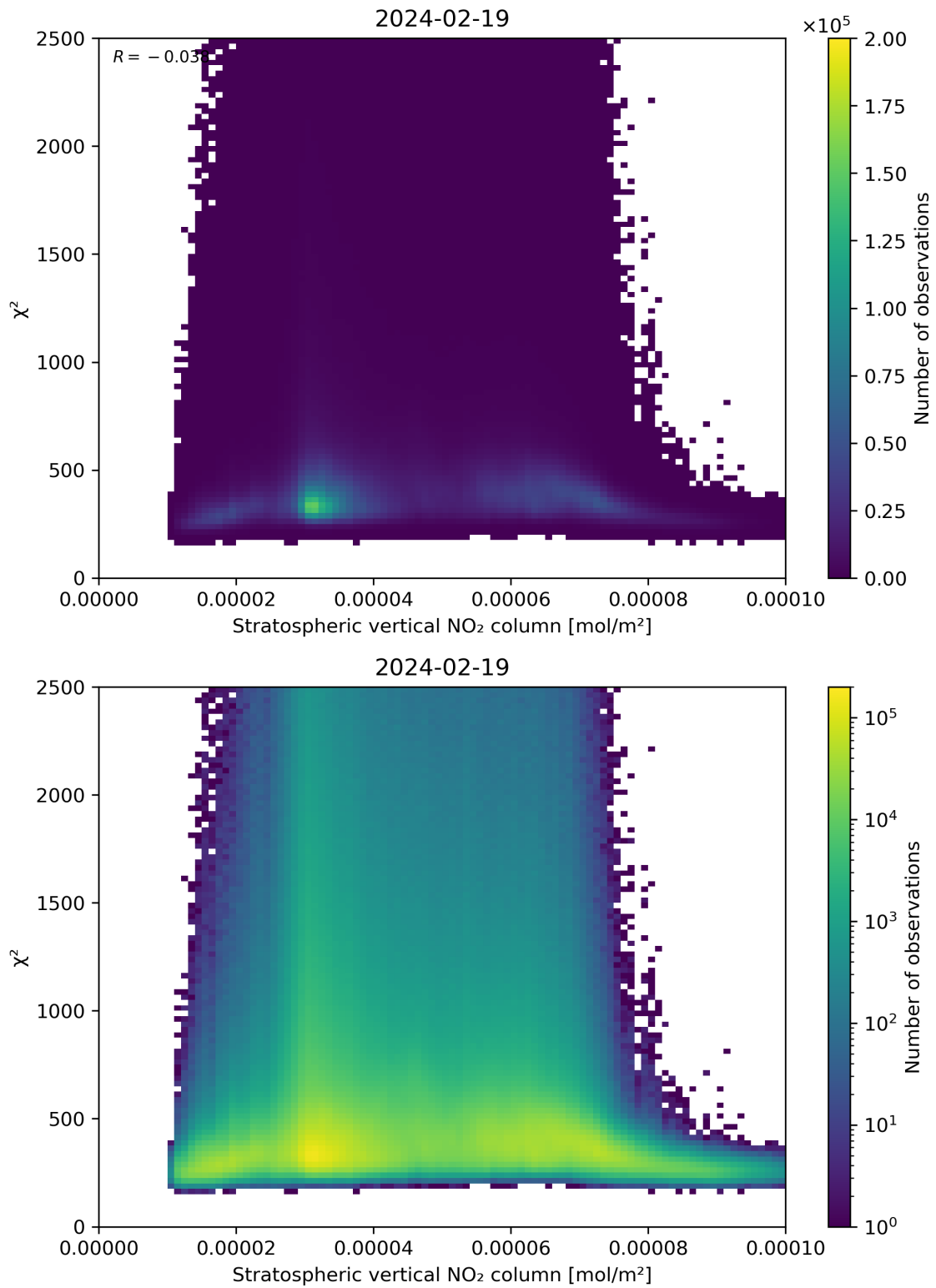
Figure 97: Scatter density plot of “Stratospheric vertical NO 2 column” against “ \chi^2 ” for 2024-02-18 to 2024-02-20.
