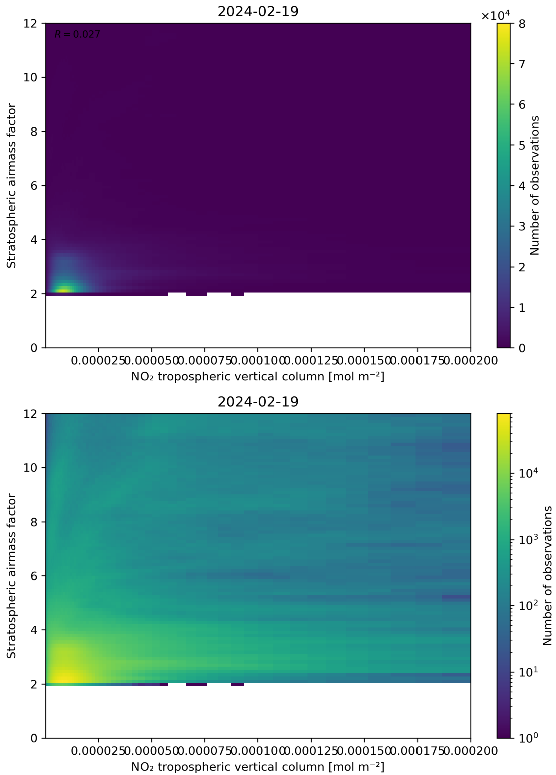
Figure 121: Scatter density plot of “NO 2 tropospheric vertical column” against “Stratospheric airmass factor” for 2024-02-18 to 2024-02-20.
