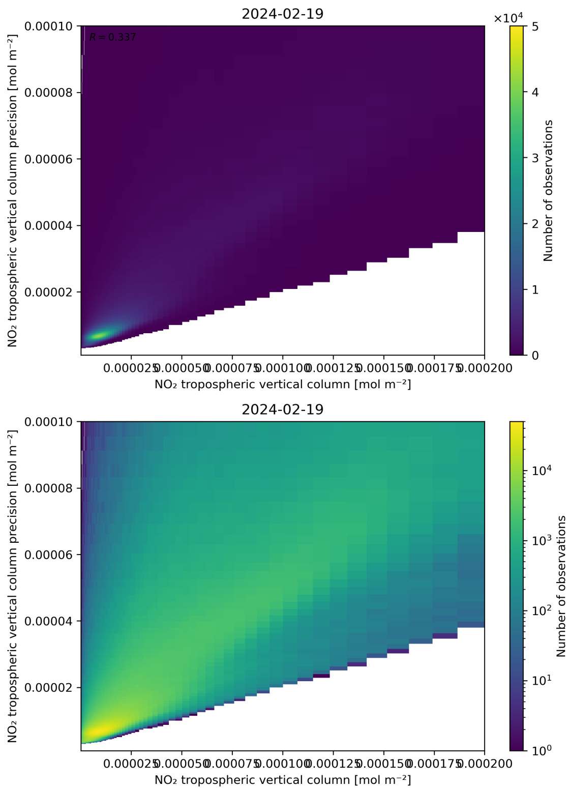
Figure 130: Scatter density plot of “NO 2 tropospheric vertical column” against “NO 2 tropospheric vertical column precision” for 2024-02-18 to 2024-02-20.
