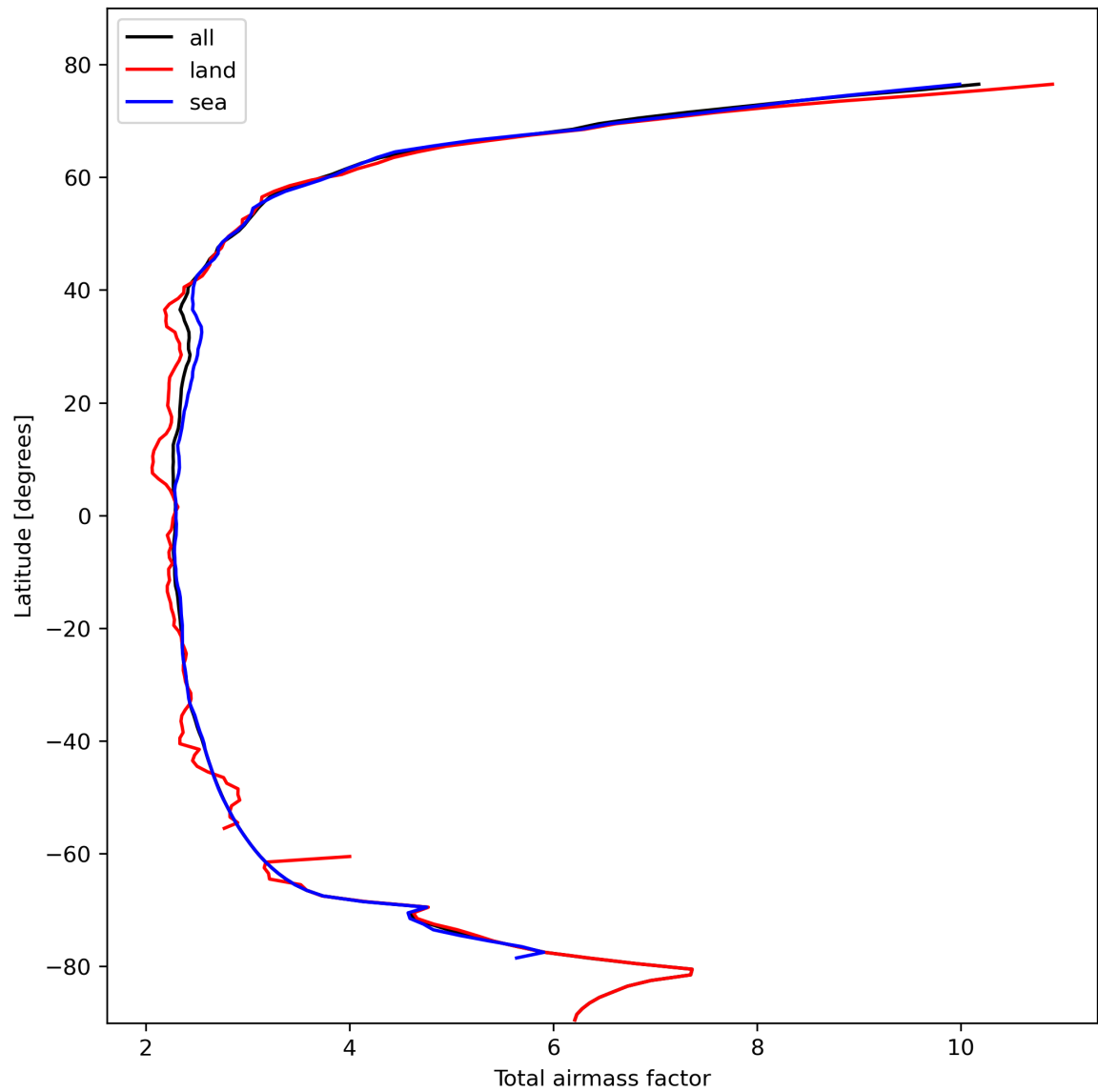
Figure 15: Zonal average of “Total airmass factor” for 2024-02-18 to 2024-02-20.
