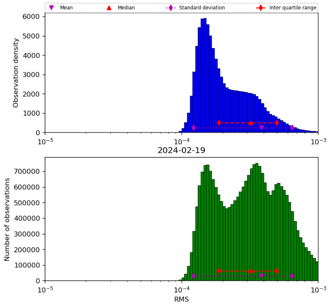
Figure 43: Histogram of “RMS” for 2024-02-18 to 2024-02-20
