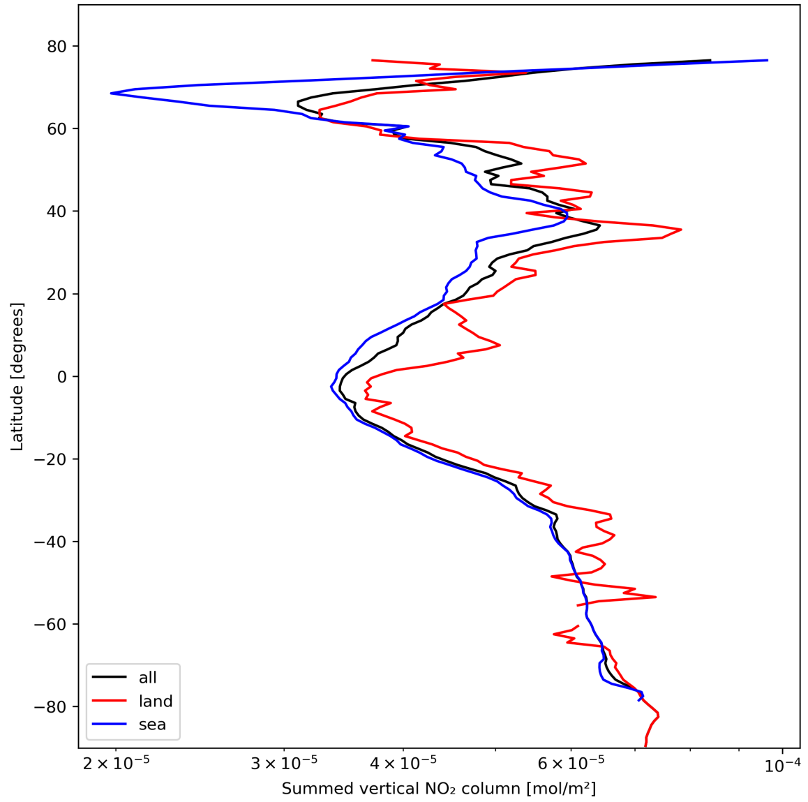
Figure 23: Zonal average of “Summed vertical NO 2 column” for 2024-02-18 to 2024-02-20.
