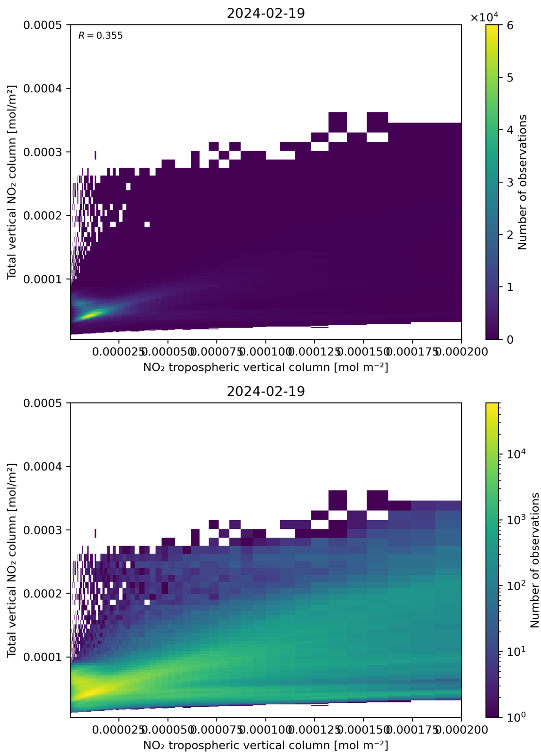
Figure 128: Scatter density plot of “NO 2 tropospheric vertical column” against “Total vertical NO 2 column” for 2024-02-18 to 2024-02-20.
