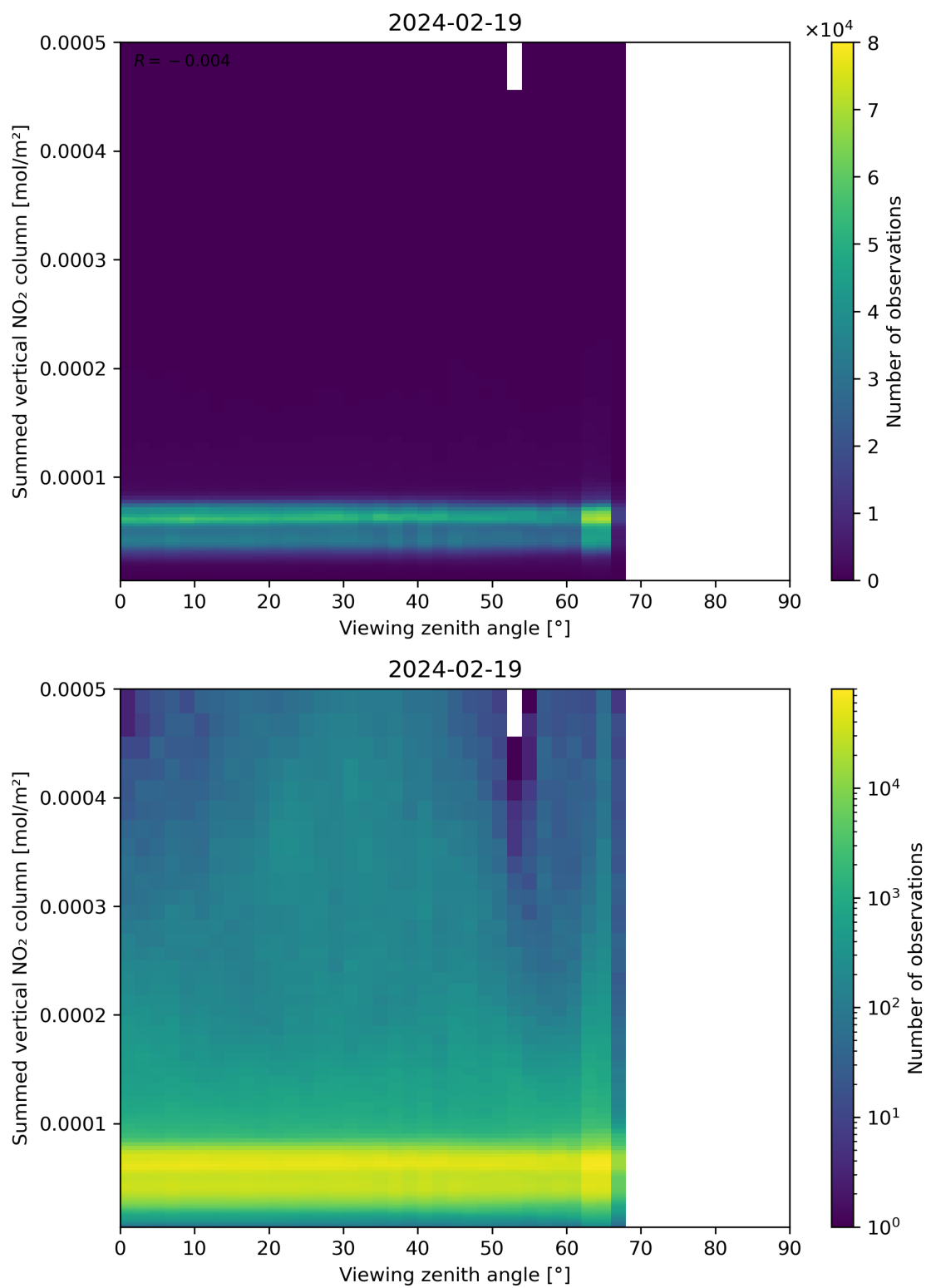
Figure 165: Scatter density plot of “Viewing zenith angle” against “Summed vertical NO 2 column” for 2024-02-18 to 2024-02-20.
