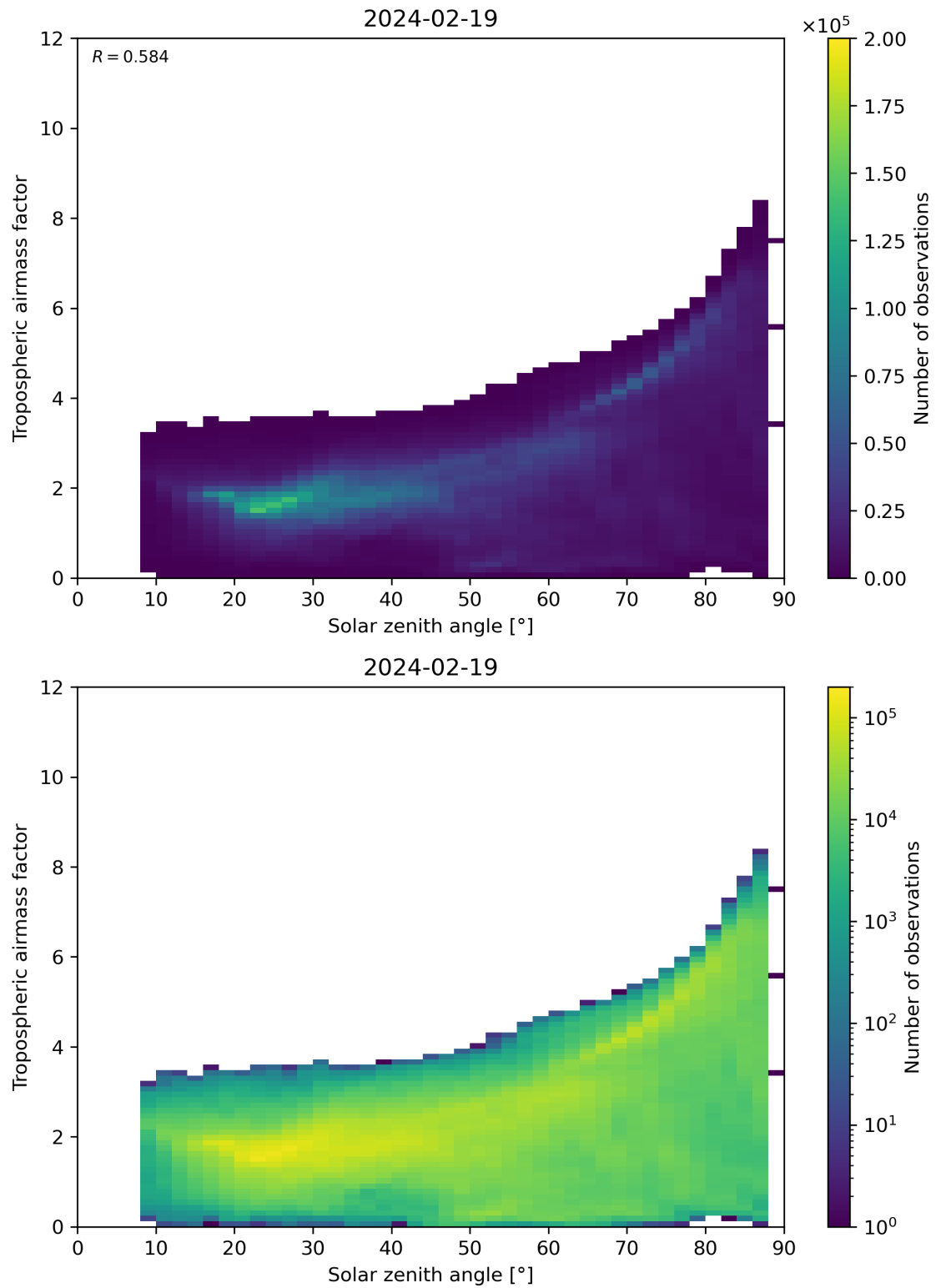
Figure 147: Scatter density plot of “Solar zenith angle” against “Tropospheric airmass factor” for 2024-02-18 to 2024-02-20.
