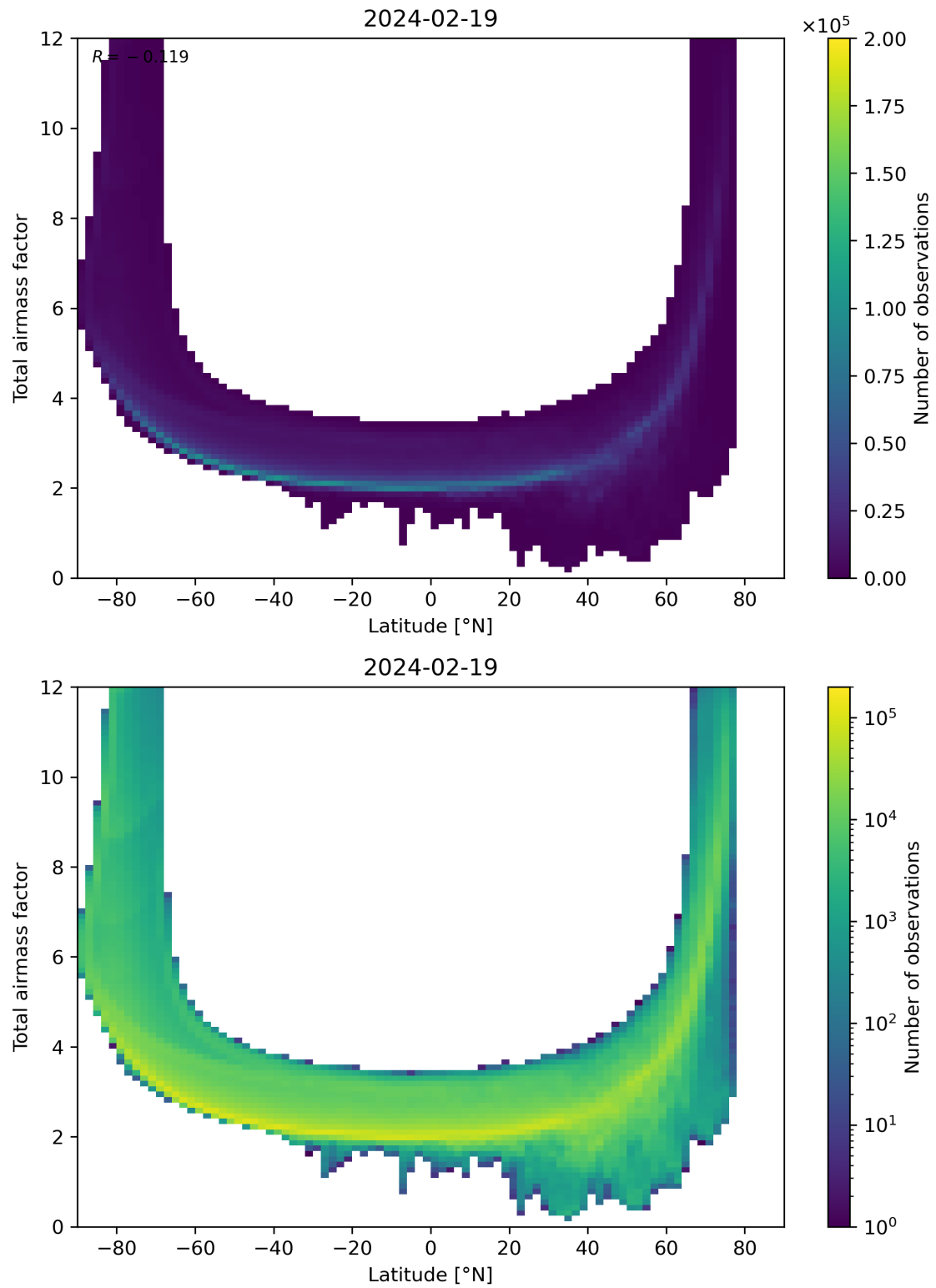
Figure 84: Scatter density plot of “Latitude” against “Total airmass factor” for 2024-02-18 to 2024-02-20.
