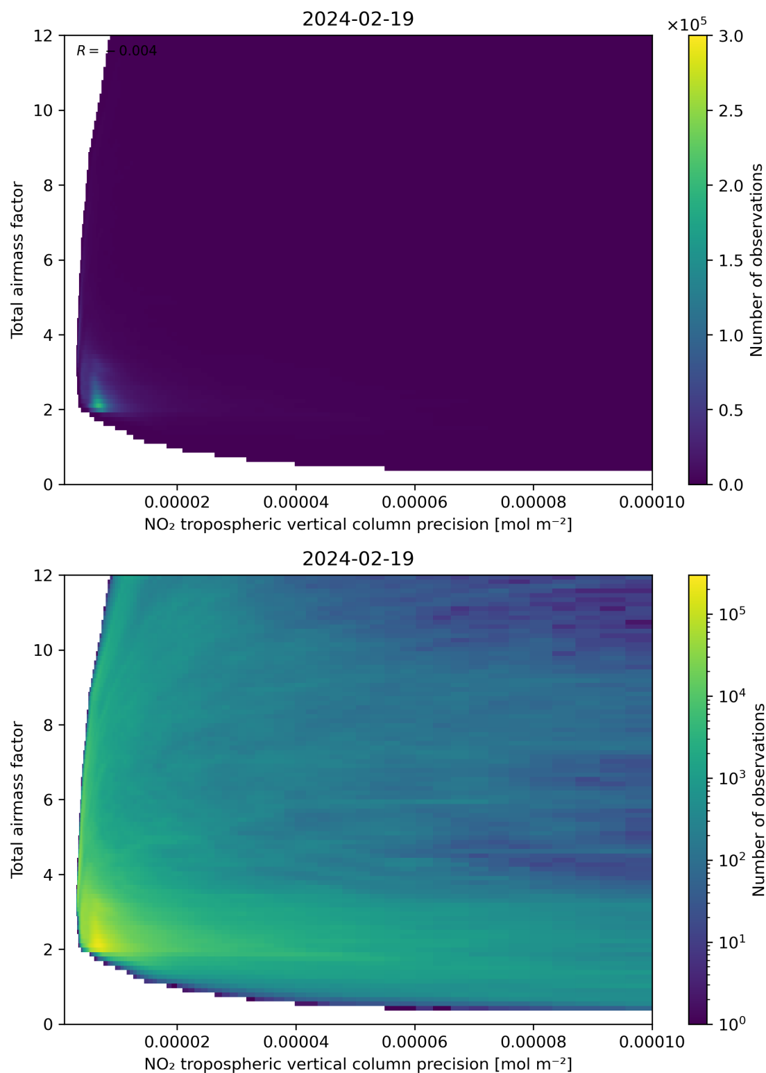
Figure 132: Scatter density plot of “NO 2 tropospheric vertical column precision” against “Total air mass factor” for 2024-02-18 to 2024-02-20.
