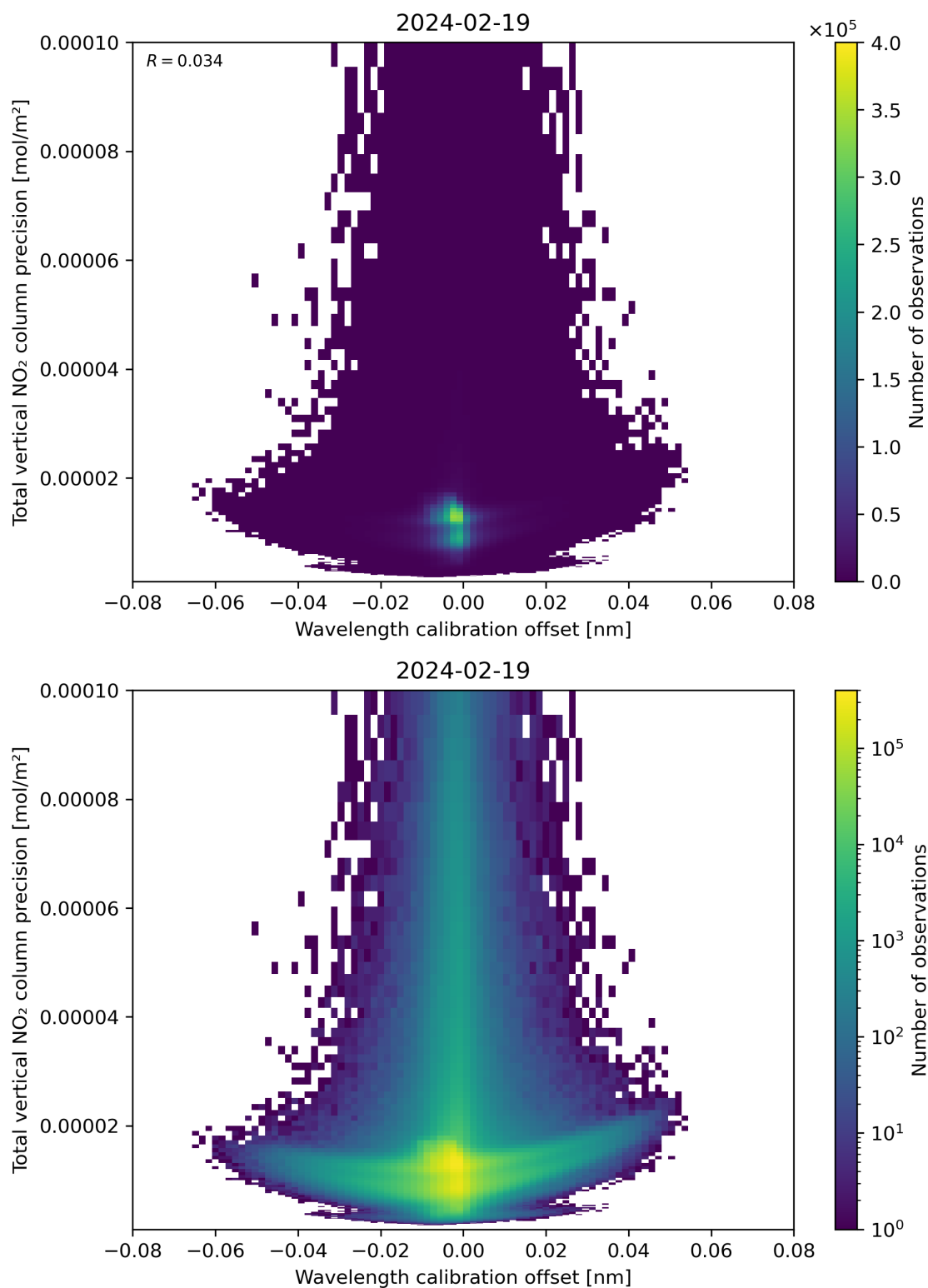
Figure 180: Scatter density plot of “Wavelength calibration offset” against “Total vertical NO 2 column precision” for 2024-02-18 to 2024-02-20.
