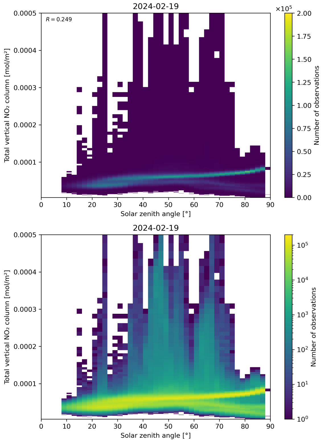
Figure 153: Scatter density plot of “Solar zenith angle” against “Total vertical NO 2 column” for 2024-02-18 to 2024-02-20.
