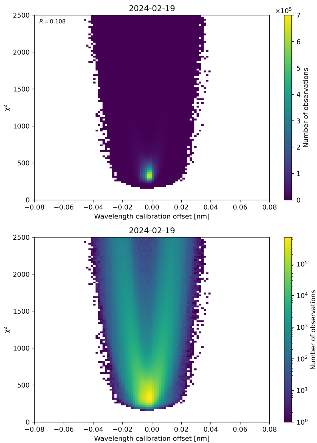
Figure 175: Scatter density plot of “Wavelength calibration offset” against “ \chi^2 ” for 2024-02-18 to 2024-02-20.
