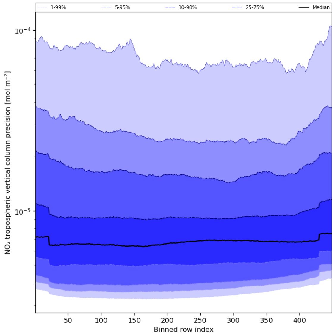
Figure 47: Along track statistics of “NO 2 tropospheric vertical column precision” for 2024-02-18 to 2024-02-20
