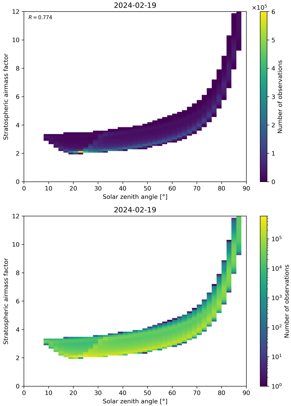
Figure 145: Scatter density plot of “Solar zenith angle” against “Stratospheric airmass factor” for 2024-02-18 to 2024-02-20.
