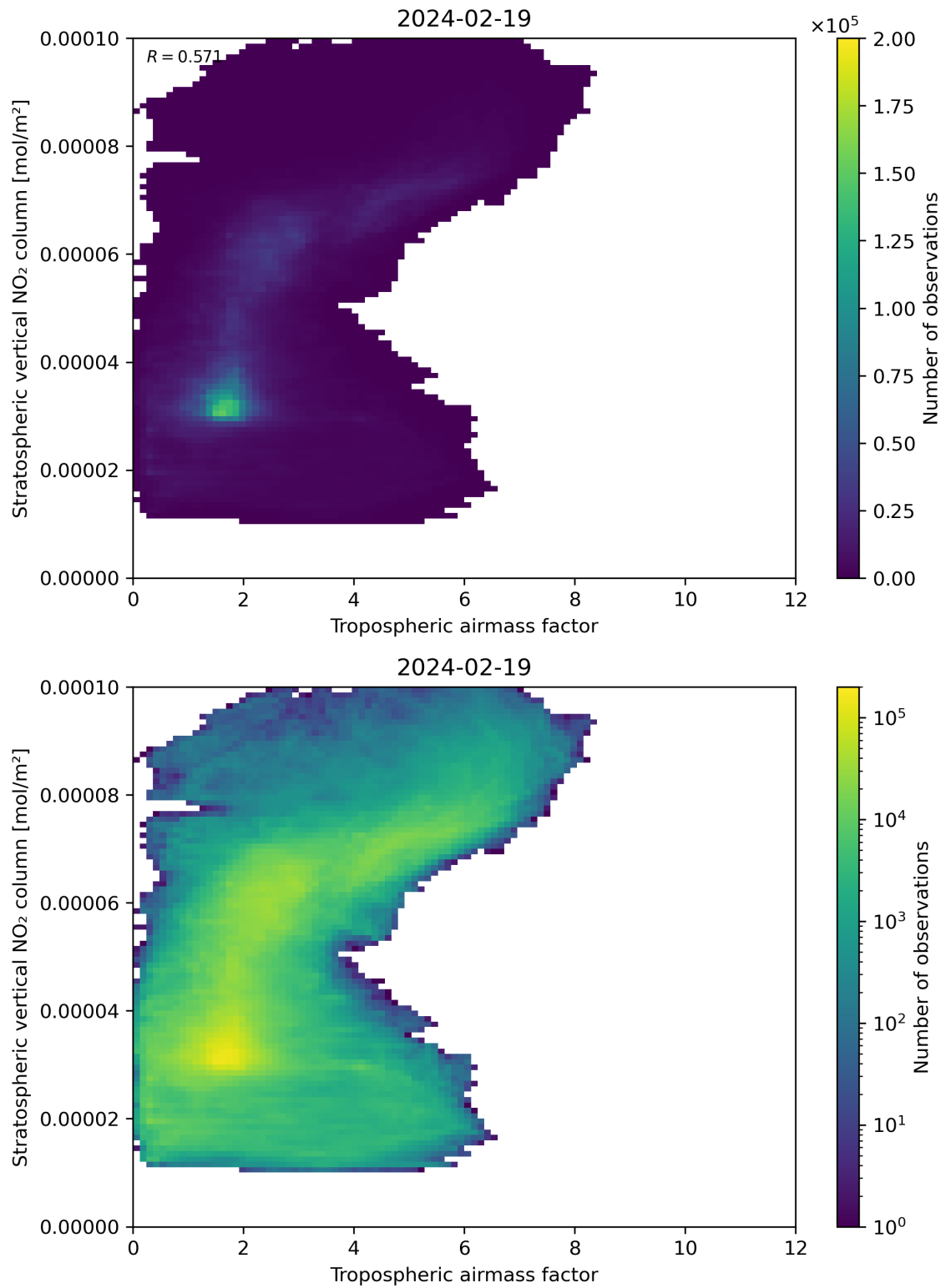
Figure 74: Scatter density plot of “Tropospheric air mass factor” against “Stratospheric vertical NO 2 column” for 2024-02-18 to 2024-02-20.
