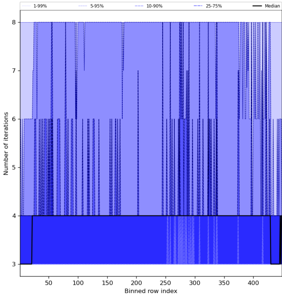
Figure 51: Along track statistics of “Number of iterations” for 2024-02-18 to 2024-02-20
