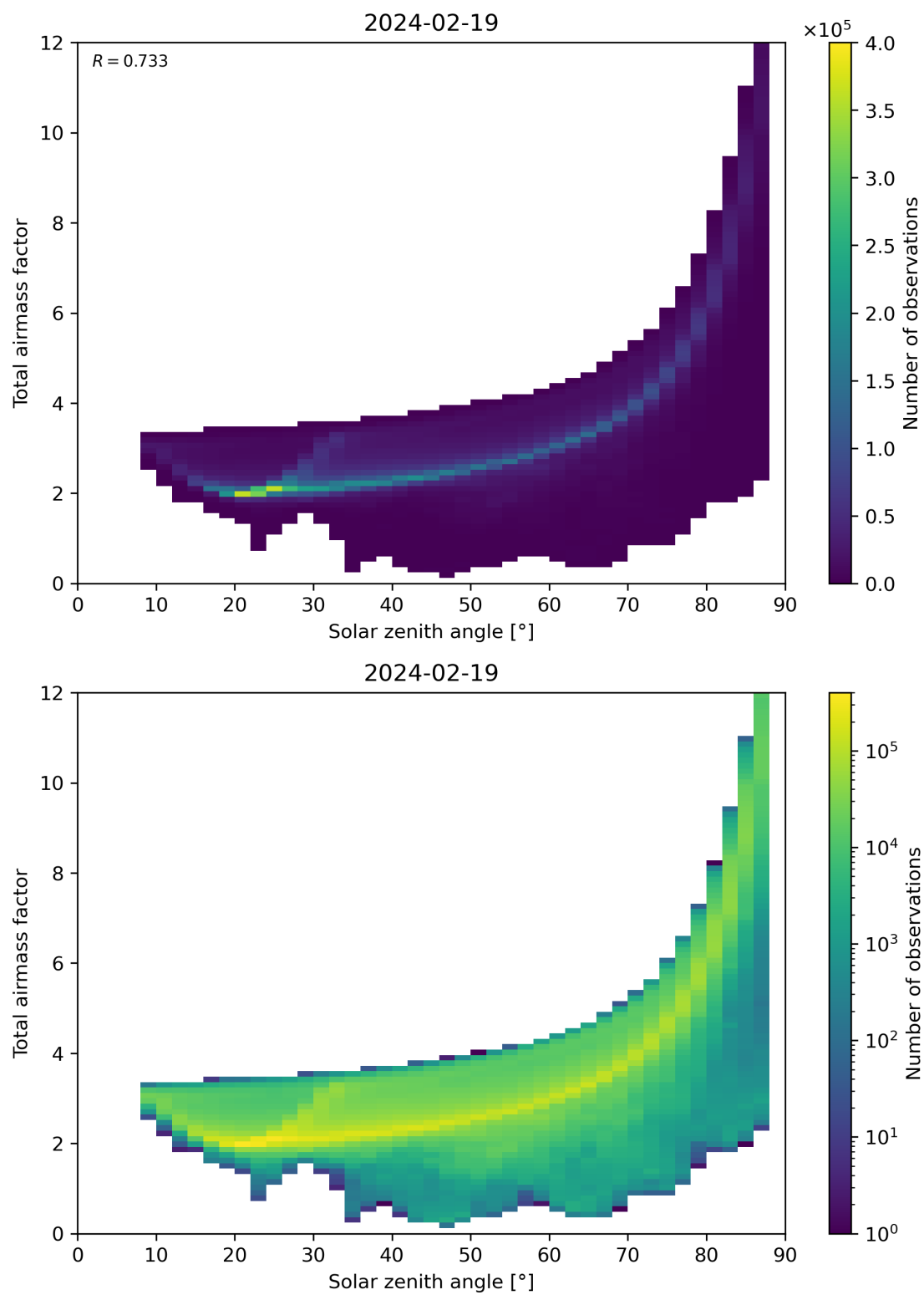
Figure 146: Scatter density plot of “Solar zenith angle” against “Total air mass factor” for 2024-02-18 to 2024-02-20.
