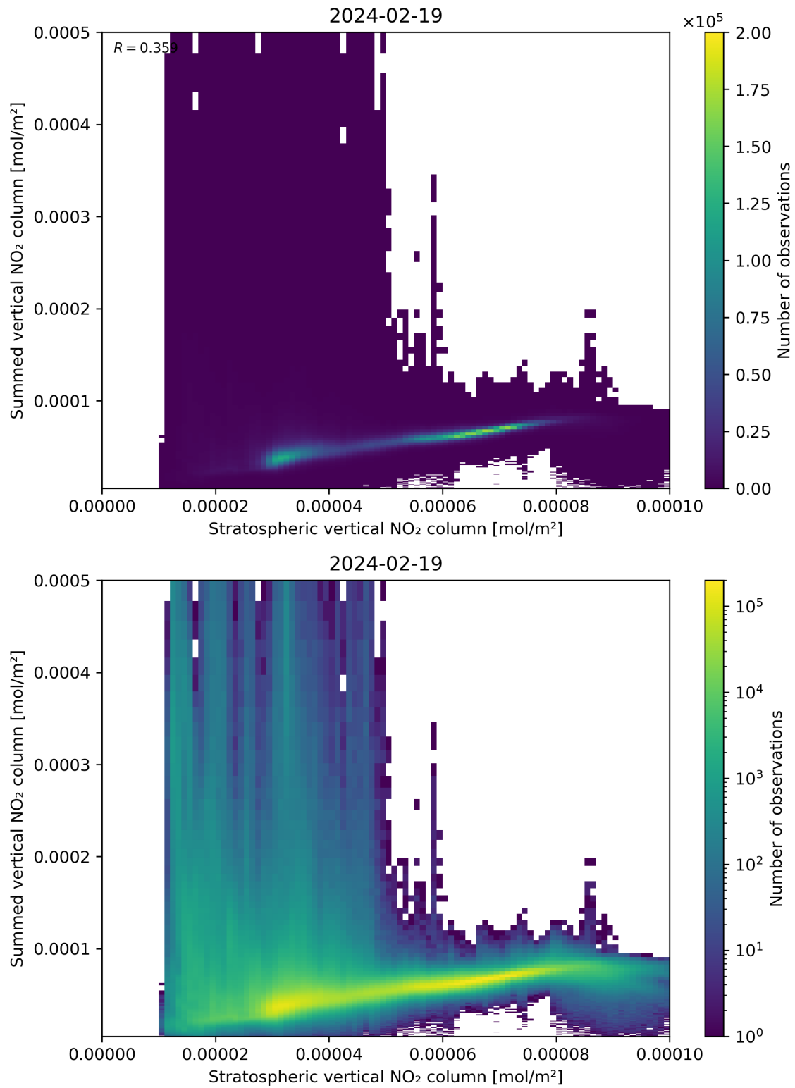
Figure 98: Scatter density plot of “Stratospheric vertical NO 2 column” against “Summed vertical NO 2 column” for 2024-02-18 to 2024-02-20.
