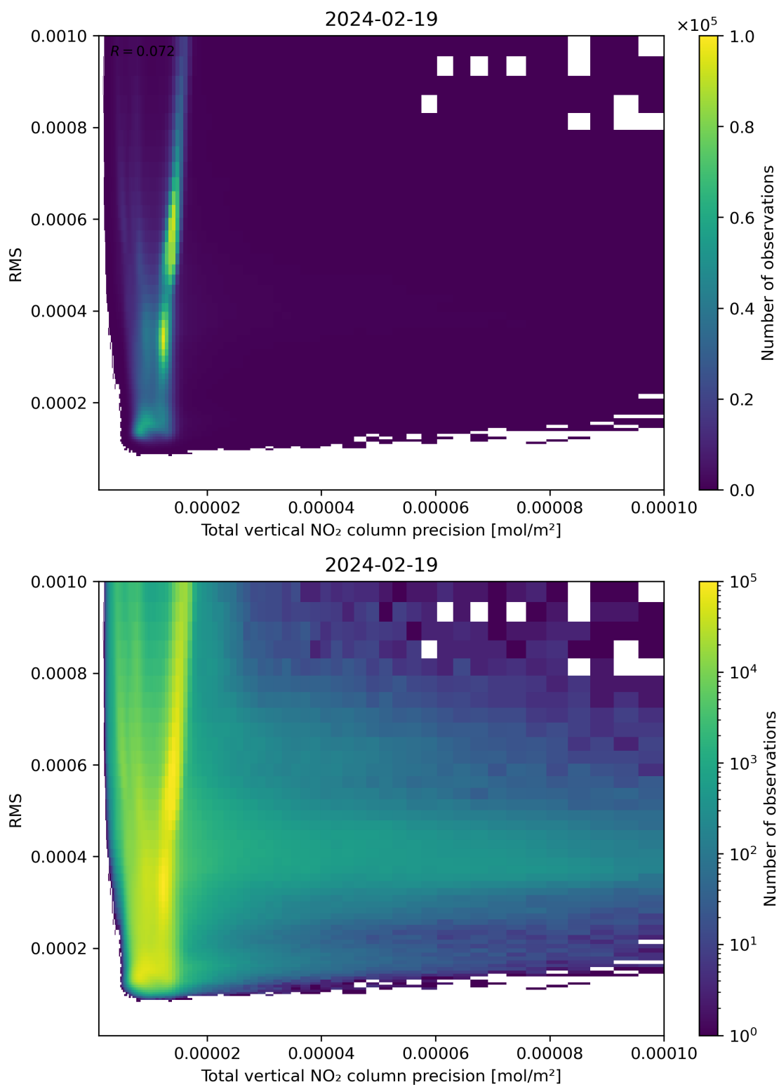
Figure 119: Scatter density plot of “Total vertical NO 2 column precision” against “RMS” for 2024-02-18 to 2024-02-20.
