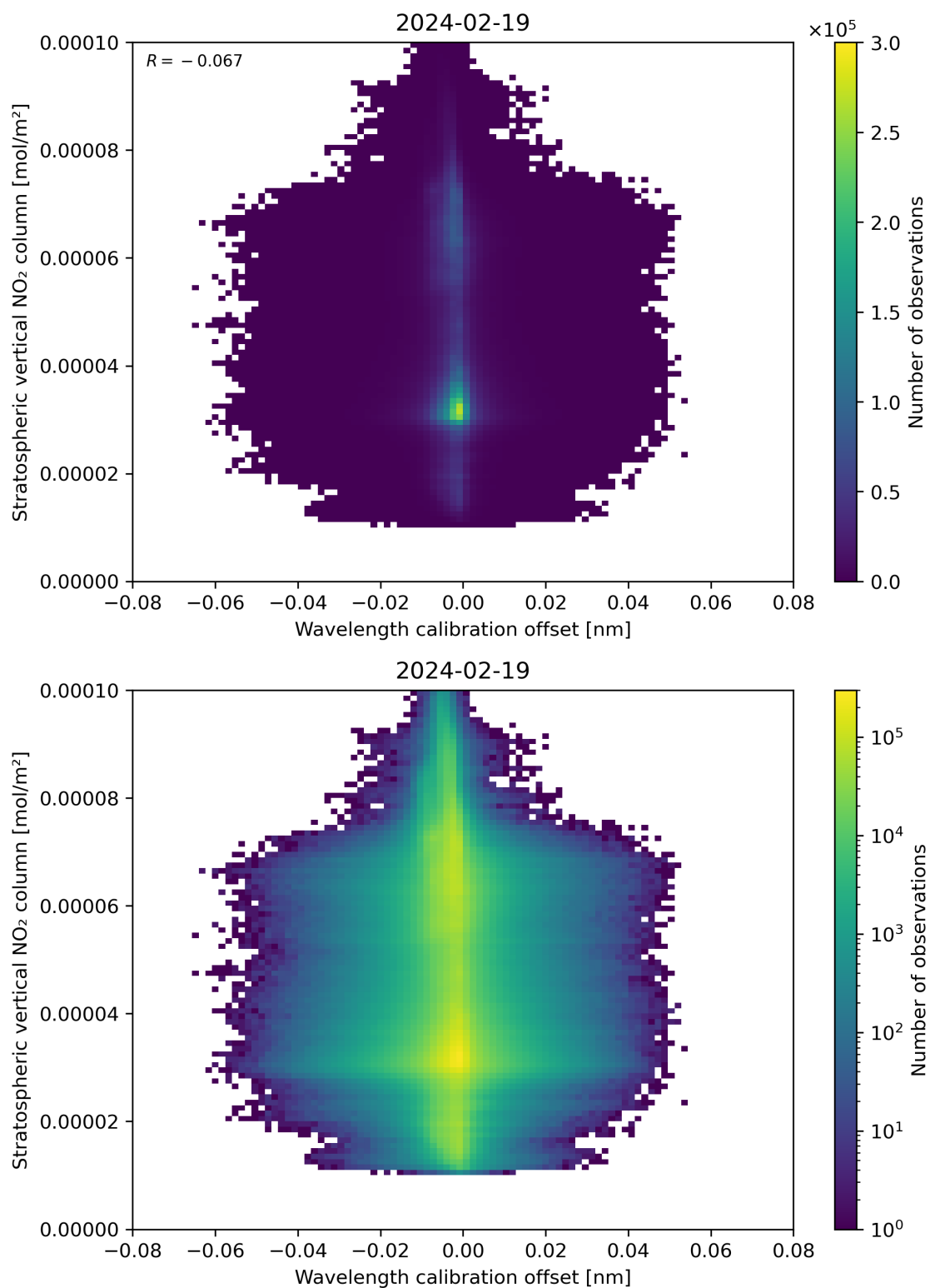
Figure 176: Scatter density plot of “Wavelength calibration offset” against “Stratospheric vertical NO 2 column” for 2024-02-18 to 2024-02-20.
