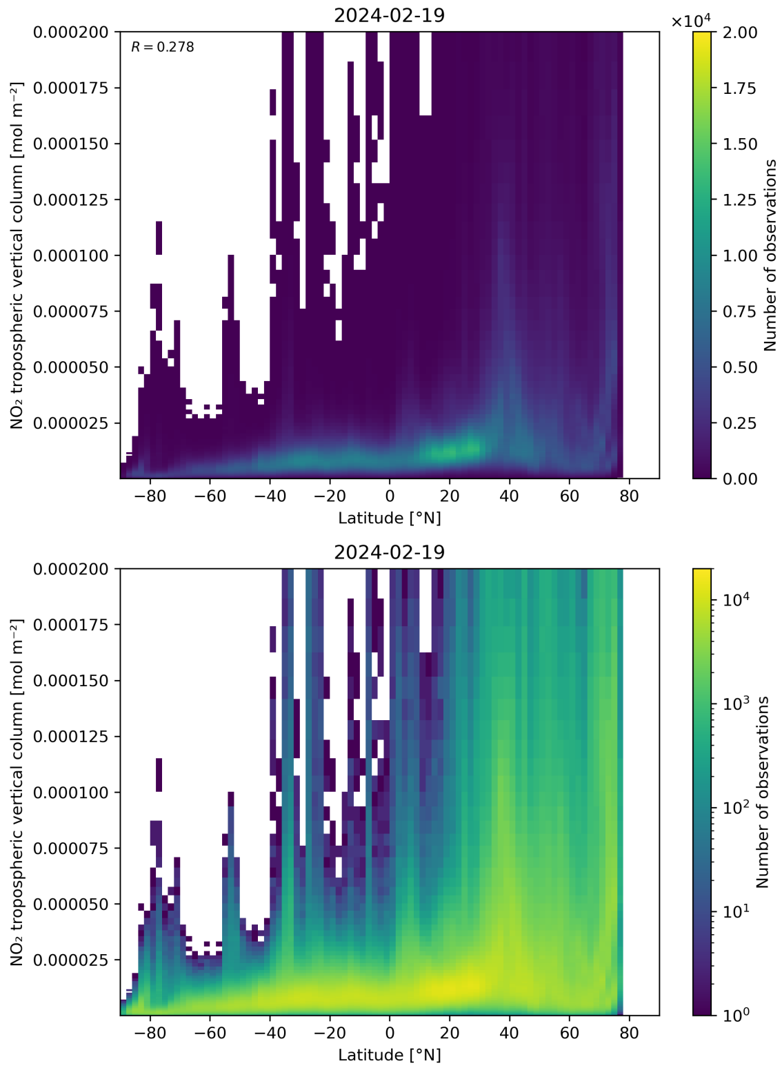
Figure 92: Scatter density plot of “Latitude” against “NO 2 tropospheric vertical column” for 2024-02-18 to 2024-02-20.
