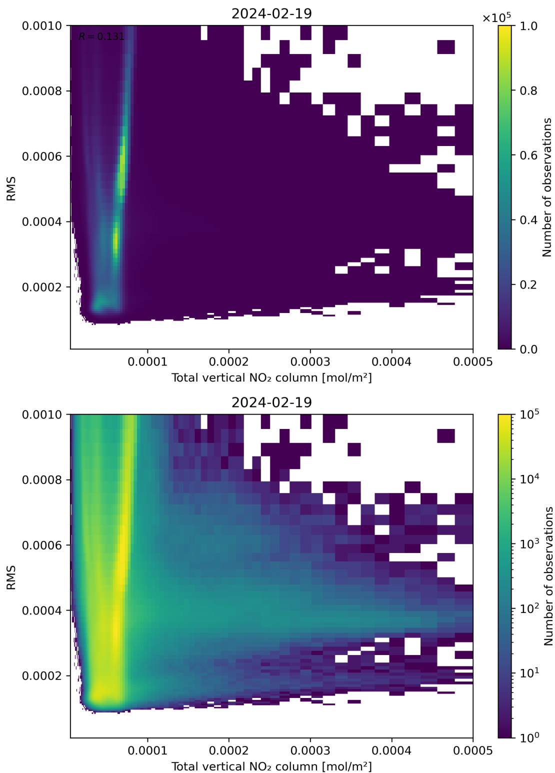
Figure 120: Scatter density plot of “Total vertical NO 2 column” against “RMS” for 2024-02-18 to 2024-02-20.
