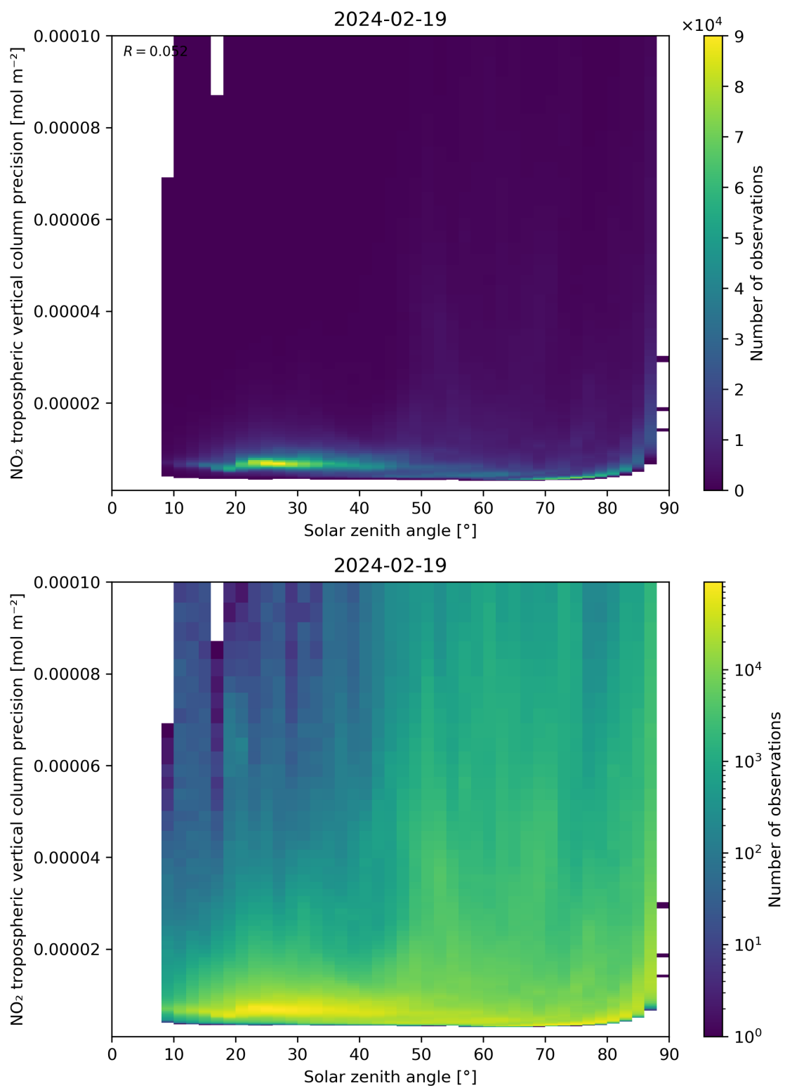
Figure 156: Scatter density plot of “Solar zenith angle” against “NO 2 tropospheric vertical column precision” for 2024-02-18 to 2024-02-20.
