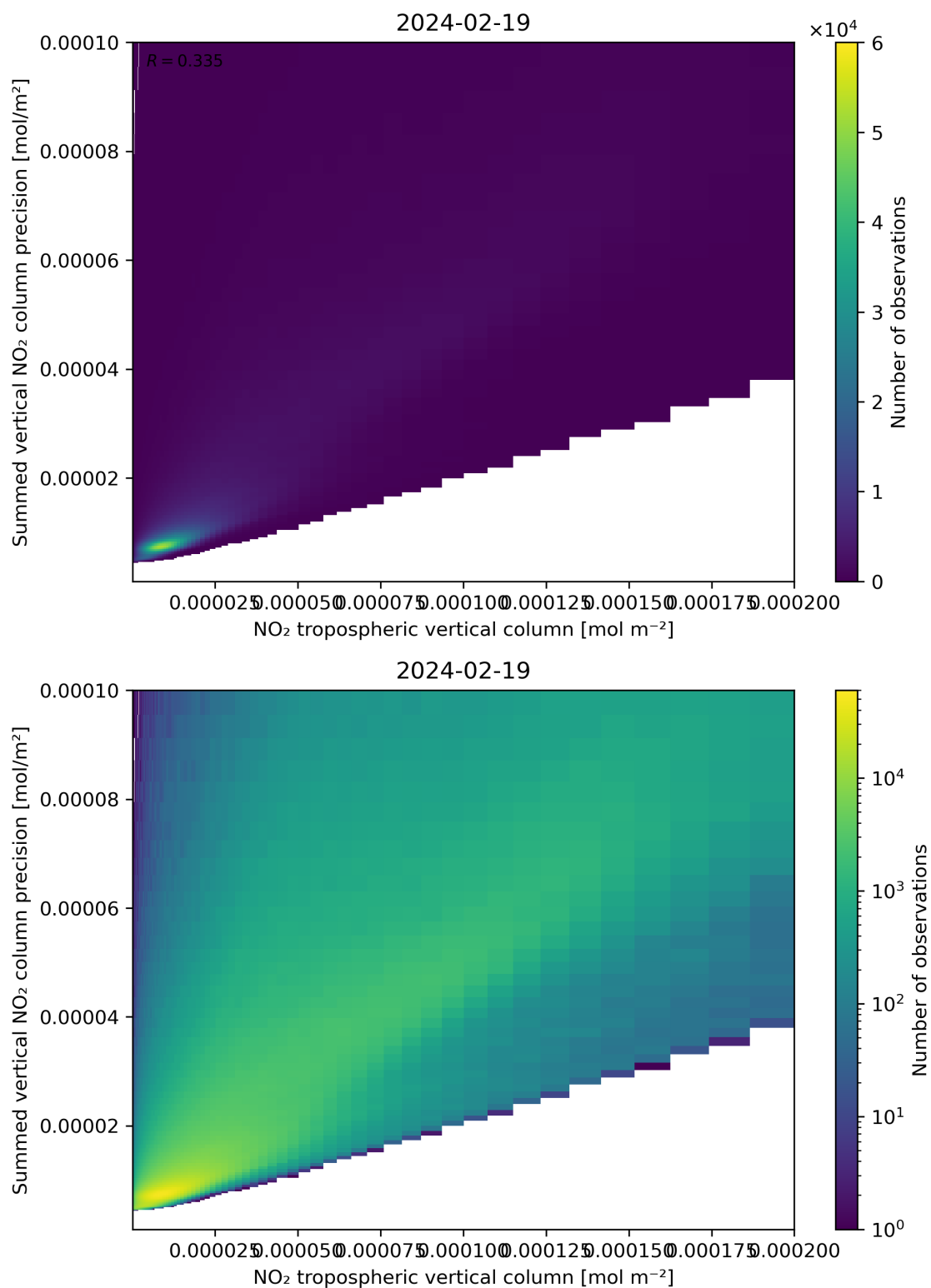
Figure 127: Scatter density plot of “NO 2 tropospheric vertical column” against “Summed vertical NO 2 column precision” for 2024-02-18 to 2024-02-20.
