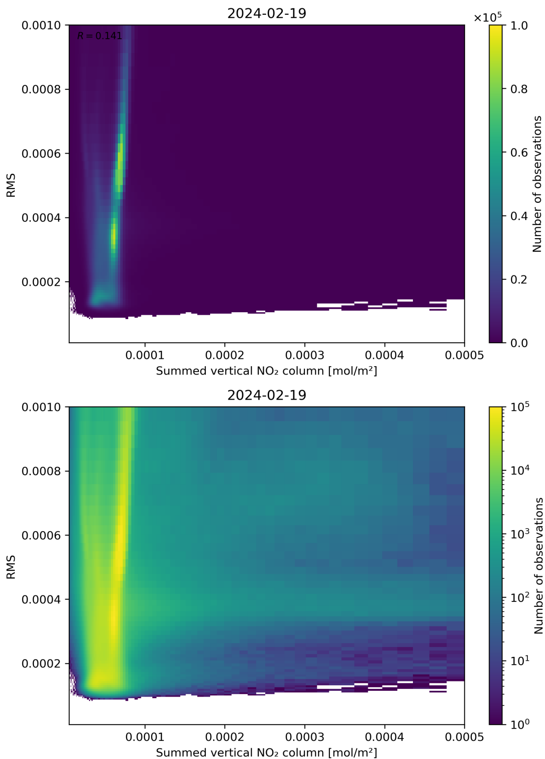
Figure 109: Scatter density plot of “Summed vertical NO 2 column” against “RMS” for 2024-02-18 to 2024-02-20.
