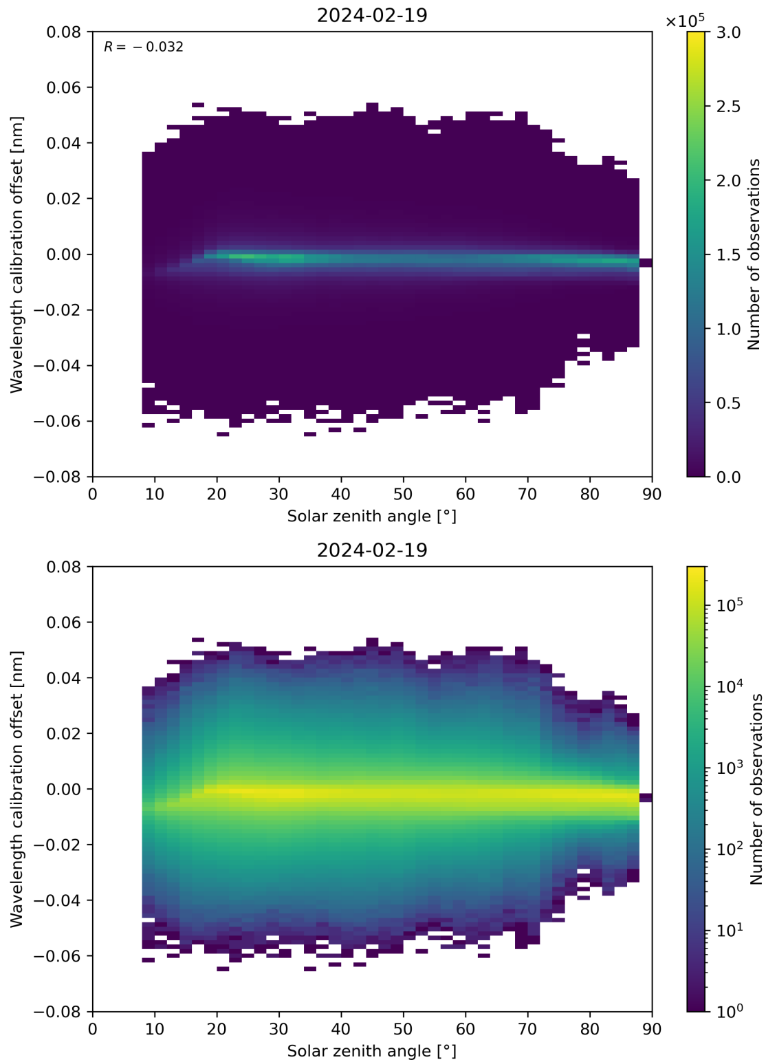
Figure 158: Scatter density plot of “Solar zenith angle” against “Wavelength calibration offset” for 2024-02-18 to 2024-02-20.
