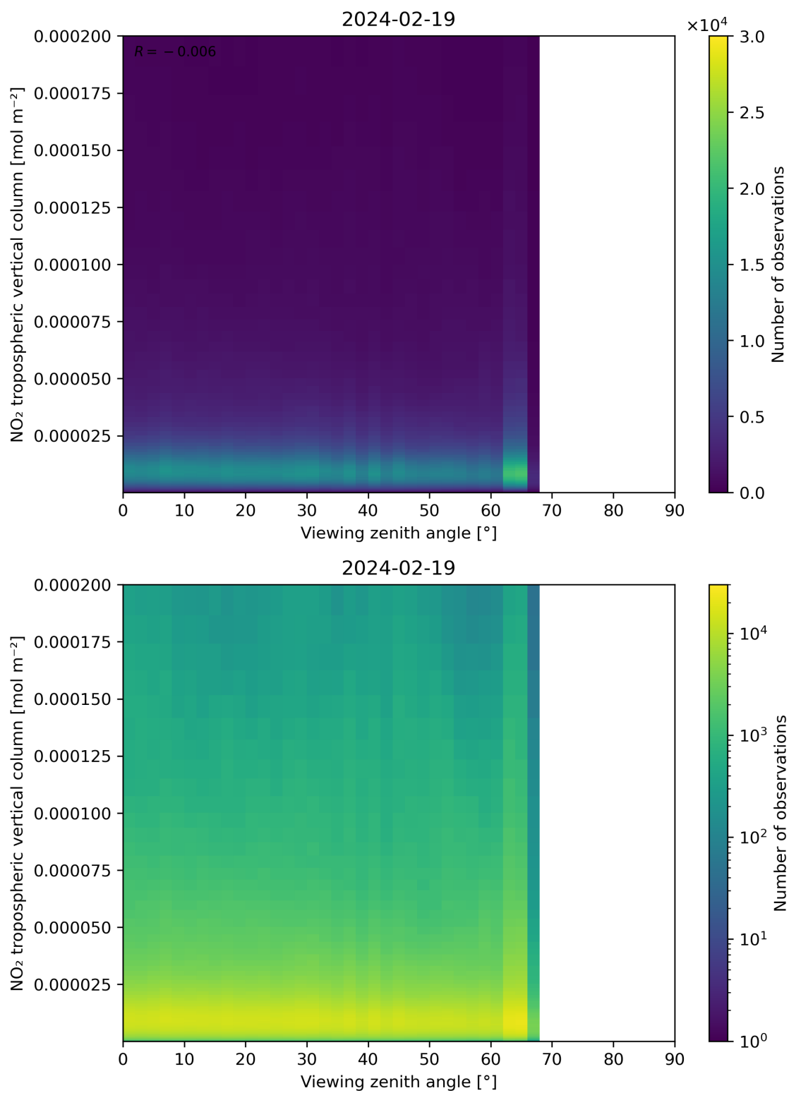
Figure 169: Scatter density plot of “Viewing zenith angle” against “NO 2 tropospheric vertical column” for 2024-02-18 to 2024-02-20.
