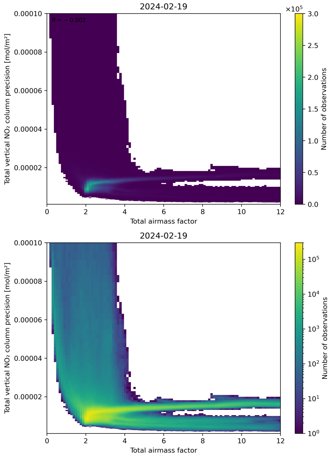
Figure 68: Scatter density plot of “Total airmass factor” against “Total vertical NO 2 column precision” for 2024-02-18 to 2024-02-20.
