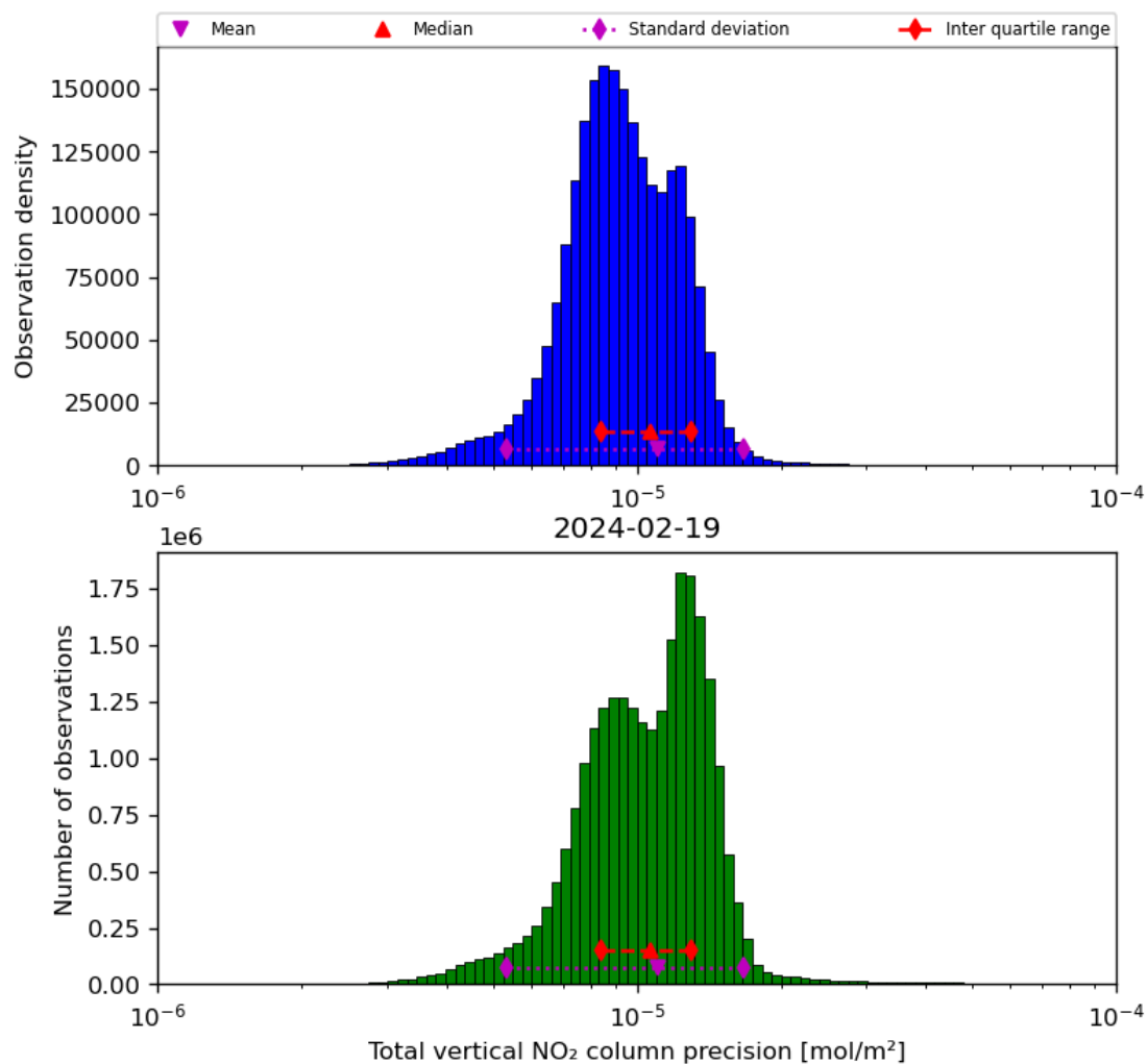
Figure 39: Histogram of “Total vertical NO 2 column precision” for 2024-02-18 to 2024-02-20
