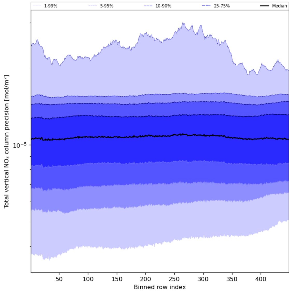
Figure 56: Along track statistics of “Total vertical NO 2 column precision” for 2024-02-18 to 2024-02-20
