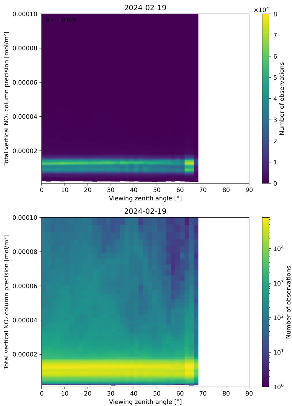
Figure 168: Scatter density plot of “Viewing zenith angle” against “Total vertical NO 2 column precision” for 2024-02-18 to 2024-02-20.
