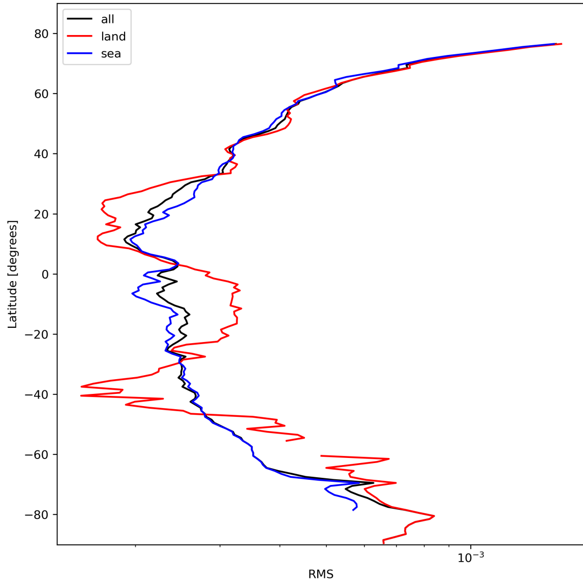
Figure 26: Zonal average of “RMS” for 2024-02-18 to 2024-02-20.
