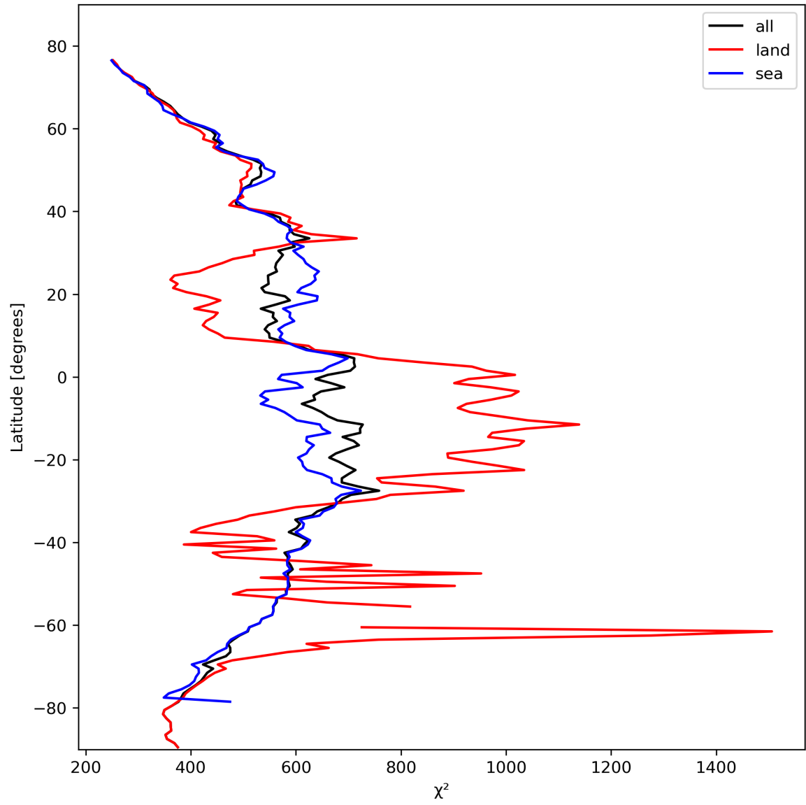
Figure 25: Zonal average of “ \chi^2 ” for 2024-02-18 to 2024-02-20.
