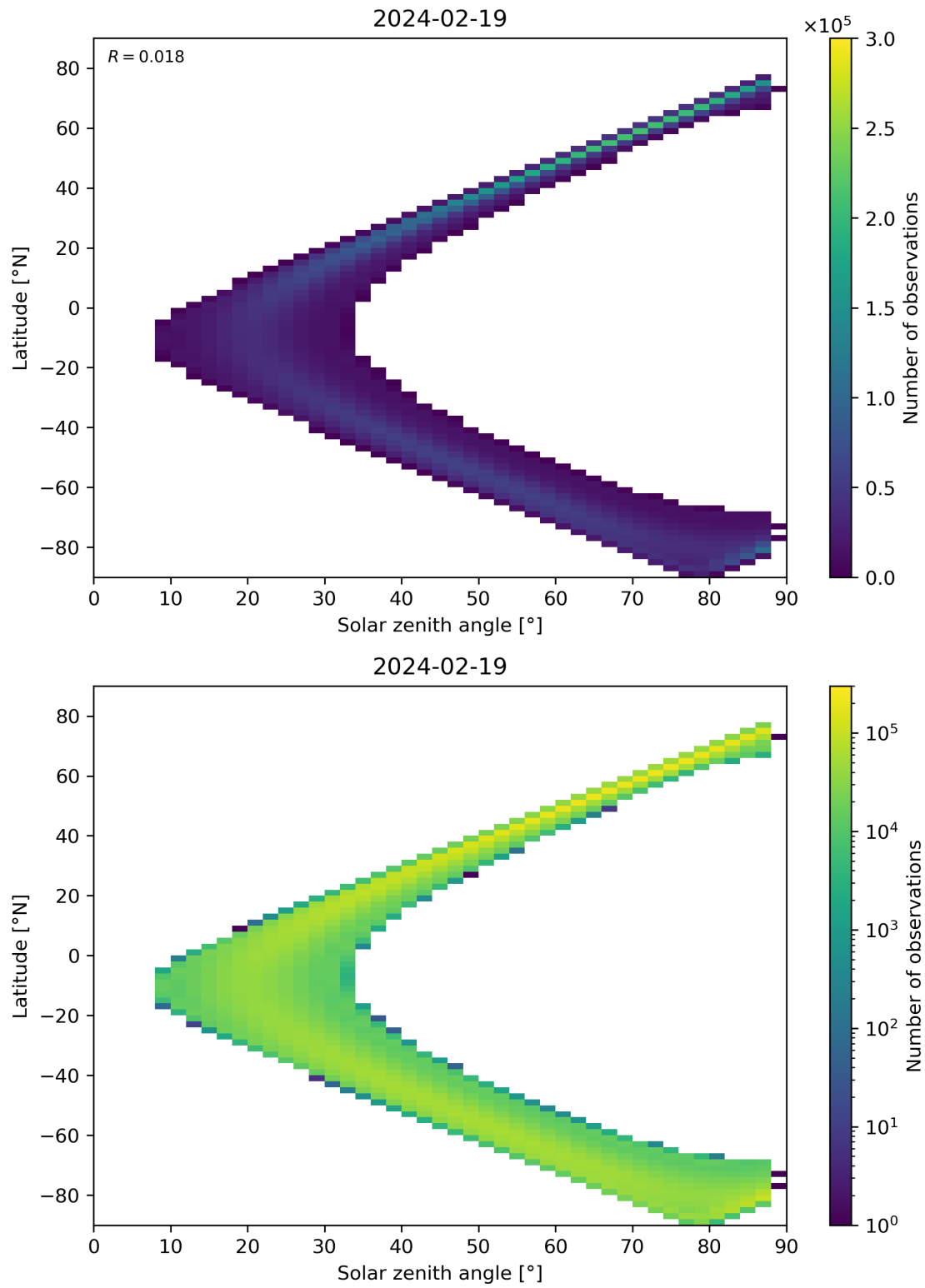
Figure 149: Scatter density plot of “Solar zenith angle” against “Latitude” for 2024-02-18 to 2024-02-20.
