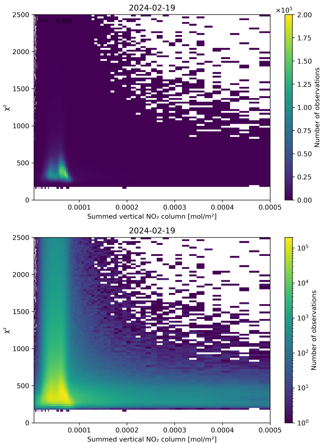
Figure 104: Scatter density plot of “Summed vertical NO 2 column” against “ \chi^2 ” for 2024-02-18 to 2024-02-20.
