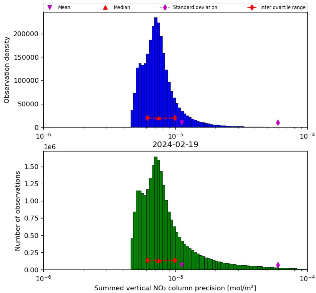
Figure 41: Histogram of “Summed vertical NO 2 column precision” for 2024-02-18 to 2024-02-20
