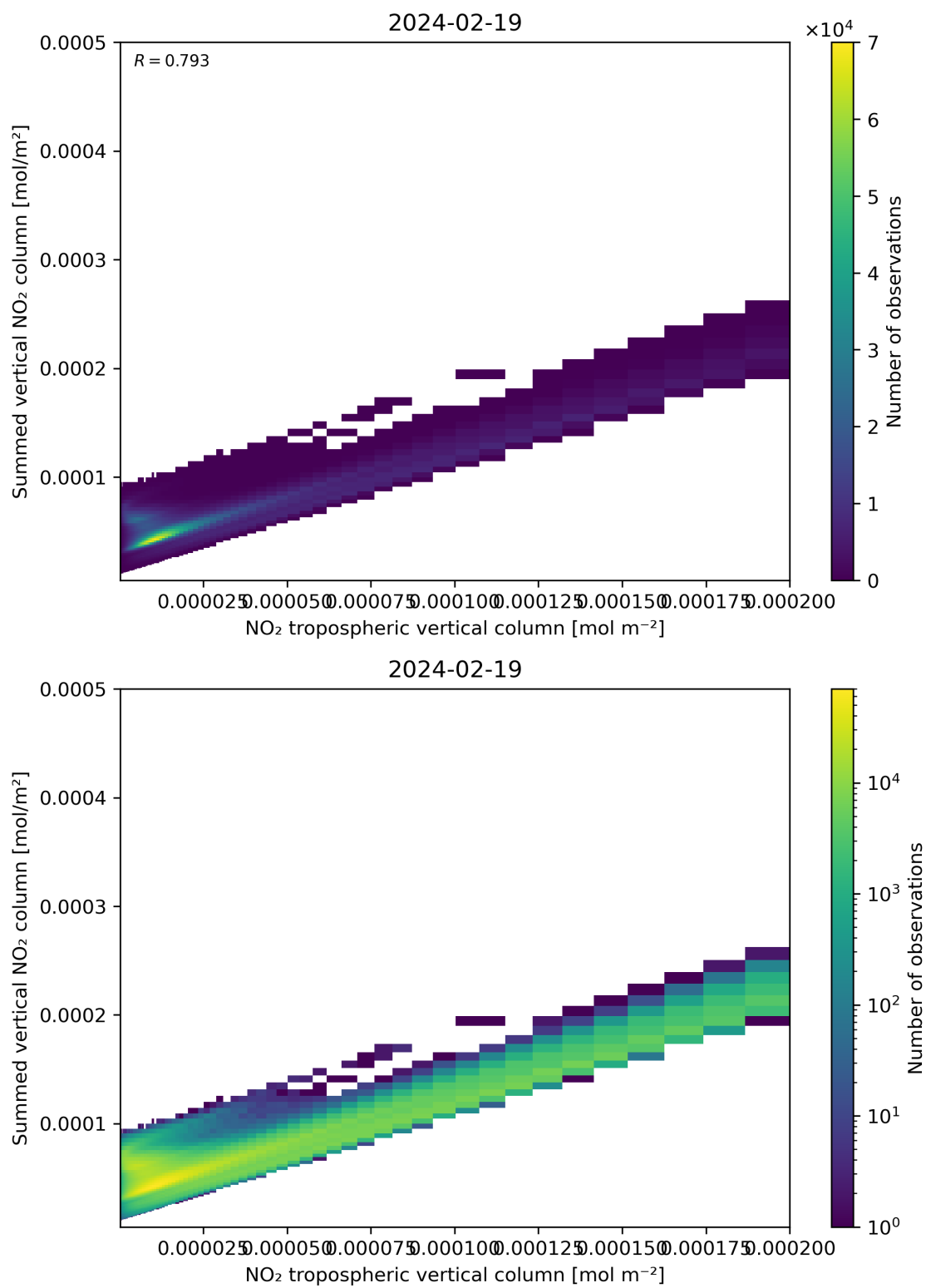
Figure 126: Scatter density plot of “NO 2 tropospheric vertical column” against “Summed vertical NO 2 column” for 2024-02-18 to 2024-02-20.
