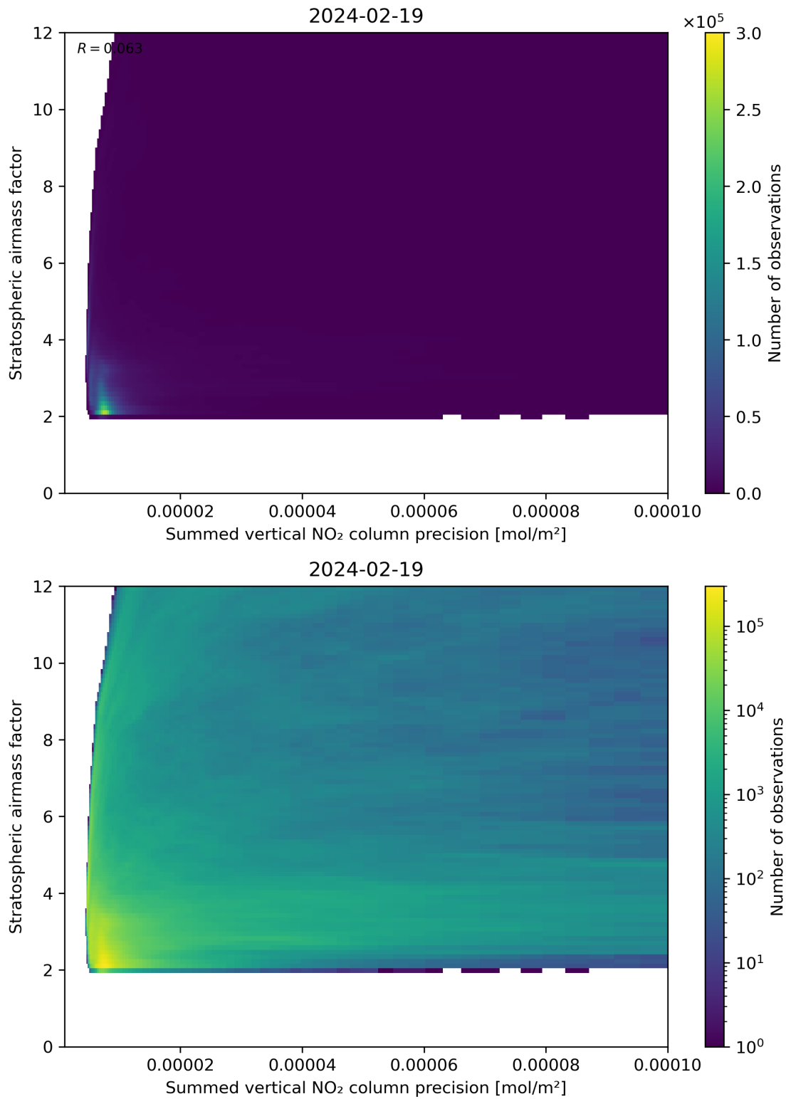
Figure 106: Scatter density plot of “Summed vertical NO 2 column precision” against “Stratospheric airmass factor” for 2024-02-18 to 2024-02-20.
