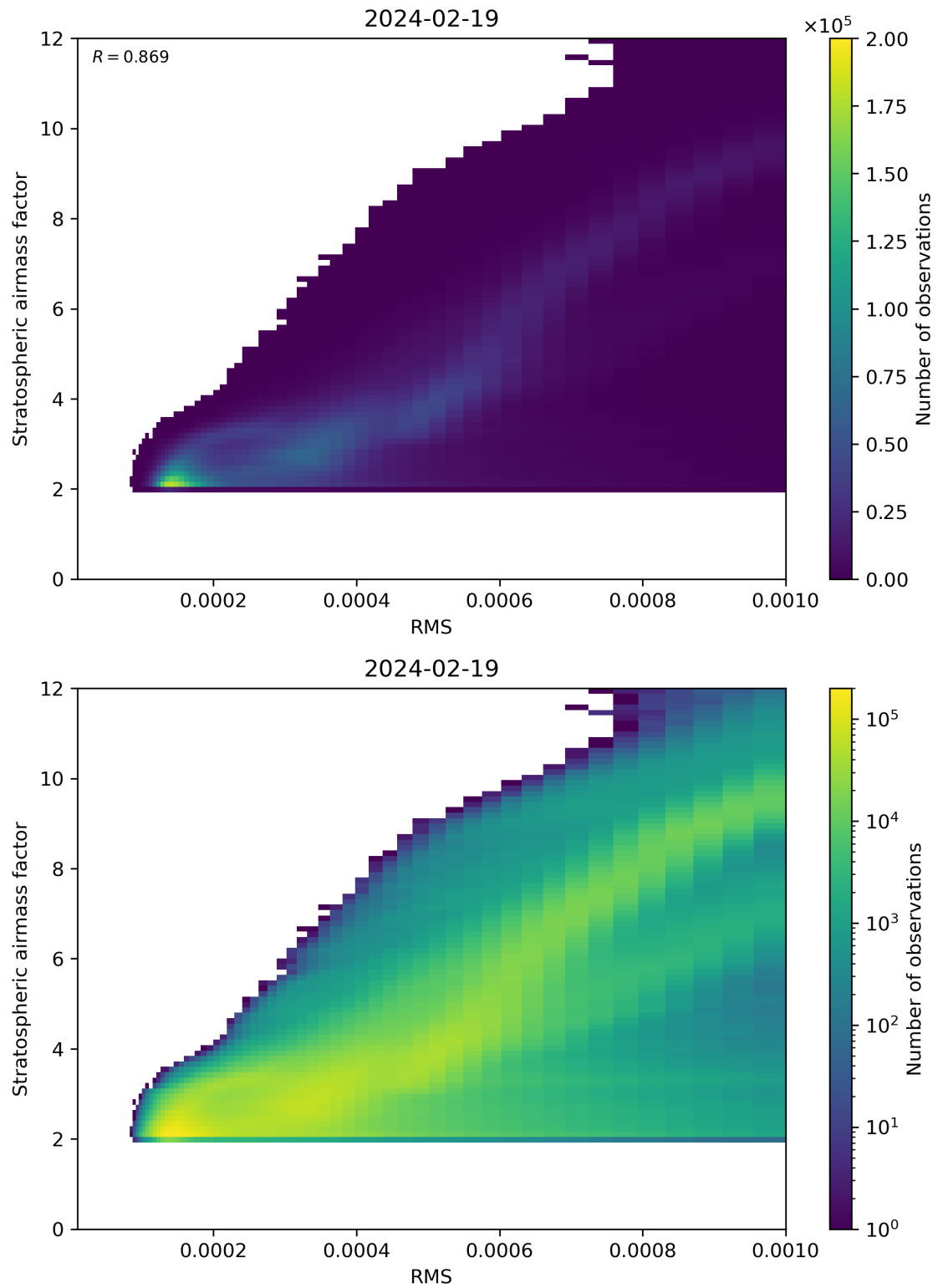
Figure 144: Scatter density plot of “RMS” against “Stratospheric airmass factor” for 2024-02-18 to 2024-02-20.
