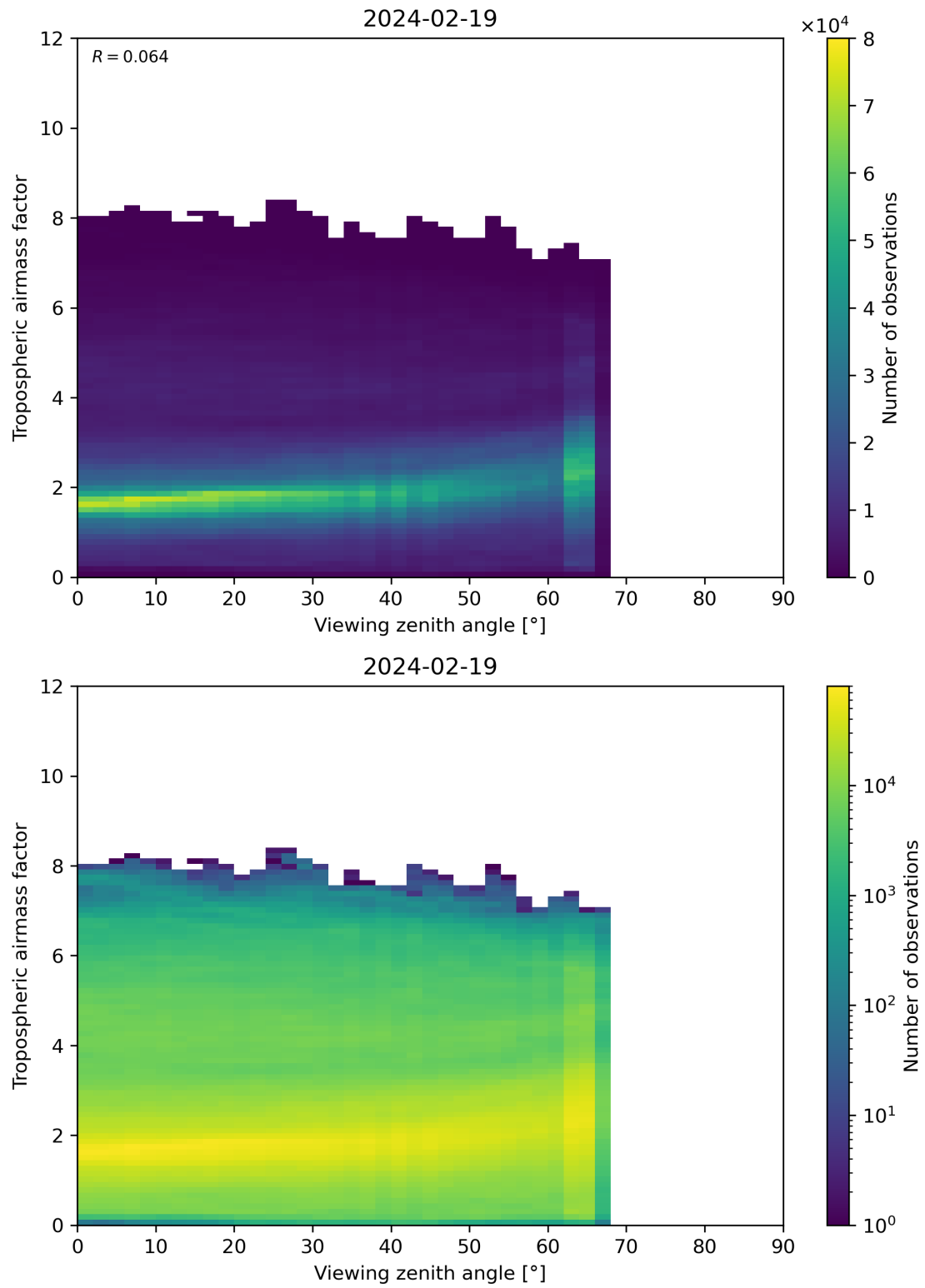
Figure 161: Scatter density plot of “Viewing zenith angle” against “Tropospheric airmass factor” for 2024-02-18 to 2024-02-20.
