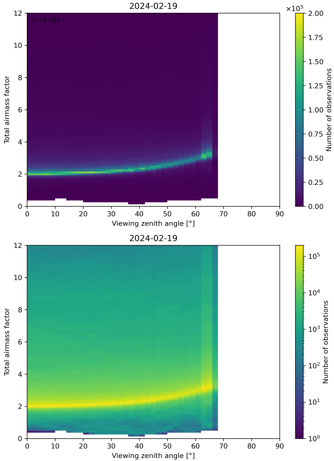
Figure 160: Scatter density plot of “Viewing zenith angle” against “Total airmass factor” for 2024-02-18 to 2024-02-20.
