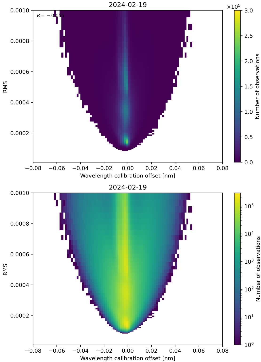
Figure 181: Scatter density plot of “Wavelength calibration offset” against “RMS” for 2024-02-18 to 2024-02-20.
