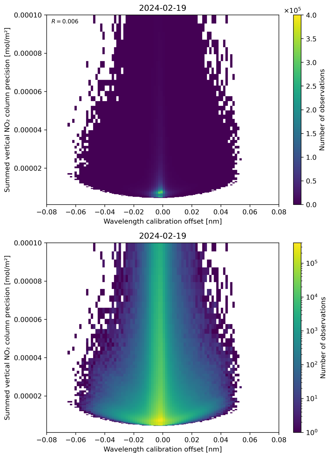
Figure 178: Scatter density plot of “Wavelength calibration offset” against “Summed vertical NO 2 column precision” for 2024-02-18 to 2024-02-20.
