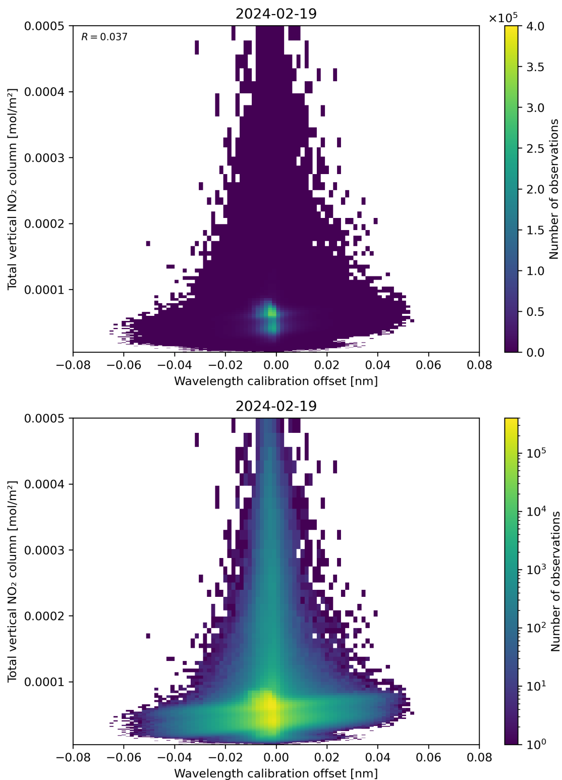
Figure 179: Scatter density plot of “Wavelength calibration offset” against “Total vertical NO 2 column” for 2024-02-18 to 2024-02-20.
