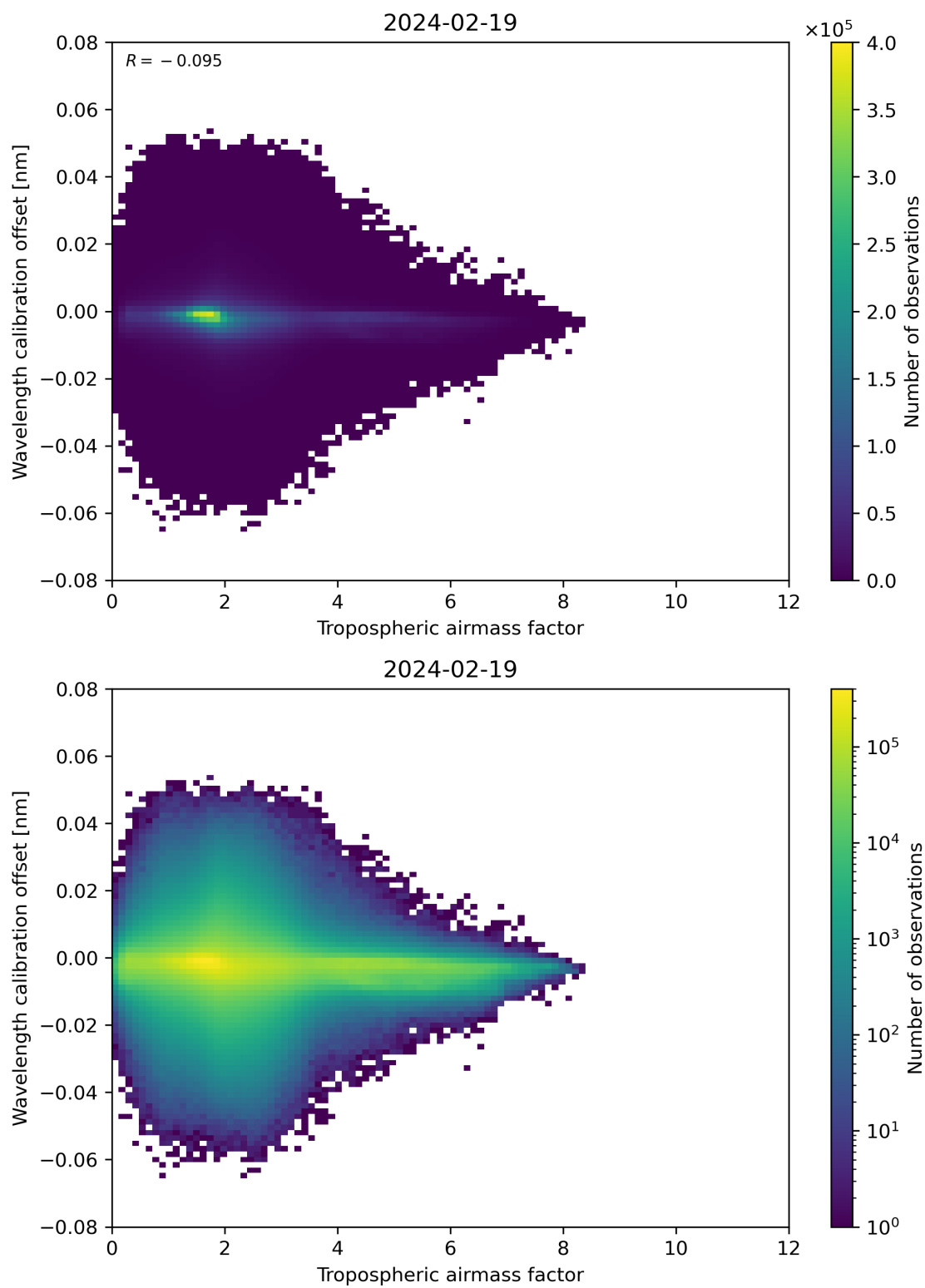
Figure 80: Scatter density plot of “Tropospheric airmass factor” against “Wavelength calibration offset” for 2024-02-18 to 2024-02-20.
