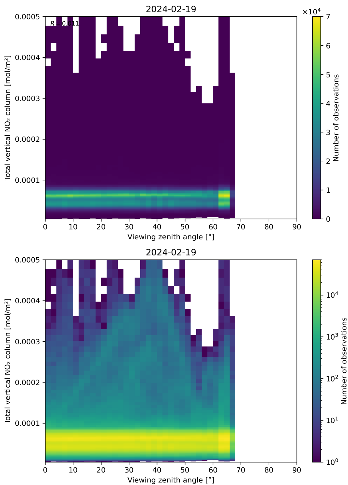
Figure 167: Scatter density plot of “Viewing zenith angle” against “Total vertical NO 2 column” for 2024-02-18 to 2024-02-20.
