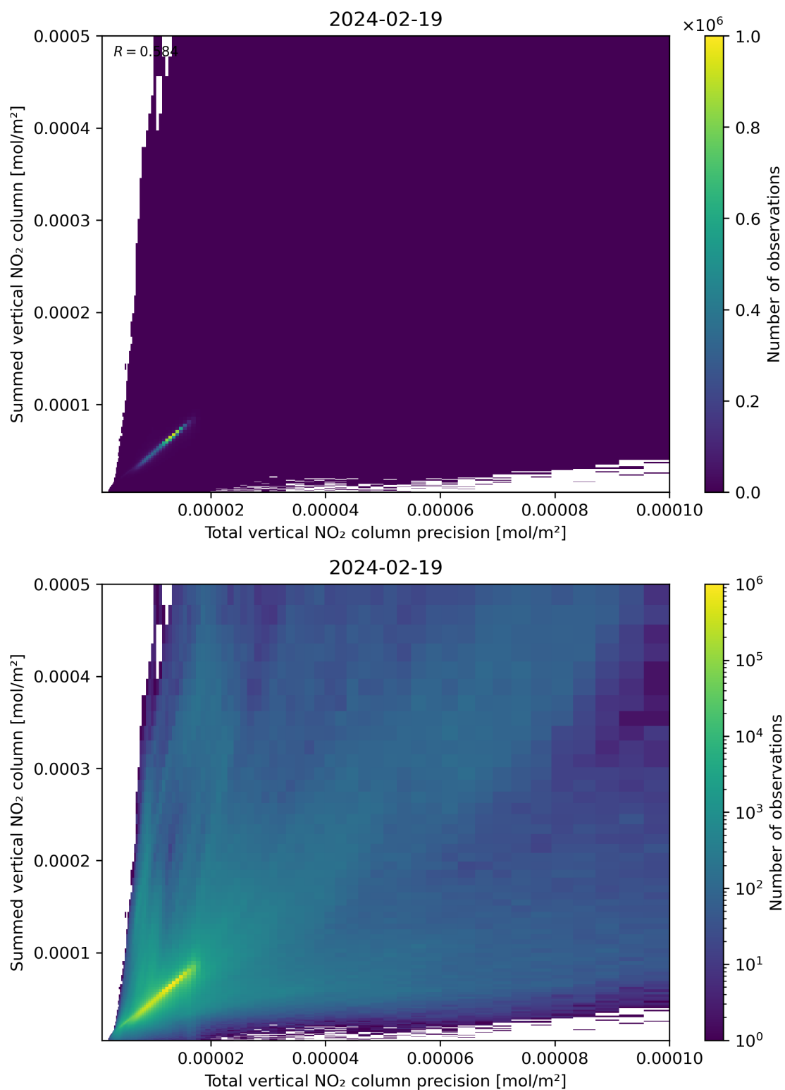
Figure 117: Scatter density plot of “Total vertical NO 2 column precision” against “Summed vertical NO 2 column” for 2024-02-18 to 2024-02-20.
