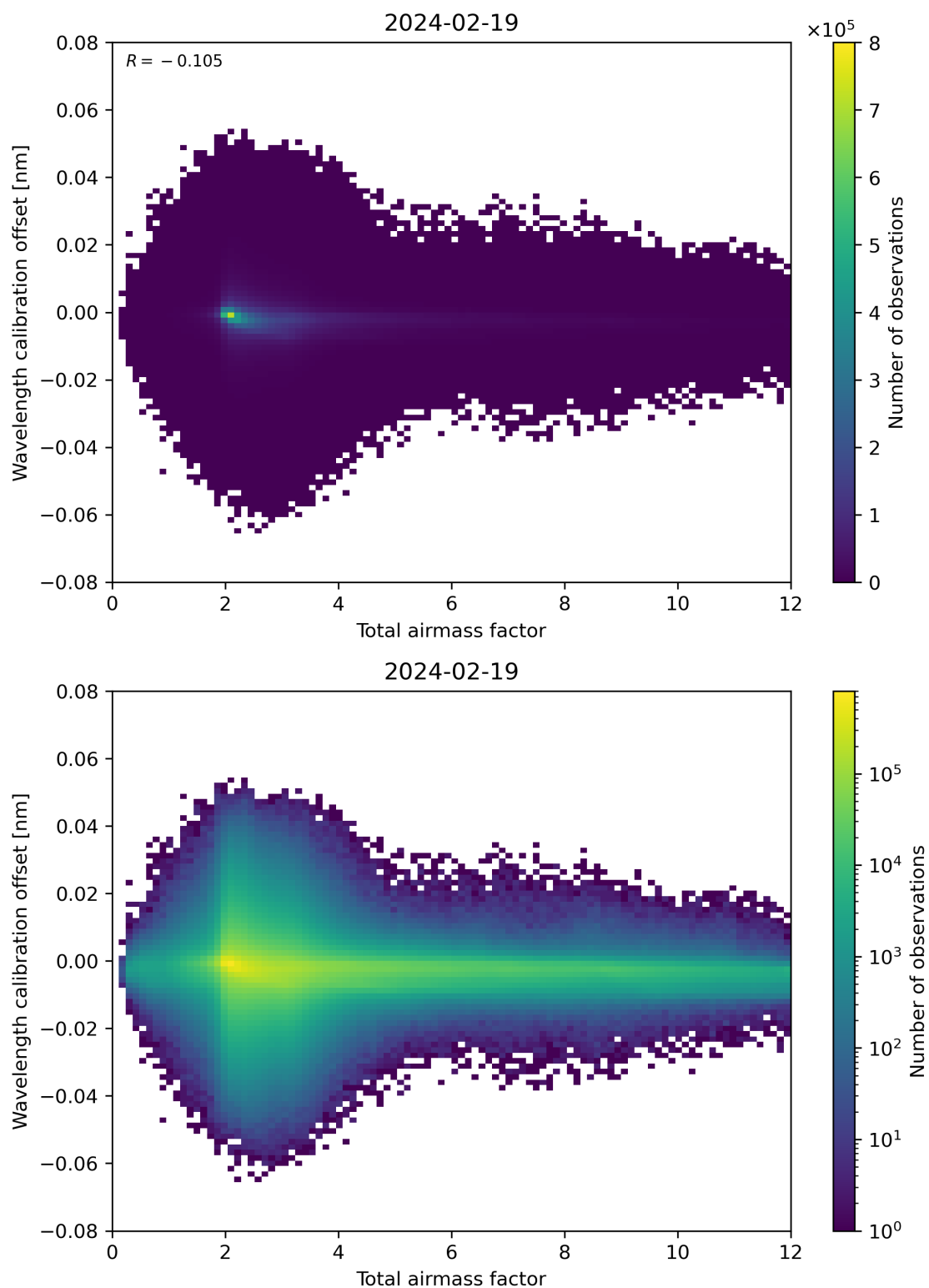
Figure 70: Scatter density plot of “Total airmass factor” against “Wavelength calibration offset” for 2024-02-18 to 2024-02-20.
