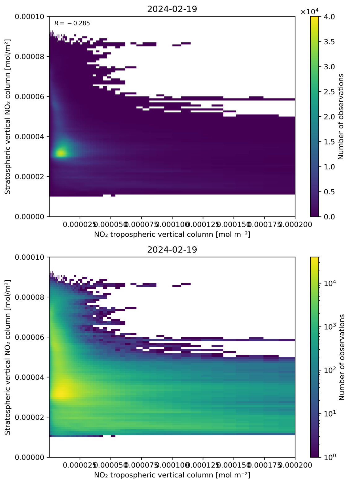
Figure 125: Scatter density plot of “NO 2 tropospheric vertical column” against “Stratospheric vertical NO 2 column” for 2024-02-18 to 2024-02-20.
