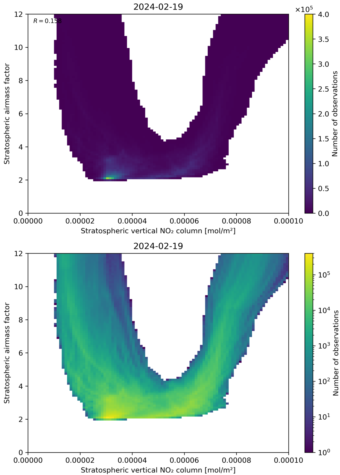
Figure 96: Scatter density plot of “Stratospheric vertical NO 2 column” against “Stratospheric airmass factor” for 2024-02-18 to 2024-02-20.
