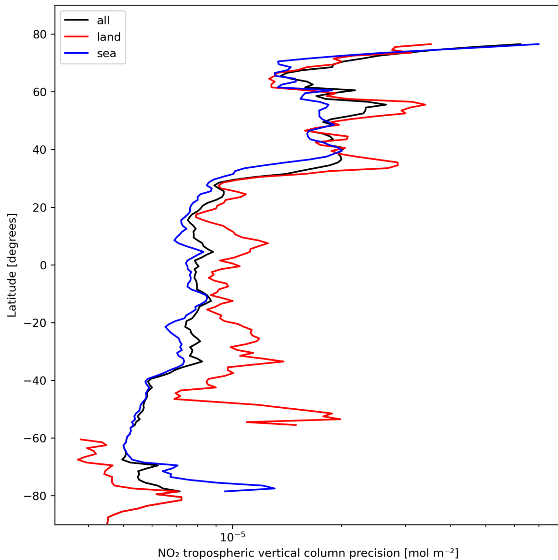
Figure 13: Zonal average of “NO 2 tropospheric vertical column precision” for 2024-02-18 to 2024-02-20.
