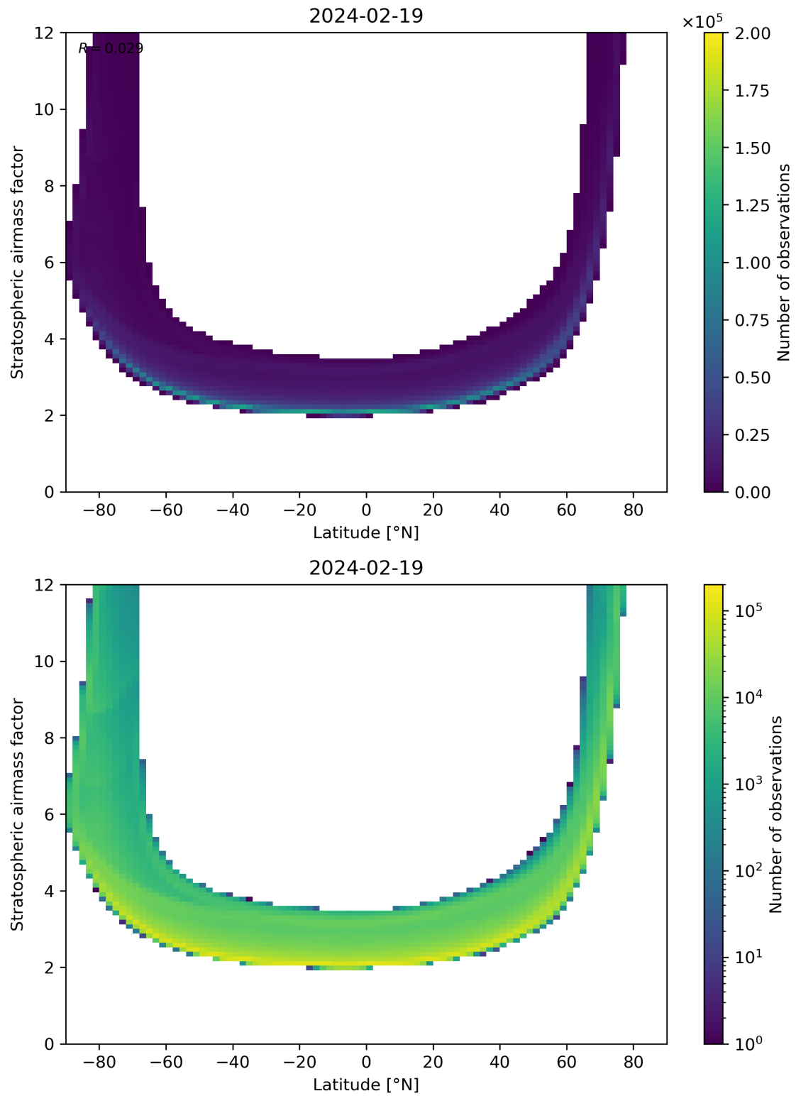
Figure 83: Scatter density plot of “Latitude” against “Stratospheric air mass factor” for 2024-02-18 to 2024-02-20.
