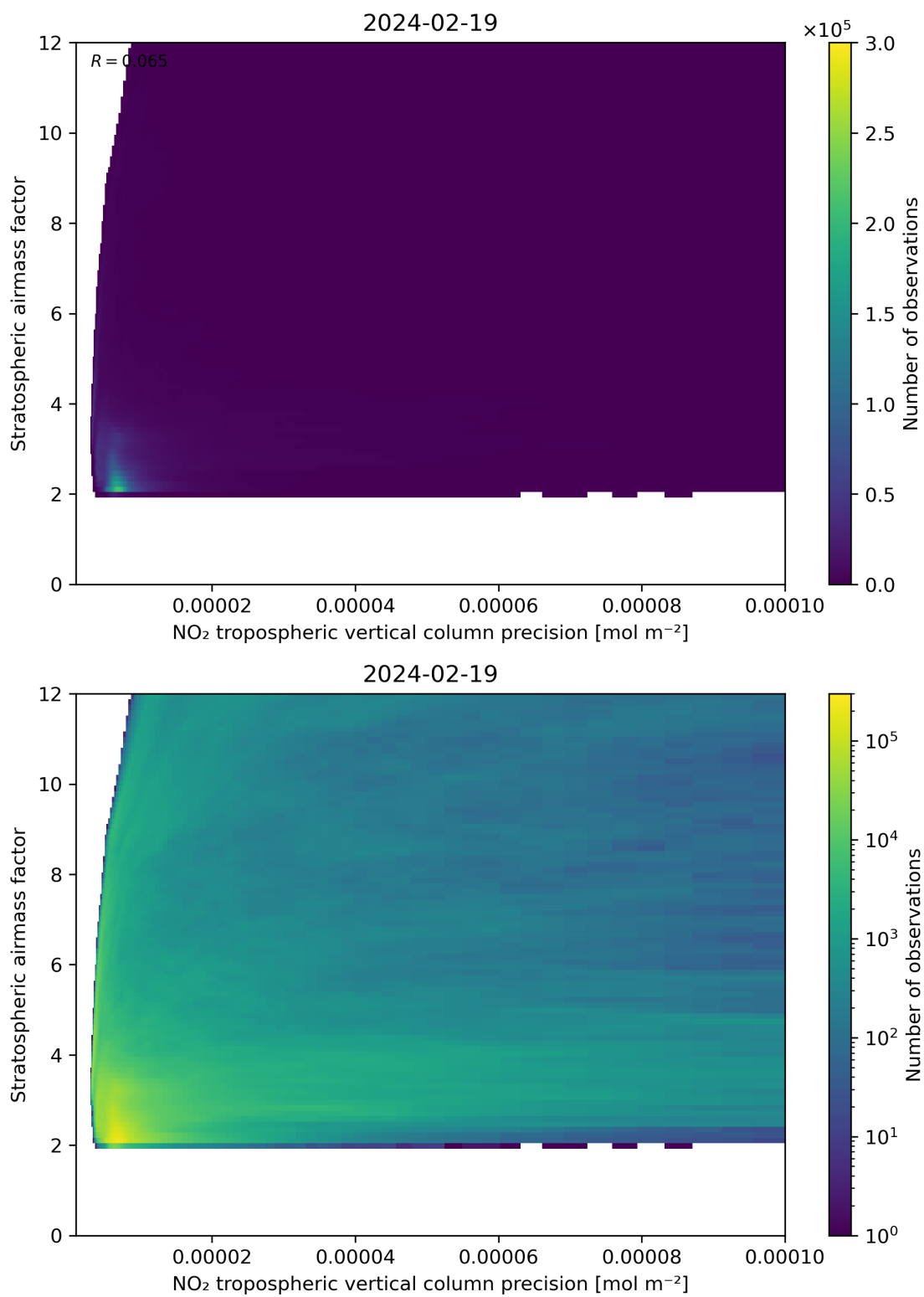
Figure 131: Scatter density plot of “NO 2 tropospheric vertical column precision” against “Stratospheric airmass factor” for 2024-02-18 to 2024-02-20.
