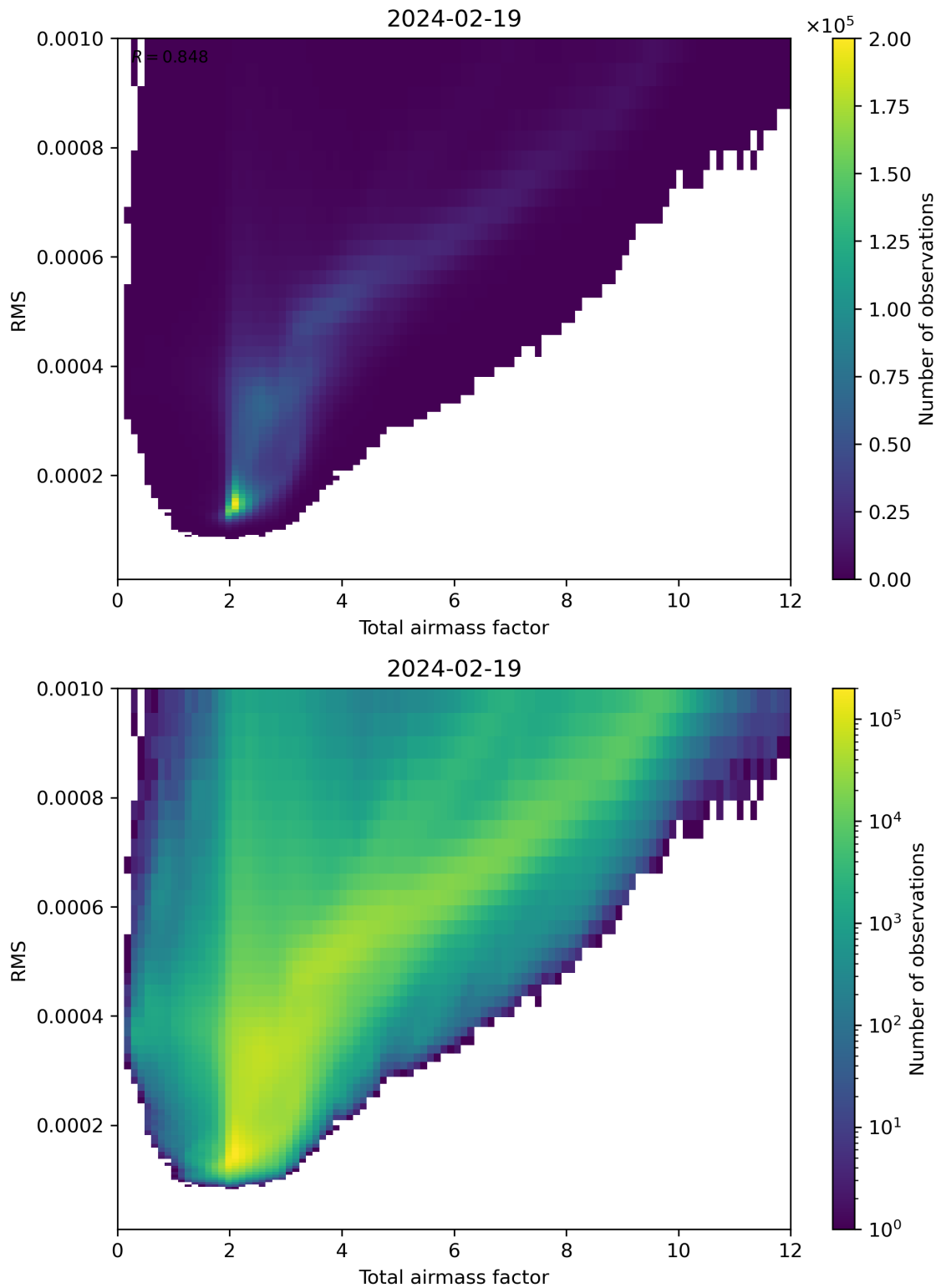
Figure 69: Scatter density plot of “Total airmass factor” against “RMS” for 2024-02-18 to 2024-02-20.
