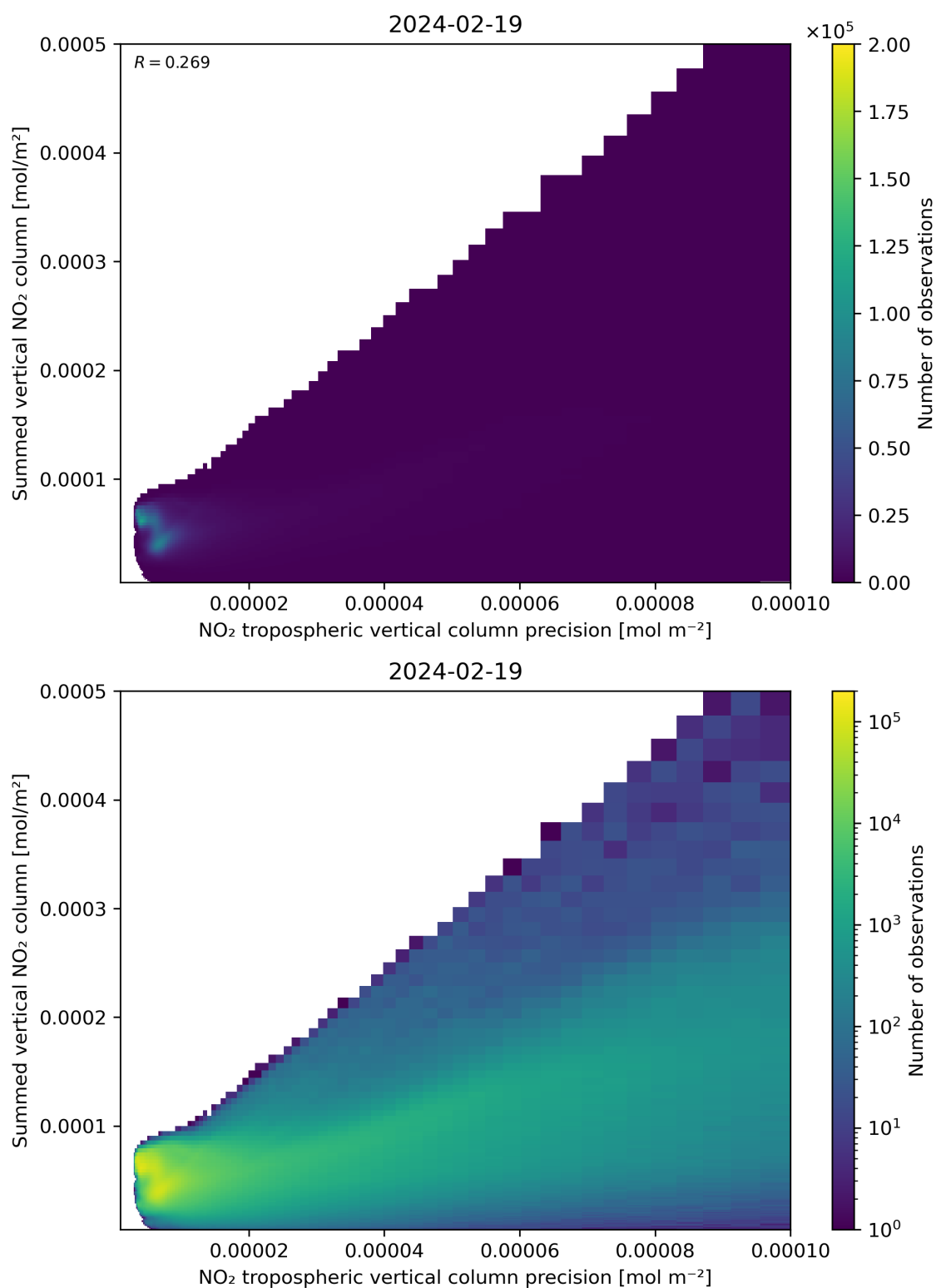
Figure 136: Scatter density plot of “NO 2 tropospheric vertical column precision” against “Summed vertical NO 2 column” for 2024-02-18 to 2024-02-20.
