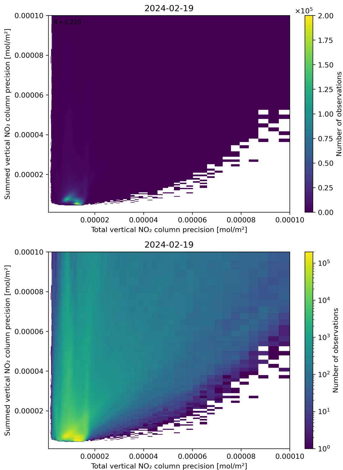
Figure 118: Scatter density plot of “Total vertical NO 2 column precision” against “Summed vertical NO 2 column precision” for 2024-02-18 to 2024-02-20.
