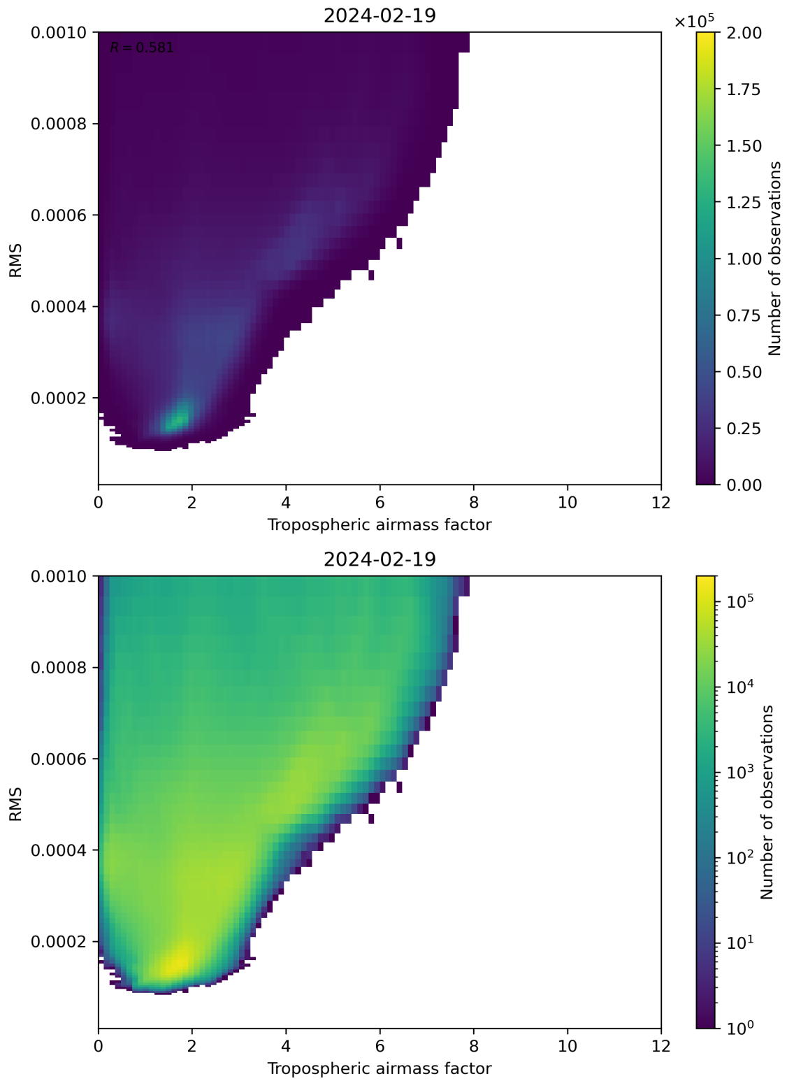
Figure 79: Scatter density plot of “Tropospheric airmass factor” against “RMS” for 2024-02-18 to 2024-02-20.
