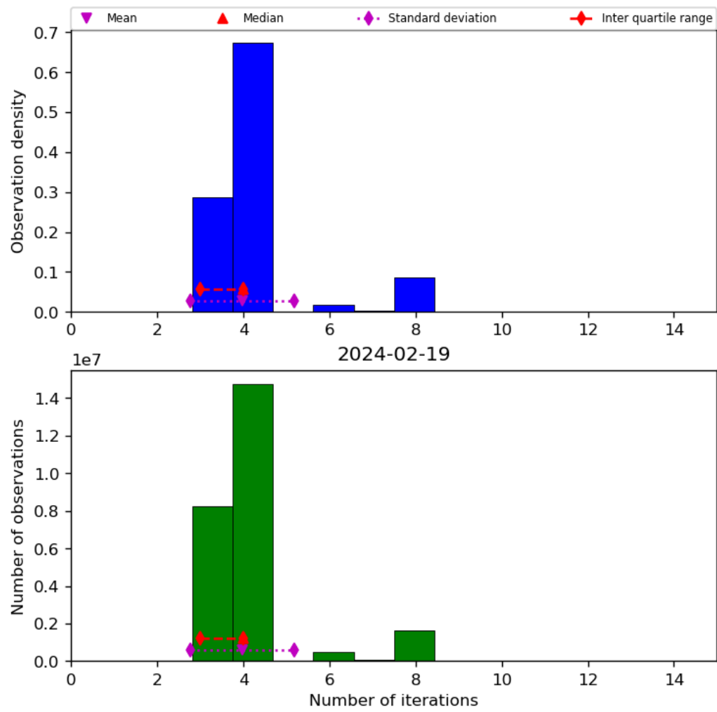
Figure 34: Histogram of “Number of iterations” for 2024-02-18 to 2024-02-20
