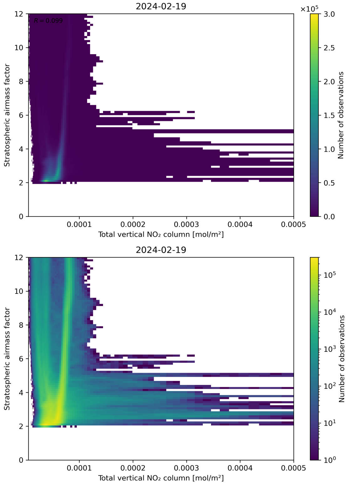
Figure 110: Scatter density plot of “Total vertical NO 2 column” against “Stratospheric airmass factor” for 2024-02-18 to 2024-02-20.
