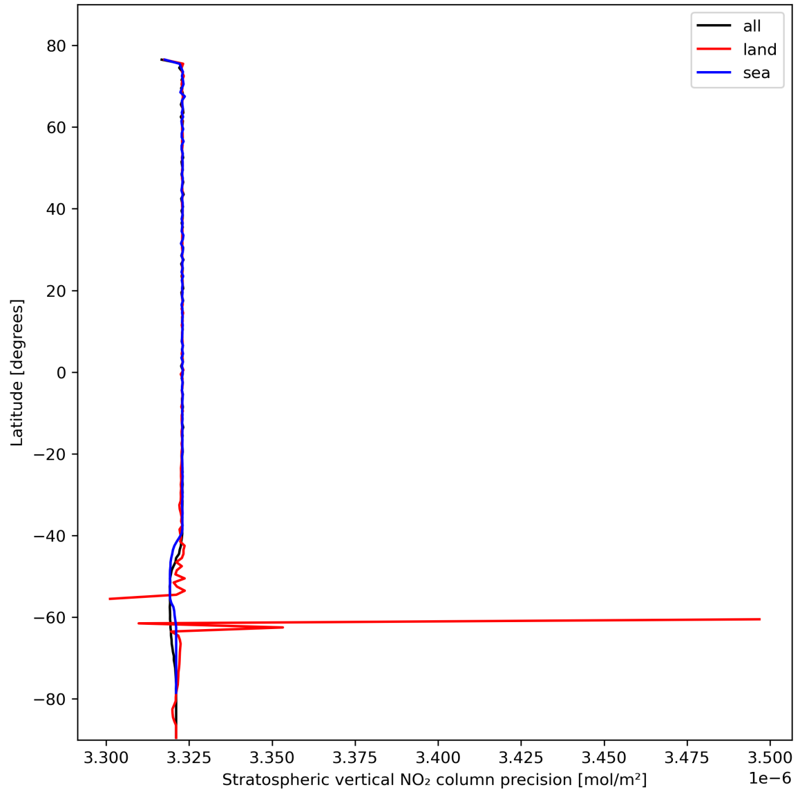
Figure 20: Zonal average of “Stratospheric vertical NO 2 column precision” for 2024-02-18 to 2024-02-20.
