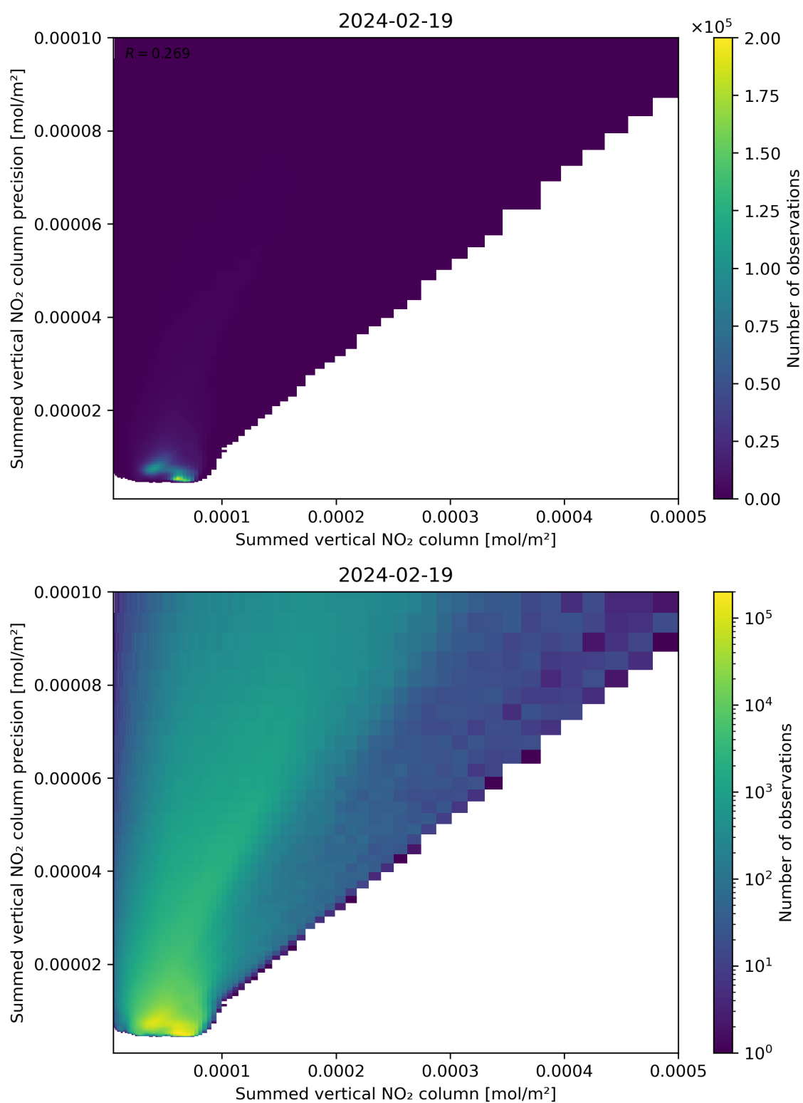
Figure 105: Scatter density plot of “Summed vertical NO 2 column” against “Summed vertical NO 2 column precision” for 2024-02-18 to 2024-02-20.
