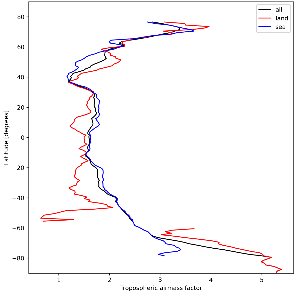
Figure 14: Zonal average of “Tropospheric airmass factor” for 2024-02-18 to 2024-02-20.
