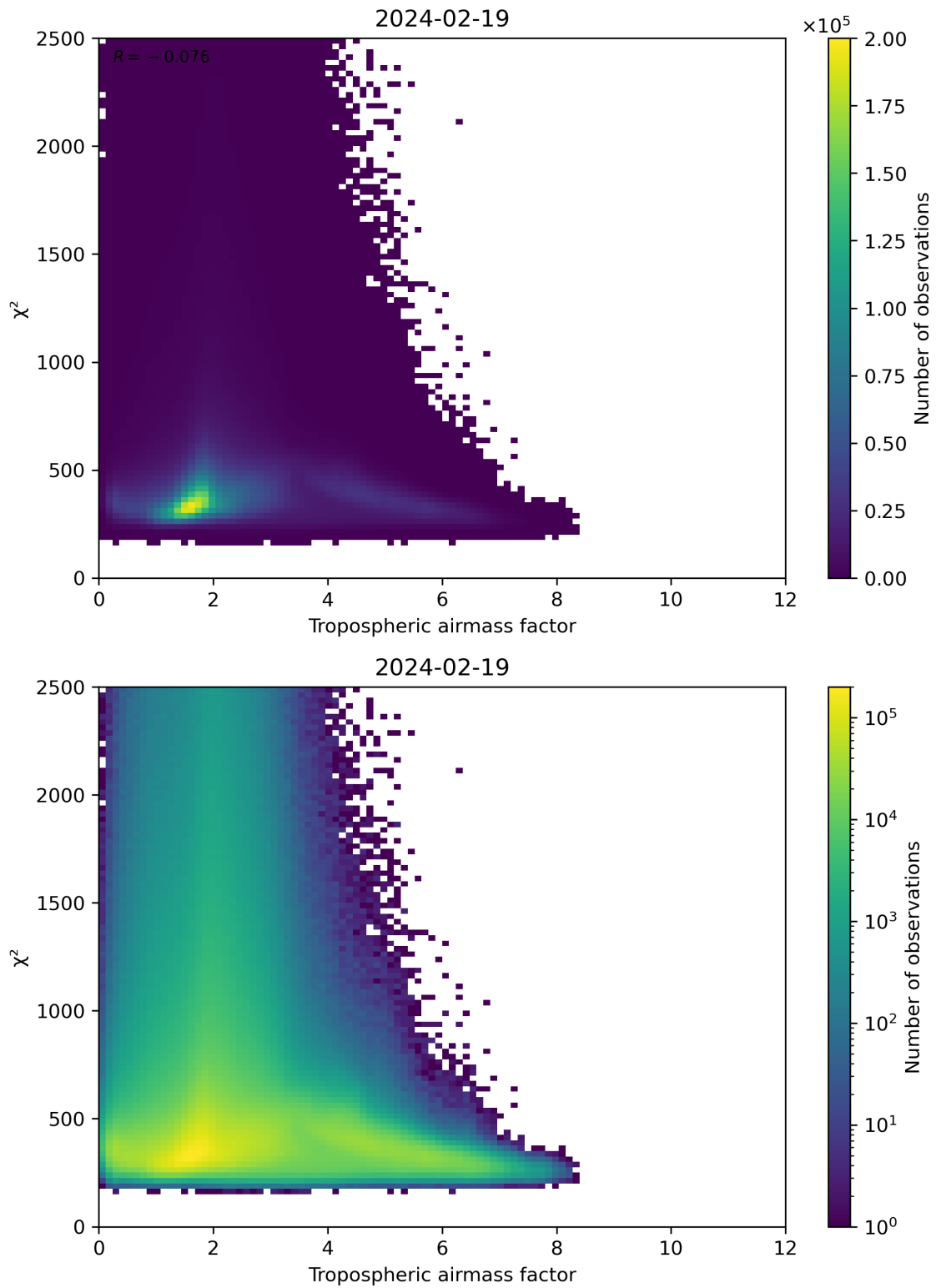
Figure 73: Scatter density plot of “Tropospheric airmass factor” against “ \chi^2 ” for 2024-02-18 to 2024-02-20.
