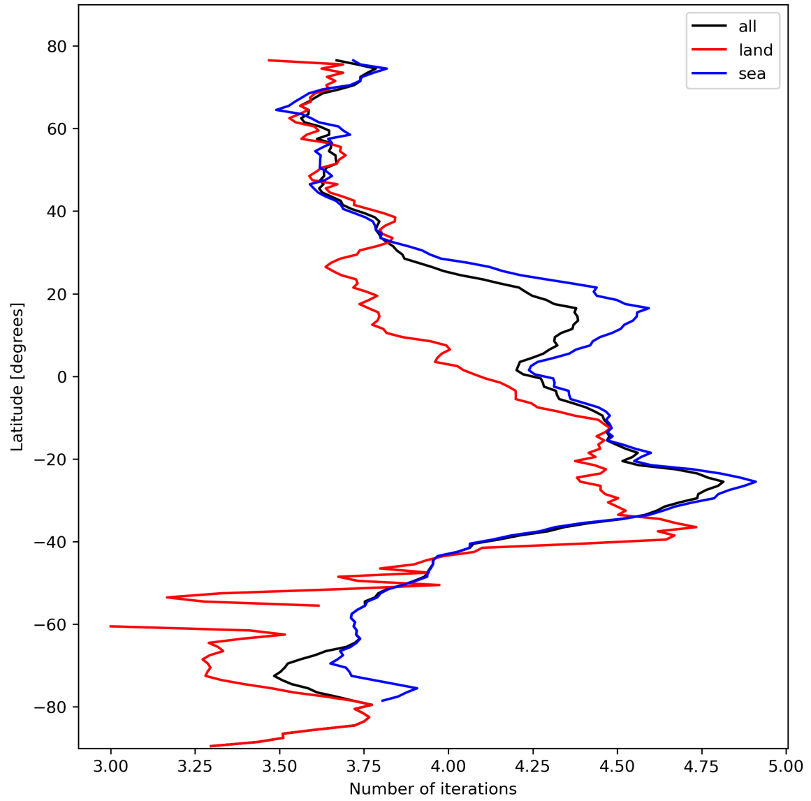
Figure 17: Zonal average of “Number of iterations” for 2024-02-18 to 2024-02-20.
