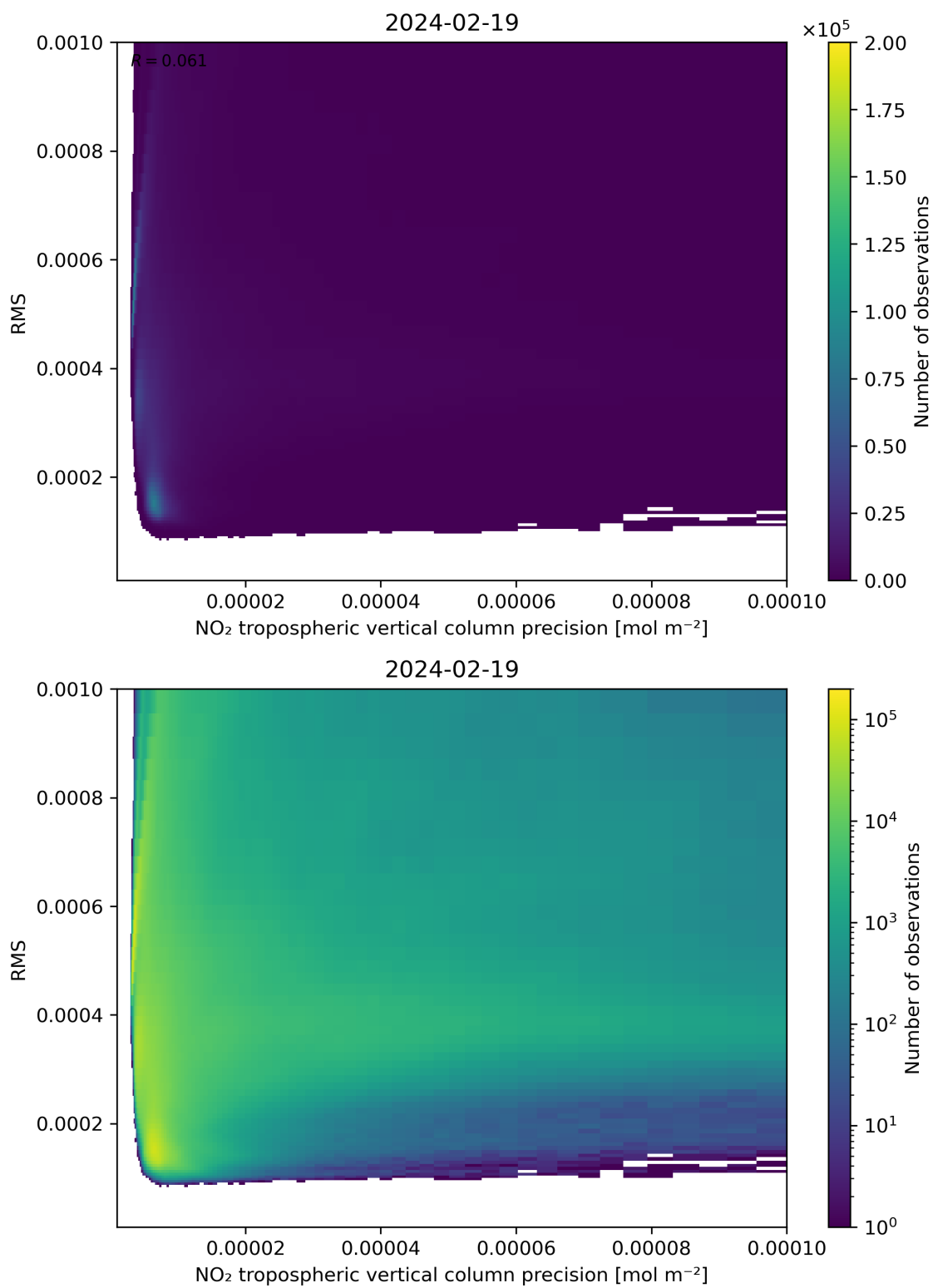
Figure 140: Scatter density plot of “NO 2 tropospheric vertical column precision” against “RMS” for 2024-02-18 to 2024-02-20.
