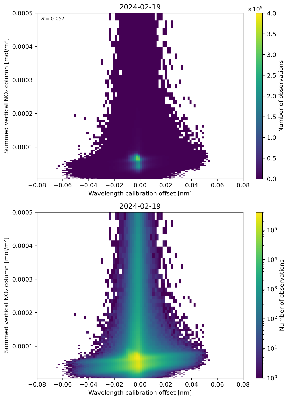
Figure 177: Scatter density plot of “Wavelength calibration offset” against “Summed vertical NO 2 column” for 2024-02-18 to 2024-02-20.
