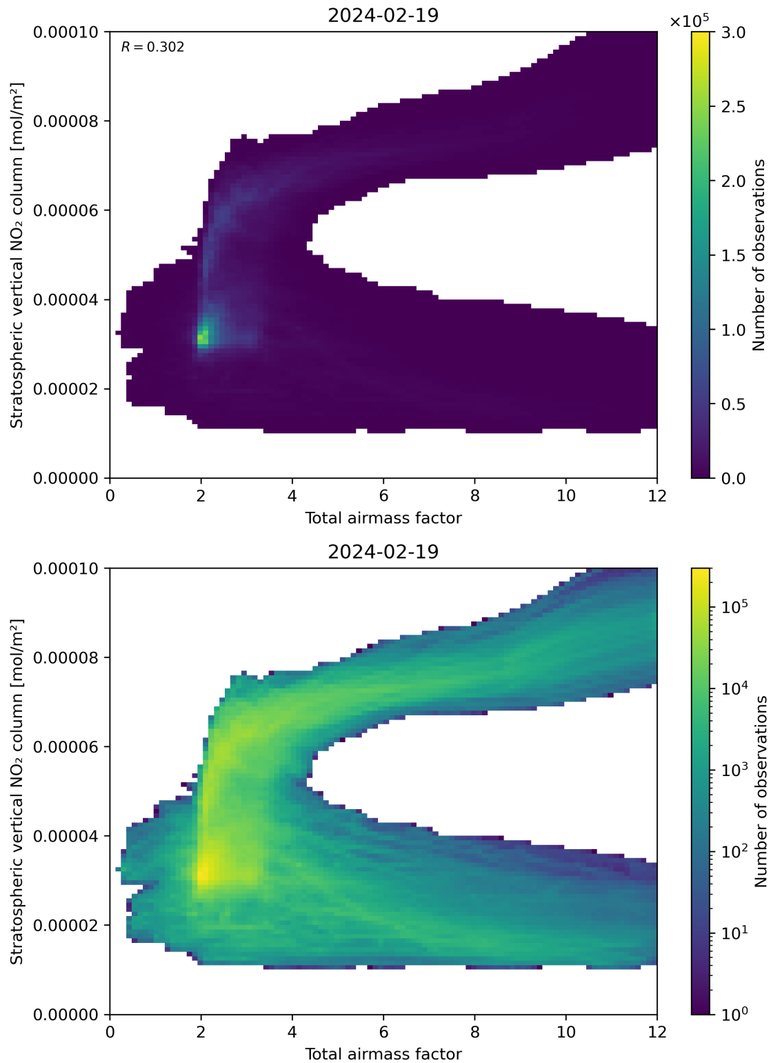
Figure 64: Scatter density plot of “Total airmass factor” against “Stratospheric vertical NO 2 column” for 2024-02-18 to 2024-02-20.
