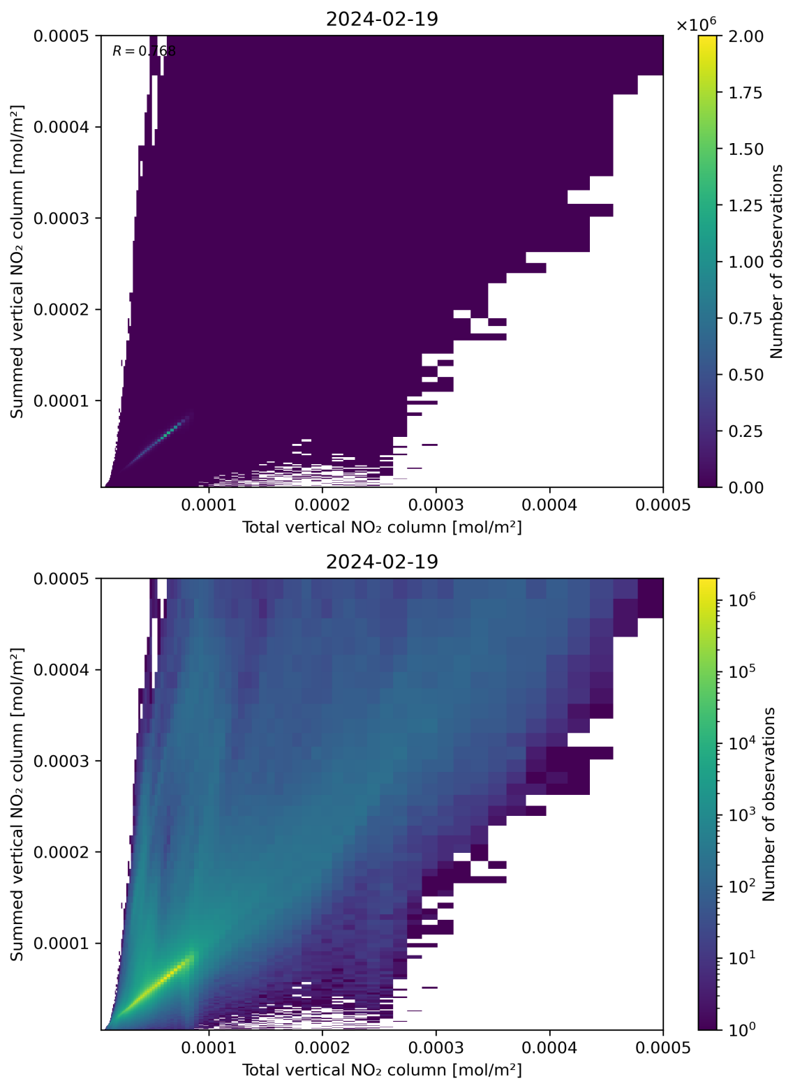
Figure 112: Scatter density plot of “Total vertical NO 2 column” against “Summed vertical NO 2 column” for 2024-02-18 to 2024-02-20.
