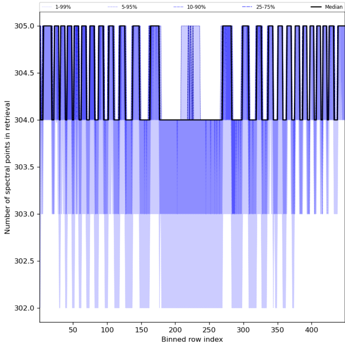
Figure 50: Along track statistics of “Number of spectral points in retrieval” for 2024-02-18 to 2024-02-20
