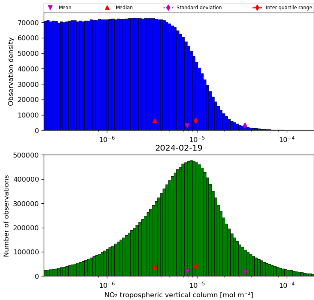
Figure 29: Histogram of “NO 2 tropospheric vertical column” for 2024-02-18 to 2024-02-20
