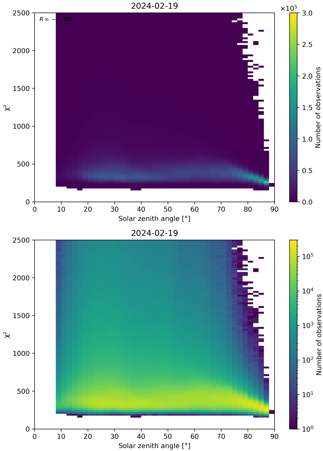
Figure 148: Scatter density plot of “Solar zenith angle” against “ \chi^2 ” for 2024-02-18 to 2024-02-20.
