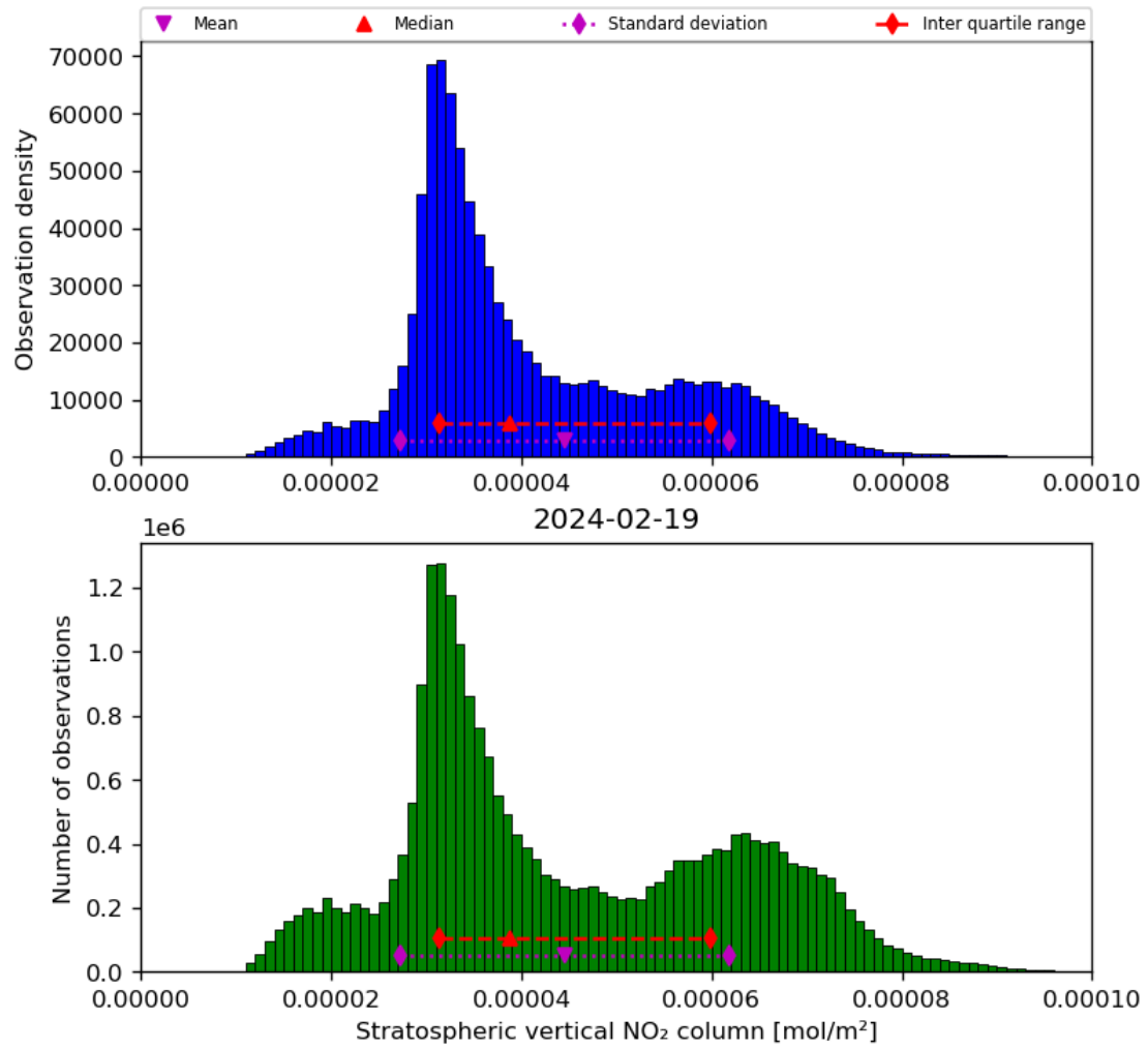
Figure 36: Histogram of “Stratospheric vertical NO 2 column” for 2024-02-18 to 2024-02-20
