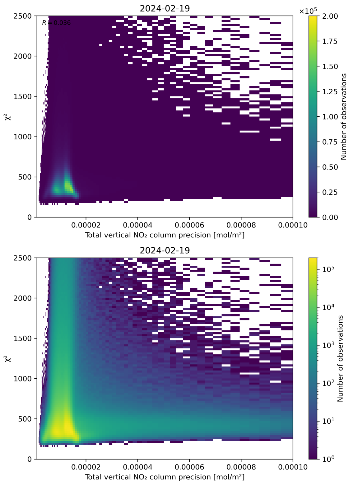
Figure 116: Scatter density plot of “Total vertical NO 2 column precision” against “ \chi^2 ” for 2024-02-18 to 2024-02-20.
