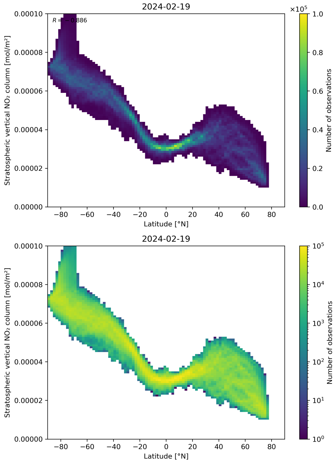
Figure 87: Scatter density plot of “Latitude” against “Stratospheric vertical NO 2 column” for 2024-02-18 to 2024-02-20.
