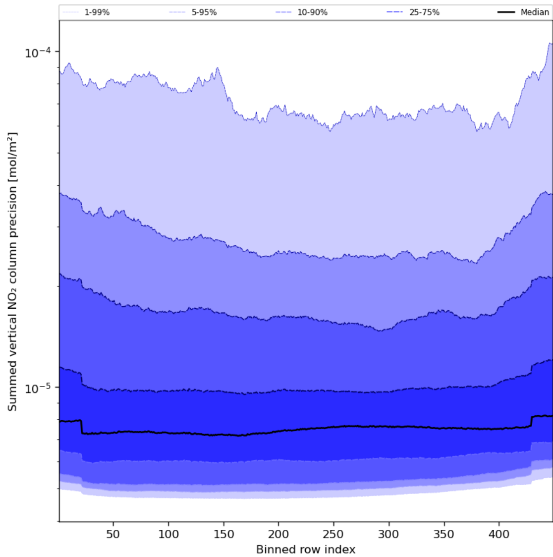
Figure 58: Along track statistics of “Summed vertical NO 2 column precision” for 2024-02-18 to 2024-02-20
