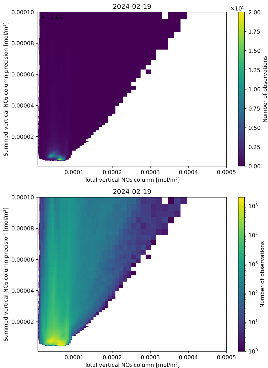
Figure 113: Scatter density plot of “Total vertical NO 2 column” against “Summed vertical NO 2 column precision” for 2024-02-18 to 2024-02-20.
