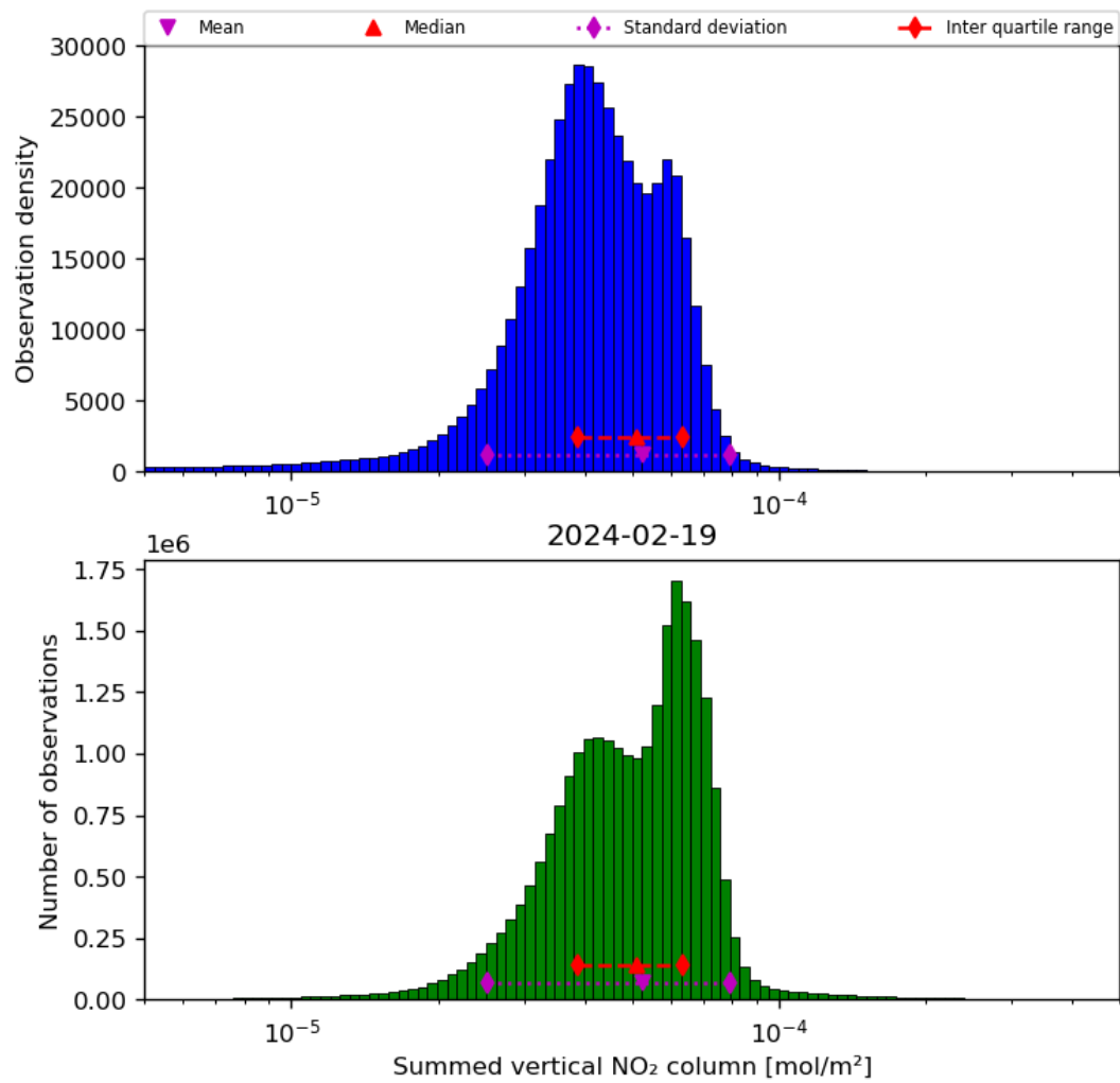
Figure 40: Histogram of “Summed vertical NO 2 column” for 2024-02-18 to 2024-02-20
