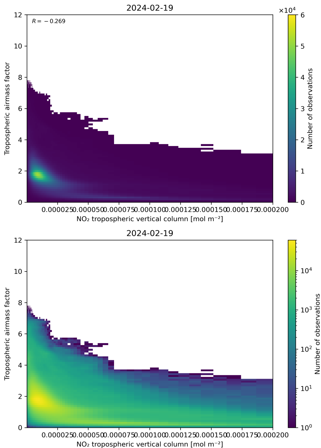
Figure 123: Scatter density plot of “NO 2 tropospheric vertical column” against “Tropospheric airmass factor” for 2024-02-18 to 2024-02-20.
