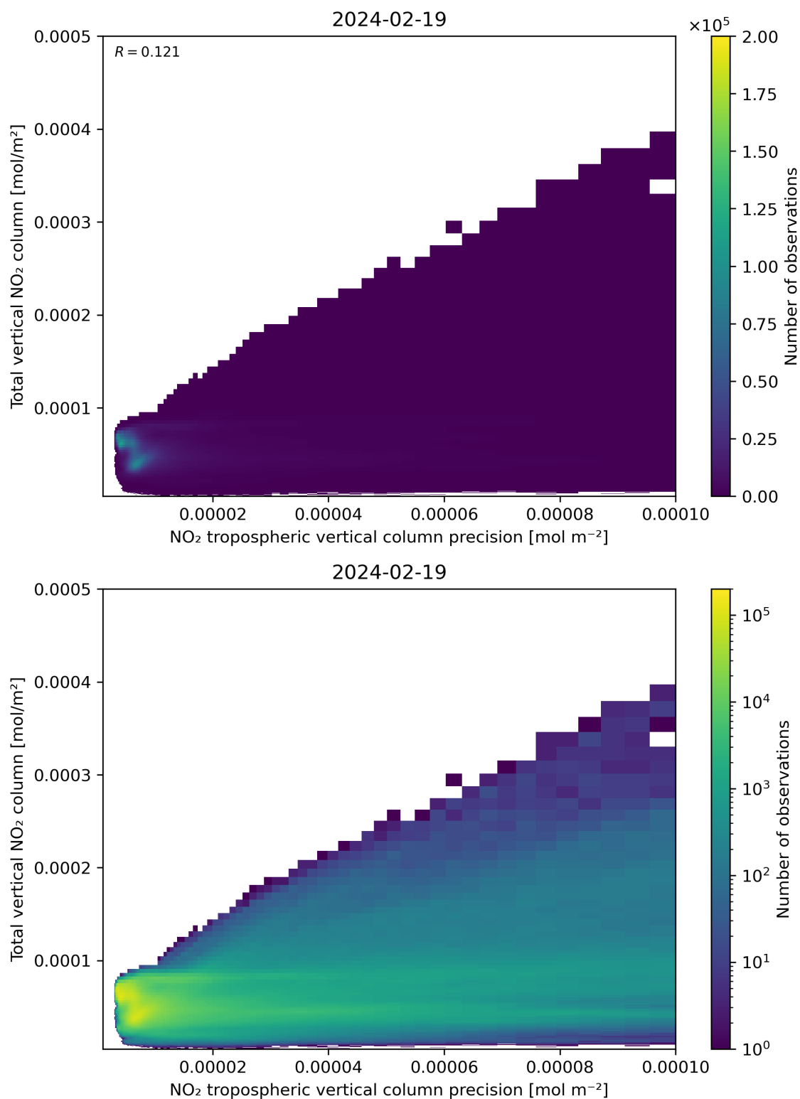
Figure 138: Scatter density plot of “NO 2 tropospheric vertical column precision” against “Total vertical NO 2 column” for 2024-02-18 to 2024-02-20.
