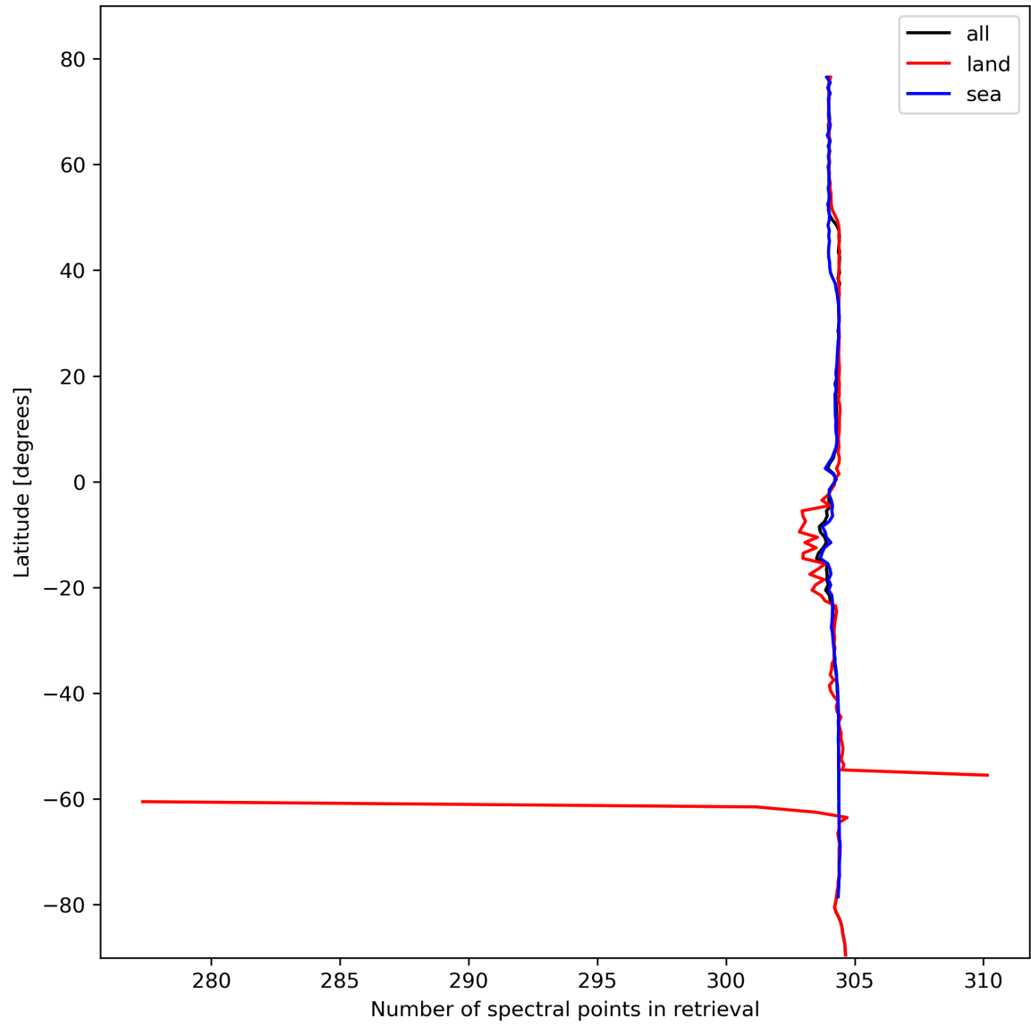
Figure 16: Zonal average of “Number of spectral points in retrieval” for 2024-02-18 to 2024-02-20.
