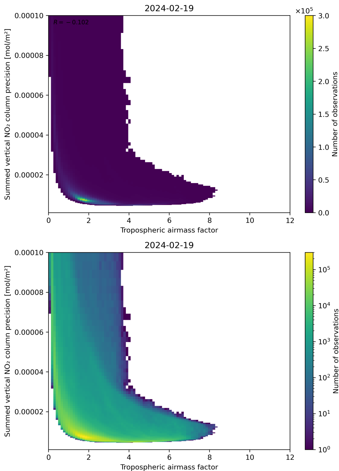
Figure 76: Scatter density plot of “Tropospheric air mass factor” against “Summed vertical NO 2 column precision” for 2024-02-18 to 2024-02-20.
