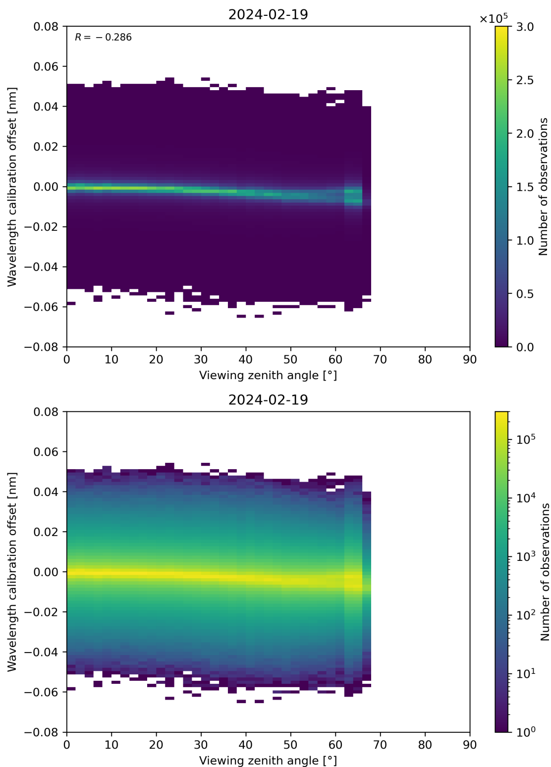
Figure 173: Scatter density plot of “Viewing zenith angle” against “Wavelength calibration offset” for 2024-02-18 to 2024-02-20.
