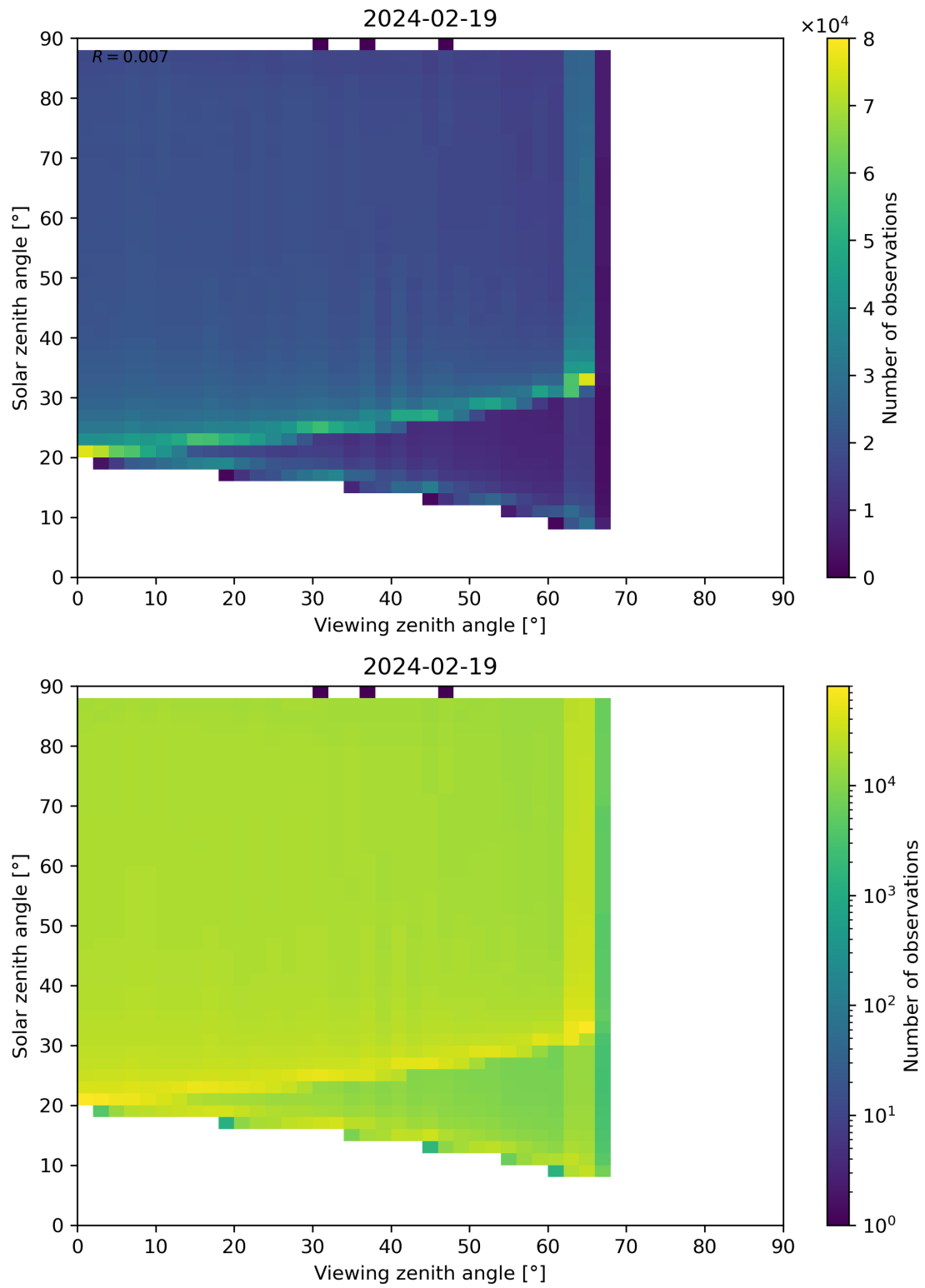
Figure 172: Scatter density plot of “Viewing zenith angle” against “Solar zenith angle” for 2024-02-18 to 2024-02-20.
