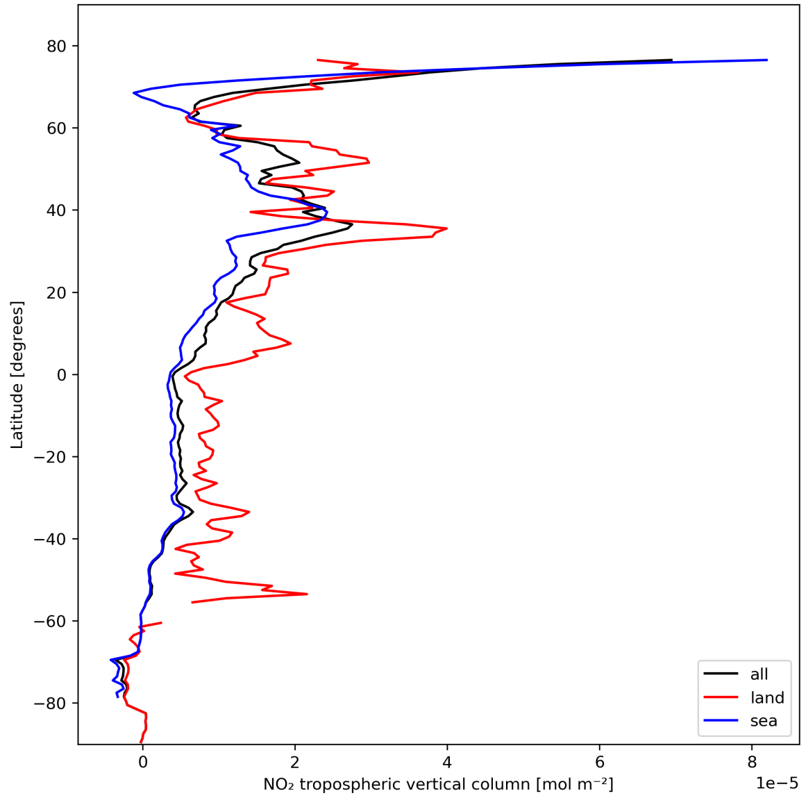
Figure 12: Zonal average of “NO 2 tropospheric vertical column” for 2024-02-18 to 2024-02-20.
