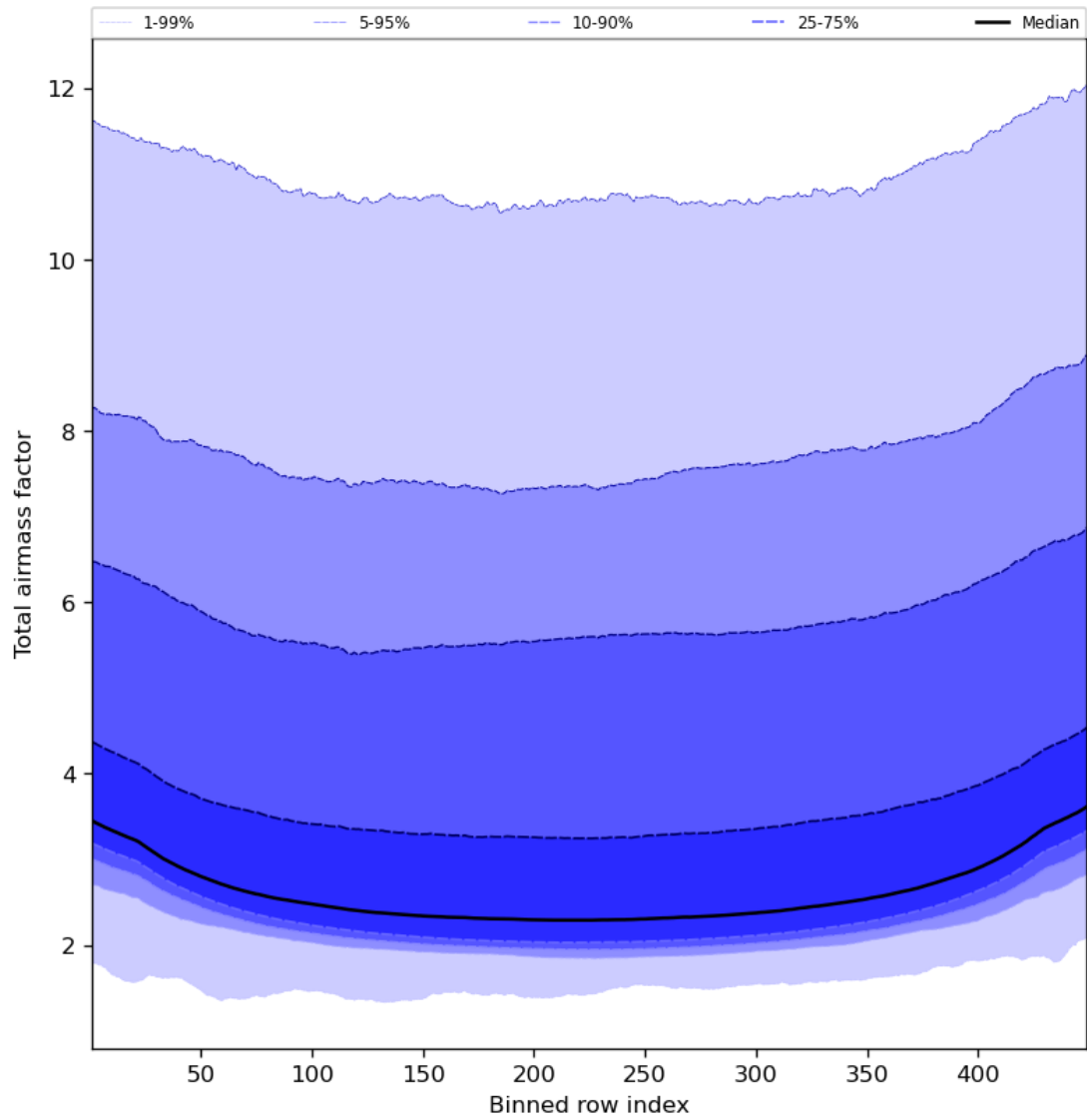
Figure 49: Along track statistics of “Total airmass factor” for 2024-02-18 to 2024-02-20
