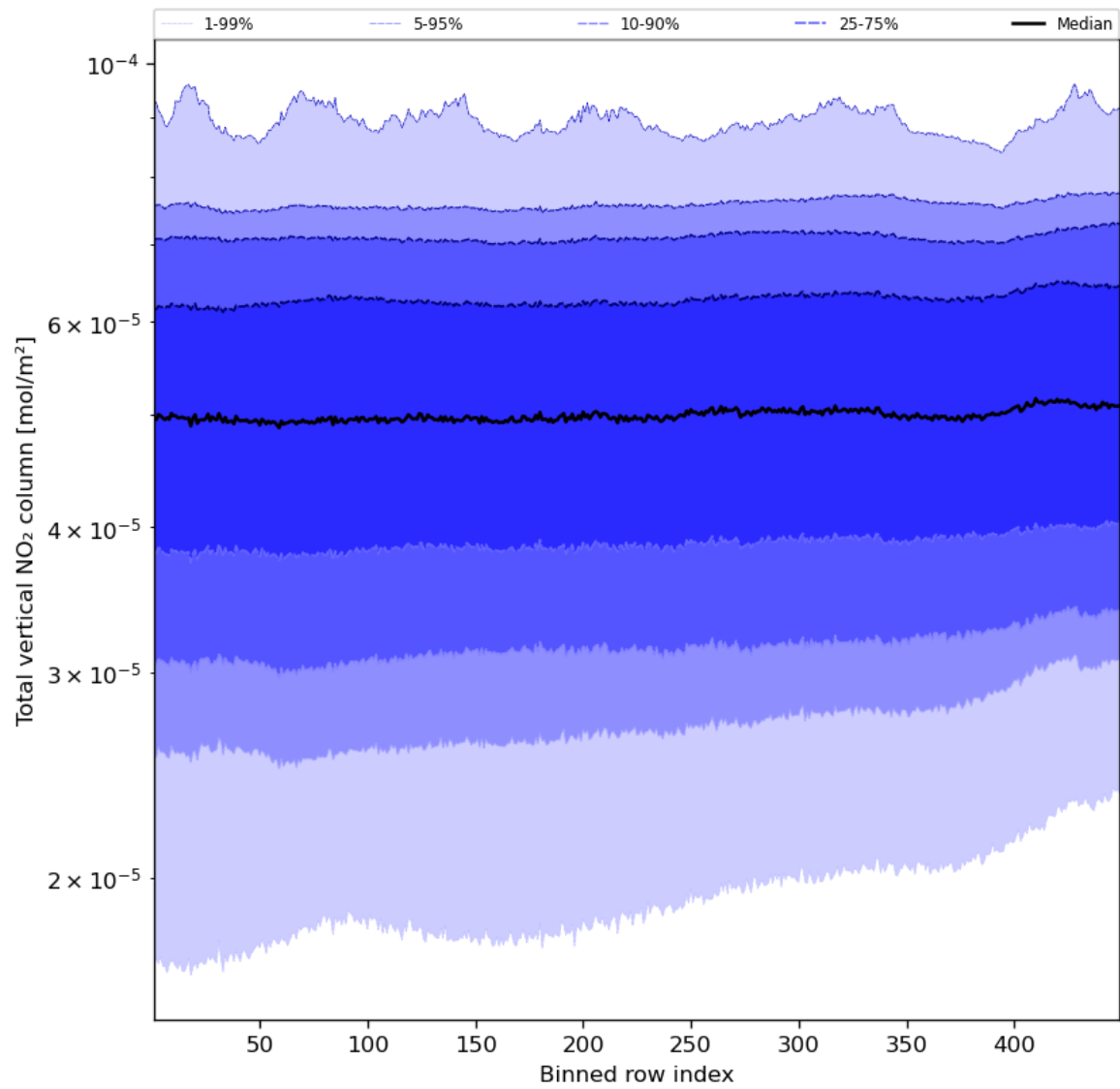
Figure 55: Along track statistics of “Total vertical NO 2 column” for 2024-02-18 to 2024-02-20
