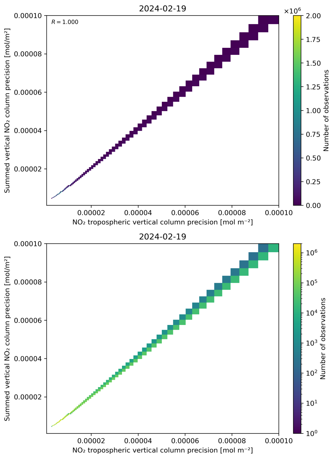
Figure 137: Scatter density plot of “NO 2 tropospheric vertical column precision” against “Summed vertical NO 2 column precision” for 2024-02-18 to 2024-02-20.
