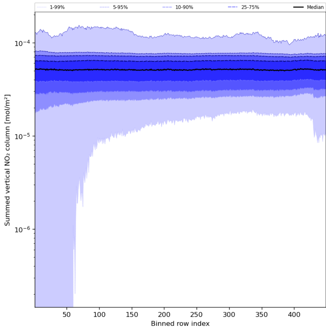
Figure 57: Along track statistics of “Summed vertical NO 2 column” for 2024-02-18 to 2024-02-20
