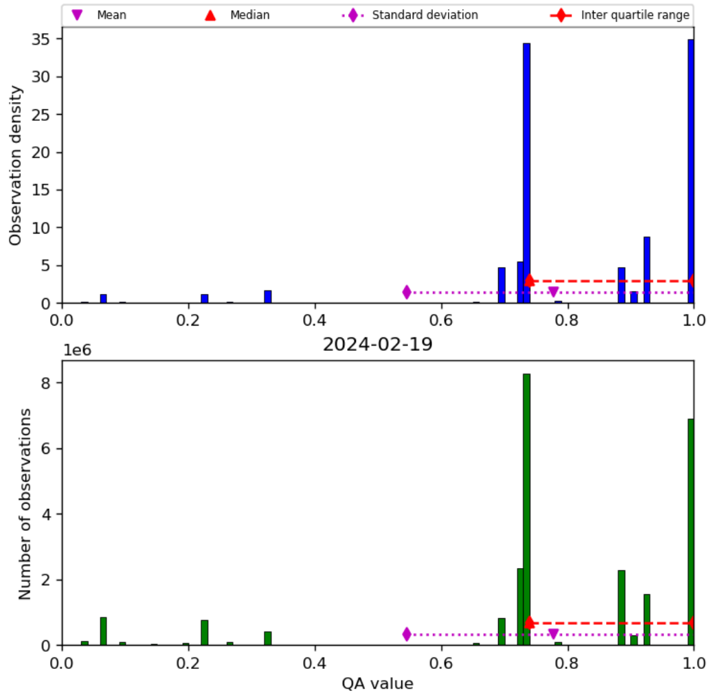
Figure 28: Histogram of “QA value” for 2024-02-18 to 2024-02-20
