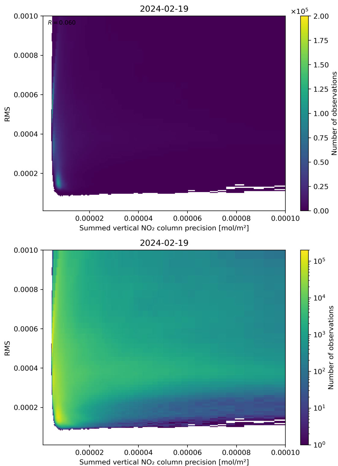
Figure 108: Scatter density plot of “Summed vertical NO 2 column precision” against “RMS” for 2024-02-18 to 2024-02-20.
