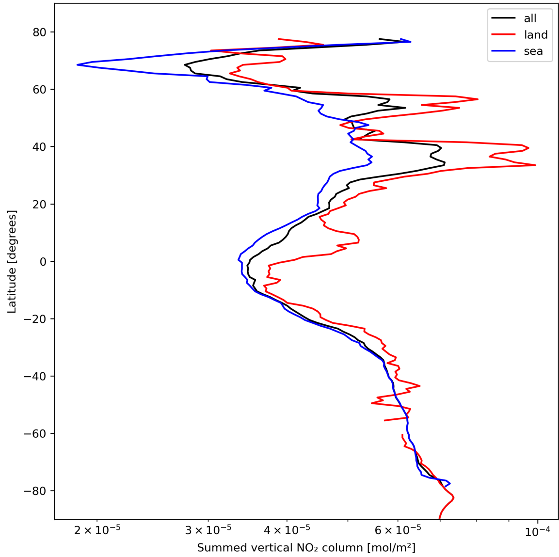
Figure 23: Zonal average of “Summed vertical NO 2 column” for 2024-02-19 to 2024-02-21.
