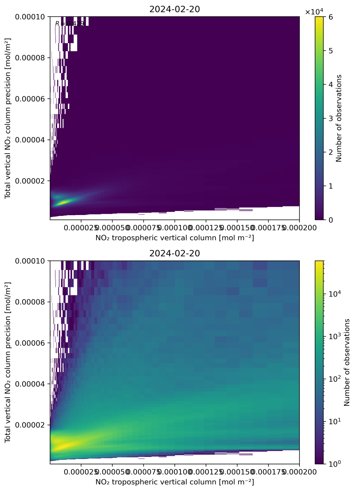
Figure 129: Scatter density plot of “NO 2 tropospheric vertical column” against “Total vertical NO 2 column precision” for 2024-02-19 to 2024-02-21.
