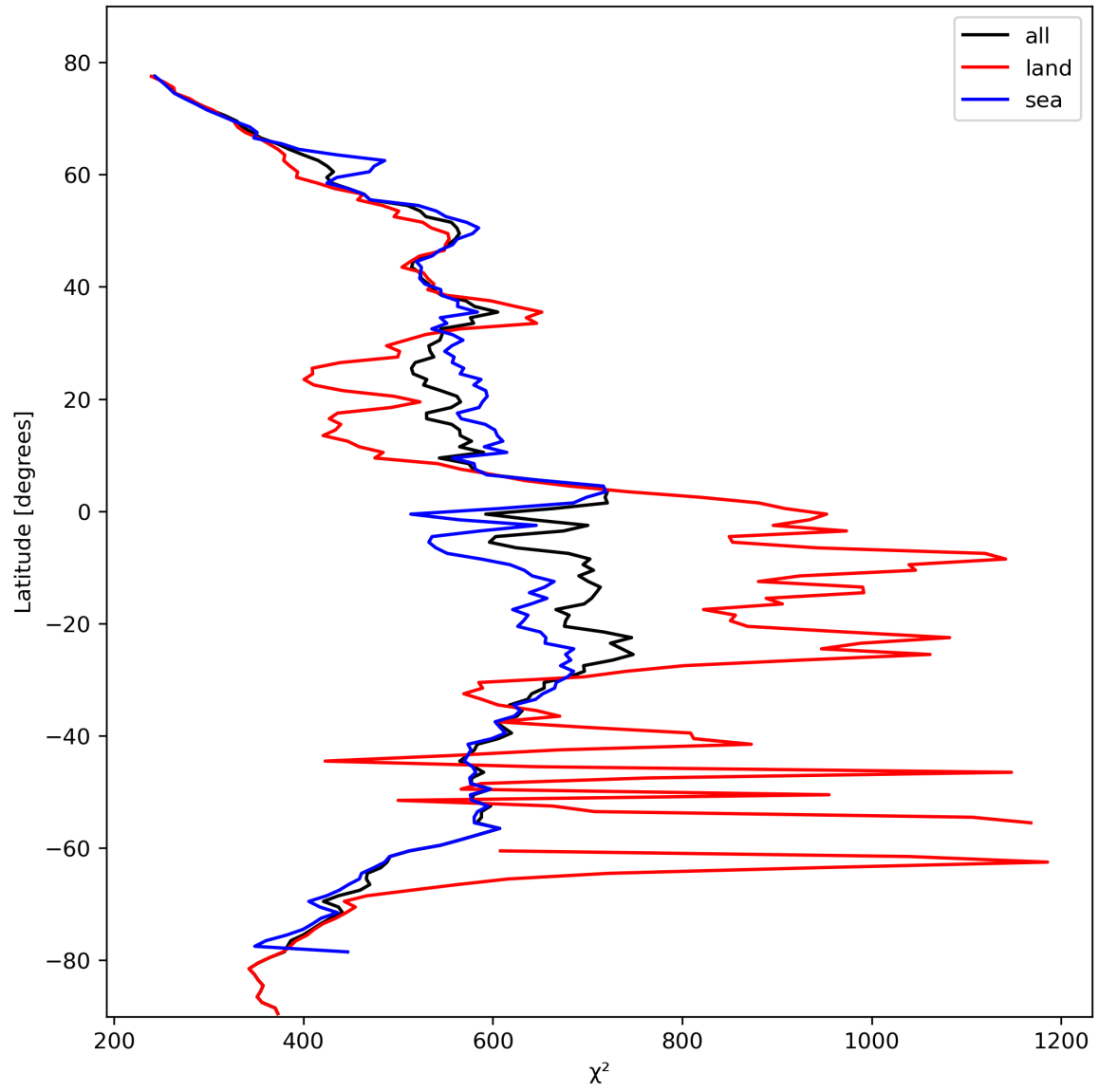
Figure 25: Zonal average of “ \chi^2 ” for 2024-02-19 to 2024-02-21.
