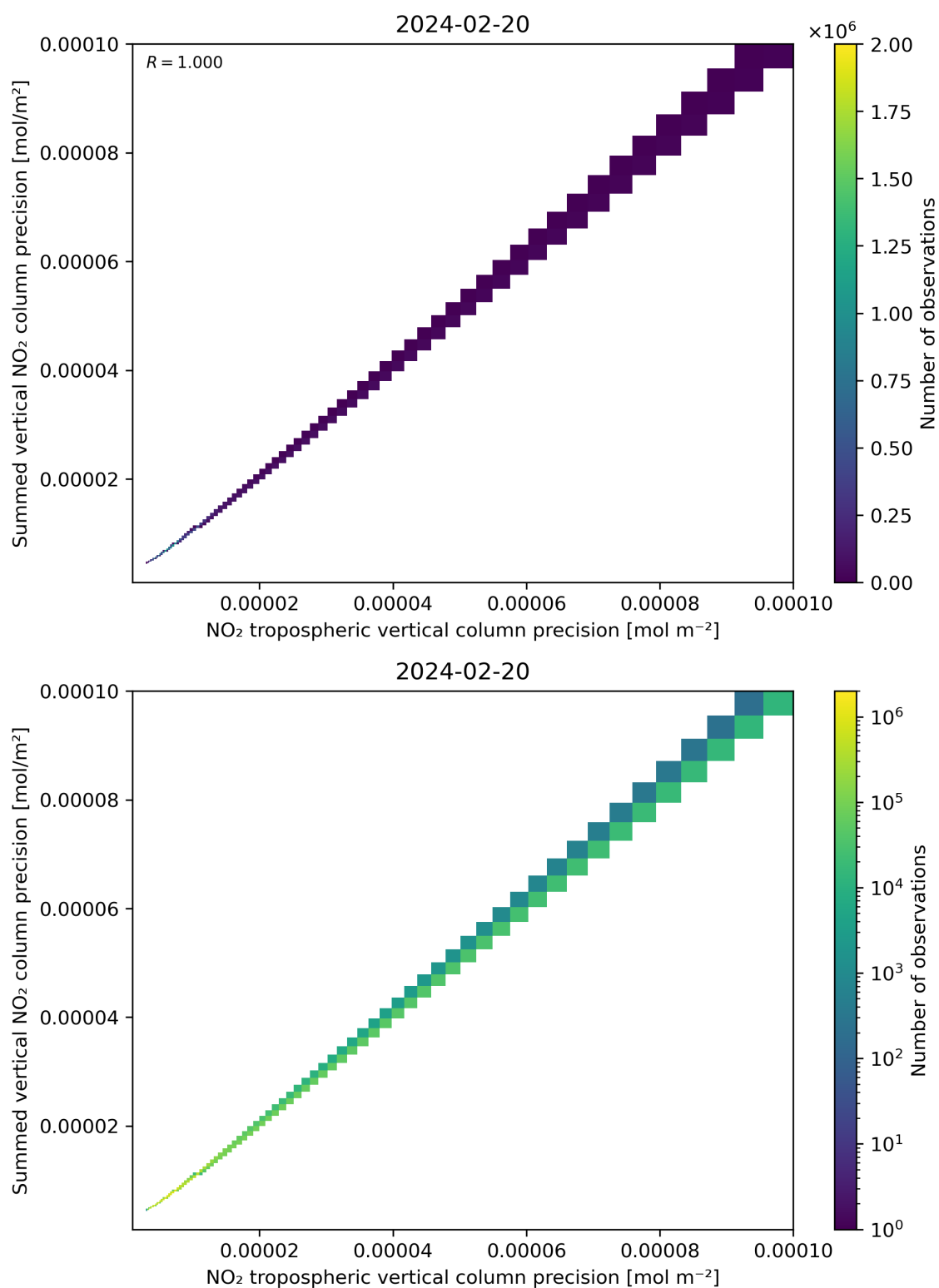
Figure 137: Scatter density plot of “NO 2 tropospheric vertical column precision” against “Summed vertical NO 2 column precision” for 2024-02-19 to 2024-02-21.
