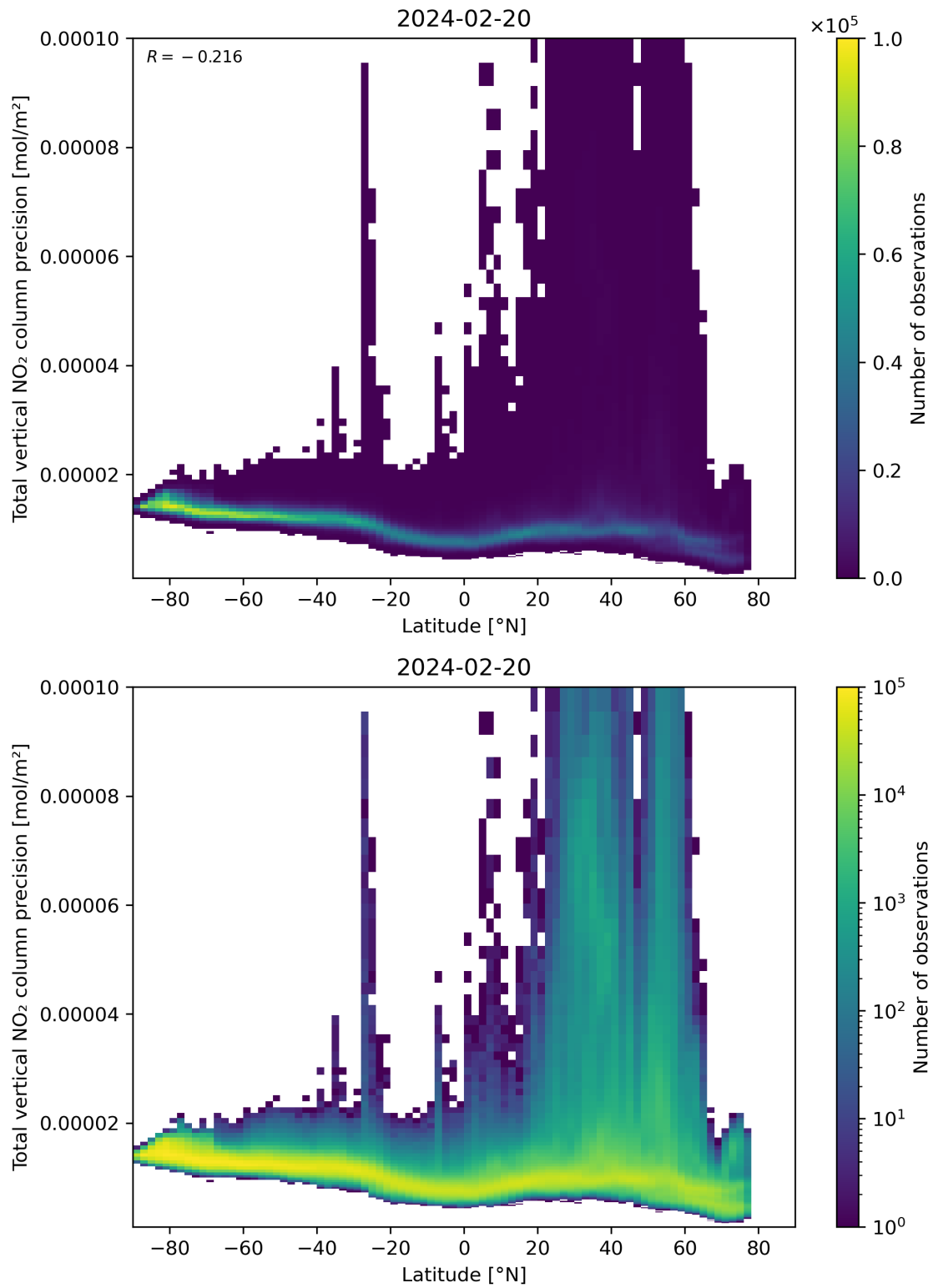
Figure 91: Scatter density plot of “Latitude” against “Total vertical NO 2 column precision” for 2024-02-19 to 2024-02-21.
