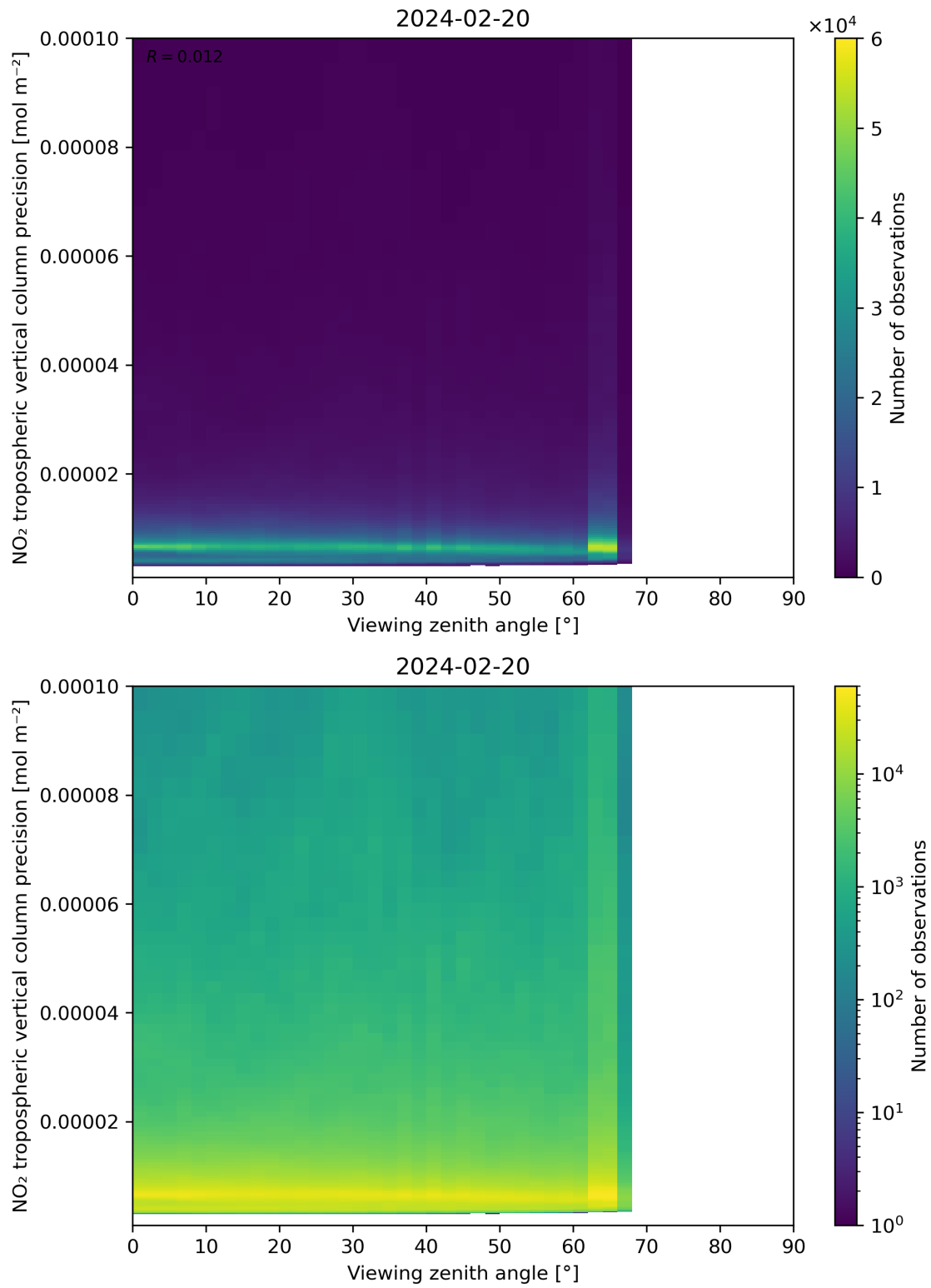
Figure 170: Scatter density plot of “Viewing zenith angle” against “NO 2 tropospheric vertical column precision” for 2024-02-19 to 2024-02-21.
