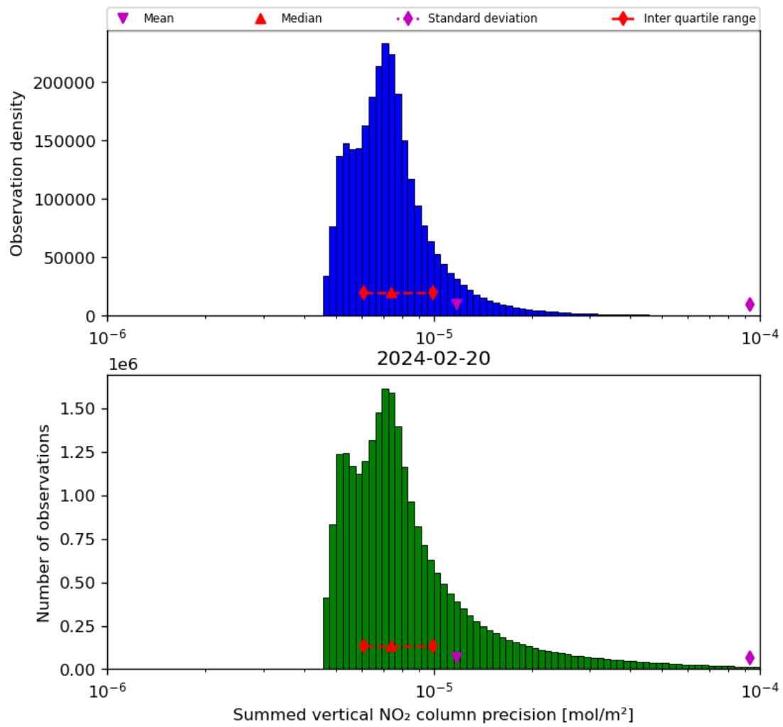
Figure 41: Histogram of “Summed vertical NO 2 column precision” for 2024-02-19 to 2024-02-21
