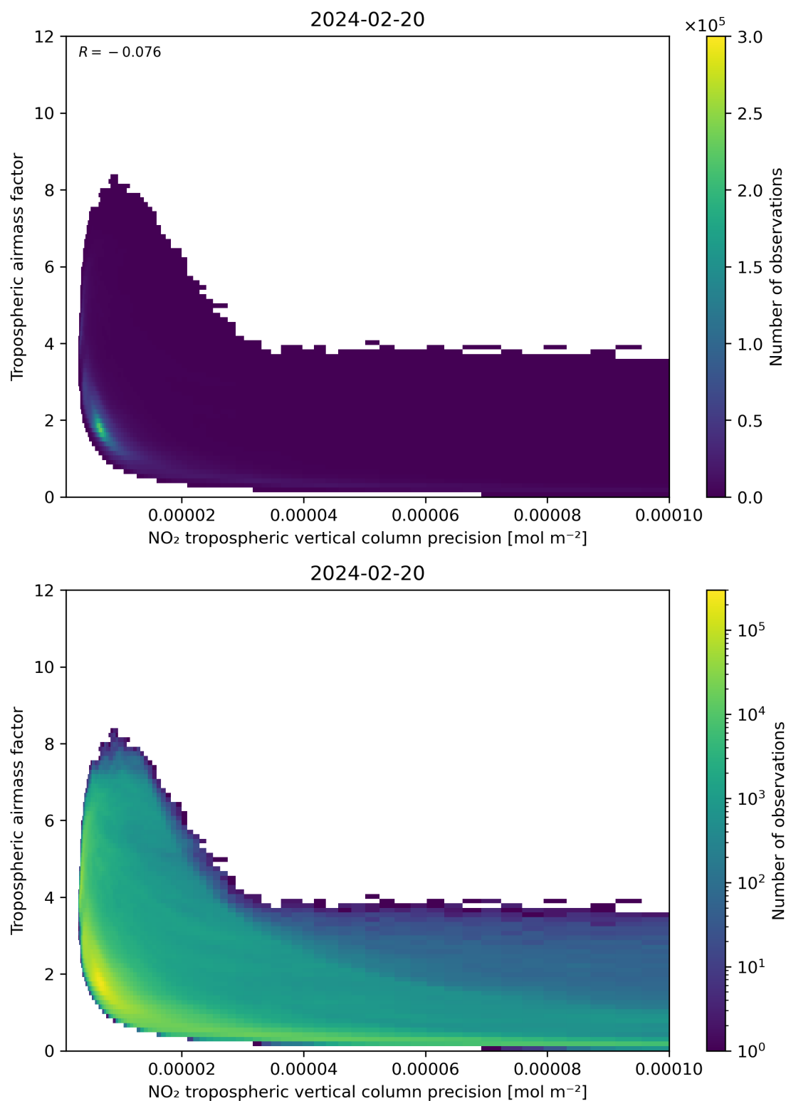
Figure 133: Scatter density plot of “NO 2 tropospheric vertical column precision” against “Tropospheric airmass factor” for 2024-02-19 to 2024-02-21.
