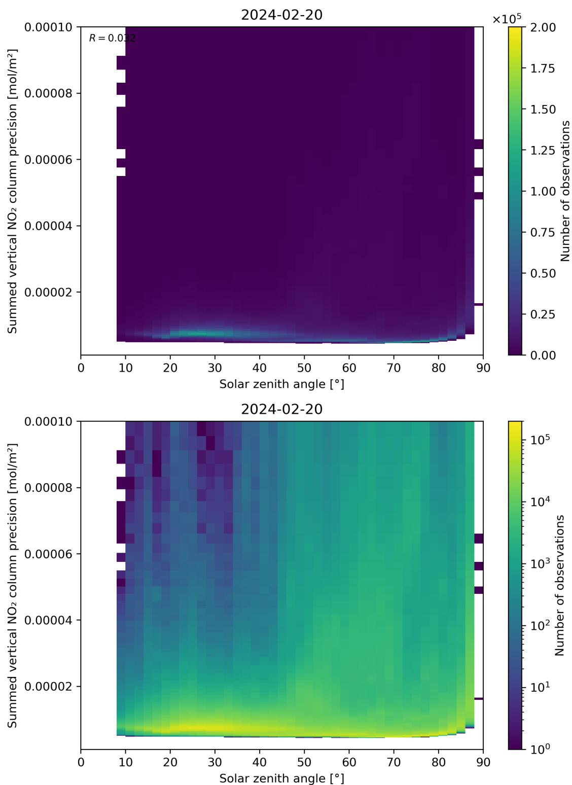
Figure 152: Scatter density plot of “Solar zenith angle” against “Summed vertical NO 2 column precision” for 2024-02-19 to 2024-02-21.
