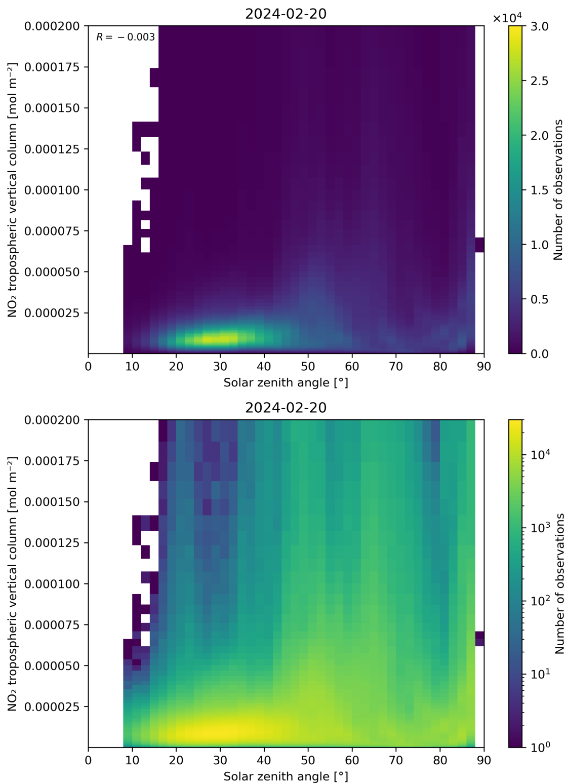
Figure 155: Scatter density plot of “Solar zenith angle” against “NO 2 tropospheric vertical column” for 2024-02-19 to 2024-02-21.
