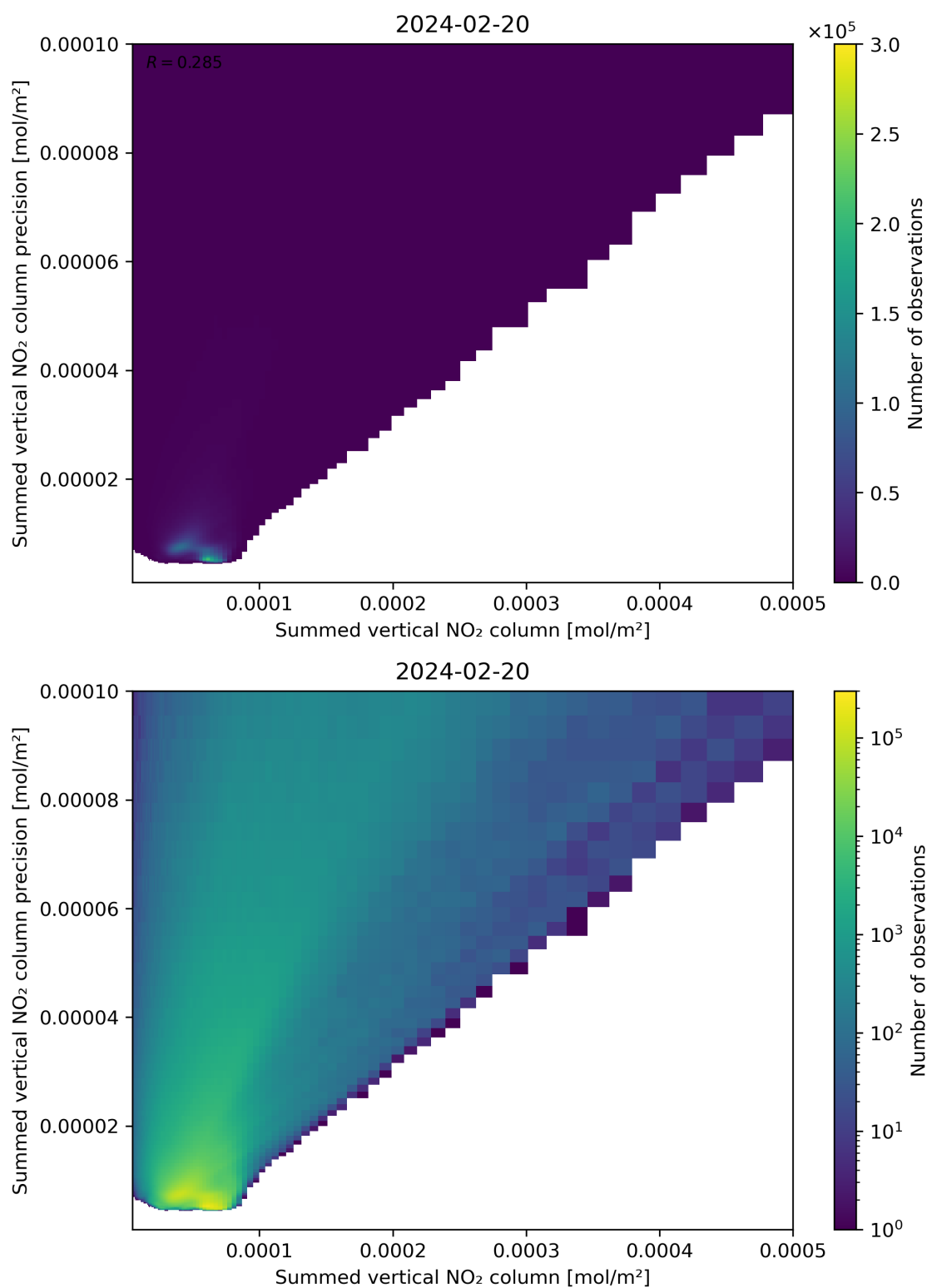
Figure 105: Scatter density plot of “Summed vertical NO 2 column” against “Summed vertical NO 2 column precision” for 2024-02-19 to 2024-02-21.
