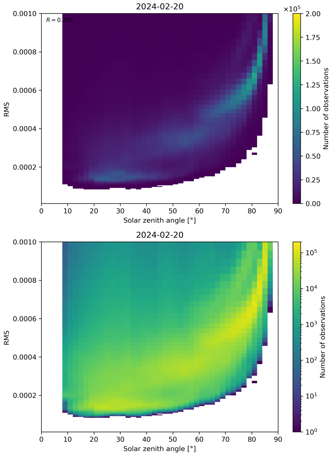
Figure 157: Scatter density plot of “Solar zenith angle” against “RMS” for 2024-02-19 to 2024-02-21.
