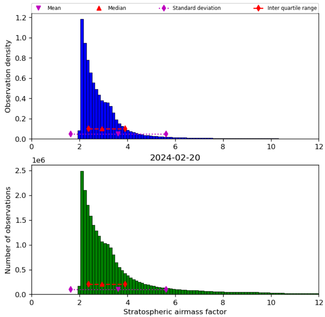
Figure 44: Histogram of “Stratospheric airmass factor” for 2024-02-19 to 2024-02-21
