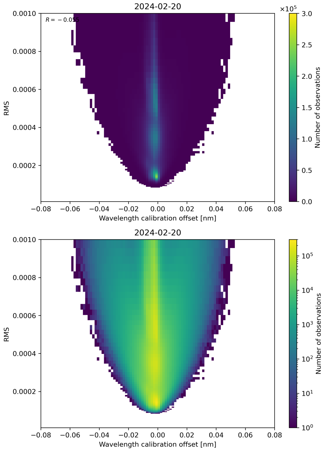
Figure 181: Scatter density plot of “Wavelength calibration offset” against “RMS” for 2024-02-19 to 2024-02-21.
