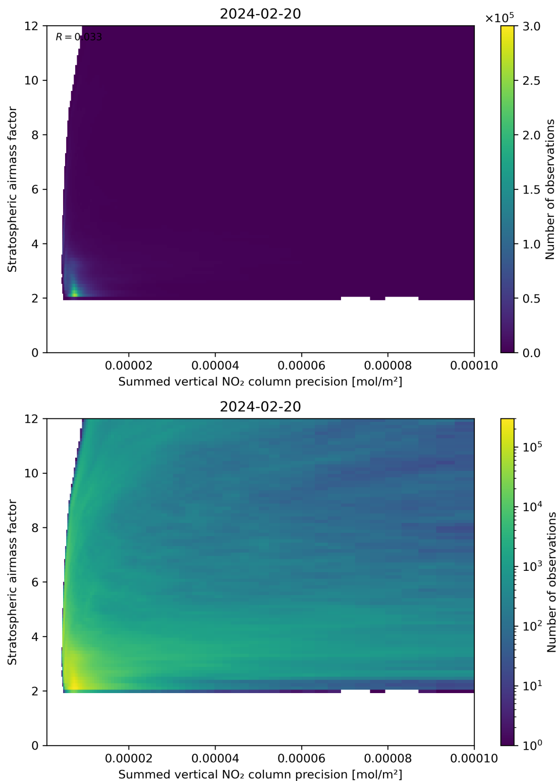
Figure 106: Scatter density plot of “Summed vertical NO 2 column precision” against “Stratospheric airmass factor” for 2024-02-19 to 2024-02-21.
