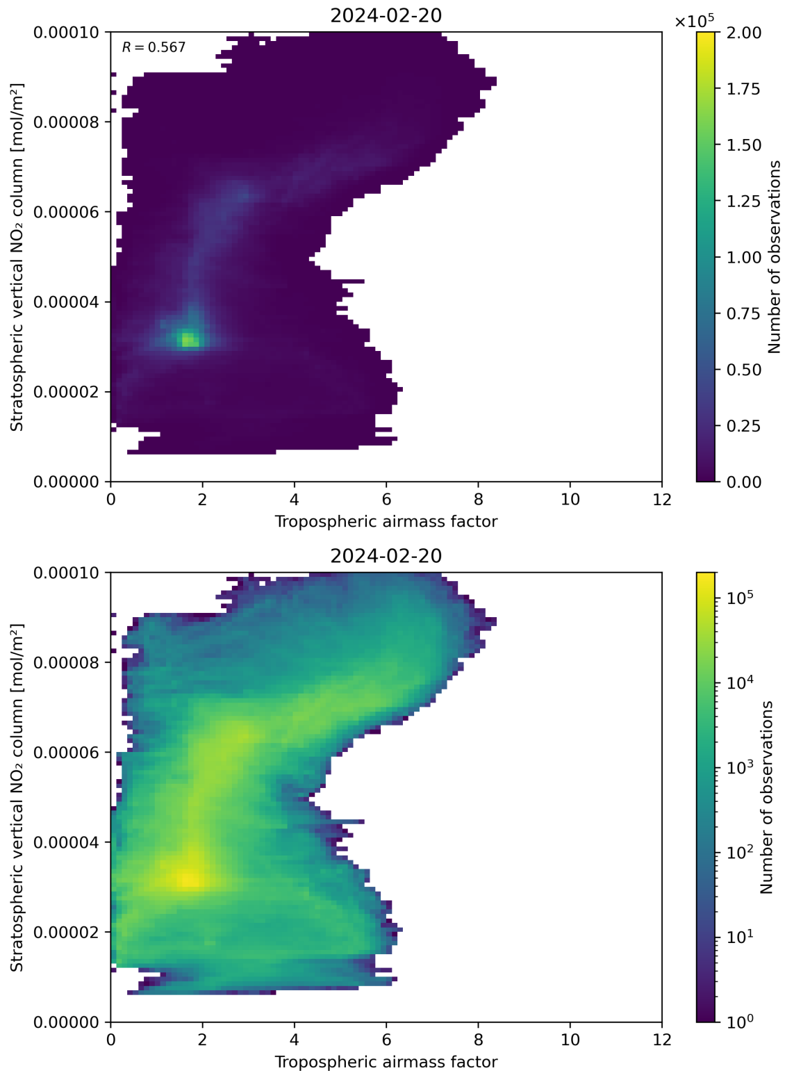
Figure 74: Scatter density plot of “Tropospheric airmass factor” against “Stratospheric vertical NO 2 column” for 2024-02-19 to 2024-02-21.
