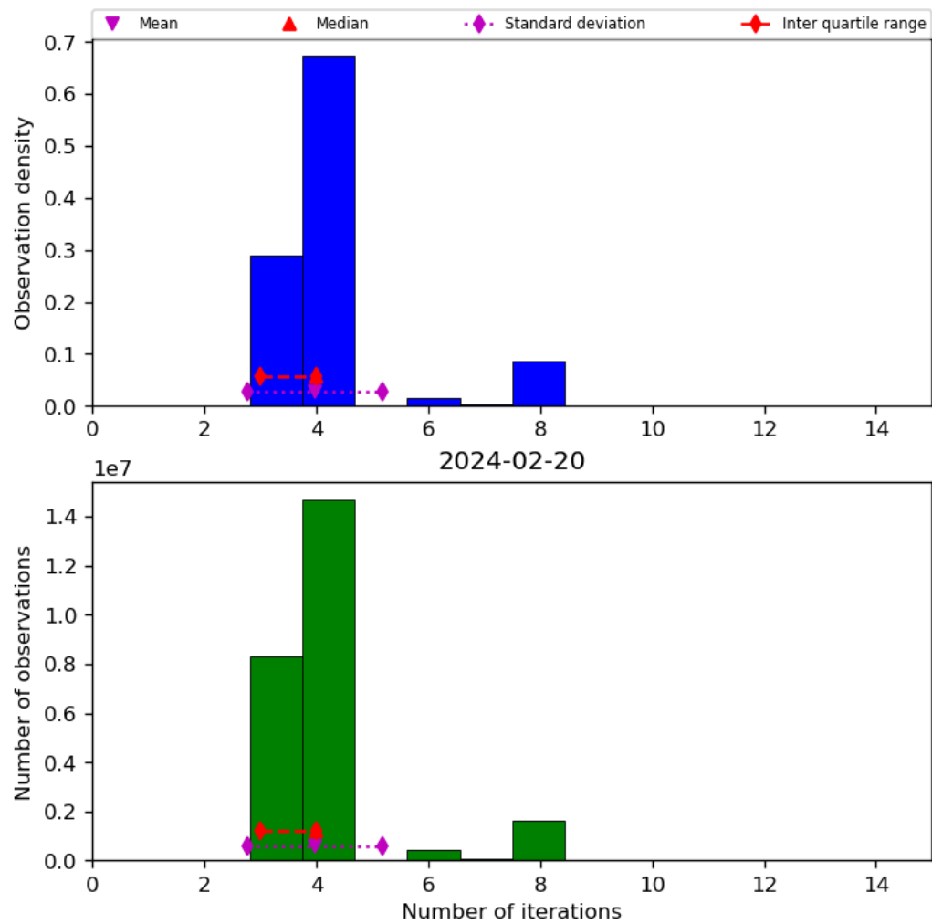
Figure 34: Histogram of “Number of iterations” for 2024-02-19 to 2024-02-21
