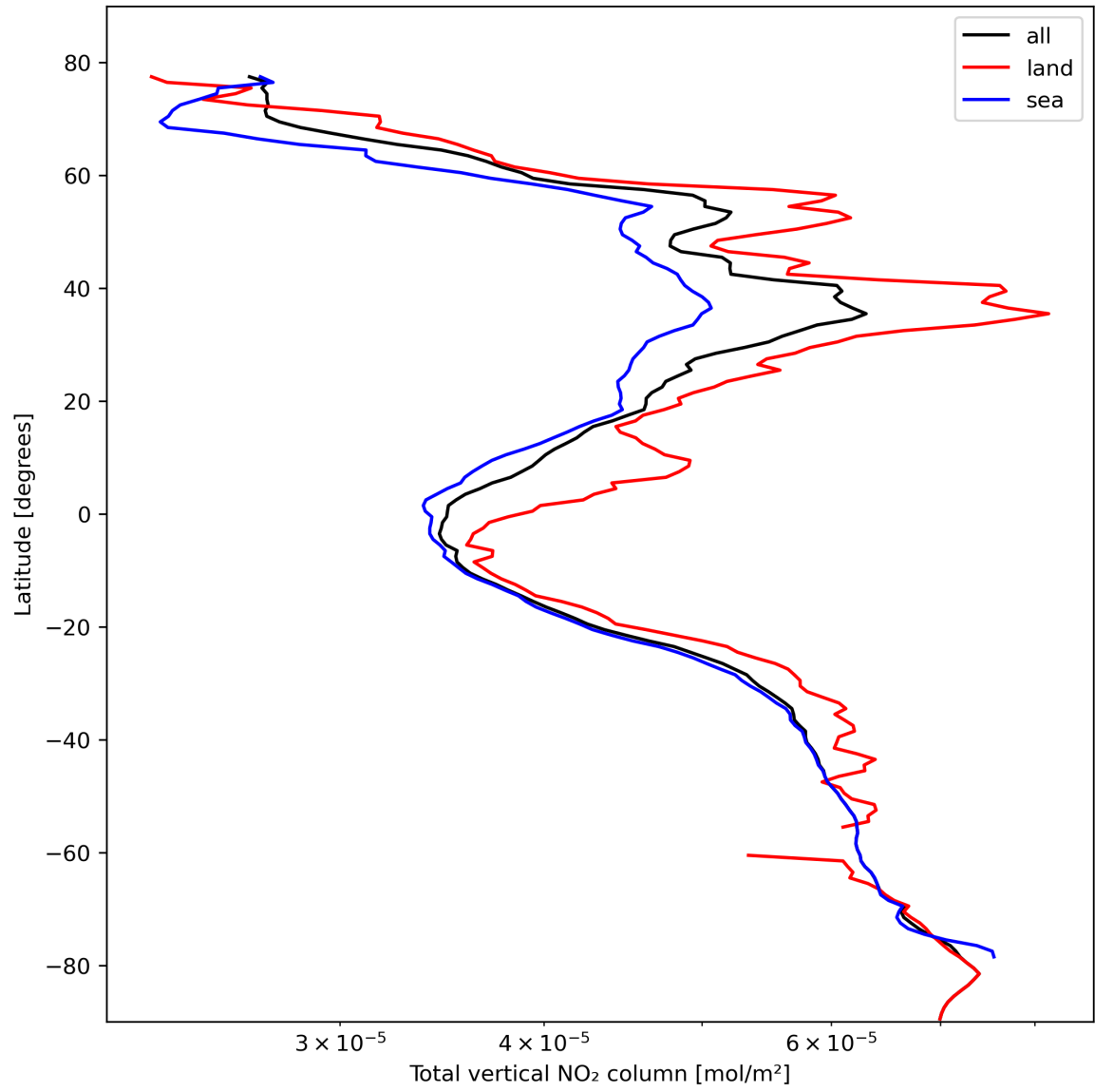
Figure 21: Zonal average of “Total vertical NO 2 column” for 2024-02-19 to 2024-02-21.
