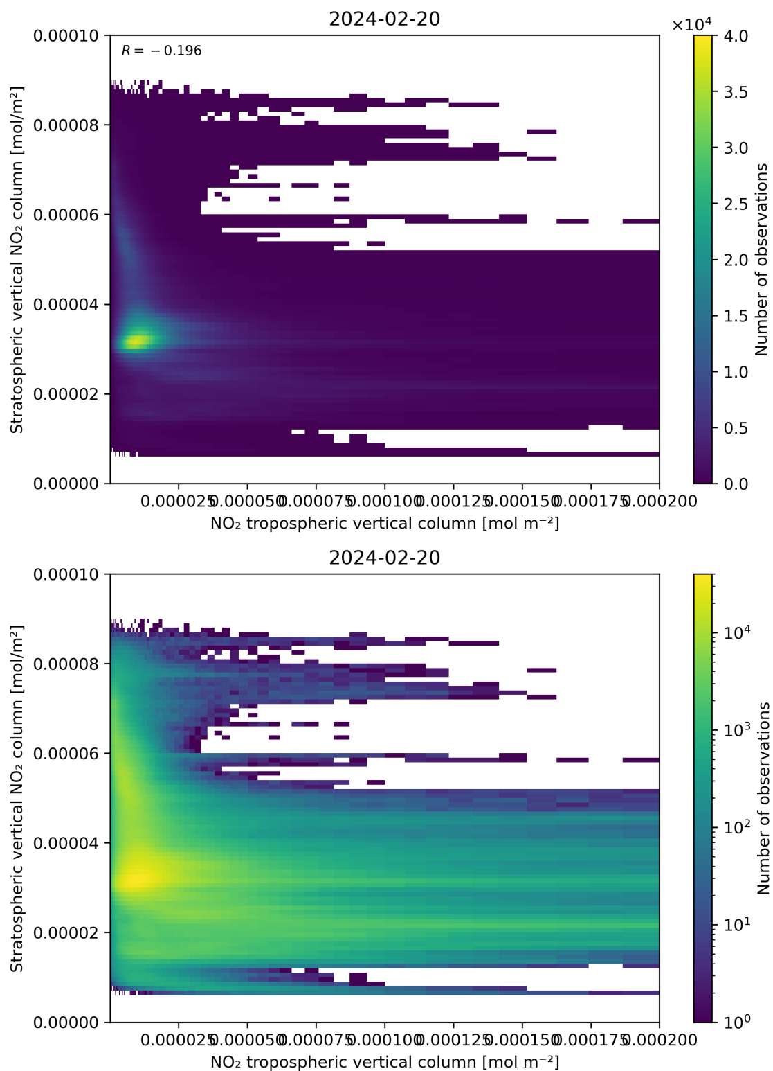
Figure 125: Scatter density plot of “NO 2 tropospheric vertical column” against “Stratospheric vertical NO 2 column” for 2024-02-19 to 2024-02-21.
