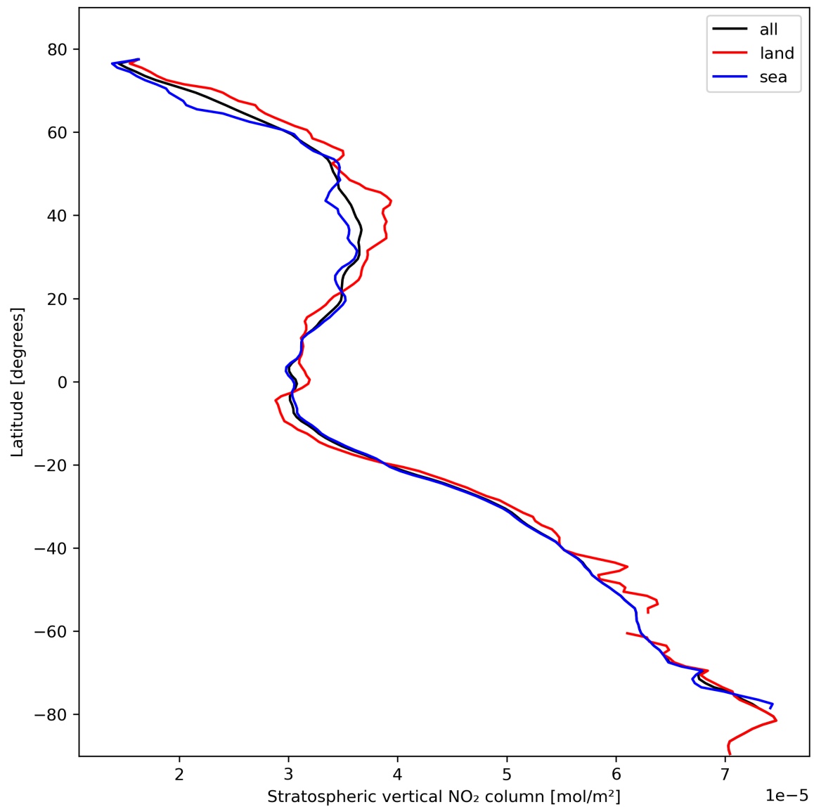
Figure 19: Zonal average of “Stratospheric vertical NO 2 column” for 2024-02-19 to 2024-02-21.
