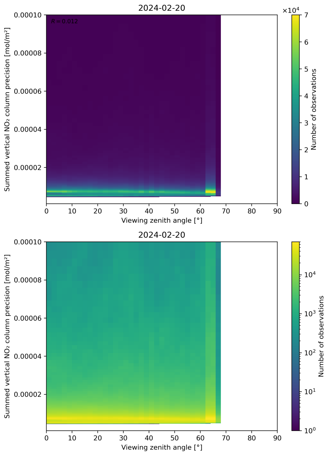
Figure 166: Scatter density plot of “Viewing zenith angle” against “Summed vertical NO 2 column precision” for 2024-02-19 to 2024-02-21.
