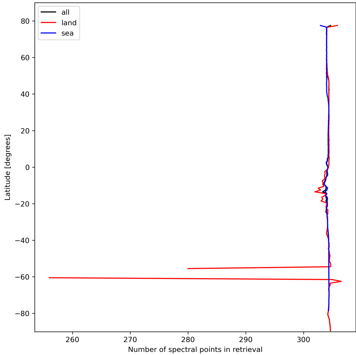
Figure 16: Zonal average of “Number of spectral points in retrieval” for 2024-02-19 to 2024-02-21.
