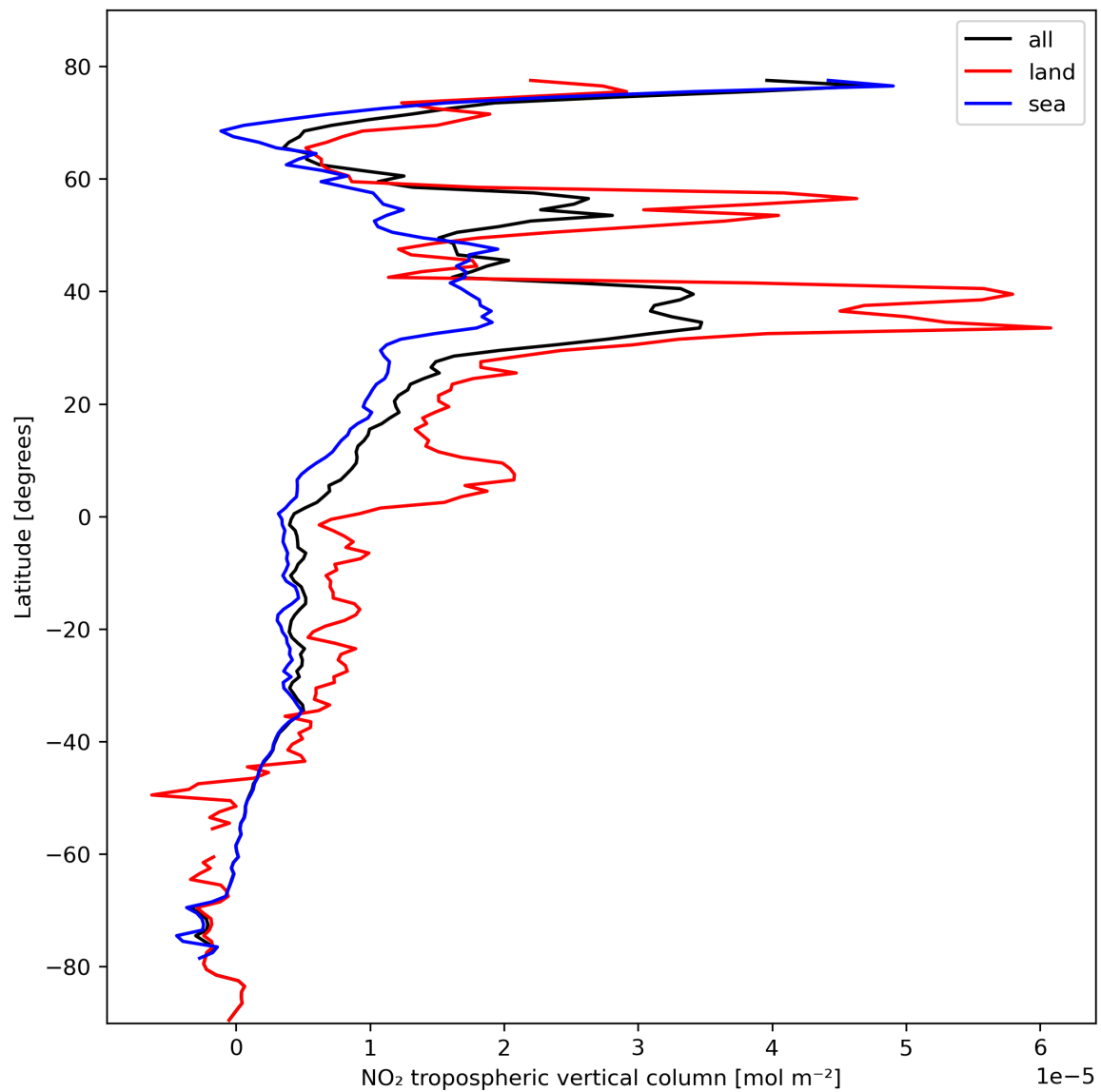
Figure 12: Zonal average of “NO 2 tropospheric vertical column” for 2024-02-19 to 2024-02-21.
