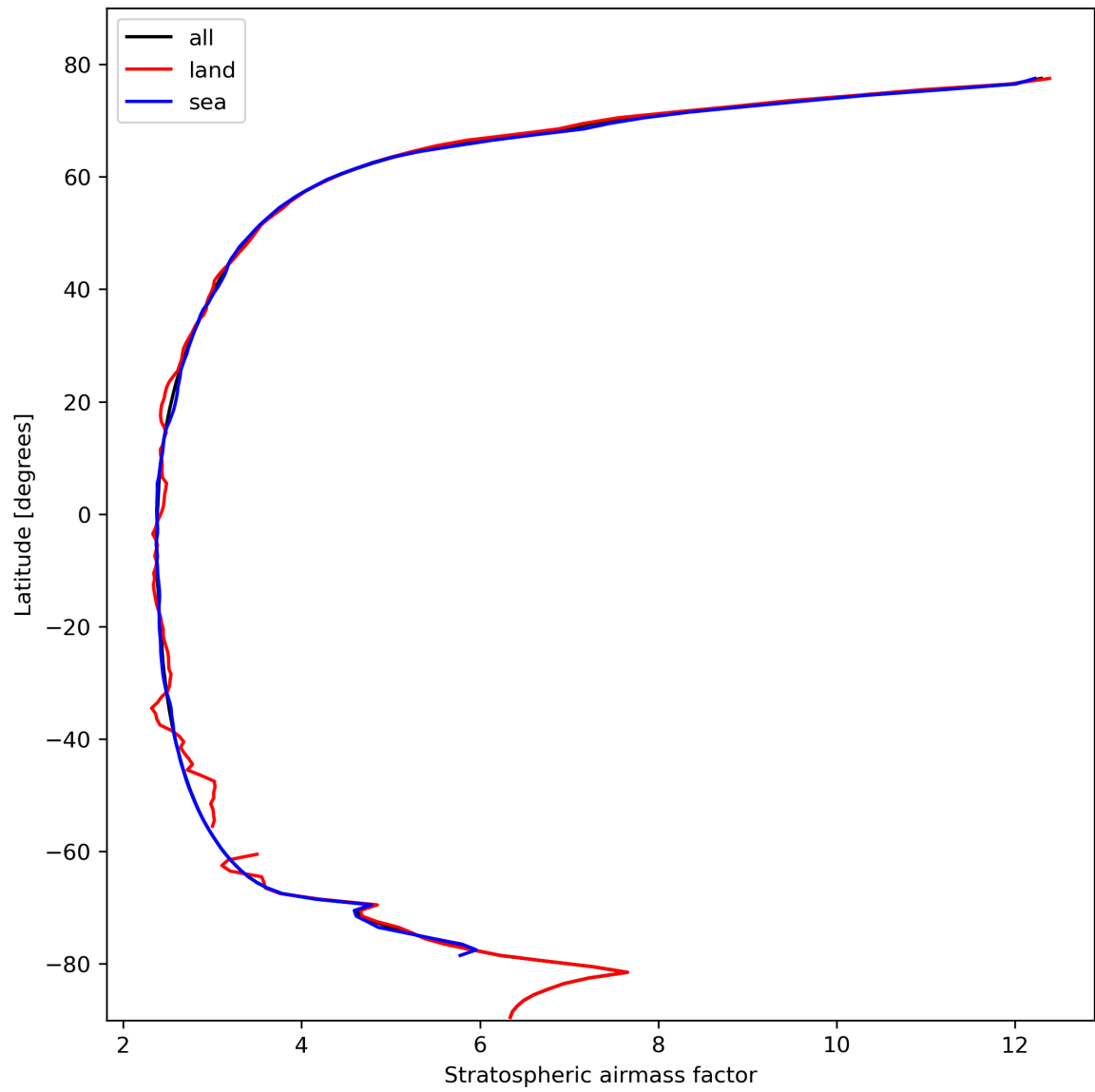
Figure 27: Zonal average of “Stratospheric airmass factor” for 2024-02-19 to 2024-02-21.
