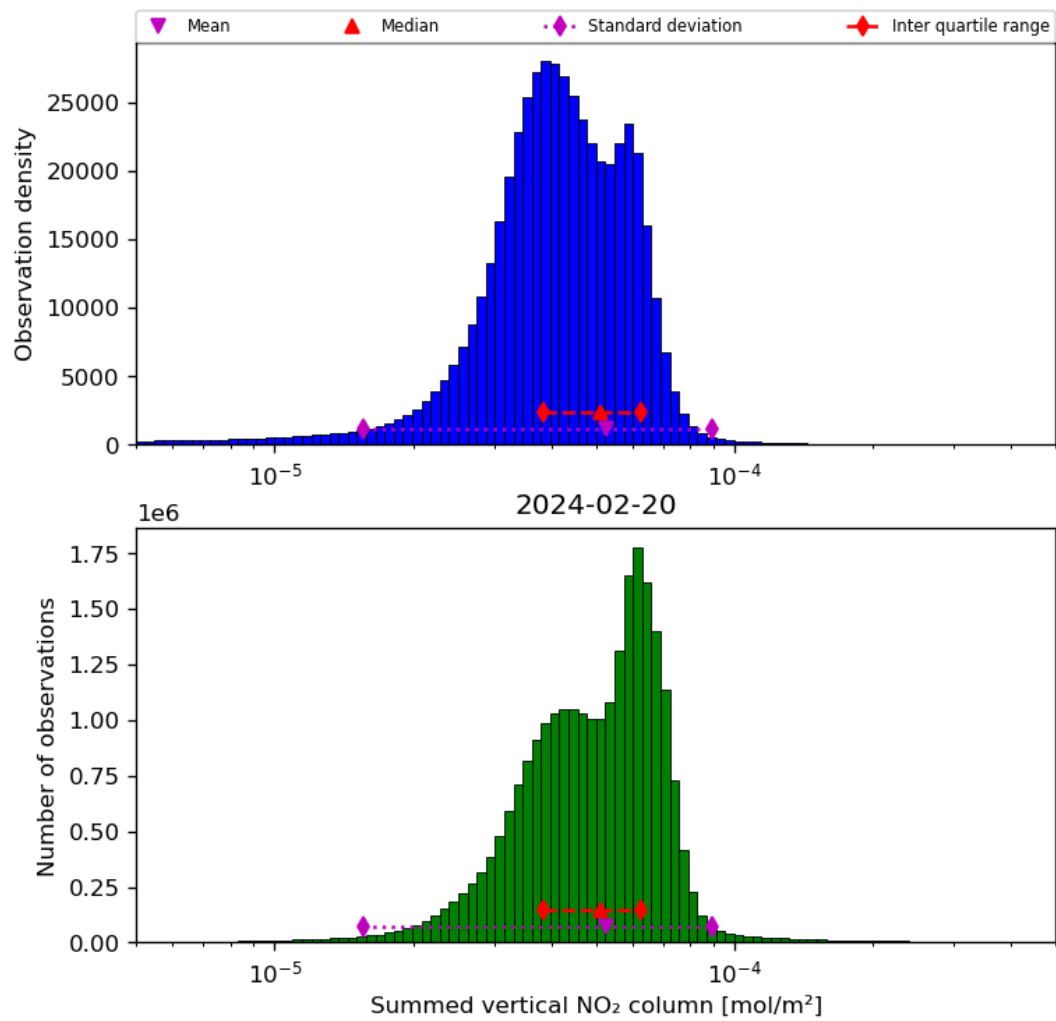
Figure 40: Histogram of “Summed vertical NO 2 column” for 2024-02-19 to 2024-02-21
