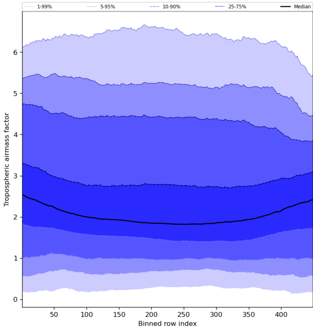
Figure 48: Along track statistics of “Tropospheric air mass factor” for 2024-02-19 to 2024-02-21
