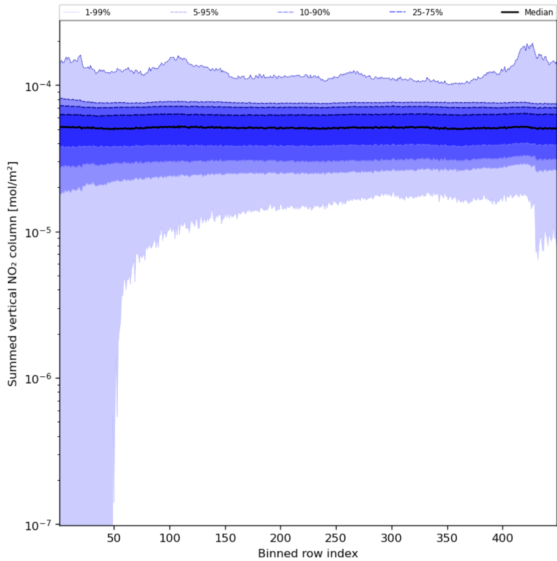
Figure 57: Along track statistics of “Summed vertical NO 2 column” for 2024-02-19 to 2024-02-21
