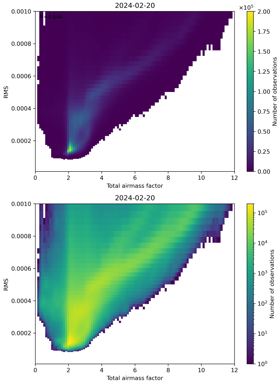
Figure 69: Scatter density plot of “Total airmass factor” against “RMS” for 2024-02-19 to 2024-02-21.
