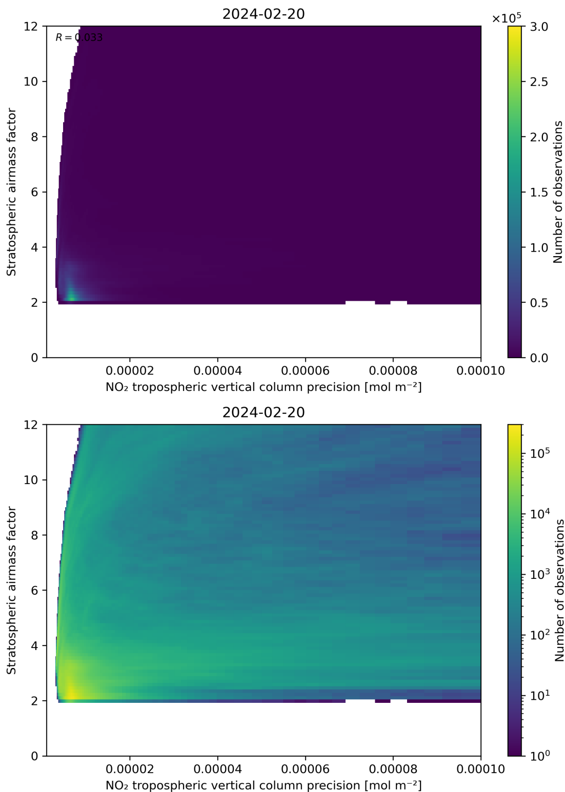
Figure 131: Scatter density plot of “NO 2 tropospheric vertical column precision” against “Stratospheric airmass factor” for 2024-02-19 to 2024-02-21.
