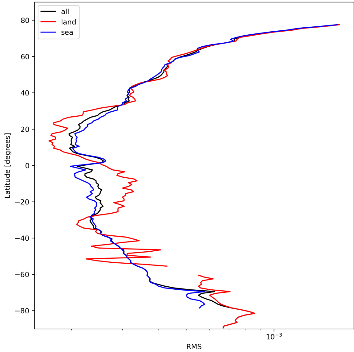
Figure 26: Zonal average of “RMS” for 2024-02-19 to 2024-02-21.
