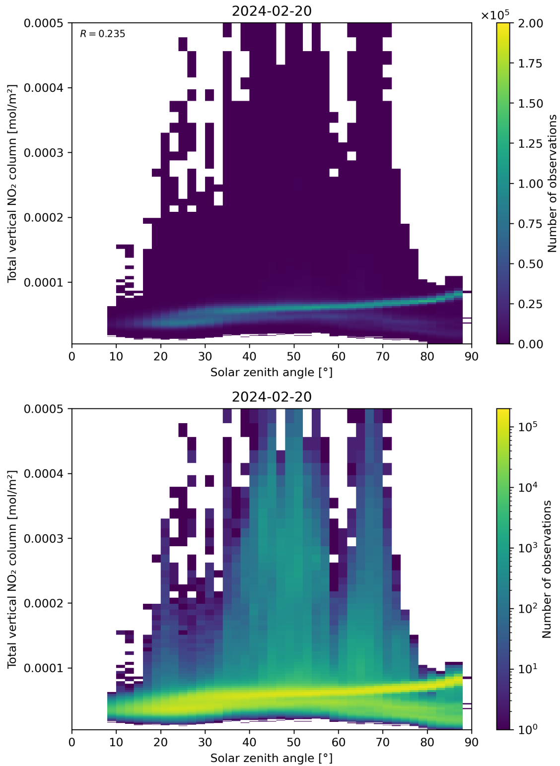
Figure 153: Scatter density plot of “Solar zenith angle” against “Total vertical NO 2 column” for 2024-02-19 to 2024-02-21.
