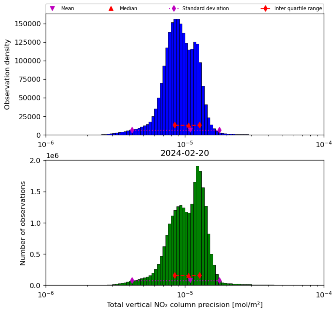
Figure 39: Histogram of "Total vertical NO 2 column precision" for 2024-02-19 to 2024-02-21
