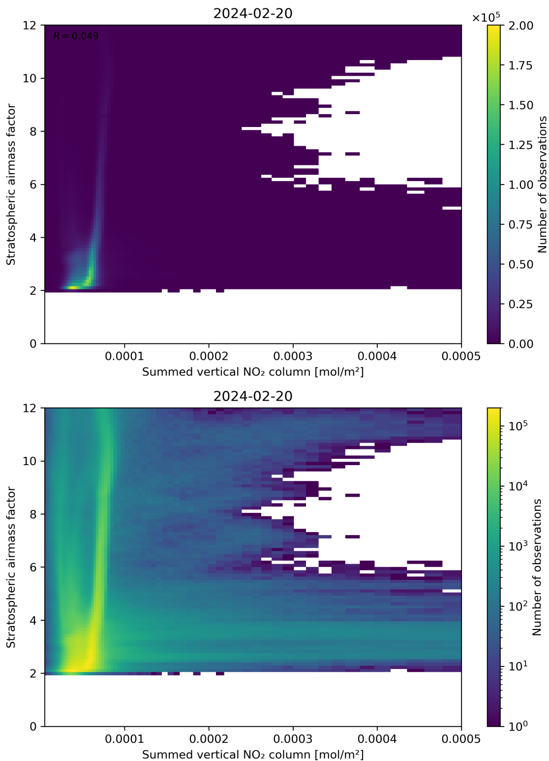
Figure 103: Scatter density plot of “Summed vertical NO 2 column” against “Stratospheric air mass factor” for 2024-02-19 to 2024-02-21.
