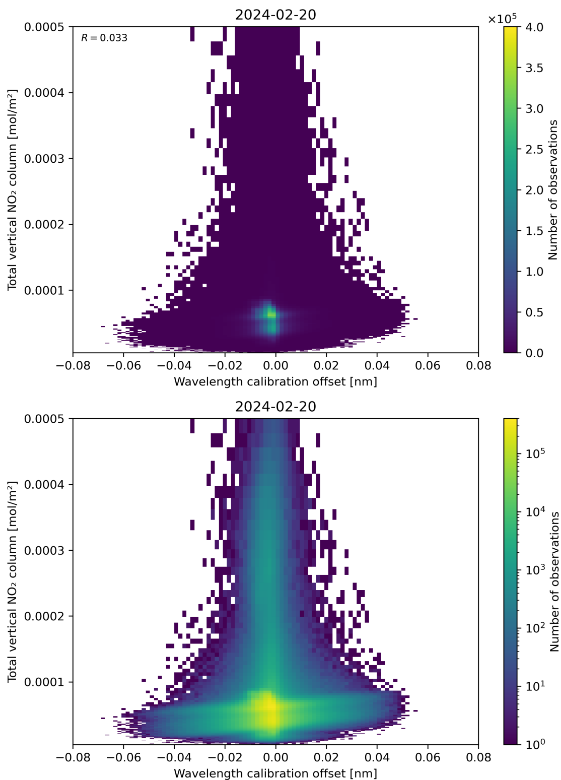
Figure 179: Scatter density plot of “Wavelength calibration offset” against “Total vertical NO 2 column” for 2024-02-19 to 2024-02-21.
