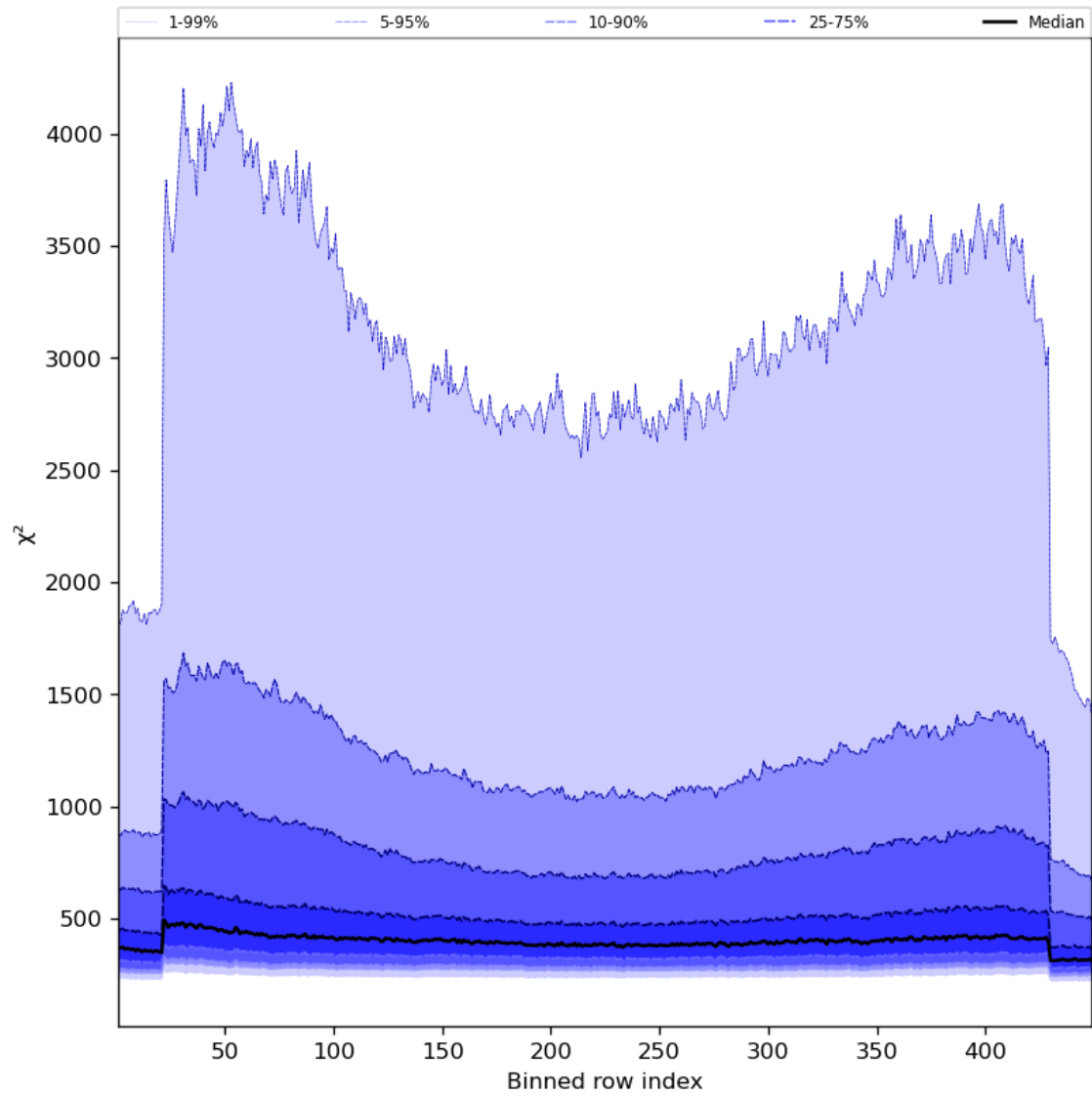
Figure 59: Along track statistics of “ \chi^2 ” for 2024-02-19 to 2024-02-21
