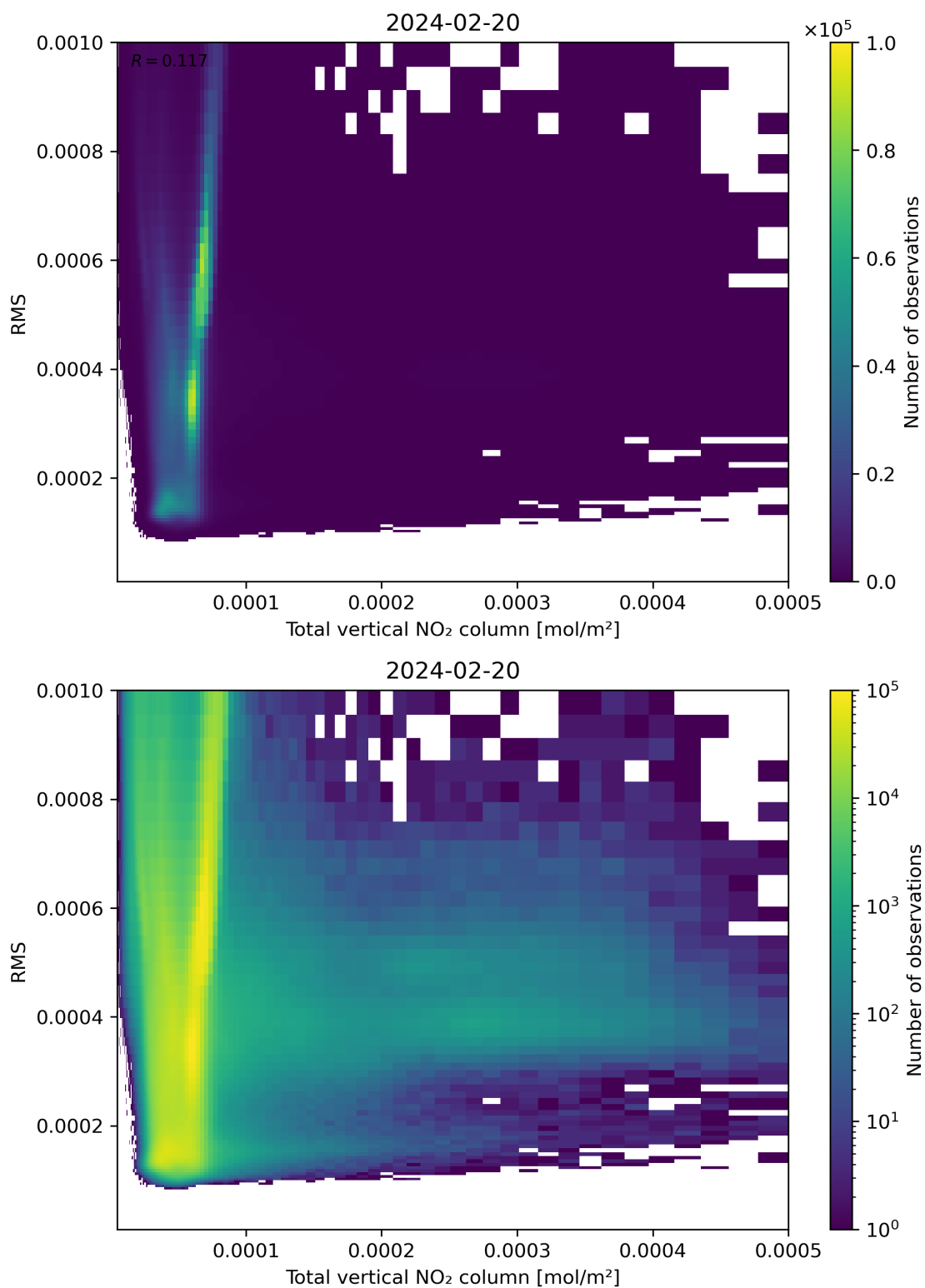
Figure 120: Scatter density plot of “Total vertical NO 2 column” against “RMS” for 2024-02-19 to 2024-02-21.
