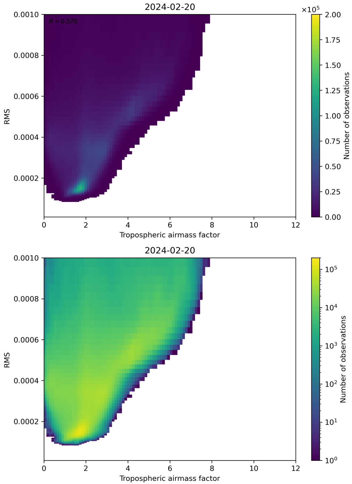
Figure 79: Scatter density plot of “Tropospheric airmass factor” against “RMS” for 2024-02-19 to 2024-02-21.
