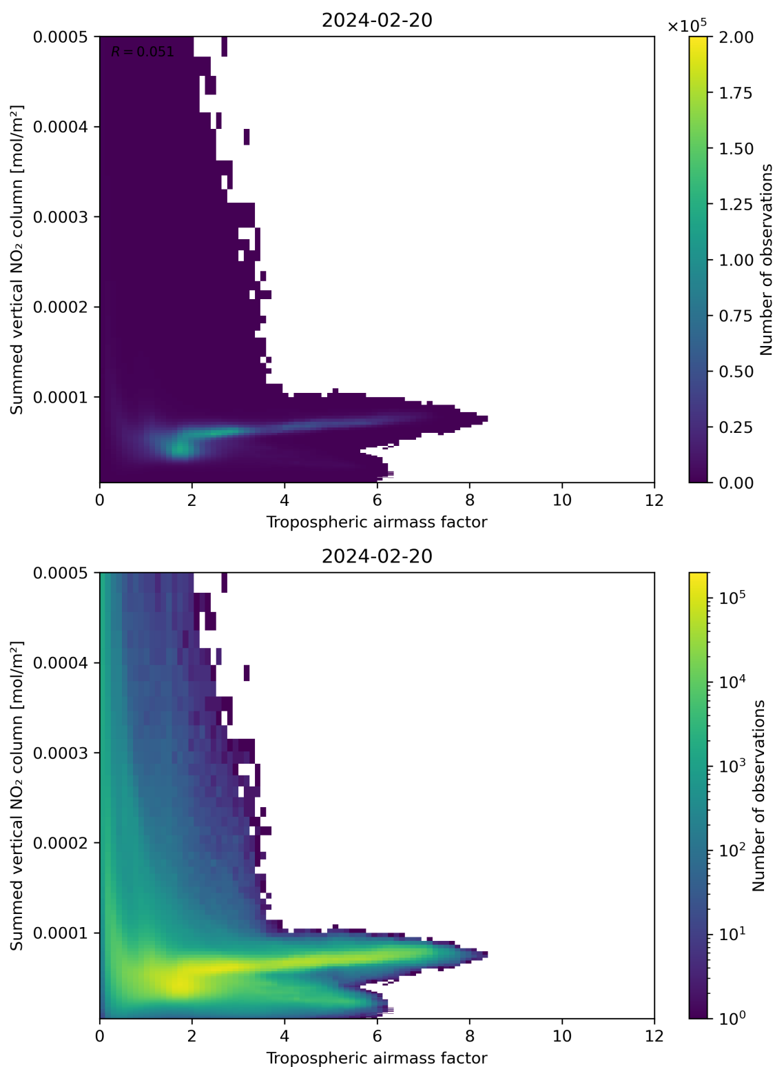
Figure 75: Scatter density plot of “Tropospheric airmass factor” against “Summed vertical NO 2 column” for 2024-02-19 to 2024-02-21.
