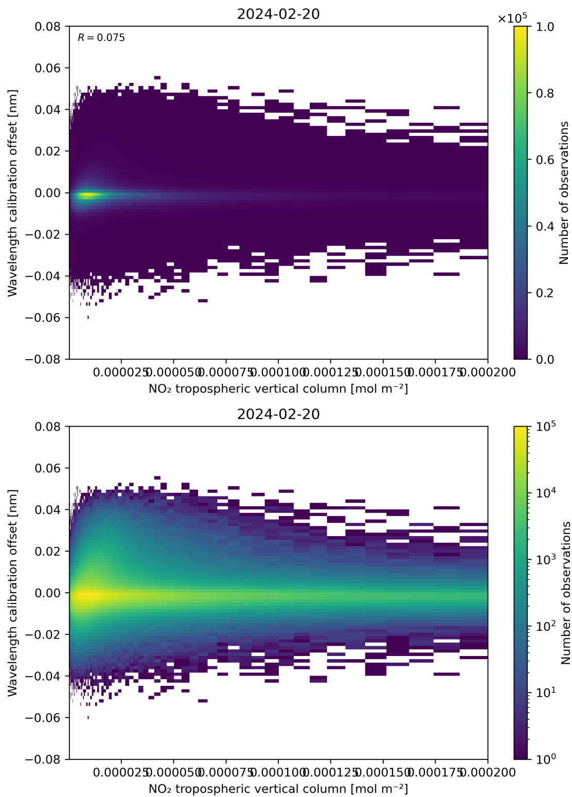
Figure 143: Scatter density plot of “NO 2 tropospheric vertical column” against “Wavelength calibration offset” for 2024-02-19 to 2024-02-21.
