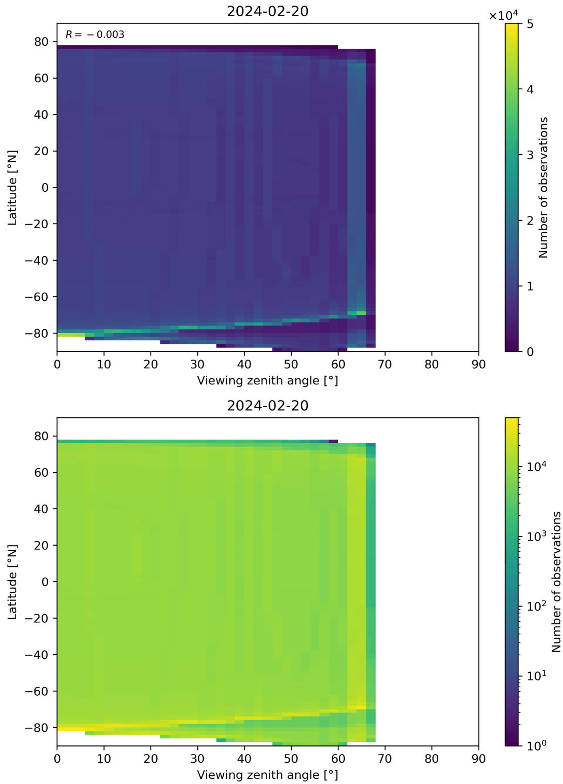
Figure 163: Scatter density plot of “Viewing zenith angle” against “Latitude” for 2024-02-19 to 2024-02-21.
