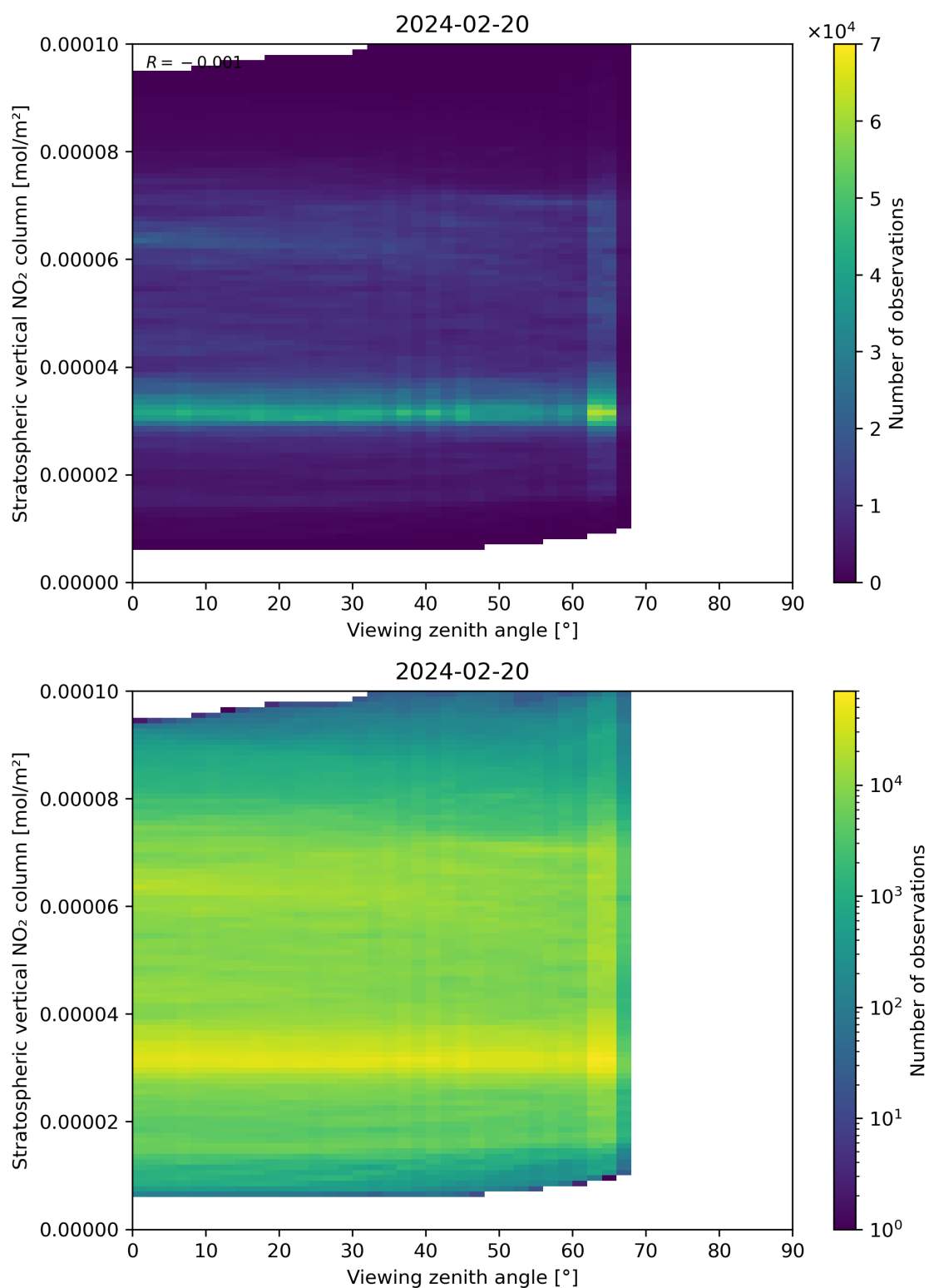
Figure 164: Scatter density plot of “Viewing zenith angle” against “Stratospheric vertical NO 2 column” for 2024-02-19 to 2024-02-21.
