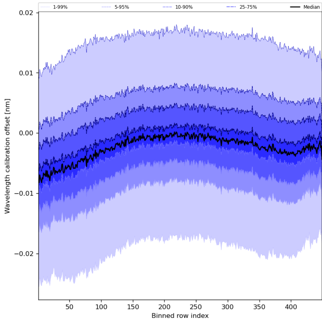
Figure 52: Along track statistics of “Wavelength calibration offset” for 2024-02-19 to 2024-02-21
