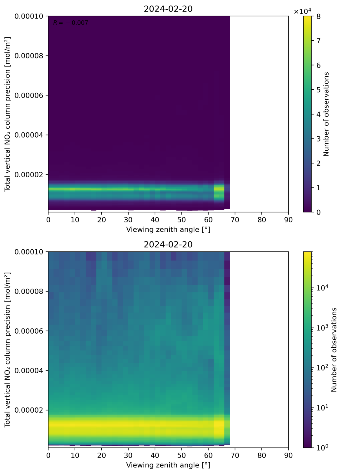
Figure 168: Scatter density plot of “Viewing zenith angle” against “Total vertical NO 2 column precision” for 2024-02-19 to 2024-02-21.
