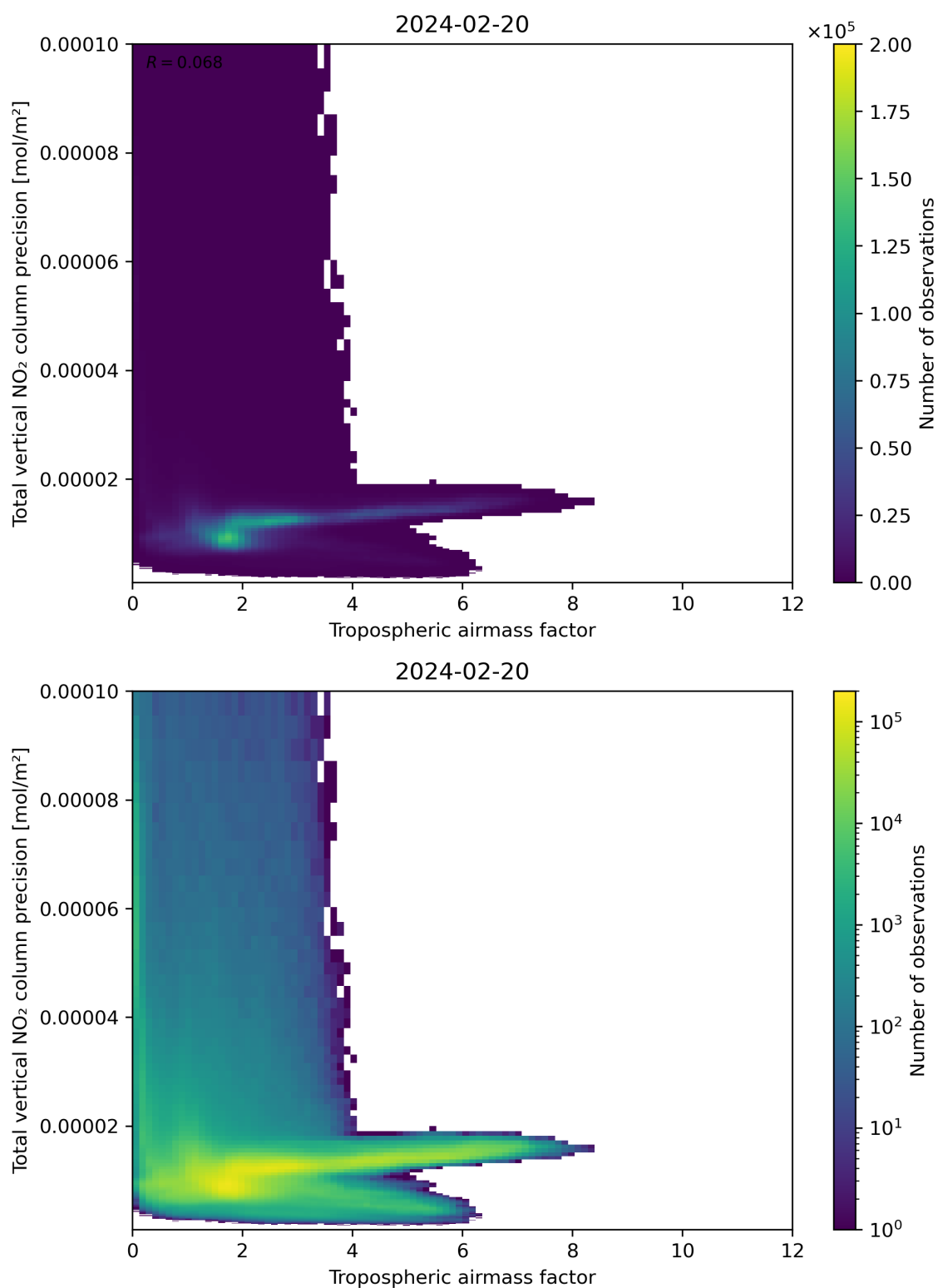
Figure 78: Scatter density plot of “Tropospheric air mass factor” against “Total vertical NO 2 column precision” for 2024-02-19 to 2024-02-21.
