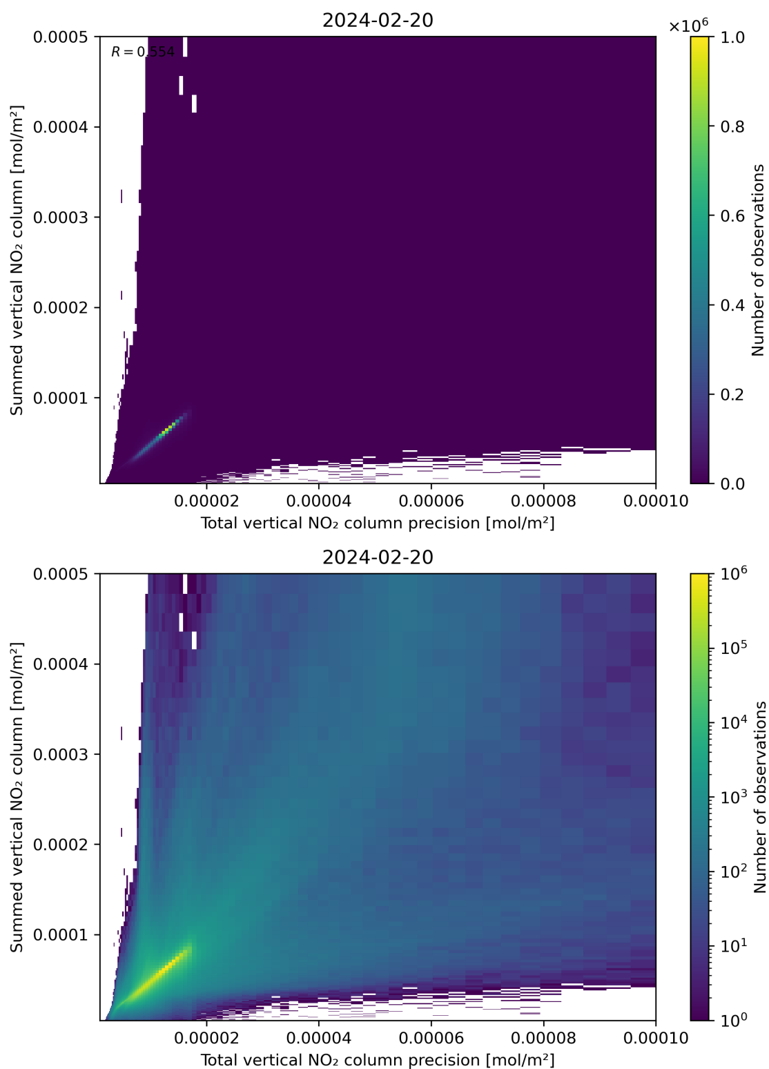
Figure 117: Scatter density plot of “Total vertical NO 2 column precision” against “Summed vertical NO 2 column” for 2024-02-19 to 2024-02-21.
