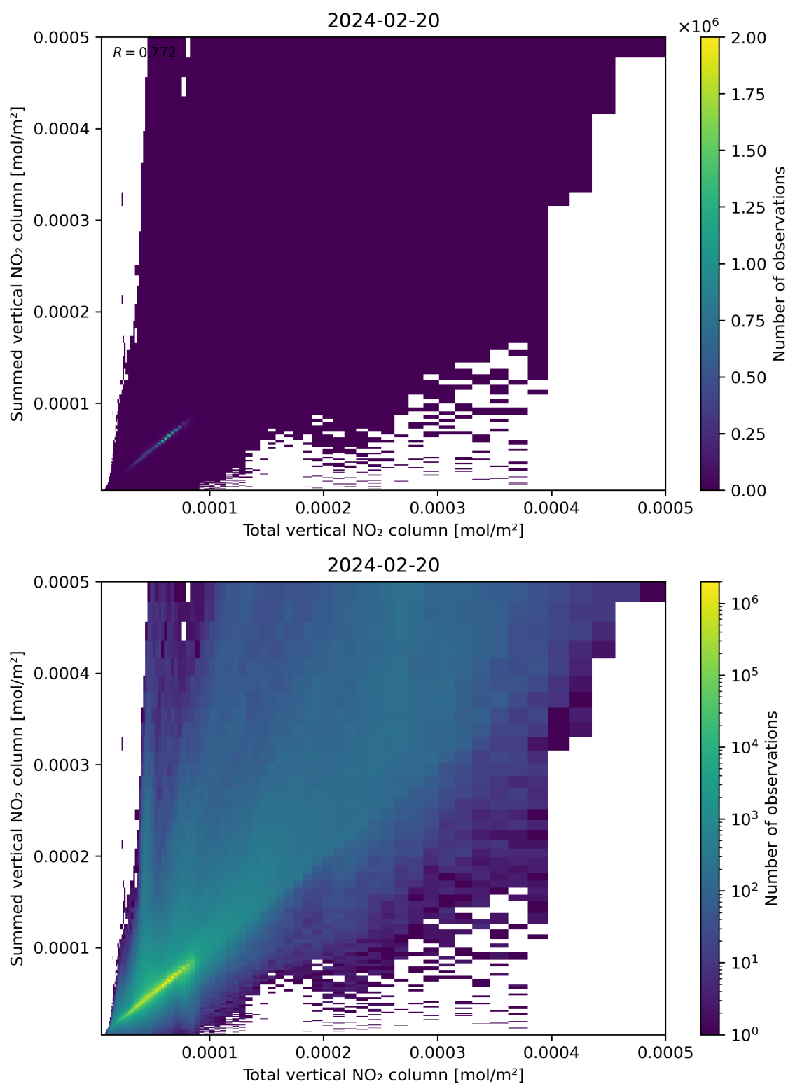
Figure 112: Scatter density plot of “Total vertical NO 2 column” against “Summed vertical NO 2 column” for 2024-02-19 to 2024-02-21.
