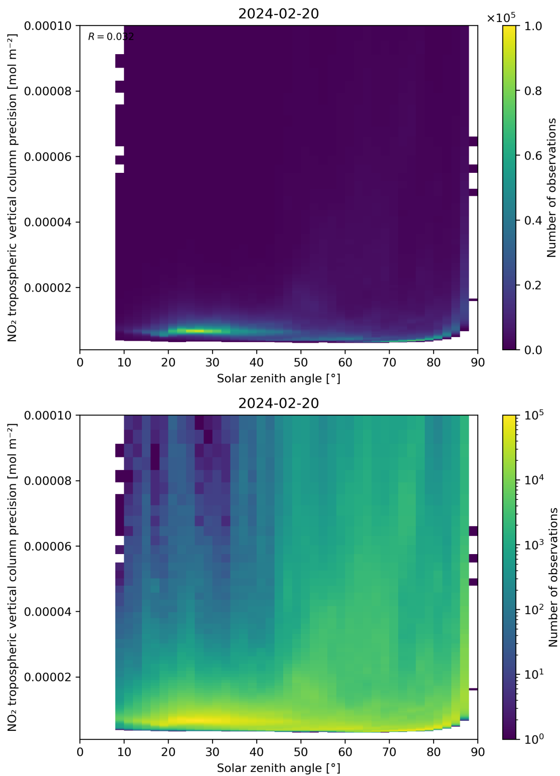
Figure 156: Scatter density plot of “Solar zenith angle” against “NO 2 tropospheric vertical column precision” for 2024-02-19 to 2024-02-21.
