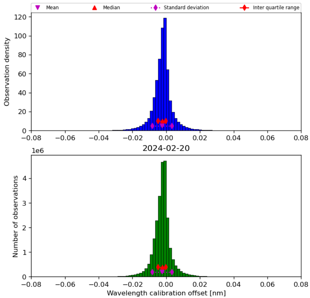
Figure 35: Histogram of “Wavelength calibration offset” for 2024-02-19 to 2024-02-21
