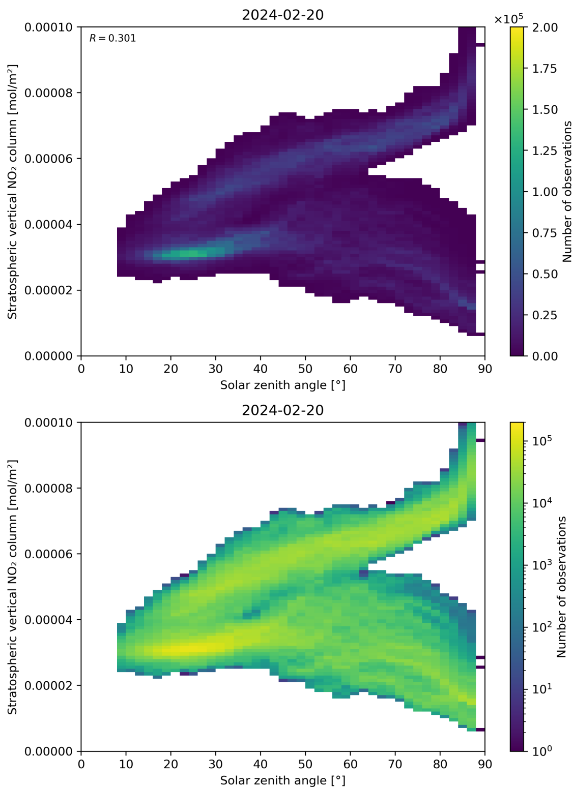
Figure 150: Scatter density plot of “Solar zenith angle” against “Stratospheric vertical NO 2 column” for 2024-02-19 to 2024-02-21.
