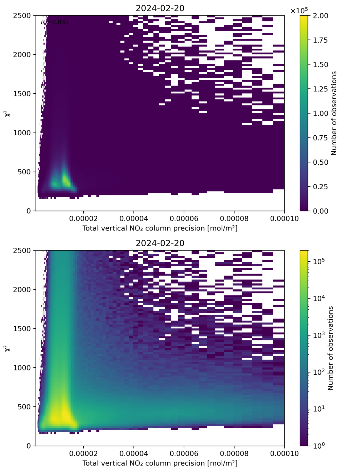
Figure 116: Scatter density plot of “Total vertical NO 2 column precision” against “ \chi^2 ” for 2024-02-19 to 2024-02-21.
