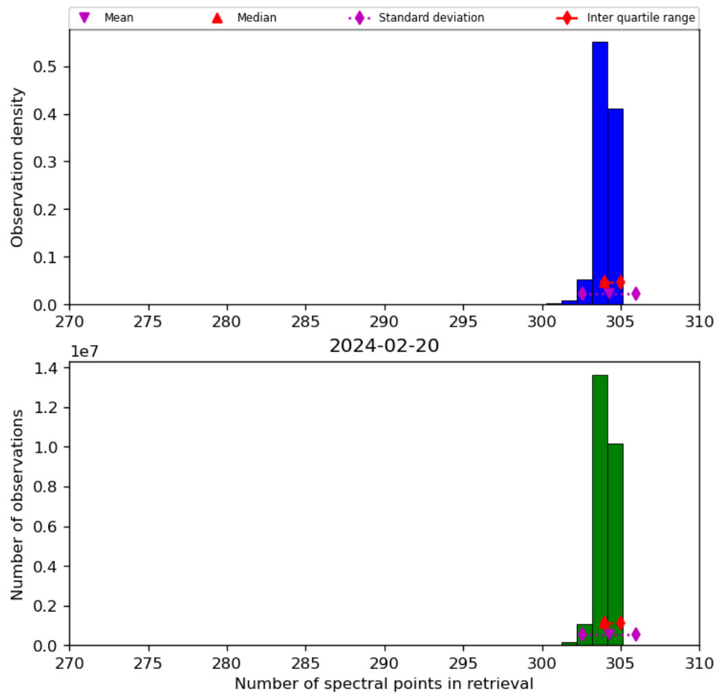
Figure 33: Histogram of “Number of spectral points in retrieval” for 2024-02-19 to 2024-02-21
