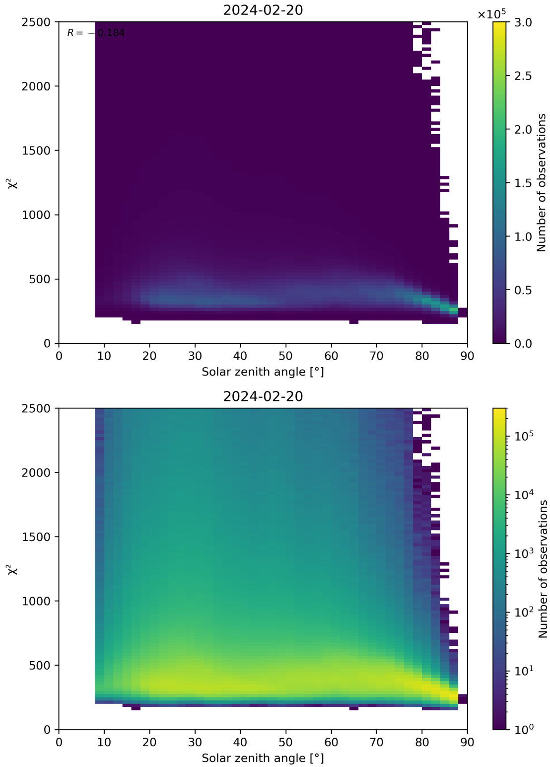
Figure 148: Scatter density plot of “Solar zenith angle” against “ \chi^2 ” for 2024-02-19 to 2024-02-21.
