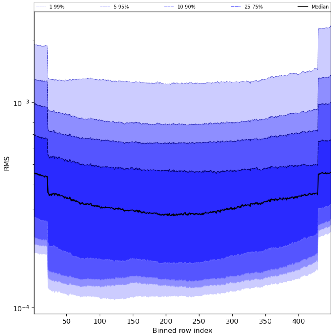
Figure 60: Along track statistics of “RMS” for 2024-02-19 to 2024-02-21
