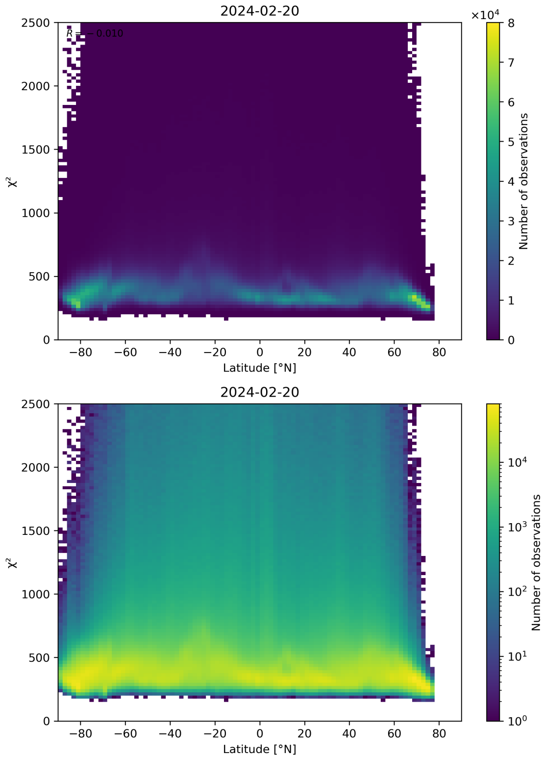
Figure 86: Scatter density plot of “Latitude” against “ \chi^2 ” for 2024-02-19 to 2024-02-21.
