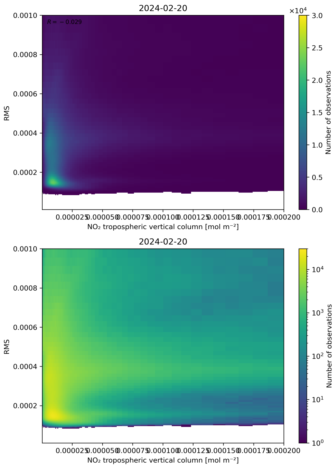
Figure 142: Scatter density plot of “NO 2 tropospheric vertical column” against “RMS” for 2024-02-19 to 2024-02-21.
