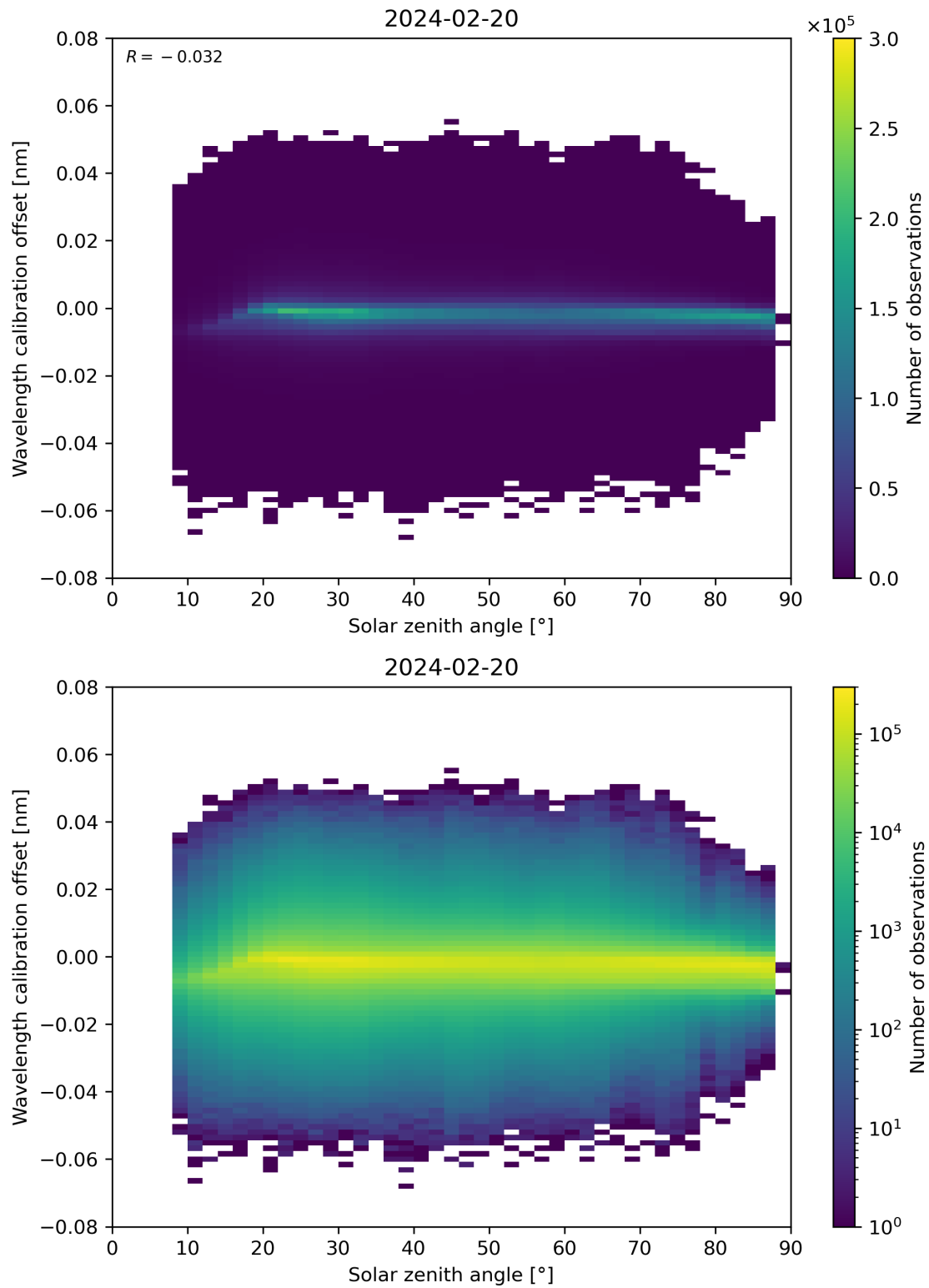
Figure 158: Scatter density plot of “Solar zenith angle” against “Wavelength calibration offset” for 2024-02-19 to 2024-02-21.
