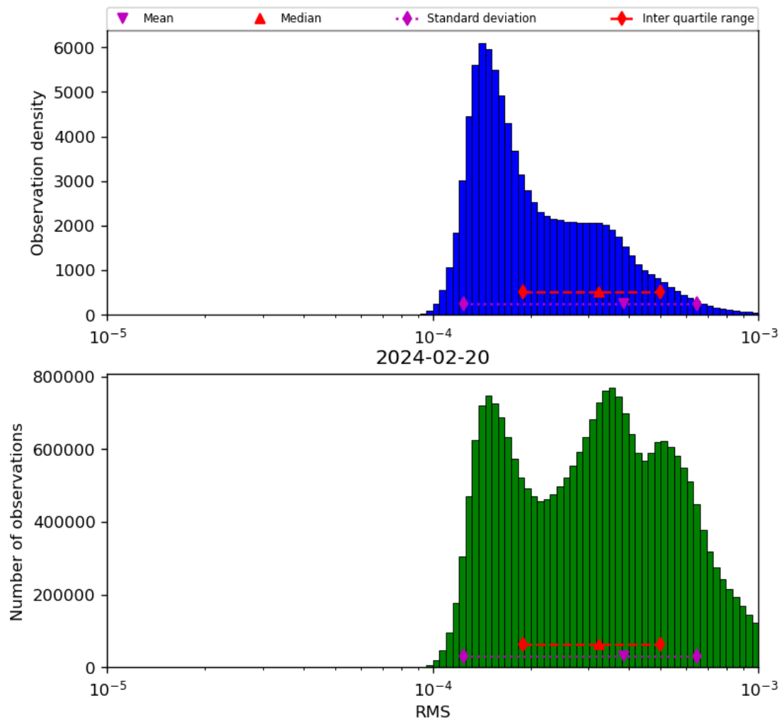
Figure 43: Histogram of “RMS” for 2024-02-19 to 2024-02-21
