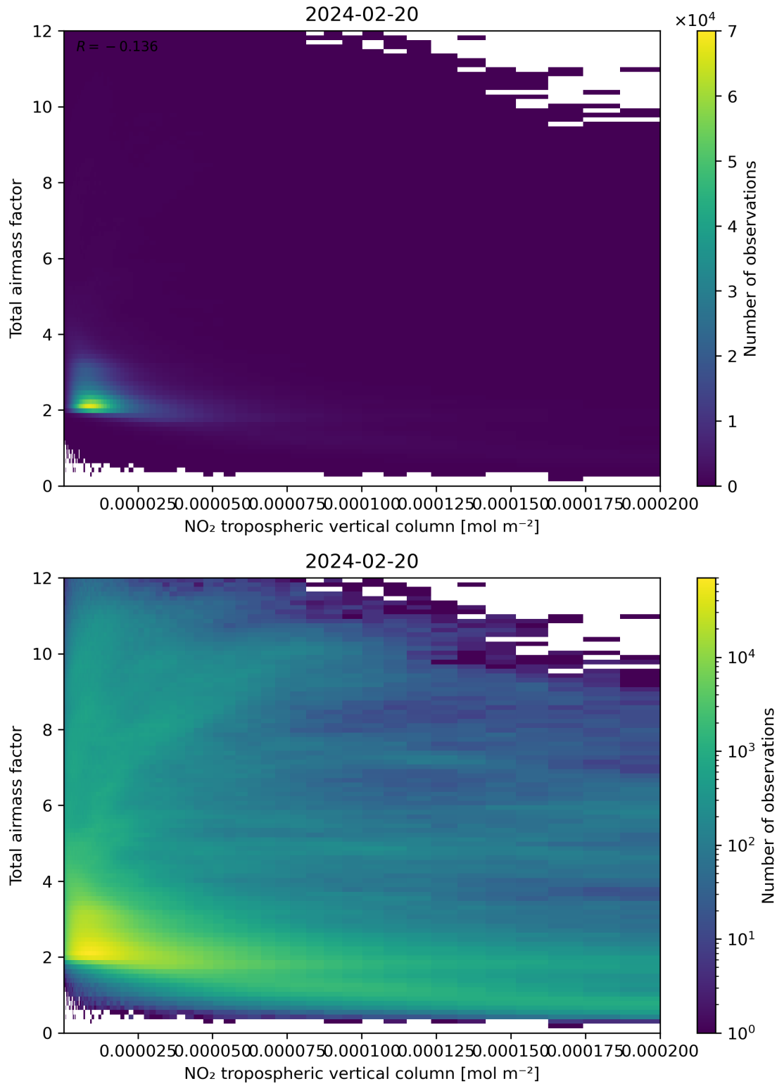
Figure 122: Scatter density plot of “NO 2 tropospheric vertical column” against “Total air mass factor” for 2024-02-19 to 2024-02-21.
