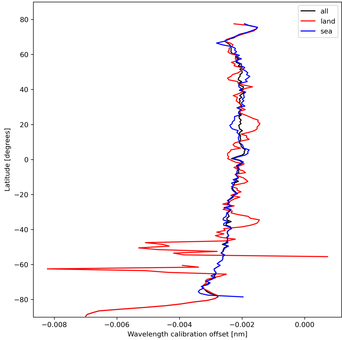
Figure 18: Zonal average of “Wavelength calibration offset” for 2024-02-19 to 2024-02-21.
