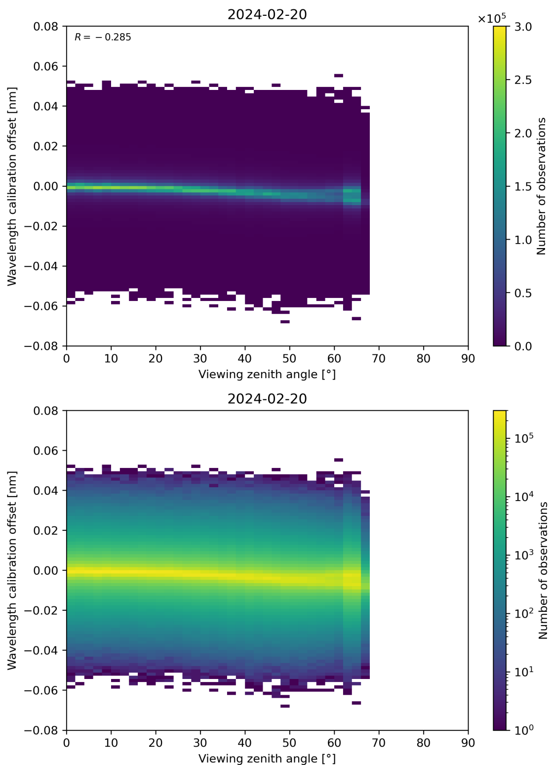
Figure 173: Scatter density plot of “Viewing zenith angle” against “Wavelength calibration offset” for 2024-02-19 to 2024-02-21.
