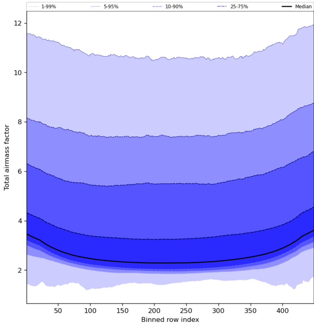
Figure 49: Along track statistics of “Total airmass factor” for 2024-02-19 to 2024-02-21
