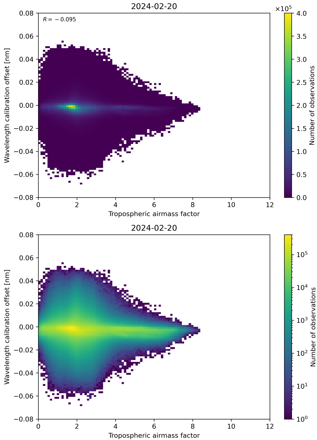
Figure 80: Scatter density plot of “Tropospheric airmass factor” against “Wavelength calibration offset” for 2024-02-19 to 2024-02-21.
