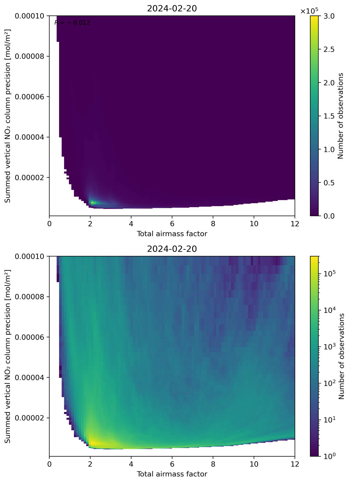
Figure 66: Scatter density plot of “Total airmass factor” against “Summed vertical NO 2 column precision” for 2024-02-19 to 2024-02-21.
