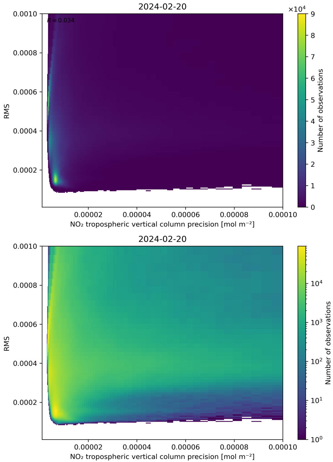
Figure 140: Scatter density plot of “NO 2 tropospheric vertical column precision” against “RMS” for 2024-02-19 to 2024-02-21.
