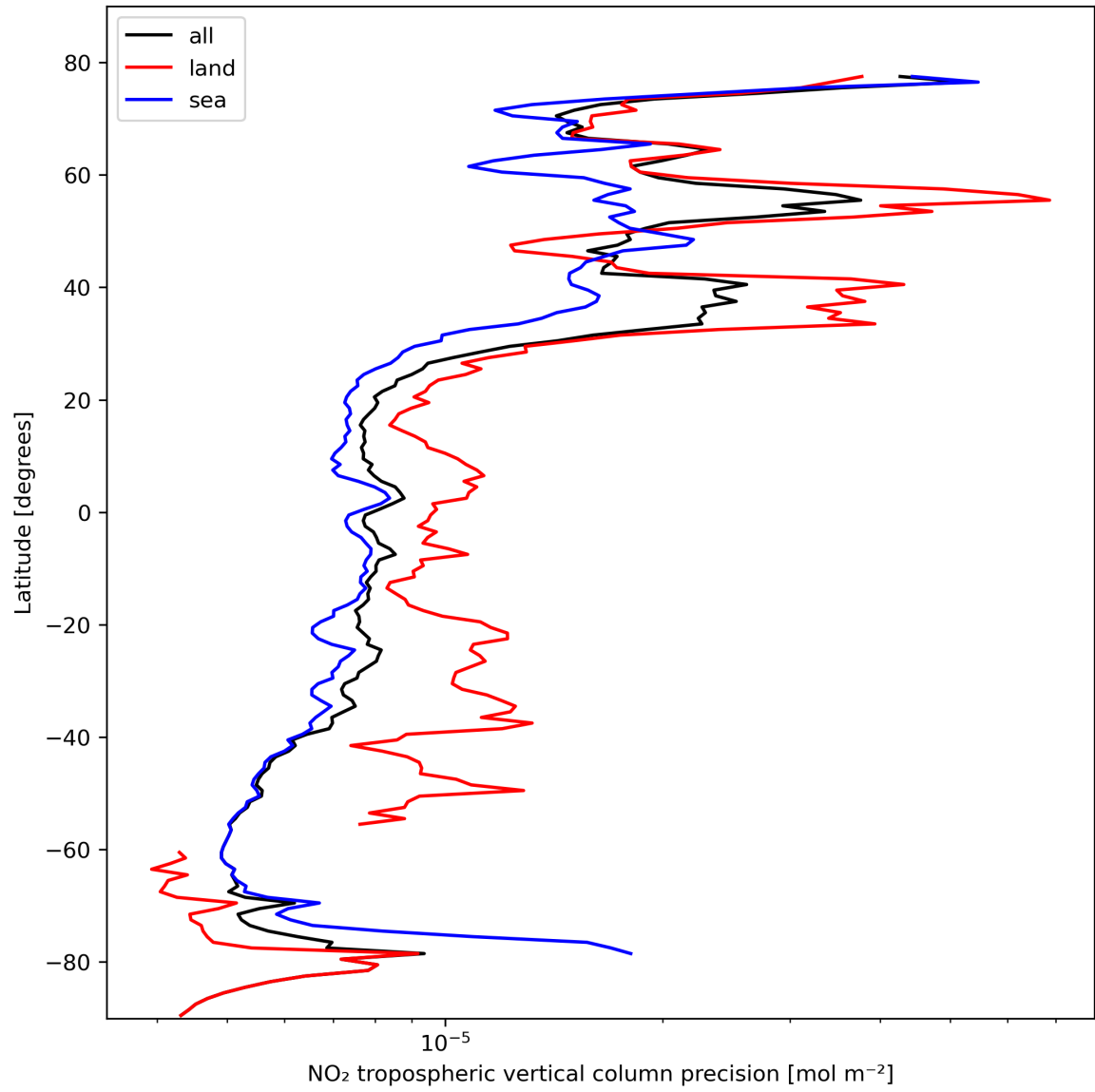
Figure 13: Zonal average of “NO 2 tropospheric vertical column precision” for 2024-02-19 to 2024-02-21.
