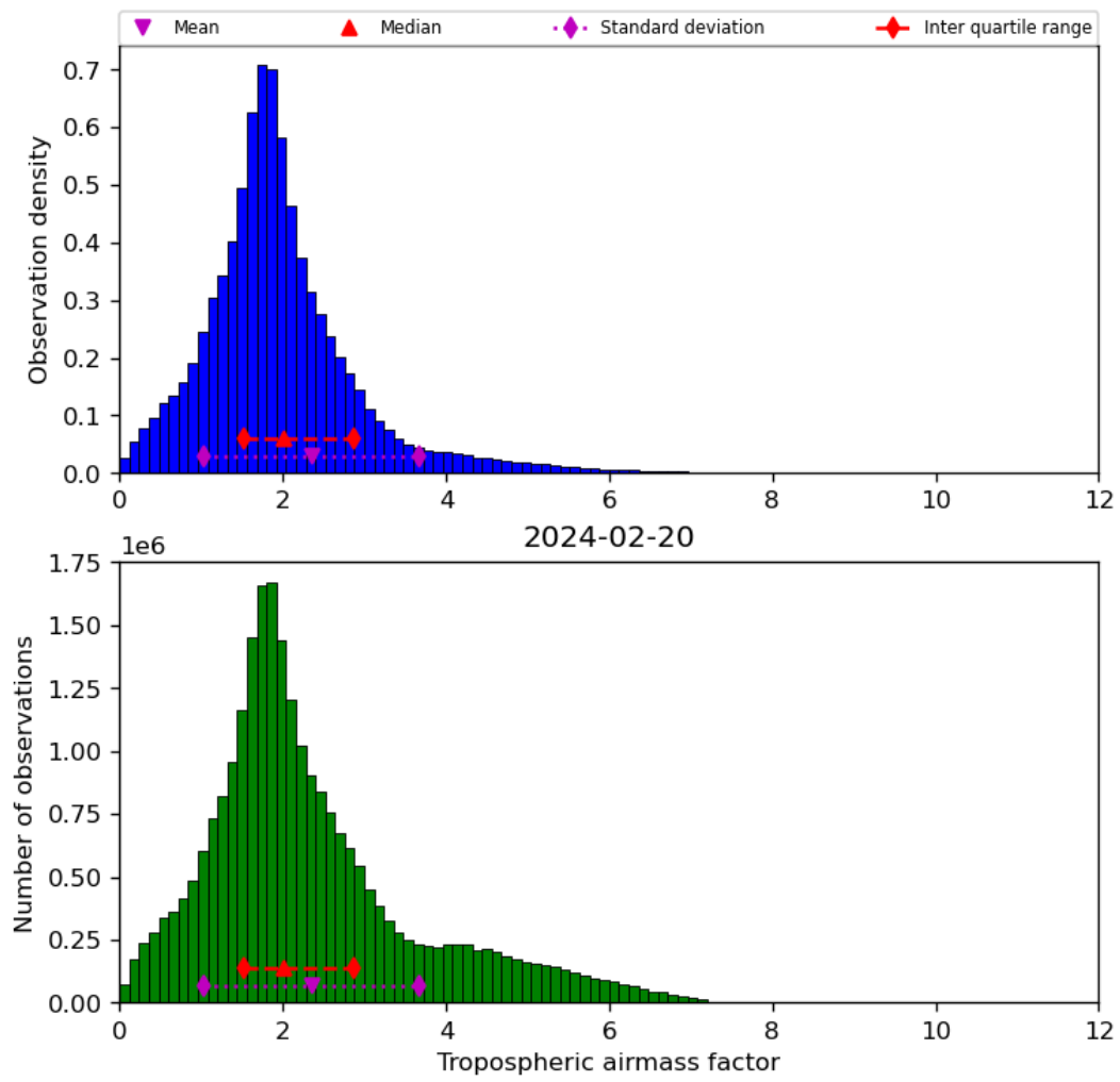
Figure 31: Histogram of “Tropospheric airmass factor” for 2024-02-19 to 2024-02-21
