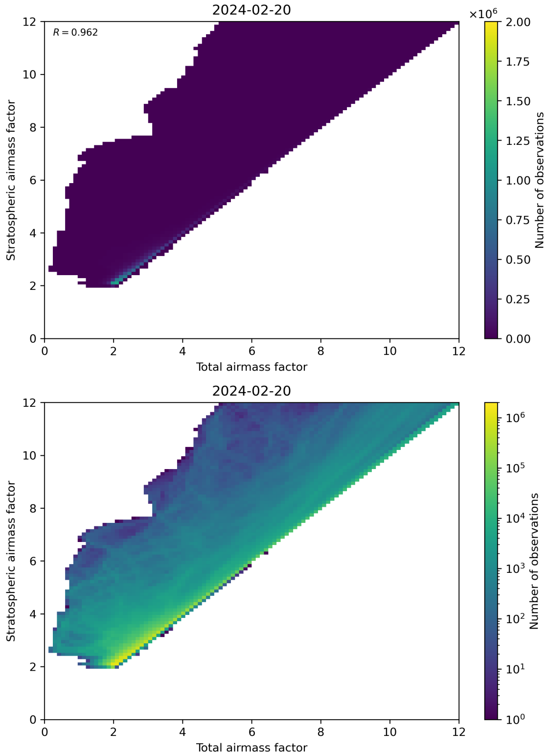
Figure 62: Scatter density plot of “Total airmass factor” against “Stratospheric airmass factor” for 2024-02-19 to 2024-02-21.
