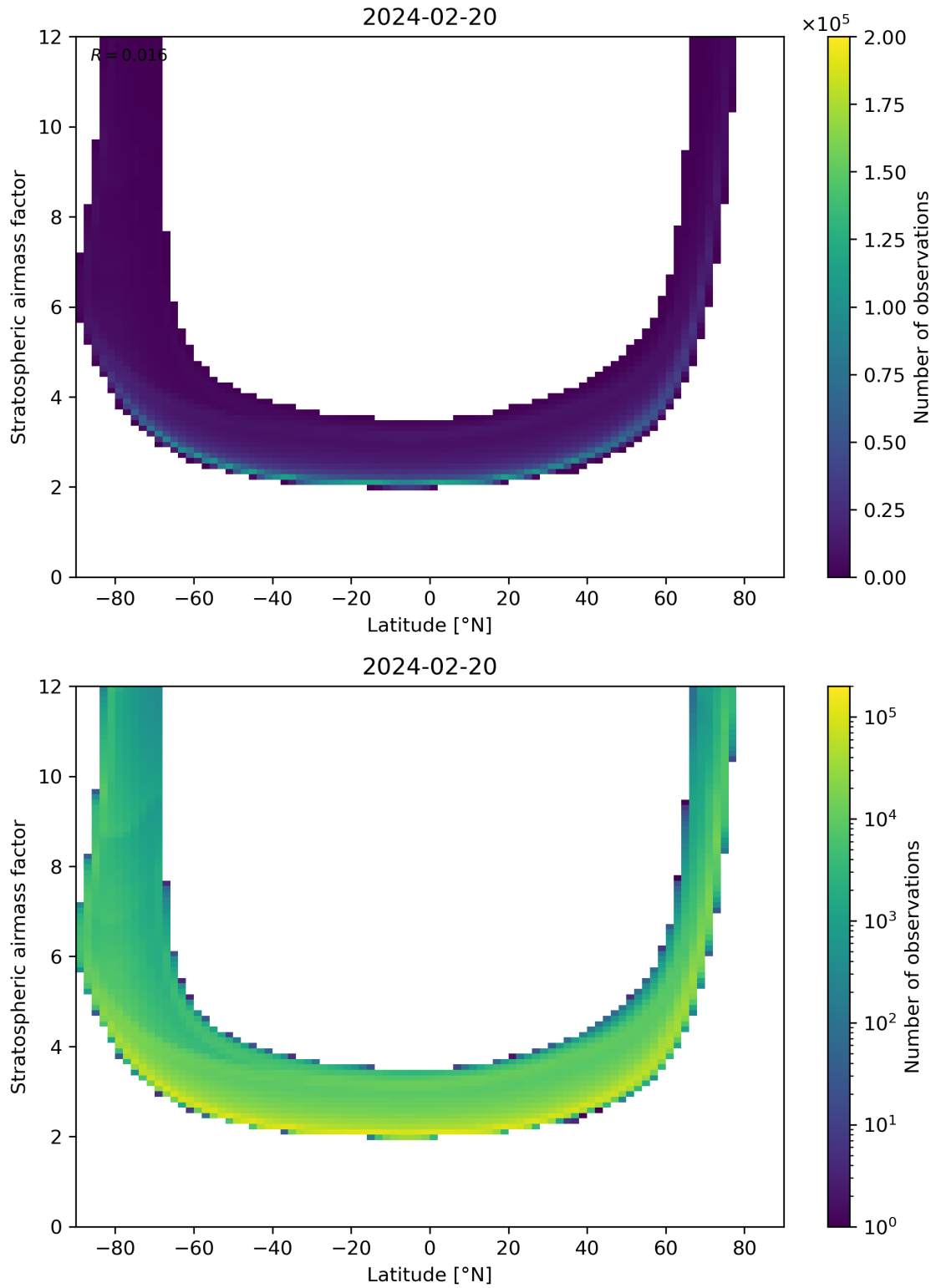
Figure 83: Scatter density plot of “Latitude” against “Stratospheric airmass factor” for 2024-02-19 to 2024-02-21.
