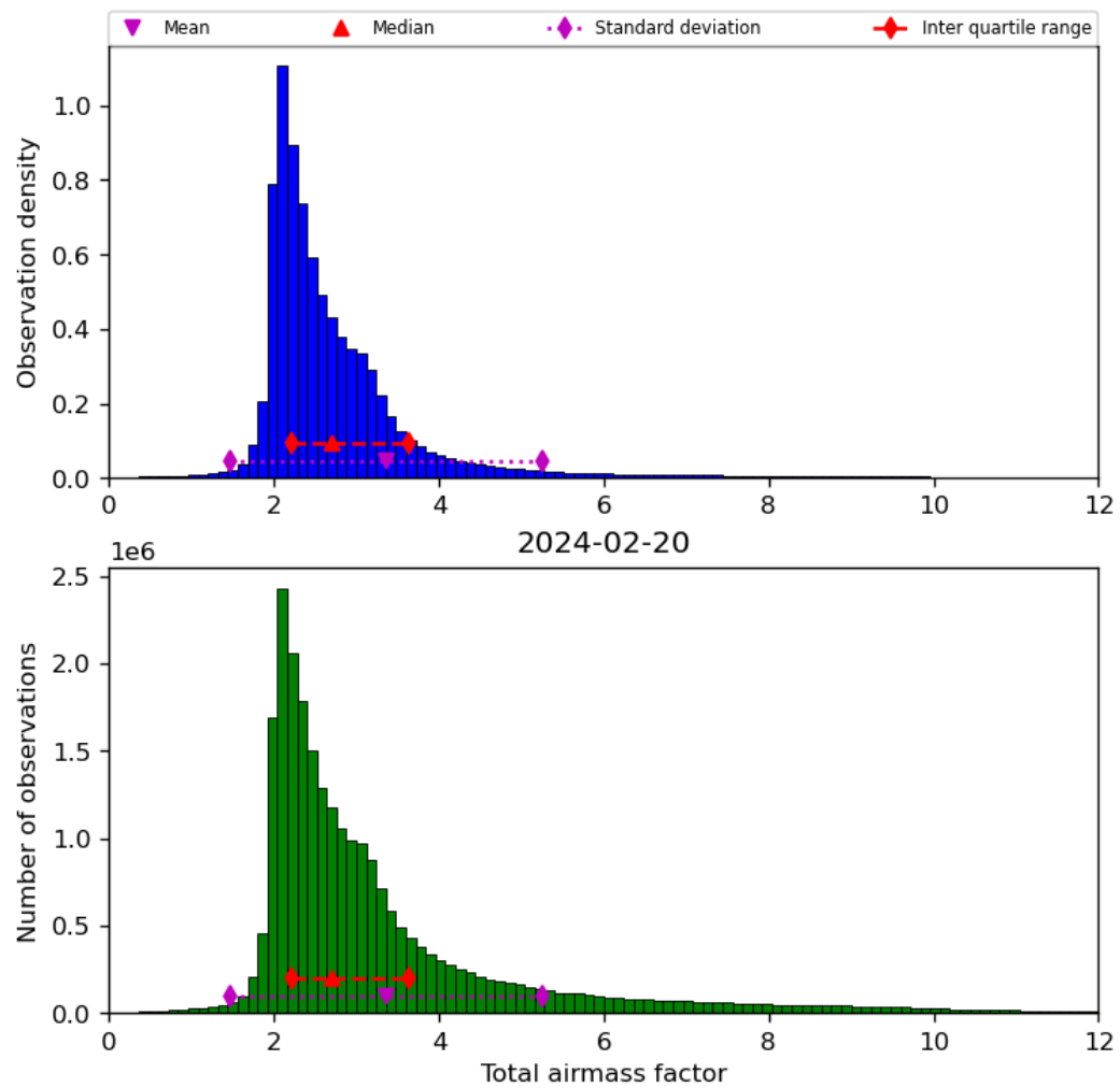
Figure 32: Histogram of “Total airmass factor” for 2024-02-19 to 2024-02-21
