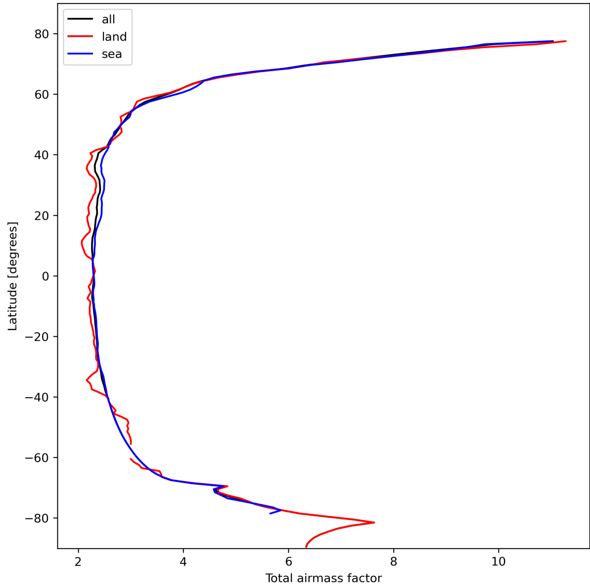
Figure 15: Zonal average of “Total airmass factor” for 2024-02-19 to 2024-02-21.
