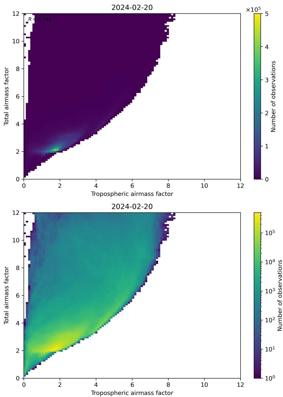
Figure 72: Scatter density plot of “Tropospheric airmass factor” against “Total airmass factor” for 2024-02-19 to 2024-02-21.
