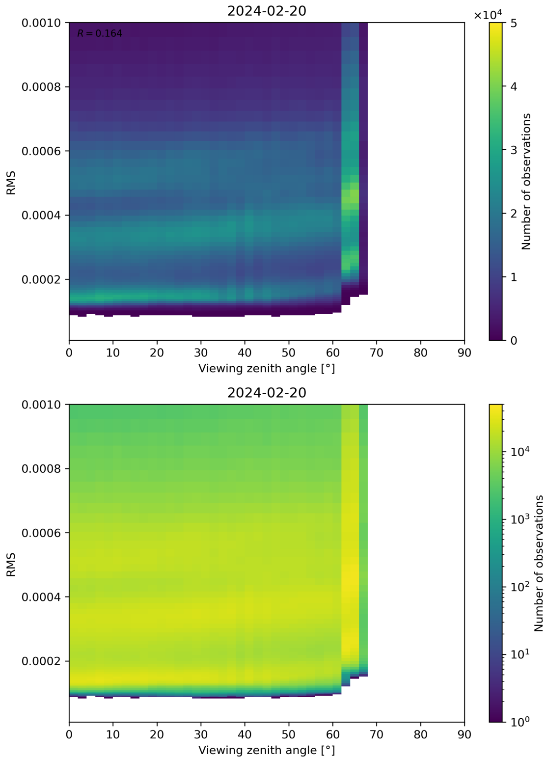
Figure 171: Scatter density plot of “Viewing zenith angle” against “RMS” for 2024-02-19 to 2024-02-21.
