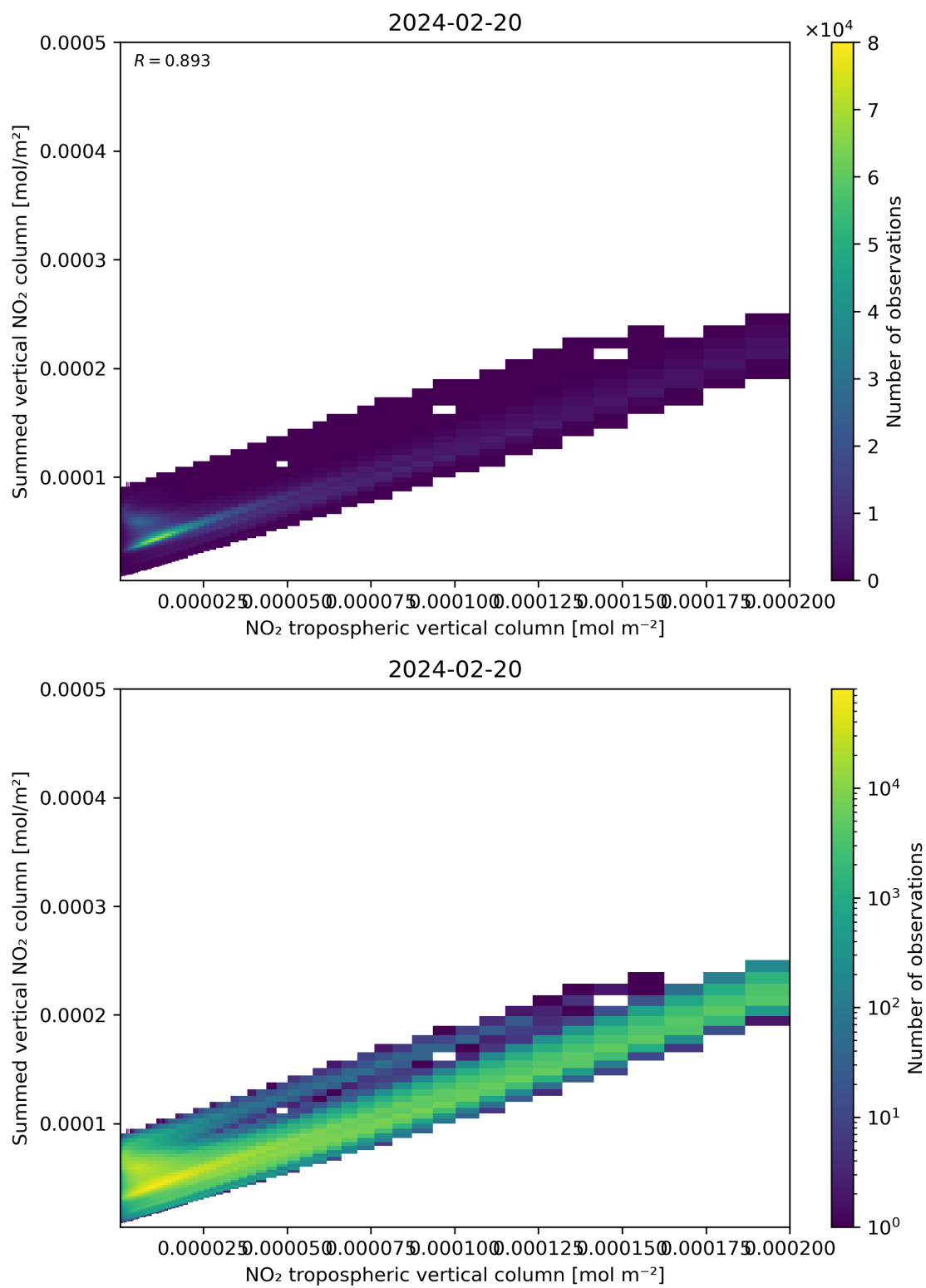
Figure 126: Scatter density plot of “NO 2 tropospheric vertical column” against “Summed vertical NO 2 column” for 2024-02-19 to 2024-02-21.
