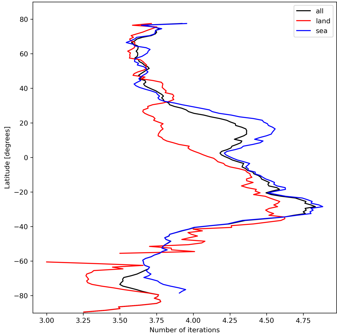
Figure 17: Zonal average of “Number of iterations” for 2024-02-19 to 2024-02-21.
