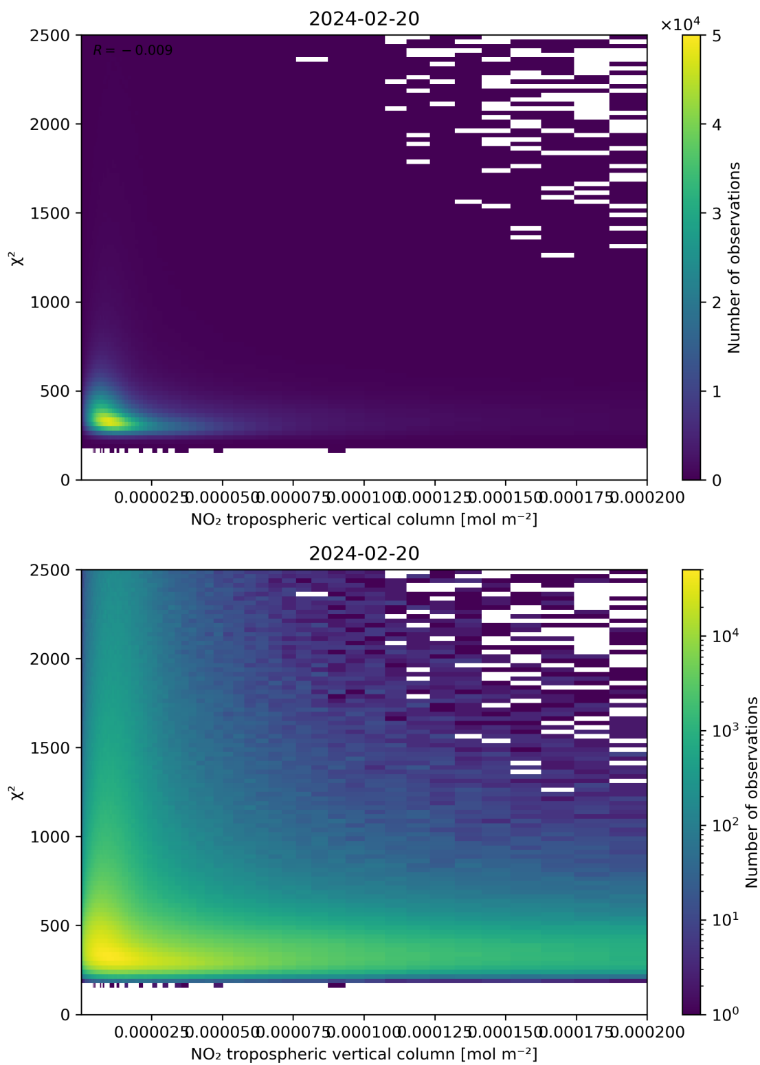
Figure 124: Scatter density plot of “NO 2 tropospheric vertical column” against “ \chi^2 ” for 2024-02-19 to 2024-02-21.
