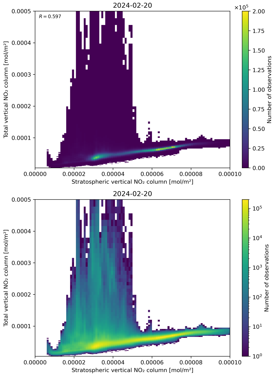
Figure 100: Scatter density plot of “Stratospheric vertical NO 2 column” against “Total vertical NO 2 column” for 2024-02-19 to 2024-02-21.
