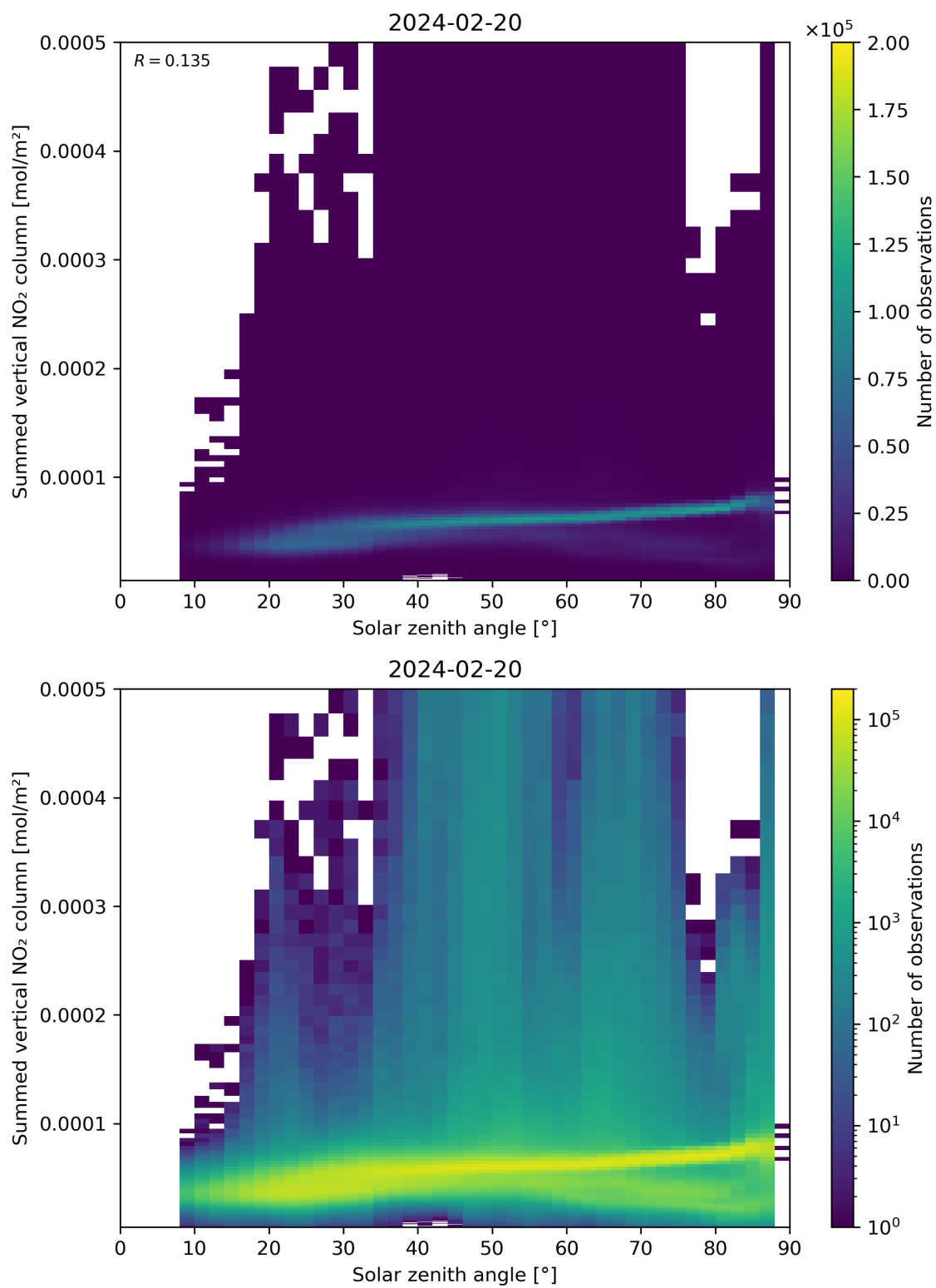
Figure 151: Scatter density plot of “Solar zenith angle” against “Summed vertical NO 2 column” for 2024-02-19 to 2024-02-21.
