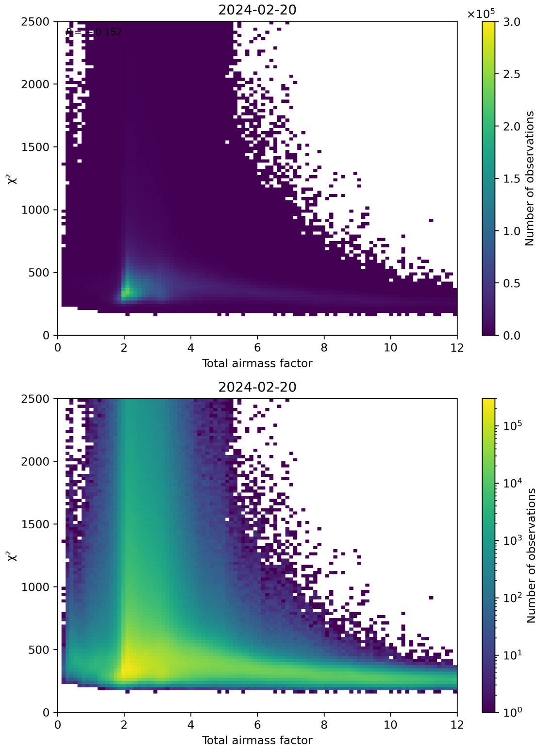
Figure 63: Scatter density plot of “Total airmass factor” against “ \chi^2 ” for 2024-02-19 to 2024-02-21.
