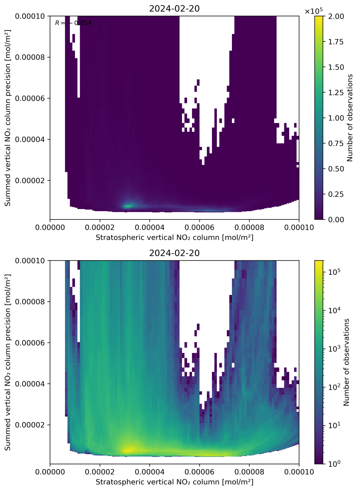
Figure 99: Scatter density plot of “Stratospheric vertical NO 2 column” against “Summed vertical NO 2 column precision” for 2024-02-19 to 2024-02-21.
