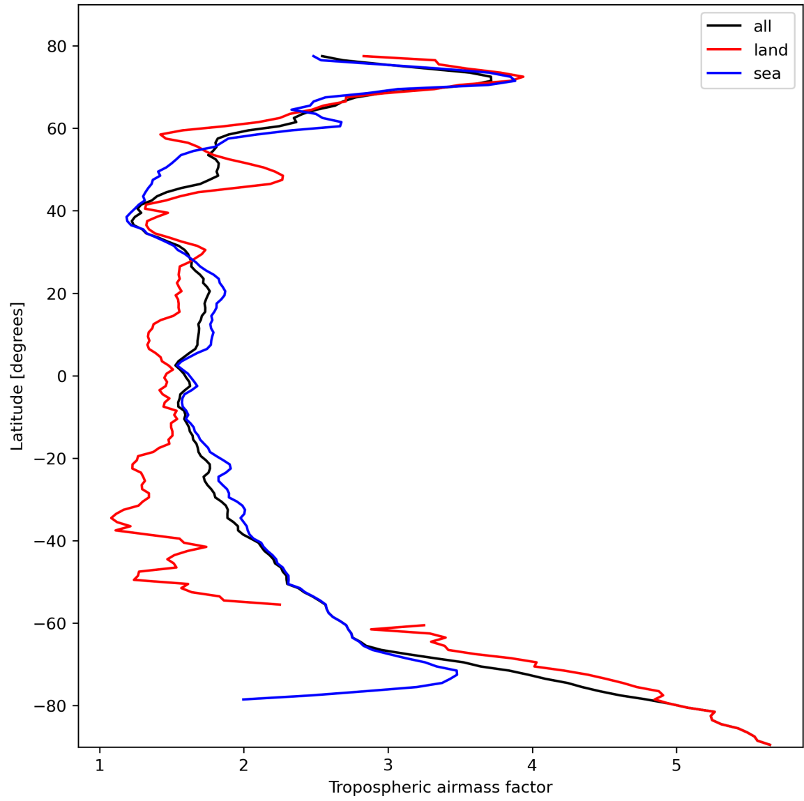
Figure 14: Zonal average of “Tropospheric airmass factor” for 2024-02-19 to 2024-02-21.
