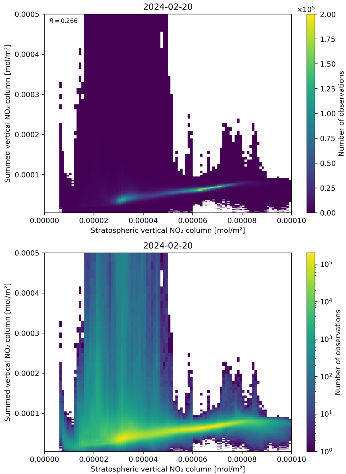
Figure 98: Scatter density plot of “Stratospheric vertical NO 2 column” against “Summed vertical NO 2 column” for 2024-02-19 to 2024-02-21.
