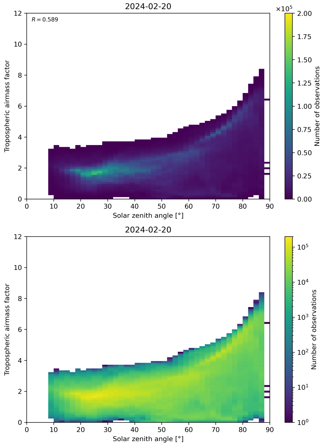
Figure 147: Scatter density plot of “Solar zenith angle” against “Tropospheric airmass factor” for 2024-02-19 to 2024-02-21.
