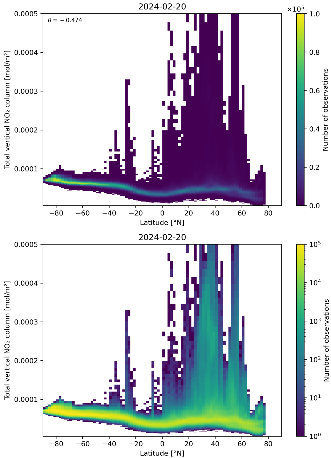
Figure 90: Scatter density plot of “Latitude” against “Total vertical NO 2 column” for 2024-02-19 to 2024-02-21.
