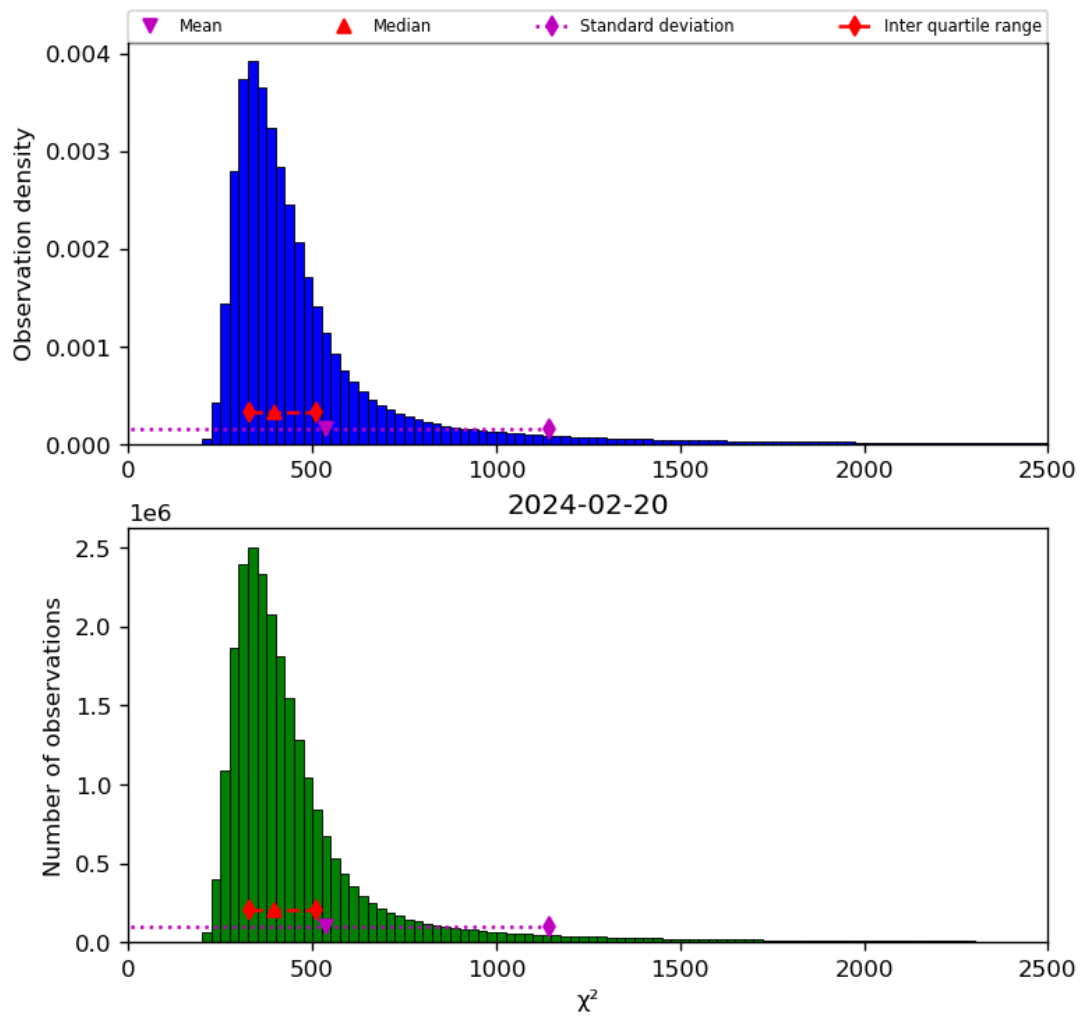
Figure 42: Histogram of “ \chi^2 ” for 2024-02-19 to 2024-02-21
