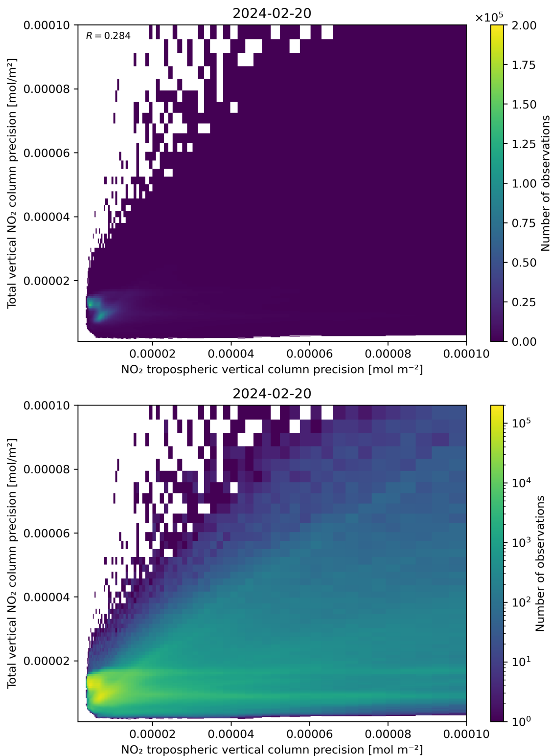
Figure 139: Scatter density plot of “NO 2 tropospheric vertical column precision” against “Total vertical NO 2 column precision” for 2024-02-19 to 2024-02-21.
