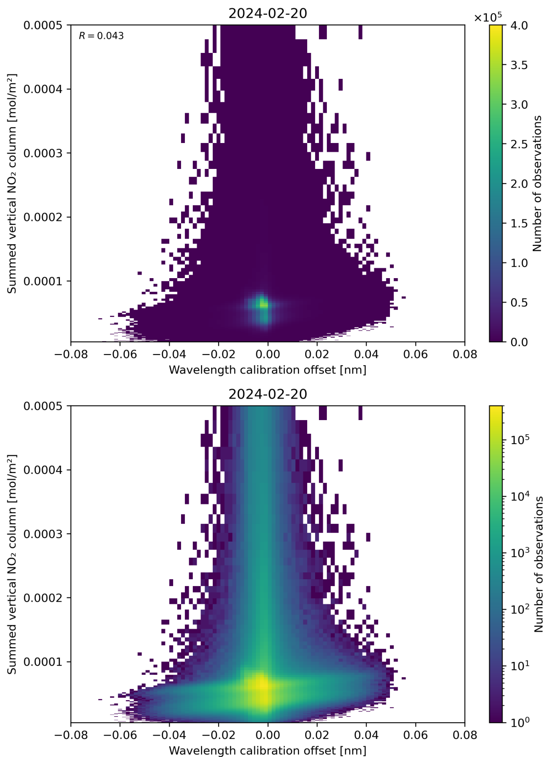
Figure 177: Scatter density plot of “Wavelength calibration offset” against “Summed vertical NO 2 column” for 2024-02-19 to 2024-02-21.
