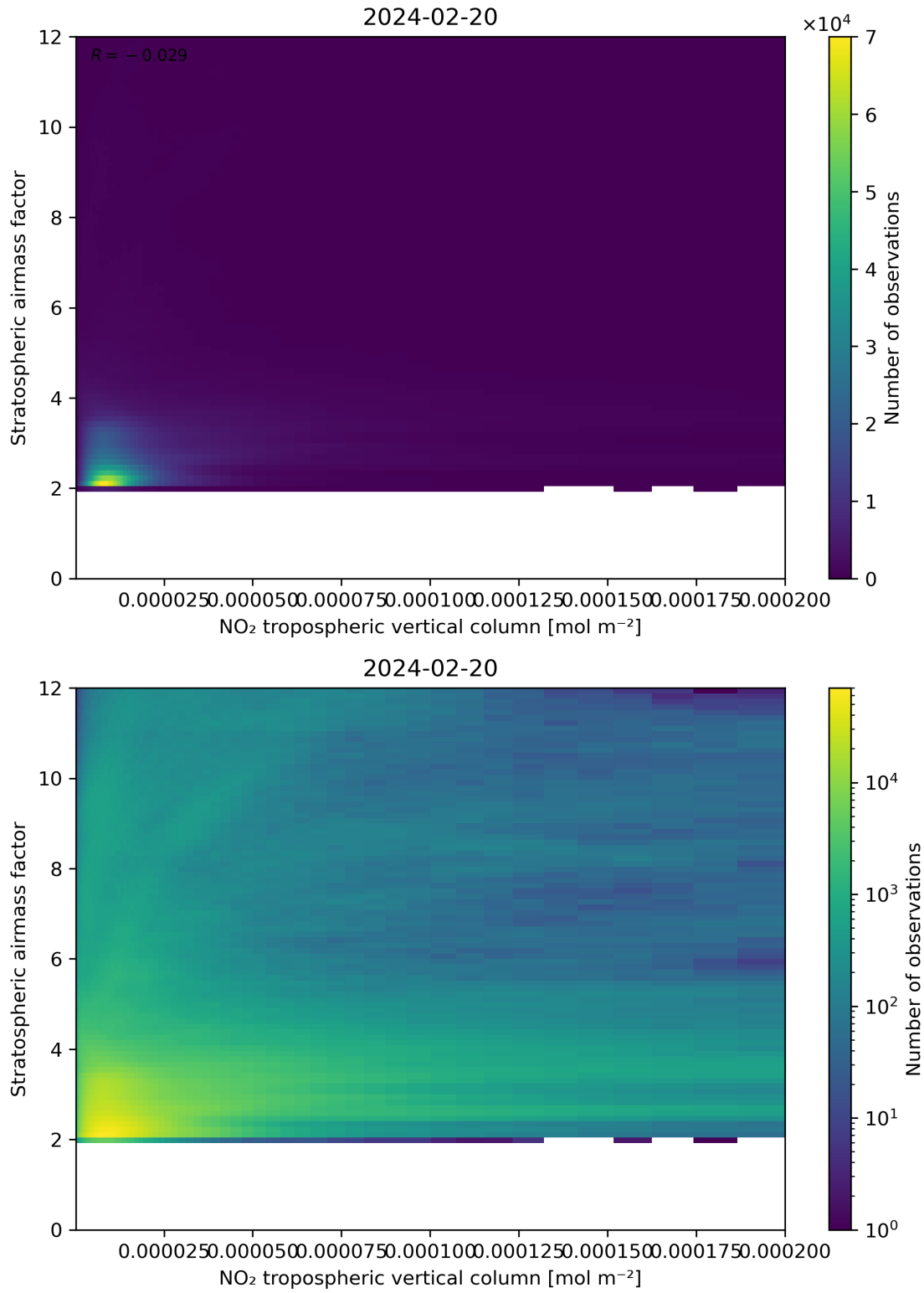
Figure 121: Scatter density plot of “NO 2 tropospheric vertical column” against “Stratospheric airmass factor” for 2024-02-19 to 2024-02-21.
