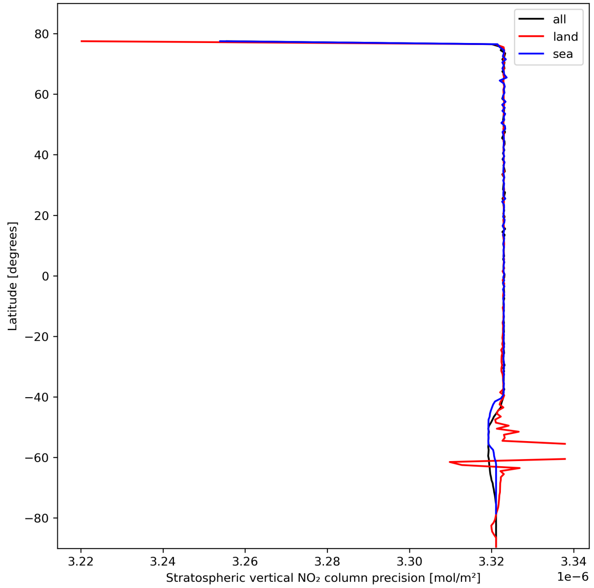
Figure 20: Zonal average of “Stratospheric vertical NO 2 column precision” for 2024-02-19 to 2024-02-21.
