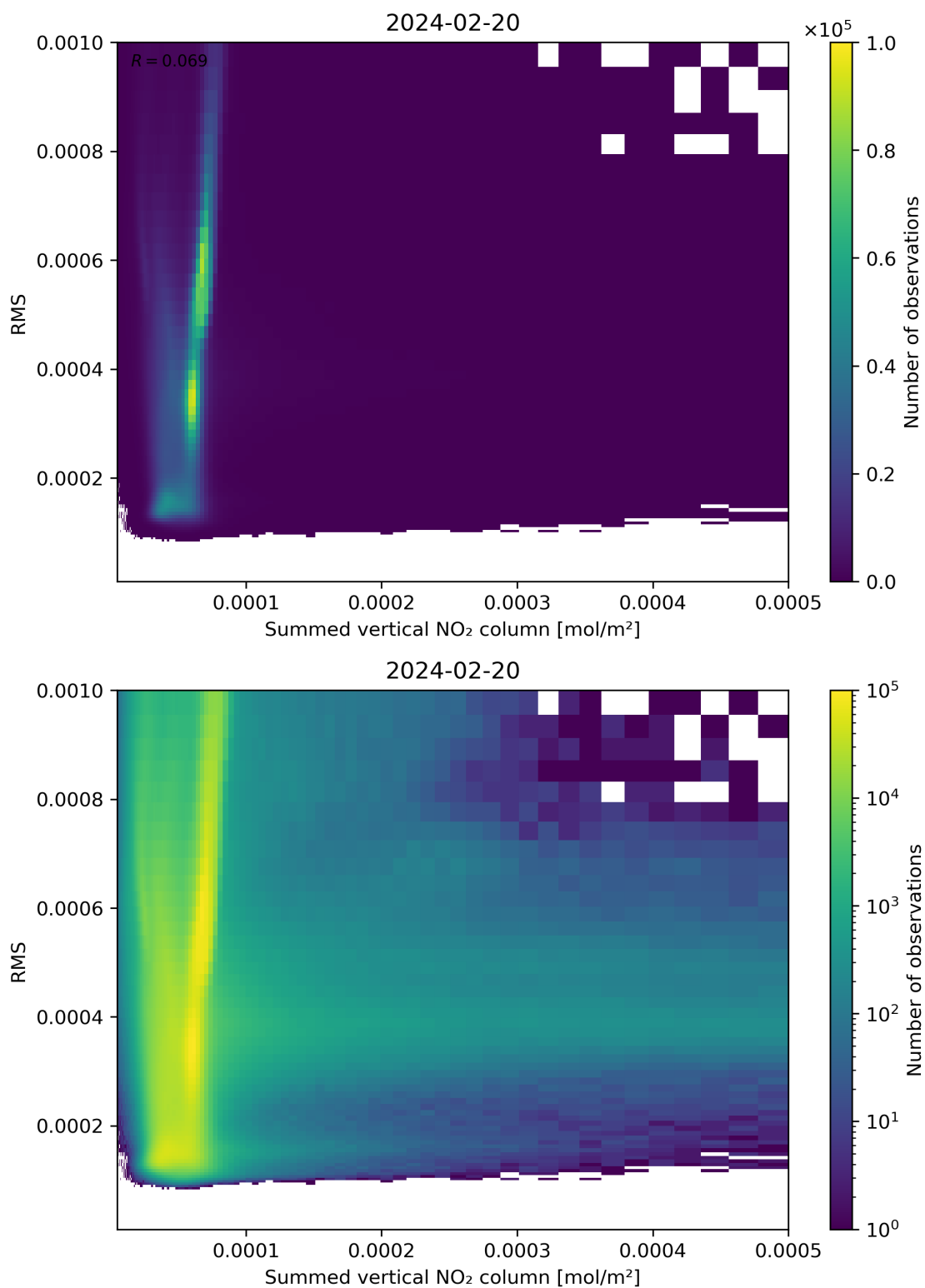
Figure 109: Scatter density plot of “Summed vertical NO 2 column” against “RMS” for 2024-02-19 to 2024-02-21.
