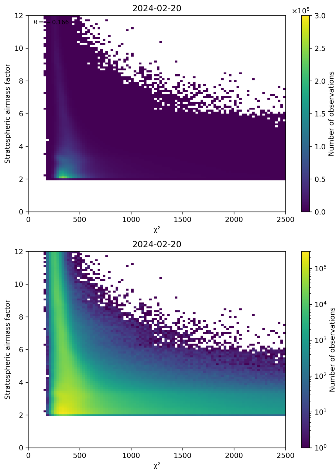
Figure 81: Scatter density plot of “ \chi^2 ” against “Stratospheric air mass factor” for 2024-02-19 to 2024-02-21.
