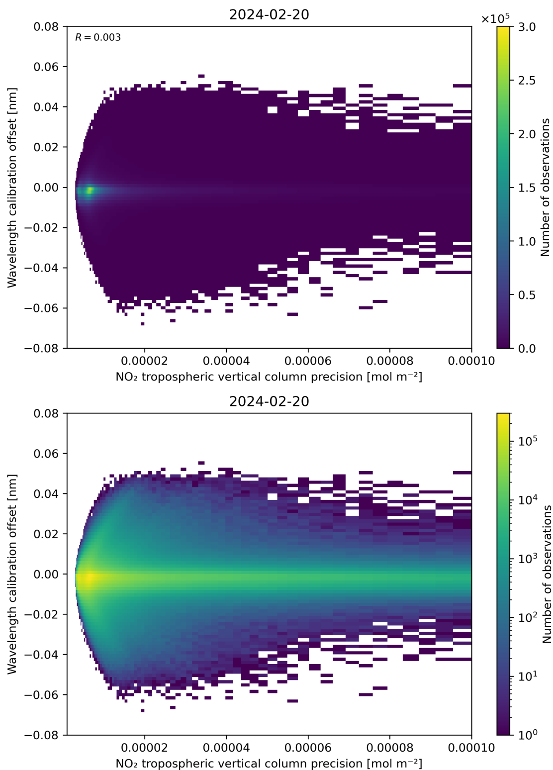
Figure 141: Scatter density plot of “NO 2 tropospheric vertical column precision” against “Wavelength calibration offset” for 2024-02-19 to 2024-02-21.
