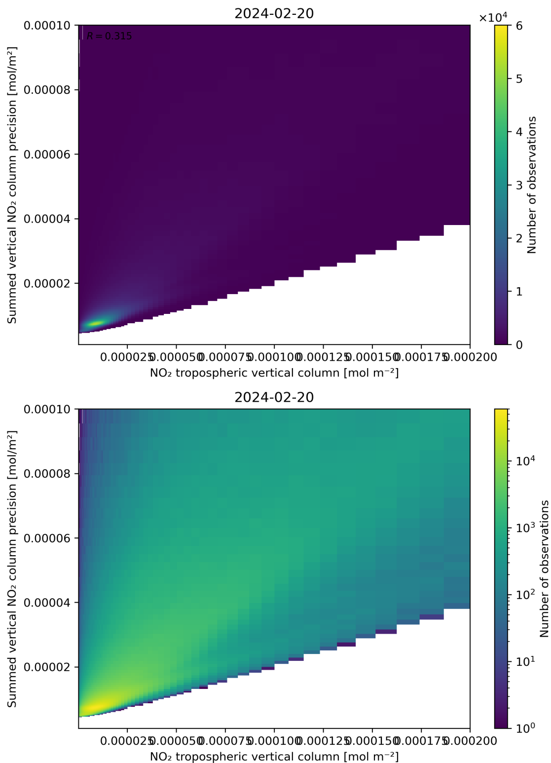
Figure 127: Scatter density plot of “NO 2 tropospheric vertical column” against “Summed vertical NO 2 column precision” for 2024-02-19 to 2024-02-21.
