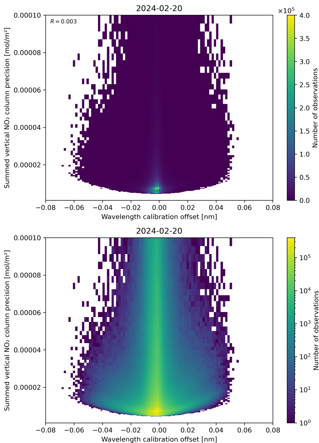
Figure 178: Scatter density plot of “Wavelength calibration offset” against “Summed vertical NO 2 column precision” for 2024-02-19 to 2024-02-21.
