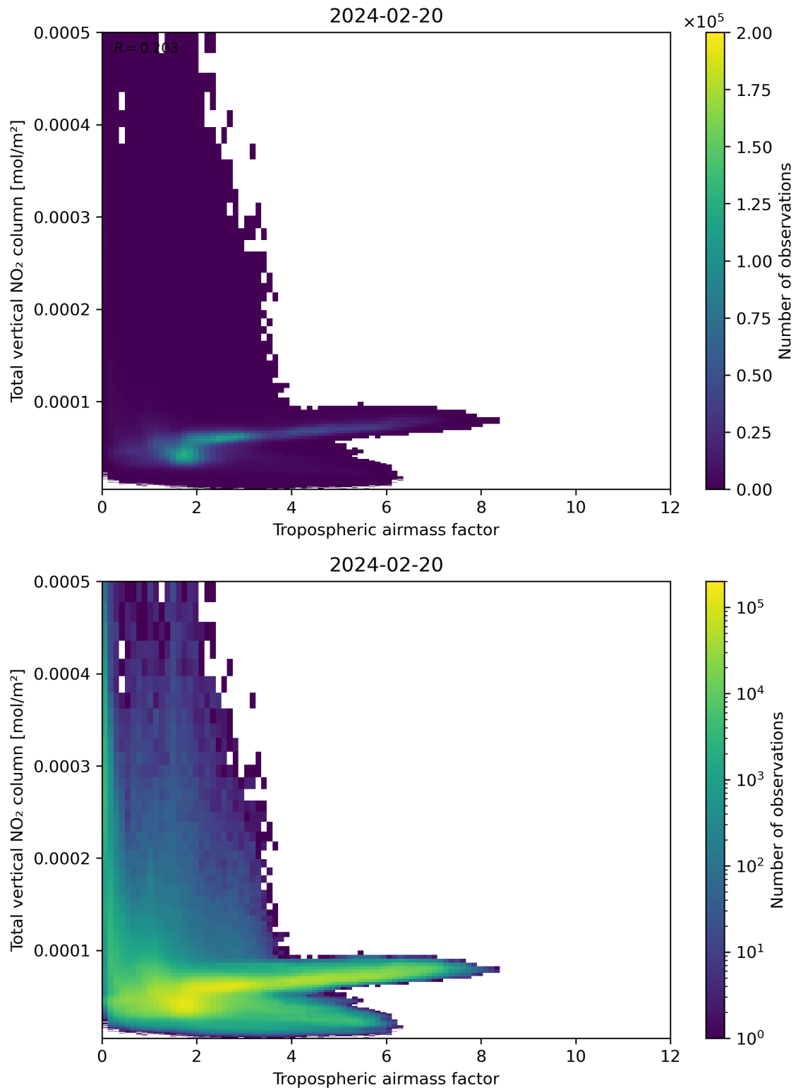
Figure 77: Scatter density plot of “Tropospheric airmass factor” against “Total vertical NO 2 column” for 2024-02-19 to 2024-02-21.
