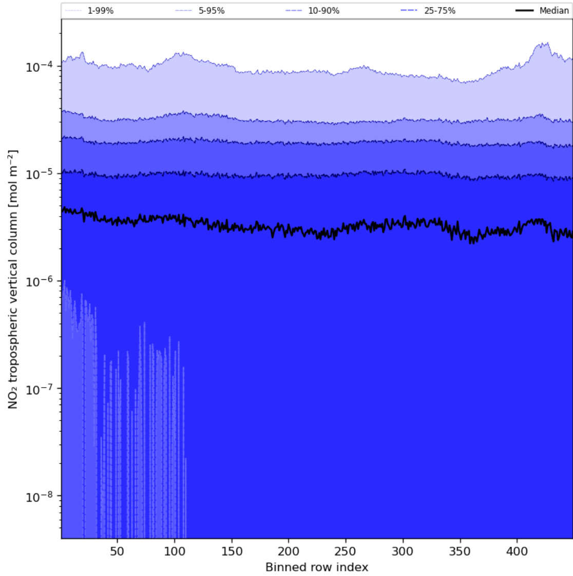
Figure 46: Along track statistics of “NO 2 tropospheric vertical column” for 2024-02-19 to 2024-02-21
