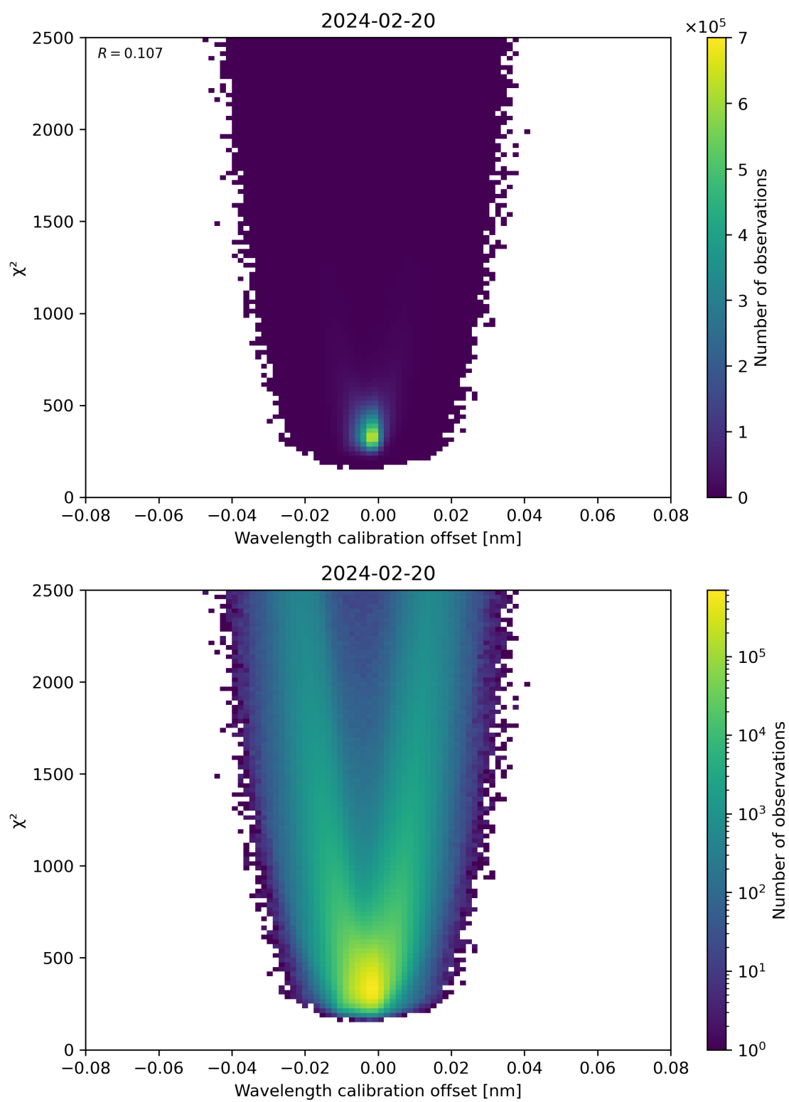
Figure 175: Scatter density plot of “Wavelength calibration offset” against “ \chi^2 ” for 2024-02-19 to 2024-02-21.
