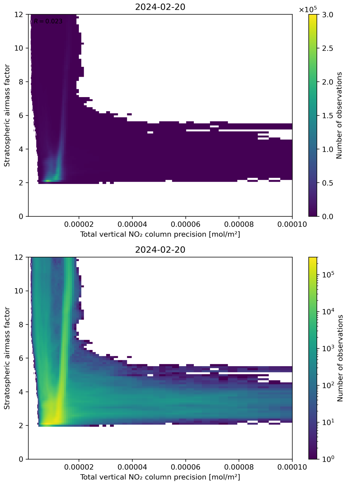
Figure 115: Scatter density plot of “Total vertical NO 2 column precision” against “Stratospheric airmass factor” for 2024-02-19 to 2024-02-21.
