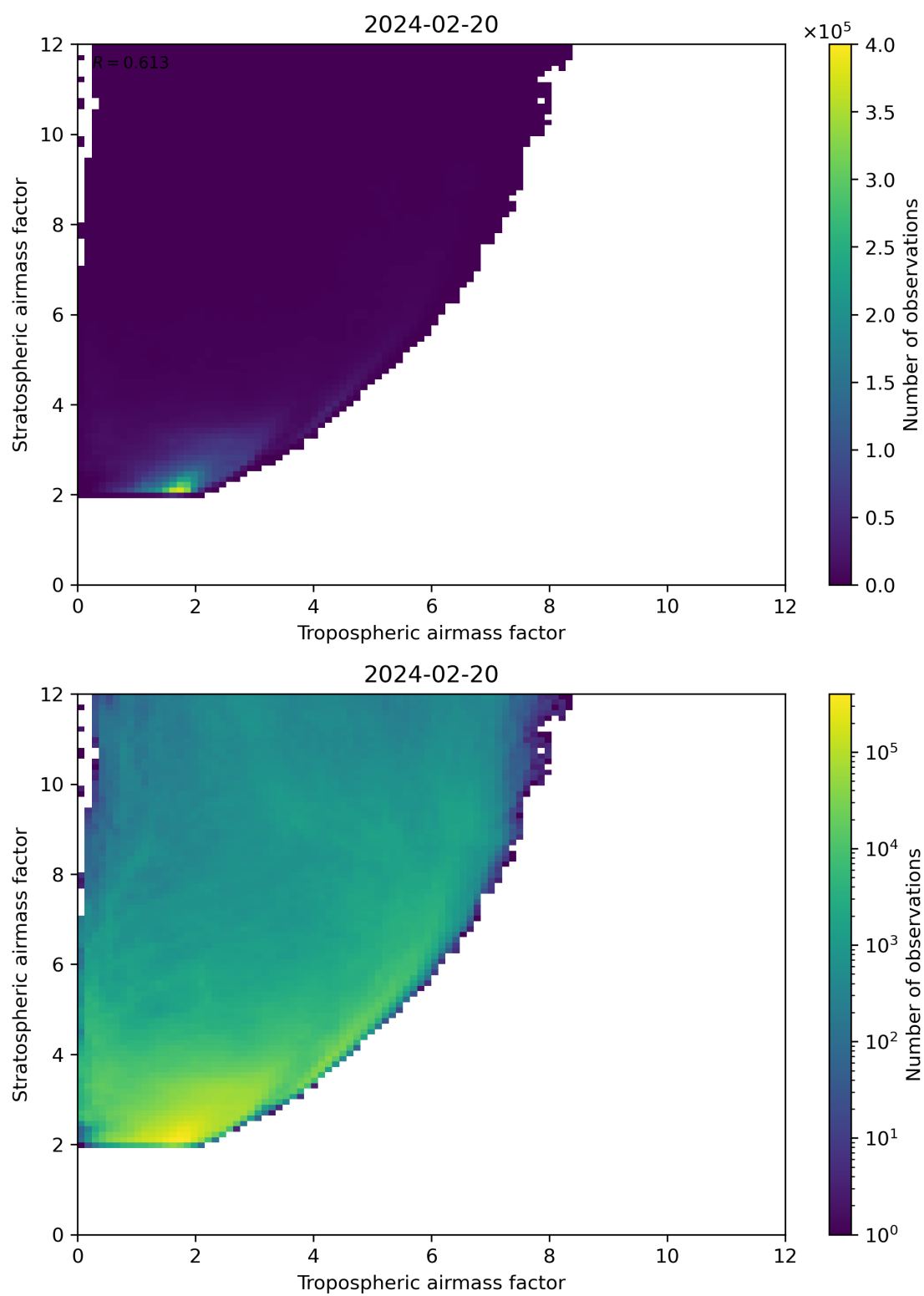
Figure 71: Scatter density plot of “Tropospheric airmass factor” against “Stratospheric airmass factor” for 2024-02-19 to 2024-02-21.
