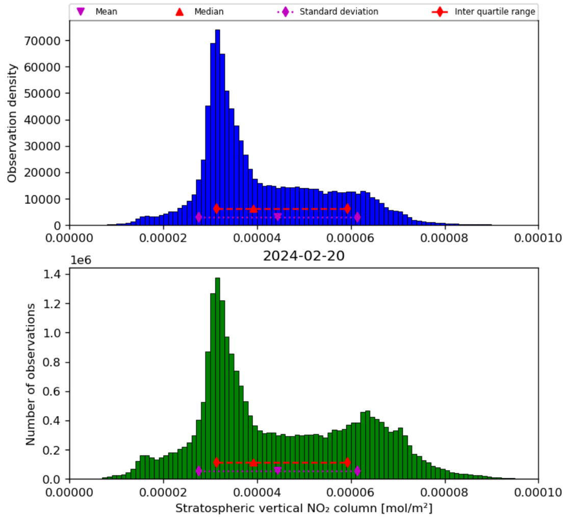
Figure 36: Histogram of “Stratospheric vertical NO 2 column” for 2024-02-19 to 2024-02-21
