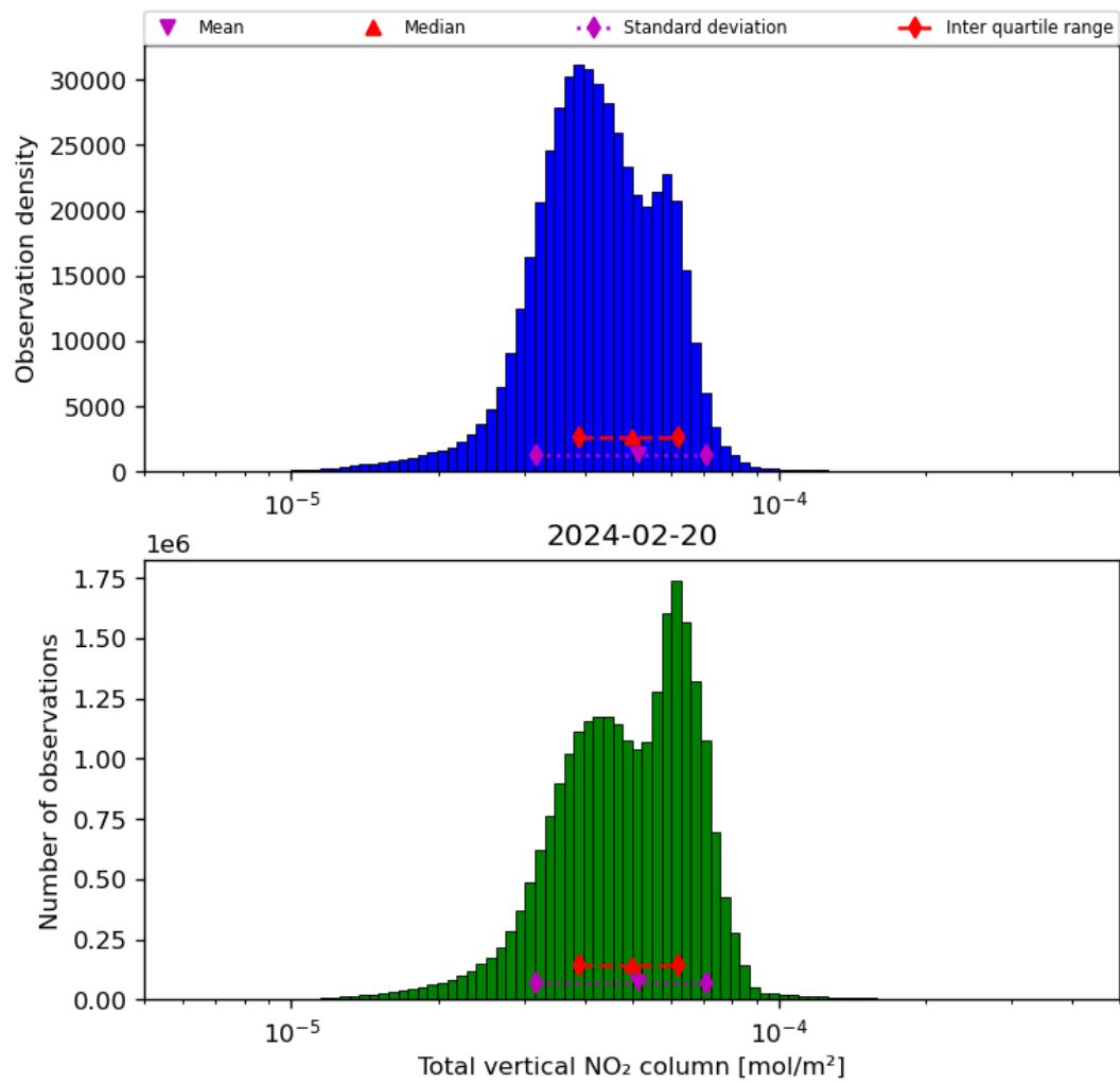
Figure 38: Histogram of “Total vertical NO 2 column” for 2024-02-19 to 2024-02-21
