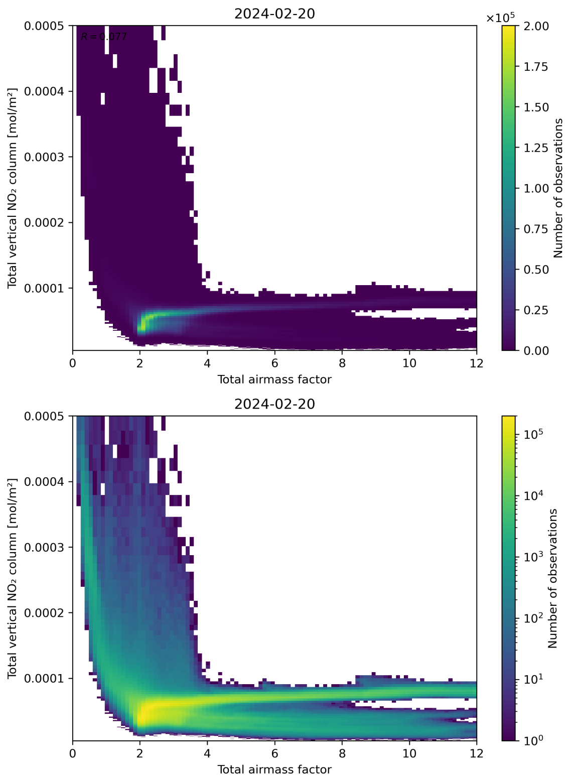
Figure 67: Scatter density plot of “Total airmass factor” against “Total vertical NO 2 column” for 2024-02-19 to 2024-02-21.
