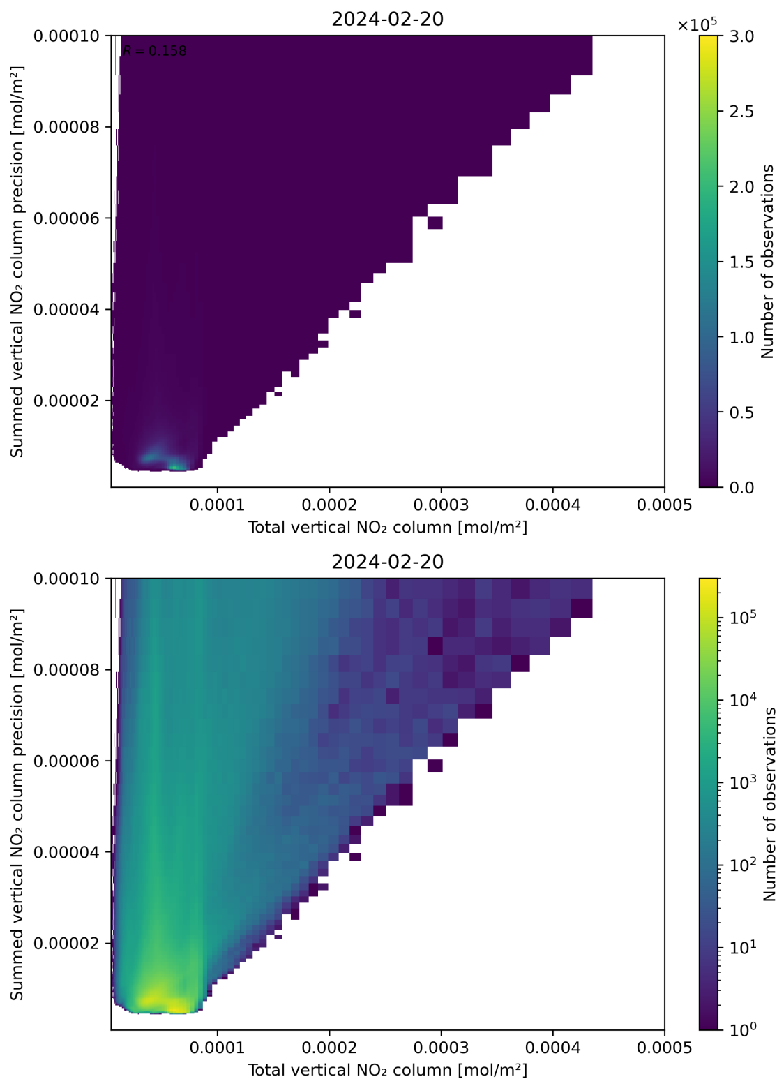
Figure 113: Scatter density plot of “Total vertical NO 2 column” against “Summed vertical NO 2 column precision” for 2024-02-19 to 2024-02-21.
