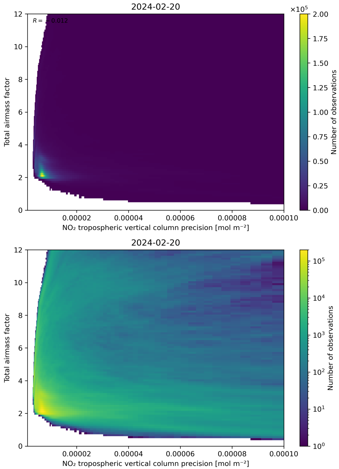
Figure 132: Scatter density plot of “NO 2 tropospheric vertical column precision” against “Total air mass factor” for 2024-02-19 to 2024-02-21.
