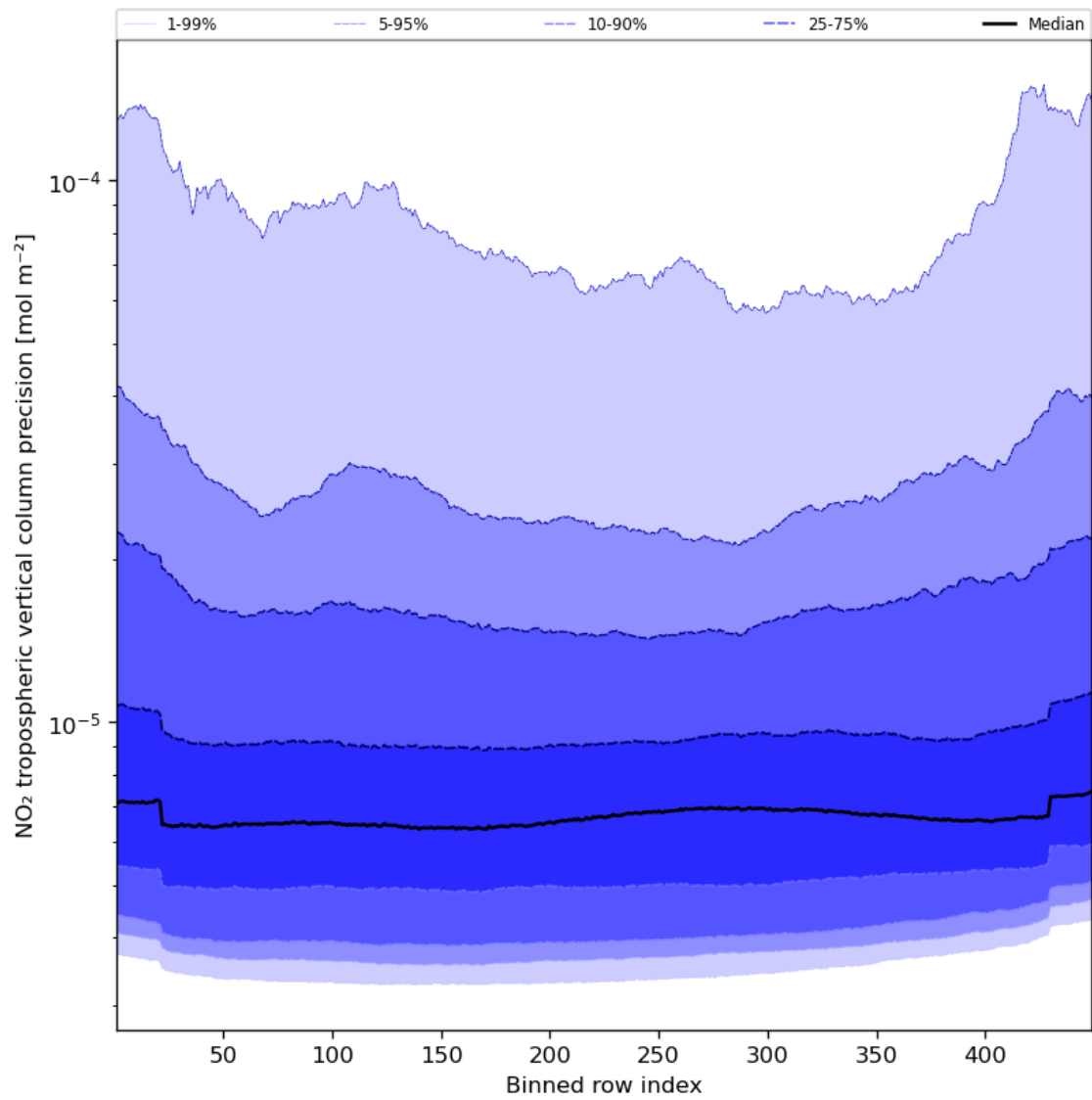
Figure 47: Along track statistics of “NO 2 tropospheric vertical column precision” for 2024-02-19 to 2024-02-21
