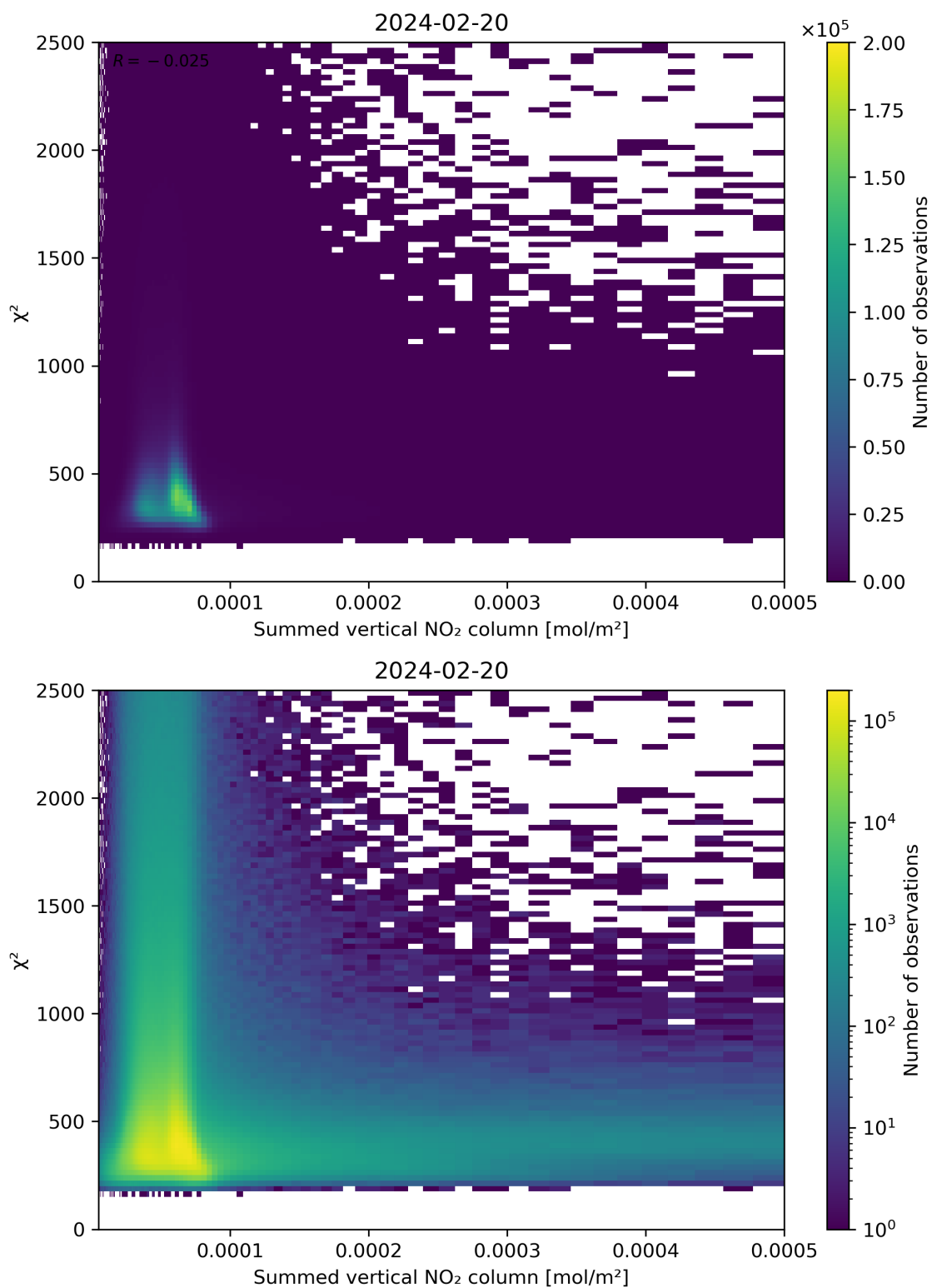
Figure 104: Scatter density plot of “Summed vertical NO 2 column” against “ \chi^2 ” for 2024-02-19 to 2024-02-21.
