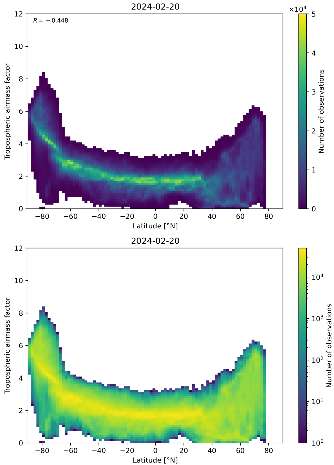
Figure 85: Scatter density plot of “Latitude” against “Tropospheric air mass factor” for 2024-02-19 to 2024-02-21.
