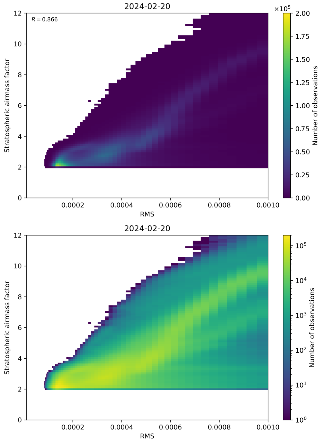
Figure 144: Scatter density plot of “RMS” against “Stratospheric airmass factor” for 2024-02-19 to 2024-02-21.
