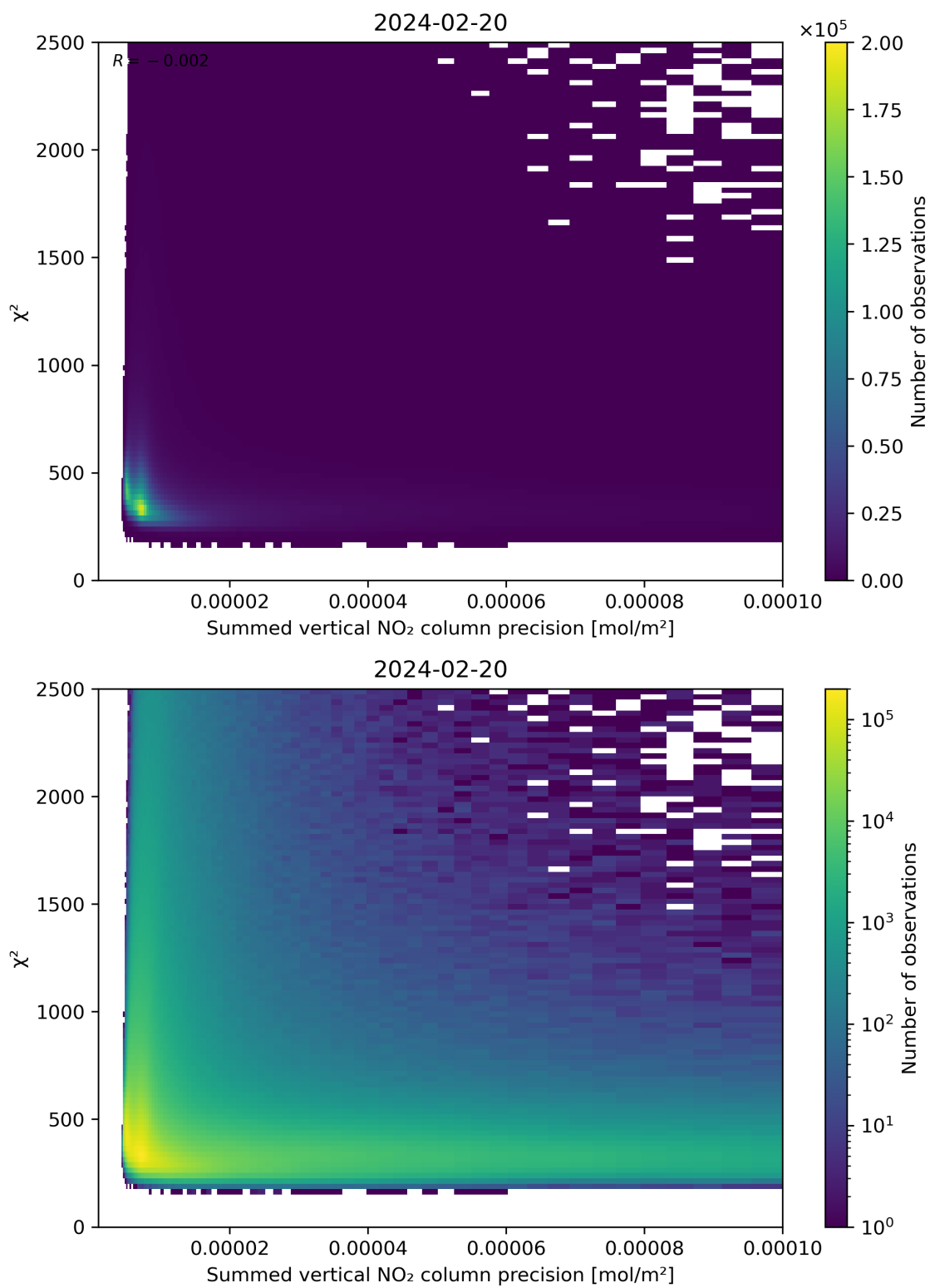
Figure 107: Scatter density plot of “Summed vertical NO 2 column precision” against “ \chi^2 ” for 2024-02-19 to 2024-02-21.
