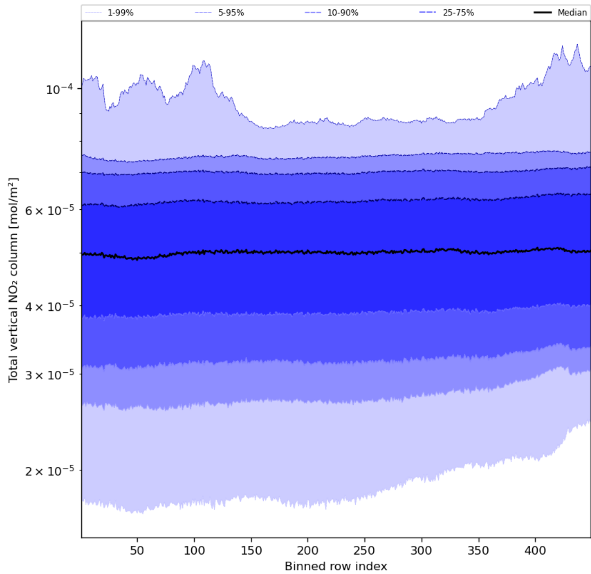
Figure 55: Along track statistics of “Total vertical NO 2 column” for 2024-02-19 to 2024-02-21
