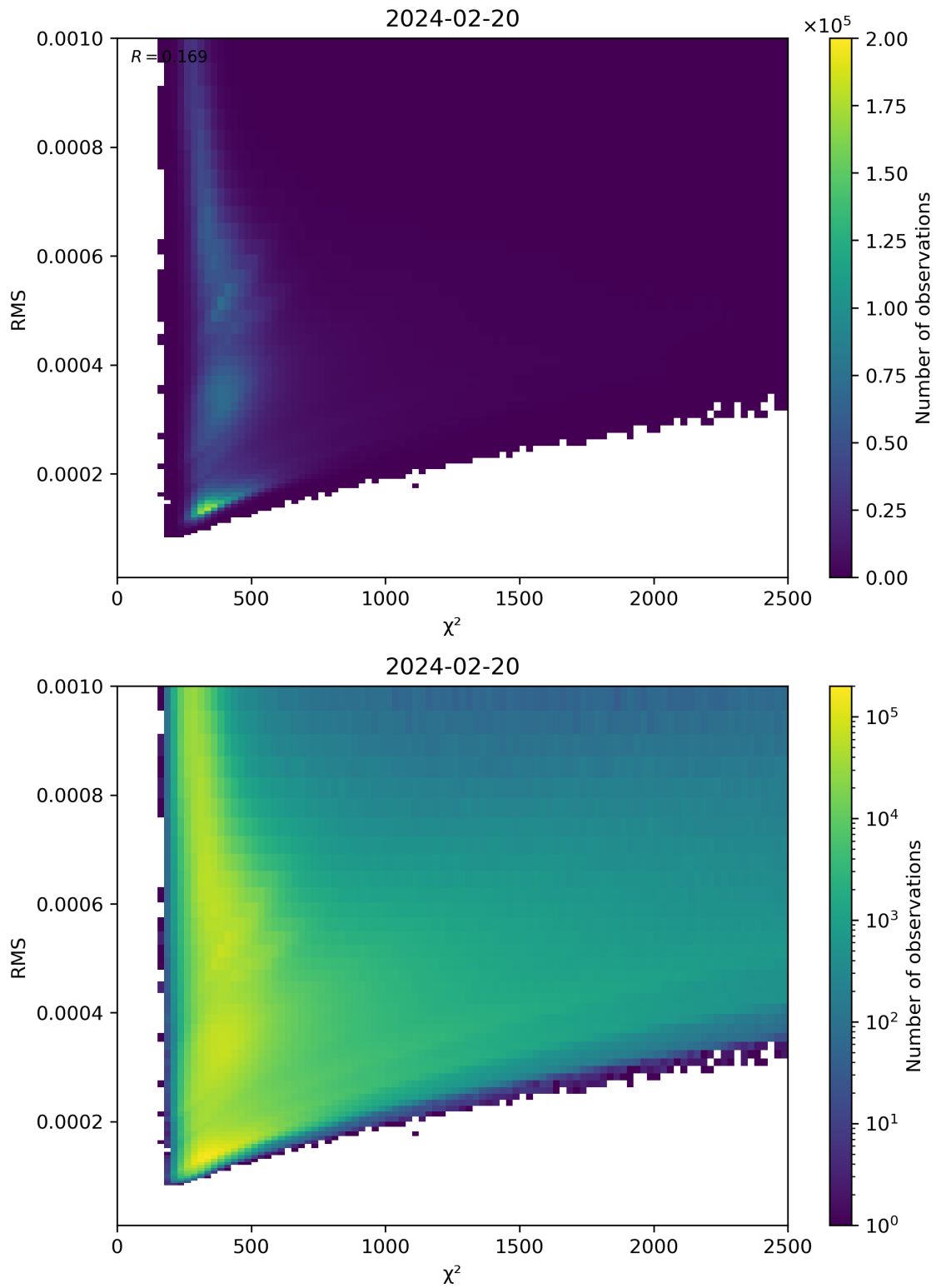
Figure 82: Scatter density plot of “ \chi^2 ” against “RMS” for 2024-02-19 to 2024-02-21.
