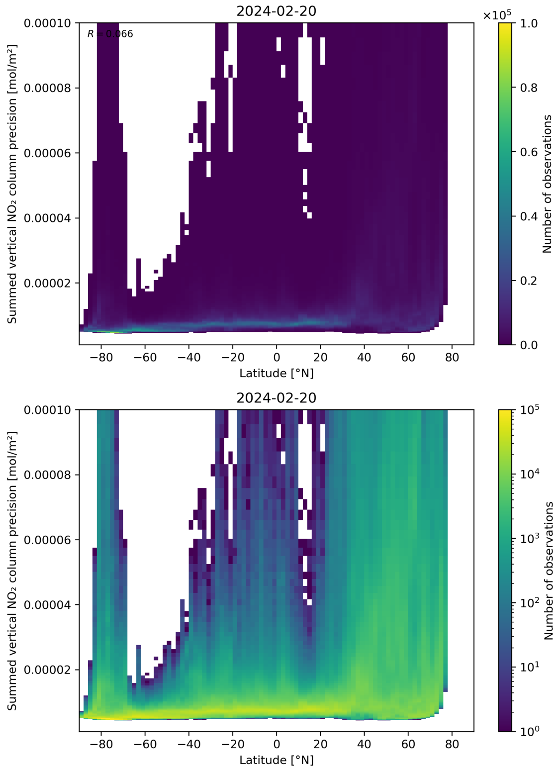
Figure 89: Scatter density plot of “Latitude” against “Summed vertical NO 2 column precision” for 2024-02-19 to 2024-02-21.
