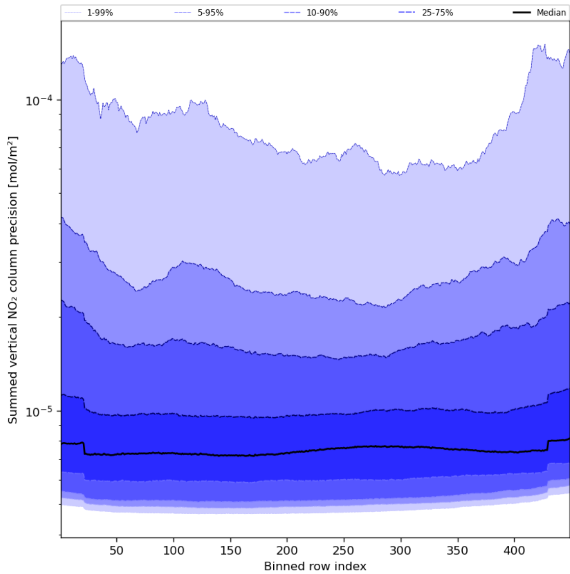
Figure 58: Along track statistics of “Summed vertical NO 2 column precision” for 2024-02-19 to 2024-02-21
