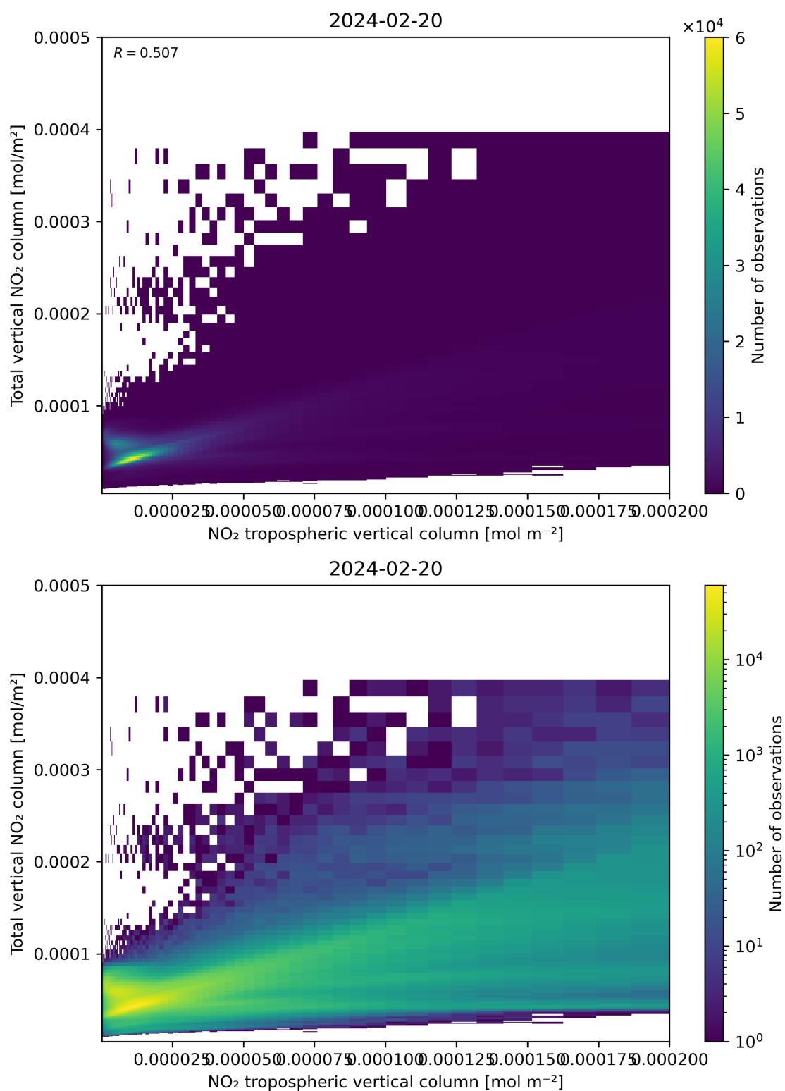
Figure 128: Scatter density plot of “NO 2 tropospheric vertical column” against “Total vertical NO 2 column” for 2024-02-19 to 2024-02-21.
