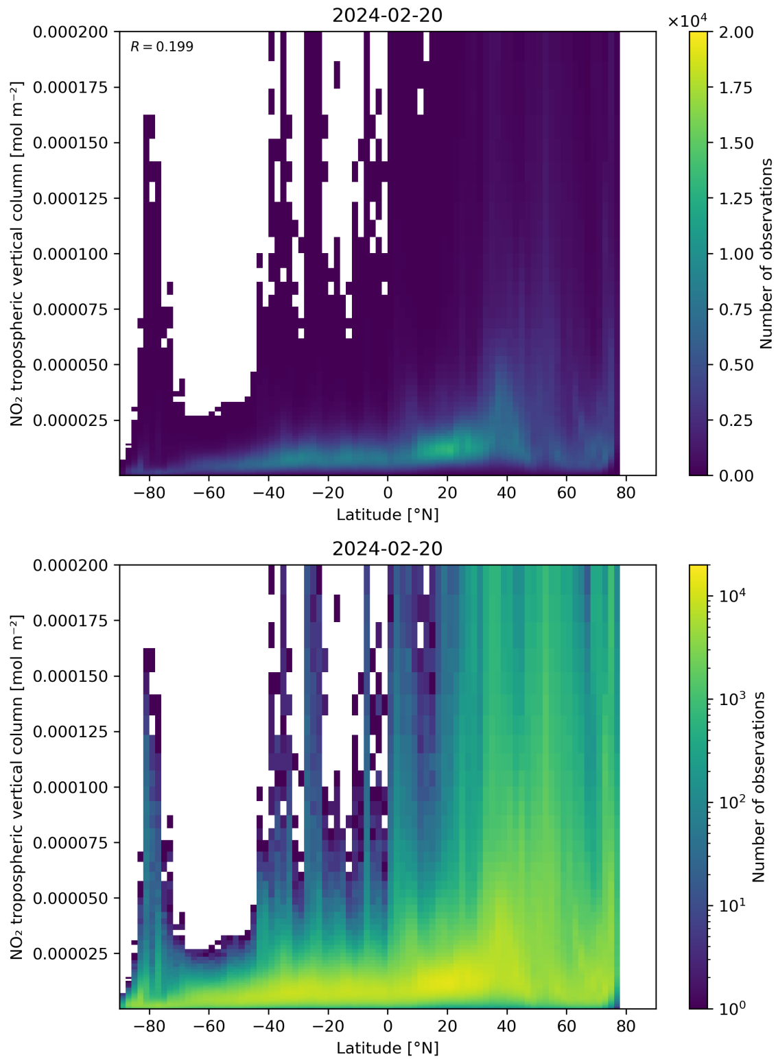
Figure 92: Scatter density plot of “Latitude” against “NO 2 tropospheric vertical column” for 2024-02-19 to 2024-02-21.
