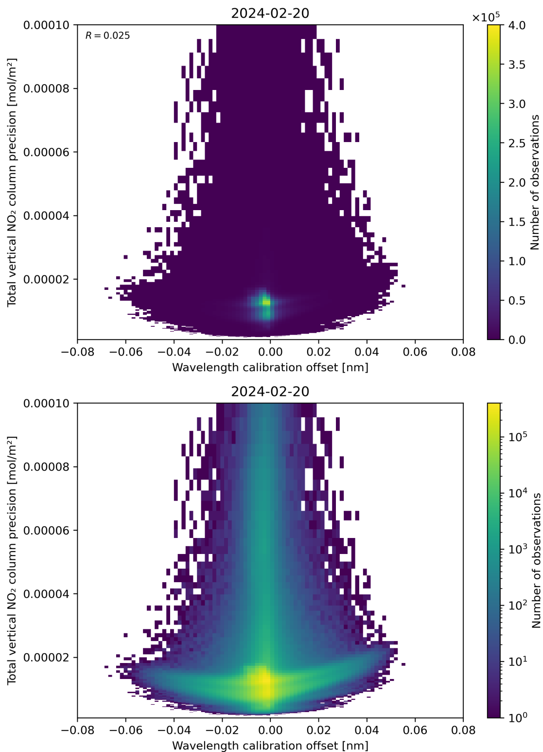
Figure 180: Scatter density plot of “Wavelength calibration offset” against “Total vertical NO 2 column precision” for 2024-02-19 to 2024-02-21.
