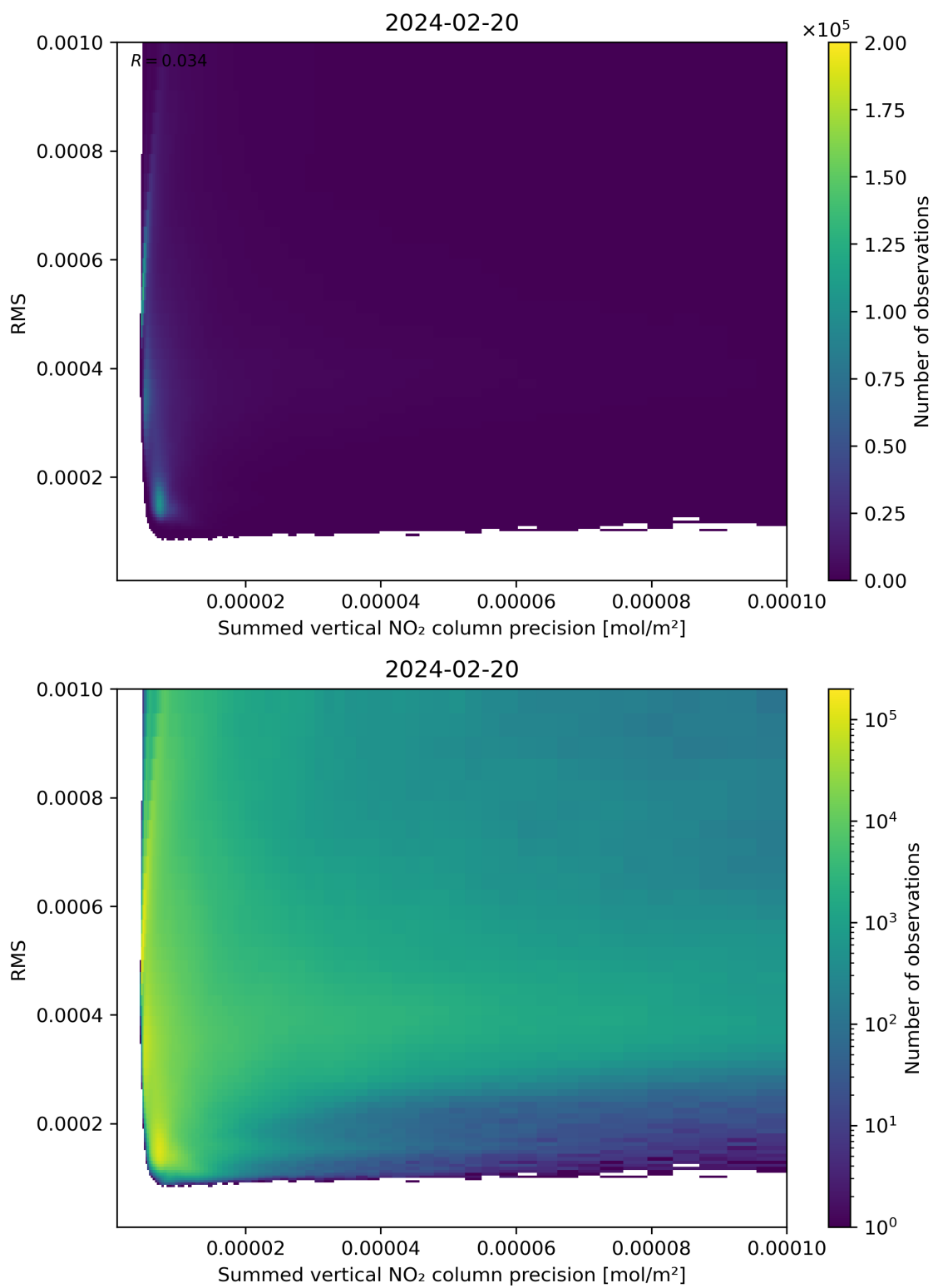
Figure 108: Scatter density plot of “Summed vertical NO 2 column precision” against “RMS” for 2024-02-19 to 2024-02-21.
