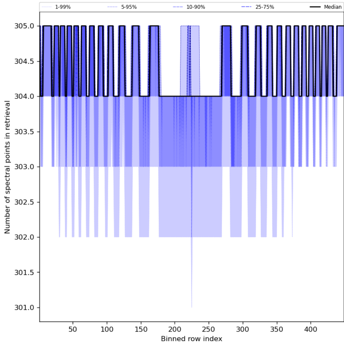
Figure 50: Along track statistics of “Number of spectral points in retrieval” for 2024-02-19 to 2024-02-21
