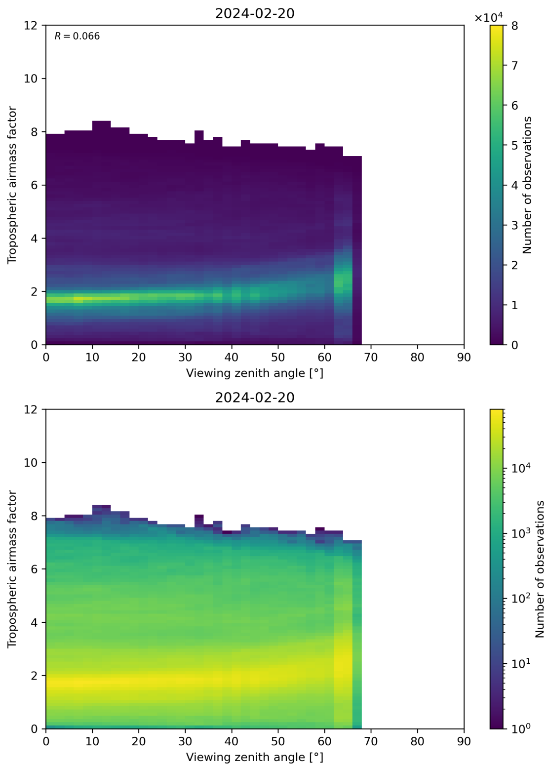
Figure 161: Scatter density plot of “Viewing zenith angle” against “Tropospheric airmass factor” for 2024-02-19 to 2024-02-21.
