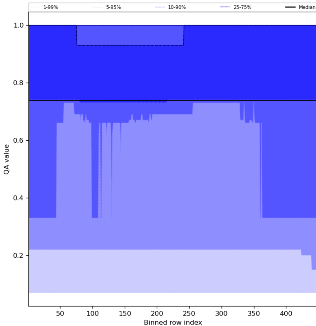
Figure 45: Along track statistics of “QA value” for 2024-02-19 to 2024-02-21
