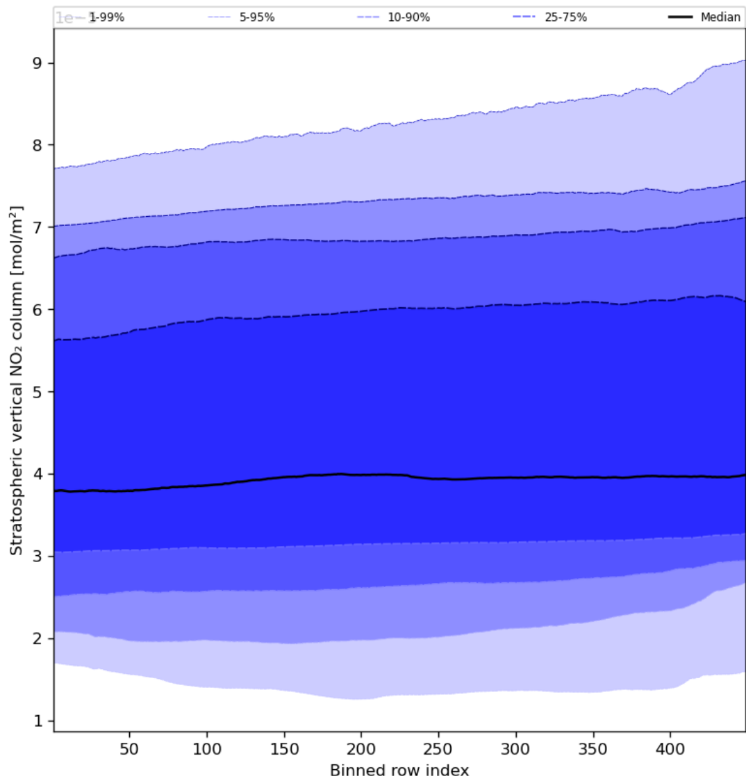
Figure 53: Along track statistics of “Stratospheric vertical NO 2 column” for 2024-02-19 to 2024-02-21
