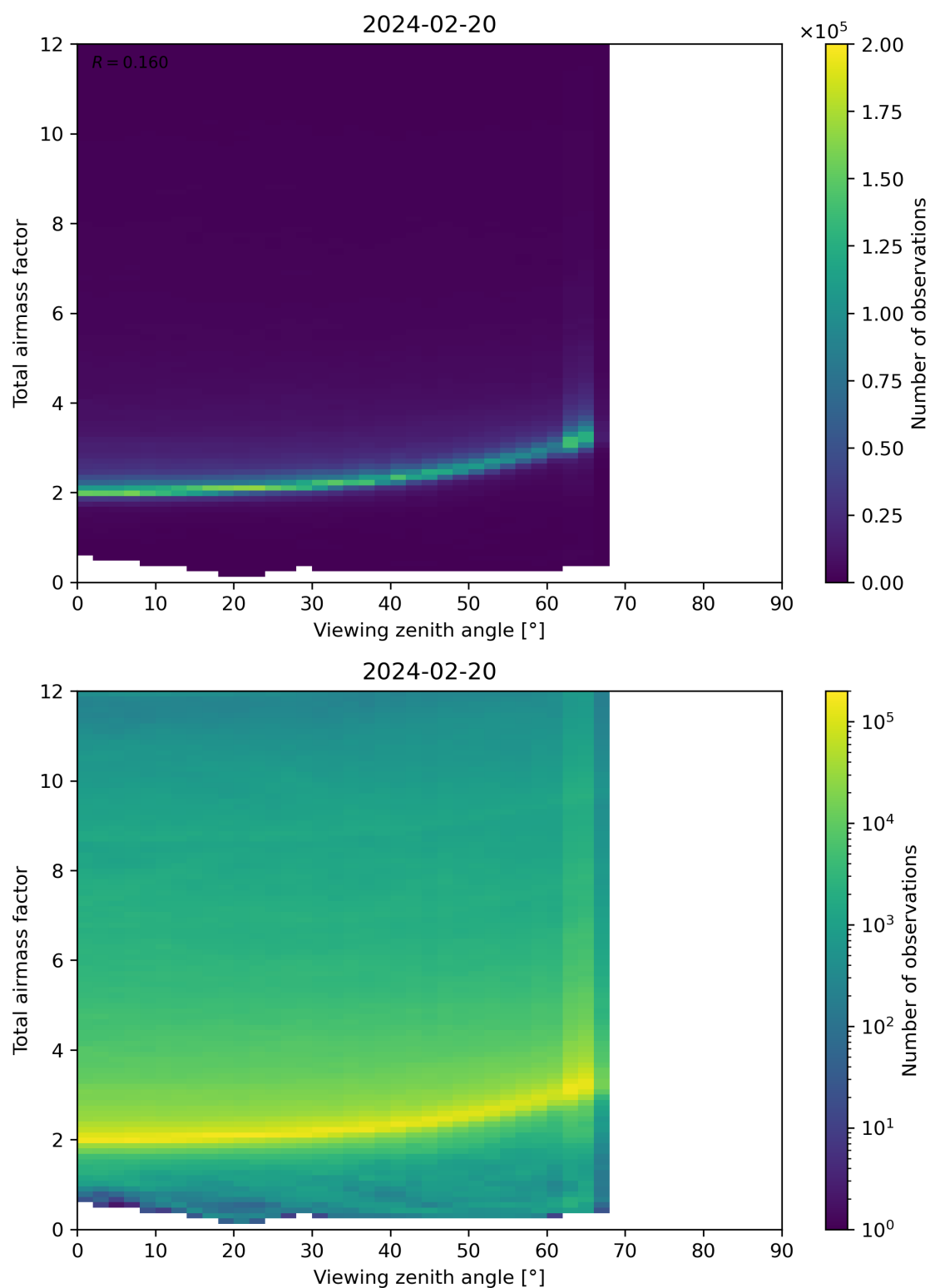
Figure 160: Scatter density plot of “Viewing zenith angle” against “Total airmass factor” for 2024-02-19 to 2024-02-21.
