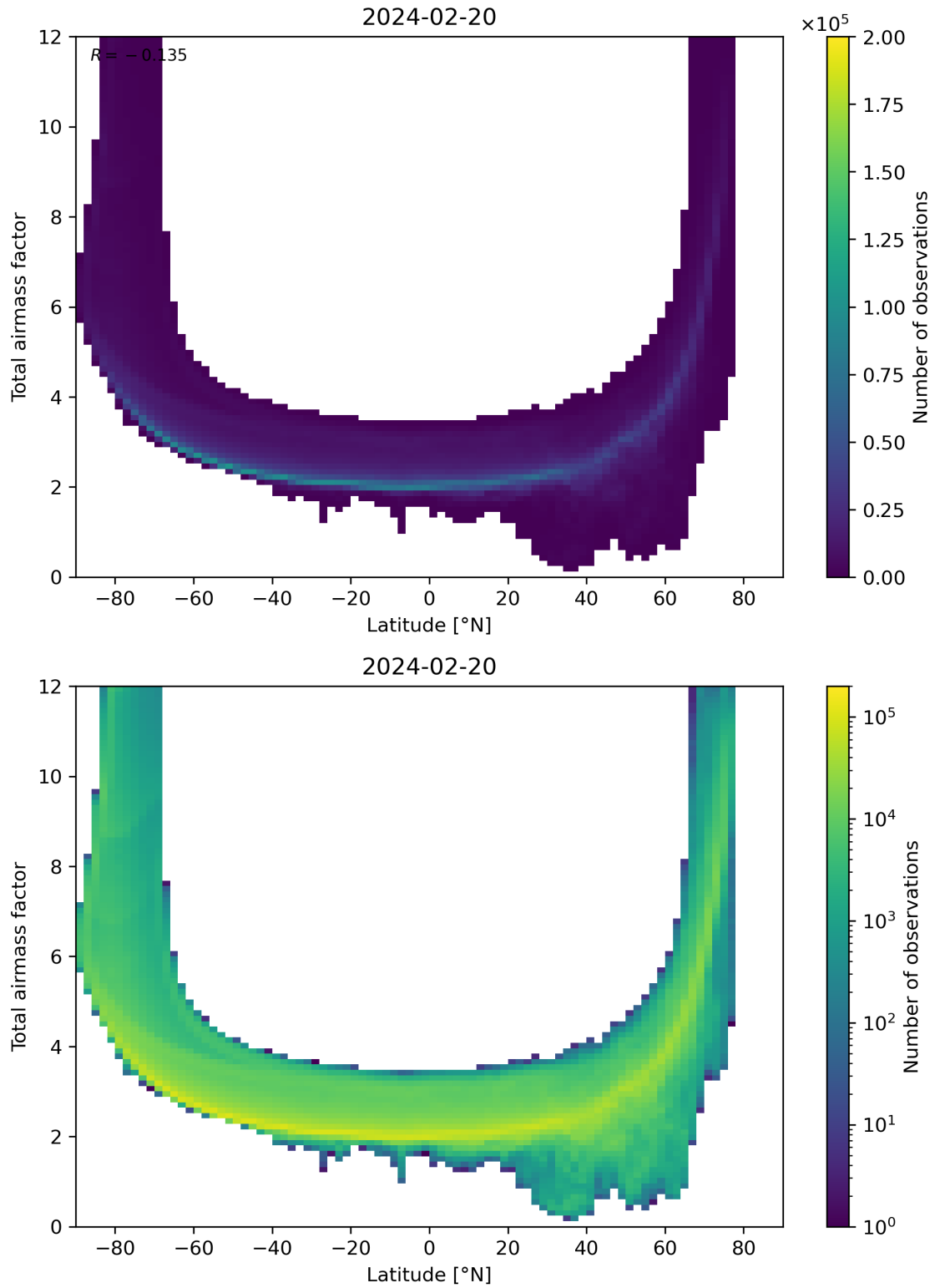
Figure 84: Scatter density plot of “Latitude” against “Total airmass factor” for 2024-02-19 to 2024-02-21.
