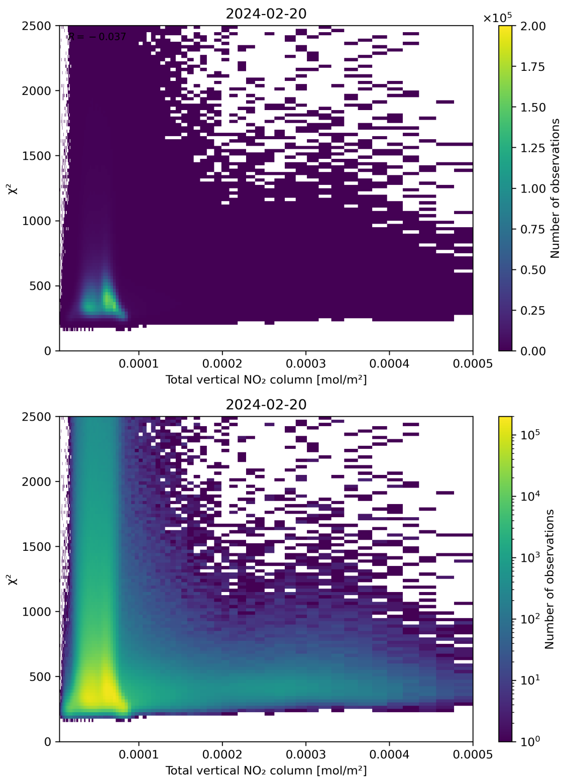
Figure 111: Scatter density plot of “Total vertical NO 2 column” against “ \chi^2 ” for 2024-02-19 to 2024-02-21.
