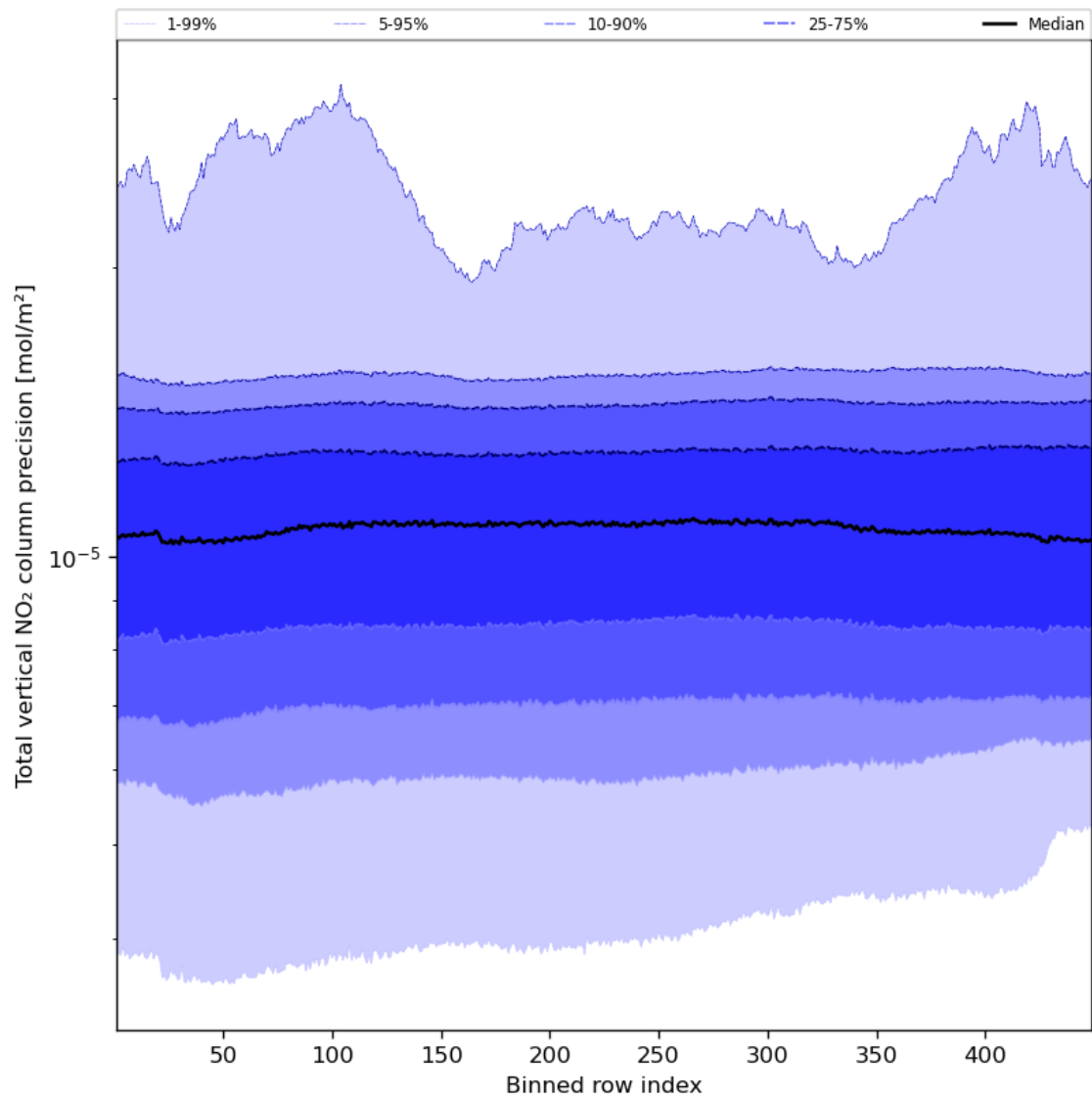
Figure 56: Along track statistics of “Total vertical NO 2 column precision” for 2024-02-19 to 2024-02-21
