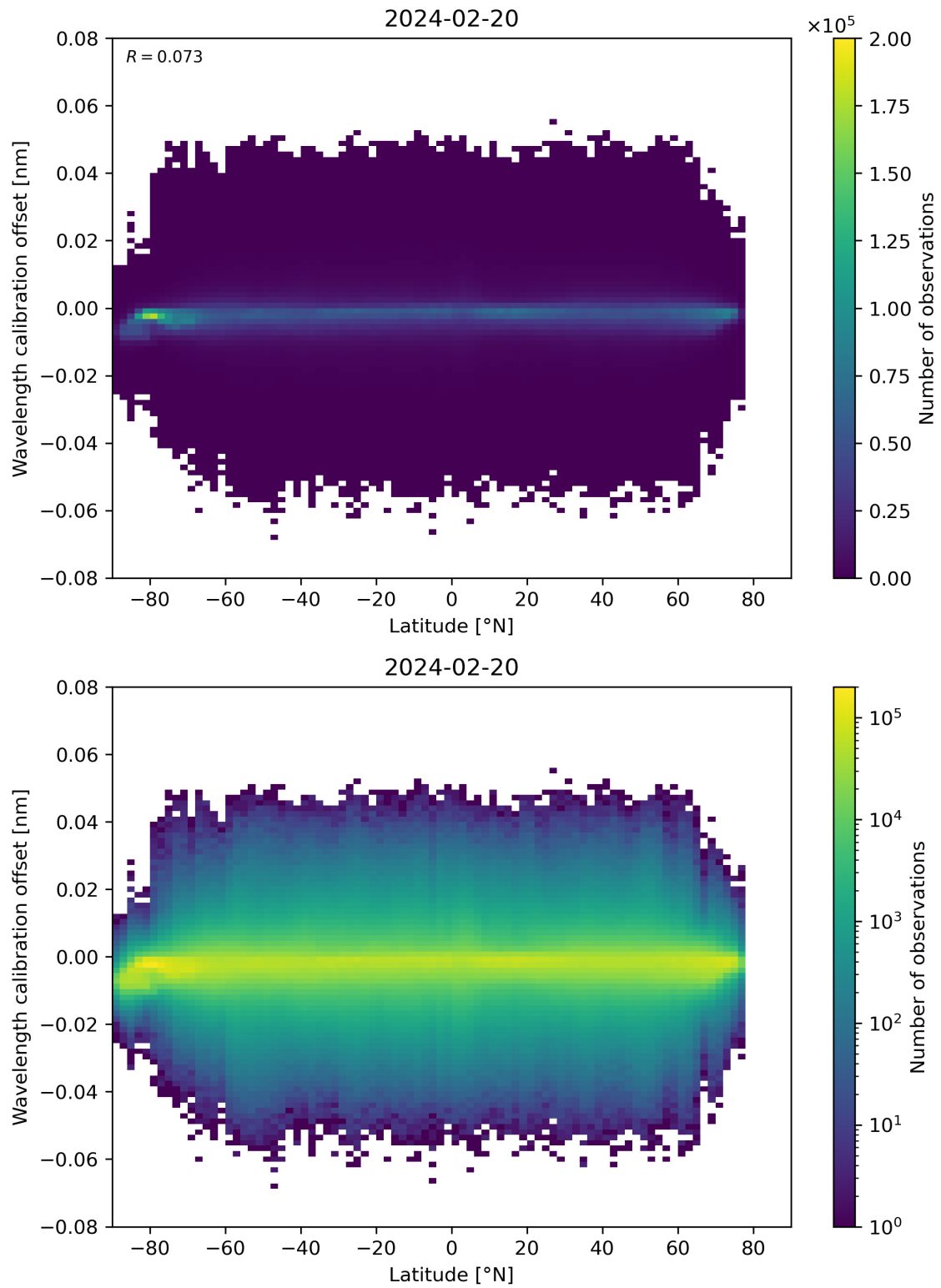
Figure 95: Scatter density plot of “Latitude” against “Wavelength calibration offset” for 2024-02-19 to 2024-02-21.
