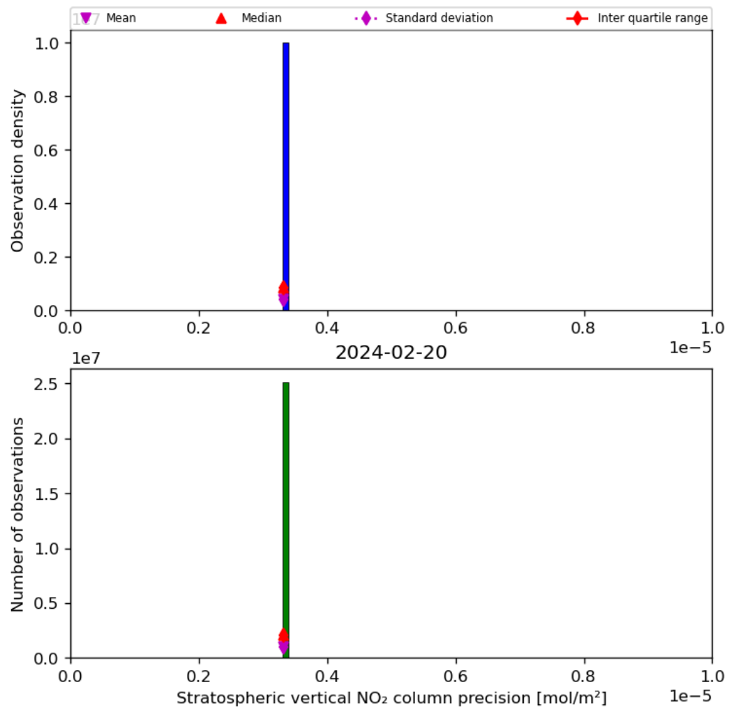
Figure 37: Histogram of “Stratospheric vertical NO 2 column precision” for 2024-02-19 to 2024-02-21
