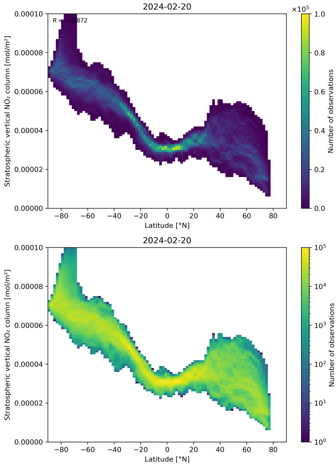
Figure 87: Scatter density plot of “Latitude” against “Stratospheric vertical NO 2 column” for 2024-02-19 to 2024-02-21.
