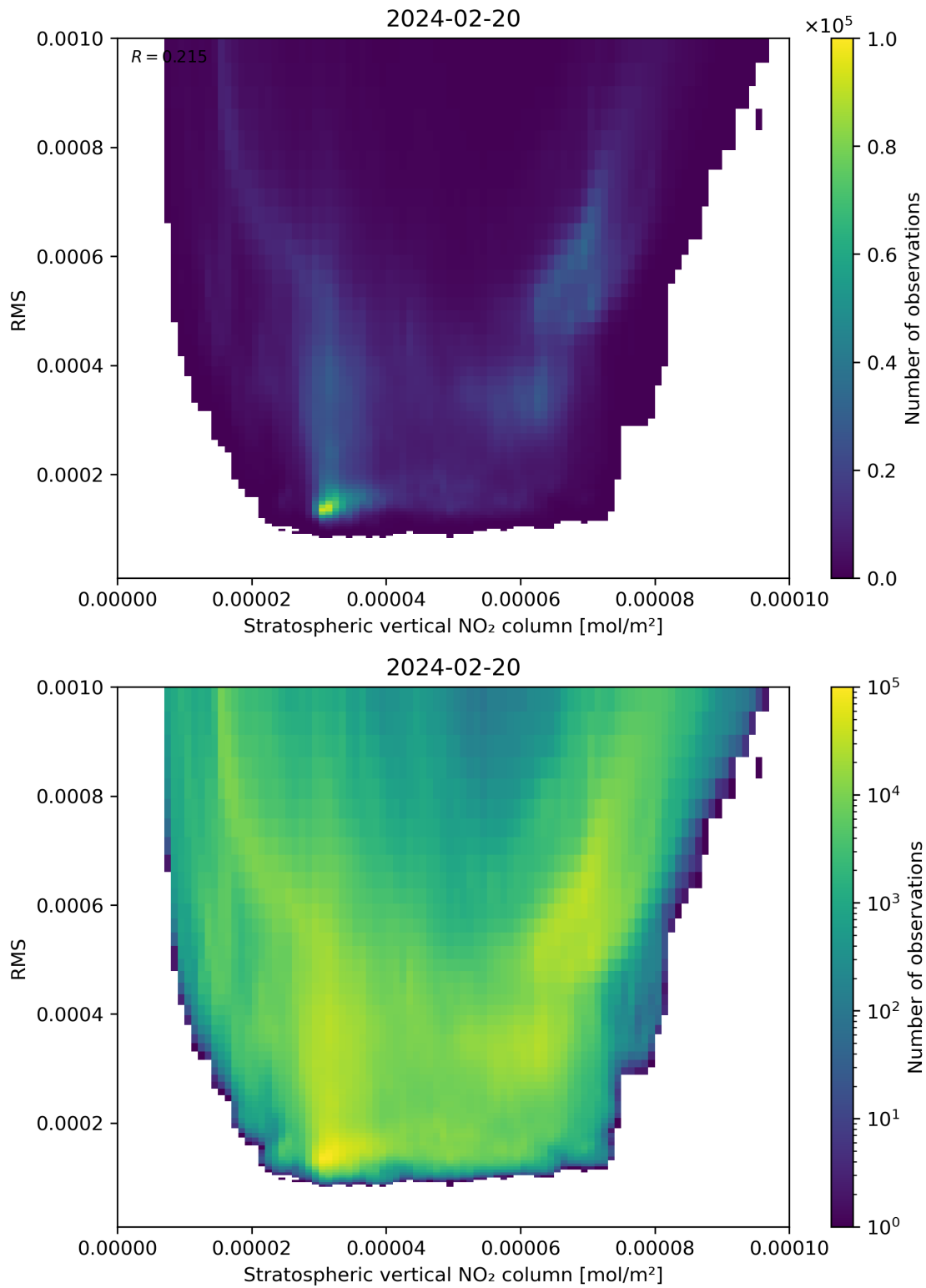
Figure 102: Scatter density plot of “Stratospheric vertical NO 2 column” against “RMS” for 2024-02-19 to 2024-02-21.
