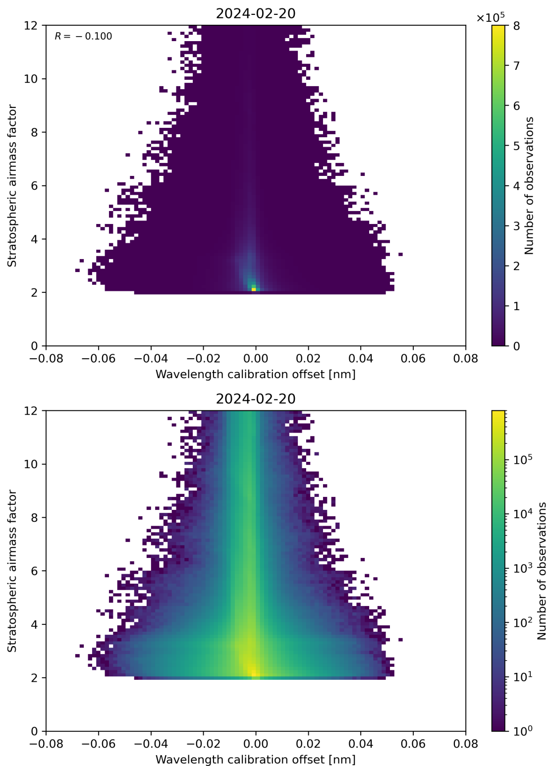
Figure 174: Scatter density plot of “Wavelength calibration offset” against “Stratospheric airmass factor” for 2024-02-19 to 2024-02-21.
