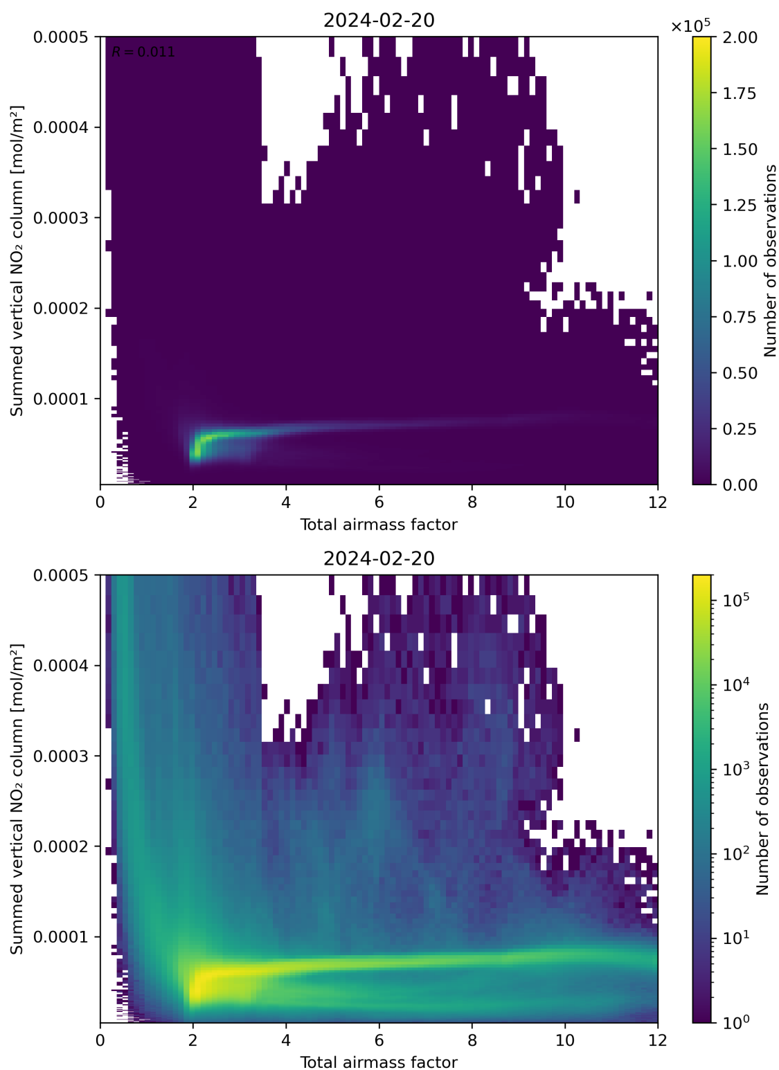
Figure 65: Scatter density plot of “Total airmass factor” against “Summed vertical NO 2 column” for 2024-02-19 to 2024-02-21.
