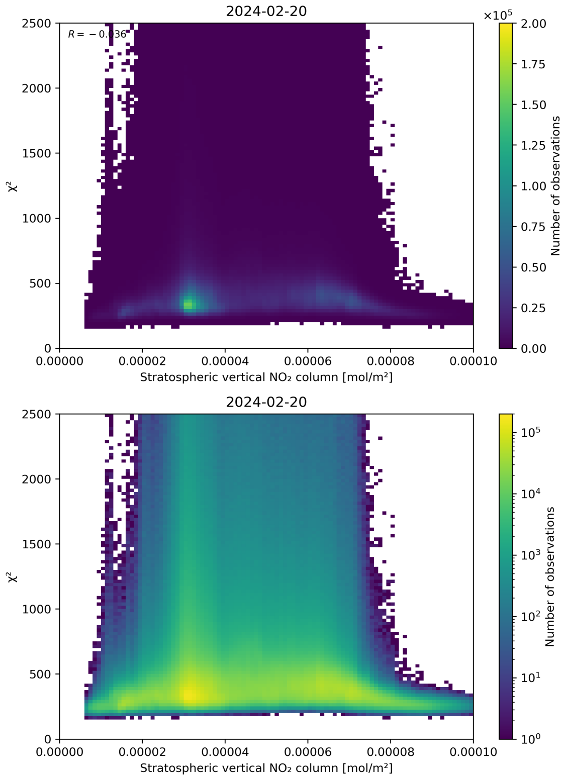
Figure 97: Scatter density plot of “Stratospheric vertical NO 2 column” against “ \chi^2 ” for 2024-02-19 to 2024-02-21.
