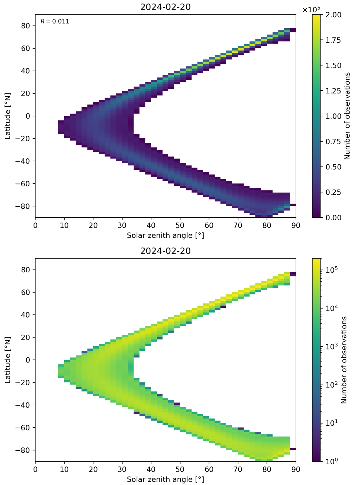
Figure 149: Scatter density plot of “Solar zenith angle” against “Latitude” for 2024-02-19 to 2024-02-21.
