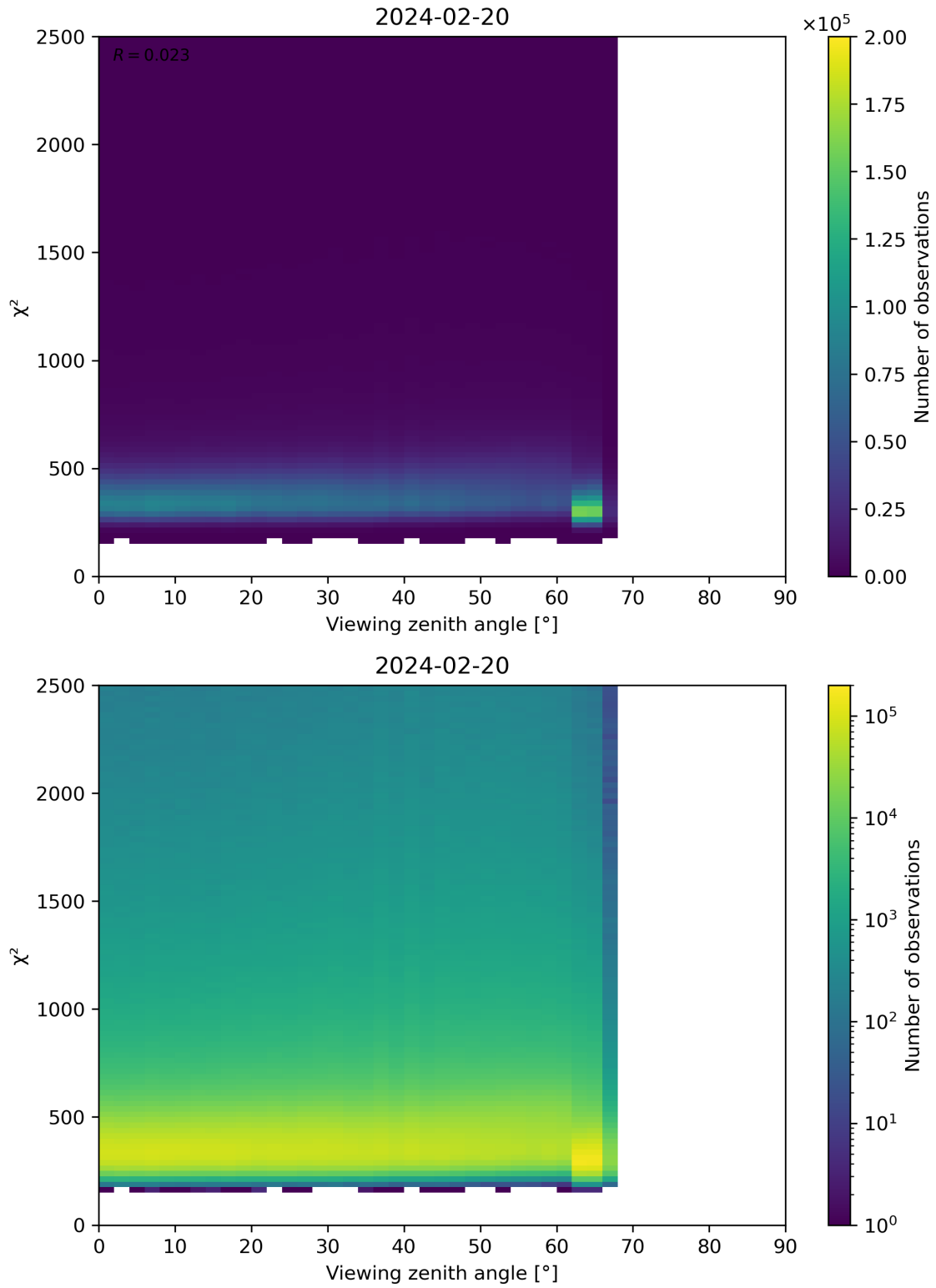
Figure 162: Scatter density plot of “Viewing zenith angle” against “ \chi^2 ” for 2024-02-19 to 2024-02-21.
