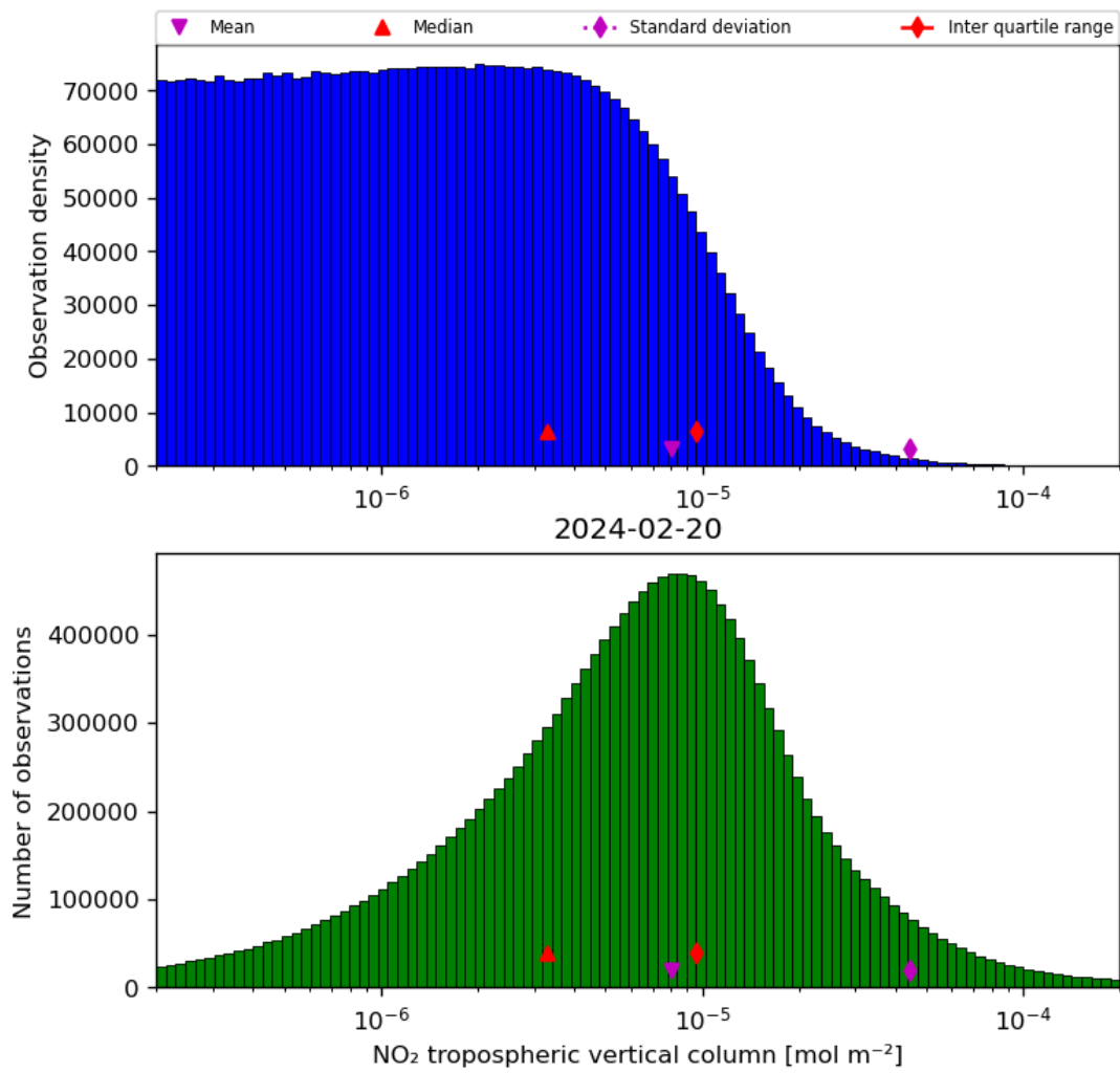
Figure 29: Histogram of “NO 2 tropospheric vertical column” for 2024-02-19 to 2024-02-21
