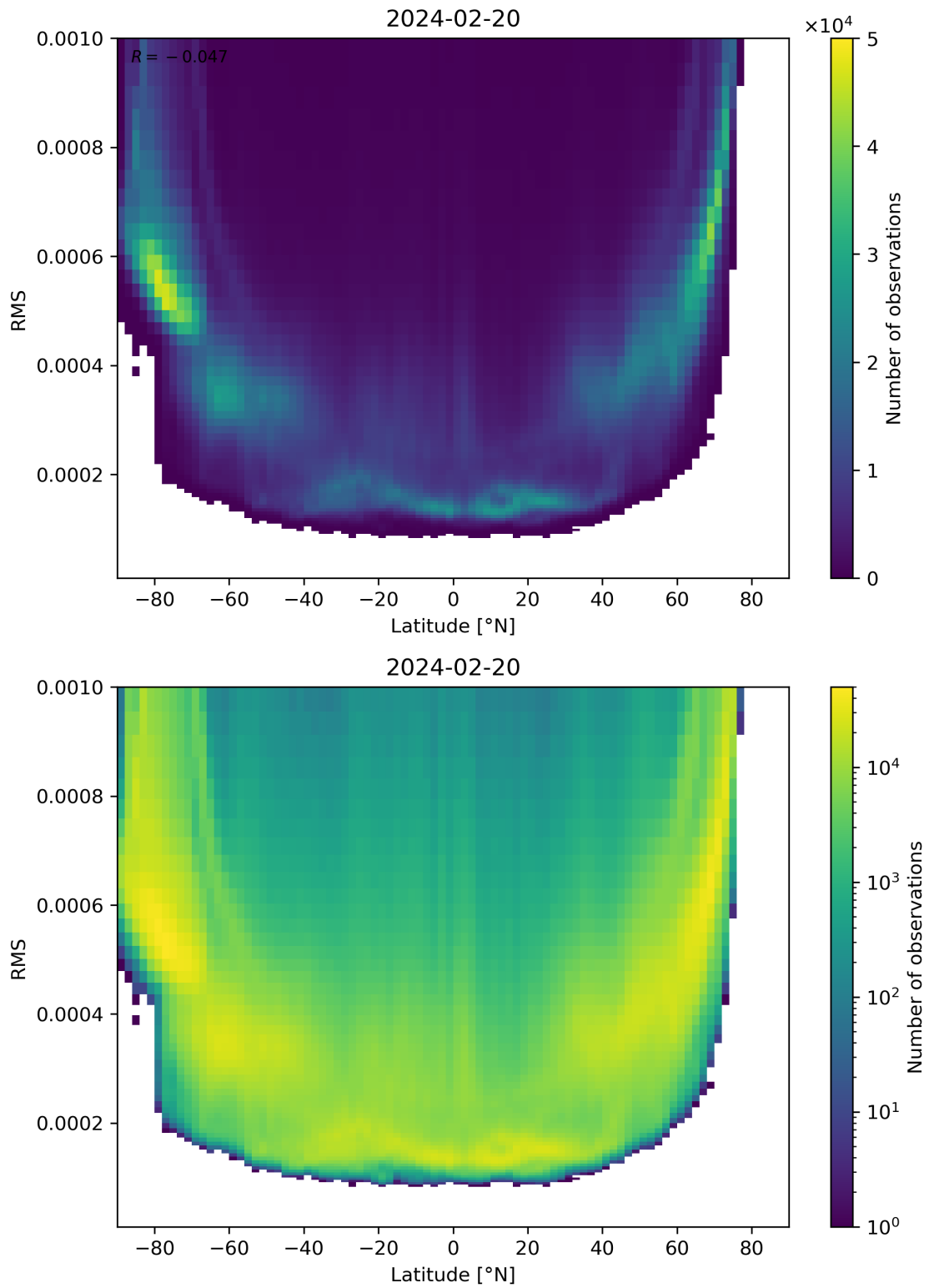
Figure 94: Scatter density plot of “Latitude” against “RMS” for 2024-02-19 to 2024-02-21.
