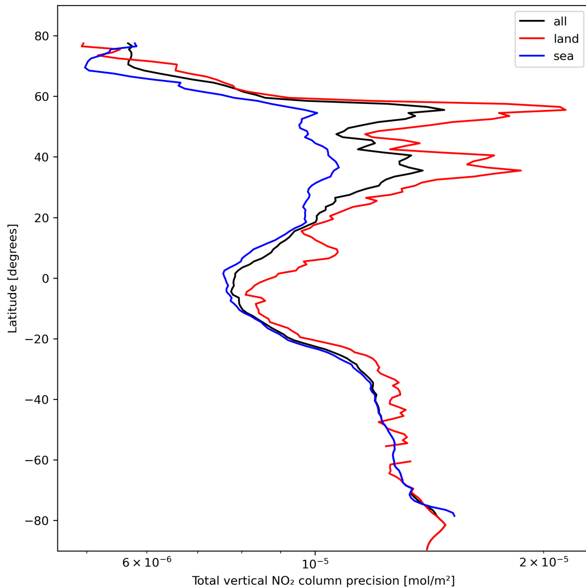
Figure 22: Zonal average of “Total vertical NO 2 column precision” for 2024-02-19 to 2024-02-21.
