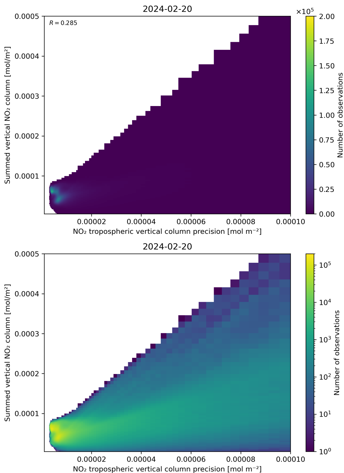
Figure 136: Scatter density plot of “NO 2 tropospheric vertical column precision” against “Summed vertical NO 2 column” for 2024-02-19 to 2024-02-21.
