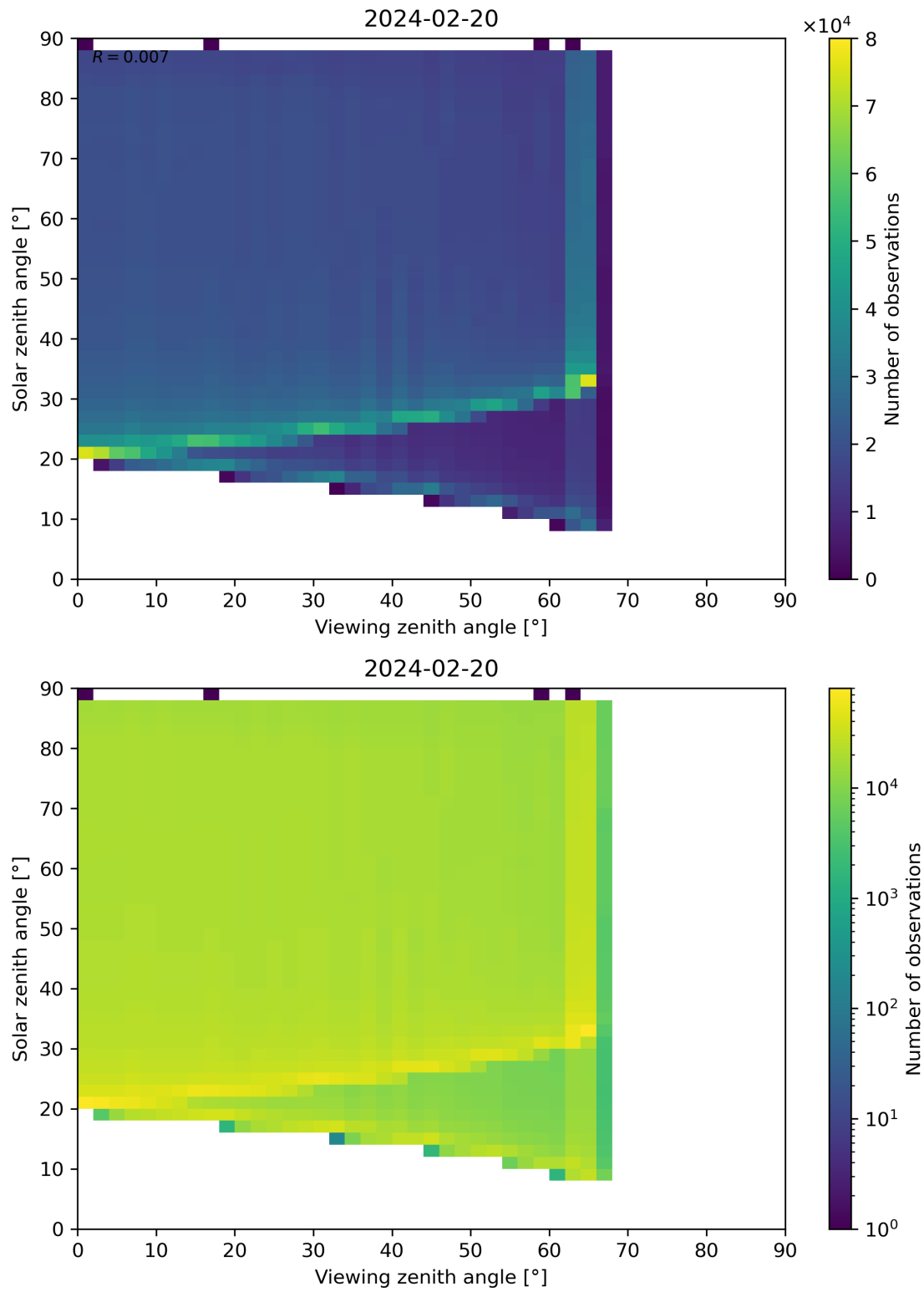
Figure 172: Scatter density plot of “Viewing zenith angle” against “Solar zenith angle” for 2024-02-19 to 2024-02-21.
