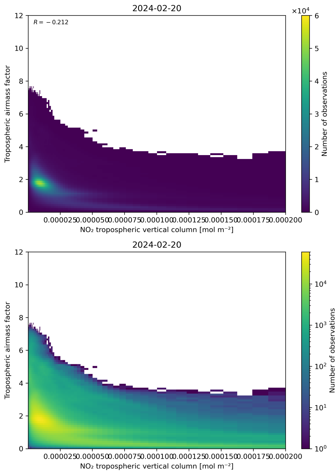
Figure 123: Scatter density plot of “NO 2 tropospheric vertical column” against “Tropospheric air mass factor” for 2024-02-19 to 2024-02-21.
