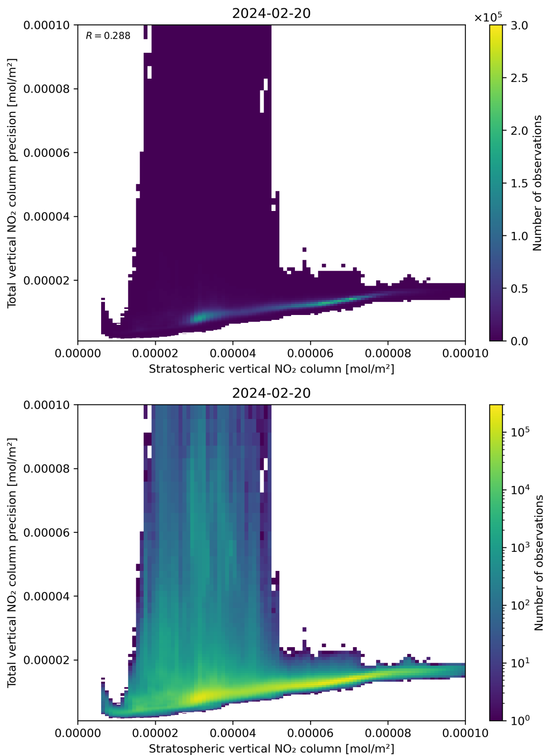
Figure 101: Scatter density plot of “Stratospheric vertical NO 2 column” against “Total vertical NO 2 column precision” for 2024-02-19 to 2024-02-21.
