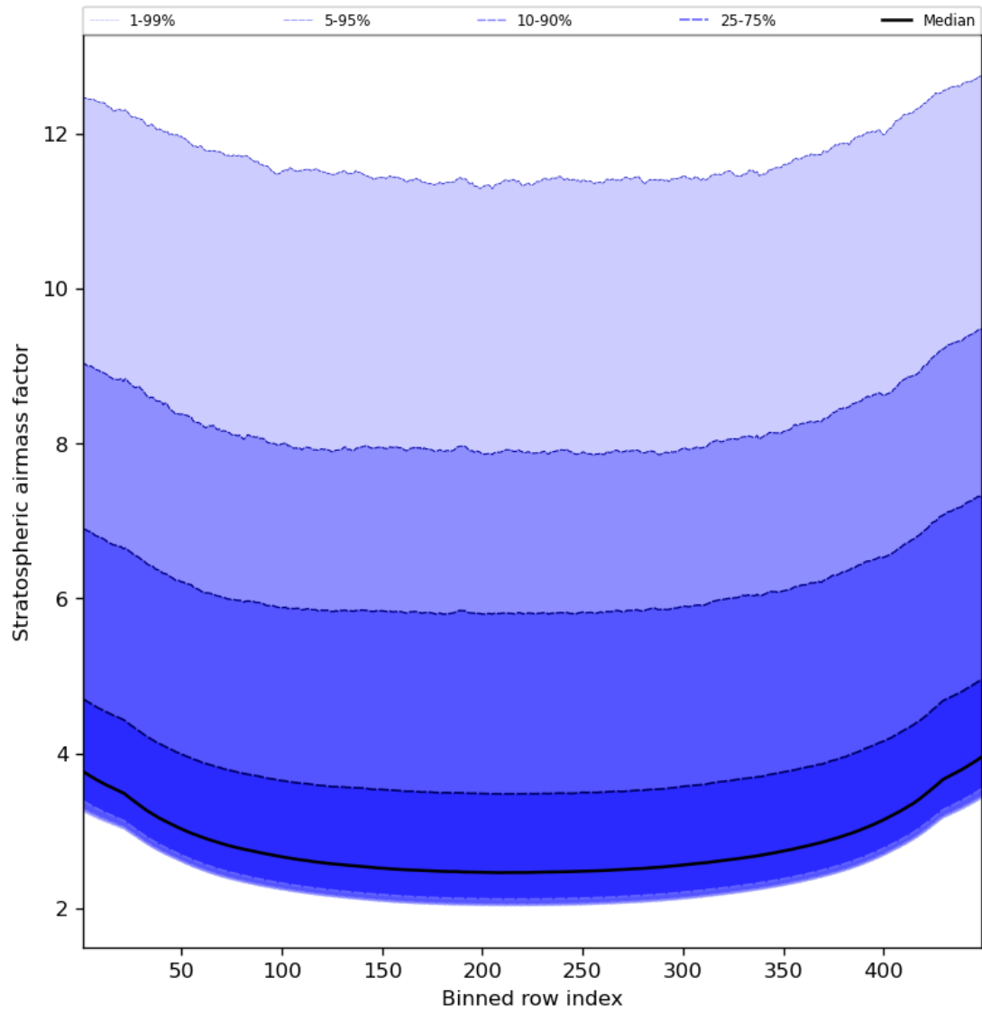
Figure 61: Along track statistics of “Stratospheric airmass factor” for 2024-02-19 to 2024-02-21
