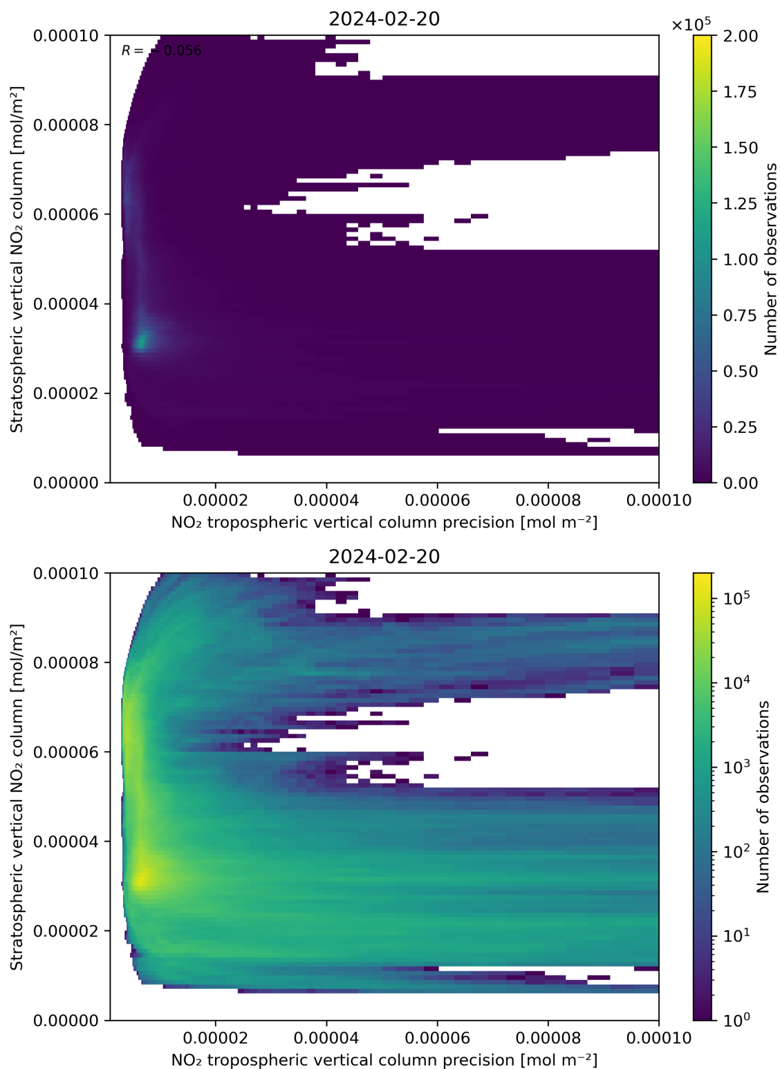
Figure 135: Scatter density plot of “NO 2 tropospheric vertical column precision” against “Stratospheric vertical NO 2 column” for 2024-02-19 to 2024-02-21.
