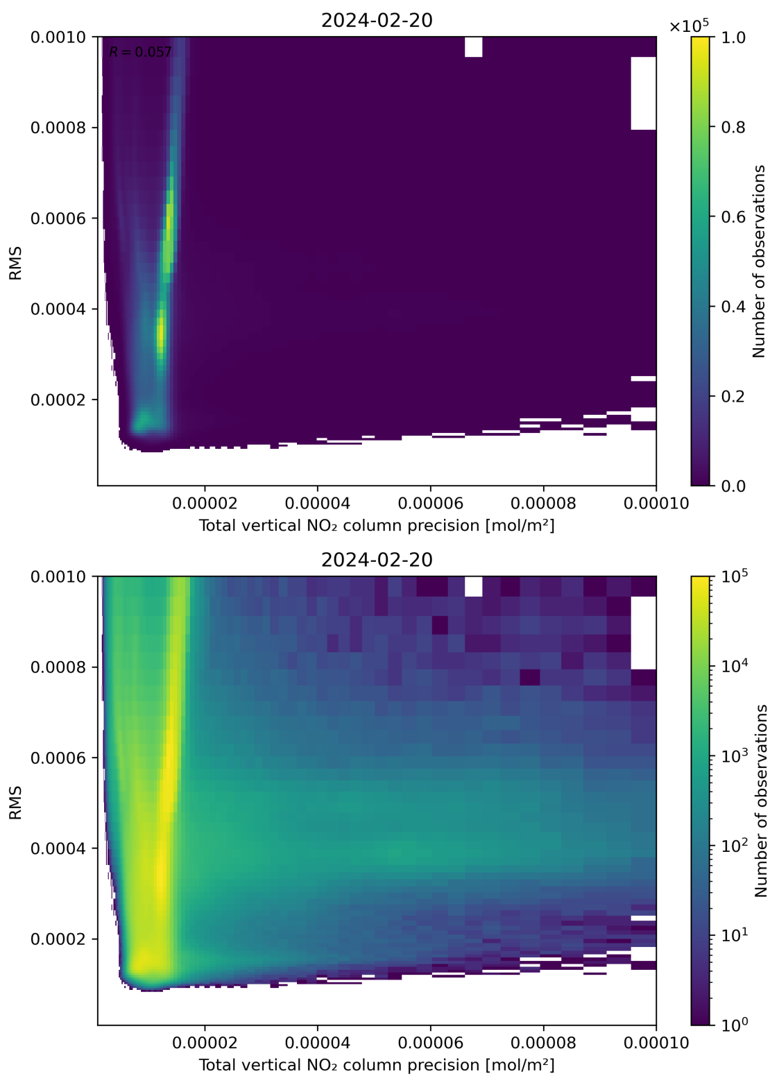
Figure 119: Scatter density plot of “Total vertical NO 2 column precision” against “RMS” for 2024-02-19 to 2024-02-21.
