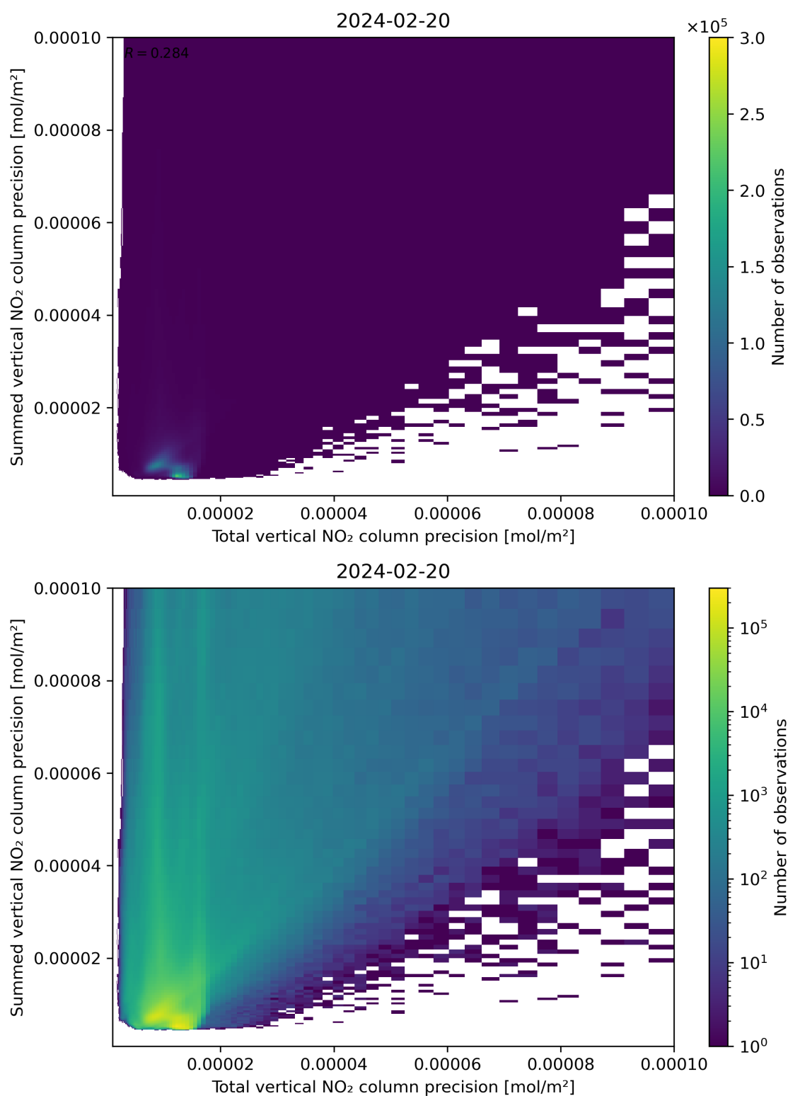
Figure 118: Scatter density plot of “Total vertical NO 2 column precision” against “Summed vertical NO 2 column precision” for 2024-02-19 to 2024-02-21.
