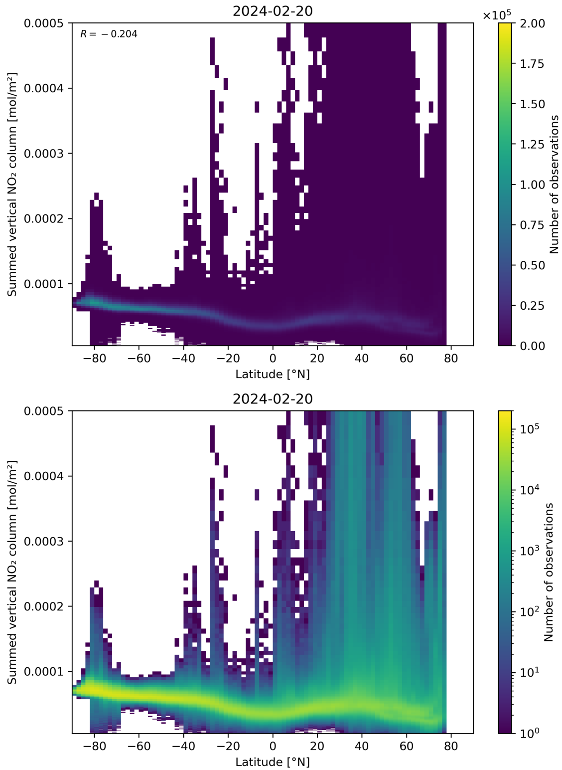
Figure 88: Scatter density plot of “Latitude” against “Summed vertical NO 2 column” for 2024-02-19 to 2024-02-21.
