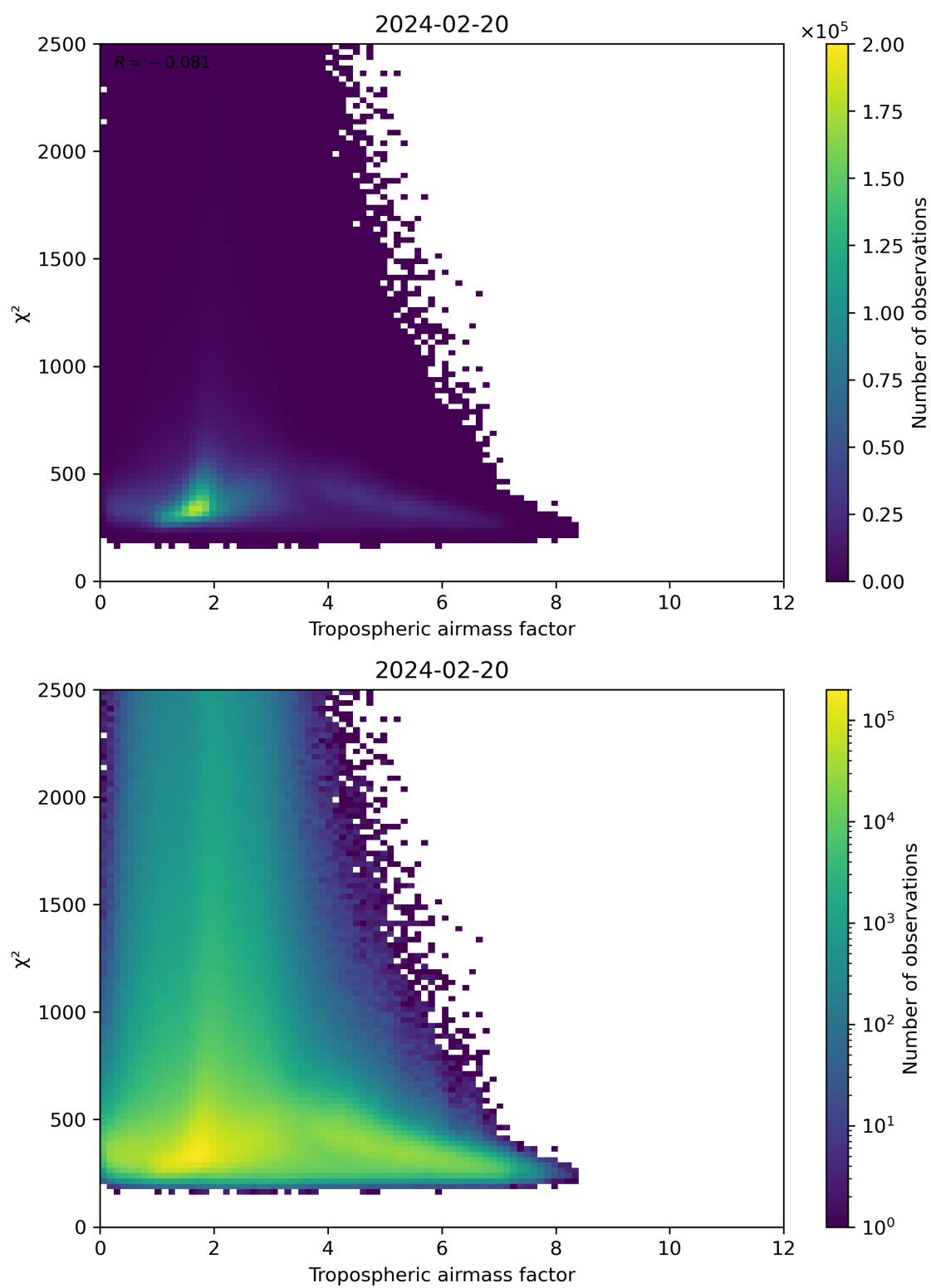
Figure 73: Scatter density plot of “Tropospheric airmass factor” against “ \chi^2 ” for 2024-02-19 to 2024-02-21.
