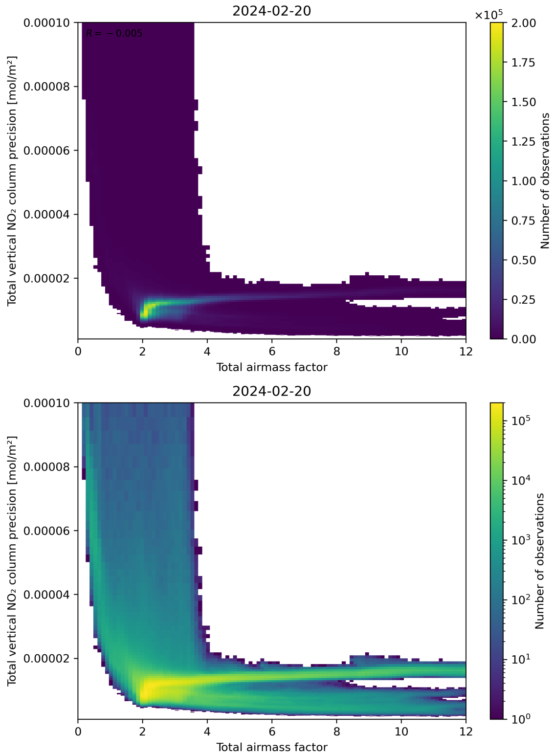
Figure 68: Scatter density plot of “Total airmass factor” against “Total vertical NO 2 column precision” for 2024-02-19 to 2024-02-21.
