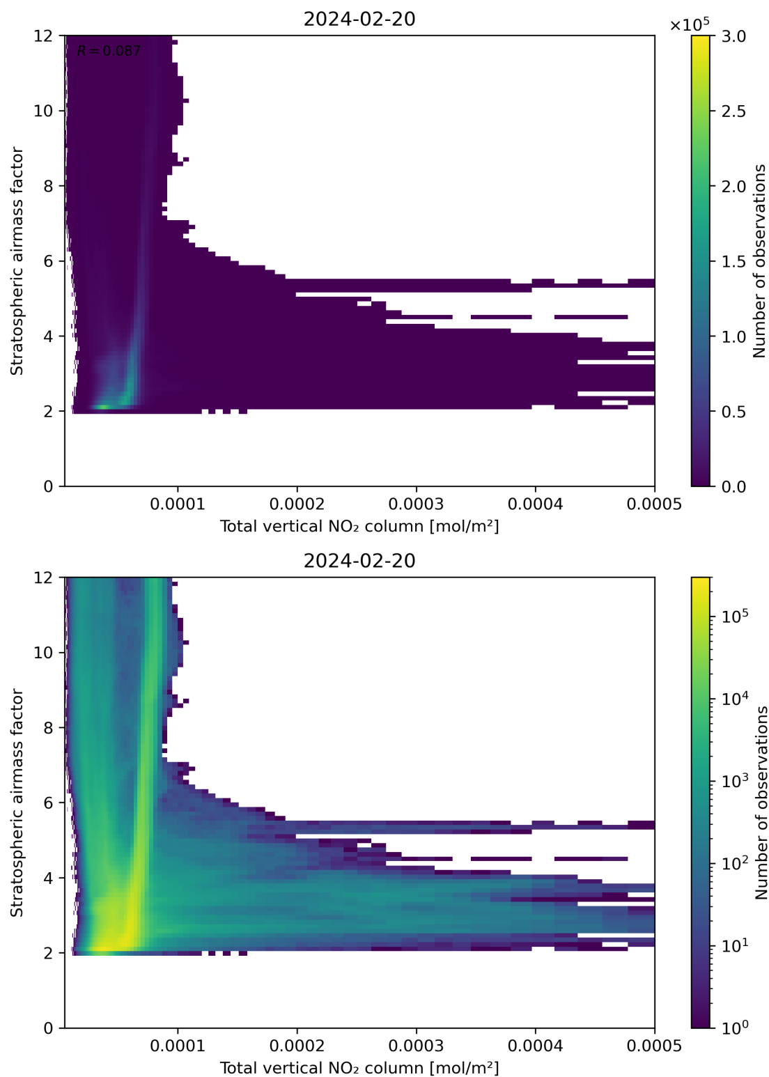
Figure 110: Scatter density plot of “Total vertical NO 2 column” against “Stratospheric airmass factor” for 2024-02-19 to 2024-02-21.
