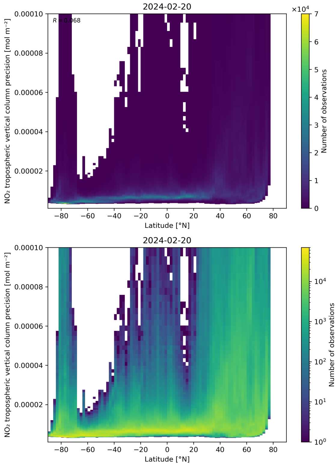
Figure 93: Scatter density plot of “Latitude” against “NO 2 tropospheric vertical column precision” for 2024-02-19 to 2024-02-21.
