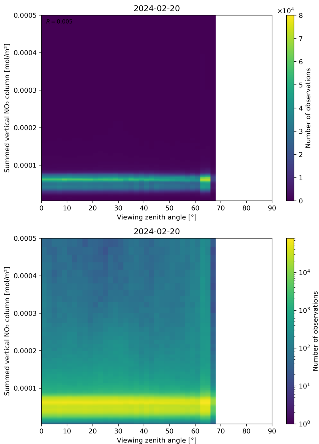
Figure 165: Scatter density plot of “Viewing zenith angle” against “Summed vertical NO 2 column” for 2024-02-19 to 2024-02-21.
