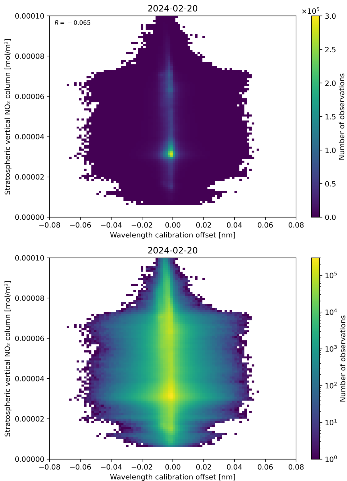
Figure 176: Scatter density plot of “Wavelength calibration offset” against “Stratospheric vertical NO 2 column” for 2024-02-19 to 2024-02-21.
