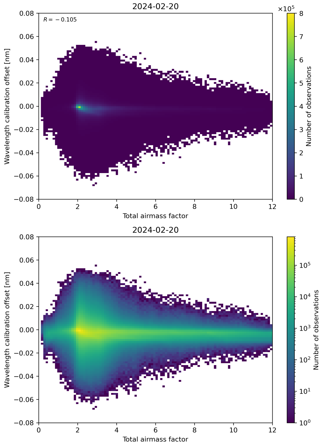
Figure 70: Scatter density plot of “Total airmass factor” against “Wavelength calibration offset” for 2024-02-19 to 2024-02-21.
