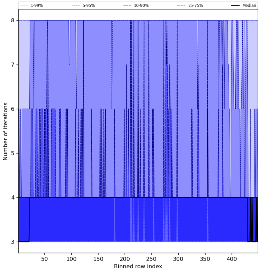
Figure 51: Along track statistics of “Number of iterations” for 2024-02-19 to 2024-02-21
