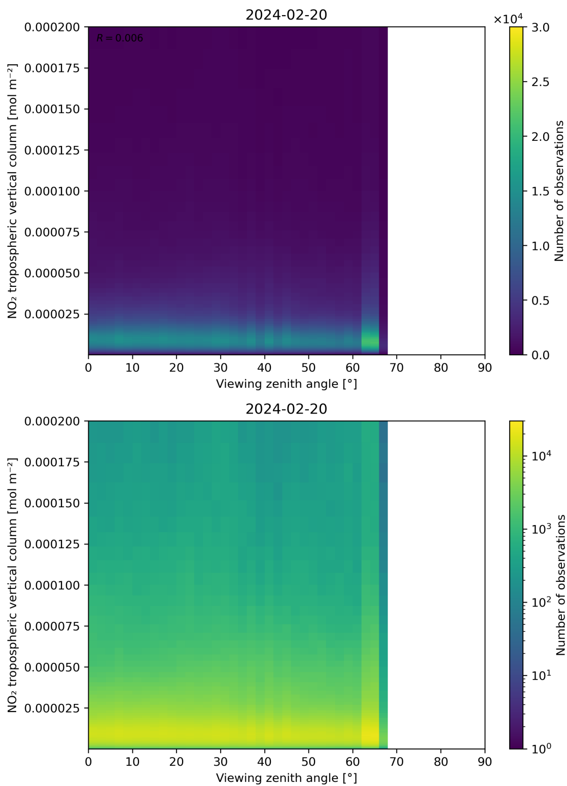
Figure 169: Scatter density plot of “Viewing zenith angle” against “NO 2 tropospheric vertical column” for 2024-02-19 to 2024-02-21.
