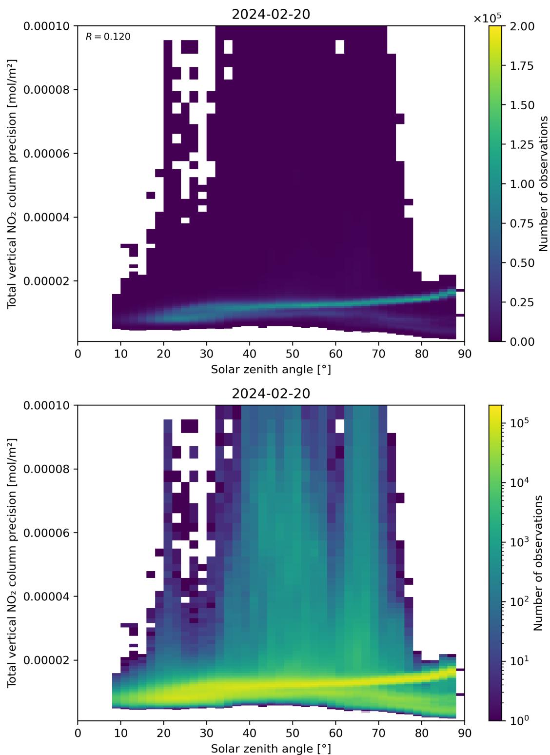
Figure 154: Scatter density plot of “Solar zenith angle” against “Total vertical NO 2 column precision” for 2024-02-19 to 2024-02-21.
