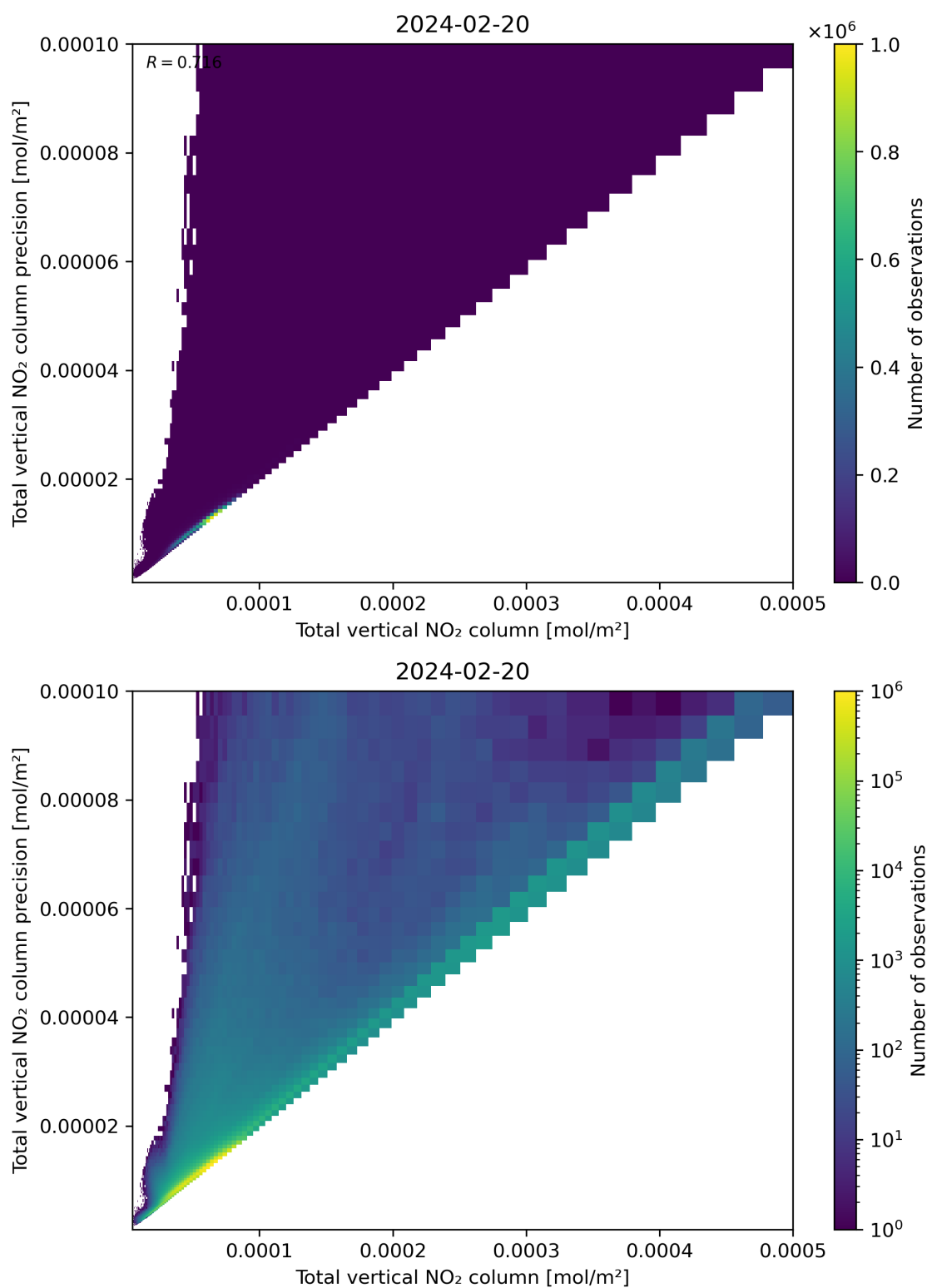
Figure 114: Scatter density plot of “Total vertical NO 2 column” against “Total vertical NO 2 column precision” for 2024-02-19 to 2024-02-21.
