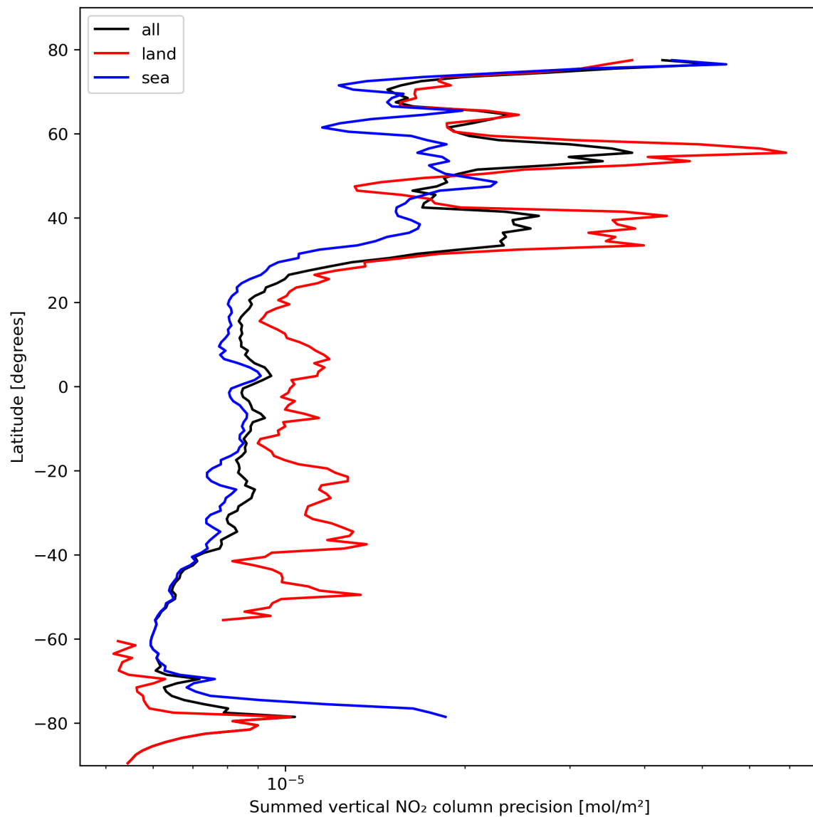
Figure 24: Zonal average of "Summed vertical NO 2 column precision" for 2024-02-19 to 2024-02-21.
