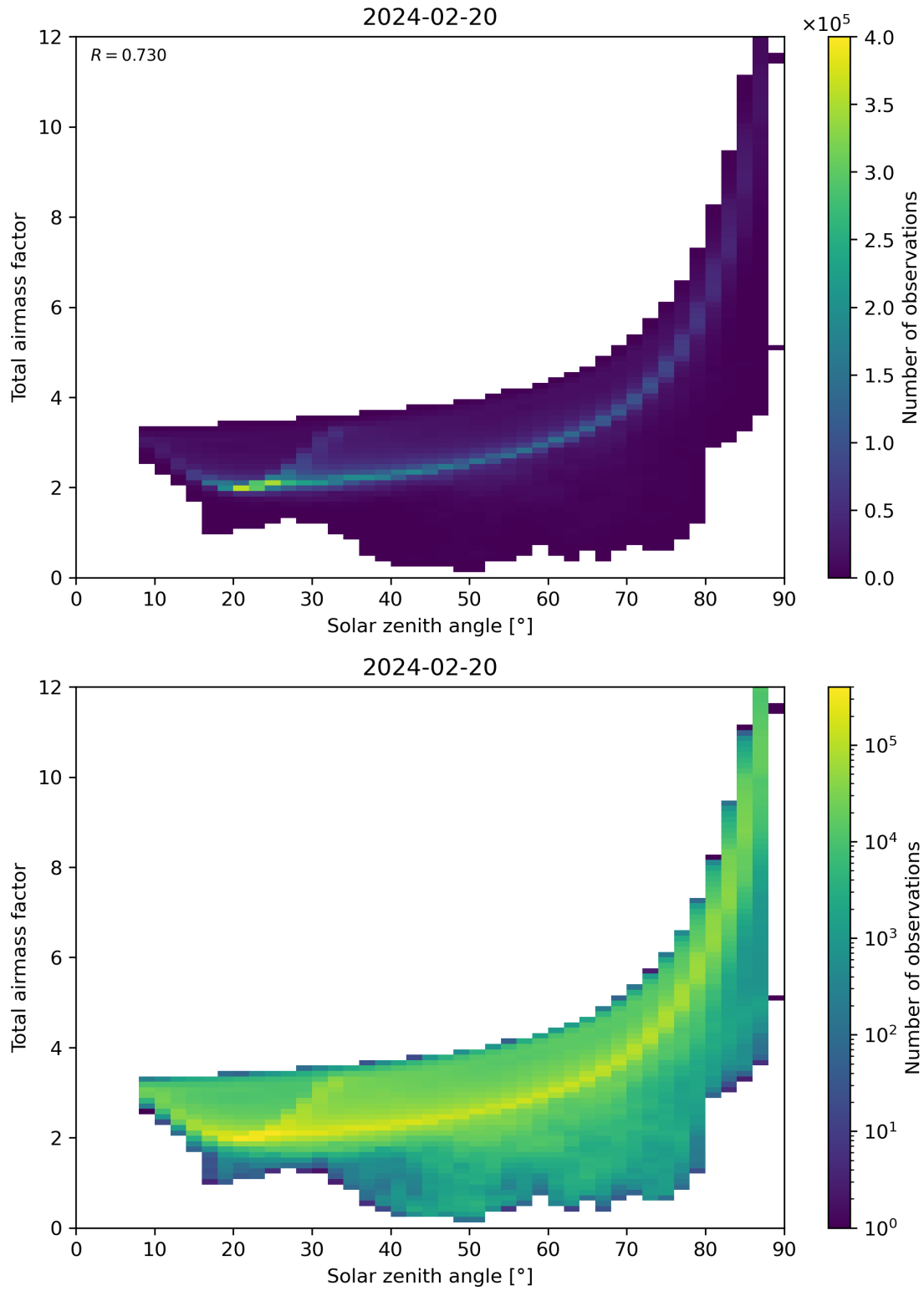
Figure 146: Scatter density plot of “Solar zenith angle” against “Total air mass factor” for 2024-02-19 to 2024-02-21.
