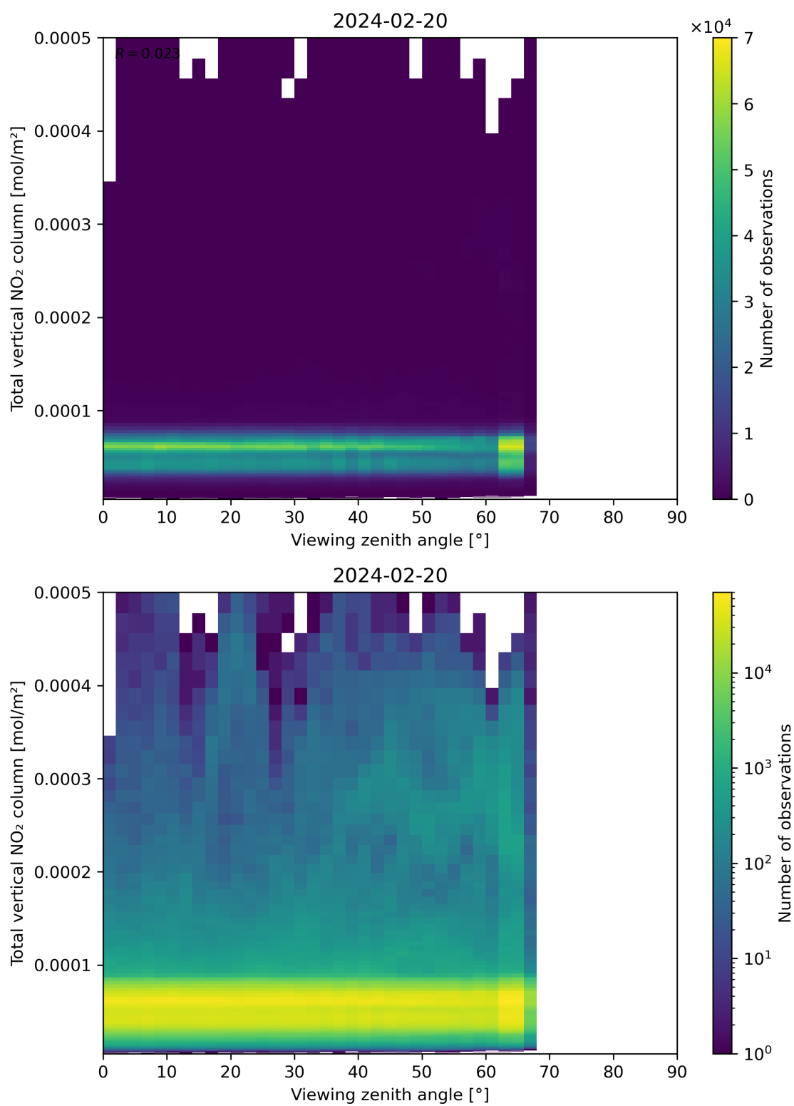
Figure 167: Scatter density plot of “Viewing zenith angle” against “Total vertical NO 2 column” for 2024-02-19 to 2024-02-21.
