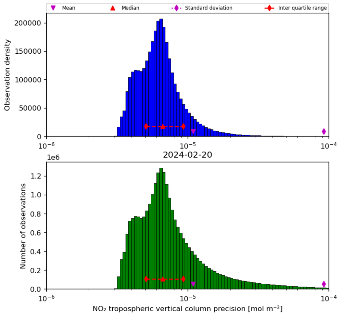
Figure 30: Histogram of “NO 2 tropospheric vertical column precision” for 2024-02-19 to 2024-02-21
