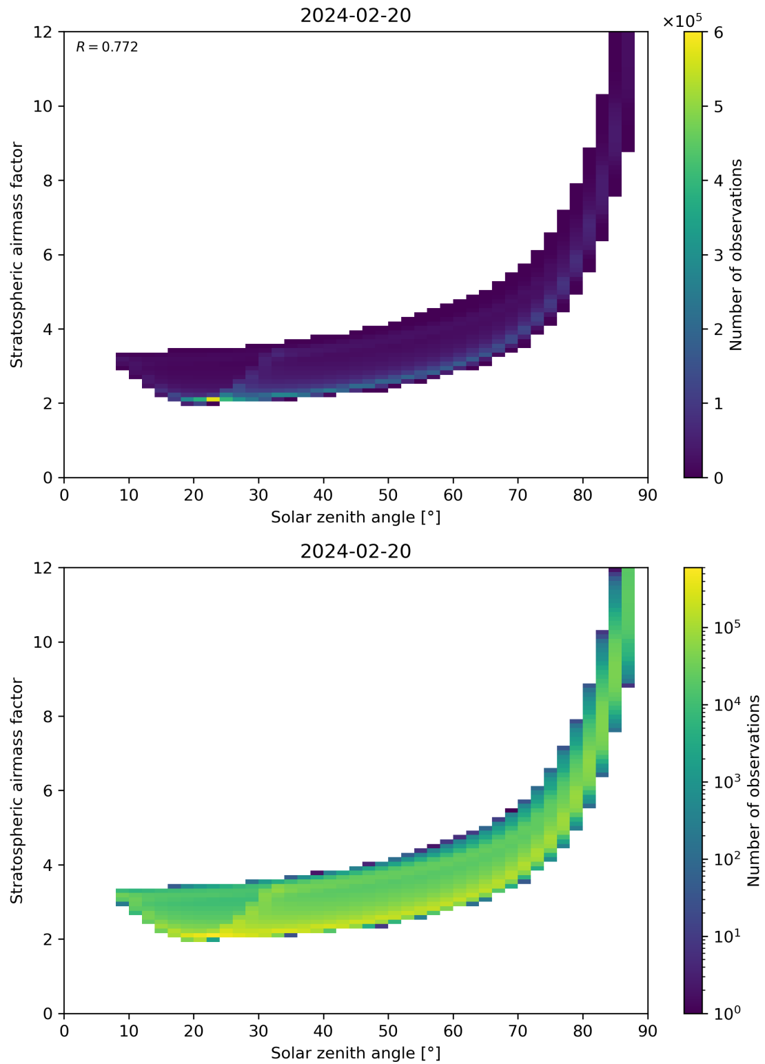
Figure 145: Scatter density plot of “Solar zenith angle” against “Stratospheric airmass factor” for 2024-02-19 to 2024-02-21.
