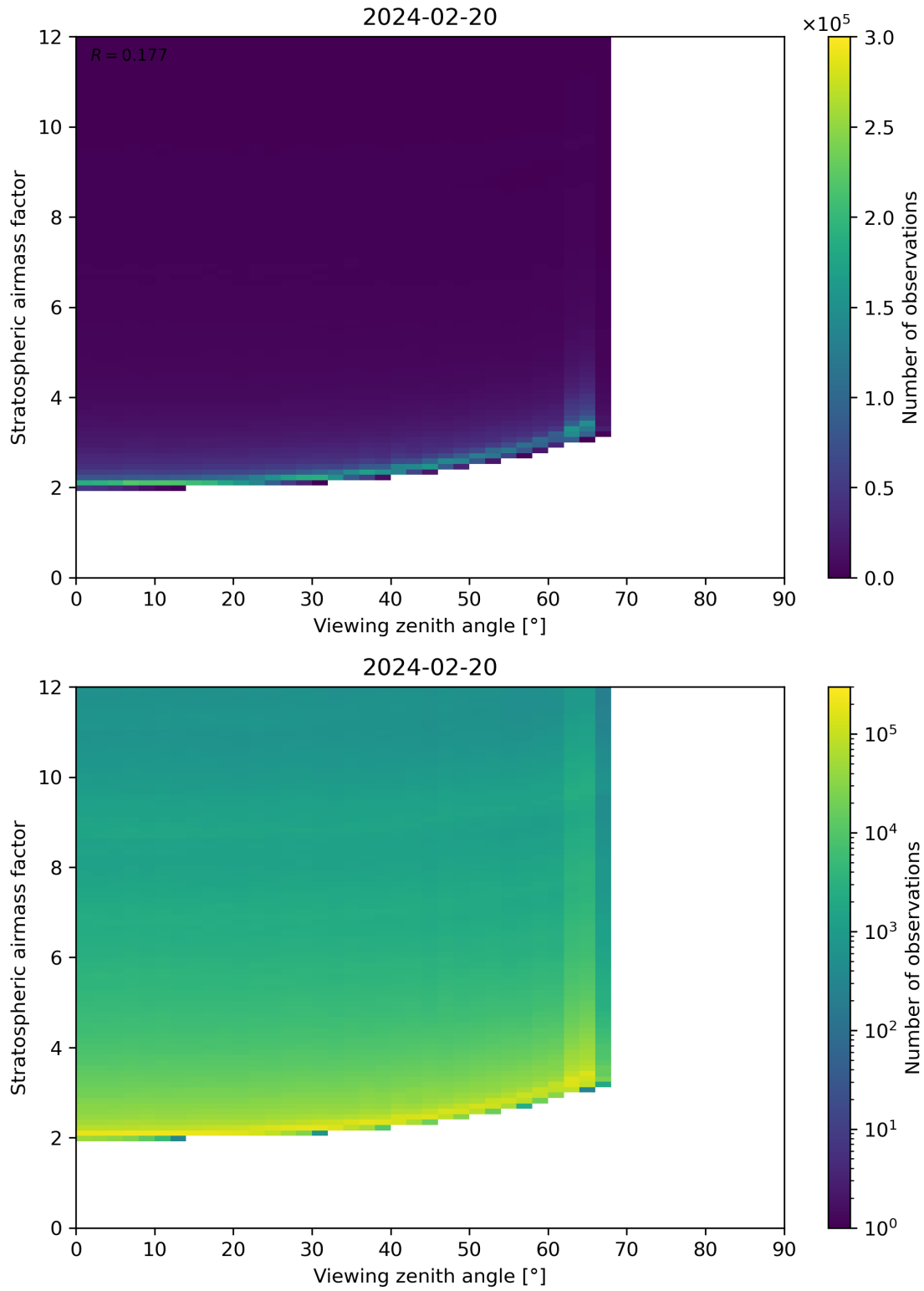
Figure 159: Scatter density plot of “Viewing zenith angle” against “Stratospheric airmass factor” for 2024-02-19 to 2024-02-21.
