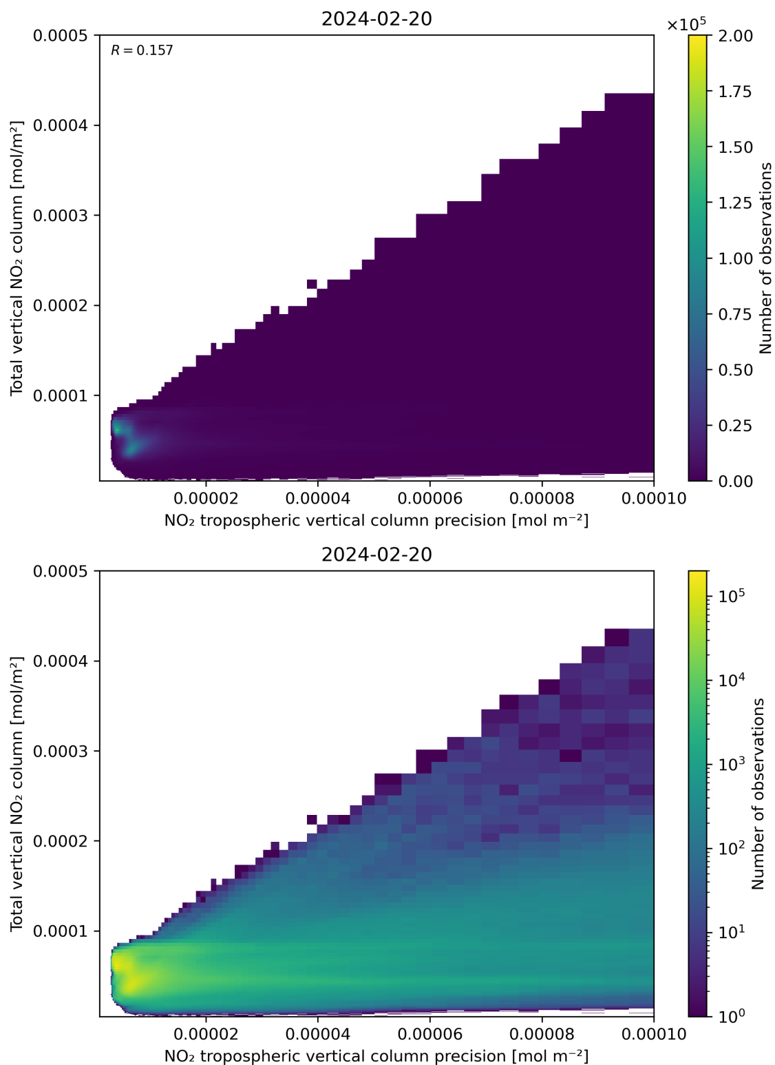
Figure 138: Scatter density plot of “NO 2 tropospheric vertical column precision” against “Total vertical NO 2 column” for 2024-02-19 to 2024-02-21.
