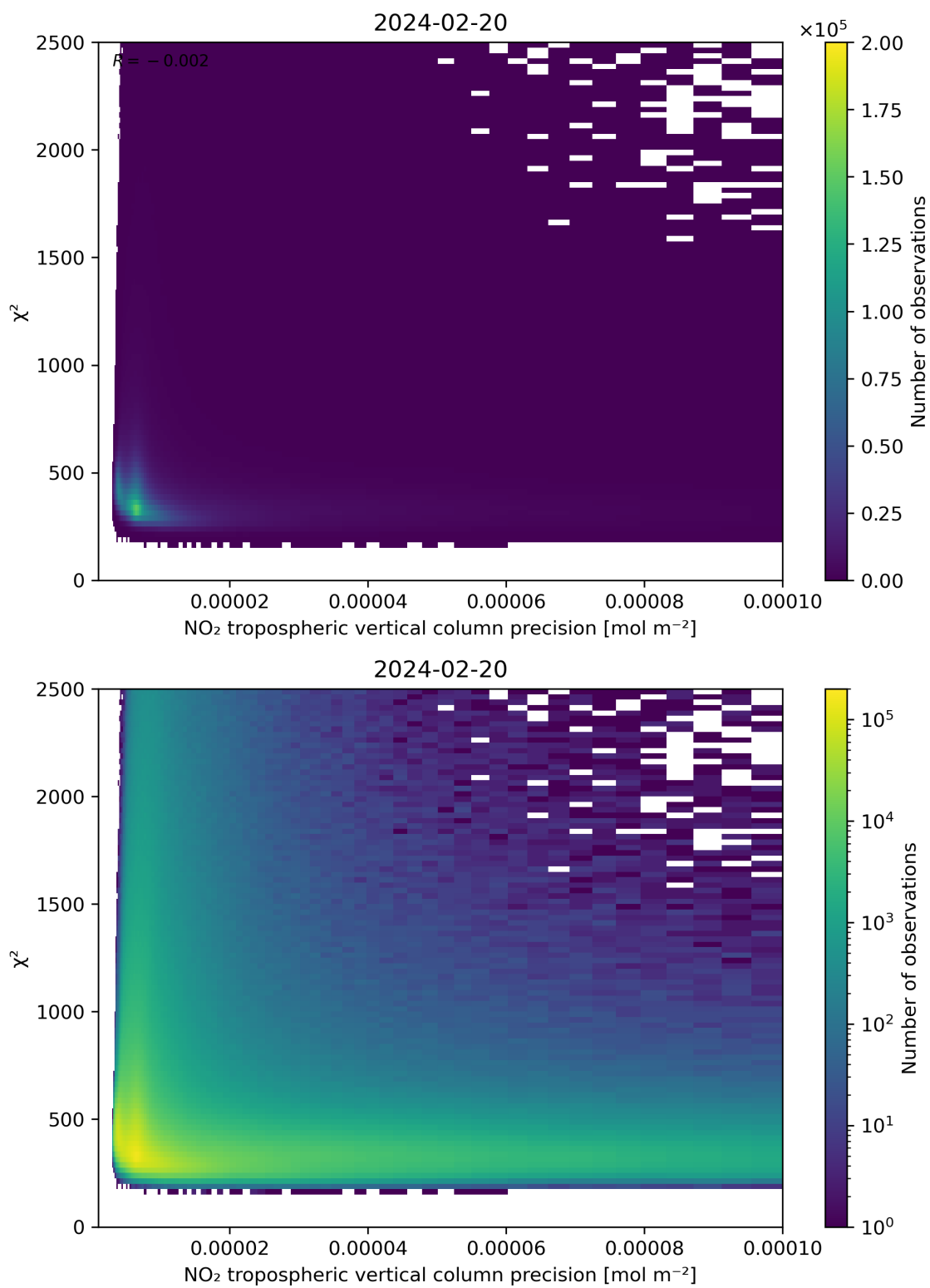
Figure 134: Scatter density plot of “NO 2 tropospheric vertical column precision” against “ \chi^2 ” for 2024-02-19 to 2024-02-21.
