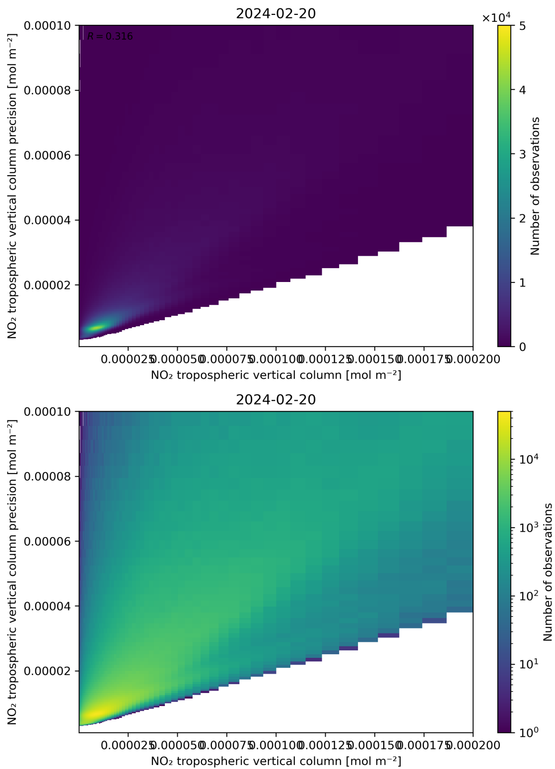
Figure 130: Scatter density plot of “NO 2 tropospheric vertical column” against “NO 2 tropospheric vertical column precision” for 2024-02-19 to 2024-02-21.
