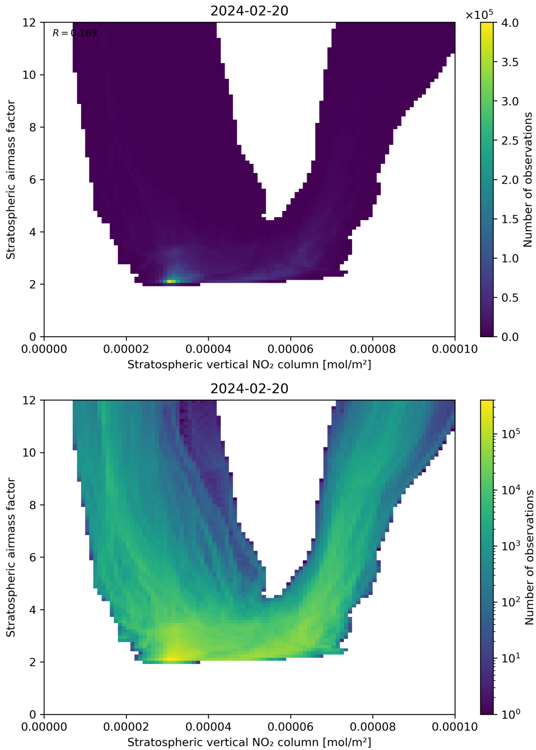
Figure 96: Scatter density plot of “Stratospheric vertical NO 2 column” against “Stratospheric airmass factor” for 2024-02-19 to 2024-02-21.
