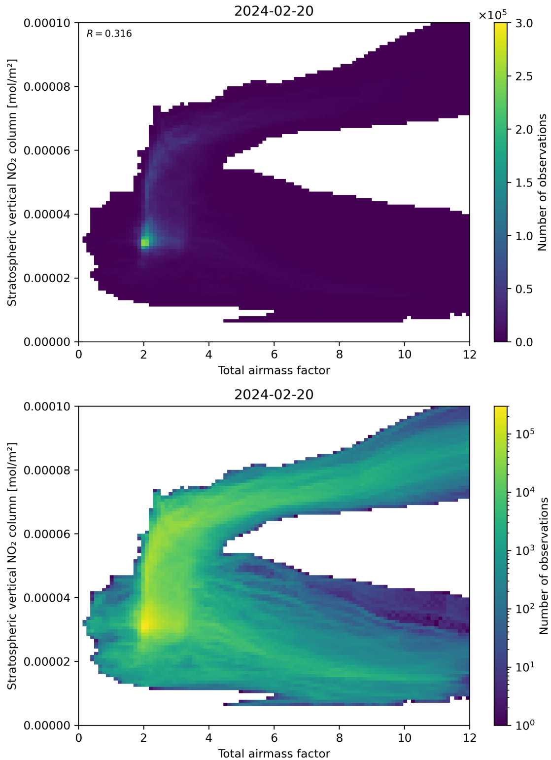
Figure 64: Scatter density plot of “Total airmass factor” against “Stratospheric vertical \text{NO}_2 column” for 2024-02-19 to 2024-02-21.
