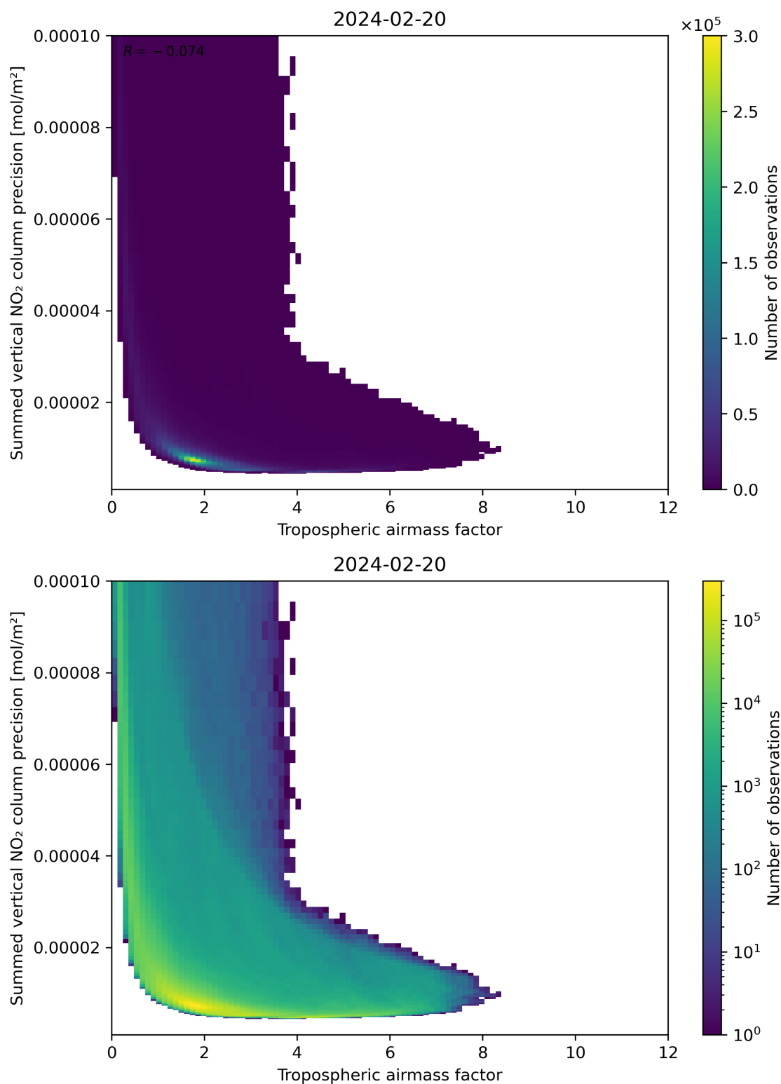
Figure 76: Scatter density plot of “Tropospheric air mass factor” against “Summed vertical NO 2 column precision” for 2024-02-19 to 2024-02-21.
