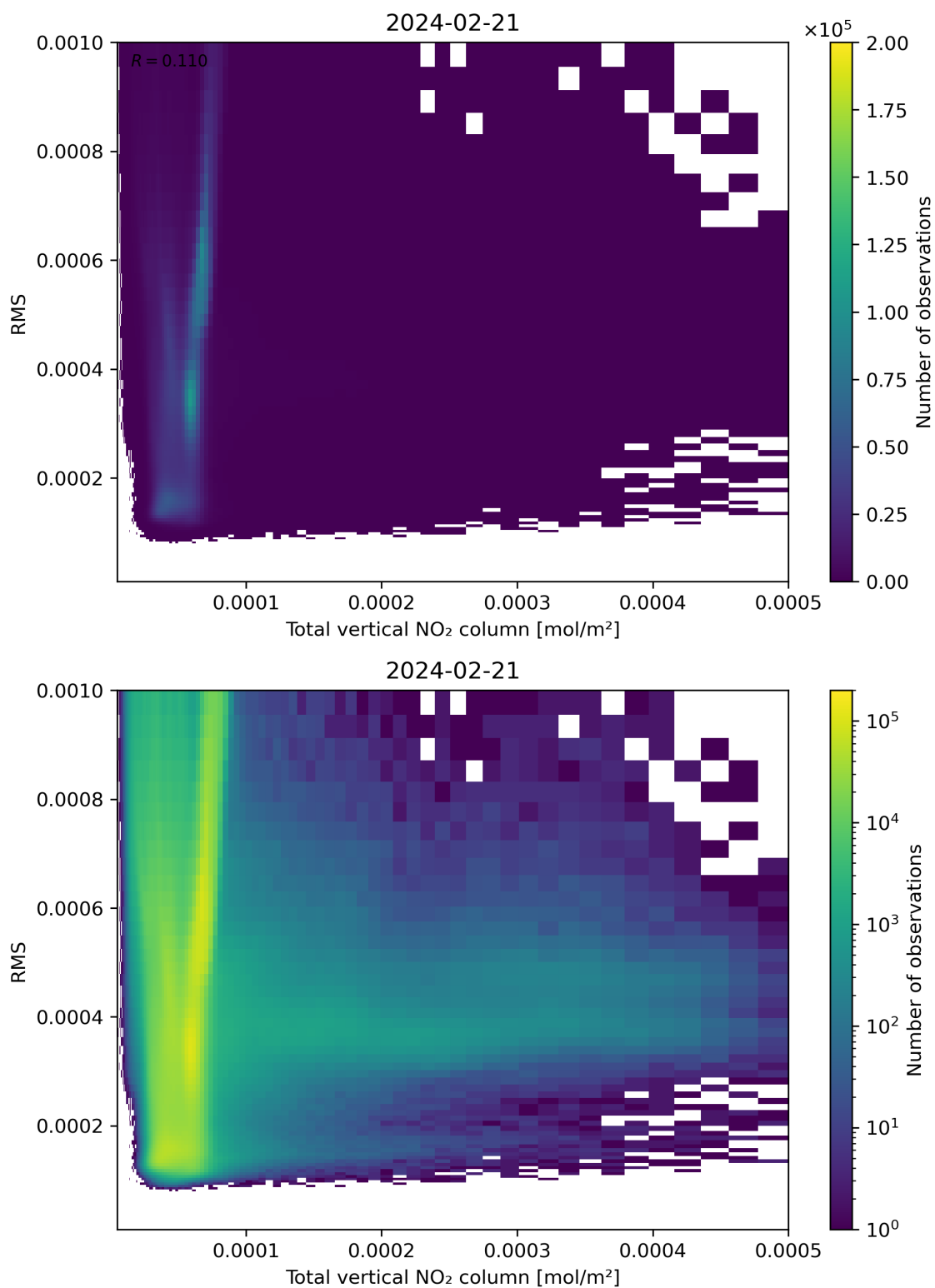
Figure 120: Scatter density plot of “Total vertical NO 2 column” against “RMS” for 2024-02-20 to 2024-02-22.
