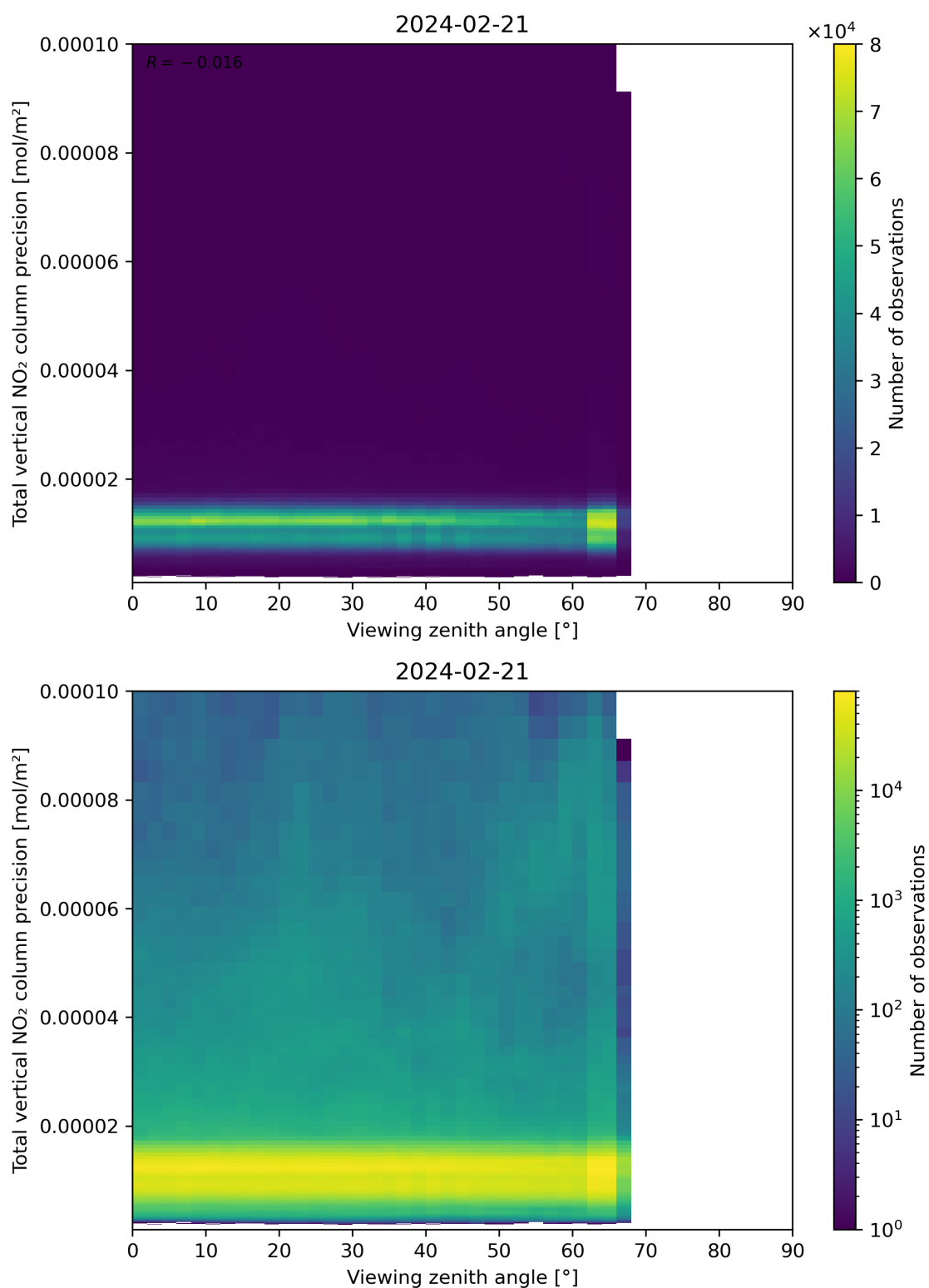
Figure 168: Scatter density plot of “Viewing zenith angle” against “Total vertical NO 2 column precision” for 2024-02-20 to 2024-02-22.
