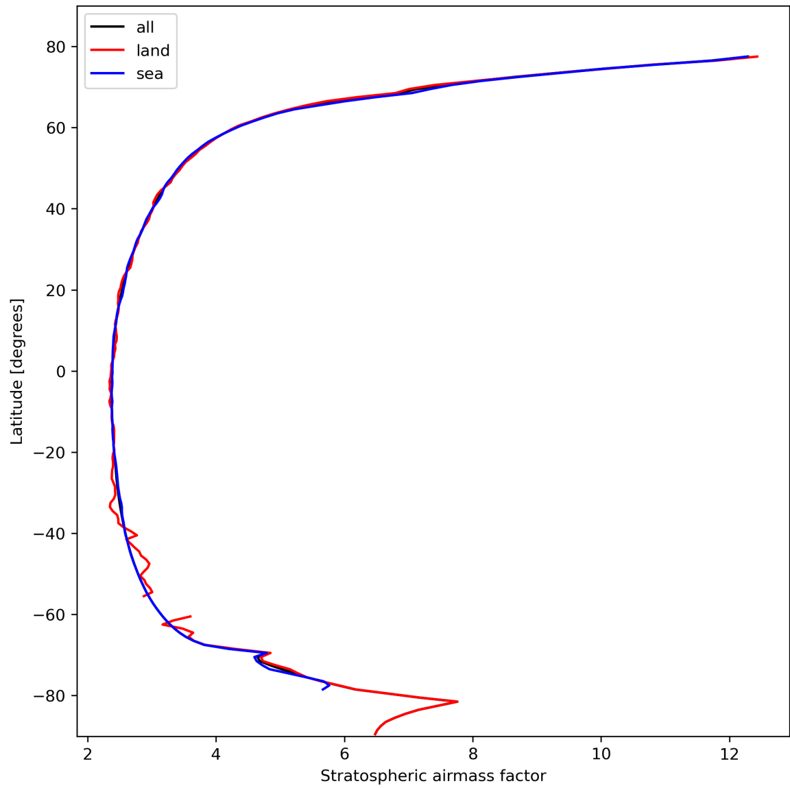
Figure 27: Zonal average of “Stratospheric airmass factor” for 2024-02-20 to 2024-02-22.
