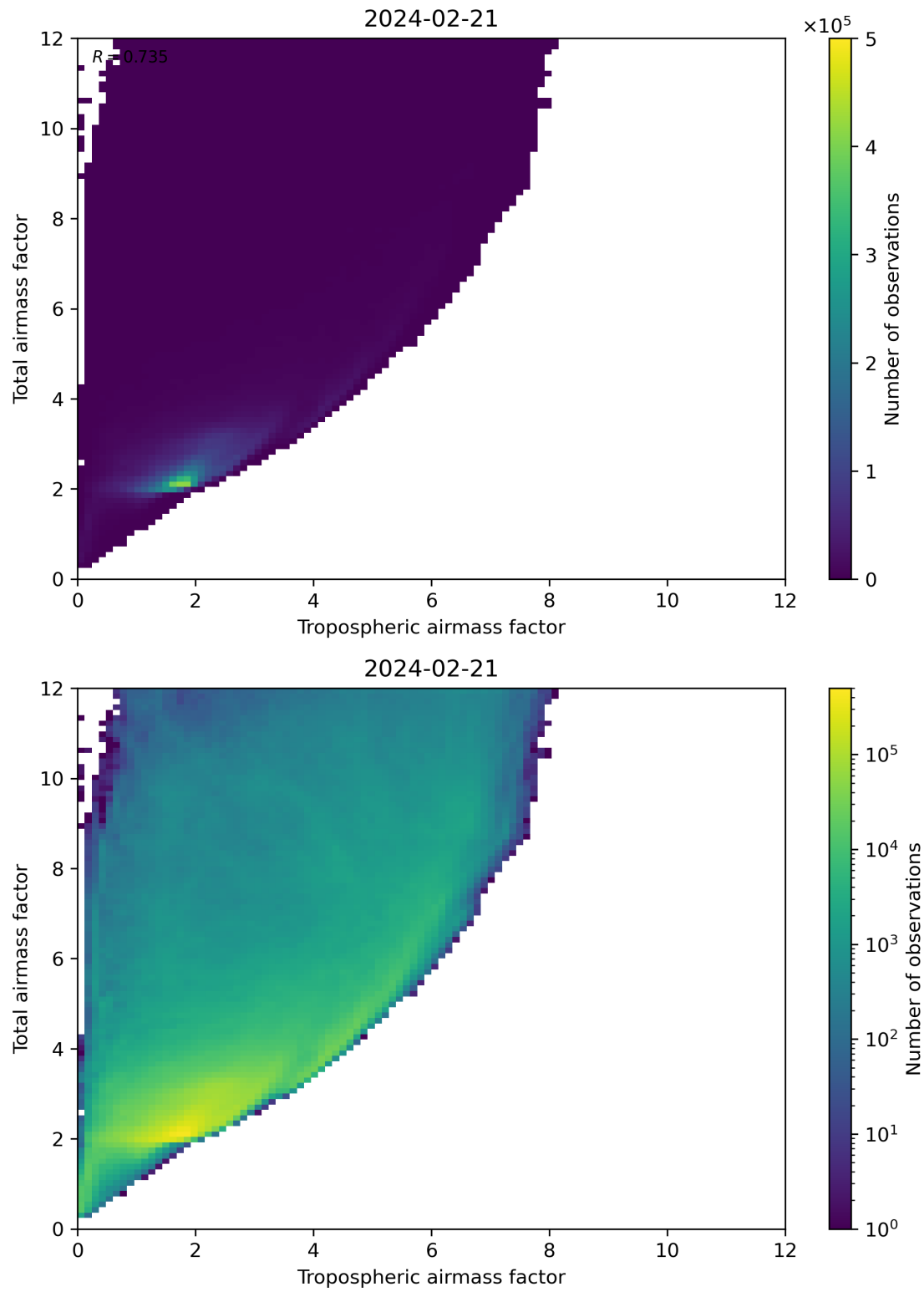
Figure 72: Scatter density plot of “Tropospheric airmass factor” against “Total airmass factor” for 2024-02-20 to 2024-02-22.
