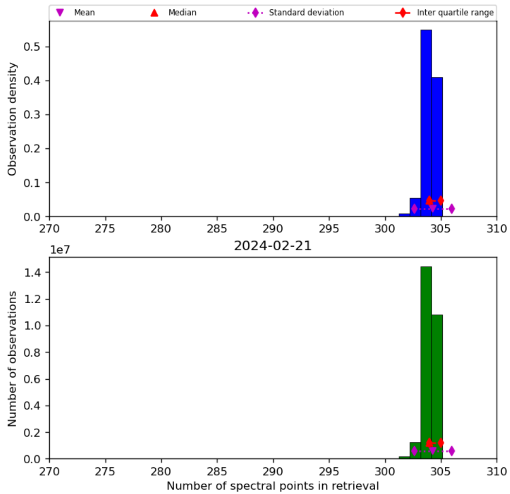
Figure 33: Histogram of “Number of spectral points in retrieval” for 2024-02-20 to 2024-02-22
