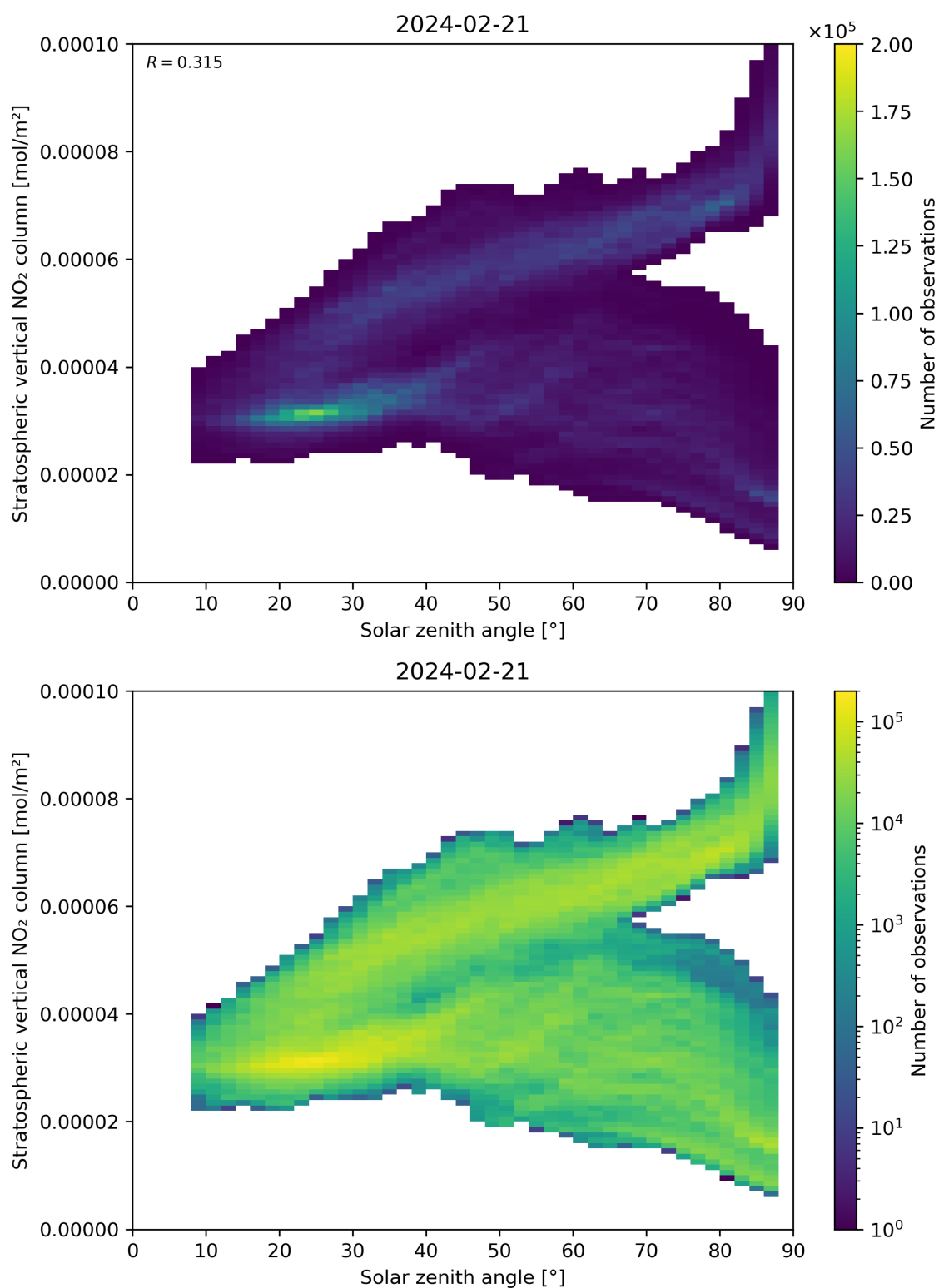
Figure 150: Scatter density plot of “Solar zenith angle” against “Stratospheric vertical NO 2 column” for 2024-02-20 to 2024-02-22.
