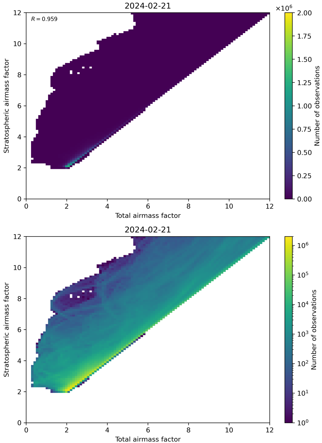
Figure 62: Scatter density plot of “Total airmass factor” against “Stratospheric airmass factor” for 2024-02-20 to 2024-02-22.
