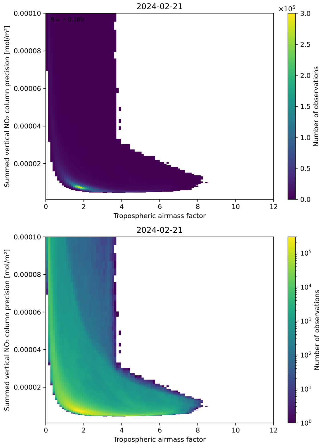
Figure 76: Scatter density plot of “Tropospheric air mass factor” against “Summed vertical NO 2 column precision” for 2024-02-20 to 2024-02-22.
