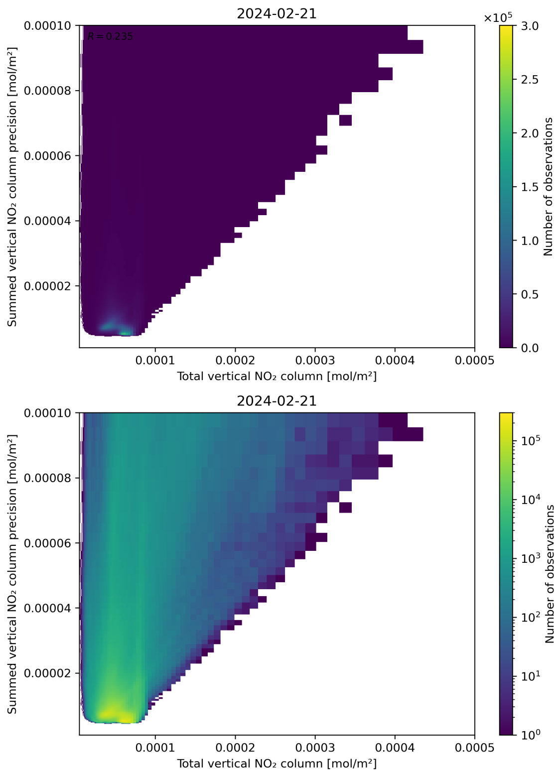
Figure 113: Scatter density plot of “Total vertical NO 2 column” against “Summed vertical NO 2 column precision” for 2024-02-20 to 2024-02-22.
