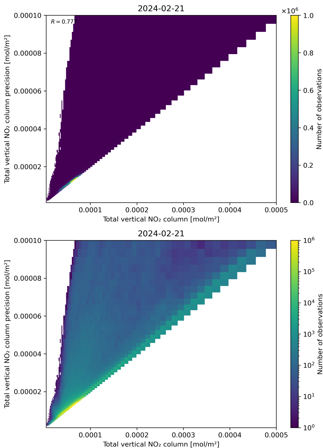
Figure 114: Scatter density plot of “Total vertical NO 2 column” against “Total vertical NO 2 column precision” for 2024-02-20 to 2024-02-22.
