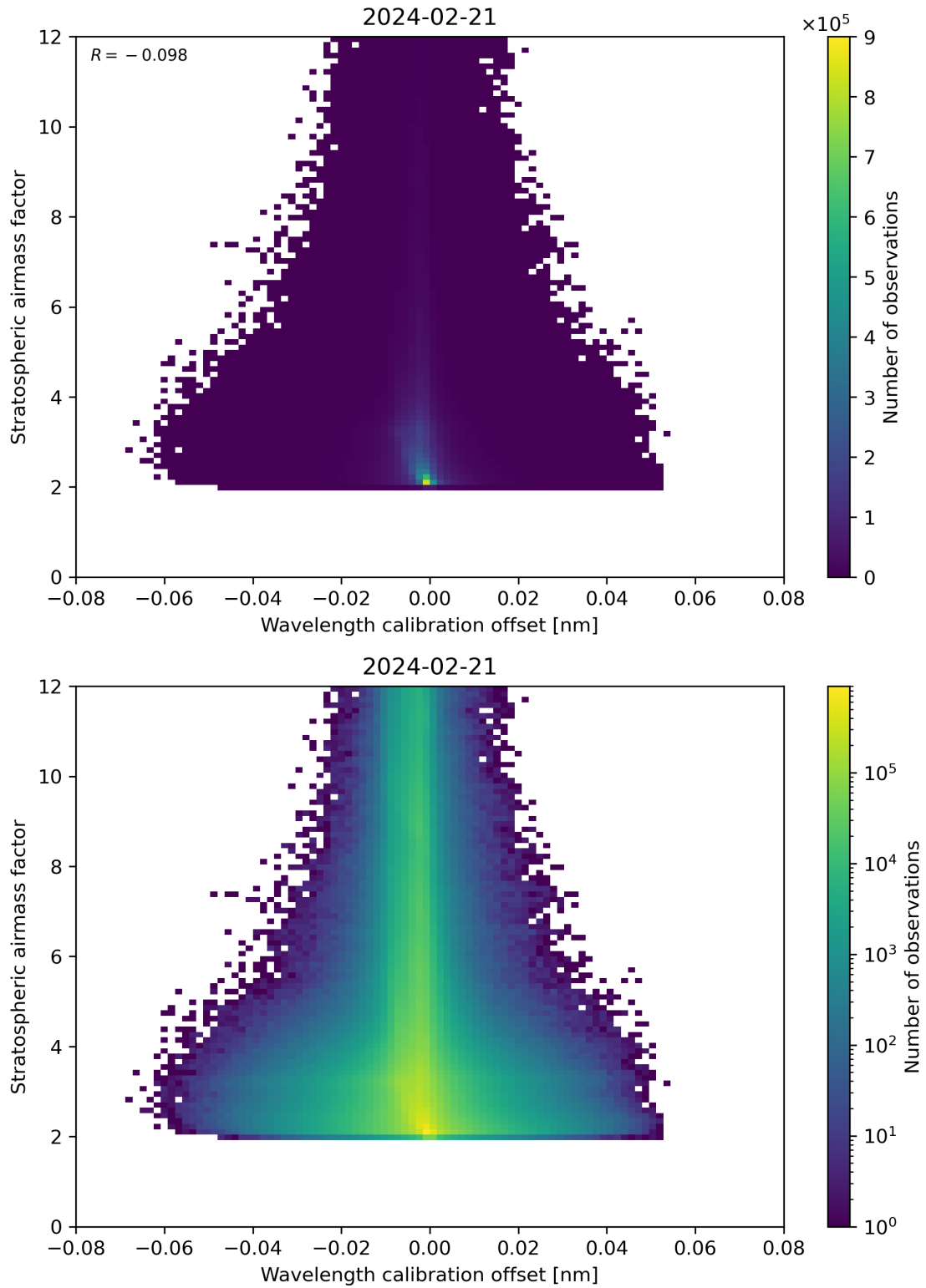
Figure 174: Scatter density plot of “Wavelength calibration offset” against “Stratospheric airmass factor” for 2024-02-20 to 2024-02-22.
