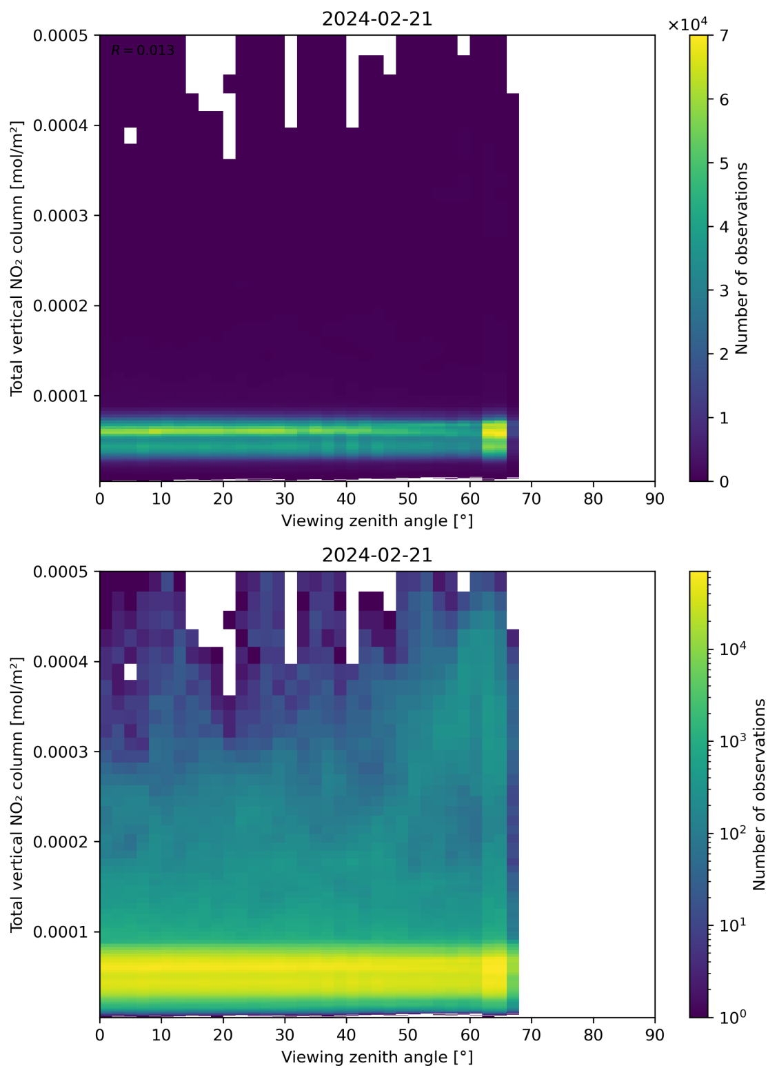
Figure 167: Scatter density plot of “Viewing zenith angle” against “Total vertical NO 2 column” for 2024-02-20 to 2024-02-22.
