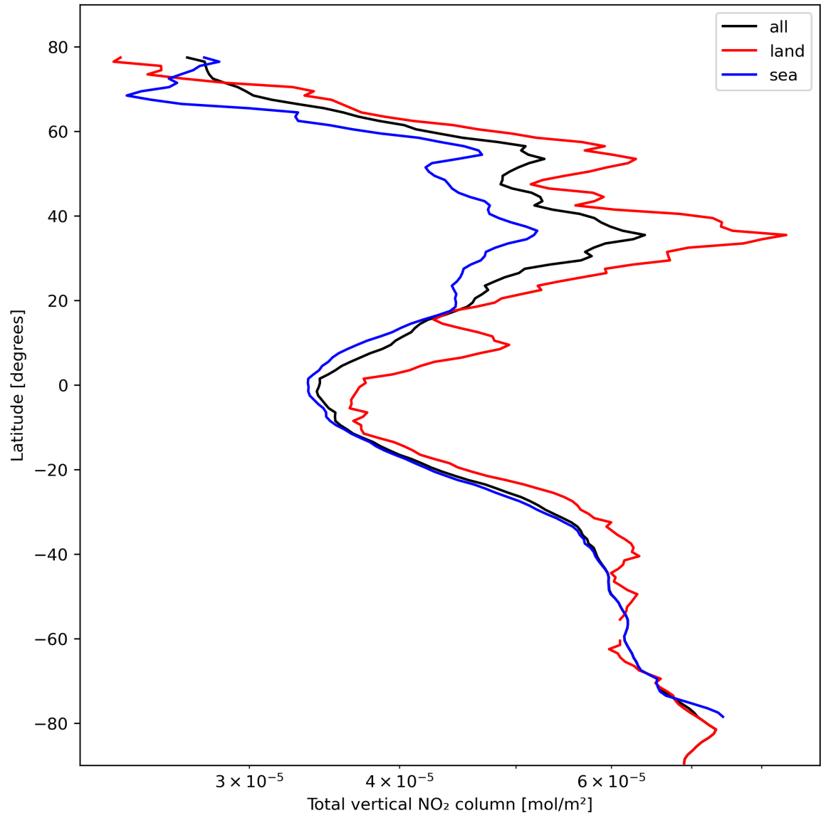
Figure 21: Zonal average of “Total vertical NO 2 column” for 2024-02-20 to 2024-02-22.
