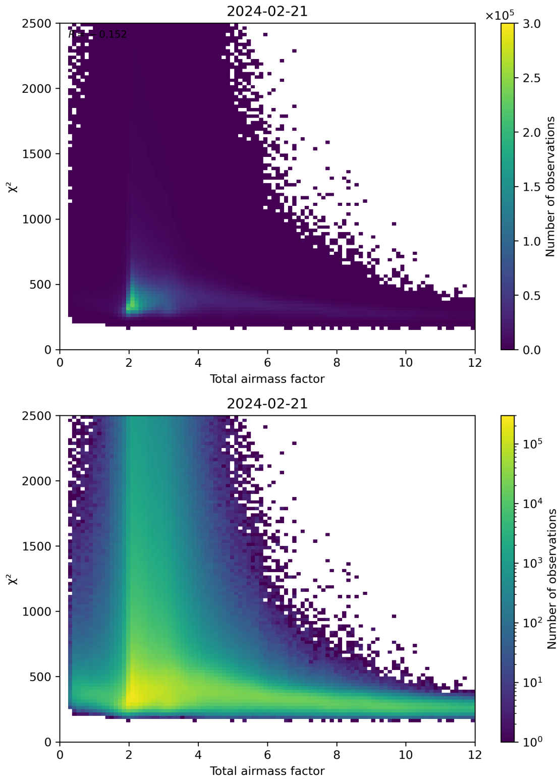
Figure 63: Scatter density plot of “Total airmass factor” against “ \chi^2 ” for 2024-02-20 to 2024-02-22.
