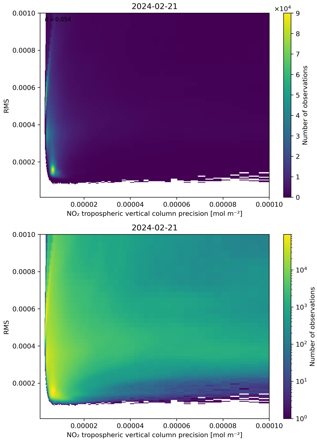
Figure 140: Scatter density plot of “NO 2 tropospheric vertical column precision” against “RMS” for 2024-02-20 to 2024-02-22.
