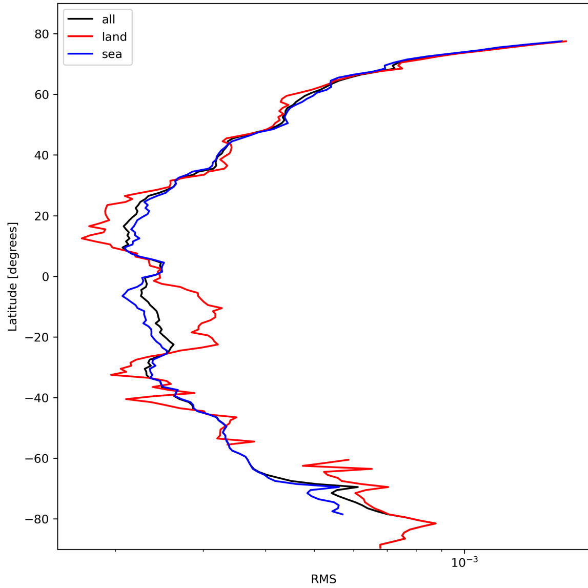
Figure 26: Zonal average of “RMS” for 2024-02-20 to 2024-02-22.
