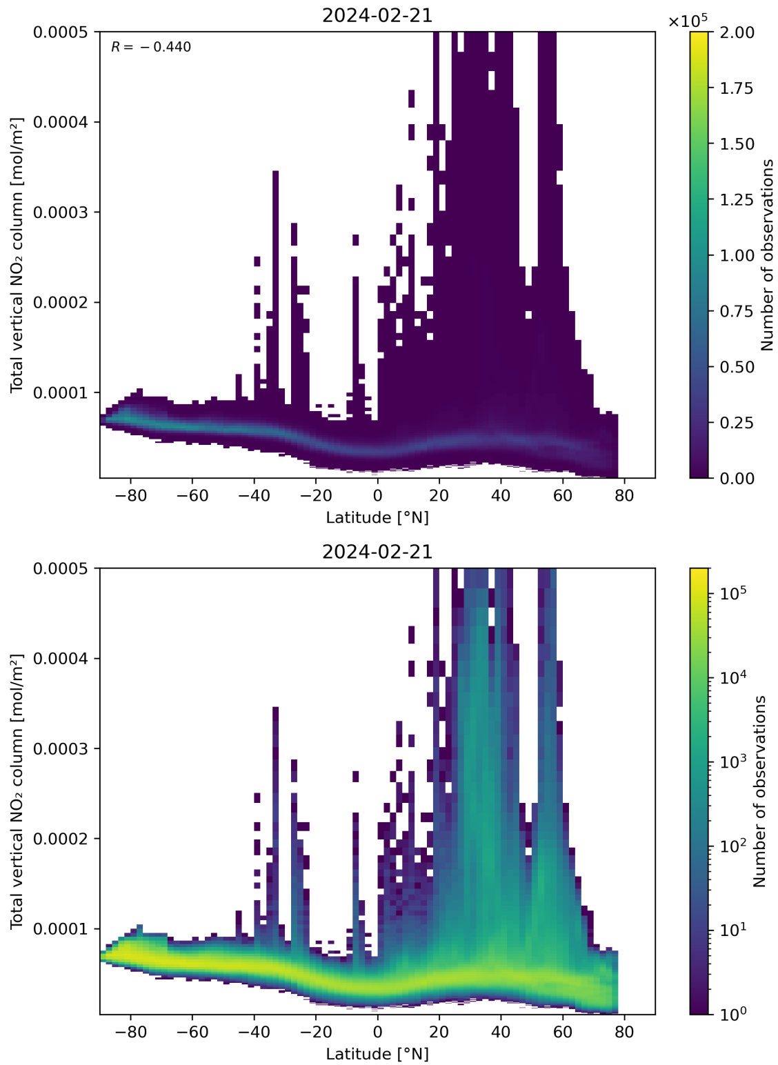
Figure 90: Scatter density plot of “Latitude” against “Total vertical NO 2 column” for 2024-02-20 to 2024-02-22.
