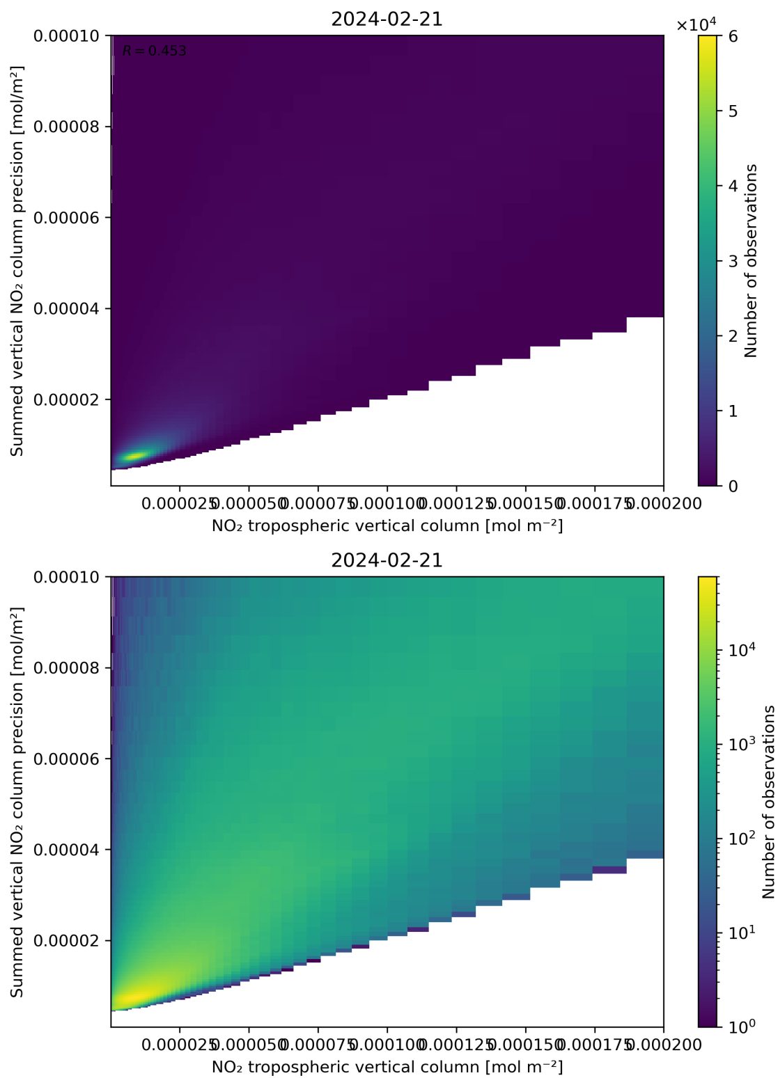
Figure 127: Scatter density plot of “NO 2 tropospheric vertical column” against “Summed vertical NO 2 column precision” for 2024-02-20 to 2024-02-22.
