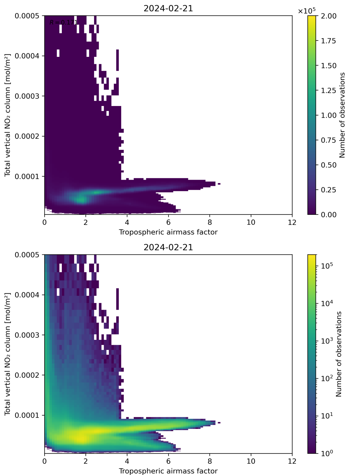
Figure 77: Scatter density plot of “Tropospheric airmass factor” against “Total vertical NO 2 column” for 2024-02-20 to 2024-02-22.
