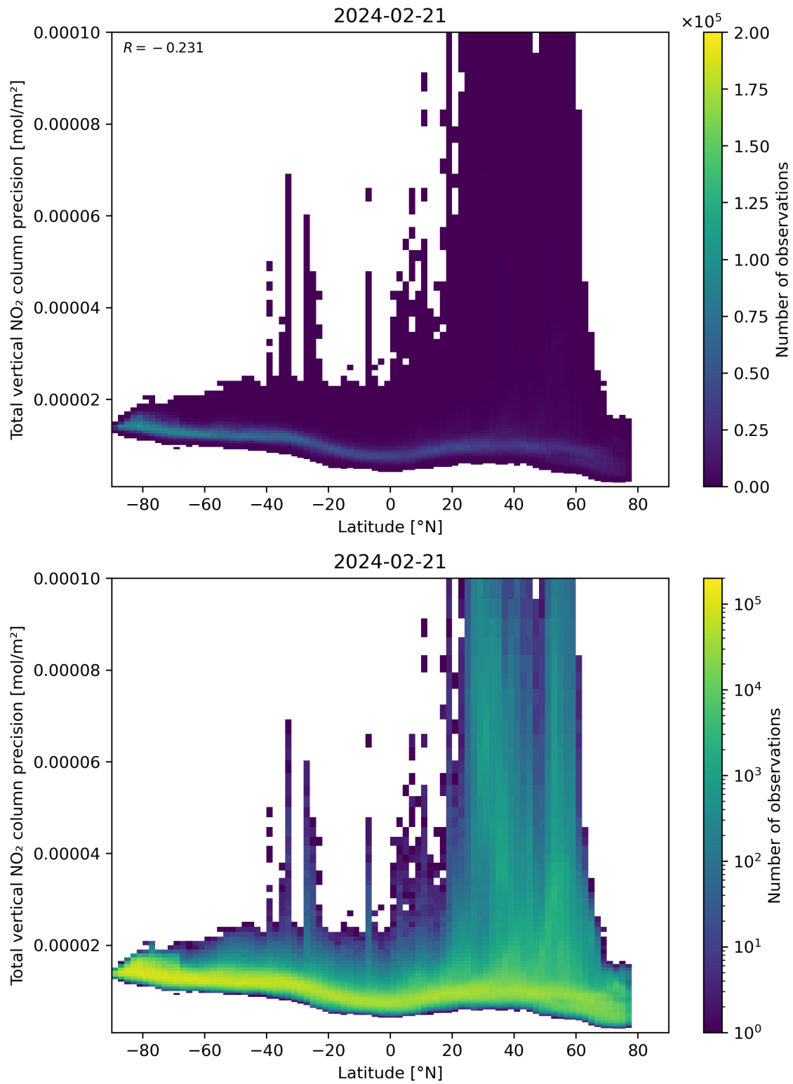
Figure 91: Scatter density plot of “Latitude” against “Total vertical NO 2 column precision” for 2024-02-20 to 2024-02-22.
