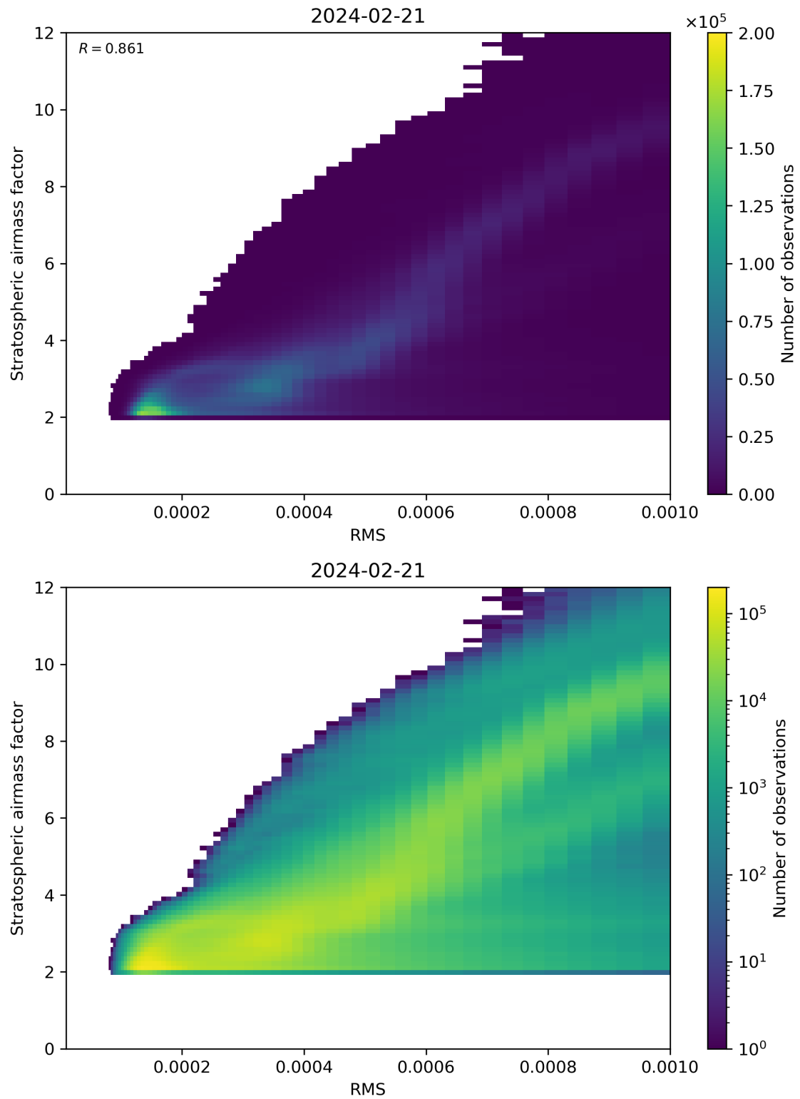
Figure 144: Scatter density plot of “RMS” against “Stratospheric airmass factor” for 2024-02-20 to 2024-02-22.
