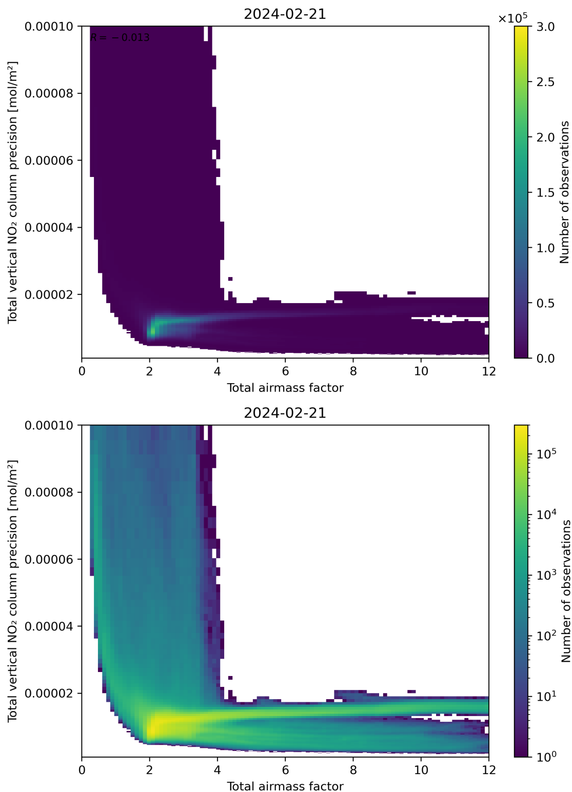
Figure 68: Scatter density plot of “Total airmass factor” against “Total vertical NO 2 column precision” for 2024-02-20 to 2024-02-22.
