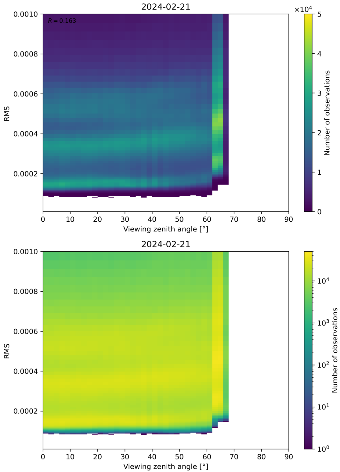
Figure 171: Scatter density plot of “Viewing zenith angle” against “RMS” for 2024-02-20 to 2024-02-22.
