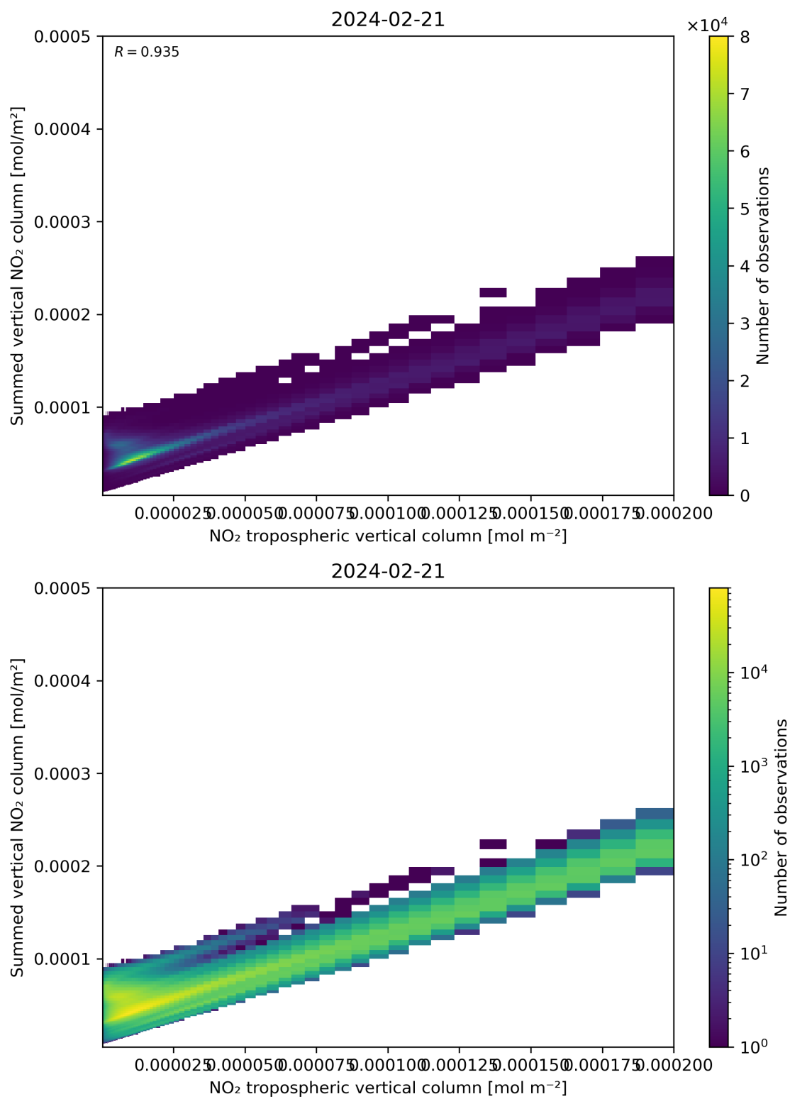
Figure 126: Scatter density plot of “NO 2 tropospheric vertical column” against “Summed vertical NO 2 column” for 2024-02-20 to 2024-02-22.
