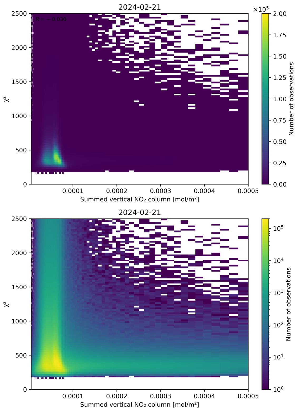
Figure 104: Scatter density plot of “Summed vertical NO 2 column” against “ \chi^2 ” for 2024-02-20 to 2024-02-22.
