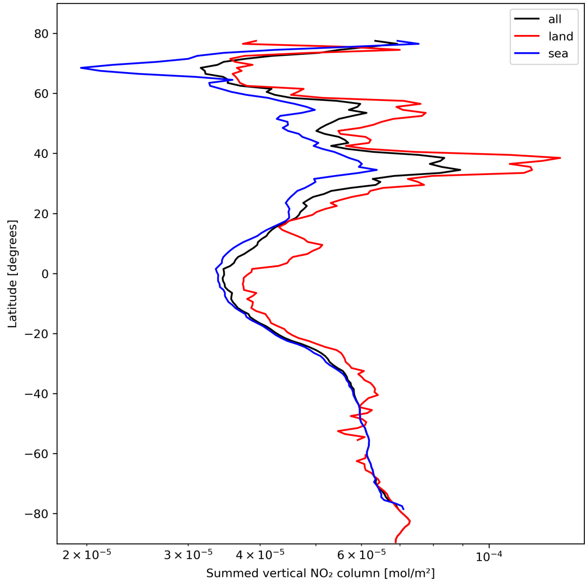
Figure 23: Zonal average of “Summed vertical NO 2 column” for 2024-02-20 to 2024-02-22.
