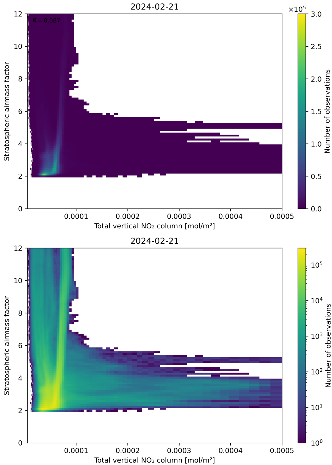
Figure 110: Scatter density plot of “Total vertical NO 2 column” against “Stratospheric airmass factor” for 2024-02-20 to 2024-02-22.
