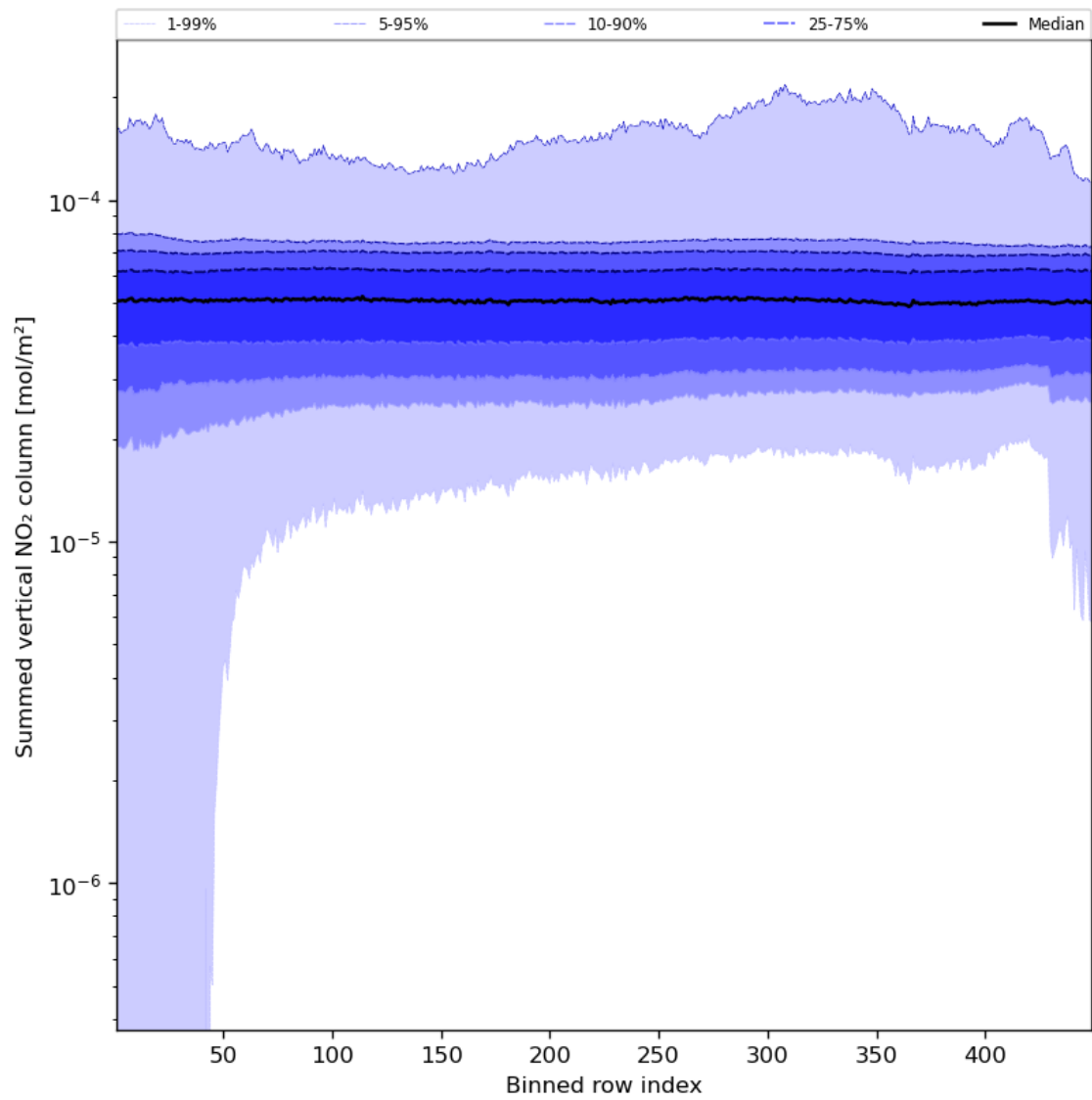
Figure 57: Along track statistics of “Summed vertical NO 2 column” for 2024-02-20 to 2024-02-22
