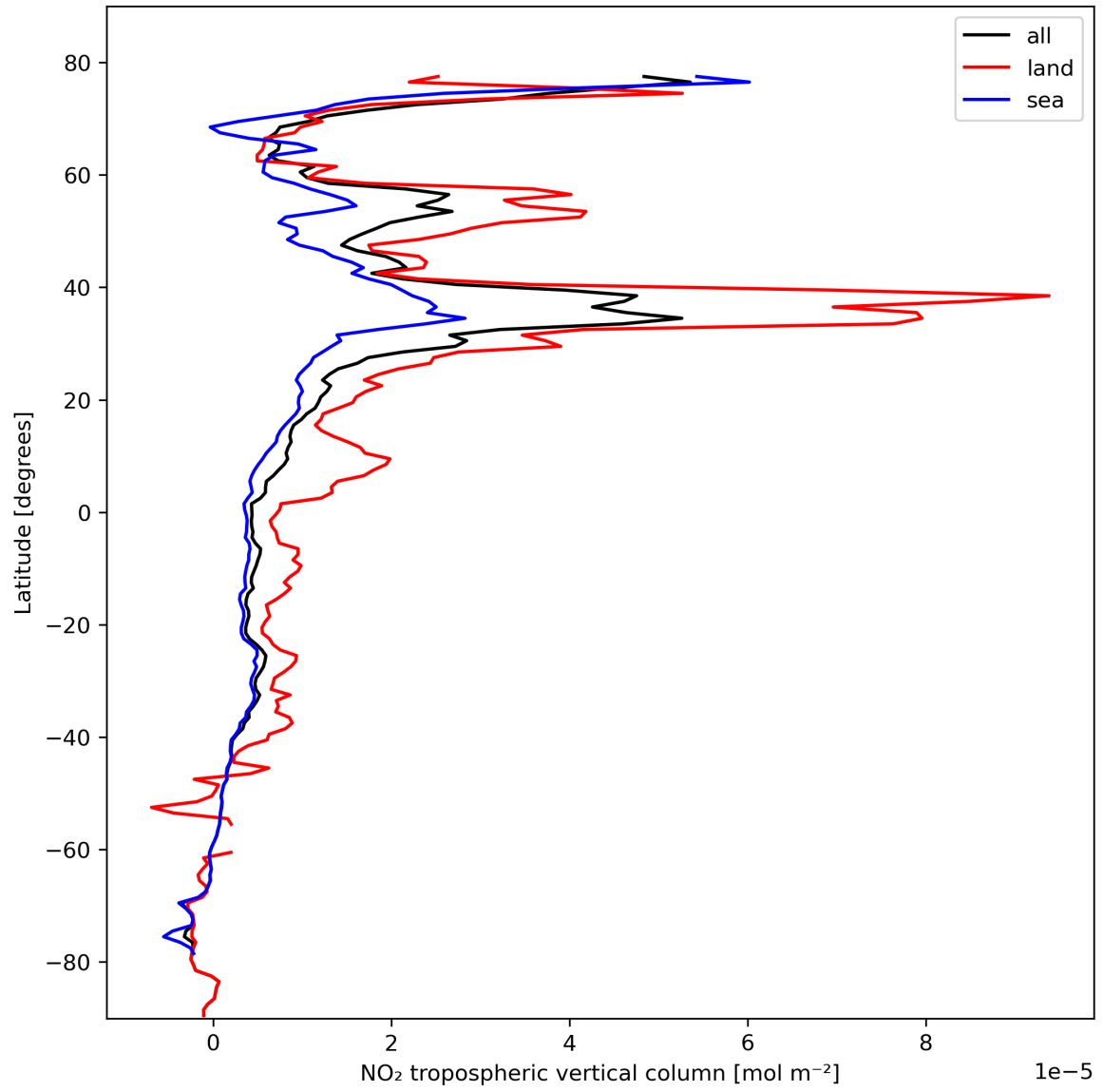
Figure 12: Zonal average of “NO 2 tropospheric vertical column” for 2024-02-20 to 2024-02-22.
