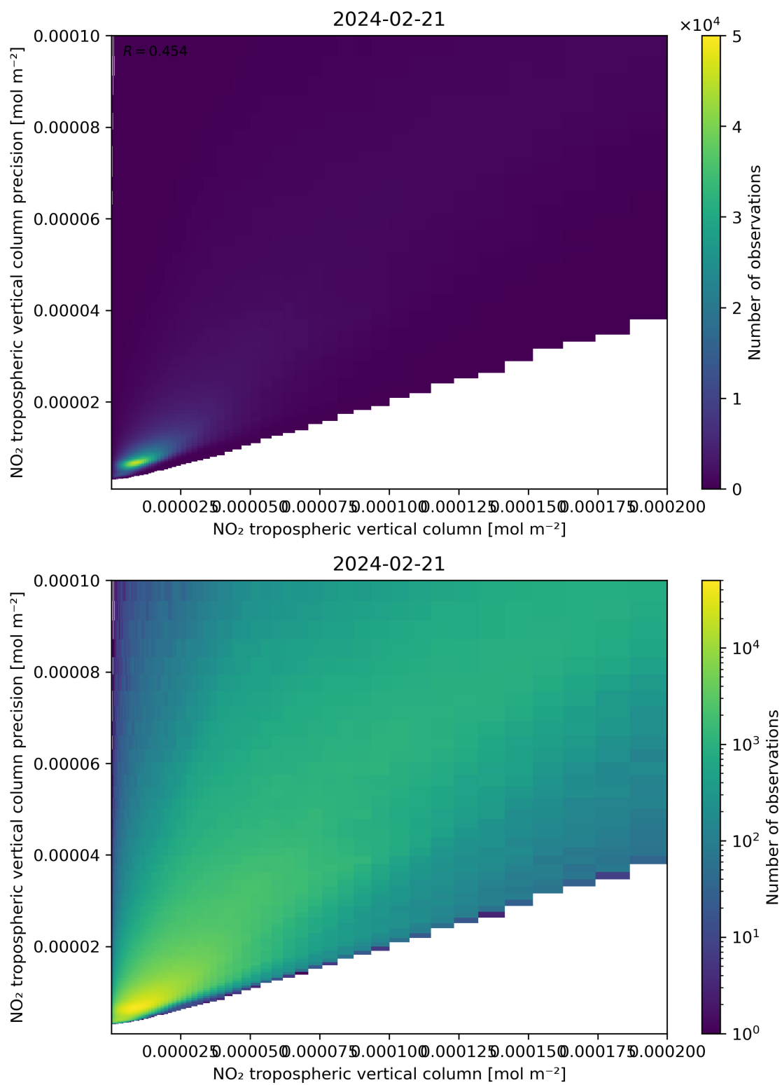
Figure 130: Scatter density plot of “NO 2 tropospheric vertical column” against “NO 2 tropospheric vertical column precision” for 2024-02-20 to 2024-02-22.
