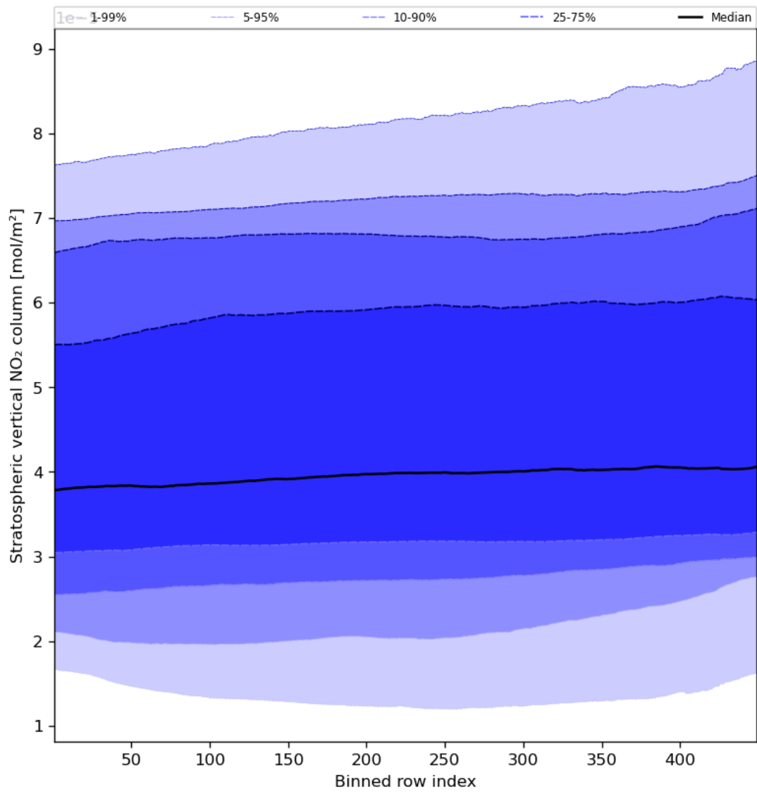
Figure 53: Along track statistics of “Stratospheric vertical NO 2 column” for 2024-02-20 to 2024-02-22
