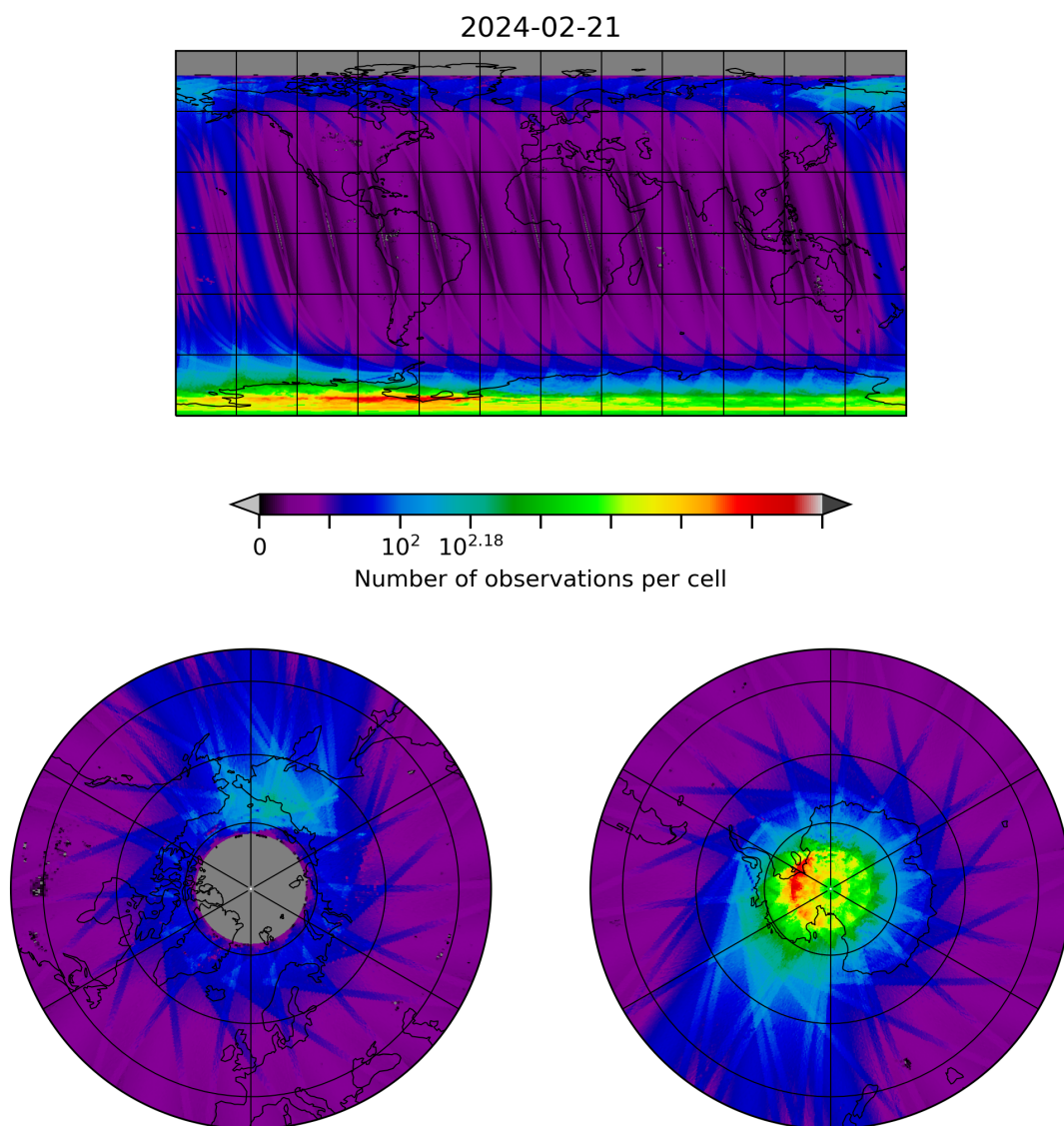
Figure 10: Map of the number of observations for 2024-02-20 to 2024-02-22
