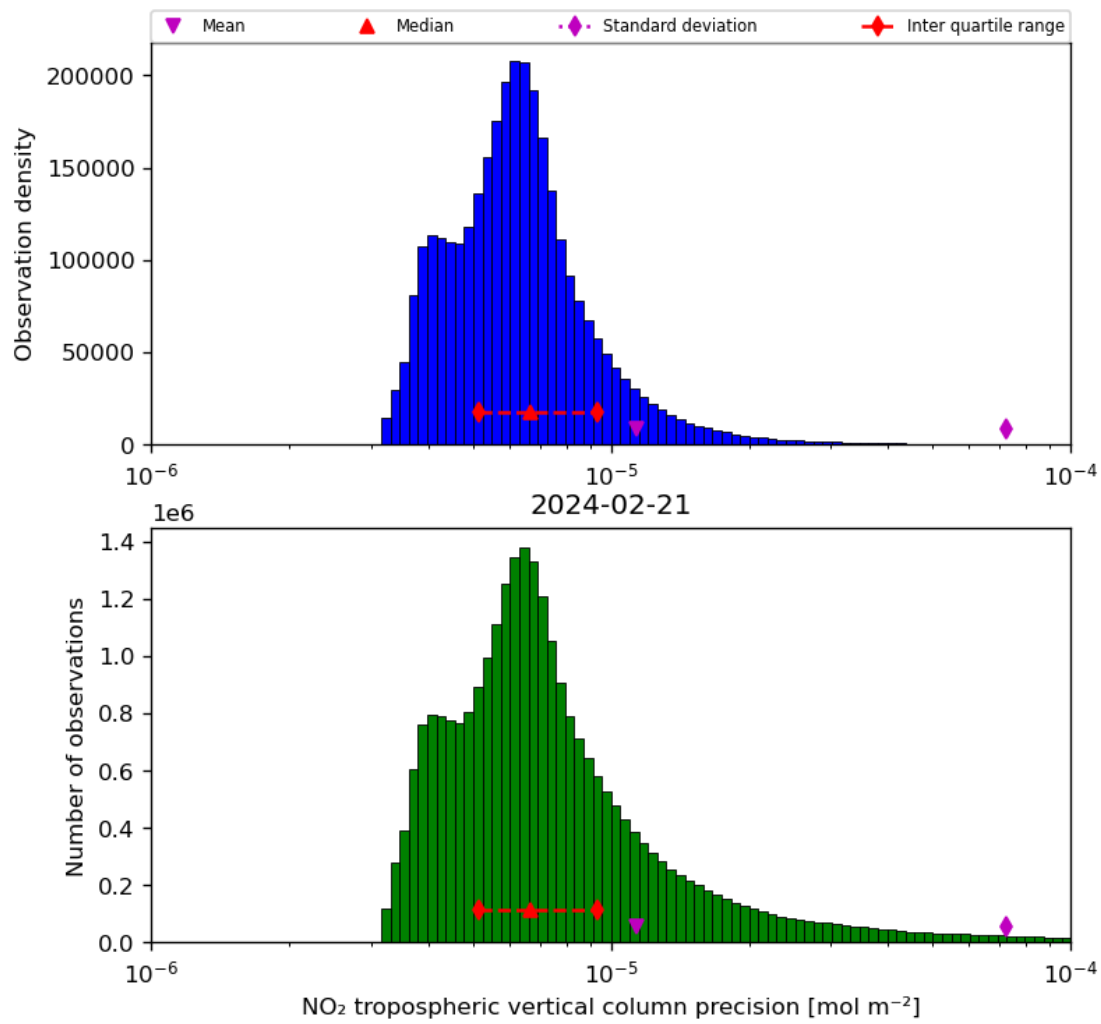
Figure 30: Histogram of “NO 2 tropospheric vertical column precision” for 2024-02-20 to 2024-02-22
