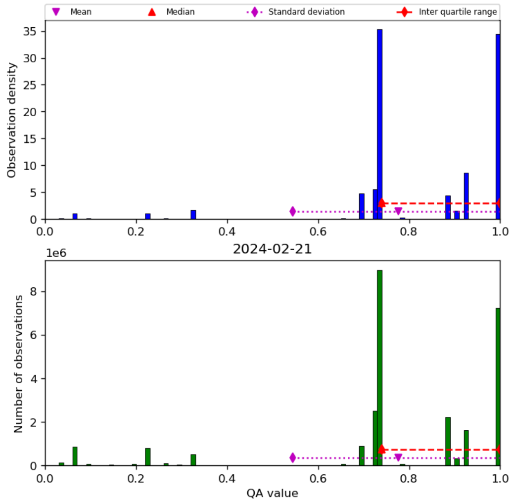
Figure 28: Histogram of “QA value” for 2024-02-20 to 2024-02-22
