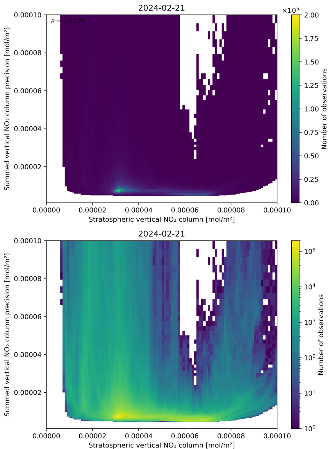
Figure 99: Scatter density plot of “Stratospheric vertical NO 2 column” against “Summed vertical NO 2 column precision” for 2024-02-20 to 2024-02-22.
