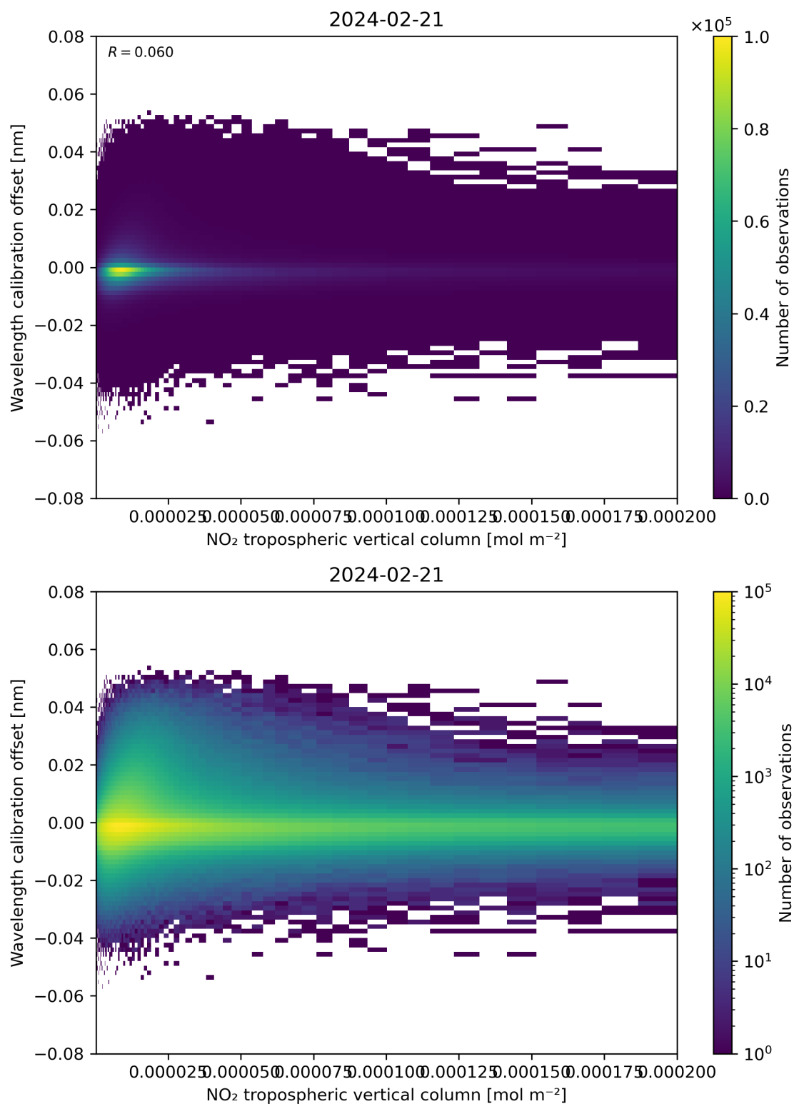
Figure 143: Scatter density plot of “NO 2 tropospheric vertical column” against “Wavelength calibration offset” for 2024-02-20 to 2024-02-22.
