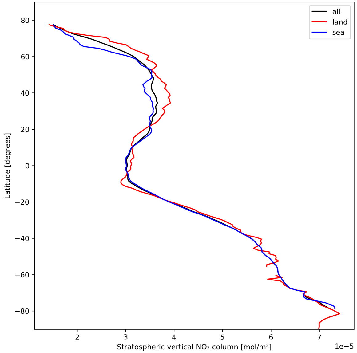
Figure 19: Zonal average of “Stratospheric vertical NO 2 column” for 2024-02-20 to 2024-02-22.
