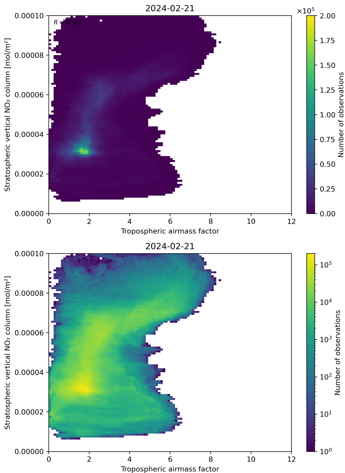
Figure 74: Scatter density plot of “Tropospheric air mass factor” against “Stratospheric vertical NO 2 column” for 2024-02-20 to 2024-02-22.
