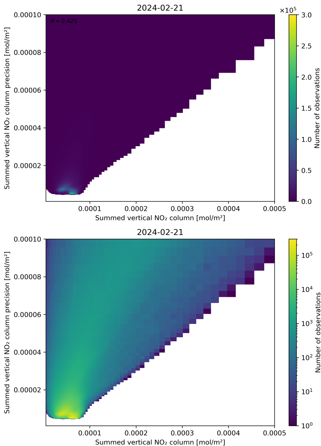
Figure 105: Scatter density plot of “Summed vertical NO 2 column” against “Summed vertical NO 2 column precision” for 2024-02-20 to 2024-02-22.
