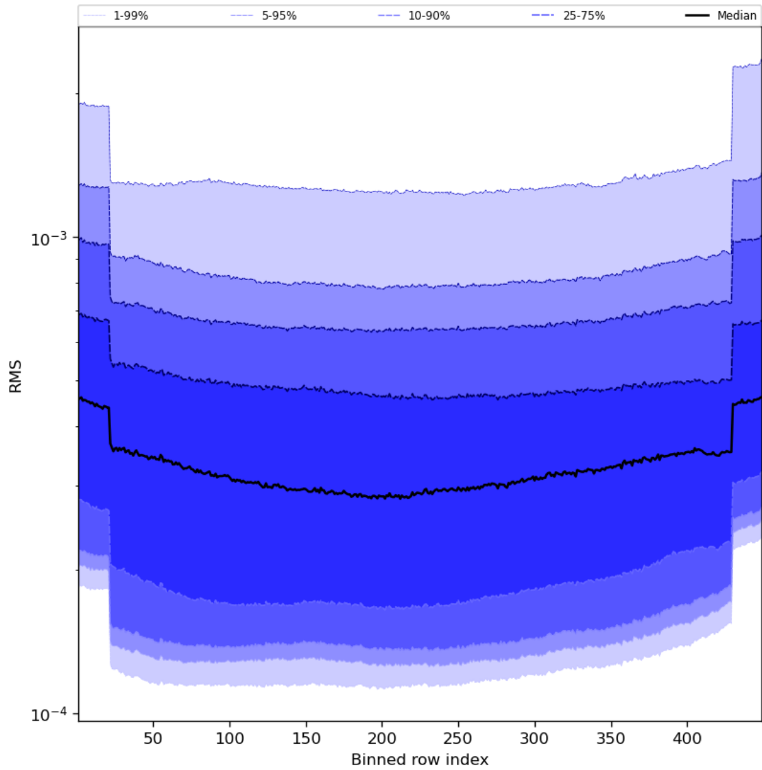
Figure 60: Along track statistics of “RMS” for 2024-02-20 to 2024-02-22
