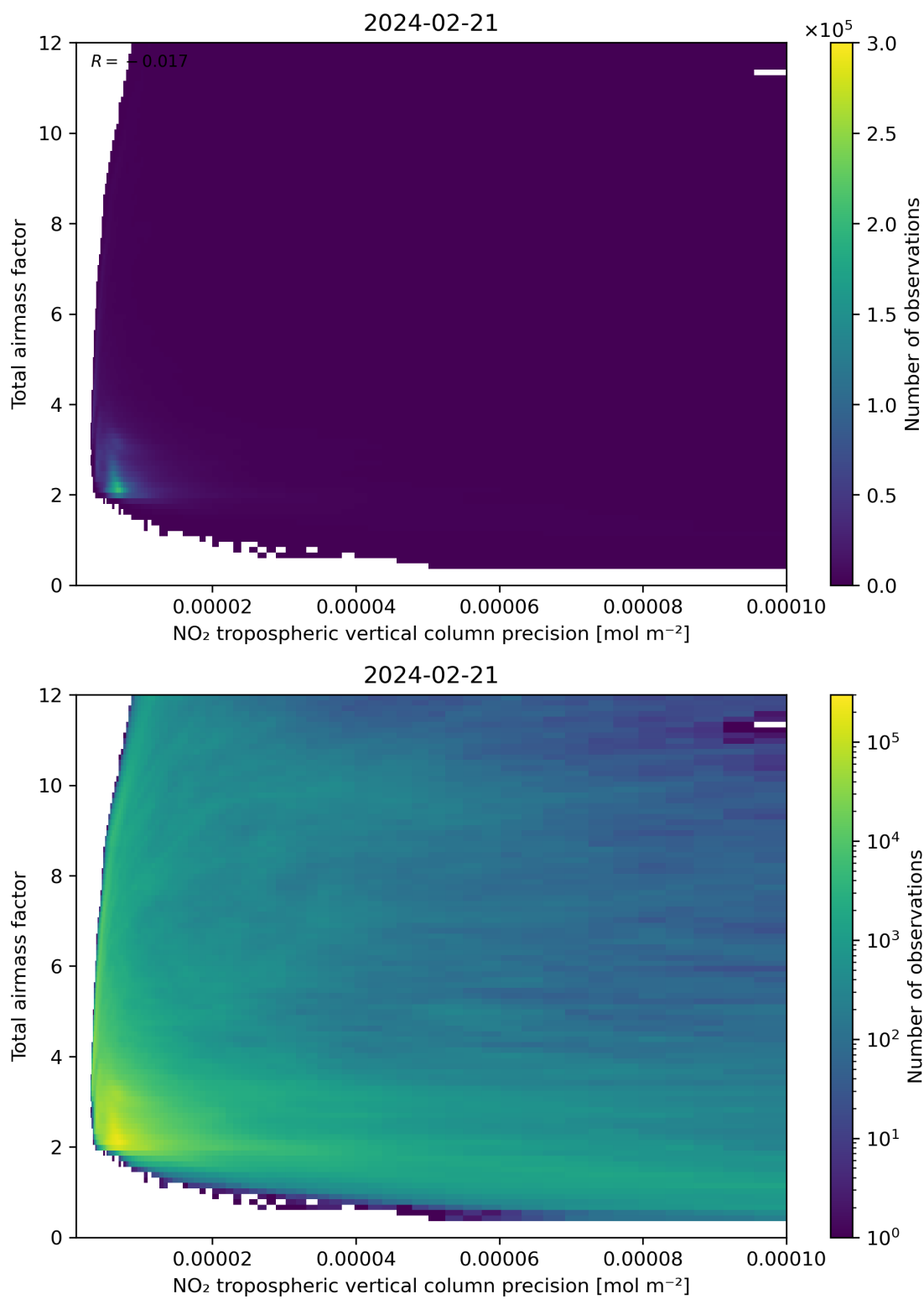
Figure 132: Scatter density plot of “NO 2 tropospheric vertical column precision” against “Total airmass factor” for 2024-02-20 to 2024-02-22.
