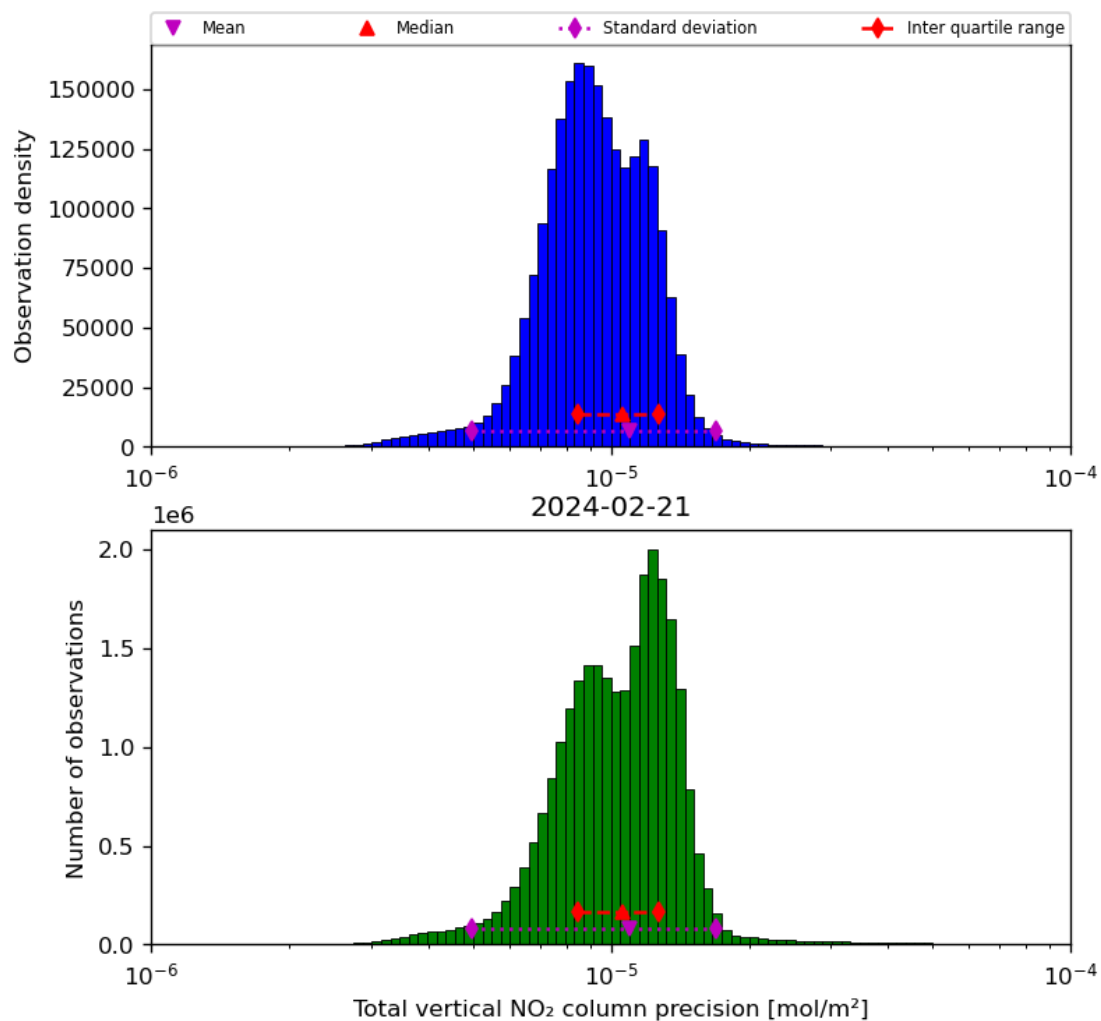
Figure 39: Histogram of “Total vertical NO 2 column precision” for 2024-02-20 to 2024-02-22
