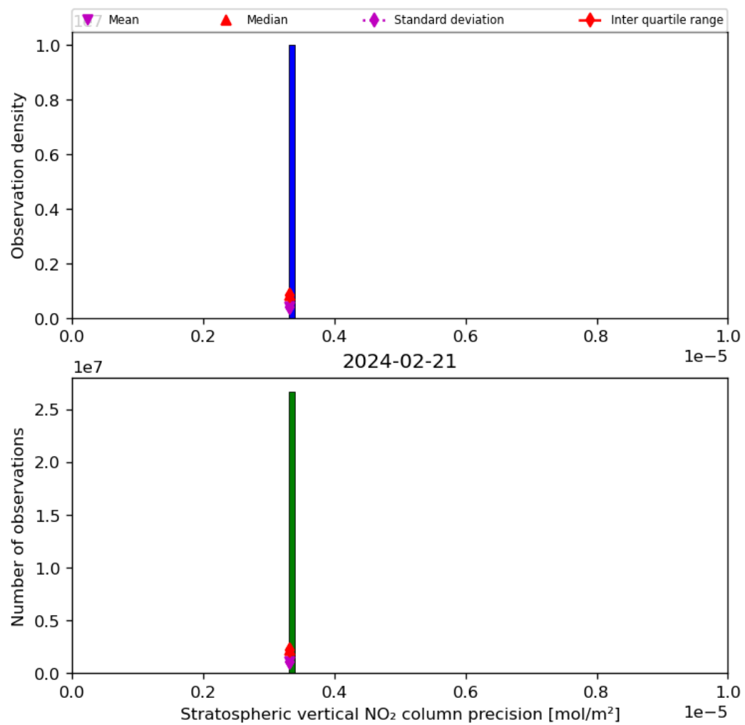
Figure 37: Histogram of “Stratospheric vertical NO 2 column precision” for 2024-02-20 to 2024-02-22
