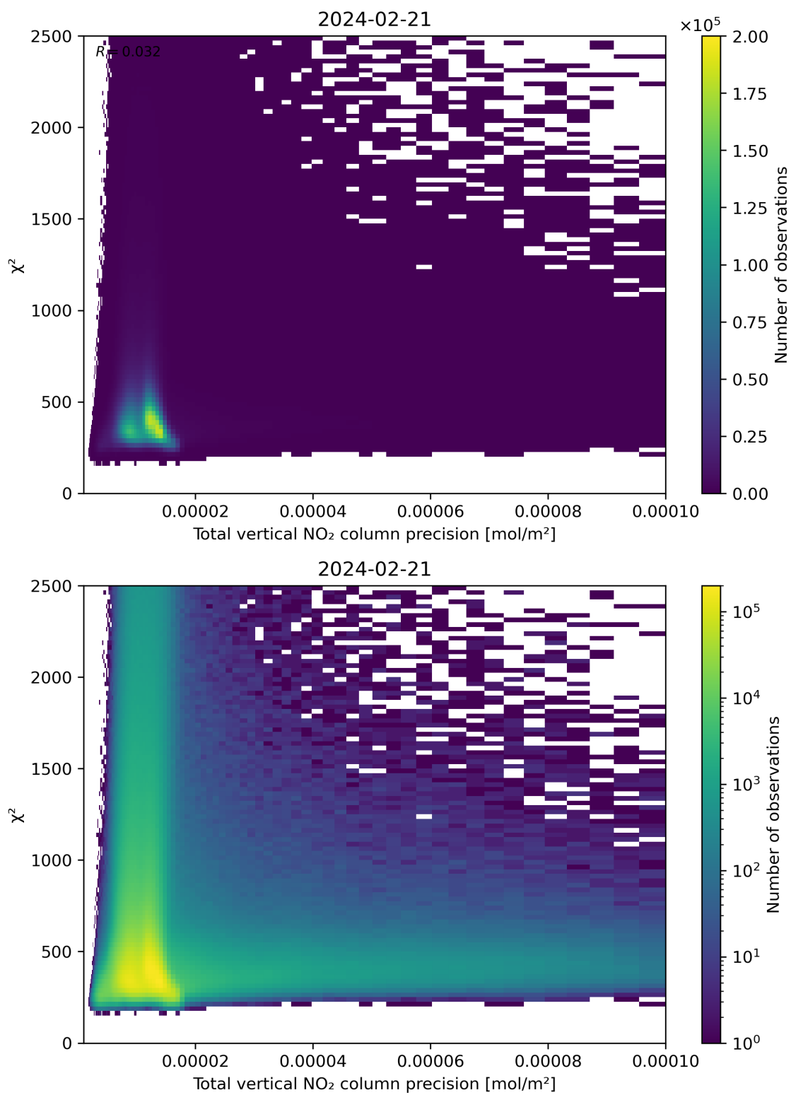
Figure 116: Scatter density plot of “Total vertical NO 2 column precision” against “ \chi^2 ” for 2024-02-20 to 2024-02-22.
