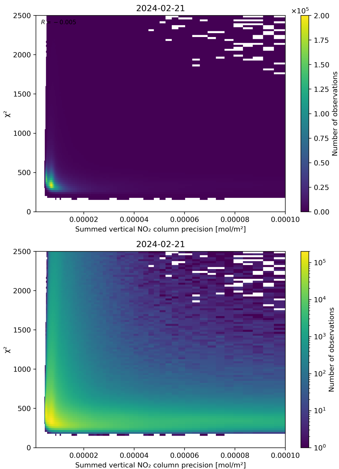
Figure 107: Scatter density plot of “Summed vertical NO 2 column precision” against “ \chi^2 ” for 2024-02-20 to 2024-02-22.
