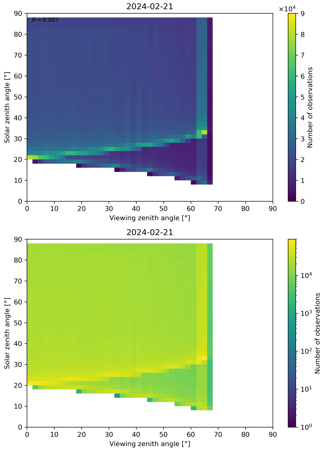
Figure 172: Scatter density plot of “Viewing zenith angle” against “Solar zenith angle” for 2024-02-20 to 2024-02-22.
