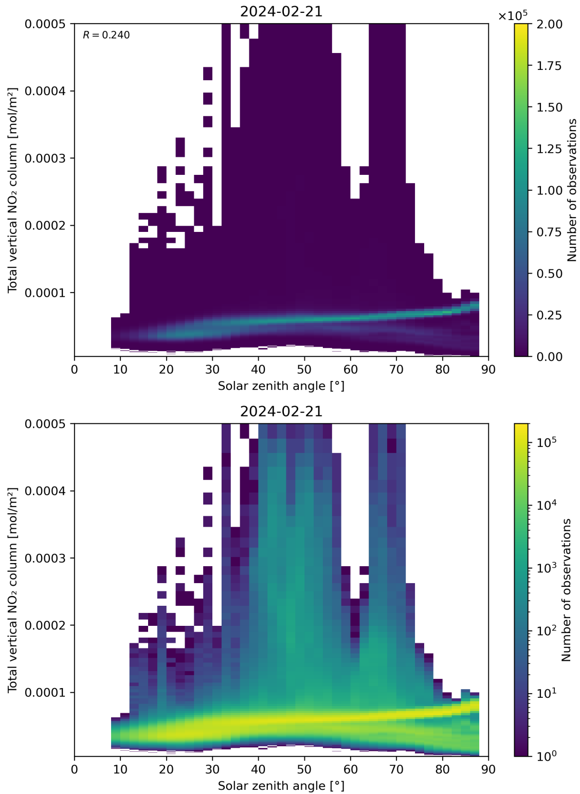
Figure 153: Scatter density plot of “Solar zenith angle” against “Total vertical NO 2 column” for 2024-02-20 to 2024-02-22.
