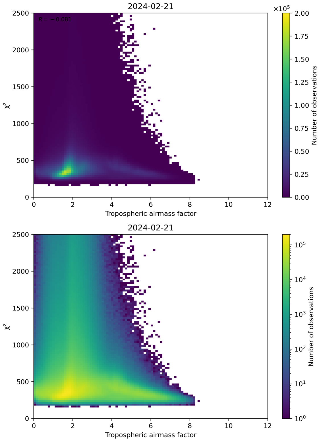
Figure 73: Scatter density plot of “Tropospheric airmass factor” against “ \chi^2 ” for 2024-02-20 to 2024-02-22.
