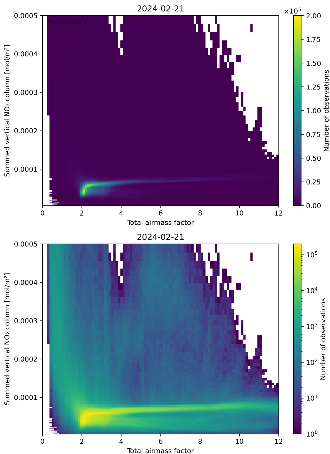
Figure 65: Scatter density plot of “Total airmass factor” against “Summed vertical NO 2 column” for 2024-02-20 to 2024-02-22.
