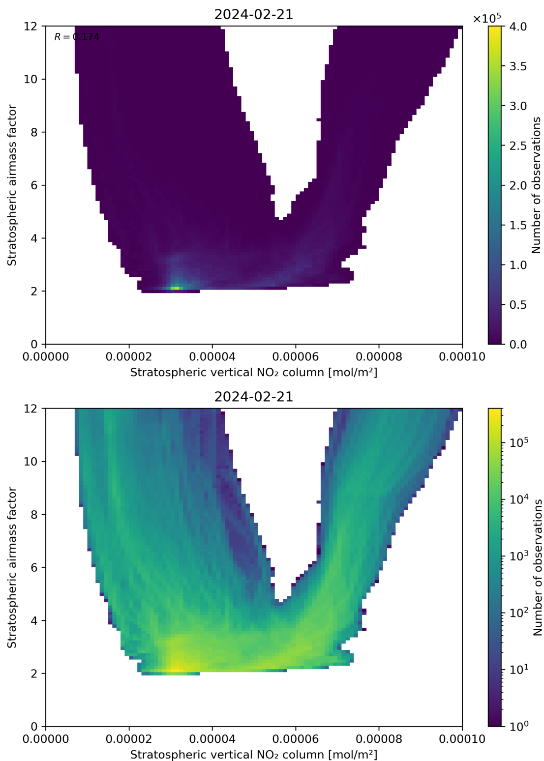
Figure 96: Scatter density plot of “Stratospheric vertical NO 2 column” against “Stratospheric airmass factor” for 2024-02-20 to 2024-02-22.
