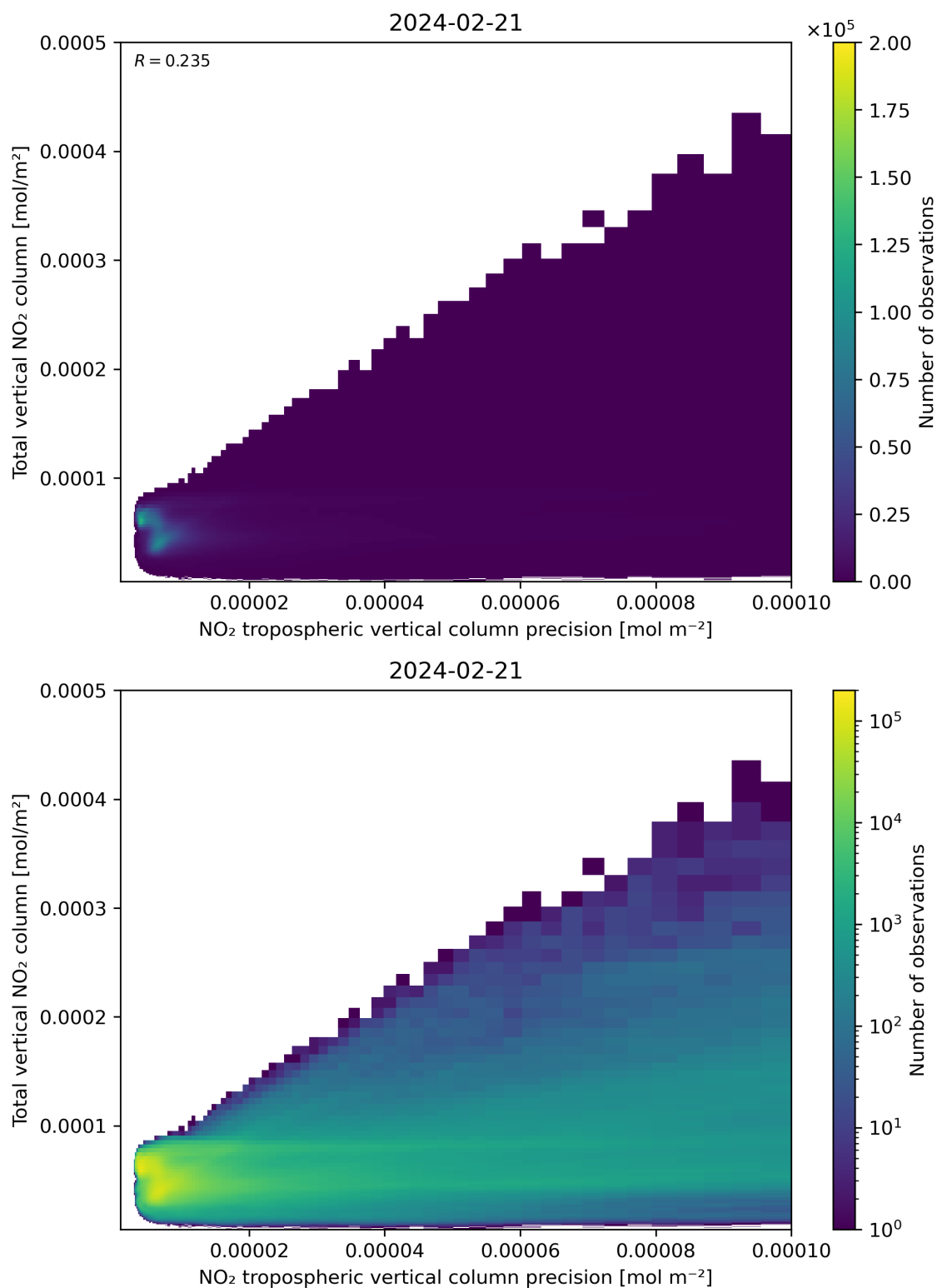
Figure 138: Scatter density plot of “NO 2 tropospheric vertical column precision” against “Total vertical NO 2 column” for 2024-02-20 to 2024-02-22.
