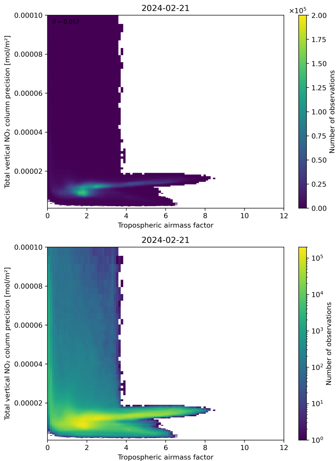
Figure 78: Scatter density plot of “Tropospheric air mass factor” against “Total vertical NO 2 column precision” for 2024-02-20 to 2024-02-22.
