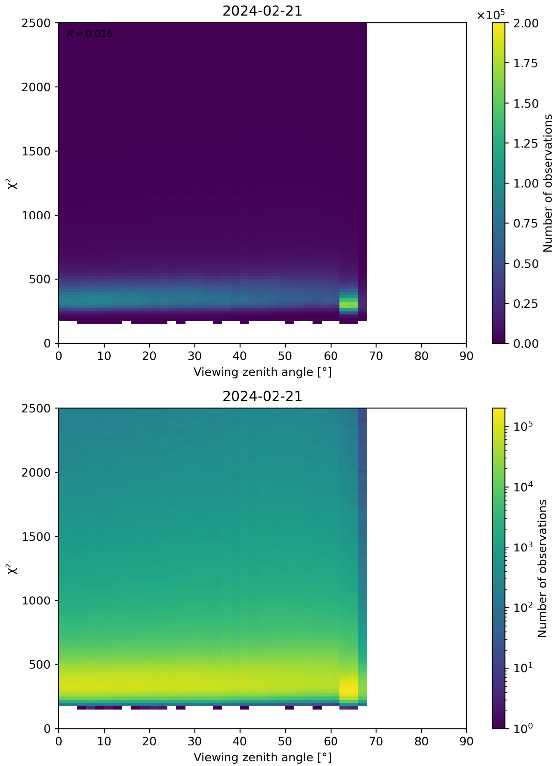
Figure 162: Scatter density plot of “Viewing zenith angle” against “ \chi^2 ” for 2024-02-20 to 2024-02-22.
