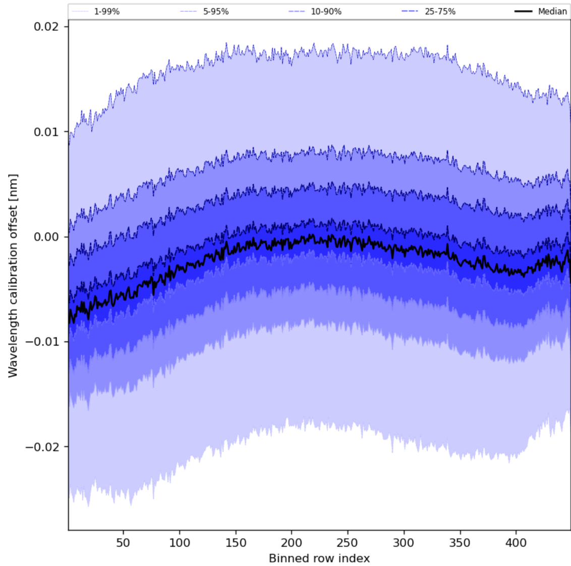
Figure 52: Along track statistics of “Wavelength calibration offset” for 2024-02-20 to 2024-02-22
