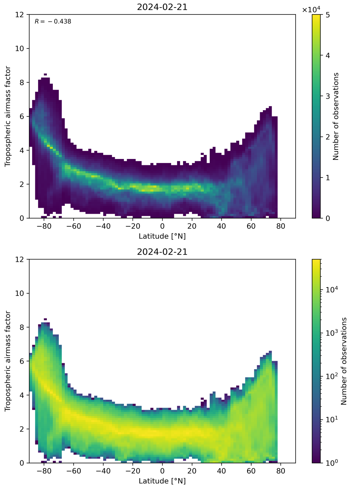
Figure 85: Scatter density plot of “Latitude” against “Tropospheric airmass factor” for 2024-02-20 to 2024-02-22.
