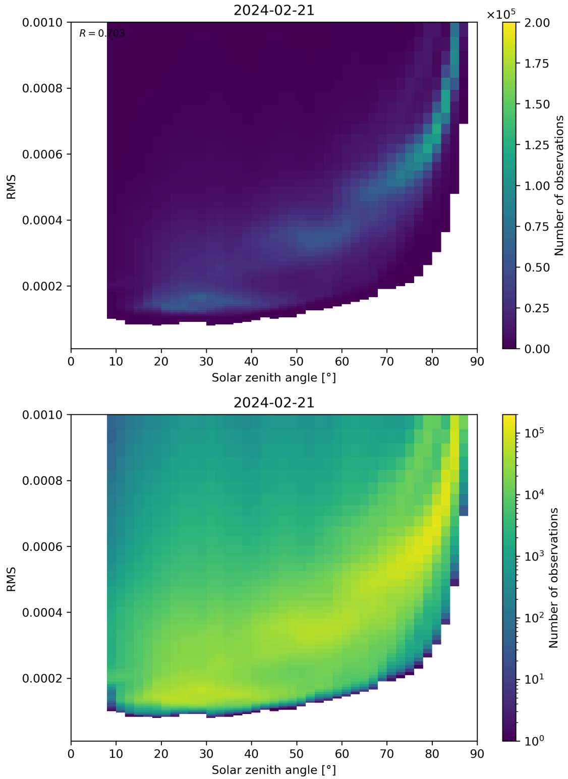
Figure 157: Scatter density plot of “Solar zenith angle” against “RMS” for 2024-02-20 to 2024-02-22.
