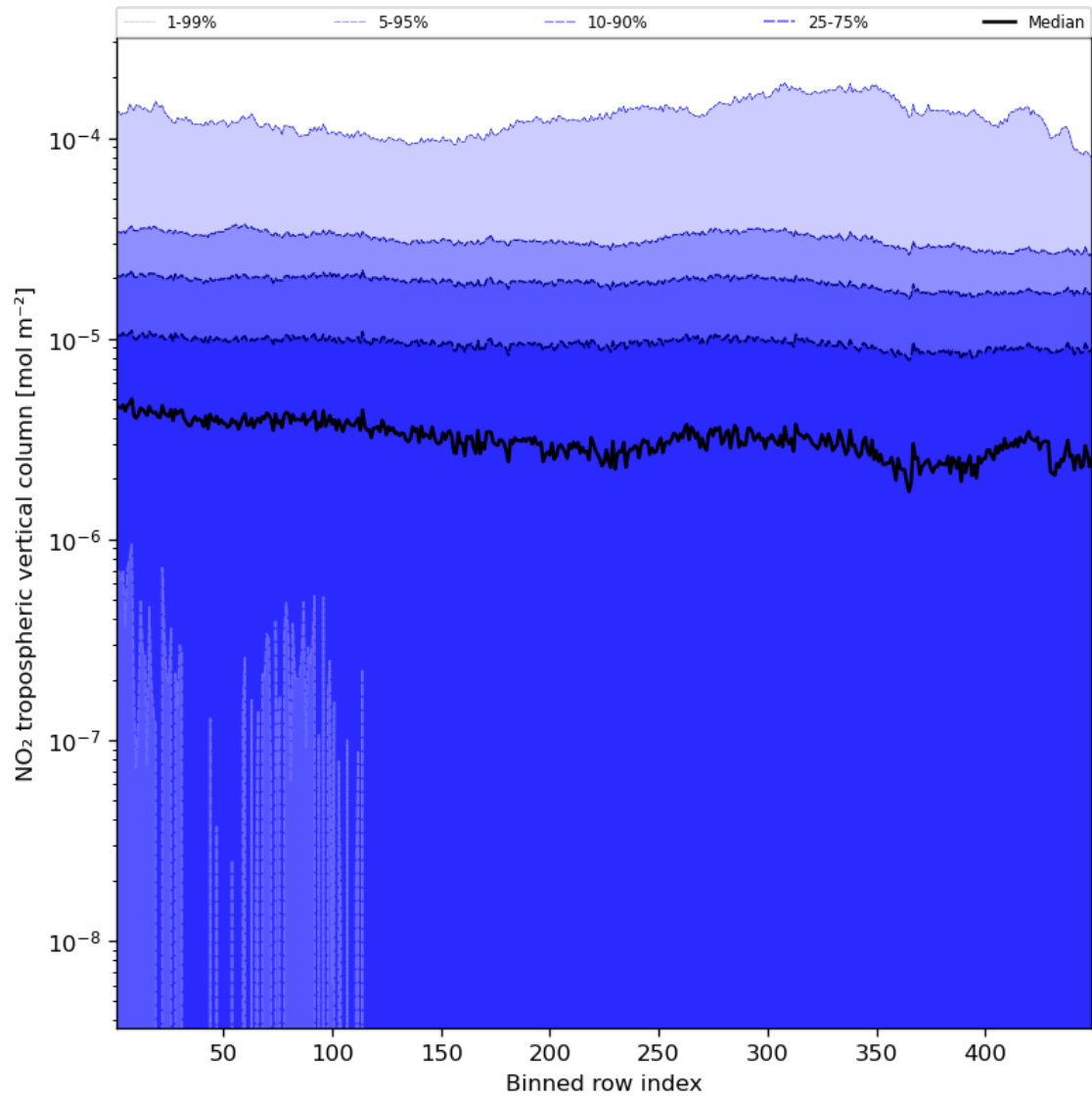
Figure 46: Along track statistics of “NO 2 tropospheric vertical column” for 2024-02-20 to 2024-02-22
