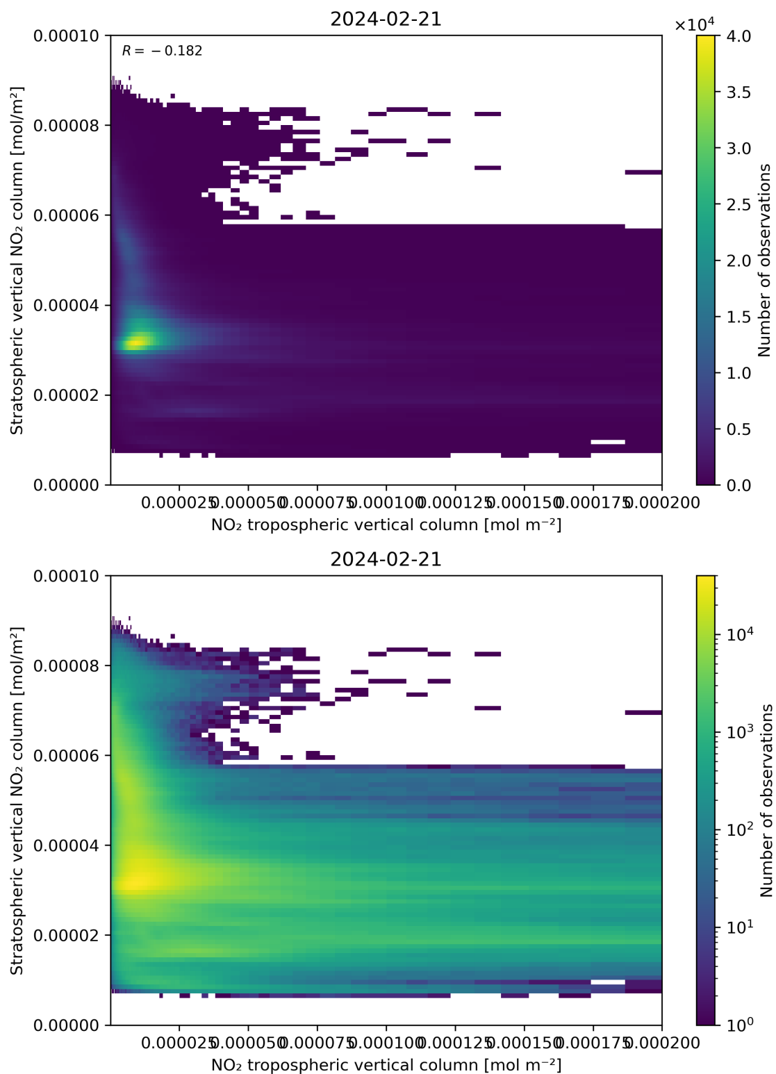
Figure 125: Scatter density plot of “NO 2 tropospheric vertical column” against “Stratospheric vertical NO 2 column” for 2024-02-20 to 2024-02-22.
