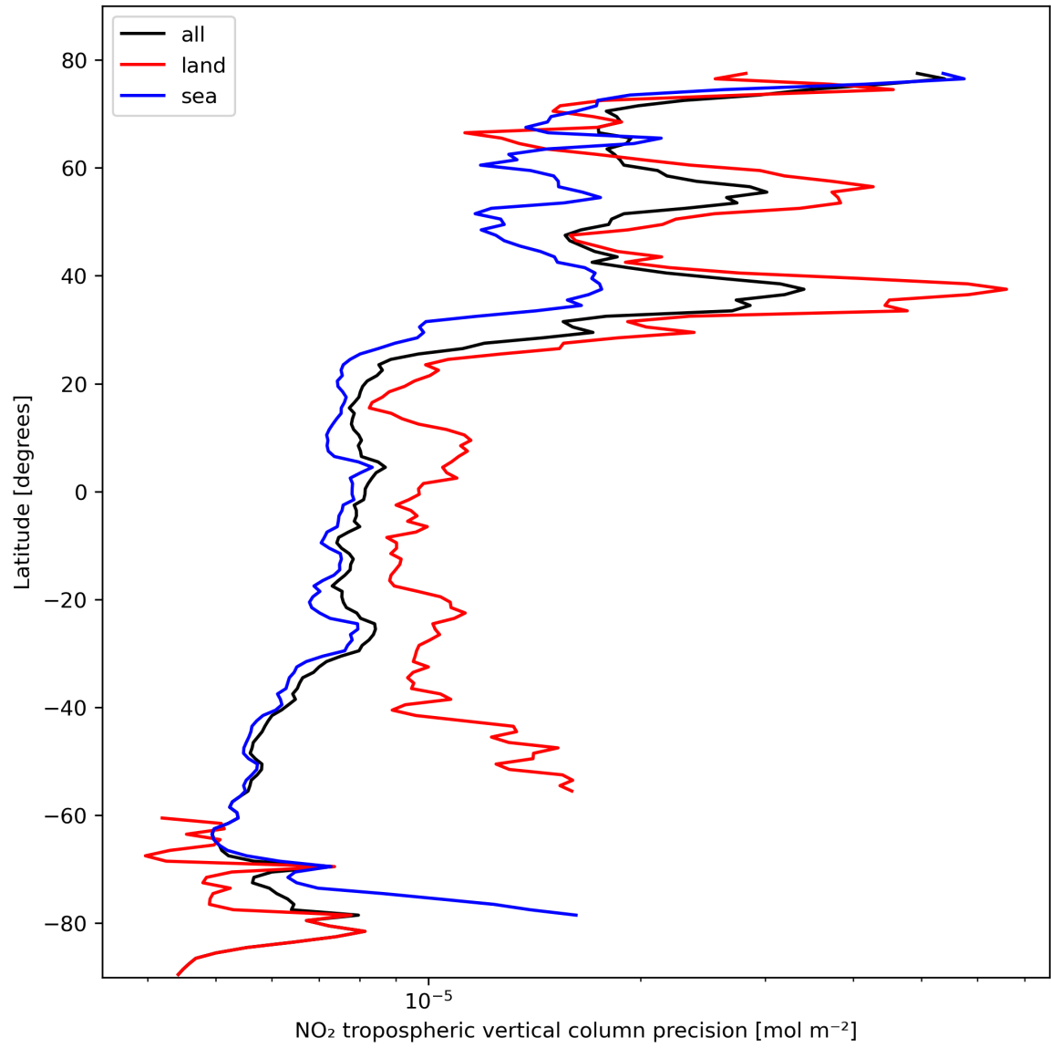
Figure 13: Zonal average of “NO 2 tropospheric vertical column precision” for 2024-02-20 to 2024-02-22.
