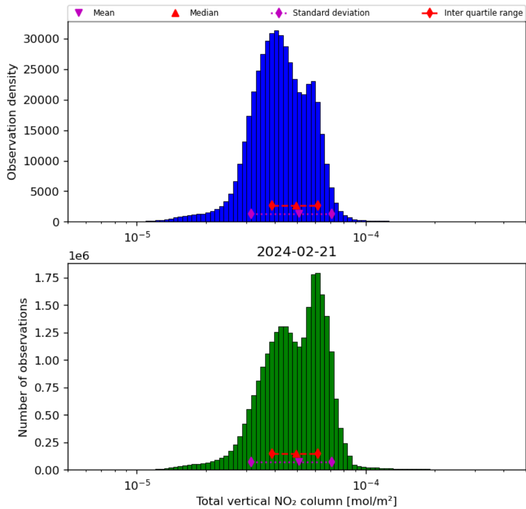
Figure 38: Histogram of “Total vertical NO 2 column” for 2024-02-20 to 2024-02-22
