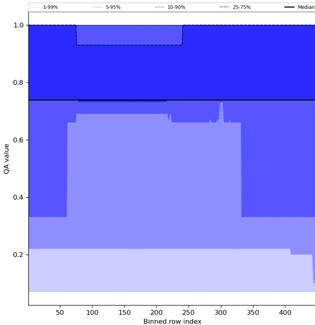
Figure 45: Along track statistics of “QA value” for 2024-02-20 to 2024-02-22
