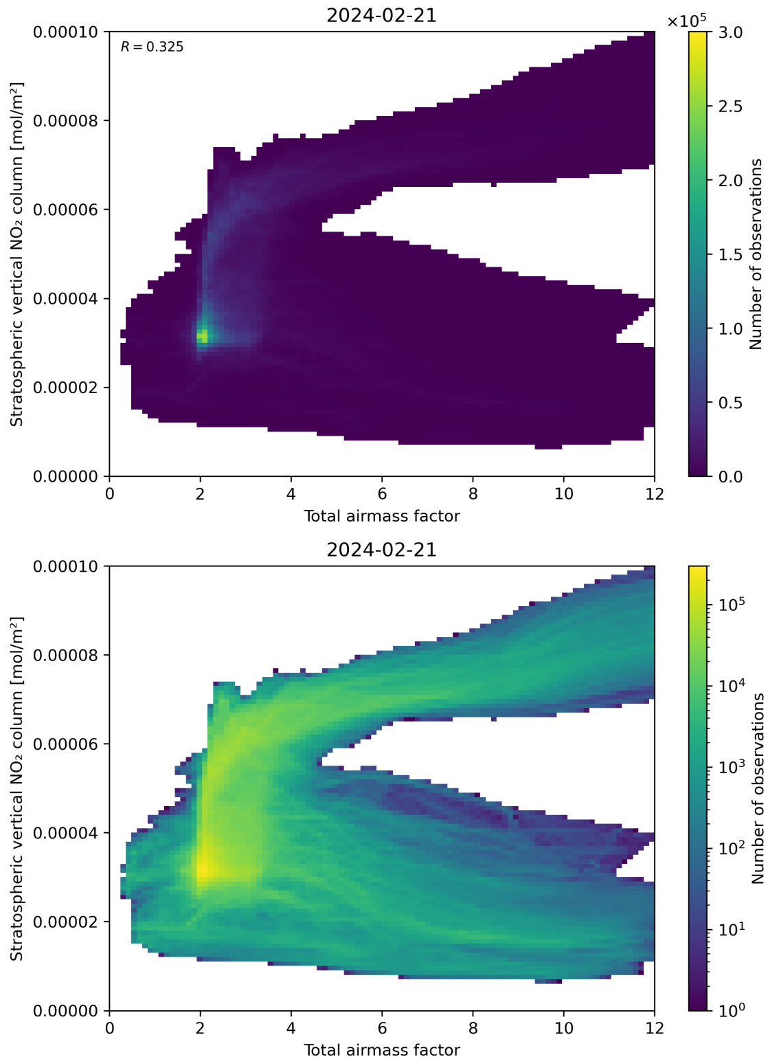
Figure 64: Scatter density plot of “Total airmass factor” against “Stratospheric vertical \text{NO}_2 column” for 2024-02-20 to 2024-02-22.
