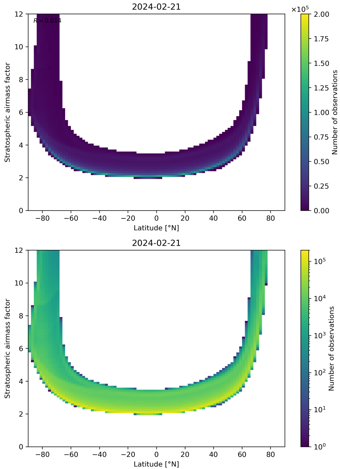
Figure 83: Scatter density plot of “Latitude” against “Stratospheric airmass factor” for 2024-02-20 to 2024-02-22.
