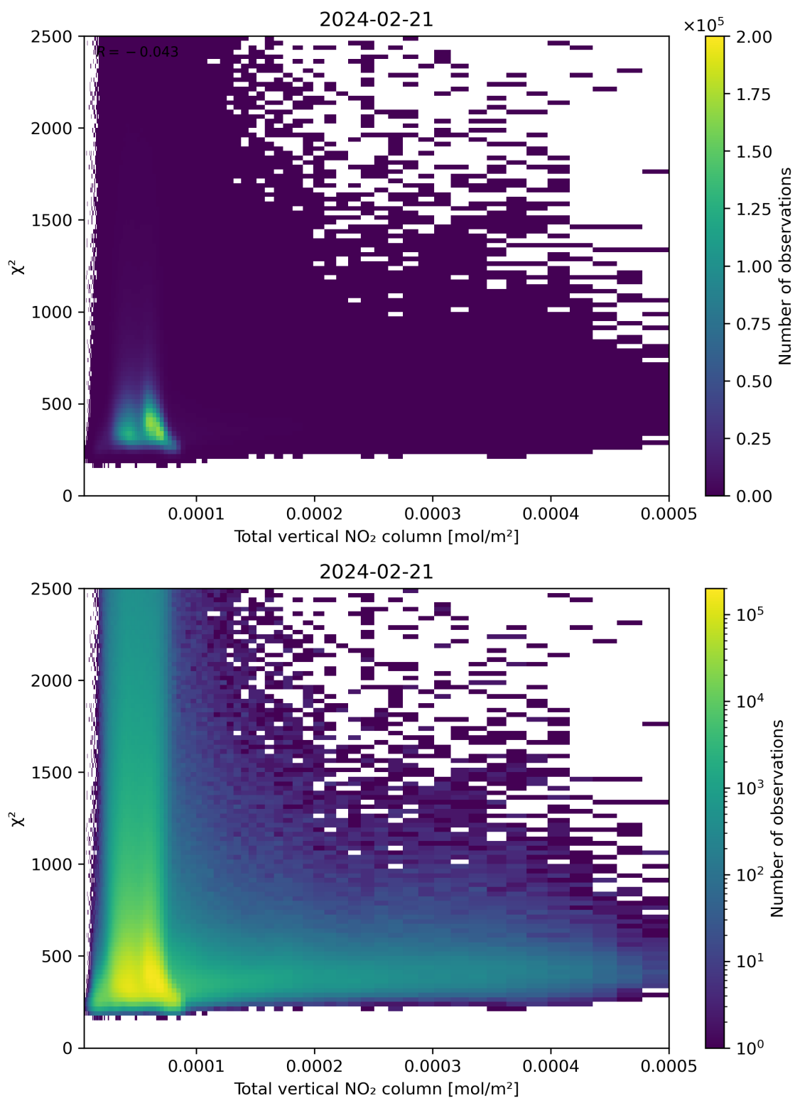
Figure 111: Scatter density plot of “Total vertical NO 2 column” against “ \chi^2 ” for 2024-02-20 to 2024-02-22.
