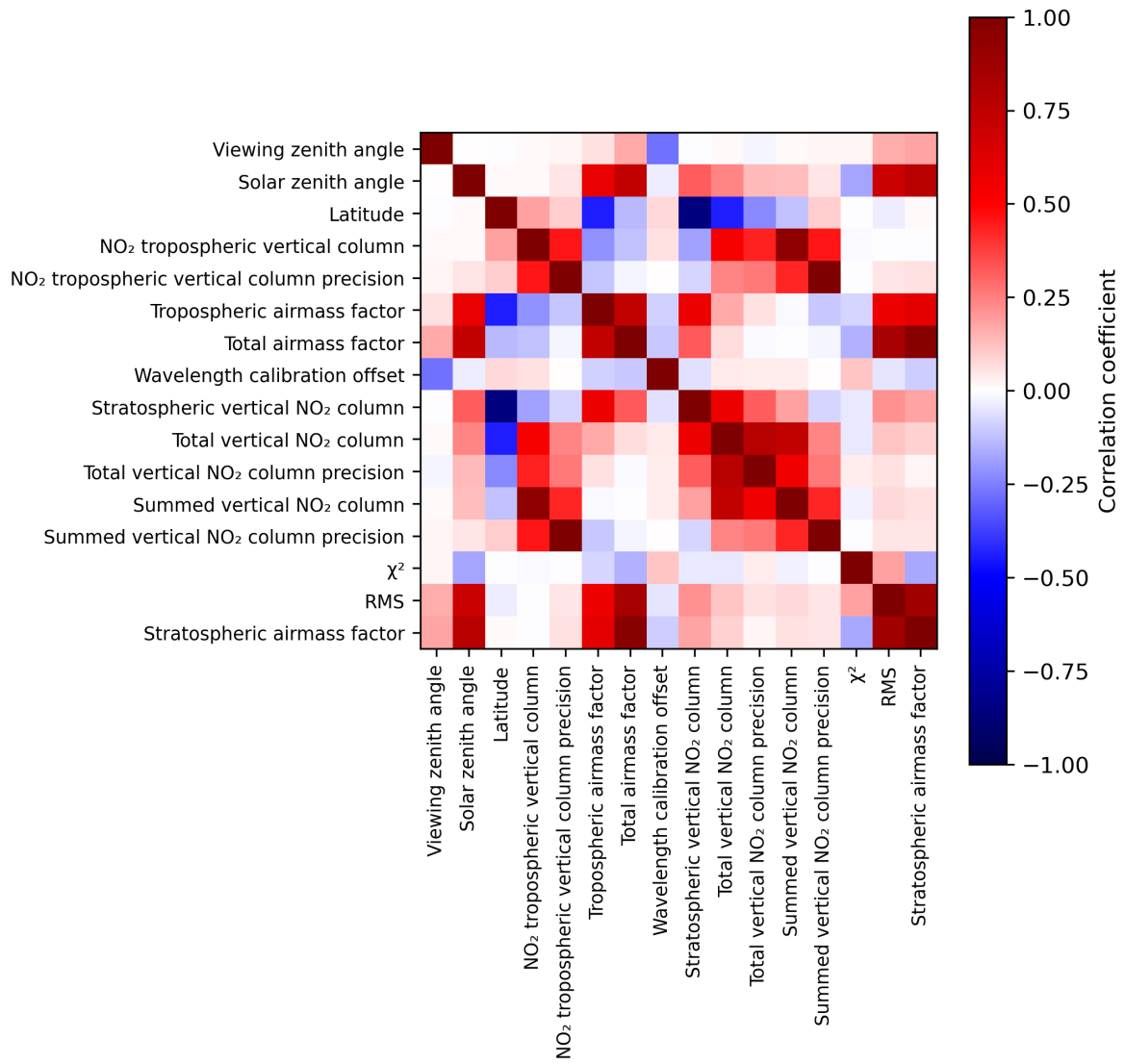
Figure 2: Map of correlation matrix for 2024-02-20 to 2024-02-22.
