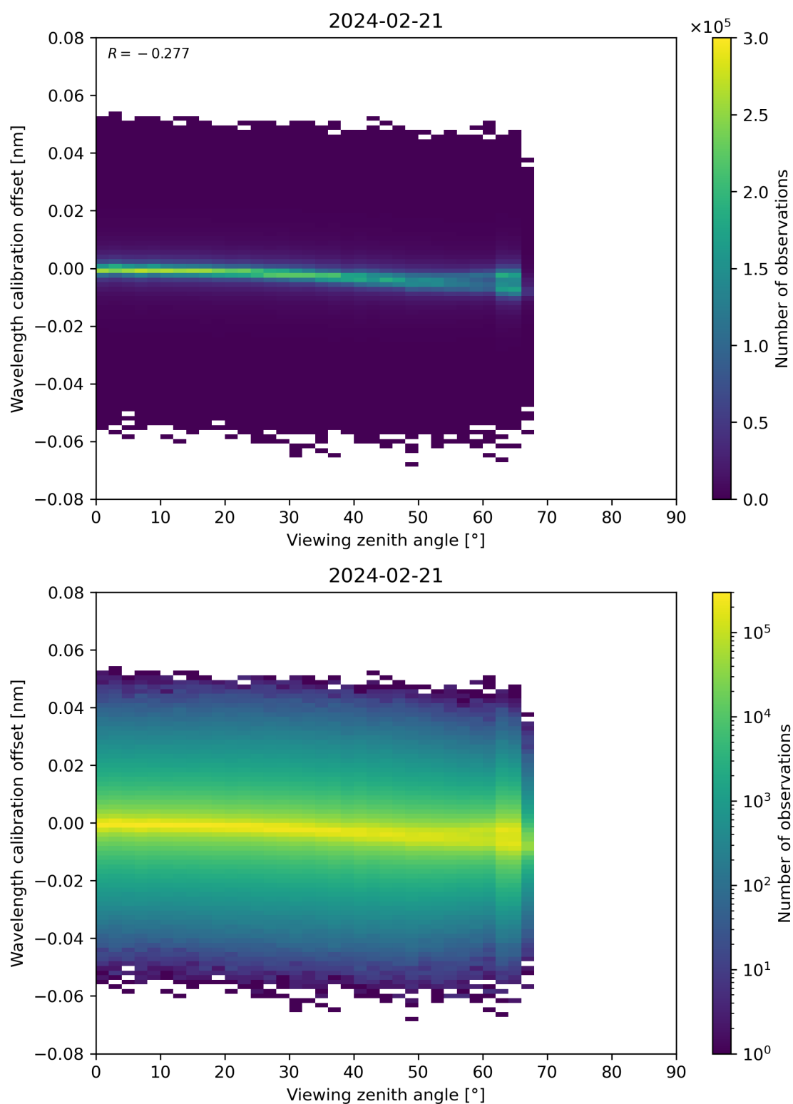
Figure 173: Scatter density plot of “Viewing zenith angle” against “Wavelength calibration offset” for 2024-02-20 to 2024-02-22.
