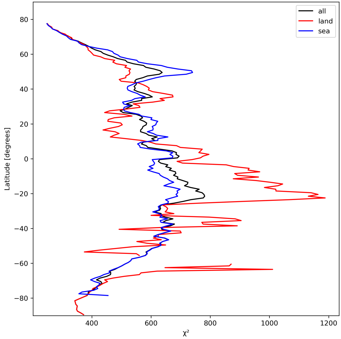
Figure 25: Zonal average of “ \chi^2 ” for 2024-02-20 to 2024-02-22.
