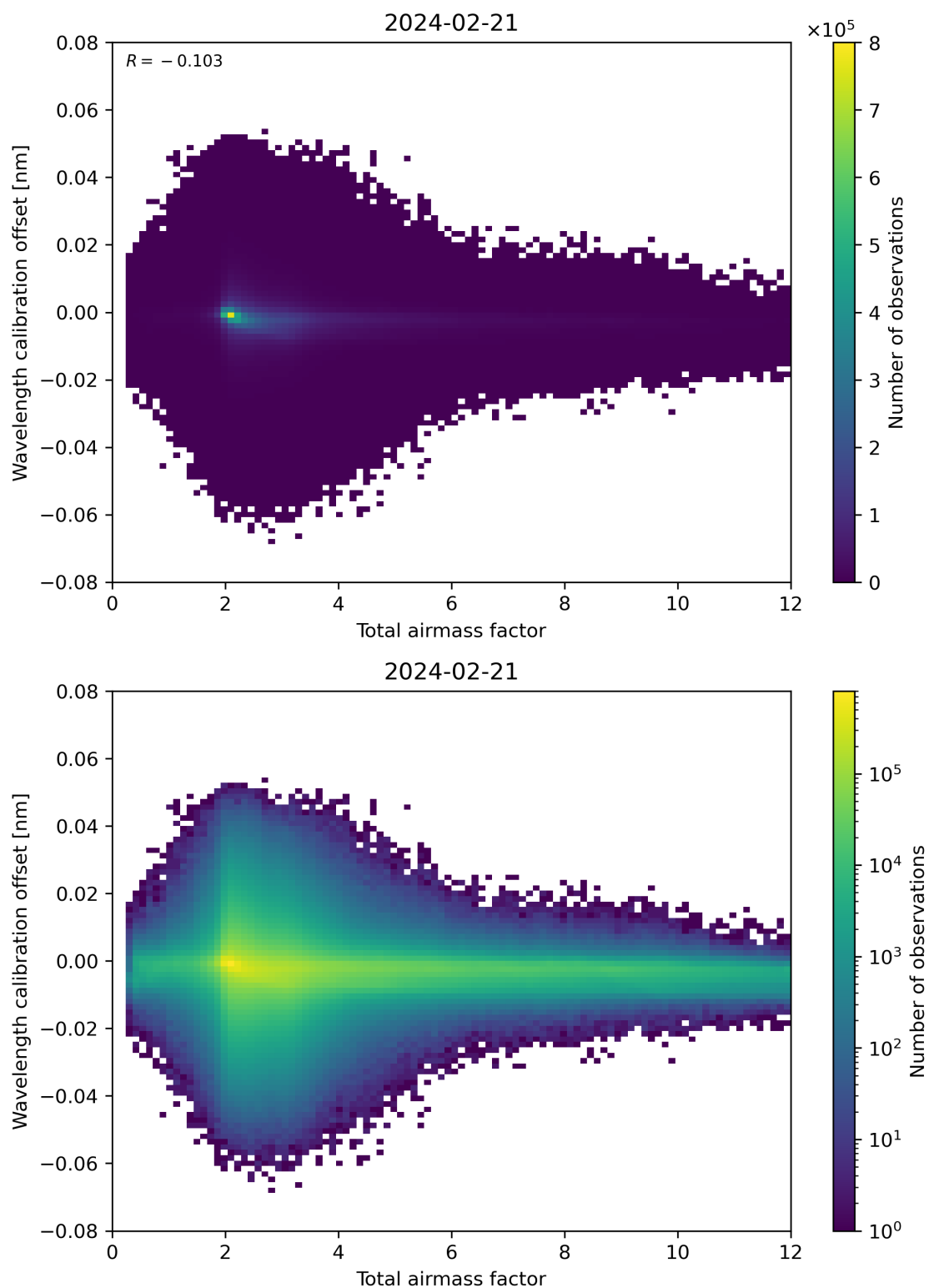
Figure 70: Scatter density plot of “Total airmass factor” against “Wavelength calibration offset” for 2024-02-20 to 2024-02-22.
