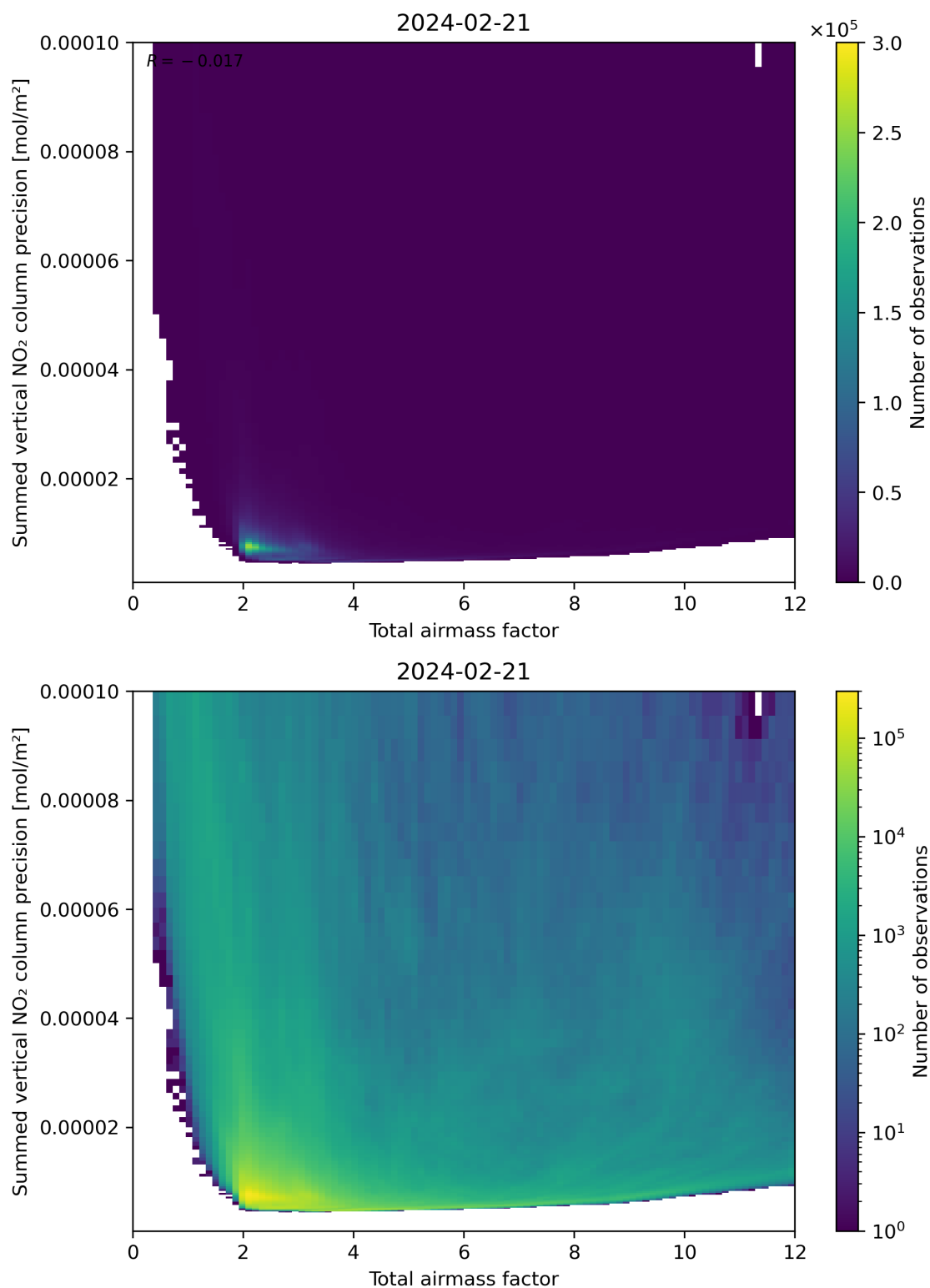
Figure 66: Scatter density plot of “Total airmass factor” against “Summed vertical NO 2 column precision” for 2024-02-20 to 2024-02-22.
