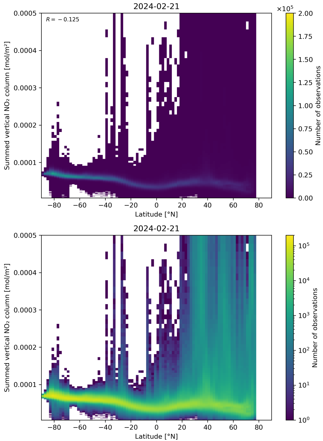
Figure 88: Scatter density plot of “Latitude” against “Summed vertical NO 2 column” for 2024-02-20 to 2024-02-22.
