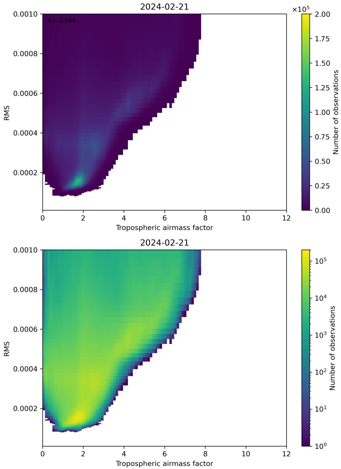
Figure 79: Scatter density plot of “Tropospheric airmass factor” against “RMS” for 2024-02-20 to 2024-02-22.
