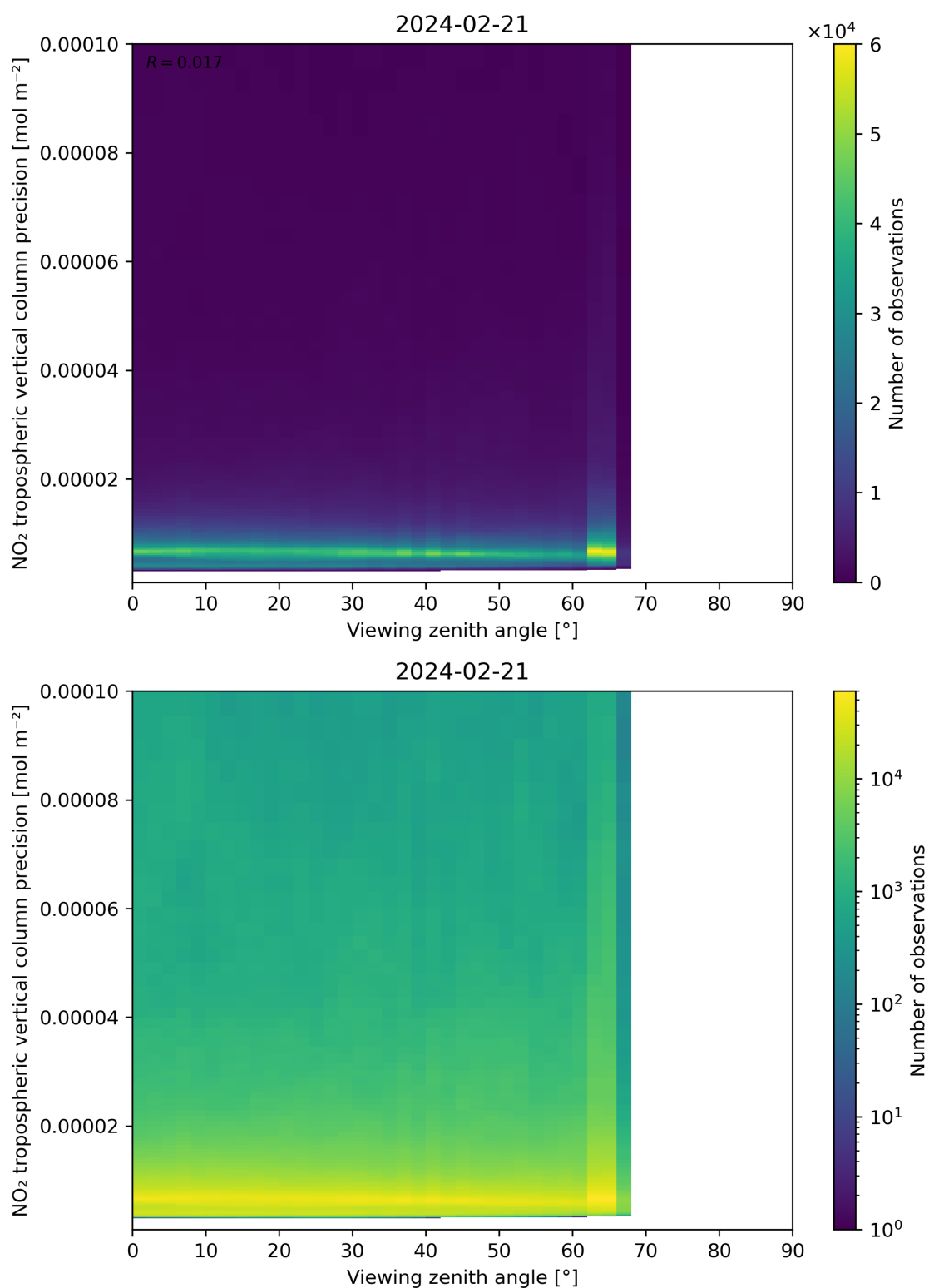
Figure 170: Scatter density plot of “Viewing zenith angle” against “NO 2 tropospheric vertical column precision” for 2024-02-20 to 2024-02-22.
