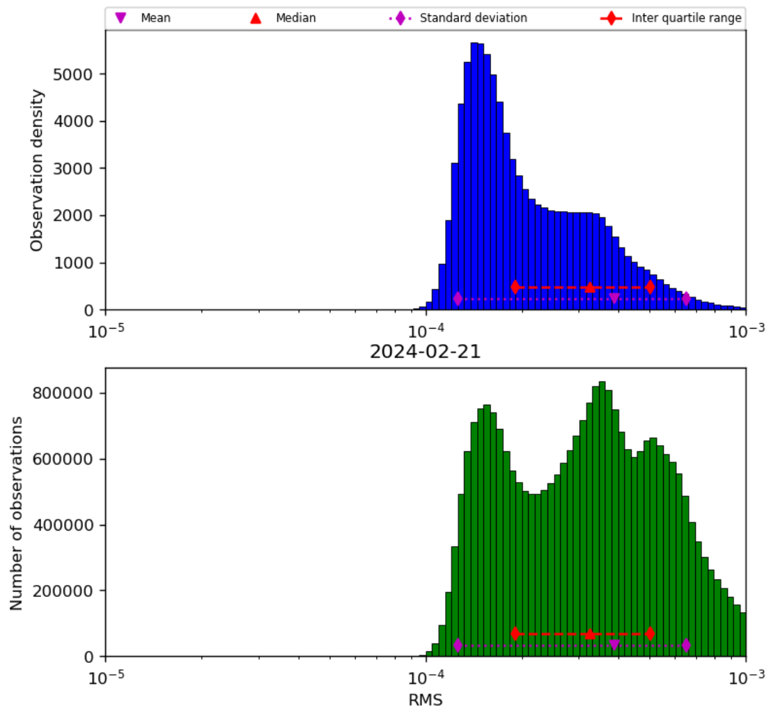
Figure 43: Histogram of “RMS” for 2024-02-20 to 2024-02-22
