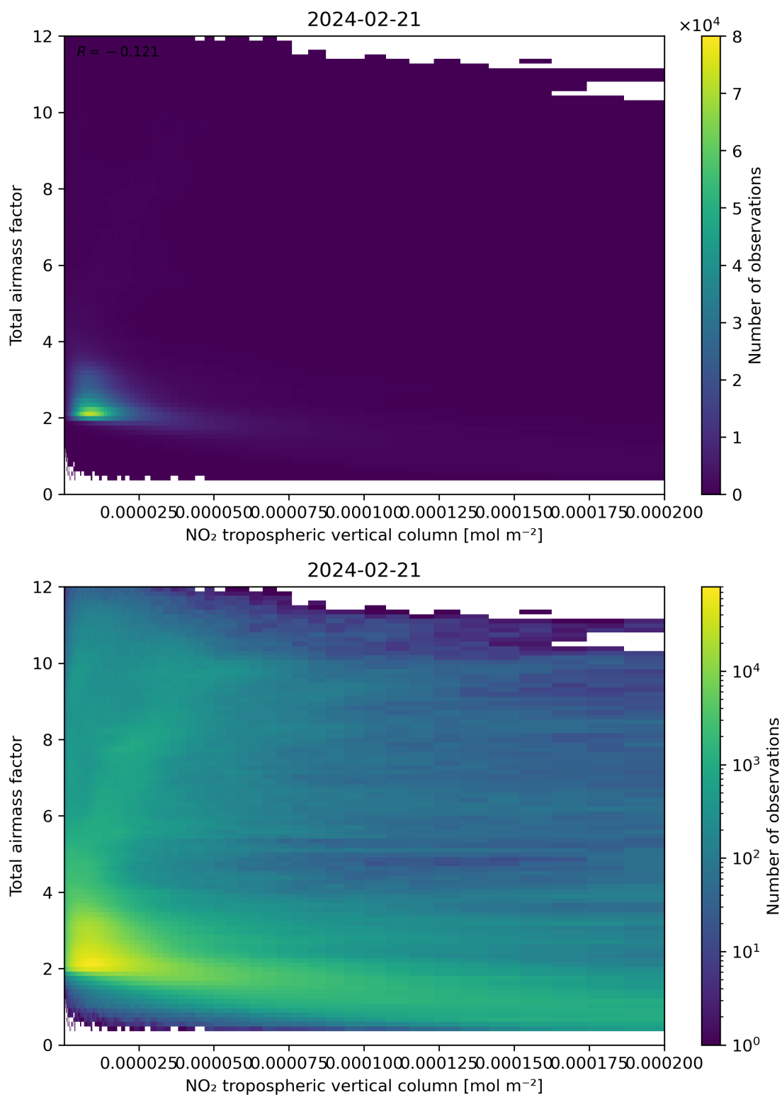
Figure 122: Scatter density plot of “NO 2 tropospheric vertical column” against “Total air mass factor” for 2024-02-20 to 2024-02-22.
