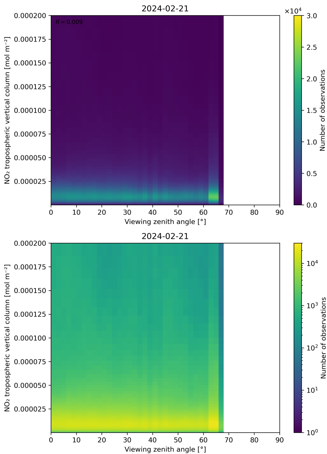
Figure 169: Scatter density plot of “Viewing zenith angle” against “NO 2 tropospheric vertical column” for 2024-02-20 to 2024-02-22.
