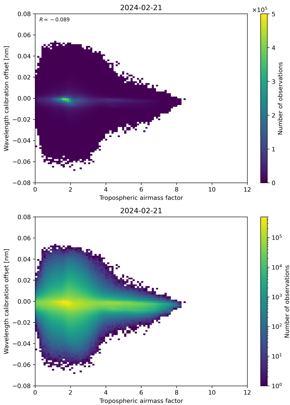
Figure 80: Scatter density plot of “Tropospheric air mass factor” against “Wavelength calibration offset” for 2024-02-20 to 2024-02-22.
