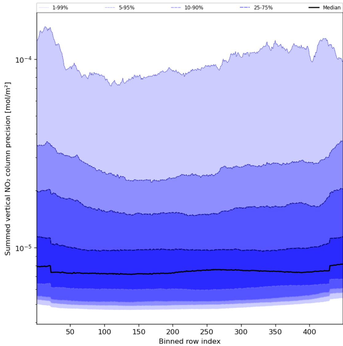
Figure 58: Along track statistics of “Summed vertical NO 2 column precision” for 2024-02-20 to 2024-02-22
