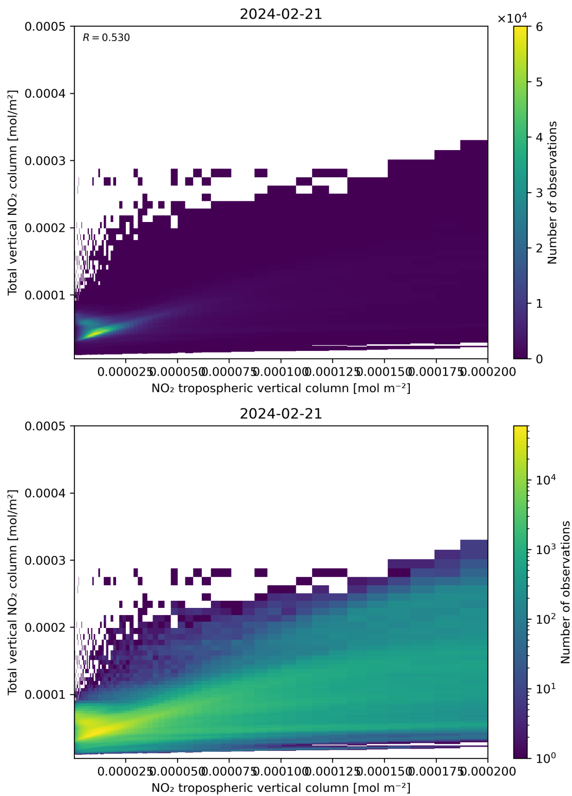
Figure 128: Scatter density plot of “NO 2 tropospheric vertical column” against “Total vertical NO 2 column” for 2024-02-20 to 2024-02-22.
