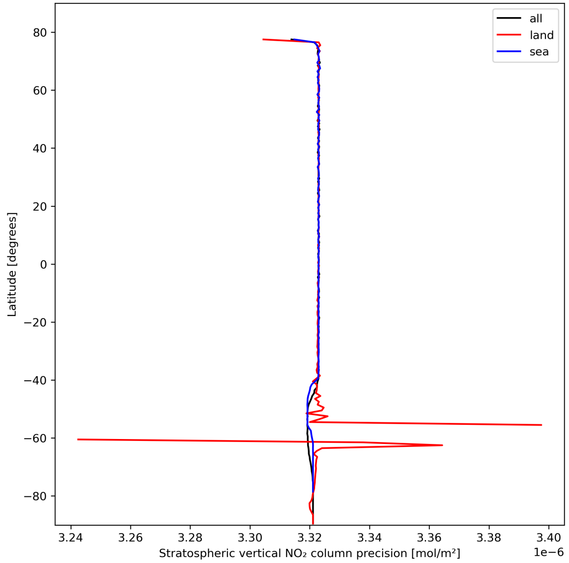
Figure 20: Zonal average of “Stratospheric vertical NO 2 column precision” for 2024-02-20 to 2024-02-22.
