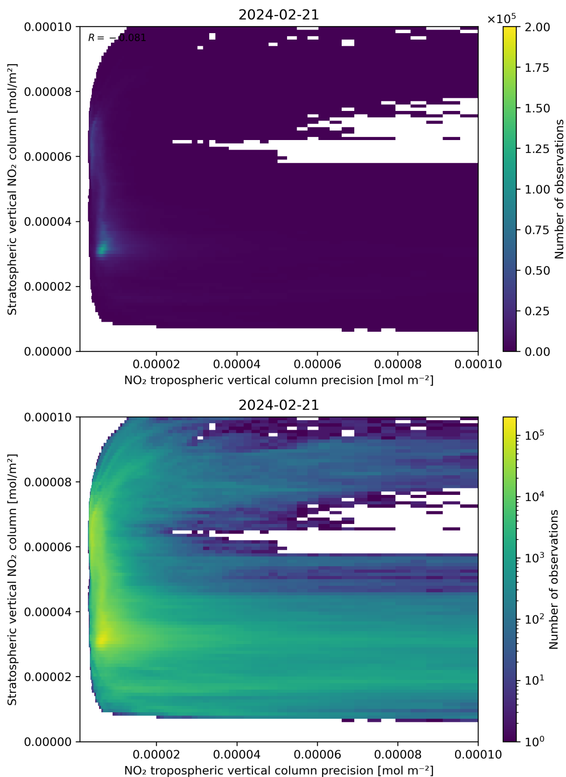
Figure 135: Scatter density plot of “NO 2 tropospheric vertical column precision” against “Stratospheric vertical NO 2 column” for 2024-02-20 to 2024-02-22.
