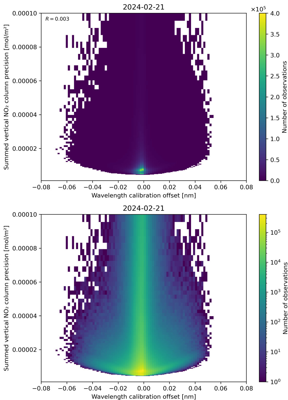
Figure 178: Scatter density plot of “Wavelength calibration offset” against “Summed vertical NO 2 column precision” for 2024-02-20 to 2024-02-22.
