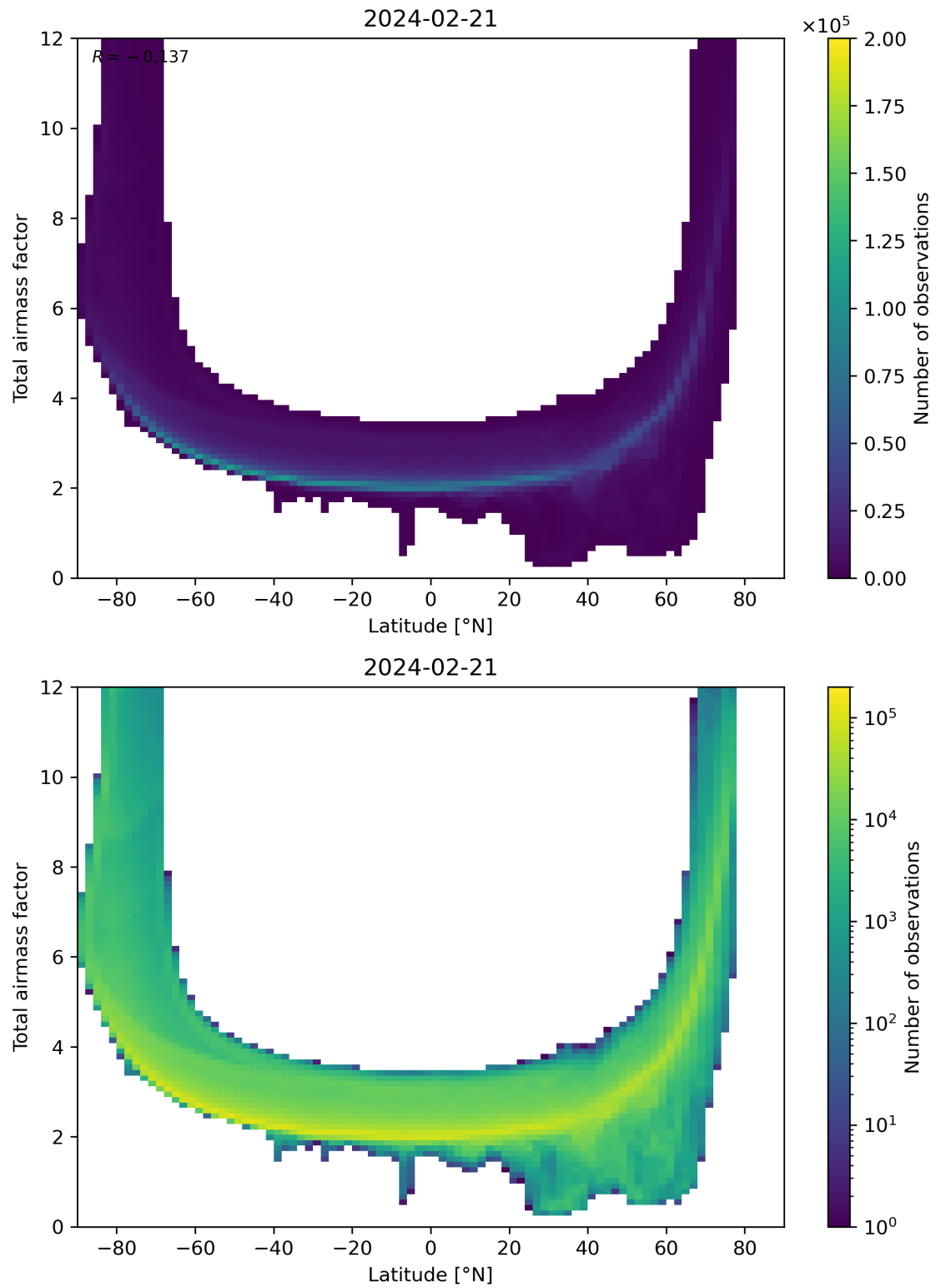
Figure 84: Scatter density plot of “Latitude” against “Total airmass factor” for 2024-02-20 to 2024-02-22.
