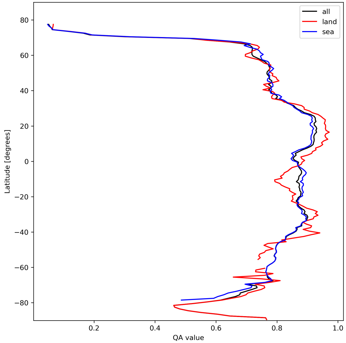
Figure 11: Zonal average of “QA value” for 2024-02-20 to 2024-02-22.
