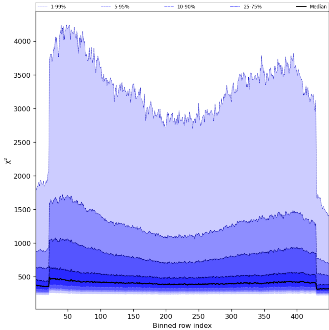
Figure 59: Along track statistics of “ \chi^2 ” for 2024-02-20 to 2024-02-22
