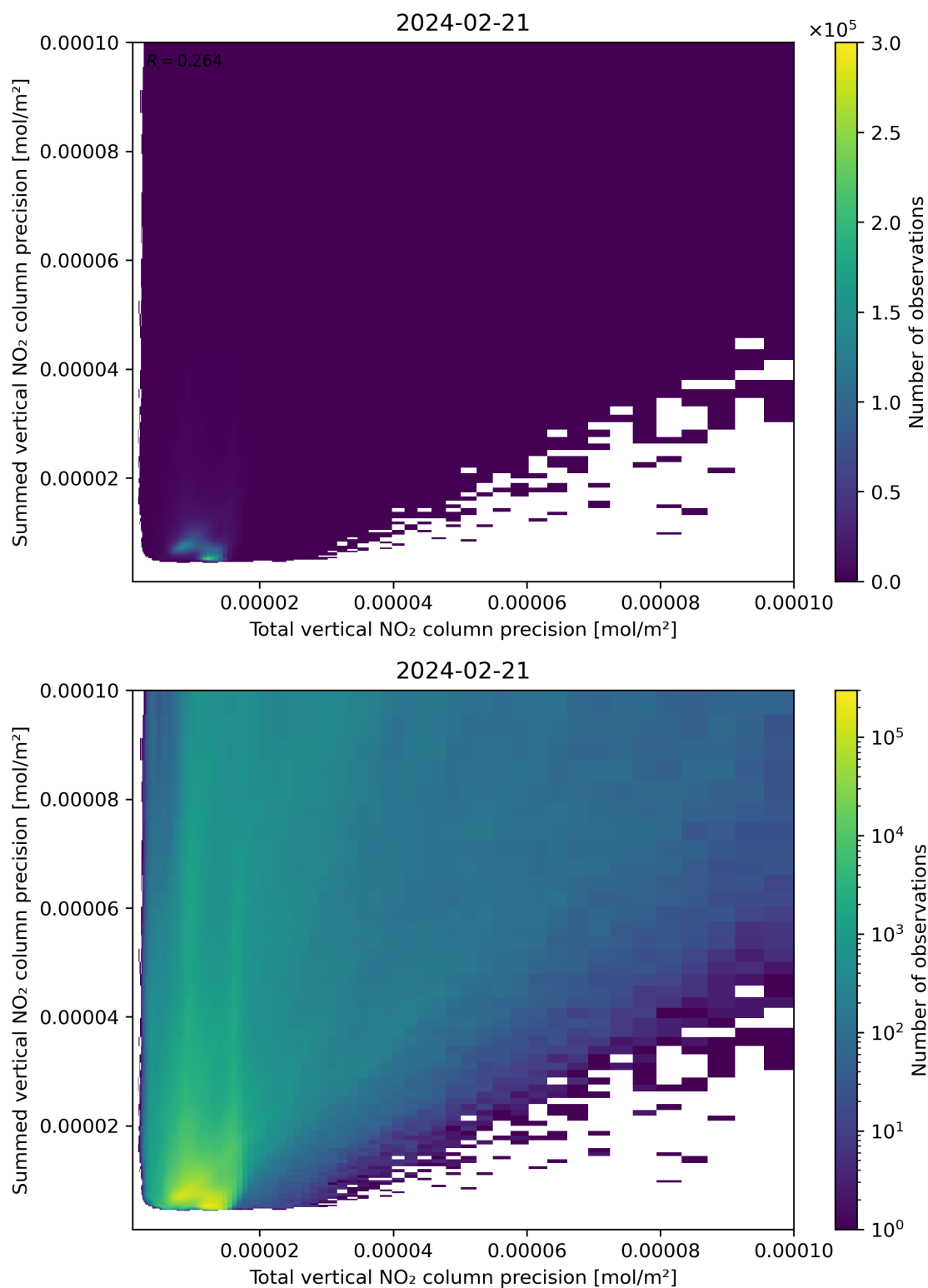
Figure 118: Scatter density plot of “Total vertical NO 2 column precision” against “Summed vertical NO 2 column precision” for 2024-02-20 to 2024-02-22.
