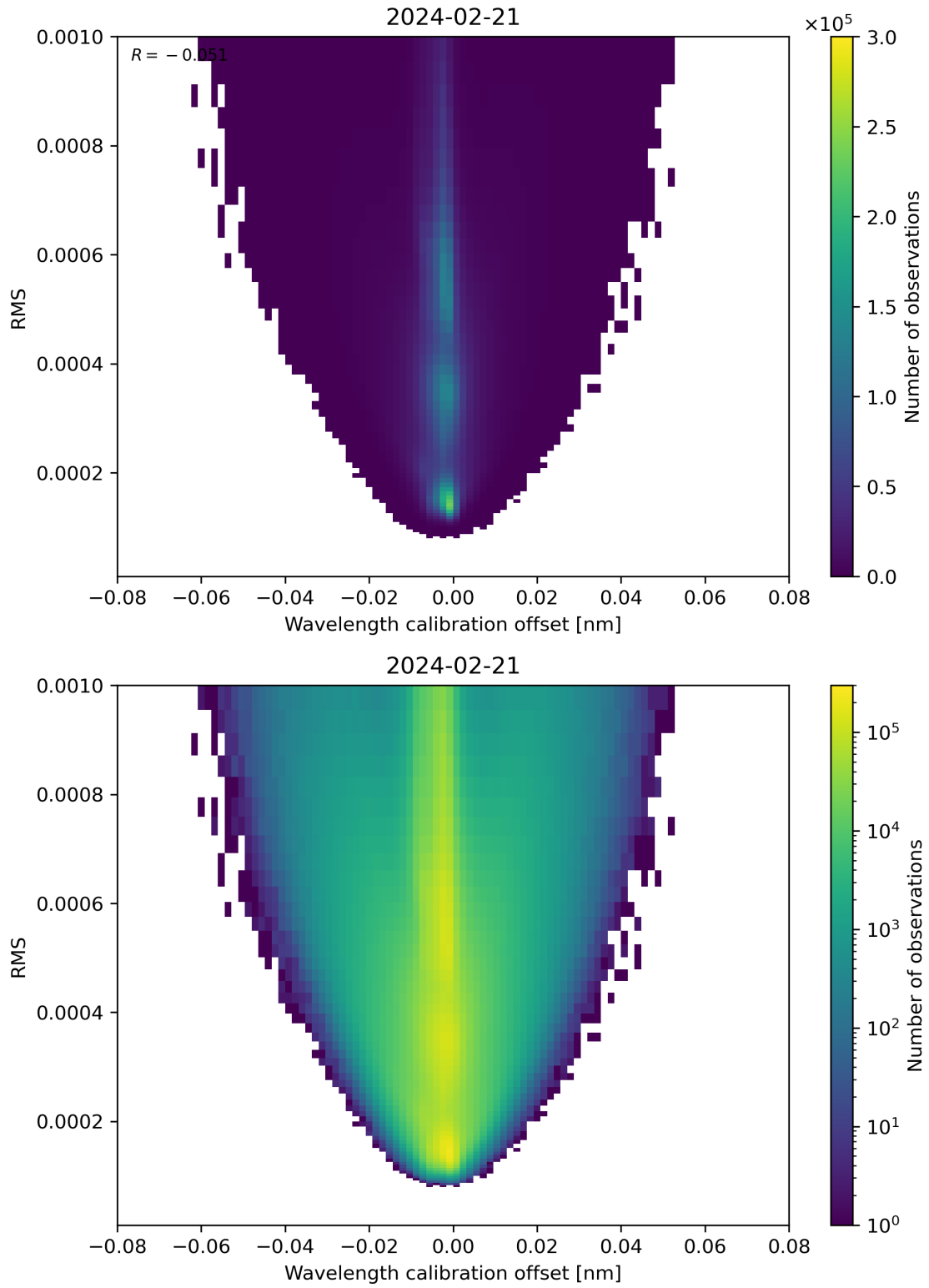
Figure 181: Scatter density plot of “Wavelength calibration offset” against “RMS” for 2024-02-20 to 2024-02-22.
