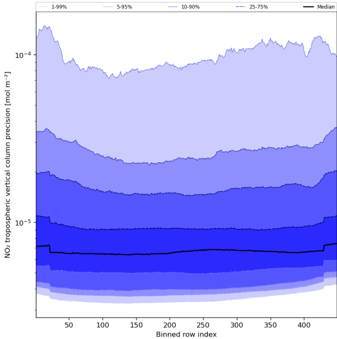
Figure 47: Along track statistics of “NO 2 tropospheric vertical column precision” for 2024-02-20 to 2024-02-22
