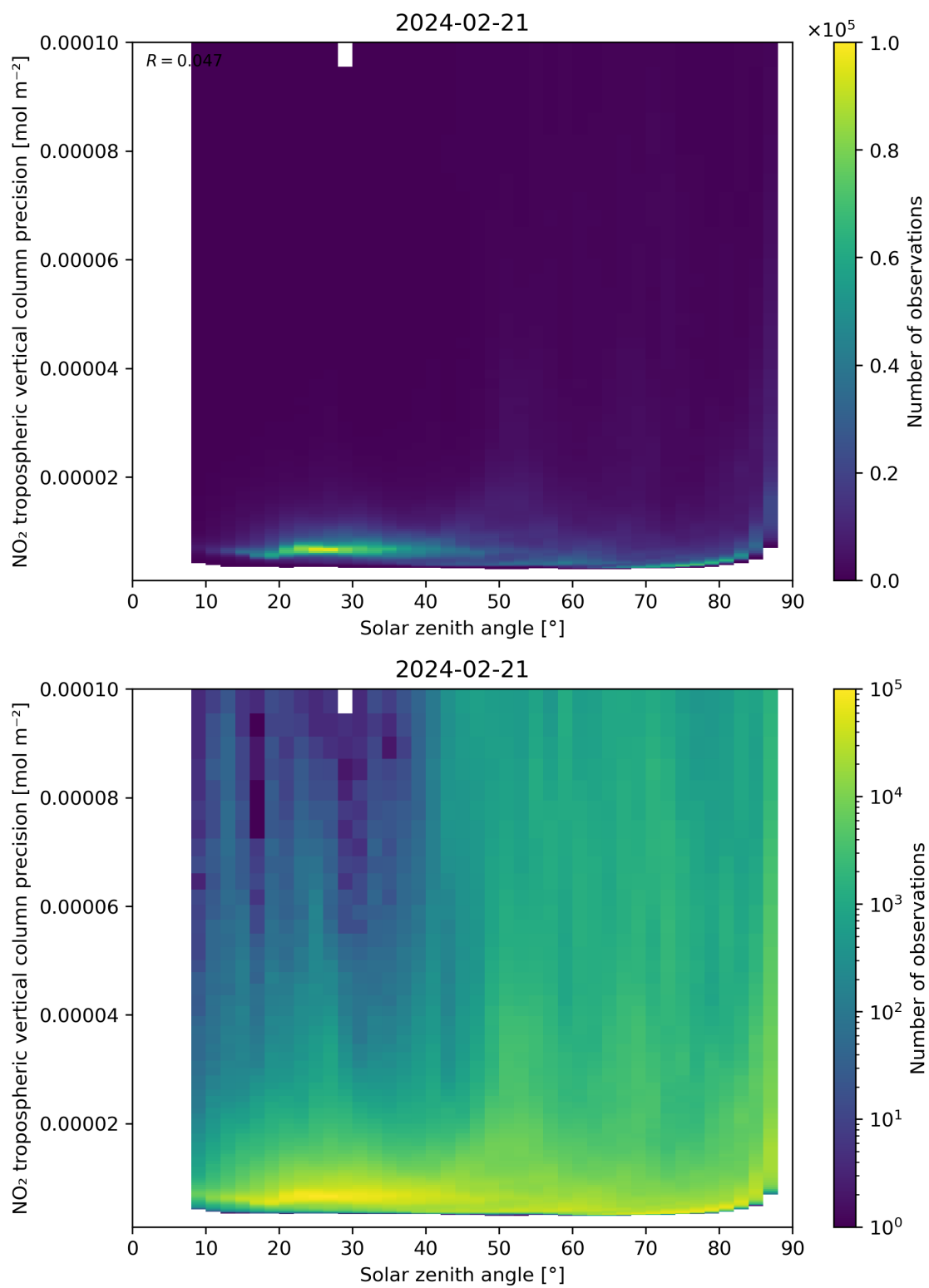
Figure 156: Scatter density plot of “Solar zenith angle” against “NO 2 tropospheric vertical column precision” for 2024-02-20 to 2024-02-22.
