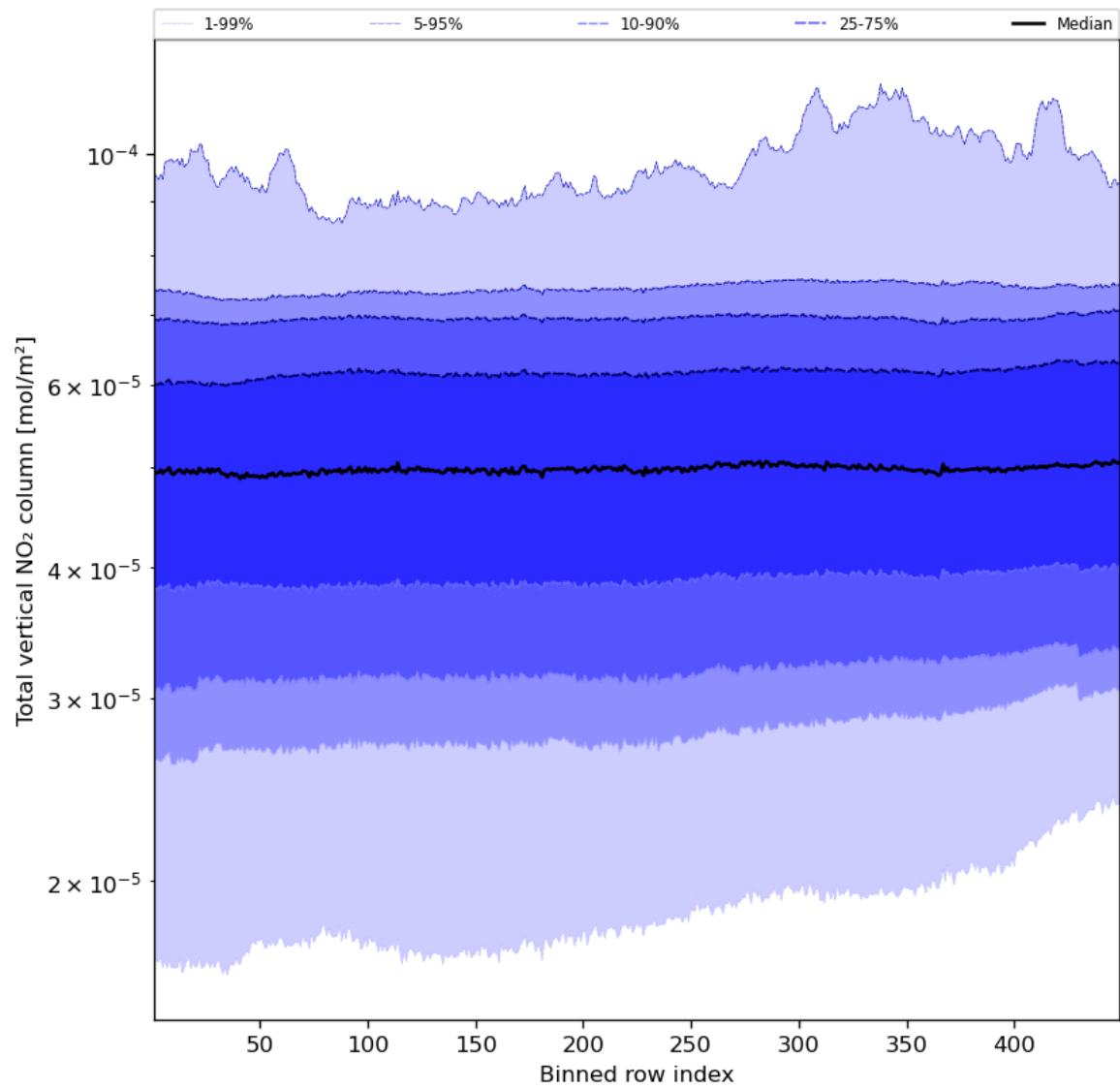
Figure 55: Along track statistics of “Total vertical NO 2 column” for 2024-02-20 to 2024-02-22
