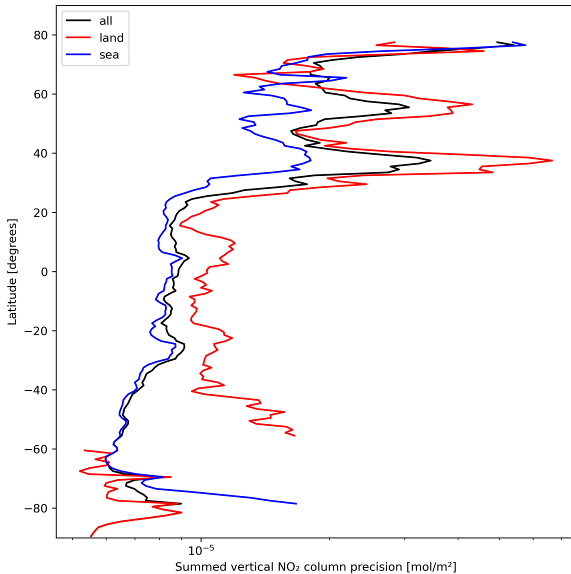
Figure 24: Zonal average of “Summed vertical NO 2 column precision” for 2024-02-20 to 2024-02-22.
