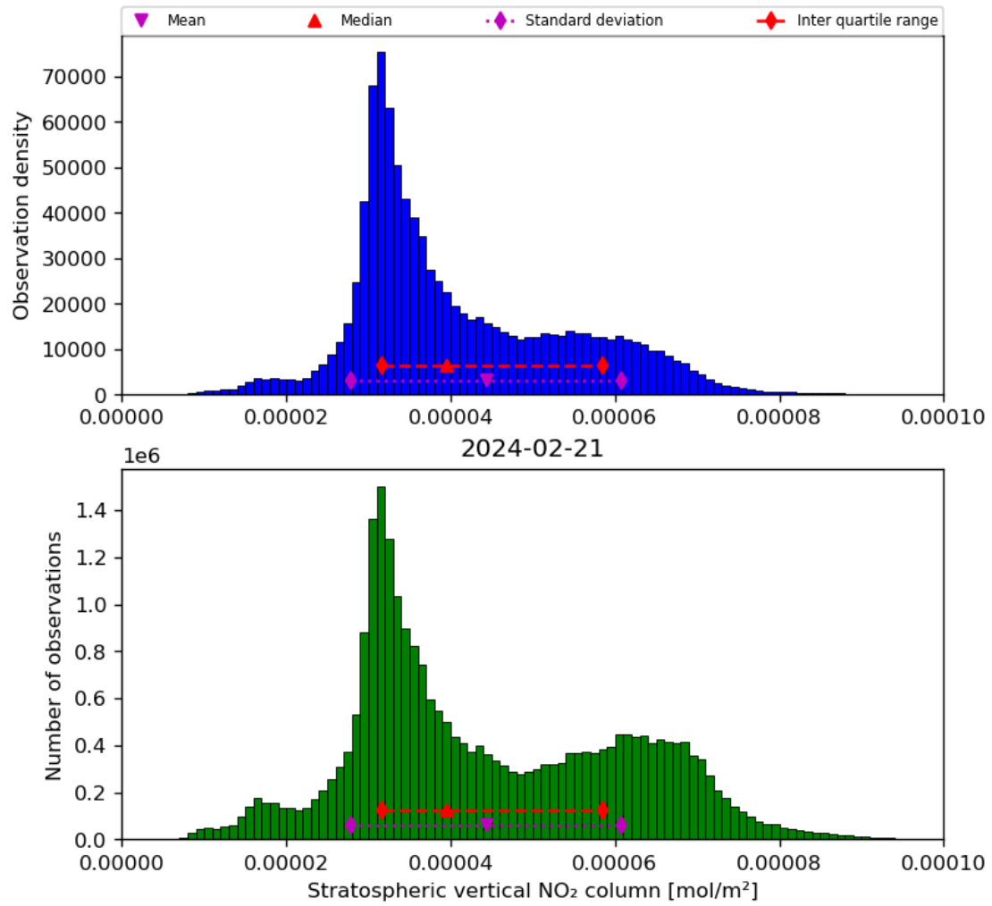
Figure 36: Histogram of “Stratospheric vertical NO 2 column” for 2024-02-20 to 2024-02-22
