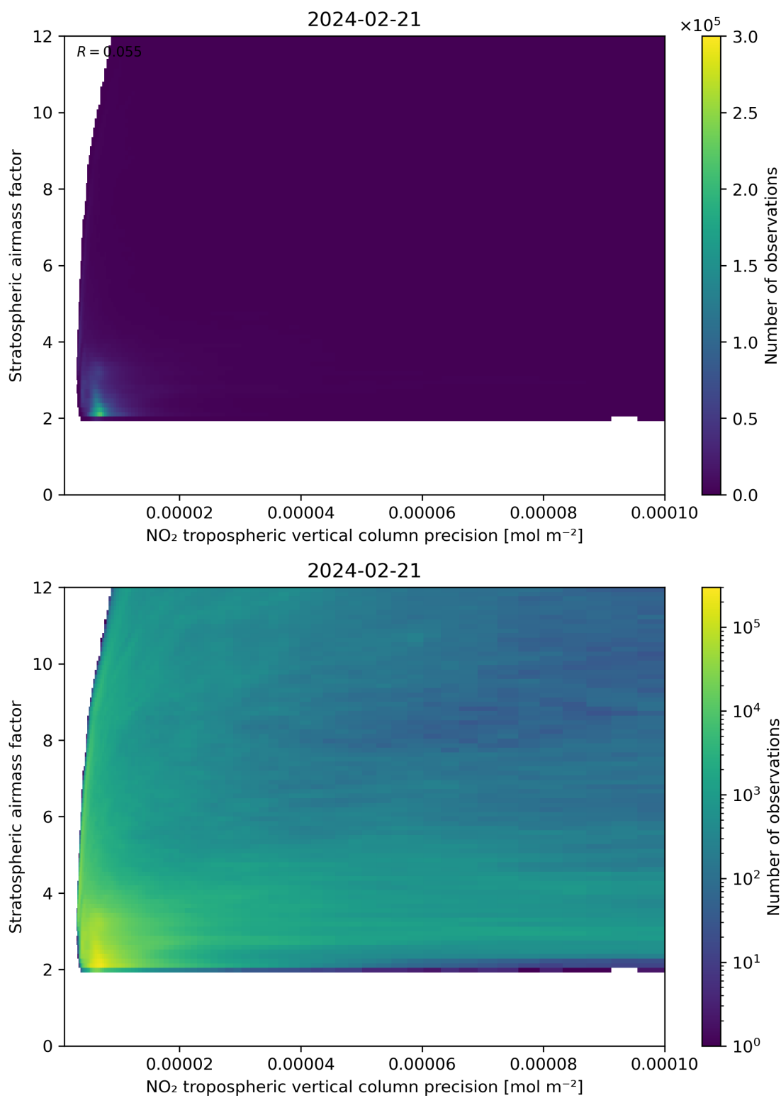
Figure 131: Scatter density plot of “NO 2 tropospheric vertical column precision” against “Stratospheric airmass factor” for 2024-02-20 to 2024-02-22.
