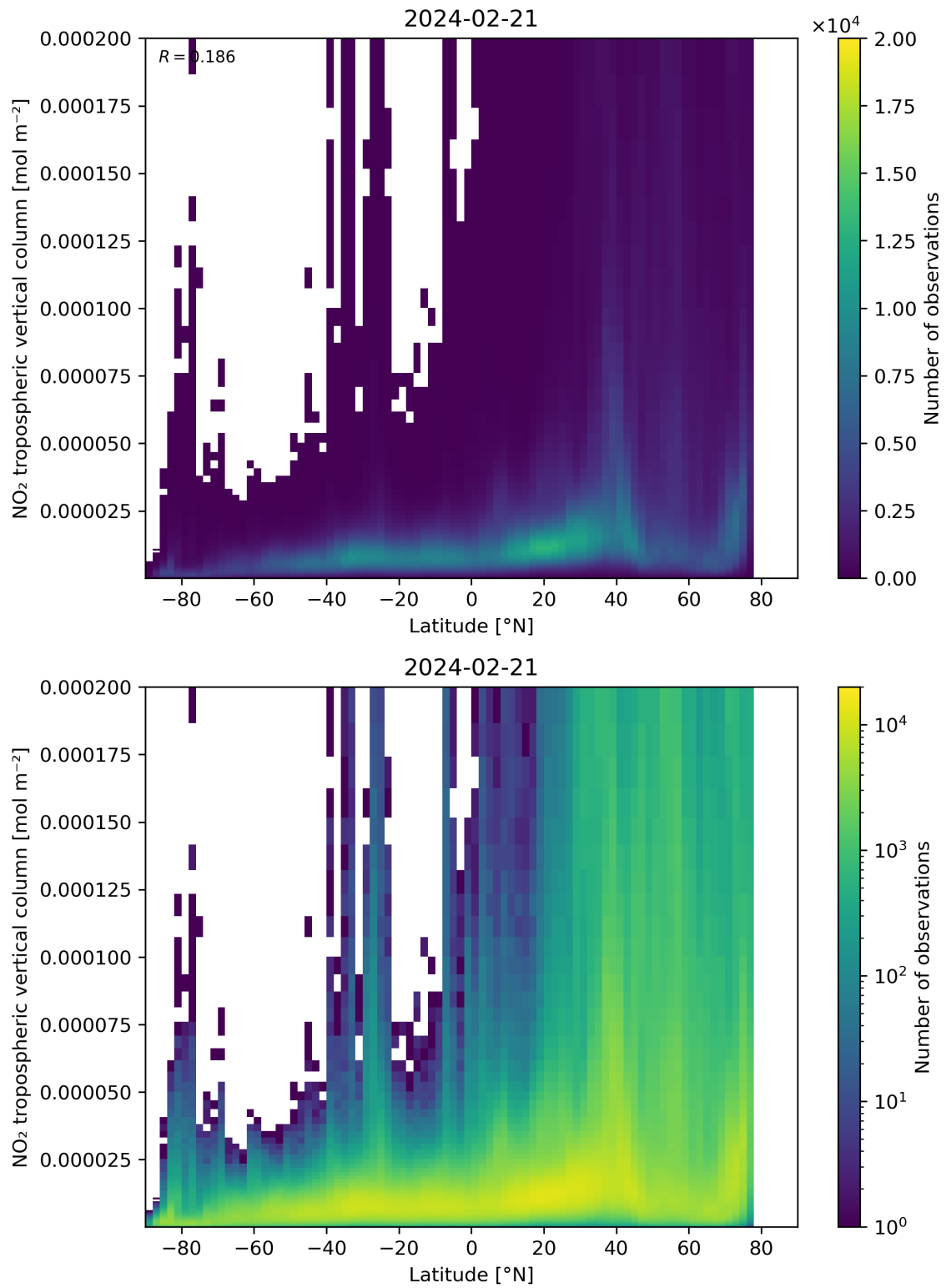
Figure 92: Scatter density plot of “Latitude” against “NO 2 tropospheric vertical column” for 2024-02-20 to 2024-02-22.
