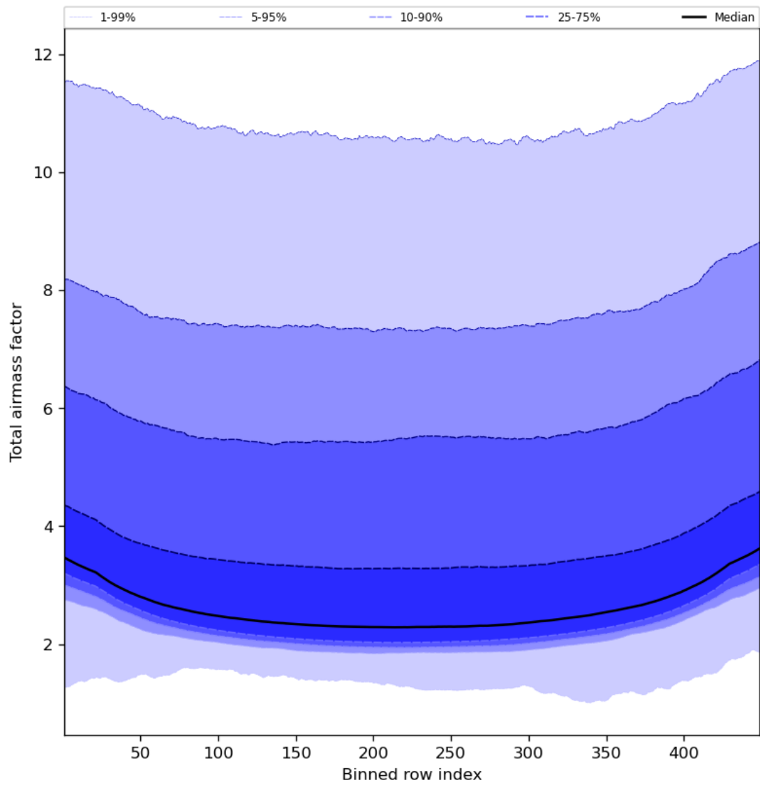
Figure 49: Along track statistics of “Total airmass factor” for 2024-02-20 to 2024-02-22
