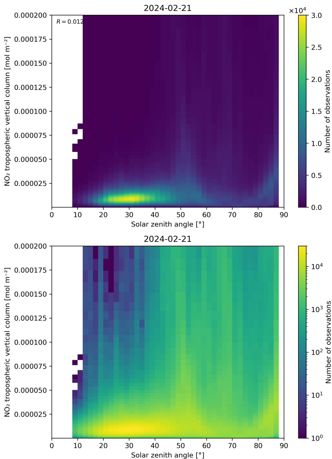
Figure 155: Scatter density plot of “Solar zenith angle” against “NO 2 tropospheric vertical column” for 2024-02-20 to 2024-02-22.
