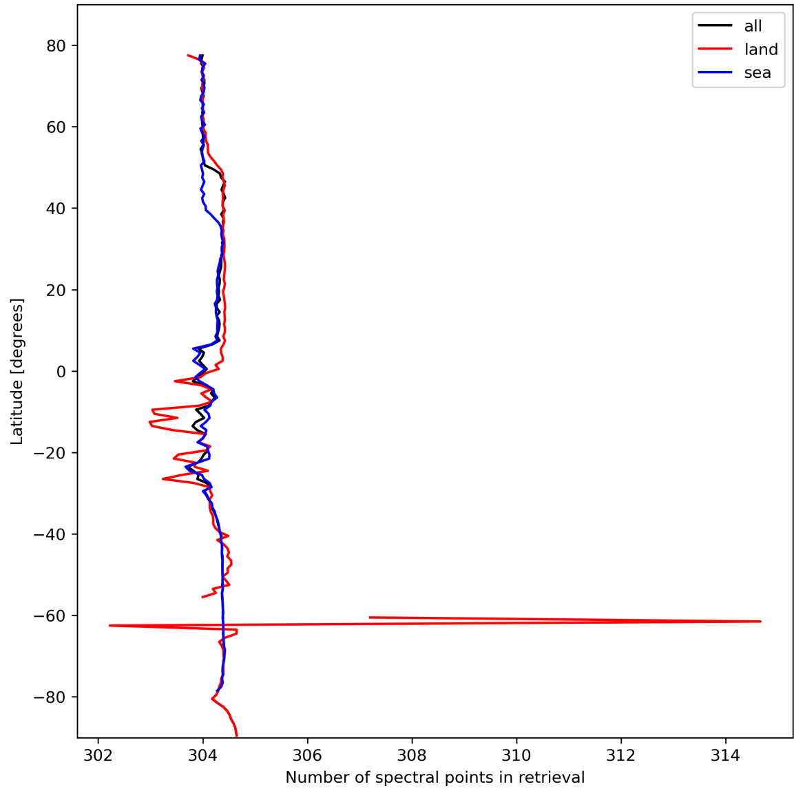
Figure 16: Zonal average of “Number of spectral points in retrieval” for 2024-02-20 to 2024-02-22.
