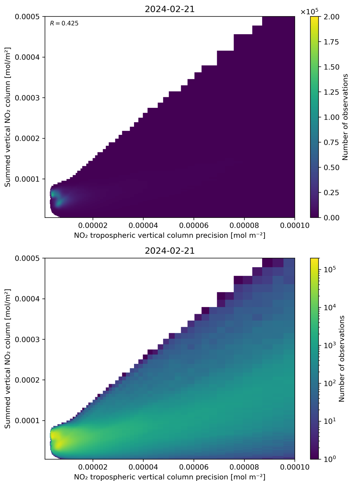
Figure 136: Scatter density plot of “NO 2 tropospheric vertical column precision” against “Summed vertical NO 2 column” for 2024-02-20 to 2024-02-22.
