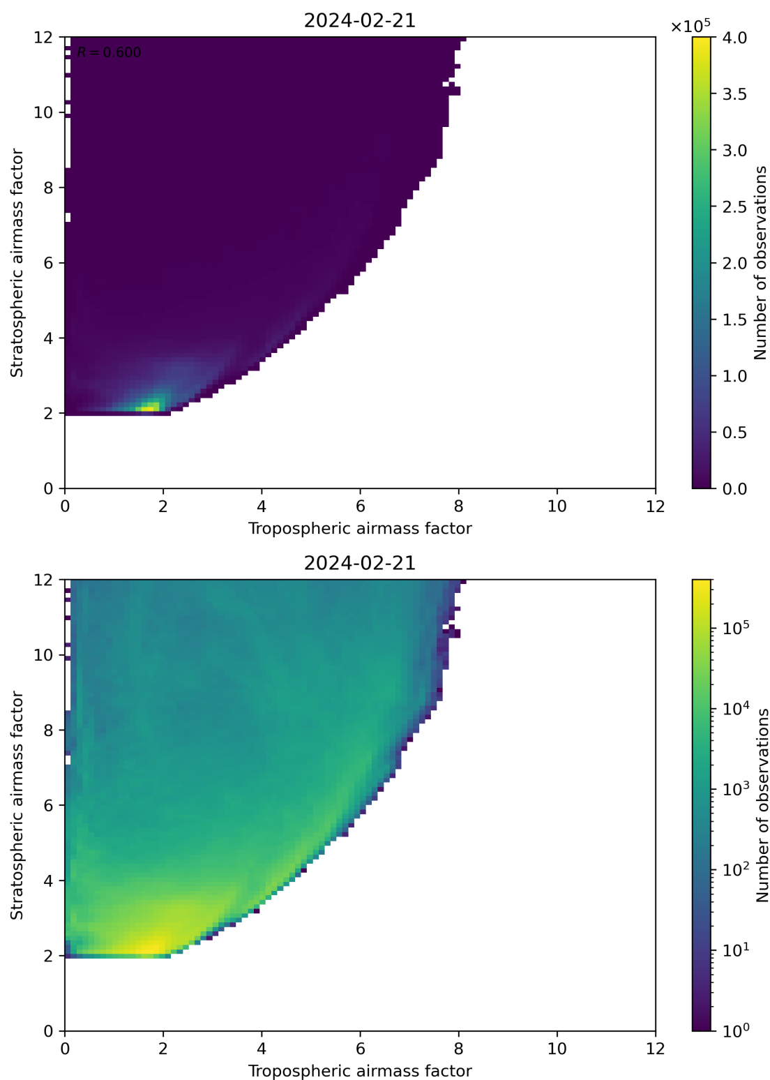
Figure 71: Scatter density plot of “Tropospheric airmass factor” against “Stratospheric airmass factor” for 2024-02-20 to 2024-02-22.
