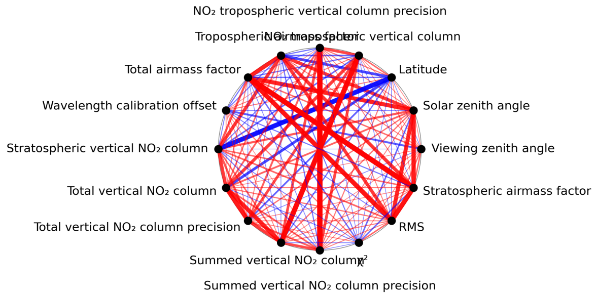
Figure 1: Map of correlation graph for 2024-02-20 to 2024-02-22.
