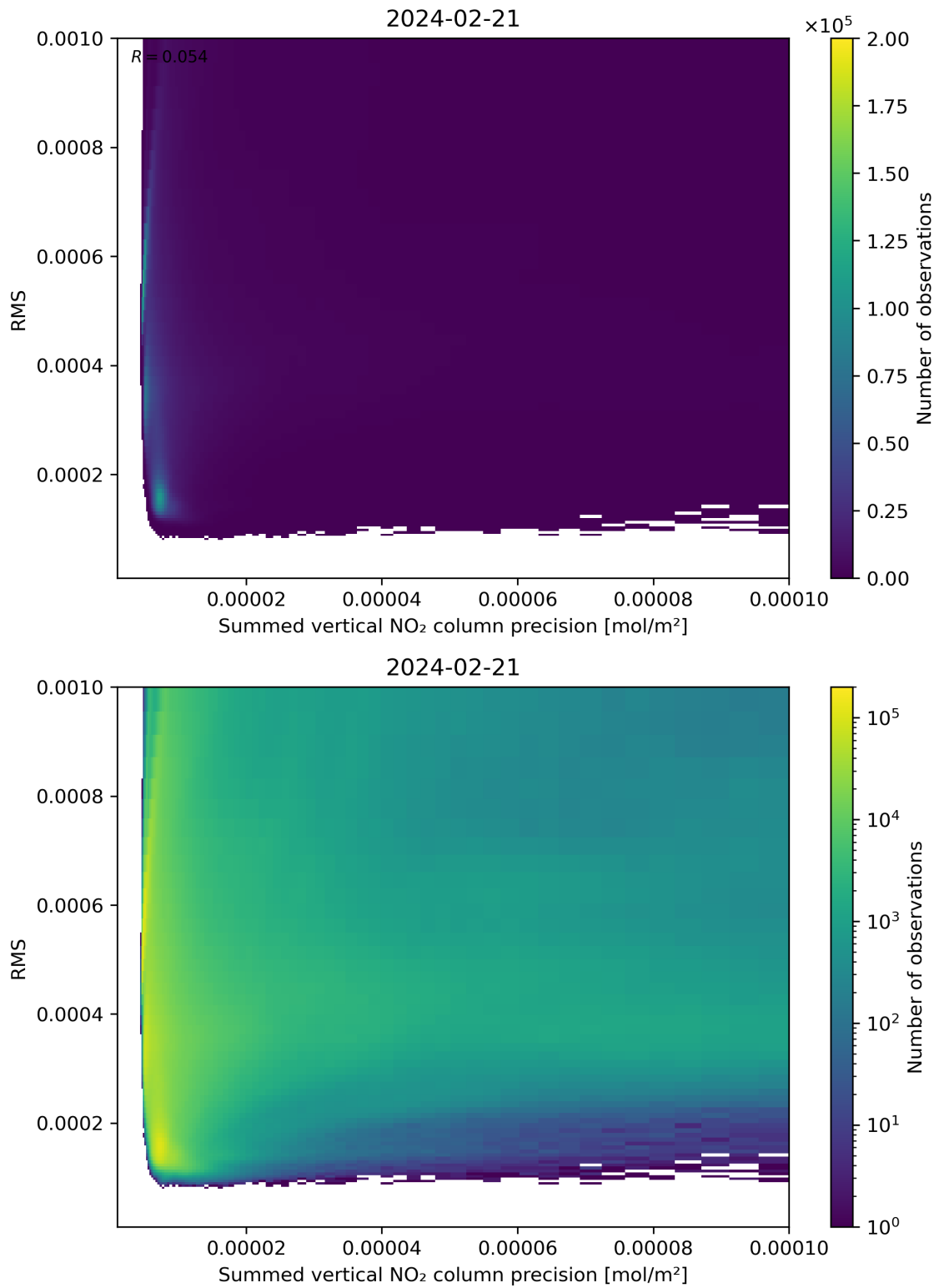
Figure 108: Scatter density plot of “Summed vertical NO 2 column precision” against “RMS” for 2024-02-20 to 2024-02-22.
