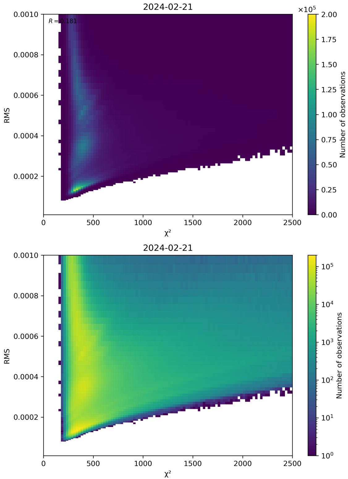
Figure 82: Scatter density plot of “ \chi^2 ” against “RMS” for 2024-02-20 to 2024-02-22.
