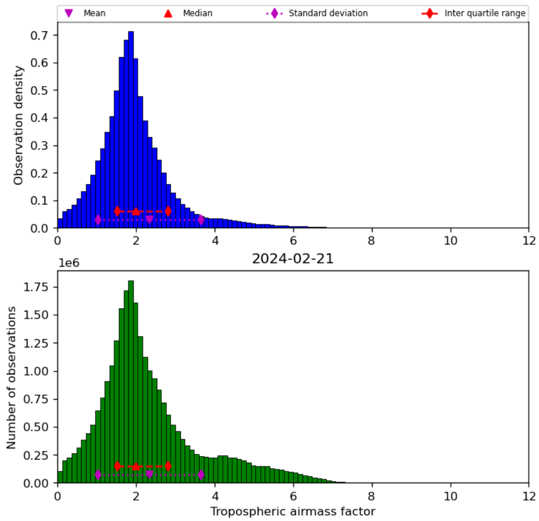
Figure 31: Histogram of “Tropospheric airmass factor” for 2024-02-20 to 2024-02-22
