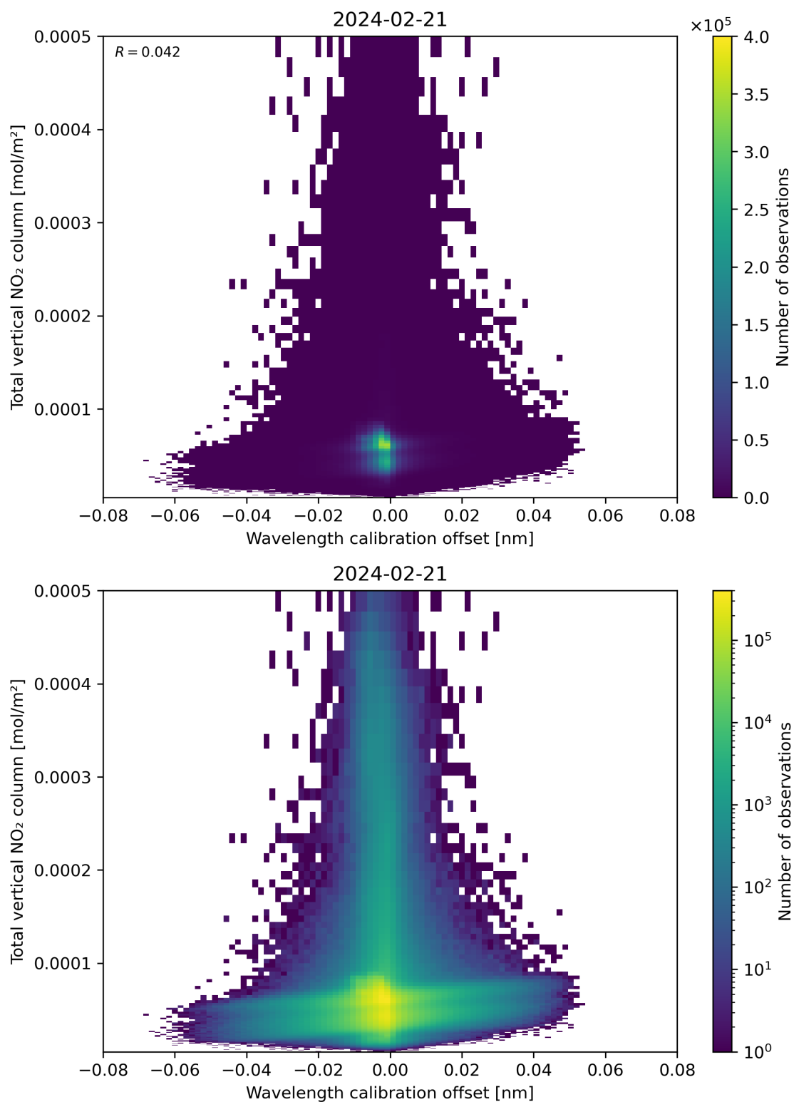
Figure 179: Scatter density plot of “Wavelength calibration offset” against “Total vertical NO 2 column” for 2024-02-20 to 2024-02-22.
