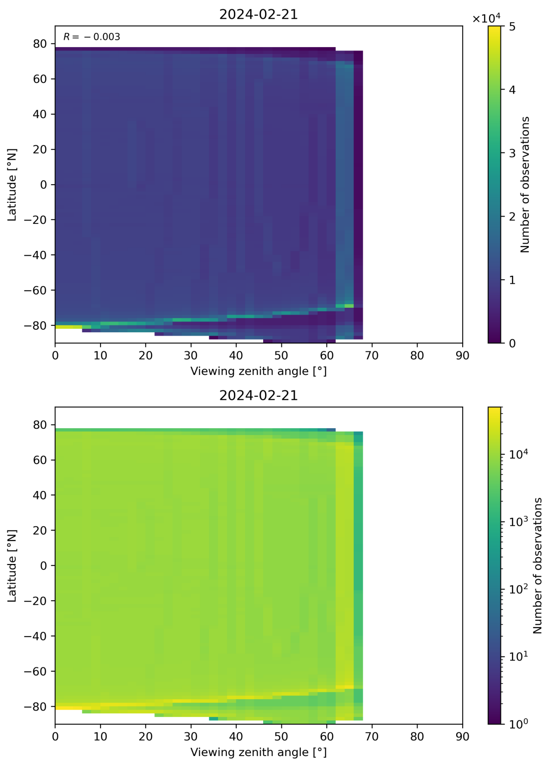
Figure 163: Scatter density plot of “Viewing zenith angle” against “Latitude” for 2024-02-20 to 2024-02-22.
