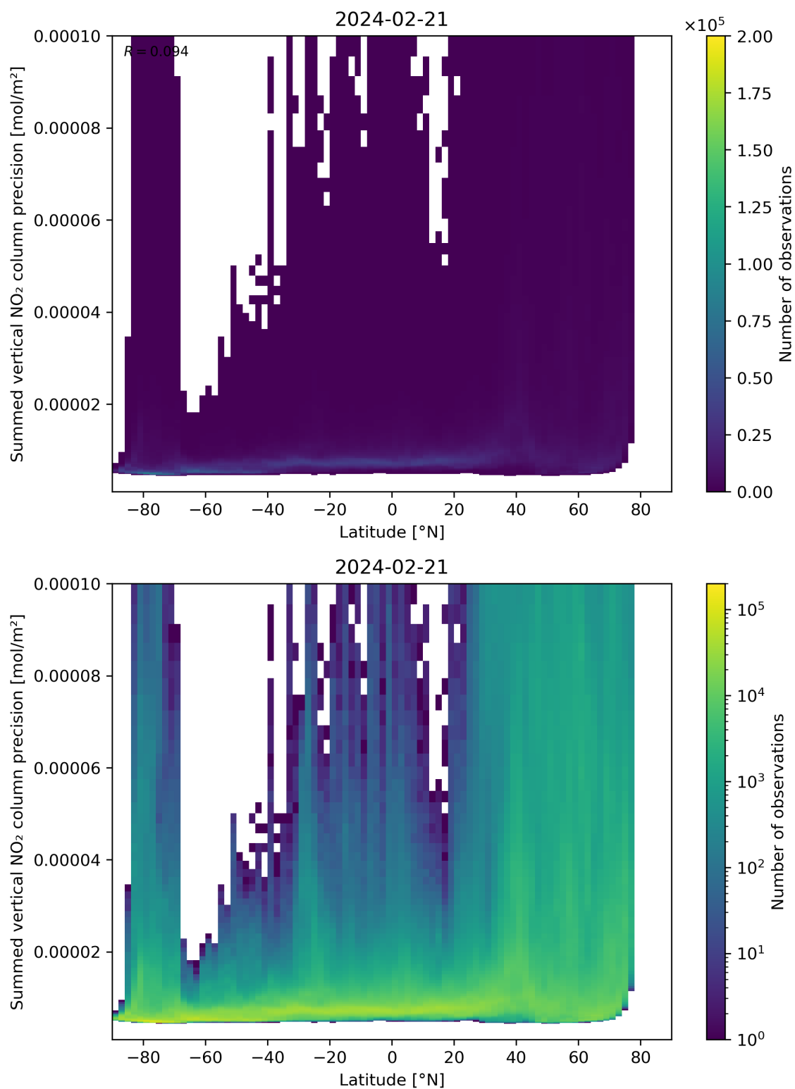
Figure 89: Scatter density plot of “Latitude” against “Summed vertical NO 2 column precision” for 2024-02-20 to 2024-02-22.
