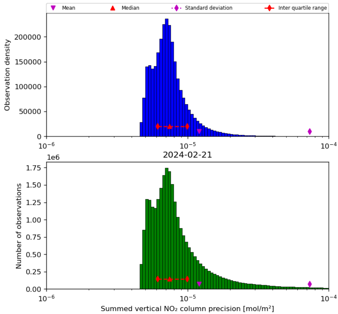
Figure 41: Histogram of “Summed vertical NO 2 column precision” for 2024-02-20 to 2024-02-22
