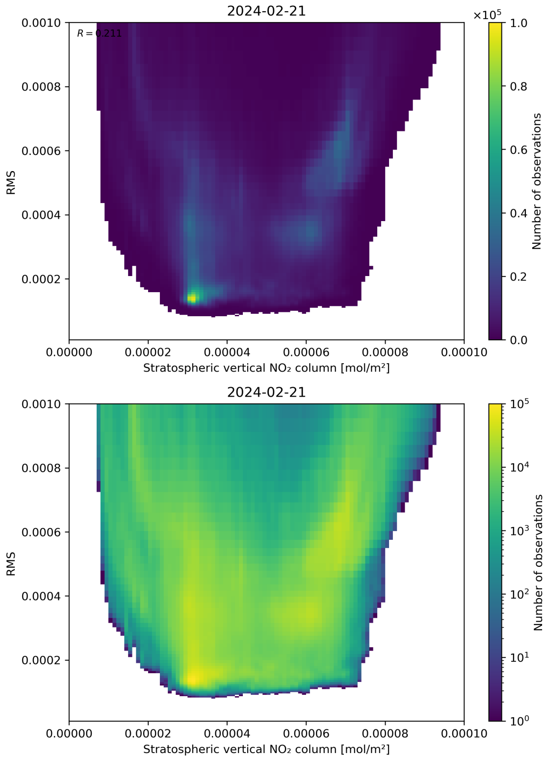
Figure 102: Scatter density plot of “Stratospheric vertical NO 2 column” against “RMS” for 2024-02-20 to 2024-02-22.
