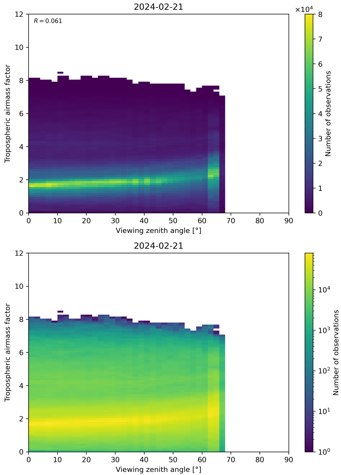
Figure 161: Scatter density plot of “Viewing zenith angle” against “Tropospheric airmass factor” for 2024-02-20 to 2024-02-22.
