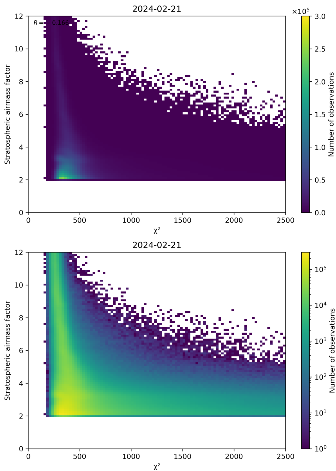
Figure 81: Scatter density plot of “ \chi^2 ” against “Stratospheric airmass factor” for 2024-02-20 to 2024-02-22.
