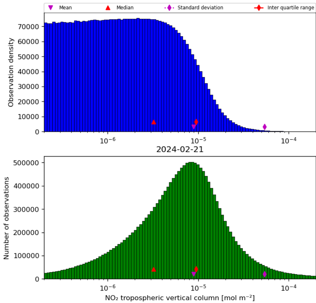
Figure 29: Histogram of “ \text{NO}_2 tropospheric vertical column” for 2024-02-20 to 2024-02-22
