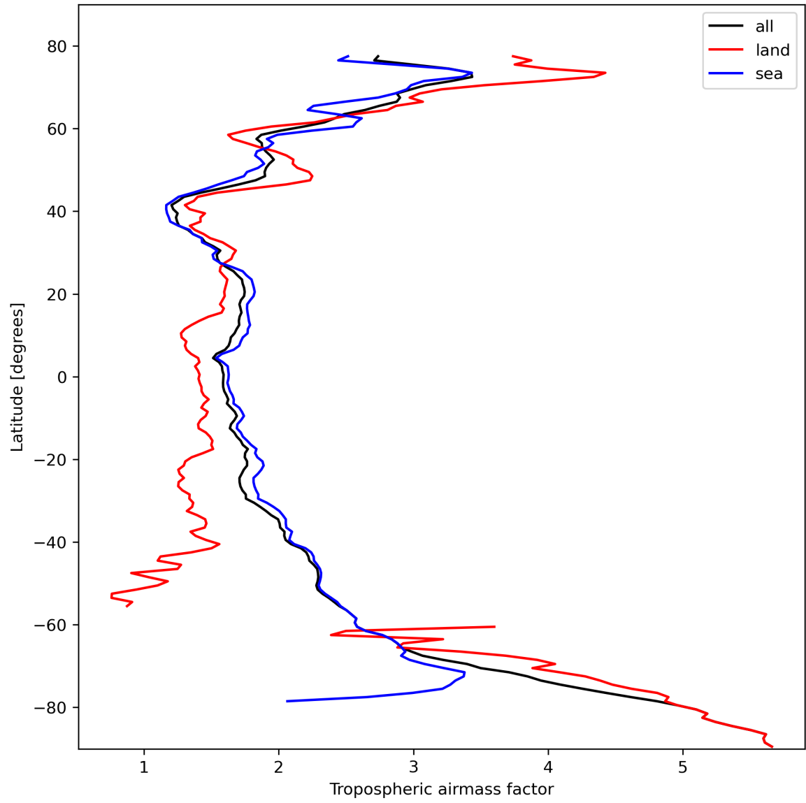
Figure 14: Zonal average of “Tropospheric airmass factor” for 2024-02-20 to 2024-02-22.
