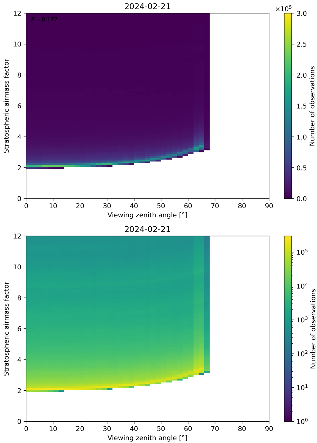
Figure 159: Scatter density plot of “Viewing zenith angle” against “Stratospheric airmass factor” for 2024-02-20 to 2024-02-22.
