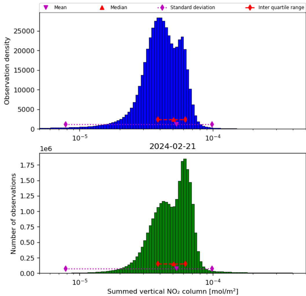
Figure 40: Histogram of “Summed vertical NO 2 column” for 2024-02-20 to 2024-02-22
