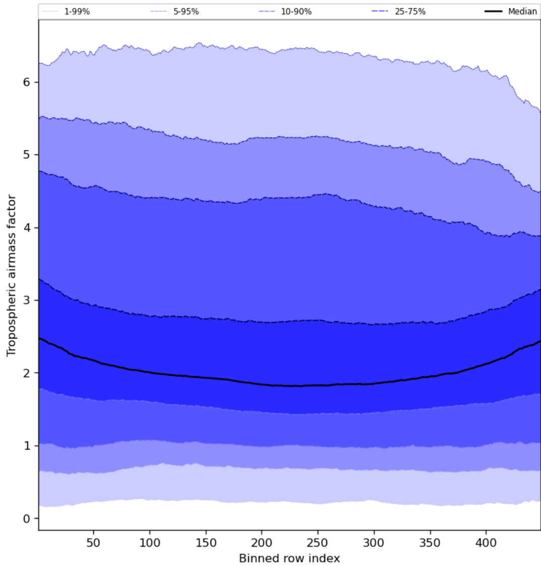
Figure 48: Along track statistics of “Tropospheric airmass factor” for 2024-02-20 to 2024-02-22
