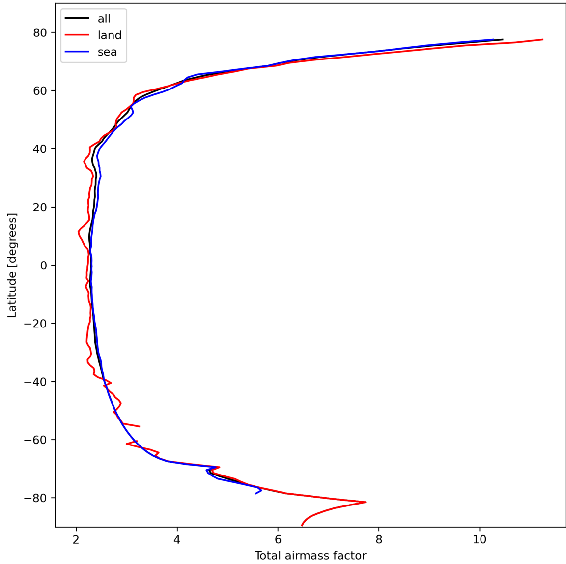
Figure 15: Zonal average of “Total airmass factor” for 2024-02-20 to 2024-02-22.
