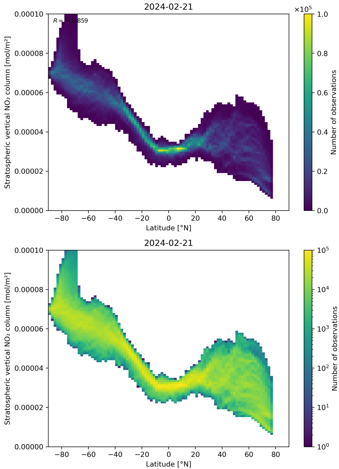
Figure 87: Scatter density plot of “Latitude” against “Stratospheric vertical NO 2 column” for 2024-02-20 to 2024-02-22.
