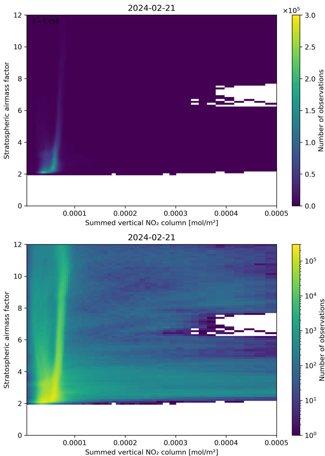
Figure 103: Scatter density plot of “Summed vertical NO 2 column” against “Stratospheric air mass factor” for 2024-02-20 to 2024-02-22.
