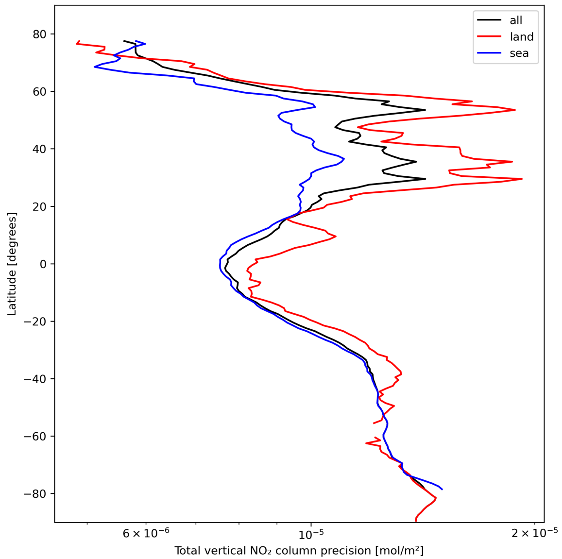
Figure 22: Zonal average of “Total vertical NO 2 column precision” for 2024-02-20 to 2024-02-22.
