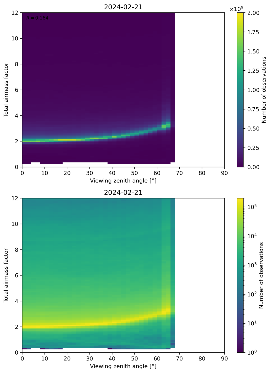
Figure 160: Scatter density plot of “Viewing zenith angle” against “Total airmass factor” for 2024-02-20 to 2024-02-22.
