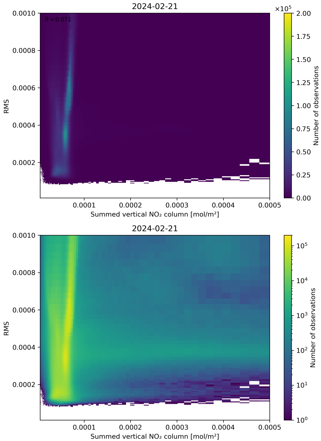
Figure 109: Scatter density plot of “Summed vertical NO 2 column” against “RMS” for 2024-02-20 to 2024-02-22.
