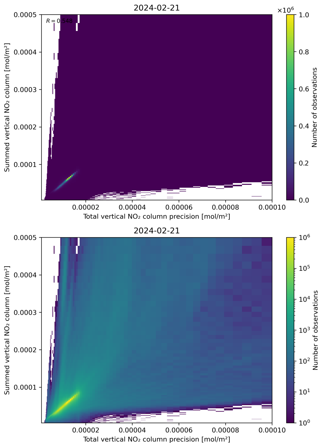
Figure 117: Scatter density plot of “Total vertical NO 2 column precision” against “Summed vertical NO 2 column” for 2024-02-20 to 2024-02-22.
