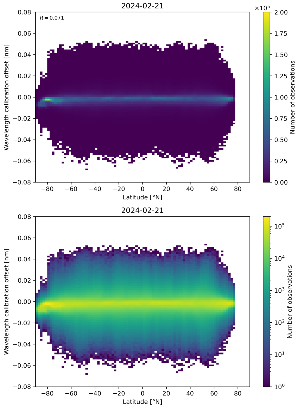
Figure 95: Scatter density plot of “Latitude” against “Wavelength calibration offset” for 2024-02-20 to 2024-02-22.
