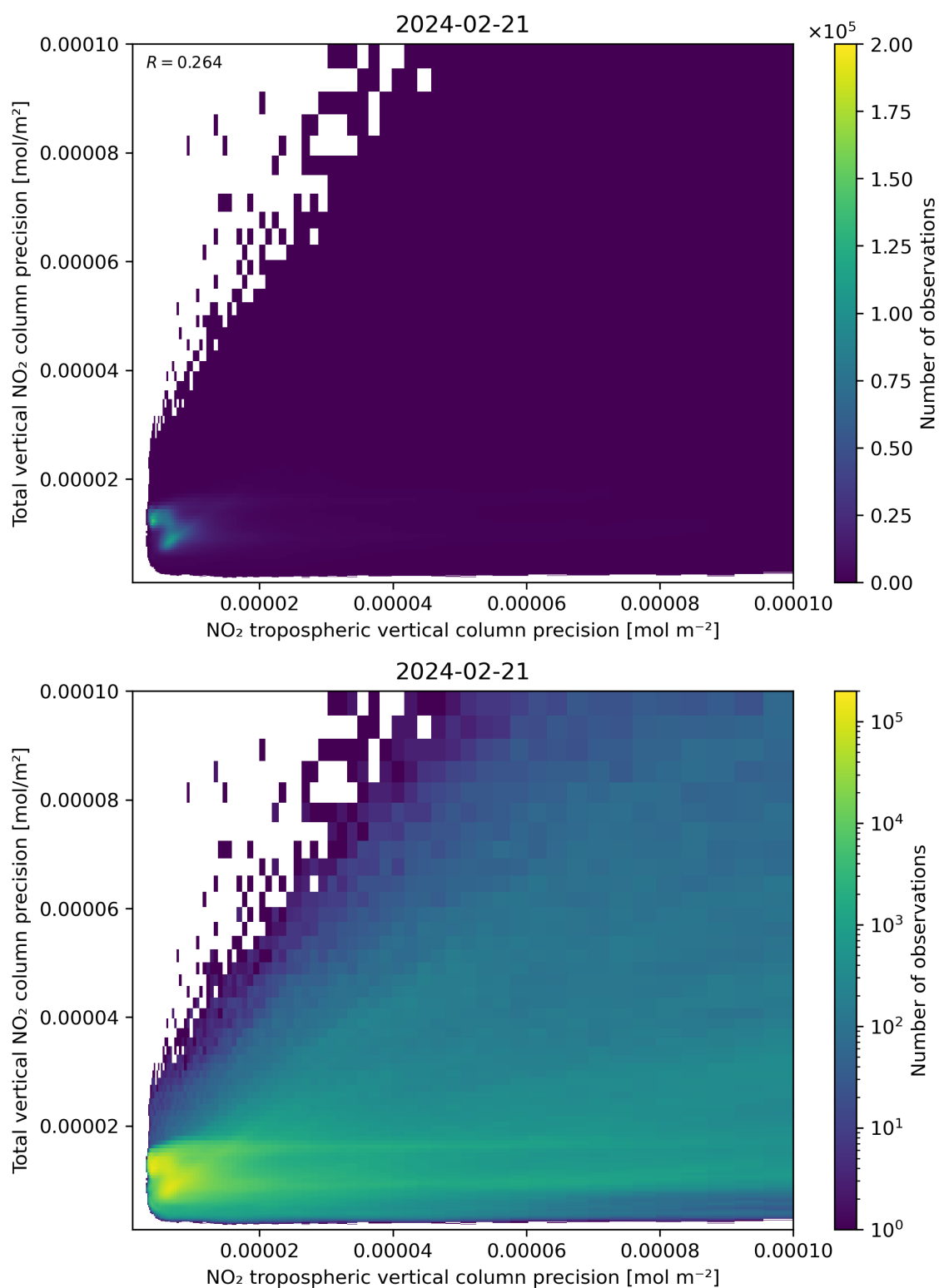
Figure 139: Scatter density plot of “NO 2 tropospheric vertical column precision” against “Total vertical NO 2 column precision” for 2024-02-20 to 2024-02-22.
