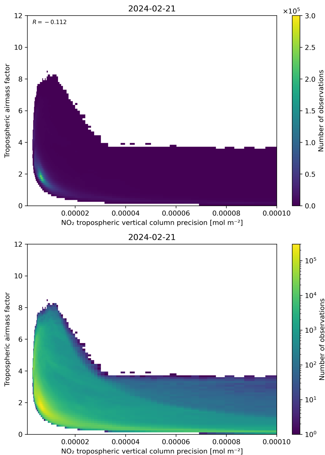
Figure 133: Scatter density plot of “NO 2 tropospheric vertical column precision” against “Tropospheric airmass factor” for 2024-02-20 to 2024-02-22.
