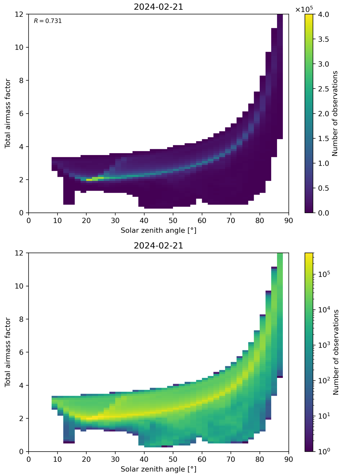
Figure 146: Scatter density plot of “Solar zenith angle” against “Total air mass factor” for 2024-02-20 to 2024-02-22.
