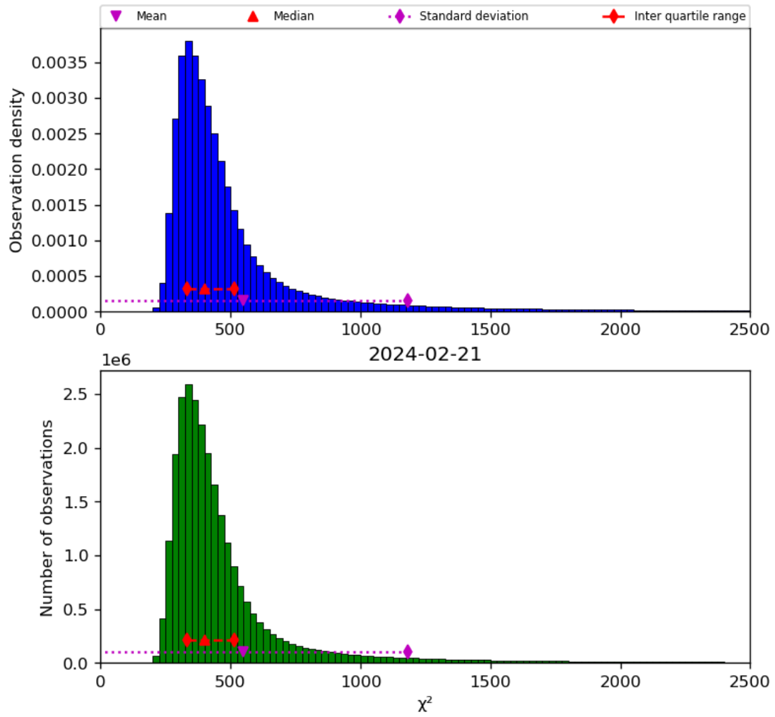
Figure 42: Histogram of “ \chi^2 ” for 2024-02-20 to 2024-02-22
