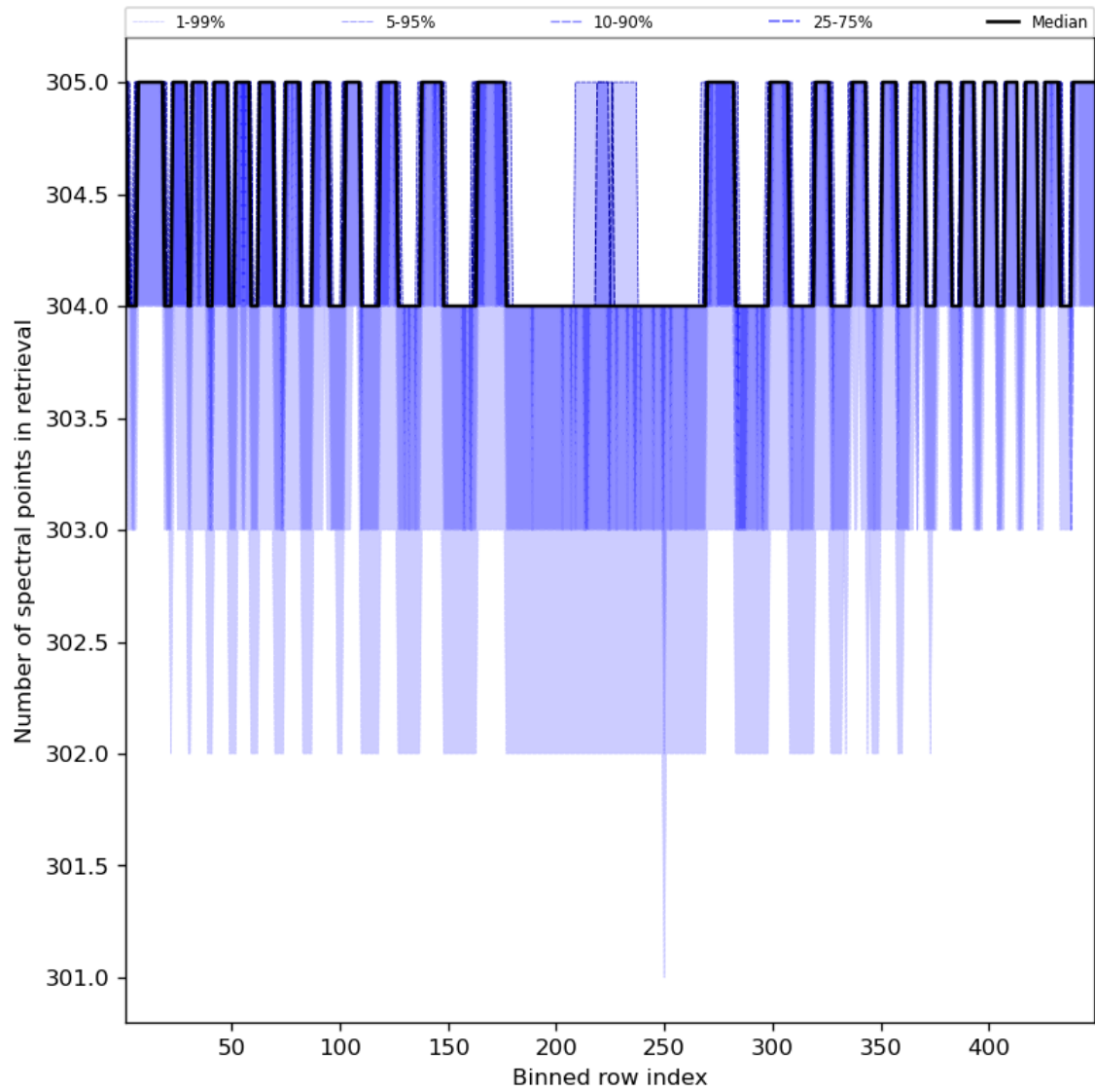
Figure 50: Along track statistics of “Number of spectral points in retrieval” for 2024-02-20 to 2024-02-22
