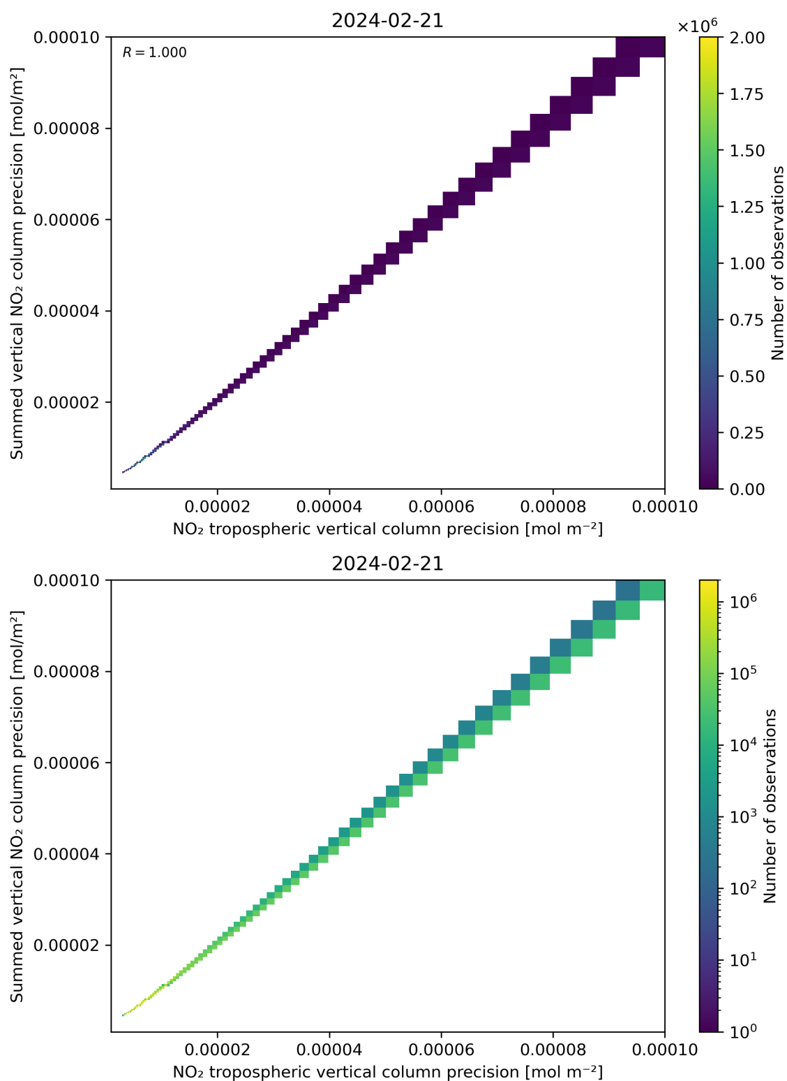
Figure 137: Scatter density plot of “NO 2 tropospheric vertical column precision” against “Summed vertical NO 2 column precision” for 2024-02-20 to 2024-02-22.
