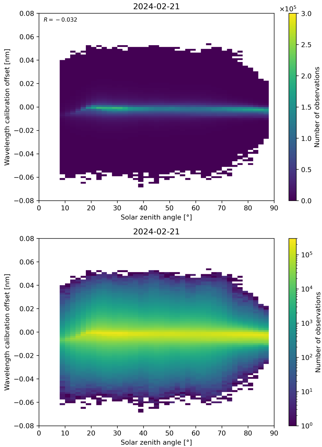
Figure 158: Scatter density plot of “Solar zenith angle” against “Wavelength calibration offset” for 2024-02-20 to 2024-02-22.
