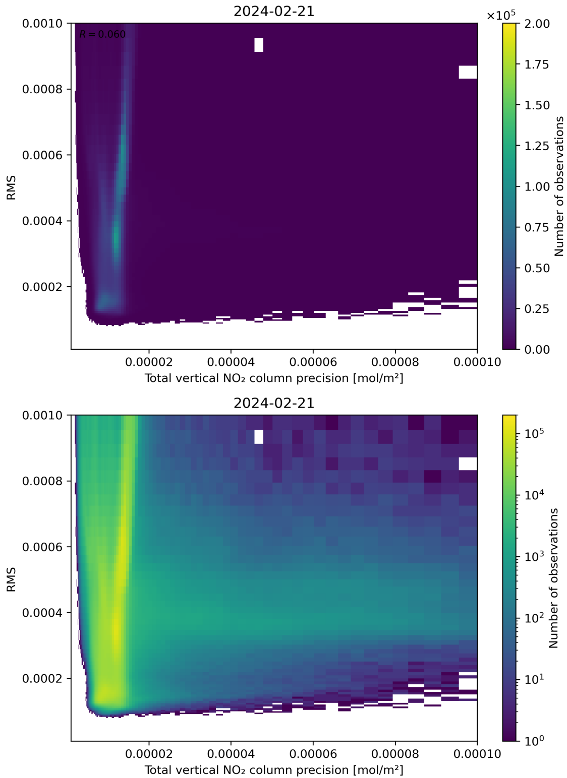
Figure 119: Scatter density plot of “Total vertical NO 2 column precision” against “RMS” for 2024-02-20 to 2024-02-22.
