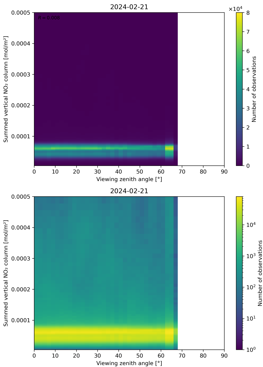
Figure 165: Scatter density plot of “Viewing zenith angle” against “Summed vertical NO 2 column” for 2024-02-20 to 2024-02-22.
