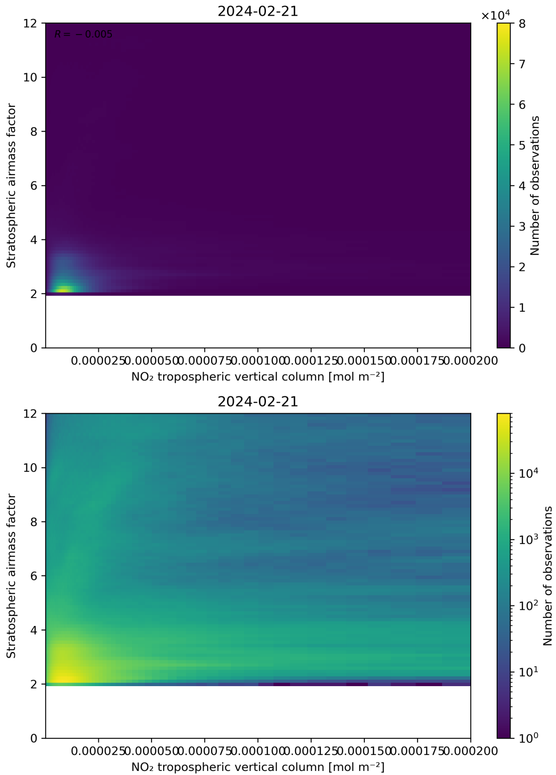
Figure 121: Scatter density plot of “NO 2 tropospheric vertical column” against “Stratospheric airmass factor” for 2024-02-20 to 2024-02-22.
