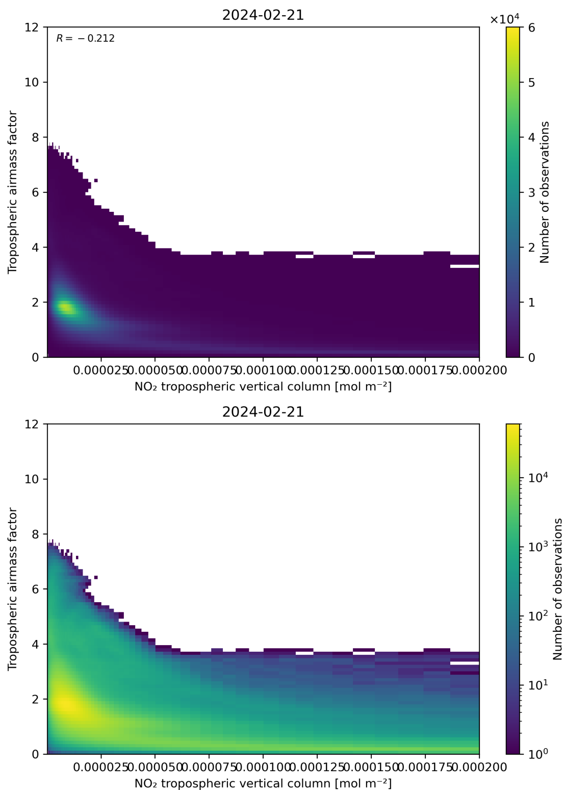
Figure 123: Scatter density plot of “NO 2 tropospheric vertical column” against “Tropospheric air mass factor” for 2024-02-20 to 2024-02-22.
