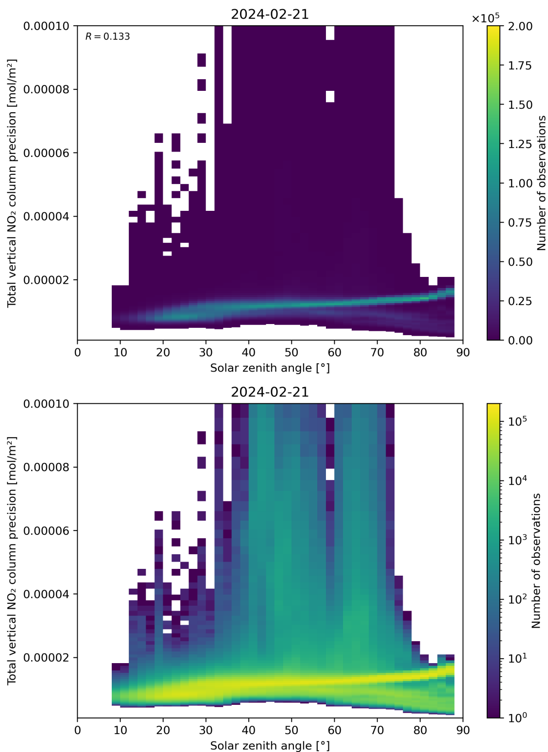
Figure 154: Scatter density plot of “Solar zenith angle” against “Total vertical NO 2 column precision” for 2024-02-20 to 2024-02-22.
