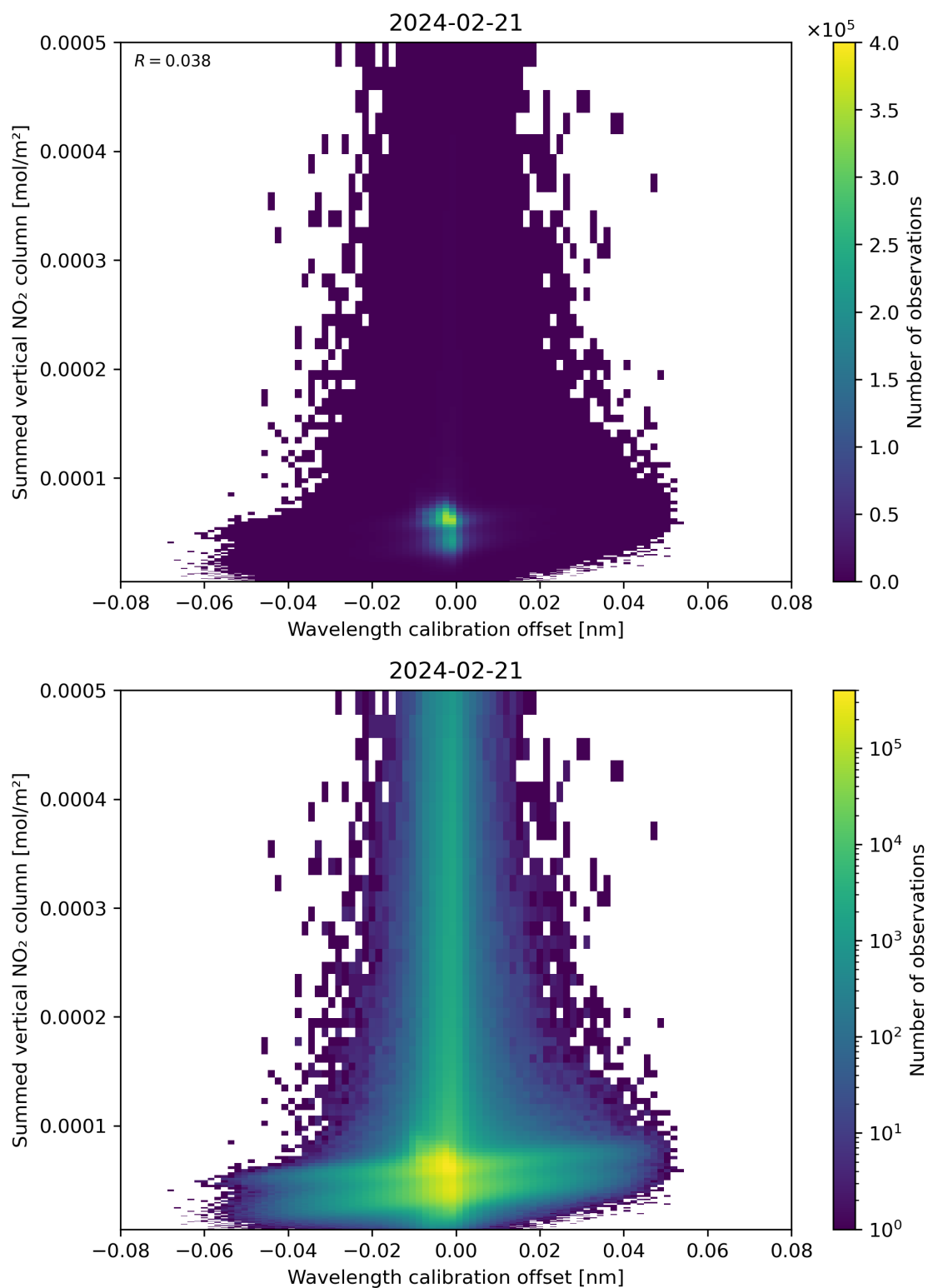
Figure 177: Scatter density plot of “Wavelength calibration offset” against “Summed vertical NO 2 column” for 2024-02-20 to 2024-02-22.
