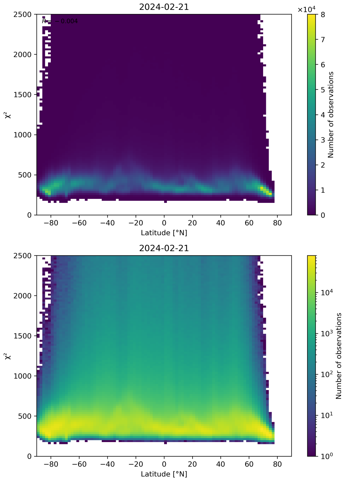
Figure 86: Scatter density plot of “Latitude” against “ \chi^2 ” for 2024-02-20 to 2024-02-22.
