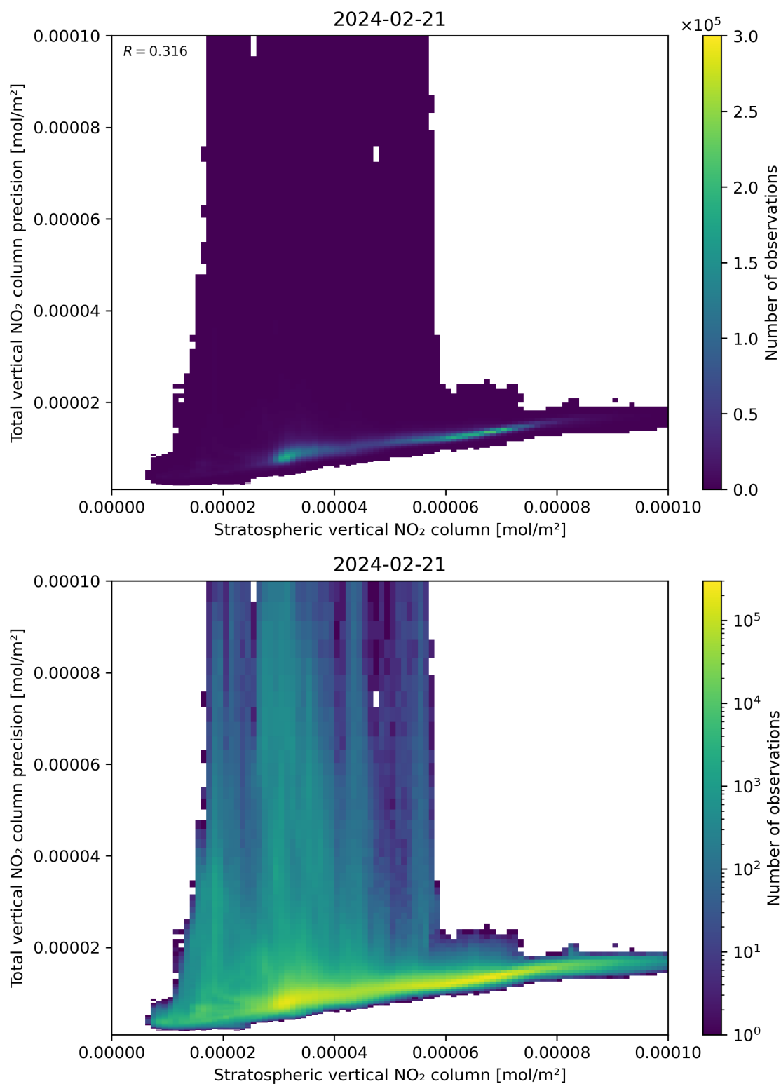
Figure 101: Scatter density plot of “Stratospheric vertical NO 2 column” against “Total vertical NO 2 column precision” for 2024-02-20 to 2024-02-22.
