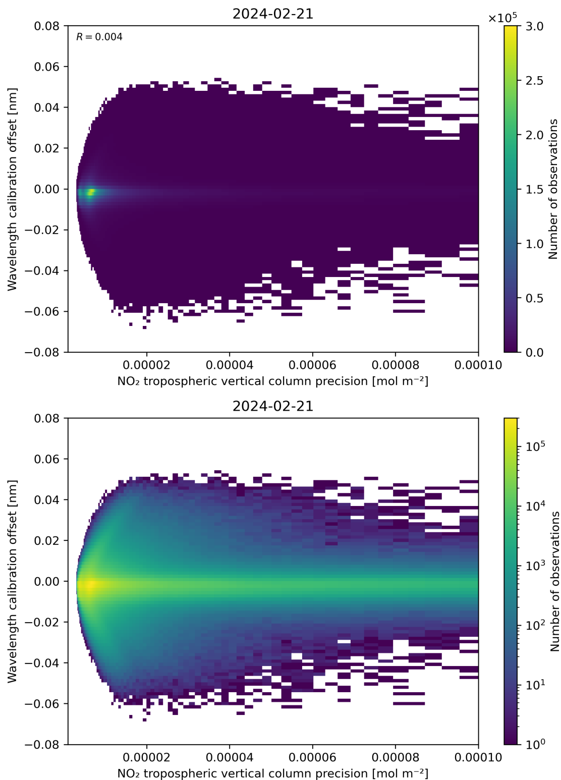
Figure 141: Scatter density plot of “NO 2 tropospheric vertical column precision” against “Wavelength calibration offset” for 2024-02-20 to 2024-02-22.
