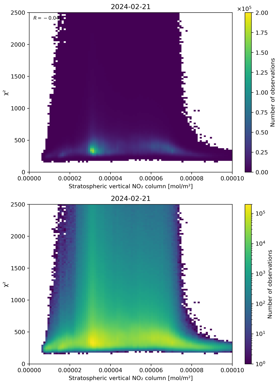
Figure 97: Scatter density plot of “Stratospheric vertical NO 2 column” against “ \chi^2 ” for 2024-02-20 to 2024-02-22.
