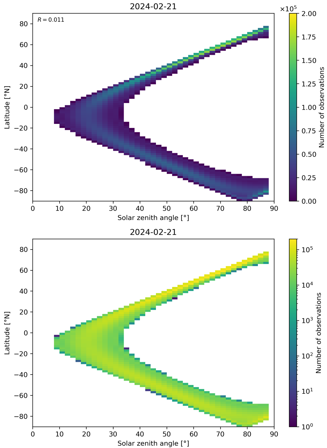
Figure 149: Scatter density plot of “Solar zenith angle” against “Latitude” for 2024-02-20 to 2024-02-22.
