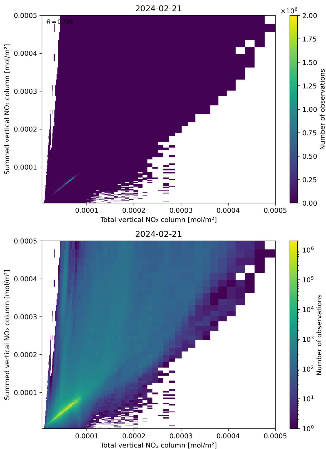
Figure 112: Scatter density plot of “Total vertical NO 2 column” against “Summed vertical NO 2 column” for 2024-02-20 to 2024-02-22.
