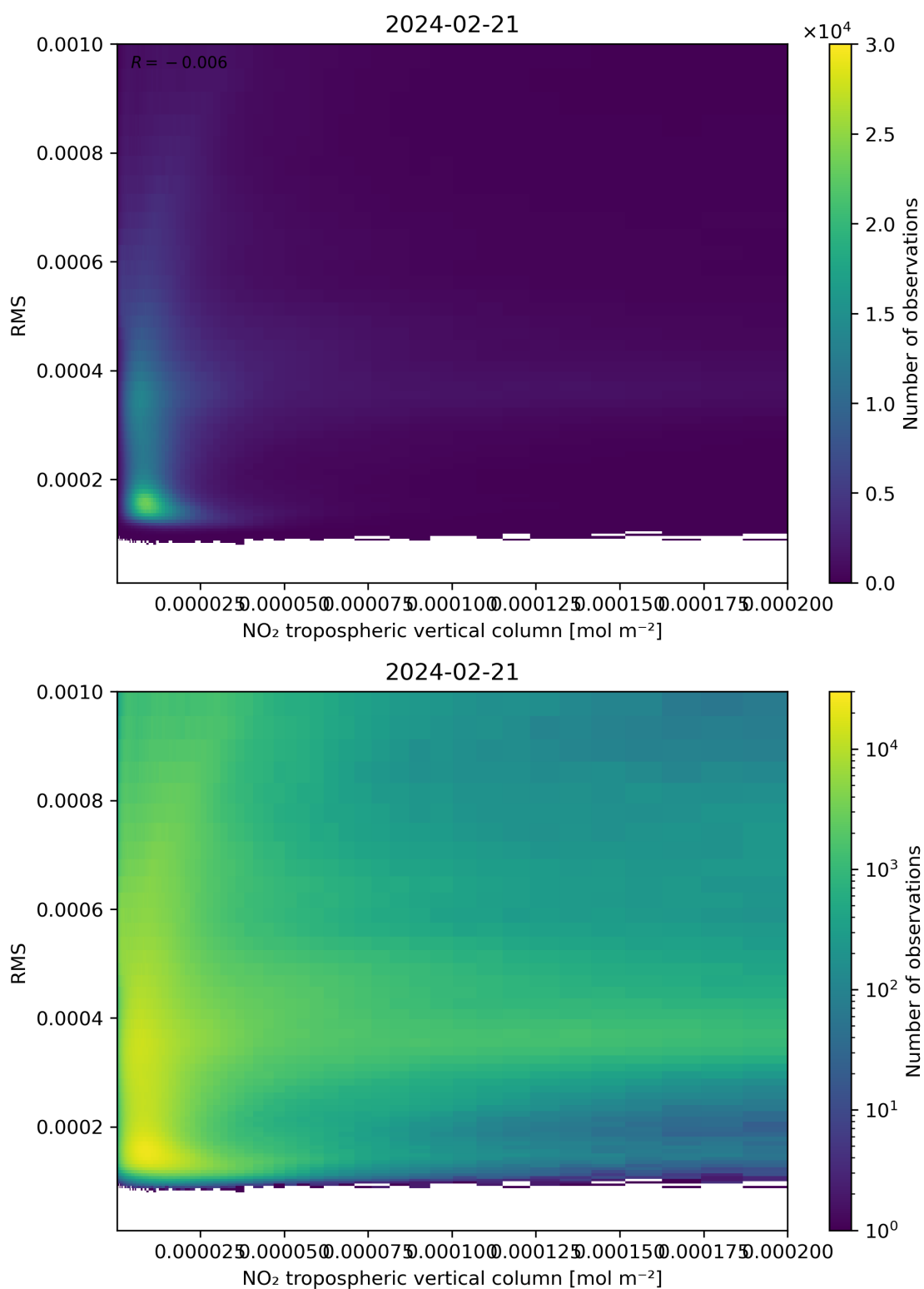
Figure 142: Scatter density plot of “NO 2 tropospheric vertical column” against “RMS” for 2024-02-20 to 2024-02-22.
