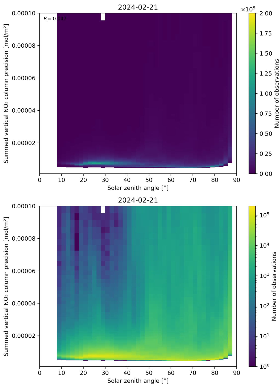
Figure 152: Scatter density plot of “Solar zenith angle” against “Summed vertical NO 2 column precision” for 2024-02-20 to 2024-02-22.
