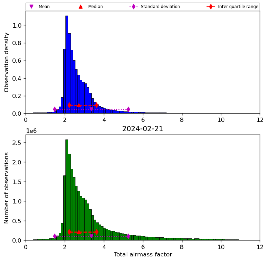
Figure 32: Histogram of “Total airmass factor” for 2024-02-20 to 2024-02-22
