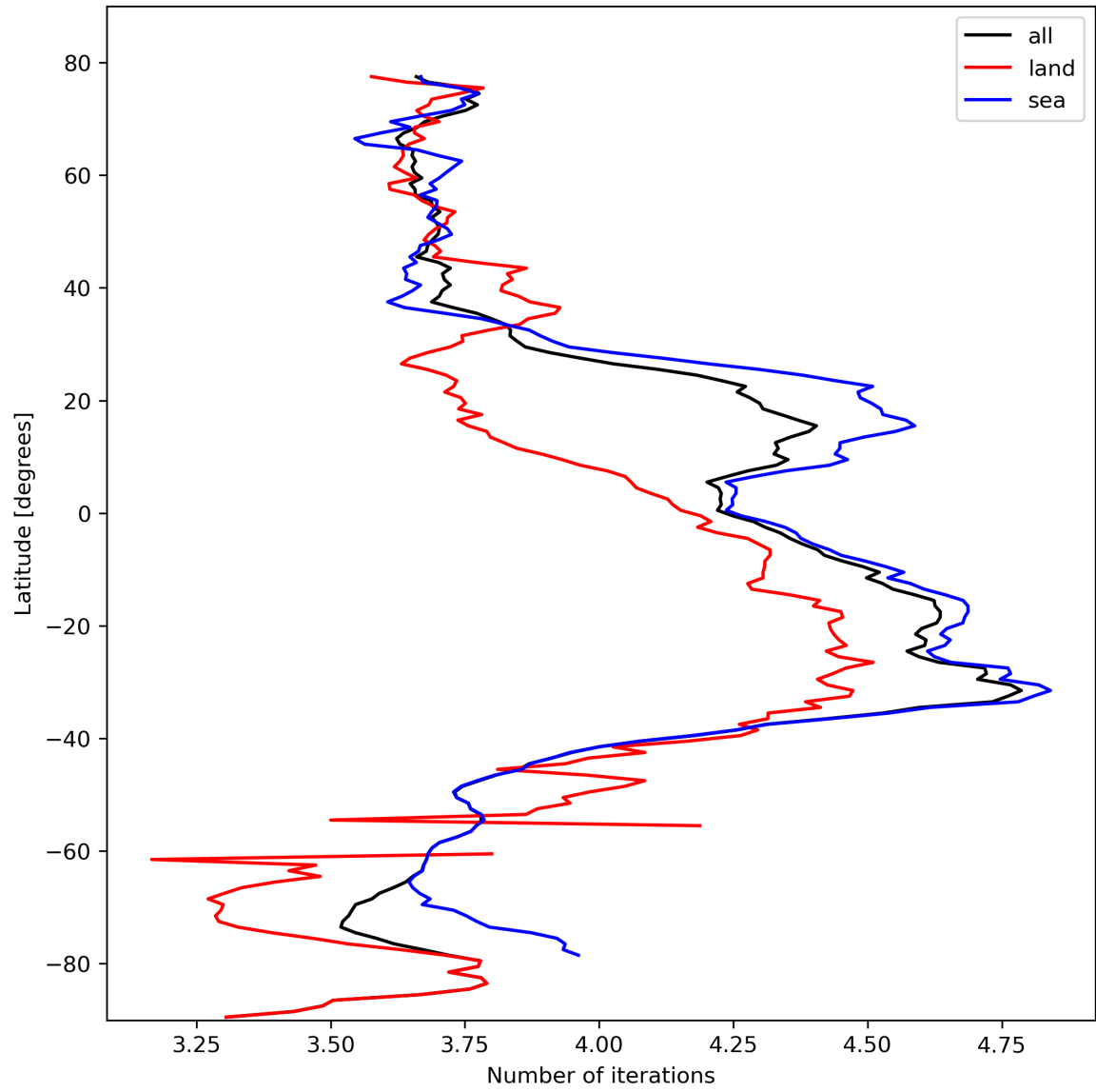
Figure 17: Zonal average of “Number of iterations” for 2024-02-20 to 2024-02-22.
