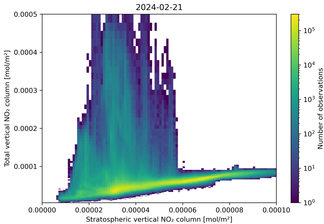
Figure 100: Scatter density plot of “Stratospheric vertical NO 2 column” against “Total vertical NO 2 column” for 2024-02-20 to 2024-02-22.
