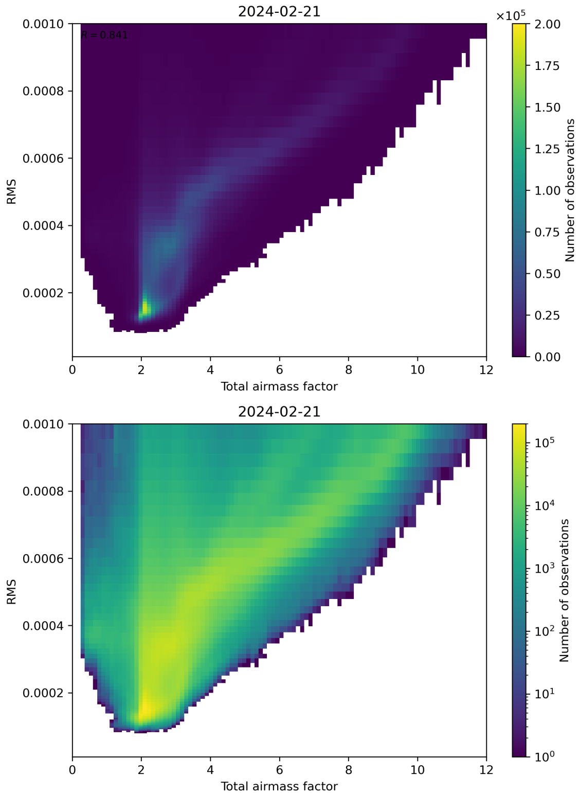
Figure 69: Scatter density plot of “Total airmass factor” against “RMS” for 2024-02-20 to 2024-02-22.
