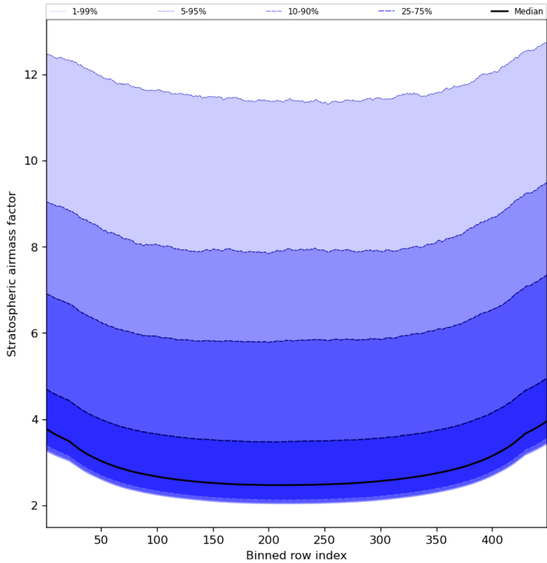
Figure 61: Along track statistics of “Stratospheric airmass factor” for 2024-02-20 to 2024-02-22
