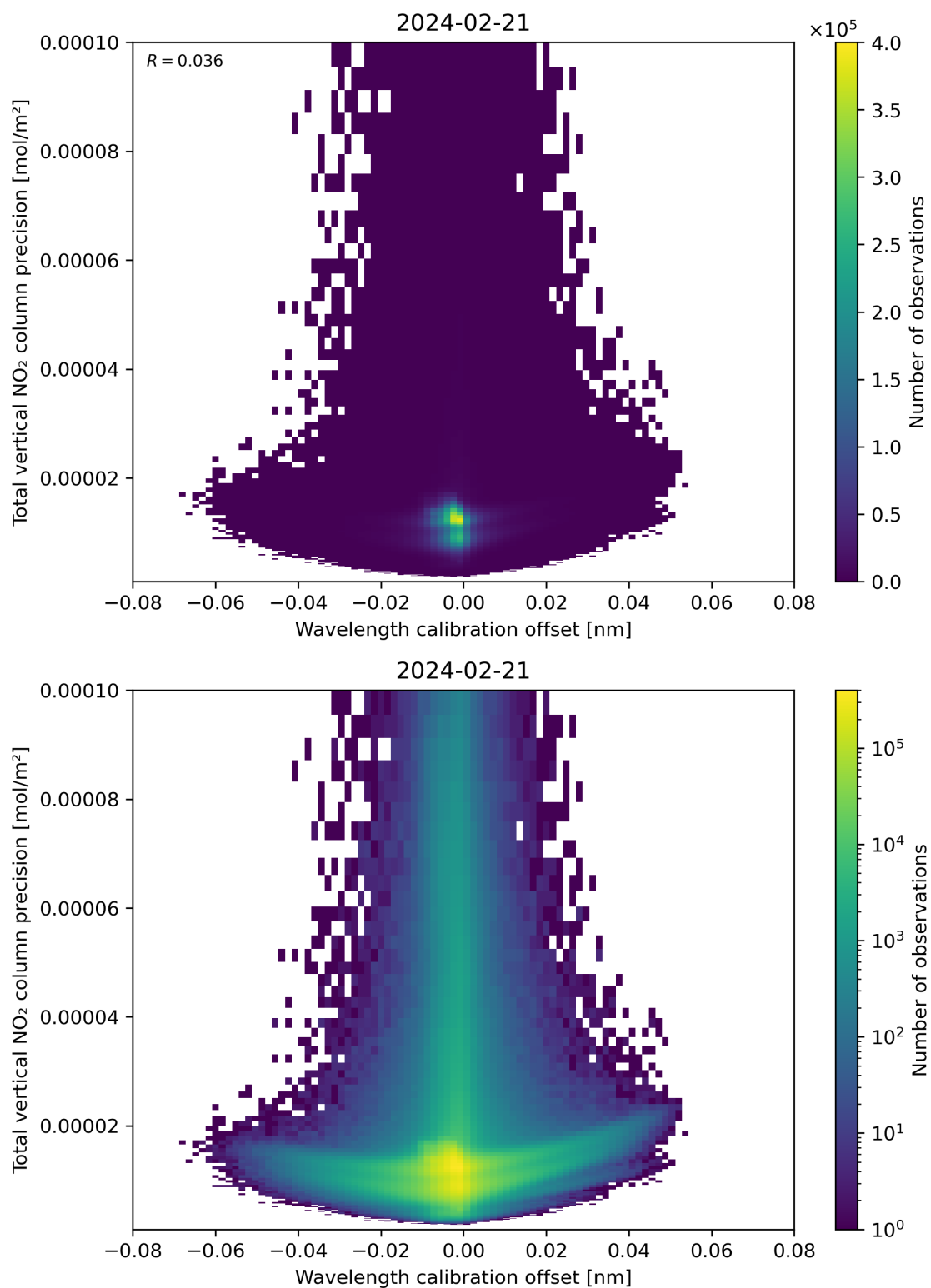
Figure 180: Scatter density plot of “Wavelength calibration offset” against “Total vertical NO 2 column precision” for 2024-02-20 to 2024-02-22.
