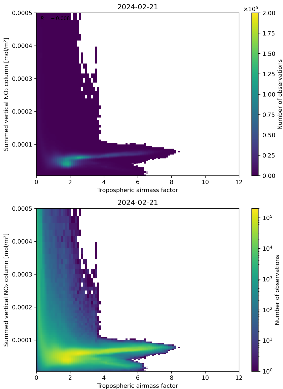
Figure 75: Scatter density plot of “Tropospheric airmass factor” against “Summed vertical NO 2 column” for 2024-02-20 to 2024-02-22.
