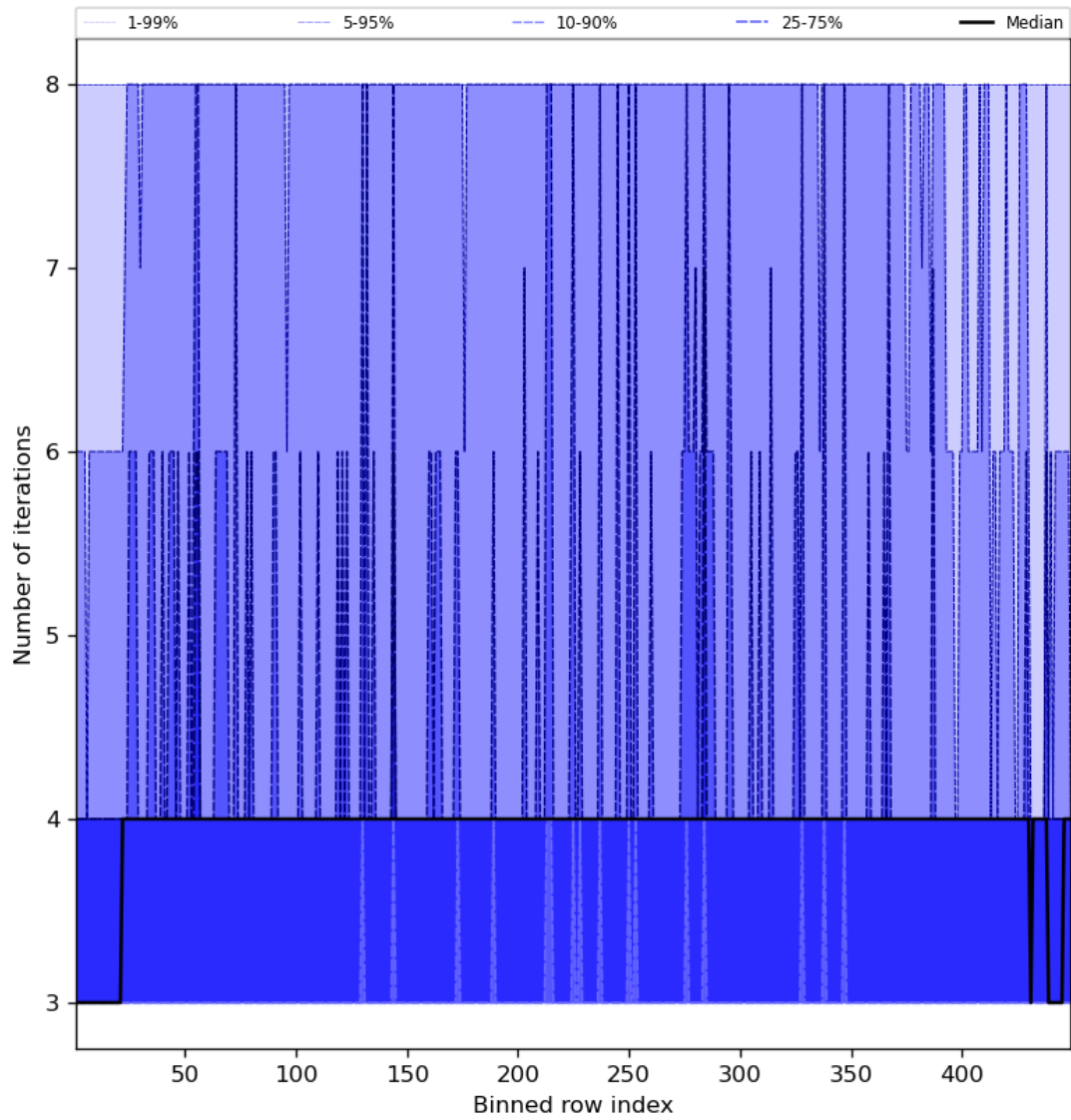
Figure 51: Along track statistics of “Number of iterations” for 2024-02-20 to 2024-02-22
