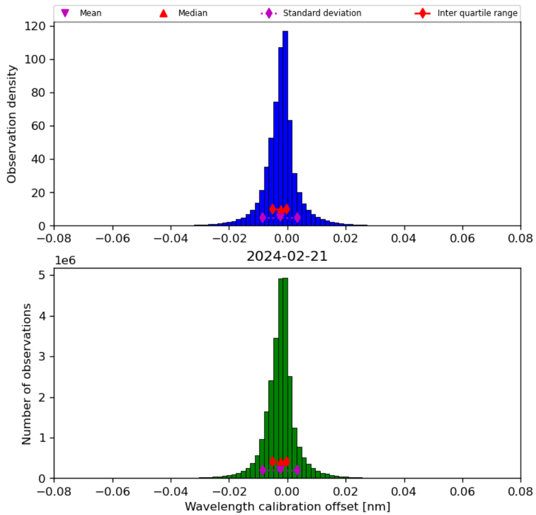
Figure 35: Histogram of “Wavelength calibration offset” for 2024-02-20 to 2024-02-22
