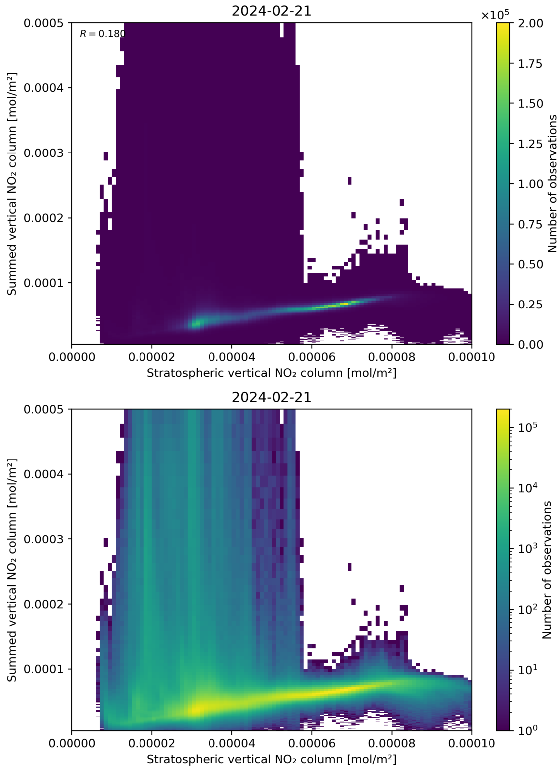
Figure 98: Scatter density plot of “Stratospheric vertical NO 2 column” against “Summed vertical NO 2 column” for 2024-02-20 to 2024-02-22.
