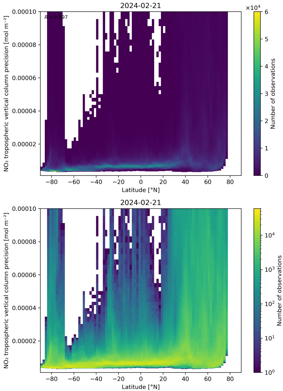
Figure 93: Scatter density plot of “Latitude” against “NO 2 tropospheric vertical column precision” for 2024-02-20 to 2024-02-22.
