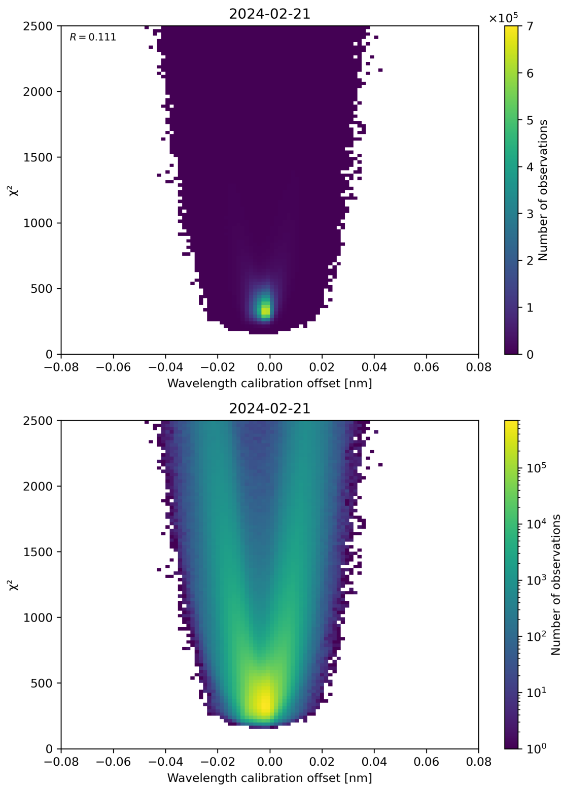
Figure 175: Scatter density plot of “Wavelength calibration offset” against “ \chi^2 ” for 2024-02-20 to 2024-02-22.
