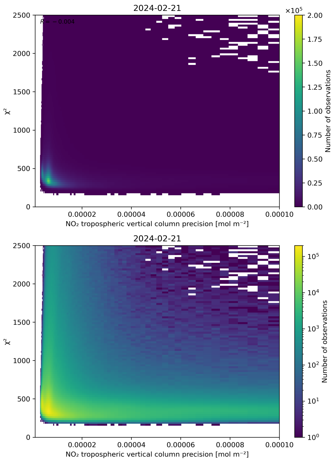
Figure 134: Scatter density plot of “NO 2 tropospheric vertical column precision” against “ \chi^2 ” for 2024-02-20 to 2024-02-22.
