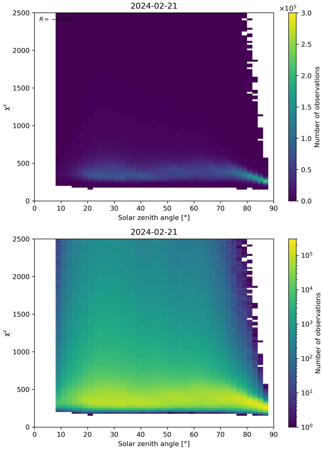
Figure 148: Scatter density plot of “Solar zenith angle” against “ \chi^2 ” for 2024-02-20 to 2024-02-22.
