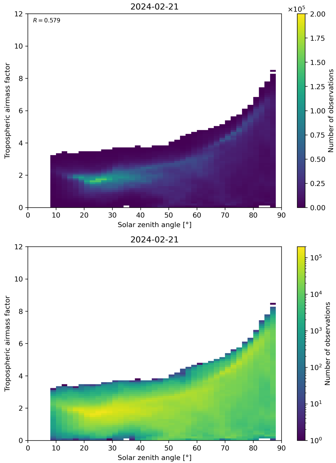
Figure 147: Scatter density plot of “Solar zenith angle” against “Tropospheric airmass factor” for 2024-02-20 to 2024-02-22.
