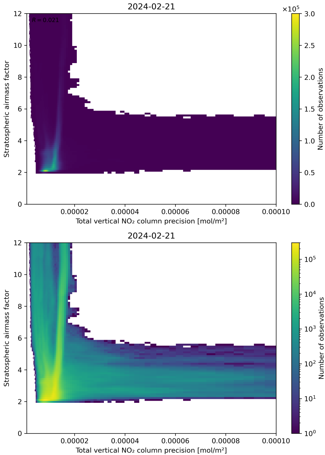
Figure 115: Scatter density plot of “Total vertical NO 2 column precision” against “Stratospheric airmass factor” for 2024-02-20 to 2024-02-22.
