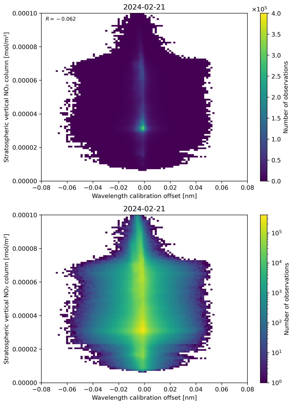
Figure 176: Scatter density plot of “Wavelength calibration offset” against “Stratospheric vertical NO 2 column” for 2024-02-20 to 2024-02-22.
