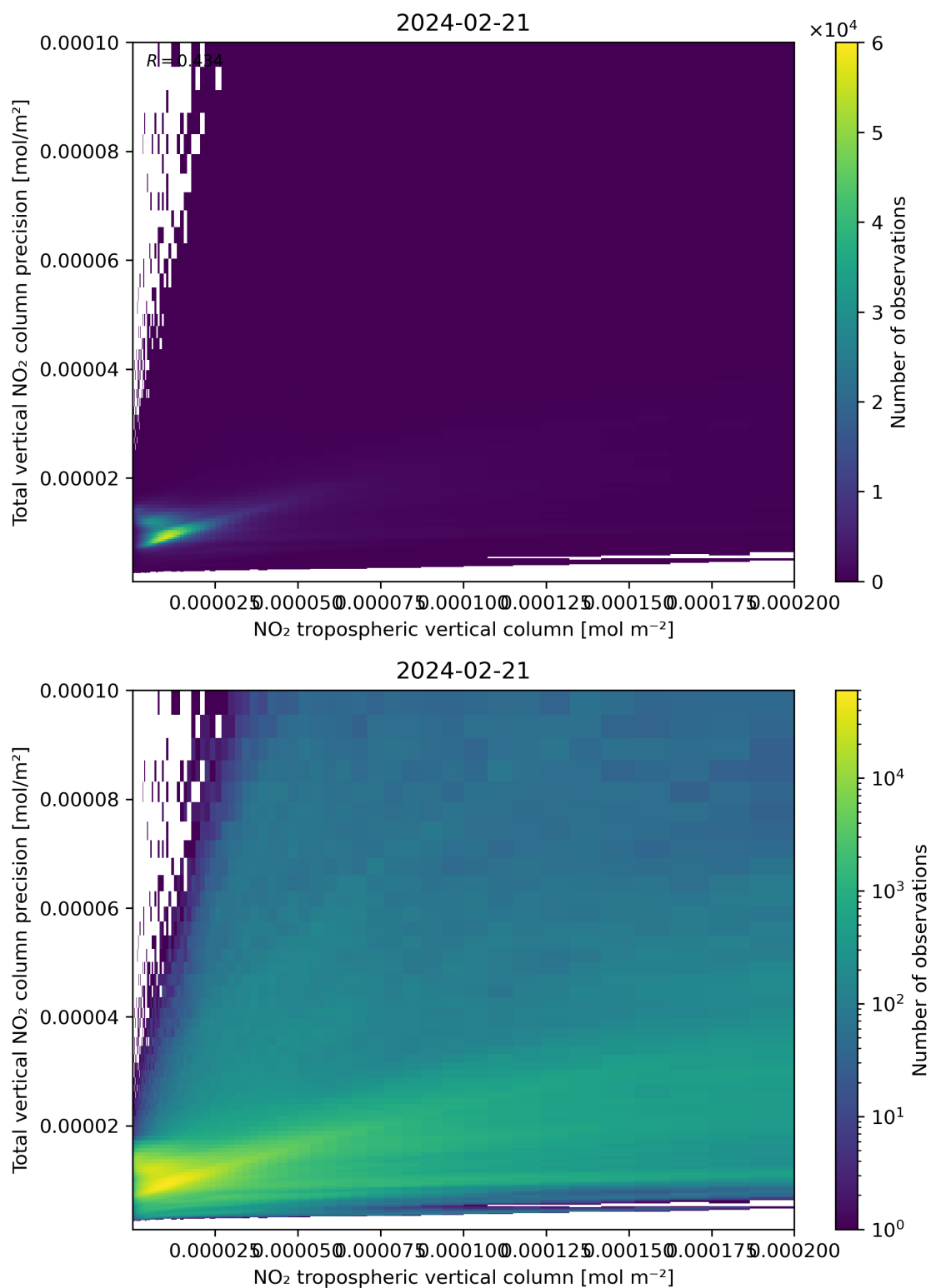
Figure 129: Scatter density plot of “NO 2 tropospheric vertical column” against “Total vertical NO 2 column precision” for 2024-02-20 to 2024-02-22.
