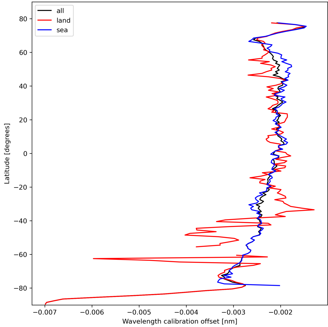
Figure 18: Zonal average of “Wavelength calibration offset” for 2024-02-20 to 2024-02-22.
