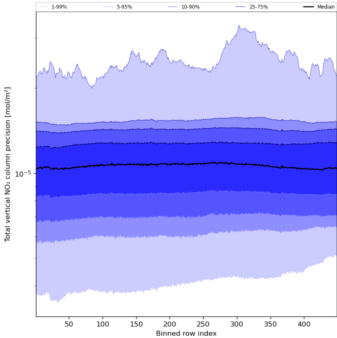
Figure 56: Along track statistics of “Total vertical NO 2 column precision” for 2024-02-20 to 2024-02-22
