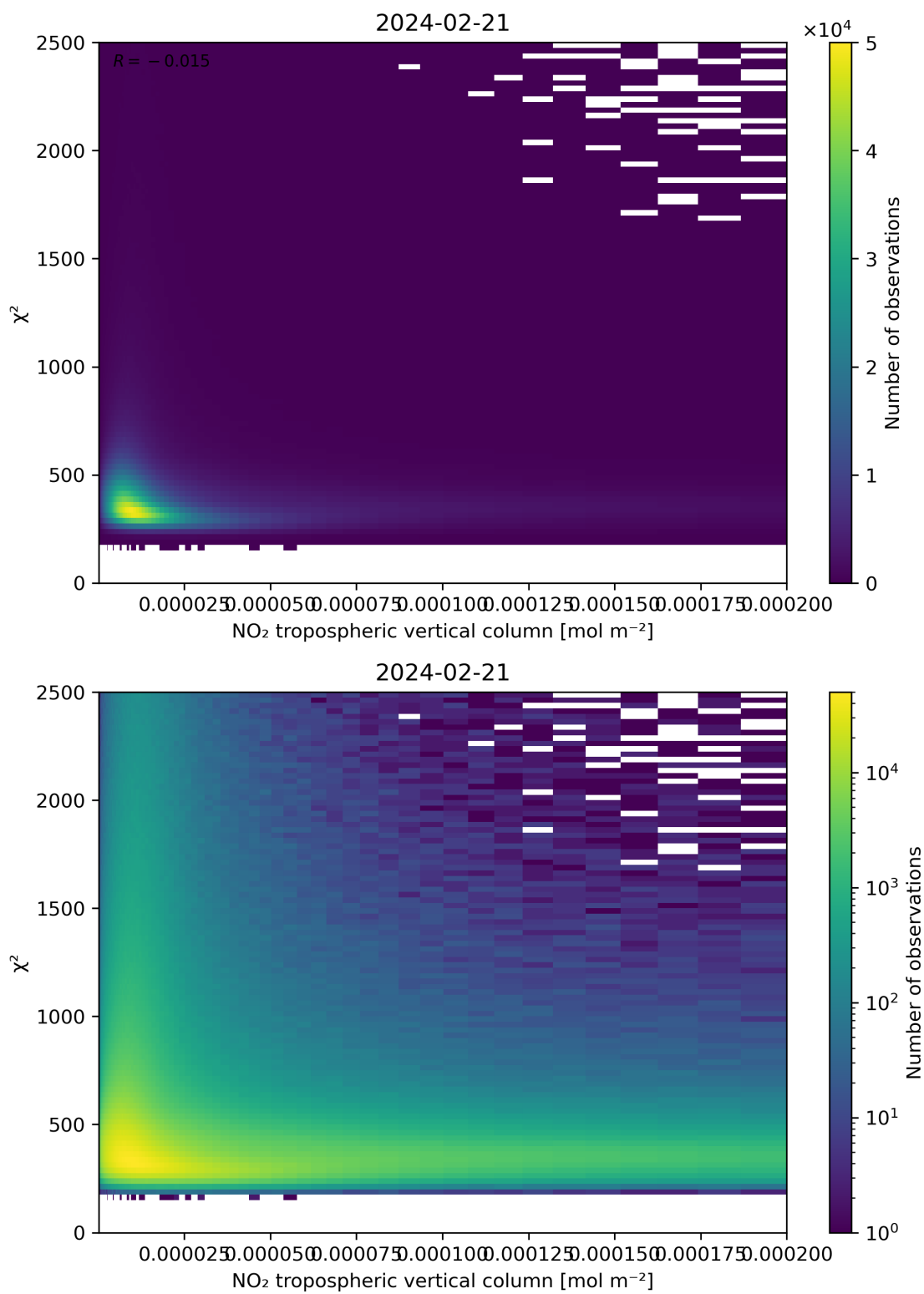
Figure 124: Scatter density plot of “NO 2 tropospheric vertical column” against “ \chi^2 ” for 2024-02-20 to 2024-02-22.
