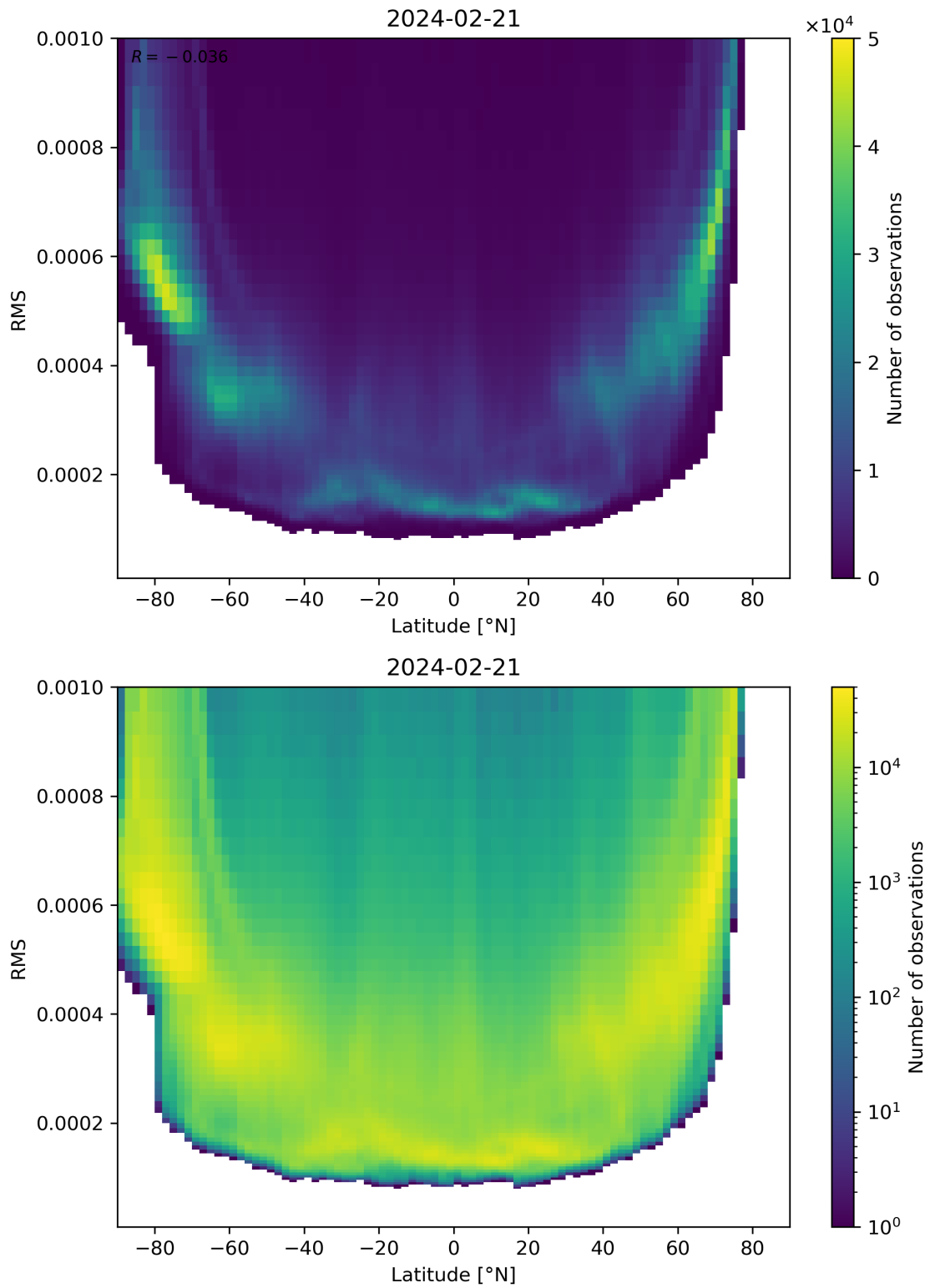
Figure 94: Scatter density plot of “Latitude” against “RMS” for 2024-02-20 to 2024-02-22.
