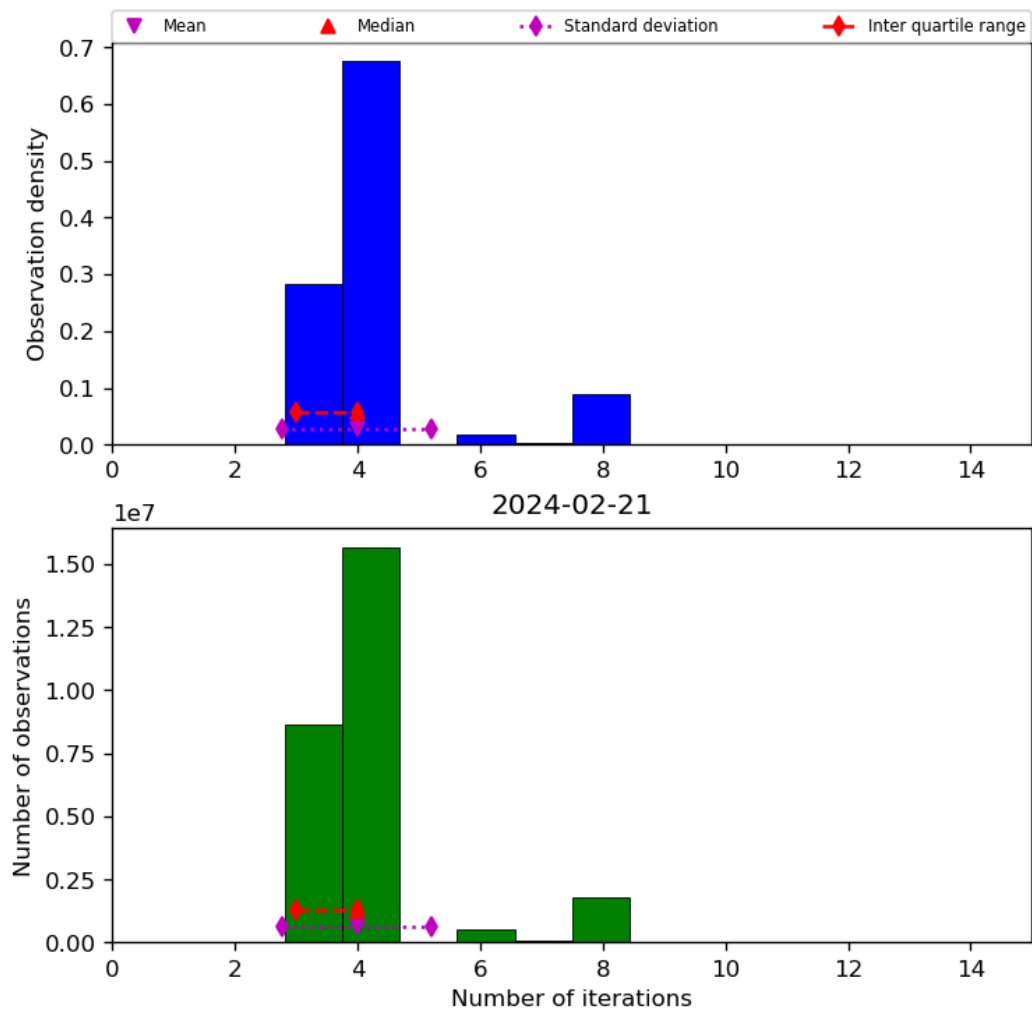
Figure 34: Histogram of “Number of iterations” for 2024-02-20 to 2024-02-22
