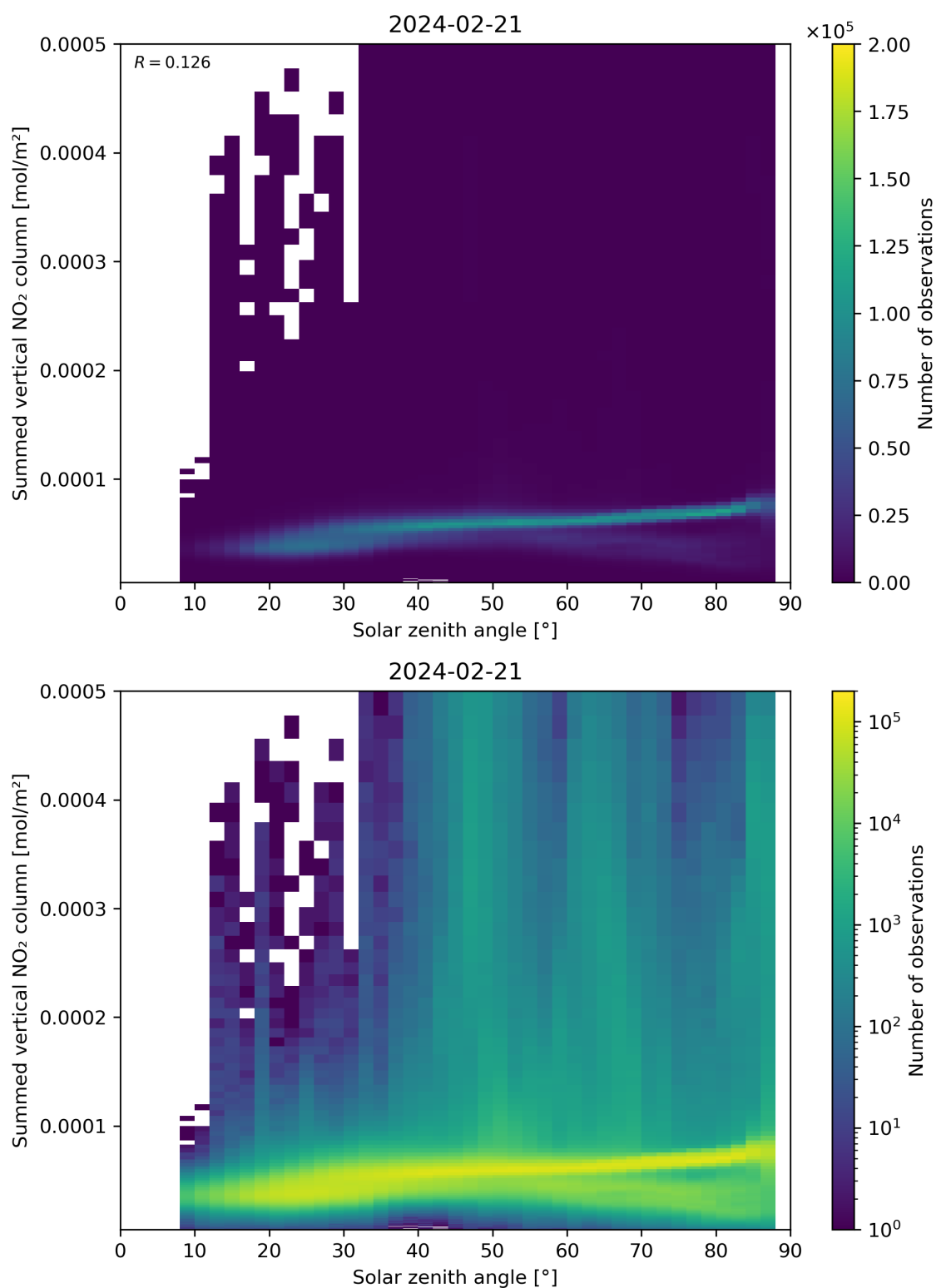
Figure 151: Scatter density plot of “Solar zenith angle” against “Summed vertical NO 2 column” for 2024-02-20 to 2024-02-22.
