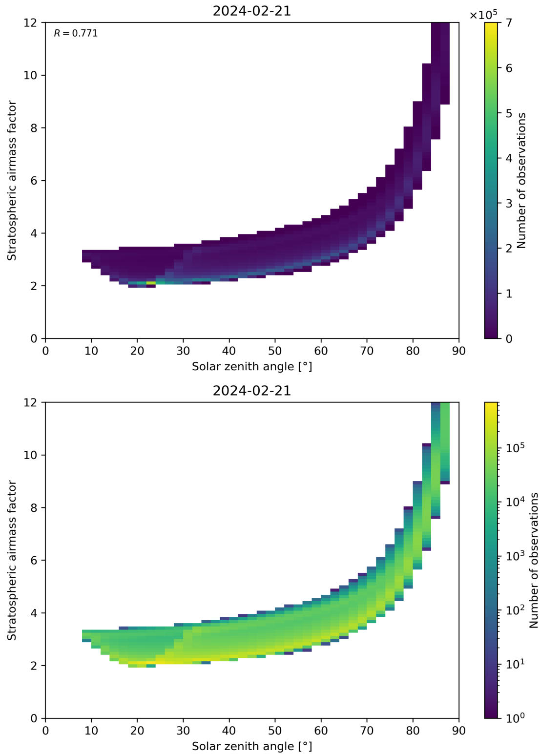
Figure 145: Scatter density plot of “Solar zenith angle” against “Stratospheric airmass factor” for 2024-02-20 to 2024-02-22.
