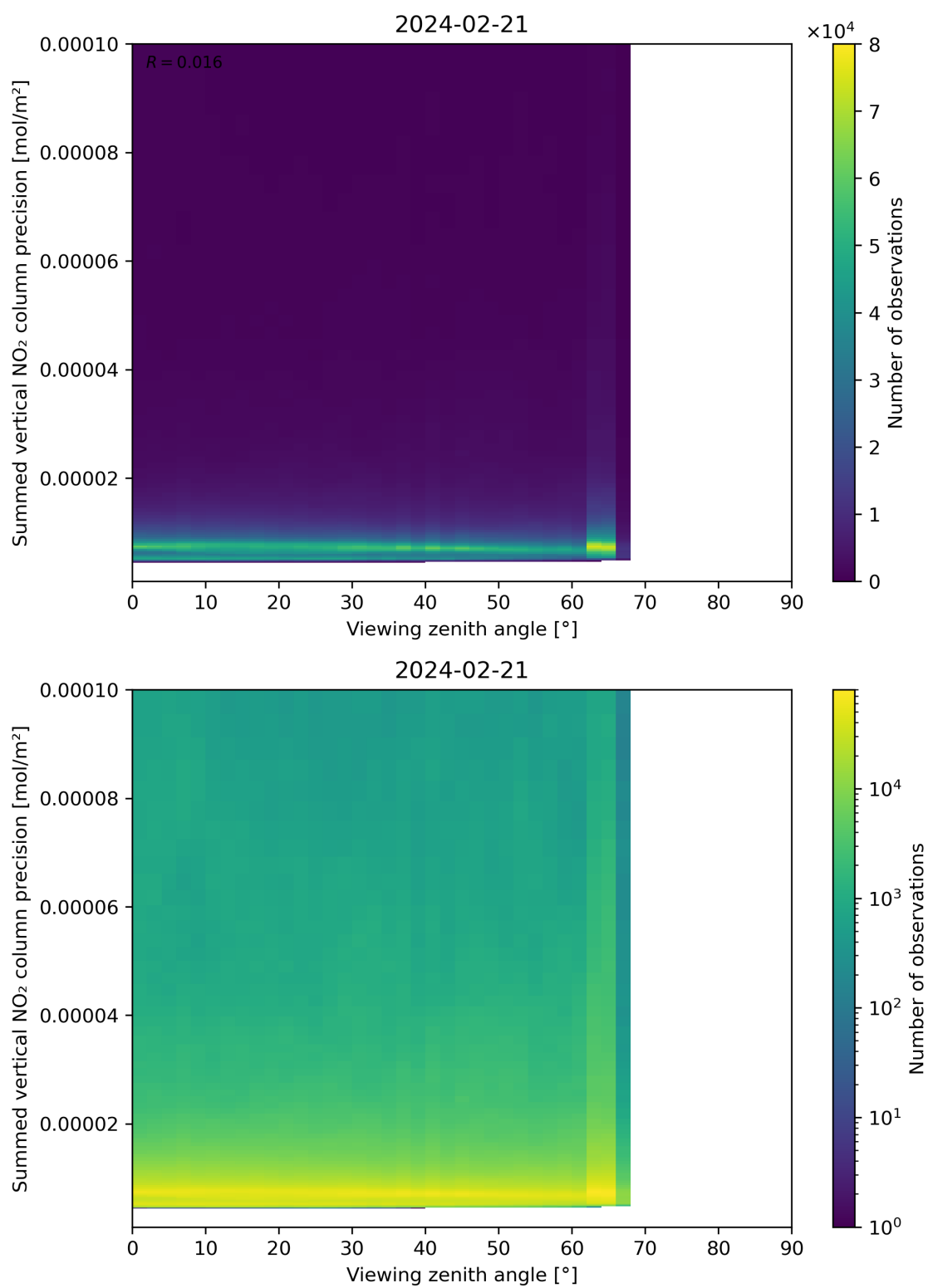
Figure 166: Scatter density plot of “Viewing zenith angle” against “Summed vertical NO 2 column precision” for 2024-02-20 to 2024-02-22.
