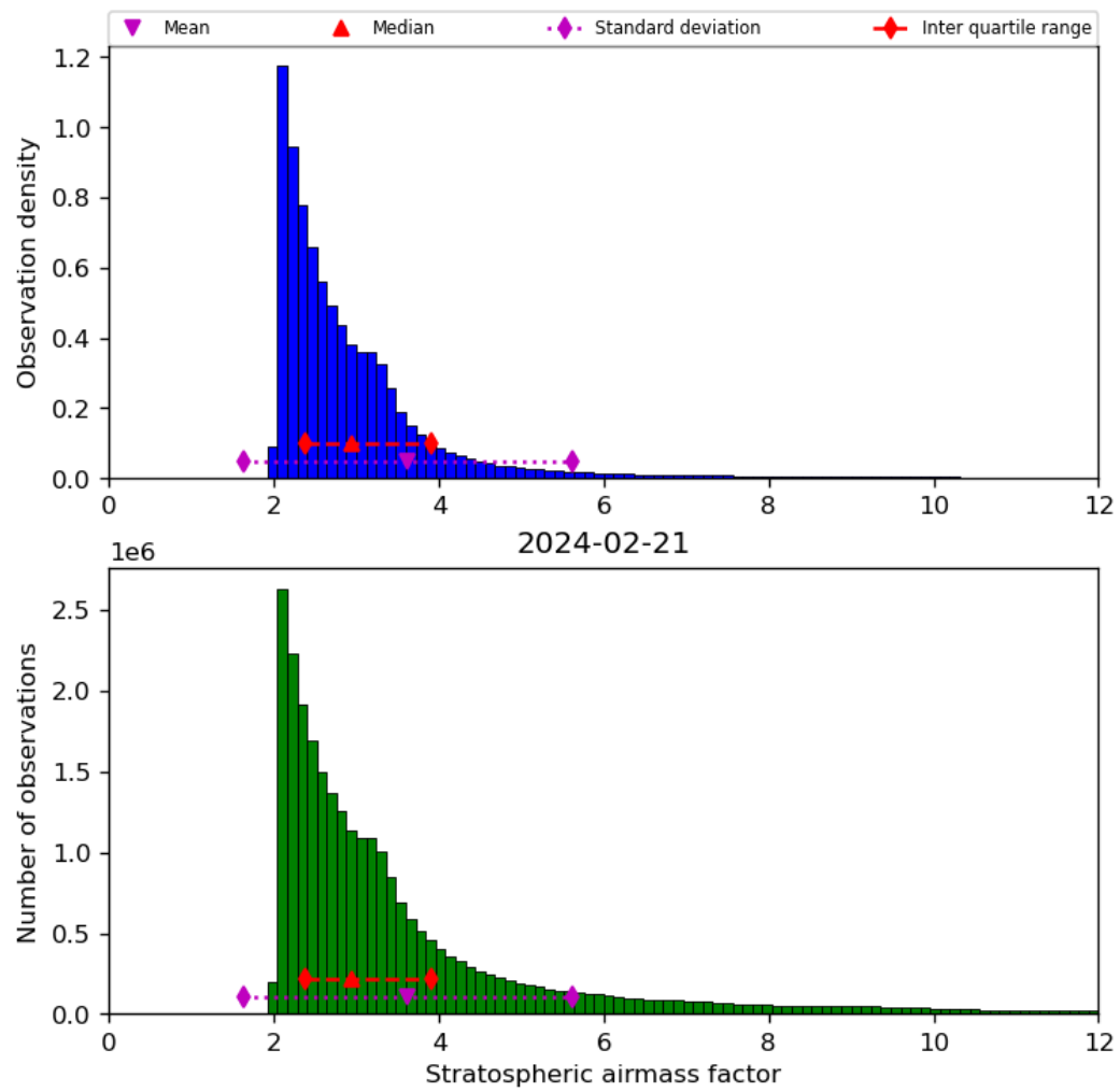
Figure 44: Histogram of “Stratospheric airmass factor” for 2024-02-20 to 2024-02-22
