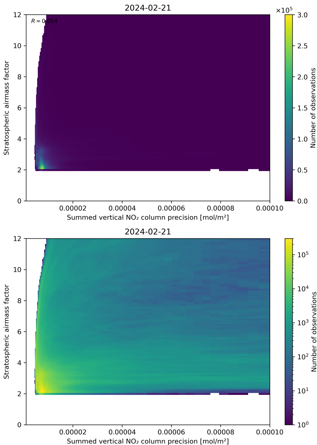
Figure 106: Scatter density plot of “Summed vertical NO 2 column precision” against “Stratospheric airmass factor” for 2024-02-20 to 2024-02-22.
