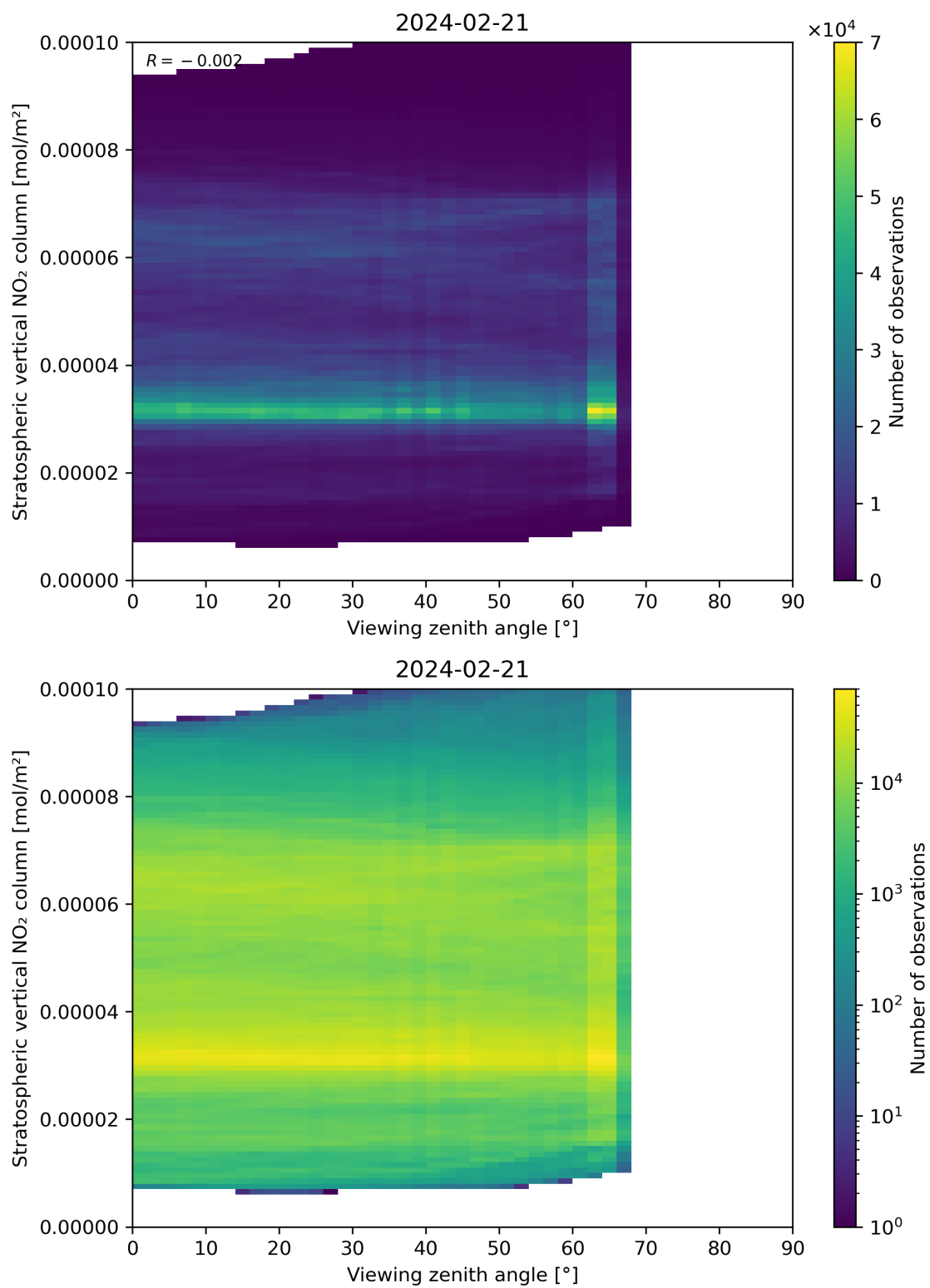
Figure 164: Scatter density plot of “Viewing zenith angle” against “Stratospheric vertical NO 2 column” for 2024-02-20 to 2024-02-22.
