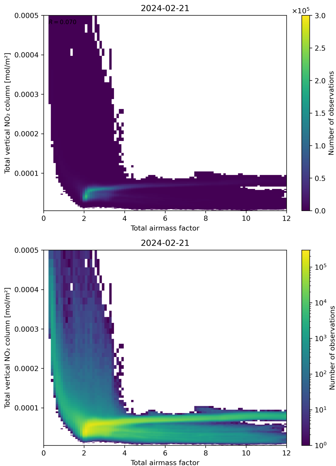
Figure 67: Scatter density plot of “Total airmass factor” against “Total vertical NO 2 column” for 2024-02-20 to 2024-02-22.
