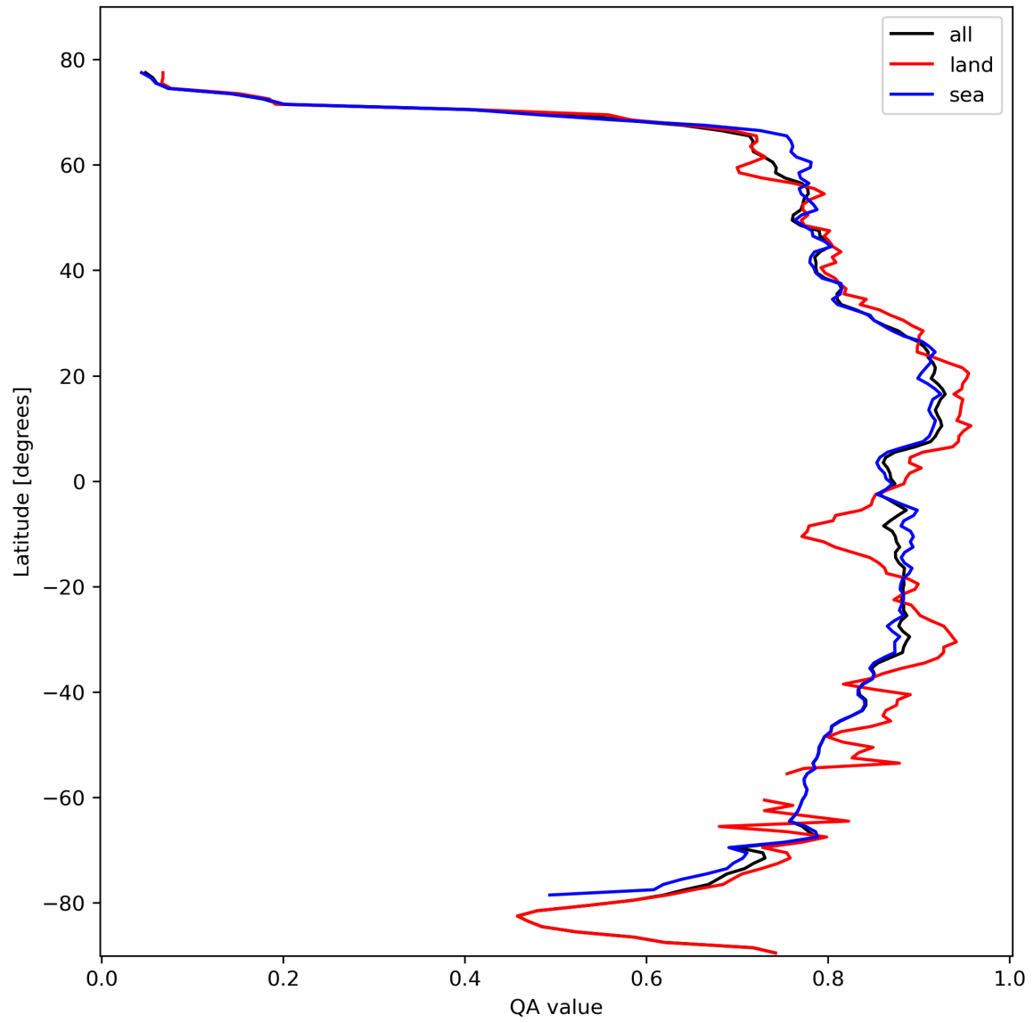
Figure 11: Zonal average of “QA value” for 2024-02-22 to 2024-02-23.
