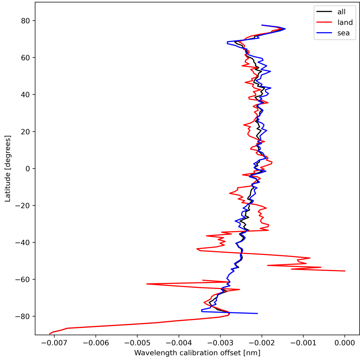
Figure 18: Zonal average of “Wavelength calibration offset” for 2024-02-22 to 2024-02-23.
