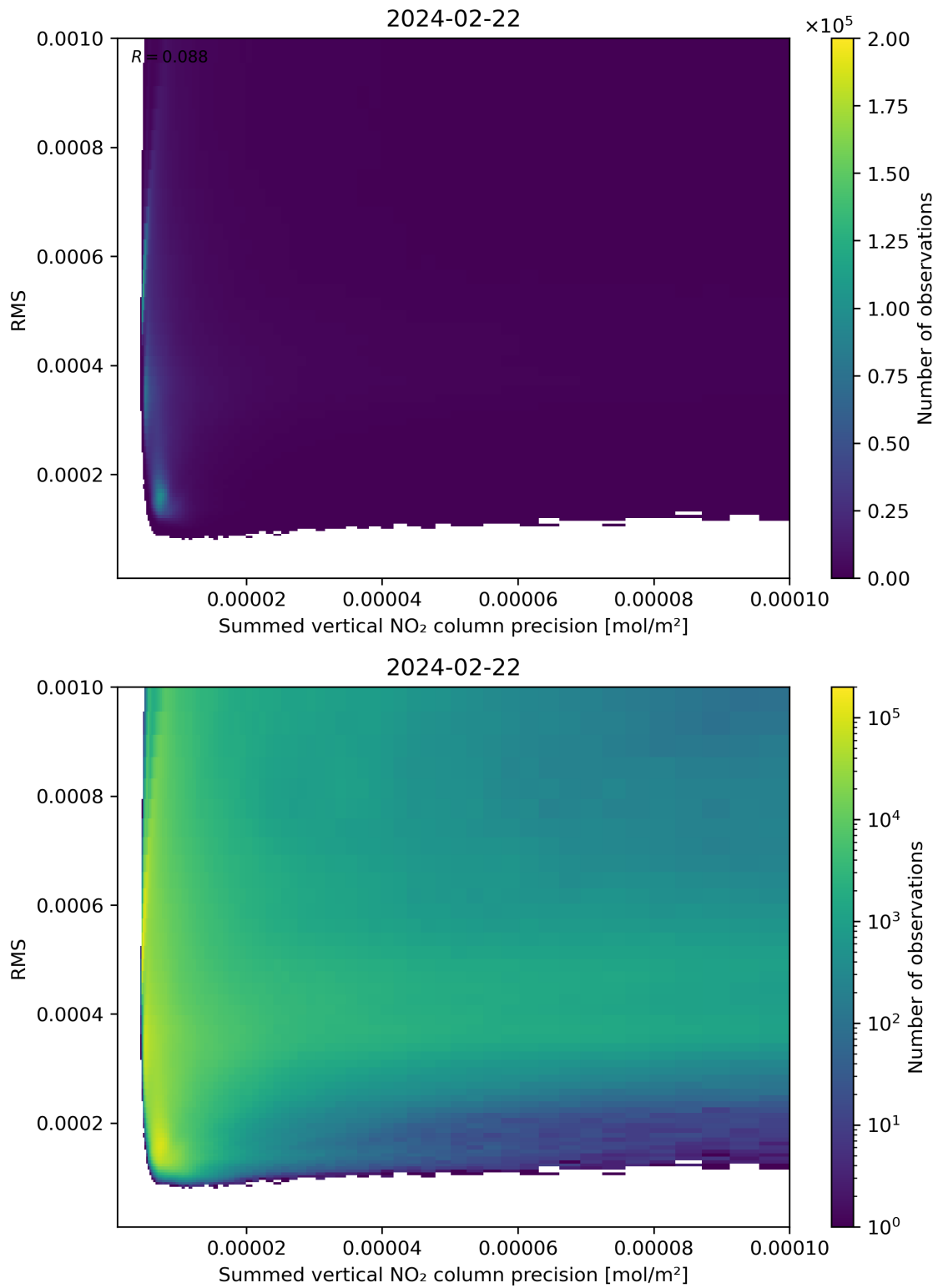
Figure 108: Scatter density plot of “Summed vertical NO 2 column precision” against “RMS” for 2024-02-22 to 2024-02-23.
