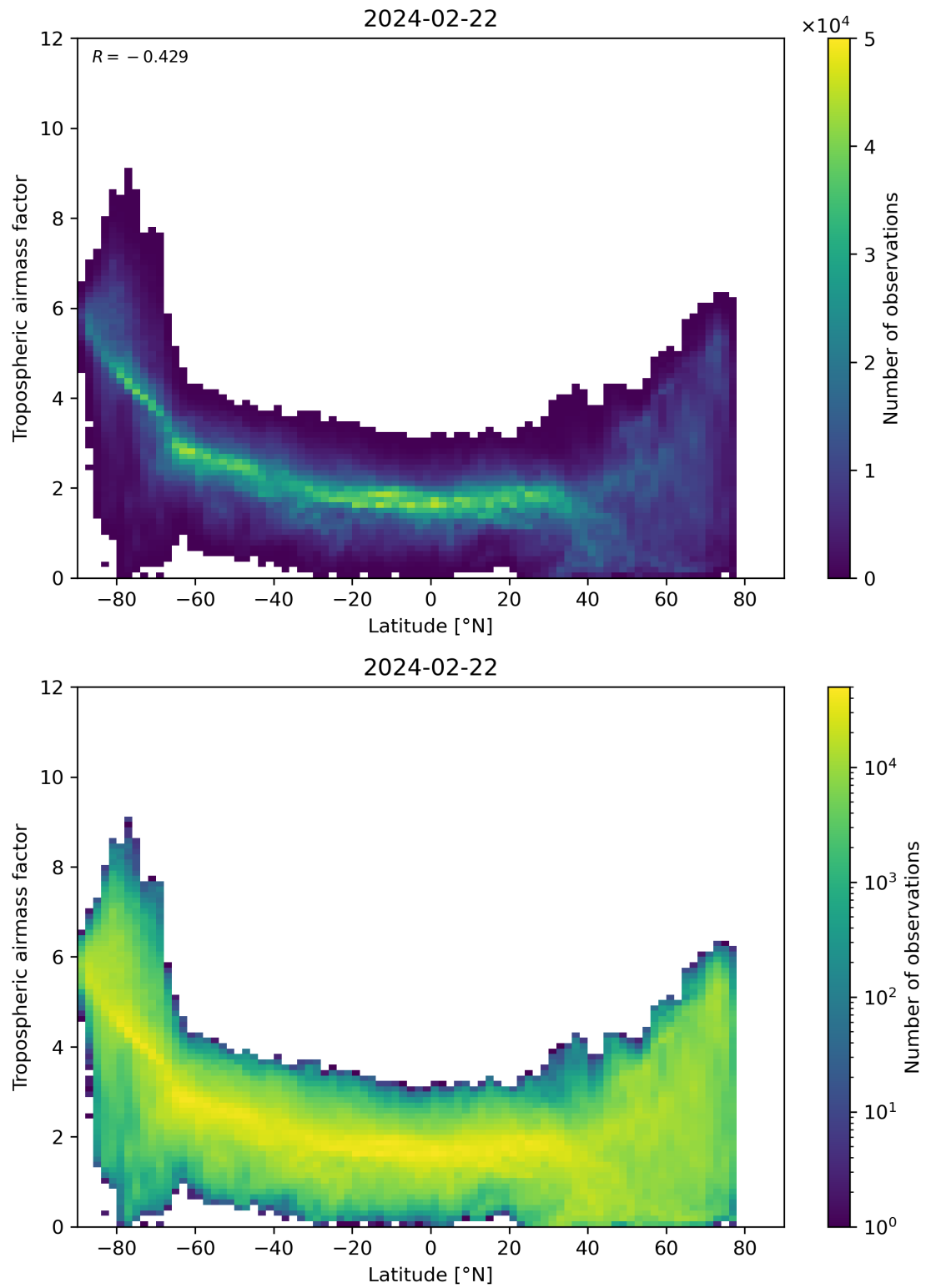
Figure 85: Scatter density plot of “Latitude” against “Tropospheric airmass factor” for 2024-02-22 to 2024-02-23.
