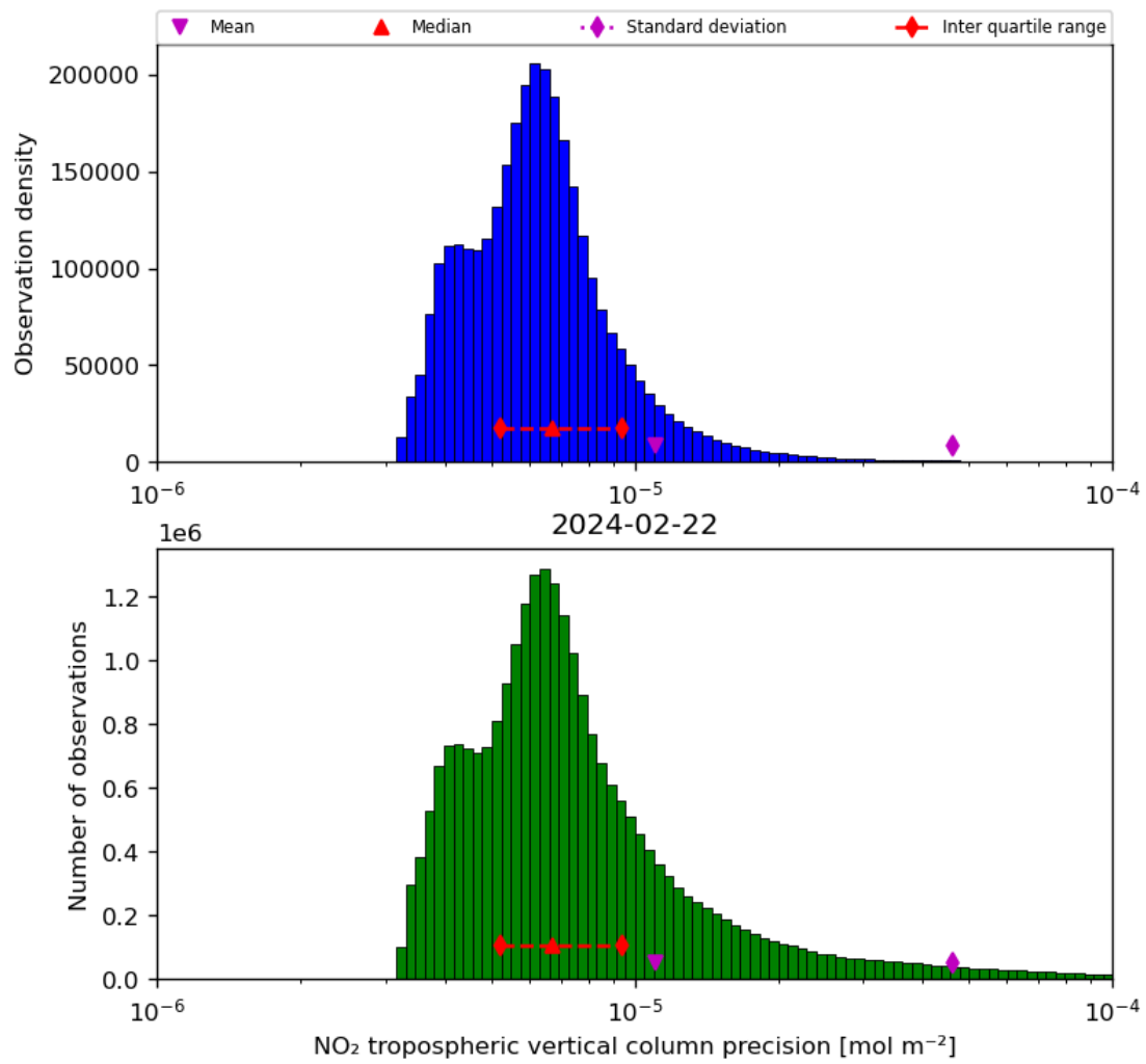
Figure 30: Histogram of "NO 2 tropospheric vertical column precision" for 2024-02-22 to 2024-02-23
