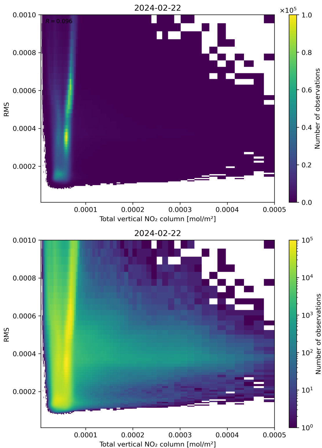
Figure 120: Scatter density plot of “Total vertical NO 2 column” against “RMS” for 2024-02-22 to 2024-02-23.
