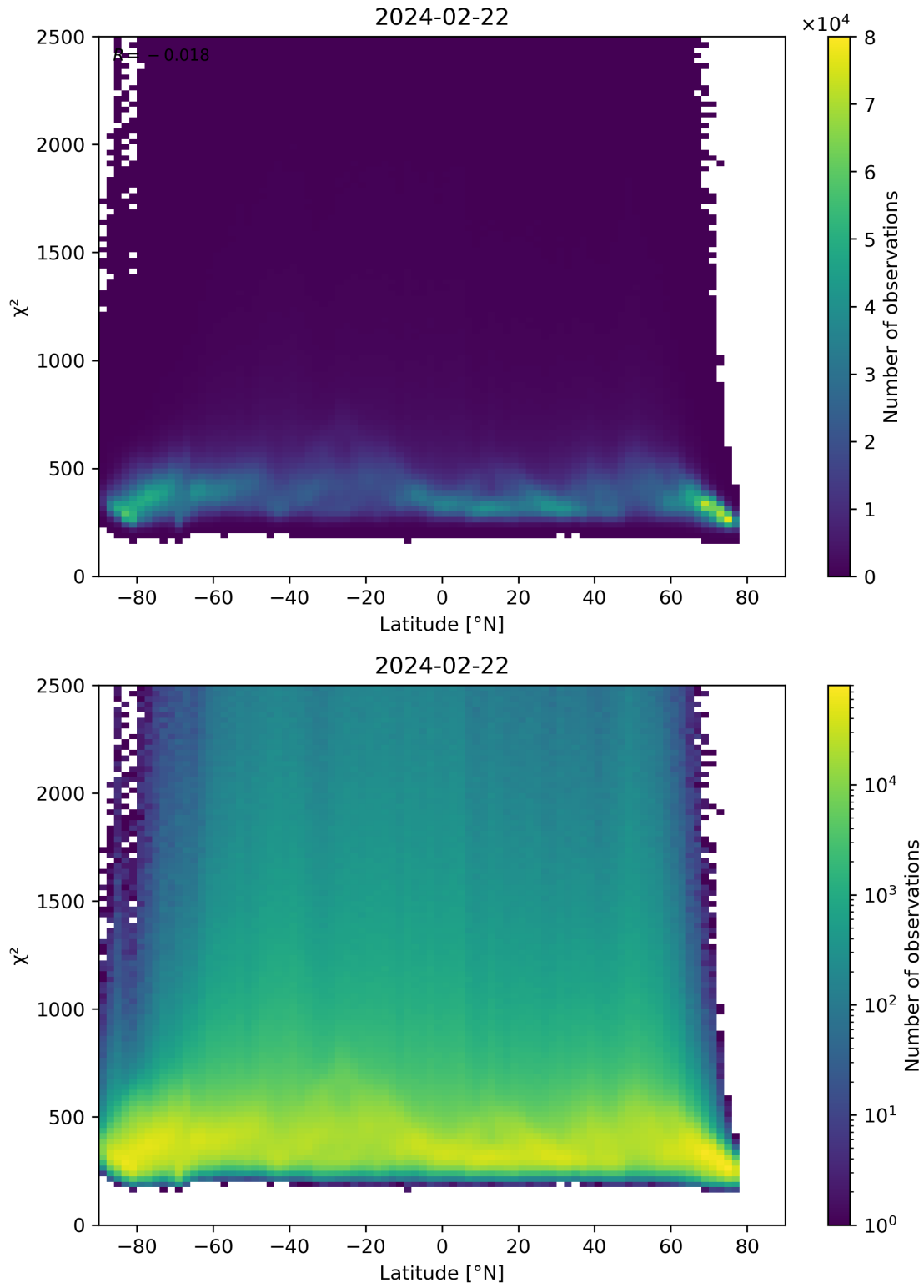
Figure 86: Scatter density plot of “Latitude” against “ \chi^2 ” for 2024-02-22 to 2024-02-23.
