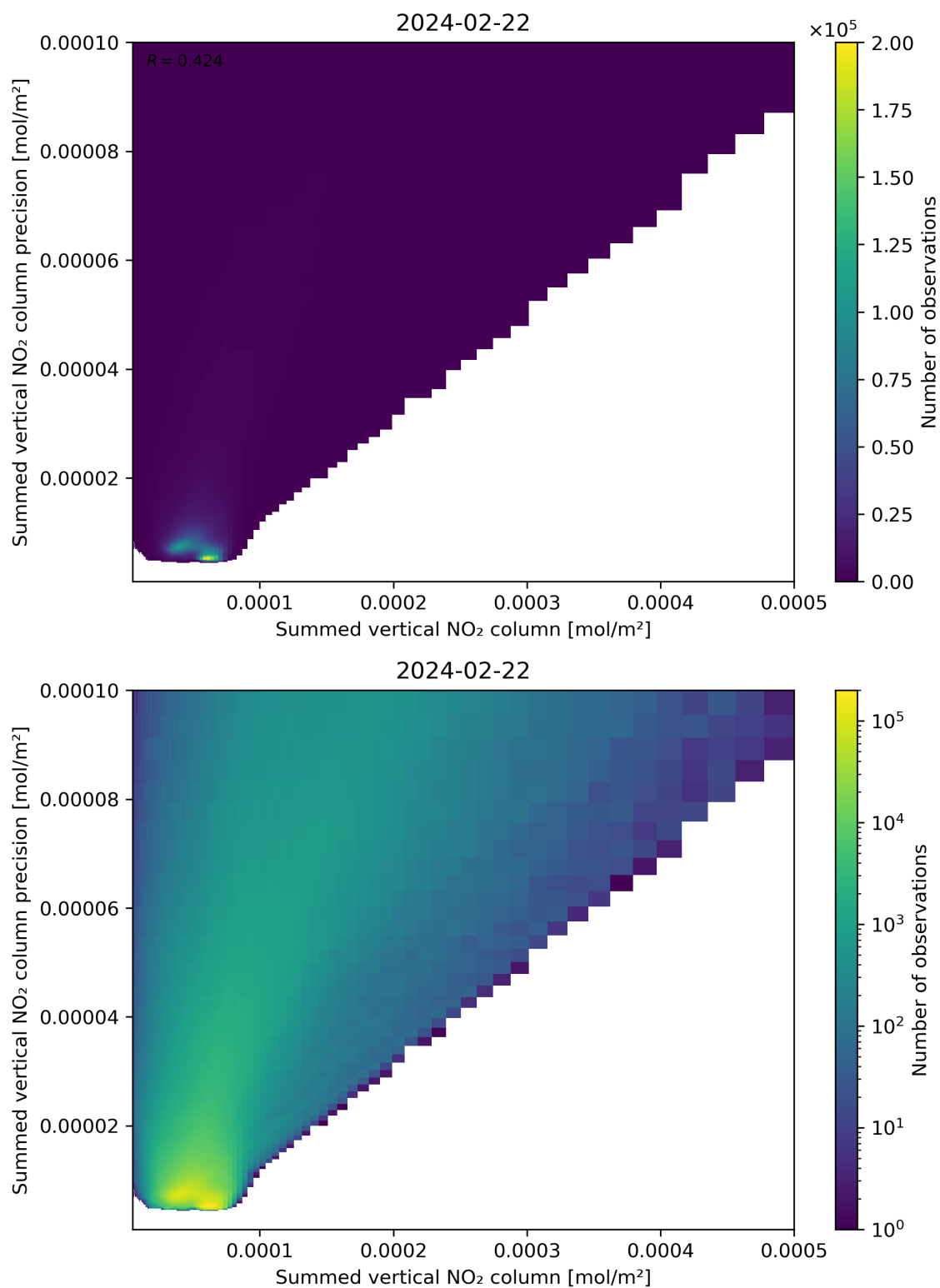
Figure 105: Scatter density plot of “Summed vertical NO 2 column” against “Summed vertical NO 2 column precision” for 2024-02-22 to 2024-02-23.
