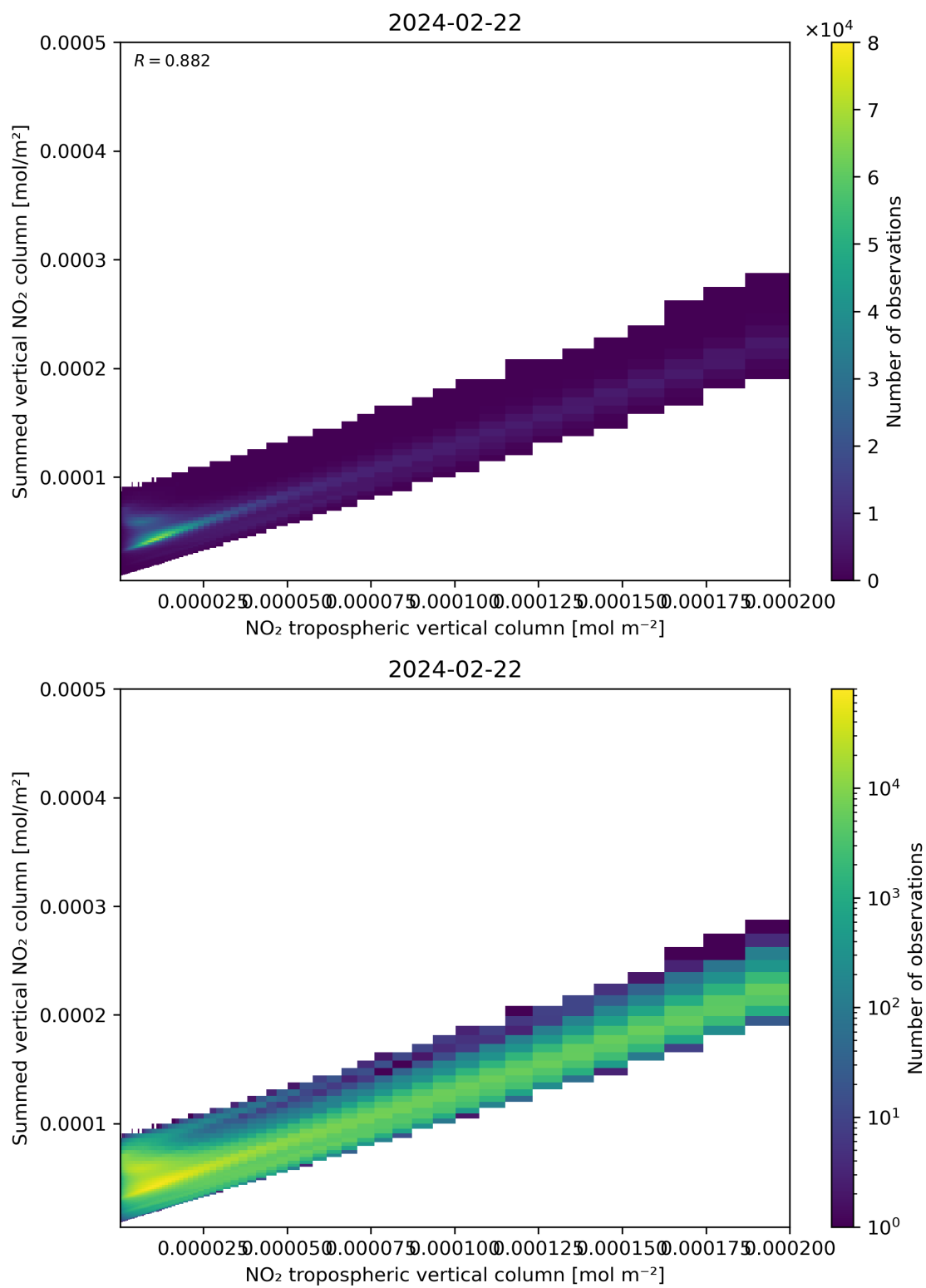
Figure 126: Scatter density plot of “NO 2 tropospheric vertical column” against “Summed vertical NO 2 column” for 2024-02-22 to 2024-02-23.
