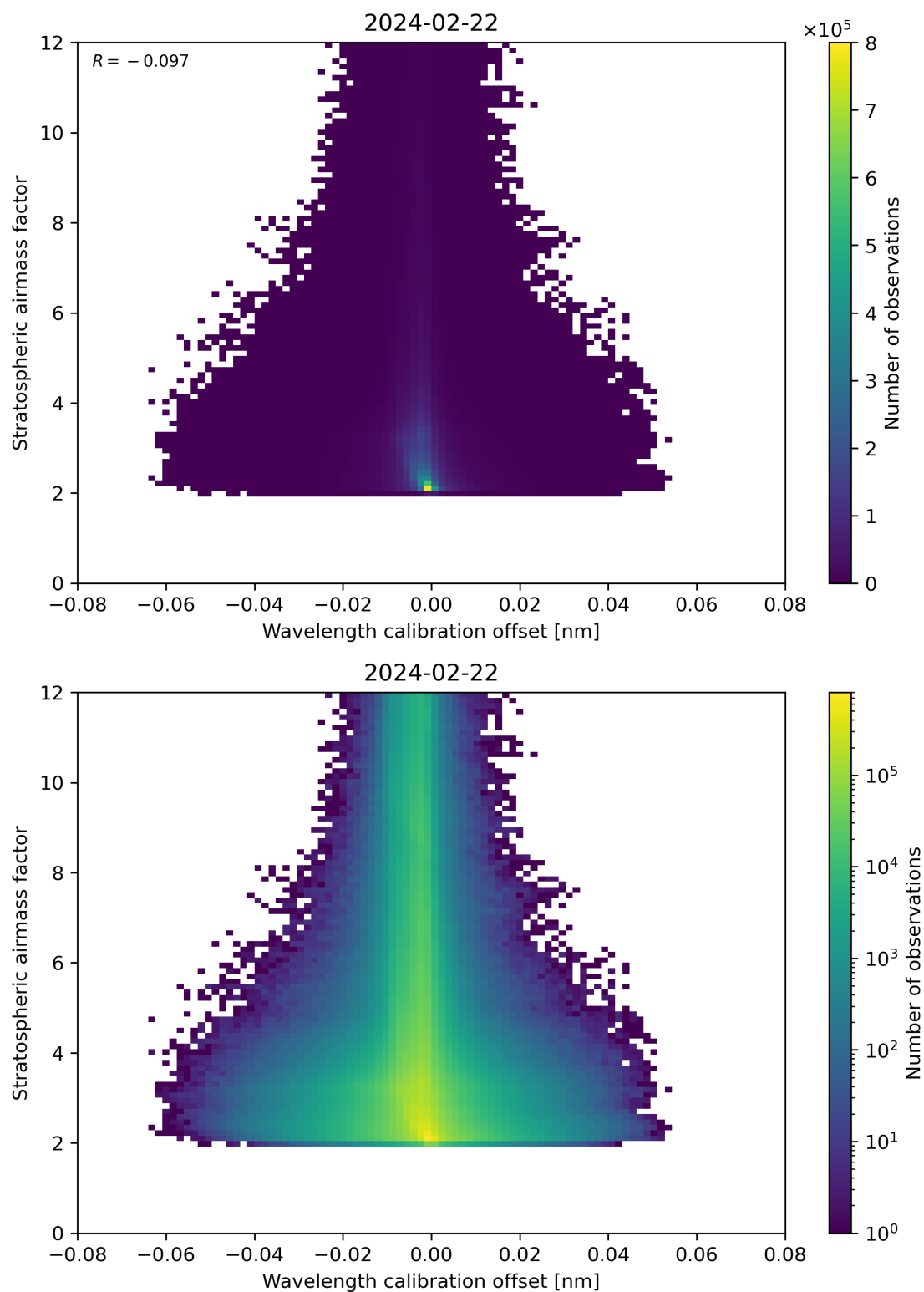
Figure 174: Scatter density plot of “Wavelength calibration offset” against “Stratospheric air mass factor” for 2024-02-22 to 2024-02-23.
