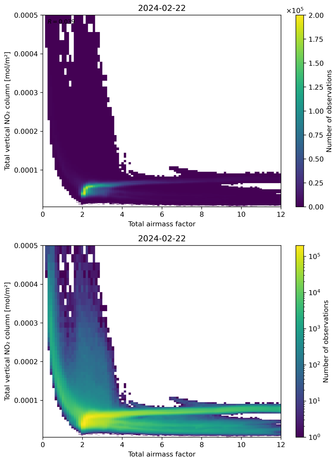
Figure 67: Scatter density plot of “Total airmass factor” against “Total vertical NO 2 column” for 2024-02-22 to 2024-02-23.
