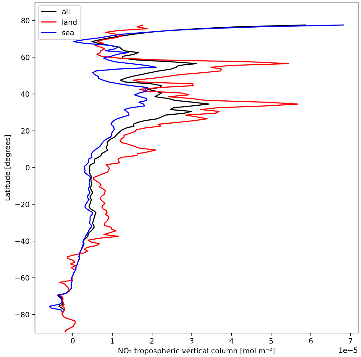
Figure 12: Zonal average of “NO 2 tropospheric vertical column” for 2024-02-22 to 2024-02-23.
