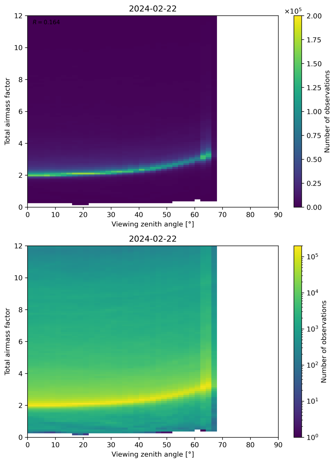
Figure 160: Scatter density plot of “Viewing zenith angle” against “Total airmass factor” for 2024-02-22 to 2024-02-23.
