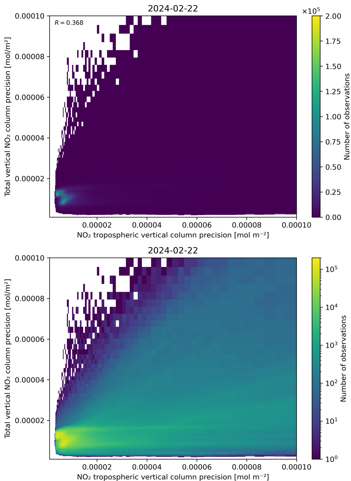
Figure 139: Scatter density plot of “NO 2 tropospheric vertical column precision” against “Total vertical NO 2 column precision” for 2024-02-22 to 2024-02-23.
