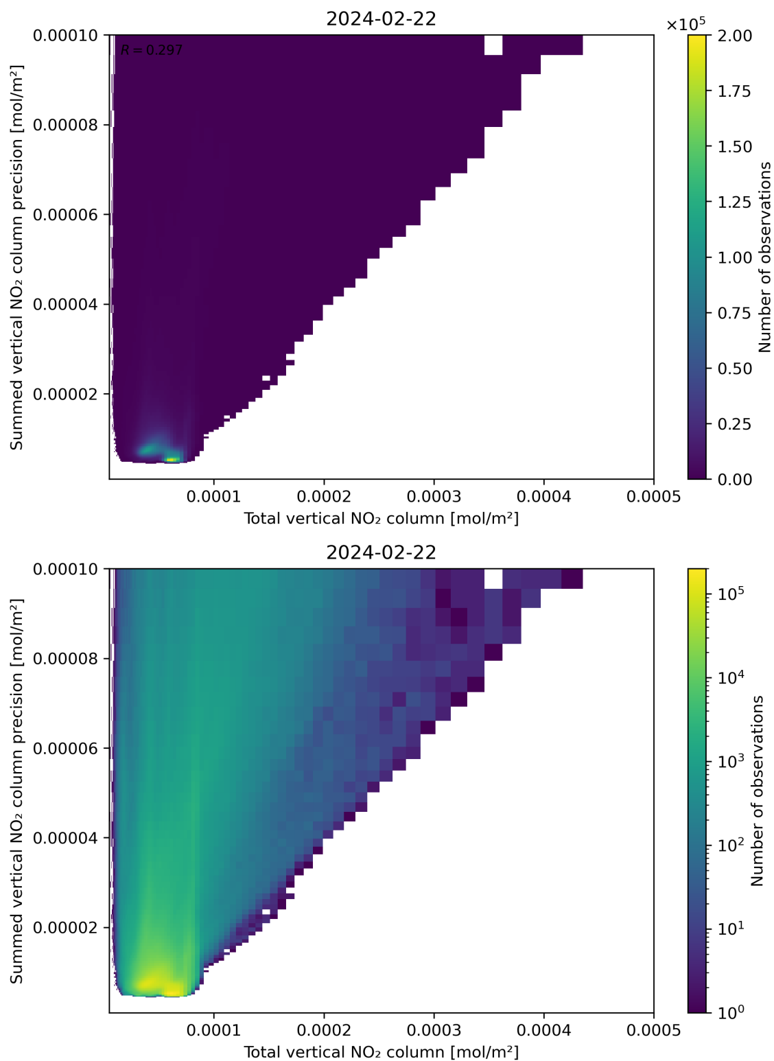
Figure 113: Scatter density plot of “Total vertical NO 2 column” against “Summed vertical NO 2 column precision” for 2024-02-22 to 2024-02-23.
