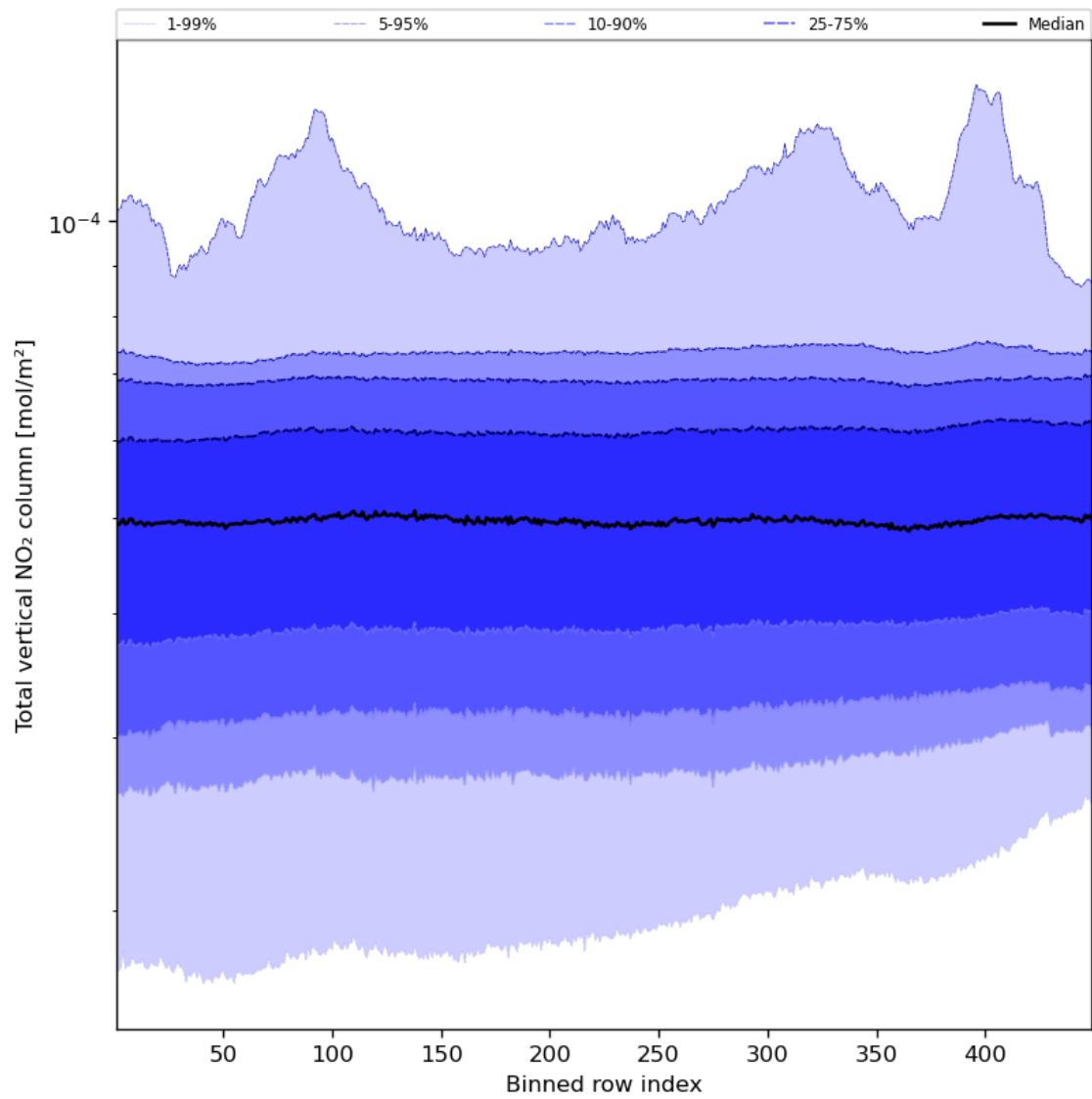
Figure 55: Along track statistics of “Total vertical NO 2 column” for 2024-02-22 to 2024-02-23
