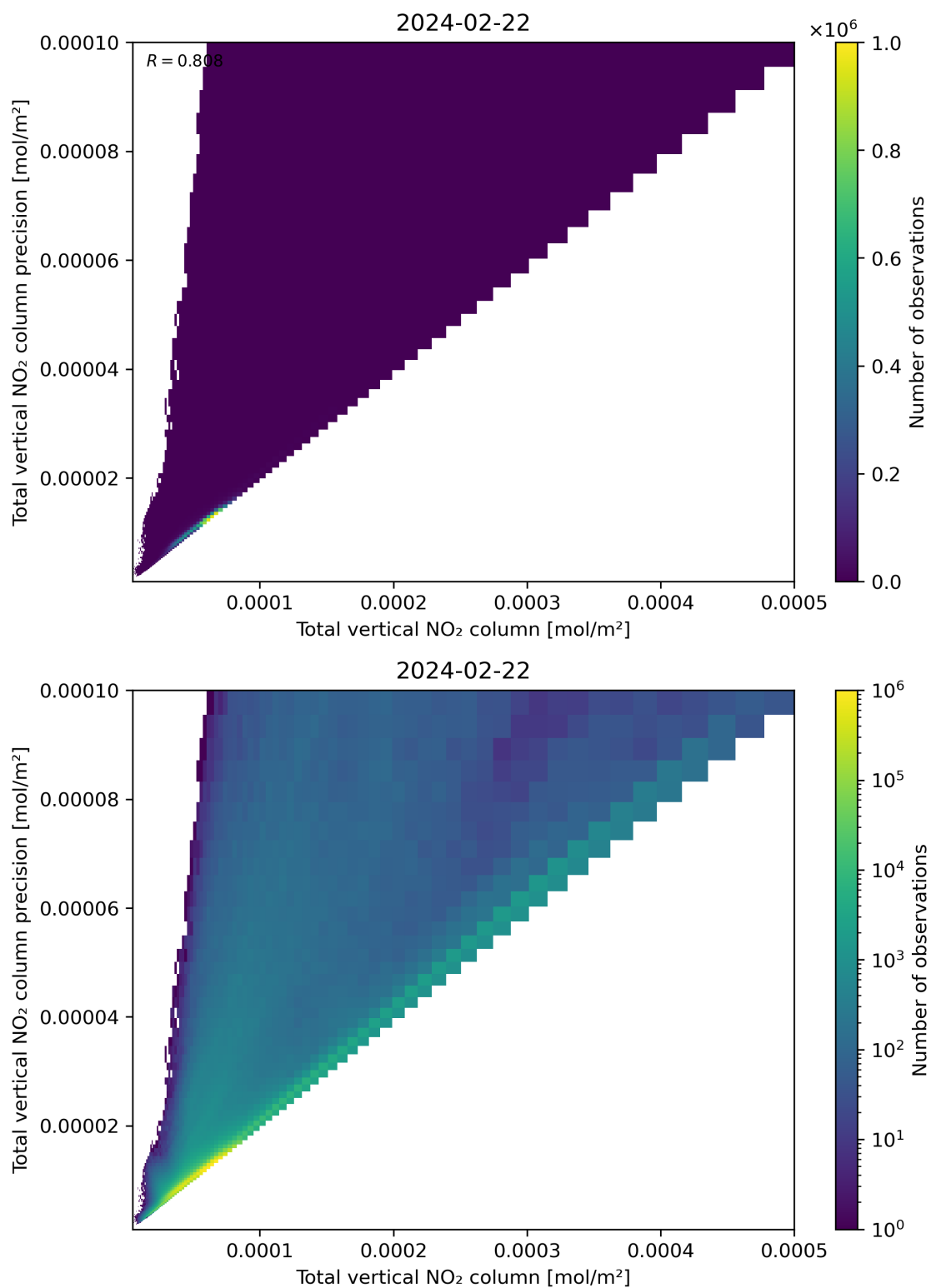
Figure 114: Scatter density plot of “Total vertical NO 2 column” against “Total vertical NO 2 column precision” for 2024-02-22 to 2024-02-23.
