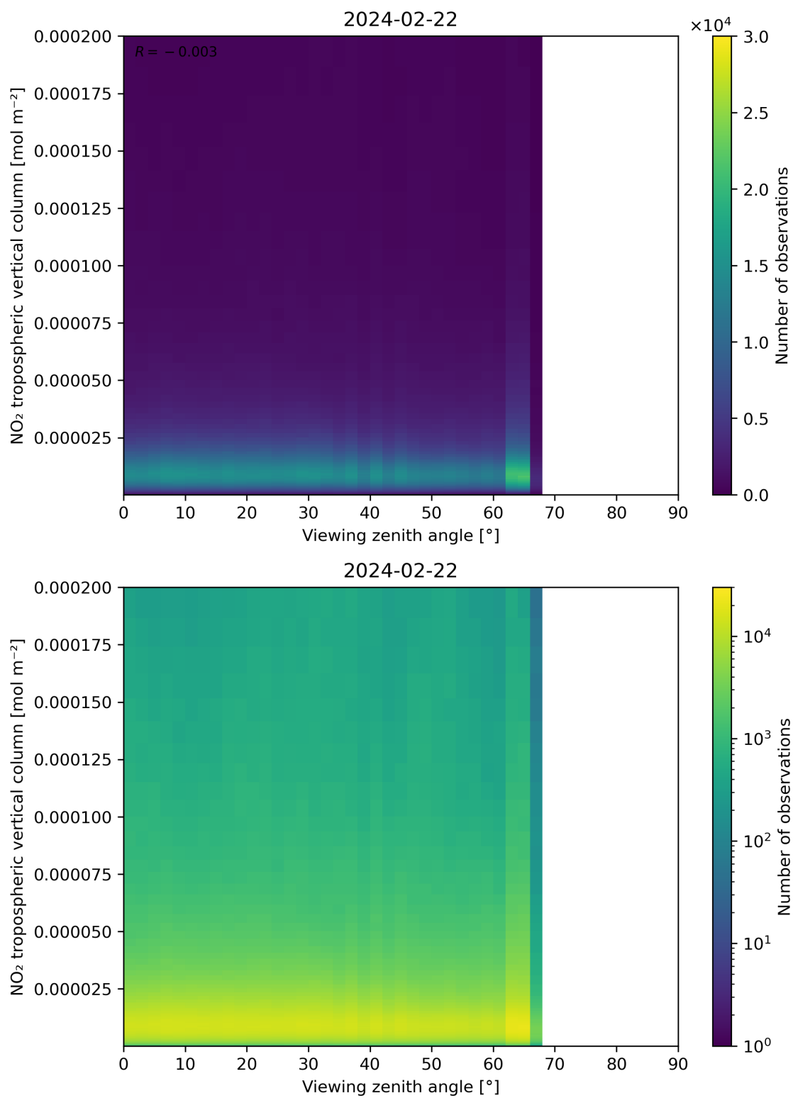
Figure 169: Scatter density plot of “Viewing zenith angle” against “NO 2 tropospheric vertical column” for 2024-02-22 to 2024-02-23.
