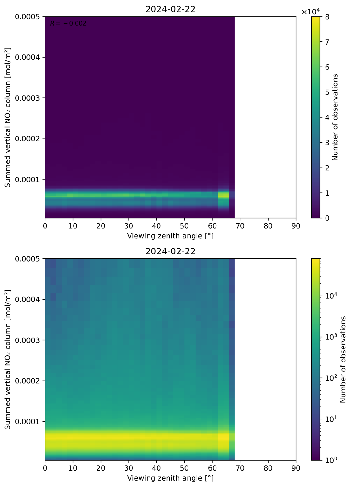
Figure 165: Scatter density plot of “Viewing zenith angle” against “Summed vertical NO 2 column” for 2024-02-22 to 2024-02-23.
