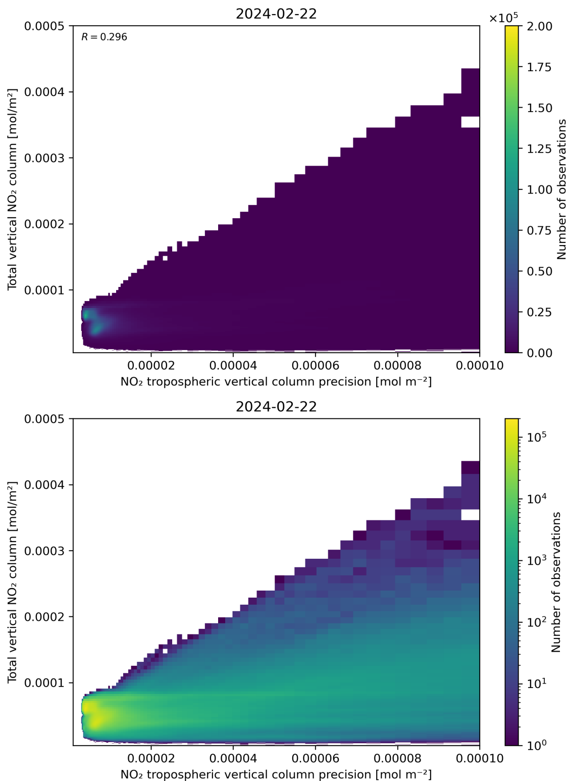
Figure 138: Scatter density plot of “NO 2 tropospheric vertical column precision” against “Total vertical NO 2 column” for 2024-02-22 to 2024-02-23.
