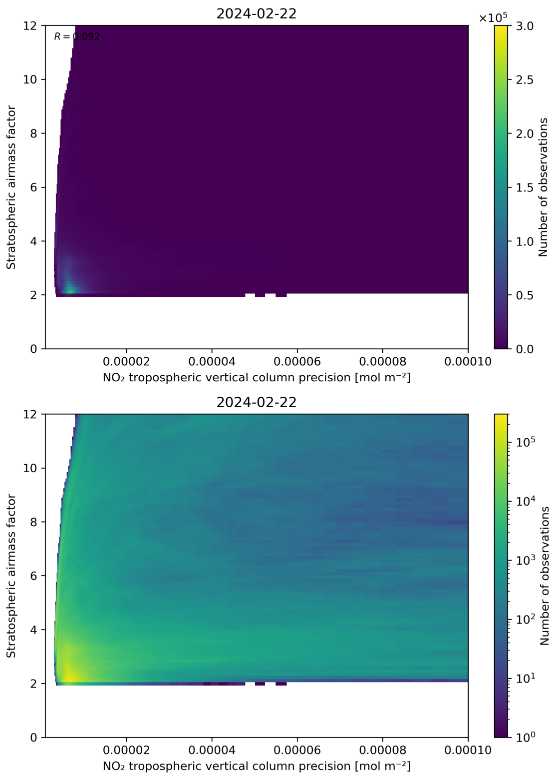
Figure 131: Scatter density plot of “NO 2 tropospheric vertical column precision” against “Stratospheric airmass factor” for 2024-02-22 to 2024-02-23.
