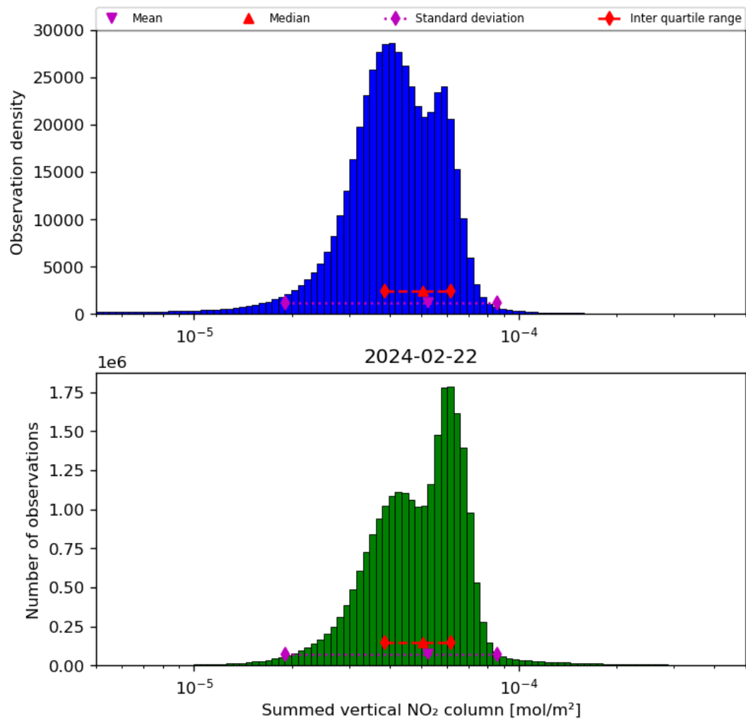
Figure 40: Histogram of “Summed vertical NO 2 column” for 2024-02-22 to 2024-02-23
