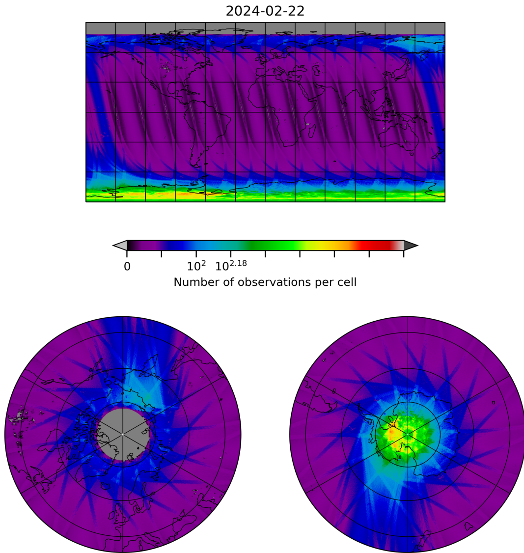
Figure 10: Map of the number of observations for 2024-02-22 to 2024-02-23
