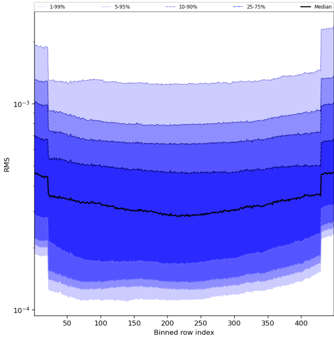
Figure 60: Along track statistics of “RMS” for 2024-02-22 to 2024-02-23
