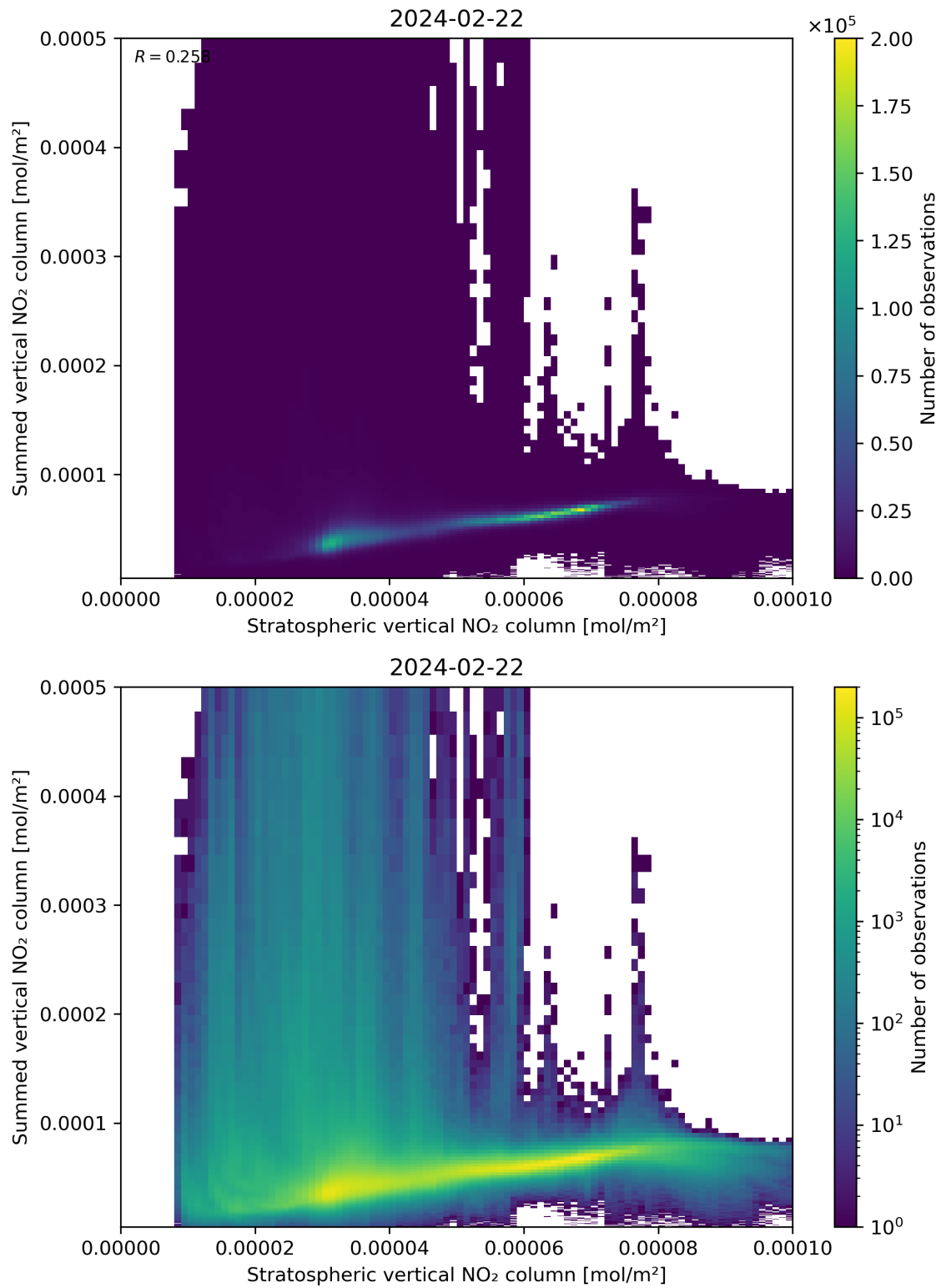
Figure 98: Scatter density plot of “Stratospheric vertical NO 2 column” against “Summed vertical NO 2 column” for 2024-02-22 to 2024-02-23.
