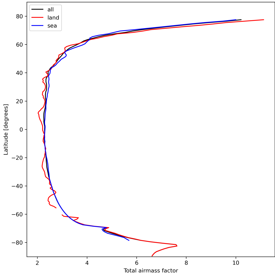
Figure 15: Zonal average of “Total airmass factor” for 2024-02-22 to 2024-02-23.
