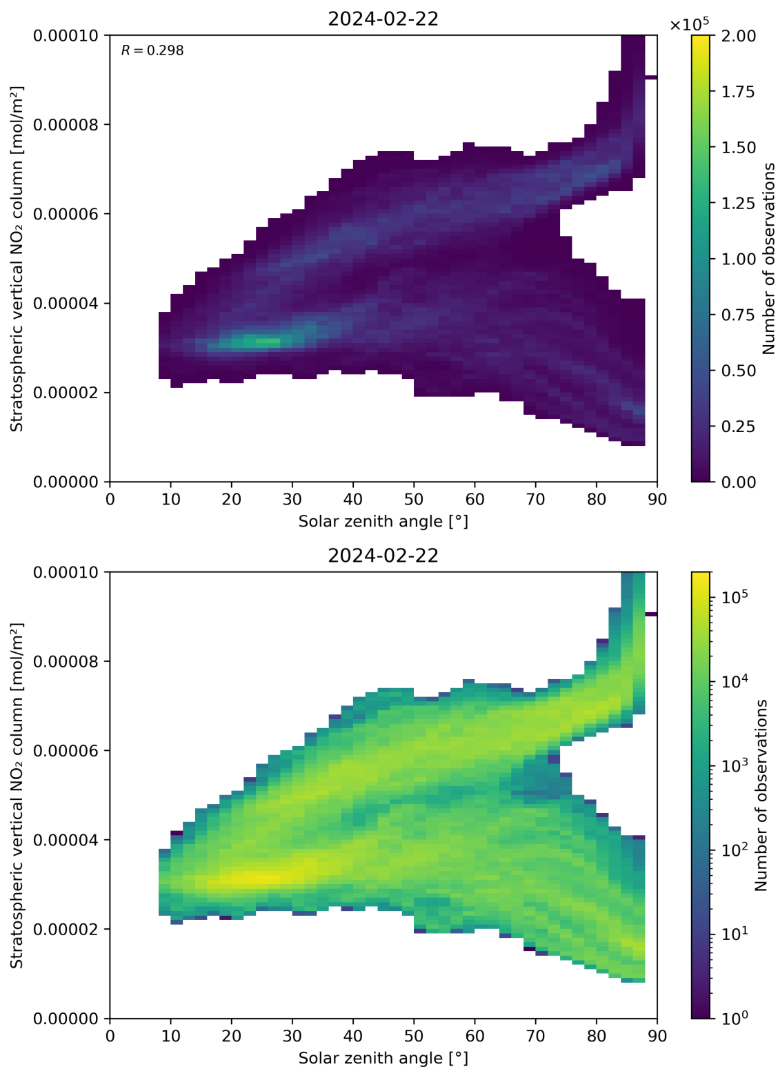
Figure 150: Scatter density plot of “Solar zenith angle” against “Stratospheric vertical NO 2 column” for 2024-02-22 to 2024-02-23.
