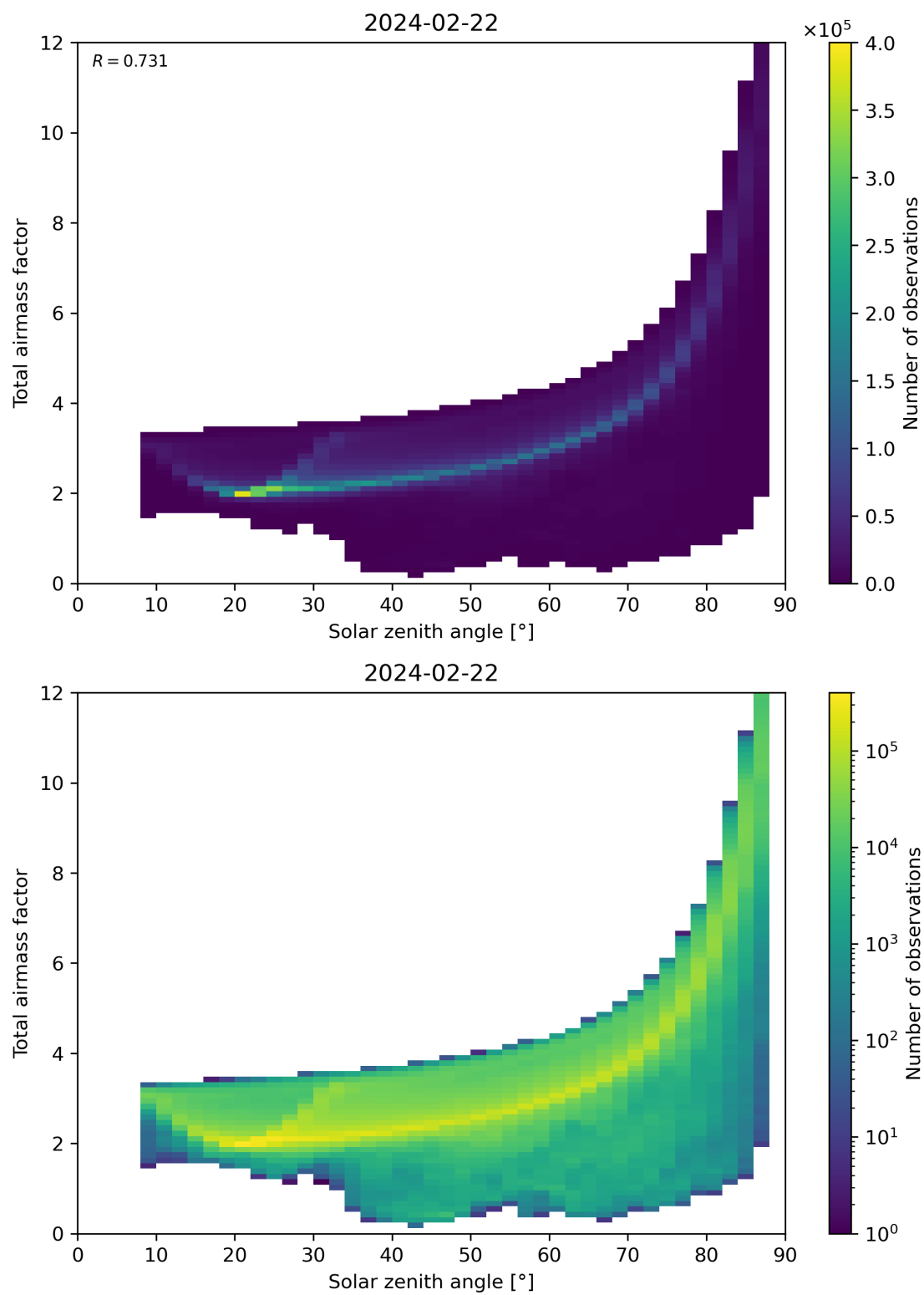
Figure 146: Scatter density plot of “Solar zenith angle” against “Total air mass factor” for 2024-02-22 to 2024-02-23.
