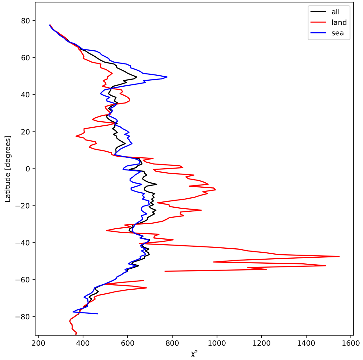
Figure 25: Zonal average of “ \chi^2 ” for 2024-02-22 to 2024-02-23.
