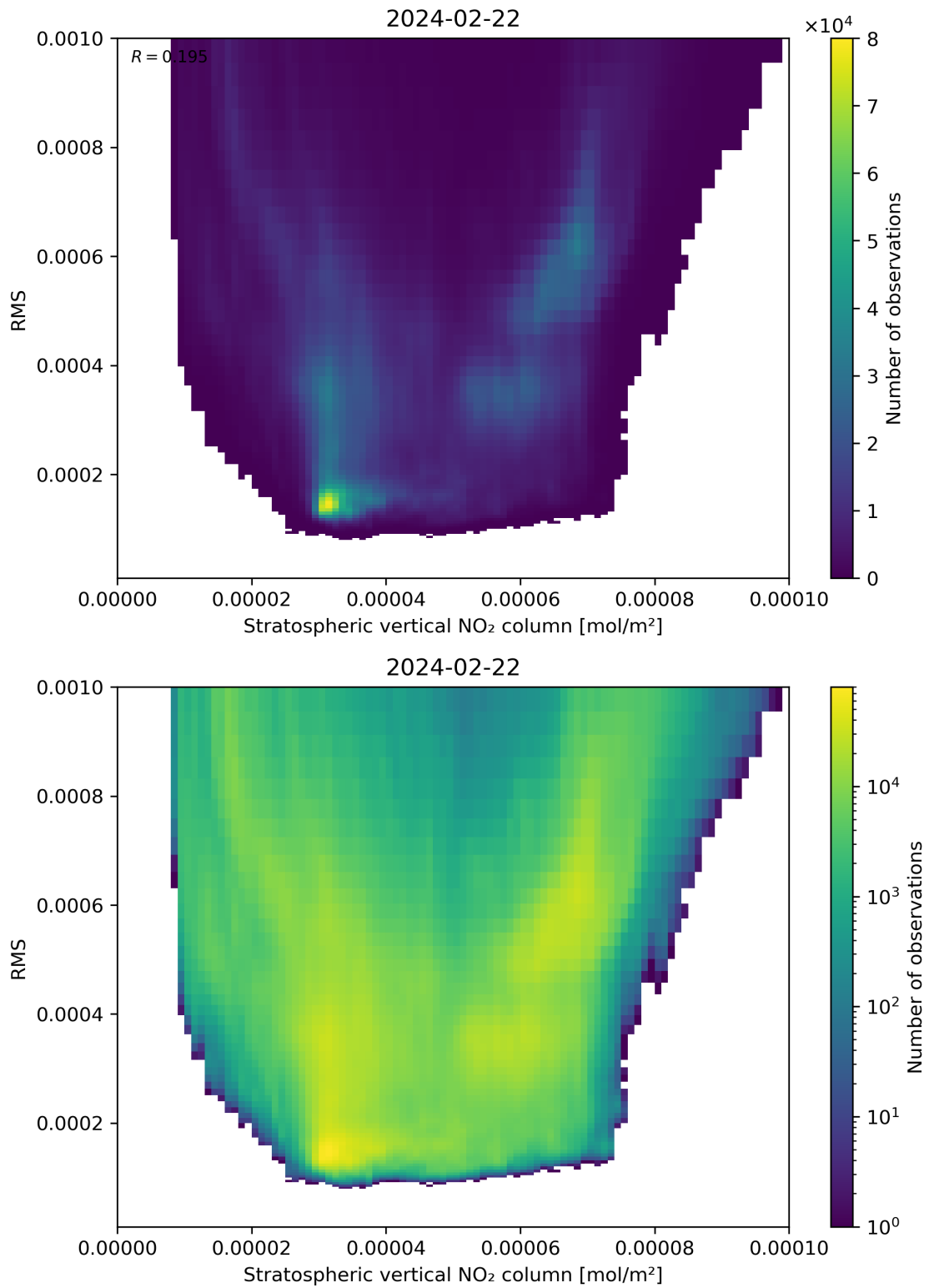
Figure 102: Scatter density plot of “Stratospheric vertical NO 2 column” against “RMS” for 2024-02-22 to 2024-02-23.
