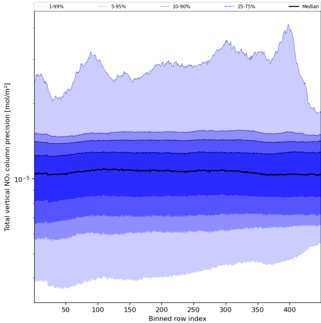
Figure 56: Along track statistics of “Total vertical NO 2 column precision” for 2024-02-22 to 2024-02-23
