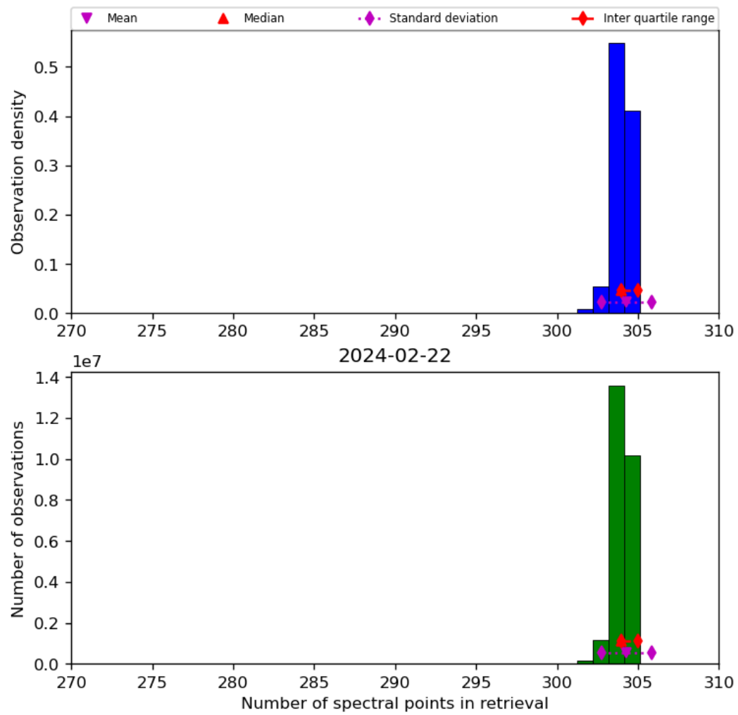
Figure 33: Histogram of “Number of spectral points in retrieval” for 2024-02-22 to 2024-02-23
