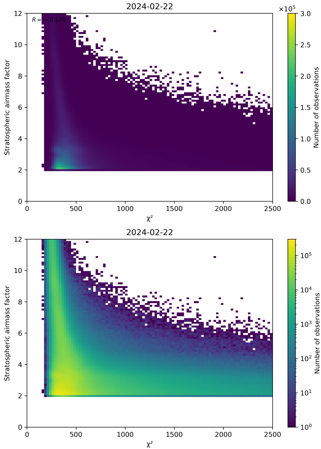
Figure 81: Scatter density plot of “ \chi^2 ” against “Stratospheric airmass factor” for 2024-02-22 to 2024-02-23.
