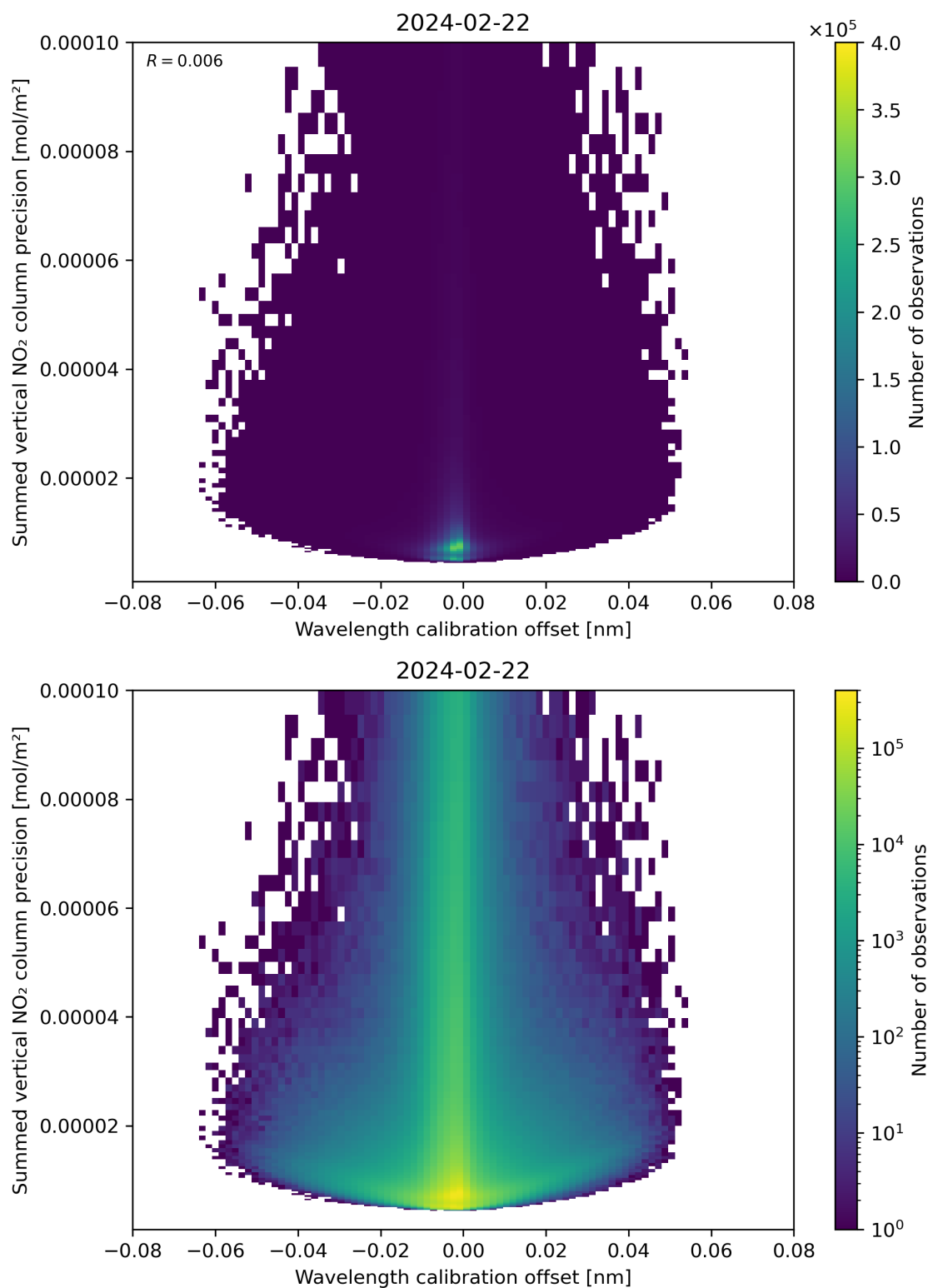
Figure 178: Scatter density plot of “Wavelength calibration offset” against “Summed vertical NO 2 column precision” for 2024-02-22 to 2024-02-23.
