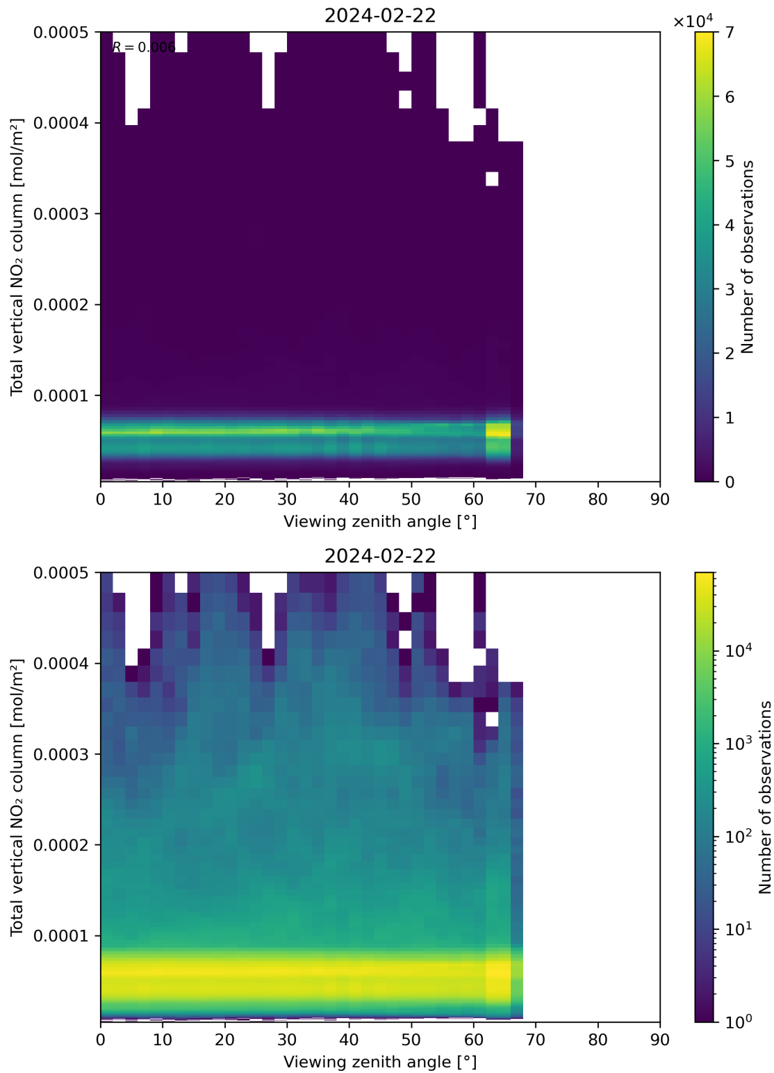
Figure 167: Scatter density plot of “Viewing zenith angle” against “Total vertical NO 2 column” for 2024-02-22 to 2024-02-23.
