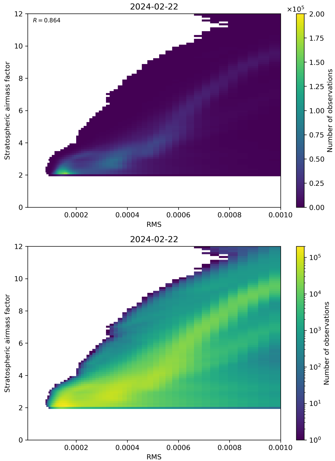
Figure 144: Scatter density plot of “RMS” against “Stratospheric airmass factor” for 2024-02-22 to 2024-02-23.
