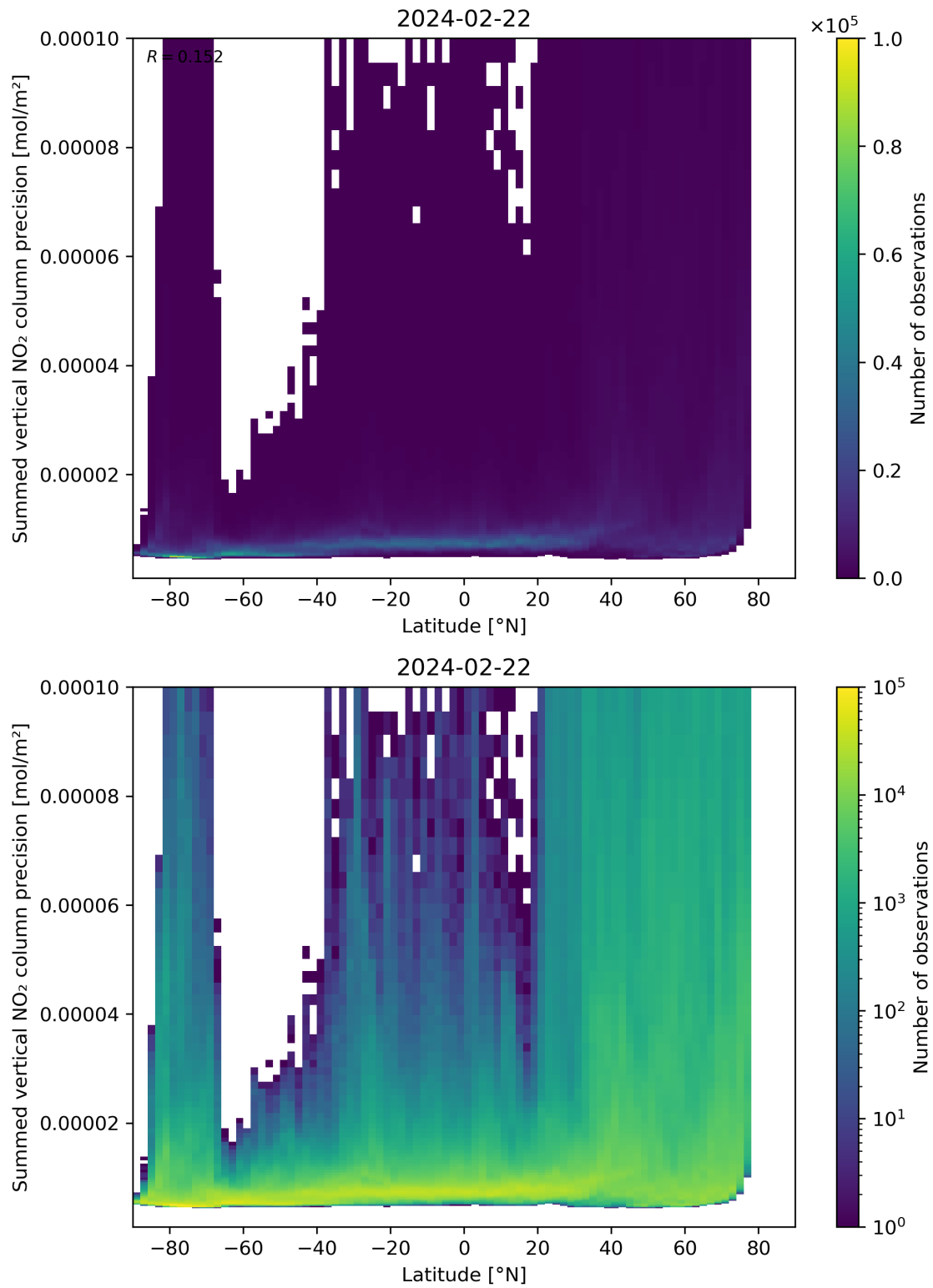
Figure 89: Scatter density plot of “Latitude” against “Summed vertical NO 2 column precision” for 2024-02-22 to 2024-02-23.
