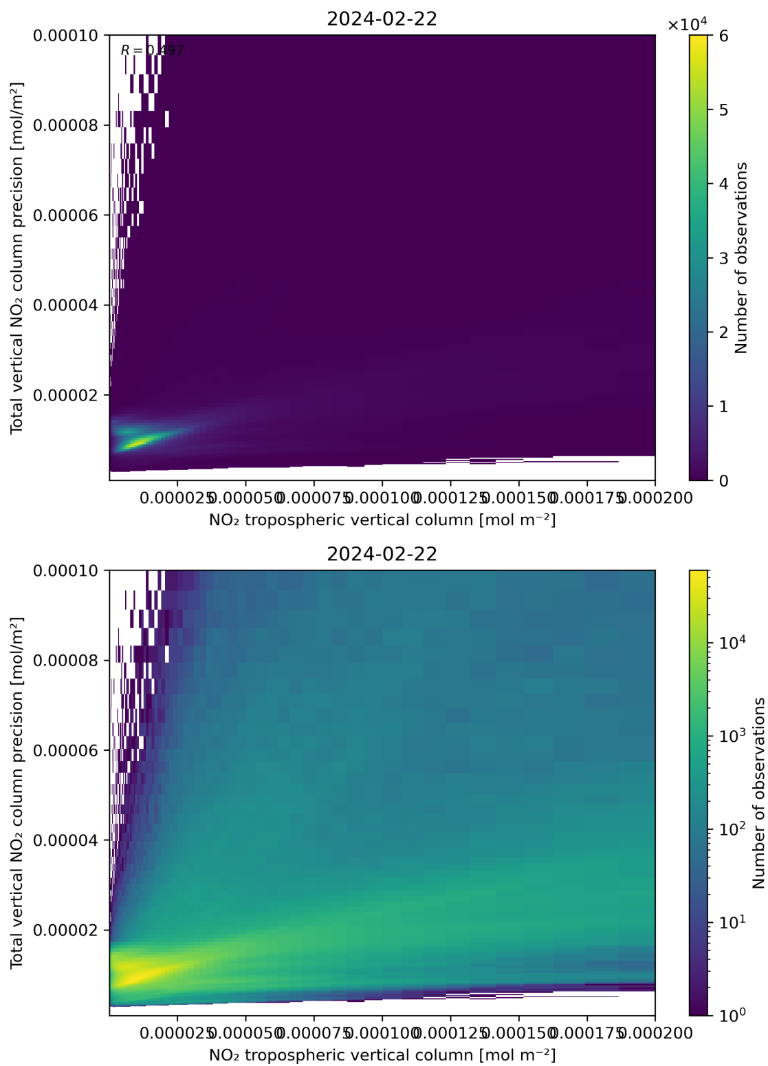
Figure 129: Scatter density plot of “NO 2 tropospheric vertical column” against “Total vertical NO 2 column precision” for 2024-02-22 to 2024-02-23.
