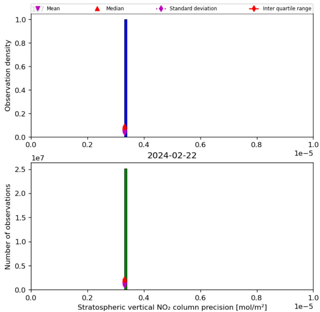
Figure 37: Histogram of “Stratospheric vertical NO 2 column precision” for 2024-02-22 to 2024-02-23
