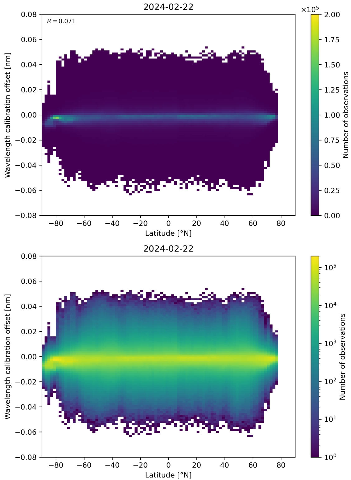
Figure 95: Scatter density plot of “Latitude” against “Wavelength calibration offset” for 2024-02-22 to 2024-02-23.
