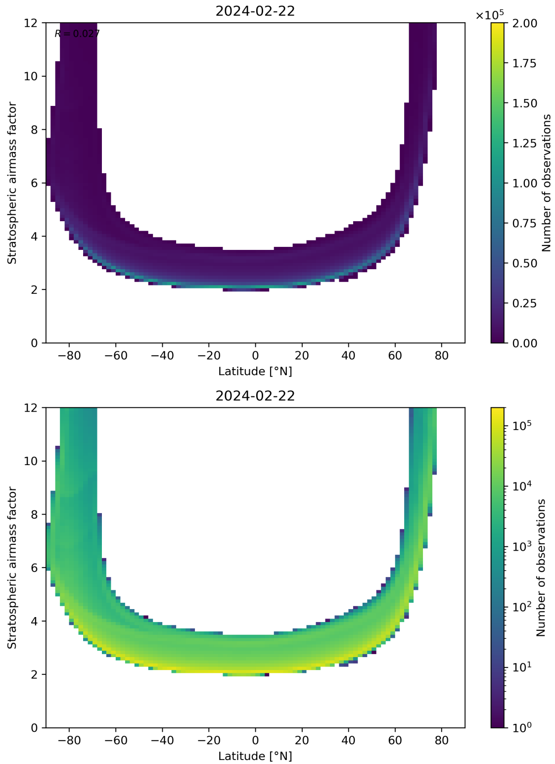
Figure 83: Scatter density plot of “Latitude” against “Stratospheric air mass factor” for 2024-02-22 to 2024-02-23.
