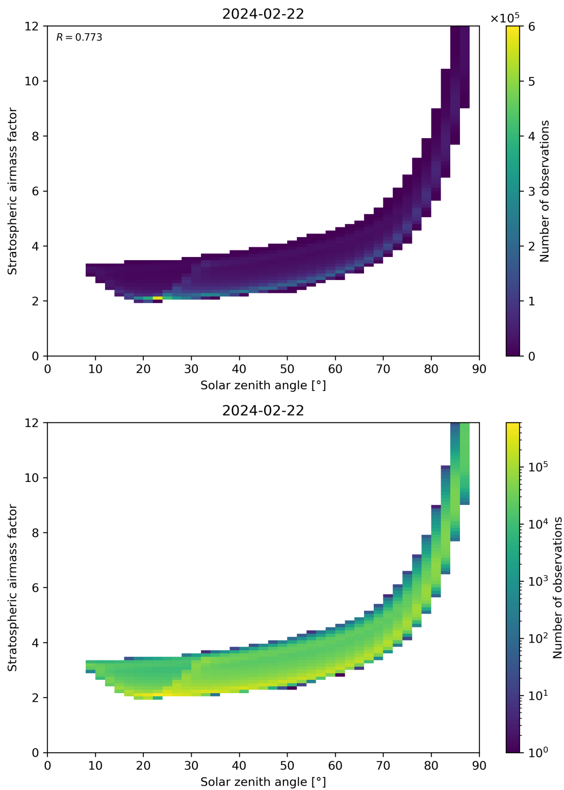
Figure 145: Scatter density plot of “Solar zenith angle” against “Stratospheric airmass factor” for 2024-02-22 to 2024-02-23.
