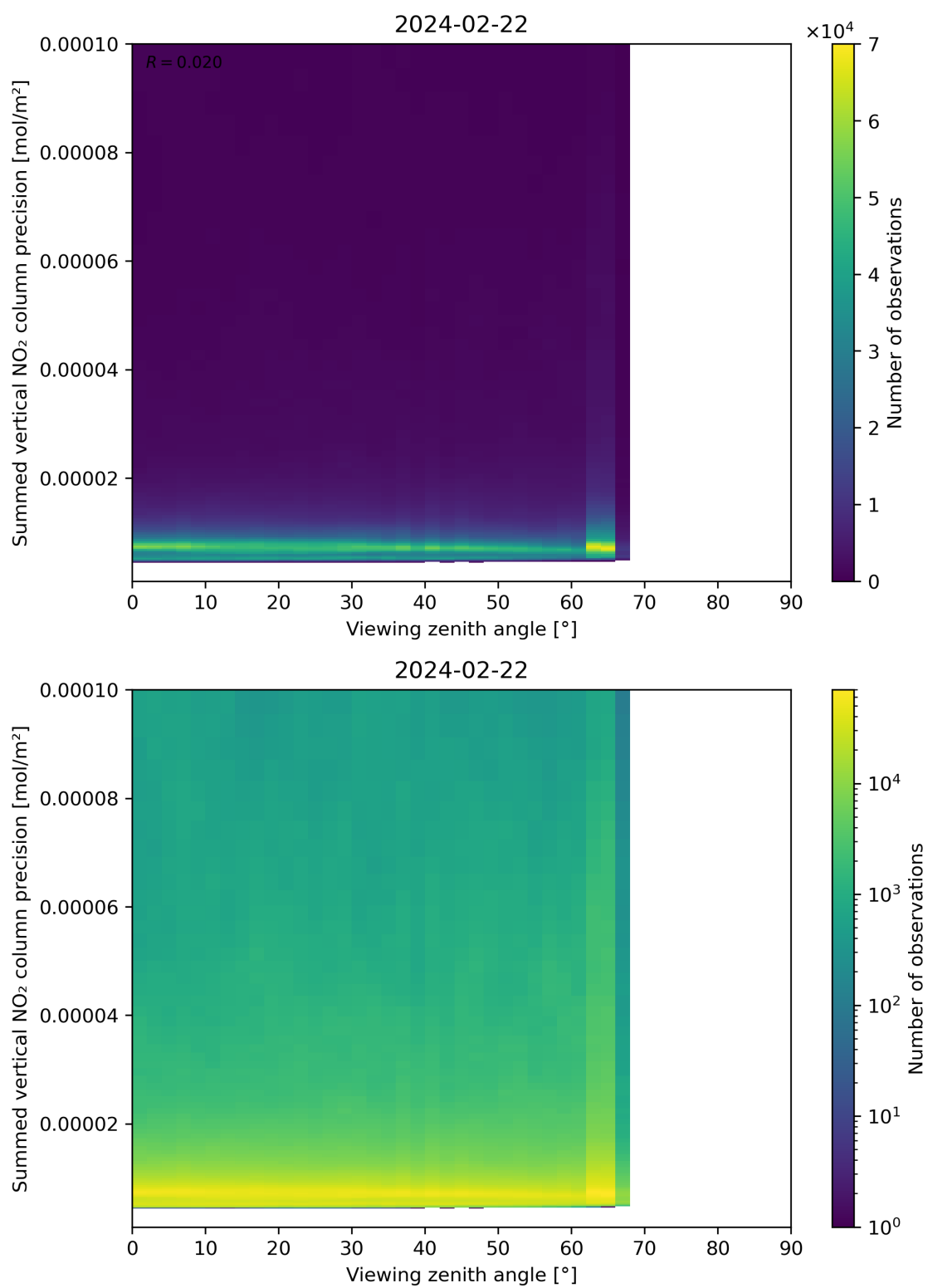
Figure 166: Scatter density plot of “Viewing zenith angle” against “Summed vertical NO 2 column precision” for 2024-02-22 to 2024-02-23.
