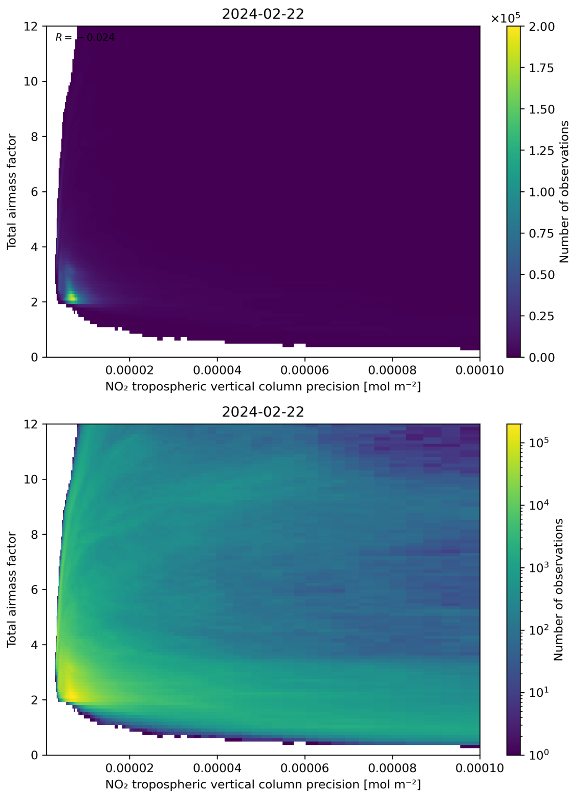
Figure 132: Scatter density plot of “NO 2 tropospheric vertical column precision” against “Total airmass factor” for 2024-02-22 to 2024-02-23.
