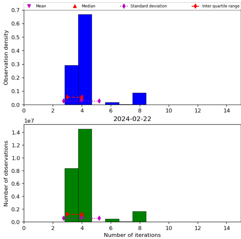
Figure 34: Histogram of “Number of iterations” for 2024-02-22 to 2024-02-23
