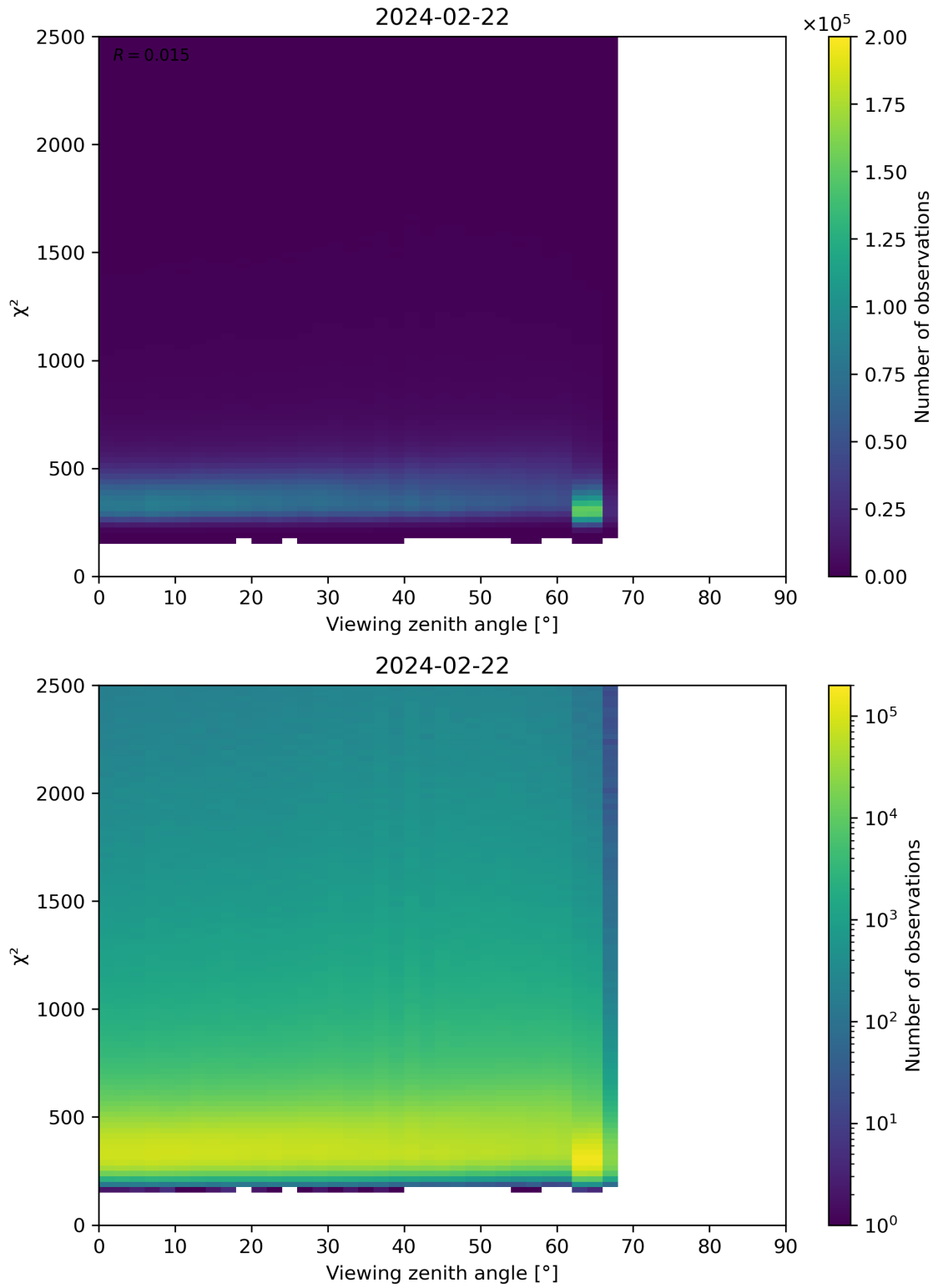
Figure 162: Scatter density plot of “Viewing zenith angle” against “ \chi^2 ” for 2024-02-22 to 2024-02-23.
