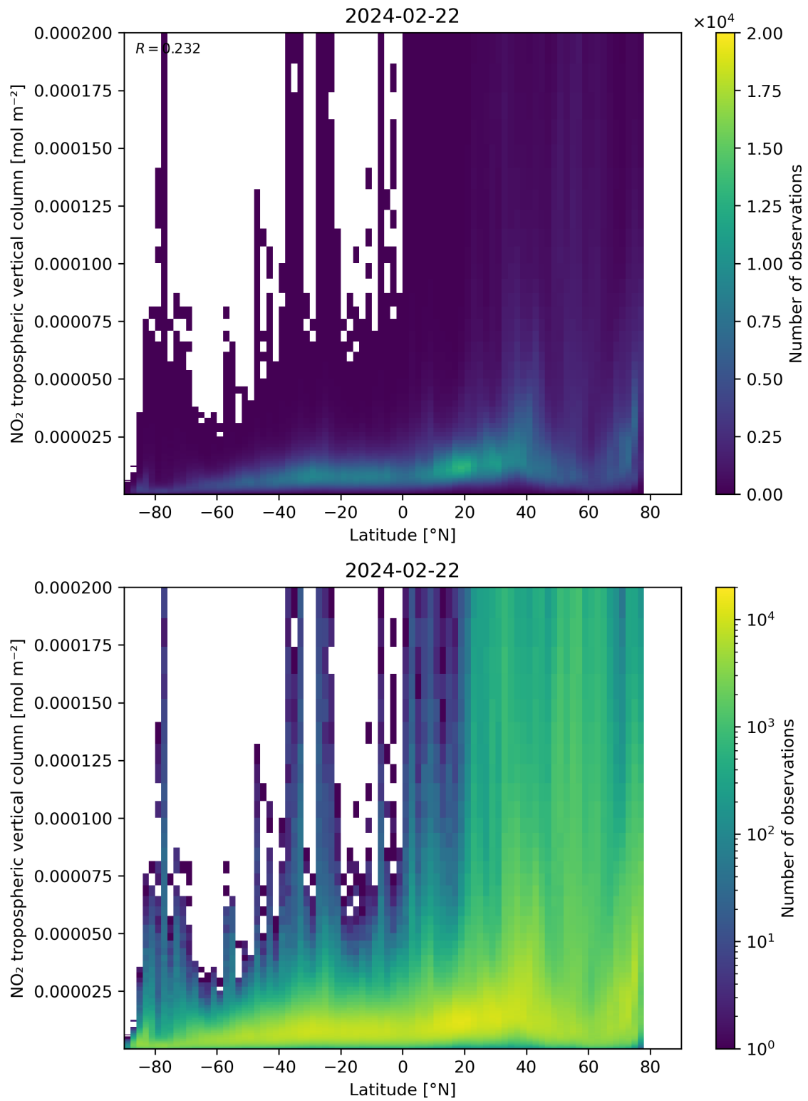
Figure 92: Scatter density plot of “Latitude” against “NO 2 tropospheric vertical column” for 2024-02-22 to 2024-02-23.
