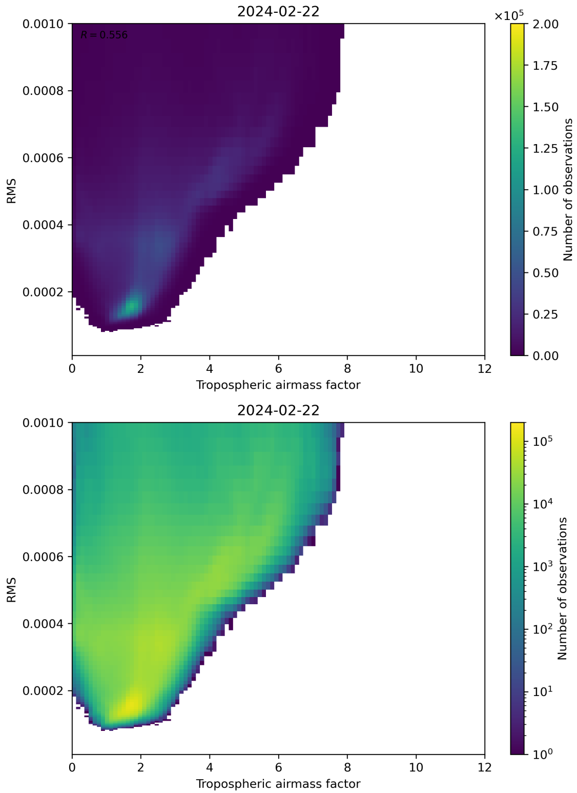
Figure 79: Scatter density plot of “Tropospheric airmass factor” against “RMS” for 2024-02-22 to 2024-02-23.
