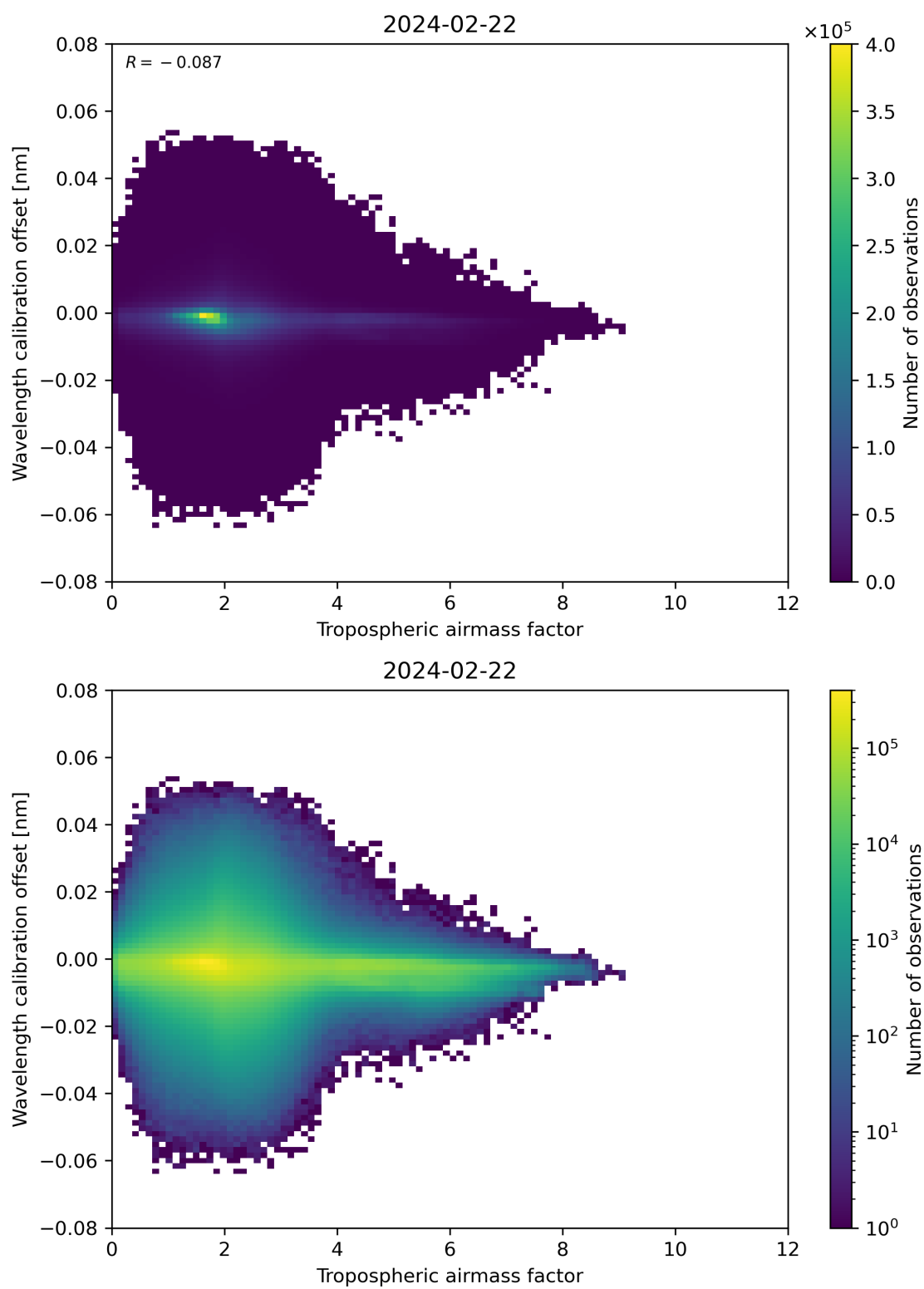
Figure 80: Scatter density plot of “Tropospheric airmass factor” against “Wavelength calibration offset” for 2024-02-22 to 2024-02-23.
