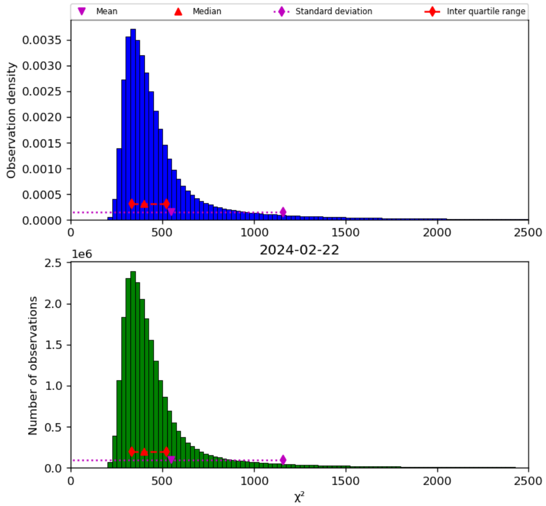
Figure 42: Histogram of “ \chi^2 ” for 2024-02-22 to 2024-02-23
