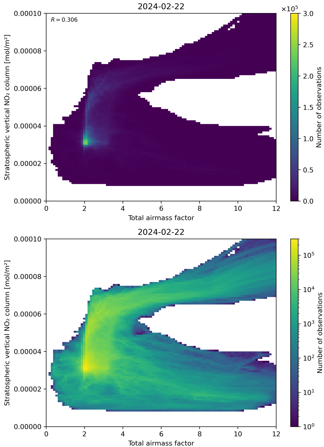
Figure 64: Scatter density plot of “Total airmass factor” against “Stratospheric vertical \text{NO}_2 column” for 2024-02-22 to 2024-02-23.
