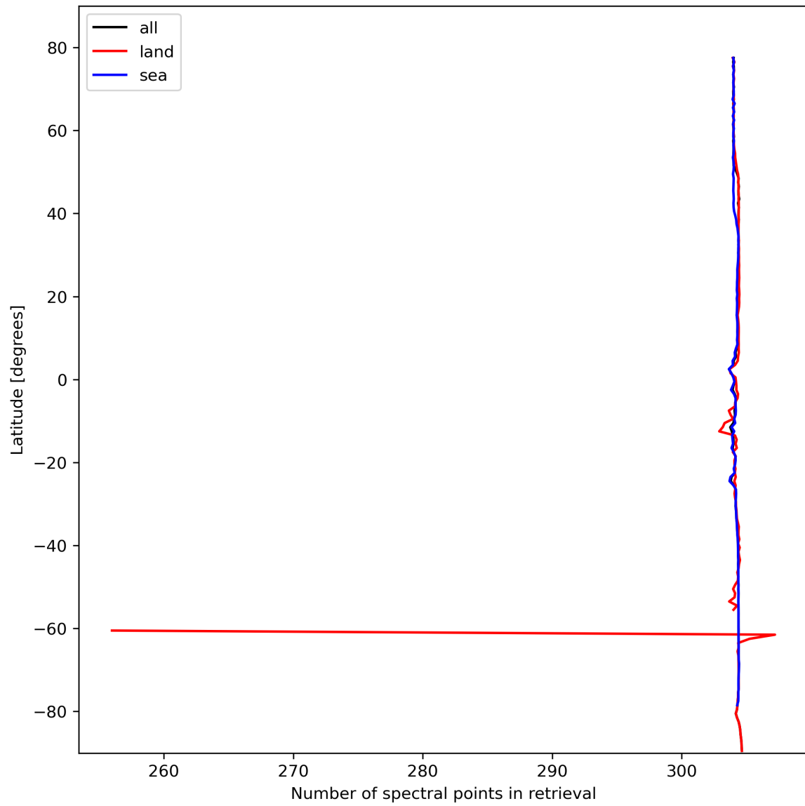
Figure 16: Zonal average of “Number of spectral points in retrieval” for 2024-02-22 to 2024-02-23.
