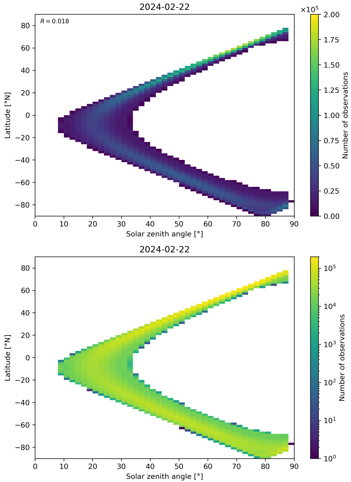
Figure 149: Scatter density plot of “Solar zenith angle” against “Latitude” for 2024-02-22 to 2024-02-23.
