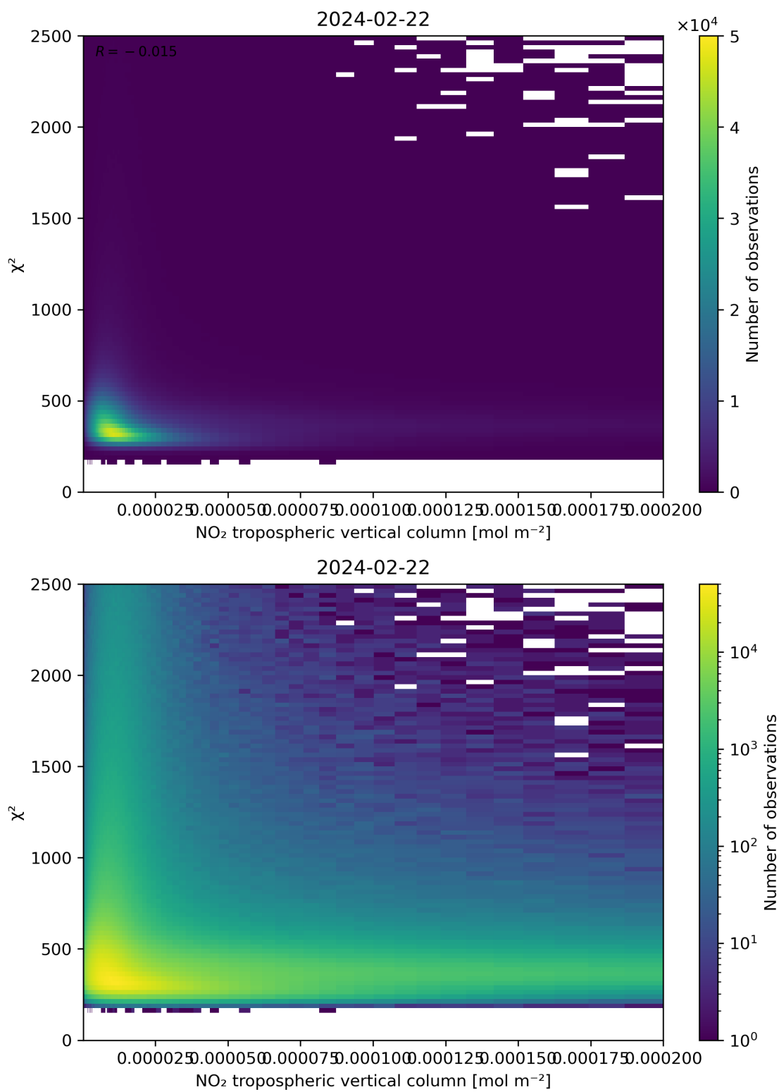
Figure 124: Scatter density plot of “NO 2 tropospheric vertical column” against “ \chi^2 ” for 2024-02-22 to 2024-02-23.
