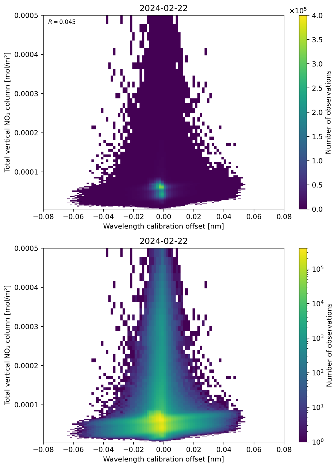
Figure 179: Scatter density plot of “Wavelength calibration offset” against “Total vertical NO 2 column” for 2024-02-22 to 2024-02-23.
