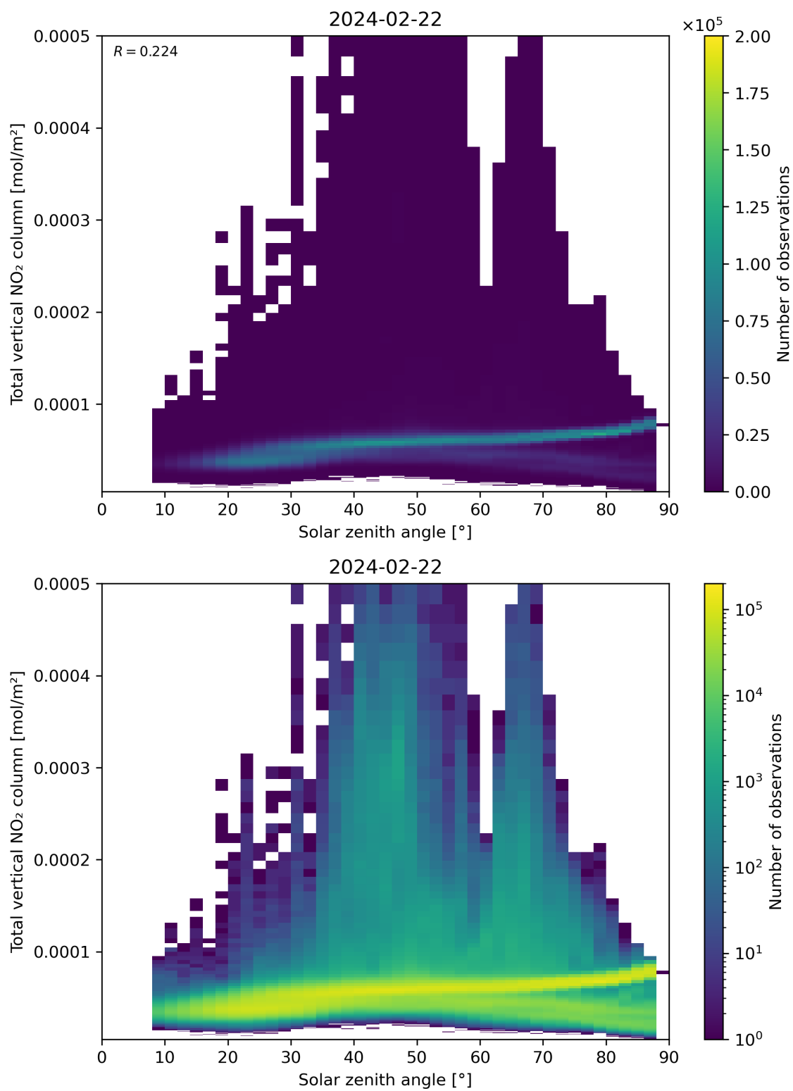
Figure 153: Scatter density plot of “Solar zenith angle” against “Total vertical NO 2 column” for 2024-02-22 to 2024-02-23.
