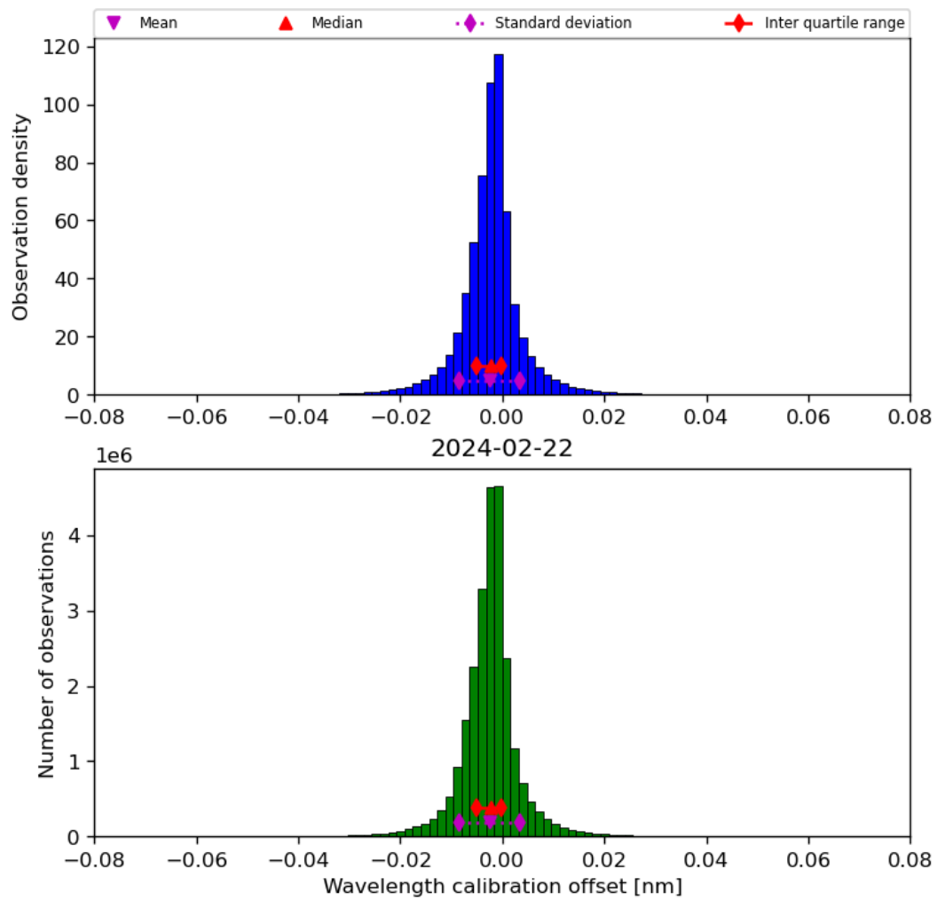
Figure 35: Histogram of “Wavelength calibration offset” for 2024-02-22 to 2024-02-23
