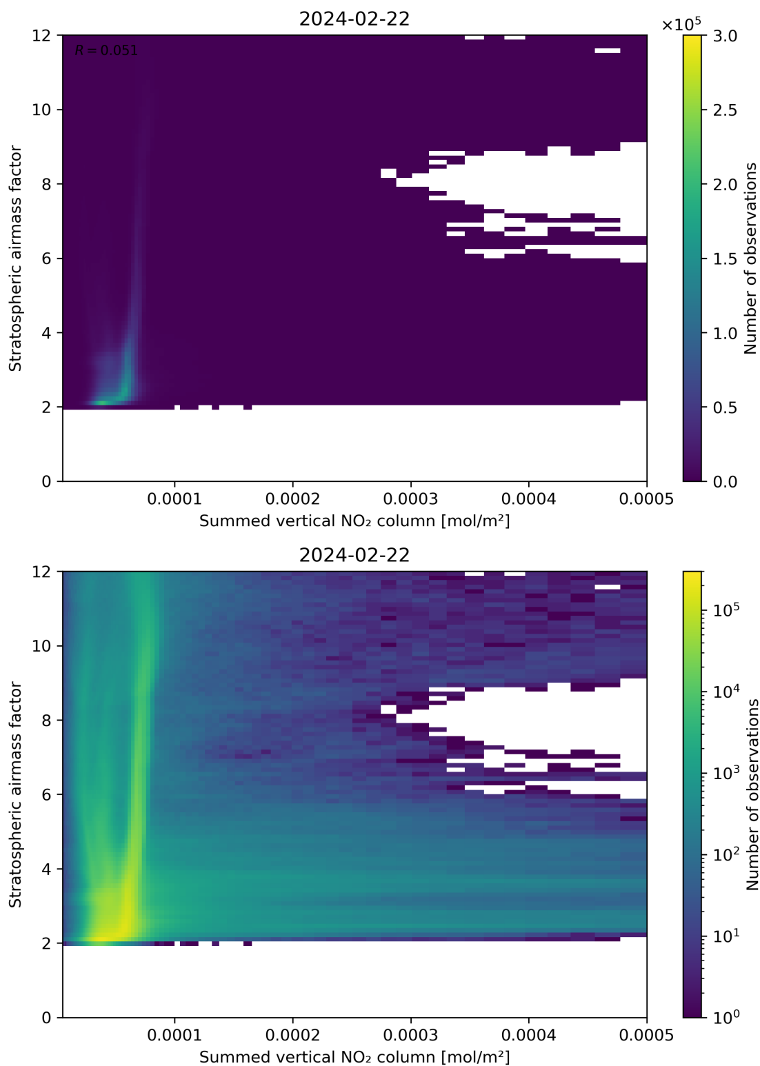
Figure 103: Scatter density plot of “Summed vertical NO 2 column” against “Stratospheric airmass factor” for 2024-02-22 to 2024-02-23.
