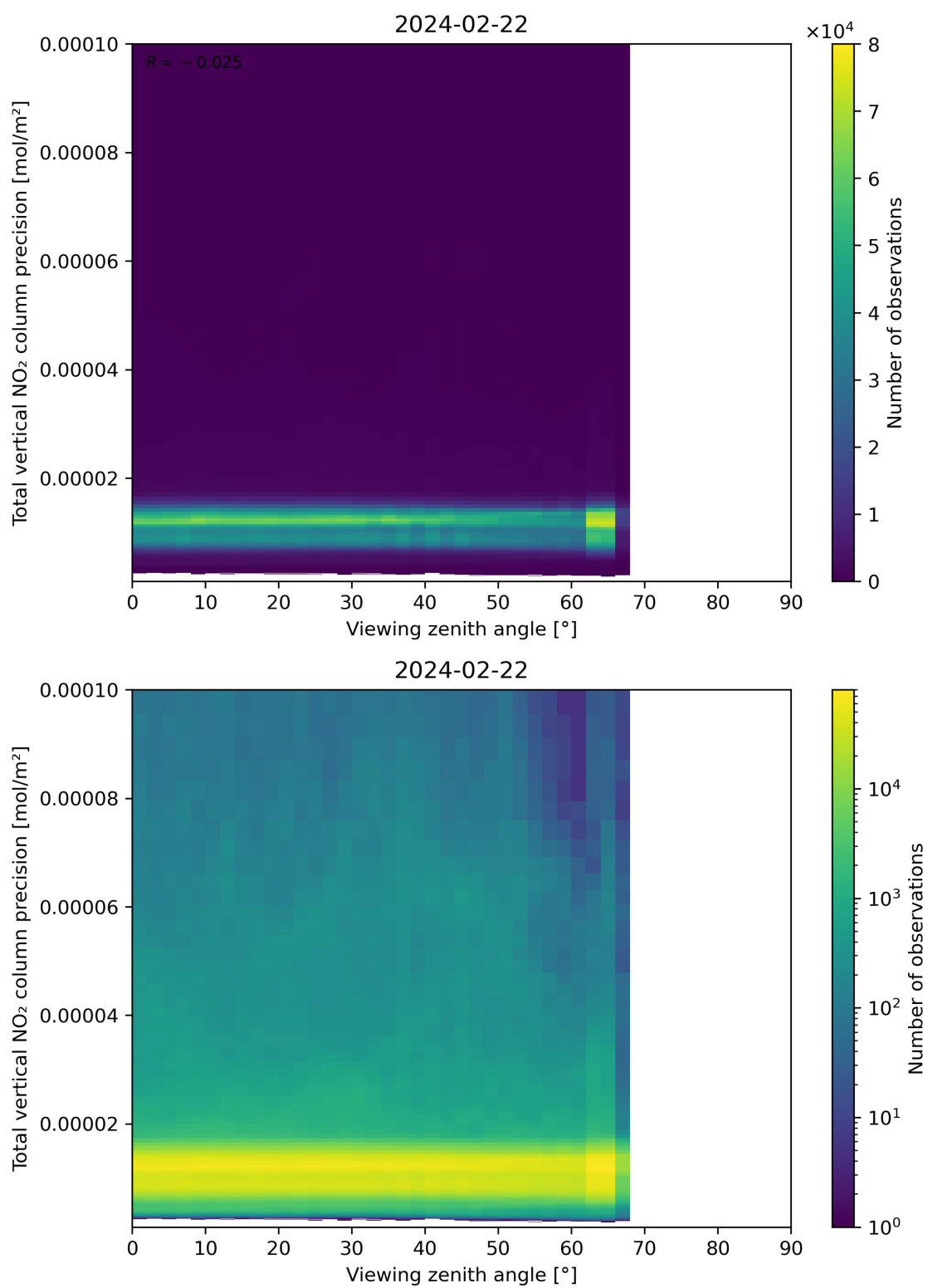
Figure 168: Scatter density plot of “Viewing zenith angle” against “Total vertical NO 2 column precision” for 2024-02-22 to 2024-02-23.
