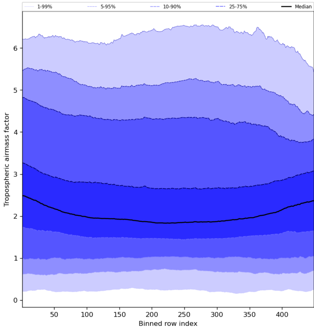
Figure 48: Along track statistics of “Tropospheric airmass factor” for 2024-02-22 to 2024-02-23
