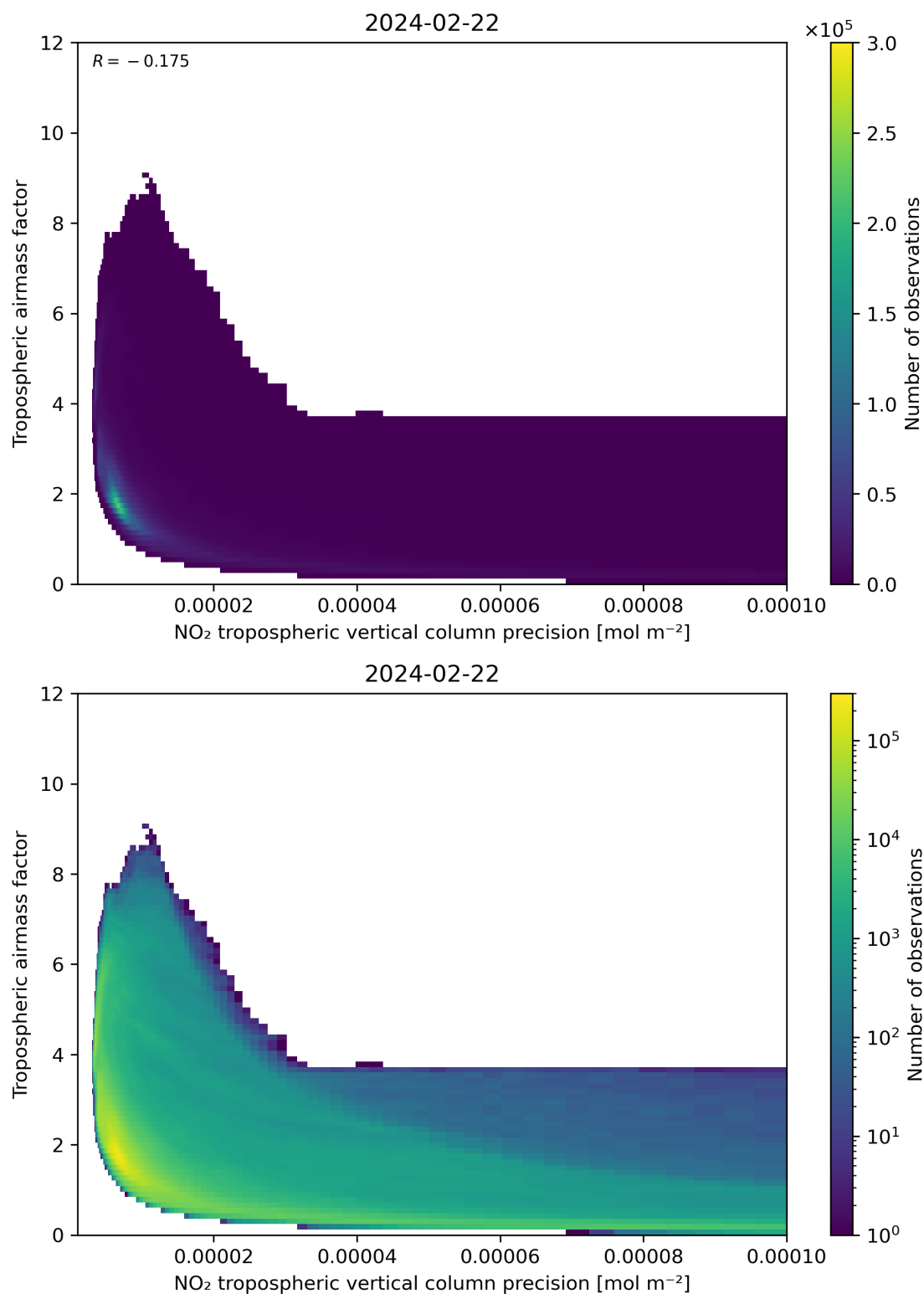
Figure 133: Scatter density plot of “NO 2 tropospheric vertical column precision” against “Tropospheric airmass factor” for 2024-02-22 to 2024-02-23.
