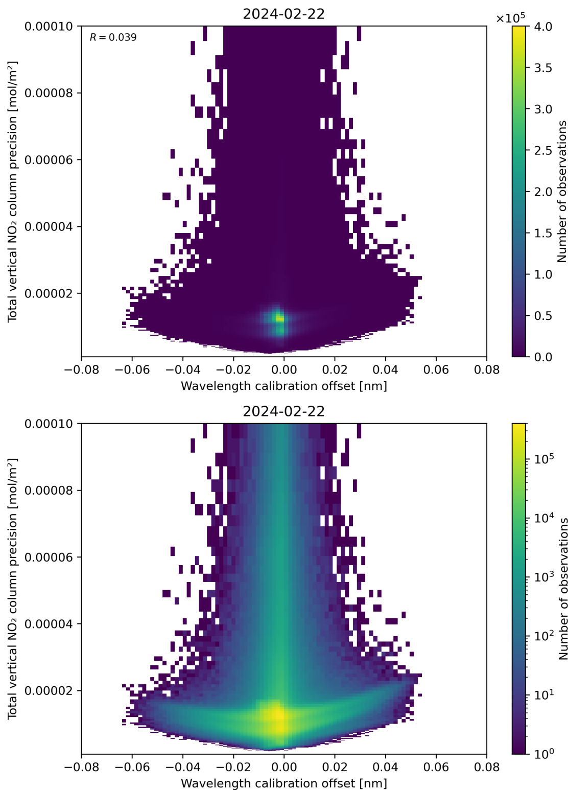
Figure 180: Scatter density plot of “Wavelength calibration offset” against “Total vertical NO 2 column precision” for 2024-02-22 to 2024-02-23.
