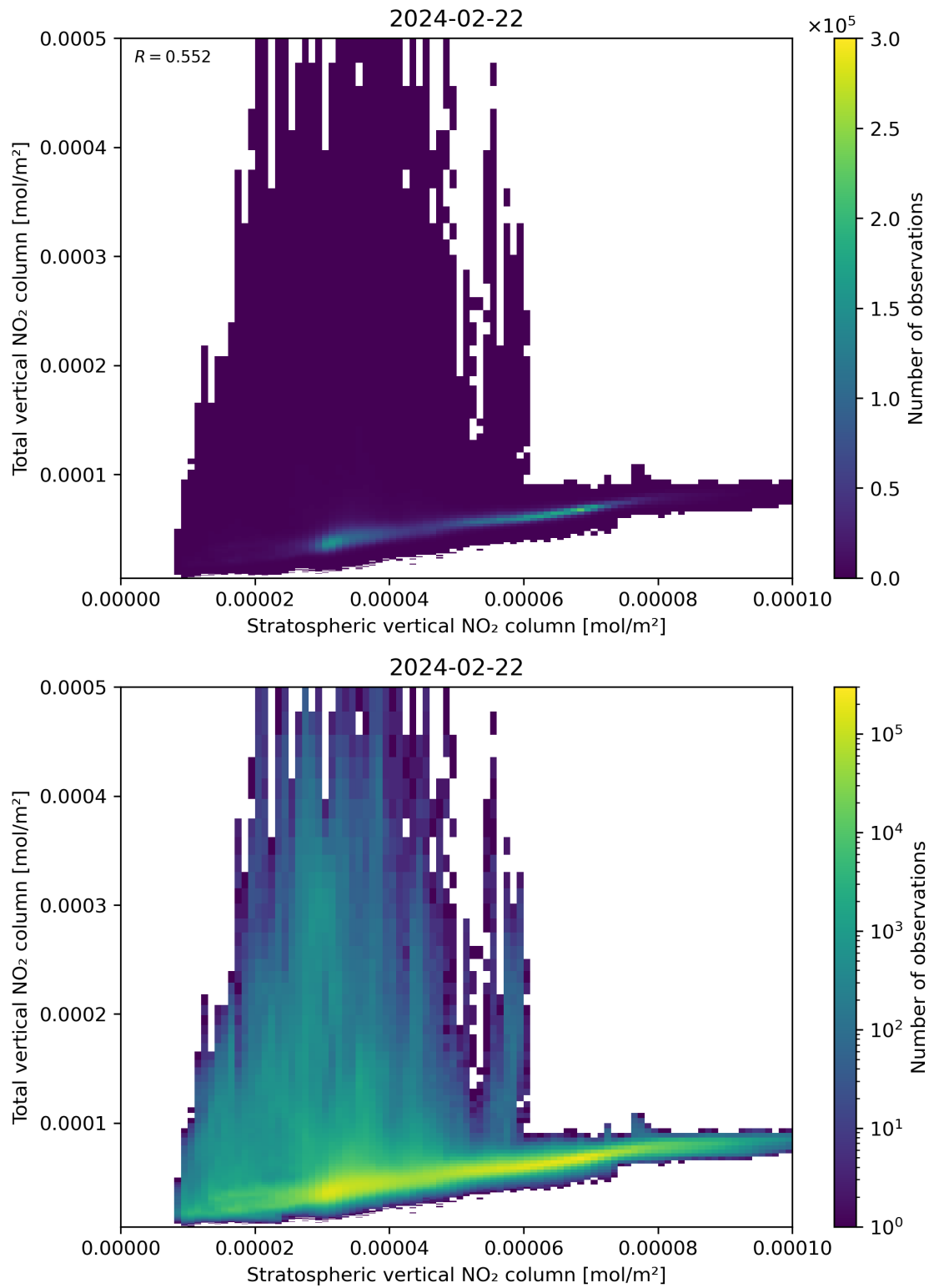
Figure 100: Scatter density plot of “Stratospheric vertical NO 2 column” against “Total vertical NO 2 column” for 2024-02-22 to 2024-02-23.
