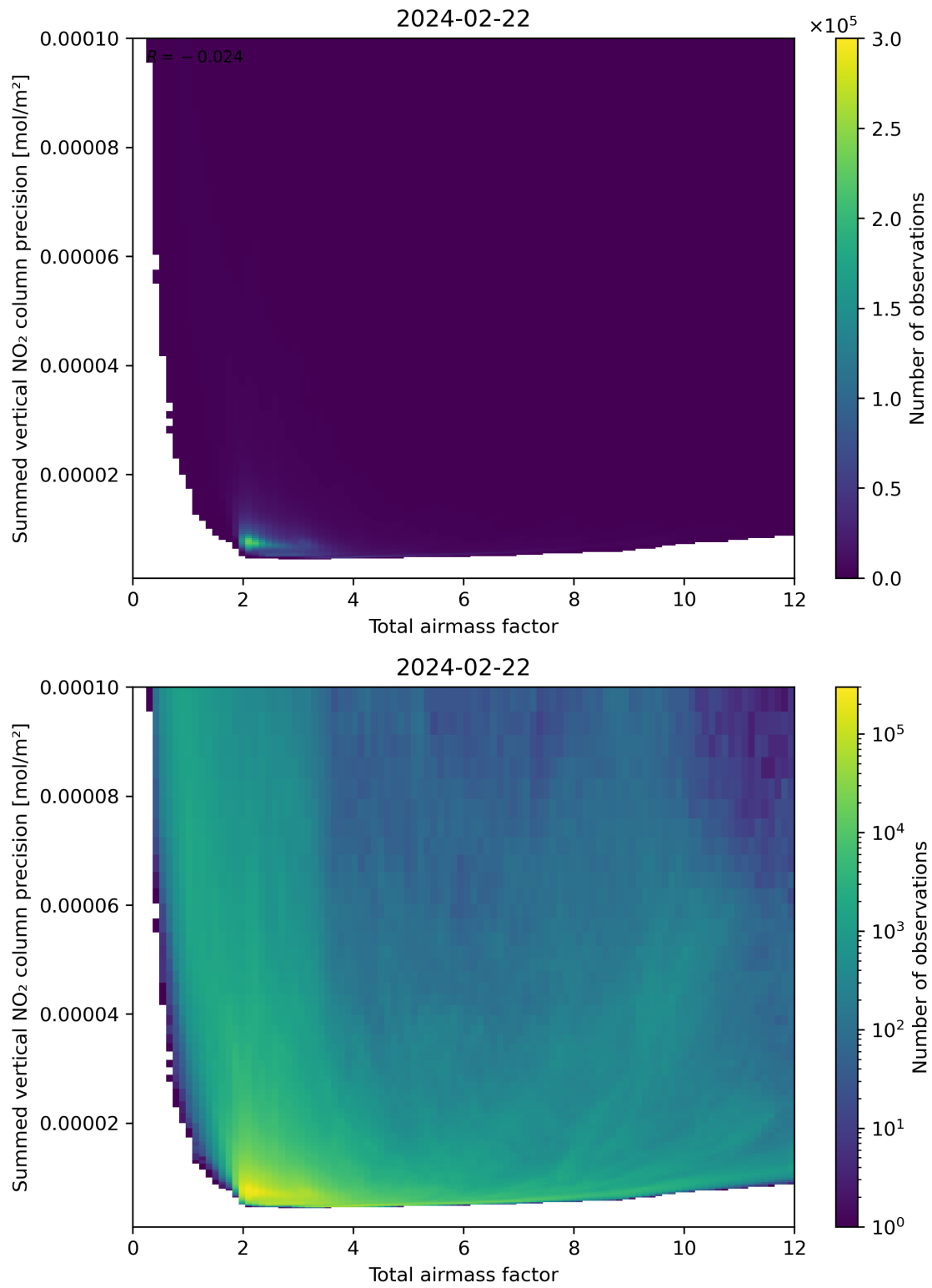
Figure 66: Scatter density plot of “Total airmass factor” against “Summed vertical NO 2 column precision” for 2024-02-22 to 2024-02-23.
