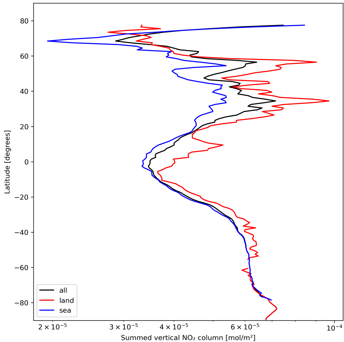
Figure 23: Zonal average of “Summed vertical NO 2 column” for 2024-02-22 to 2024-02-23.
