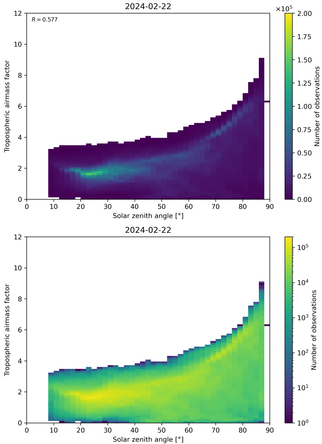
Figure 147: Scatter density plot of “Solar zenith angle” against “Tropospheric airmass factor” for 2024-02-22 to 2024-02-23.
