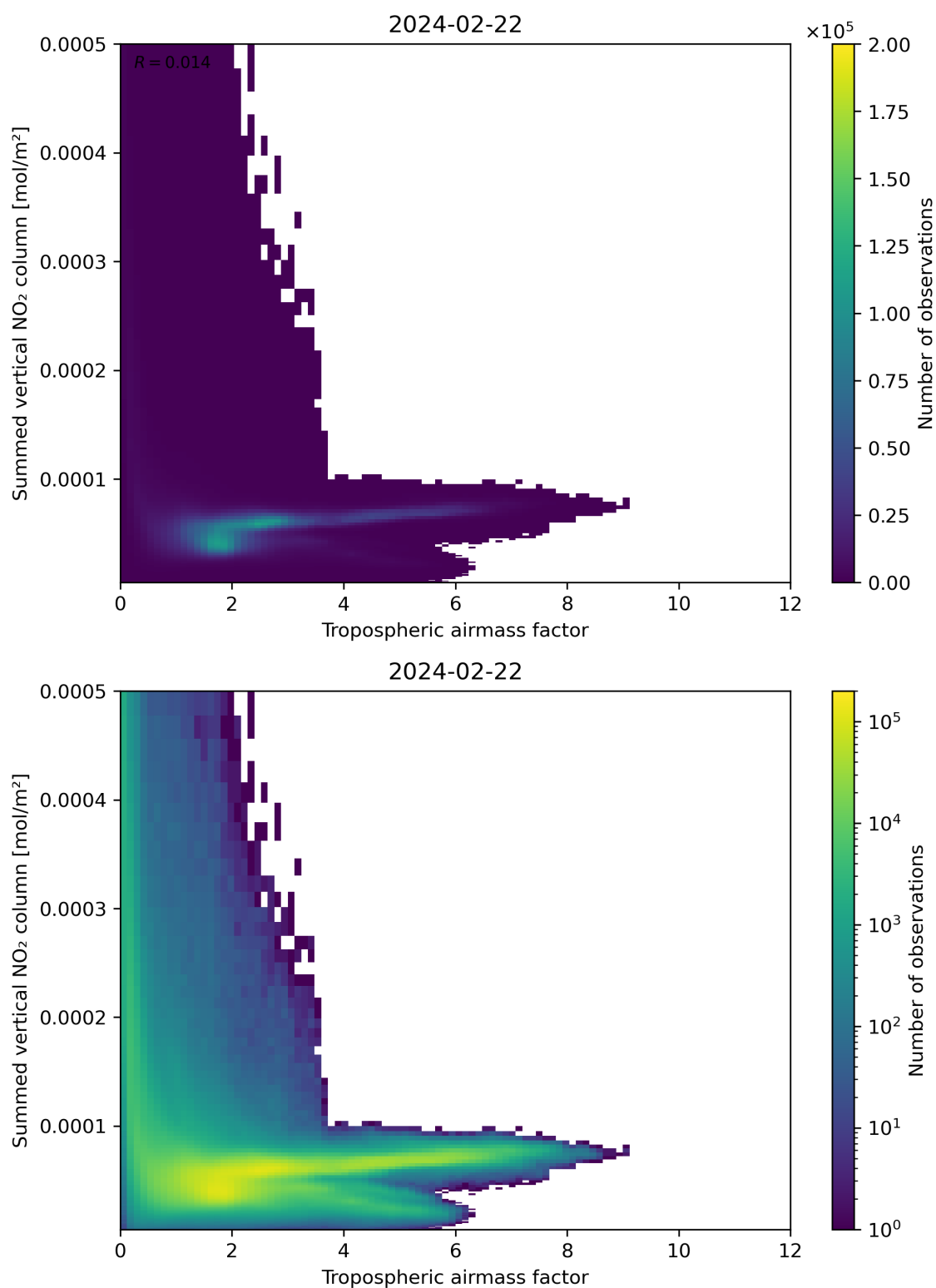
Figure 75: Scatter density plot of “Tropospheric airmass factor” against “Summed vertical NO 2 column” for 2024-02-22 to 2024-02-23.
