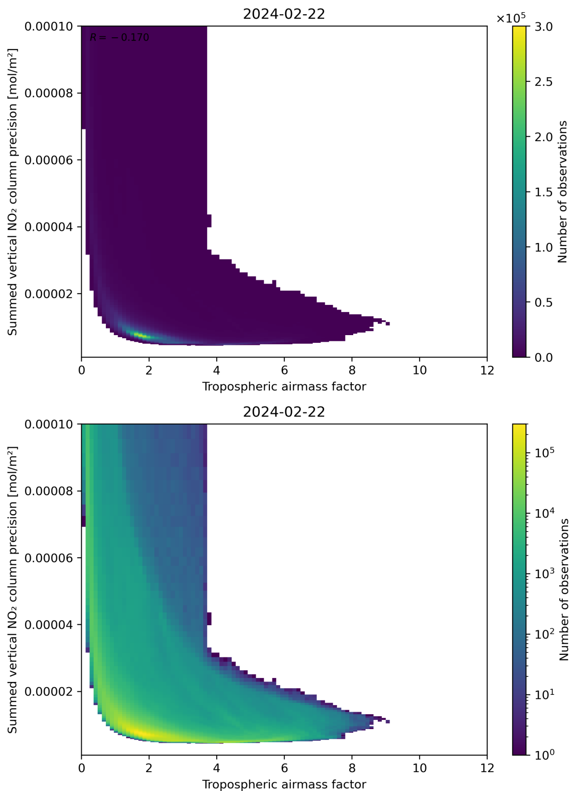
Figure 76: Scatter density plot of “Tropospheric air mass factor” against “Summed vertical NO 2 column precision” for 2024-02-22 to 2024-02-23.
