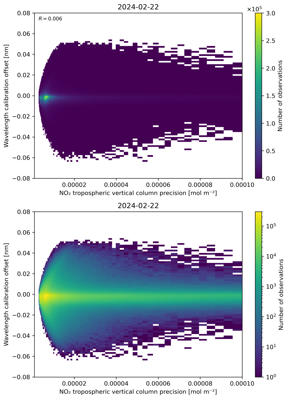
Figure 141: Scatter density plot of “NO 2 tropospheric vertical column precision” against “Wavelength calibration offset” for 2024-02-22 to 2024-02-23.
