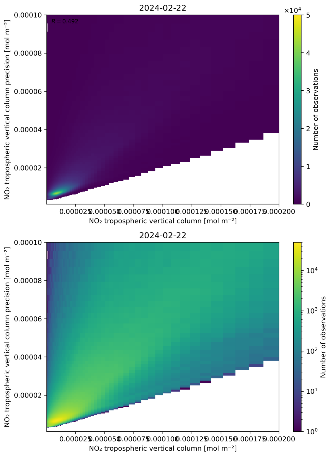
Figure 130: Scatter density plot of “NO 2 tropospheric vertical column” against “NO 2 tropospheric vertical column precision” for 2024-02-22 to 2024-02-23.
