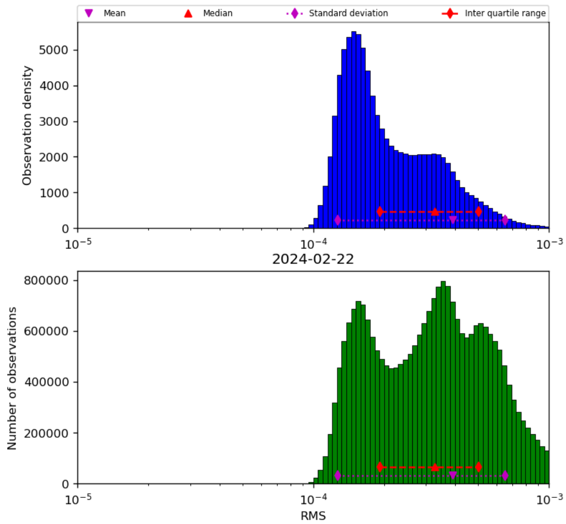
Figure 43: Histogram of “RMS” for 2024-02-22 to 2024-02-23
