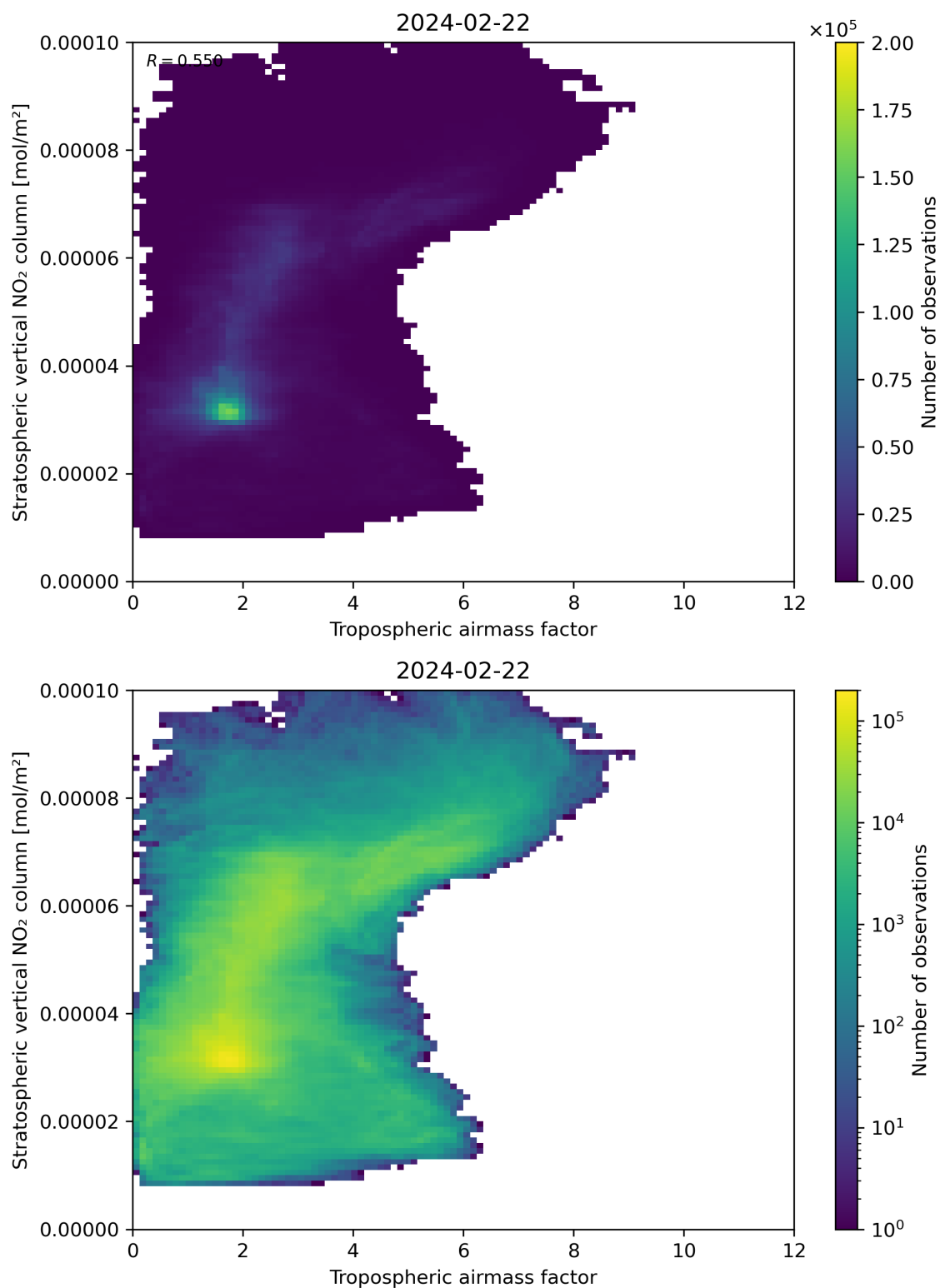
Figure 74: Scatter density plot of “Tropospheric airmass factor” against “Stratospheric vertical NO 2 column” for 2024-02-22 to 2024-02-23.
