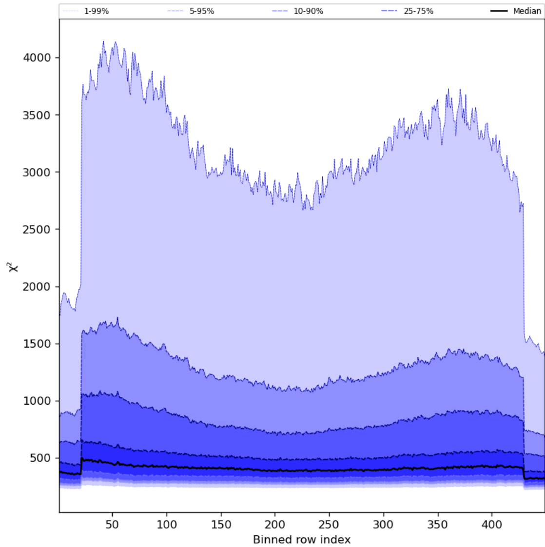
Figure 59: Along track statistics of “ \chi^2 ” for 2024-02-22 to 2024-02-23
