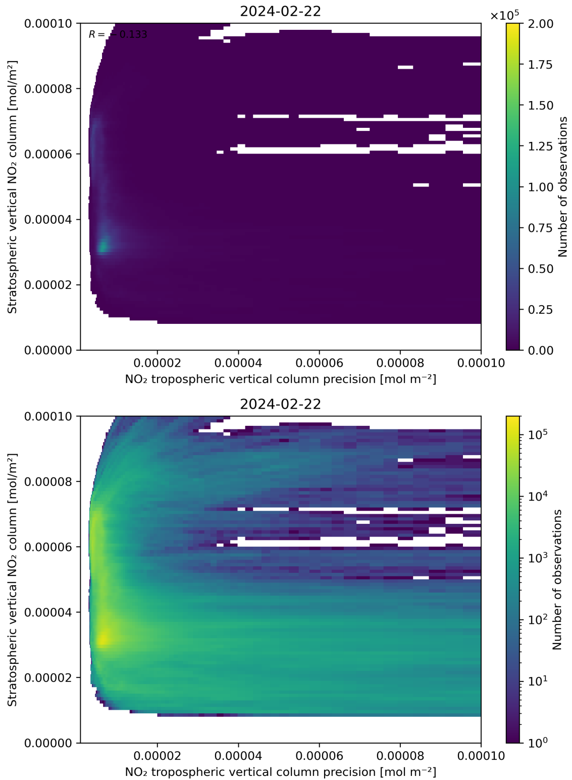
Figure 135: Scatter density plot of “NO 2 tropospheric vertical column precision” against “Stratospheric vertical NO 2 column” for 2024-02-22 to 2024-02-23.
