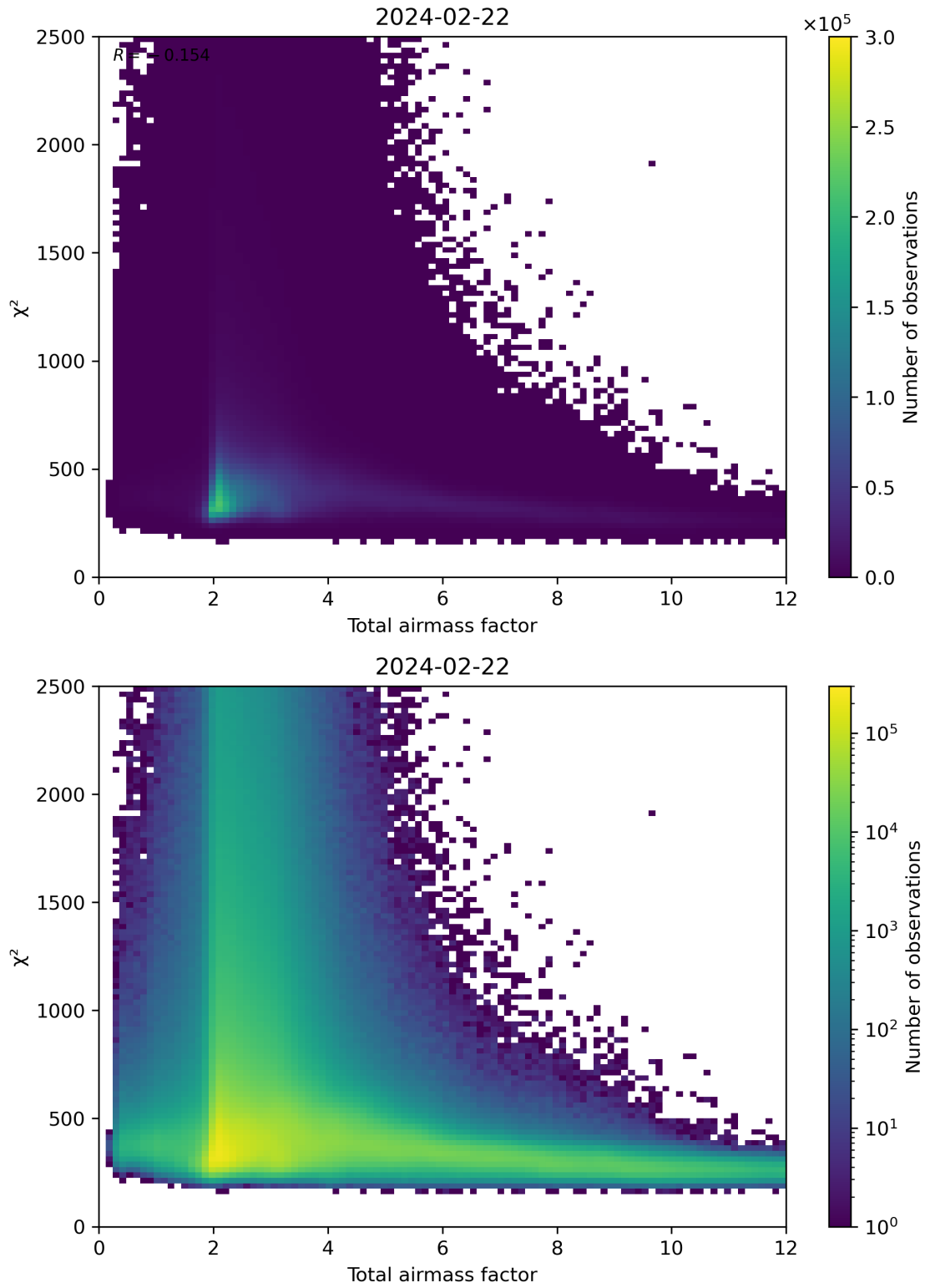
Figure 63: Scatter density plot of “Total airmass factor” against “ \chi^2 ” for 2024-02-22 to 2024-02-23.
