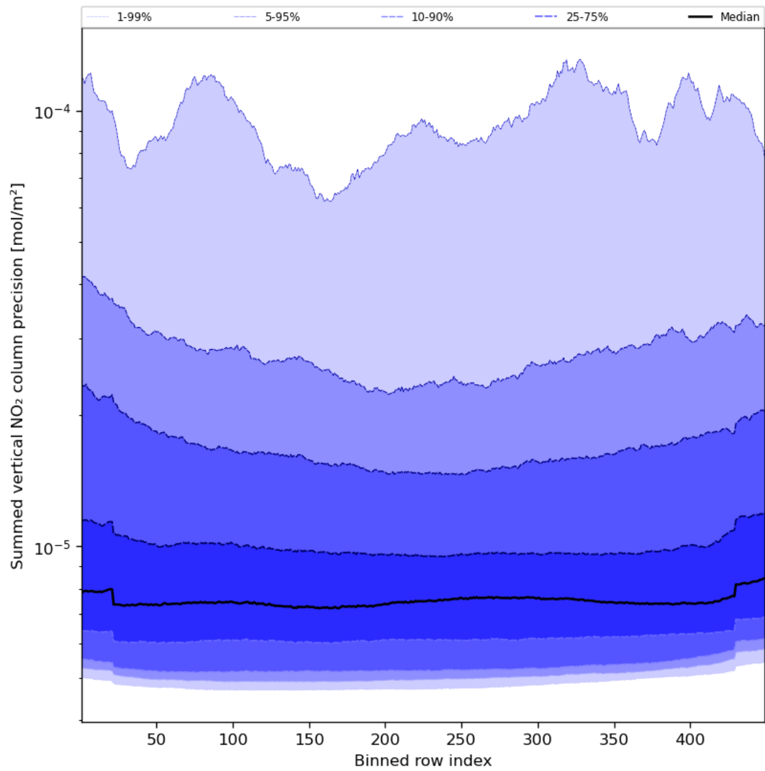
Figure 58: Along track statistics of “Summed vertical NO 2 column precision” for 2024-02-22 to 2024-02-23
