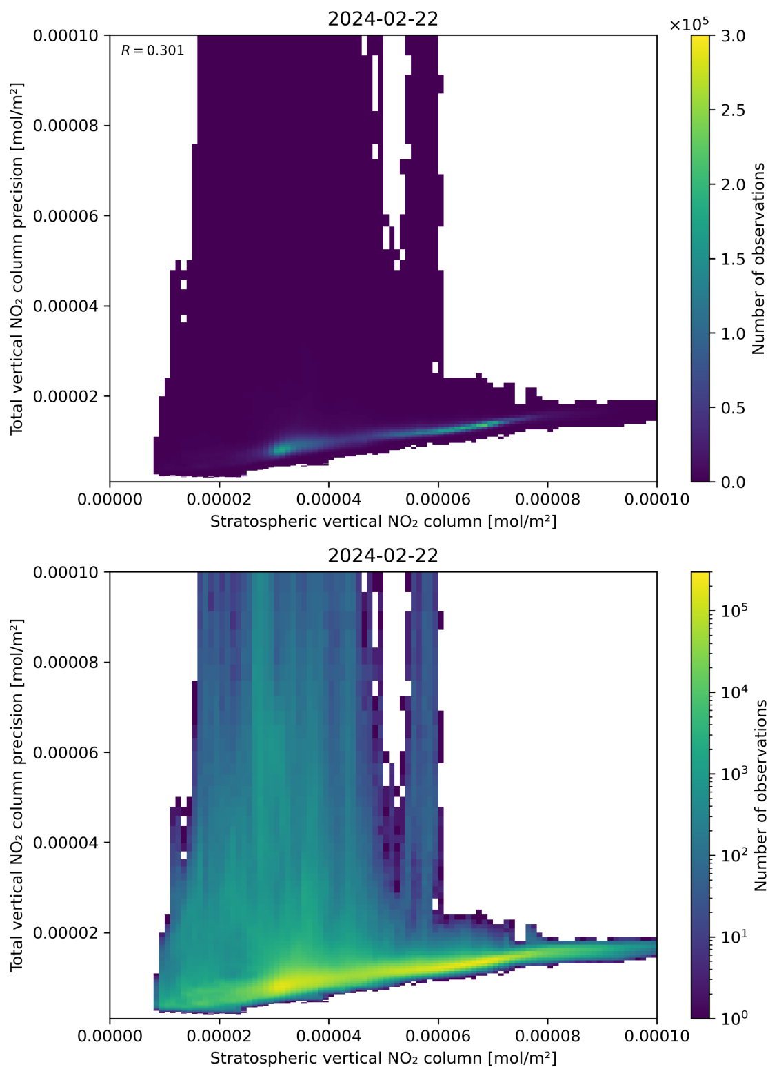
Figure 101: Scatter density plot of “Stratospheric vertical NO 2 column” against “Total vertical NO 2 column precision” for 2024-02-22 to 2024-02-23.
