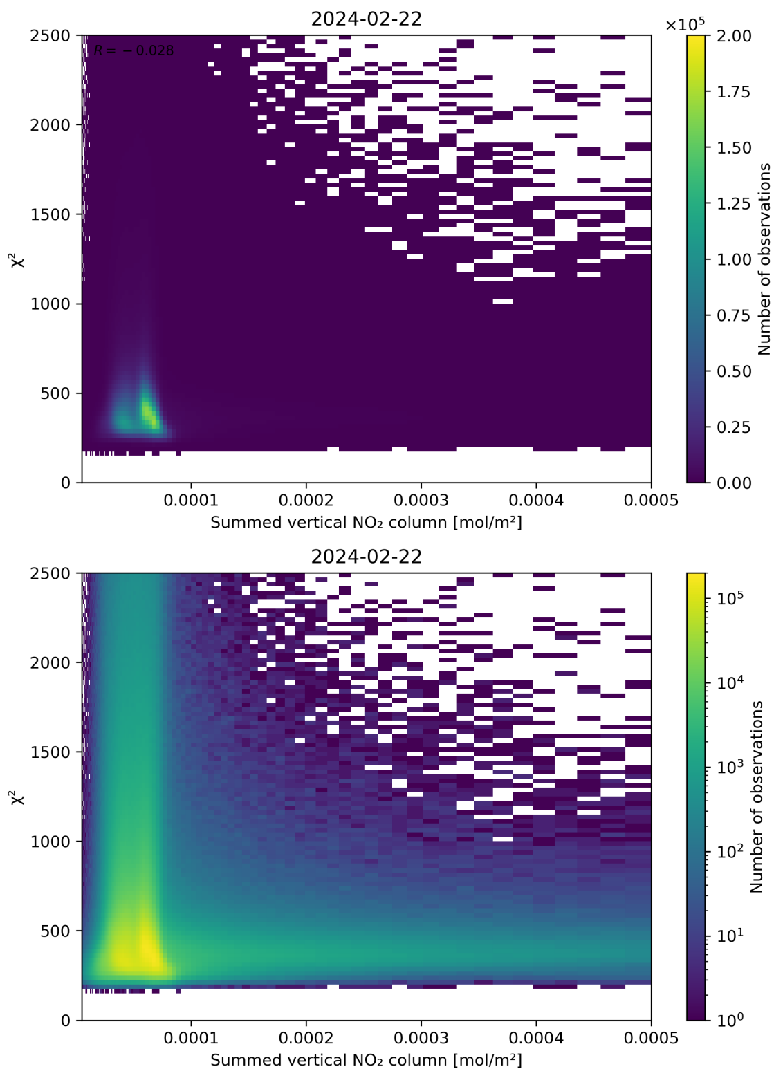
Figure 104: Scatter density plot of “Summed vertical NO 2 column” against “ \chi^2 ” for 2024-02-22 to 2024-02-23.
