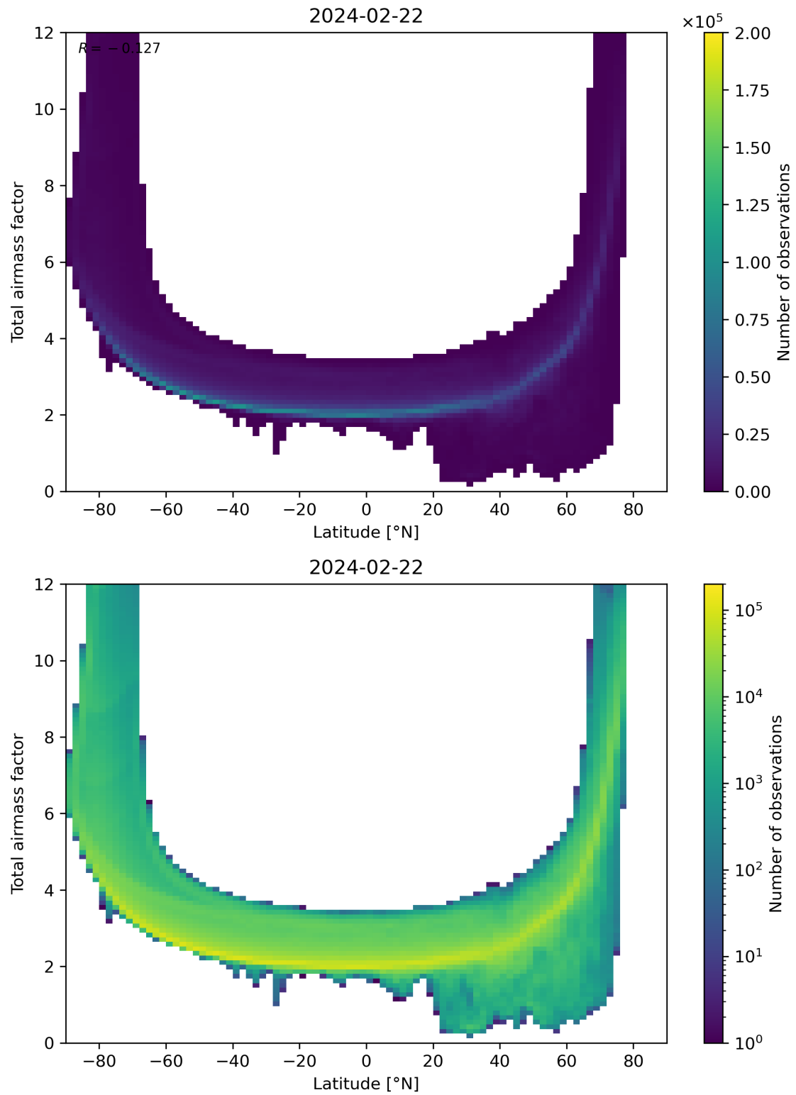
Figure 84: Scatter density plot of “Latitude” against “Total airmass factor” for 2024-02-22 to 2024-02-23.
