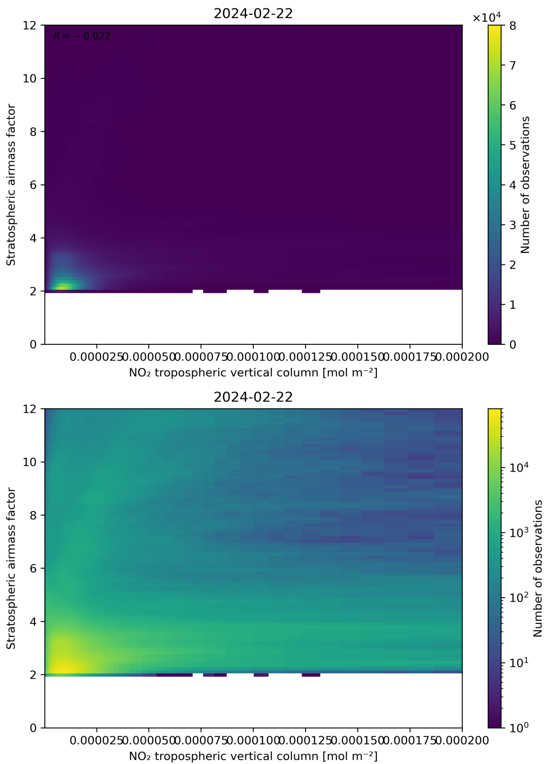
Figure 121: Scatter density plot of “NO 2 tropospheric vertical column” against “Stratospheric airmass factor” for 2024-02-22 to 2024-02-23.
