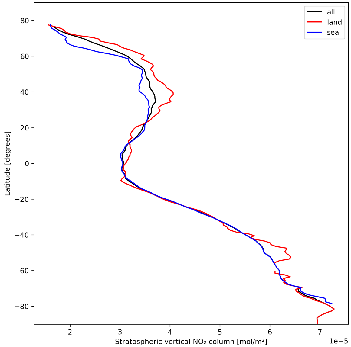
Figure 19: Zonal average of “Stratospheric vertical NO 2 column” for 2024-02-22 to 2024-02-23.
