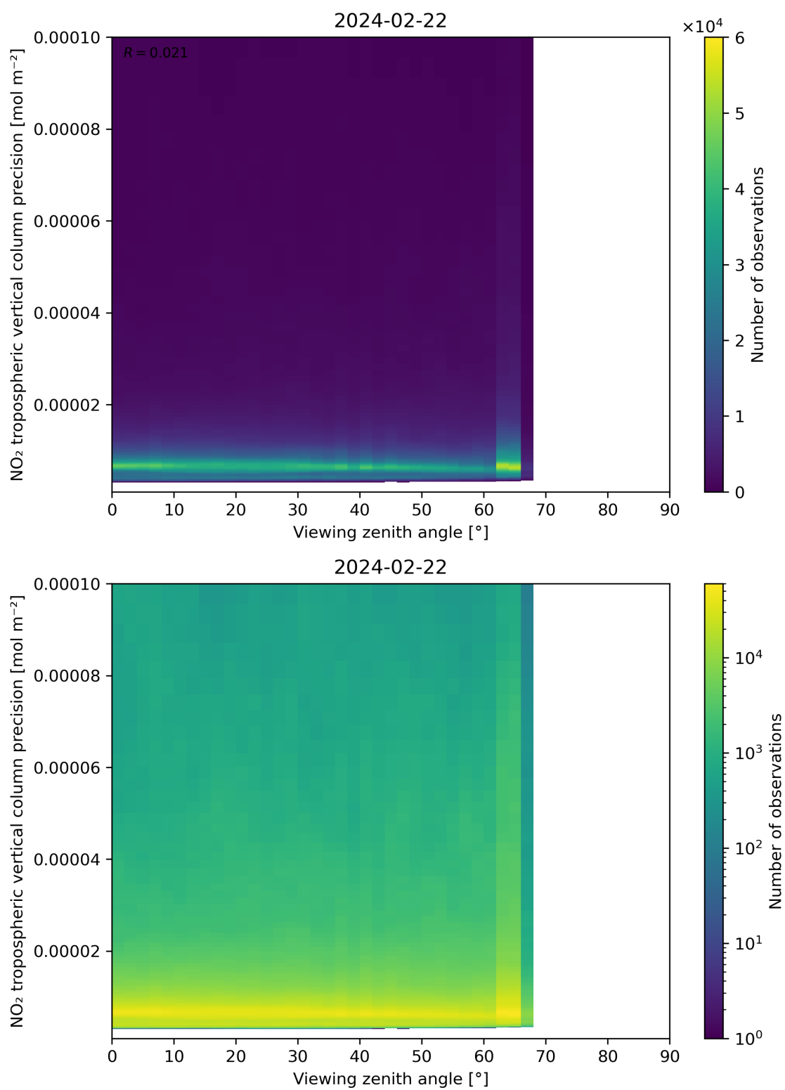
Figure 170: Scatter density plot of “Viewing zenith angle” against “NO 2 tropospheric vertical column precision” for 2024-02-22 to 2024-02-23.
