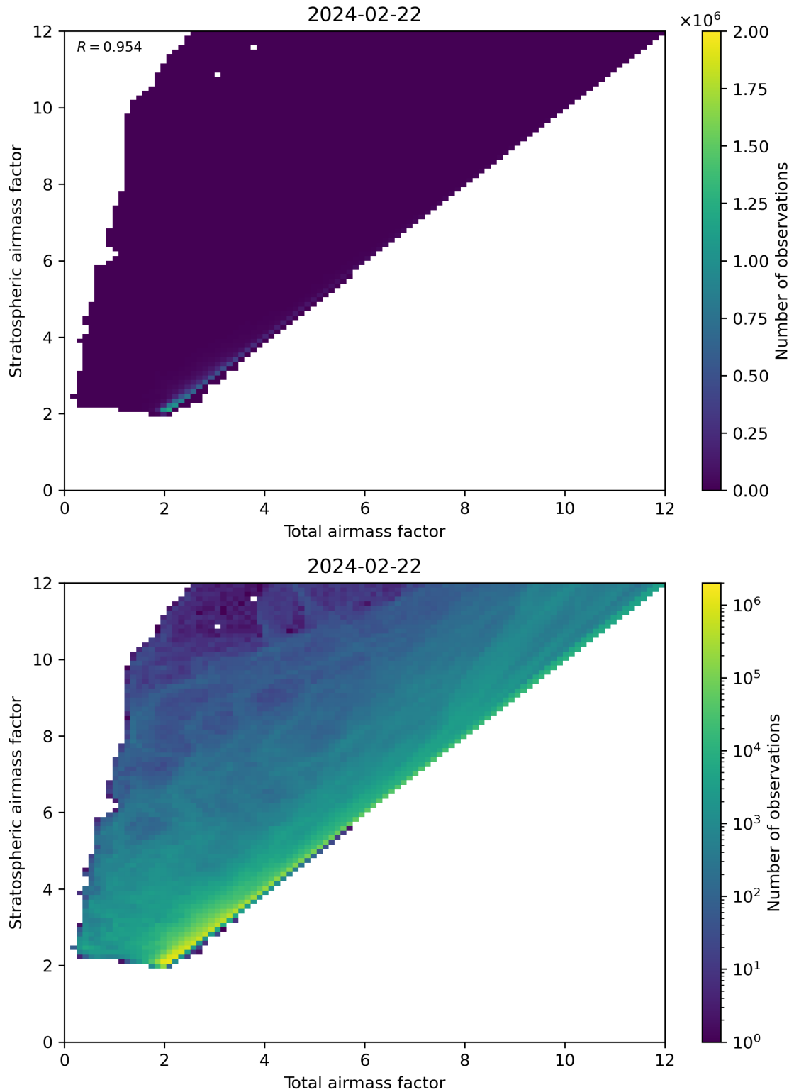
Figure 62: Scatter density plot of “Total airmass factor” against “Stratospheric airmass factor” for 2024-02-22 to 2024-02-23.
