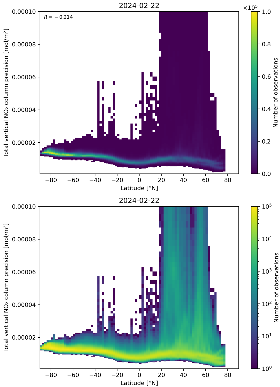
Figure 91: Scatter density plot of “Latitude” against “Total vertical NO 2 column precision” for 2024-02-22 to 2024-02-23.
