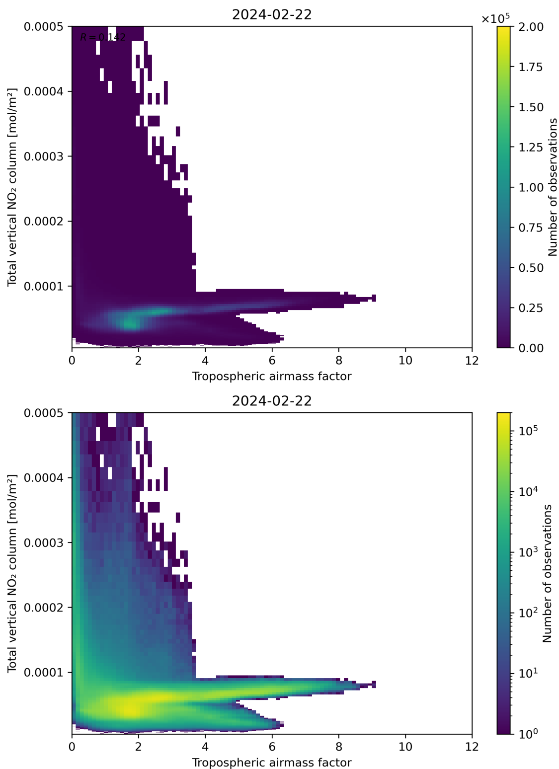
Figure 77: Scatter density plot of “Tropospheric airmass factor” against “Total vertical NO 2 column” for 2024-02-22 to 2024-02-23.
