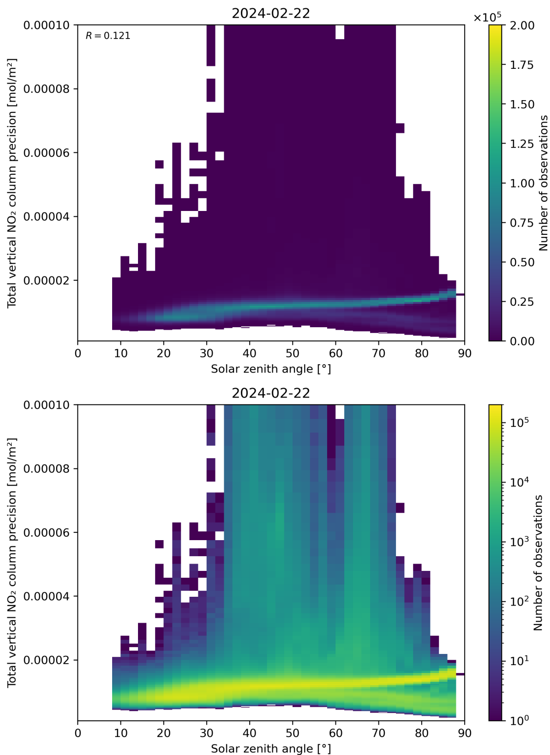
Figure 154: Scatter density plot of “Solar zenith angle” against “Total vertical NO 2 column precision” for 2024-02-22 to 2024-02-23.
