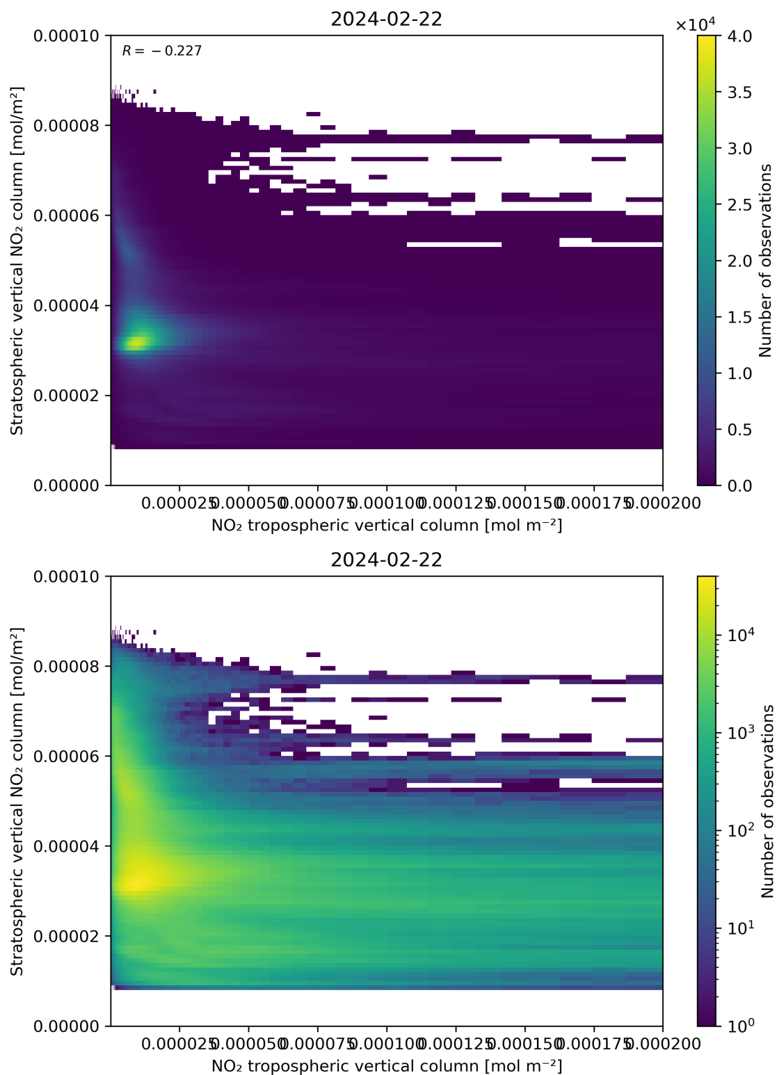
Figure 125: Scatter density plot of “NO 2 tropospheric vertical column” against “Stratospheric vertical NO 2 column” for 2024-02-22 to 2024-02-23.
