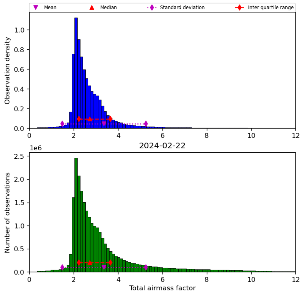
Figure 32: Histogram of “Total airmass factor” for 2024-02-22 to 2024-02-23
