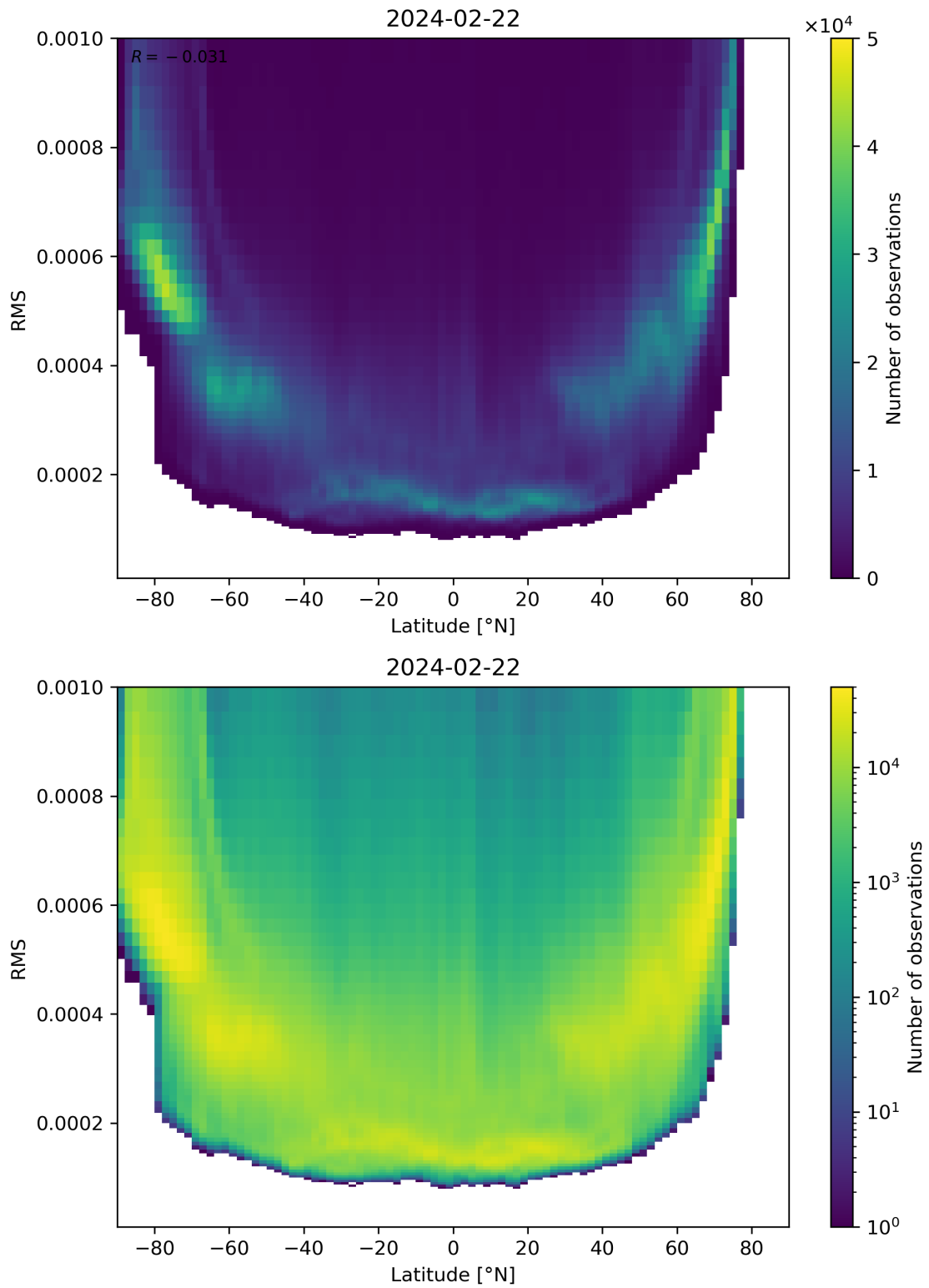
Figure 94: Scatter density plot of “Latitude” against “RMS” for 2024-02-22 to 2024-02-23.
