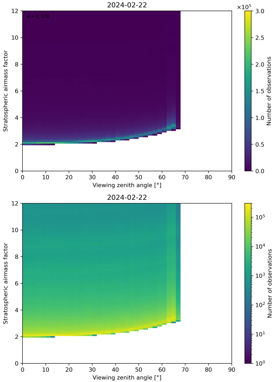
Figure 159: Scatter density plot of “Viewing zenith angle” against “Stratospheric airmass factor” for 2024-02-22 to 2024-02-23.
