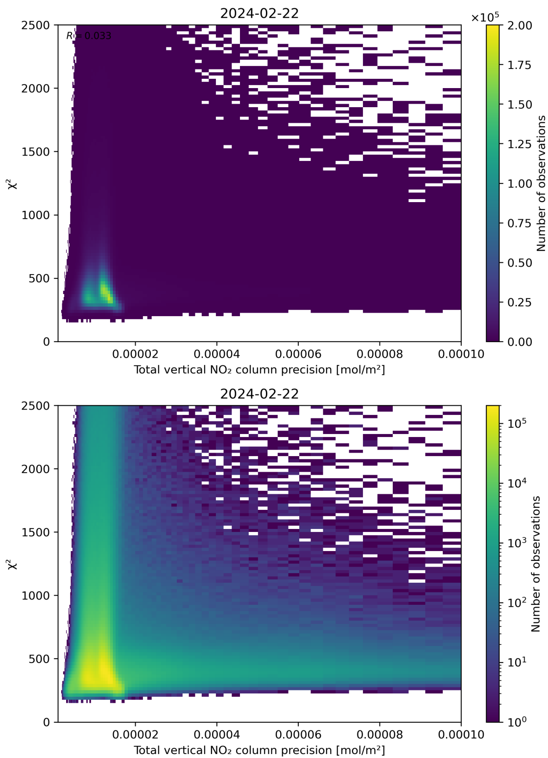
Figure 116: Scatter density plot of “Total vertical NO 2 column precision” against “ \chi^2 ” for 2024-02-22 to 2024-02-23.
