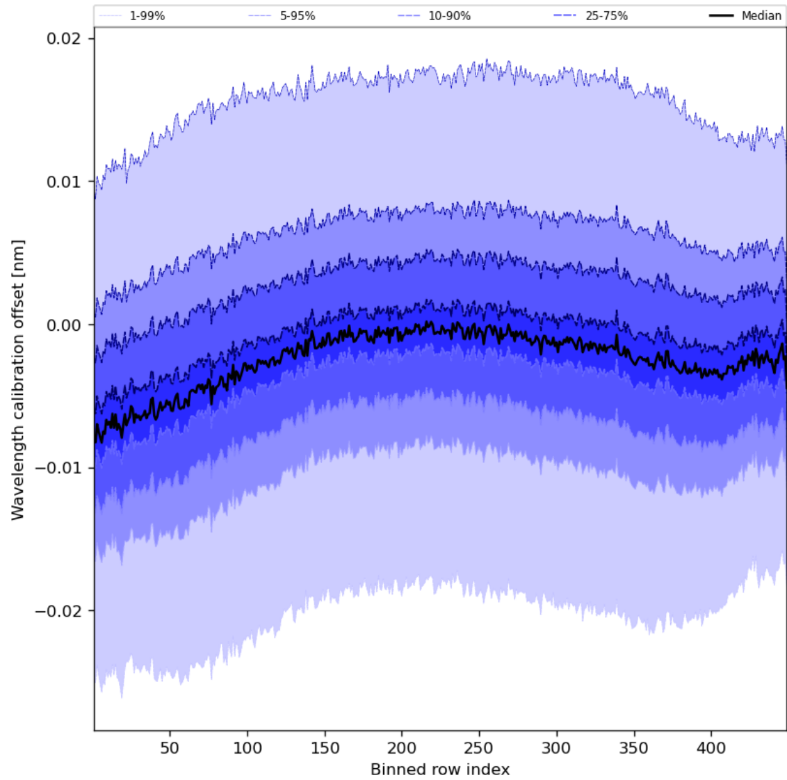
Figure 52: Along track statistics of “Wavelength calibration offset” for 2024-02-22 to 2024-02-23
