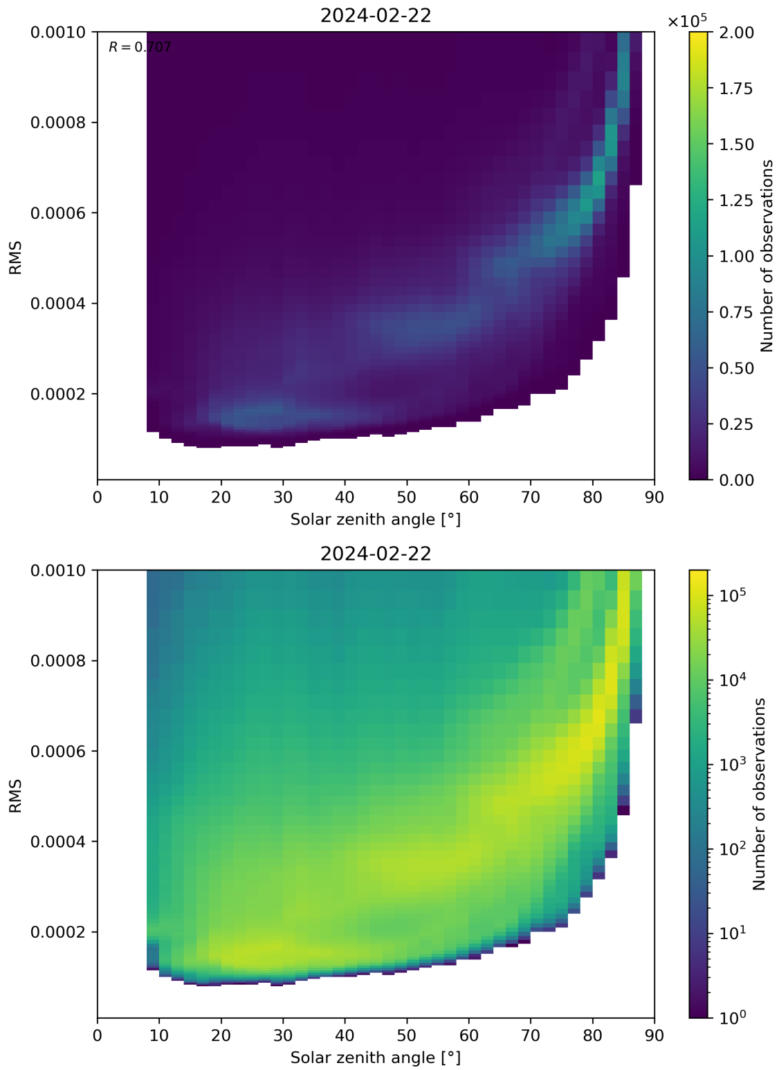
Figure 157: Scatter density plot of “Solar zenith angle” against “RMS” for 2024-02-22 to 2024-02-23.
