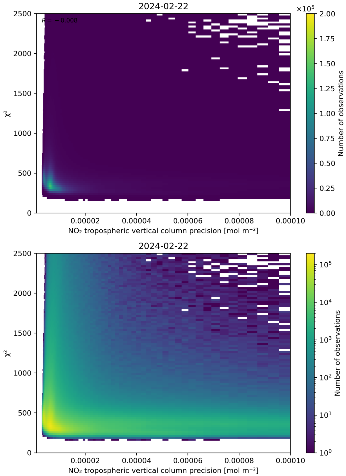
Figure 134: Scatter density plot of “NO 2 tropospheric vertical column precision” against “ \chi^2 ” for 2024-02-22 to 2024-02-23.
