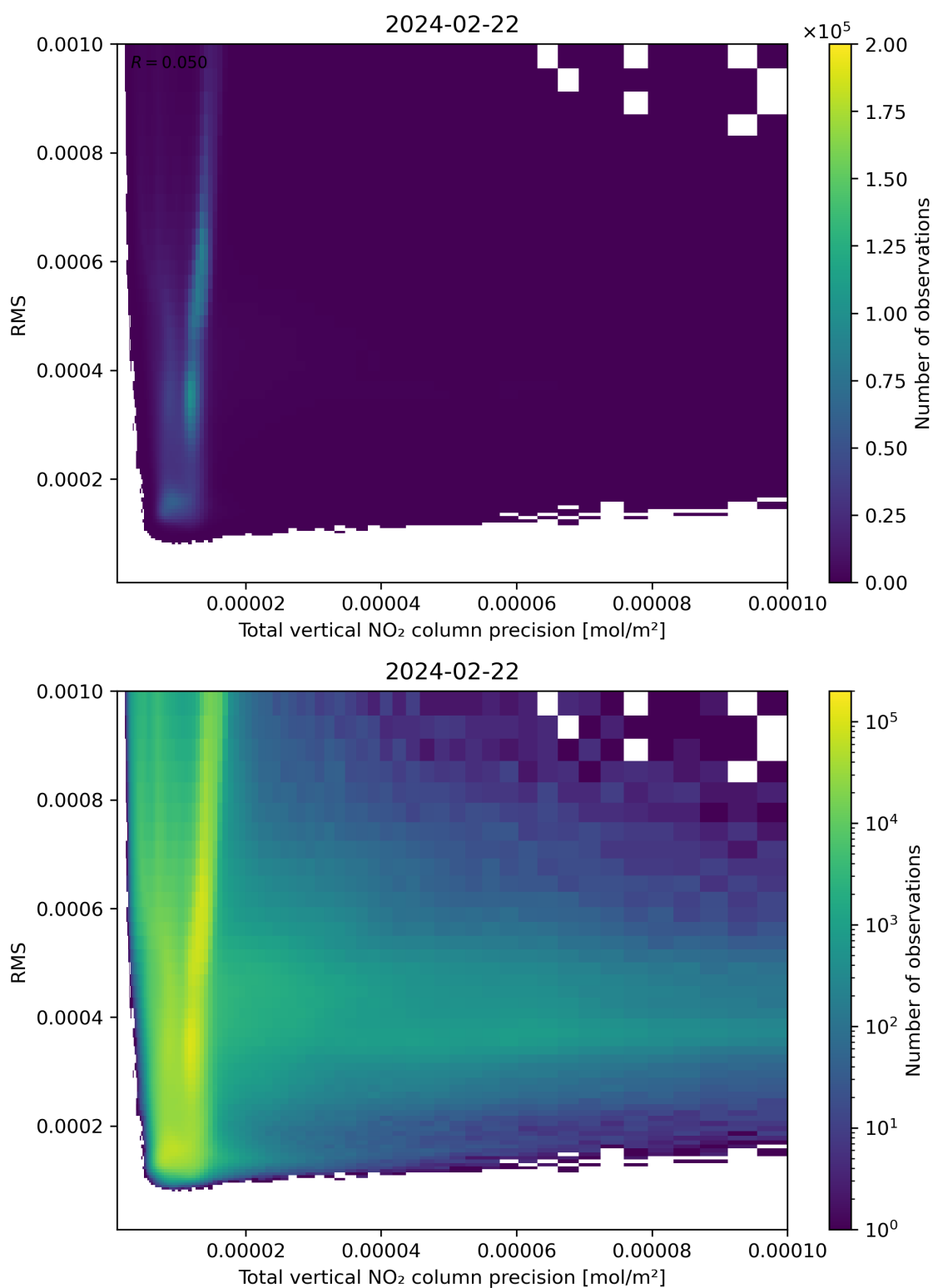
Figure 119: Scatter density plot of “Total vertical NO 2 column precision” against “RMS” for 2024-02-22 to 2024-02-23.
