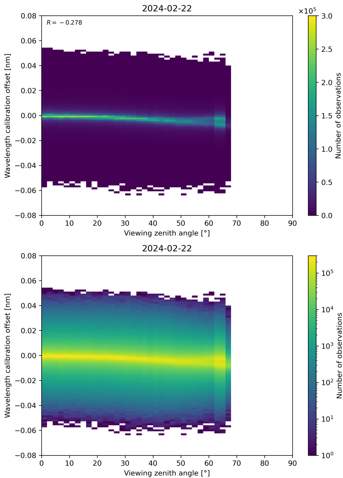
Figure 173: Scatter density plot of “Viewing zenith angle” against “Wavelength calibration offset” for 2024-02-22 to 2024-02-23.
