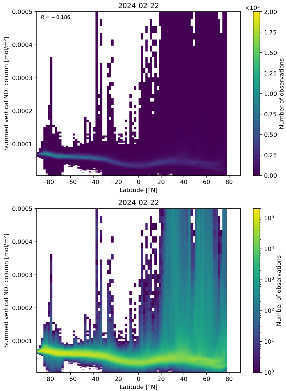
Figure 88: Scatter density plot of “Latitude” against “Summed vertical NO 2 column” for 2024-02-22 to 2024-02-23.
