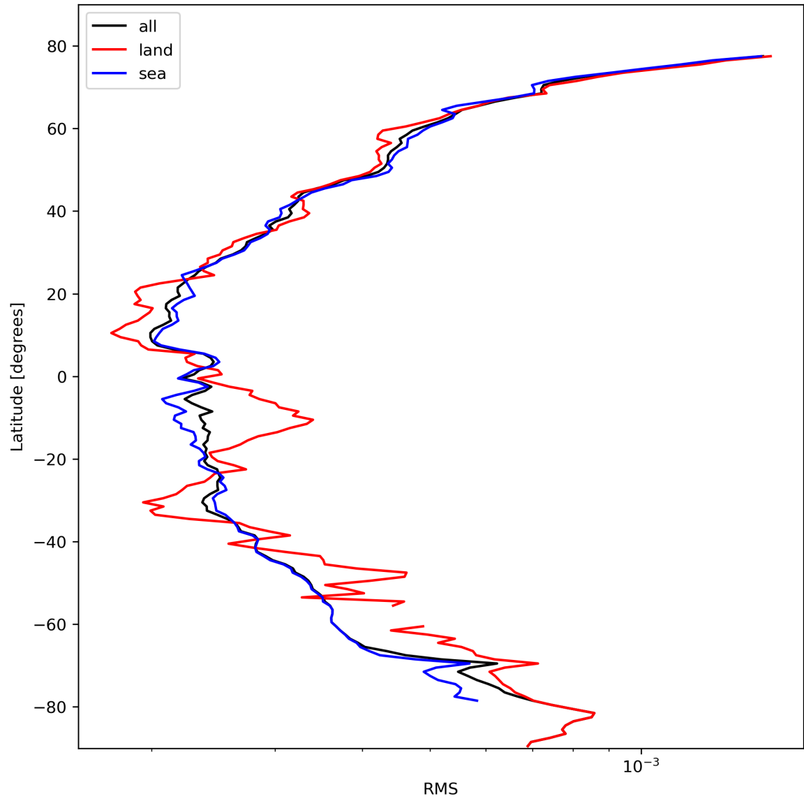
Figure 26: Zonal average of “RMS” for 2024-02-22 to 2024-02-23.
