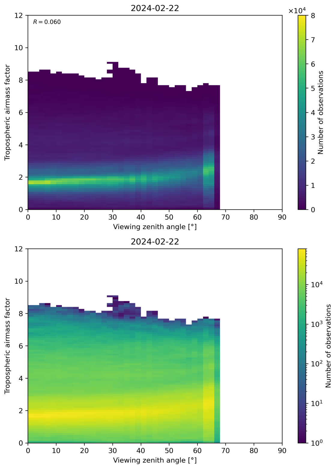
Figure 161: Scatter density plot of “Viewing zenith angle” against “Tropospheric airmass factor” for 2024-02-22 to 2024-02-23.
