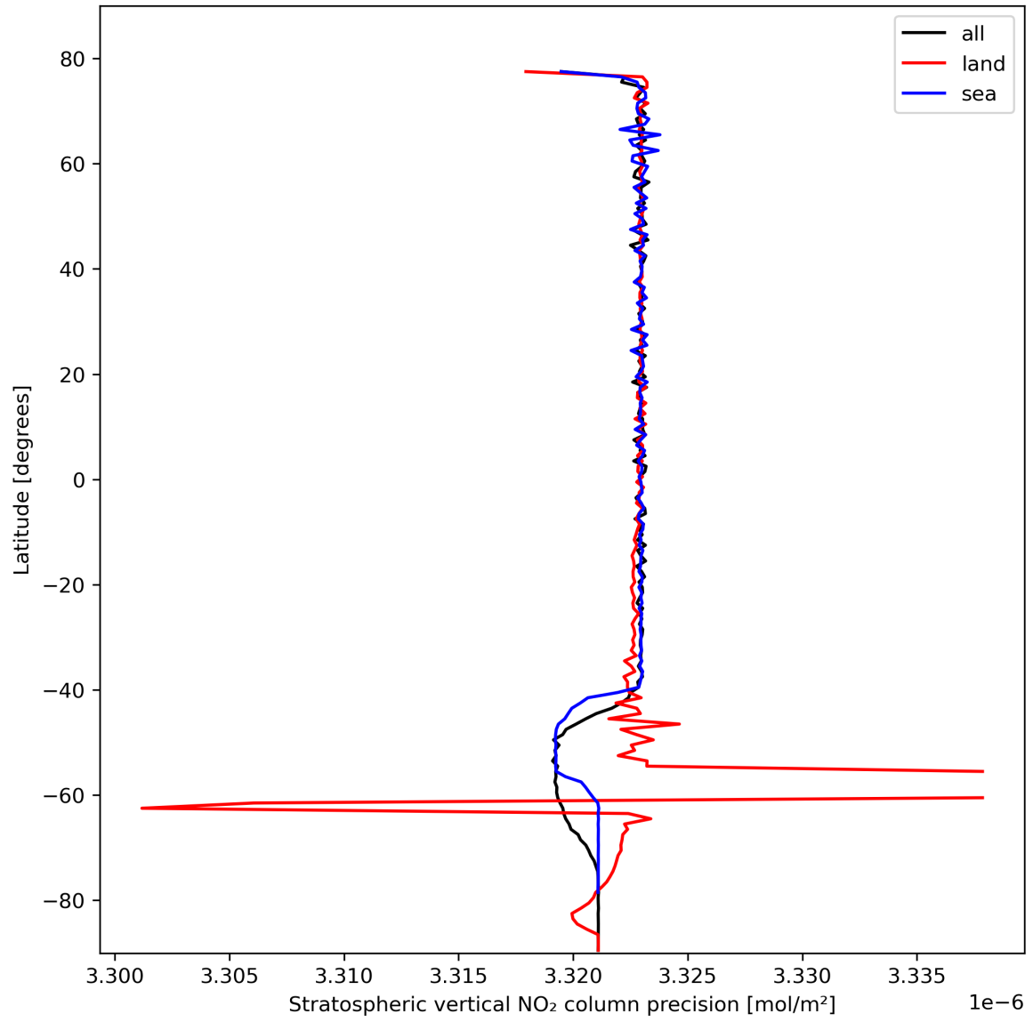
Figure 20: Zonal average of “Stratospheric vertical NO 2 column precision” for 2024-02-22 to 2024-02-23.
