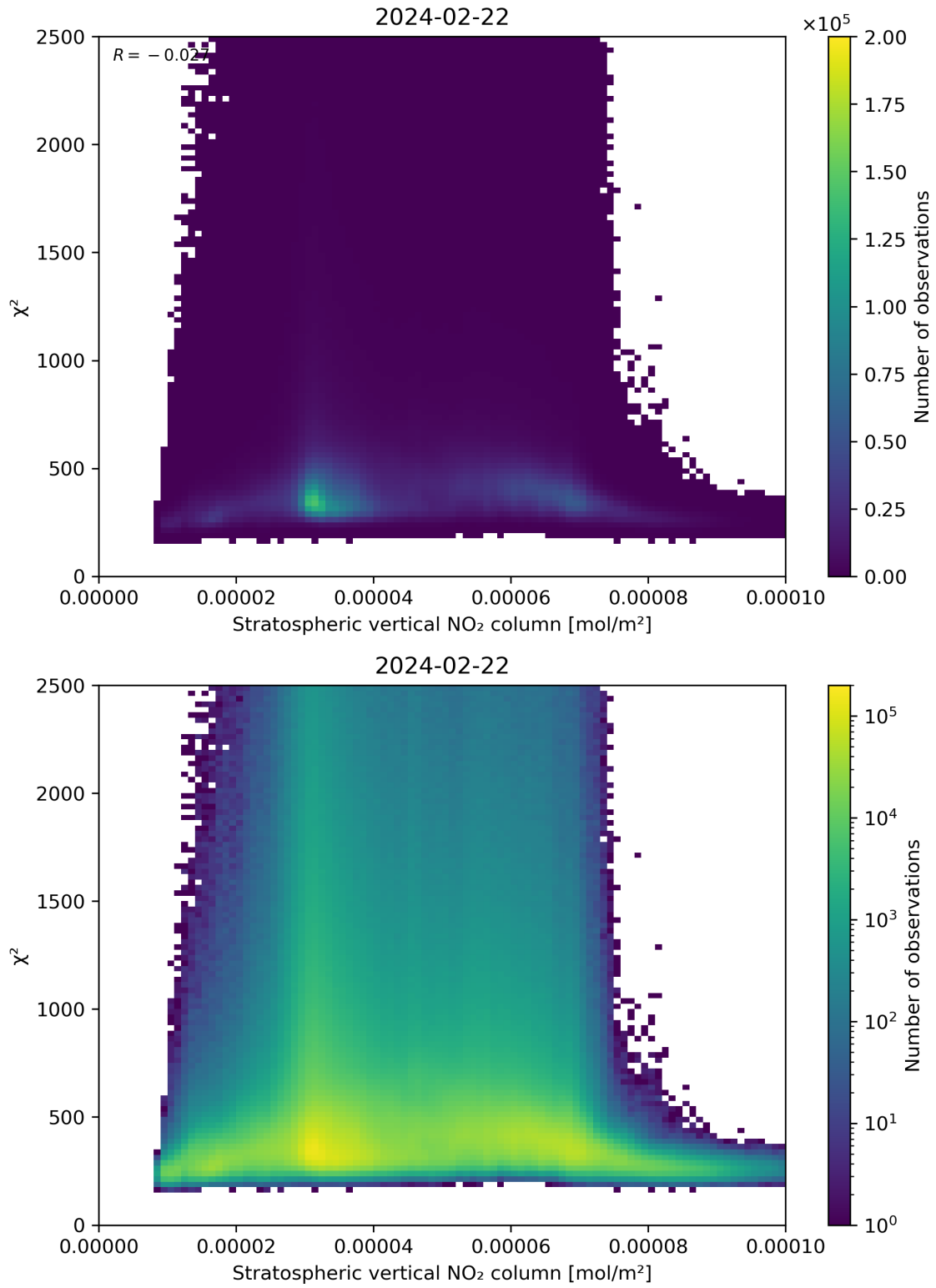
Figure 97: Scatter density plot of “Stratospheric vertical NO 2 column” against “ \chi^2 ” for 2024-02-22 to 2024-02-23.
