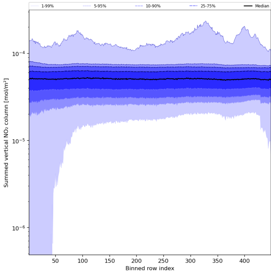
Figure 57: Along track statistics of “Summed vertical NO 2 column” for 2024-02-22 to 2024-02-23
