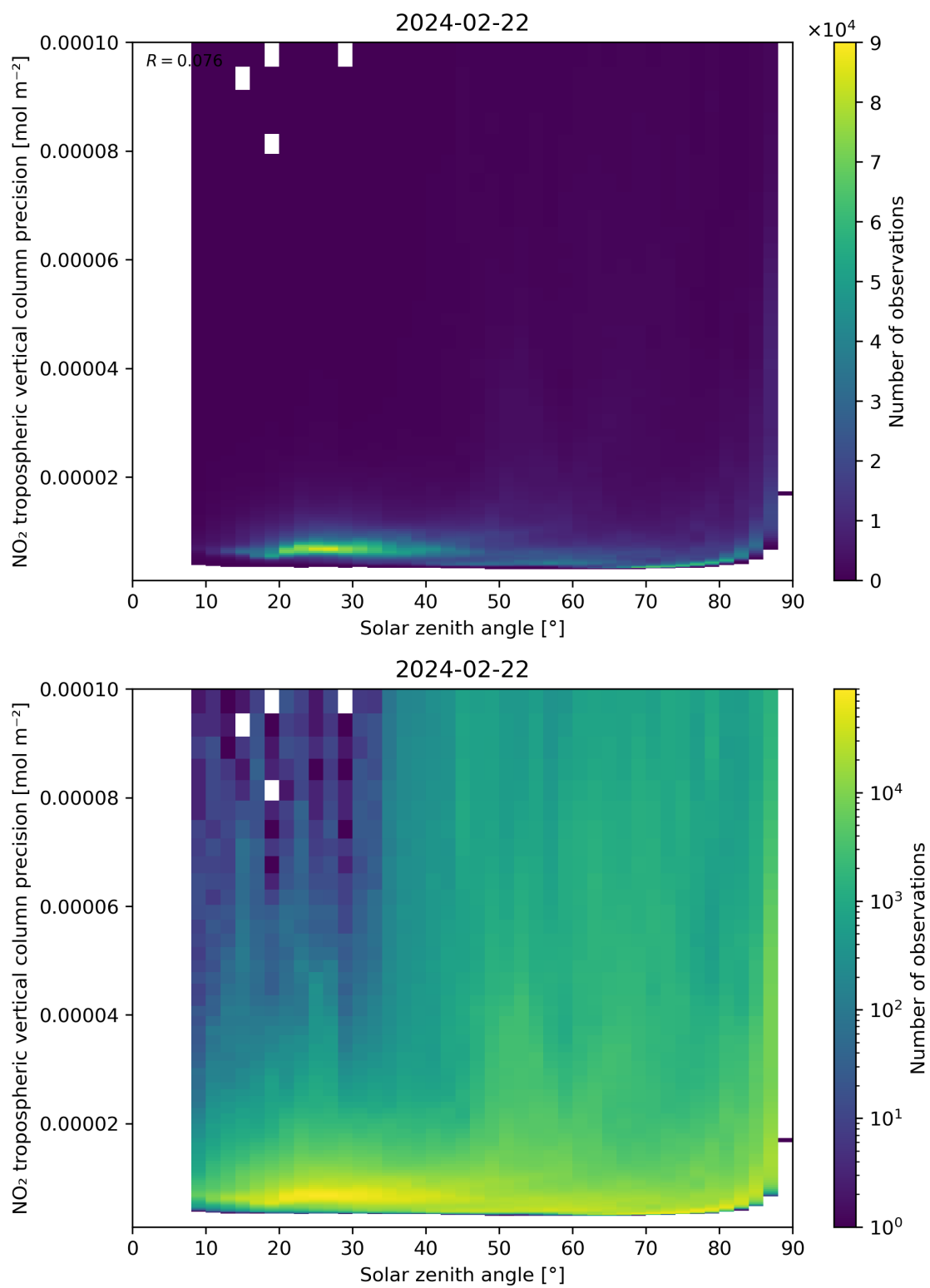
Figure 156: Scatter density plot of “Solar zenith angle” against “NO 2 tropospheric vertical column precision” for 2024-02-22 to 2024-02-23.
