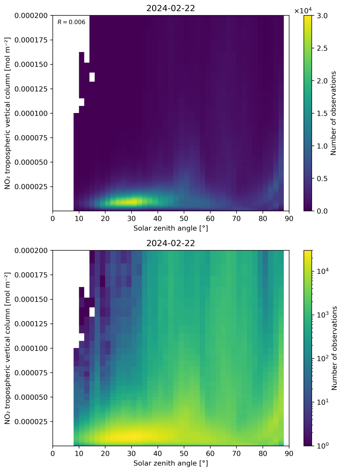
Figure 155: Scatter density plot of “Solar zenith angle” against “NO 2 tropospheric vertical column” for 2024-02-22 to 2024-02-23.
