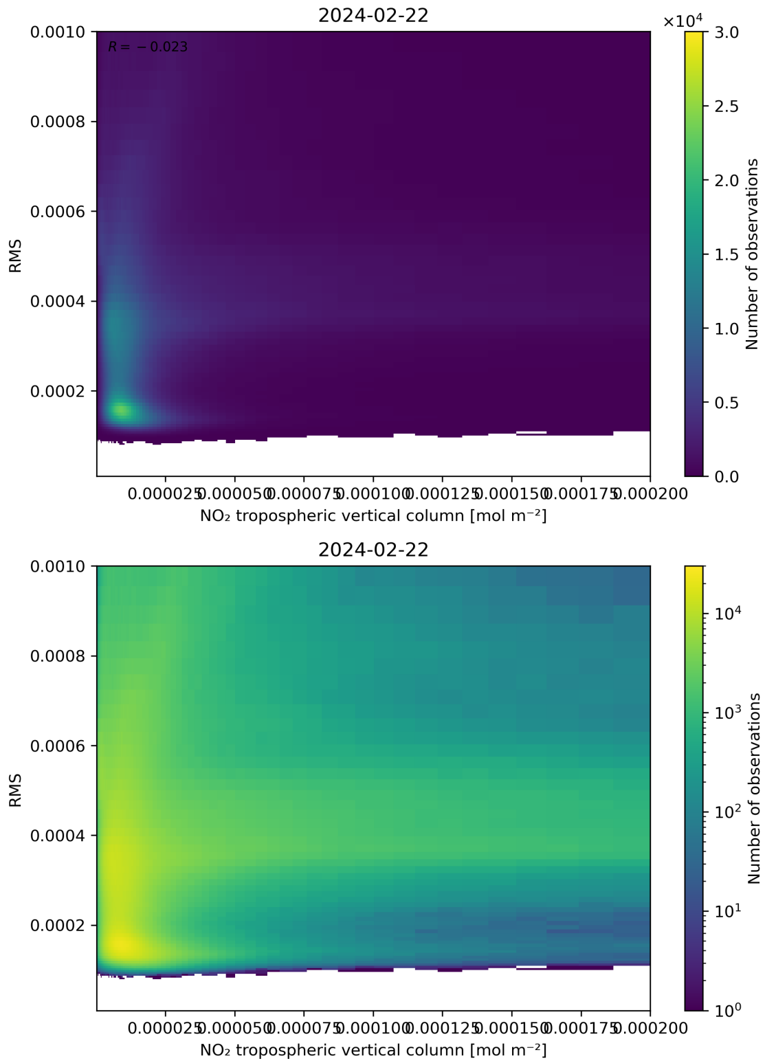
Figure 142: Scatter density plot of “NO 2 tropospheric vertical column” against “RMS” for 2024-02-22 to 2024-02-23.
