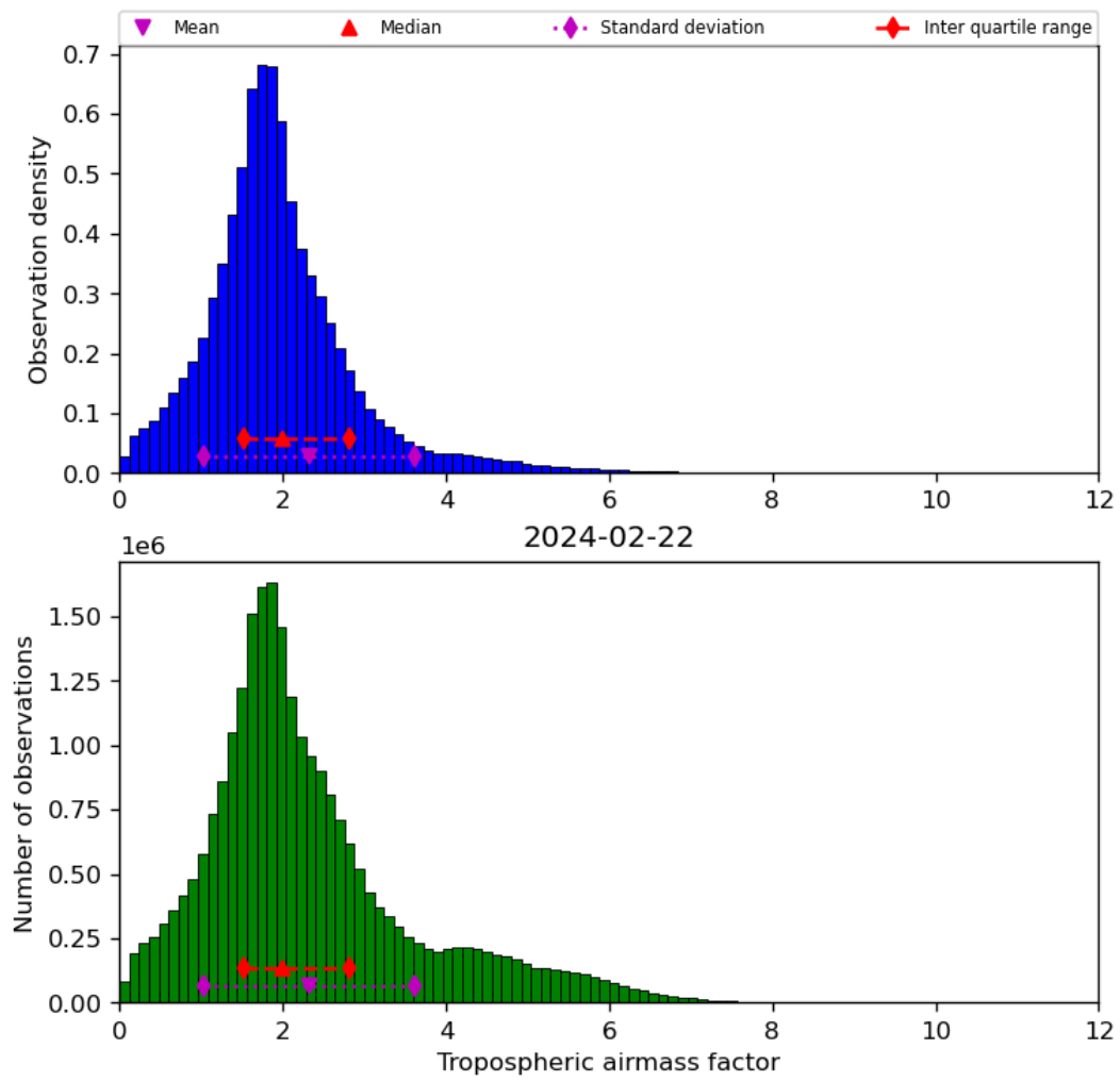
Figure 31: Histogram of “Tropospheric airmass factor” for 2024-02-22 to 2024-02-23
