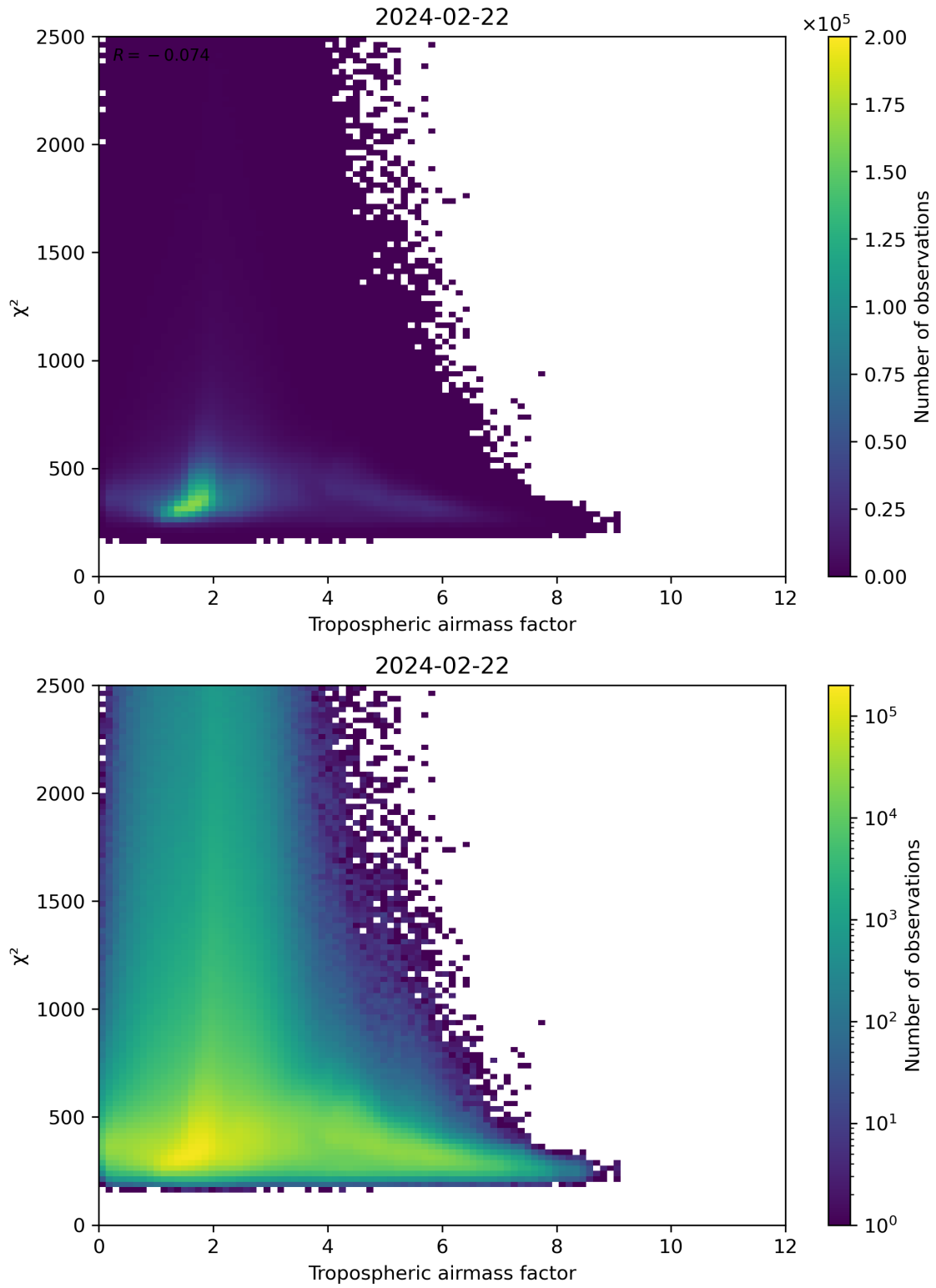
Figure 73: Scatter density plot of “Tropospheric airmass factor” against “ \chi^2 ” for 2024-02-22 to 2024-02-23.
