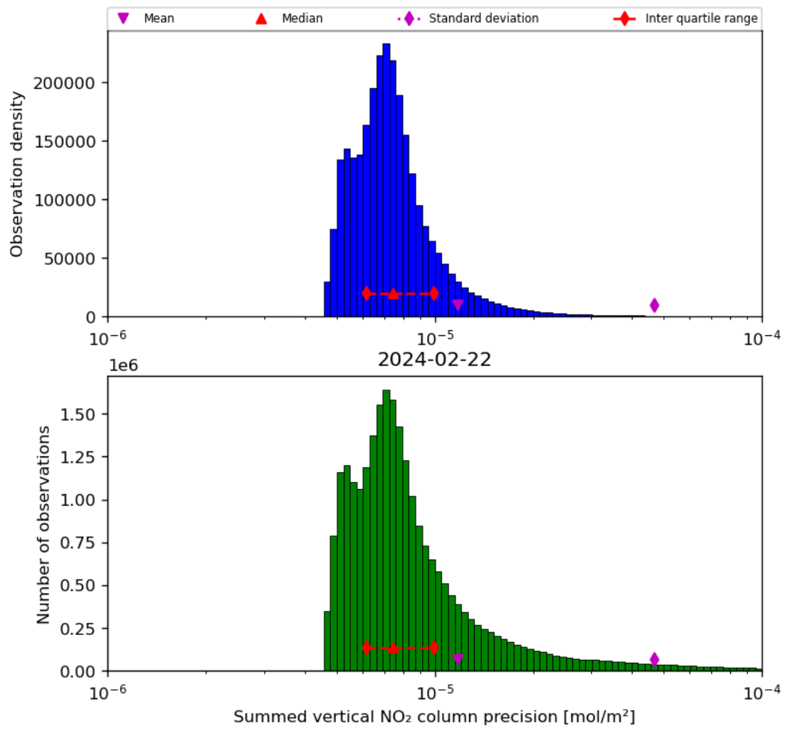
Figure 41: Histogram of “Summed vertical NO 2 column precision” for 2024-02-22 to 2024-02-23
