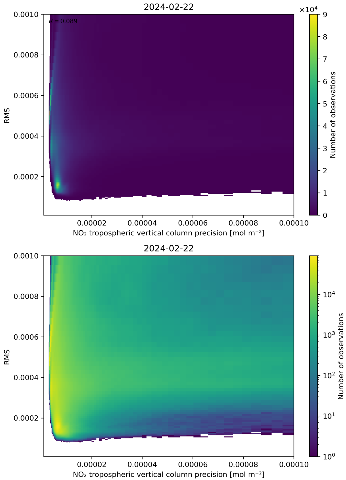
Figure 140: Scatter density plot of “NO 2 tropospheric vertical column precision” against “RMS” for 2024-02-22 to 2024-02-23.
