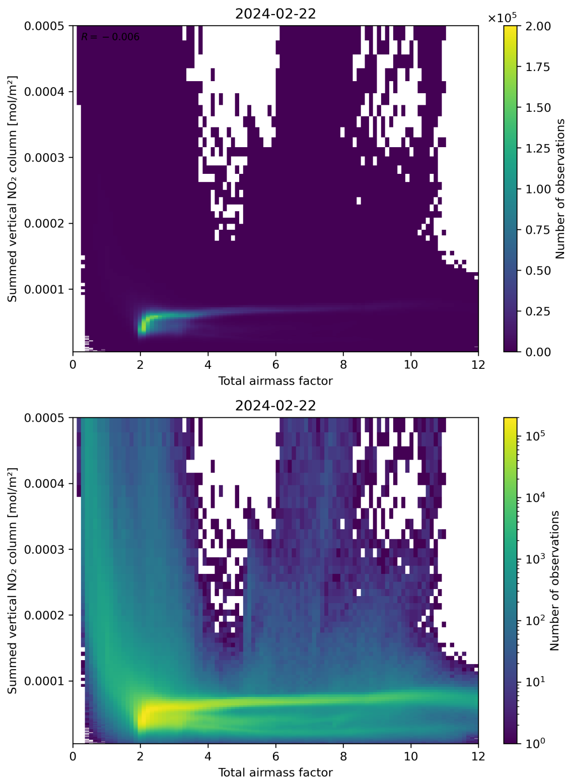
Figure 65: Scatter density plot of “Total airmass factor” against “Summed vertical NO 2 column” for 2024-02-22 to 2024-02-23.
