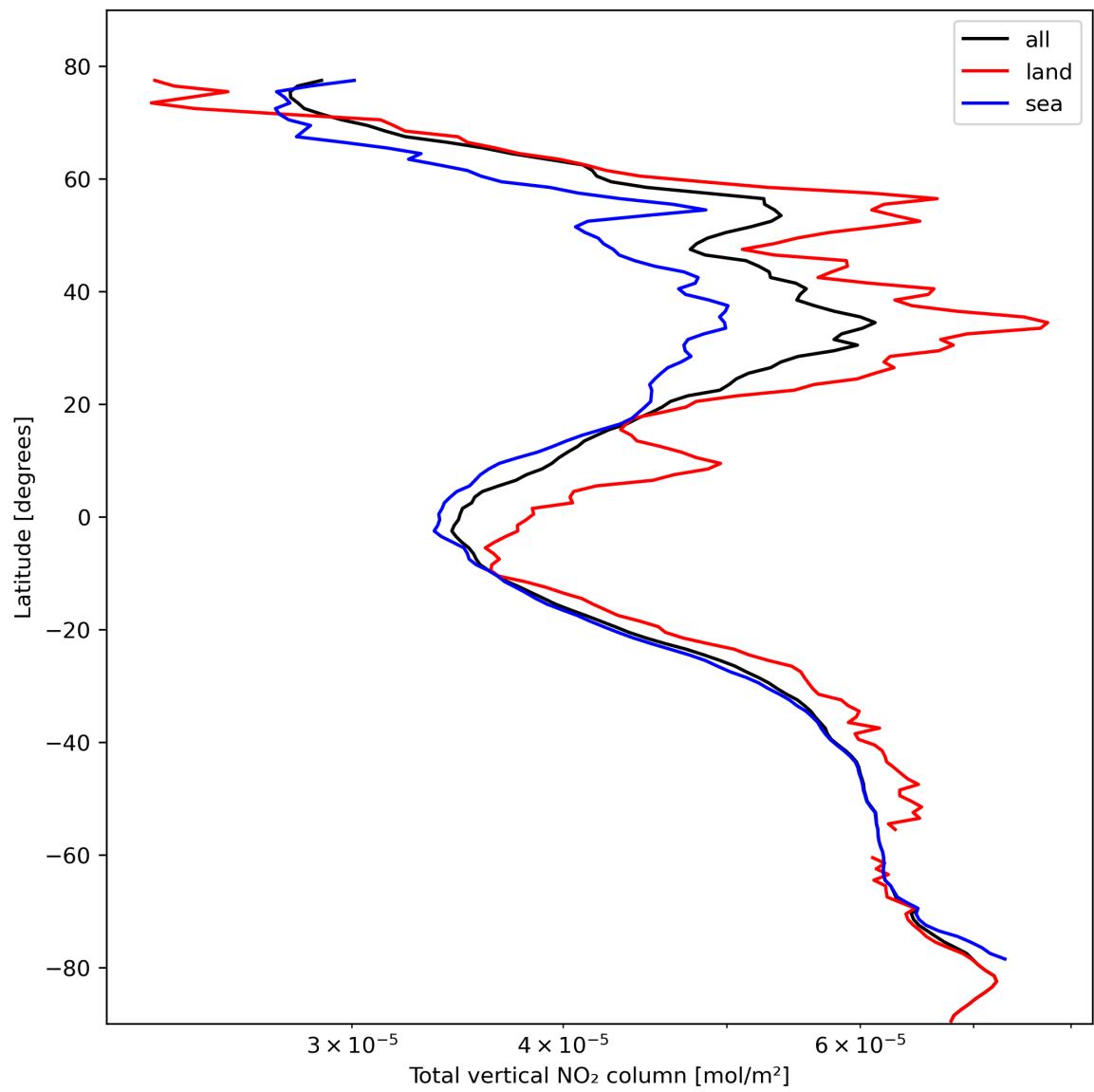
Figure 21: Zonal average of “Total vertical NO 2 column” for 2024-02-22 to 2024-02-23.
