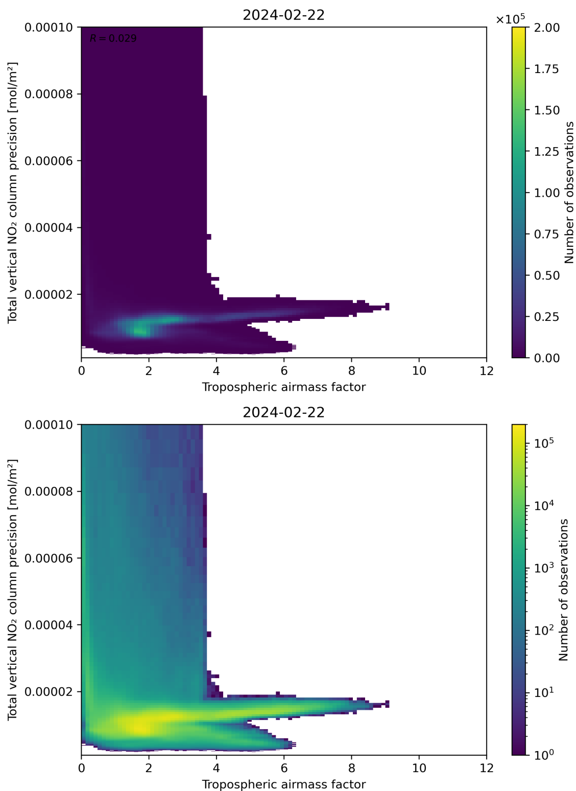
Figure 78: Scatter density plot of “Tropospheric air mass factor” against “Total vertical NO 2 column precision” for 2024-02-22 to 2024-02-23.
