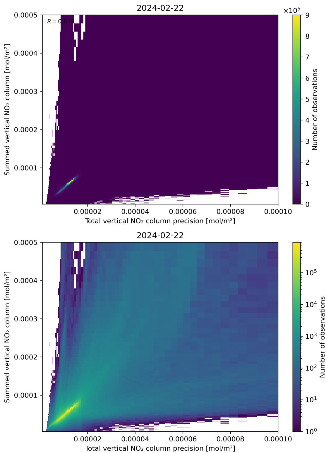
Figure 117: Scatter density plot of “Total vertical NO 2 column precision” against “Summed vertical NO 2 column” for 2024-02-22 to 2024-02-23.
