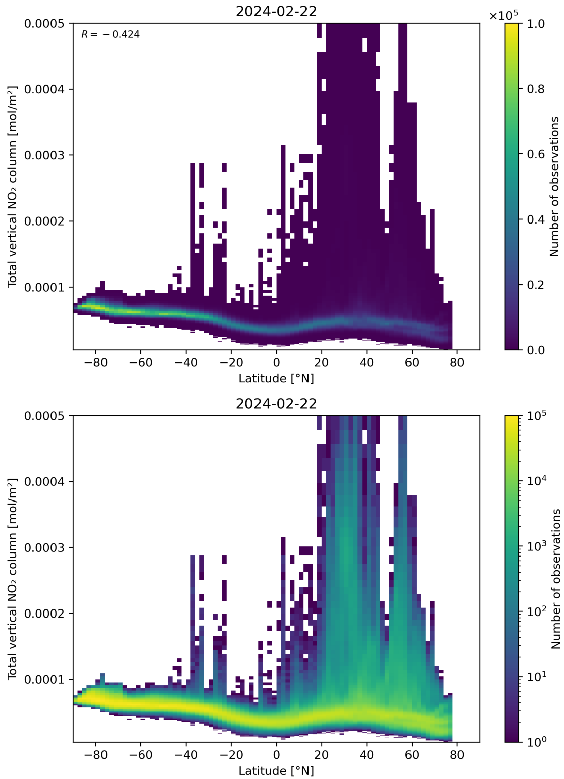
Figure 90: Scatter density plot of “Latitude” against “Total vertical NO 2 column” for 2024-02-22 to 2024-02-23.
