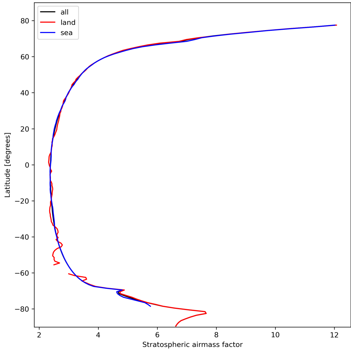
Figure 27: Zonal average of “Stratospheric air mass factor” for 2024-02-22 to 2024-02-23.
