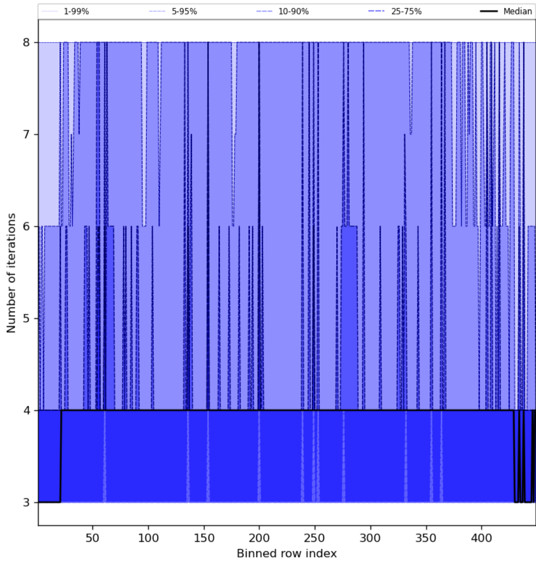
Figure 51: Along track statistics of “Number of iterations” for 2024-02-22 to 2024-02-23
