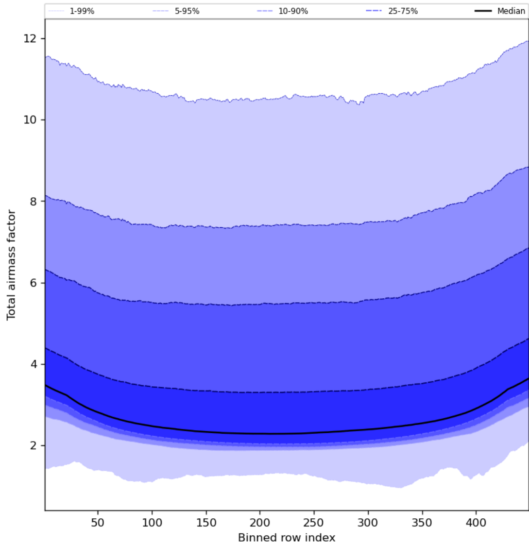
Figure 49: Along track statistics of “Total airmass factor” for 2024-02-22 to 2024-02-23
