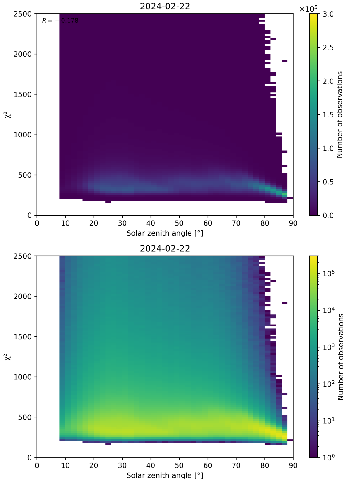
Figure 148: Scatter density plot of “Solar zenith angle” against “ \chi^2 ” for 2024-02-22 to 2024-02-23.
