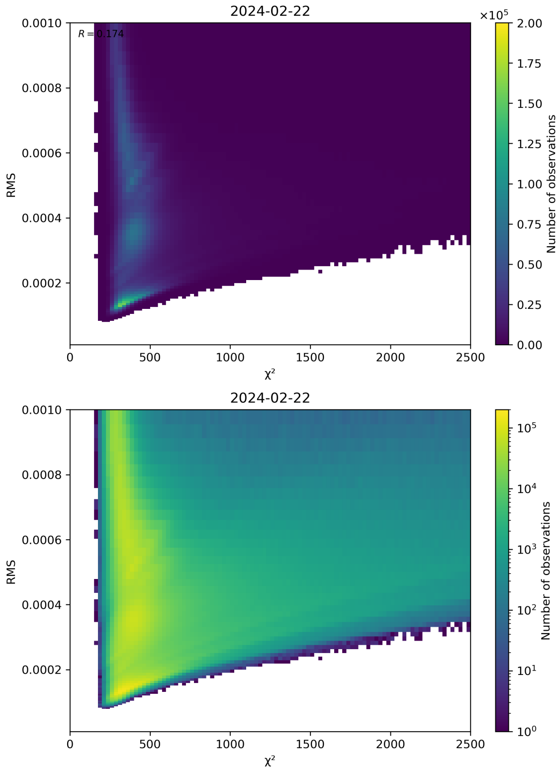
Figure 82: Scatter density plot of “ \chi^2 ” against “RMS” for 2024-02-22 to 2024-02-23.
