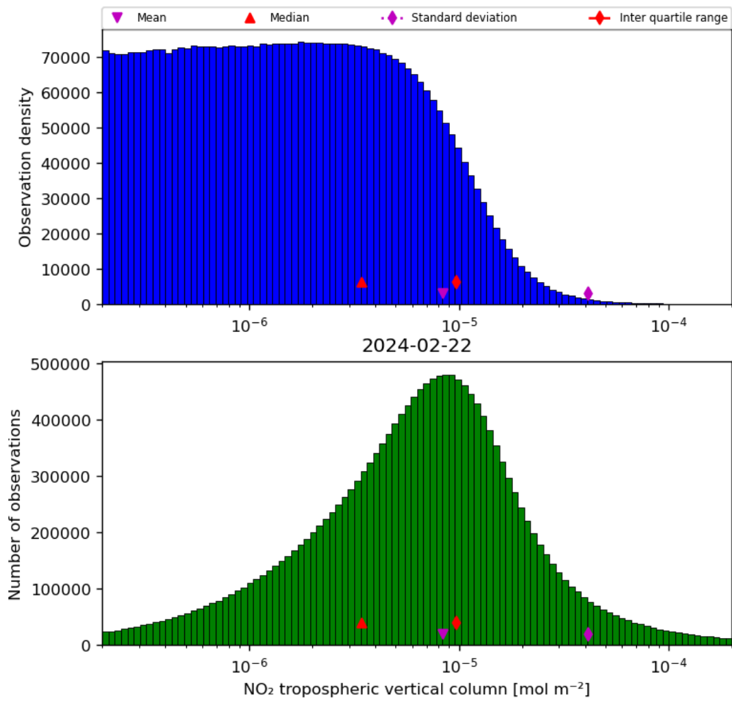
Figure 29: Histogram of “NO 2 tropospheric vertical column” for 2024-02-22 to 2024-02-23
