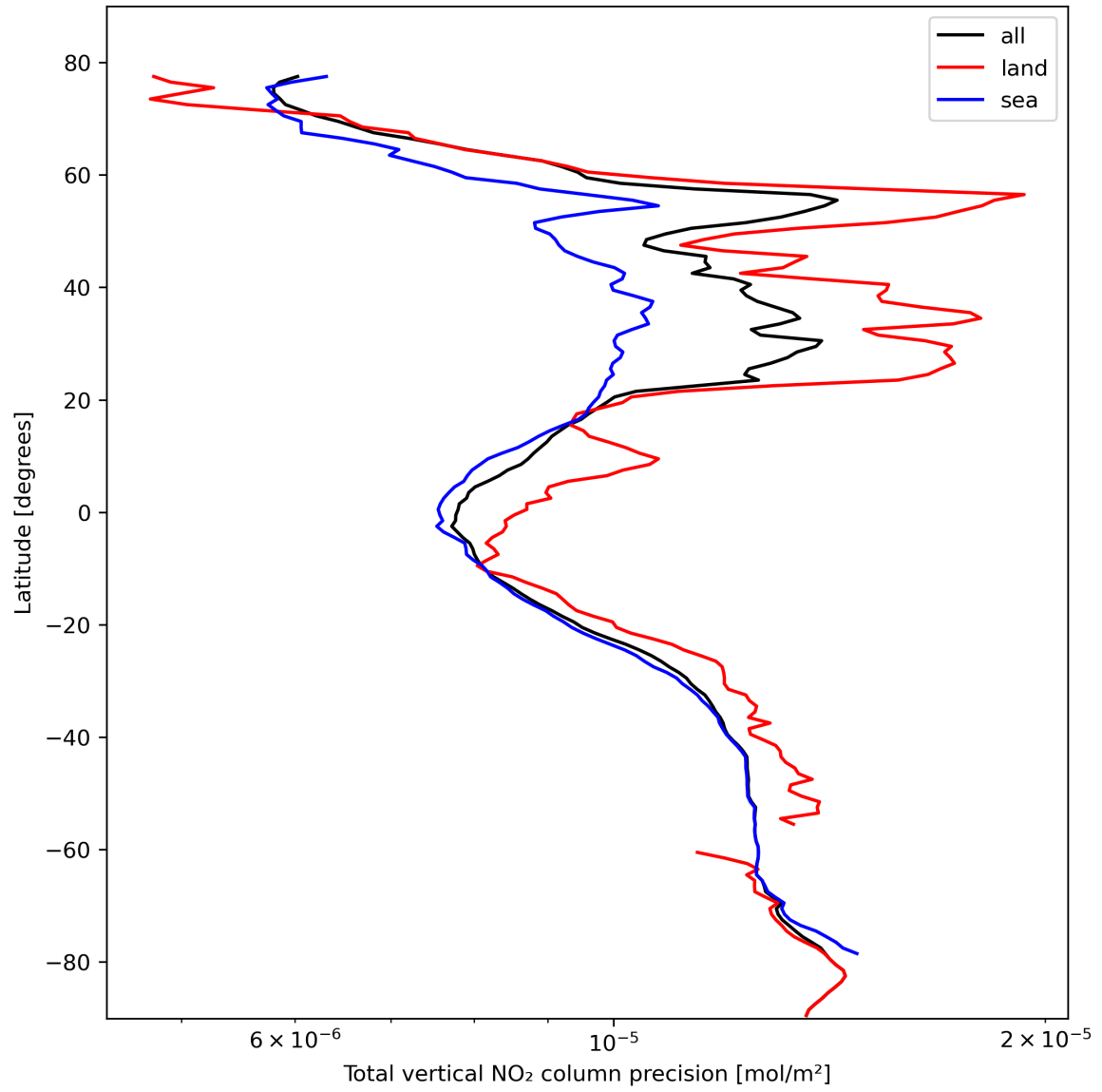
Figure 22: Zonal average of “Total vertical NO 2 column precision” for 2024-02-22 to 2024-02-23.
