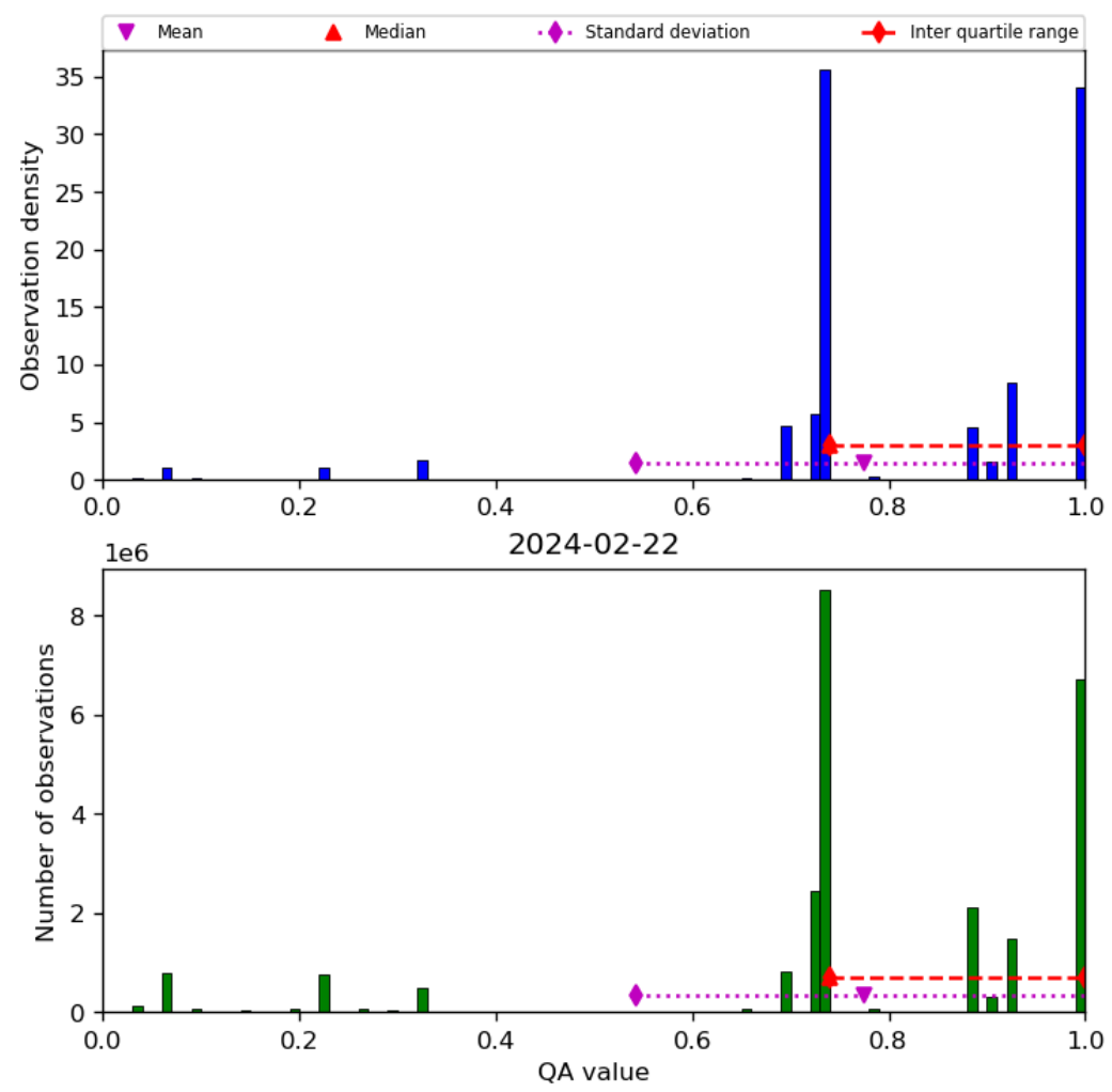
Figure 28: Histogram of “QA value” for 2024-02-22 to 2024-02-23
