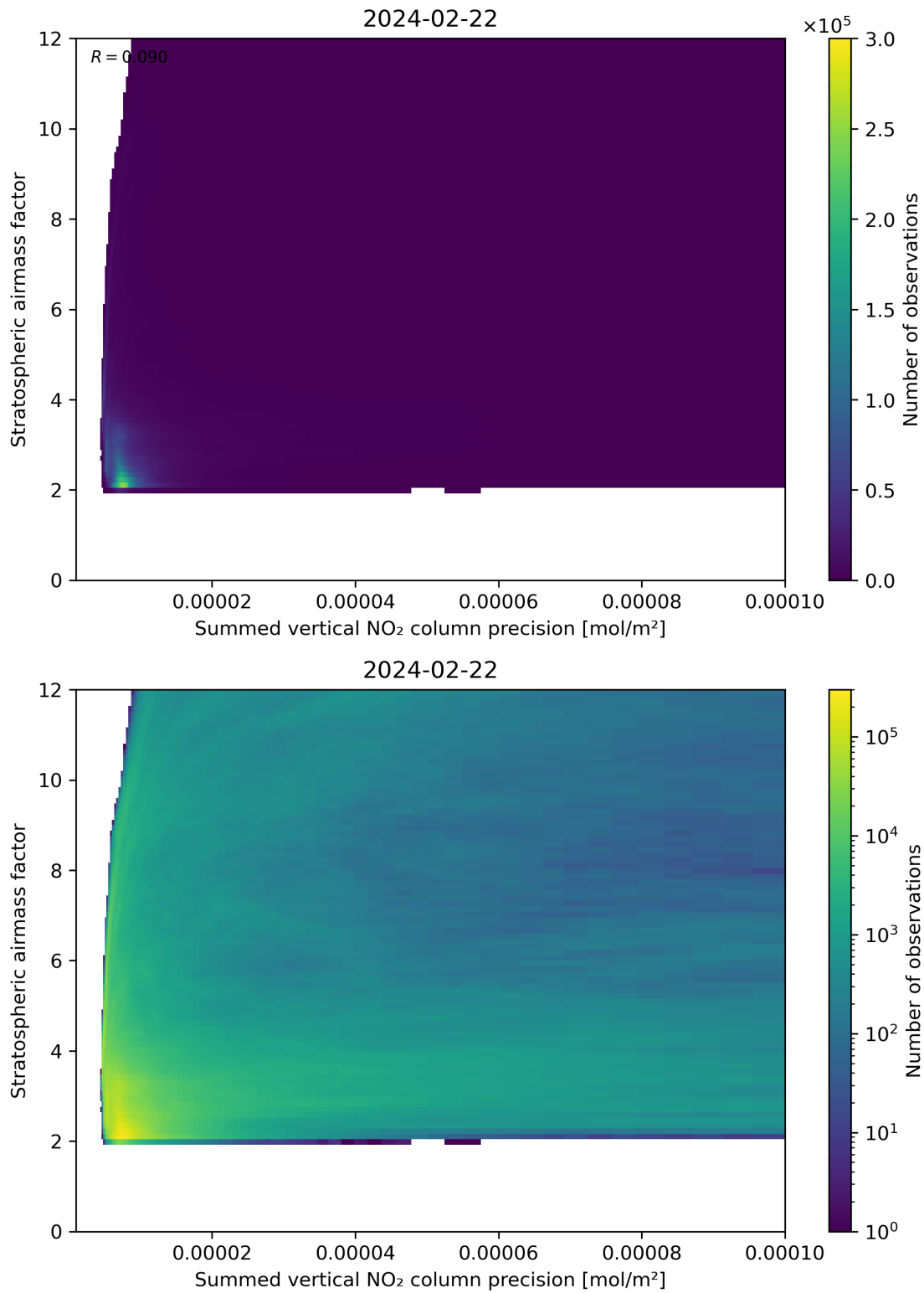
Figure 106: Scatter density plot of “Summed vertical NO 2 column precision” against “Stratospheric airmass factor” for 2024-02-22 to 2024-02-23.
