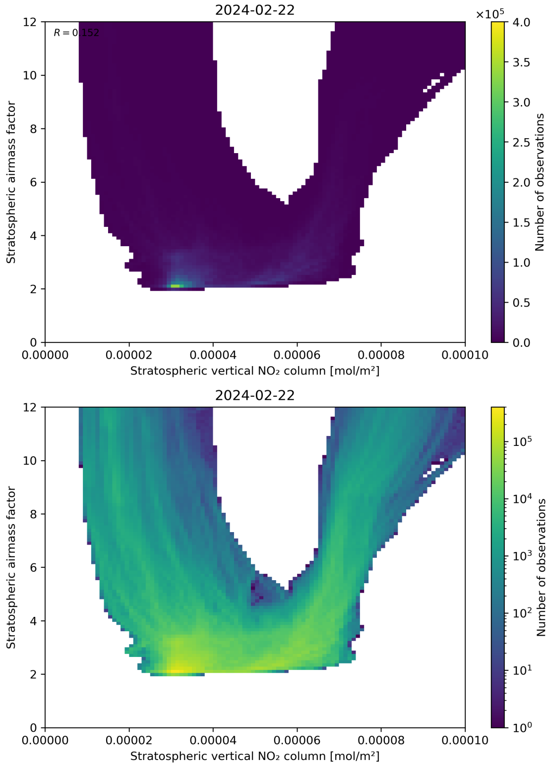
Figure 96: Scatter density plot of “Stratospheric vertical NO 2 column” against “Stratospheric airmass factor” for 2024-02-22 to 2024-02-23.
