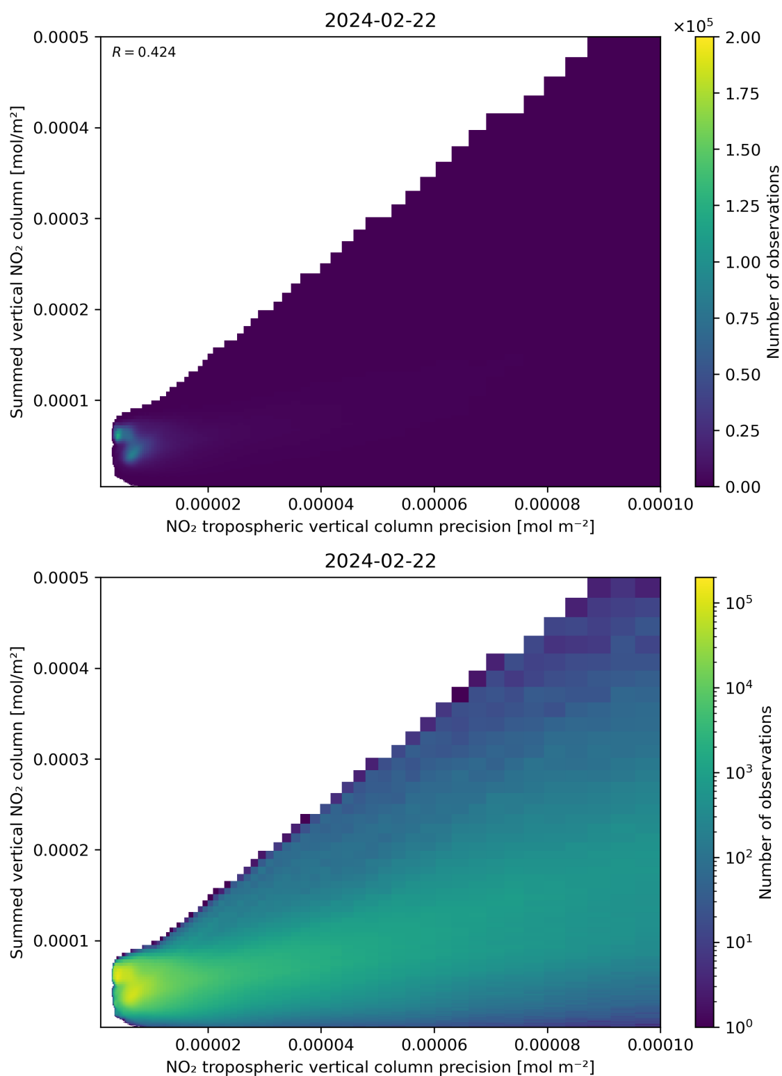
Figure 136: Scatter density plot of “NO 2 tropospheric vertical column precision” against “Summed vertical NO 2 column” for 2024-02-22 to 2024-02-23.
