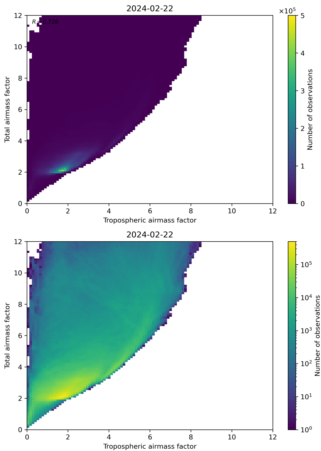
Figure 72: Scatter density plot of “Tropospheric airmass factor” against “Total airmass factor” for 2024-02-22 to 2024-02-23.
