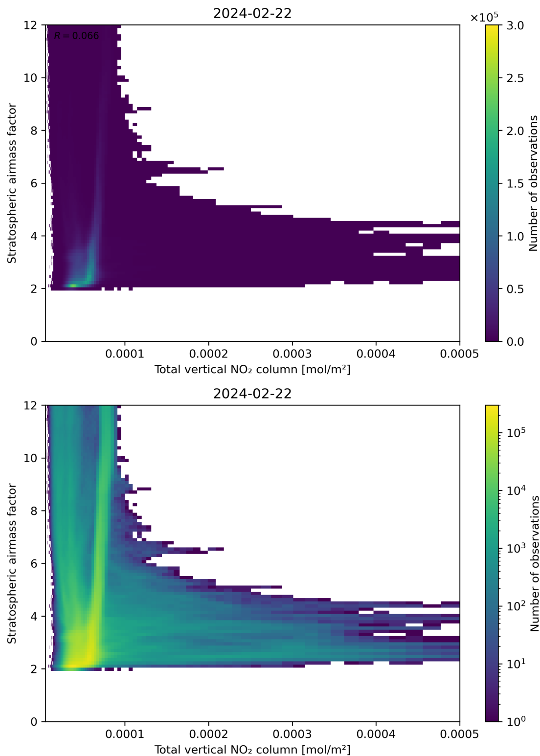
Figure 110: Scatter density plot of “Total vertical NO 2 column” against “Stratospheric airmass factor” for 2024-02-22 to 2024-02-23.
