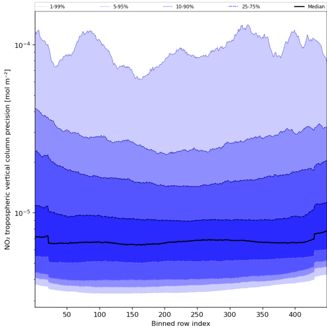
Figure 47: Along track statistics of “NO 2 tropospheric vertical column precision” for 2024-02-22 to 2024-02-23
