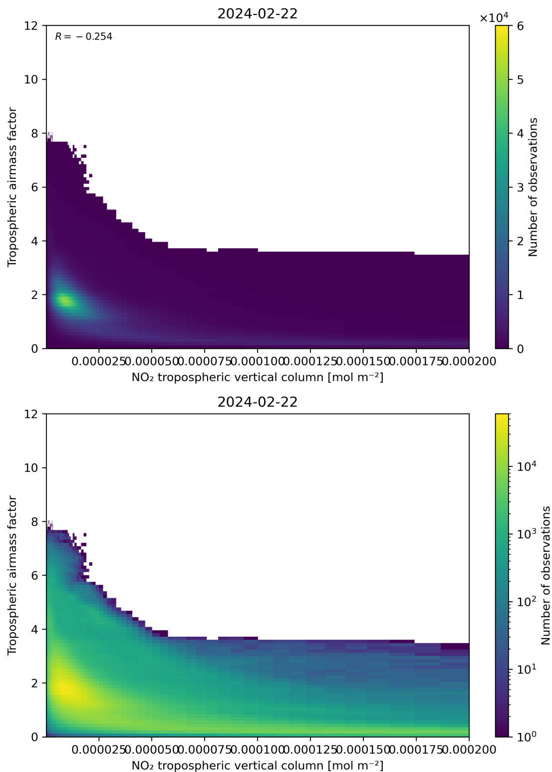
Figure 123: Scatter density plot of “NO 2 tropospheric vertical column” against “Tropospheric airmass factor” for 2024-02-22 to 2024-02-23.
