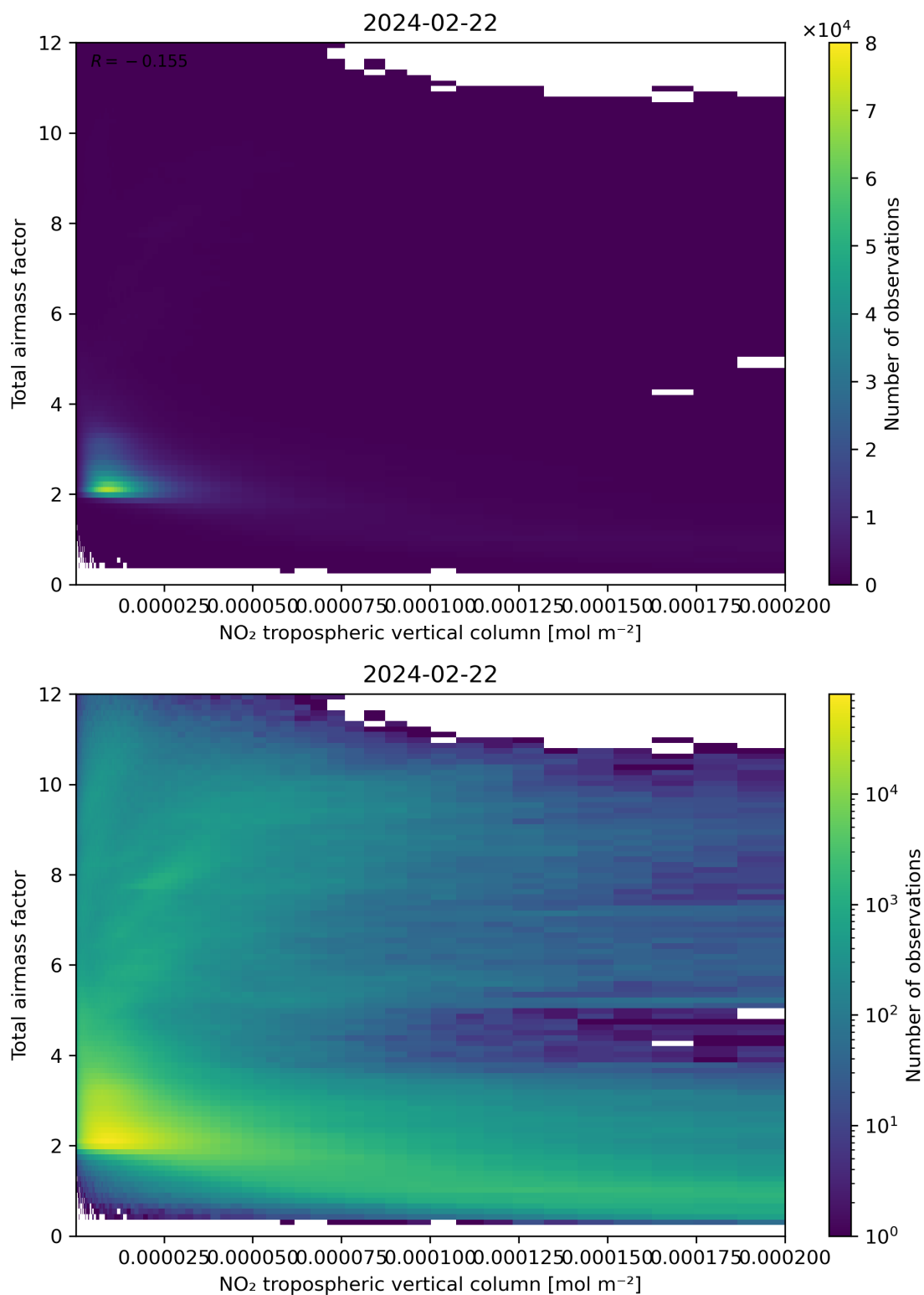
Figure 122: Scatter density plot of “NO 2 tropospheric vertical column” against “Total air mass factor” for 2024-02-22 to 2024-02-23.
