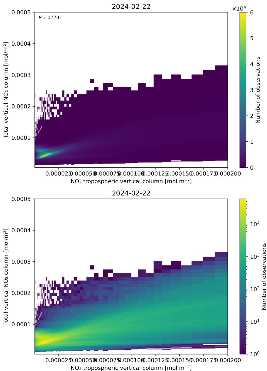
Figure 128: Scatter density plot of “NO 2 tropospheric vertical column” against “Total vertical NO 2 column” for 2024-02-22 to 2024-02-23.
