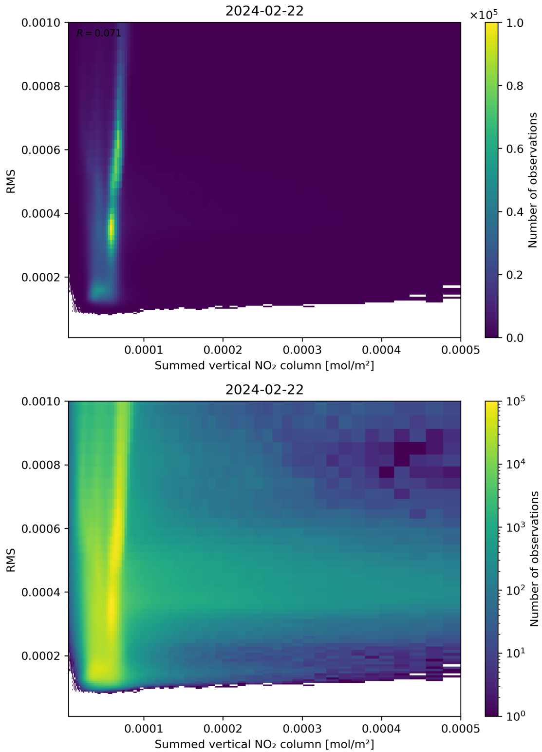
Figure 109: Scatter density plot of “Summed vertical NO 2 column” against “RMS” for 2024-02-22 to 2024-02-23.
