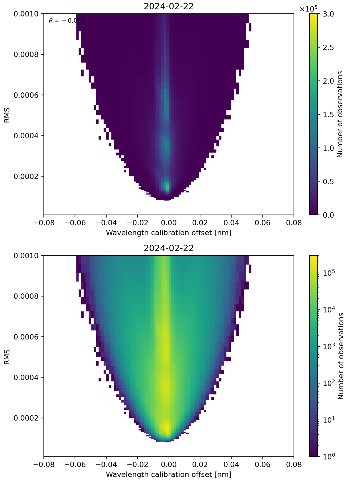
Figure 181: Scatter density plot of “Wavelength calibration offset” against “RMS” for 2024-02-22 to 2024-02-23.
