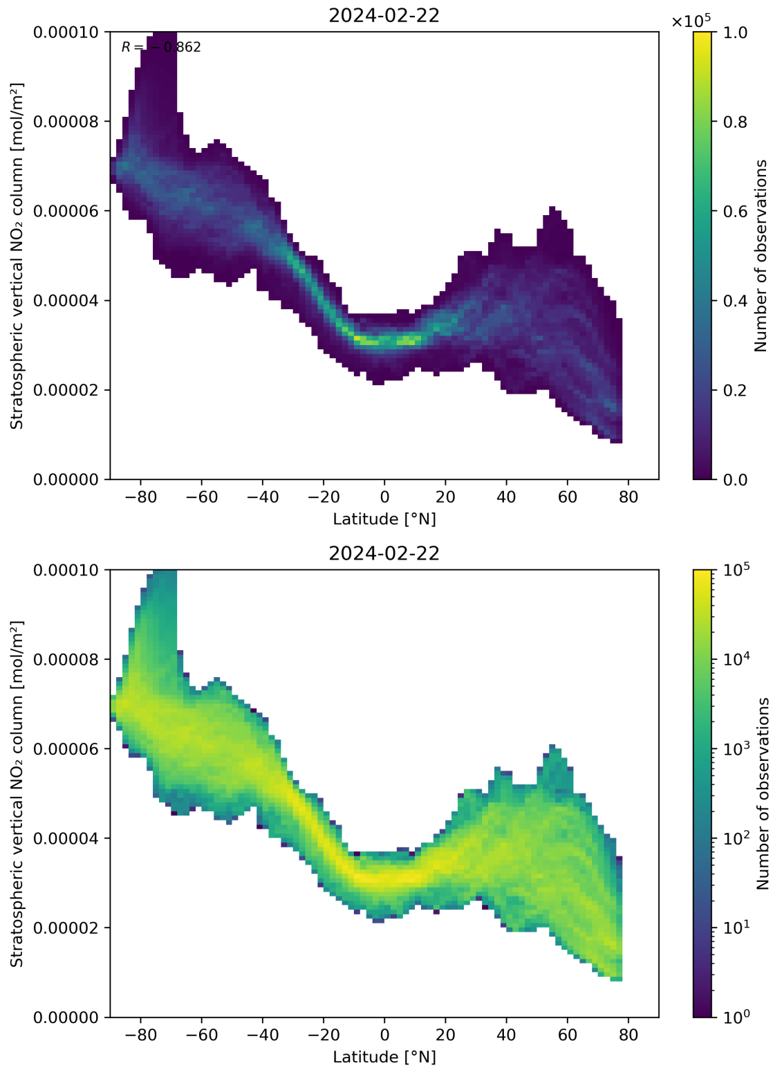
Figure 87: Scatter density plot of “Latitude” against “Stratospheric vertical NO 2 column” for 2024-02-22 to 2024-02-23.
