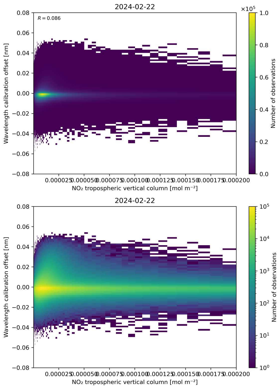
Figure 143: Scatter density plot of “NO 2 tropospheric vertical column” against “Wavelength calibration offset” for 2024-02-22 to 2024-02-23.
