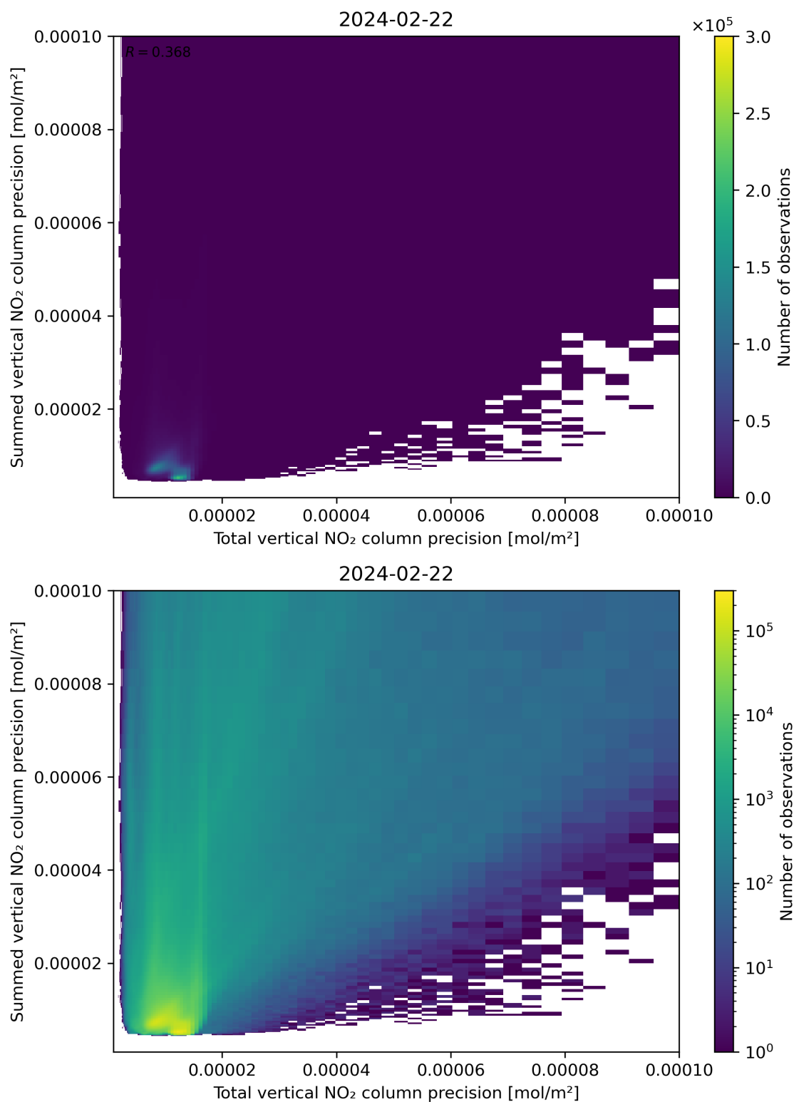
Figure 118: Scatter density plot of “Total vertical NO 2 column precision” against “Summed vertical NO 2 column precision” for 2024-02-22 to 2024-02-23.
