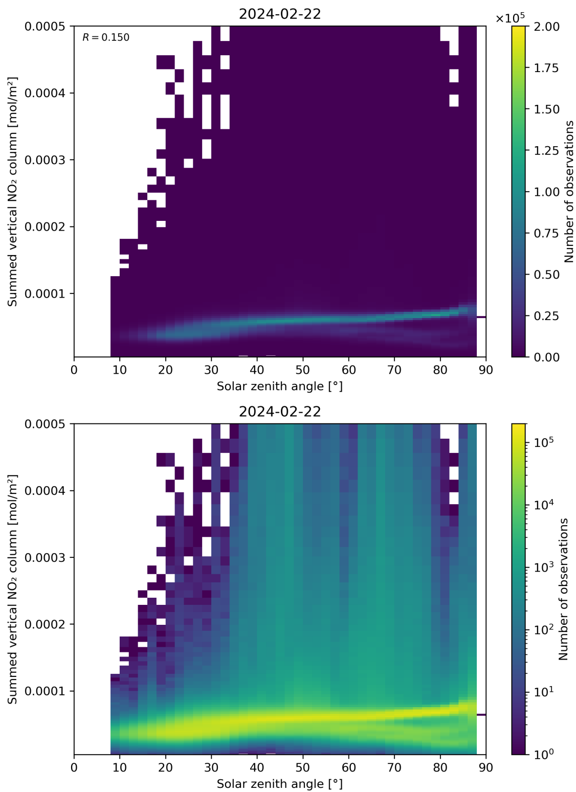
Figure 151: Scatter density plot of “Solar zenith angle” against “Summed vertical NO 2 column” for 2024-02-22 to 2024-02-23.
