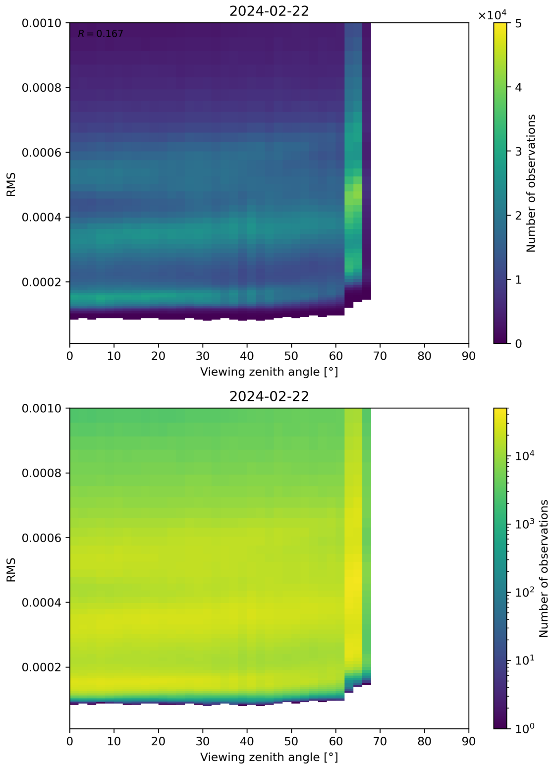
Figure 171: Scatter density plot of “Viewing zenith angle” against “RMS” for 2024-02-22 to 2024-02-23.
