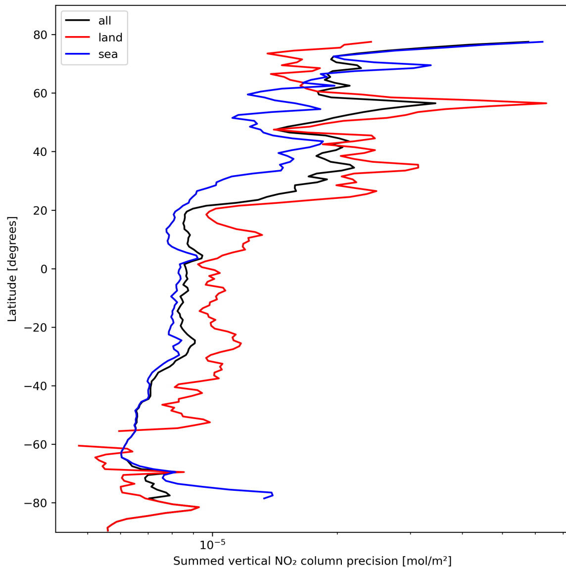
Figure 24: Zonal average of “Summed vertical NO 2 column precision” for 2024-02-22 to 2024-02-23.
