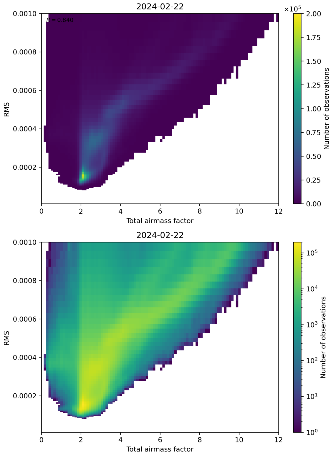
Figure 69: Scatter density plot of “Total airmass factor” against “RMS” for 2024-02-22 to 2024-02-23.
