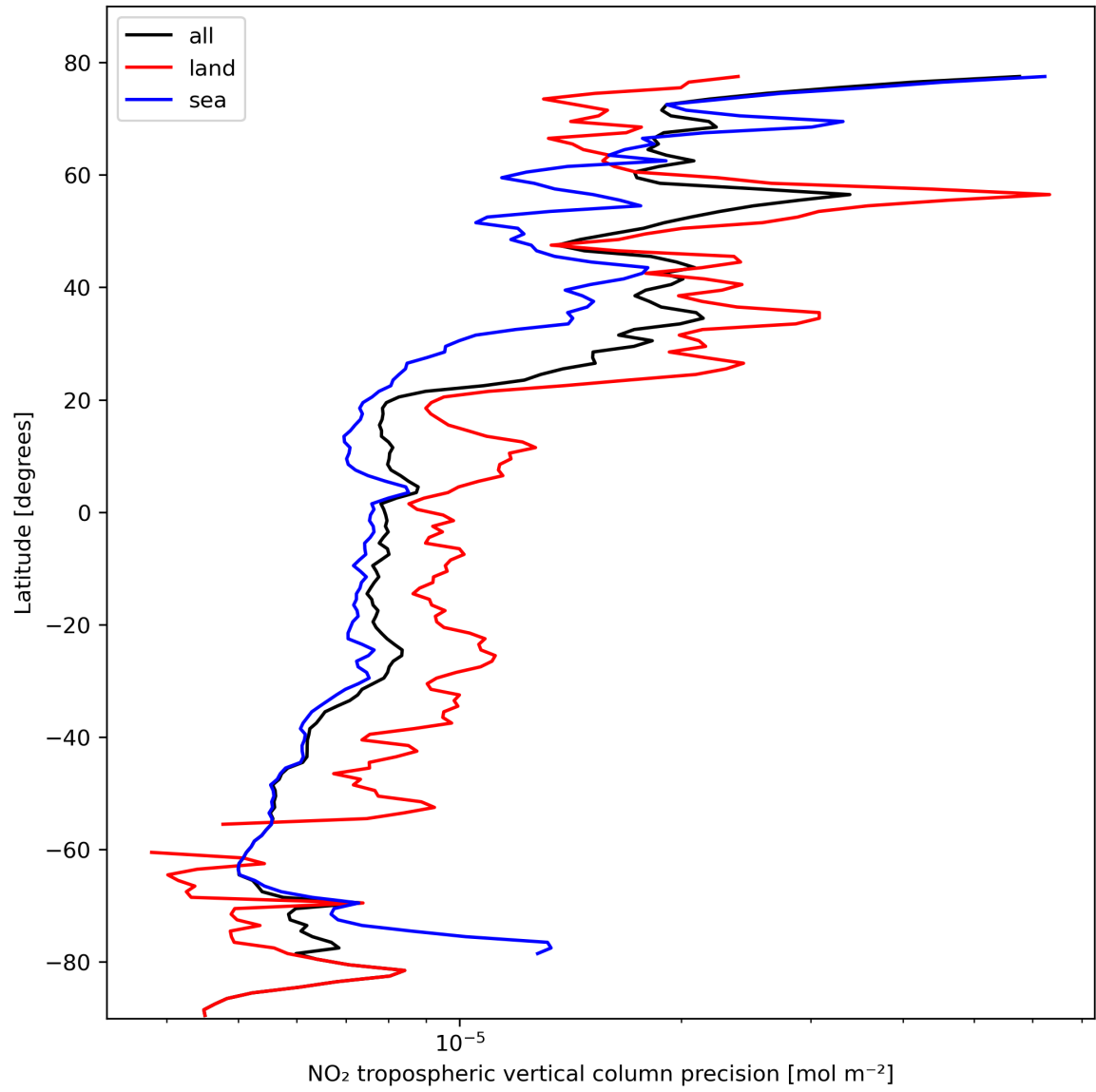
Figure 13: Zonal average of “NO 2 tropospheric vertical column precision” for 2024-02-22 to 2024-02-23.
