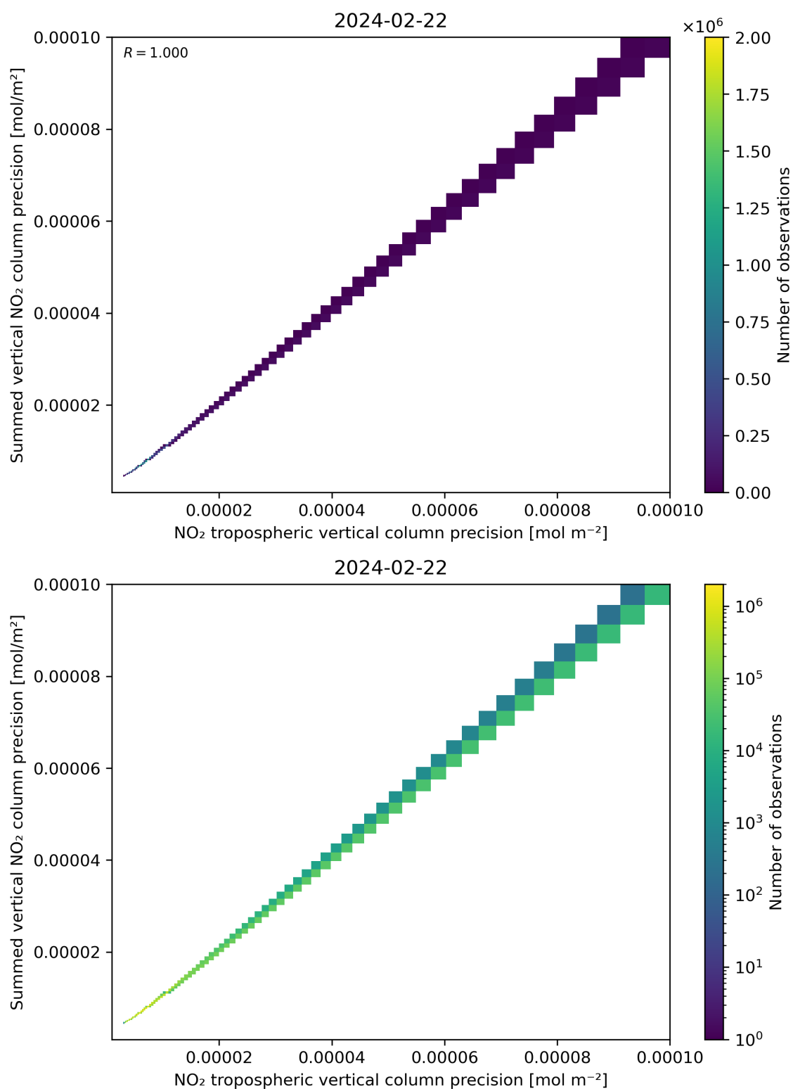
Figure 137: Scatter density plot of “NO 2 tropospheric vertical column precision” against “Summed vertical NO 2 column precision” for 2024-02-22 to 2024-02-23.
