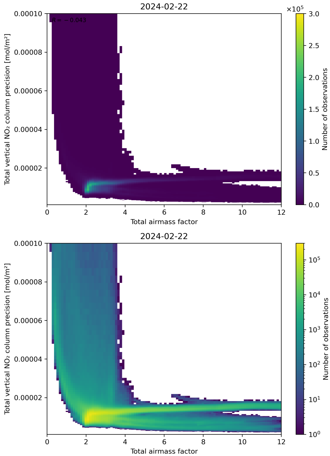
Figure 68: Scatter density plot of “Total airmass factor” against “Total vertical NO 2 column precision” for 2024-02-22 to 2024-02-23.
