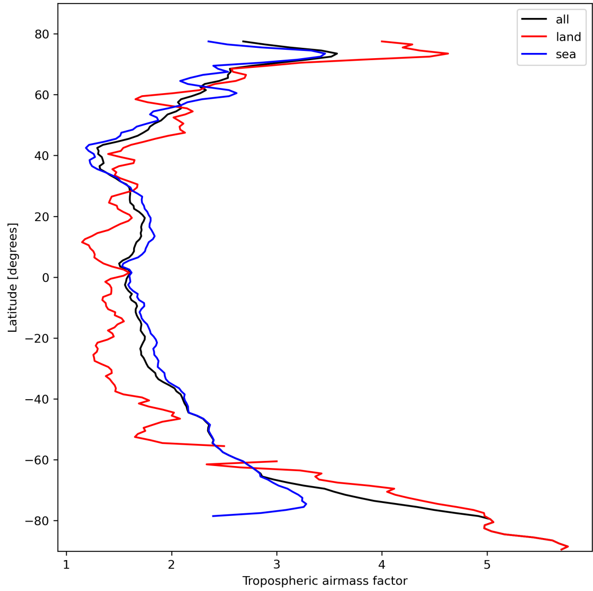
Figure 14: Zonal average of “Tropospheric airmass factor” for 2024-02-22 to 2024-02-23.
