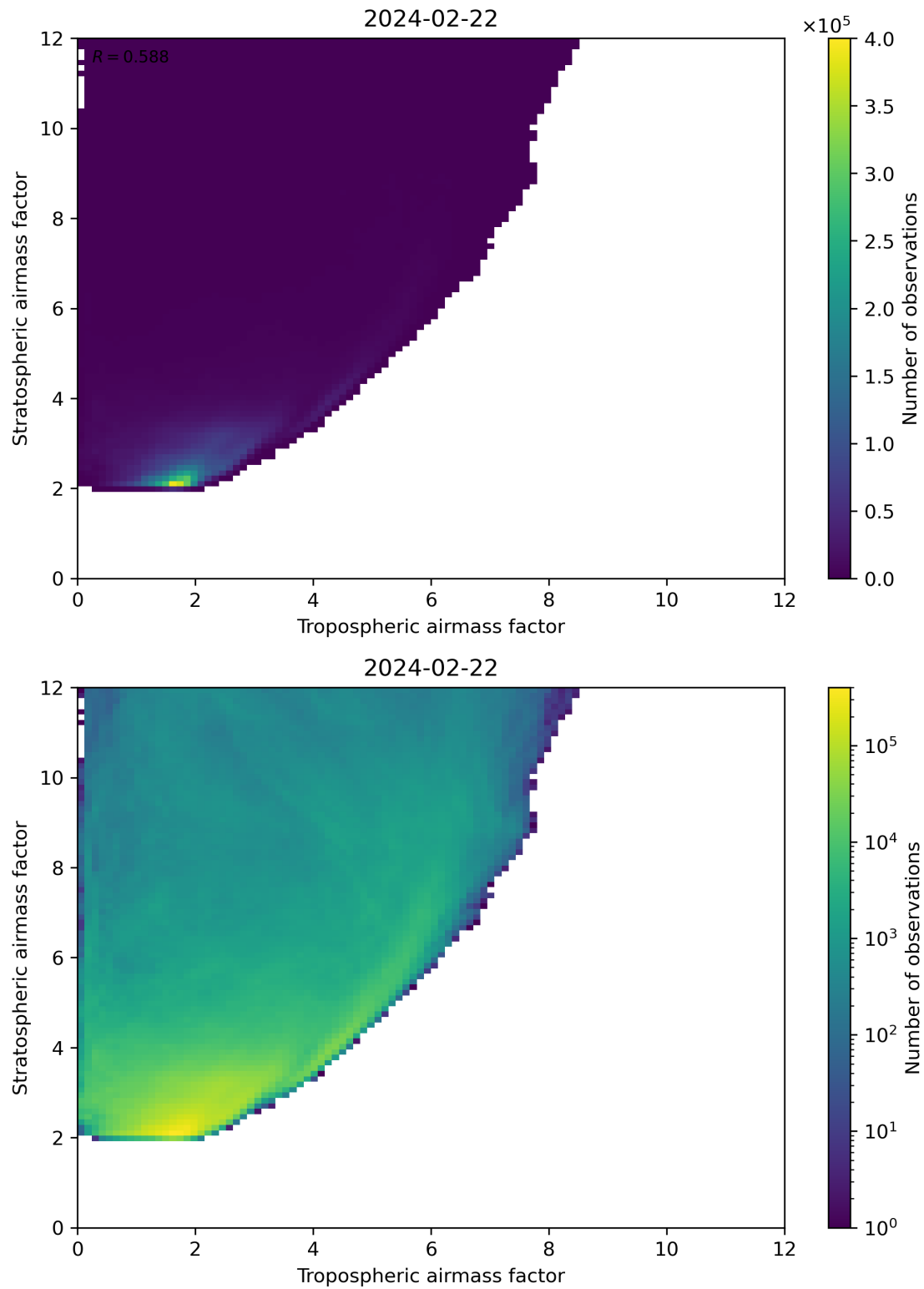
Figure 71: Scatter density plot of “Tropospheric airmass factor” against “Stratospheric airmass factor” for 2024-02-22 to 2024-02-23.
