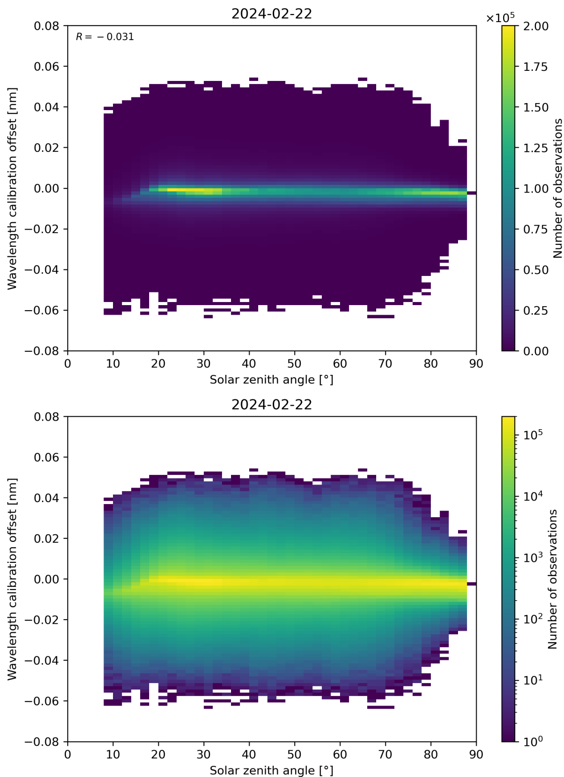
Figure 158: Scatter density plot of “Solar zenith angle” against “Wavelength calibration offset” for 2024-02-22 to 2024-02-23.
