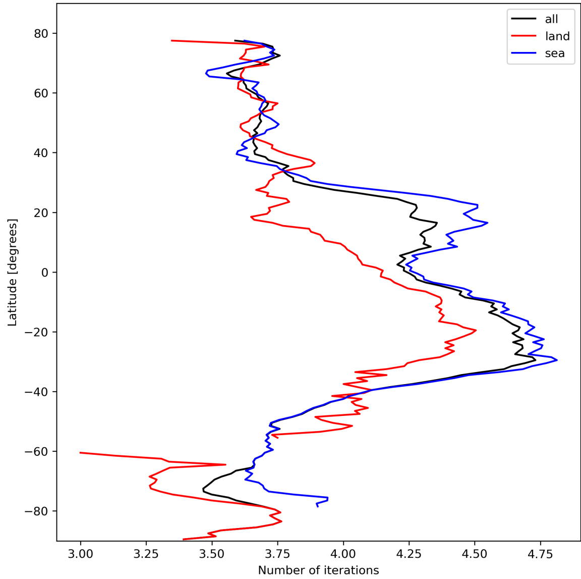
Figure 17: Zonal average of “Number of iterations” for 2024-02-22 to 2024-02-23.
