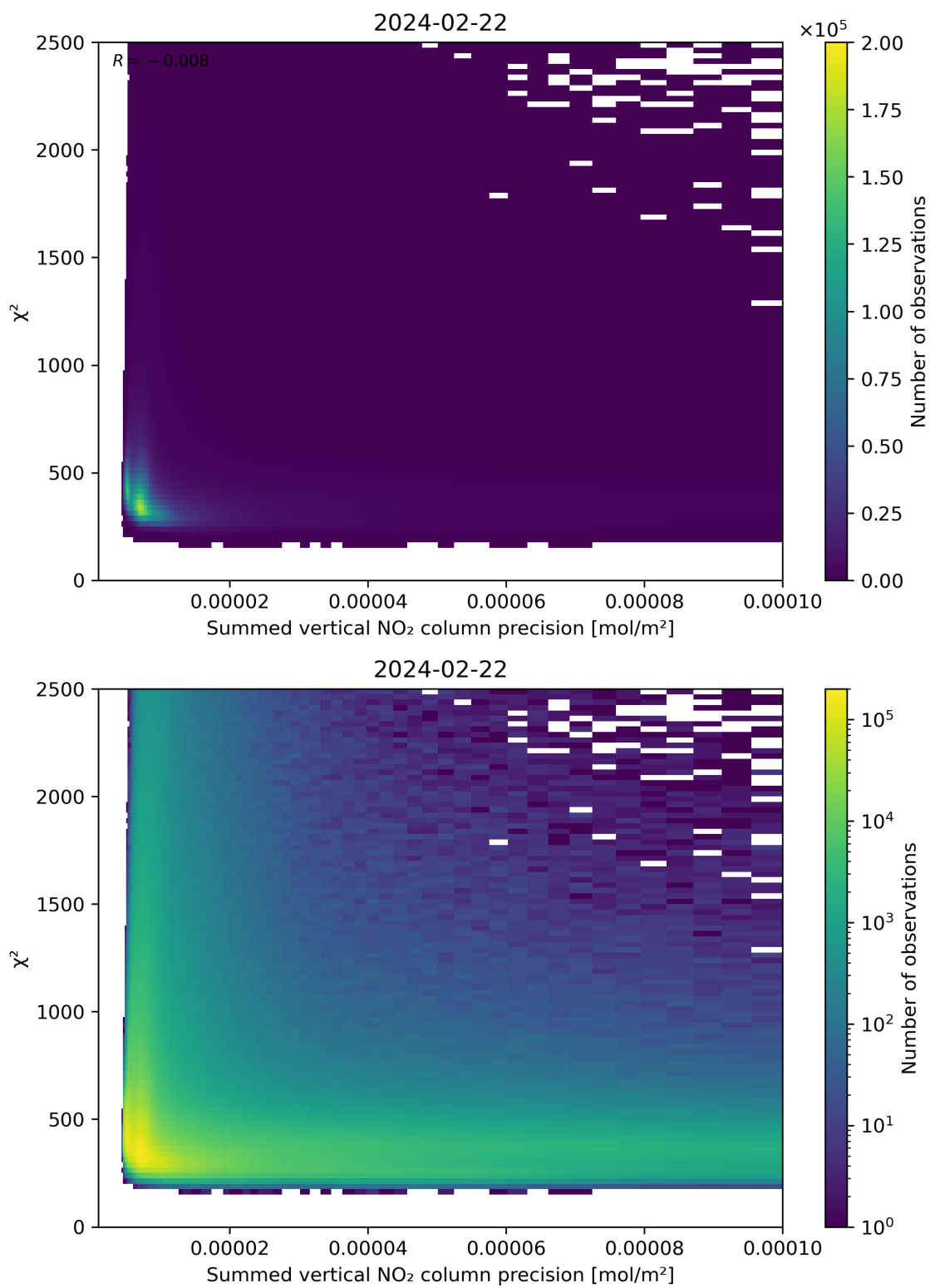
Figure 107: Scatter density plot of “Summed vertical NO 2 column precision” against “ \chi^2 ” for 2024-02-22 to 2024-02-23.
