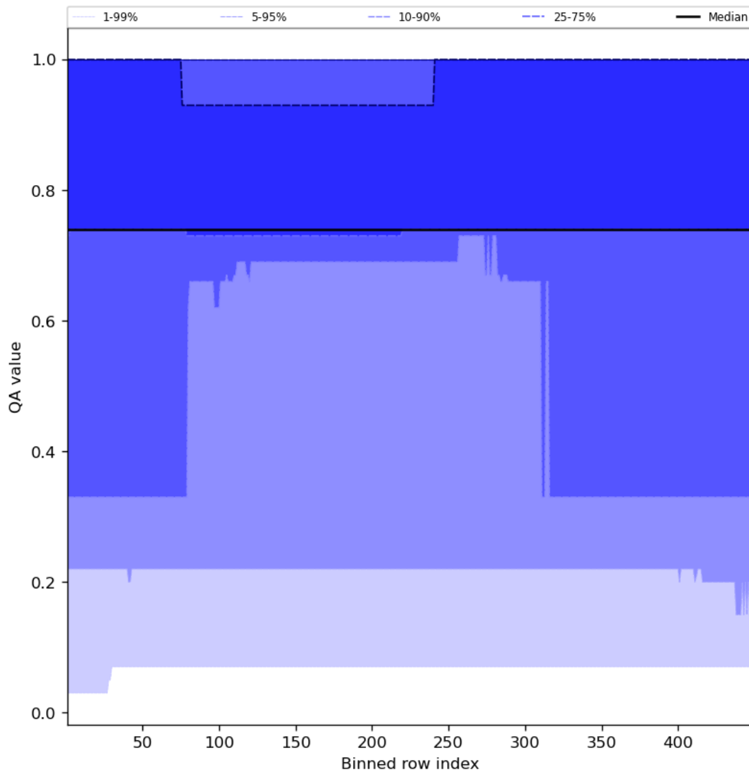
Figure 45: Along track statistics of “QA value” for 2024-02-22 to 2024-02-23
