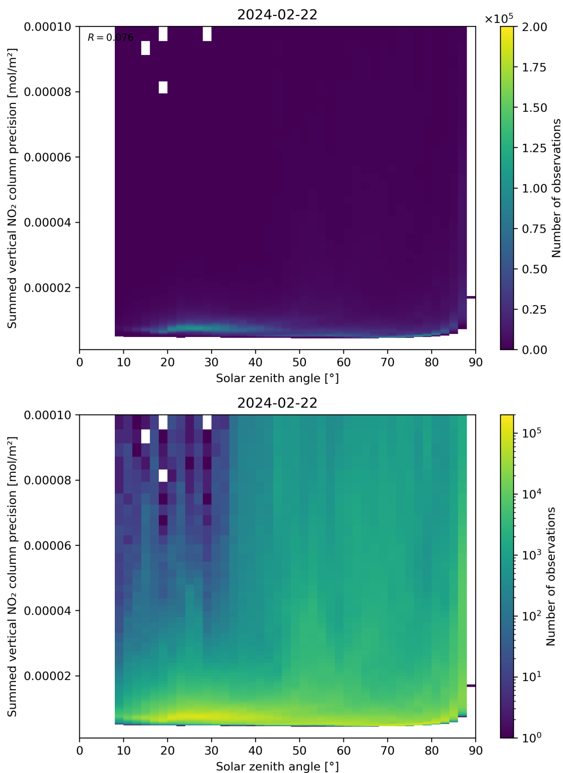
Figure 152: Scatter density plot of “Solar zenith angle” against “Summed vertical NO 2 column precision” for 2024-02-22 to 2024-02-23.
