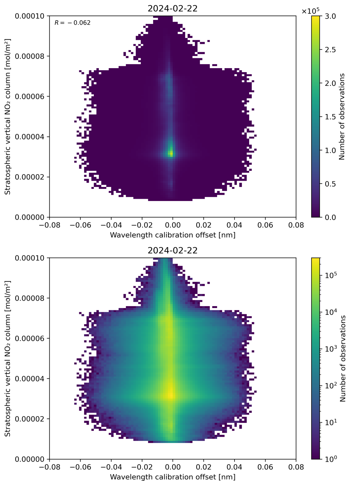
Figure 176: Scatter density plot of “Wavelength calibration offset” against “Stratospheric vertical NO 2 column” for 2024-02-22 to 2024-02-23.
