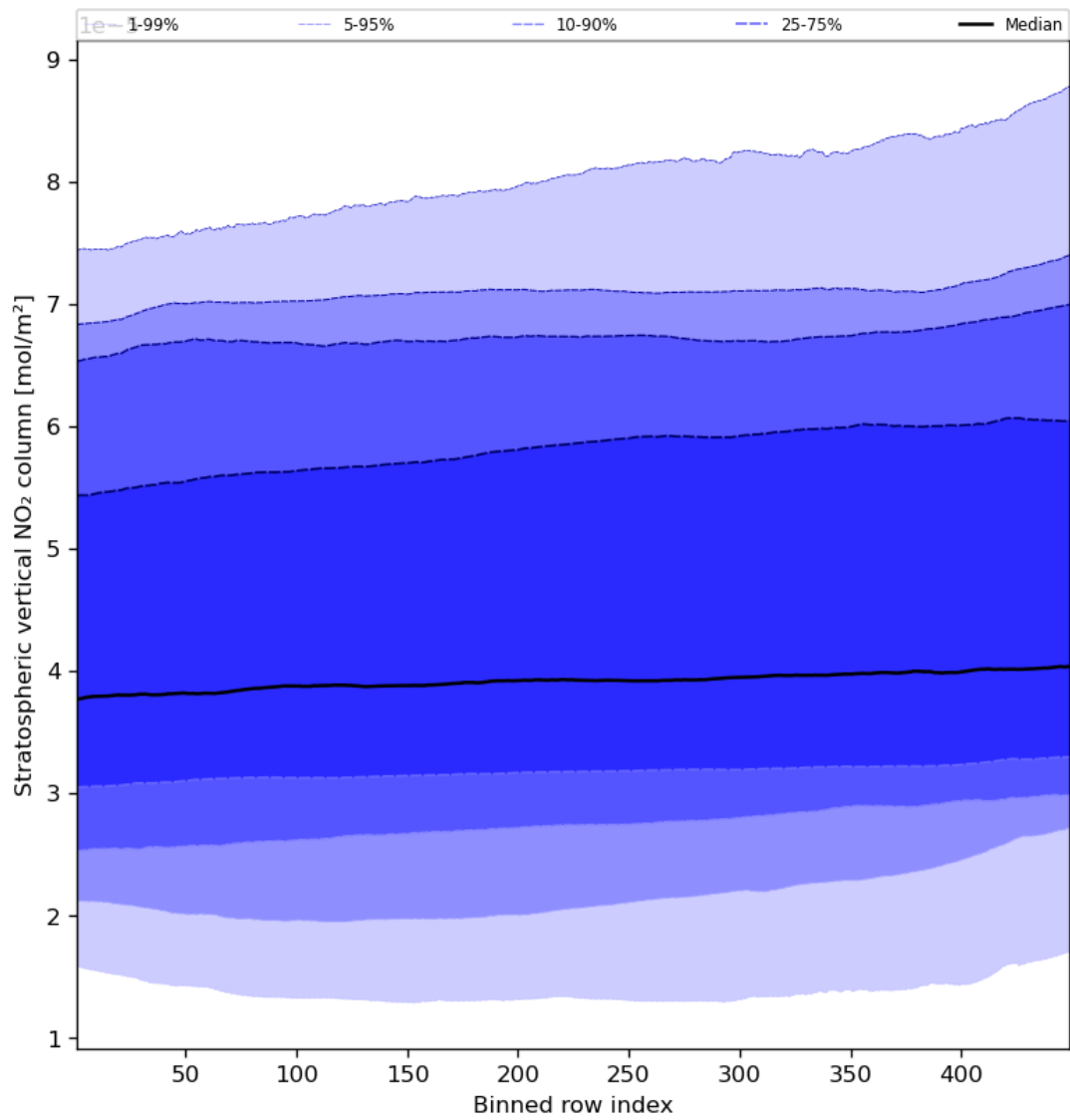
Figure 53: Along track statistics of “Stratospheric vertical NO 2 column” for 2024-02-22 to 2024-02-23
