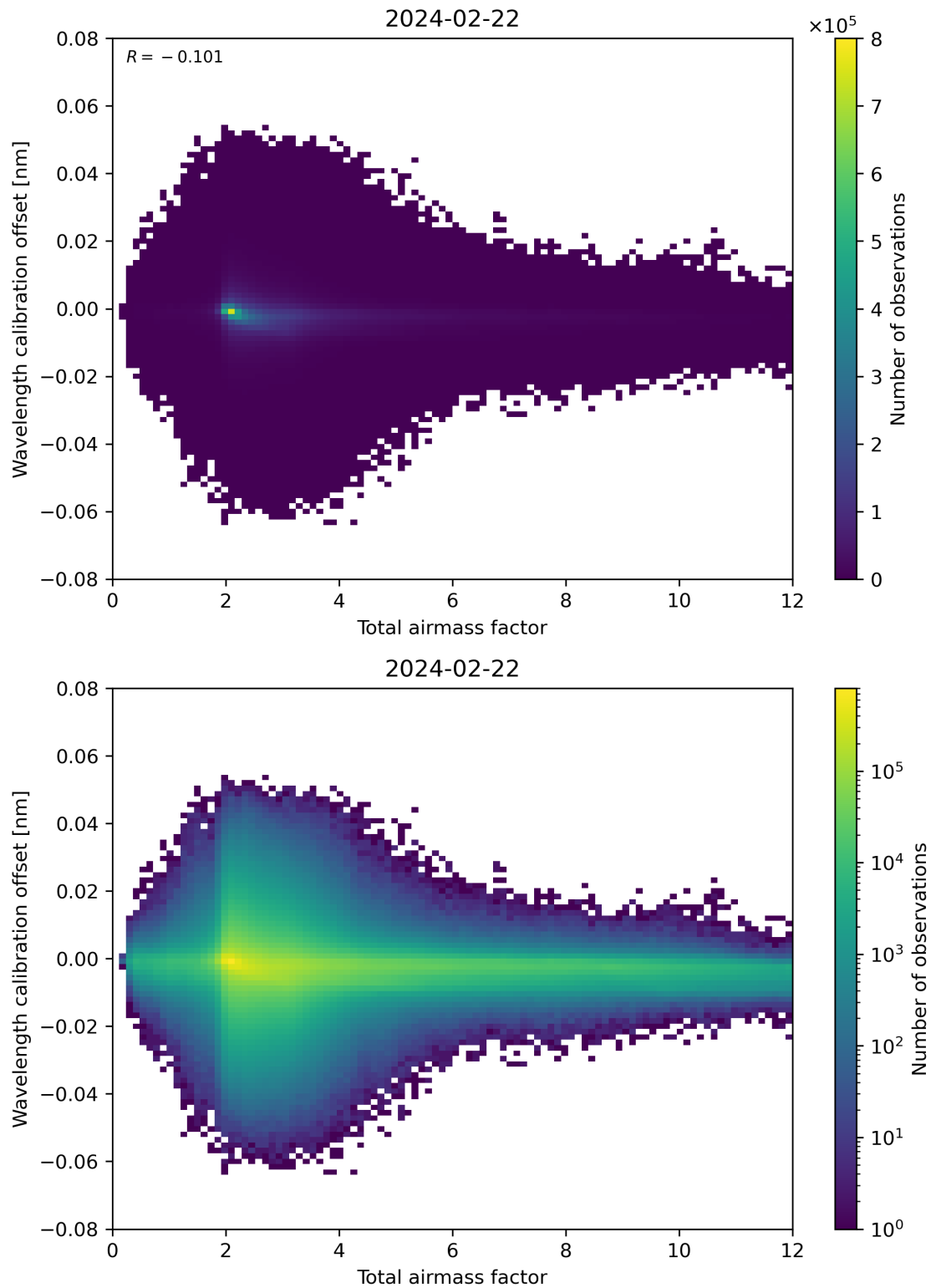
Figure 70: Scatter density plot of “Total airmass factor” against “Wavelength calibration offset” for 2024-02-22 to 2024-02-23.
