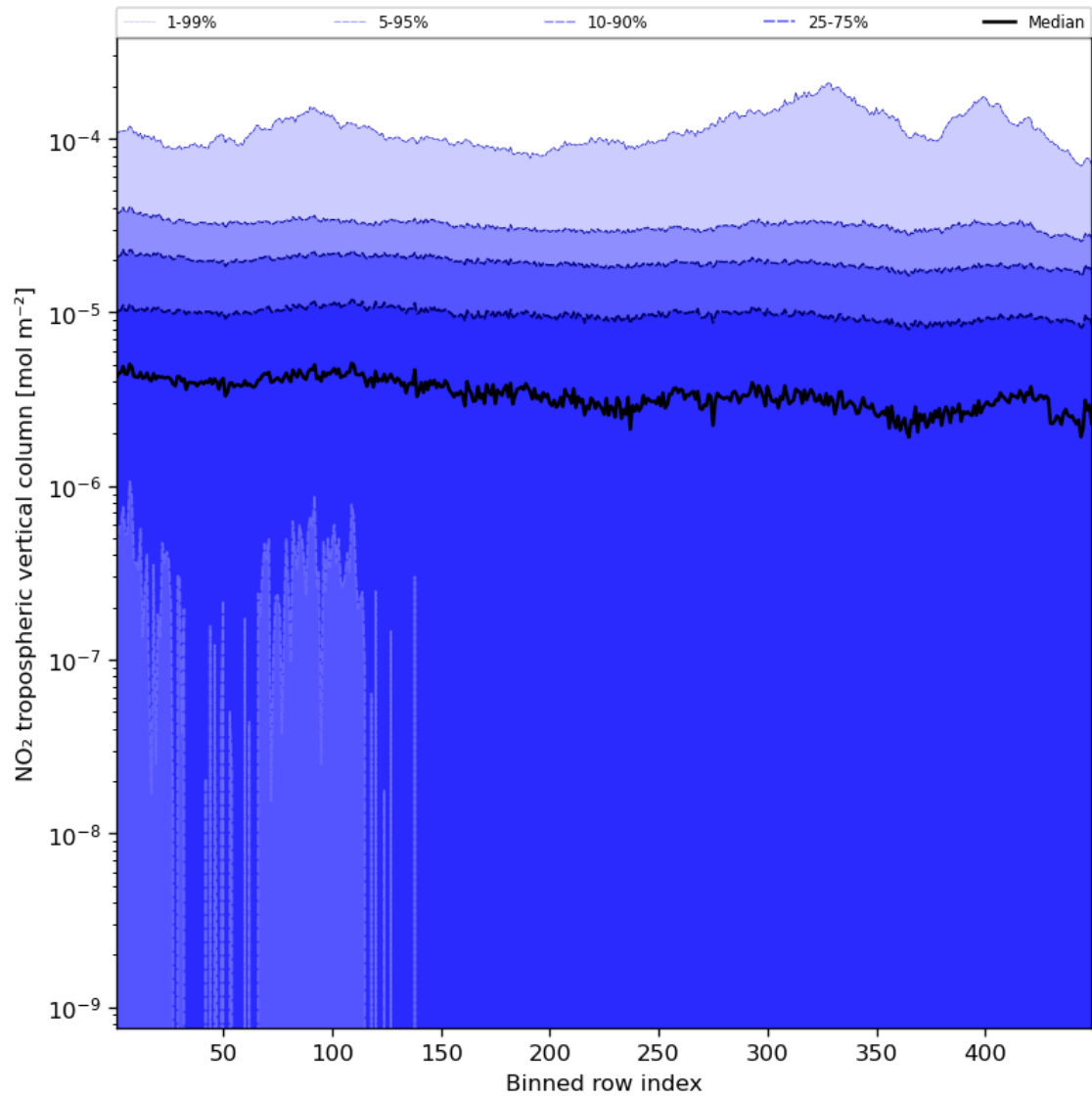
Figure 46: Along track statistics of “NO 2 tropospheric vertical column” for 2024-02-22 to 2024-02-23
