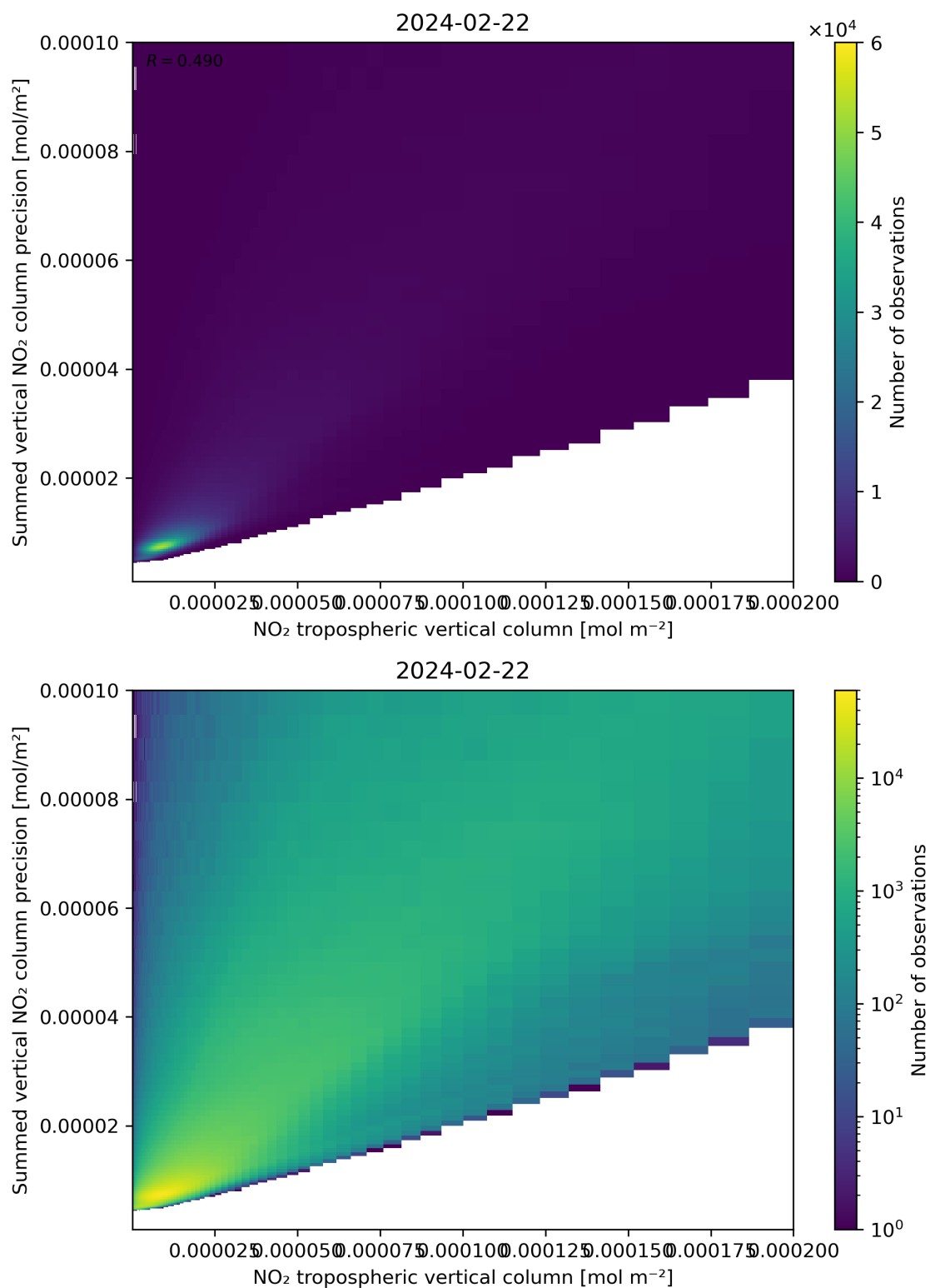
Figure 127: Scatter density plot of “NO 2 tropospheric vertical column” against “Summed vertical NO 2 column precision” for 2024-02-22 to 2024-02-23.
