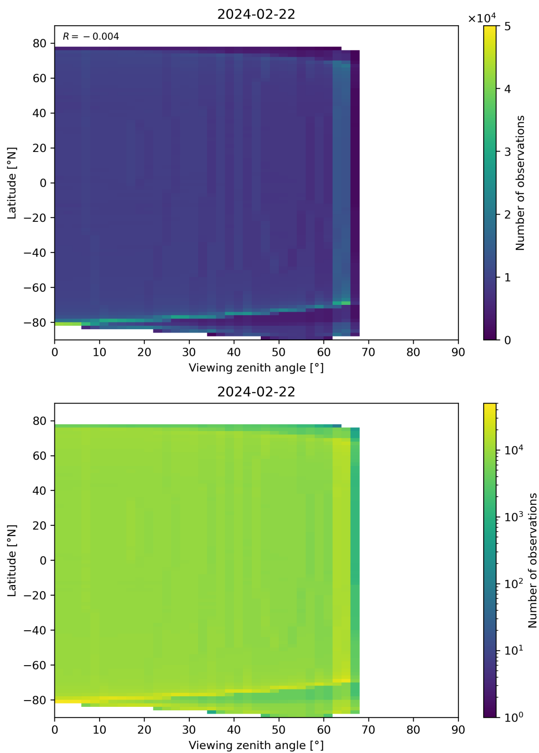
Figure 163: Scatter density plot of “Viewing zenith angle” against “Latitude” for 2024-02-22 to 2024-02-23.
