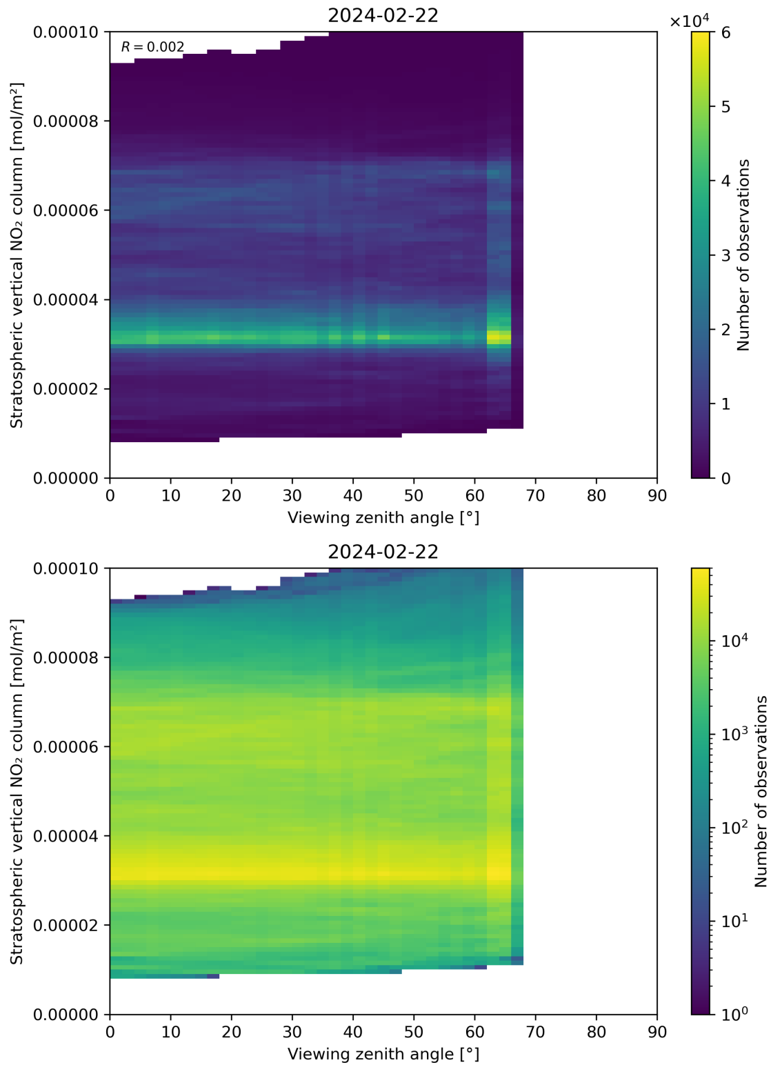
Figure 164: Scatter density plot of “Viewing zenith angle” against “Stratospheric vertical NO 2 column” for 2024-02-22 to 2024-02-23.
