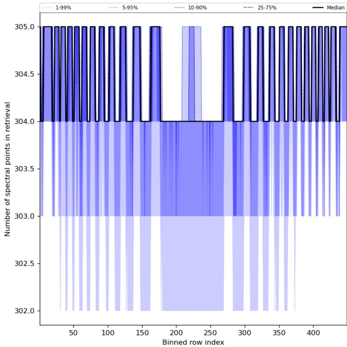
Figure 50: Along track statistics of “Number of spectral points in retrieval” for 2024-02-22 to 2024-02-23
