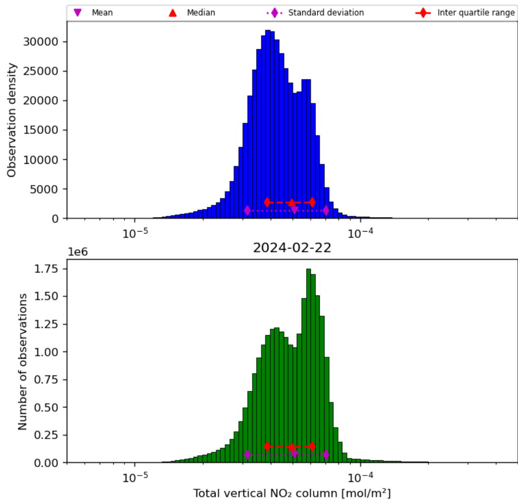
Figure 38: Histogram of “Total vertical NO 2 column” for 2024-02-22 to 2024-02-23
