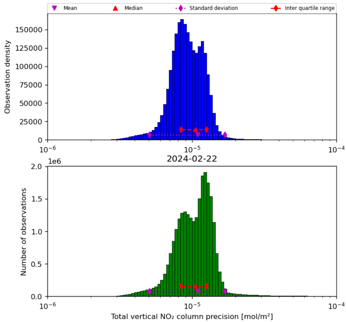
Figure 39: Histogram of “Total vertical NO 2 column precision” for 2024-02-22 to 2024-02-23
