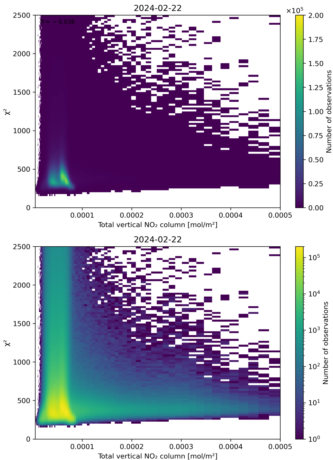
Figure 111: Scatter density plot of “Total vertical NO 2 column” against “ \chi^2 ” for 2024-02-22 to 2024-02-23.
