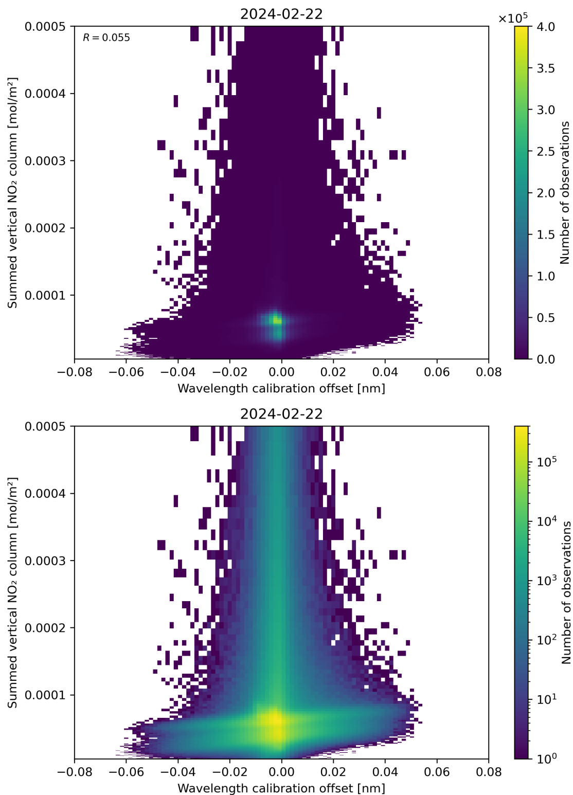
Figure 177: Scatter density plot of “Wavelength calibration offset” against “Summed vertical NO 2 column” for 2024-02-22 to 2024-02-23.
