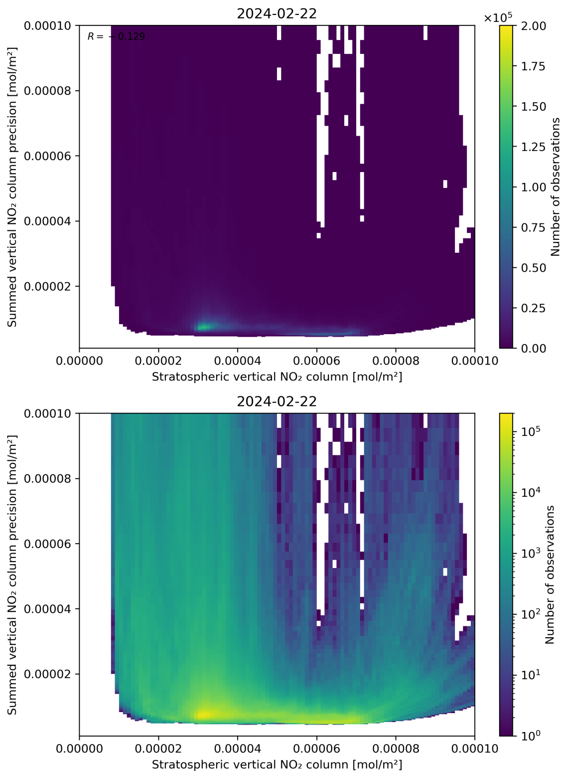
Figure 99: Scatter density plot of “Stratospheric vertical NO 2 column” against “Summed vertical NO 2 column precision” for 2024-02-22 to 2024-02-23.
