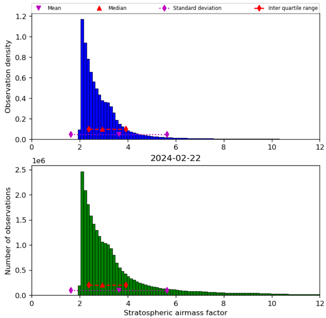
Figure 44: Histogram of “Stratospheric airmass factor” for 2024-02-22 to 2024-02-23
