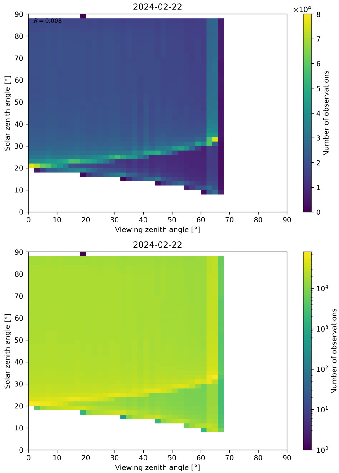
Figure 172: Scatter density plot of “Viewing zenith angle” against “Solar zenith angle” for 2024-02-22 to 2024-02-23.
