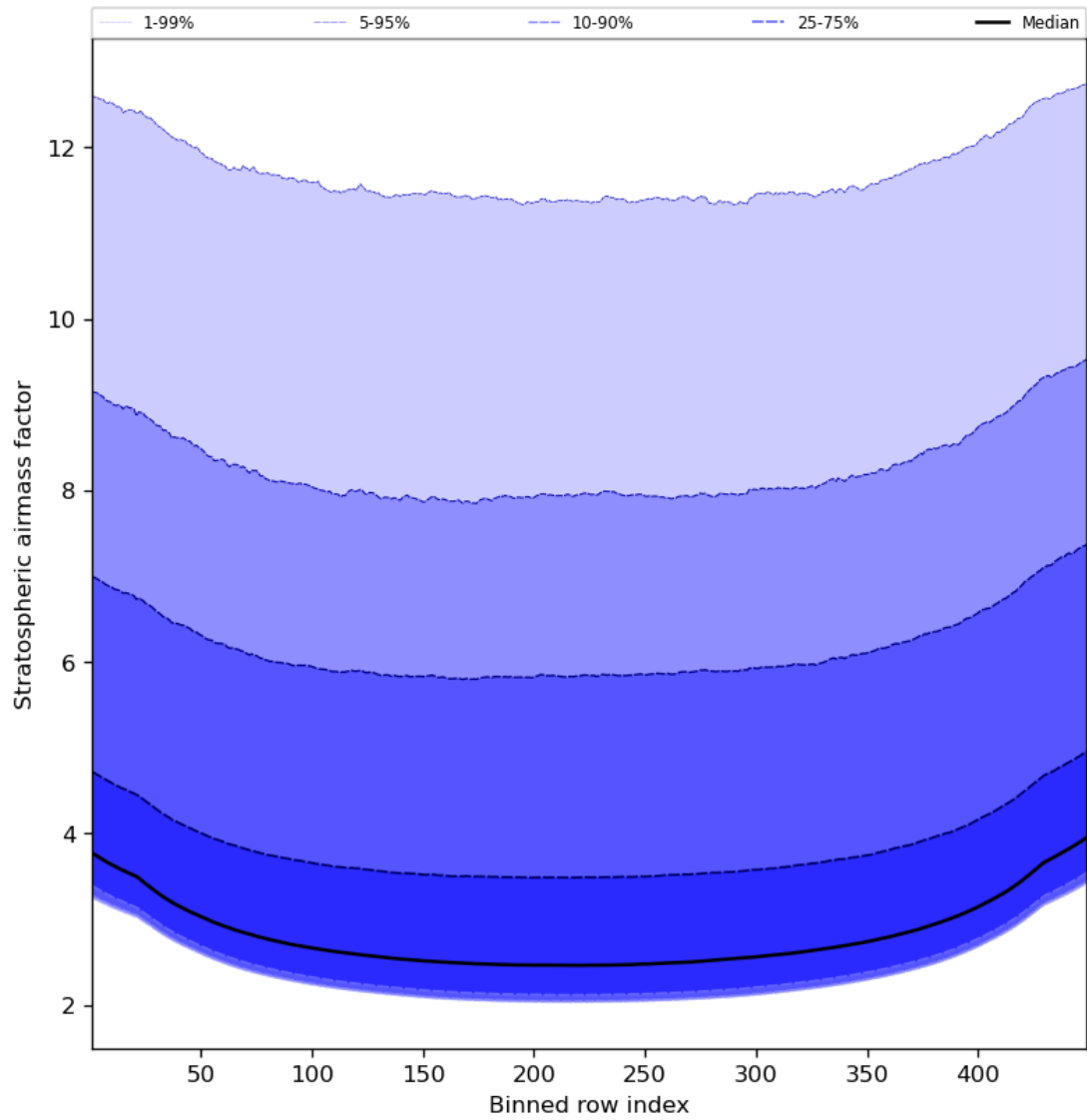
Figure 61: Along track statistics of “Stratospheric airmass factor” for 2024-02-22 to 2024-02-23
