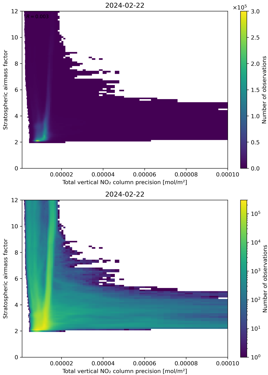
Figure 115: Scatter density plot of “Total vertical NO 2 column precision” against “Stratospheric air mass factor” for 2024-02-22 to 2024-02-23.
