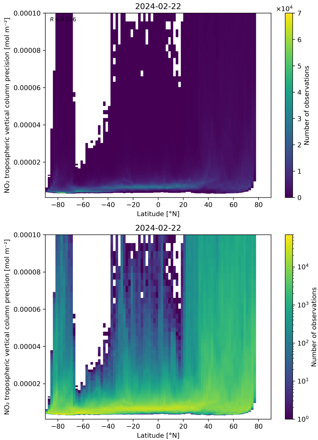
Figure 93: Scatter density plot of “Latitude” against “NO 2 tropospheric vertical column precision” for 2024-02-22 to 2024-02-23.
