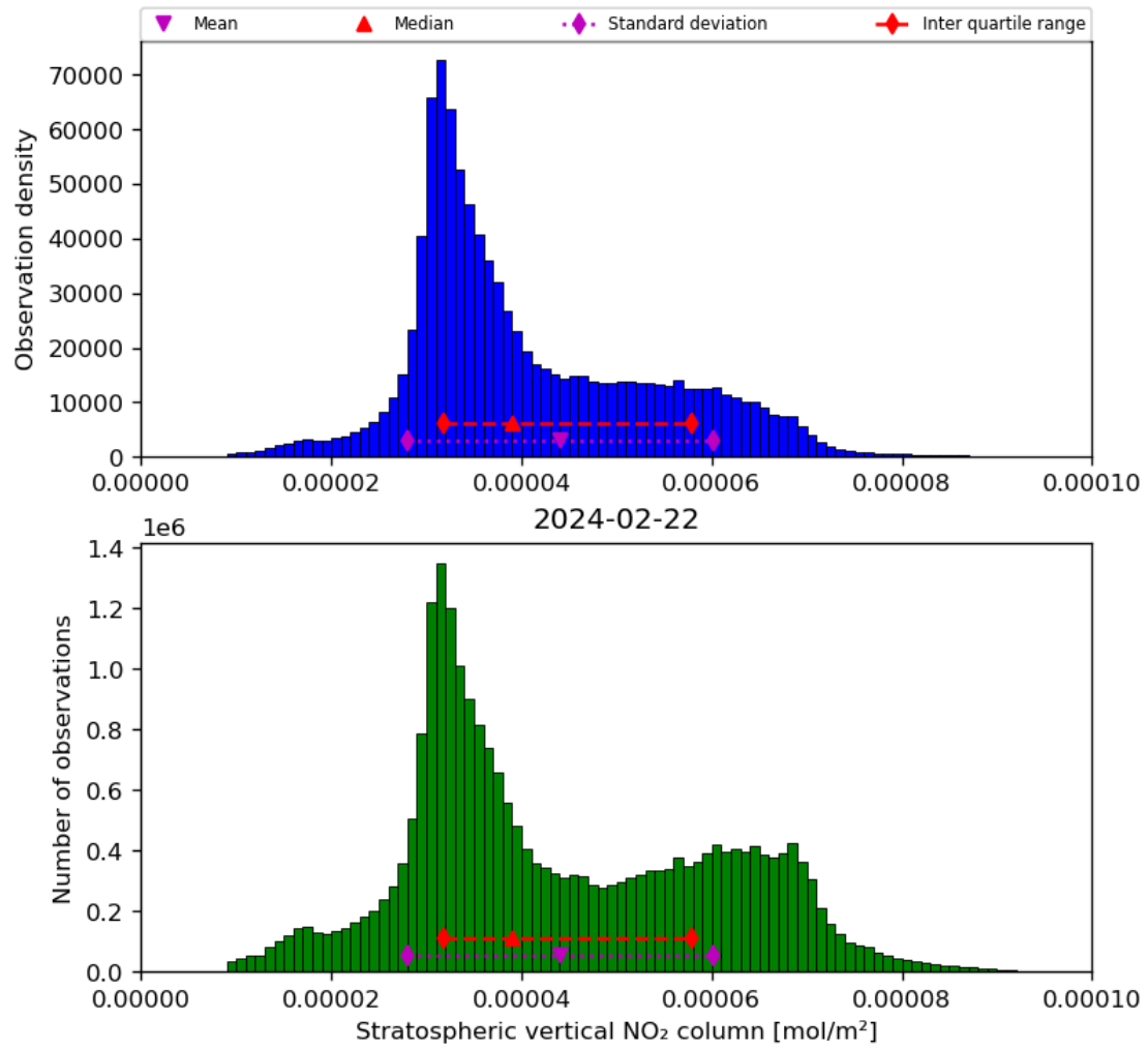
Figure 36: Histogram of “Stratospheric vertical NO 2 column” for 2024-02-22 to 2024-02-23
