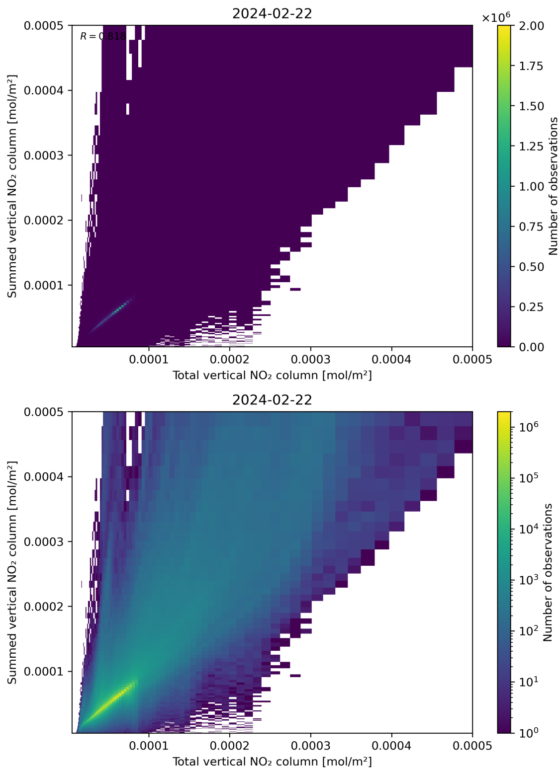
Figure 112: Scatter density plot of “Total vertical NO 2 column” against “Summed vertical NO 2 column” for 2024-02-22 to 2024-02-23.
