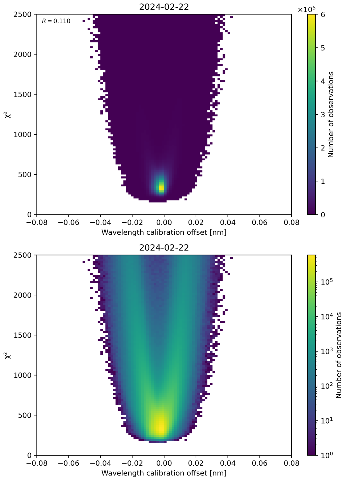
Figure 175: Scatter density plot of “Wavelength calibration offset” against “ \chi^2 ” for 2024-02-22 to 2024-02-23.
