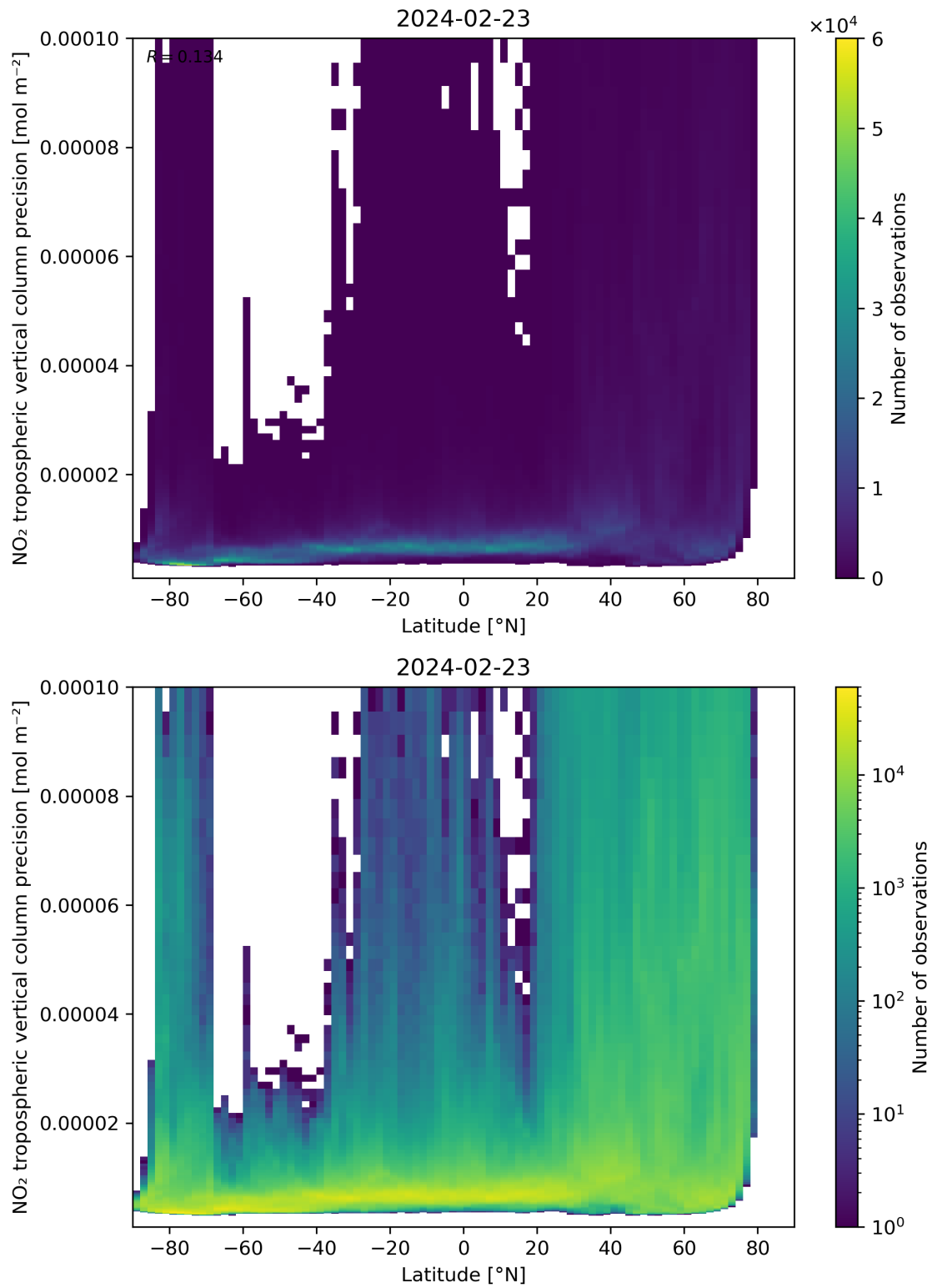
Figure 93: Scatter density plot of “Latitude” against “NO 2 tropospheric vertical column precision” for 2024-02-22 to 2024-02-24.
