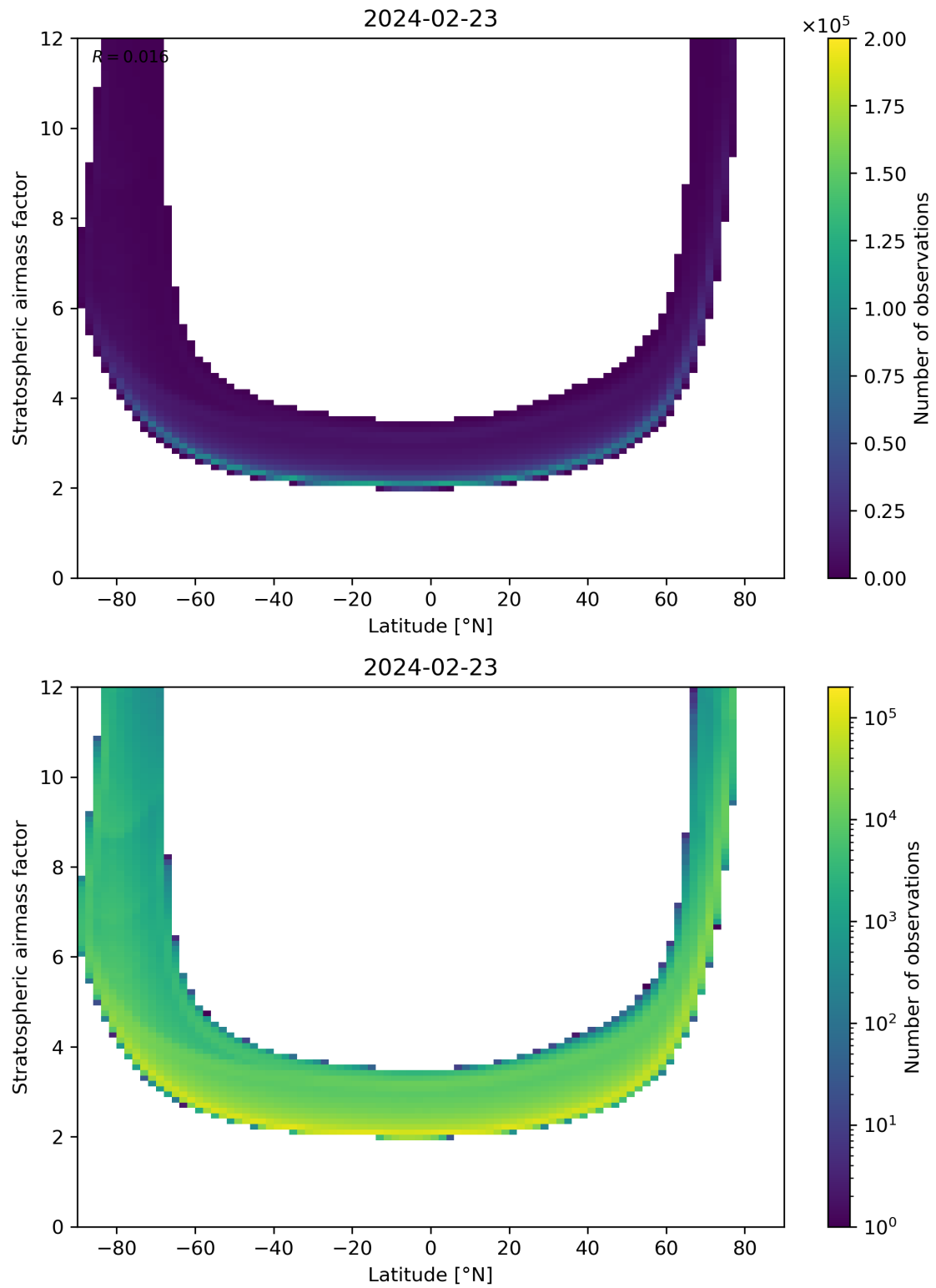
Figure 83: Scatter density plot of “Latitude” against “Stratospheric air mass factor” for 2024-02-22 to 2024-02-24.
