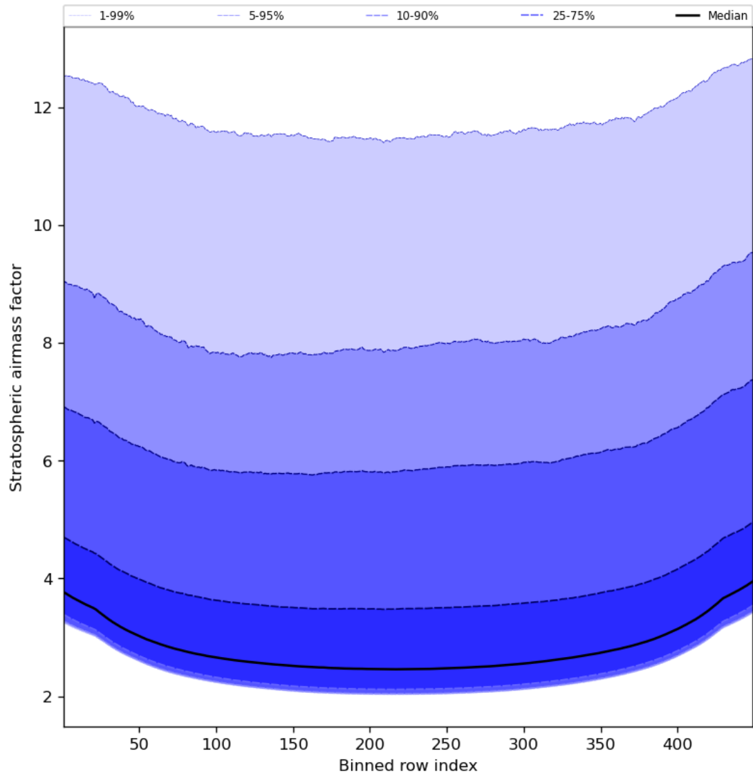
Figure 61: Along track statistics of “Stratospheric airmass factor” for 2024-02-22 to 2024-02-24
