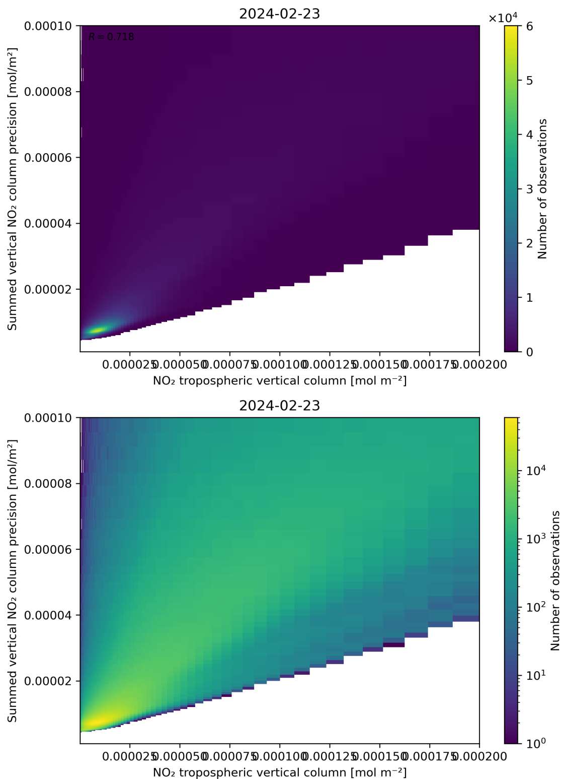
Figure 127: Scatter density plot of “NO 2 tropospheric vertical column” against “Summed vertical NO 2 column precision” for 2024-02-22 to 2024-02-24.
