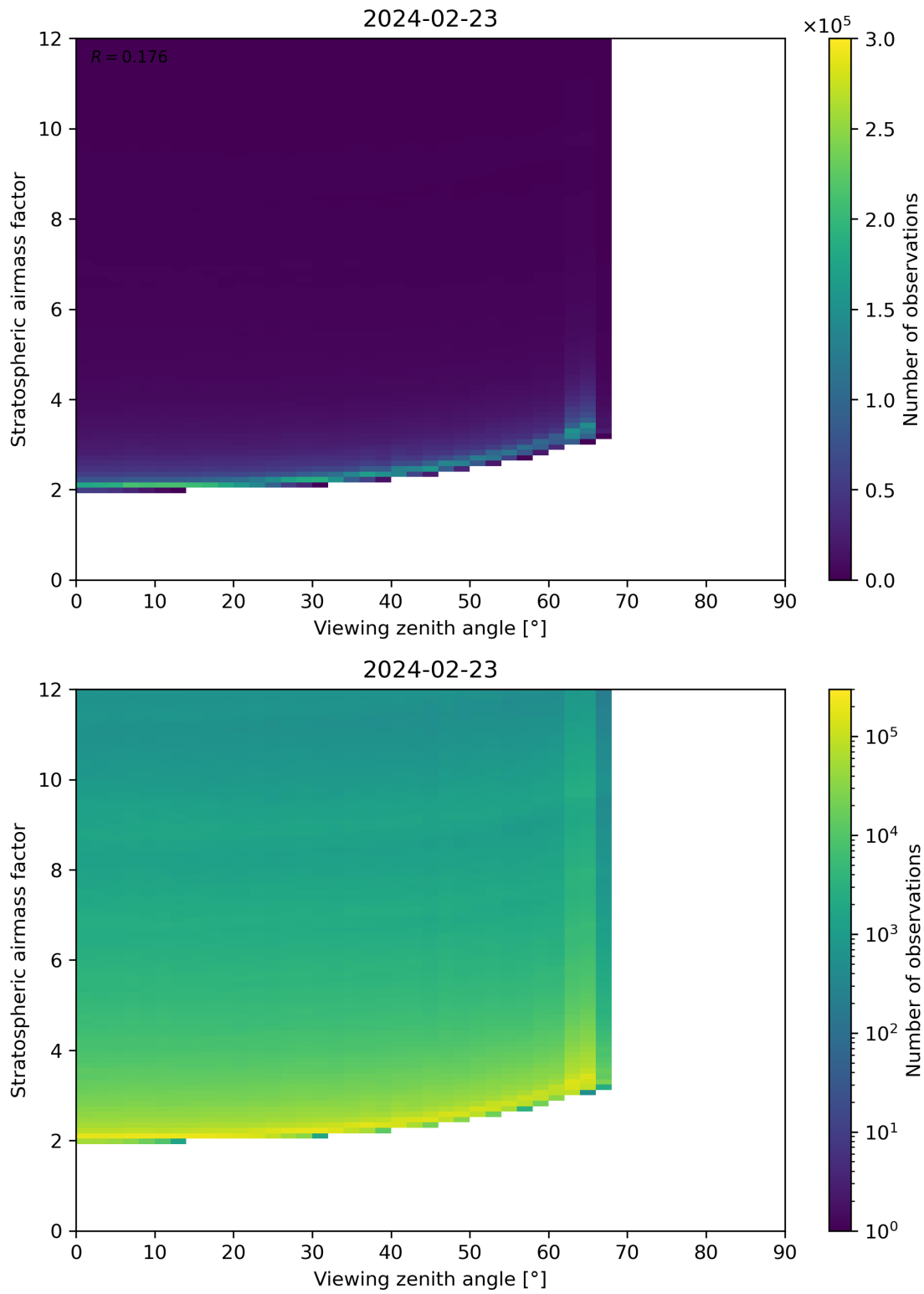
Figure 159: Scatter density plot of “Viewing zenith angle” against “Stratospheric airmass factor” for 2024-02-22 to 2024-02-24.
