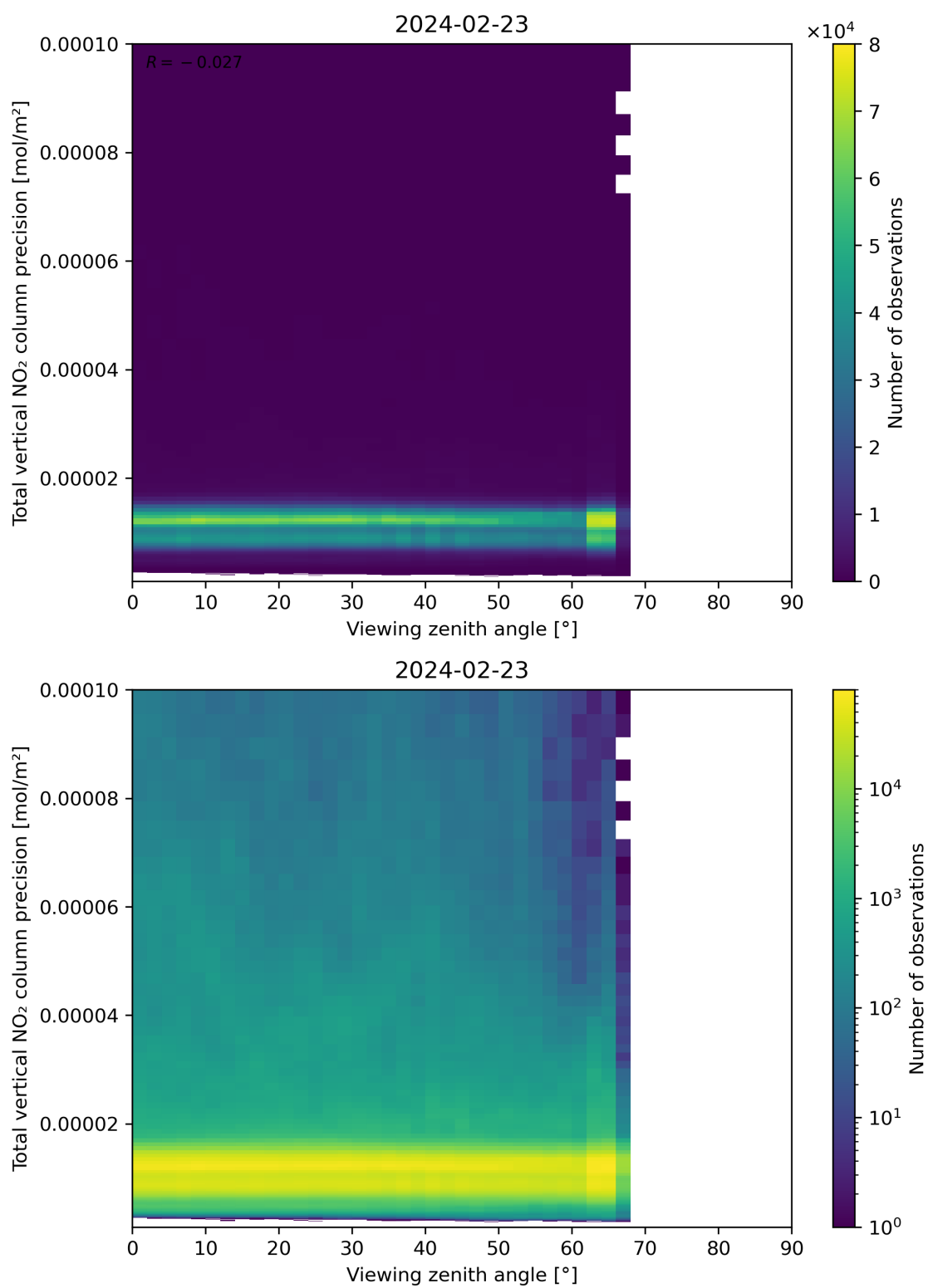
Figure 168: Scatter density plot of “Viewing zenith angle” against “Total vertical NO 2 column precision” for 2024-02-22 to 2024-02-24.
