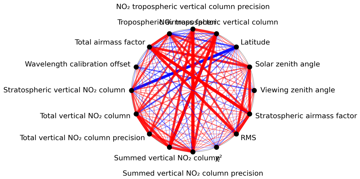
Figure 1: Map of correlation graph for 2024-02-22 to 2024-02-24.
