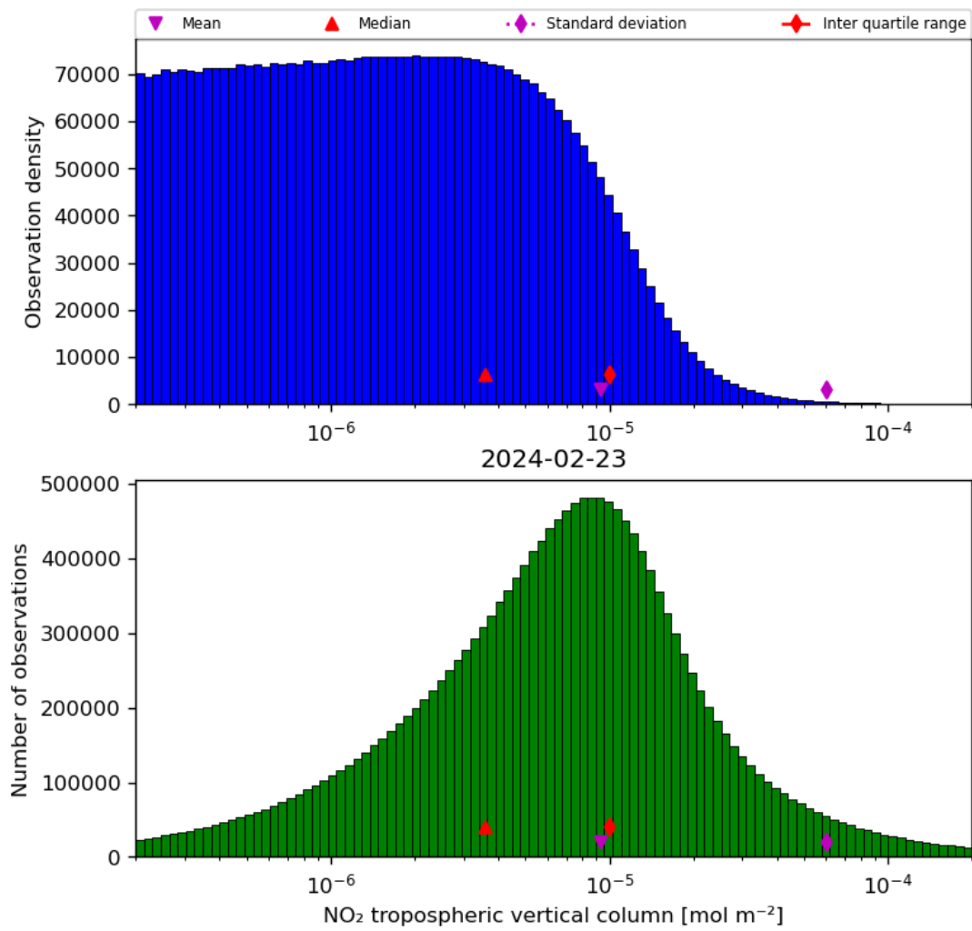
Figure 29: Histogram of “ \text{NO}_2 tropospheric vertical column” for 2024-02-22 to 2024-02-24
