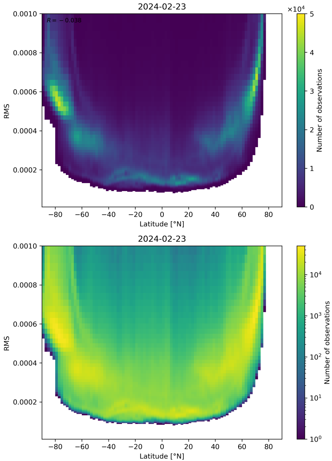
Figure 94: Scatter density plot of “Latitude” against “RMS” for 2024-02-22 to 2024-02-24.
