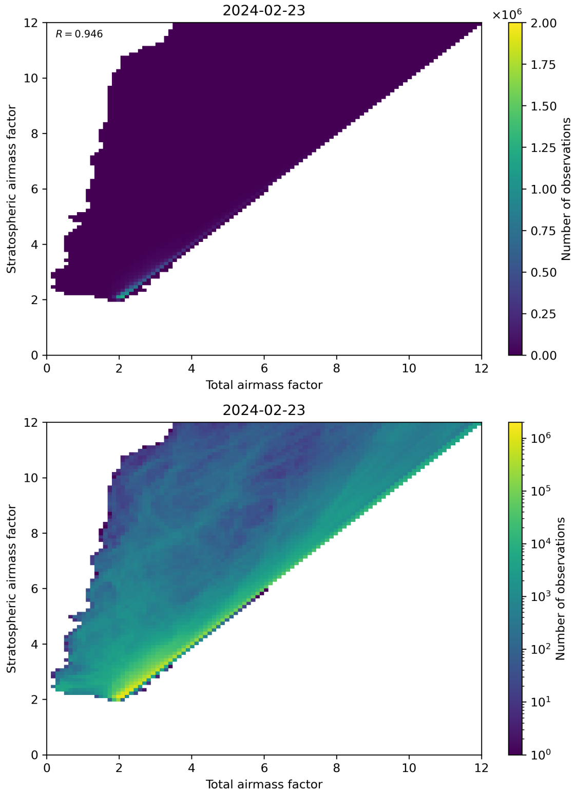
Figure 62: Scatter density plot of “Total airmass factor” against “Stratospheric airmass factor” for 2024-02-22 to 2024-02-24.
