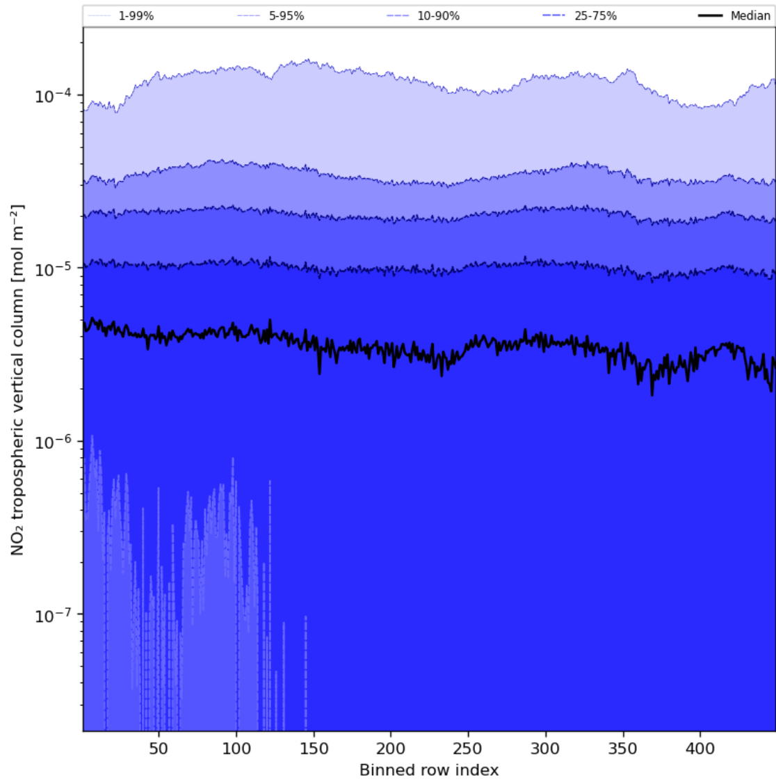
Figure 46: Along track statistics of “NO 2 tropospheric vertical column” for 2024-02-22 to 2024-02-24
