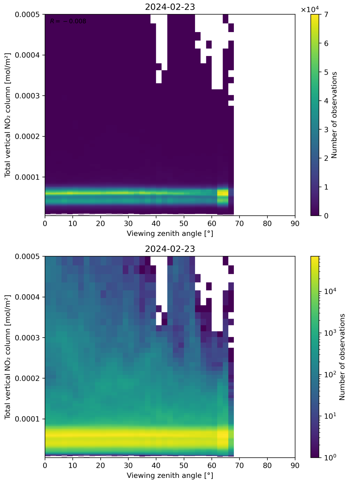
Figure 167: Scatter density plot of “Viewing zenith angle” against “Total vertical NO 2 column” for 2024-02-22 to 2024-02-24.
