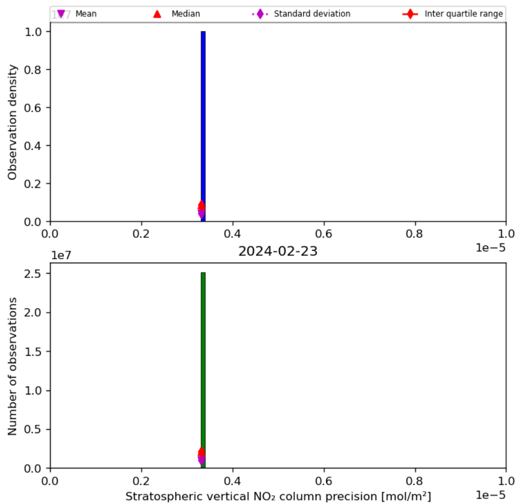
Figure 37: Histogram of “Stratospheric vertical NO 2 column precision” for 2024-02-22 to 2024-02-24
