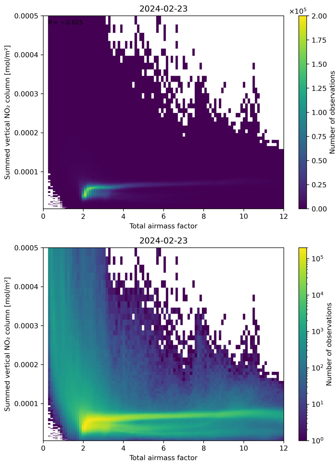
Figure 65: Scatter density plot of “Total airmass factor” against “Summed vertical NO 2 column” for 2024-02-22 to 2024-02-24.
