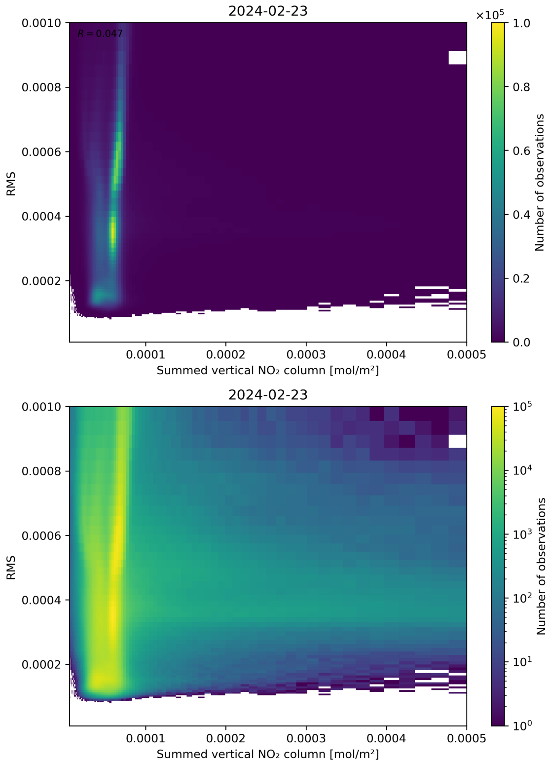
Figure 109: Scatter density plot of “Summed vertical NO 2 column” against “RMS” for 2024-02-22 to 2024-02-24.
