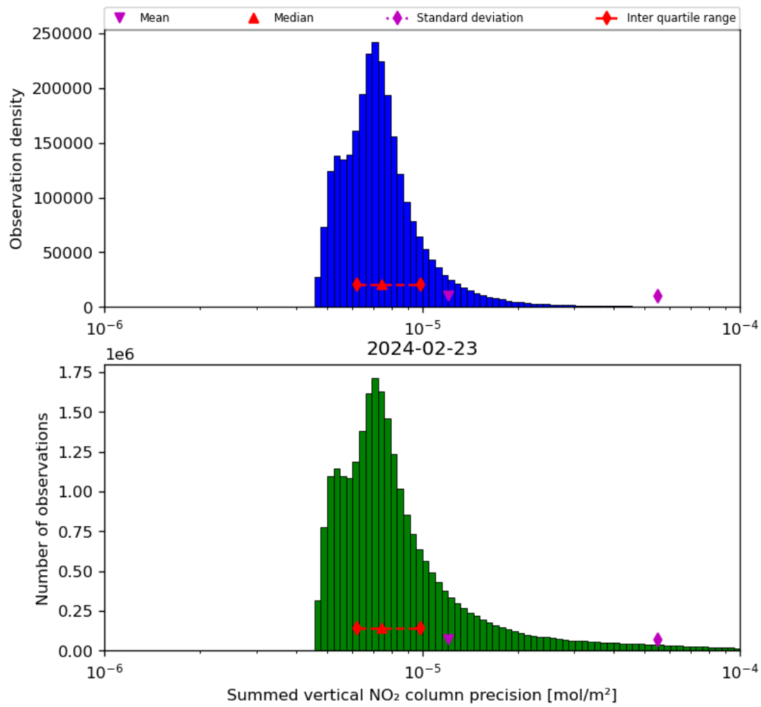
Figure 41: Histogram of “Summed vertical NO 2 column precision” for 2024-02-22 to 2024-02-24
