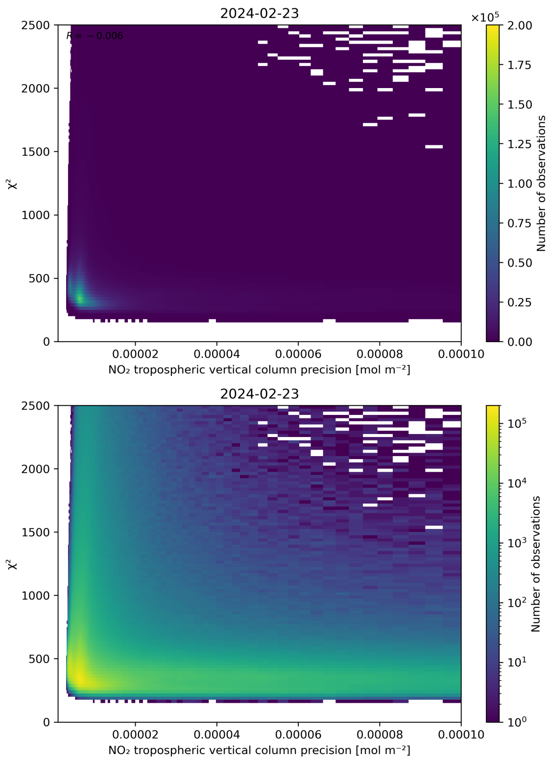
Figure 134: Scatter density plot of “NO 2 tropospheric vertical column precision” against “ \chi^2 ” for 2024-02-22 to 2024-02-24.
