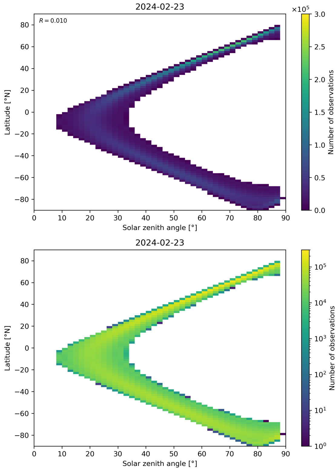
Figure 149: Scatter density plot of “Solar zenith angle” against “Latitude” for 2024-02-22 to 2024-02-24.
