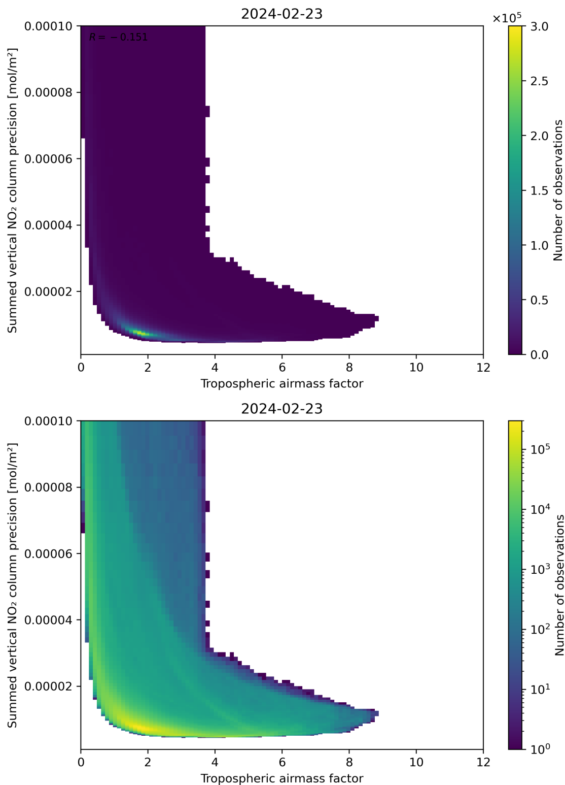
Figure 76: Scatter density plot of “Tropospheric air mass factor” against “Summed vertical NO 2 column precision” for 2024-02-22 to 2024-02-24.
