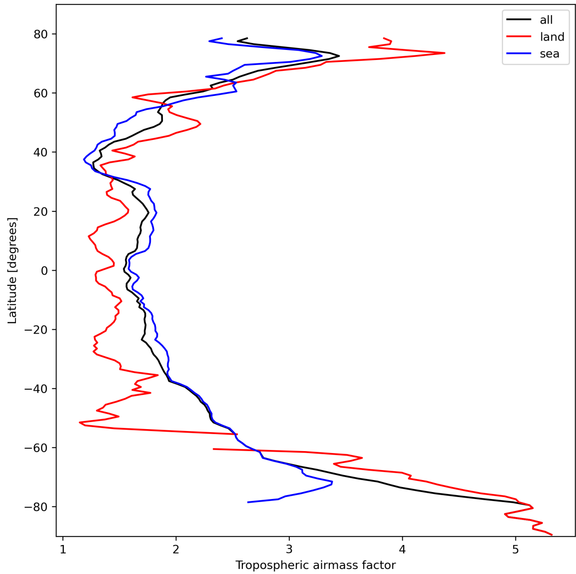
Figure 14: Zonal average of “Tropospheric airmass factor” for 2024-02-22 to 2024-02-24.
