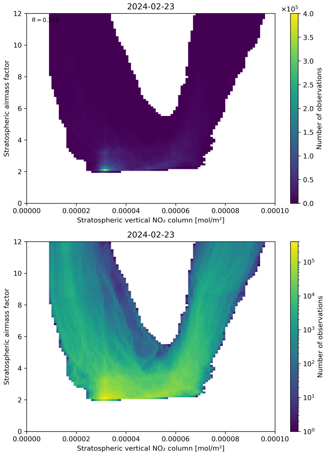
Figure 96: Scatter density plot of “Stratospheric vertical NO 2 column” against “Stratospheric airmass factor” for 2024-02-22 to 2024-02-24.
