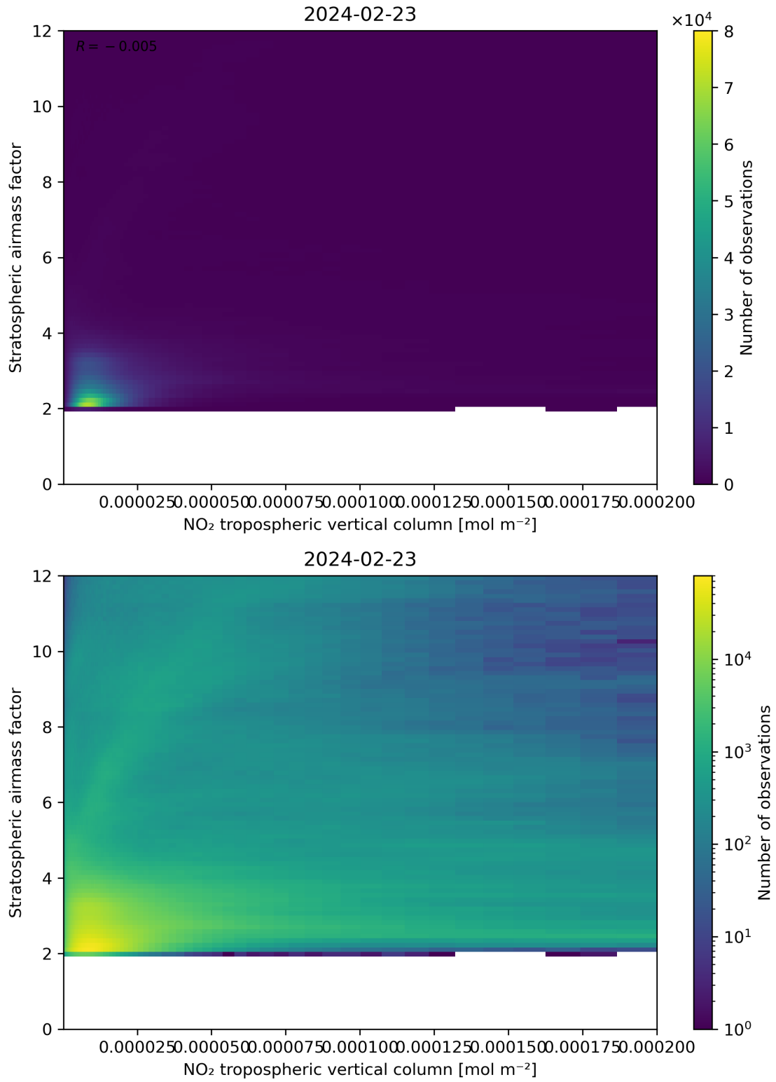
Figure 121: Scatter density plot of “NO 2 tropospheric vertical column” against “Stratospheric airmass factor” for 2024-02-22 to 2024-02-24.
