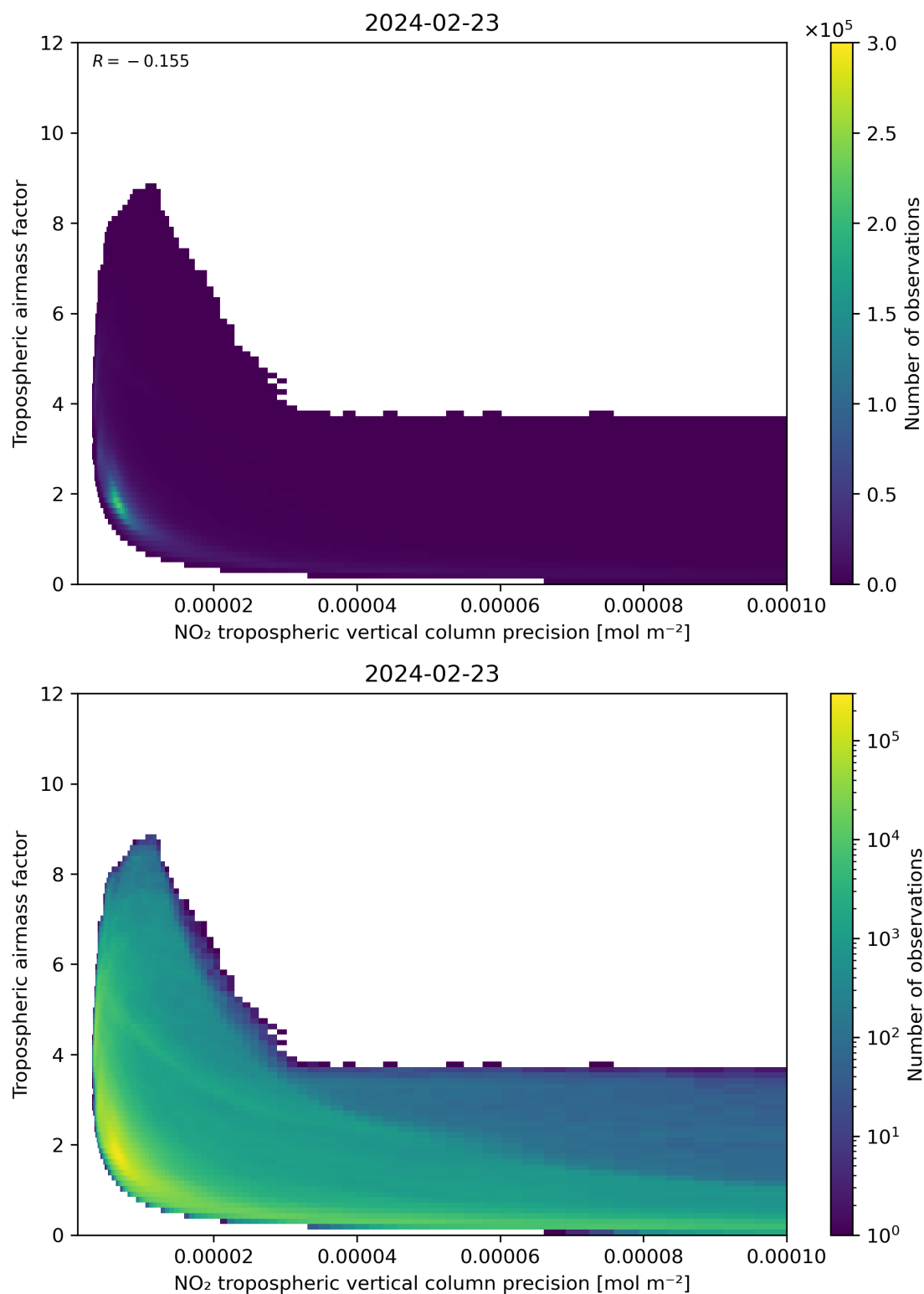
Figure 133: Scatter density plot of “NO 2 tropospheric vertical column precision” against “Tropospheric airmass factor” for 2024-02-22 to 2024-02-24.
