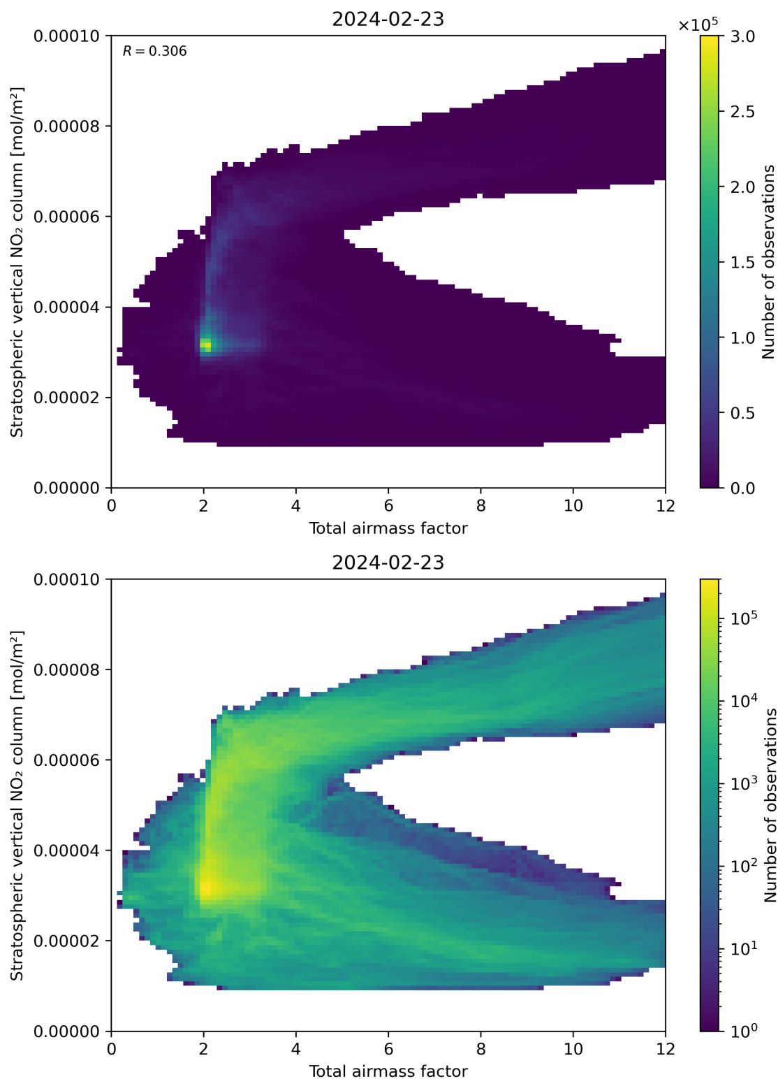
Figure 64: Scatter density plot of “Total airmass factor” against “Stratospheric vertical \text{NO}_2 column” for 2024-02-22 to 2024-02-24.
