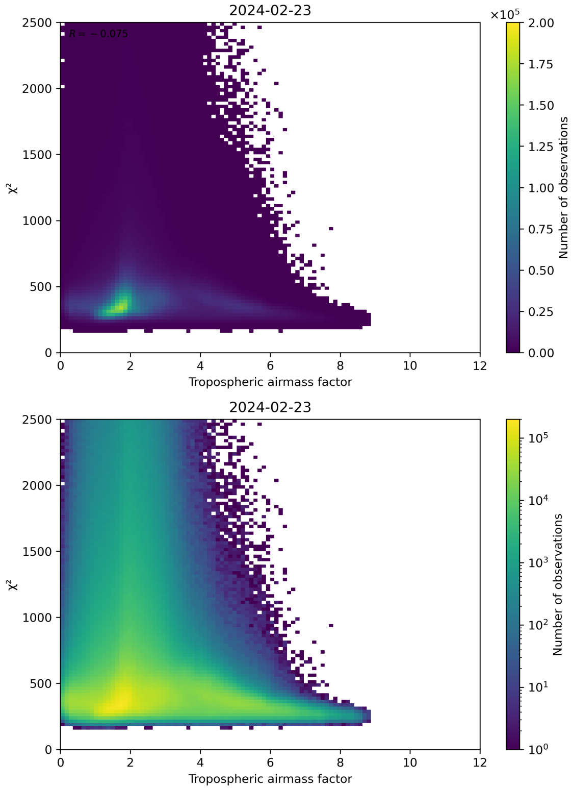
Figure 73: Scatter density plot of “Tropospheric airmass factor” against “ \chi^2 ” for 2024-02-22 to 2024-02-24.
