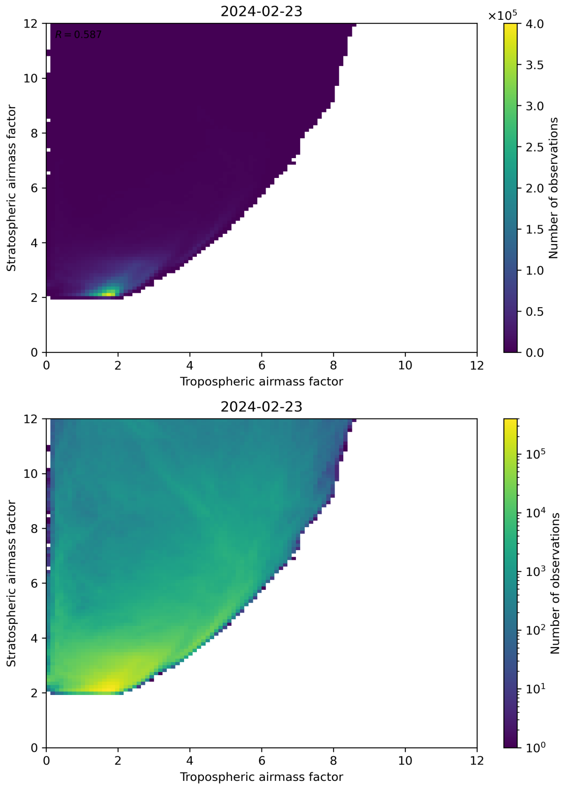
Figure 71: Scatter density plot of “Tropospheric airmass factor” against “Stratospheric airmass factor” for 2024-02-22 to 2024-02-24.
