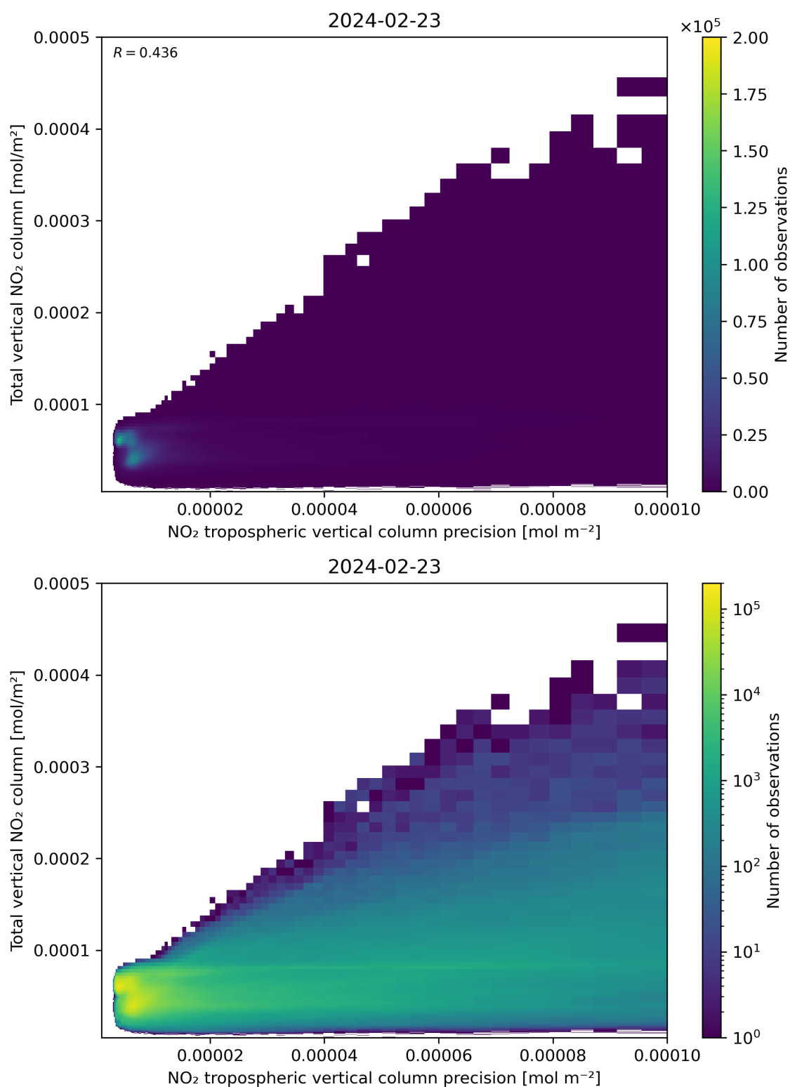
Figure 138: Scatter density plot of “NO 2 tropospheric vertical column precision” against “Total vertical NO 2 column” for 2024-02-22 to 2024-02-24.
