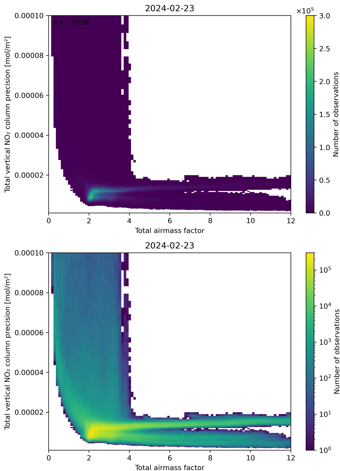
Figure 68: Scatter density plot of “Total airmass factor” against “Total vertical NO 2 column precision” for 2024-02-22 to 2024-02-24.
