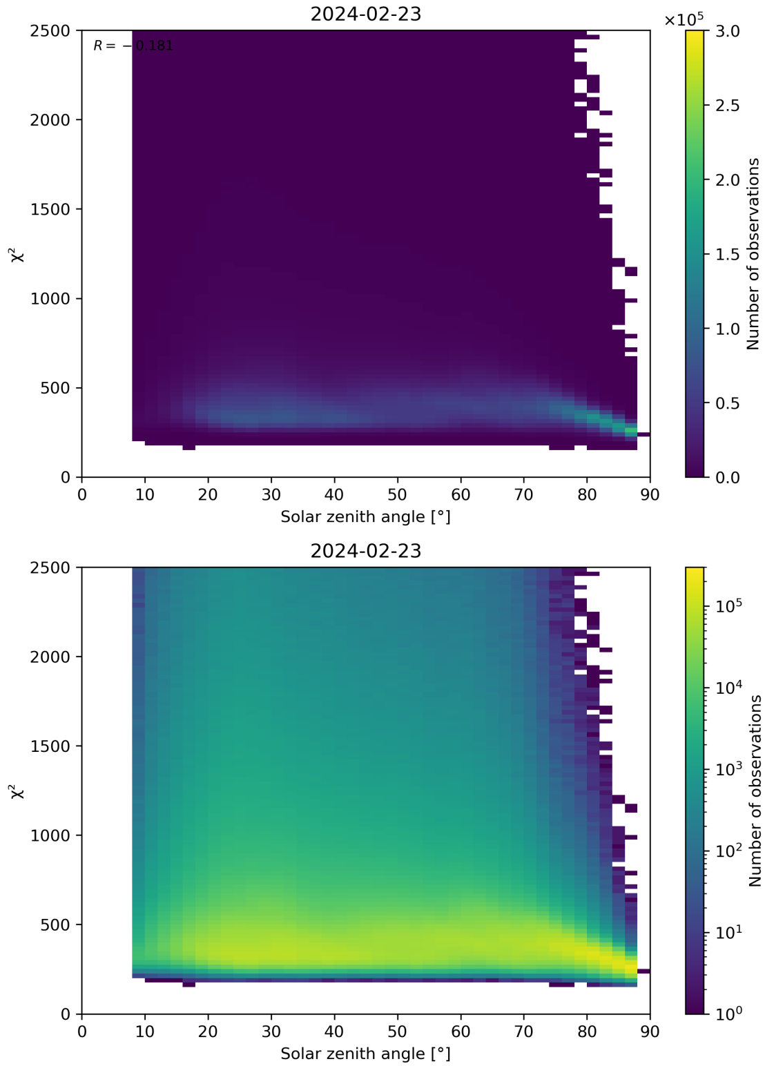
Figure 148: Scatter density plot of “Solar zenith angle” against “ \chi^2 ” for 2024-02-22 to 2024-02-24.
