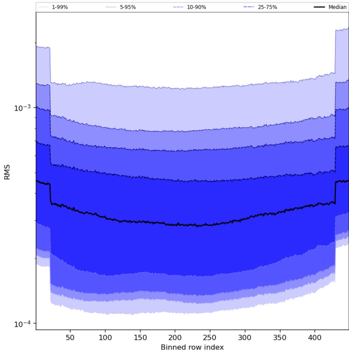
Figure 60: Along track statistics of “RMS” for 2024-02-22 to 2024-02-24
