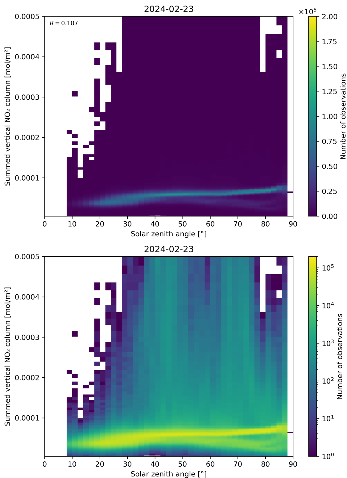
Figure 151: Scatter density plot of “Solar zenith angle” against “Summed vertical NO 2 column” for 2024-02-22 to 2024-02-24.
