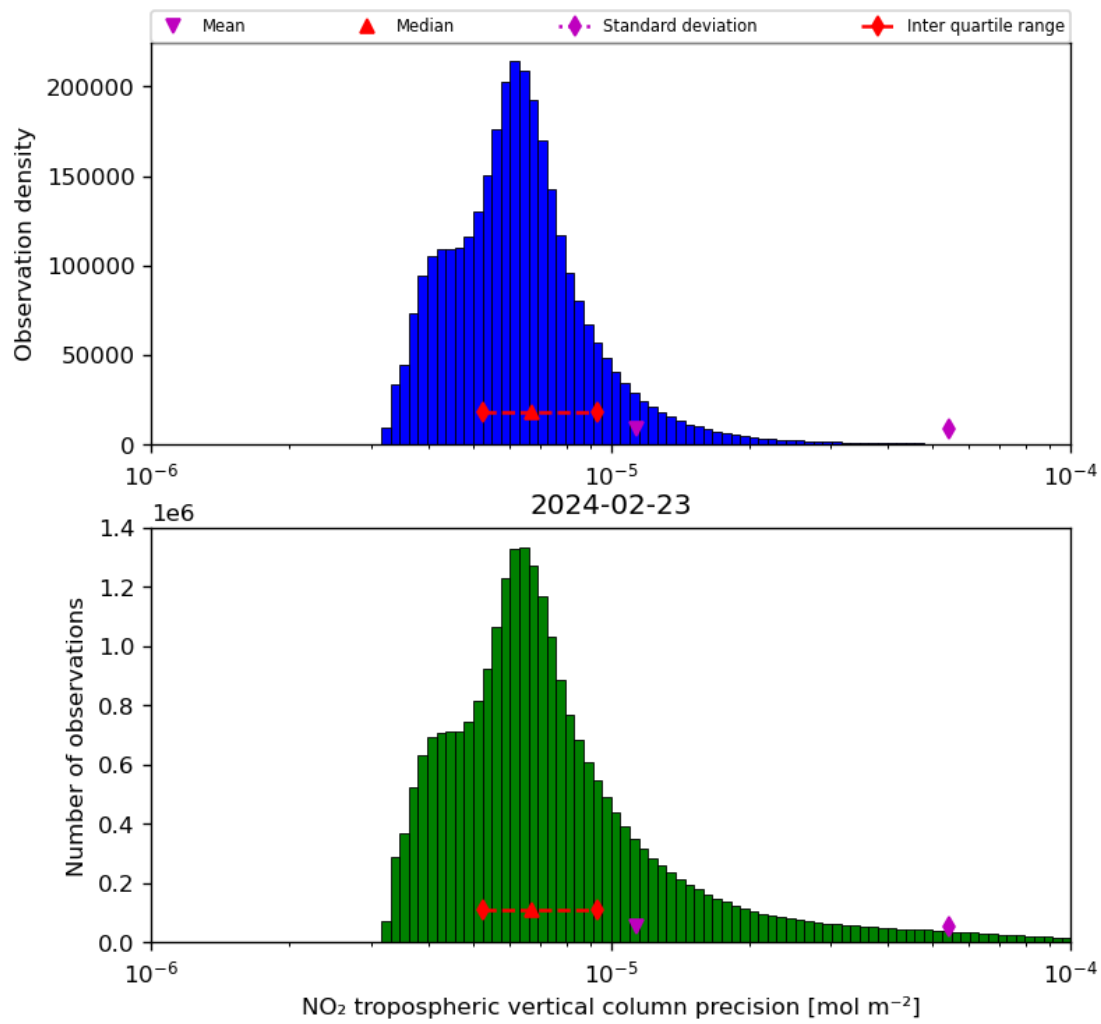
Figure 30: Histogram of “NO 2 tropospheric vertical column precision” for 2024-02-22 to 2024-02-24
