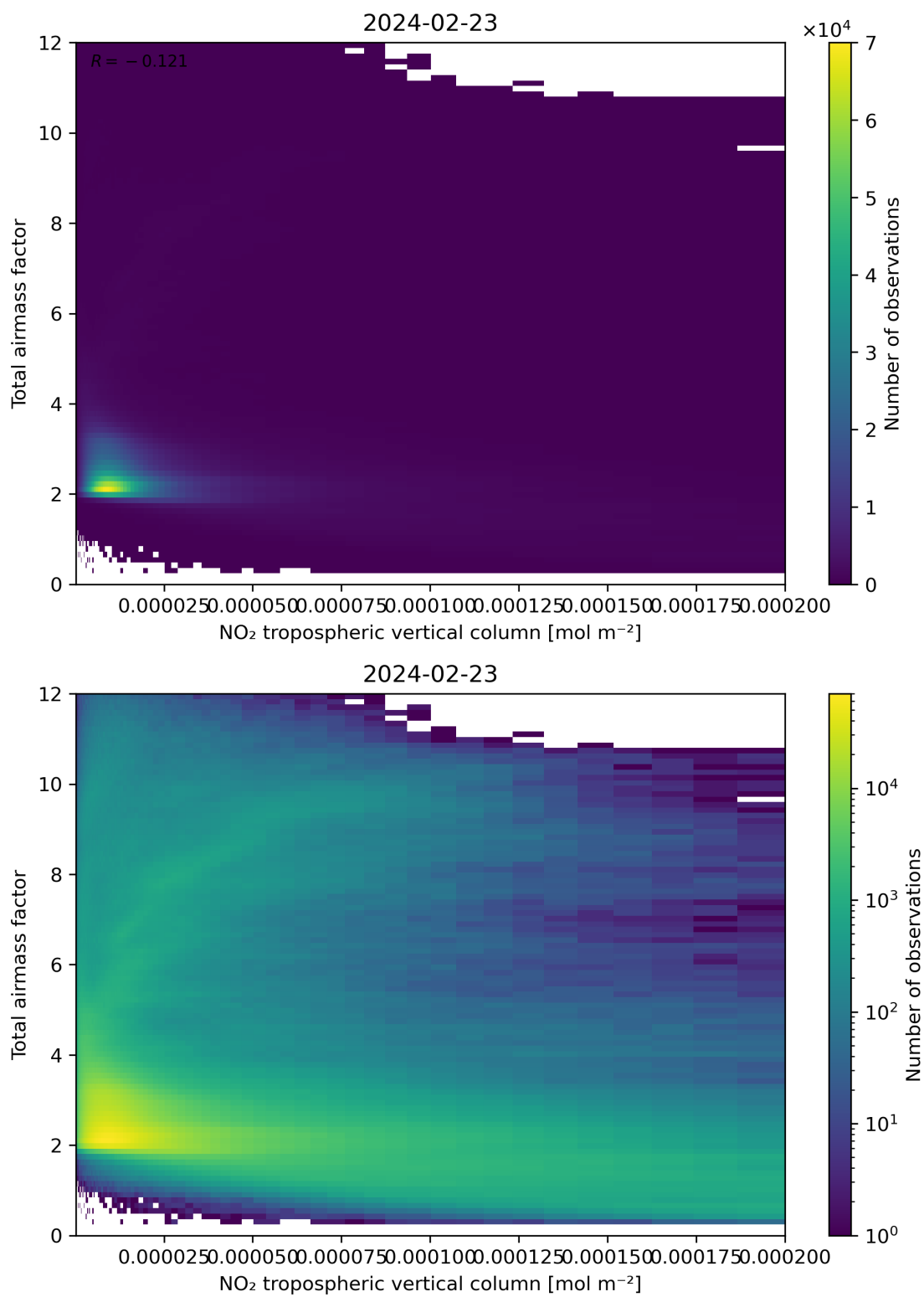
Figure 122: Scatter density plot of “NO 2 tropospheric vertical column” against “Total air mass factor” for 2024-02-22 to 2024-02-24.
