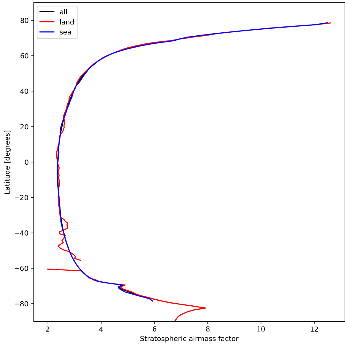
Figure 27: Zonal average of “Stratospheric air mass factor” for 2024-02-22 to 2024-02-24.
