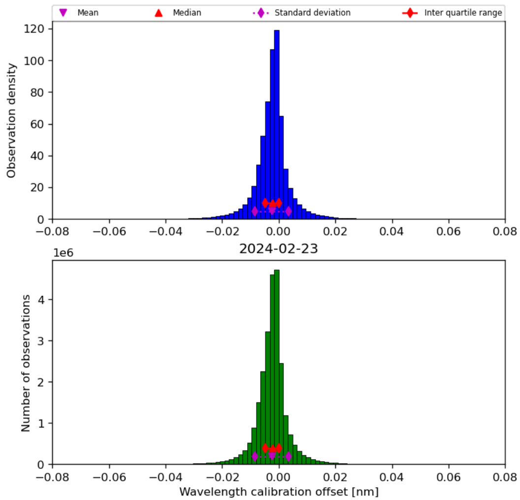
Figure 35: Histogram of “Wavelength calibration offset” for 2024-02-22 to 2024-02-24
