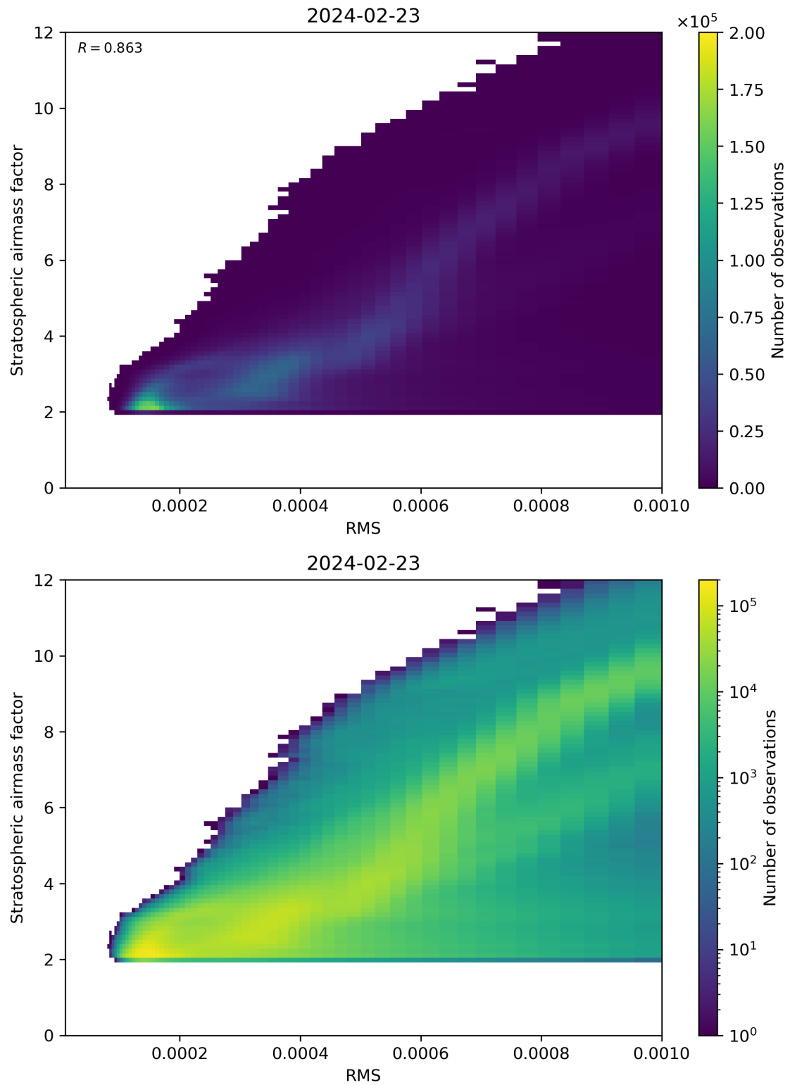
Figure 144: Scatter density plot of “RMS” against “Stratospheric airmass factor” for 2024-02-22 to 2024-02-24.
