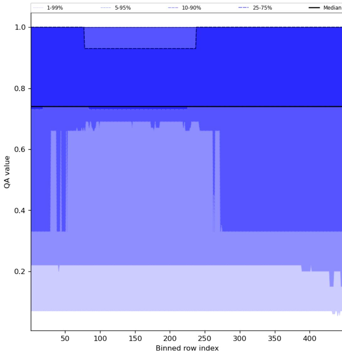
Figure 45: Along track statistics of “QA value” for 2024-02-22 to 2024-02-24
