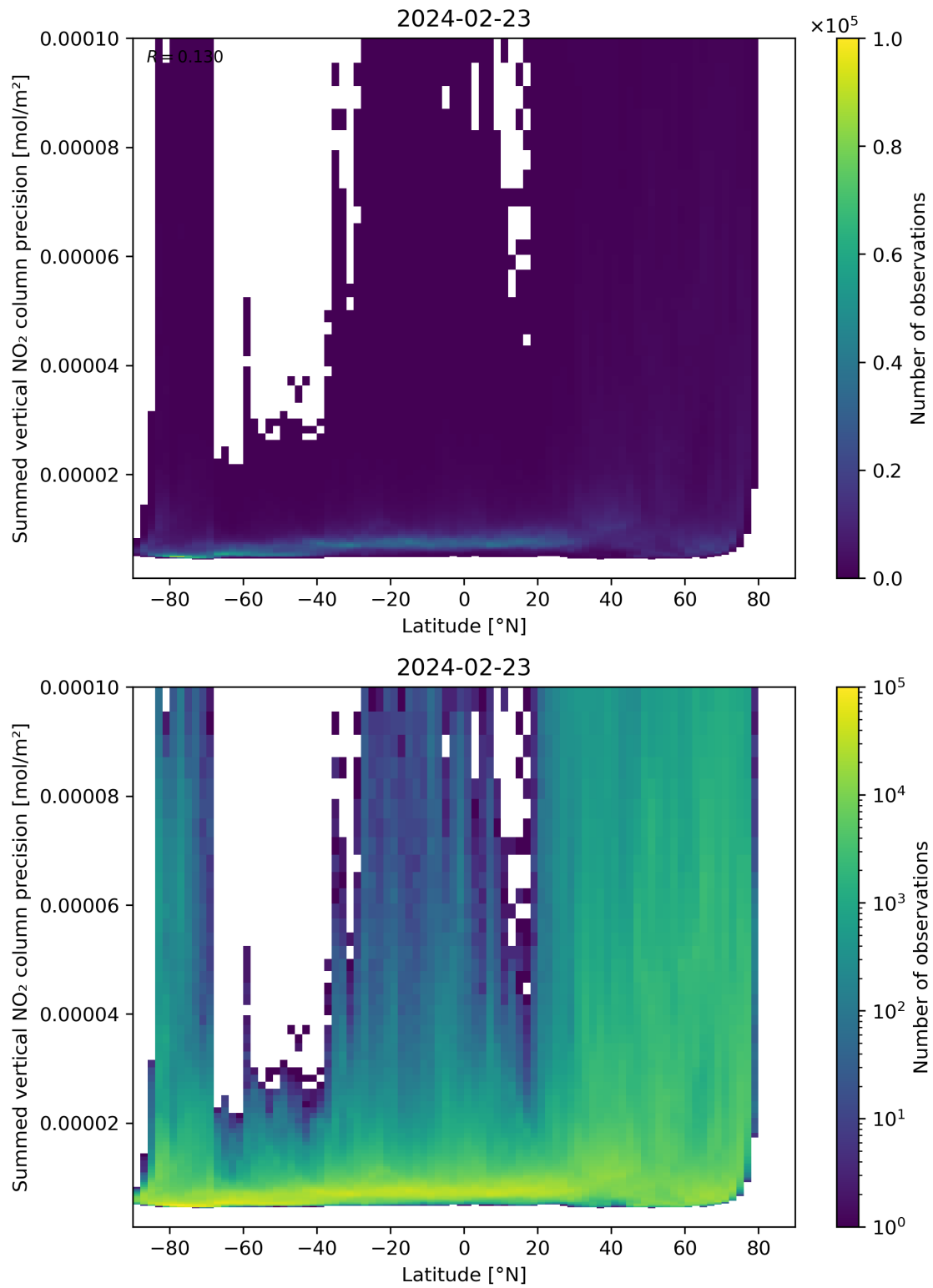
Figure 89: Scatter density plot of “Latitude” against “Summed vertical NO 2 column precision” for 2024-02-22 to 2024-02-24.
