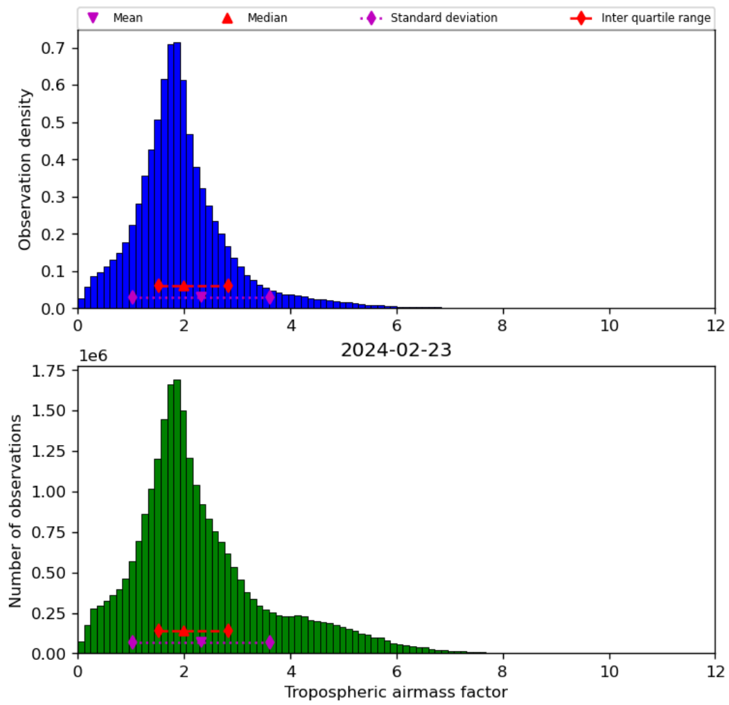
Figure 31: Histogram of “Tropospheric airmass factor” for 2024-02-22 to 2024-02-24
