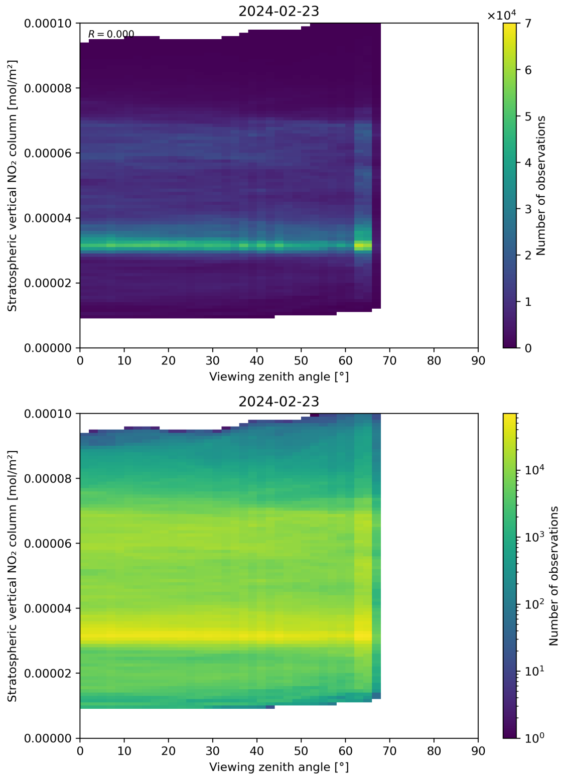
Figure 164: Scatter density plot of “Viewing zenith angle” against “Stratospheric vertical NO 2 column” for 2024-02-22 to 2024-02-24.
