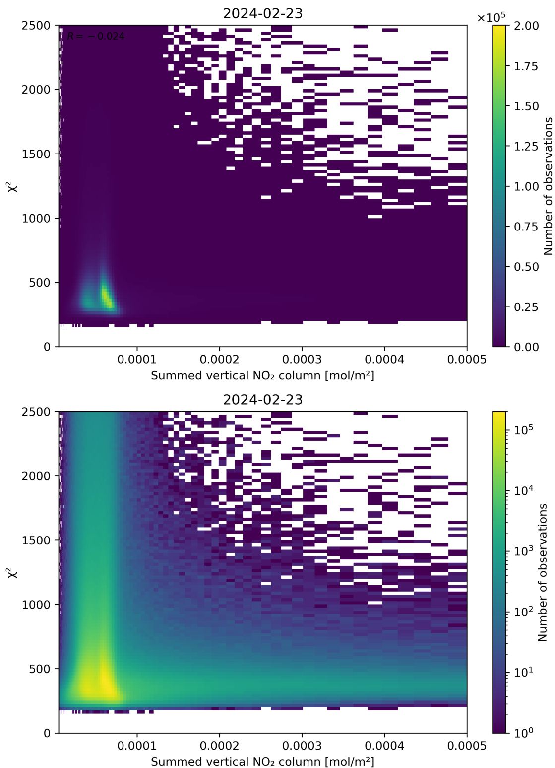
Figure 104: Scatter density plot of “Summed vertical NO 2 column” against “ \chi^2 ” for 2024-02-22 to 2024-02-24.
