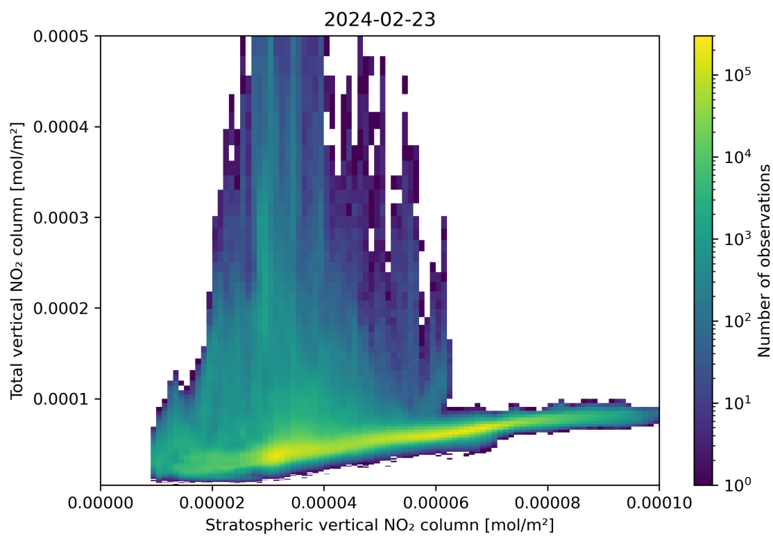
Figure 100: Scatter density plot of “Stratospheric vertical NO 2 column” against “Total vertical NO 2 column” for 2024-02-22 to 2024-02-24.
