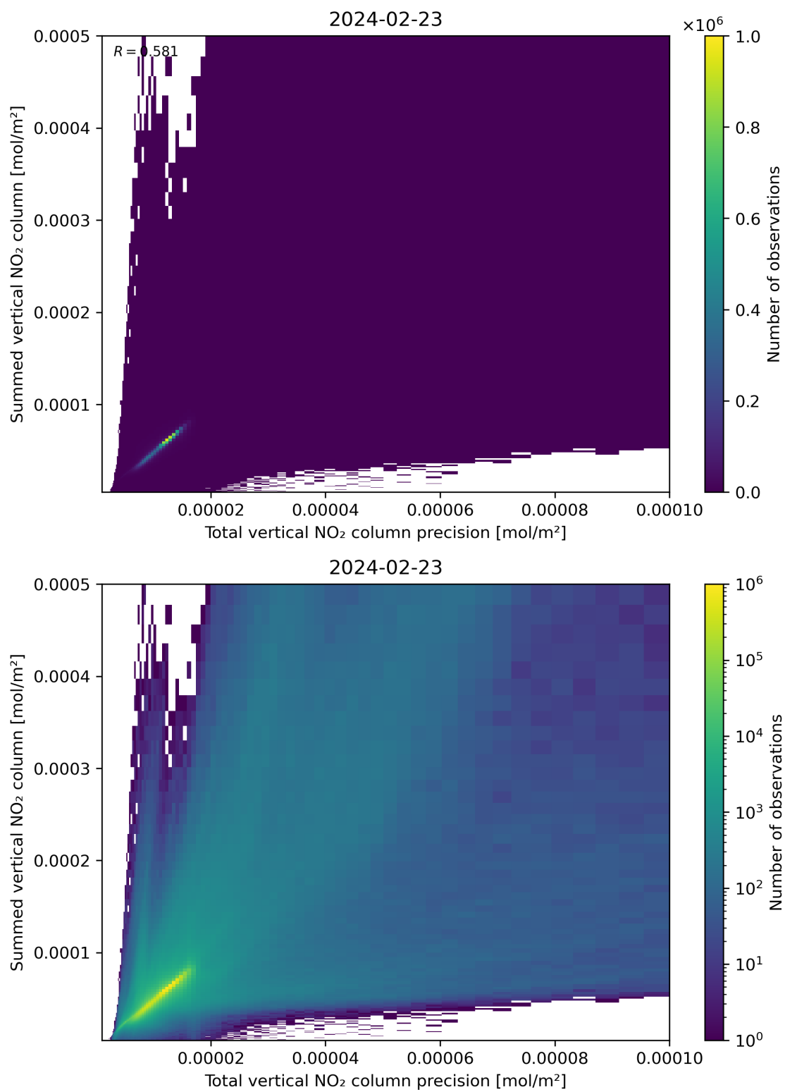
Figure 117: Scatter density plot of “Total vertical NO 2 column precision” against “Summed vertical NO 2 column” for 2024-02-22 to 2024-02-24.
