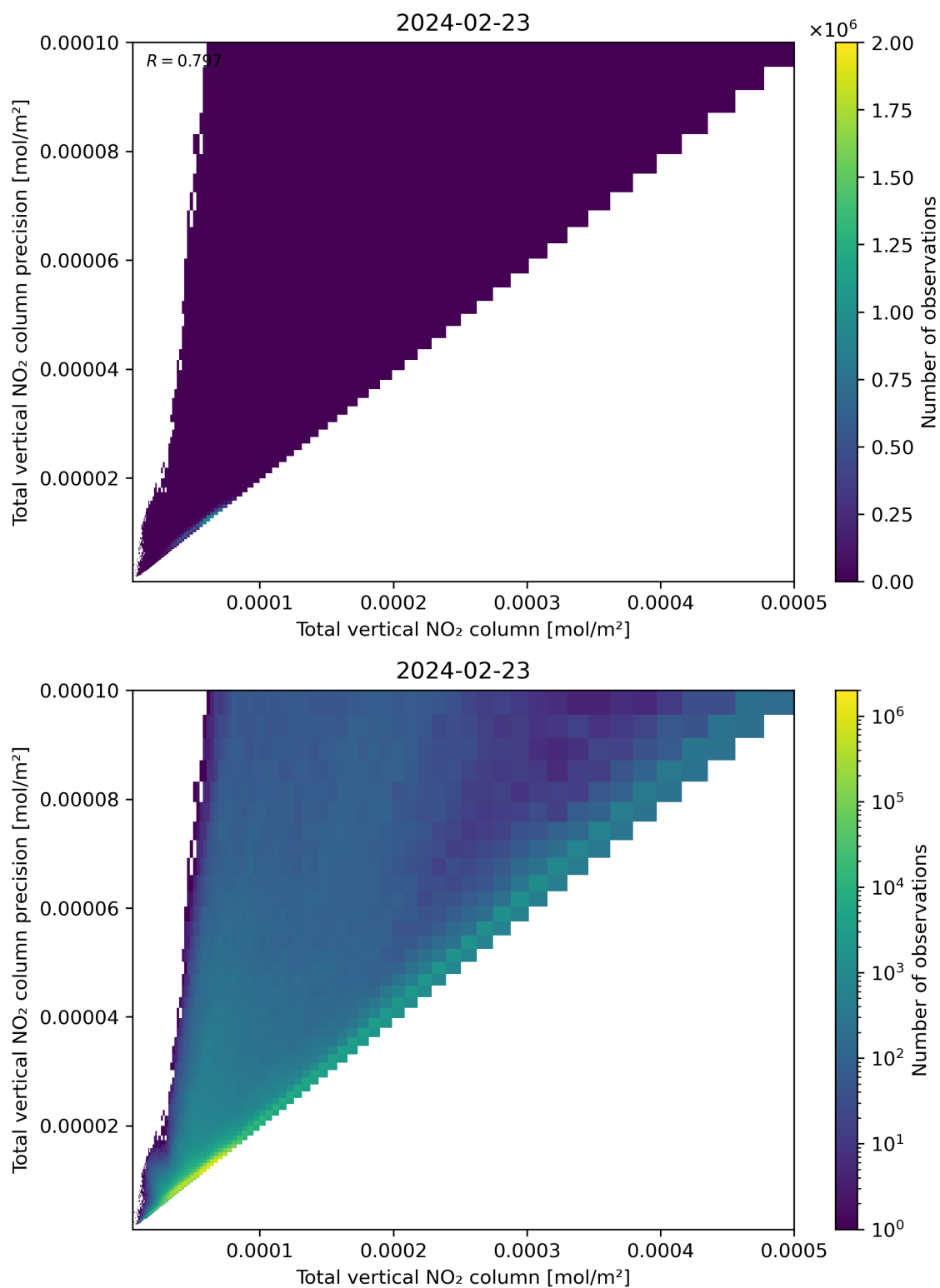
Figure 114: Scatter density plot of “Total vertical NO 2 column” against “Total vertical NO 2 column precision” for 2024-02-22 to 2024-02-24.
