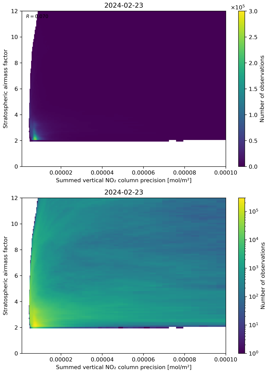
Figure 106: Scatter density plot of “Summed vertical NO 2 column precision” against “Stratospheric airmass factor” for 2024-02-22 to 2024-02-24.
