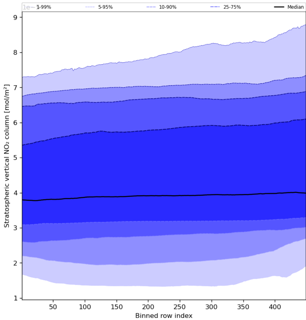
Figure 53: Along track statistics of “Stratospheric vertical NO 2 column” for 2024-02-22 to 2024-02-24
