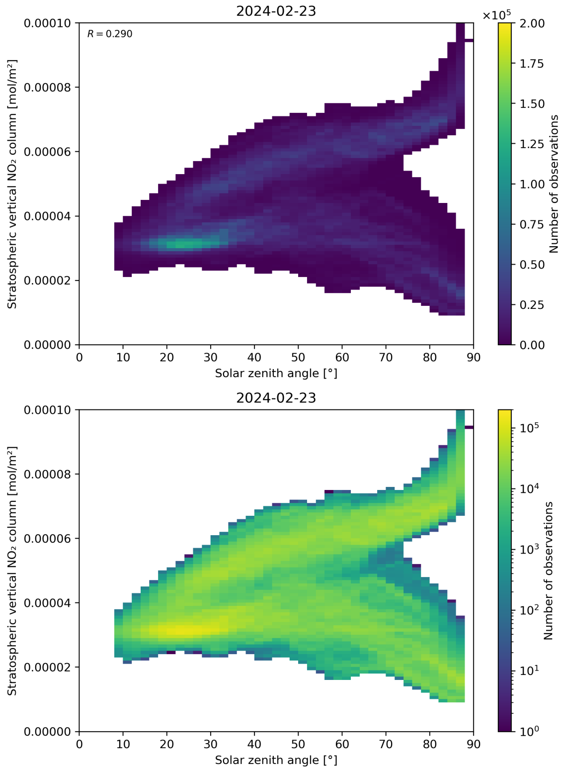
Figure 150: Scatter density plot of “Solar zenith angle” against “Stratospheric vertical NO 2 column” for 2024-02-22 to 2024-02-24.
