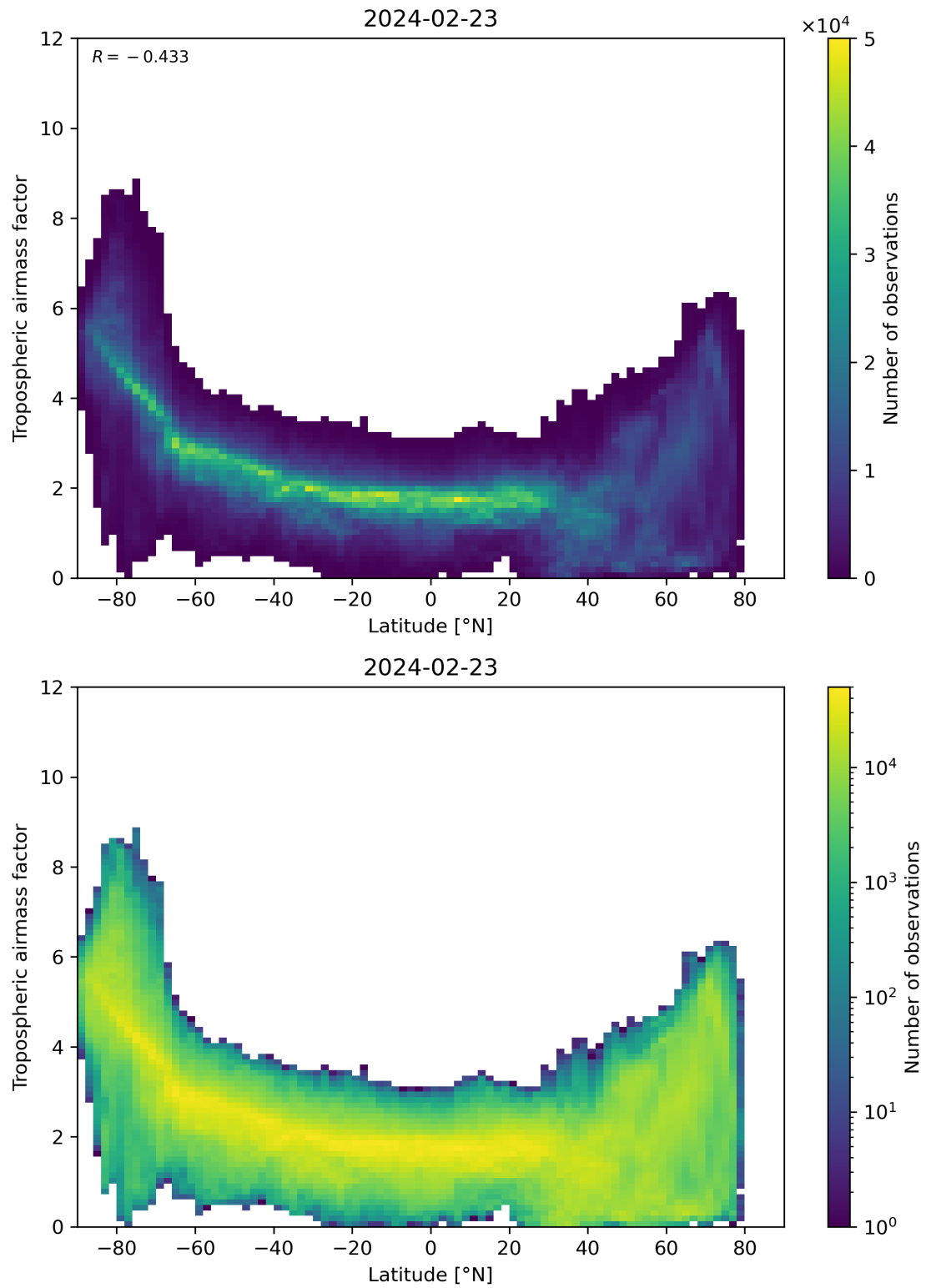
Figure 85: Scatter density plot of “Latitude” against “Tropospheric airmass factor” for 2024-02-22 to 2024-02-24.
