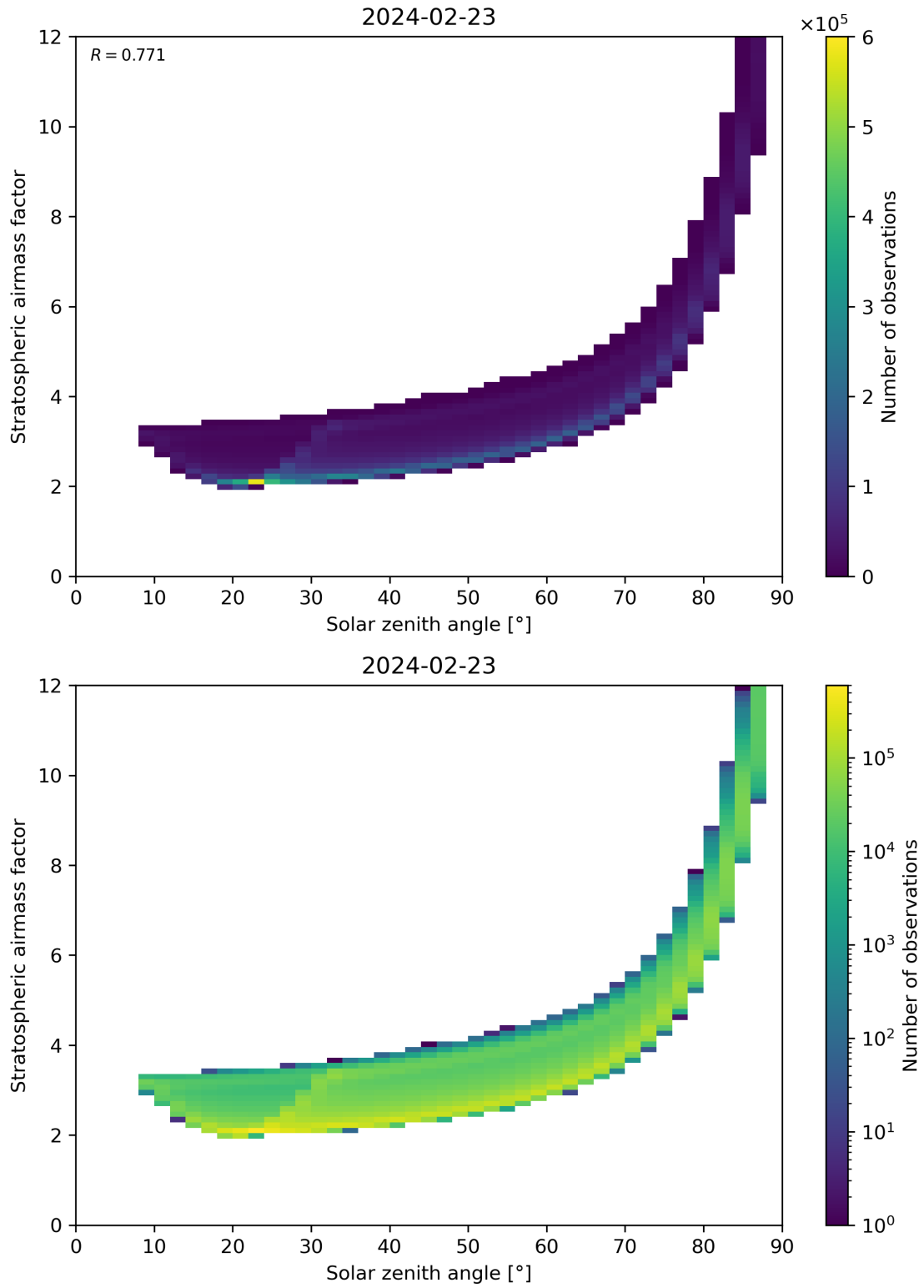
Figure 145: Scatter density plot of “Solar zenith angle” against “Stratospheric airmass factor” for 2024-02-22 to 2024-02-24.
