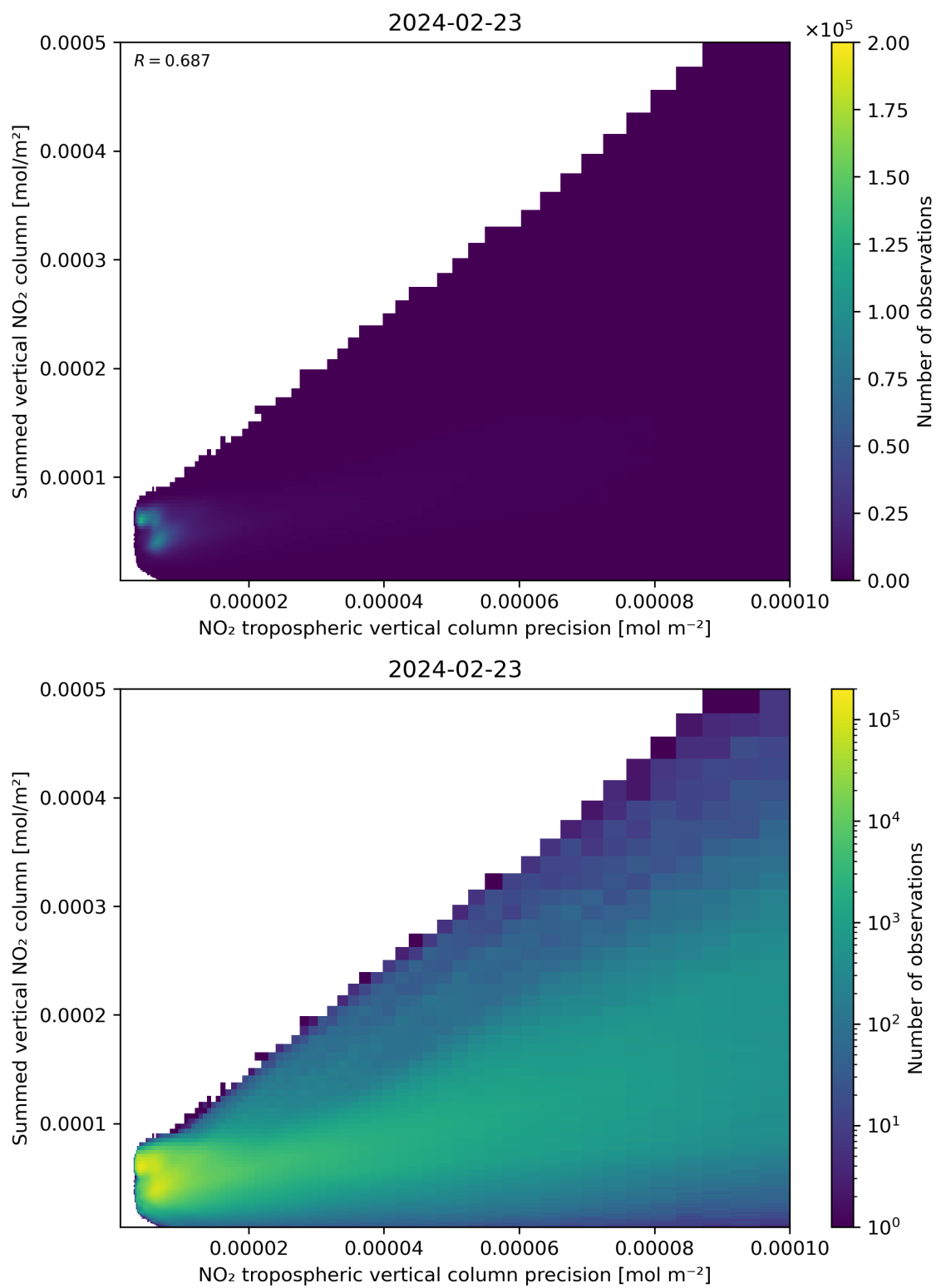
Figure 136: Scatter density plot of “NO 2 tropospheric vertical column precision” against “Summed vertical NO 2 column” for 2024-02-22 to 2024-02-24.
