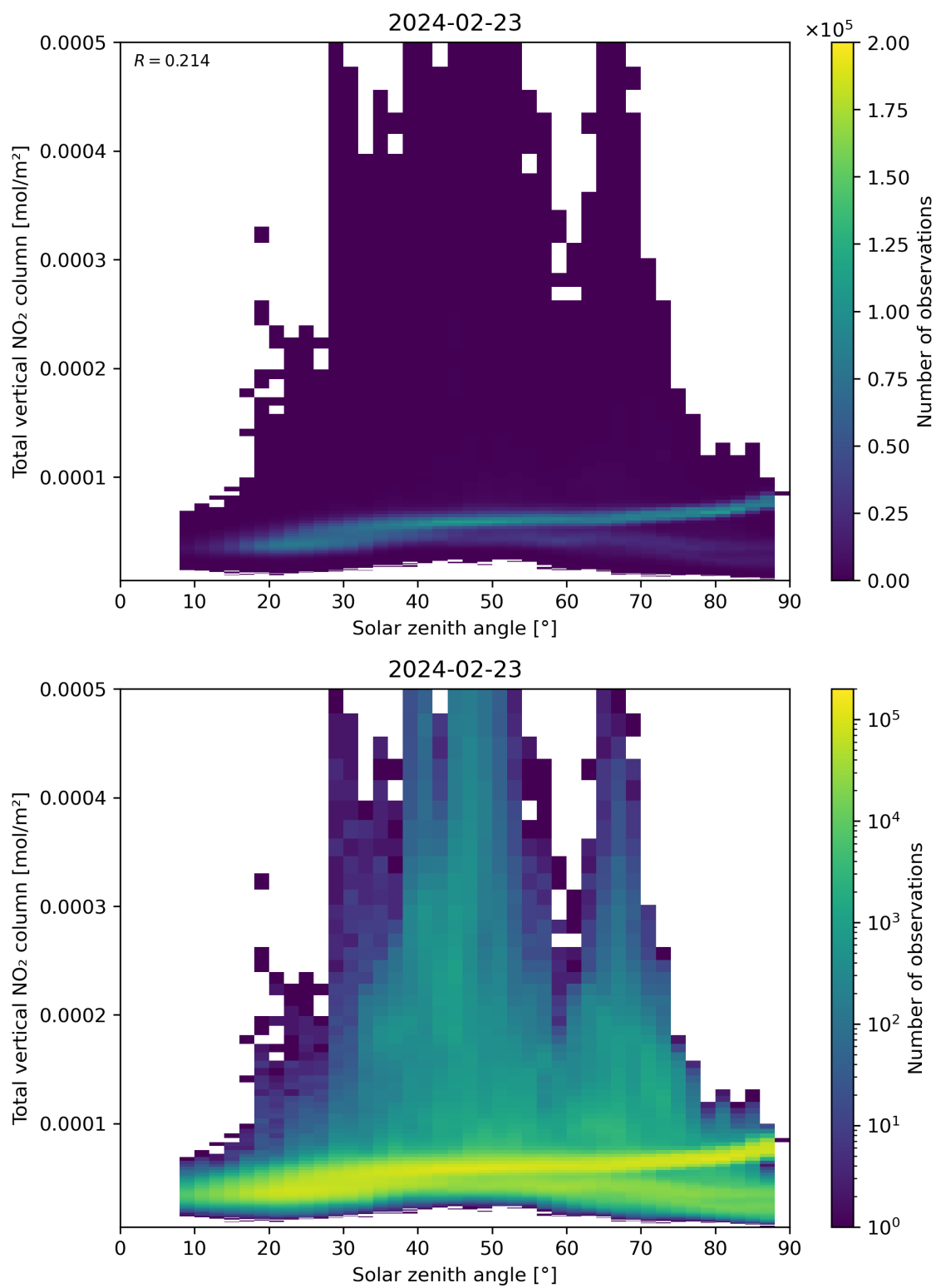
Figure 153: Scatter density plot of “Solar zenith angle” against “Total vertical NO 2 column” for 2024-02-22 to 2024-02-24.
