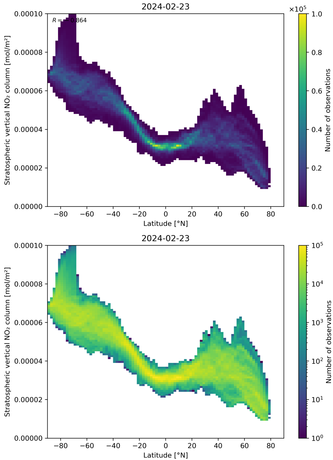
Figure 87: Scatter density plot of “Latitude” against “Stratospheric vertical NO 2 column” for 2024-02-22 to 2024-02-24.
