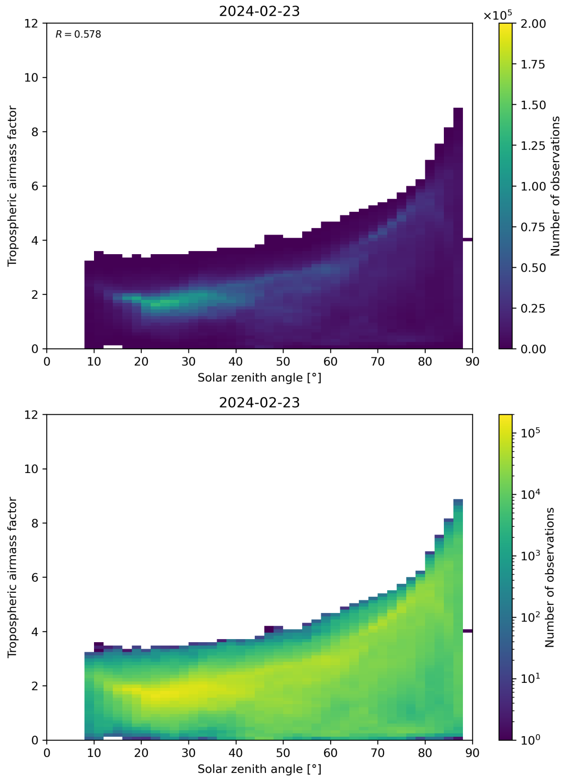
Figure 147: Scatter density plot of “Solar zenith angle” against “Tropospheric airmass factor” for 2024-02-22 to 2024-02-24.
