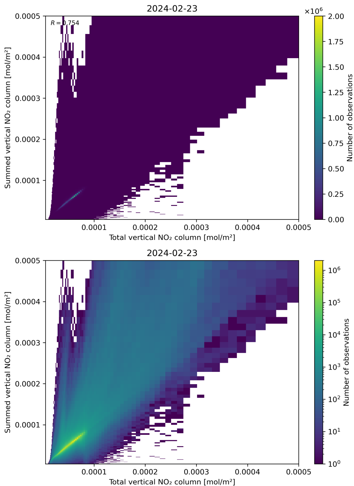
Figure 112: Scatter density plot of “Total vertical NO 2 column” against “Summed vertical NO 2 column” for 2024-02-22 to 2024-02-24.
