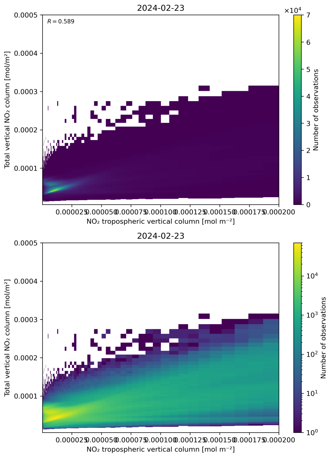
Figure 128: Scatter density plot of “NO 2 tropospheric vertical column” against “Total vertical NO 2 column” for 2024-02-22 to 2024-02-24.
