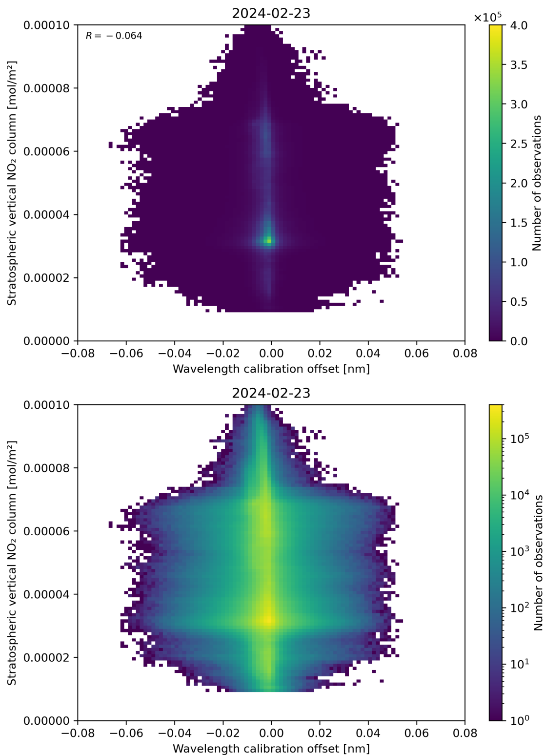
Figure 176: Scatter density plot of “Wavelength calibration offset” against “Stratospheric vertical NO 2 column” for 2024-02-22 to 2024-02-24.
