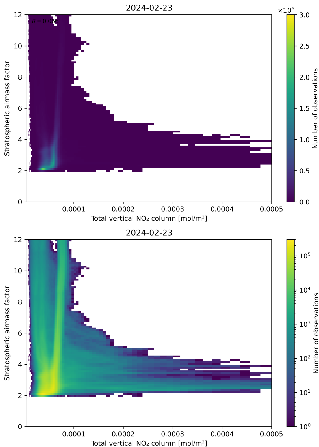
Figure 110: Scatter density plot of “Total vertical NO 2 column” against “Stratospheric airmass factor” for 2024-02-22 to 2024-02-24.
