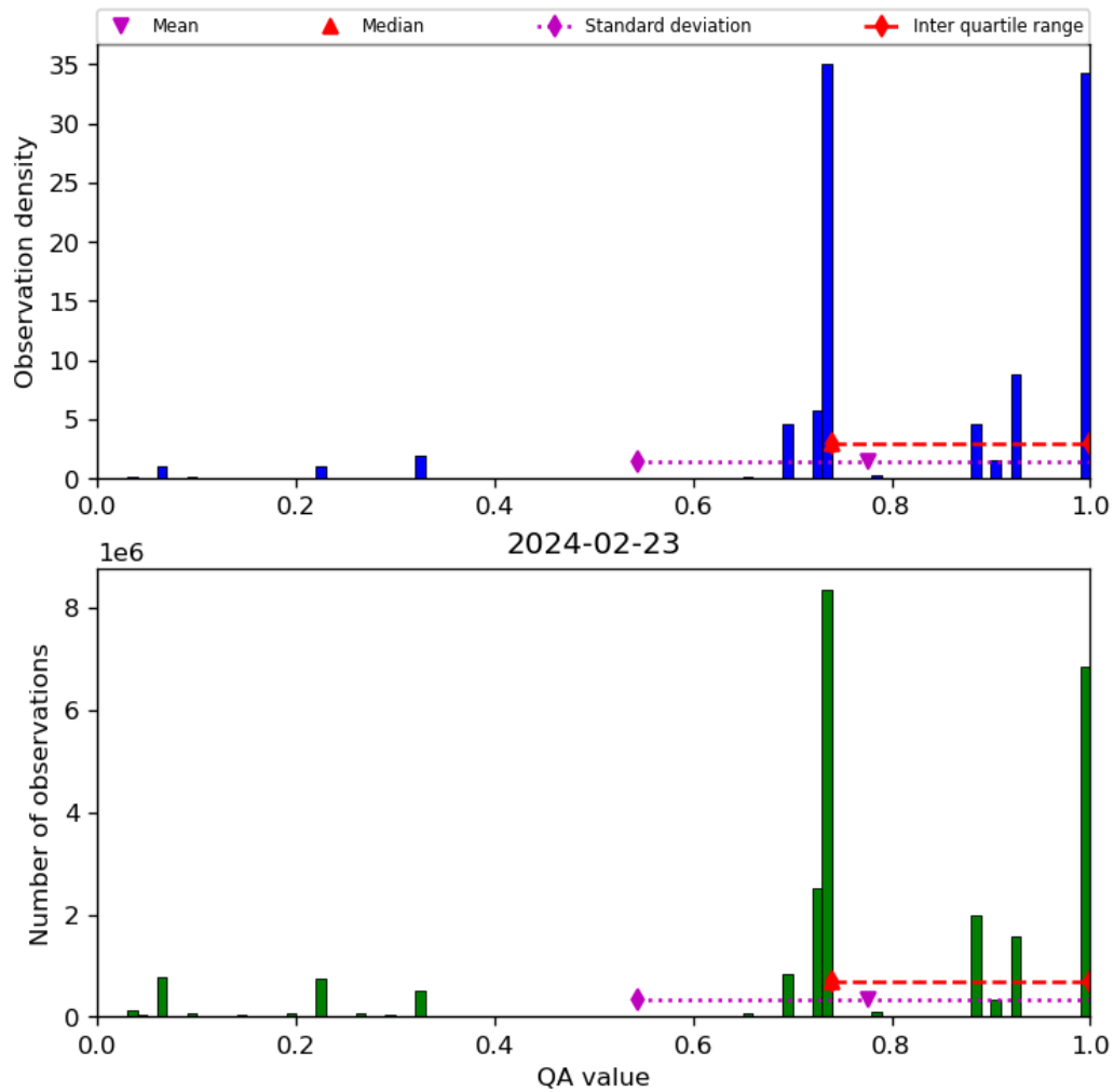
Figure 28: Histogram of “QA value” for 2024-02-22 to 2024-02-24
