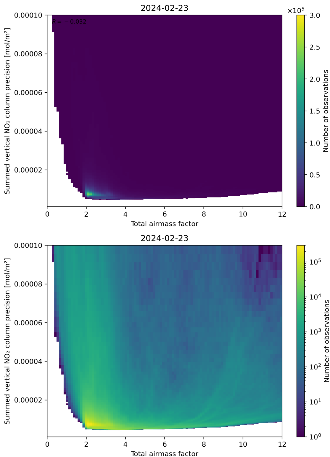
Figure 66: Scatter density plot of “Total airmass factor” against “Summed vertical NO 2 column precision” for 2024-02-22 to 2024-02-24.
