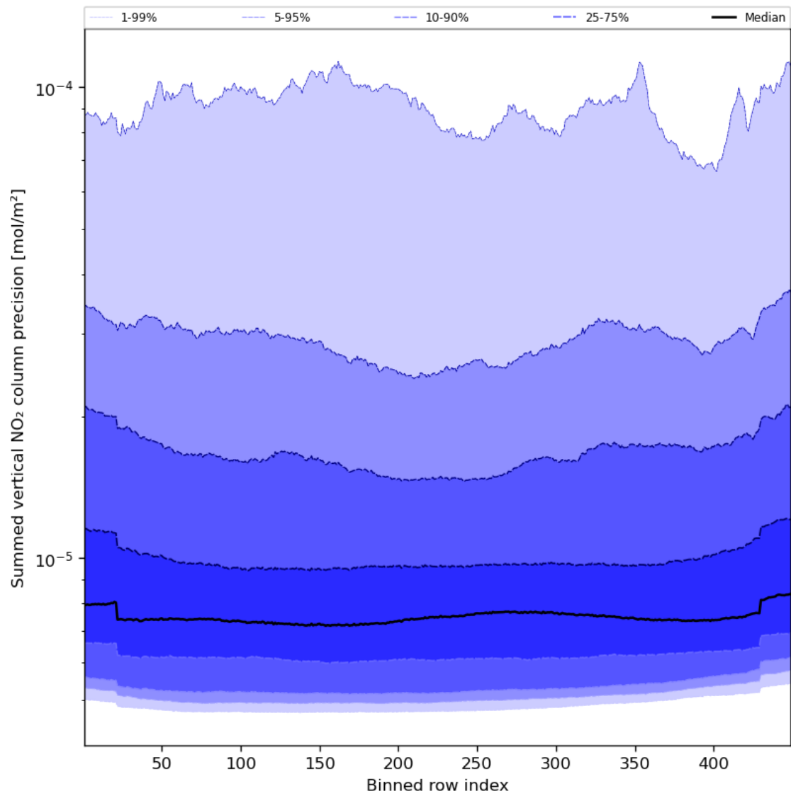
Figure 58: Along track statistics of “Summed vertical NO 2 column precision” for 2024-02-22 to 2024-02-24
