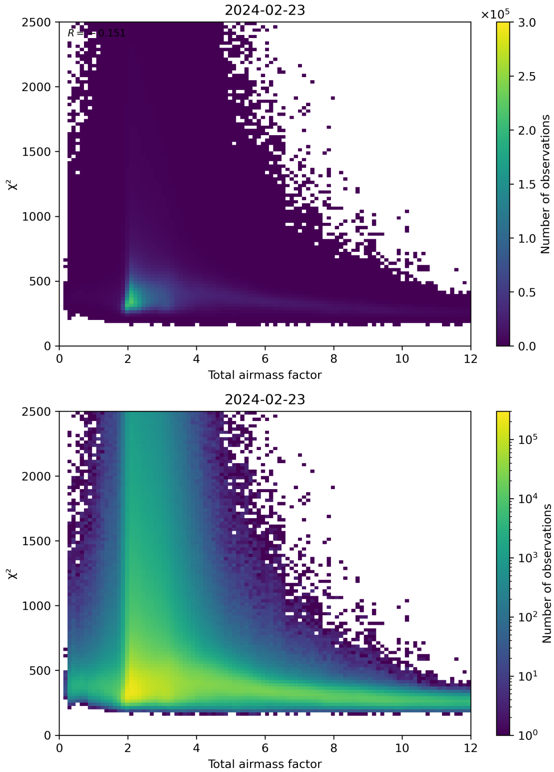
Figure 63: Scatter density plot of “Total airmass factor” against “ \chi^2 ” for 2024-02-22 to 2024-02-24.
