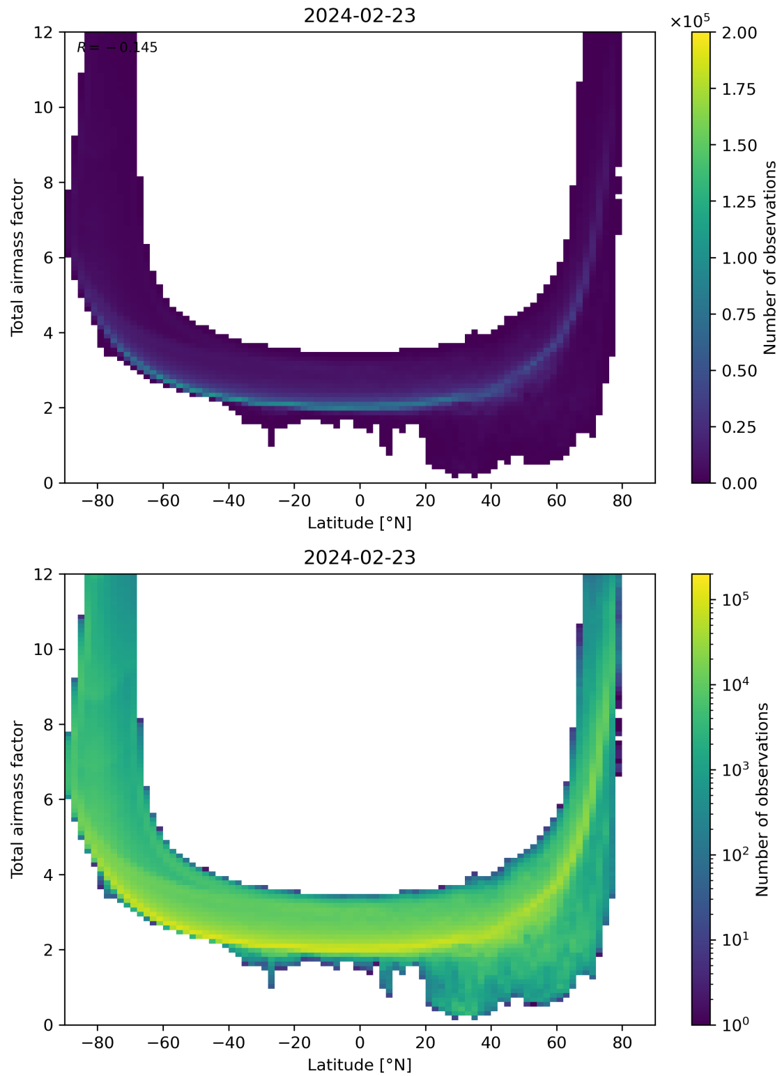
Figure 84: Scatter density plot of “Latitude” against “Total airmass factor” for 2024-02-22 to 2024-02-24.
