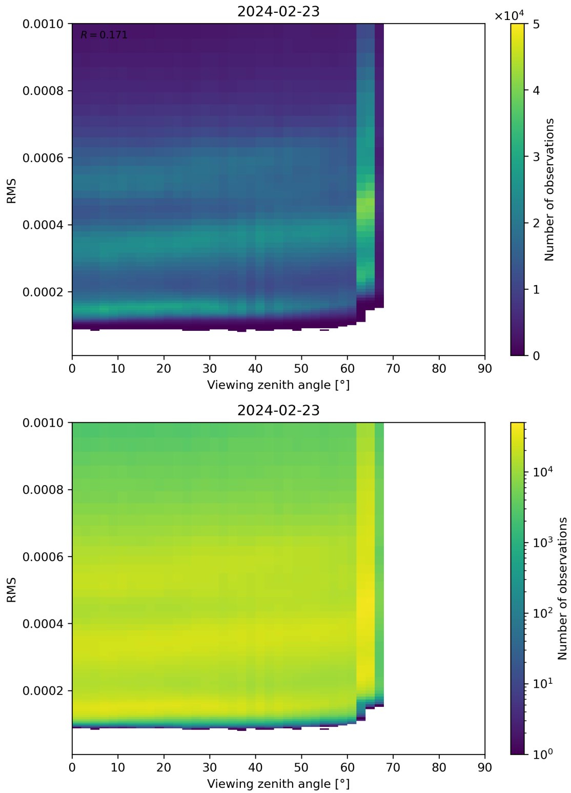
Figure 171: Scatter density plot of “Viewing zenith angle” against “RMS” for 2024-02-22 to 2024-02-24.
