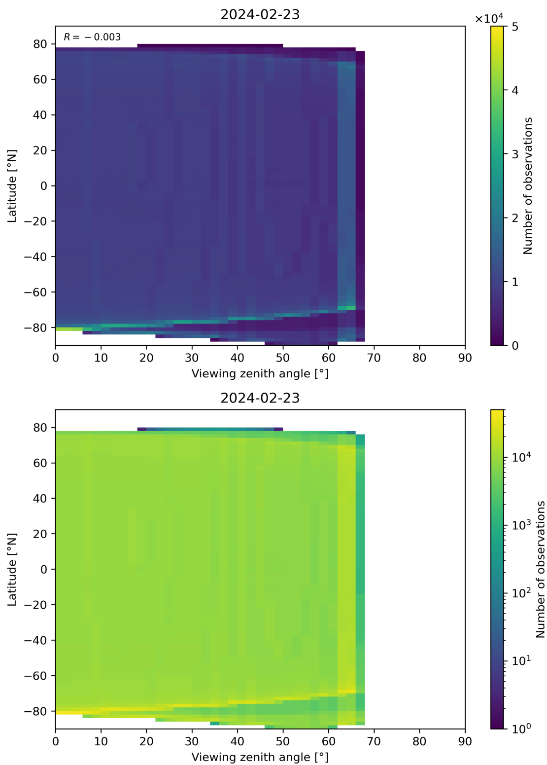
Figure 163: Scatter density plot of “Viewing zenith angle” against “Latitude” for 2024-02-22 to 2024-02-24.
