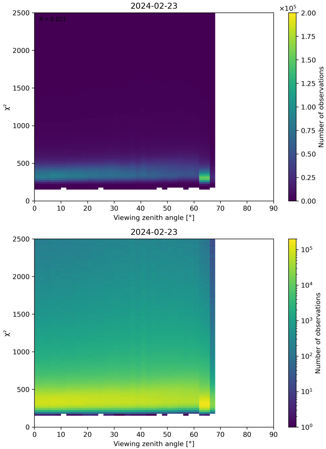
Figure 162: Scatter density plot of “Viewing zenith angle” against “ \chi^2 ” for 2024-02-22 to 2024-02-24.
