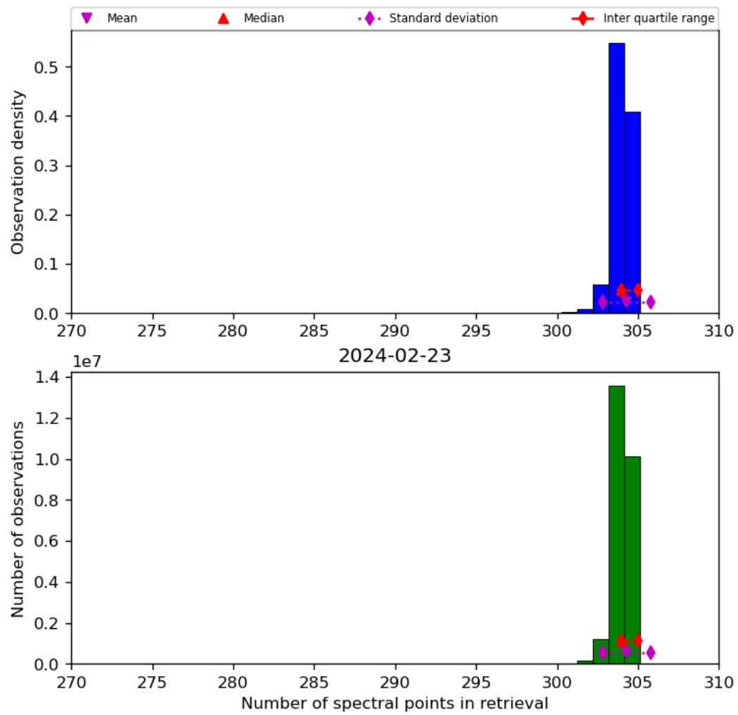
Figure 33: Histogram of “Number of spectral points in retrieval” for 2024-02-22 to 2024-02-24
