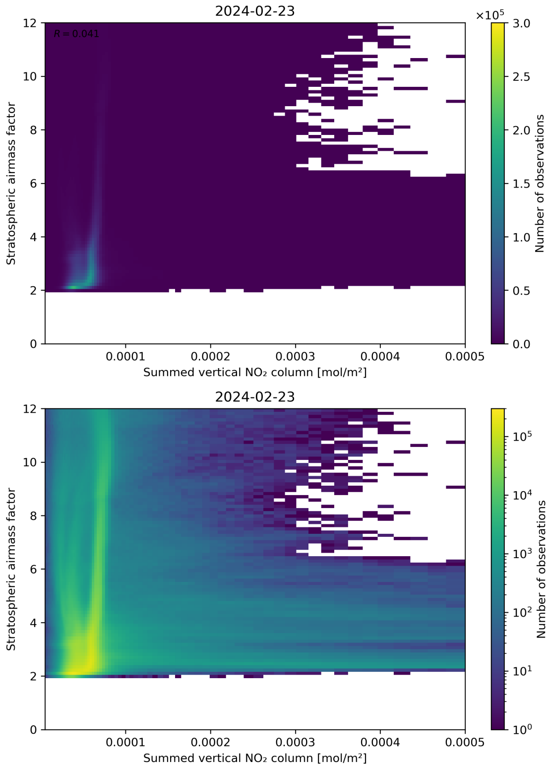
Figure 103: Scatter density plot of “Summed vertical NO 2 column” against “Stratospheric airmass factor” for 2024-02-22 to 2024-02-24.
