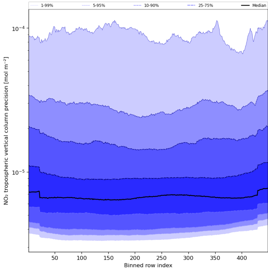
Figure 47: Along track statistics of “NO 2 tropospheric vertical column precision” for 2024-02-22 to 2024-02-24
