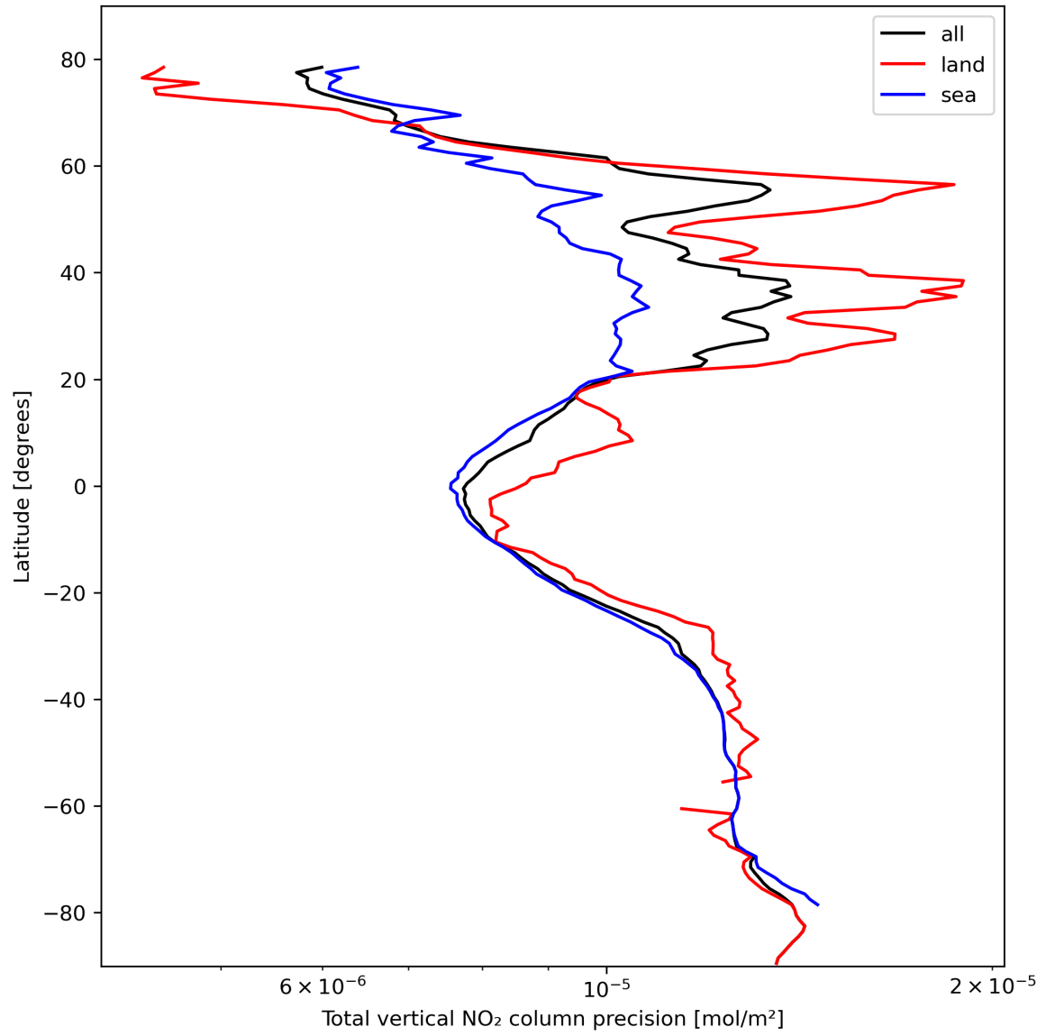
Figure 22: Zonal average of “Total vertical NO 2 column precision” for 2024-02-22 to 2024-02-24.
