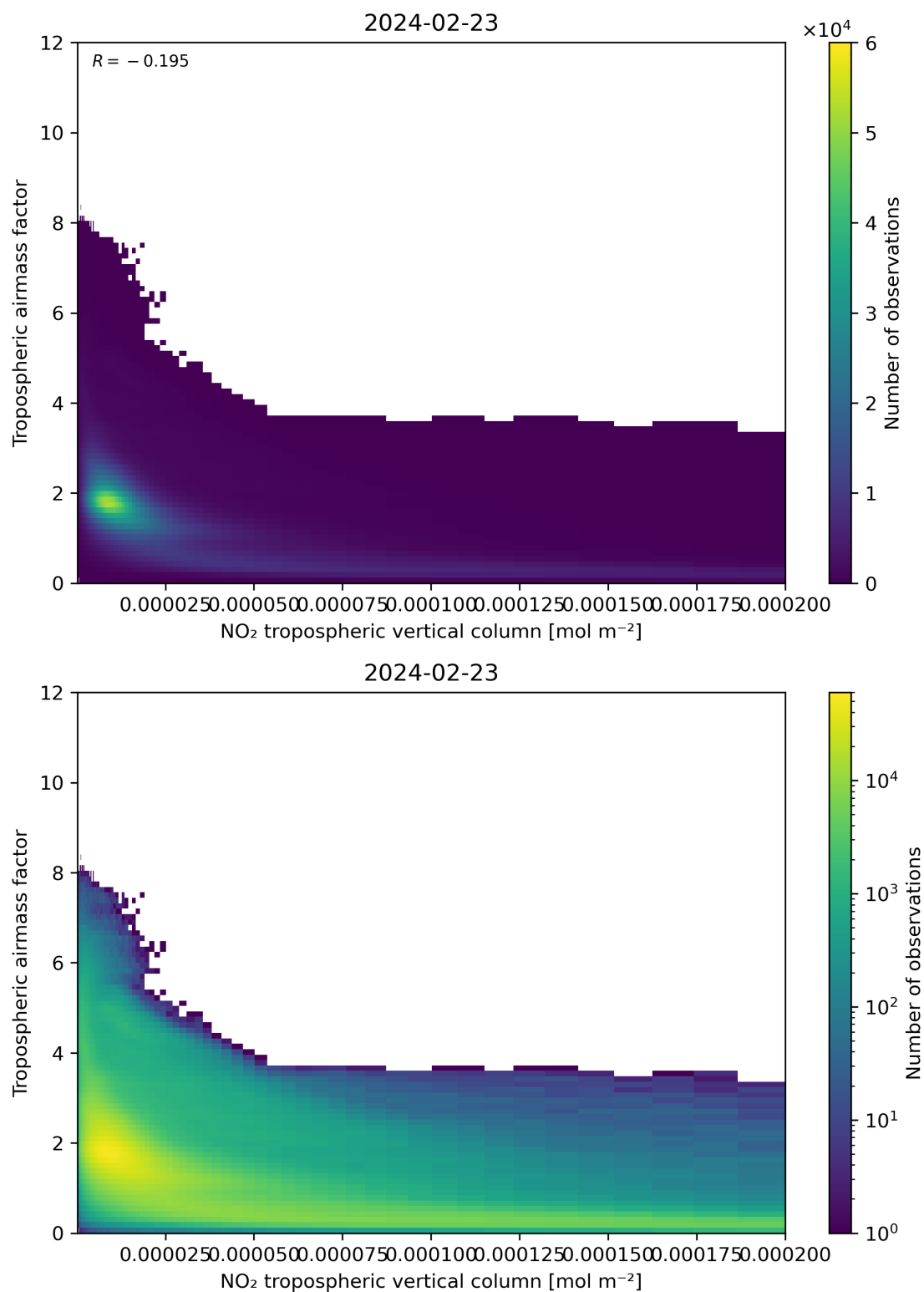
Figure 123: Scatter density plot of “NO 2 tropospheric vertical column” against “Tropospheric airmass factor” for 2024-02-22 to 2024-02-24.
