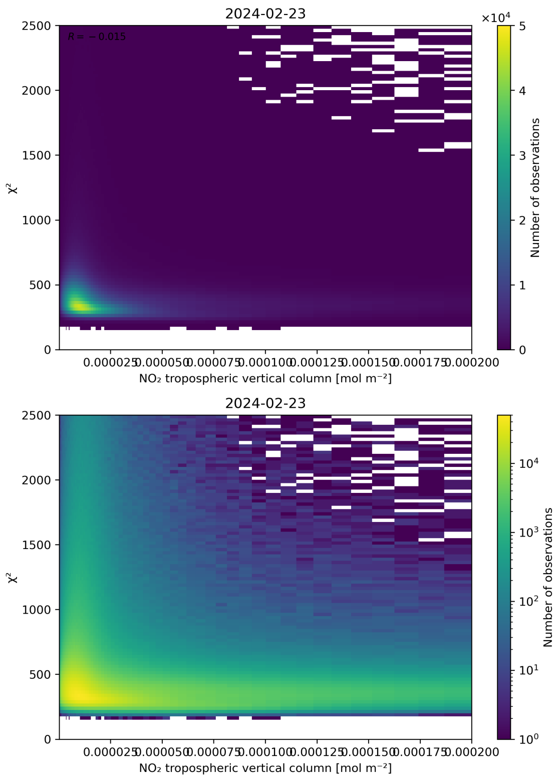
Figure 124: Scatter density plot of “NO 2 tropospheric vertical column” against “ \chi^2 ” for 2024-02-22 to 2024-02-24.
