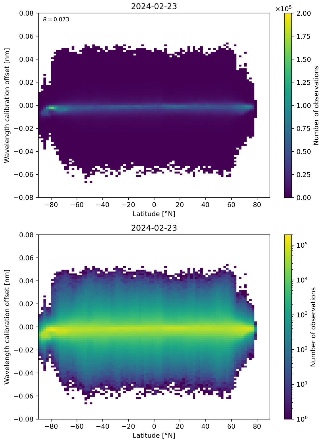
Figure 95: Scatter density plot of “Latitude” against “Wavelength calibration offset” for 2024-02-22 to 2024-02-24.
