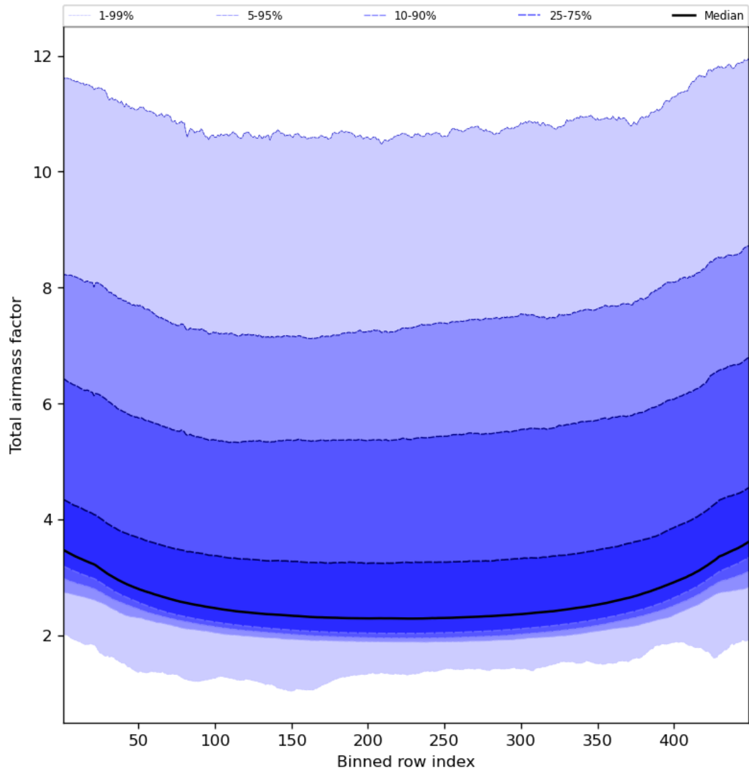
Figure 49: Along track statistics of “Total airmass factor” for 2024-02-22 to 2024-02-24
