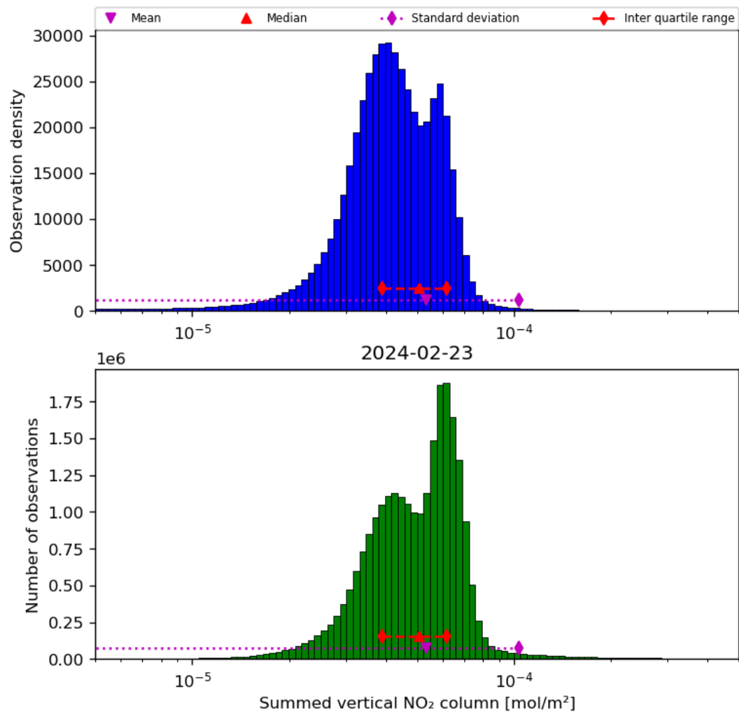
Figure 40: Histogram of “Summed vertical NO 2 column” for 2024-02-22 to 2024-02-24
