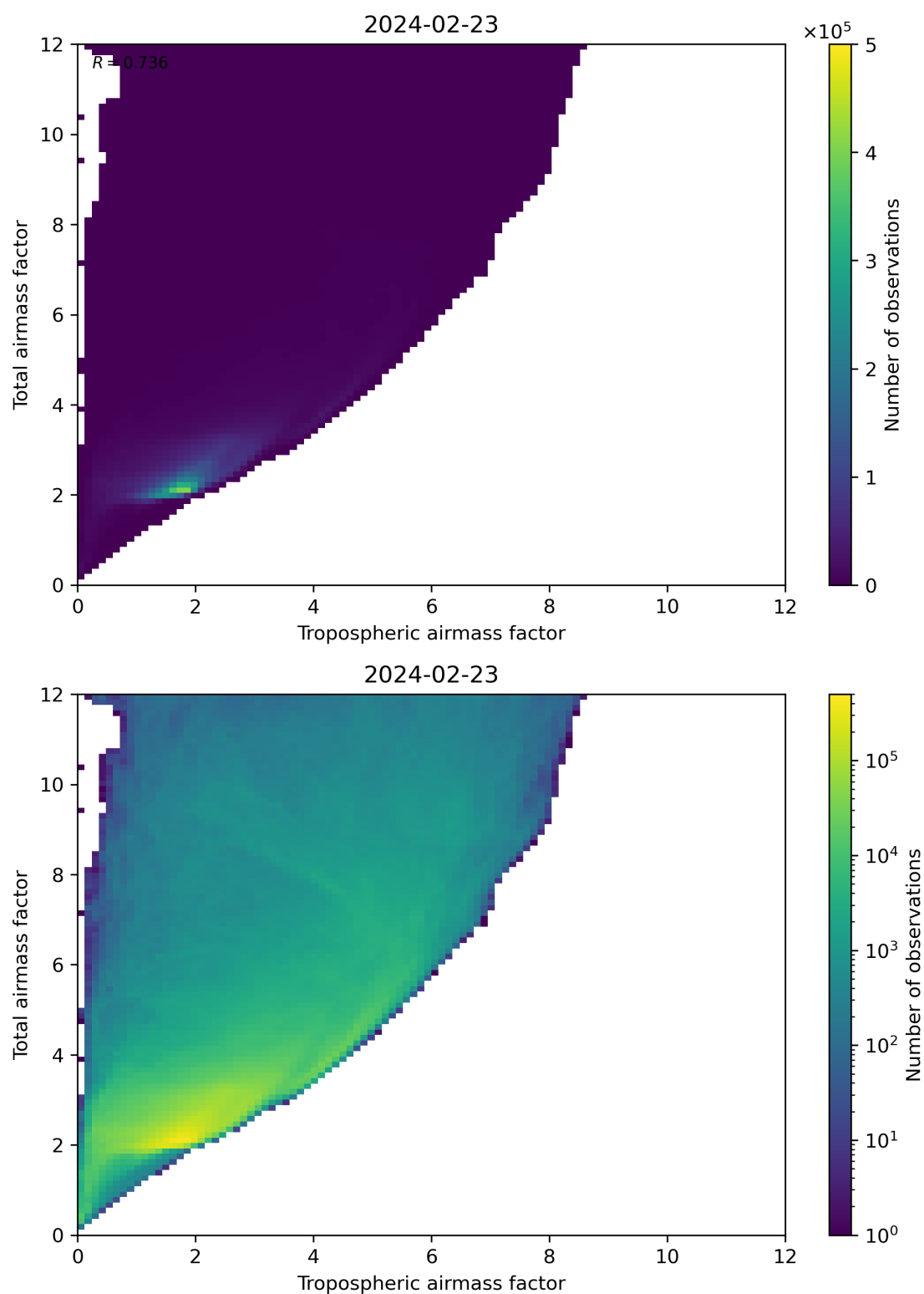
Figure 72: Scatter density plot of “Tropospheric airmass factor” against “Total airmass factor” for 2024-02-22 to 2024-02-24.
