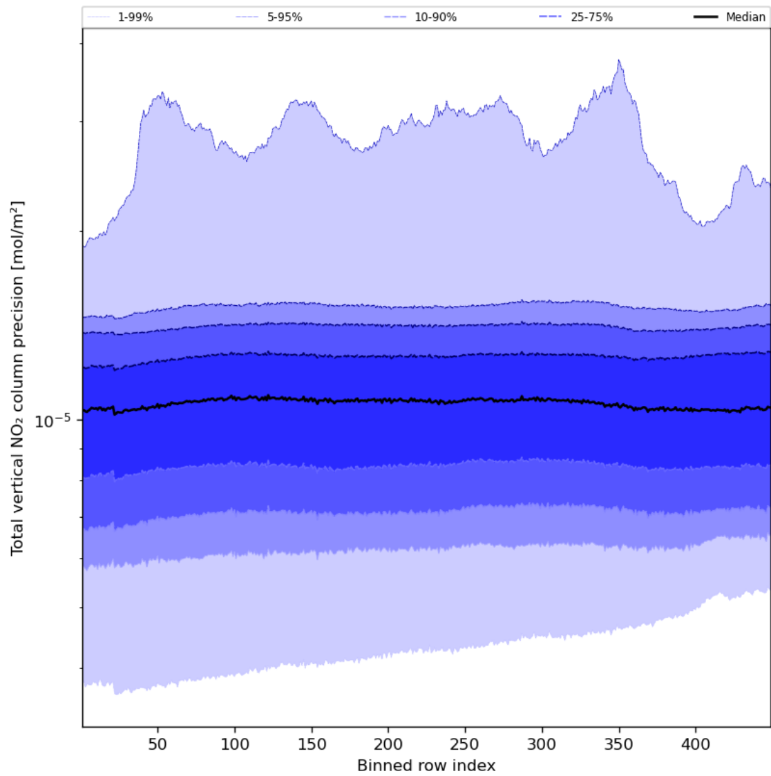
Figure 56: Along track statistics of “Total vertical NO 2 column precision” for 2024-02-22 to 2024-02-24
