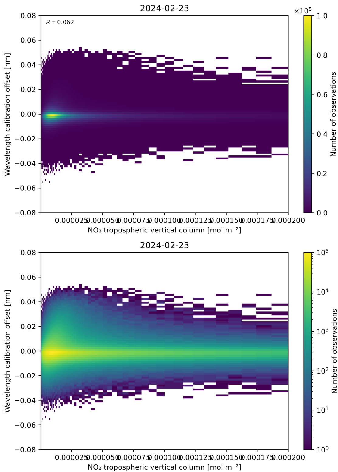
Figure 143: Scatter density plot of “NO 2 tropospheric vertical column” against “Wavelength calibration offset” for 2024-02-22 to 2024-02-24.
