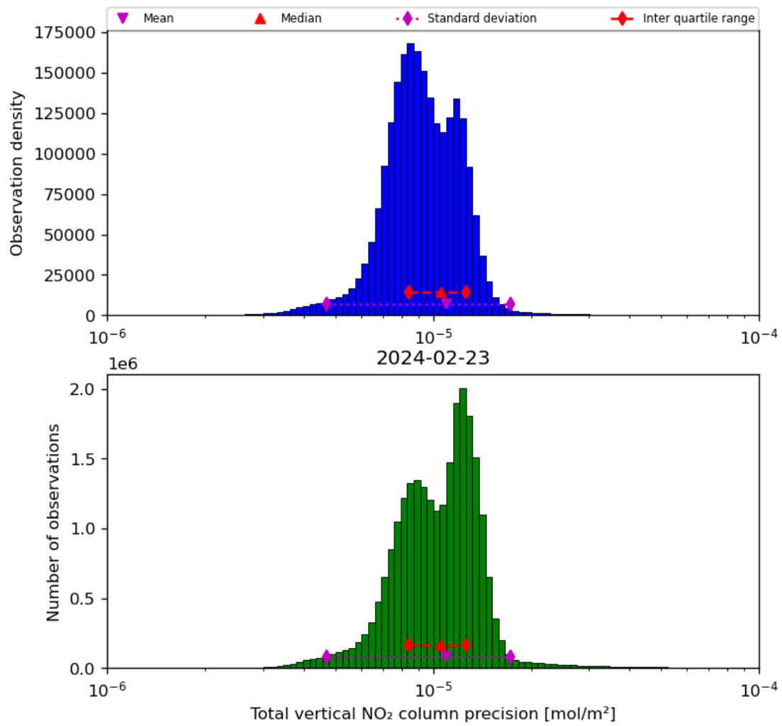
Figure 39: Histogram of “Total vertical NO 2 column precision” for 2024-02-22 to 2024-02-24
