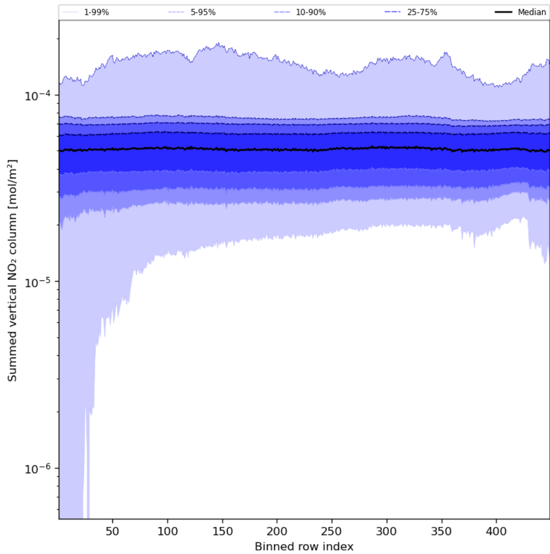
Figure 57: Along track statistics of “Summed vertical NO 2 column” for 2024-02-22 to 2024-02-24
