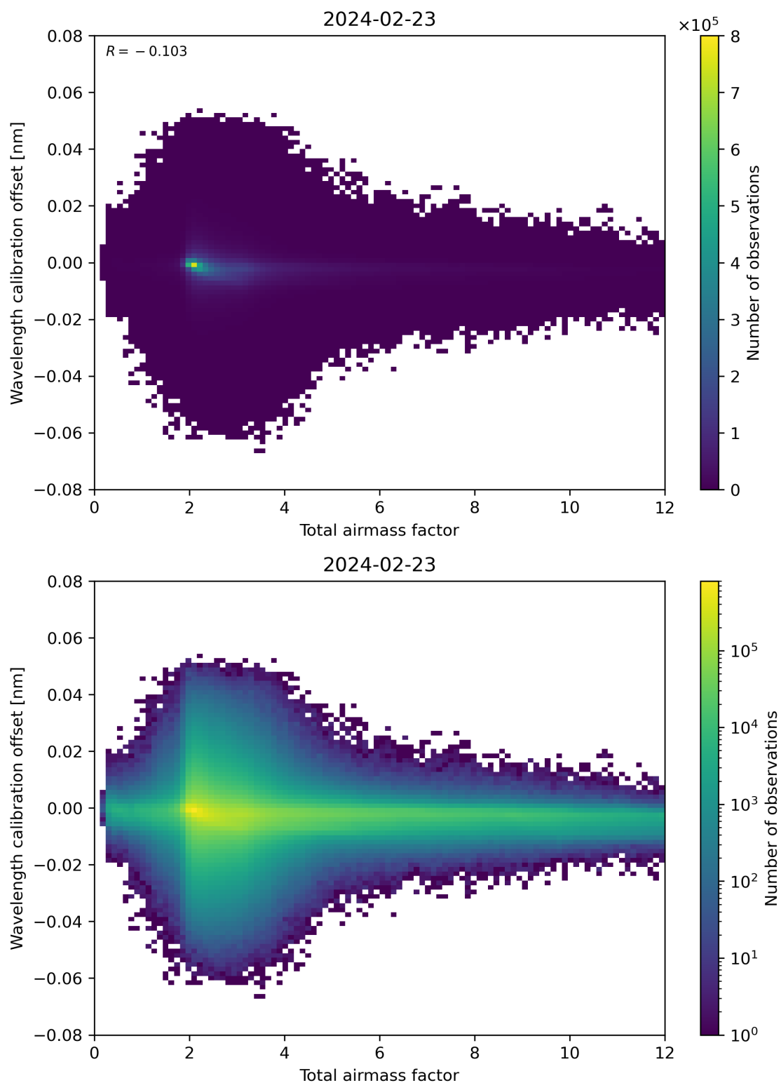
Figure 70: Scatter density plot of “Total airmass factor” against “Wavelength calibration offset” for 2024-02-22 to 2024-02-24.
