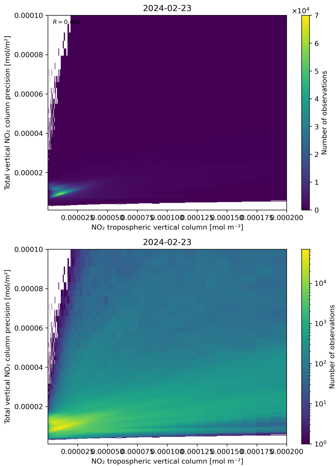
Figure 129: Scatter density plot of “NO 2 tropospheric vertical column” against “Total vertical NO 2 column precision” for 2024-02-22 to 2024-02-24.
