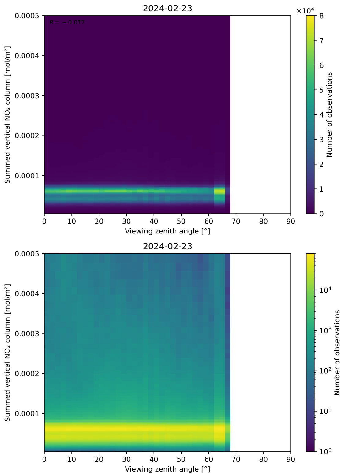
Figure 165: Scatter density plot of “Viewing zenith angle” against “Summed vertical NO 2 column” for 2024-02-22 to 2024-02-24.
