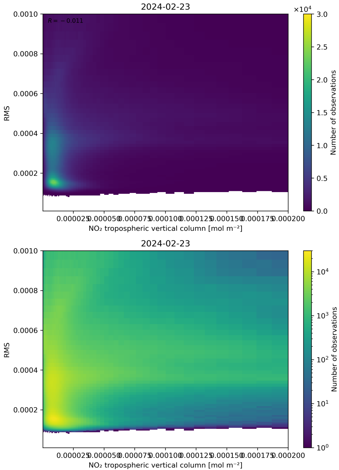
Figure 142: Scatter density plot of “NO 2 tropospheric vertical column” against “RMS” for 2024-02-22 to 2024-02-24.
