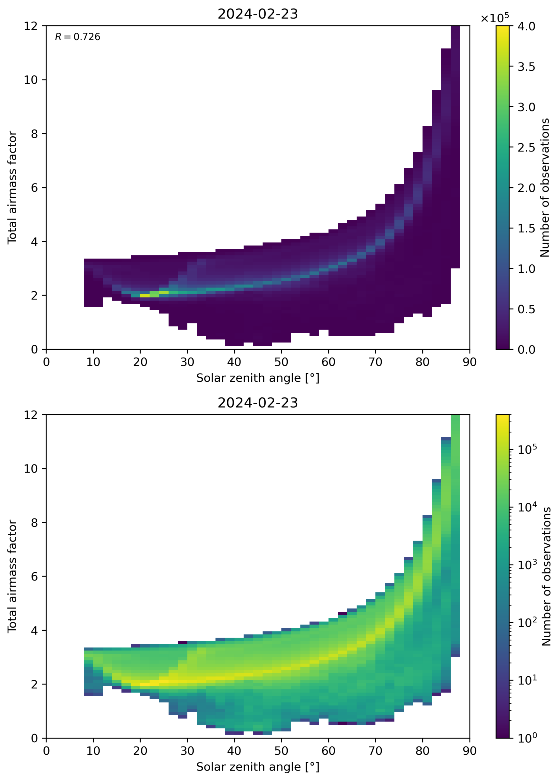
Figure 146: Scatter density plot of “Solar zenith angle” against “Total air mass factor” for 2024-02-22 to 2024-02-24.
