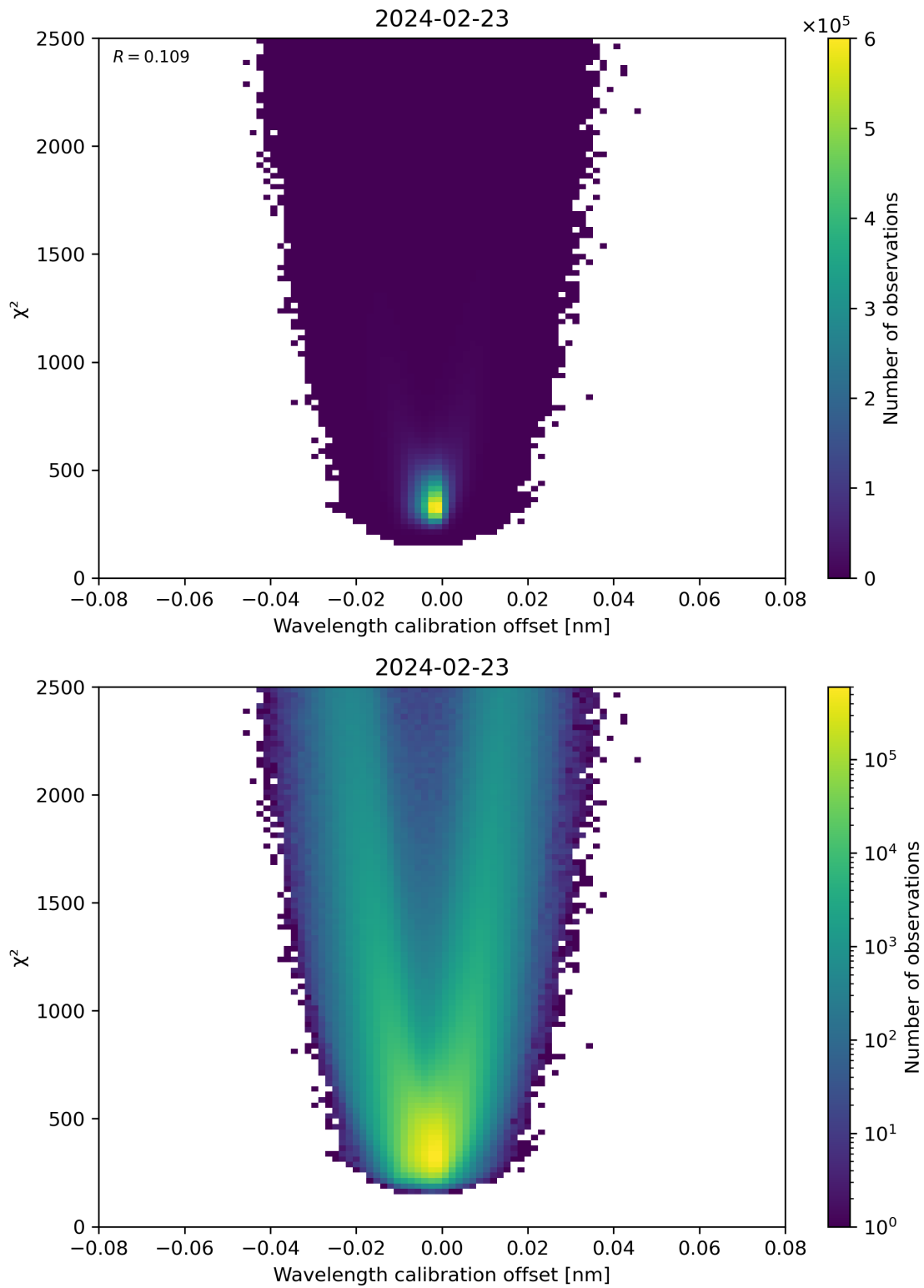
Figure 175: Scatter density plot of “Wavelength calibration offset” against “ \chi^2 ” for 2024-02-22 to 2024-02-24.
