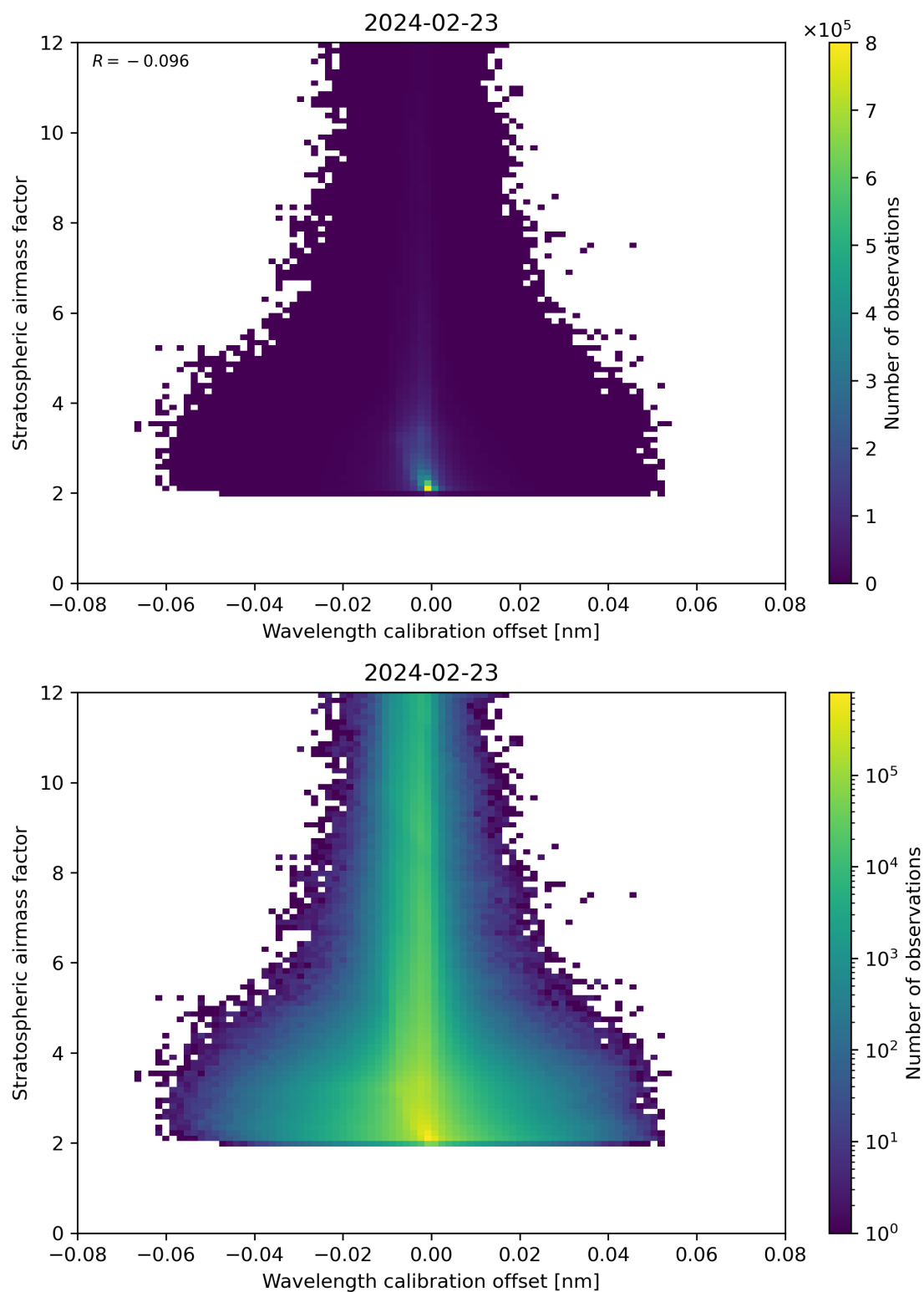
Figure 174: Scatter density plot of “Wavelength calibration offset” against “Stratospheric airmass factor” for 2024-02-22 to 2024-02-24.
