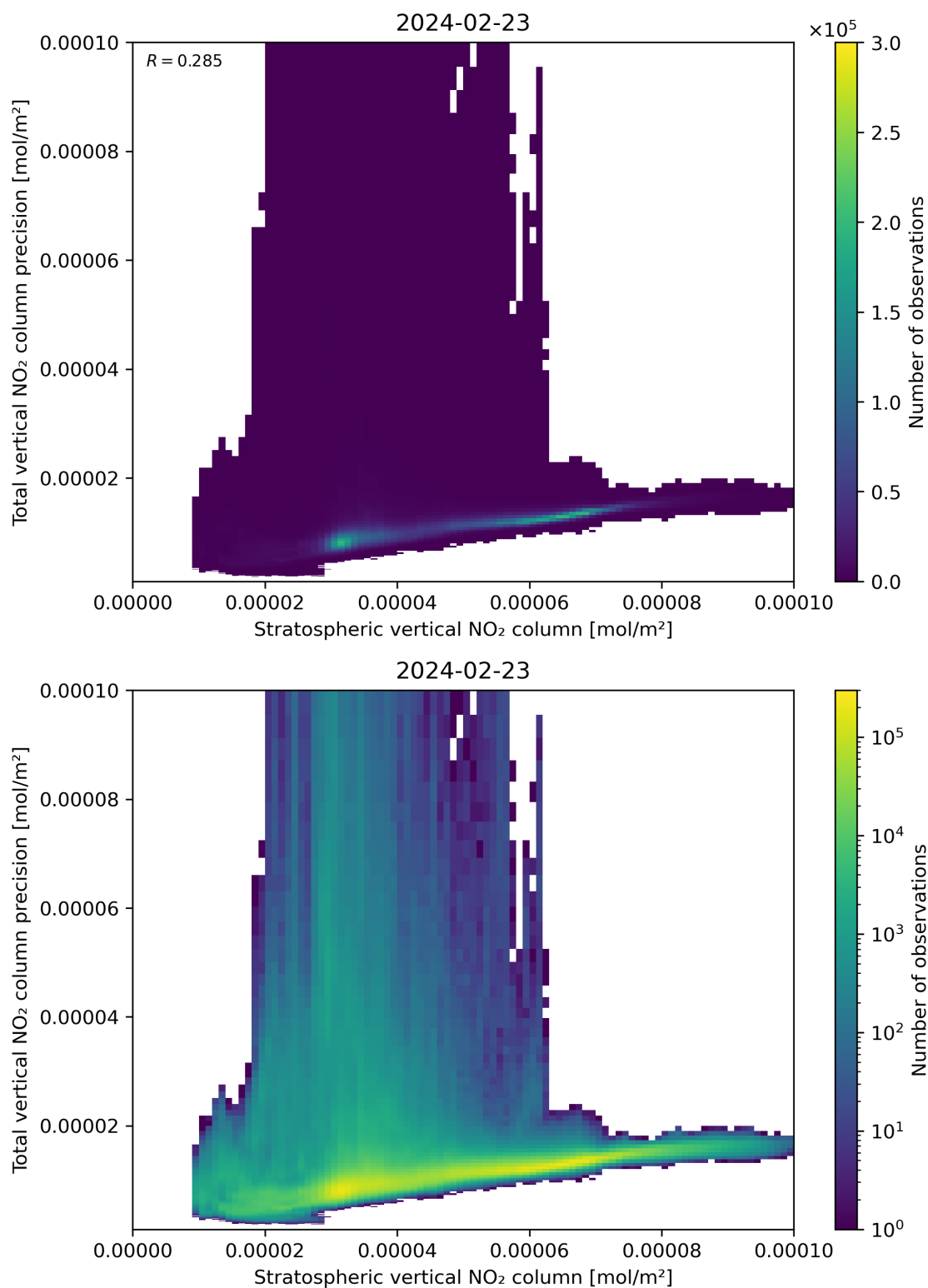
Figure 101: Scatter density plot of “Stratospheric vertical NO 2 column” against “Total vertical NO 2 column precision” for 2024-02-22 to 2024-02-24.
