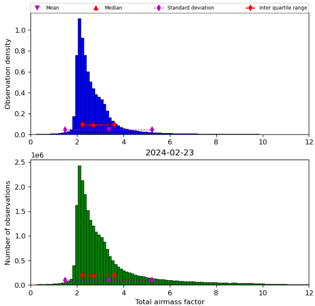
Figure 32: Histogram of “Total airmass factor” for 2024-02-22 to 2024-02-24
