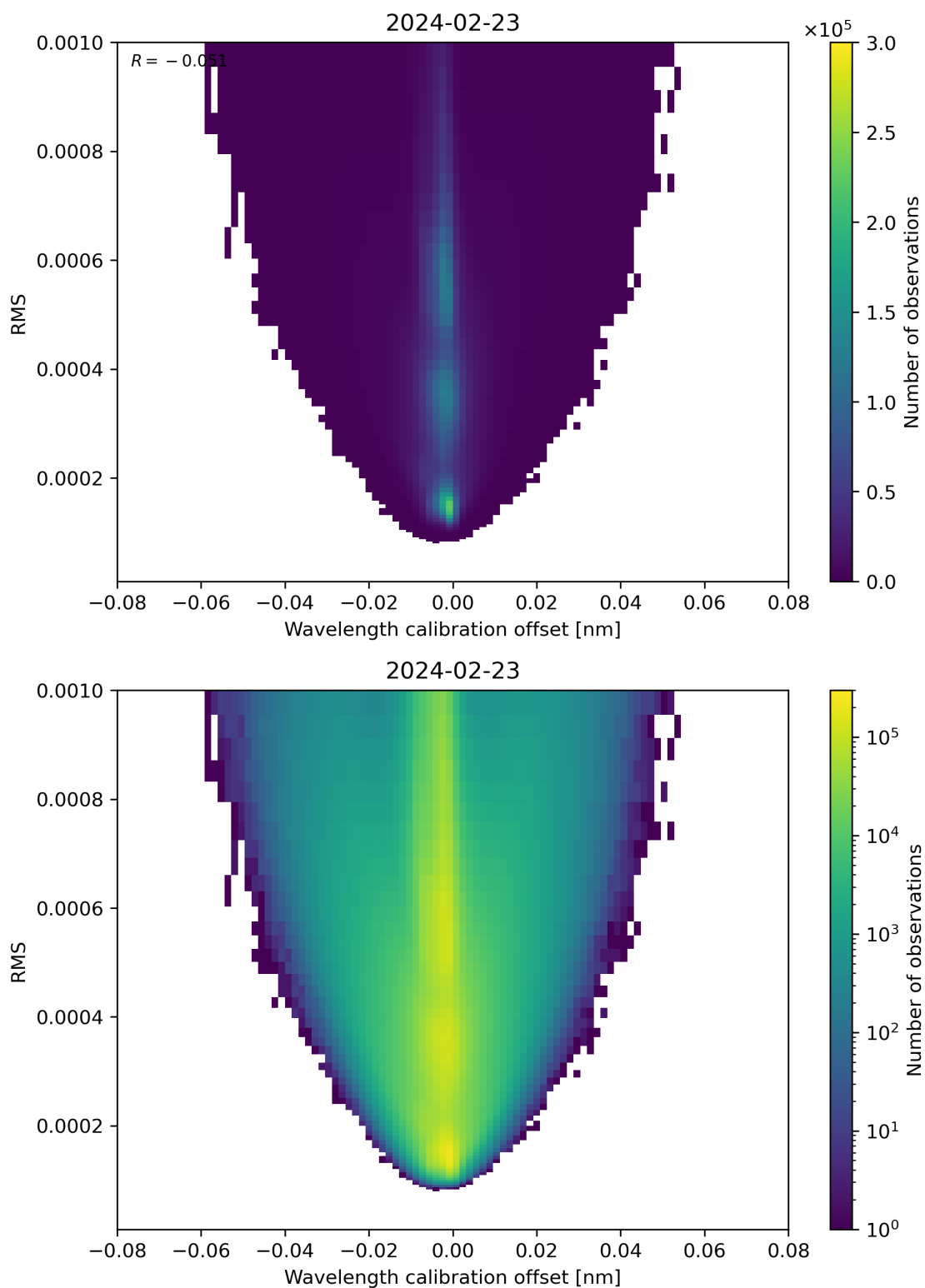
Figure 181: Scatter density plot of “Wavelength calibration offset” against “RMS” for 2024-02-22 to 2024-02-24.
