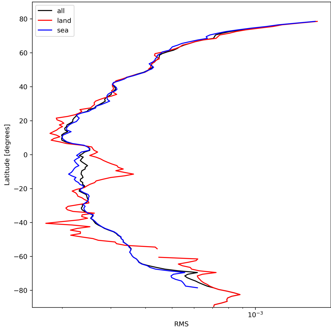
Figure 26: Zonal average of “RMS” for 2024-02-22 to 2024-02-24.
