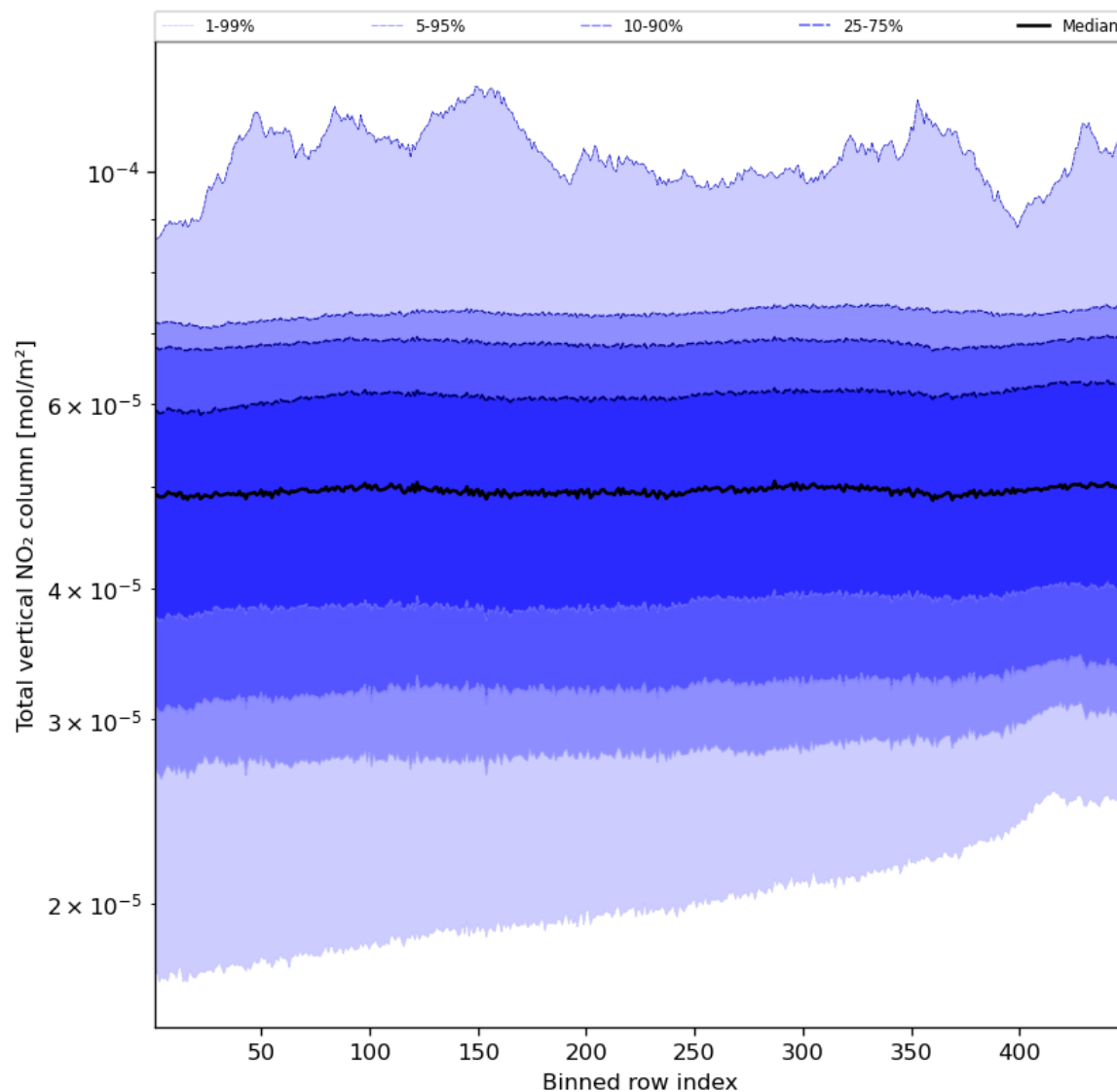
Figure 55: Along track statistics of “Total vertical NO 2 column” for 2024-02-22 to 2024-02-24
