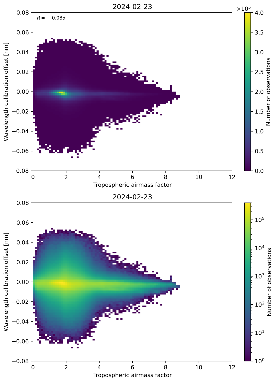
Figure 80: Scatter density plot of “Tropospheric airmass factor” against “Wavelength calibration offset” for 2024-02-22 to 2024-02-24.
