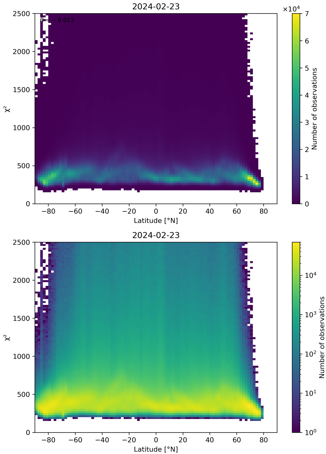
Figure 86: Scatter density plot of “Latitude” against “ \chi^2 ” for 2024-02-22 to 2024-02-24.
