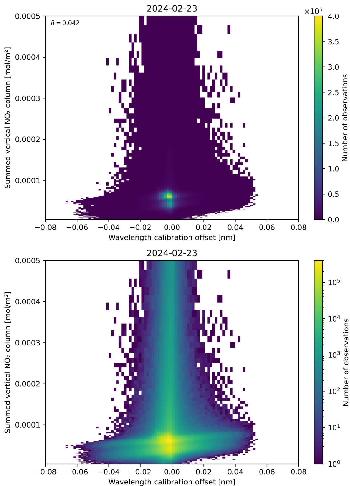
Figure 177: Scatter density plot of “Wavelength calibration offset” against “Summed vertical NO 2 column” for 2024-02-22 to 2024-02-24.
