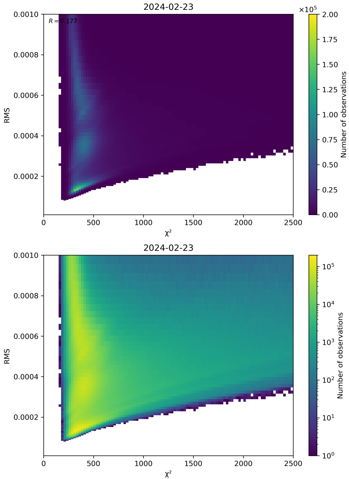
Figure 82: Scatter density plot of “ \chi^2 ” against “RMS” for 2024-02-22 to 2024-02-24.
