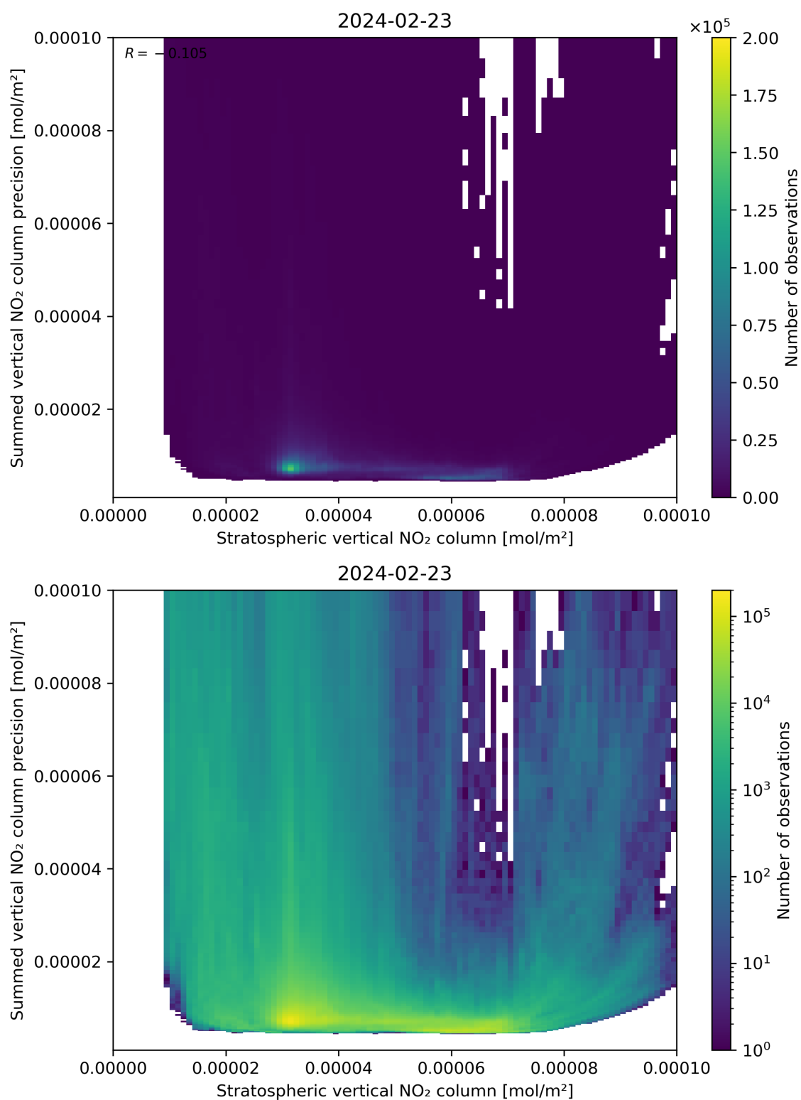
Figure 99: Scatter density plot of “Stratospheric vertical NO 2 column” against “Summed vertical NO 2 column precision” for 2024-02-22 to 2024-02-24.
