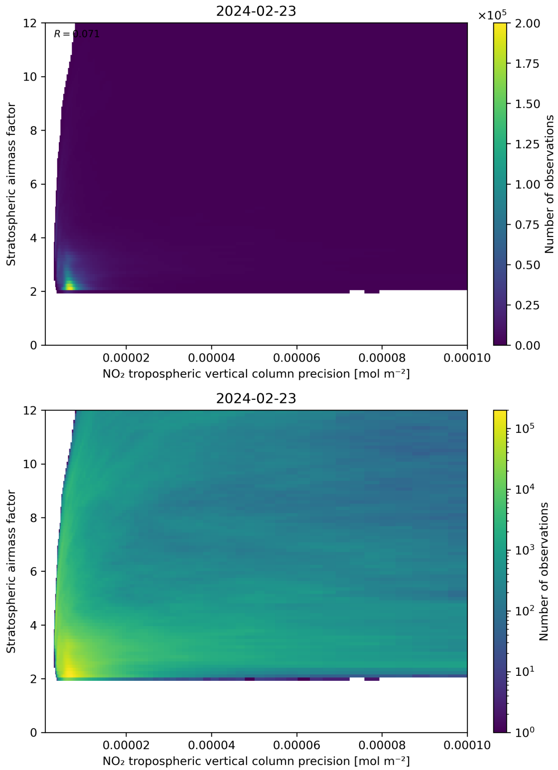
Figure 131: Scatter density plot of “NO 2 tropospheric vertical column precision” against “Stratospheric airmass factor” for 2024-02-22 to 2024-02-24.
