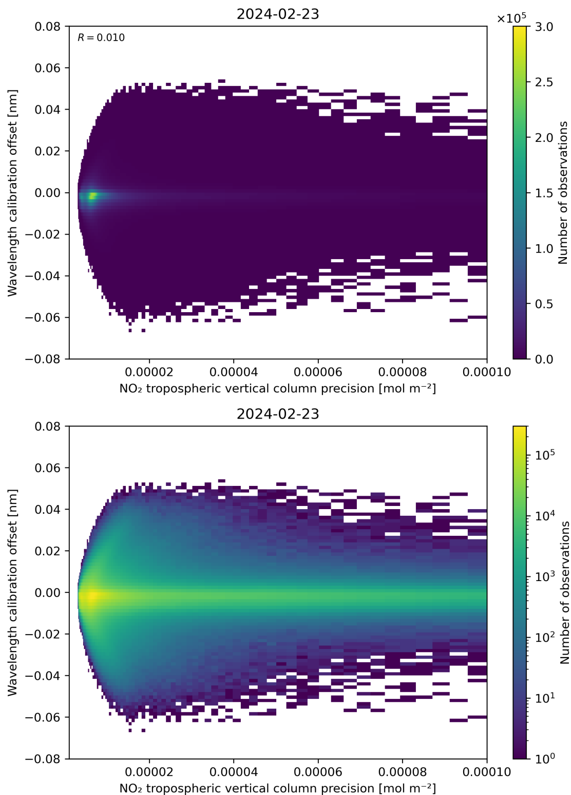
Figure 141: Scatter density plot of “NO 2 tropospheric vertical column precision” against “Wavelength calibration offset” for 2024-02-22 to 2024-02-24.
