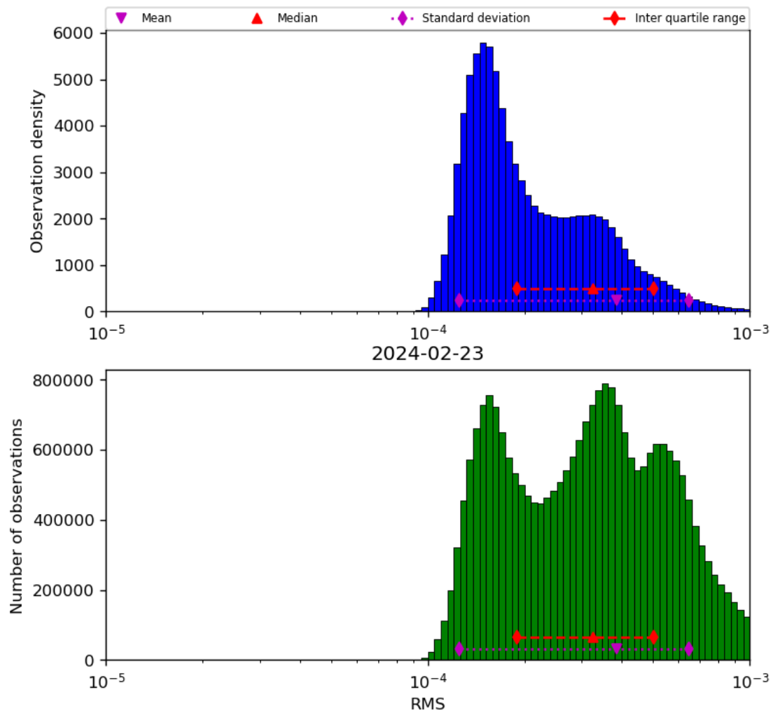
Figure 43: Histogram of “RMS” for 2024-02-22 to 2024-02-24
