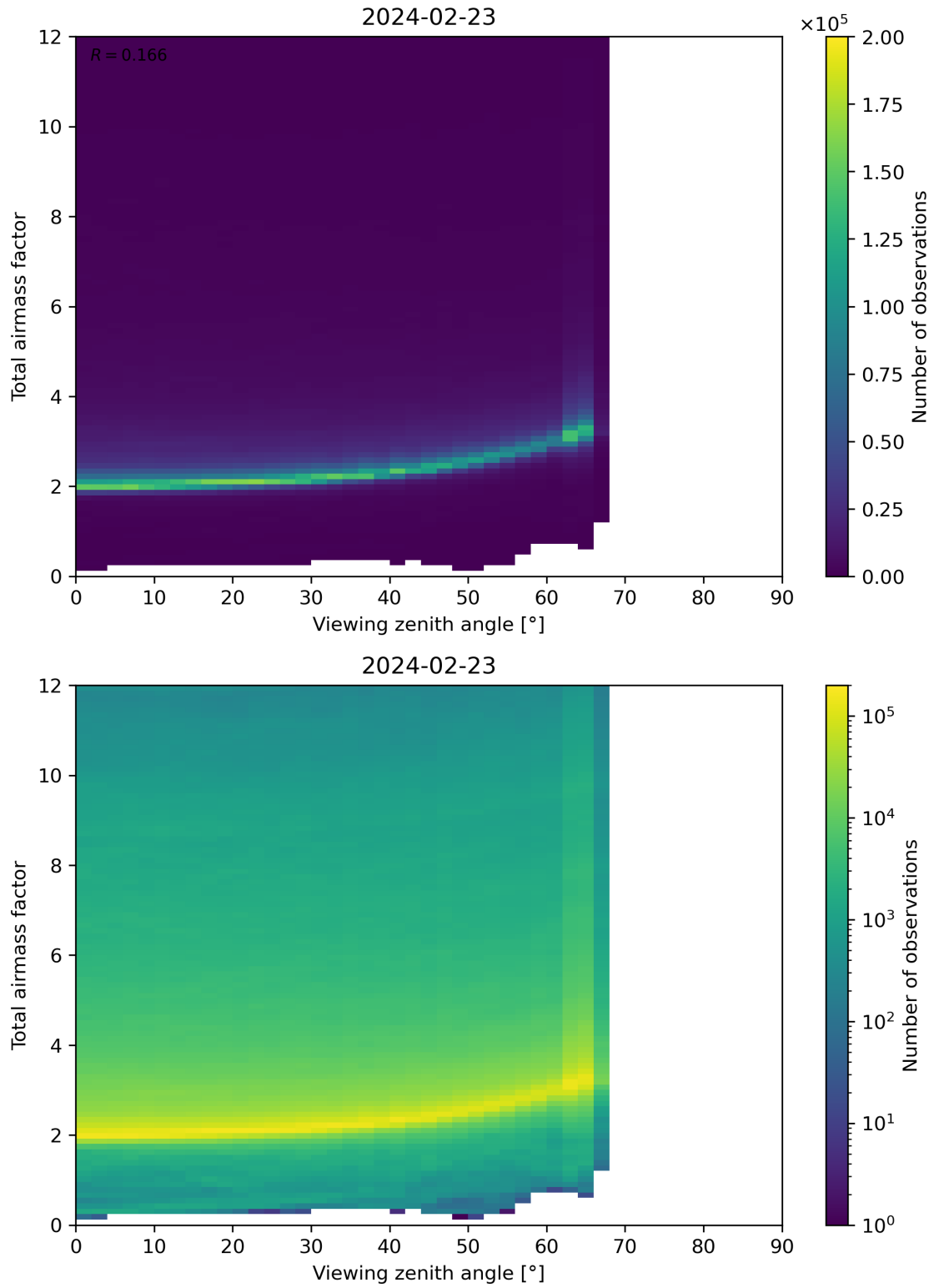
Figure 160: Scatter density plot of “Viewing zenith angle” against “Total airmass factor” for 2024-02-22 to 2024-02-24.
