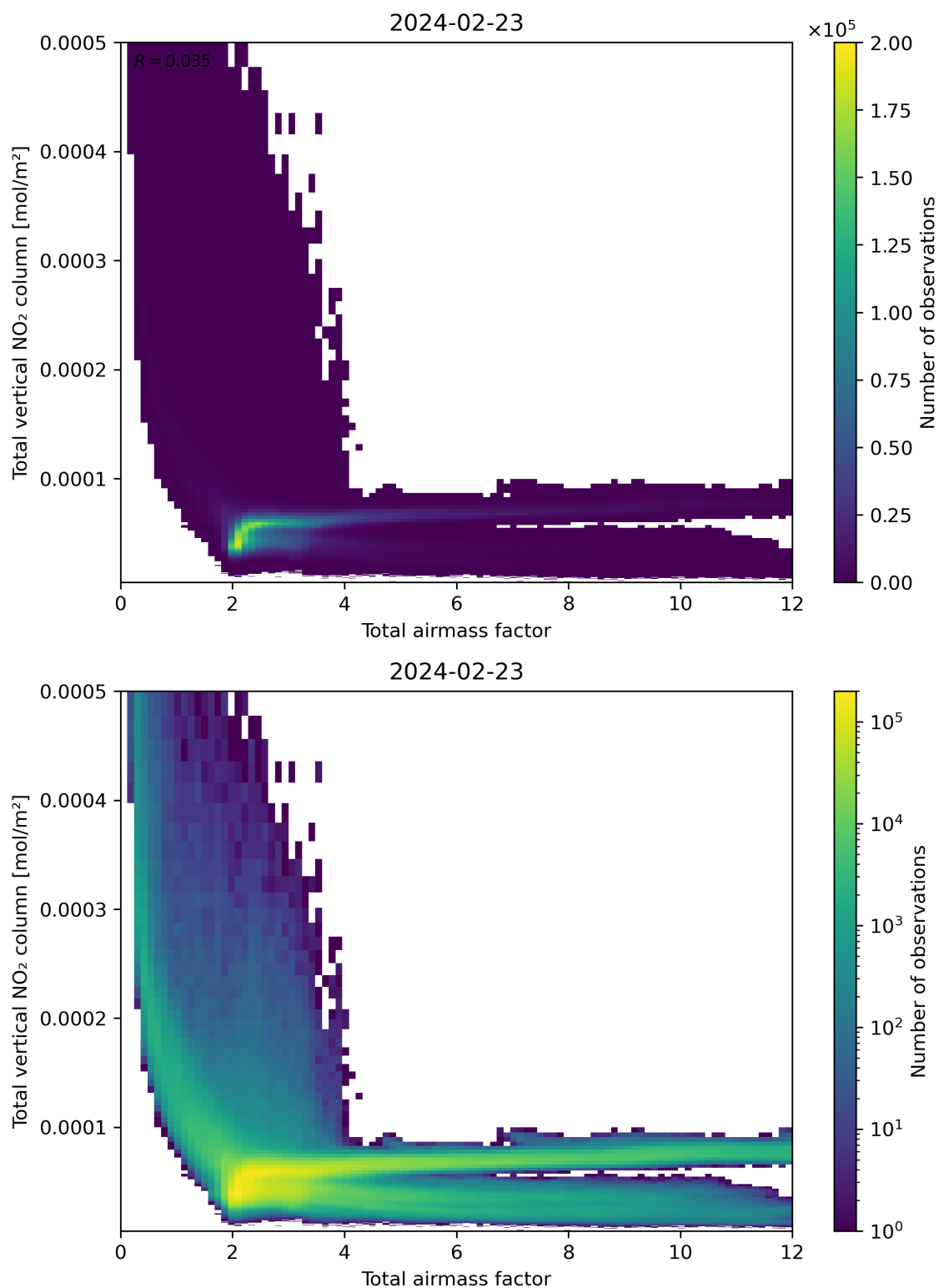
Figure 67: Scatter density plot of “Total airmass factor” against “Total vertical NO 2 column” for 2024-02-22 to 2024-02-24.
