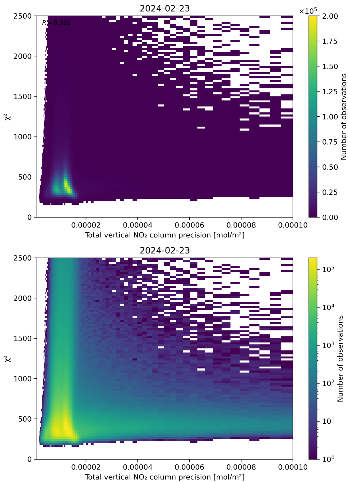
Figure 116: Scatter density plot of "Total vertical NO 2 column precision" against " \chi^2 " for 2024-02-22 to 2024-02-24.
