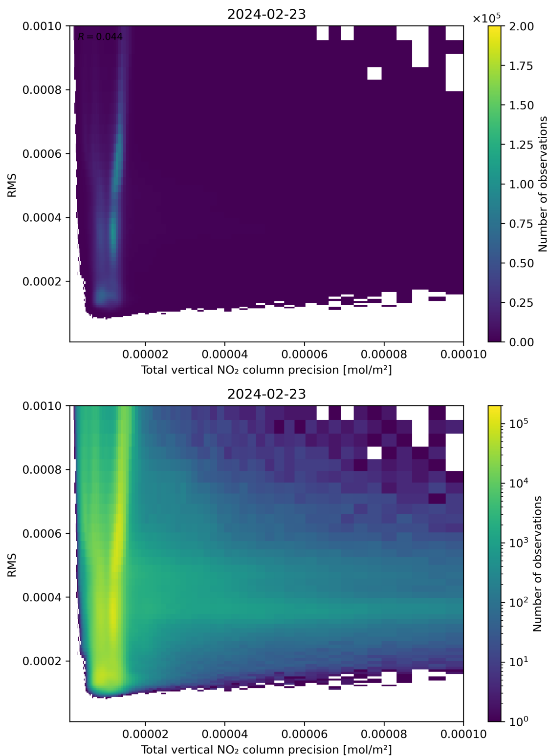
Figure 119: Scatter density plot of “Total vertical NO 2 column precision” against “RMS” for 2024-02-22 to 2024-02-24.
