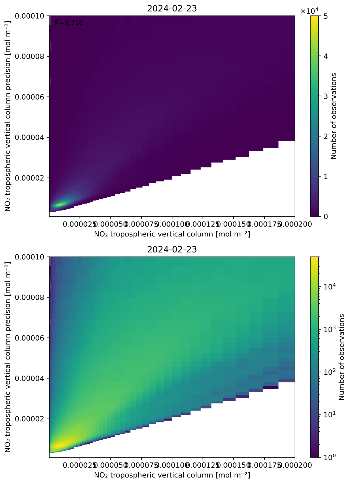
Figure 130: Scatter density plot of “NO 2 tropospheric vertical column” against “NO 2 tropospheric vertical column precision” for 2024-02-22 to 2024-02-24.
