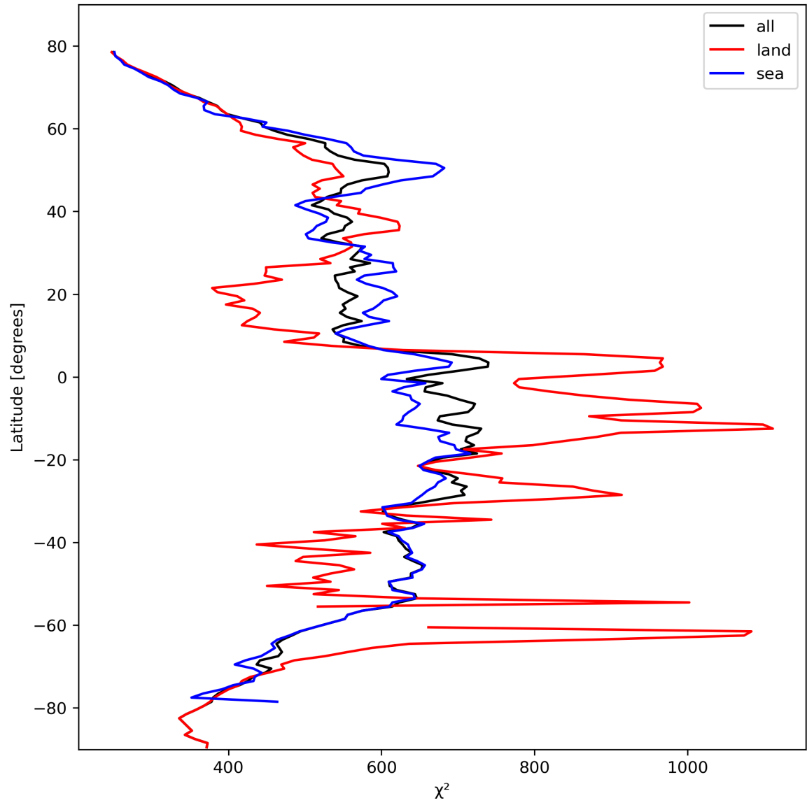
Figure 25: Zonal average of “ \chi^2 ” for 2024-02-22 to 2024-02-24.
