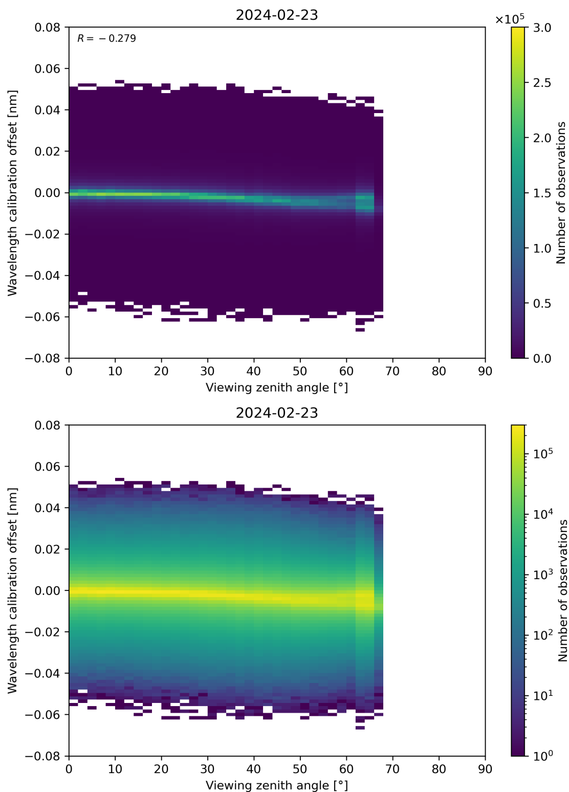
Figure 173: Scatter density plot of “Viewing zenith angle” against “Wavelength calibration offset” for 2024-02-22 to 2024-02-24.
