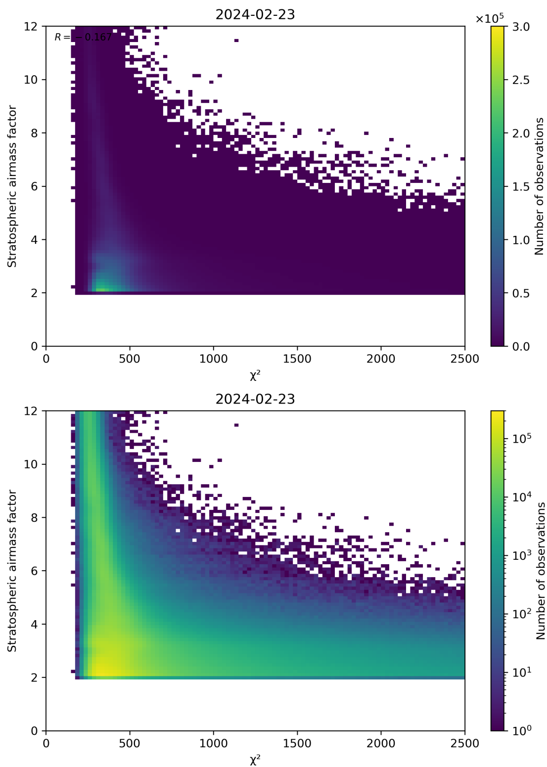
Figure 81: Scatter density plot of “ \chi^2 ” against “Stratospheric airmass factor” for 2024-02-22 to 2024-02-24.
