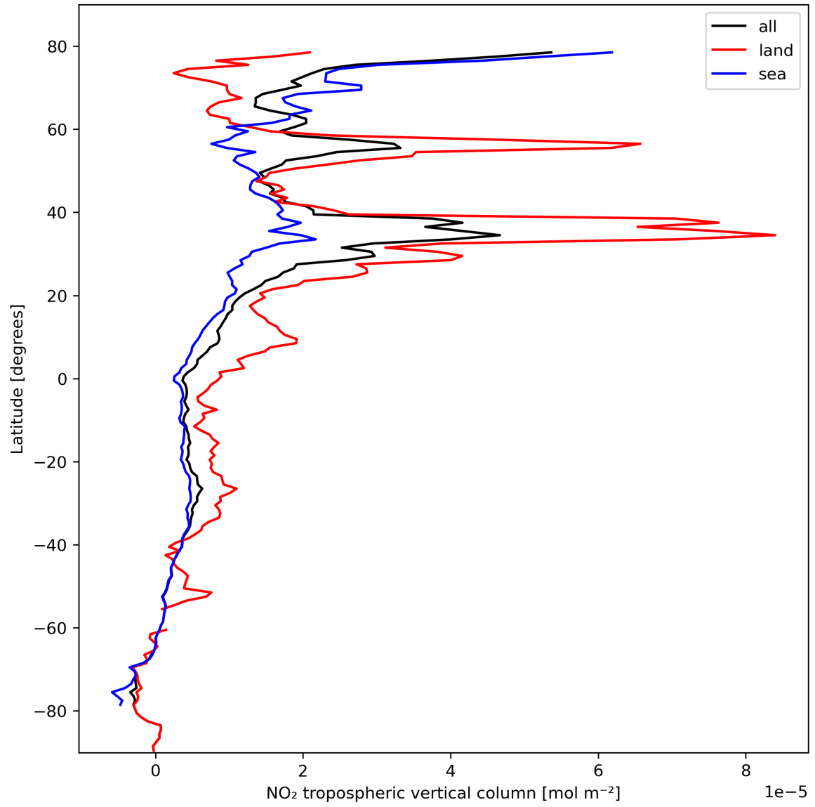
Figure 12: Zonal average of “NO 2 tropospheric vertical column” for 2024-02-22 to 2024-02-24.
