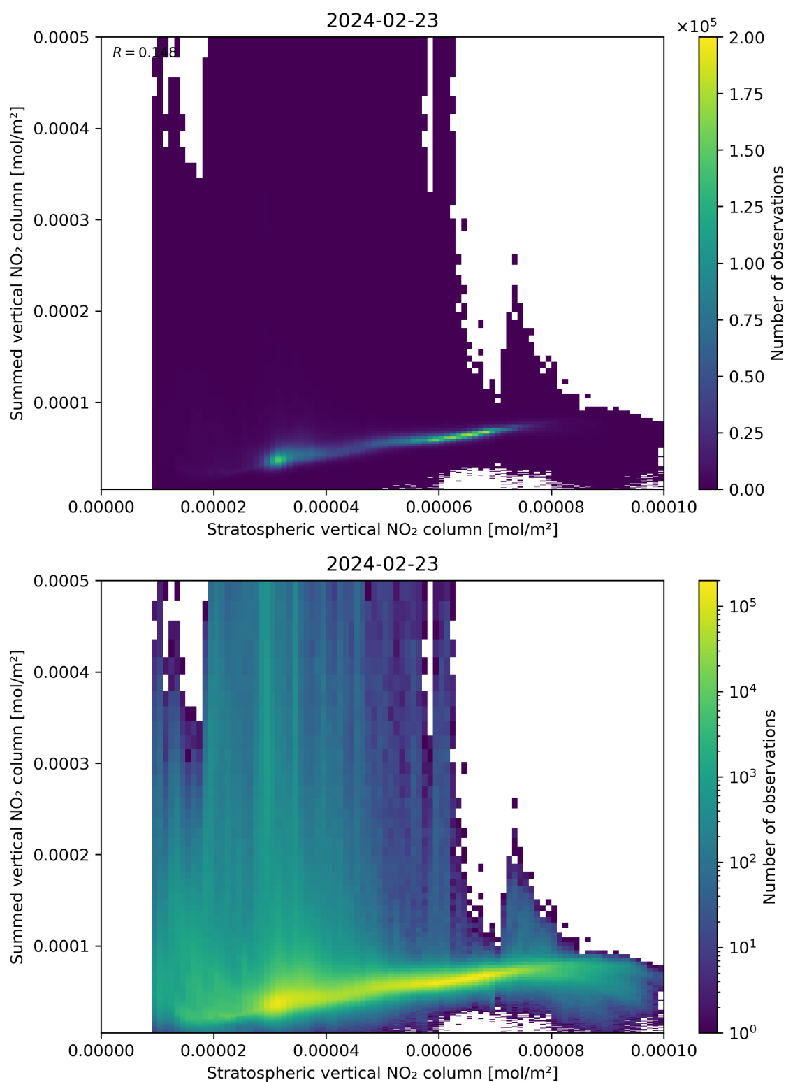
Figure 98: Scatter density plot of “Stratospheric vertical NO 2 column” against “Summed vertical NO 2 column” for 2024-02-22 to 2024-02-24.
