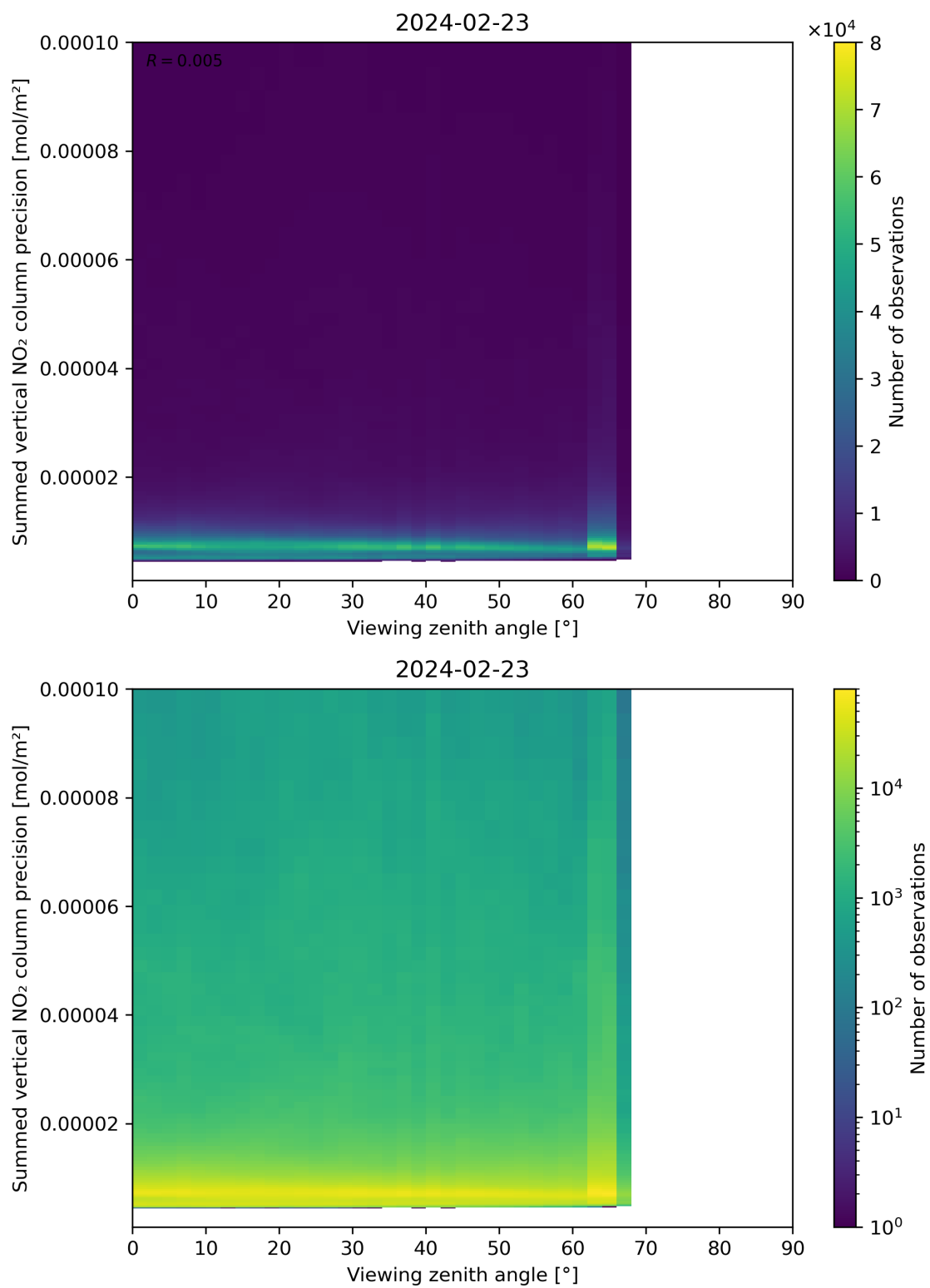
Figure 166: Scatter density plot of “Viewing zenith angle” against “Summed vertical NO 2 column precision” for 2024-02-22 to 2024-02-24.
