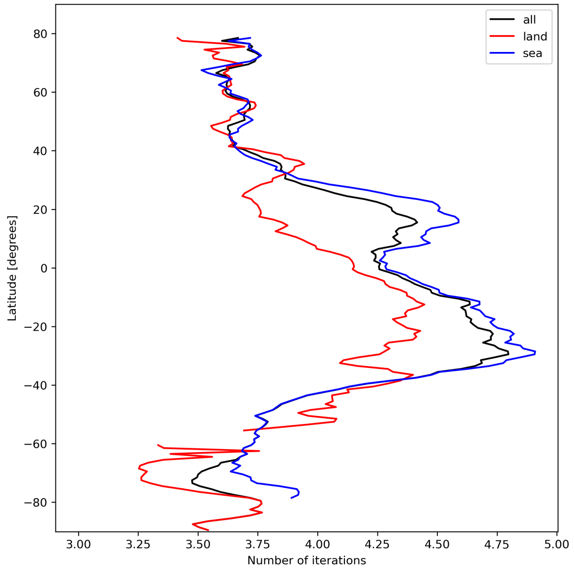
Figure 17: Zonal average of “Number of iterations” for 2024-02-22 to 2024-02-24.
