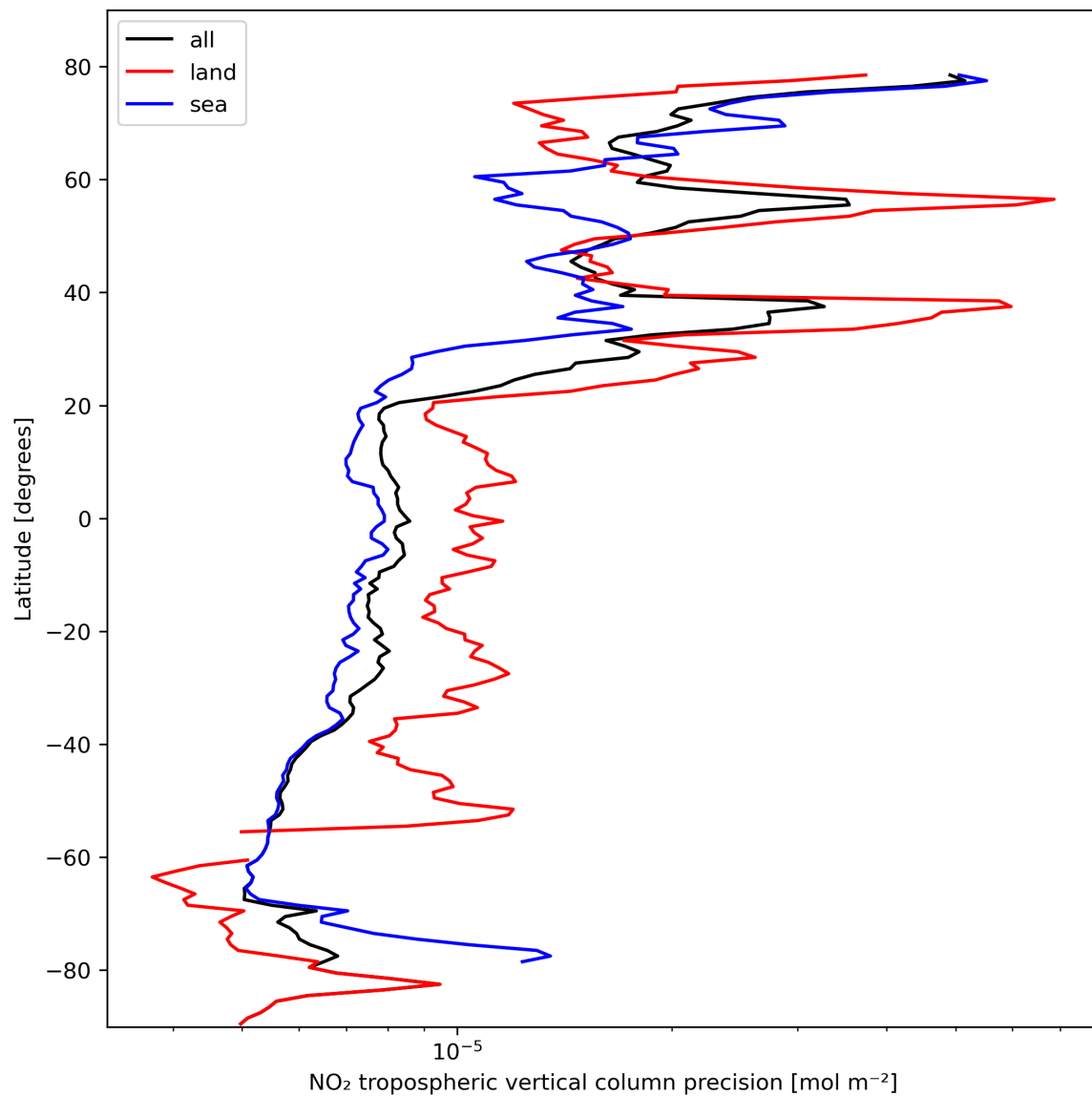
Figure 13: Zonal average of “NO 2 tropospheric vertical column precision” for 2024-02-22 to 2024-02-24.
