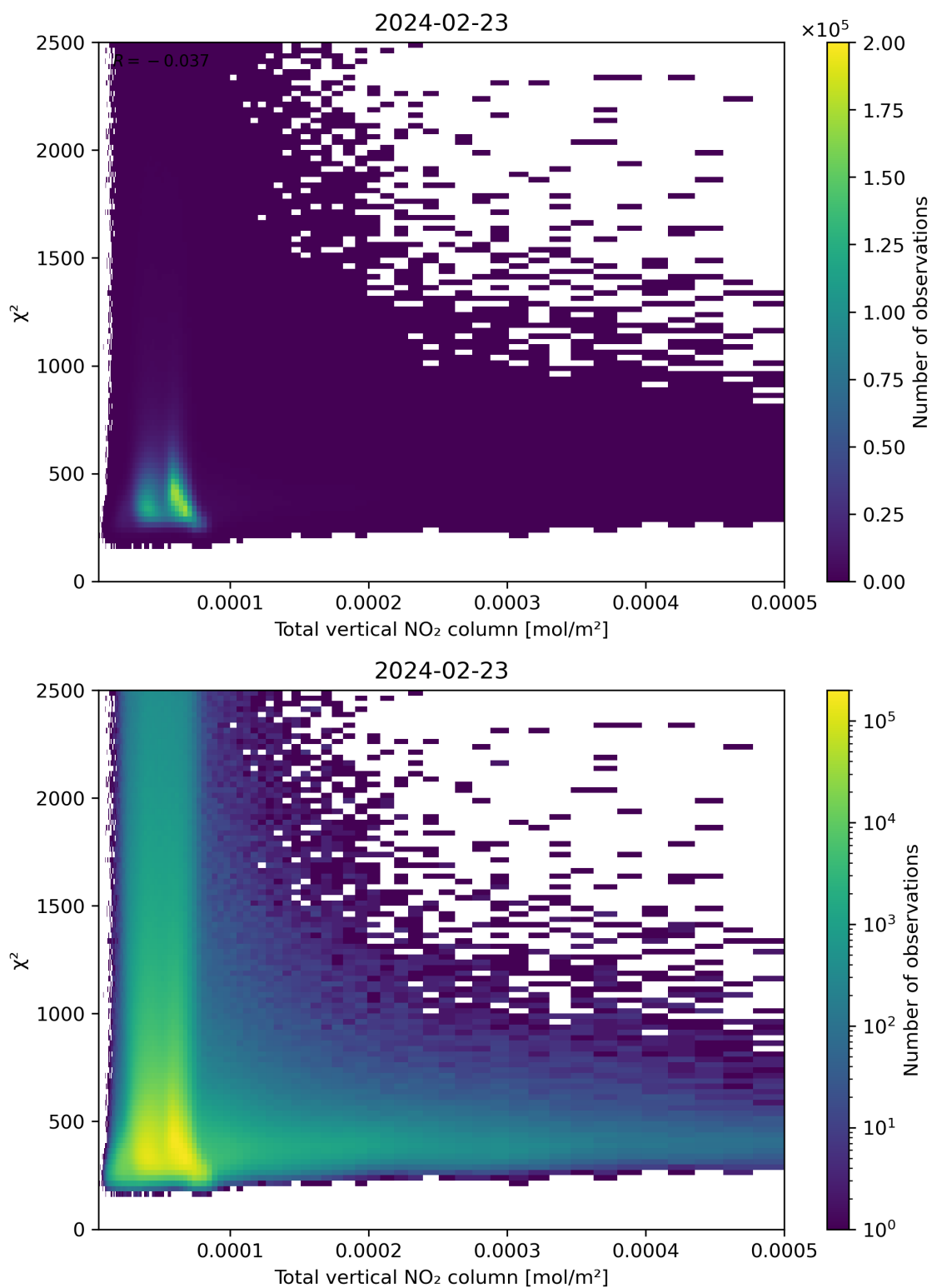
Figure 111: Scatter density plot of “Total vertical NO 2 column” against “ \chi^2 ” for 2024-02-22 to 2024-02-24.
