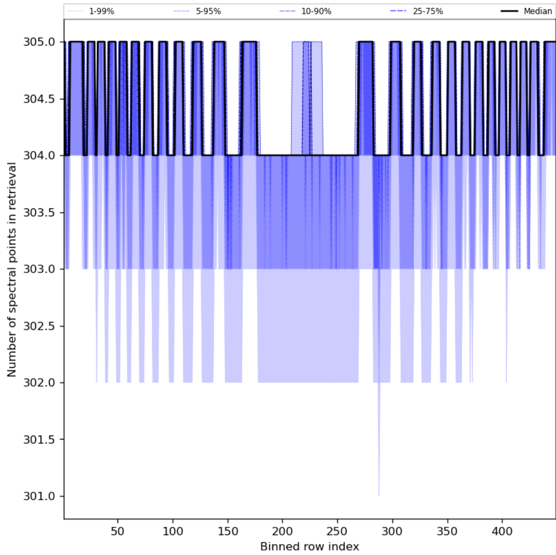
Figure 50: Along track statistics of “Number of spectral points in retrieval” for 2024-02-22 to 2024-02-24
