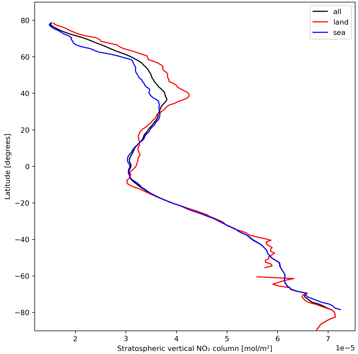
Figure 19: Zonal average of “Stratospheric vertical NO 2 column” for 2024-02-22 to 2024-02-24.
