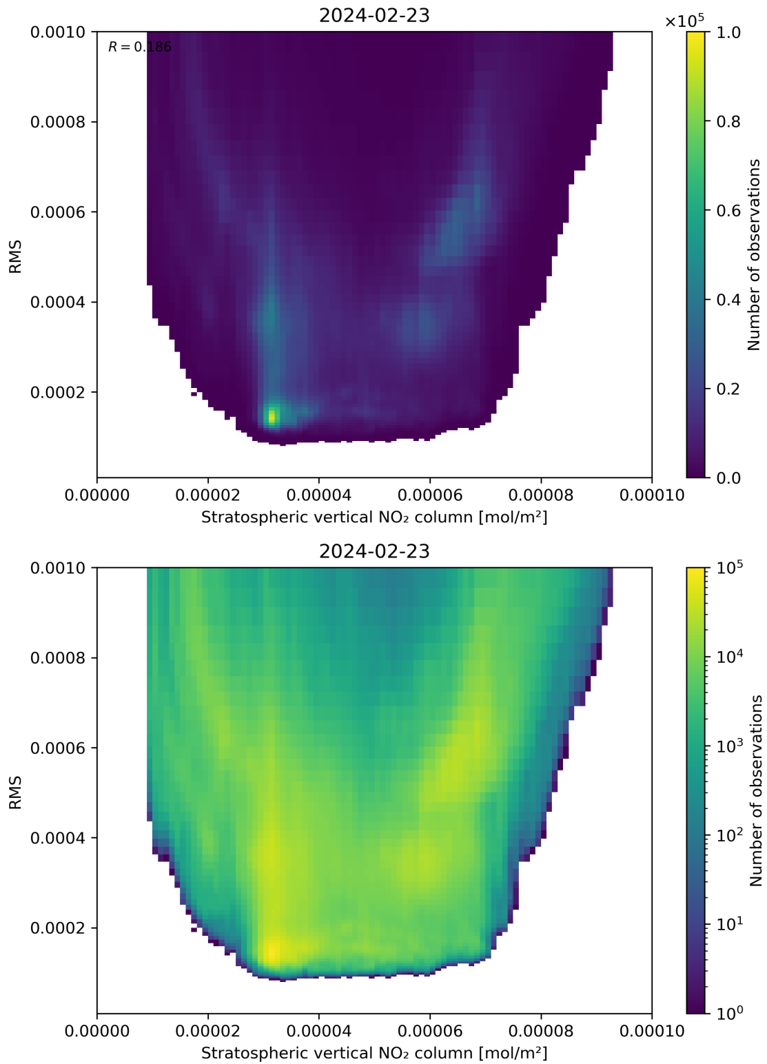
Figure 102: Scatter density plot of “Stratospheric vertical NO 2 column” against “RMS” for 2024-02-22 to 2024-02-24.
