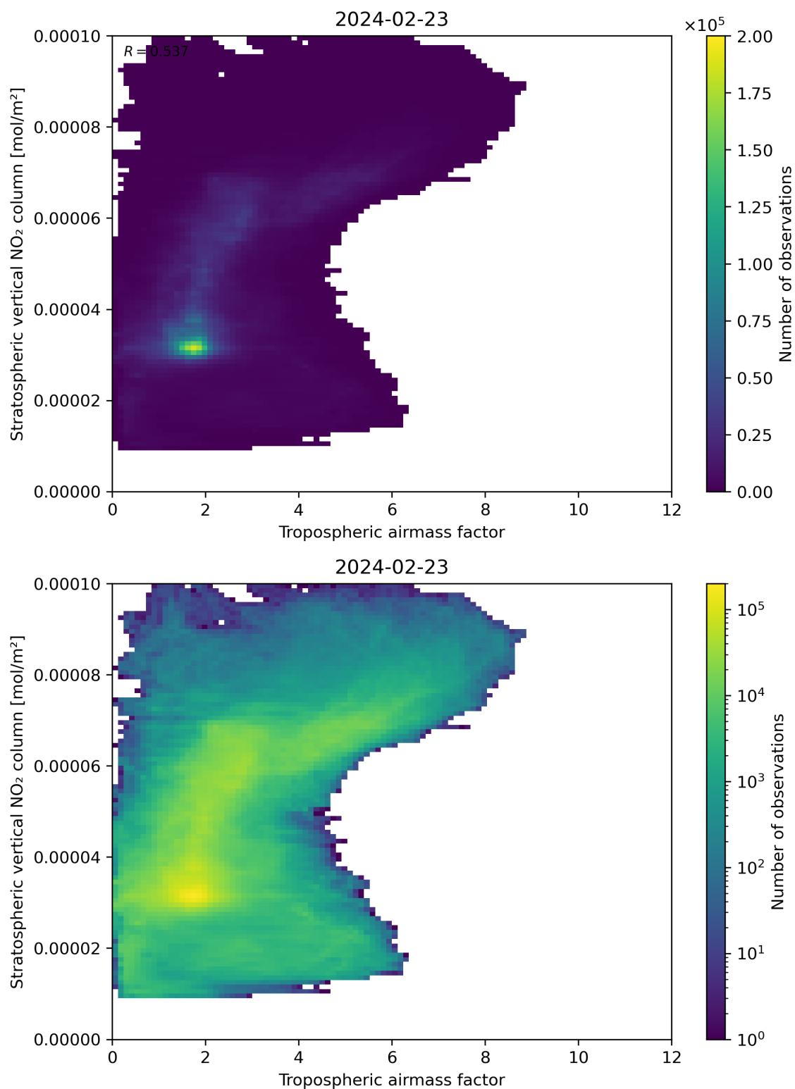
Figure 74: Scatter density plot of “Tropospheric airmass factor” against “Stratospheric vertical NO 2 column” for 2024-02-22 to 2024-02-24.
