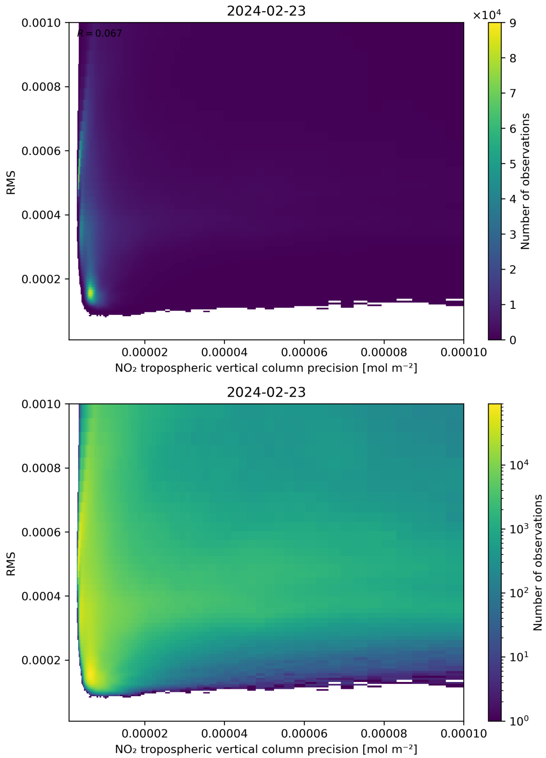
Figure 140: Scatter density plot of “NO 2 tropospheric vertical column precision” against “RMS” for 2024-02-22 to 2024-02-24.
