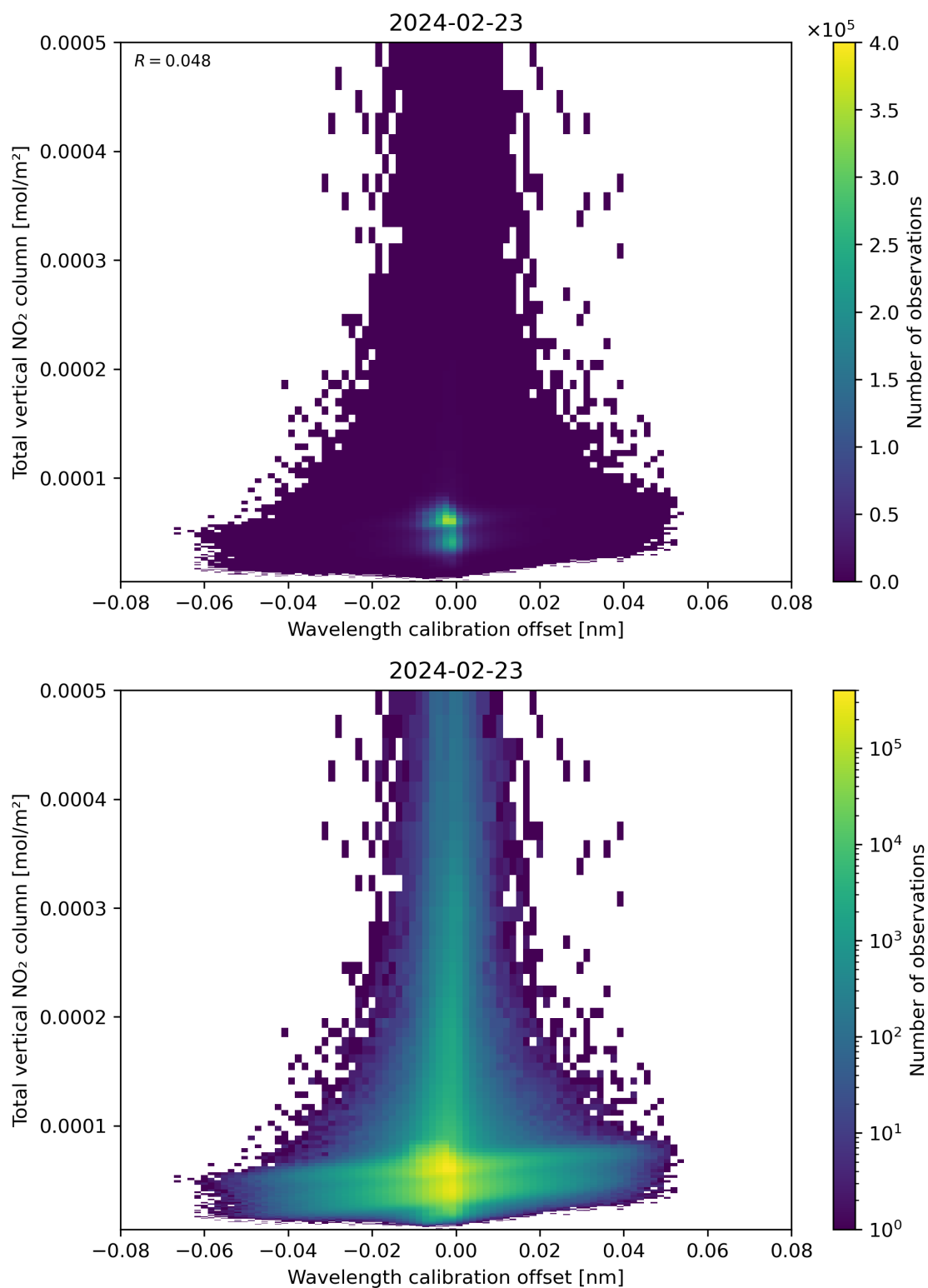
Figure 179: Scatter density plot of “Wavelength calibration offset” against “Total vertical NO 2 column” for 2024-02-22 to 2024-02-24.
