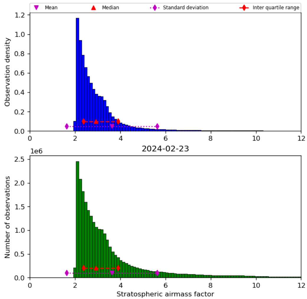
Figure 44: Histogram of “Stratospheric airmass factor” for 2024-02-22 to 2024-02-24
