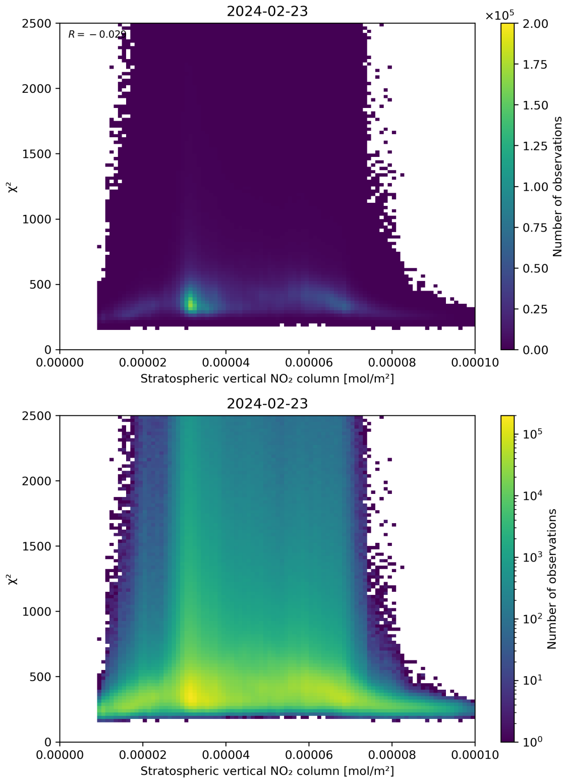
Figure 97: Scatter density plot of “Stratospheric vertical NO 2 column” against “ \chi^2 ” for 2024-02-22 to 2024-02-24.
