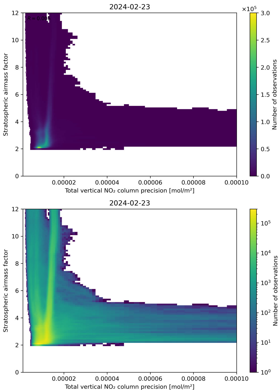
Figure 115: Scatter density plot of “Total vertical NO 2 column precision” against “Stratospheric air mass factor” for 2024-02-22 to 2024-02-24.
