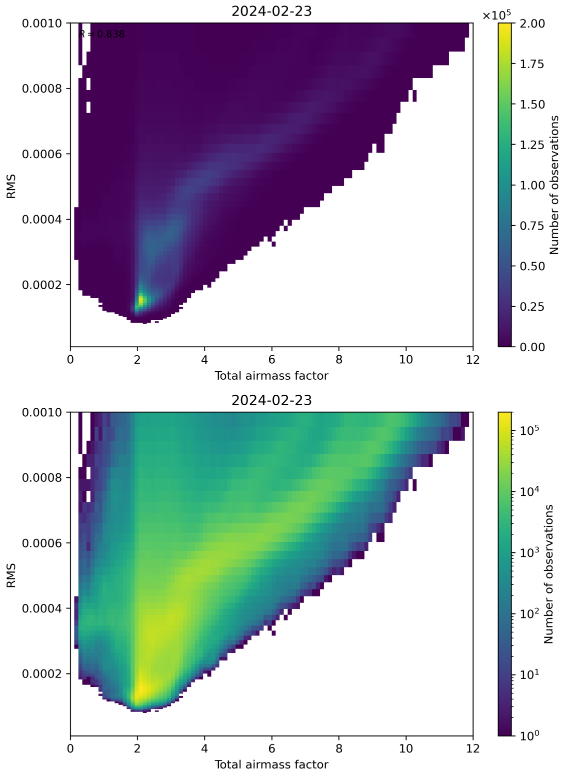
Figure 69: Scatter density plot of “Total airmass factor” against “RMS” for 2024-02-22 to 2024-02-24.
