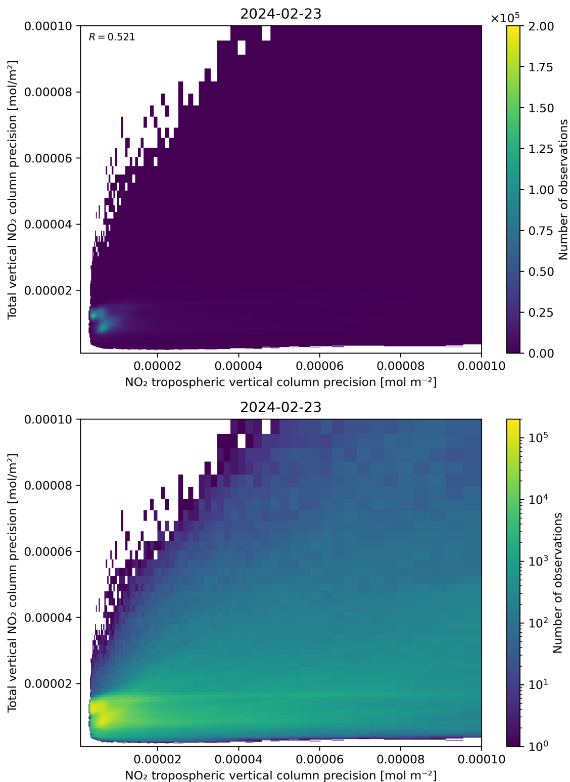
Figure 139: Scatter density plot of “NO 2 tropospheric vertical column precision” against “Total vertical NO 2 column precision” for 2024-02-22 to 2024-02-24.
