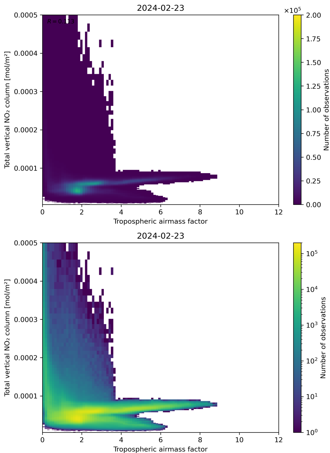
Figure 77: Scatter density plot of “Tropospheric airmass factor” against “Total vertical NO 2 column” for 2024-02-22 to 2024-02-24.
