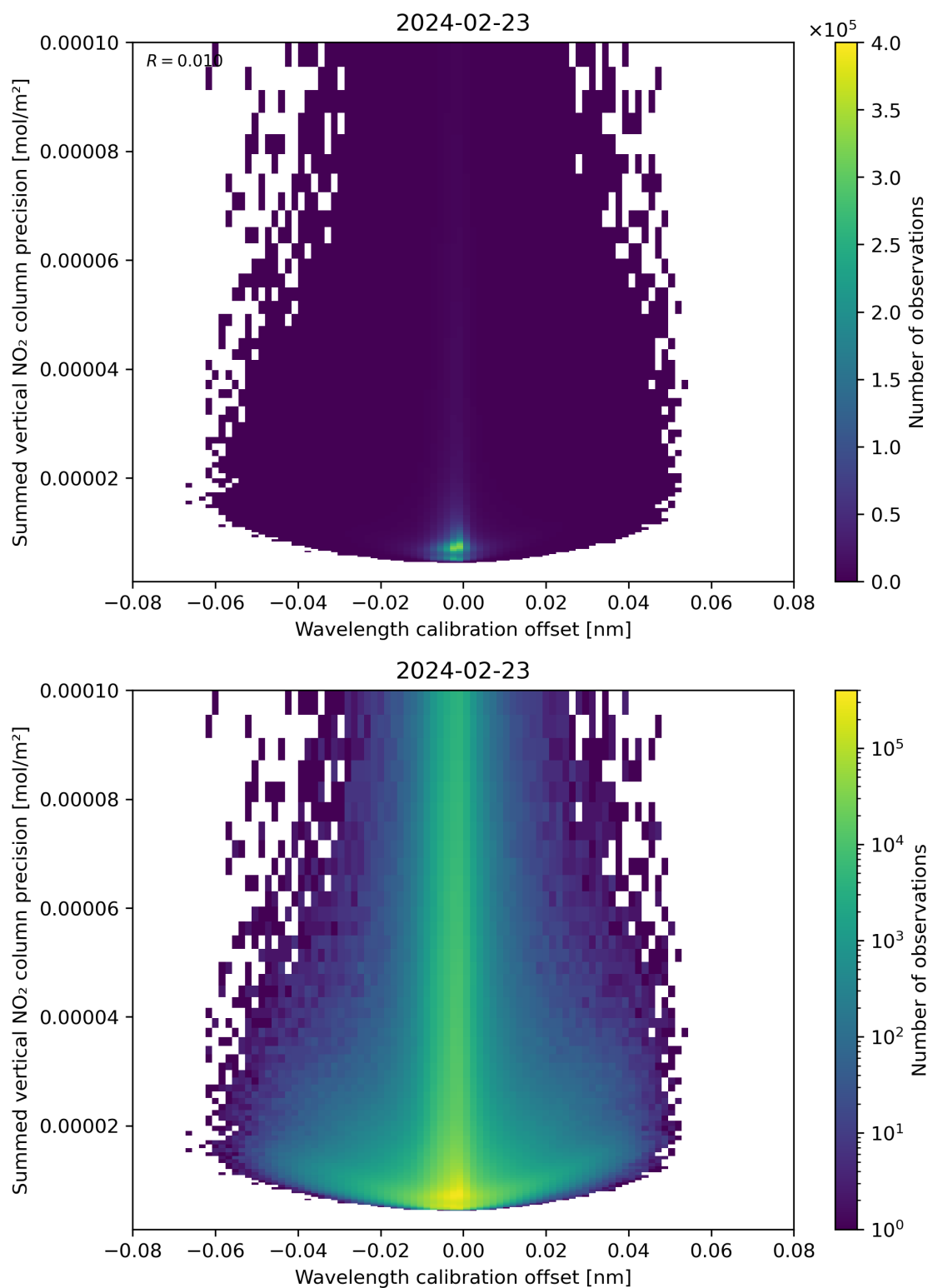
Figure 178: Scatter density plot of “Wavelength calibration offset” against “Summed vertical NO 2 column precision” for 2024-02-22 to 2024-02-24.
