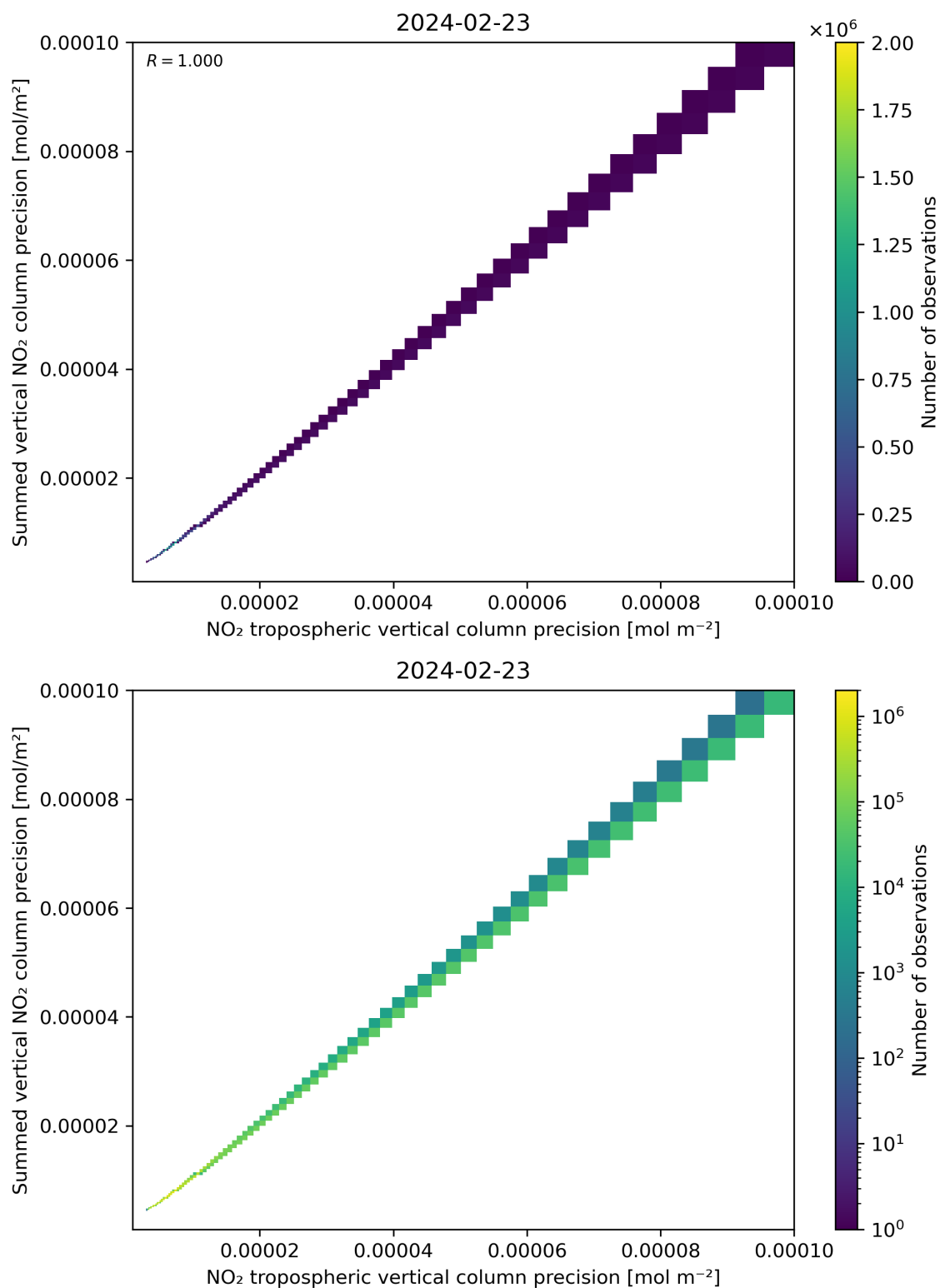
Figure 137: Scatter density plot of “NO 2 tropospheric vertical column precision” against “Summed vertical NO 2 column precision” for 2024-02-22 to 2024-02-24.
