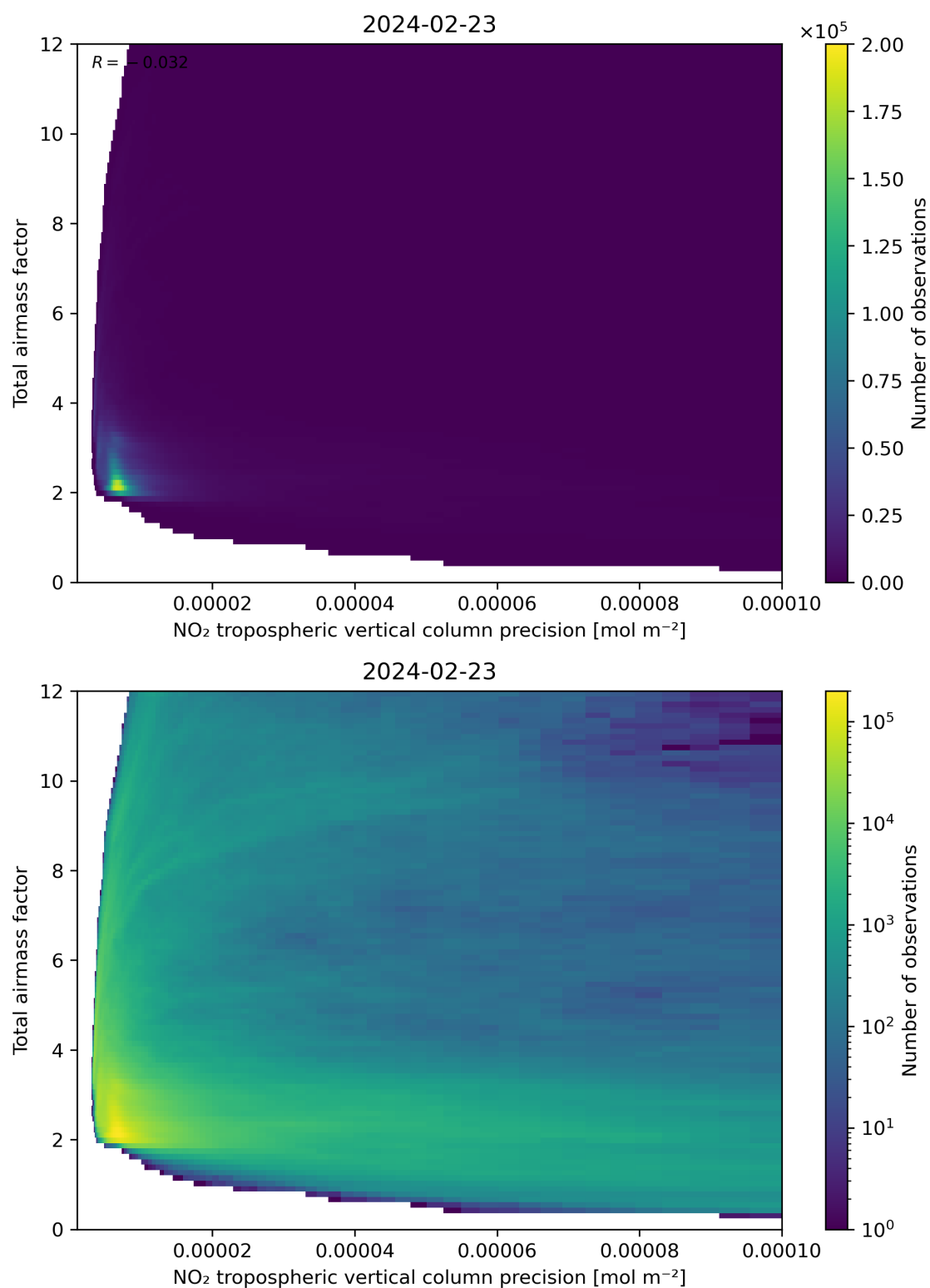
Figure 132: Scatter density plot of “NO 2 tropospheric vertical column precision” against “Total air mass factor” for 2024-02-22 to 2024-02-24.
