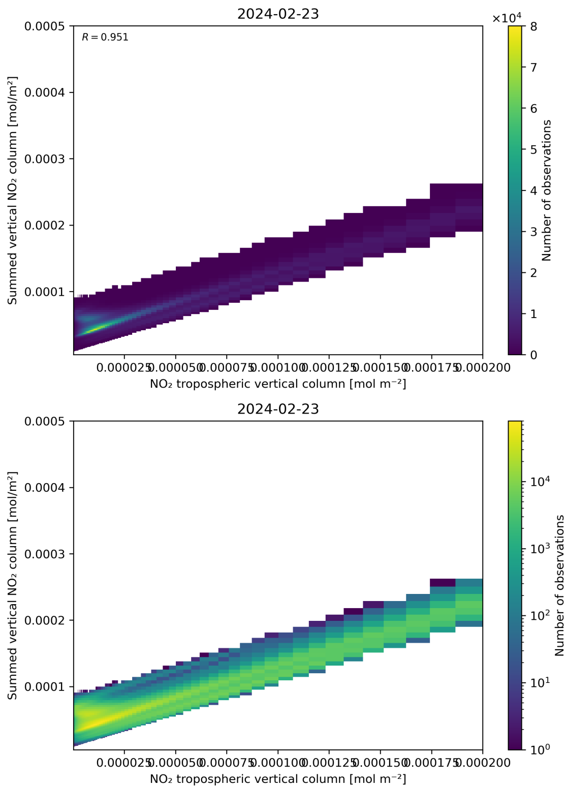
Figure 126: Scatter density plot of “NO 2 tropospheric vertical column” against “Summed vertical NO 2 column” for 2024-02-22 to 2024-02-24.
