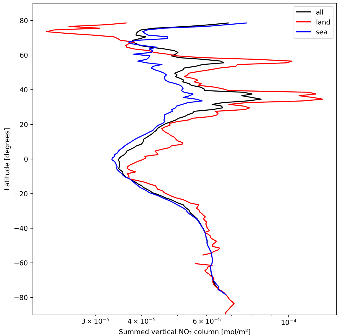
Figure 23: Zonal average of “Summed vertical NO 2 column” for 2024-02-22 to 2024-02-24.
