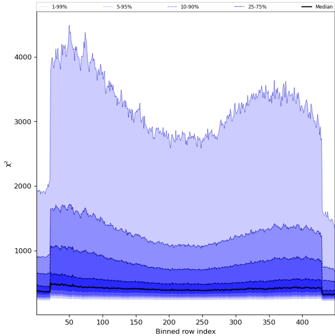
Figure 59: Along track statistics of “ \chi^2 ” for 2024-02-22 to 2024-02-24
