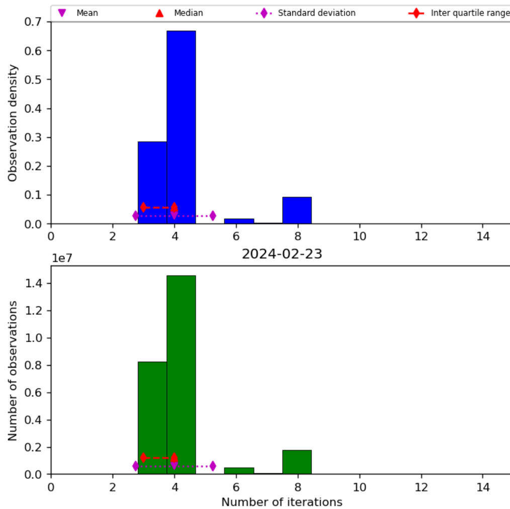
Figure 34: Histogram of “Number of iterations” for 2024-02-22 to 2024-02-24
