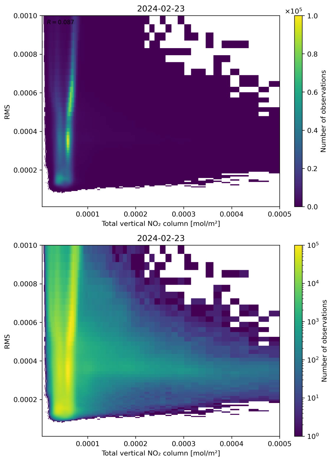
Figure 120: Scatter density plot of “Total vertical NO 2 column” against “RMS” for 2024-02-22 to 2024-02-24.
