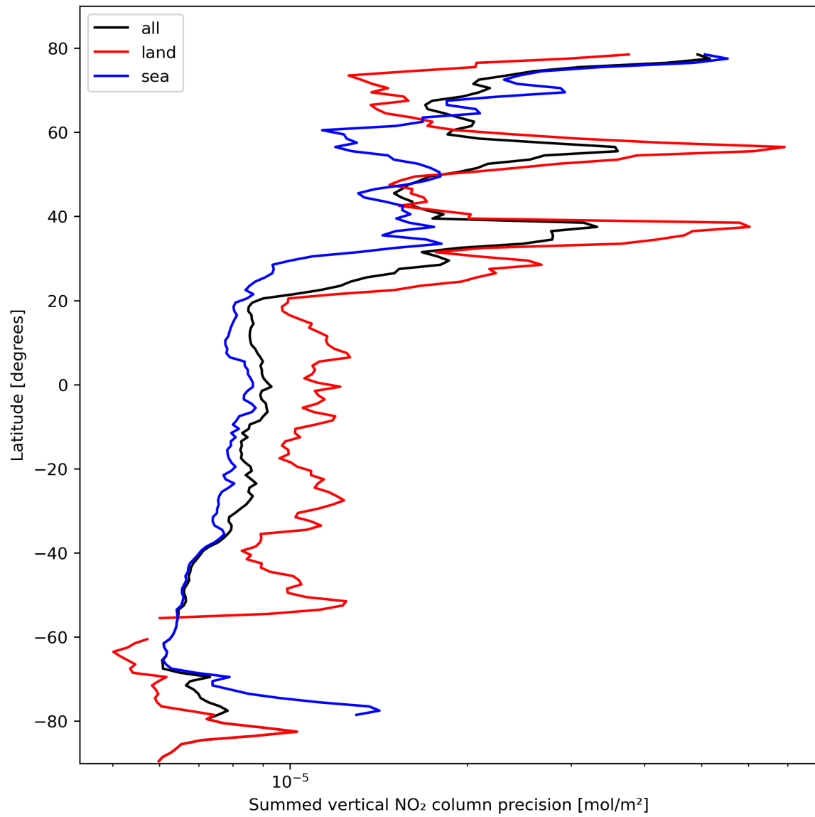
Figure 24: Zonal average of “Summed vertical NO 2 column precision” for 2024-02-22 to 2024-02-24.
