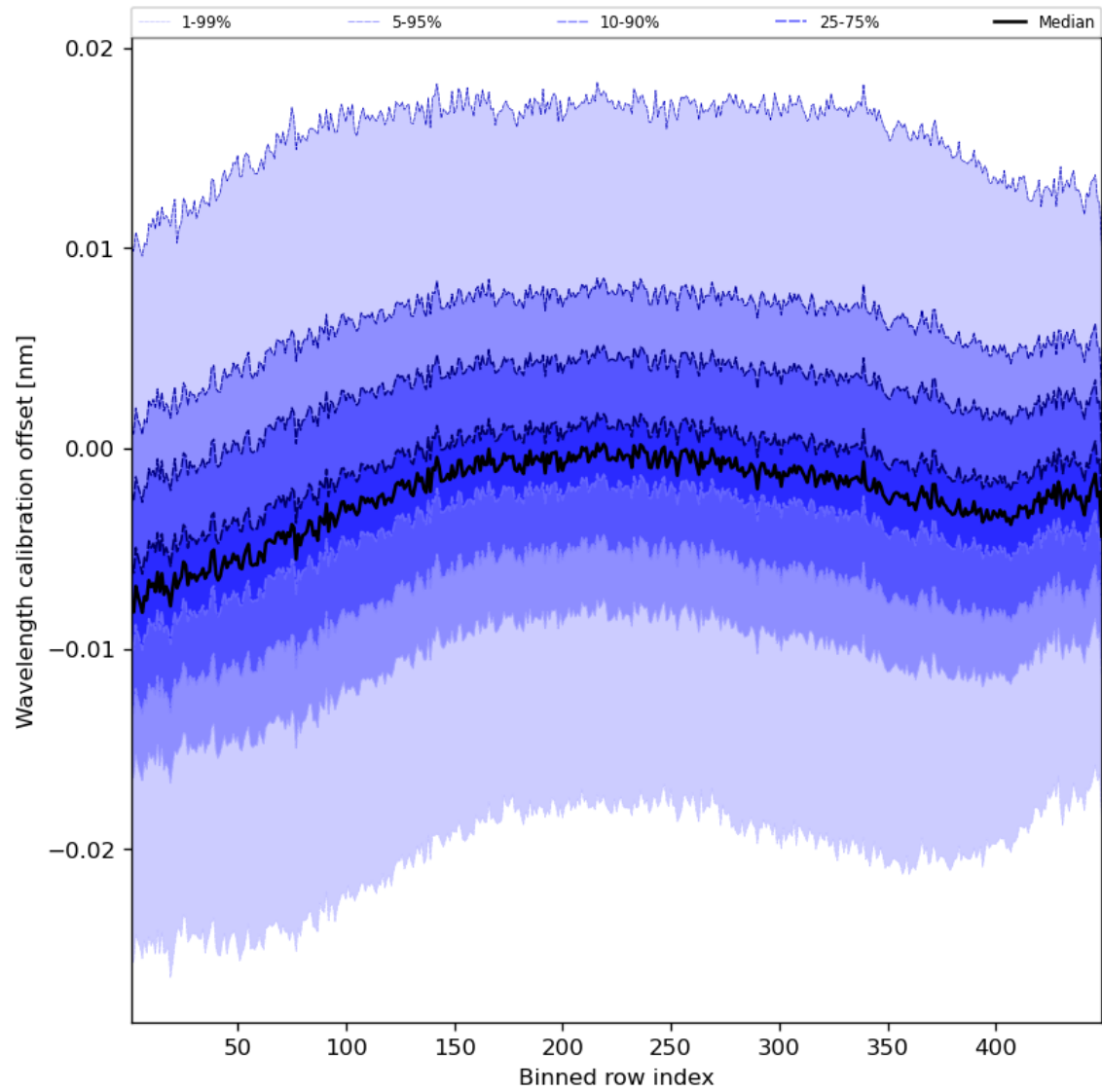
Figure 52: Along track statistics of “Wavelength calibration offset” for 2024-02-22 to 2024-02-24
