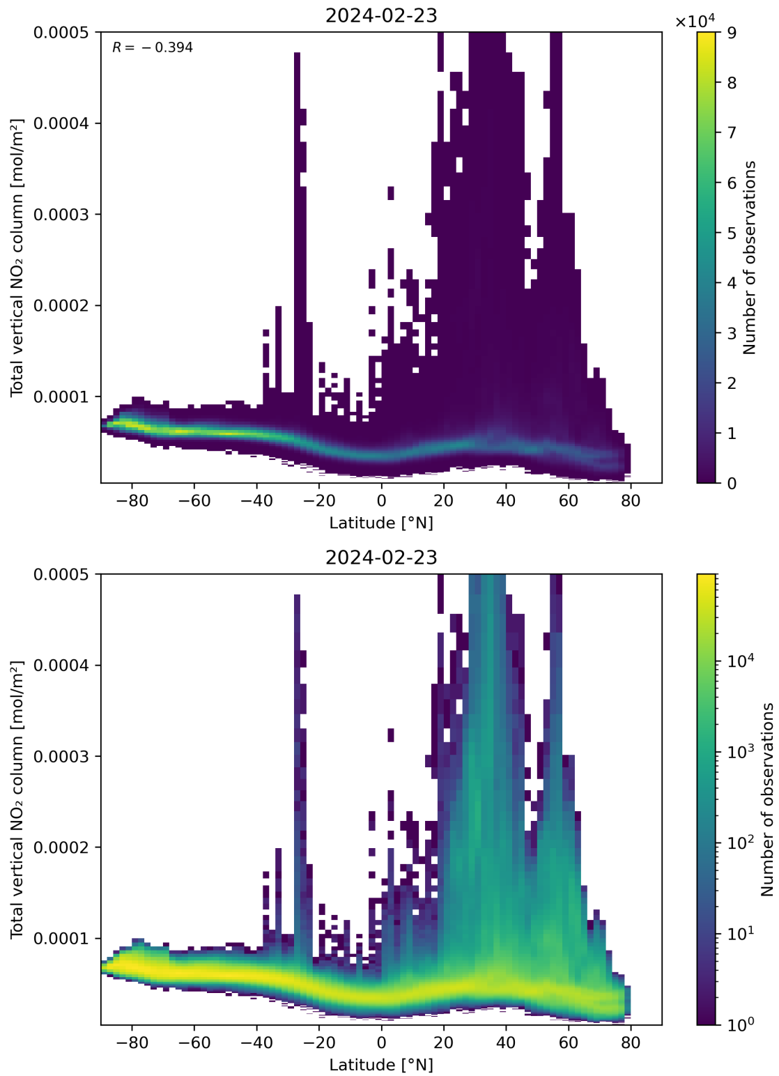
Figure 90: Scatter density plot of “Latitude” against “Total vertical NO 2 column” for 2024-02-22 to 2024-02-24.
