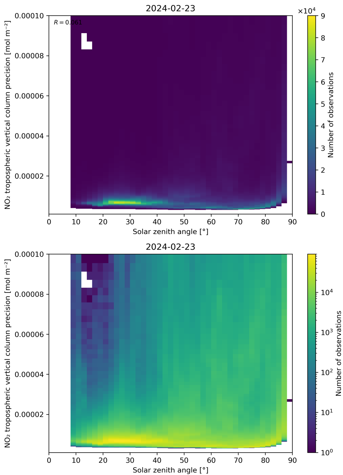
Figure 156: Scatter density plot of “Solar zenith angle” against “NO 2 tropospheric vertical column precision” for 2024-02-22 to 2024-02-24.
