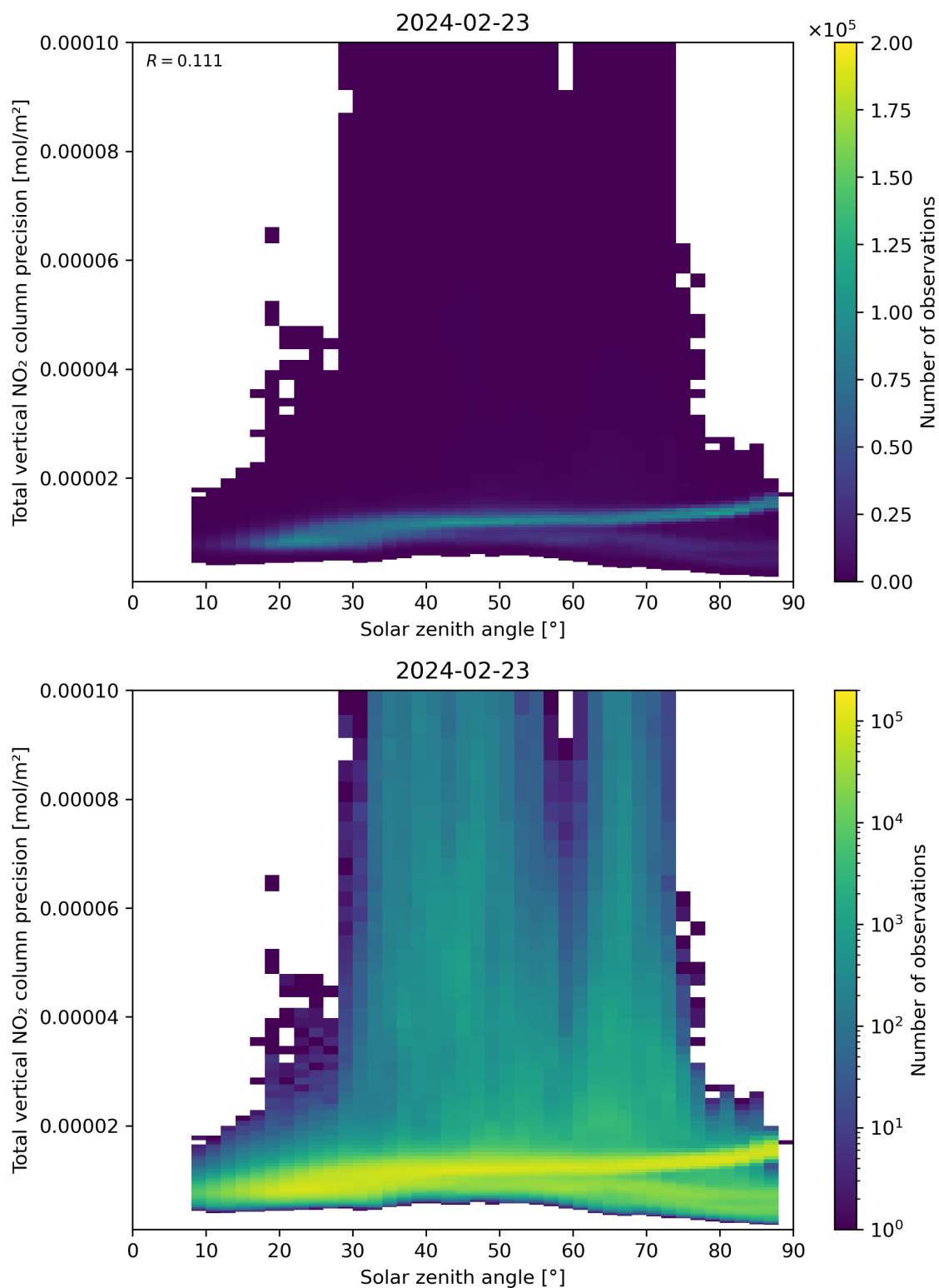
Figure 154: Scatter density plot of “Solar zenith angle” against “Total vertical NO 2 column precision” for 2024-02-22 to 2024-02-24.
