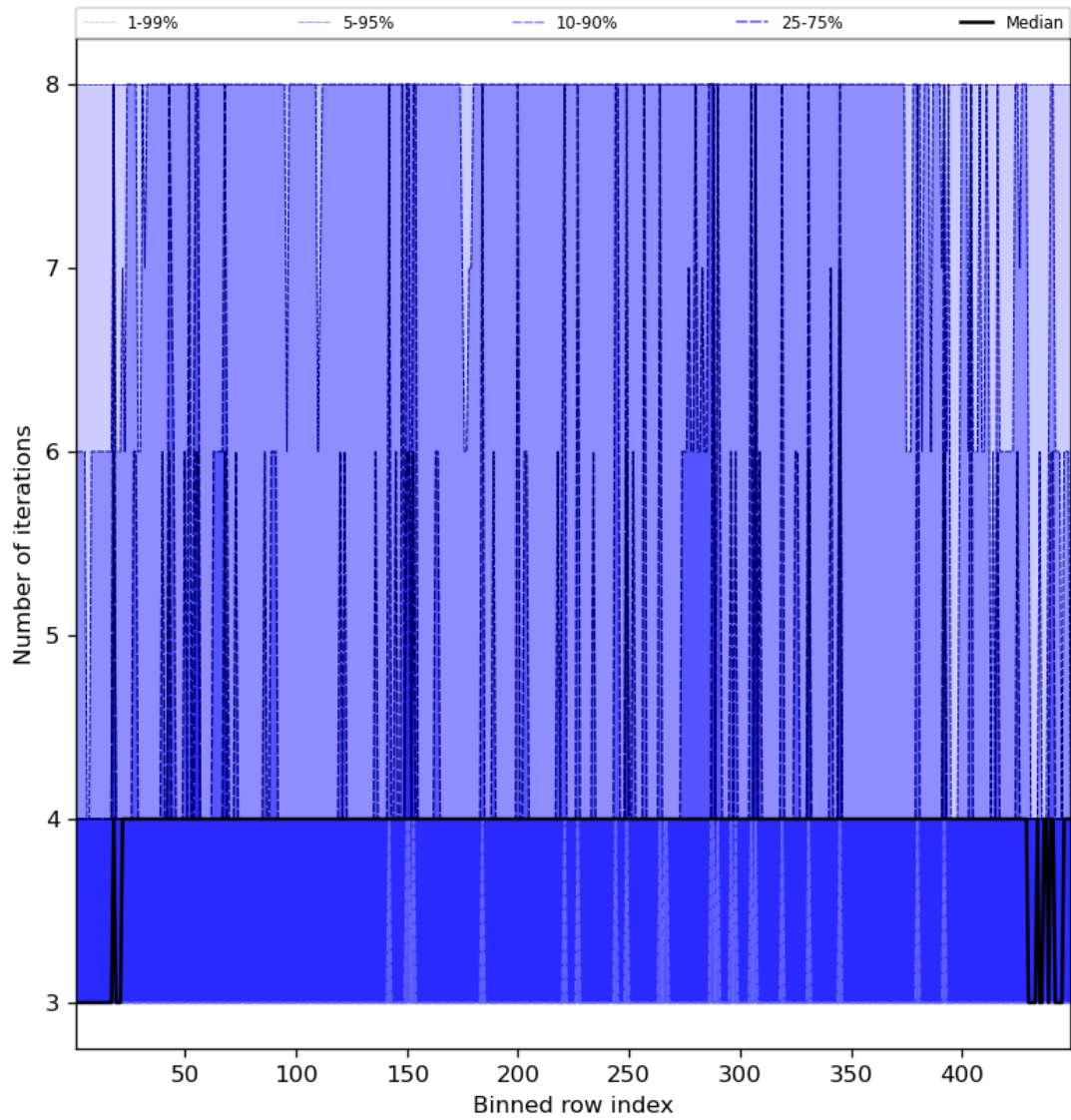
Figure 51: Along track statistics of “Number of iterations” for 2024-02-22 to 2024-02-24
