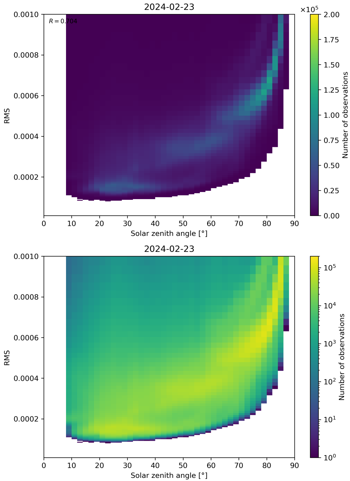
Figure 157: Scatter density plot of “Solar zenith angle” against “RMS” for 2024-02-22 to 2024-02-24.
