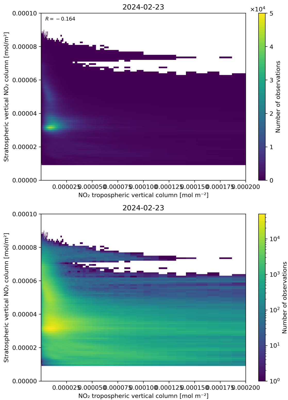
Figure 125: Scatter density plot of “NO 2 tropospheric vertical column” against “Stratospheric vertical NO 2 column” for 2024-02-22 to 2024-02-24.
