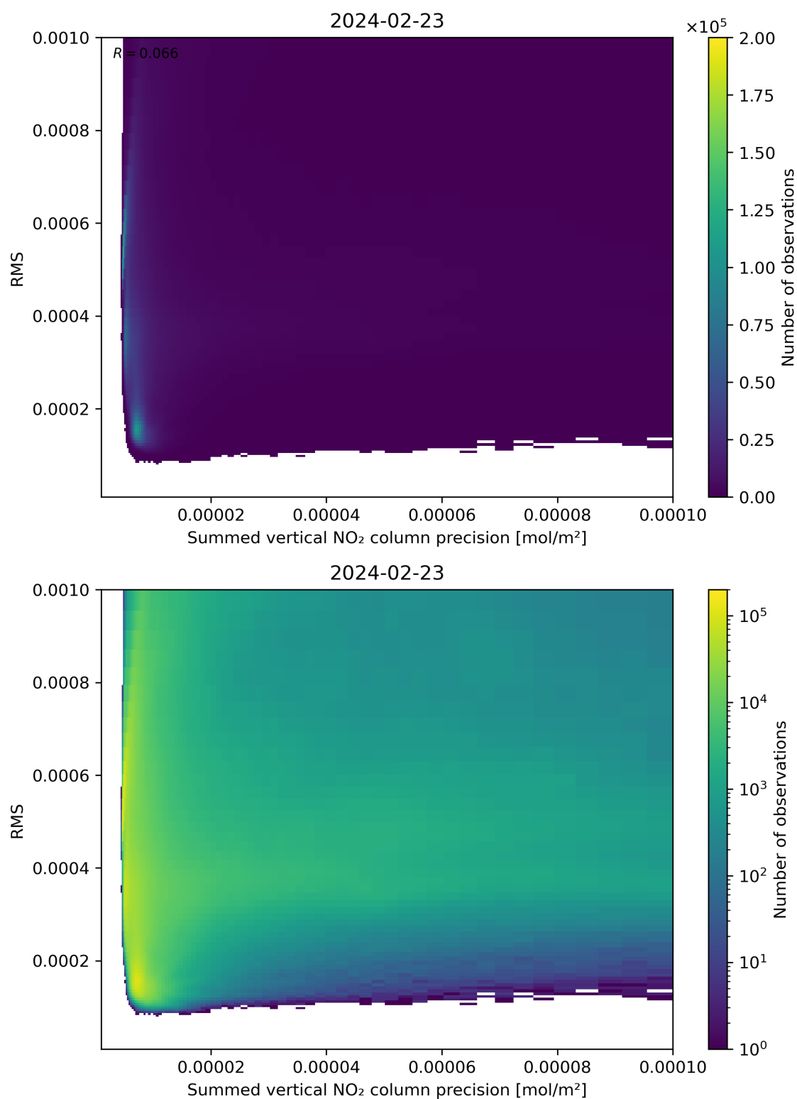
Figure 108: Scatter density plot of “Summed vertical NO 2 column precision” against “RMS” for 2024-02-22 to 2024-02-24.
