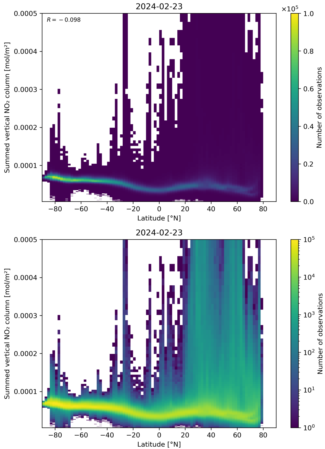
Figure 88: Scatter density plot of “Latitude” against “Summed vertical NO 2 column” for 2024-02-22 to 2024-02-24.
