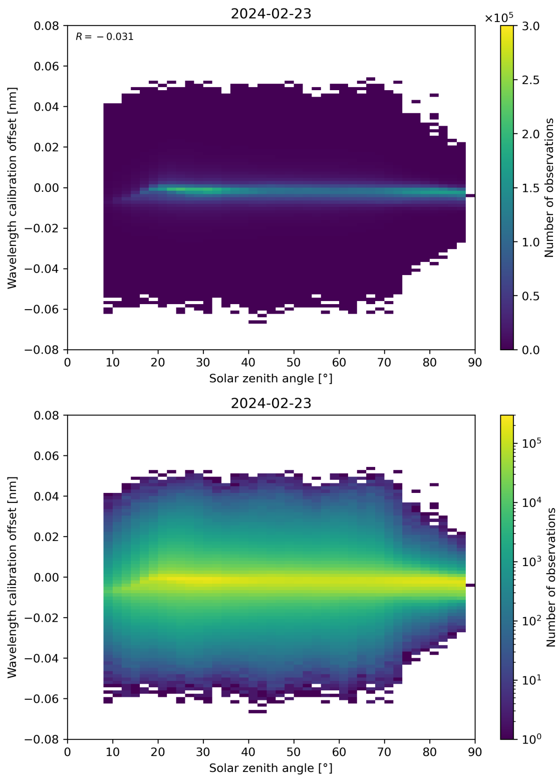
Figure 158: Scatter density plot of “Solar zenith angle” against “Wavelength calibration offset” for 2024-02-22 to 2024-02-24.
