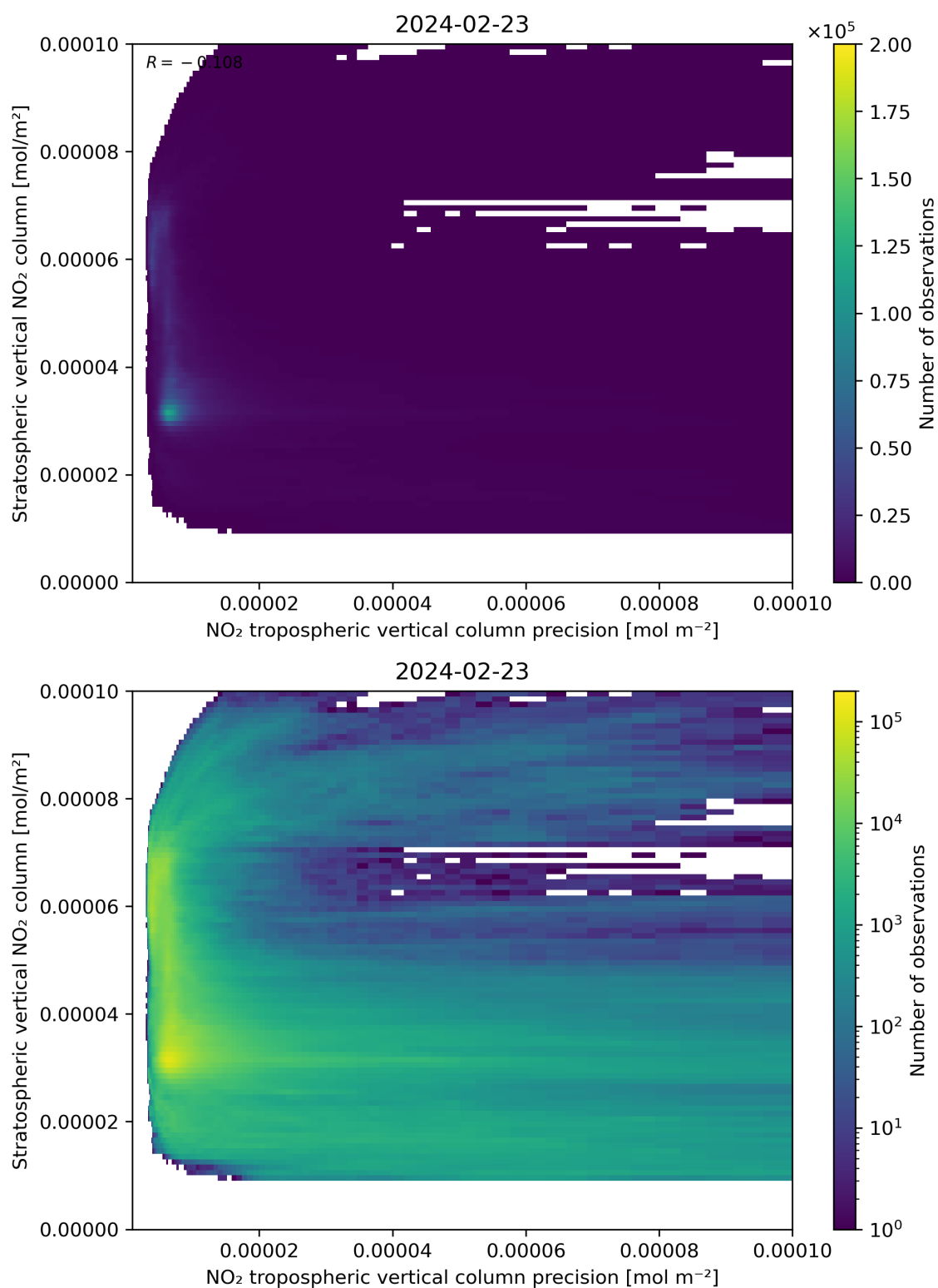
Figure 135: Scatter density plot of “NO 2 tropospheric vertical column precision” against “Stratospheric vertical NO 2 column” for 2024-02-22 to 2024-02-24.
