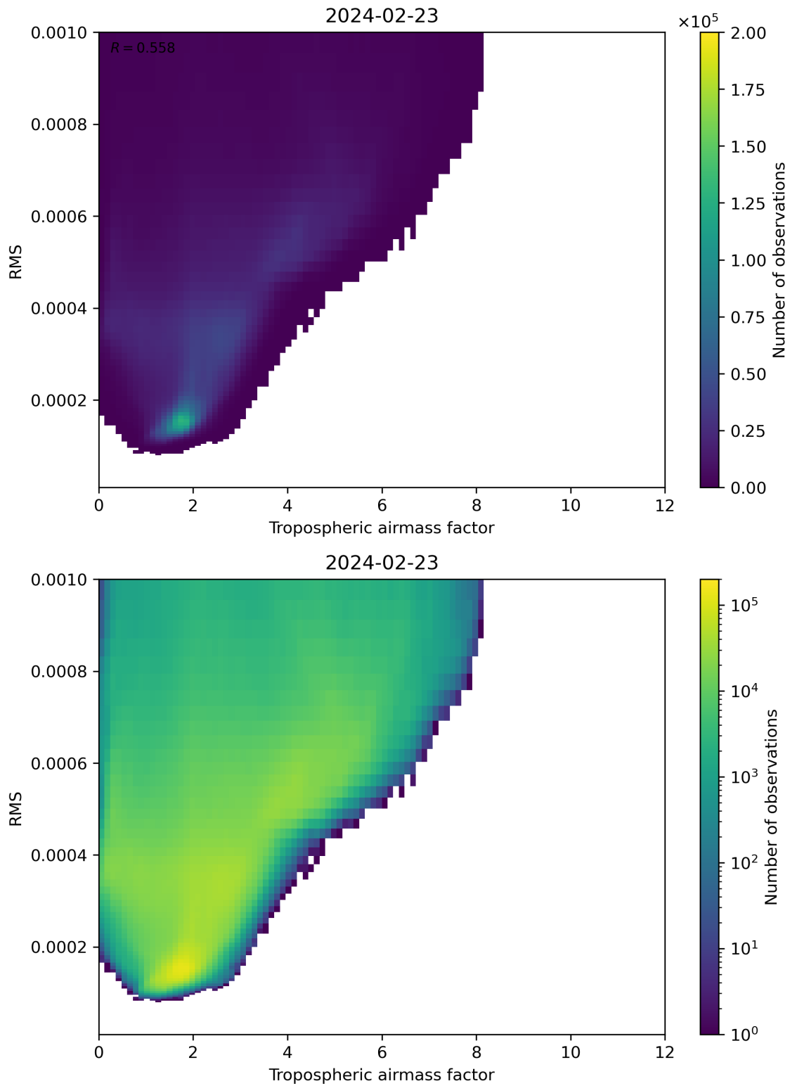
Figure 79: Scatter density plot of “Tropospheric airmass factor” against “RMS” for 2024-02-22 to 2024-02-24.
