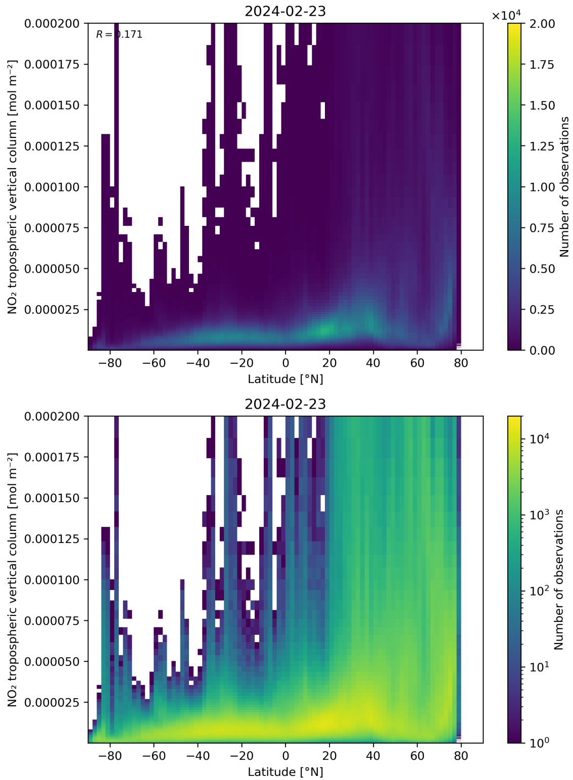
Figure 92: Scatter density plot of “Latitude” against “NO 2 tropospheric vertical column” for 2024-02-22 to 2024-02-24.
