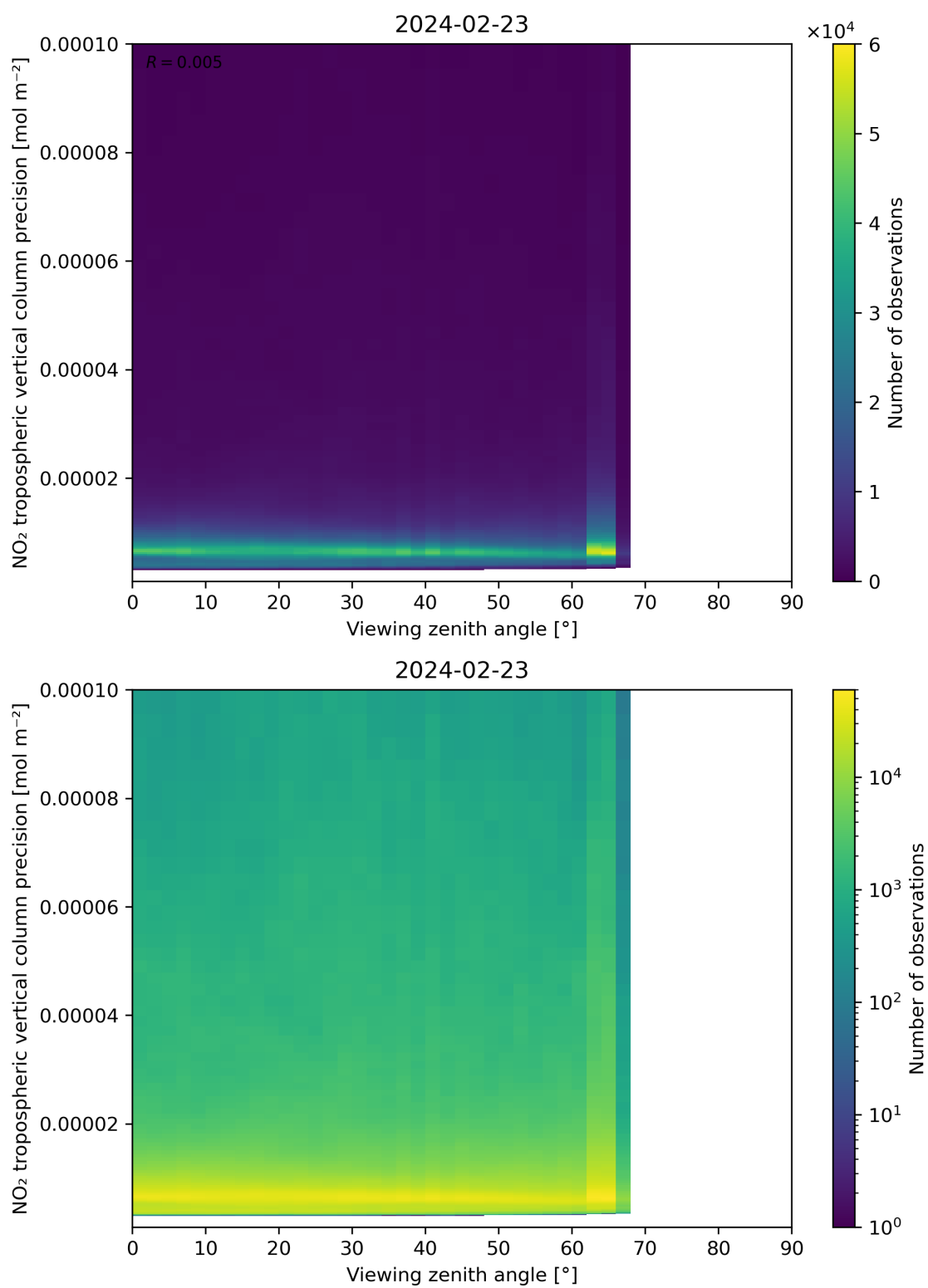
Figure 170: Scatter density plot of “Viewing zenith angle” against “NO 2 tropospheric vertical column precision” for 2024-02-22 to 2024-02-24.
