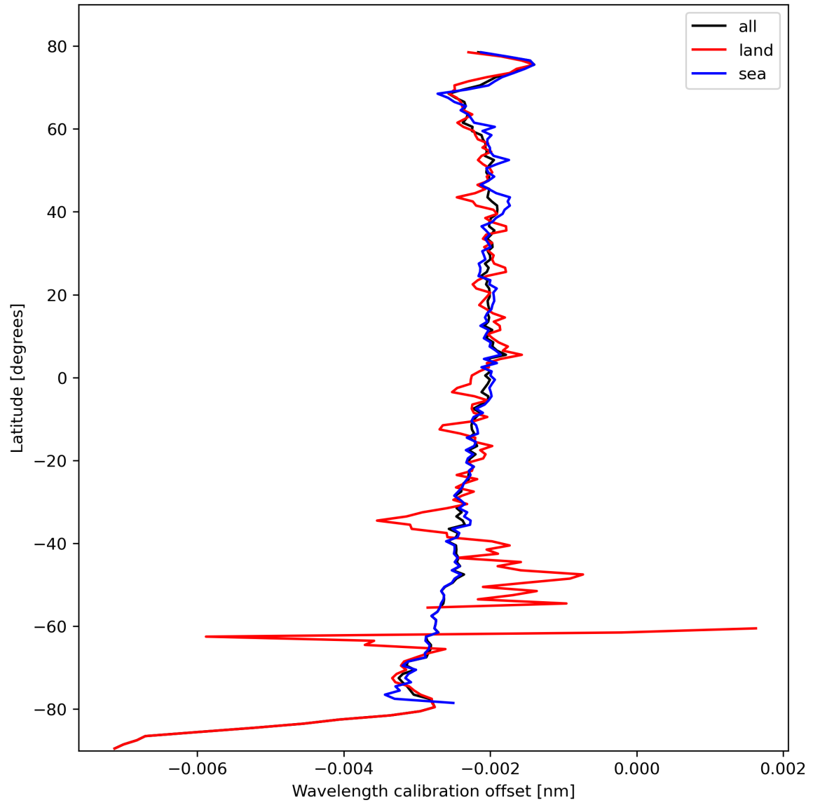
Figure 18: Zonal average of “Wavelength calibration offset” for 2024-02-22 to 2024-02-24.
