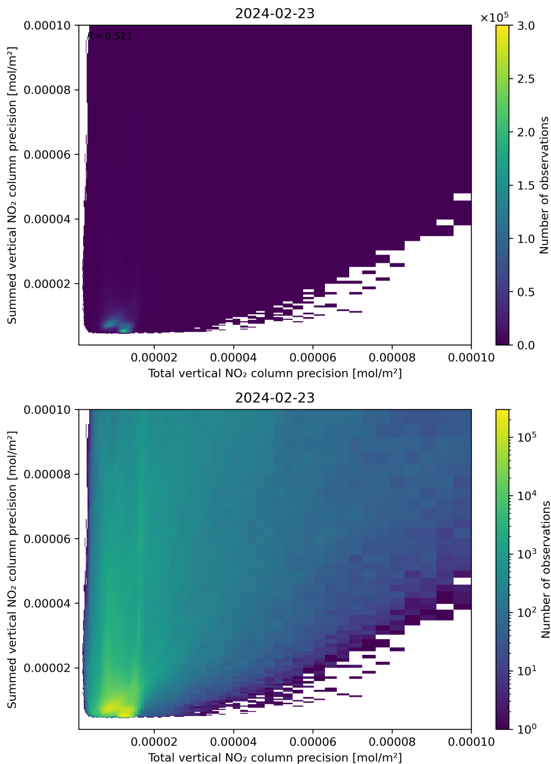
Figure 118: Scatter density plot of “Total vertical NO 2 column precision” against “Summed vertical NO 2 column precision” for 2024-02-22 to 2024-02-24.
