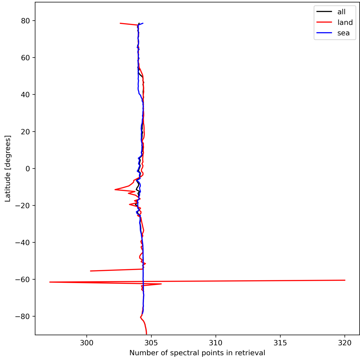
Figure 16: Zonal average of “Number of spectral points in retrieval” for 2024-02-22 to 2024-02-24.
