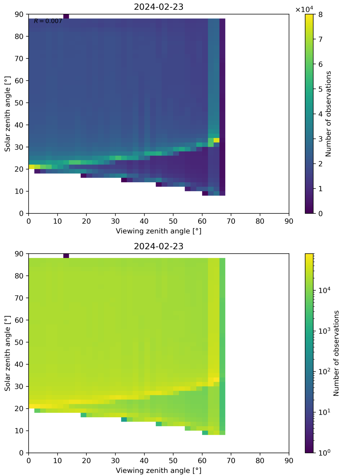
Figure 172: Scatter density plot of “Viewing zenith angle” against “Solar zenith angle” for 2024-02-22 to 2024-02-24.
