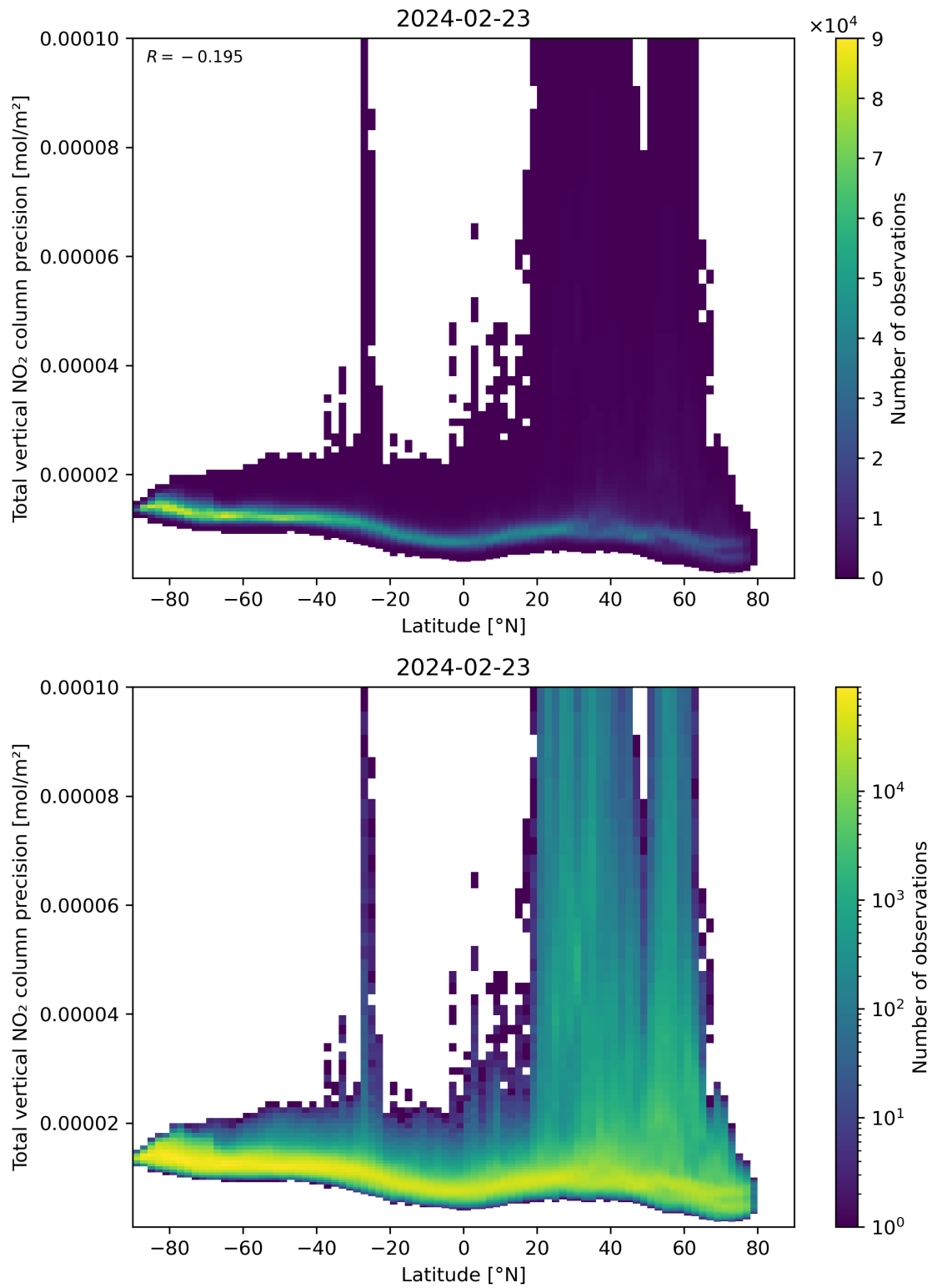
Figure 91: Scatter density plot of “Latitude” against “Total vertical NO 2 column precision” for 2024-02-22 to 2024-02-24.
