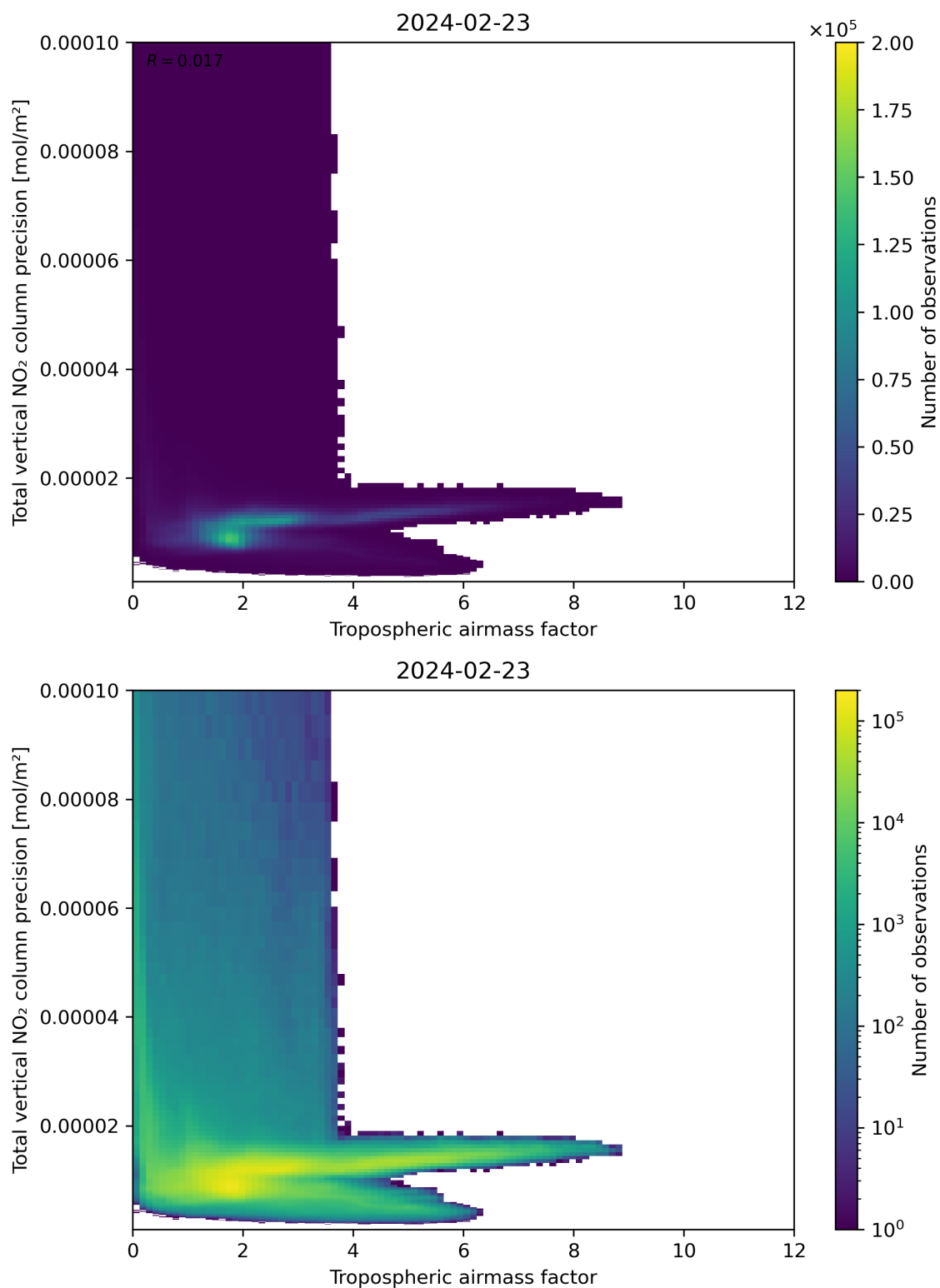
Figure 78: Scatter density plot of “Tropospheric air mass factor” against “Total vertical NO 2 column precision” for 2024-02-22 to 2024-02-24.
