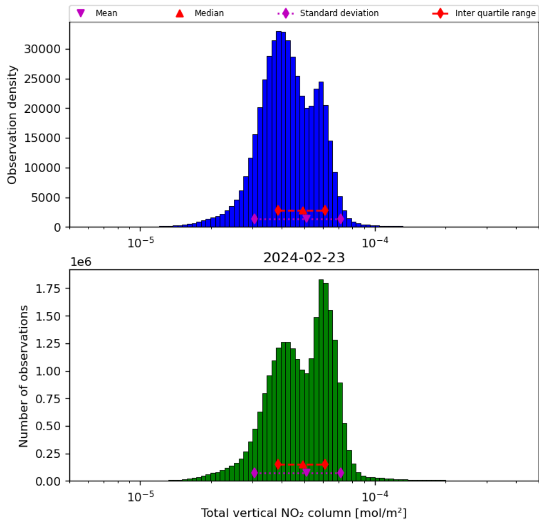
Figure 38: Histogram of “Total vertical NO 2 column” for 2024-02-22 to 2024-02-24
