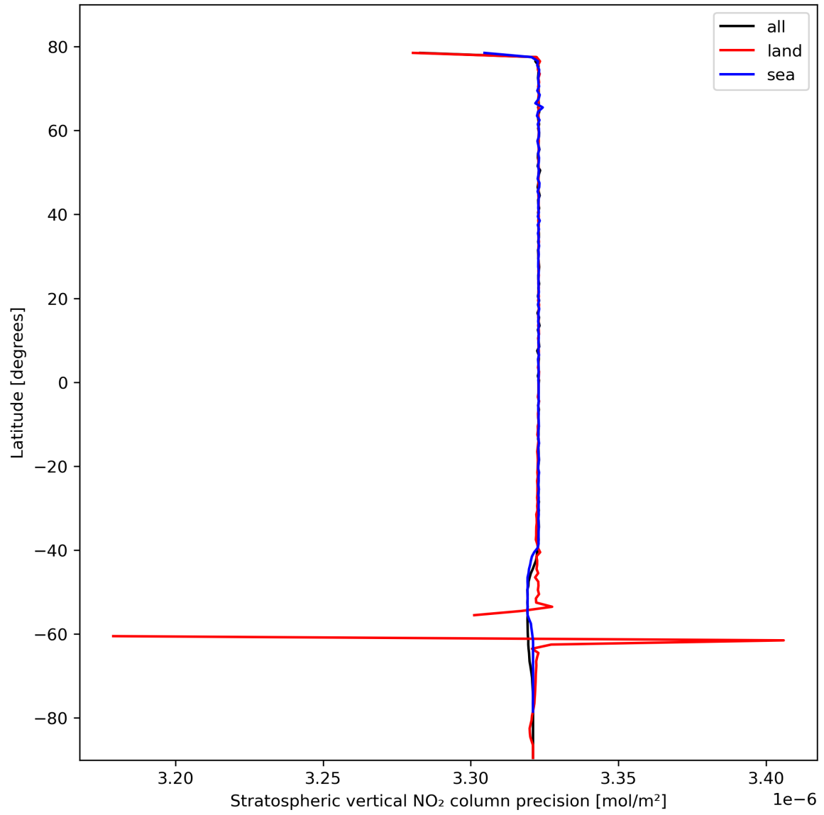
Figure 20: Zonal average of “Stratospheric vertical NO 2 column precision” for 2024-02-22 to 2024-02-24.
