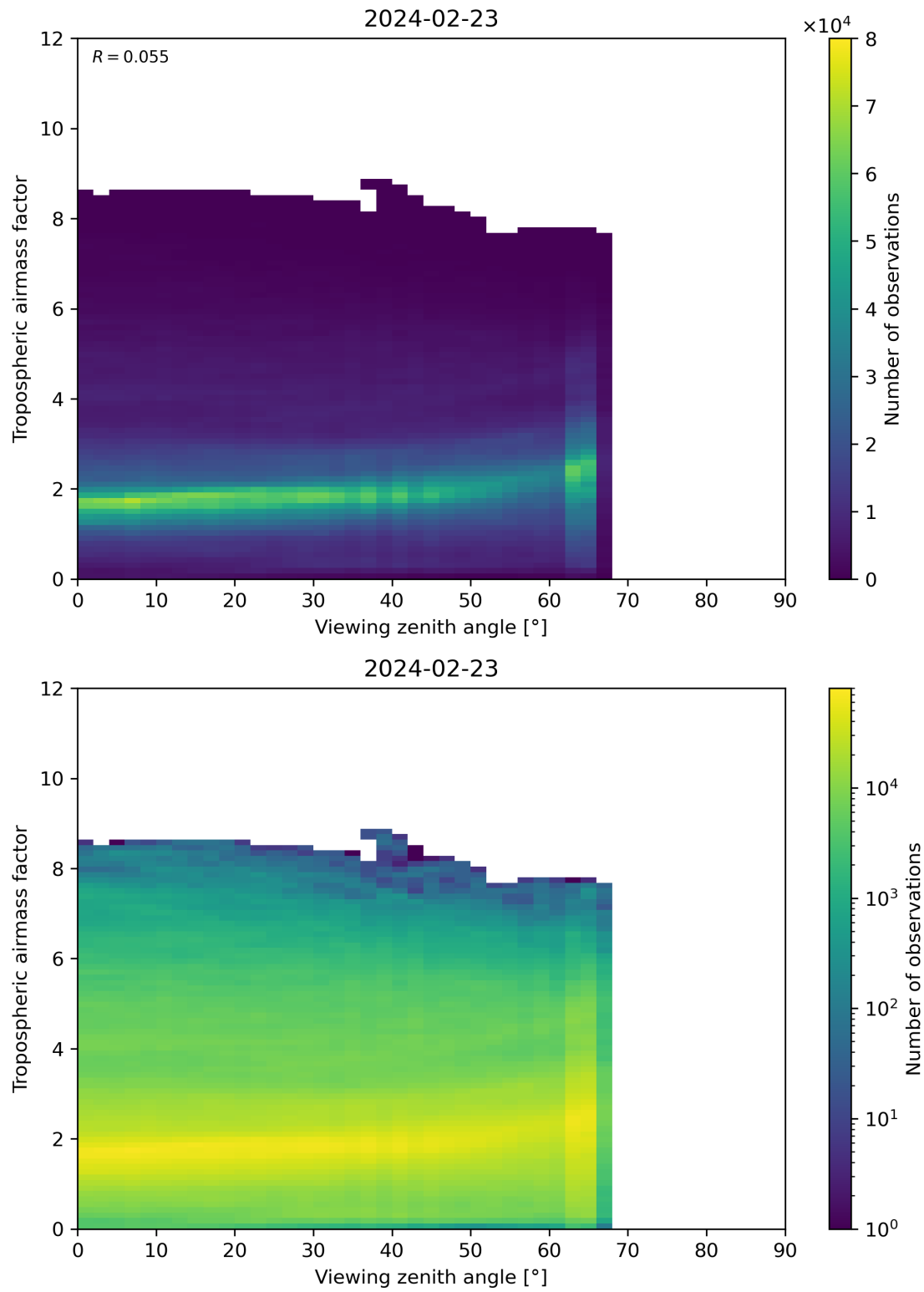
Figure 161: Scatter density plot of “Viewing zenith angle” against “Tropospheric airmass factor” for 2024-02-22 to 2024-02-24.
