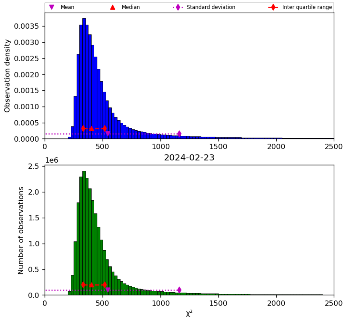
Figure 42: Histogram of “ \chi^2 ” for 2024-02-22 to 2024-02-24
