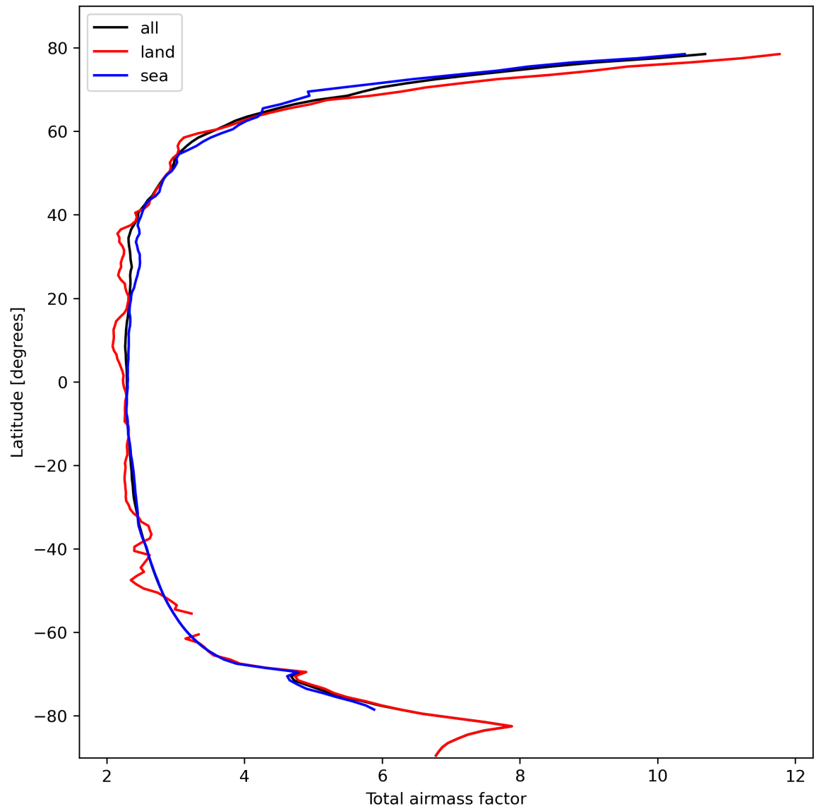
Figure 15: Zonal average of “Total airmass factor” for 2024-02-22 to 2024-02-24.
