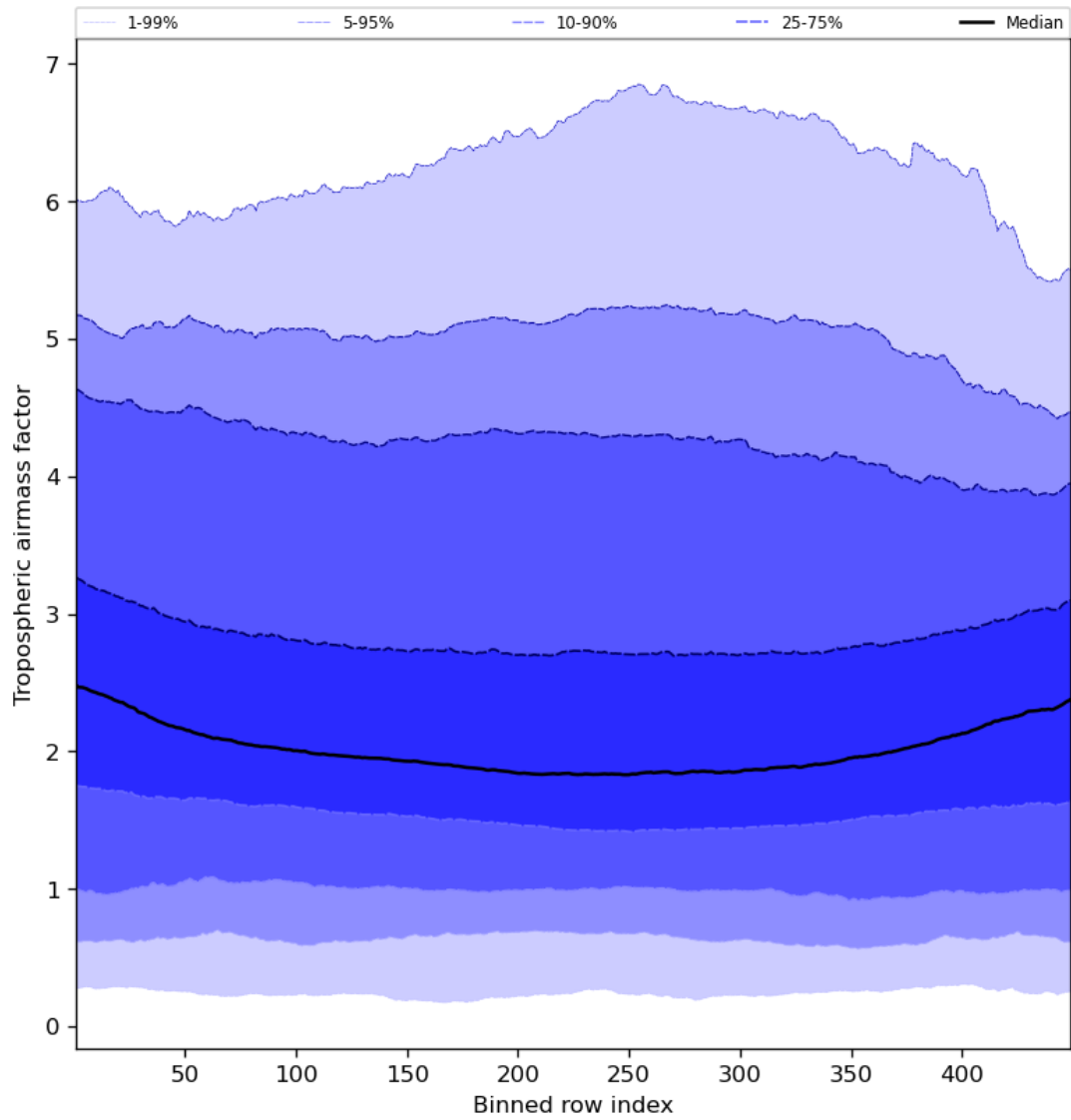
Figure 48: Along track statistics of “Tropospheric air mass factor” for 2024-02-22 to 2024-02-24
