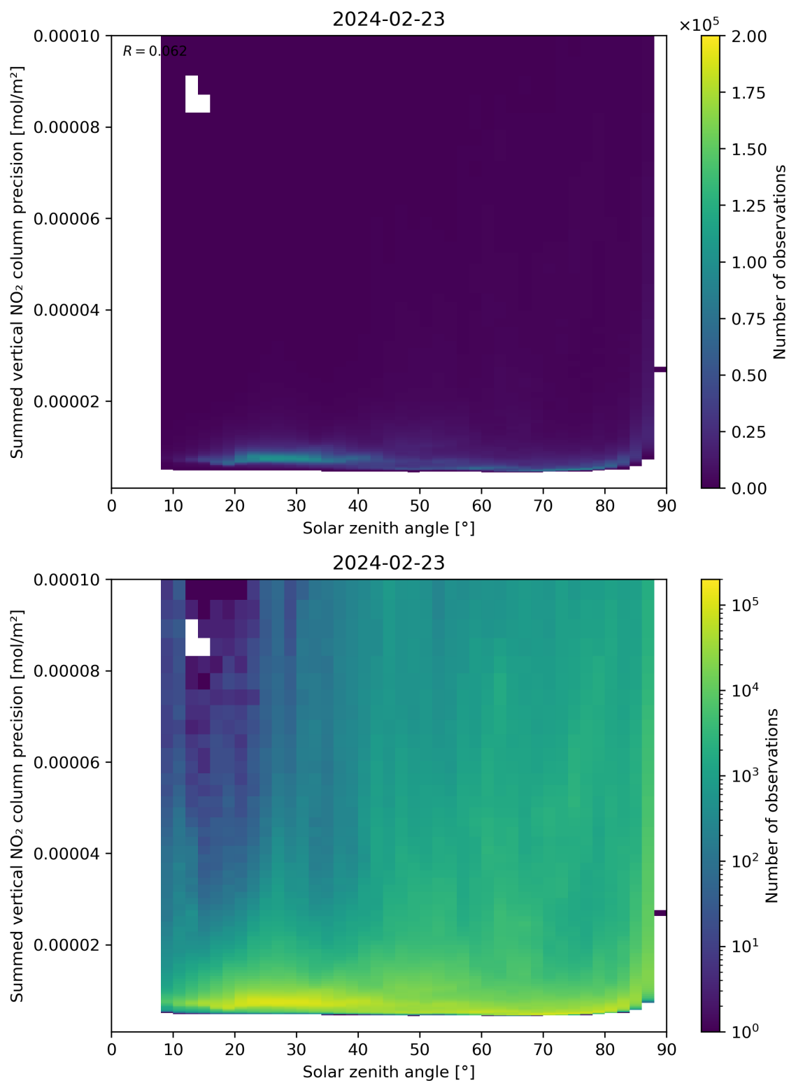
Figure 152: Scatter density plot of “Solar zenith angle” against “Summed vertical NO 2 column precision” for 2024-02-22 to 2024-02-24.
