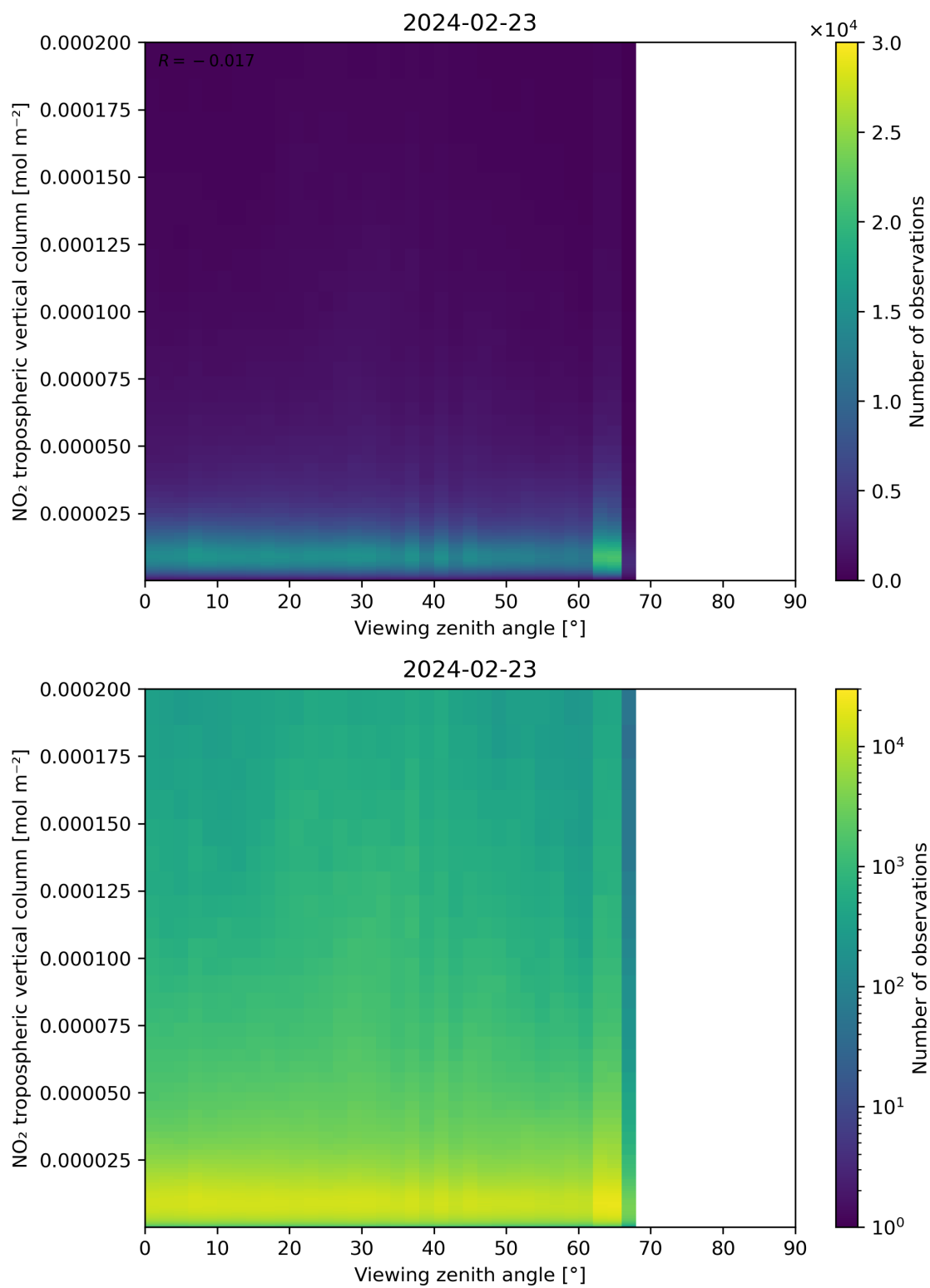
Figure 169: Scatter density plot of “Viewing zenith angle” against “NO 2 tropospheric vertical column” for 2024-02-22 to 2024-02-24.
