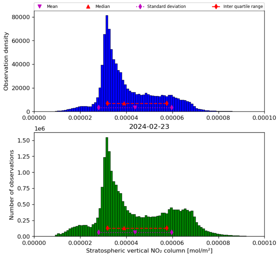
Figure 36: Histogram of “Stratospheric vertical NO 2 column” for 2024-02-22 to 2024-02-24
