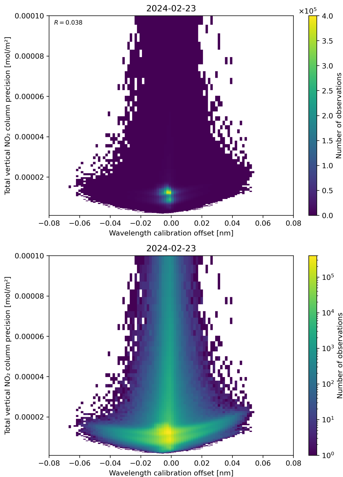
Figure 180: Scatter density plot of “Wavelength calibration offset” against “Total vertical NO 2 column precision” for 2024-02-22 to 2024-02-24.
