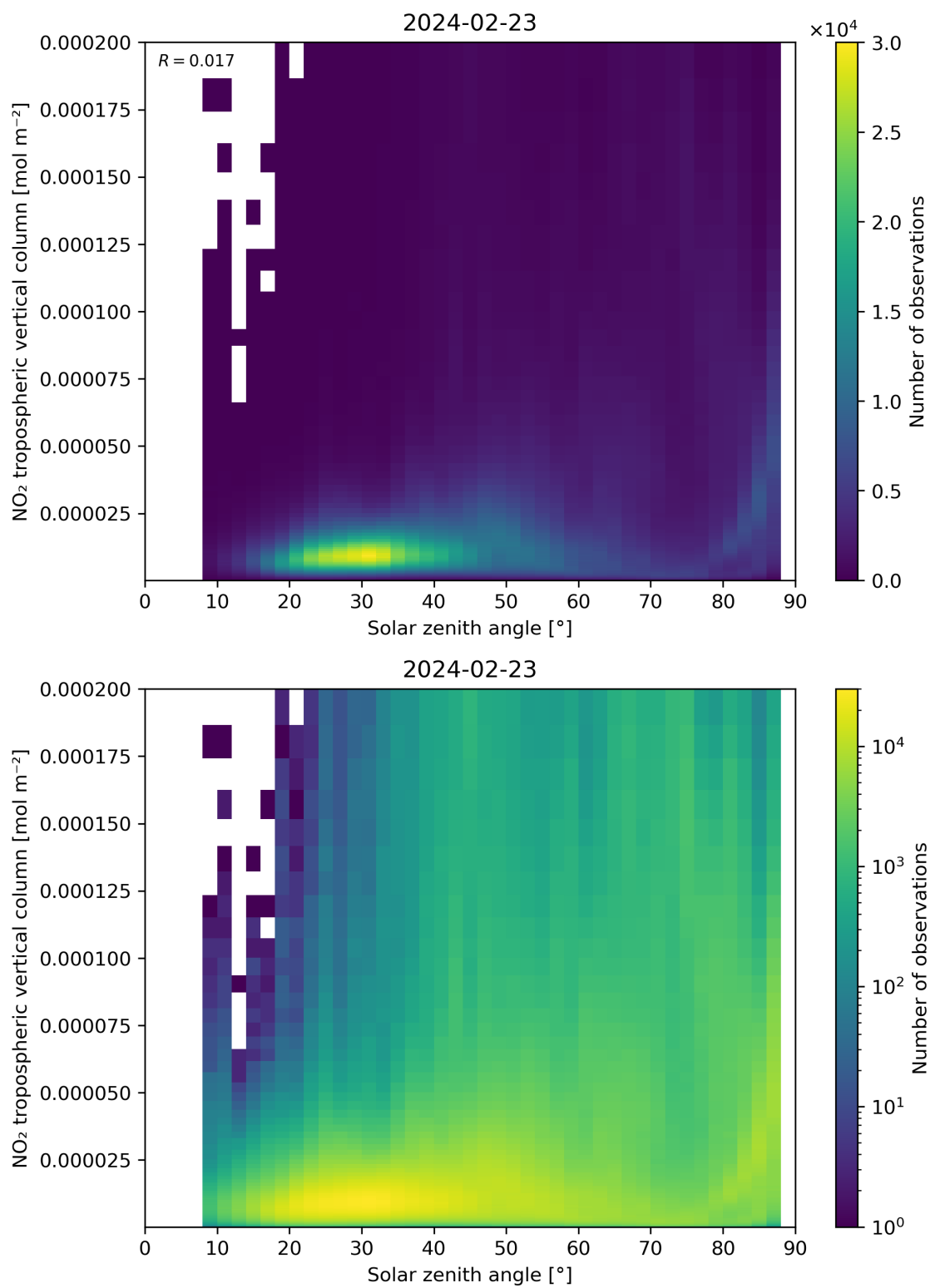
Figure 155: Scatter density plot of “Solar zenith angle” against “NO 2 tropospheric vertical column” for 2024-02-22 to 2024-02-24.
