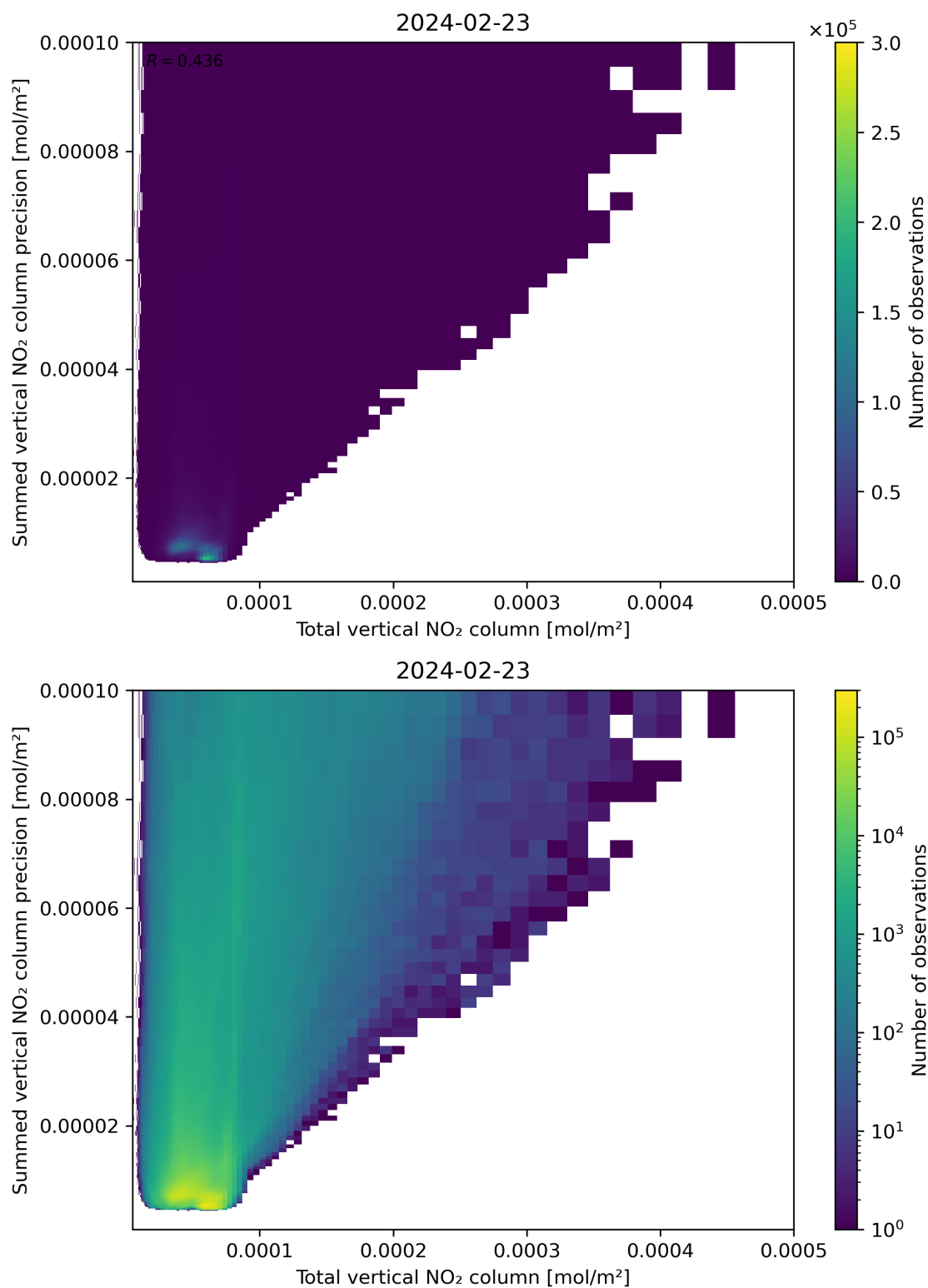
Figure 113: Scatter density plot of “Total vertical NO 2 column” against “Summed vertical NO 2 column precision” for 2024-02-22 to 2024-02-24.
