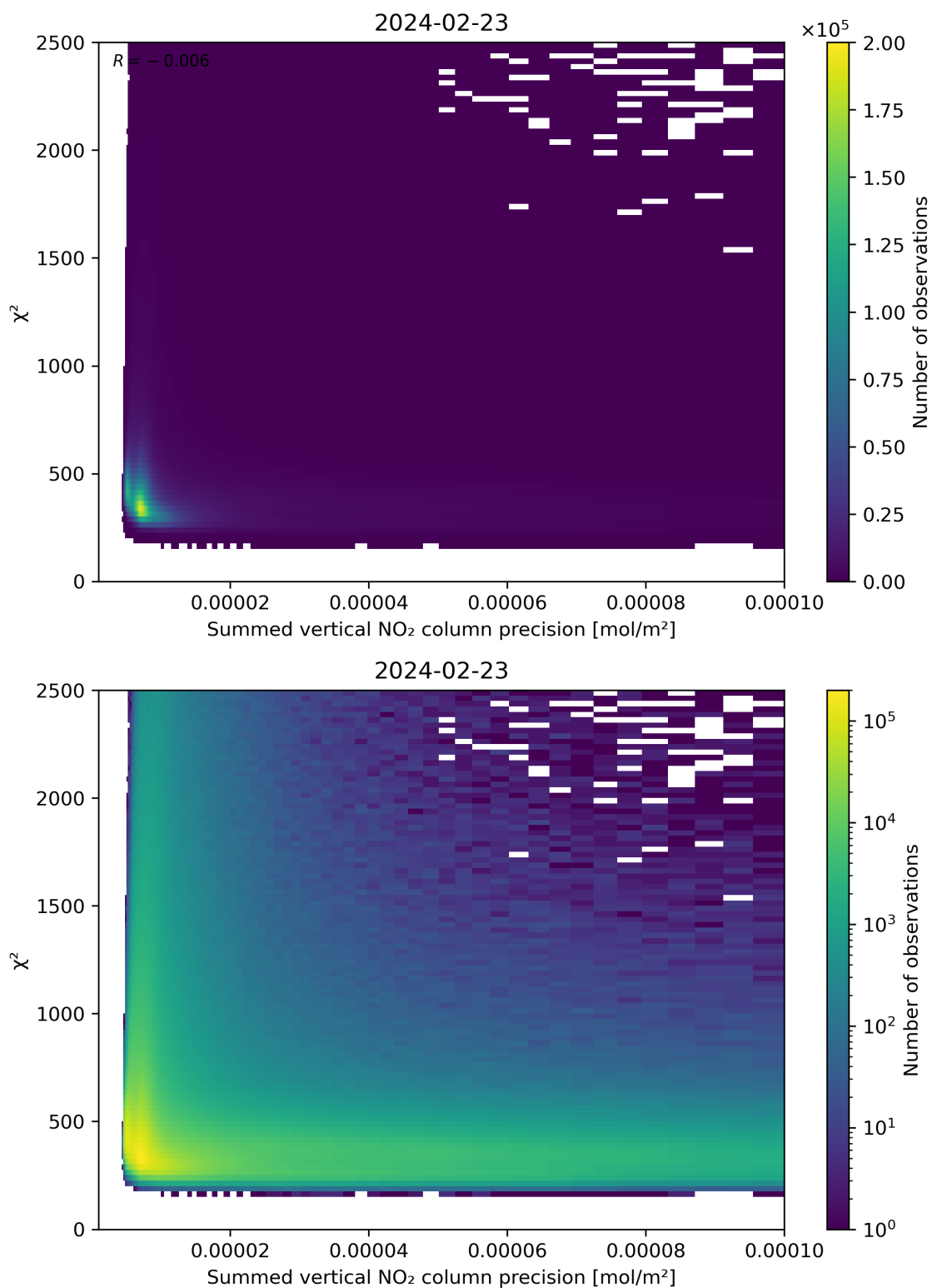
Figure 107: Scatter density plot of “Summed vertical NO 2 column precision” against “ \chi^2 ” for 2024-02-22 to 2024-02-24.
