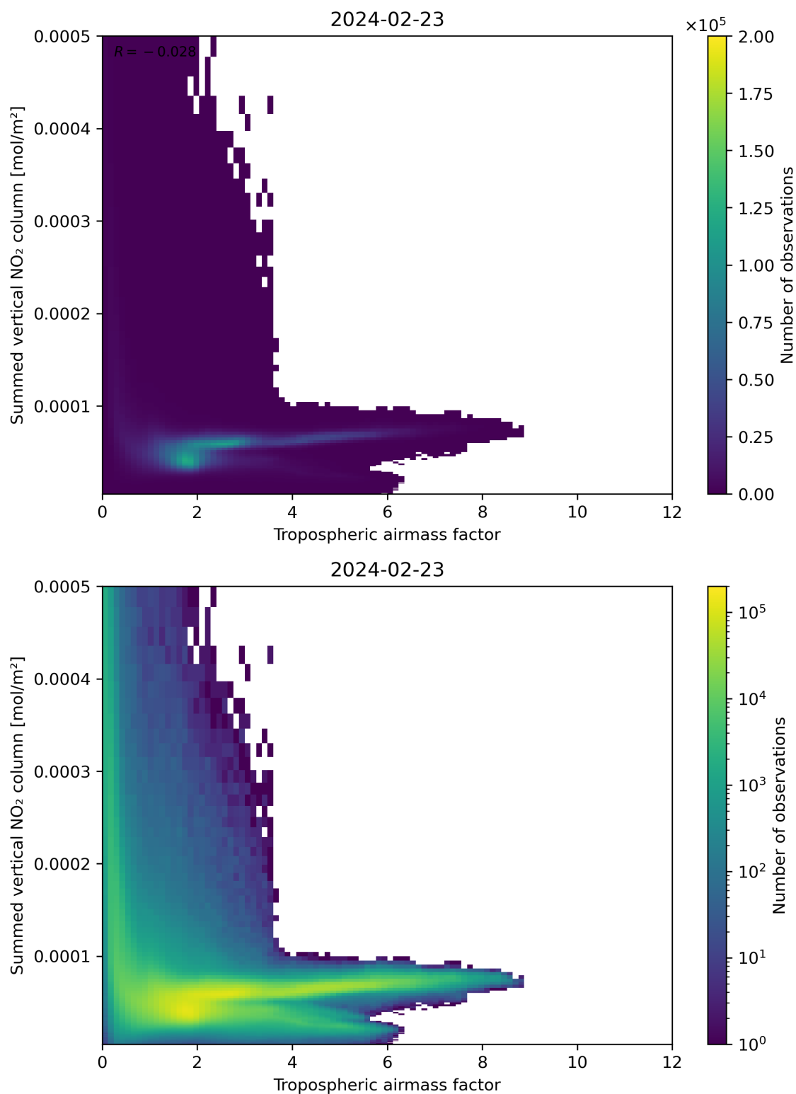
Figure 75: Scatter density plot of “Tropospheric air mass factor” against “Summed vertical NO 2 column” for 2024-02-22 to 2024-02-24.
