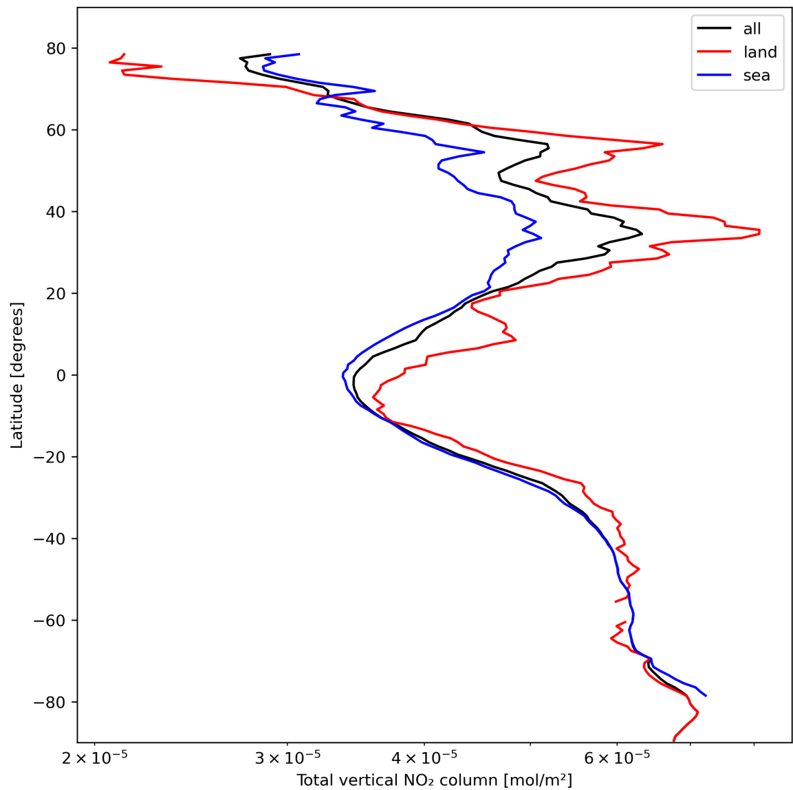
Figure 21: Zonal average of “Total vertical NO 2 column” for 2024-02-22 to 2024-02-24.
