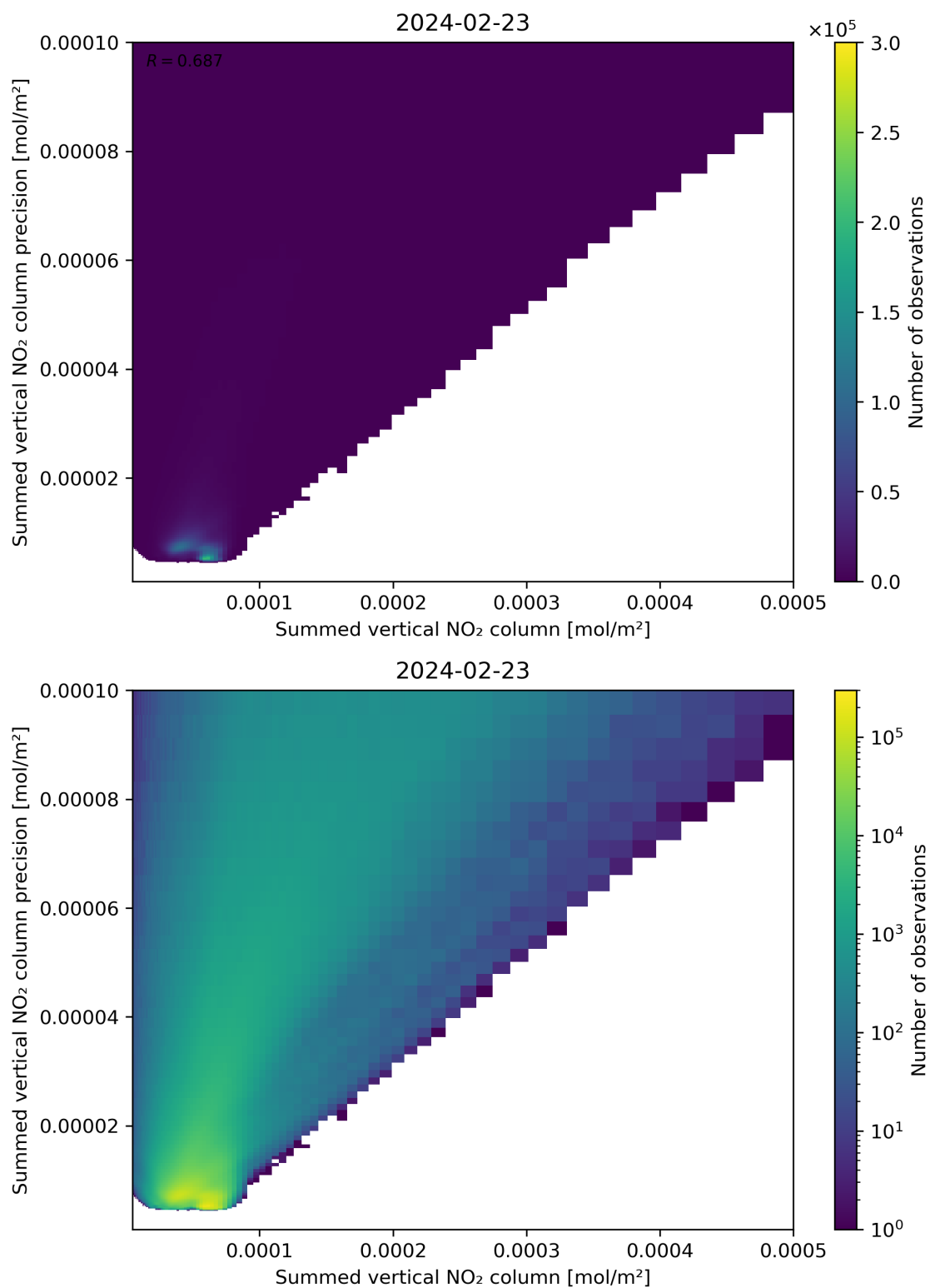
Figure 105: Scatter density plot of “Summed vertical NO 2 column” against “Summed vertical NO 2 column precision” for 2024-02-22 to 2024-02-24.
