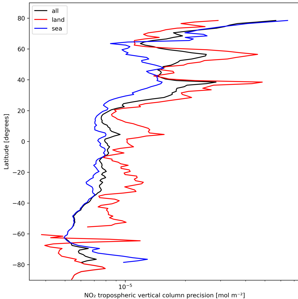
Figure 13: Zonal average of “NO 2 tropospheric vertical column precision” for 2024-02-23 to 2024-02-25.
