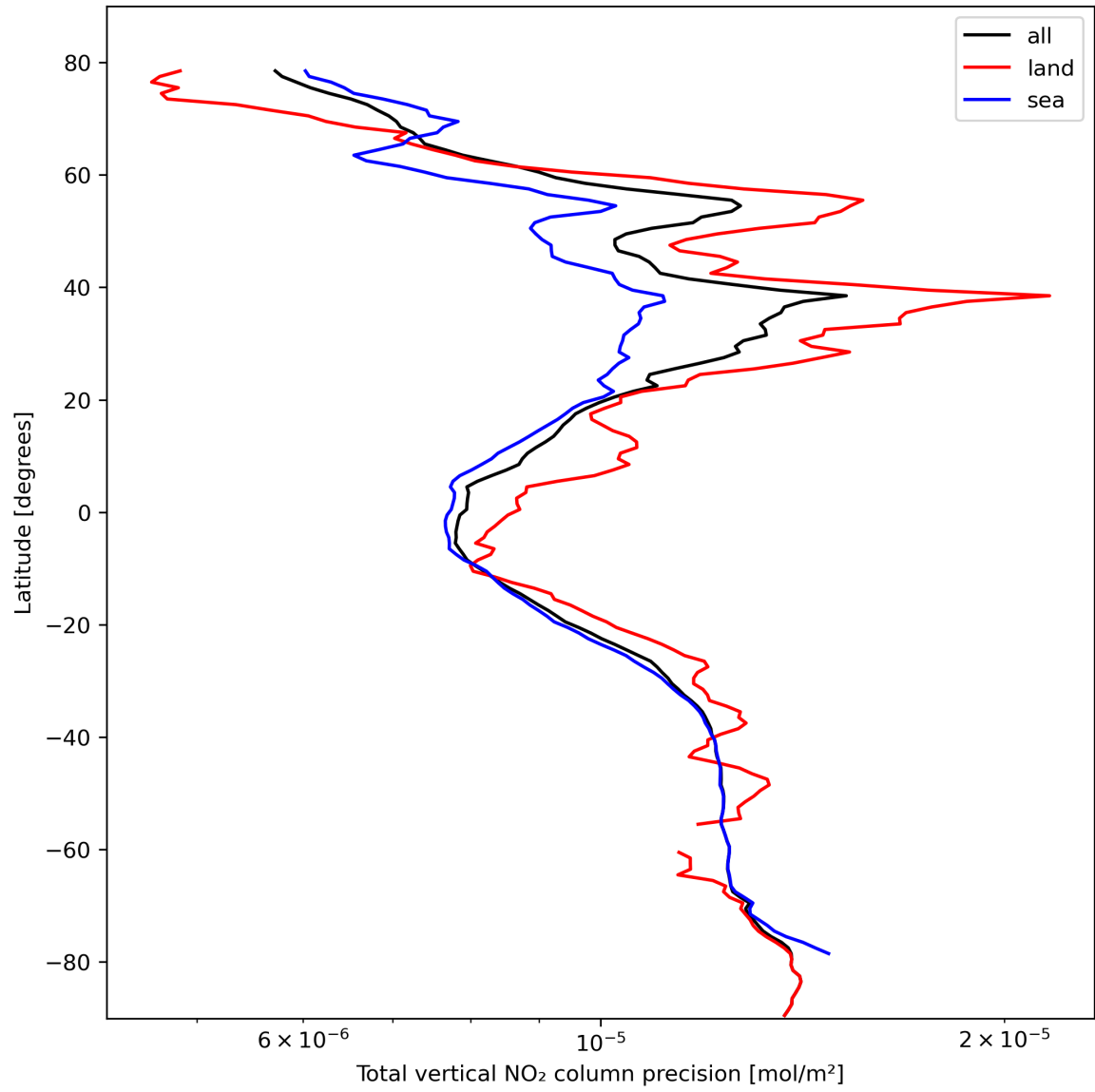
Figure 22: Zonal average of “Total vertical NO 2 column precision” for 2024-02-23 to 2024-02-25.
