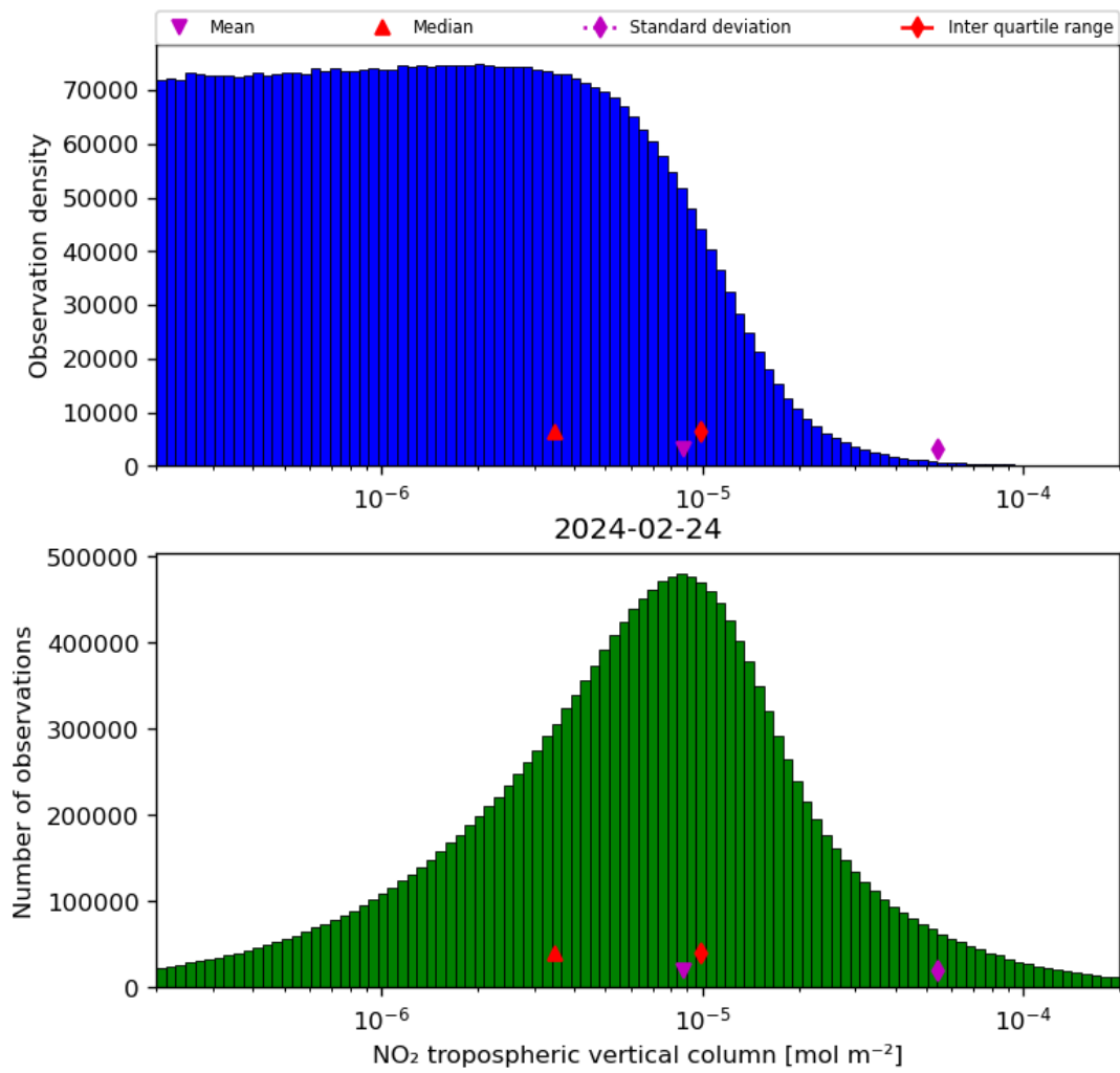
Figure 29: Histogram of “NO 2 tropospheric vertical column” for 2024-02-23 to 2024-02-25
