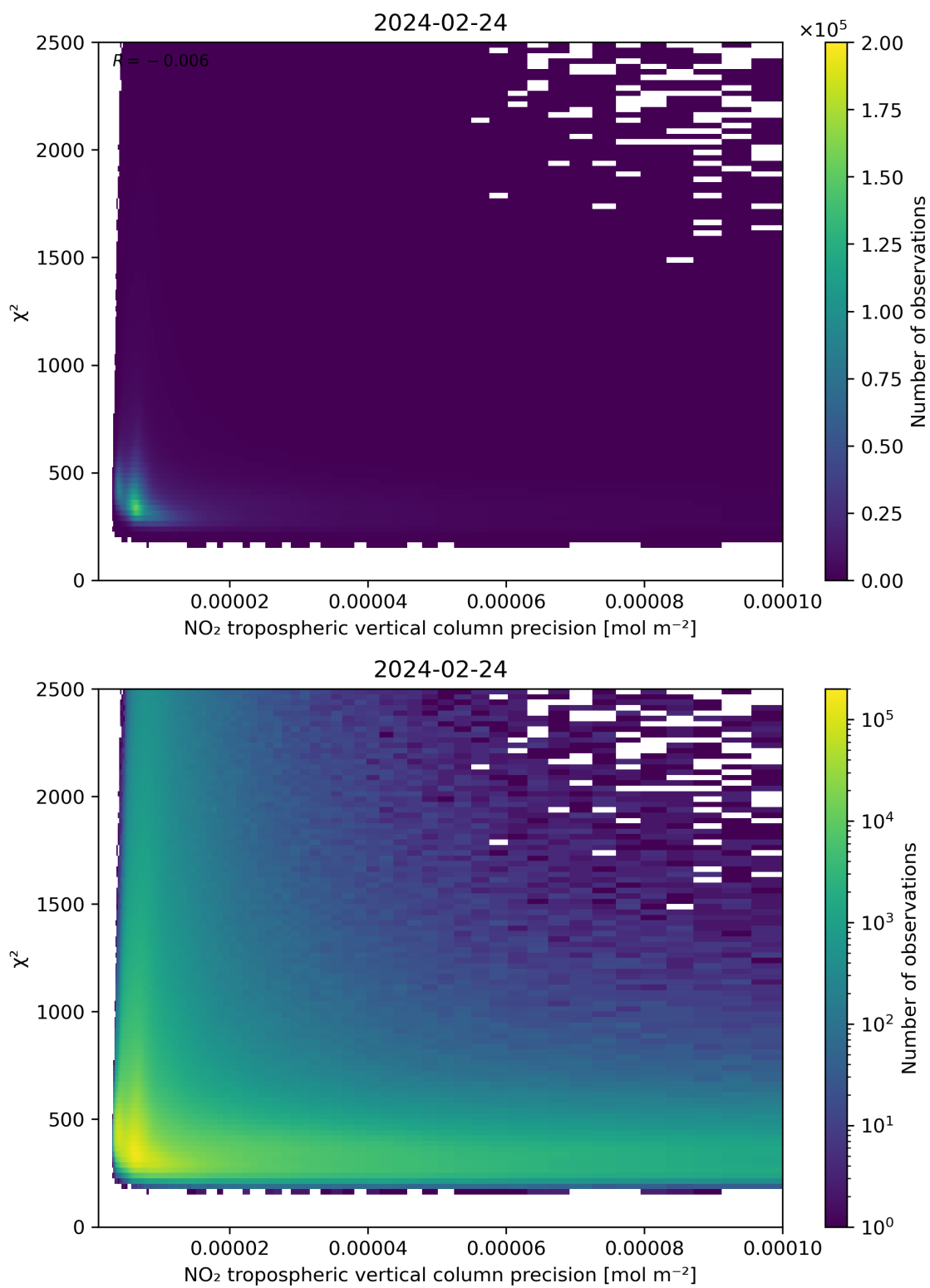
Figure 134: Scatter density plot of “NO 2 tropospheric vertical column precision” against “ \chi^2 ” for 2024-02-23 to 2024-02-25.
