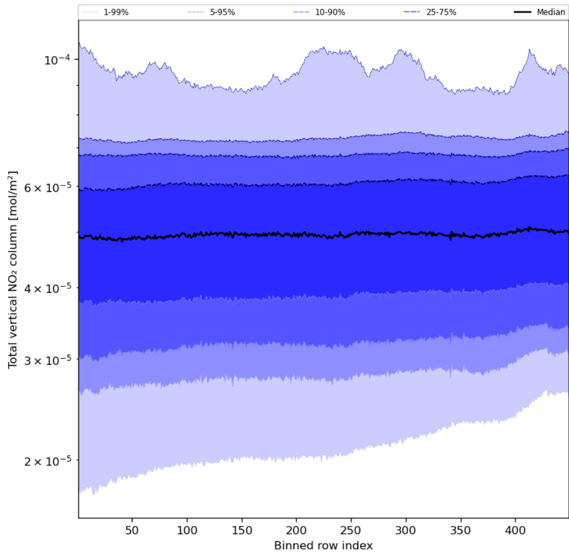
Figure 55: Along track statistics of “Total vertical NO 2 column” for 2024-02-23 to 2024-02-25
