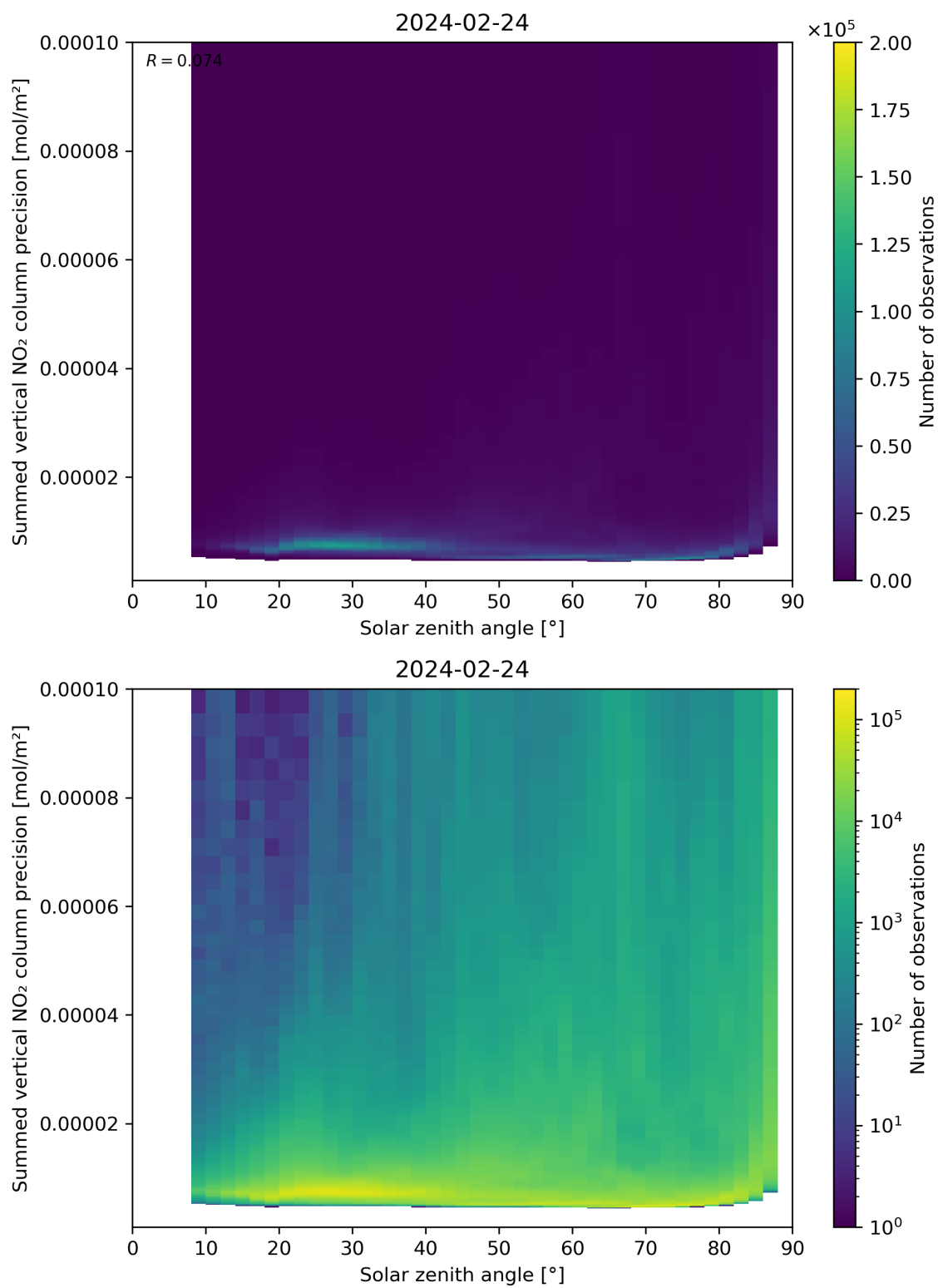
Figure 152: Scatter density plot of “Solar zenith angle” against “Summed vertical NO 2 column precision” for 2024-02-23 to 2024-02-25.
