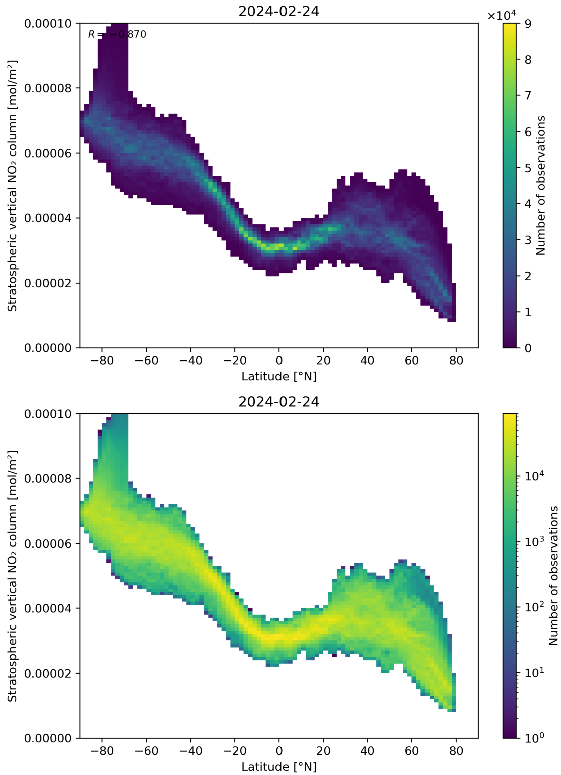
Figure 87: Scatter density plot of “Latitude” against “Stratospheric vertical NO 2 column” for 2024-02-23 to 2024-02-25.
