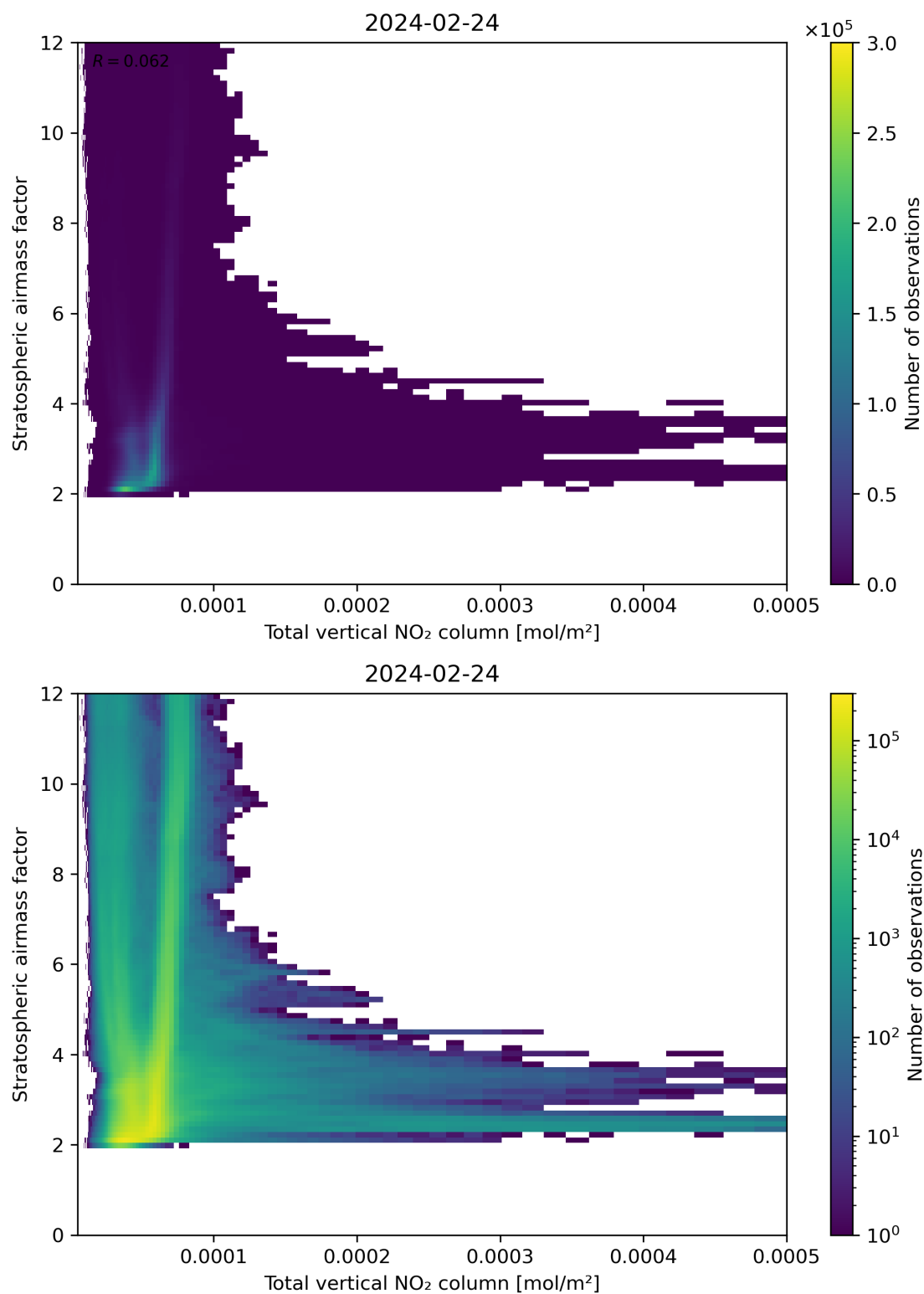
Figure 110: Scatter density plot of “Total vertical NO 2 column” against “Stratospheric airmass factor” for 2024-02-23 to 2024-02-25.
