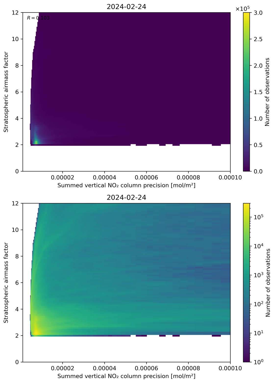
Figure 106: Scatter density plot of “Summed vertical NO 2 column precision” against “Stratospheric airmass factor” for 2024-02-23 to 2024-02-25.
