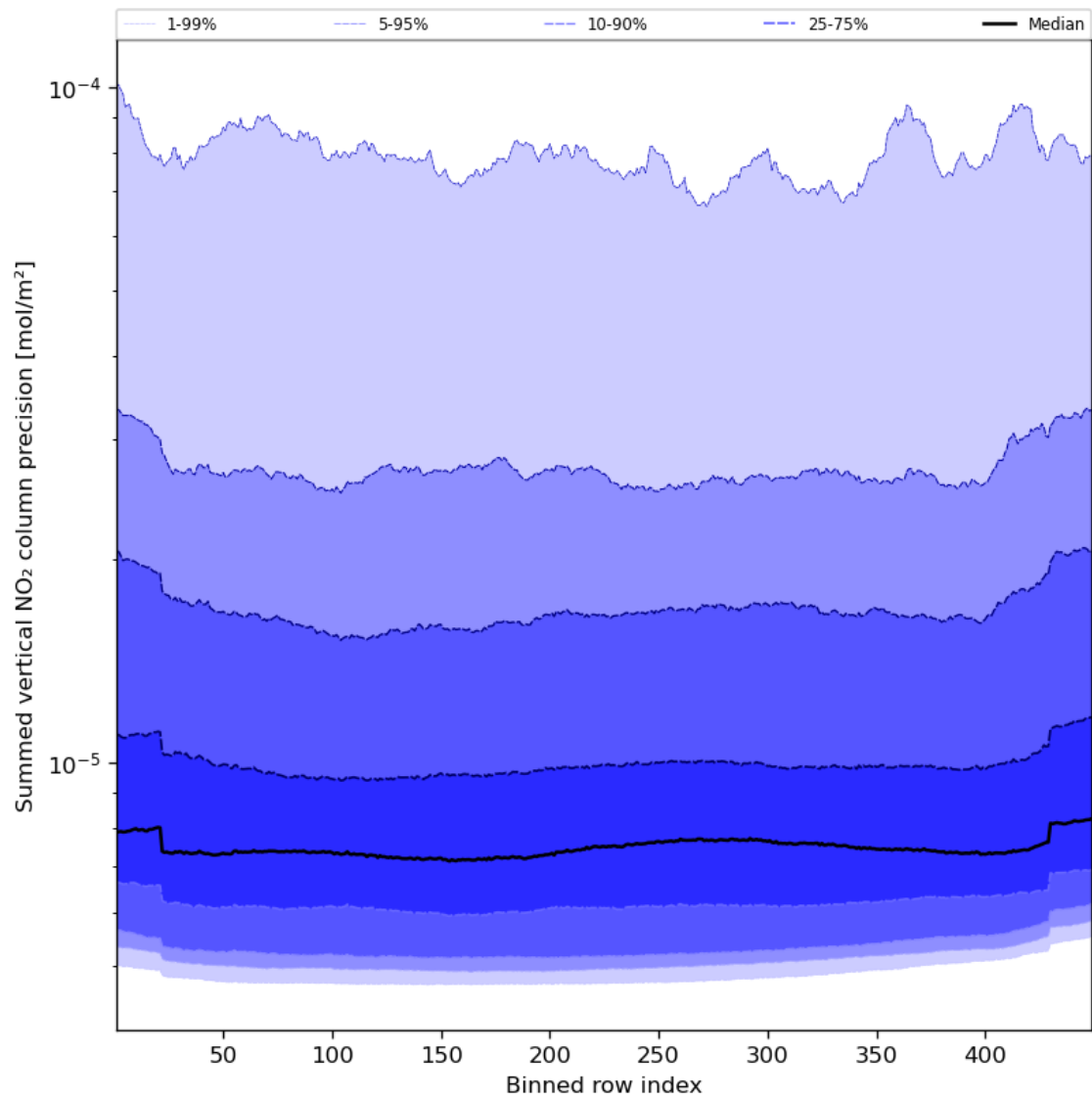
Figure 58: Along track statistics of “Summed vertical NO 2 column precision” for 2024-02-23 to 2024-02-25
