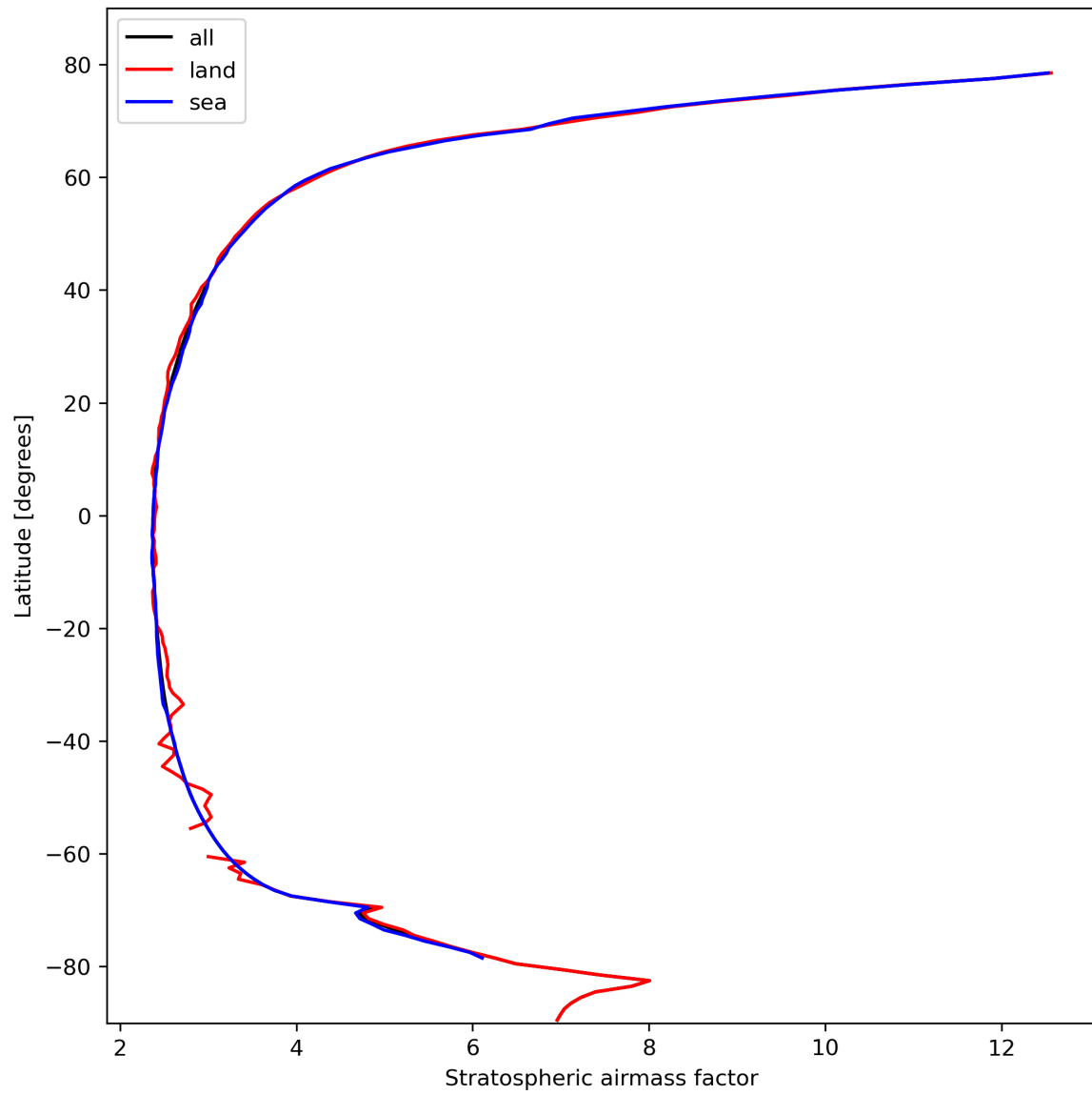
Figure 27: Zonal average of “Stratospheric airmass factor” for 2024-02-23 to 2024-02-25.
