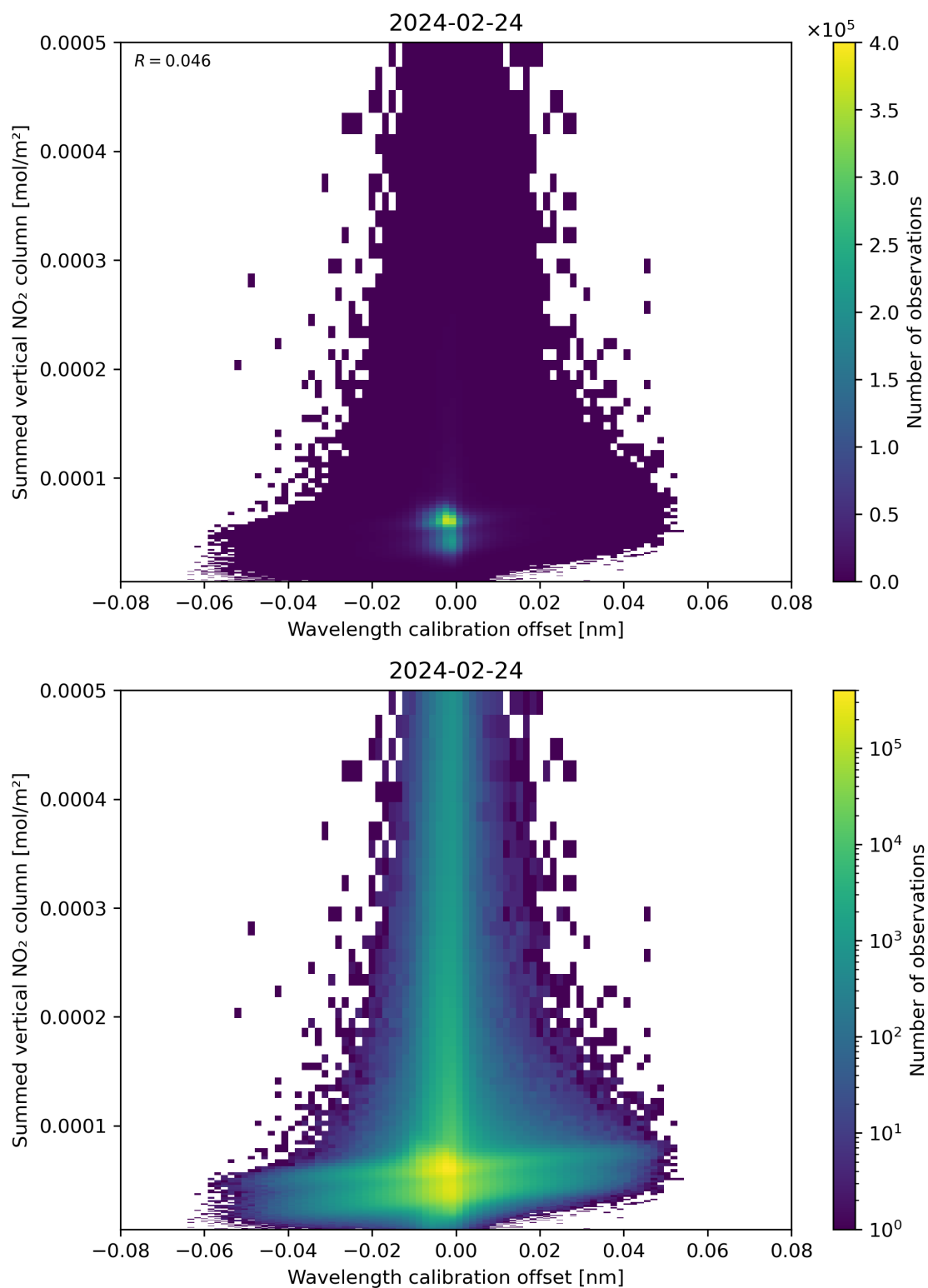
Figure 177: Scatter density plot of “Wavelength calibration offset” against “Summed vertical NO 2 column” for 2024-02-23 to 2024-02-25.
