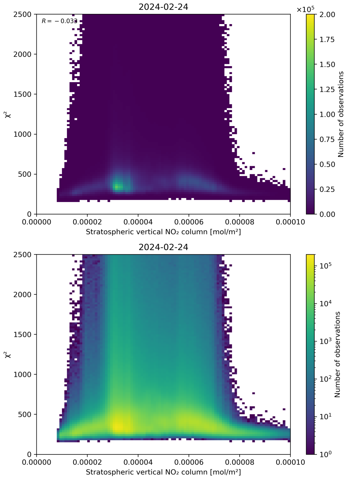
Figure 97: Scatter density plot of “Stratospheric vertical NO 2 column” against “ \chi^2 ” for 2024-02-23 to 2024-02-25.
