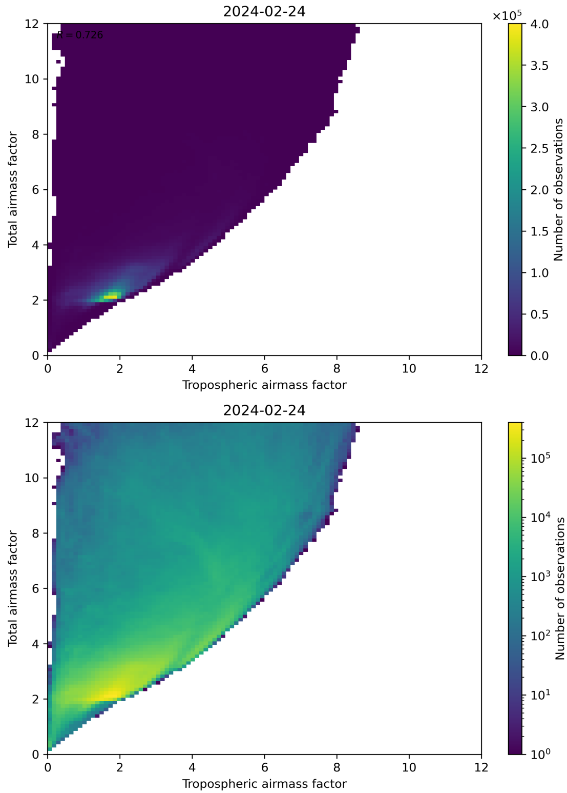
Figure 72: Scatter density plot of “Tropospheric airmass factor” against “Total airmass factor” for 2024-02-23 to 2024-02-25.
