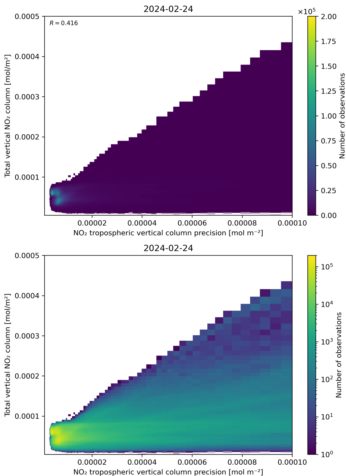
Figure 138: Scatter density plot of “NO 2 tropospheric vertical column precision” against “Total vertical NO 2 column” for 2024-02-23 to 2024-02-25.
