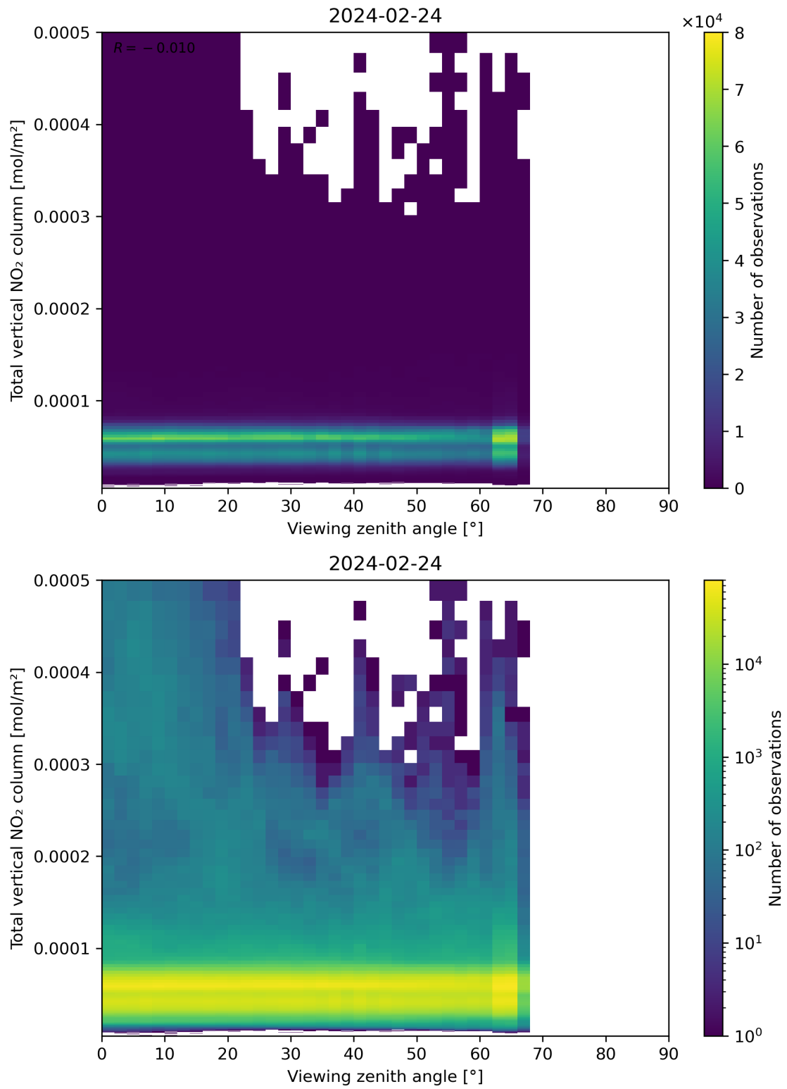
Figure 167: Scatter density plot of “Viewing zenith angle” against “Total vertical NO 2 column” for 2024-02-23 to 2024-02-25.
