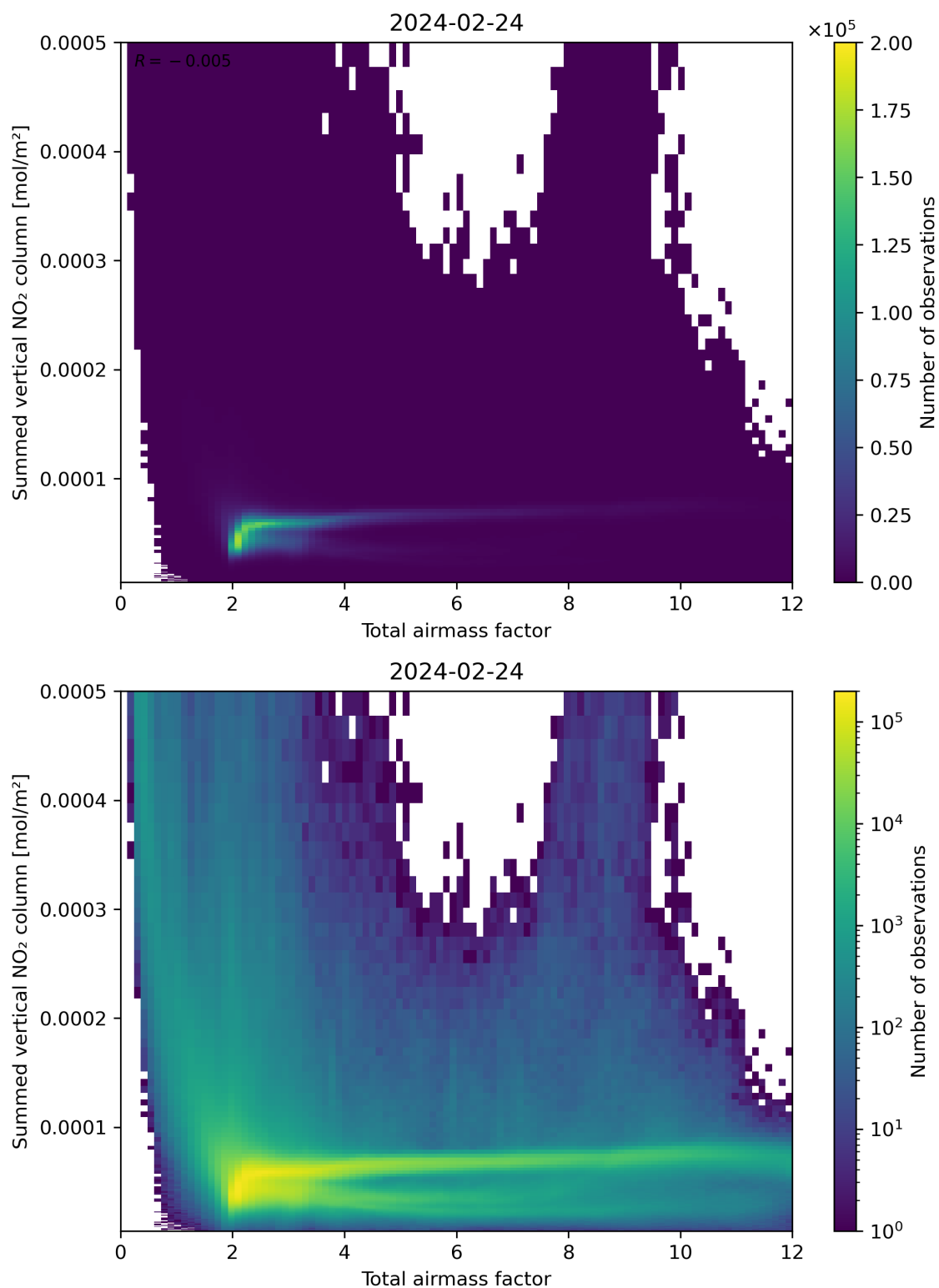
Figure 65: Scatter density plot of “Total airmass factor” against “Summed vertical NO 2 column” for 2024-02-23 to 2024-02-25.
