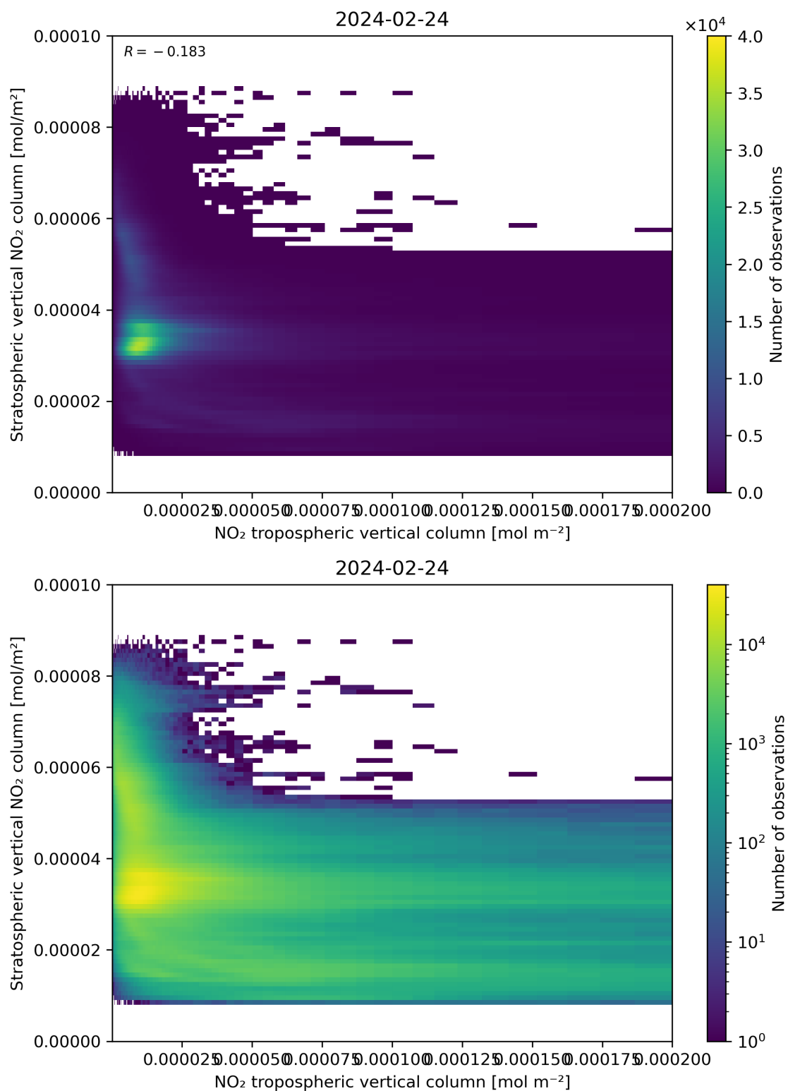
Figure 125: Scatter density plot of “NO 2 tropospheric vertical column” against “Stratospheric vertical NO 2 column” for 2024-02-23 to 2024-02-25.
