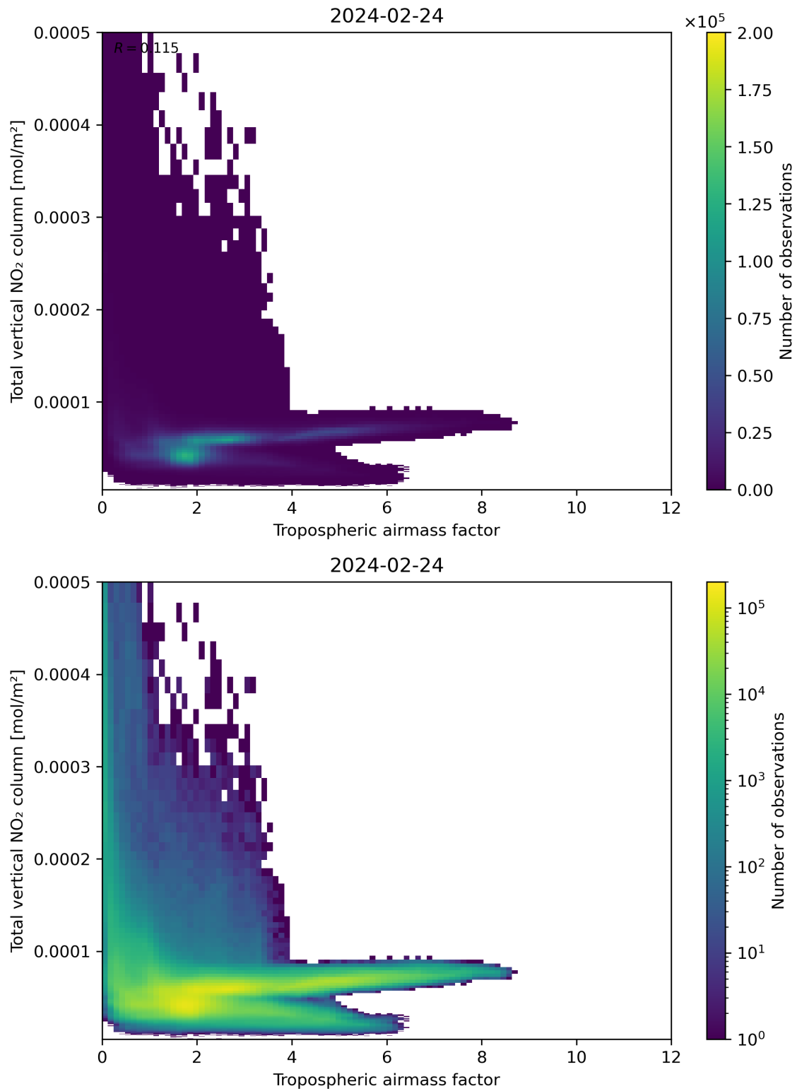
Figure 77: Scatter density plot of “Tropospheric airmass factor” against “Total vertical NO 2 column” for 2024-02-23 to 2024-02-25.
