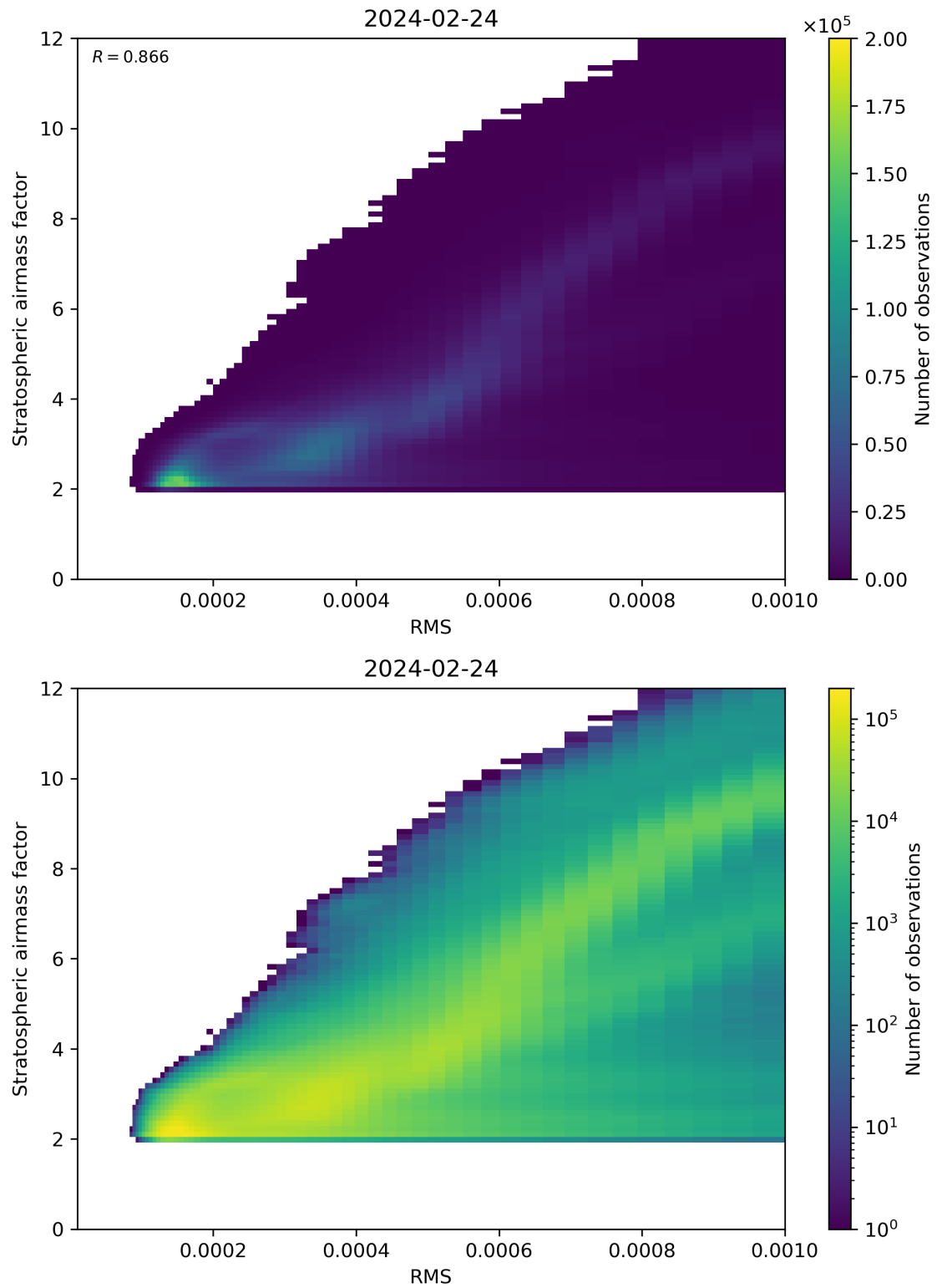
Figure 144: Scatter density plot of “RMS” against “Stratospheric airmass factor” for 2024-02-23 to 2024-02-25.
