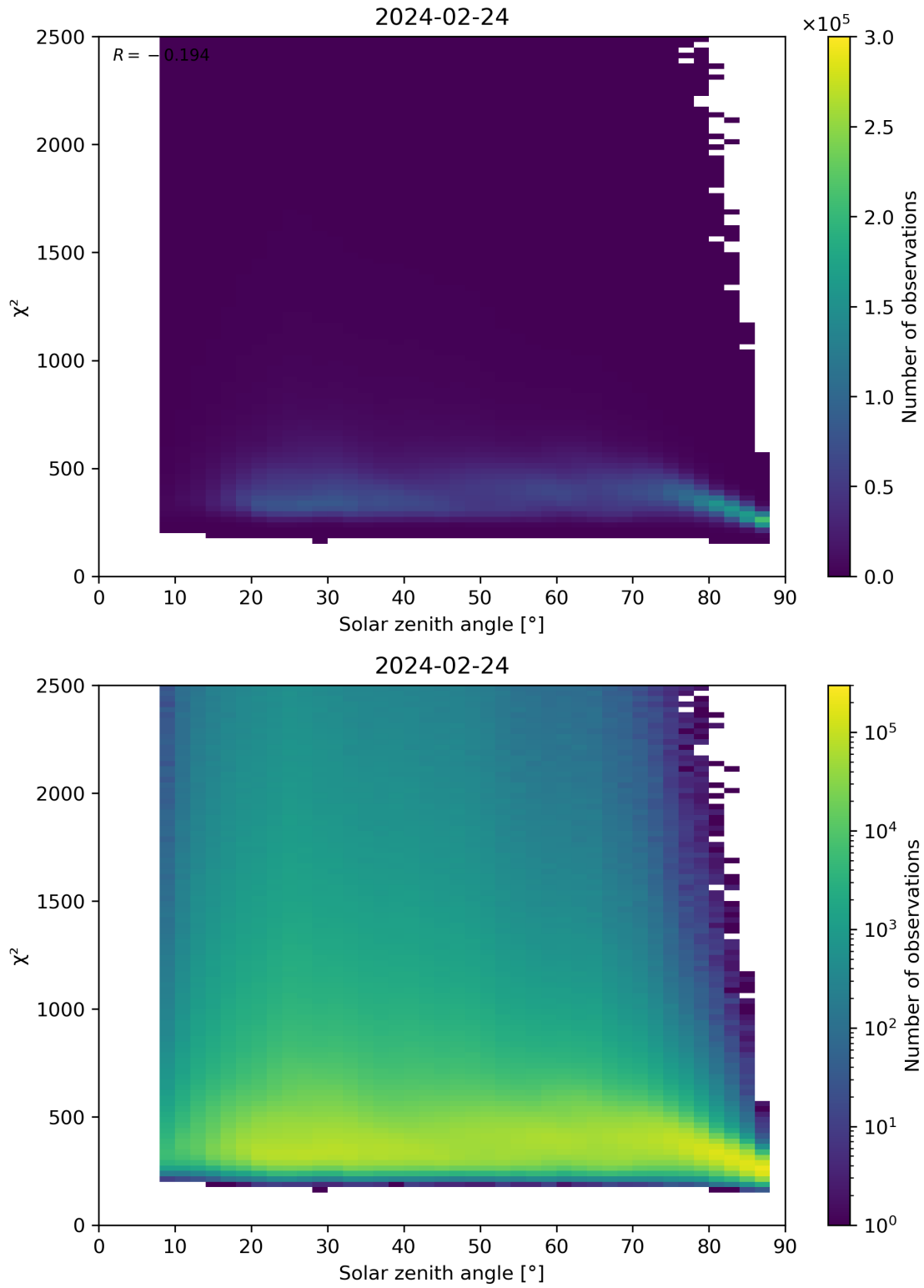
Figure 148: Scatter density plot of “Solar zenith angle” against “ \chi^2 ” for 2024-02-23 to 2024-02-25.
