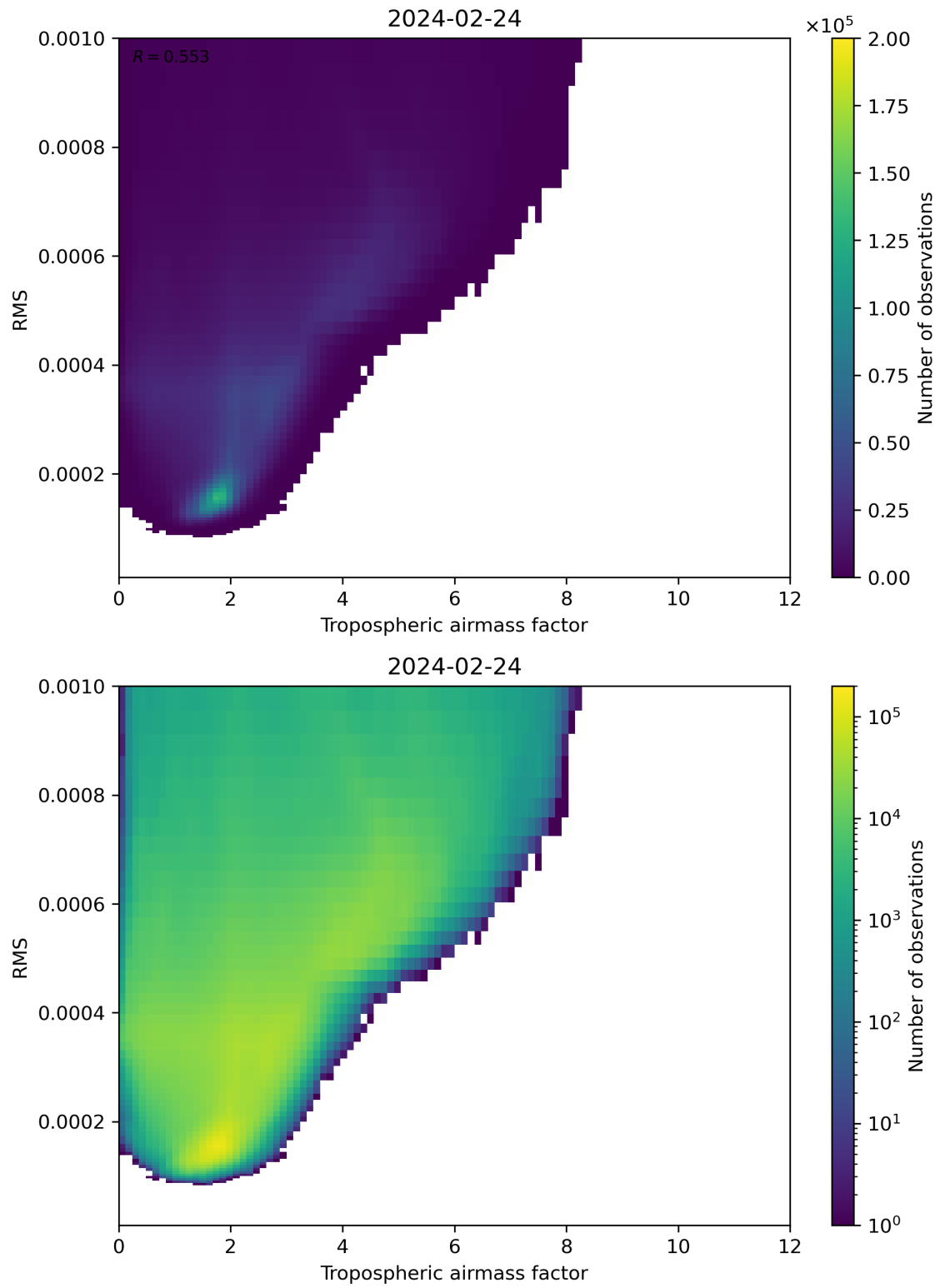
Figure 79: Scatter density plot of “Tropospheric airmass factor” against “RMS” for 2024-02-23 to 2024-02-25.
