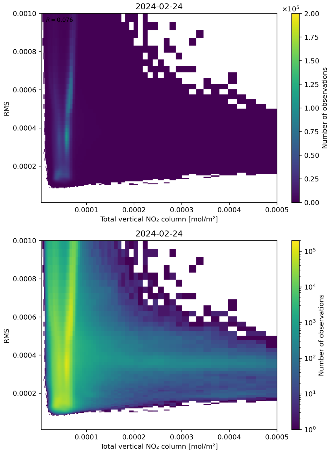
Figure 120: Scatter density plot of “Total vertical NO 2 column” against “RMS” for 2024-02-23 to 2024-02-25.
