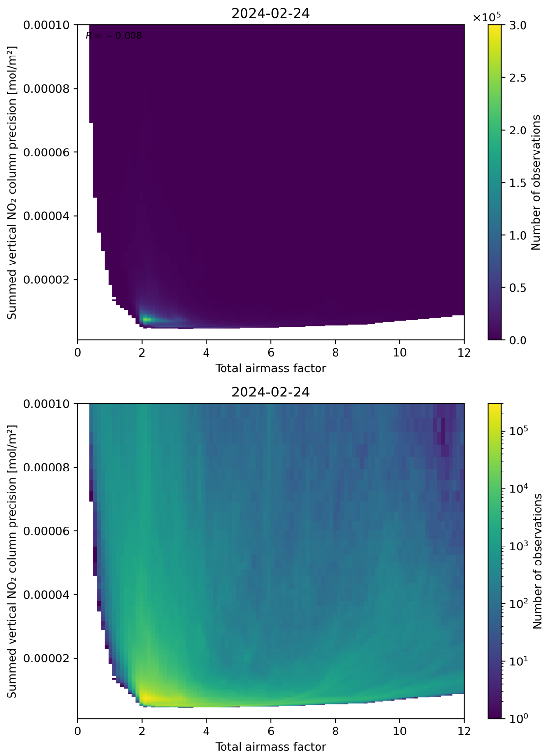
Figure 66: Scatter density plot of “Total airmass factor” against “Summed vertical NO 2 column precision” for 2024-02-23 to 2024-02-25.
