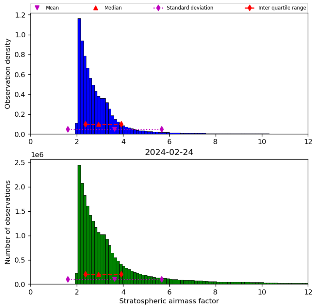
Figure 44: Histogram of “Stratospheric airmass factor” for 2024-02-23 to 2024-02-25
