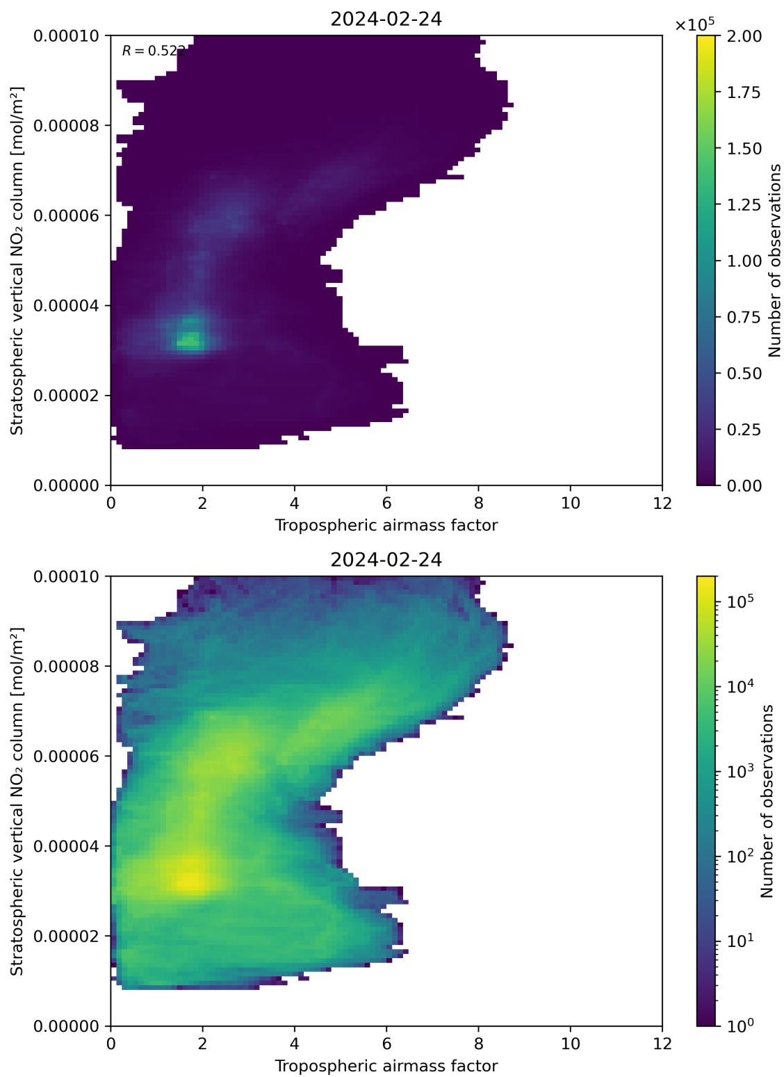
Figure 74: Scatter density plot of “Tropospheric air mass factor” against “Stratospheric vertical NO 2 column” for 2024-02-23 to 2024-02-25.
