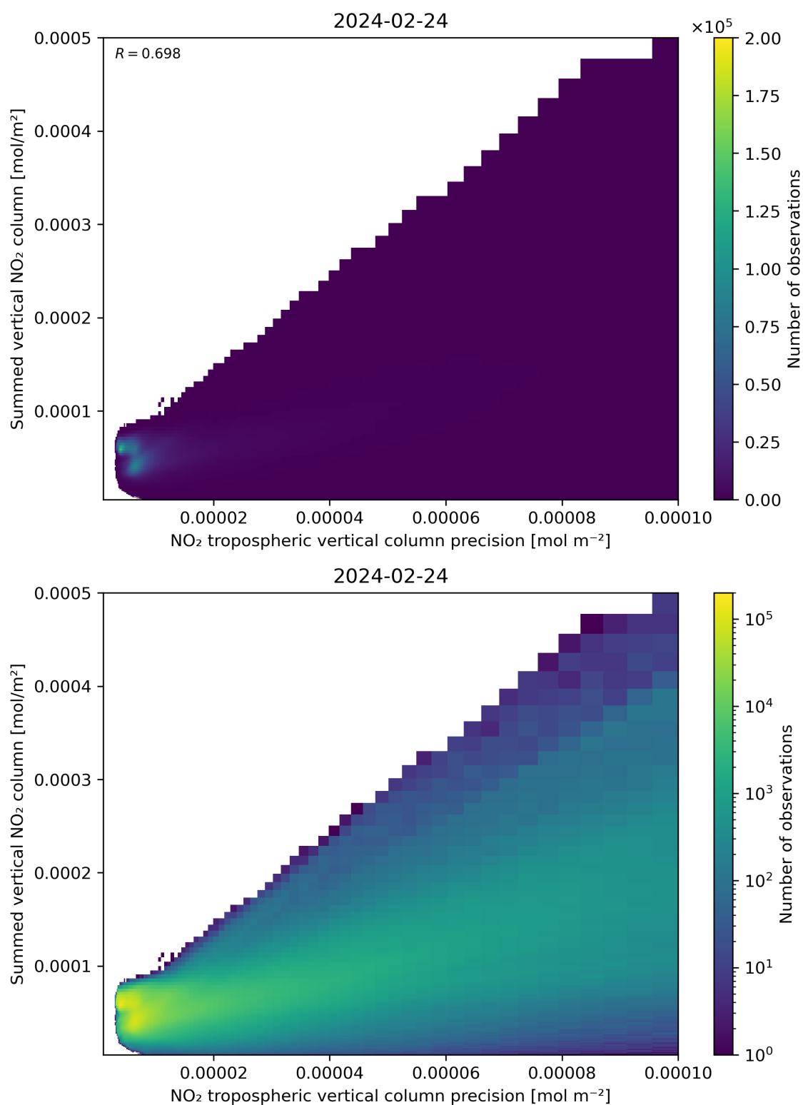
Figure 136: Scatter density plot of “NO 2 tropospheric vertical column precision” against “Summed vertical NO 2 column” for 2024-02-23 to 2024-02-25.
