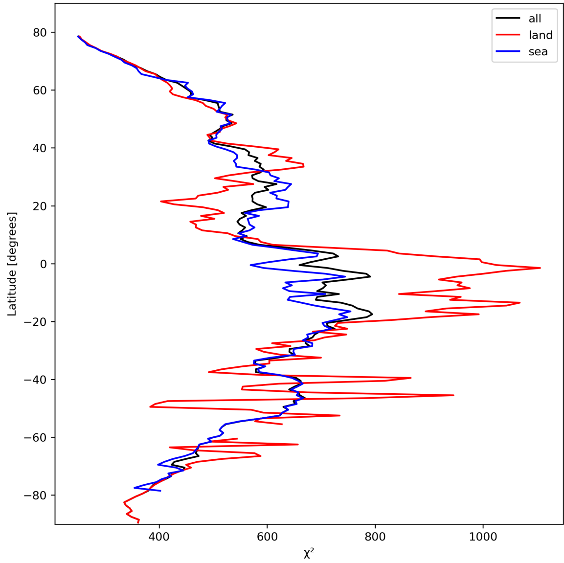
Figure 25: Zonal average of “ \chi^2 ” for 2024-02-23 to 2024-02-25.
