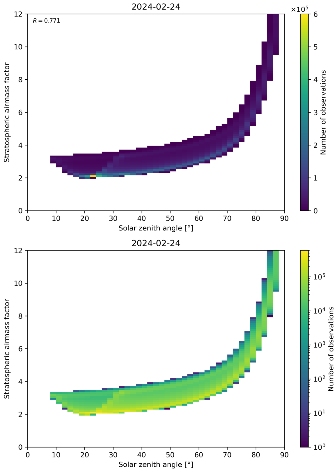
Figure 145: Scatter density plot of “Solar zenith angle” against “Stratospheric airmass factor” for 2024-02-23 to 2024-02-25.
