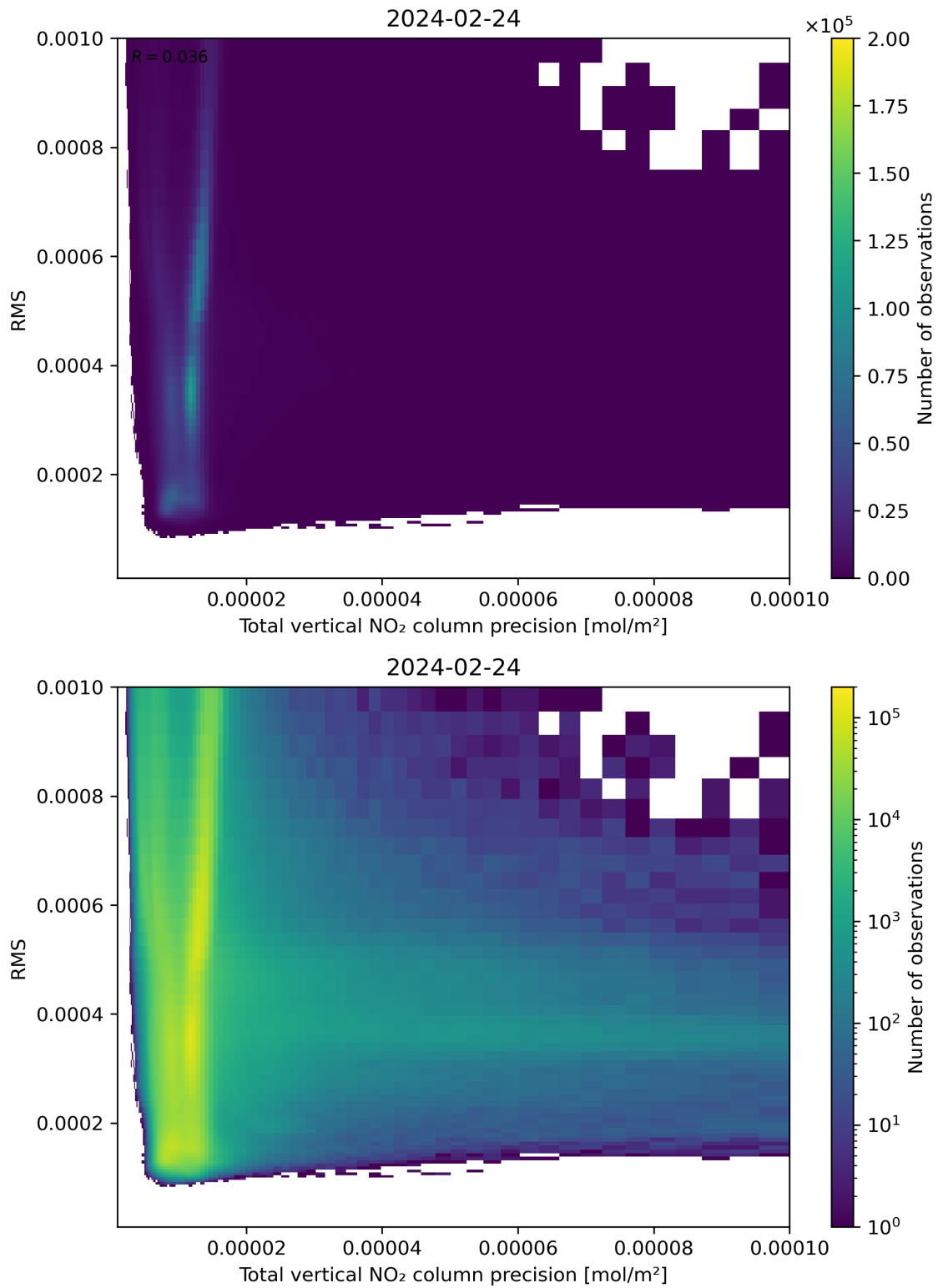
Figure 119: Scatter density plot of “Total vertical NO 2 column precision” against “RMS” for 2024-02-23 to 2024-02-25.
