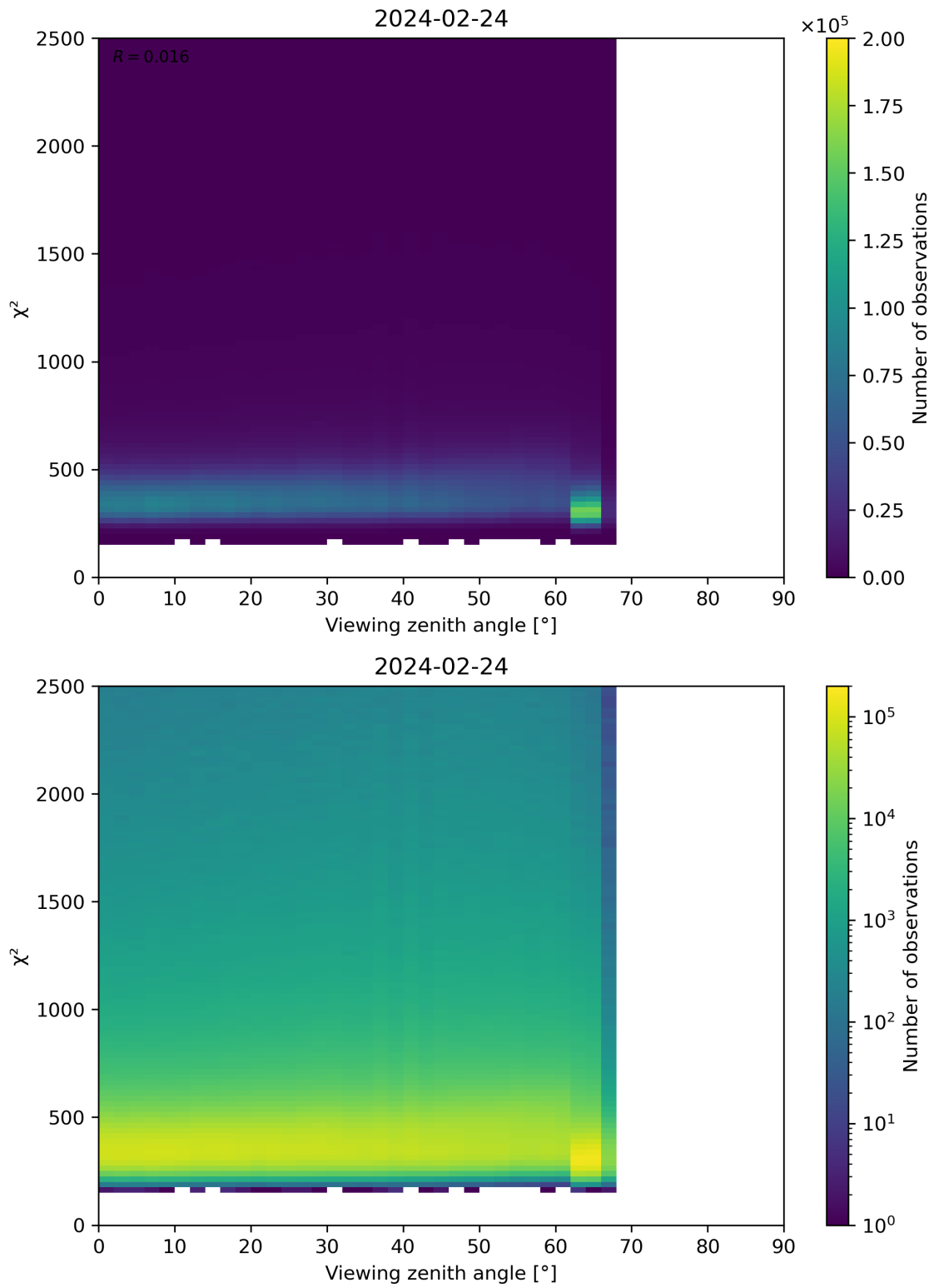
Figure 162: Scatter density plot of “Viewing zenith angle” against “ \chi^2 ” for 2024-02-23 to 2024-02-25.
