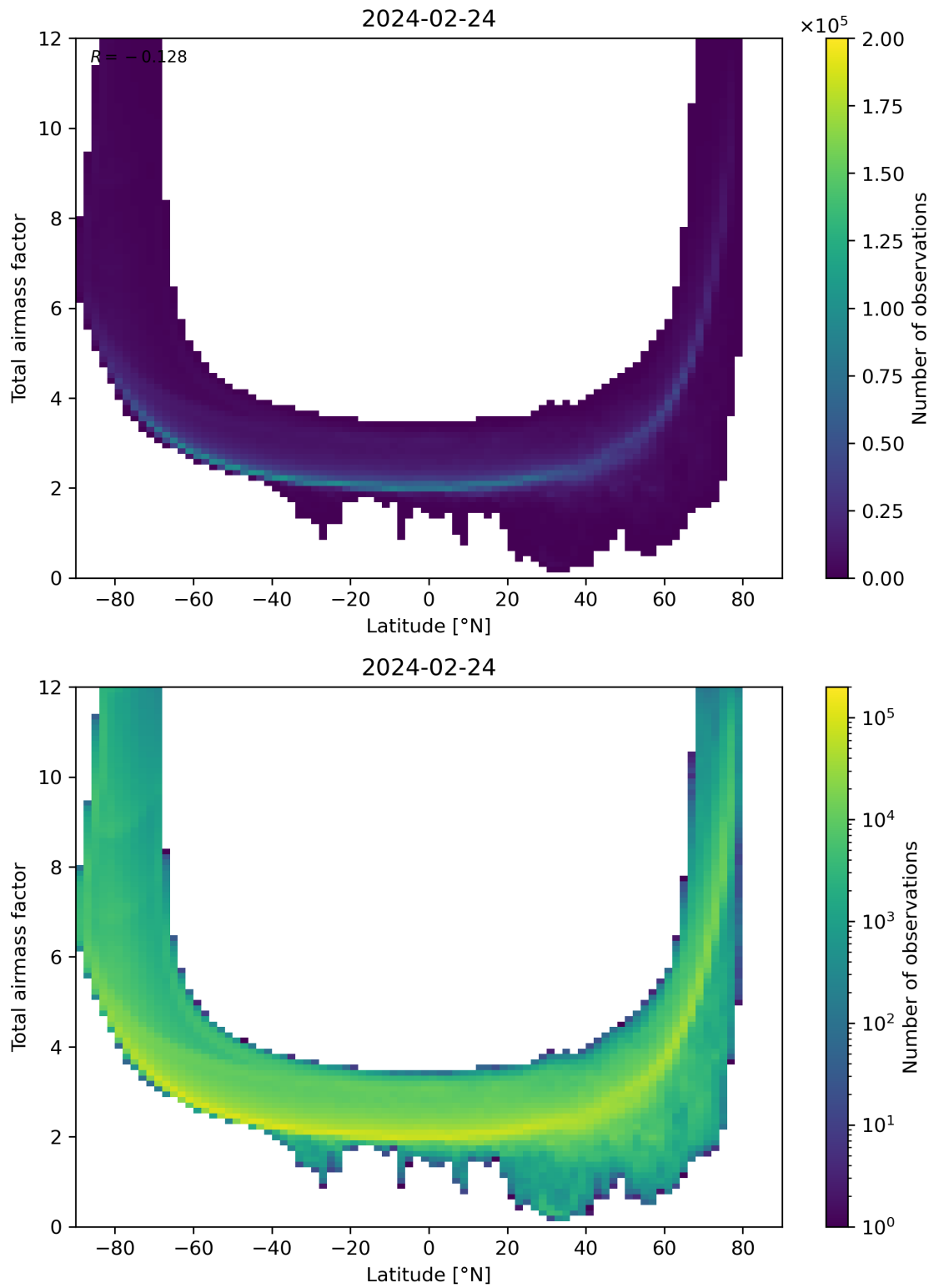
Figure 84: Scatter density plot of “Latitude” against “Total airmass factor” for 2024-02-23 to 2024-02-25.
