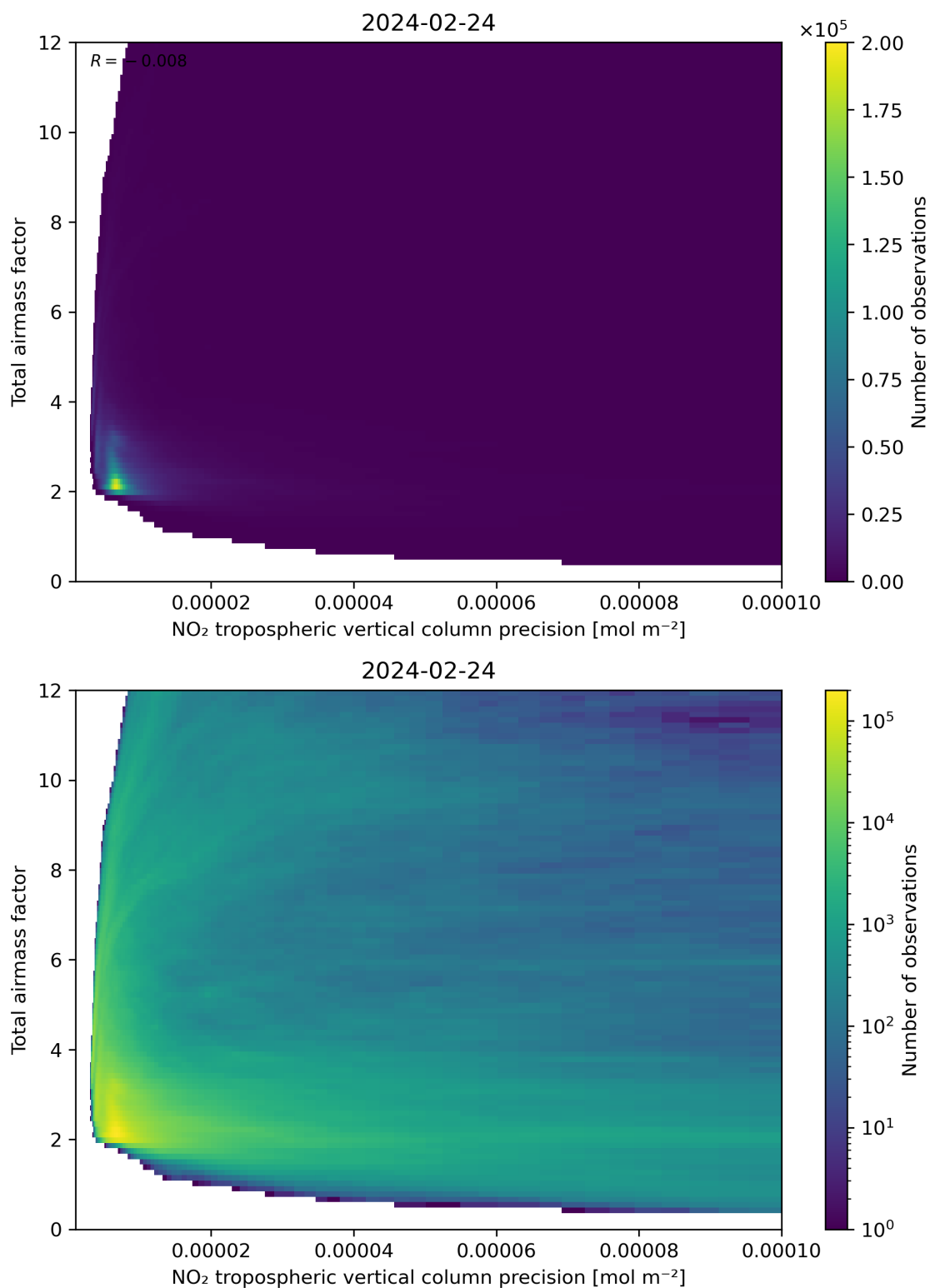
Figure 132: Scatter density plot of “NO 2 tropospheric vertical column precision” against “Total air mass factor” for 2024-02-23 to 2024-02-25.
