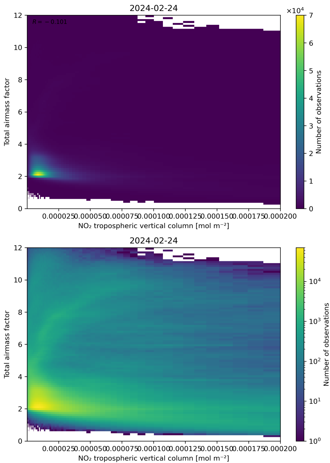
Figure 122: Scatter density plot of “NO 2 tropospheric vertical column” against “Total air mass factor” for 2024-02-23 to 2024-02-25.
