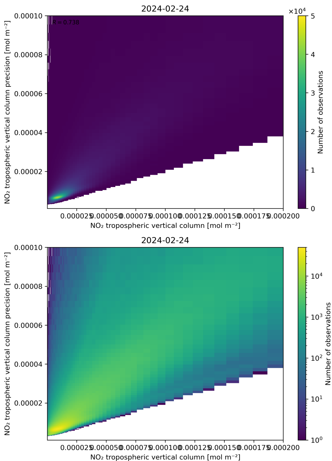
Figure 130: Scatter density plot of “NO 2 tropospheric vertical column” against “NO 2 tropospheric vertical column precision” for 2024-02-23 to 2024-02-25.
