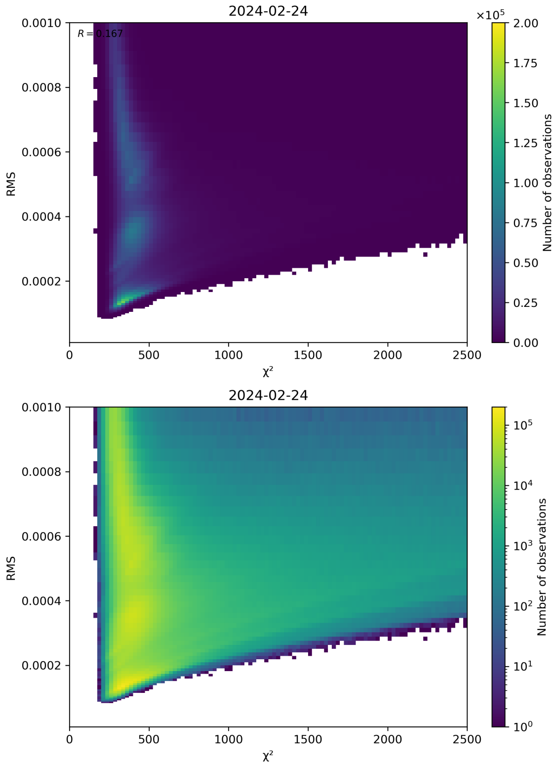
Figure 82: Scatter density plot of “ \chi^2 ” against “RMS” for 2024-02-23 to 2024-02-25.
