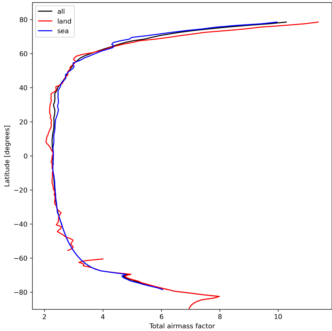
Figure 15: Zonal average of “Total airmass factor” for 2024-02-23 to 2024-02-25.
