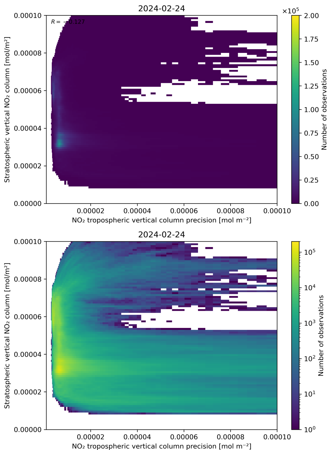
Figure 135: Scatter density plot of “ \text{NO}_2 tropospheric vertical column precision” against “Stratospheric vertical \text{NO}_2 column” for 2024-02-23 to 2024-02-25.
