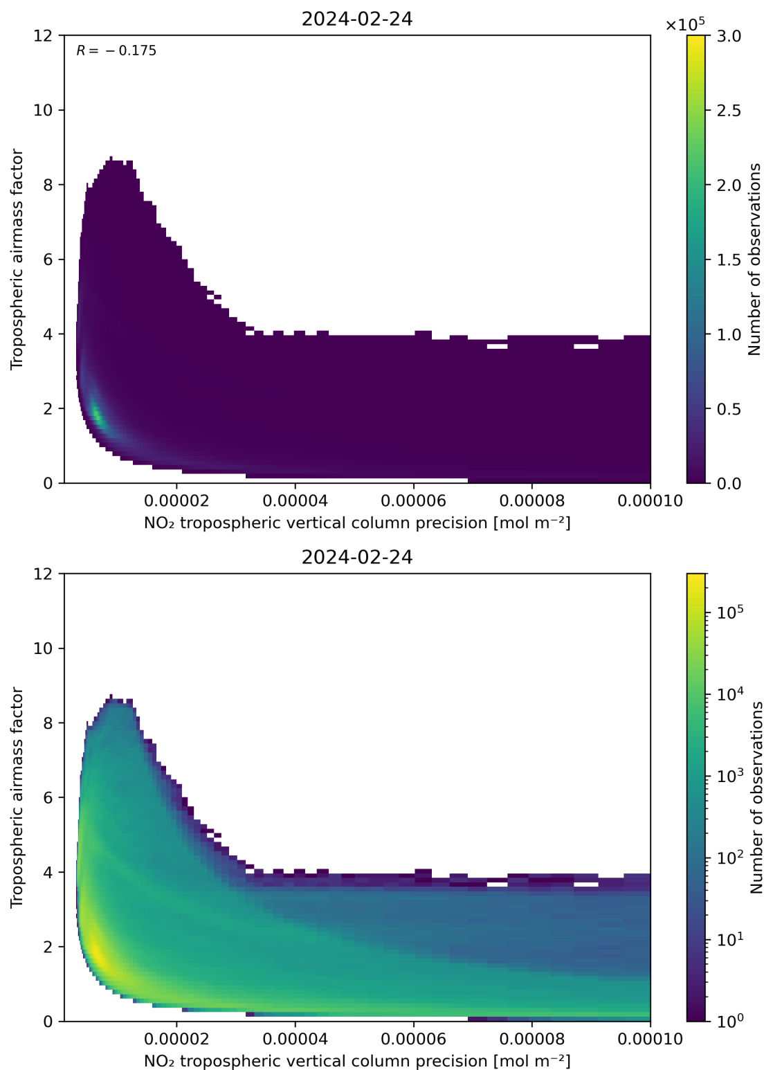
Figure 133: Scatter density plot of “NO 2 tropospheric vertical column precision” against “Tropospheric airmass factor” for 2024-02-23 to 2024-02-25.
