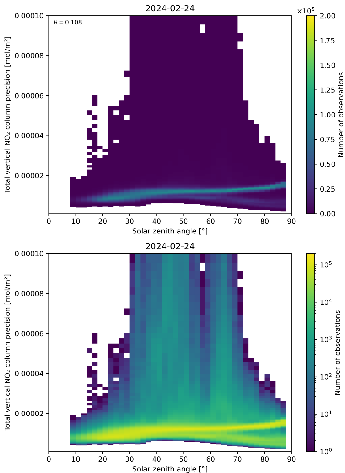
Figure 154: Scatter density plot of “Solar zenith angle” against “Total vertical NO 2 column precision” for 2024-02-23 to 2024-02-25.
