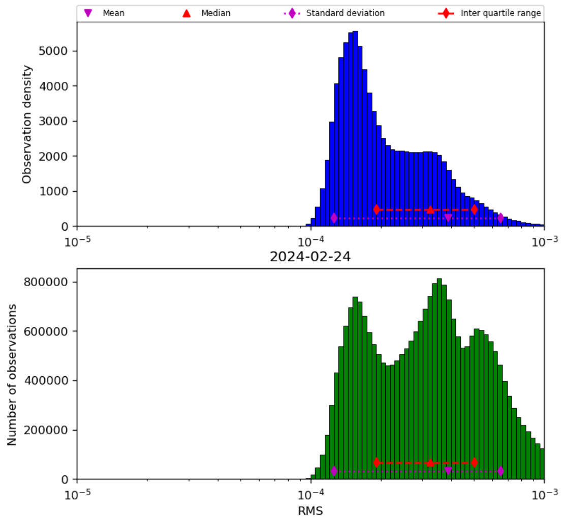
Figure 43: Histogram of “RMS” for 2024-02-23 to 2024-02-25
