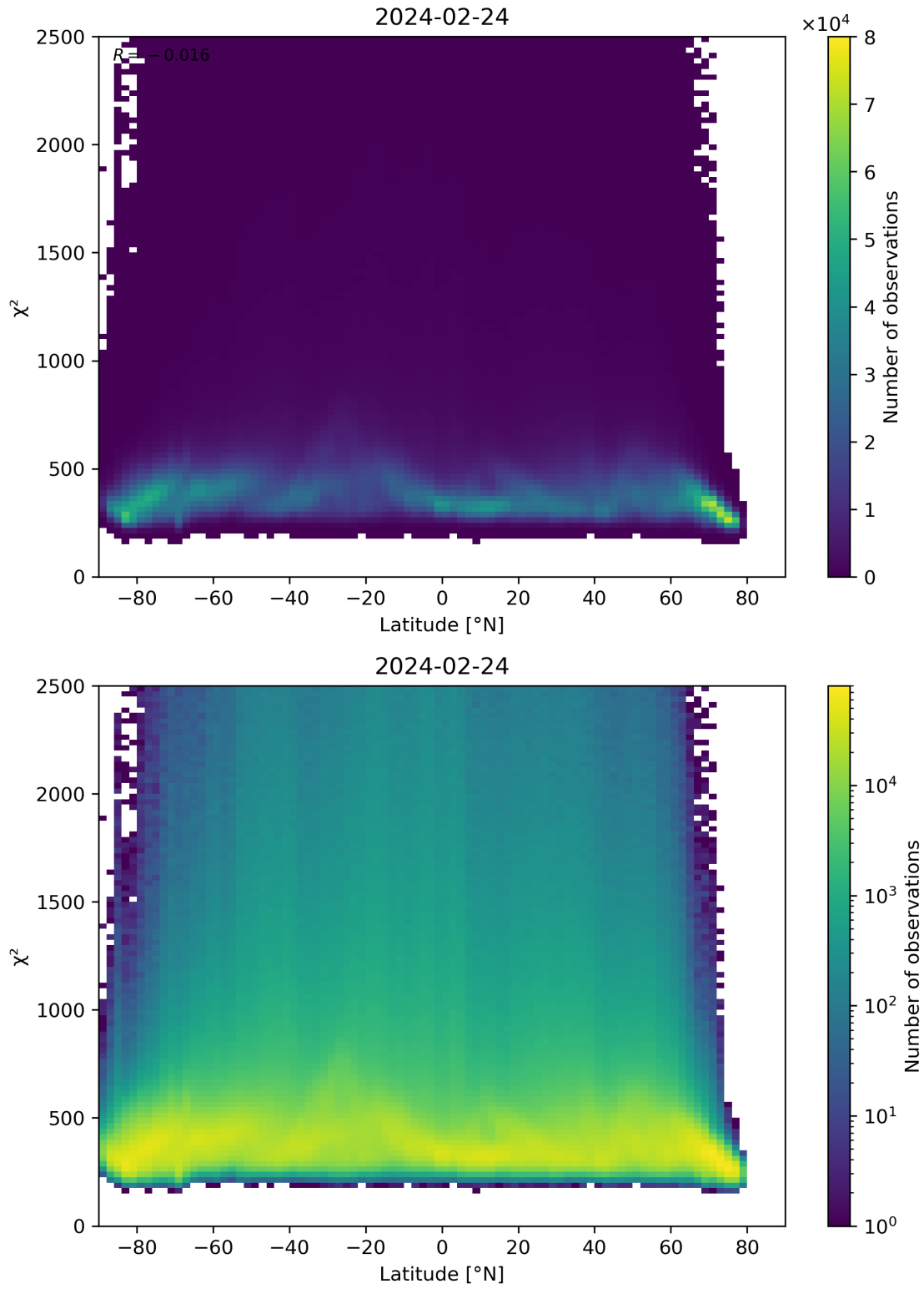
Figure 86: Scatter density plot of “Latitude” against “ \chi^2 ” for 2024-02-23 to 2024-02-25.
