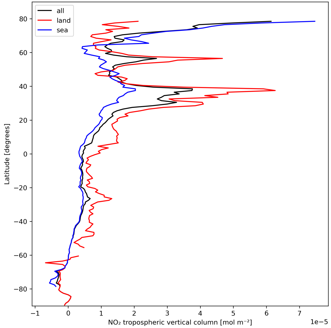
Figure 12: Zonal average of “NO 2 tropospheric vertical column” for 2024-02-23 to 2024-02-25.
