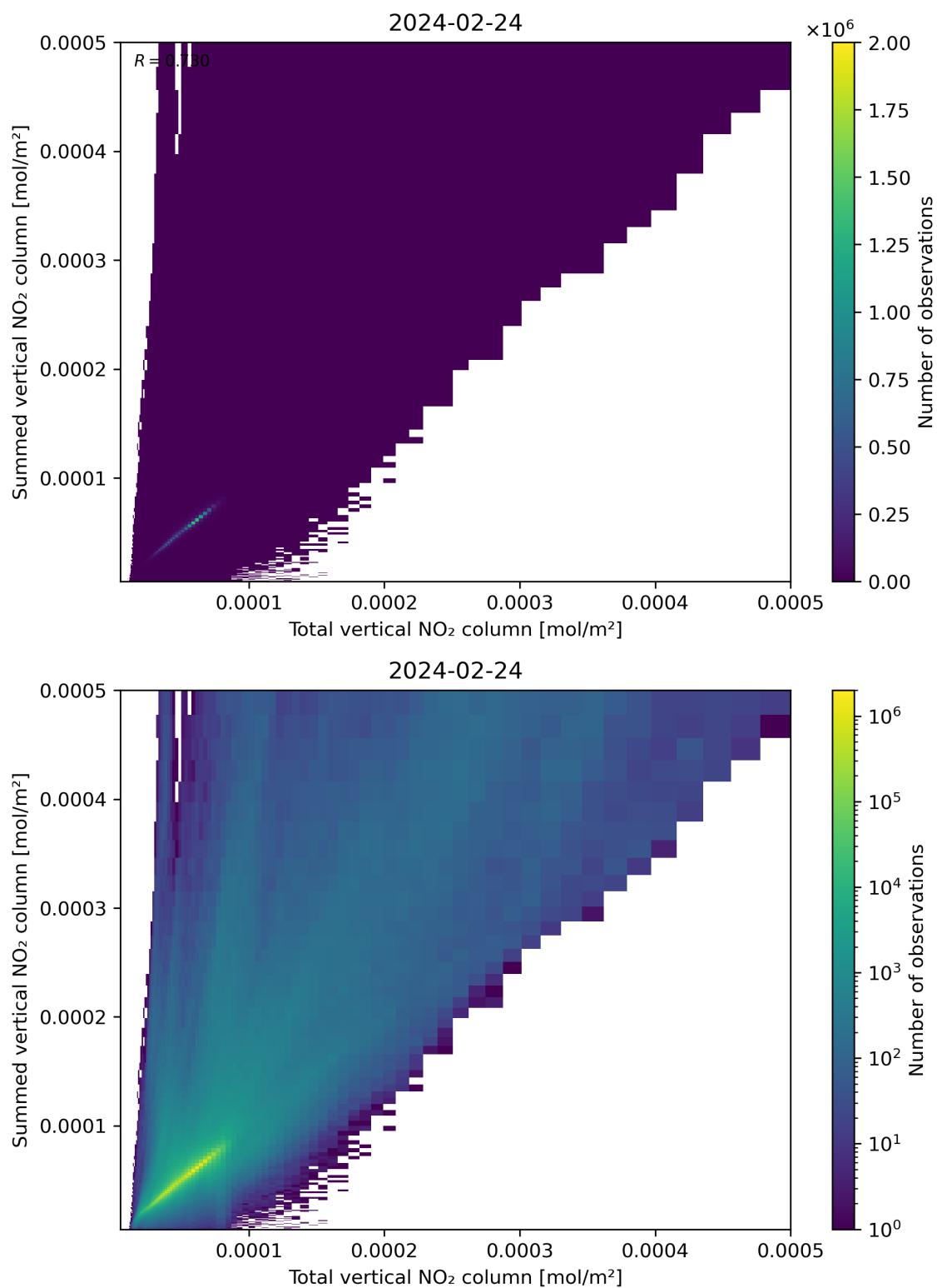
Figure 112: Scatter density plot of “Total vertical NO 2 column” against “Summed vertical NO 2 column” for 2024-02-23 to 2024-02-25.
