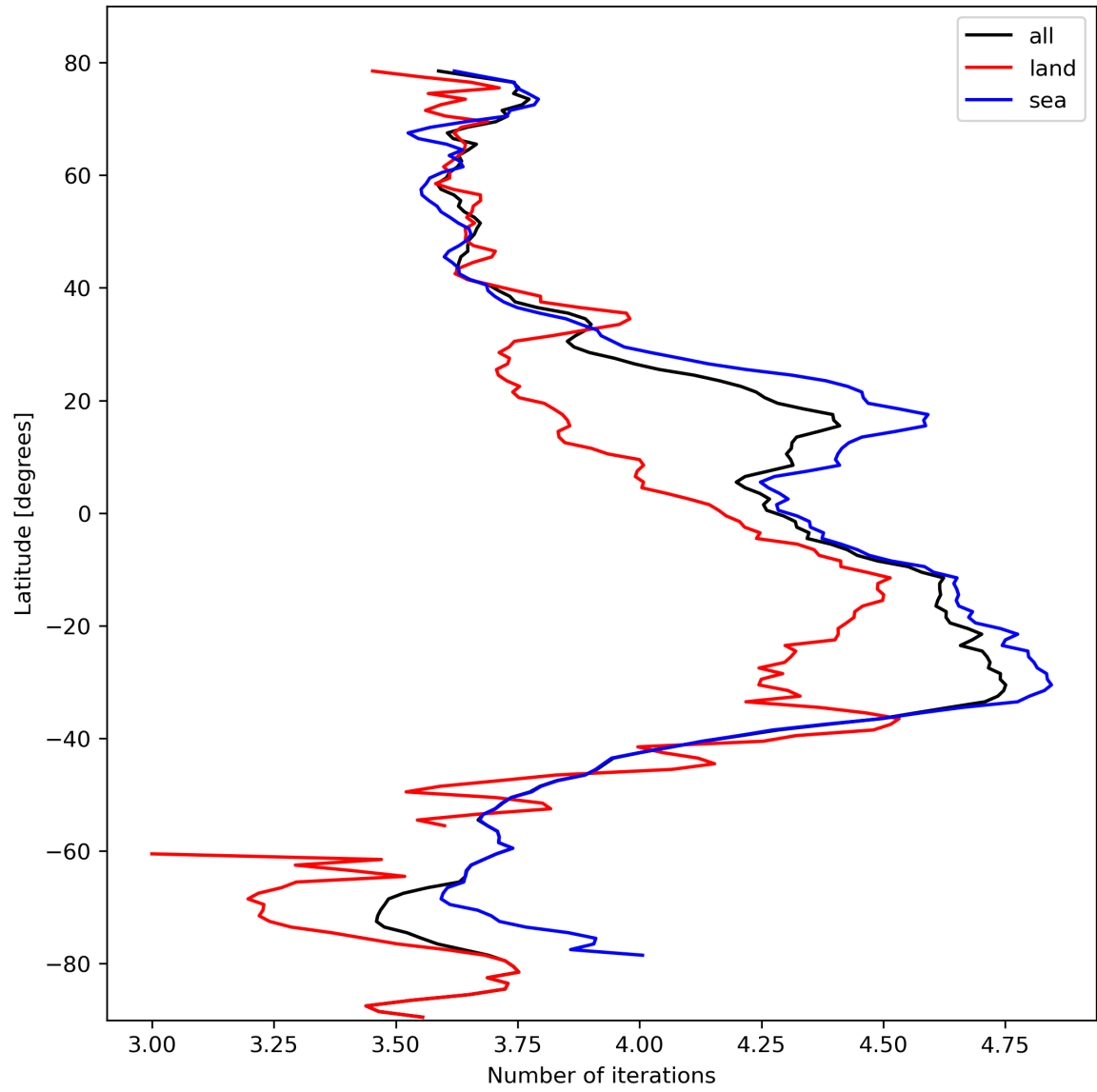
Figure 17: Zonal average of “Number of iterations” for 2024-02-23 to 2024-02-25.
