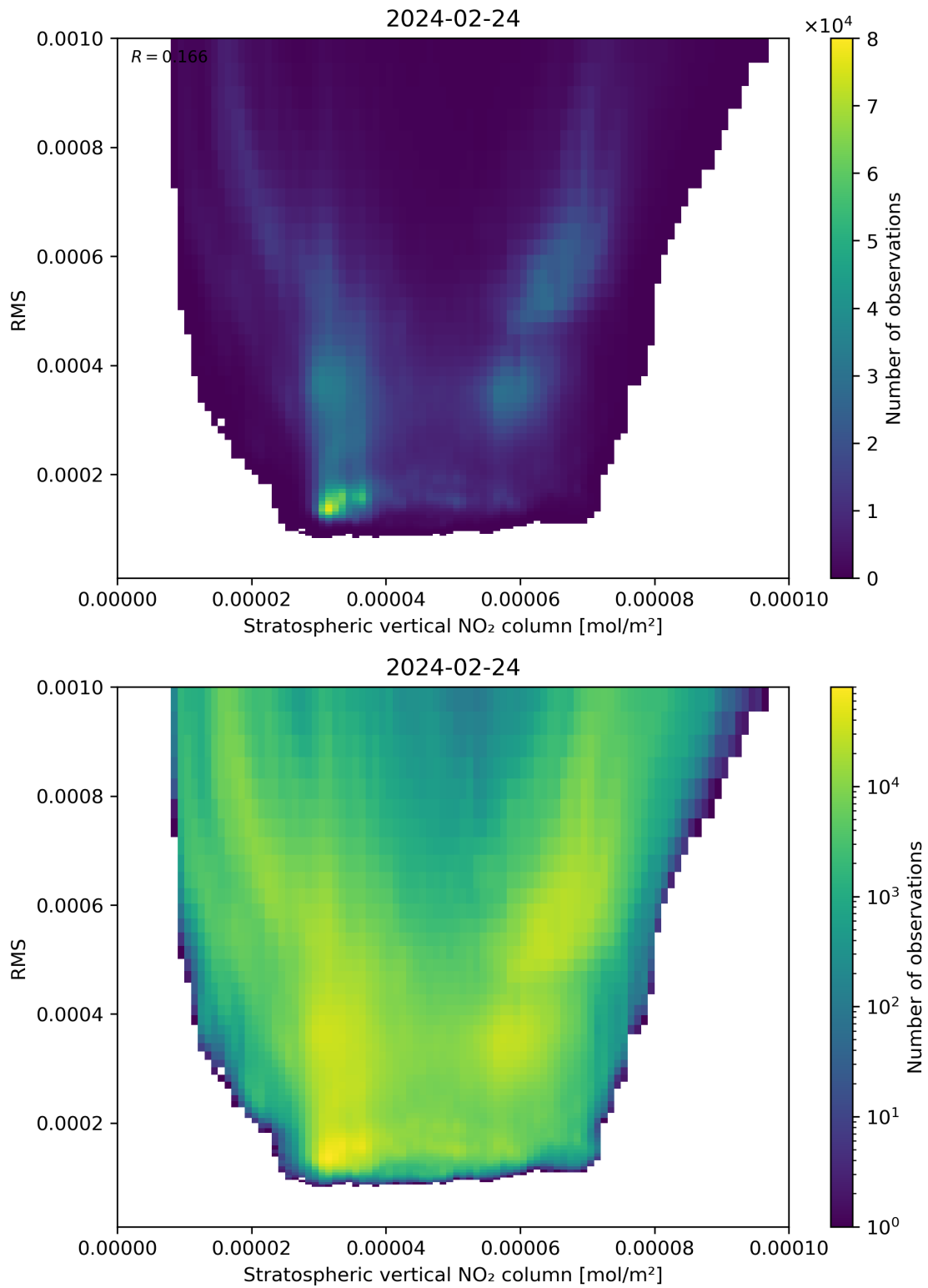
Figure 102: Scatter density plot of “Stratospheric vertical NO 2 column” against “RMS” for 2024-02-23 to 2024-02-25.
