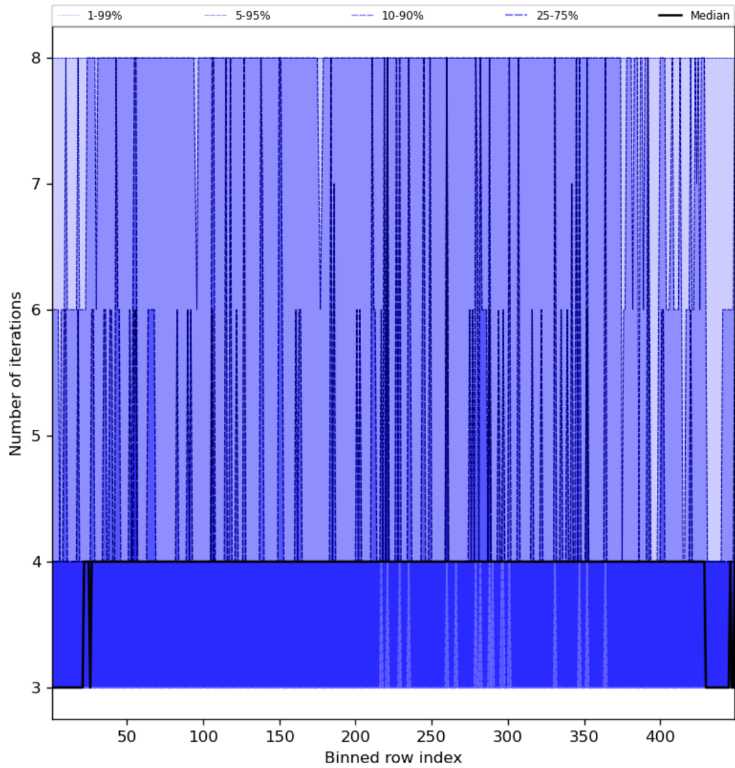
Figure 51: Along track statistics of “Number of iterations” for 2024-02-23 to 2024-02-25
