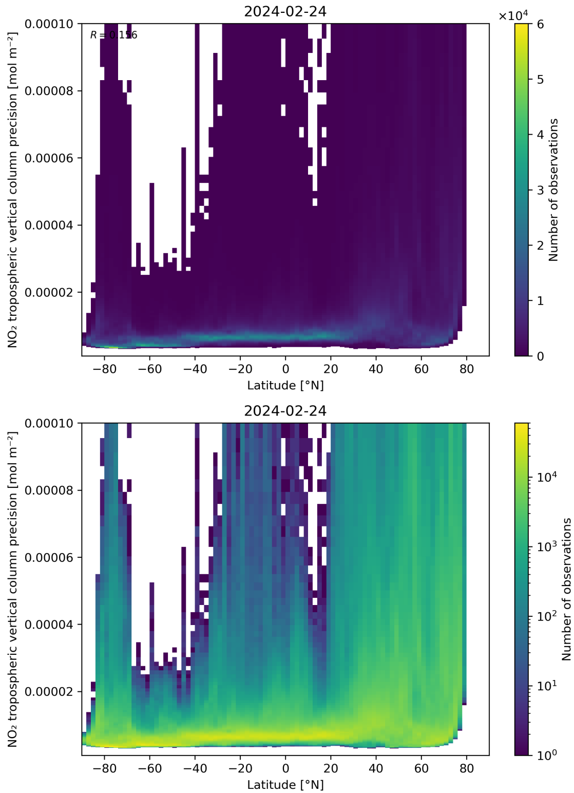
Figure 93: Scatter density plot of “Latitude” against “NO 2 tropospheric vertical column precision” for 2024-02-23 to 2024-02-25.
