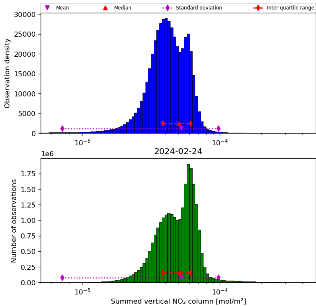
Figure 40: Histogram of “Summed vertical NO 2 column” for 2024-02-23 to 2024-02-25
