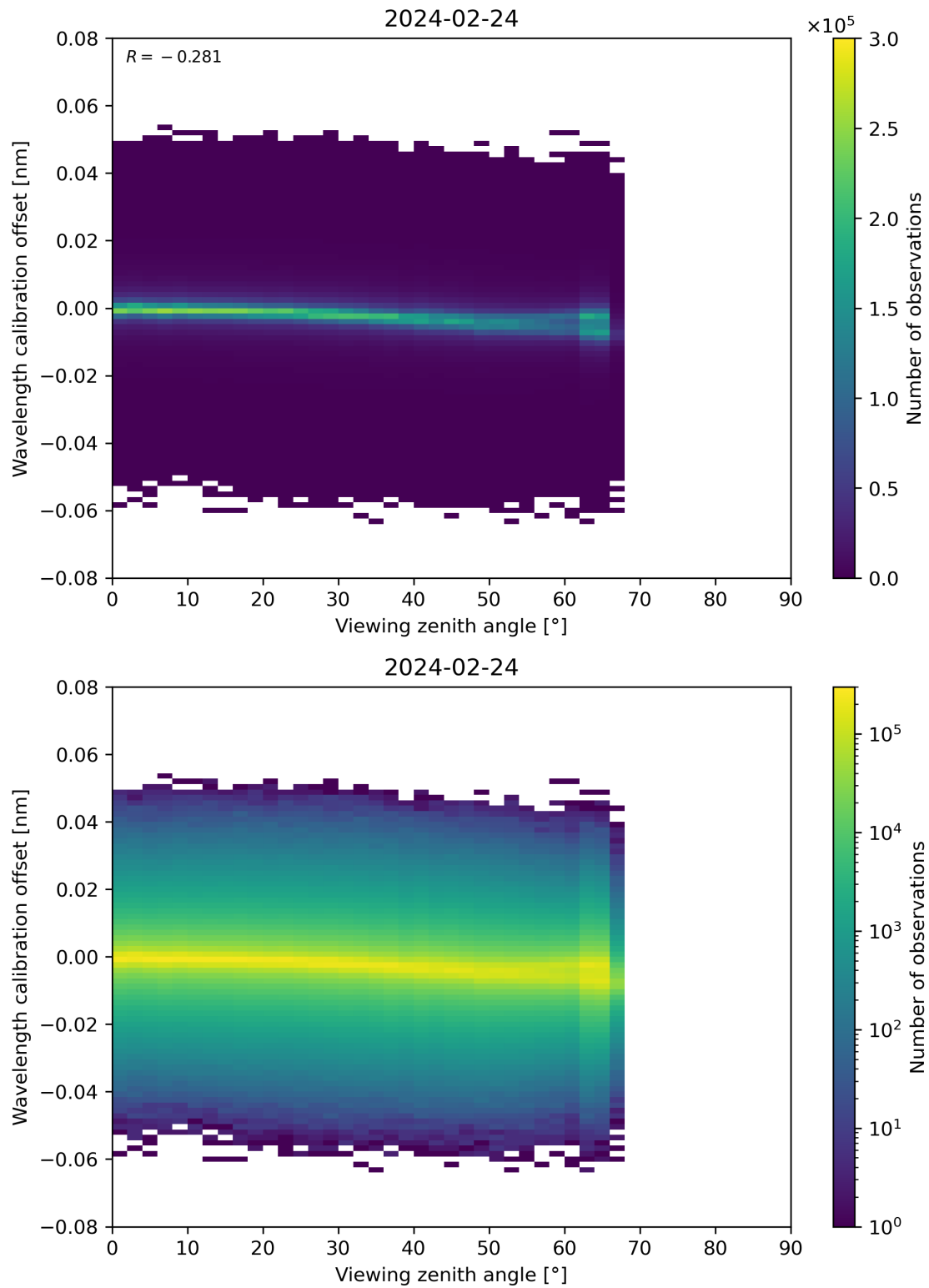
Figure 173: Scatter density plot of “Viewing zenith angle” against “Wavelength calibration offset” for 2024-02-23 to 2024-02-25.
