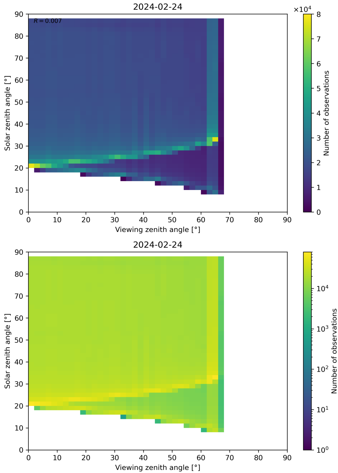
Figure 172: Scatter density plot of “Viewing zenith angle” against “Solar zenith angle” for 2024-02-23 to 2024-02-25.
