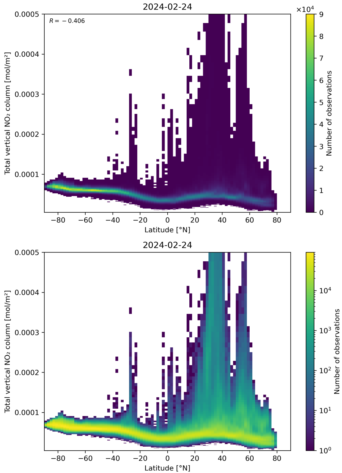
Figure 90: Scatter density plot of “Latitude” against “Total vertical NO 2 column” for 2024-02-23 to 2024-02-25.
