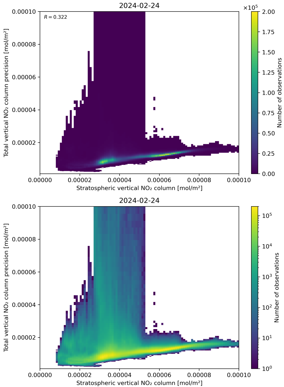
Figure 101: Scatter density plot of “Stratospheric vertical NO 2 column” against “Total vertical NO 2 column precision” for 2024-02-23 to 2024-02-25.
