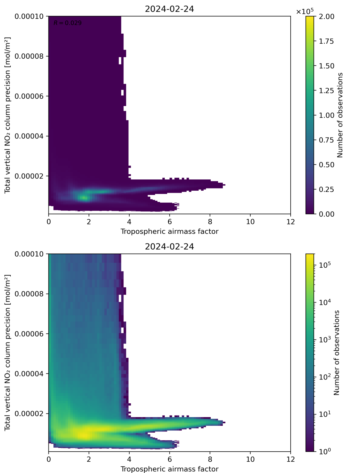
Figure 78: Scatter density plot of “Tropospheric air mass factor” against “Total vertical NO 2 column precision” for 2024-02-23 to 2024-02-25.
