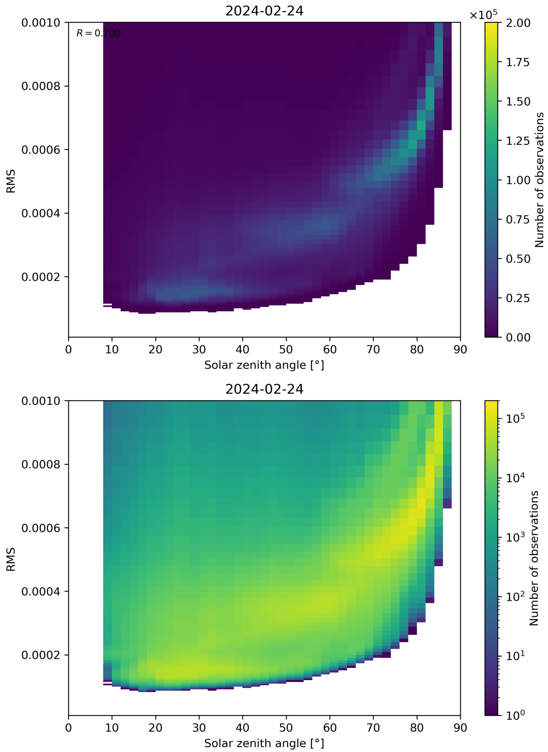
Figure 157: Scatter density plot of “Solar zenith angle” against “RMS” for 2024-02-23 to 2024-02-25.
