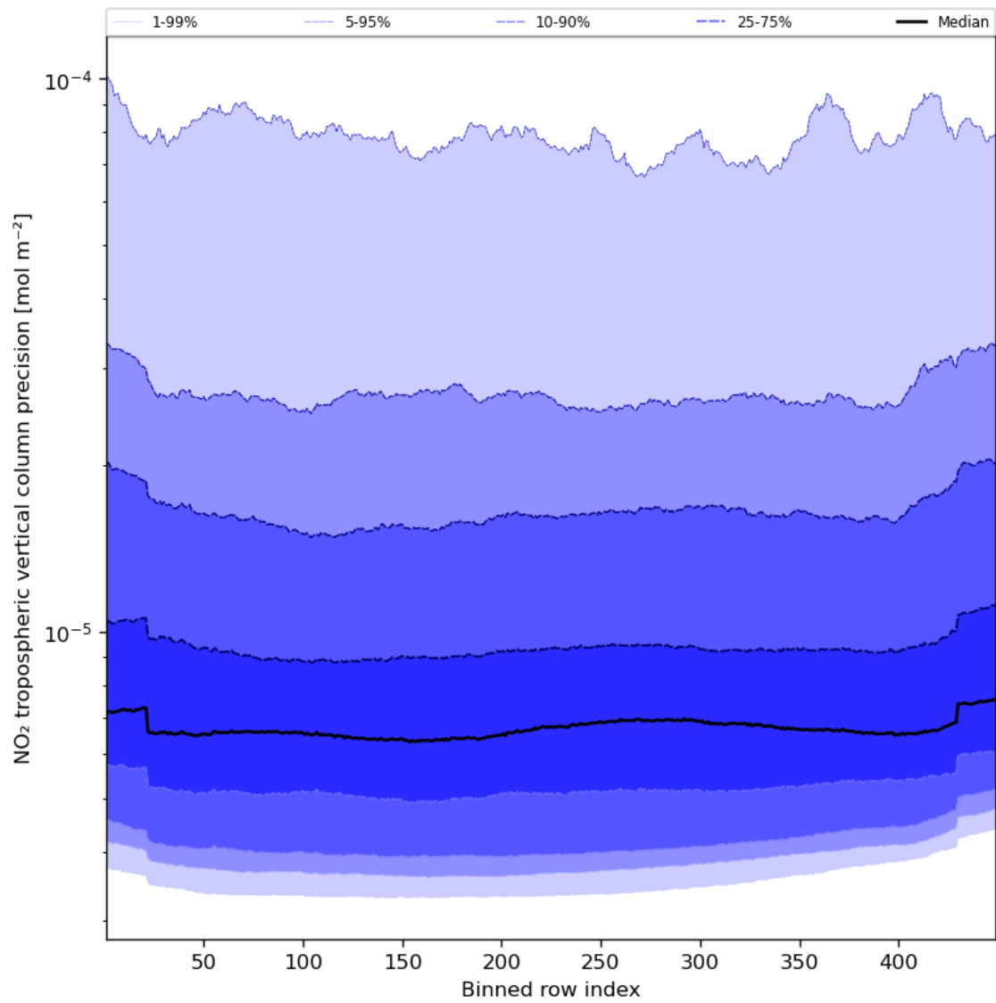
Figure 47: Along track statistics of “NO 2 tropospheric vertical column precision” for 2024-02-23 to 2024-02-25
