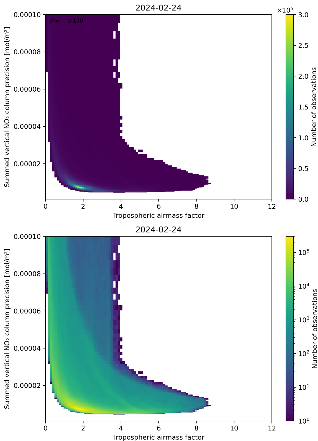
Figure 76: Scatter density plot of “Tropospheric airmass factor” against “Summed vertical NO 2 column precision” for 2024-02-23 to 2024-02-25.
