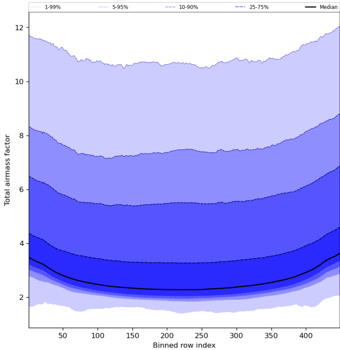
Figure 49: Along track statistics of “Total airmass factor” for 2024-02-23 to 2024-02-25
