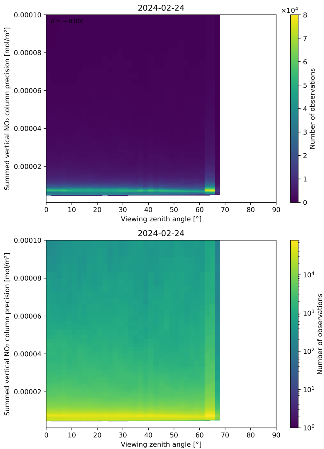
Figure 166: Scatter density plot of “Viewing zenith angle” against “Summed vertical NO 2 column precision” for 2024-02-23 to 2024-02-25.
