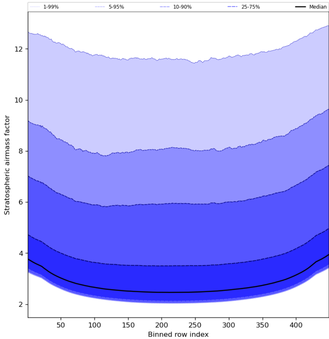
Figure 61: Along track statistics of “Stratospheric airmass factor” for 2024-02-23 to 2024-02-25
