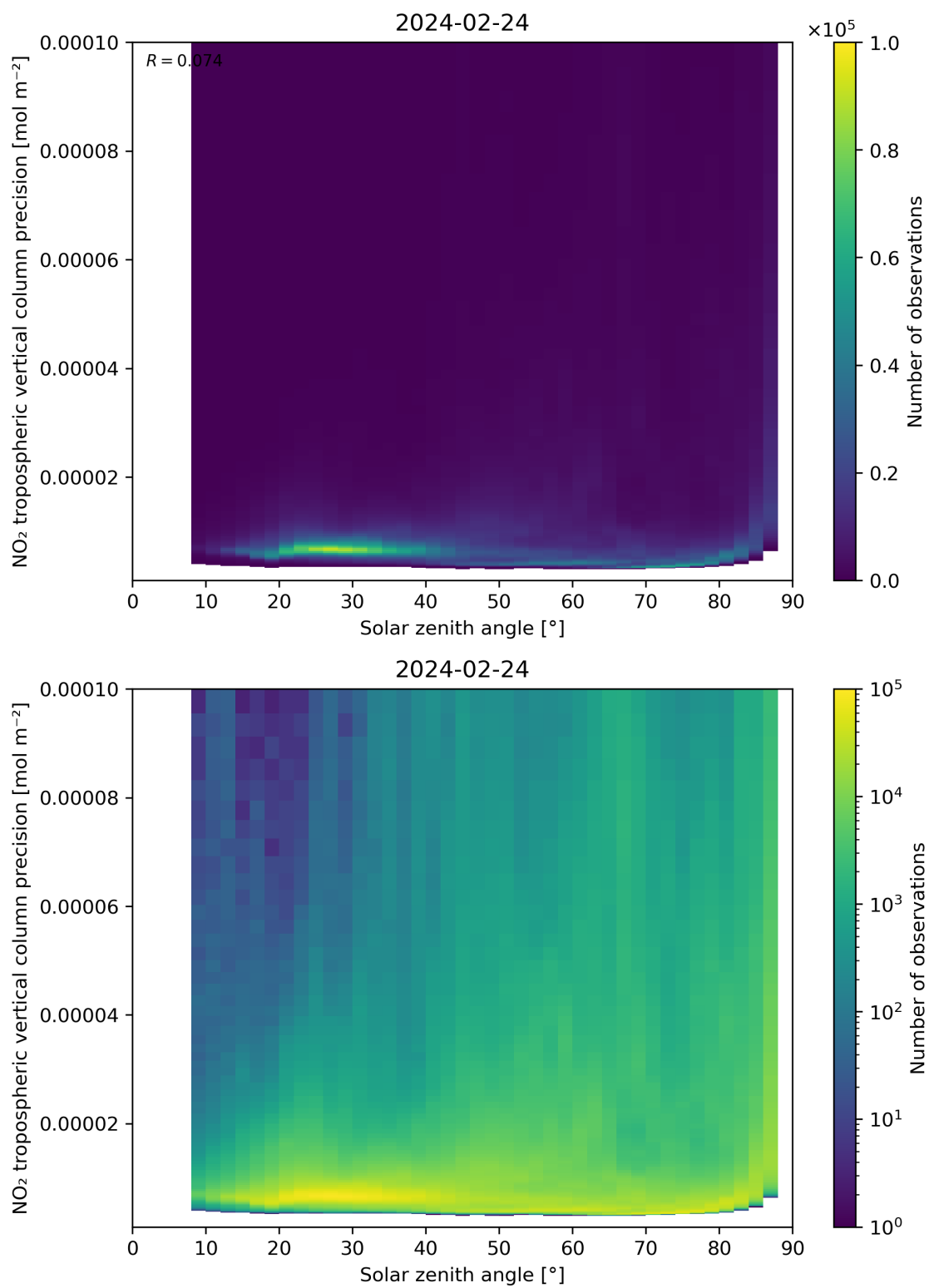
Figure 156: Scatter density plot of “Solar zenith angle” against “NO 2 tropospheric vertical column precision” for 2024-02-23 to 2024-02-25.
