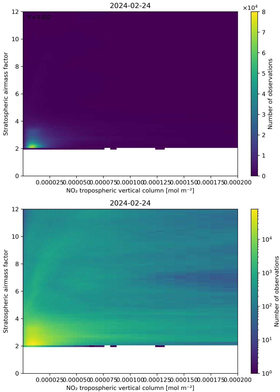
Figure 121: Scatter density plot of “NO 2 tropospheric vertical column” against “Stratospheric airmass factor” for 2024-02-23 to 2024-02-25.
