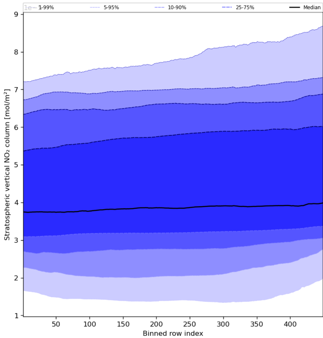
Figure 53: Along track statistics of “Stratospheric vertical NO 2 column” for 2024-02-23 to 2024-02-25
