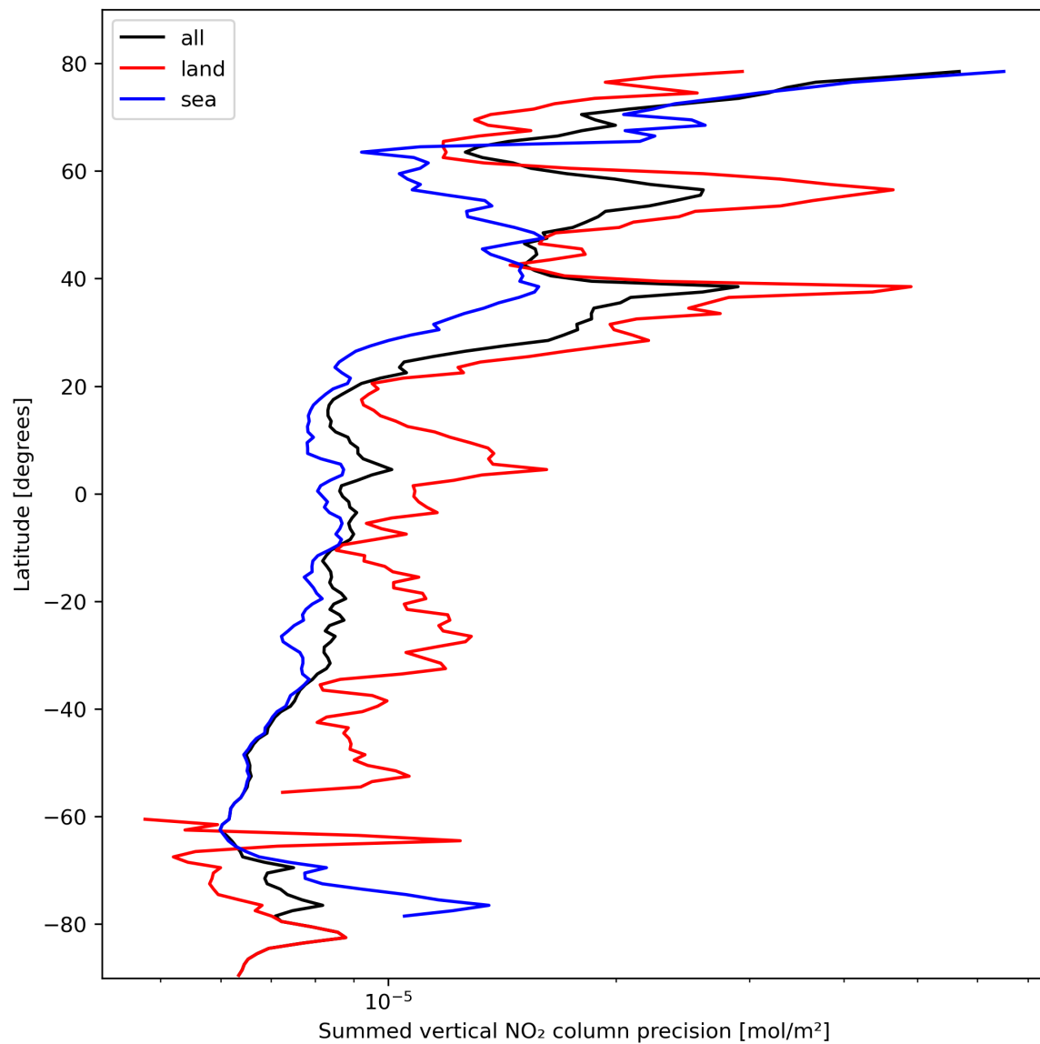
Figure 24: Zonal average of “Summed vertical NO 2 column precision” for 2024-02-23 to 2024-02-25.
