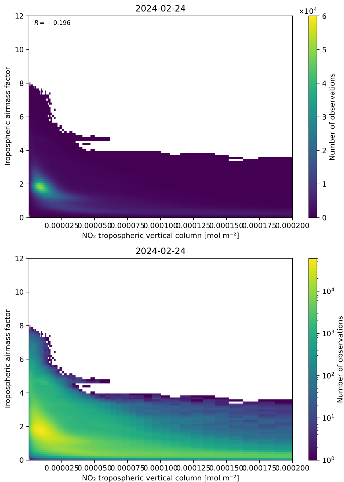
Figure 123: Scatter density plot of “NO 2 tropospheric vertical column” against “Tropospheric airmass factor” for 2024-02-23 to 2024-02-25.
