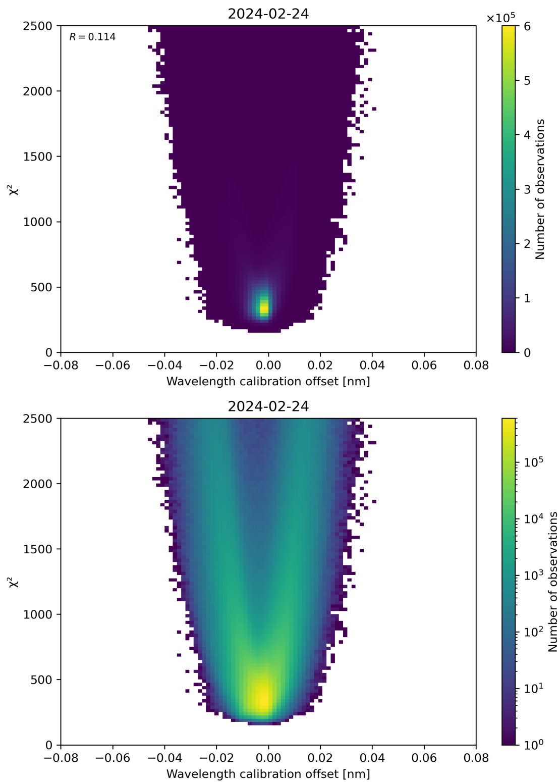
Figure 175: Scatter density plot of “Wavelength calibration offset” against “ \chi^2 ” for 2024-02-23 to 2024-02-25.
