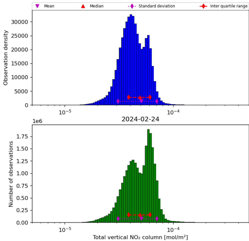
Figure 38: Histogram of “Total vertical NO 2 column” for 2024-02-23 to 2024-02-25
