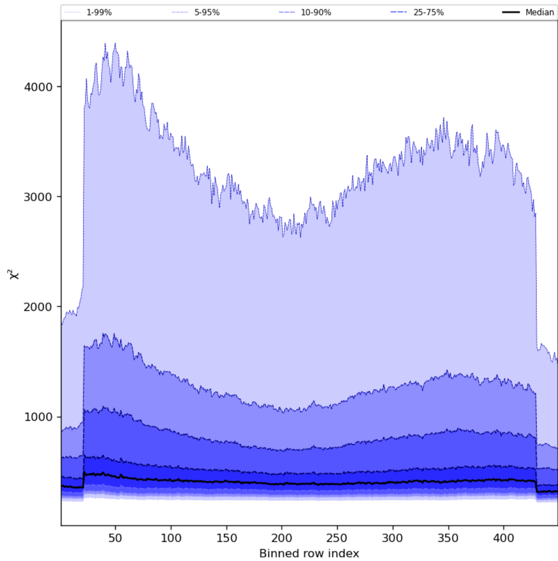
Figure 59: Along track statistics of “ \chi^2 ” for 2024-02-23 to 2024-02-25
