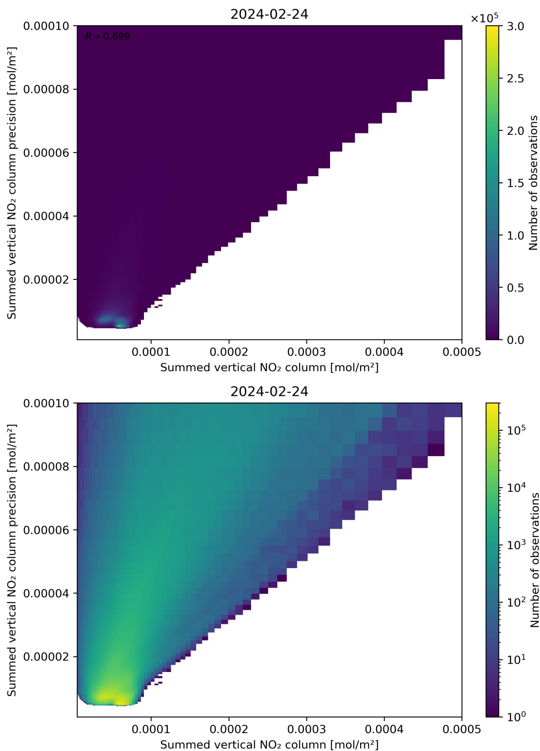
Figure 105: Scatter density plot of “Summed vertical NO 2 column” against “Summed vertical NO 2 column precision” for 2024-02-23 to 2024-02-25.
