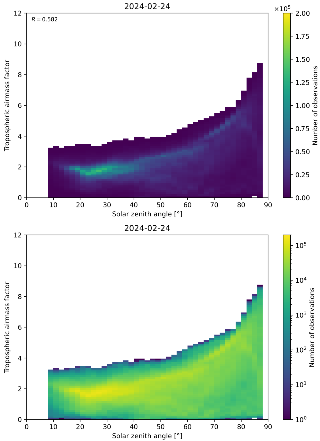
Figure 147: Scatter density plot of “Solar zenith angle” against “Tropospheric airmass factor” for 2024-02-23 to 2024-02-25.
