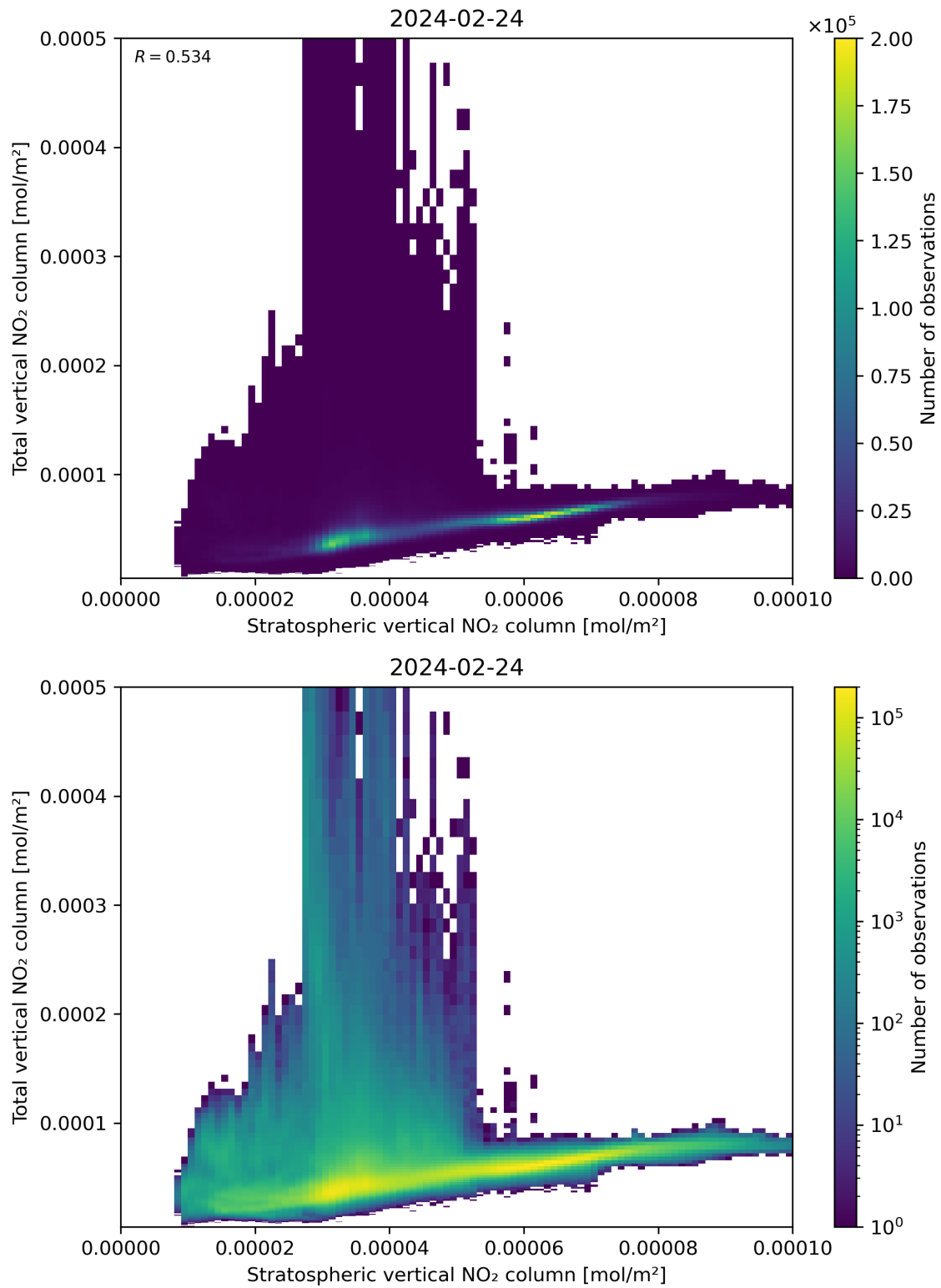
Figure 100: Scatter density plot of “Stratospheric vertical NO 2 column” against “Total vertical NO 2 column” for 2024-02-23 to 2024-02-25.
