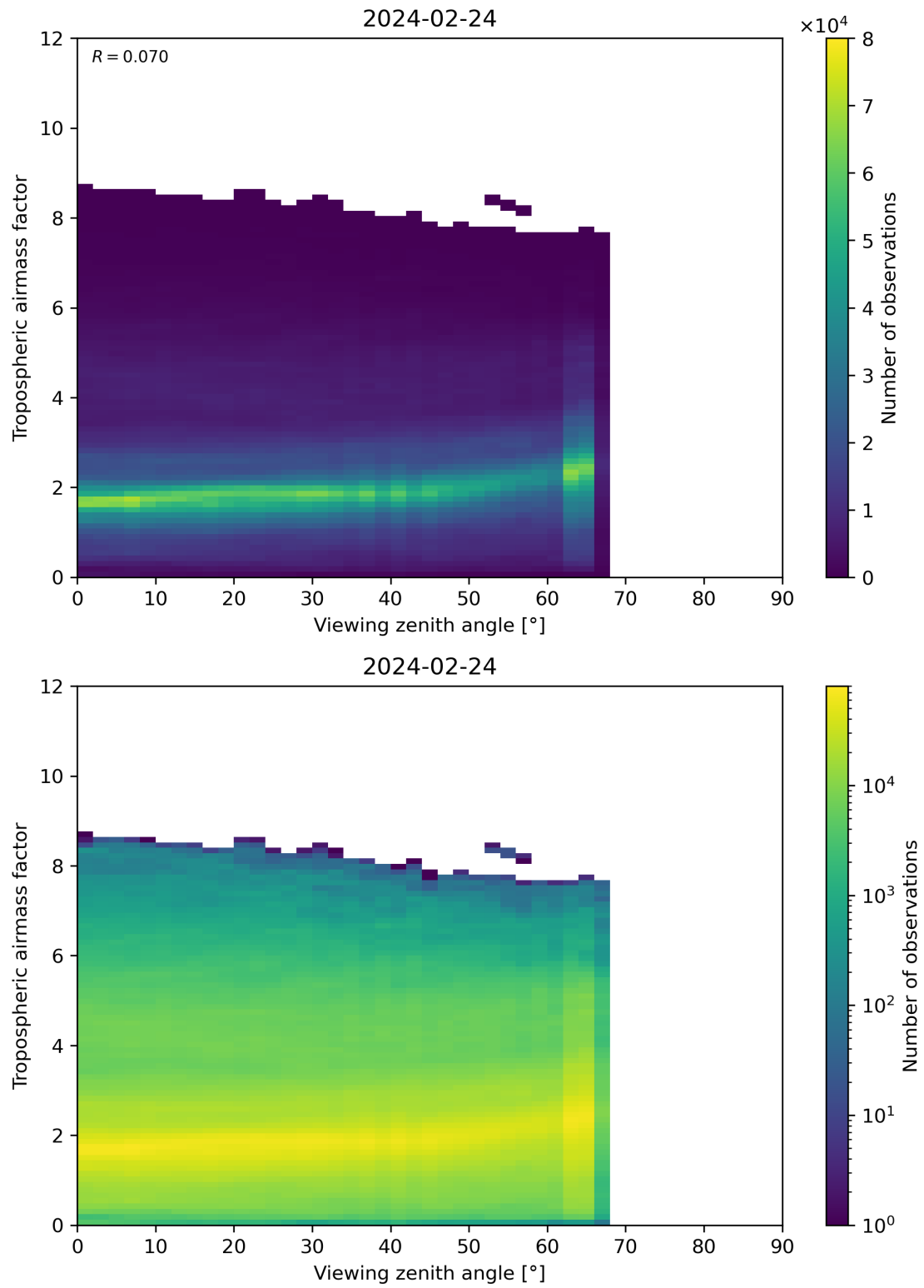
Figure 161: Scatter density plot of “Viewing zenith angle” against “Tropospheric airmass factor” for 2024-02-23 to 2024-02-25.
