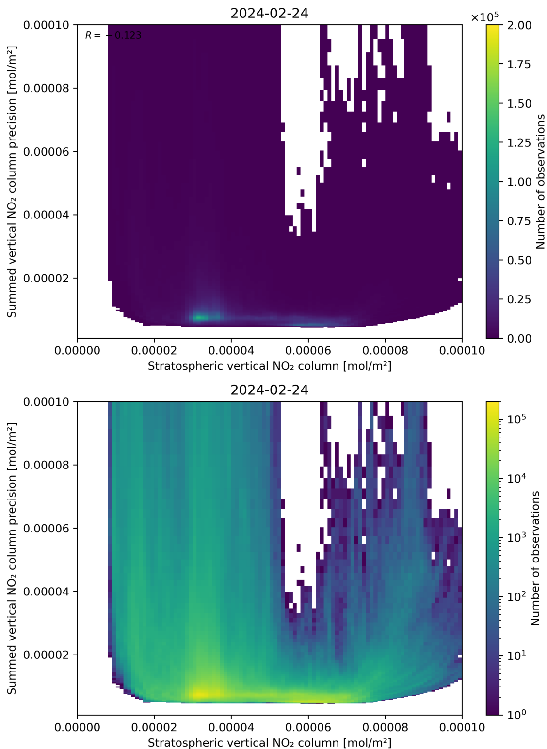
Figure 99: Scatter density plot of “Stratospheric vertical NO 2 column” against “Summed vertical NO 2 column precision” for 2024-02-23 to 2024-02-25.
