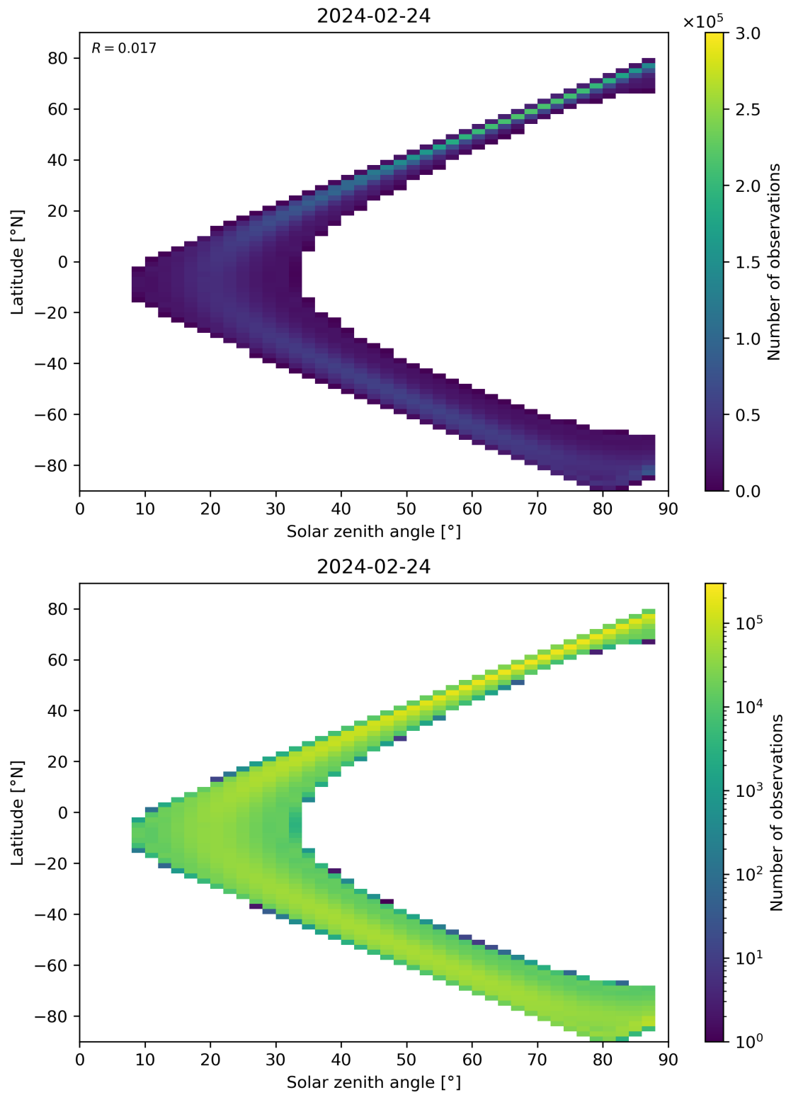
Figure 149: Scatter density plot of “Solar zenith angle” against “Latitude” for 2024-02-23 to 2024-02-25.
