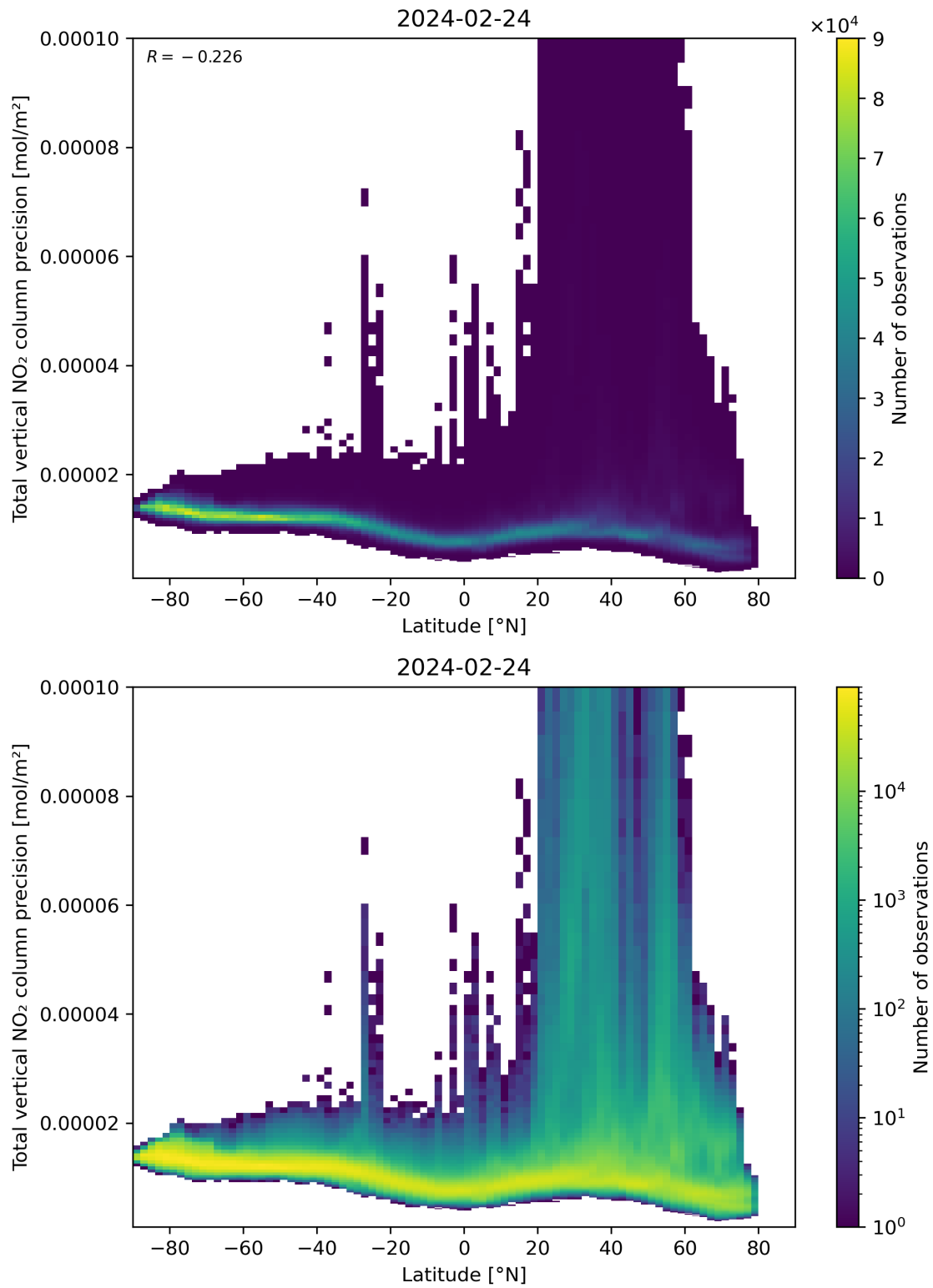
Figure 91: Scatter density plot of “Latitude” against “Total vertical NO 2 column precision” for 2024-02-23 to 2024-02-25.
