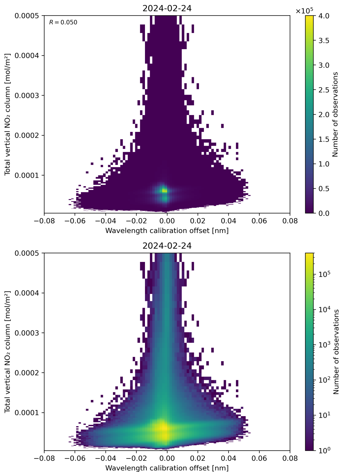
Figure 179: Scatter density plot of “Wavelength calibration offset” against “Total vertical NO 2 column” for 2024-02-23 to 2024-02-25.
