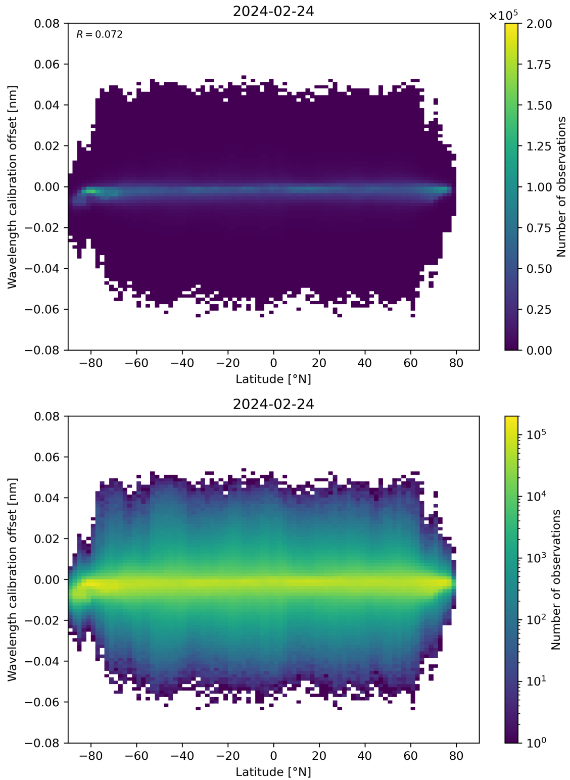
Figure 95: Scatter density plot of “Latitude” against “Wavelength calibration offset” for 2024-02-23 to 2024-02-25.
