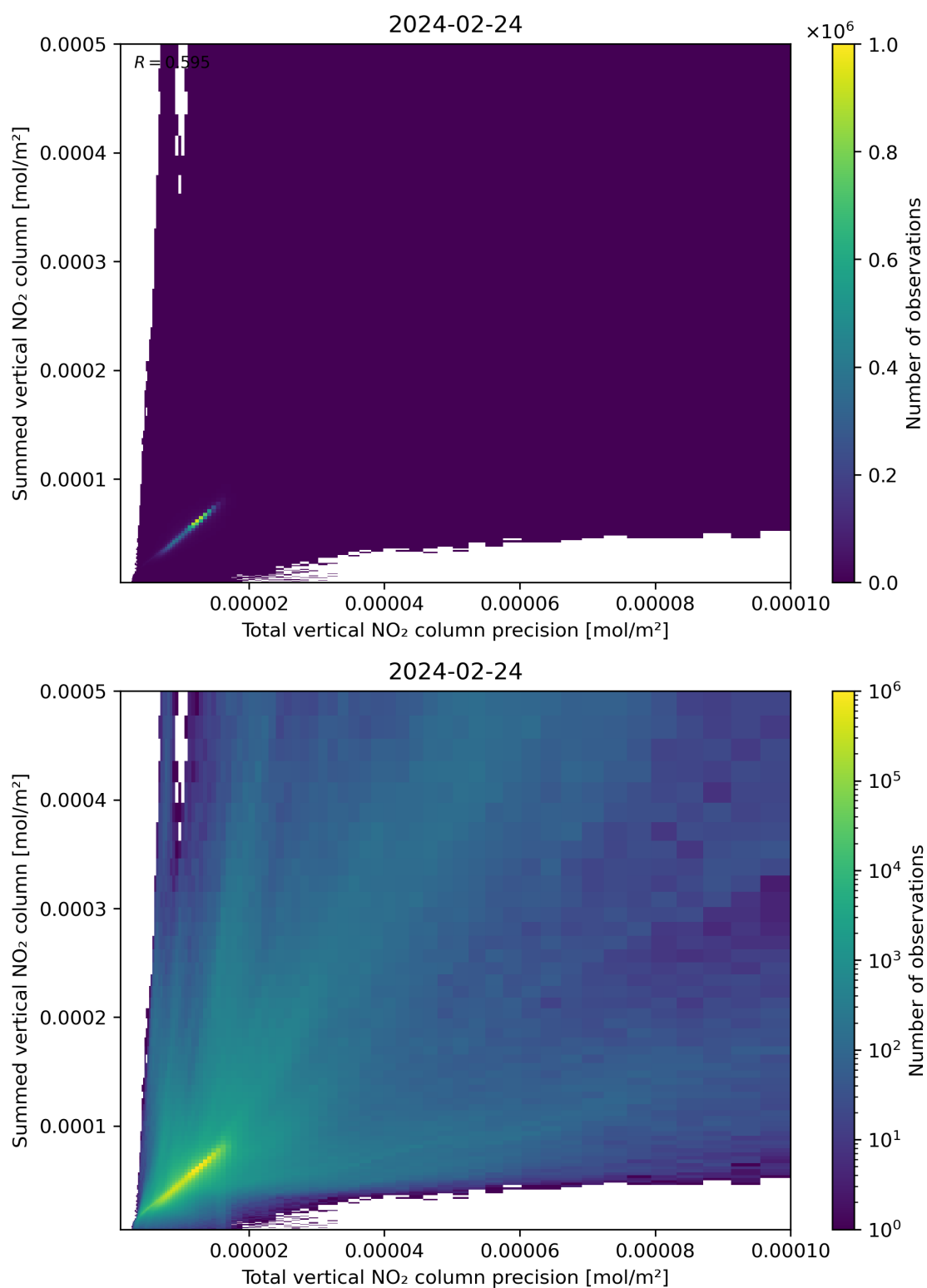
Figure 117: Scatter density plot of “Total vertical NO 2 column precision” against “Summed vertical NO 2 column” for 2024-02-23 to 2024-02-25.
