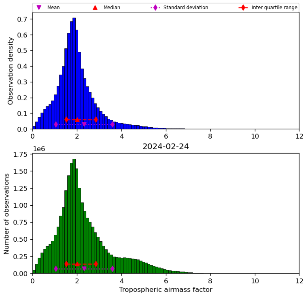
Figure 31: Histogram of “Tropospheric airmass factor” for 2024-02-23 to 2024-02-25
