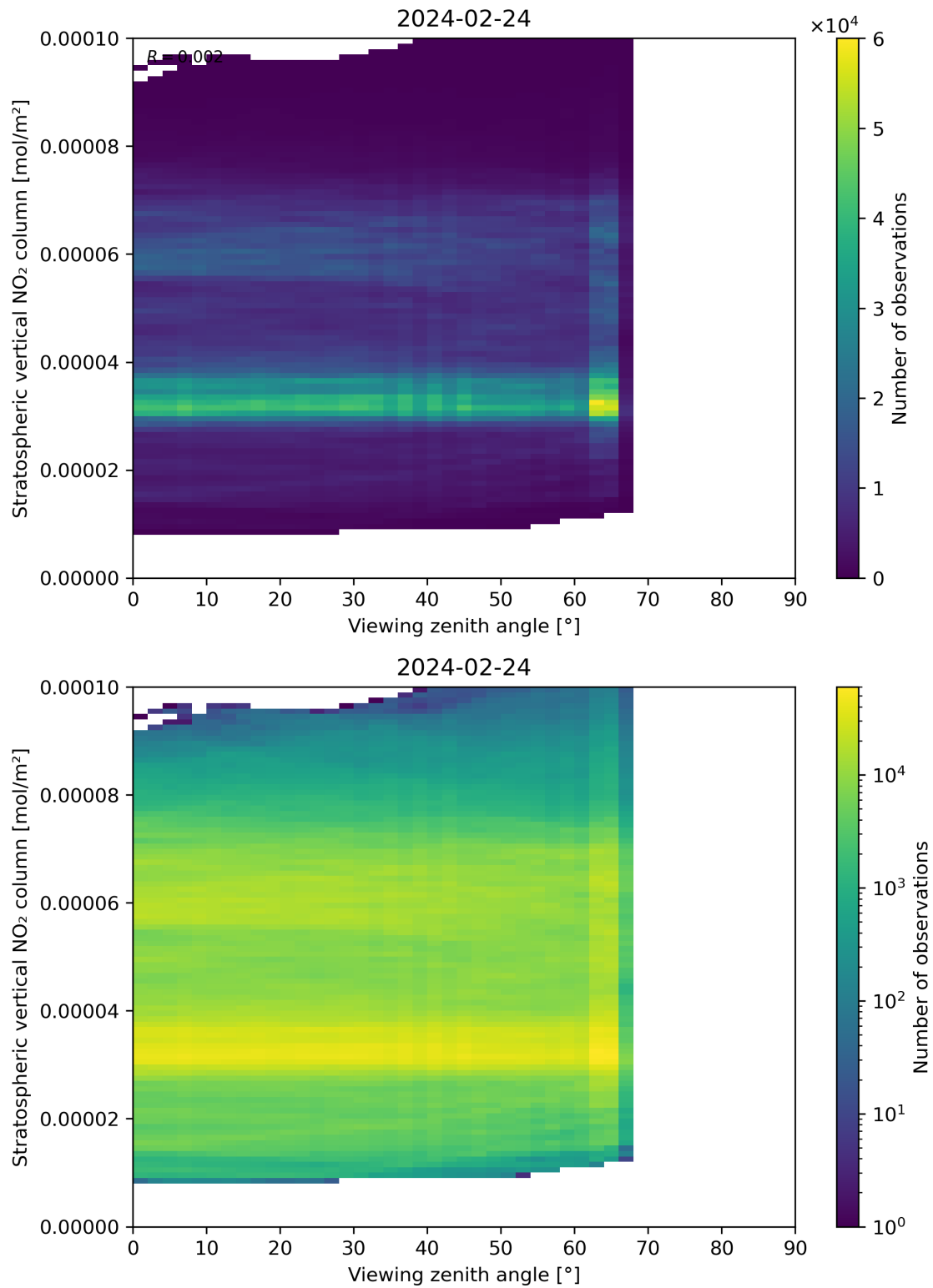
Figure 164: Scatter density plot of “Viewing zenith angle” against “Stratospheric vertical NO 2 column” for 2024-02-23 to 2024-02-25.
