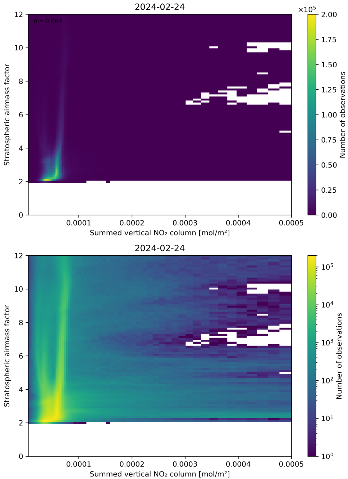
Figure 103: Scatter density plot of “Summed vertical NO 2 column” against “Stratospheric airmass factor” for 2024-02-23 to 2024-02-25.
