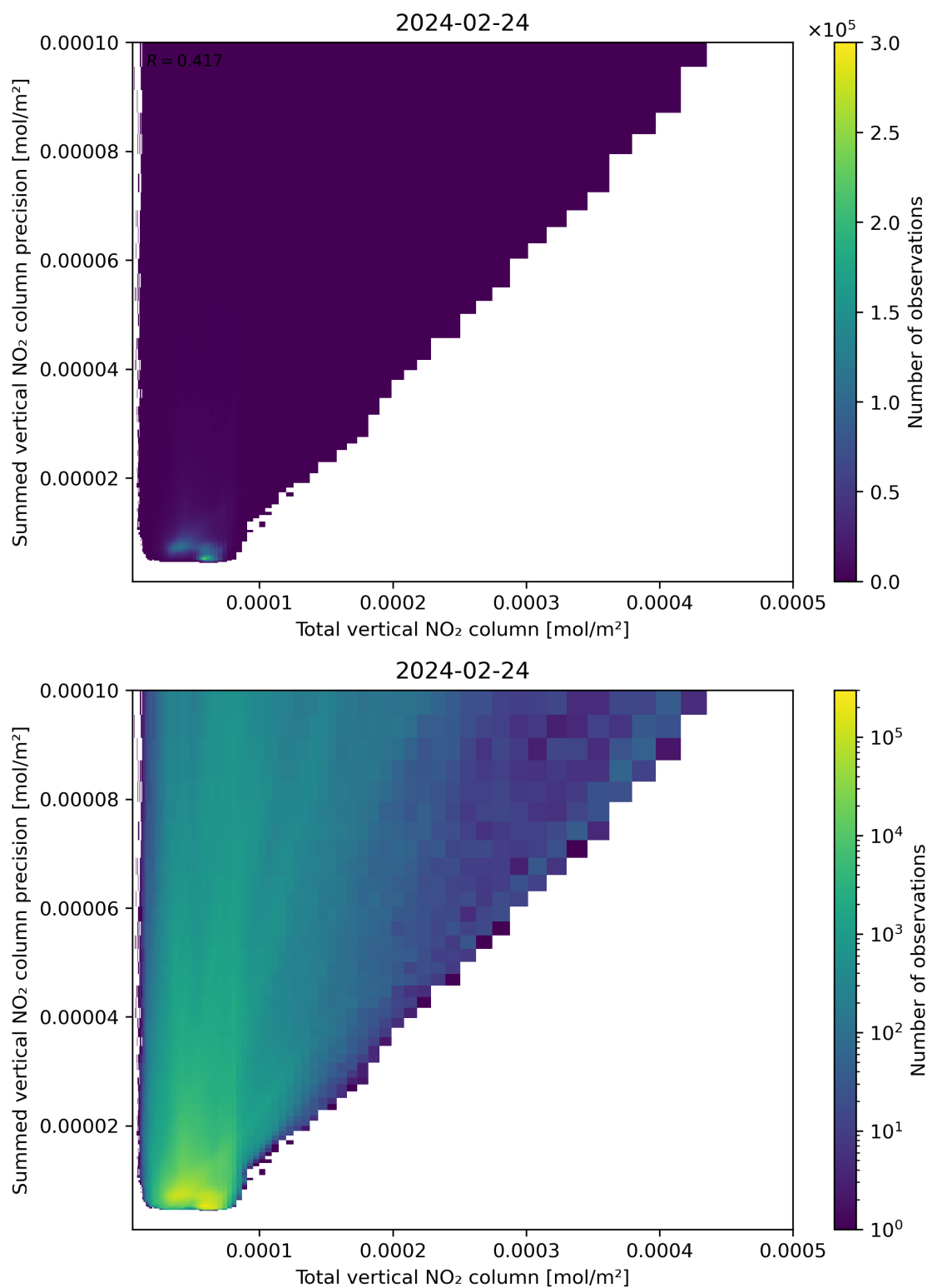
Figure 113: Scatter density plot of “Total vertical NO 2 column” against “Summed vertical NO 2 column precision” for 2024-02-23 to 2024-02-25.
