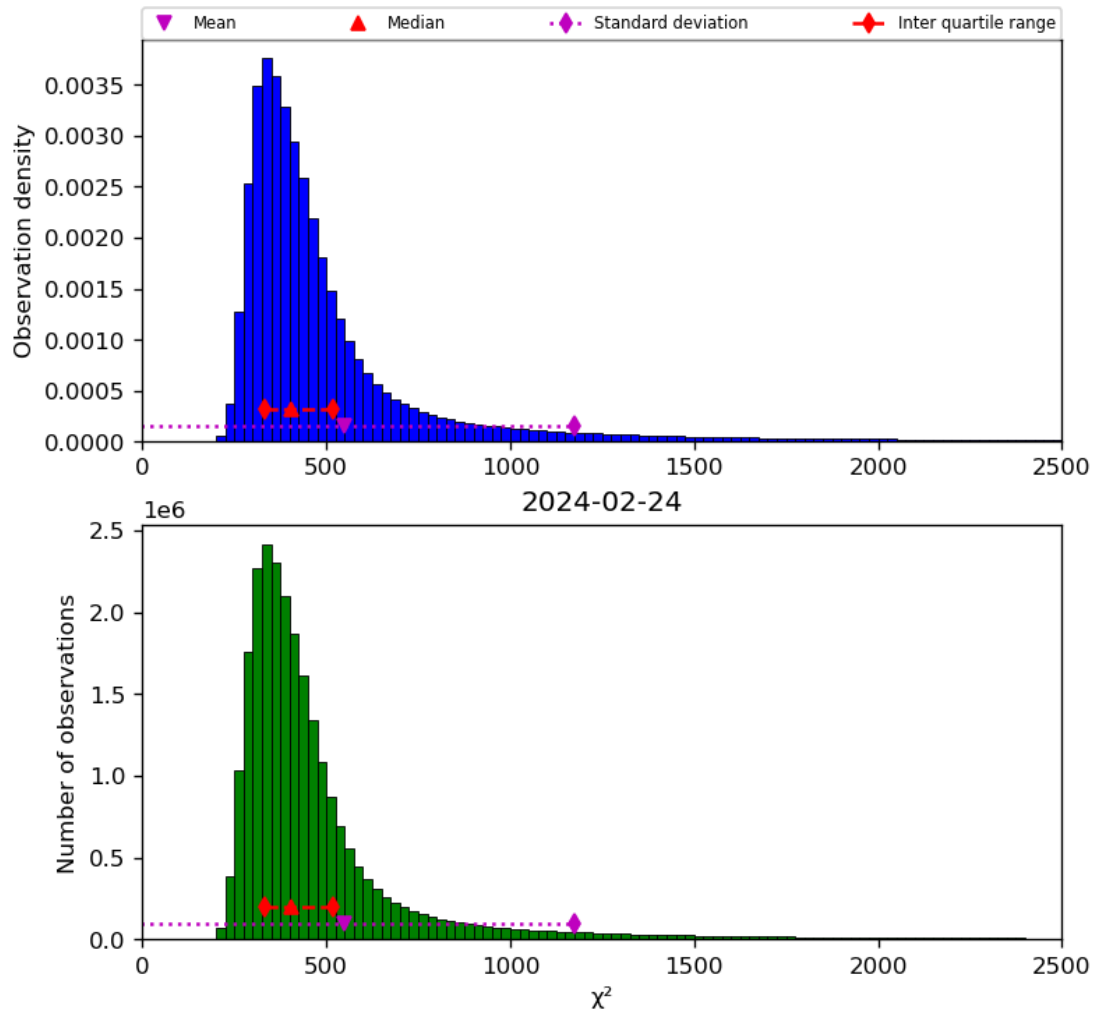
Figure 42: Histogram of “ \chi^2 ” for 2024-02-23 to 2024-02-25
