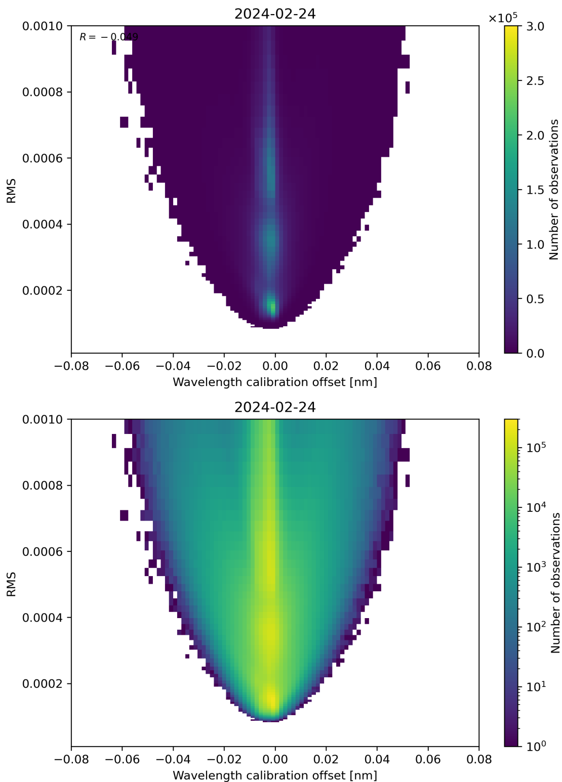
Figure 181: Scatter density plot of “Wavelength calibration offset” against “RMS” for 2024-02-23 to 2024-02-25.
