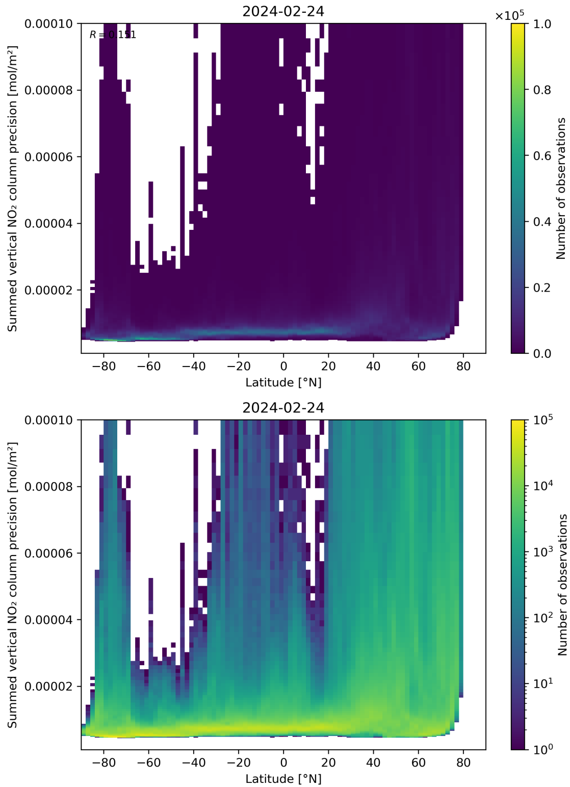
Figure 89: Scatter density plot of “Latitude” against “Summed vertical NO 2 column precision” for 2024-02-23 to 2024-02-25.
