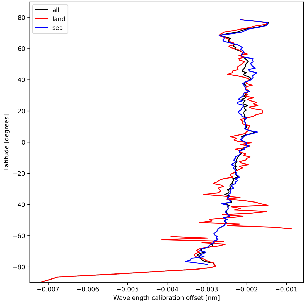
Figure 18: Zonal average of “Wavelength calibration offset” for 2024-02-23 to 2024-02-25.
