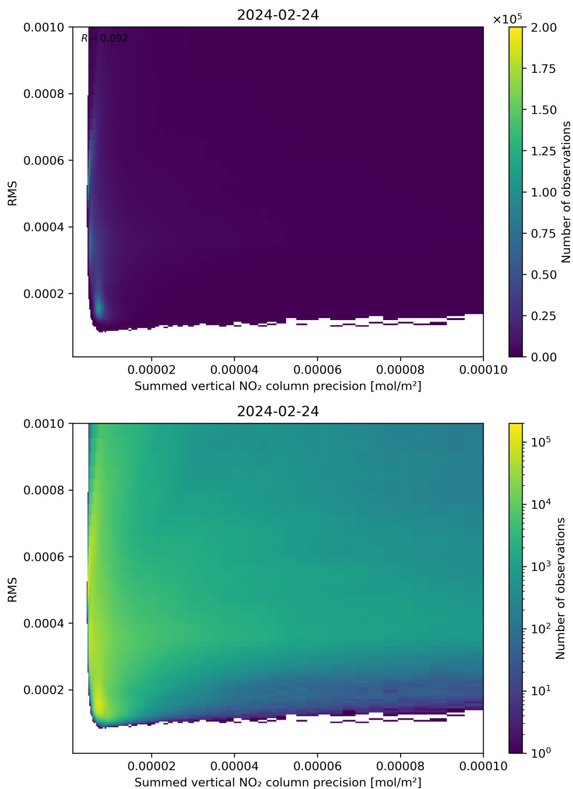
Figure 108: Scatter density plot of “Summed vertical NO 2 column precision” against “RMS” for 2024-02-23 to 2024-02-25.
