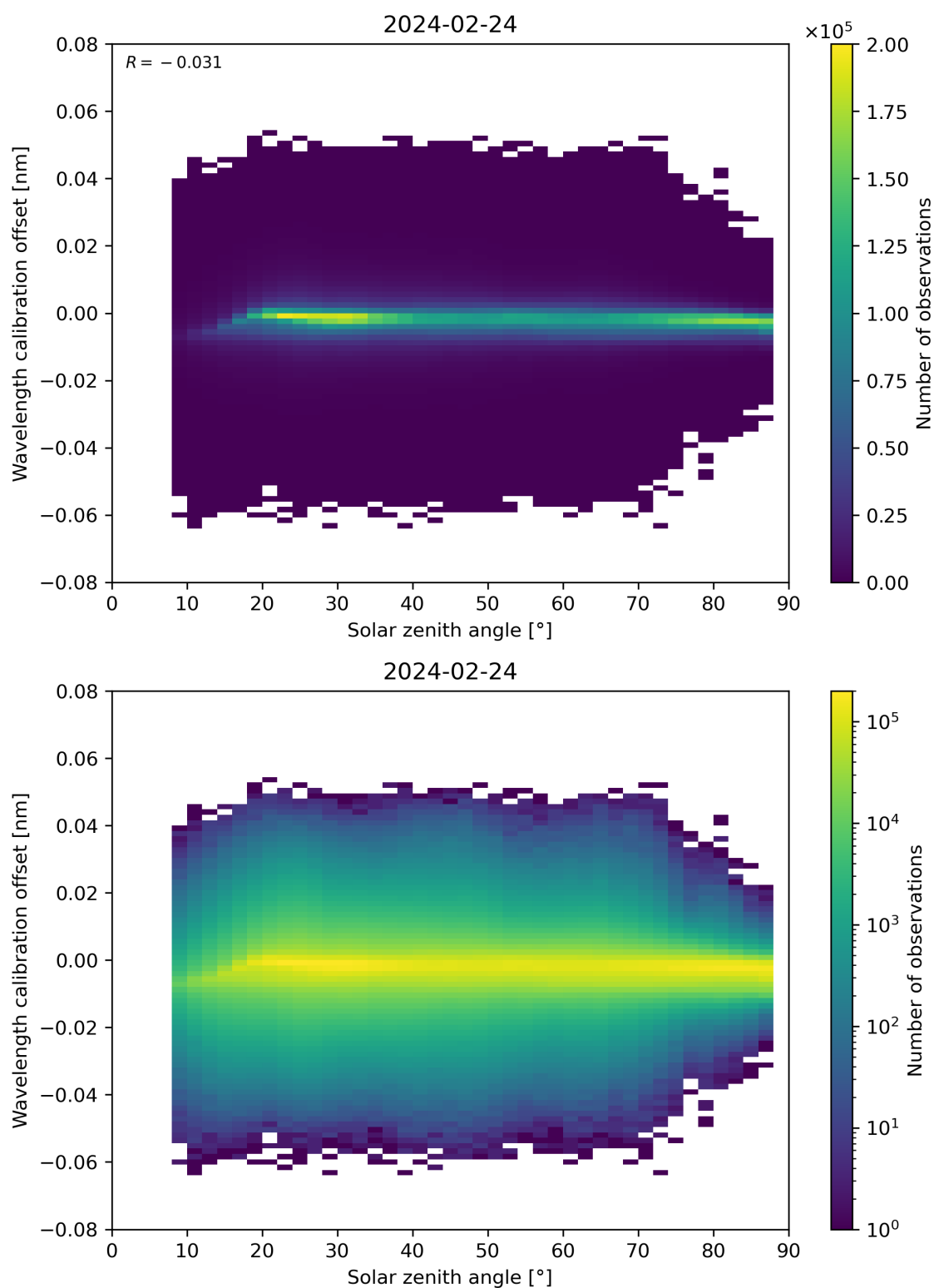
Figure 158: Scatter density plot of “Solar zenith angle” against “Wavelength calibration offset” for 2024-02-23 to 2024-02-25.
