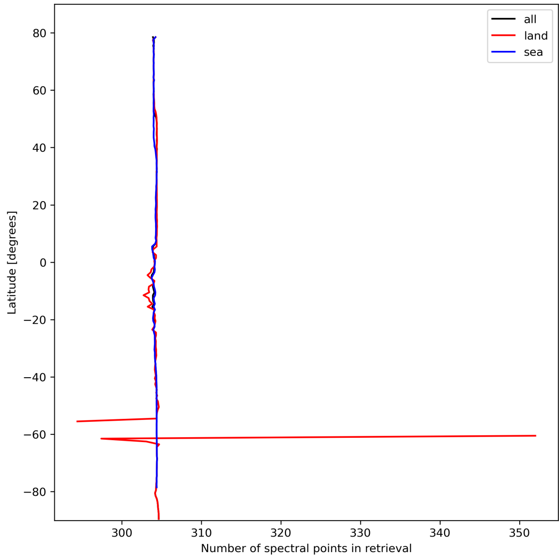
Figure 16: Zonal average of “Number of spectral points in retrieval” for 2024-02-23 to 2024-02-25.
