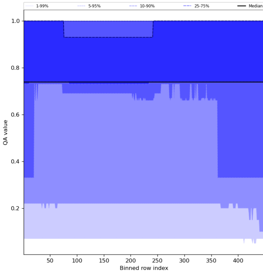
Figure 45: Along track statistics of “QA value” for 2024-02-23 to 2024-02-25
