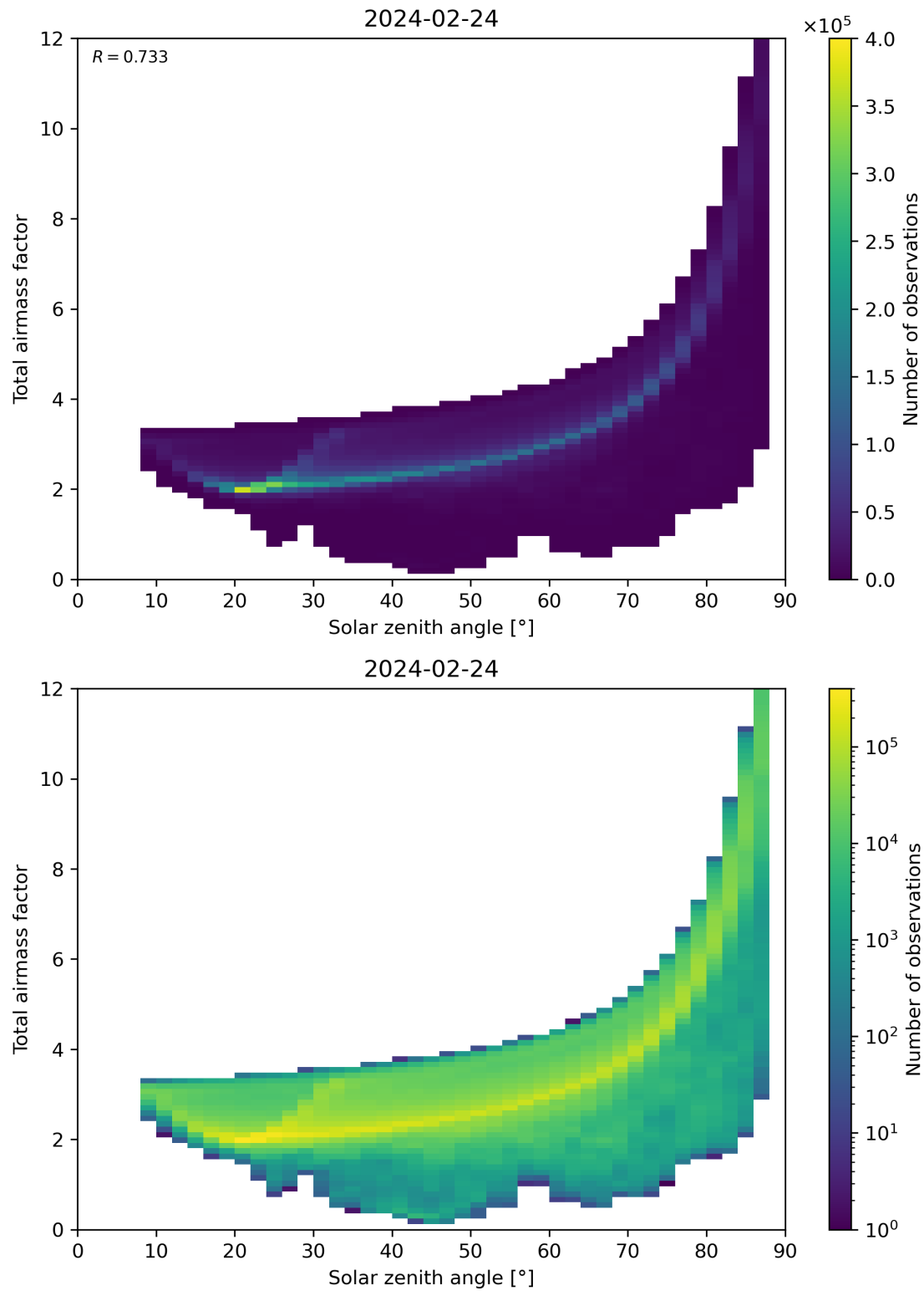
Figure 146: Scatter density plot of “Solar zenith angle” against “Total air mass factor” for 2024-02-23 to 2024-02-25.
