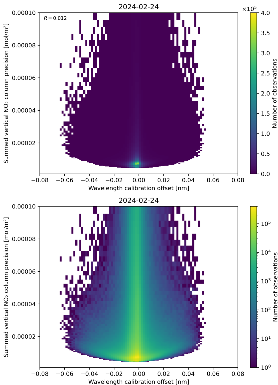
Figure 178: Scatter density plot of “Wavelength calibration offset” against “Summed vertical NO 2 column precision” for 2024-02-23 to 2024-02-25.
