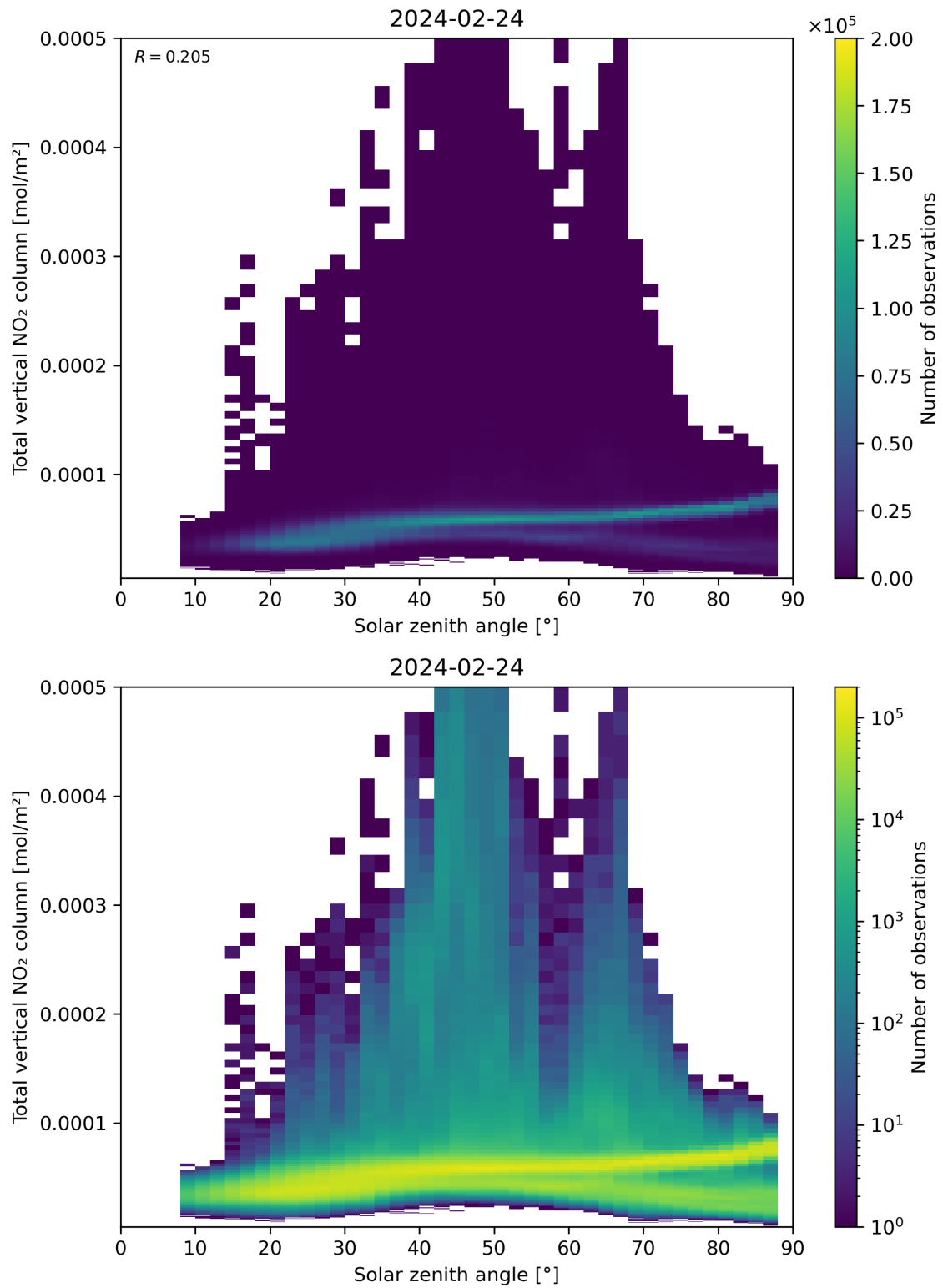
Figure 153: Scatter density plot of “Solar zenith angle” against “Total vertical NO 2 column” for 2024-02-23 to 2024-02-25.
