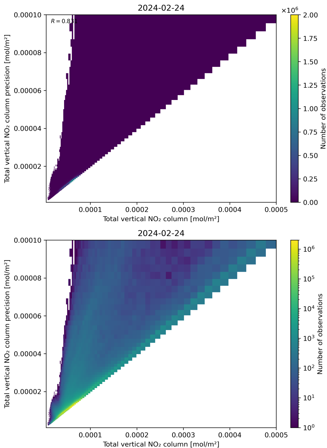
Figure 114: Scatter density plot of “Total vertical NO 2 column” against “Total vertical NO 2 column precision” for 2024-02-23 to 2024-02-25.
