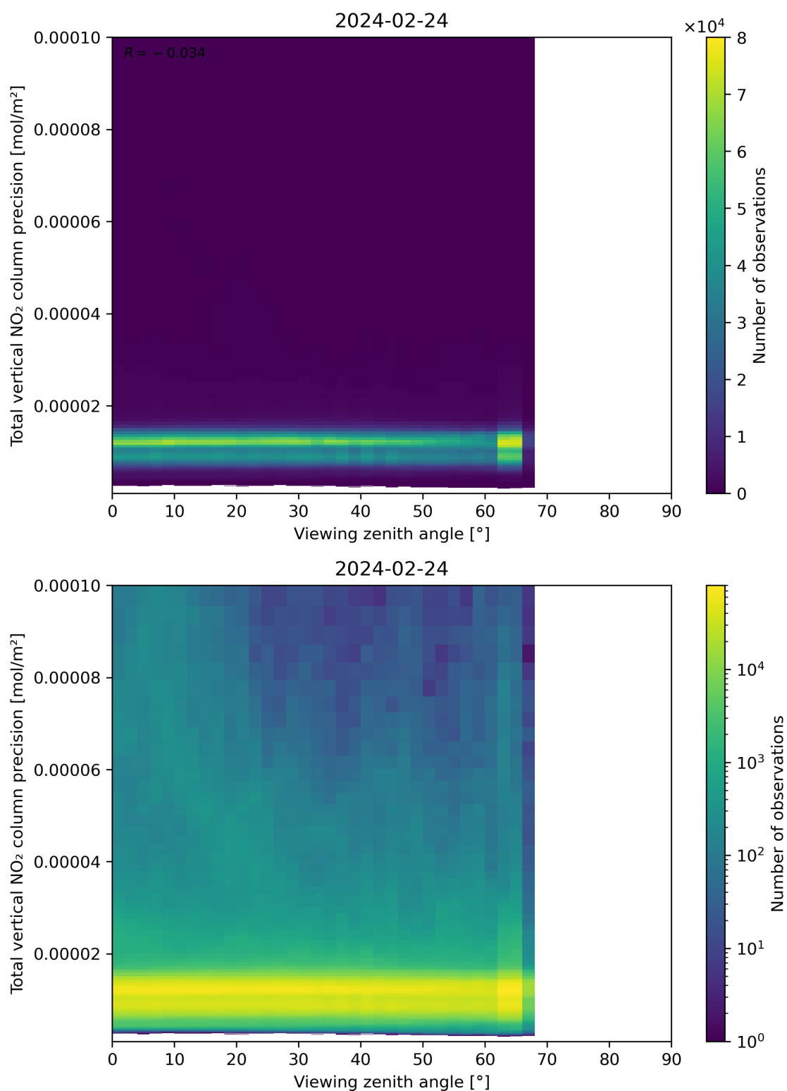
Figure 168: Scatter density plot of “Viewing zenith angle” against “Total vertical NO 2 column precision” for 2024-02-23 to 2024-02-25.
