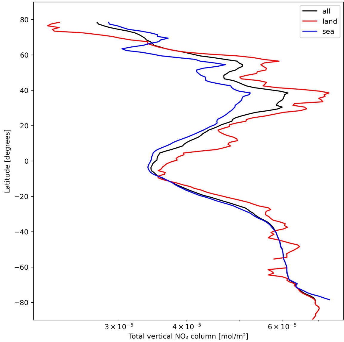
Figure 21: Zonal average of “Total vertical NO 2 column” for 2024-02-23 to 2024-02-25.
