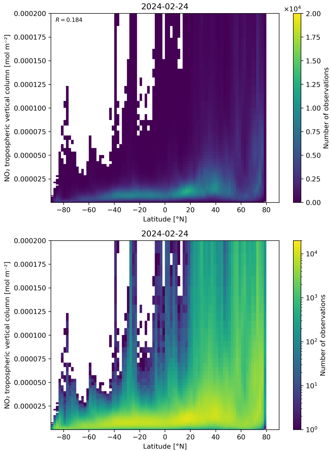
Figure 92: Scatter density plot of “Latitude” against “NO 2 tropospheric vertical column” for 2024-02-23 to 2024-02-25.
