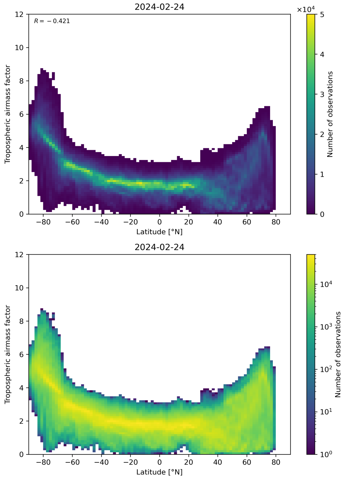
Figure 85: Scatter density plot of “Latitude” against “Tropospheric airmass factor” for 2024-02-23 to 2024-02-25.
