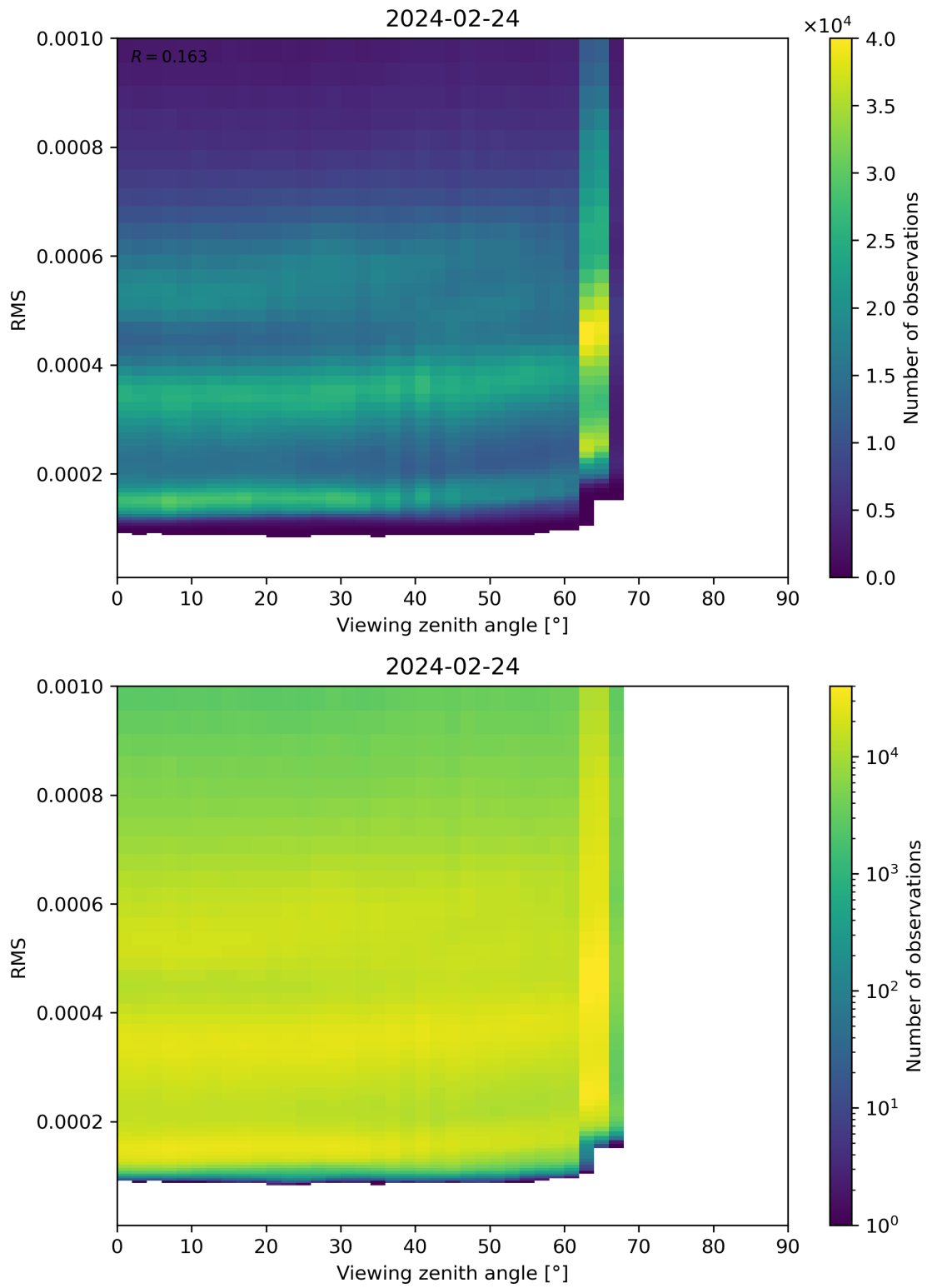
Figure 171: Scatter density plot of “Viewing zenith angle” against “RMS” for 2024-02-23 to 2024-02-25.
