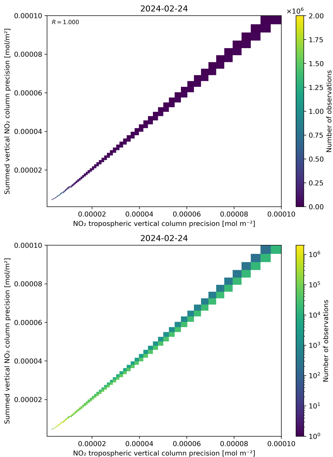
Figure 137: Scatter density plot of “NO 2 tropospheric vertical column precision” against “Summed vertical NO 2 column precision” for 2024-02-23 to 2024-02-25.
