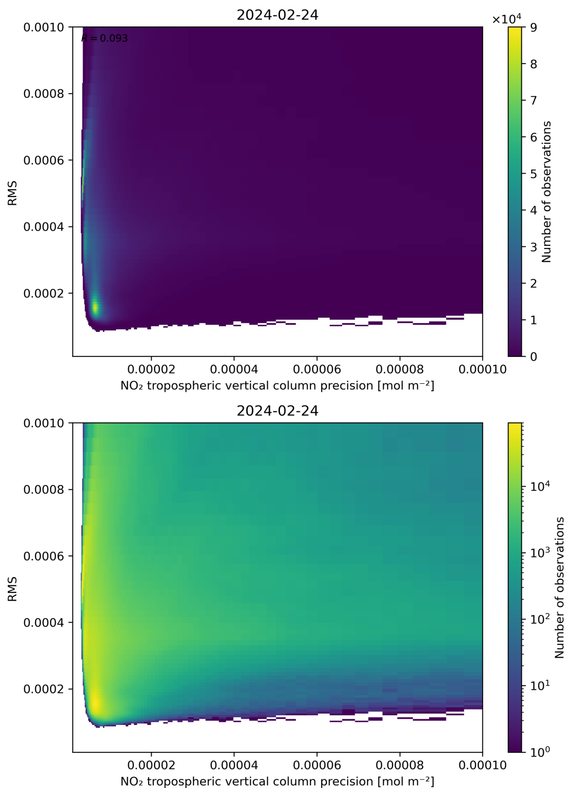
Figure 140: Scatter density plot of “NO 2 tropospheric vertical column precision” against “RMS” for 2024-02-23 to 2024-02-25.
