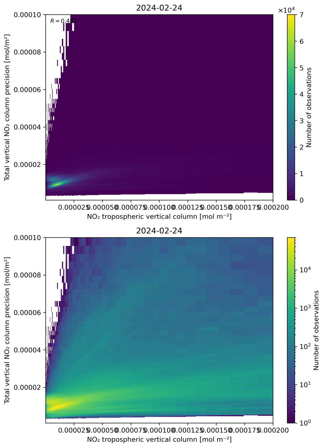
Figure 129: Scatter density plot of “NO 2 tropospheric vertical column” against “Total vertical NO 2 column precision” for 2024-02-23 to 2024-02-25.
