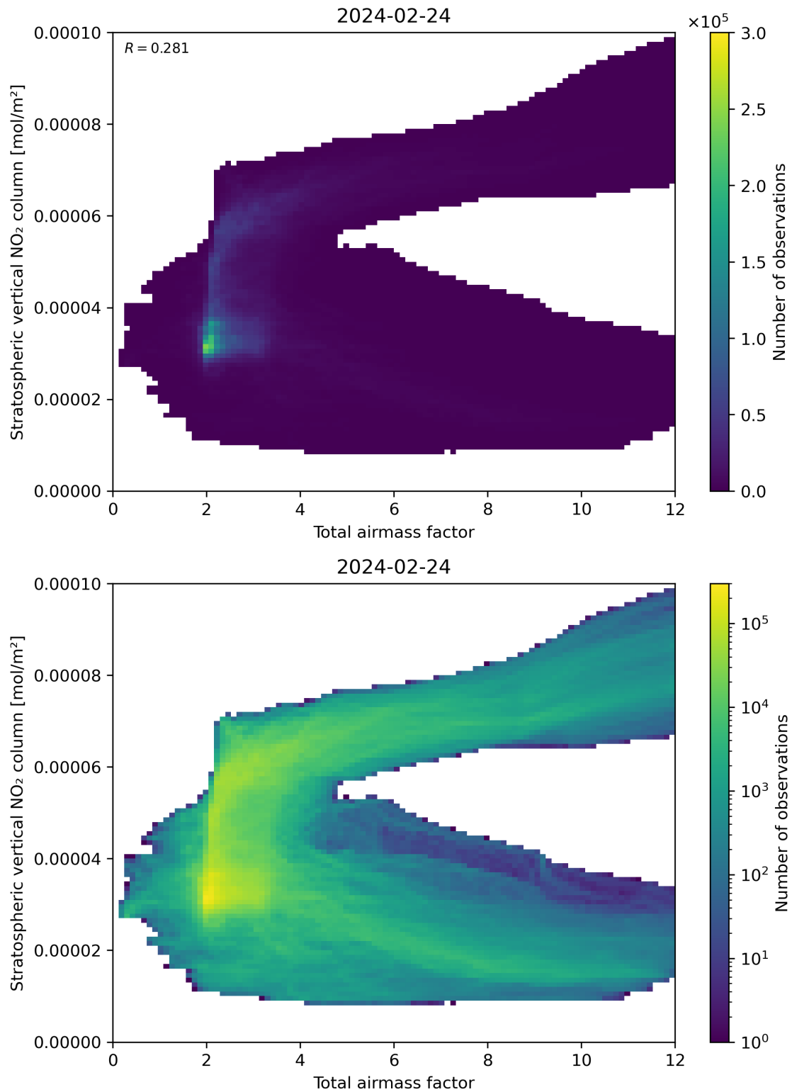
Figure 64: Scatter density plot of “Total airmass factor” against “Stratospheric vertical \text{NO}_2 column” for 2024-02-23 to 2024-02-25.
