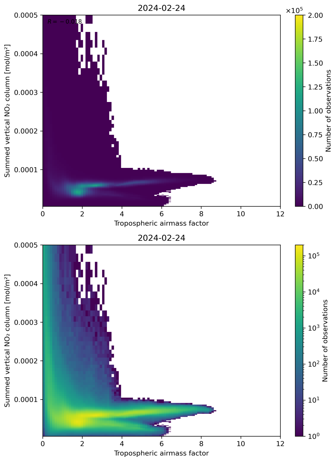
Figure 75: Scatter density plot of “Tropospheric airmass factor” against “Summed vertical NO 2 column” for 2024-02-23 to 2024-02-25.
