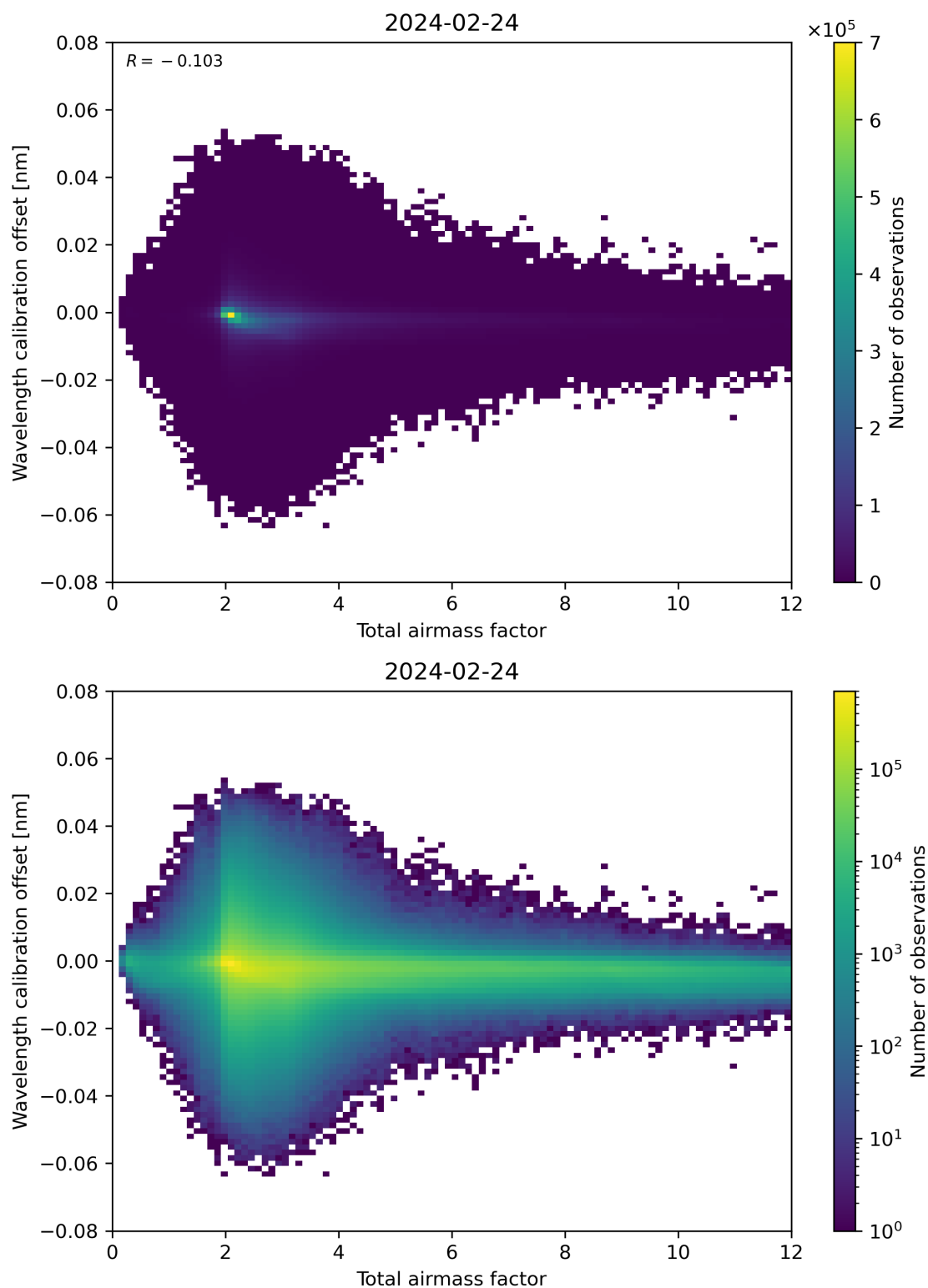
Figure 70: Scatter density plot of “Total airmass factor” against “Wavelength calibration offset” for 2024-02-23 to 2024-02-25.
