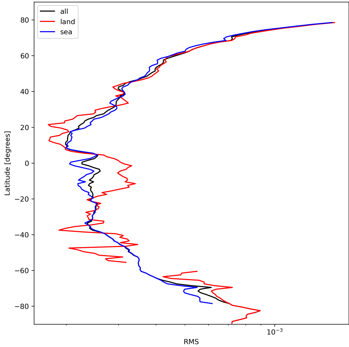
Figure 26: Zonal average of “RMS” for 2024-02-23 to 2024-02-25.
