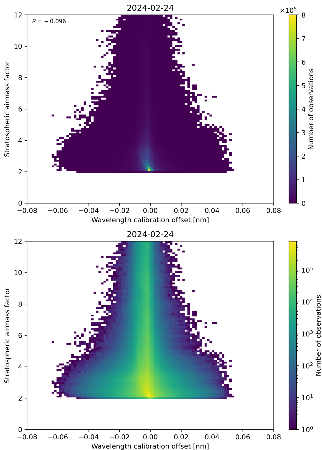
Figure 174: Scatter density plot of “Wavelength calibration offset” against “Stratospheric airmass factor” for 2024-02-23 to 2024-02-25.
