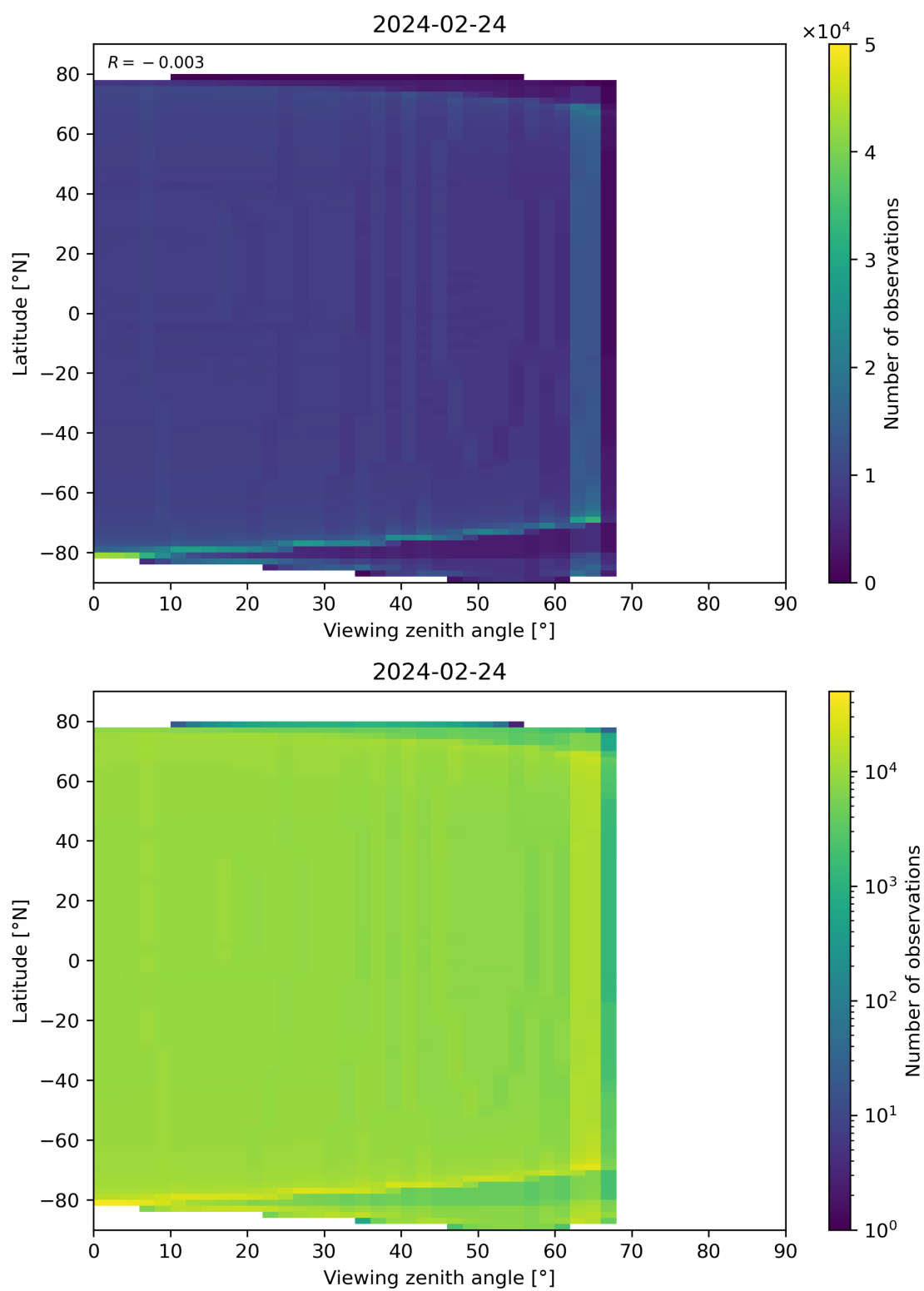
Figure 163: Scatter density plot of “Viewing zenith angle” against “Latitude” for 2024-02-23 to 2024-02-25.
