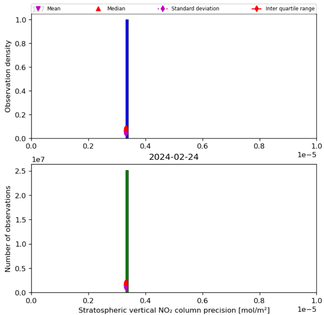
Figure 37: Histogram of “Stratospheric vertical NO 2 column precision” for 2024-02-23 to 2024-02-25
