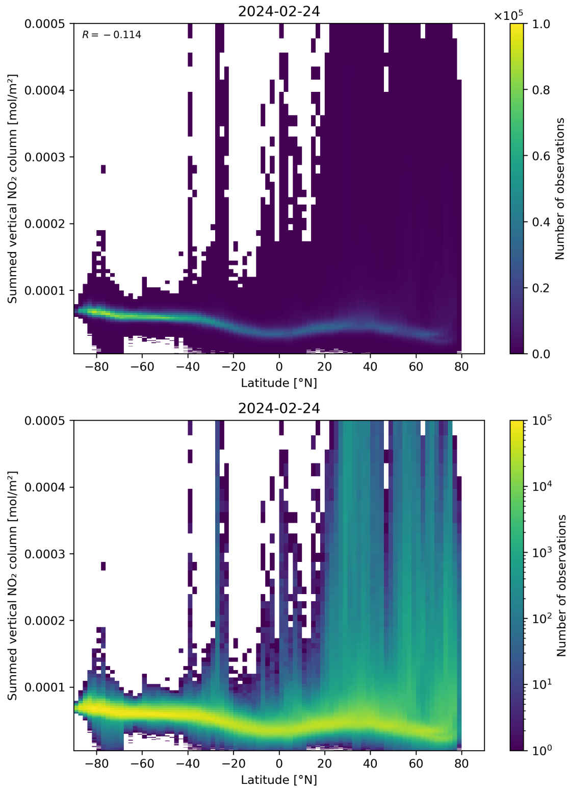
Figure 88: Scatter density plot of “Latitude” against “Summed vertical NO 2 column” for 2024-02-23 to 2024-02-25.
