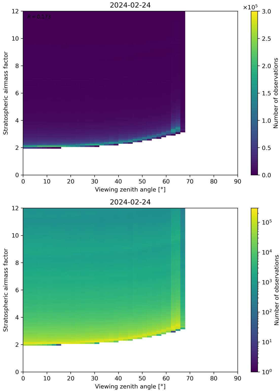
Figure 159: Scatter density plot of “Viewing zenith angle” against “Stratospheric airmass factor” for 2024-02-23 to 2024-02-25.
