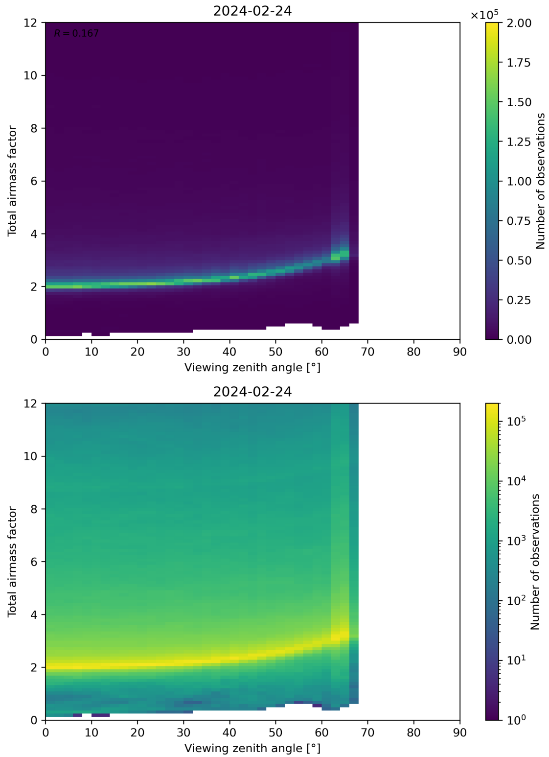
Figure 160: Scatter density plot of “Viewing zenith angle” against “Total airmass factor” for 2024-02-23 to 2024-02-25.
