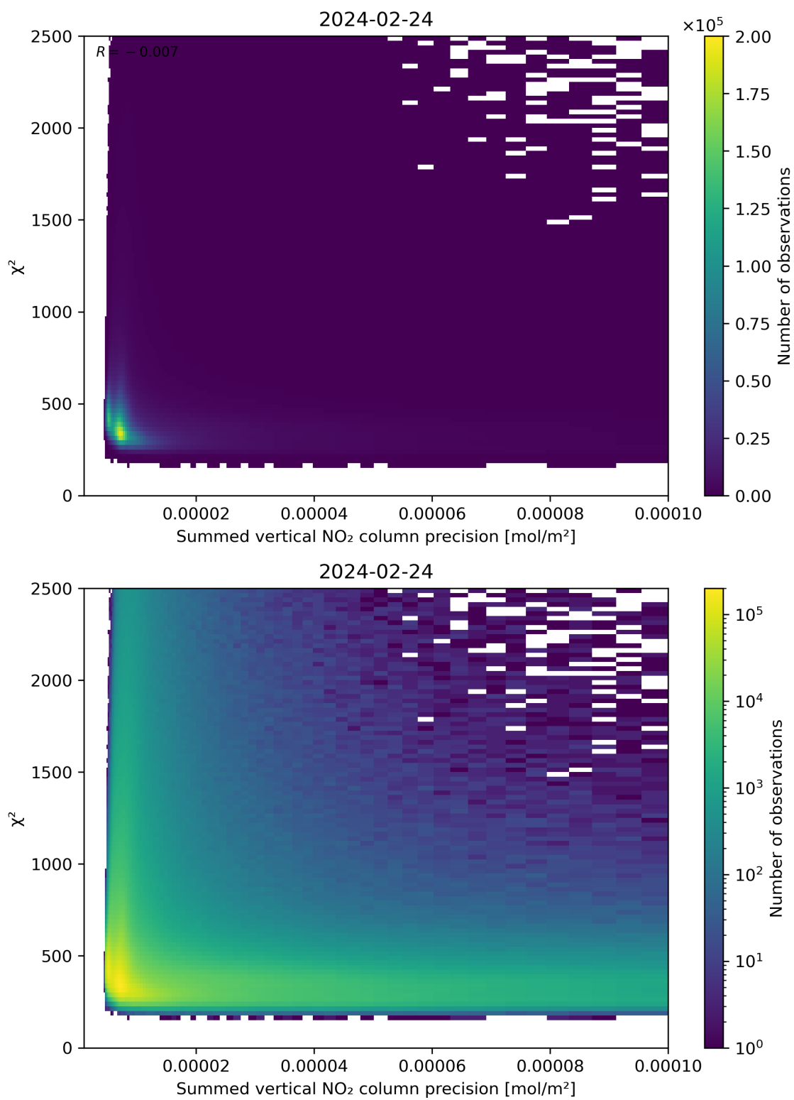
Figure 107: Scatter density plot of “Summed vertical NO 2 column precision” against “ \chi^2 ” for 2024-02-23 to 2024-02-25.
