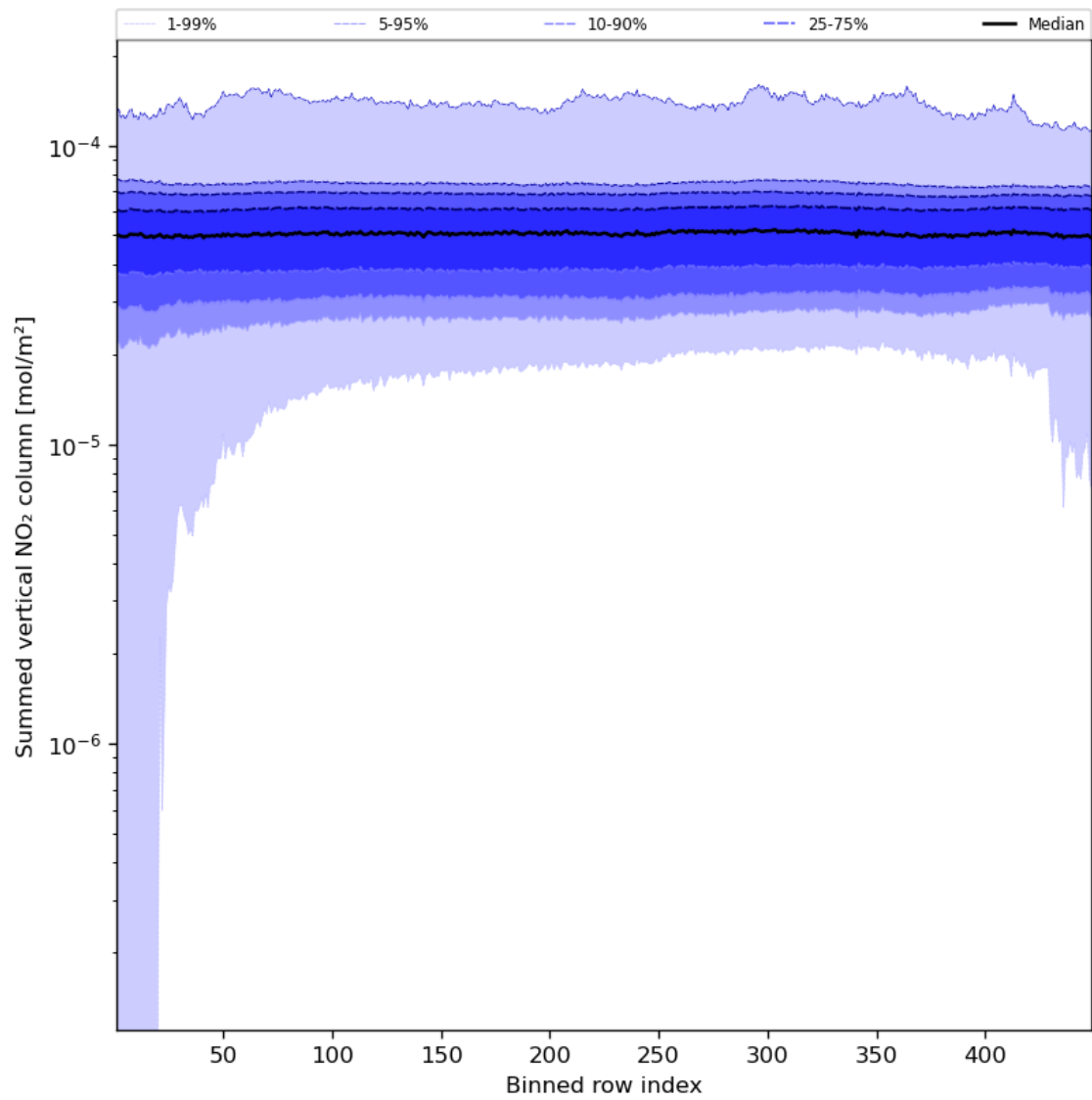
Figure 57: Along track statistics of “Summed vertical NO 2 column” for 2024-02-23 to 2024-02-25
