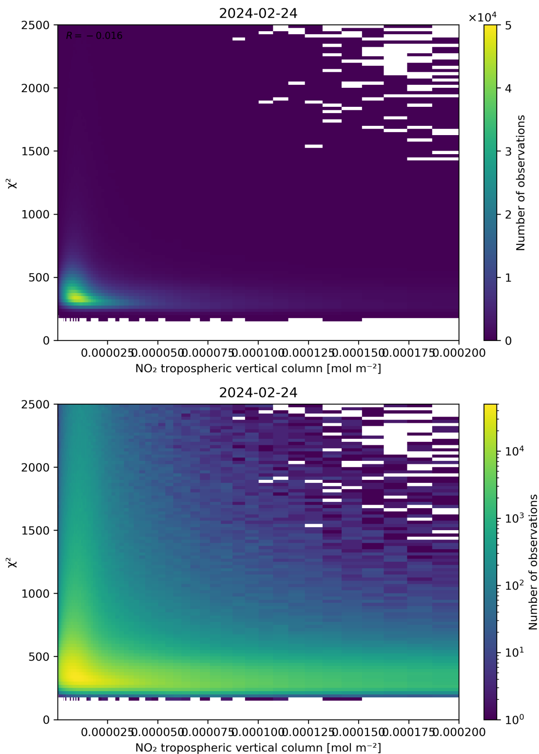
Figure 124: Scatter density plot of “NO 2 tropospheric vertical column” against “ \chi^2 ” for 2024-02-23 to 2024-02-25.
