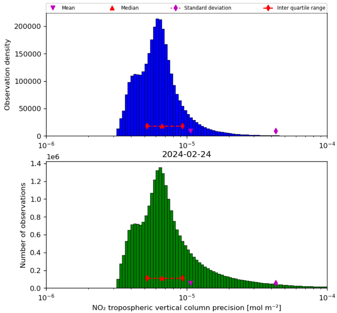
Figure 30: Histogram of “NO 2 tropospheric vertical column precision” for 2024-02-23 to 2024-02-25
