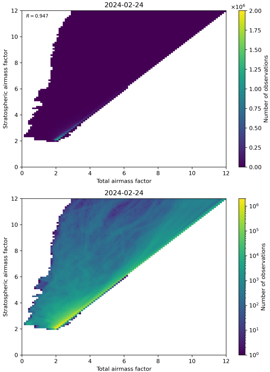
Figure 62: Scatter density plot of “Total airmass factor” against “Stratospheric airmass factor” for 2024-02-23 to 2024-02-25.
