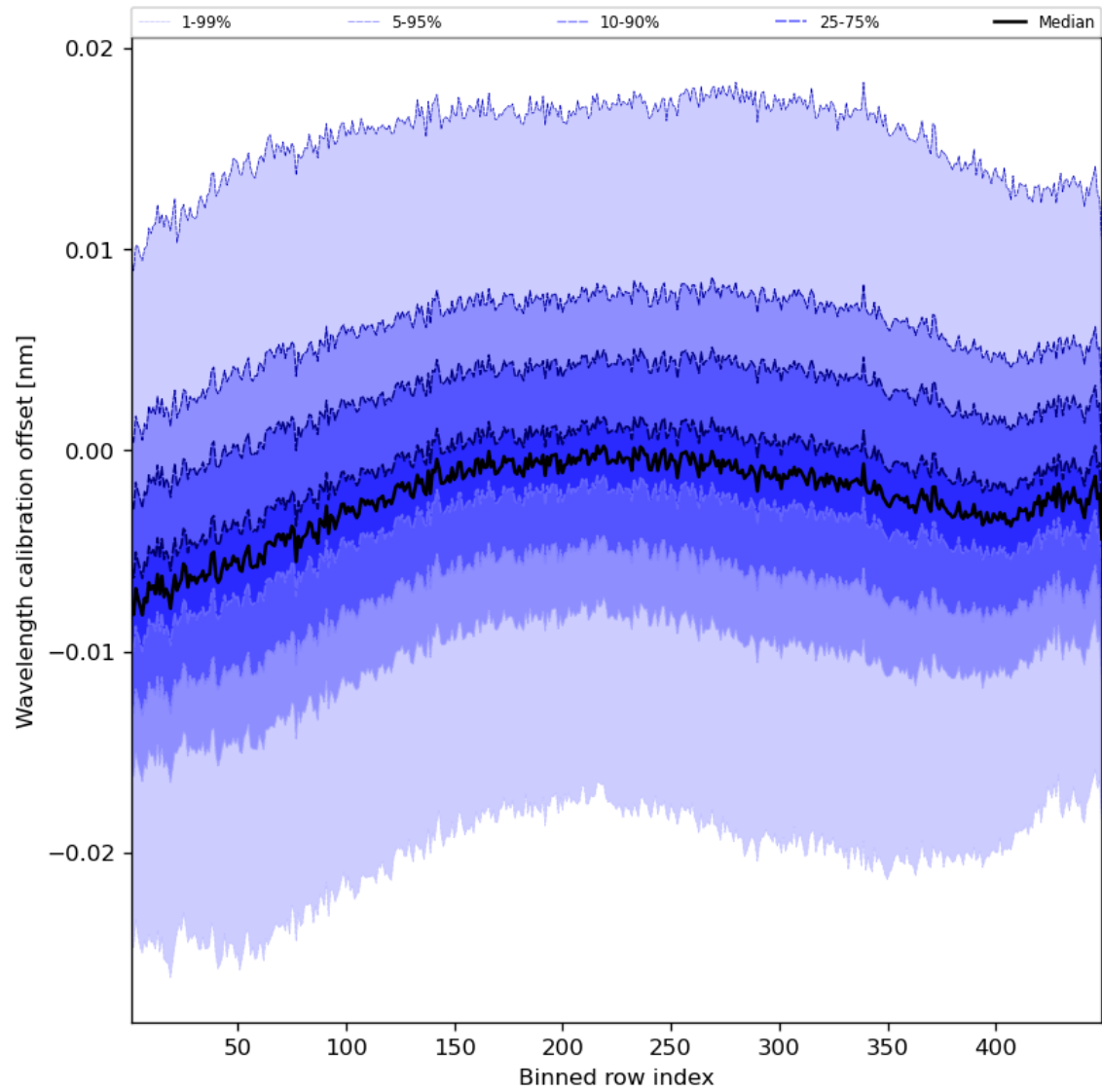
Figure 52: Along track statistics of “Wavelength calibration offset” for 2024-02-23 to 2024-02-25
