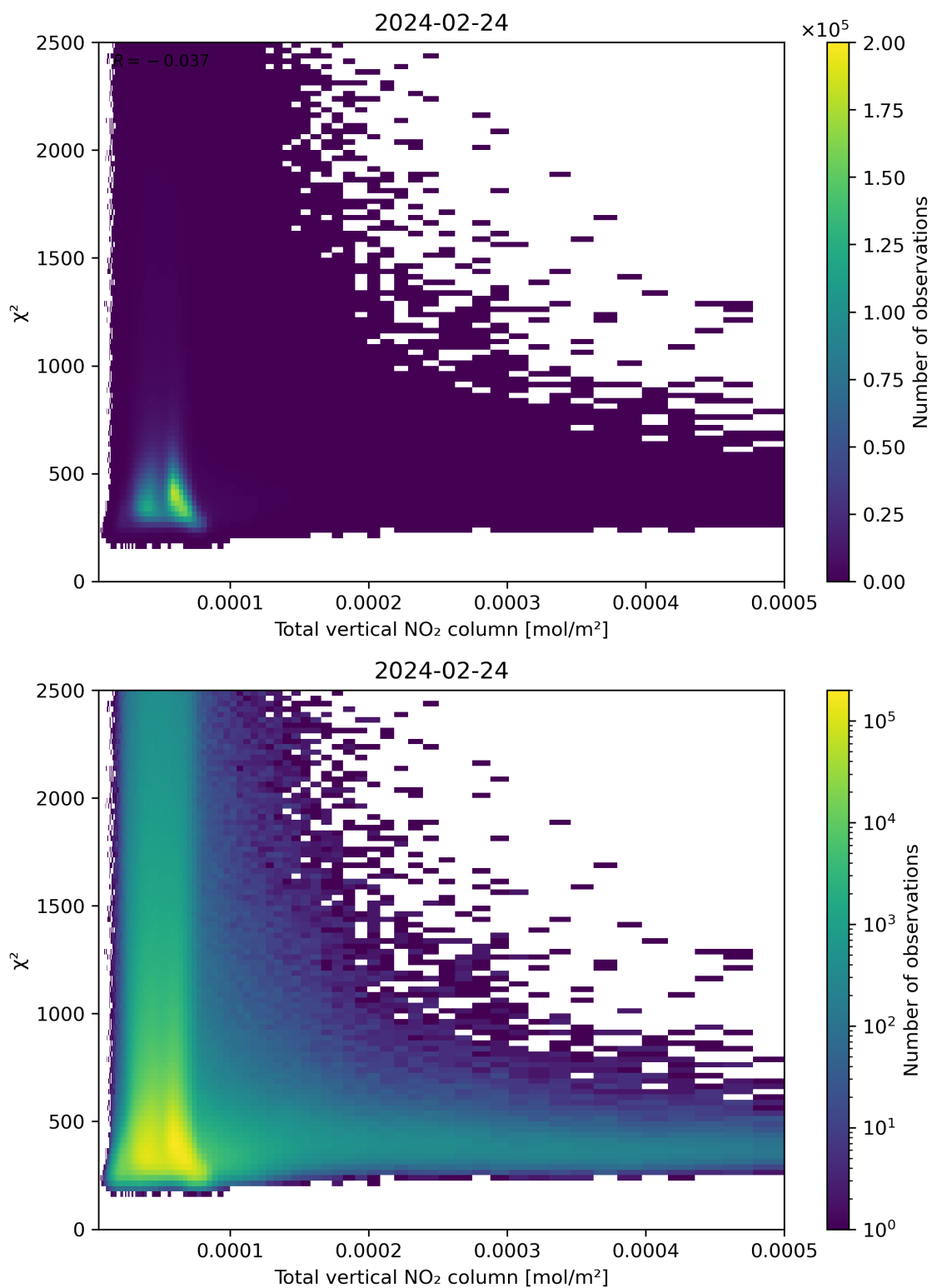
Figure 111: Scatter density plot of “Total vertical NO 2 column” against “ \chi^2 ” for 2024-02-23 to 2024-02-25.
