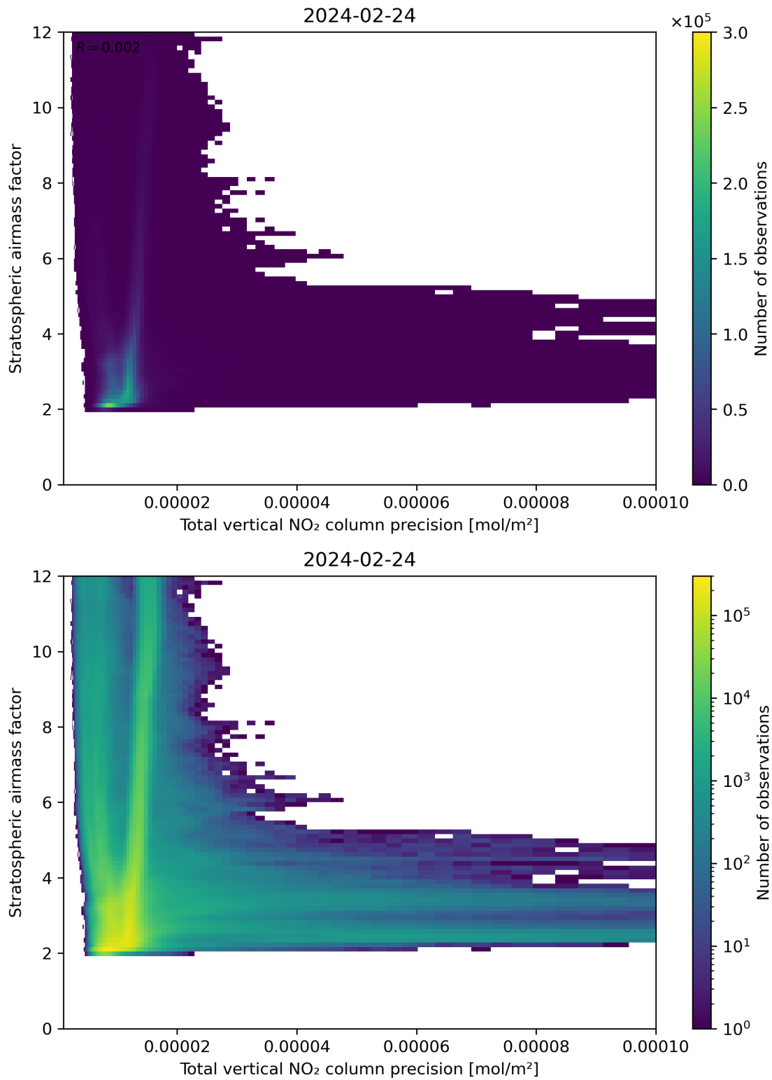
Figure 115: Scatter density plot of “Total vertical NO 2 column precision” against “Stratospheric air mass factor” for 2024-02-23 to 2024-02-25.
