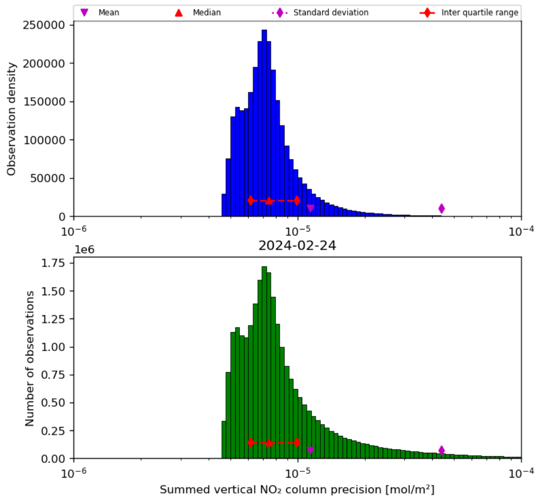
Figure 41: Histogram of “Summed vertical NO 2 column precision” for 2024-02-23 to 2024-02-25
