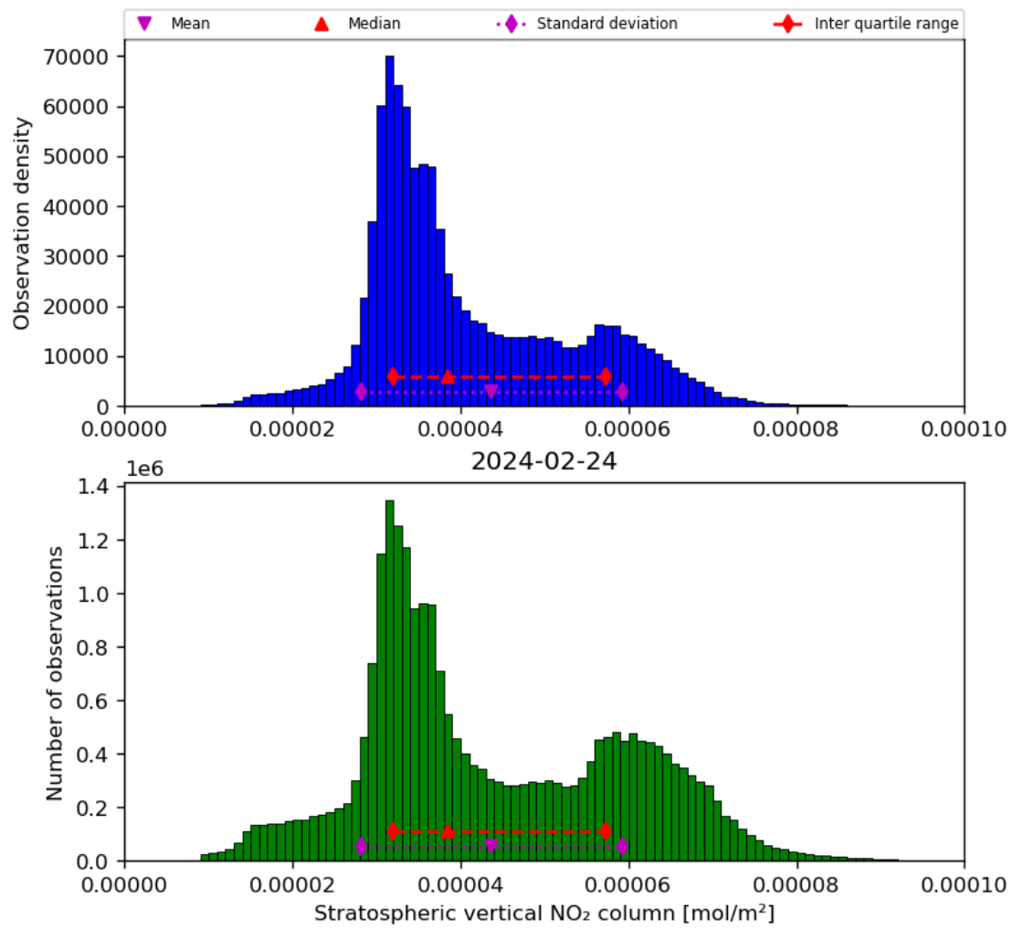
Figure 36: Histogram of “Stratospheric vertical NO 2 column” for 2024-02-23 to 2024-02-25
