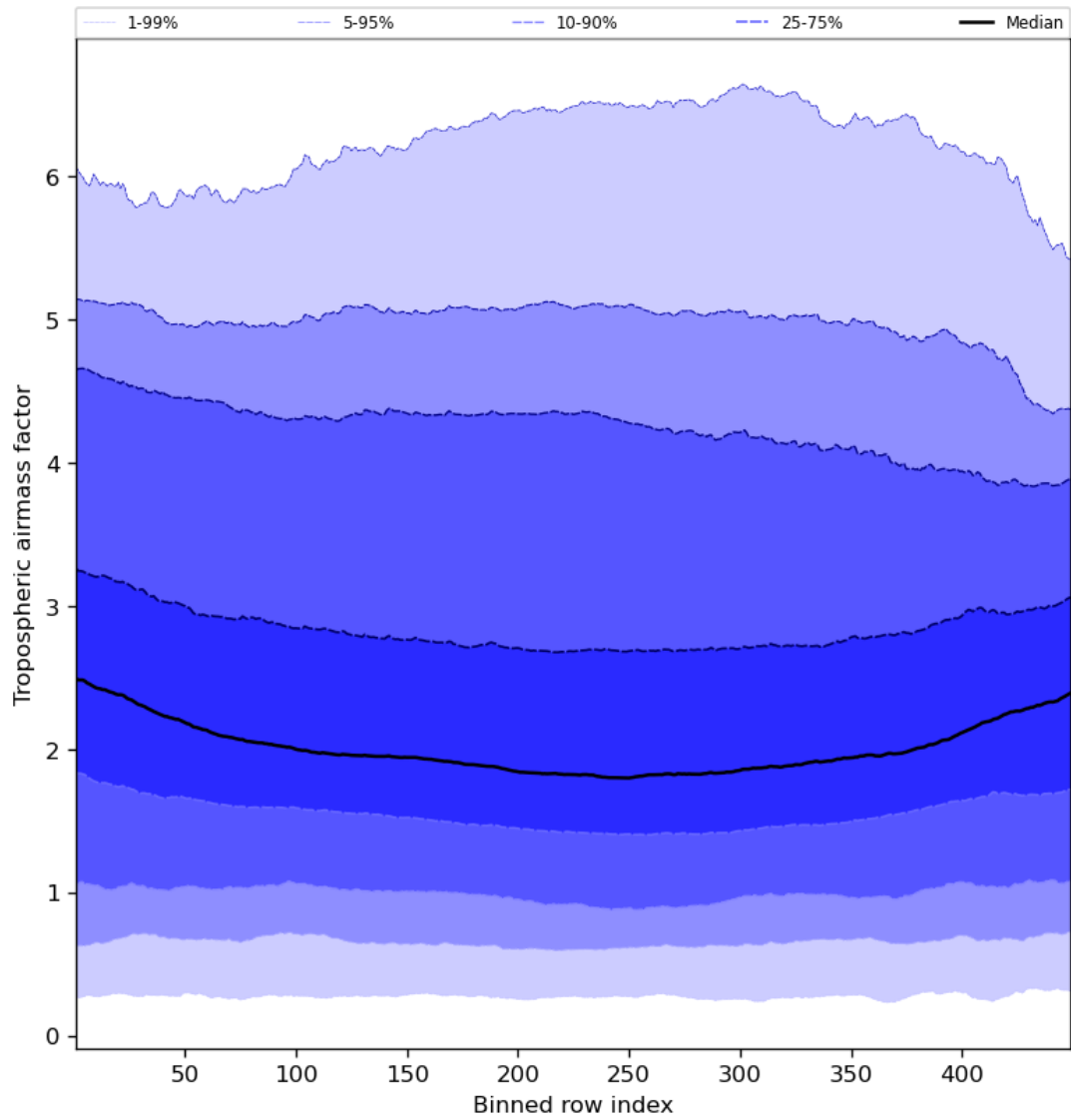
Figure 48: Along track statistics of “Tropospheric airmass factor” for 2024-02-23 to 2024-02-25
