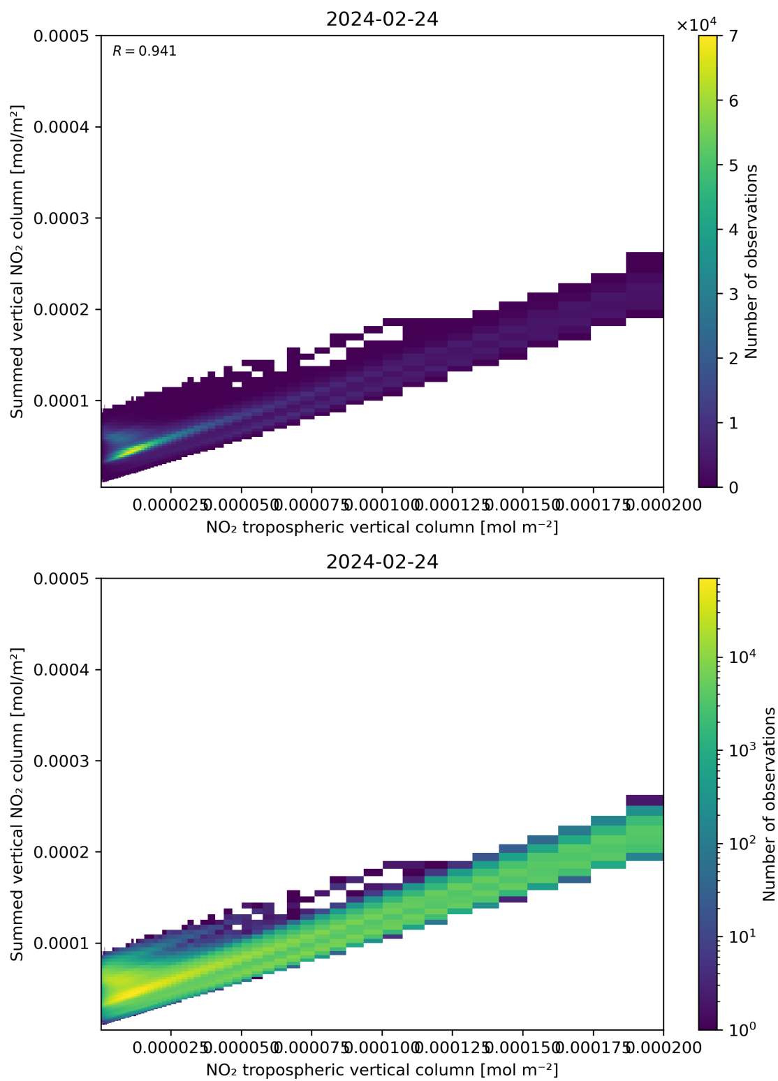
Figure 126: Scatter density plot of “NO 2 tropospheric vertical column” against “Summed vertical NO 2 column” for 2024-02-23 to 2024-02-25.
