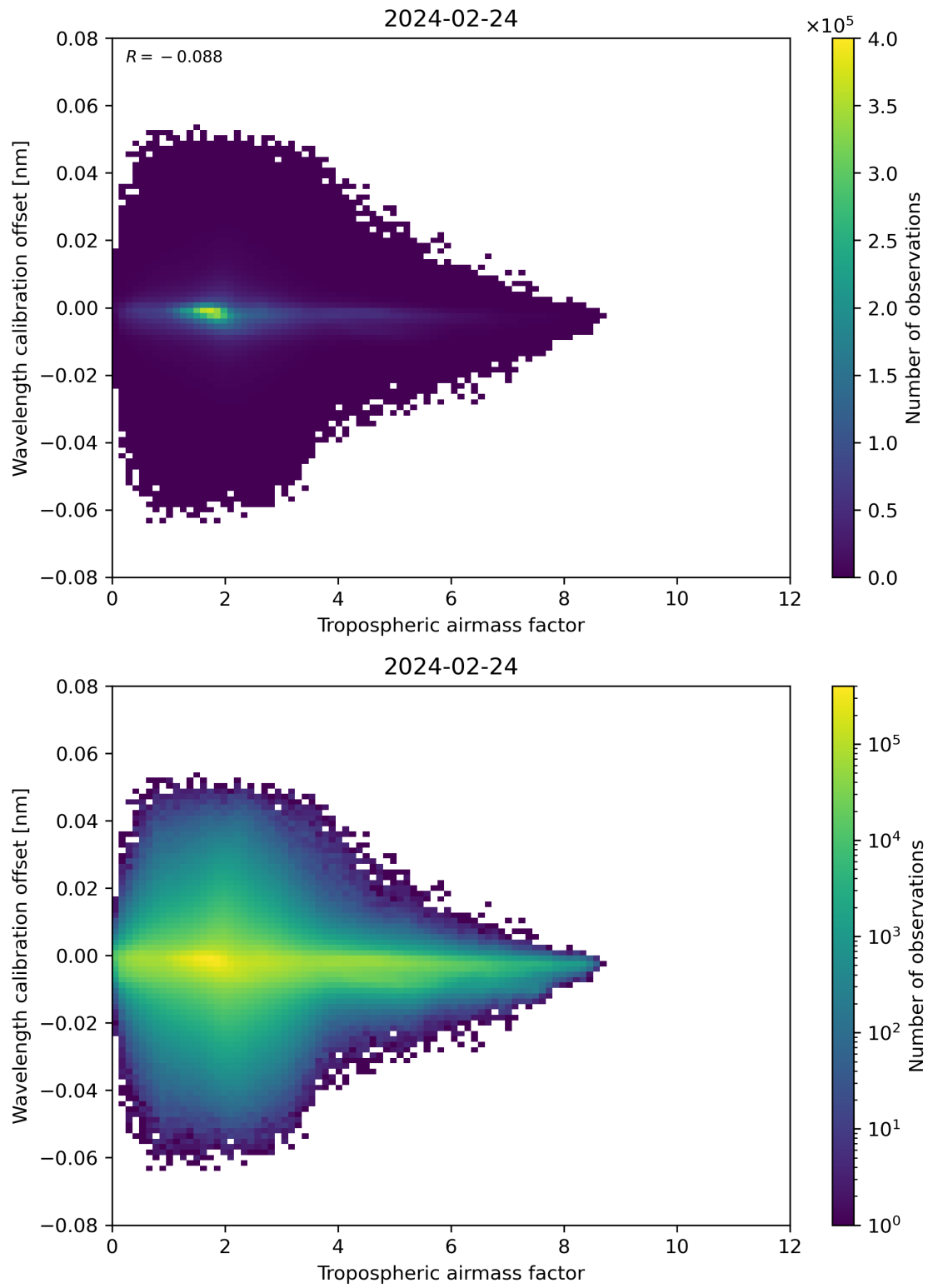
Figure 80: Scatter density plot of “Tropospheric airmass factor” against “Wavelength calibration offset” for 2024-02-23 to 2024-02-25.
