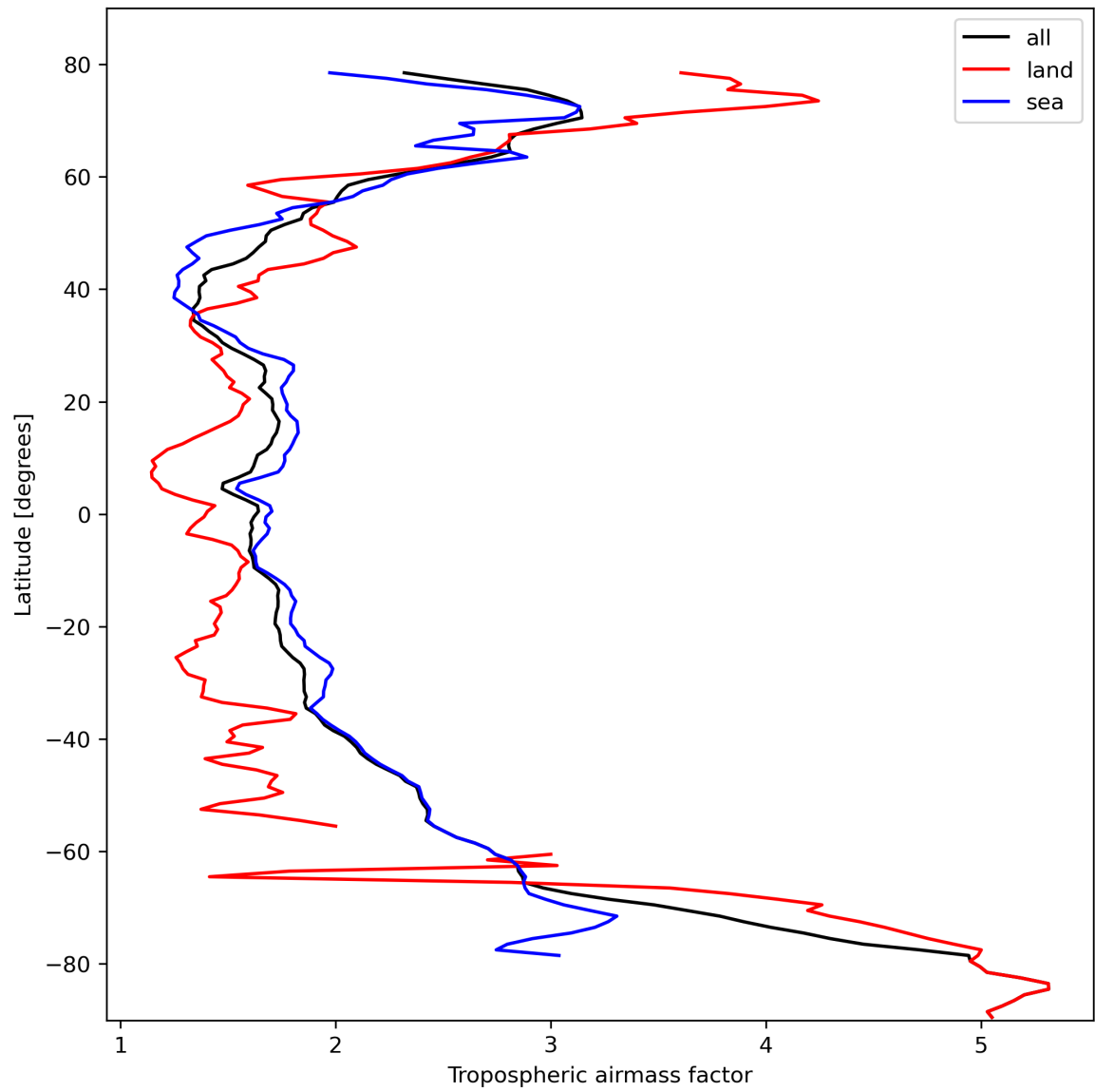
Figure 14: Zonal average of “Tropospheric airmass factor” for 2024-02-23 to 2024-02-25.
