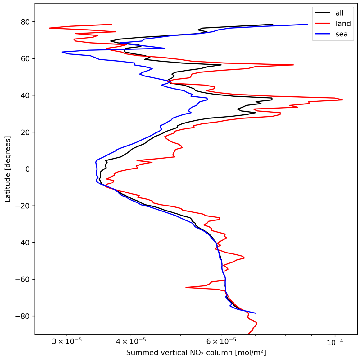
Figure 23: Zonal average of “Summed vertical NO 2 column” for 2024-02-23 to 2024-02-25.
