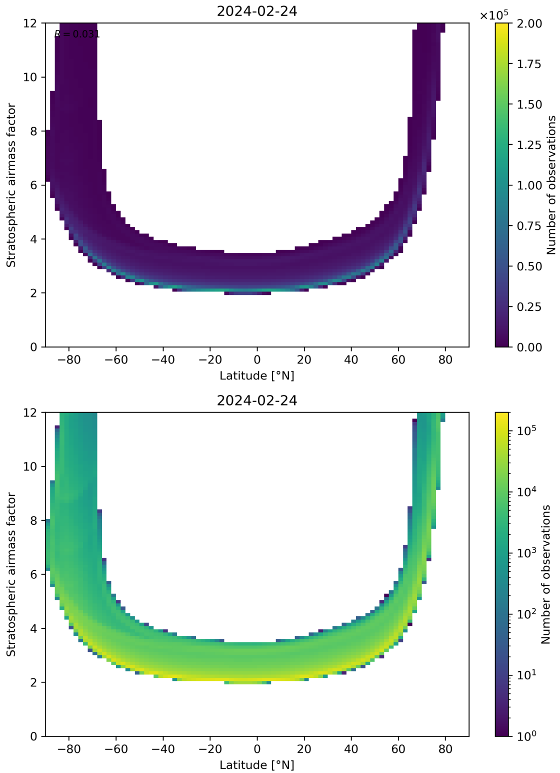
Figure 83: Scatter density plot of “Latitude” against “Stratospheric airmass factor” for 2024-02-23 to 2024-02-25.
