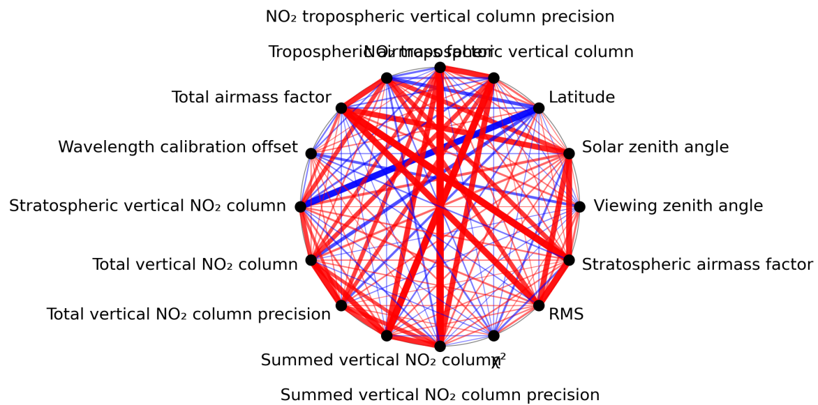
Figure 1: Map of correlation graph for 2024-02-23 to 2024-02-25.
