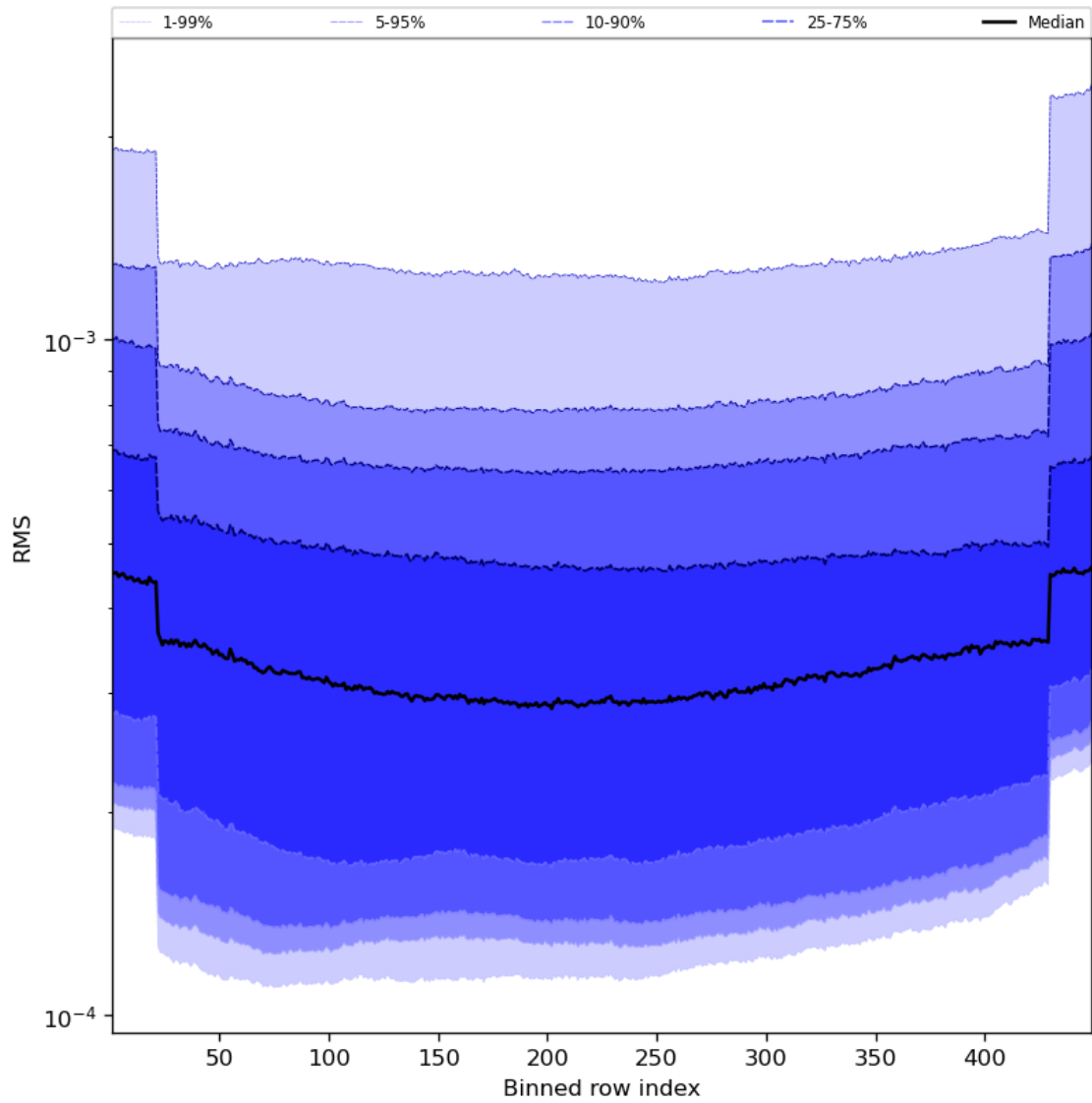
Figure 60: Along track statistics of “RMS” for 2024-02-23 to 2024-02-25
