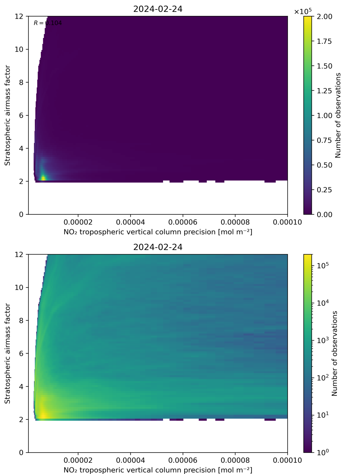
Figure 131: Scatter density plot of “NO 2 tropospheric vertical column precision” against “Stratospheric airmass factor” for 2024-02-23 to 2024-02-25.
