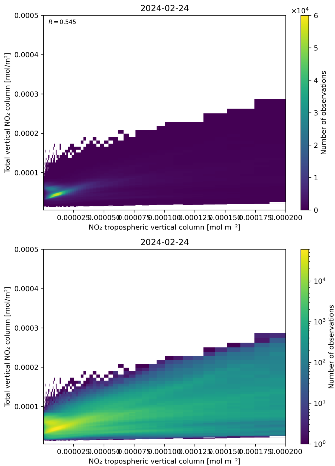
Figure 128: Scatter density plot of “NO 2 tropospheric vertical column” against “Total vertical NO 2 column” for 2024-02-23 to 2024-02-25.
