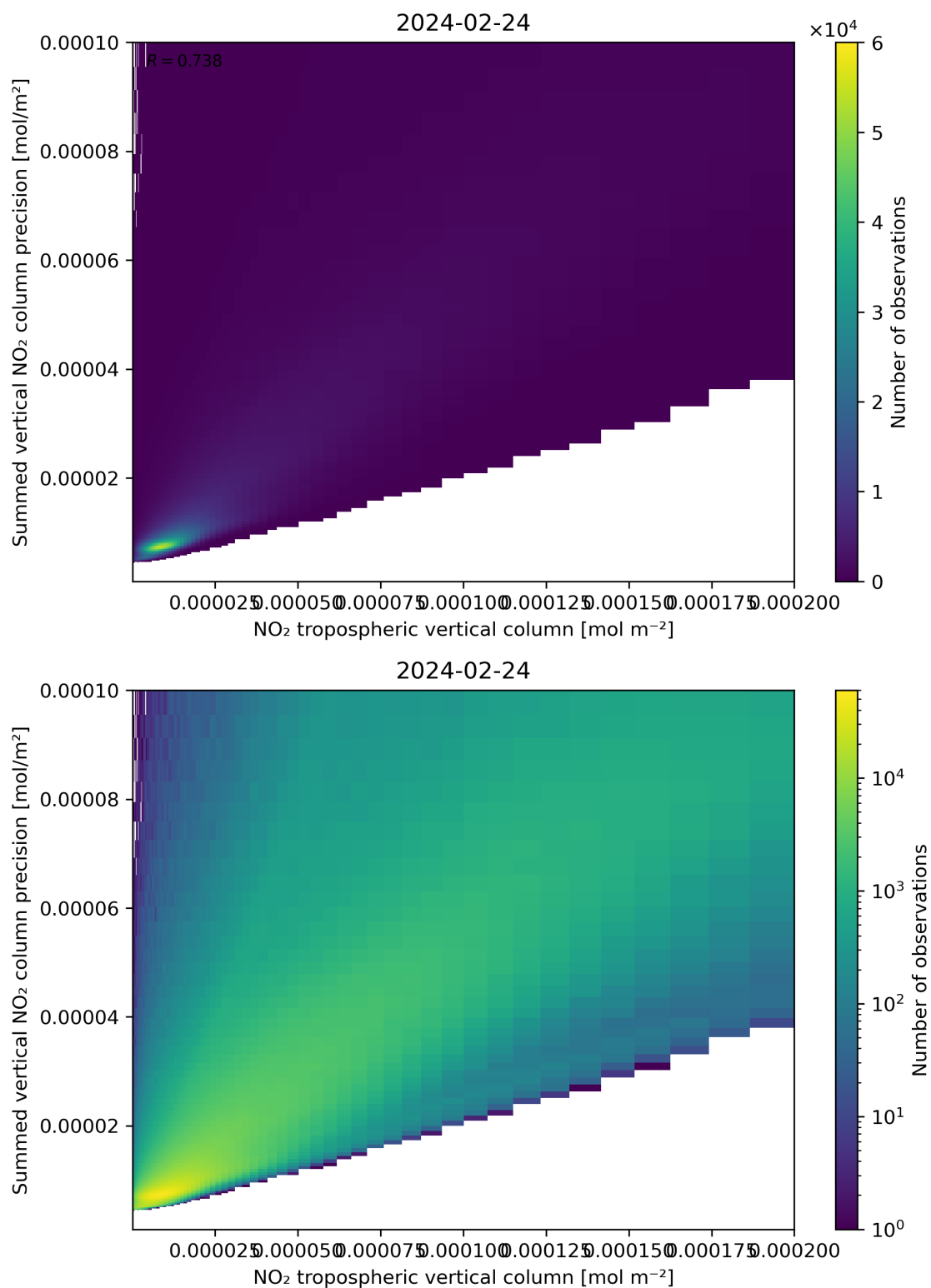
Figure 127: Scatter density plot of “NO 2 tropospheric vertical column” against “Summed vertical NO 2 column precision” for 2024-02-23 to 2024-02-25.
