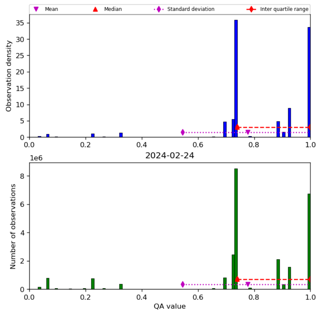
Figure 28: Histogram of “QA value” for 2024-02-23 to 2024-02-25
