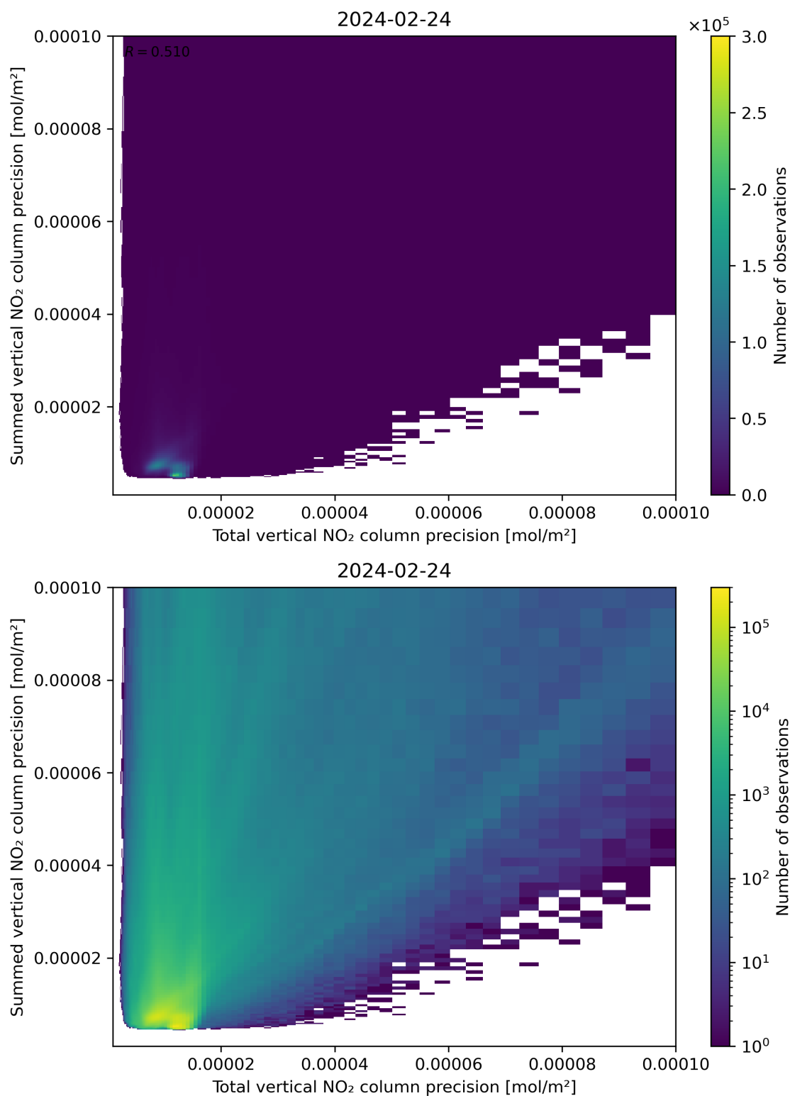
Figure 118: Scatter density plot of “Total vertical NO 2 column precision” against “Summed vertical NO 2 column precision” for 2024-02-23 to 2024-02-25.
