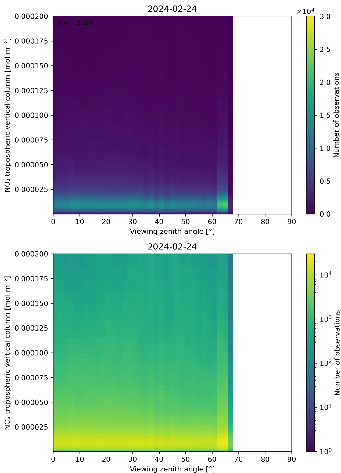
Figure 169: Scatter density plot of “Viewing zenith angle” against “NO 2 tropospheric vertical column” for 2024-02-23 to 2024-02-25.
