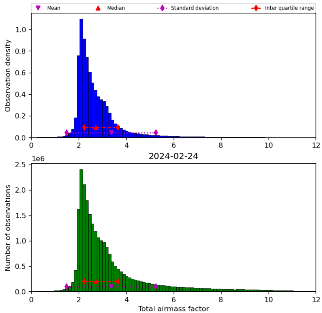
Figure 32: Histogram of “Total airmass factor” for 2024-02-23 to 2024-02-25
