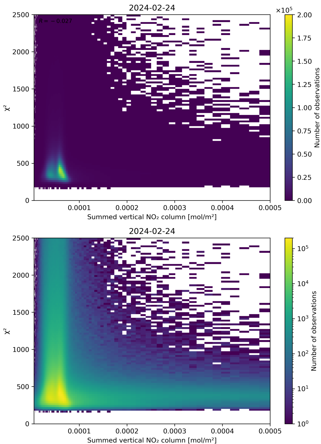
Figure 104: Scatter density plot of “Summed vertical NO 2 column” against “ \chi^2 ” for 2024-02-23 to 2024-02-25.
