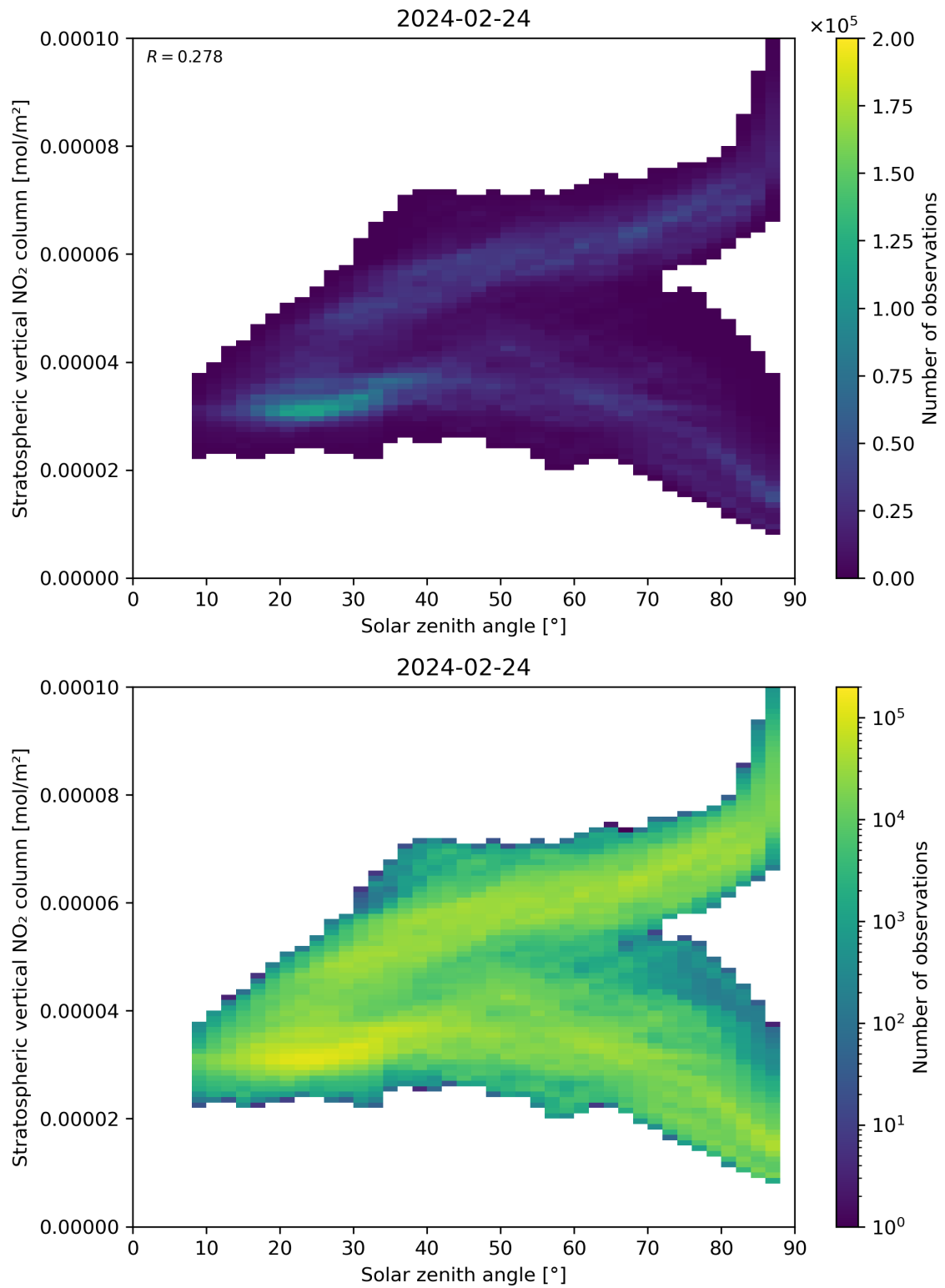
Figure 150: Scatter density plot of “Solar zenith angle” against “Stratospheric vertical NO 2 column” for 2024-02-23 to 2024-02-25.
