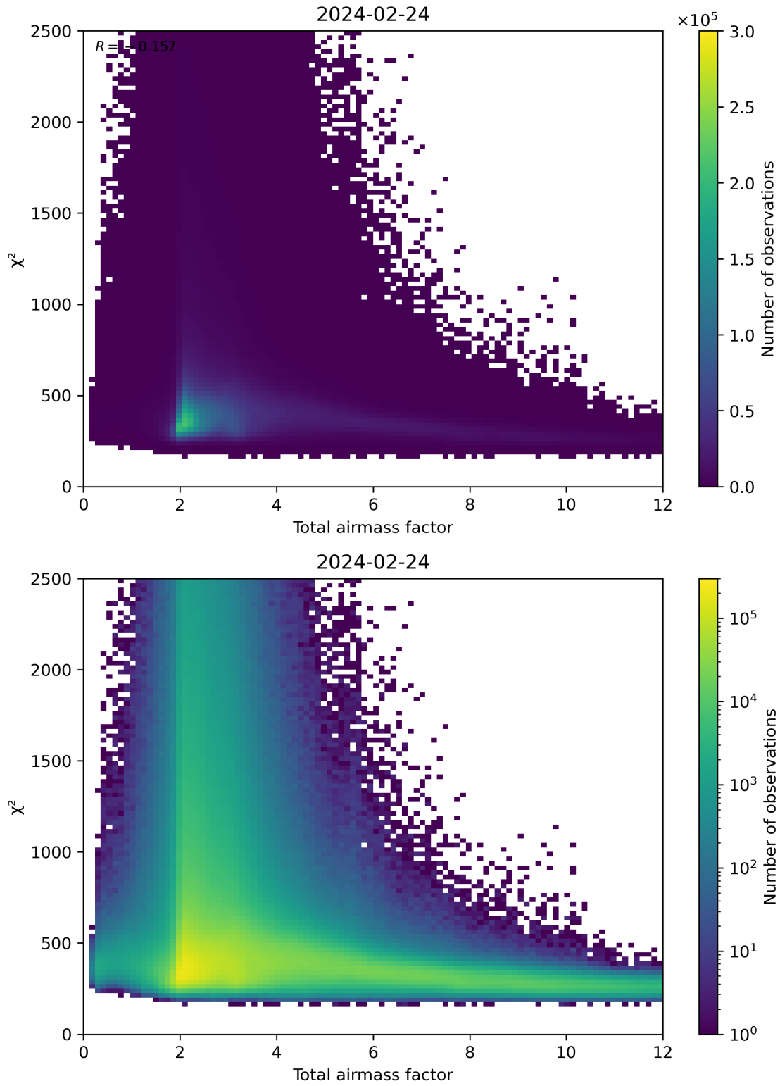
Figure 63: Scatter density plot of “Total airmass factor” against “ \chi^2 ” for 2024-02-23 to 2024-02-25.
