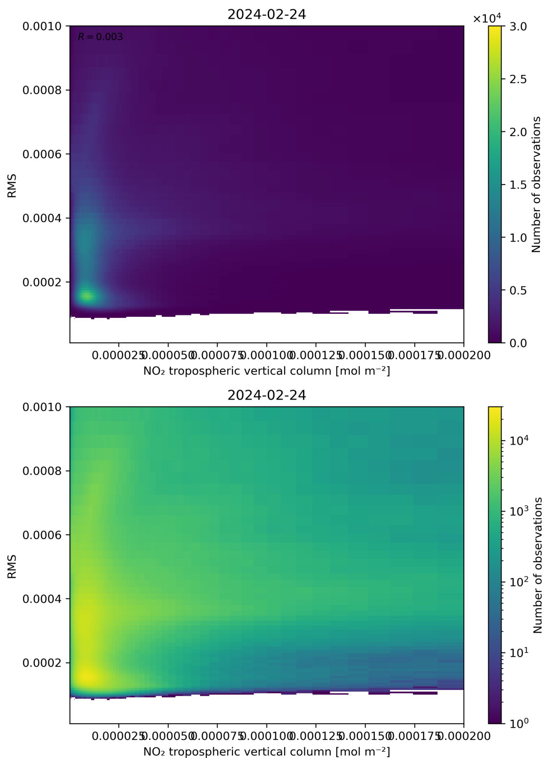
Figure 142: Scatter density plot of “NO 2 tropospheric vertical column” against “RMS” for 2024-02-23 to 2024-02-25.
