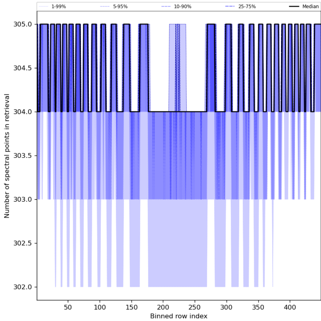
Figure 50: Along track statistics of “Number of spectral points in retrieval” for 2024-02-23 to 2024-02-25
