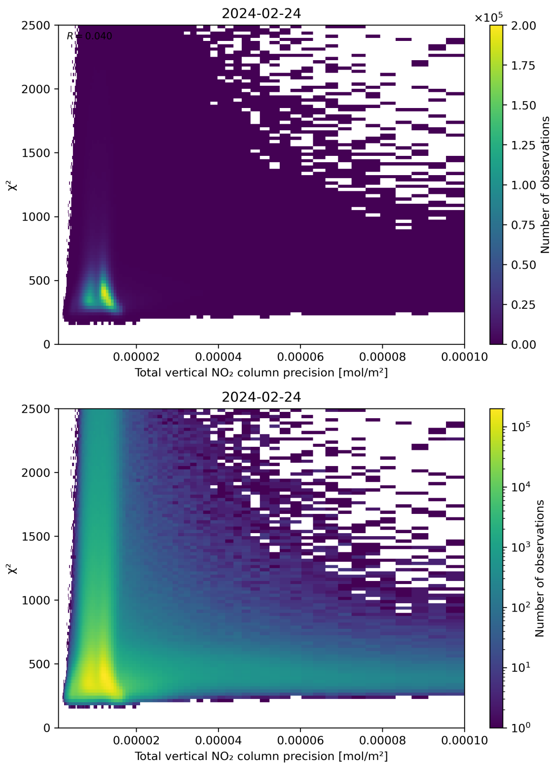
Figure 116: Scatter density plot of “Total vertical NO 2 column precision” against “ \chi^2 ” for 2024-02-23 to 2024-02-25.
