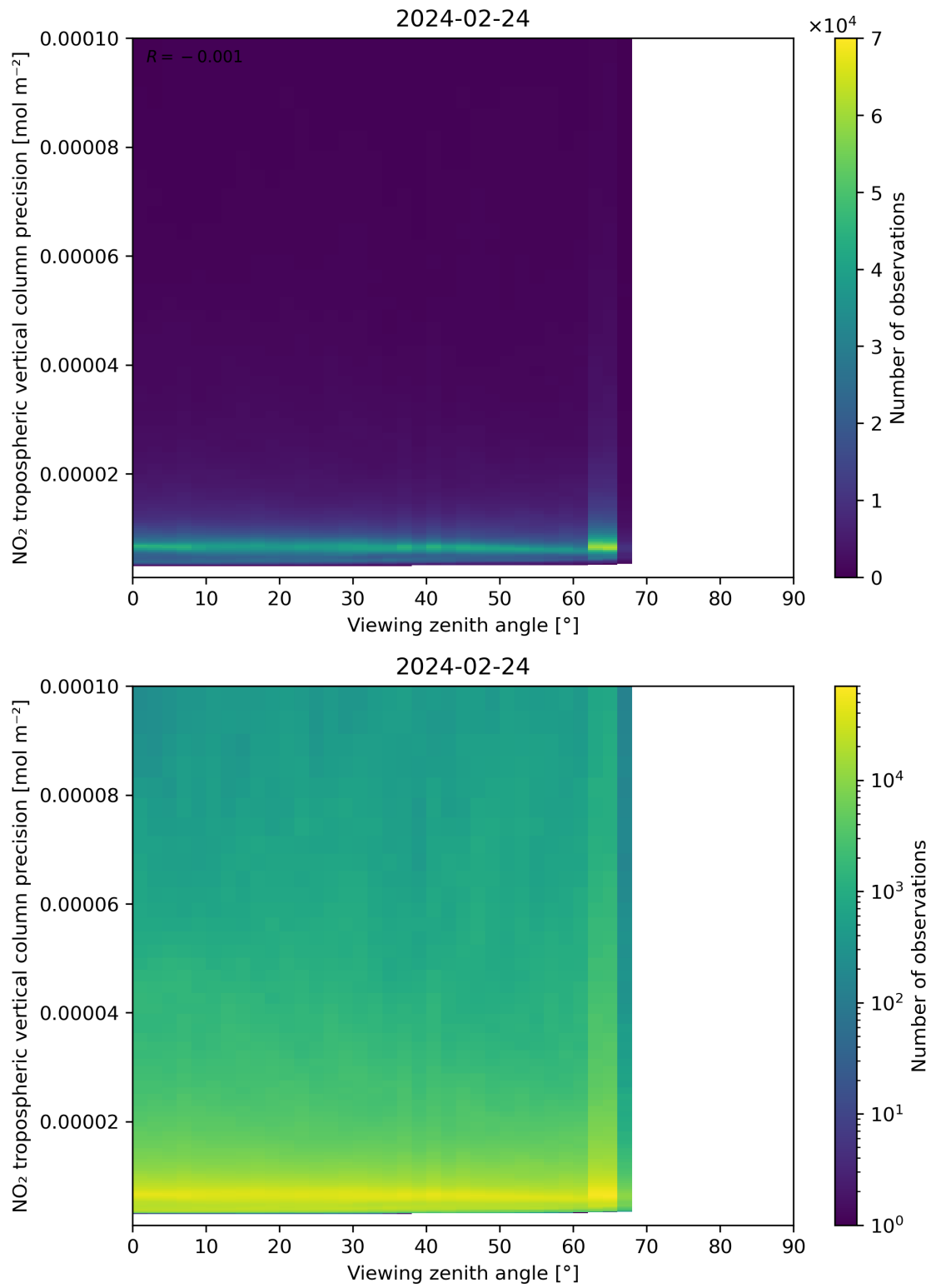
Figure 170: Scatter density plot of “Viewing zenith angle” against “NO 2 tropospheric vertical column precision” for 2024-02-23 to 2024-02-25.
