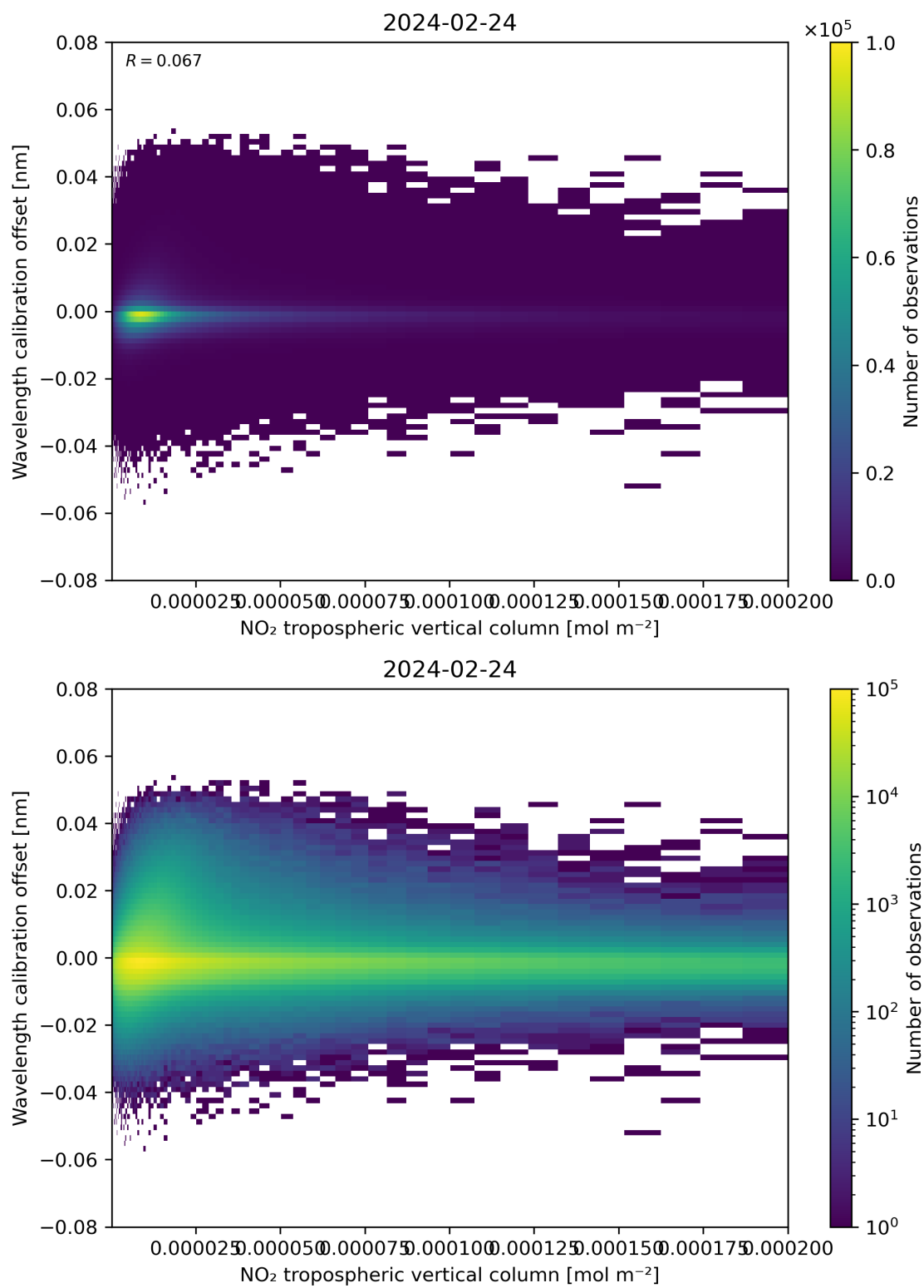
Figure 143: Scatter density plot of “NO 2 tropospheric vertical column” against “Wavelength calibration offset” for 2024-02-23 to 2024-02-25.
