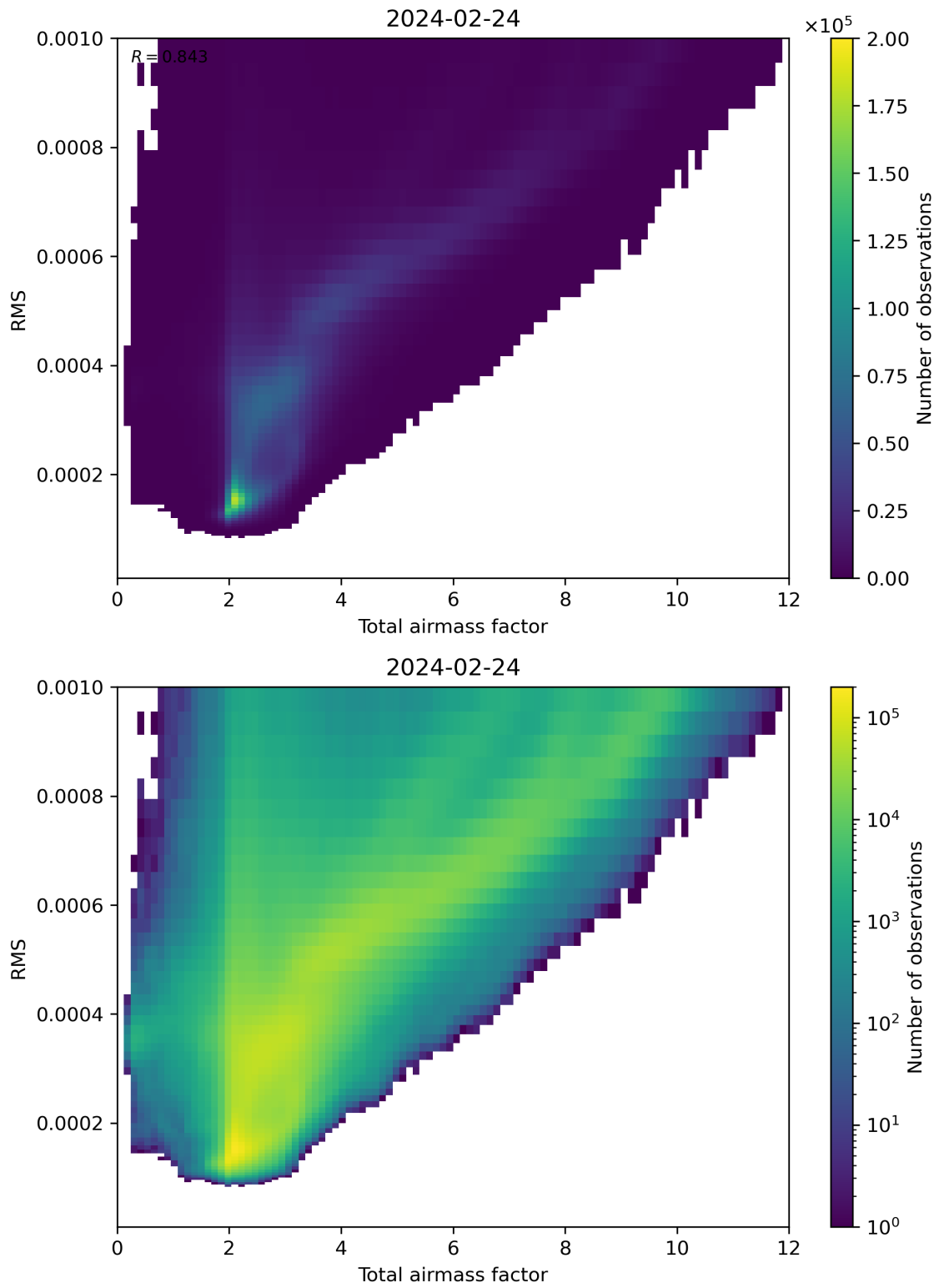
Figure 69: Scatter density plot of “Total airmass factor” against “RMS” for 2024-02-23 to 2024-02-25.
