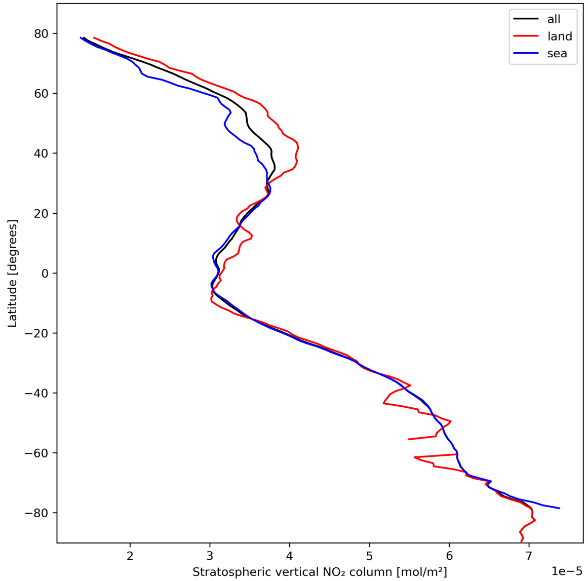
Figure 19: Zonal average of “Stratospheric vertical NO 2 column” for 2024-02-23 to 2024-02-25.
