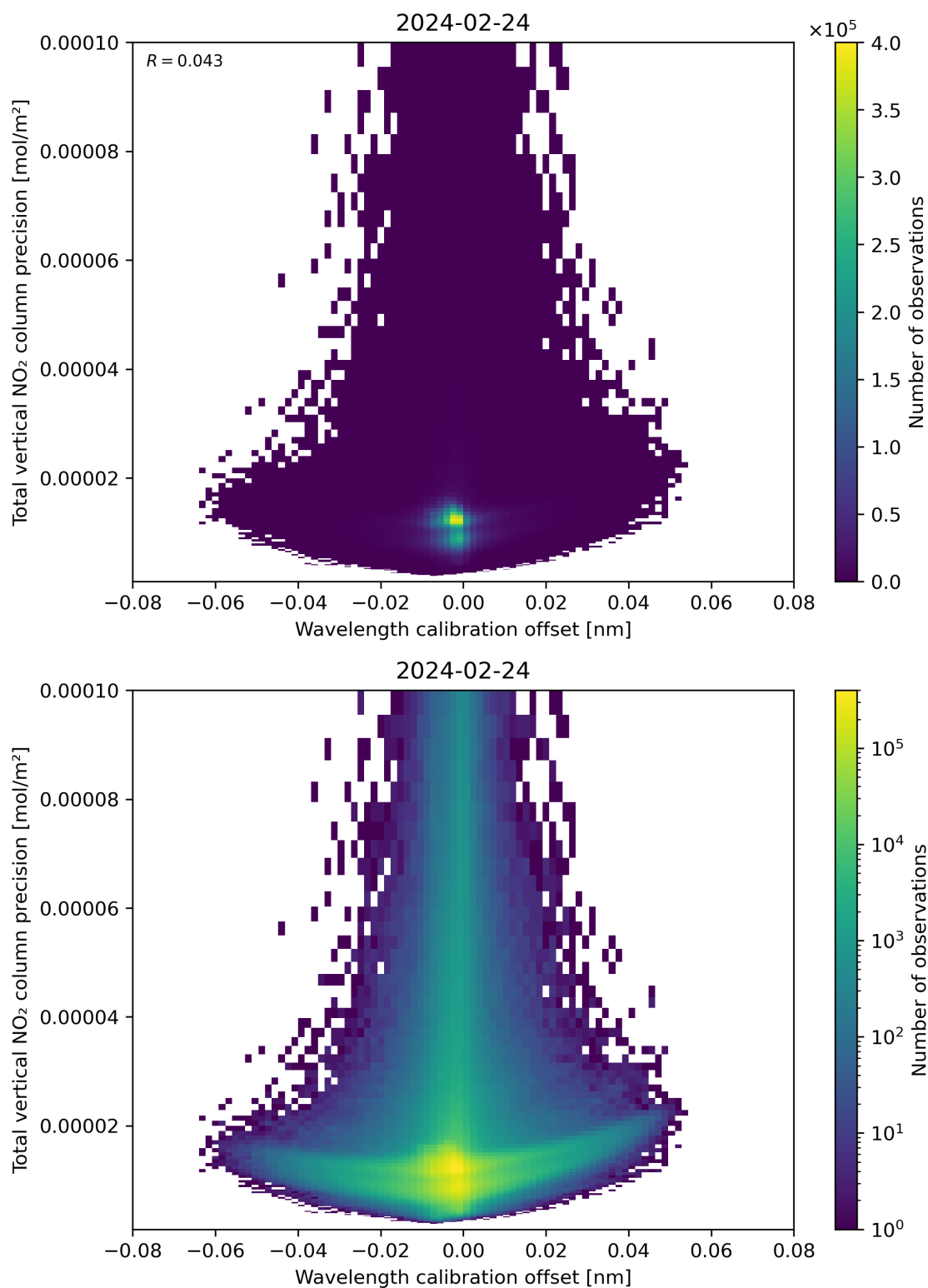
Figure 180: Scatter density plot of “Wavelength calibration offset” against “Total vertical NO 2 column precision” for 2024-02-23 to 2024-02-25.
