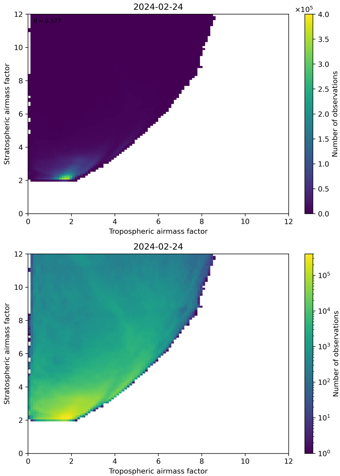
Figure 71: Scatter density plot of “Tropospheric airmass factor” against “Stratospheric airmass factor” for 2024-02-23 to 2024-02-25.
