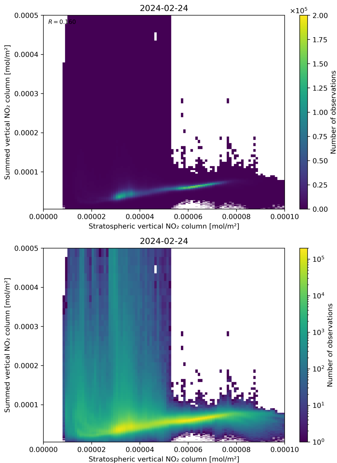
Figure 98: Scatter density plot of “Stratospheric vertical NO 2 column” against “Summed vertical NO 2 column” for 2024-02-23 to 2024-02-25.
