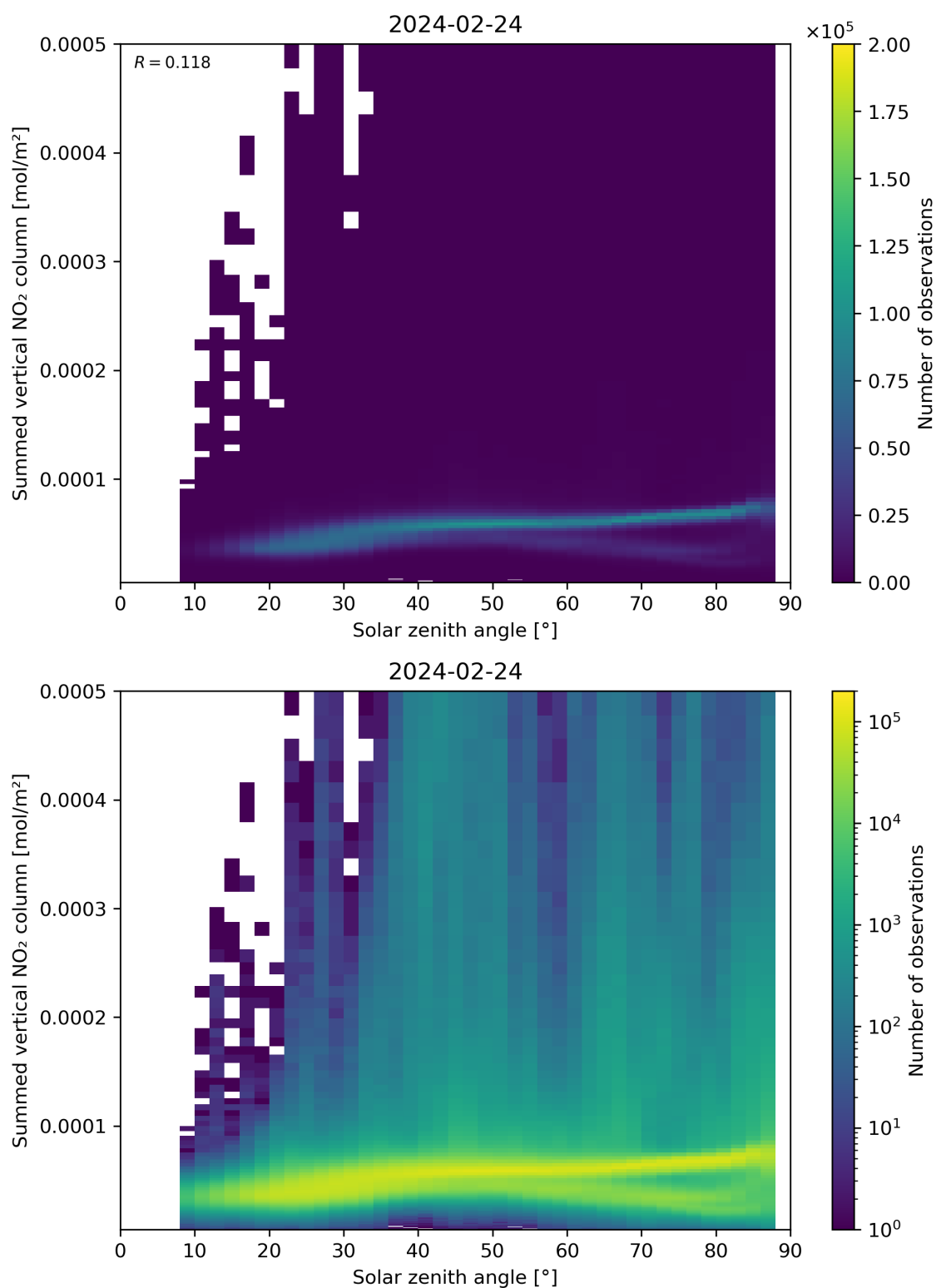
Figure 151: Scatter density plot of “Solar zenith angle” against “Summed vertical NO 2 column” for 2024-02-23 to 2024-02-25.
