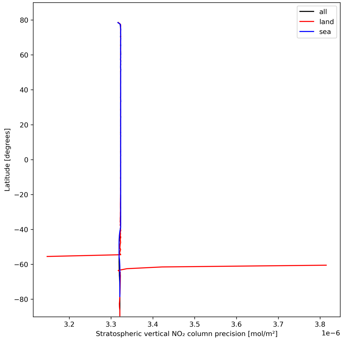
Figure 20: Zonal average of “Stratospheric vertical NO 2 column precision” for 2024-02-23 to 2024-02-25.
