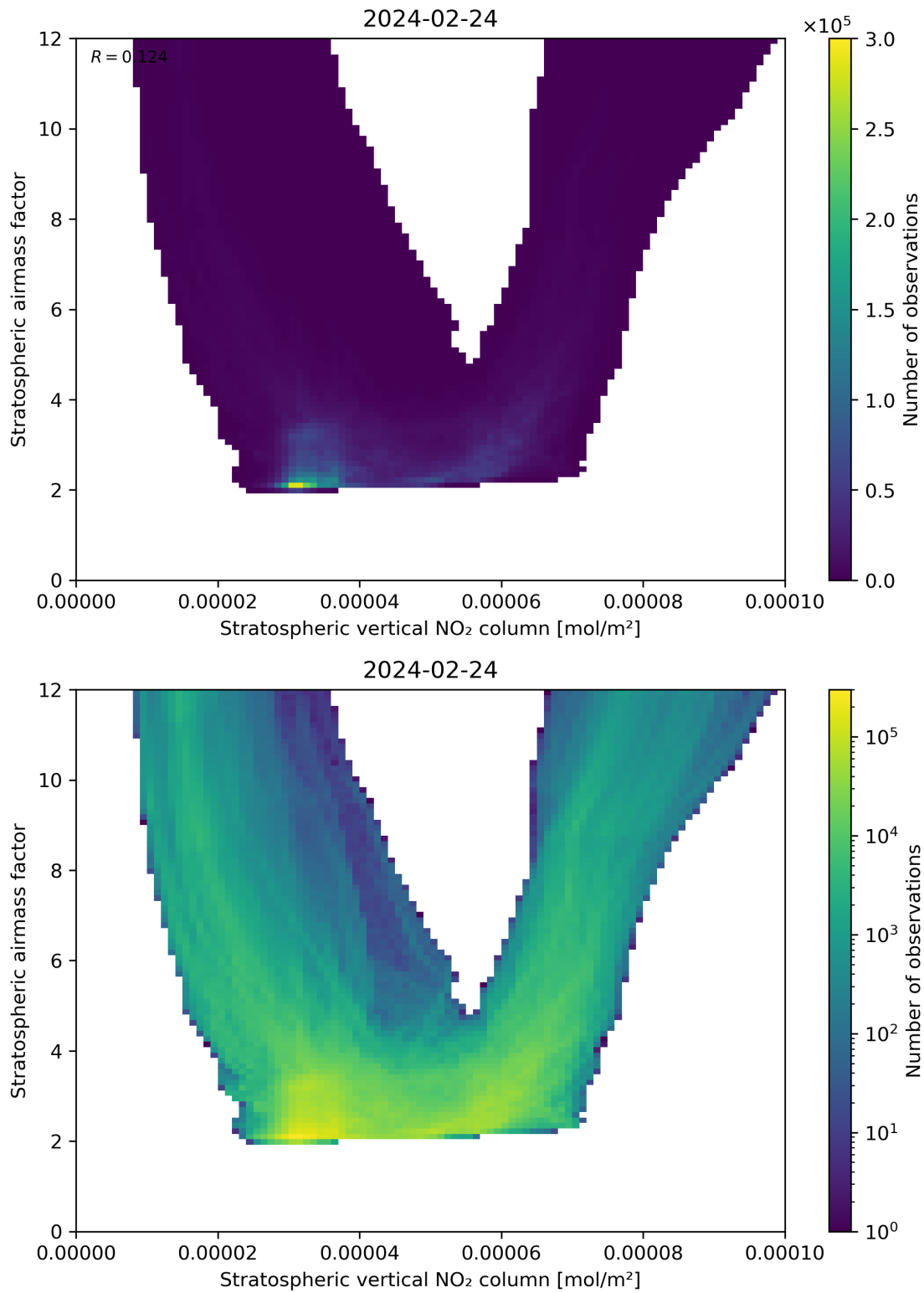
Figure 96: Scatter density plot of “Stratospheric vertical NO 2 column” against “Stratospheric airmass factor” for 2024-02-23 to 2024-02-25.
