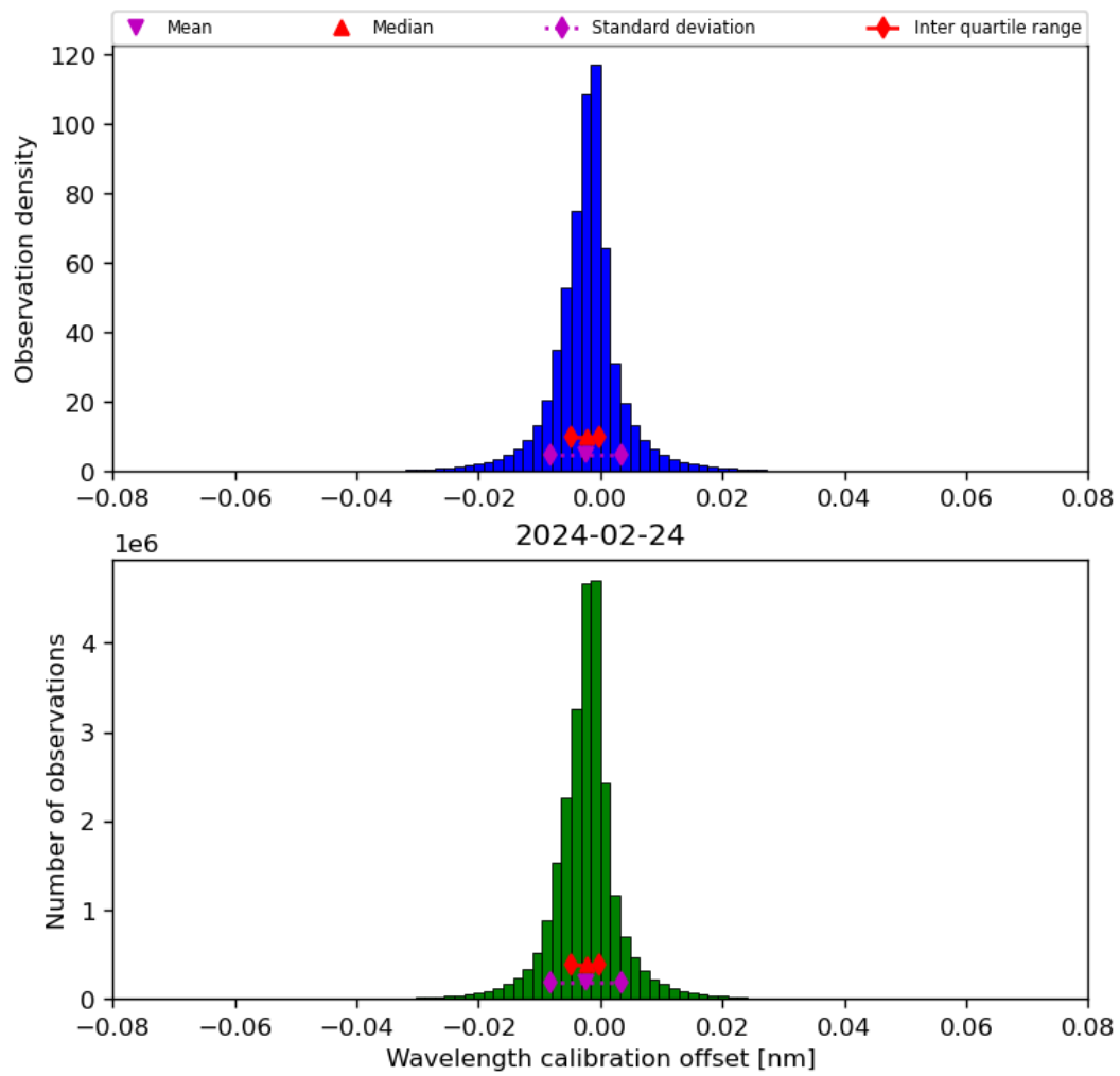
Figure 35: Histogram of “Wavelength calibration offset” for 2024-02-23 to 2024-02-25
