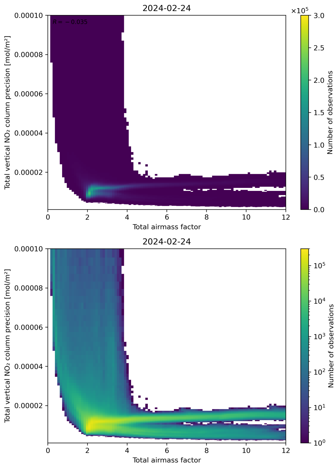
Figure 68: Scatter density plot of “Total airmass factor” against “Total vertical NO 2 column precision” for 2024-02-23 to 2024-02-25.
