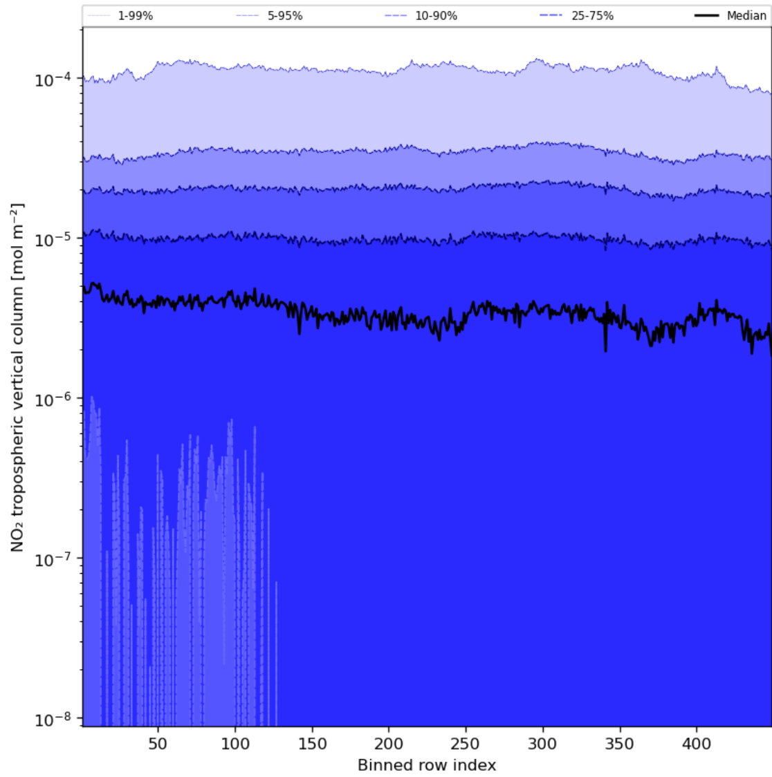
Figure 46: Along track statistics of “NO 2 tropospheric vertical column” for 2024-02-23 to 2024-02-25
