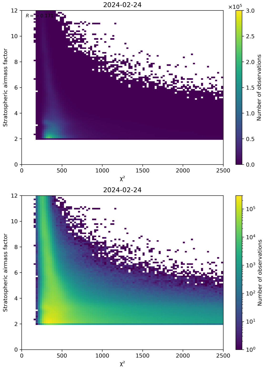
Figure 81: Scatter density plot of “ \chi^2 ” against “Stratospheric airmass factor” for 2024-02-23 to 2024-02-25.
