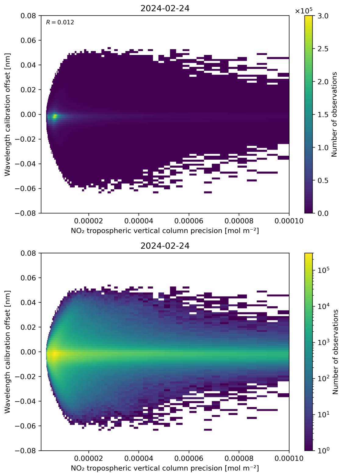
Figure 141: Scatter density plot of “NO 2 tropospheric vertical column precision” against “Wavelength calibration offset” for 2024-02-23 to 2024-02-25.
