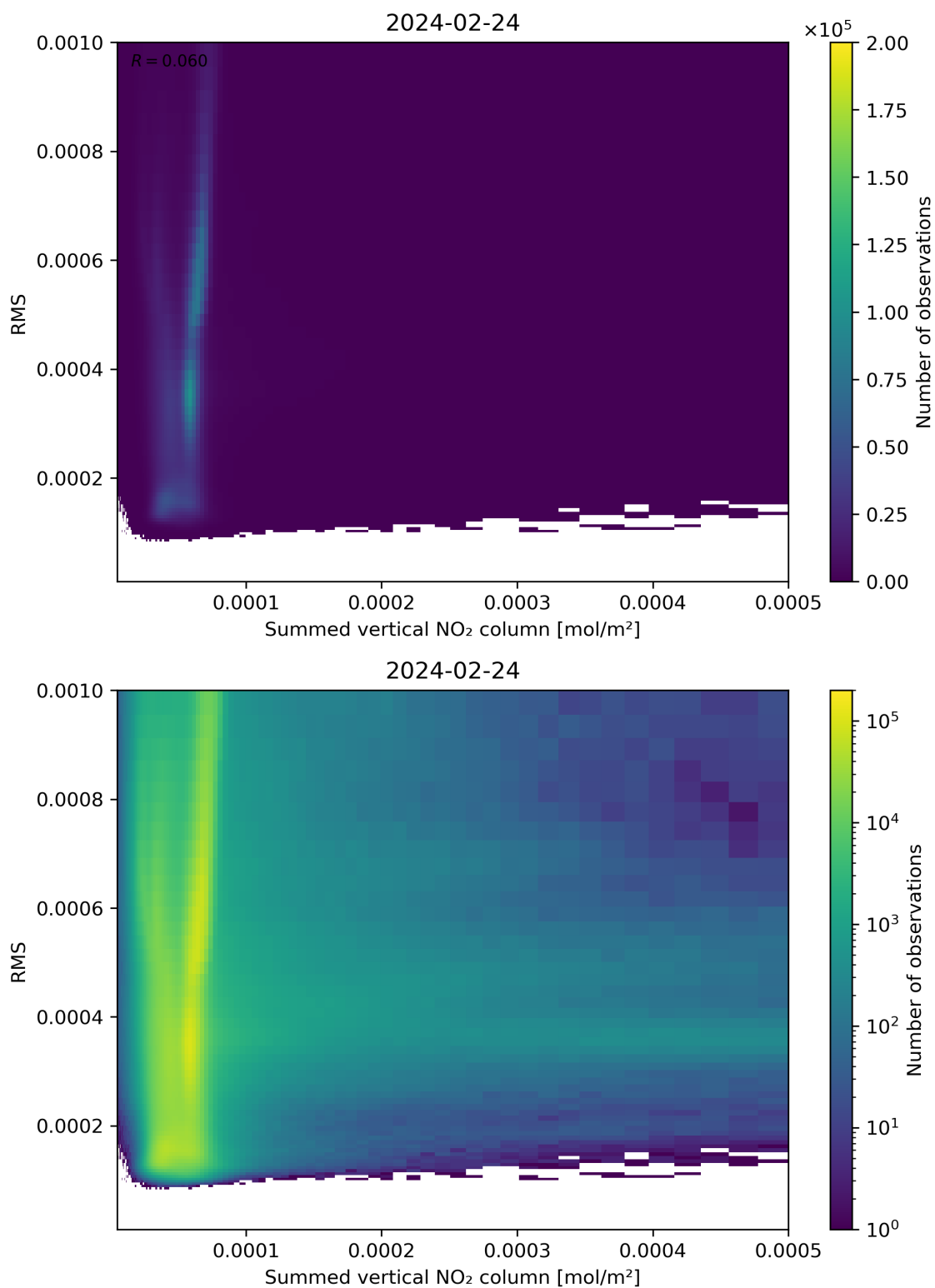
Figure 109: Scatter density plot of “Summed vertical NO 2 column” against “RMS” for 2024-02-23 to 2024-02-25.
