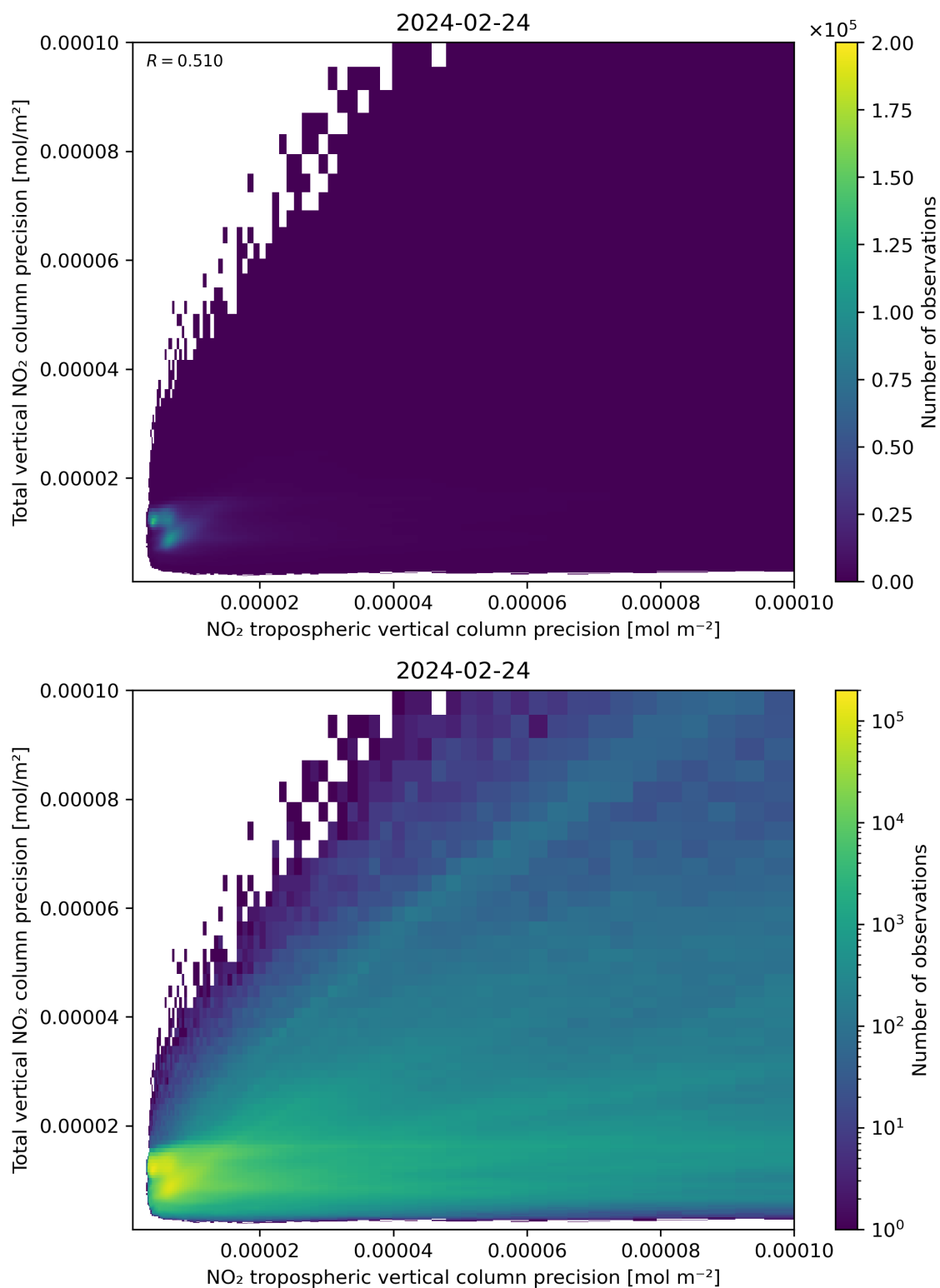
Figure 139: Scatter density plot of “NO 2 tropospheric vertical column precision” against “Total vertical NO 2 column precision” for 2024-02-23 to 2024-02-25.
