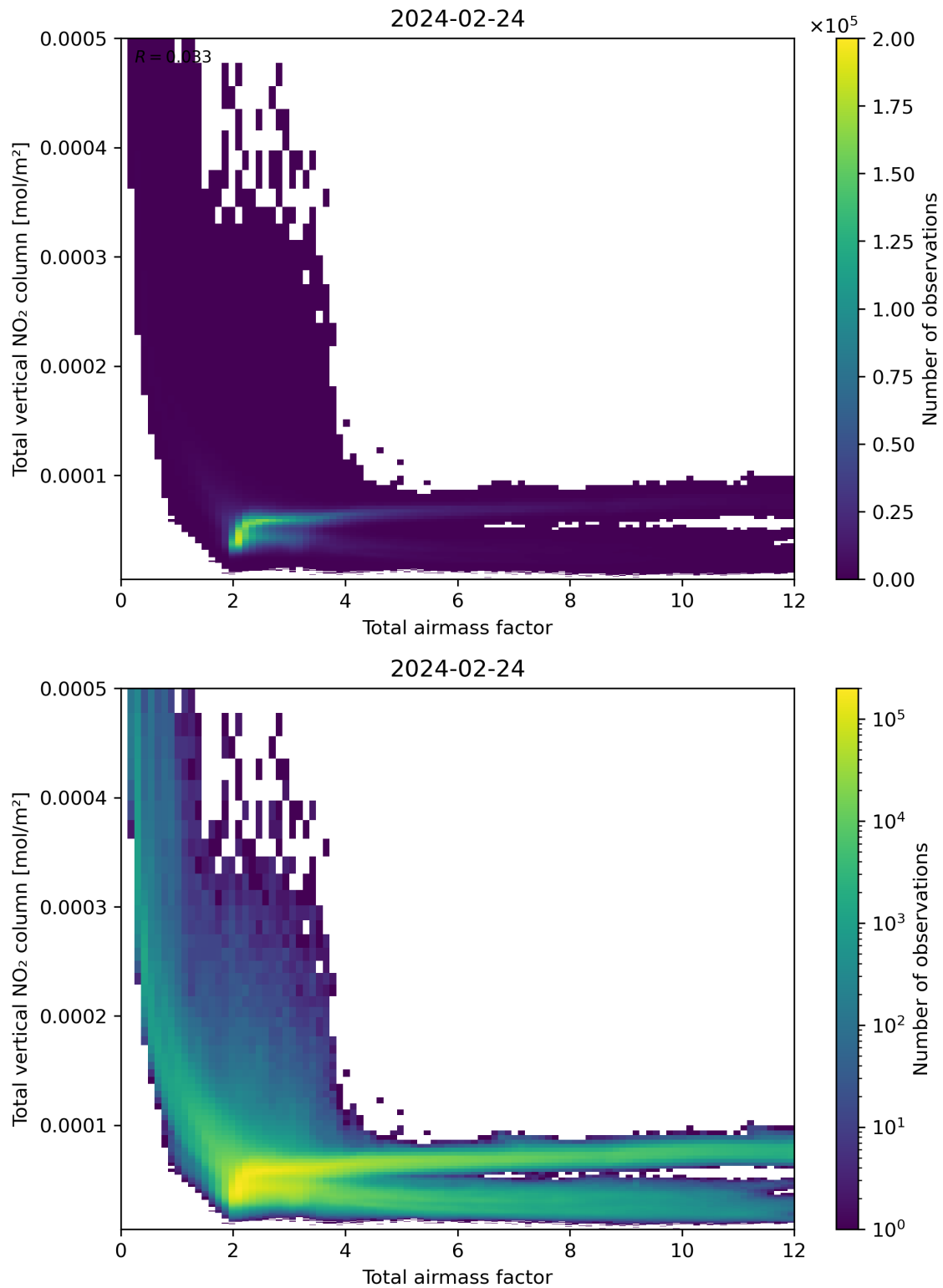
Figure 67: Scatter density plot of “Total airmass factor” against “Total vertical NO 2 column” for 2024-02-23 to 2024-02-25.
