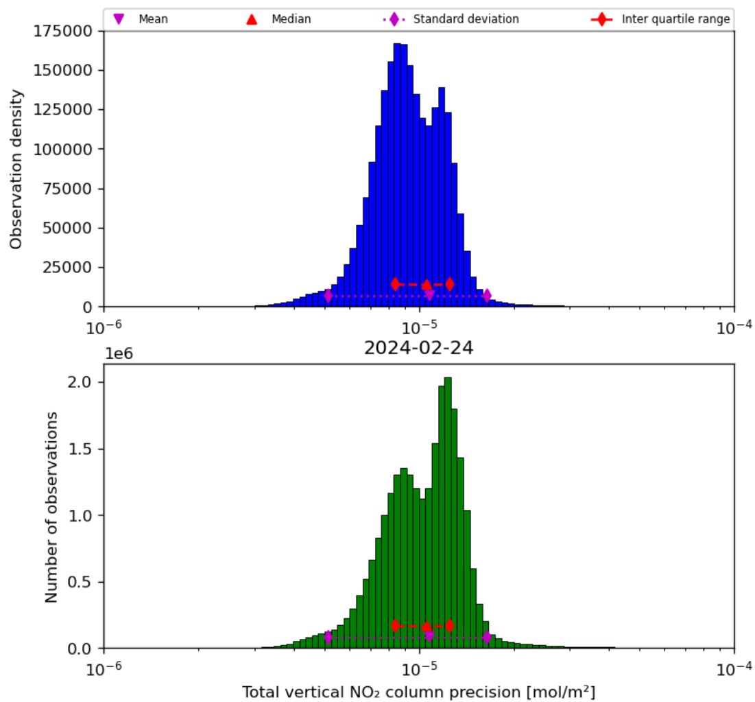
Figure 39: Histogram of “Total vertical NO 2 column precision” for 2024-02-23 to 2024-02-25
