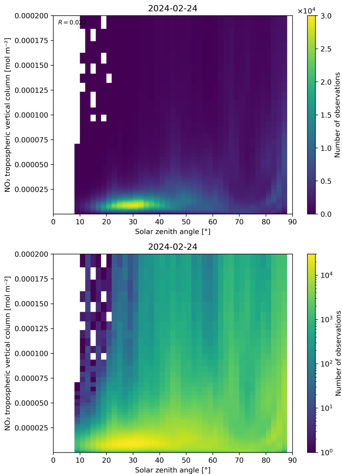
Figure 155: Scatter density plot of “Solar zenith angle” against “NO 2 tropospheric vertical column” for 2024-02-23 to 2024-02-25.
