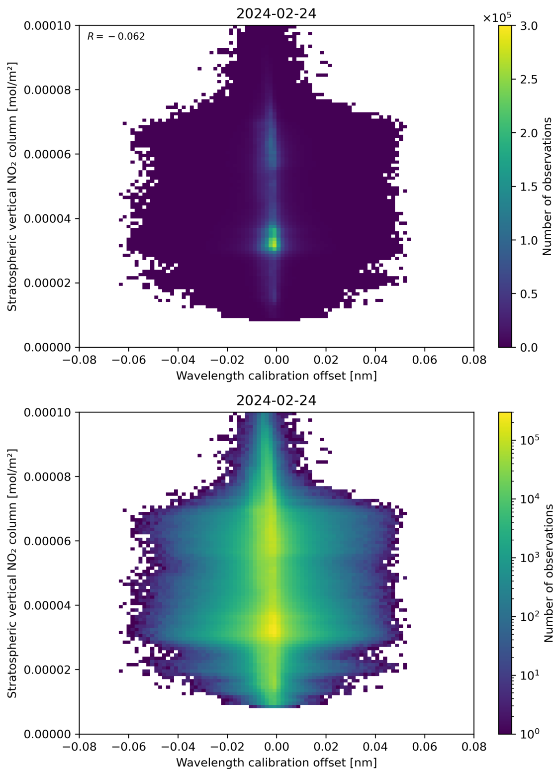
Figure 176: Scatter density plot of “Wavelength calibration offset” against “Stratospheric vertical NO 2 column” for 2024-02-23 to 2024-02-25.
