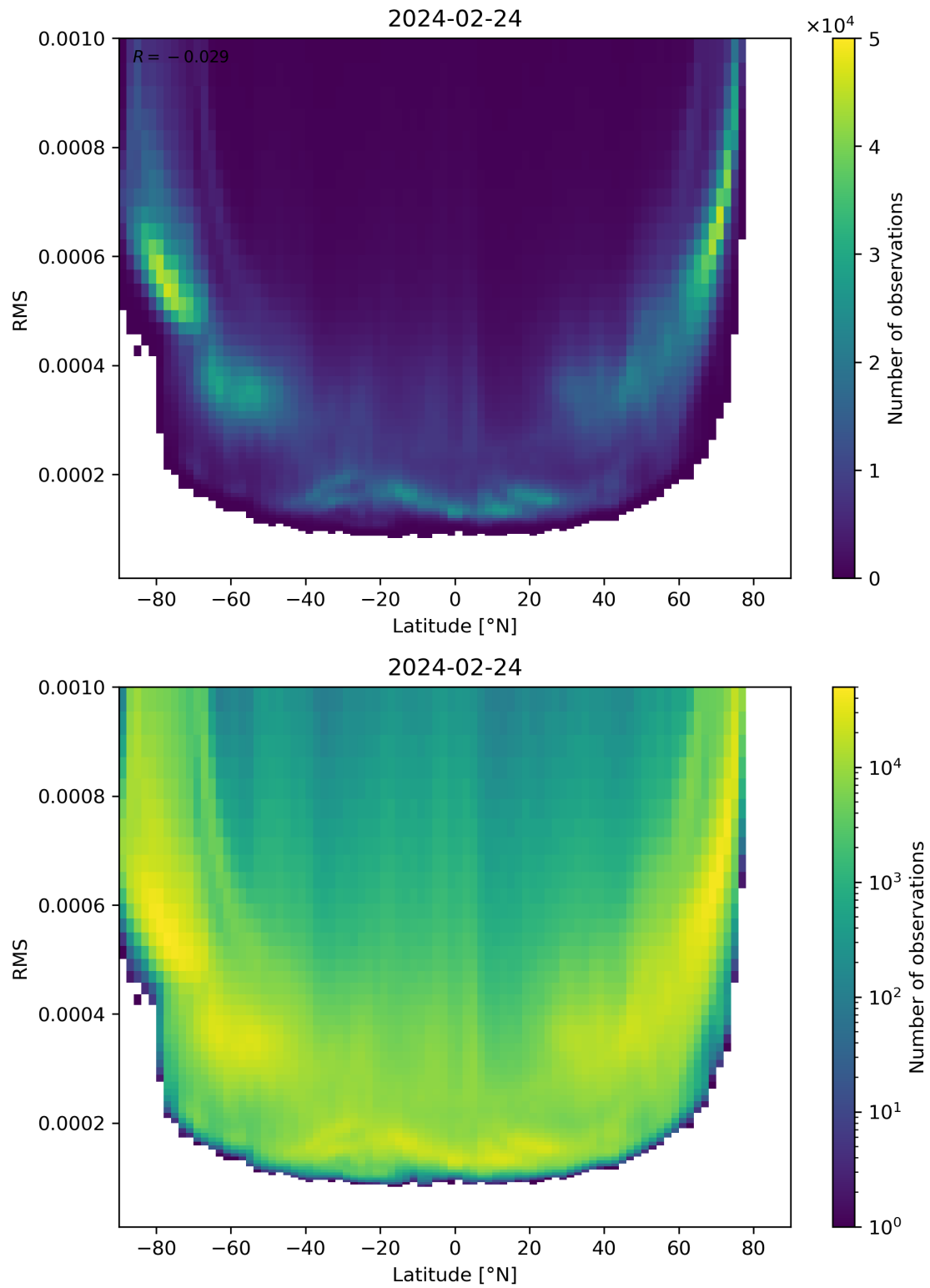
Figure 94: Scatter density plot of “Latitude” against “RMS” for 2024-02-23 to 2024-02-25.
