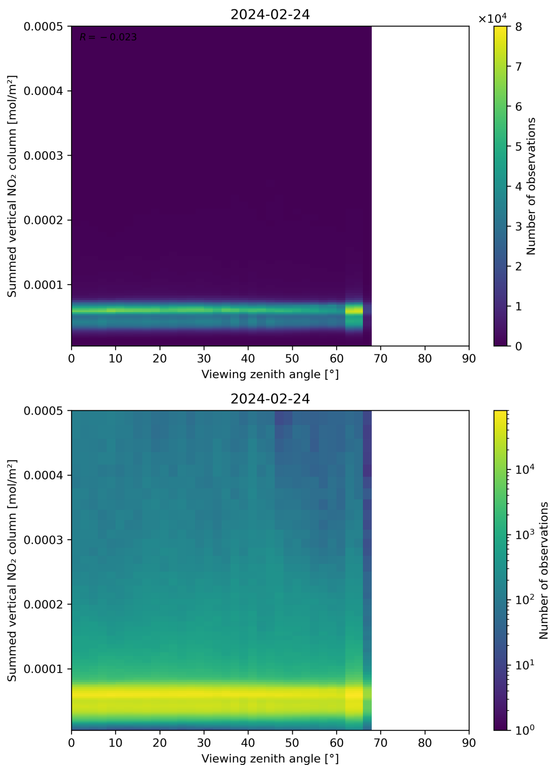
Figure 165: Scatter density plot of “Viewing zenith angle” against “Summed vertical NO 2 column” for 2024-02-23 to 2024-02-25.
