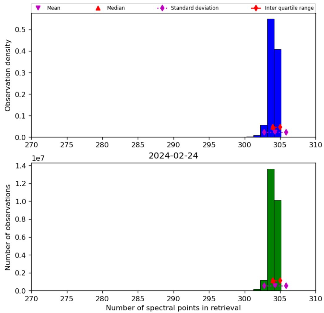
Figure 33: Histogram of “Number of spectral points in retrieval” for 2024-02-23 to 2024-02-25
