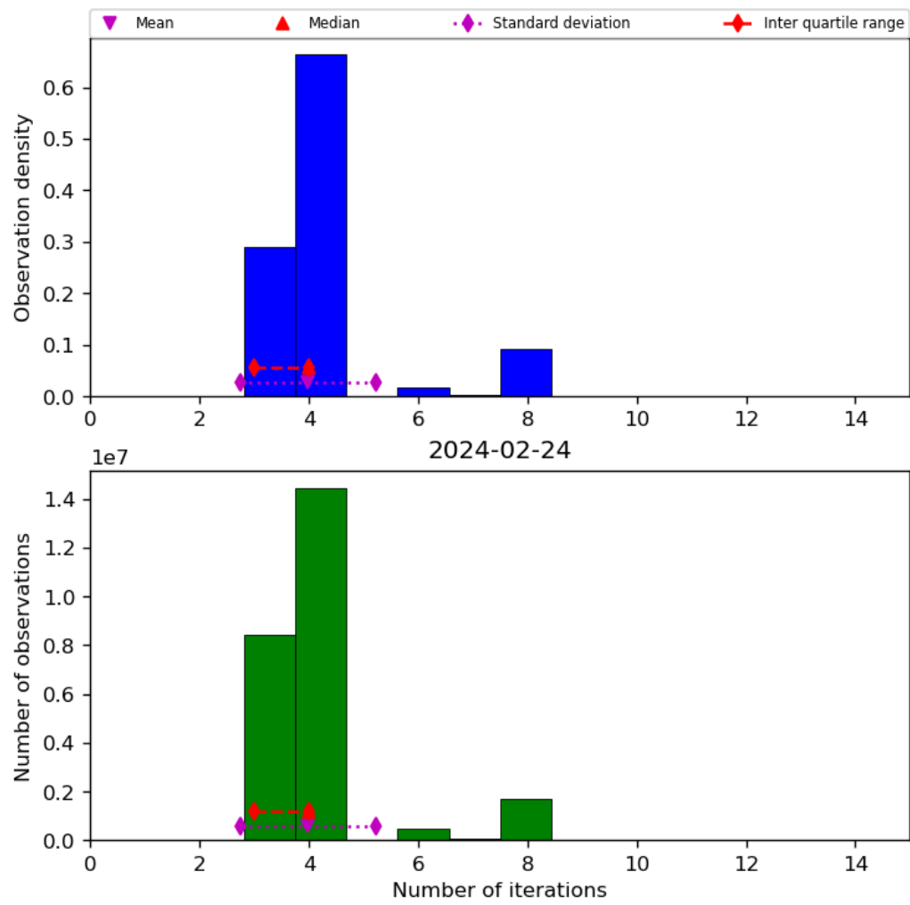
Figure 34: Histogram of “Number of iterations” for 2024-02-23 to 2024-02-25
