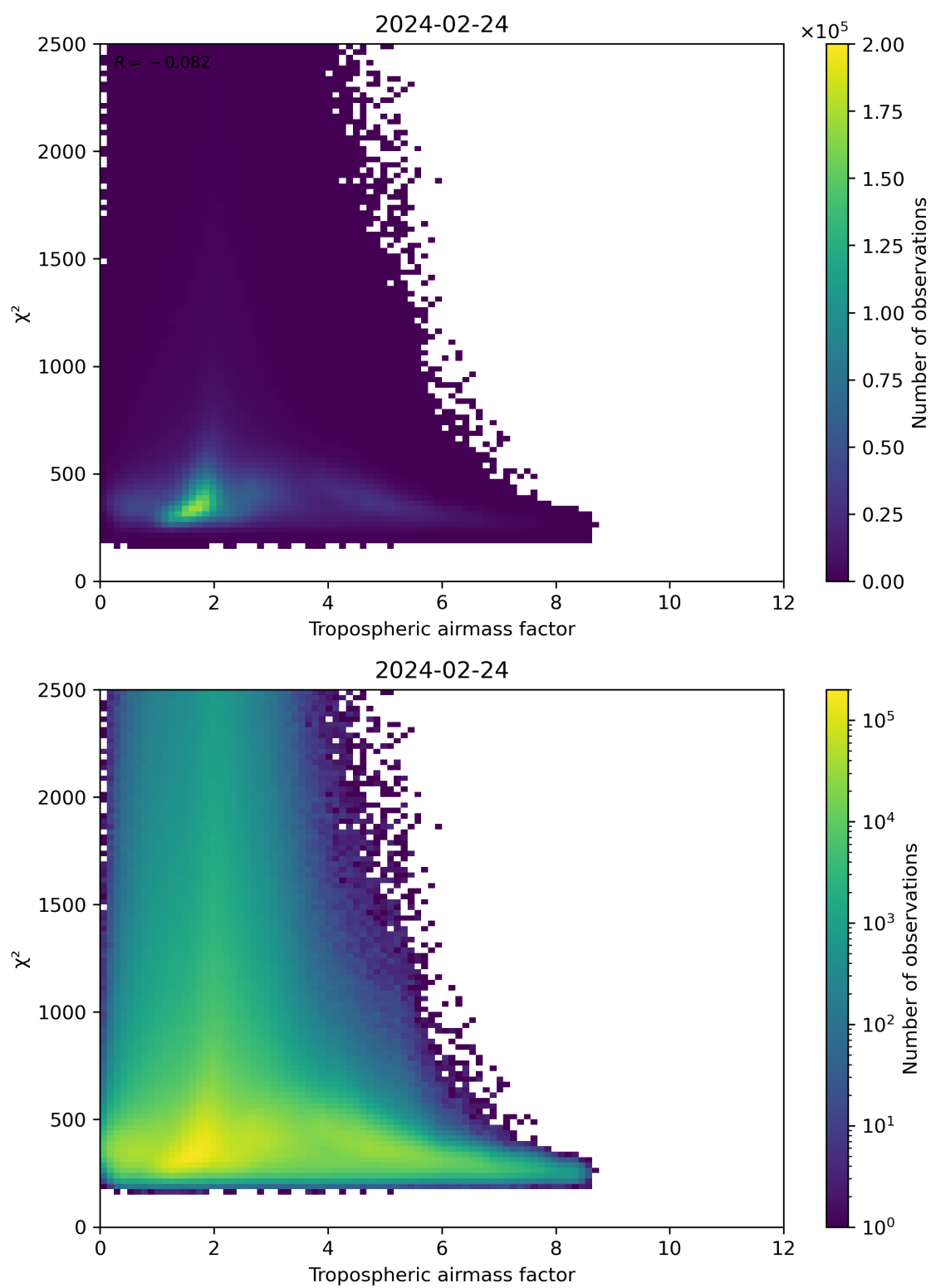
Figure 73: Scatter density plot of “Tropospheric airmass factor” against “ \chi^2 ” for 2024-02-23 to 2024-02-25.
