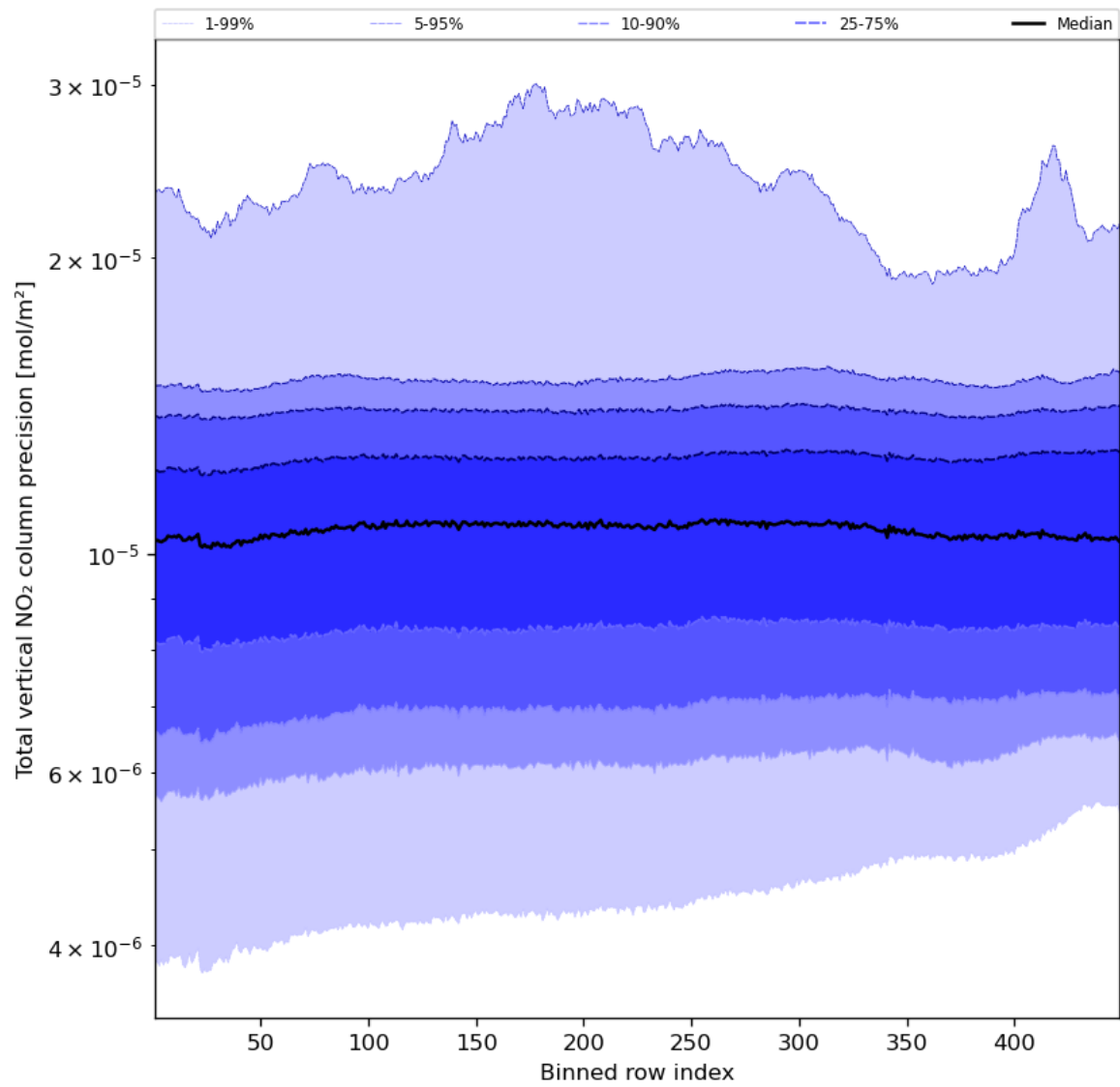
Figure 56: Along track statistics of "Total vertical NO 2 column precision" for 2024-02-23 to 2024-02-25
