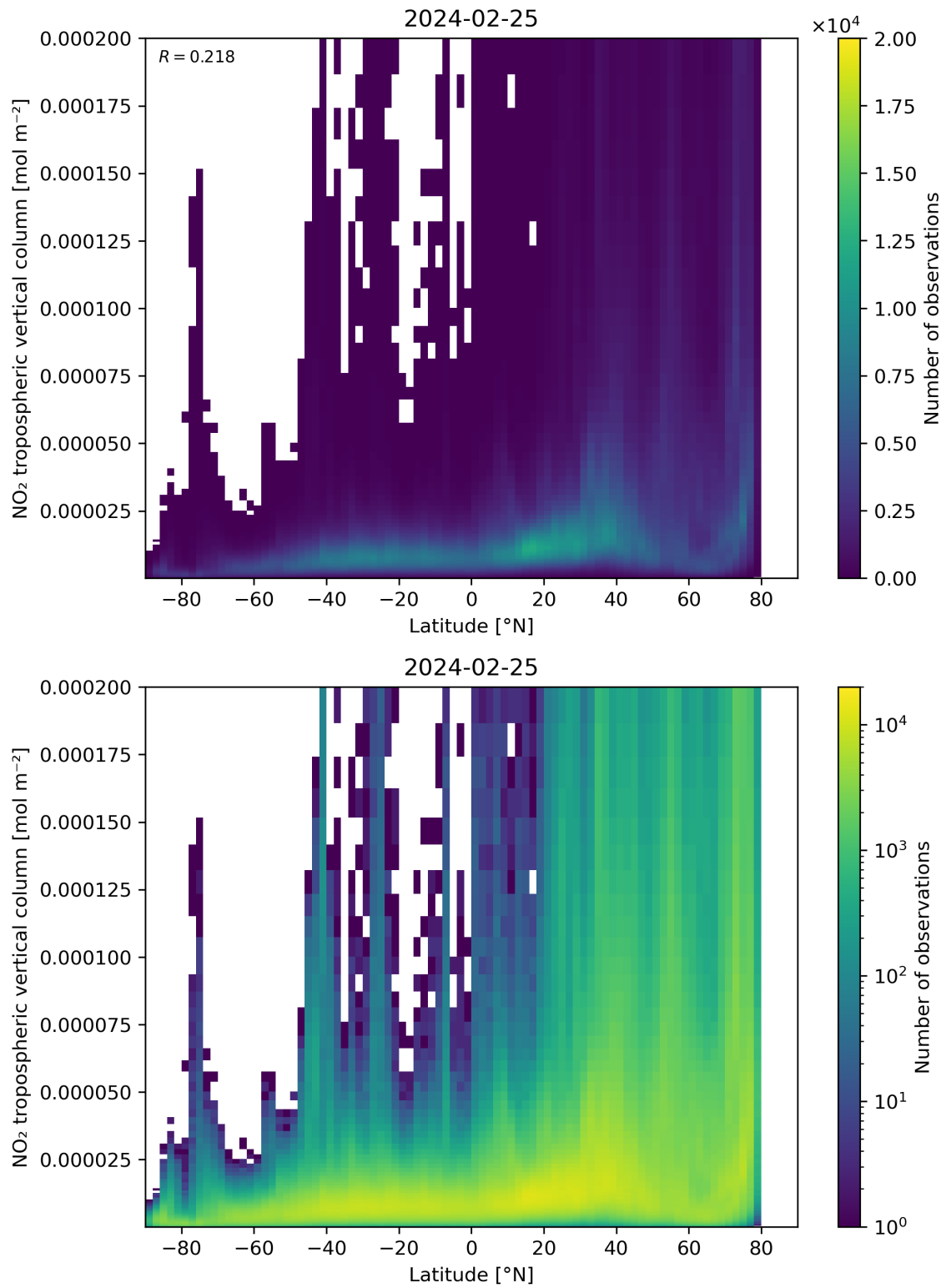
Figure 92: Scatter density plot of “Latitude” against “NO 2 tropospheric vertical column” for 2024-02-24 to 2024-02-26.
