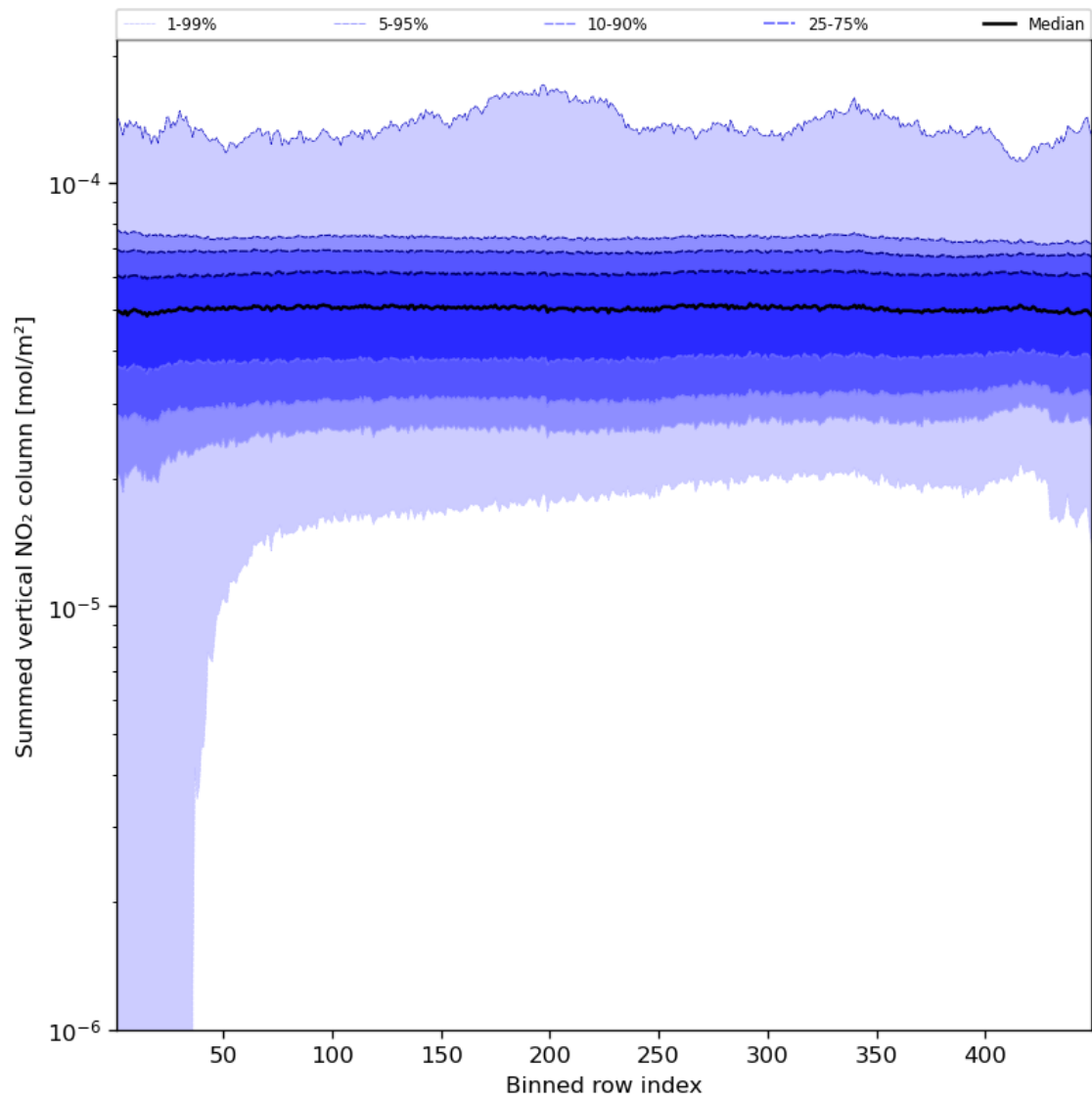
Figure 57: Along track statistics of “Summed vertical NO 2 column” for 2024-02-24 to 2024-02-26
