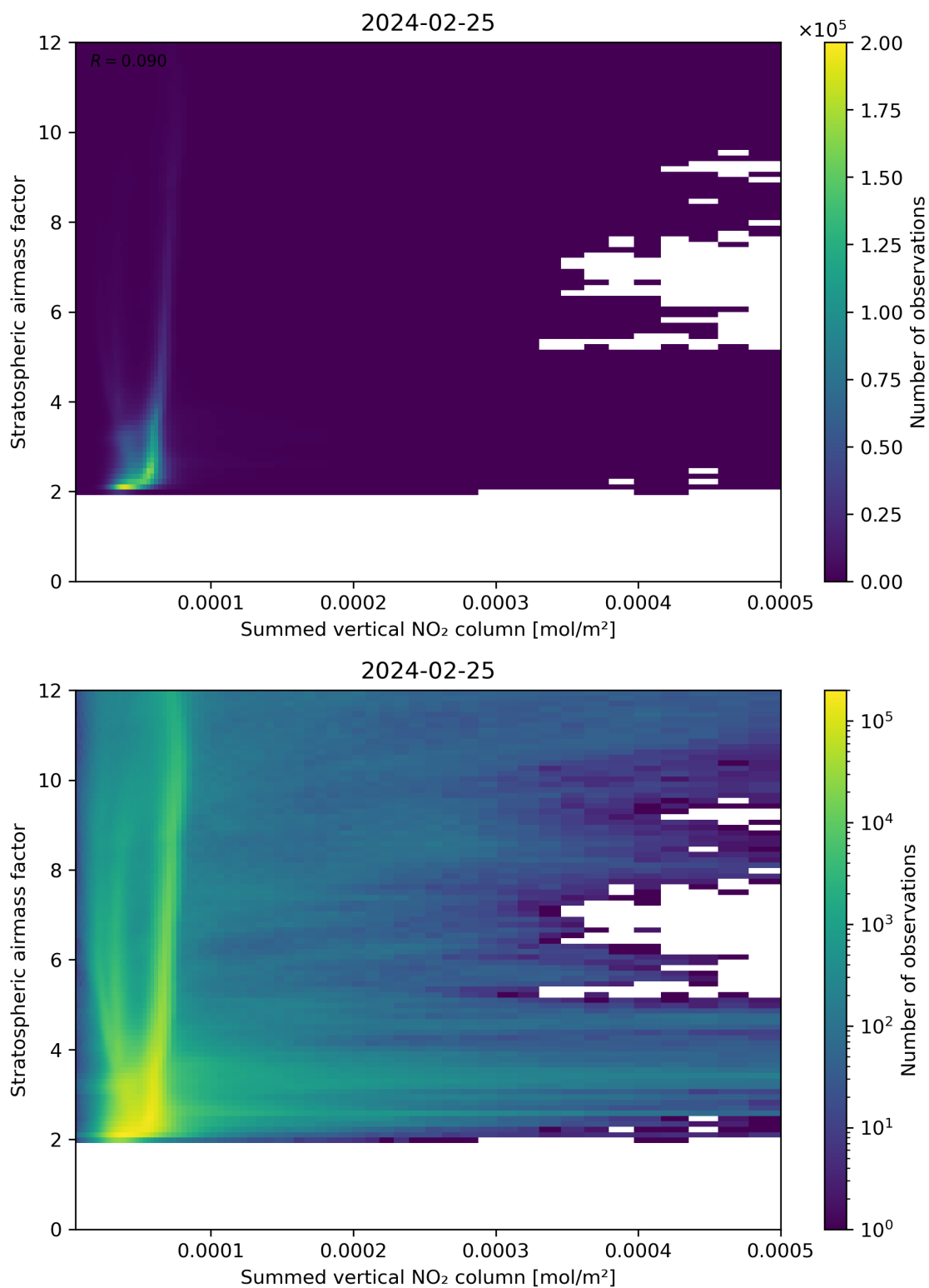
Figure 103: Scatter density plot of “Summed vertical NO 2 column” against “Stratospheric airmass factor” for 2024-02-24 to 2024-02-26.
