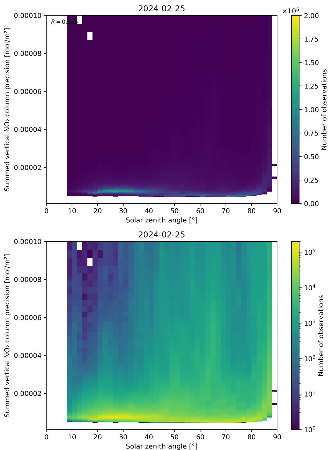
Figure 152: Scatter density plot of “Solar zenith angle” against “Summed vertical NO 2 column precision” for 2024-02-24 to 2024-02-26.
