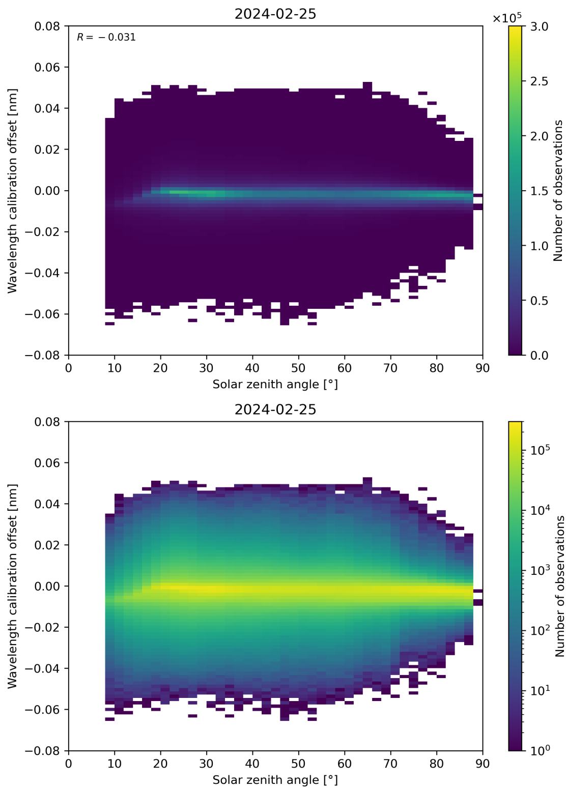
Figure 158: Scatter density plot of “Solar zenith angle” against “Wavelength calibration offset” for 2024-02-24 to 2024-02-26.
