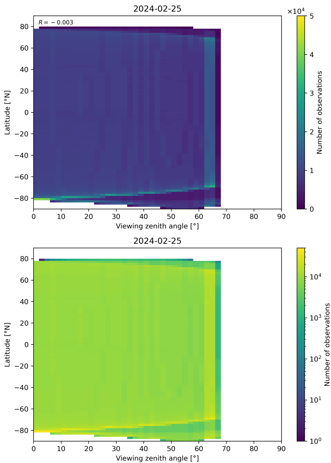
Figure 163: Scatter density plot of “Viewing zenith angle” against “Latitude” for 2024-02-24 to 2024-02-26.
