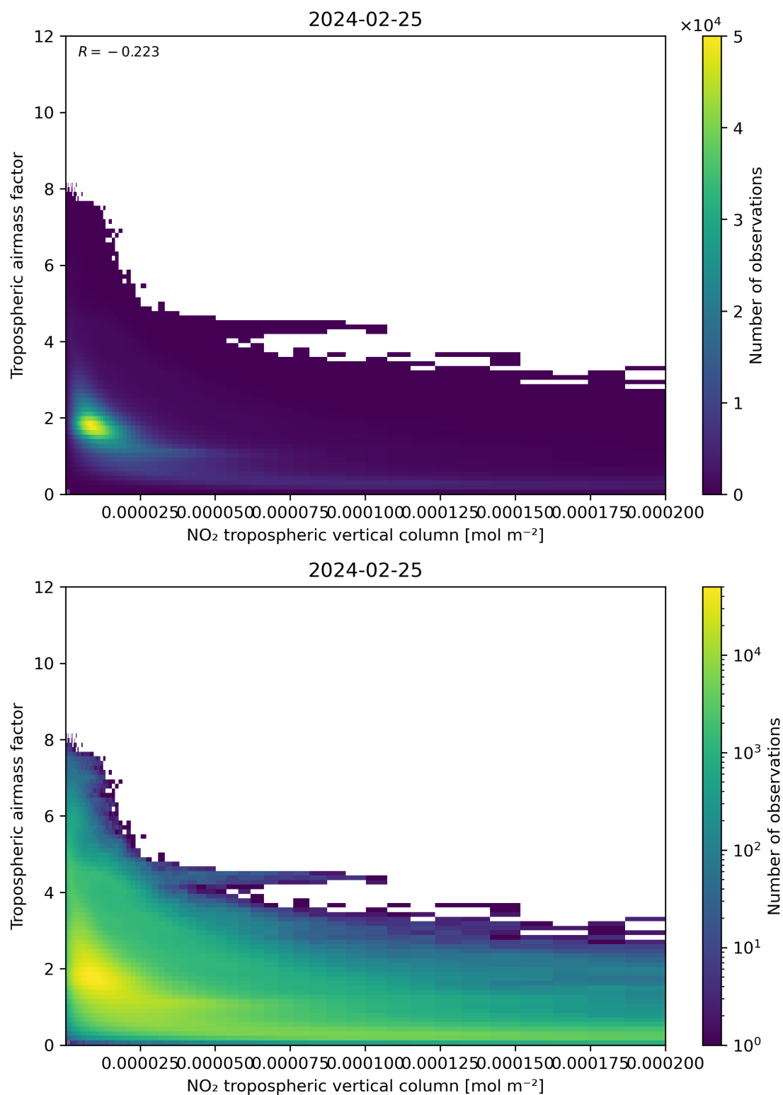
Figure 123: Scatter density plot of “NO 2 tropospheric vertical column” against “Tropospheric air mass factor” for 2024-02-24 to 2024-02-26.
