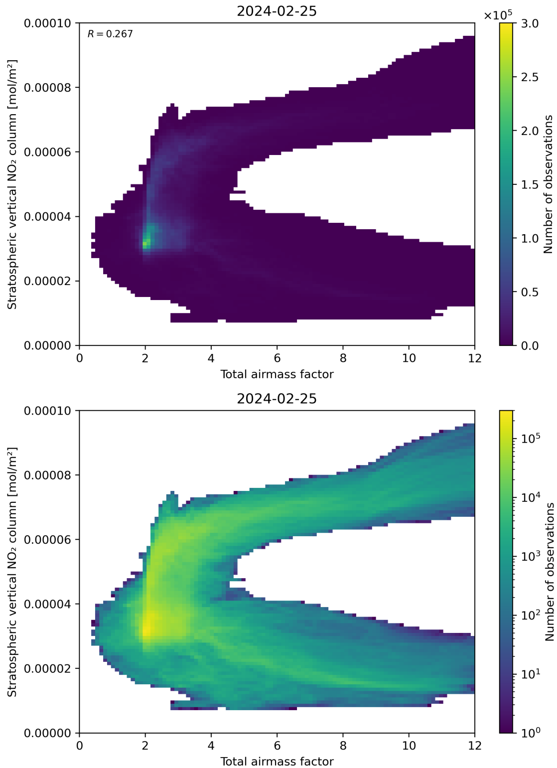
Figure 64: Scatter density plot of “Total airmass factor” against “Stratospheric vertical NO 2 column” for 2024-02-24 to 2024-02-26.
