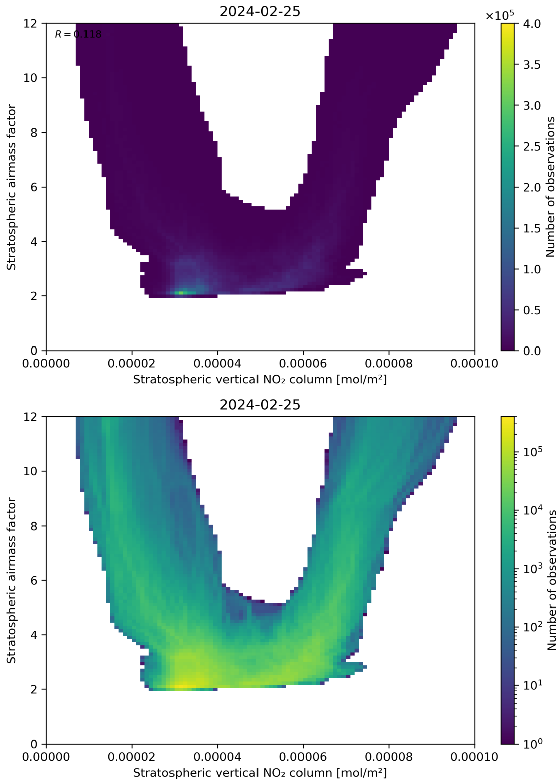
Figure 96: Scatter density plot of “Stratospheric vertical NO 2 column” against “Stratospheric airmass factor” for 2024-02-24 to 2024-02-26.
