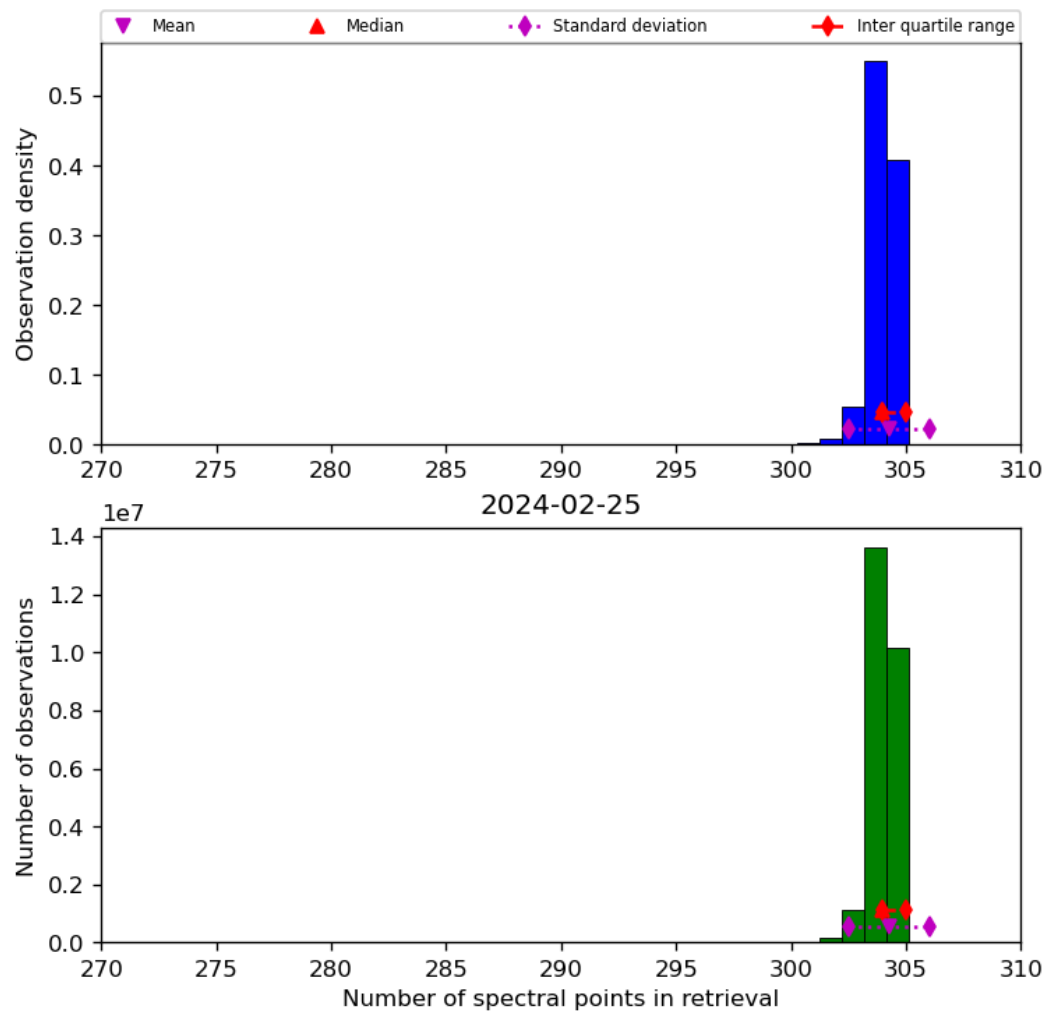
Figure 33: Histogram of “Number of spectral points in retrieval” for 2024-02-24 to 2024-02-26
