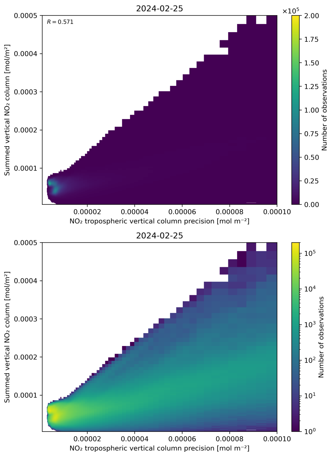
Figure 136: Scatter density plot of “NO 2 tropospheric vertical column precision” against “Summed vertical NO 2 column” for 2024-02-24 to 2024-02-26.
