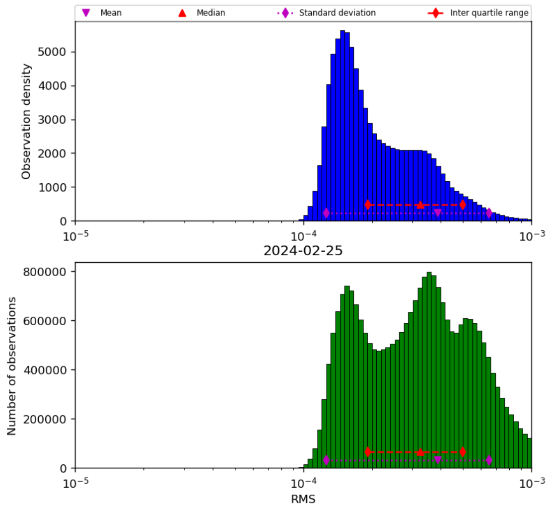
Figure 43: Histogram of “RMS” for 2024-02-24 to 2024-02-26
