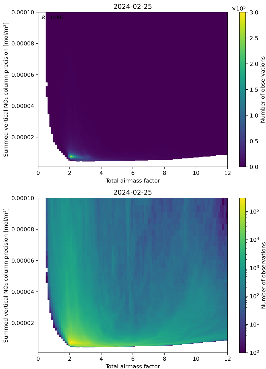
Figure 66: Scatter density plot of “Total airmass factor” against “Summed vertical NO 2 column precision” for 2024-02-24 to 2024-02-26.
