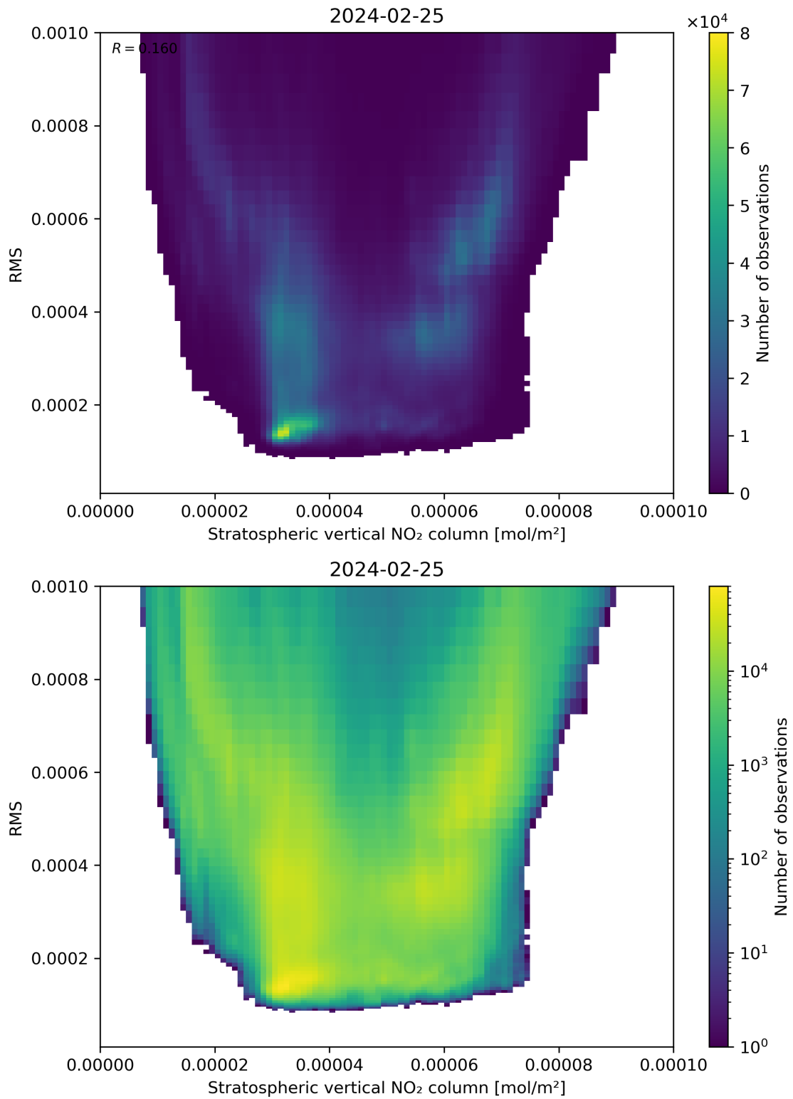
Figure 102: Scatter density plot of “Stratospheric vertical NO 2 column” against “RMS” for 2024-02-24 to 2024-02-26.
