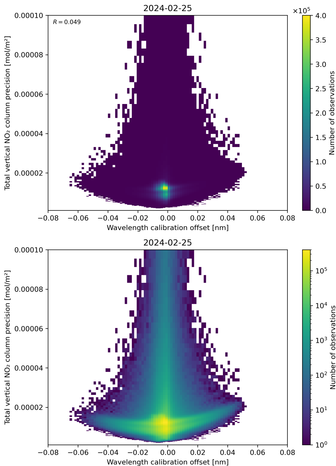
Figure 180: Scatter density plot of “Wavelength calibration offset” against “Total vertical NO 2 column precision” for 2024-02-24 to 2024-02-26.
