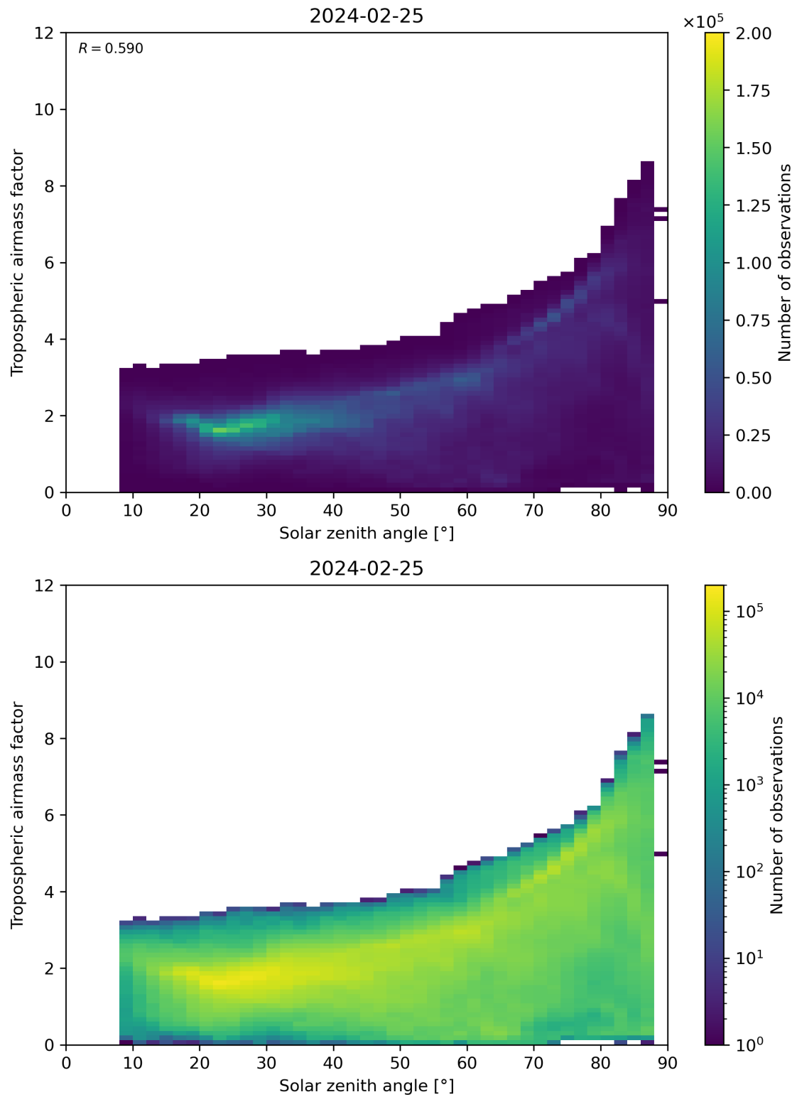
Figure 147: Scatter density plot of “Solar zenith angle” against “Tropospheric airmass factor” for 2024-02-24 to 2024-02-26.
