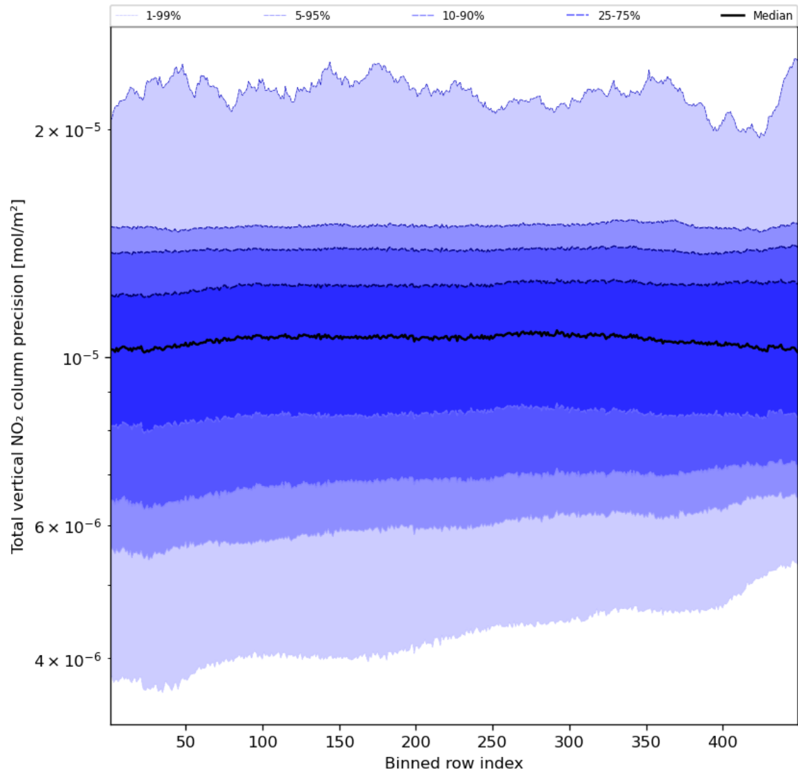
Figure 56: Along track statistics of “Total vertical NO 2 column precision” for 2024-02-24 to 2024-02-26
