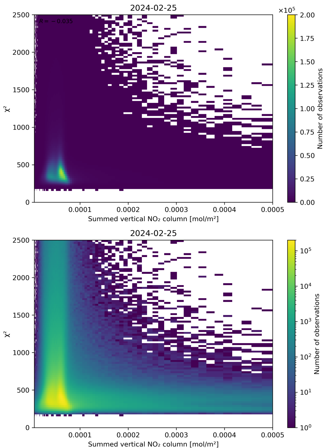
Figure 104: Scatter density plot of “Summed vertical NO 2 column” against “ \chi^2 ” for 2024-02-24 to 2024-02-26.
