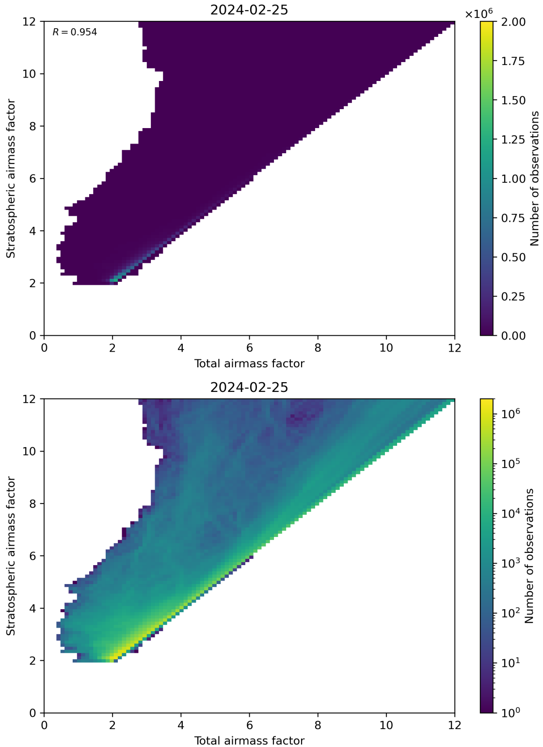
Figure 62: Scatter density plot of “Total airmass factor” against “Stratospheric airmass factor” for 2024-02-24 to 2024-02-26.
