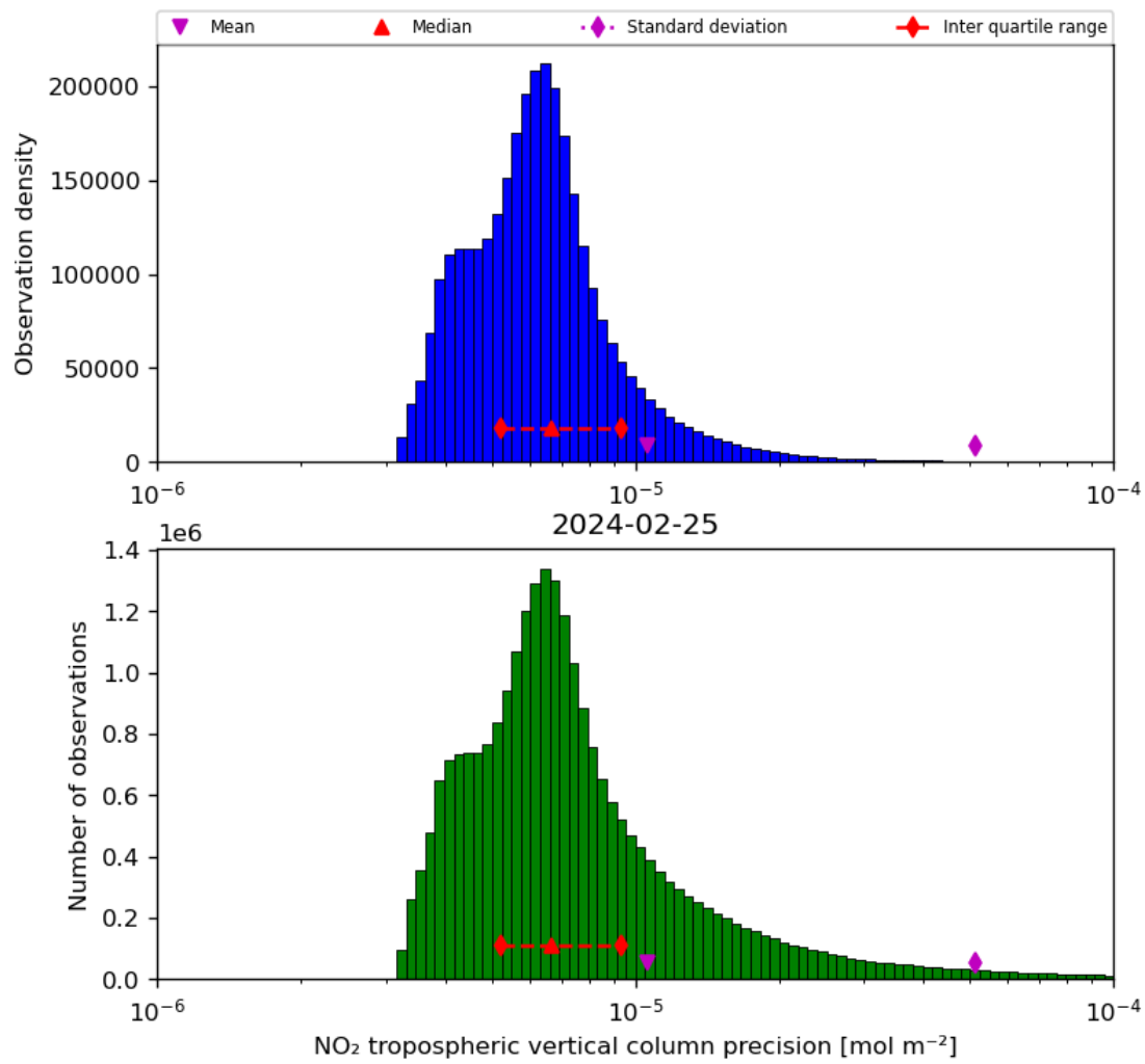
Figure 30: Histogram of “NO 2 tropospheric vertical column precision” for 2024-02-24 to 2024-02-26
