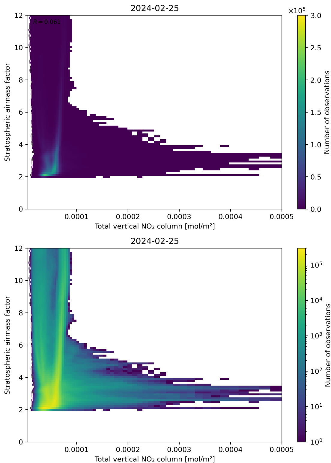
Figure 110: Scatter density plot of “Total vertical NO 2 column” against “Stratospheric air mass factor” for 2024-02-24 to 2024-02-26.
