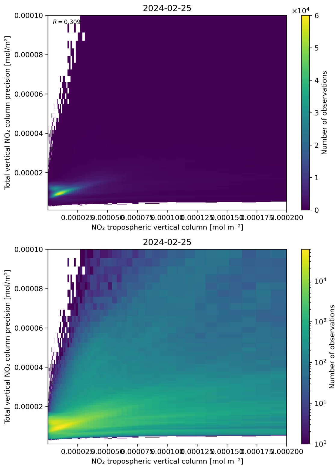
Figure 129: Scatter density plot of “NO 2 tropospheric vertical column” against “Total vertical NO 2 column precision” for 2024-02-24 to 2024-02-26.
