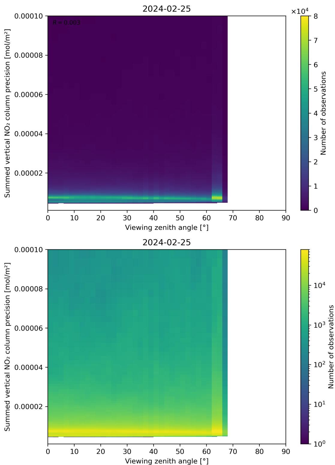
Figure 166: Scatter density plot of “Viewing zenith angle” against “Summed vertical NO 2 column precision” for 2024-02-24 to 2024-02-26.
