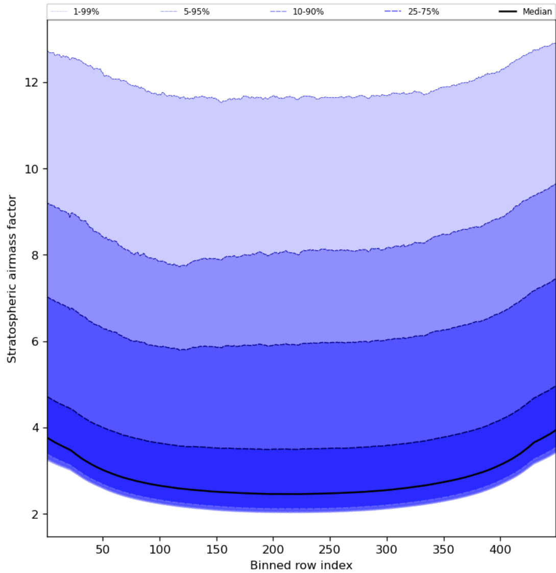
Figure 61: Along track statistics of “Stratospheric airmass factor” for 2024-02-24 to 2024-02-26
