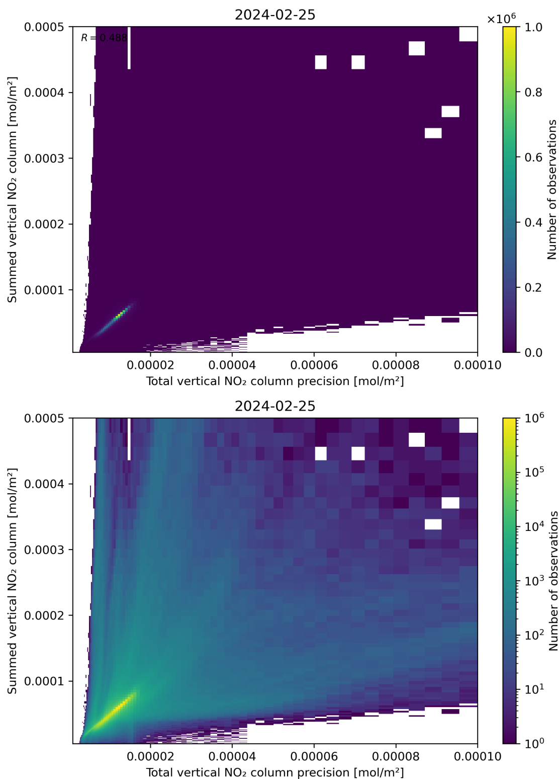
Figure 117: Scatter density plot of “Total vertical NO 2 column precision” against “Summed vertical NO 2 column” for 2024-02-24 to 2024-02-26.
