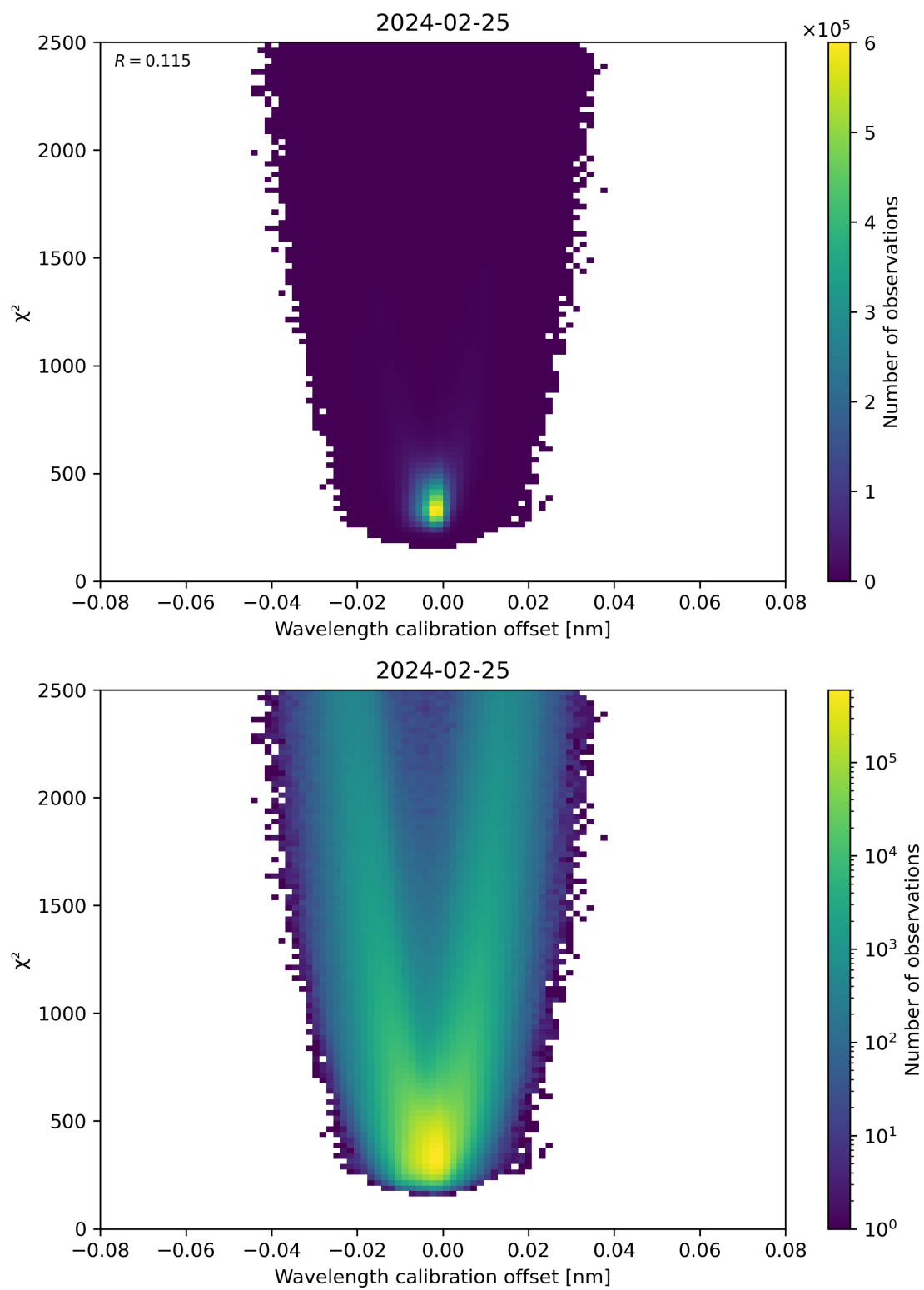
Figure 175: Scatter density plot of “Wavelength calibration offset” against “ \chi^2 ” for 2024-02-24 to 2024-02-26.
