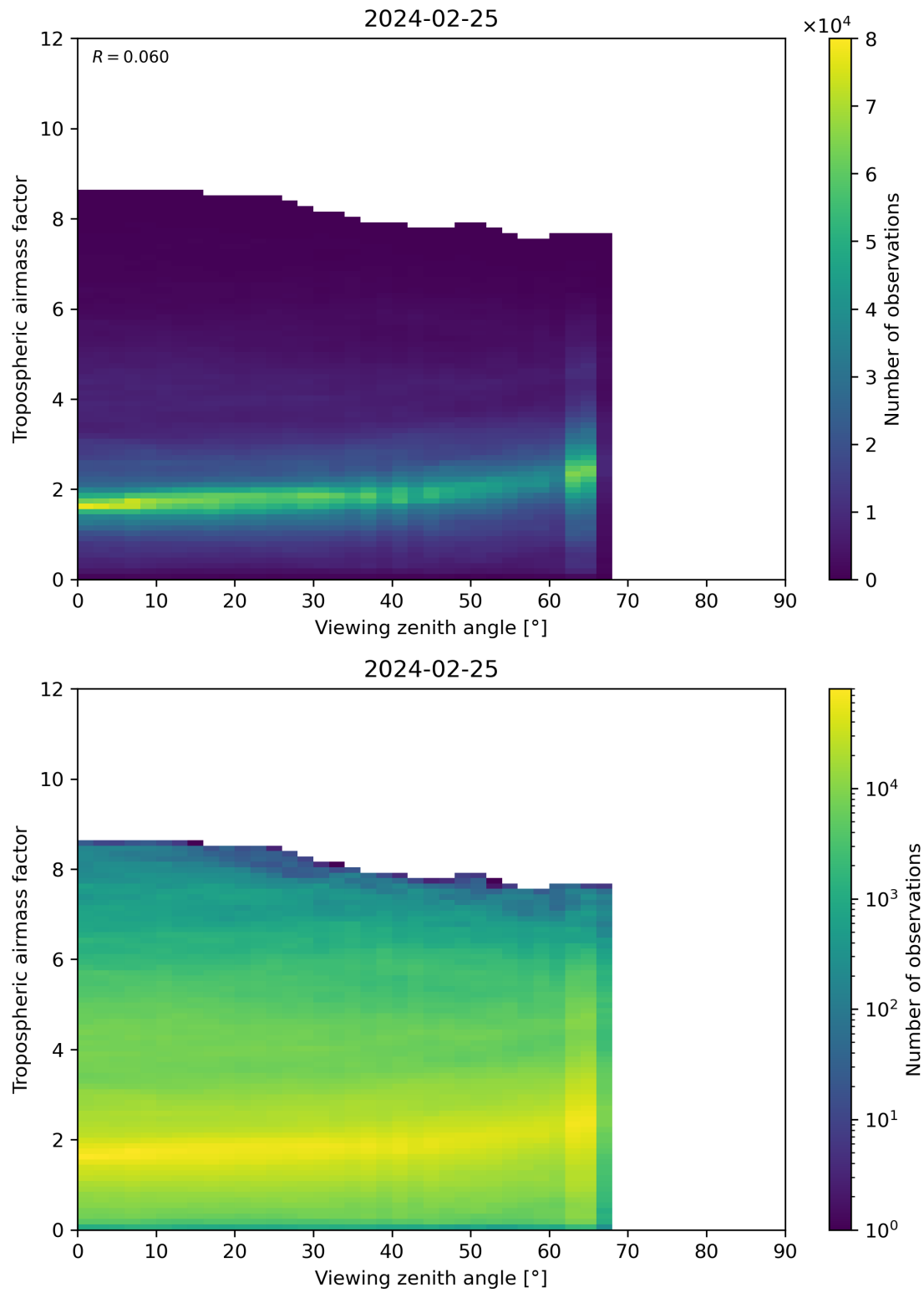
Figure 161: Scatter density plot of “Viewing zenith angle” against “Tropospheric airmass factor” for 2024-02-24 to 2024-02-26.
