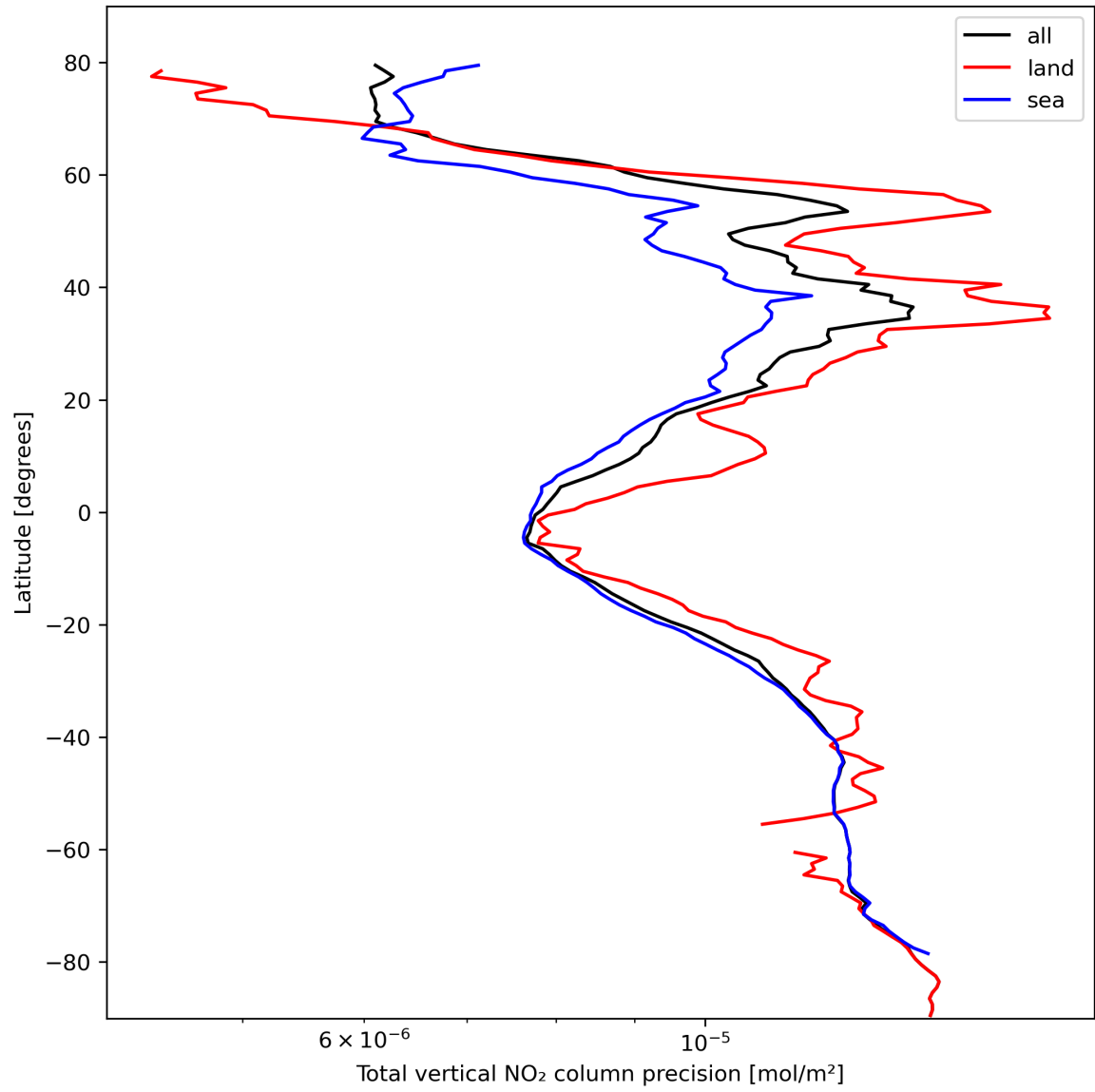
Figure 22: Zonal average of “Total vertical NO 2 column precision” for 2024-02-24 to 2024-02-26.
