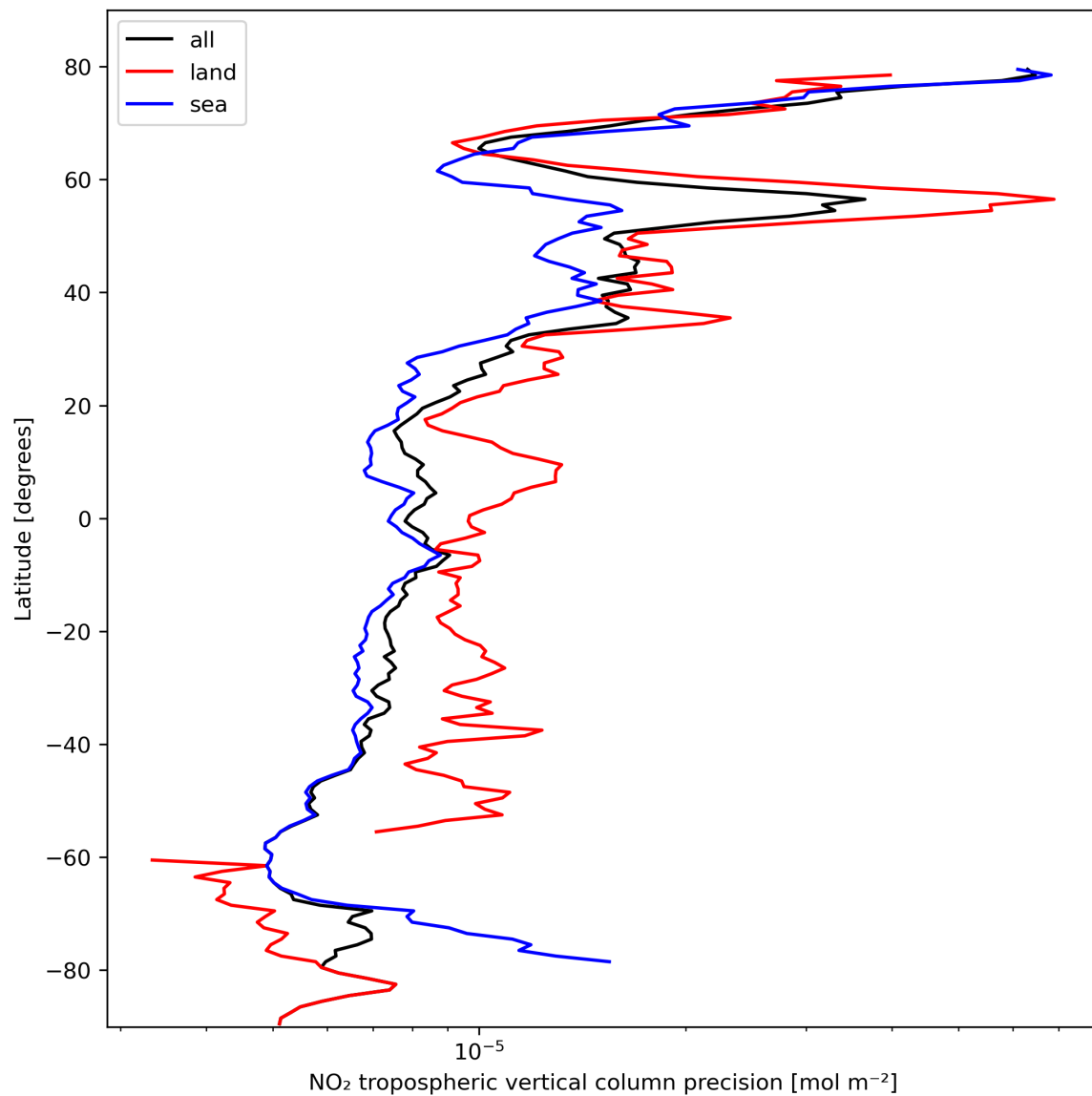
Figure 13: Zonal average of “NO 2 tropospheric vertical column precision” for 2024-02-24 to 2024-02-26.
