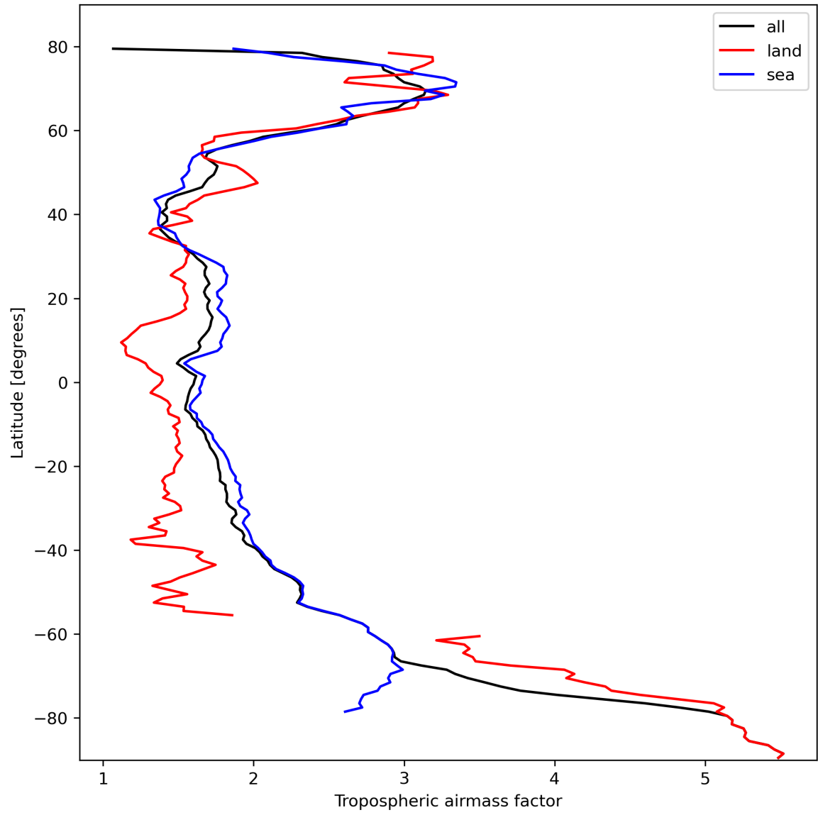
Figure 14: Zonal average of “Tropospheric airmass factor” for 2024-02-24 to 2024-02-26.
