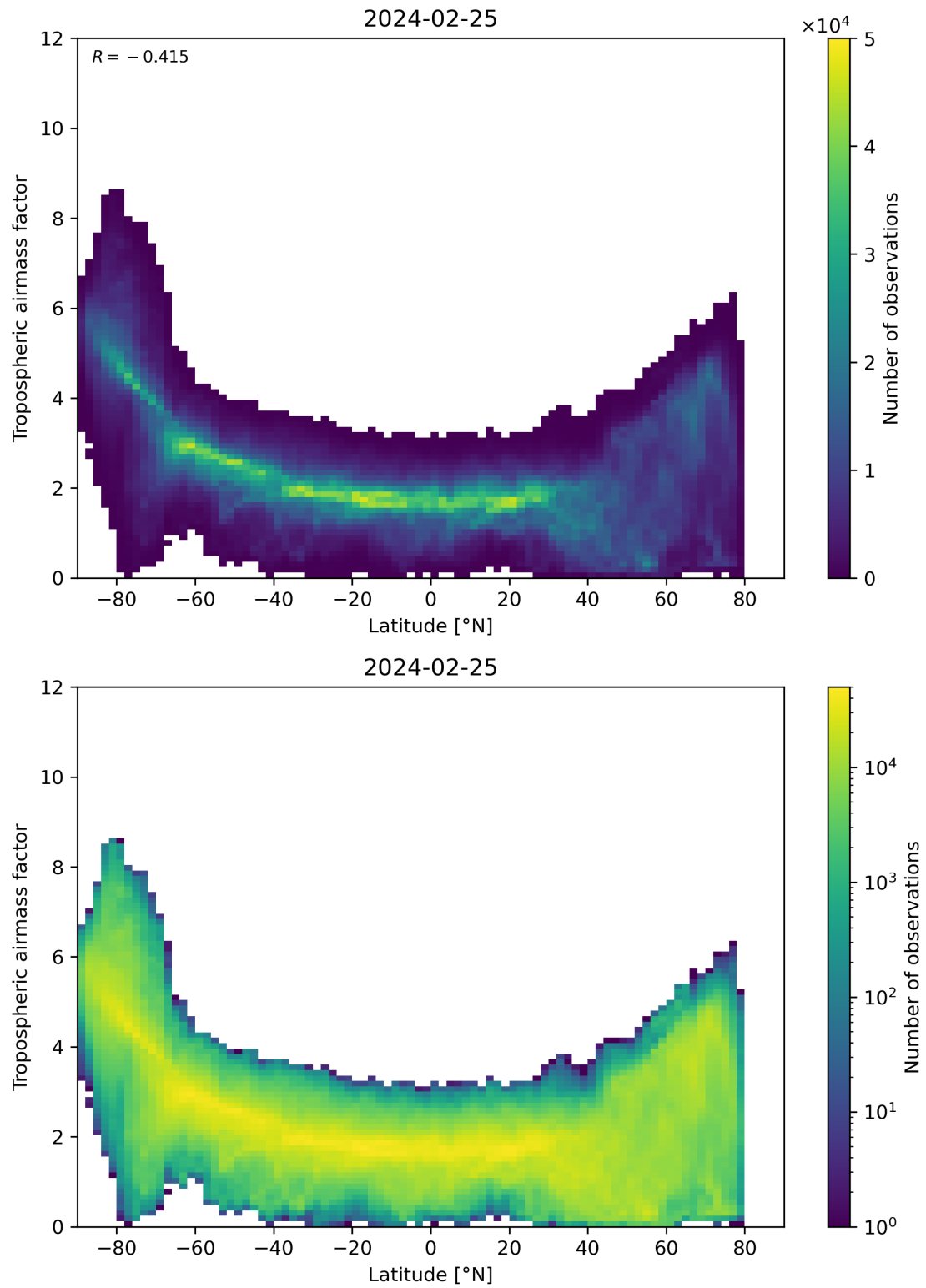
Figure 85: Scatter density plot of “Latitude” against “Tropospheric airmass factor” for 2024-02-24 to 2024-02-26.
