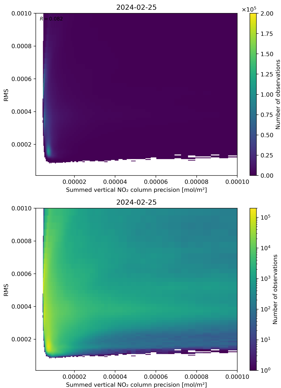
Figure 108: Scatter density plot of “Summed vertical NO 2 column precision” against “RMS” for 2024-02-24 to 2024-02-26.
