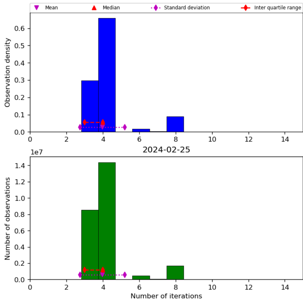
Figure 34: Histogram of “Number of iterations” for 2024-02-24 to 2024-02-26
