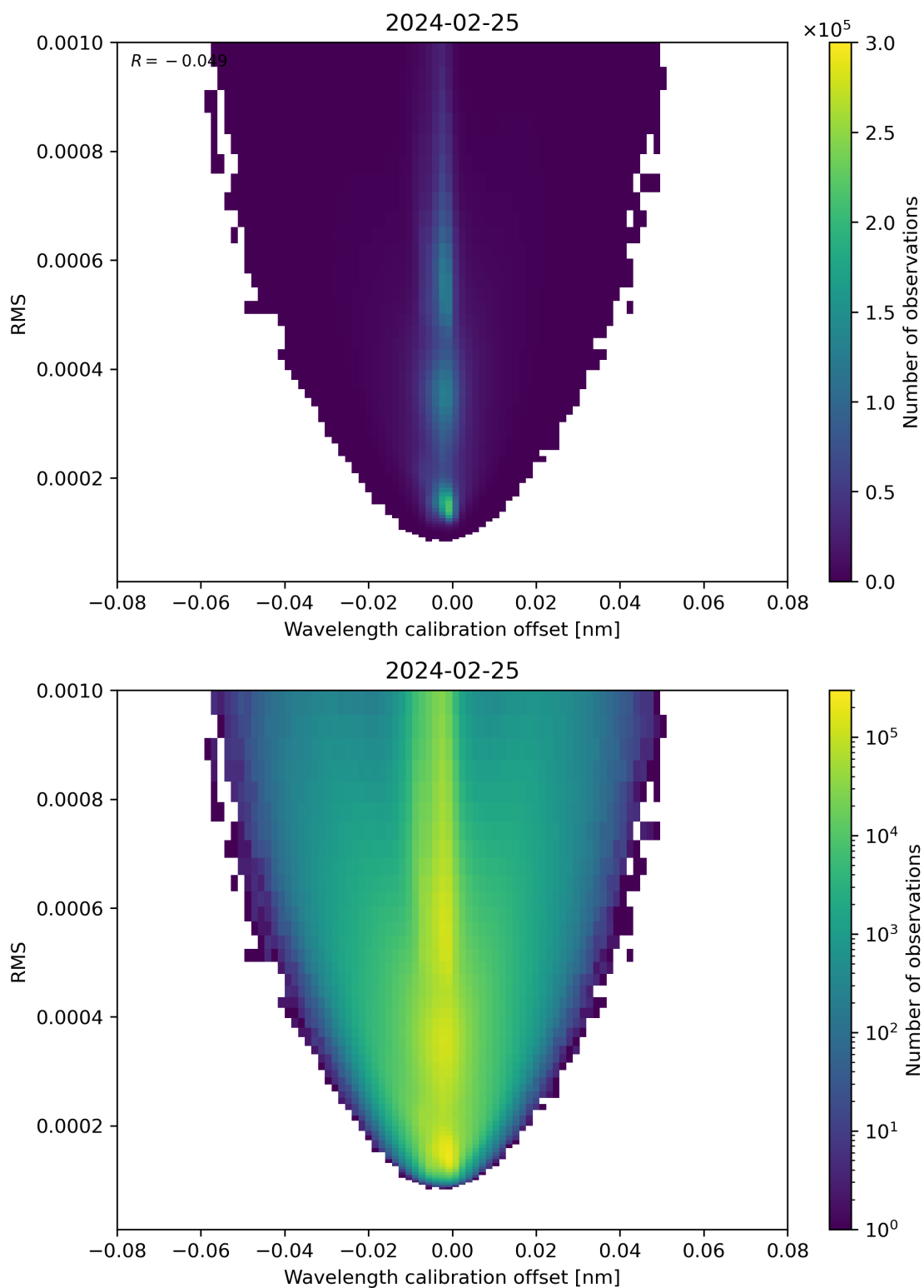
Figure 181: Scatter density plot of “Wavelength calibration offset” against “RMS” for 2024-02-24 to 2024-02-26.
