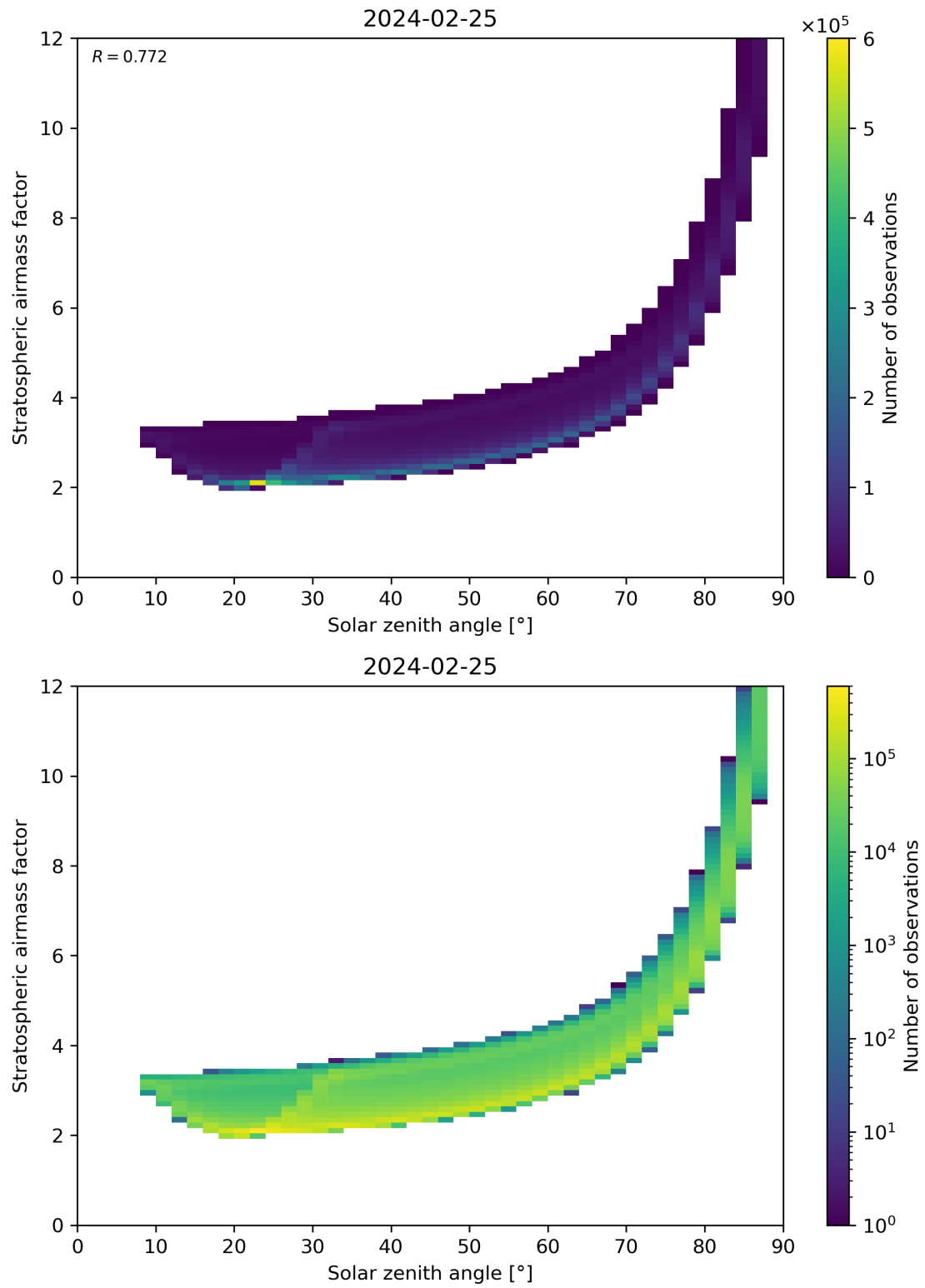
Figure 145: Scatter density plot of “Solar zenith angle” against “Stratospheric airmass factor” for 2024-02-24 to 2024-02-26.
