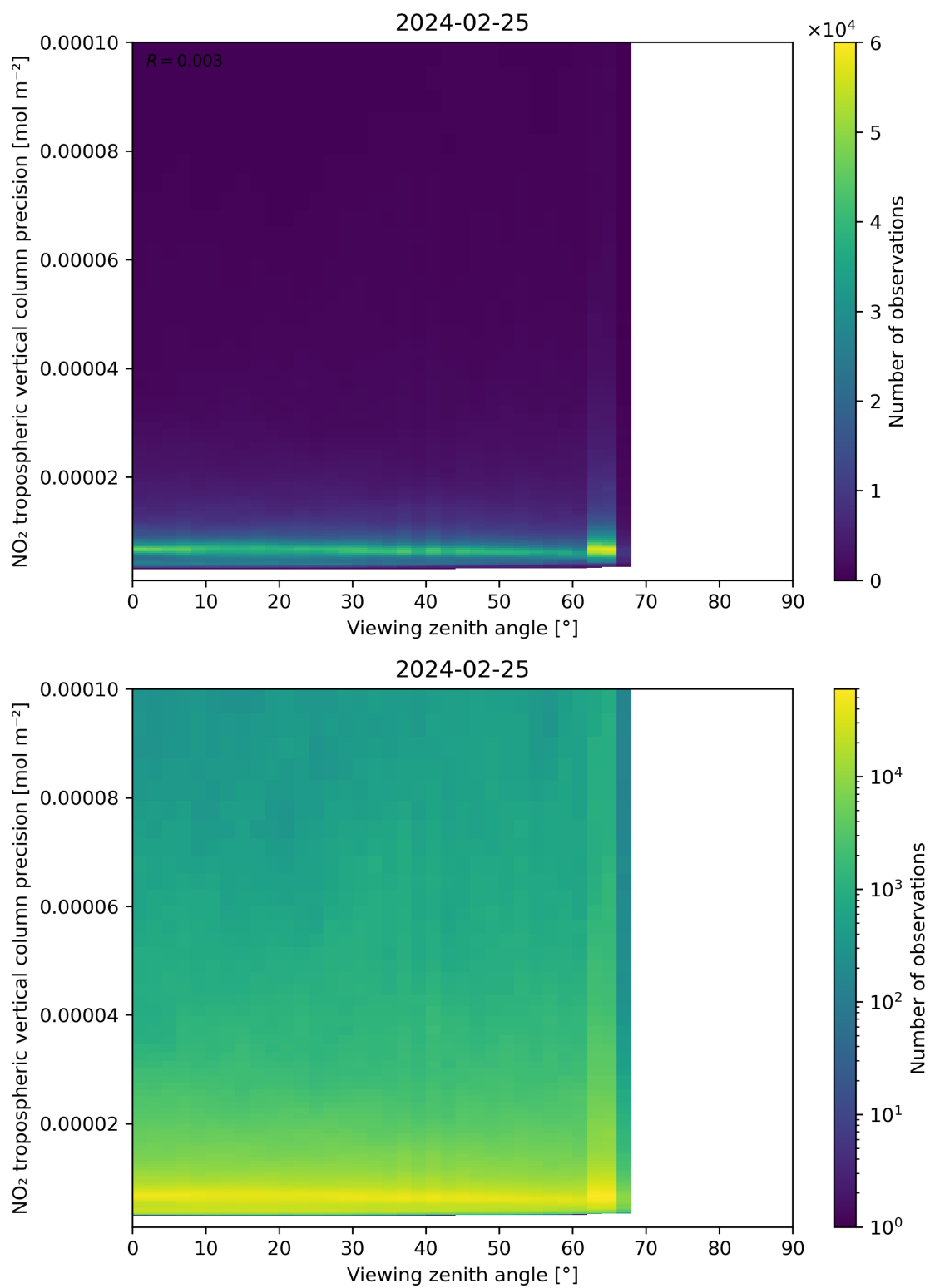
Figure 170: Scatter density plot of “Viewing zenith angle” against “NO 2 tropospheric vertical column precision” for 2024-02-24 to 2024-02-26.
