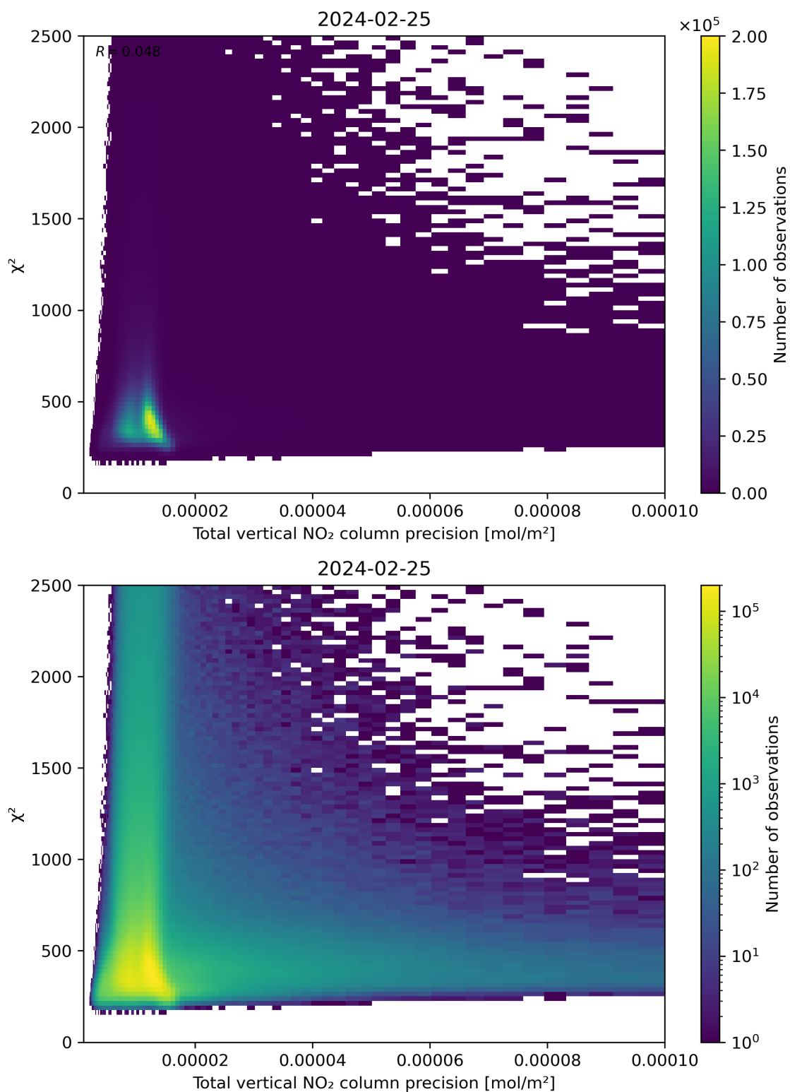
Figure 116: Scatter density plot of “Total vertical NO 2 column precision” against “ \chi^2 ” for 2024-02-24 to 2024-02-26.
