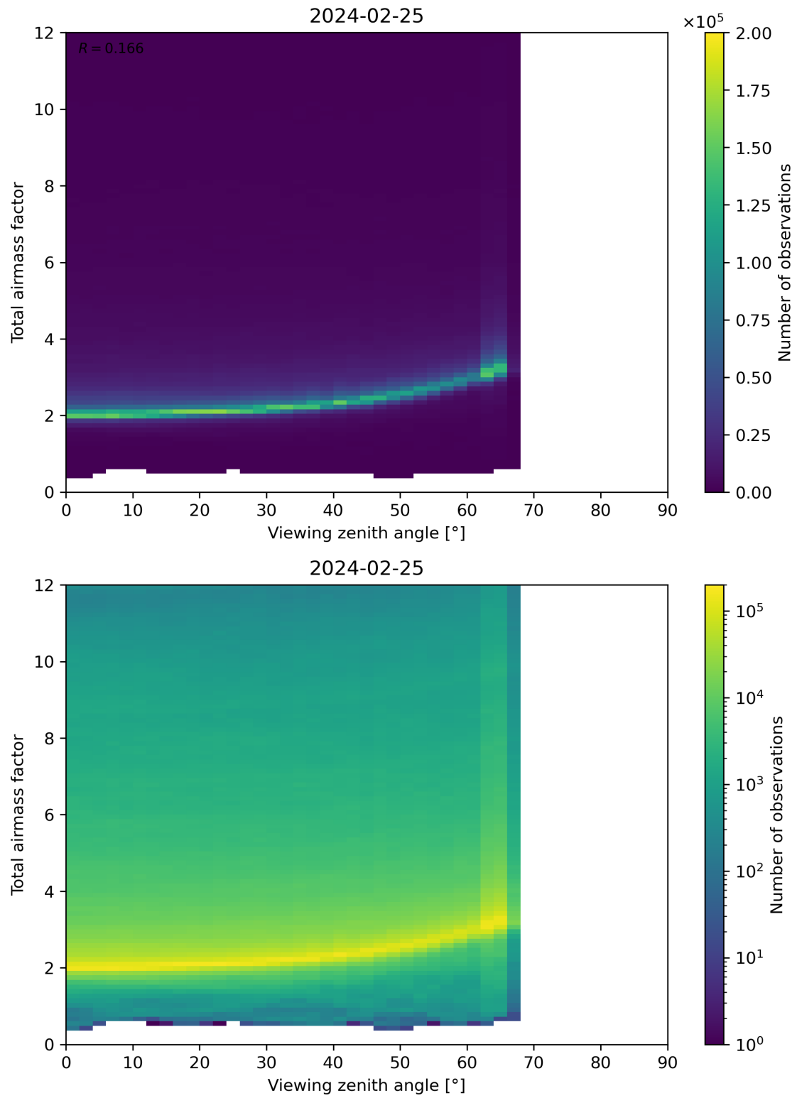
Figure 160: Scatter density plot of “Viewing zenith angle” against “Total airmass factor” for 2024-02-24 to 2024-02-26.
