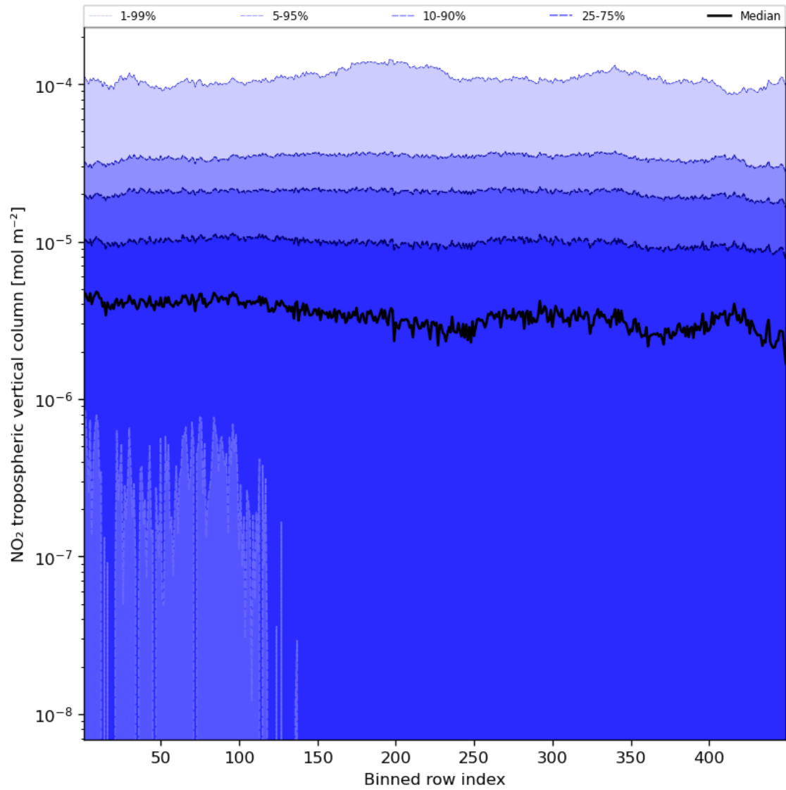
Figure 46: Along track statistics of "NO 2 tropospheric vertical column" for 2024-02-24 to 2024-02-26
