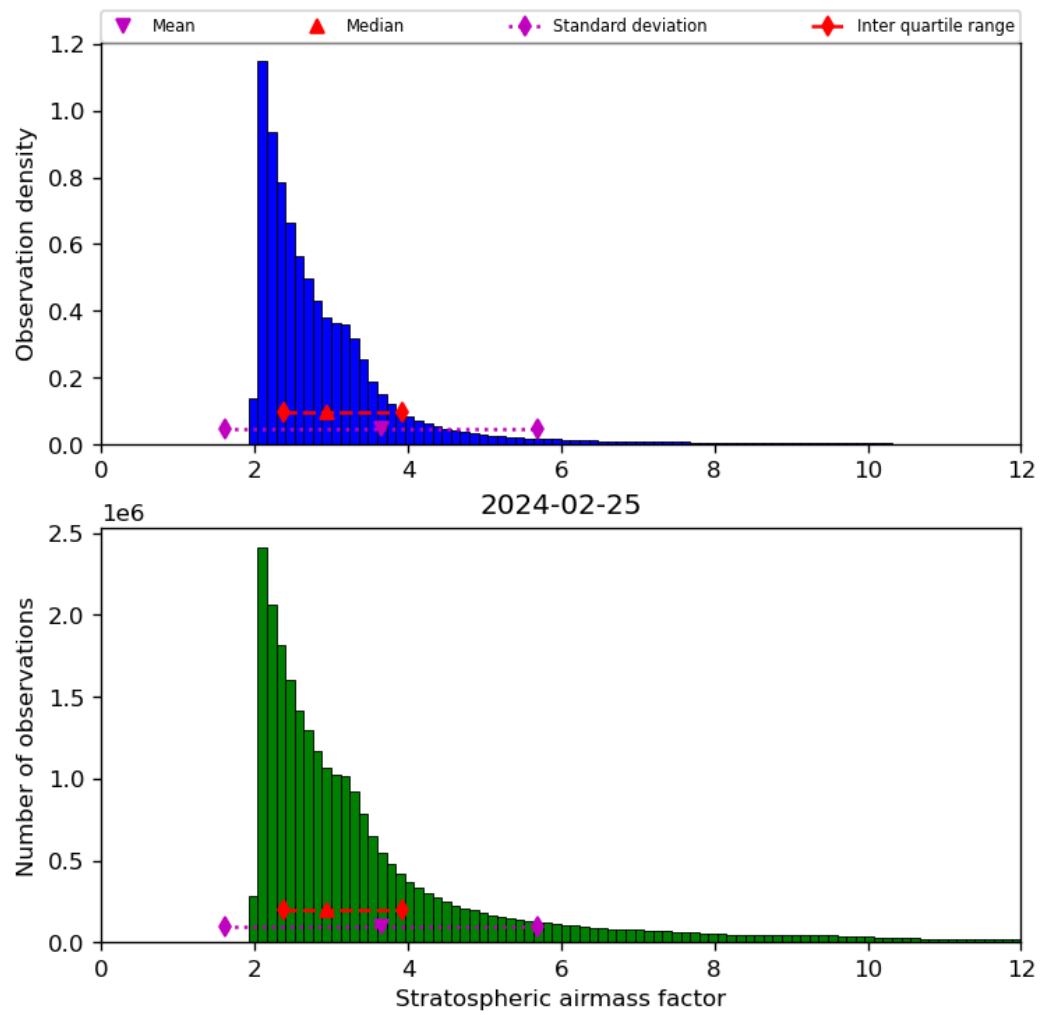
Figure 44: Histogram of “Stratospheric airmass factor” for 2024-02-24 to 2024-02-26
