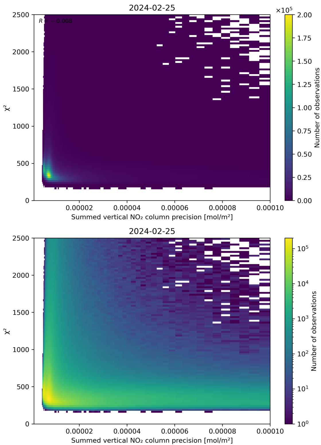
Figure 107: Scatter density plot of “Summed vertical NO 2 column precision” against “ \chi^2 ” for 2024-02-24 to 2024-02-26.
