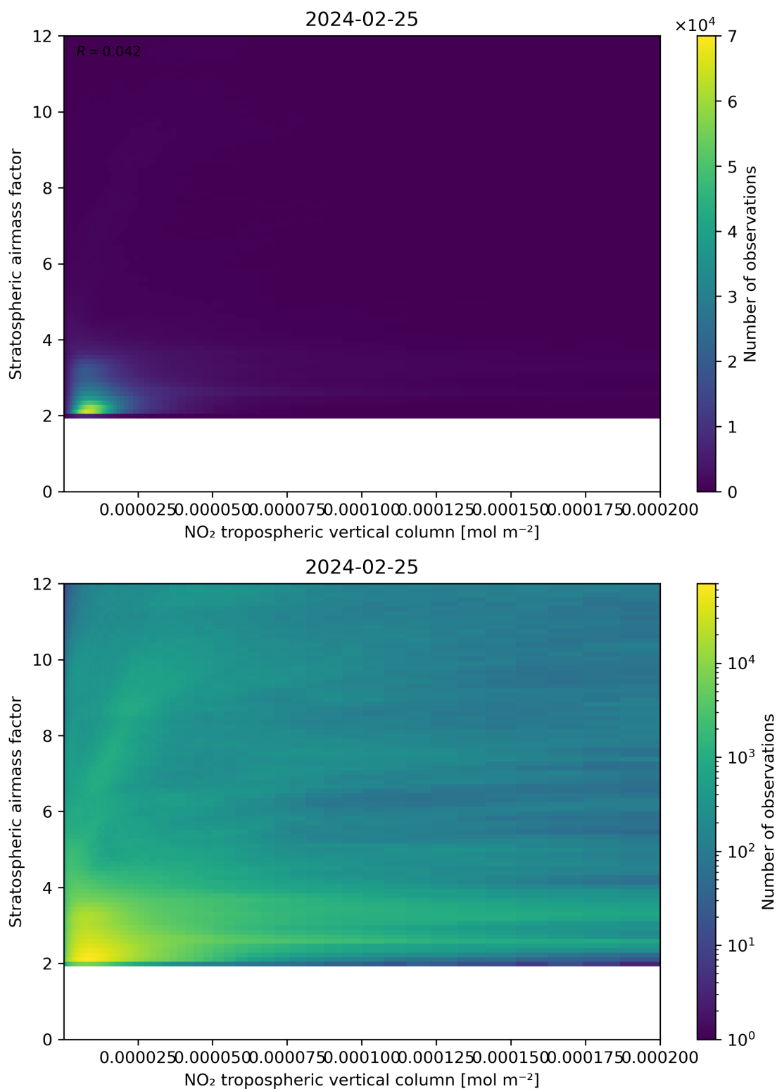
Figure 121: Scatter density plot of “NO 2 tropospheric vertical column” against “Stratospheric airmass factor” for 2024-02-24 to 2024-02-26.
