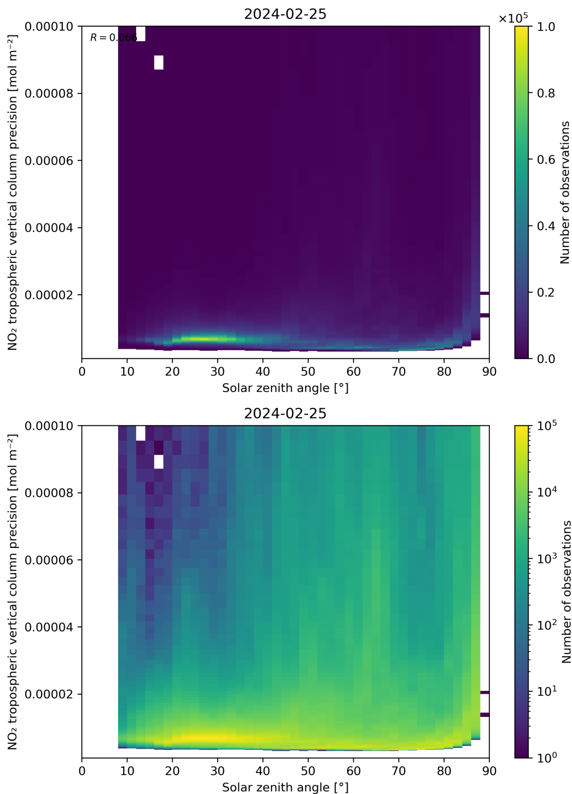
Figure 156: Scatter density plot of “Solar zenith angle” against “NO 2 tropospheric vertical column precision” for 2024-02-24 to 2024-02-26.
