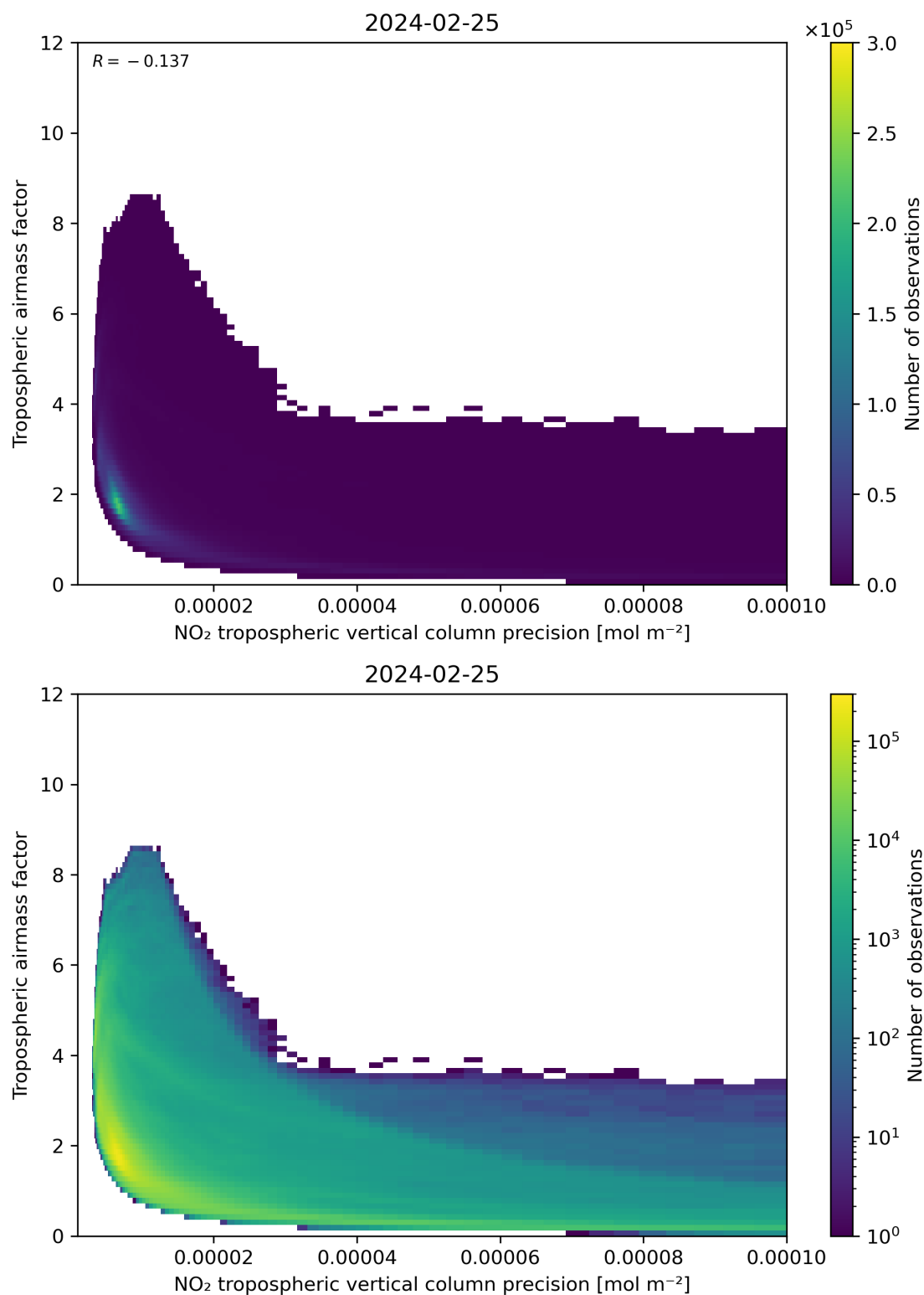
Figure 133: Scatter density plot of “NO 2 tropospheric vertical column precision” against “Tropospheric airmass factor” for 2024-02-24 to 2024-02-26.
