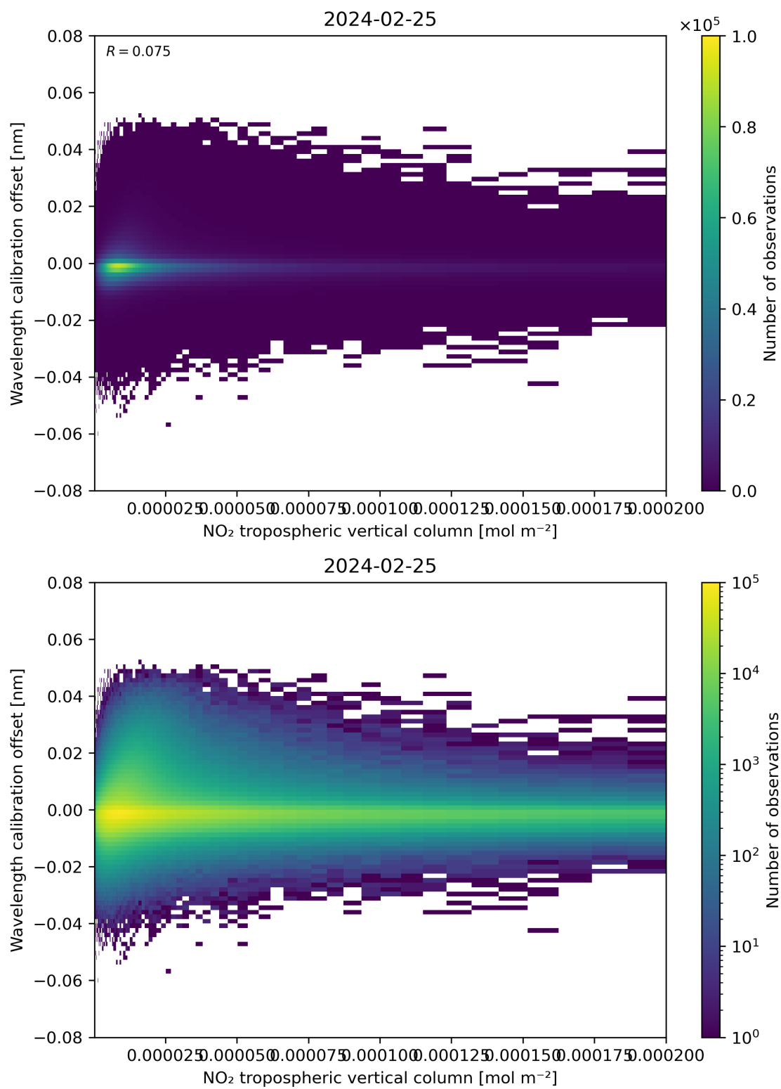
Figure 143: Scatter density plot of “NO 2 tropospheric vertical column” against “Wavelength calibration offset” for 2024-02-24 to 2024-02-26.
