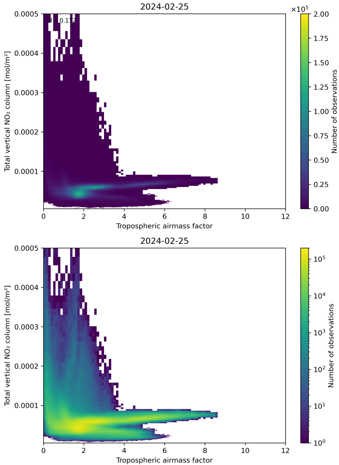
Figure 77: Scatter density plot of “Tropospheric airmass factor” against “Total vertical NO 2 column” for 2024-02-24 to 2024-02-26.
