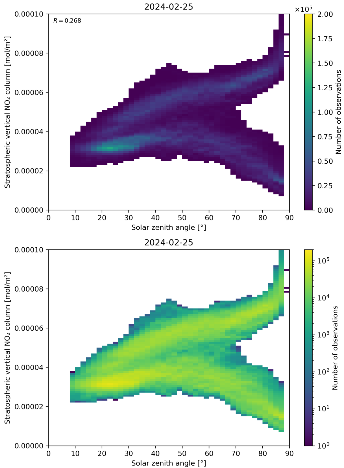
Figure 150: Scatter density plot of “Solar zenith angle” against “Stratospheric vertical NO 2 column” for 2024-02-24 to 2024-02-26.
