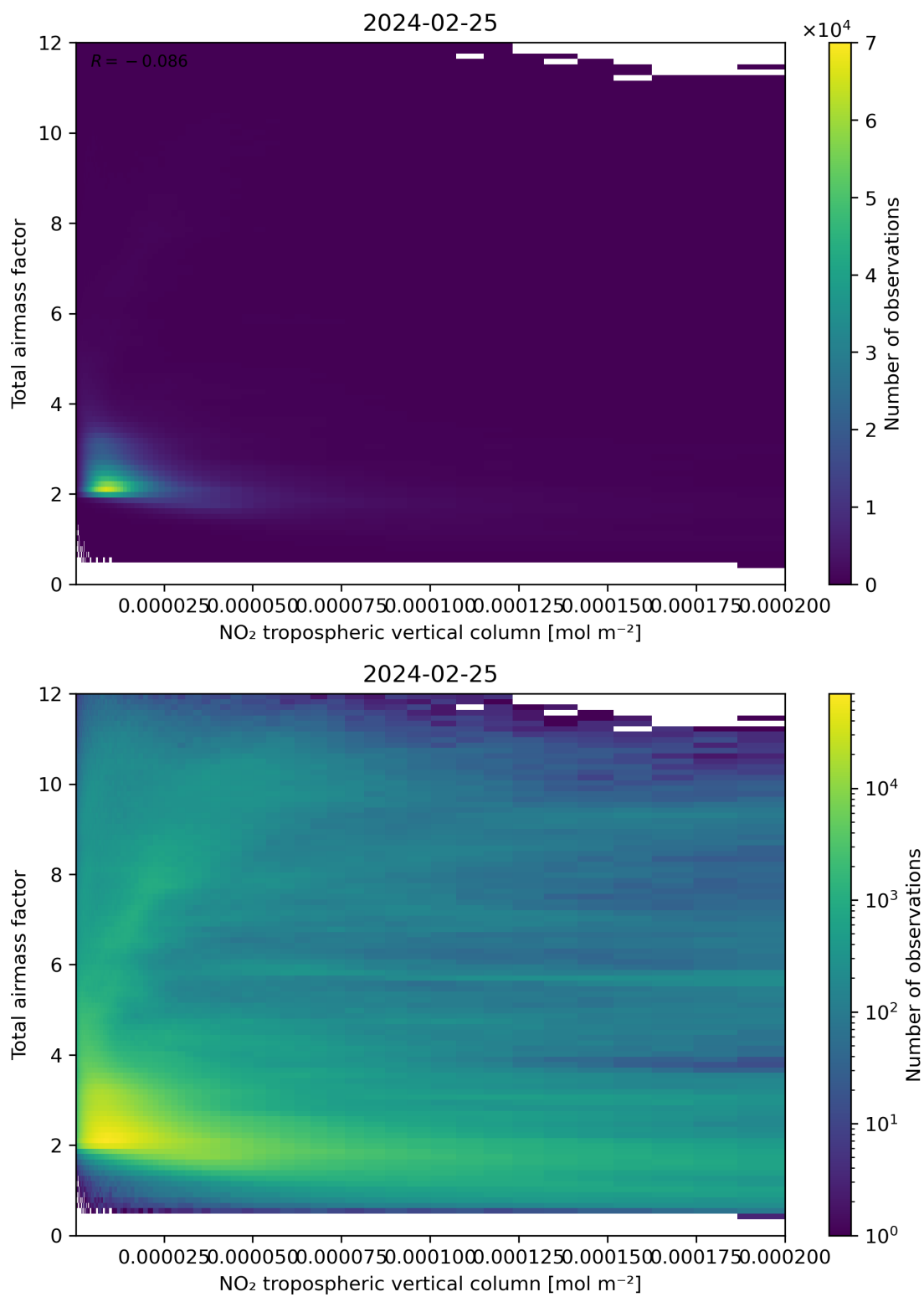
Figure 122: Scatter density plot of “NO 2 tropospheric vertical column” against “Total air mass factor” for 2024-02-24 to 2024-02-26.
