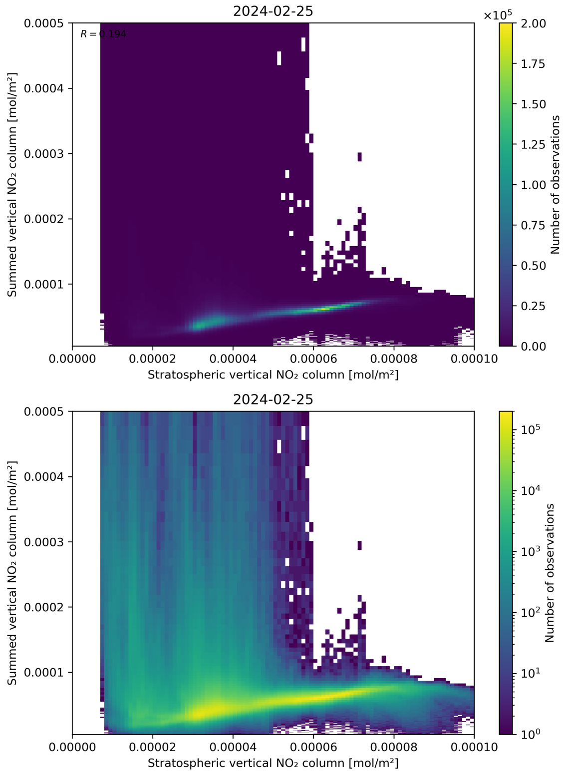
Figure 98: Scatter density plot of “Stratospheric vertical NO 2 column” against “Summed vertical NO 2 column” for 2024-02-24 to 2024-02-26.
