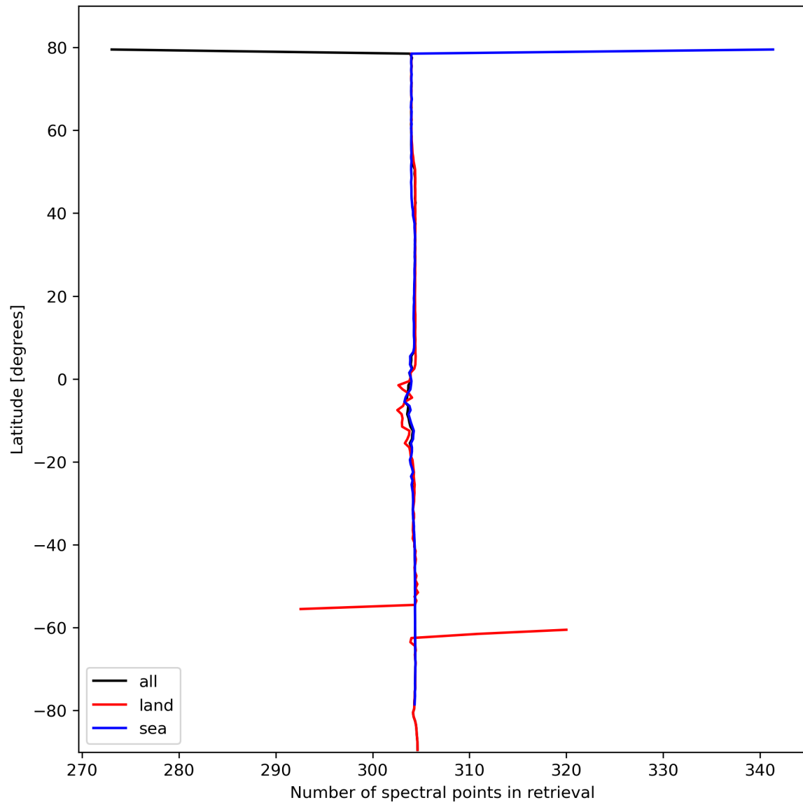
Figure 16: Zonal average of “Number of spectral points in retrieval” for 2024-02-24 to 2024-02-26.
