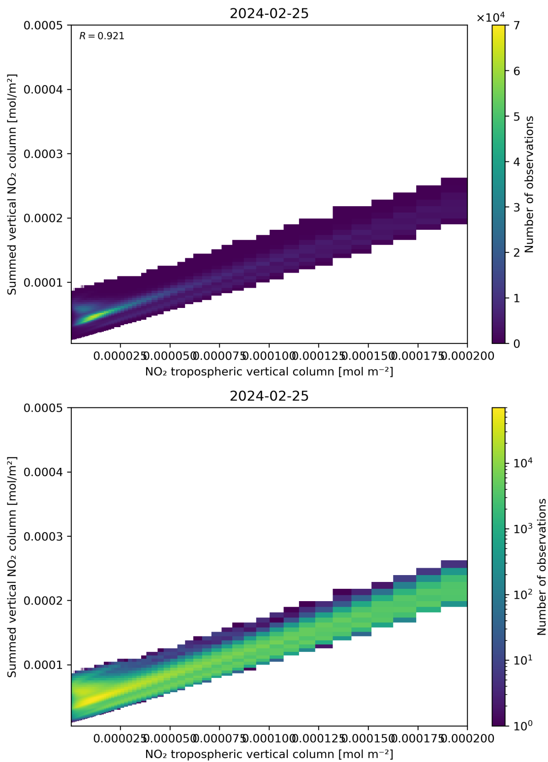
Figure 126: Scatter density plot of “NO 2 tropospheric vertical column” against “Summed vertical NO 2 column” for 2024-02-24 to 2024-02-26.
