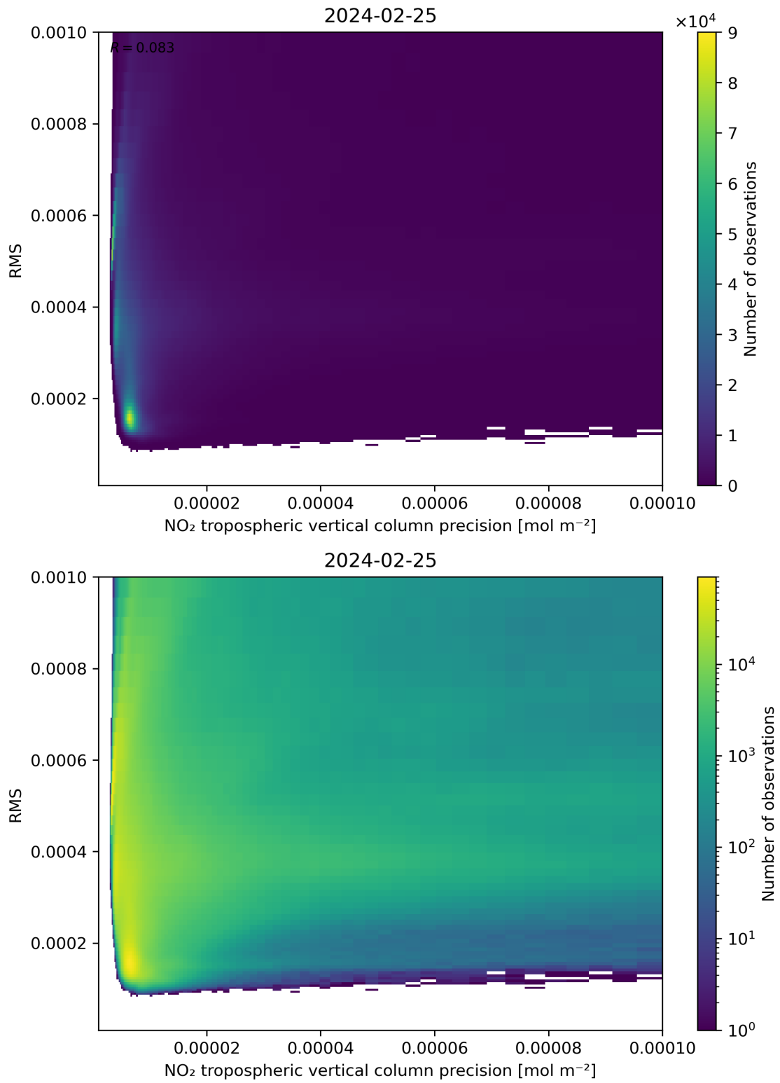
Figure 140: Scatter density plot of “NO 2 tropospheric vertical column precision” against “RMS” for 2024-02-24 to 2024-02-26.
