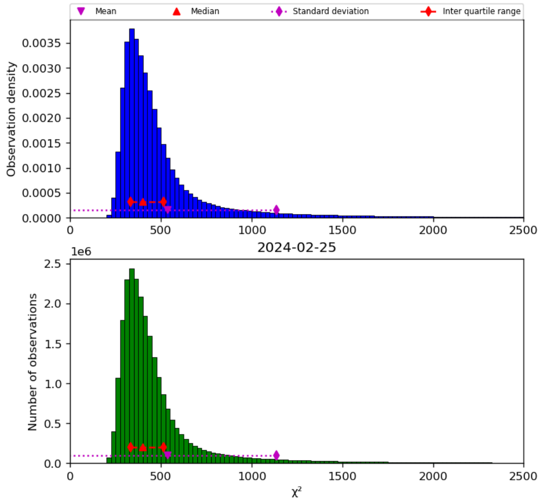
Figure 42: Histogram of “ \chi^2 ” for 2024-02-24 to 2024-02-26
