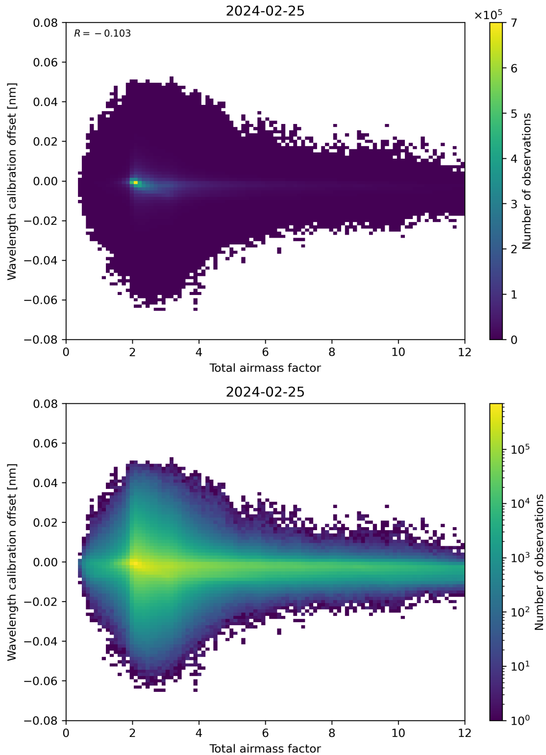
Figure 70: Scatter density plot of “Total airmass factor” against “Wavelength calibration offset” for 2024-02-24 to 2024-02-26.
