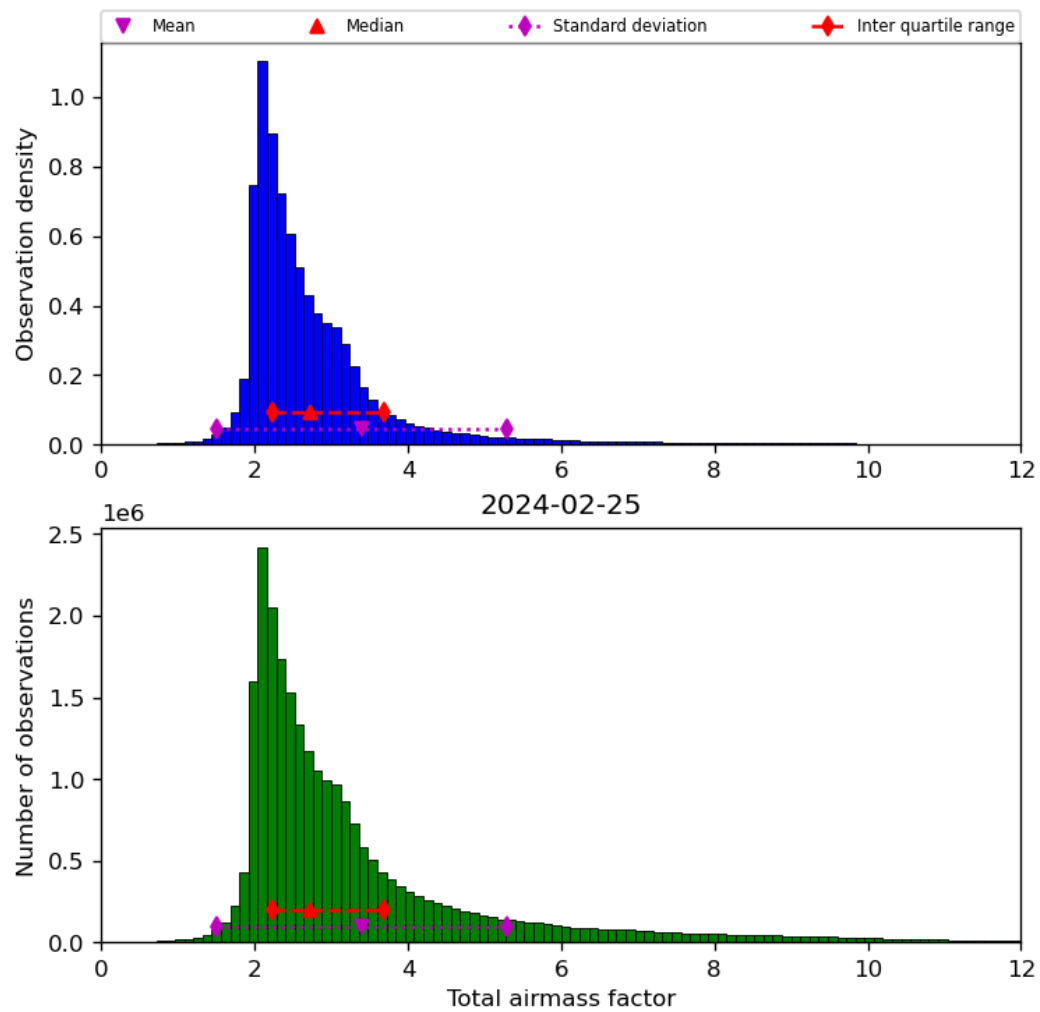
Figure 32: Histogram of “Total airmass factor” for 2024-02-24 to 2024-02-26
