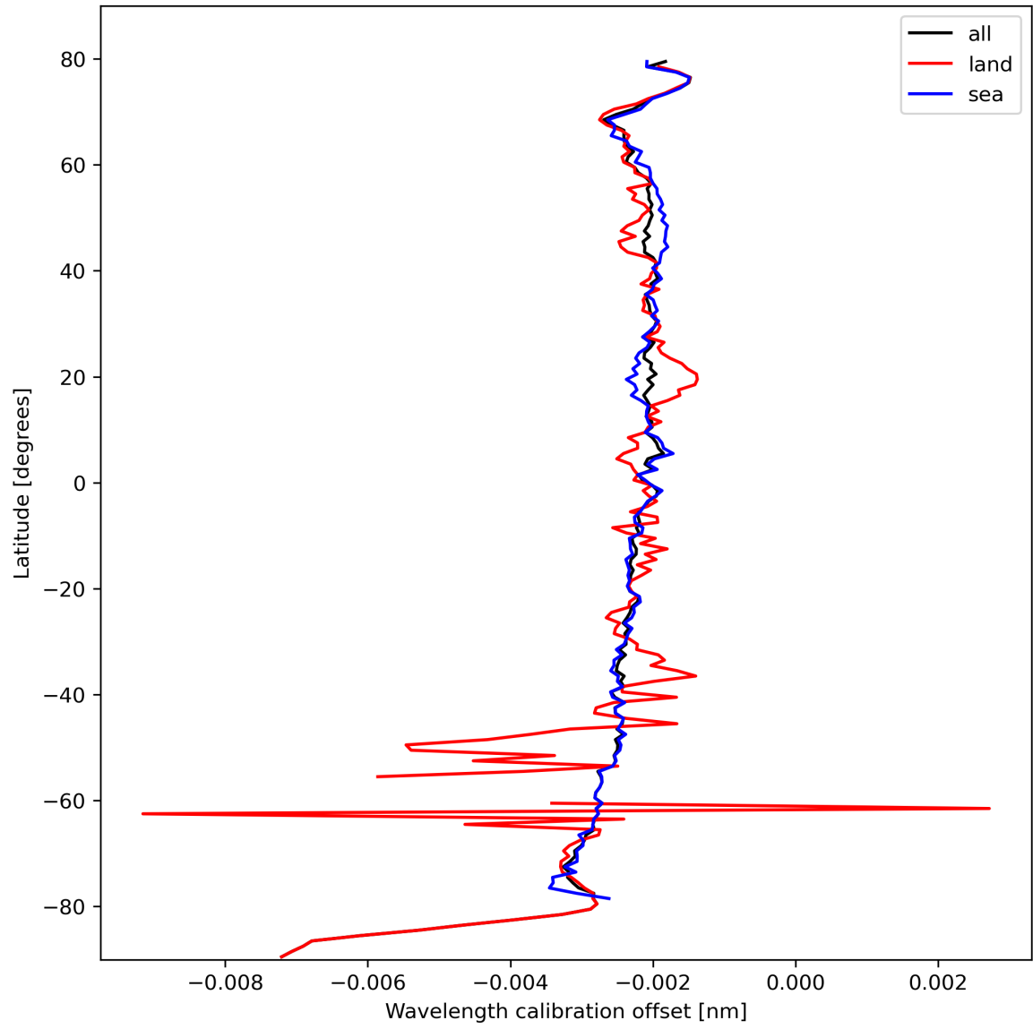
Figure 18: Zonal average of “Wavelength calibration offset” for 2024-02-24 to 2024-02-26.
