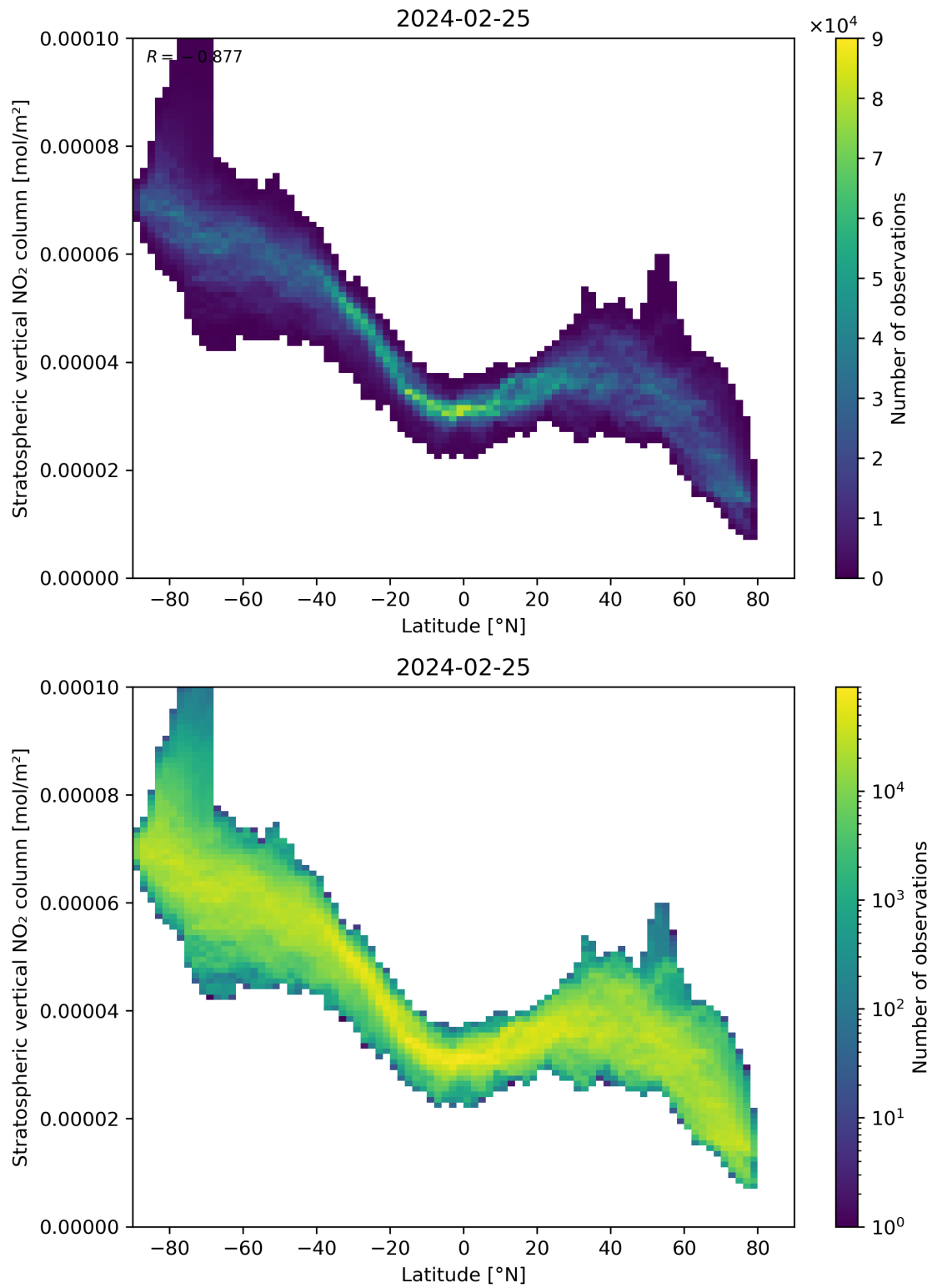
Figure 87: Scatter density plot of “Latitude” against “Stratospheric vertical NO 2 column” for 2024-02-24 to 2024-02-26.
