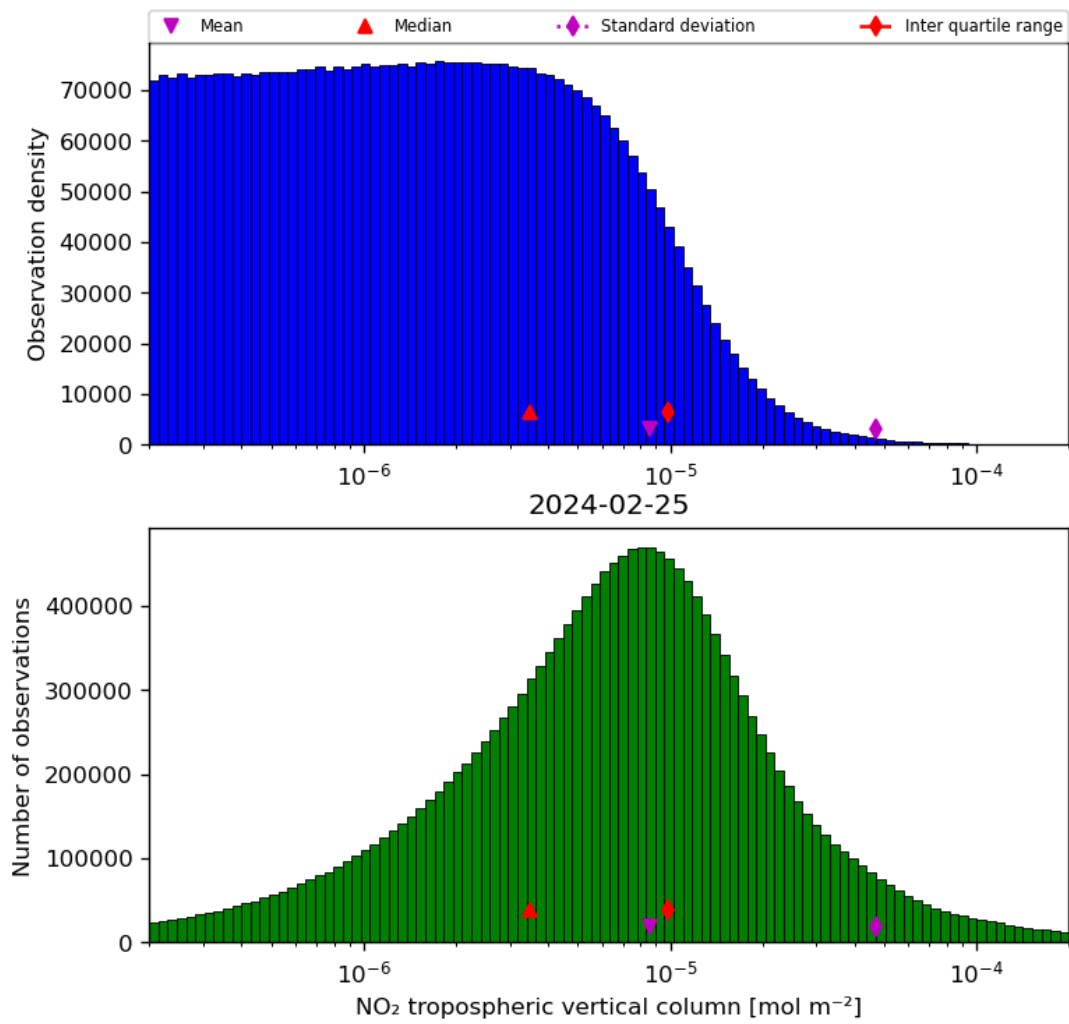
Figure 29: Histogram of “NO 2 tropospheric vertical column” for 2024-02-24 to 2024-02-26
