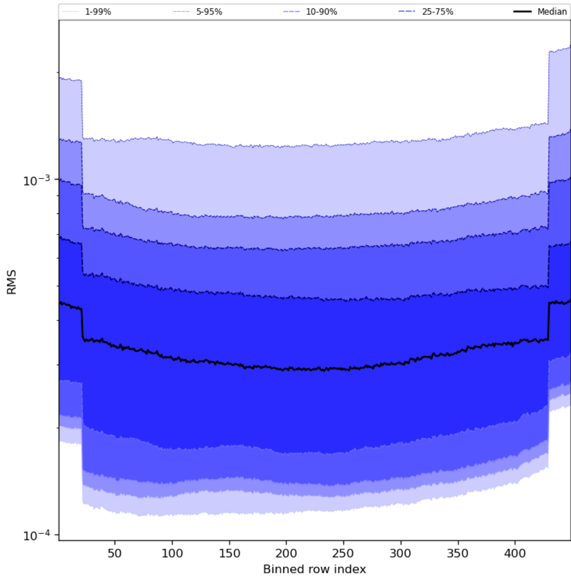
Figure 60: Along track statistics of “RMS” for 2024-02-24 to 2024-02-26
