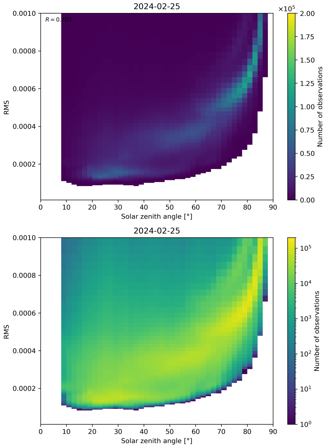
Figure 157: Scatter density plot of “Solar zenith angle” against “RMS” for 2024-02-24 to 2024-02-26.
