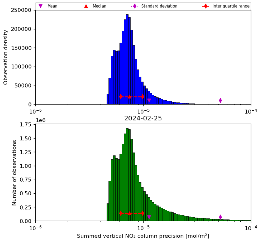
Figure 41: Histogram of “Summed vertical NO 2 column precision” for 2024-02-24 to 2024-02-26
