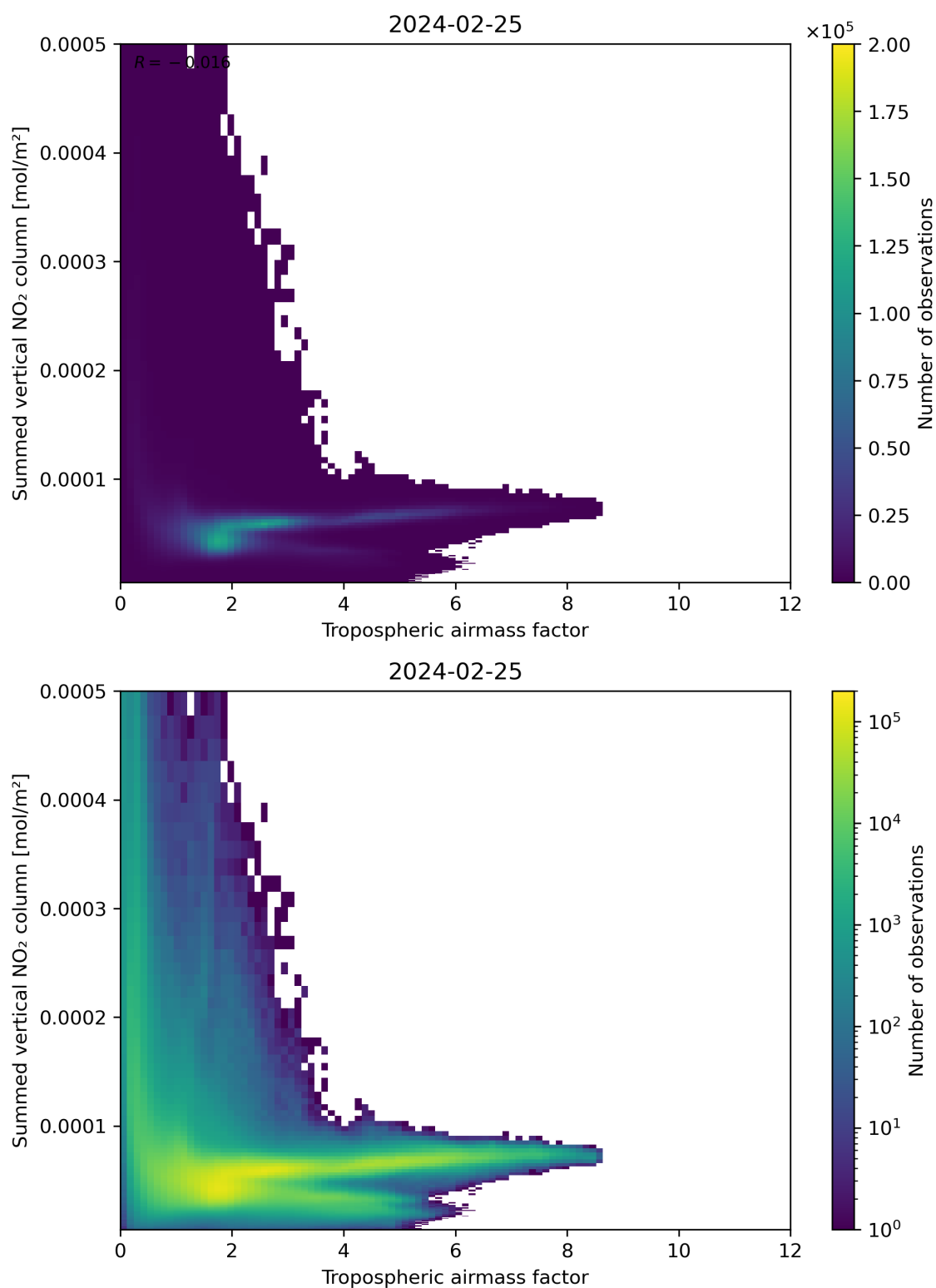
Figure 75: Scatter density plot of “Tropospheric airmass factor” against “Summed vertical NO 2 column” for 2024-02-24 to 2024-02-26.
