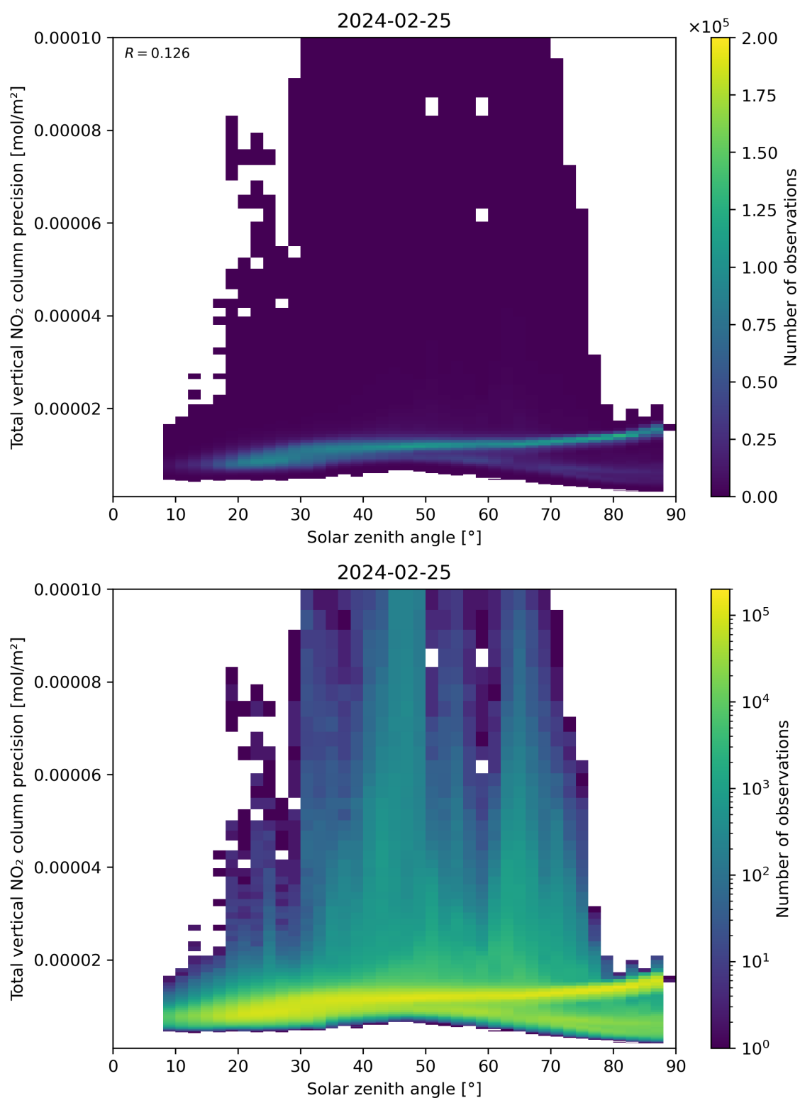
Figure 154: Scatter density plot of “Solar zenith angle” against “Total vertical NO 2 column precision” for 2024-02-24 to 2024-02-26.
