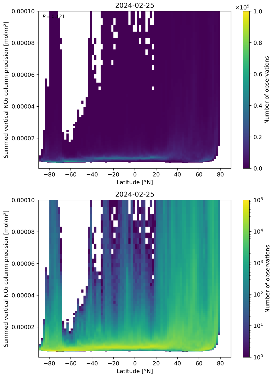
Figure 89: Scatter density plot of “Latitude” against “Summed vertical NO 2 column precision” for 2024-02-24 to 2024-02-26.
