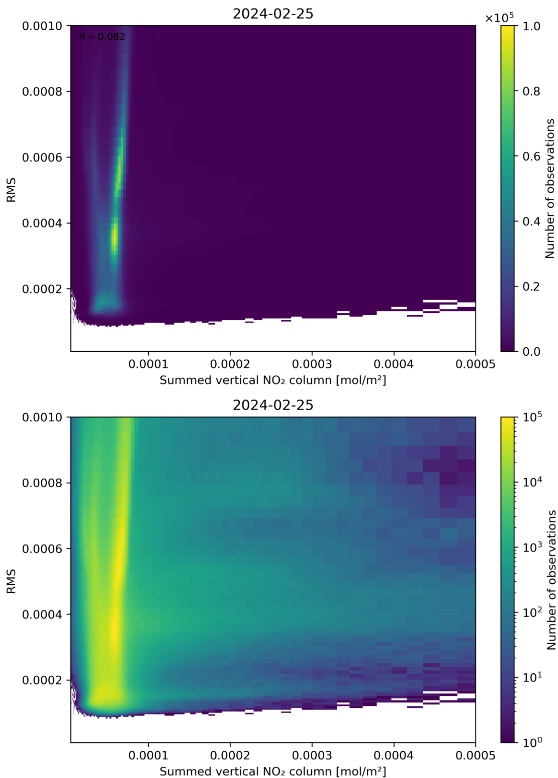
Figure 109: Scatter density plot of “Summed vertical NO 2 column” against “RMS” for 2024-02-24 to 2024-02-26.
