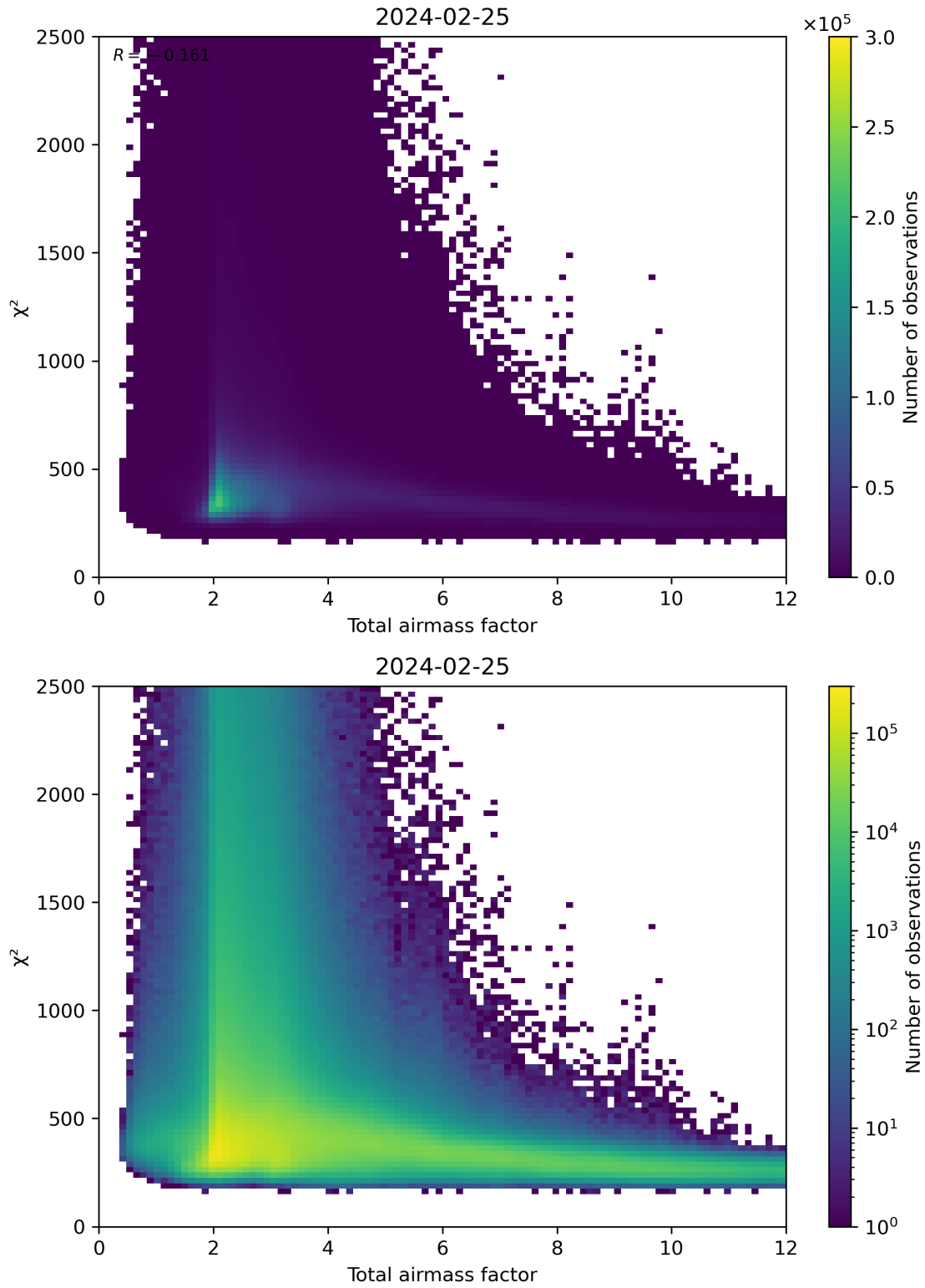
Figure 63: Scatter density plot of “Total airmass factor” against “ \chi^2 ” for 2024-02-24 to 2024-02-26.
