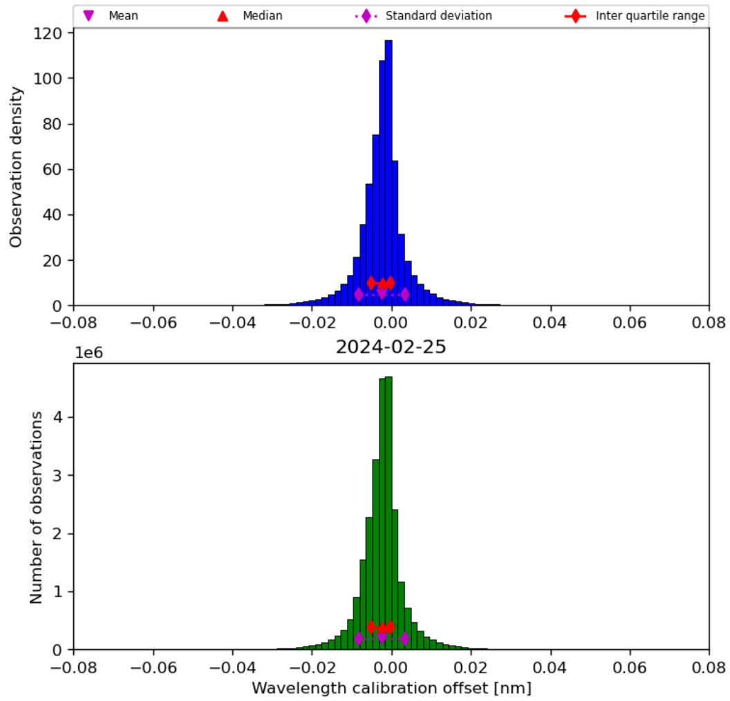
Figure 35: Histogram of “Wavelength calibration offset” for 2024-02-24 to 2024-02-26
