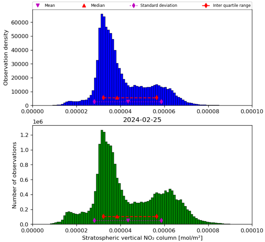
Figure 36: Histogram of “Stratospheric vertical NO 2 column” for 2024-02-24 to 2024-02-26
