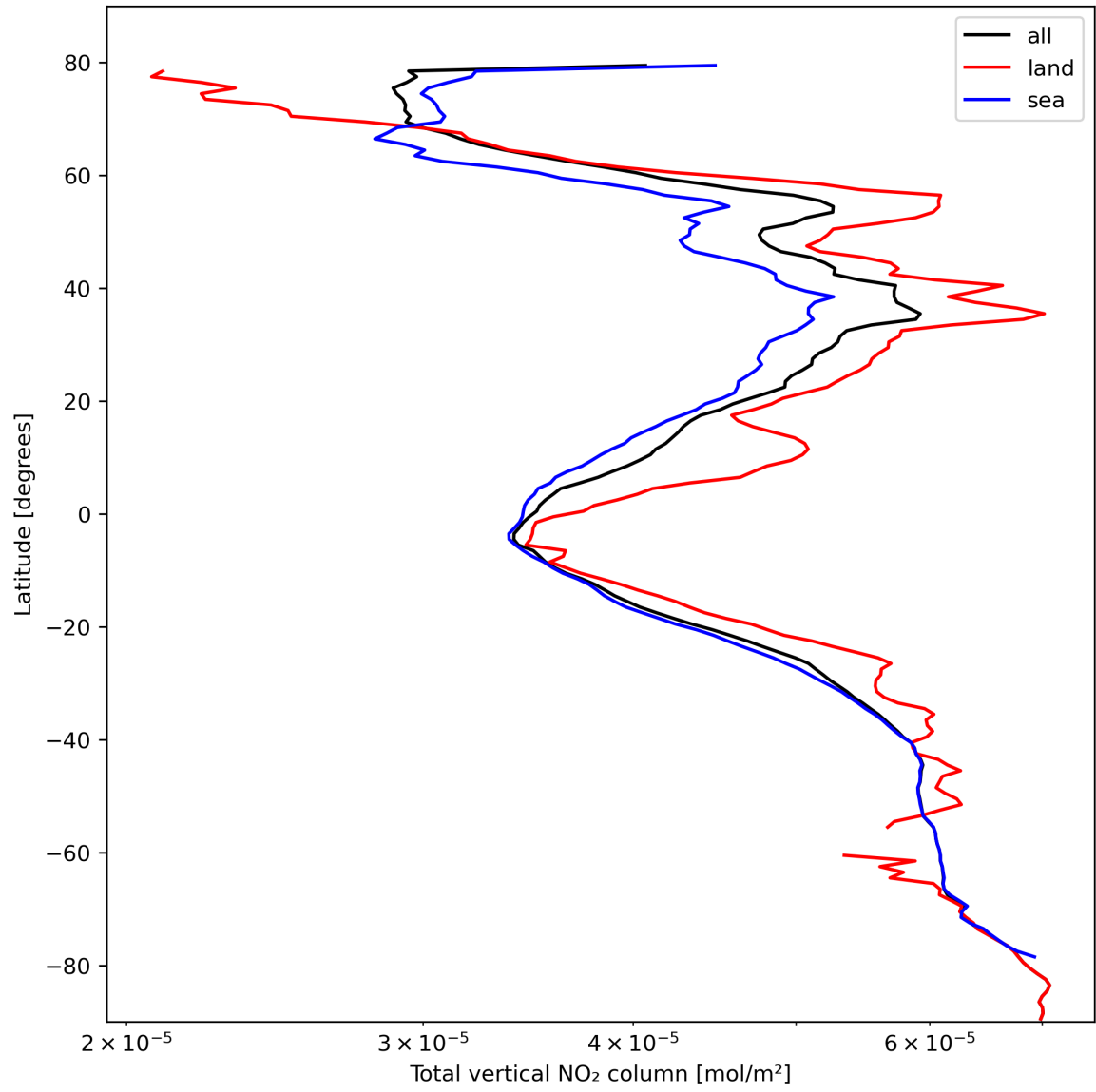
Figure 21: Zonal average of “Total vertical NO 2 column” for 2024-02-24 to 2024-02-26.
