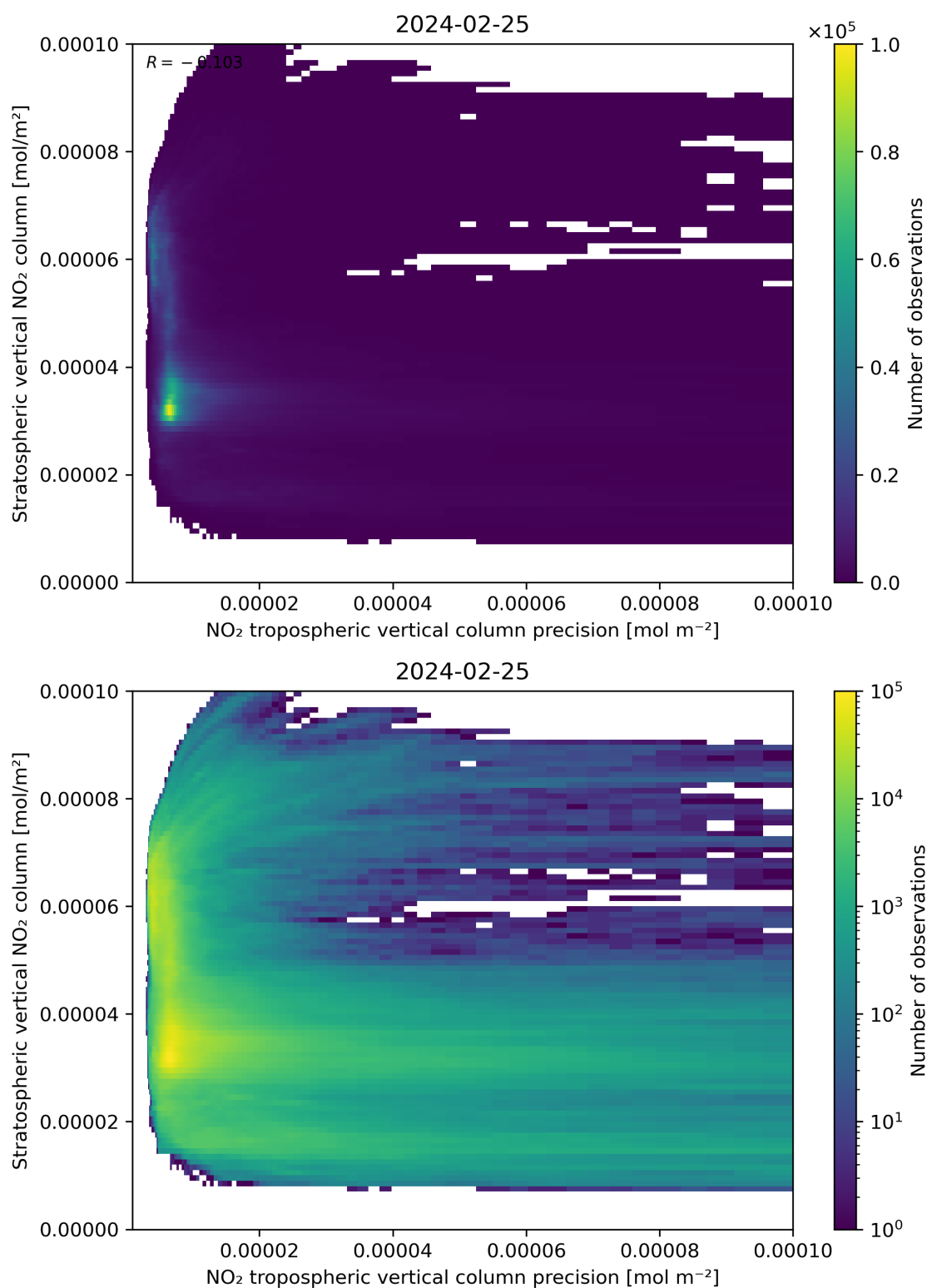
Figure 135: Scatter density plot of “NO 2 tropospheric vertical column precision” against “Stratospheric vertical NO 2 column” for 2024-02-24 to 2024-02-26.
