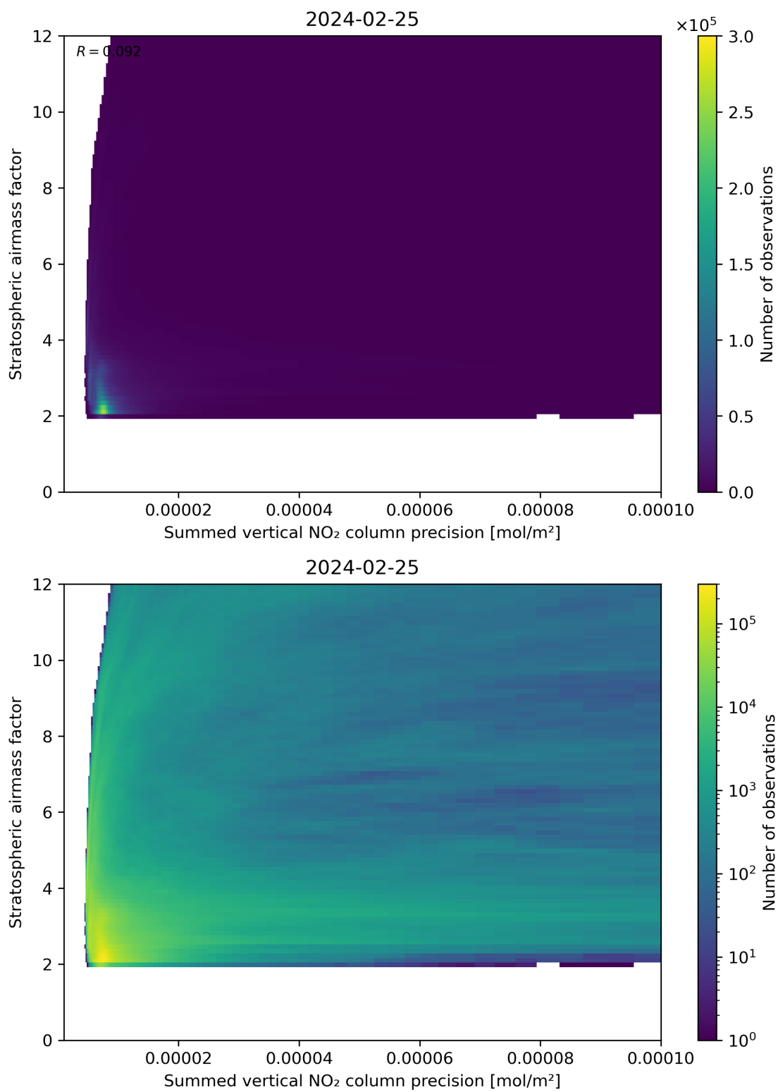
Figure 106: Scatter density plot of “Summed vertical NO 2 column precision” against “Stratospheric airmass factor” for 2024-02-24 to 2024-02-26.
