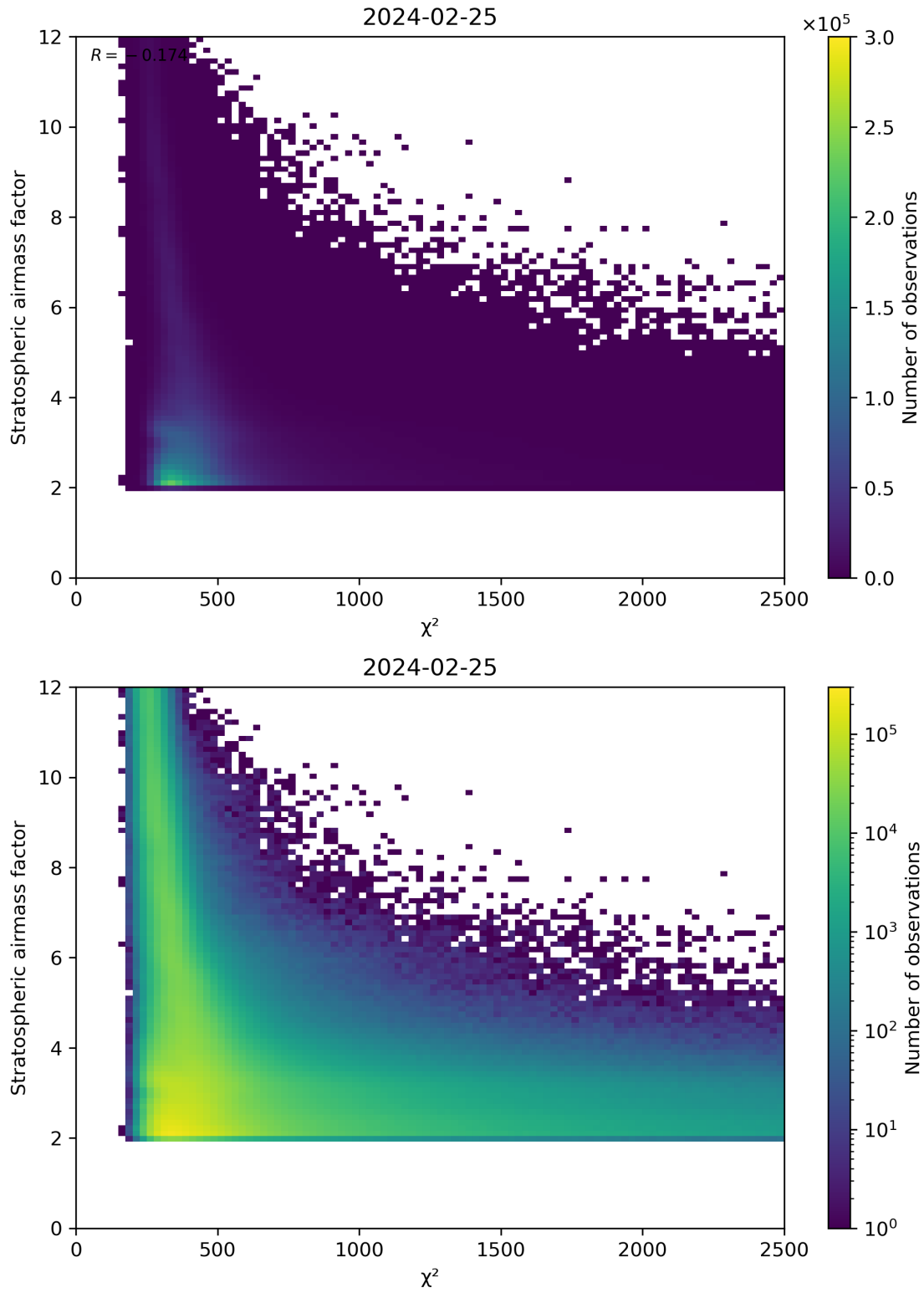
Figure 81: Scatter density plot of “ \chi^2 ” against “Stratospheric air mass factor” for 2024-02-24 to 2024-02-26.
