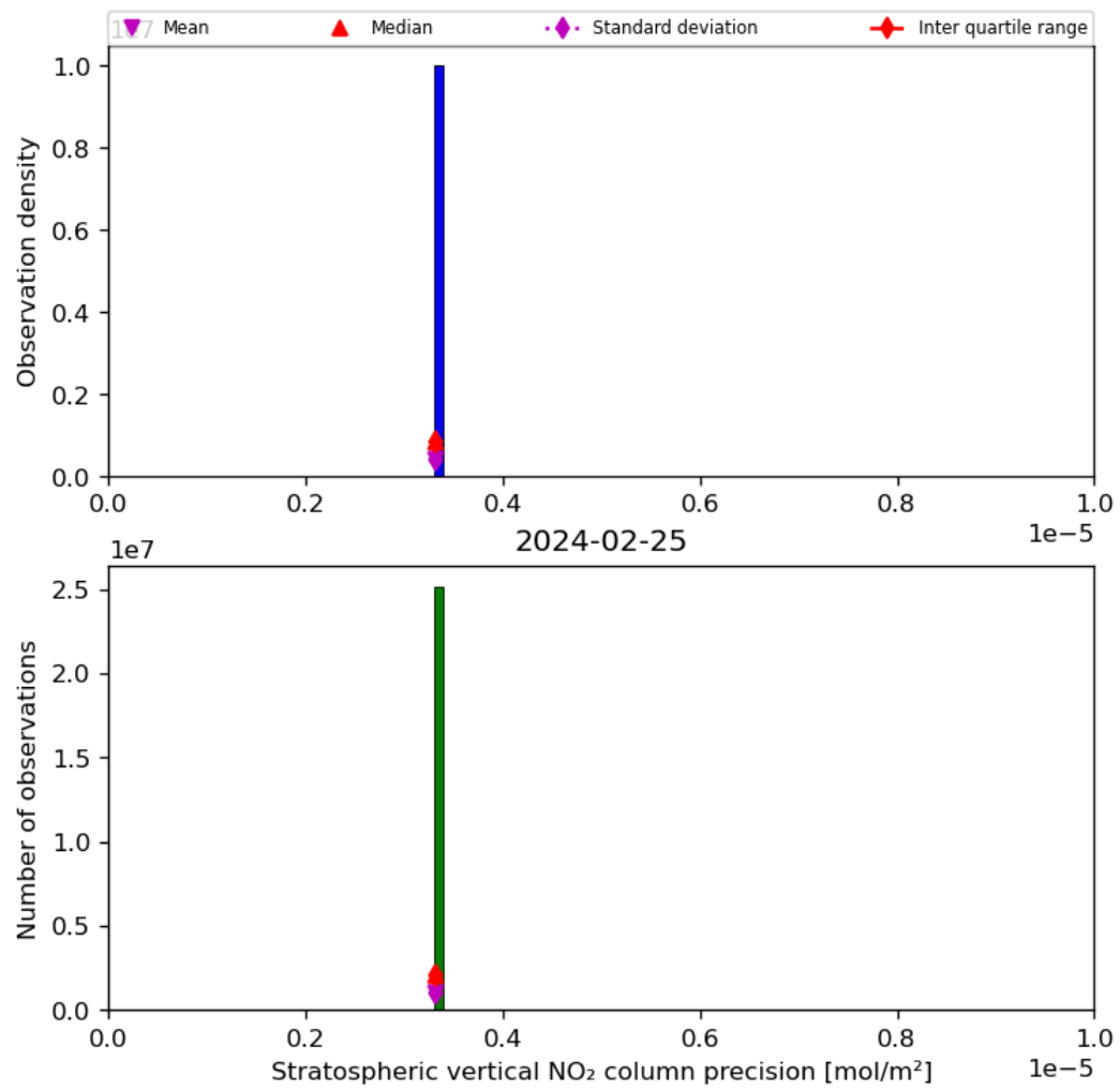
Figure 37: Histogram of “Stratospheric vertical NO 2 column precision” for 2024-02-24 to 2024-02-26
