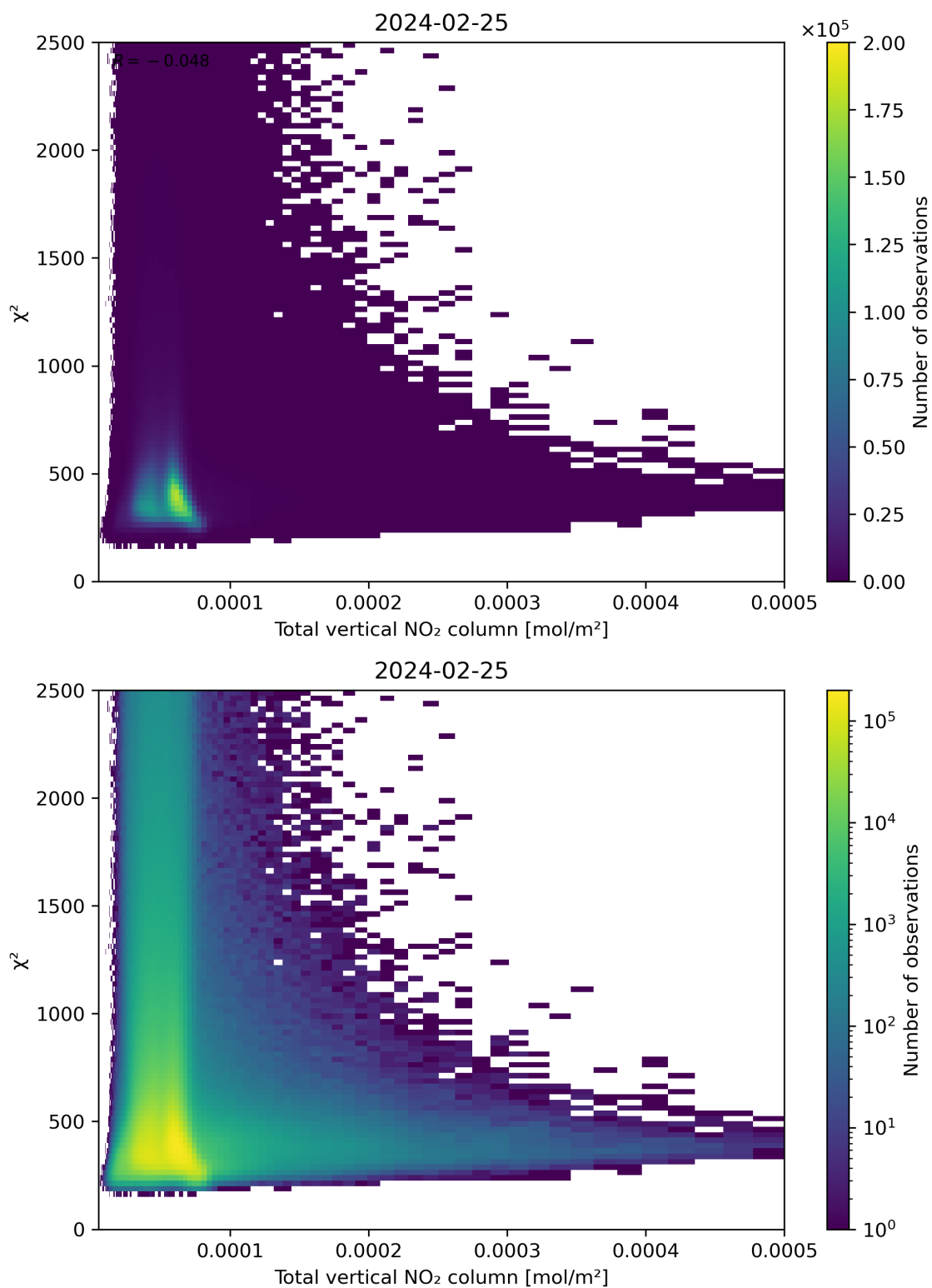
Figure 111: Scatter density plot of “Total vertical NO 2 column” against “ \chi^2 ” for 2024-02-24 to 2024-02-26.
