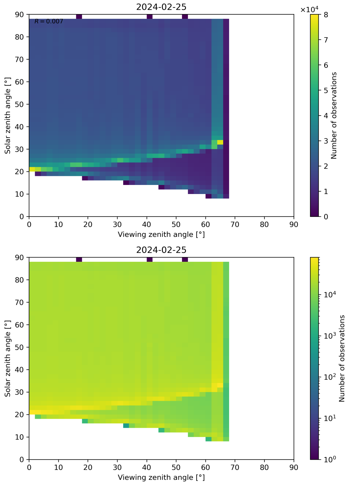
Figure 172: Scatter density plot of “Viewing zenith angle” against “Solar zenith angle” for 2024-02-24 to 2024-02-26.
