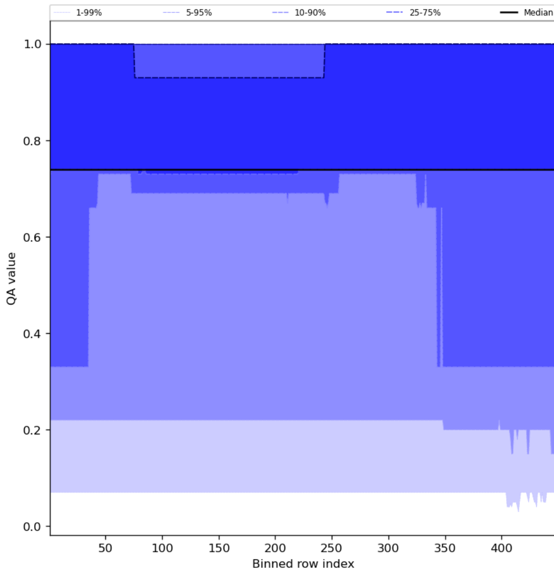
Figure 45: Along track statistics of “QA value” for 2024-02-24 to 2024-02-26
