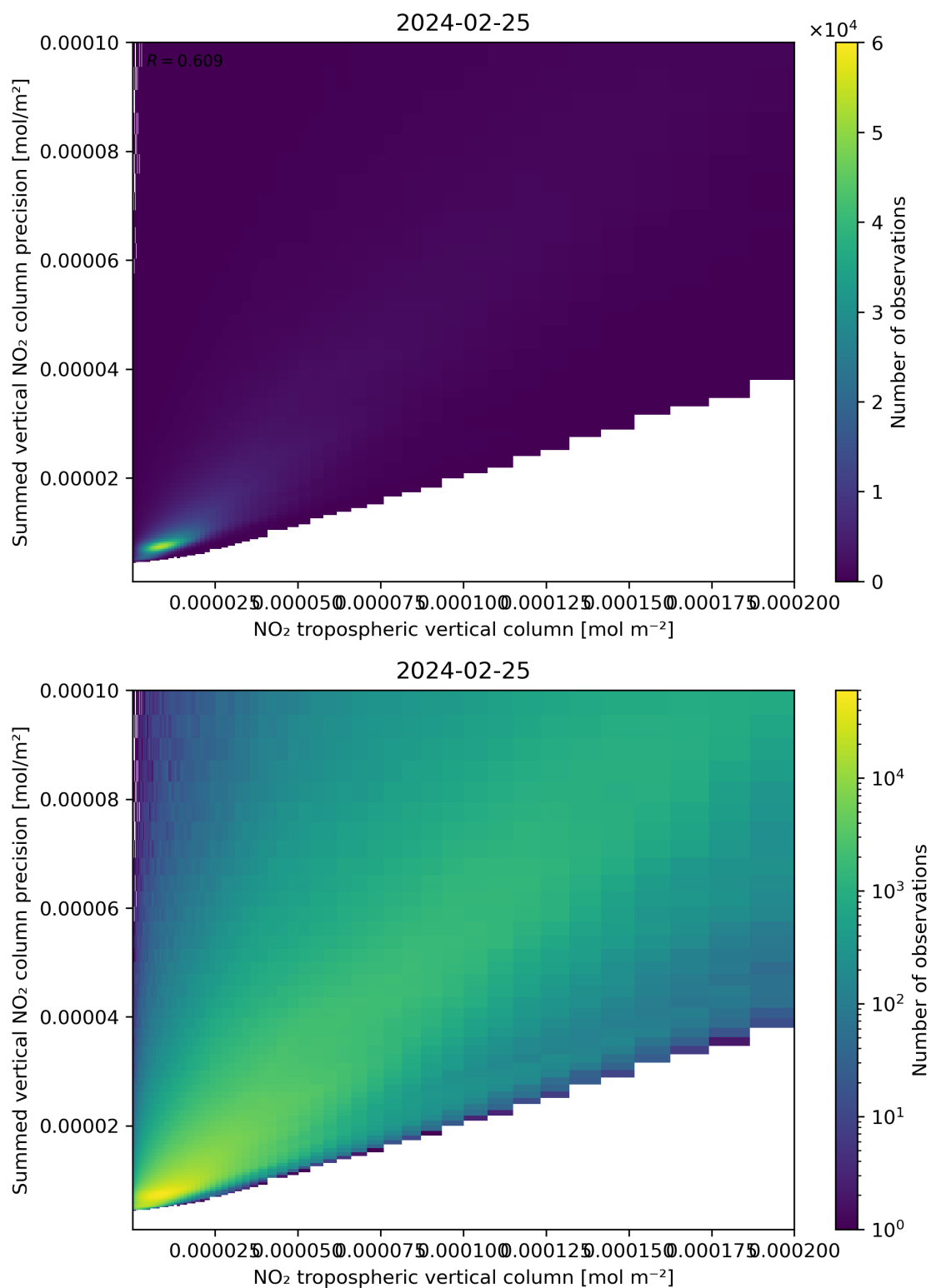
Figure 127: Scatter density plot of “NO 2 tropospheric vertical column” against “Summed vertical NO 2 column precision” for 2024-02-24 to 2024-02-26.
