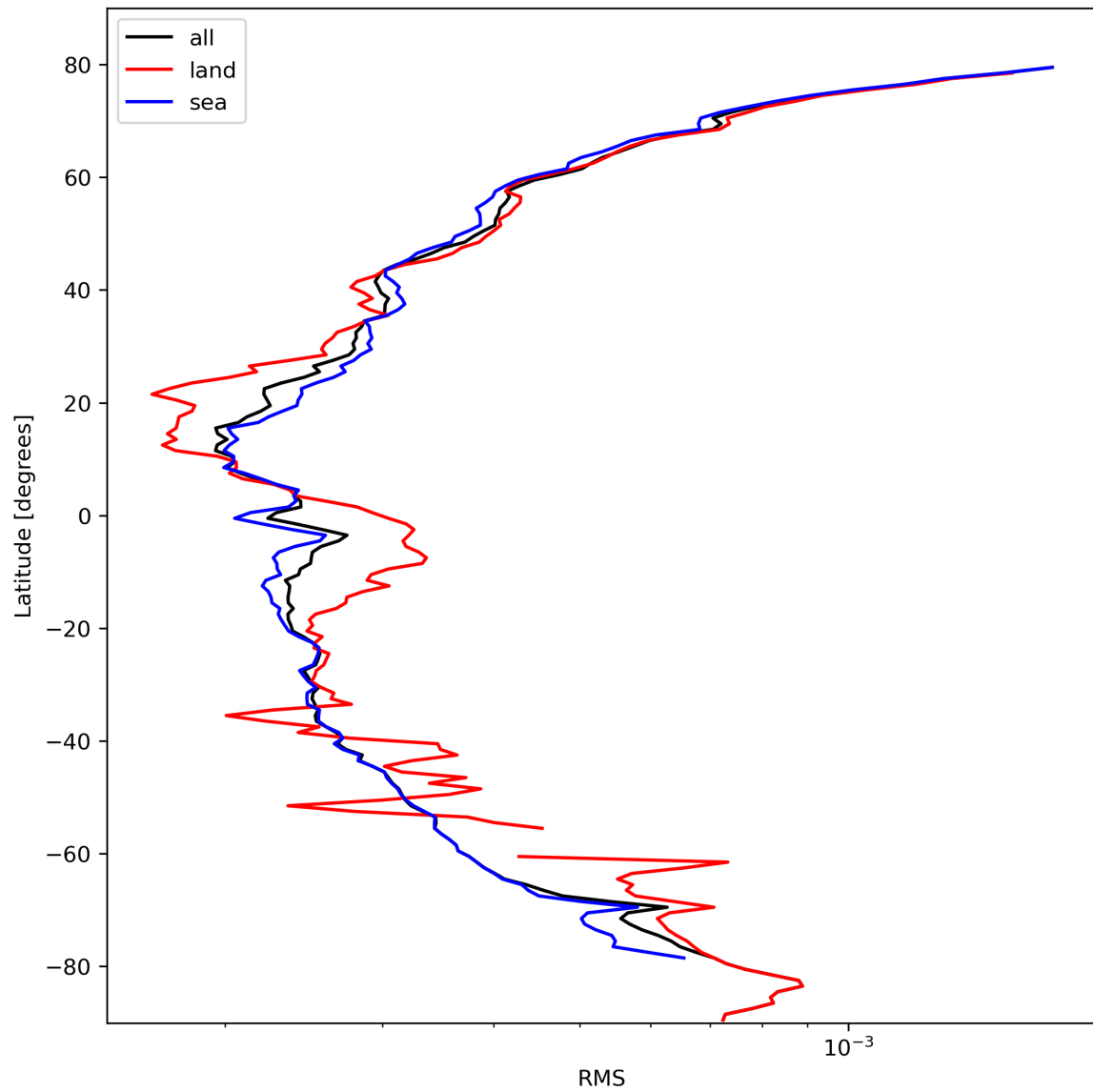
Figure 26: Zonal average of “RMS” for 2024-02-24 to 2024-02-26.
