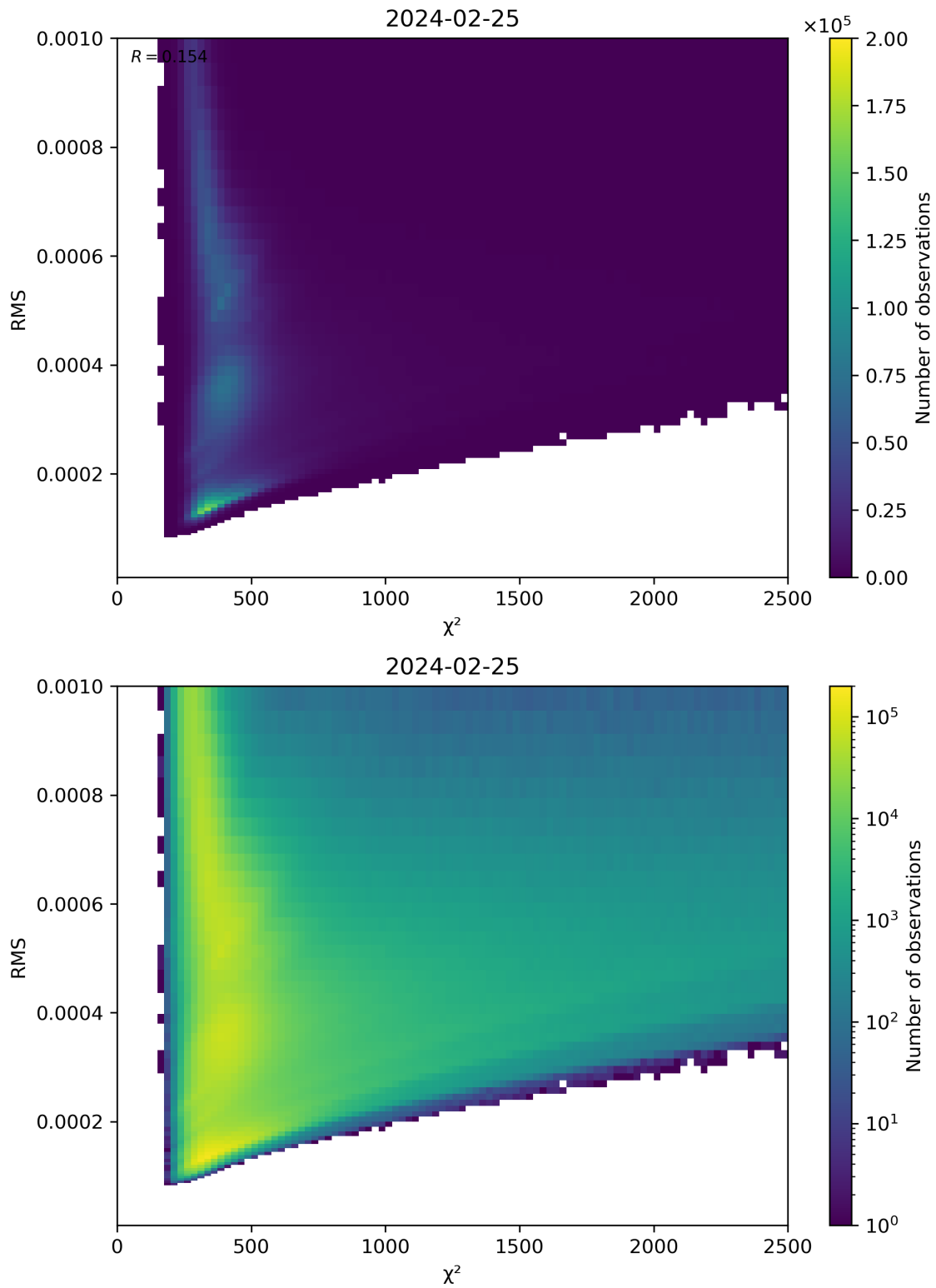
Figure 82: Scatter density plot of “ \chi^2 ” against “RMS” for 2024-02-24 to 2024-02-26.
