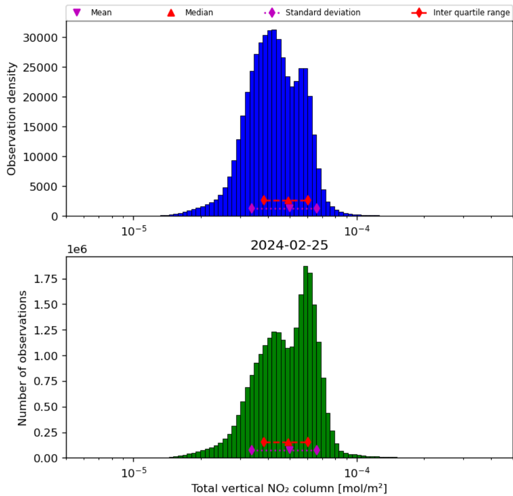
Figure 38: Histogram of “Total vertical NO 2 column” for 2024-02-24 to 2024-02-26
