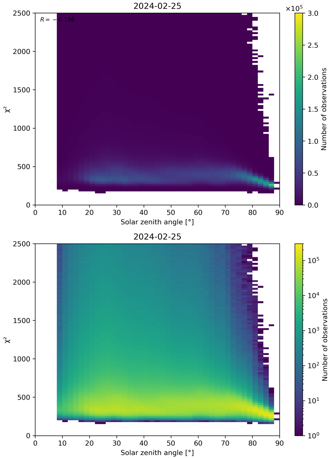
Figure 148: Scatter density plot of “Solar zenith angle” against “ \chi^2 ” for 2024-02-24 to 2024-02-26.
