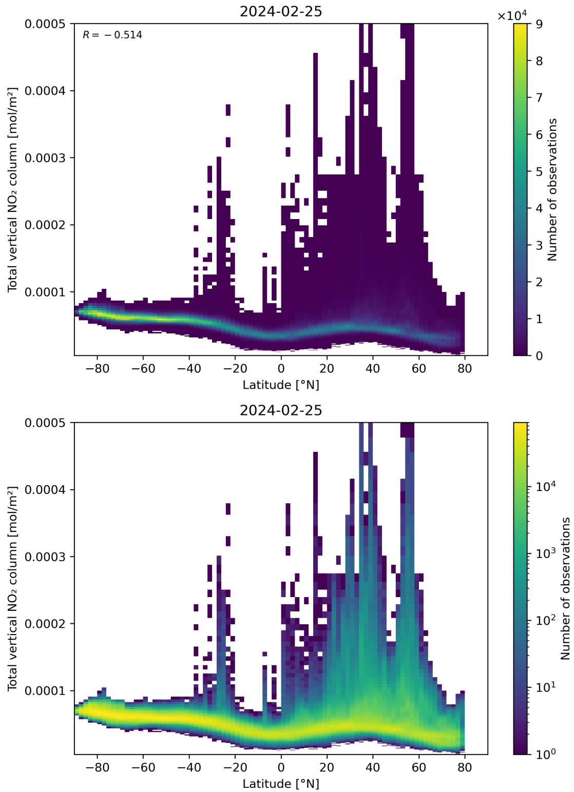
Figure 90: Scatter density plot of “Latitude” against “Total vertical NO 2 column” for 2024-02-24 to 2024-02-26.
