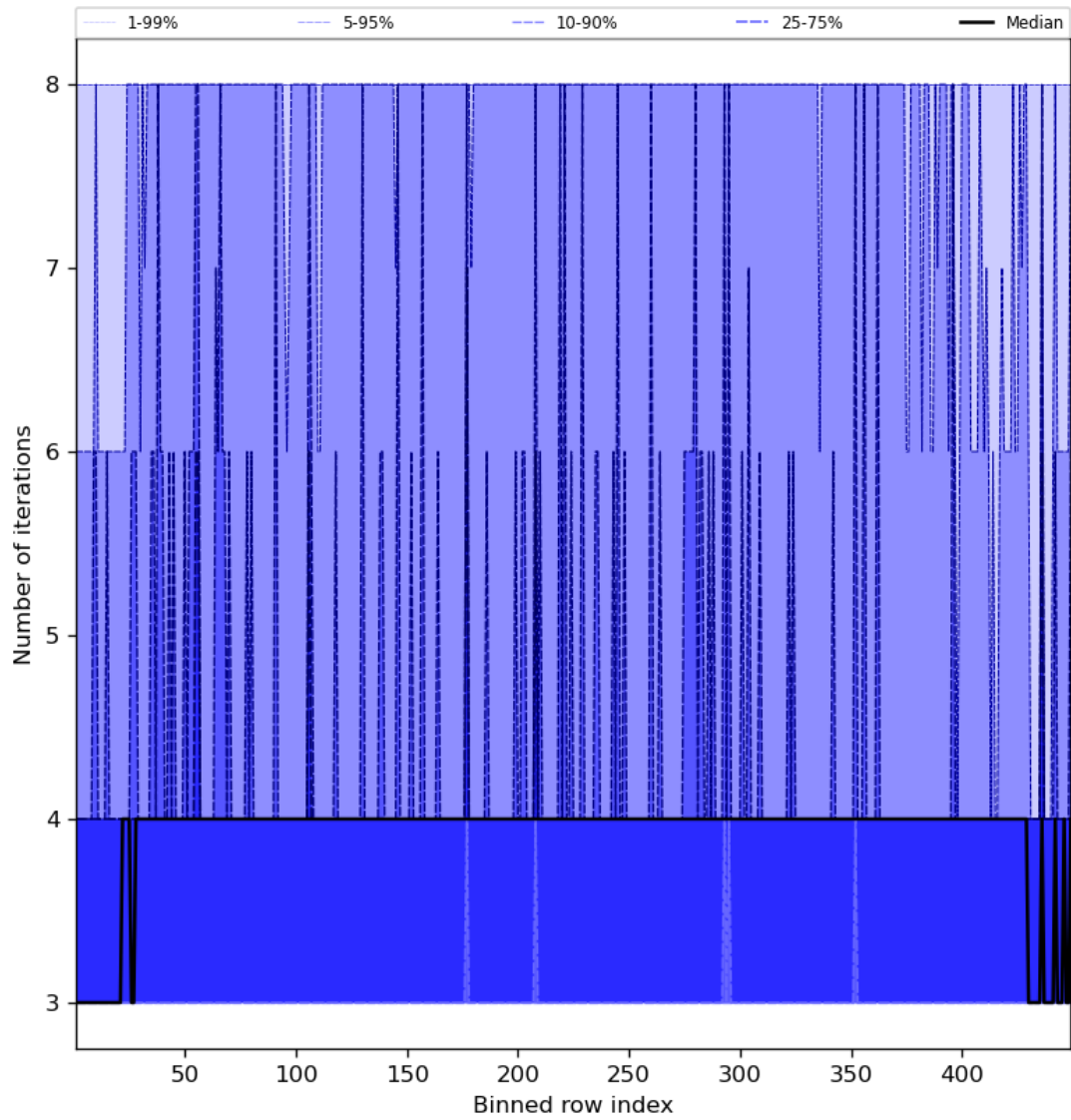
Figure 51: Along track statistics of “Number of iterations” for 2024-02-24 to 2024-02-26
