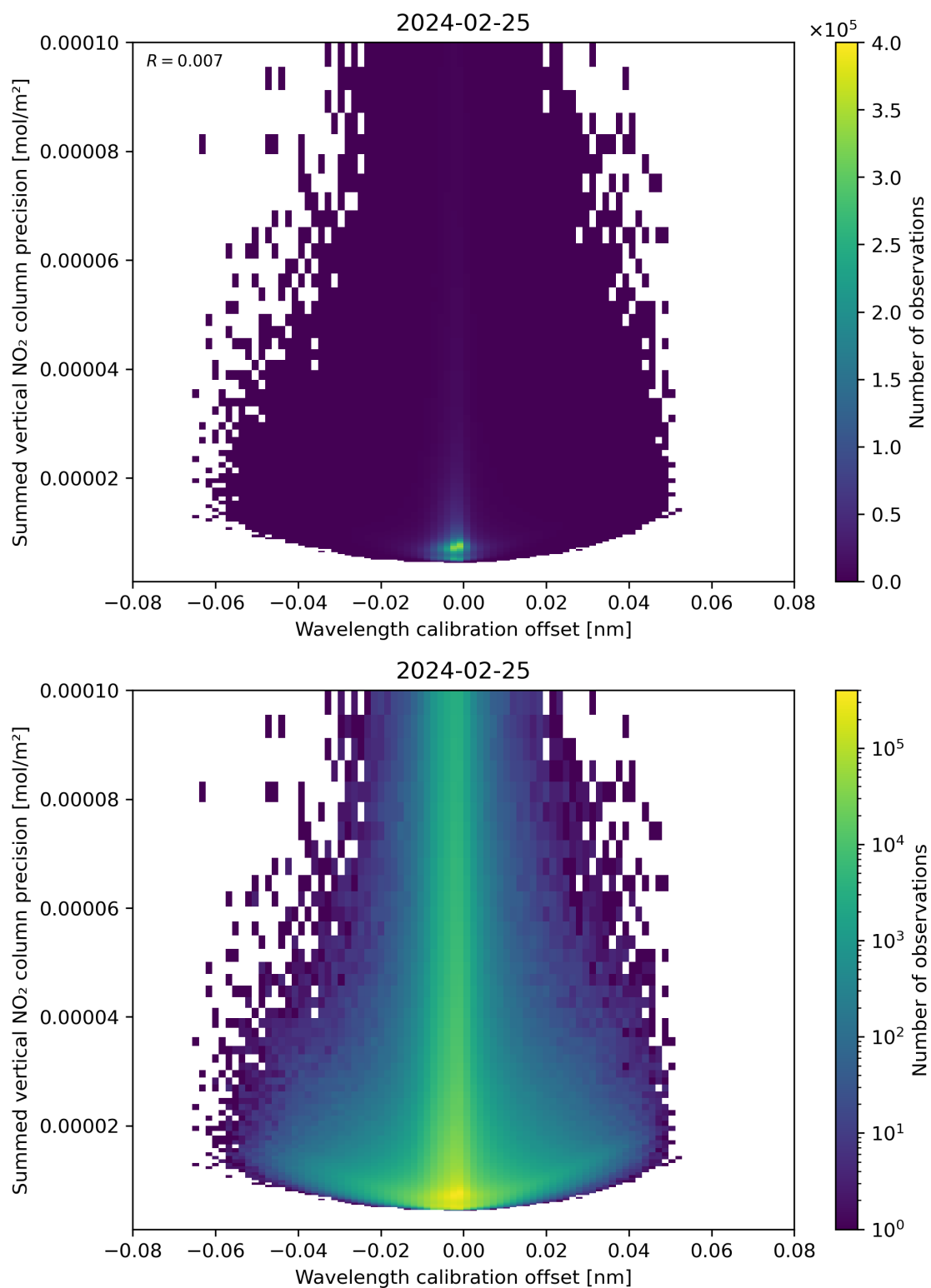
Figure 178: Scatter density plot of “Wavelength calibration offset” against “Summed vertical NO 2 column precision” for 2024-02-24 to 2024-02-26.
