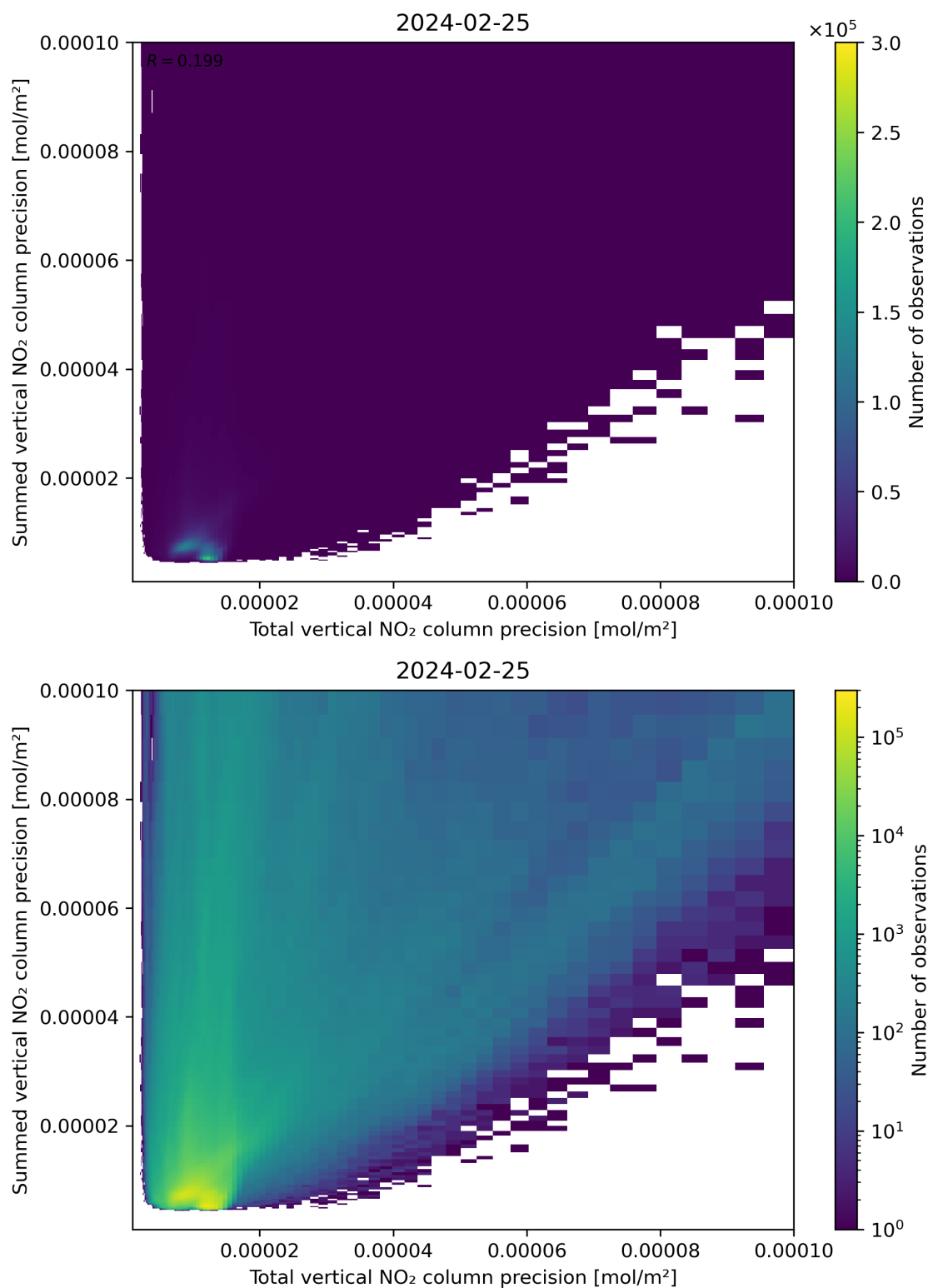
Figure 118: Scatter density plot of “Total vertical NO 2 column precision” against “Summed vertical NO 2 column precision” for 2024-02-24 to 2024-02-26.
