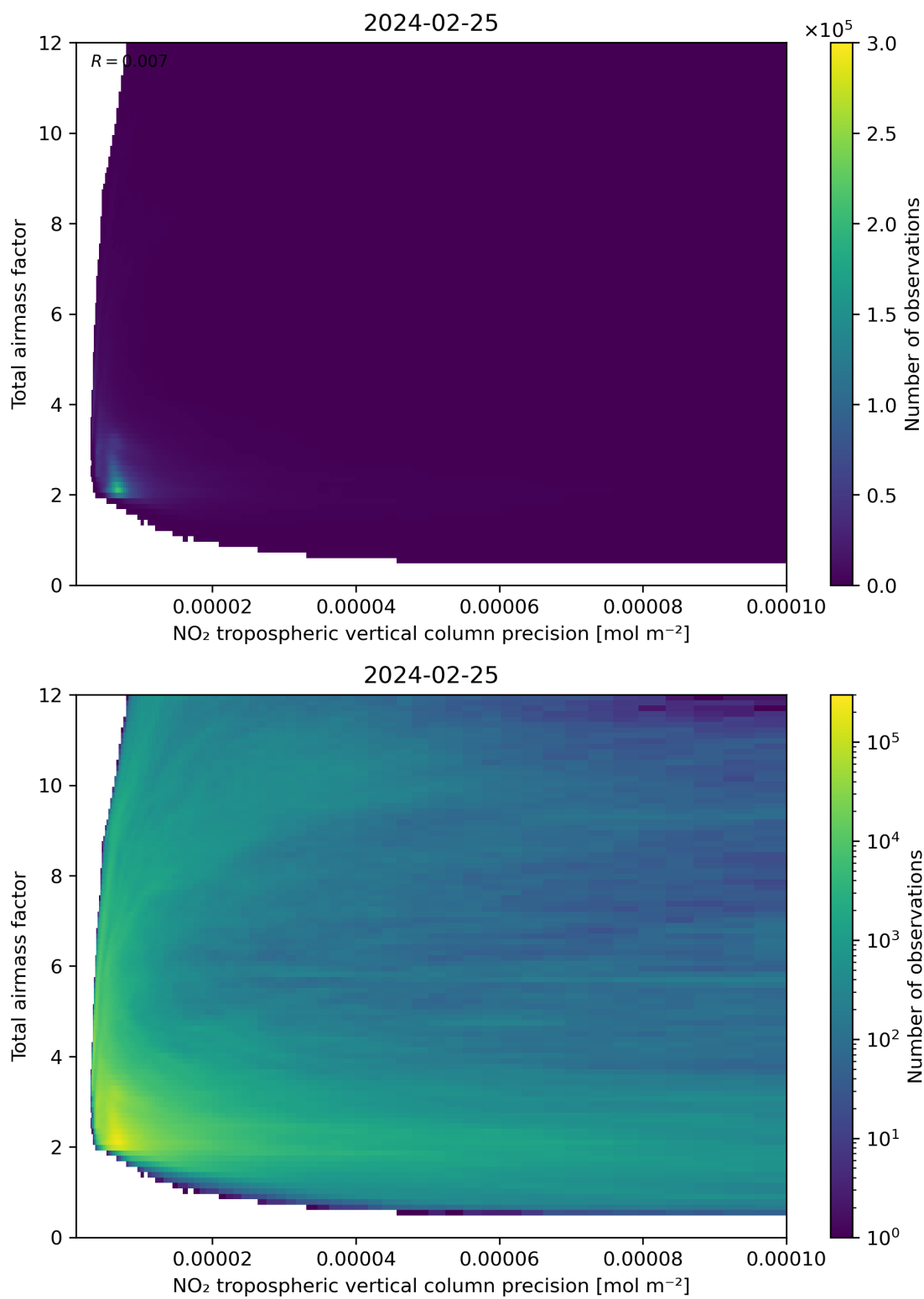
Figure 132: Scatter density plot of “NO 2 tropospheric vertical column precision” against “Total air mass factor” for 2024-02-24 to 2024-02-26.
