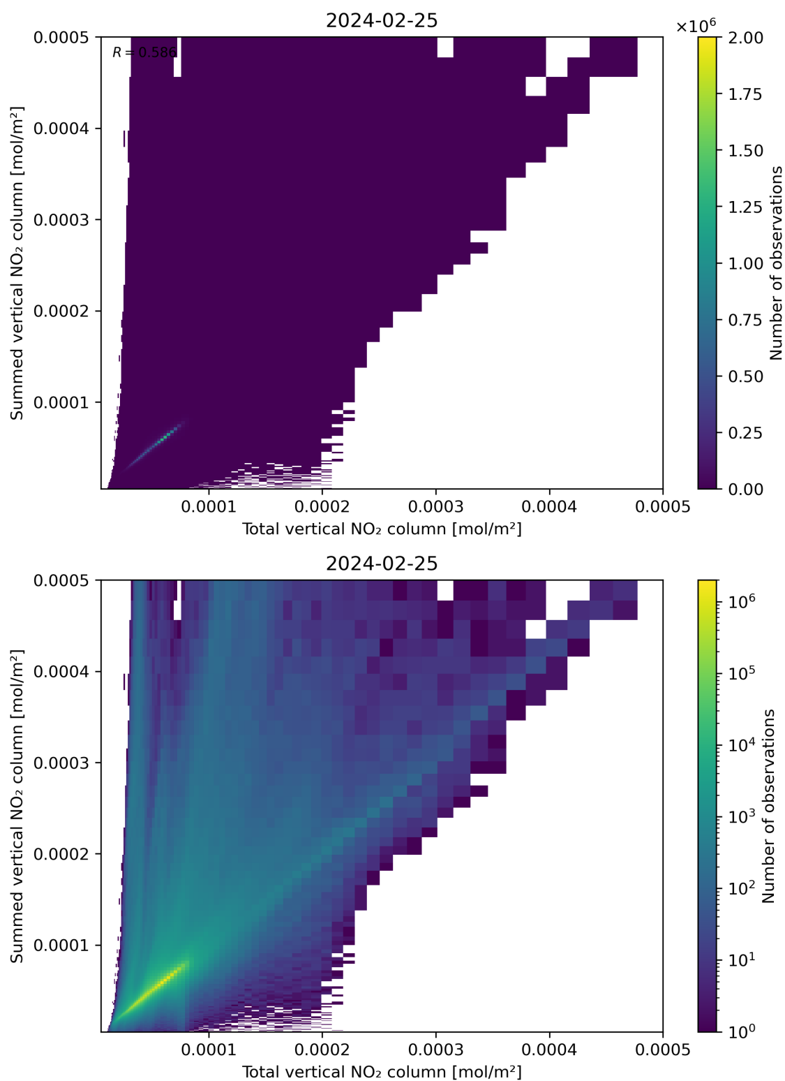
Figure 112: Scatter density plot of “Total vertical NO 2 column” against “Summed vertical NO 2 column” for 2024-02-24 to 2024-02-26.
