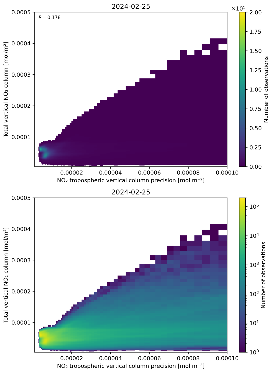
Figure 138: Scatter density plot of “NO 2 tropospheric vertical column precision” against “Total vertical NO 2 column” for 2024-02-24 to 2024-02-26.
