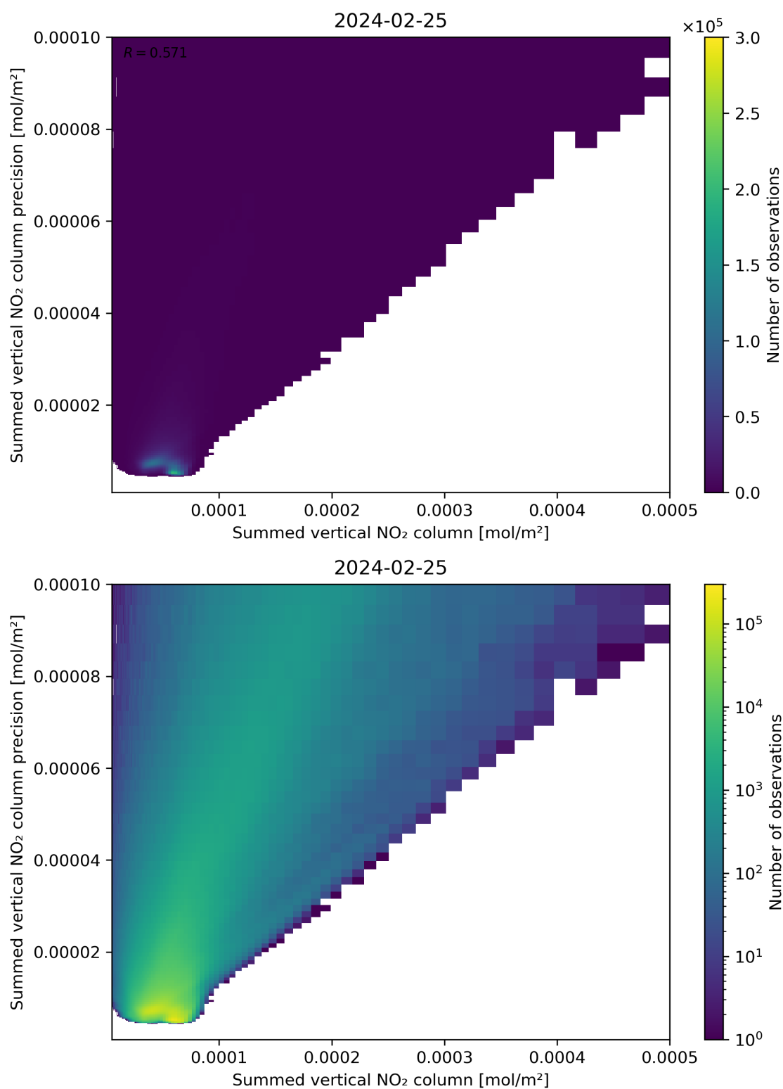
Figure 105: Scatter density plot of “Summed vertical NO 2 column” against “Summed vertical NO 2 column precision” for 2024-02-24 to 2024-02-26.
