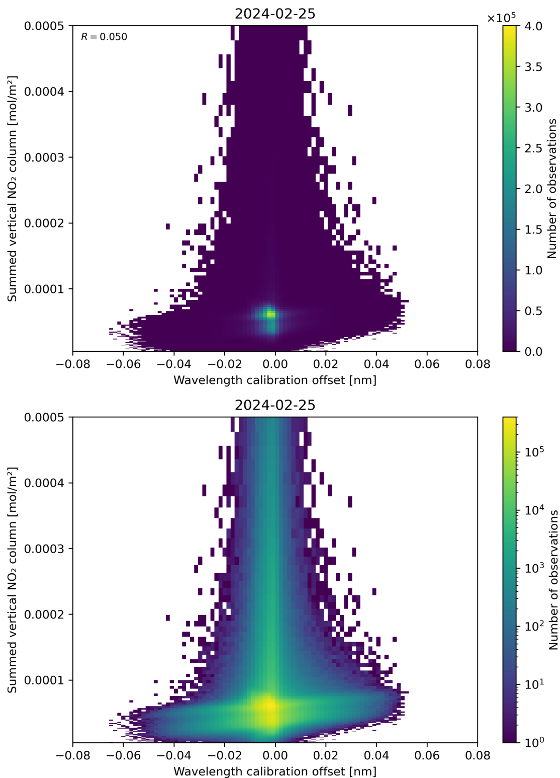
Figure 177: Scatter density plot of “Wavelength calibration offset” against “Summed vertical NO 2 column” for 2024-02-24 to 2024-02-26.
