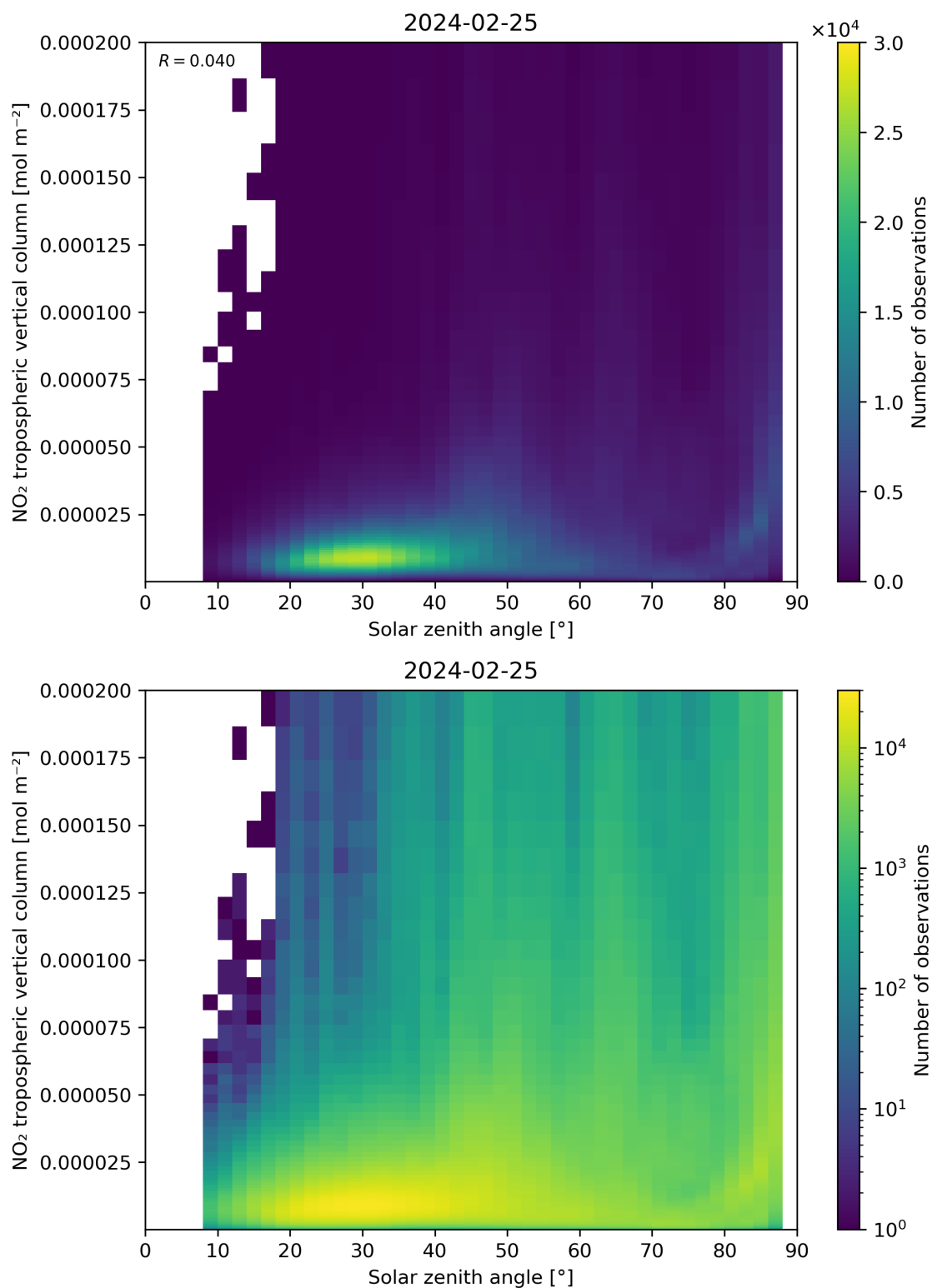
Figure 155: Scatter density plot of “Solar zenith angle” against “NO 2 tropospheric vertical column” for 2024-02-24 to 2024-02-26.
