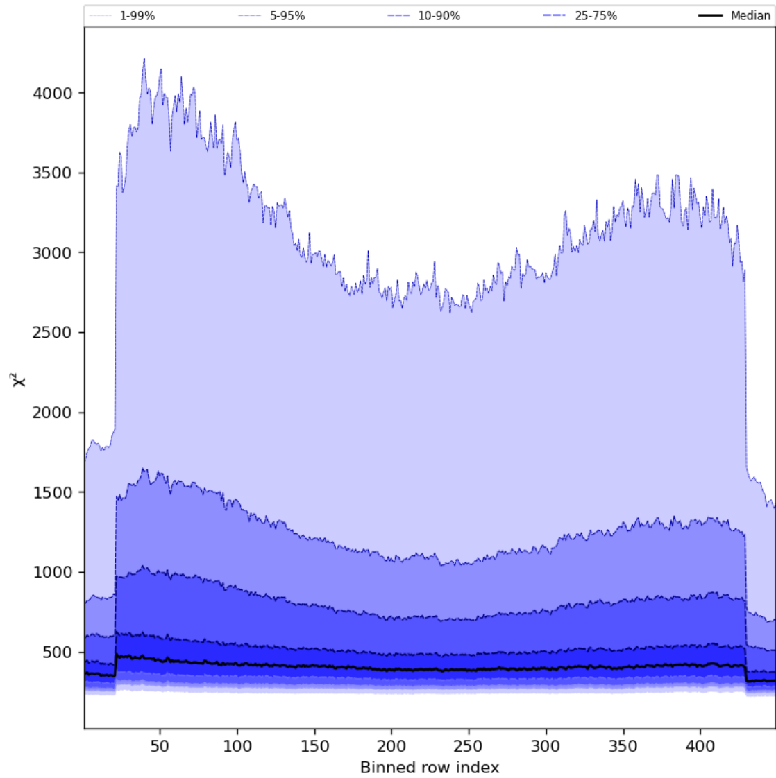
Figure 59: Along track statistics of “ \chi^2 ” for 2024-02-24 to 2024-02-26
