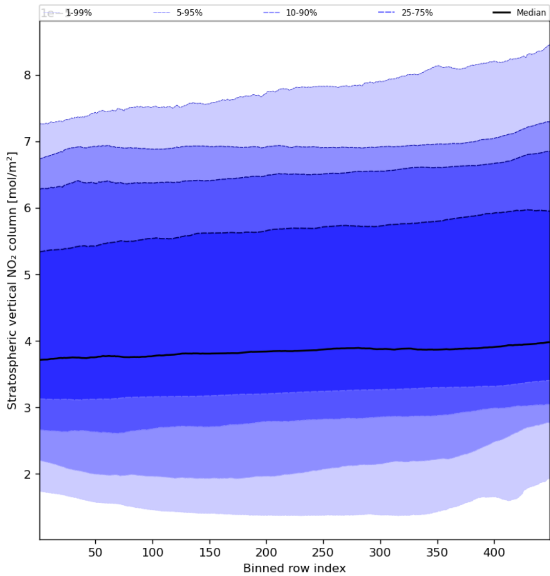
Figure 53: Along track statistics of “Stratospheric vertical NO 2 column” for 2024-02-24 to 2024-02-26
