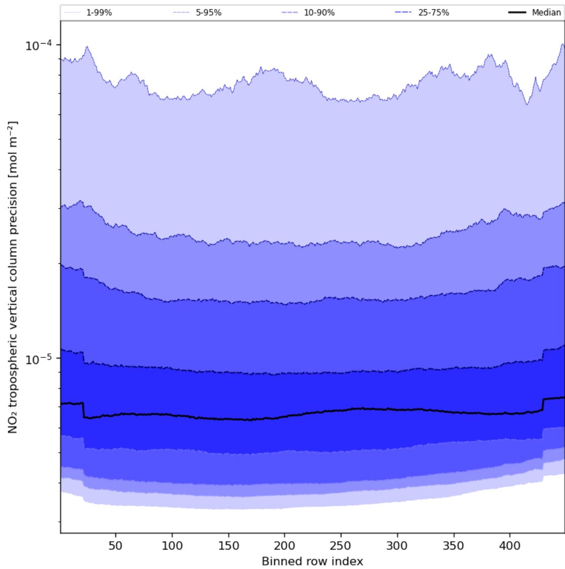
Figure 47: Along track statistics of “NO 2 tropospheric vertical column precision” for 2024-02-24 to 2024-02-26
