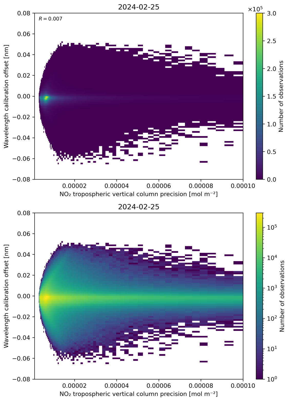
Figure 141: Scatter density plot of “NO 2 tropospheric vertical column precision” against “Wavelength calibration offset” for 2024-02-24 to 2024-02-26.
