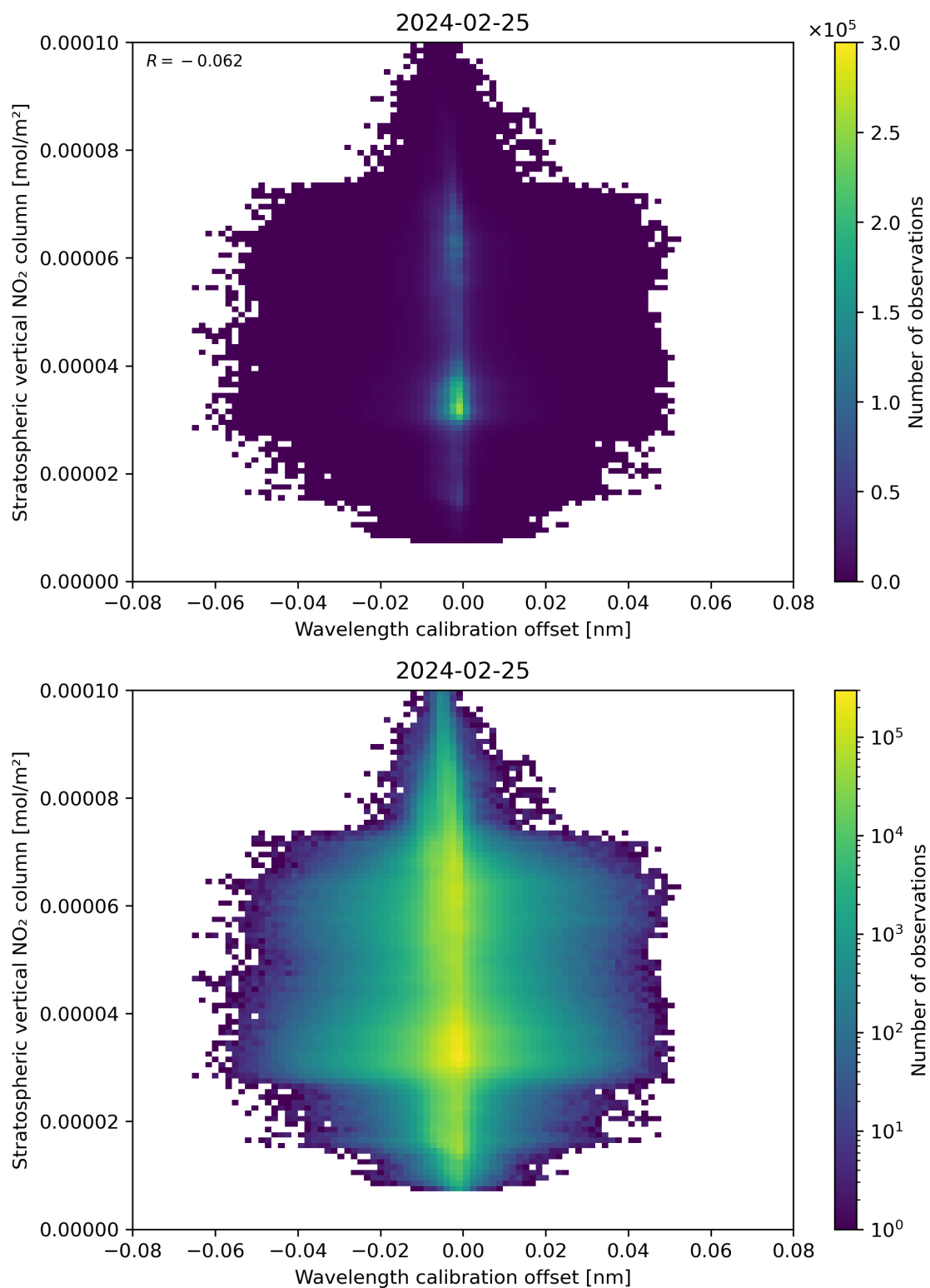
Figure 176: Scatter density plot of “Wavelength calibration offset” against “Stratospheric vertical NO 2 column” for 2024-02-24 to 2024-02-26.
