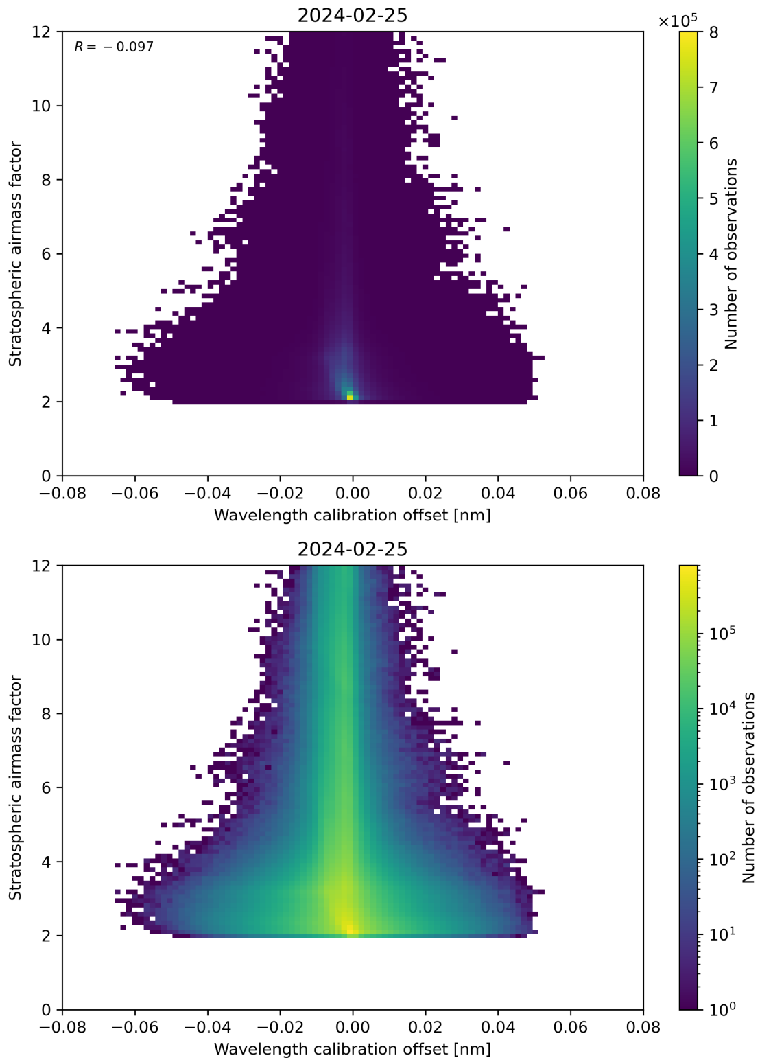
Figure 174: Scatter density plot of “Wavelength calibration offset” against “Stratospheric airmass factor” for 2024-02-24 to 2024-02-26.
