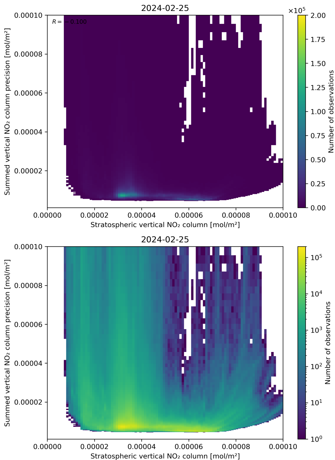
Figure 99: Scatter density plot of “Stratospheric vertical NO 2 column” against “Summed vertical NO 2 column precision” for 2024-02-24 to 2024-02-26.
