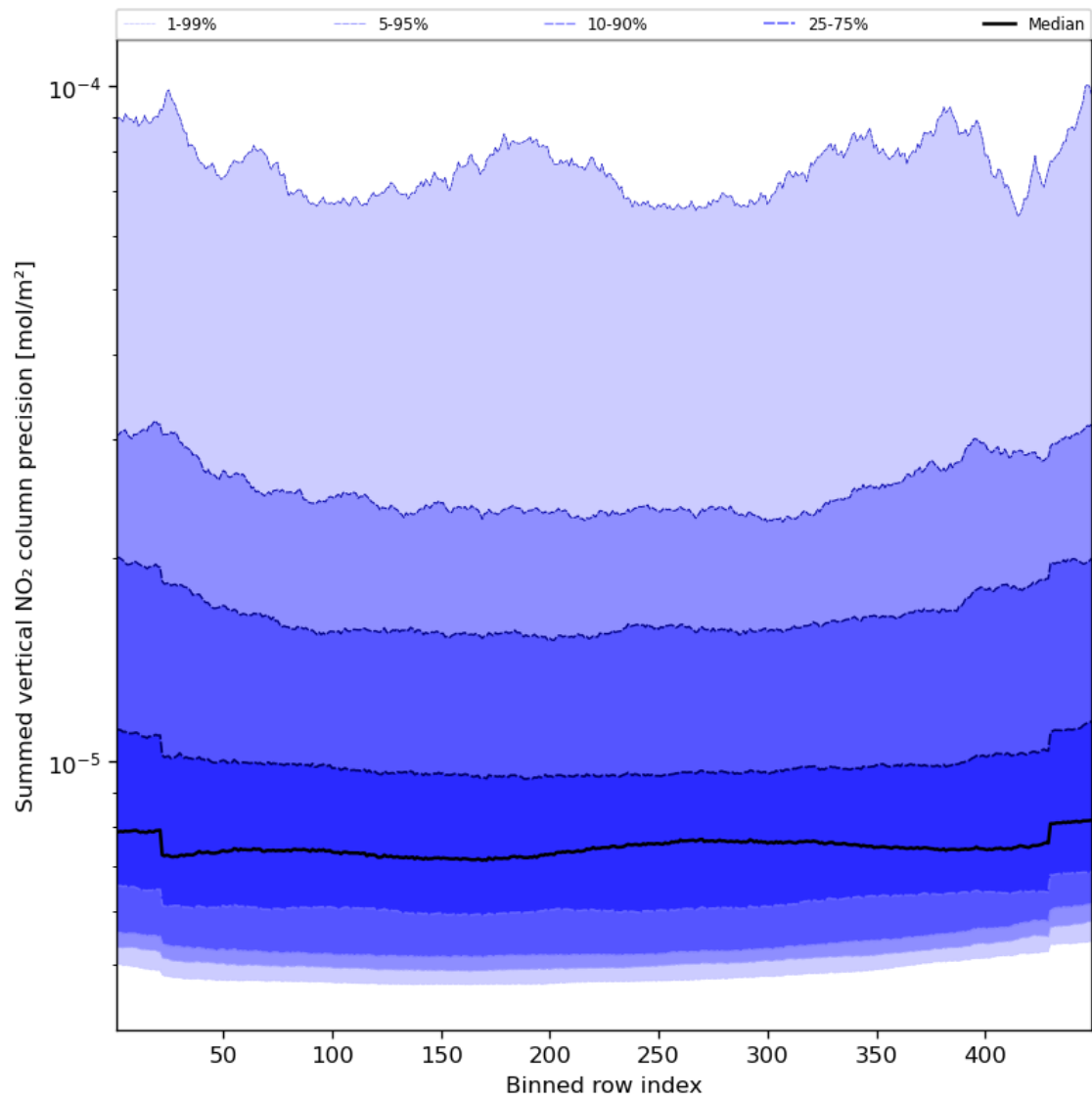
Figure 58: Along track statistics of “Summed vertical NO 2 column precision” for 2024-02-24 to 2024-02-26
