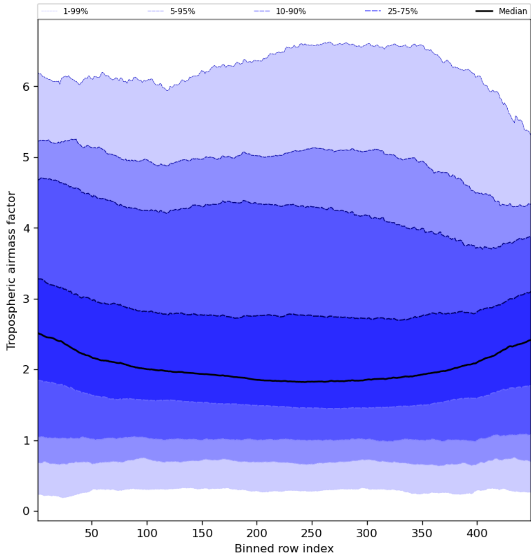
Figure 48: Along track statistics of “Tropospheric airmass factor” for 2024-02-24 to 2024-02-26
