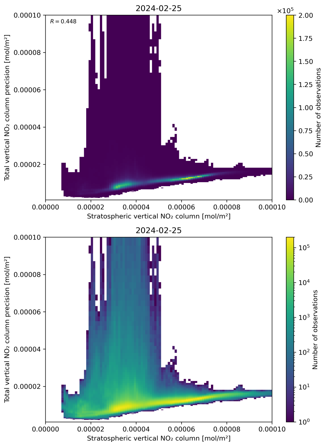
Figure 101: Scatter density plot of “Stratospheric vertical NO 2 column” against “Total vertical NO 2 column precision” for 2024-02-24 to 2024-02-26.
