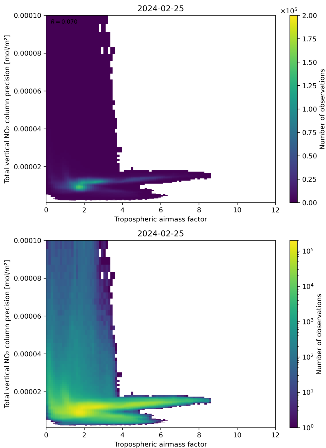
Figure 78: Scatter density plot of “Tropospheric air mass factor” against “Total vertical NO 2 column precision” for 2024-02-24 to 2024-02-26.
