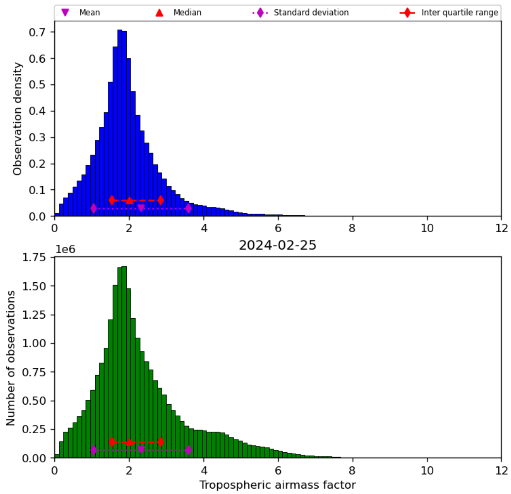
Figure 31: Histogram of “Tropospheric airmass factor” for 2024-02-24 to 2024-02-26
