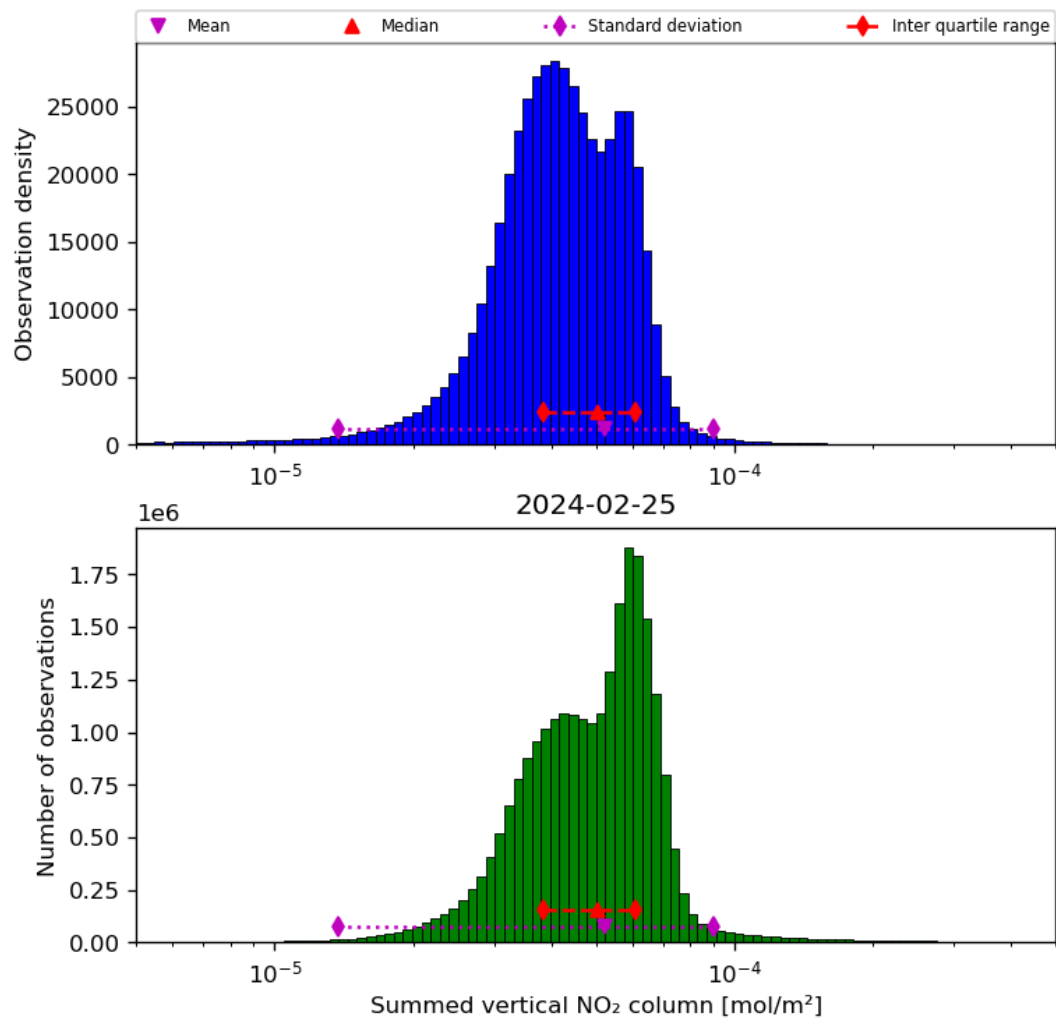
Figure 40: Histogram of “Summed vertical NO 2 column” for 2024-02-24 to 2024-02-26
