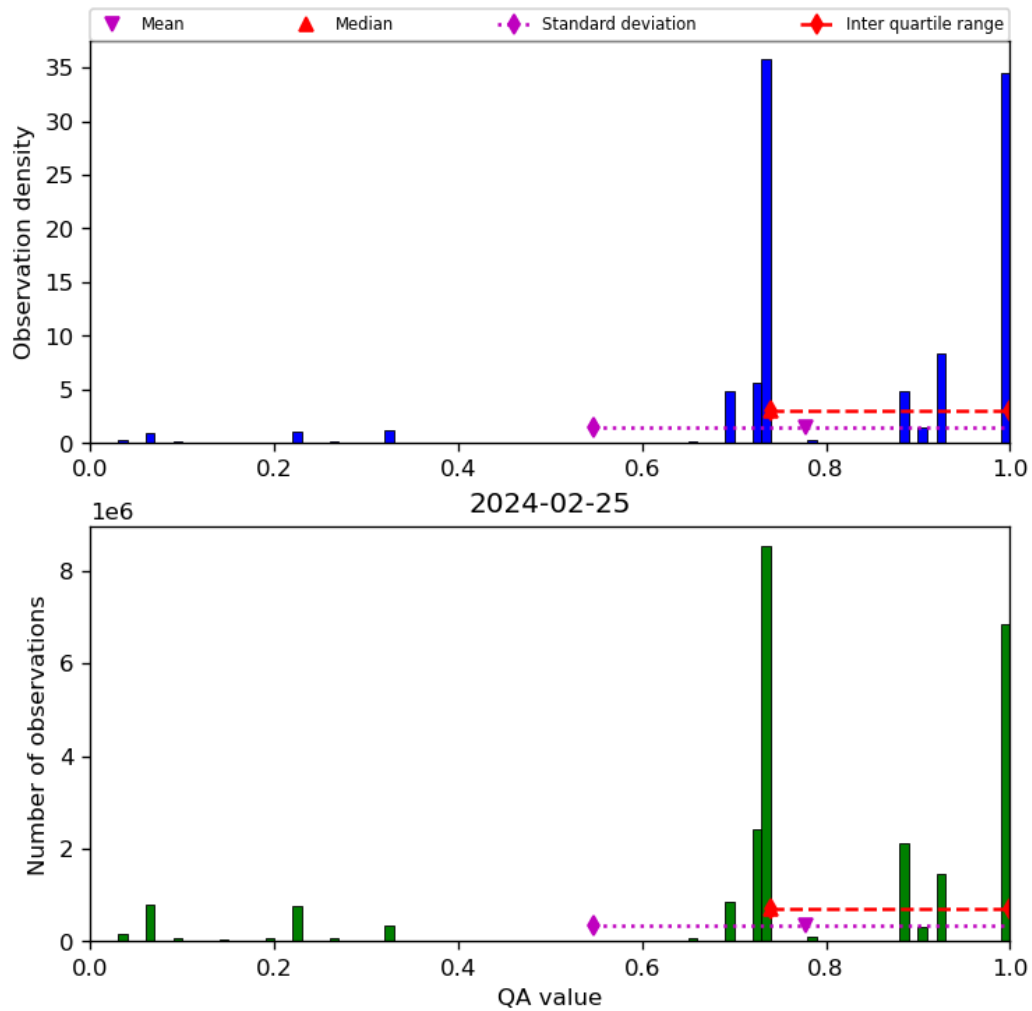
Figure 28: Histogram of “QA value” for 2024-02-24 to 2024-02-26
