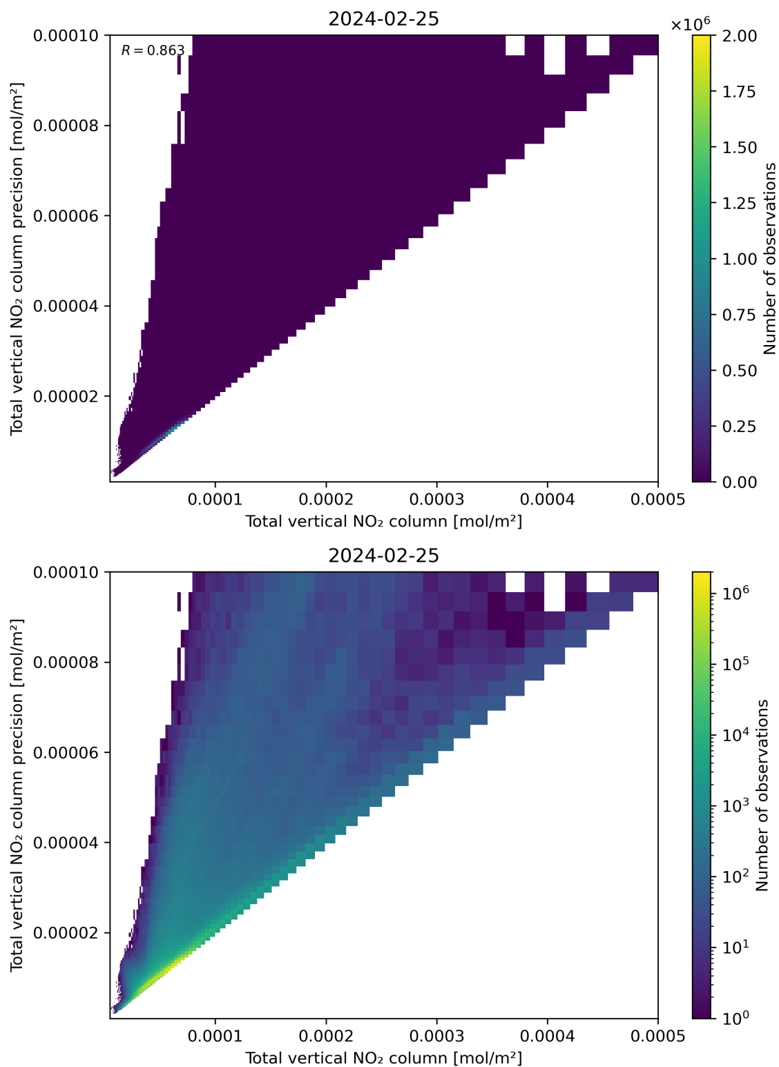
Figure 114: Scatter density plot of “Total vertical NO 2 column” against “Total vertical NO 2 column precision” for 2024-02-24 to 2024-02-26.
