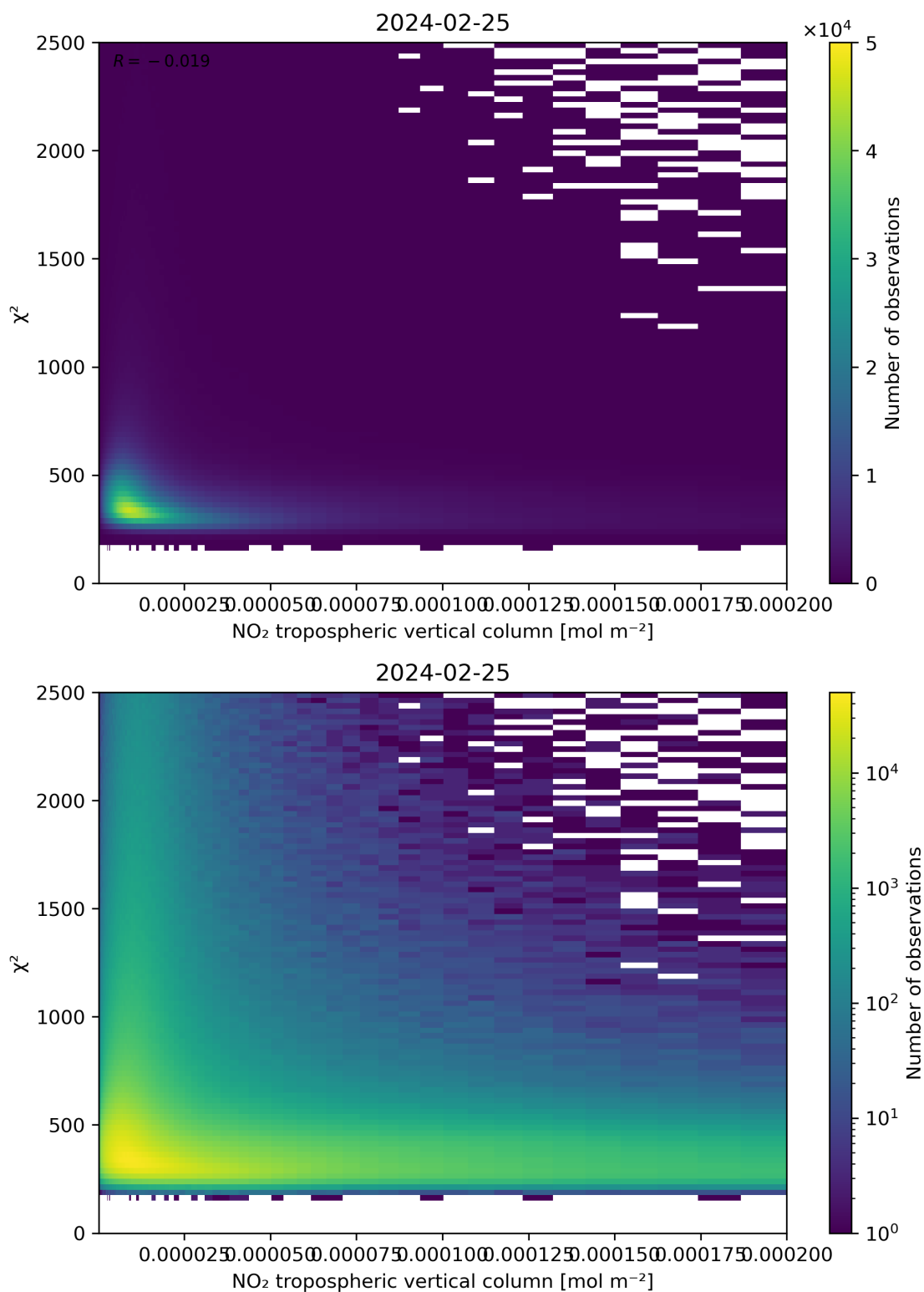
Figure 124: Scatter density plot of “NO 2 tropospheric vertical column” against “ \chi^2 ” for 2024-02-24 to 2024-02-26.
