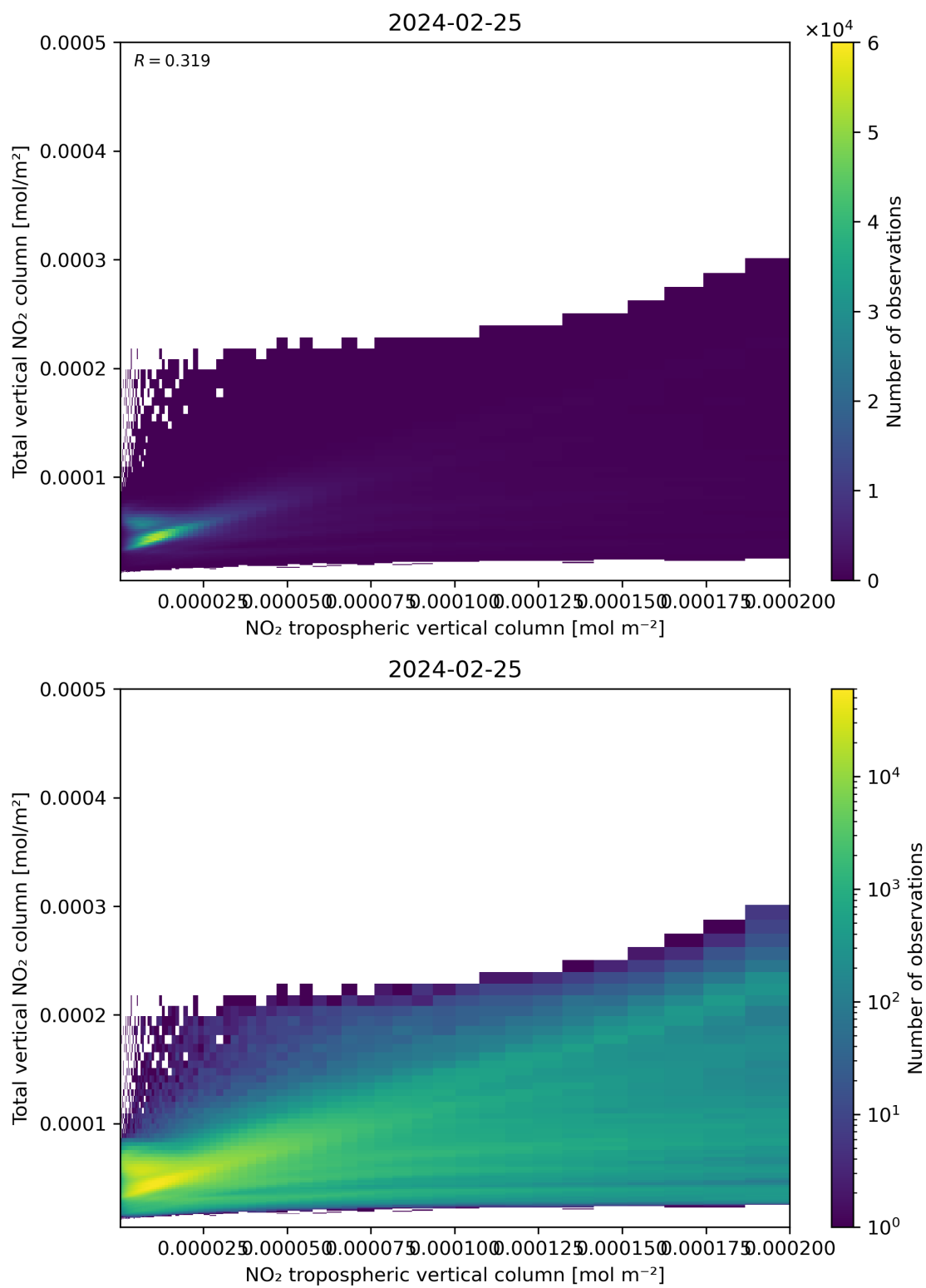
Figure 128: Scatter density plot of “NO 2 tropospheric vertical column” against “Total vertical NO 2 column” for 2024-02-24 to 2024-02-26.
