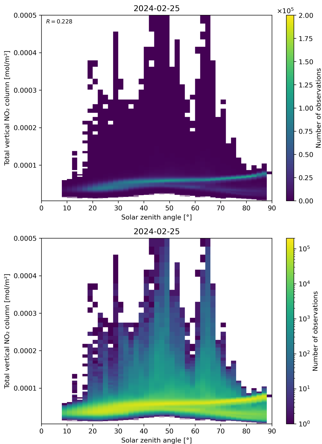
Figure 153: Scatter density plot of “Solar zenith angle” against “Total vertical NO 2 column” for 2024-02-24 to 2024-02-26.
