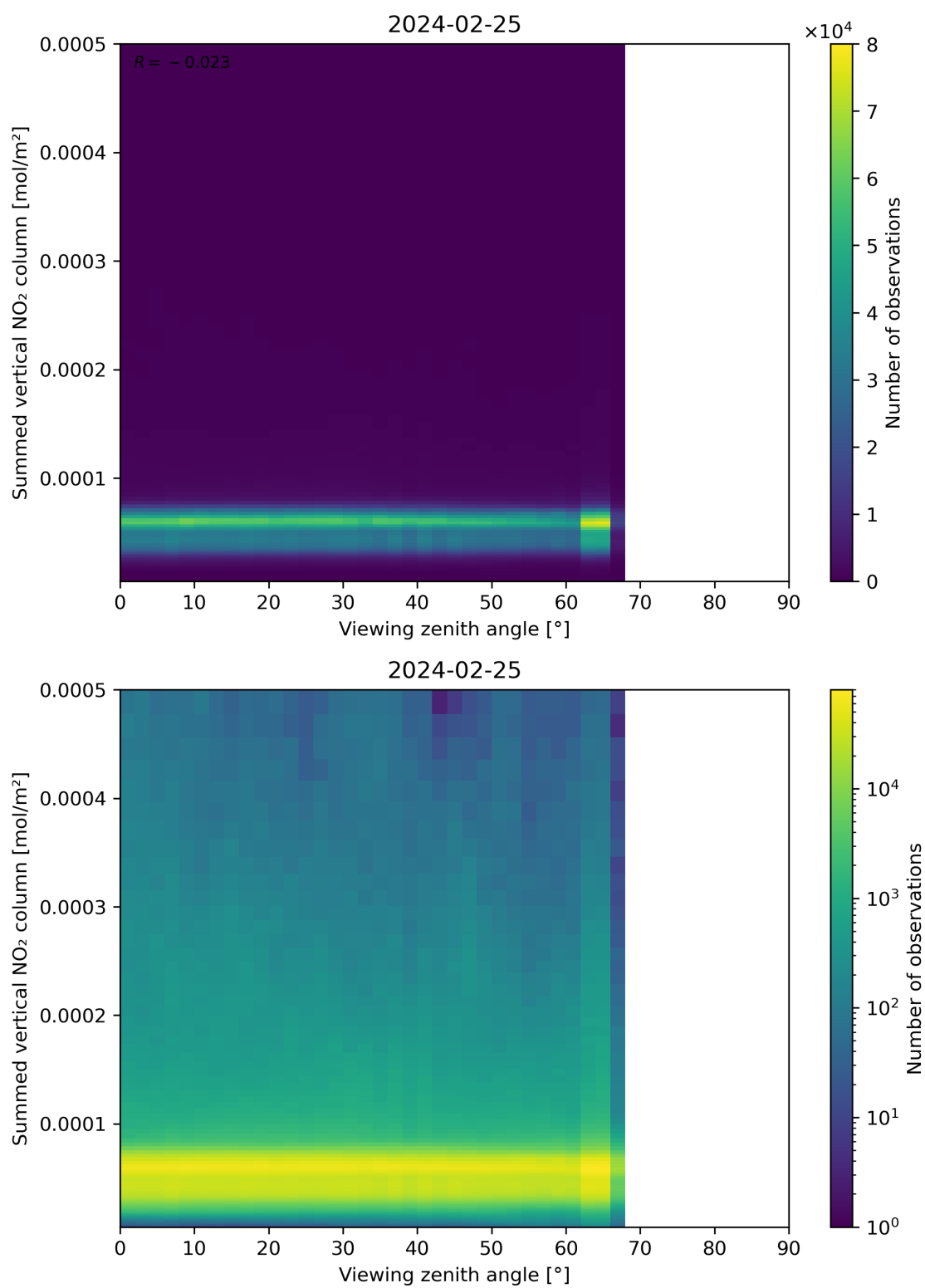
Figure 165: Scatter density plot of “Viewing zenith angle” against “Summed vertical NO 2 column” for 2024-02-24 to 2024-02-26.
