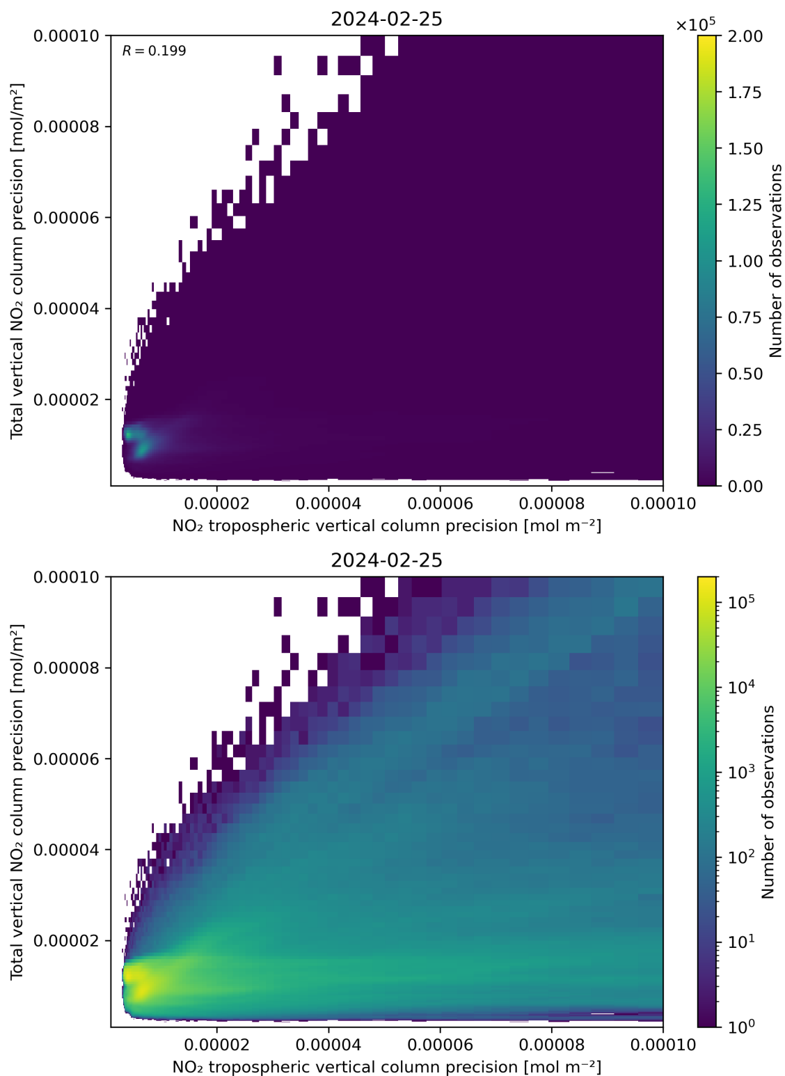
Figure 139: Scatter density plot of “NO 2 tropospheric vertical column precision” against “Total vertical NO 2 column precision” for 2024-02-24 to 2024-02-26.
