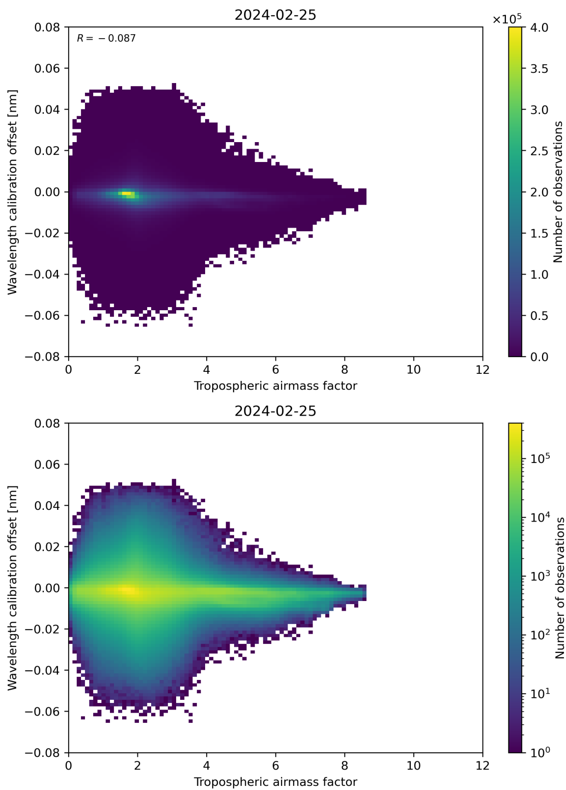
Figure 80: Scatter density plot of “Tropospheric airmass factor” against “Wavelength calibration offset” for 2024-02-24 to 2024-02-26.
