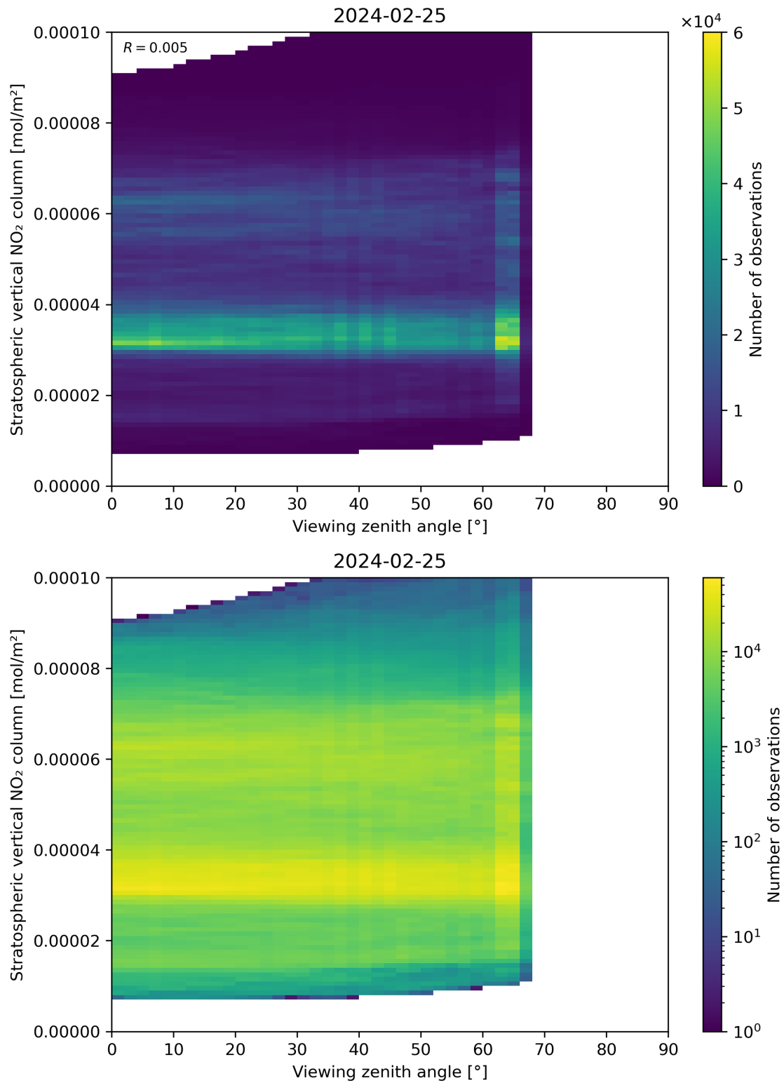
Figure 164: Scatter density plot of “Viewing zenith angle” against “Stratospheric vertical NO 2 column” for 2024-02-24 to 2024-02-26.
