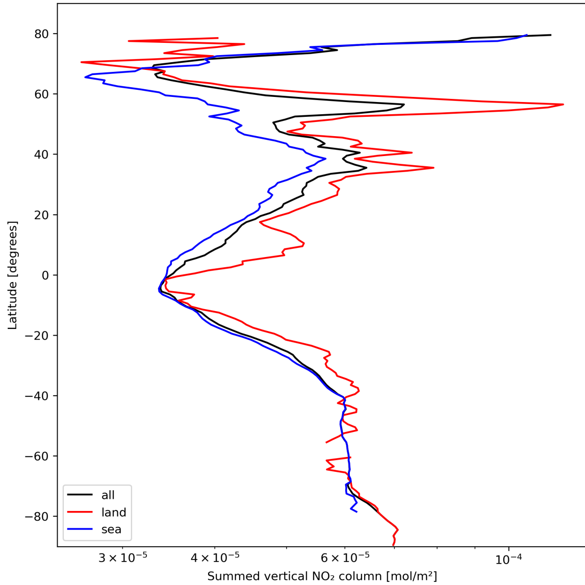
Figure 23: Zonal average of “Summed vertical NO 2 column” for 2024-02-24 to 2024-02-26.
