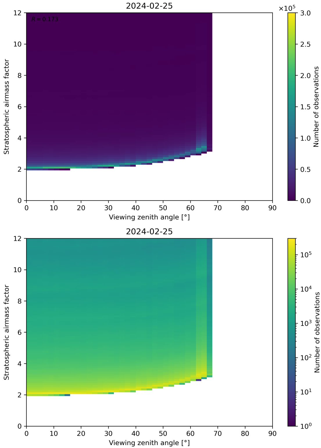
Figure 159: Scatter density plot of “Viewing zenith angle” against “Stratospheric airmass factor” for 2024-02-24 to 2024-02-26.
