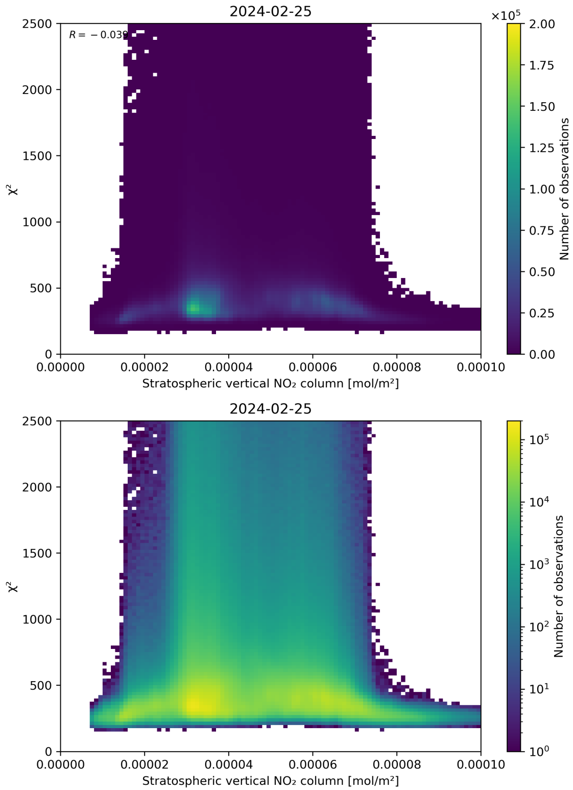
Figure 97: Scatter density plot of “Stratospheric vertical NO 2 column” against “ \chi^2 ” for 2024-02-24 to 2024-02-26.
