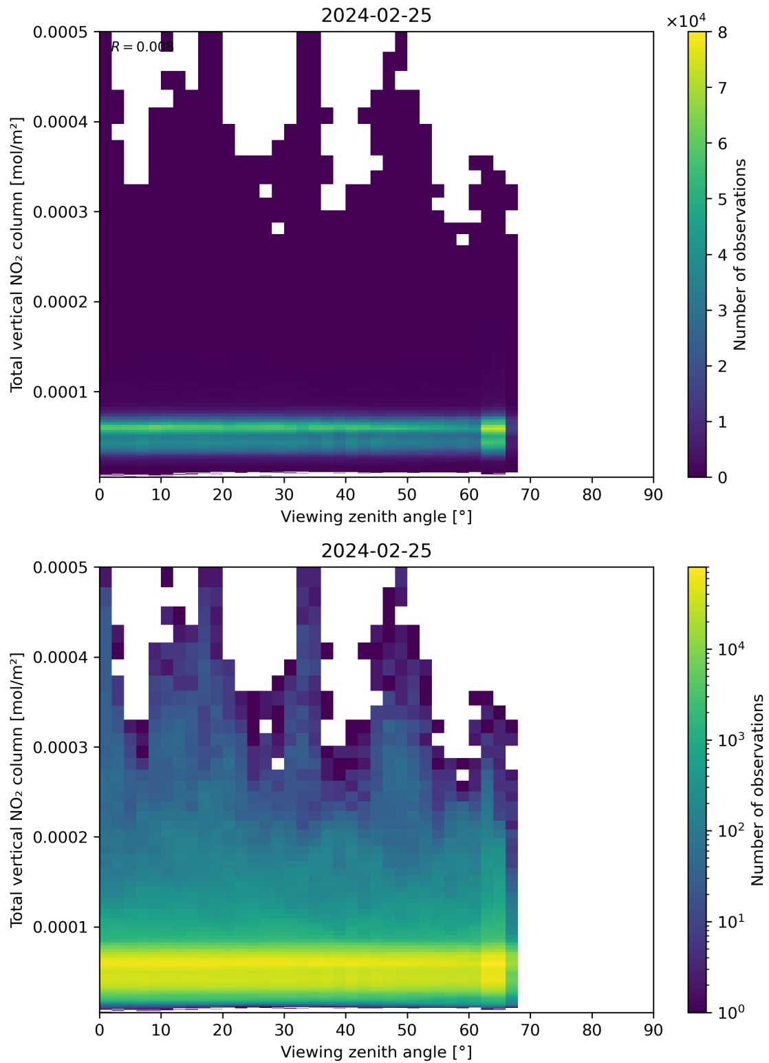
Figure 167: Scatter density plot of “Viewing zenith angle” against “Total vertical NO 2 column” for 2024-02-24 to 2024-02-26.
