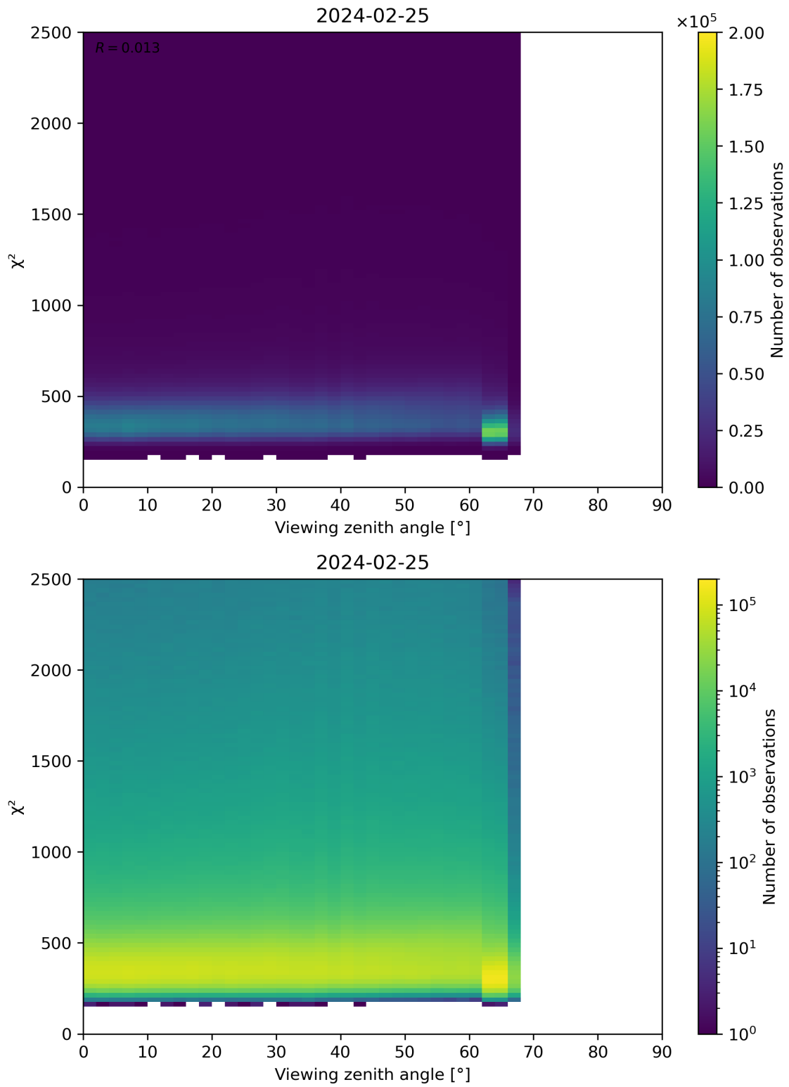
Figure 162: Scatter density plot of “Viewing zenith angle” against “ \chi^2 ” for 2024-02-24 to 2024-02-26.
