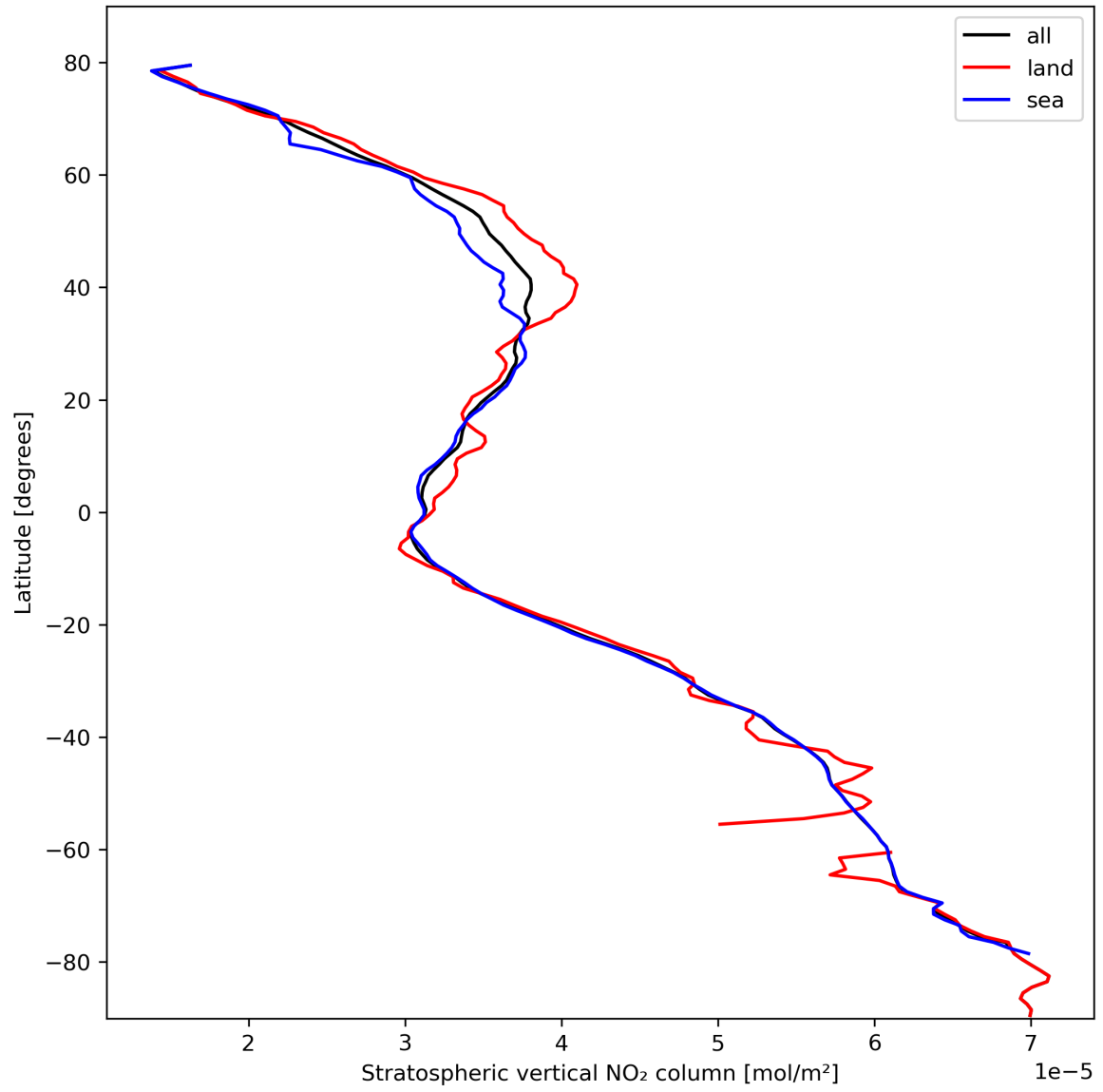
Figure 19: Zonal average of “Stratospheric vertical NO 2 column” for 2024-02-24 to 2024-02-26.
