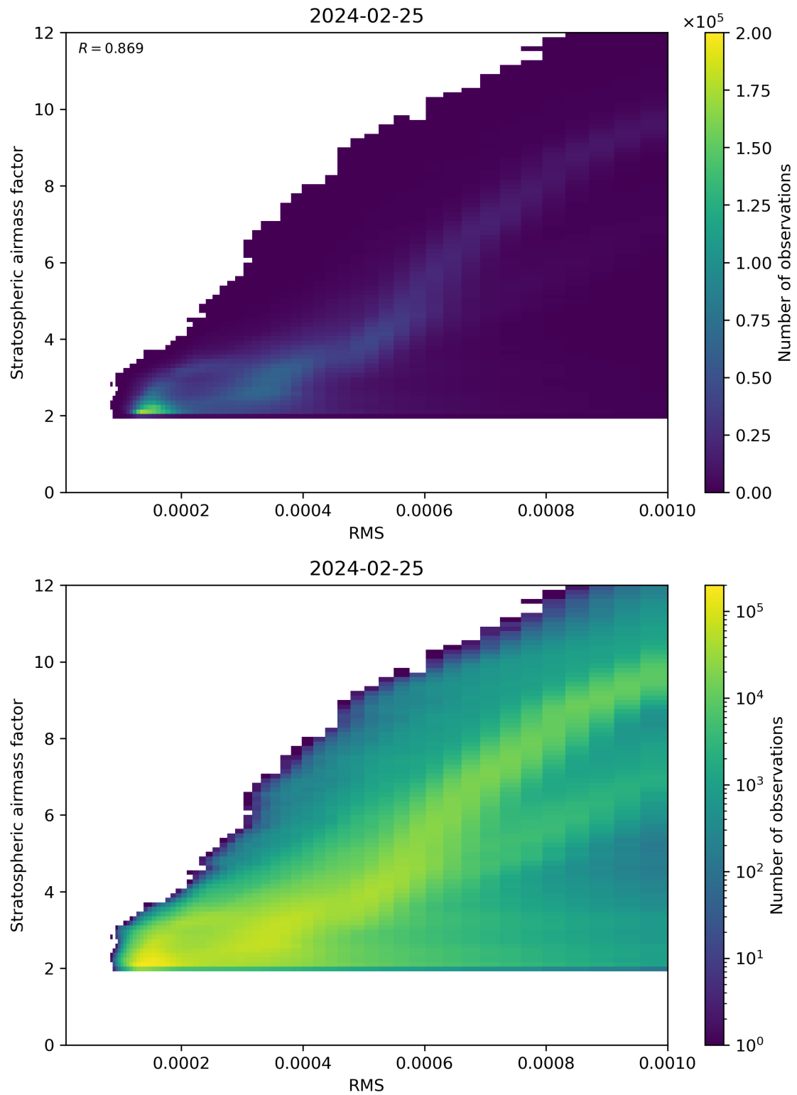
Figure 144: Scatter density plot of “RMS” against “Stratospheric airmass factor” for 2024-02-24 to 2024-02-26.
