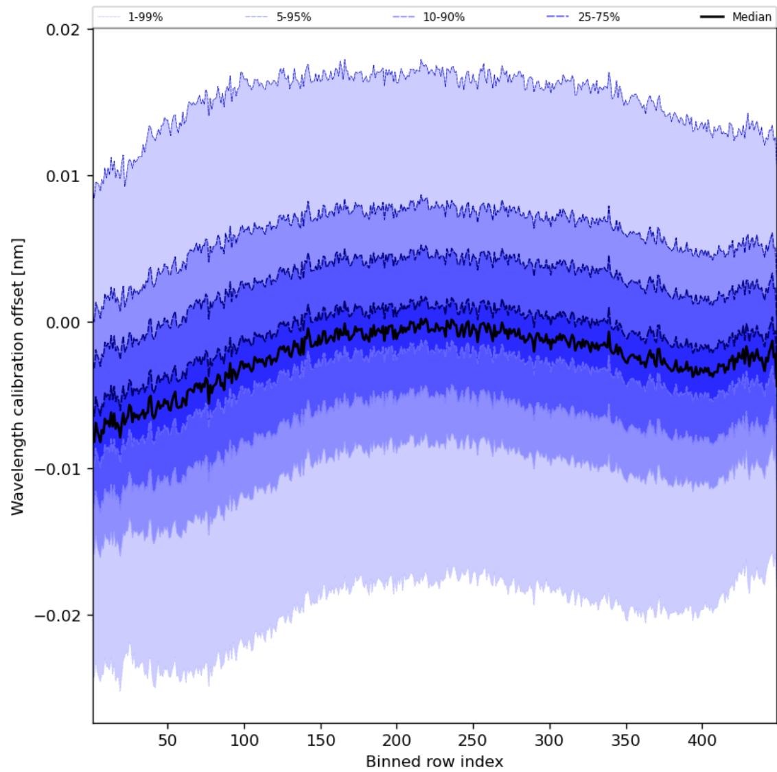
Figure 52: Along track statistics of “Wavelength calibration offset” for 2024-02-24 to 2024-02-26
