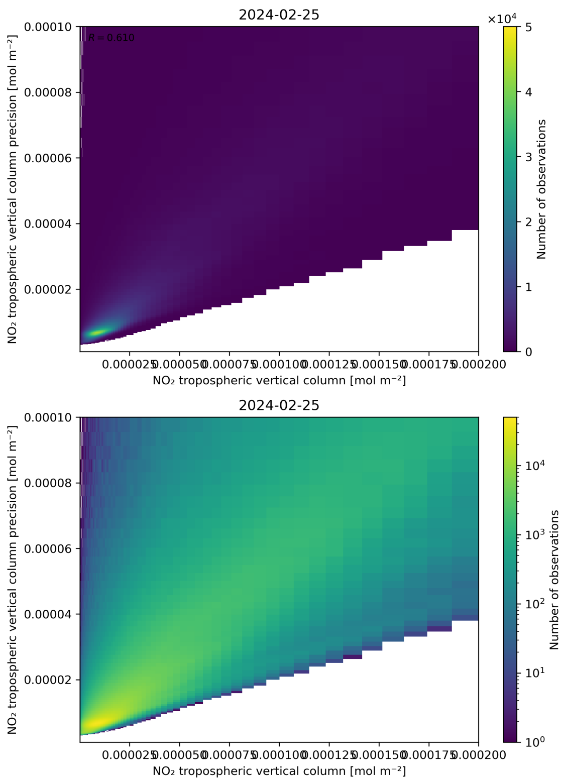
Figure 130: Scatter density plot of “NO 2 tropospheric vertical column” against “NO 2 tropospheric vertical column precision” for 2024-02-24 to 2024-02-26.
