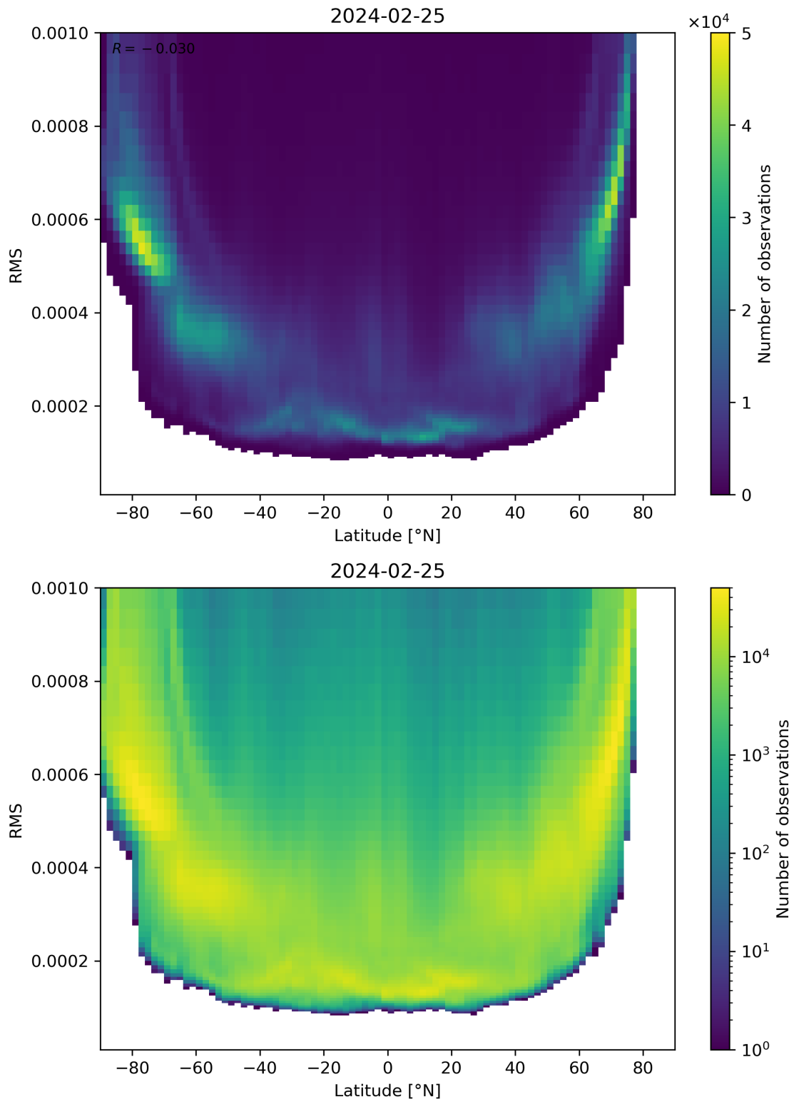
Figure 94: Scatter density plot of “Latitude” against “RMS” for 2024-02-24 to 2024-02-26.
