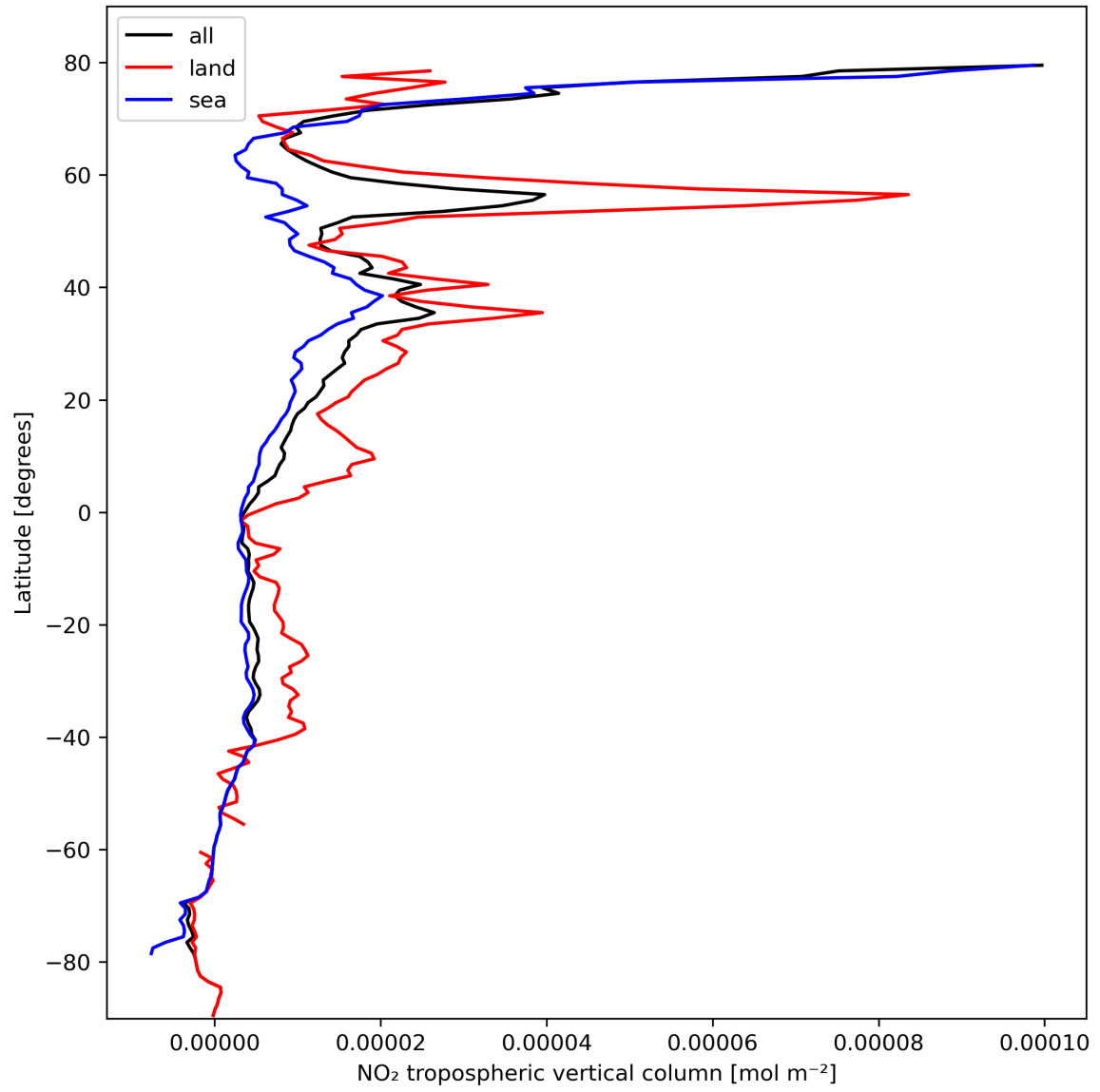
Figure 12: Zonal average of “NO 2 tropospheric vertical column” for 2024-02-24 to 2024-02-26.
