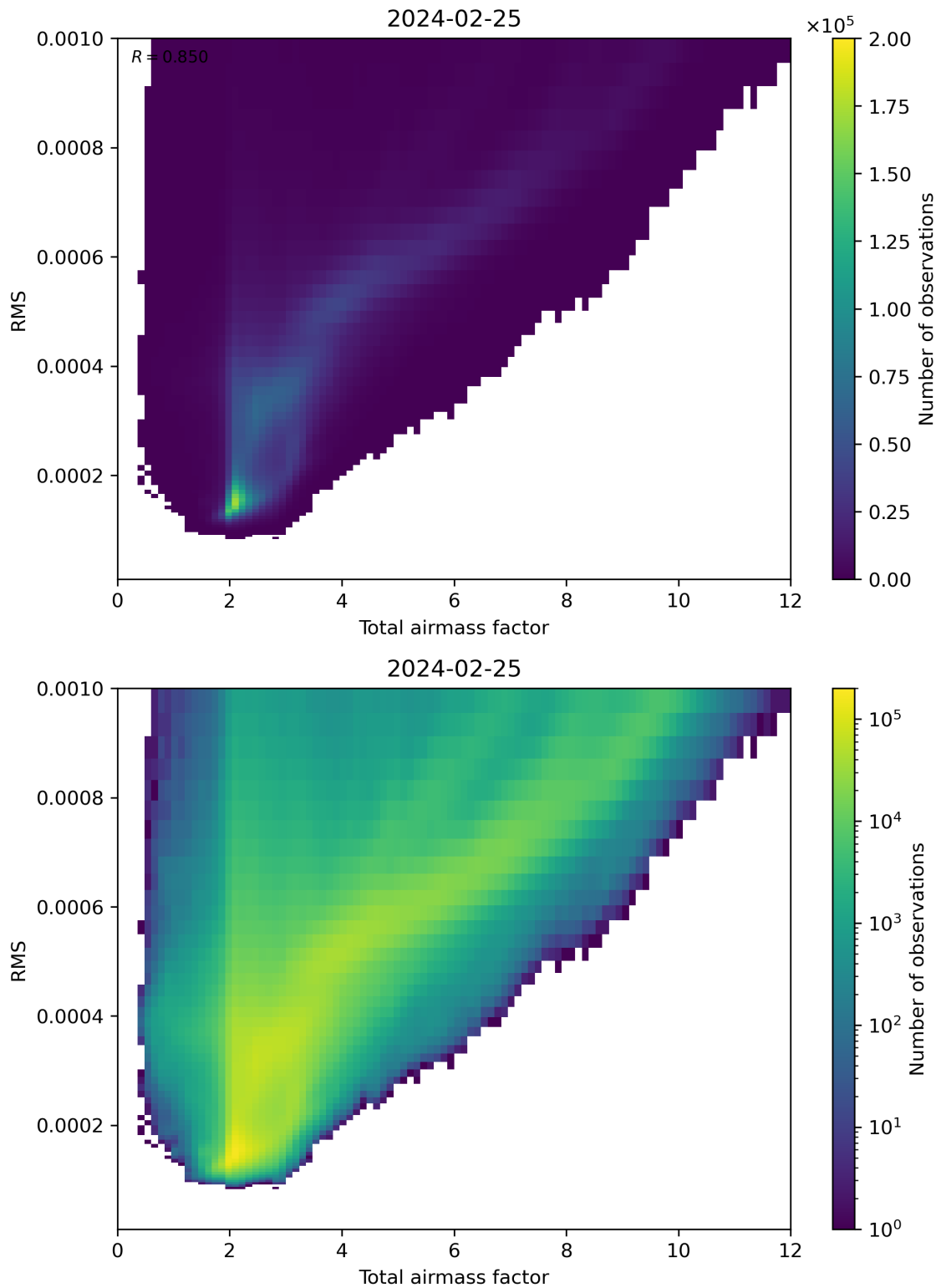
Figure 69: Scatter density plot of “Total airmass factor” against “RMS” for 2024-02-24 to 2024-02-26.
