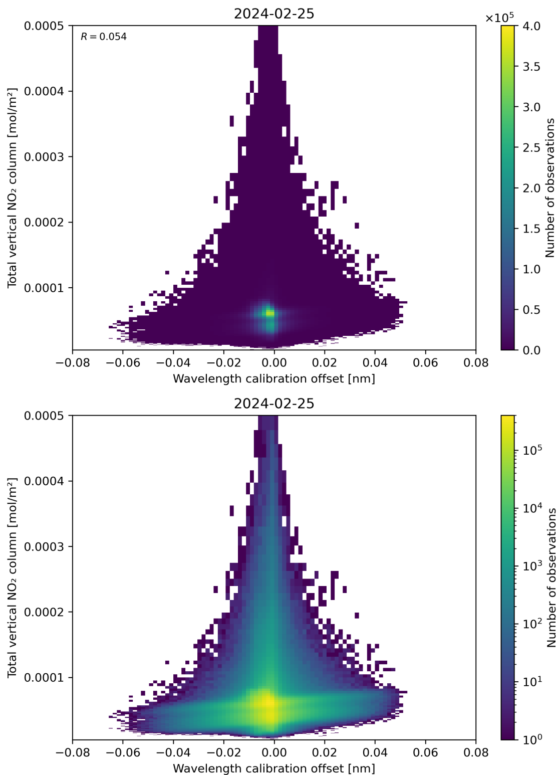
Figure 179: Scatter density plot of “Wavelength calibration offset” against “Total vertical NO 2 column” for 2024-02-24 to 2024-02-26.
