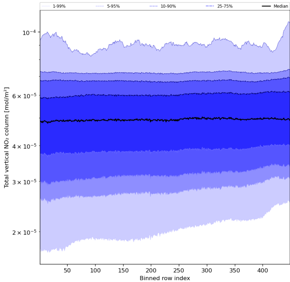
Figure 55: Along track statistics of “Total vertical NO 2 column” for 2024-02-24 to 2024-02-26
