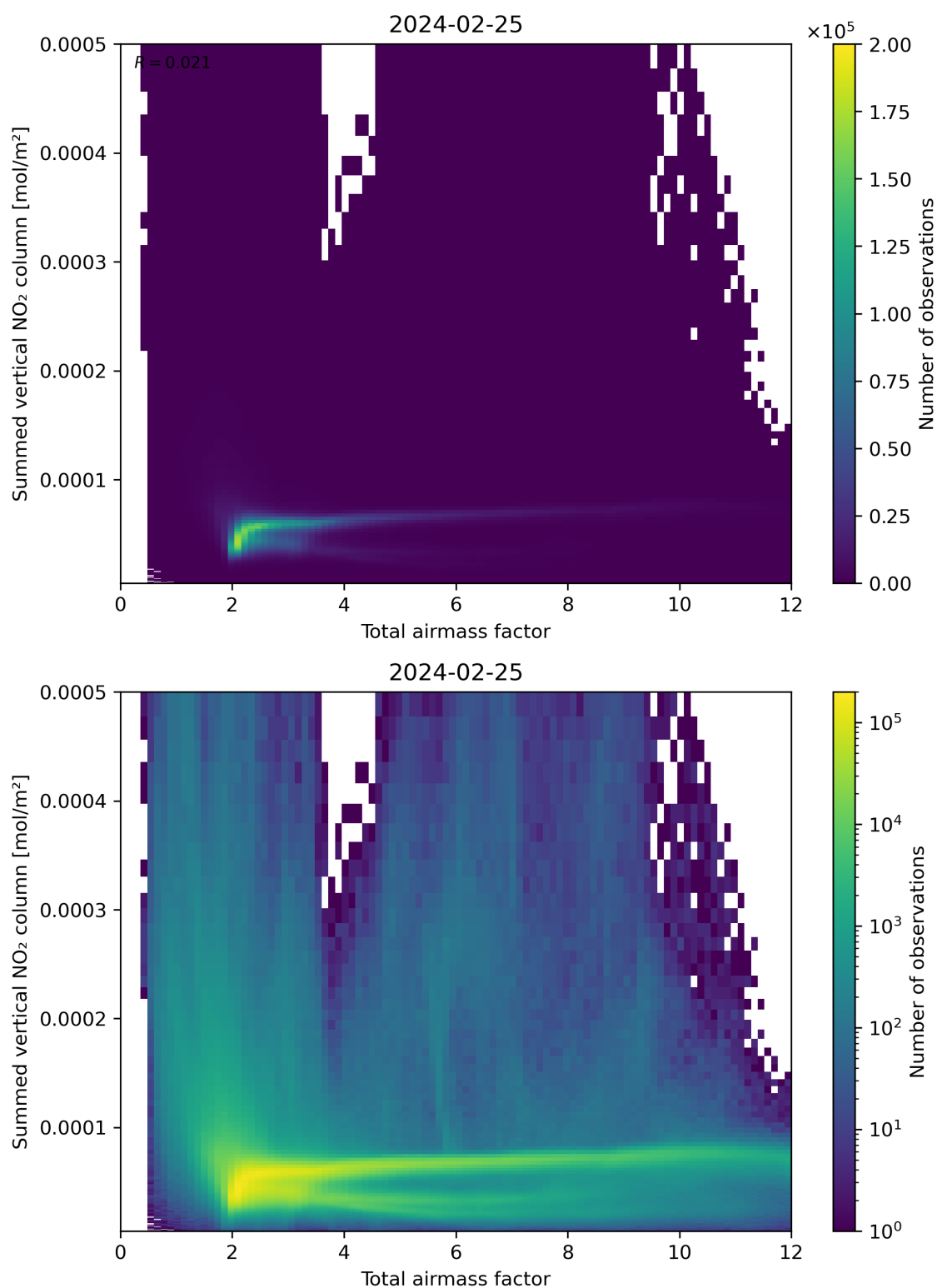
Figure 65: Scatter density plot of “Total airmass factor” against “Summed vertical NO 2 column” for 2024-02-24 to 2024-02-26.
