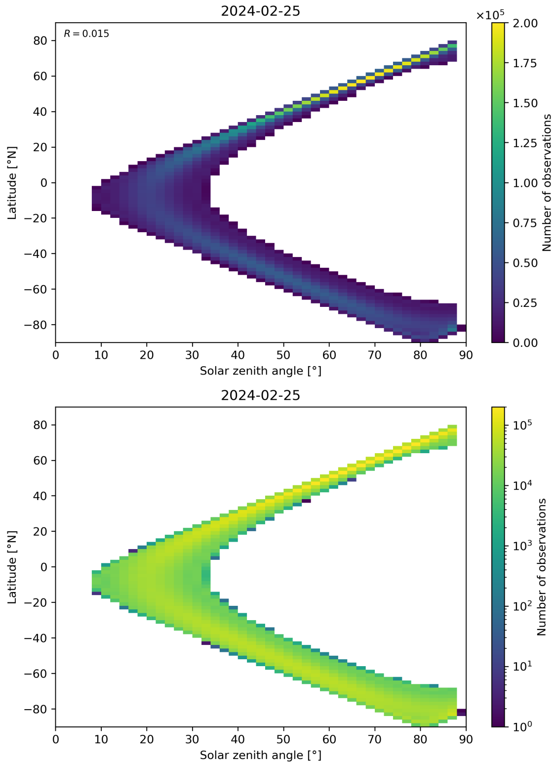
Figure 149: Scatter density plot of “Solar zenith angle” against “Latitude” for 2024-02-24 to 2024-02-26.
