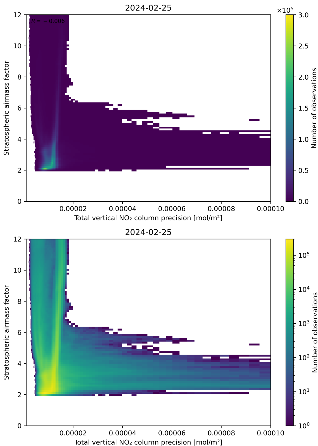
Figure 115: Scatter density plot of “Total vertical NO 2 column precision” against “Stratospheric air mass factor” for 2024-02-24 to 2024-02-26.
