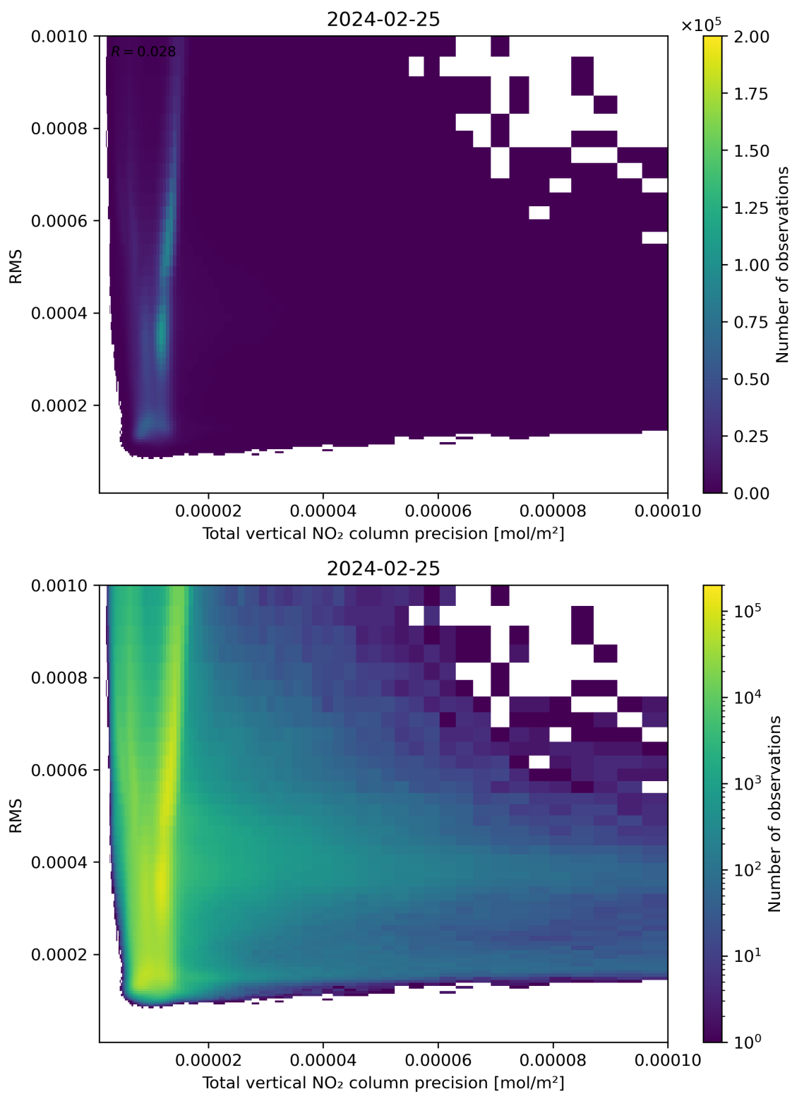
Figure 119: Scatter density plot of “Total vertical NO 2 column precision” against “RMS” for 2024-02-24 to 2024-02-26.
