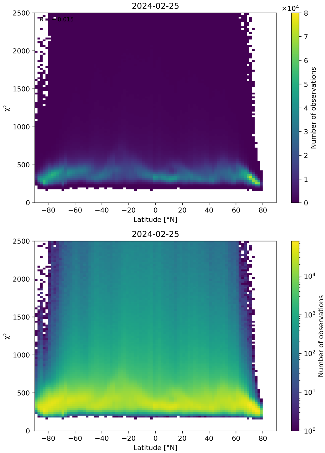
Figure 86: Scatter density plot of “Latitude” against “ \chi^2 ” for 2024-02-24 to 2024-02-26.
