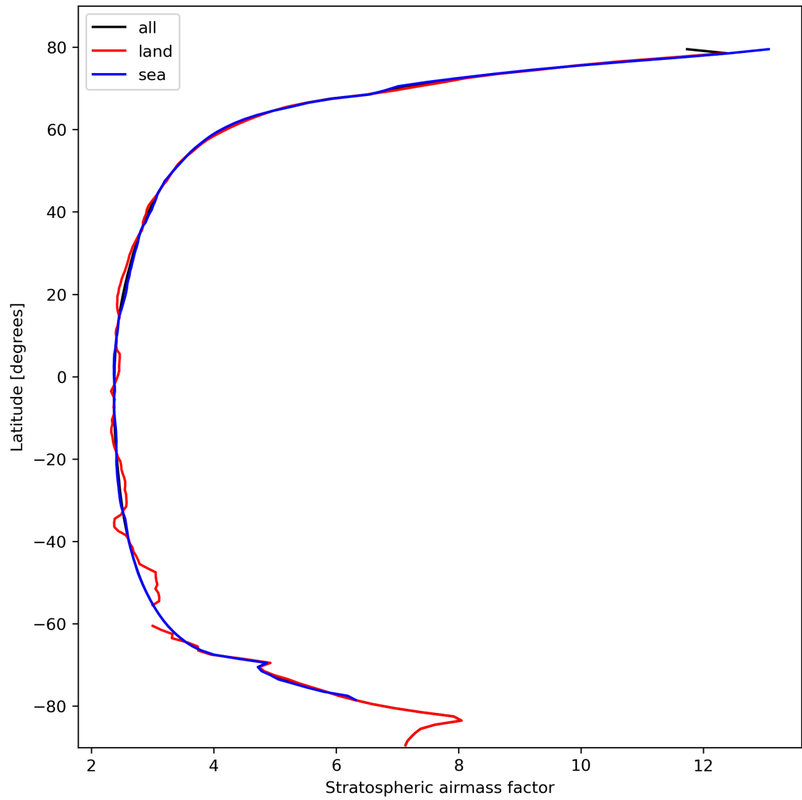
Figure 27: Zonal average of “Stratospheric airmass factor” for 2024-02-24 to 2024-02-26.
