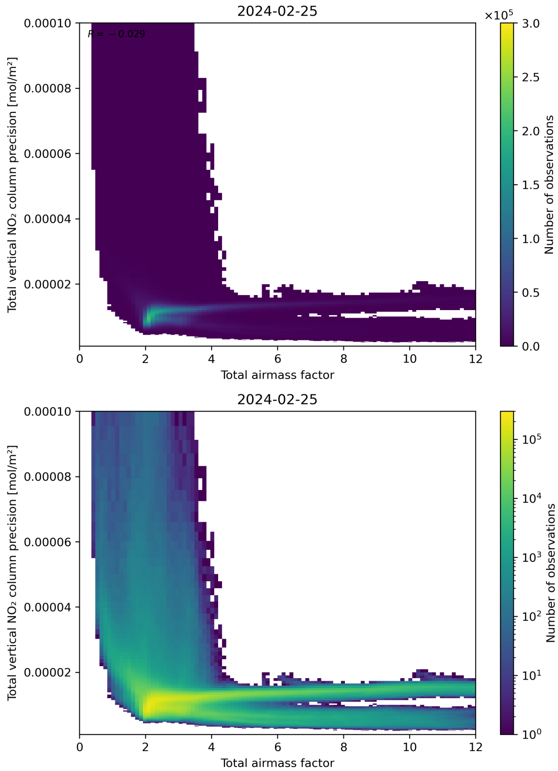
Figure 68: Scatter density plot of “Total airmass factor” against “Total vertical NO 2 column precision” for 2024-02-24 to 2024-02-26.
