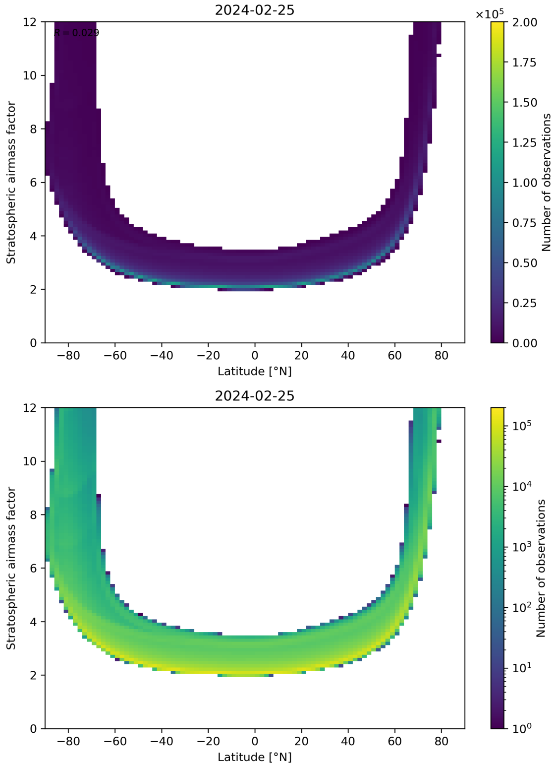
Figure 83: Scatter density plot of “Latitude” against “Stratospheric airmass factor” for 2024-02-24 to 2024-02-26.
