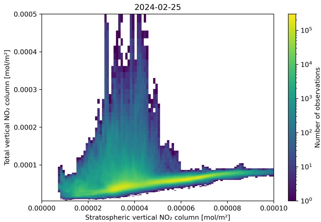
Figure 100: Scatter density plot of “Stratospheric vertical NO 2 column” against “Total vertical NO 2 column” for 2024-02-24 to 2024-02-26.
