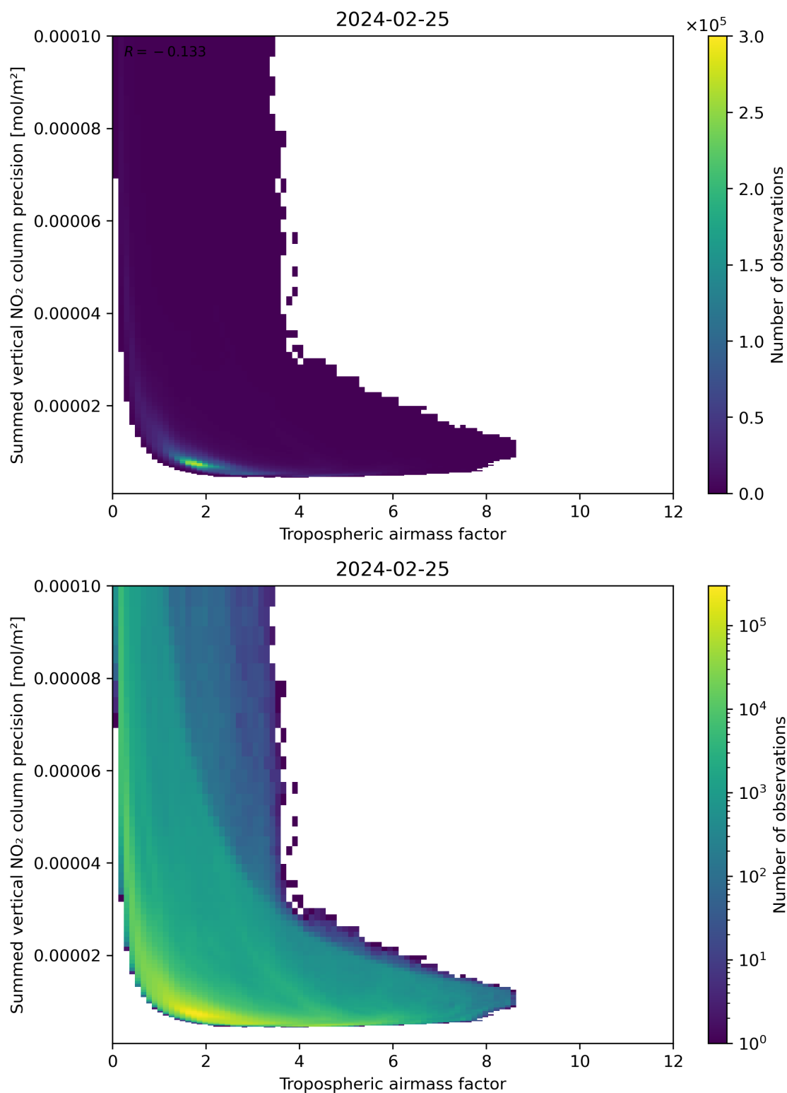
Figure 76: Scatter density plot of “Tropospheric air mass factor” against “Summed vertical NO 2 column precision” for 2024-02-24 to 2024-02-26.
