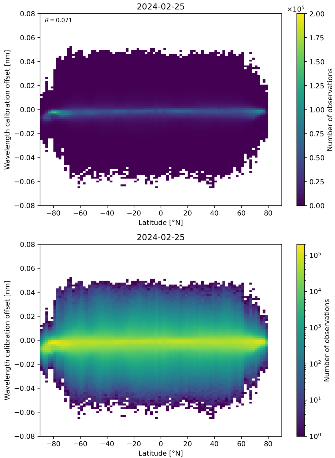
Figure 95: Scatter density plot of “Latitude” against “Wavelength calibration offset” for 2024-02-24 to 2024-02-26.
