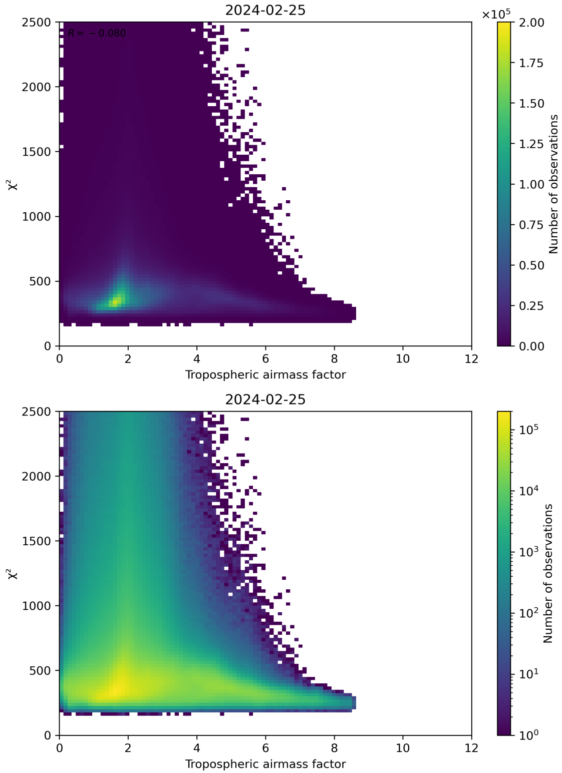
Figure 73: Scatter density plot of “Tropospheric airmass factor” against “ \chi^2 ” for 2024-02-24 to 2024-02-26.
