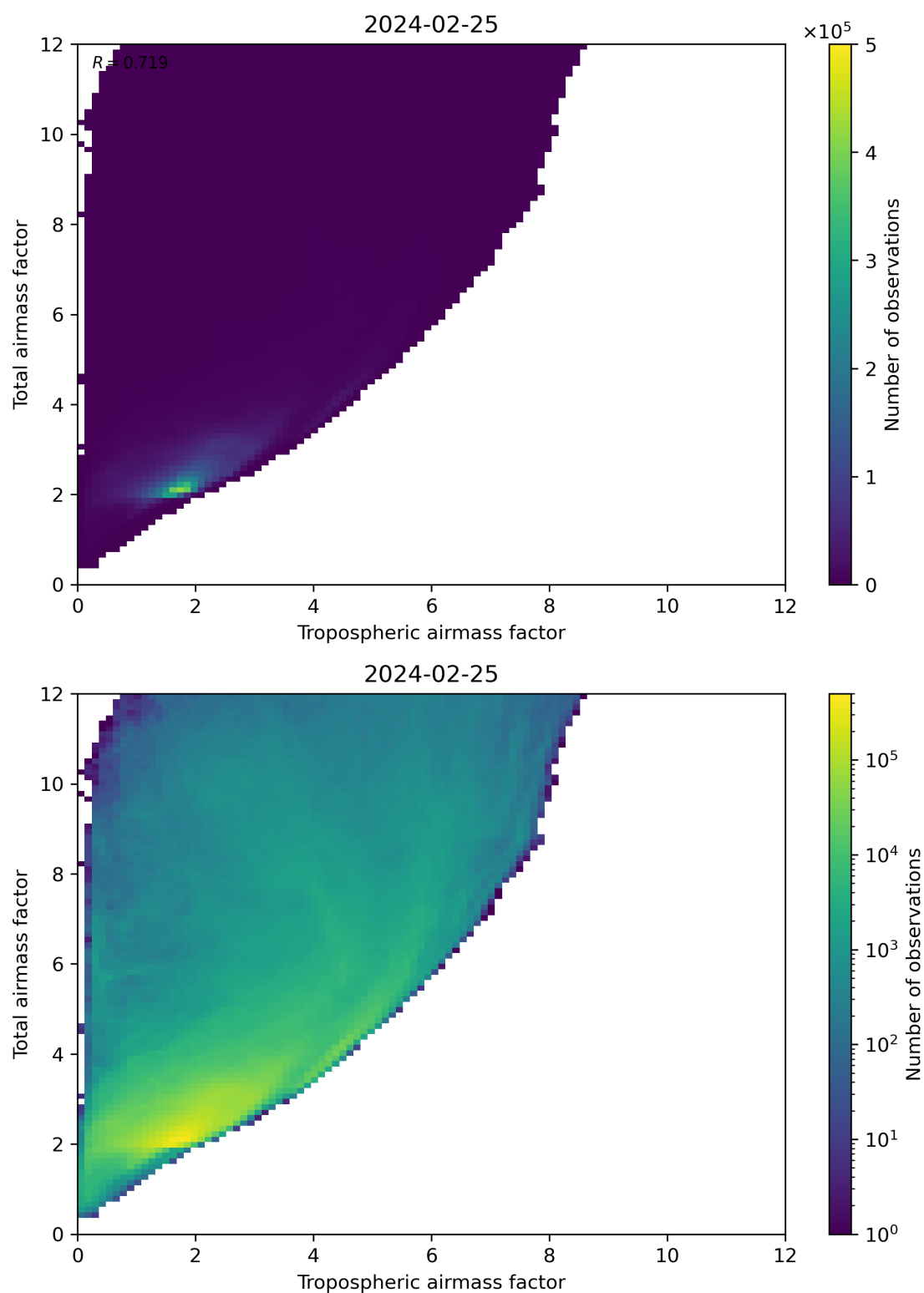
Figure 72: Scatter density plot of “Tropospheric airmass factor” against “Total airmass factor” for 2024-02-24 to 2024-02-26.
