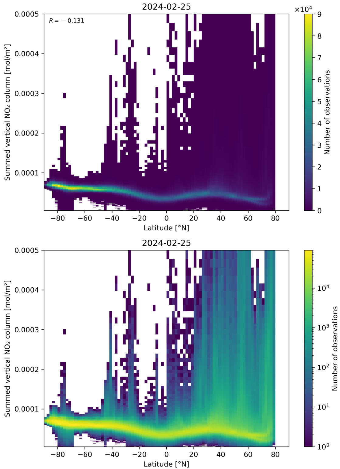
Figure 88: Scatter density plot of “Latitude” against “Summed vertical NO 2 column” for 2024-02-24 to 2024-02-26.
