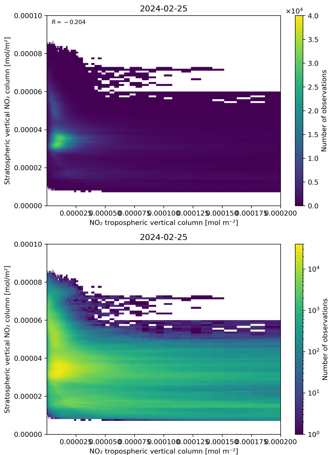
Figure 125: Scatter density plot of “NO 2 tropospheric vertical column” against “Stratospheric vertical NO 2 column” for 2024-02-24 to 2024-02-26.
