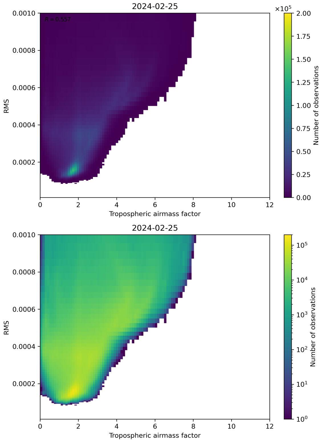
Figure 79: Scatter density plot of “Tropospheric airmass factor” against “RMS” for 2024-02-24 to 2024-02-26.
