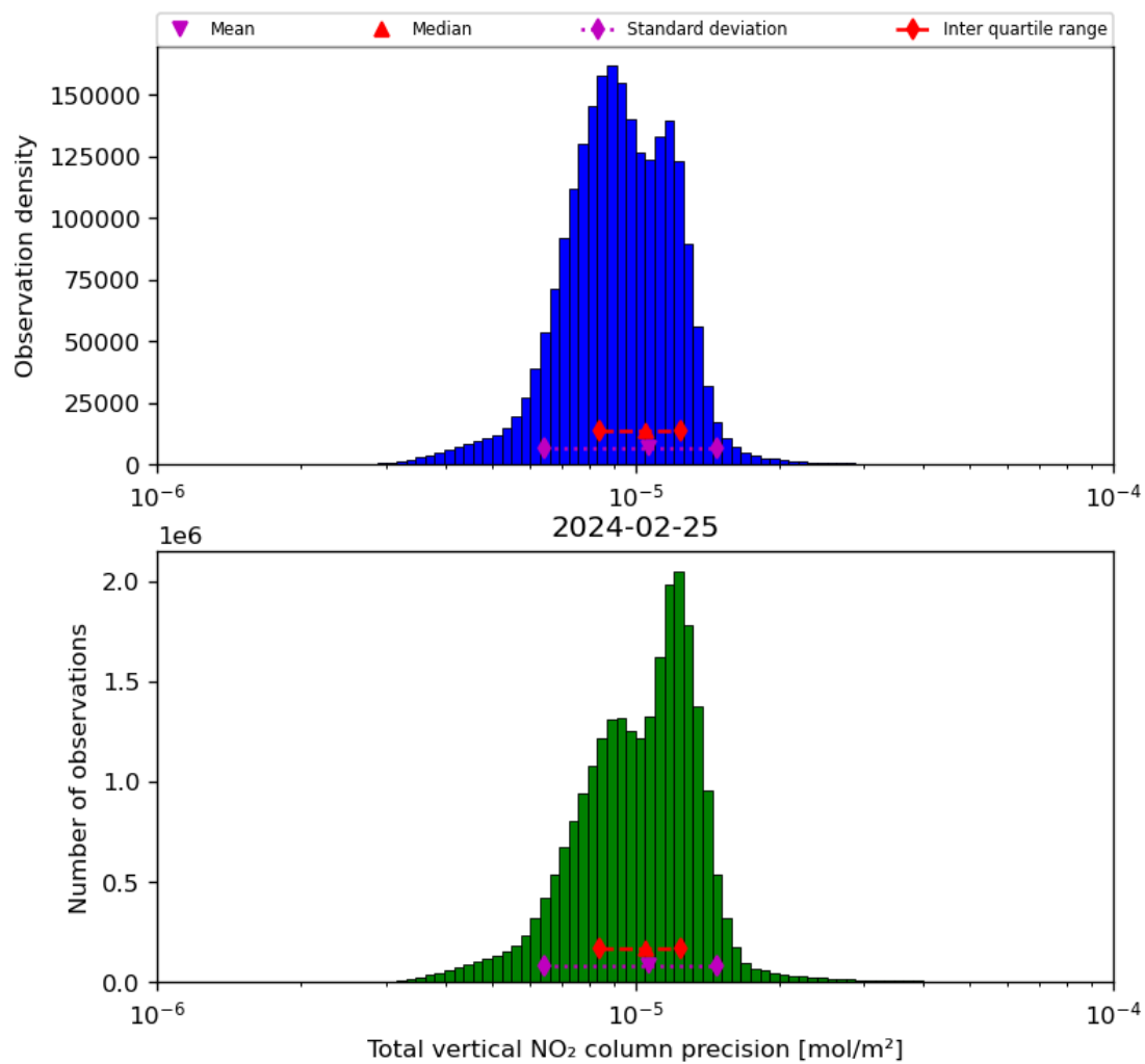
Figure 39: Histogram of “Total vertical NO 2 column precision” for 2024-02-24 to 2024-02-26
