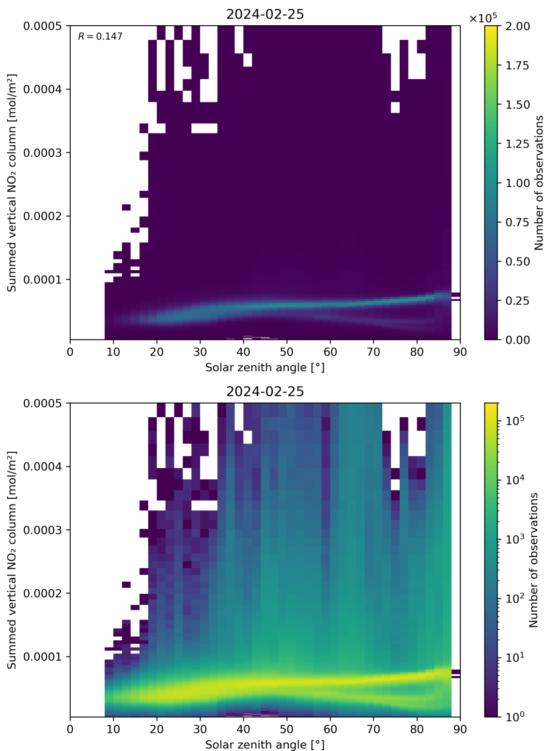
Figure 151: Scatter density plot of “Solar zenith angle” against “Summed vertical NO 2 column” for 2024-02-24 to 2024-02-26.
