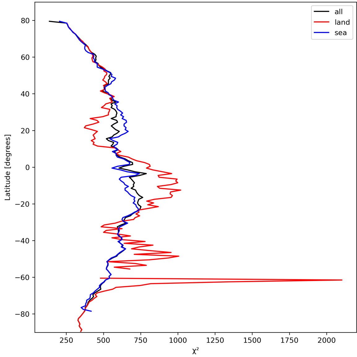
Figure 25: Zonal average of “ \chi^2 ” for 2024-02-24 to 2024-02-26.
