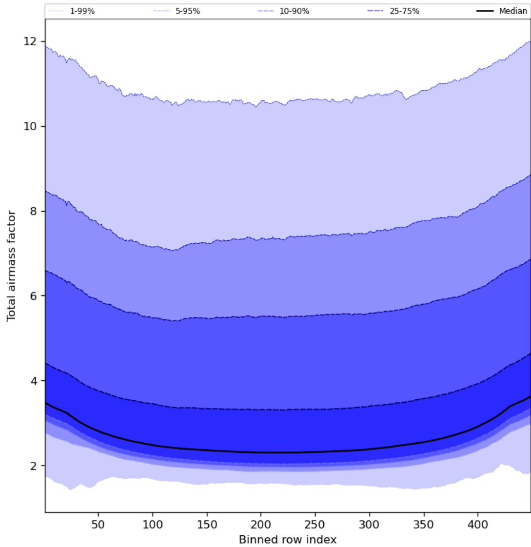
Figure 49: Along track statistics of “Total airmass factor” for 2024-02-24 to 2024-02-26
