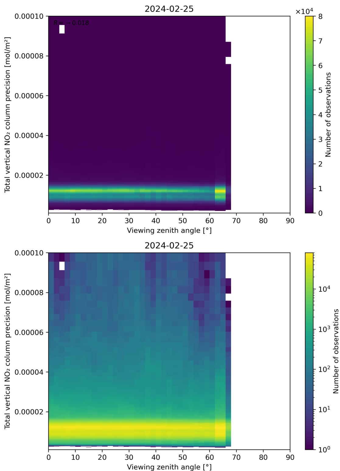
Figure 168: Scatter density plot of “Viewing zenith angle” against “Total vertical NO 2 column precision” for 2024-02-24 to 2024-02-26.
