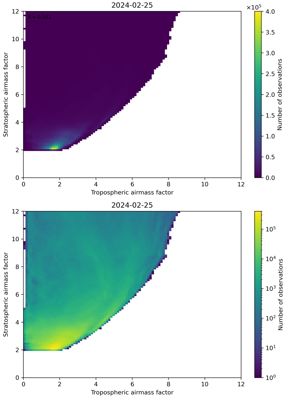
Figure 71: Scatter density plot of “Tropospheric airmass factor” against “Stratospheric airmass factor” for 2024-02-24 to 2024-02-26.
