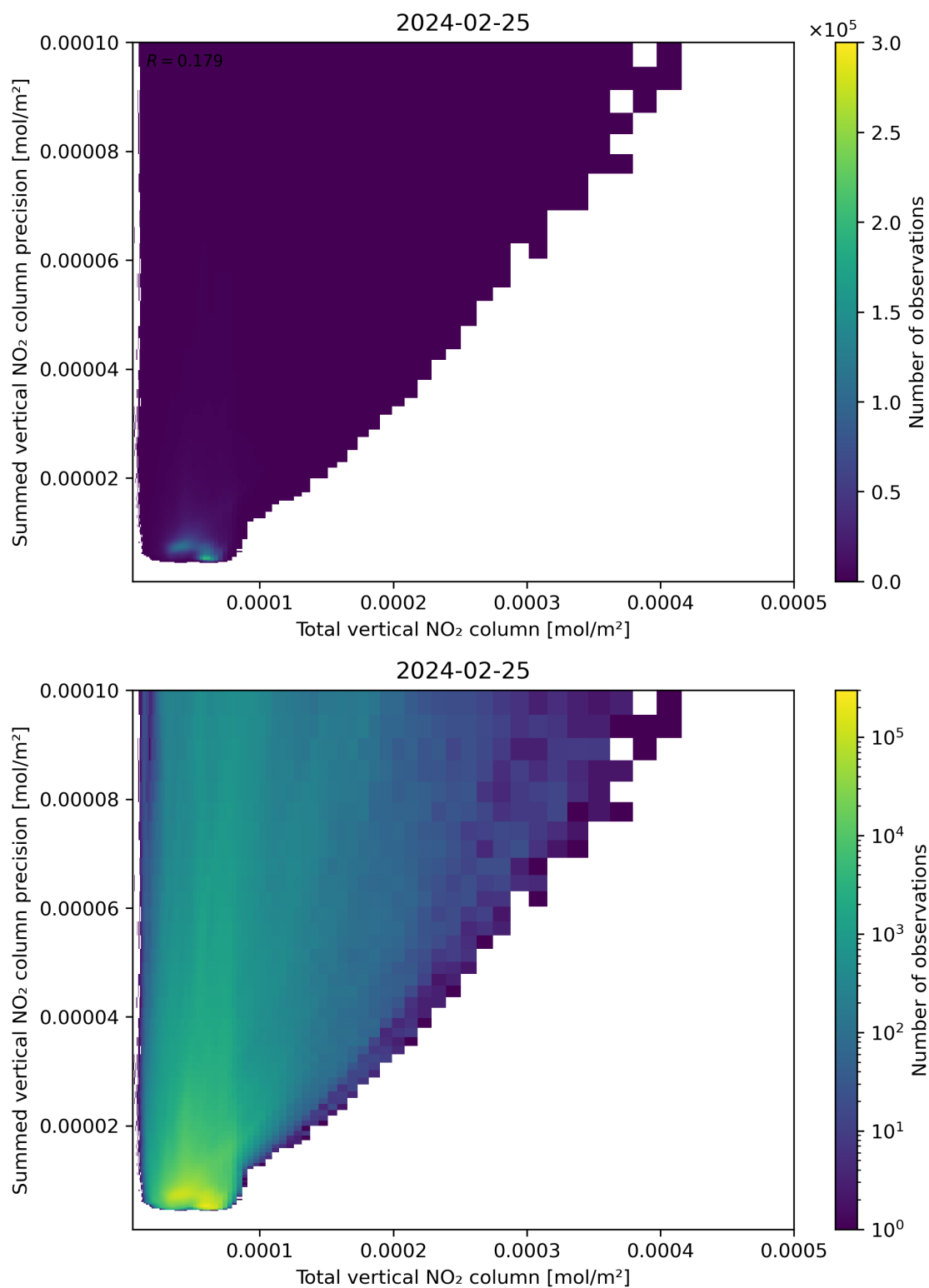
Figure 113: Scatter density plot of “Total vertical NO 2 column” against “Summed vertical NO 2 column precision” for 2024-02-24 to 2024-02-26.
