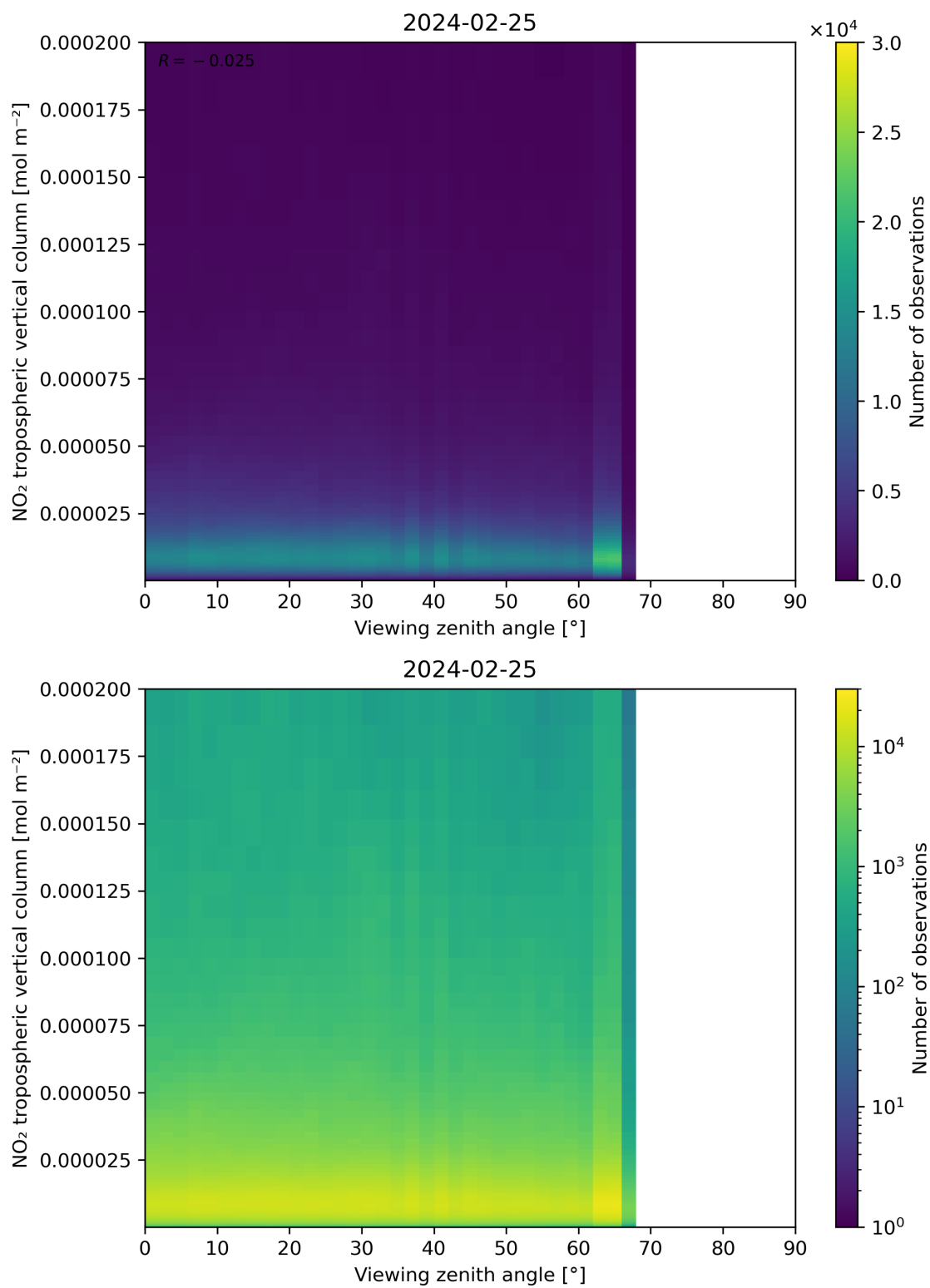
Figure 169: Scatter density plot of “Viewing zenith angle” against “NO 2 tropospheric vertical column” for 2024-02-24 to 2024-02-26.
