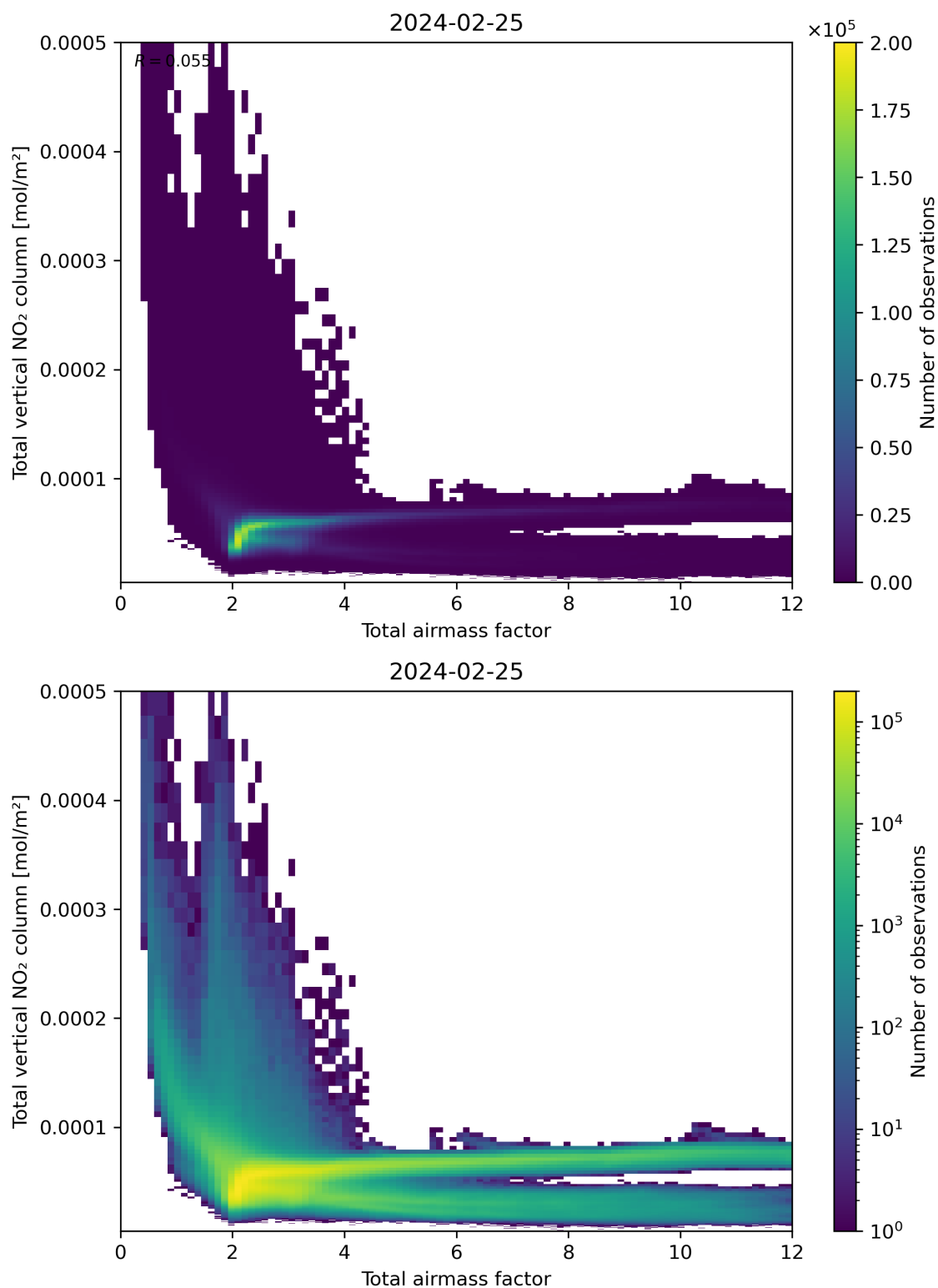
Figure 67: Scatter density plot of “Total airmass factor” against “Total vertical NO 2 column” for 2024-02-24 to 2024-02-26.
