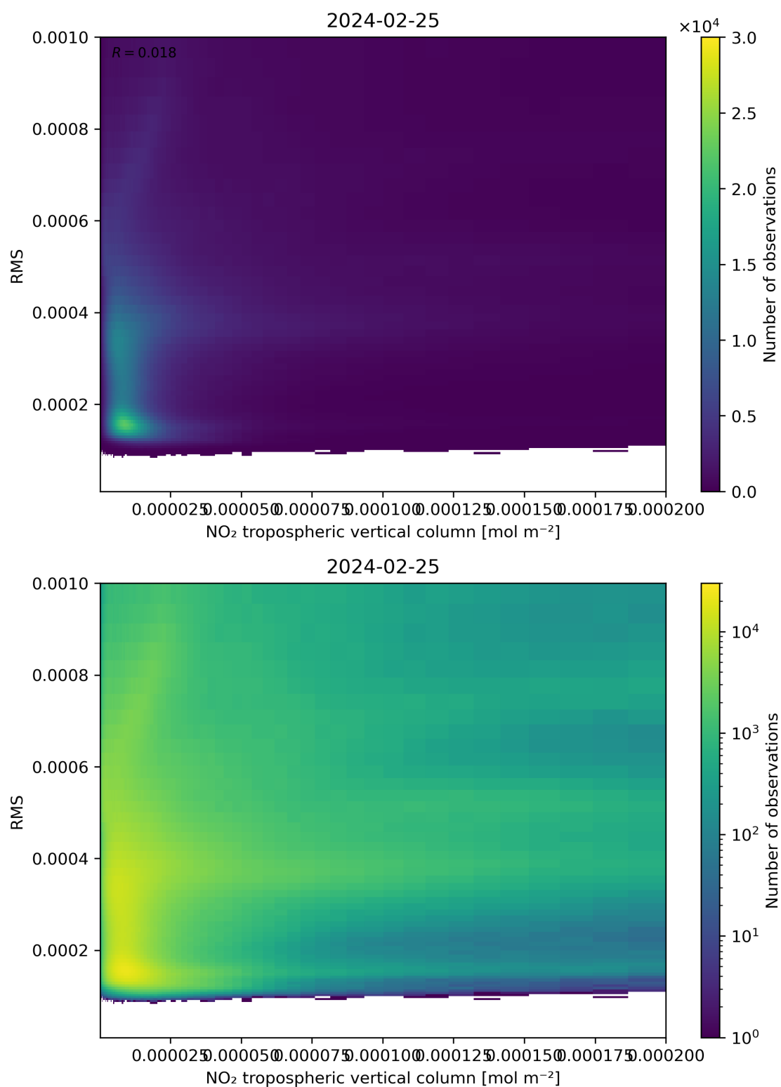
Figure 142: Scatter density plot of “NO 2 tropospheric vertical column” against “RMS” for 2024-02-24 to 2024-02-26.
