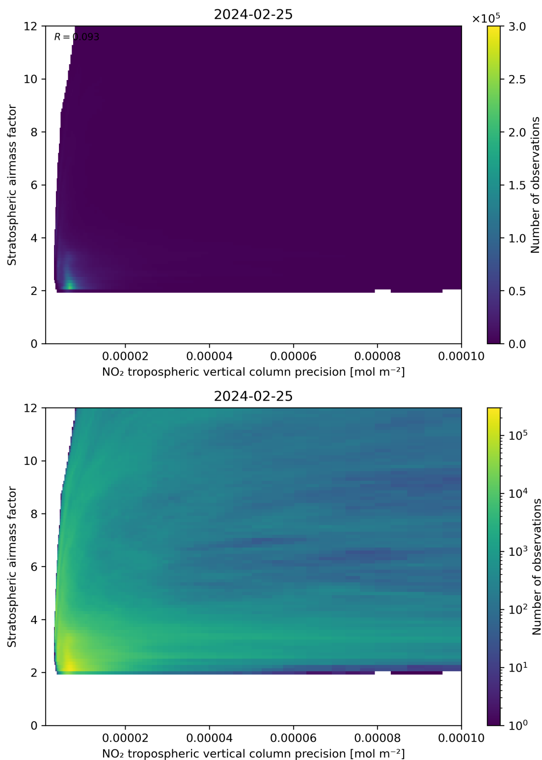
Figure 131: Scatter density plot of “NO 2 tropospheric vertical column precision” against “Stratospheric airmass factor” for 2024-02-24 to 2024-02-26.
