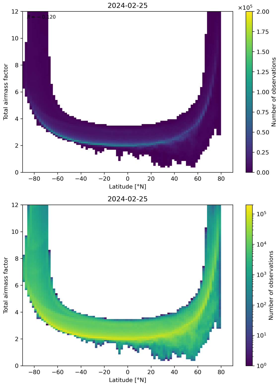
Figure 84: Scatter density plot of “Latitude” against “Total airmass factor” for 2024-02-24 to 2024-02-26.
