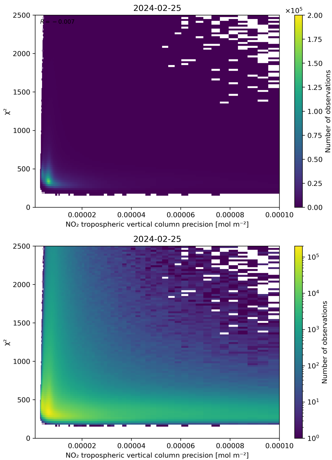
Figure 134: Scatter density plot of “NO 2 tropospheric vertical column precision” against “ \chi^2 ” for 2024-02-24 to 2024-02-26.
