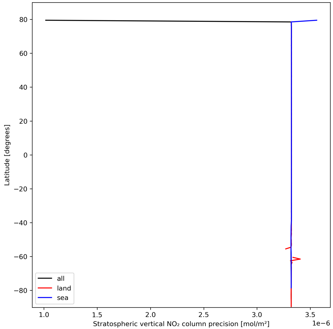
Figure 20: Zonal average of “Stratospheric vertical NO 2 column precision” for 2024-02-24 to 2024-02-26.
