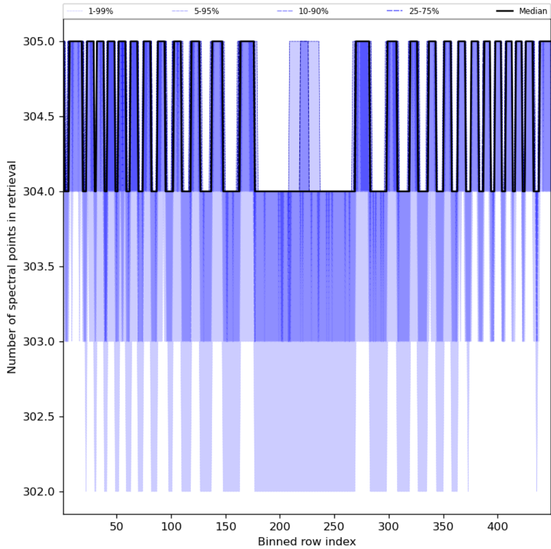
Figure 50: Along track statistics of “Number of spectral points in retrieval” for 2024-02-24 to 2024-02-26
