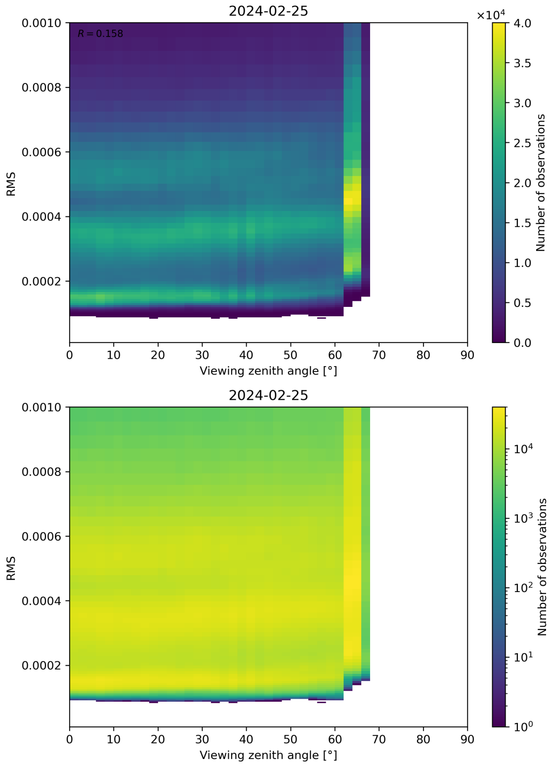
Figure 171: Scatter density plot of “Viewing zenith angle” against “RMS” for 2024-02-24 to 2024-02-26.
