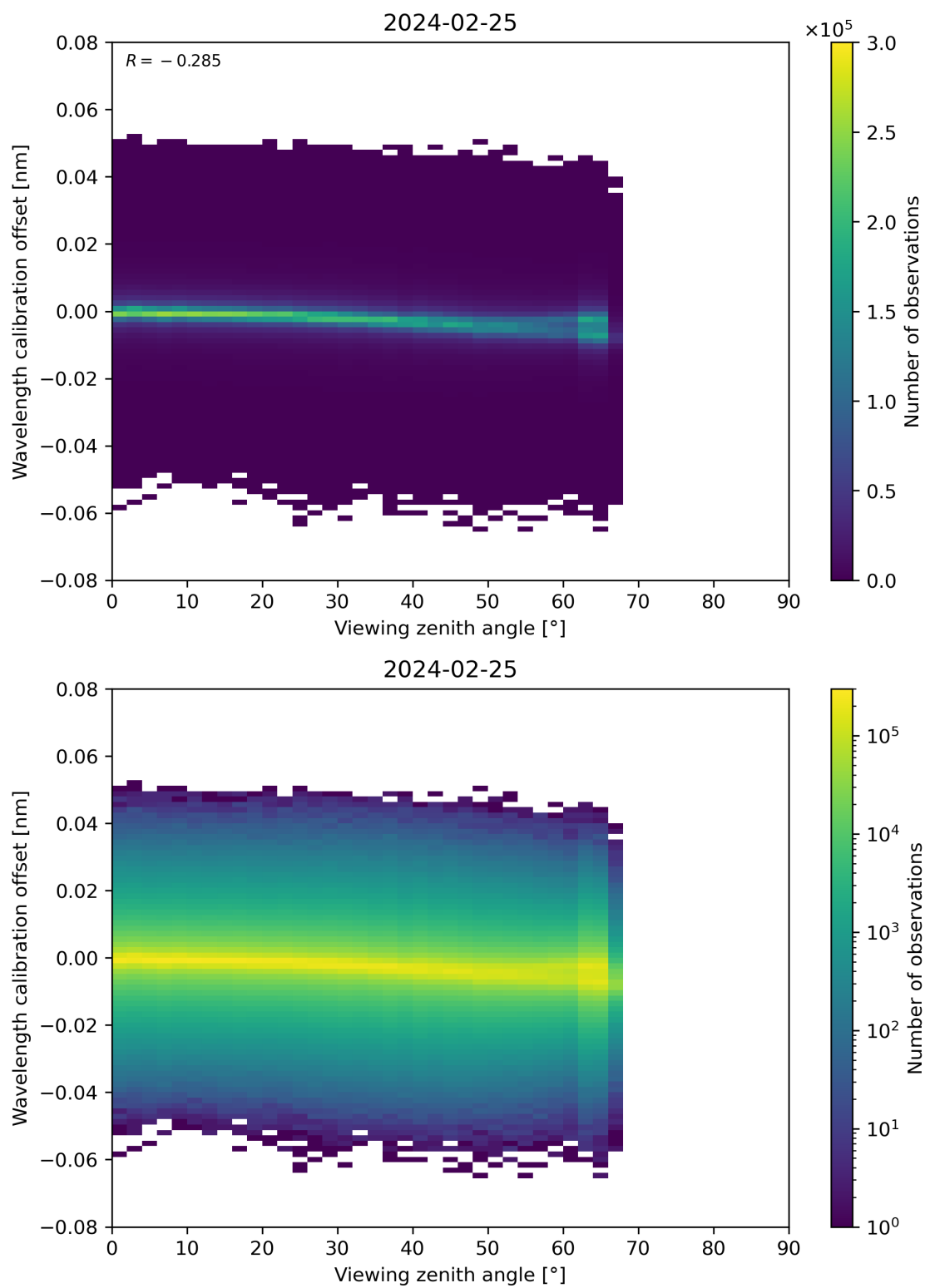
Figure 173: Scatter density plot of “Viewing zenith angle” against “Wavelength calibration offset” for 2024-02-24 to 2024-02-26.
