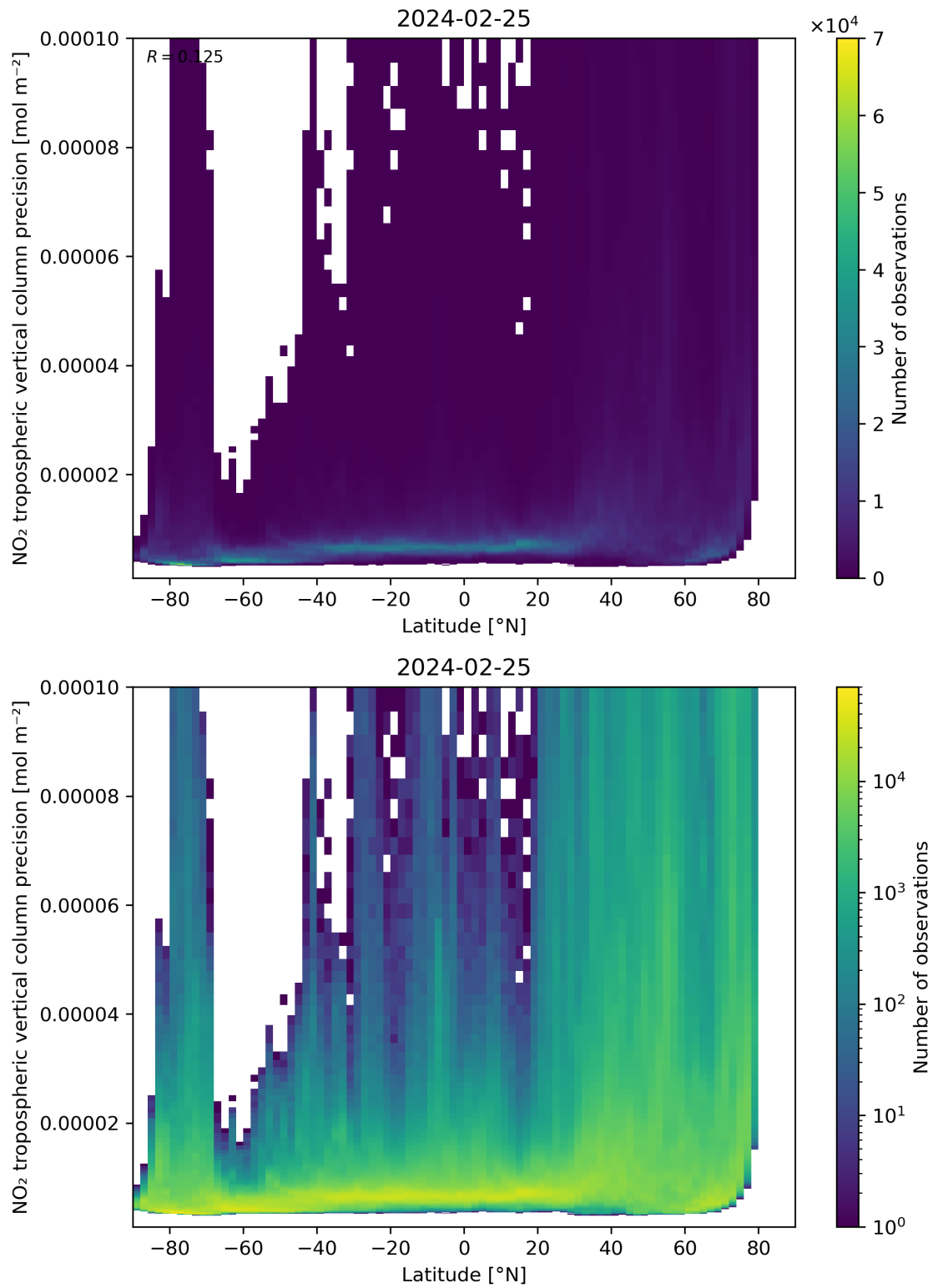
Figure 93: Scatter density plot of “Latitude” against “NO 2 tropospheric vertical column precision” for 2024-02-24 to 2024-02-26.
