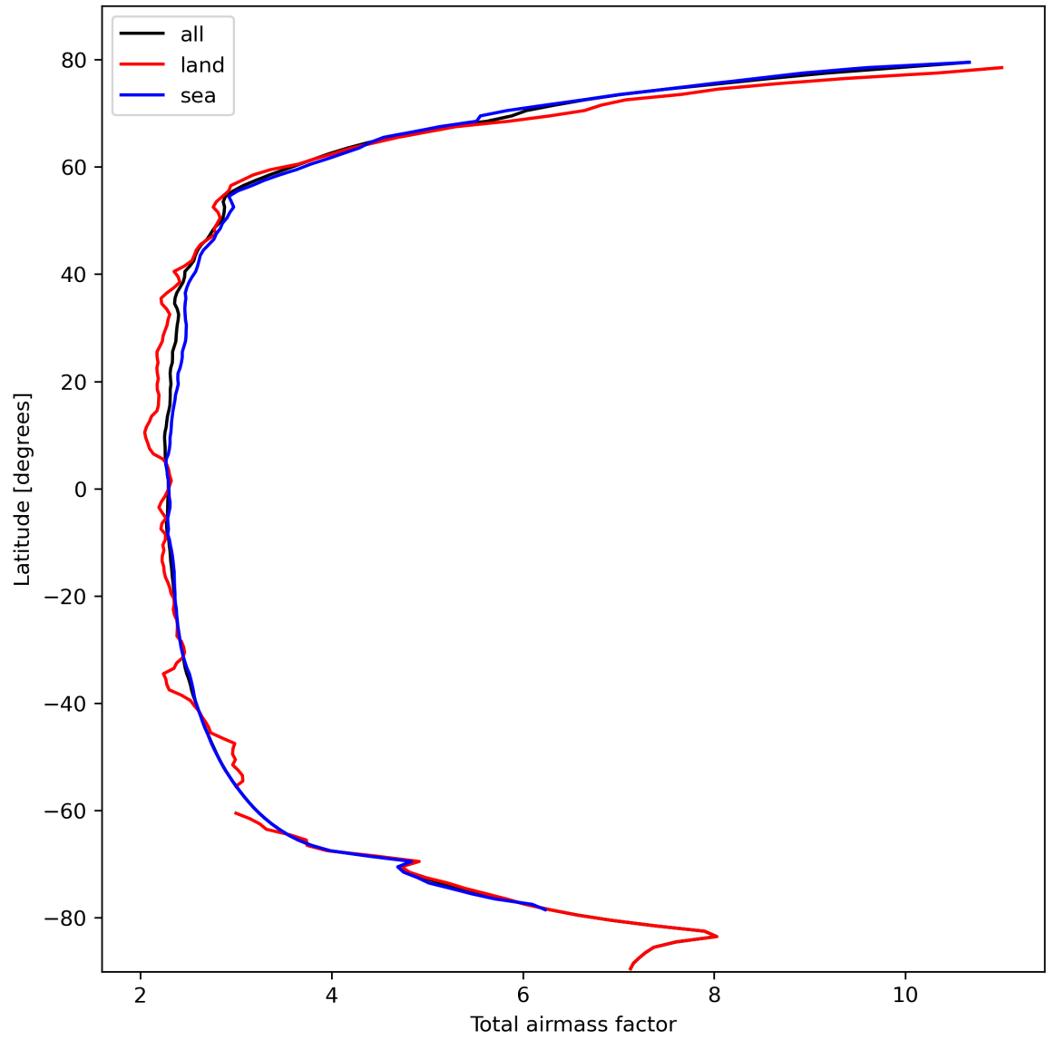
Figure 15: Zonal average of “Total airmass factor” for 2024-02-24 to 2024-02-26.
