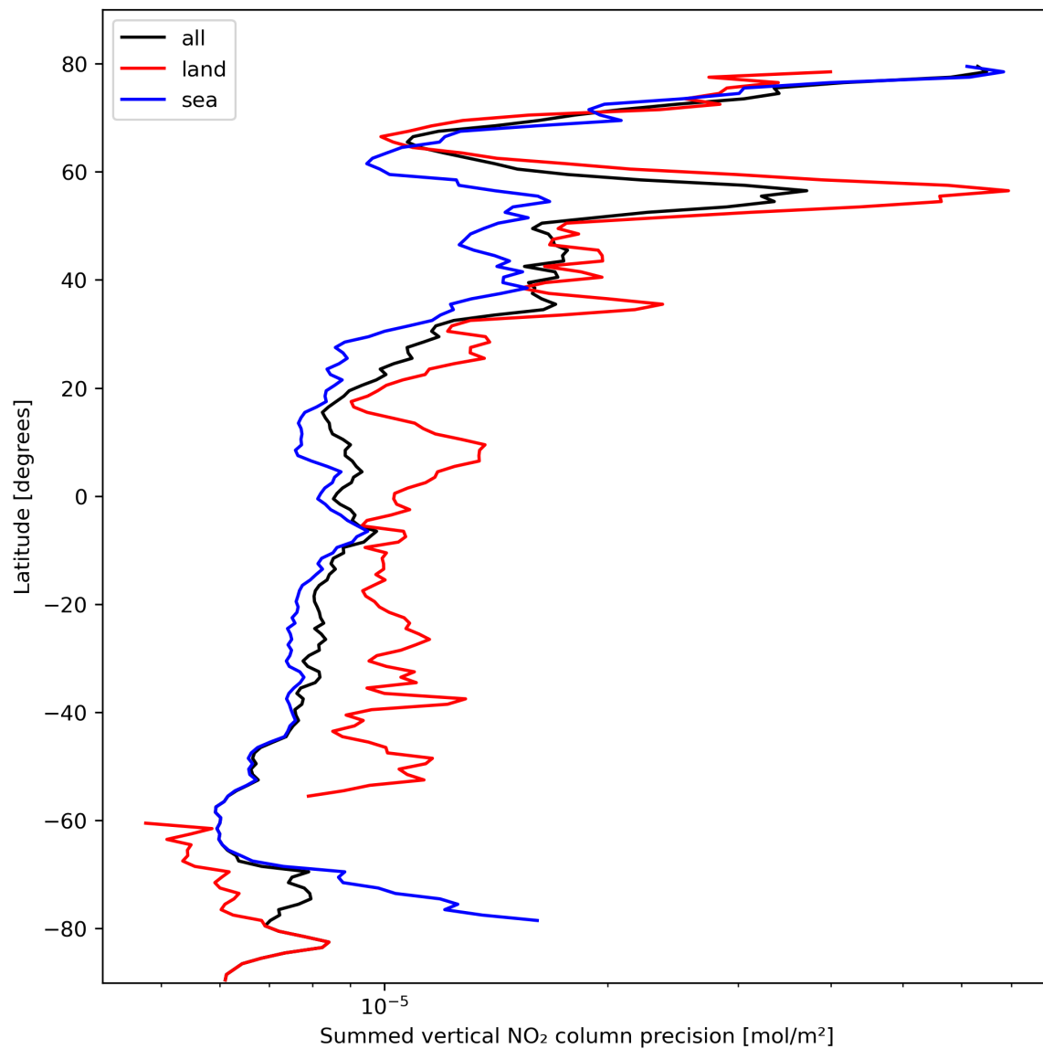
Figure 24: Zonal average of “Summed vertical NO 2 column precision” for 2024-02-24 to 2024-02-26.
