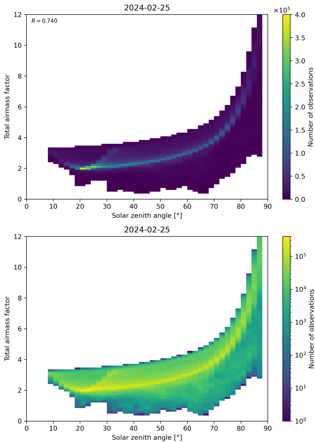
Figure 146: Scatter density plot of “Solar zenith angle” against “Total air mass factor” for 2024-02-24 to 2024-02-26.
