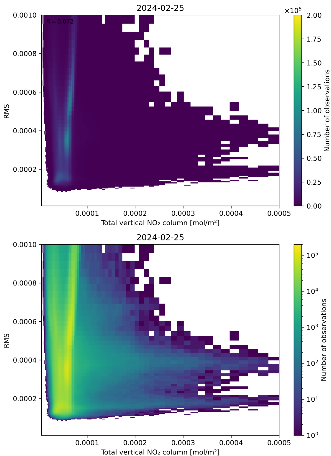
Figure 120: Scatter density plot of “Total vertical NO 2 column” against “RMS” for 2024-02-24 to 2024-02-26.
