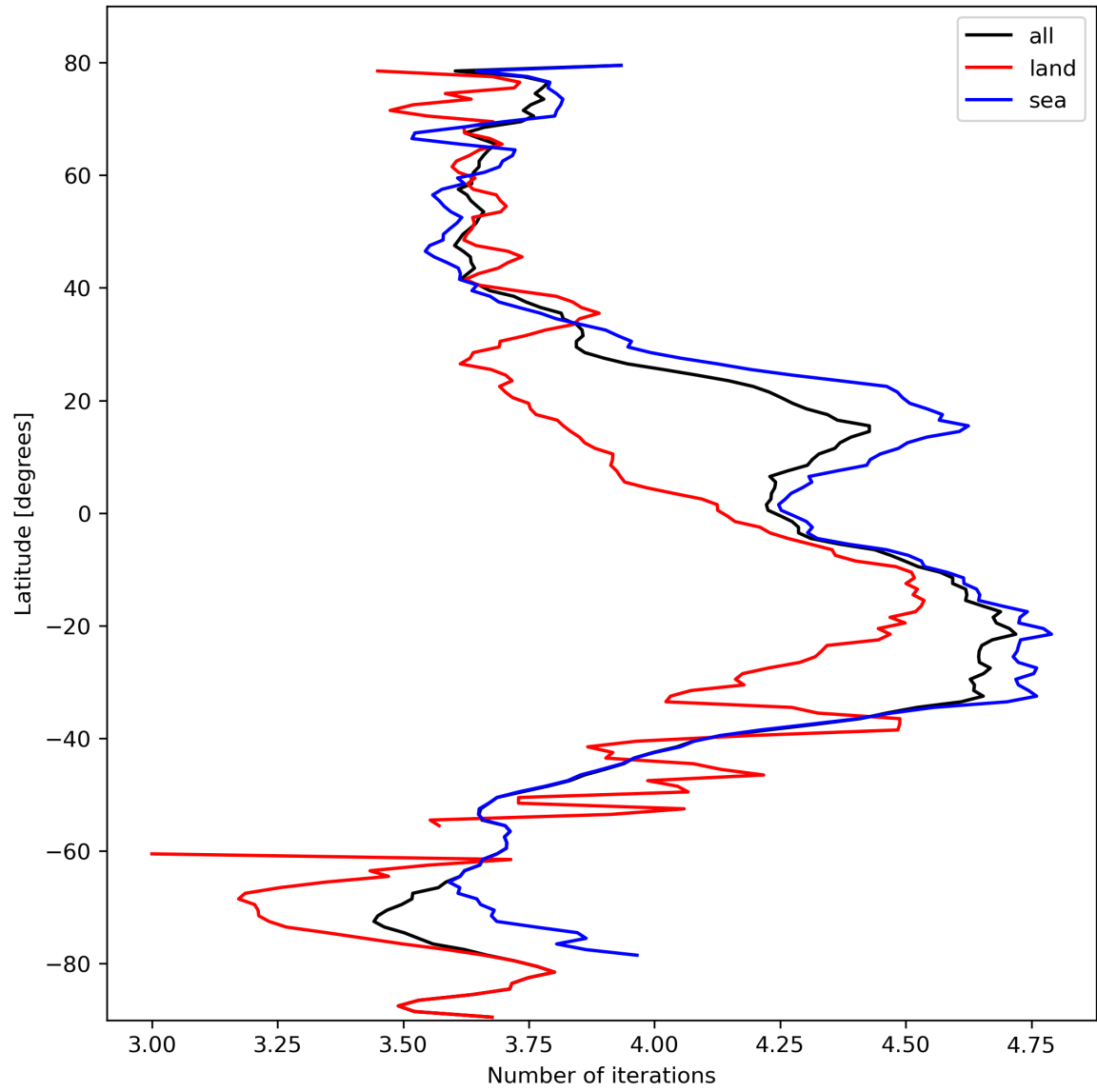
Figure 17: Zonal average of “Number of iterations” for 2024-02-24 to 2024-02-26.
