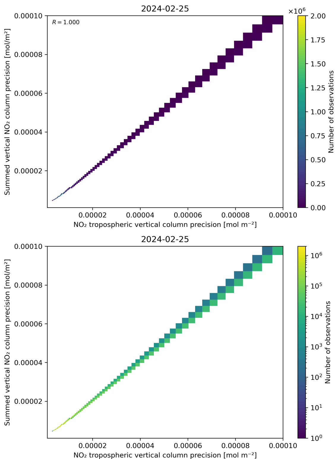
Figure 137: Scatter density plot of “NO 2 tropospheric vertical column precision” against “Summed vertical NO 2 column precision” for 2024-02-24 to 2024-02-26.
