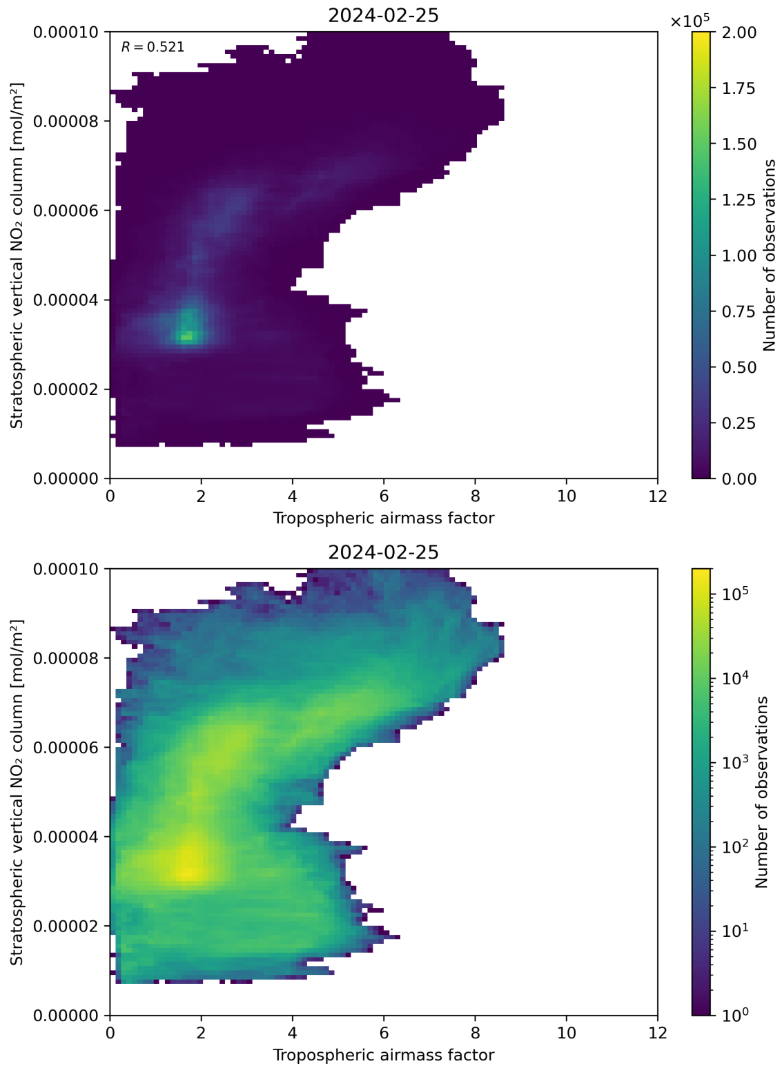
Figure 74: Scatter density plot of “Tropospheric air mass factor” against “Stratospheric vertical NO 2 column” for 2024-02-24 to 2024-02-26.
