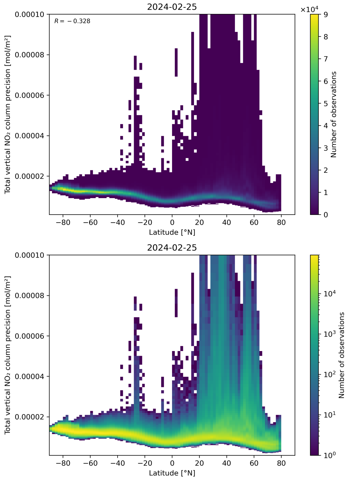
Figure 91: Scatter density plot of “Latitude” against “Total vertical NO 2 column precision” for 2024-02-24 to 2024-02-26.
