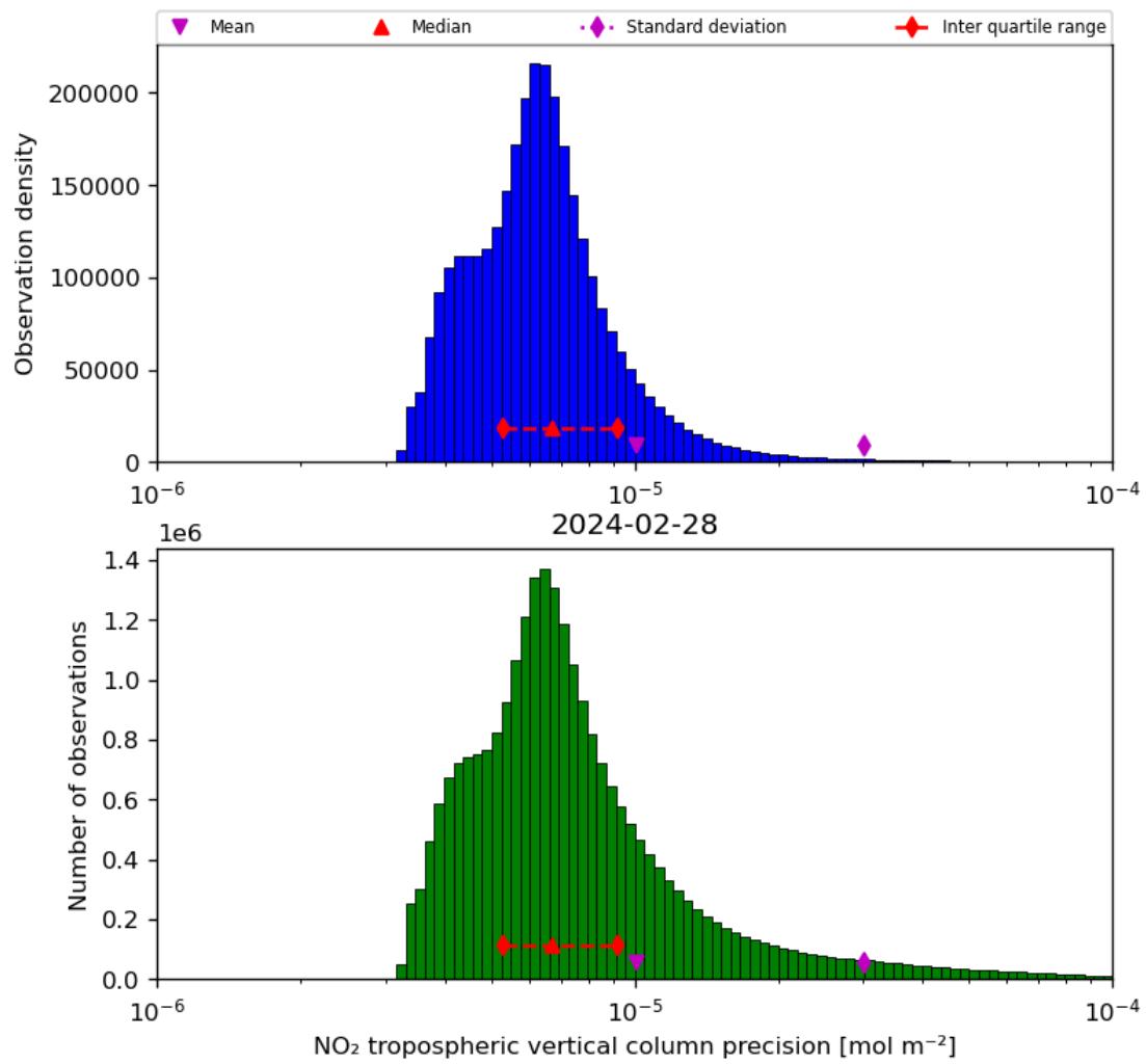
Figure 30: Histogram of “NO 2 tropospheric vertical column precision” for 2024-02-27 to 2024-02-29
