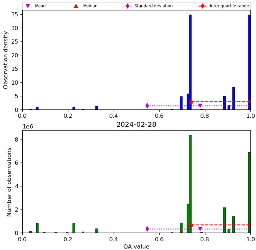
Figure 28: Histogram of “QA value” for 2024-02-27 to 2024-02-29
