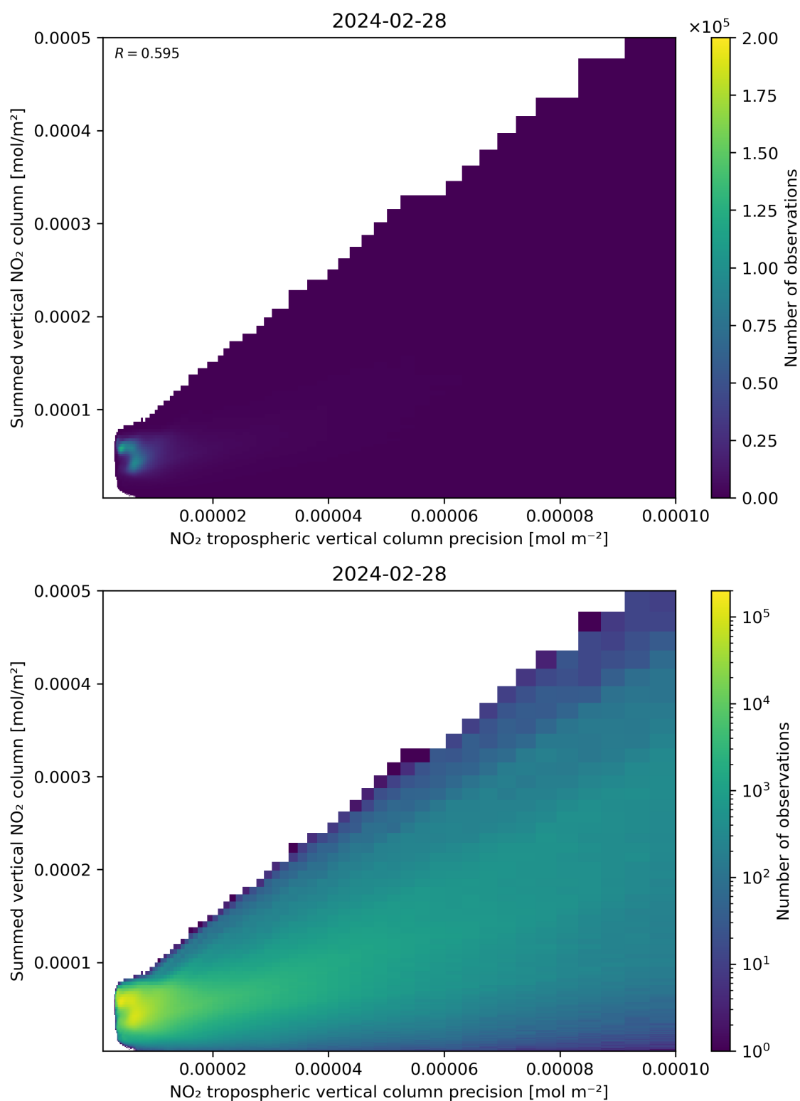
Figure 136: Scatter density plot of “NO 2 tropospheric vertical column precision” against “Summed vertical NO 2 column” for 2024-02-27 to 2024-02-29.
