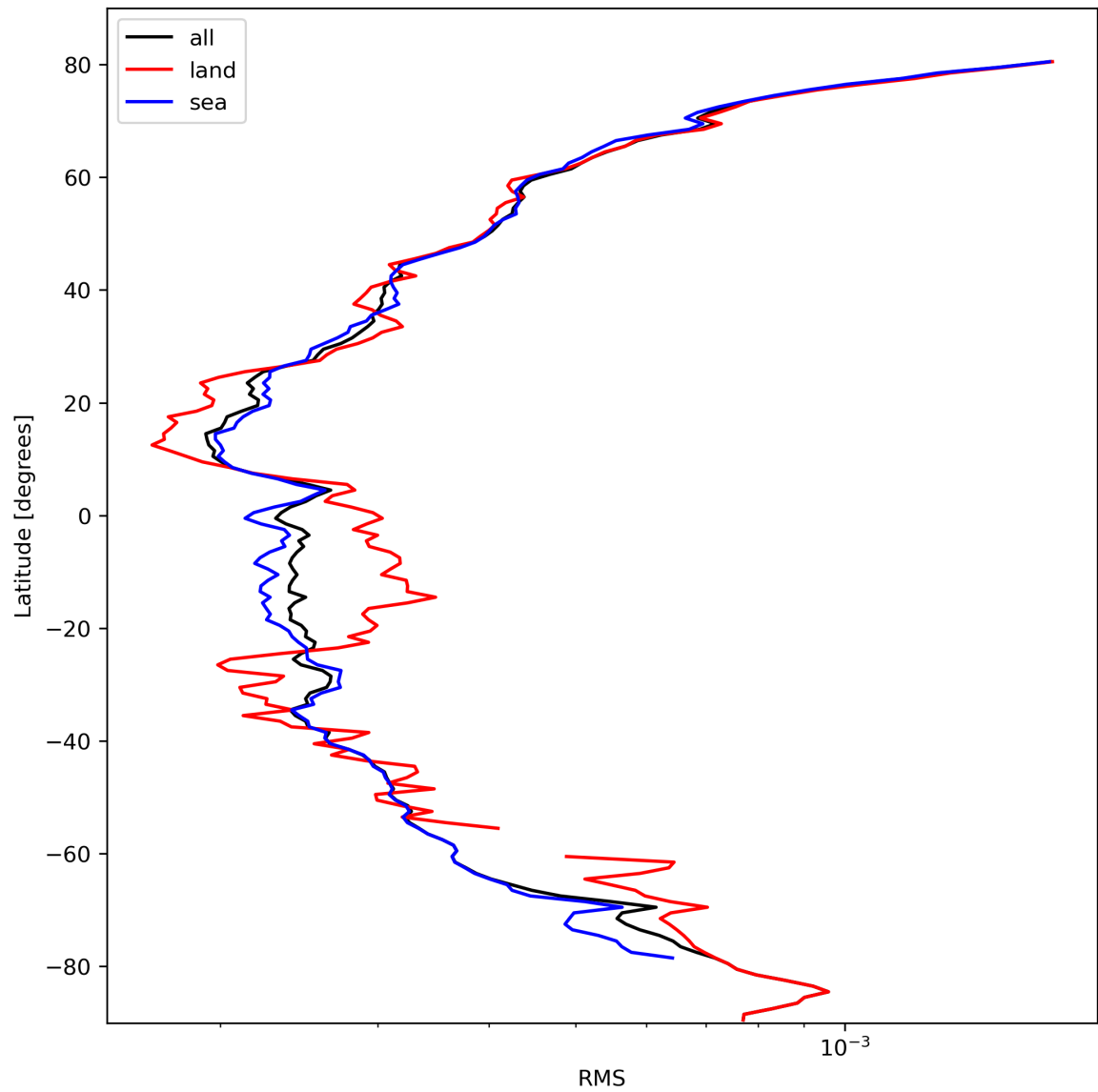
Figure 26: Zonal average of “RMS” for 2024-02-27 to 2024-02-29.
