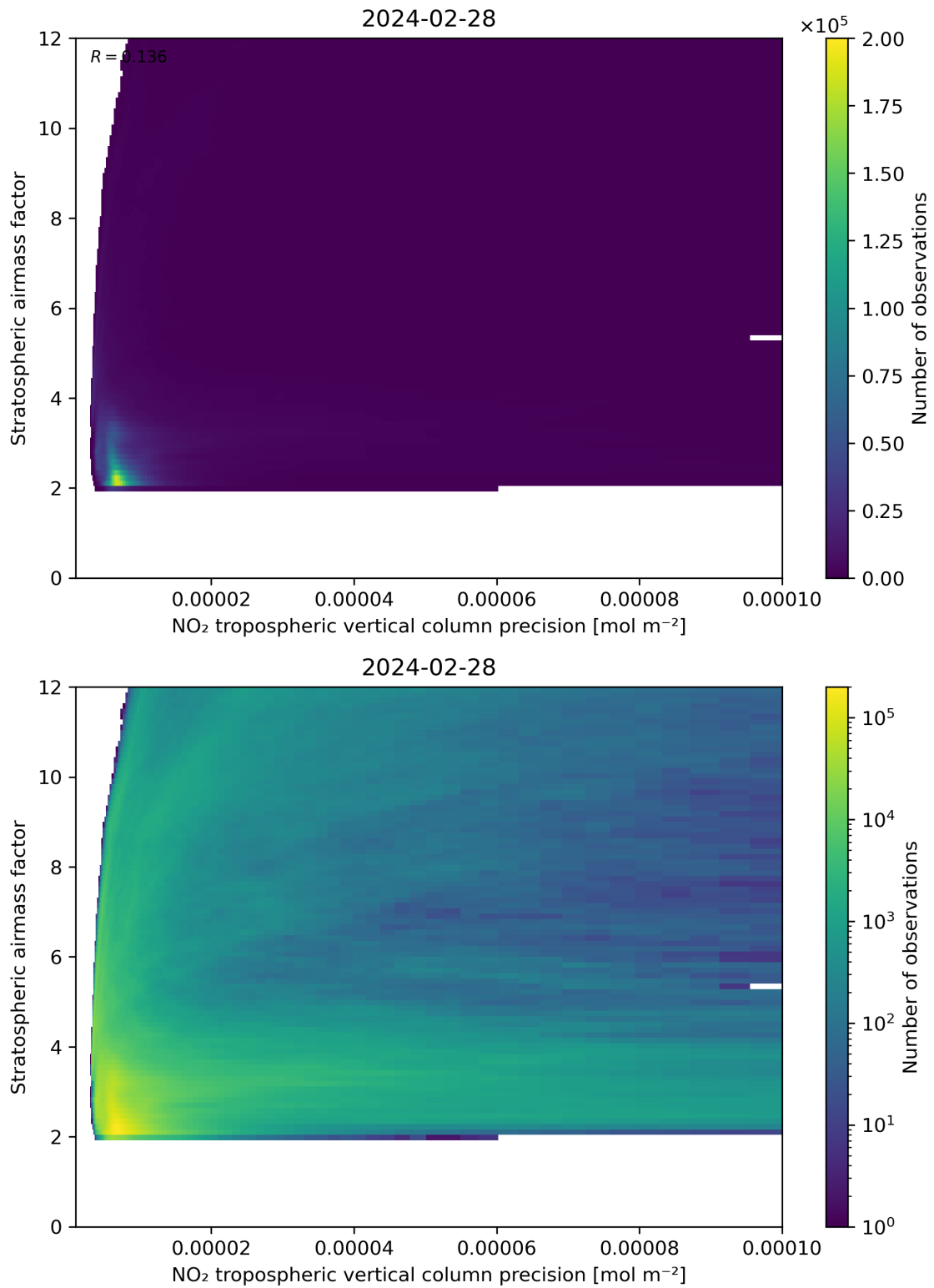
Figure 131: Scatter density plot of “NO 2 tropospheric vertical column precision” against “Stratospheric airmass factor” for 2024-02-27 to 2024-02-29.
