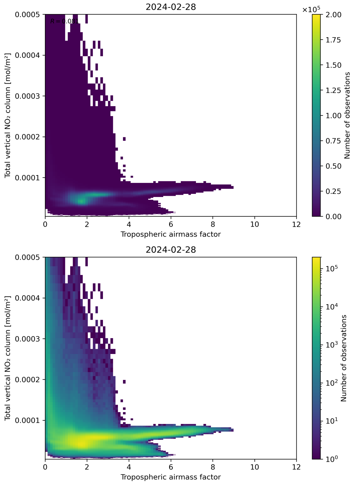
Figure 77: Scatter density plot of “Tropospheric airmass factor” against “Total vertical NO 2 column” for 2024-02-27 to 2024-02-29.
