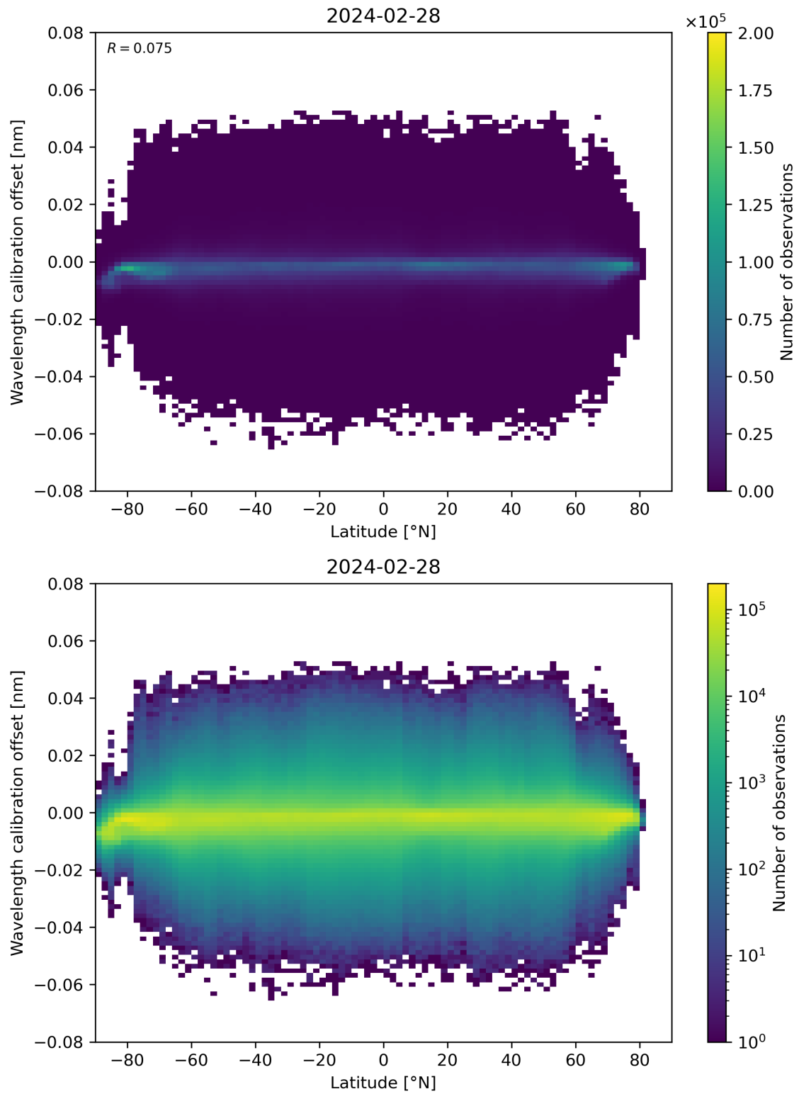
Figure 95: Scatter density plot of “Latitude” against “Wavelength calibration offset” for 2024-02-27 to 2024-02-29.
