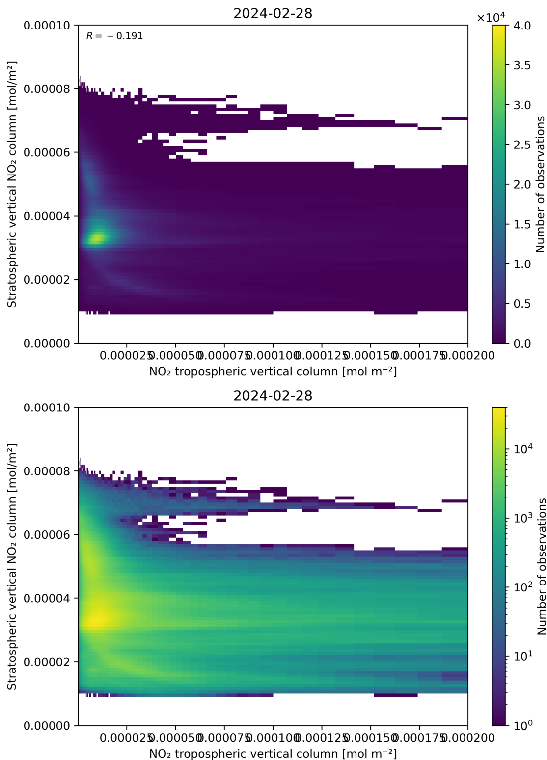
Figure 125: Scatter density plot of “NO 2 tropospheric vertical column” against “Stratospheric vertical NO 2 column” for 2024-02-27 to 2024-02-29.
