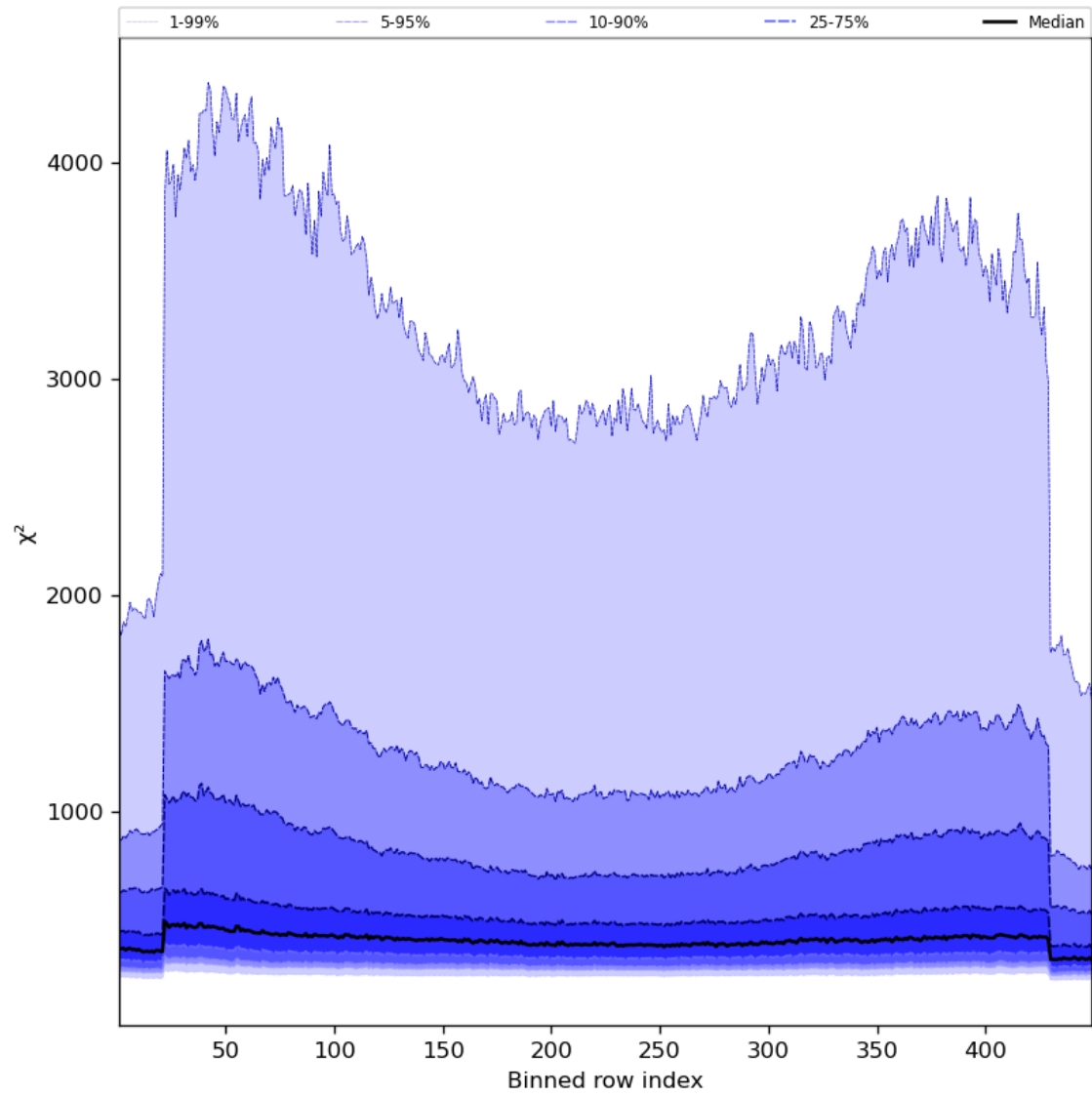
Figure 59: Along track statistics of “ \chi^2 ” for 2024-02-27 to 2024-02-29
