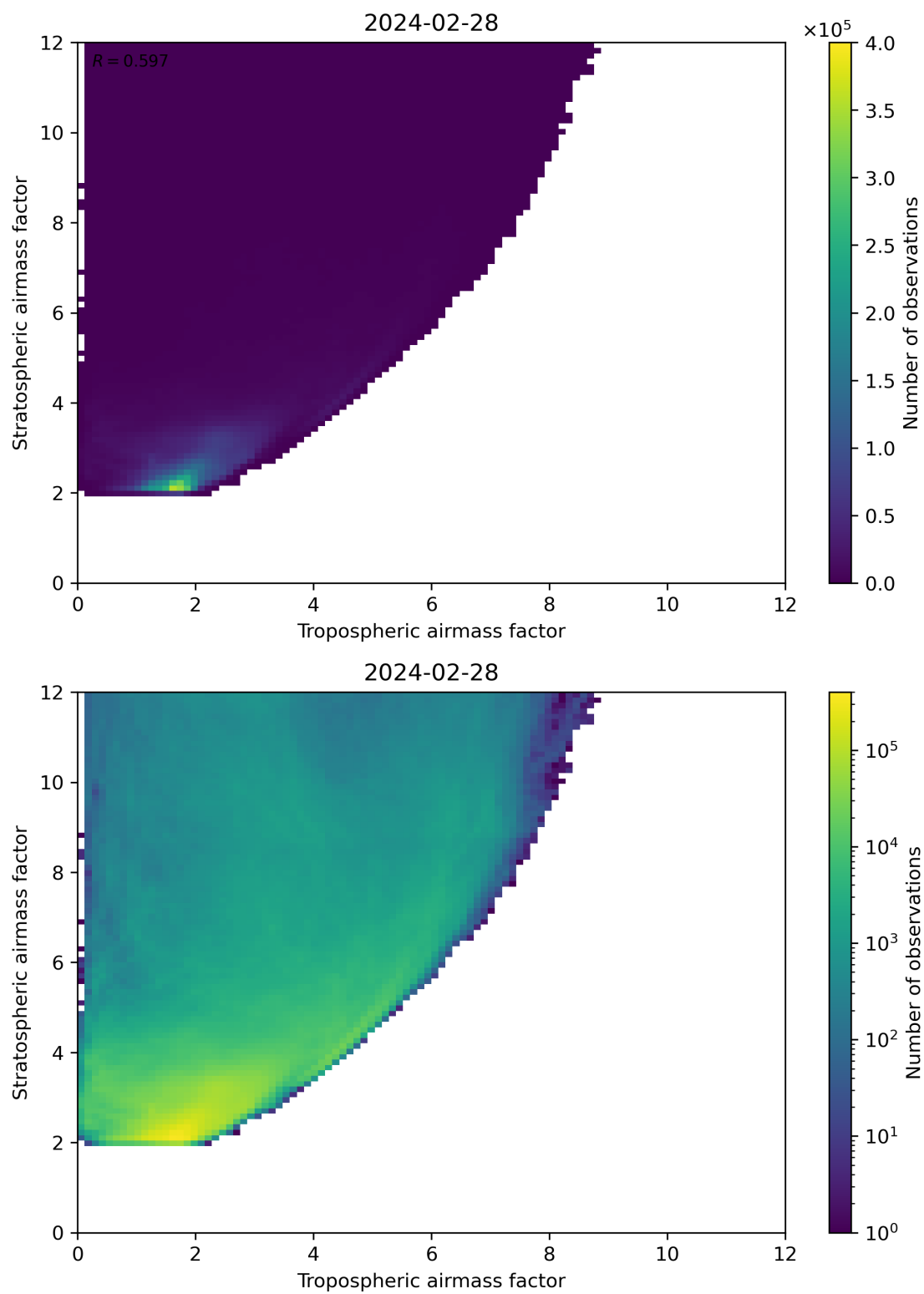
Figure 71: Scatter density plot of “Tropospheric airmass factor” against “Stratospheric airmass factor” for 2024-02-27 to 2024-02-29.
