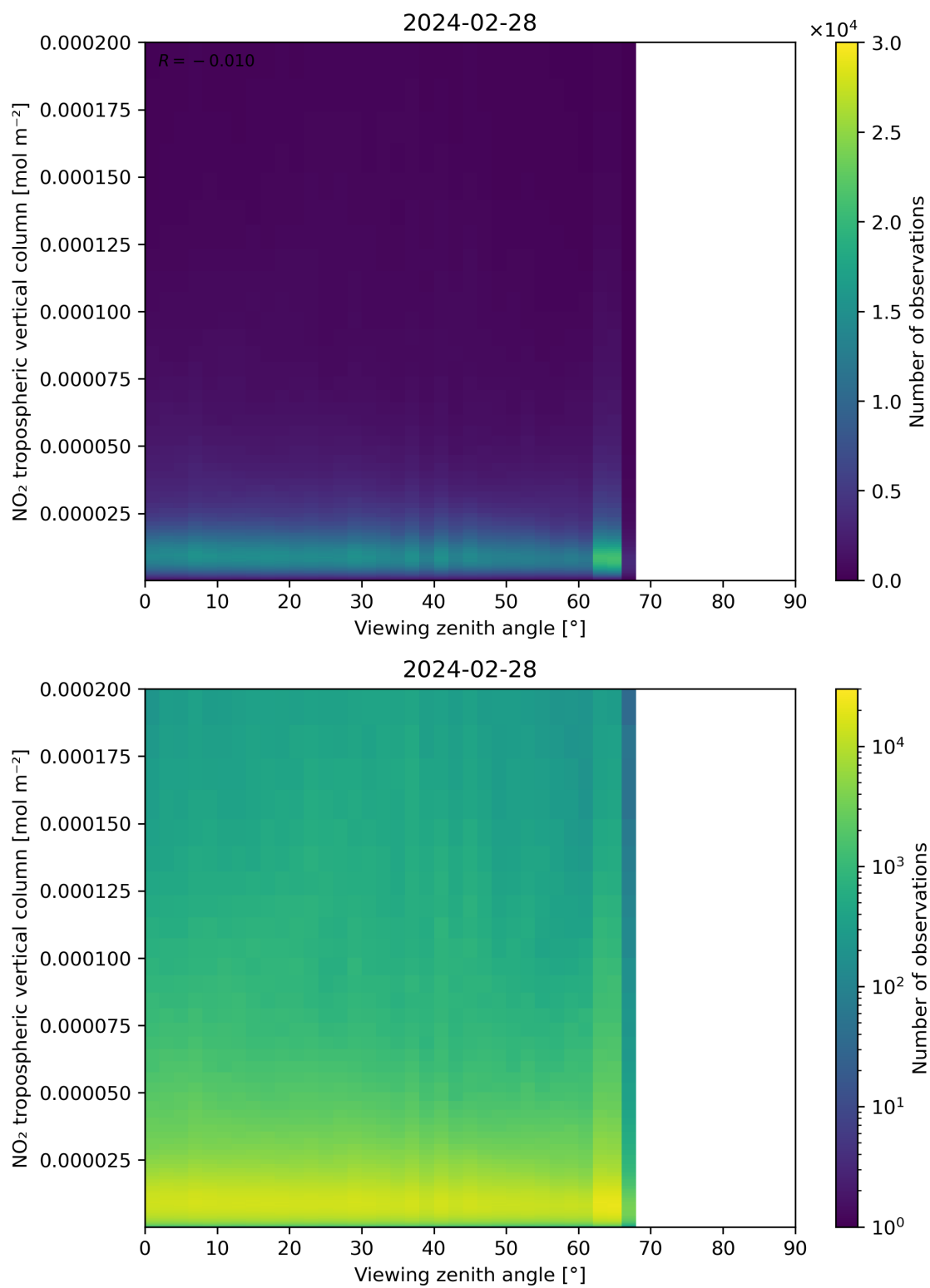
Figure 169: Scatter density plot of “Viewing zenith angle” against “NO 2 tropospheric vertical column” for 2024-02-27 to 2024-02-29.
