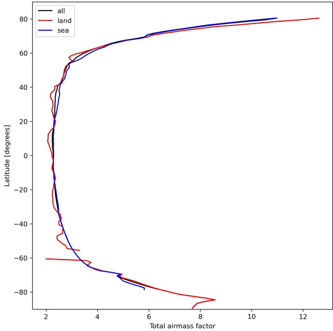
Figure 15: Zonal average of “Total airmass factor” for 2024-02-27 to 2024-02-29.
