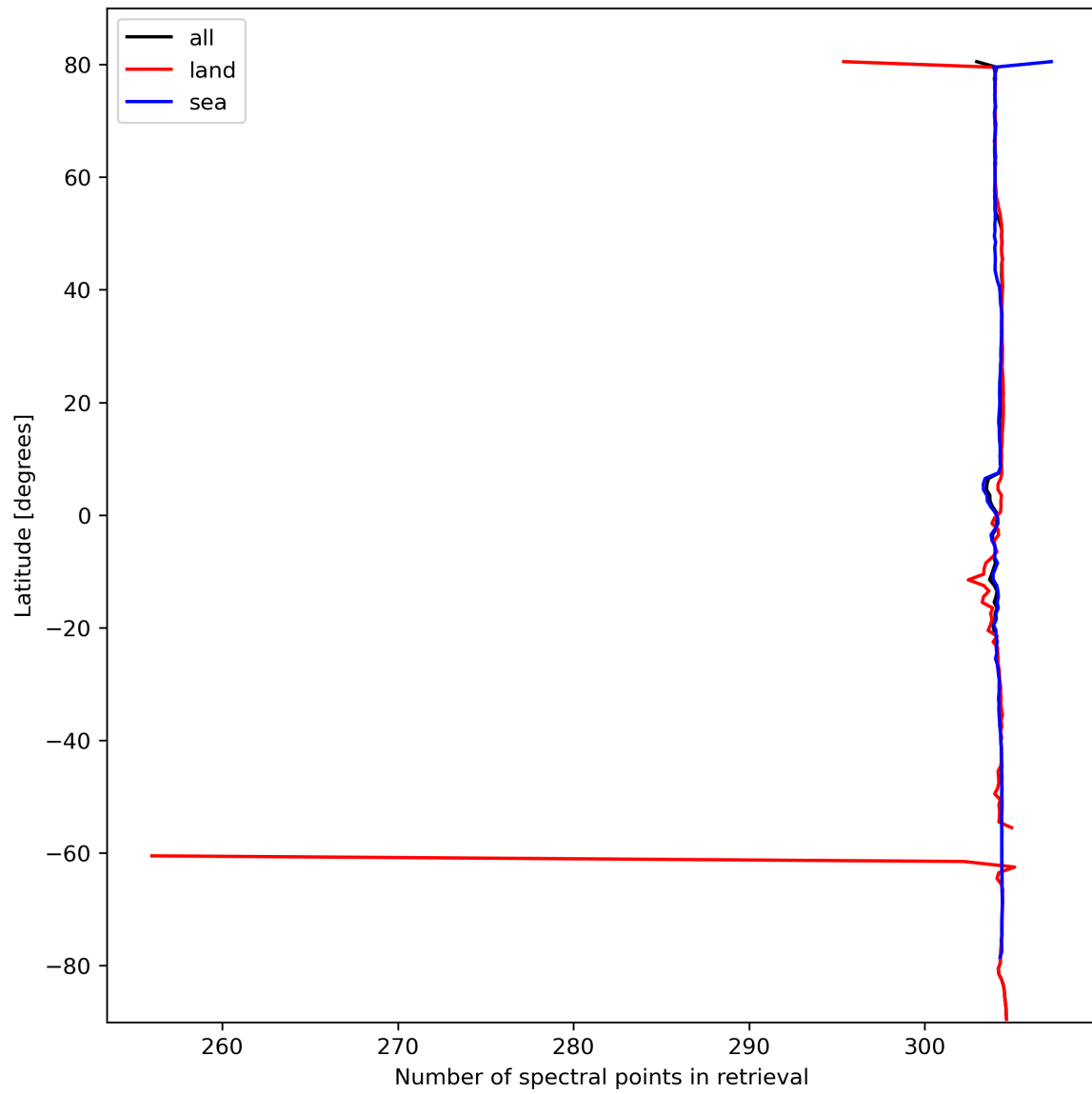
Figure 16: Zonal average of “Number of spectral points in retrieval” for 2024-02-27 to 2024-02-29.
