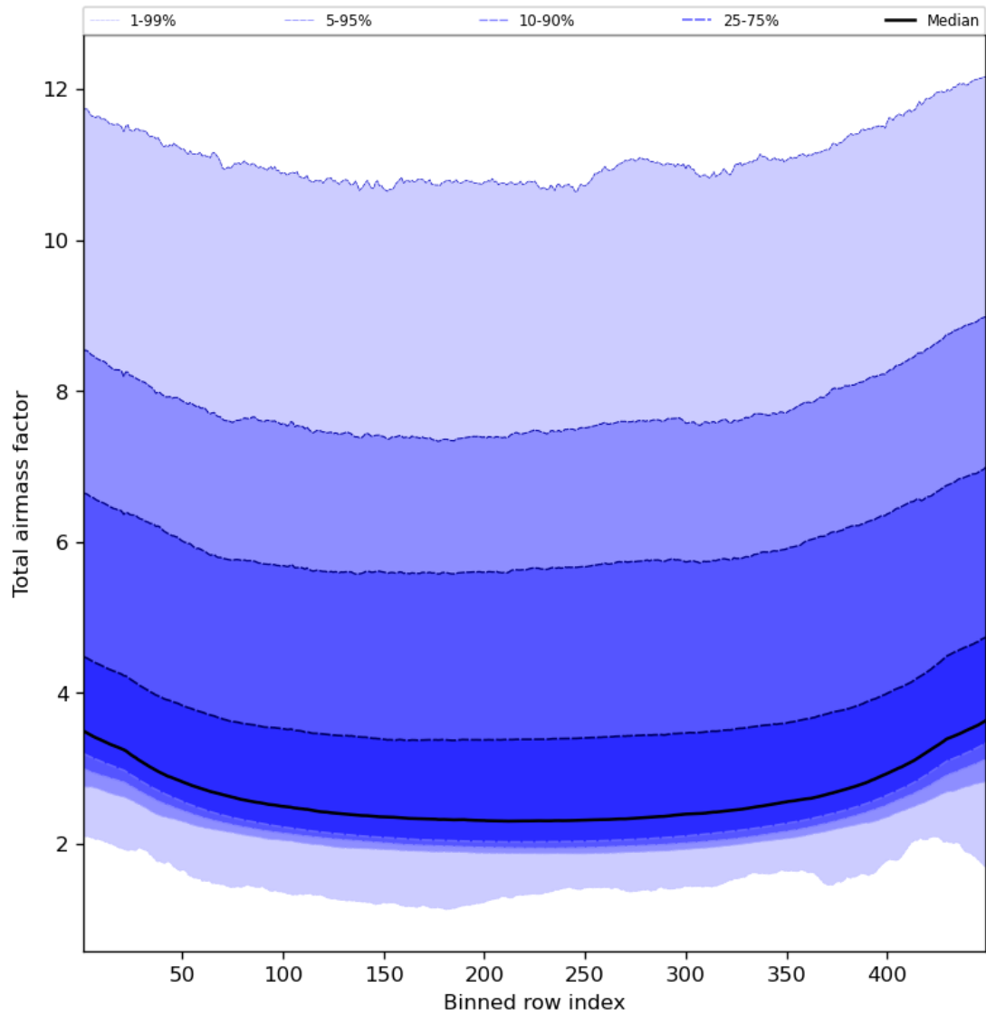
Figure 49: Along track statistics of “Total airmass factor” for 2024-02-27 to 2024-02-29
