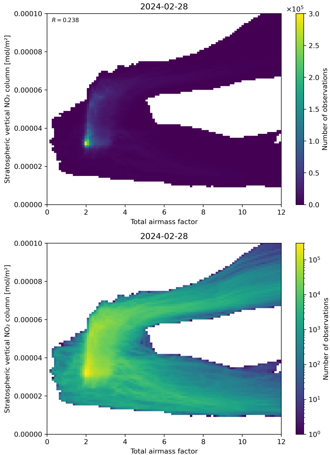
Figure 64: Scatter density plot of “Total airmass factor” against “Stratospheric vertical NO 2 column” for 2024-02-27 to 2024-02-29.
