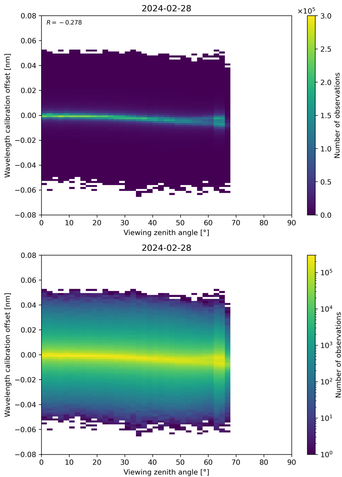
Figure 173: Scatter density plot of “Viewing zenith angle” against “Wavelength calibration offset” for 2024-02-27 to 2024-02-29.
