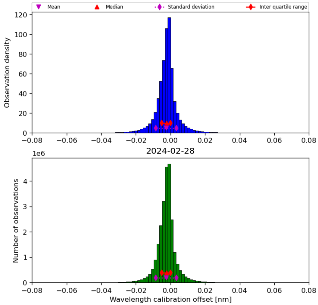
Figure 35: Histogram of “Wavelength calibration offset” for 2024-02-27 to 2024-02-29
