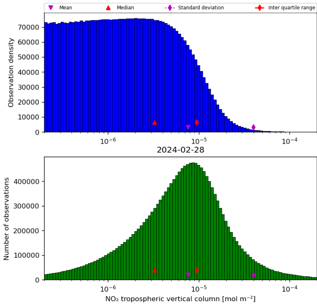
Figure 29: Histogram of “NO 2 tropospheric vertical column” for 2024-02-27 to 2024-02-29
