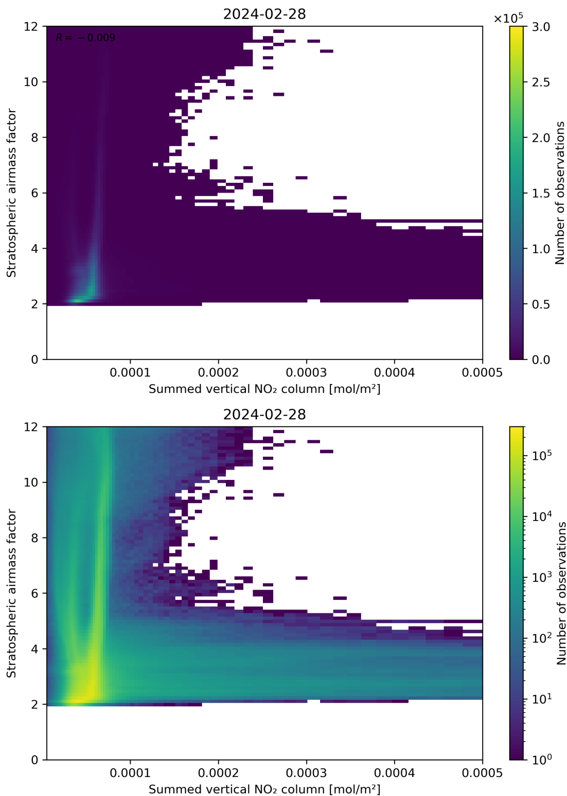
Figure 103: Scatter density plot of “Summed vertical NO 2 column” against “Stratospheric airmass factor” for 2024-02-27 to 2024-02-29.
