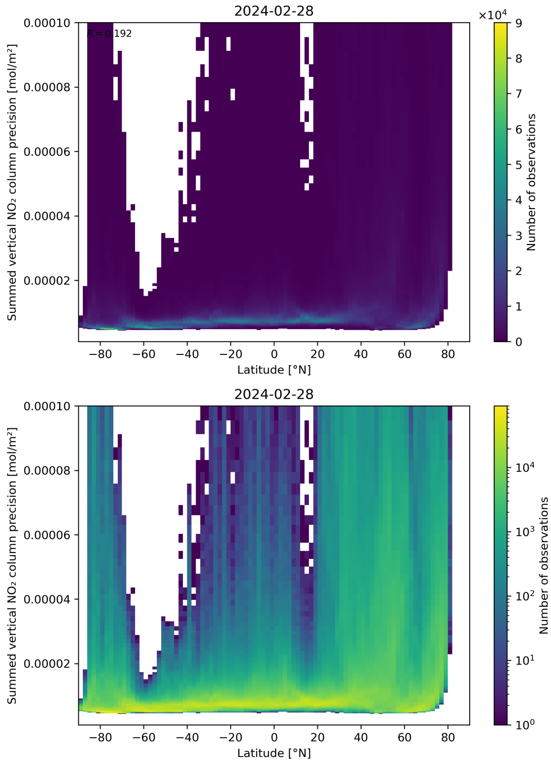
Figure 89: Scatter density plot of “Latitude” against “Summed vertical NO 2 column precision” for 2024-02-27 to 2024-02-29.
