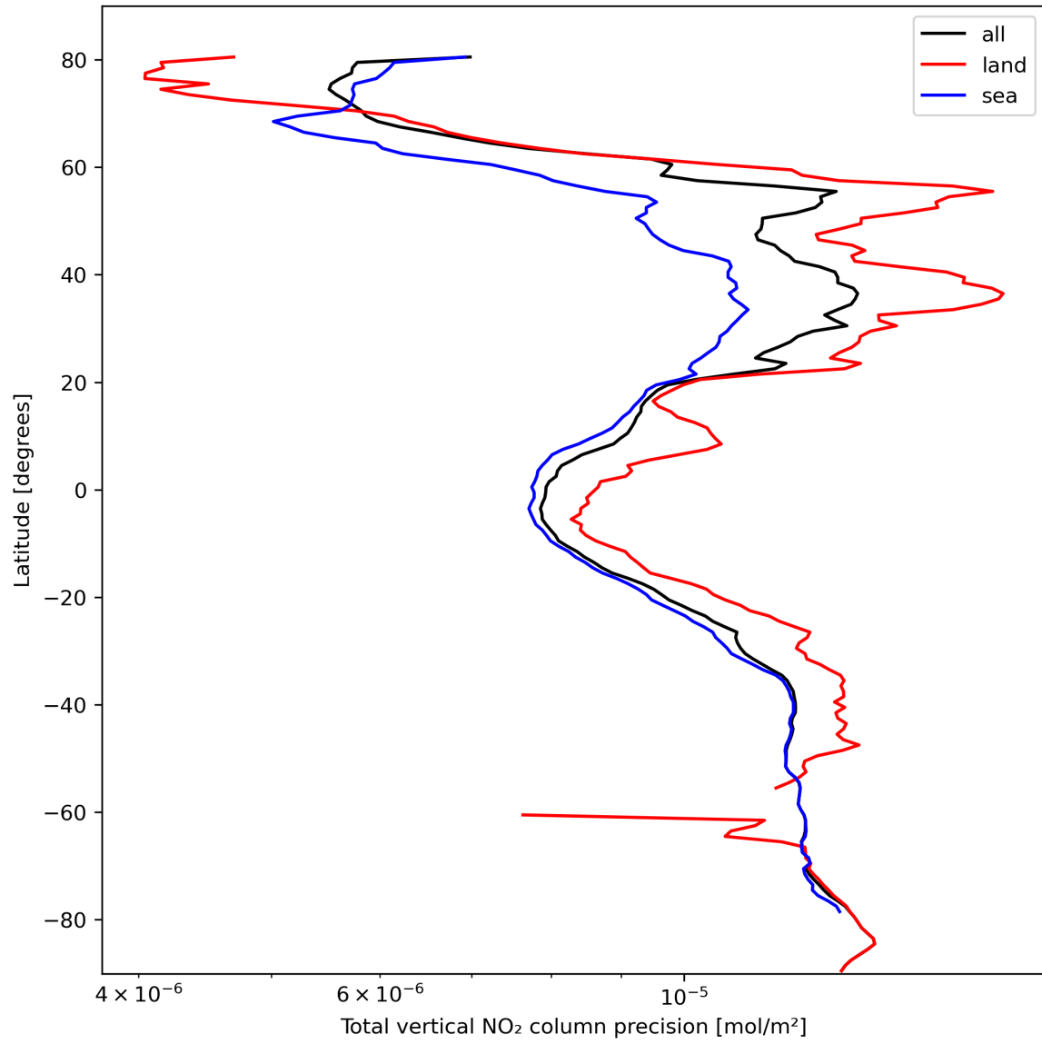
Figure 22: Zonal average of "Total vertical NO 2 column precision" for 2024-02-27 to 2024-02-29.
