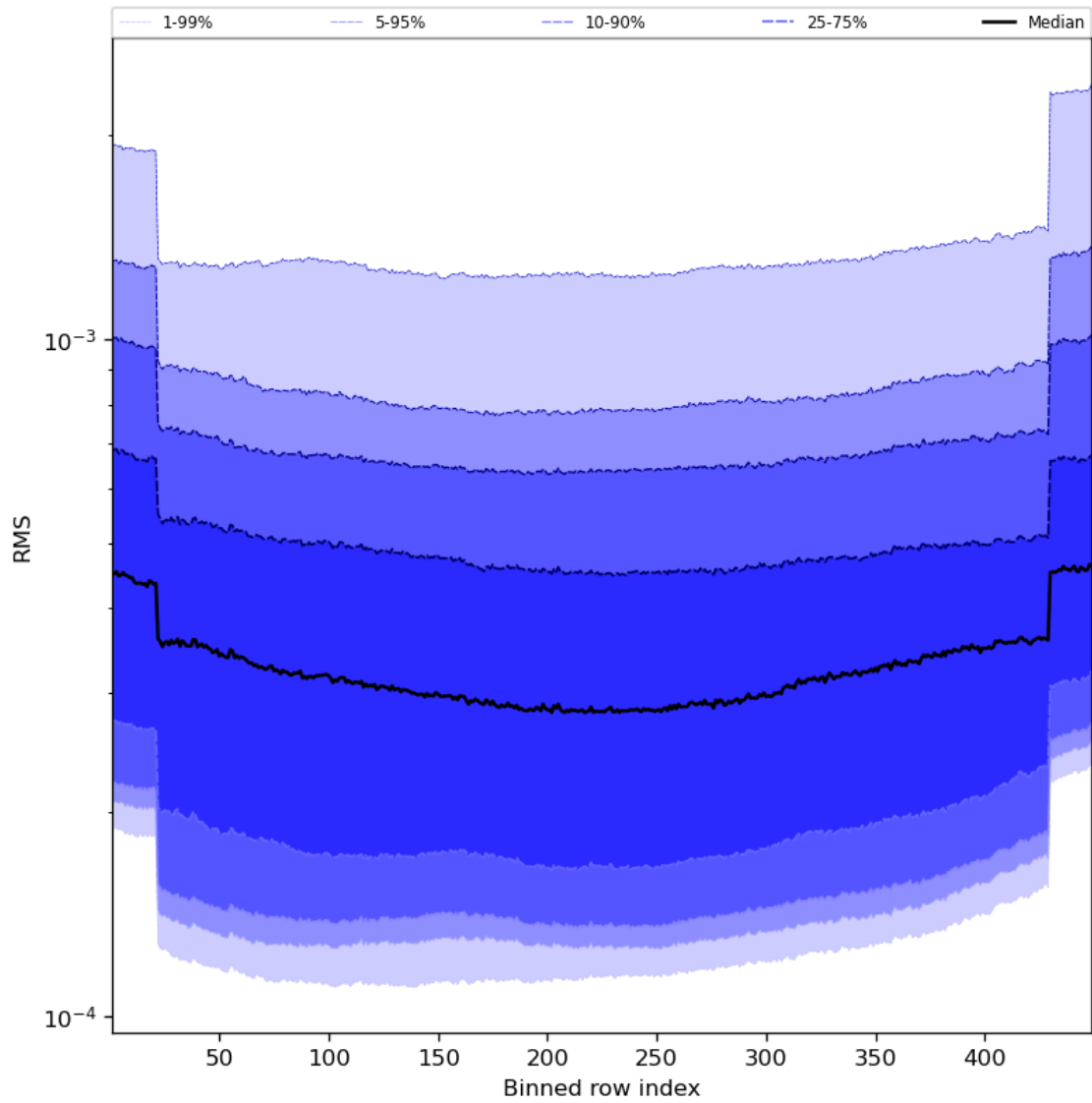
Figure 60: Along track statistics of “RMS” for 2024-02-27 to 2024-02-29
