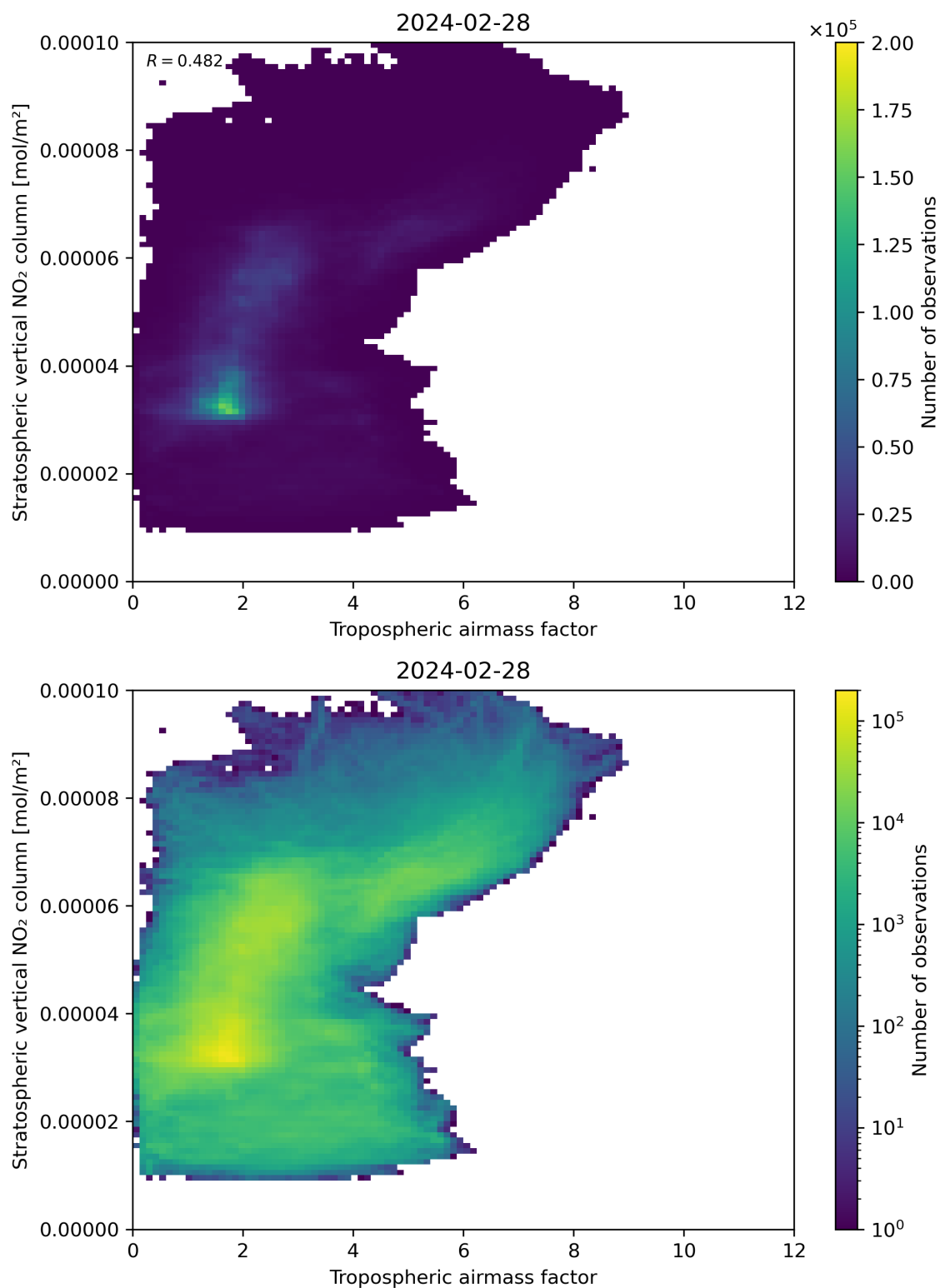
Figure 74: Scatter density plot of “Tropospheric air mass factor” against “Stratospheric vertical NO 2 column” for 2024-02-27 to 2024-02-29.
