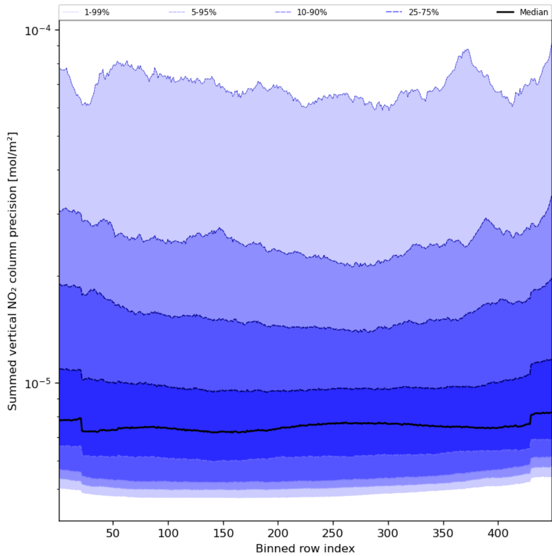
Figure 58: Along track statistics of “Summed vertical NO 2 column precision” for 2024-02-27 to 2024-02-29
