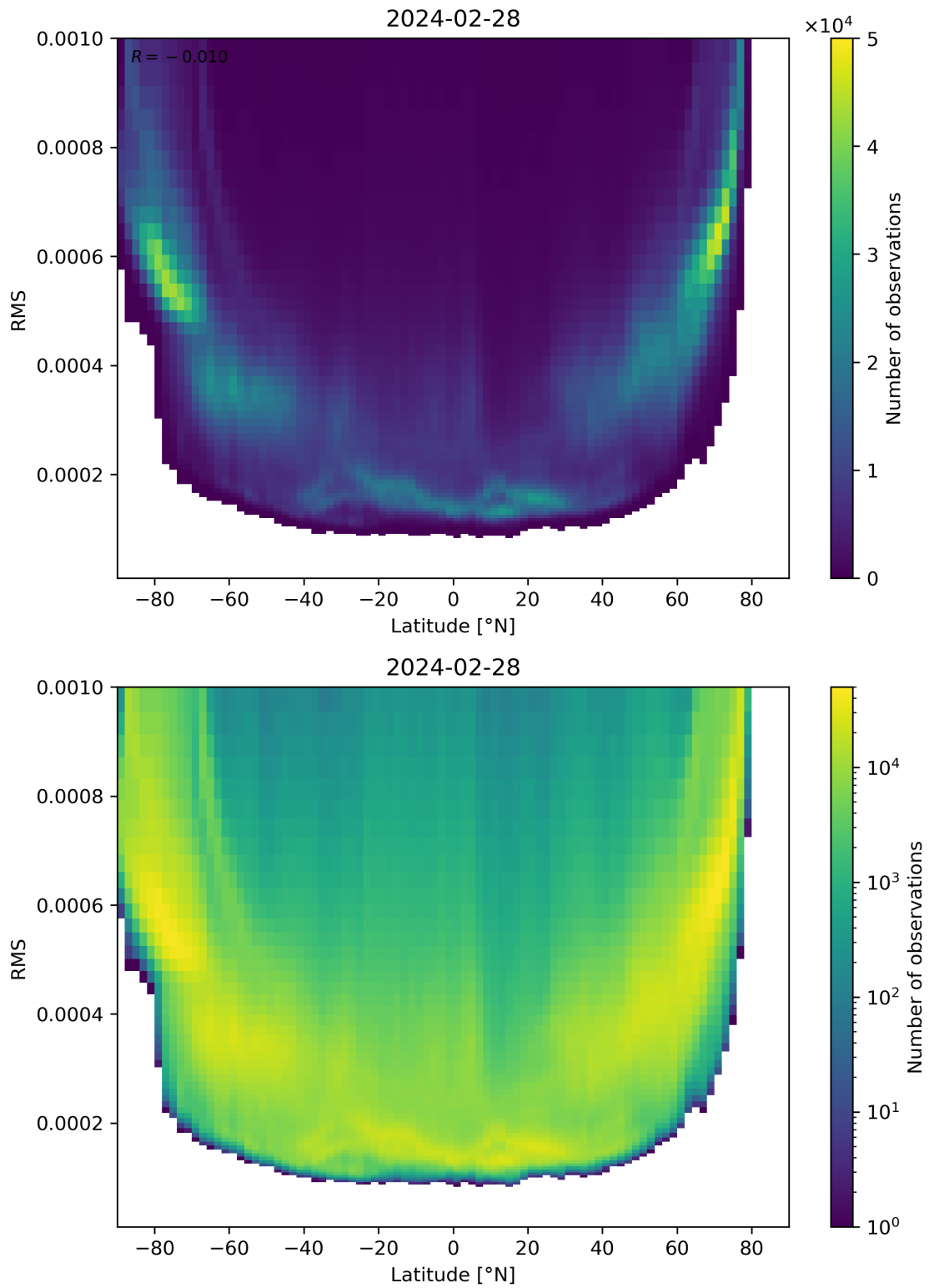
Figure 94: Scatter density plot of “Latitude” against “RMS” for 2024-02-27 to 2024-02-29.
