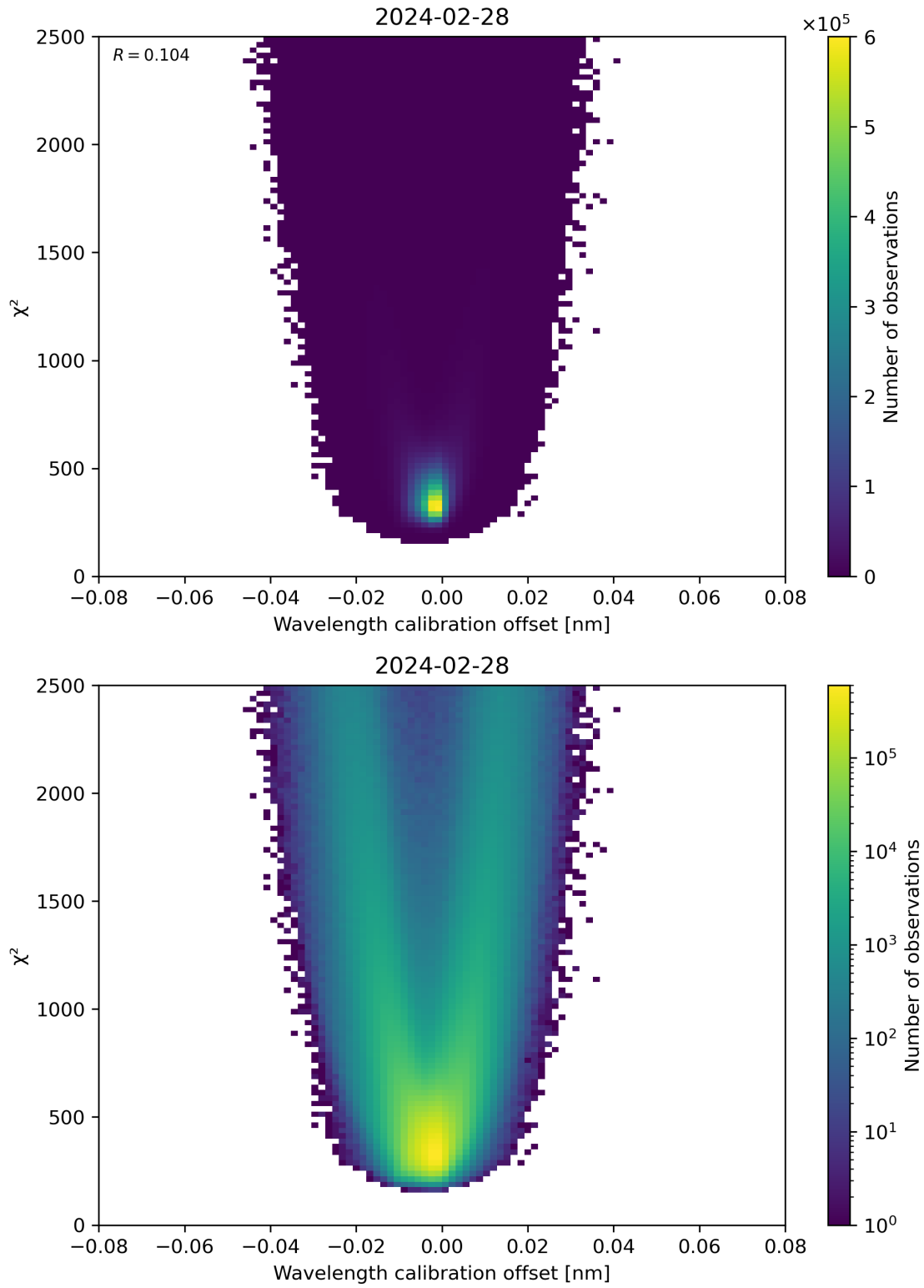
Figure 175: Scatter density plot of “Wavelength calibration offset” against “ \chi^2 ” for 2024-02-27 to 2024-02-29.
