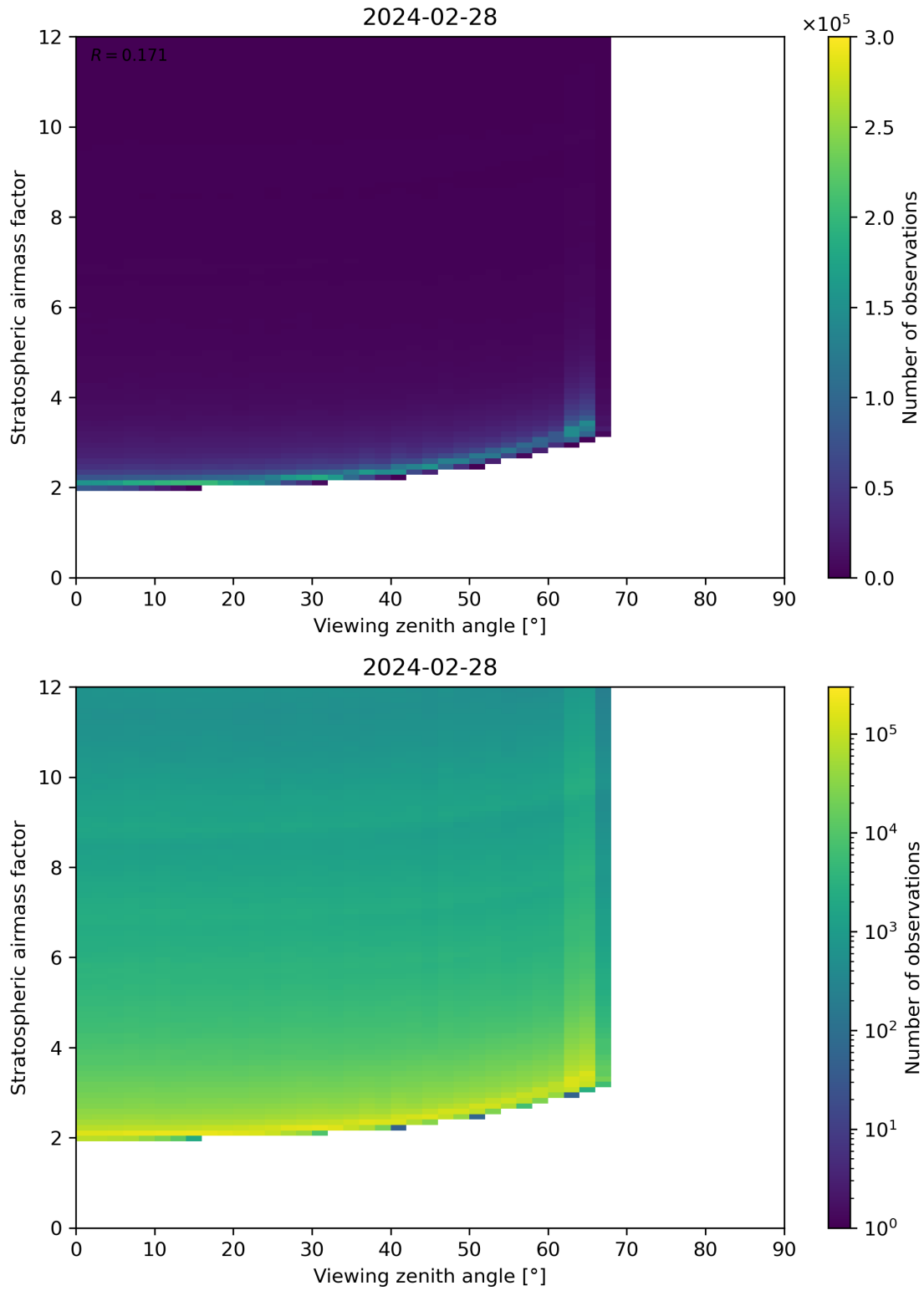
Figure 159: Scatter density plot of “Viewing zenith angle” against “Stratospheric airmass factor” for 2024-02-27 to 2024-02-29.
