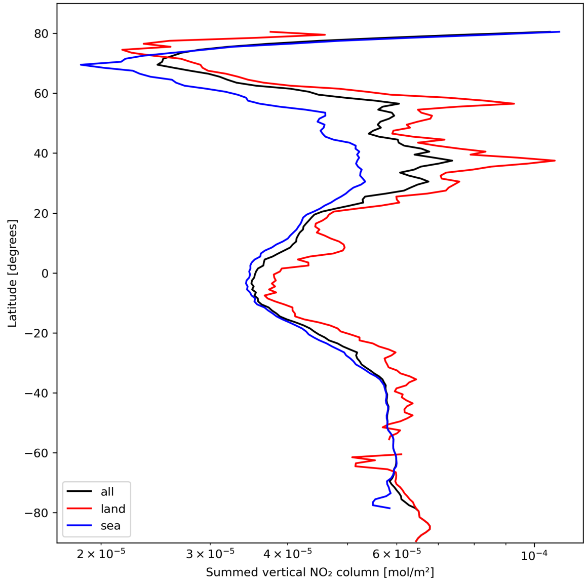
Figure 23: Zonal average of “Summed vertical NO 2 column” for 2024-02-27 to 2024-02-29.
