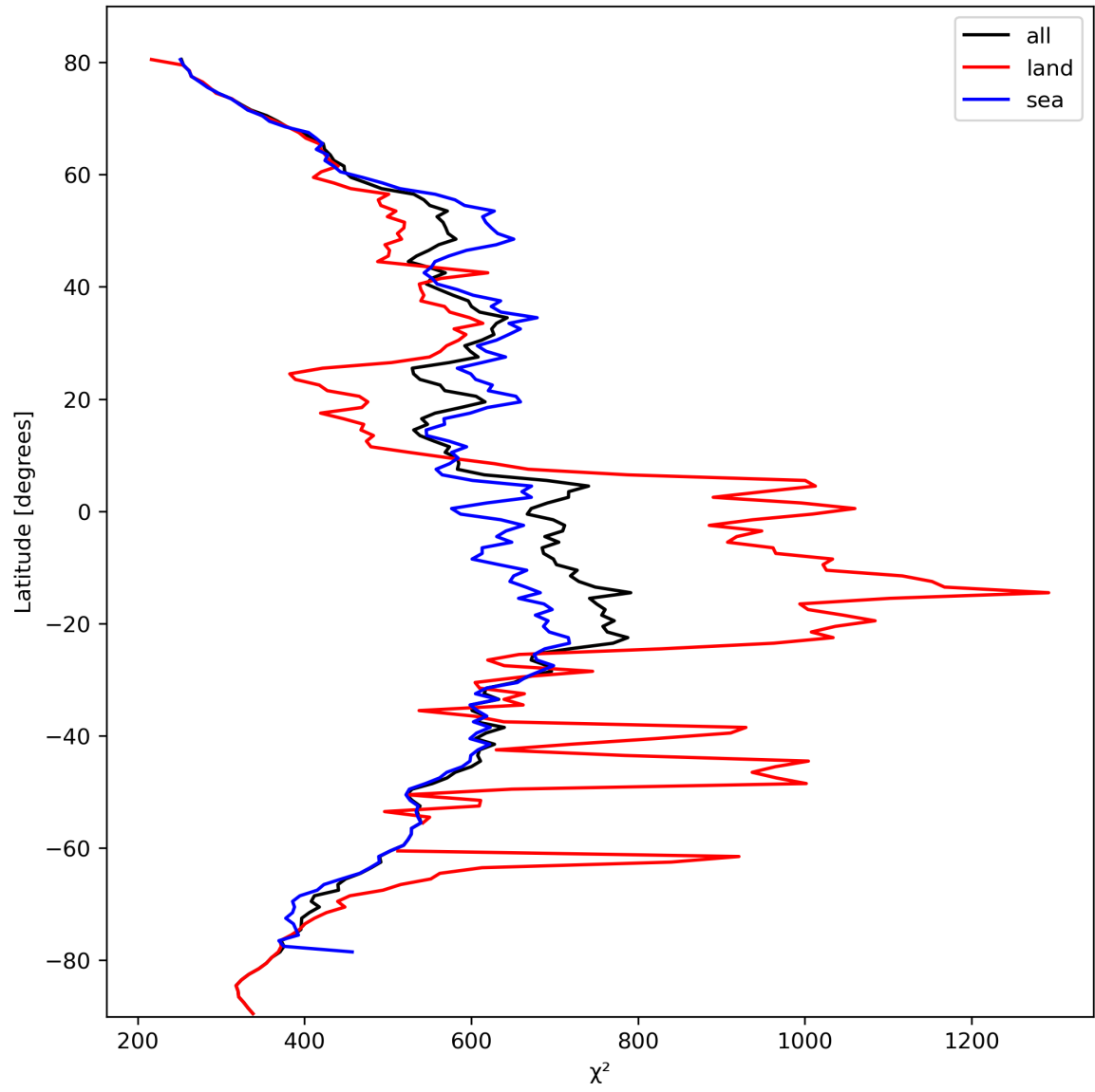
Figure 25: Zonal average of “ \chi^2 ” for 2024-02-27 to 2024-02-29.
