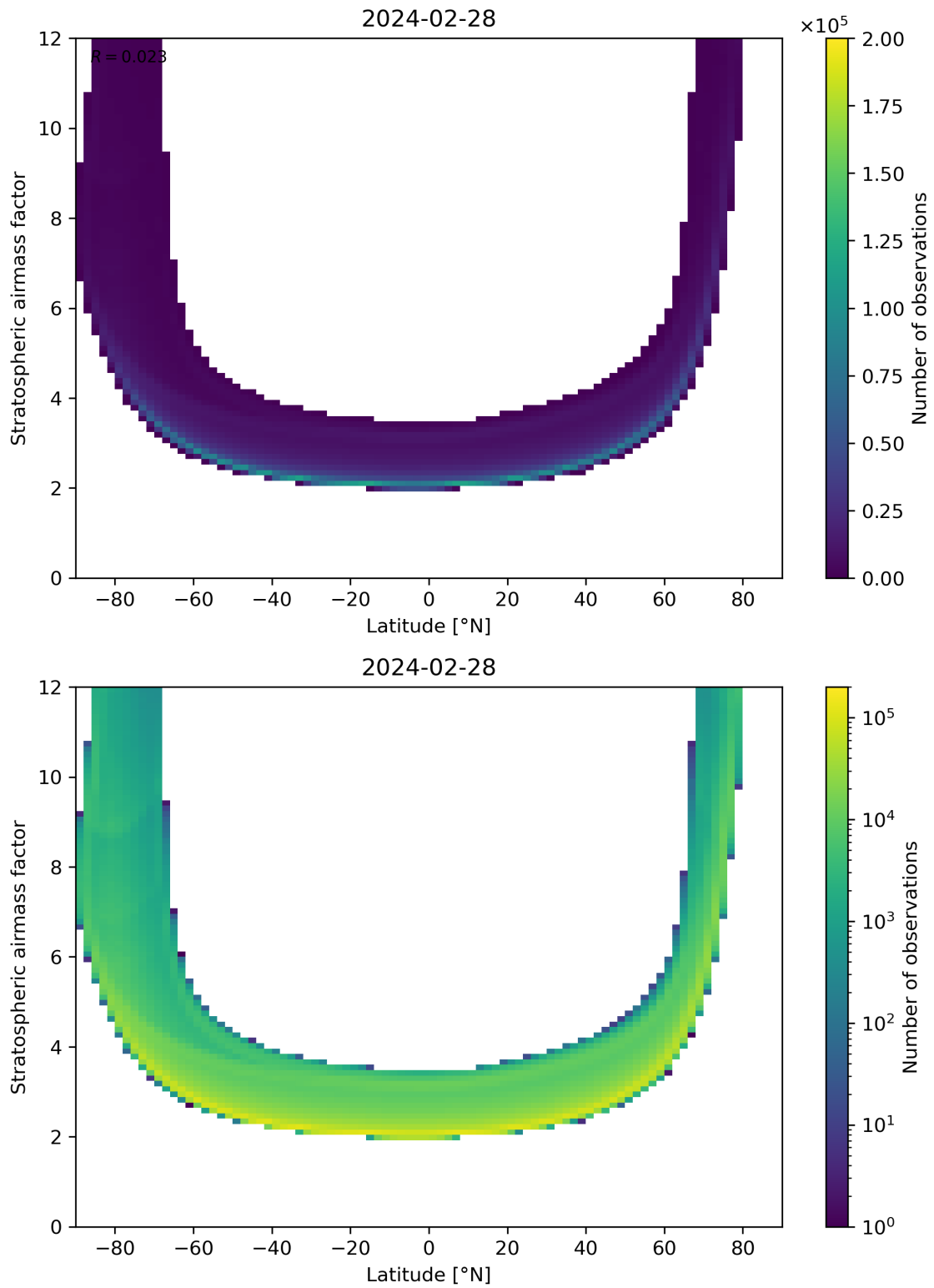
Figure 83: Scatter density plot of “Latitude” against “Stratospheric air mass factor” for 2024-02-27 to 2024-02-29.
