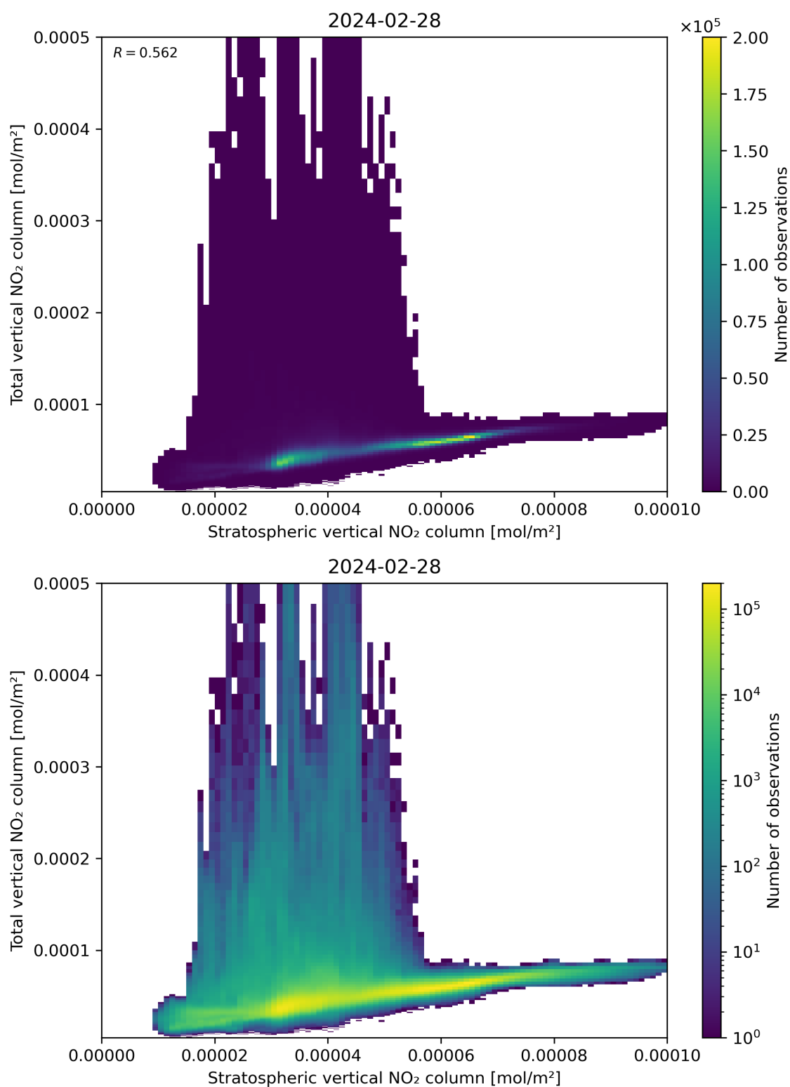
Figure 100: Scatter density plot of “Stratospheric vertical NO 2 column” against “Total vertical NO 2 column” for 2024-02-27 to 2024-02-29.
