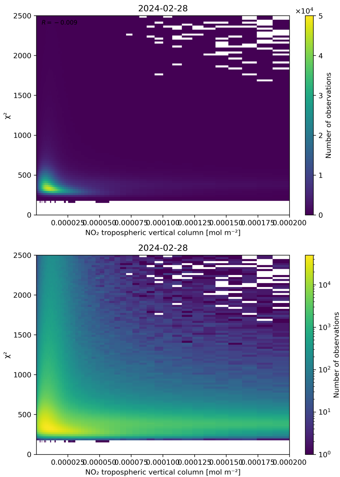
Figure 124: Scatter density plot of “NO 2 tropospheric vertical column” against “ \chi^2 ” for 2024-02-27 to 2024-02-29.
