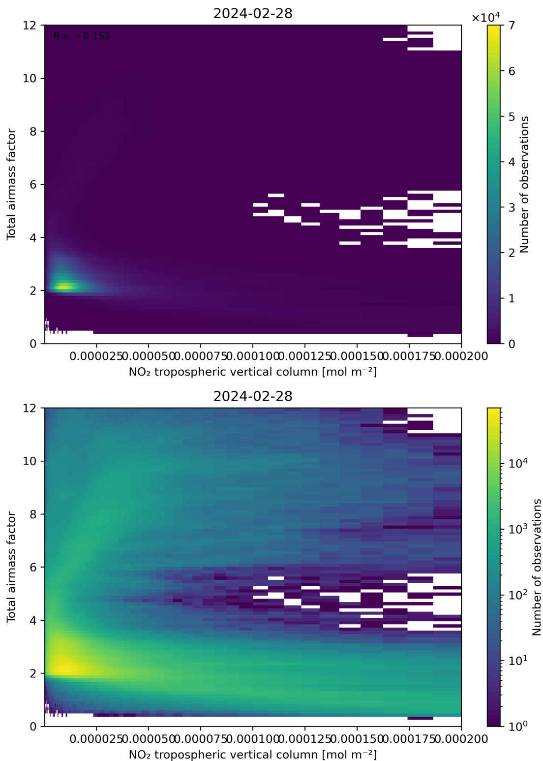
Figure 122: Scatter density plot of “NO 2 tropospheric vertical column” against “Total air mass factor” for 2024-02-27 to 2024-02-29.
