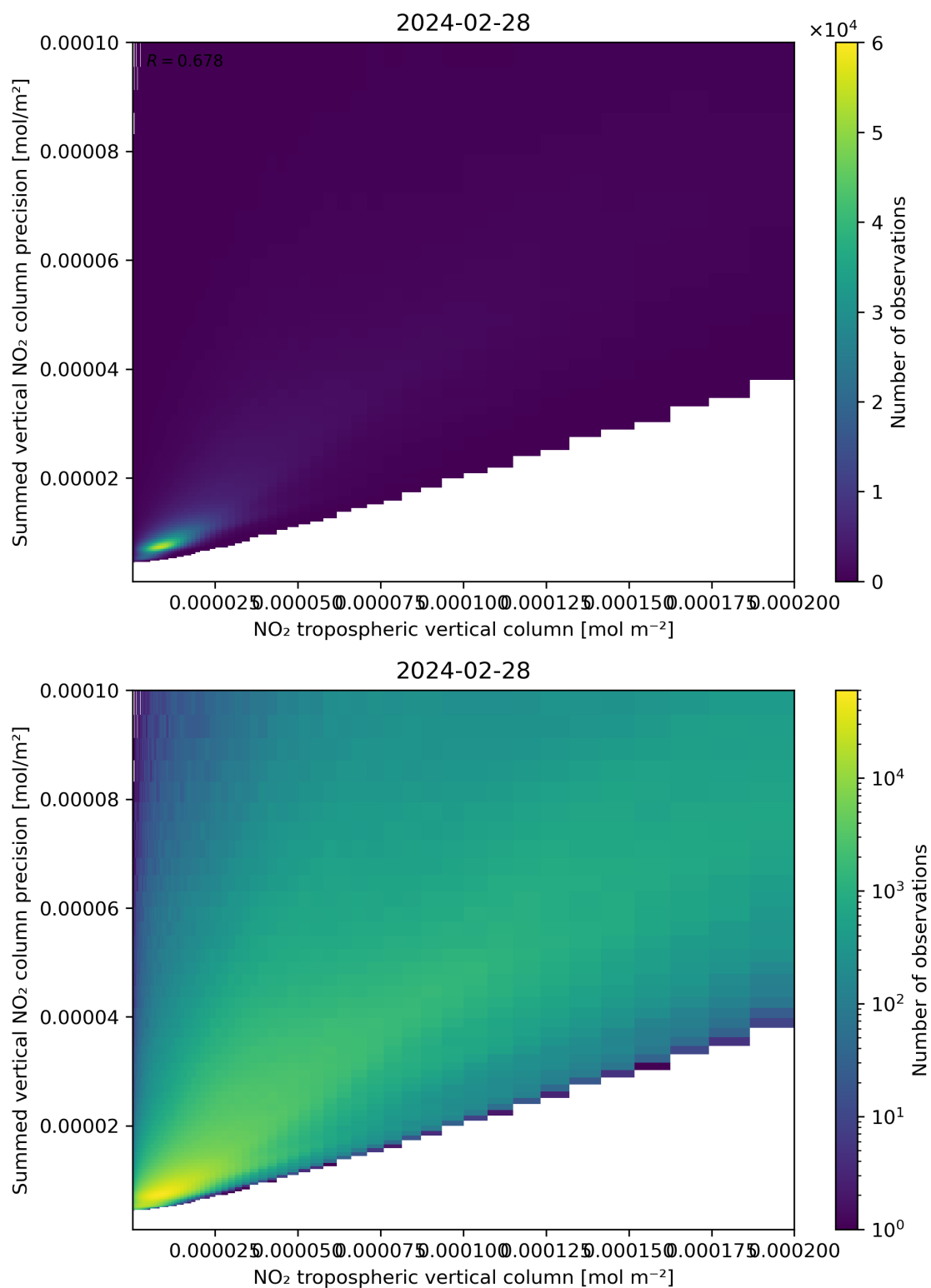
Figure 127: Scatter density plot of “NO 2 tropospheric vertical column” against “Summed vertical NO 2 column precision” for 2024-02-27 to 2024-02-29.
