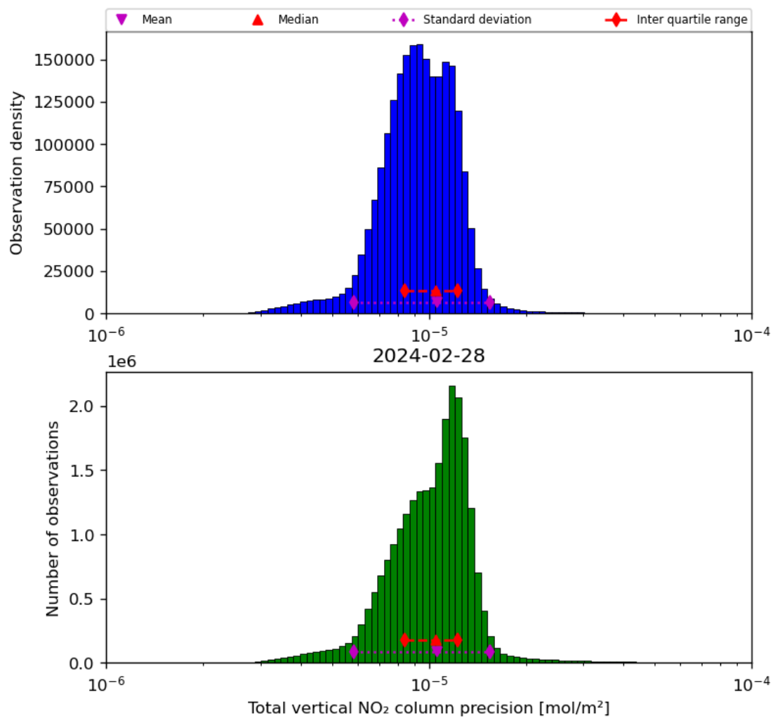
Figure 39: Histogram of “Total vertical NO 2 column precision” for 2024-02-27 to 2024-02-29
