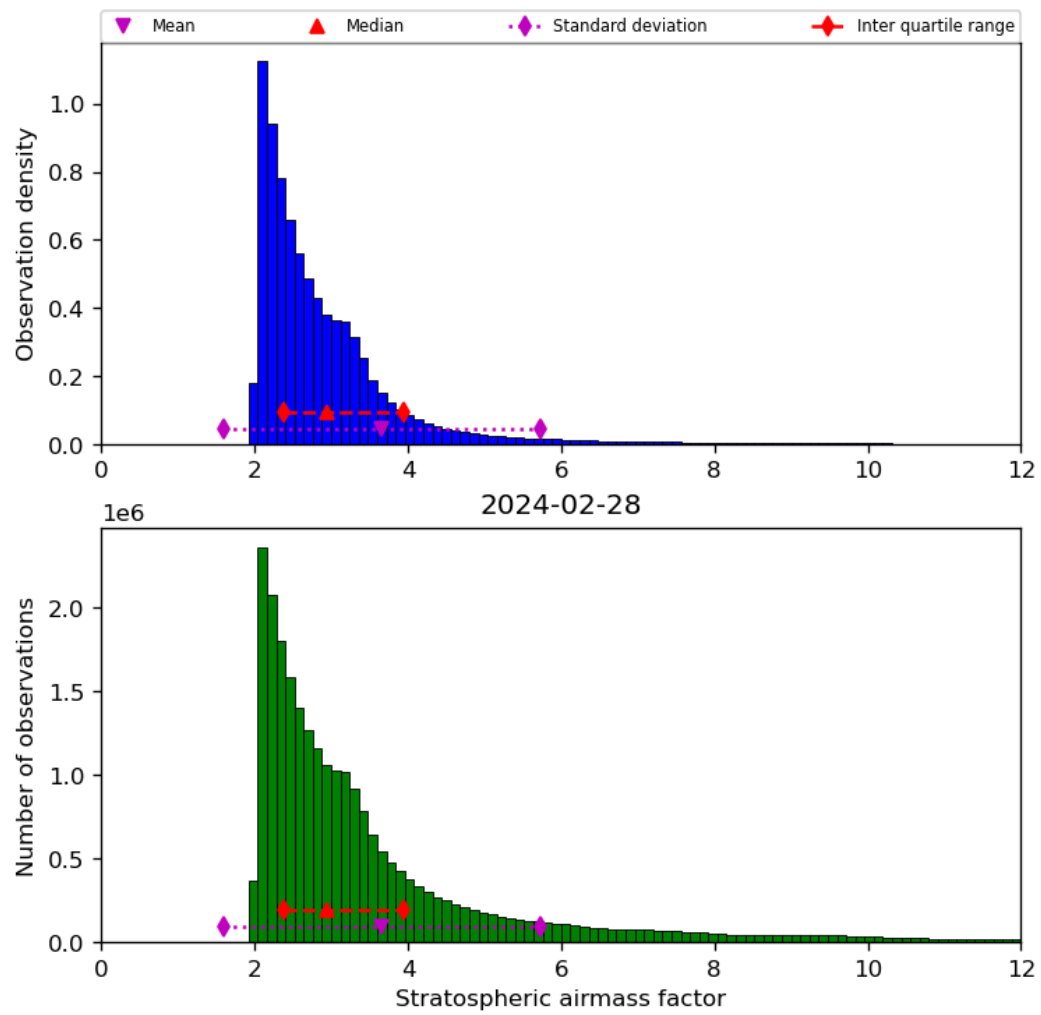
Figure 44: Histogram of “Stratospheric airmass factor” for 2024-02-27 to 2024-02-29
