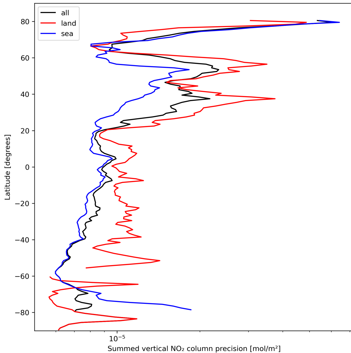
Figure 24: Zonal average of “Summed vertical NO 2 column precision” for 2024-02-27 to 2024-02-29.
