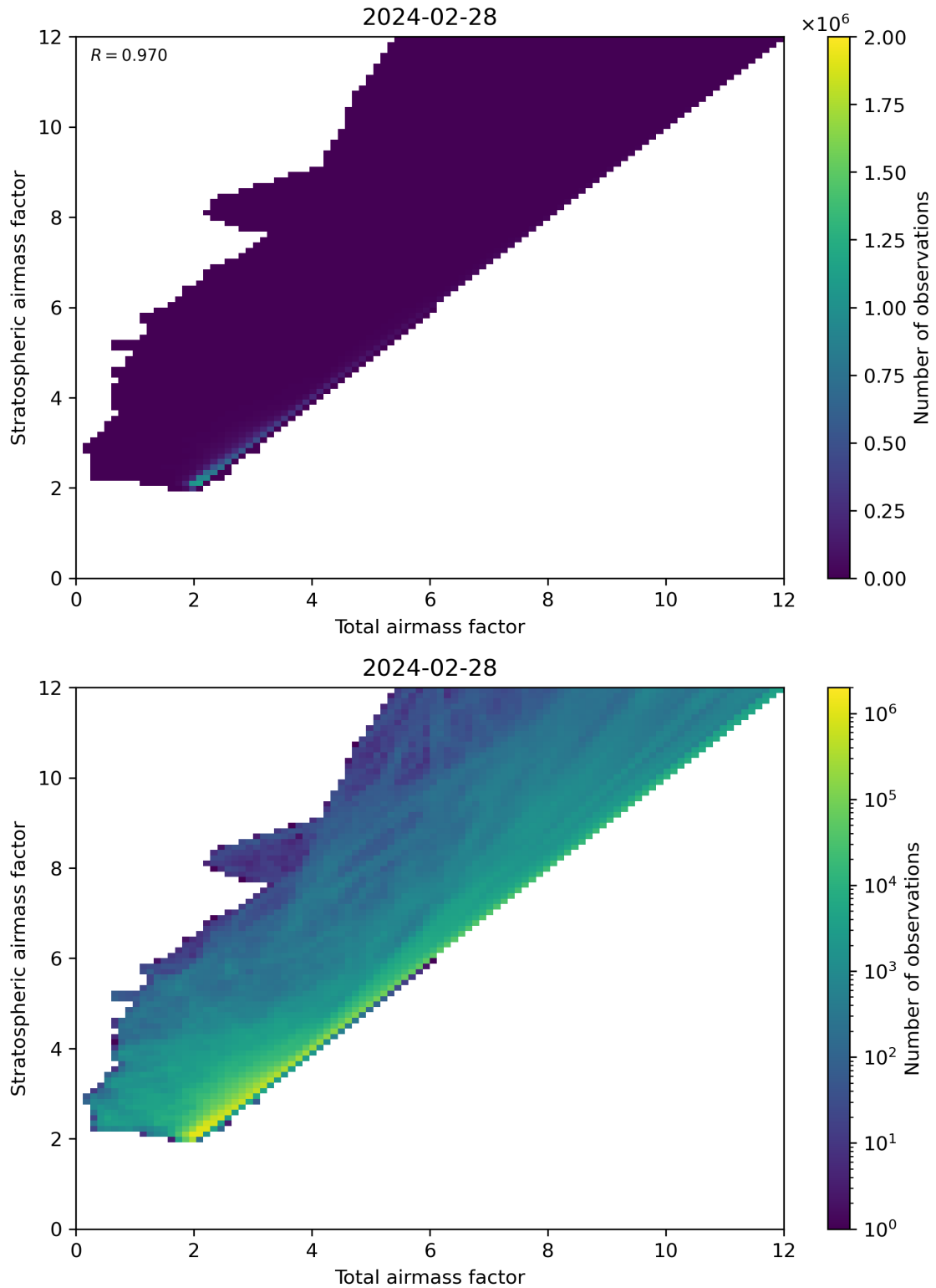
Figure 62: Scatter density plot of “Total airmass factor” against “Stratospheric airmass factor” for 2024-02-27 to 2024-02-29.
