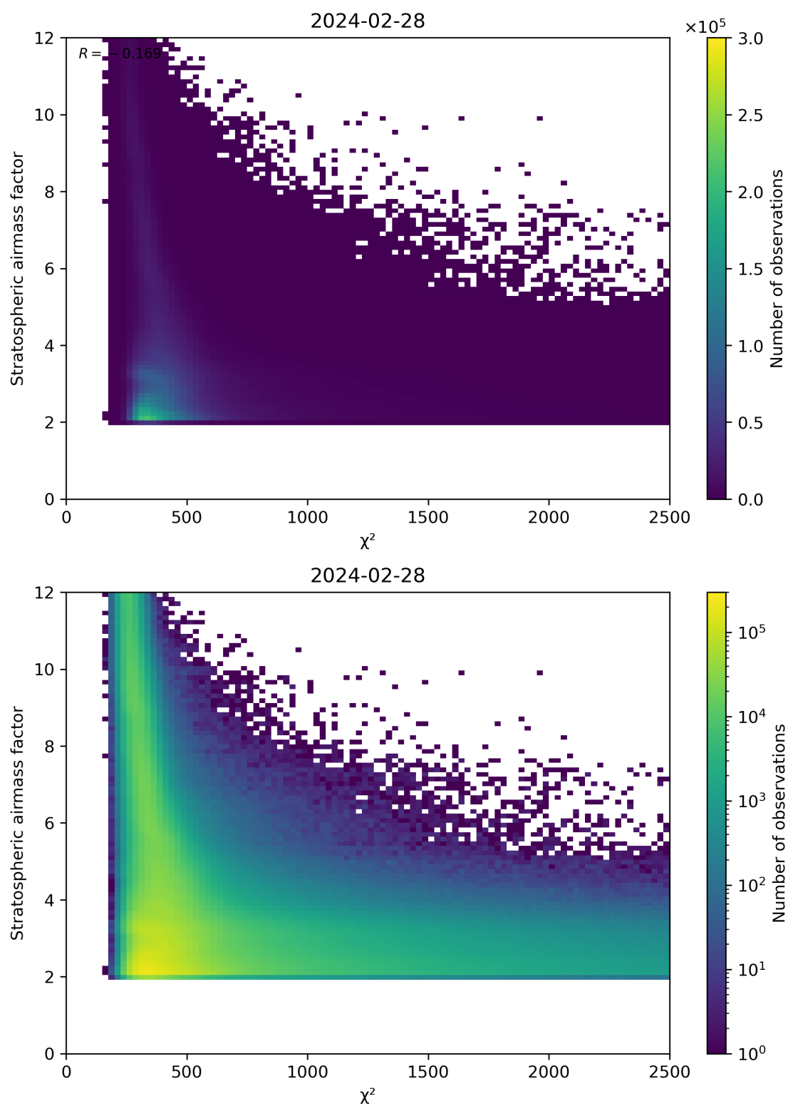
Figure 81: Scatter density plot of “ \chi^2 ” against “Stratospheric airmass factor” for 2024-02-27 to 2024-02-29.
