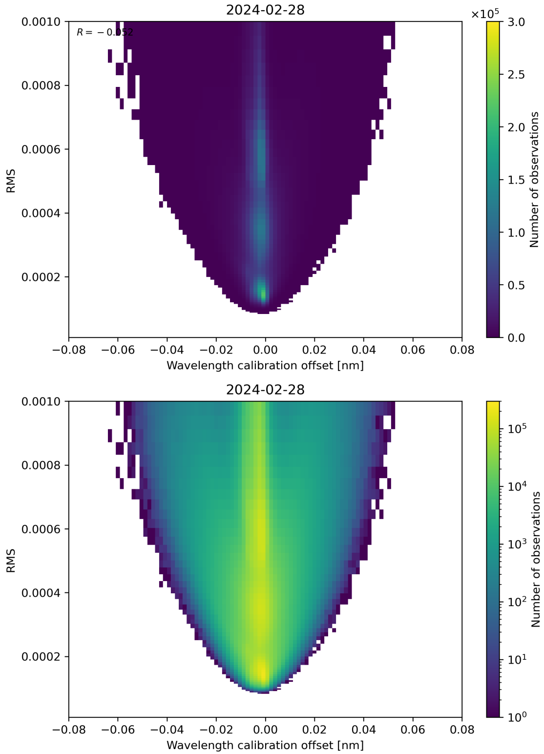
Figure 181: Scatter density plot of “Wavelength calibration offset” against “RMS” for 2024-02-27 to 2024-02-29.
