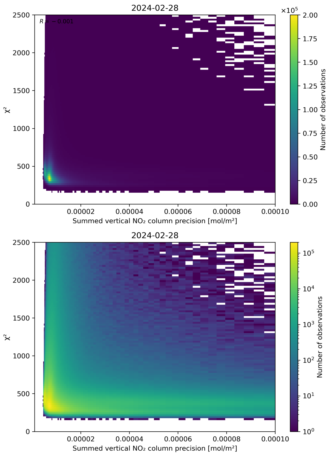
Figure 107: Scatter density plot of “Summed vertical NO 2 column precision” against “ \chi^2 ” for 2024-02-27 to 2024-02-29.
