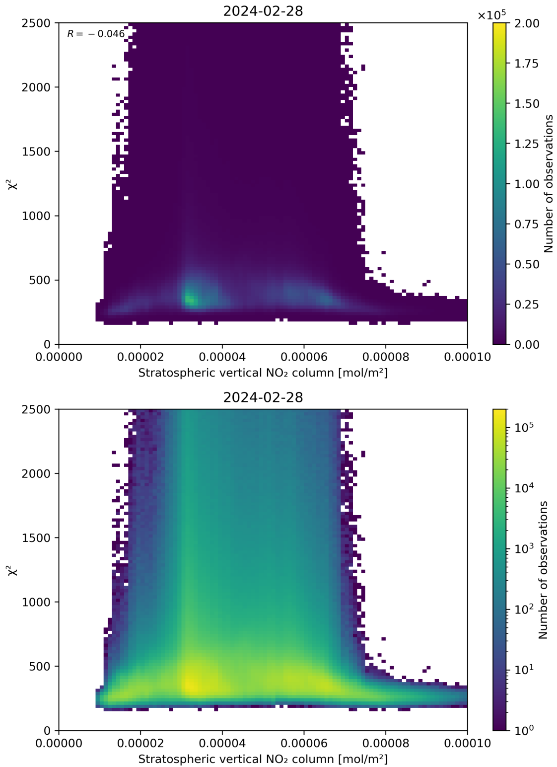
Figure 97: Scatter density plot of “Stratospheric vertical NO 2 column” against “ \chi^2 ” for 2024-02-27 to 2024-02-29.
