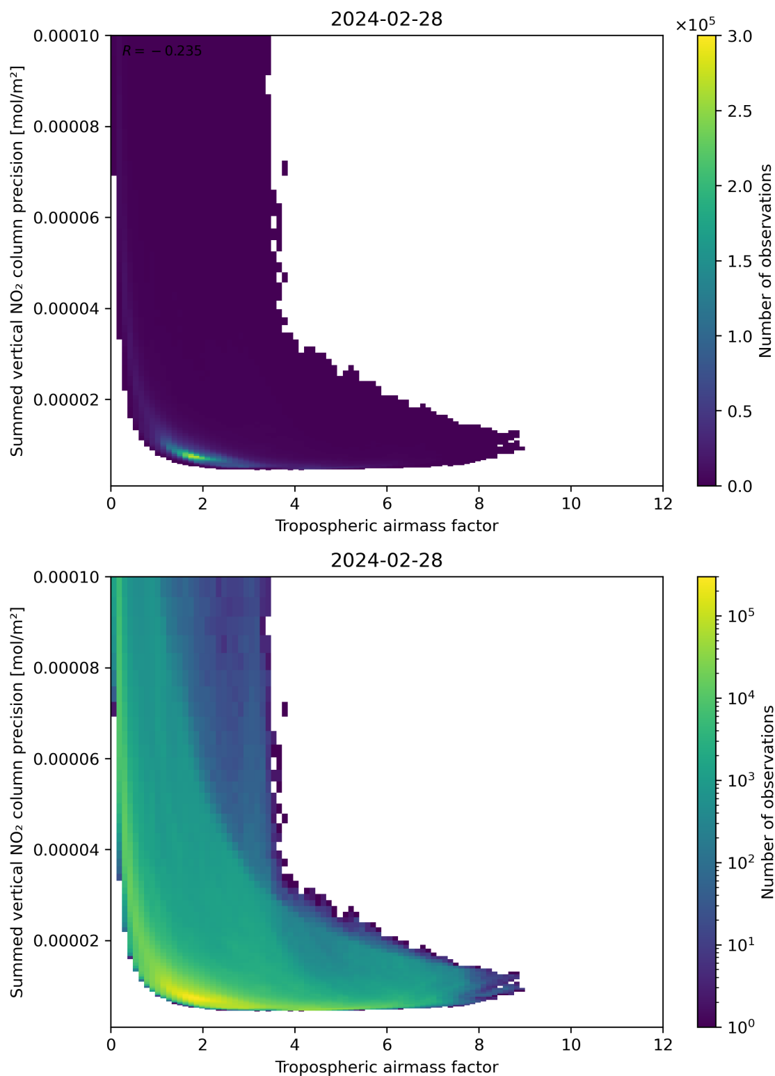
Figure 76: Scatter density plot of “Tropospheric air mass factor” against “Summed vertical NO 2 column precision” for 2024-02-27 to 2024-02-29.
