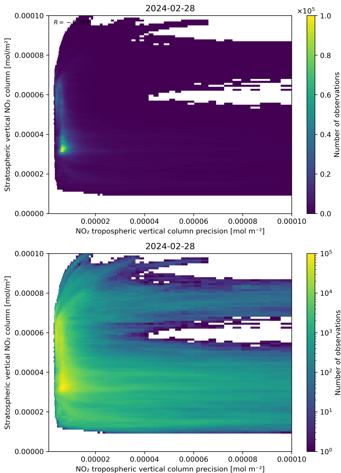
Figure 135: Scatter density plot of “NO 2 tropospheric vertical column precision” against “Stratospheric vertical NO 2 column” for 2024-02-27 to 2024-02-29.
