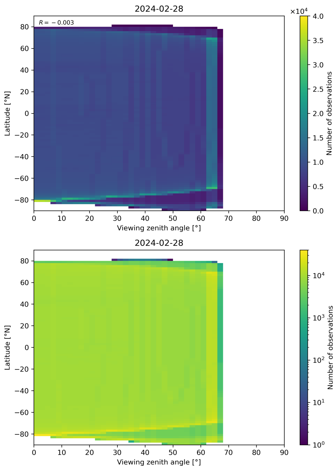
Figure 163: Scatter density plot of “Viewing zenith angle” against “Latitude” for 2024-02-27 to 2024-02-29.
