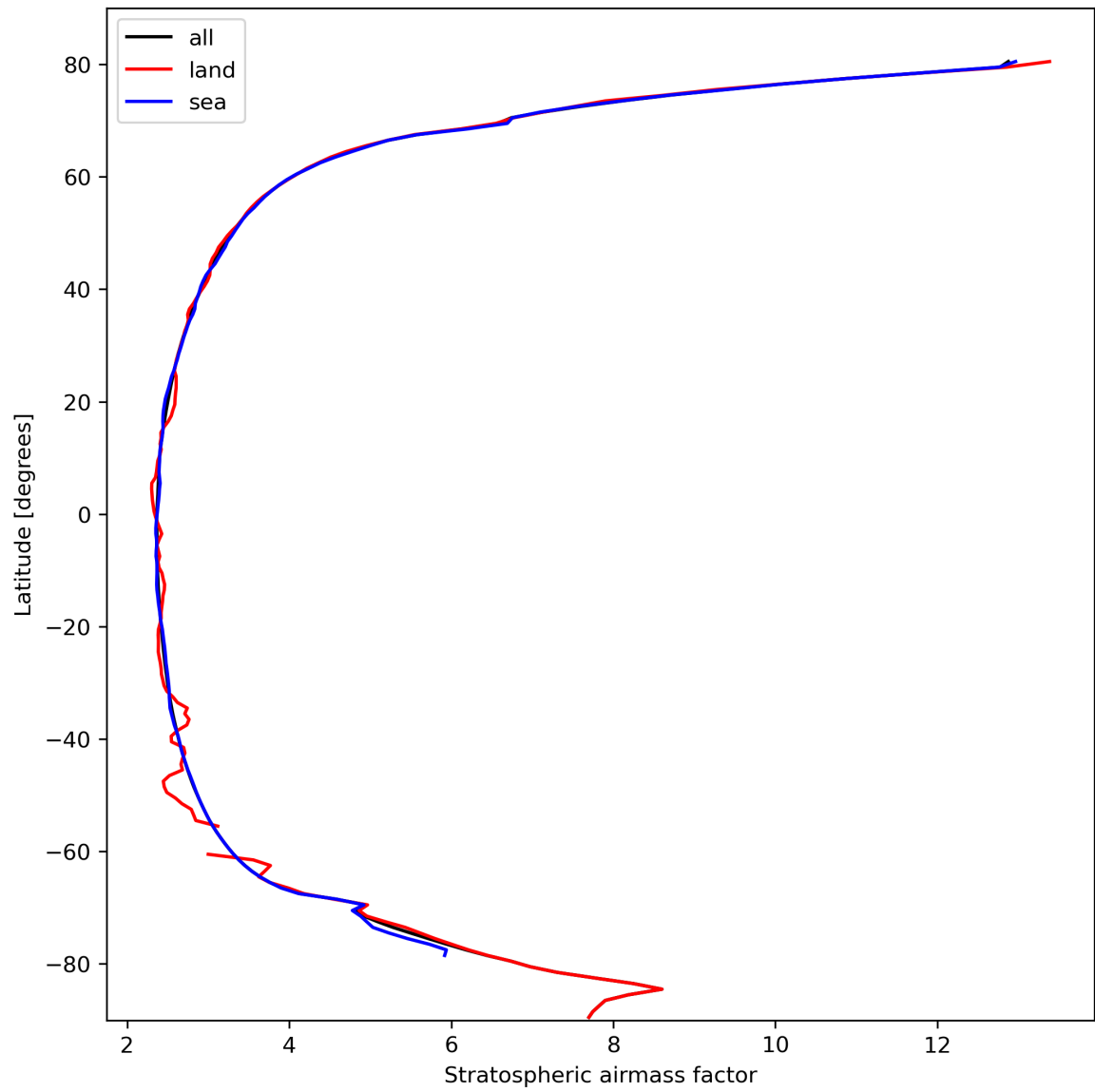
Figure 27: Zonal average of “Stratospheric air mass factor” for 2024-02-27 to 2024-02-29.
