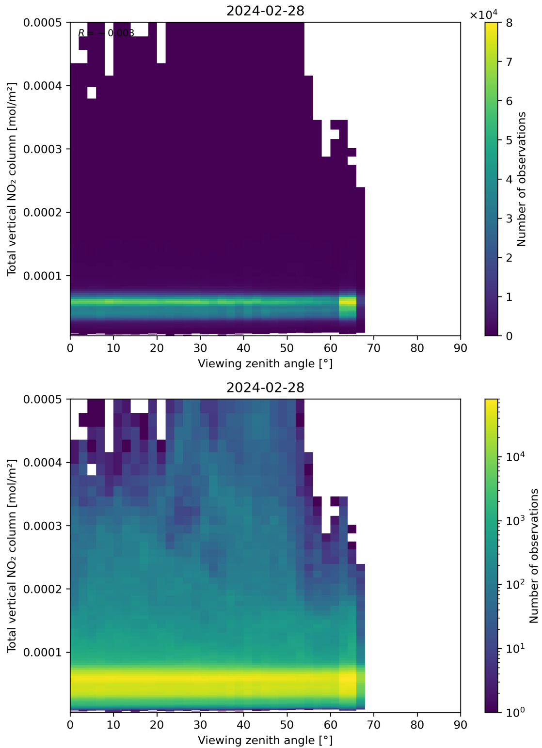
Figure 167: Scatter density plot of “Viewing zenith angle” against “Total vertical NO 2 column” for 2024-02-27 to 2024-02-29.
