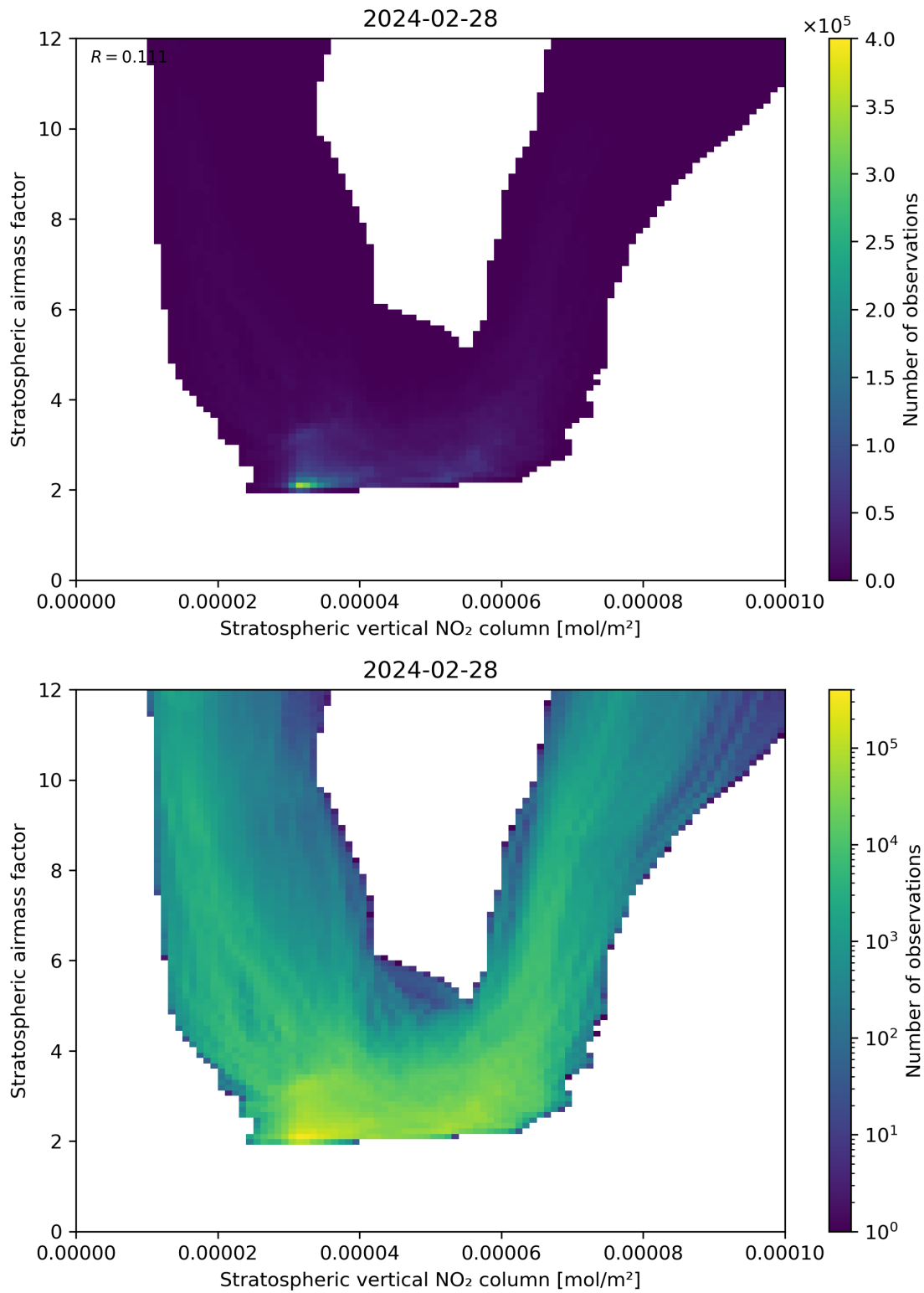
Figure 96: Scatter density plot of “Stratospheric vertical NO 2 column” against “Stratospheric airmass factor” for 2024-02-27 to 2024-02-29.
