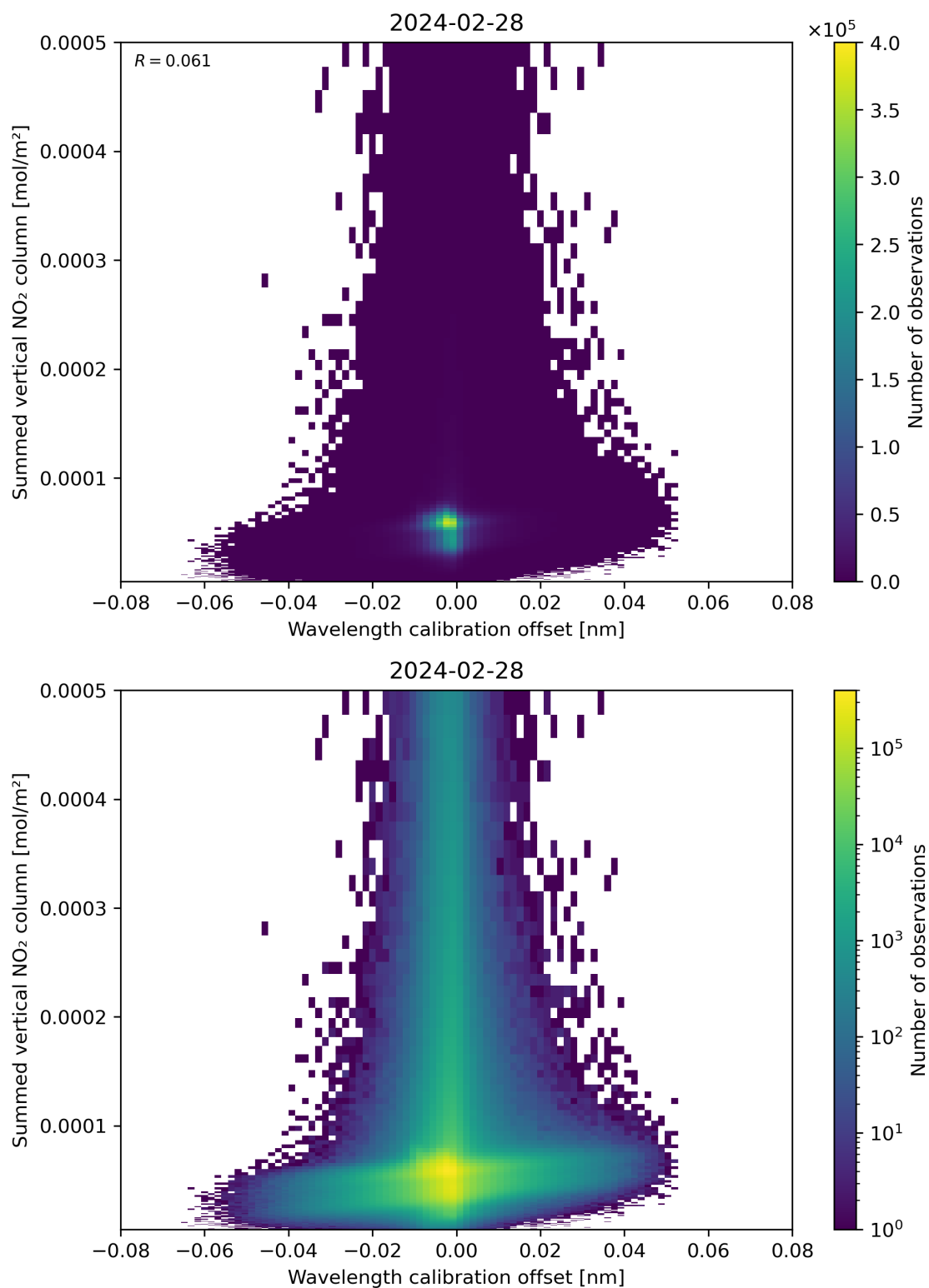
Figure 177: Scatter density plot of “Wavelength calibration offset” against “Summed vertical NO 2 column” for 2024-02-27 to 2024-02-29.
