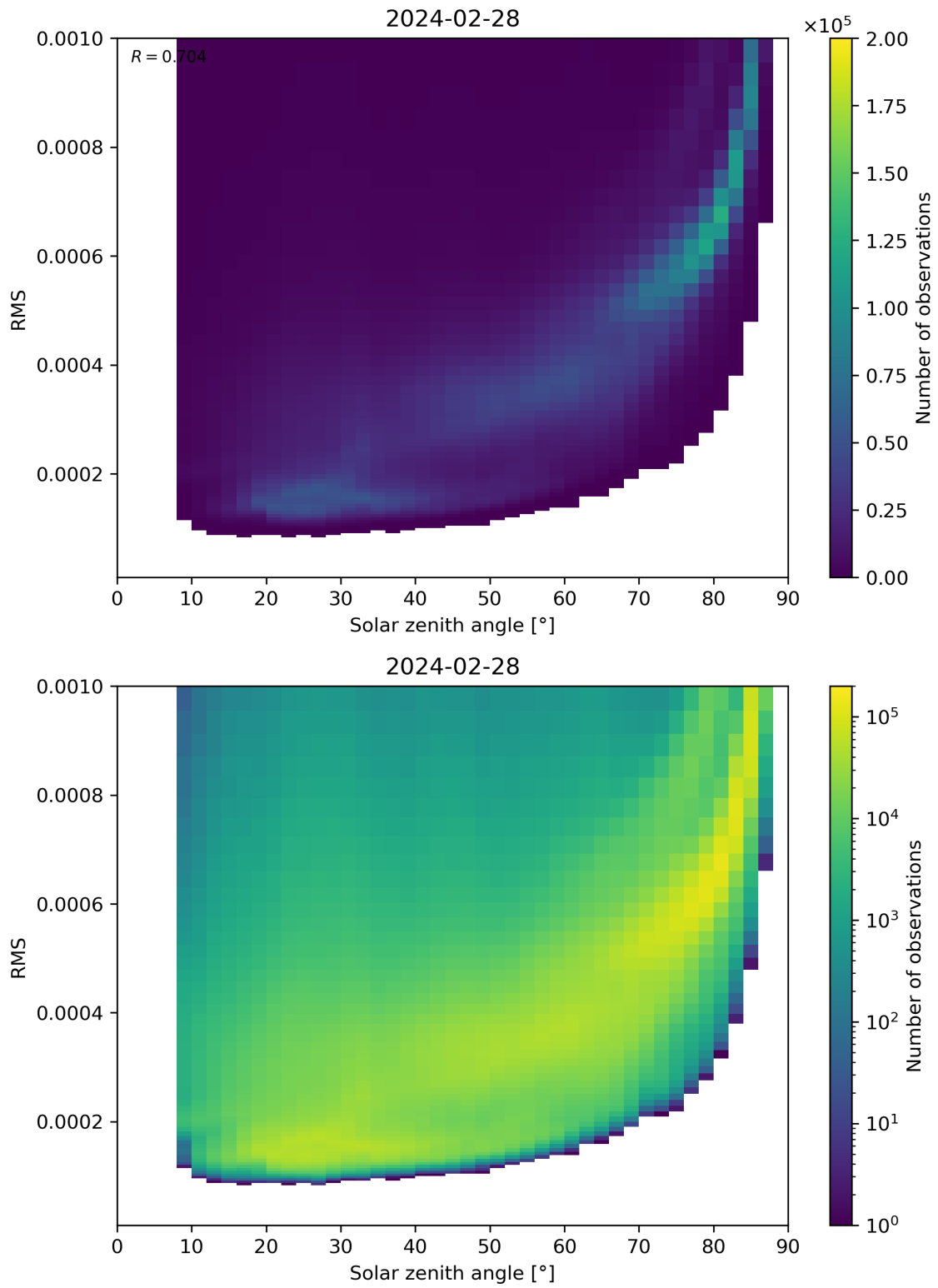
Figure 157: Scatter density plot of “Solar zenith angle” against “RMS” for 2024-02-27 to 2024-02-29.
