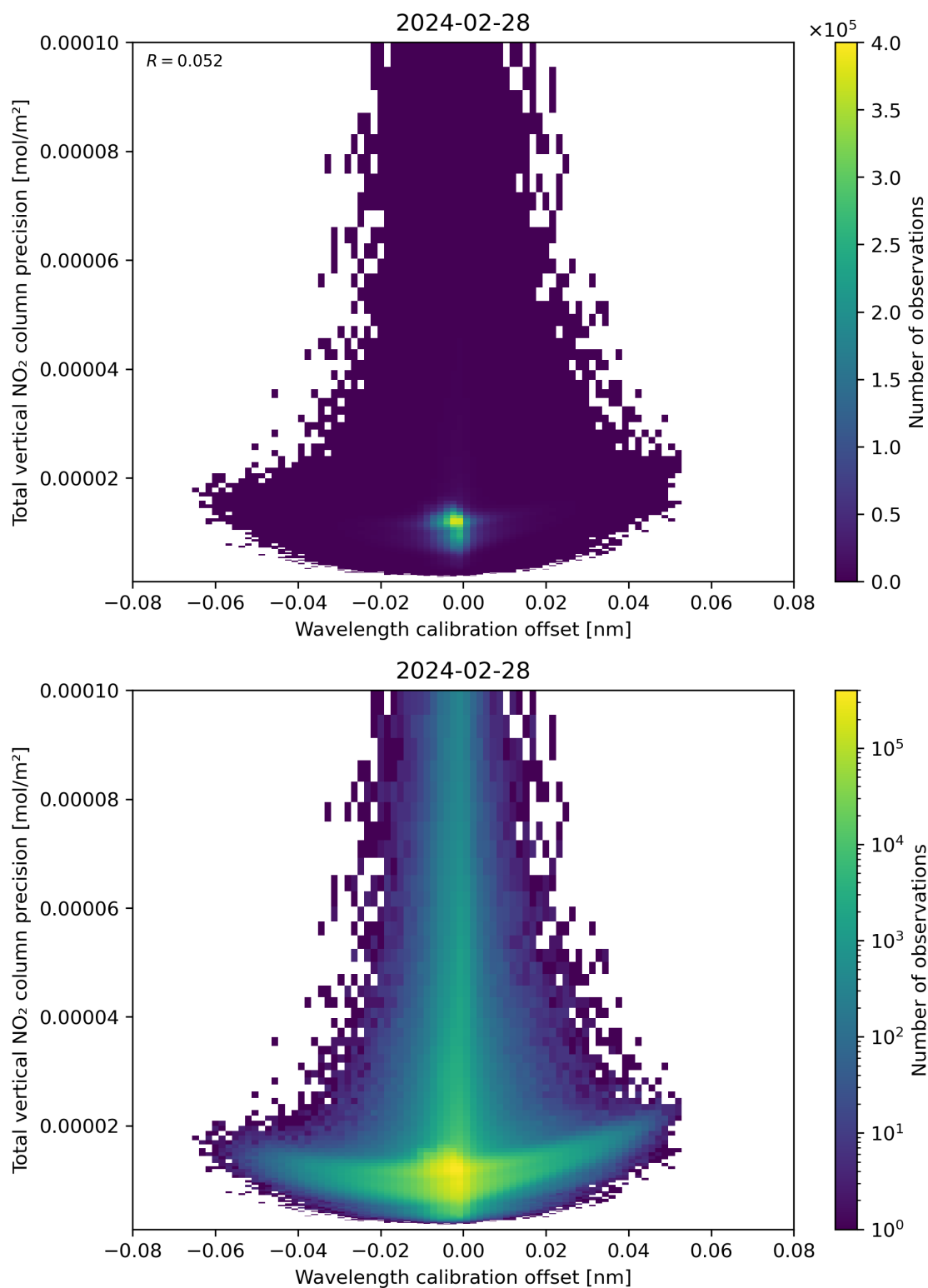
Figure 180: Scatter density plot of “Wavelength calibration offset” against “Total vertical NO 2 column precision” for 2024-02-27 to 2024-02-29.
