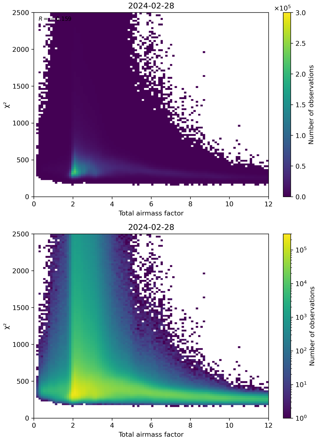
Figure 63: Scatter density plot of “Total airmass factor” against “ \chi^2 ” for 2024-02-27 to 2024-02-29.
