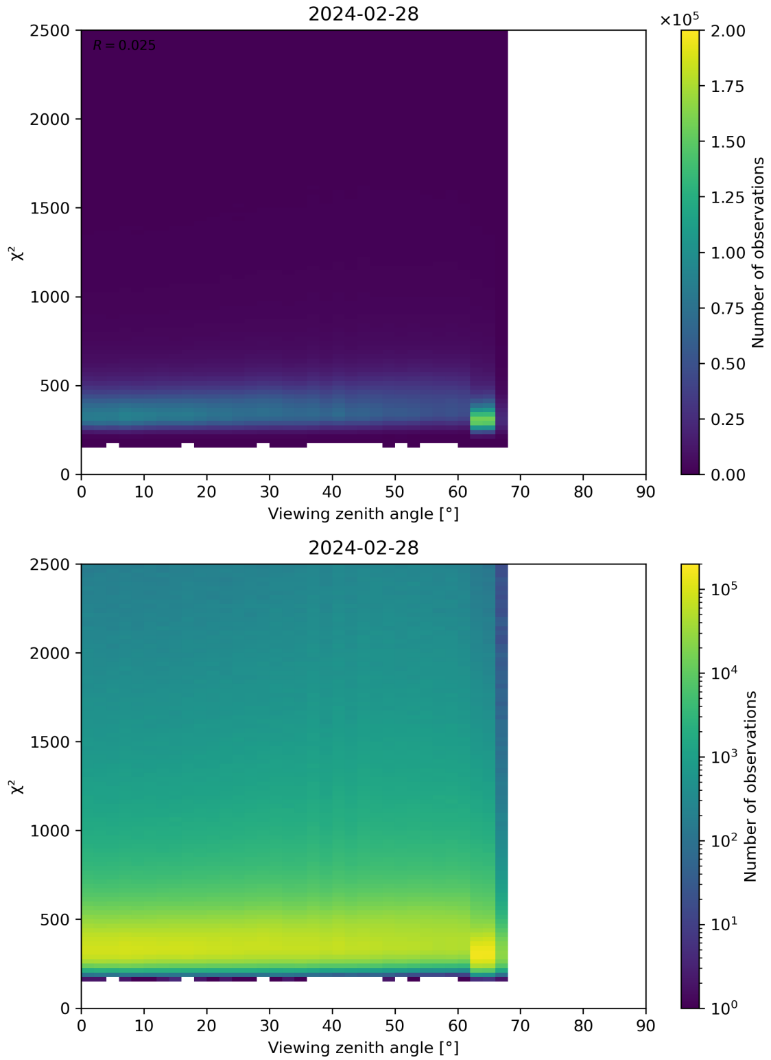
Figure 162: Scatter density plot of “Viewing zenith angle” against “ \chi^2 ” for 2024-02-27 to 2024-02-29.
