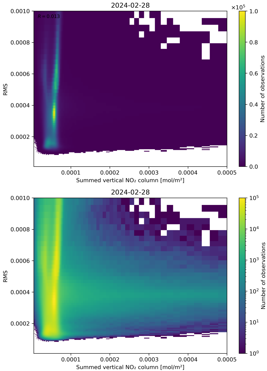
Figure 109: Scatter density plot of “Summed vertical NO 2 column” against “RMS” for 2024-02-27 to 2024-02-29.
