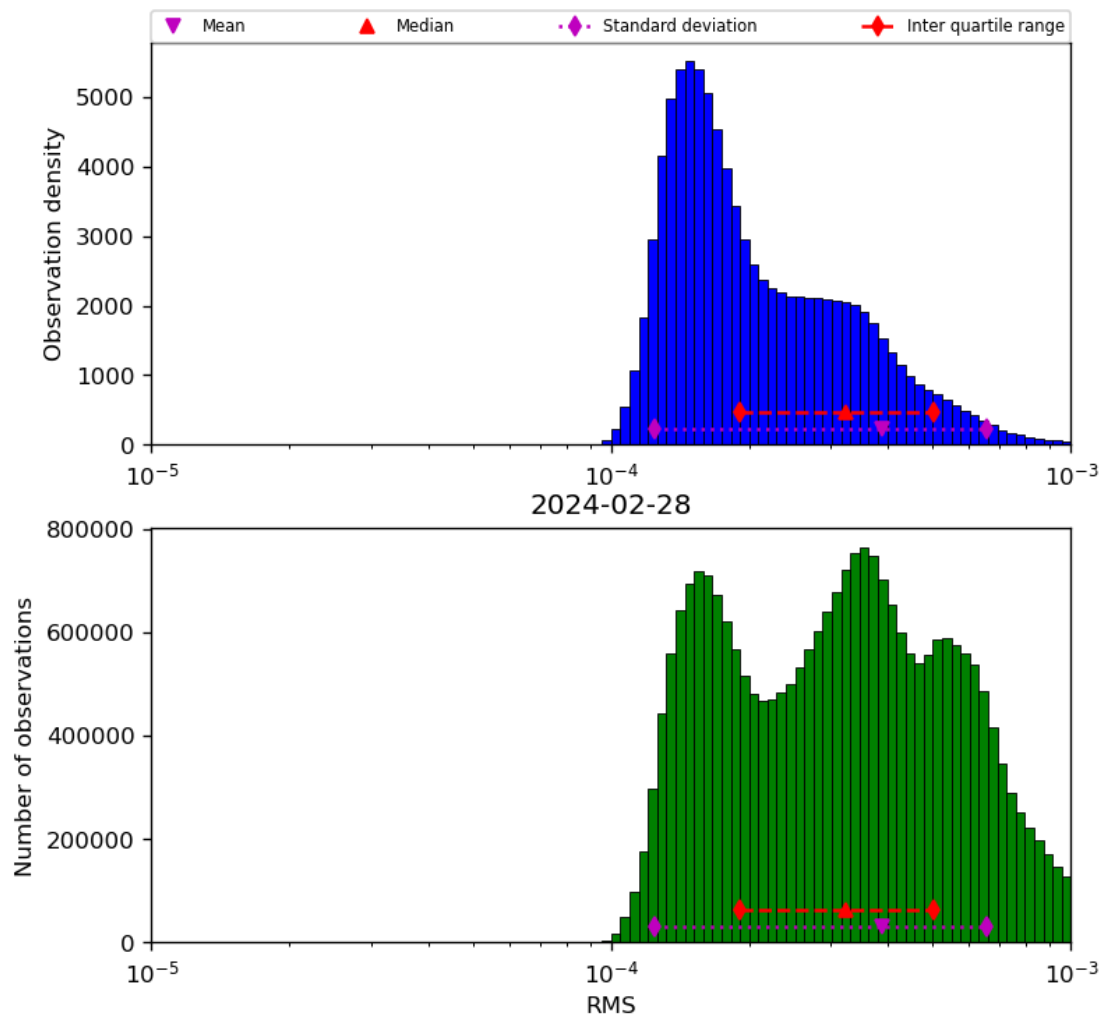
Figure 43: Histogram of “RMS” for 2024-02-27 to 2024-02-29
