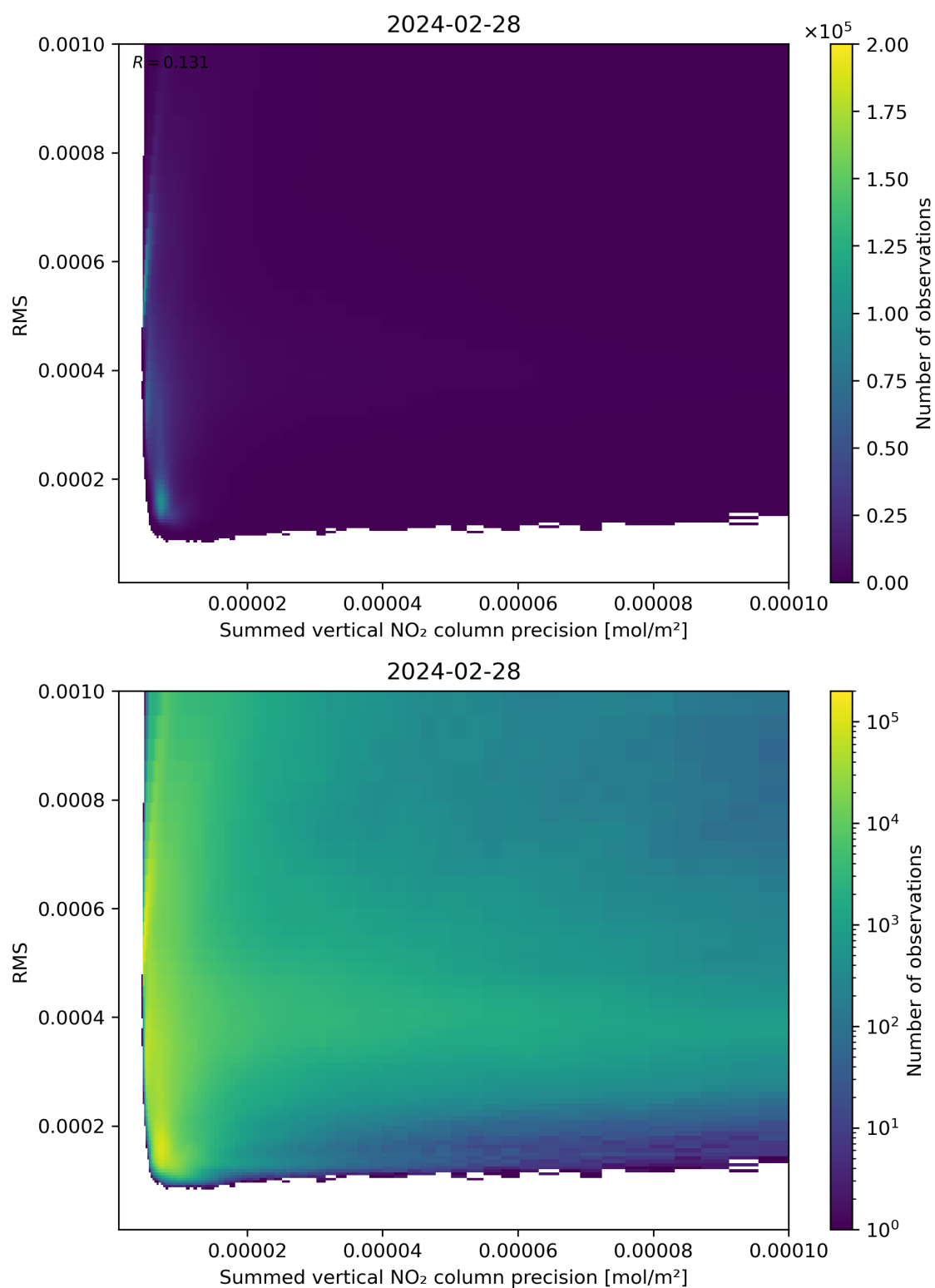
Figure 108: Scatter density plot of “Summed vertical NO 2 column precision” against “RMS” for 2024-02-27 to 2024-02-29.
