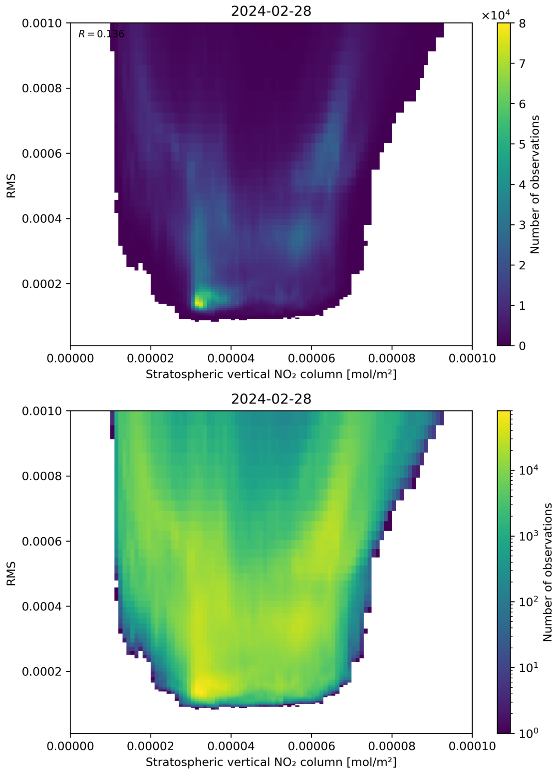
Figure 102: Scatter density plot of “Stratospheric vertical NO 2 column” against “RMS” for 2024-02-27 to 2024-02-29.
