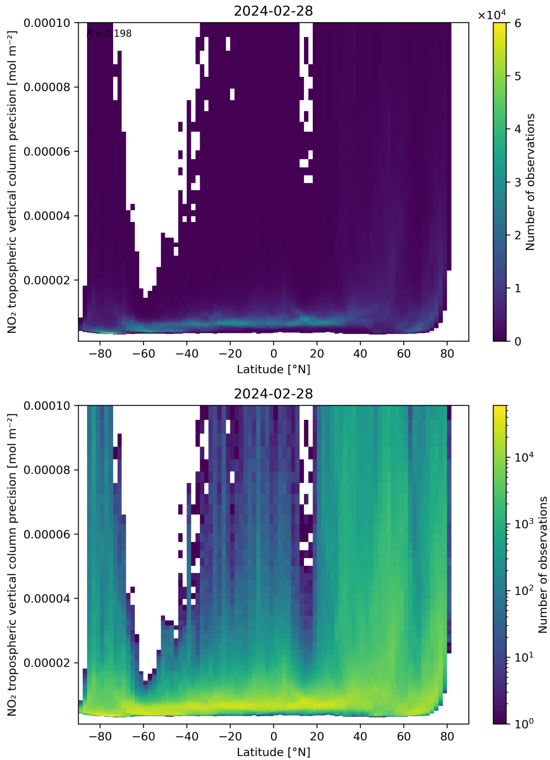
Figure 93: Scatter density plot of “Latitude” against “NO 2 tropospheric vertical column precision” for 2024-02-27 to 2024-02-29.
