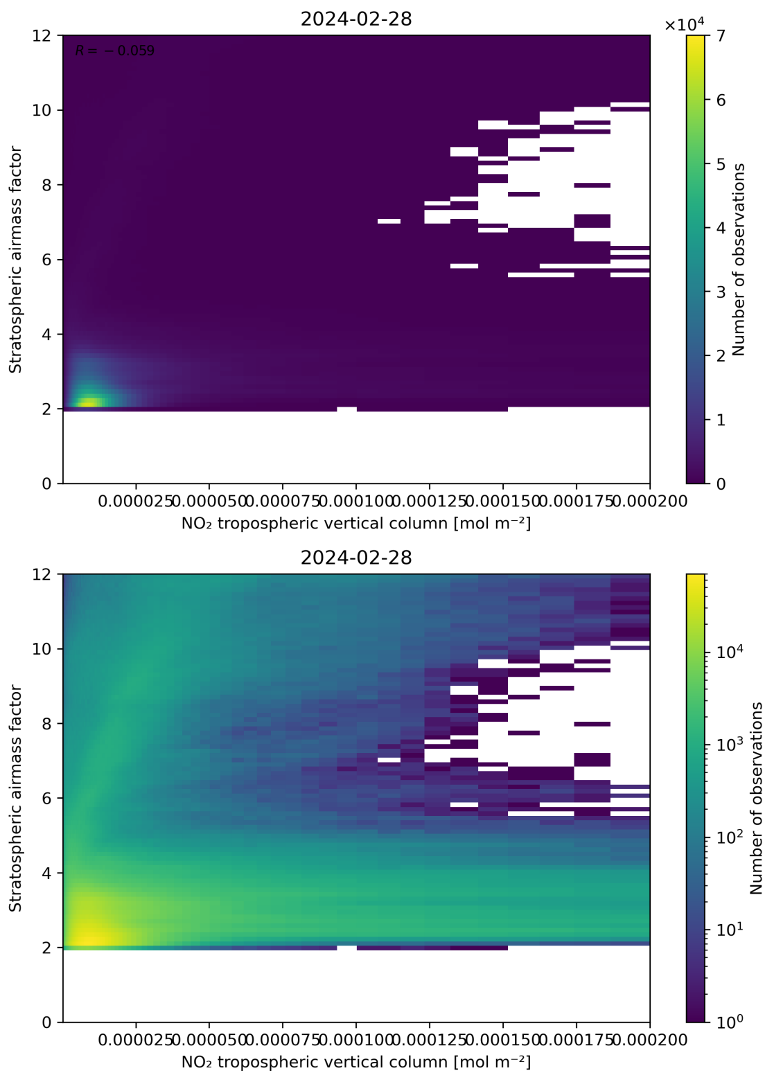
Figure 121: Scatter density plot of “NO 2 tropospheric vertical column” against “Stratospheric air mass factor” for 2024-02-27 to 2024-02-29.
