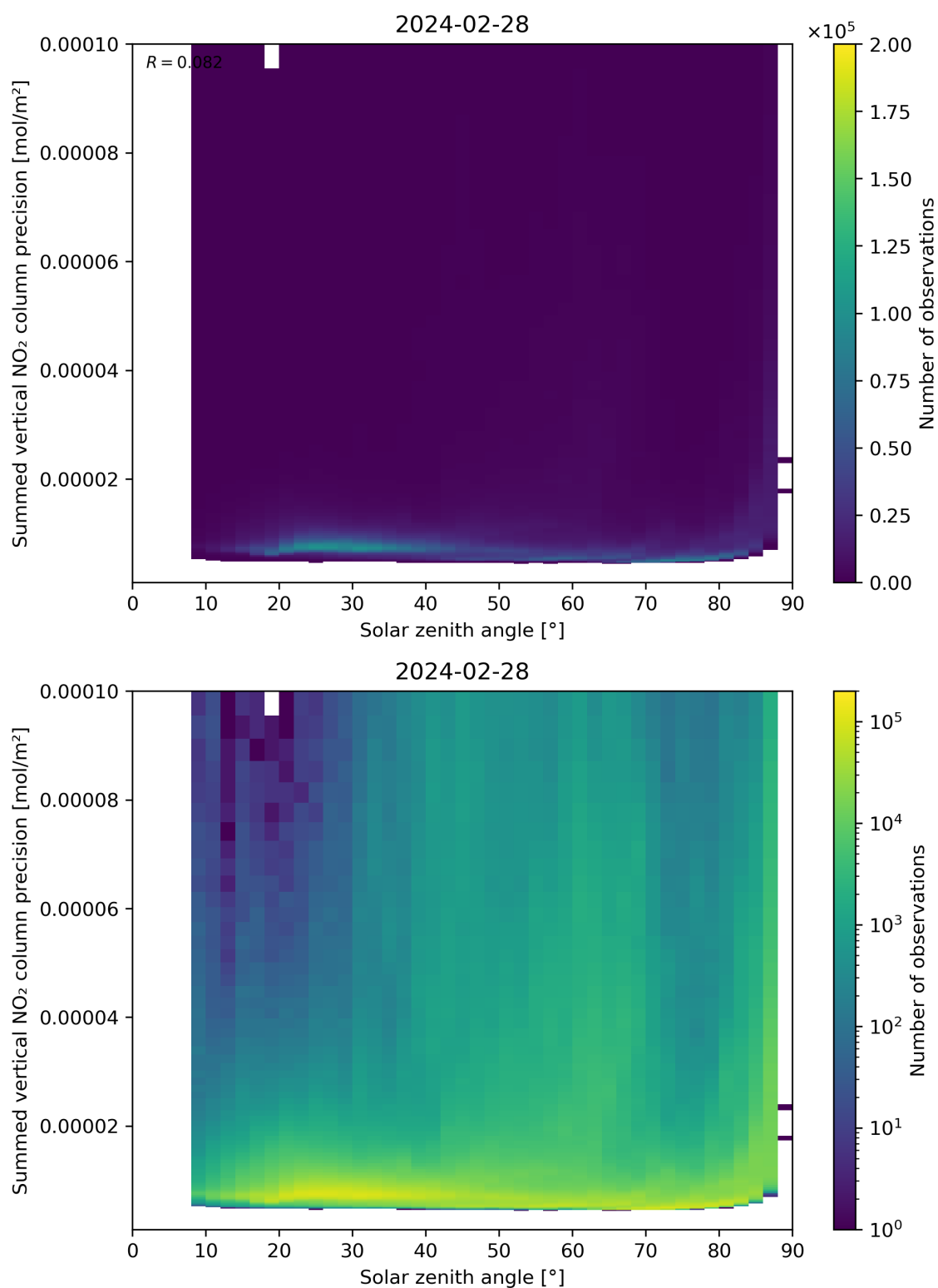
Figure 152: Scatter density plot of “Solar zenith angle” against “Summed vertical NO 2 column precision” for 2024-02-27 to 2024-02-29.
