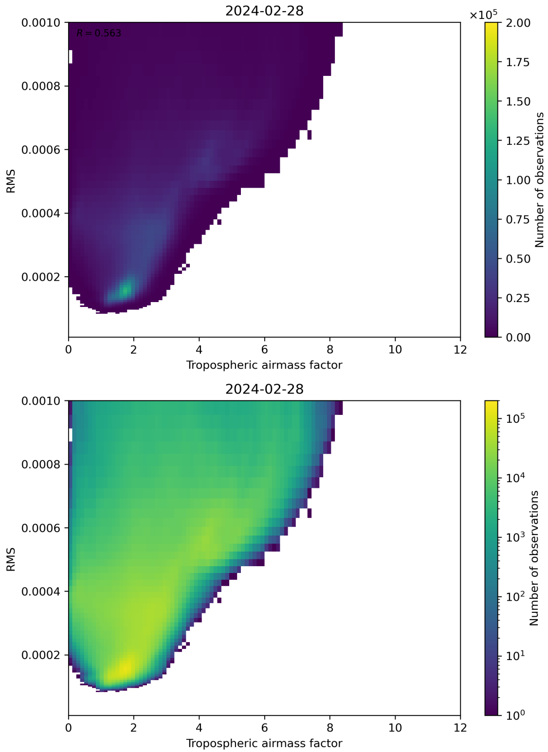
Figure 79: Scatter density plot of “Tropospheric airmass factor” against “RMS” for 2024-02-27 to 2024-02-29.
