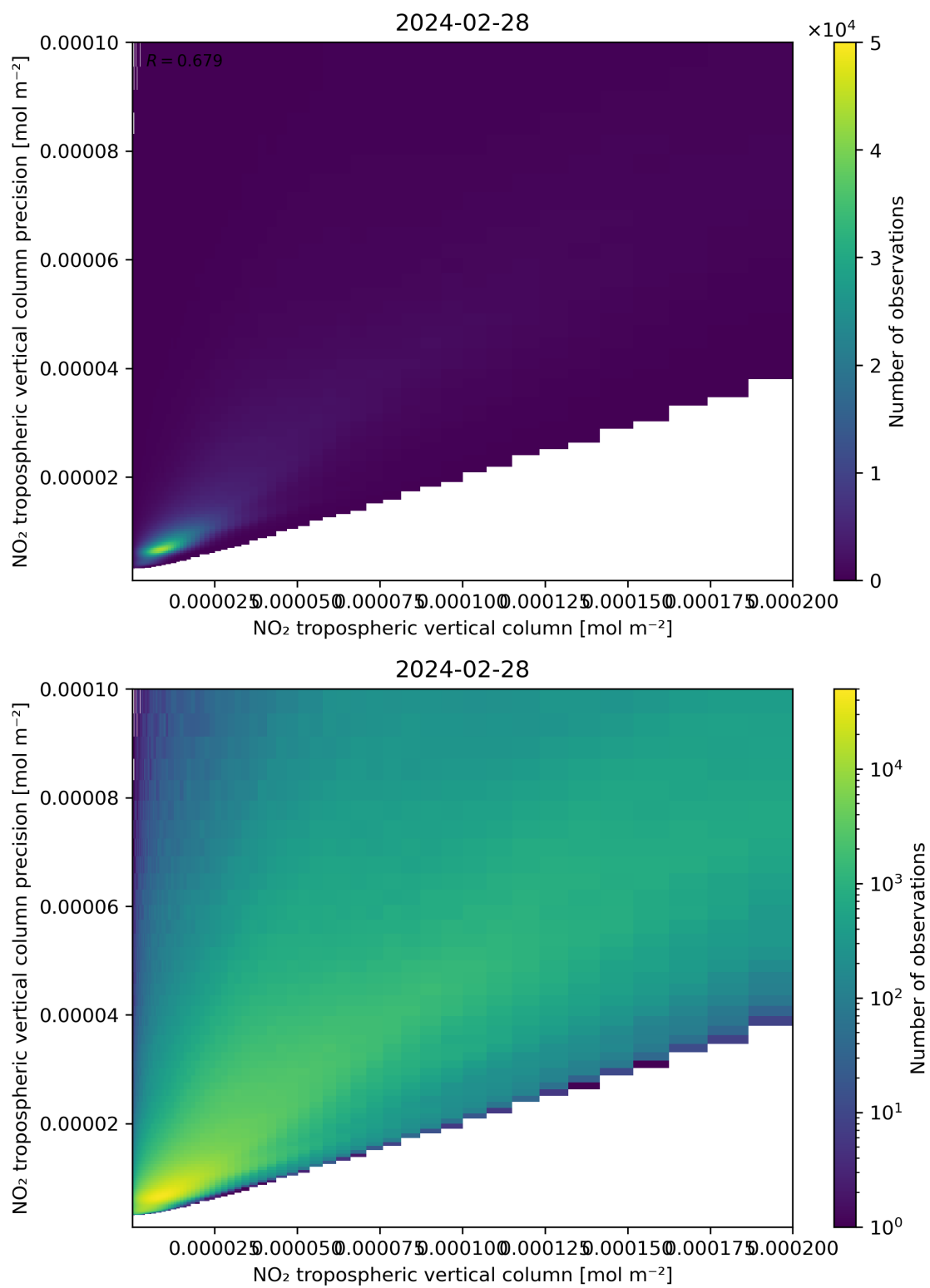
Figure 130: Scatter density plot of “NO 2 tropospheric vertical column” against “NO 2 tropospheric vertical column precision” for 2024-02-27 to 2024-02-29.
