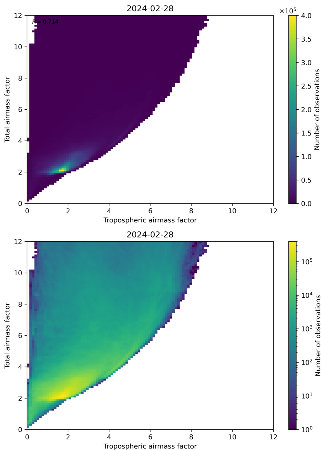
Figure 72: Scatter density plot of “Tropospheric airmass factor” against “Total airmass factor” for 2024-02-27 to 2024-02-29.
