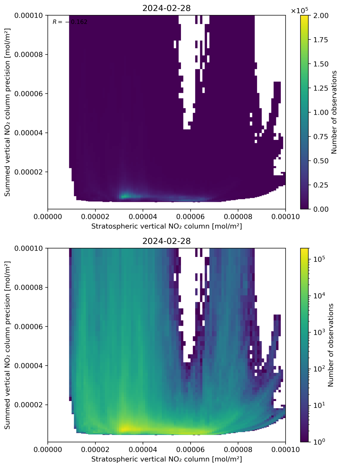
Figure 99: Scatter density plot of “Stratospheric vertical NO 2 column” against “Summed vertical NO 2 column precision” for 2024-02-27 to 2024-02-29.
