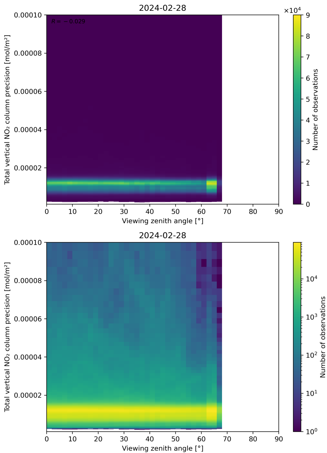
Figure 168: Scatter density plot of “Viewing zenith angle” against “Total vertical NO 2 column precision” for 2024-02-27 to 2024-02-29.
