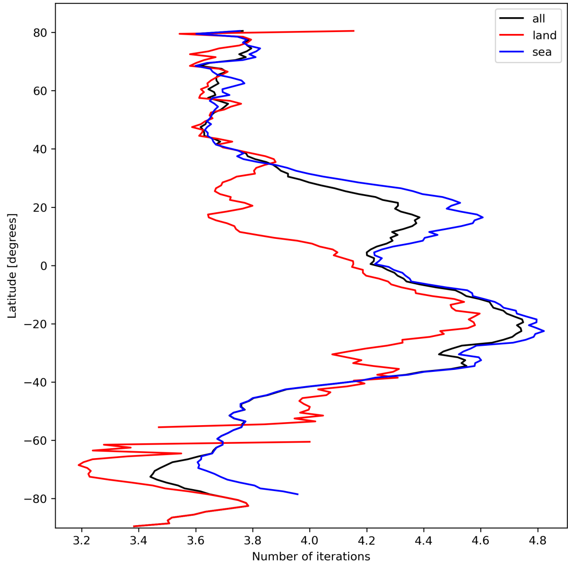
Figure 17: Zonal average of “Number of iterations” for 2024-02-27 to 2024-02-29.
