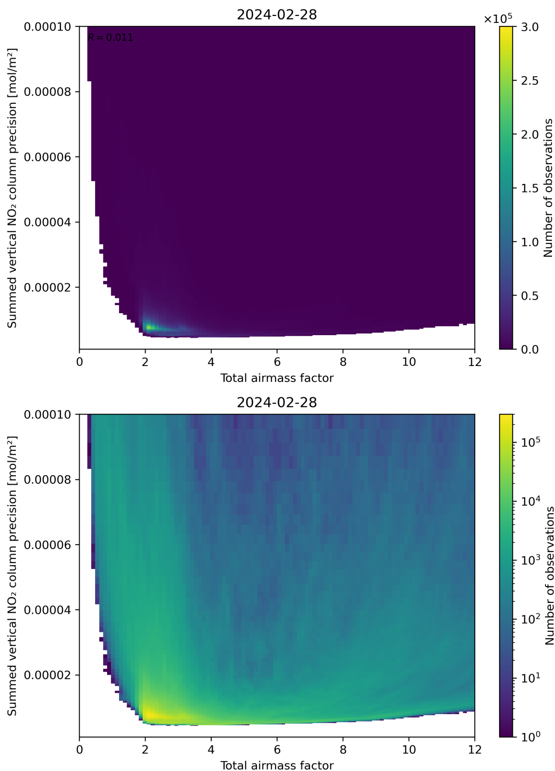
Figure 66: Scatter density plot of “Total airmass factor” against “Summed vertical NO 2 column precision” for 2024-02-27 to 2024-02-29.
