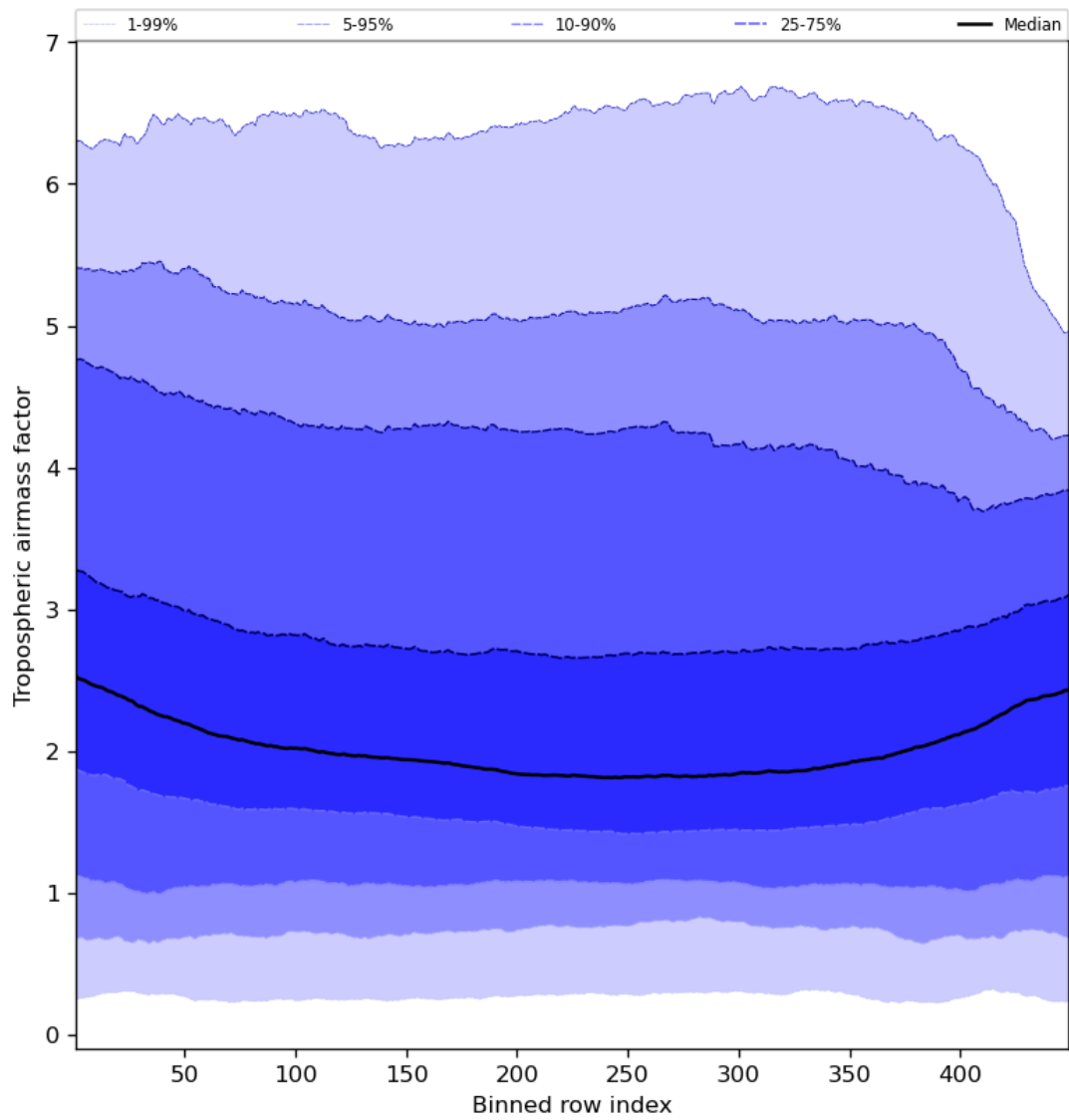
Figure 48: Along track statistics of “Tropospheric air mass factor” for 2024-02-27 to 2024-02-29
