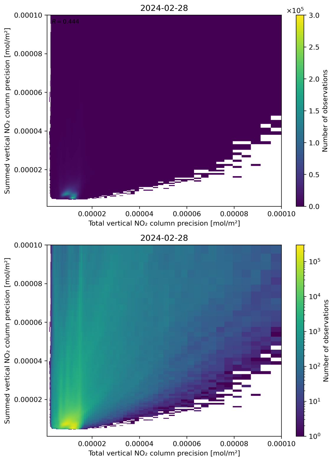
Figure 118: Scatter density plot of “Total vertical NO 2 column precision” against “Summed vertical NO 2 column precision” for 2024-02-27 to 2024-02-29.
