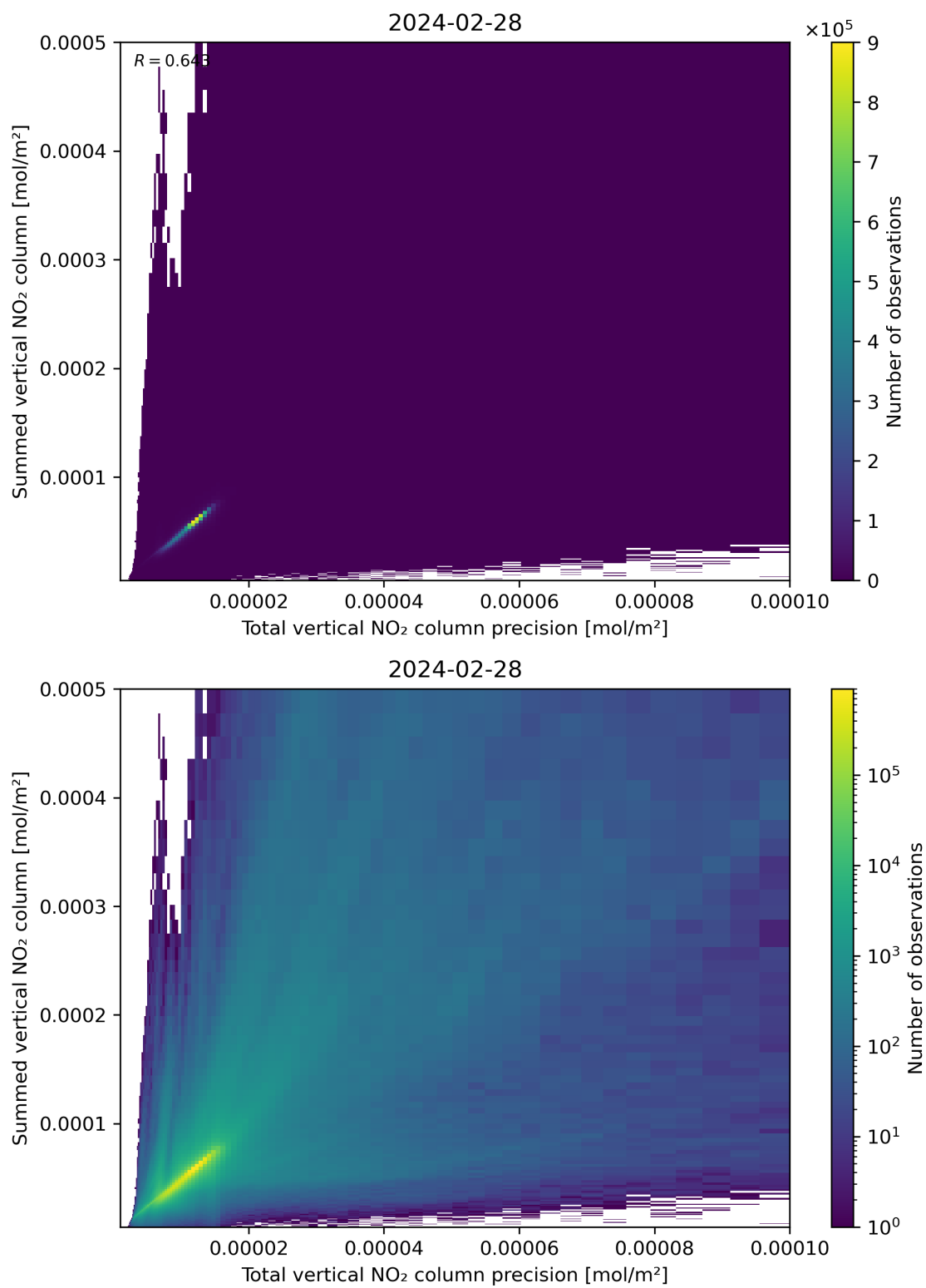
Figure 117: Scatter density plot of “Total vertical NO 2 column precision” against “Summed vertical NO 2 column” for 2024-02-27 to 2024-02-29.
