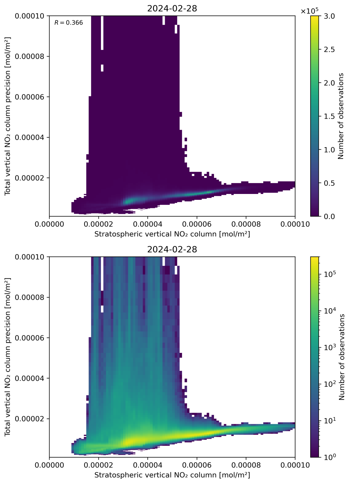
Figure 101: Scatter density plot of “Stratospheric vertical NO 2 column” against “Total vertical NO 2 column precision” for 2024-02-27 to 2024-02-29.
