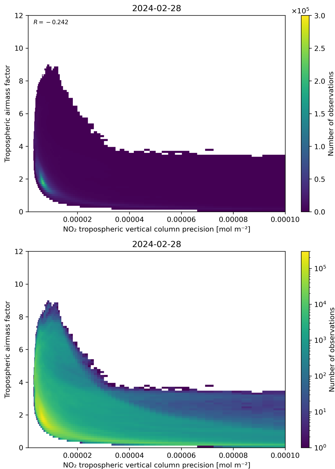
Figure 133: Scatter density plot of “NO 2 tropospheric vertical column precision” against “Tropospheric airmass factor” for 2024-02-27 to 2024-02-29.
