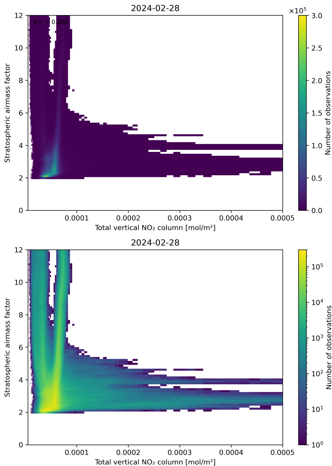
Figure 110: Scatter density plot of “Total vertical NO 2 column” against “Stratospheric air mass factor” for 2024-02-27 to 2024-02-29.
