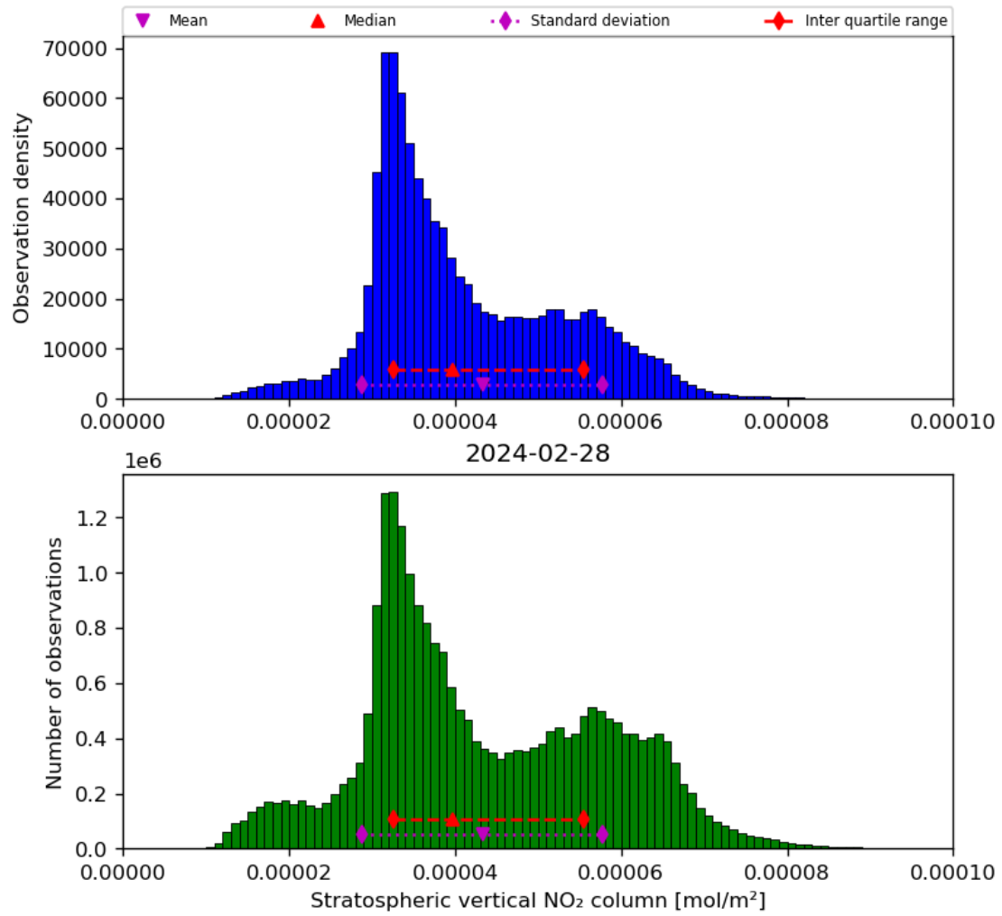
Figure 36: Histogram of “Stratospheric vertical NO 2 column” for 2024-02-27 to 2024-02-29
