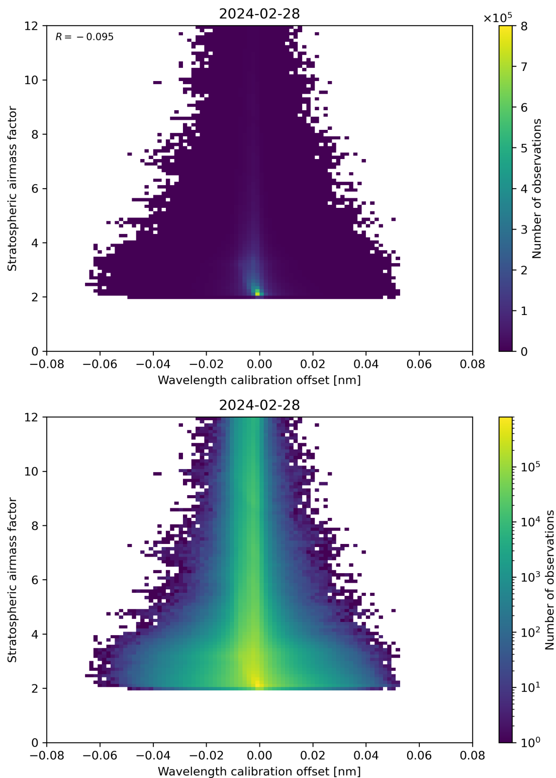
Figure 174: Scatter density plot of “Wavelength calibration offset” against “Stratospheric airmass factor” for 2024-02-27 to 2024-02-29.
