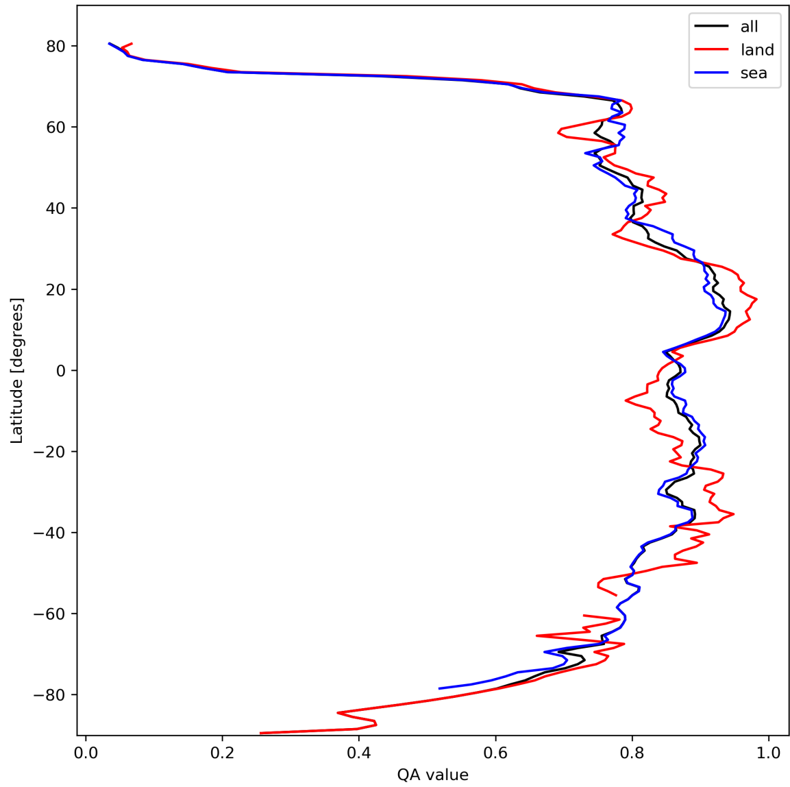
Figure 11: Zonal average of “QA value” for 2024-02-27 to 2024-02-29.
