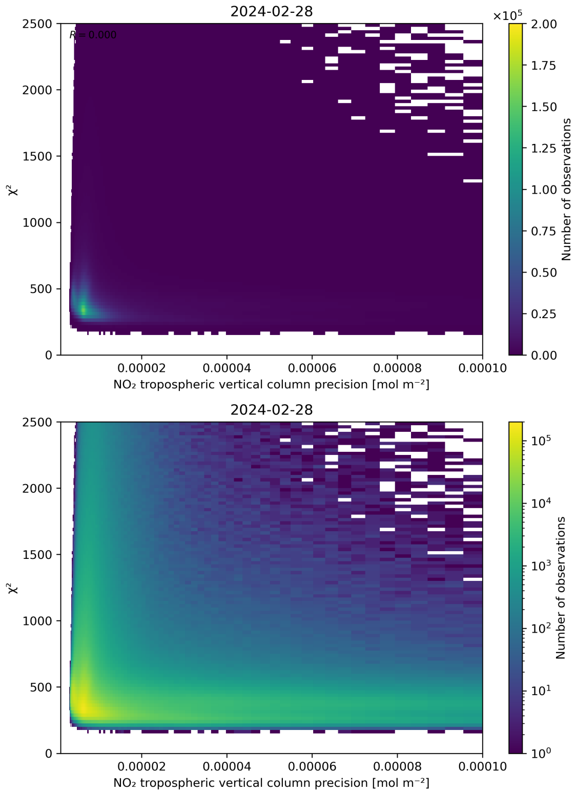
Figure 134: Scatter density plot of “NO 2 tropospheric vertical column precision” against “ \chi^2 ” for 2024-02-27 to 2024-02-29.
