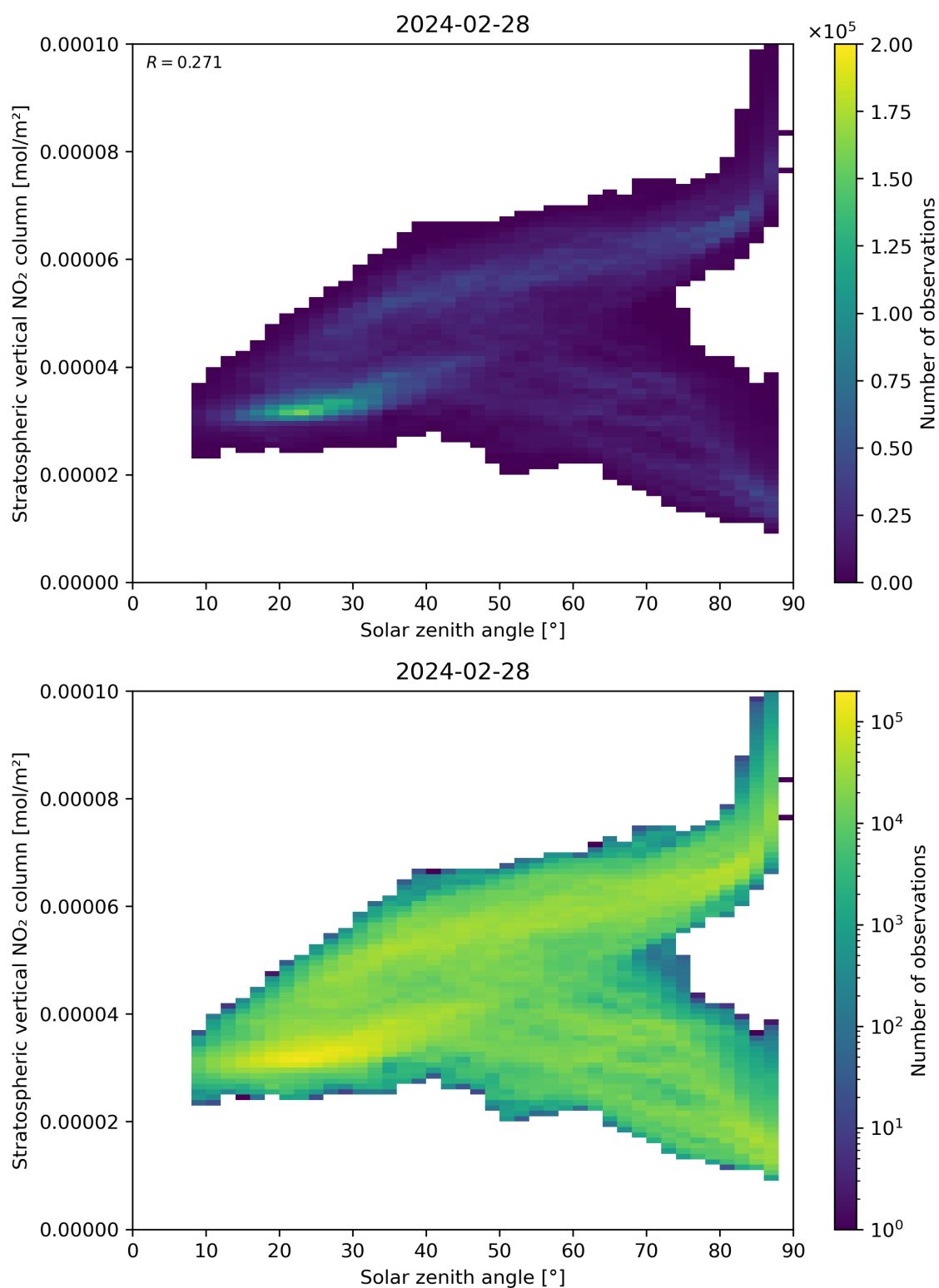
Figure 150: Scatter density plot of “Solar zenith angle” against “Stratospheric vertical NO 2 column” for 2024-02-27 to 2024-02-29.
