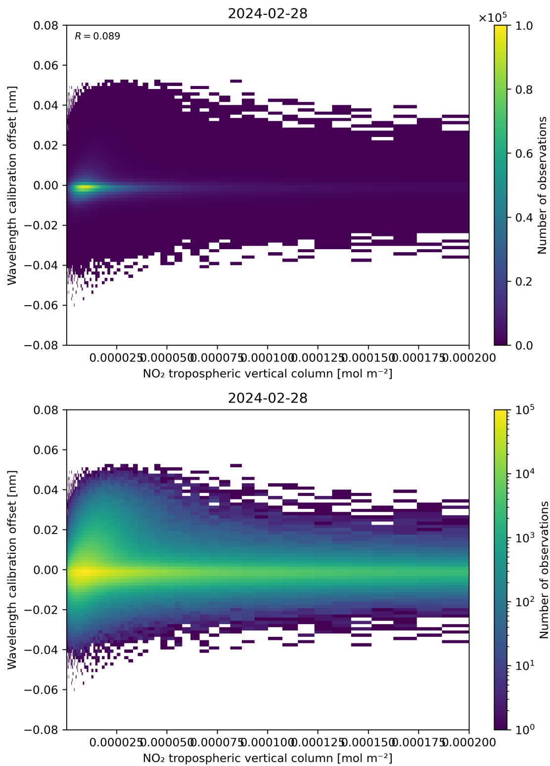
Figure 143: Scatter density plot of “NO 2 tropospheric vertical column” against “Wavelength calibration offset” for 2024-02-27 to 2024-02-29.
