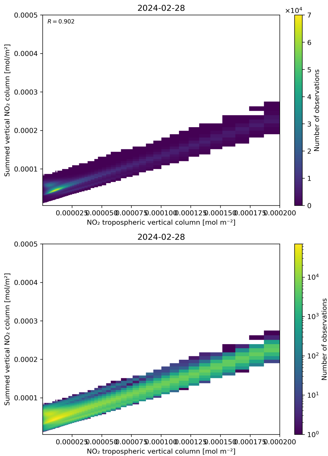
Figure 126: Scatter density plot of “NO 2 tropospheric vertical column” against “Summed vertical NO 2 column” for 2024-02-27 to 2024-02-29.
