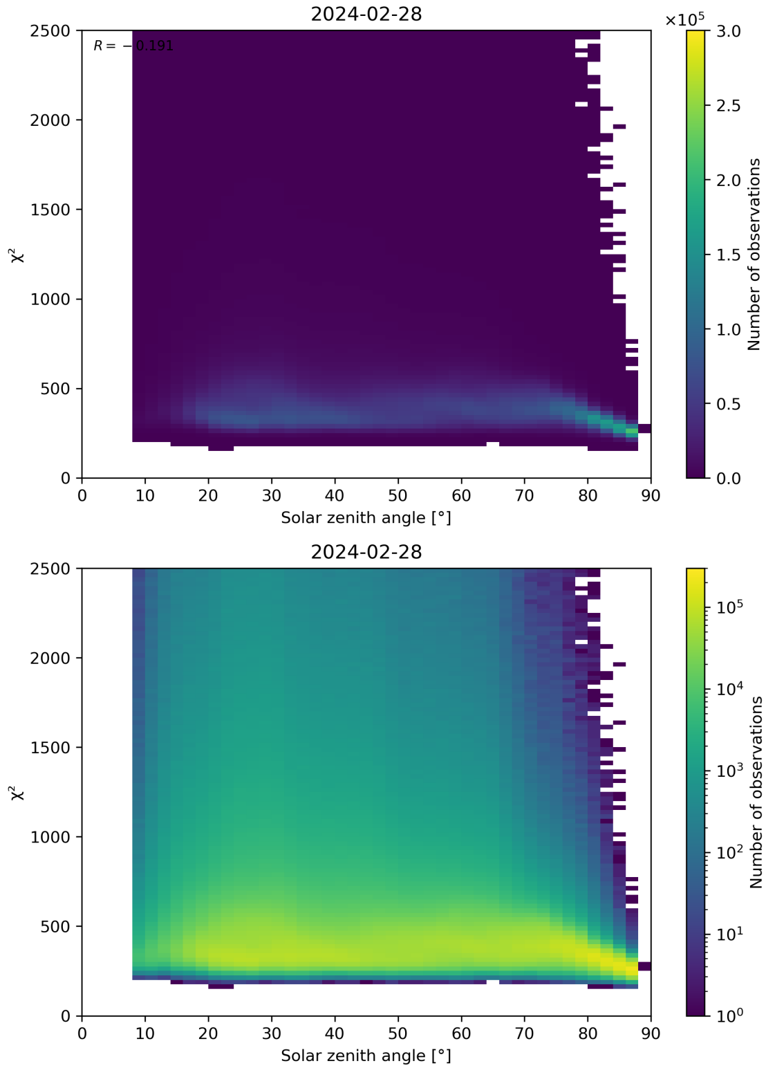
Figure 148: Scatter density plot of “Solar zenith angle” against “ \chi^2 ” for 2024-02-27 to 2024-02-29.
