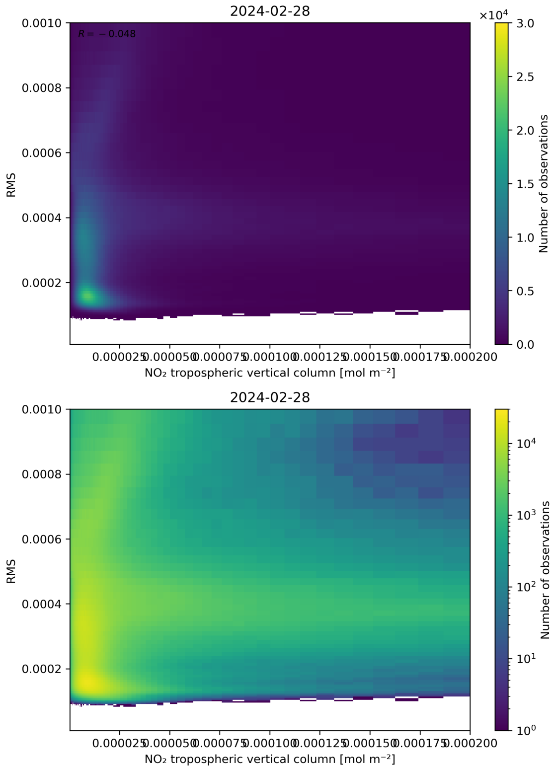
Figure 142: Scatter density plot of “NO 2 tropospheric vertical column” against “RMS” for 2024-02-27 to 2024-02-29.
