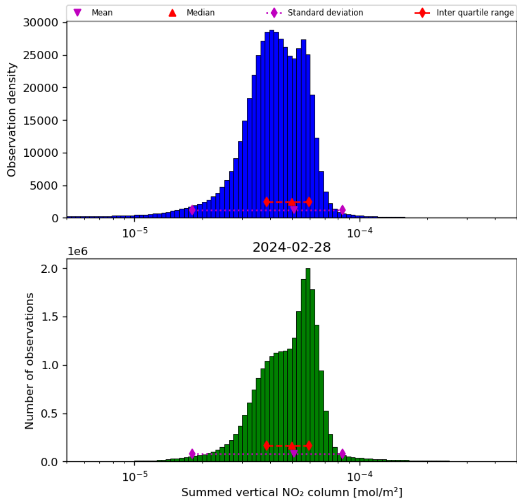
Figure 40: Histogram of “Summed vertical NO 2 column” for 2024-02-27 to 2024-02-29
