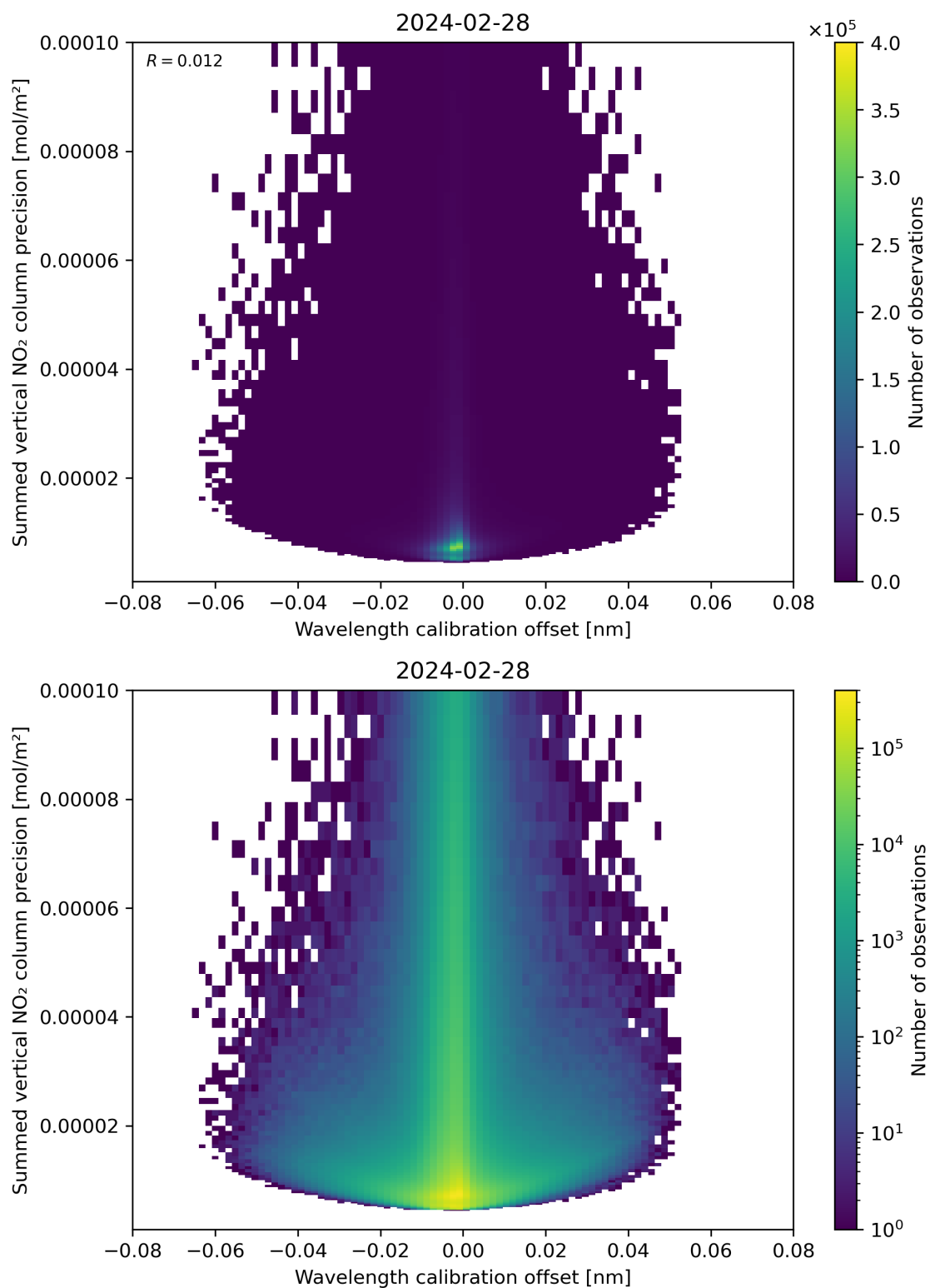
Figure 178: Scatter density plot of “Wavelength calibration offset” against “Summed vertical NO 2 column precision” for 2024-02-27 to 2024-02-29.
