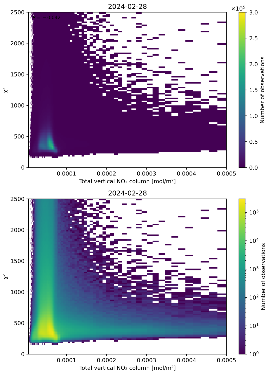
Figure 111: Scatter density plot of “Total vertical NO 2 column” against “ \chi^2 ” for 2024-02-27 to 2024-02-29.
