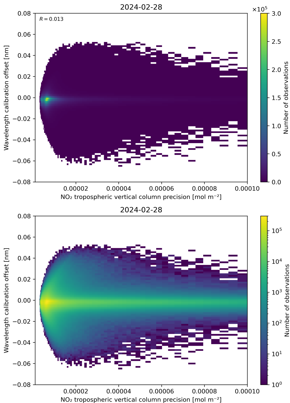
Figure 141: Scatter density plot of “NO 2 tropospheric vertical column precision” against “Wavelength calibration offset” for 2024-02-27 to 2024-02-29.
