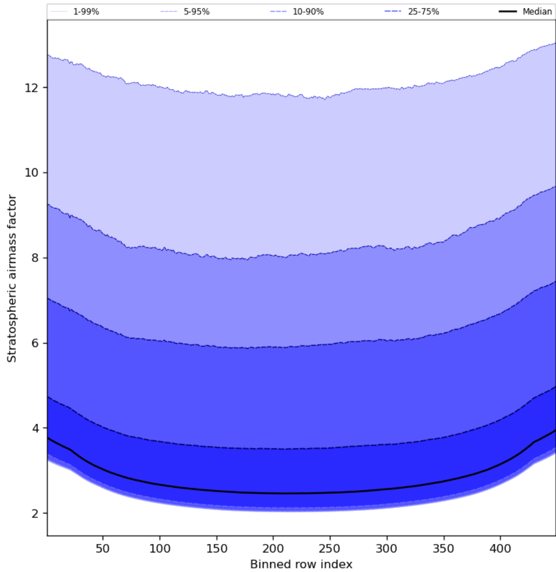
Figure 61: Along track statistics of “Stratospheric airmass factor” for 2024-02-27 to 2024-02-29
