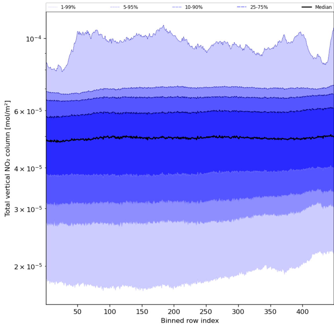
Figure 55: Along track statistics of “Total vertical NO 2 column” for 2024-02-27 to 2024-02-29
