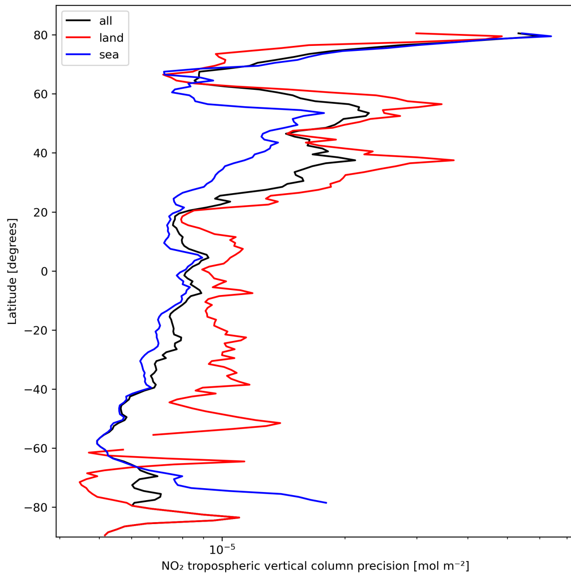
Figure 13: Zonal average of “NO 2 tropospheric vertical column precision” for 2024-02-27 to 2024-02-29.
