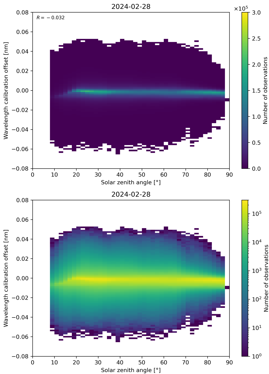
Figure 158: Scatter density plot of “Solar zenith angle” against “Wavelength calibration offset” for 2024-02-27 to 2024-02-29.
