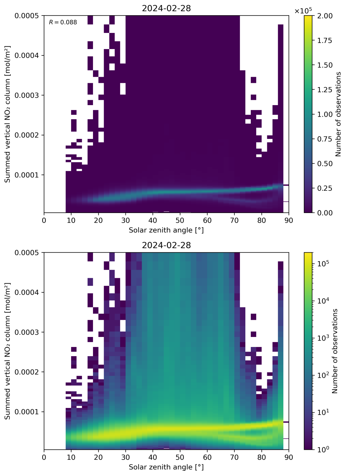
Figure 151: Scatter density plot of “Solar zenith angle” against “Summed vertical NO 2 column” for 2024-02-27 to 2024-02-29.
