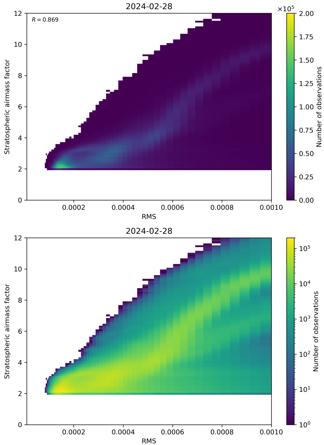
Figure 144: Scatter density plot of “RMS” against “Stratospheric airmass factor” for 2024-02-27 to 2024-02-29.
