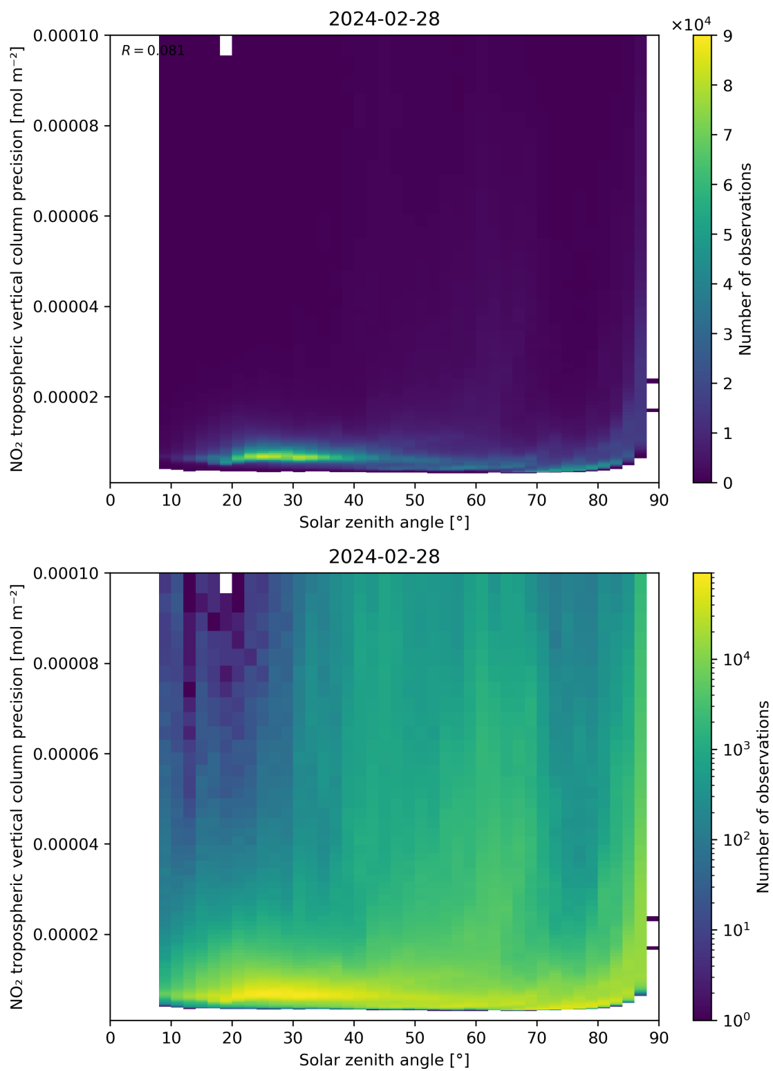
Figure 156: Scatter density plot of “Solar zenith angle” against “NO 2 tropospheric vertical column precision” for 2024-02-27 to 2024-02-29.
