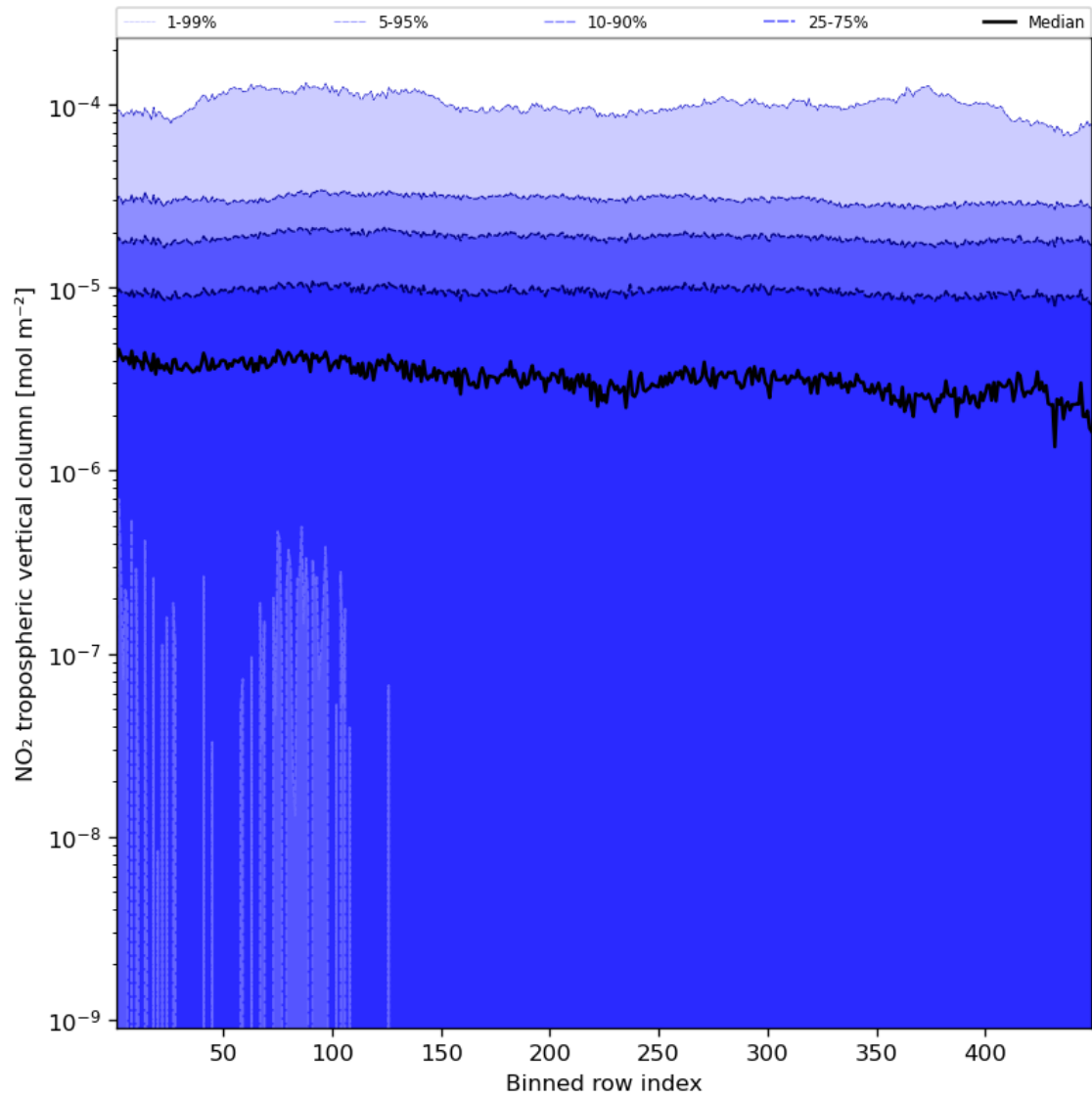
Figure 46: Along track statistics of “NO 2 tropospheric vertical column” for 2024-02-27 to 2024-02-29
