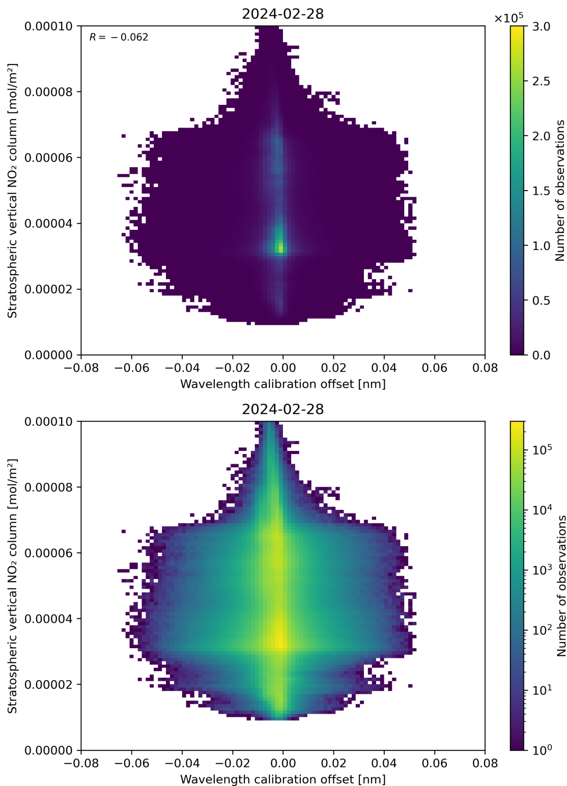
Figure 176: Scatter density plot of “Wavelength calibration offset” against “Stratospheric vertical NO 2 column” for 2024-02-27 to 2024-02-29.
