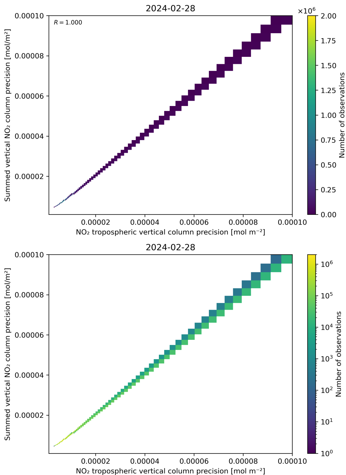
Figure 137: Scatter density plot of “NO 2 tropospheric vertical column precision” against “Summed vertical NO 2 column precision” for 2024-02-27 to 2024-02-29.
