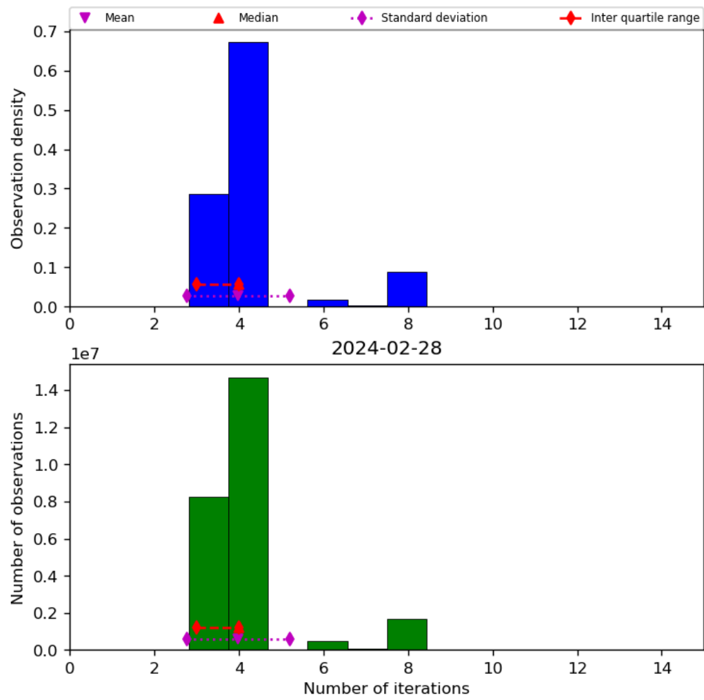
Figure 34: Histogram of “Number of iterations” for 2024-02-27 to 2024-02-29
