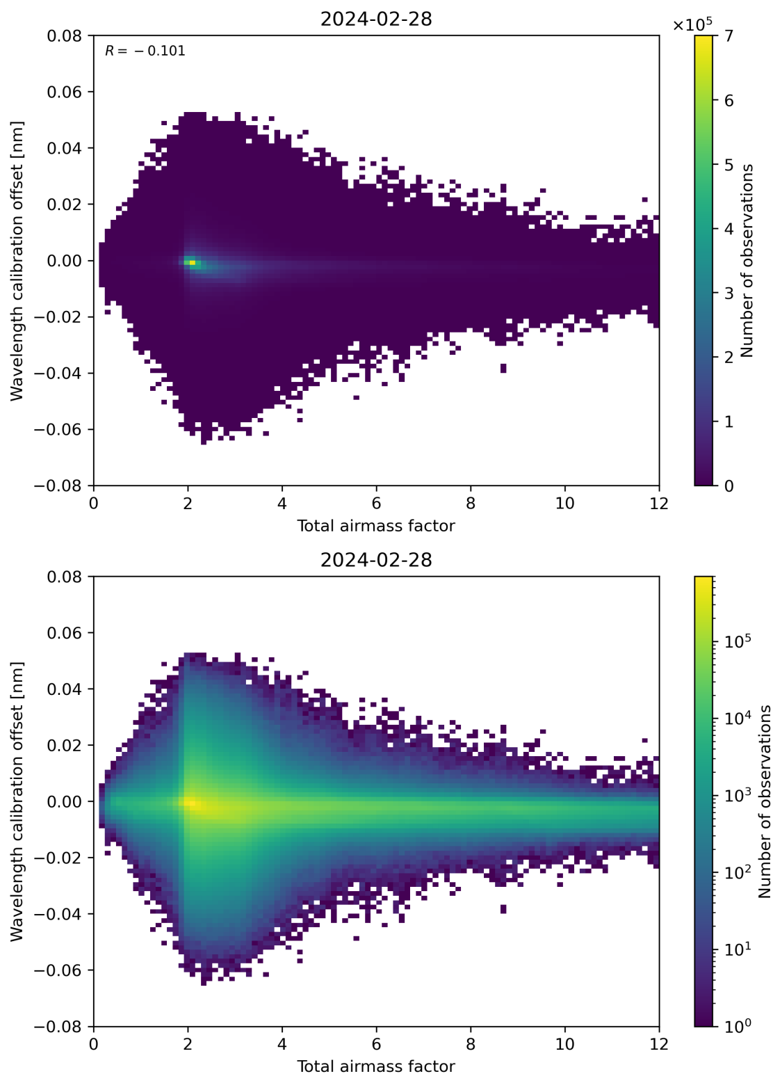
Figure 70: Scatter density plot of “Total airmass factor” against “Wavelength calibration offset” for 2024-02-27 to 2024-02-29.
