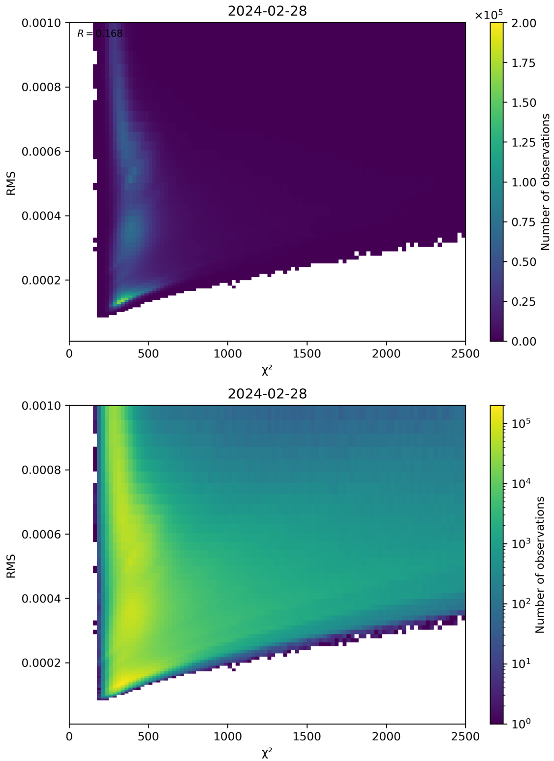
Figure 82: Scatter density plot of “ \chi^2 ” against “RMS” for 2024-02-27 to 2024-02-29.
