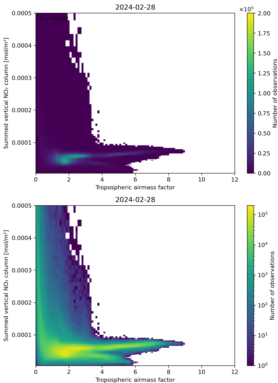
Figure 75: Scatter density plot of “Tropospheric airmass factor” against “Summed vertical NO 2 column” for 2024-02-27 to 2024-02-29.
