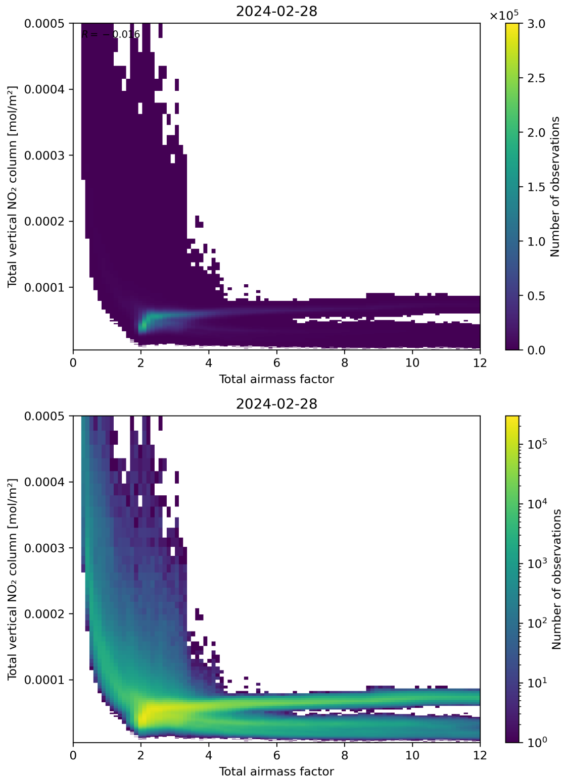
Figure 67: Scatter density plot of “Total airmass factor” against “Total vertical NO 2 column” for 2024-02-27 to 2024-02-29.
