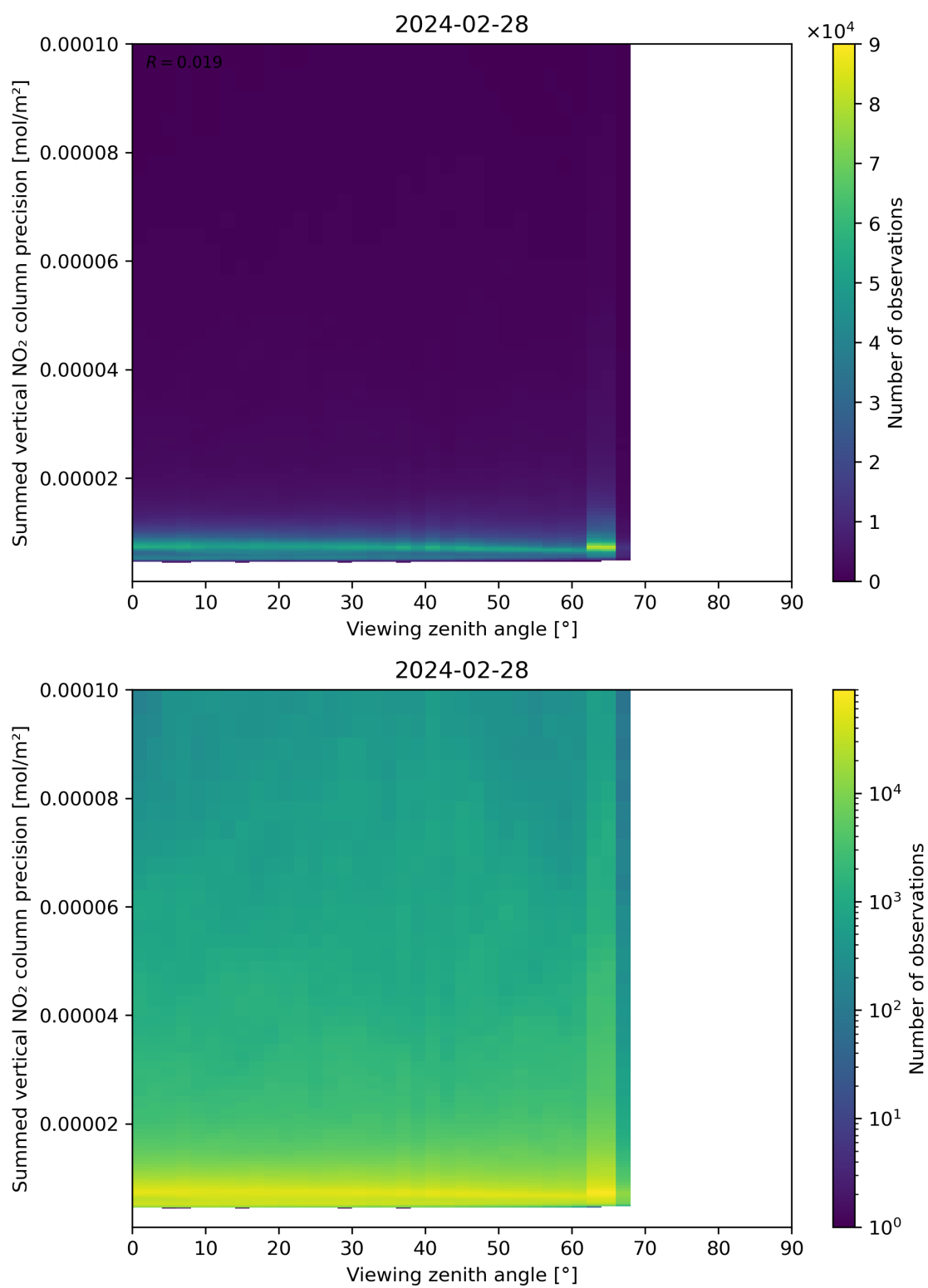
Figure 166: Scatter density plot of “Viewing zenith angle” against “Summed vertical NO 2 column precision” for 2024-02-27 to 2024-02-29.
