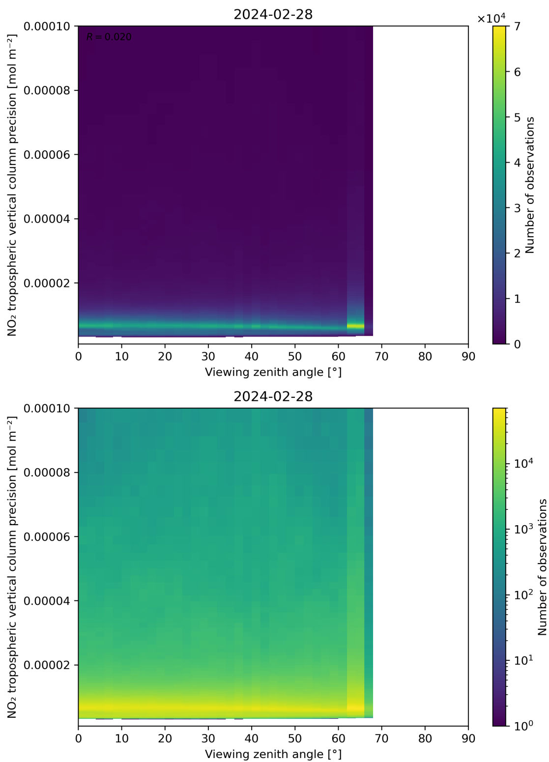
Figure 170: Scatter density plot of “Viewing zenith angle” against “NO 2 tropospheric vertical column precision” for 2024-02-27 to 2024-02-29.
