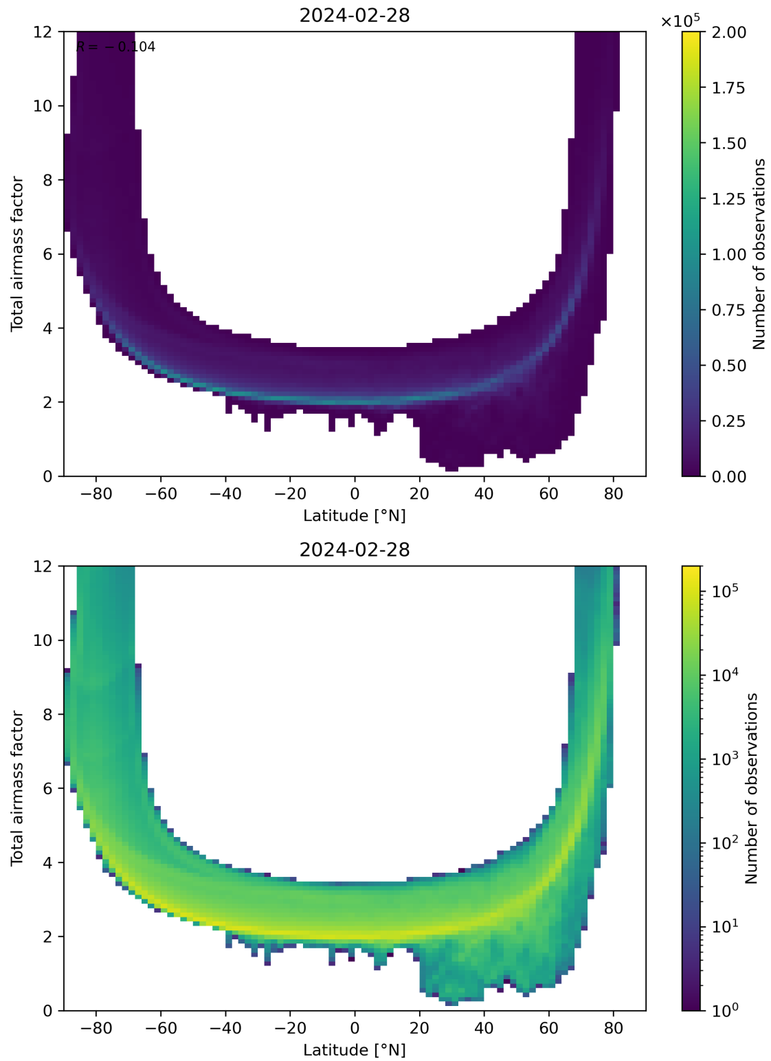
Figure 84: Scatter density plot of “Latitude” against “Total airmass factor” for 2024-02-27 to 2024-02-29.
