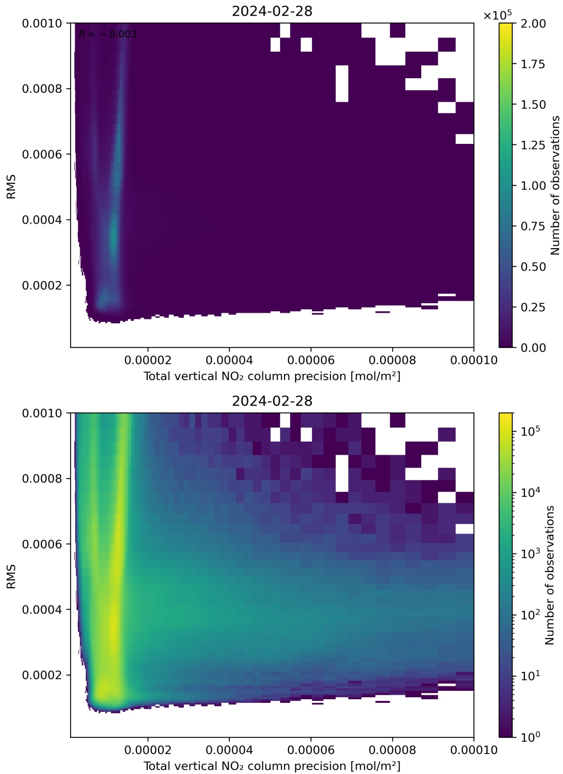
Figure 119: Scatter density plot of “Total vertical NO 2 column precision” against “RMS” for 2024-02-27 to 2024-02-29.
