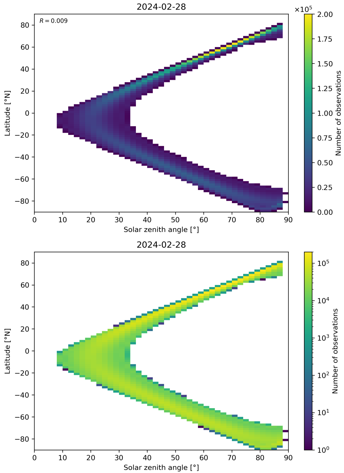
Figure 149: Scatter density plot of “Solar zenith angle” against “Latitude” for 2024-02-27 to 2024-02-29.
