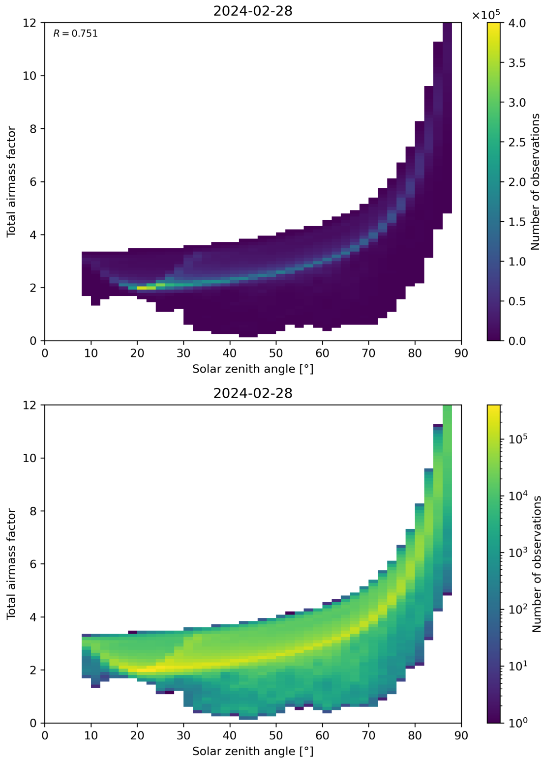
Figure 146: Scatter density plot of “Solar zenith angle” against “Total airmass factor” for 2024-02-27 to 2024-02-29.
