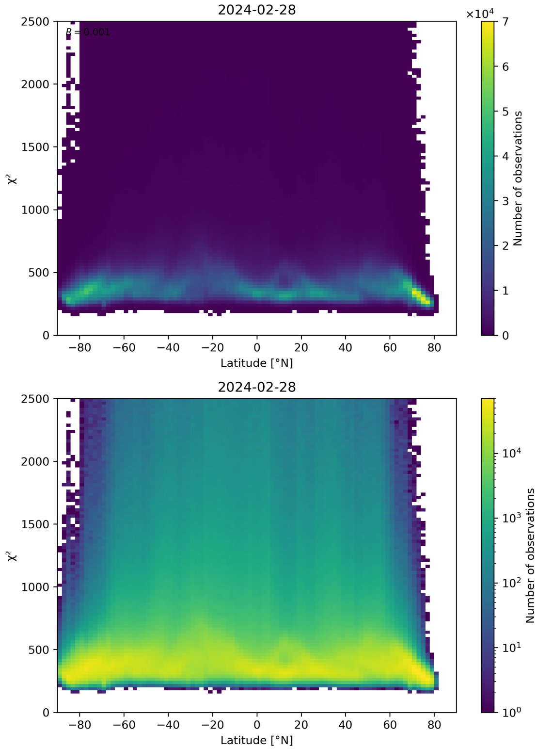
Figure 86: Scatter density plot of “Latitude” against “ \chi^2 ” for 2024-02-27 to 2024-02-29.
