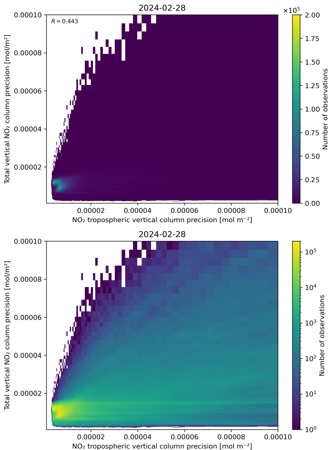
Figure 139: Scatter density plot of “NO 2 tropospheric vertical column precision” against “Total vertical NO 2 column precision” for 2024-02-27 to 2024-02-29.
