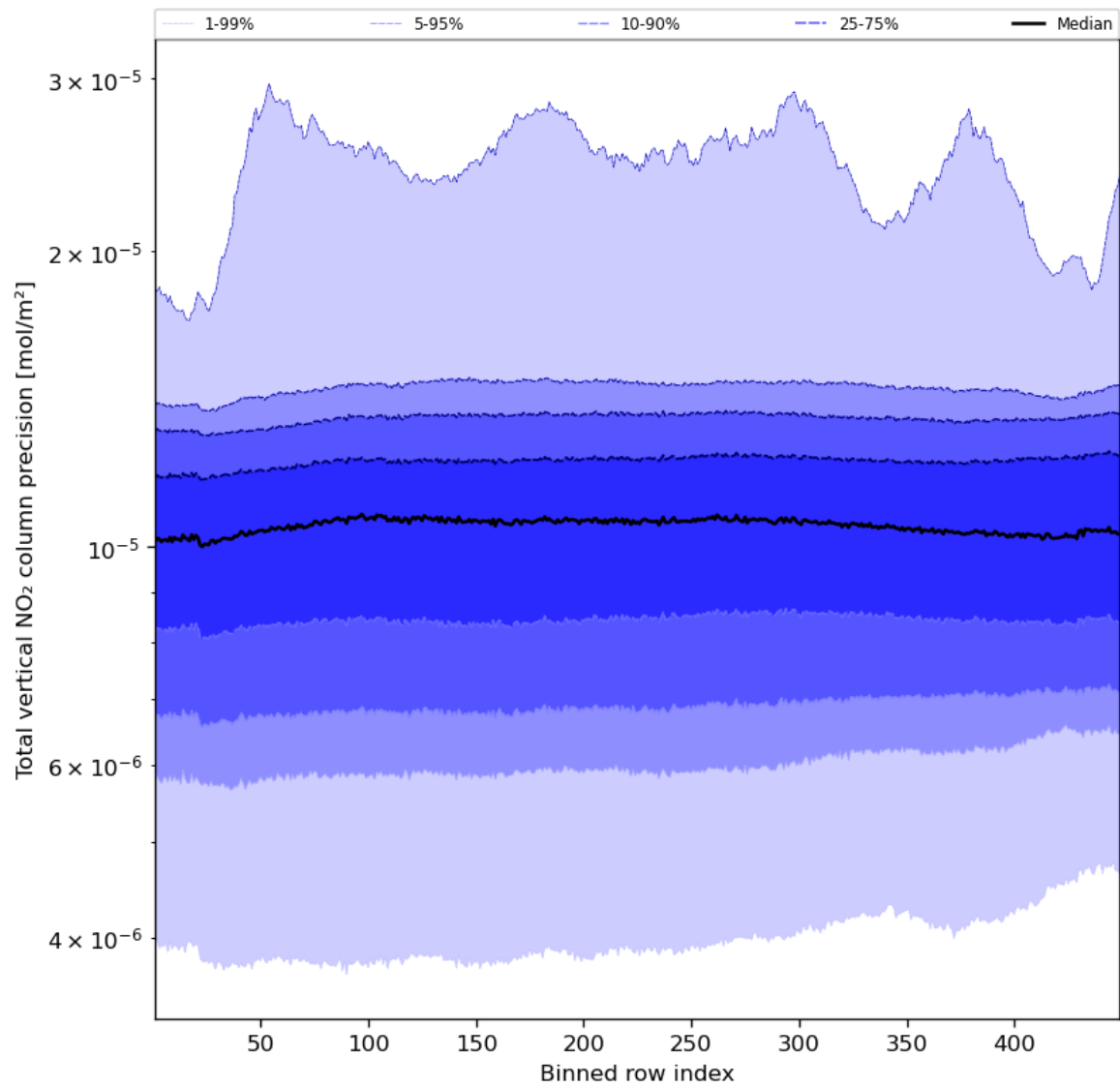
Figure 56: Along track statistics of “Total vertical NO 2 column precision” for 2024-02-27 to 2024-02-29
