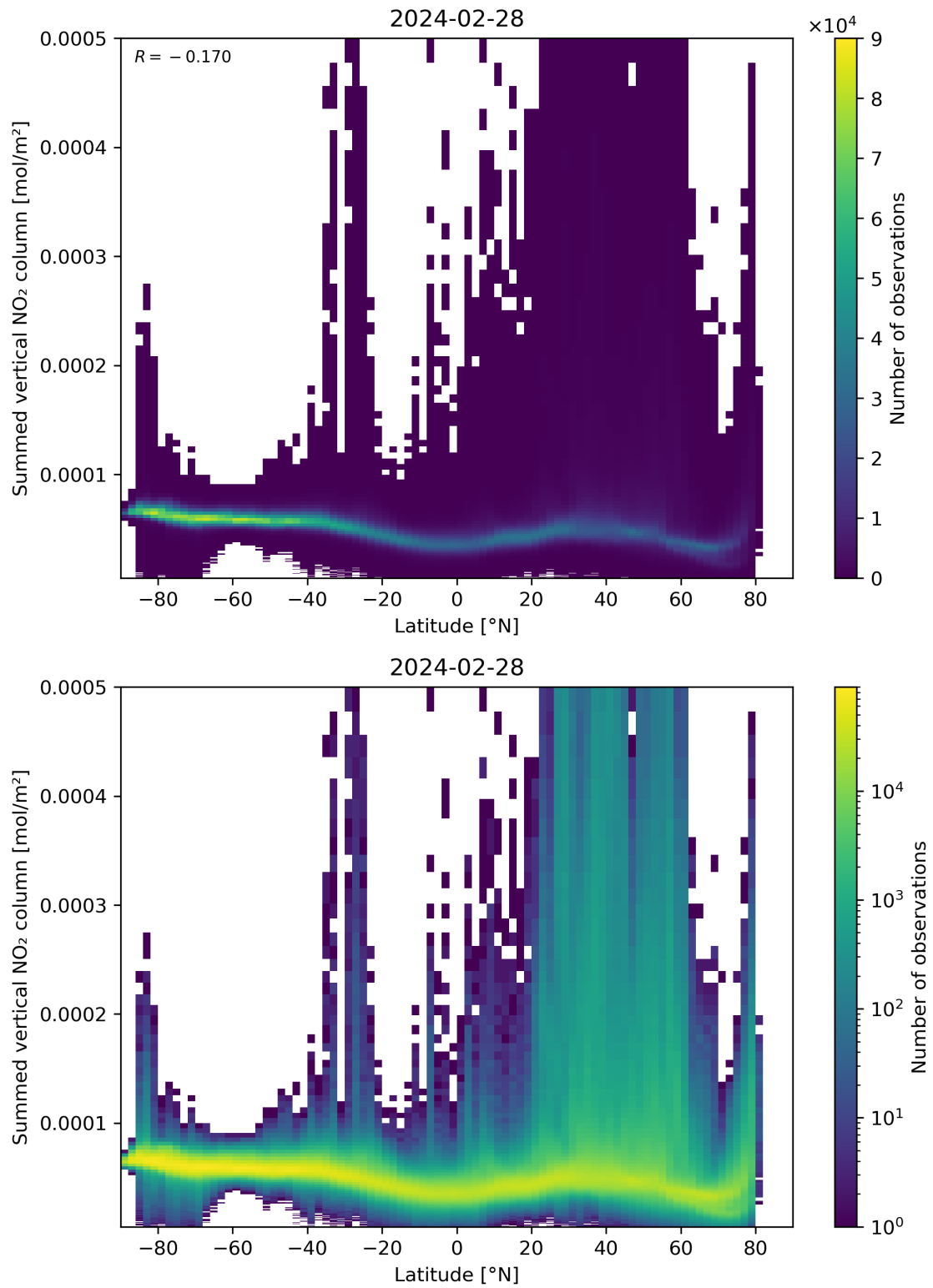
Figure 88: Scatter density plot of “Latitude” against “Summed vertical NO 2 column” for 2024-02-27 to 2024-02-29.
