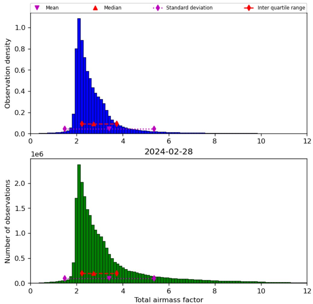
Figure 32: Histogram of “Total airmass factor” for 2024-02-27 to 2024-02-29
