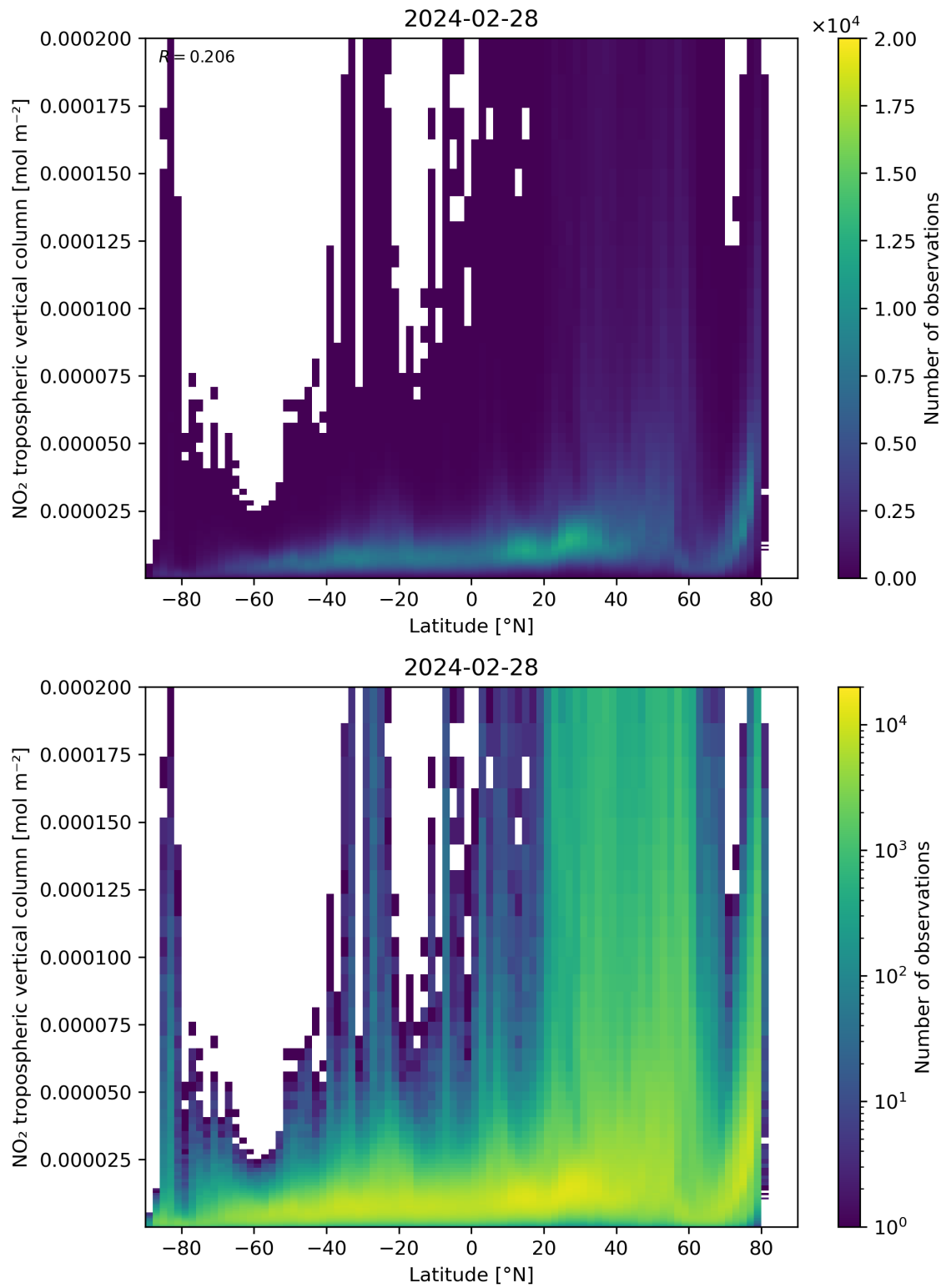
Figure 92: Scatter density plot of “Latitude” against “NO 2 tropospheric vertical column” for 2024-02-27 to 2024-02-29.
