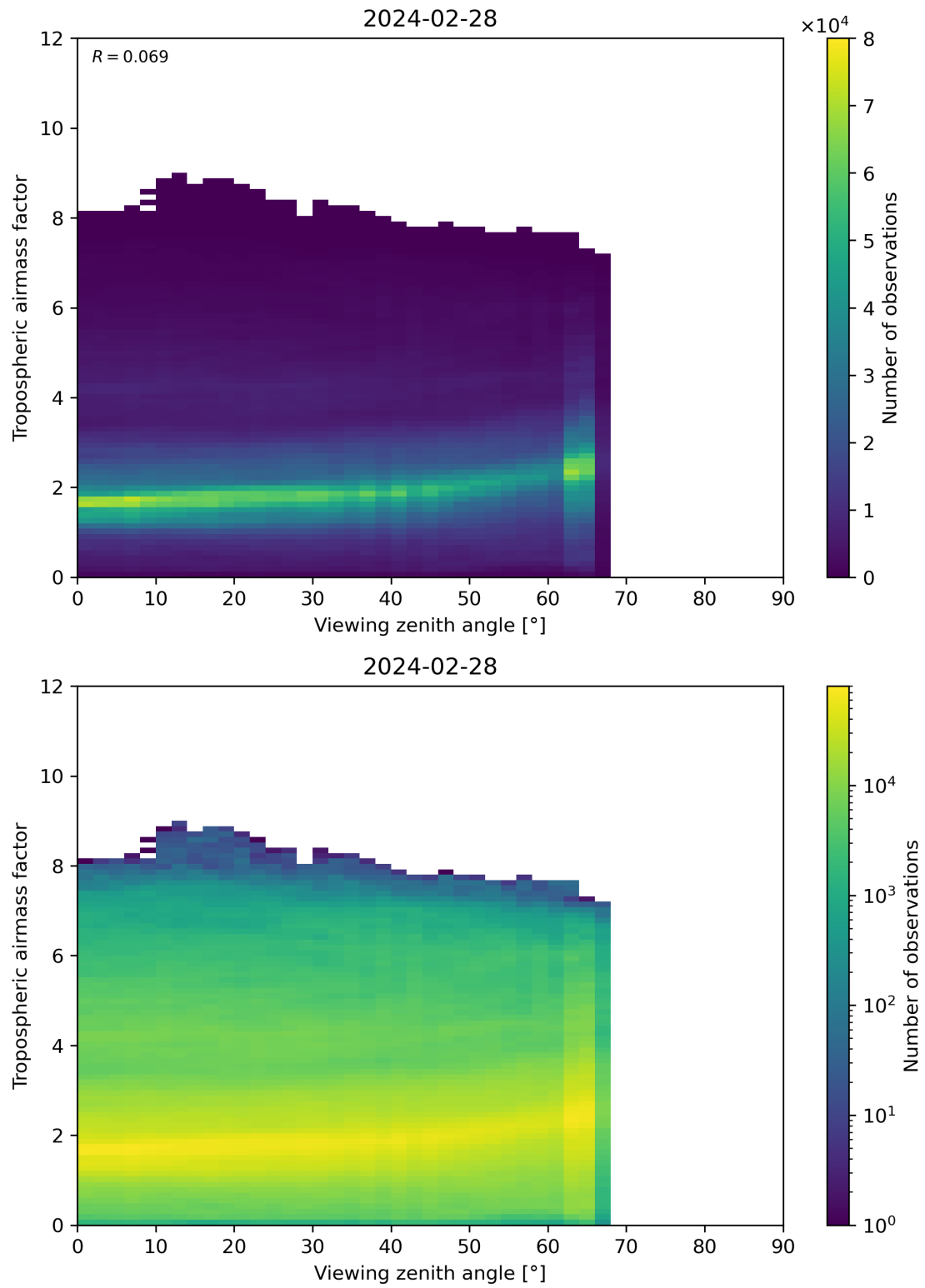
Figure 161: Scatter density plot of “Viewing zenith angle” against “Tropospheric airmass factor” for 2024-02-27 to 2024-02-29.
