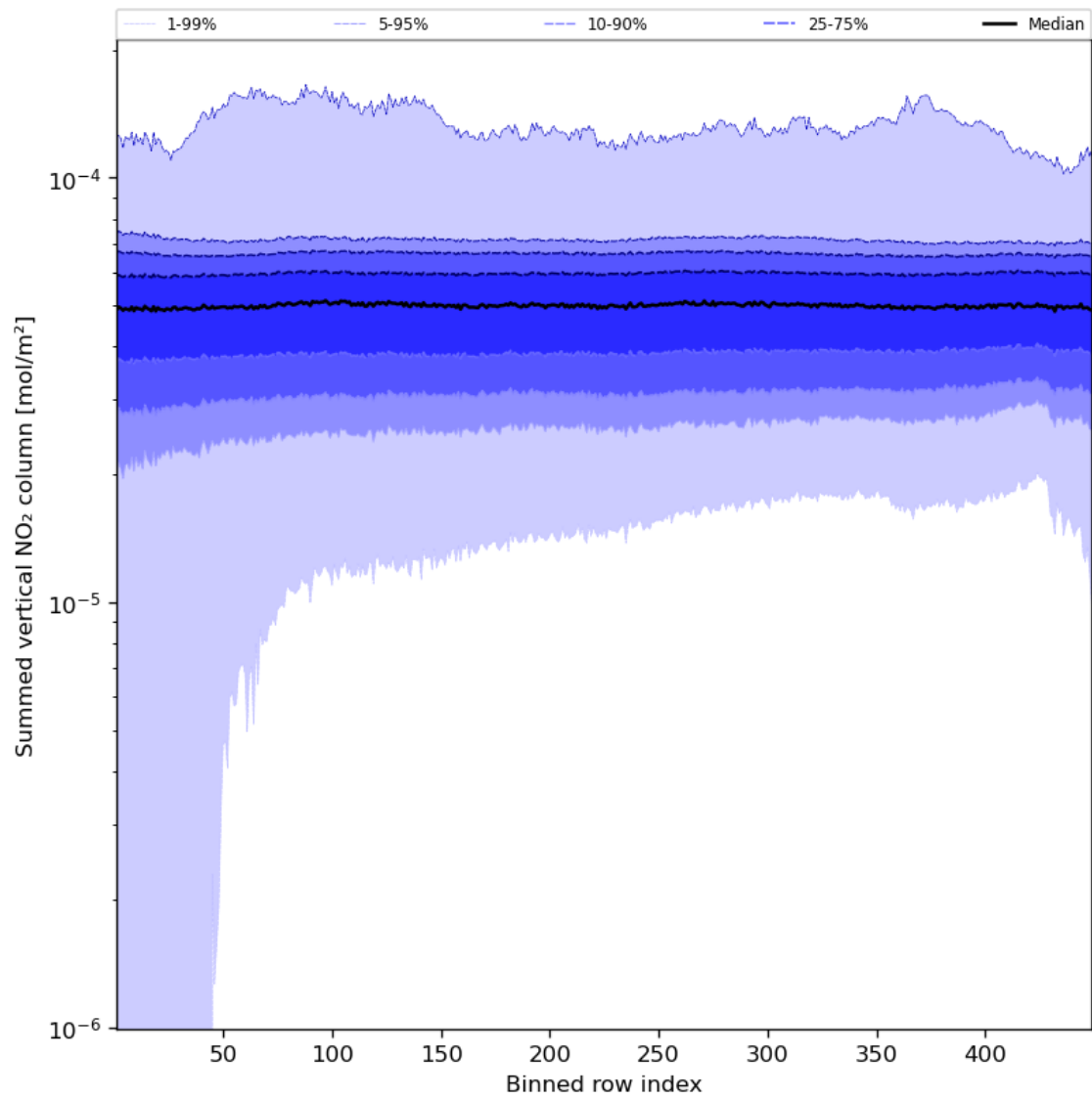
Figure 57: Along track statistics of “Summed vertical NO 2 column” for 2024-02-27 to 2024-02-29
