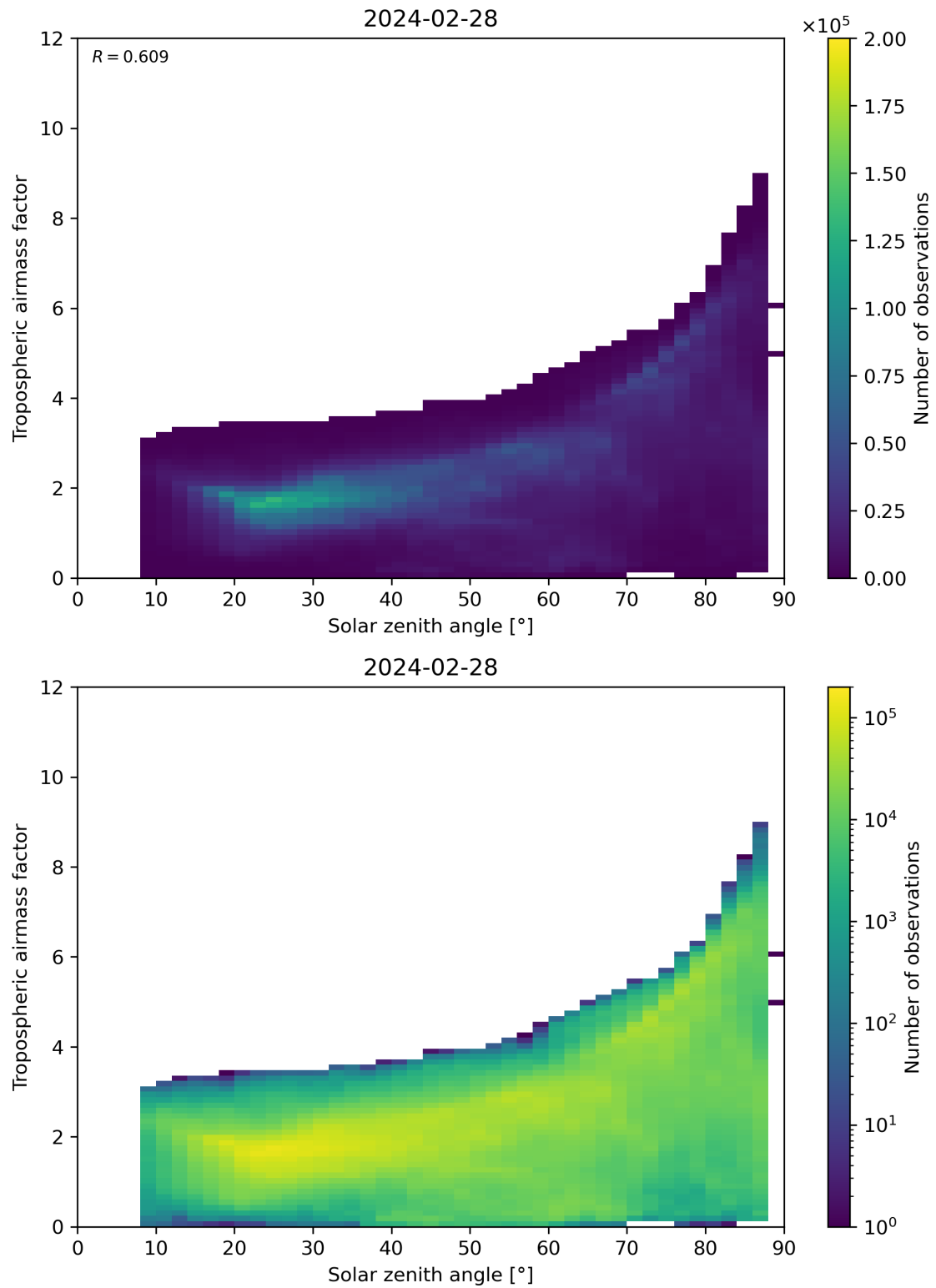
Figure 147: Scatter density plot of “Solar zenith angle” against “Tropospheric airmass factor” for 2024-02-27 to 2024-02-29.
