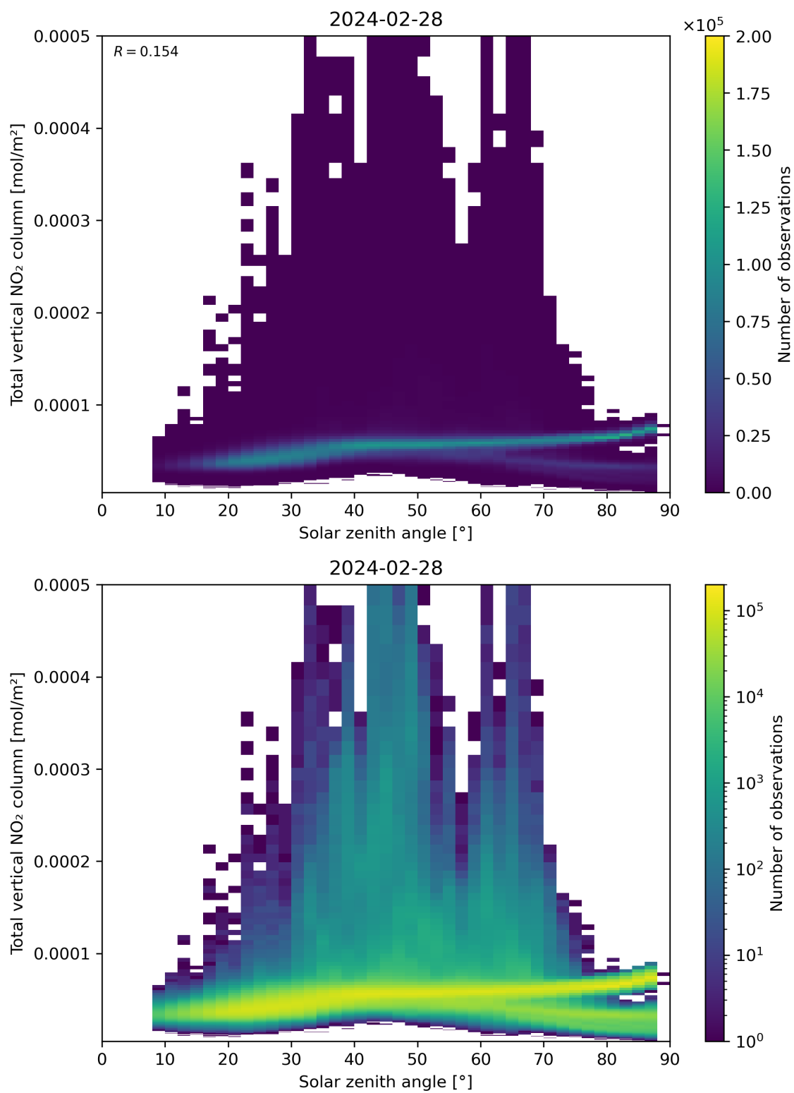
Figure 153: Scatter density plot of “Solar zenith angle” against “Total vertical NO 2 column” for 2024-02-27 to 2024-02-29.
