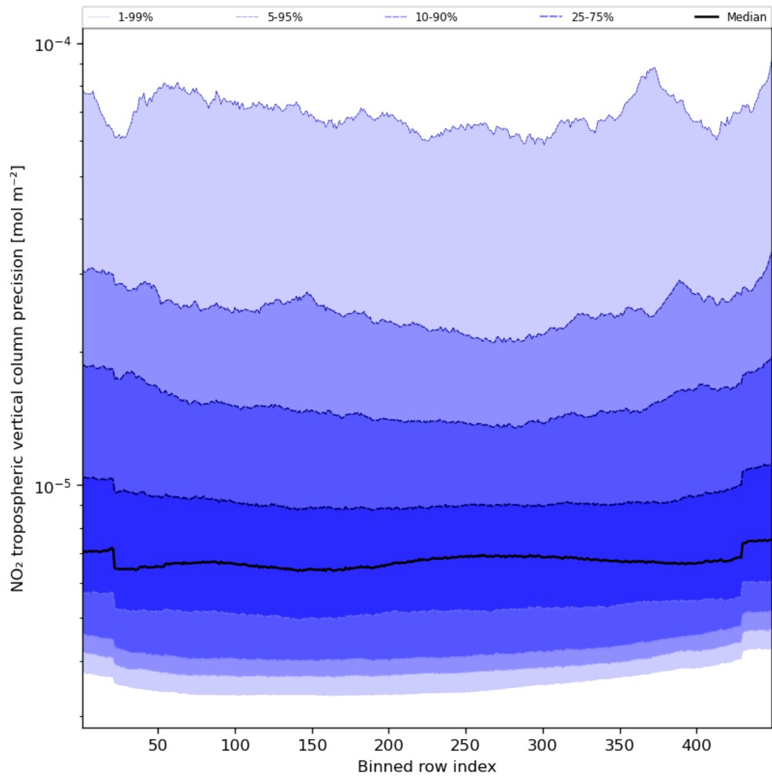
Figure 47: Along track statistics of “NO 2 tropospheric vertical column precision” for 2024-02-27 to 2024-02-29
