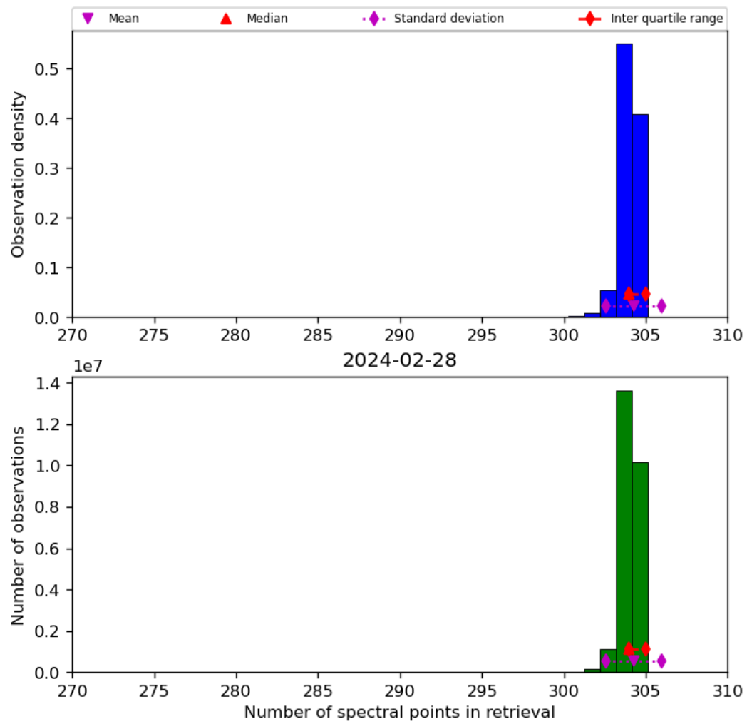
Figure 33: Histogram of “Number of spectral points in retrieval” for 2024-02-27 to 2024-02-29
