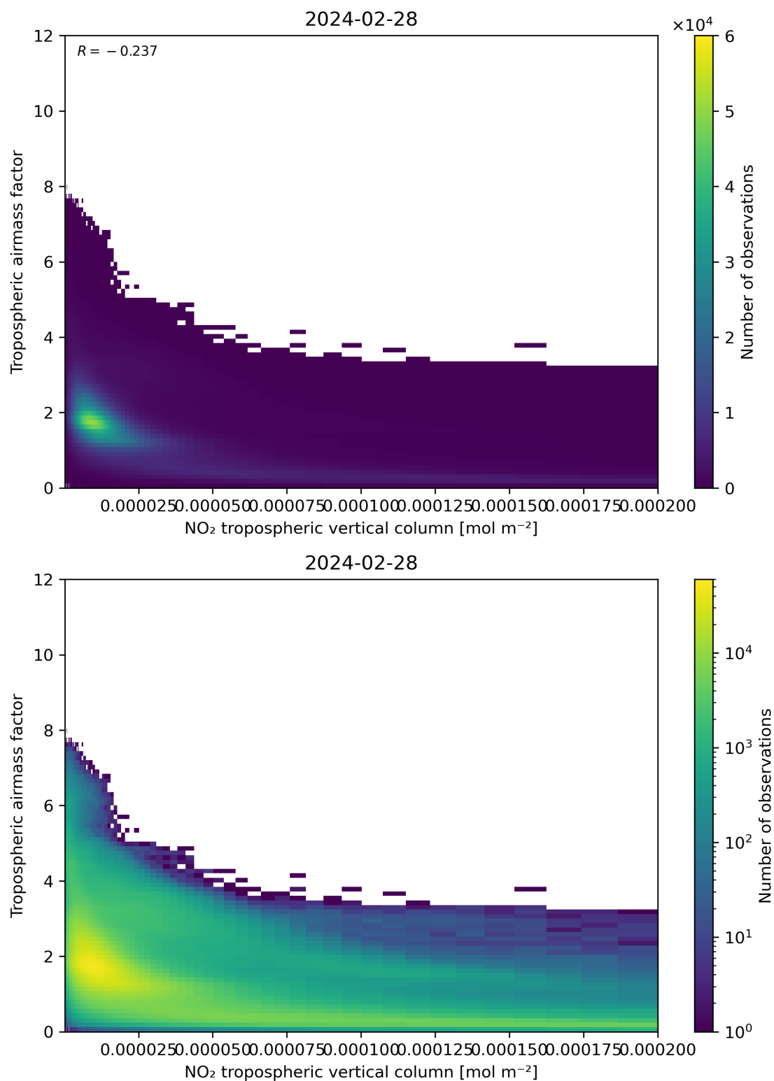
Figure 123: Scatter density plot of “NO 2 tropospheric vertical column” against “Tropospheric air mass factor” for 2024-02-27 to 2024-02-29.
