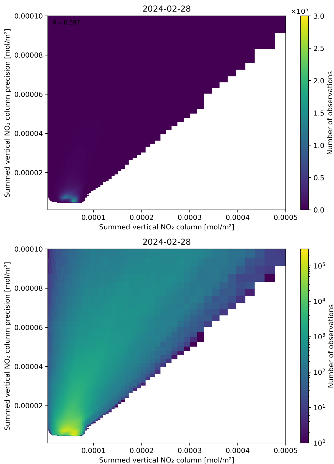
Figure 105: Scatter density plot of “Summed vertical NO 2 column” against “Summed vertical NO 2 column precision” for 2024-02-27 to 2024-02-29.
