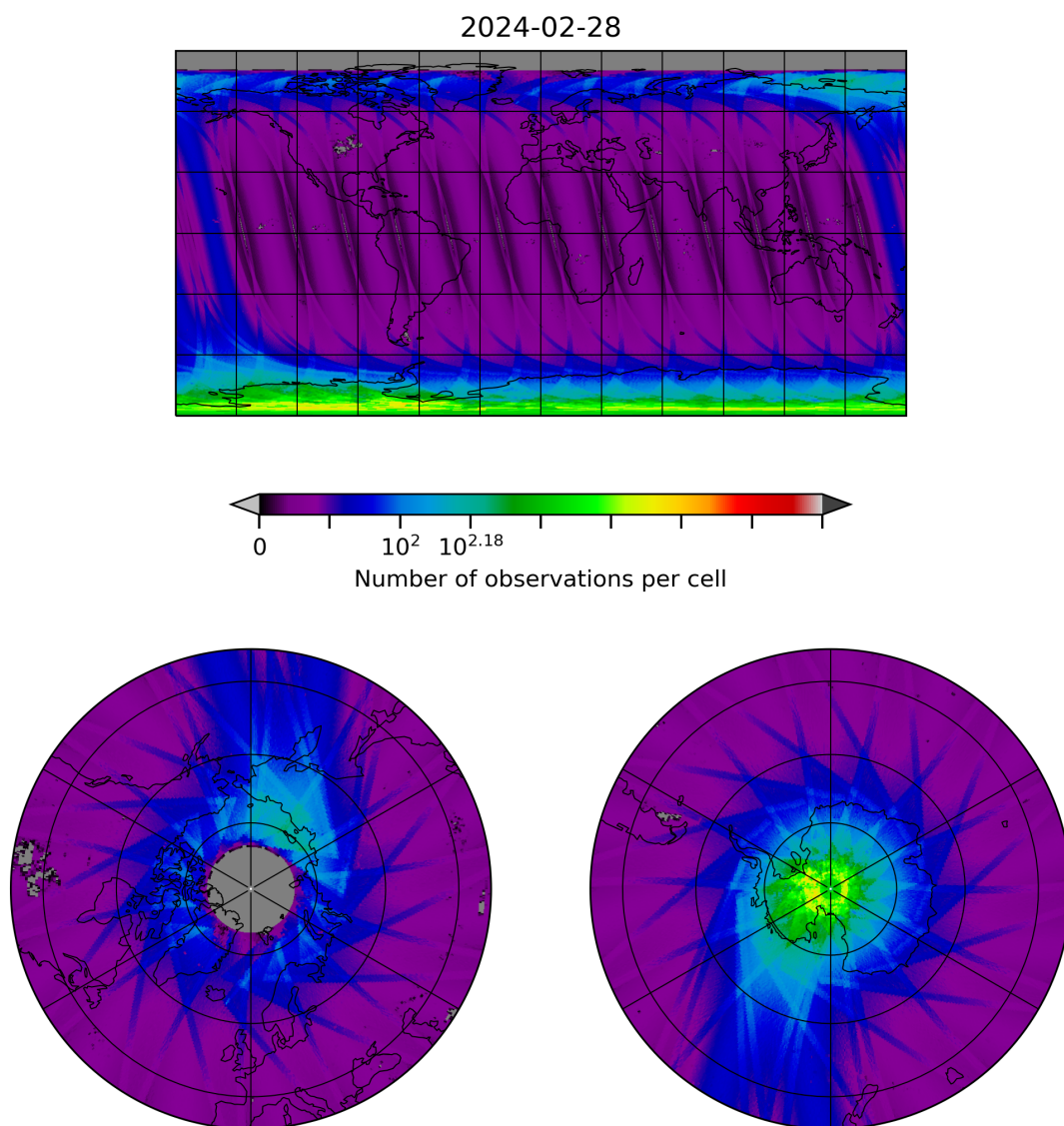
Figure 10: Map of the number of observations for 2024-02-27 to 2024-02-29
