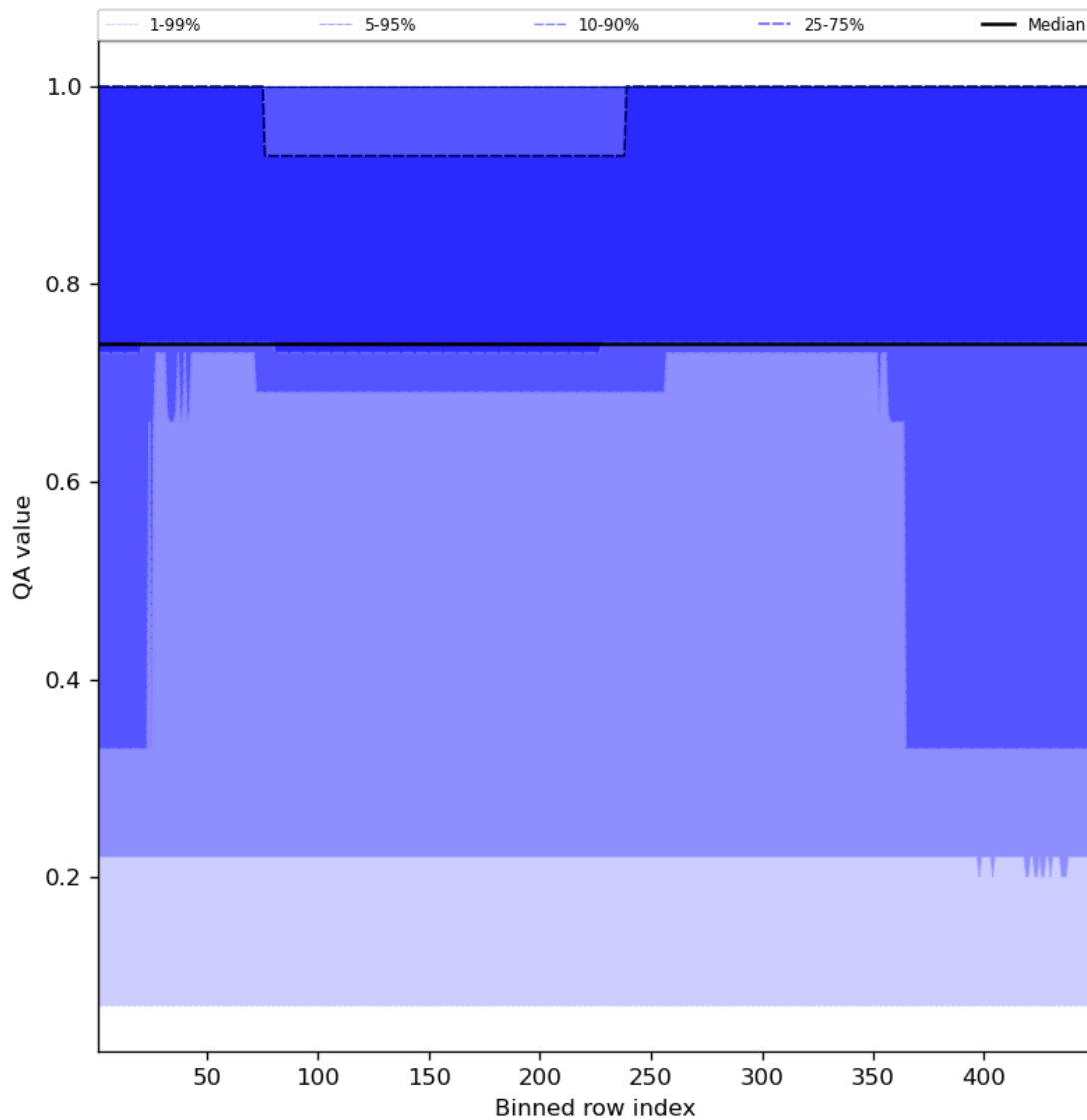
Figure 45: Along track statistics of “QA value” for 2024-02-27 to 2024-02-29
