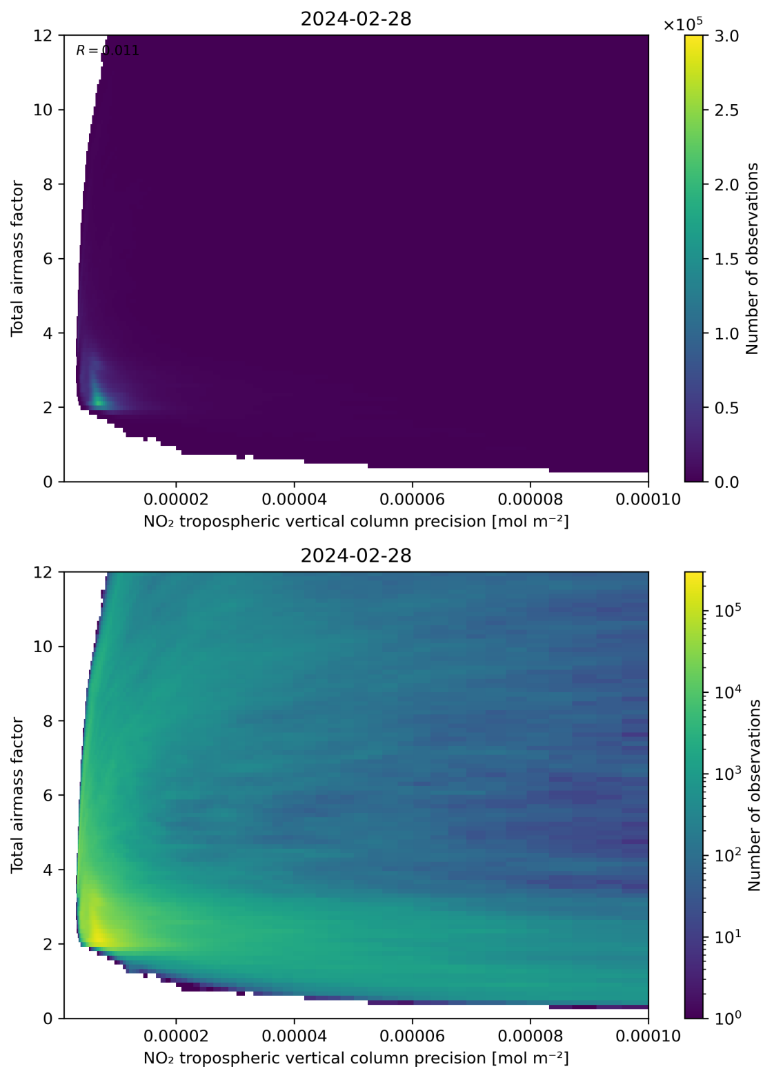
Figure 132: Scatter density plot of “NO 2 tropospheric vertical column precision” against “Total air mass factor” for 2024-02-27 to 2024-02-29.
