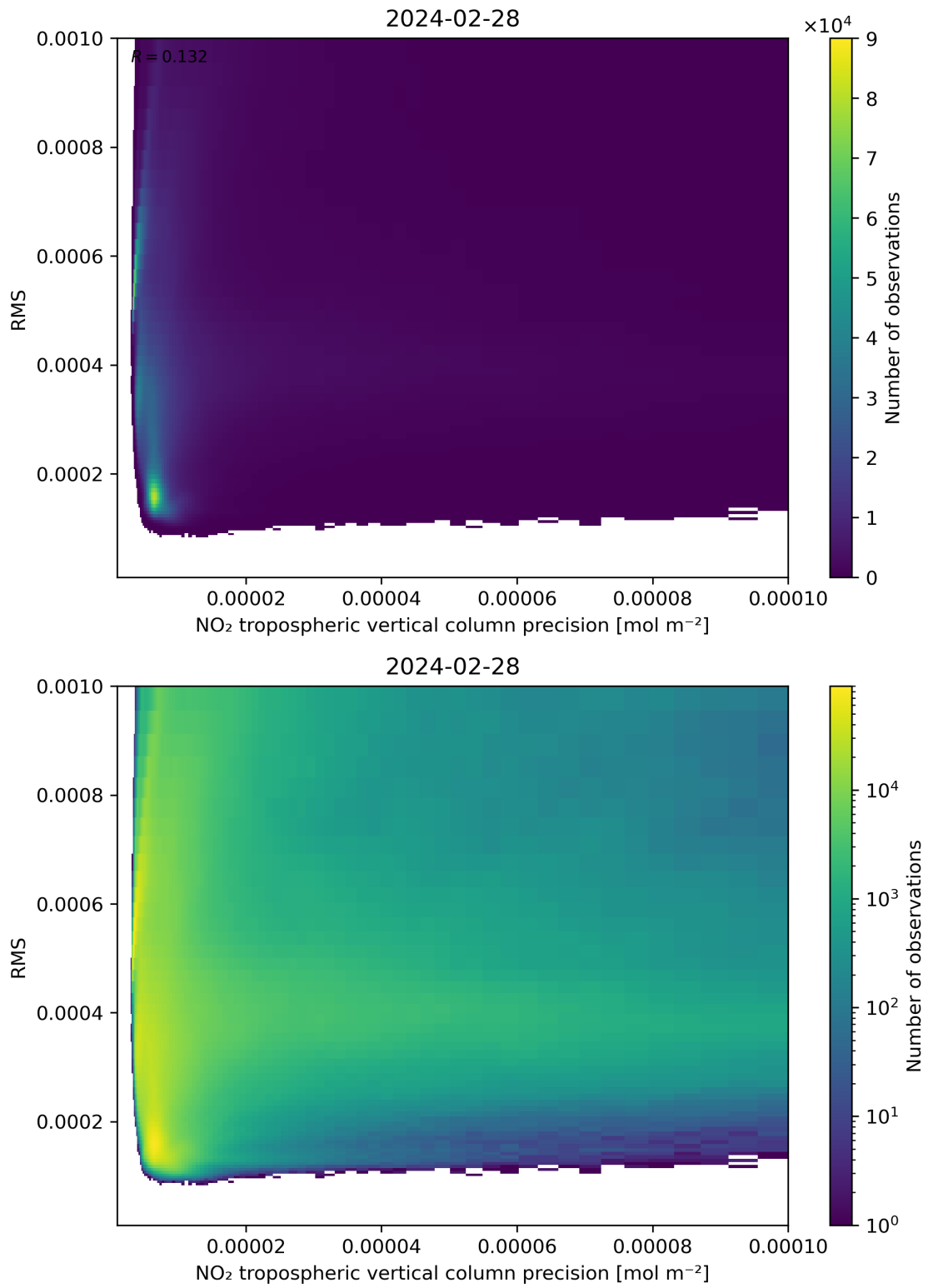
Figure 140: Scatter density plot of “NO 2 tropospheric vertical column precision” against “RMS” for 2024-02-27 to 2024-02-29.
