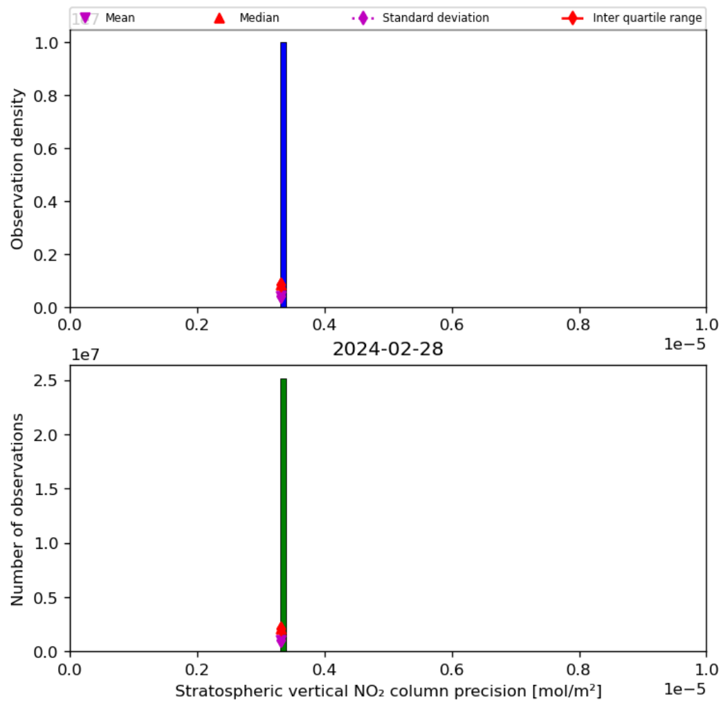
Figure 37: Histogram of “Stratospheric vertical NO 2 column precision” for 2024-02-27 to 2024-02-29
