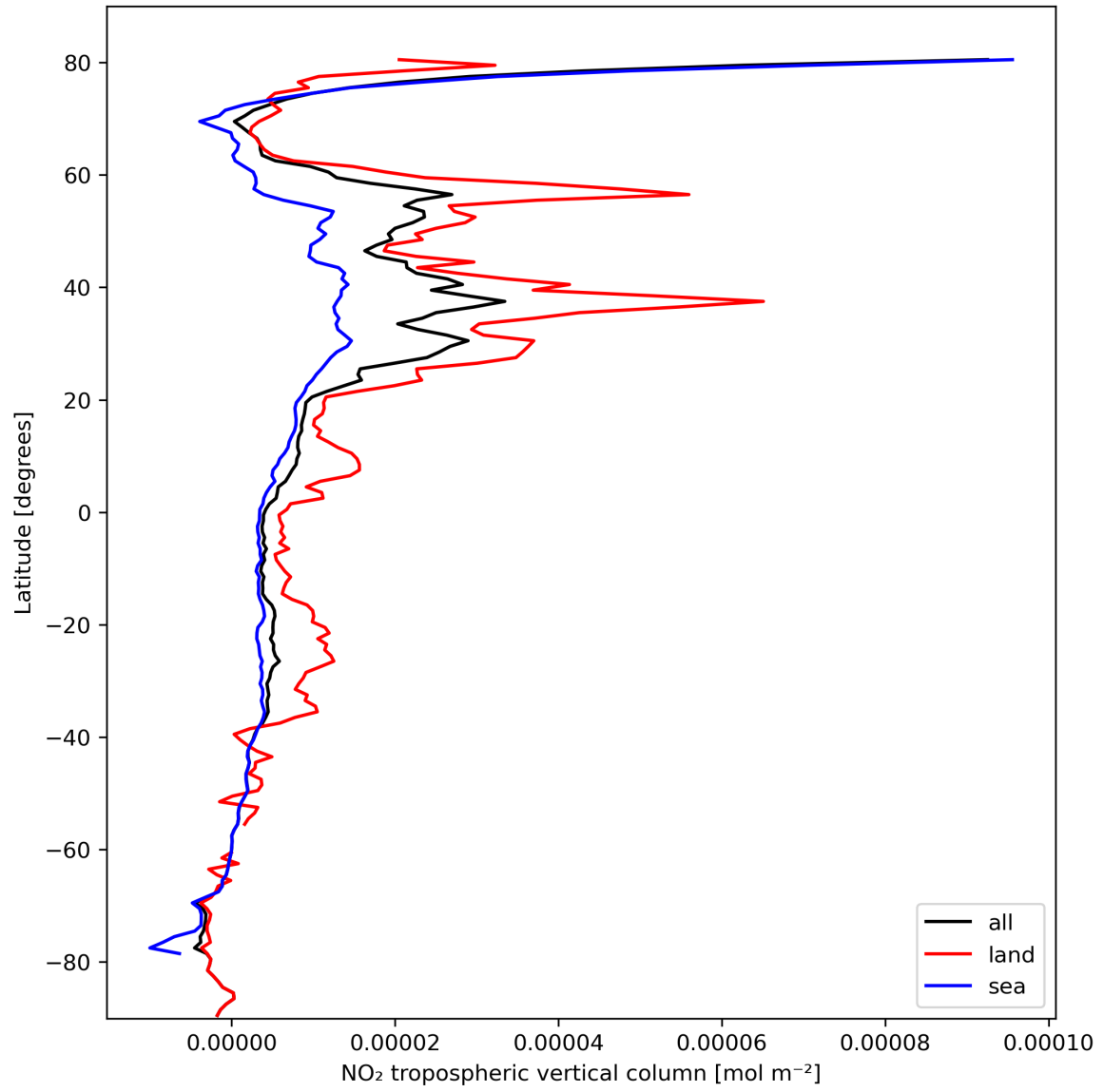
Figure 12: Zonal average of “NO 2 tropospheric vertical column” for 2024-02-27 to 2024-02-29.
