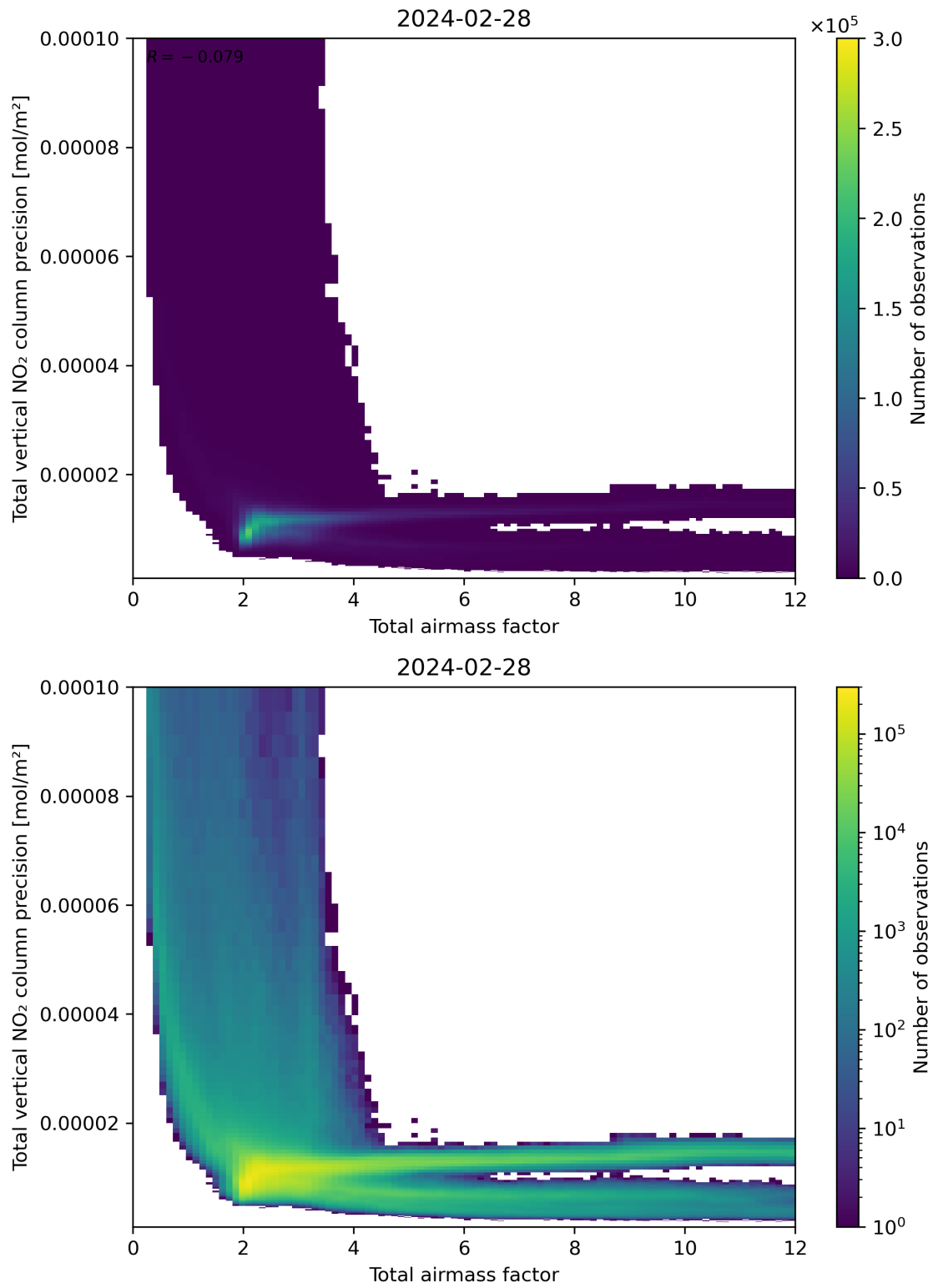
Figure 68: Scatter density plot of “Total airmass factor” against “Total vertical NO 2 column precision” for 2024-02-27 to 2024-02-29.
