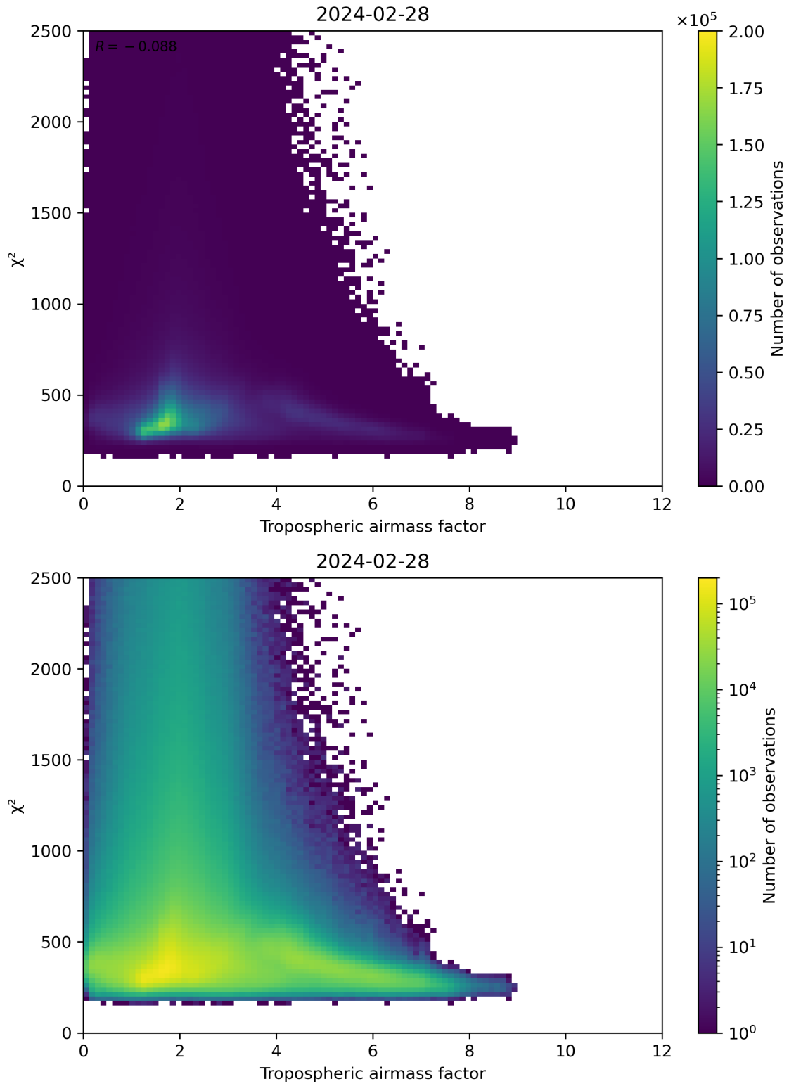
Figure 73: Scatter density plot of “Tropospheric airmass factor” against “ \chi^2 ” for 2024-02-27 to 2024-02-29.
