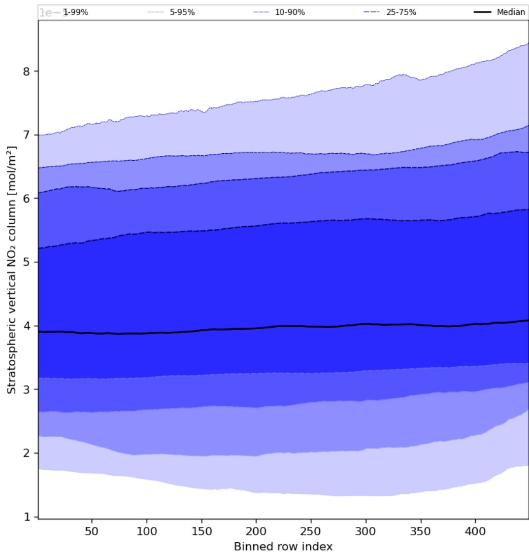
Figure 53: Along track statistics of “Stratospheric vertical NO 2 column” for 2024-02-27 to 2024-02-29
