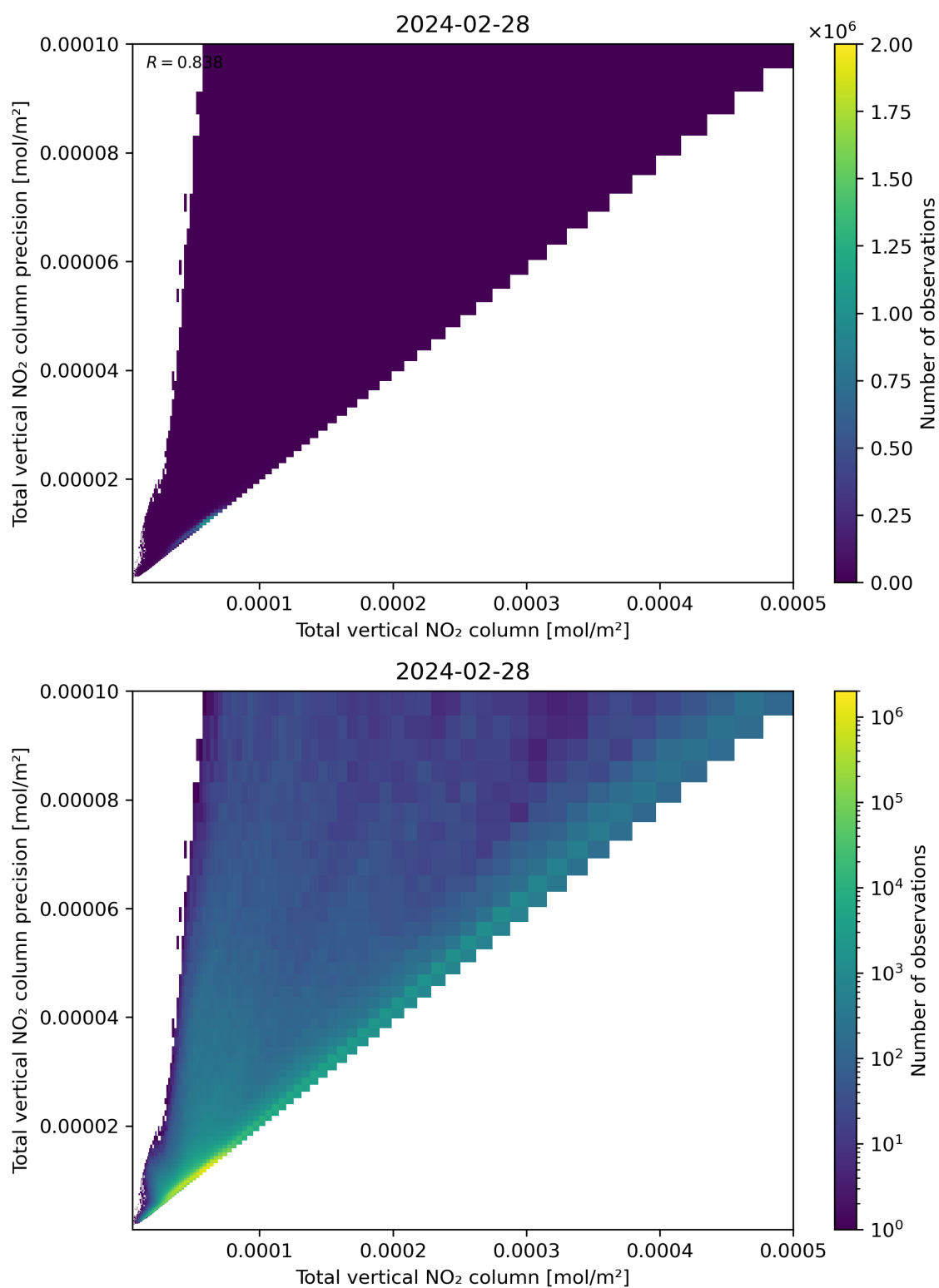
Figure 114: Scatter density plot of “Total vertical NO 2 column” against “Total vertical NO 2 column precision” for 2024-02-27 to 2024-02-29.
