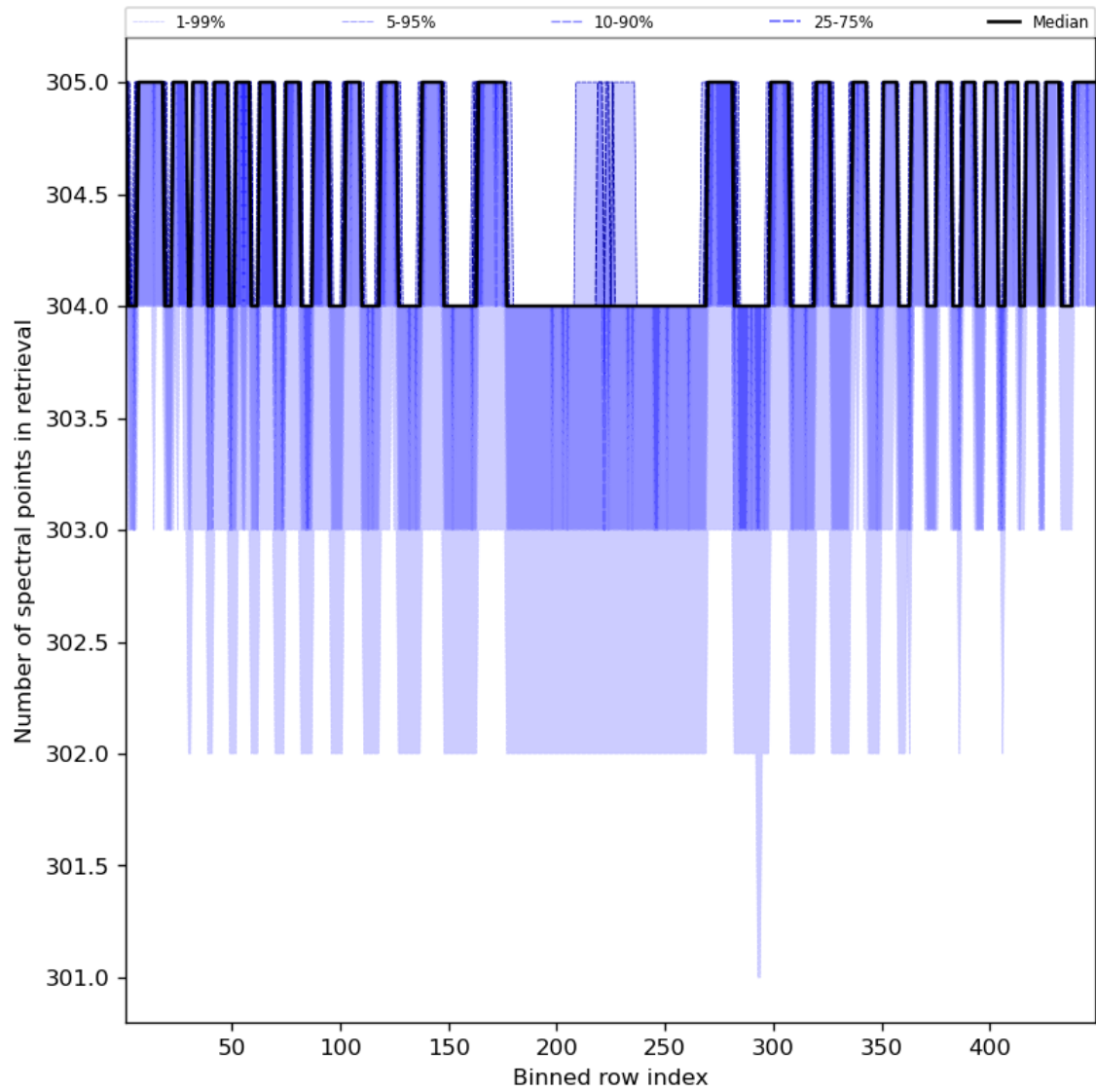
Figure 50: Along track statistics of “Number of spectral points in retrieval” for 2024-02-27 to 2024-02-29
