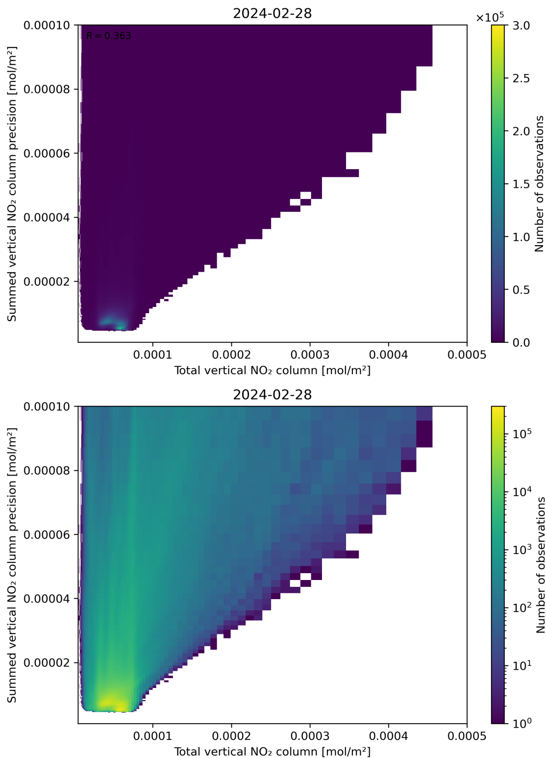
Figure 113: Scatter density plot of “Total vertical NO 2 column” against “Summed vertical NO 2 column precision” for 2024-02-27 to 2024-02-29.
