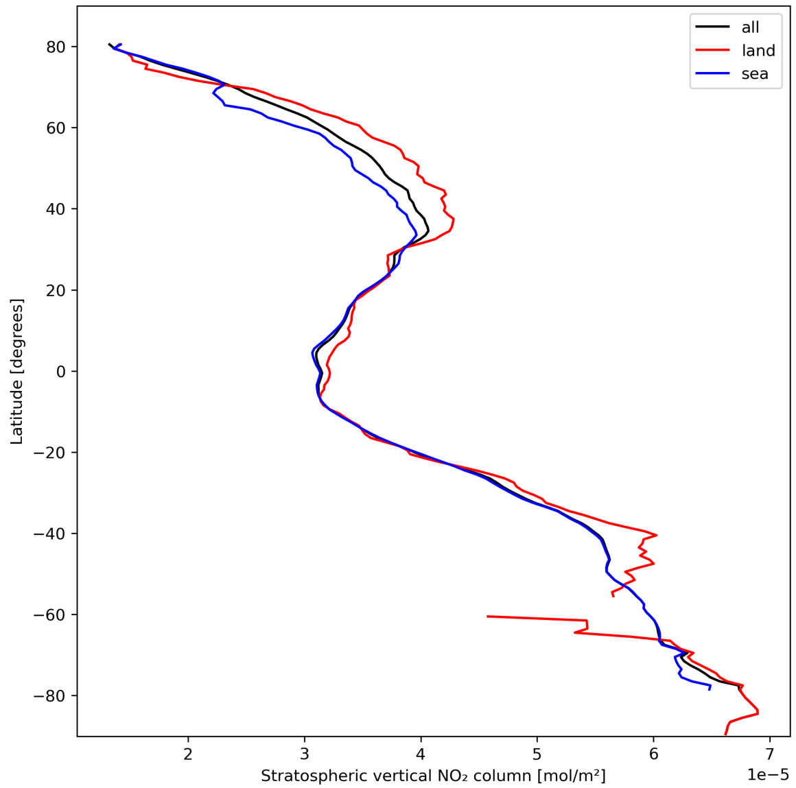
Figure 19: Zonal average of “Stratospheric vertical NO 2 column” for 2024-02-27 to 2024-02-29.
