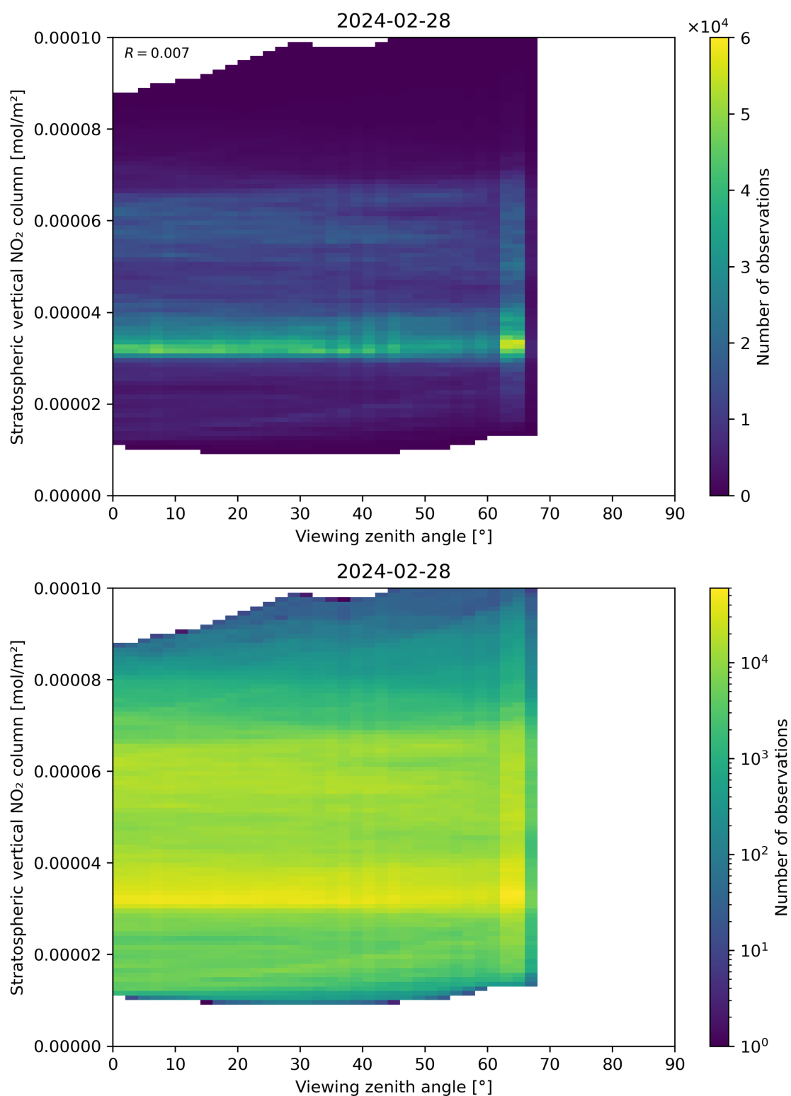
Figure 164: Scatter density plot of “Viewing zenith angle” against “Stratospheric vertical NO 2 column” for 2024-02-27 to 2024-02-29.
