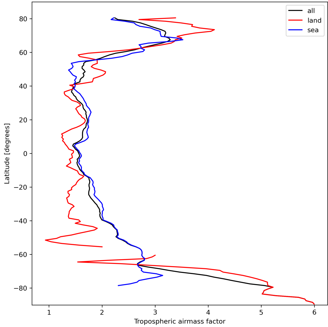
Figure 14: Zonal average of “Tropospheric airmass factor” for 2024-02-27 to 2024-02-29.
