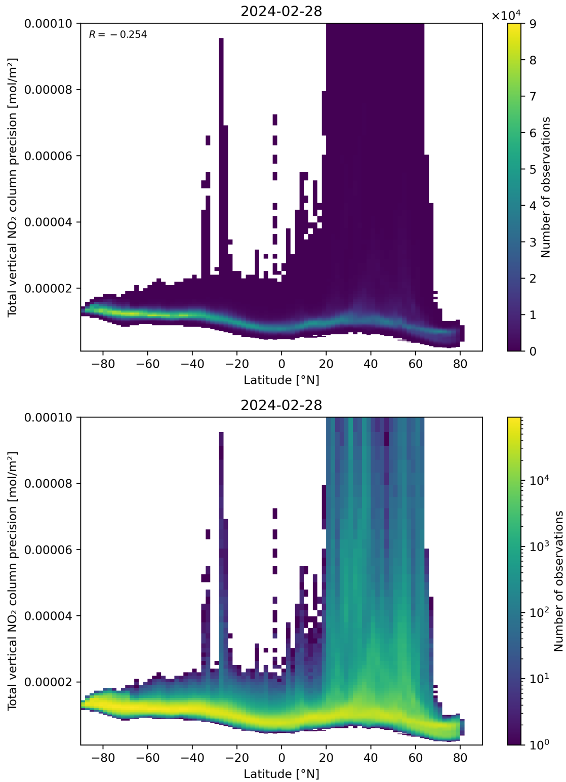
Figure 91: Scatter density plot of “Latitude” against “Total vertical NO 2 column precision” for 2024-02-27 to 2024-02-29.
