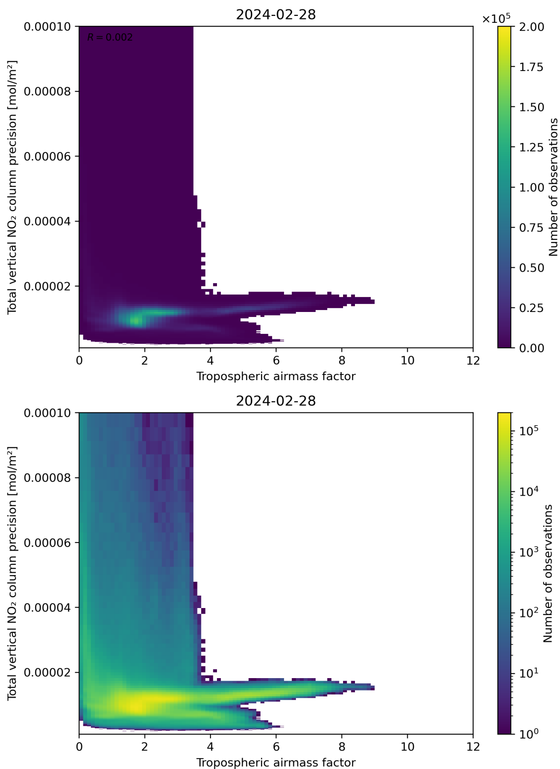
Figure 78: Scatter density plot of “Tropospheric air mass factor” against “Total vertical NO 2 column precision” for 2024-02-27 to 2024-02-29.
