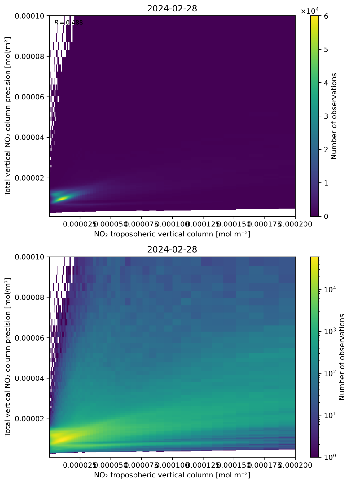
Figure 129: Scatter density plot of “NO 2 tropospheric vertical column” against “Total vertical NO 2 column precision” for 2024-02-27 to 2024-02-29.
