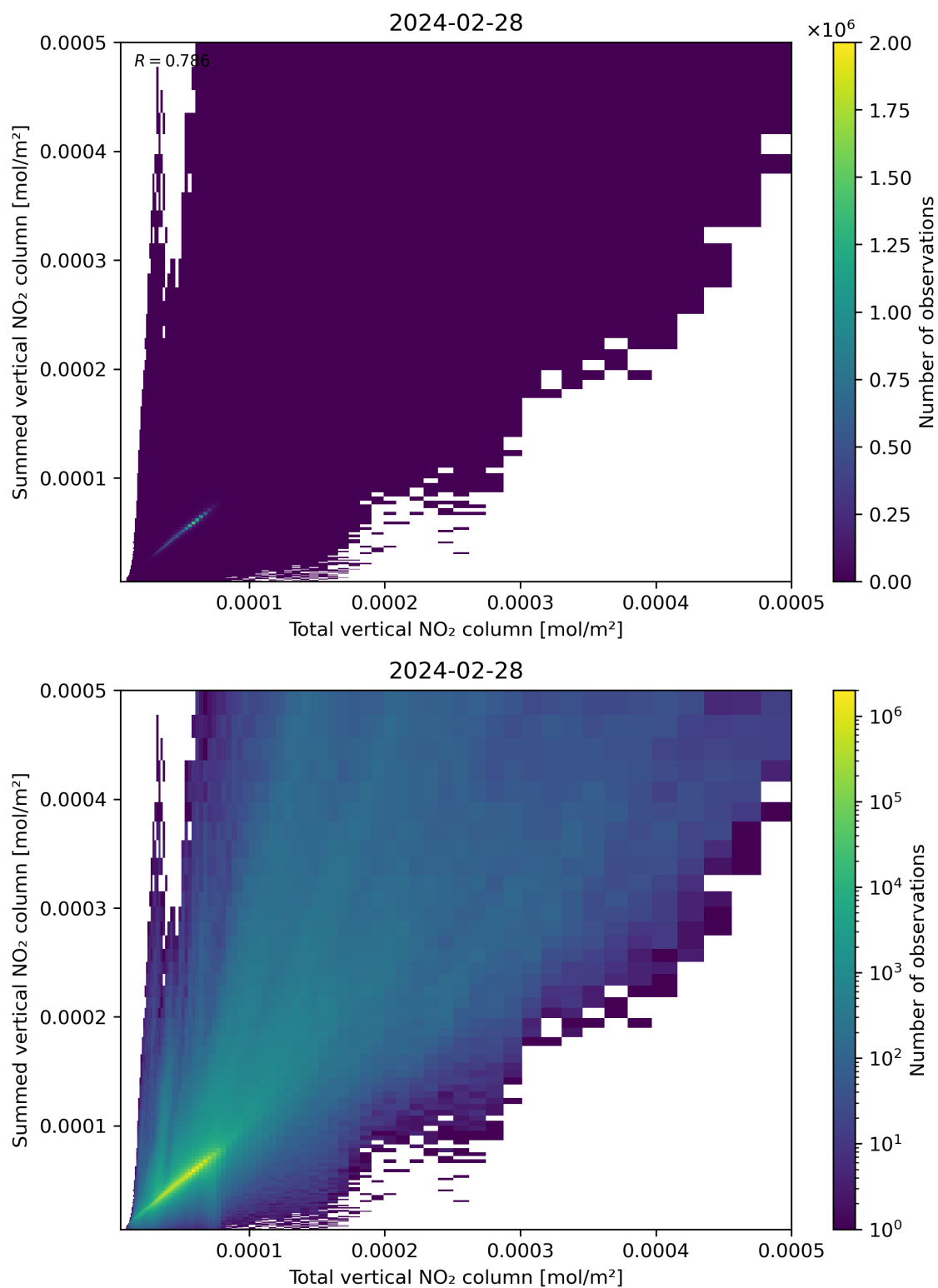
Figure 112: Scatter density plot of “Total vertical NO 2 column” against “Summed vertical NO 2 column” for 2024-02-27 to 2024-02-29.
