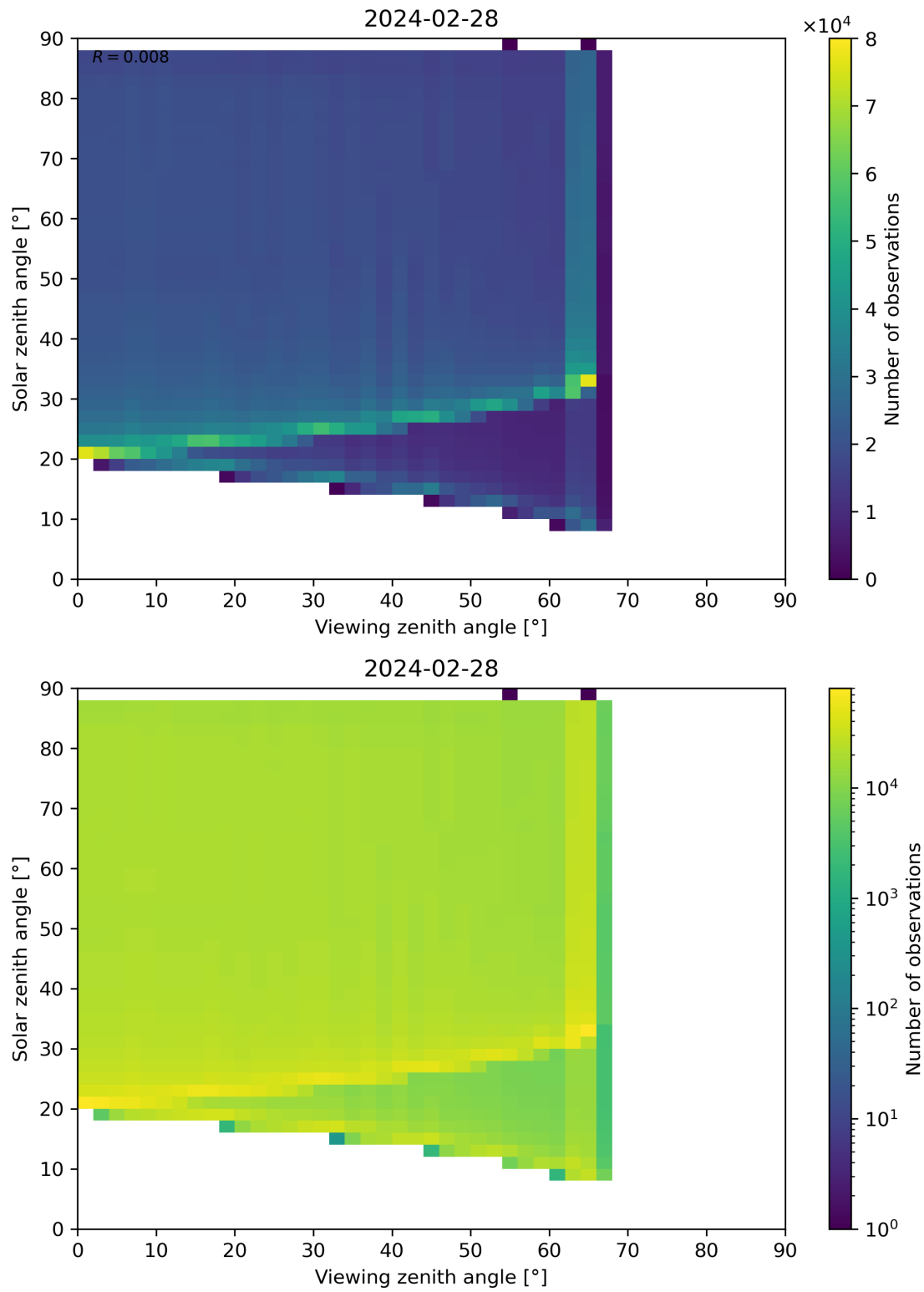
Figure 172: Scatter density plot of “Viewing zenith angle” against “Solar zenith angle” for 2024-02-27 to 2024-02-29.
