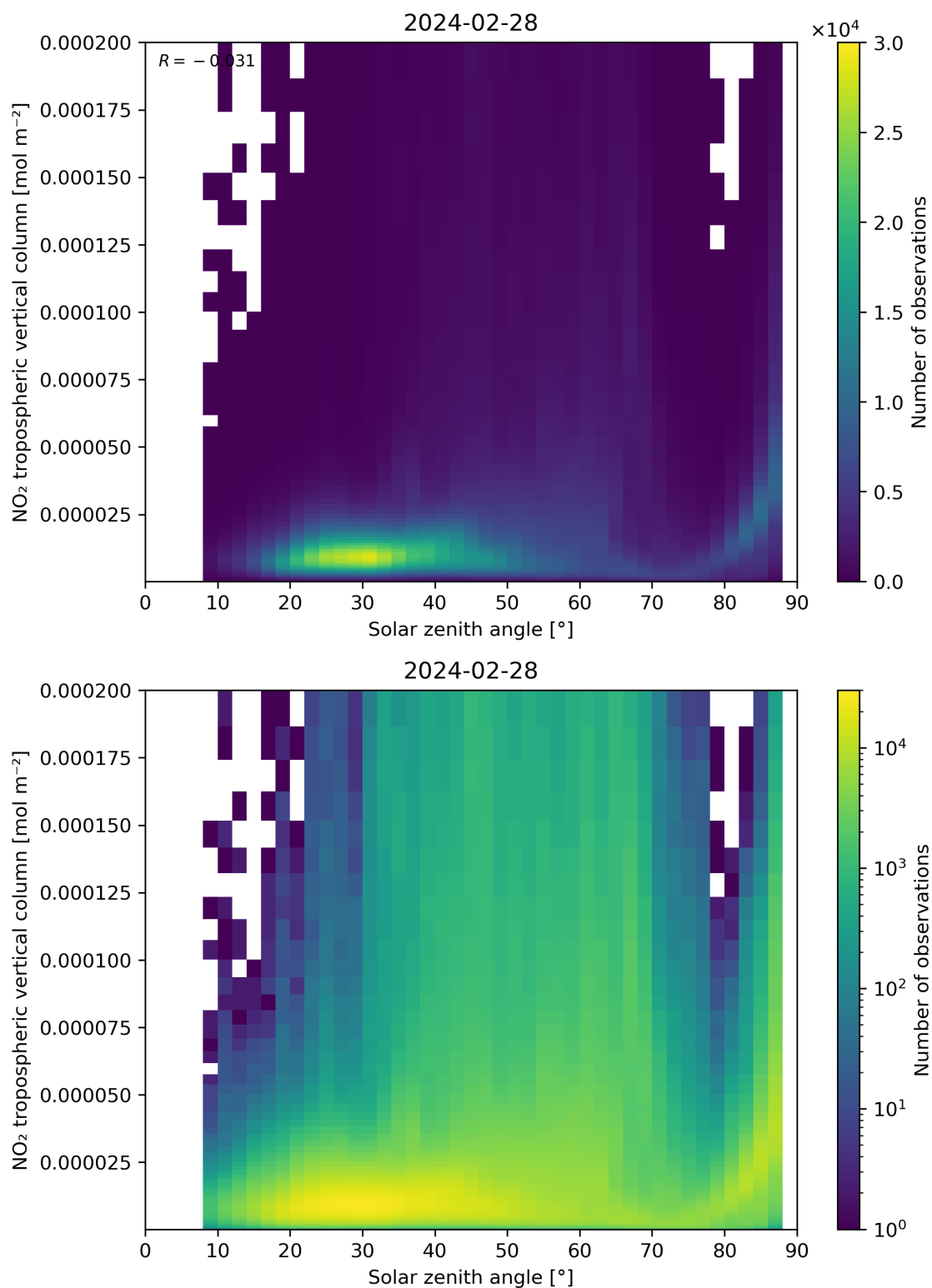
Figure 155: Scatter density plot of “Solar zenith angle” against “NO 2 tropospheric vertical column” for 2024-02-27 to 2024-02-29.
