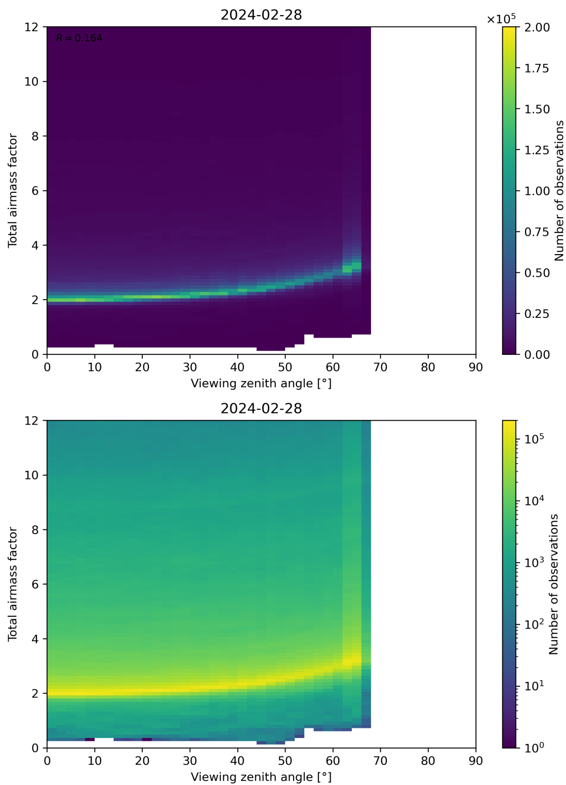
Figure 160: Scatter density plot of “Viewing zenith angle” against “Total airmass factor” for 2024-02-27 to 2024-02-29.
