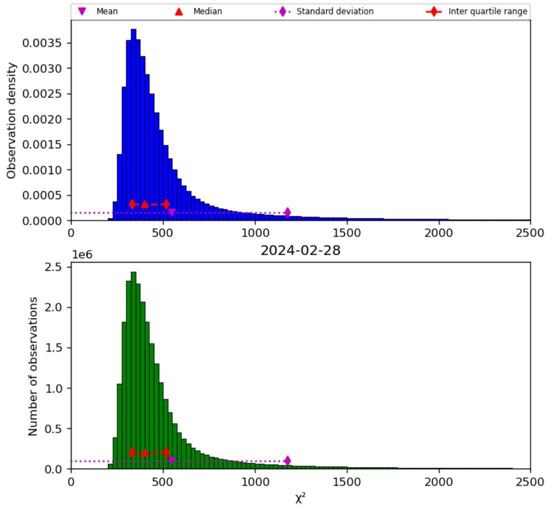
Figure 42: Histogram of “ \chi^2 ” for 2024-02-27 to 2024-02-29
