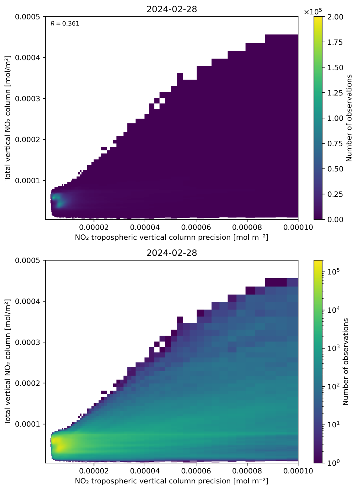
Figure 138: Scatter density plot of “NO 2 tropospheric vertical column precision” against “Total vertical NO 2 column” for 2024-02-27 to 2024-02-29.
