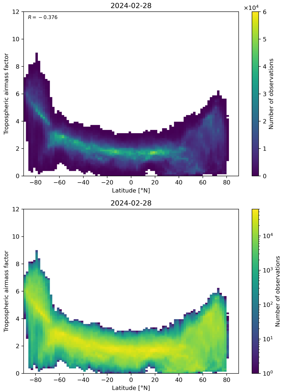
Figure 85: Scatter density plot of “Latitude” against “Tropospheric airmass factor” for 2024-02-27 to 2024-02-29.
