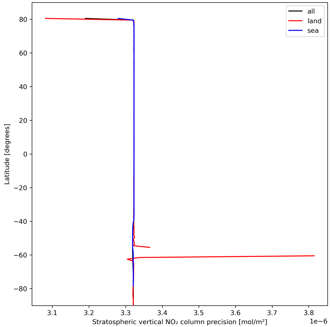
Figure 20: Zonal average of “Stratospheric vertical NO 2 column precision” for 2024-02-27 to 2024-02-29.
