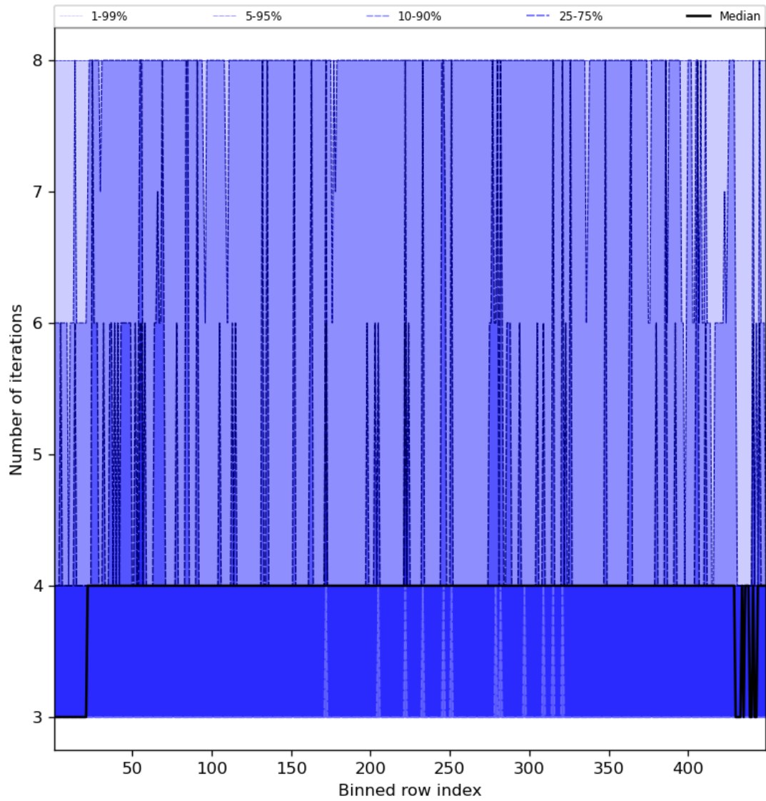
Figure 51: Along track statistics of “Number of iterations” for 2024-02-27 to 2024-02-29
