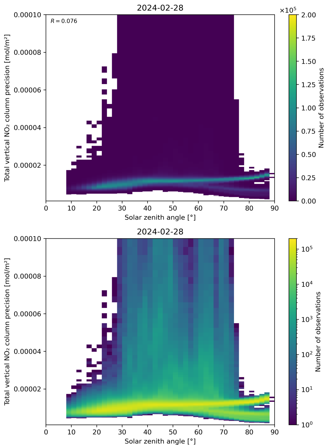
Figure 154: Scatter density plot of “Solar zenith angle” against “Total vertical NO 2 column precision” for 2024-02-27 to 2024-02-29.
