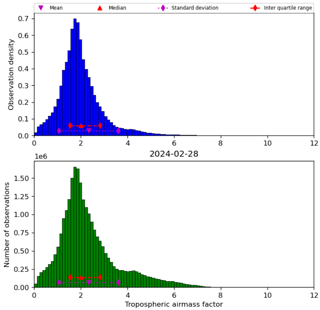
Figure 31: Histogram of “Tropospheric airmass factor” for 2024-02-27 to 2024-02-29
