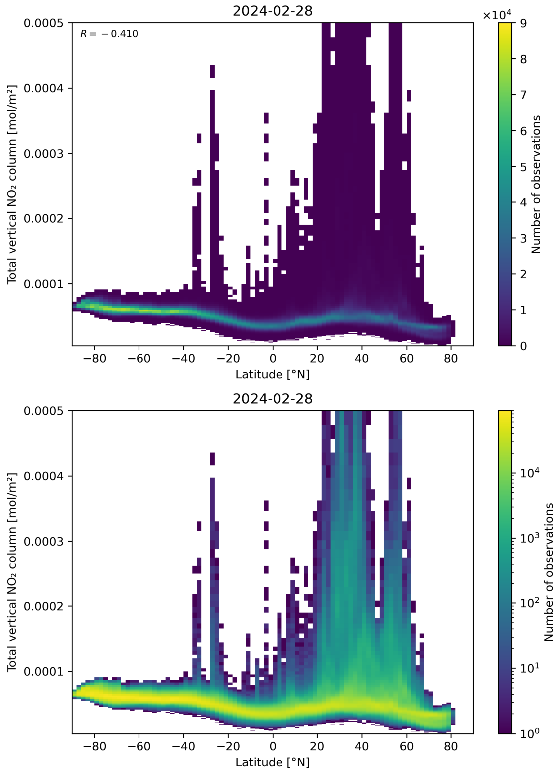
Figure 90: Scatter density plot of “Latitude” against “Total vertical NO 2 column” for 2024-02-27 to 2024-02-29.
