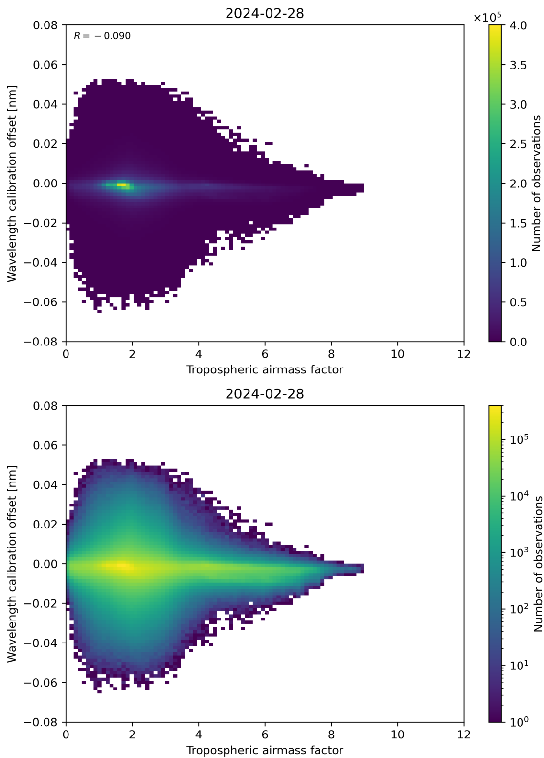
Figure 80: Scatter density plot of “Tropospheric airmass factor” against “Wavelength calibration offset” for 2024-02-27 to 2024-02-29.
