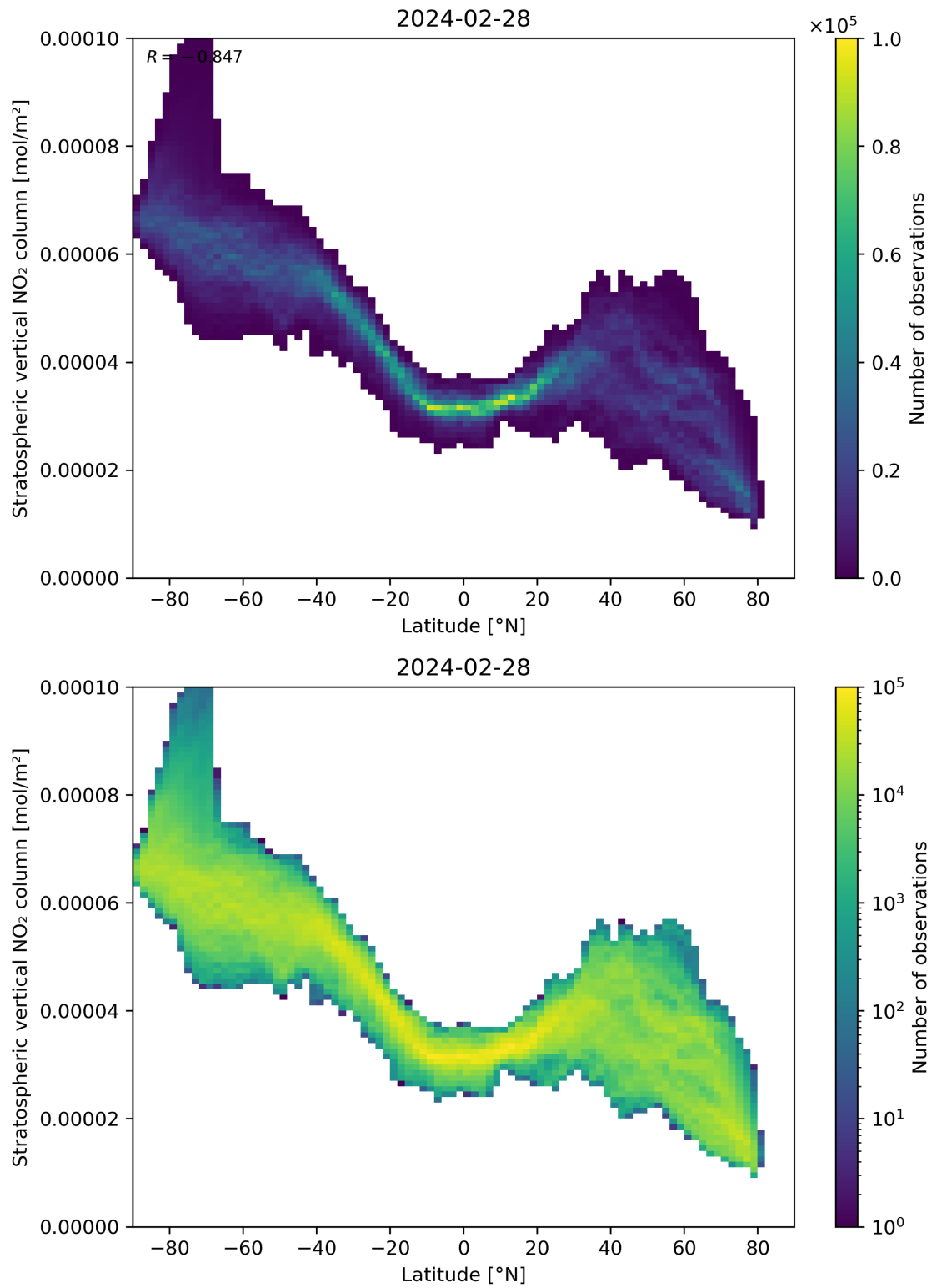
Figure 87: Scatter density plot of “Latitude” against “Stratospheric vertical NO 2 column” for 2024-02-27 to 2024-02-29.
