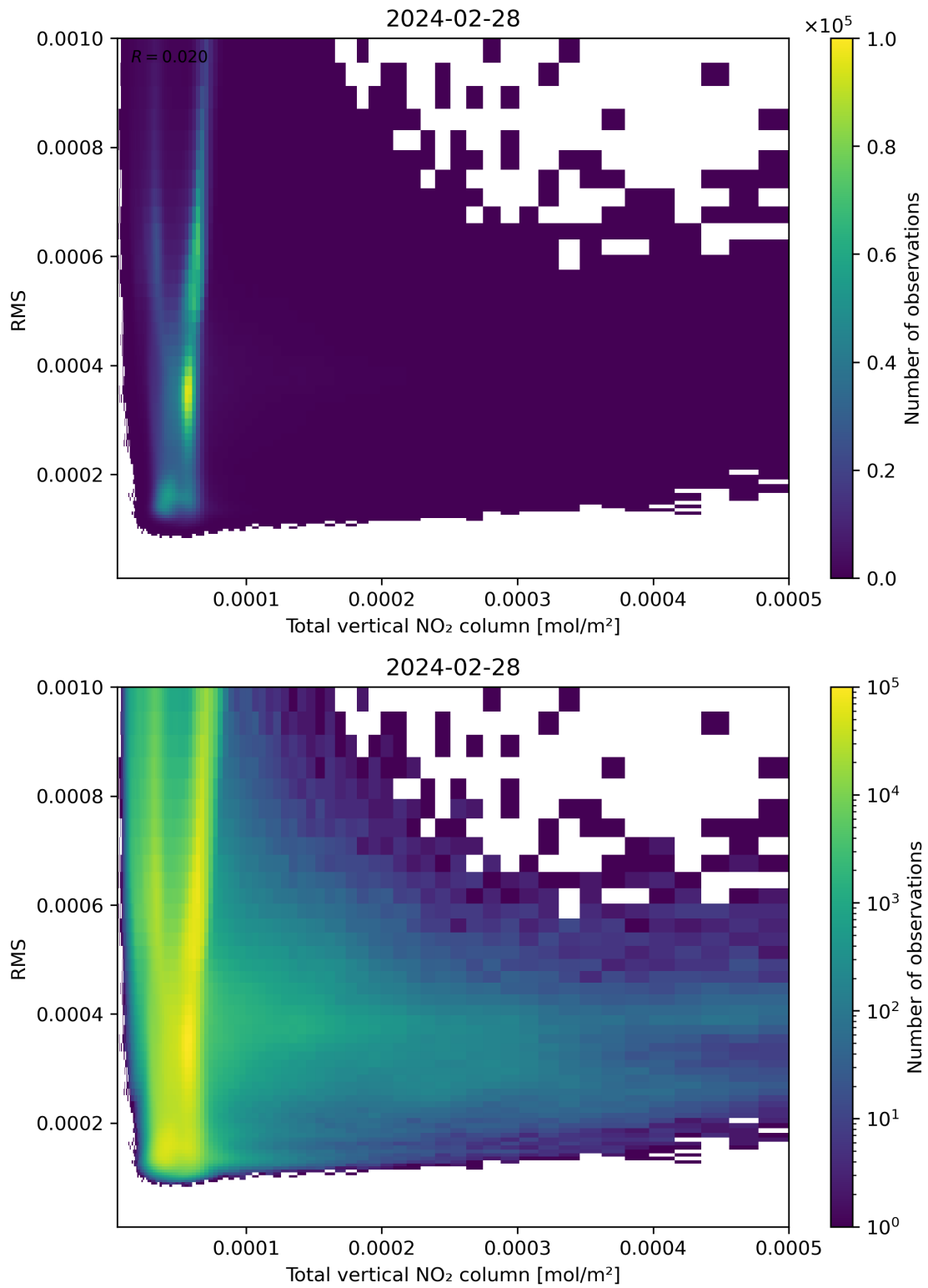
Figure 120: Scatter density plot of “Total vertical NO 2 column” against “RMS” for 2024-02-27 to 2024-02-29.
