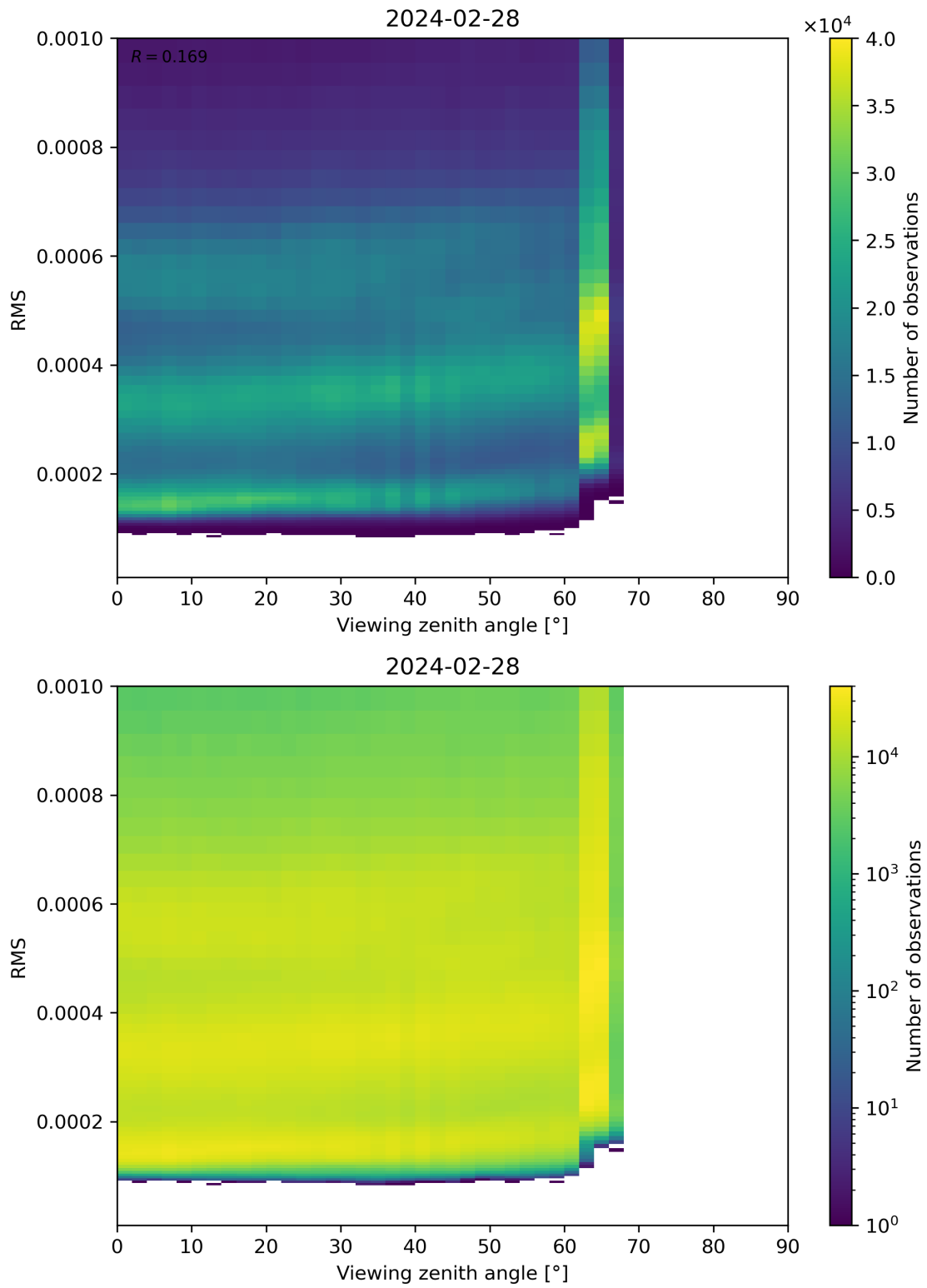
Figure 171: Scatter density plot of “Viewing zenith angle” against “RMS” for 2024-02-27 to 2024-02-29.
