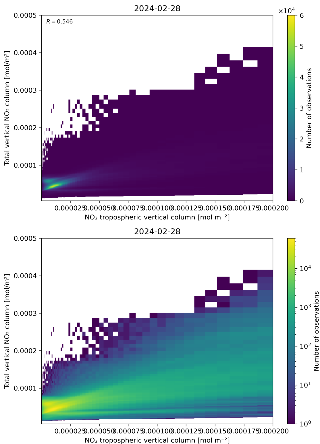
Figure 128: Scatter density plot of “NO 2 tropospheric vertical column” against “Total vertical NO 2 column” for 2024-02-27 to 2024-02-29.
