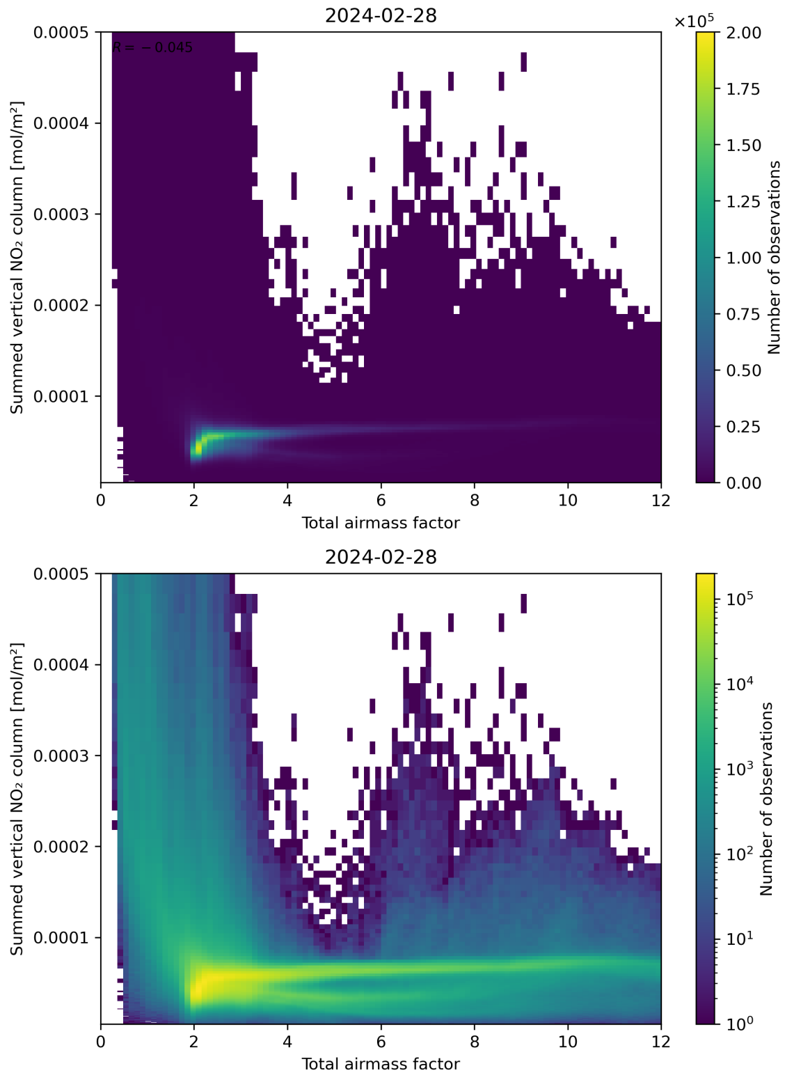
Figure 65: Scatter density plot of “Total airmass factor” against “Summed vertical NO 2 column” for 2024-02-27 to 2024-02-29.
