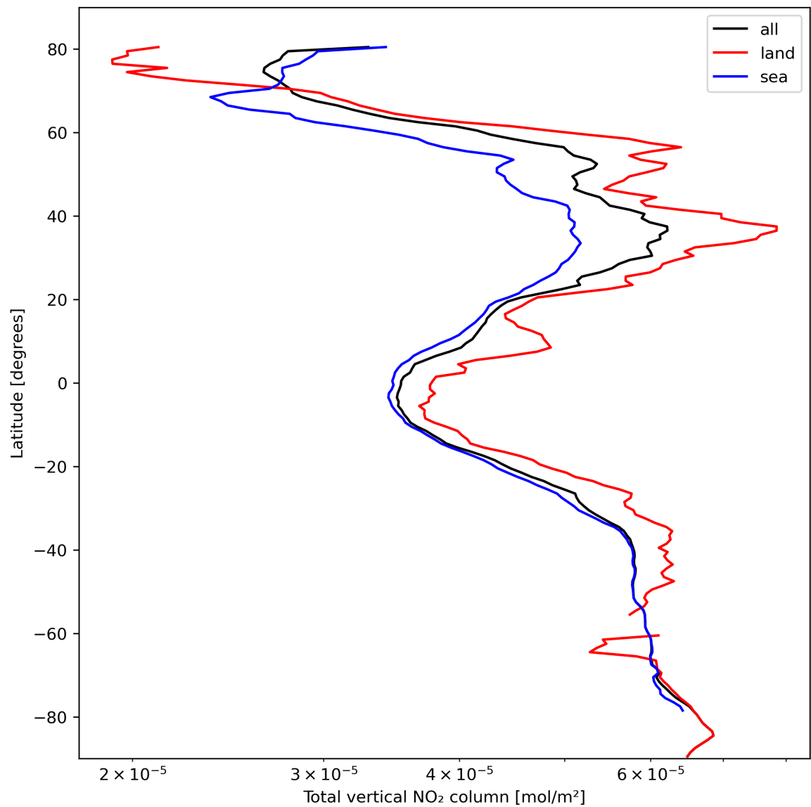
Figure 21: Zonal average of “Total vertical NO 2 column” for 2024-02-27 to 2024-02-29.
