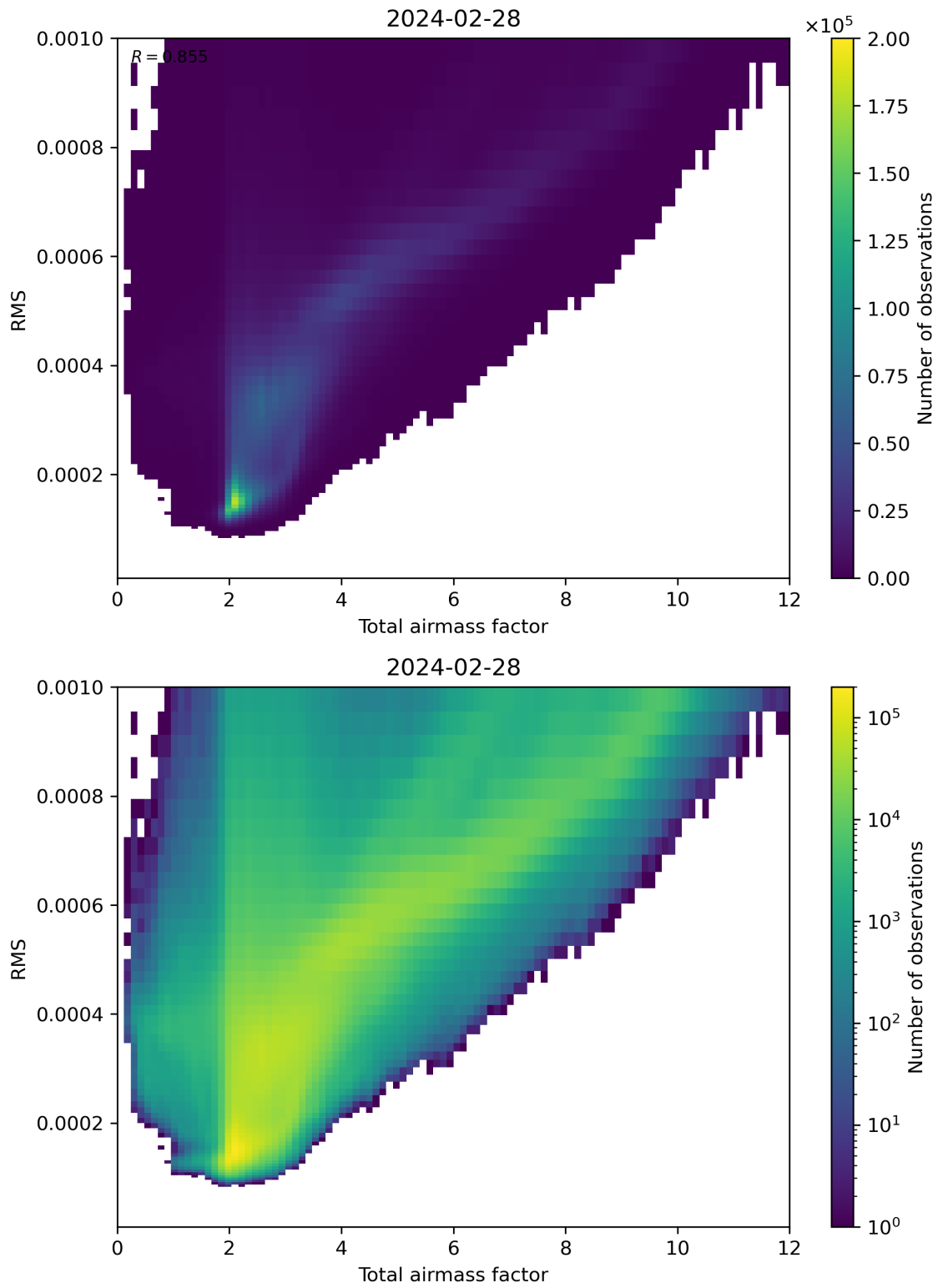
Figure 69: Scatter density plot of “Total airmass factor” against “RMS” for 2024-02-27 to 2024-02-29.
