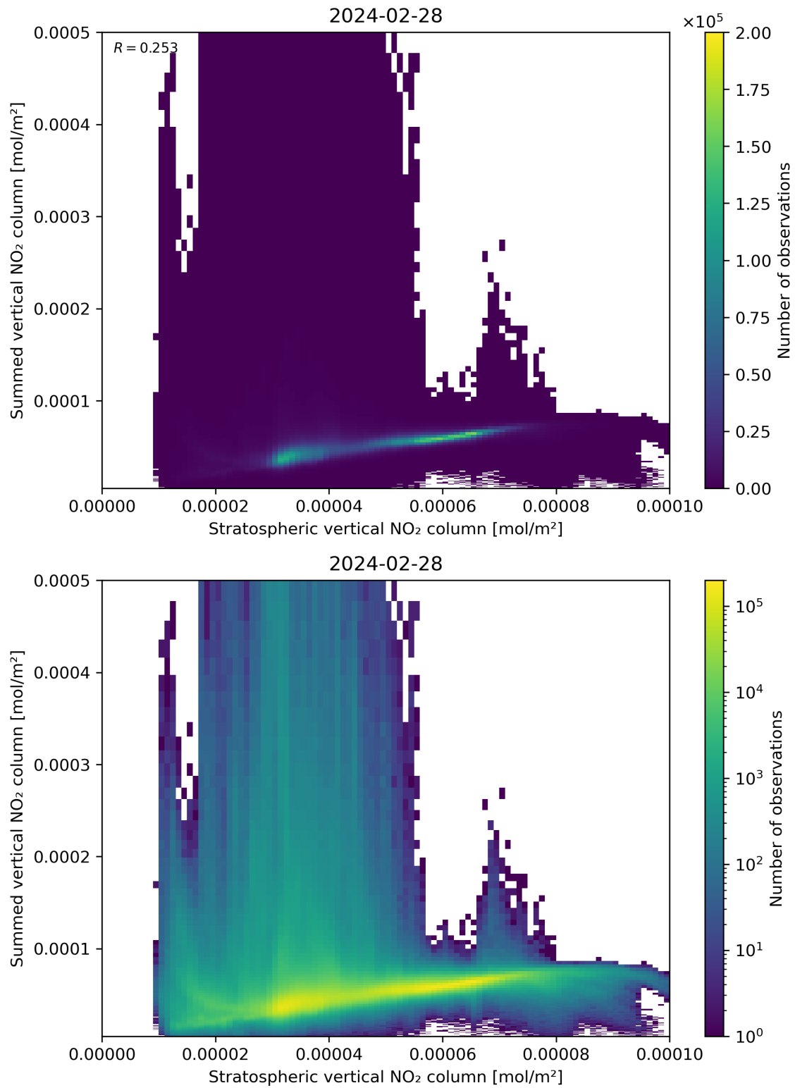
Figure 98: Scatter density plot of “Stratospheric vertical NO 2 column” against “Summed vertical NO 2 column” for 2024-02-27 to 2024-02-29.
