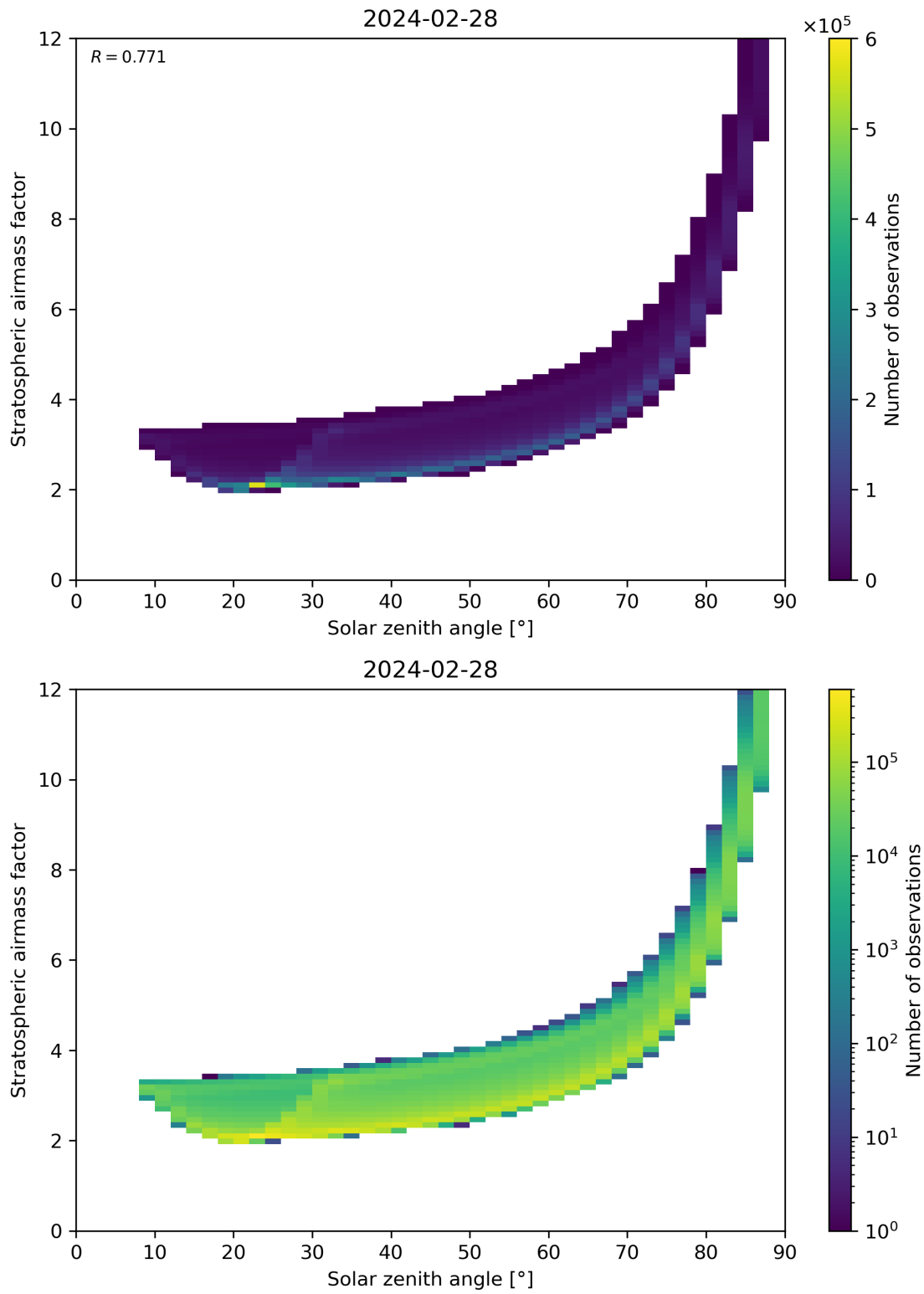
Figure 145: Scatter density plot of “Solar zenith angle” against “Stratospheric airmass factor” for 2024-02-27 to 2024-02-29.
