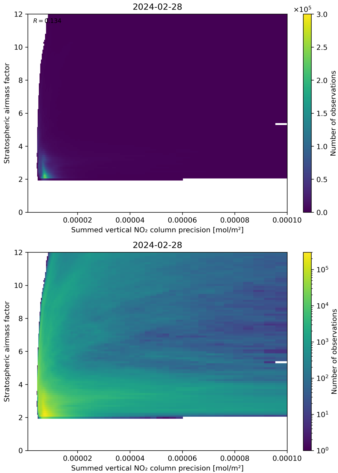
Figure 106: Scatter density plot of “Summed vertical NO 2 column precision” against “Stratospheric airmass factor” for 2024-02-27 to 2024-02-29.
