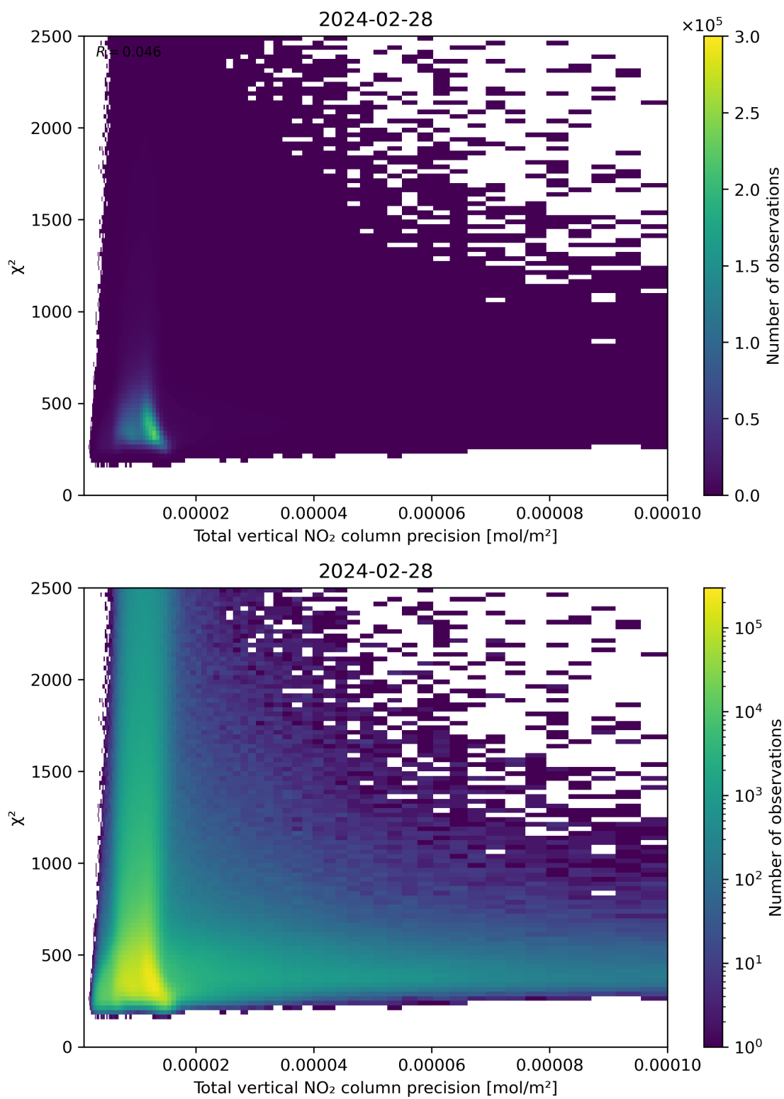
Figure 116: Scatter density plot of “Total vertical NO 2 column precision” against “ \chi^2 ” for 2024-02-27 to 2024-02-29.
