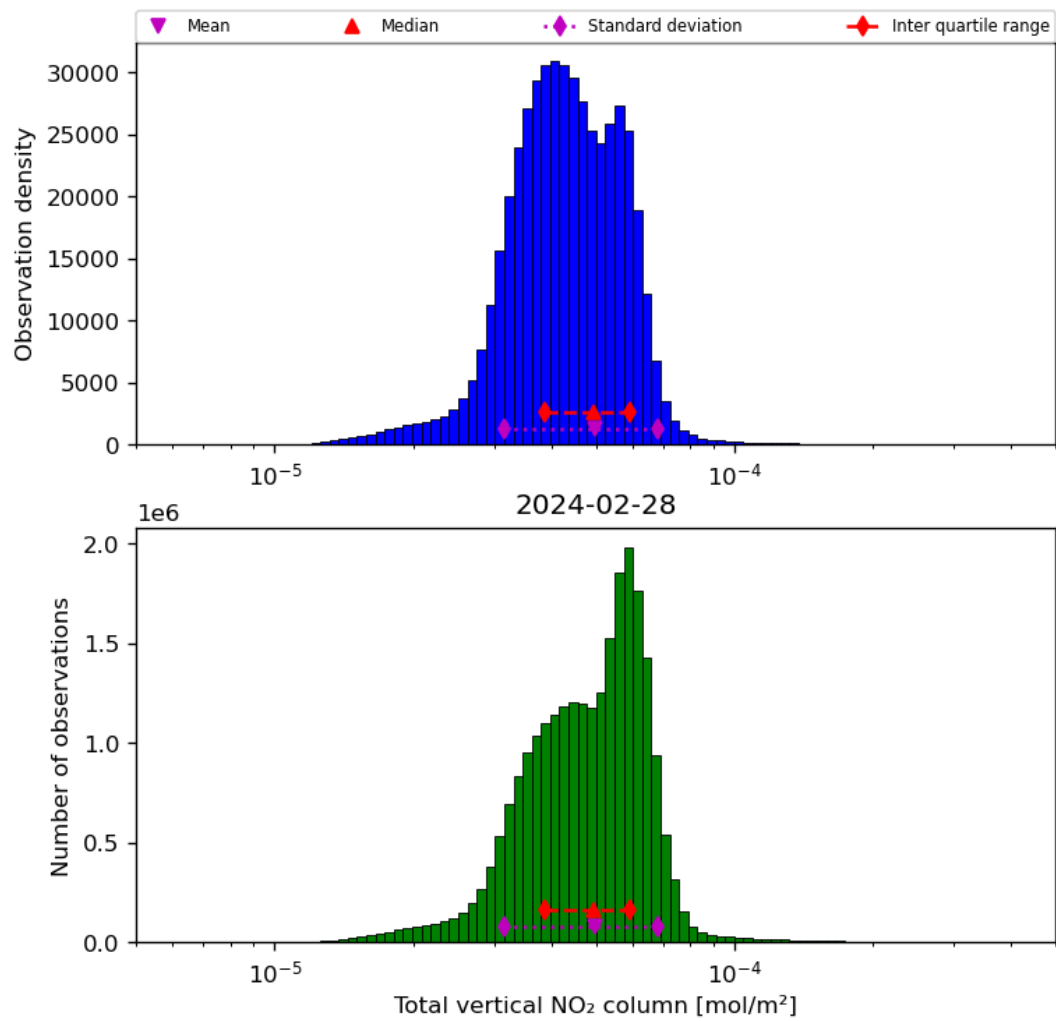
Figure 38: Histogram of “Total vertical NO 2 column” for 2024-02-27 to 2024-02-29
