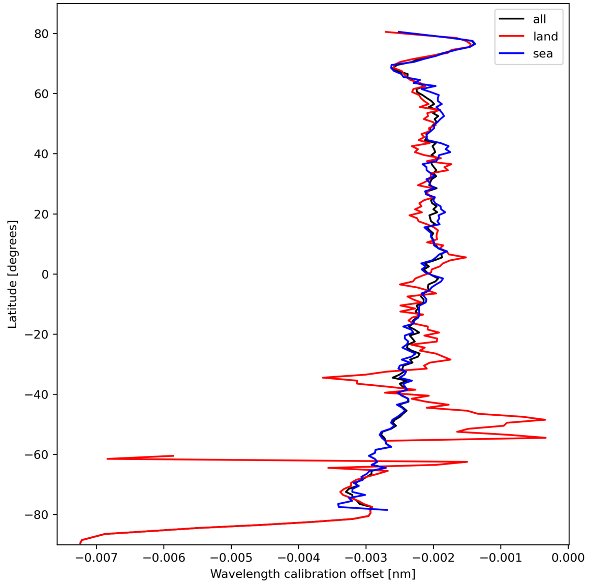
Figure 18: Zonal average of “Wavelength calibration offset” for 2024-02-27 to 2024-02-29.
