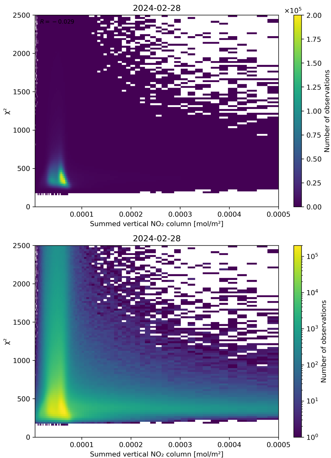
Figure 104: Scatter density plot of “Summed vertical NO 2 column” against “ \chi^2 ” for 2024-02-27 to 2024-02-29.
