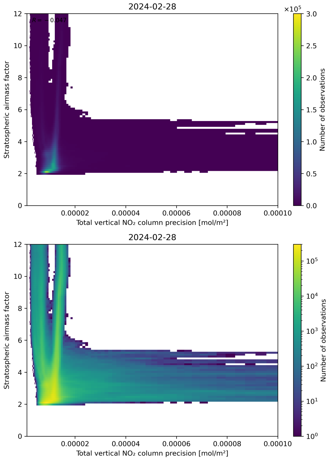
Figure 115: Scatter density plot of “Total vertical NO 2 column precision” against “Stratospheric air mass factor” for 2024-02-27 to 2024-02-29.
