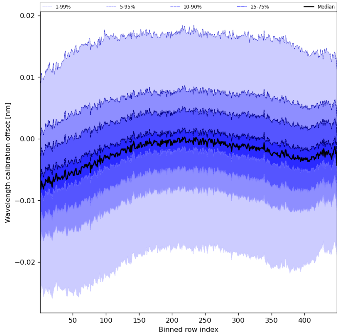
Figure 52: Along track statistics of “Wavelength calibration offset” for 2024-02-27 to 2024-02-29
