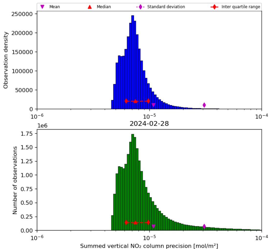
Figure 41: Histogram of “Summed vertical NO 2 column precision” for 2024-02-27 to 2024-02-29
