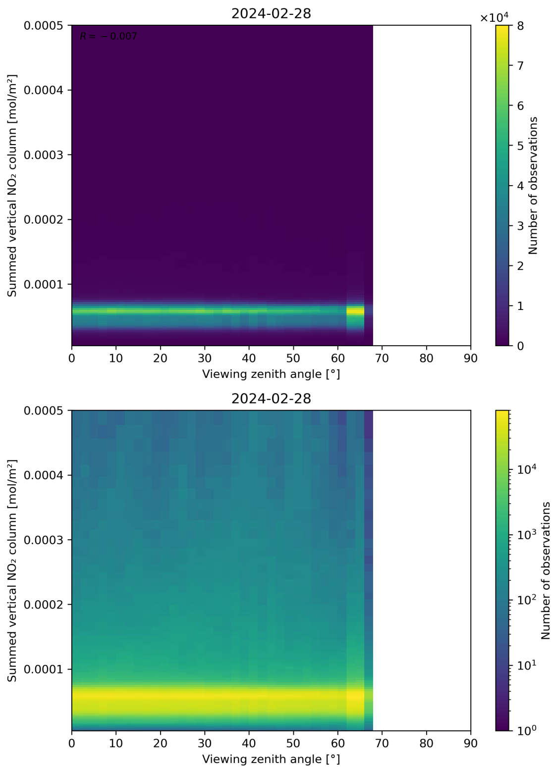
Figure 165: Scatter density plot of “Viewing zenith angle” against “Summed vertical NO 2 column” for 2024-02-27 to 2024-02-29.
