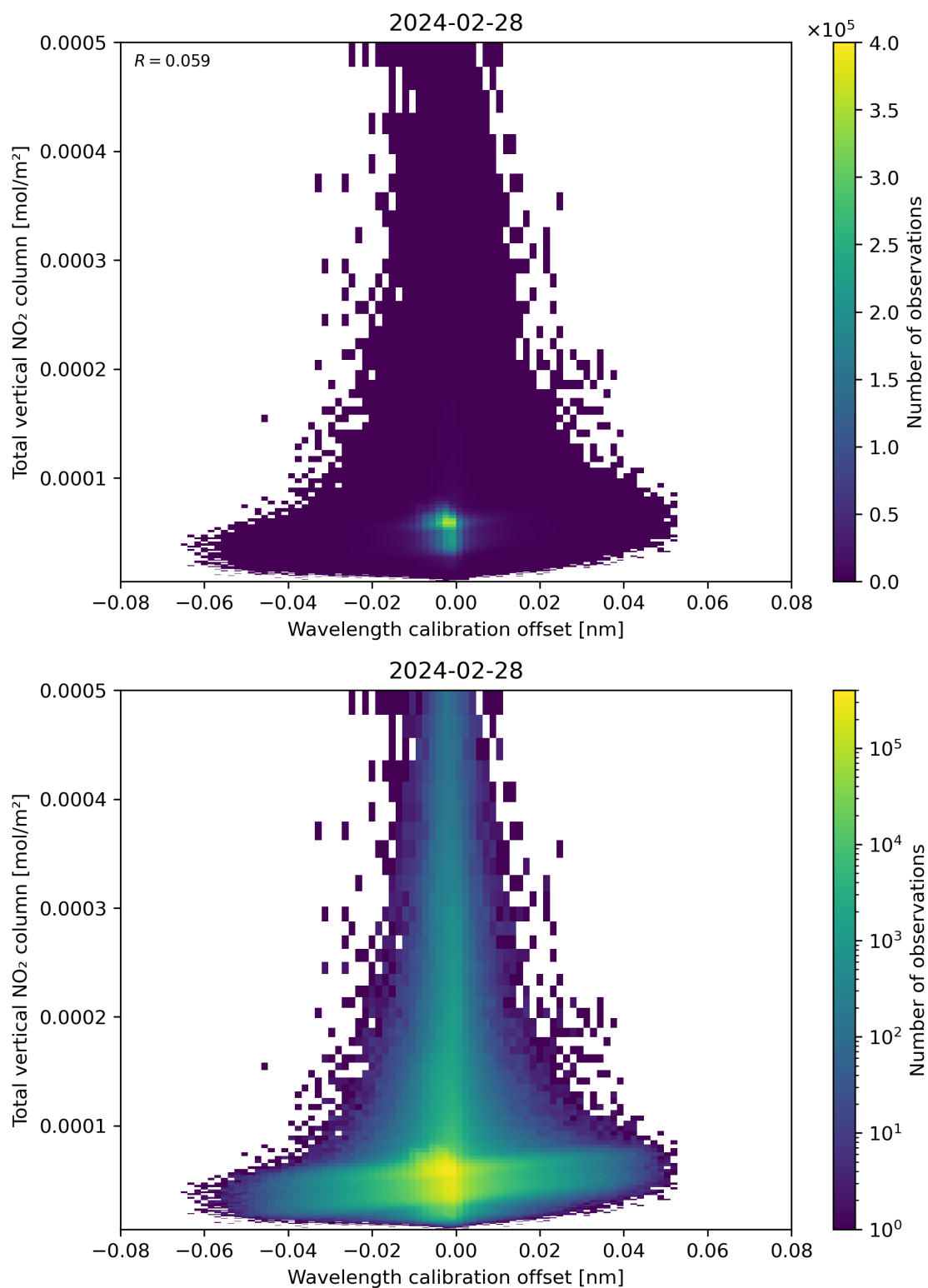
Figure 179: Scatter density plot of “Wavelength calibration offset” against “Total vertical NO 2 column” for 2024-02-27 to 2024-02-29.
