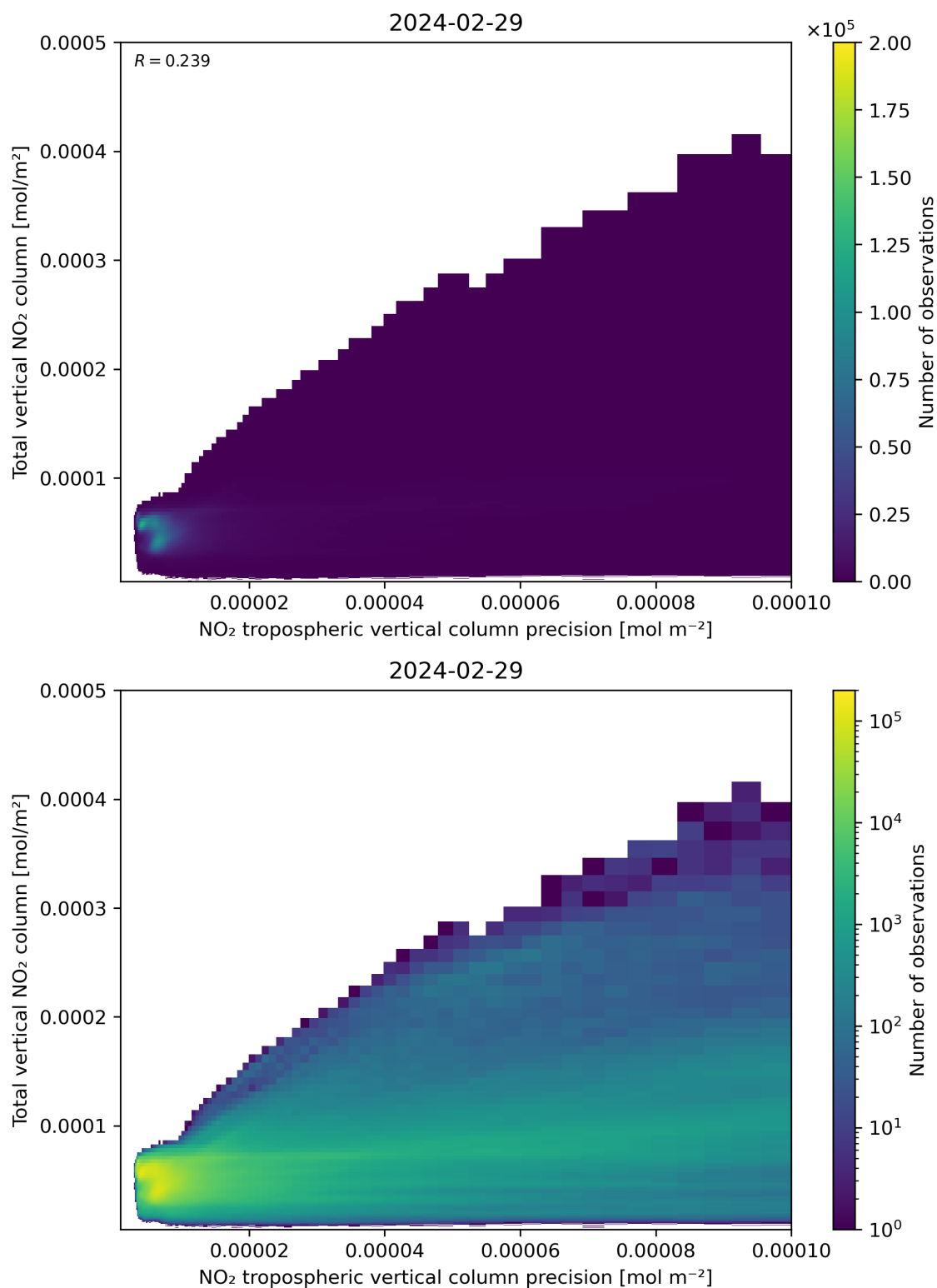
Figure 138: Scatter density plot of “NO 2 tropospheric vertical column precision” against “Total vertical NO 2 column” for 2024-02-28 to 2024-03-01.
