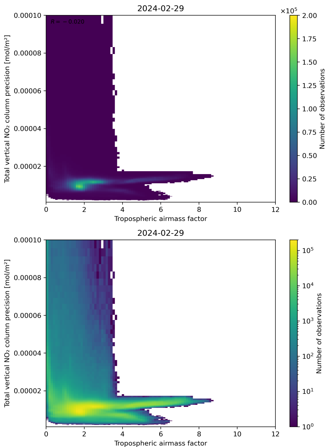
Figure 78: Scatter density plot of “Tropospheric airmass factor” against “Total vertical NO 2 column precision” for 2024-02-28 to 2024-03-01.
