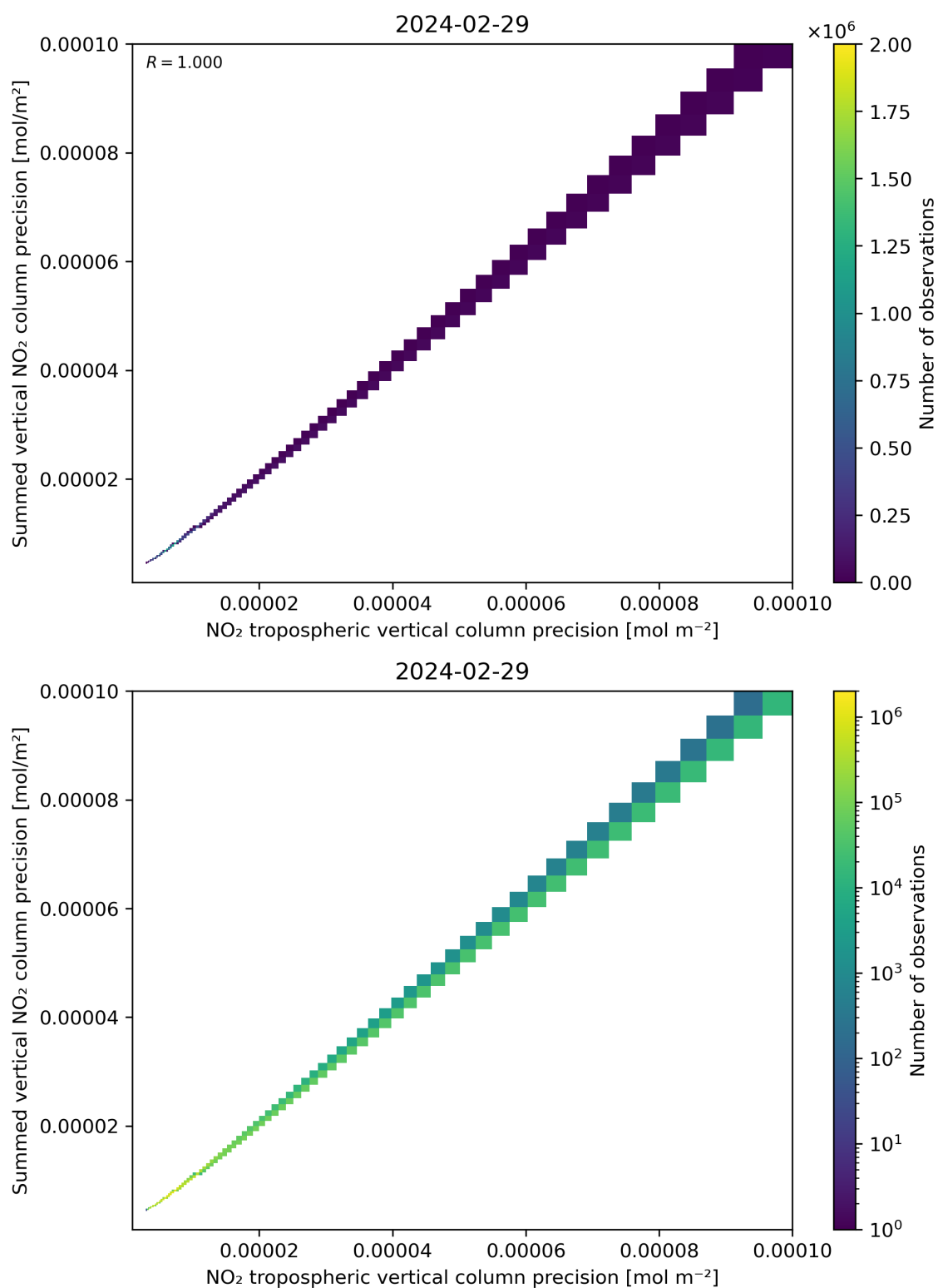
Figure 137: Scatter density plot of “NO 2 tropospheric vertical column precision” against “Summed vertical NO 2 column precision” for 2024-02-28 to 2024-03-01.
