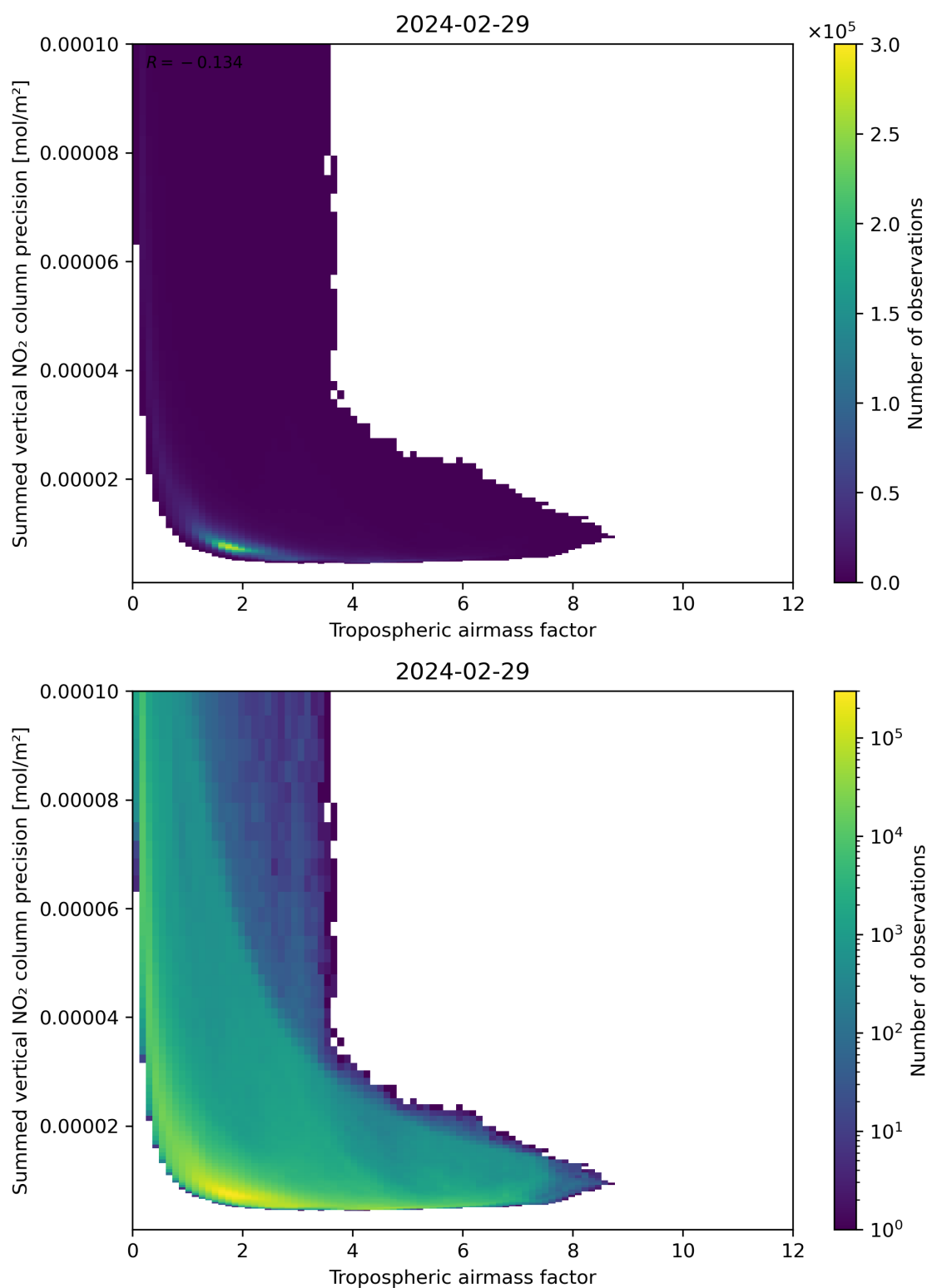
Figure 76: Scatter density plot of “Tropospheric air mass factor” against “Summed vertical NO 2 column precision” for 2024-02-28 to 2024-03-01.
