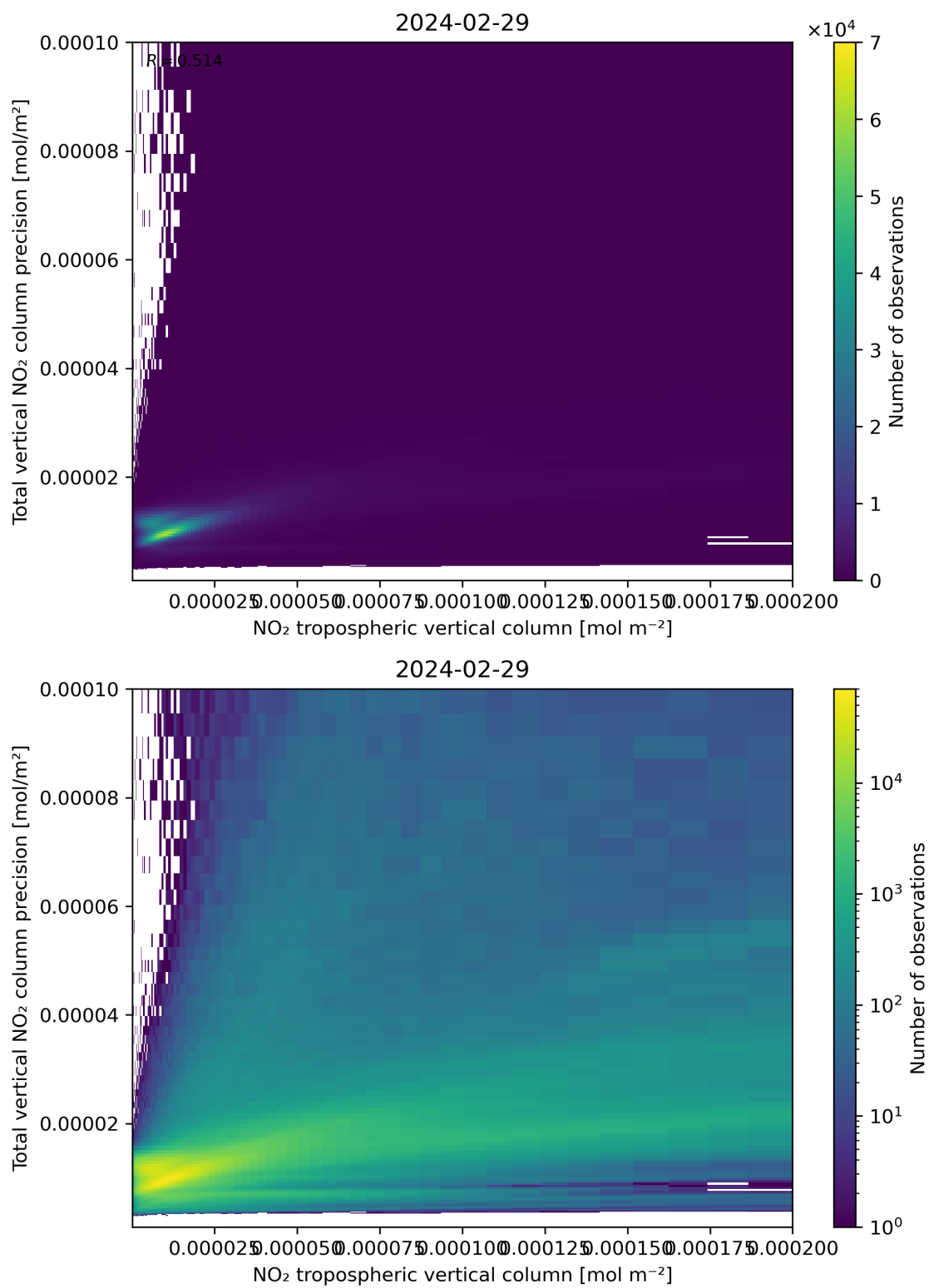
Figure 129: Scatter density plot of “NO 2 tropospheric vertical column” against “Total vertical NO 2 column precision” for 2024-02-28 to 2024-03-01.
