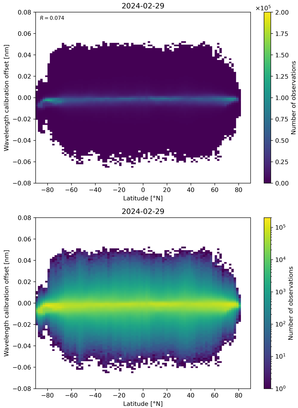
Figure 95: Scatter density plot of “Latitude” against “Wavelength calibration offset” for 2024-02-28 to 2024-03-01.
