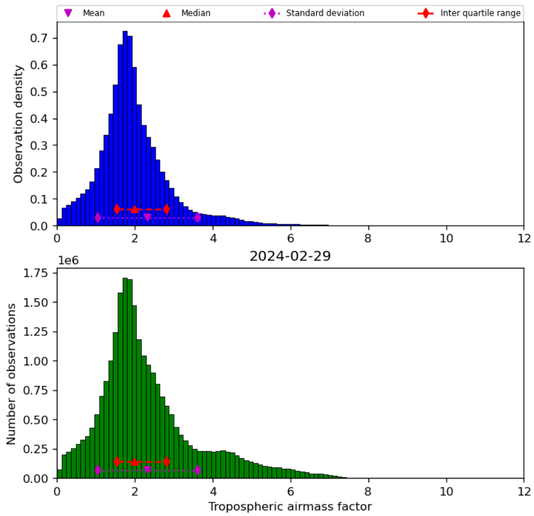
Figure 31: Histogram of “Tropospheric airmass factor” for 2024-02-28 to 2024-03-01
