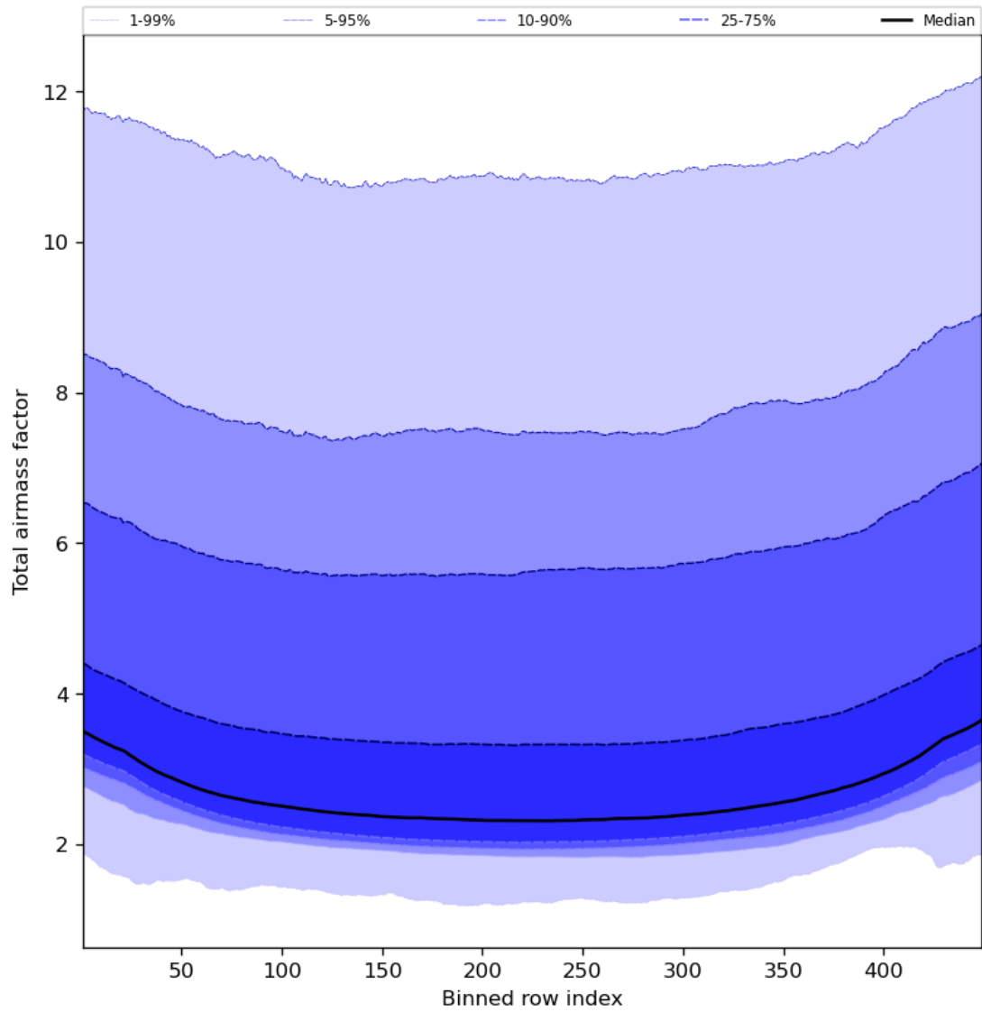
Figure 49: Along track statistics of “Total airmass factor” for 2024-02-28 to 2024-03-01
