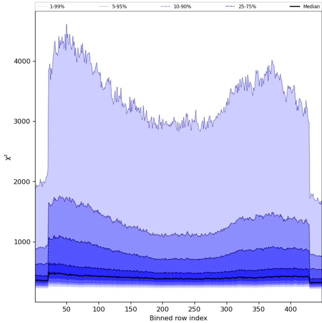
Figure 59: Along track statistics of “ \chi^2 ” for 2024-02-28 to 2024-03-01
