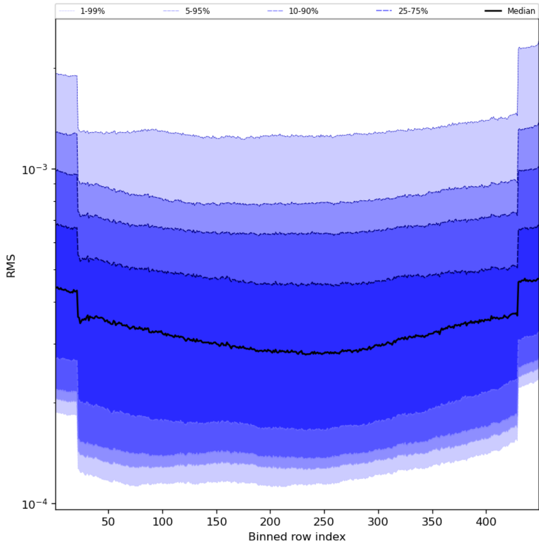
Figure 60: Along track statistics of “RMS” for 2024-02-28 to 2024-03-01
