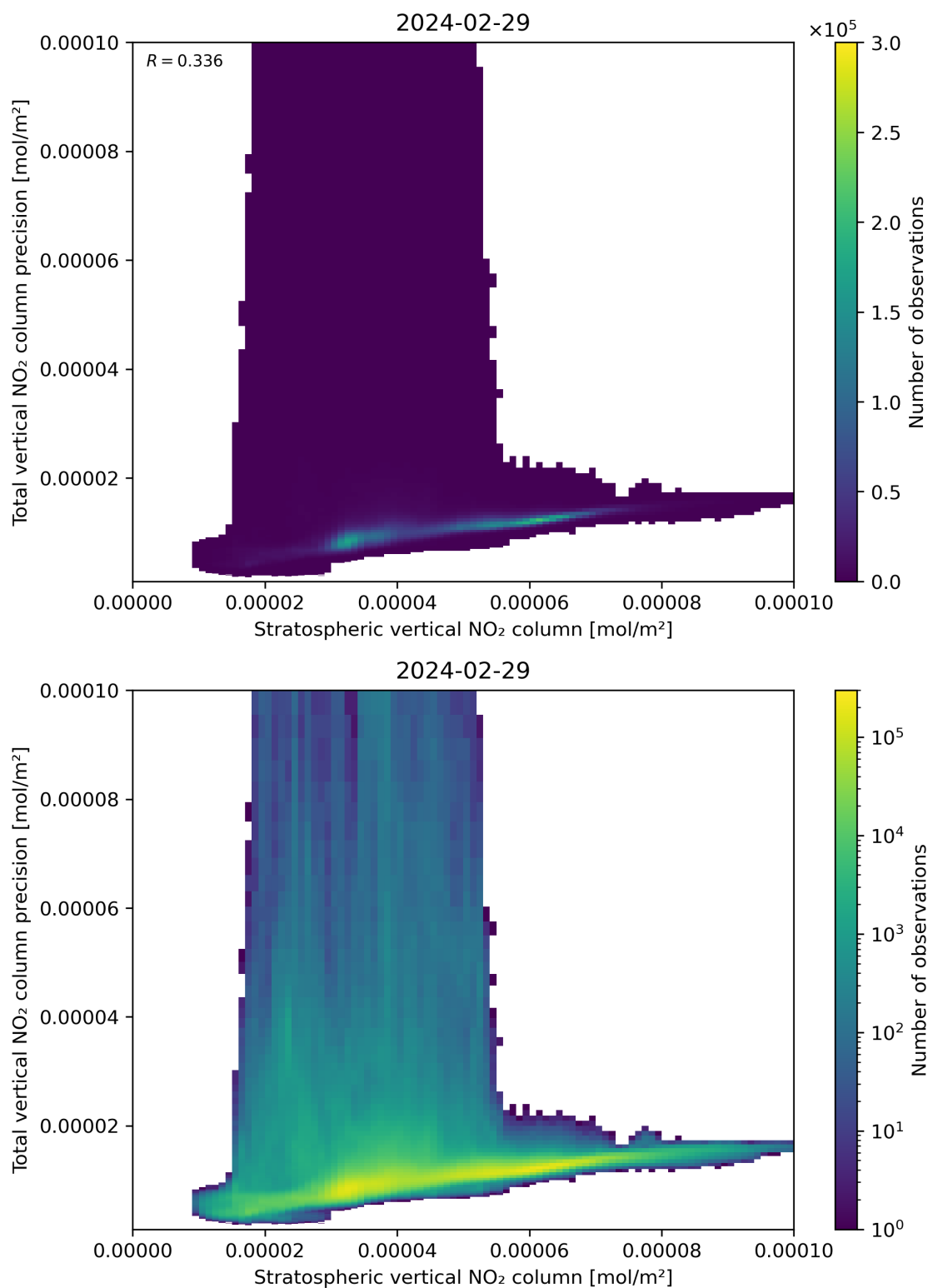
Figure 101: Scatter density plot of “Stratospheric vertical NO 2 column” against “Total vertical NO 2 column precision” for 2024-02-28 to 2024-03-01.
