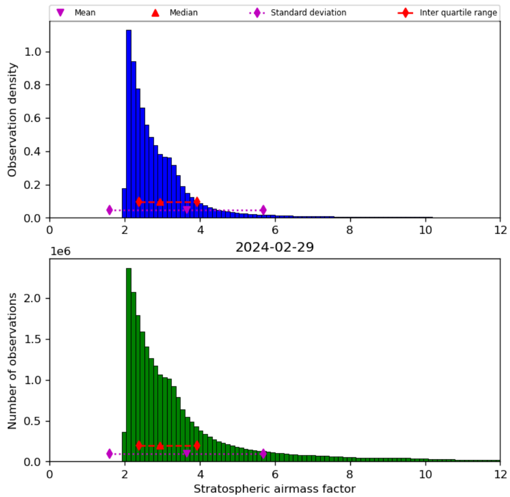
Figure 44: Histogram of “Stratospheric airmass factor” for 2024-02-28 to 2024-03-01
