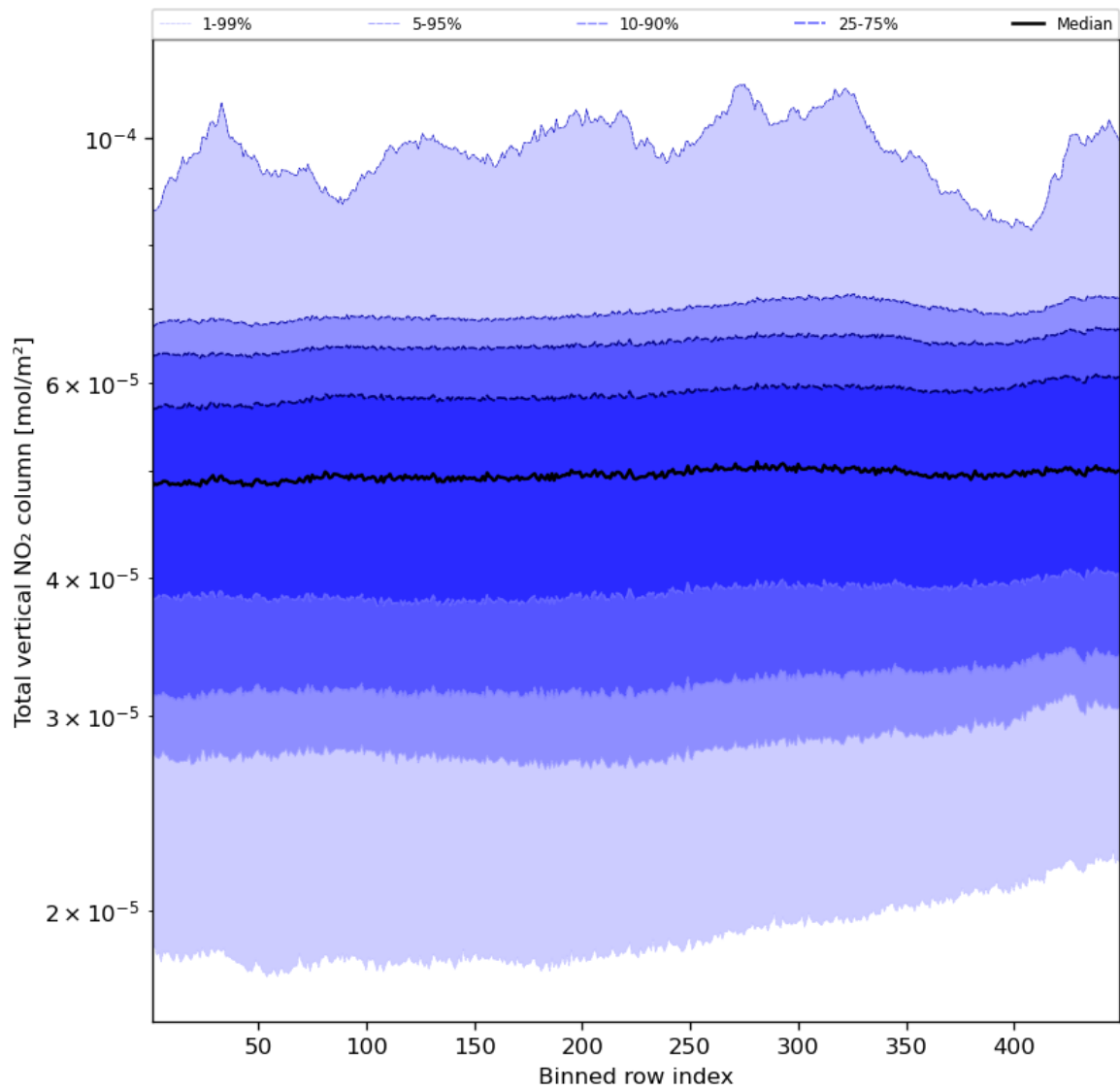
Figure 55: Along track statistics of “Total vertical NO 2 column” for 2024-02-28 to 2024-03-01
