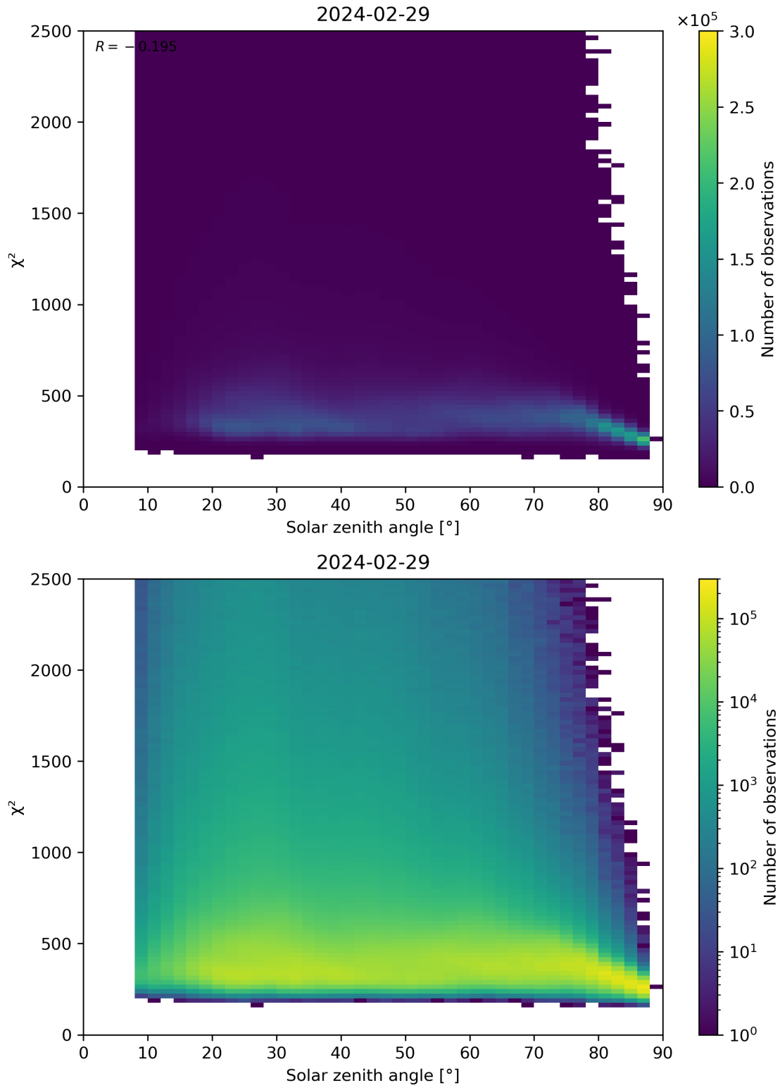
Figure 148: Scatter density plot of “Solar zenith angle” against “ \chi^2 ” for 2024-02-28 to 2024-03-01.
