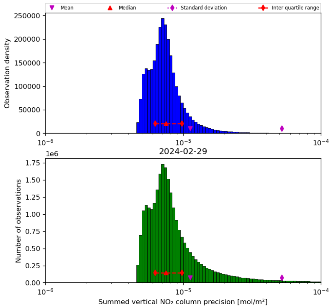
Figure 41: Histogram of "Summed vertical NO 2 column precision" for 2024-02-28 to 2024-03-01
