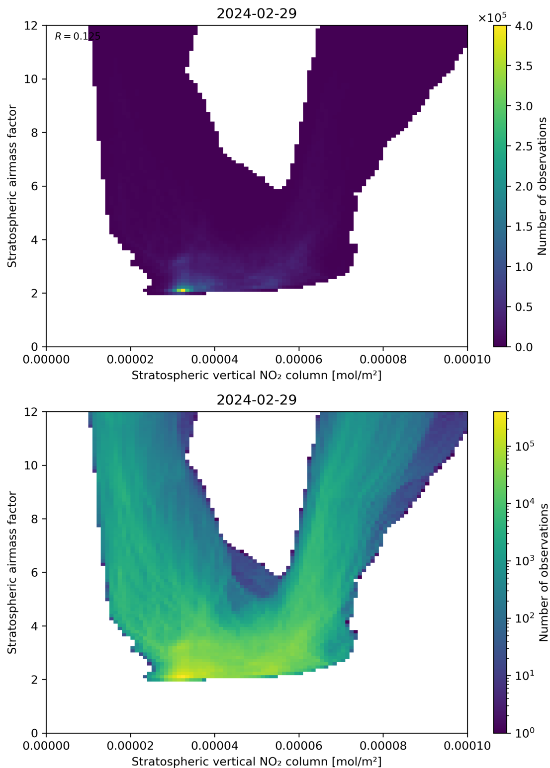
Figure 96: Scatter density plot of “Stratospheric vertical NO 2 column” against “Stratospheric airmass factor” for 2024-02-28 to 2024-03-01.
