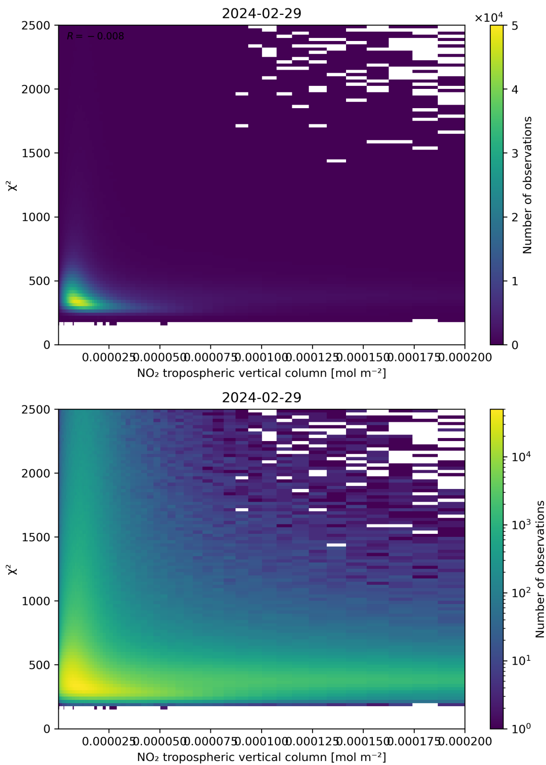
Figure 124: Scatter density plot of “NO 2 tropospheric vertical column” against “ \chi^2 ” for 2024-02-28 to 2024-03-01.
