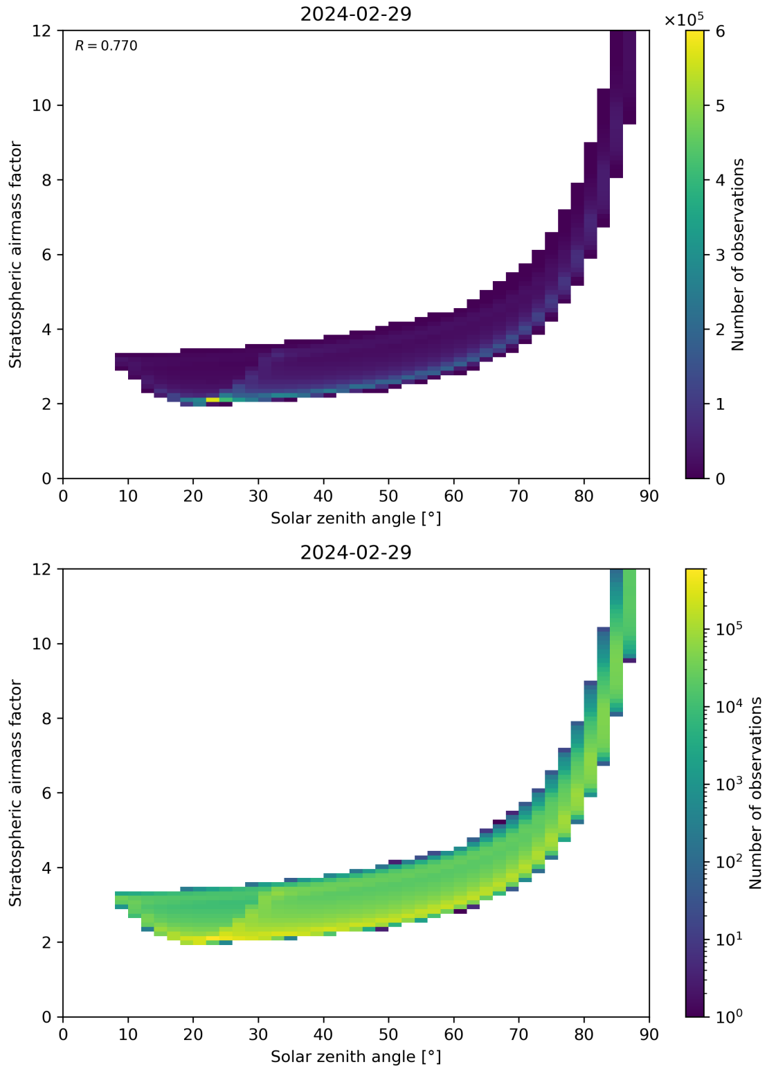
Figure 145: Scatter density plot of “Solar zenith angle” against “Stratospheric airmass factor” for 2024-02-28 to 2024-03-01.
