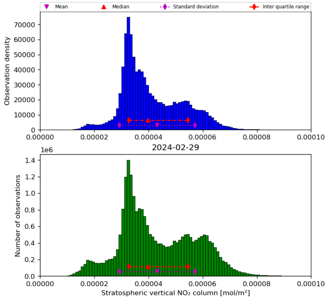
Figure 36: Histogram of “Stratospheric vertical NO 2 column” for 2024-02-28 to 2024-03-01
