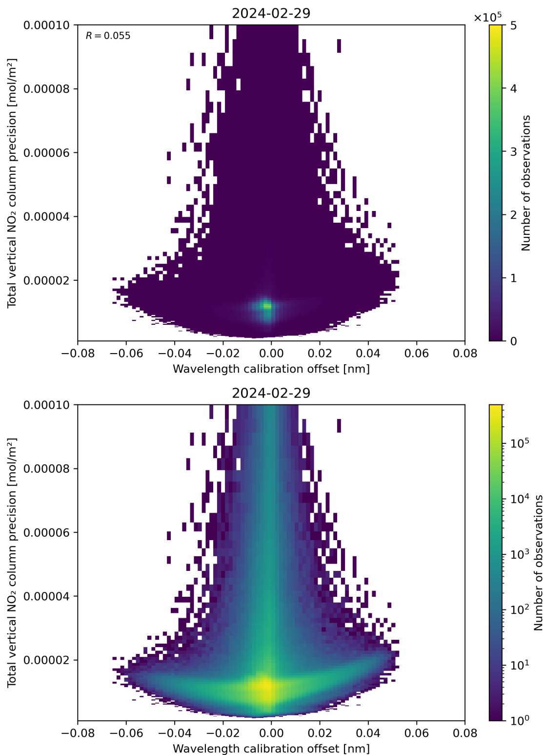
Figure 180: Scatter density plot of “Wavelength calibration offset” against “Total vertical NO 2 column precision” for 2024-02-28 to 2024-03-01.
