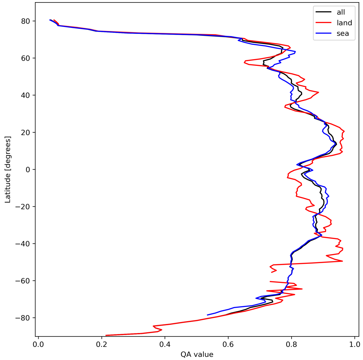
Figure 11: Zonal average of “QA value” for 2024-02-28 to 2024-03-01.
