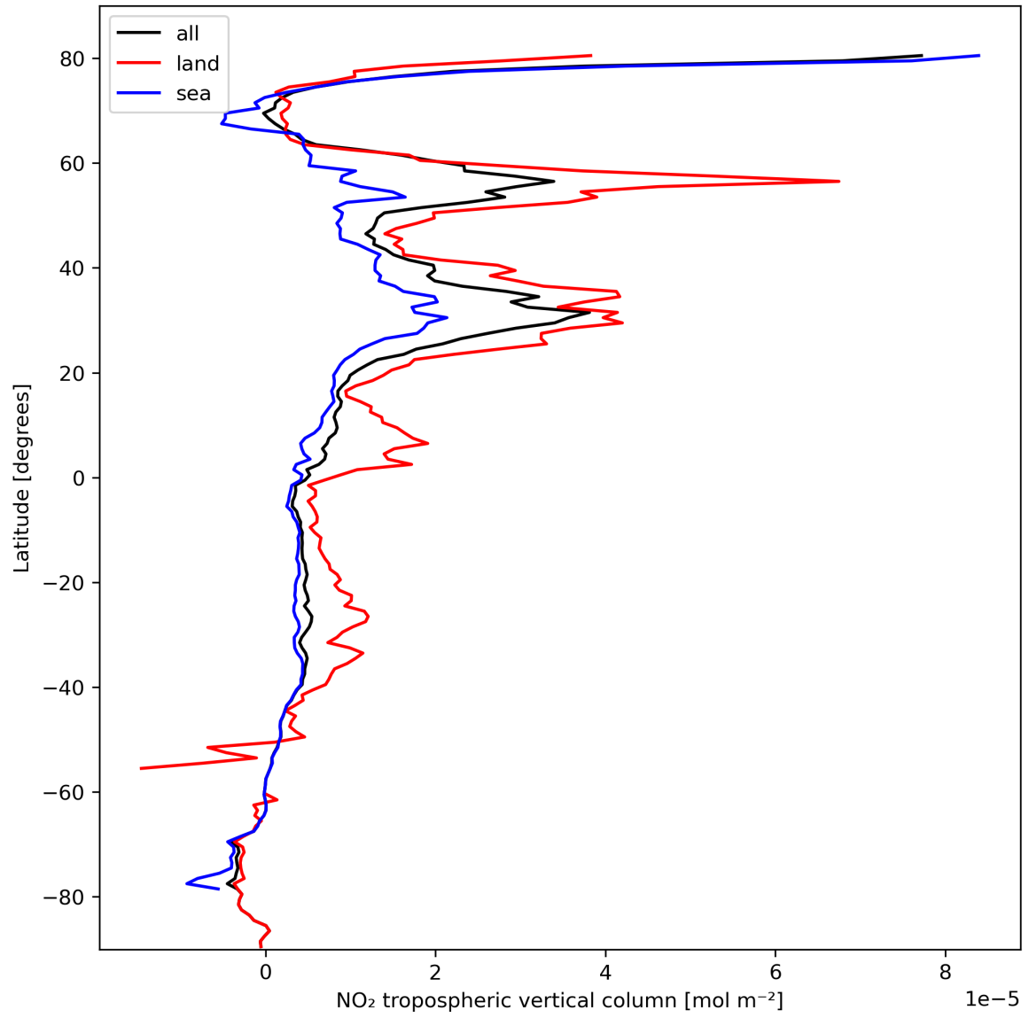
Figure 12: Zonal average of “NO 2 tropospheric vertical column” for 2024-02-28 to 2024-03-01.
