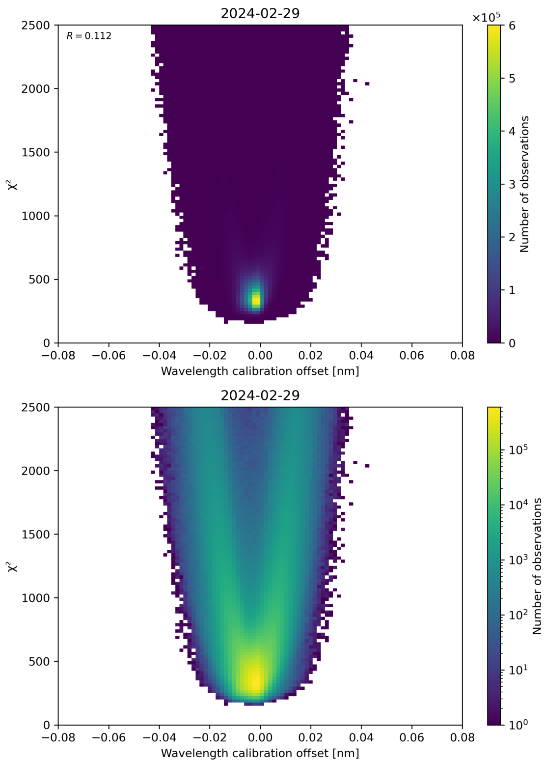
Figure 175: Scatter density plot of “Wavelength calibration offset” against “ \chi^2 ” for 2024-02-28 to 2024-03-01.
