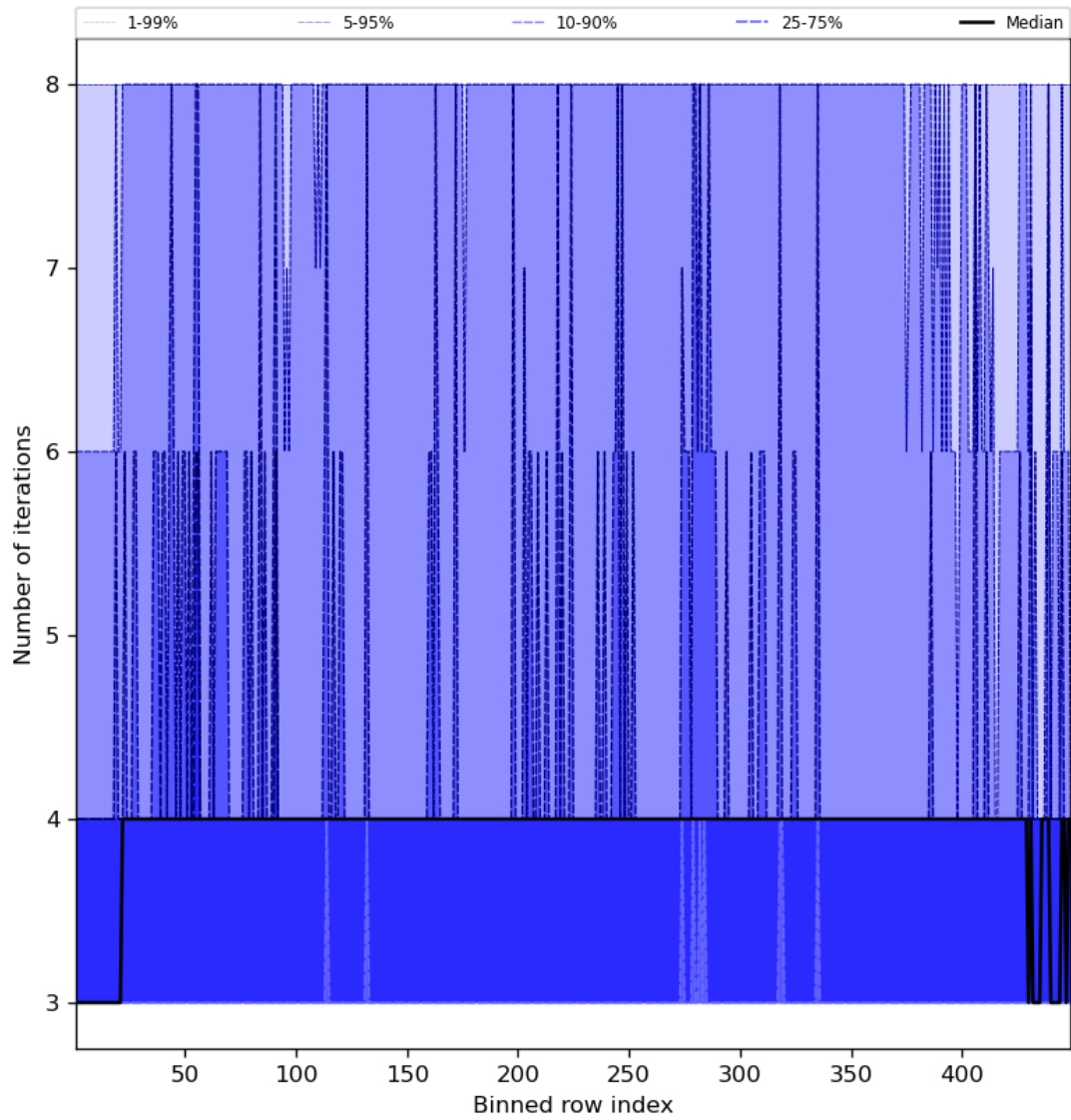
Figure 51: Along track statistics of "Number of iterations" for 2024-02-28 to 2024-03-01
