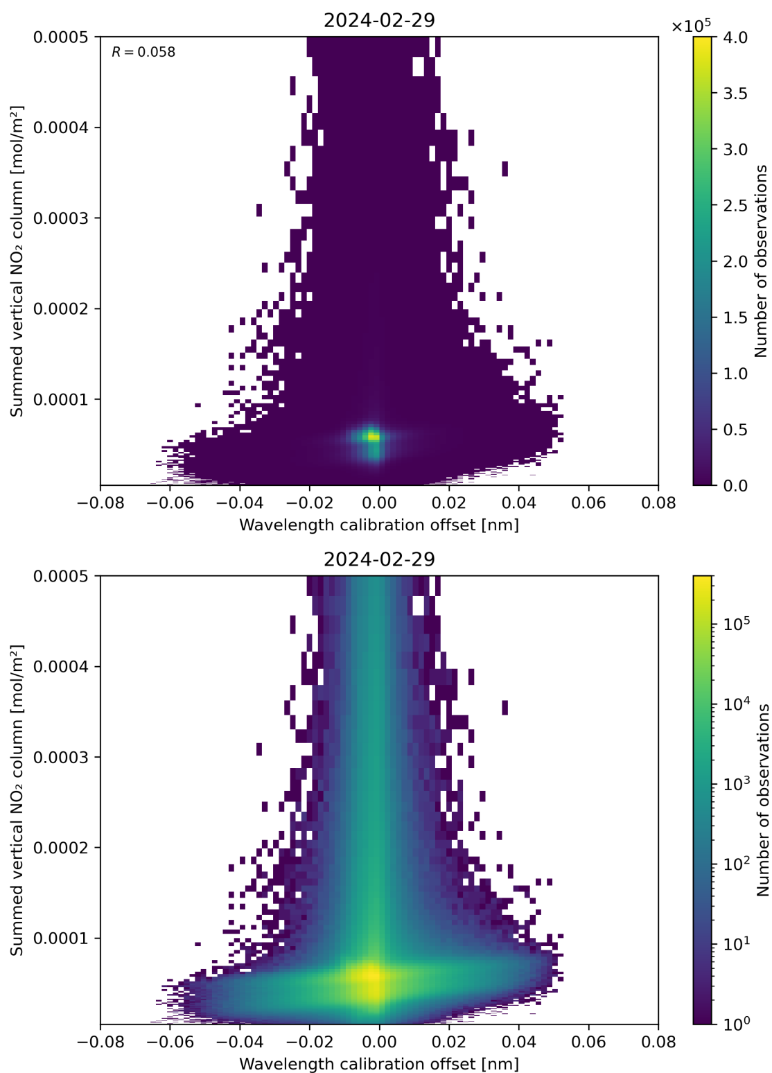
Figure 177: Scatter density plot of “Wavelength calibration offset” against “Summed vertical NO 2 column” for 2024-02-28 to 2024-03-01.
