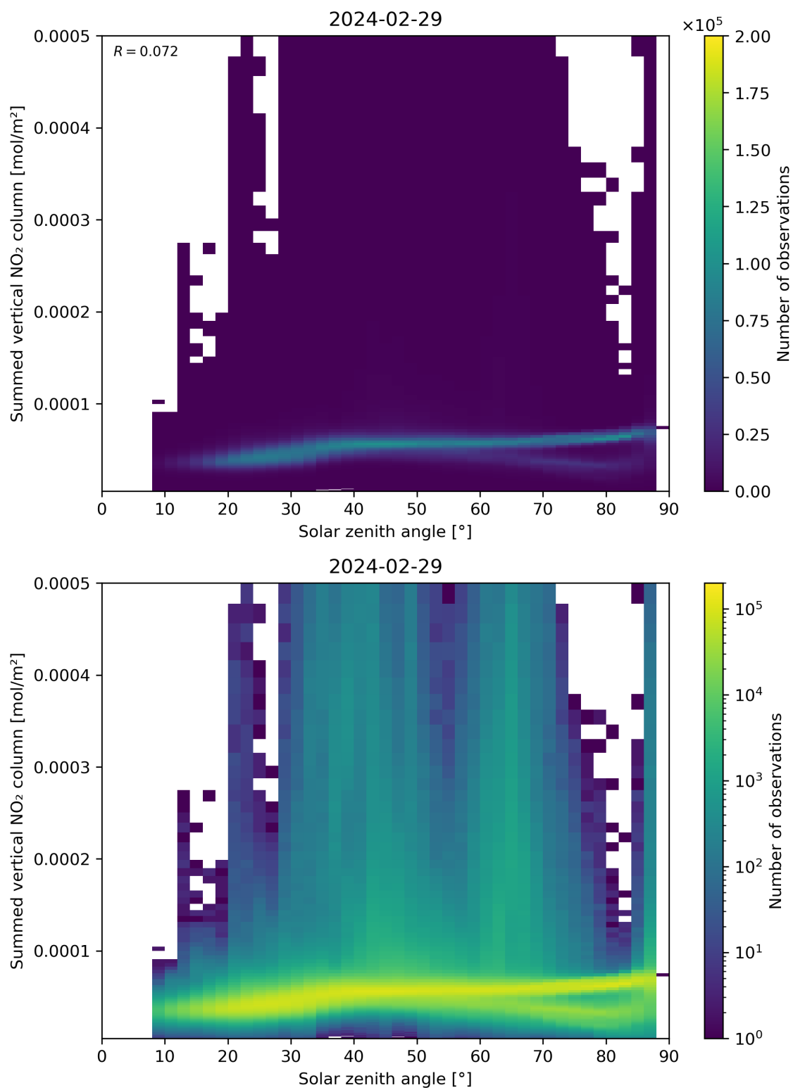
Figure 151: Scatter density plot of “Solar zenith angle” against “Summed vertical NO 2 column” for 2024-02-28 to 2024-03-01.
