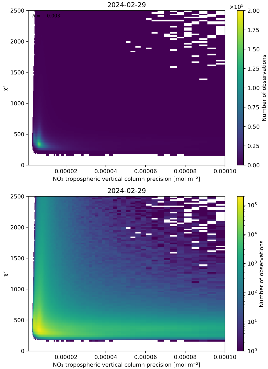
Figure 134: Scatter density plot of “NO 2 tropospheric vertical column precision” against “ \chi^2 ” for 2024-02-28 to 2024-03-01.
