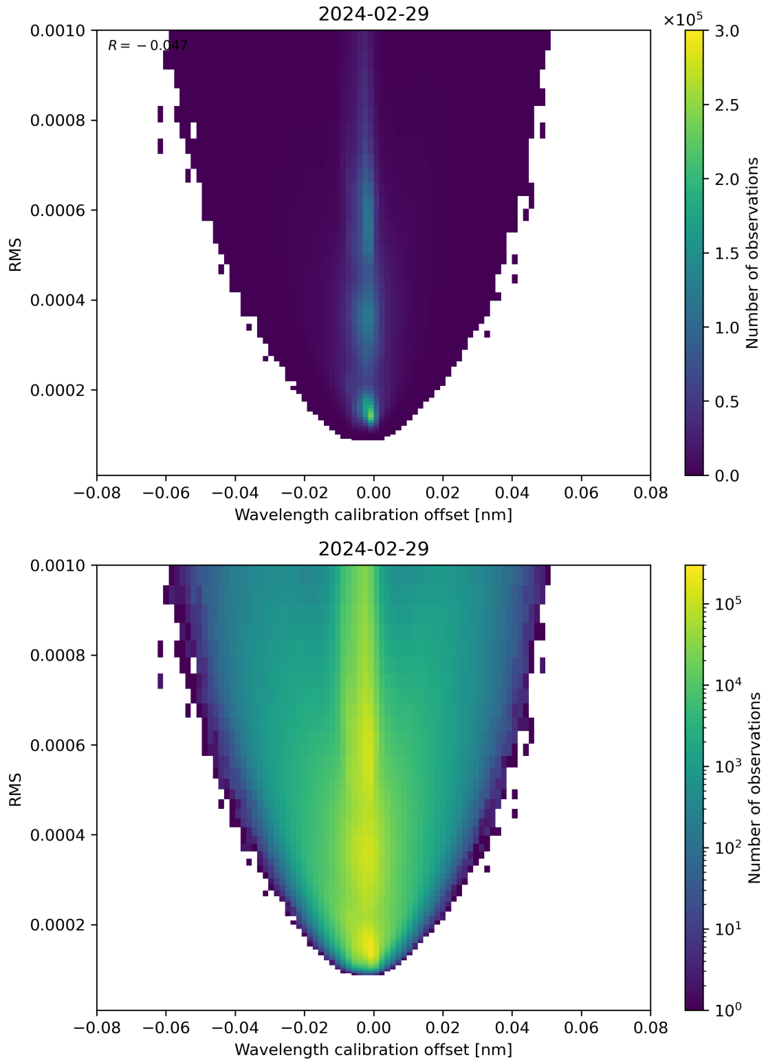
Figure 181: Scatter density plot of “Wavelength calibration offset” against “RMS” for 2024-02-28 to 2024-03-01.
