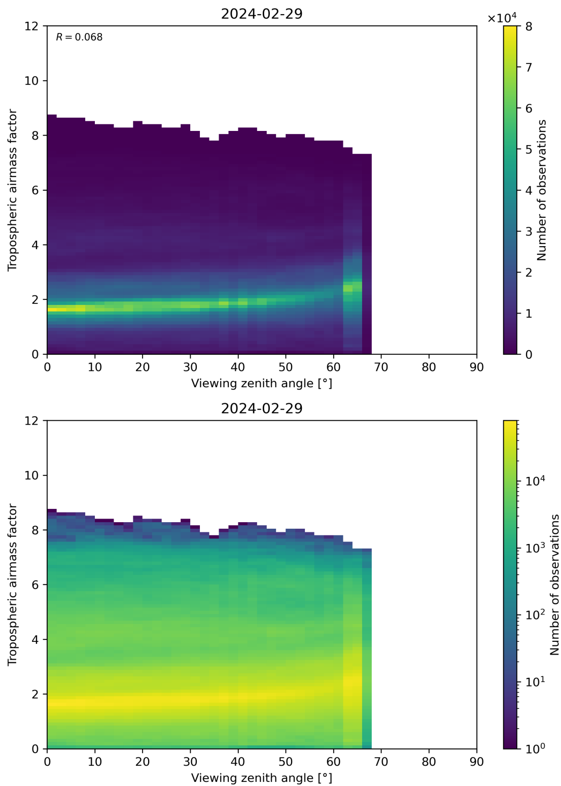
Figure 161: Scatter density plot of “Viewing zenith angle” against “Tropospheric airmass factor” for 2024-02-28 to 2024-03-01.
