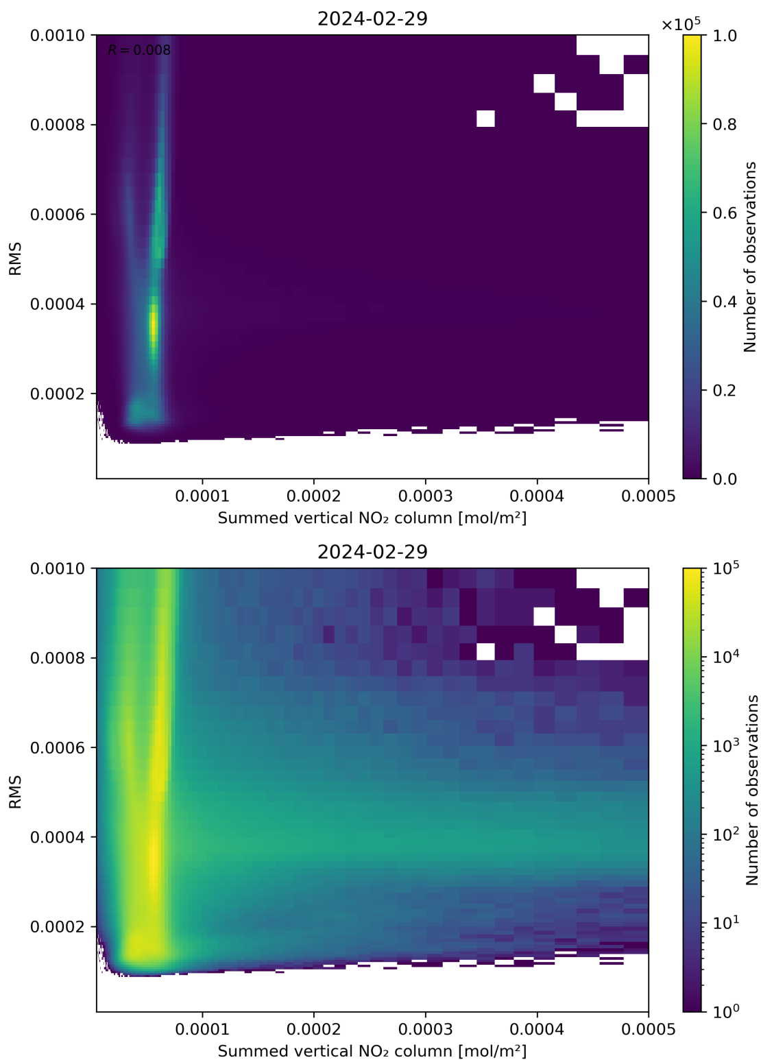
Figure 109: Scatter density plot of “Summed vertical NO 2 column” against “RMS” for 2024-02-28 to 2024-03-01.
