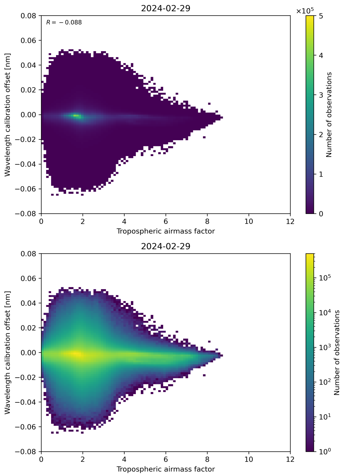
Figure 80: Scatter density plot of “Tropospheric air mass factor” against “Wavelength calibration offset” for 2024-02-28 to 2024-03-01.
