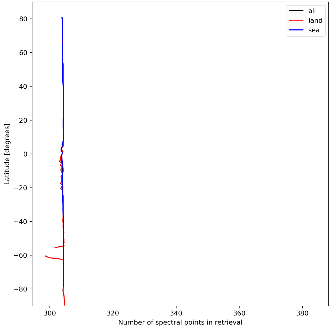
Figure 16: Zonal average of “Number of spectral points in retrieval” for 2024-02-28 to 2024-03-01.
