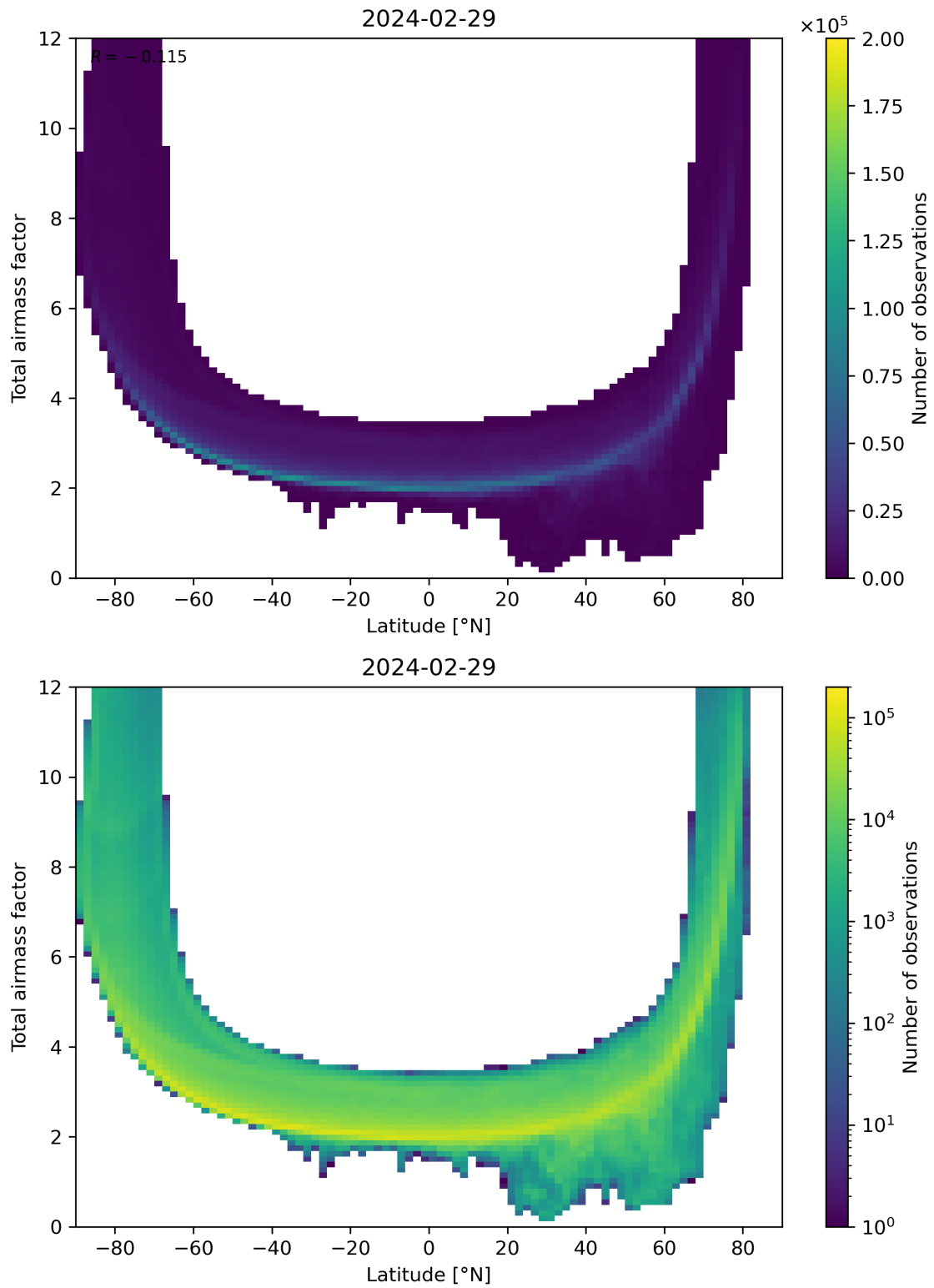
Figure 84: Scatter density plot of “Latitude” against “Total airmass factor” for 2024-02-28 to 2024-03-01.
