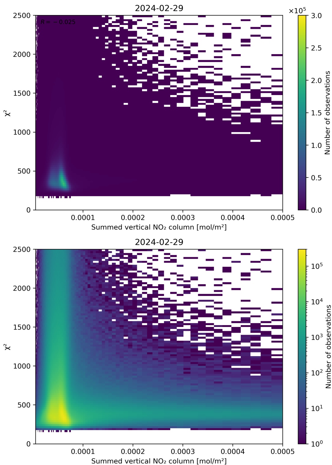
Figure 104: Scatter density plot of “Summed vertical NO 2 column” against “ \chi^2 ” for 2024-02-28 to 2024-03-01.
