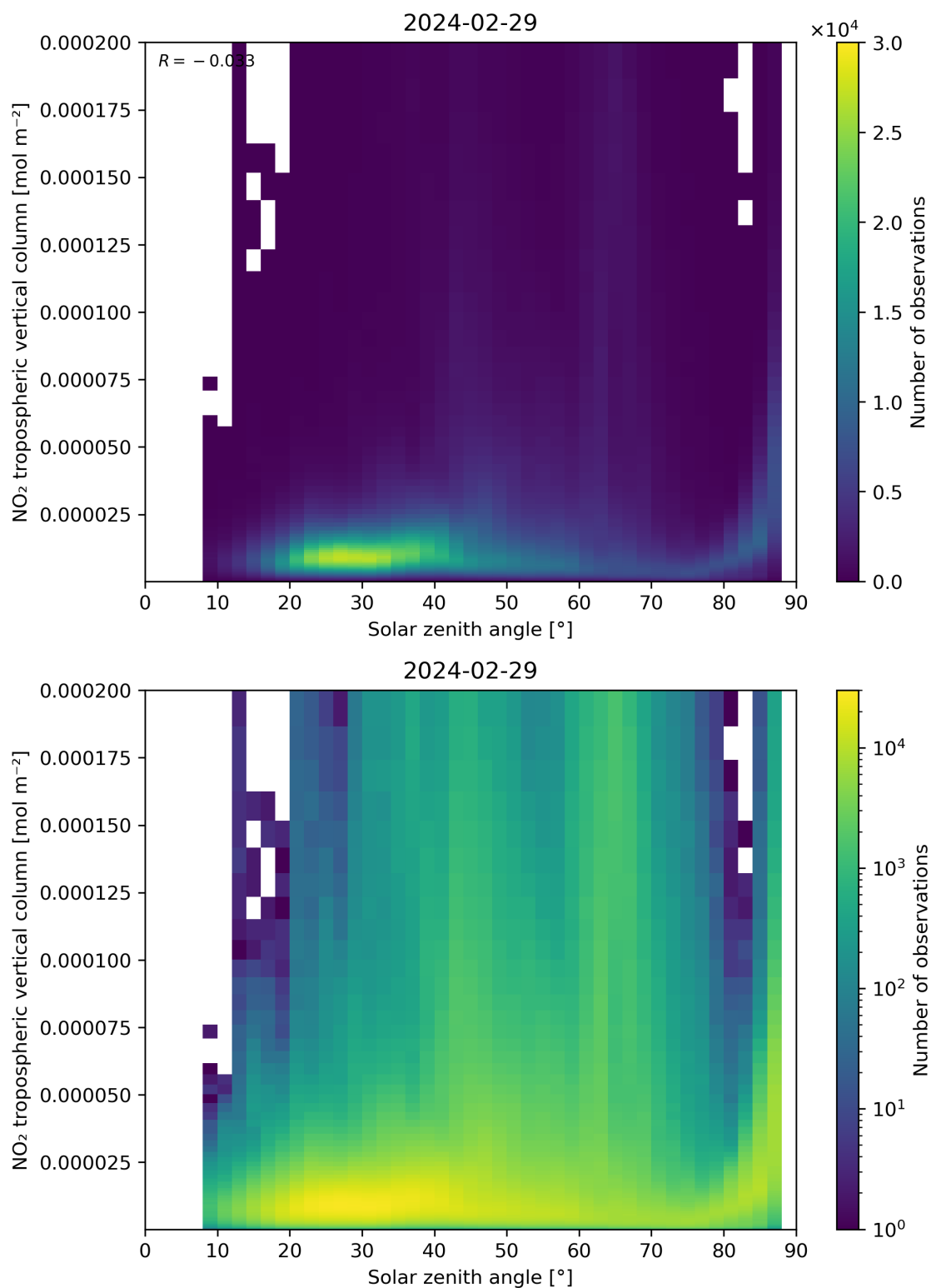
Figure 155: Scatter density plot of “Solar zenith angle” against “NO 2 tropospheric vertical column” for 2024-02-28 to 2024-03-01.
