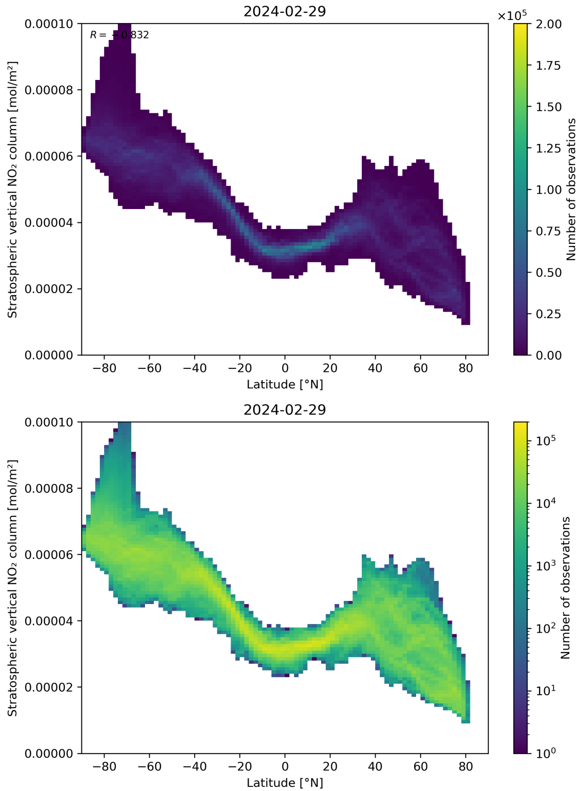
Figure 87: Scatter density plot of “Latitude” against “Stratospheric vertical NO 2 column” for 2024-02-28 to 2024-03-01.
