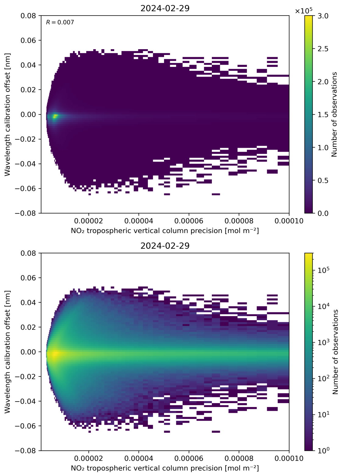
Figure 141: Scatter density plot of “NO 2 tropospheric vertical column precision” against “Wavelength calibration offset” for 2024-02-28 to 2024-03-01.
