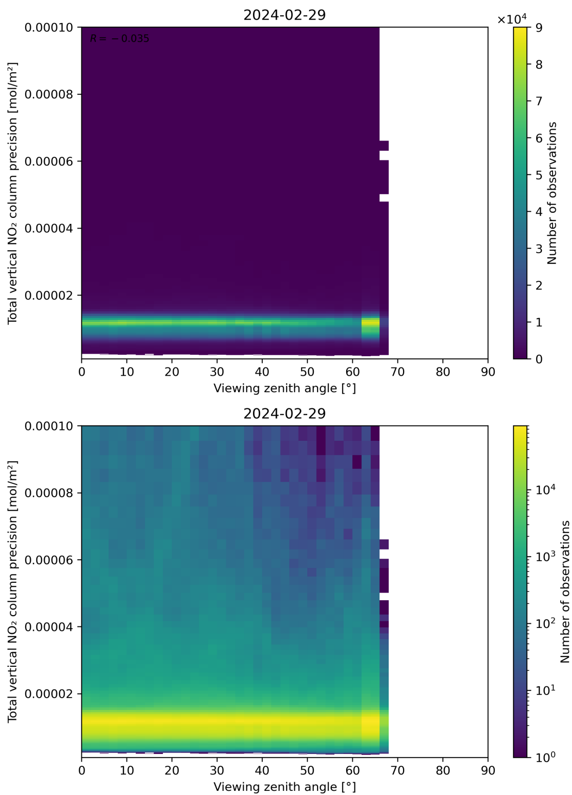
Figure 168: Scatter density plot of “Viewing zenith angle” against “Total vertical NO 2 column precision” for 2024-02-28 to 2024-03-01.
