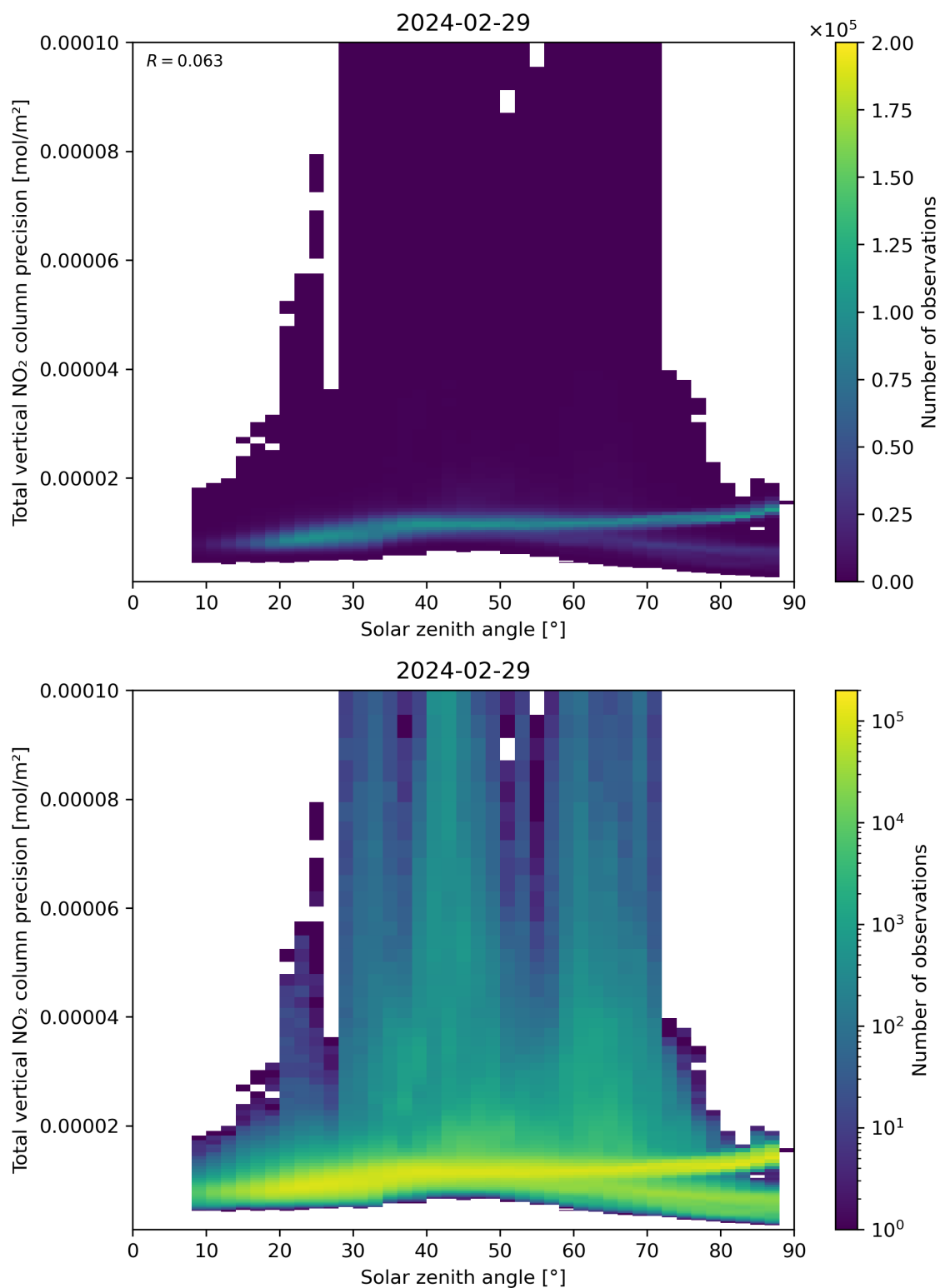
Figure 154: Scatter density plot of “Solar zenith angle” against “Total vertical NO 2 column precision” for 2024-02-28 to 2024-03-01.
