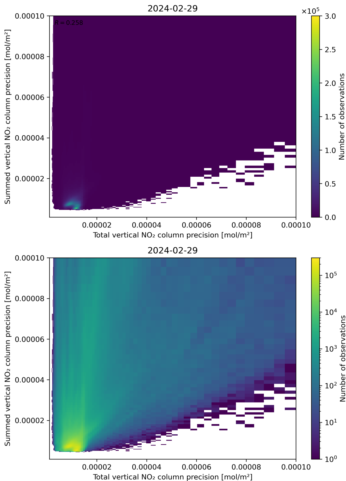
Figure 118: Scatter density plot of “Total vertical NO 2 column precision” against “Summed vertical NO 2 column precision” for 2024-02-28 to 2024-03-01.
