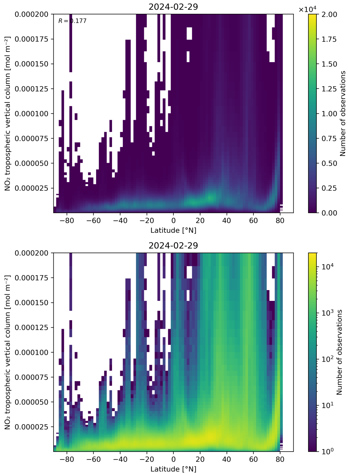
Figure 92: Scatter density plot of “Latitude” against “NO 2 tropospheric vertical column” for 2024-02-28 to 2024-03-01.
