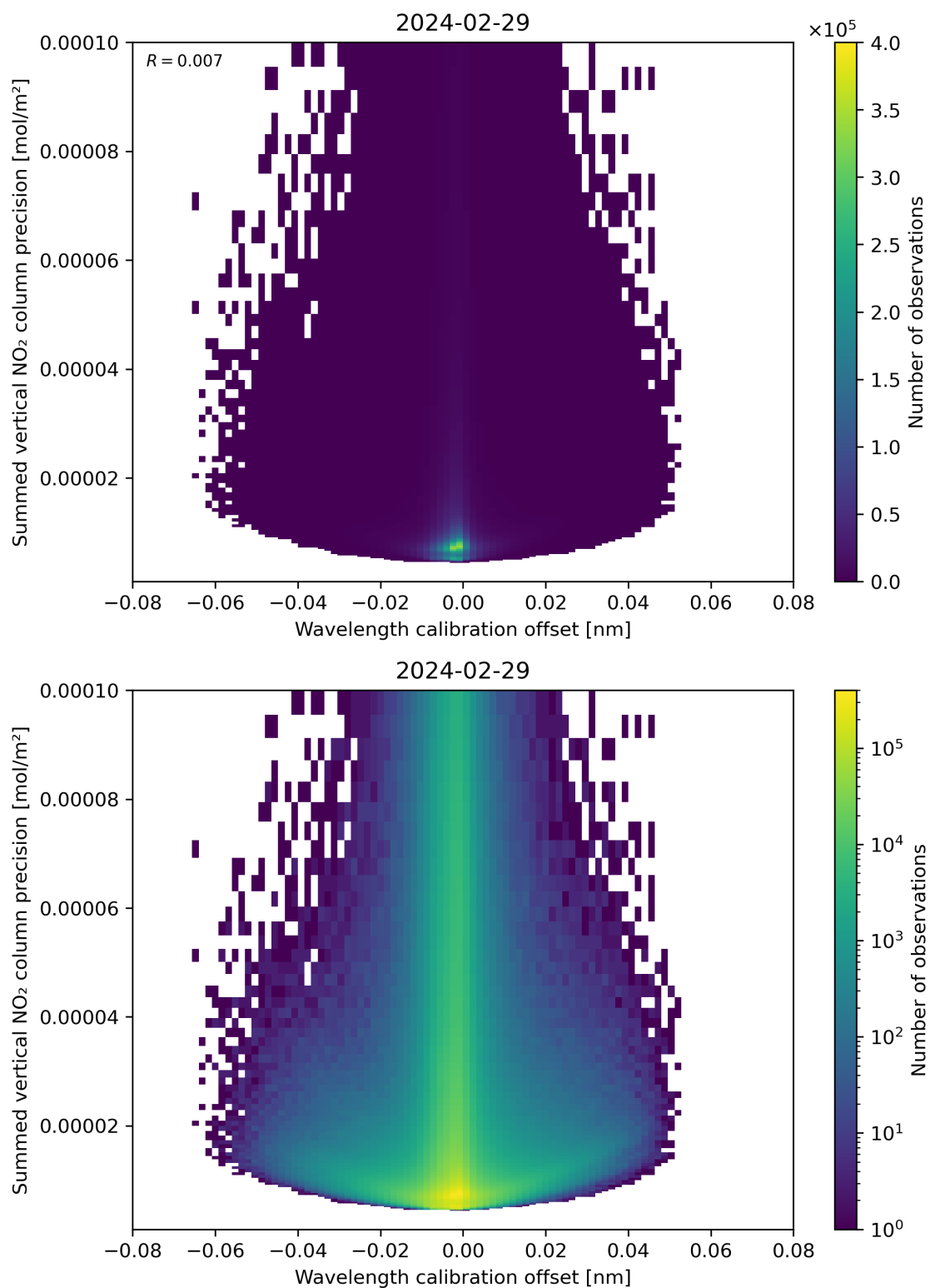
Figure 178: Scatter density plot of “Wavelength calibration offset” against “Summed vertical NO 2 column precision” for 2024-02-28 to 2024-03-01.
