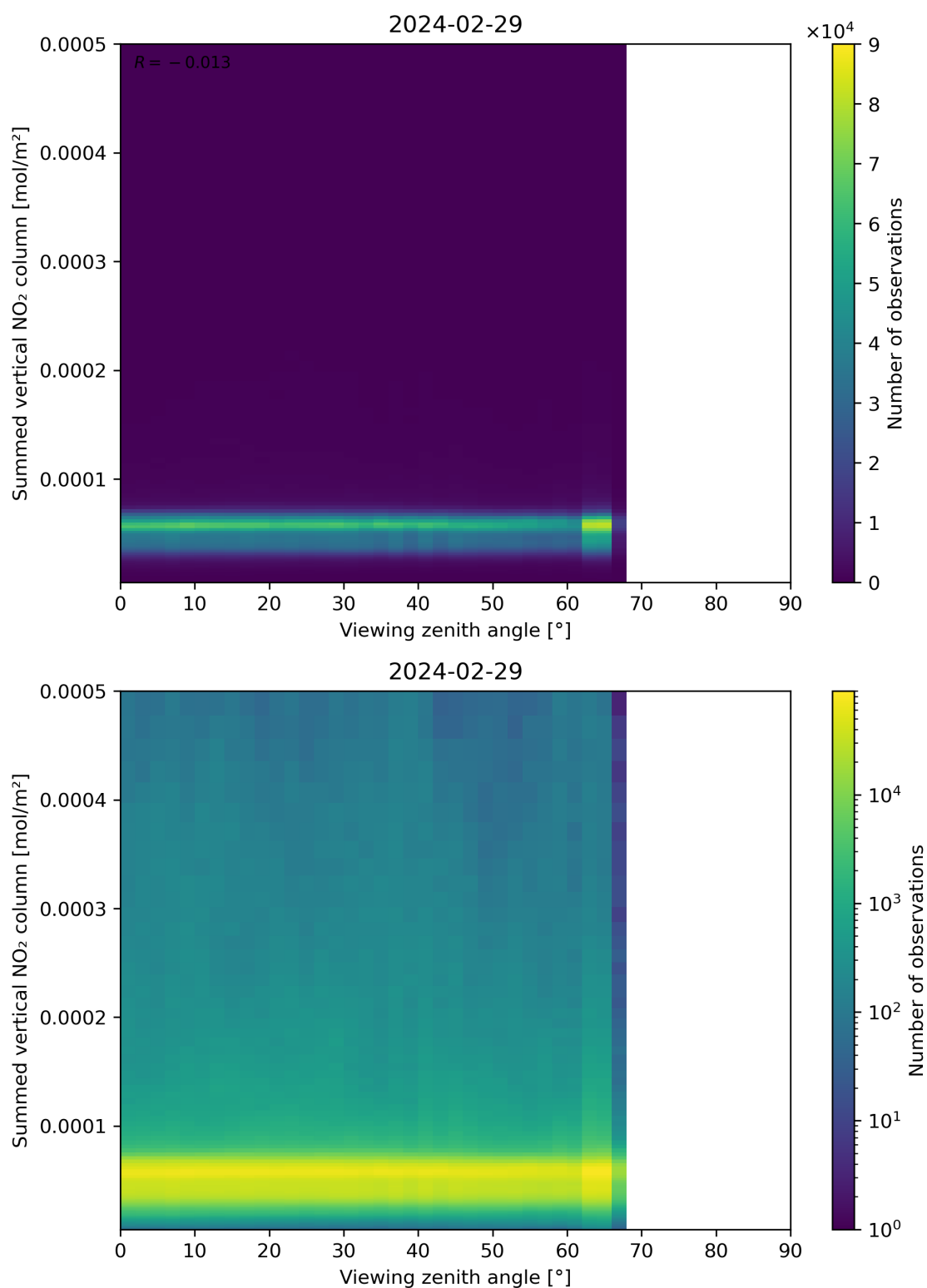
Figure 165: Scatter density plot of “Viewing zenith angle” against “Summed vertical NO 2 column” for 2024-02-28 to 2024-03-01.
