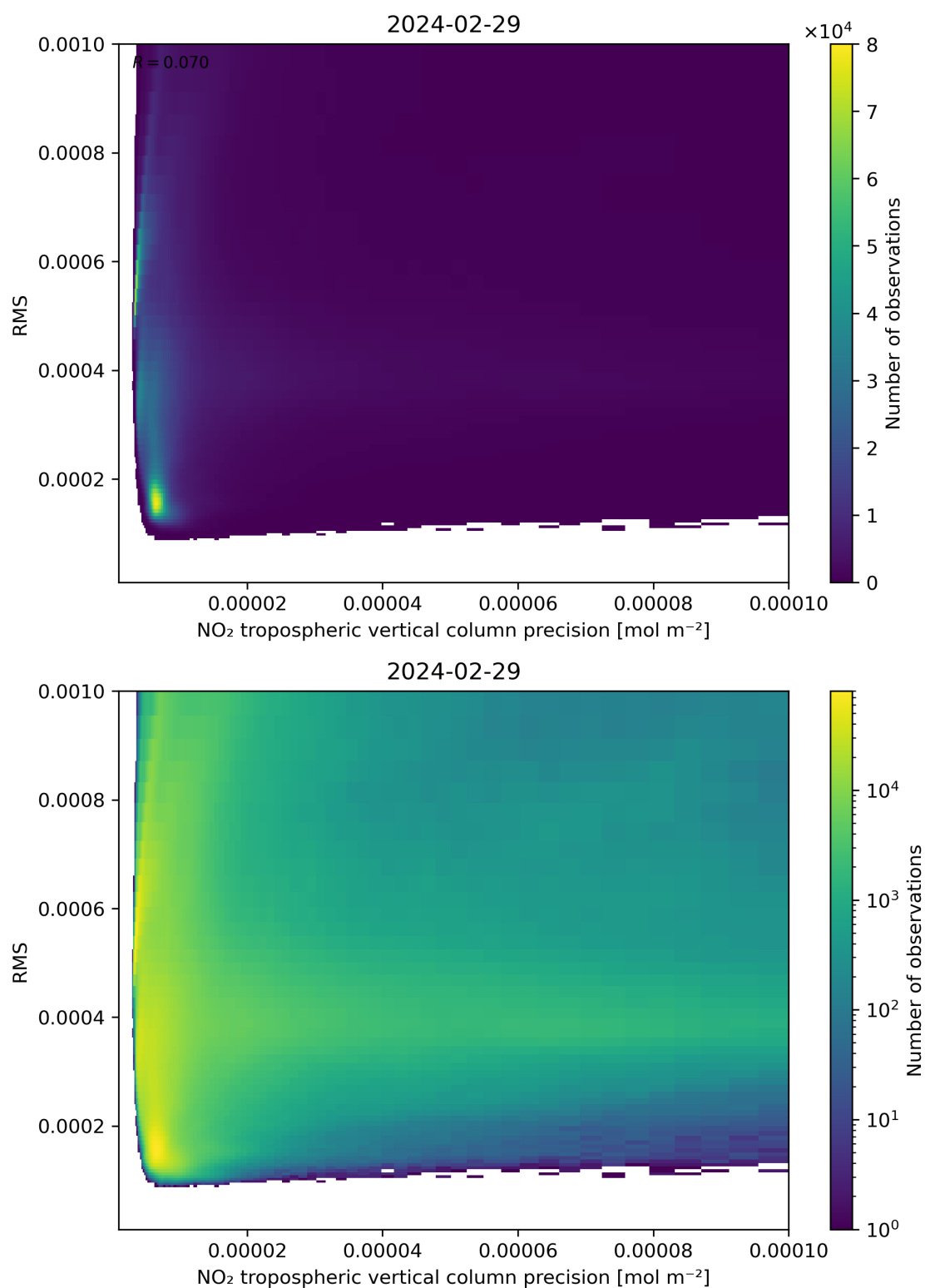
Figure 140: Scatter density plot of “NO 2 tropospheric vertical column precision” against “RMS” for 2024-02-28 to 2024-03-01.
