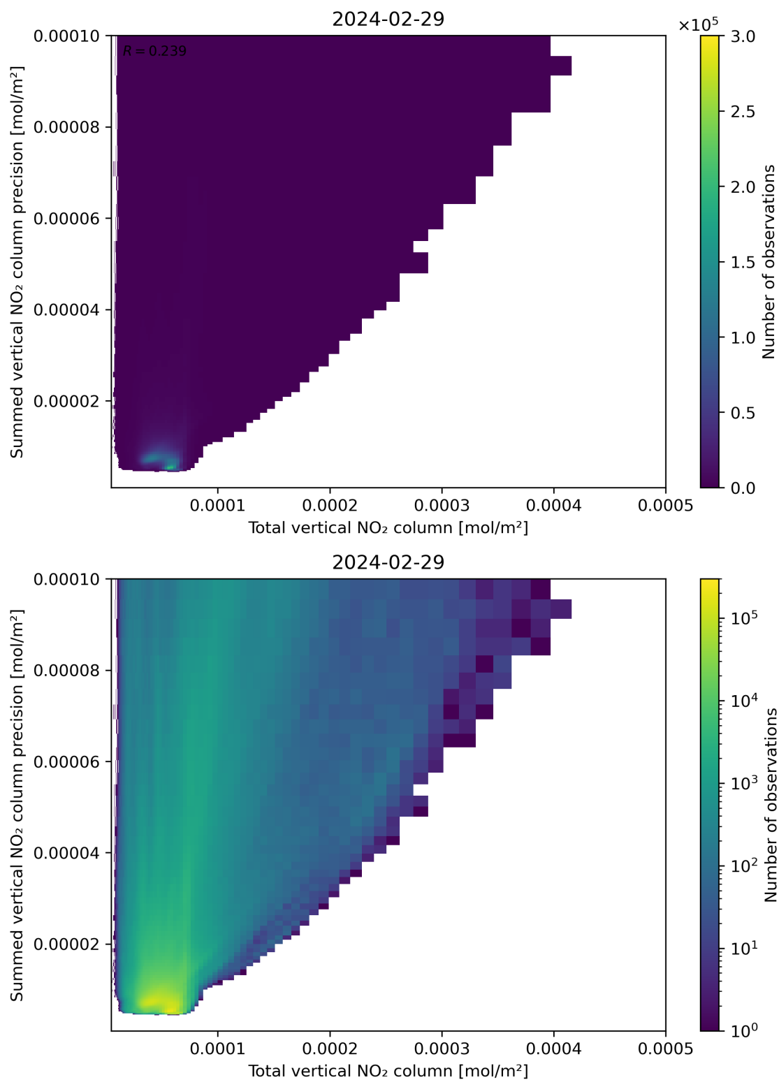
Figure 113: Scatter density plot of “Total vertical NO 2 column” against “Summed vertical NO 2 column precision” for 2024-02-28 to 2024-03-01.
