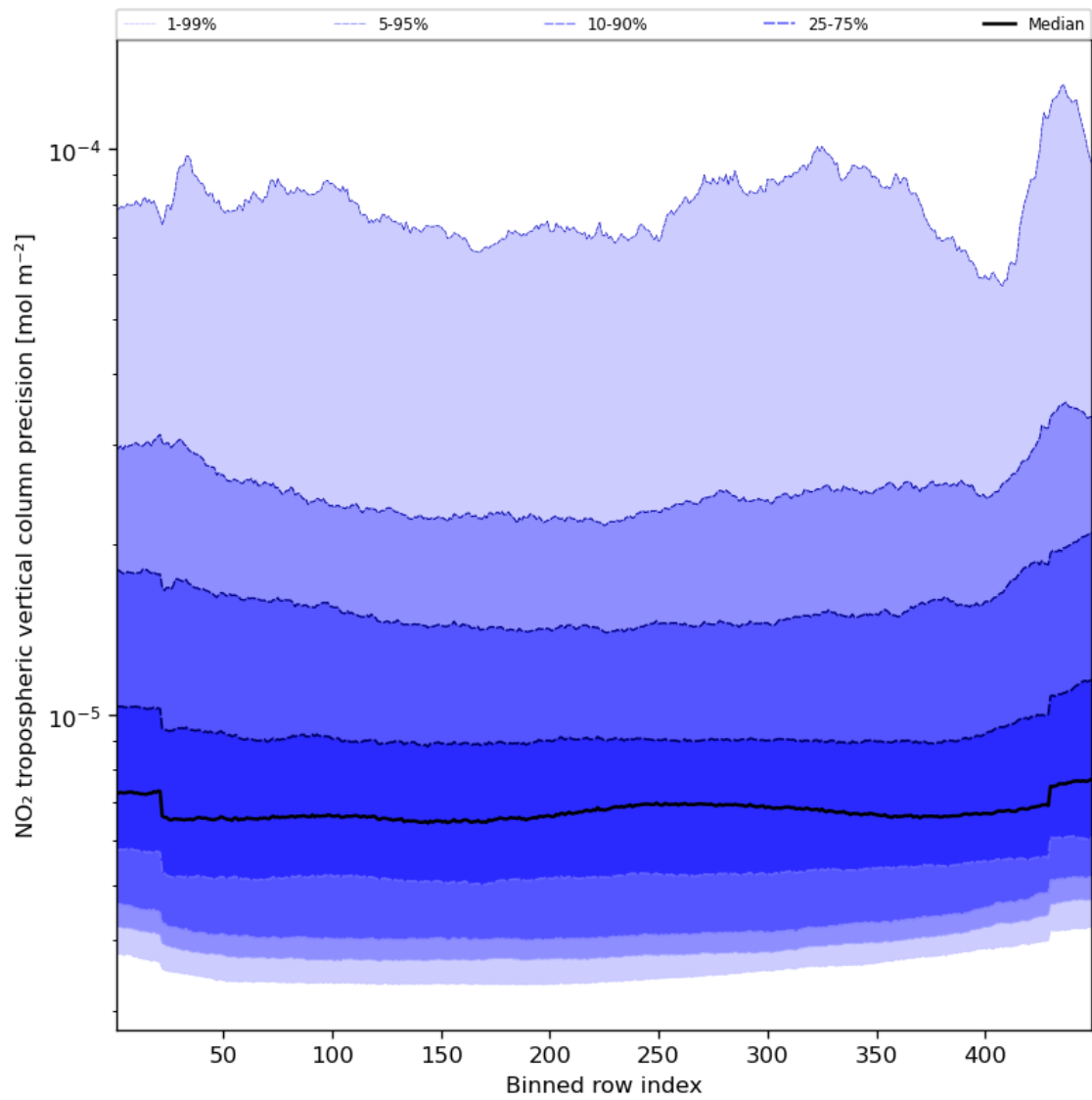
Figure 47: Along track statistics of “NO 2 tropospheric vertical column precision” for 2024-02-28 to 2024-03-01
