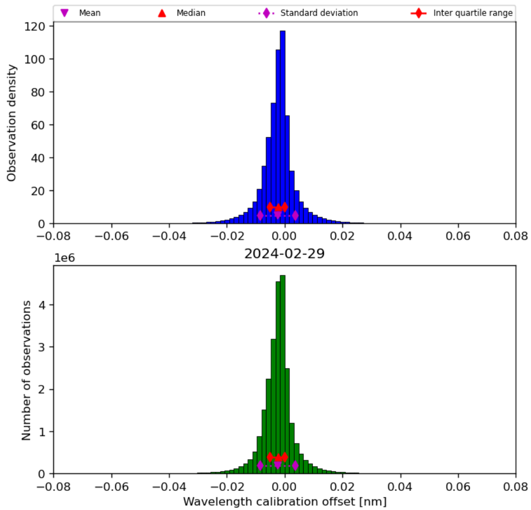
Figure 35: Histogram of “Wavelength calibration offset” for 2024-02-28 to 2024-03-01
