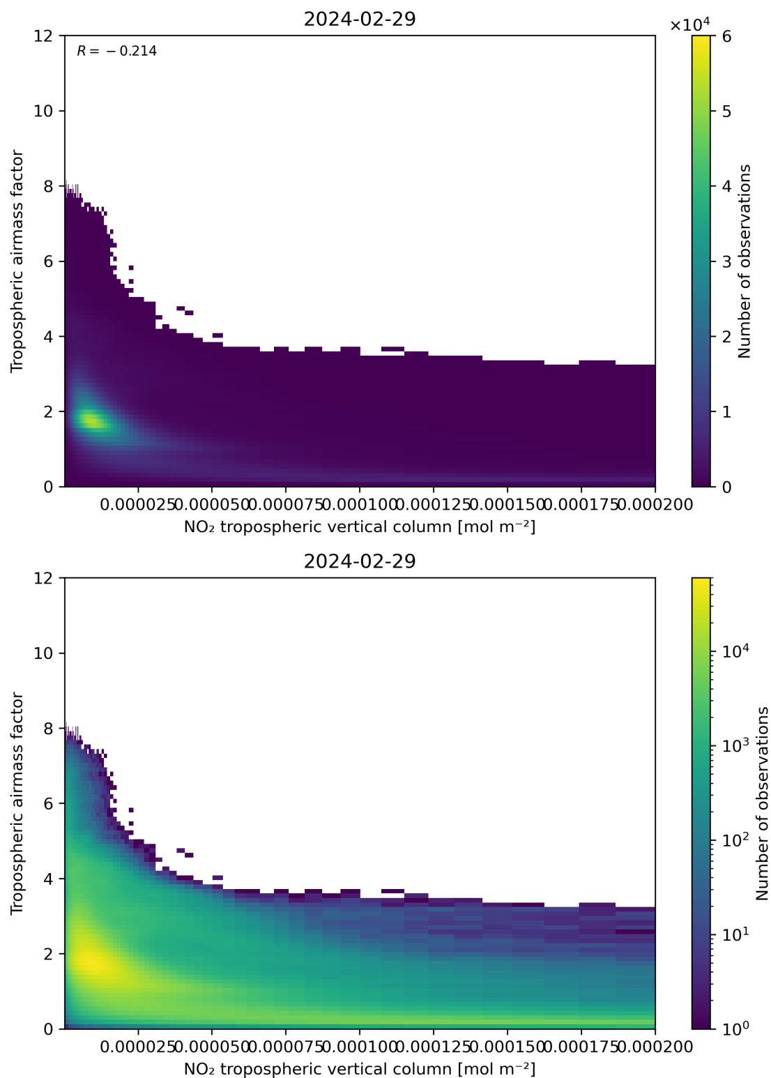
Figure 123: Scatter density plot of “NO 2 tropospheric vertical column” against “Tropospheric airmass factor” for 2024-02-28 to 2024-03-01.
