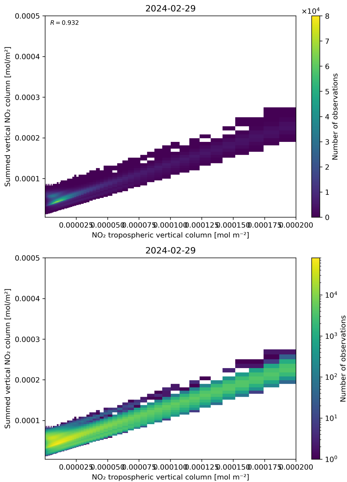
Figure 126: Scatter density plot of “NO 2 tropospheric vertical column” against “Summed vertical NO 2 column” for 2024-02-28 to 2024-03-01.
