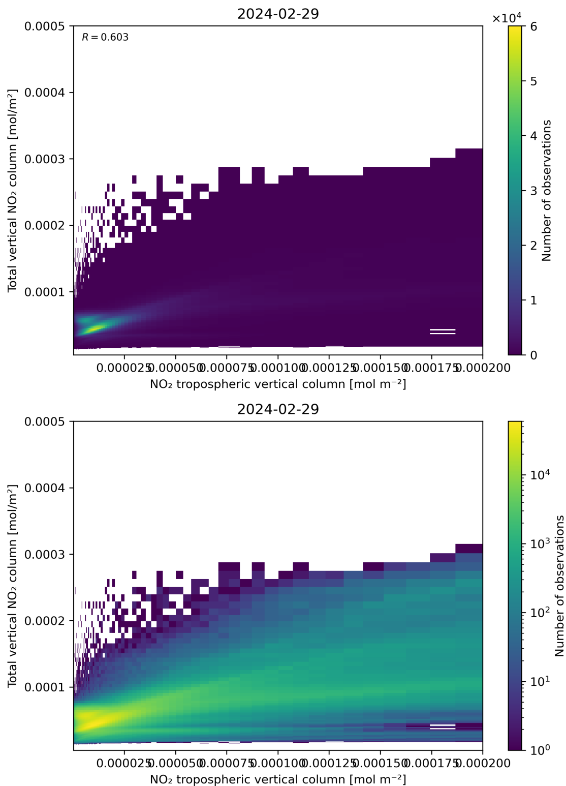
Figure 128: Scatter density plot of “NO 2 tropospheric vertical column” against “Total vertical NO 2 column” for 2024-02-28 to 2024-03-01.
