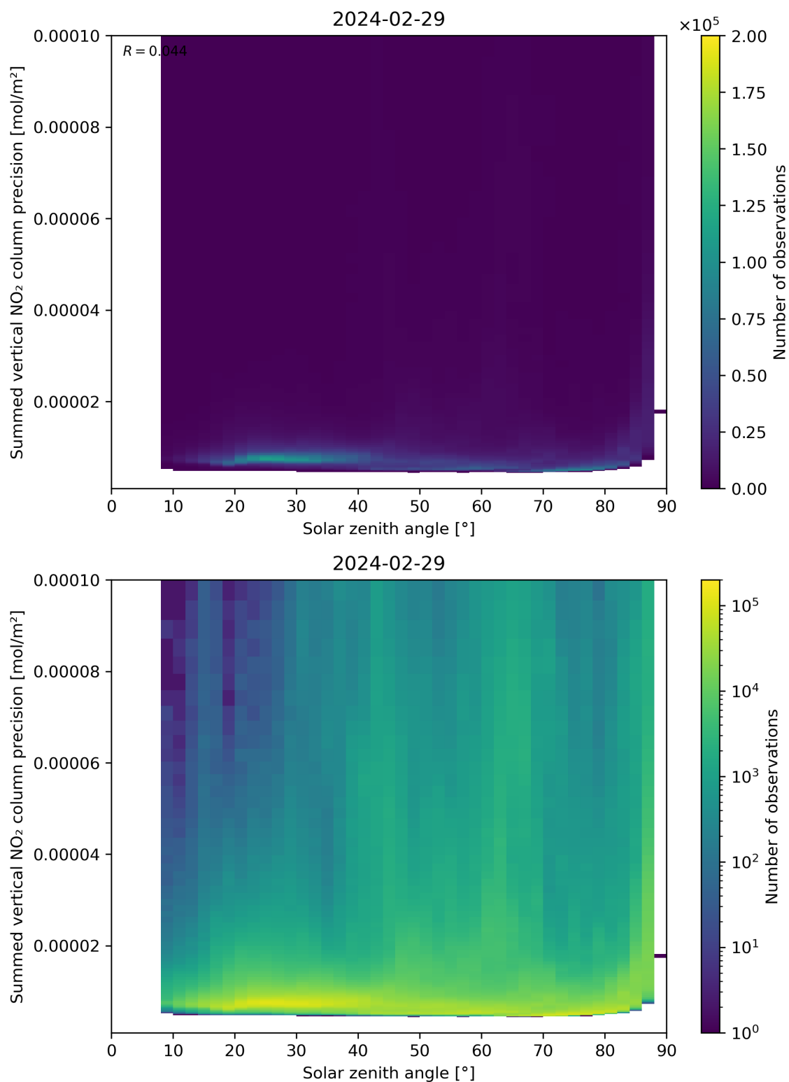
Figure 152: Scatter density plot of “Solar zenith angle” against “Summed vertical NO 2 column precision” for 2024-02-28 to 2024-03-01.
