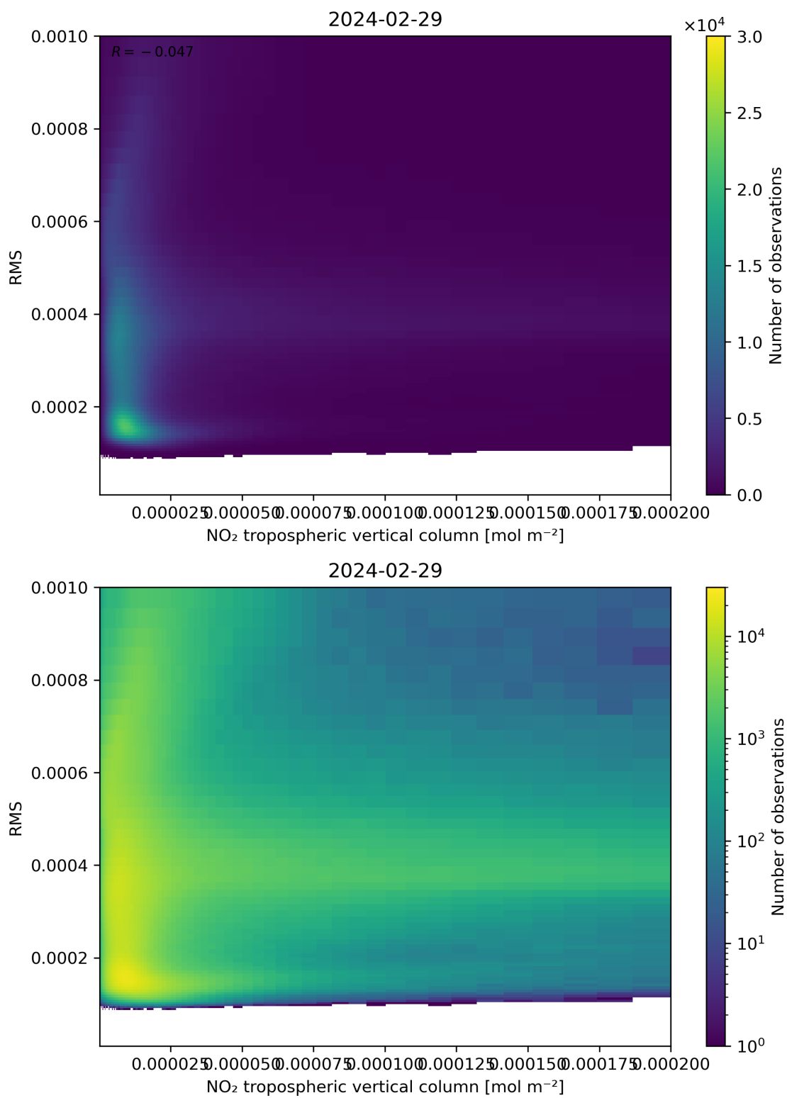
Figure 142: Scatter density plot of “NO 2 tropospheric vertical column” against “RMS” for 2024-02-28 to 2024-03-01.
