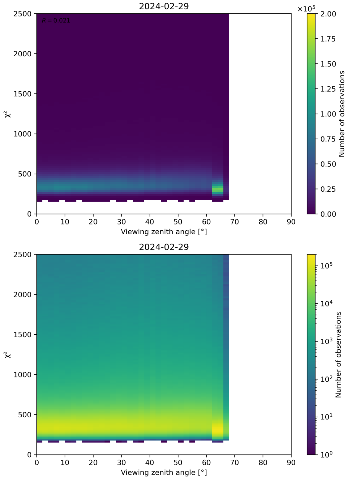
Figure 162: Scatter density plot of “Viewing zenith angle” against “ \chi^2 ” for 2024-02-28 to 2024-03-01.
