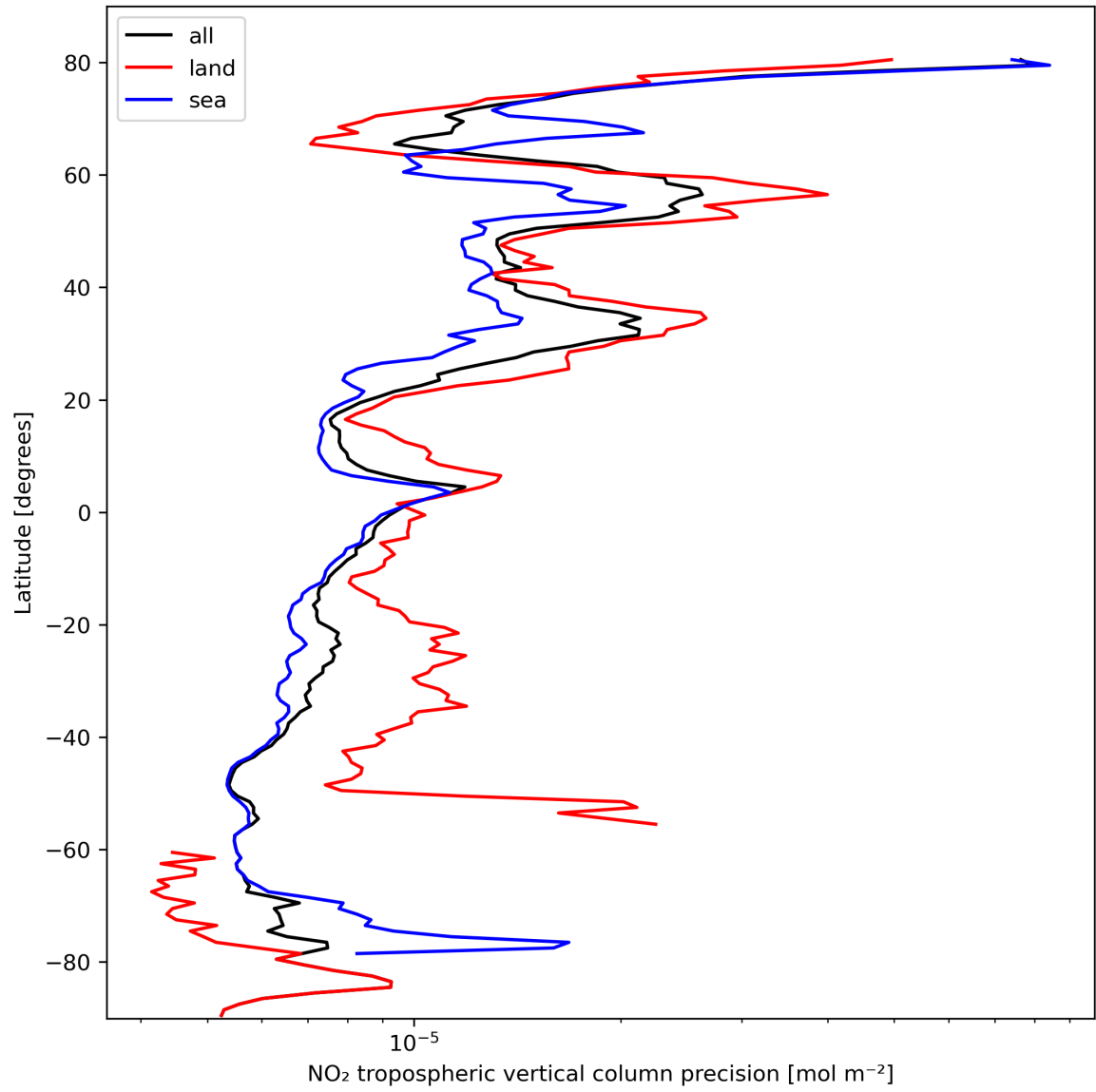
Figure 13: Zonal average of “NO 2 tropospheric vertical column precision” for 2024-02-28 to 2024-03-01.
