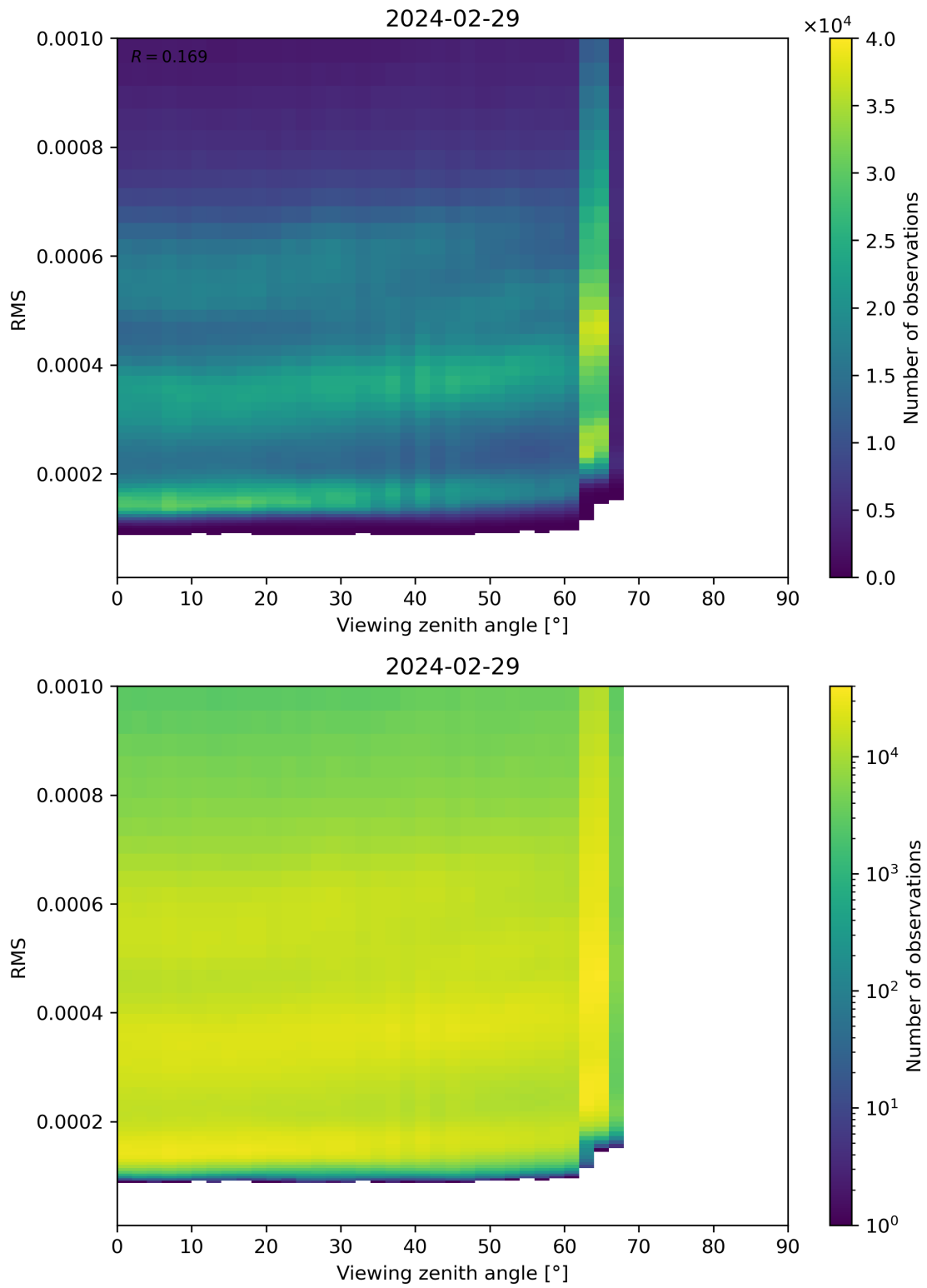
Figure 171: Scatter density plot of “Viewing zenith angle” against “RMS” for 2024-02-28 to 2024-03-01.
