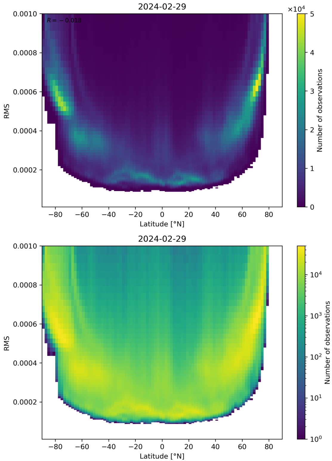
Figure 94: Scatter density plot of “Latitude” against “RMS” for 2024-02-28 to 2024-03-01.
