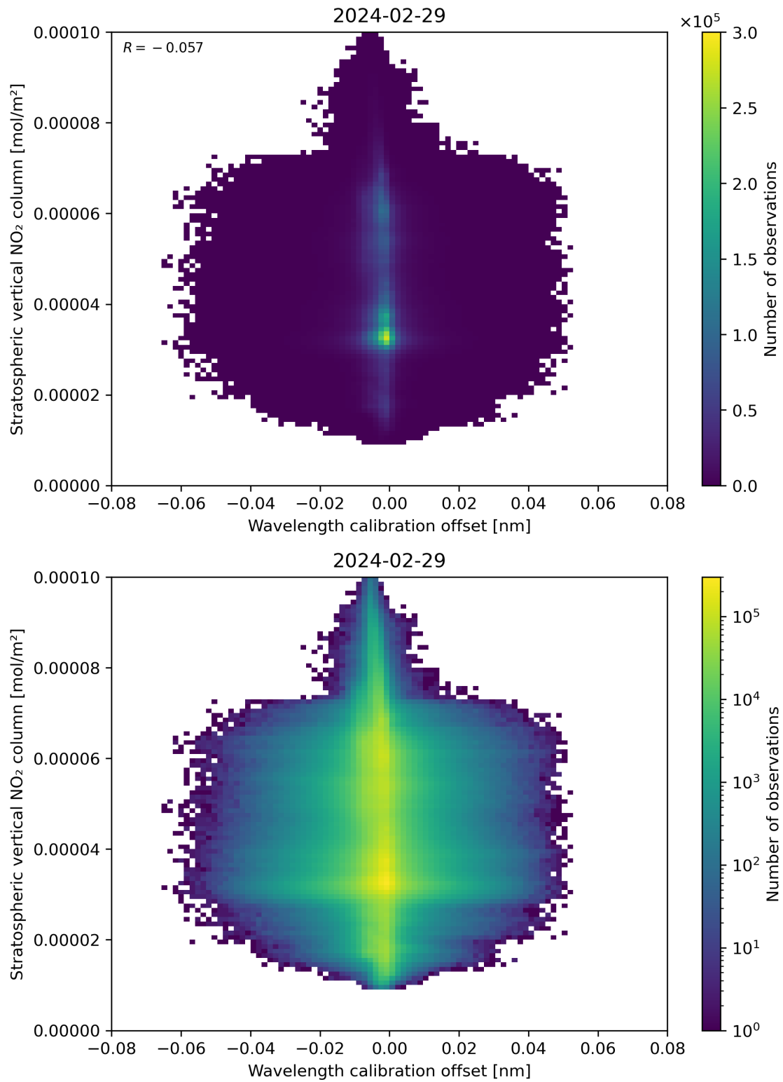
Figure 176: Scatter density plot of “Wavelength calibration offset” against “Stratospheric vertical NO 2 column” for 2024-02-28 to 2024-03-01.
