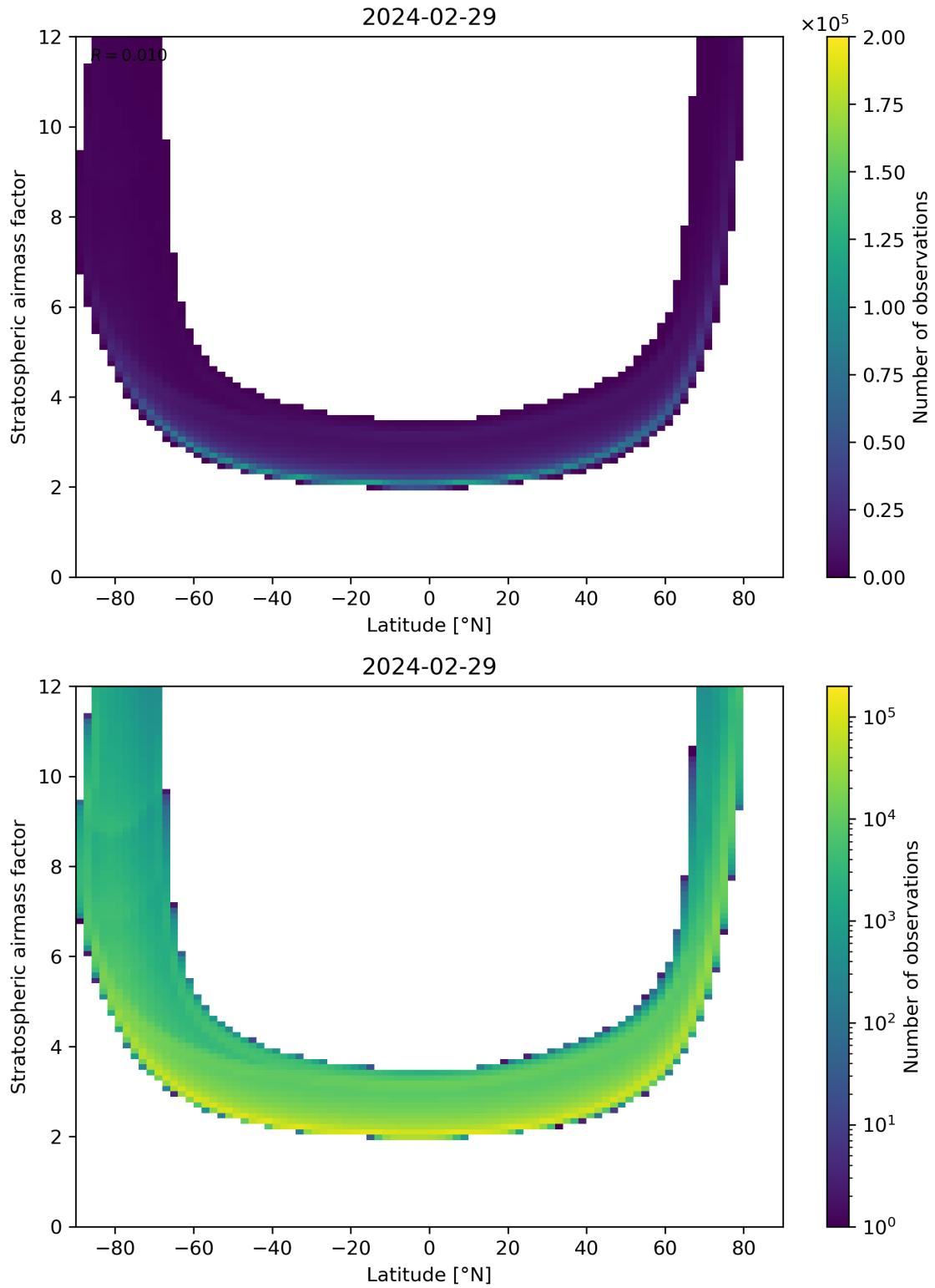
Figure 83: Scatter density plot of “Latitude” against “Stratospheric air mass factor” for 2024-02-28 to 2024-03-01.
