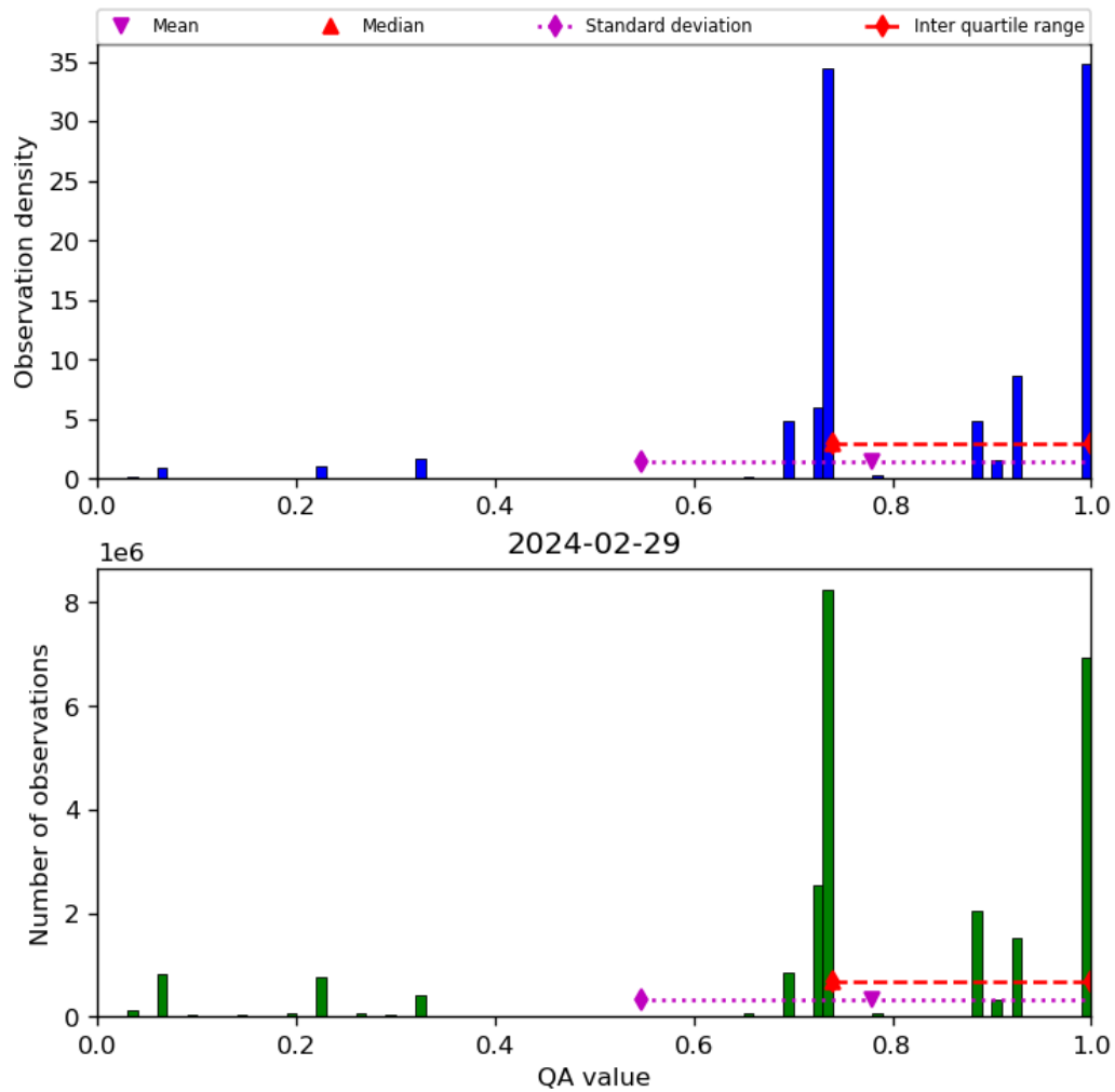
Figure 28: Histogram of “QA value” for 2024-02-28 to 2024-03-01
