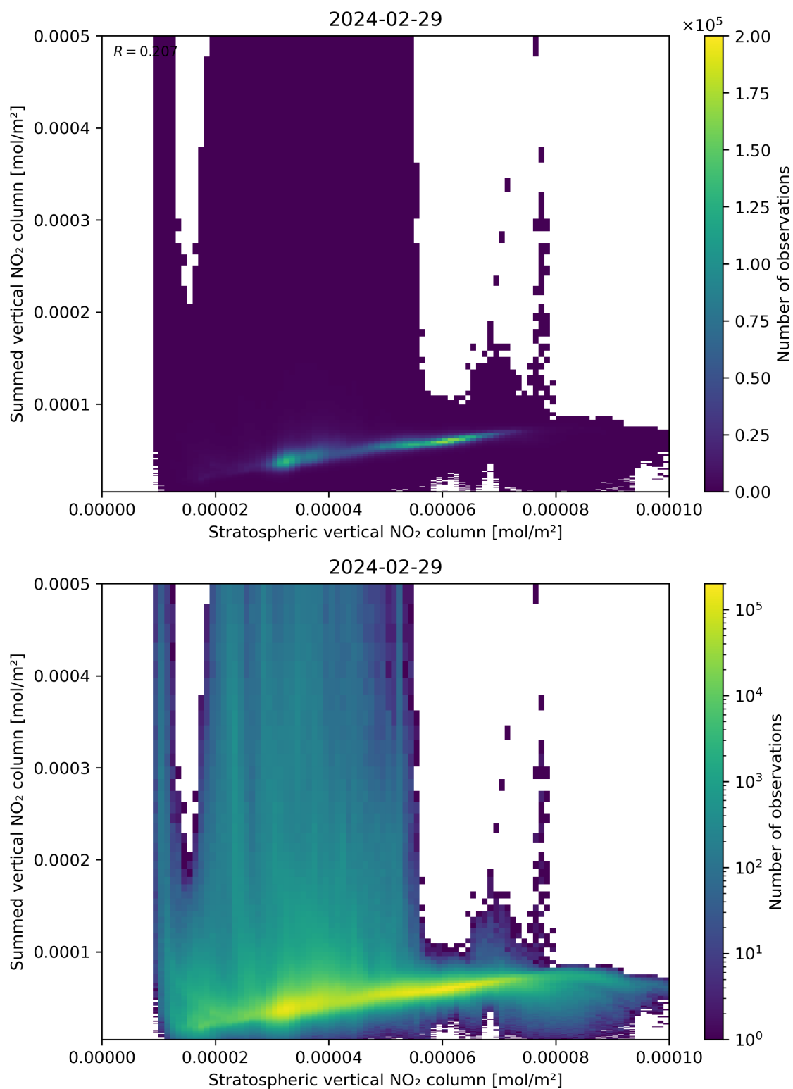
Figure 98: Scatter density plot of “Stratospheric vertical NO 2 column” against “Summed vertical NO 2 column” for 2024-02-28 to 2024-03-01.
