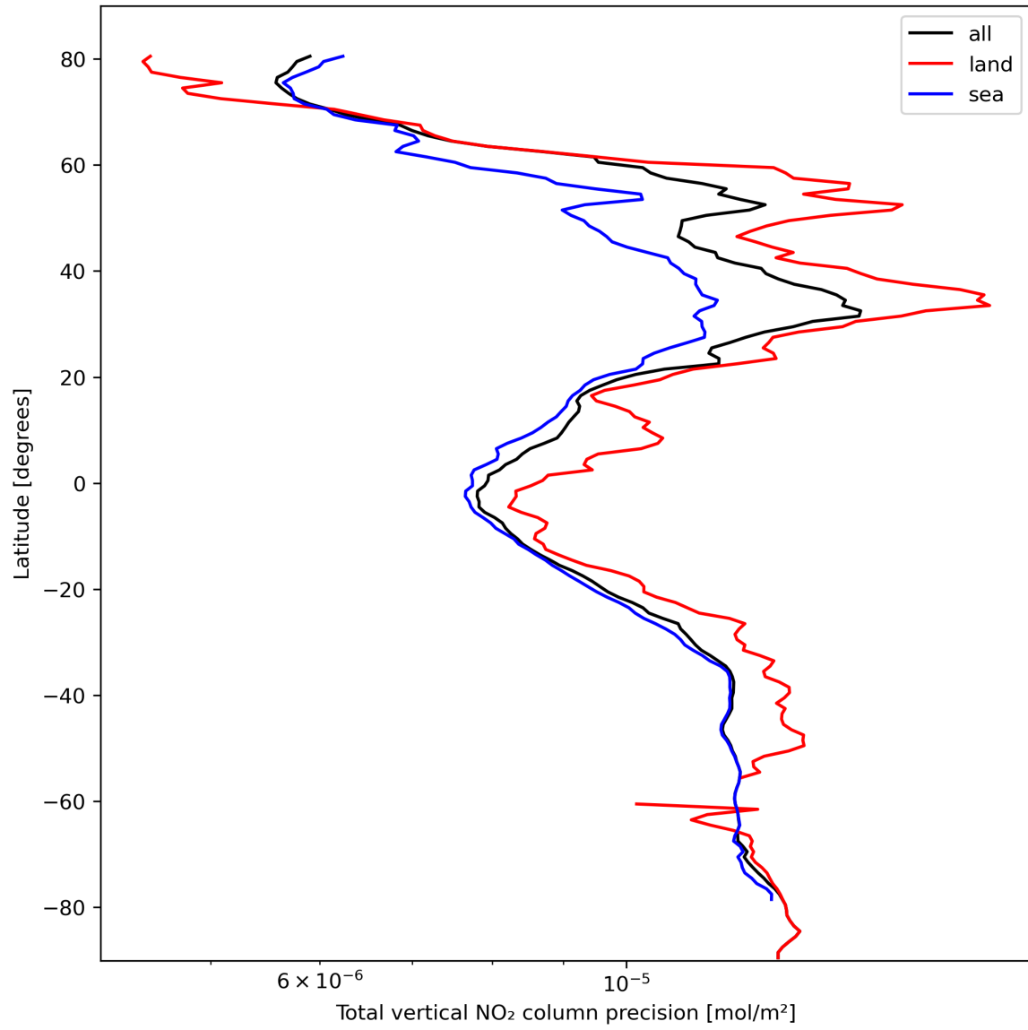
Figure 22: Zonal average of “Total vertical NO 2 column precision” for 2024-02-28 to 2024-03-01.
