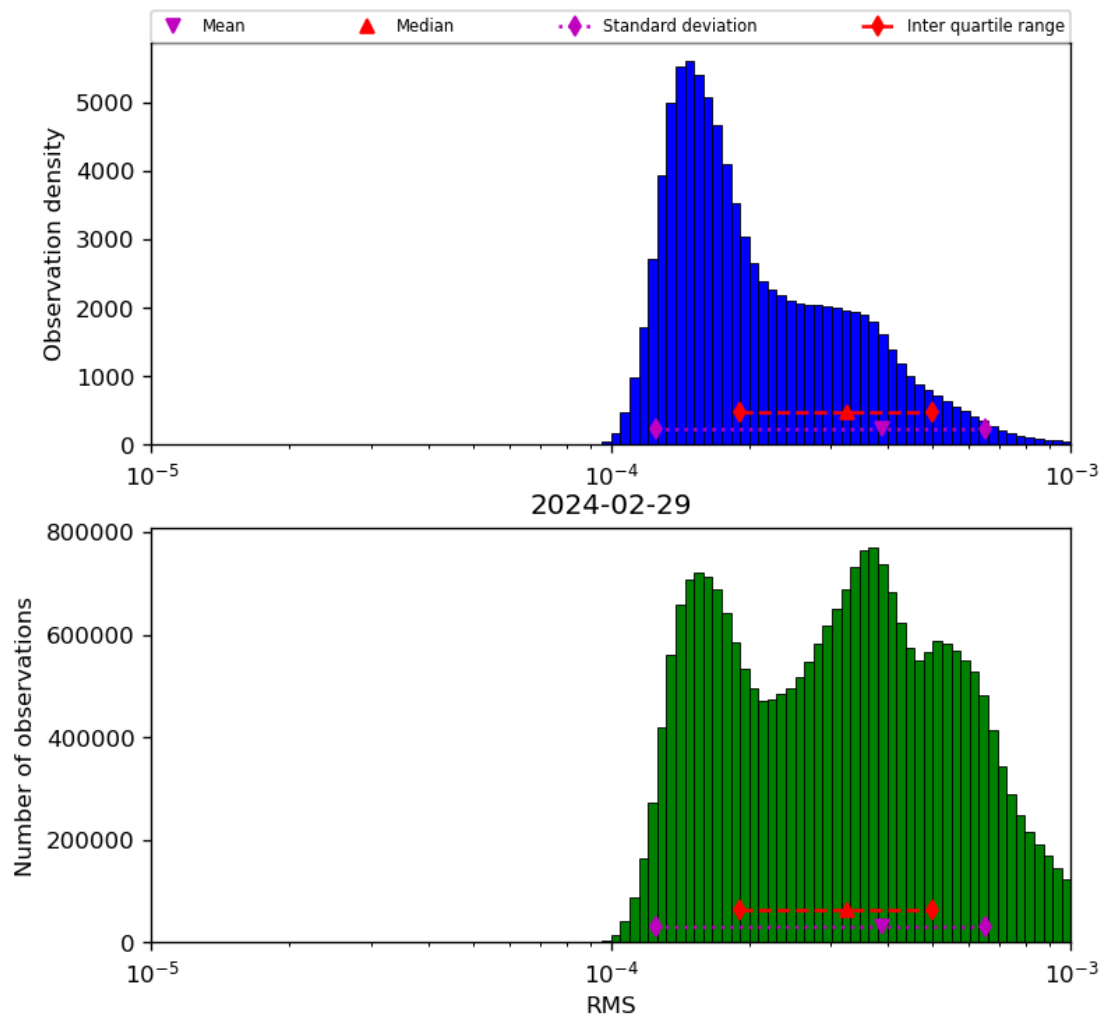
Figure 43: Histogram of “RMS” for 2024-02-28 to 2024-03-01
