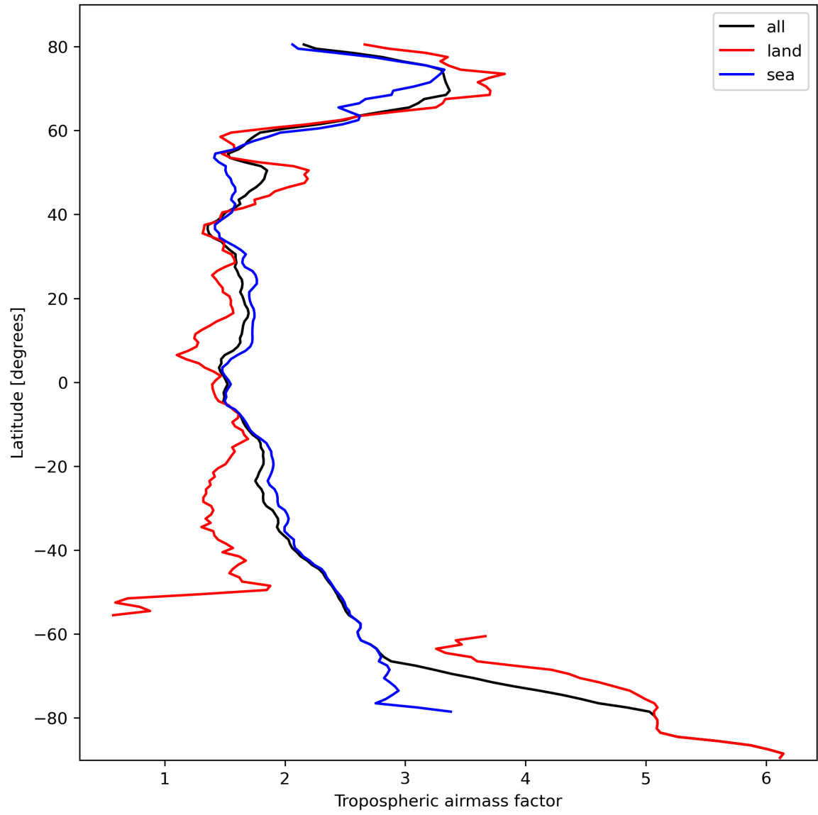
Figure 14: Zonal average of “Tropospheric airmass factor” for 2024-02-28 to 2024-03-01.
