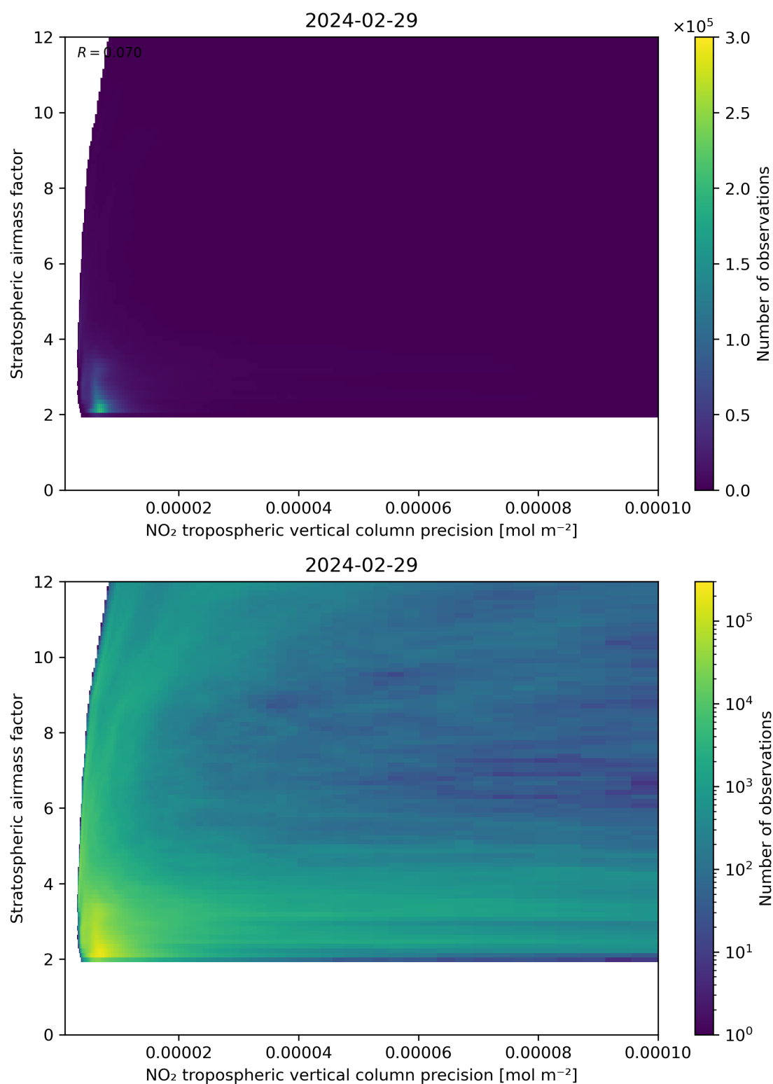
Figure 131: Scatter density plot of “NO 2 tropospheric vertical column precision” against “Stratospheric airmass factor” for 2024-02-28 to 2024-03-01.
