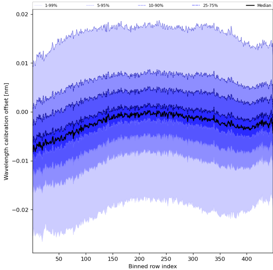
Figure 52: Along track statistics of “Wavelength calibration offset” for 2024-02-28 to 2024-03-01
