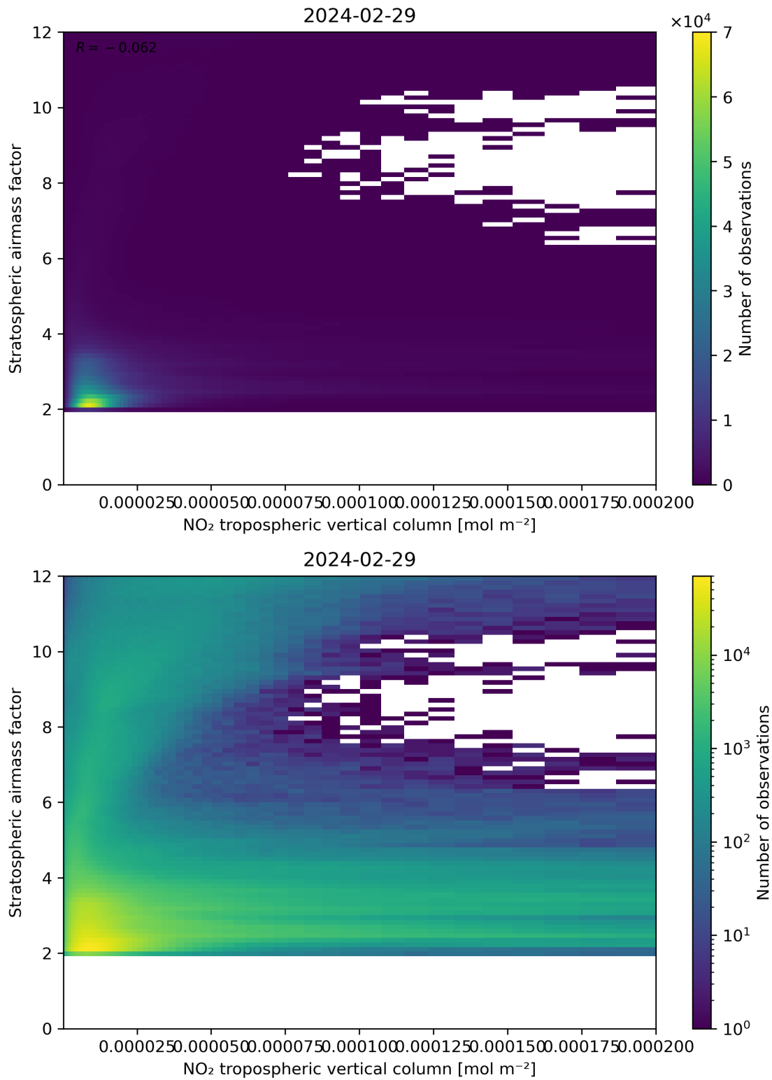
Figure 121: Scatter density plot of “NO 2 tropospheric vertical column” against “Stratospheric airmass factor” for 2024-02-28 to 2024-03-01.
