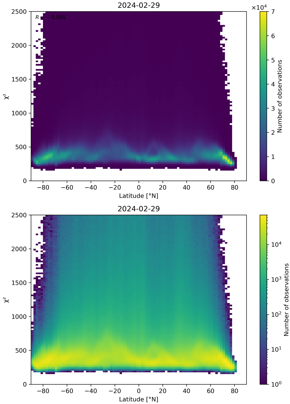
Figure 86: Scatter density plot of “Latitude” against “ \chi^2 ” for 2024-02-28 to 2024-03-01.
