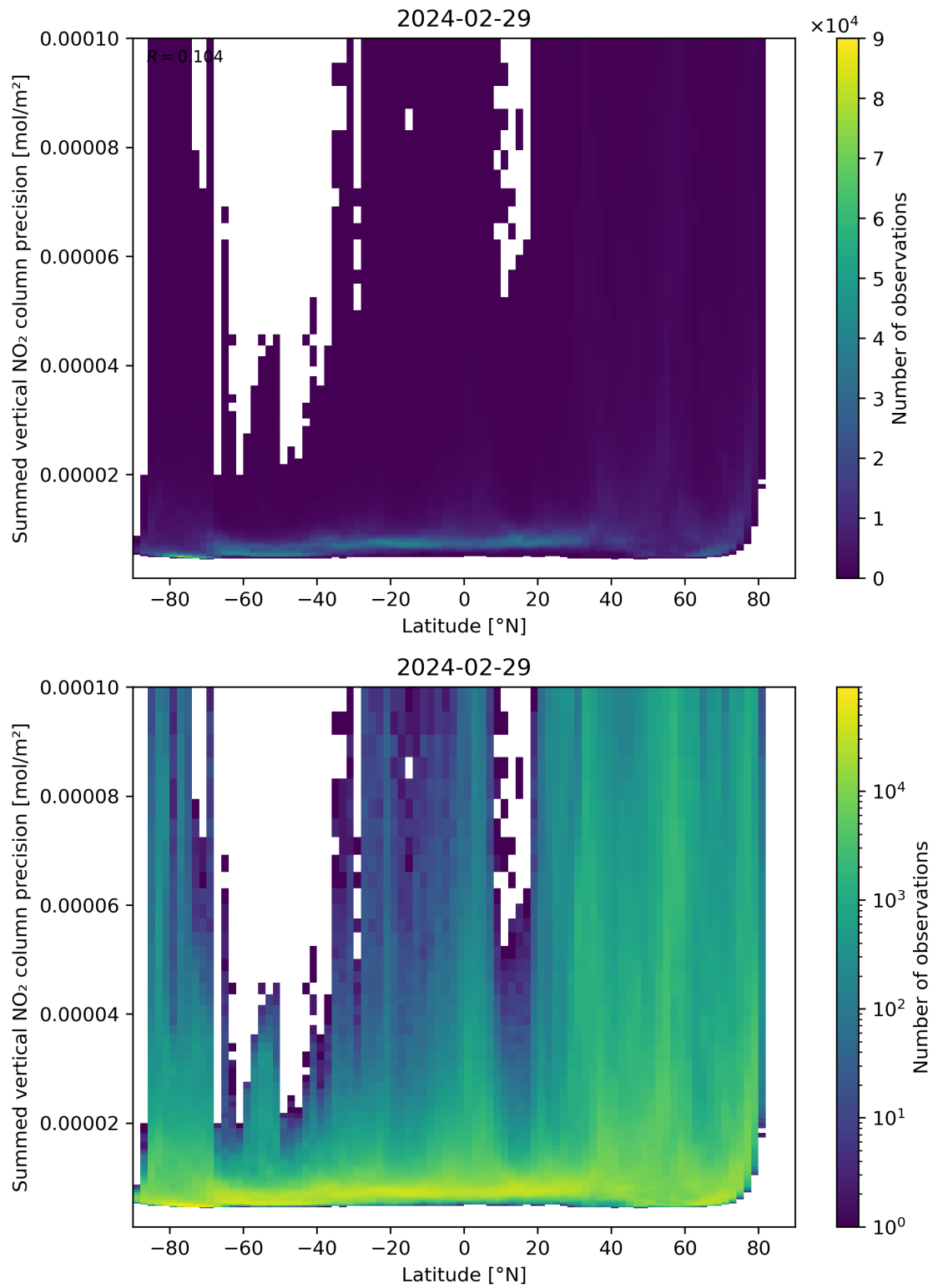
Figure 89: Scatter density plot of “Latitude” against “Summed vertical NO 2 column precision” for 2024-02-28 to 2024-03-01.
