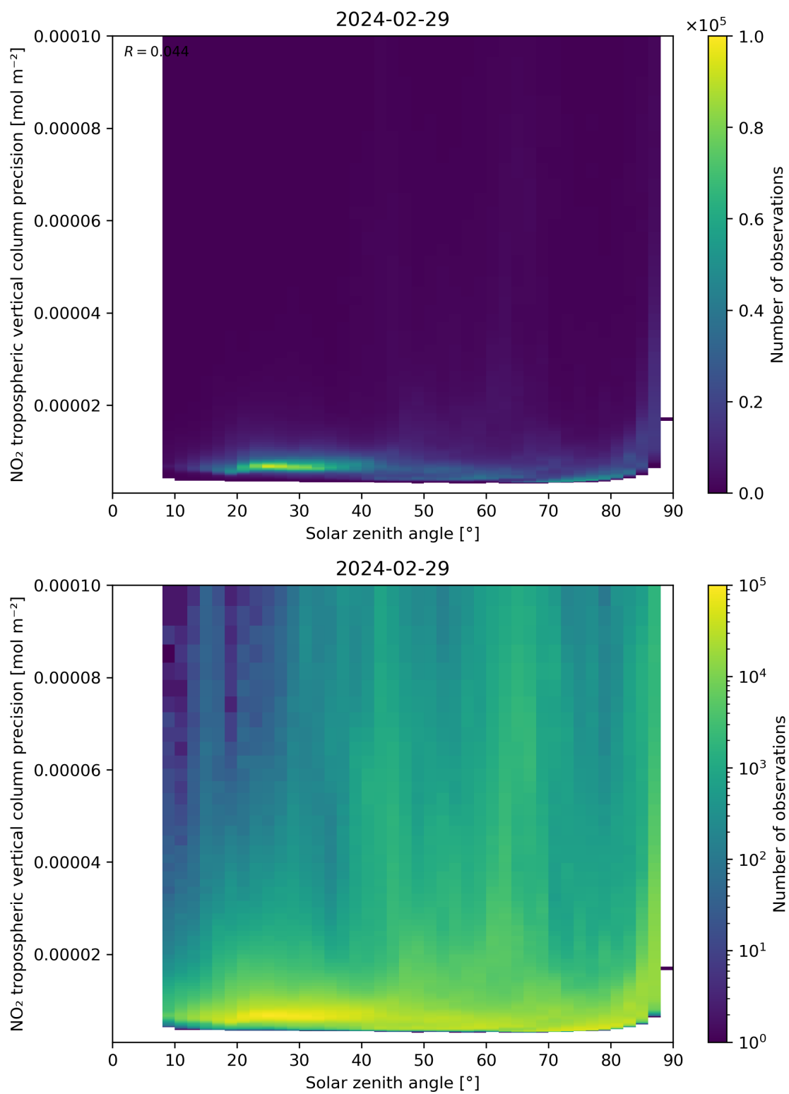
Figure 156: Scatter density plot of “Solar zenith angle” against “NO 2 tropospheric vertical column precision” for 2024-02-28 to 2024-03-01.
