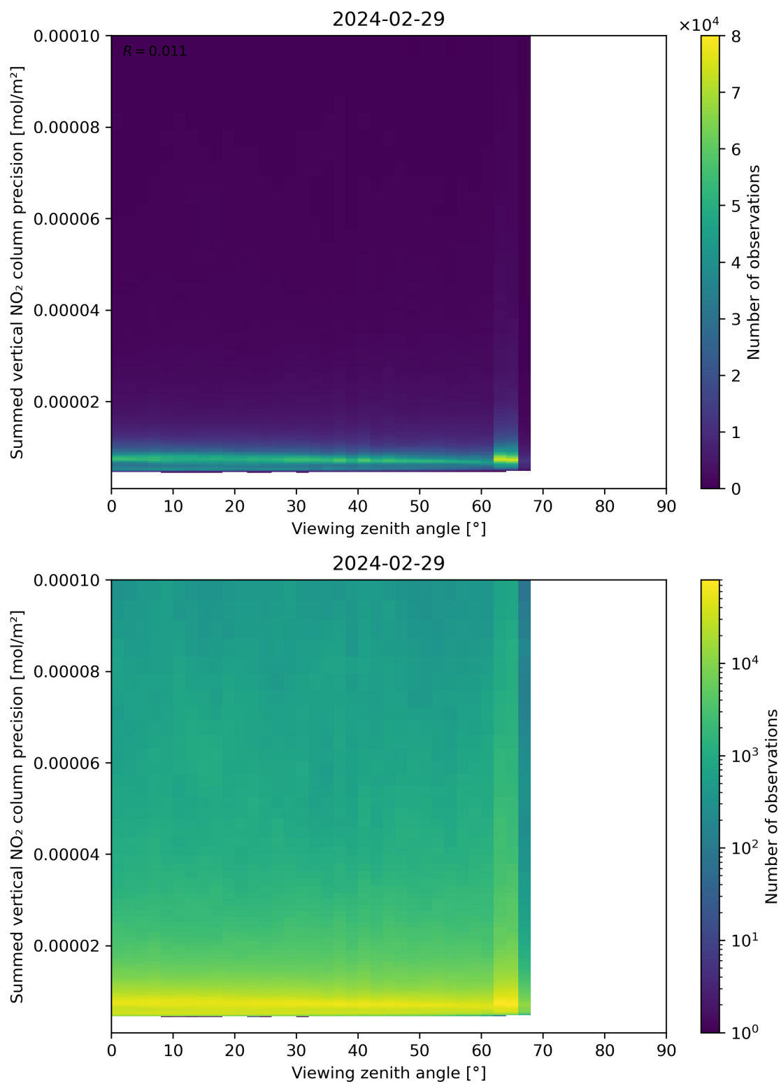
Figure 166: Scatter density plot of “Viewing zenith angle” against “Summed vertical NO 2 column precision” for 2024-02-28 to 2024-03-01.
