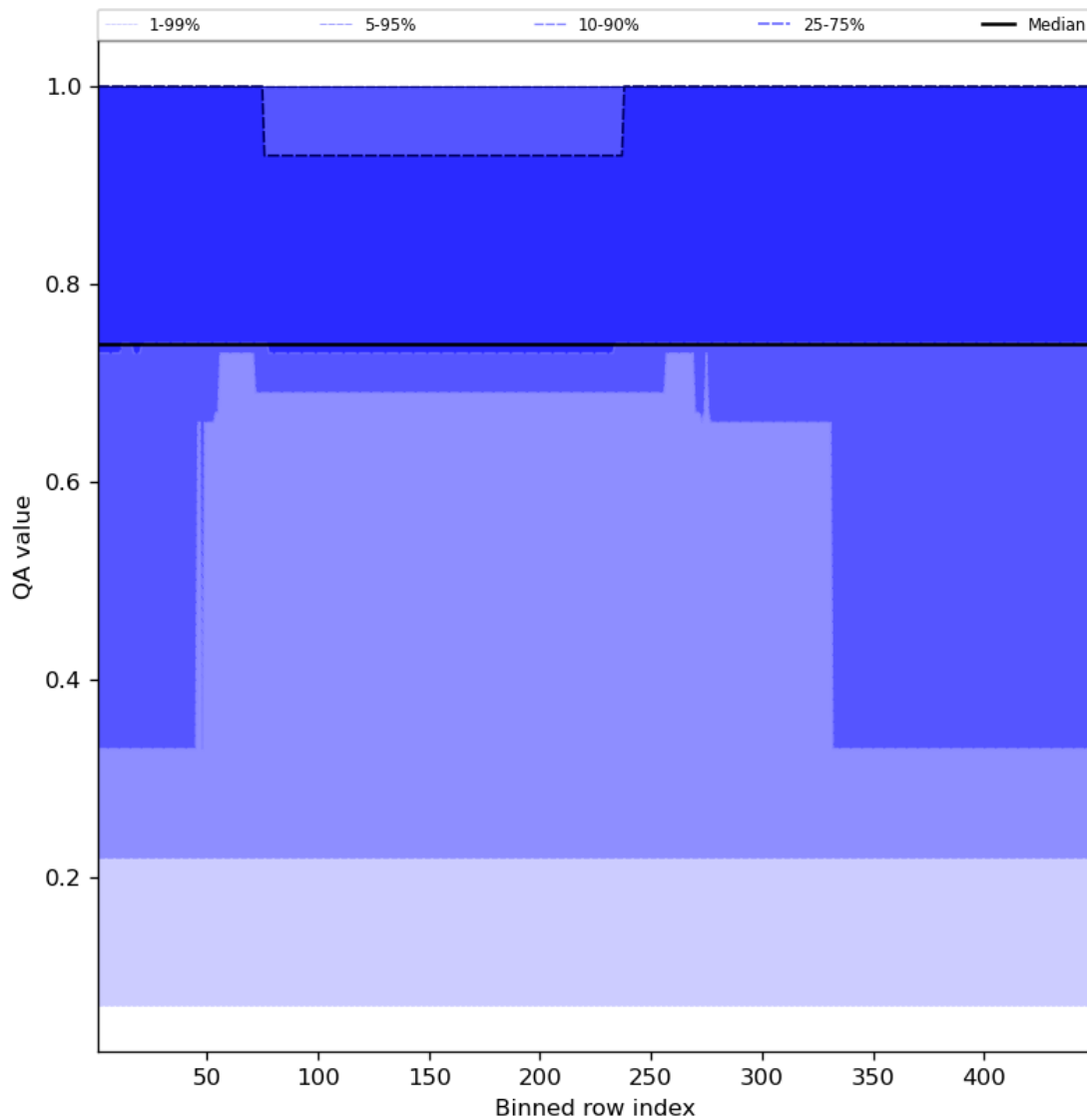
Figure 45: Along track statistics of “QA value” for 2024-02-28 to 2024-03-01
