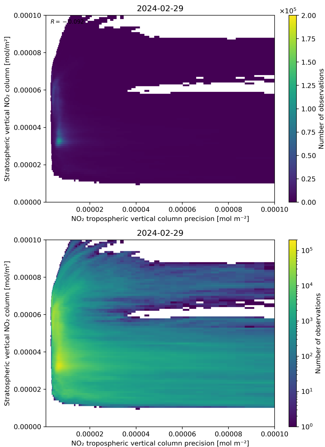
Figure 135: Scatter density plot of “NO 2 tropospheric vertical column precision” against “Stratospheric vertical NO 2 column” for 2024-02-28 to 2024-03-01.
