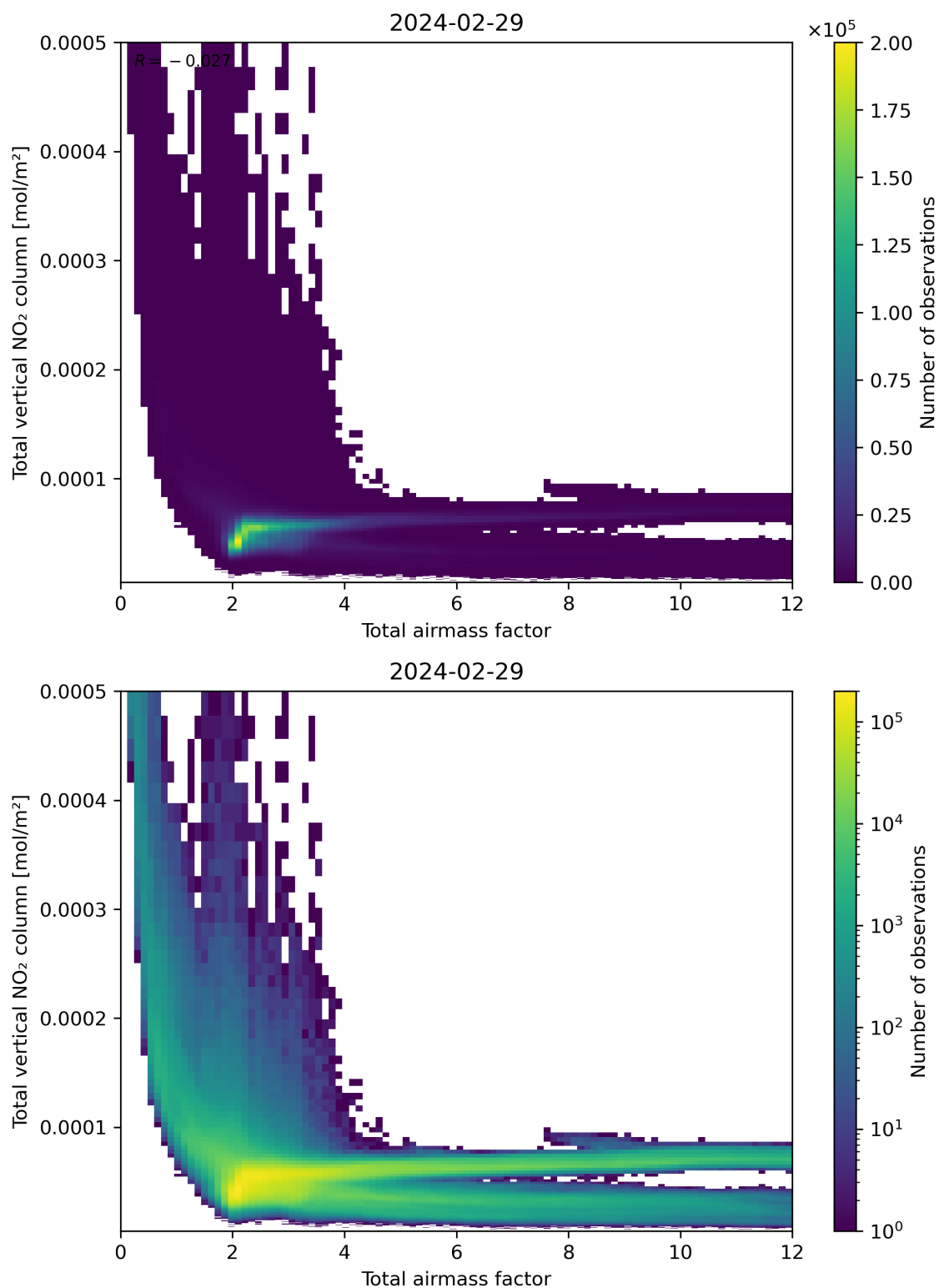
Figure 67: Scatter density plot of “Total airmass factor” against “Total vertical NO 2 column” for 2024-02-28 to 2024-03-01.
