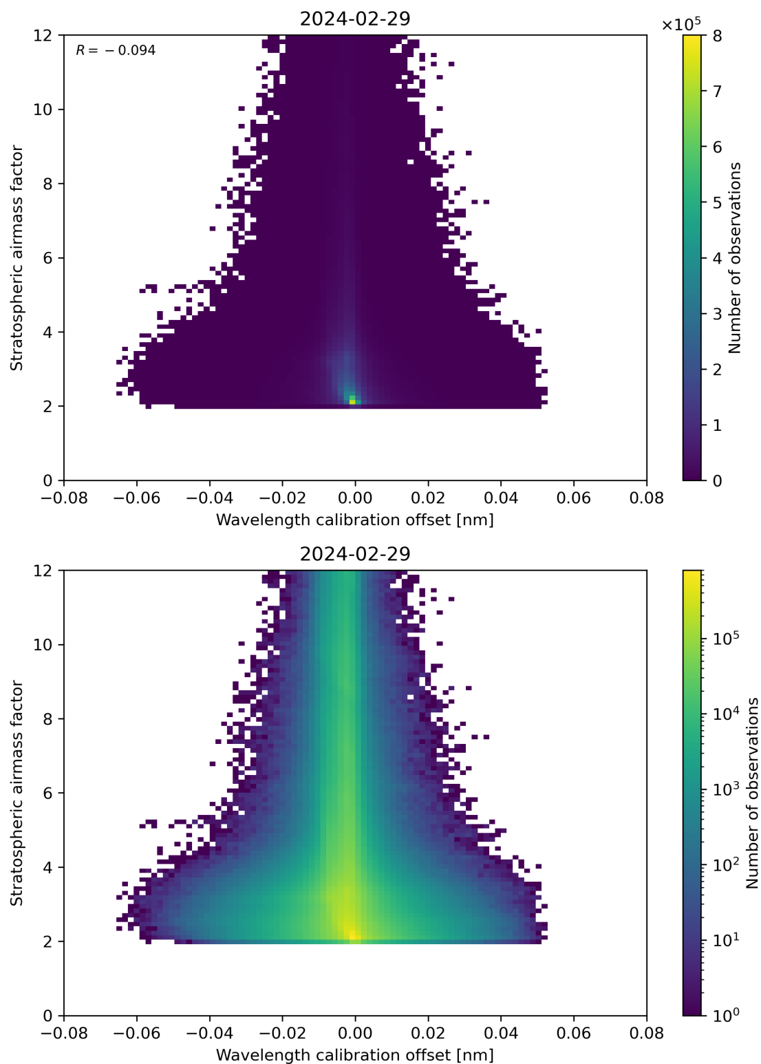
Figure 174: Scatter density plot of “Wavelength calibration offset” against “Stratospheric airmass factor” for 2024-02-28 to 2024-03-01.
