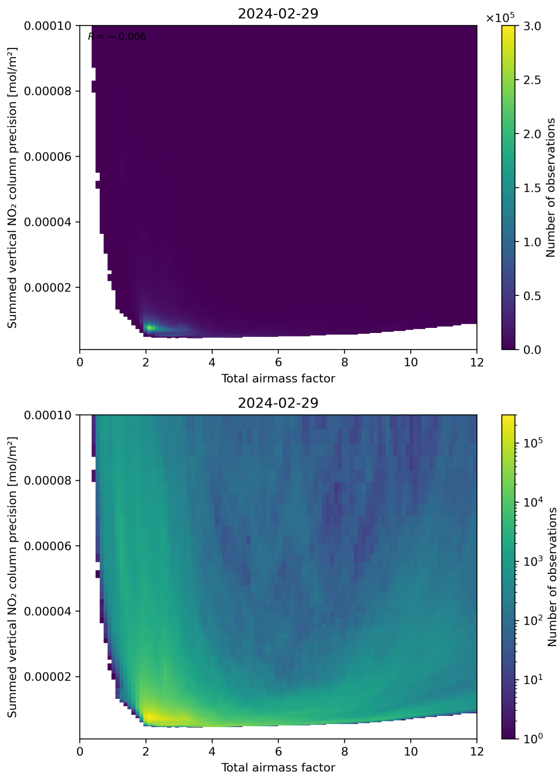
Figure 66: Scatter density plot of “Total airmass factor” against “Summed vertical NO 2 column precision” for 2024-02-28 to 2024-03-01.
