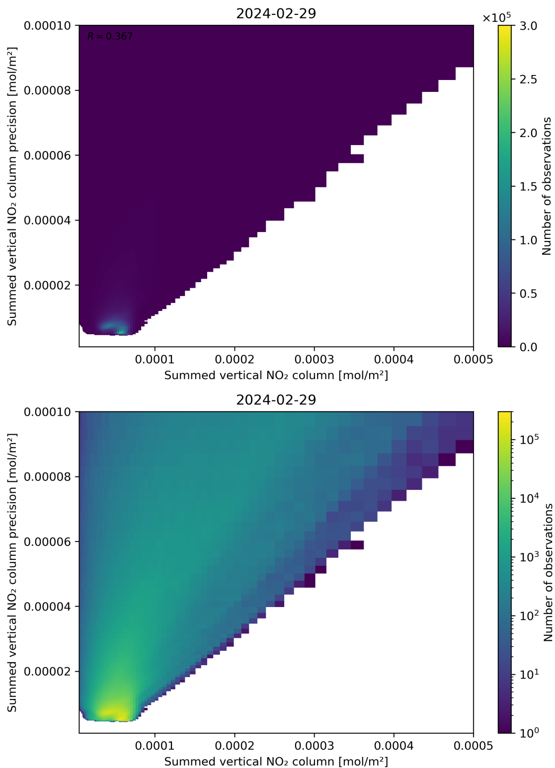
Figure 105: Scatter density plot of “Summed vertical NO 2 column” against “Summed vertical NO 2 column precision” for 2024-02-28 to 2024-03-01.
