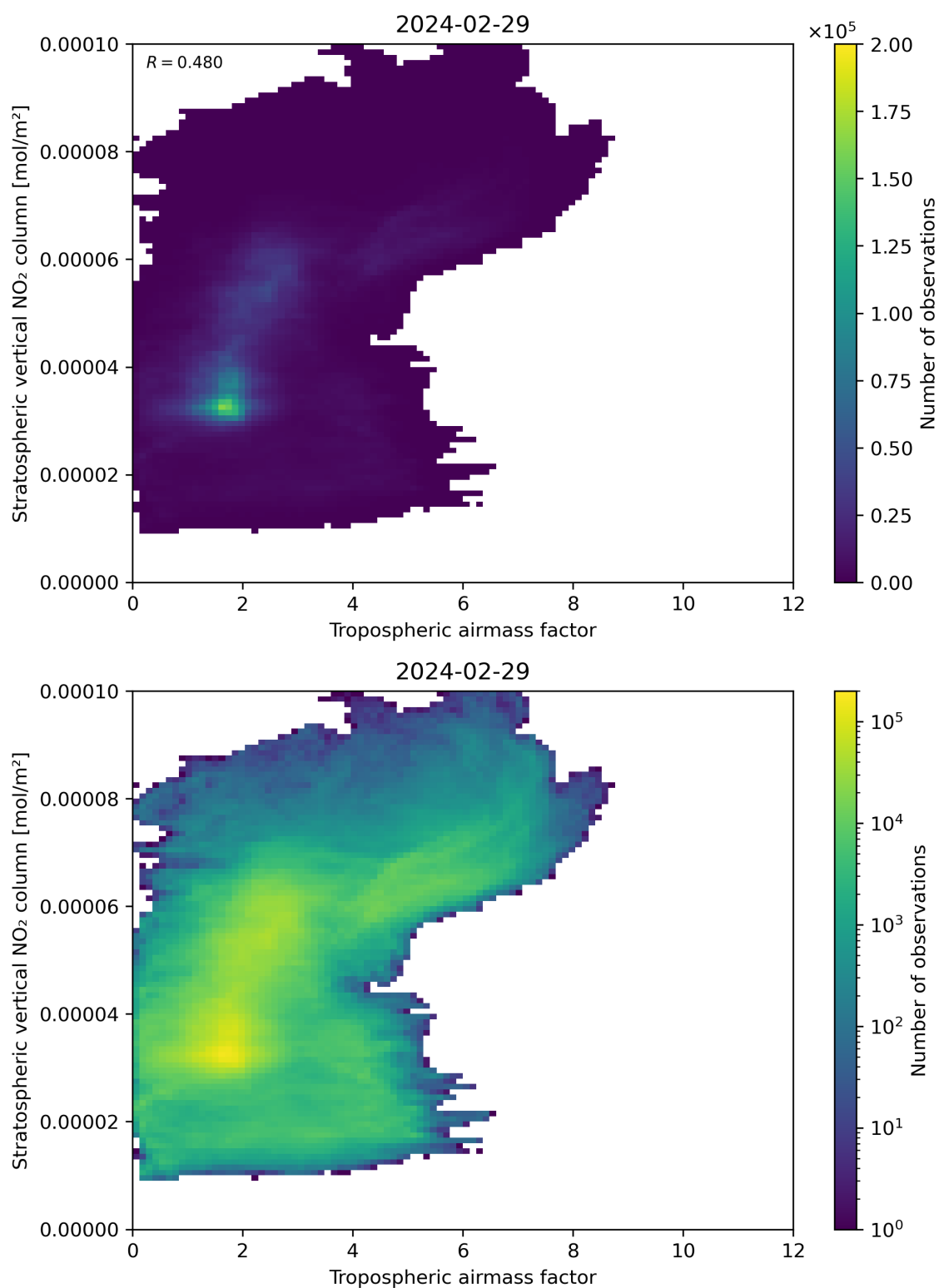
Figure 74: Scatter density plot of “Tropospheric air mass factor” against “Stratospheric vertical NO 2 column” for 2024-02-28 to 2024-03-01.
