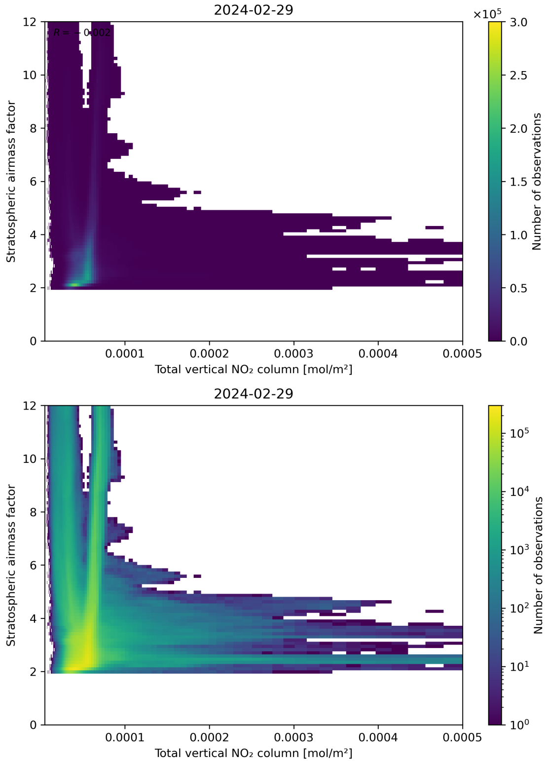
Figure 110: Scatter density plot of “Total vertical NO 2 column” against “Stratospheric airmass factor” for 2024-02-28 to 2024-03-01.
