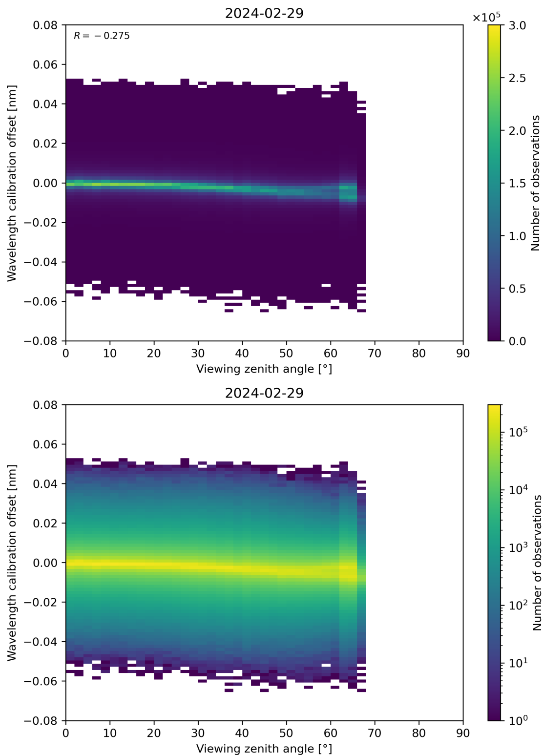
Figure 173: Scatter density plot of “Viewing zenith angle” against “Wavelength calibration offset” for 2024-02-28 to 2024-03-01.
