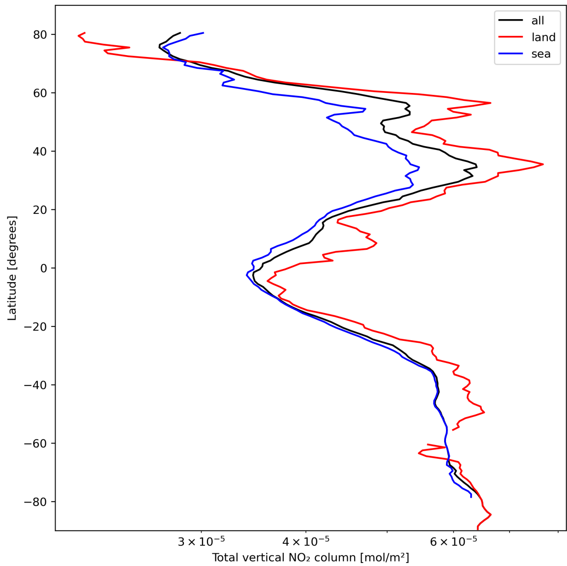
Figure 21: Zonal average of “Total vertical NO 2 column” for 2024-02-28 to 2024-03-01.
