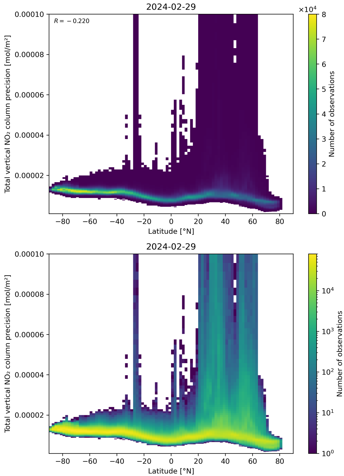
Figure 91: Scatter density plot of “Latitude” against “Total vertical NO 2 column precision” for 2024-02-28 to 2024-03-01.
