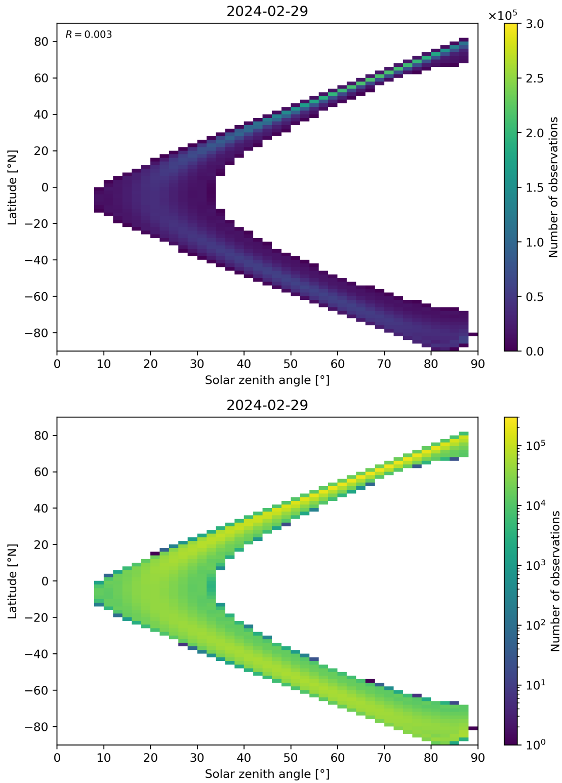
Figure 149: Scatter density plot of “Solar zenith angle” against “Latitude” for 2024-02-28 to 2024-03-01.
