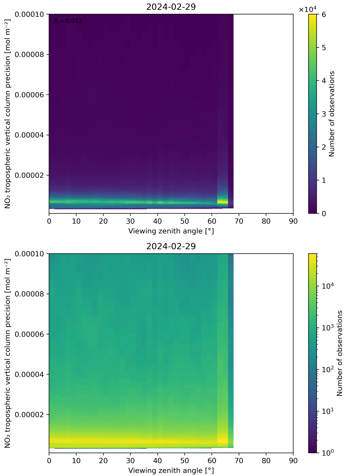
Figure 170: Scatter density plot of “Viewing zenith angle” against “NO 2 tropospheric vertical column precision” for 2024-02-28 to 2024-03-01.
