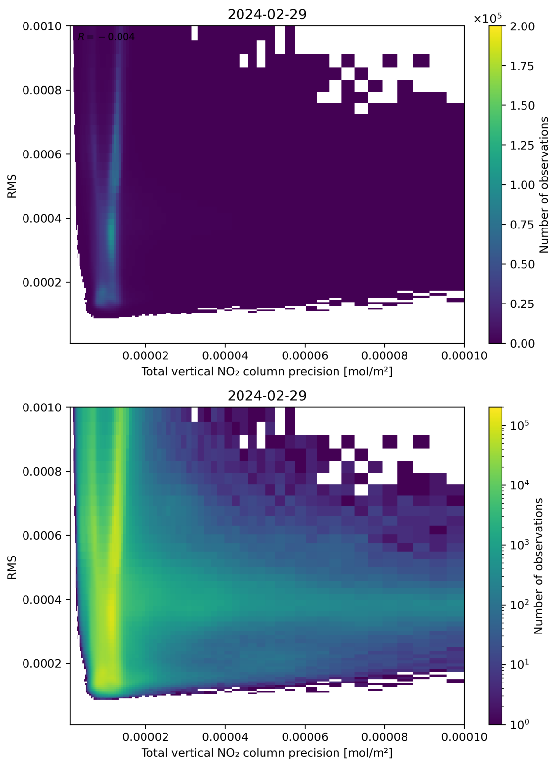
Figure 119: Scatter density plot of “Total vertical NO 2 column precision” against “RMS” for 2024-02-28 to 2024-03-01.
