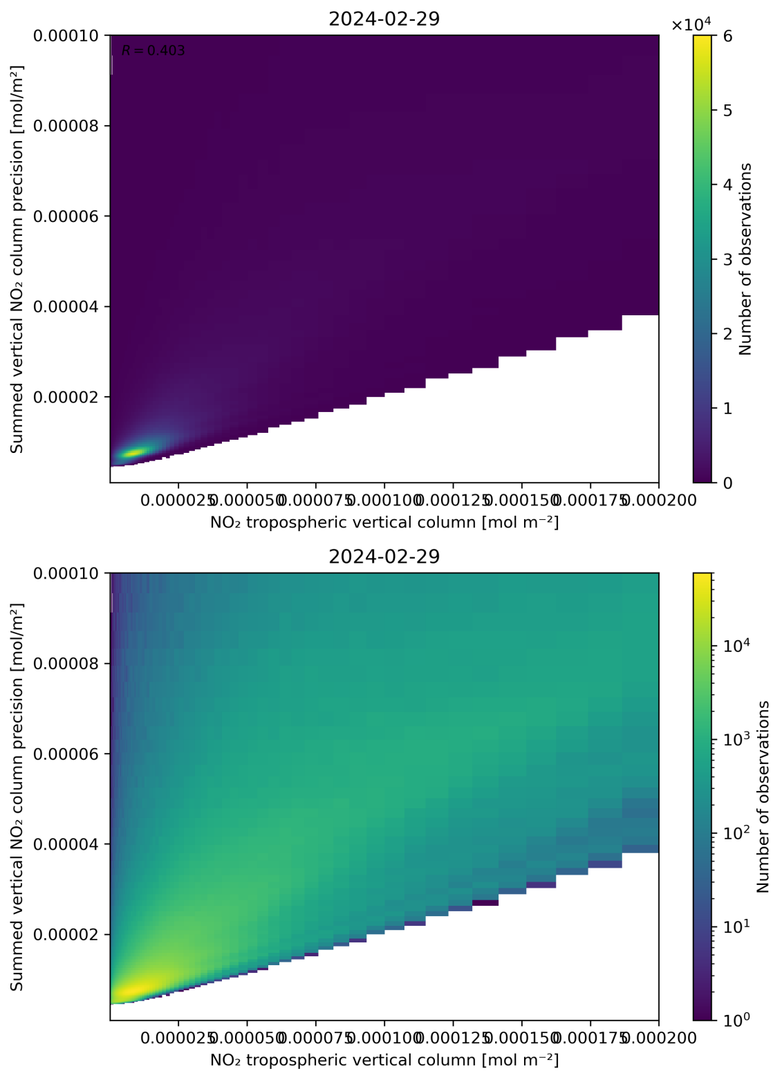
Figure 127: Scatter density plot of “NO 2 tropospheric vertical column” against “Summed vertical NO 2 column precision” for 2024-02-28 to 2024-03-01.
