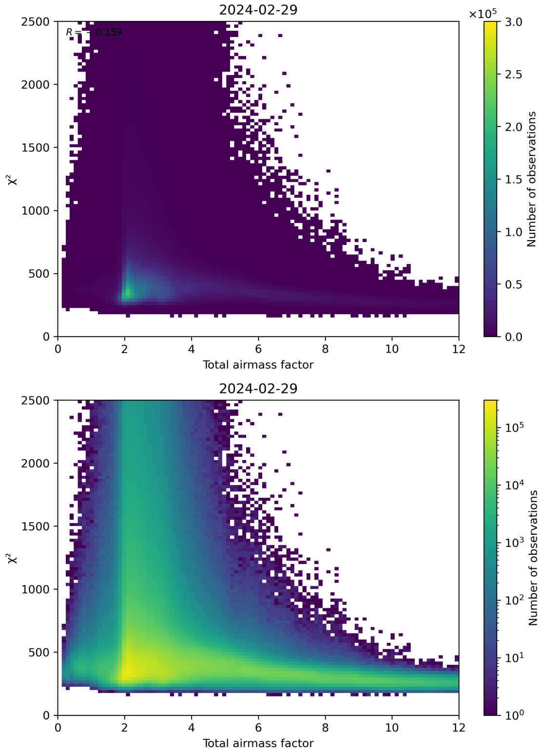
Figure 63: Scatter density plot of “Total airmass factor” against “ \chi^2 ” for 2024-02-28 to 2024-03-01.
