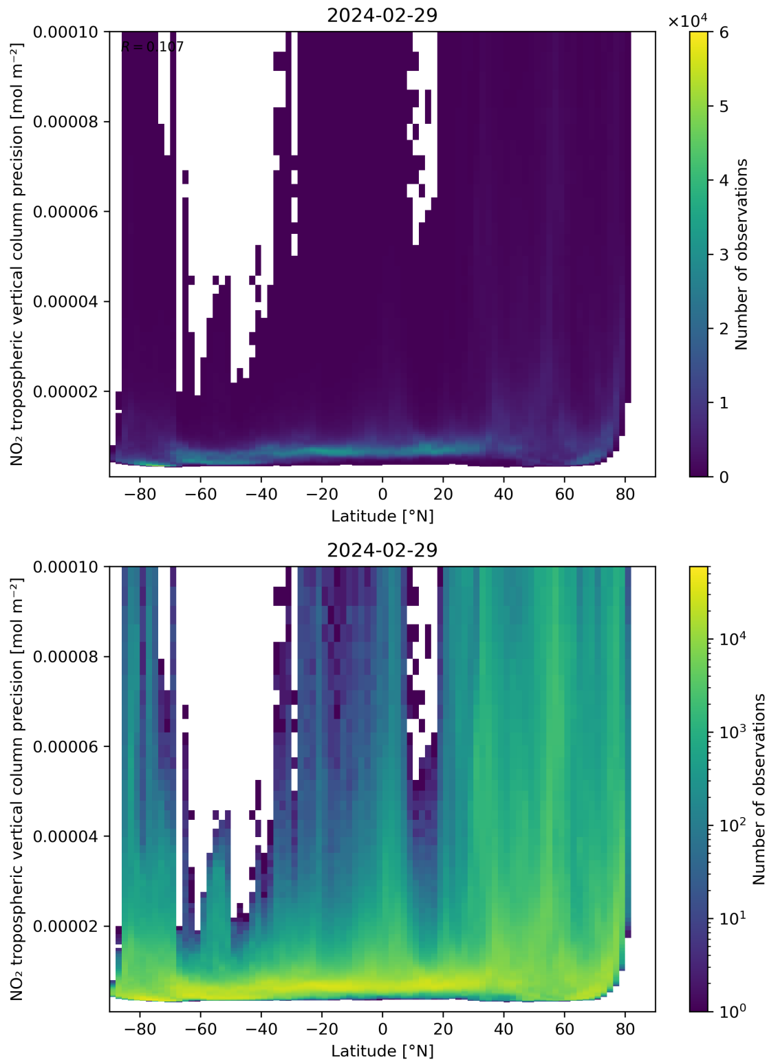
Figure 93: Scatter density plot of “Latitude” against “NO 2 tropospheric vertical column precision” for 2024-02-28 to 2024-03-01.
