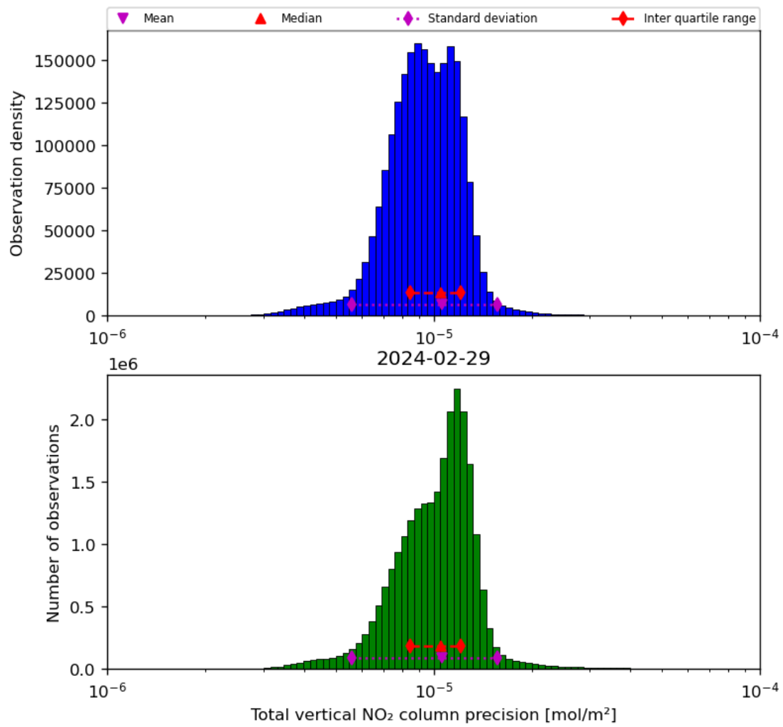
Figure 39: Histogram of “Total vertical NO 2 column precision” for 2024-02-28 to 2024-03-01
