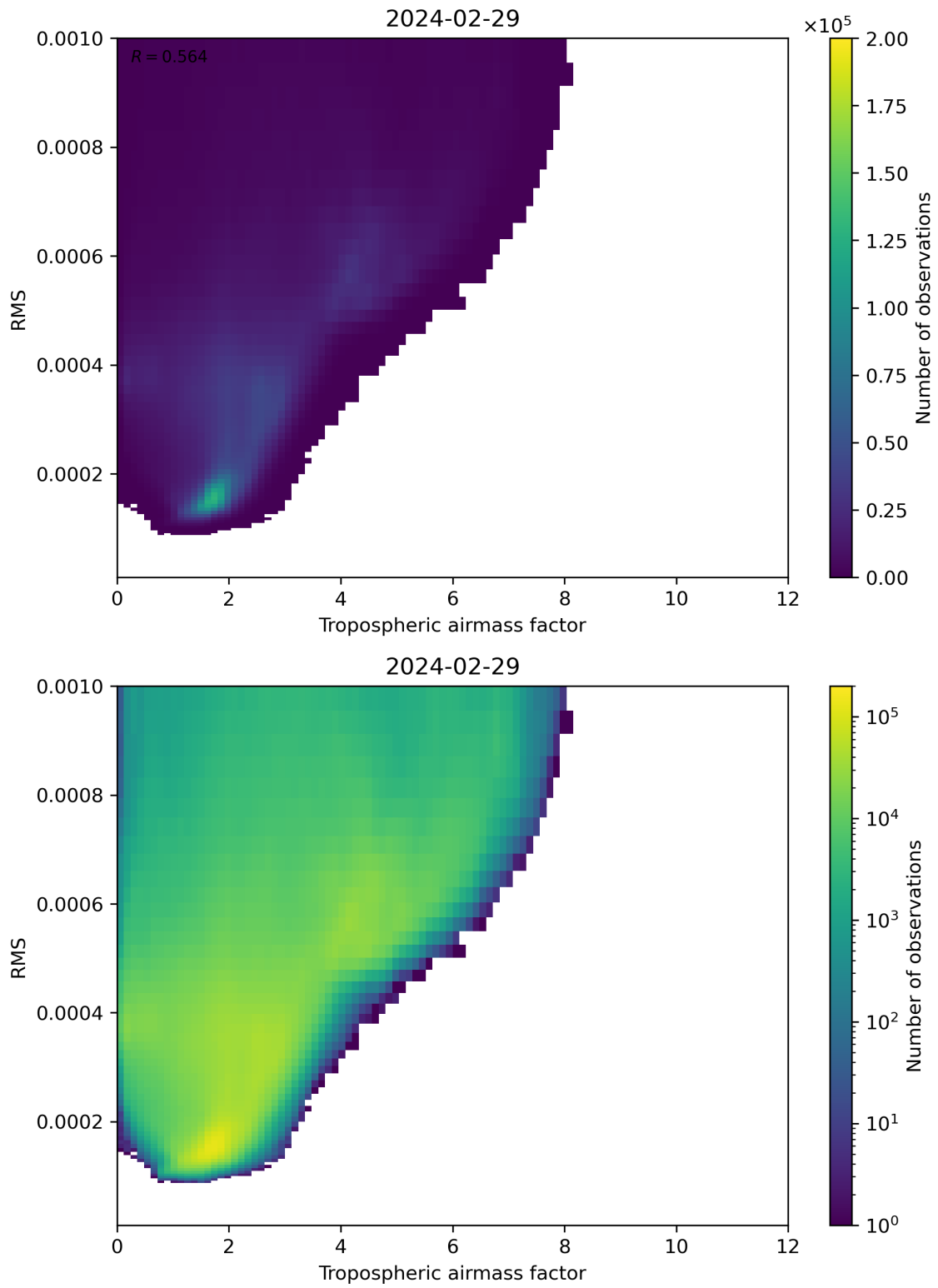
Figure 79: Scatter density plot of “Tropospheric airmass factor” against “RMS” for 2024-02-28 to 2024-03-01.
