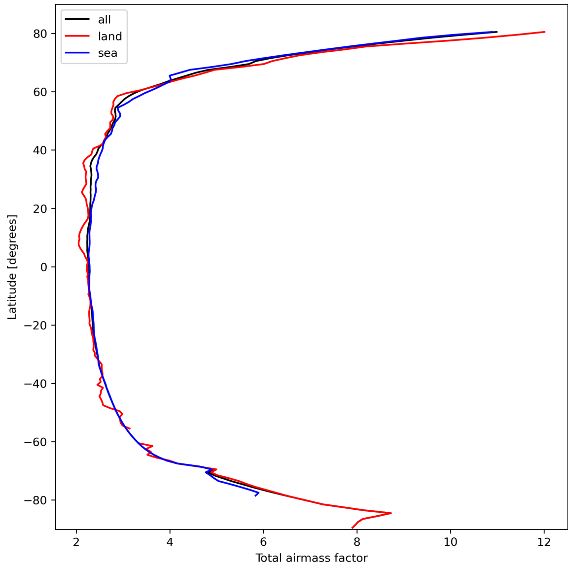
Figure 15: Zonal average of “Total airmass factor” for 2024-02-28 to 2024-03-01.
