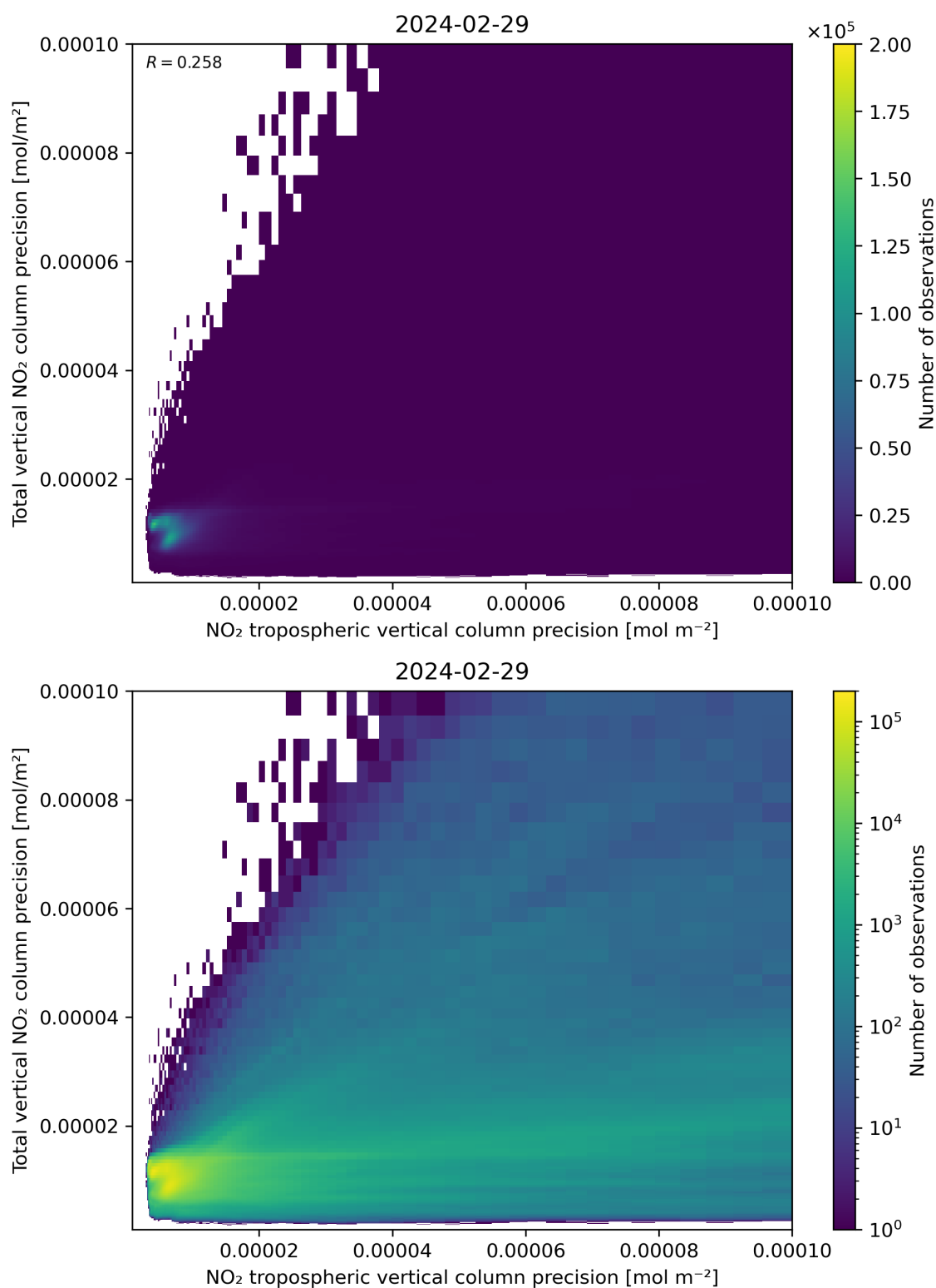
Figure 139: Scatter density plot of “NO 2 tropospheric vertical column precision” against “Total vertical NO 2 column precision” for 2024-02-28 to 2024-03-01.
