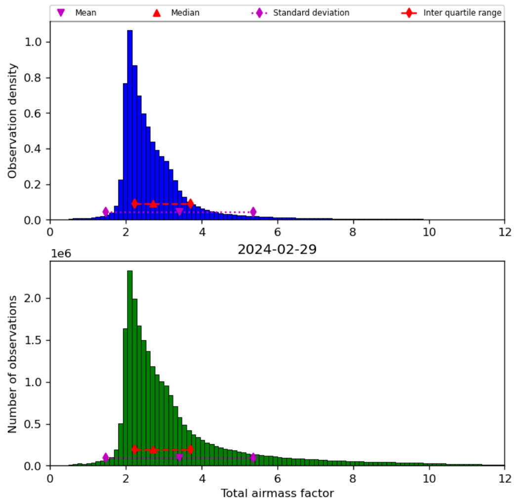
Figure 32: Histogram of “Total airmass factor” for 2024-02-28 to 2024-03-01
