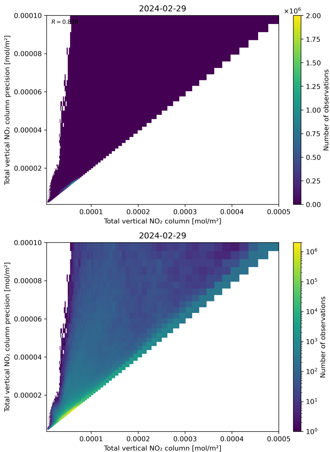
Figure 114: Scatter density plot of “Total vertical NO 2 column” against “Total vertical NO 2 column precision” for 2024-02-28 to 2024-03-01.
