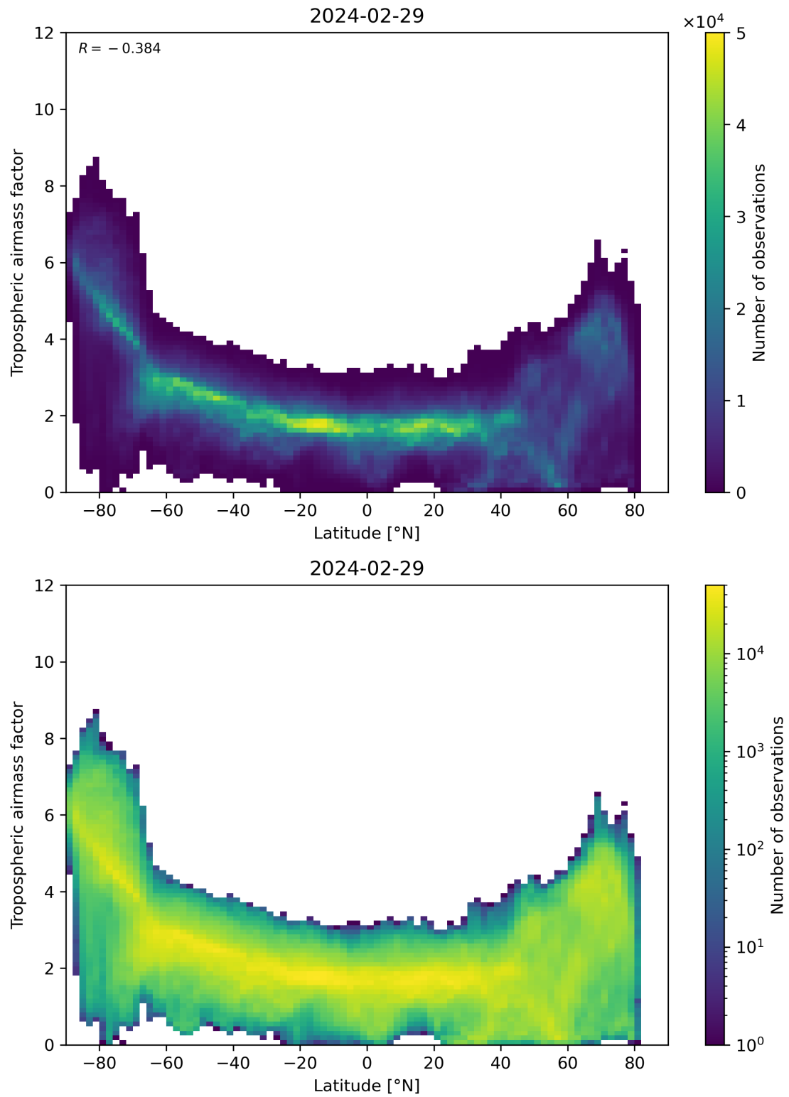
Figure 85: Scatter density plot of “Latitude” against “Tropospheric airmass factor” for 2024-02-28 to 2024-03-01.
