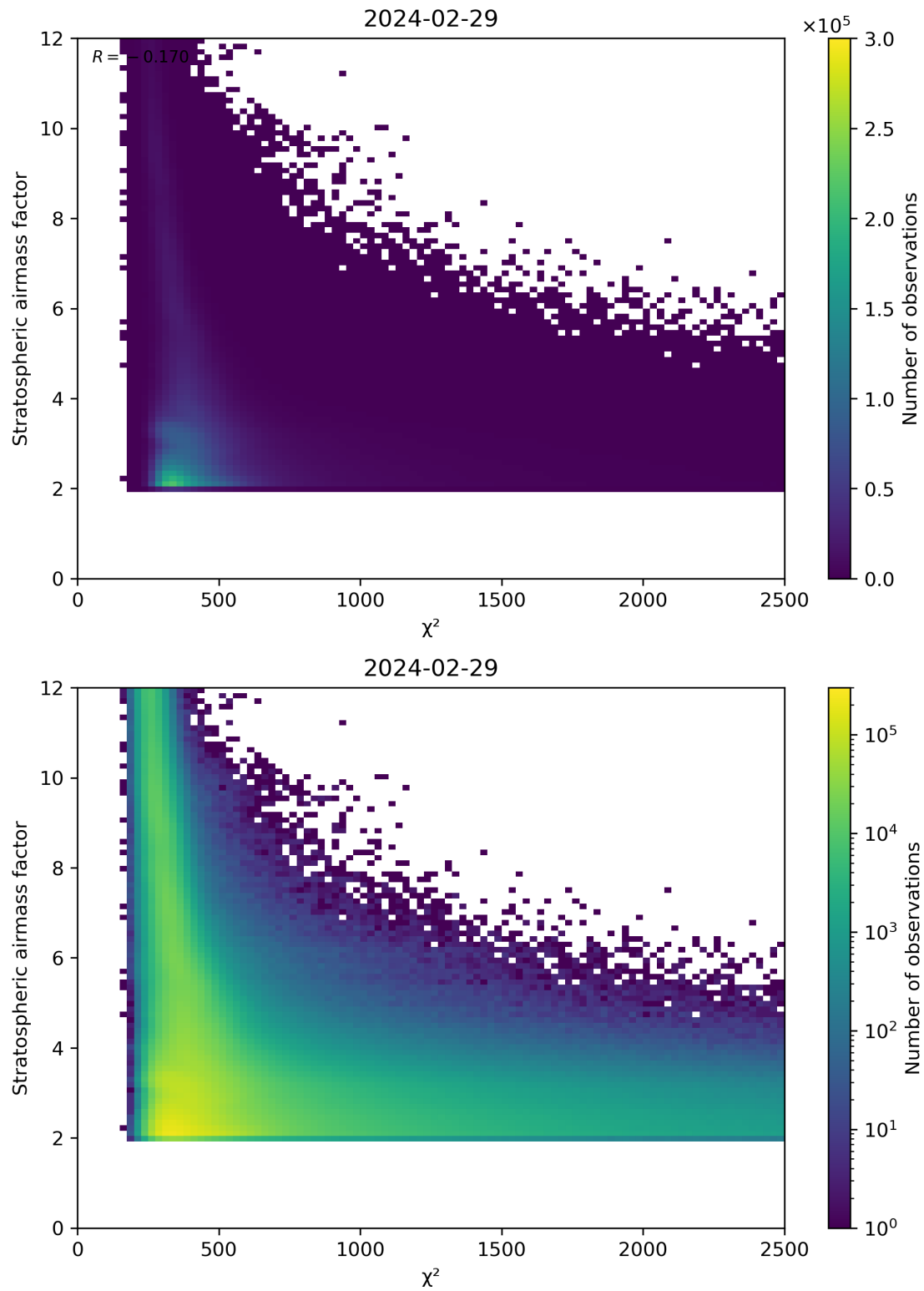
Figure 81: Scatter density plot of “ \chi^2 ” against “Stratospheric airmass factor” for 2024-02-28 to 2024-03-01.
