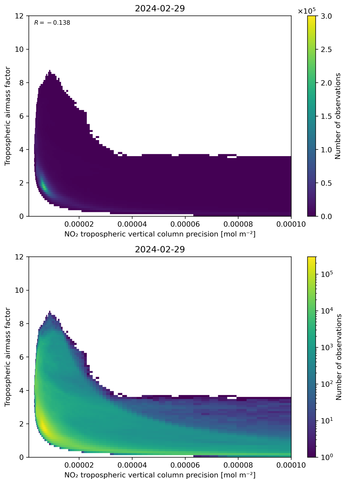
Figure 133: Scatter density plot of “NO 2 tropospheric vertical column precision” against “Tropospheric airmass factor” for 2024-02-28 to 2024-03-01.
