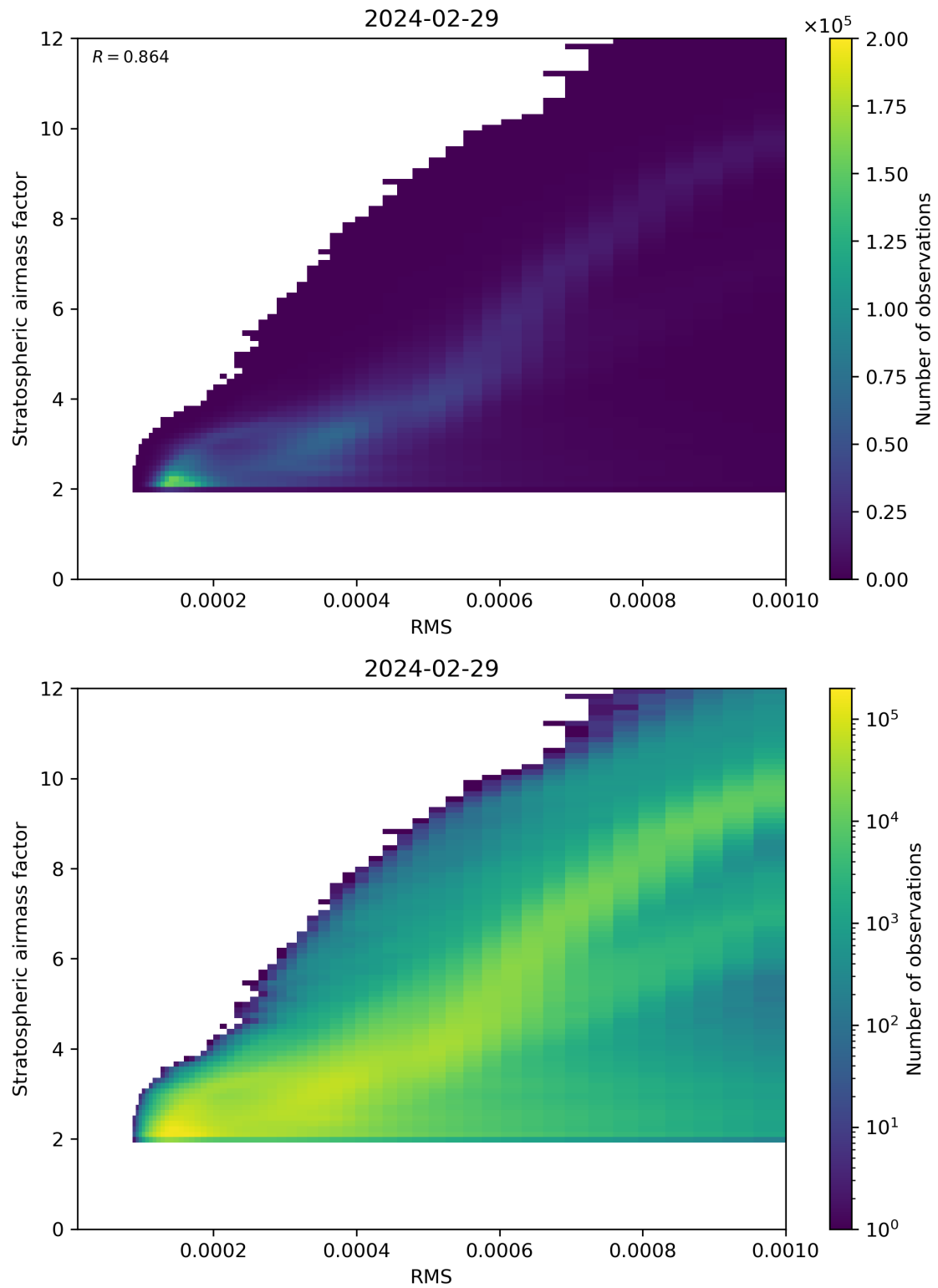
Figure 144: Scatter density plot of “RMS” against “Stratospheric airmass factor” for 2024-02-28 to 2024-03-01.
