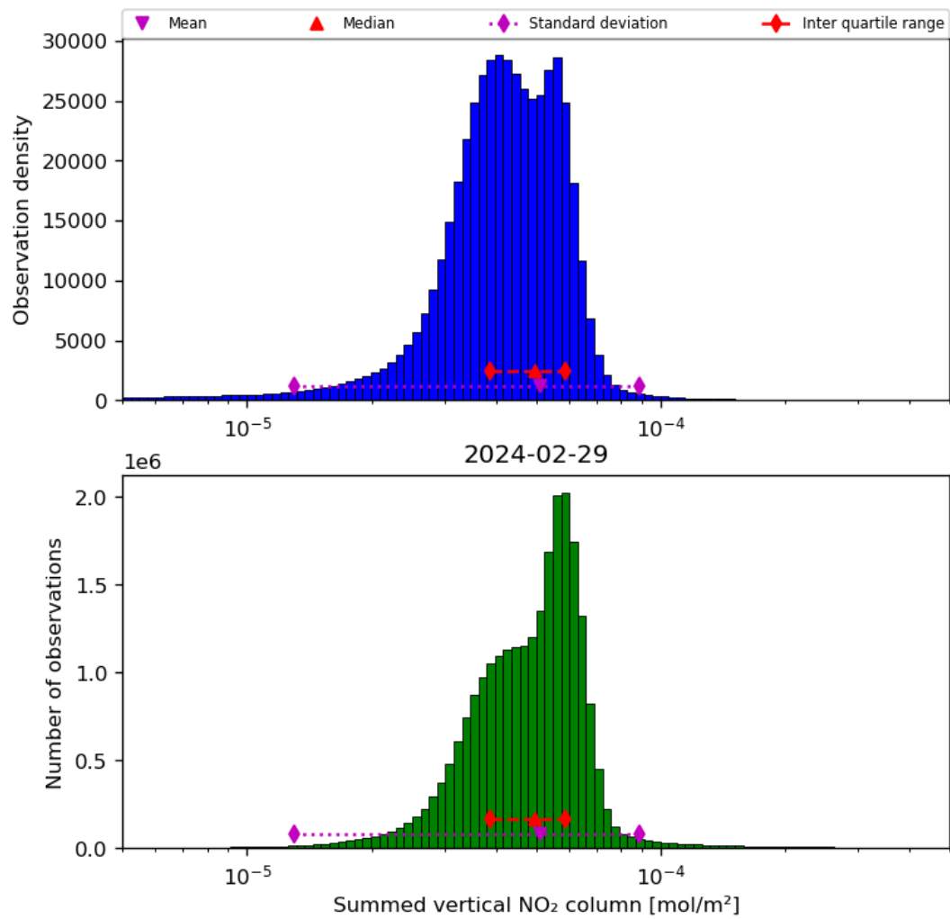
Figure 40: Histogram of “Summed vertical NO 2 column” for 2024-02-28 to 2024-03-01
