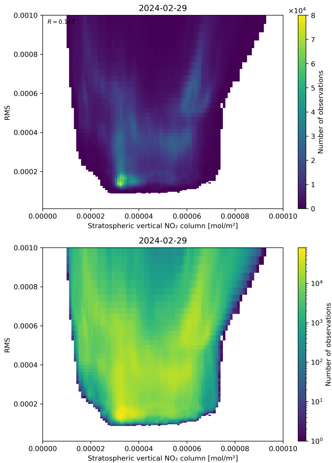
Figure 102: Scatter density plot of “Stratospheric vertical NO 2 column” against “RMS” for 2024-02-28 to 2024-03-01.
