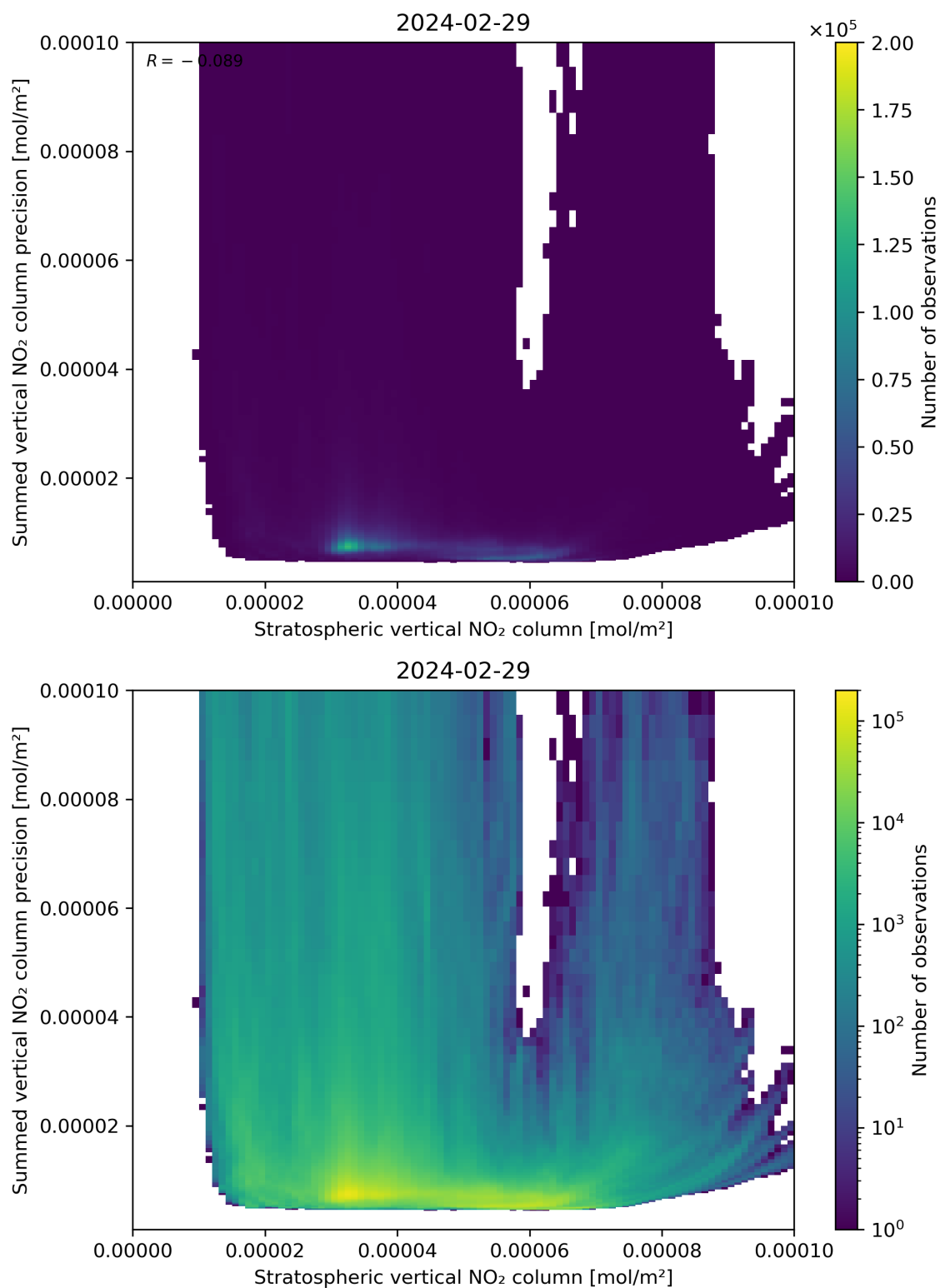
Figure 99: Scatter density plot of “Stratospheric vertical NO 2 column” against “Summed vertical NO 2 column precision” for 2024-02-28 to 2024-03-01.
