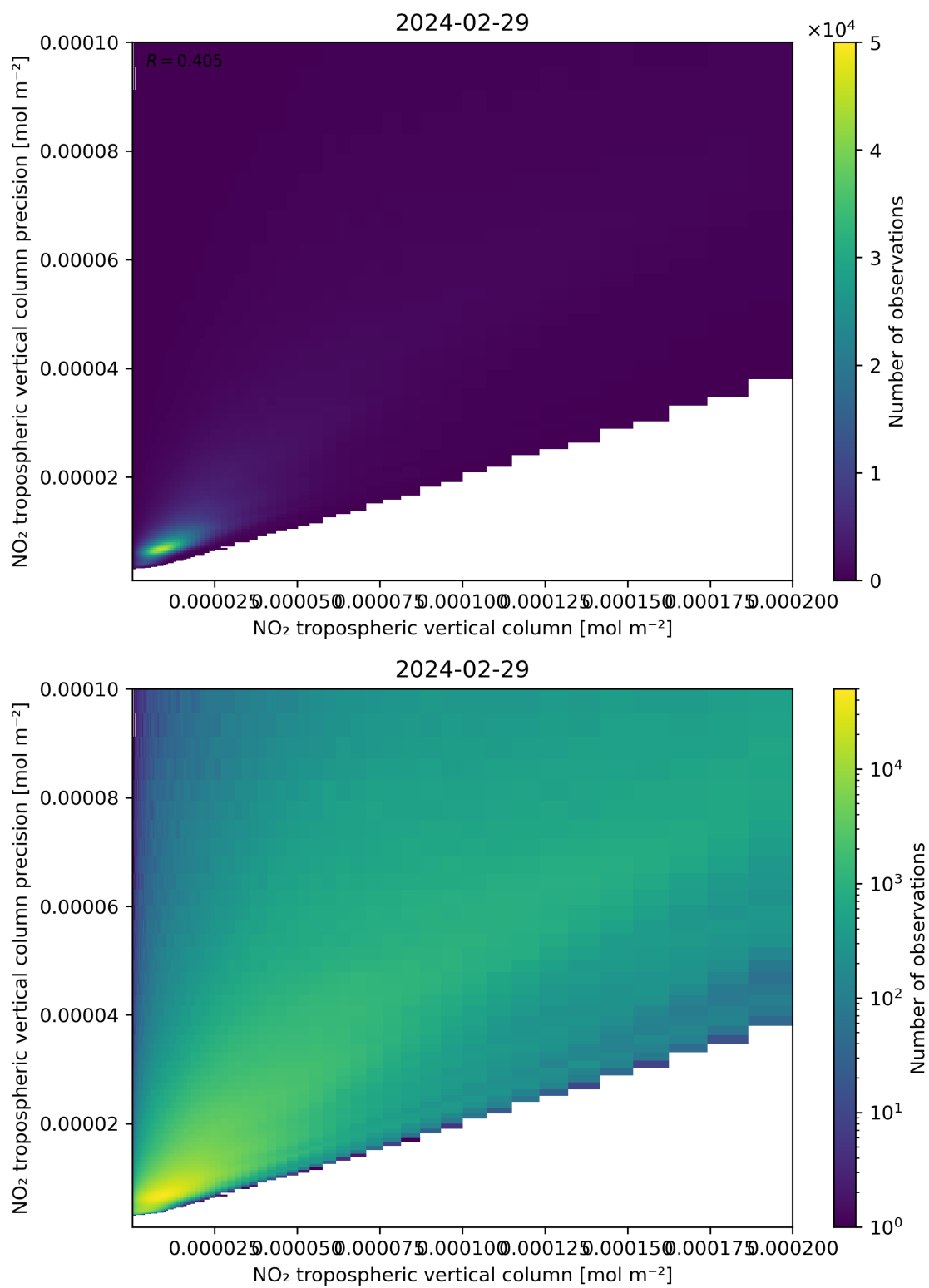
Figure 130: Scatter density plot of “NO 2 tropospheric vertical column” against “NO 2 tropospheric vertical column precision” for 2024-02-28 to 2024-03-01.
