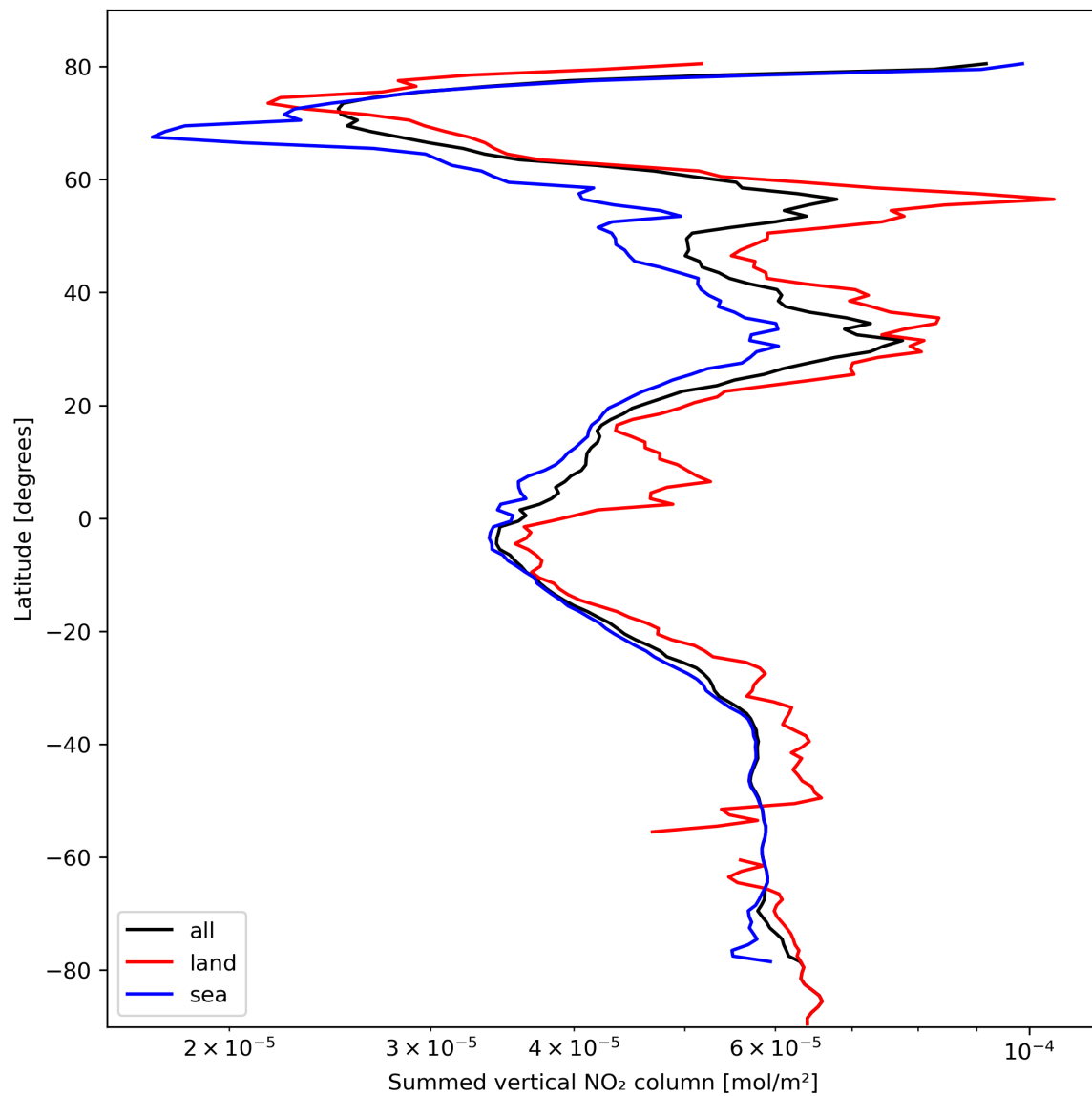
Figure 23: Zonal average of “Summed vertical NO 2 column” for 2024-02-28 to 2024-03-01.
