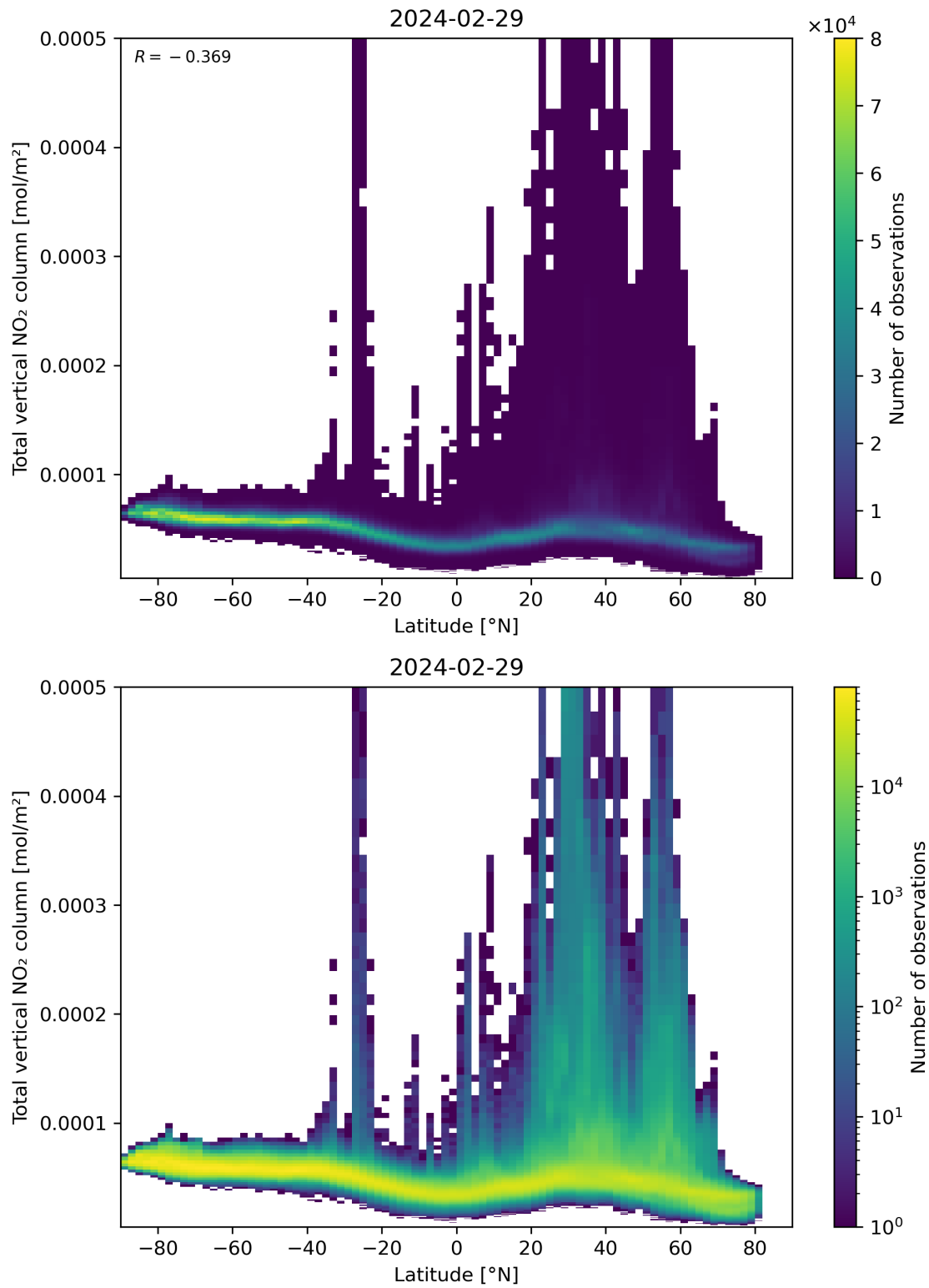
Figure 90: Scatter density plot of “Latitude” against “Total vertical NO 2 column” for 2024-02-28 to 2024-03-01.
