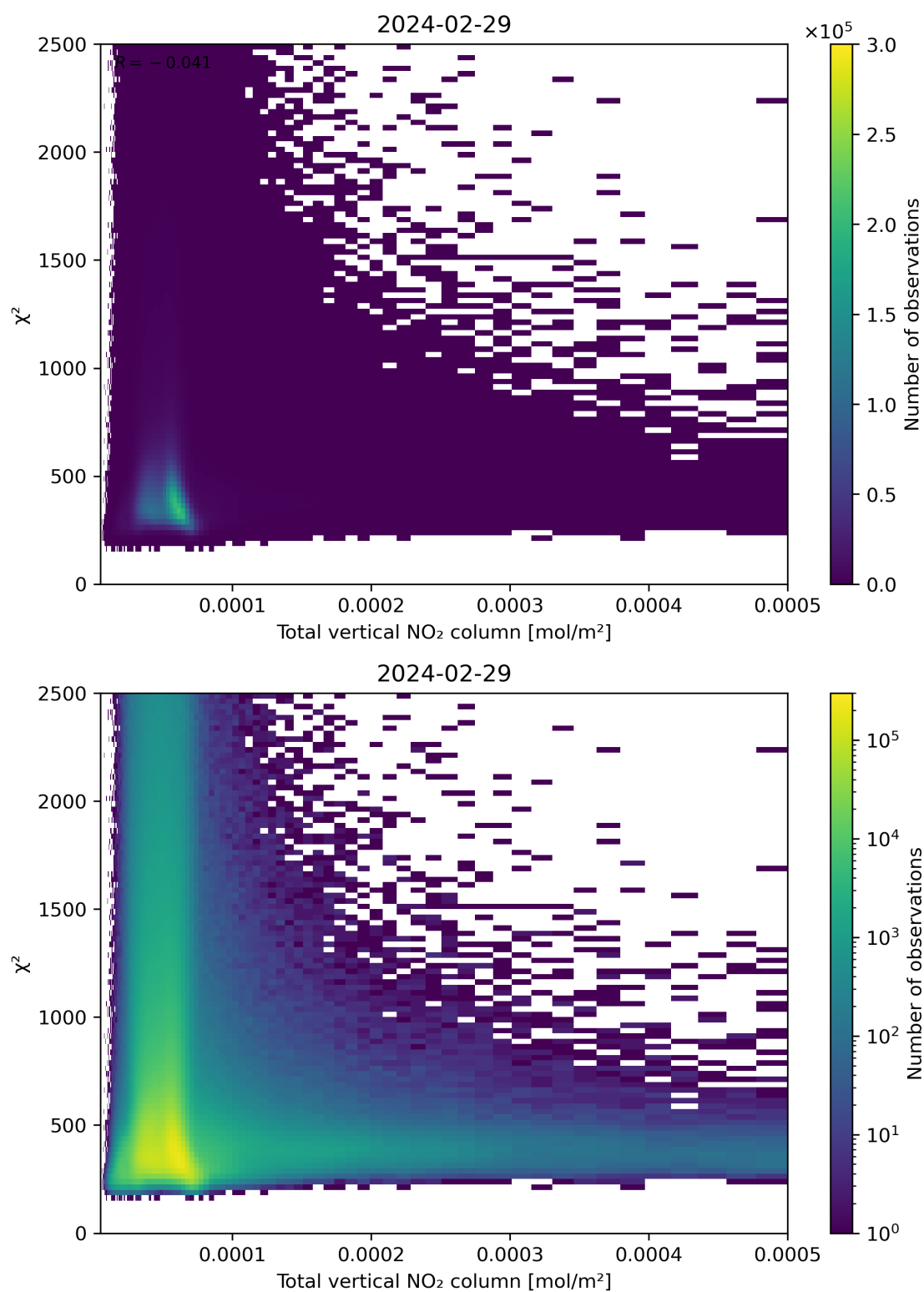
Figure 111: Scatter density plot of “Total vertical NO 2 column” against “ \chi^2 ” for 2024-02-28 to 2024-03-01.
