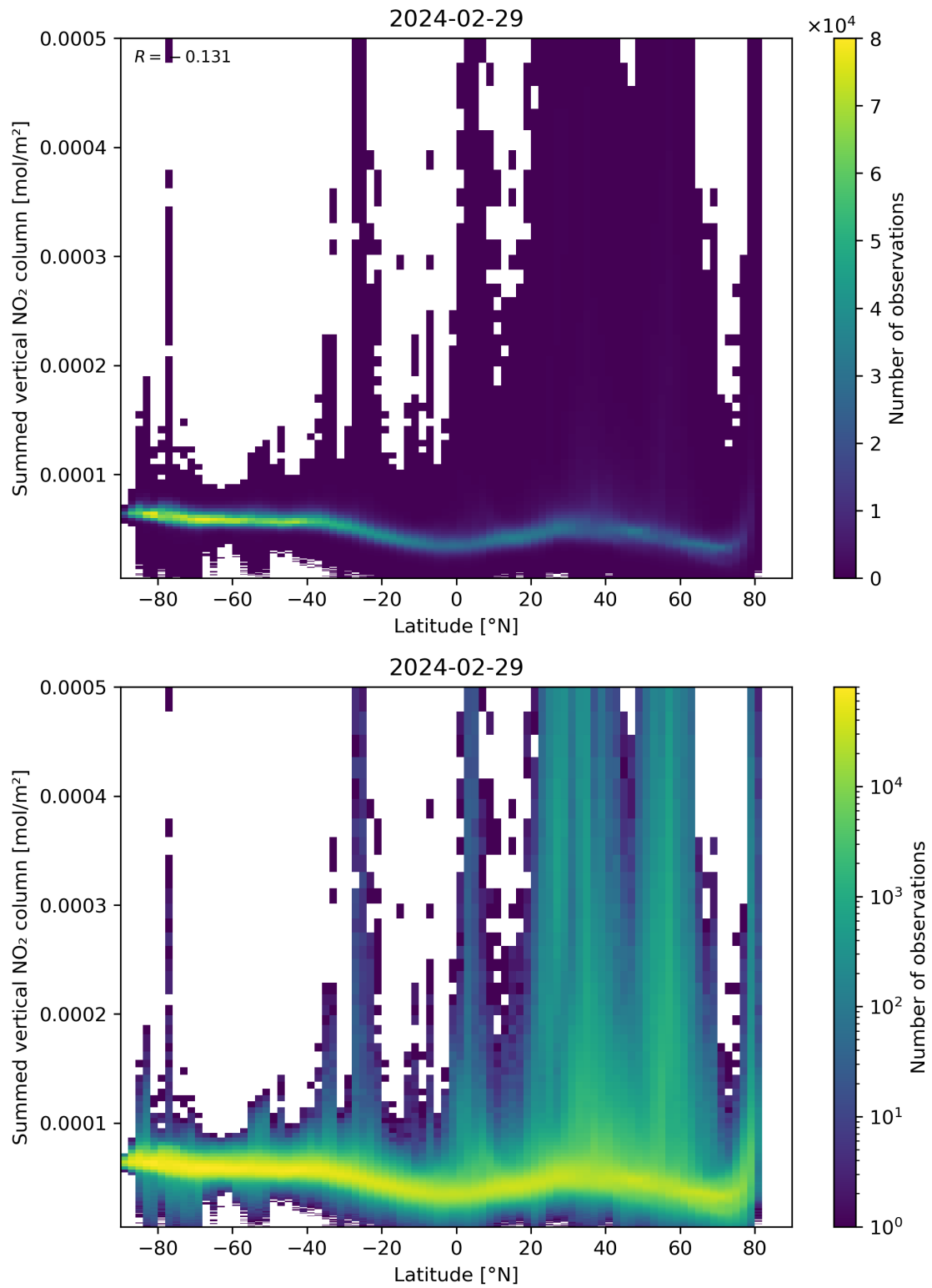
Figure 88: Scatter density plot of “Latitude” against “Summed vertical NO 2 column” for 2024-02-28 to 2024-03-01.
