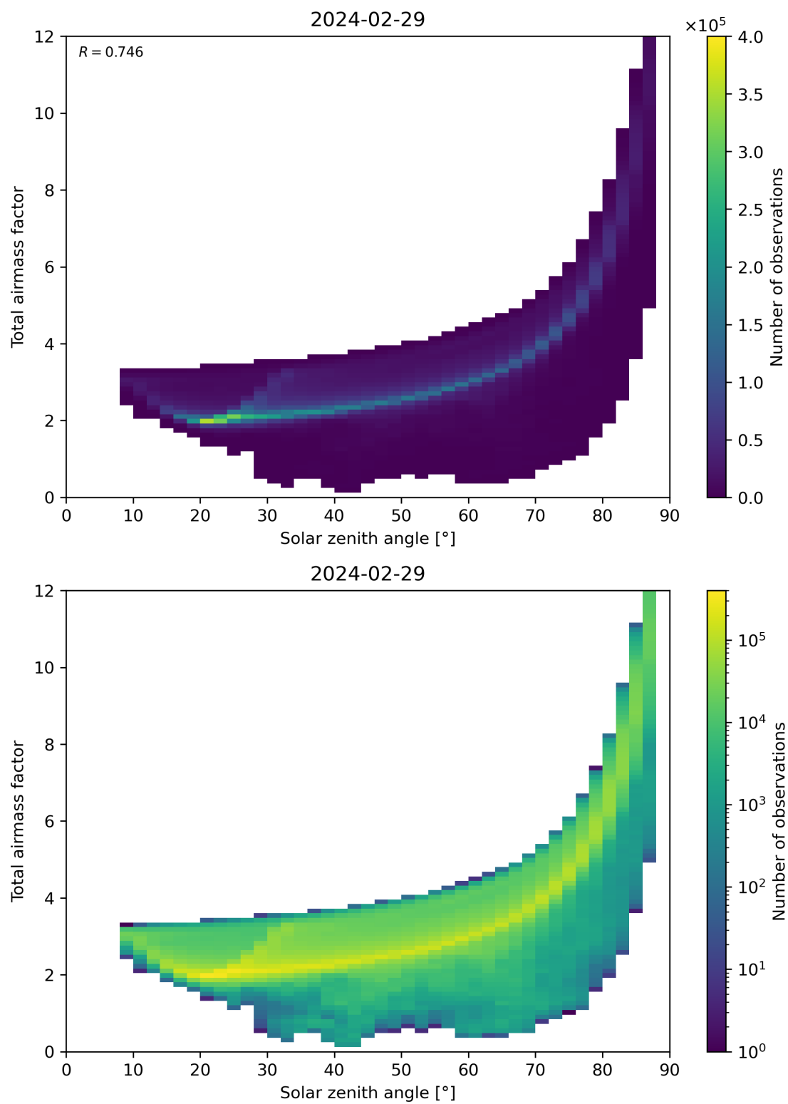
Figure 146: Scatter density plot of “Solar zenith angle” against “Total air mass factor” for 2024-02-28 to 2024-03-01.
