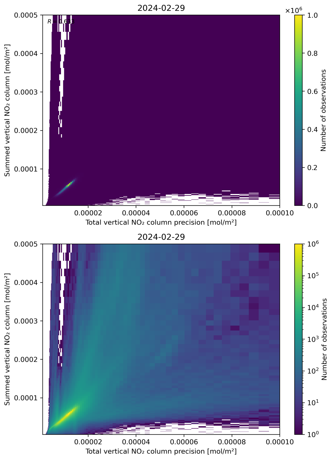
Figure 117: Scatter density plot of “Total vertical NO 2 column precision” against “Summed vertical NO 2 column” for 2024-02-28 to 2024-03-01.
