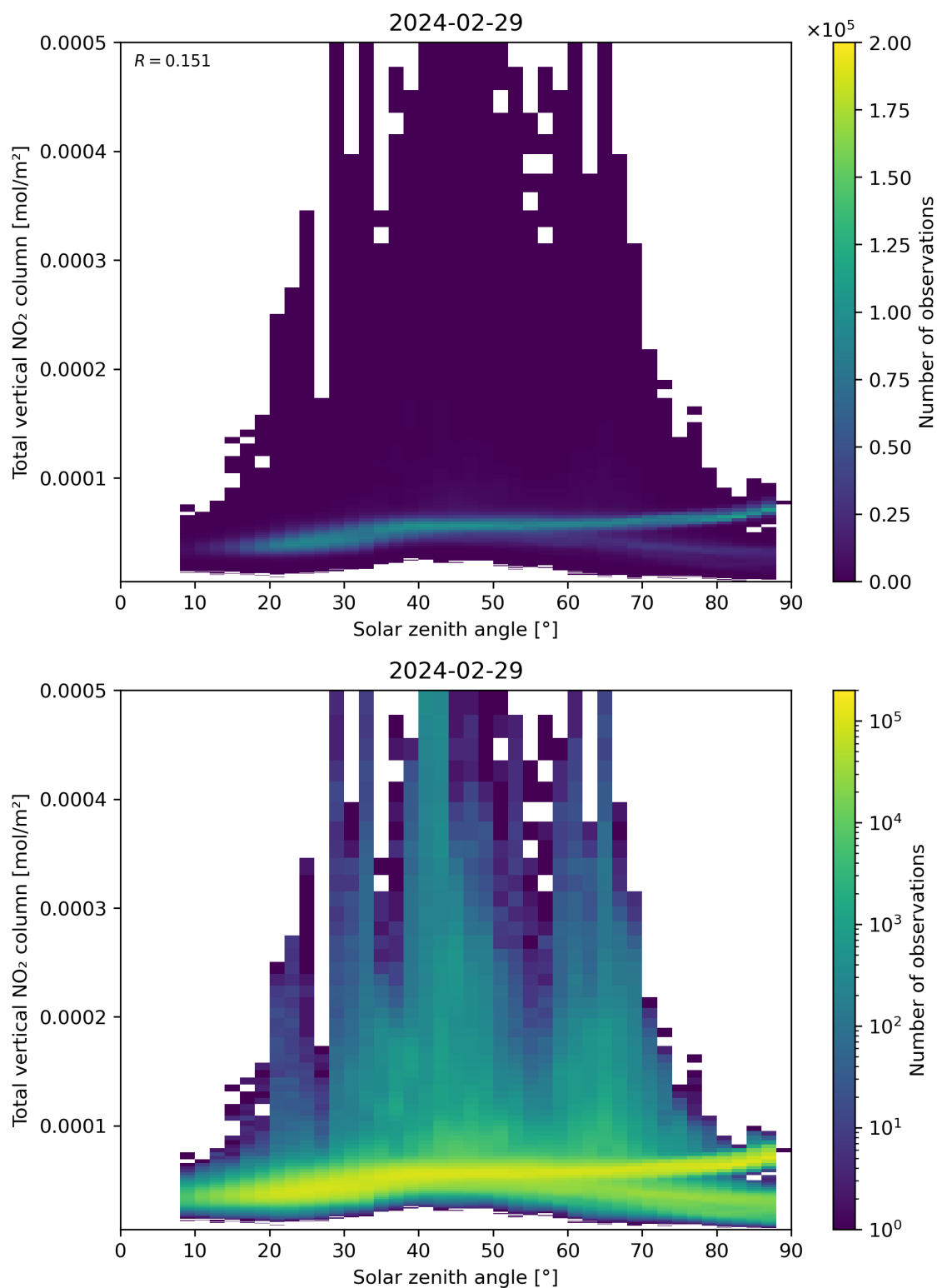
Figure 153: Scatter density plot of “Solar zenith angle” against “Total vertical NO 2 column” for 2024-02-28 to 2024-03-01.
