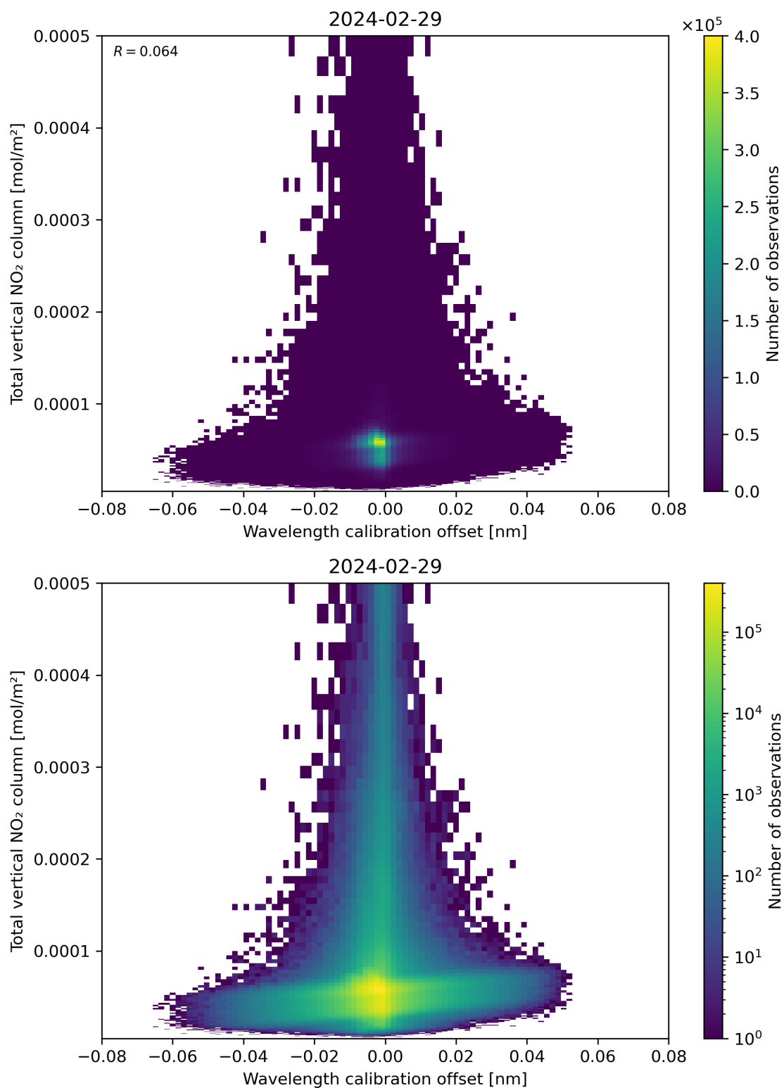
Figure 179: Scatter density plot of “Wavelength calibration offset” against “Total vertical NO 2 column” for 2024-02-28 to 2024-03-01.
