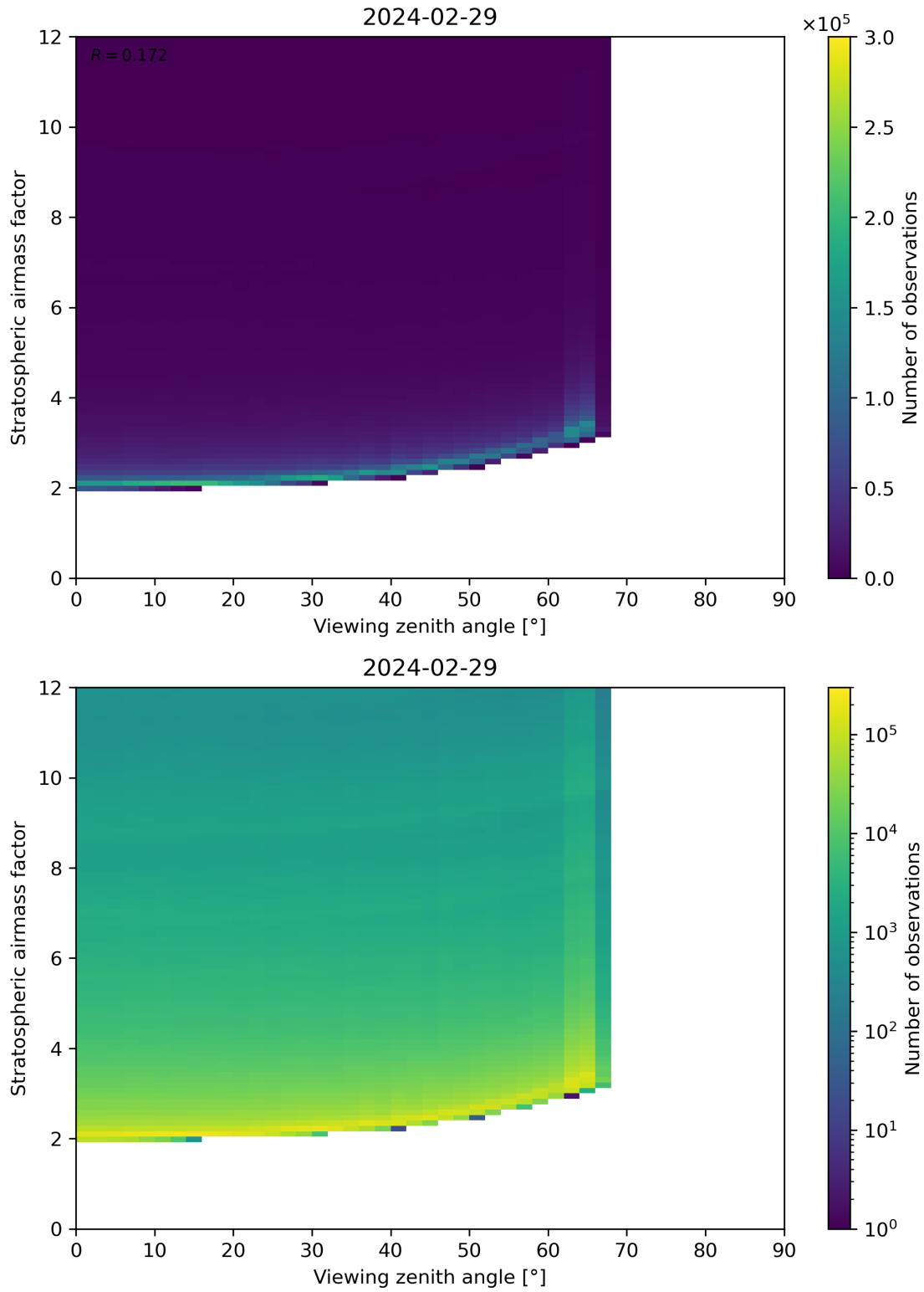
Figure 159: Scatter density plot of “Viewing zenith angle” against “Stratospheric airmass factor” for 2024-02-28 to 2024-03-01.
