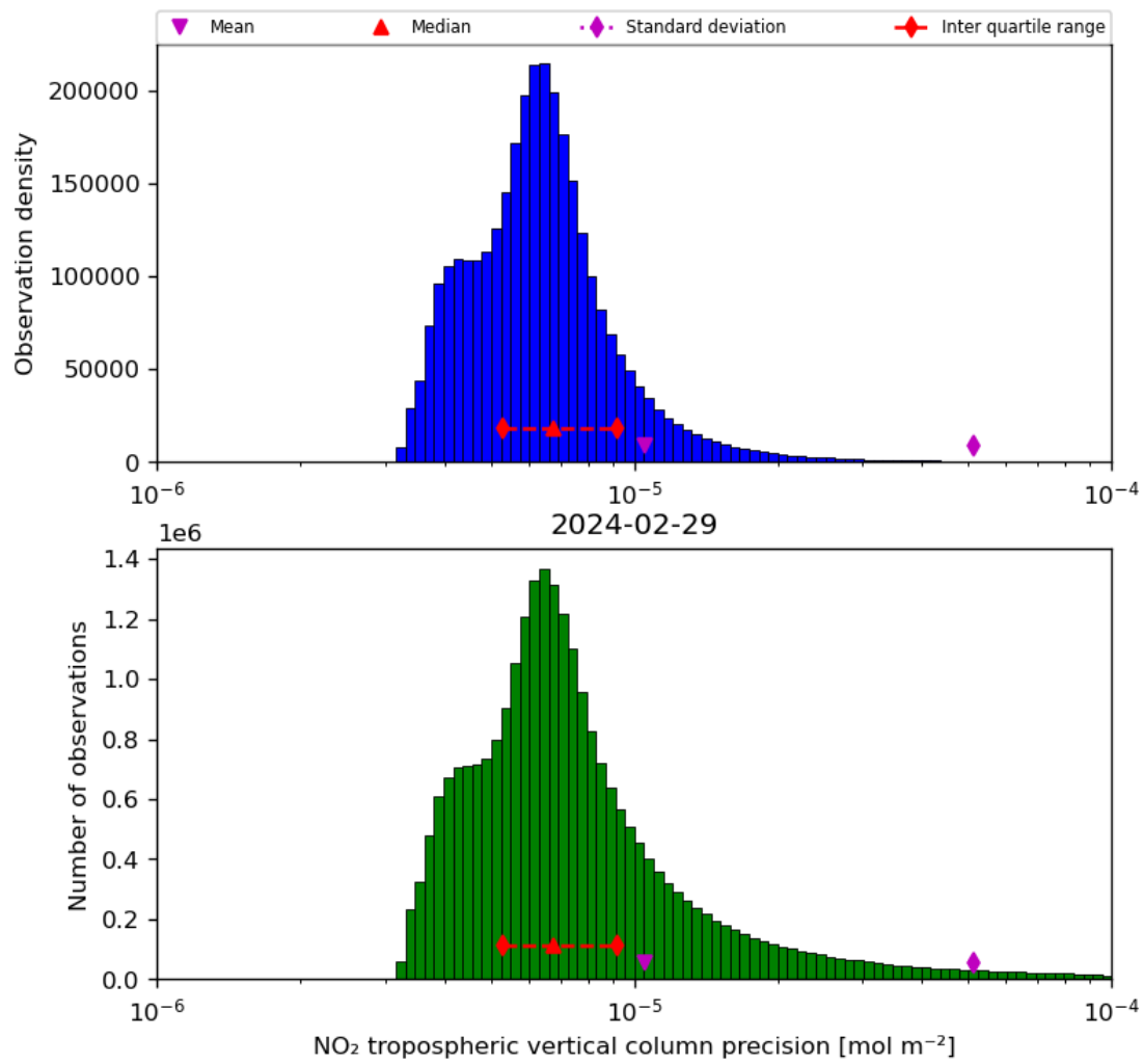
Figure 30: Histogram of “NO 2 tropospheric vertical column precision” for 2024-02-28 to 2024-03-01
