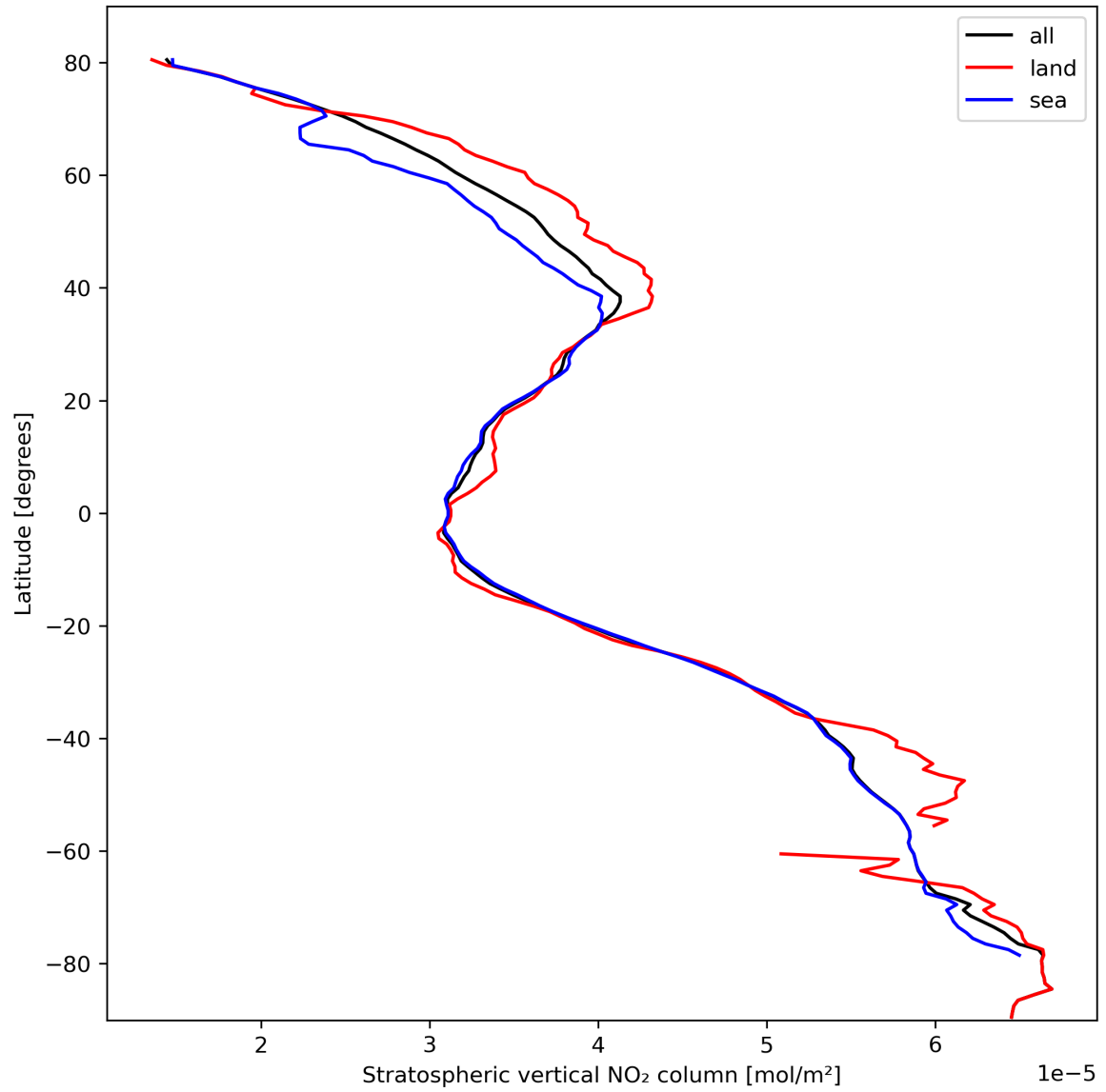
Figure 19: Zonal average of “Stratospheric vertical NO 2 column” for 2024-02-28 to 2024-03-01.
