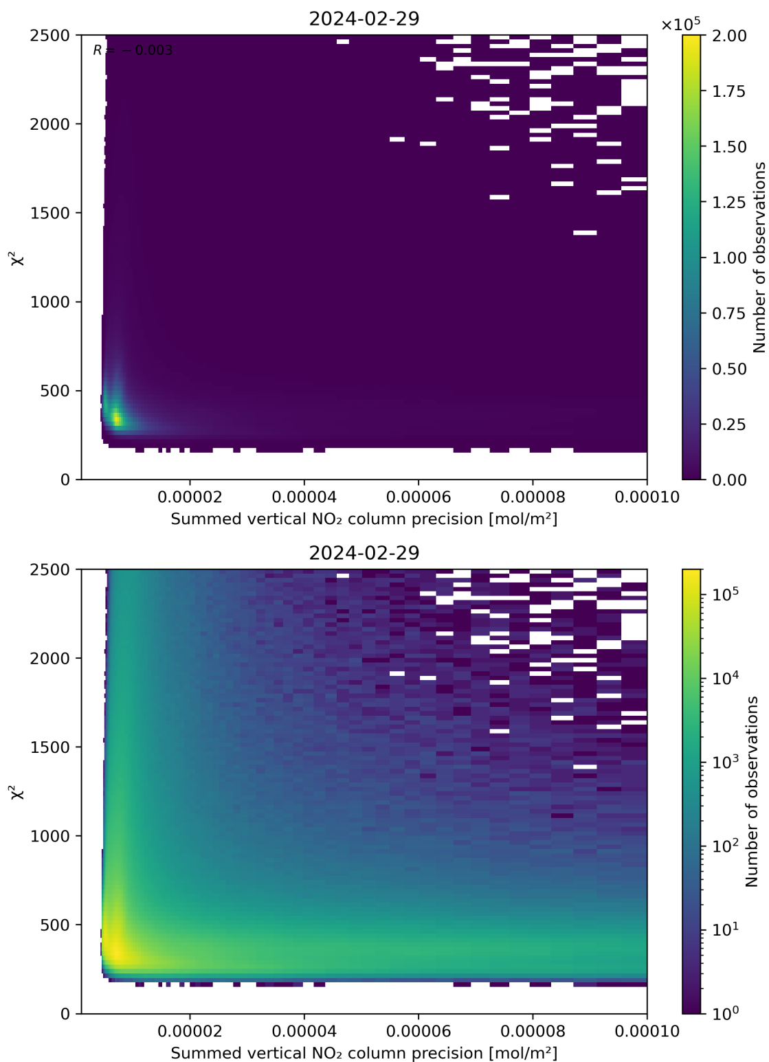
Figure 107: Scatter density plot of “Summed vertical NO 2 column precision” against “ \chi^2 ” for 2024-02-28 to 2024-03-01.
