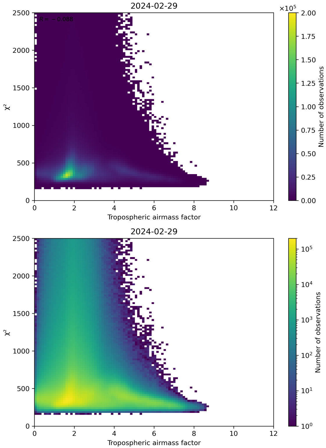
Figure 73: Scatter density plot of “Tropospheric airmass factor” against “ \chi^2 ” for 2024-02-28 to 2024-03-01.
