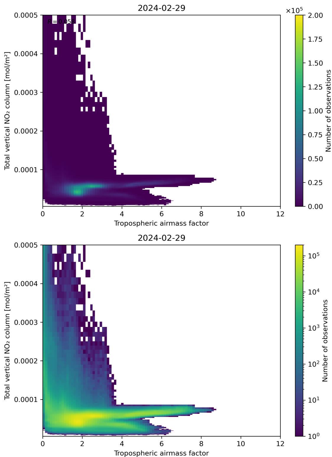
Figure 77: Scatter density plot of “Tropospheric airmass factor” against “Total vertical NO 2 column” for 2024-02-28 to 2024-03-01.
