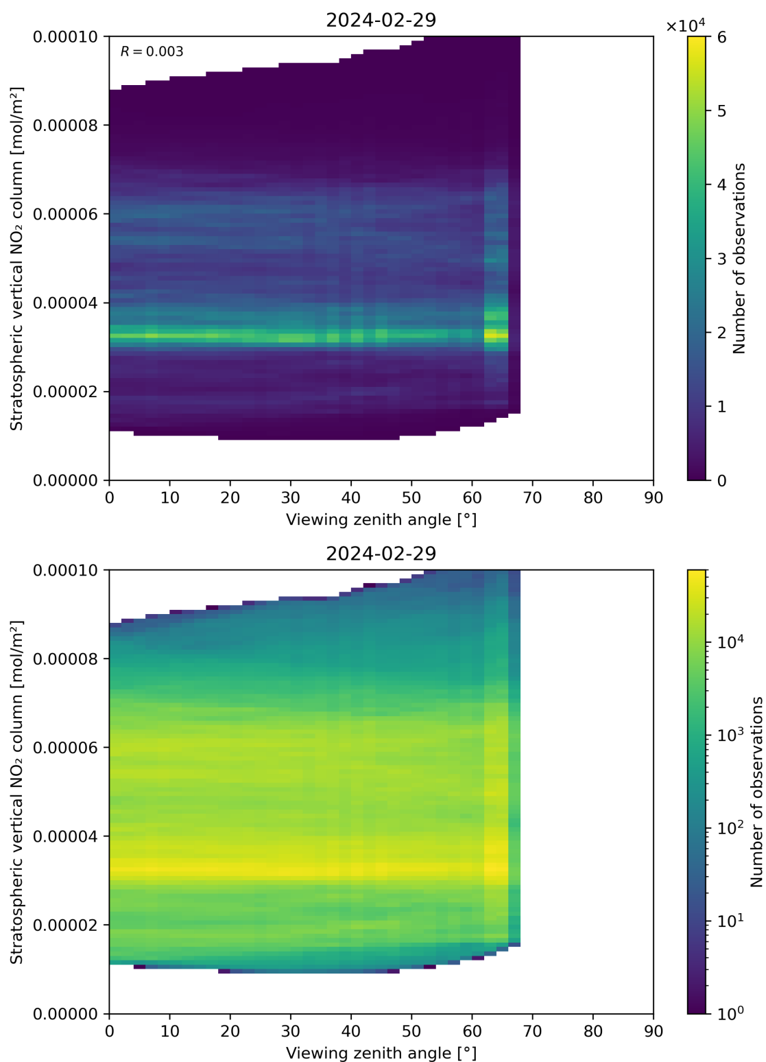
Figure 164: Scatter density plot of “Viewing zenith angle” against “Stratospheric vertical NO 2 column” for 2024-02-28 to 2024-03-01.
