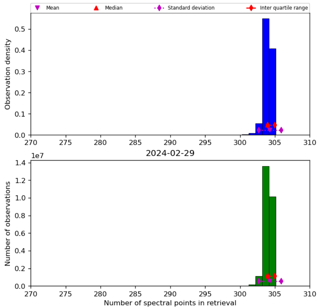
Figure 33: Histogram of “Number of spectral points in retrieval” for 2024-02-28 to 2024-03-01
