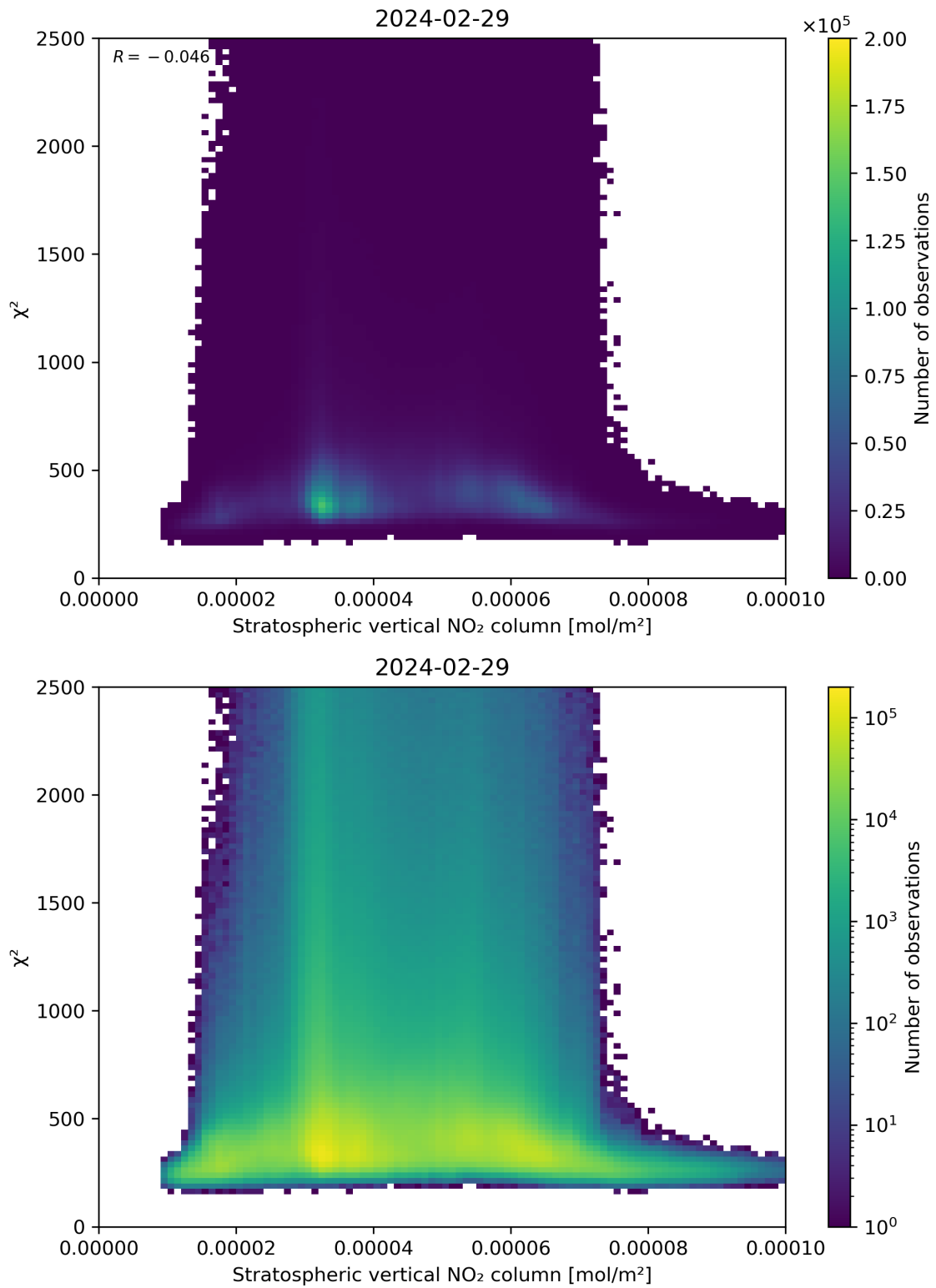
Figure 97: Scatter density plot of “Stratospheric vertical NO 2 column” against “ \chi^2 ” for 2024-02-28 to 2024-03-01.
