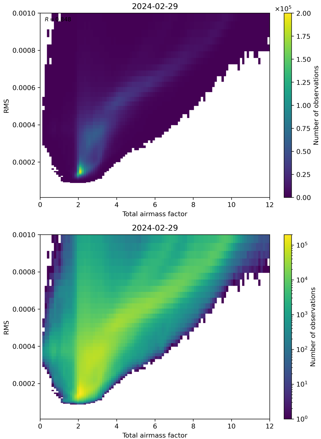
Figure 69: Scatter density plot of “Total airmass factor” against “RMS” for 2024-02-28 to 2024-03-01.
