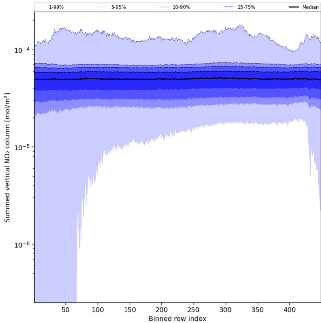
Figure 57: Along track statistics of “Summed vertical NO 2 column” for 2024-02-28 to 2024-03-01
