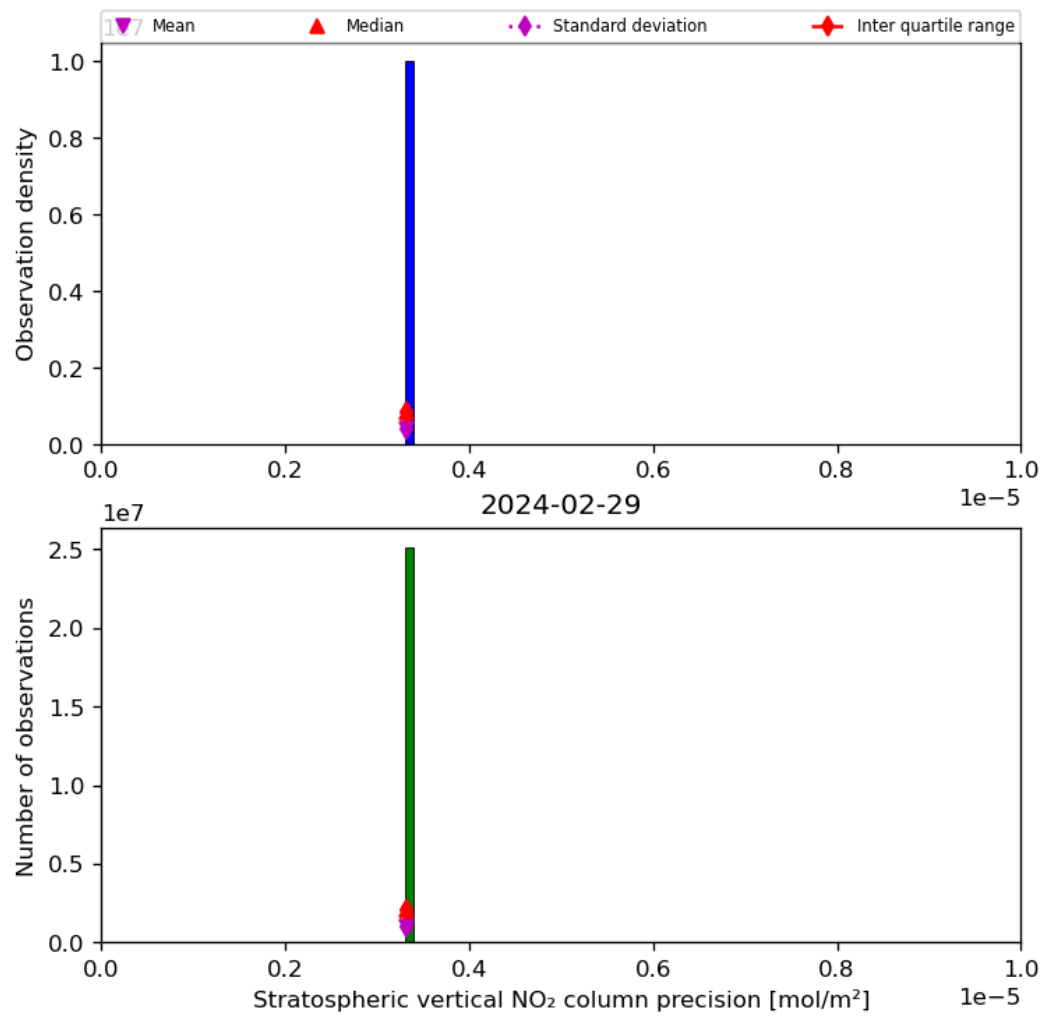
Figure 37: Histogram of “Stratospheric vertical NO 2 column precision” for 2024-02-28 to 2024-03-01
