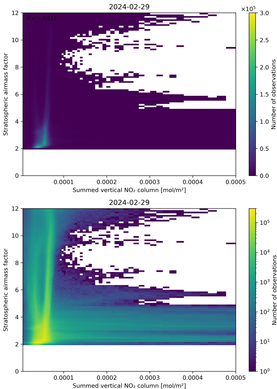
Figure 103: Scatter density plot of “Summed vertical NO 2 column” against “Stratospheric air mass factor” for 2024-02-28 to 2024-03-01.
