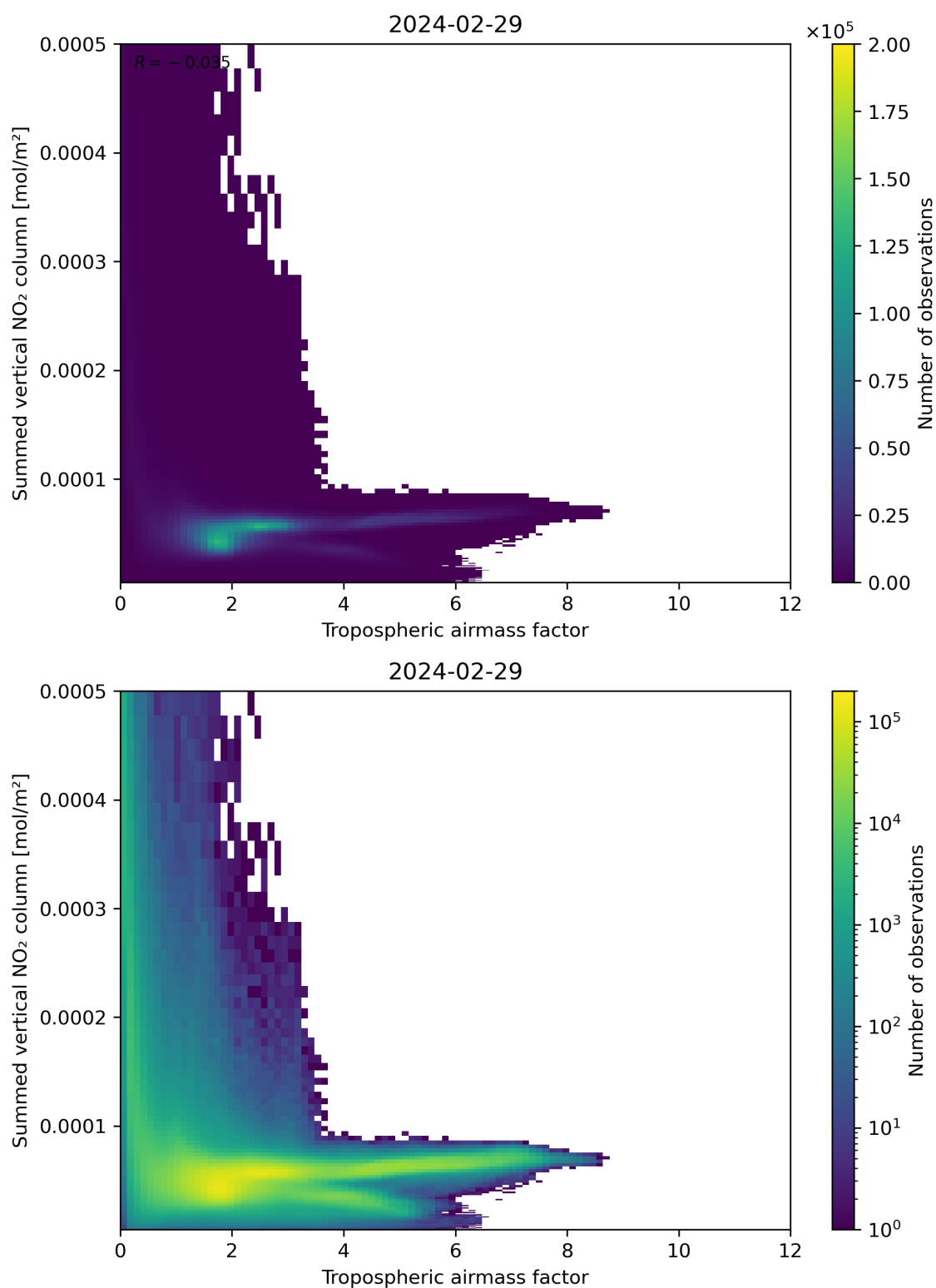
Figure 75: Scatter density plot of “Tropospheric airmass factor” against “Summed vertical NO 2 column” for 2024-02-28 to 2024-03-01.
