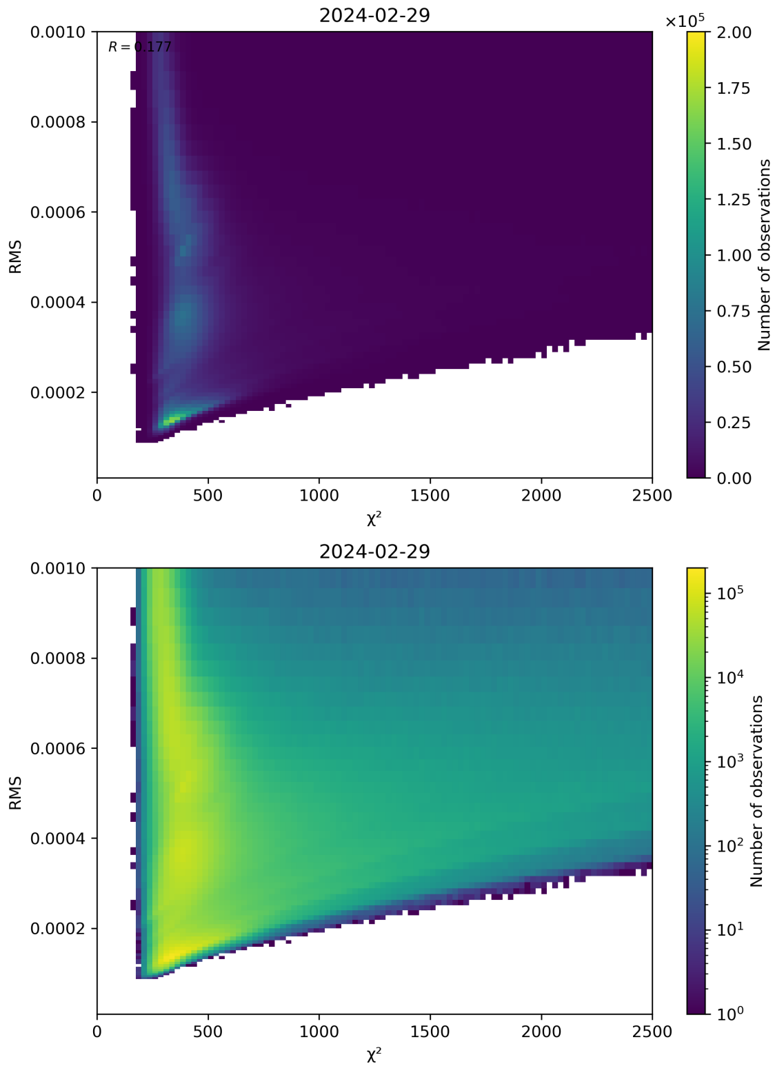
Figure 82: Scatter density plot of “ \chi^2 ” against “RMS” for 2024-02-28 to 2024-03-01.
