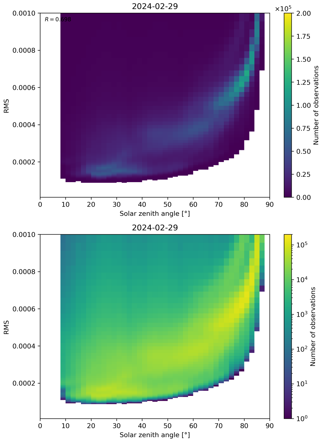
Figure 157: Scatter density plot of “Solar zenith angle” against “RMS” for 2024-02-28 to 2024-03-01.
