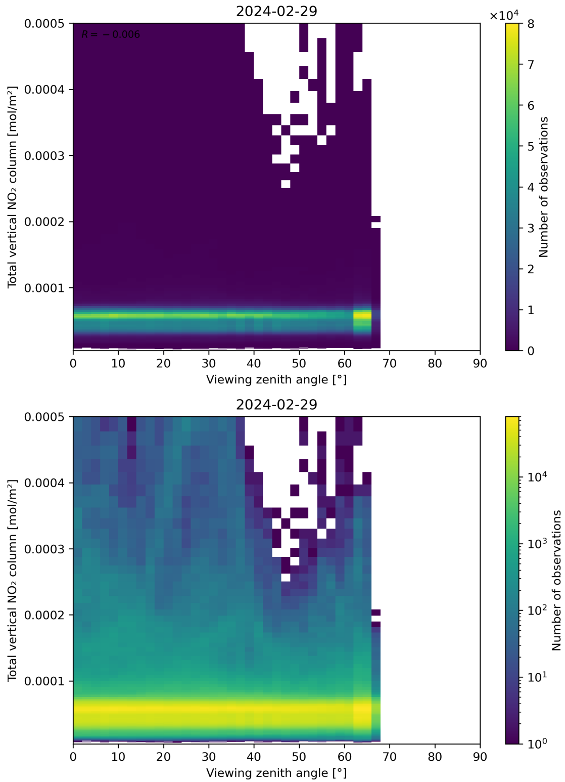
Figure 167: Scatter density plot of “Viewing zenith angle” against “Total vertical NO 2 column” for 2024-02-28 to 2024-03-01.
