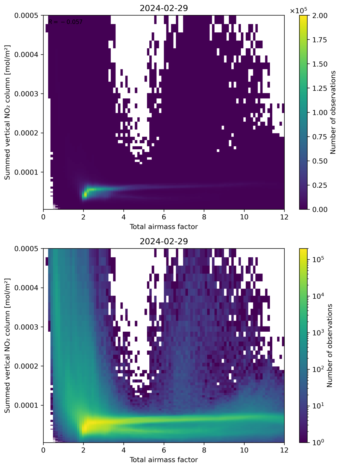
Figure 65: Scatter density plot of “Total airmass factor” against “Summed vertical NO 2 column” for 2024-02-28 to 2024-03-01.
