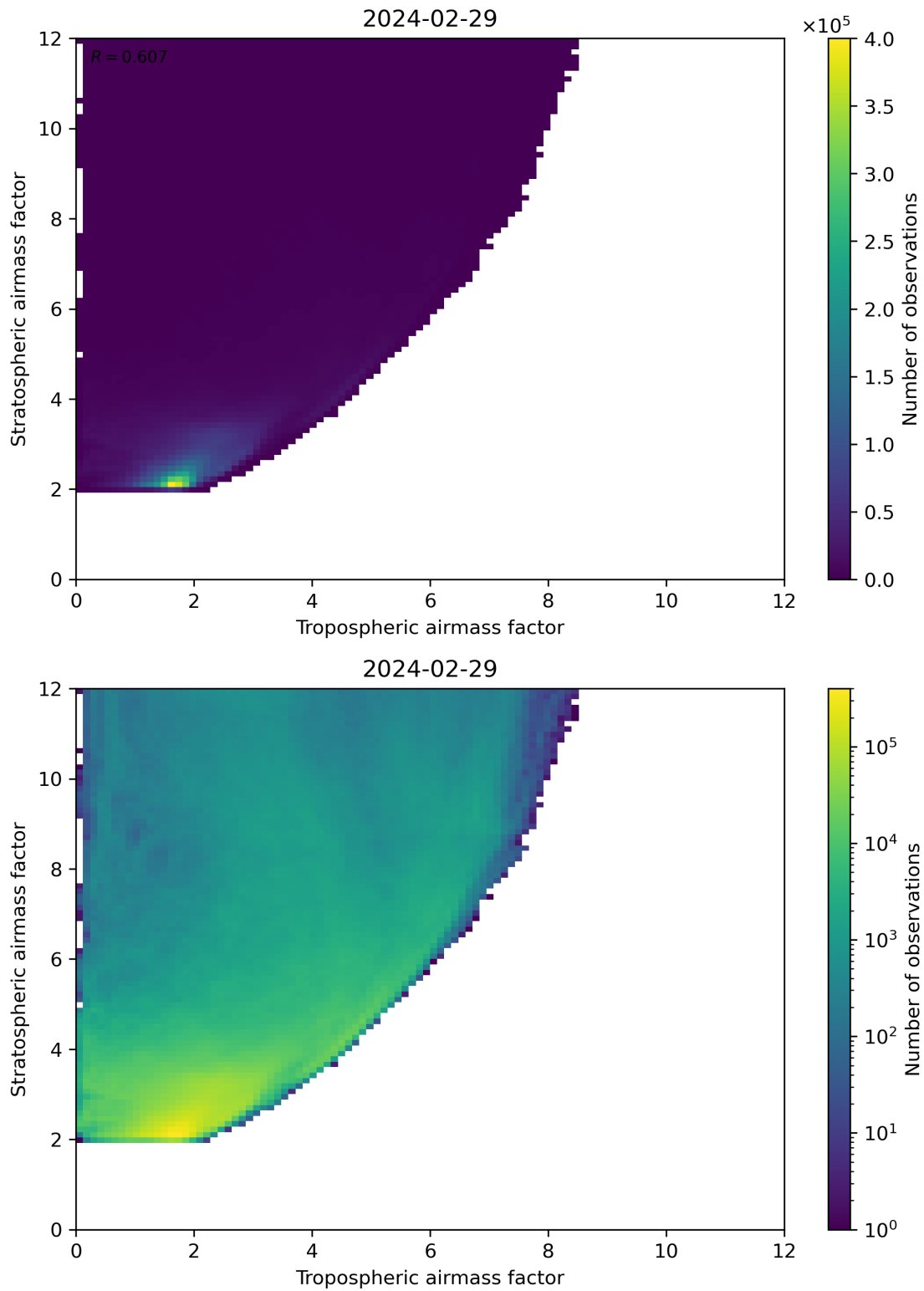
Figure 71: Scatter density plot of “Tropospheric airmass factor” against “Stratospheric airmass factor” for 2024-02-28 to 2024-03-01.
