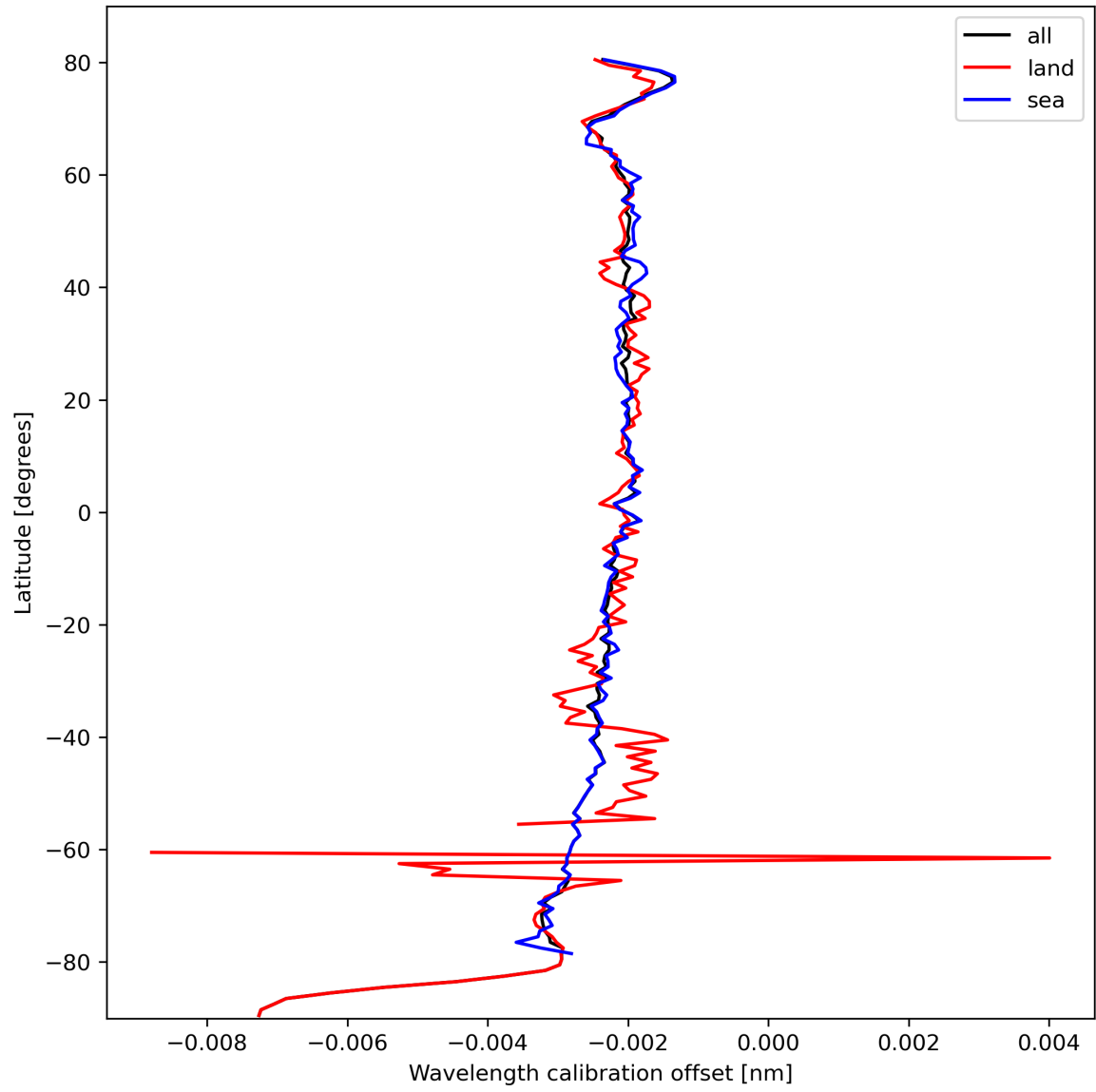
Figure 18: Zonal average of “Wavelength calibration offset” for 2024-02-28 to 2024-03-01.
