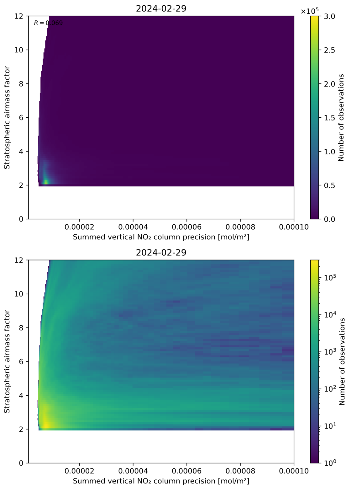
Figure 106: Scatter density plot of “Summed vertical NO 2 column precision” against “Stratospheric airmass factor” for 2024-02-28 to 2024-03-01.
