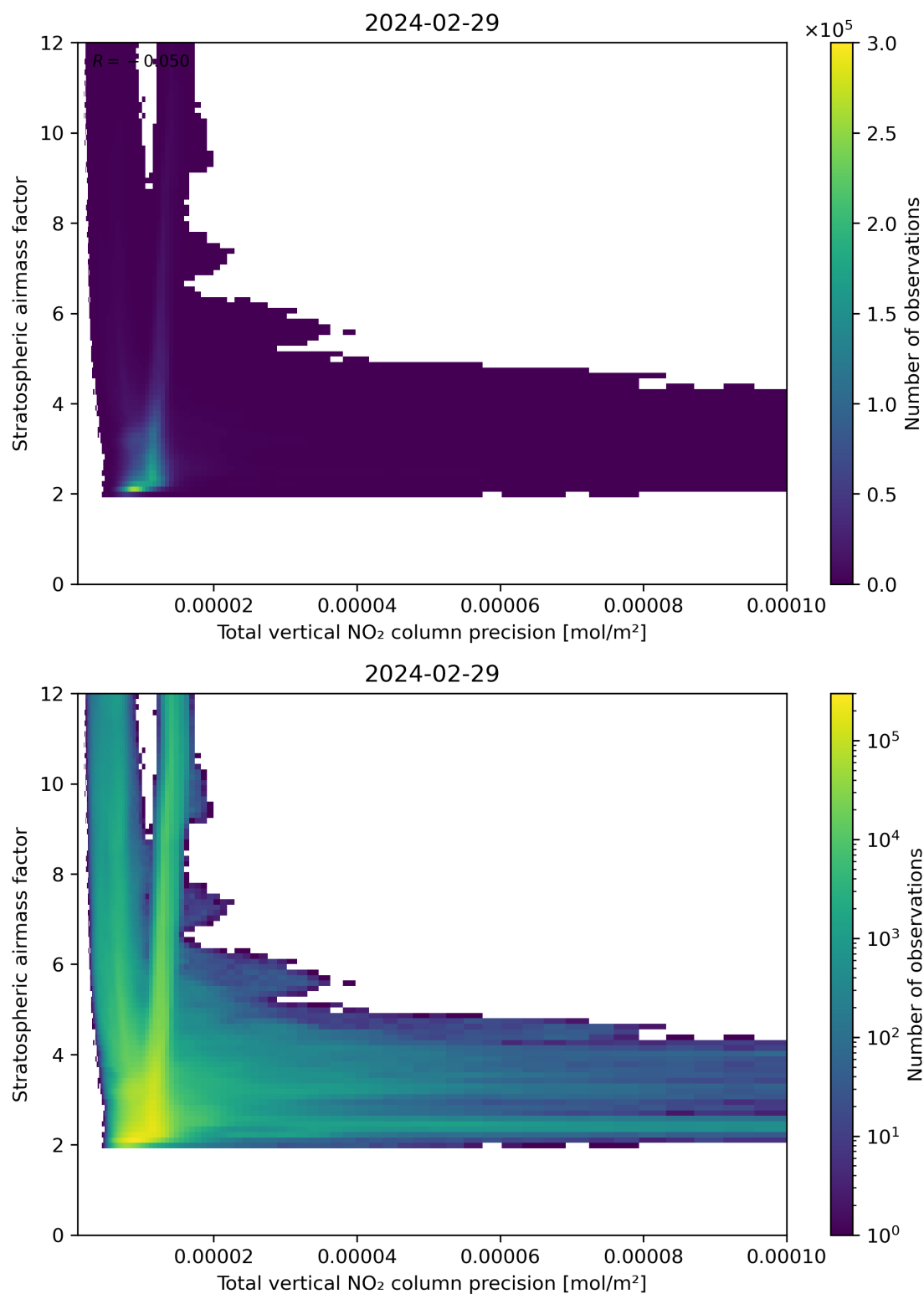
Figure 115: Scatter density plot of “Total vertical NO 2 column precision” against “Stratospheric air mass factor” for 2024-02-28 to 2024-03-01.
