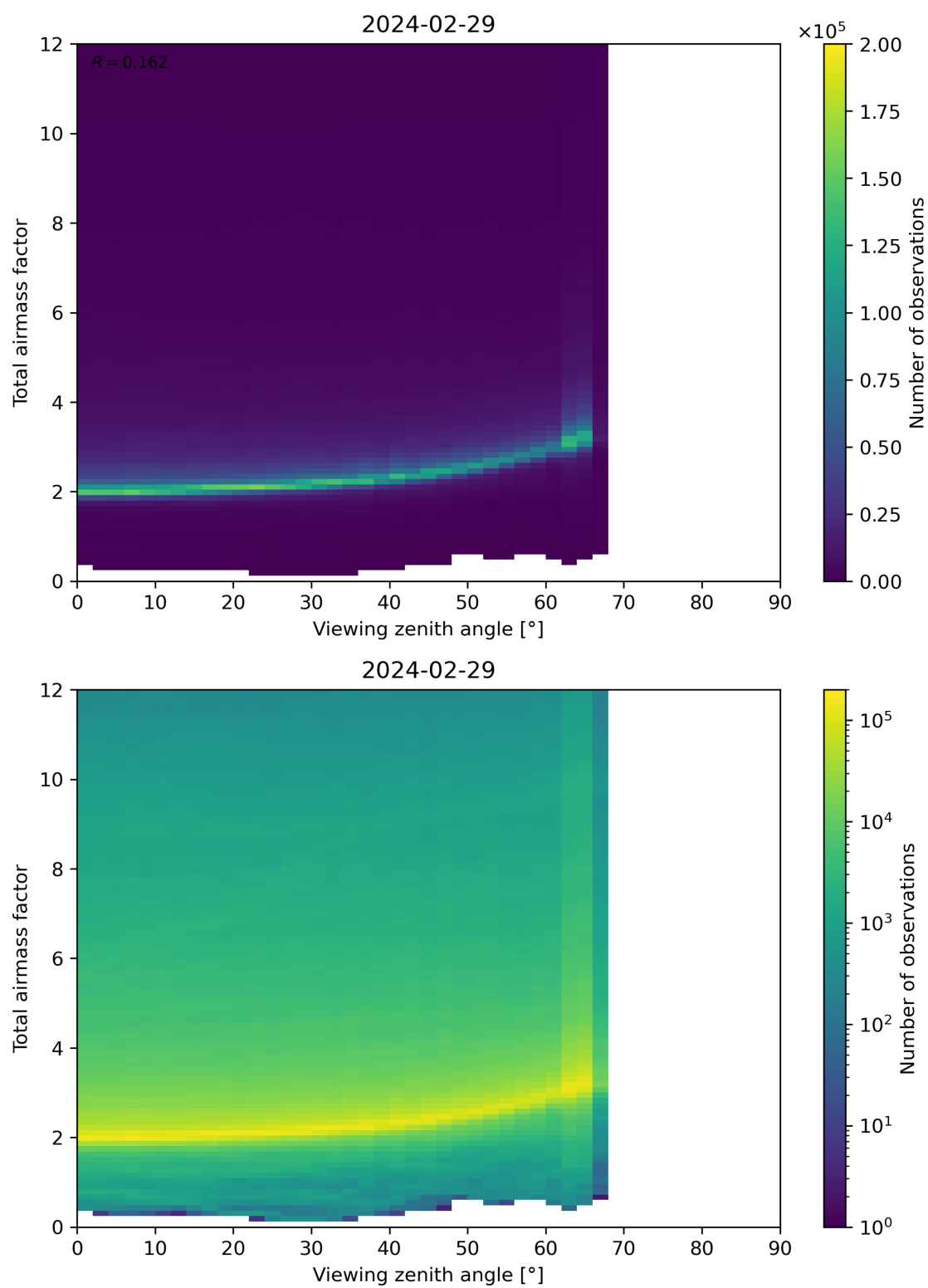
Figure 160: Scatter density plot of “Viewing zenith angle” against “Total airmass factor” for 2024-02-28 to 2024-03-01.
