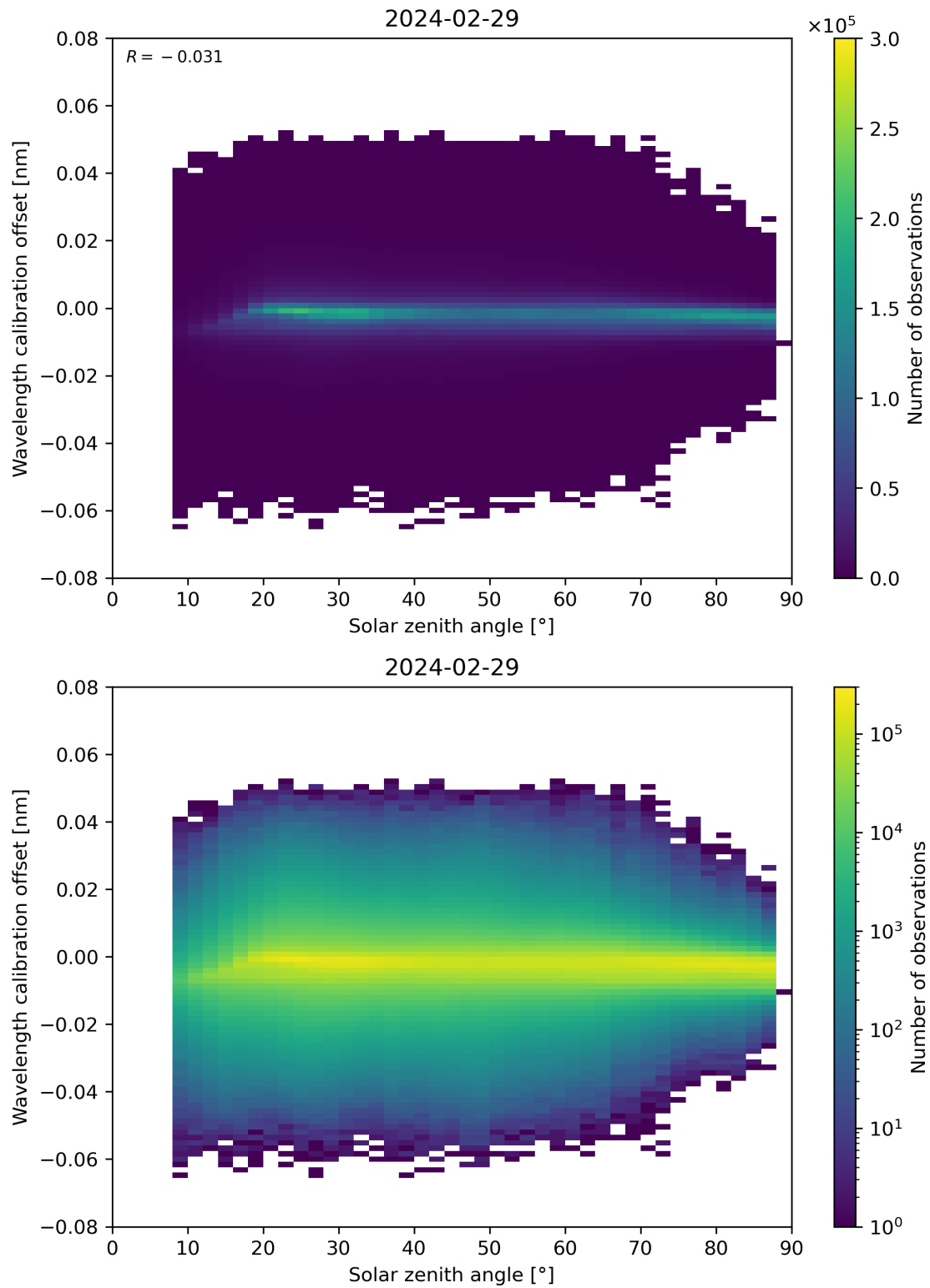
Figure 158: Scatter density plot of “Solar zenith angle” against “Wavelength calibration offset” for 2024-02-28 to 2024-03-01.
