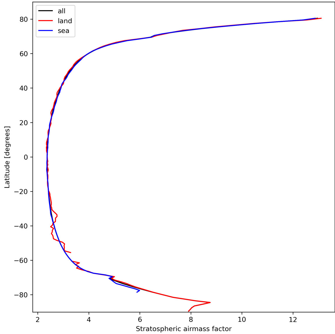
Figure 27: Zonal average of “Stratospheric air mass factor” for 2024-02-28 to 2024-03-01.
