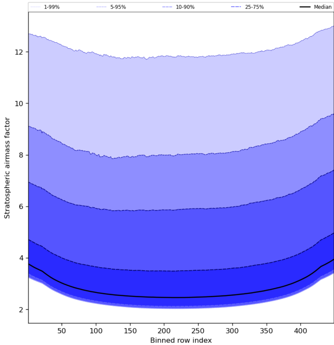
Figure 61: Along track statistics of “Stratospheric airmass factor” for 2024-02-28 to 2024-03-01
