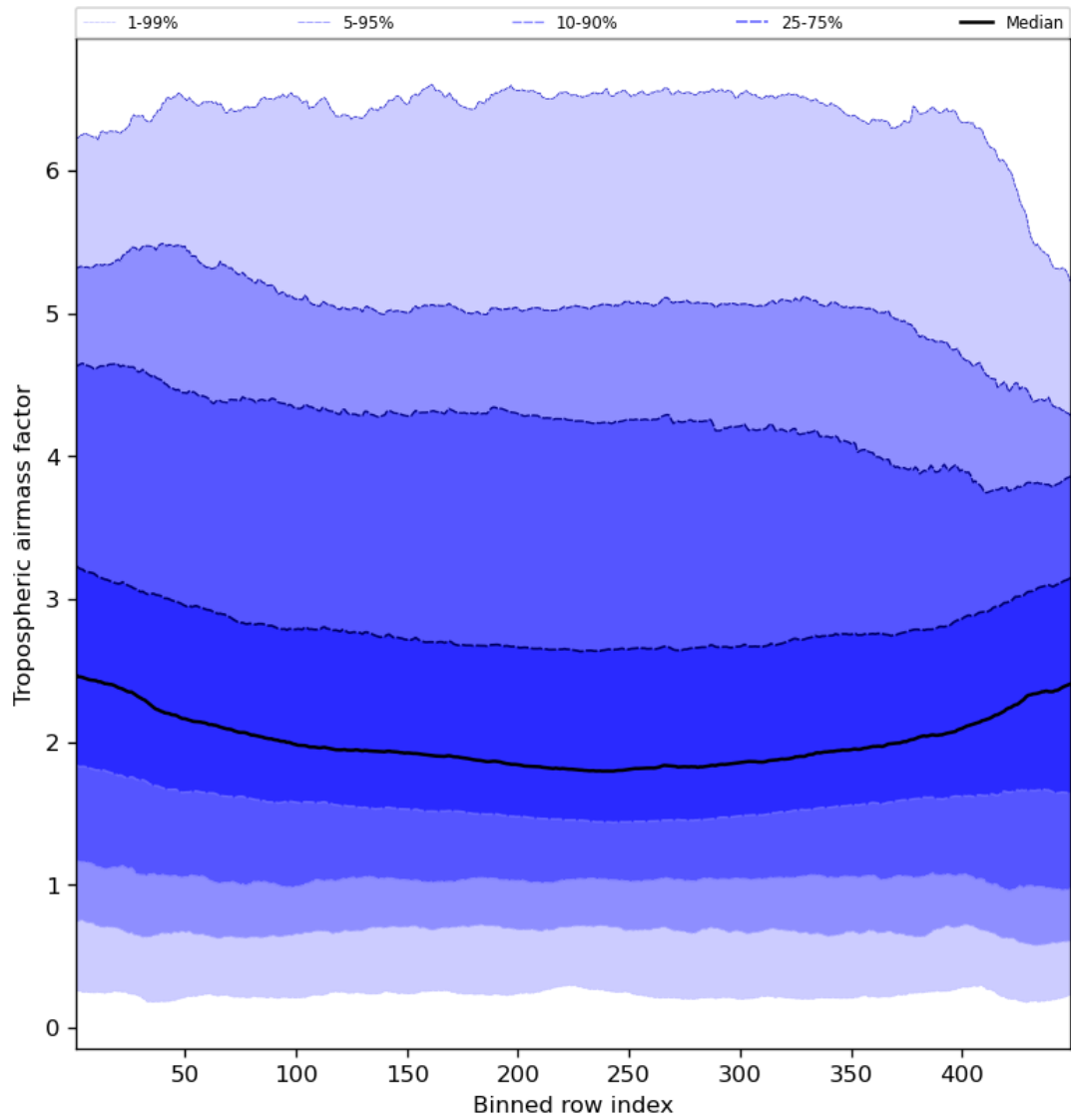
Figure 48: Along track statistics of “Tropospheric airmass factor” for 2024-02-28 to 2024-03-01
