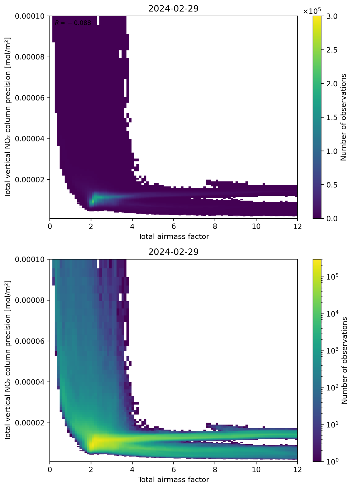
Figure 68: Scatter density plot of “Total airmass factor” against “Total vertical NO 2 column precision” for 2024-02-28 to 2024-03-01.
