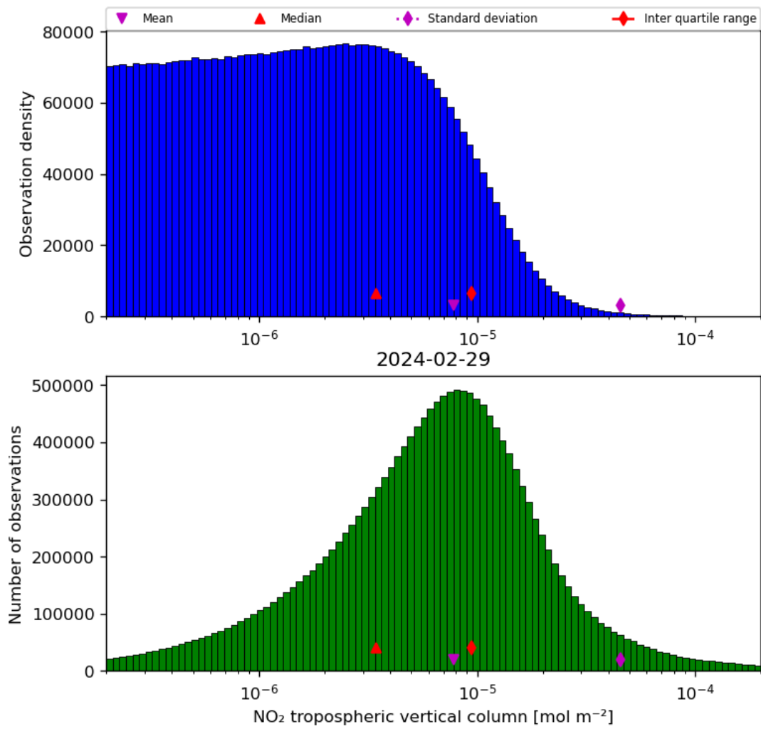
Figure 29: Histogram of “NO 2 tropospheric vertical column” for 2024-02-28 to 2024-03-01
