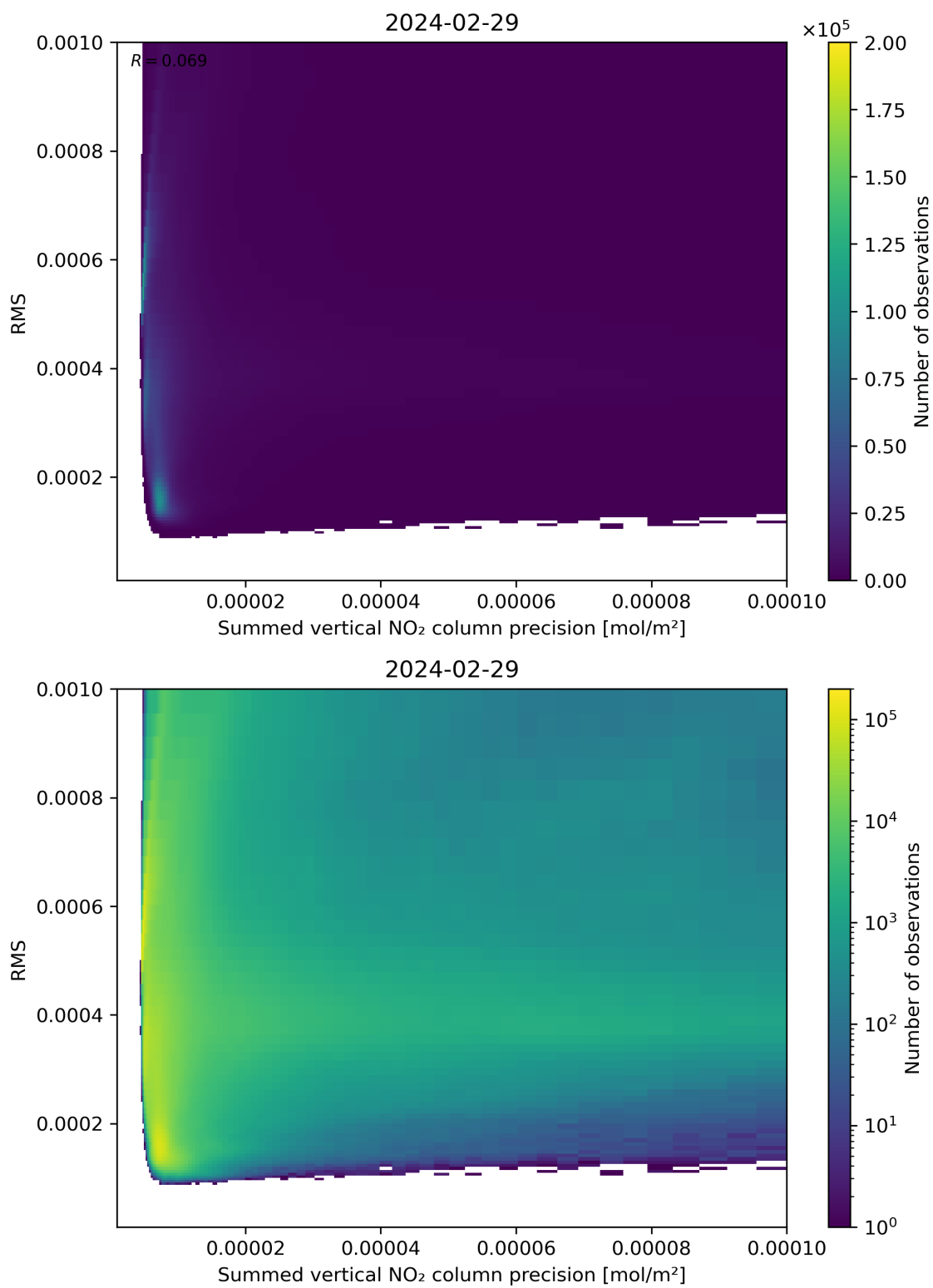
Figure 108: Scatter density plot of “Summed vertical NO 2 column precision” against “RMS” for 2024-02-28 to 2024-03-01.
