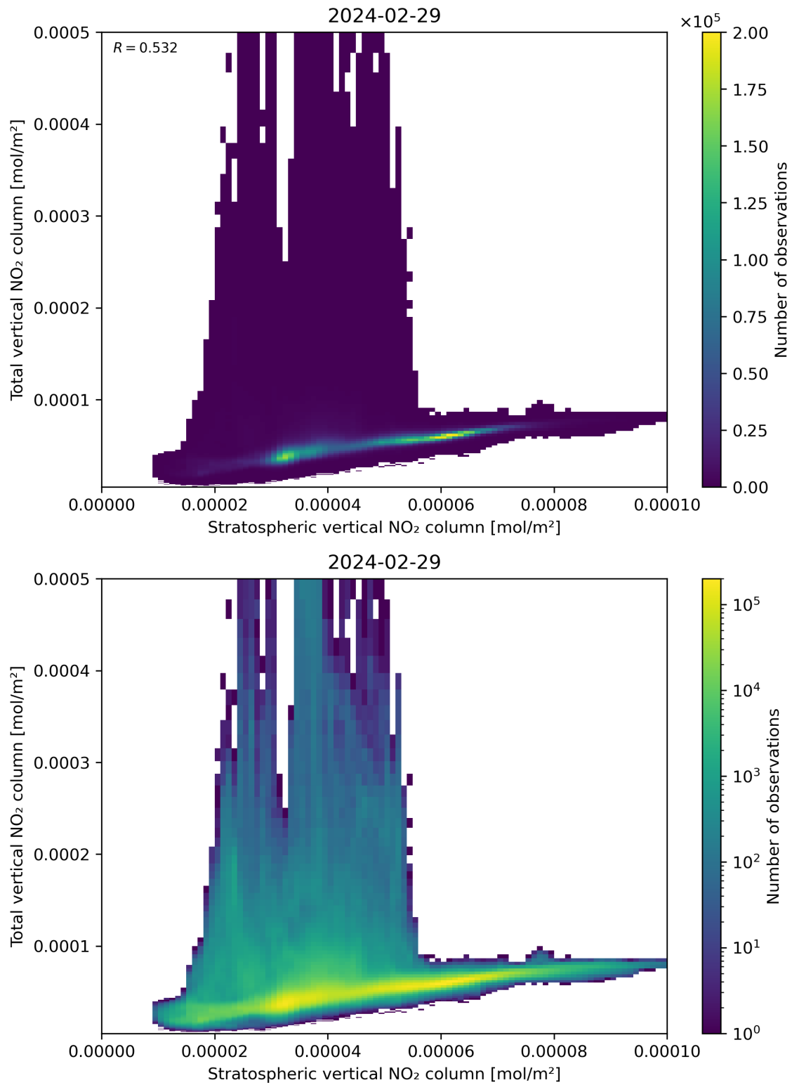
Figure 100: Scatter density plot of “Stratospheric vertical NO 2 column” against “Total vertical NO 2 column” for 2024-02-28 to 2024-03-01.
