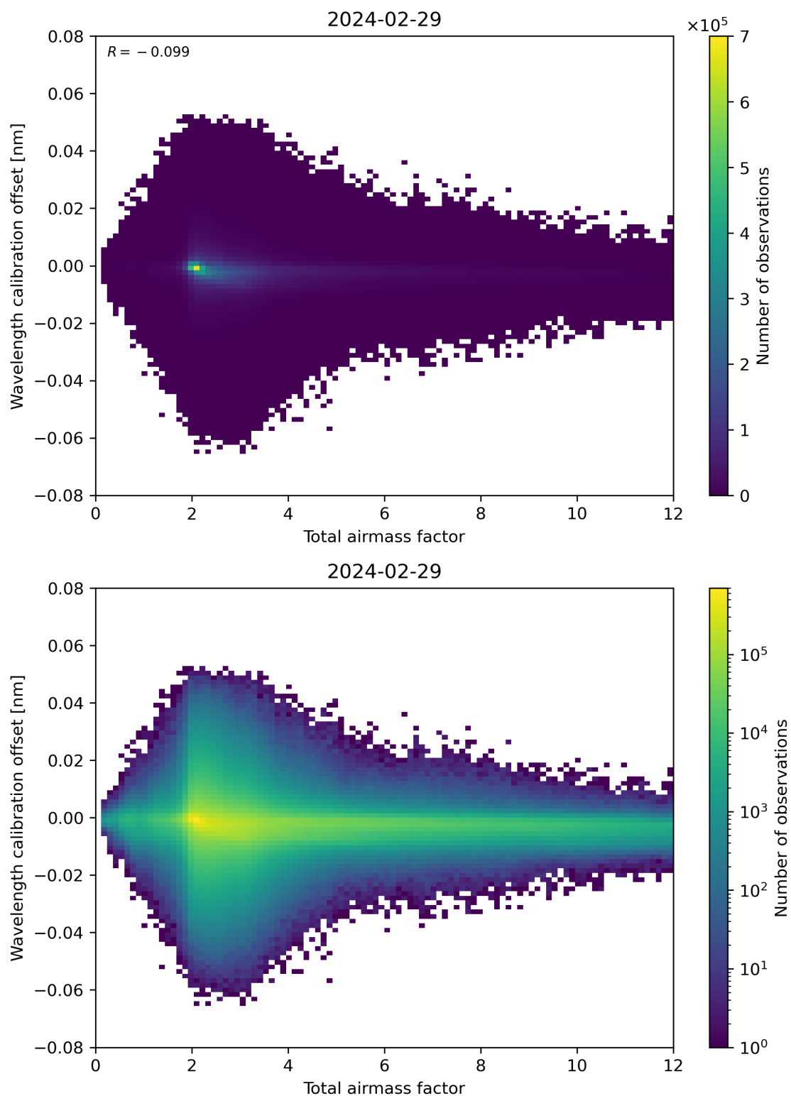
Figure 70: Scatter density plot of “Total airmass factor” against “Wavelength calibration offset” for 2024-02-28 to 2024-03-01.
