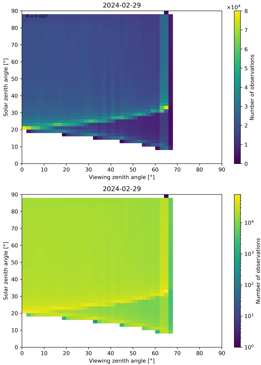
Figure 172: Scatter density plot of “Viewing zenith angle” against “Solar zenith angle” for 2024-02-28 to 2024-03-01.
