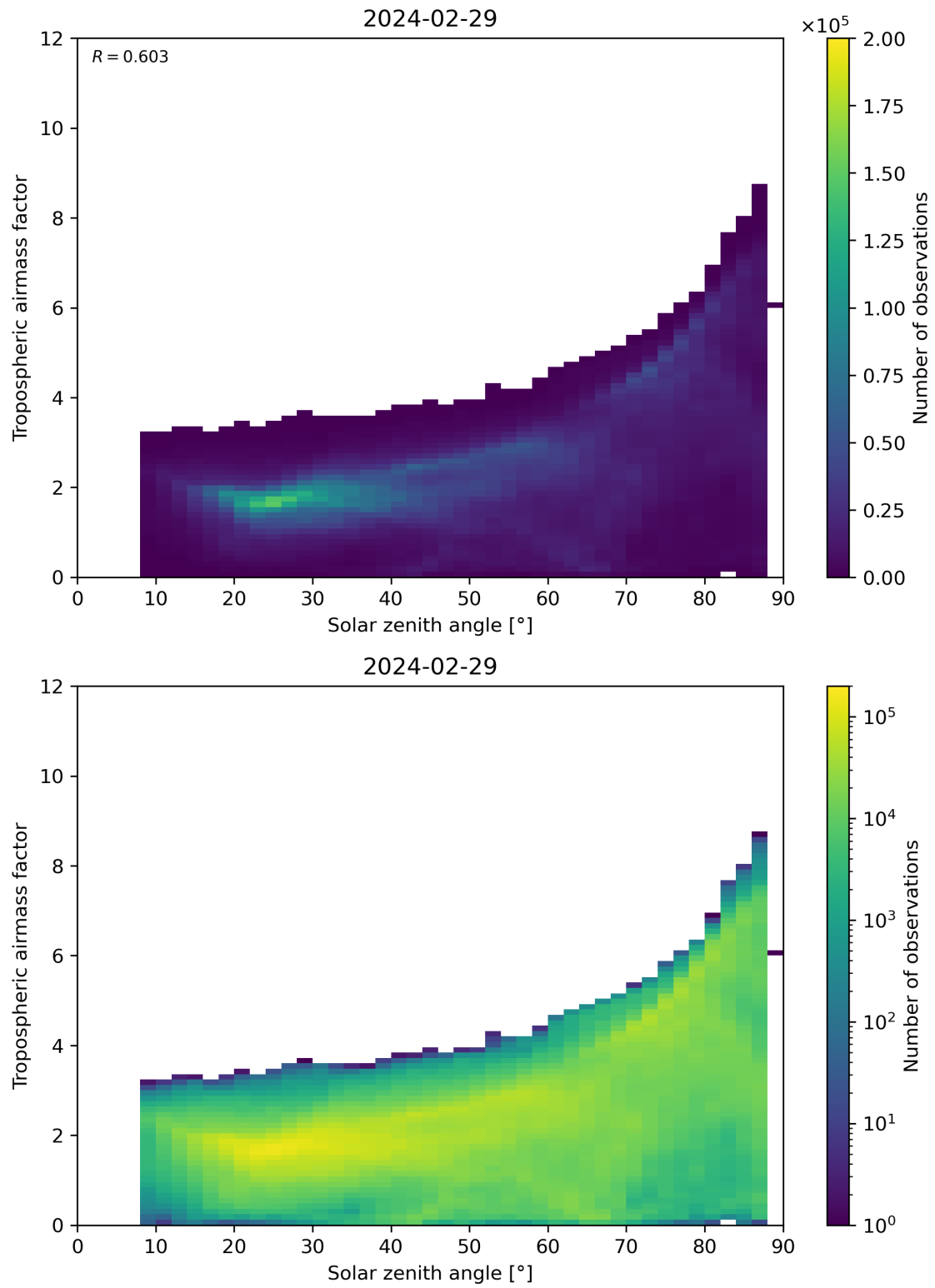
Figure 147: Scatter density plot of “Solar zenith angle” against “Tropospheric airmass factor” for 2024-02-28 to 2024-03-01.
