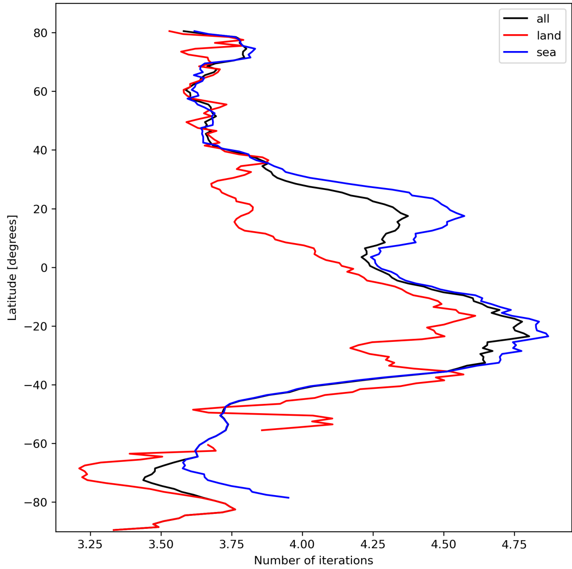
Figure 17: Zonal average of “Number of iterations” for 2024-02-28 to 2024-03-01.
