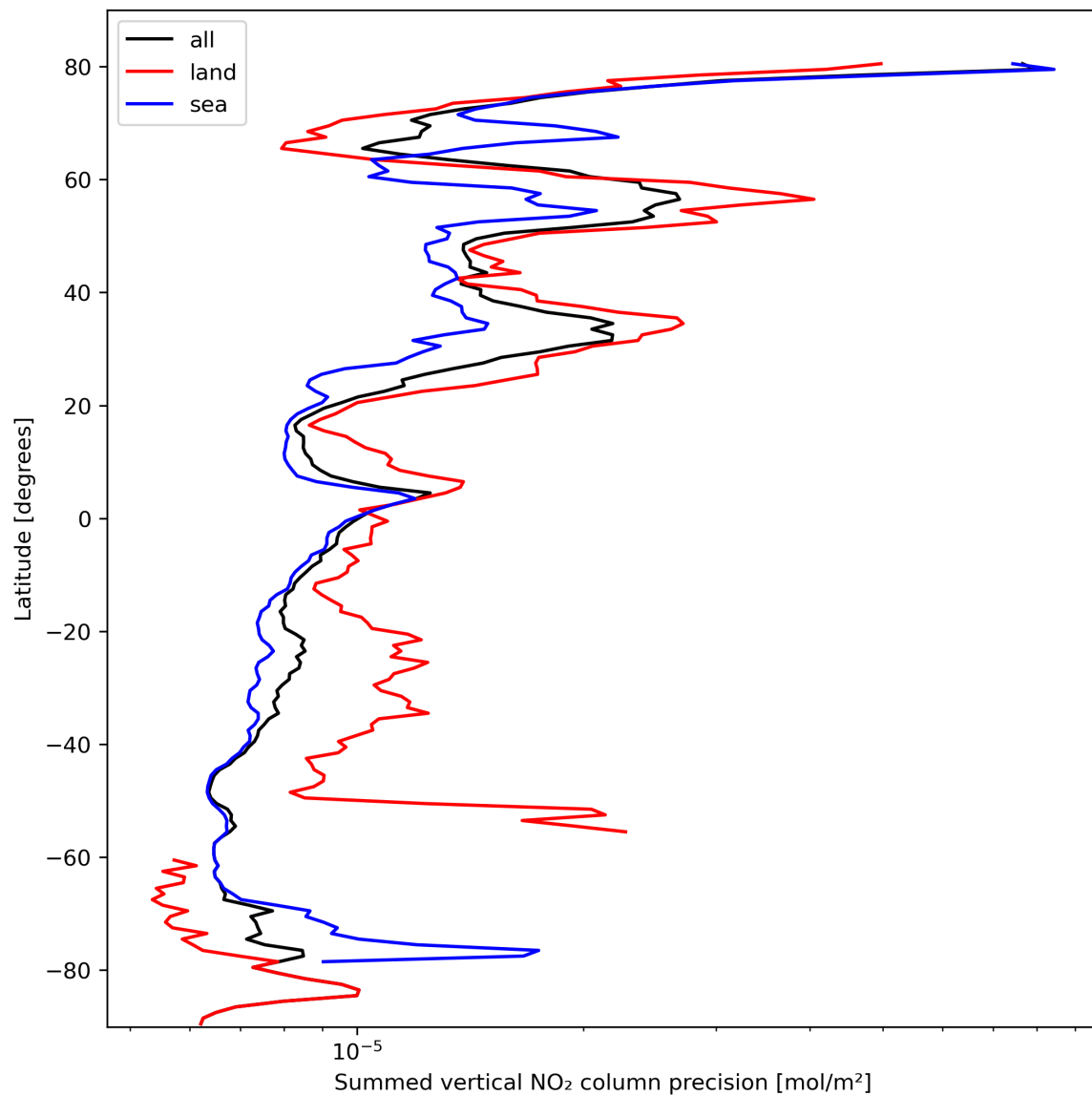
Figure 24: Zonal average of “Summed vertical NO 2 column precision” for 2024-02-28 to 2024-03-01.
