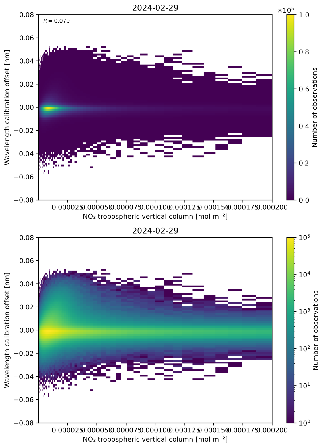
Figure 143: Scatter density plot of “NO 2 tropospheric vertical column” against “Wavelength calibration offset” for 2024-02-28 to 2024-03-01.
