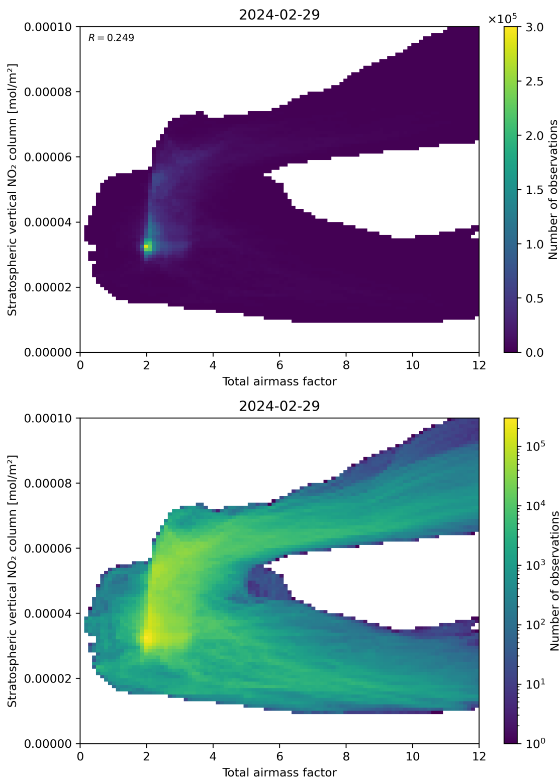
Figure 64: Scatter density plot of “Total airmass factor” against “Stratospheric vertical \text{NO}_2 column” for 2024-02-28 to 2024-03-01.
