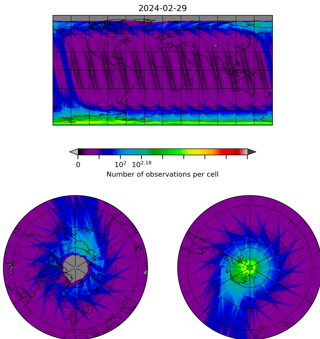
Figure 10: Map of the number of observations for 2024-02-28 to 2024-03-01
