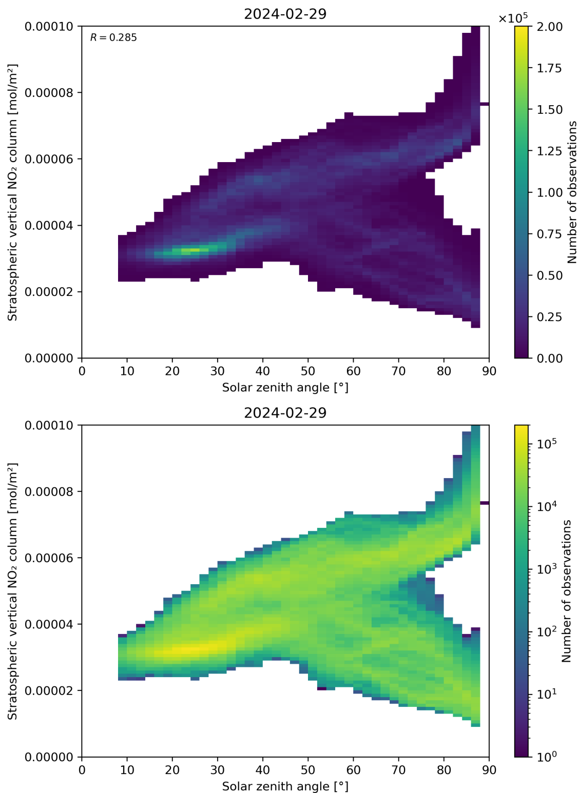
Figure 150: Scatter density plot of “Solar zenith angle” against “Stratospheric vertical NO 2 column” for 2024-02-28 to 2024-03-01.
