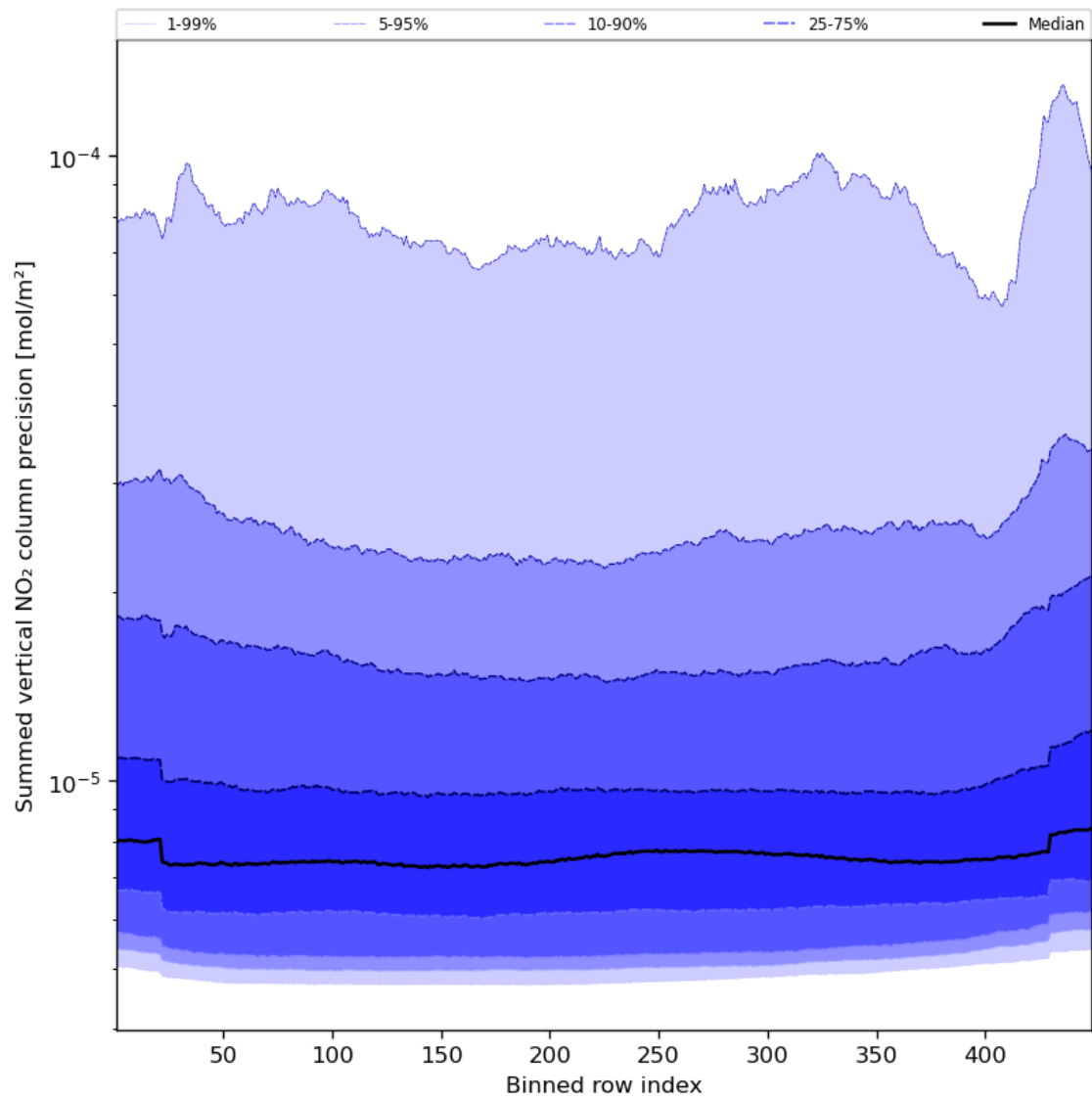
Figure 58: Along track statistics of “Summed vertical NO 2 column precision” for 2024-02-28 to 2024-03-01
