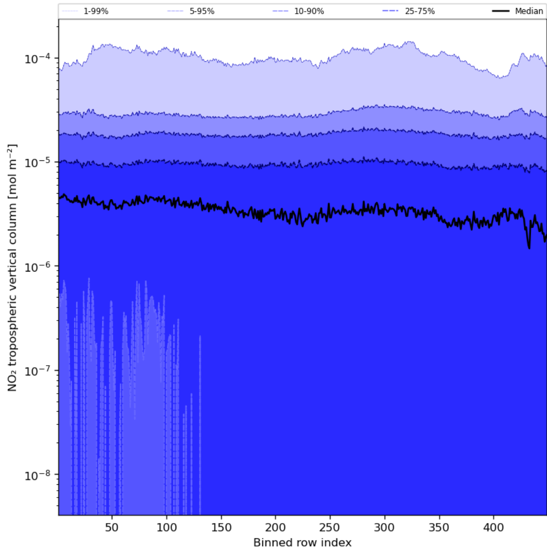
Figure 46: Along track statistics of “NO 2 tropospheric vertical column” for 2024-02-28 to 2024-03-01
