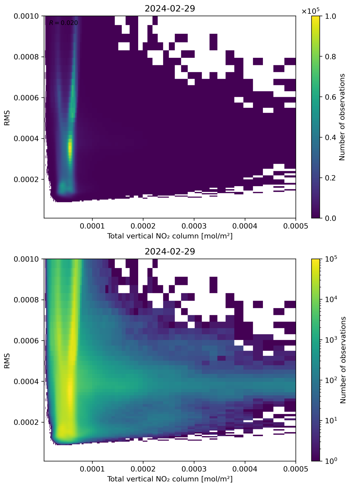
Figure 120: Scatter density plot of “Total vertical NO 2 column” against “RMS” for 2024-02-28 to 2024-03-01.
