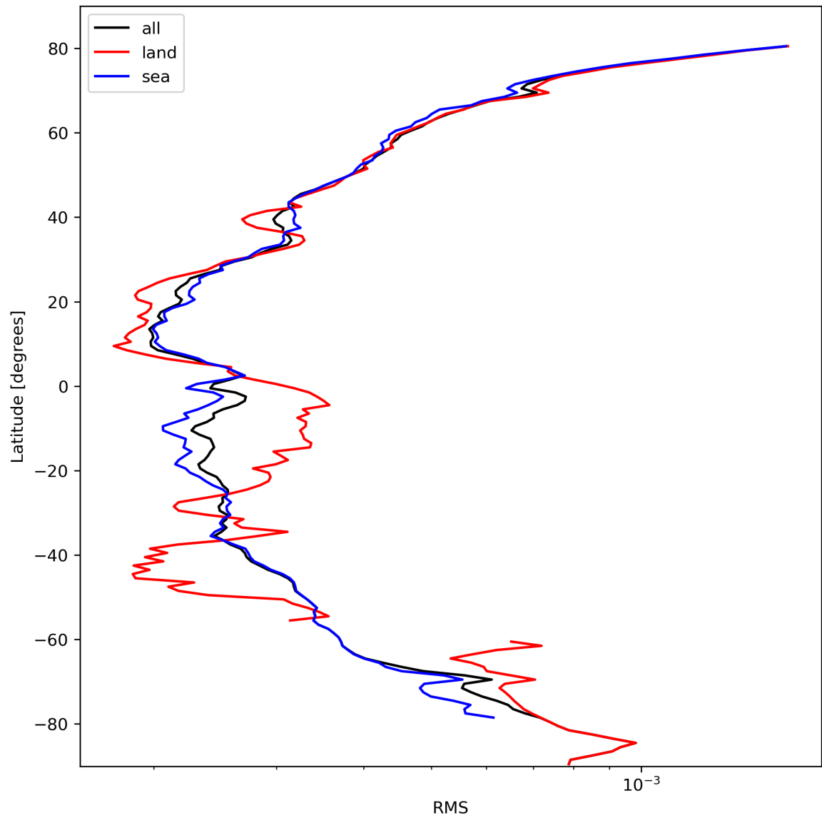
Figure 26: Zonal average of “RMS” for 2024-02-28 to 2024-03-01.
