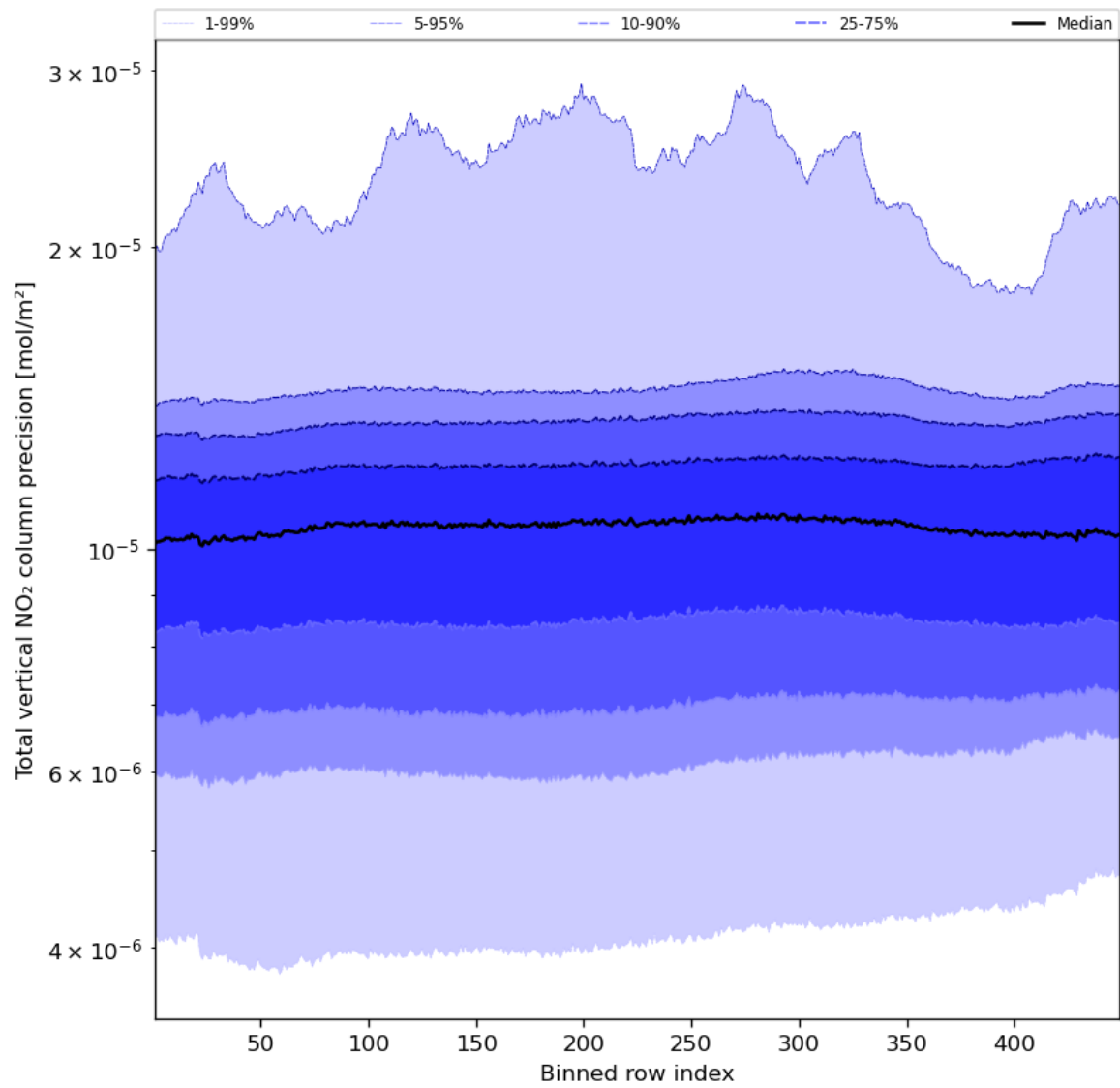
Figure 56: Along track statistics of “Total vertical NO 2 column precision” for 2024-02-28 to 2024-03-01
