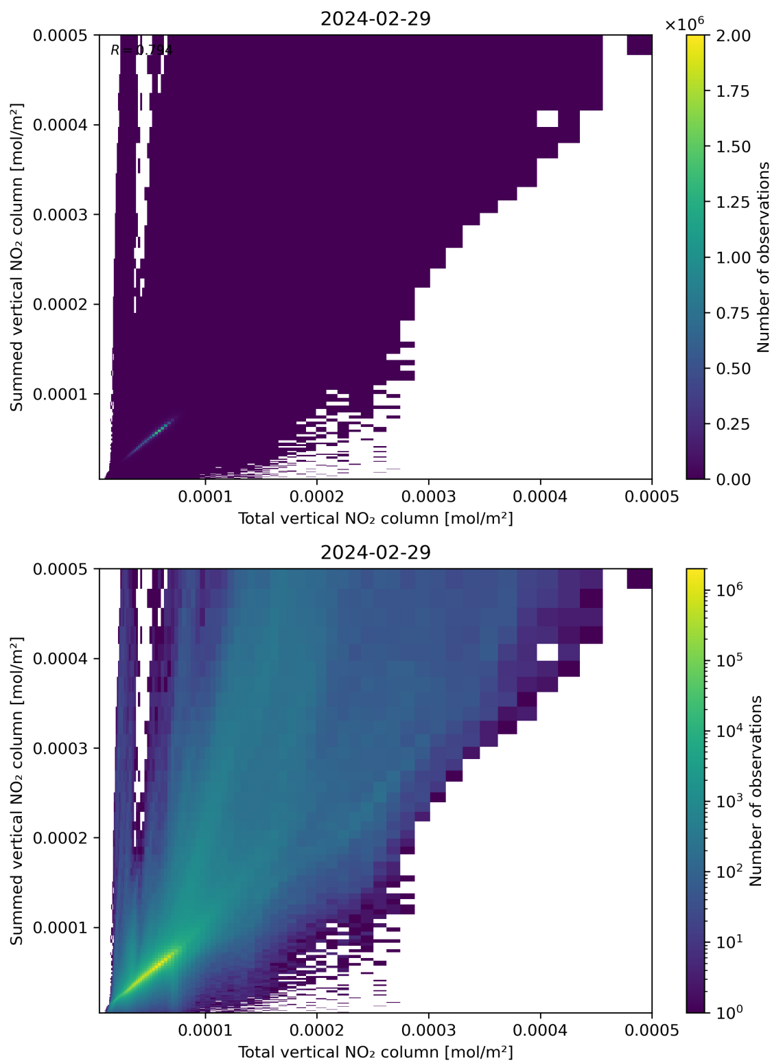
Figure 112: Scatter density plot of “Total vertical NO 2 column” against “Summed vertical NO 2 column” for 2024-02-28 to 2024-03-01.
