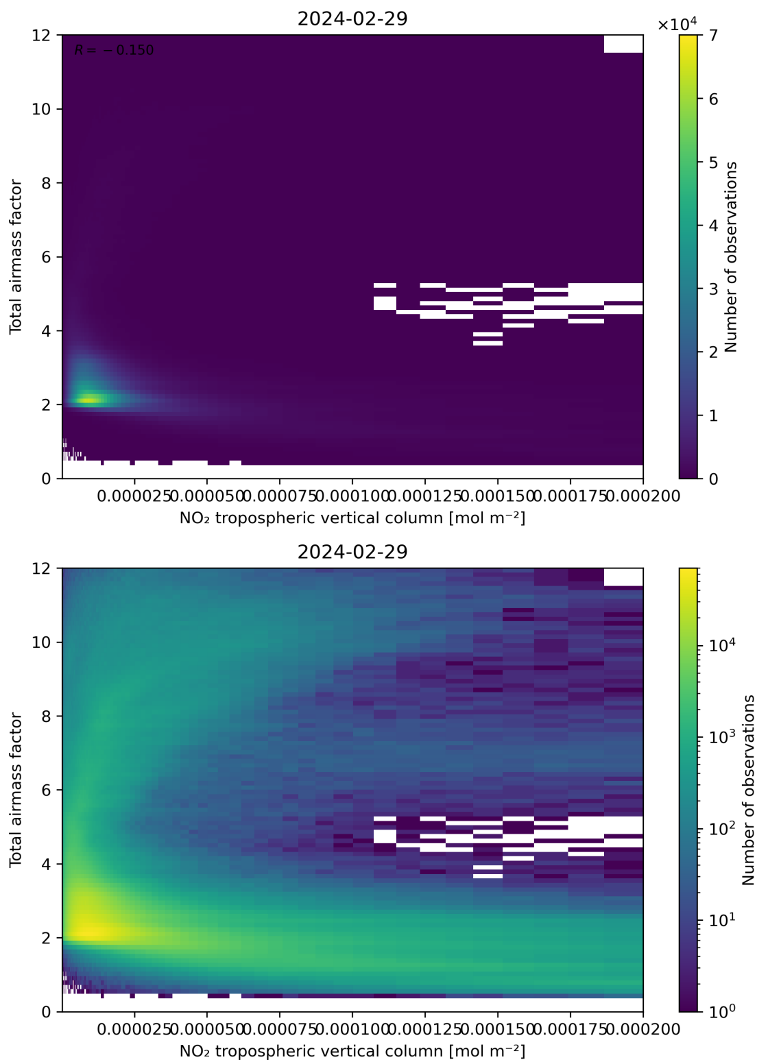
Figure 122: Scatter density plot of “NO 2 tropospheric vertical column” against “Total air mass factor” for 2024-02-28 to 2024-03-01.
