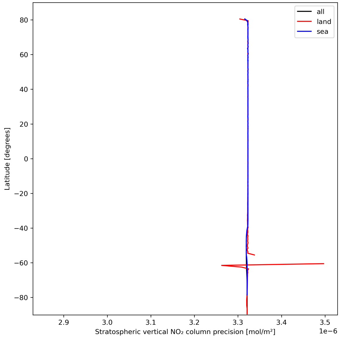
Figure 20: Zonal average of “Stratospheric vertical NO 2 column precision” for 2024-02-28 to 2024-03-01.
