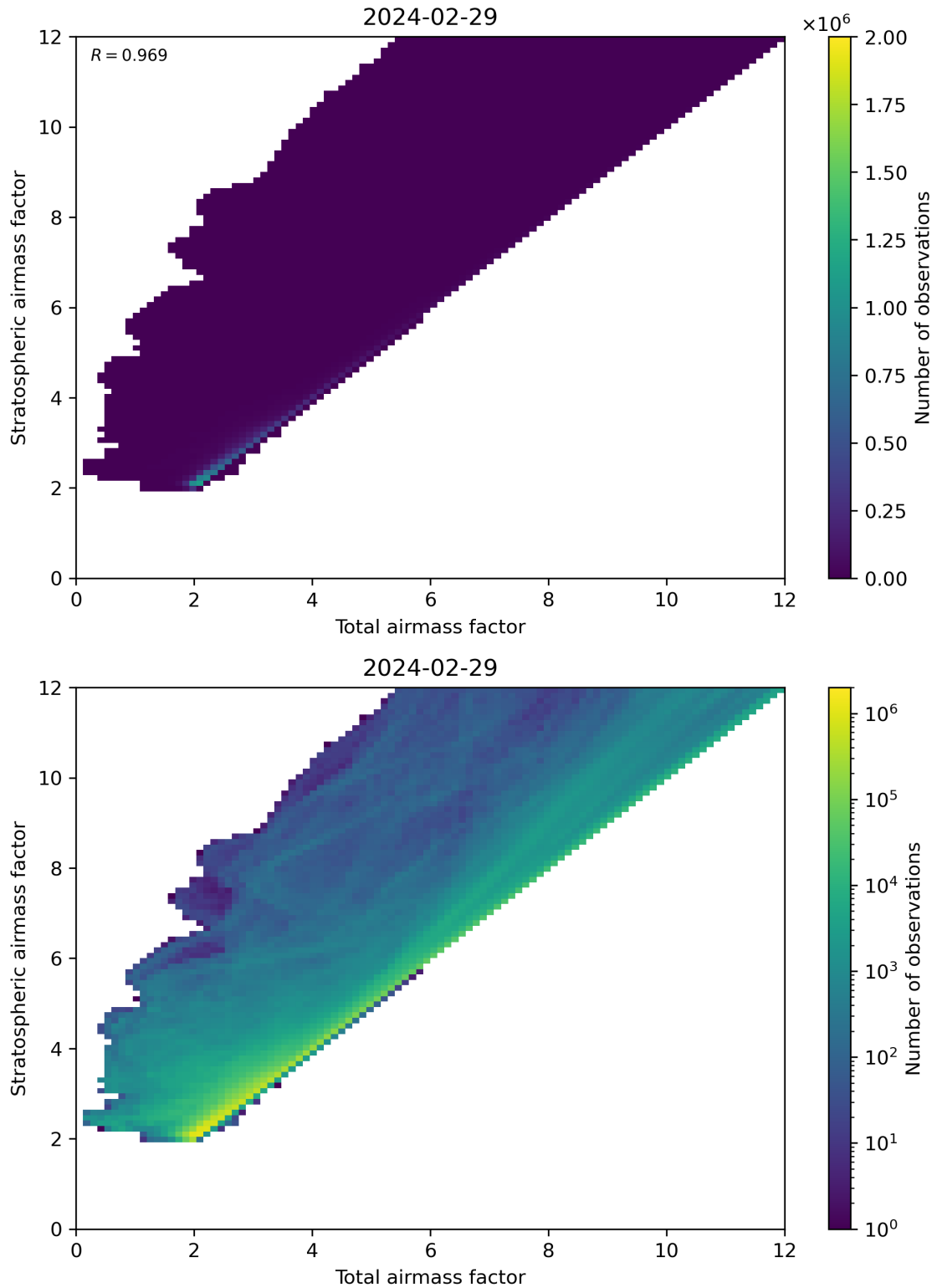
Figure 62: Scatter density plot of “Total airmass factor” against “Stratospheric airmass factor” for 2024-02-28 to 2024-03-01.
