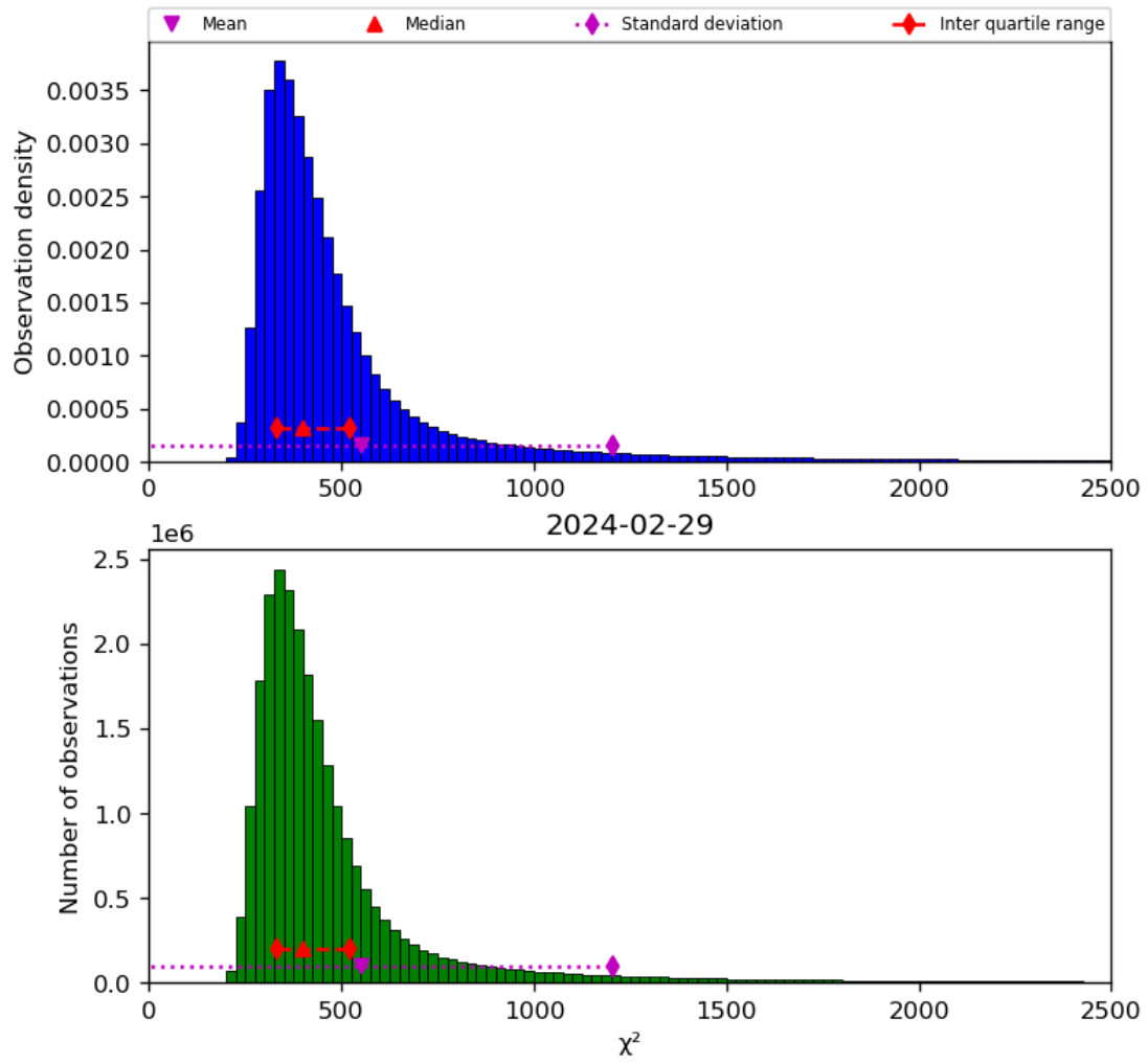
Figure 42: Histogram of “ \chi^2 ” for 2024-02-28 to 2024-03-01
