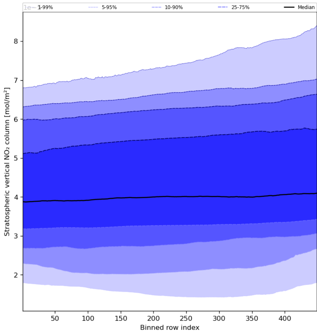
Figure 53: Along track statistics of “Stratospheric vertical NO 2 column” for 2024-02-28 to 2024-03-01
