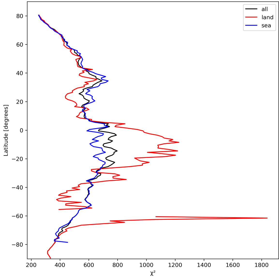
Figure 25: Zonal average of “ \chi^2 ” for 2024-02-28 to 2024-03-01.
