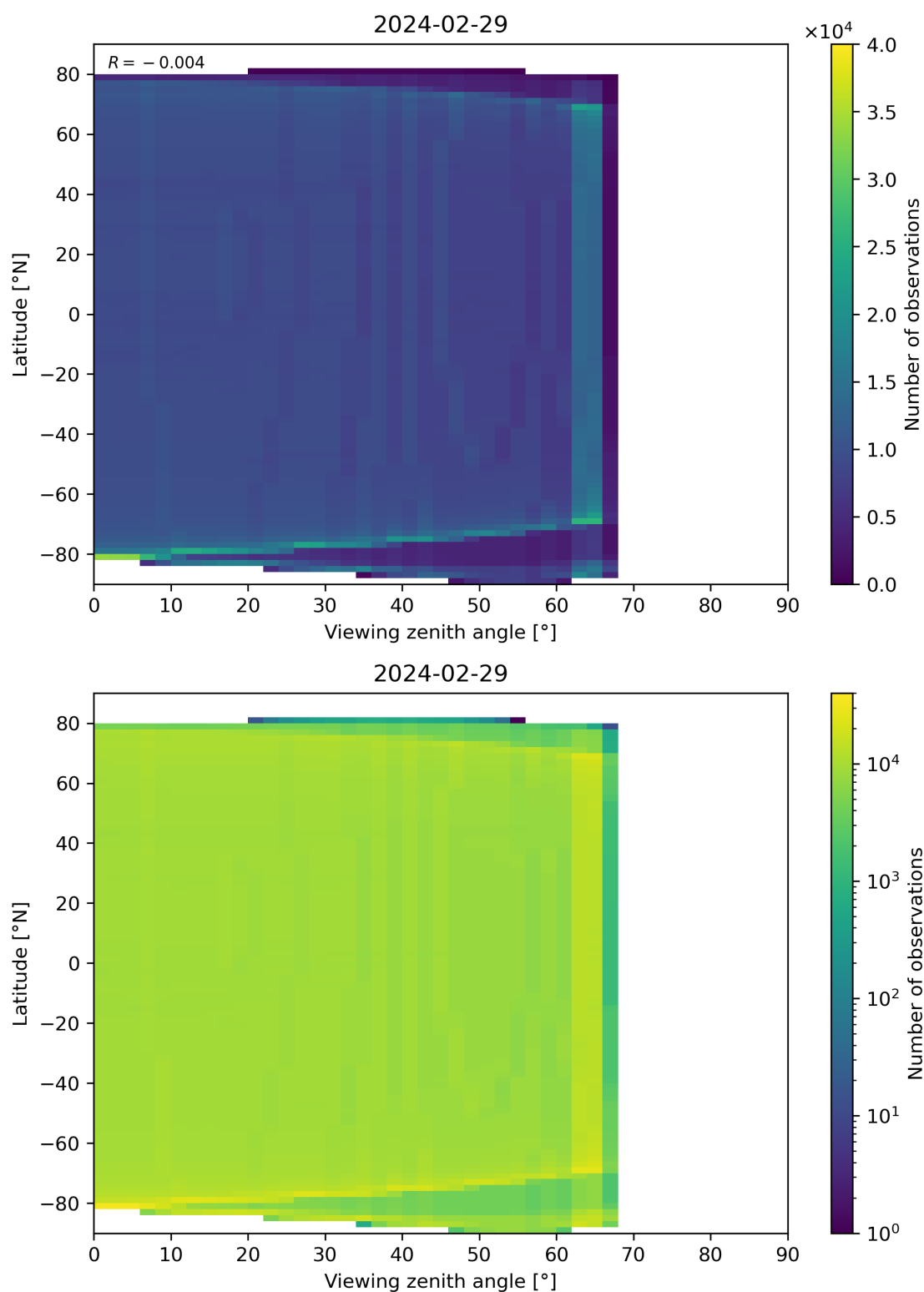
Figure 163: Scatter density plot of “Viewing zenith angle” against “Latitude” for 2024-02-28 to 2024-03-01.
