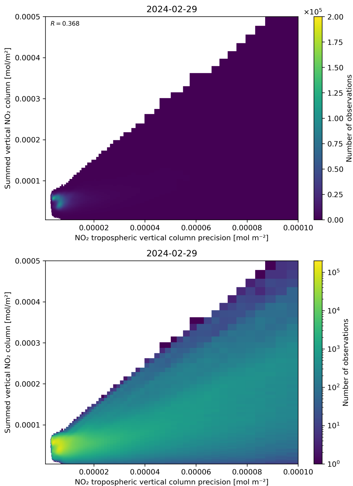
Figure 136: Scatter density plot of “NO 2 tropospheric vertical column precision” against “Summed vertical NO 2 column” for 2024-02-28 to 2024-03-01.
