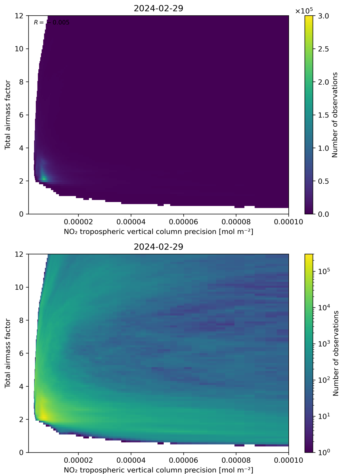
Figure 132: Scatter density plot of “NO 2 tropospheric vertical column precision” against “Total air mass factor” for 2024-02-28 to 2024-03-01.
