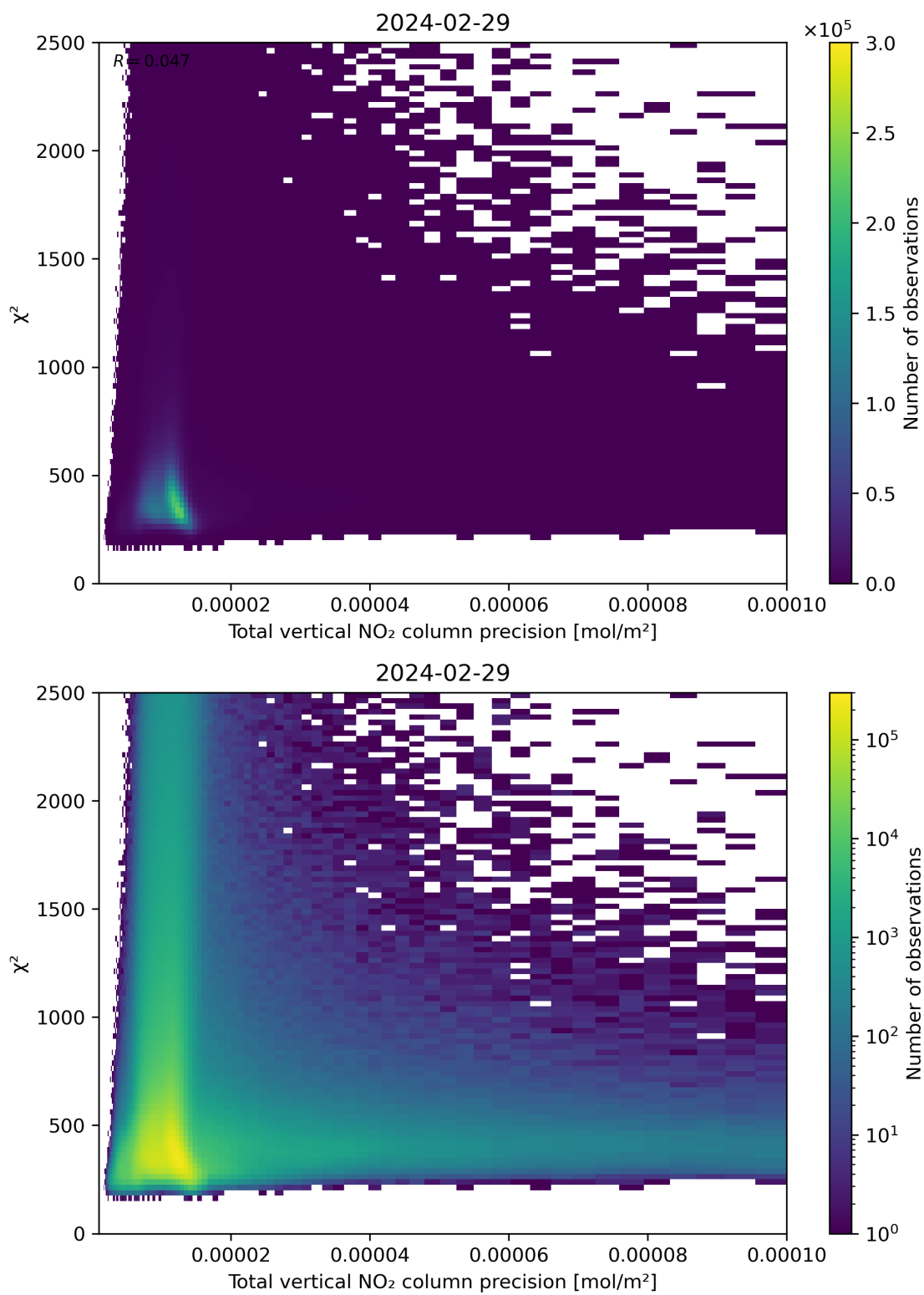
Figure 116: Scatter density plot of “Total vertical NO 2 column precision” against “ \chi^2 ” for 2024-02-28 to 2024-03-01.
