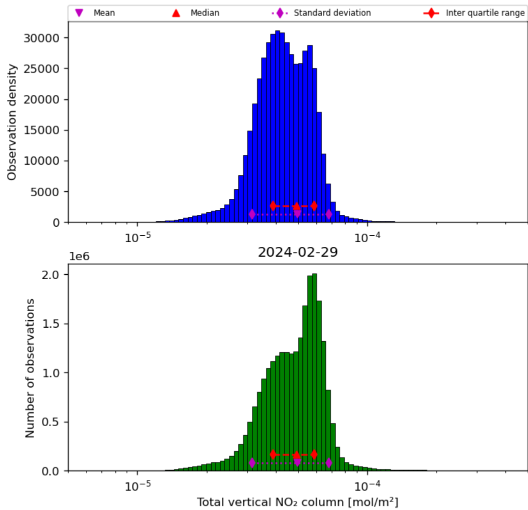
Figure 38: Histogram of “Total vertical NO 2 column” for 2024-02-28 to 2024-03-01
