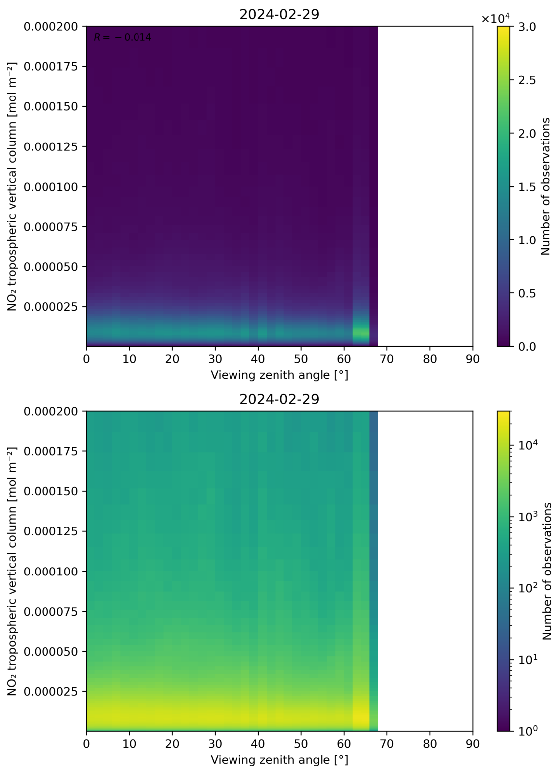
Figure 169: Scatter density plot of “Viewing zenith angle” against “NO 2 tropospheric vertical column” for 2024-02-28 to 2024-03-01.
