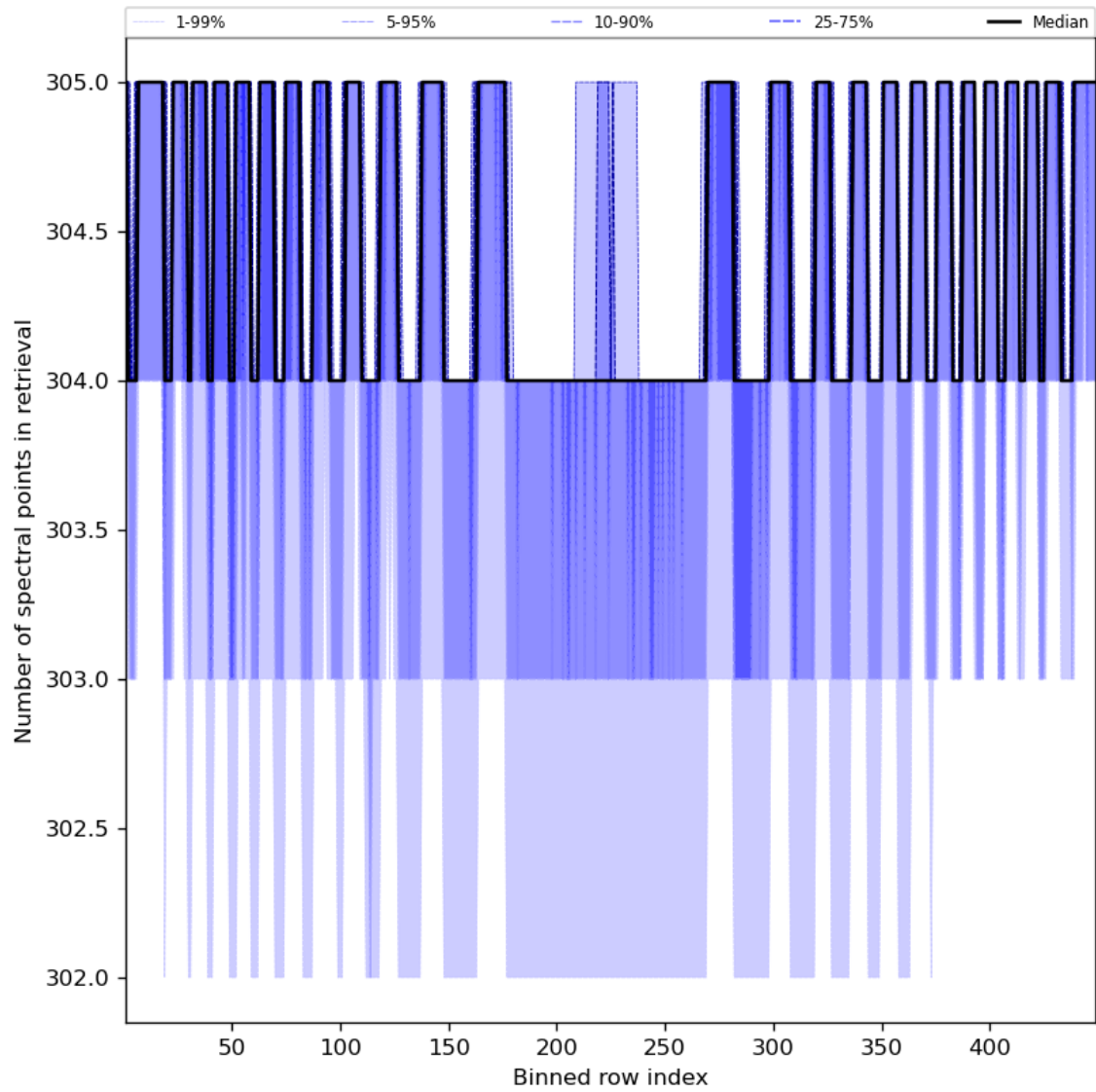
Figure 50: Along track statistics of “Number of spectral points in retrieval” for 2024-02-28 to 2024-03-01
