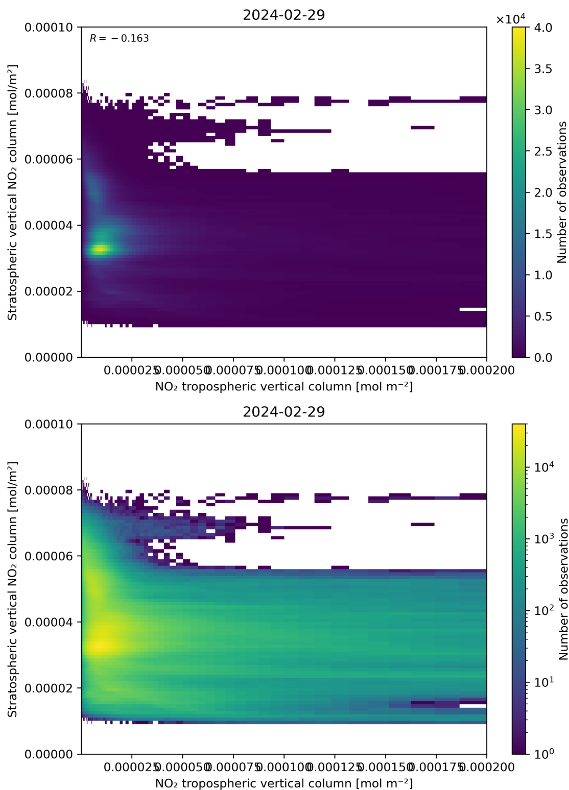
Figure 125: Scatter density plot of “NO 2 tropospheric vertical column” against “Stratospheric vertical NO 2 column” for 2024-02-28 to 2024-03-01.
