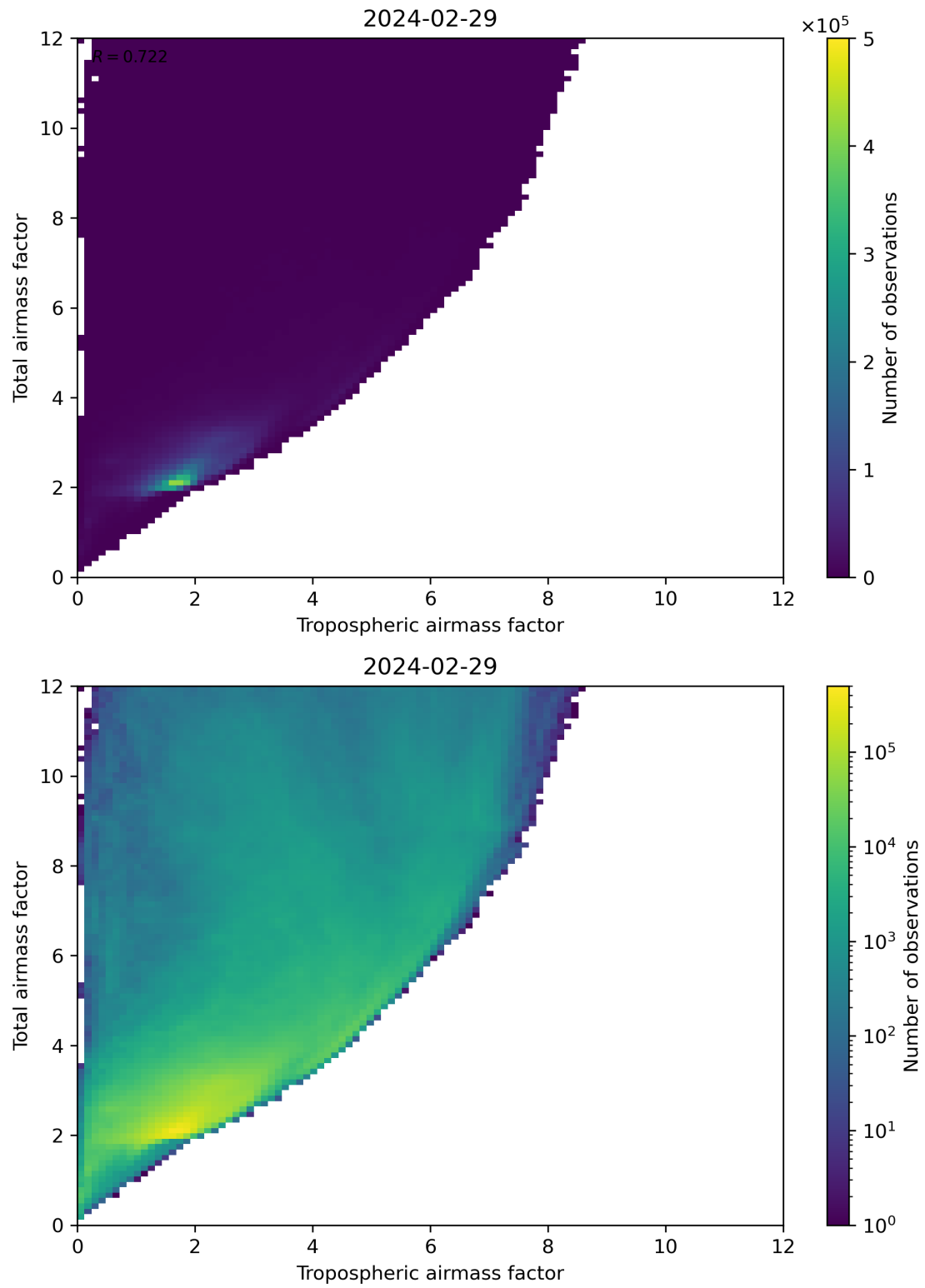
Figure 72: Scatter density plot of “Tropospheric airmass factor” against “Total airmass factor” for 2024-02-28 to 2024-03-01.
