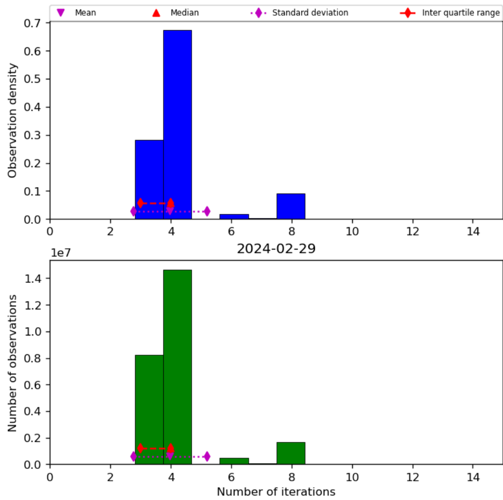
Figure 34: Histogram of “Number of iterations” for 2024-02-28 to 2024-03-01
