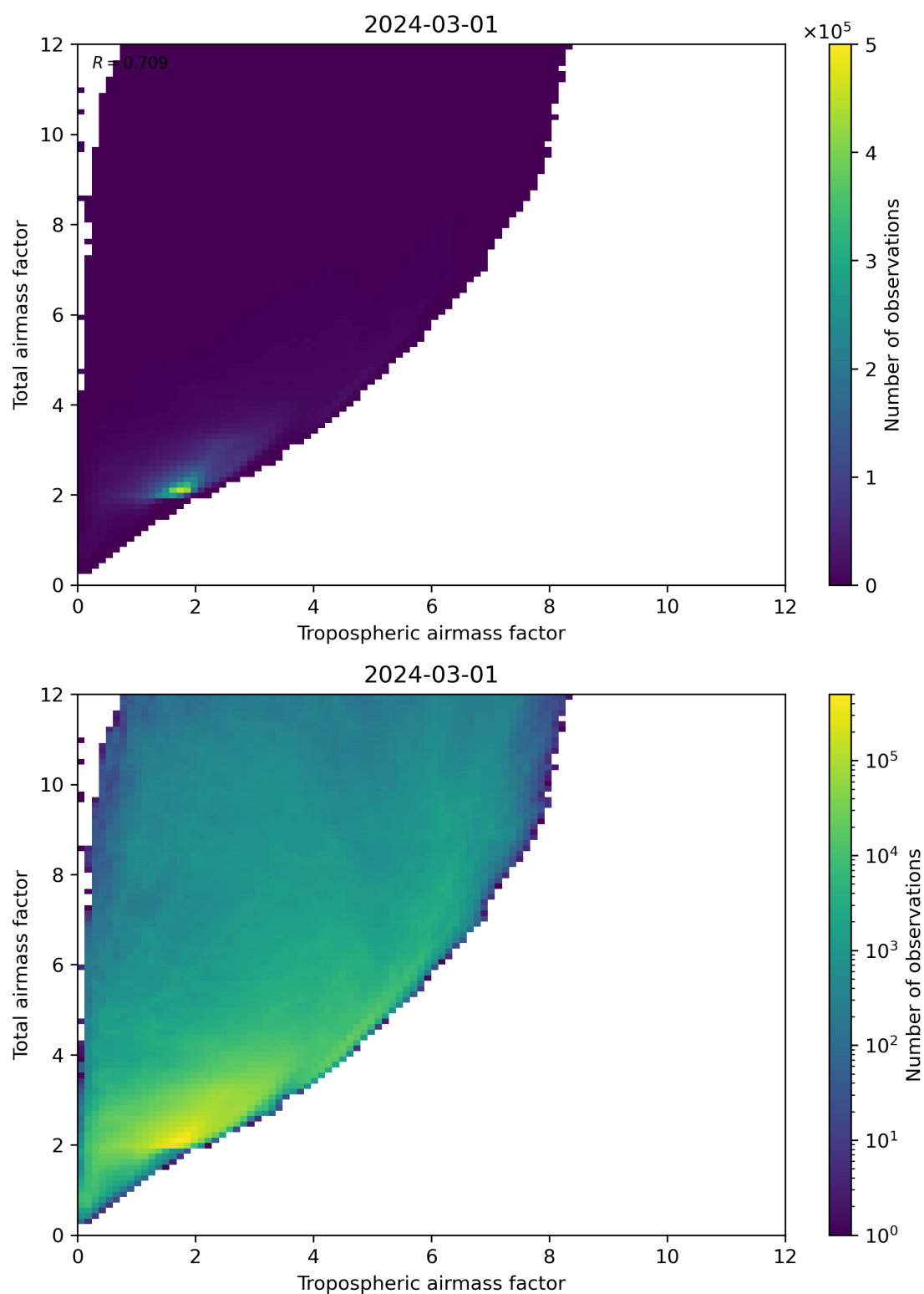
Figure 72: Scatter density plot of “Tropospheric airmass factor” against “Total airmass factor” for 2024-02-29 to 2024-03-02.
