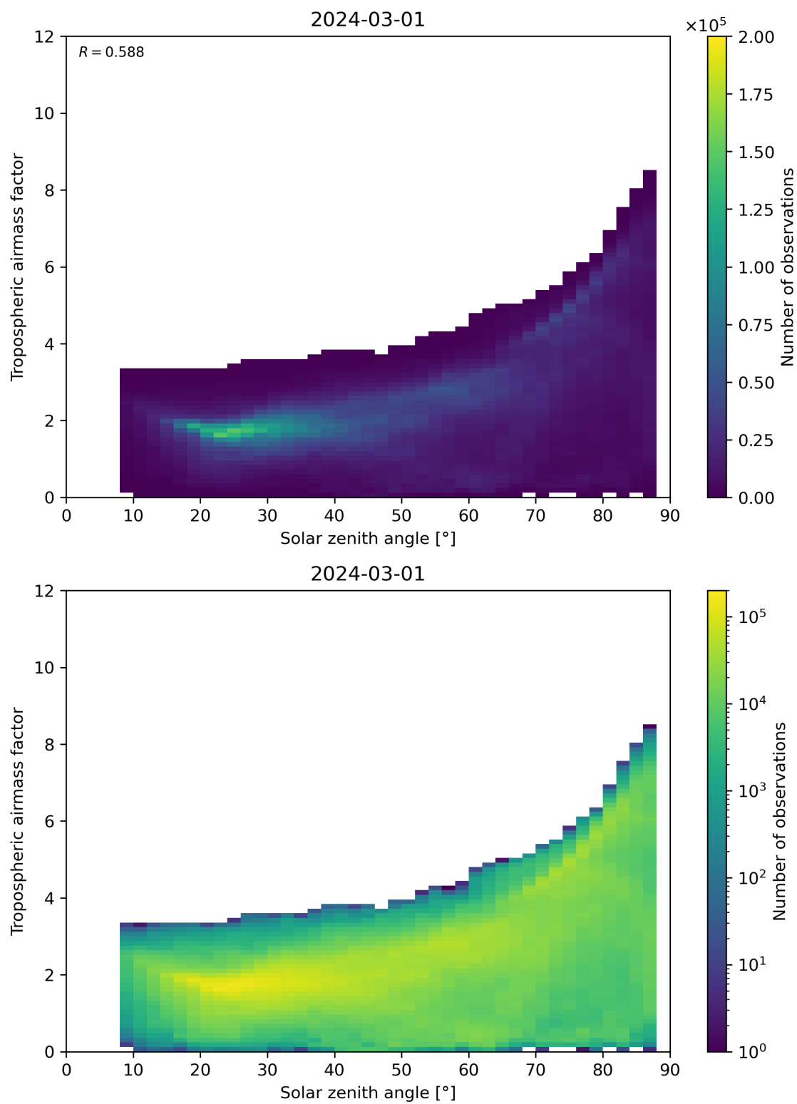
Figure 147: Scatter density plot of “Solar zenith angle” against “Tropospheric airmass factor” for 2024-02-29 to 2024-03-02.
