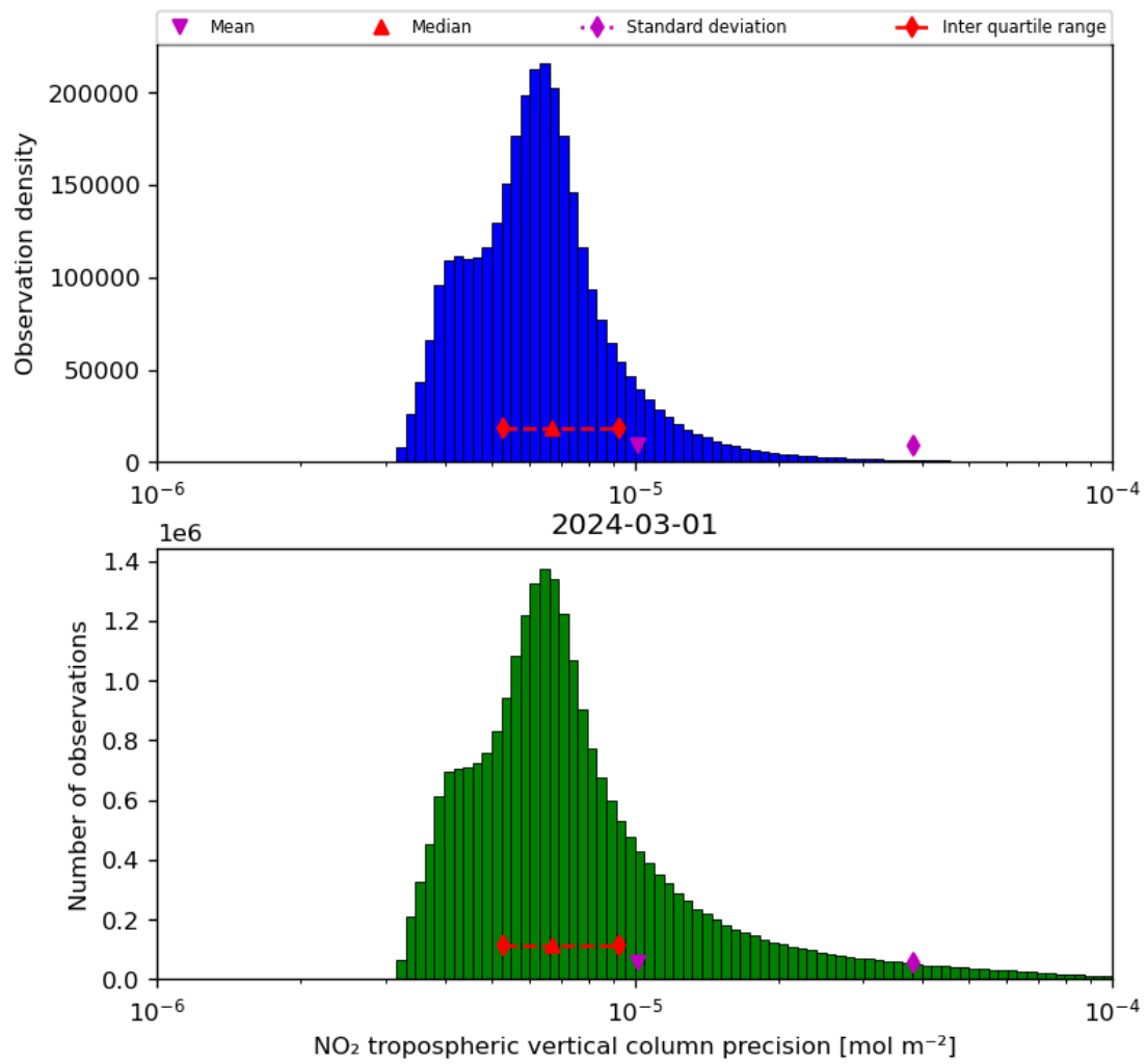
Figure 30: Histogram of “NO 2 tropospheric vertical column precision” for 2024-02-29 to 2024-03-02
