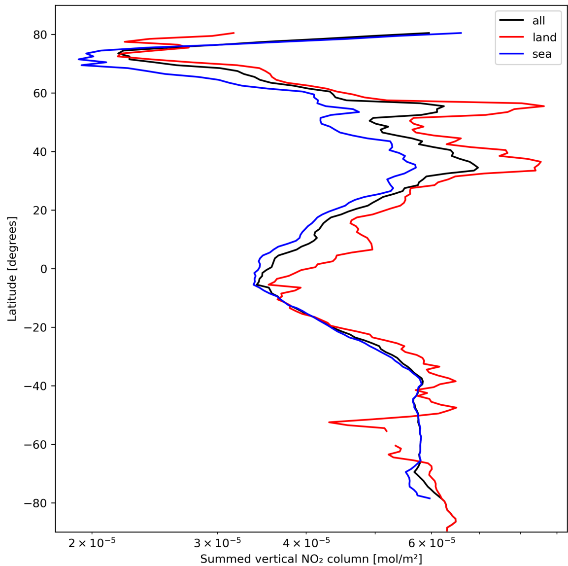
Figure 23: Zonal average of “Summed vertical NO 2 column” for 2024-02-29 to 2024-03-02.
