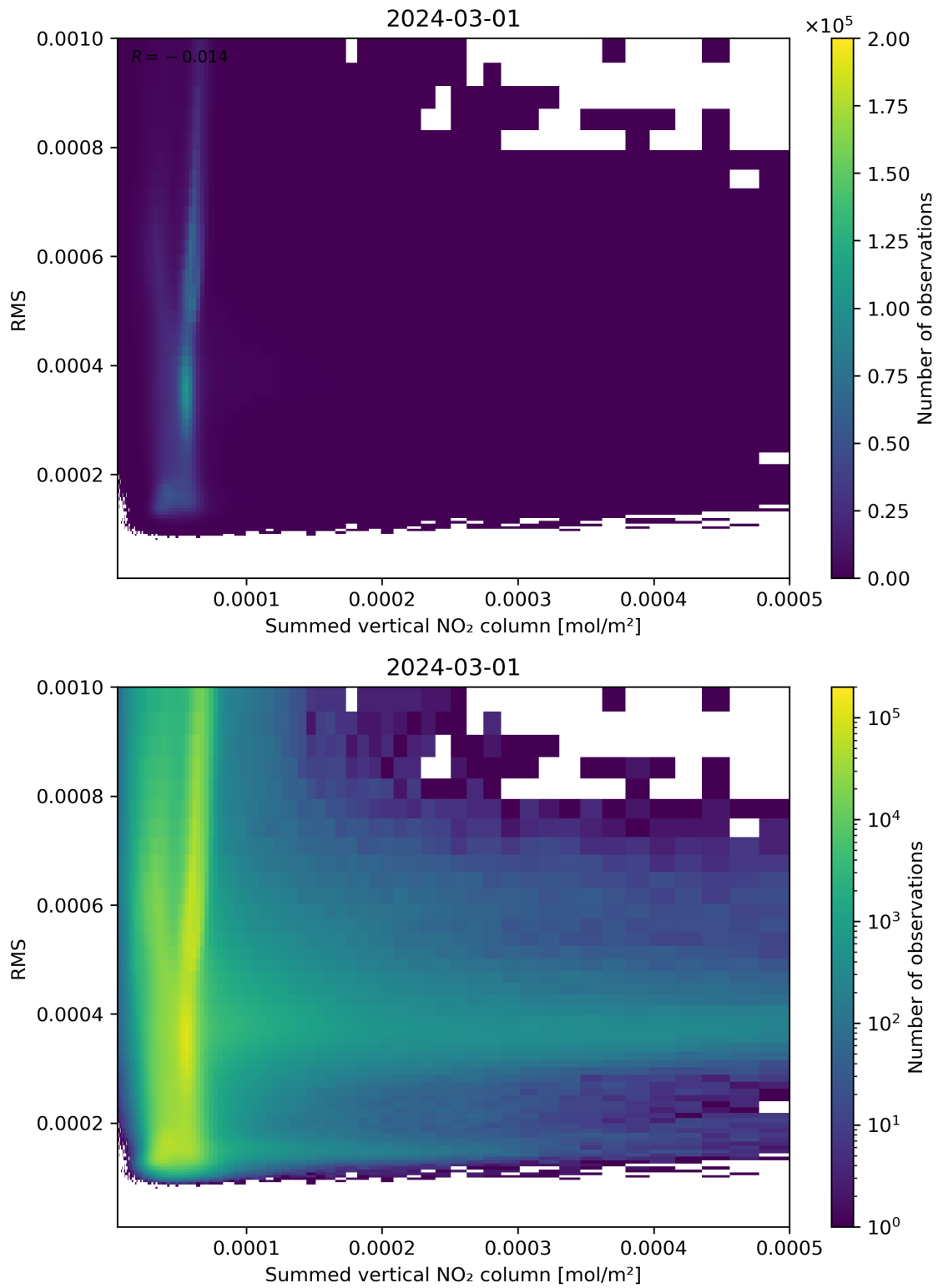
Figure 109: Scatter density plot of “Summed vertical NO 2 column” against “RMS” for 2024-02-29 to 2024-03-02.
