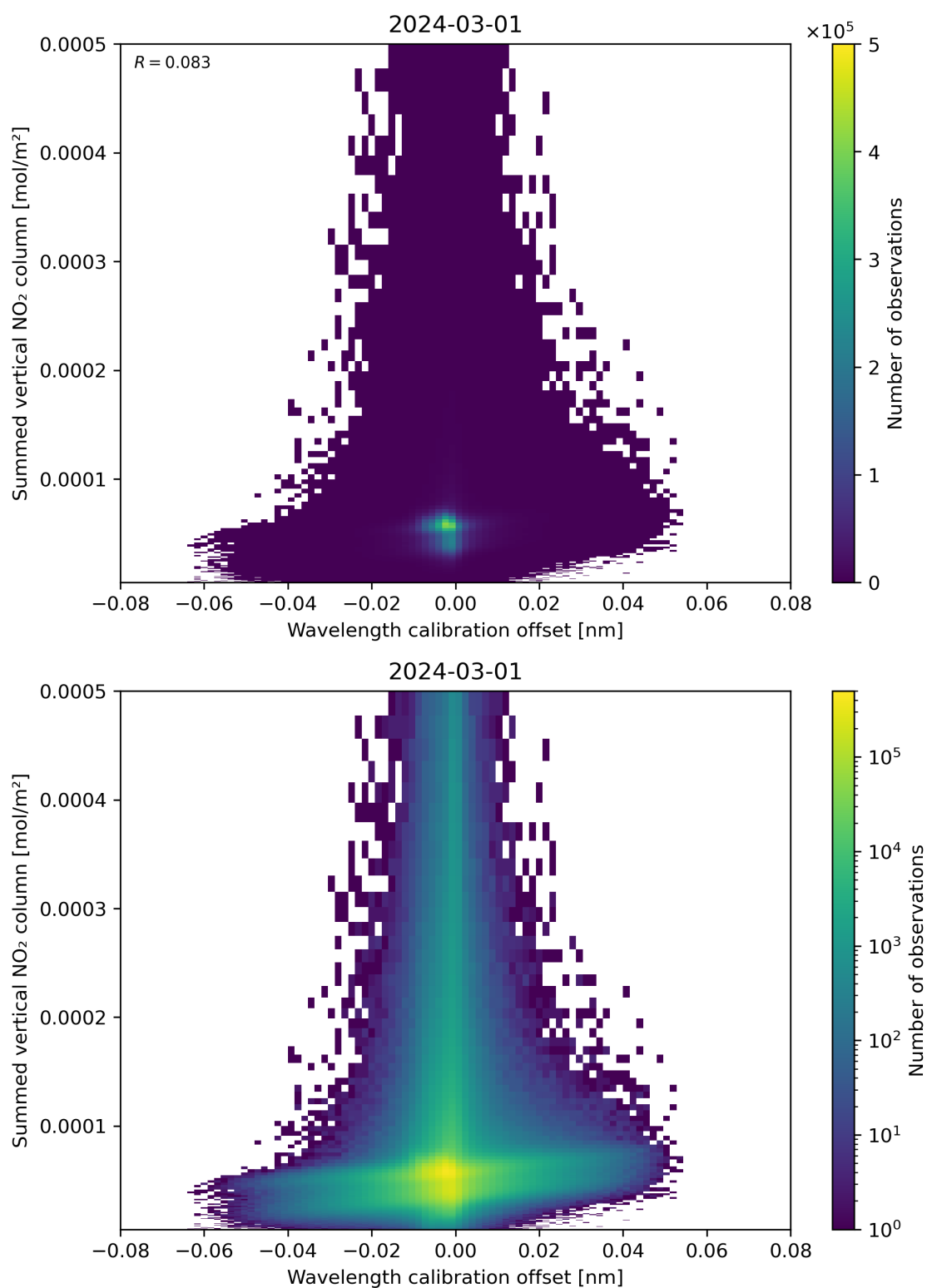
Figure 177: Scatter density plot of “Wavelength calibration offset” against “Summed vertical NO 2 column” for 2024-02-29 to 2024-03-02.
