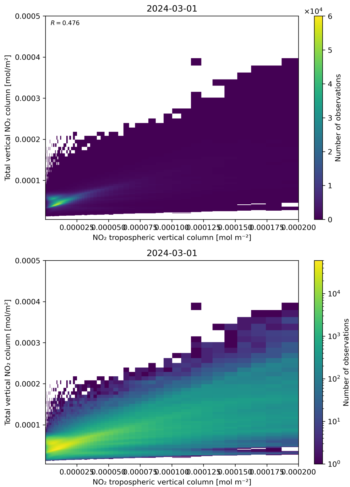
Figure 128: Scatter density plot of “NO 2 tropospheric vertical column” against “Total vertical NO 2 column” for 2024-02-29 to 2024-03-02.
