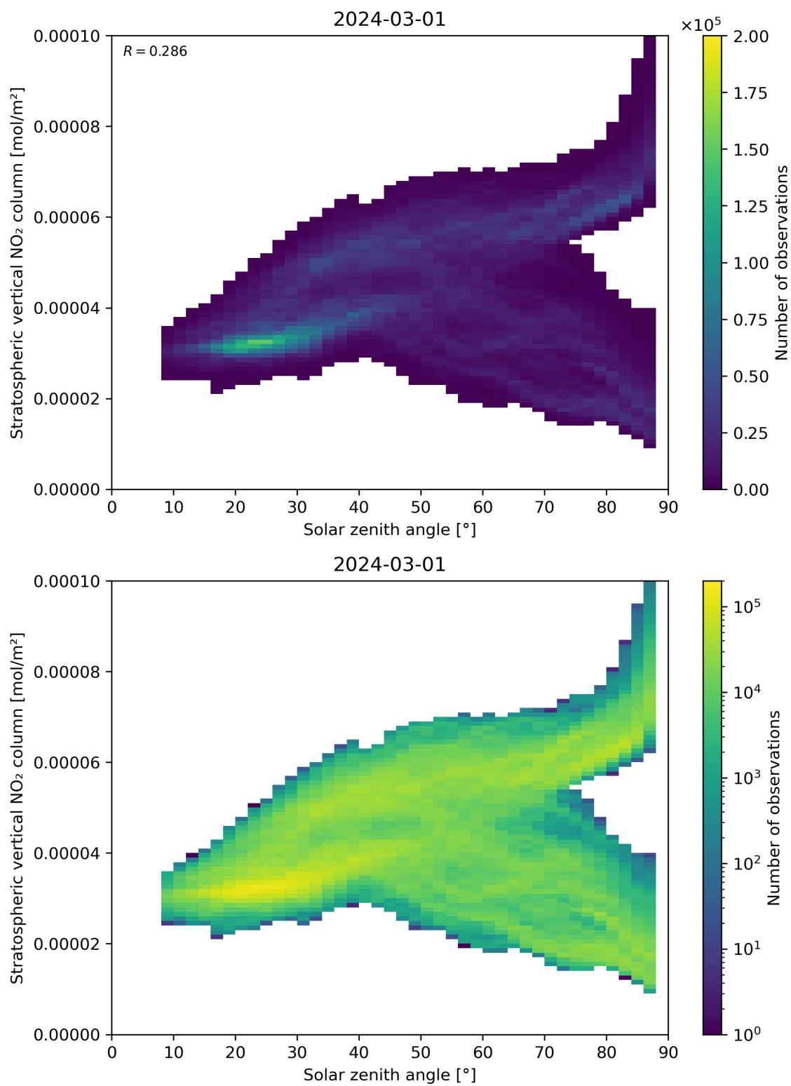
Figure 150: Scatter density plot of “Solar zenith angle” against “Stratospheric vertical NO 2 column” for 2024-02-29 to 2024-03-02.
