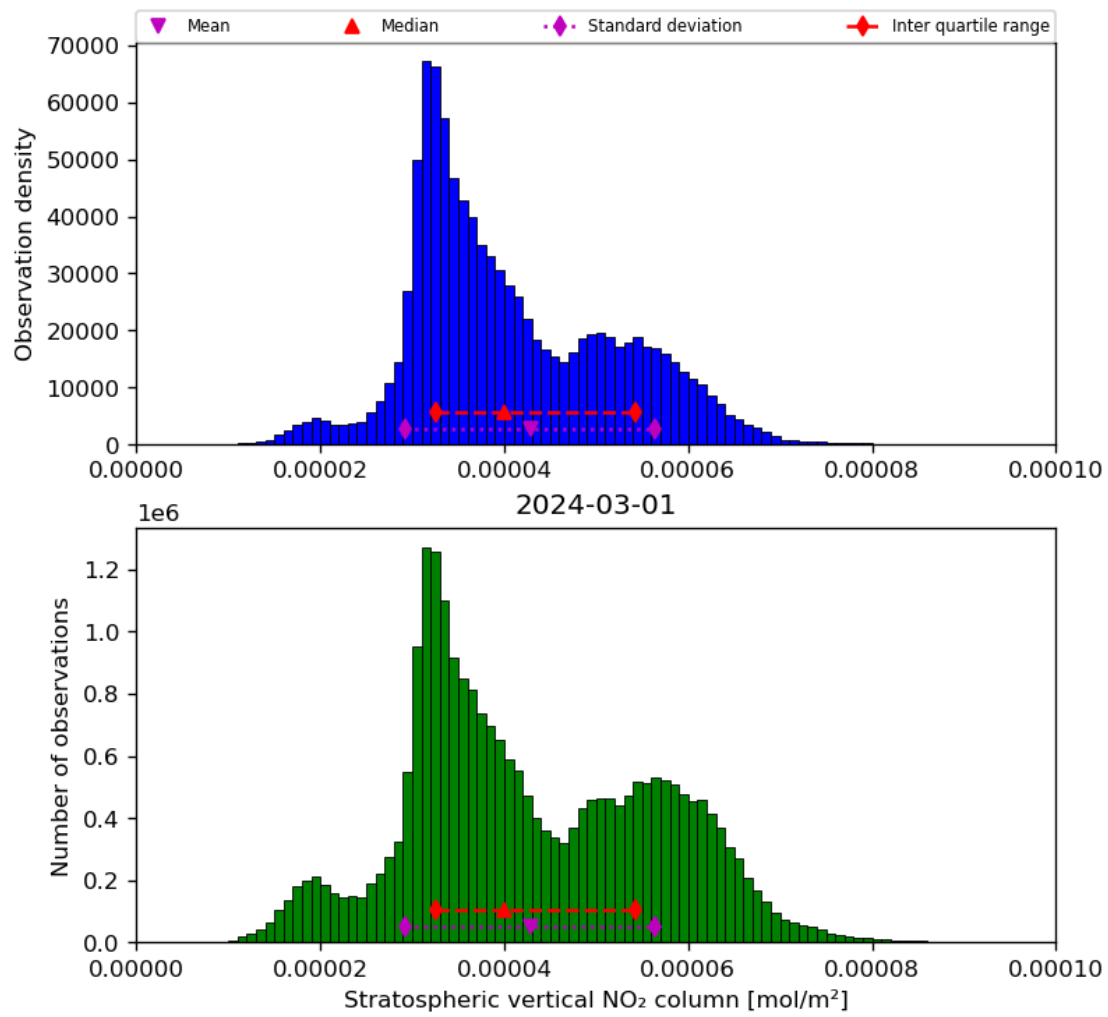
Figure 36: Histogram of “Stratospheric vertical NO 2 column” for 2024-02-29 to 2024-03-02
