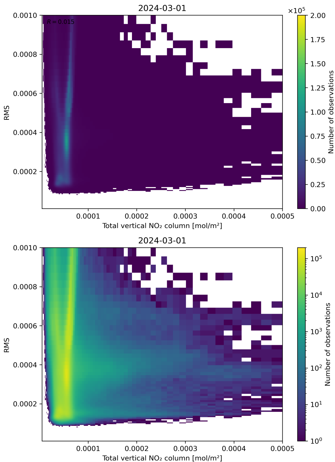
Figure 120: Scatter density plot of “Total vertical NO 2 column” against “RMS” for 2024-02-29 to 2024-03-02.
