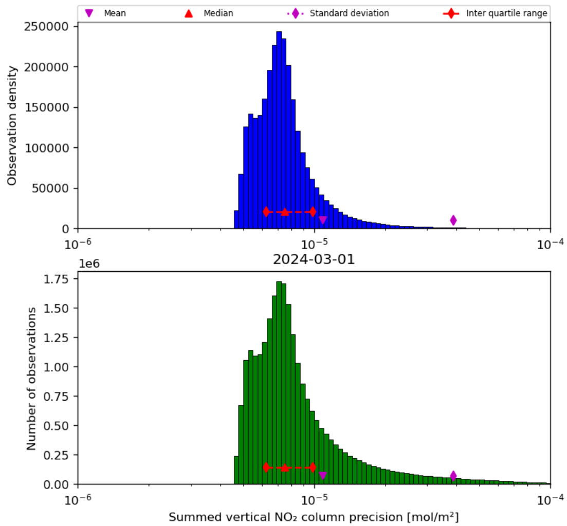
Figure 41: Histogram of “Summed vertical NO 2 column precision” for 2024-02-29 to 2024-03-02
