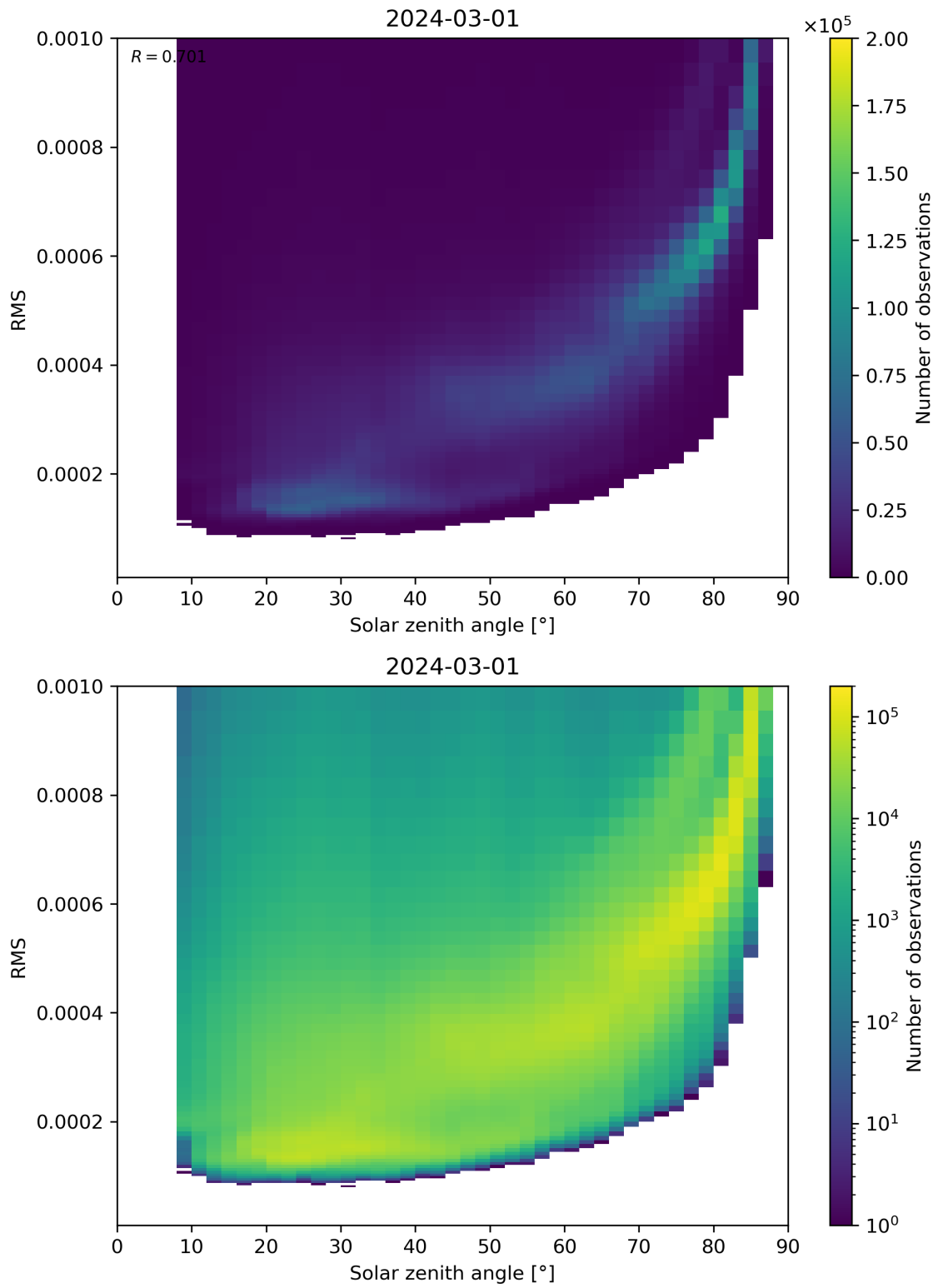
Figure 157: Scatter density plot of “Solar zenith angle” against “RMS” for 2024-02-29 to 2024-03-02.
