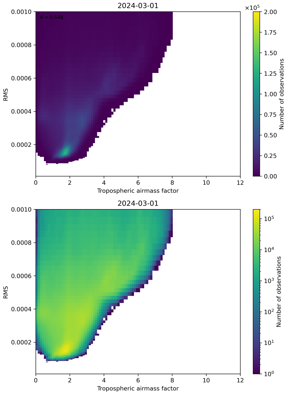
Figure 79: Scatter density plot of “Tropospheric airmass factor” against “RMS” for 2024-02-29 to 2024-03-02.
