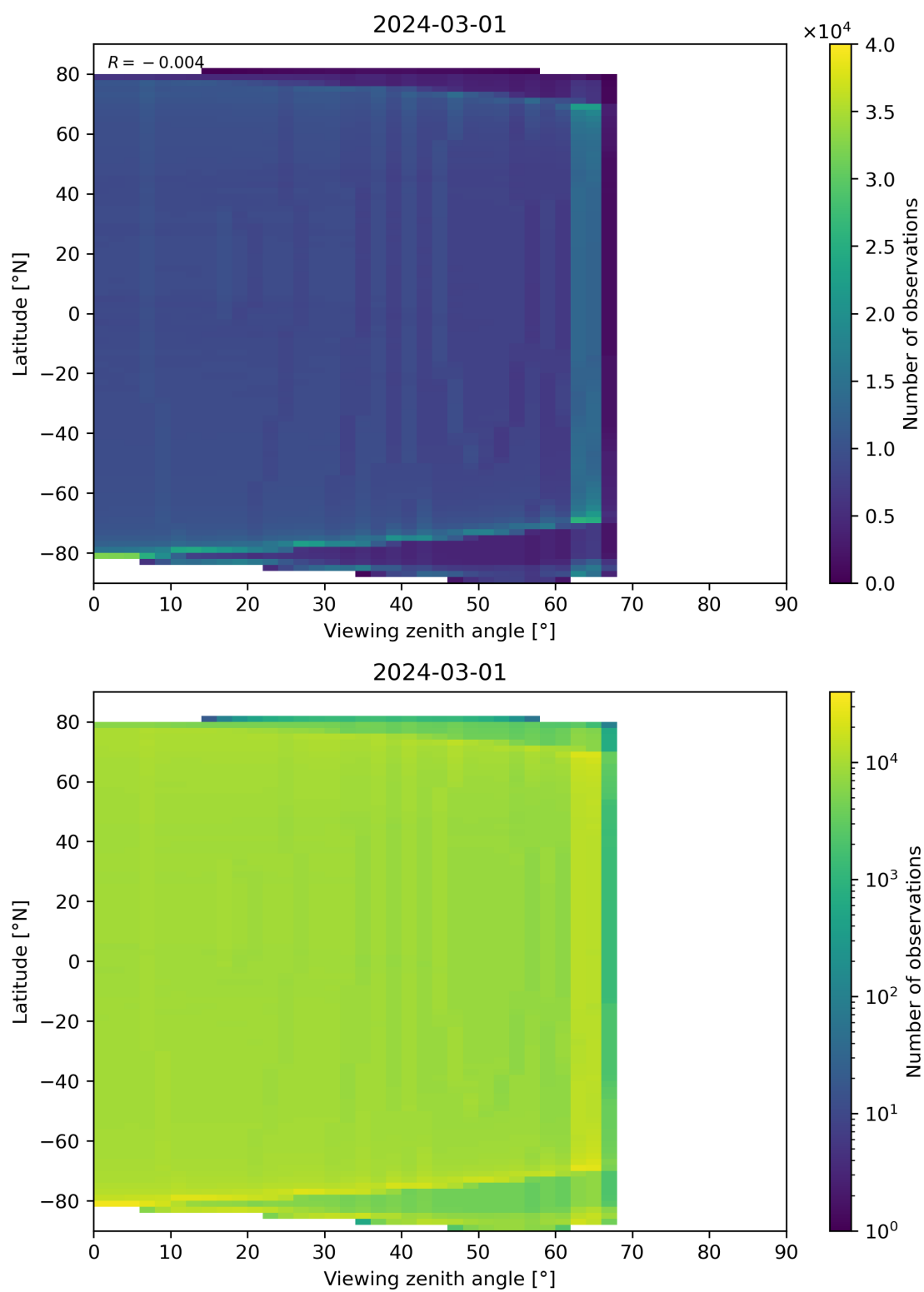
Figure 163: Scatter density plot of “Viewing zenith angle” against “Latitude” for 2024-02-29 to 2024-03-02.
