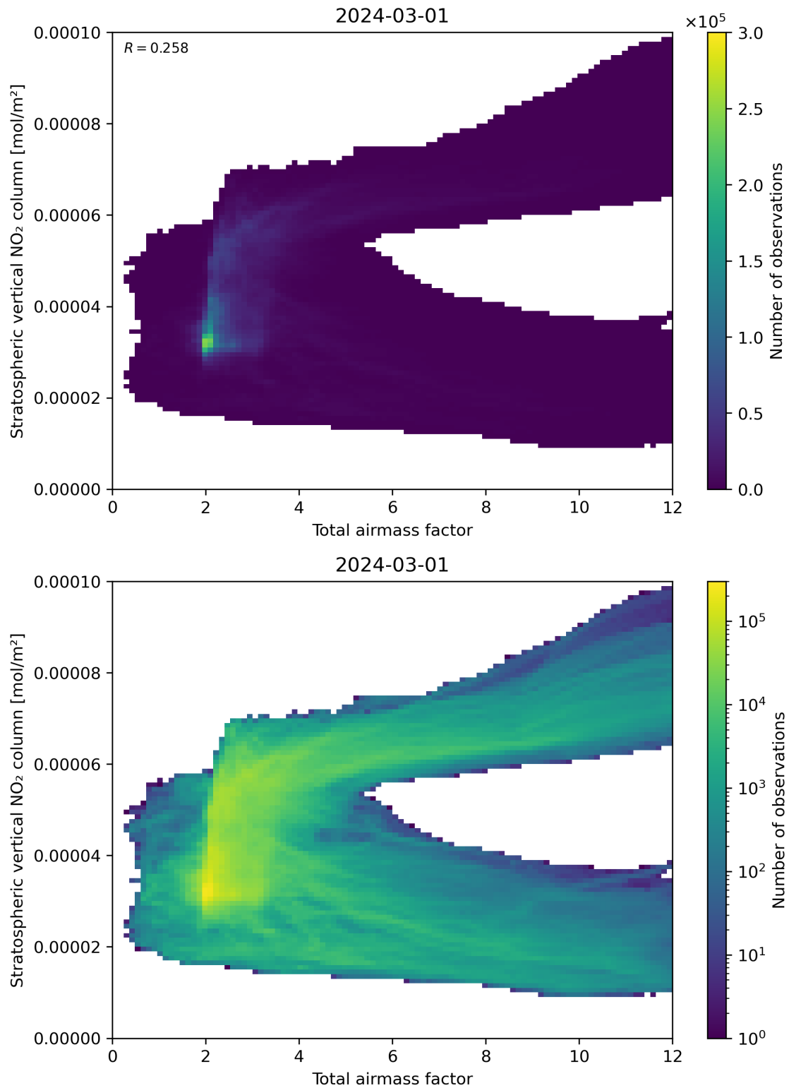
Figure 64: Scatter density plot of “Total airmass factor” against “Stratospheric vertical NO 2 column” for 2024-02-29 to 2024-03-02.
