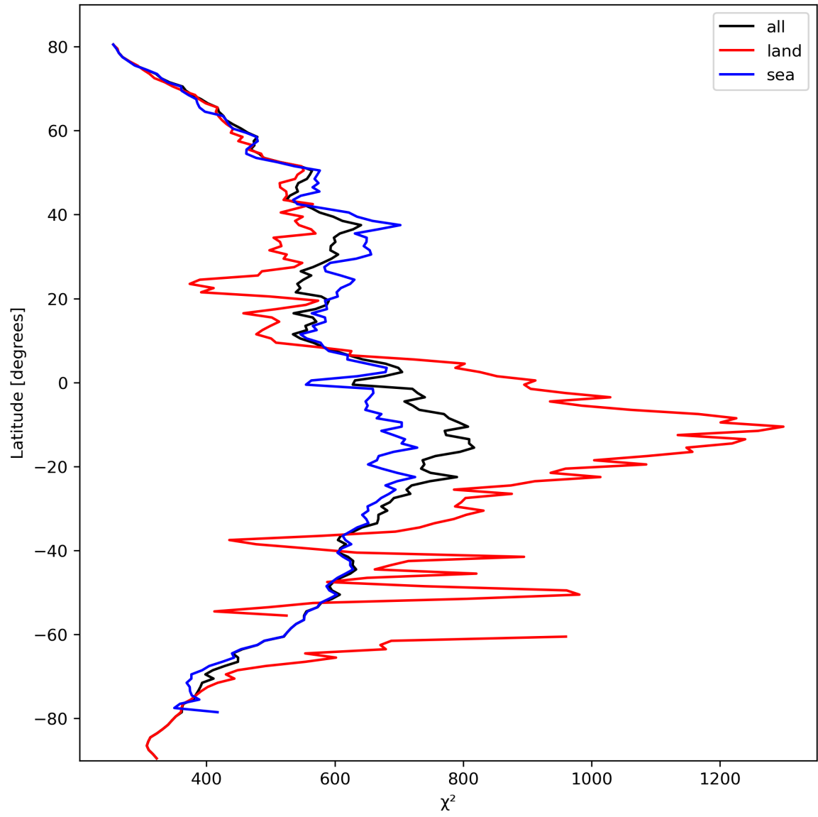
Figure 25: Zonal average of “ \chi^2 ” for 2024-02-29 to 2024-03-02.
