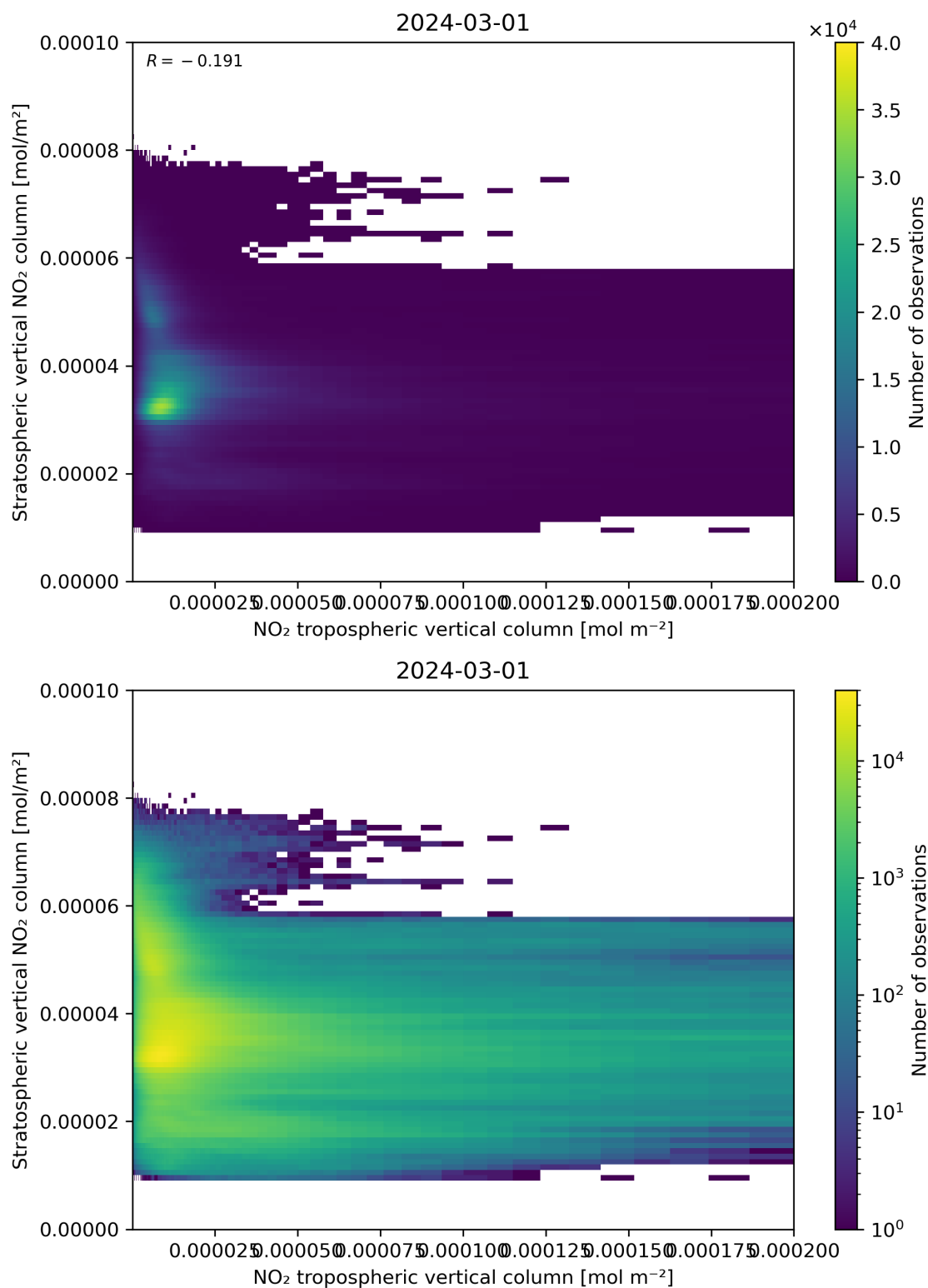
Figure 125: Scatter density plot of “NO 2 tropospheric vertical column” against “Stratospheric vertical NO 2 column” for 2024-02-29 to 2024-03-02.
