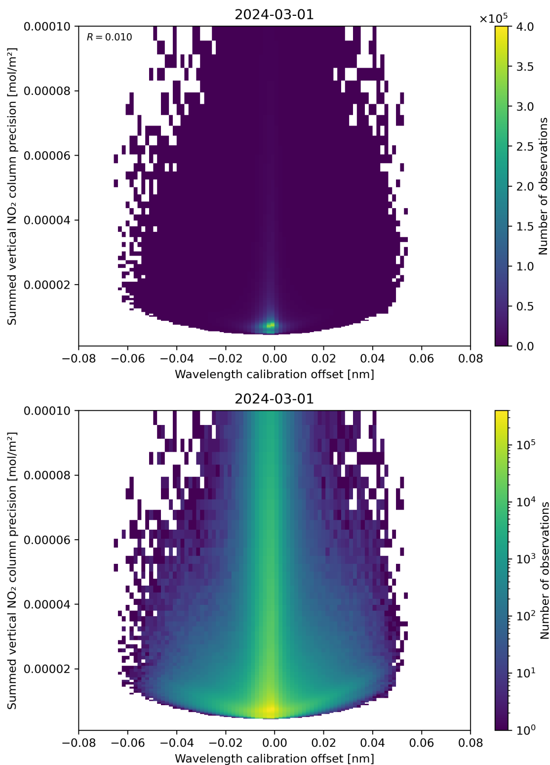
Figure 178: Scatter density plot of “Wavelength calibration offset” against “Summed vertical NO 2 column precision” for 2024-02-29 to 2024-03-02.
