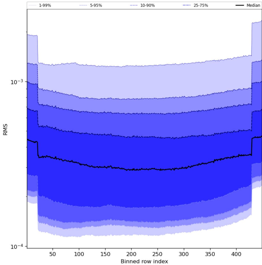
Figure 60: Along track statistics of “RMS” for 2024-02-29 to 2024-03-02
