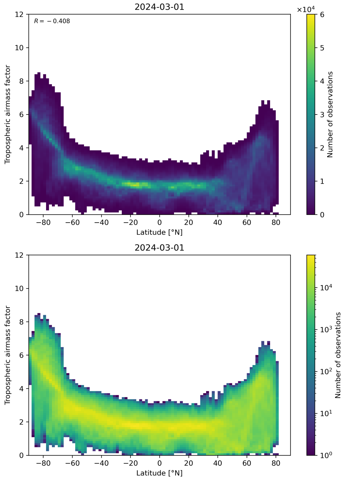
Figure 85: Scatter density plot of “Latitude” against “Tropospheric airmass factor” for 2024-02-29 to 2024-03-02.
