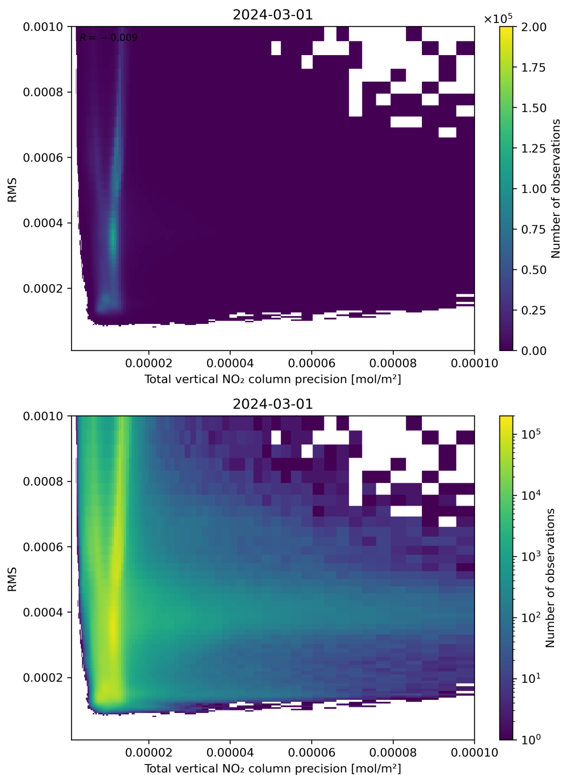
Figure 119: Scatter density plot of “Total vertical NO 2 column precision” against “RMS” for 2024-02-29 to 2024-03-02.
