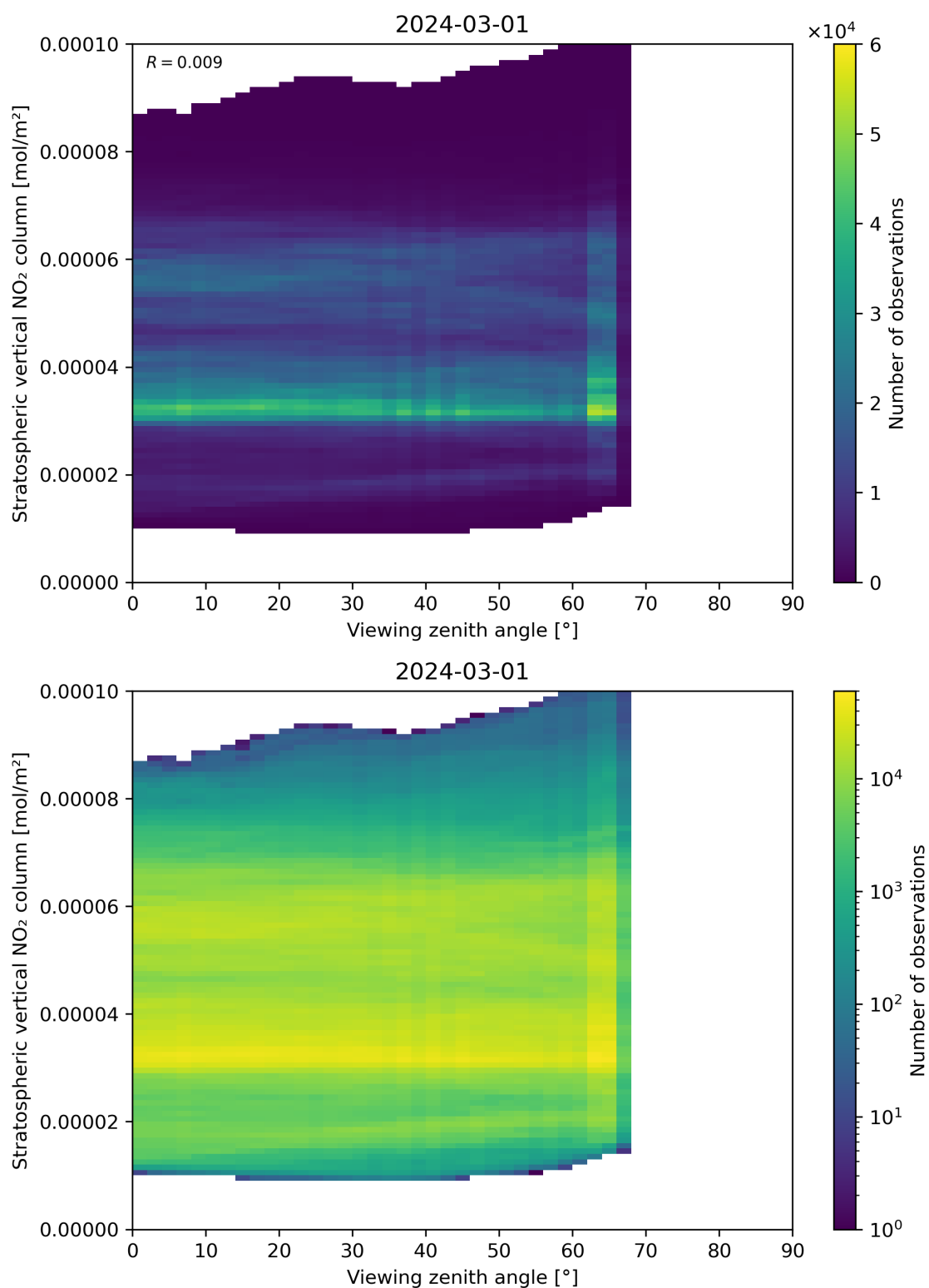
Figure 164: Scatter density plot of “Viewing zenith angle” against “Stratospheric vertical NO 2 column” for 2024-02-29 to 2024-03-02.
