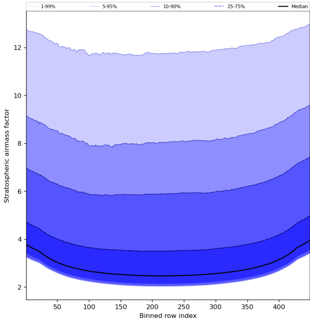
Figure 61: Along track statistics of “Stratospheric airmass factor” for 2024-02-29 to 2024-03-02
