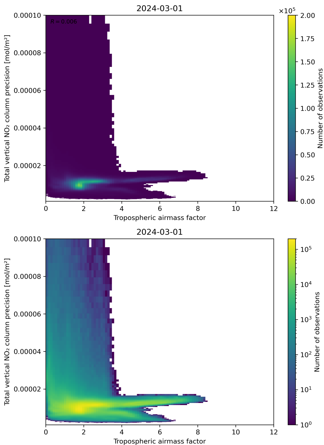
Figure 78: Scatter density plot of “Tropospheric air mass factor” against “Total vertical NO 2 column precision” for 2024-02-29 to 2024-03-02.
