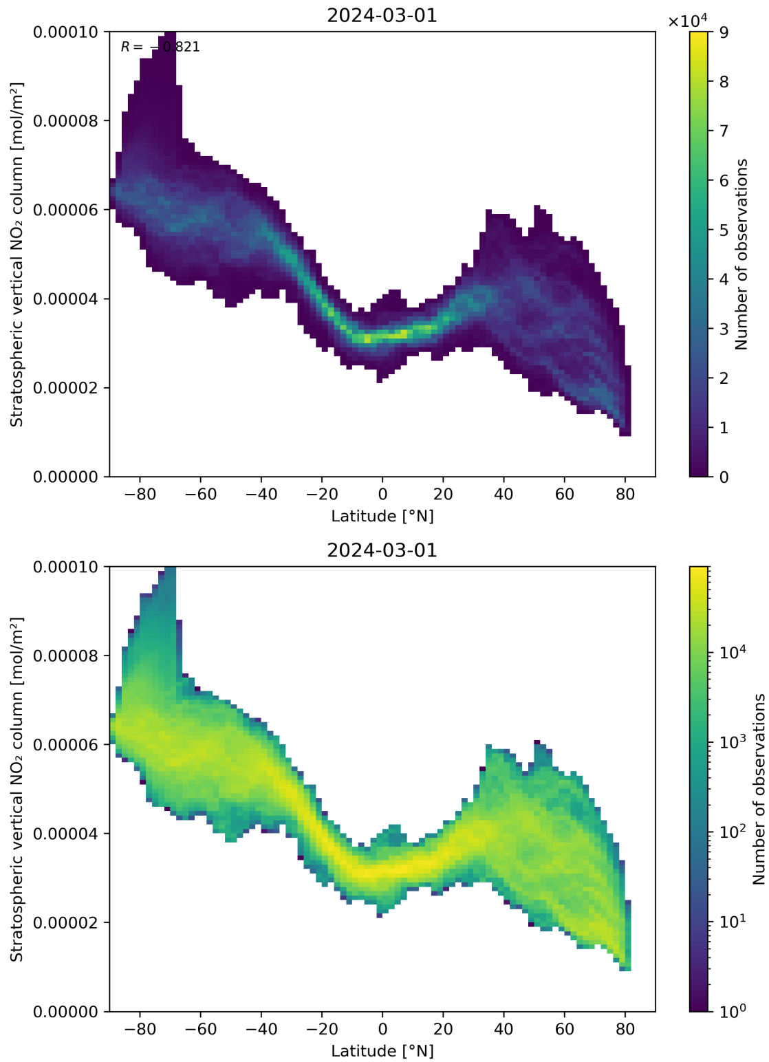
Figure 87: Scatter density plot of “Latitude” against “Stratospheric vertical NO 2 column” for 2024-02-29 to 2024-03-02.
