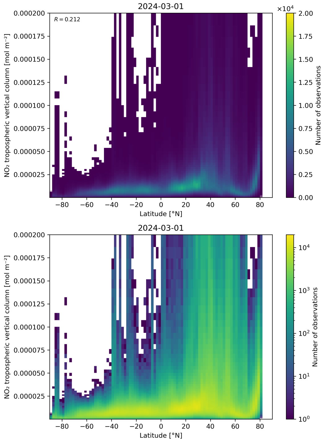
Figure 92: Scatter density plot of “Latitude” against “NO 2 tropospheric vertical column” for 2024-02-29 to 2024-03-02.
