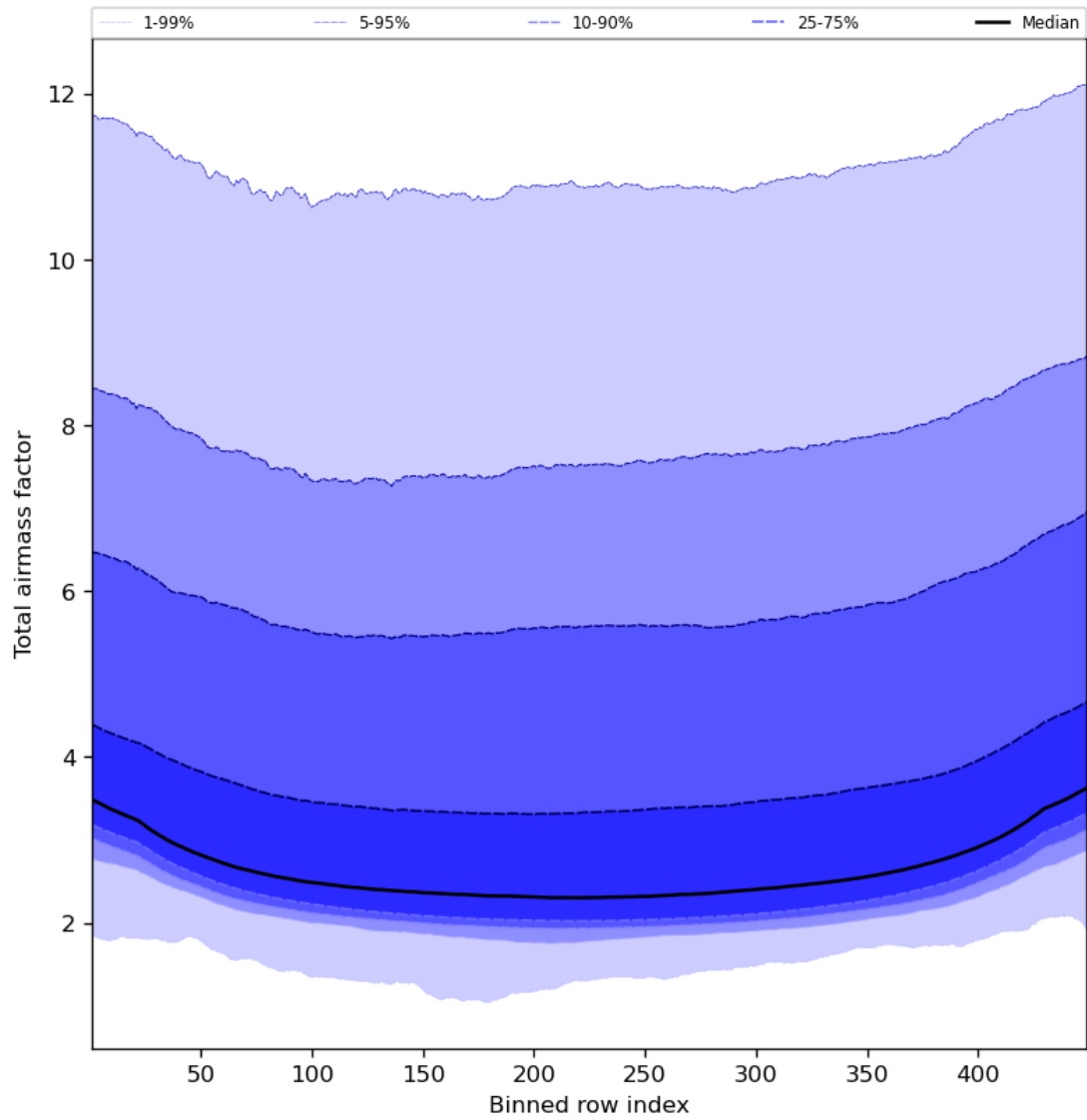
Figure 49: Along track statistics of “Total airmass factor” for 2024-02-29 to 2024-03-02
