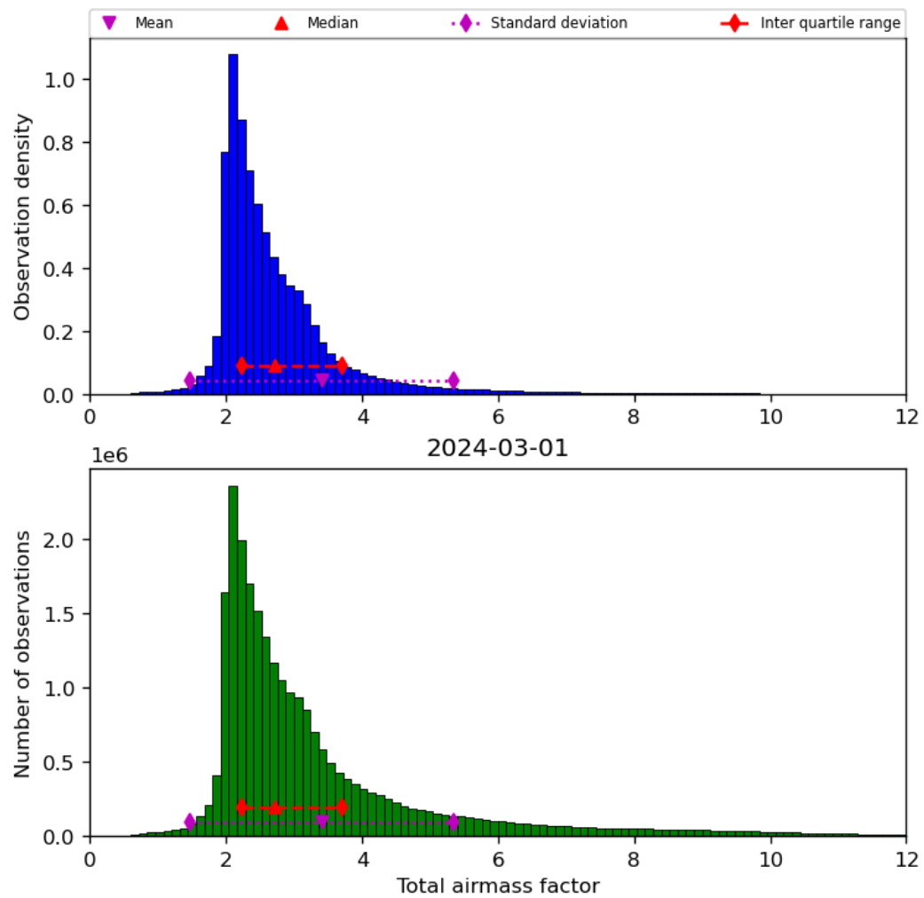
Figure 32: Histogram of “Total airmass factor” for 2024-02-29 to 2024-03-02
