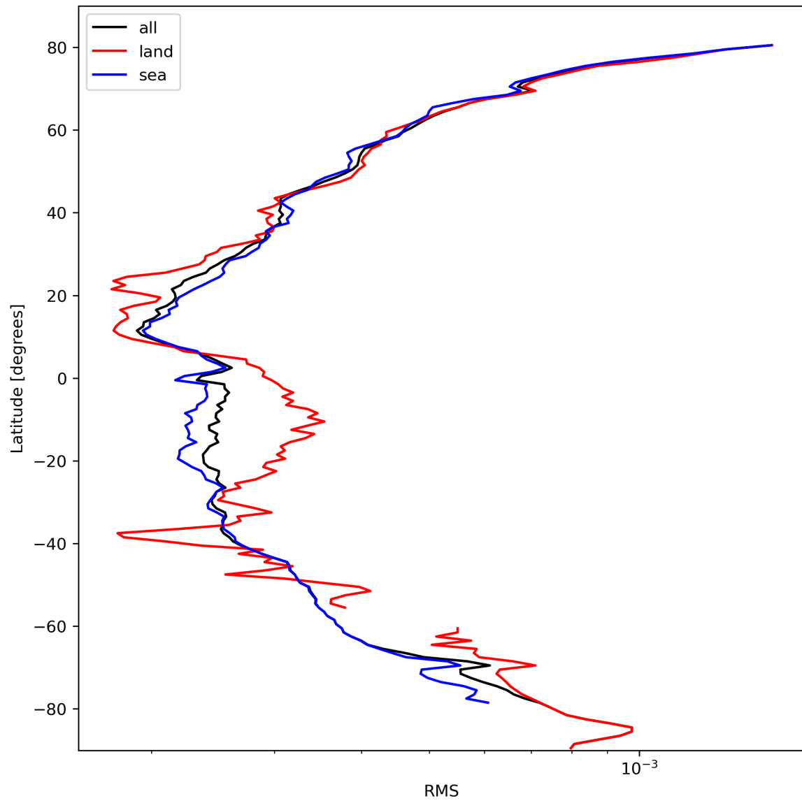
Figure 26: Zonal average of “RMS” for 2024-02-29 to 2024-03-02.
