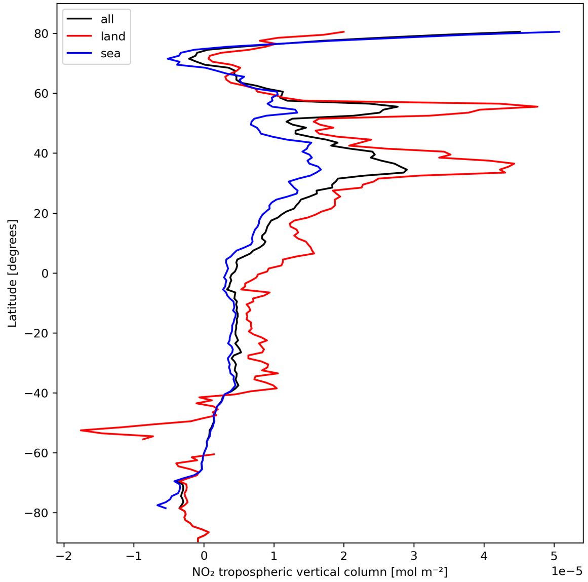
Figure 12: Zonal average of “NO 2 tropospheric vertical column” for 2024-02-29 to 2024-03-02.
