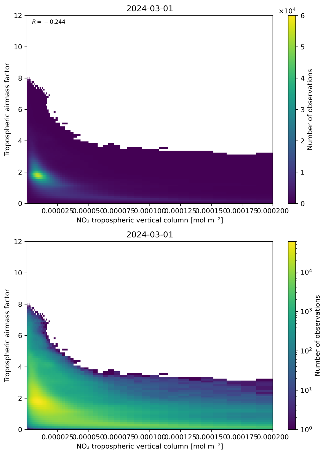
Figure 123: Scatter density plot of “NO 2 tropospheric vertical column” against “Tropospheric air mass factor” for 2024-02-29 to 2024-03-02.
