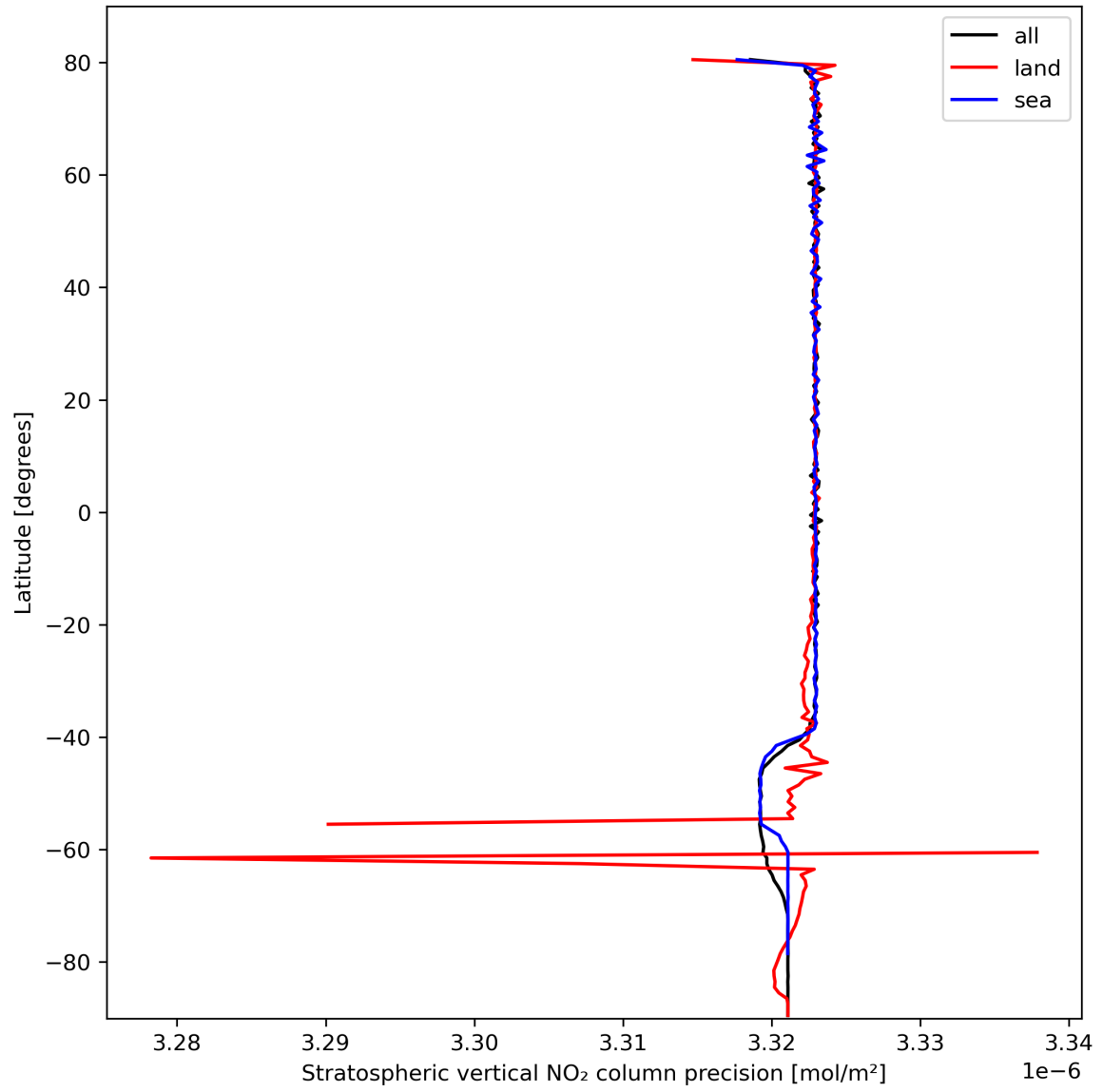
Figure 20: Zonal average of “Stratospheric vertical NO 2 column precision” for 2024-02-29 to 2024-03-02.
