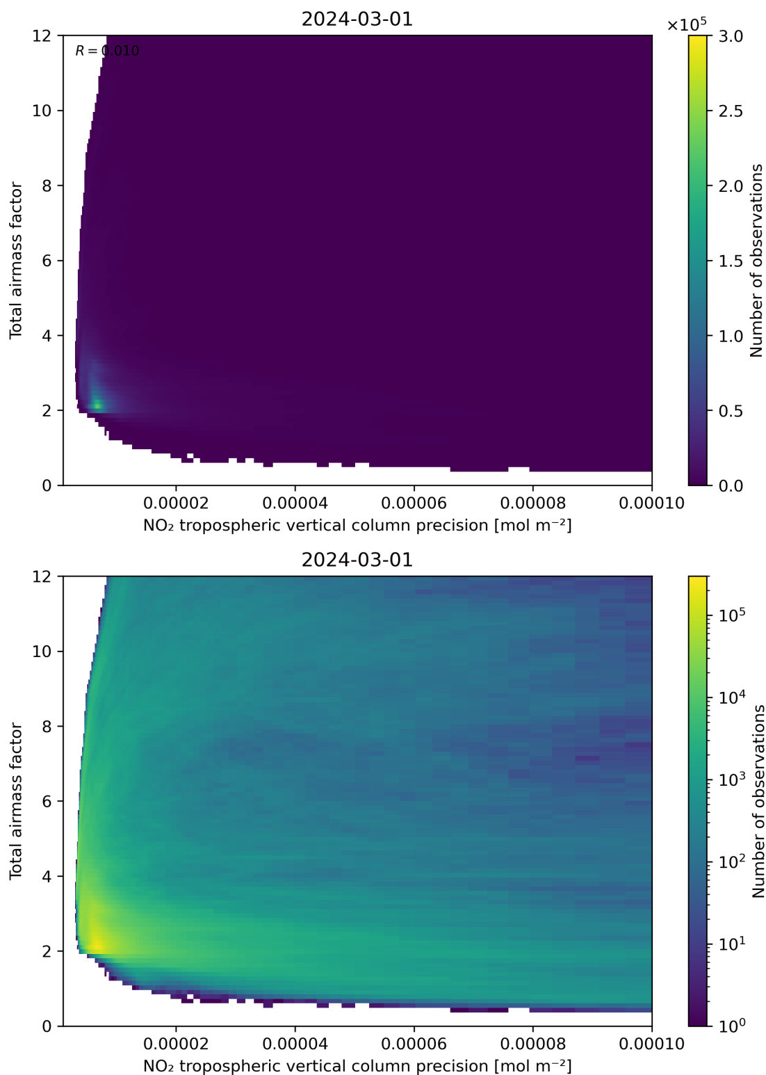
Figure 132: Scatter density plot of “NO 2 tropospheric vertical column precision” against “Total air mass factor” for 2024-02-29 to 2024-03-02.
