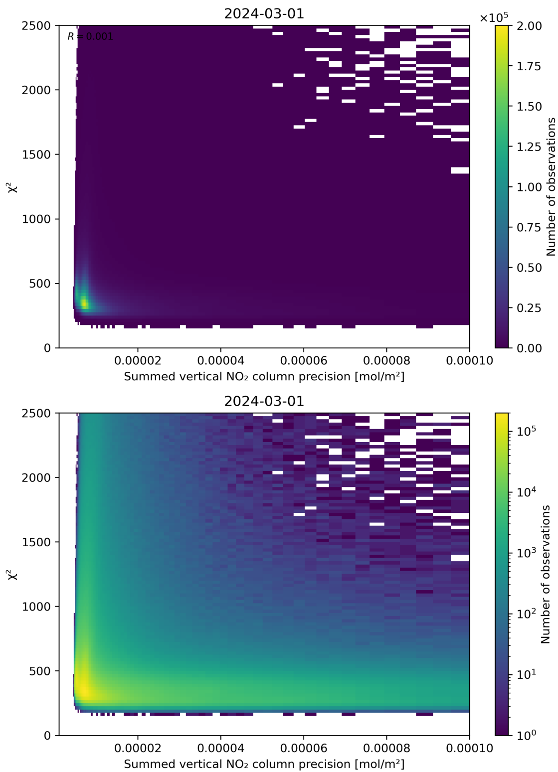
Figure 107: Scatter density plot of “Summed vertical NO 2 column precision” against “ \chi^2 ” for 2024-02-29 to 2024-03-02.
