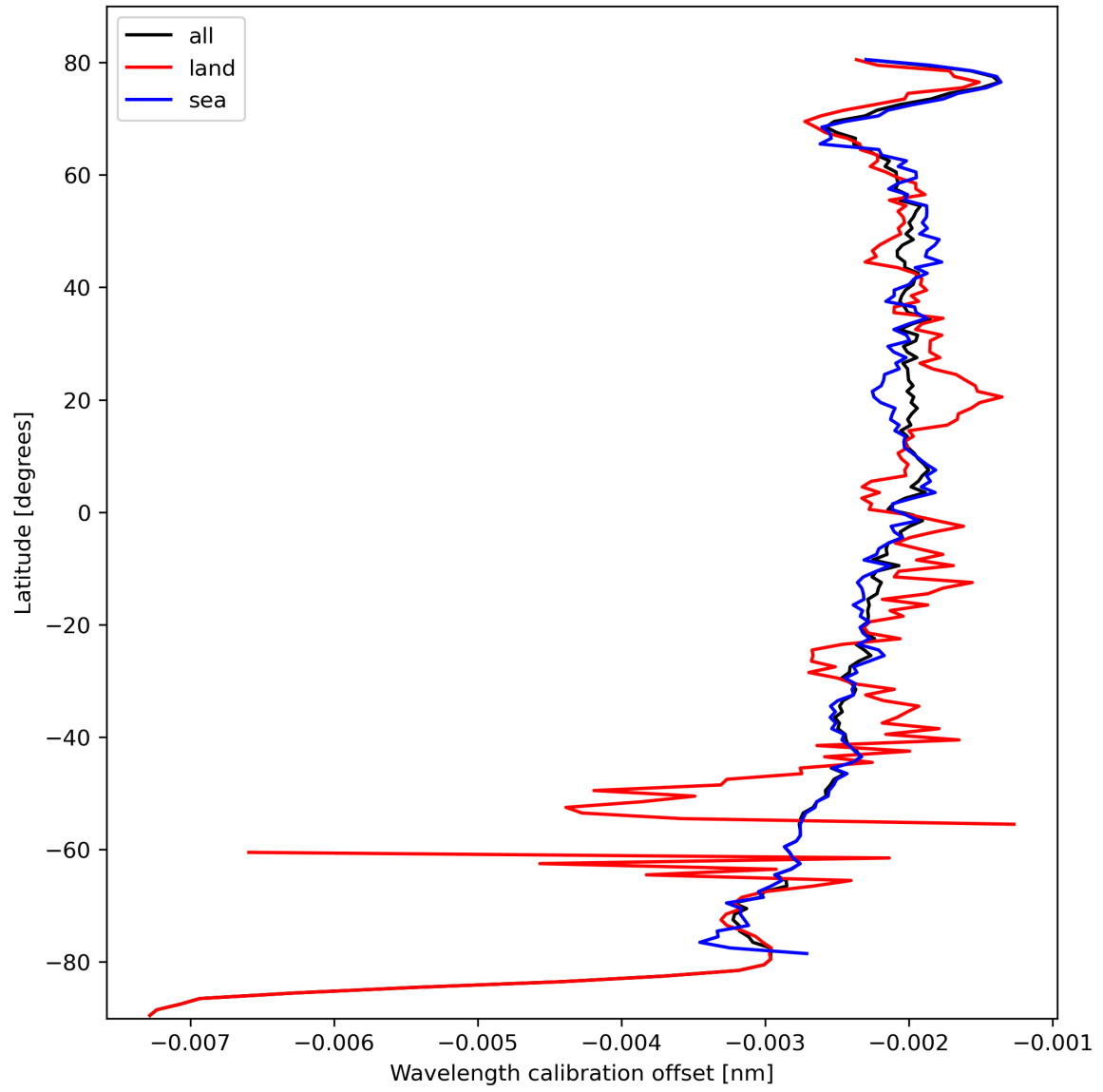
Figure 18: Zonal average of “Wavelength calibration offset” for 2024-02-29 to 2024-03-02.
