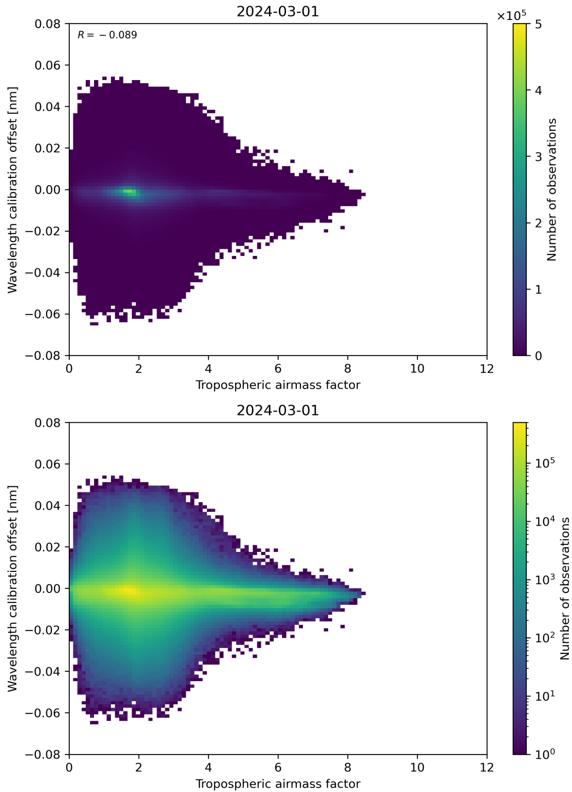
Figure 80: Scatter density plot of “Tropospheric air mass factor” against “Wavelength calibration offset” for 2024-02-29 to 2024-03-02.
