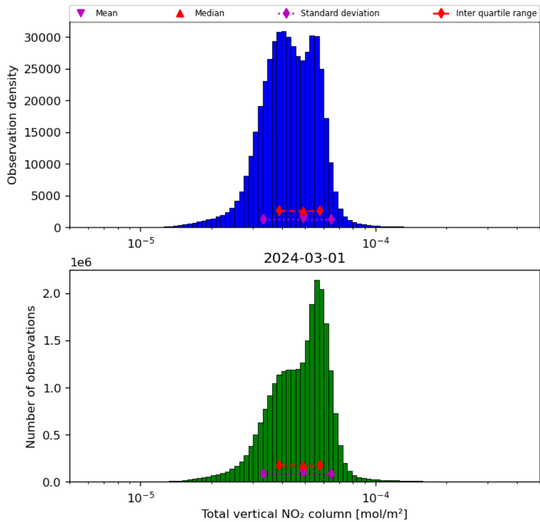
Figure 38: Histogram of "Total vertical NO 2 column" for 2024-02-29 to 2024-03-02
