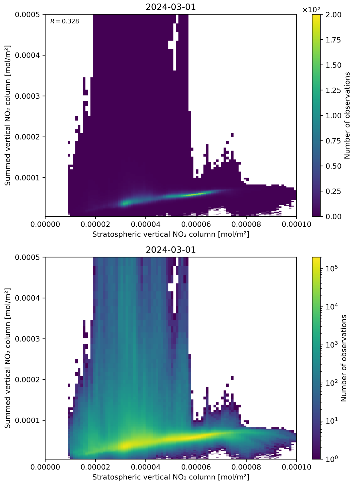
Figure 98: Scatter density plot of “Stratospheric vertical NO 2 column” against “Summed vertical NO 2 column” for 2024-02-29 to 2024-03-02.
