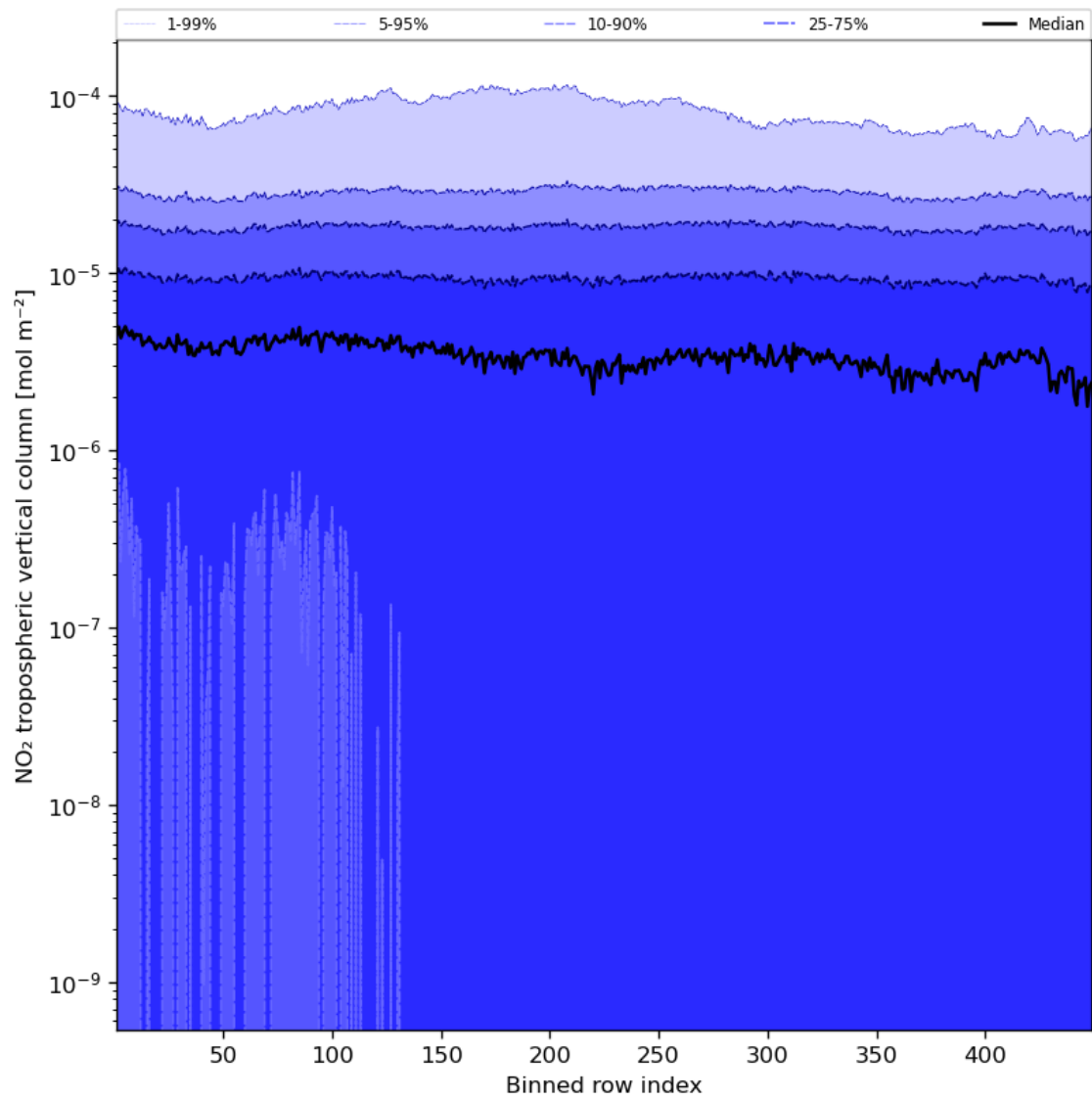
Figure 46: Along track statistics of “NO 2 tropospheric vertical column” for 2024-02-29 to 2024-03-02
