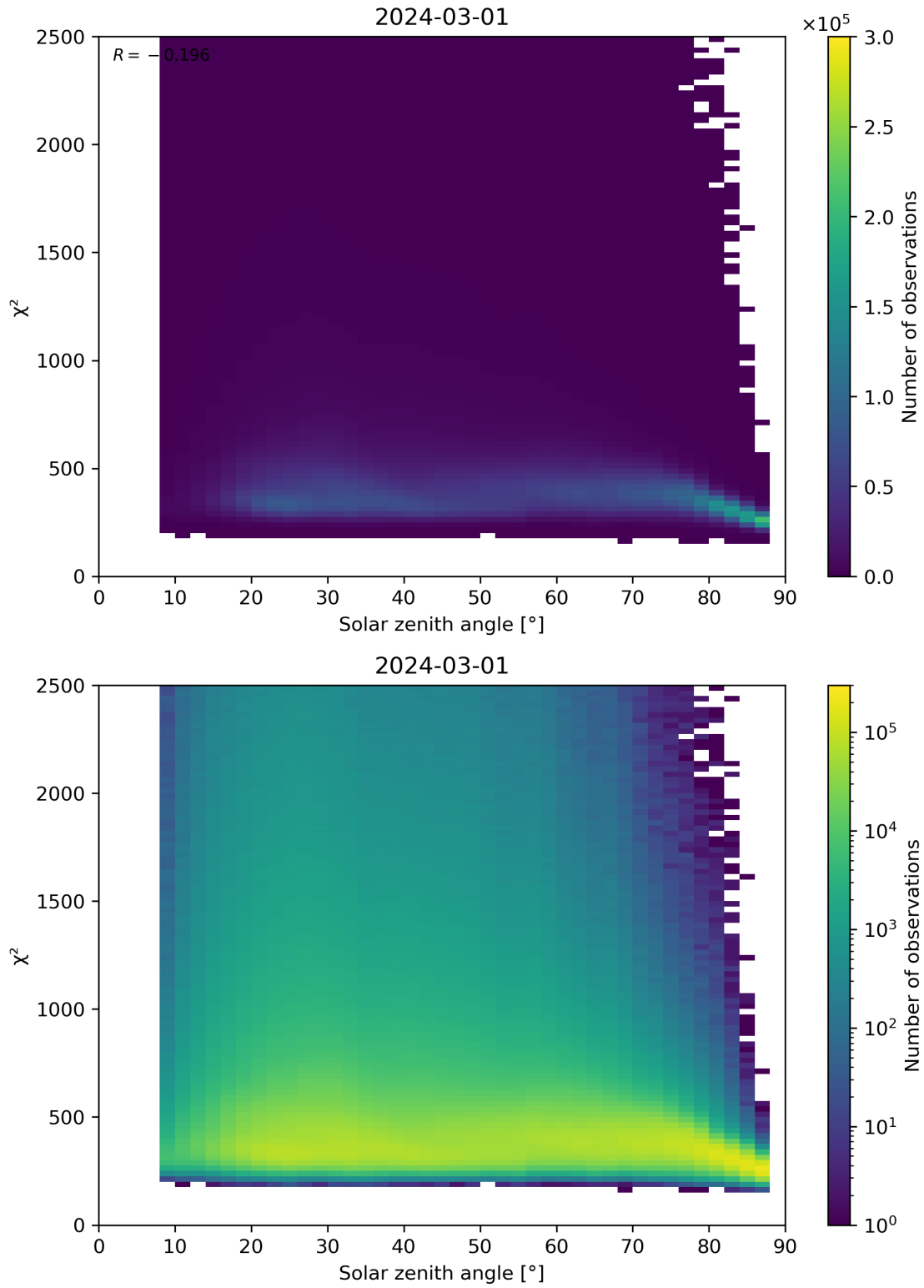
Figure 148: Scatter density plot of “Solar zenith angle” against “ \chi^2 ” for 2024-02-29 to 2024-03-02.
