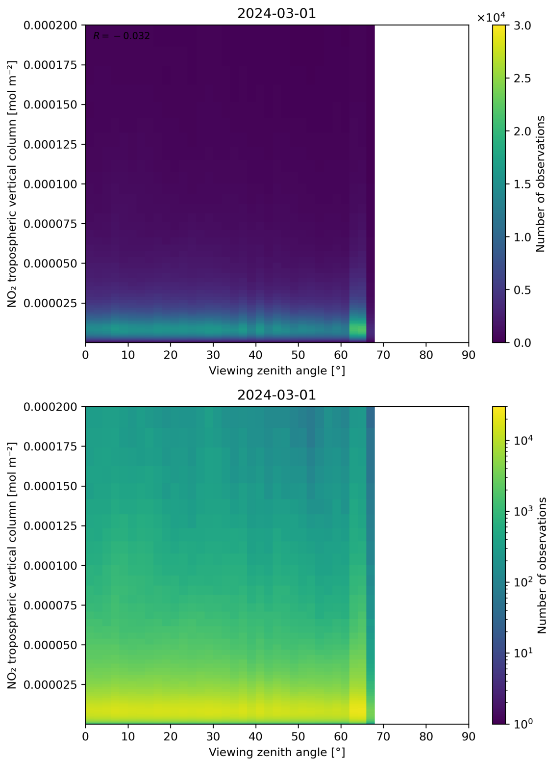
Figure 169: Scatter density plot of “Viewing zenith angle” against “NO 2 tropospheric vertical column” for 2024-02-29 to 2024-03-02.
