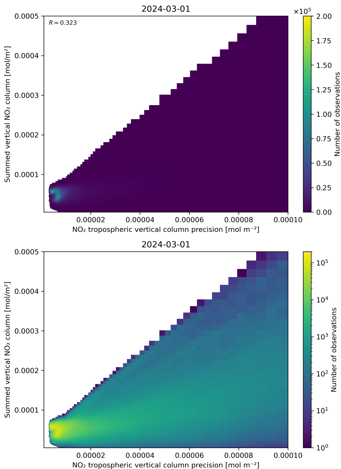
Figure 136: Scatter density plot of “NO 2 tropospheric vertical column precision” against “Summed vertical NO 2 column” for 2024-02-29 to 2024-03-02.
