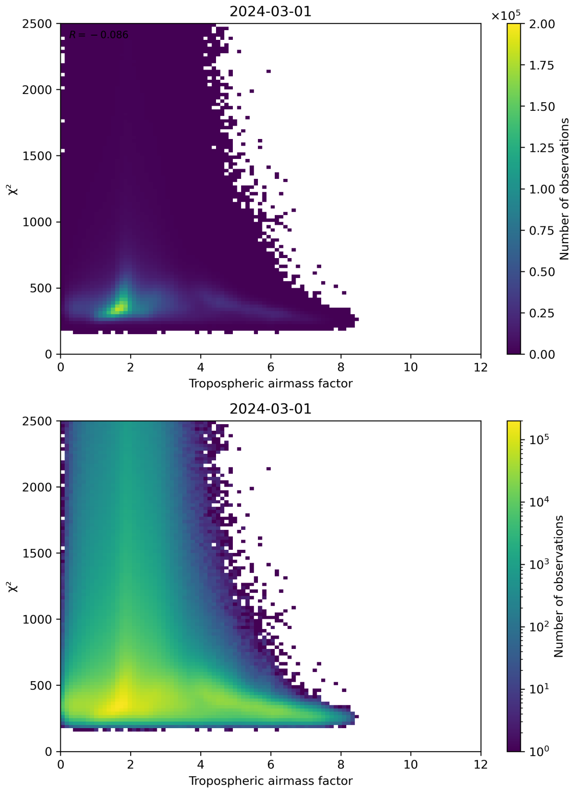
Figure 73: Scatter density plot of “Tropospheric airmass factor” against “ \chi^2 ” for 2024-02-29 to 2024-03-02.
