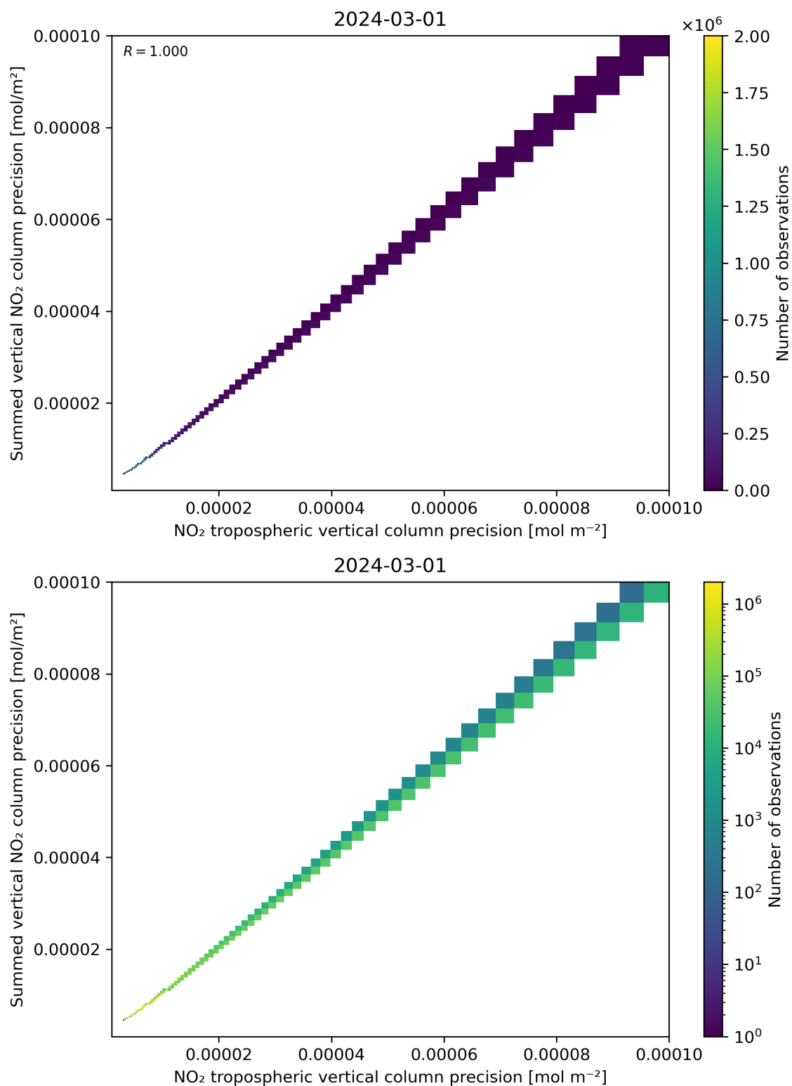
Figure 137: Scatter density plot of “NO 2 tropospheric vertical column precision” against “Summed vertical NO 2 column precision” for 2024-02-29 to 2024-03-02.
