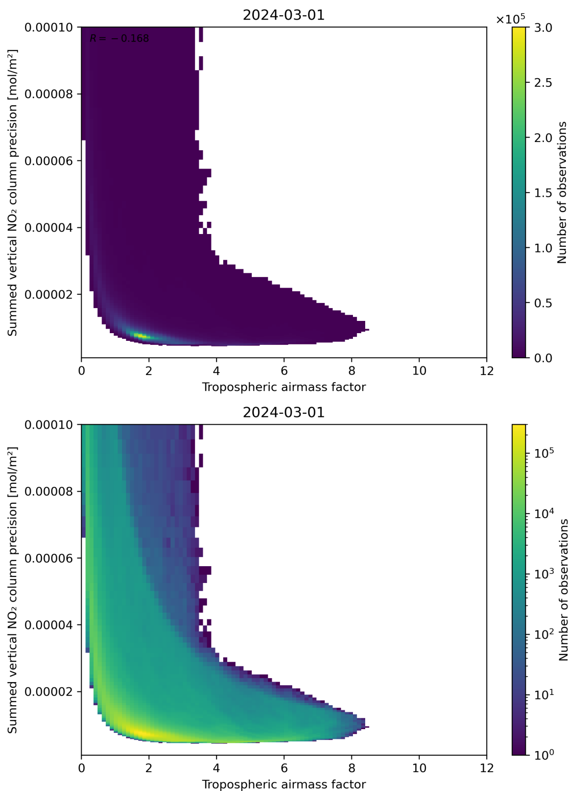
Figure 76: Scatter density plot of “Tropospheric airmass factor” against “Summed vertical NO 2 column precision” for 2024-02-29 to 2024-03-02.
