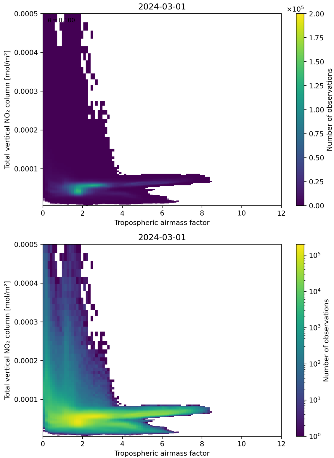
Figure 77: Scatter density plot of “Tropospheric airmass factor” against “Total vertical NO 2 column” for 2024-02-29 to 2024-03-02.
