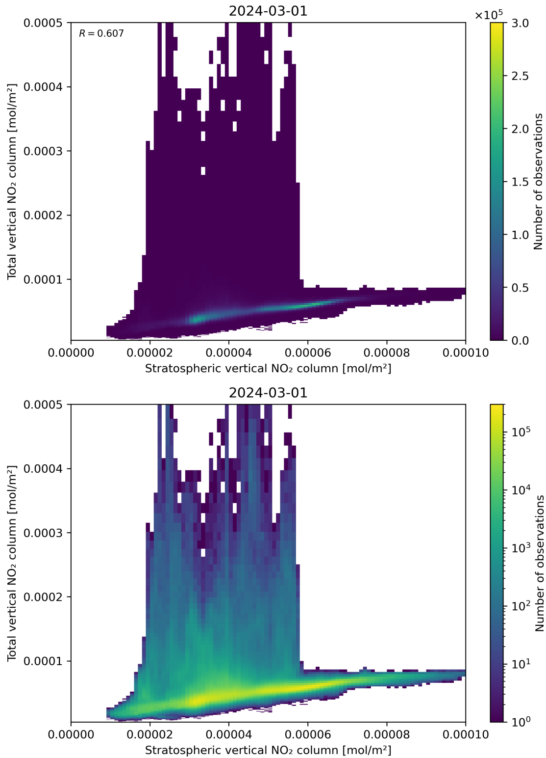
Figure 100: Scatter density plot of “Stratospheric vertical NO 2 column” against “Total vertical NO 2 column” for 2024-02-29 to 2024-03-02.
