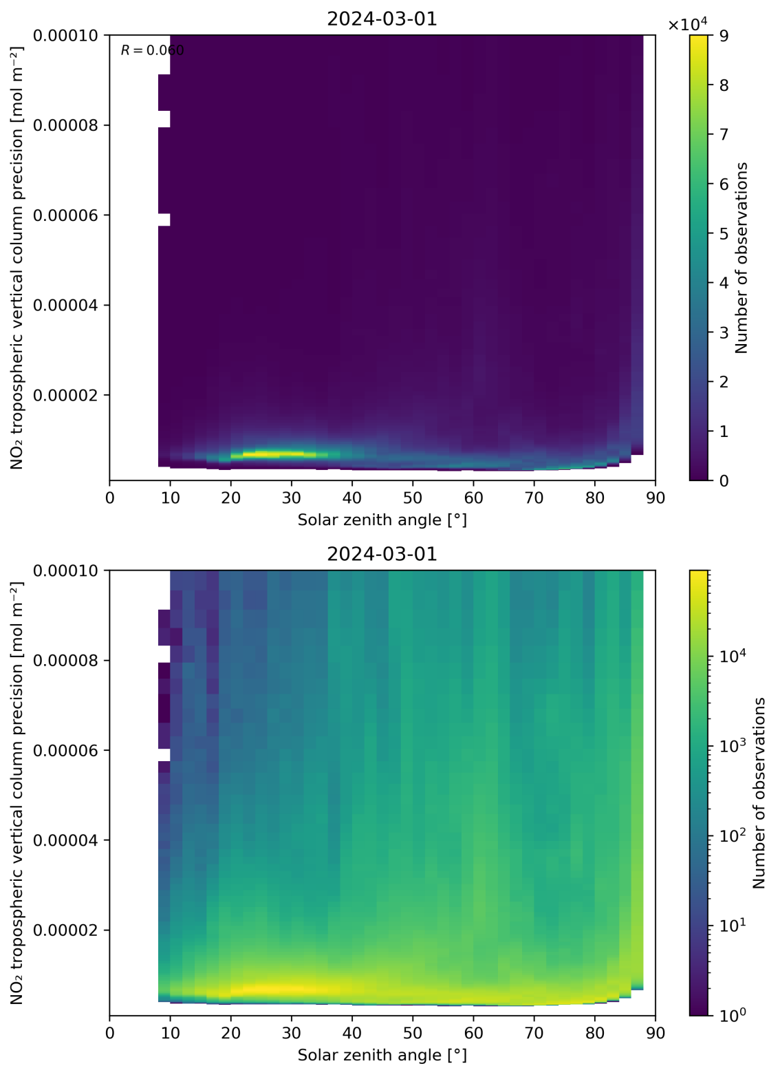
Figure 156: Scatter density plot of “Solar zenith angle” against “NO 2 tropospheric vertical column precision” for 2024-02-29 to 2024-03-02.
