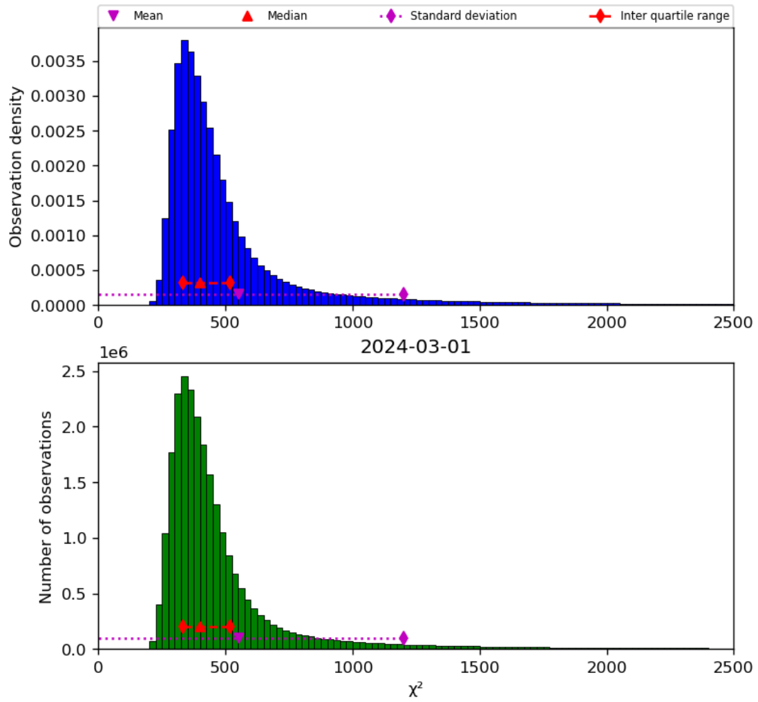
Figure 42: Histogram of “ \chi^2 ” for 2024-02-29 to 2024-03-02
