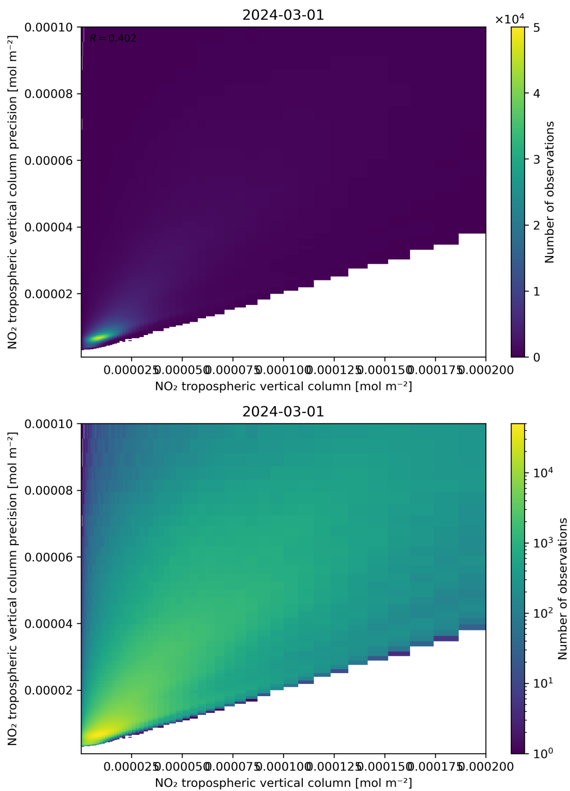
Figure 130: Scatter density plot of “NO 2 tropospheric vertical column” against “NO 2 tropospheric vertical column precision” for 2024-02-29 to 2024-03-02.
