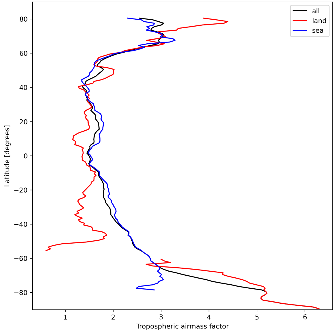
Figure 14: Zonal average of “Tropospheric airmass factor” for 2024-02-29 to 2024-03-02.
