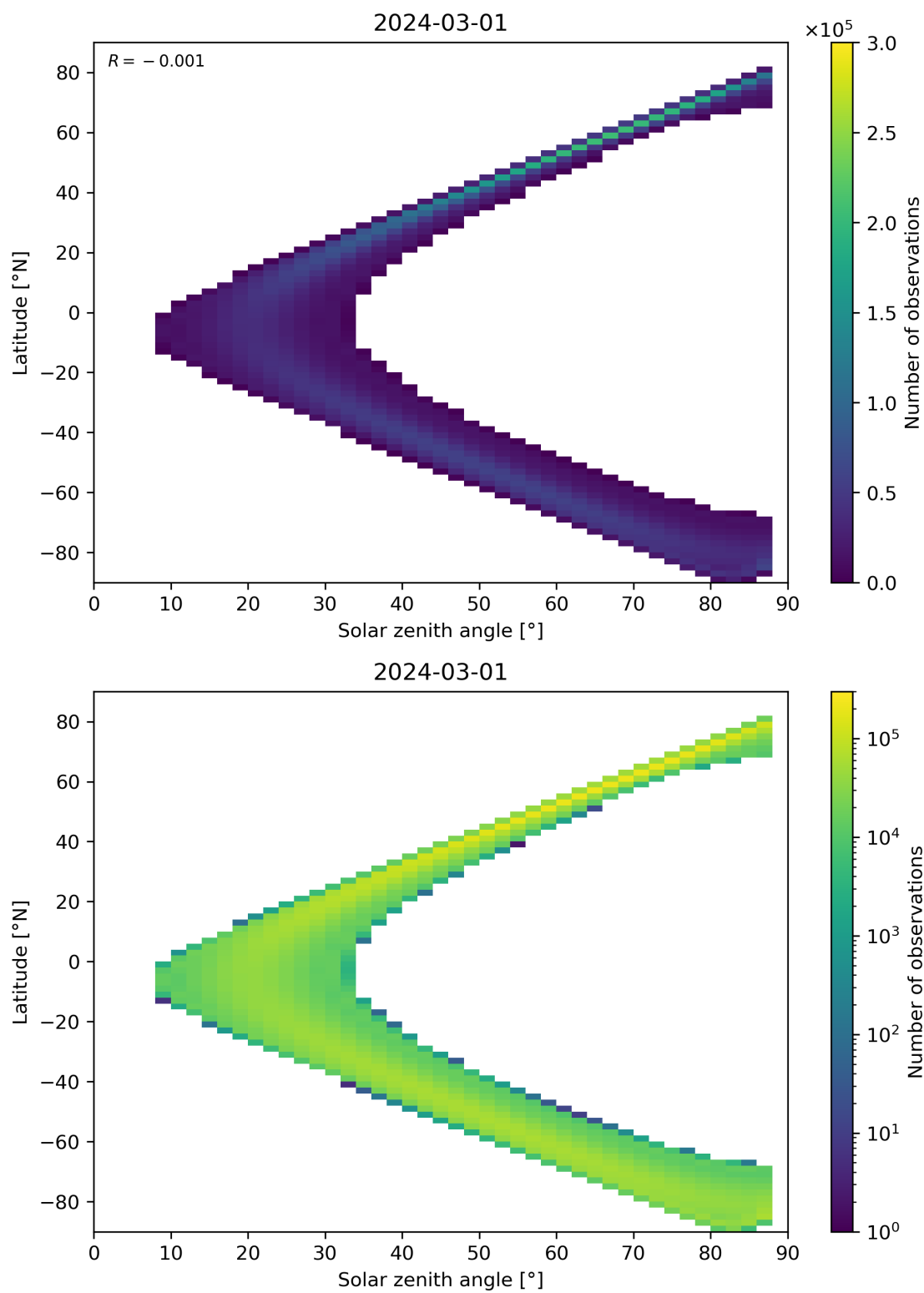
Figure 149: Scatter density plot of “Solar zenith angle” against “Latitude” for 2024-02-29 to 2024-03-02.
