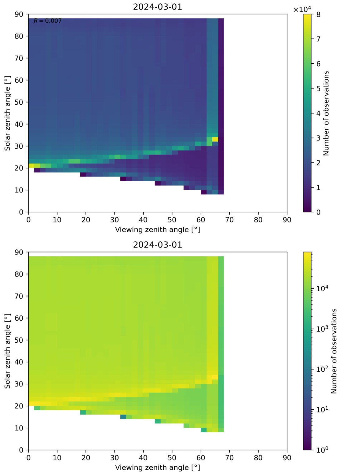
Figure 172: Scatter density plot of “Viewing zenith angle” against “Solar zenith angle” for 2024-02-29 to 2024-03-02.
