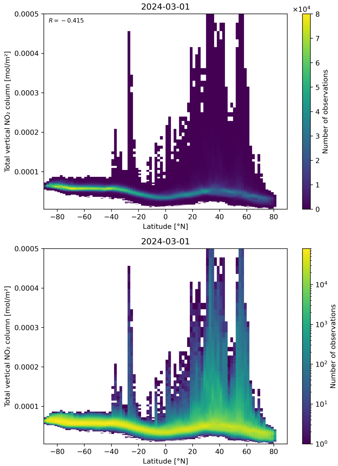
Figure 90: Scatter density plot of “Latitude” against “Total vertical NO 2 column” for 2024-02-29 to 2024-03-02.
