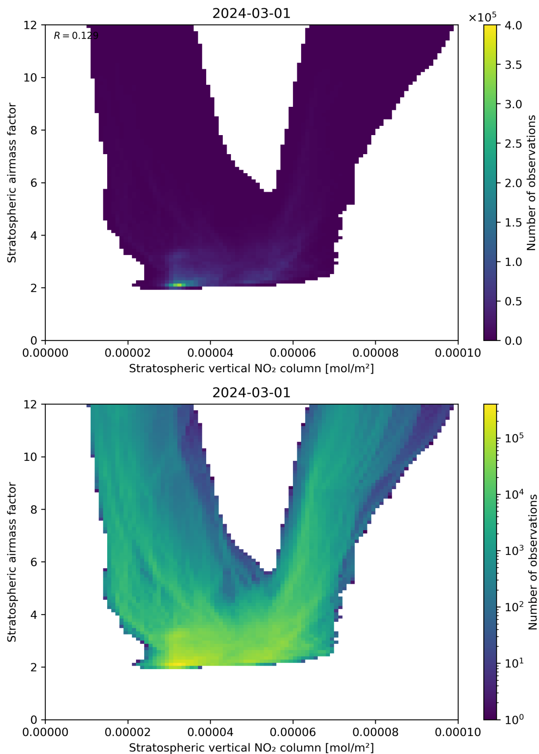
Figure 96: Scatter density plot of “Stratospheric vertical NO 2 column” against “Stratospheric airmass factor” for 2024-02-29 to 2024-03-02.
