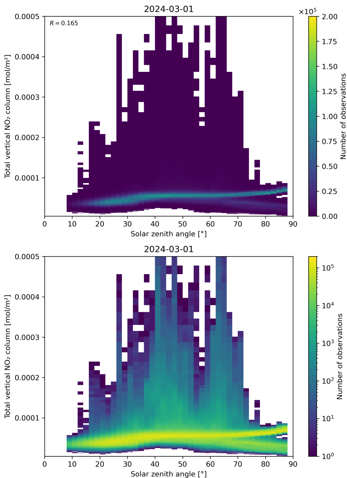
Figure 153: Scatter density plot of “Solar zenith angle” against “Total vertical NO 2 column” for 2024-02-29 to 2024-03-02.
