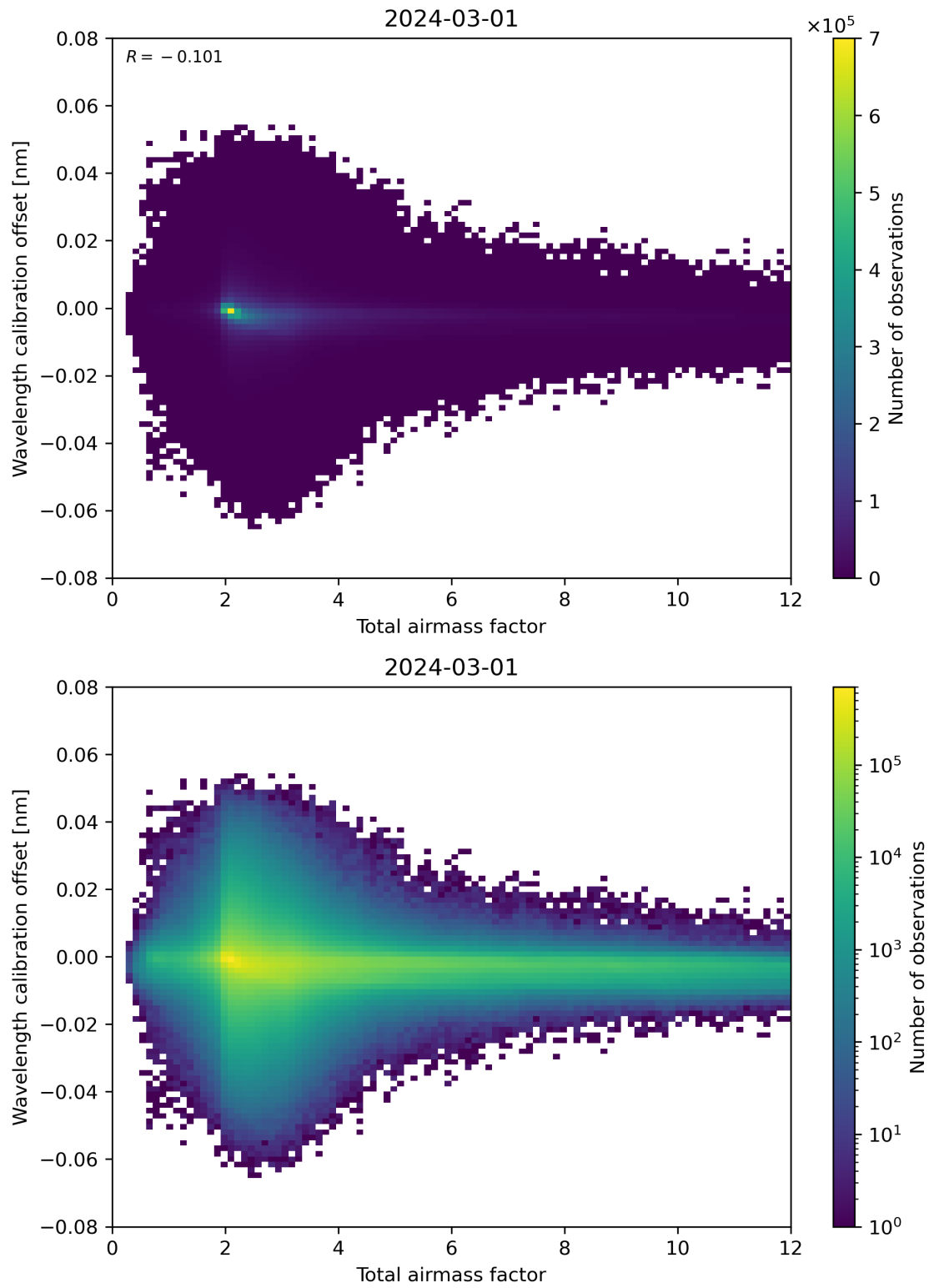
Figure 70: Scatter density plot of “Total airmass factor” against “Wavelength calibration offset” for 2024-02-29 to 2024-03-02.
