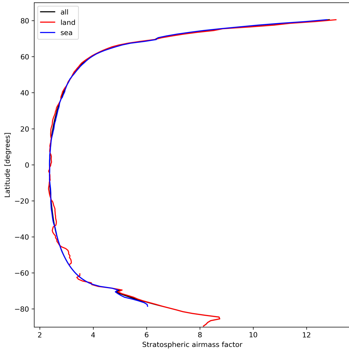
Figure 27: Zonal average of “Stratospheric airmass factor” for 2024-02-29 to 2024-03-02.
