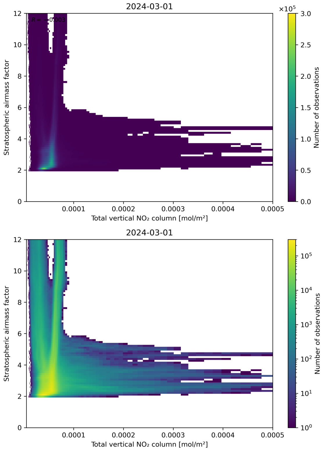
Figure 110: Scatter density plot of “Total vertical NO 2 column” against “Stratospheric airmass factor” for 2024-02-29 to 2024-03-02.
