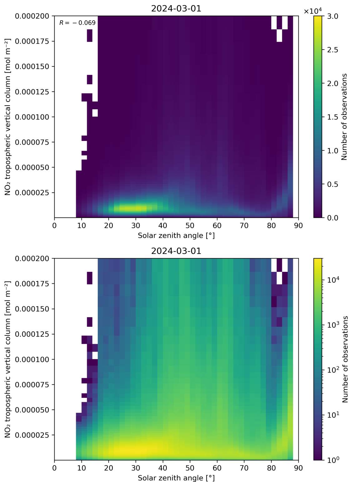
Figure 155: Scatter density plot of “Solar zenith angle” against “NO 2 tropospheric vertical column” for 2024-02-29 to 2024-03-02.
