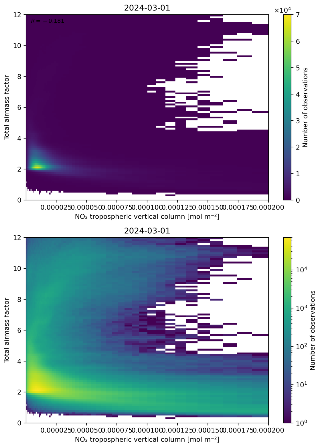
Figure 122: Scatter density plot of “NO 2 tropospheric vertical column” against “Total air mass factor” for 2024-02-29 to 2024-03-02.
