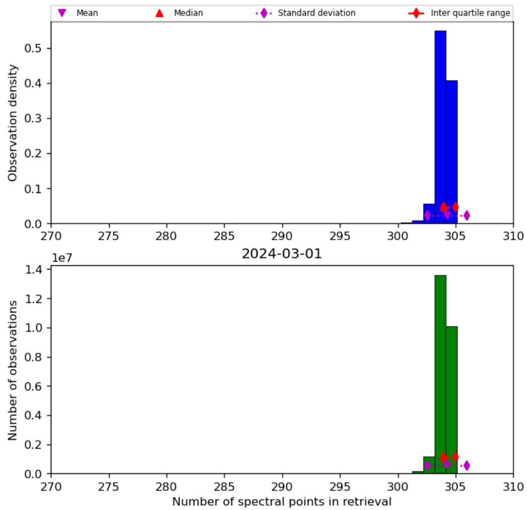
Figure 33: Histogram of “Number of spectral points in retrieval” for 2024-02-29 to 2024-03-02
