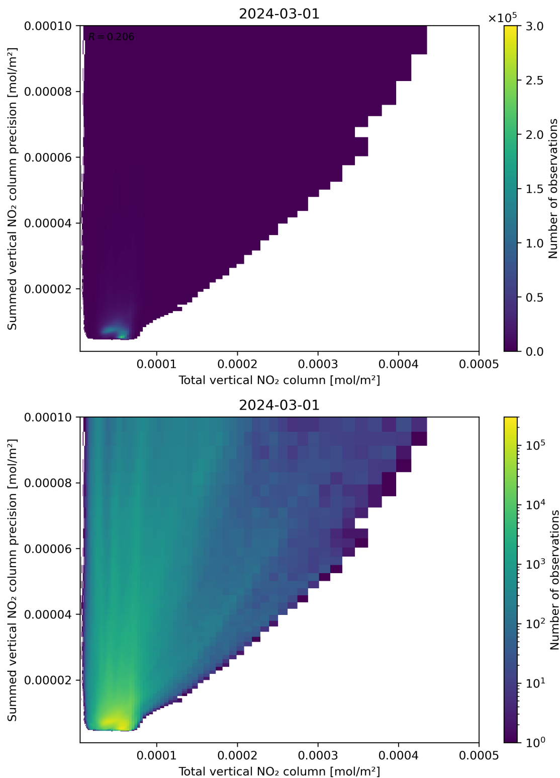
Figure 113: Scatter density plot of “Total vertical NO 2 column” against “Summed vertical NO 2 column precision” for 2024-02-29 to 2024-03-02.
