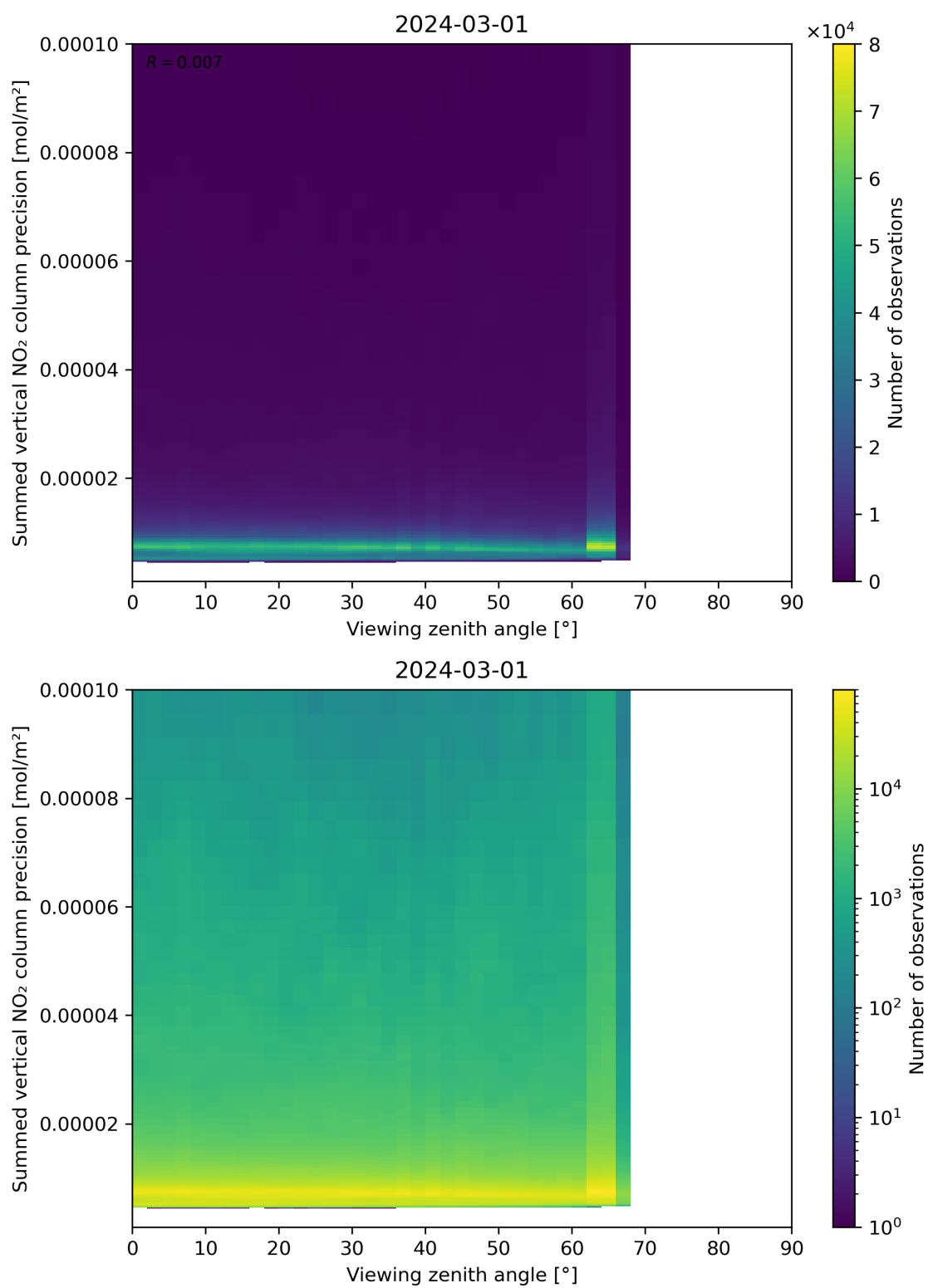
Figure 166: Scatter density plot of “Viewing zenith angle” against “Summed vertical NO 2 column precision” for 2024-02-29 to 2024-03-02.
