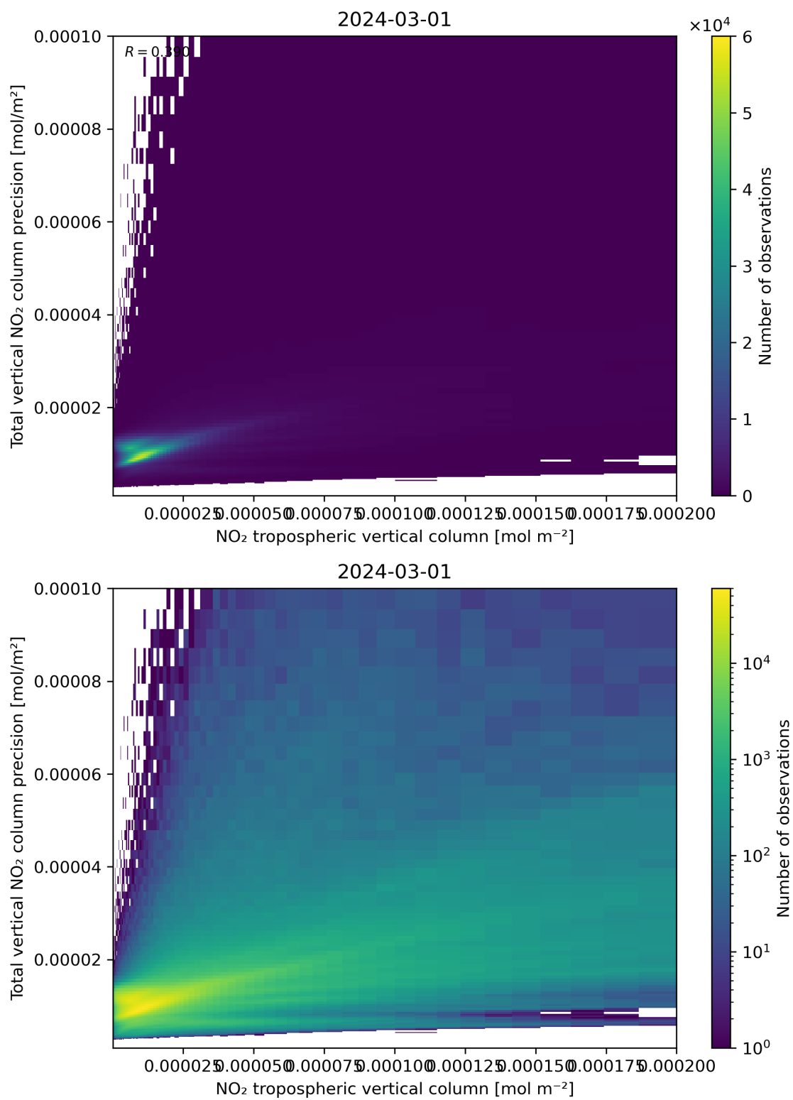
Figure 129: Scatter density plot of “NO 2 tropospheric vertical column” against “Total vertical NO 2 column precision” for 2024-02-29 to 2024-03-02.
