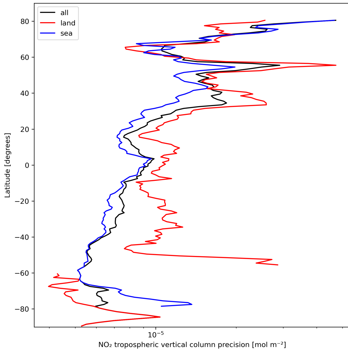
Figure 13: Zonal average of “NO 2 tropospheric vertical column precision” for 2024-02-29 to 2024-03-02.
