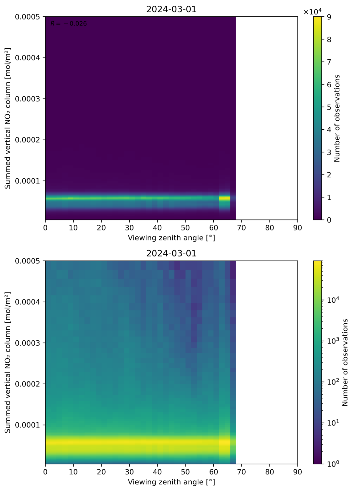
Figure 165: Scatter density plot of “Viewing zenith angle” against “Summed vertical NO 2 column” for 2024-02-29 to 2024-03-02.
