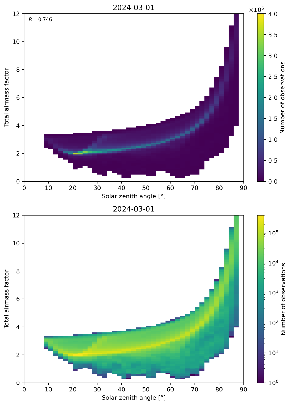
Figure 146: Scatter density plot of “Solar zenith angle” against “Total airmass factor” for 2024-02-29 to 2024-03-02.
