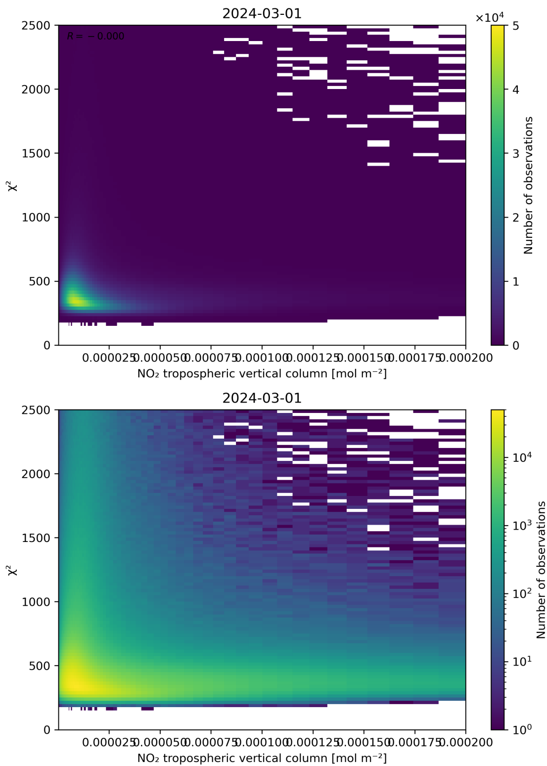
Figure 124: Scatter density plot of “NO 2 tropospheric vertical column” against “ \chi^2 ” for 2024-02-29 to 2024-03-02.
