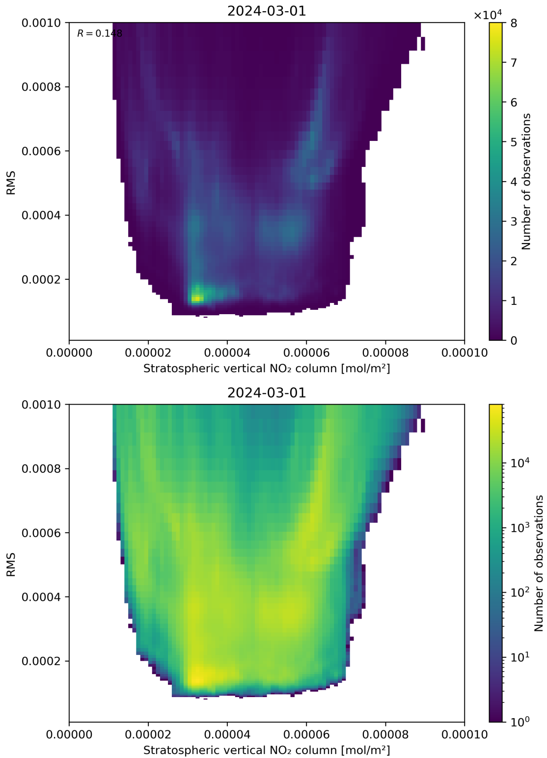
Figure 102: Scatter density plot of “Stratospheric vertical NO 2 column” against “RMS” for 2024-02-29 to 2024-03-02.
