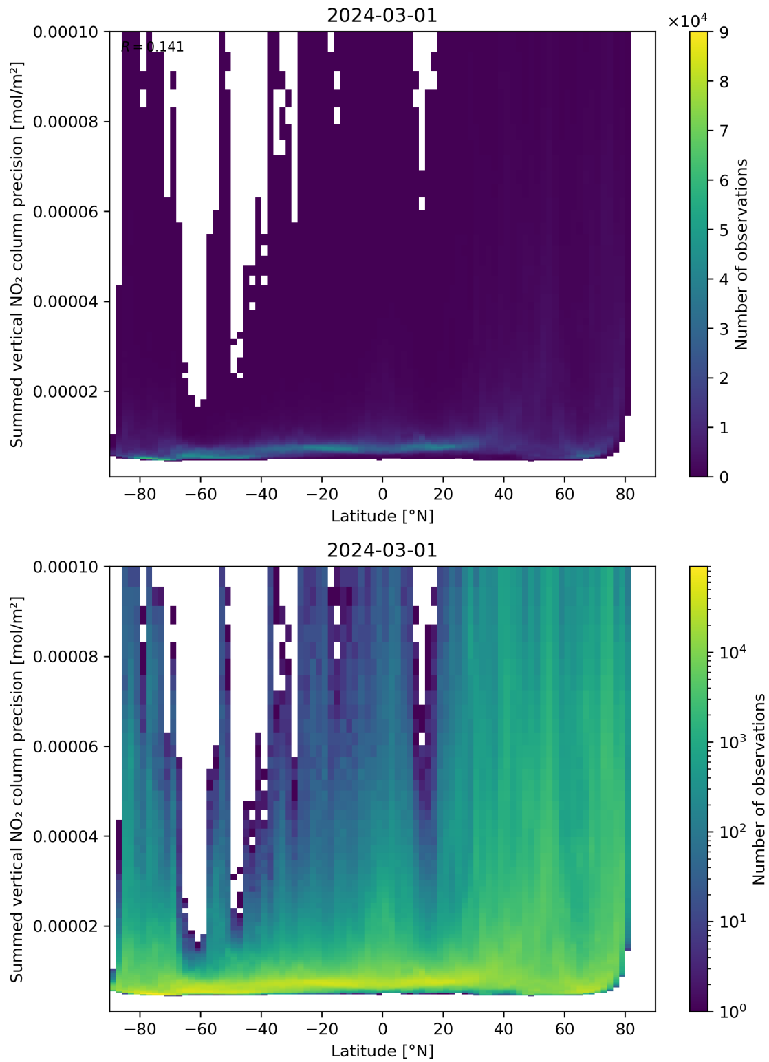
Figure 89: Scatter density plot of “Latitude” against “Summed vertical NO 2 column precision” for 2024-02-29 to 2024-03-02.
