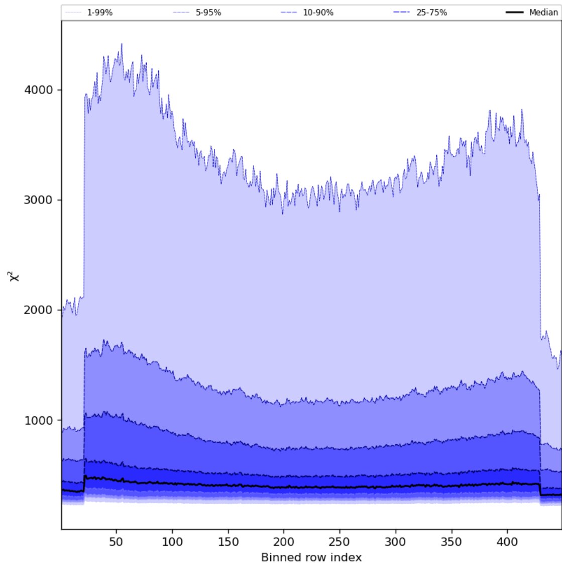
Figure 59: Along track statistics of “ \chi^2 ” for 2024-02-29 to 2024-03-02
