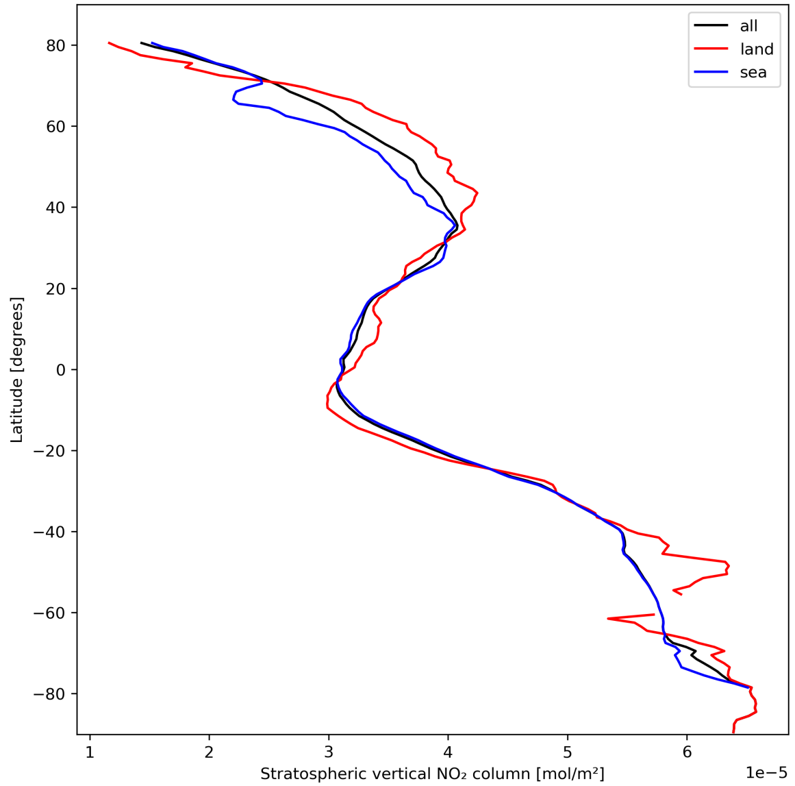
Figure 19: Zonal average of “Stratospheric vertical NO 2 column” for 2024-02-29 to 2024-03-02.
