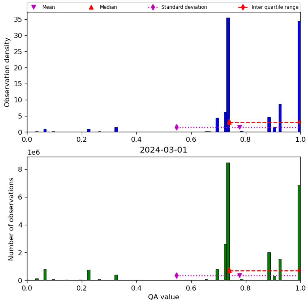
Figure 28: Histogram of “QA value” for 2024-02-29 to 2024-03-02
