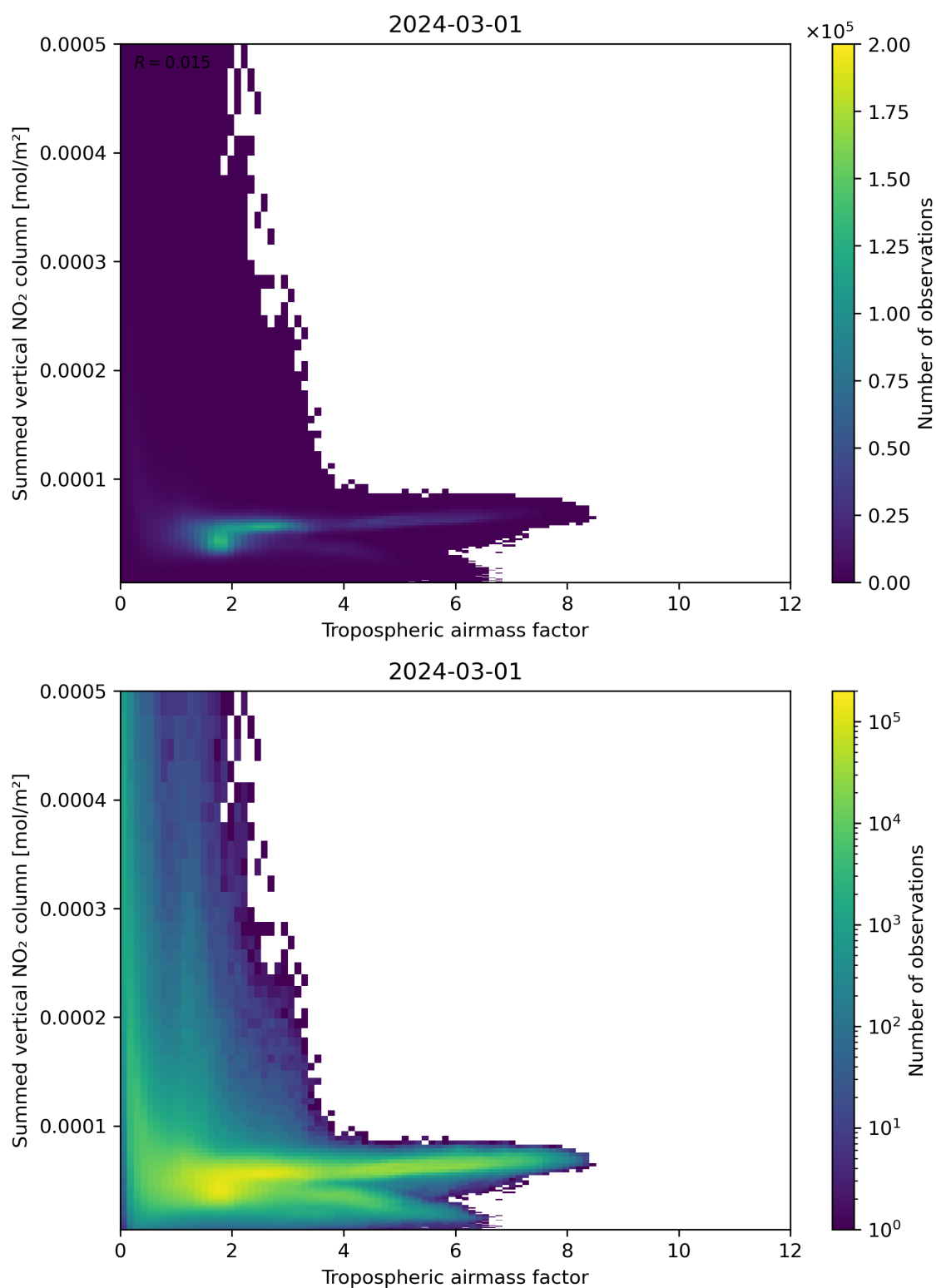
Figure 75: Scatter density plot of “Tropospheric air mass factor” against “Summed vertical NO 2 column” for 2024-02-29 to 2024-03-02.
