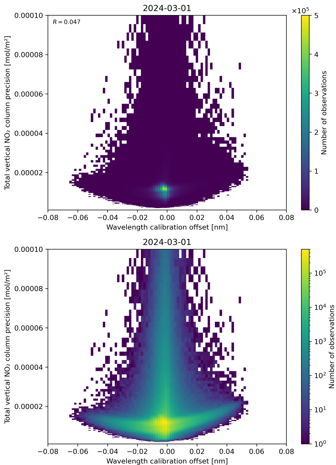
Figure 180: Scatter density plot of “Wavelength calibration offset” against “Total vertical NO 2 column precision” for 2024-02-29 to 2024-03-02.
