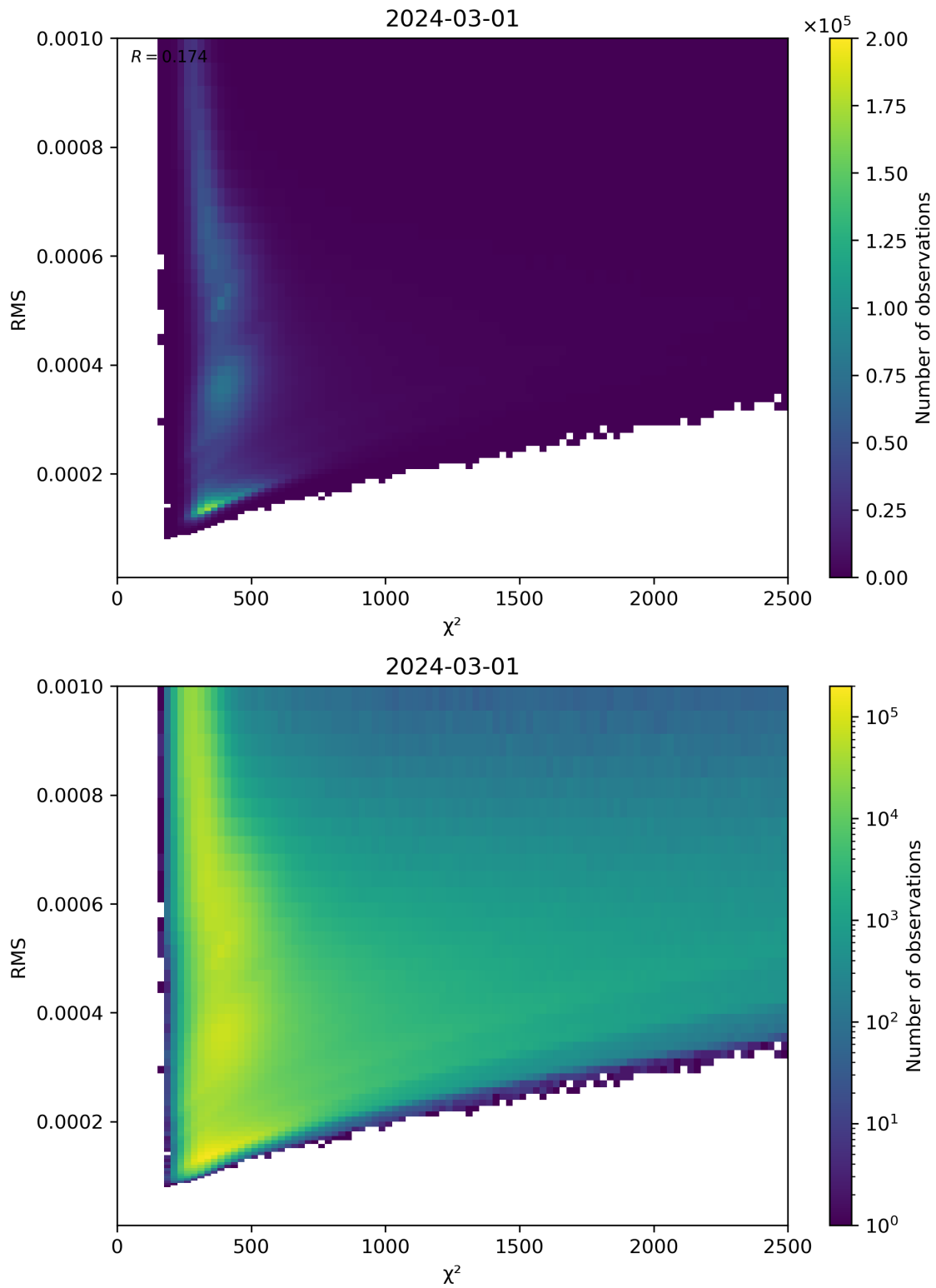
Figure 82: Scatter density plot of “ \chi^2 ” against “RMS” for 2024-02-29 to 2024-03-02.
