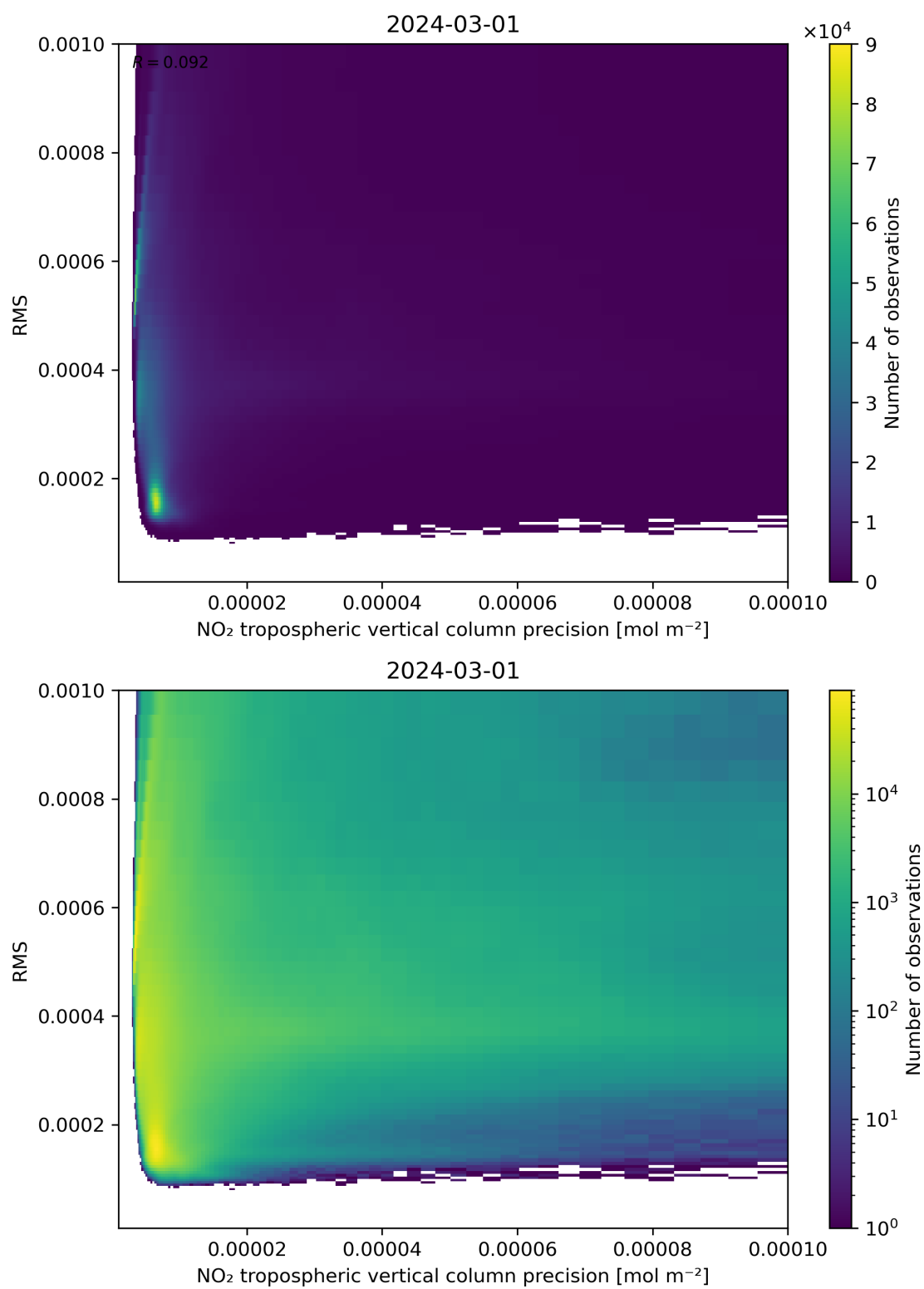
Figure 140: Scatter density plot of “NO 2 tropospheric vertical column precision” against “RMS” for 2024-02-29 to 2024-03-02.
