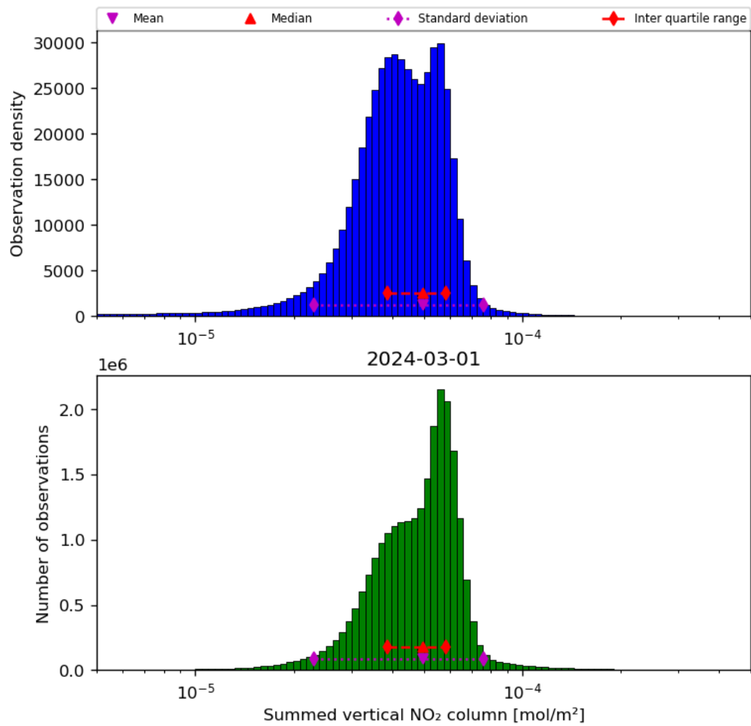
Figure 40: Histogram of “Summed vertical NO 2 column” for 2024-02-29 to 2024-03-02
