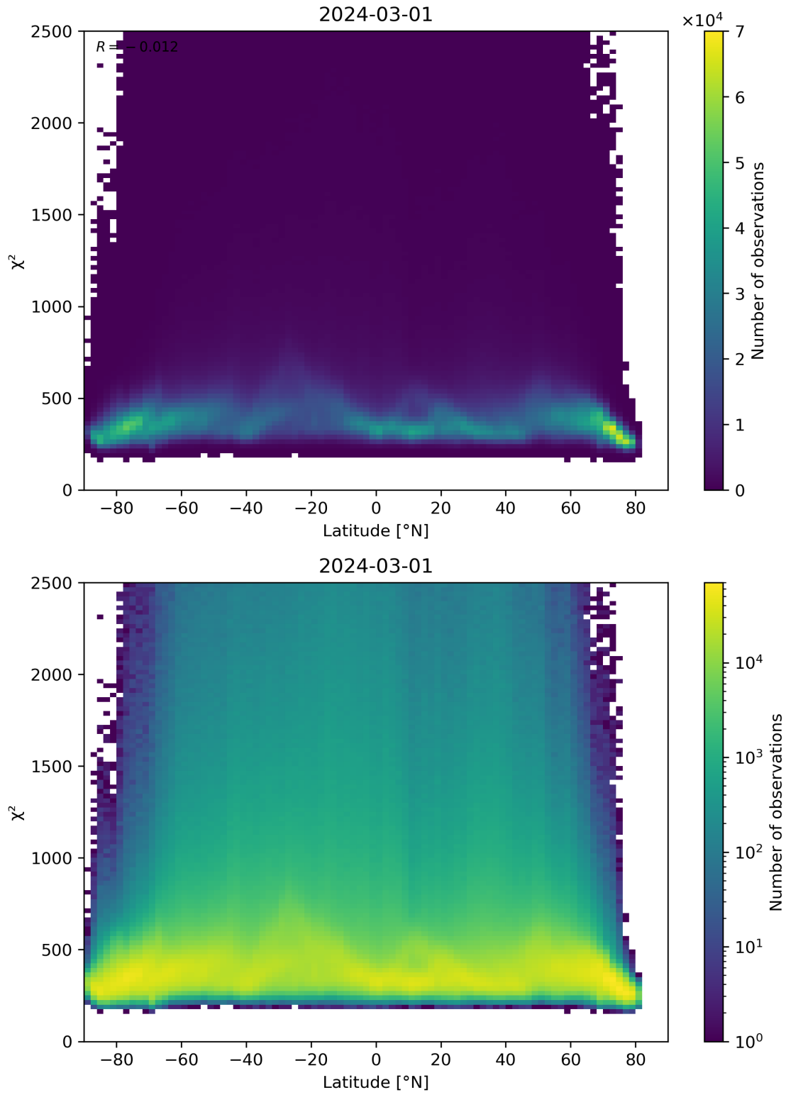
Figure 86: Scatter density plot of “Latitude” against “ \chi^2 ” for 2024-02-29 to 2024-03-02.
