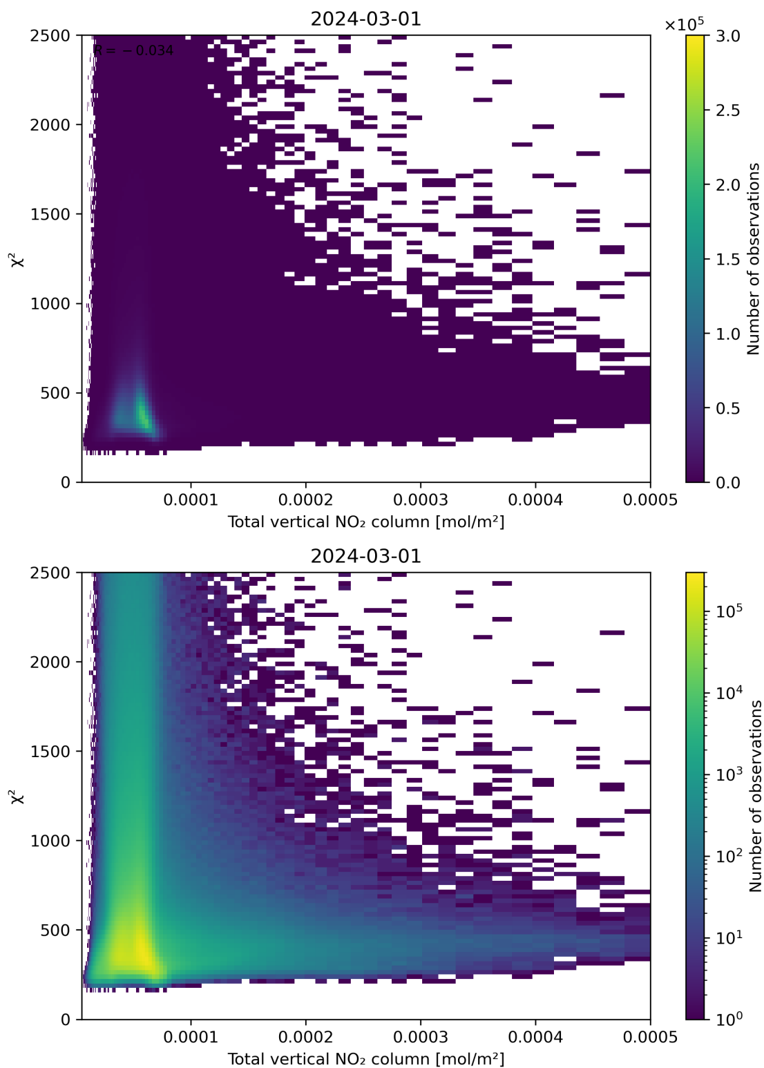
Figure 111: Scatter density plot of “Total vertical NO 2 column” against “ \chi^2 ” for 2024-02-29 to 2024-03-02.
