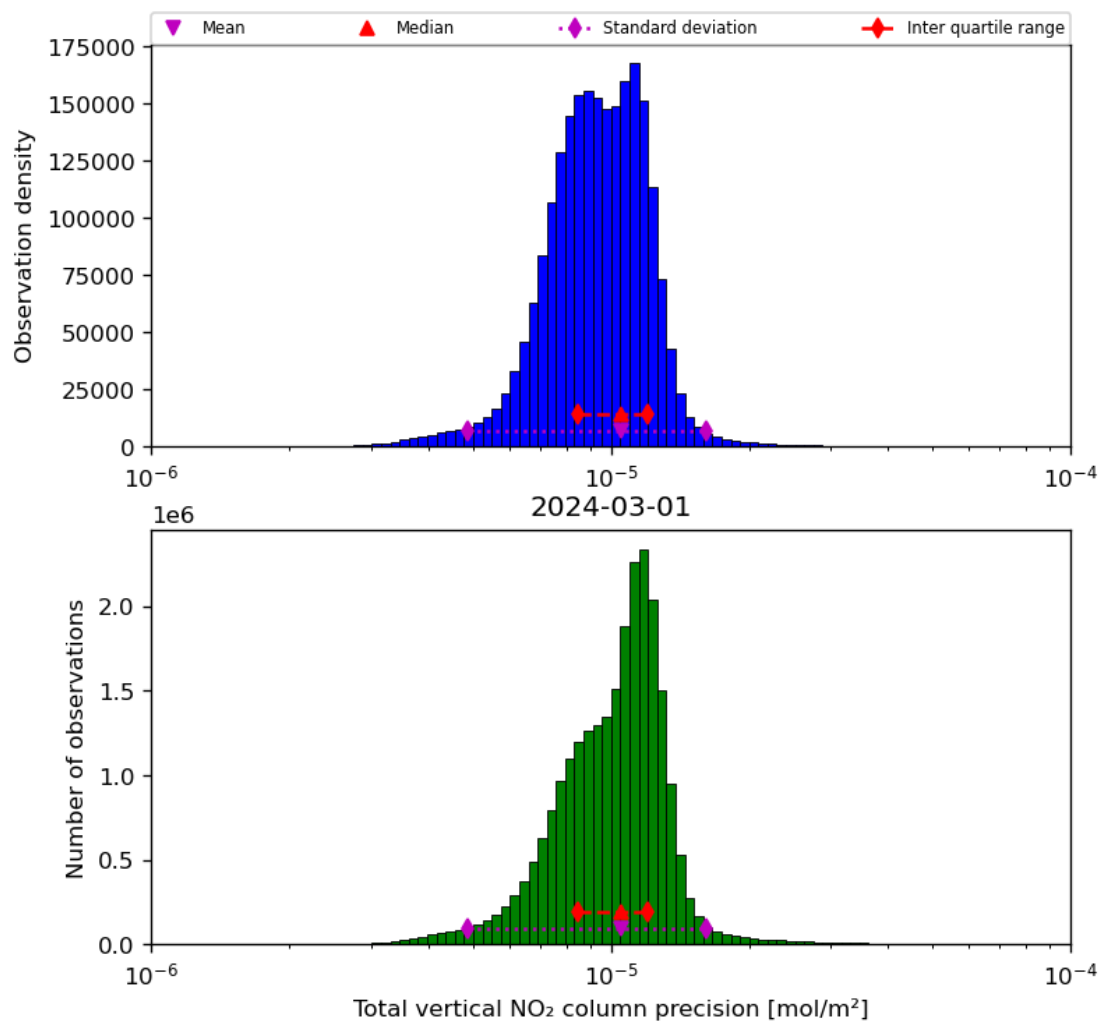
Figure 39: Histogram of “Total vertical NO 2 column precision” for 2024-02-29 to 2024-03-02
