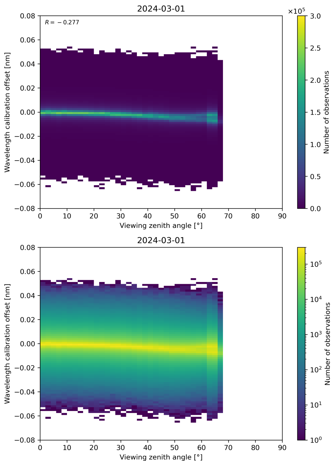
Figure 173: Scatter density plot of “Viewing zenith angle” against “Wavelength calibration offset” for 2024-02-29 to 2024-03-02.
