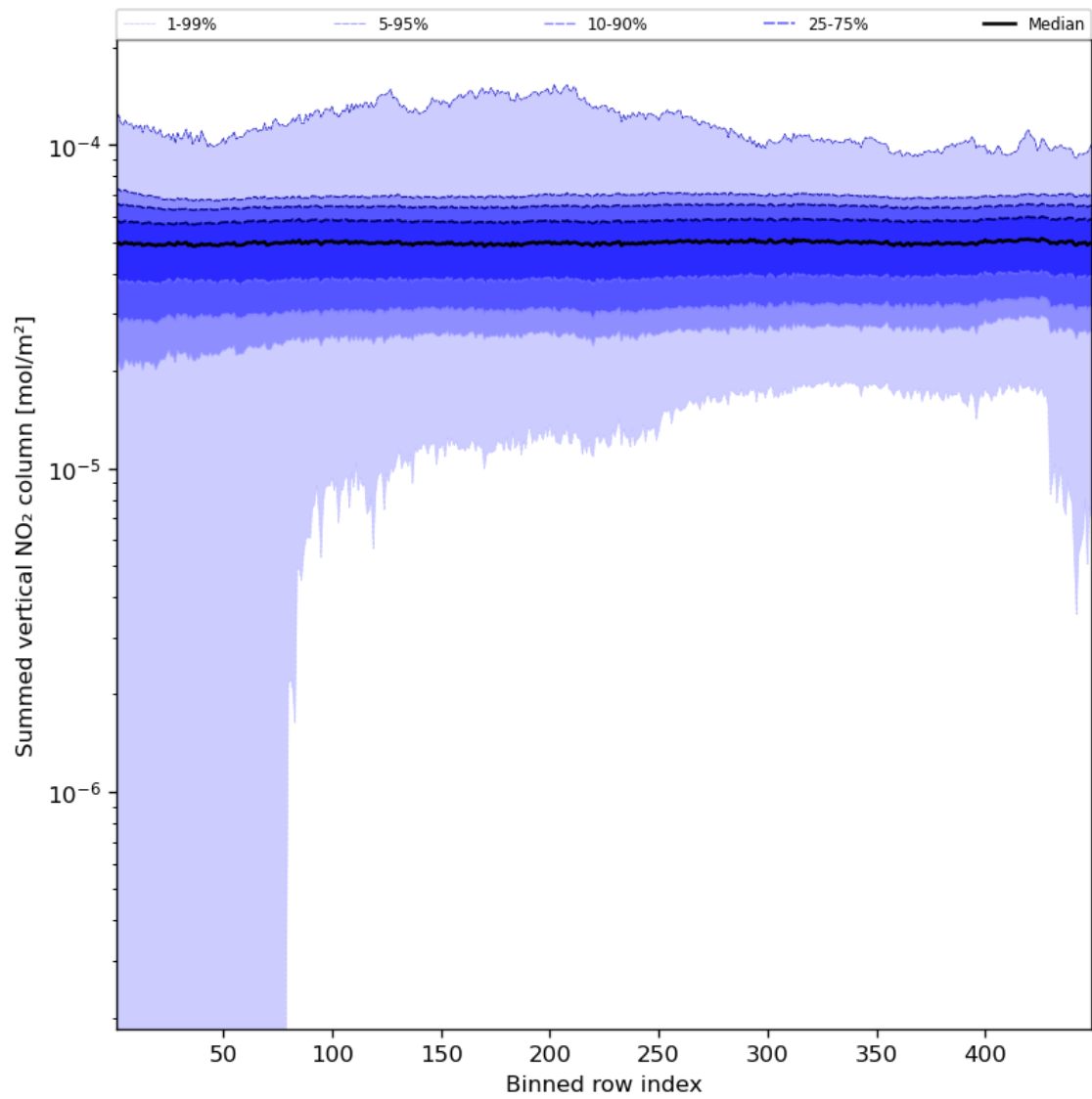
Figure 57: Along track statistics of “Summed vertical NO 2 column” for 2024-02-29 to 2024-03-02
