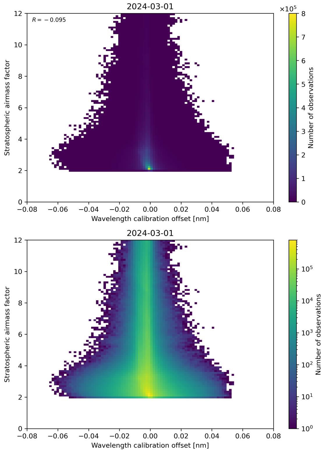
Figure 174: Scatter density plot of “Wavelength calibration offset” against “Stratospheric air mass factor” for 2024-02-29 to 2024-03-02.
