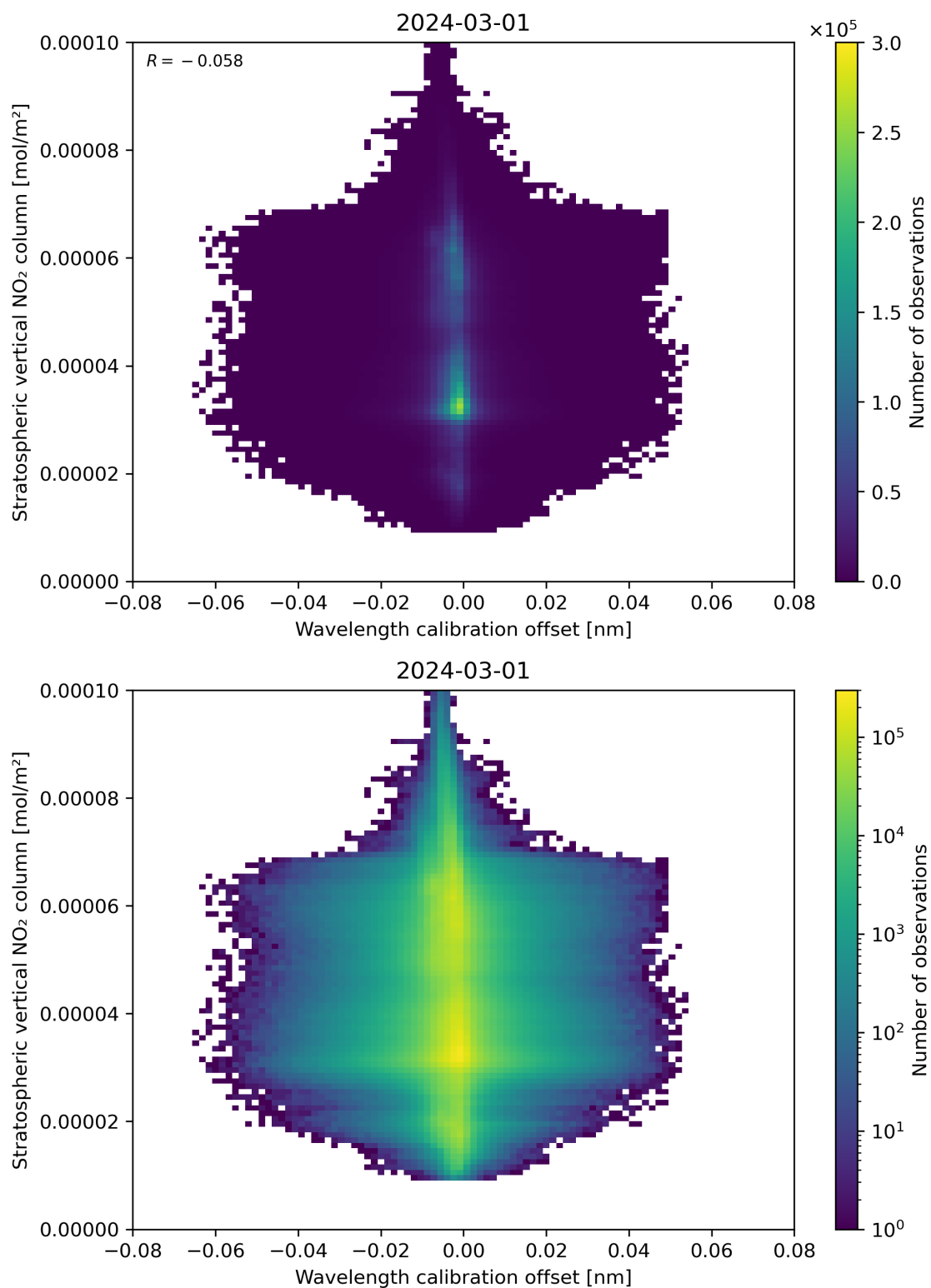
Figure 176: Scatter density plot of “Wavelength calibration offset” against “Stratospheric vertical NO 2 column” for 2024-02-29 to 2024-03-02.
