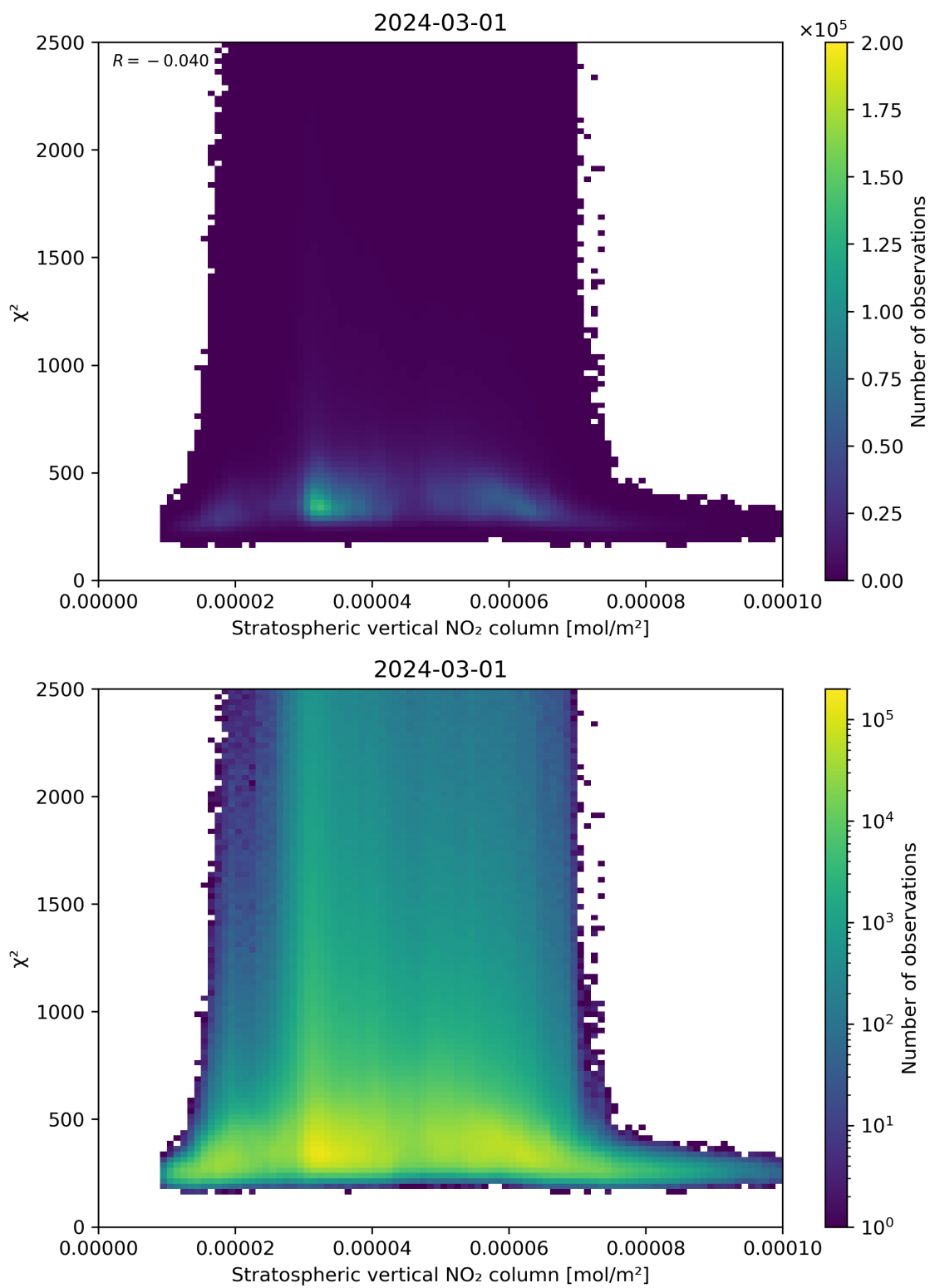
Figure 97: Scatter density plot of “Stratospheric vertical NO 2 column” against “ \chi^2 ” for 2024-02-29 to 2024-03-02.
