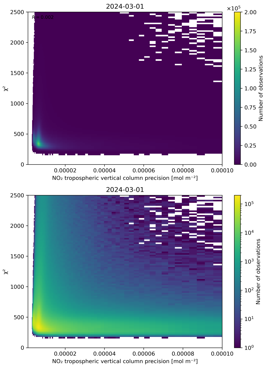
Figure 134: Scatter density plot of “NO 2 tropospheric vertical column precision” against “ \chi^2 ” for 2024-02-29 to 2024-03-02.
