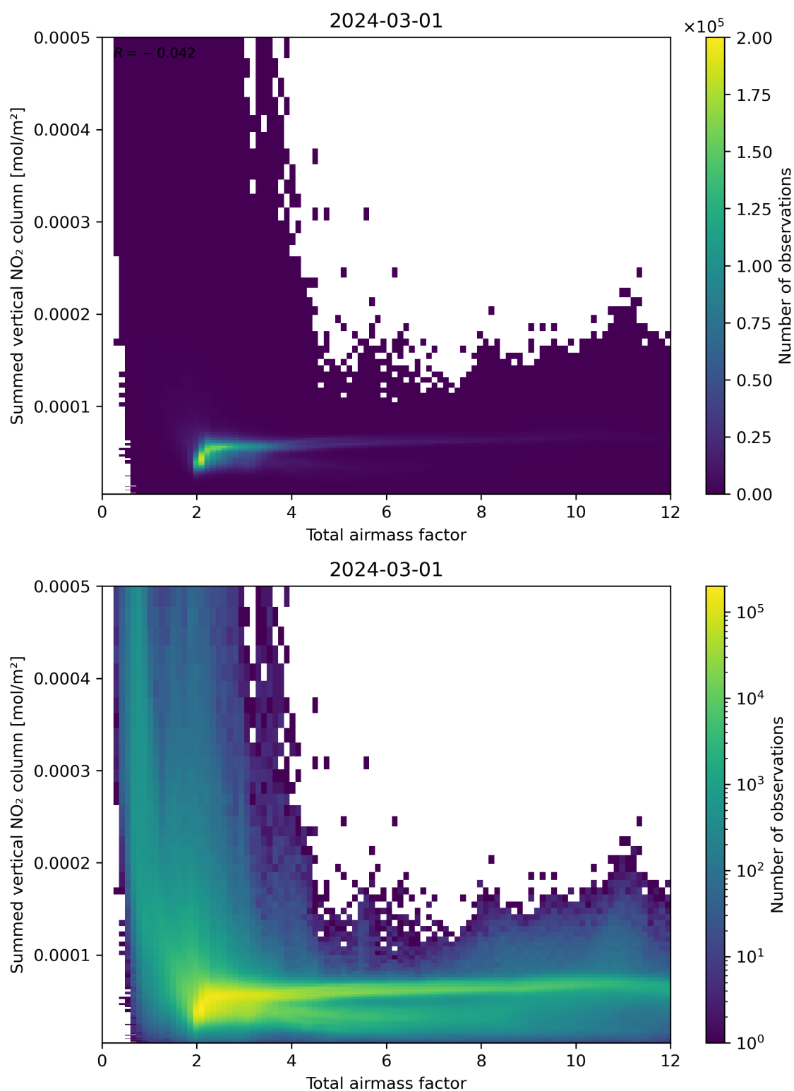
Figure 65: Scatter density plot of “Total airmass factor” against “Summed vertical NO 2 column” for 2024-02-29 to 2024-03-02.
