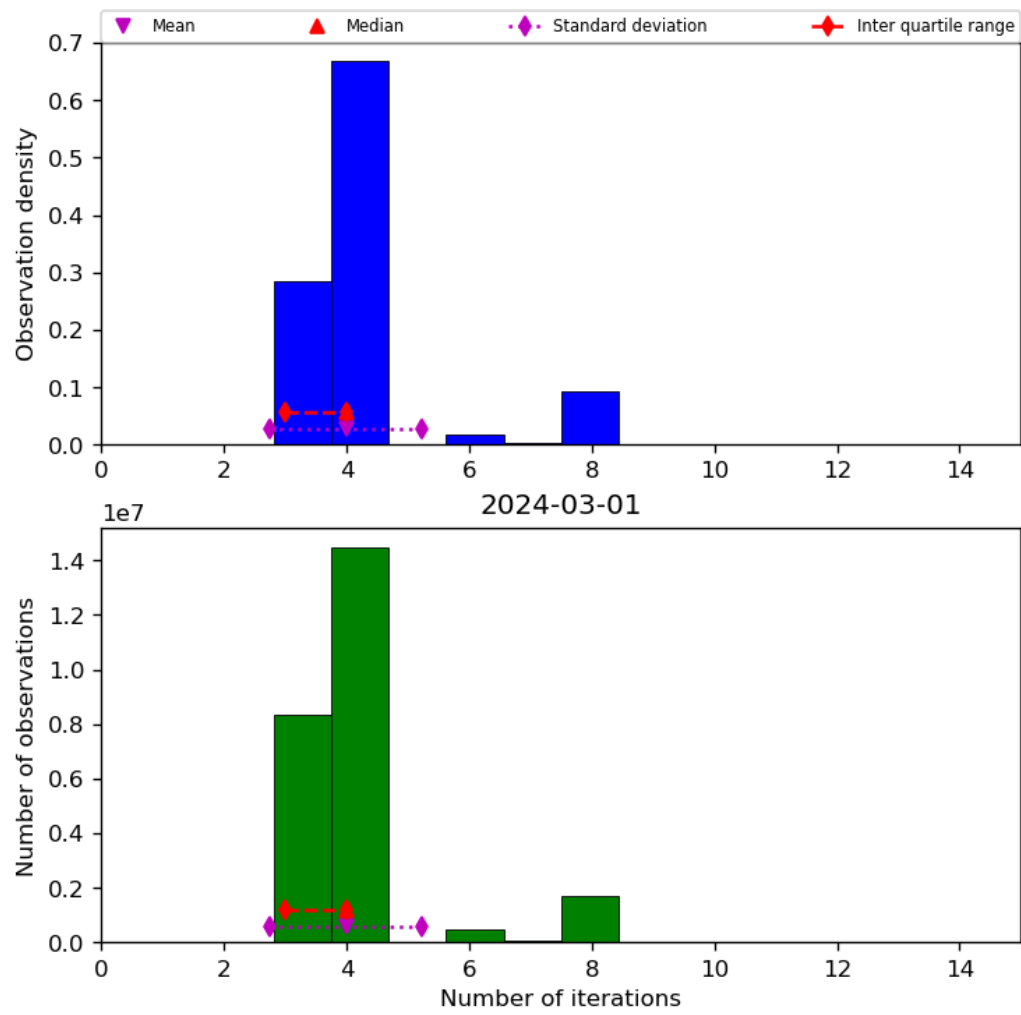
Figure 34: Histogram of “Number of iterations” for 2024-02-29 to 2024-03-02
