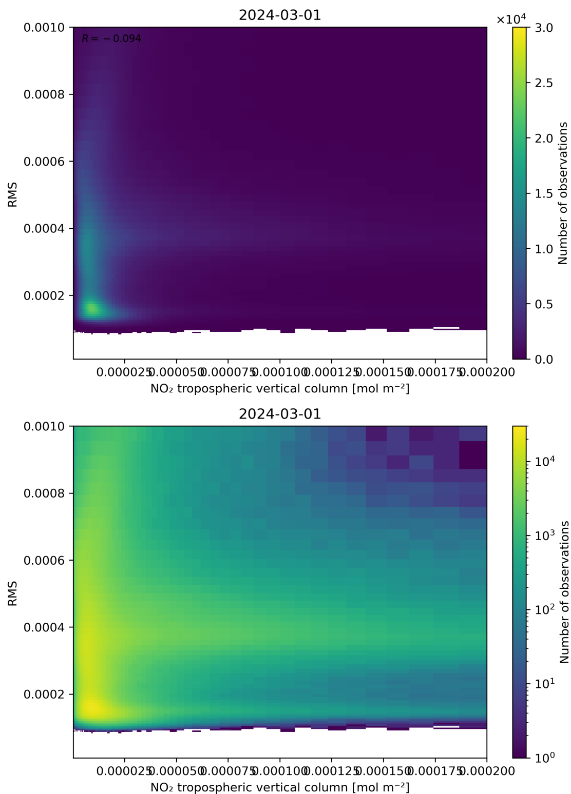
Figure 142: Scatter density plot of “NO 2 tropospheric vertical column” against “RMS” for 2024-02-29 to 2024-03-02.
