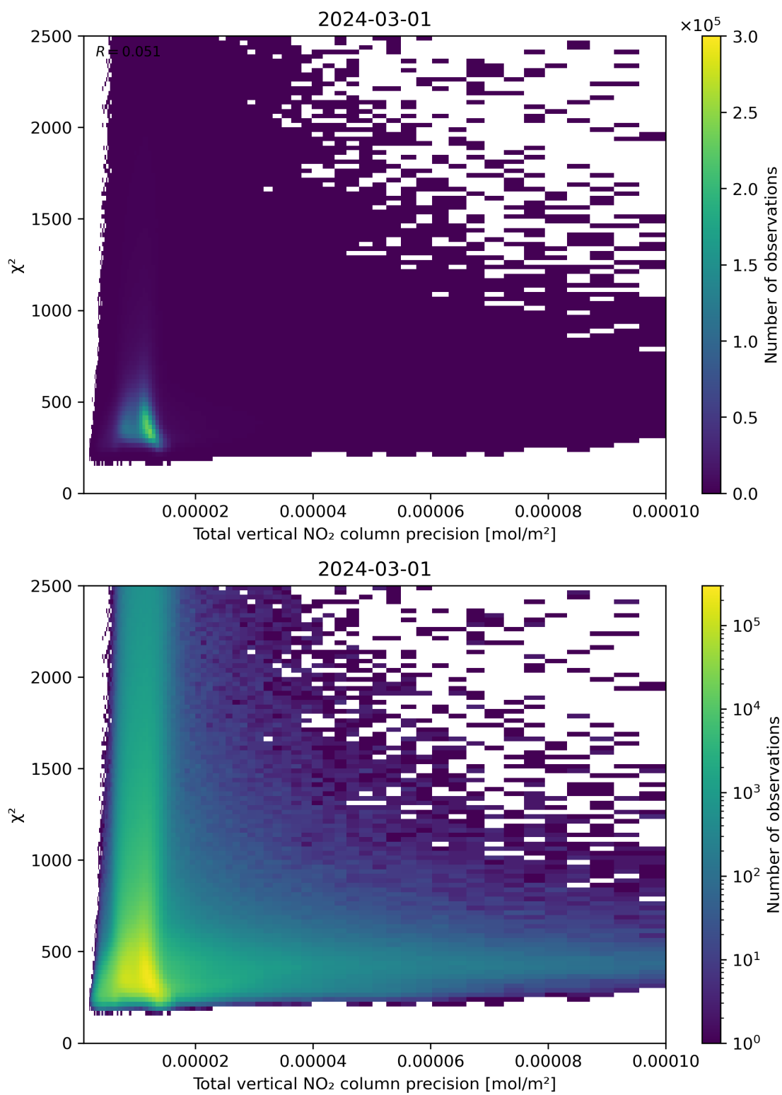
Figure 116: Scatter density plot of “Total vertical NO 2 column precision” against “ \chi^2 ” for 2024-02-29 to 2024-03-02.
