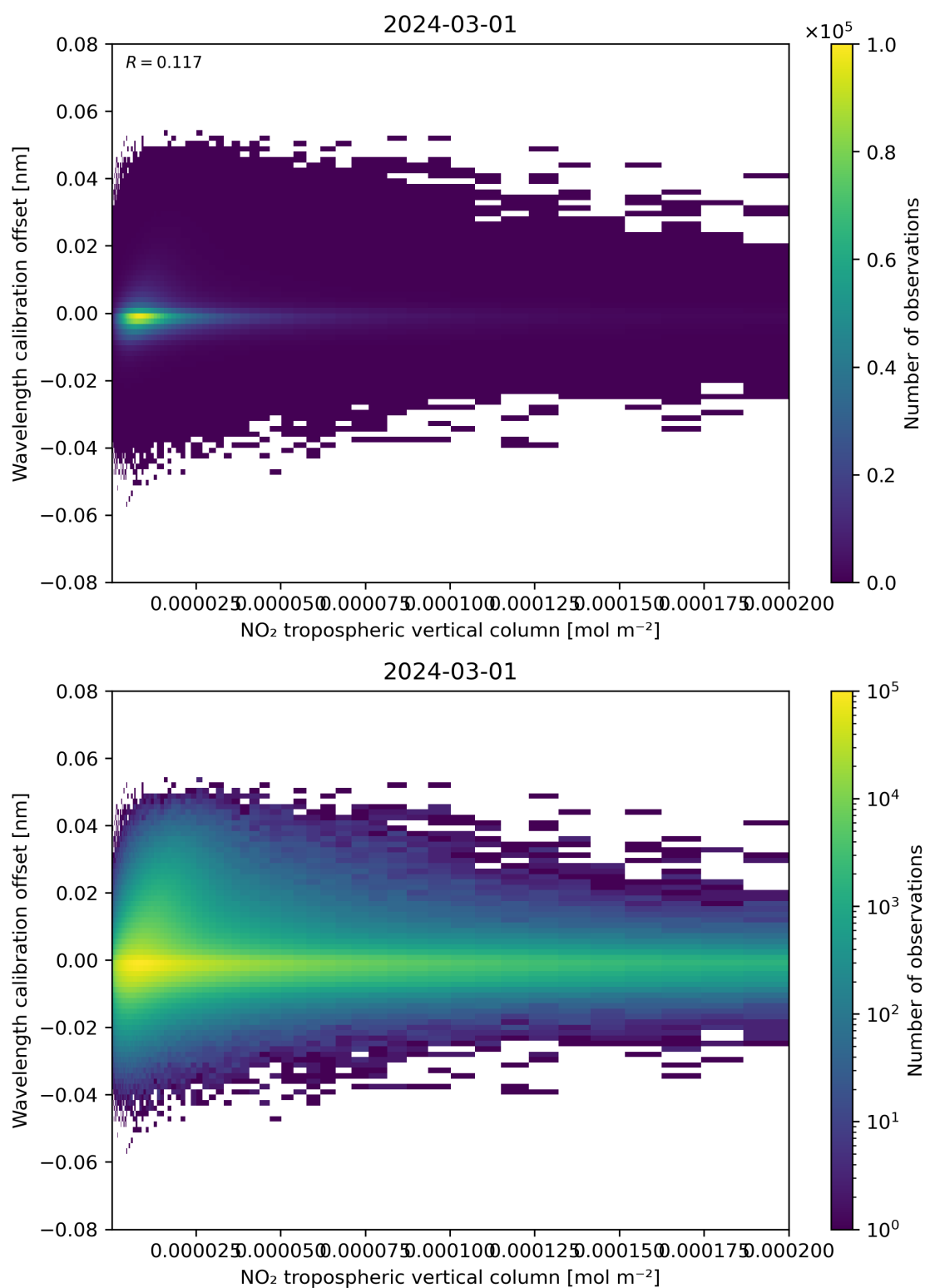
Figure 143: Scatter density plot of “NO 2 tropospheric vertical column” against “Wavelength calibration offset” for 2024-02-29 to 2024-03-02.
