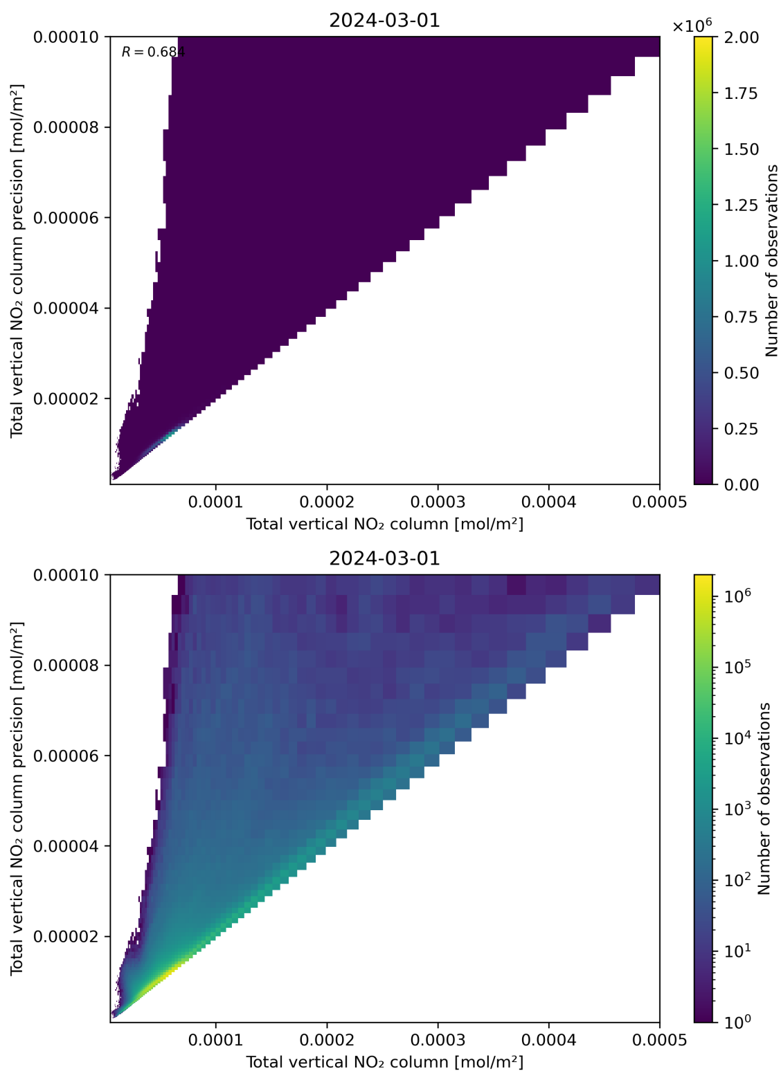
Figure 114: Scatter density plot of “Total vertical NO 2 column” against “Total vertical NO 2 column precision” for 2024-02-29 to 2024-03-02.
