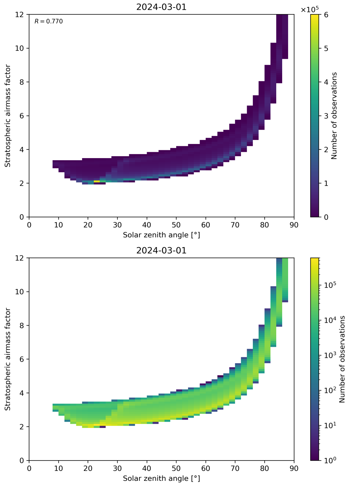
Figure 145: Scatter density plot of “Solar zenith angle” against “Stratospheric airmass factor” for 2024-02-29 to 2024-03-02.
