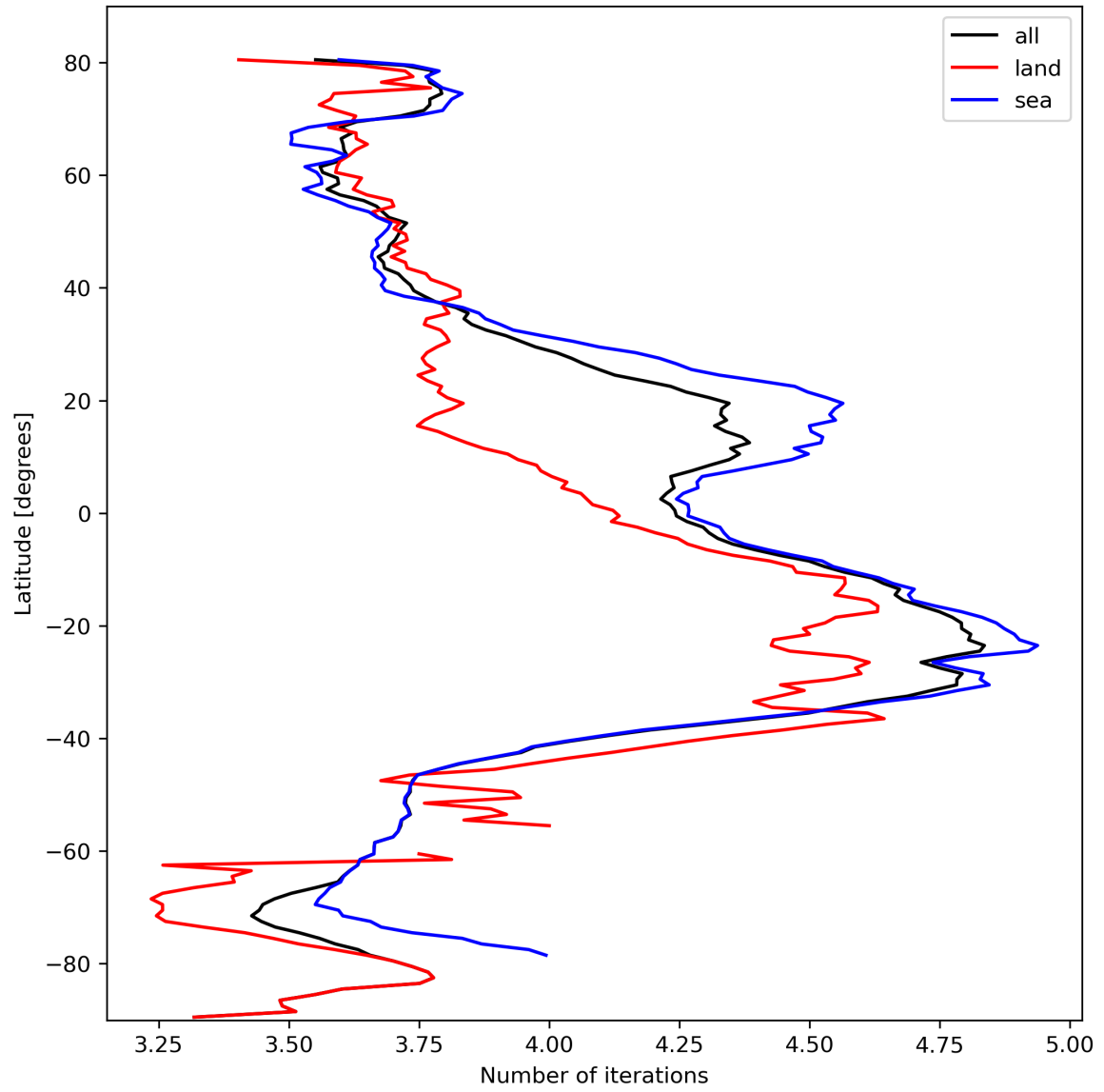
Figure 17: Zonal average of “Number of iterations” for 2024-02-29 to 2024-03-02.
