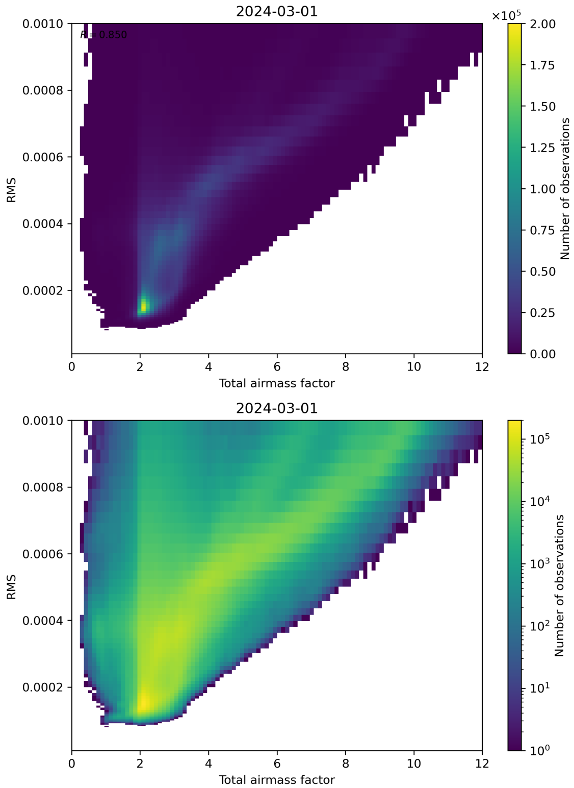
Figure 69: Scatter density plot of “Total airmass factor” against “RMS” for 2024-02-29 to 2024-03-02.
