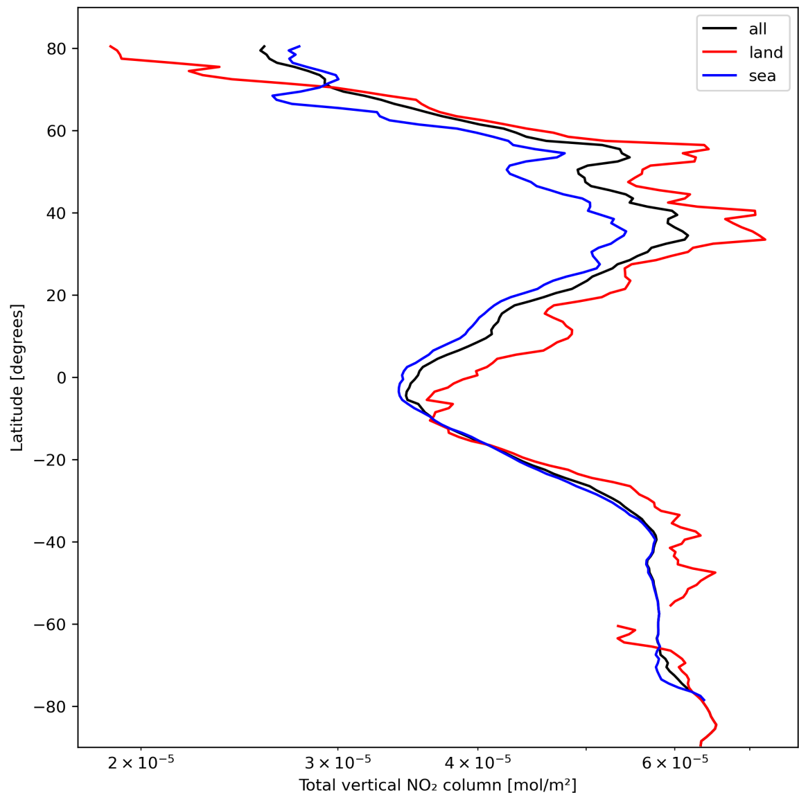
Figure 21: Zonal average of “Total vertical NO 2 column” for 2024-02-29 to 2024-03-02.
