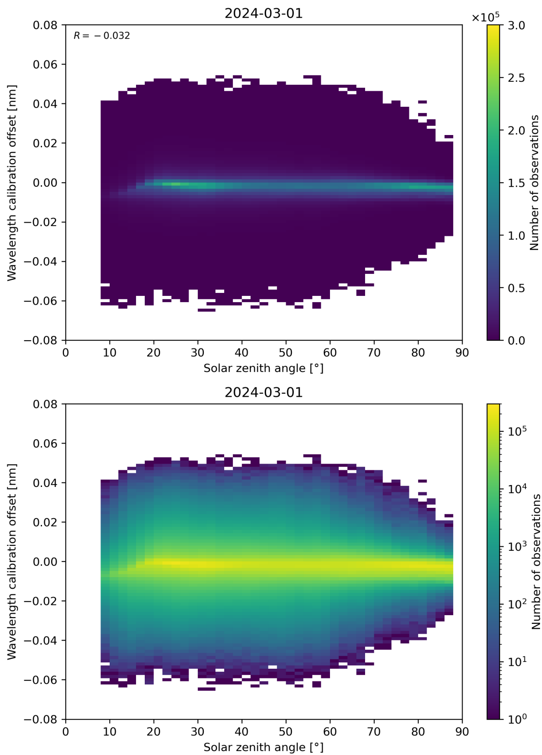
Figure 158: Scatter density plot of “Solar zenith angle” against “Wavelength calibration offset” for 2024-02-29 to 2024-03-02.
