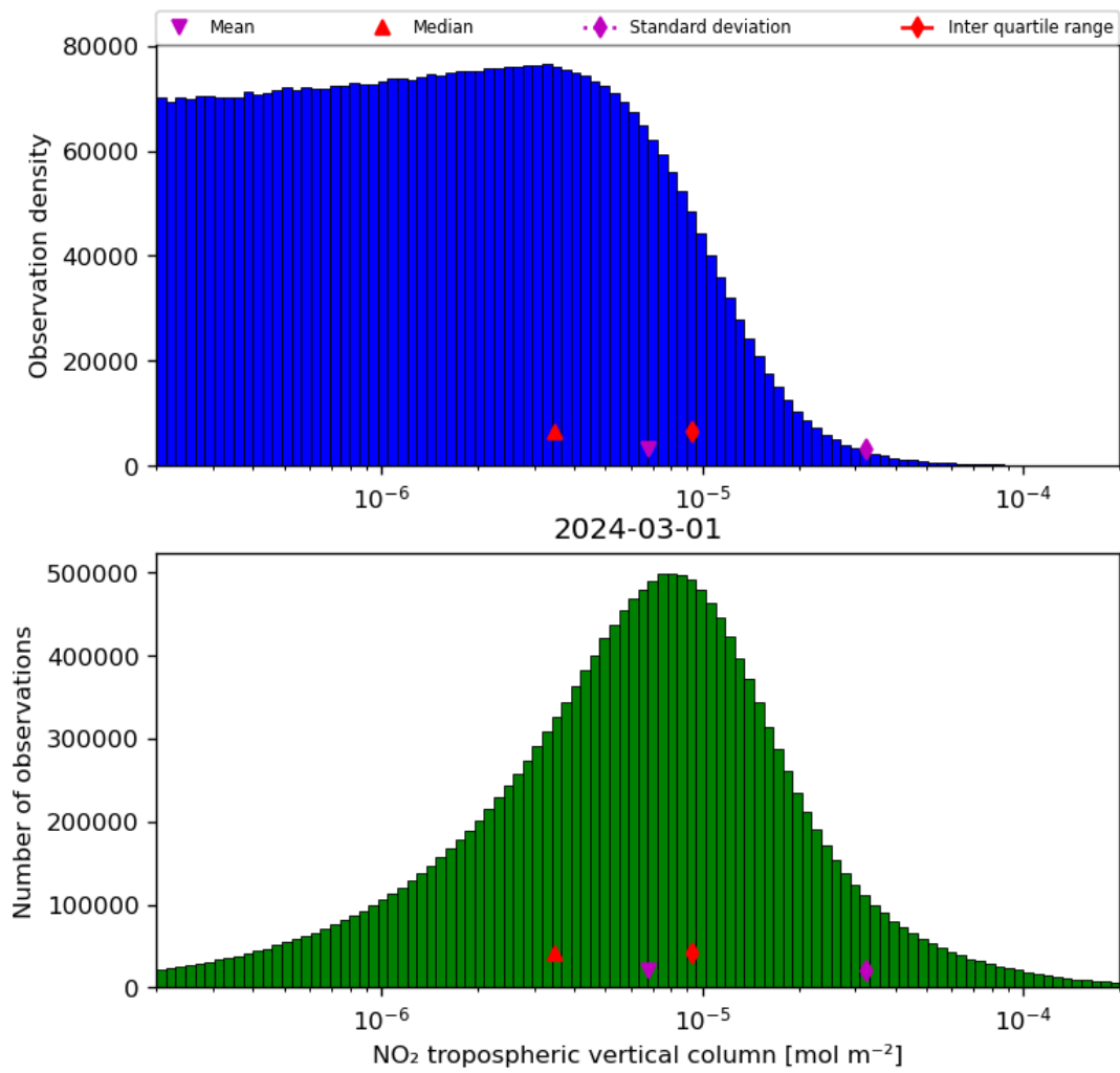
Figure 29: Histogram of “NO 2 tropospheric vertical column” for 2024-02-29 to 2024-03-02
