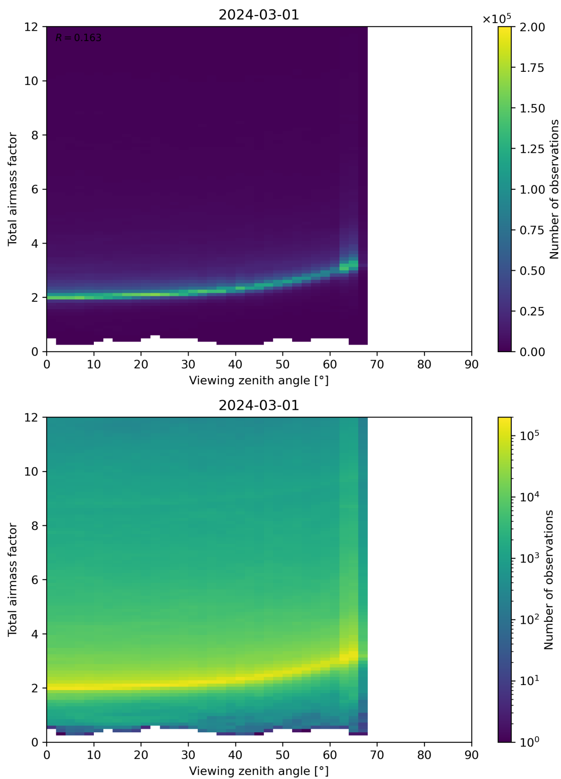
Figure 160: Scatter density plot of “Viewing zenith angle” against “Total airmass factor” for 2024-02-29 to 2024-03-02.
