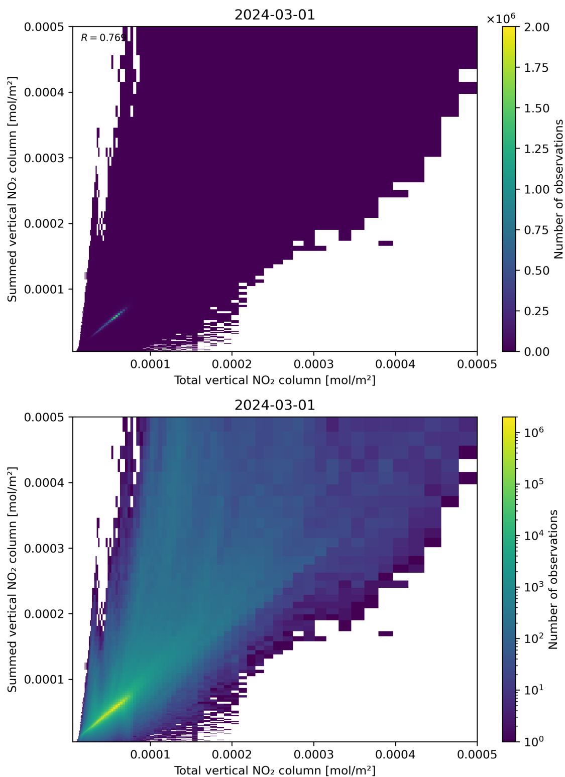
Figure 112: Scatter density plot of “Total vertical NO 2 column” against “Summed vertical NO 2 column” for 2024-02-29 to 2024-03-02.
