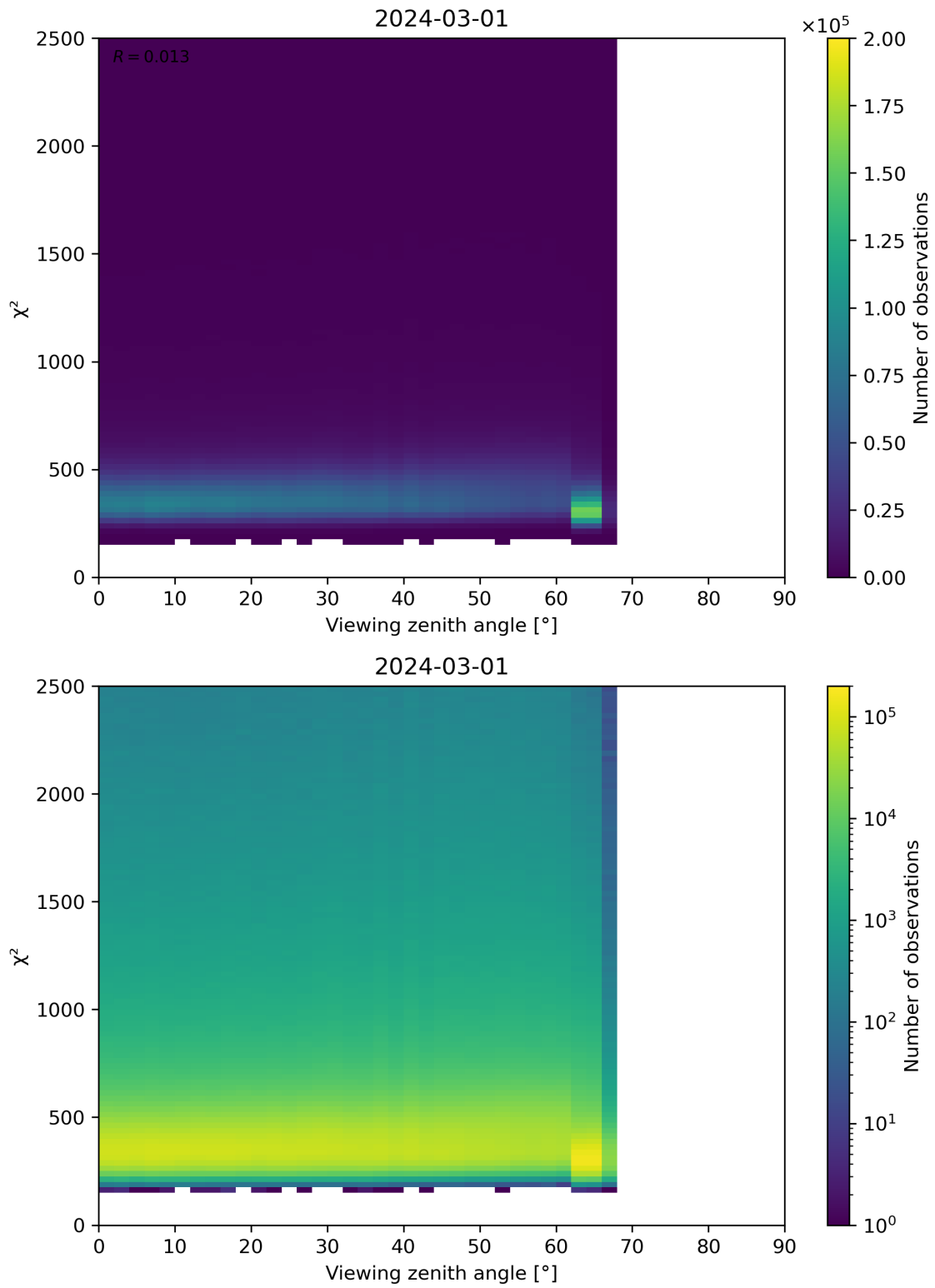
Figure 162: Scatter density plot of “Viewing zenith angle” against “ \chi^2 ” for 2024-02-29 to 2024-03-02.
