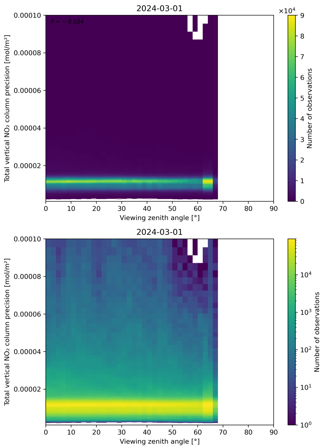
Figure 168: Scatter density plot of “Viewing zenith angle” against “Total vertical NO 2 column precision” for 2024-02-29 to 2024-03-02.
