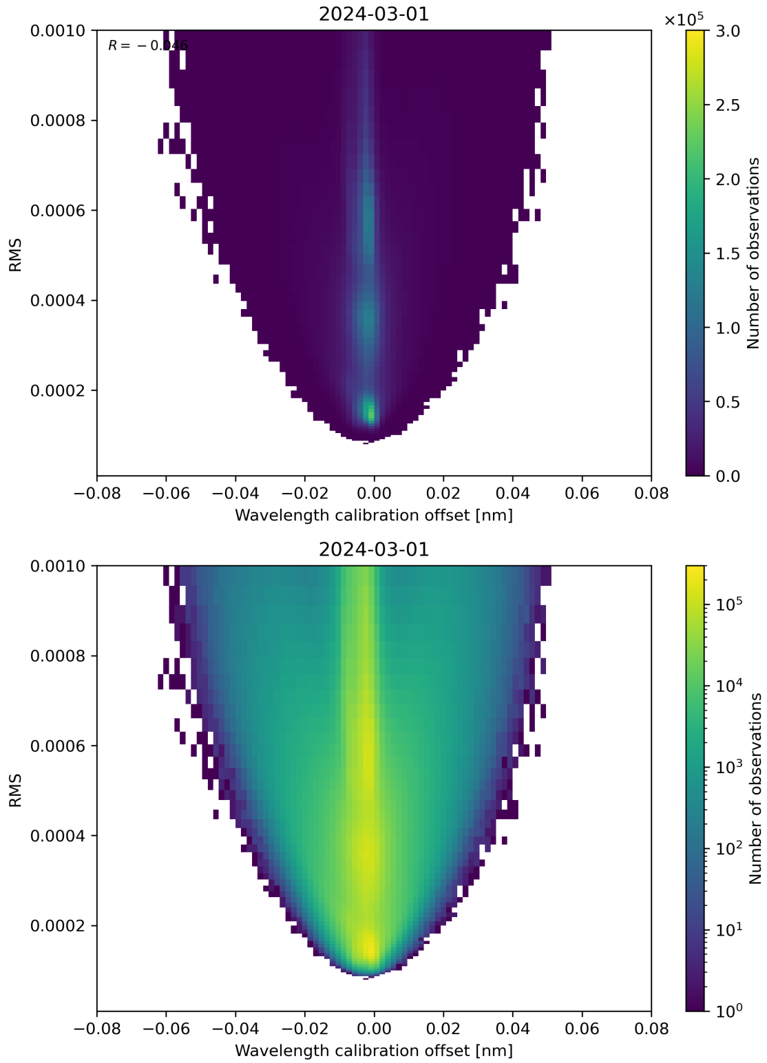
Figure 181: Scatter density plot of “Wavelength calibration offset” against “RMS” for 2024-02-29 to 2024-03-02.
