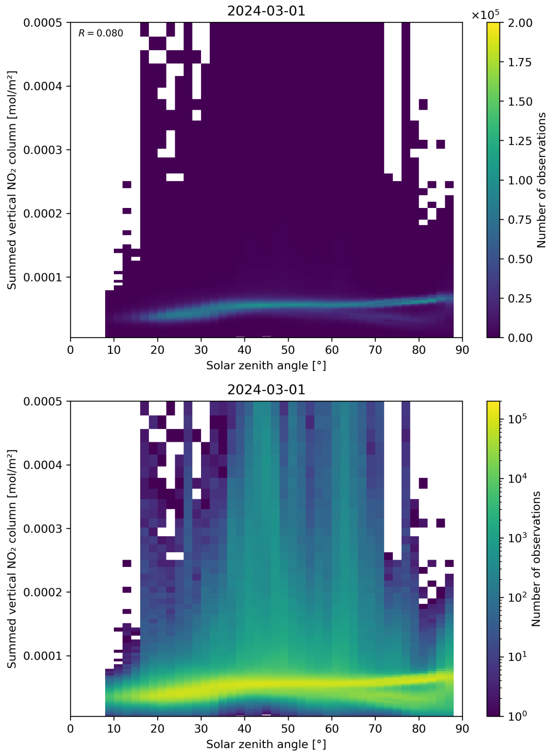
Figure 151: Scatter density plot of “Solar zenith angle” against “Summed vertical NO 2 column” for 2024-02-29 to 2024-03-02.
