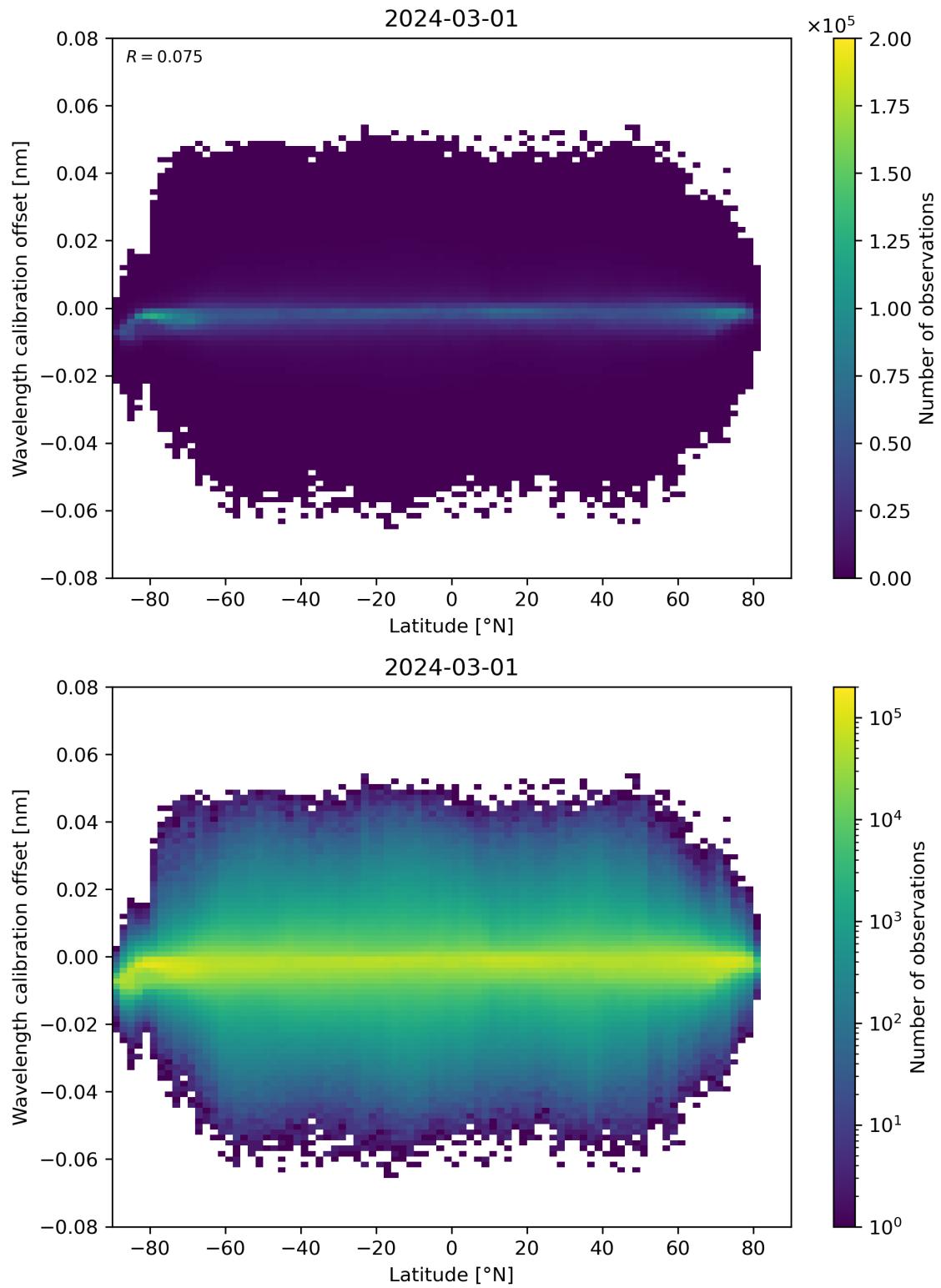
Figure 95: Scatter density plot of “Latitude” against “Wavelength calibration offset” for 2024-02-29 to 2024-03-02.
