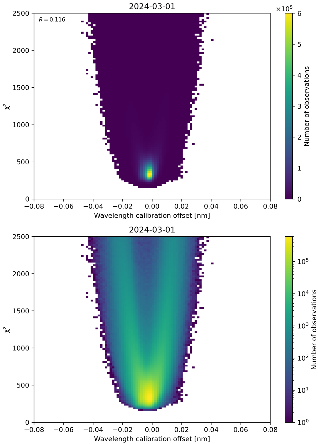
Figure 175: Scatter density plot of “Wavelength calibration offset” against “ \chi^2 ” for 2024-02-29 to 2024-03-02.
