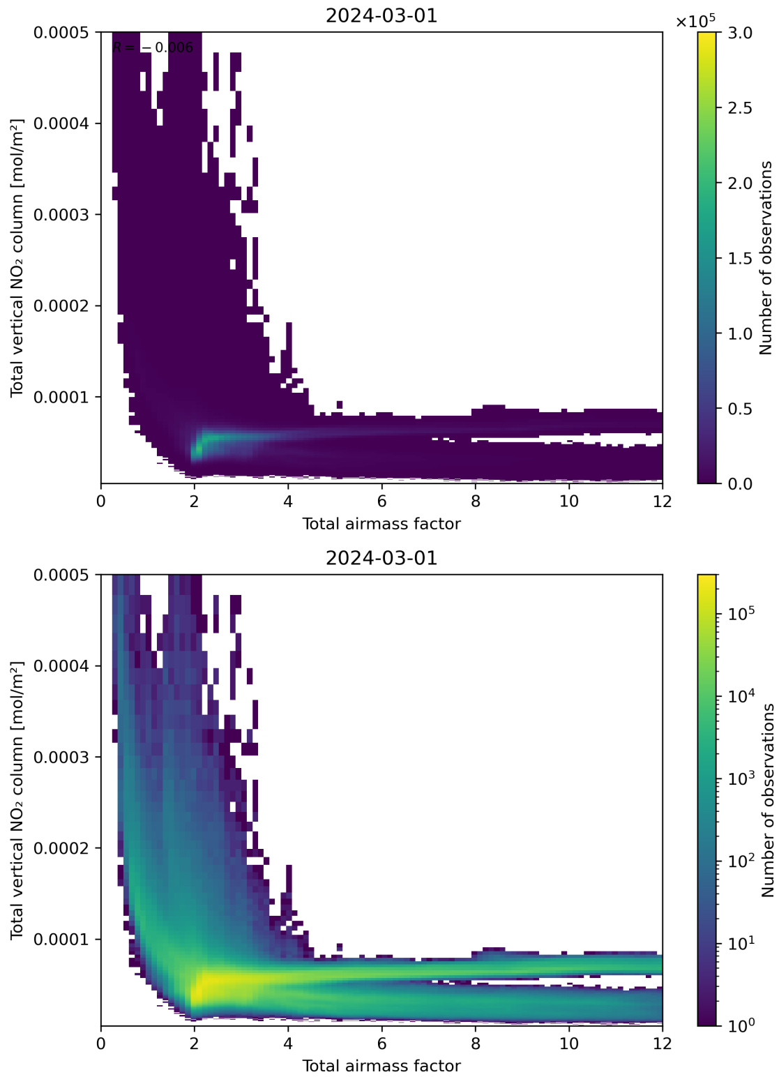
Figure 67: Scatter density plot of “Total airmass factor” against “Total vertical NO 2 column” for 2024-02-29 to 2024-03-02.
