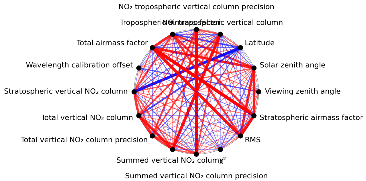
Figure 1: Map of correlation graph for 2024-02-29 to 2024-03-02.
