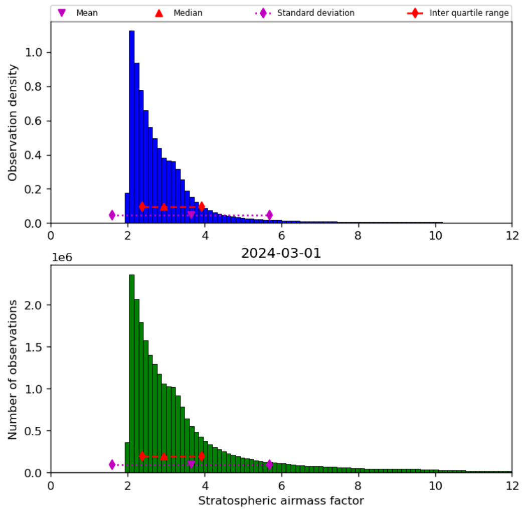
Figure 44: Histogram of “Stratospheric airmass factor” for 2024-02-29 to 2024-03-02
