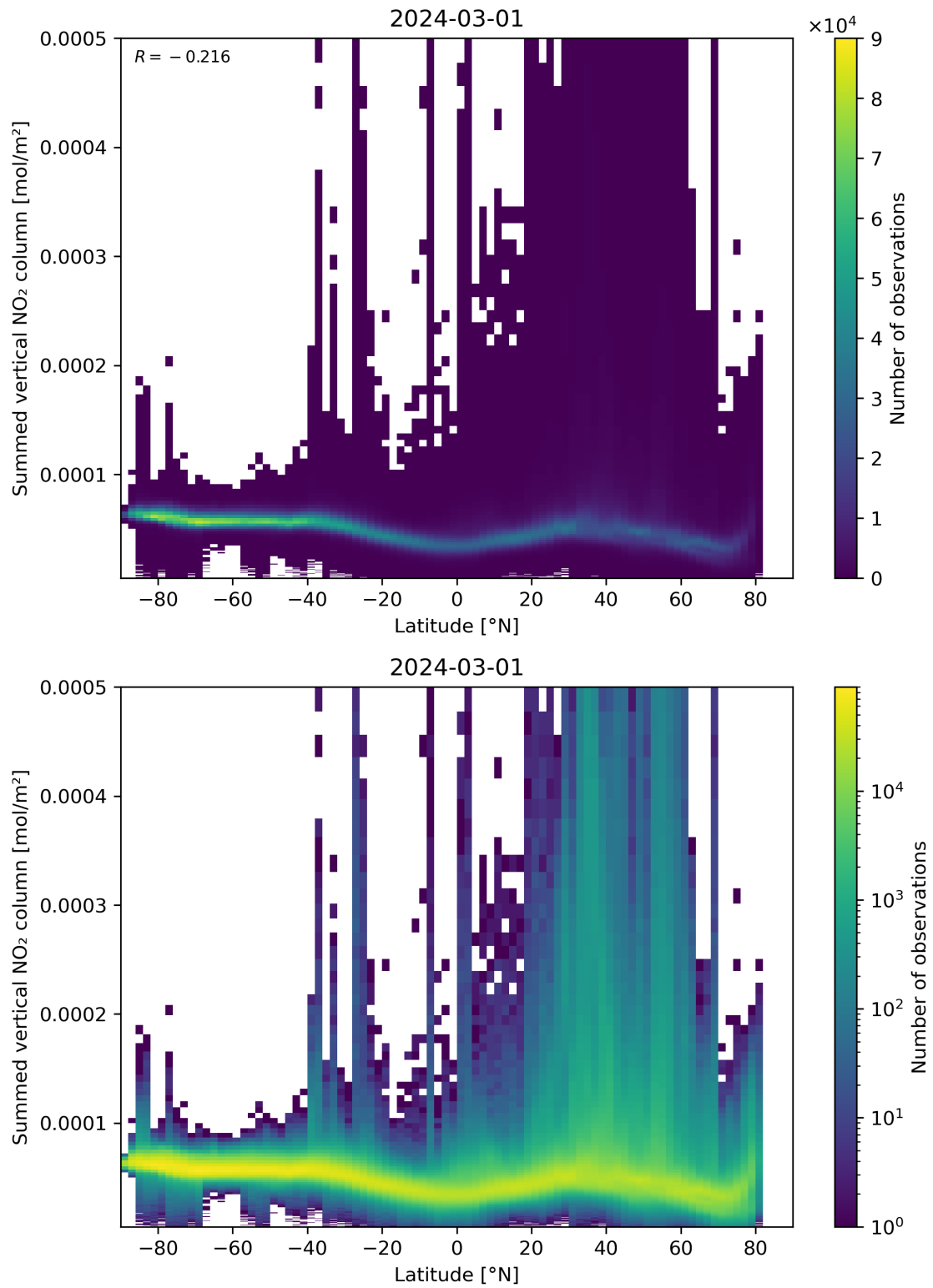
Figure 88: Scatter density plot of “Latitude” against “Summed vertical NO 2 column” for 2024-02-29 to 2024-03-02.
