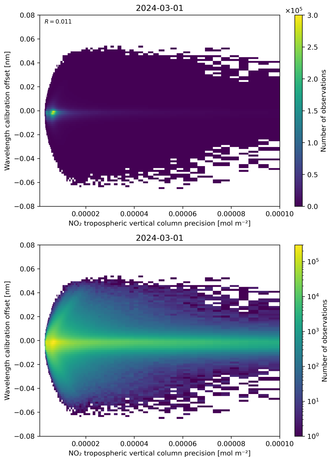
Figure 141: Scatter density plot of “NO 2 tropospheric vertical column precision” against “Wavelength calibration offset” for 2024-02-29 to 2024-03-02.
