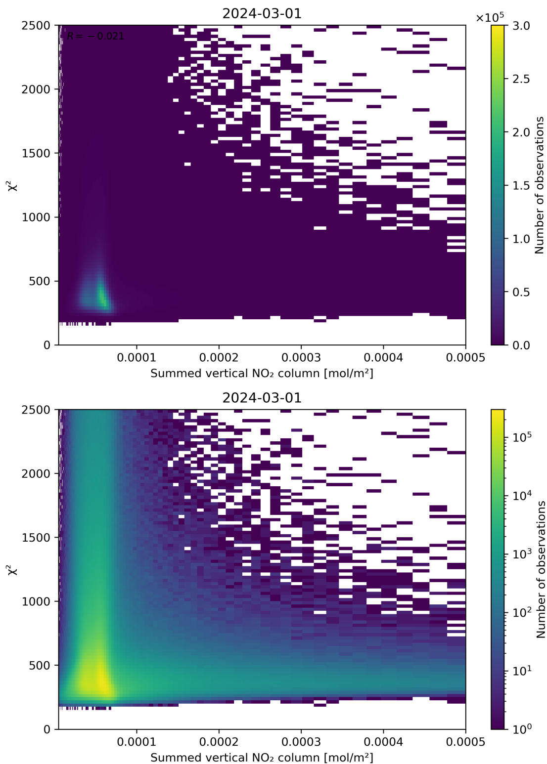
Figure 104: Scatter density plot of “Summed vertical NO 2 column” against “ \chi^2 ” for 2024-02-29 to 2024-03-02.
