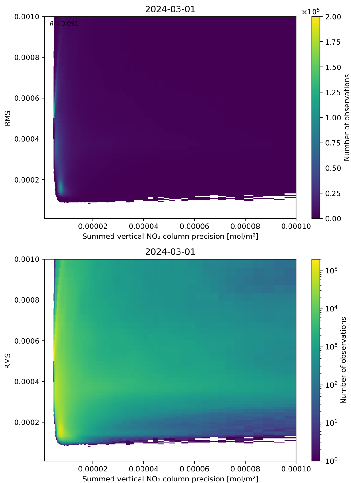
Figure 108: Scatter density plot of “Summed vertical NO 2 column precision” against “RMS” for 2024-02-29 to 2024-03-02.
