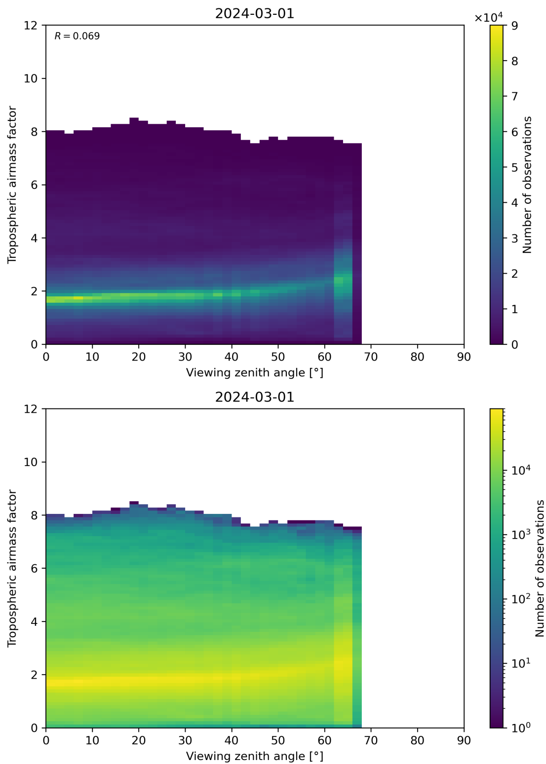
Figure 161: Scatter density plot of “Viewing zenith angle” against “Tropospheric airmass factor” for 2024-02-29 to 2024-03-02.
