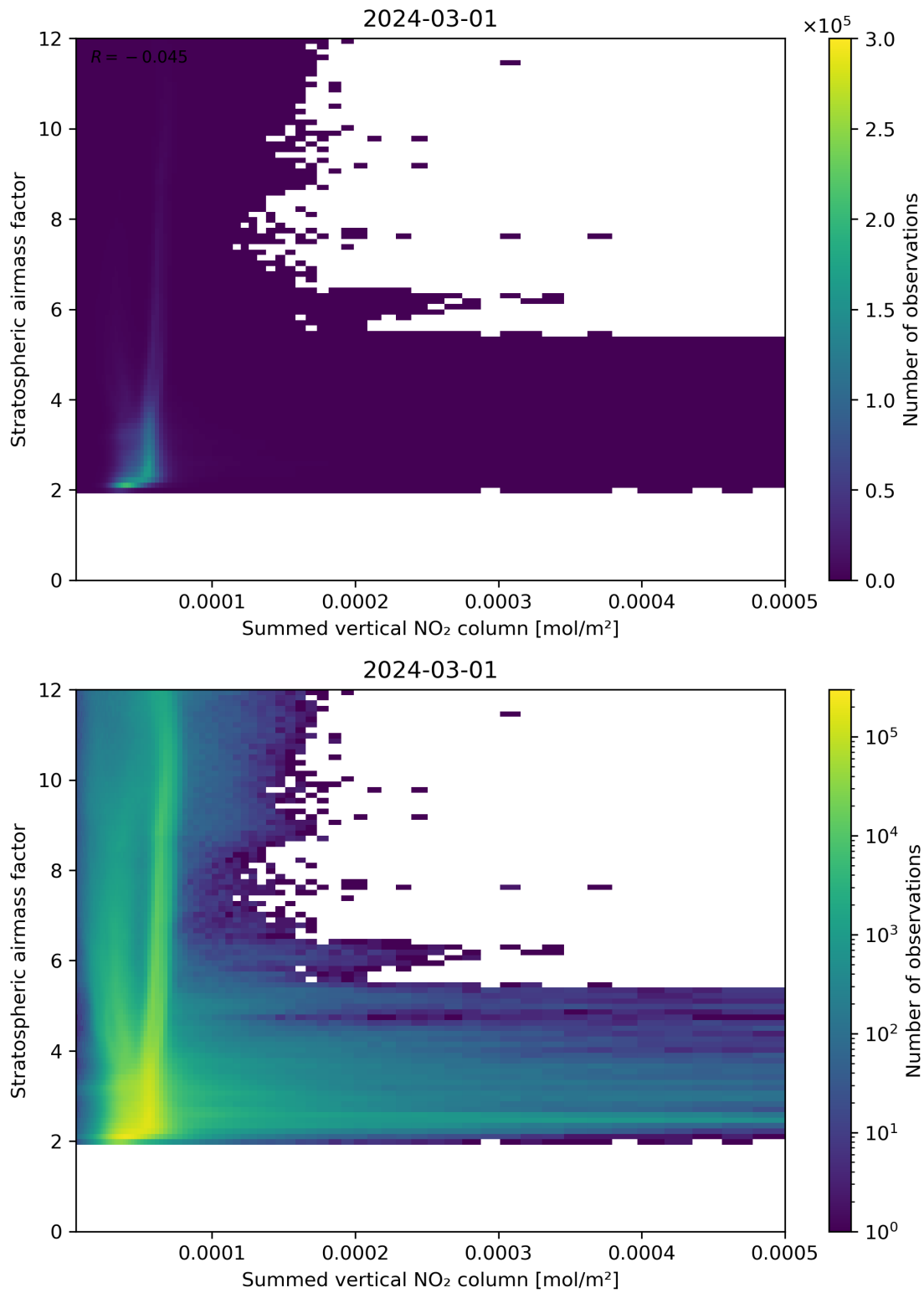
Figure 103: Scatter density plot of “Summed vertical NO 2 column” against “Stratospheric air mass factor” for 2024-02-29 to 2024-03-02.
