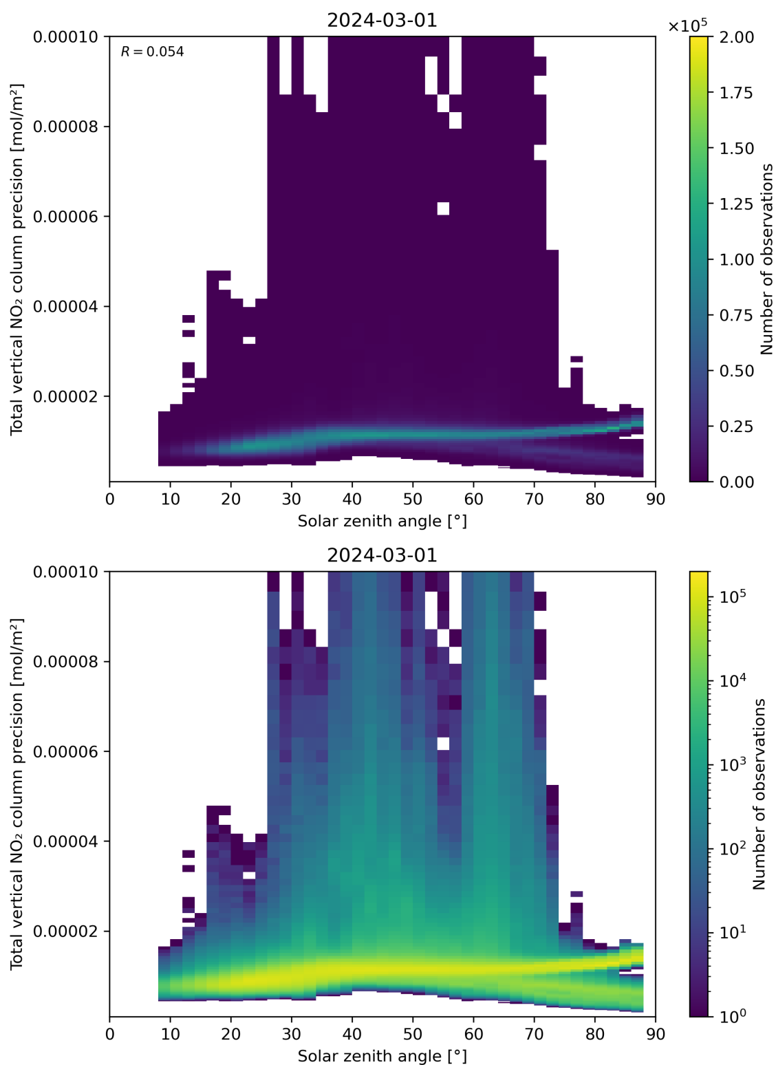
Figure 154: Scatter density plot of “Solar zenith angle” against “Total vertical NO 2 column precision” for 2024-02-29 to 2024-03-02.
