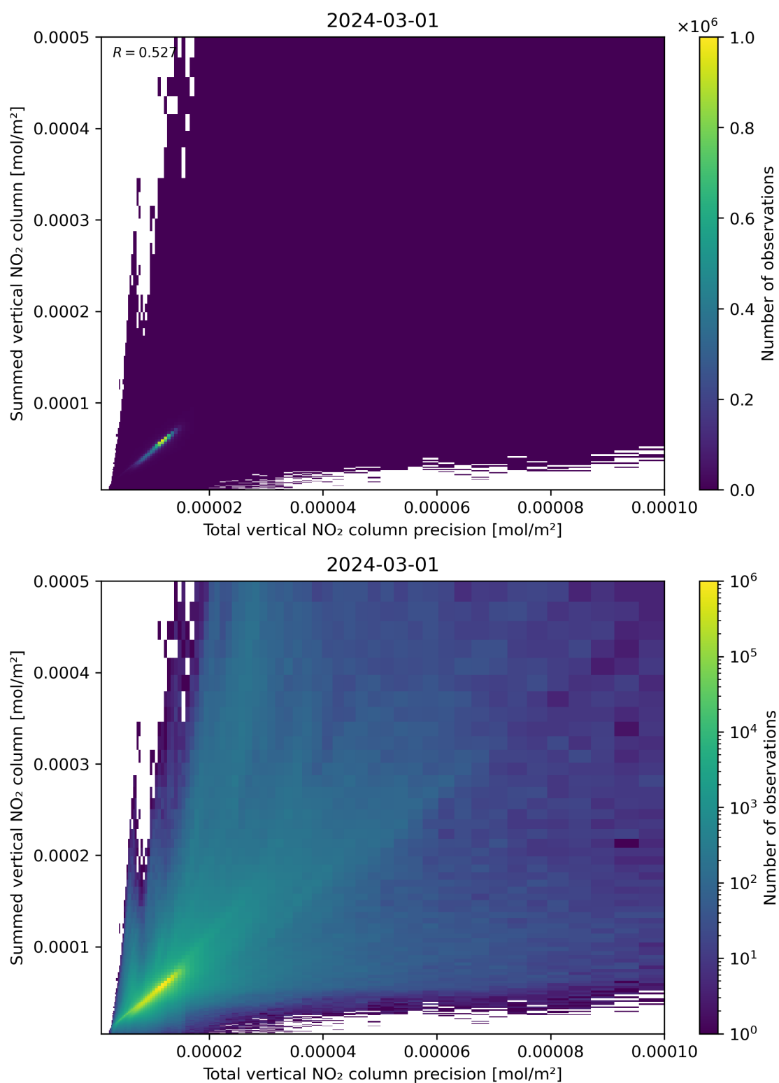
Figure 117: Scatter density plot of “Total vertical NO 2 column precision” against “Summed vertical NO 2 column” for 2024-02-29 to 2024-03-02.
