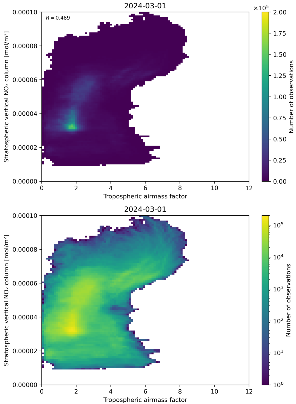
Figure 74: Scatter density plot of “Tropospheric air mass factor” against “Stratospheric vertical NO 2 column” for 2024-02-29 to 2024-03-02.
