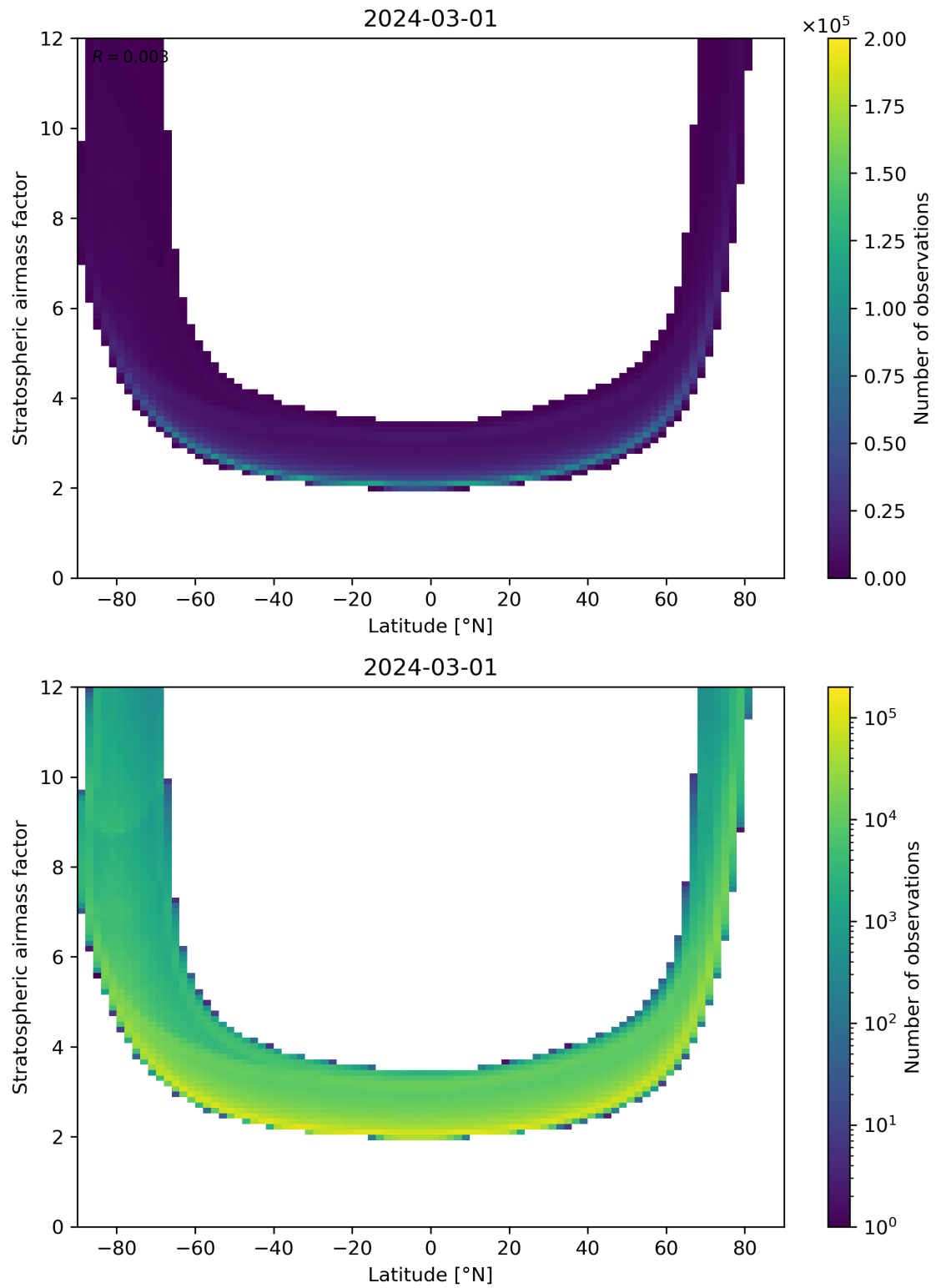
Figure 83: Scatter density plot of “Latitude” against “Stratospheric air mass factor” for 2024-02-29 to 2024-03-02.
