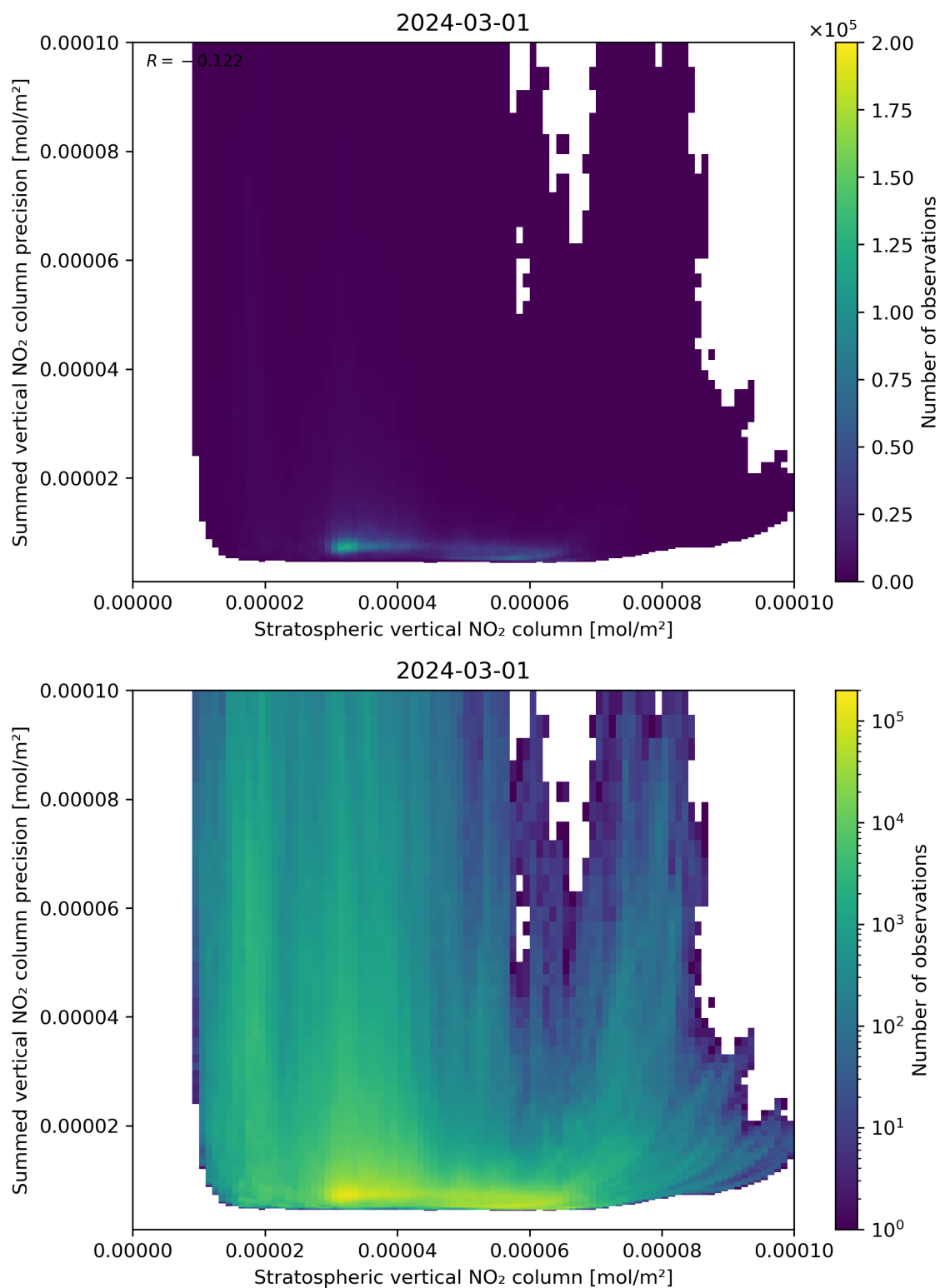
Figure 99: Scatter density plot of “Stratospheric vertical NO 2 column” against “Summed vertical NO 2 column precision” for 2024-02-29 to 2024-03-02.
