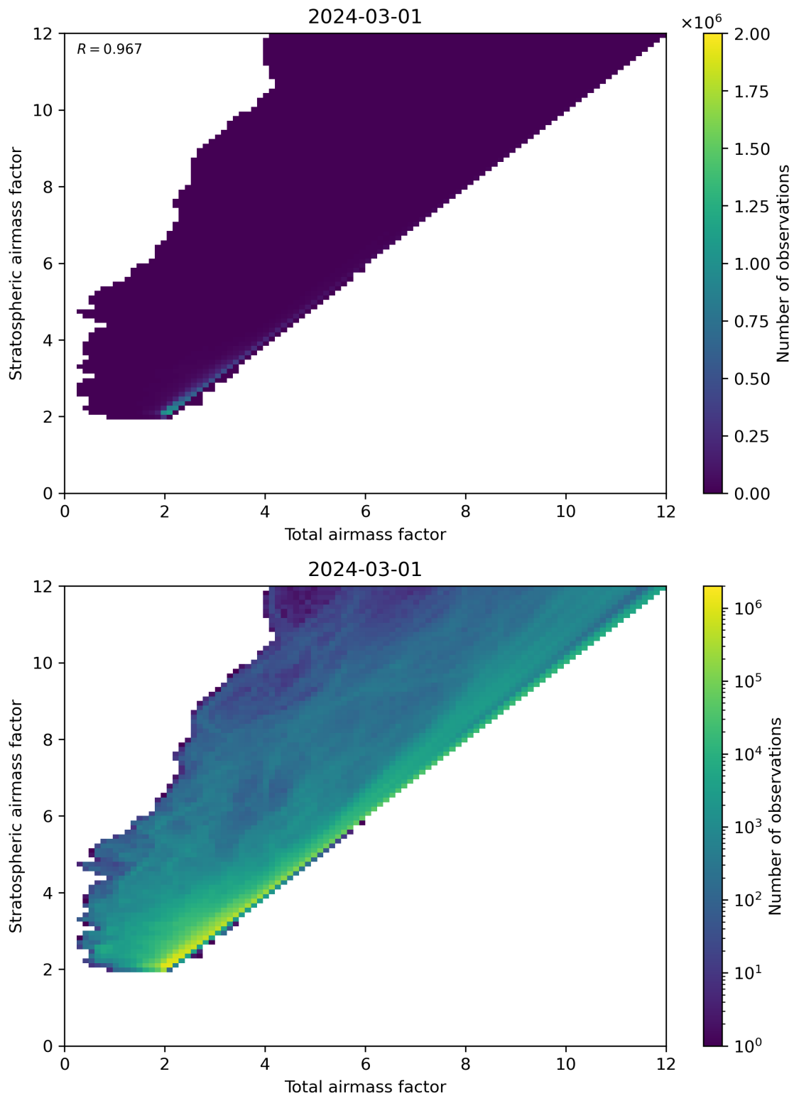
Figure 62: Scatter density plot of “Total airmass factor” against “Stratospheric airmass factor” for 2024-02-29 to 2024-03-02.
