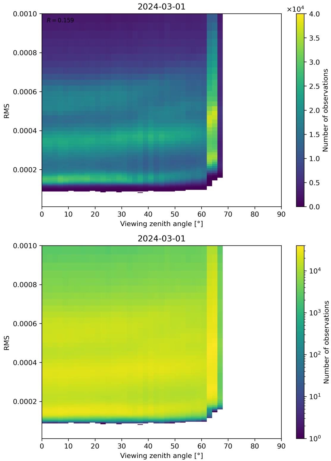
Figure 171: Scatter density plot of “Viewing zenith angle” against “RMS” for 2024-02-29 to 2024-03-02.
