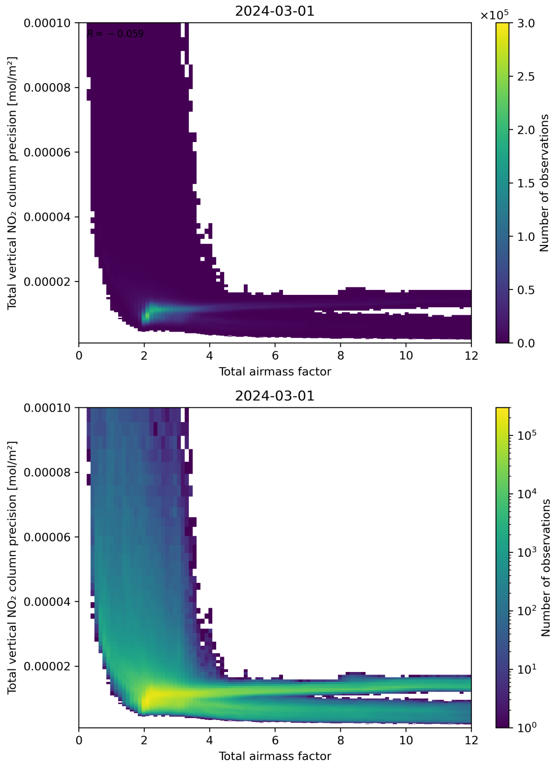
Figure 68: Scatter density plot of “Total airmass factor” against “Total vertical NO 2 column precision” for 2024-02-29 to 2024-03-02.
