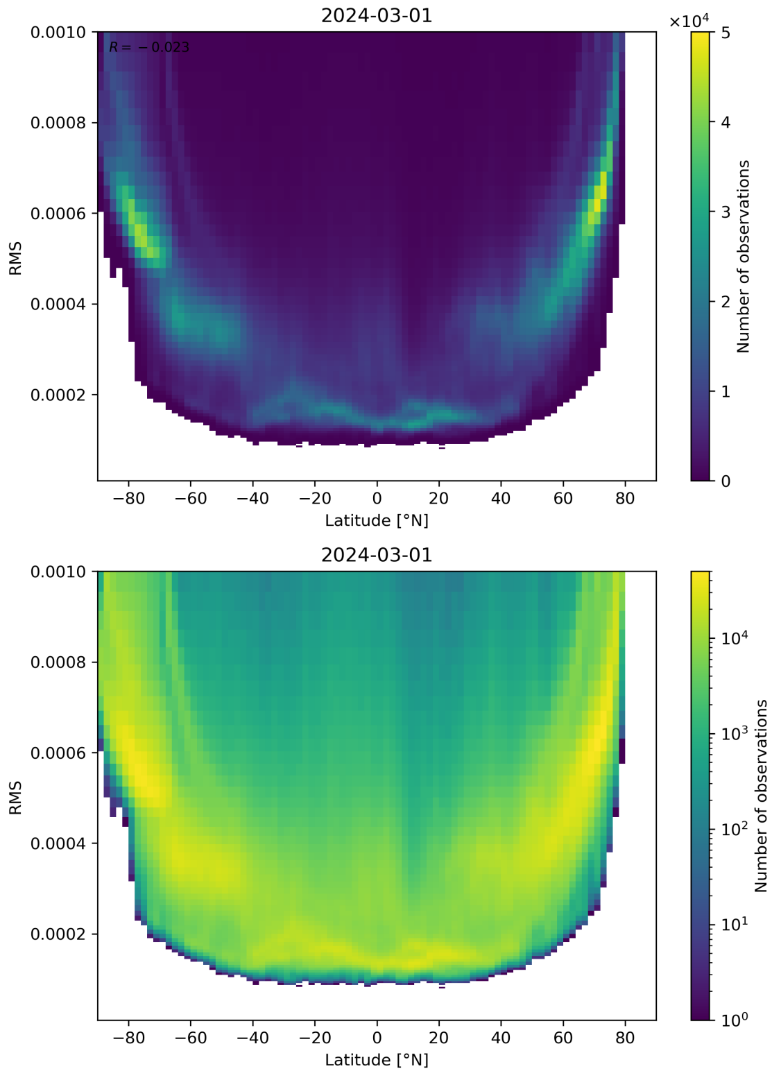
Figure 94: Scatter density plot of “Latitude” against “RMS” for 2024-02-29 to 2024-03-02.
