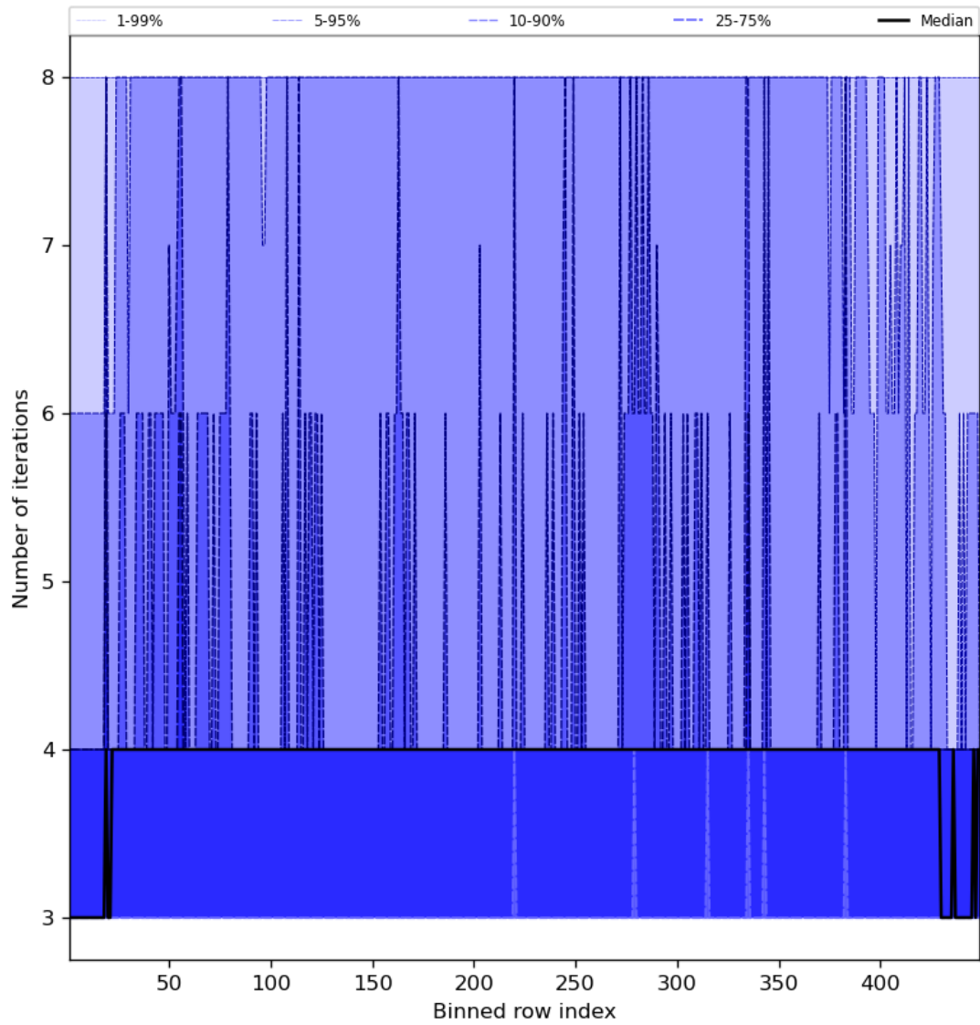
Figure 51: Along track statistics of “Number of iterations” for 2024-02-29 to 2024-03-02
