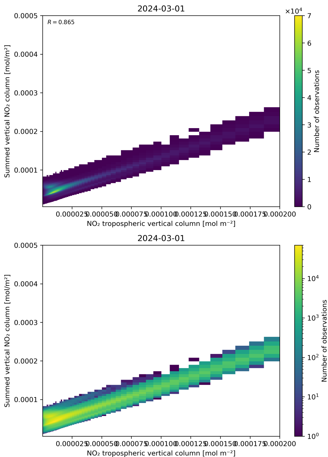
Figure 126: Scatter density plot of “NO 2 tropospheric vertical column” against “Summed vertical NO 2 column” for 2024-02-29 to 2024-03-02.
