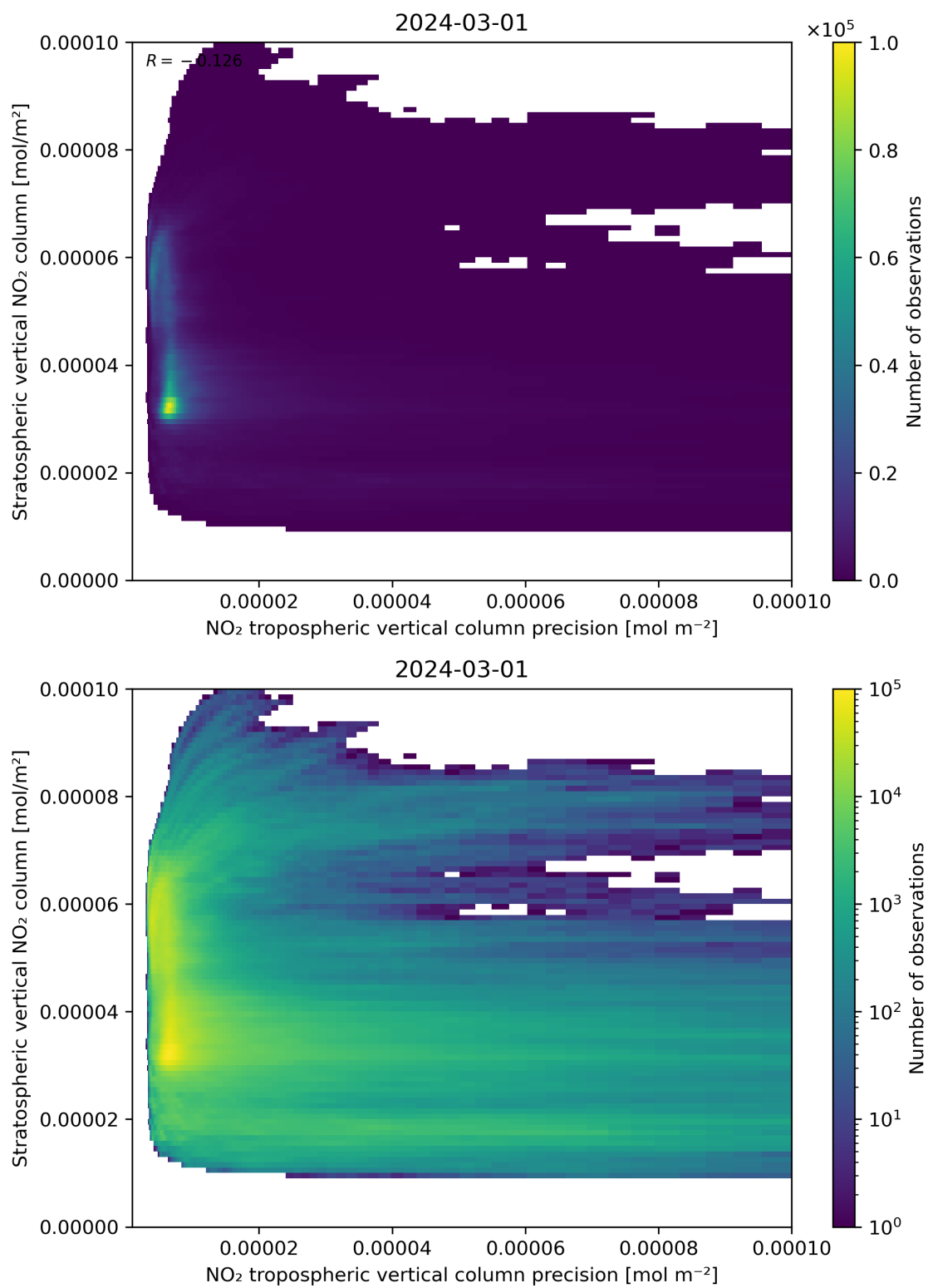
Figure 135: Scatter density plot of “NO 2 tropospheric vertical column precision” against “Stratospheric vertical NO 2 column” for 2024-02-29 to 2024-03-02.
