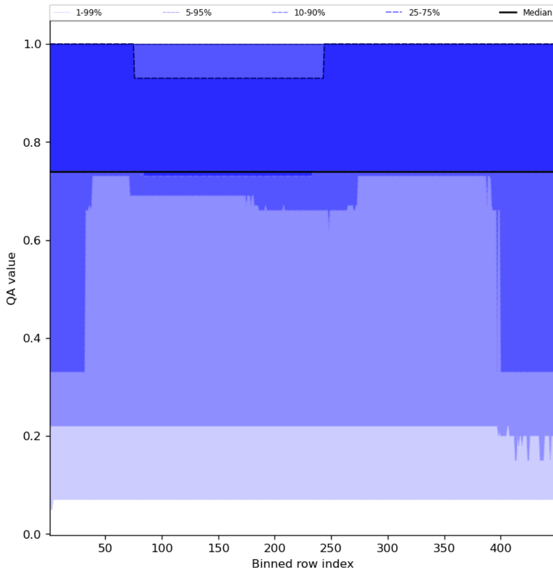
Figure 45: Along track statistics of “QA value” for 2024-02-29 to 2024-03-02
