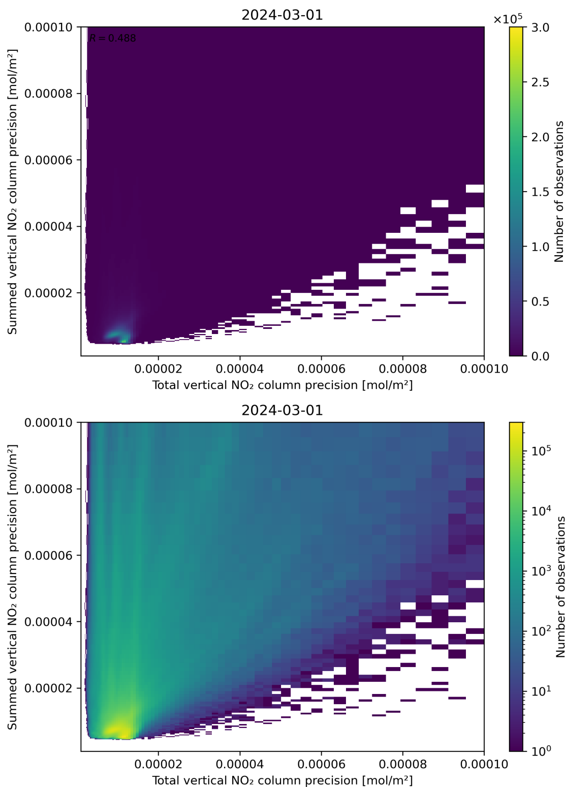
Figure 118: Scatter density plot of “Total vertical NO 2 column precision” against “Summed vertical NO 2 column precision” for 2024-02-29 to 2024-03-02.
