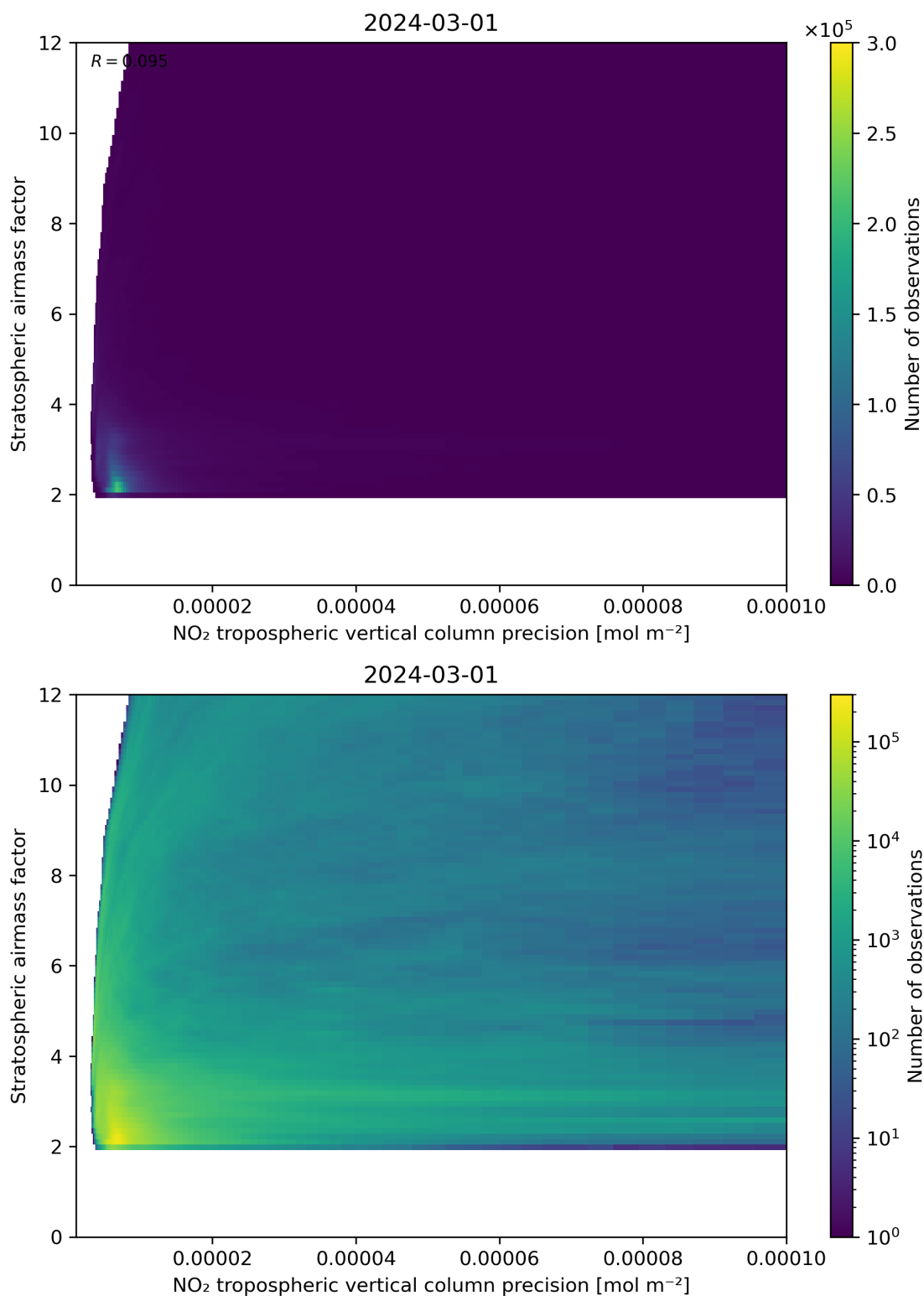
Figure 131: Scatter density plot of “NO 2 tropospheric vertical column precision” against “Stratospheric airmass factor” for 2024-02-29 to 2024-03-02.
