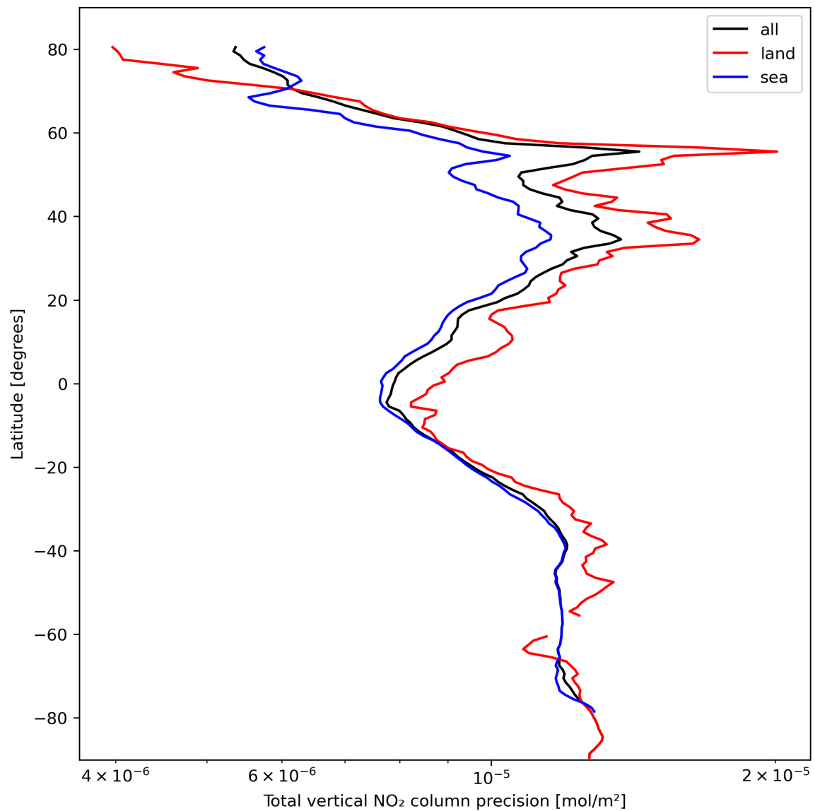
Figure 22: Zonal average of “Total vertical NO 2 column precision” for 2024-02-29 to 2024-03-02.
