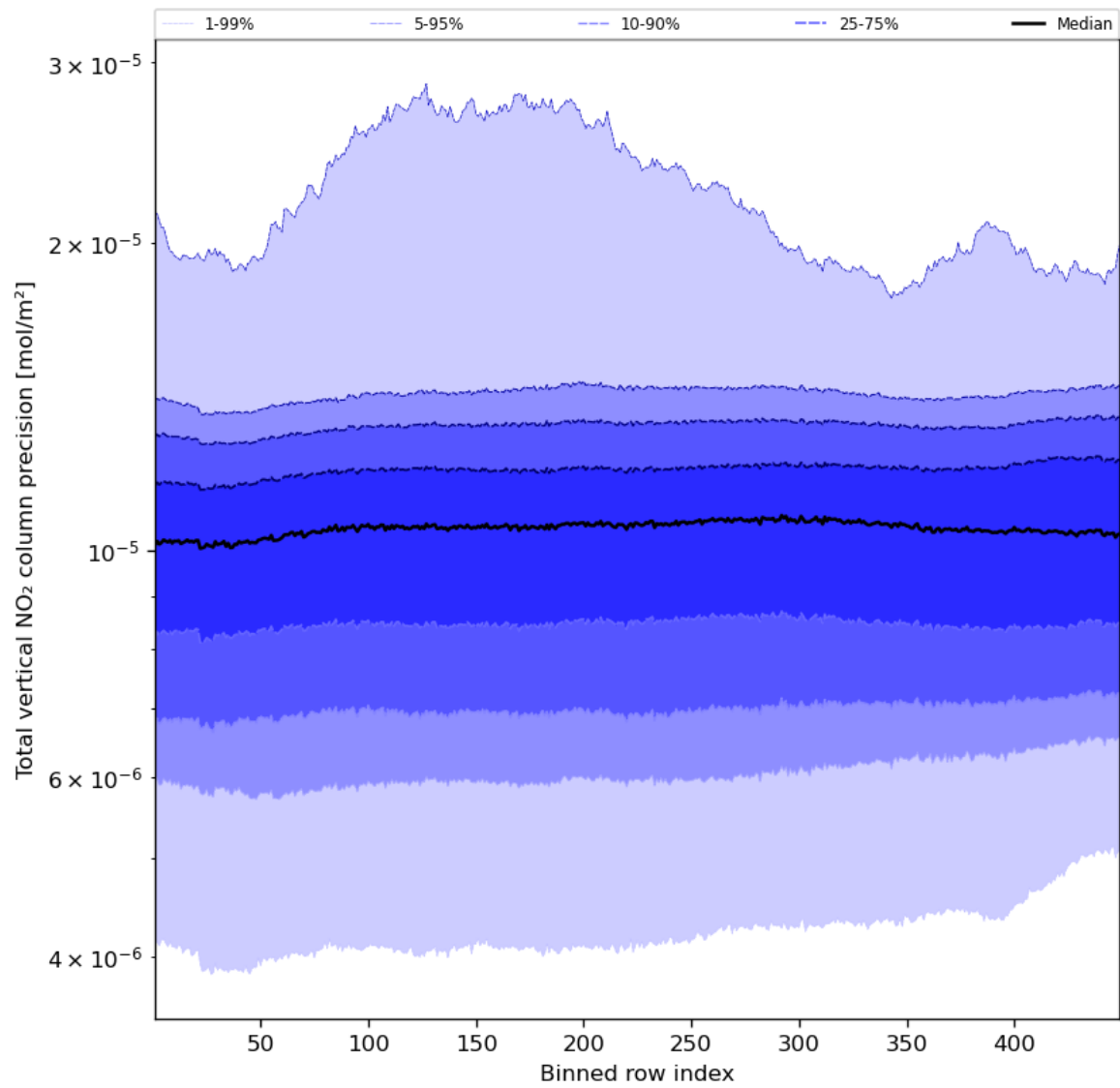
Figure 56: Along track statistics of “Total vertical NO 2 column precision” for 2024-02-29 to 2024-03-02
