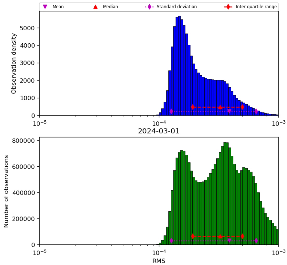
Figure 43: Histogram of “RMS” for 2024-02-29 to 2024-03-02
