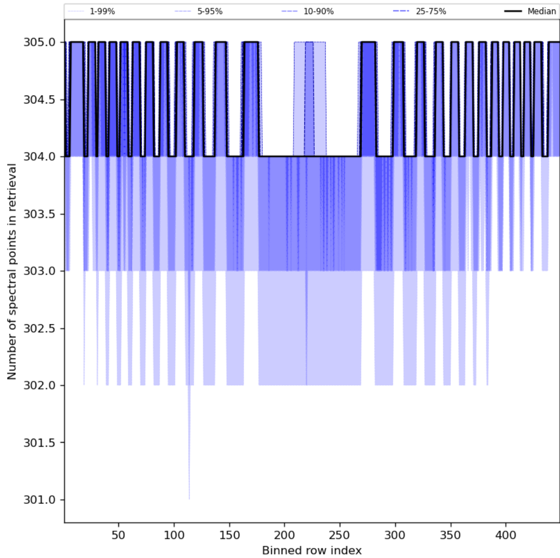
Figure 50: Along track statistics of “Number of spectral points in retrieval” for 2024-02-29 to 2024-03-02
