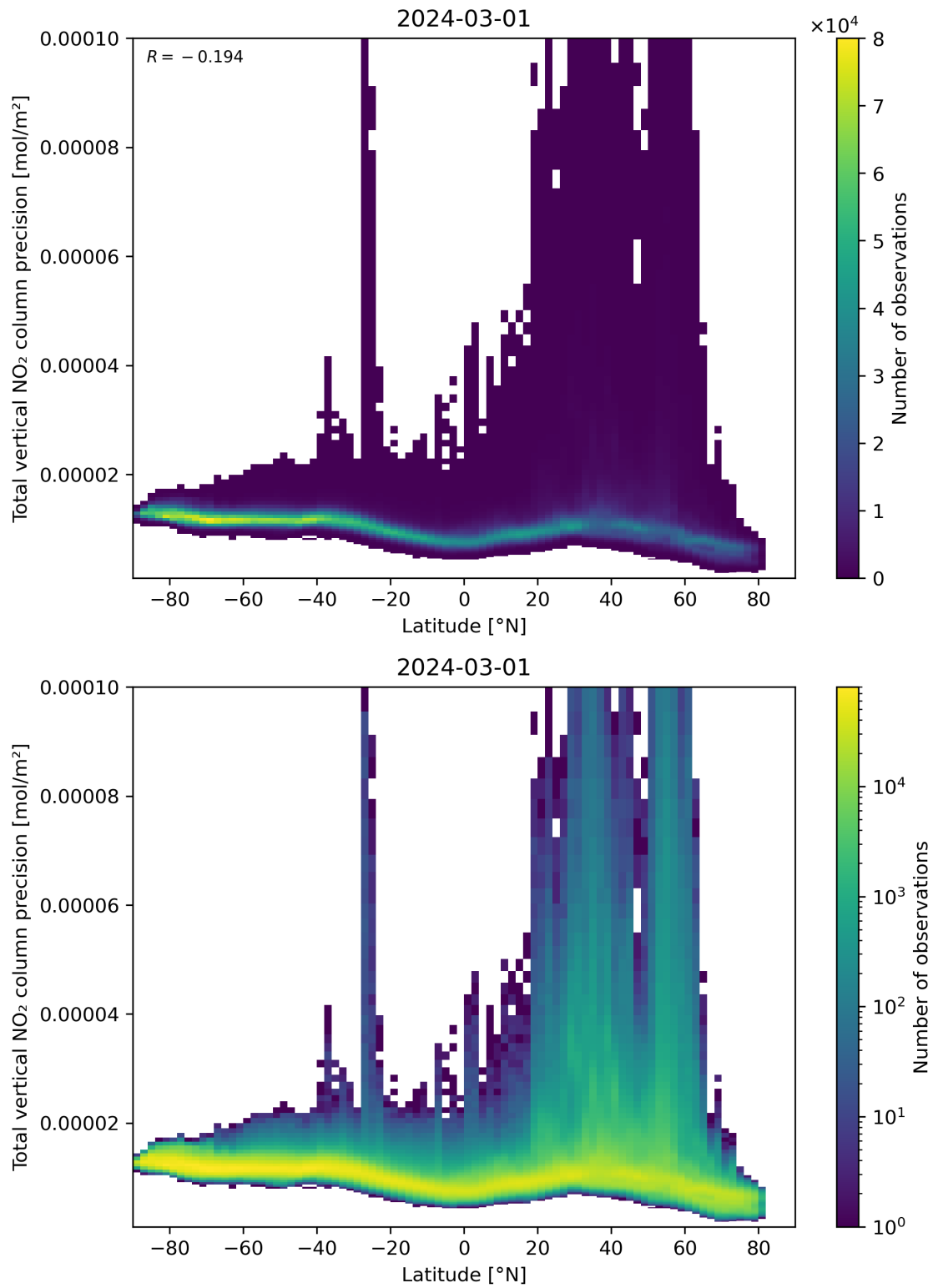
Figure 91: Scatter density plot of “Latitude” against “Total vertical NO 2 column precision” for 2024-02-29 to 2024-03-02.
