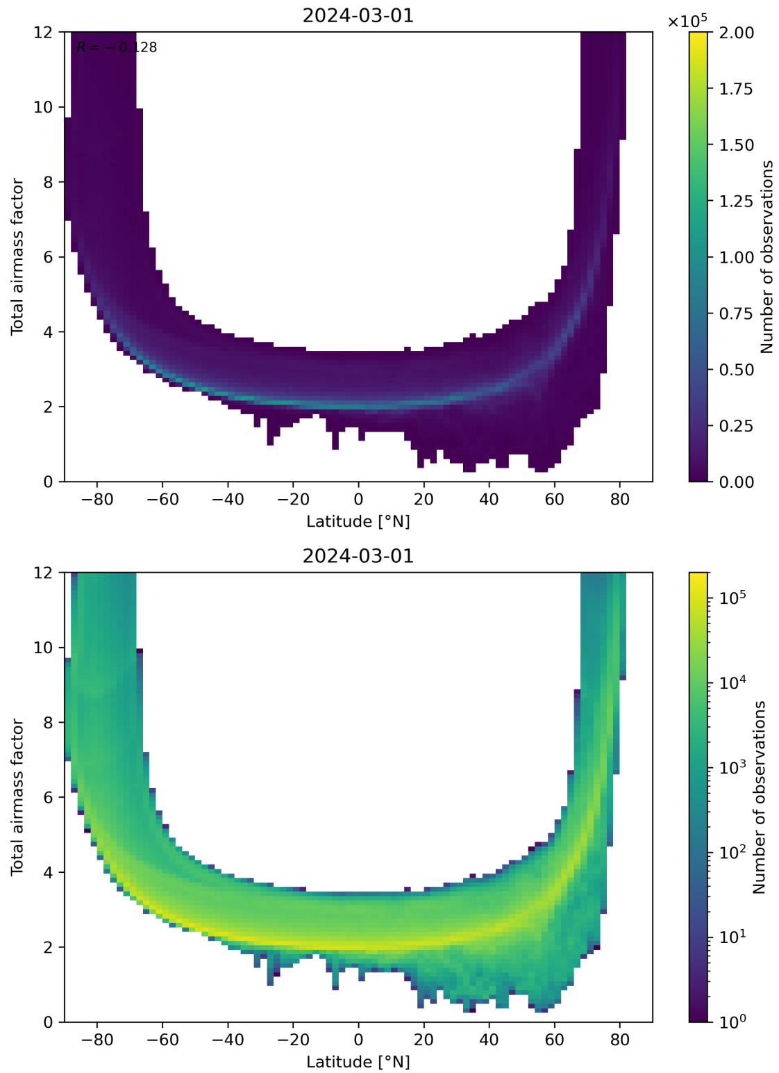
Figure 84: Scatter density plot of “Latitude” against “Total airmass factor” for 2024-02-29 to 2024-03-02.
