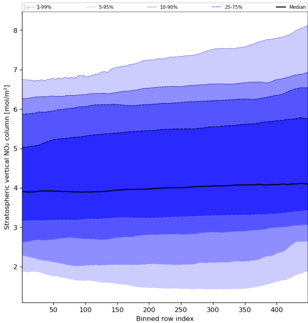
Figure 53: Along track statistics of “Stratospheric vertical NO 2 column” for 2024-02-29 to 2024-03-02
