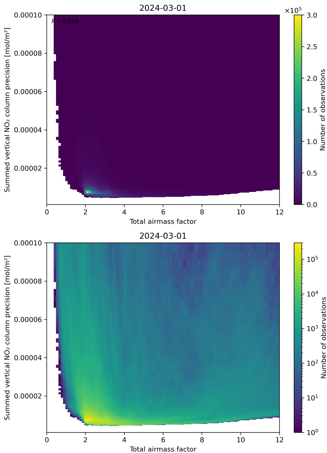
Figure 66: Scatter density plot of “Total airmass factor” against “Summed vertical NO 2 column precision” for 2024-02-29 to 2024-03-02.
