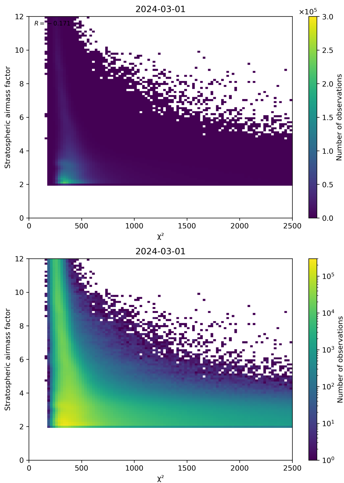
Figure 81: Scatter density plot of “ \chi^2 ” against “Stratospheric airmass factor” for 2024-02-29 to 2024-03-02.
