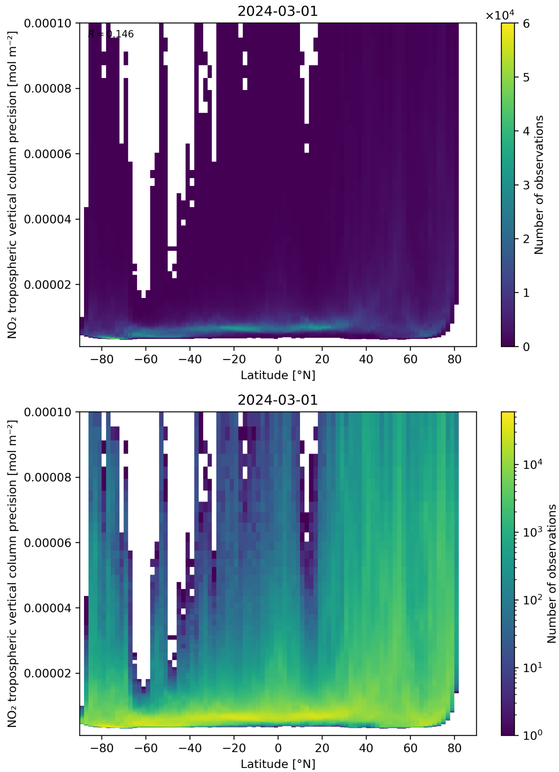
Figure 93: Scatter density plot of “Latitude” against “NO 2 tropospheric vertical column precision” for 2024-02-29 to 2024-03-02.
