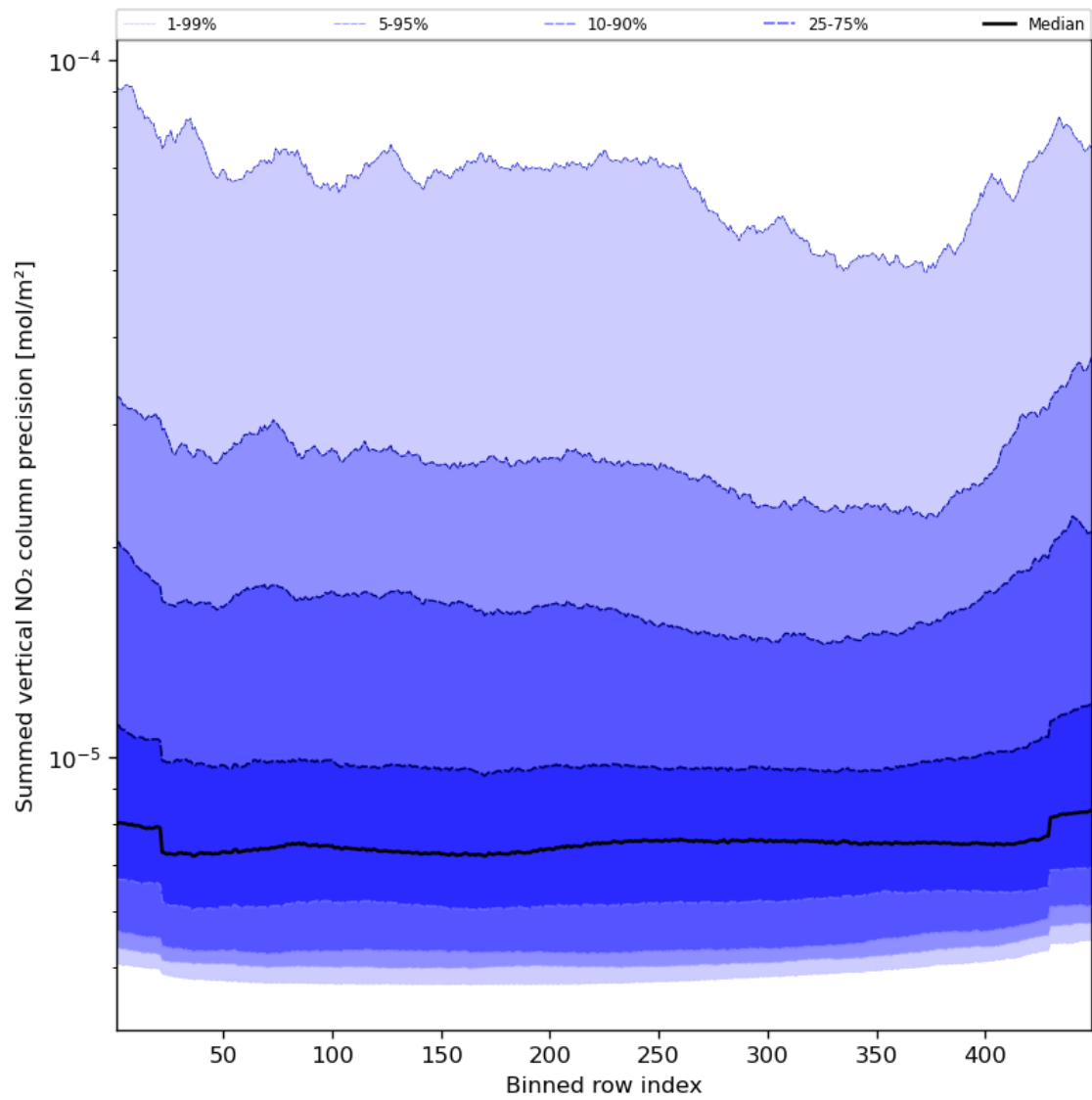
Figure 58: Along track statistics of “Summed vertical NO 2 column precision” for 2024-02-29 to 2024-03-02
