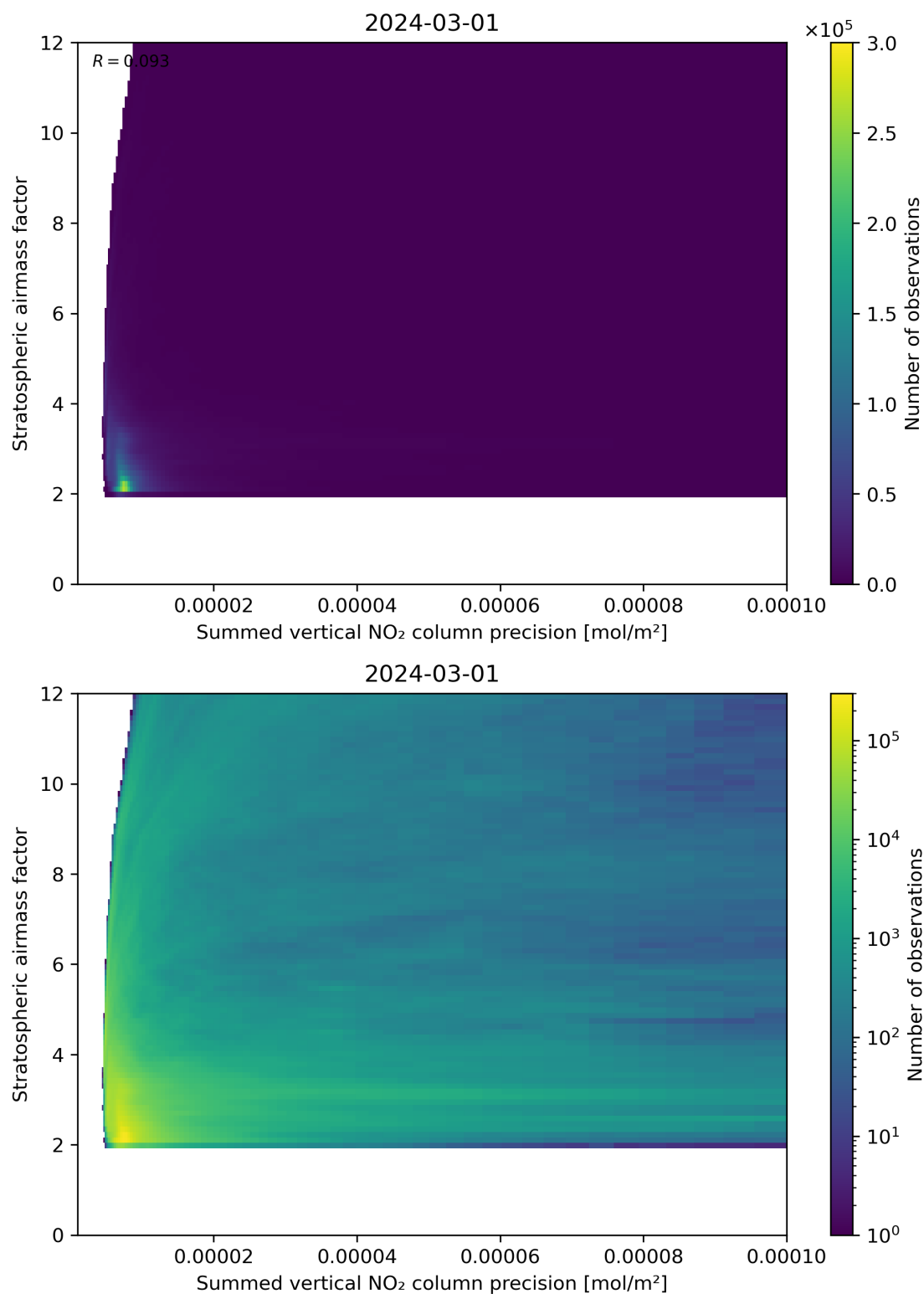
Figure 106: Scatter density plot of “Summed vertical NO 2 column precision” against “Stratospheric airmass factor” for 2024-02-29 to 2024-03-02.
