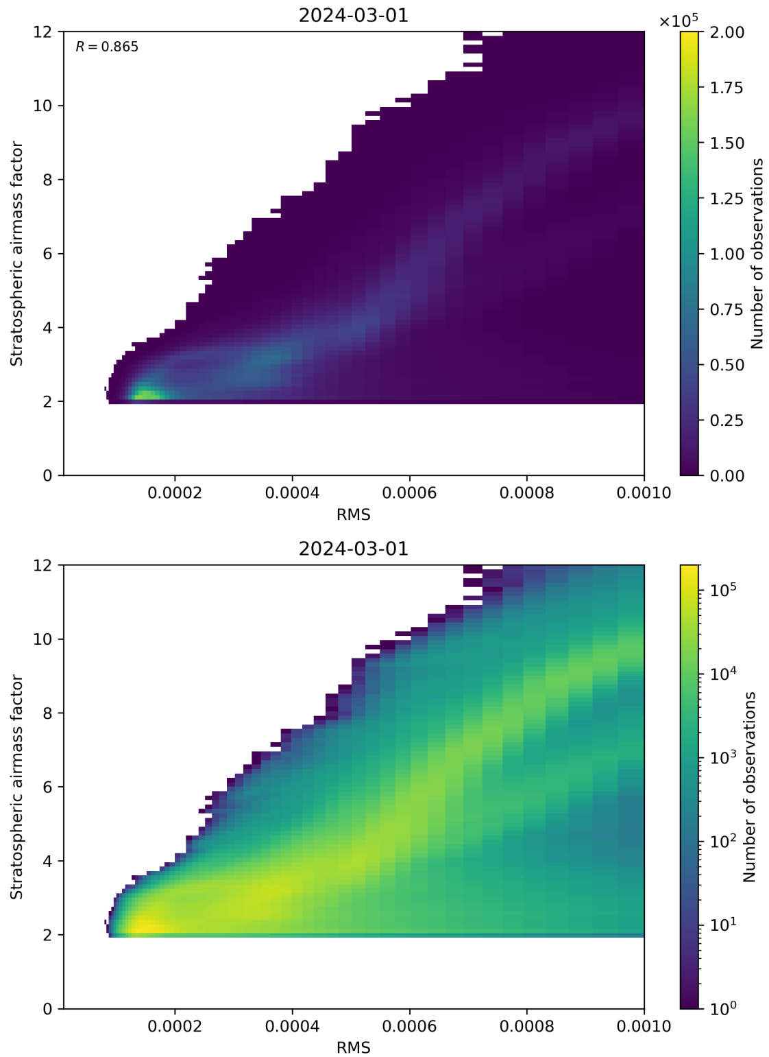
Figure 144: Scatter density plot of “RMS” against “Stratospheric airmass factor” for 2024-02-29 to 2024-03-02.
