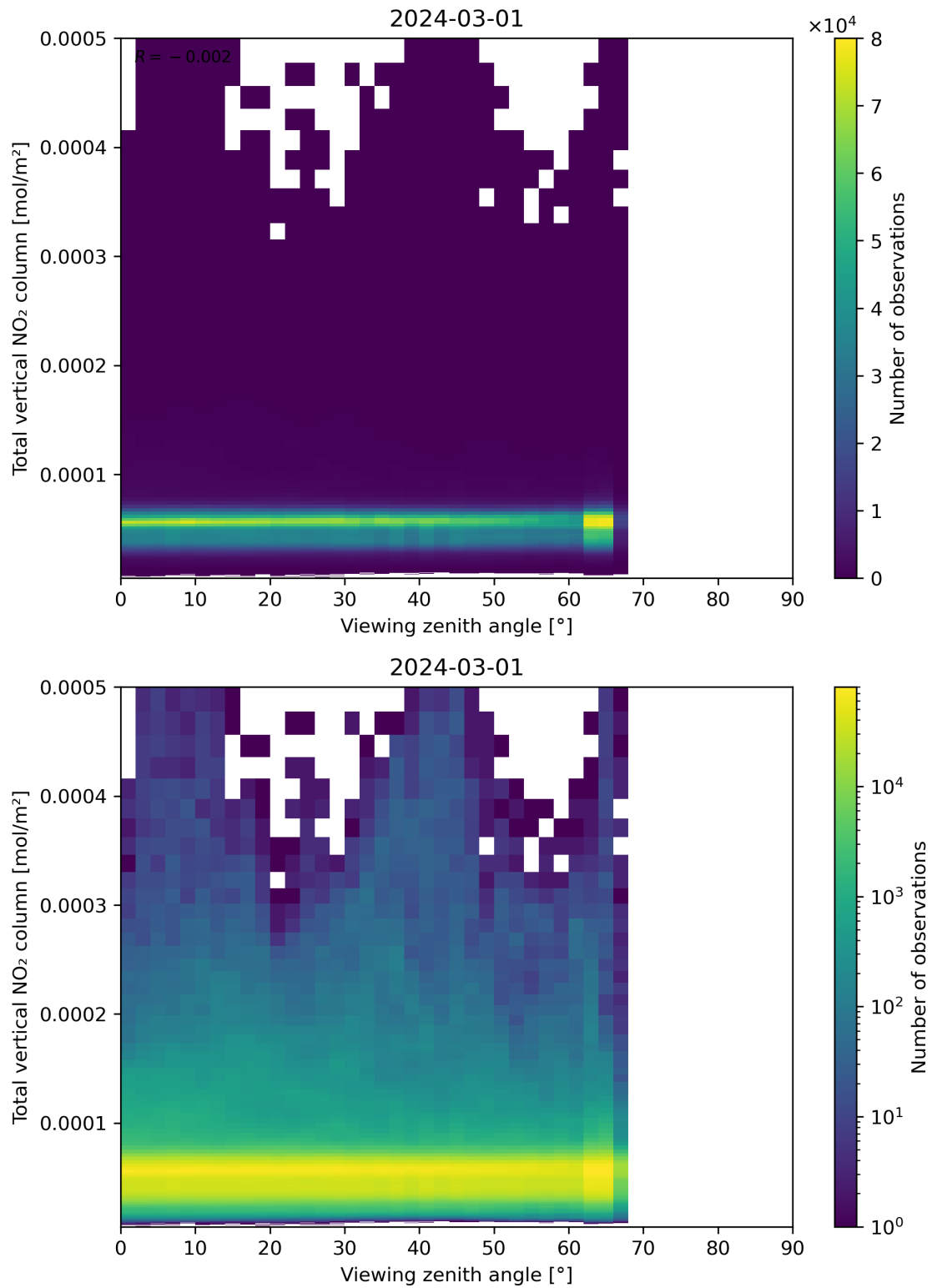
Figure 167: Scatter density plot of “Viewing zenith angle” against “Total vertical NO 2 column” for 2024-02-29 to 2024-03-02.
