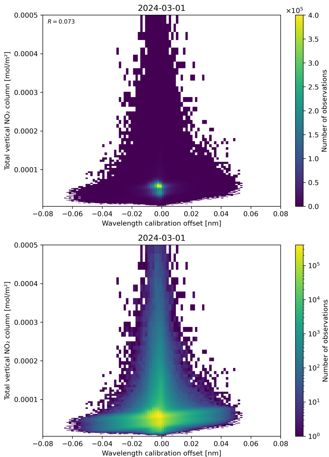
Figure 179: Scatter density plot of “Wavelength calibration offset” against “Total vertical NO 2 column” for 2024-02-29 to 2024-03-02.
