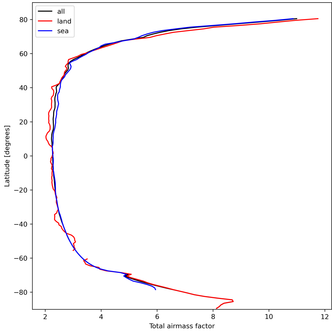
Figure 15: Zonal average of “Total airmass factor” for 2024-02-29 to 2024-03-02.
