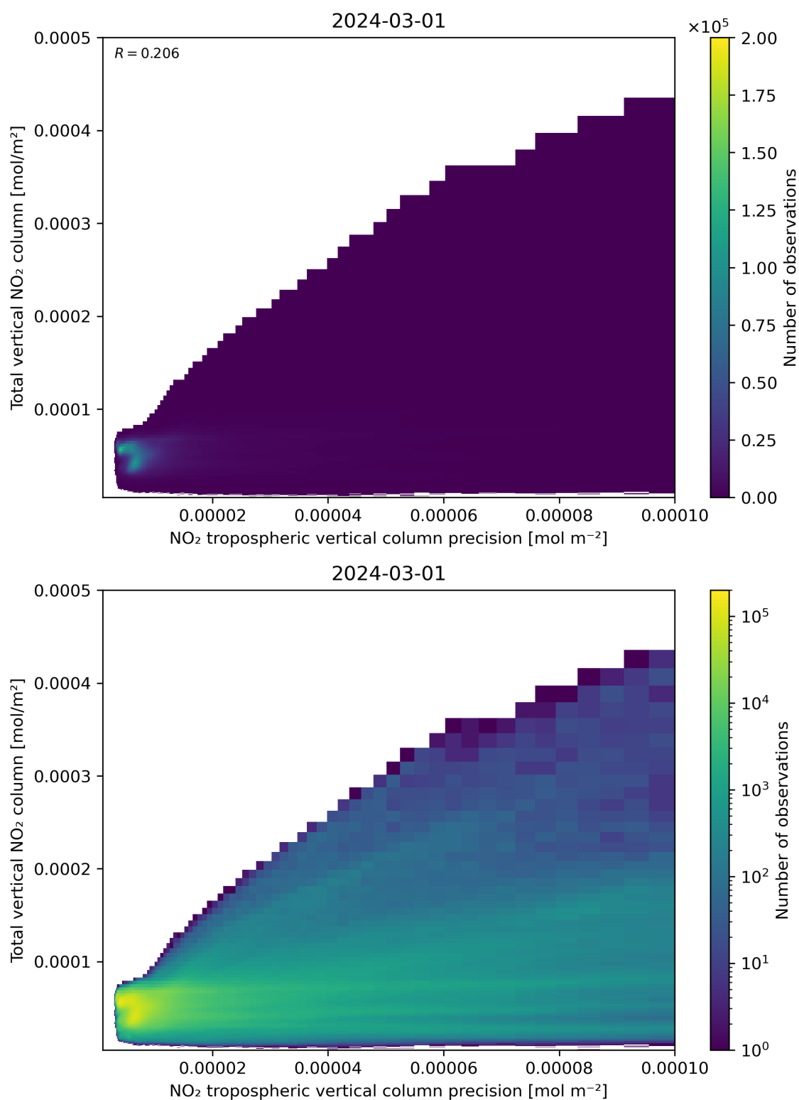
Figure 138: Scatter density plot of “NO 2 tropospheric vertical column precision” against “Total vertical NO 2 column” for 2024-02-29 to 2024-03-02.
