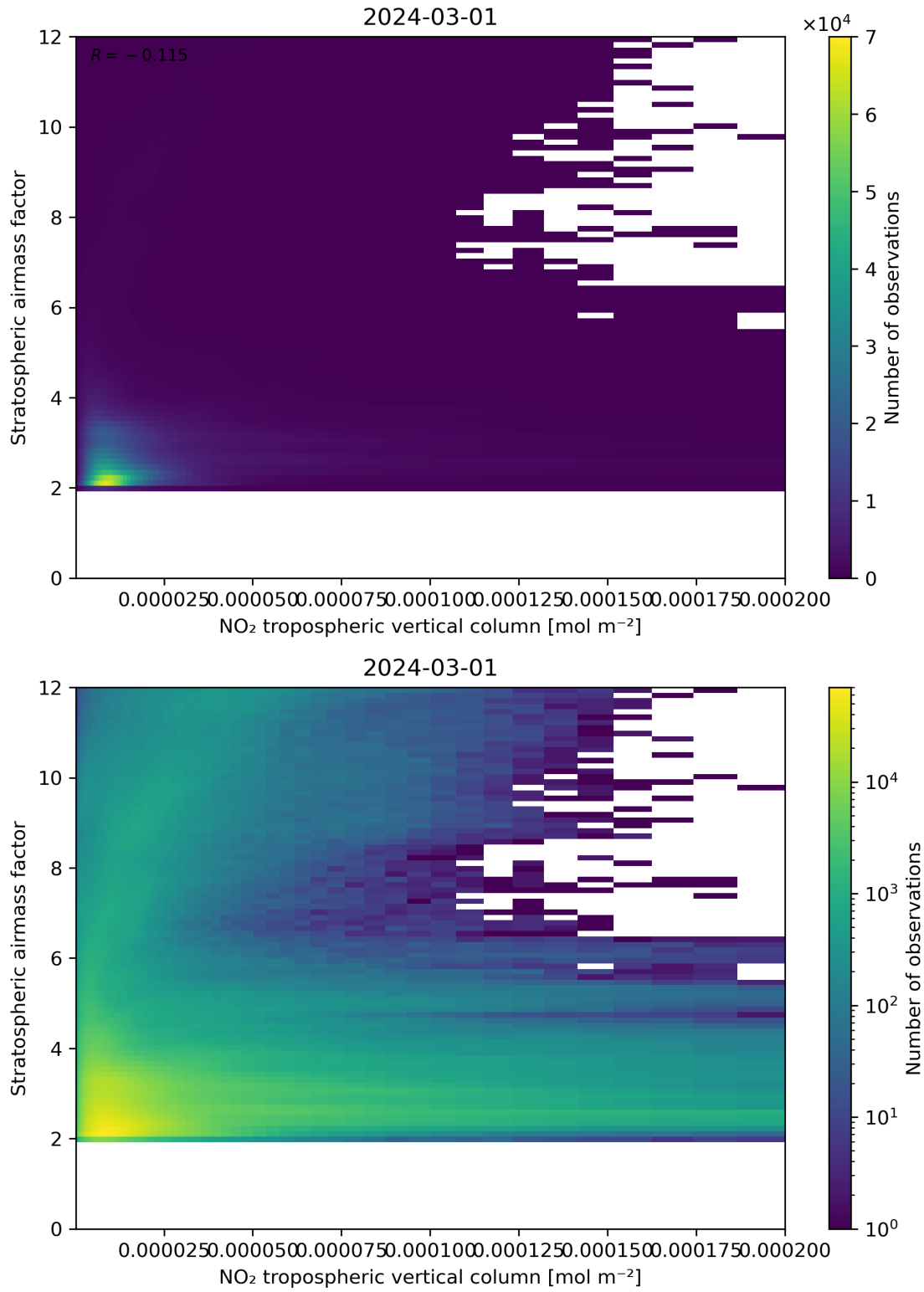
Figure 121: Scatter density plot of “NO 2 tropospheric vertical column” against “Stratospheric air mass factor” for 2024-02-29 to 2024-03-02.
