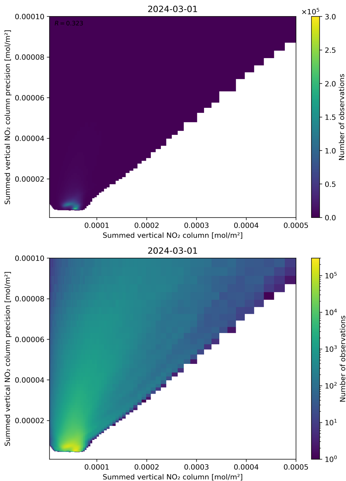
Figure 105: Scatter density plot of “Summed vertical NO 2 column” against “Summed vertical NO 2 column precision” for 2024-02-29 to 2024-03-02.
