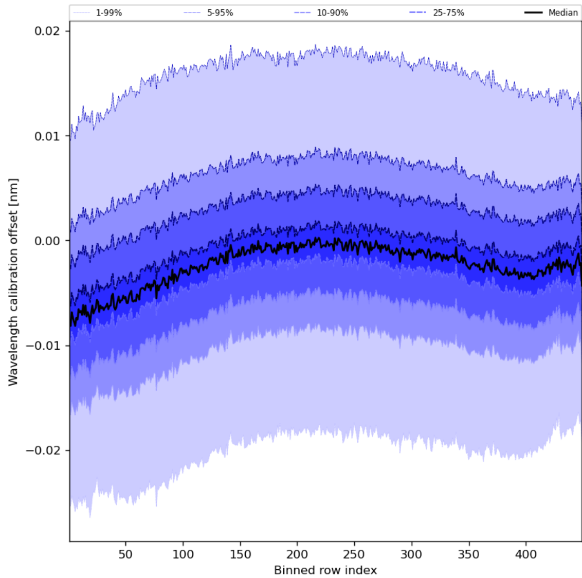
Figure 52: Along track statistics of “Wavelength calibration offset” for 2024-02-29 to 2024-03-02
