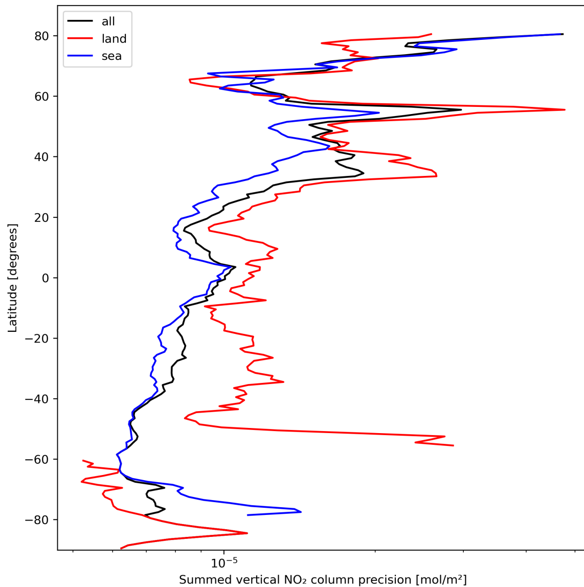
Figure 24: Zonal average of “Summed vertical NO 2 column precision” for 2024-02-29 to 2024-03-02.
