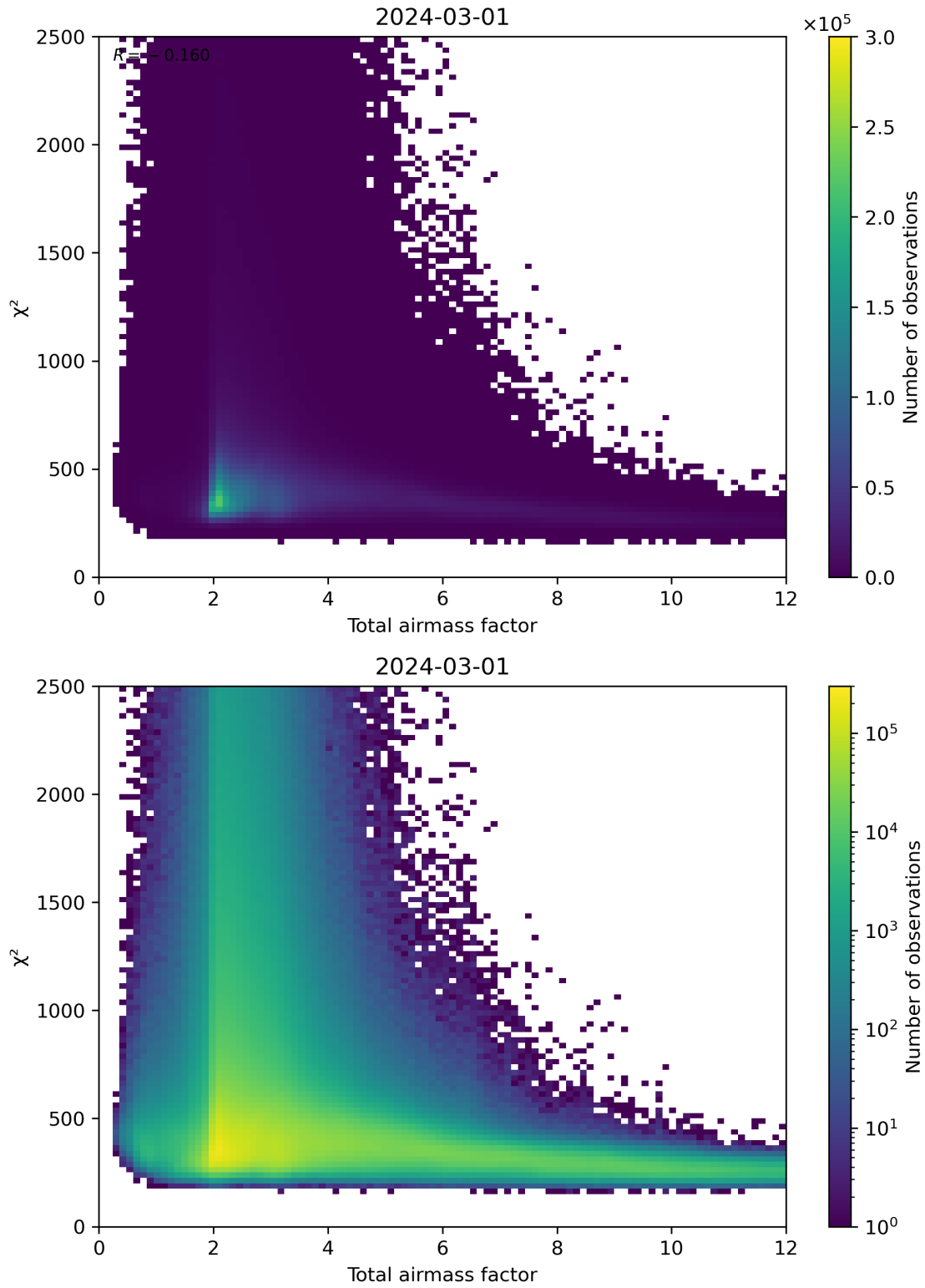
Figure 63: Scatter density plot of “Total airmass factor” against “ \chi^2 ” for 2024-02-29 to 2024-03-02.
