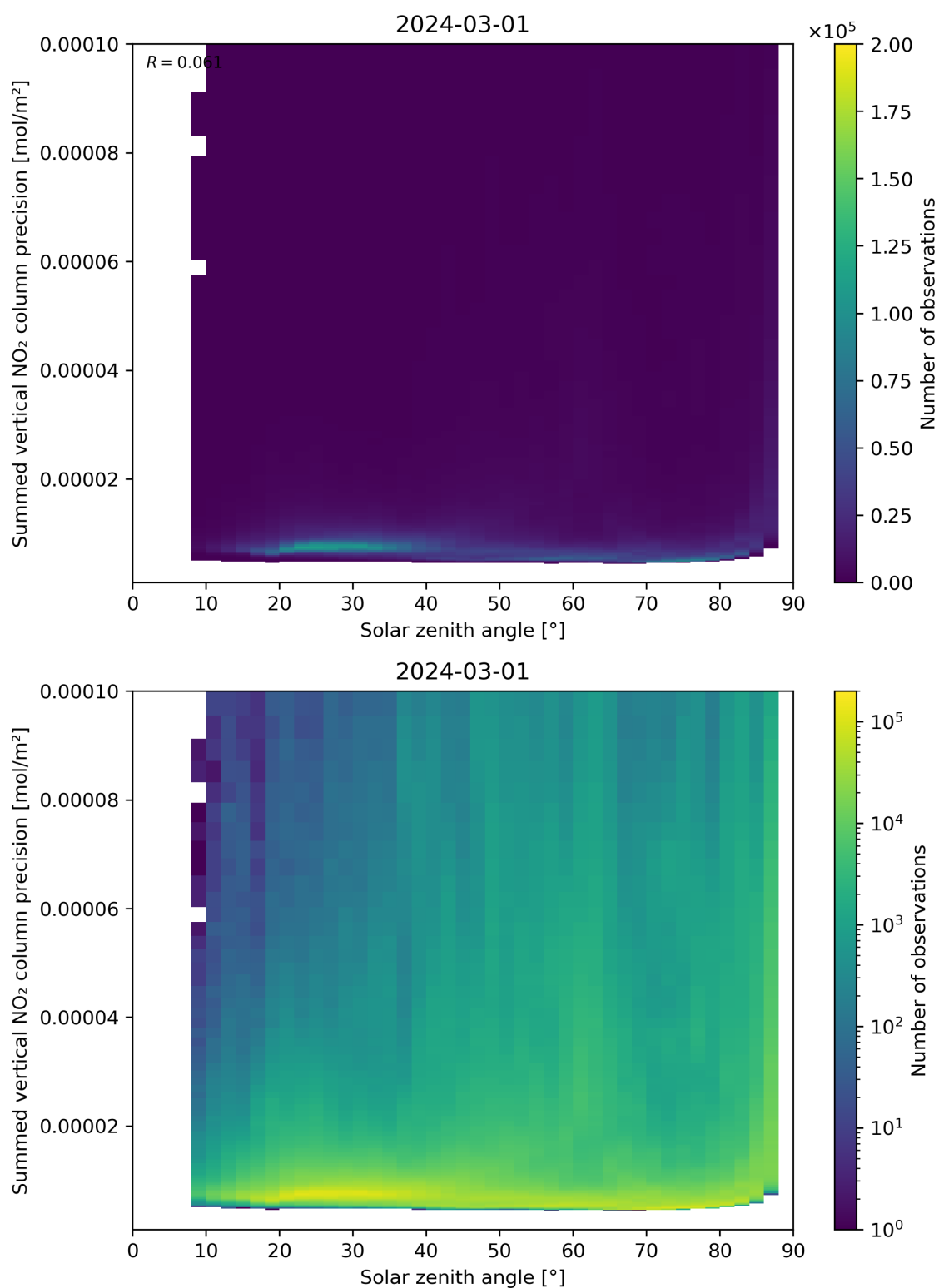
Figure 152: Scatter density plot of “Solar zenith angle” against “Summed vertical NO 2 column precision” for 2024-02-29 to 2024-03-02.
