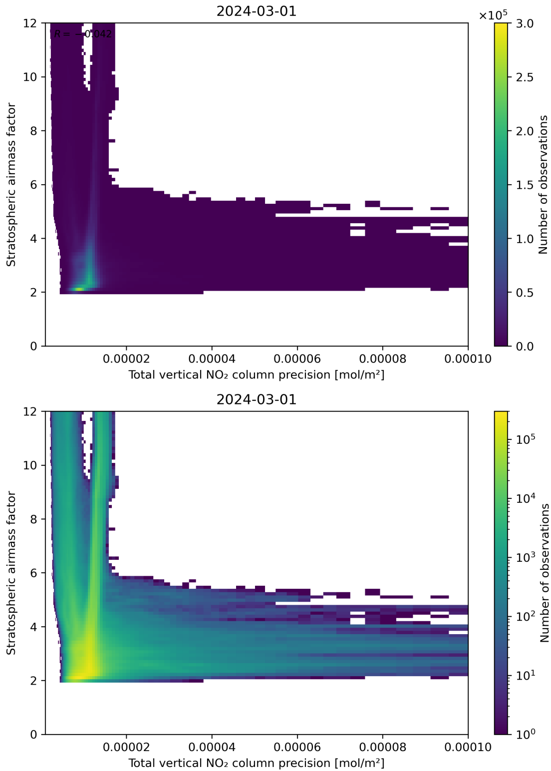
Figure 115: Scatter density plot of “Total vertical NO 2 column precision” against “Stratospheric air mass factor” for 2024-02-29 to 2024-03-02.
