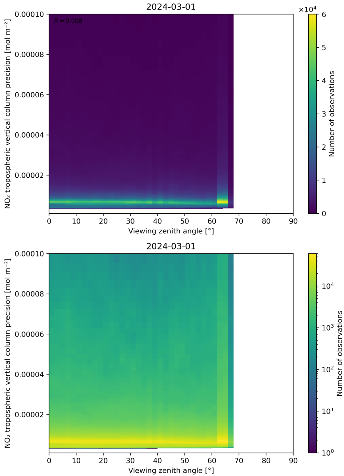
Figure 170: Scatter density plot of “Viewing zenith angle” against “NO 2 tropospheric vertical column precision” for 2024-02-29 to 2024-03-02.
