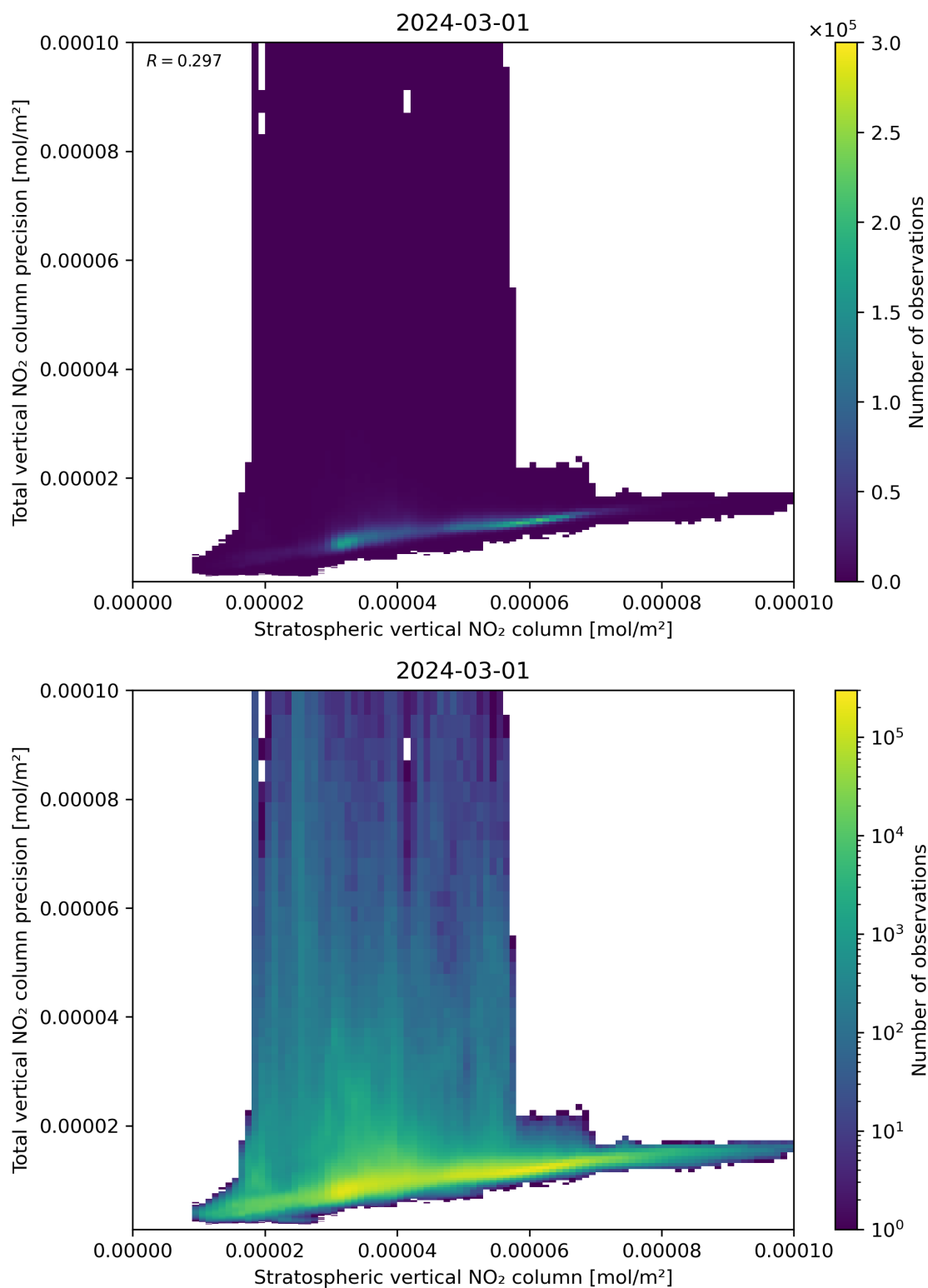
Figure 101: Scatter density plot of “Stratospheric vertical NO 2 column” against “Total vertical NO 2 column precision” for 2024-02-29 to 2024-03-02.
