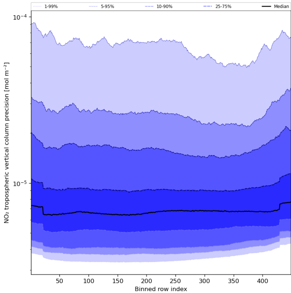
Figure 47: Along track statistics of “NO 2 tropospheric vertical column precision” for 2024-02-29 to 2024-03-02
