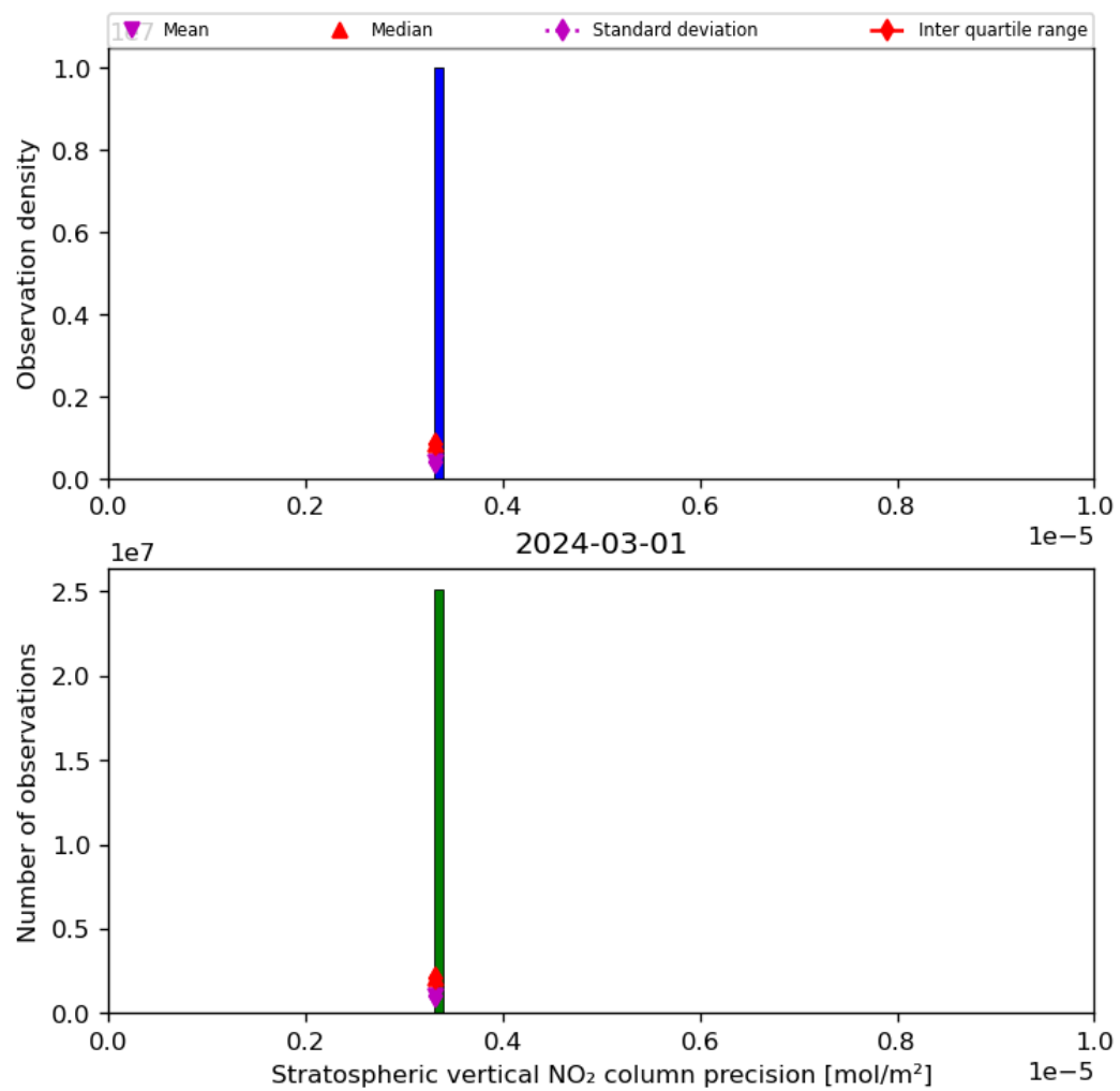
Figure 37: Histogram of “Stratospheric vertical NO 2 column precision” for 2024-02-29 to 2024-03-02
