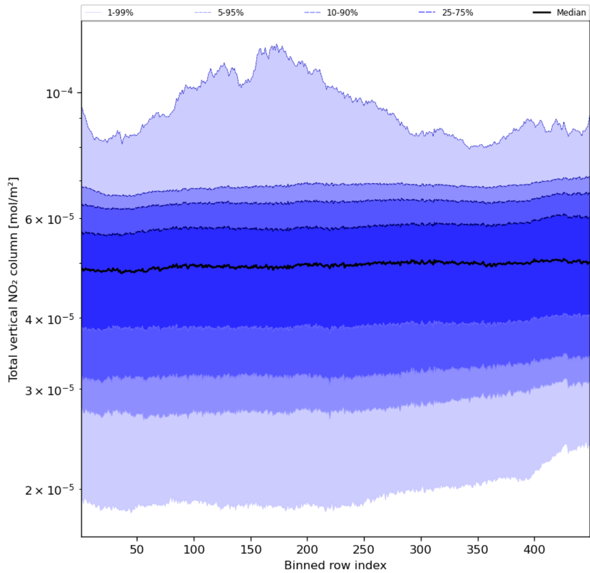
Figure 55: Along track statistics of “Total vertical NO 2 column” for 2024-02-29 to 2024-03-02
