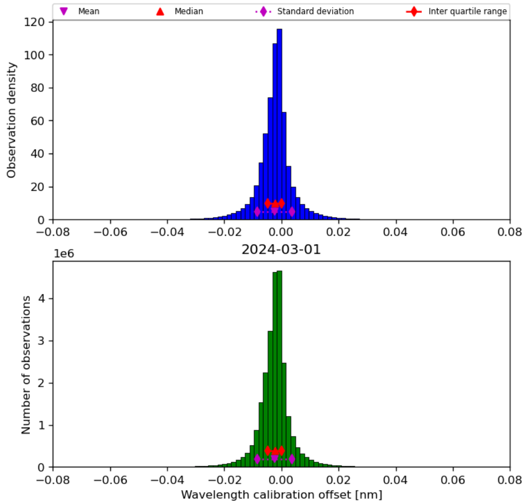
Figure 35: Histogram of “Wavelength calibration offset” for 2024-02-29 to 2024-03-02
