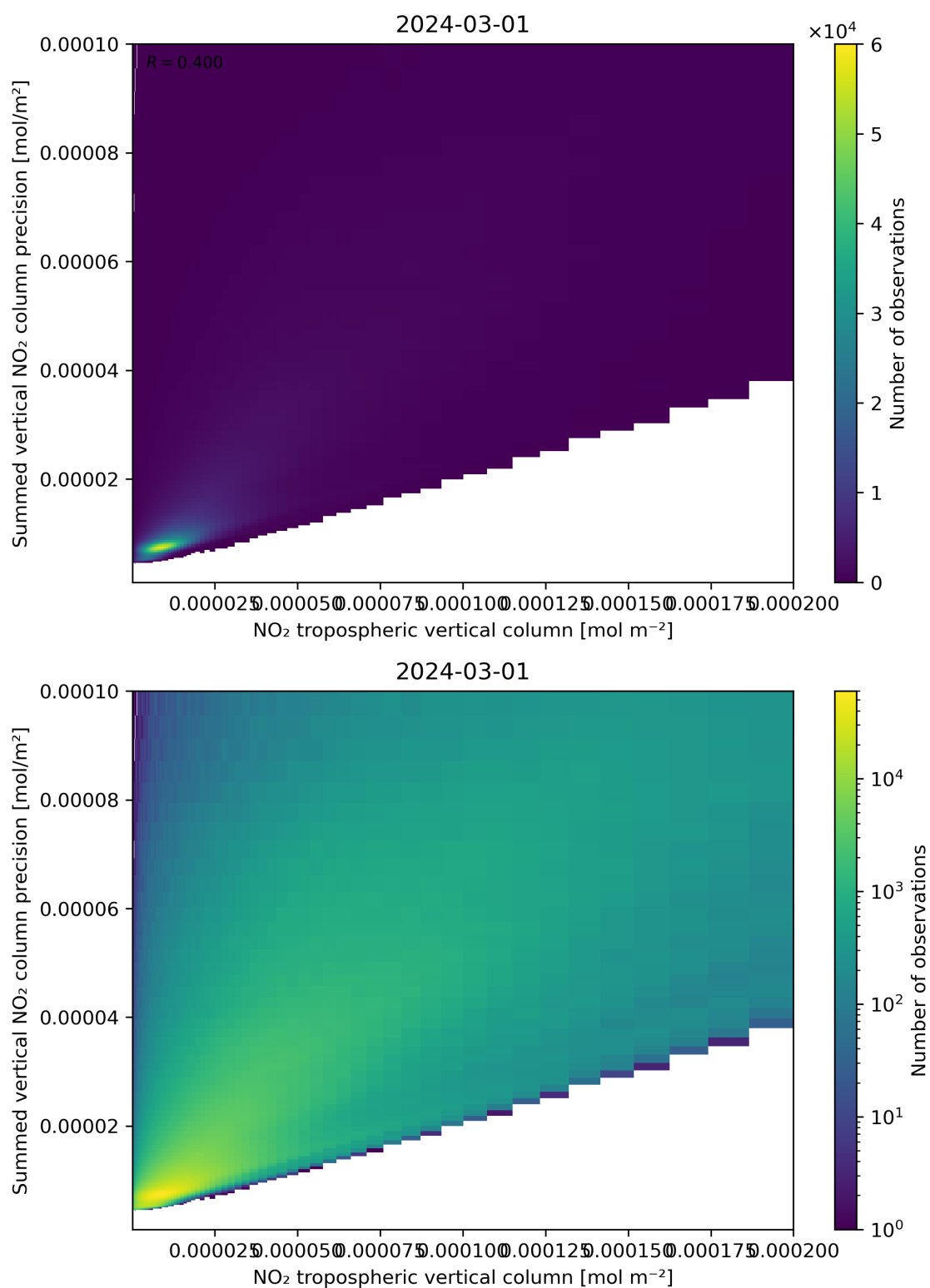
Figure 127: Scatter density plot of “NO 2 tropospheric vertical column” against “Summed vertical NO 2 column precision” for 2024-02-29 to 2024-03-02.
