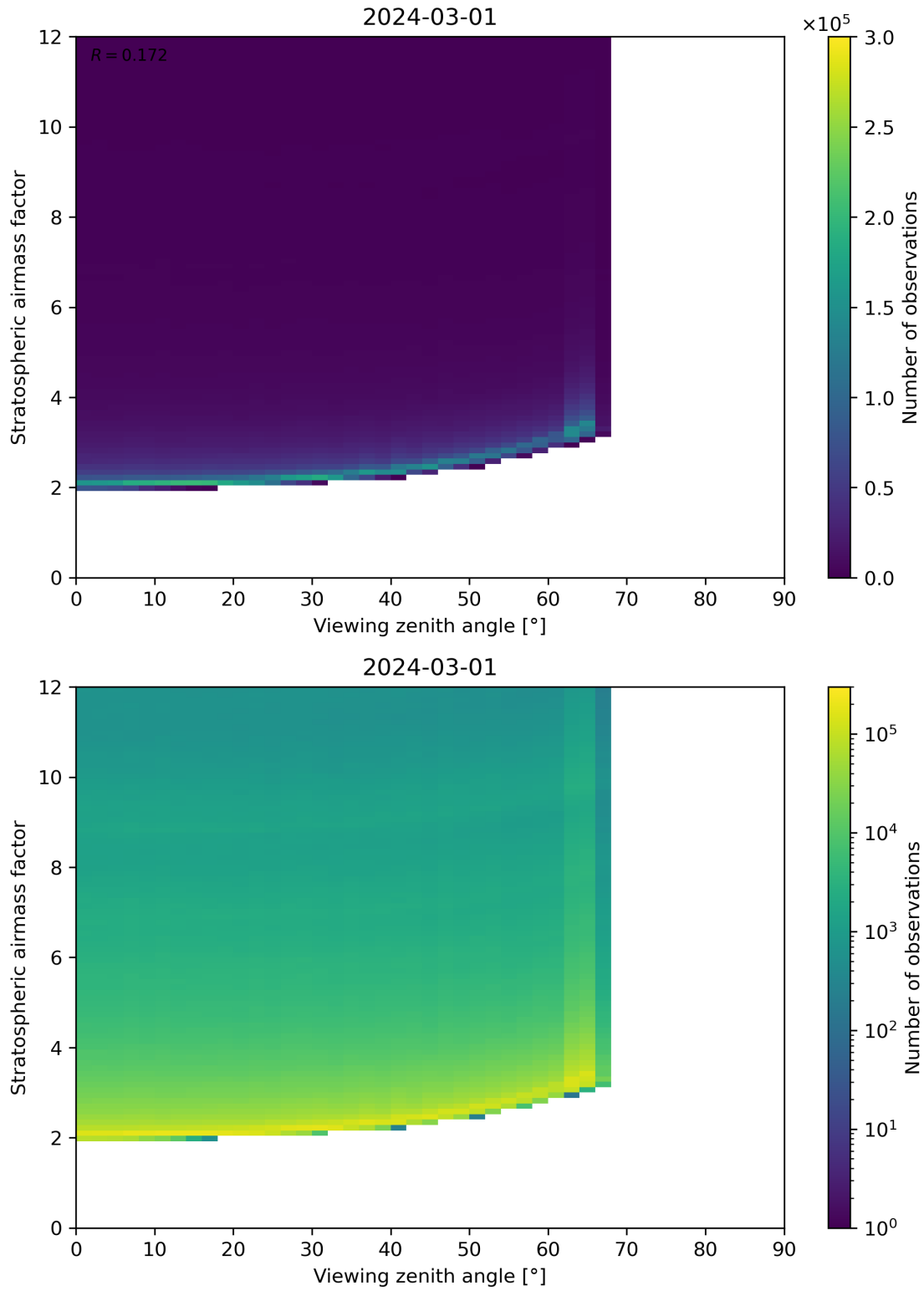
Figure 159: Scatter density plot of “Viewing zenith angle” against “Stratospheric airmass factor” for 2024-02-29 to 2024-03-02.
