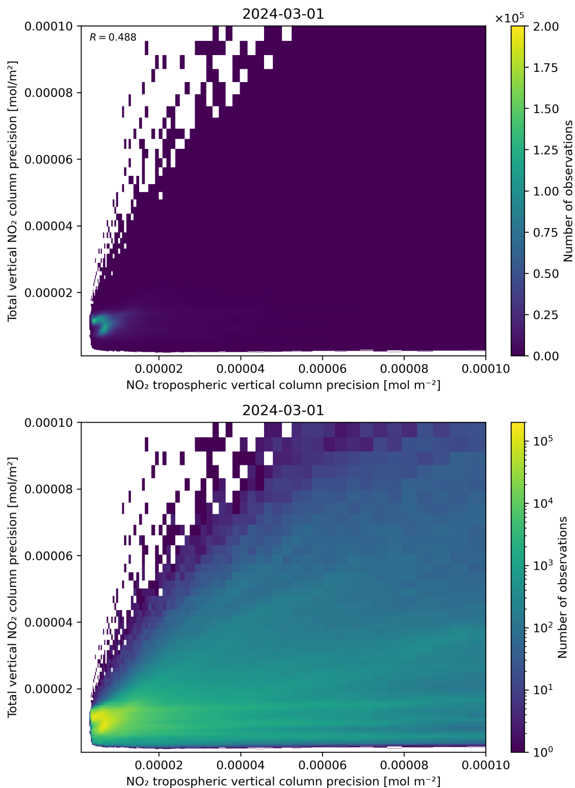
Figure 139: Scatter density plot of “NO 2 tropospheric vertical column precision” against “Total vertical NO 2 column precision” for 2024-02-29 to 2024-03-02.
