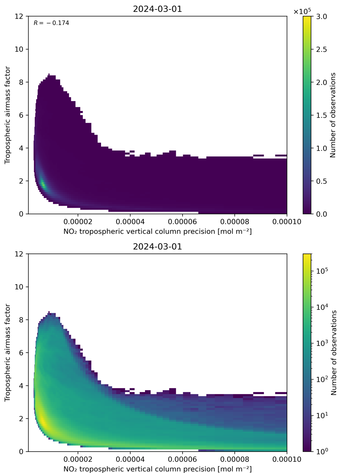
Figure 133: Scatter density plot of “NO 2 tropospheric vertical column precision” against “Tropospheric airmass factor” for 2024-02-29 to 2024-03-02.
