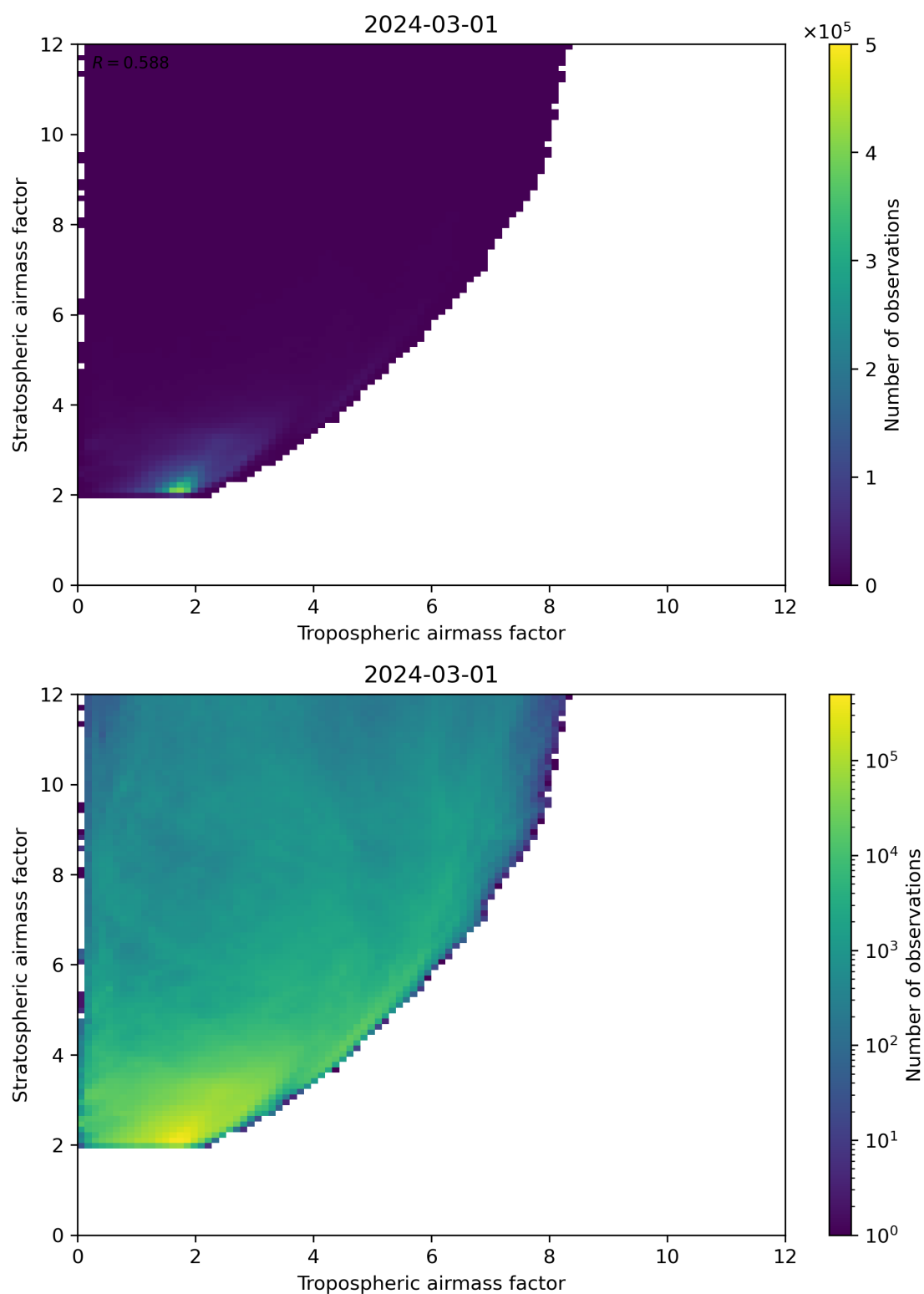
Figure 71: Scatter density plot of “Tropospheric airmass factor” against “Stratospheric airmass factor” for 2024-02-29 to 2024-03-02.
