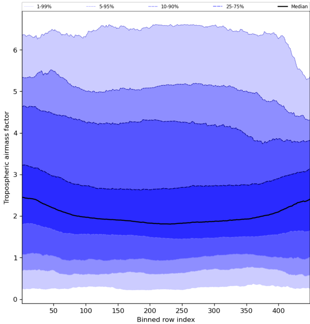
Figure 48: Along track statistics of “Tropospheric airmass factor” for 2024-02-29 to 2024-03-02
