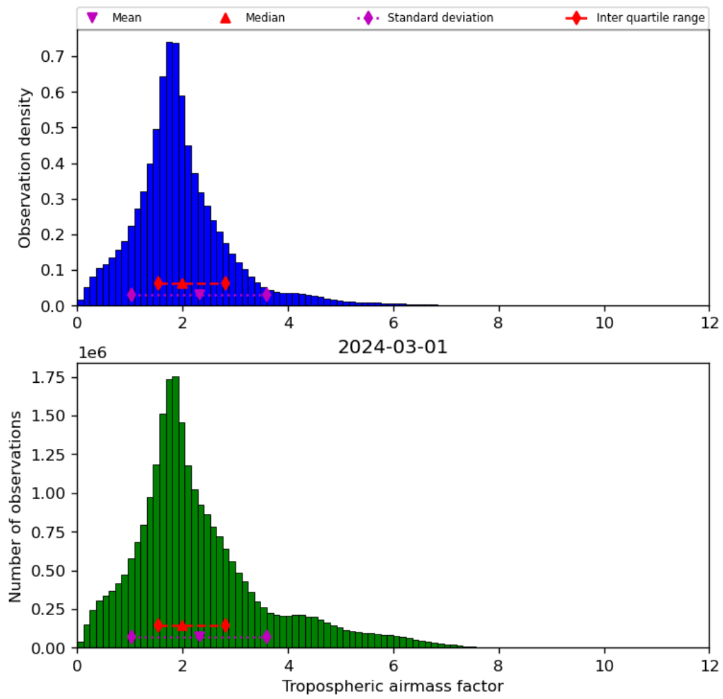
Figure 31: Histogram of “Tropospheric airmass factor” for 2024-02-29 to 2024-03-02
