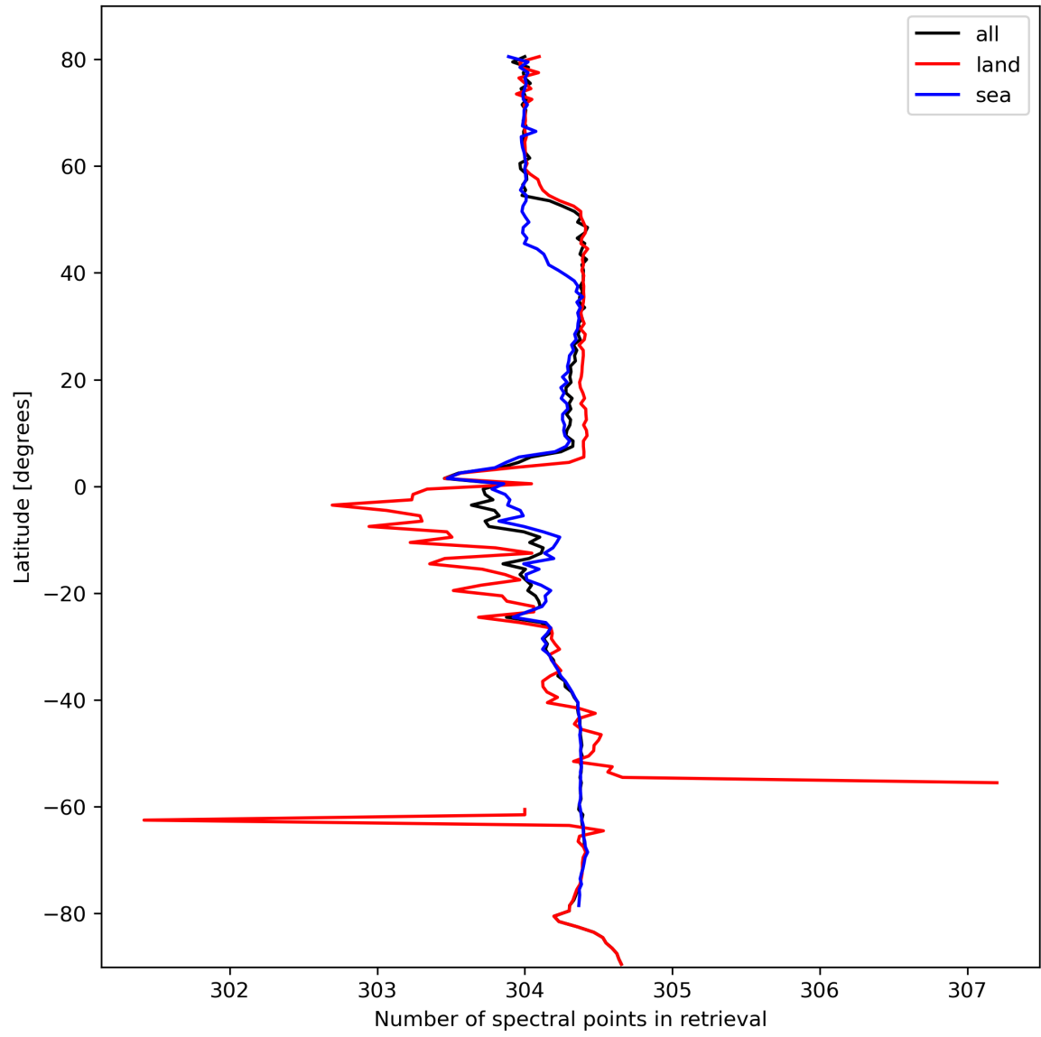
Figure 16: Zonal average of “Number of spectral points in retrieval” for 2024-02-29 to 2024-03-02.
