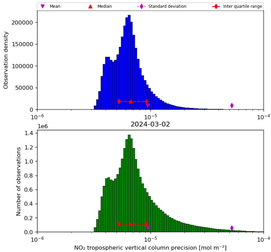
Figure 30: Histogram of “NO 2 tropospheric vertical column precision” for 2024-03-01 to 2024-03-03
