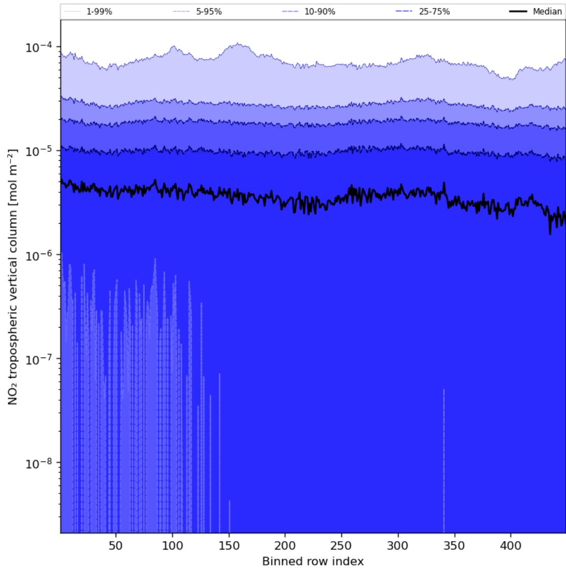
Figure 46: Along track statistics of “NO 2 tropospheric vertical column” for 2024-03-01 to 2024-03-03
