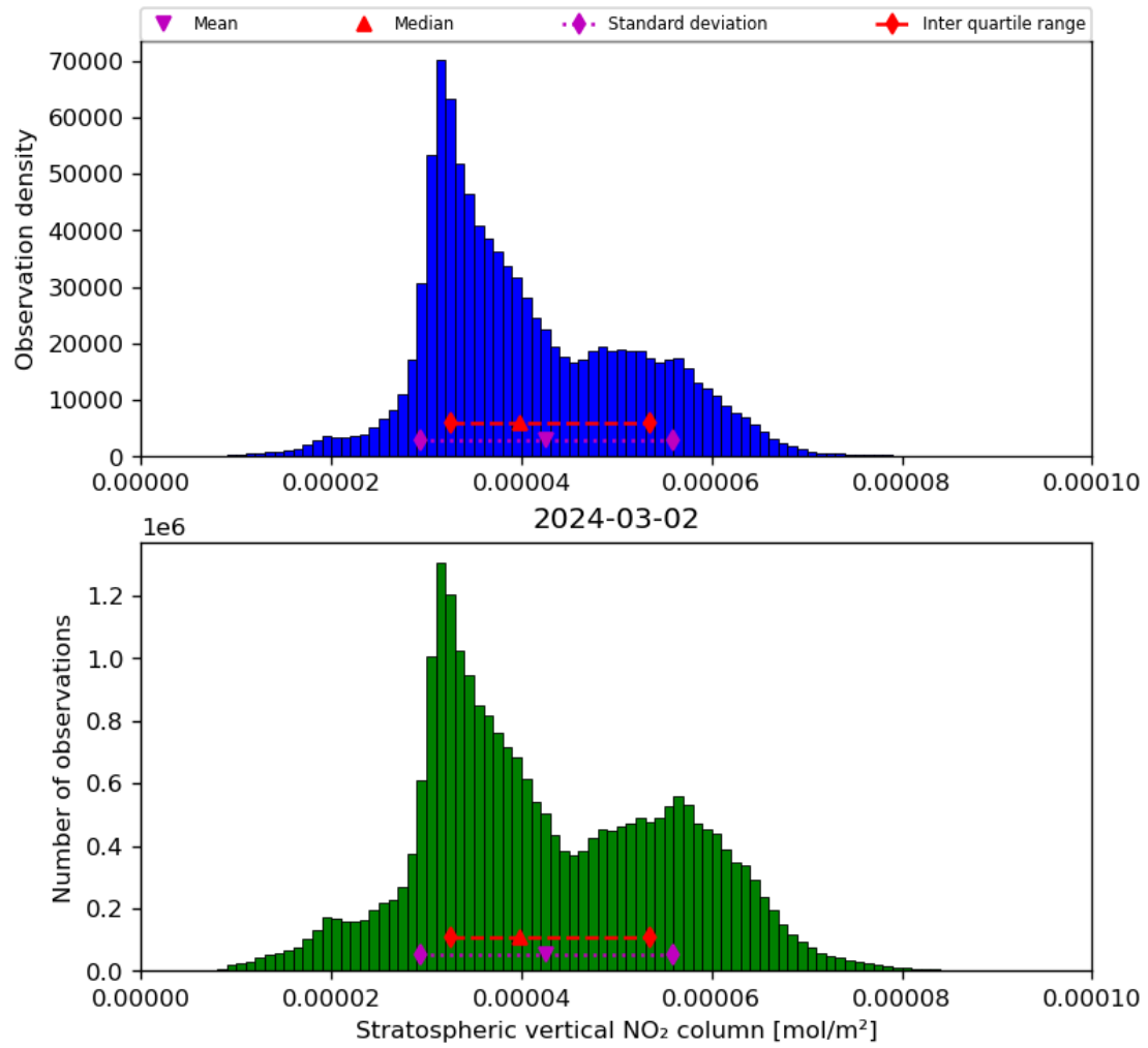
Figure 36: Histogram of “Stratospheric vertical NO 2 column” for 2024-03-01 to 2024-03-03
