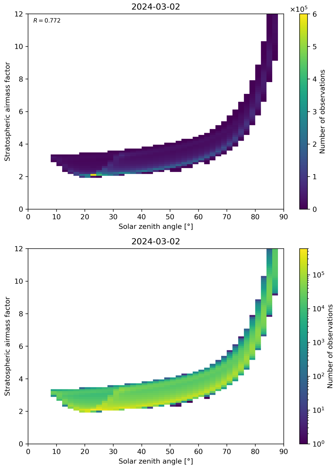
Figure 145: Scatter density plot of “Solar zenith angle” against “Stratospheric airmass factor” for 2024-03-01 to 2024-03-03.
