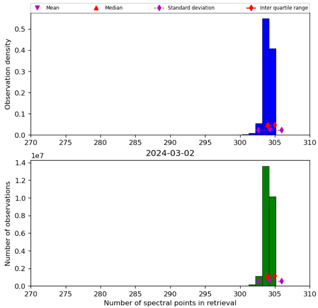
Figure 33: Histogram of “Number of spectral points in retrieval” for 2024-03-01 to 2024-03-03
