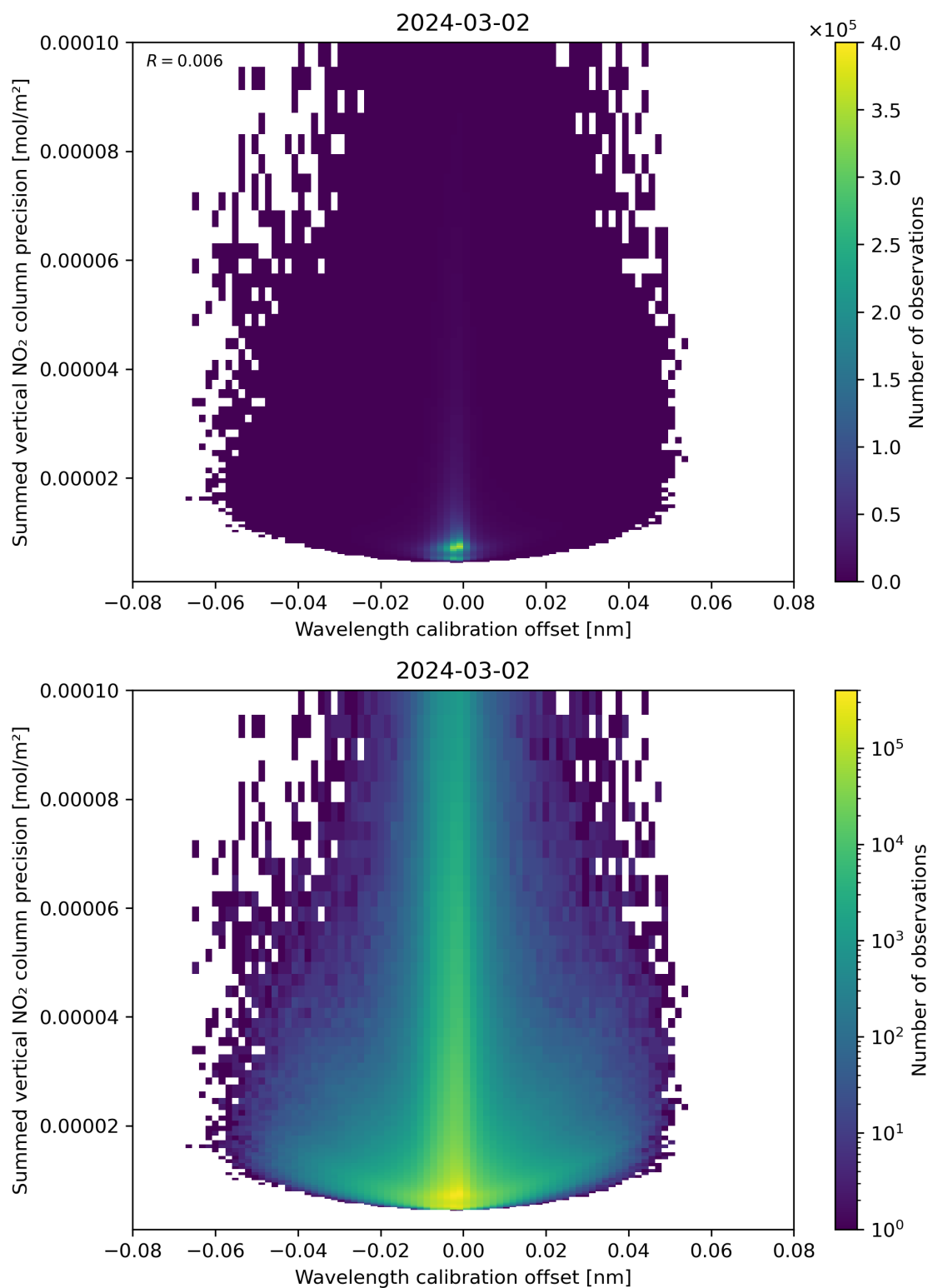
Figure 178: Scatter density plot of “Wavelength calibration offset” against “Summed vertical NO 2 column precision” for 2024-03-01 to 2024-03-03.
