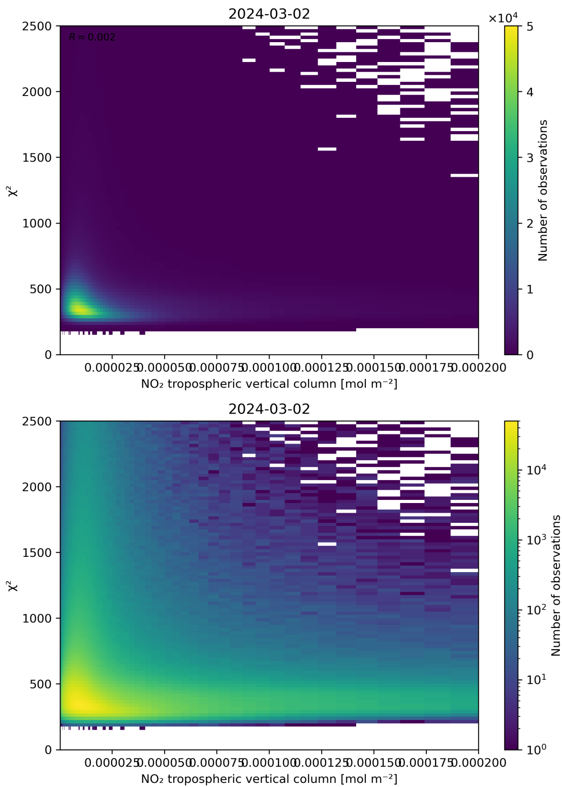
Figure 124: Scatter density plot of “NO 2 tropospheric vertical column” against “ \chi^2 ” for 2024-03-01 to 2024-03-03.
