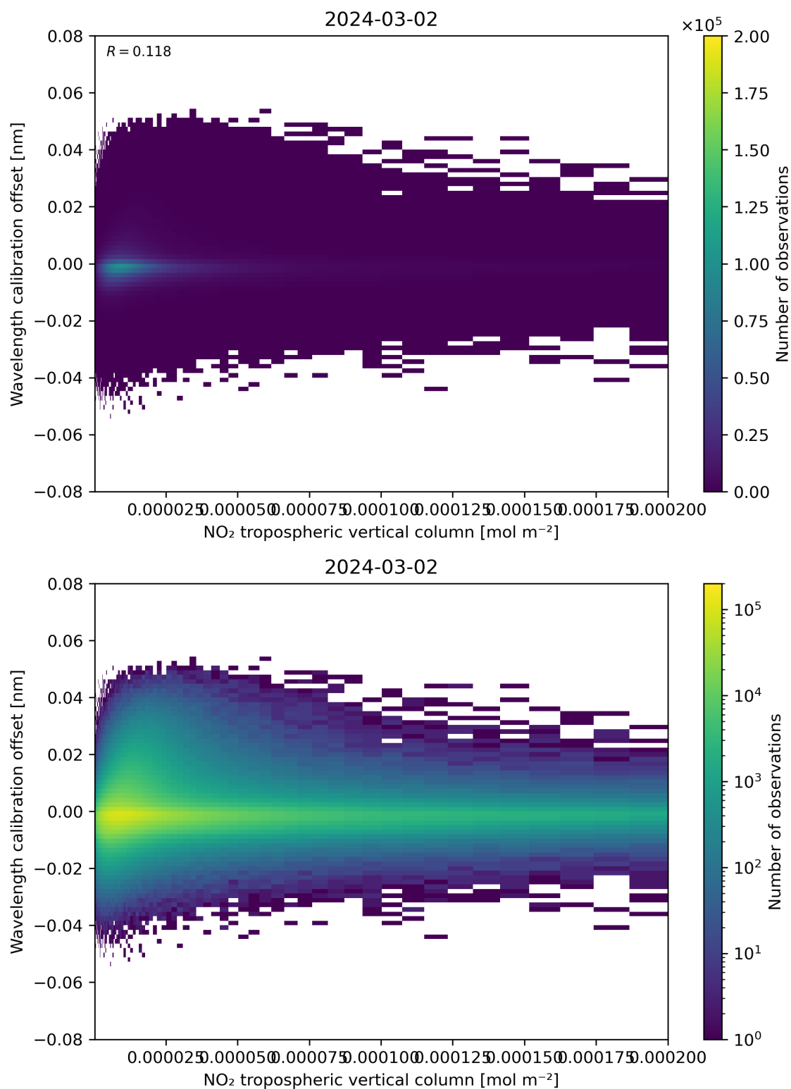
Figure 143: Scatter density plot of “NO 2 tropospheric vertical column” against “Wavelength calibration offset” for 2024-03-01 to 2024-03-03.
