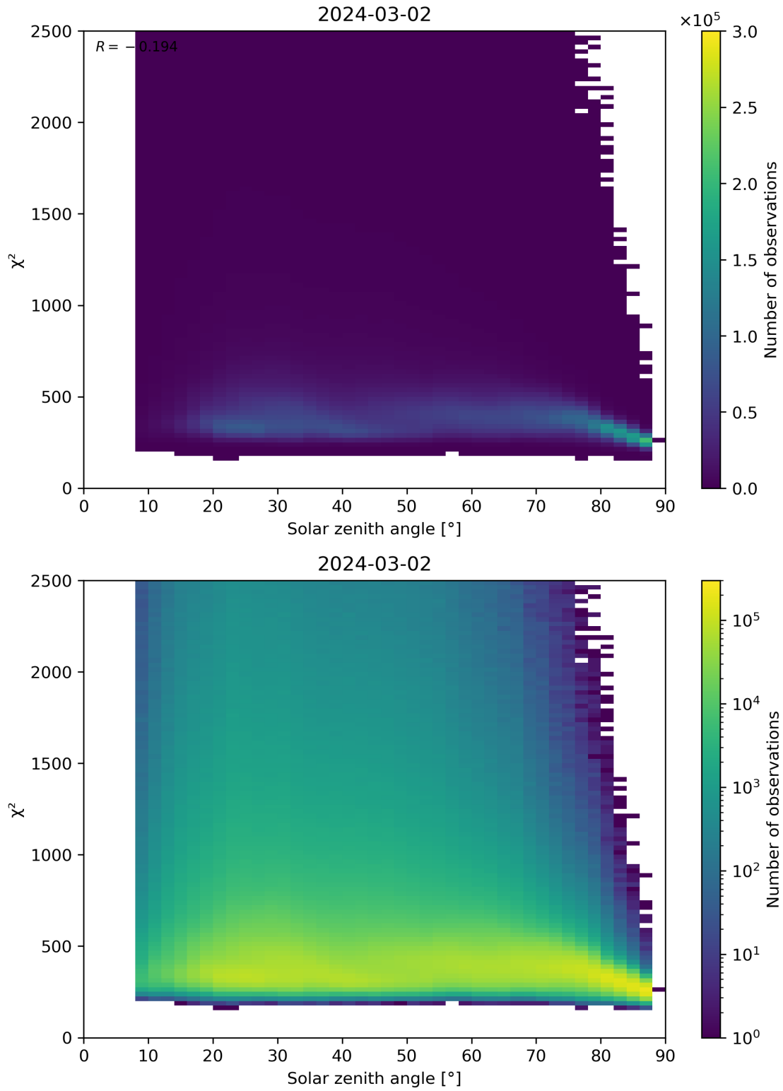
Figure 148: Scatter density plot of “Solar zenith angle” against “ \chi^2 ” for 2024-03-01 to 2024-03-03.
