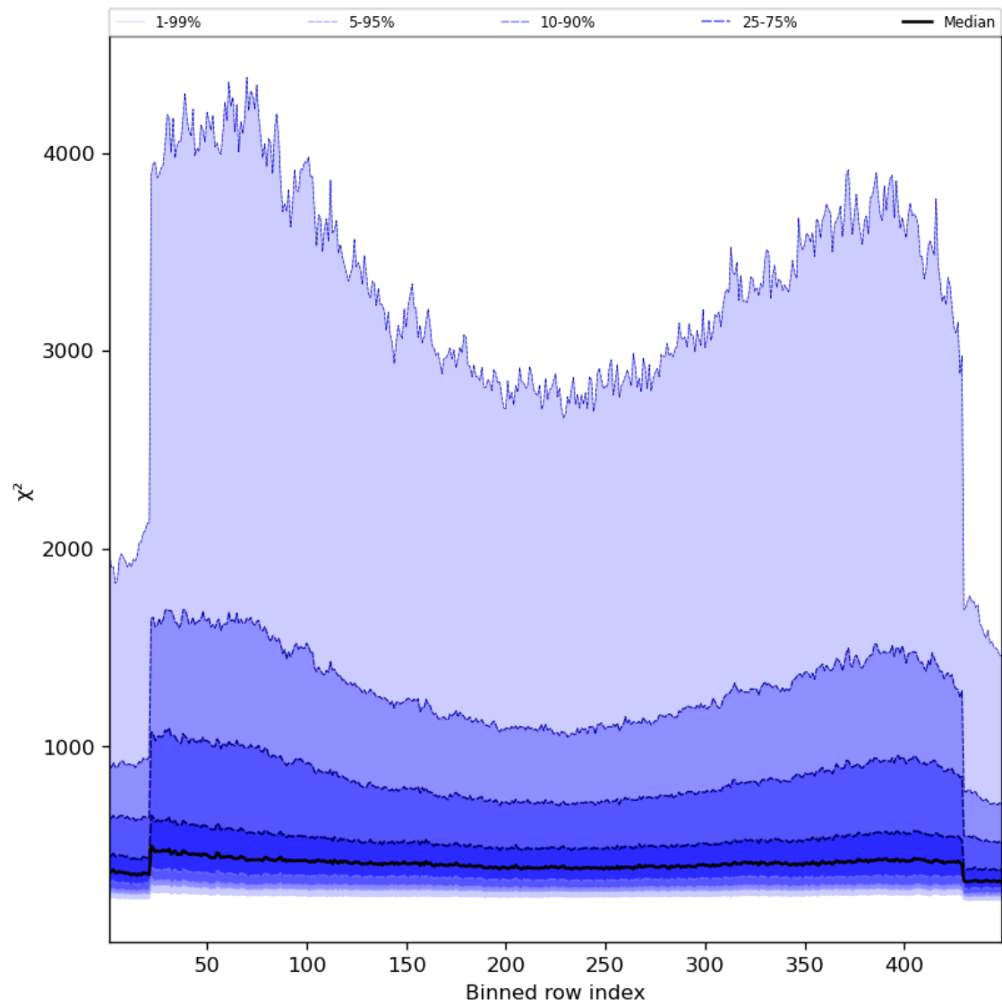
Figure 59: Along track statistics of “ \chi^2 ” for 2024-03-01 to 2024-03-03
