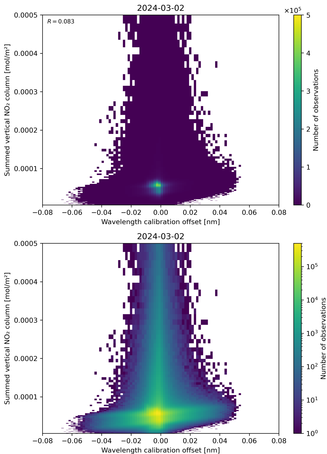
Figure 177: Scatter density plot of “Wavelength calibration offset” against “Summed vertical NO 2 column” for 2024-03-01 to 2024-03-03.
