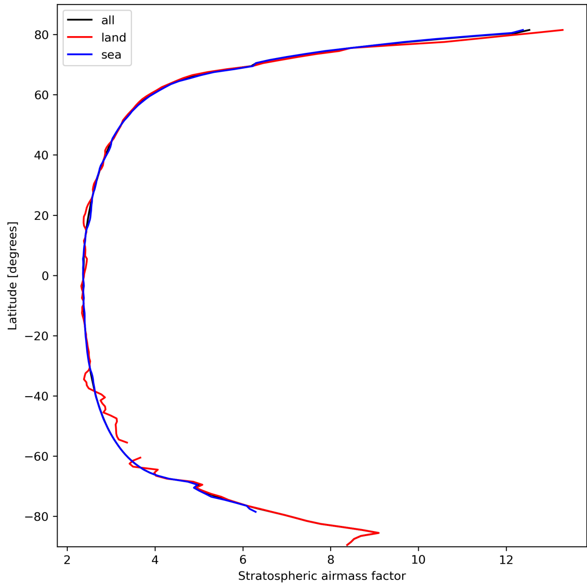
Figure 27: Zonal average of “Stratospheric air mass factor” for 2024-03-01 to 2024-03-03.
