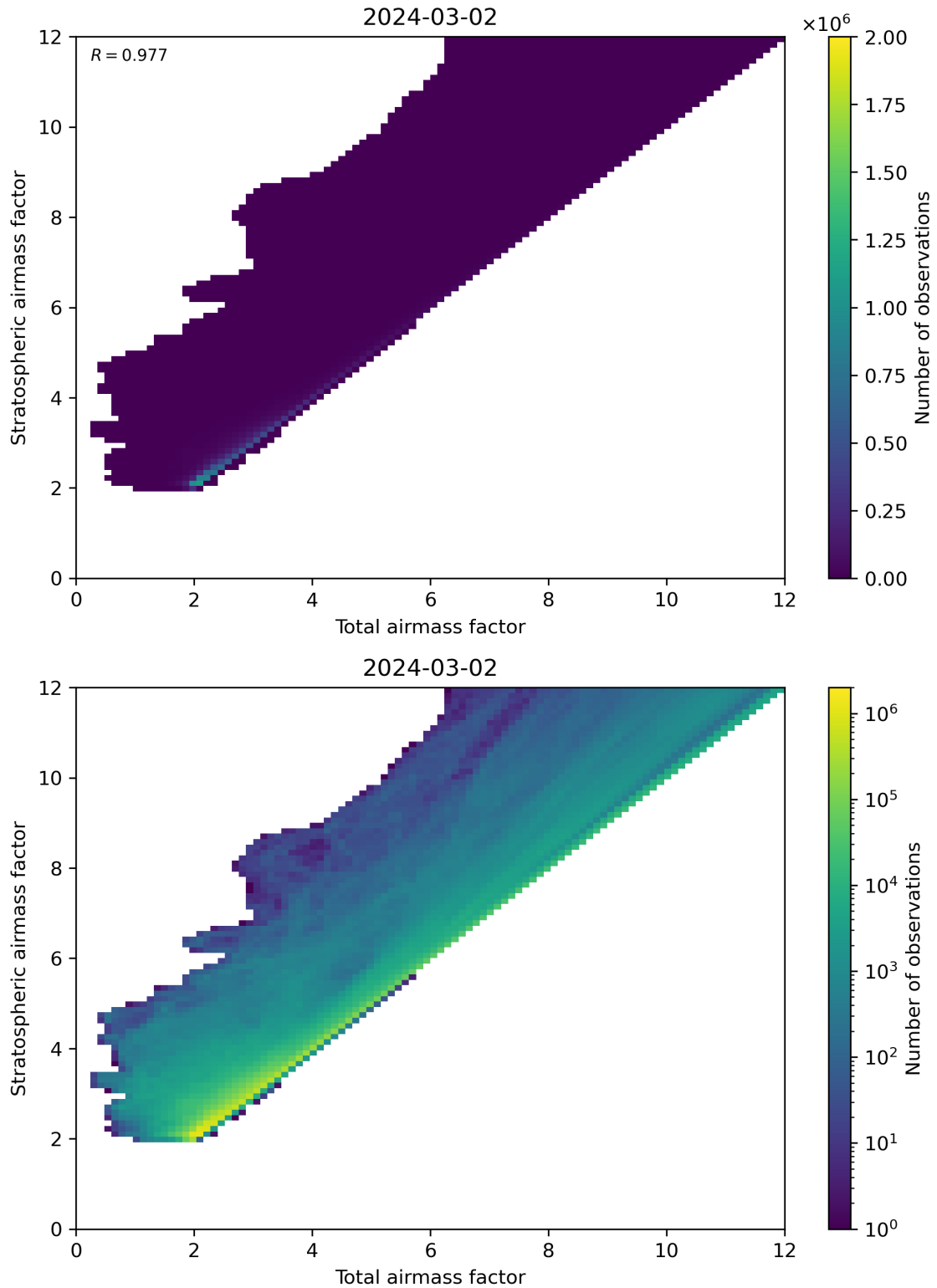
Figure 62: Scatter density plot of “Total airmass factor” against “Stratospheric airmass factor” for 2024-03-01 to 2024-03-03.
