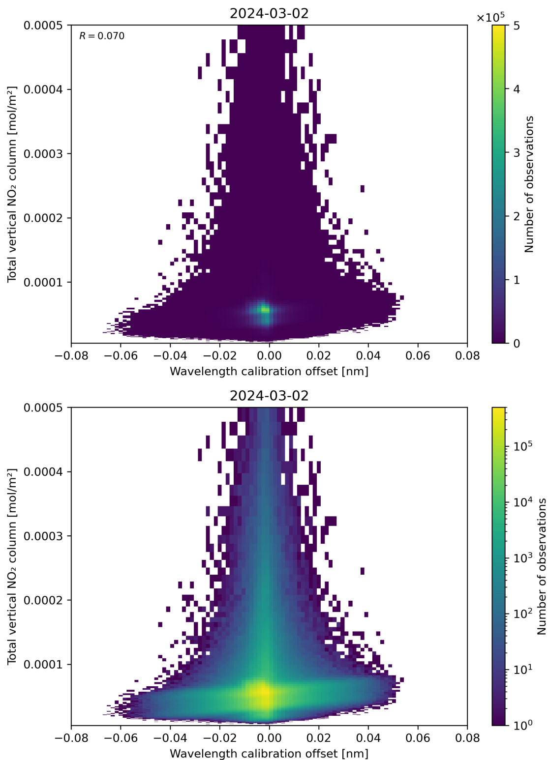
Figure 179: Scatter density plot of “Wavelength calibration offset” against “Total vertical NO 2 column” for 2024-03-01 to 2024-03-03.
