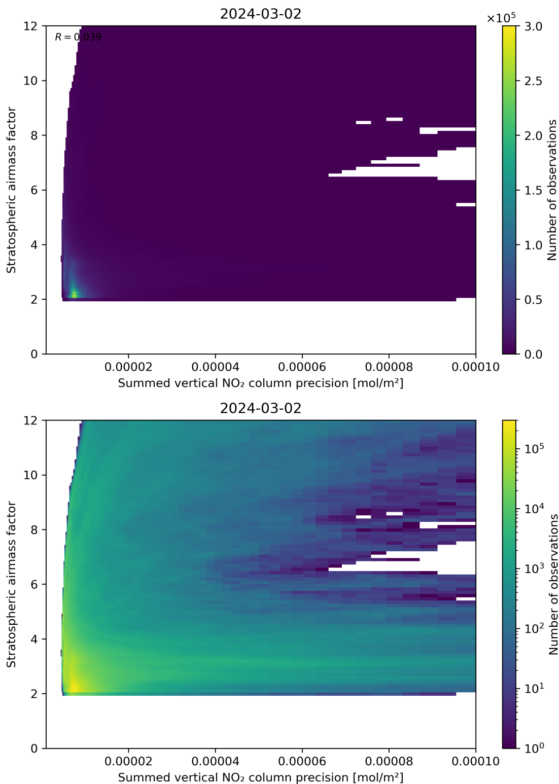
Figure 106: Scatter density plot of “Summed vertical NO 2 column precision” against “Stratospheric airmass factor” for 2024-03-01 to 2024-03-03.
