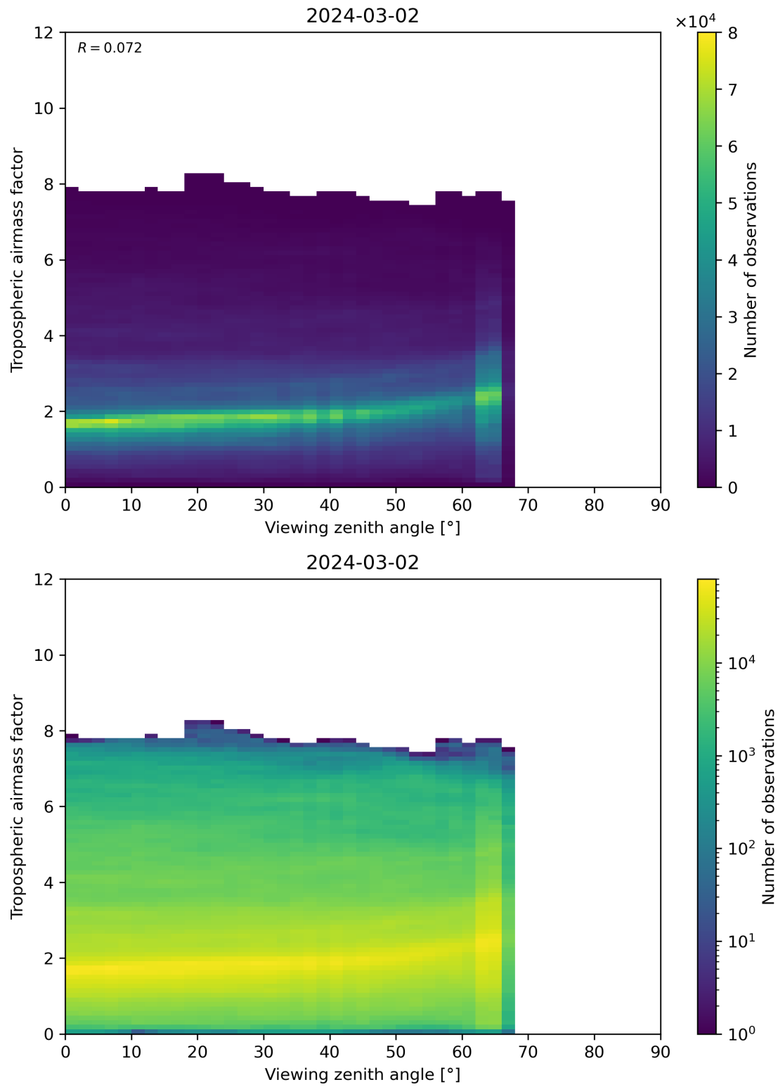
Figure 161: Scatter density plot of “Viewing zenith angle” against “Tropospheric airmass factor” for 2024-03-01 to 2024-03-03.
