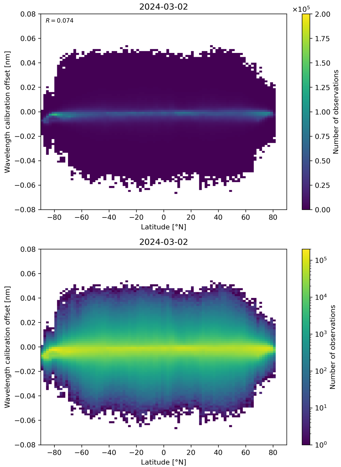
Figure 95: Scatter density plot of “Latitude” against “Wavelength calibration offset” for 2024-03-01 to 2024-03-03.
