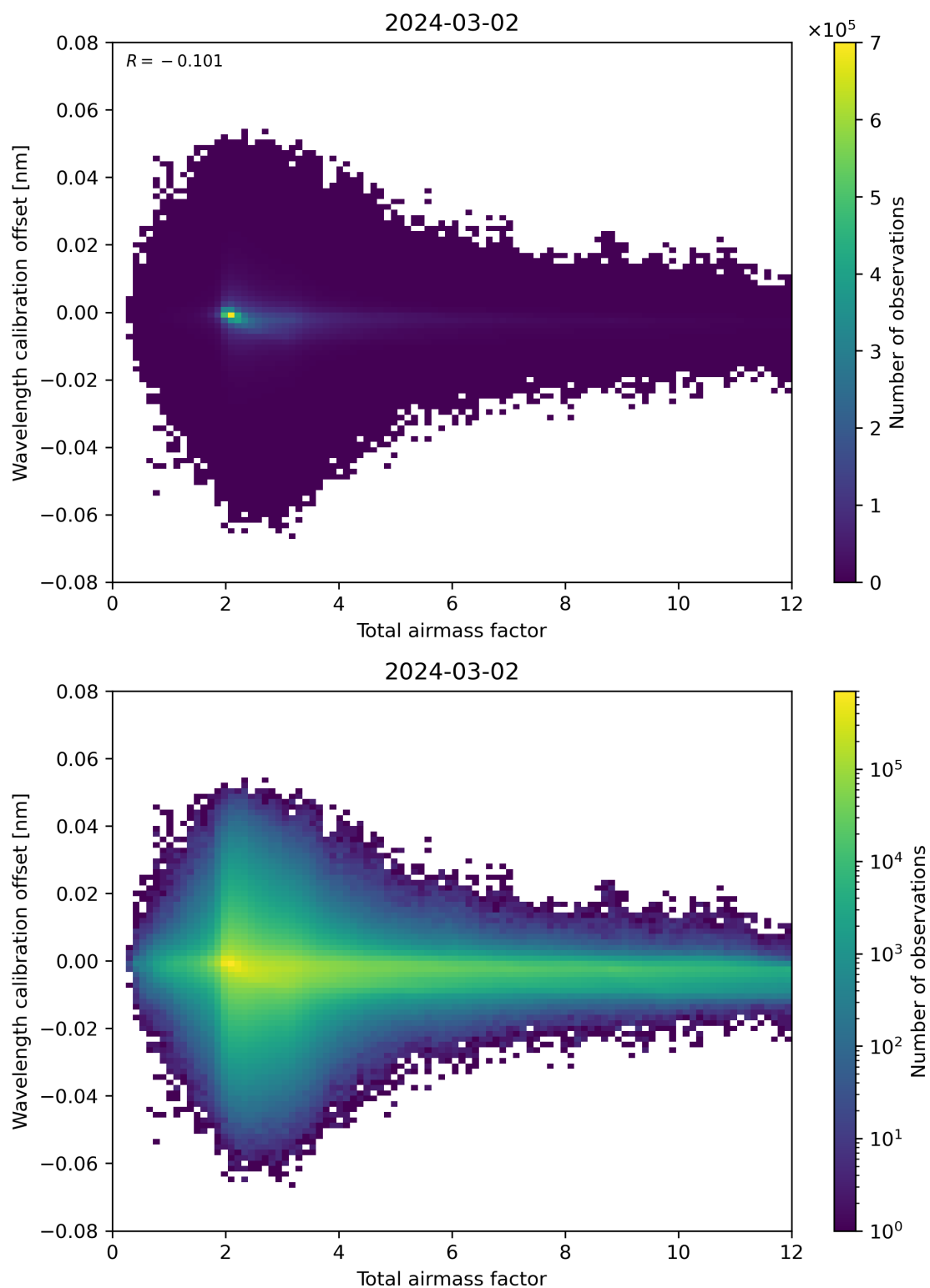
Figure 70: Scatter density plot of “Total airmass factor” against “Wavelength calibration offset” for 2024-03-01 to 2024-03-03.
