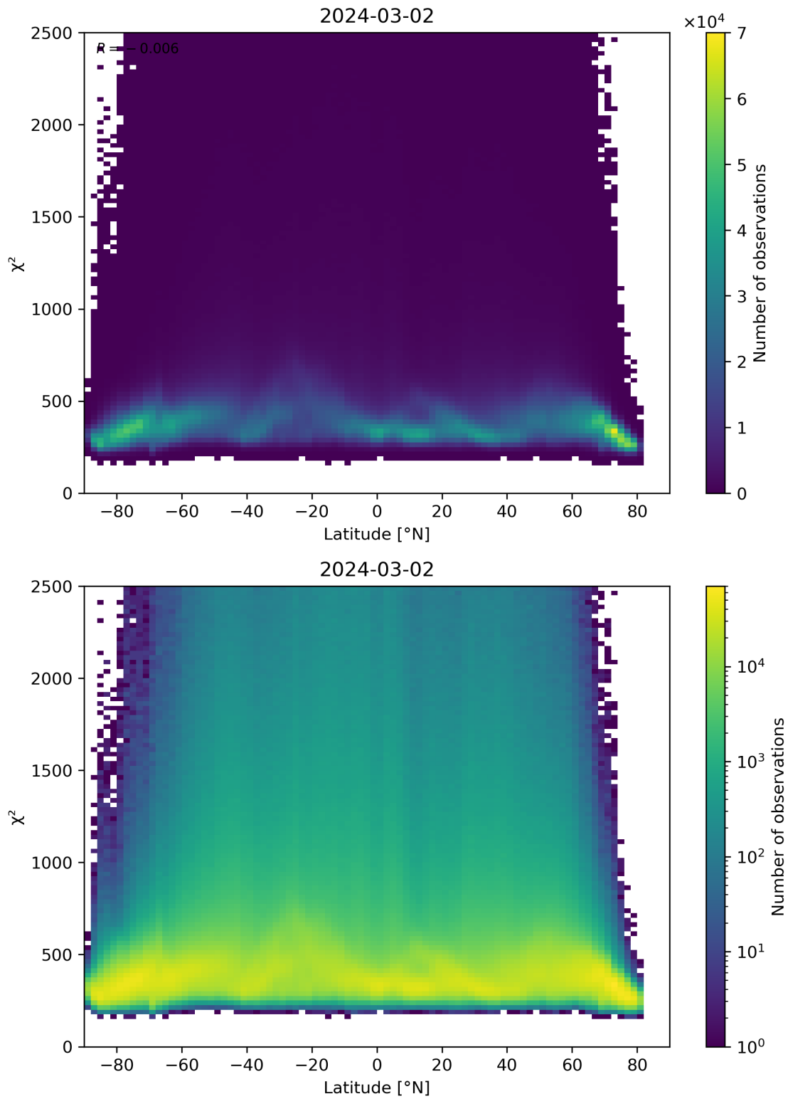
Figure 86: Scatter density plot of “Latitude” against “ \chi^2 ” for 2024-03-01 to 2024-03-03.
