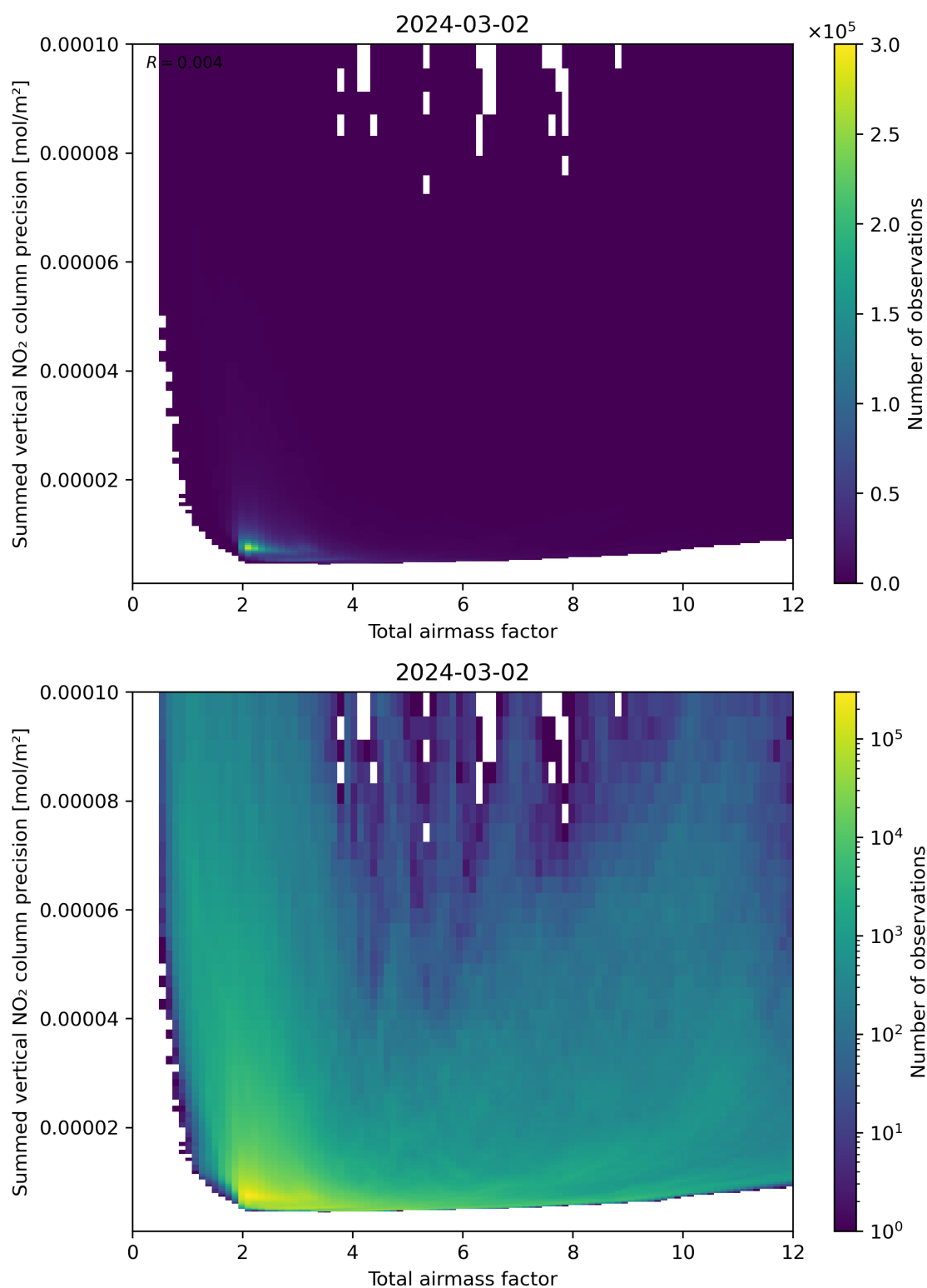
Figure 66: Scatter density plot of “Total airmass factor” against “Summed vertical NO 2 column precision” for 2024-03-01 to 2024-03-03.
