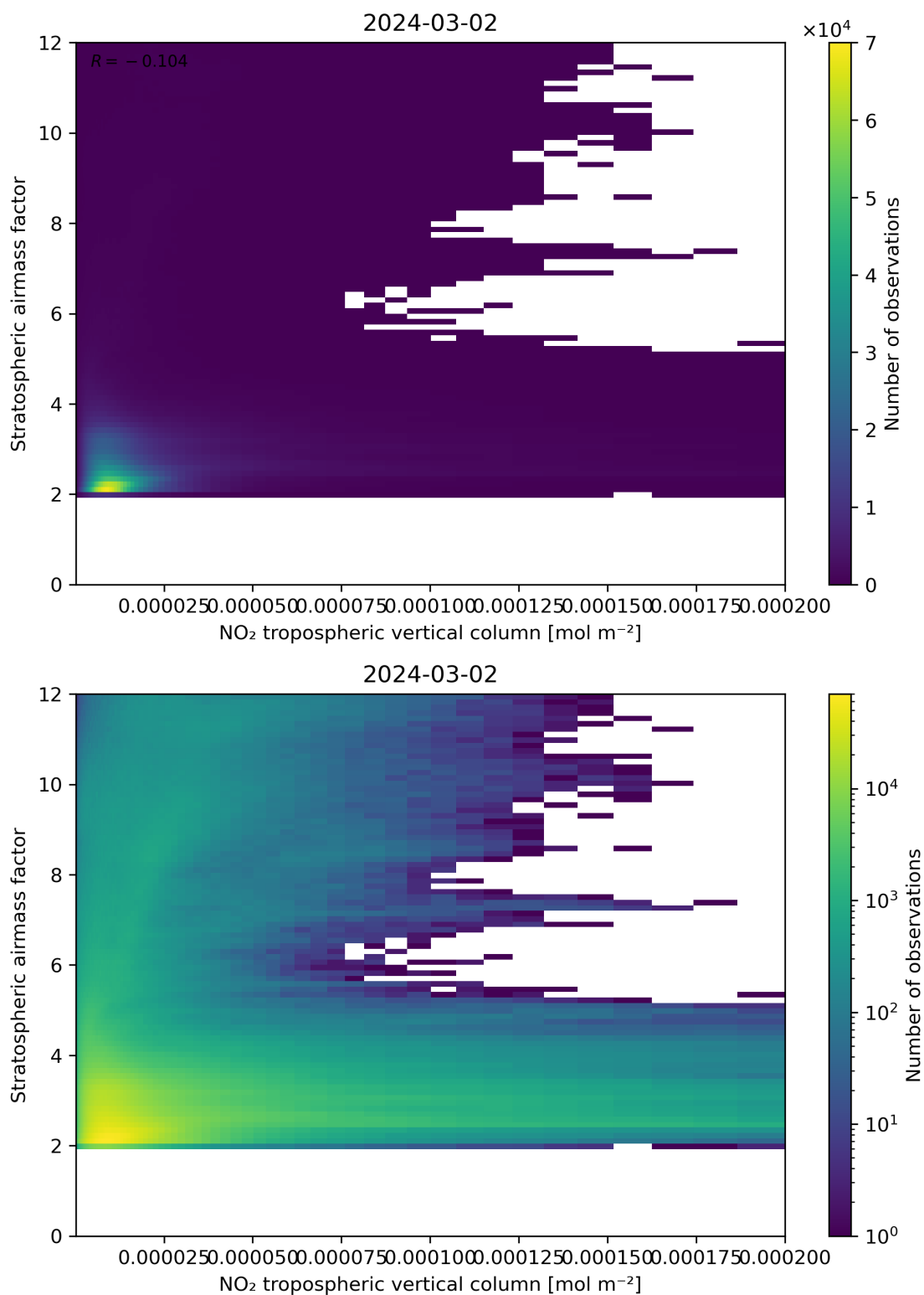
Figure 121: Scatter density plot of “NO 2 tropospheric vertical column” against “Stratospheric air mass factor” for 2024-03-01 to 2024-03-03.
