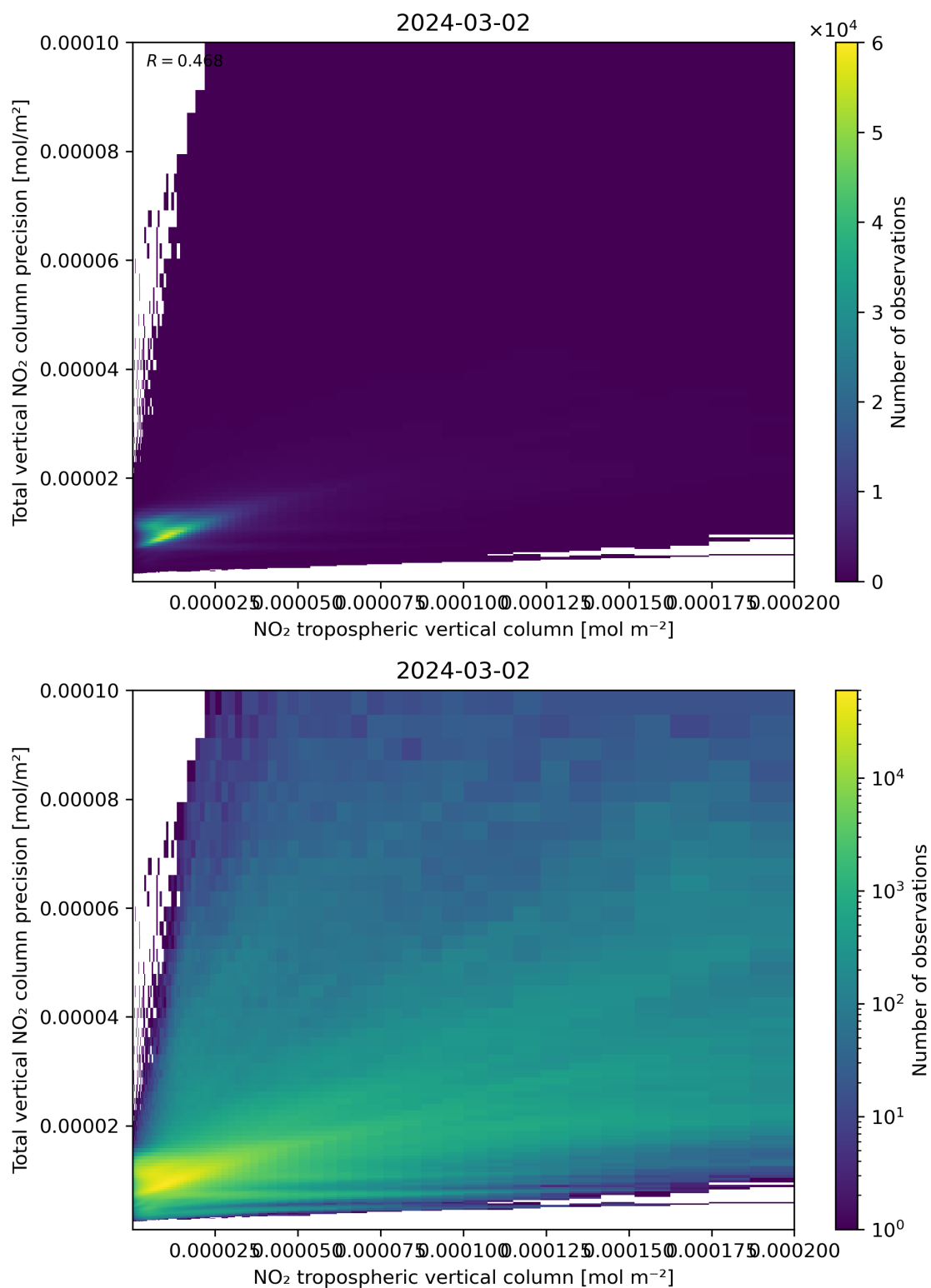
Figure 129: Scatter density plot of “NO 2 tropospheric vertical column” against “Total vertical NO 2 column precision” for 2024-03-01 to 2024-03-03.
