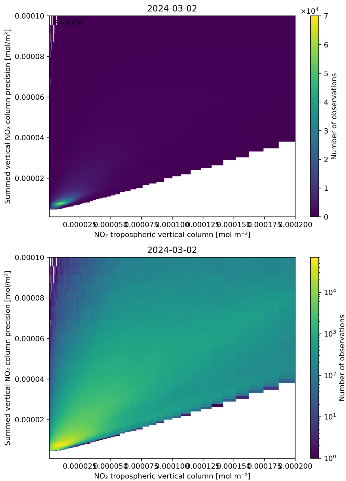
Figure 127: Scatter density plot of “NO 2 tropospheric vertical column” against “Summed vertical NO 2 column precision” for 2024-03-01 to 2024-03-03.
