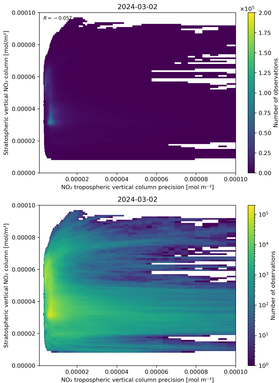
Figure 135: Scatter density plot of “NO 2 tropospheric vertical column precision” against “Stratospheric vertical NO 2 column” for 2024-03-01 to 2024-03-03.
