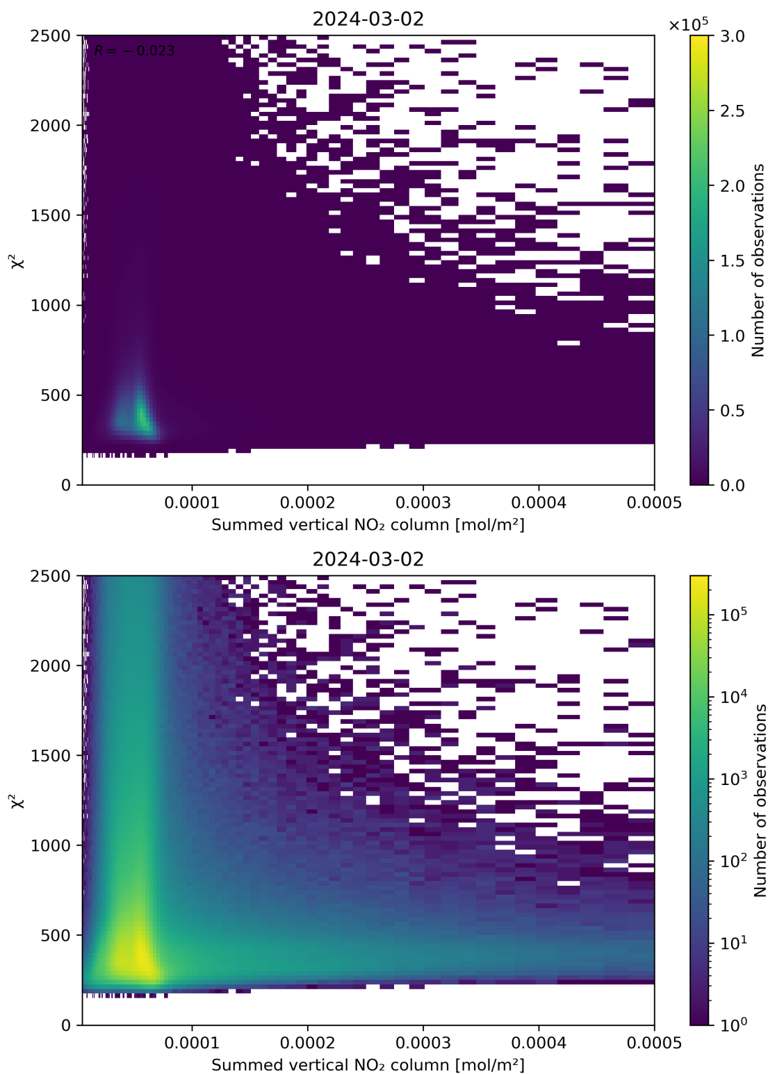
Figure 104: Scatter density plot of “Summed vertical NO 2 column” against “ \chi^2 ” for 2024-03-01 to 2024-03-03.
