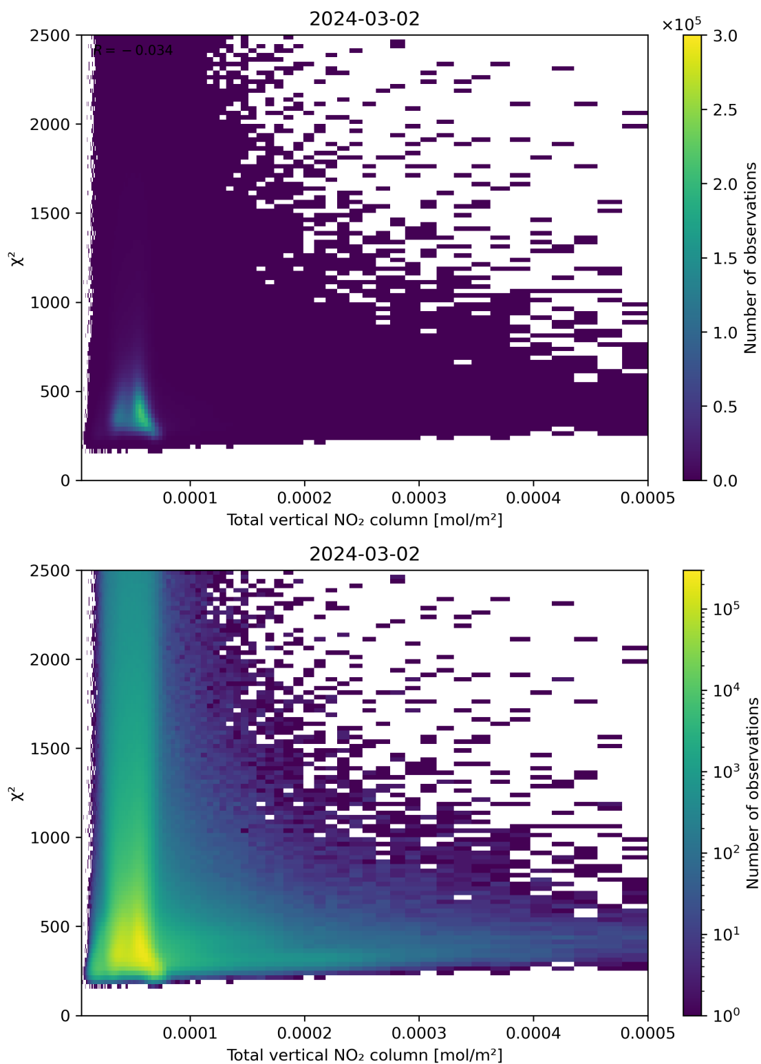
Figure 111: Scatter density plot of “Total vertical NO 2 column” against “ \chi^2 ” for 2024-03-01 to 2024-03-03.
