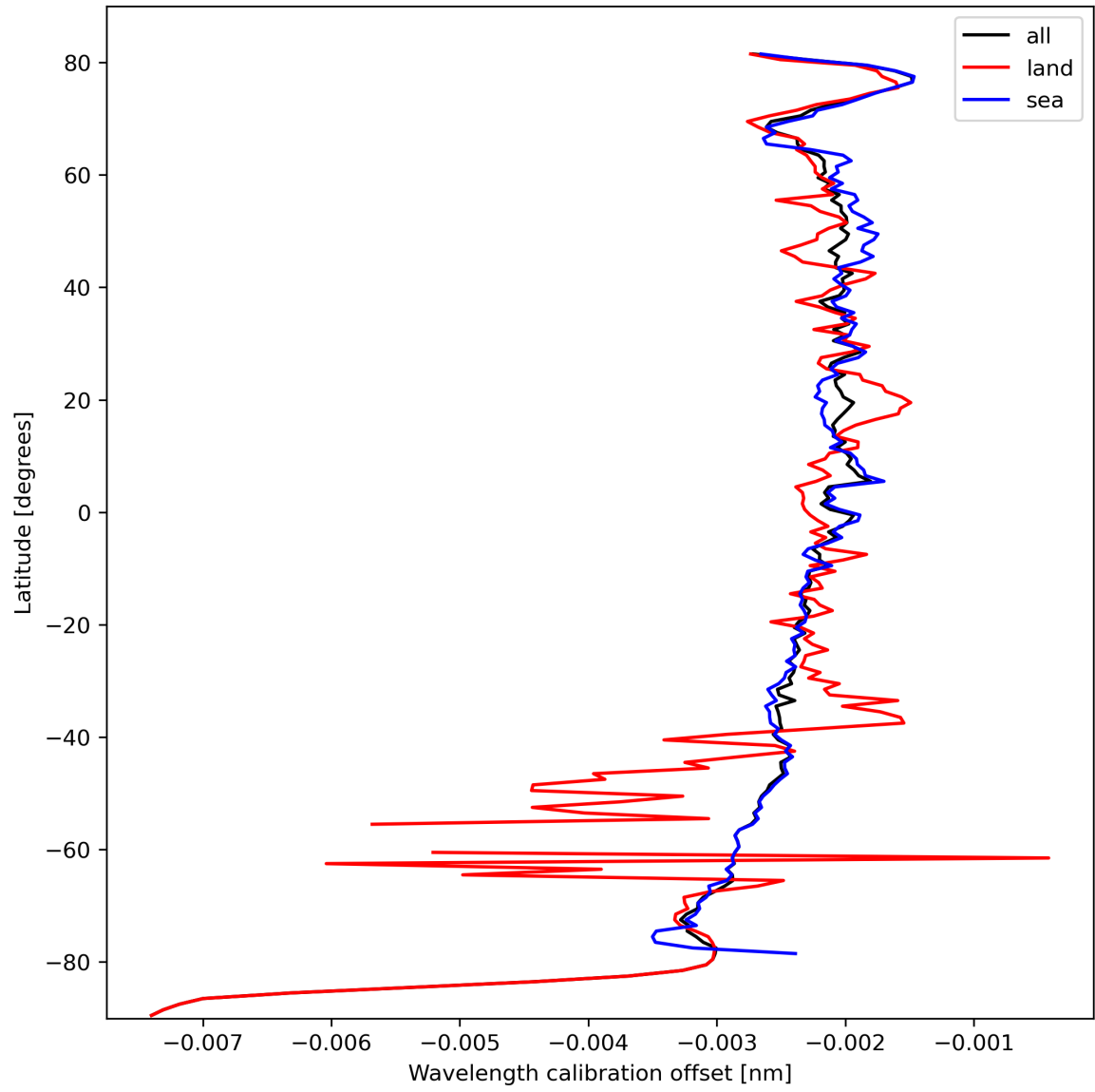
Figure 18: Zonal average of “Wavelength calibration offset” for 2024-03-01 to 2024-03-03.
