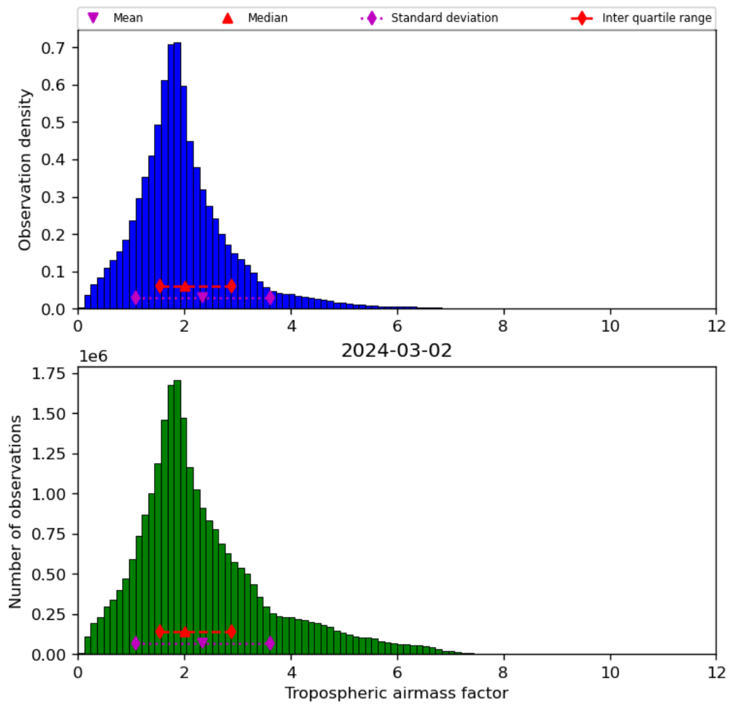
Figure 31: Histogram of “Tropospheric airmass factor” for 2024-03-01 to 2024-03-03
