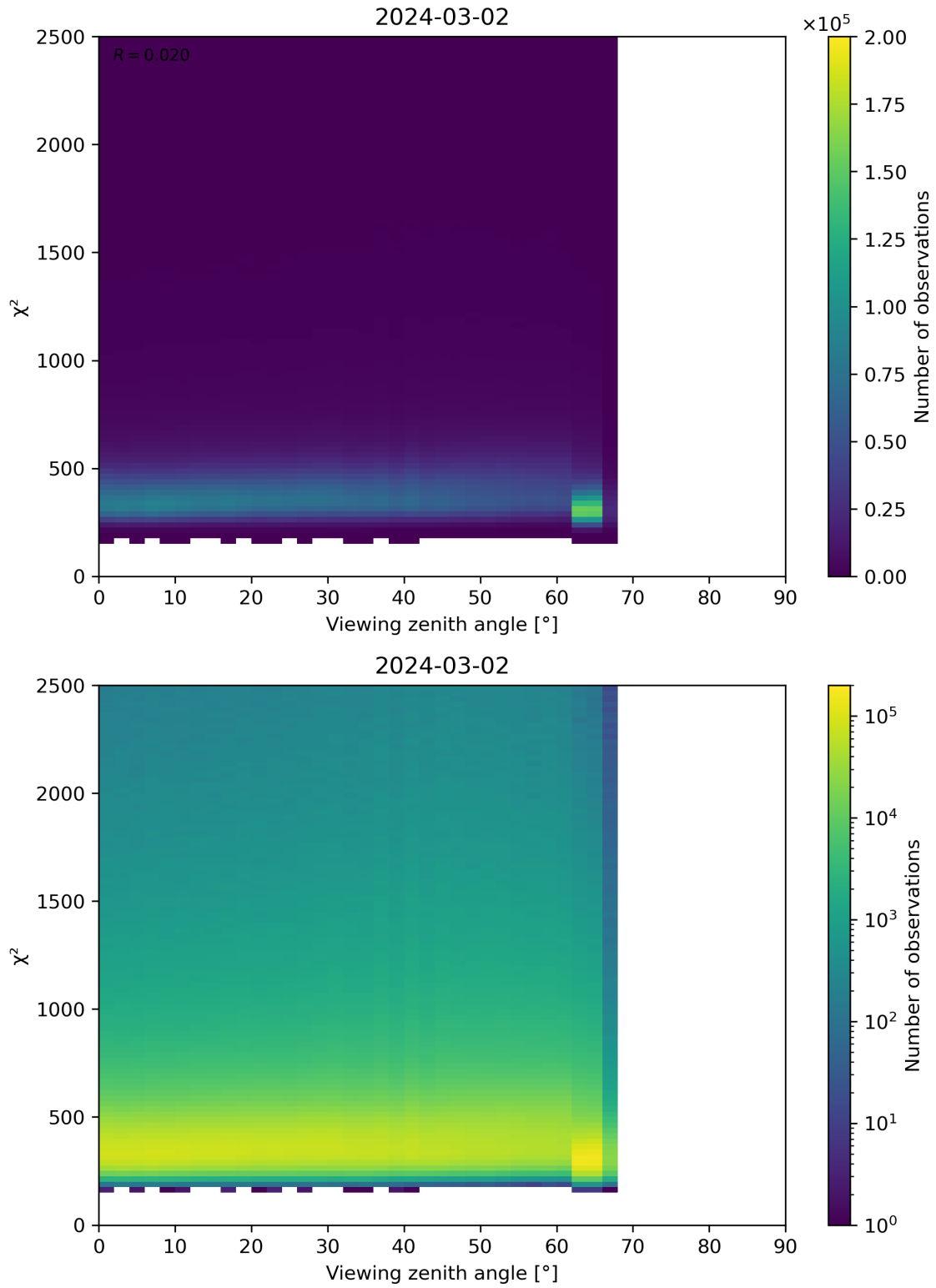
Figure 162: Scatter density plot of “Viewing zenith angle” against “ \chi^2 ” for 2024-03-01 to 2024-03-03.
