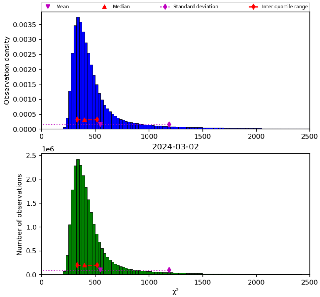
Figure 42: Histogram of “ \chi^2 ” for 2024-03-01 to 2024-03-03
