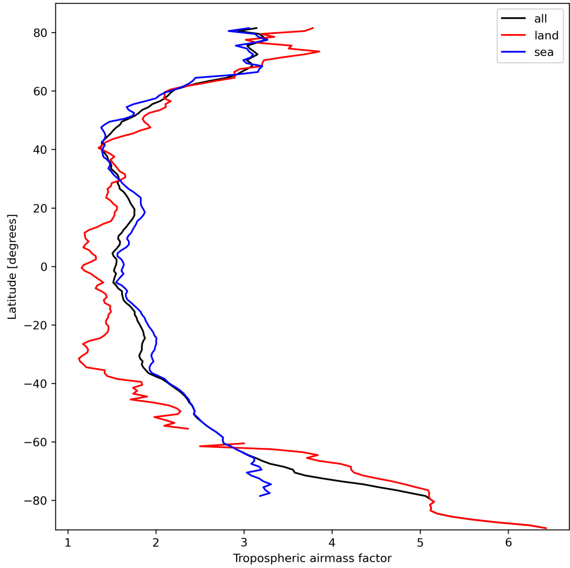
Figure 14: Zonal average of “Tropospheric airmass factor” for 2024-03-01 to 2024-03-03.
