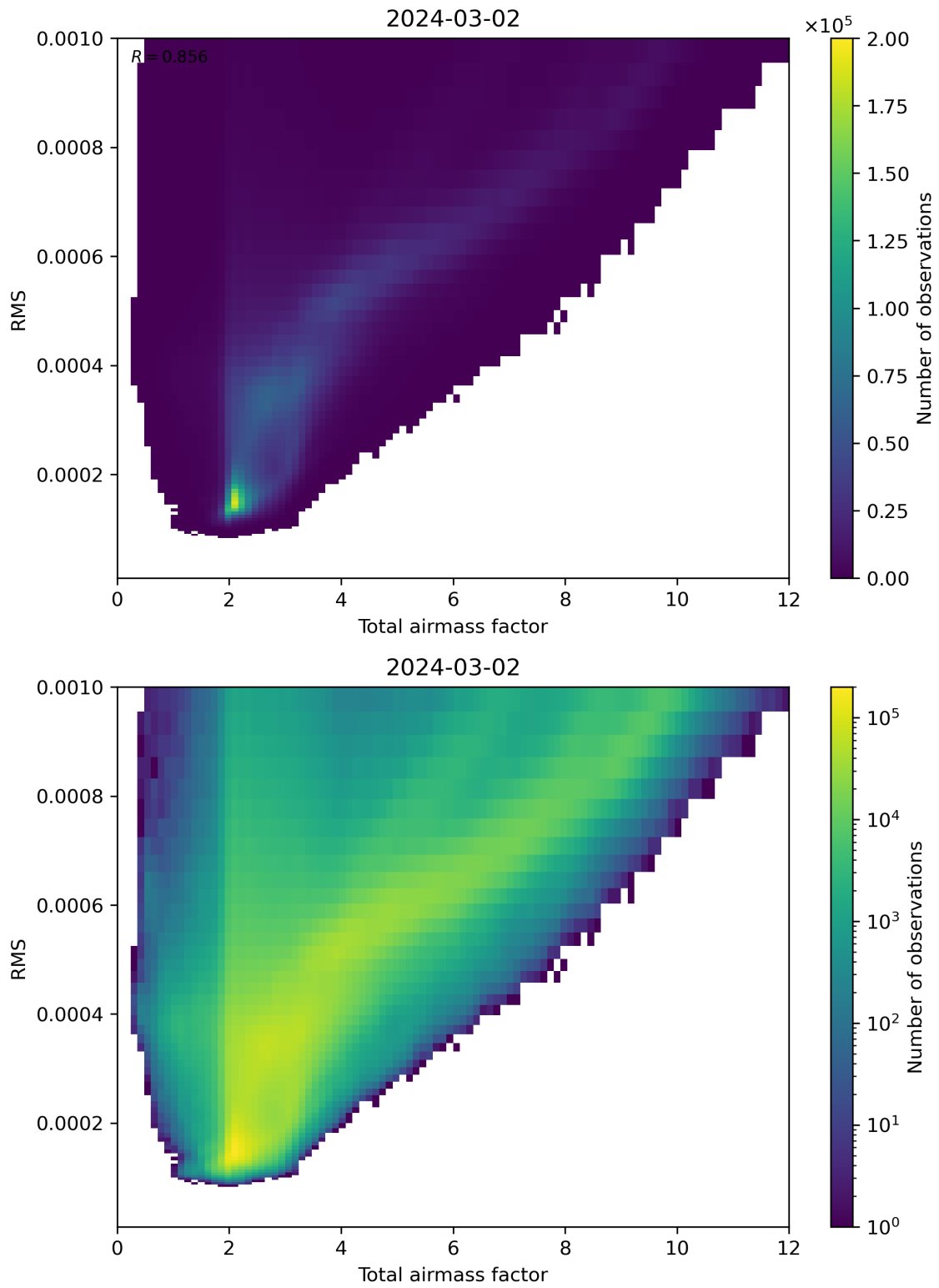
Figure 69: Scatter density plot of “Total airmass factor” against “RMS” for 2024-03-01 to 2024-03-03.
