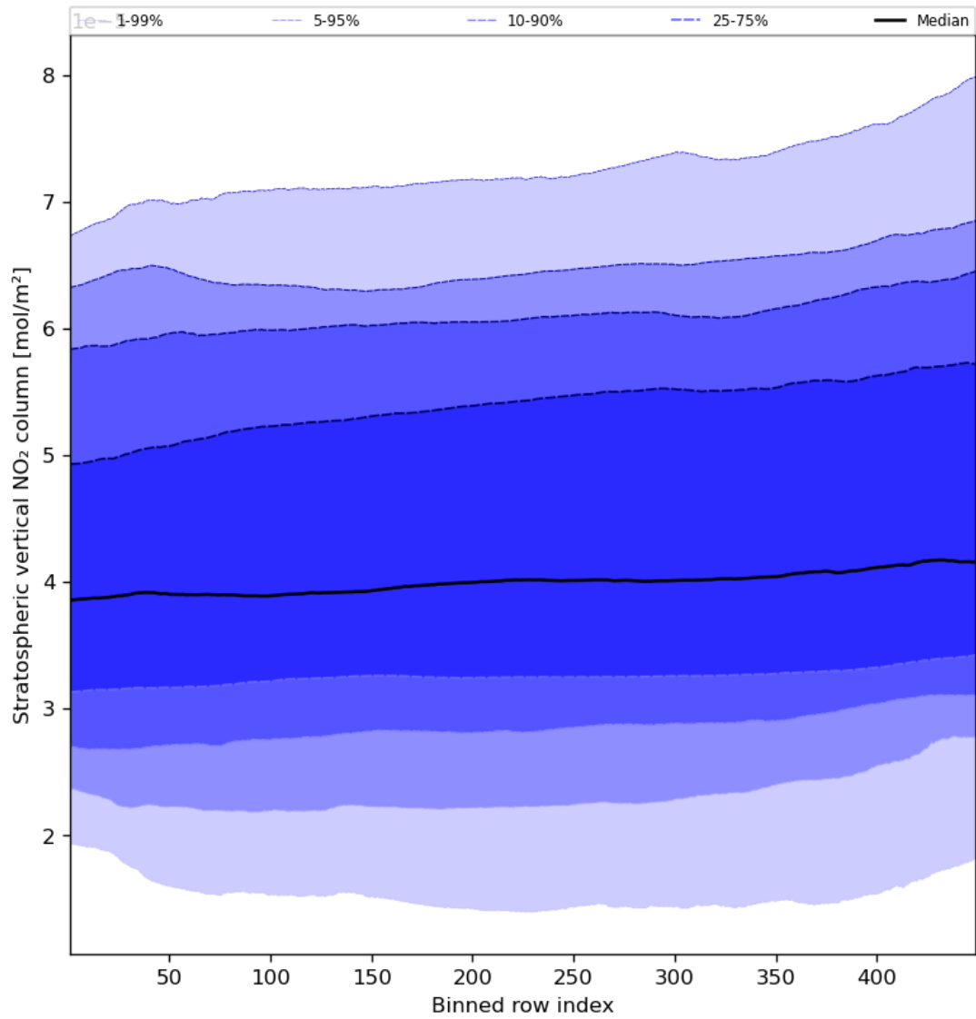
Figure 53: Along track statistics of “Stratospheric vertical NO 2 column” for 2024-03-01 to 2024-03-03
