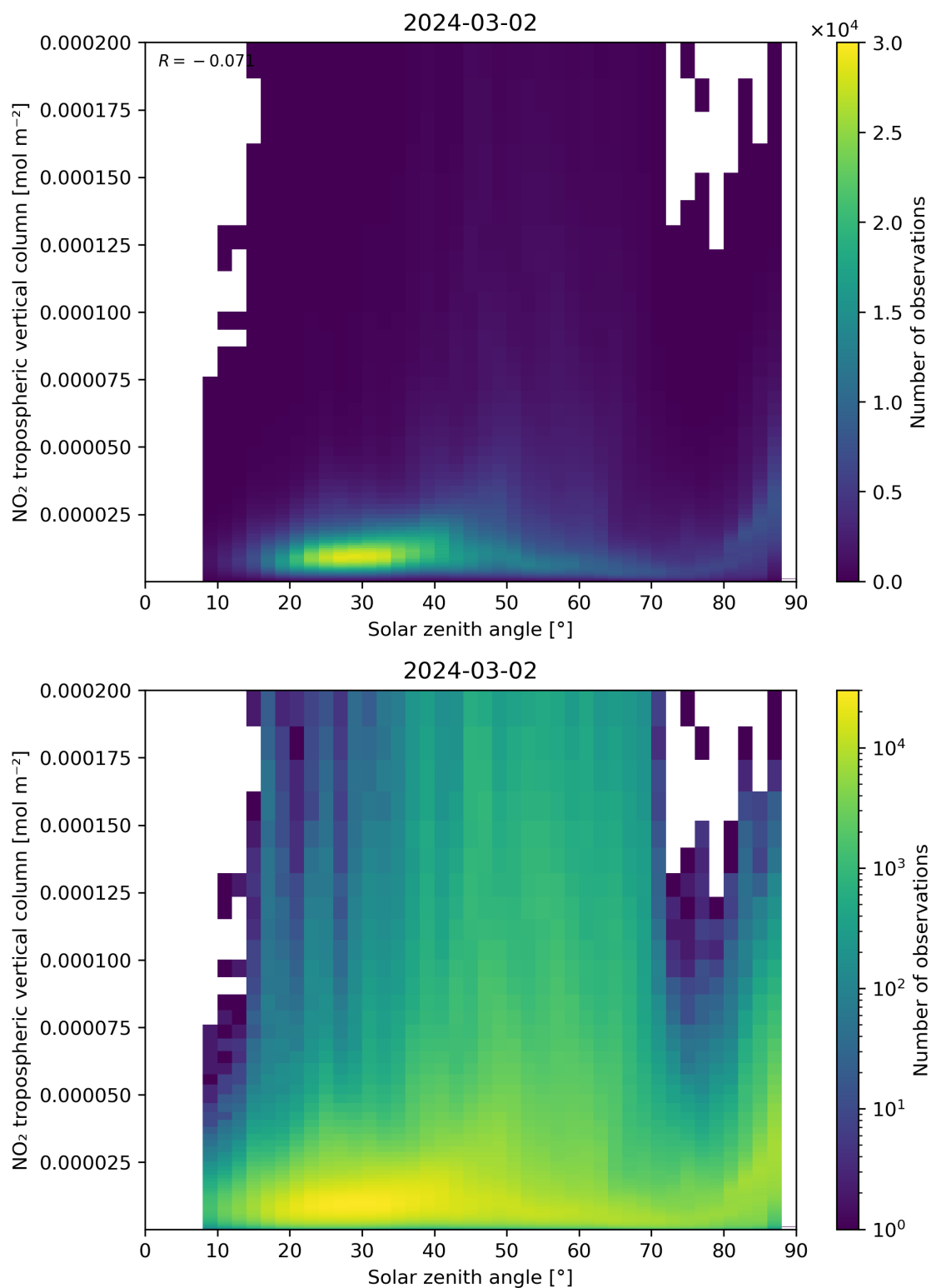
Figure 155: Scatter density plot of “Solar zenith angle” against “NO 2 tropospheric vertical column” for 2024-03-01 to 2024-03-03.
