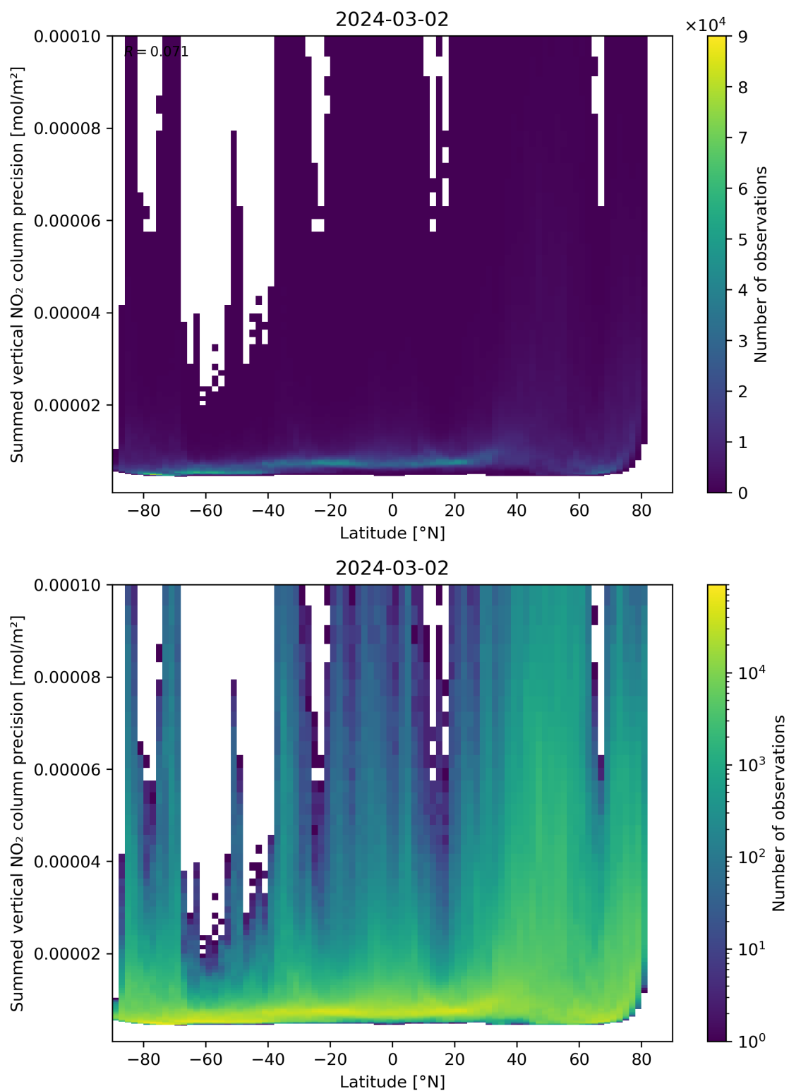
Figure 89: Scatter density plot of “Latitude” against “Summed vertical NO 2 column precision” for 2024-03-01 to 2024-03-03.
