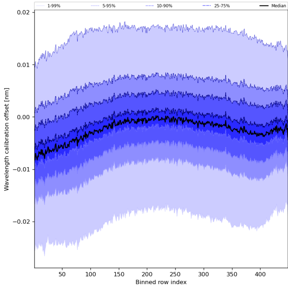
Figure 52: Along track statistics of “Wavelength calibration offset” for 2024-03-01 to 2024-03-03
