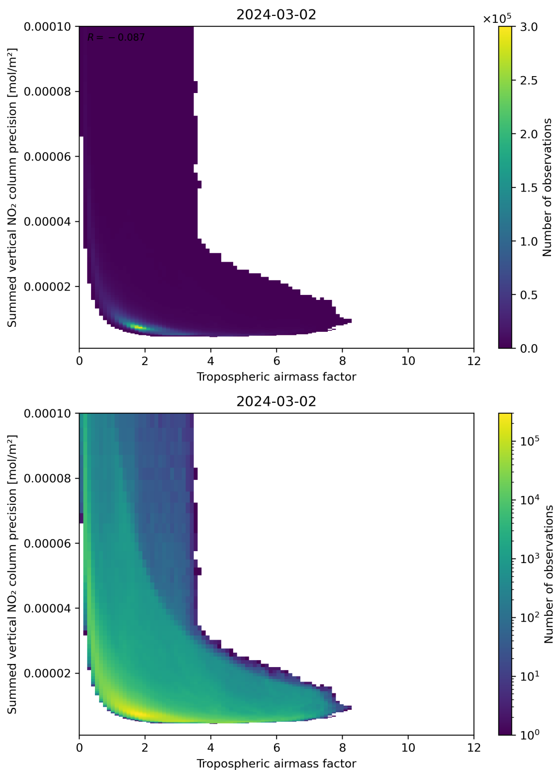
Figure 76: Scatter density plot of “Tropospheric air mass factor” against “Summed vertical NO 2 column precision” for 2024-03-01 to 2024-03-03.
