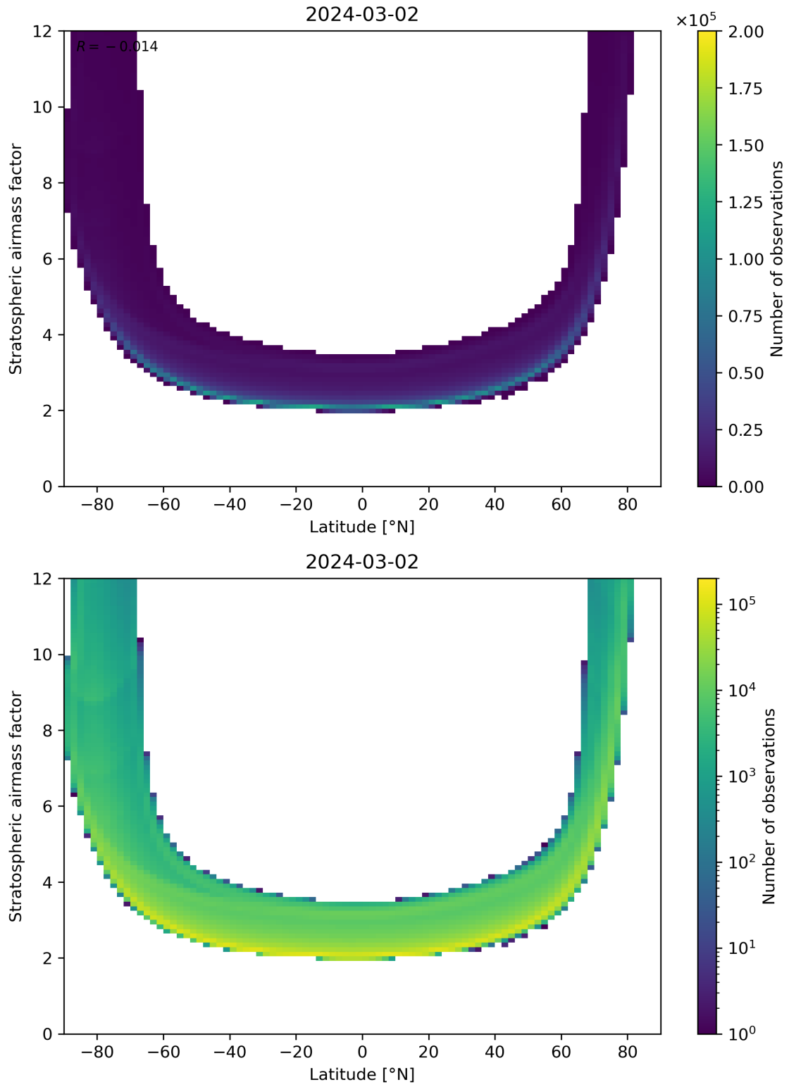
Figure 83: Scatter density plot of “Latitude” against “Stratospheric airmass factor” for 2024-03-01 to 2024-03-03.
