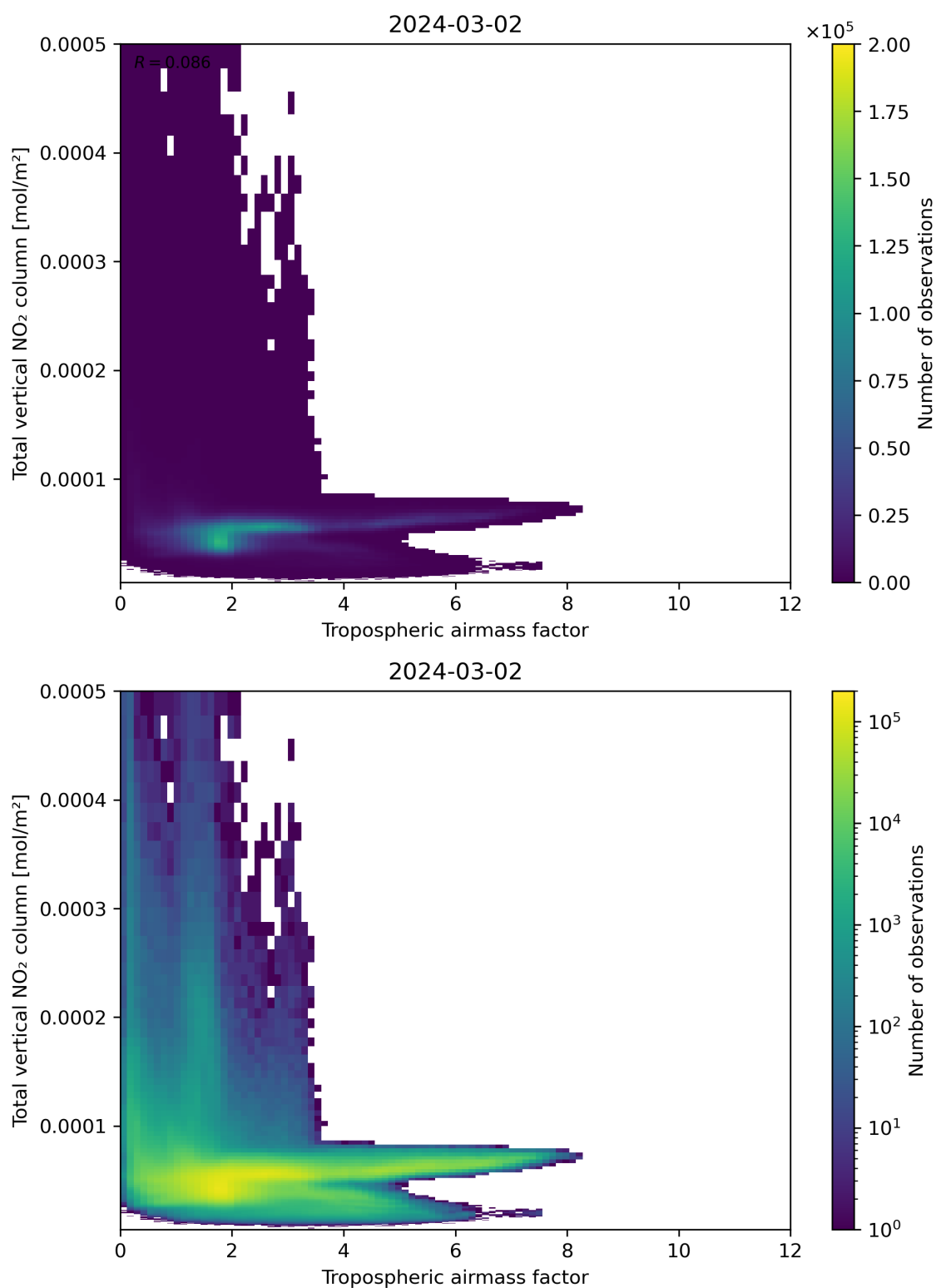
Figure 77: Scatter density plot of “Tropospheric airmass factor” against “Total vertical NO 2 column” for 2024-03-01 to 2024-03-03.
