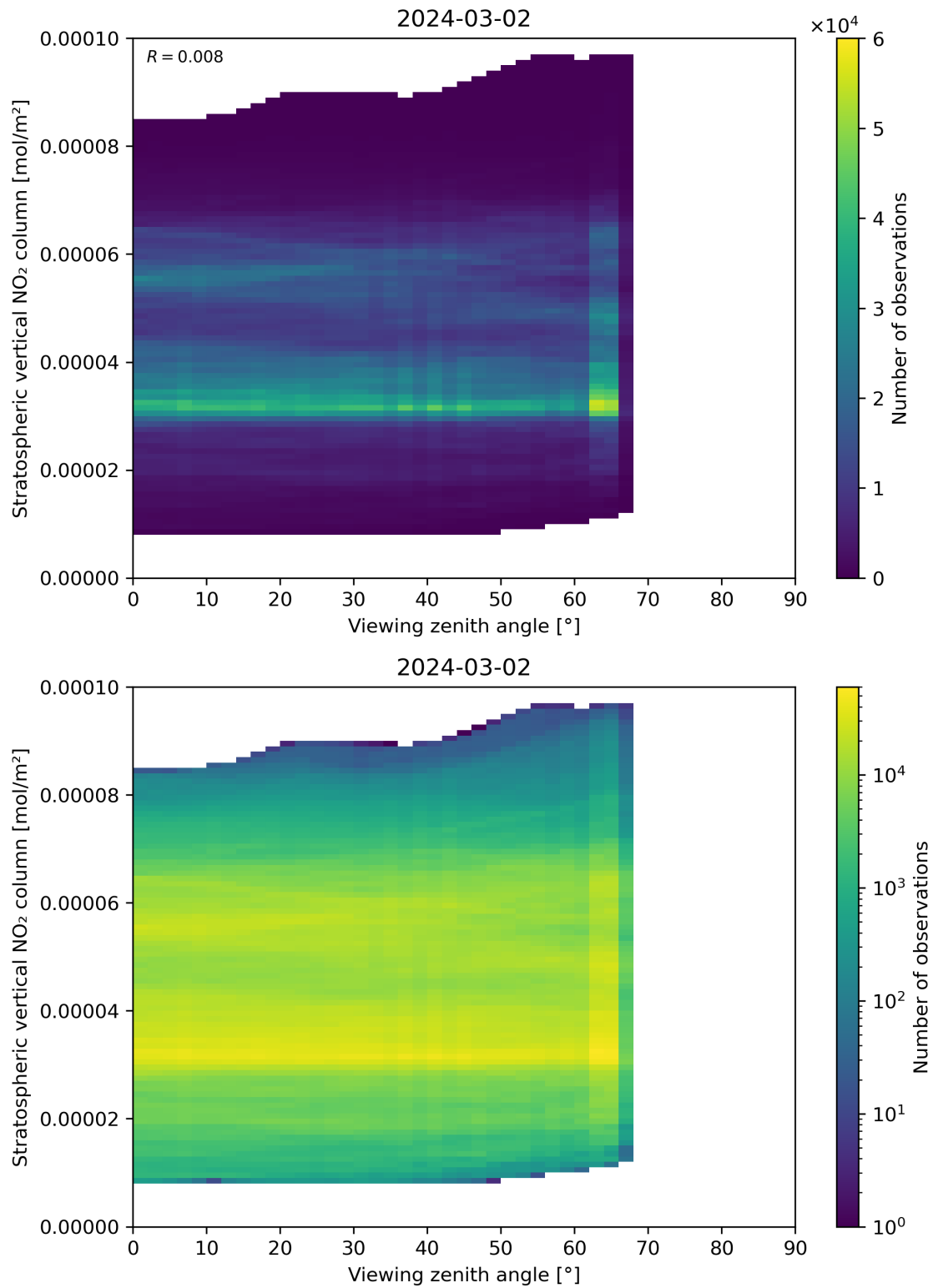
Figure 164: Scatter density plot of “Viewing zenith angle” against “Stratospheric vertical NO 2 column” for 2024-03-01 to 2024-03-03.
