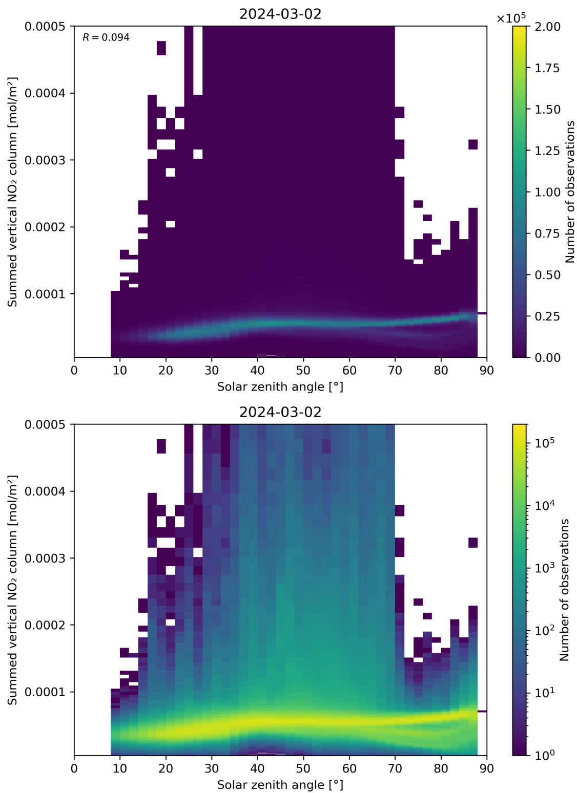
Figure 151: Scatter density plot of “Solar zenith angle” against “Summed vertical NO 2 column” for 2024-03-01 to 2024-03-03.
