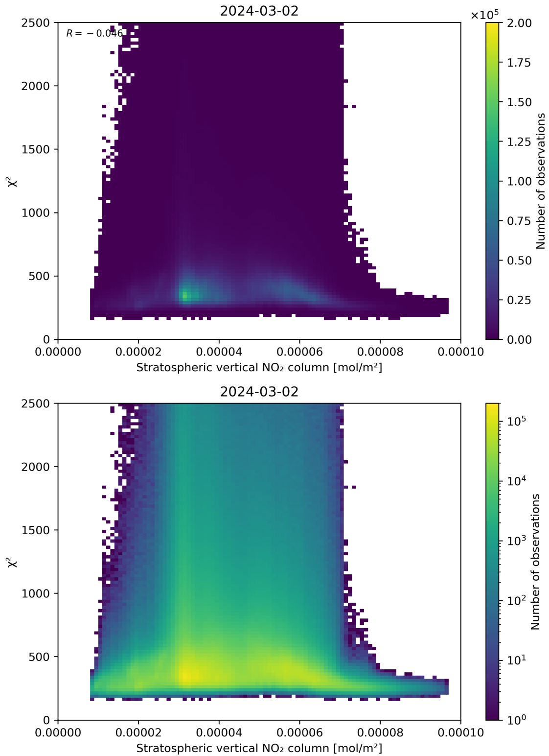
Figure 97: Scatter density plot of “Stratospheric vertical NO 2 column” against “ \chi^2 ” for 2024-03-01 to 2024-03-03.
