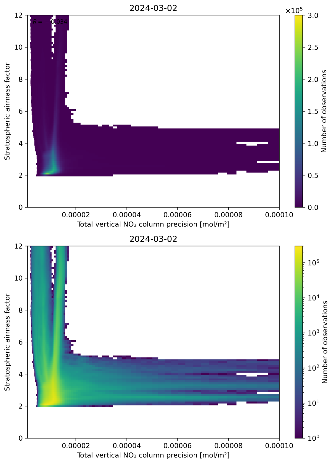
Figure 115: Scatter density plot of “Total vertical NO 2 column precision” against “Stratospheric air mass factor” for 2024-03-01 to 2024-03-03.
