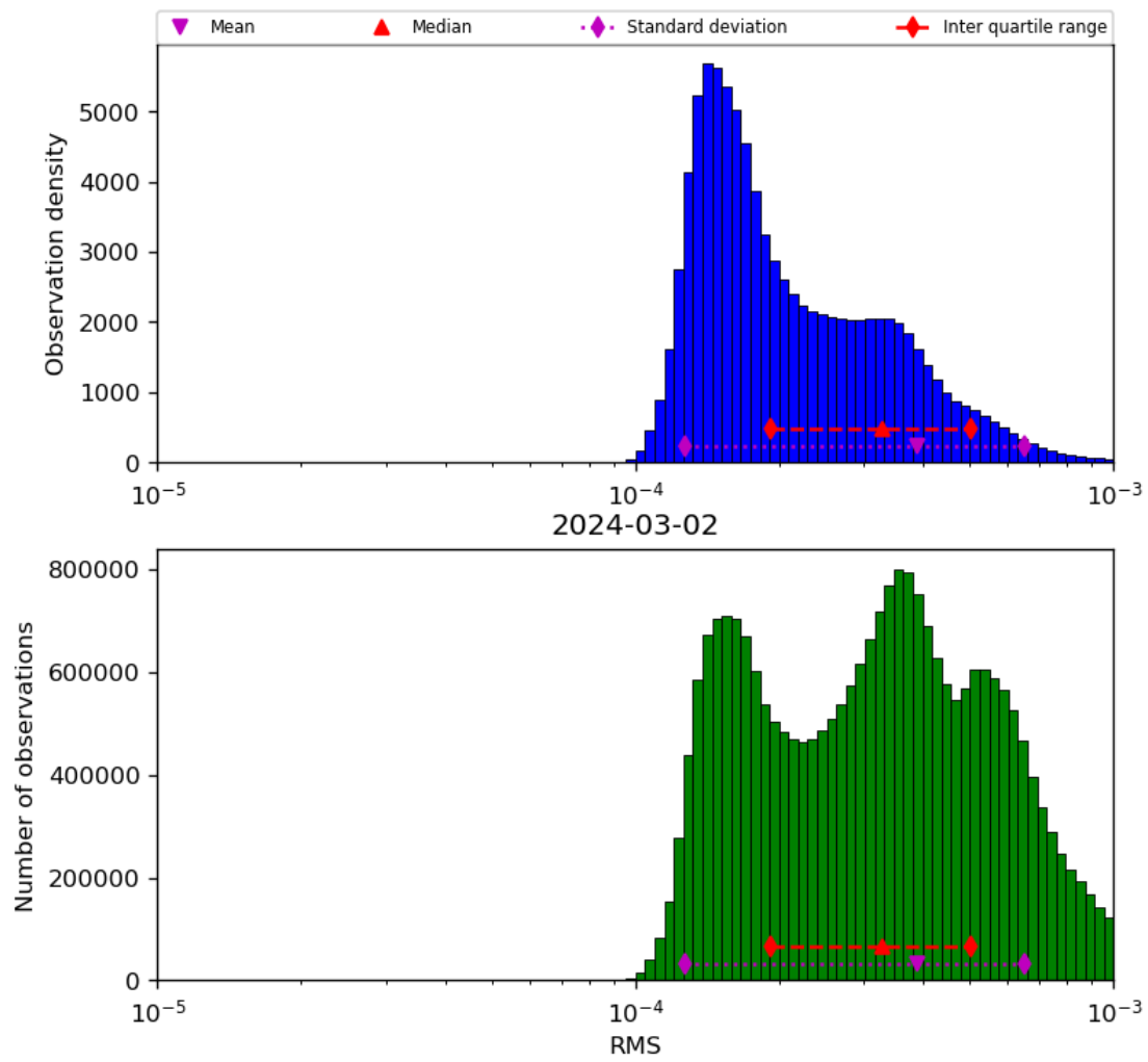
Figure 43: Histogram of “RMS” for 2024-03-01 to 2024-03-03
