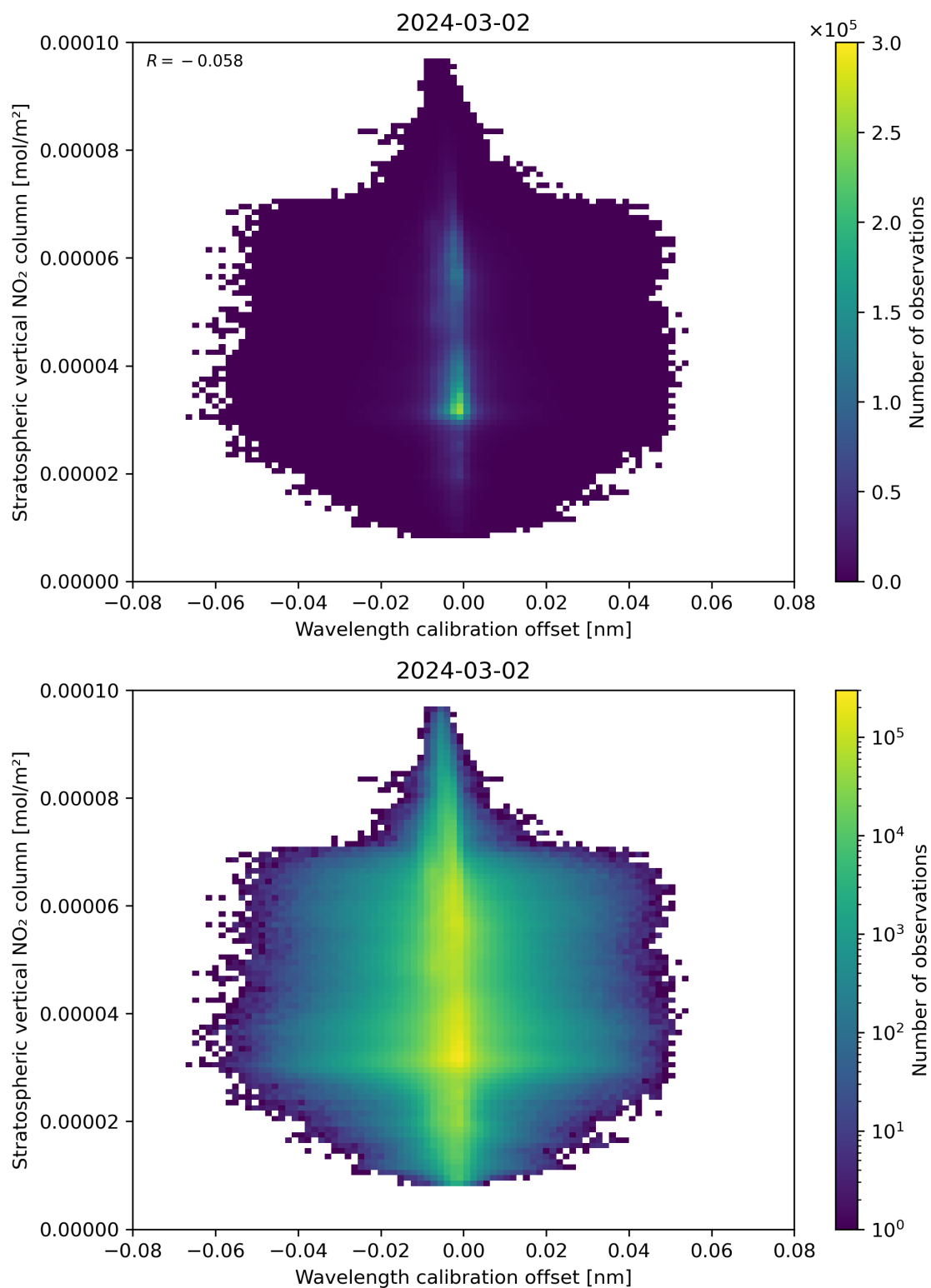
Figure 176: Scatter density plot of “Wavelength calibration offset” against “Stratospheric vertical NO 2 column” for 2024-03-01 to 2024-03-03.
