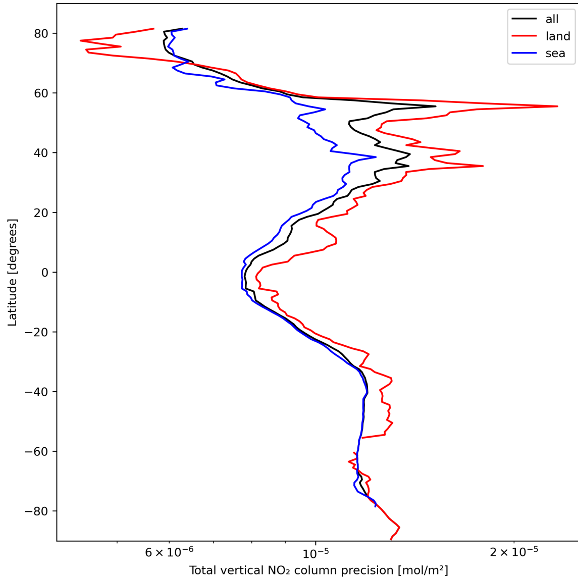
Figure 22: Zonal average of “Total vertical NO 2 column precision” for 2024-03-01 to 2024-03-03.
