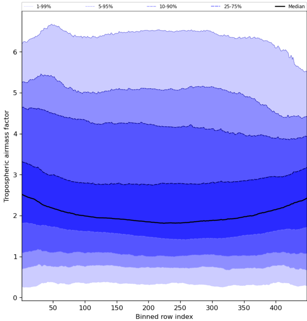
Figure 48: Along track statistics of “Tropospheric air mass factor” for 2024-03-01 to 2024-03-03
