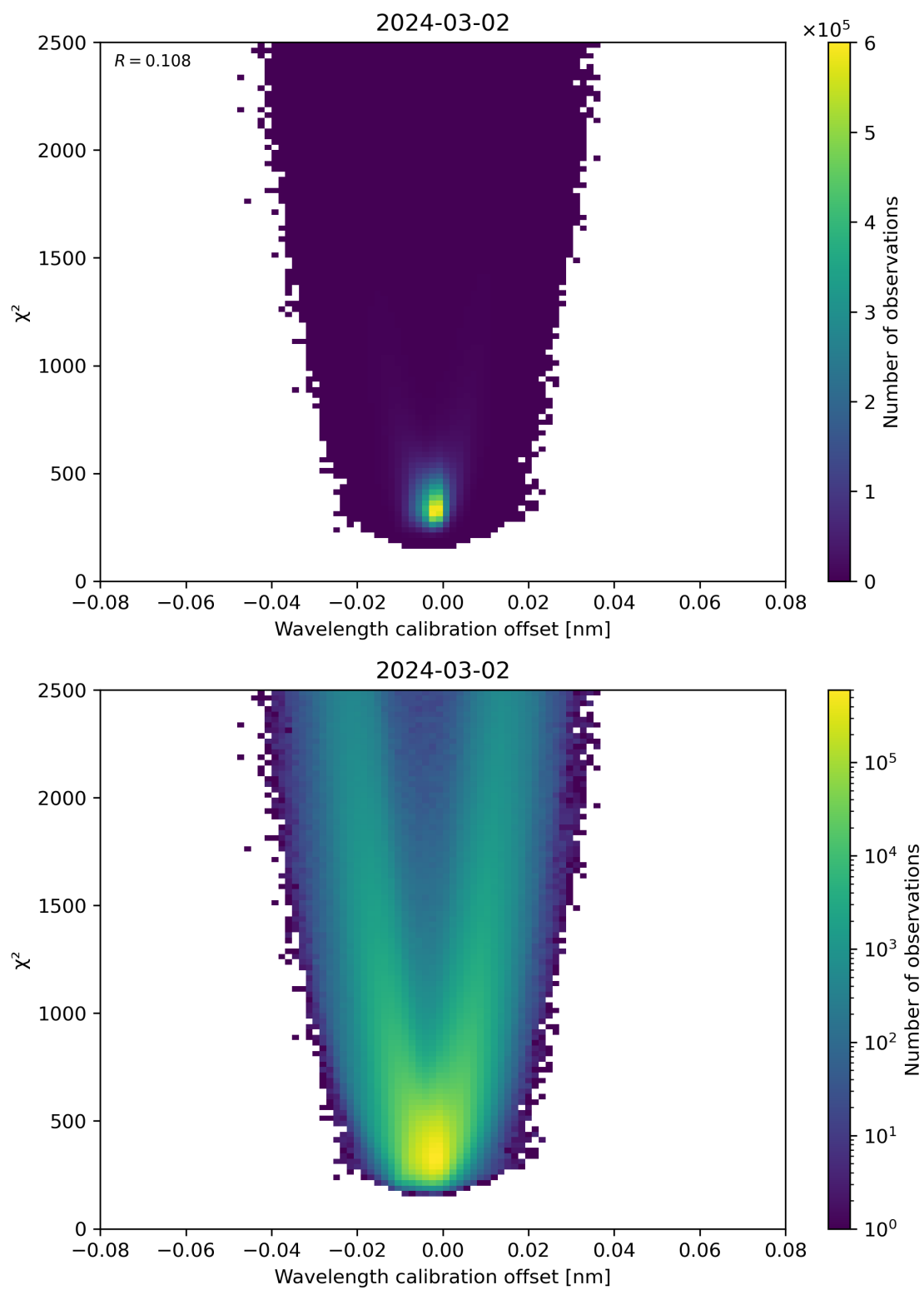
Figure 175: Scatter density plot of “Wavelength calibration offset” against “ \chi^2 ” for 2024-03-01 to 2024-03-03.
