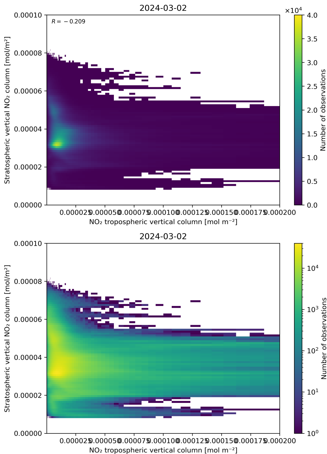
Figure 125: Scatter density plot of “NO 2 tropospheric vertical column” against “Stratospheric vertical NO 2 column” for 2024-03-01 to 2024-03-03.
