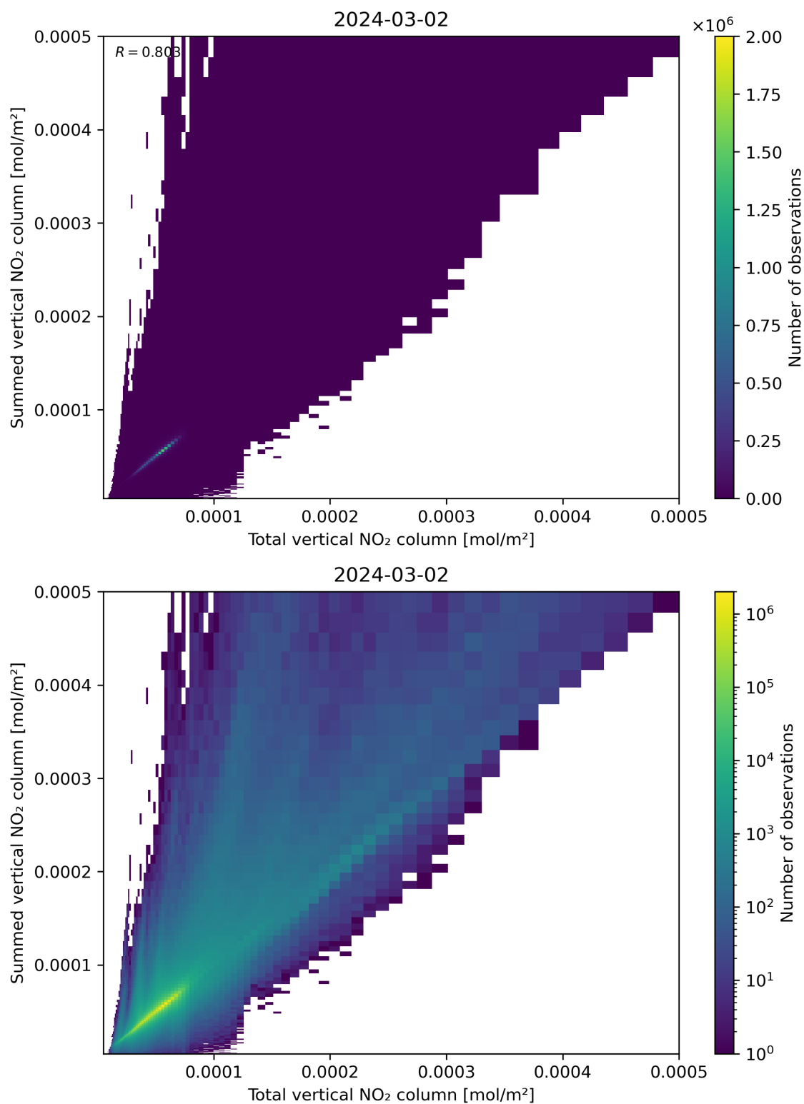
Figure 112: Scatter density plot of “Total vertical NO 2 column” against “Summed vertical NO 2 column” for 2024-03-01 to 2024-03-03.
