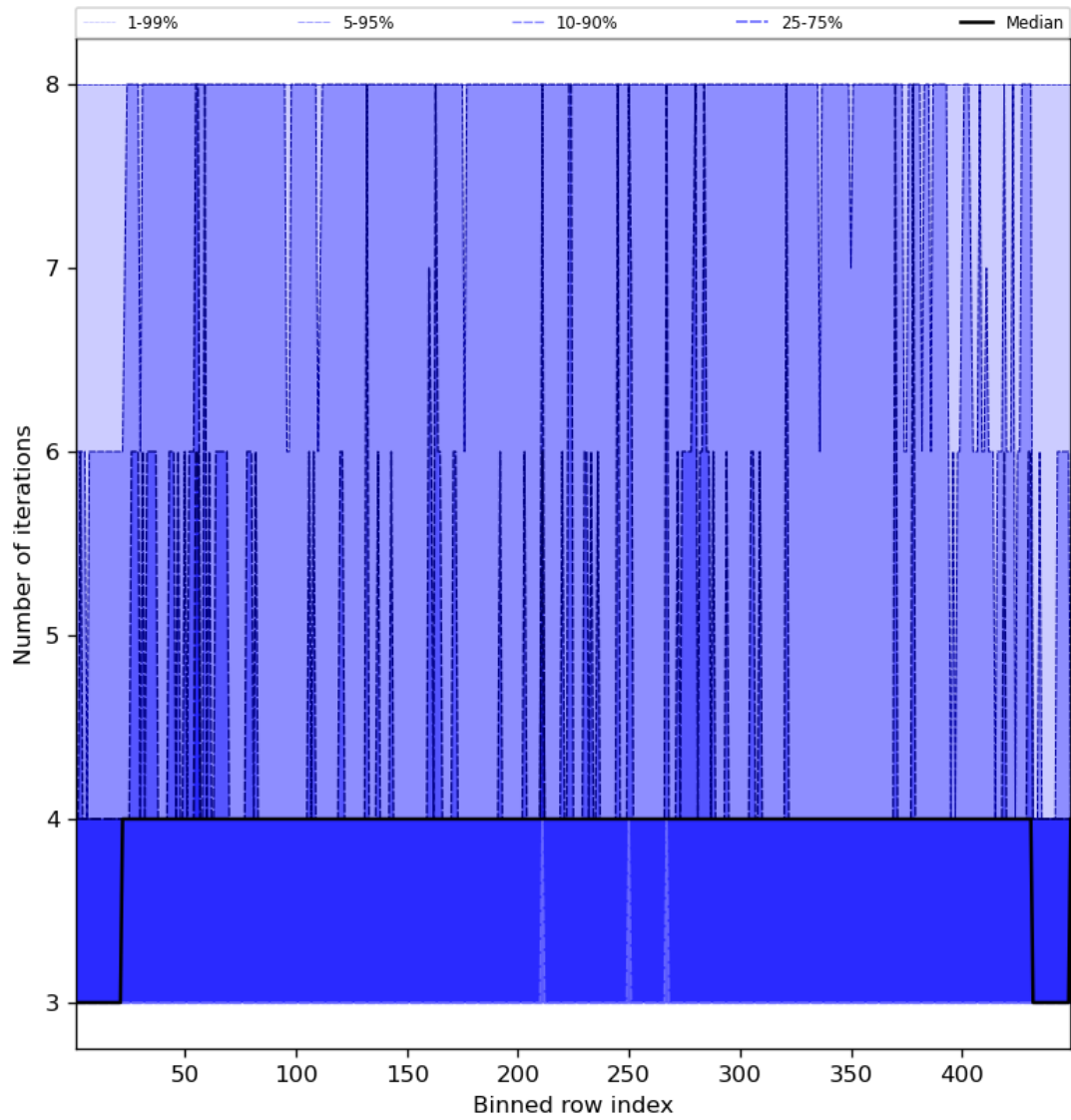
Figure 51: Along track statistics of “Number of iterations” for 2024-03-01 to 2024-03-03
