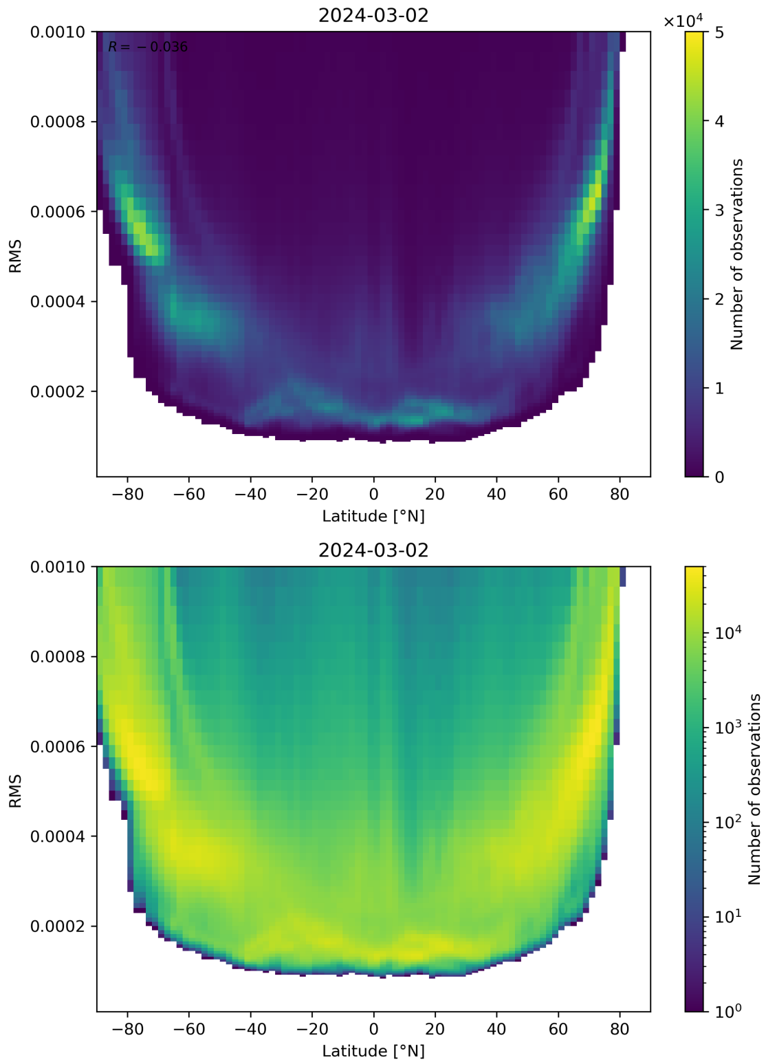
Figure 94: Scatter density plot of “Latitude” against “RMS” for 2024-03-01 to 2024-03-03.
