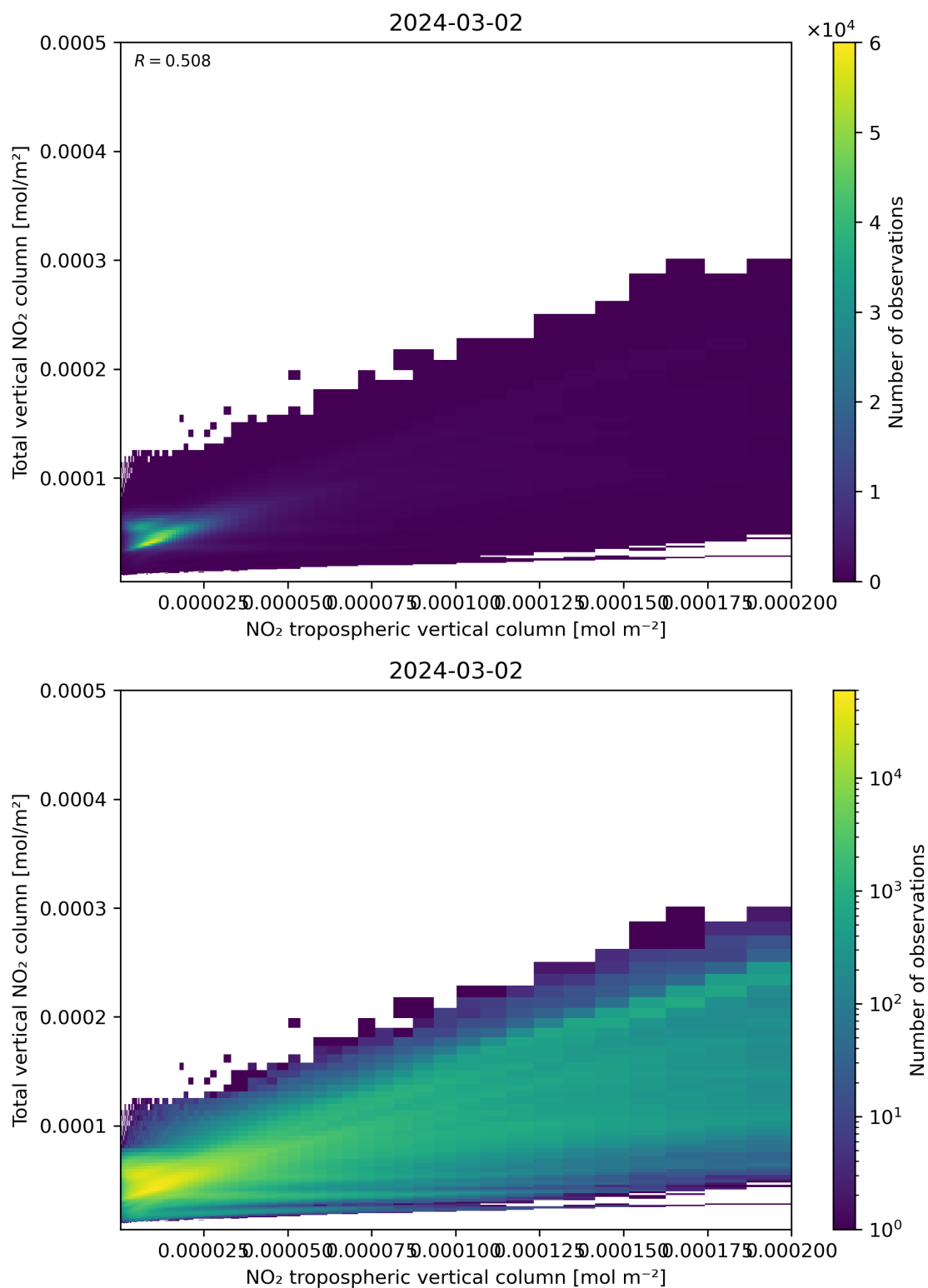
Figure 128: Scatter density plot of “NO 2 tropospheric vertical column” against “Total vertical NO 2 column” for 2024-03-01 to 2024-03-03.
