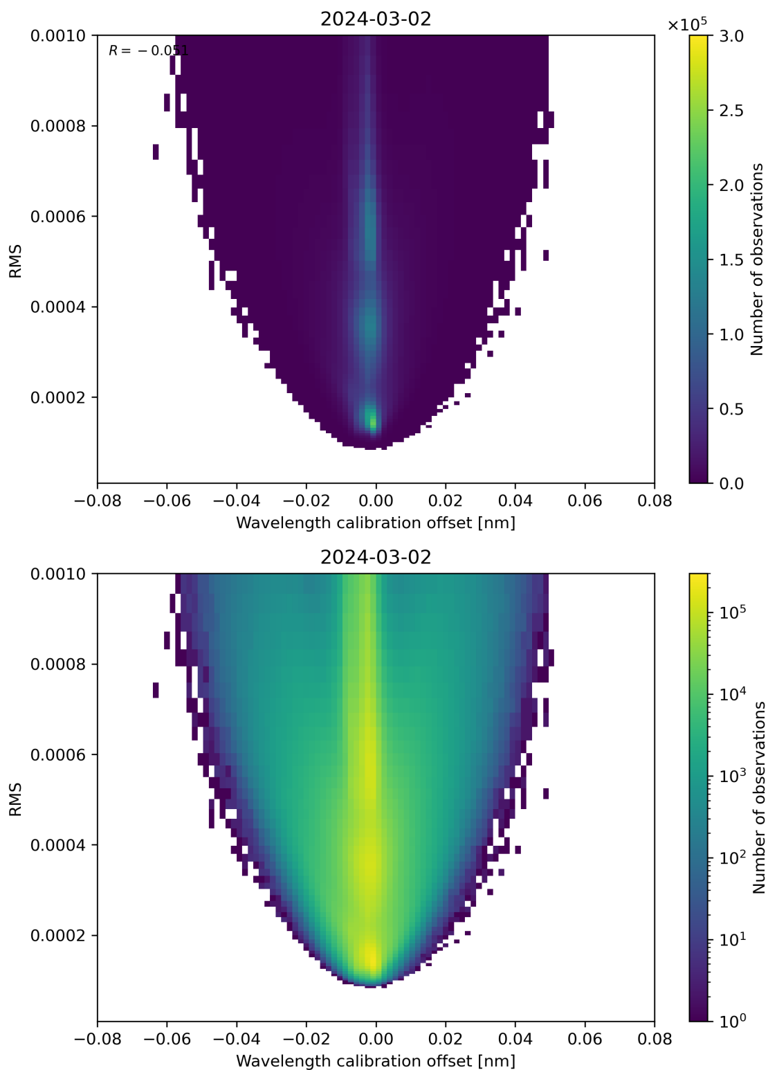
Figure 181: Scatter density plot of “Wavelength calibration offset” against “RMS” for 2024-03-01 to 2024-03-03.
