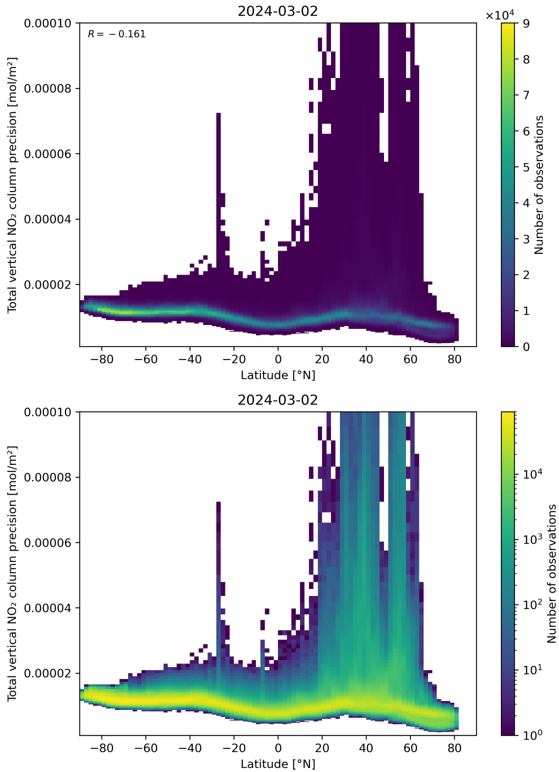
Figure 91: Scatter density plot of “Latitude” against “Total vertical NO 2 column precision” for 2024-03-01 to 2024-03-03.
