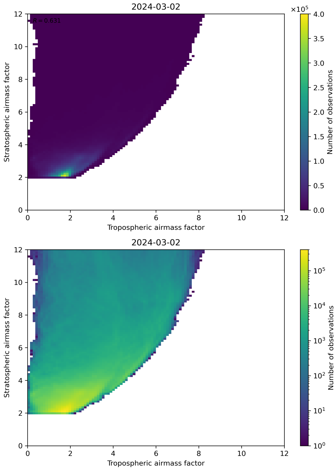
Figure 71: Scatter density plot of “Tropospheric airmass factor” against “Stratospheric airmass factor” for 2024-03-01 to 2024-03-03.
