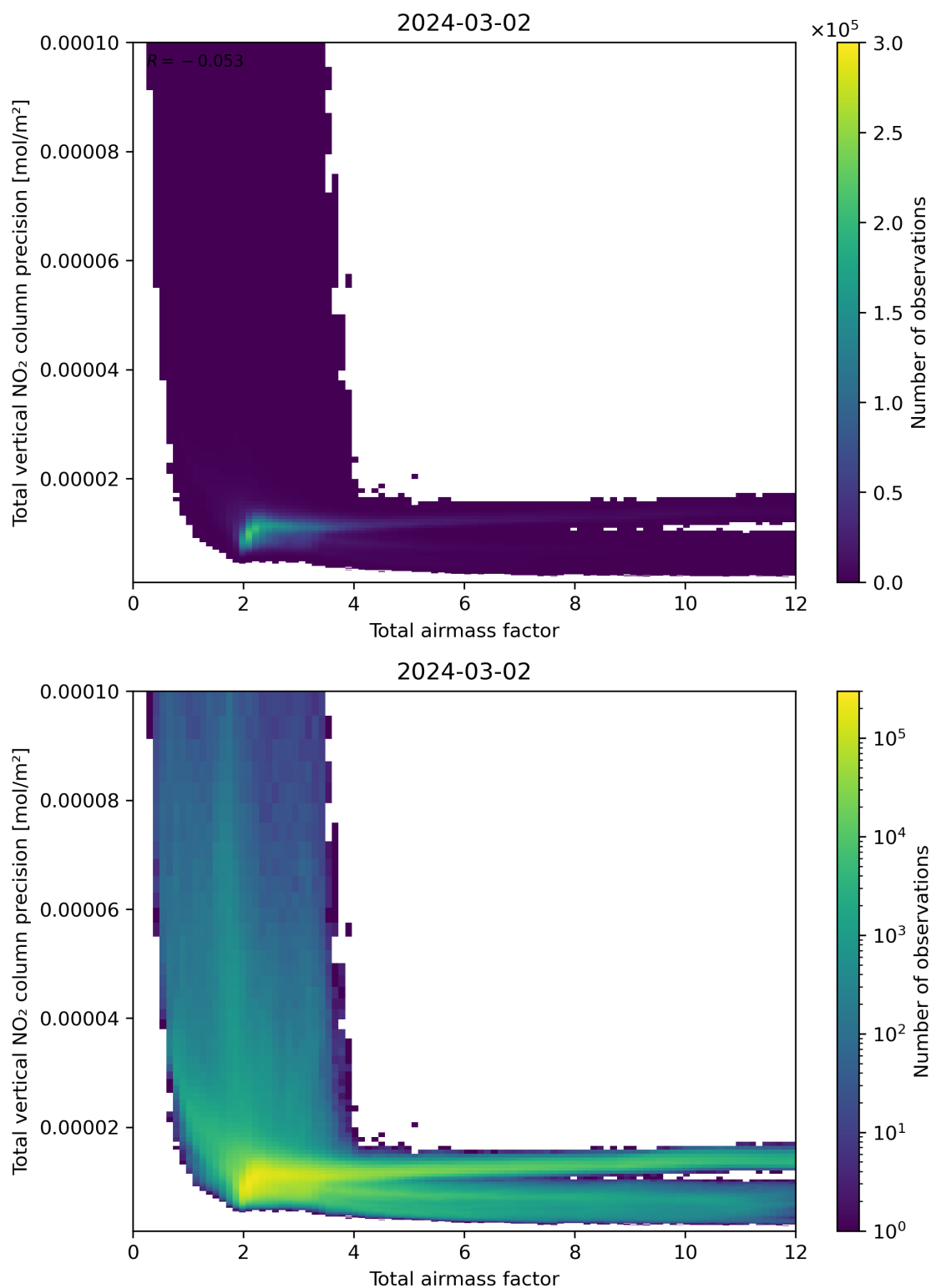
Figure 68: Scatter density plot of “Total airmass factor” against “Total vertical NO 2 column precision” for 2024-03-01 to 2024-03-03.
