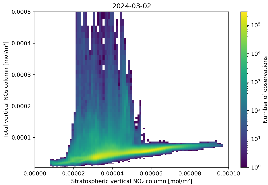
Figure 100: Scatter density plot of “Stratospheric vertical NO 2 column” against “Total vertical NO 2 column” for 2024-03-01 to 2024-03-03.
