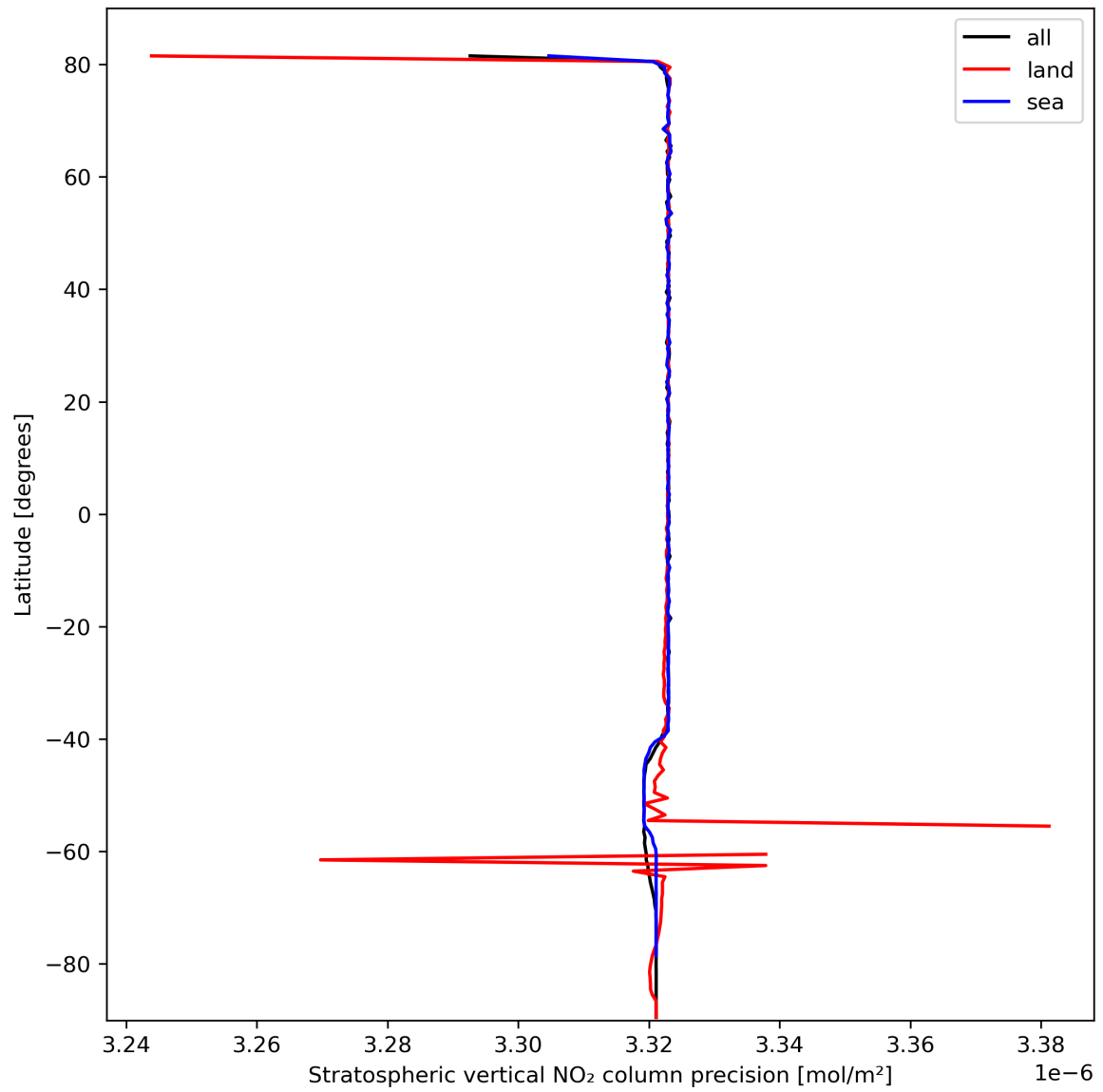
Figure 20: Zonal average of “Stratospheric vertical NO 2 column precision” for 2024-03-01 to 2024-03-03.
