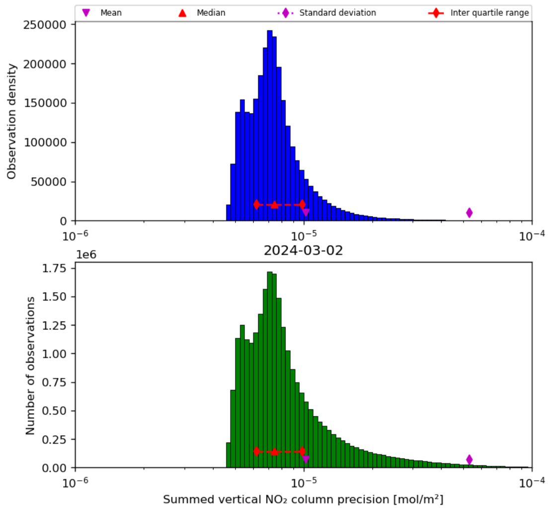
Figure 41: Histogram of “Summed vertical NO 2 column precision” for 2024-03-01 to 2024-03-03
