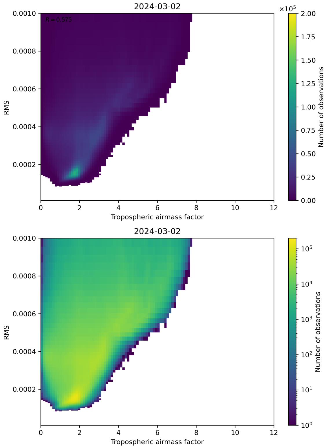
Figure 79: Scatter density plot of “Tropospheric airmass factor” against “RMS” for 2024-03-01 to 2024-03-03.
