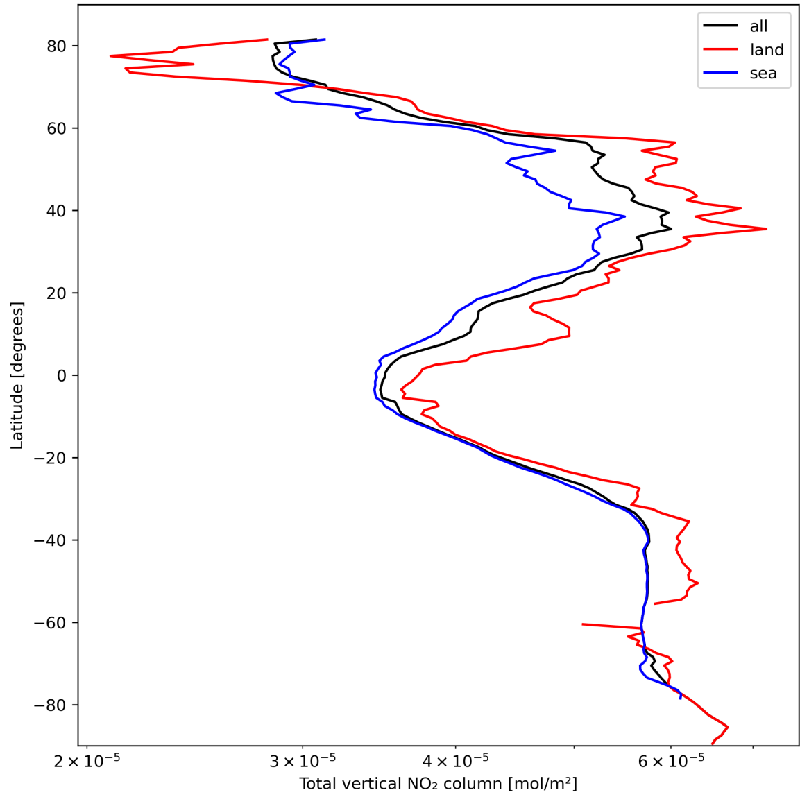
Figure 21: Zonal average of “Total vertical NO 2 column” for 2024-03-01 to 2024-03-03.
