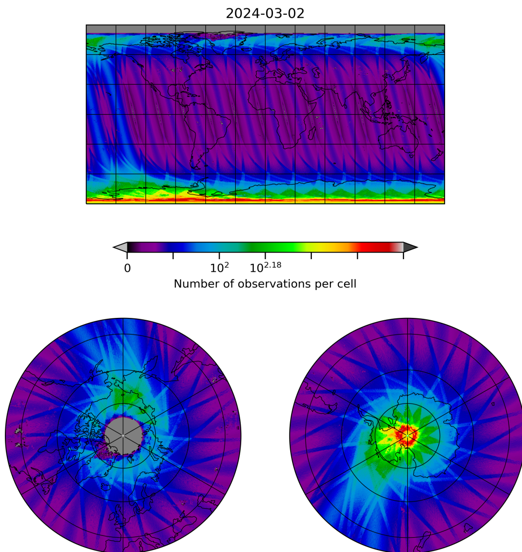
Figure 10: Map of the number of observations for 2024-03-01 to 2024-03-03
