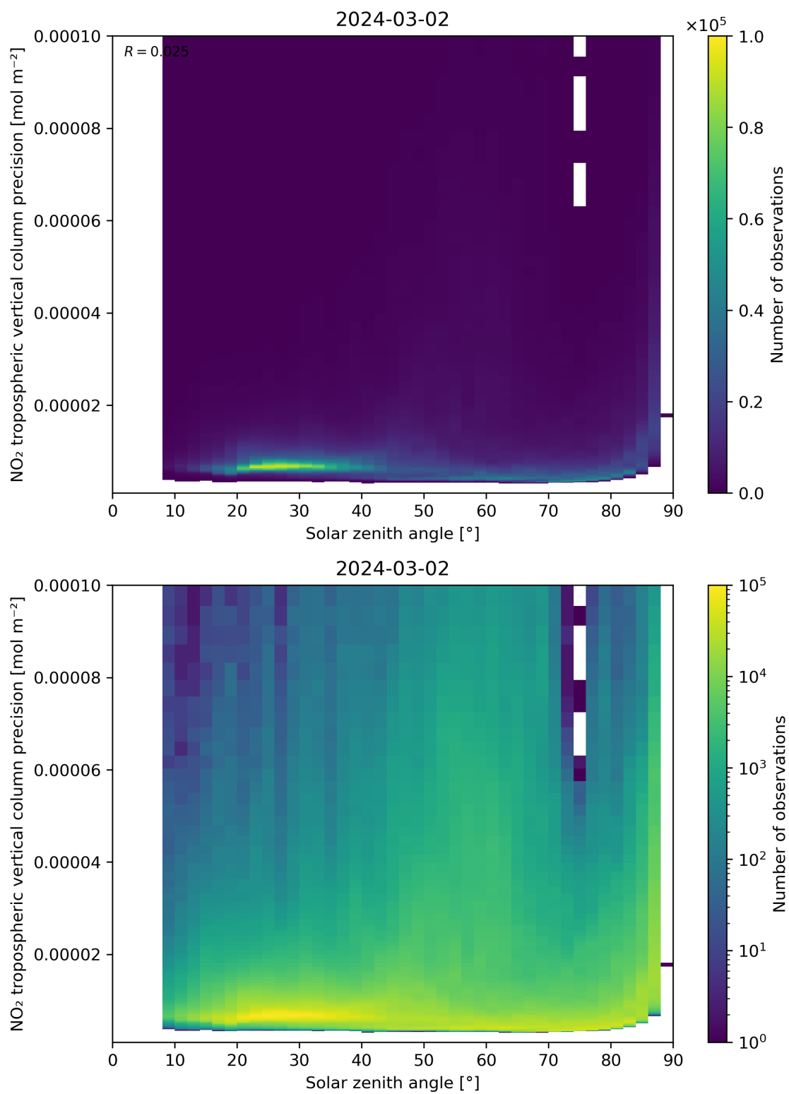
Figure 156: Scatter density plot of “Solar zenith angle” against “NO 2 tropospheric vertical column precision” for 2024-03-01 to 2024-03-03.
