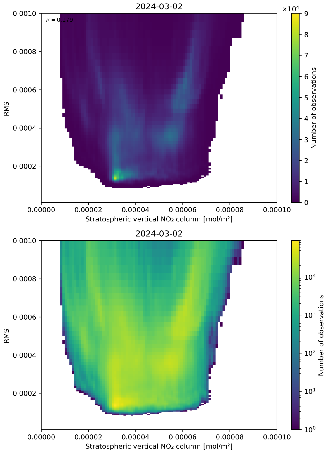
Figure 102: Scatter density plot of “Stratospheric vertical NO 2 column” against “RMS” for 2024-03-01 to 2024-03-03.
