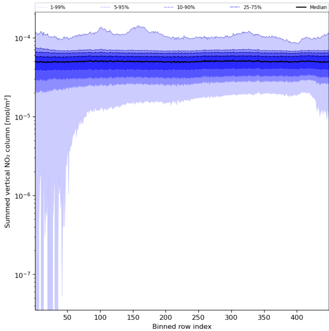
Figure 57: Along track statistics of “Summed vertical NO 2 column” for 2024-03-01 to 2024-03-03
