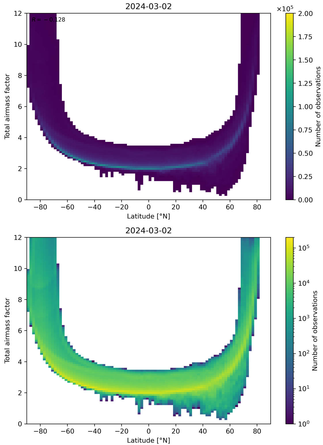
Figure 84: Scatter density plot of “Latitude” against “Total airmass factor” for 2024-03-01 to 2024-03-03.
