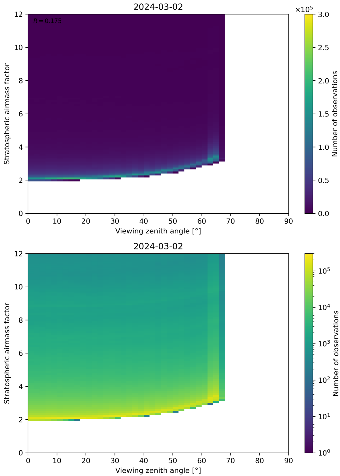
Figure 159: Scatter density plot of “Viewing zenith angle” against “Stratospheric airmass factor” for 2024-03-01 to 2024-03-03.
