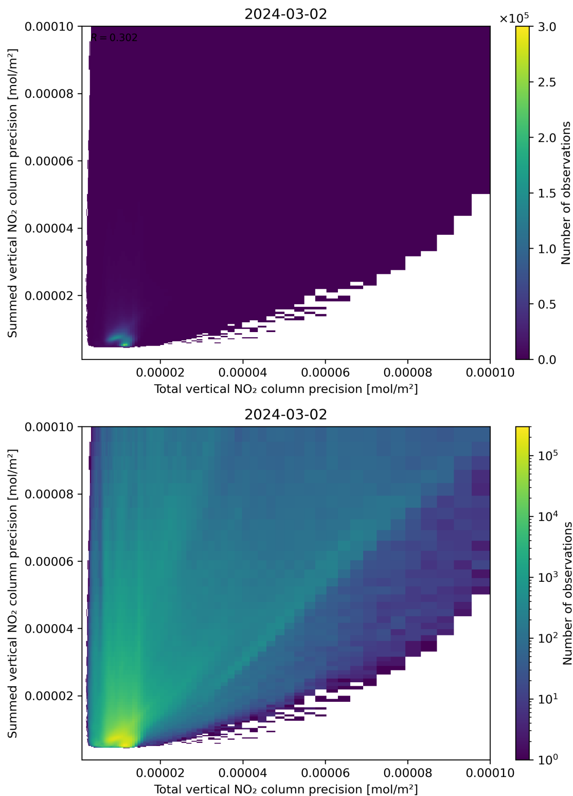
Figure 118: Scatter density plot of “Total vertical NO 2 column precision” against “Summed vertical NO 2 column precision” for 2024-03-01 to 2024-03-03.
