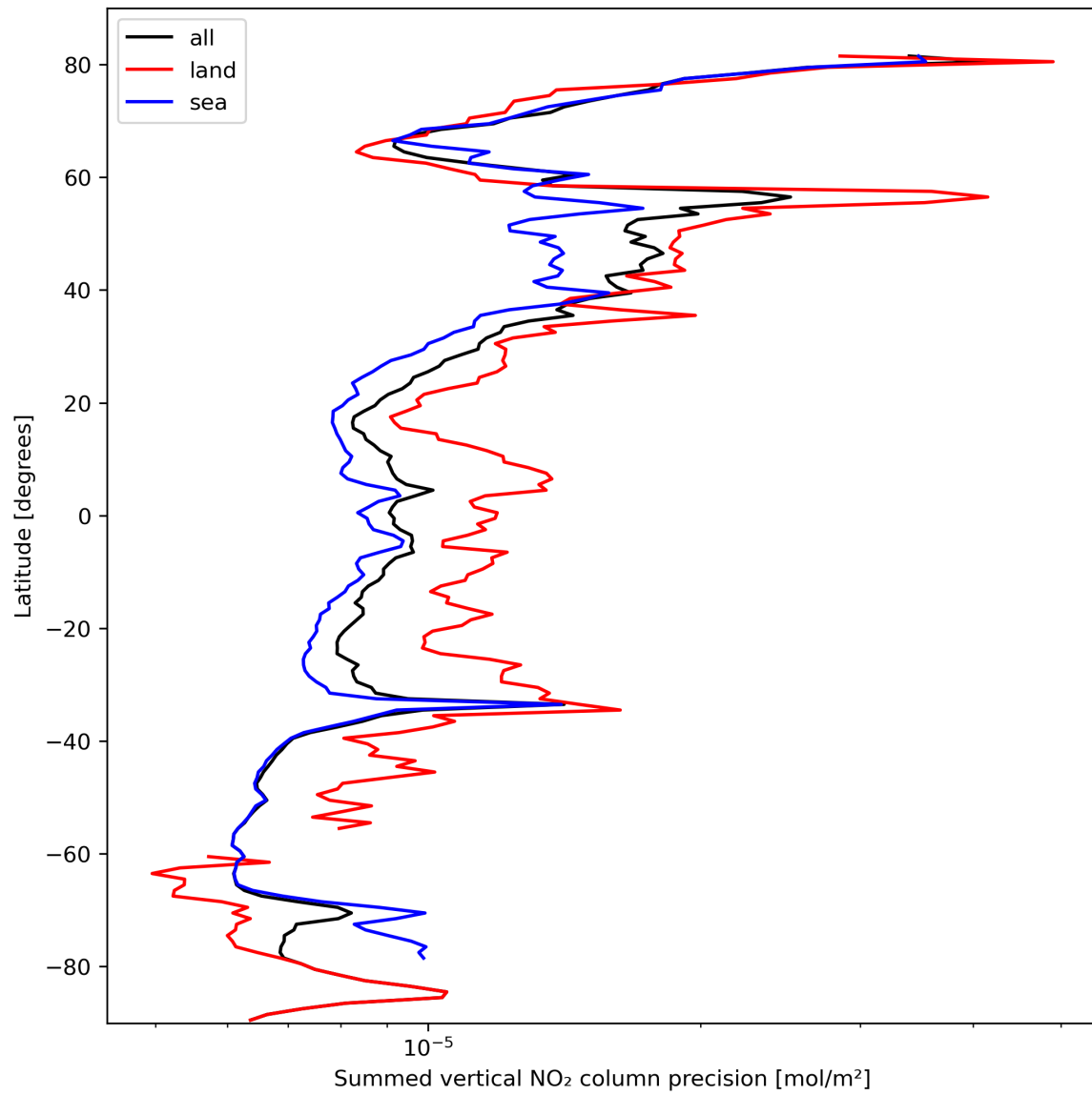
Figure 24: Zonal average of “Summed vertical NO 2 column precision” for 2024-03-01 to 2024-03-03.
