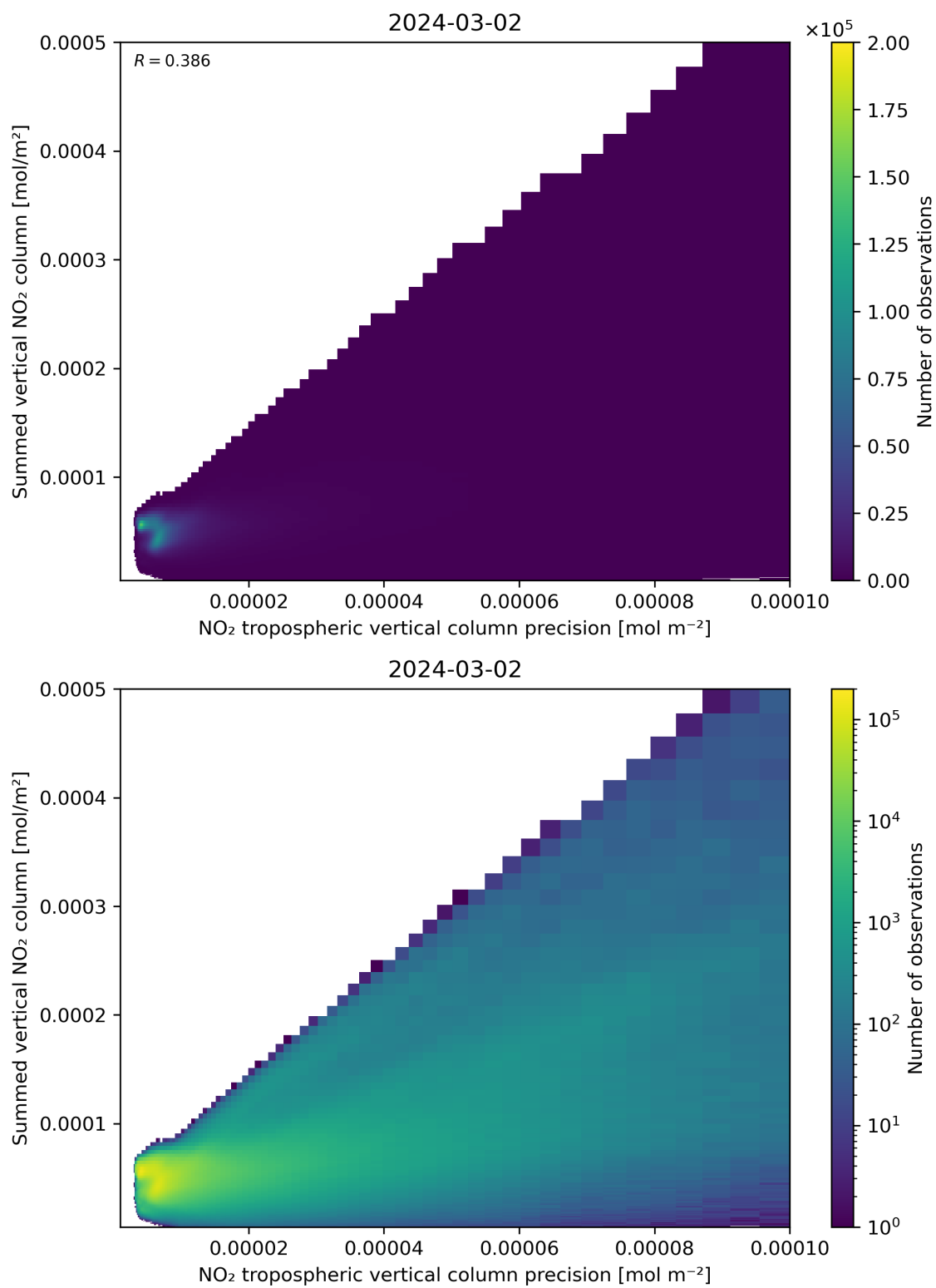
Figure 136: Scatter density plot of “NO 2 tropospheric vertical column precision” against “Summed vertical NO 2 column” for 2024-03-01 to 2024-03-03.
