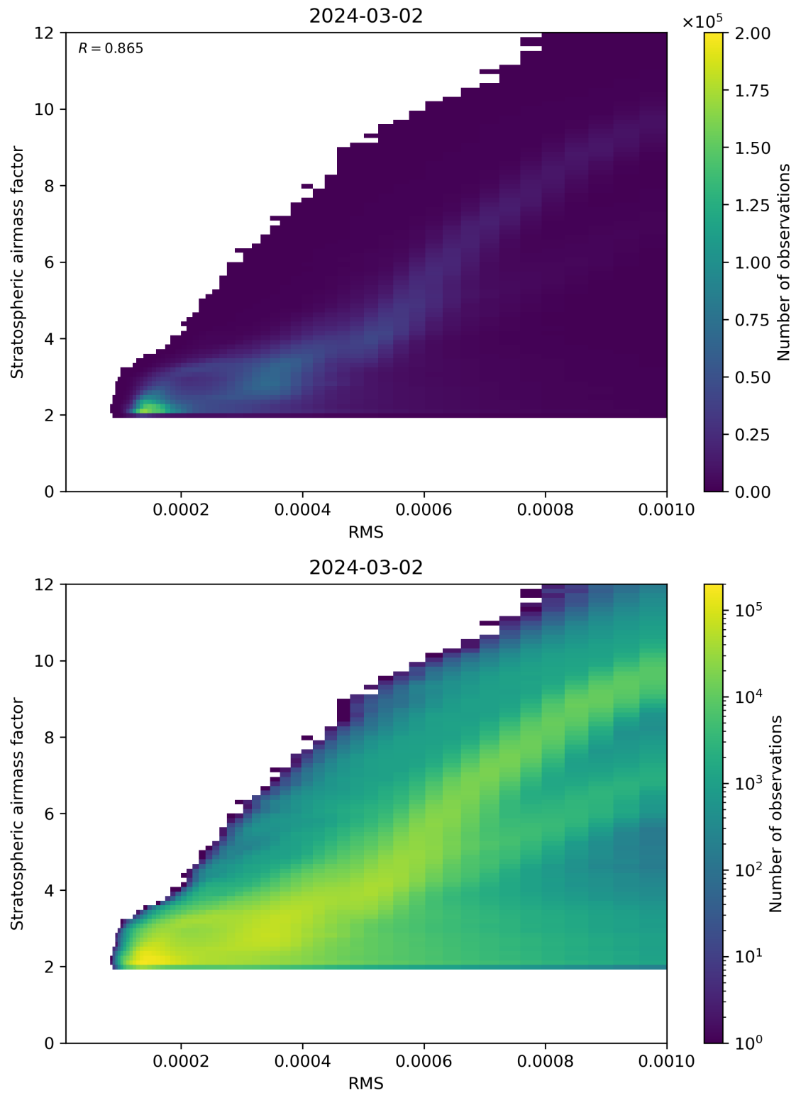
Figure 144: Scatter density plot of “RMS” against “Stratospheric airmass factor” for 2024-03-01 to 2024-03-03.
