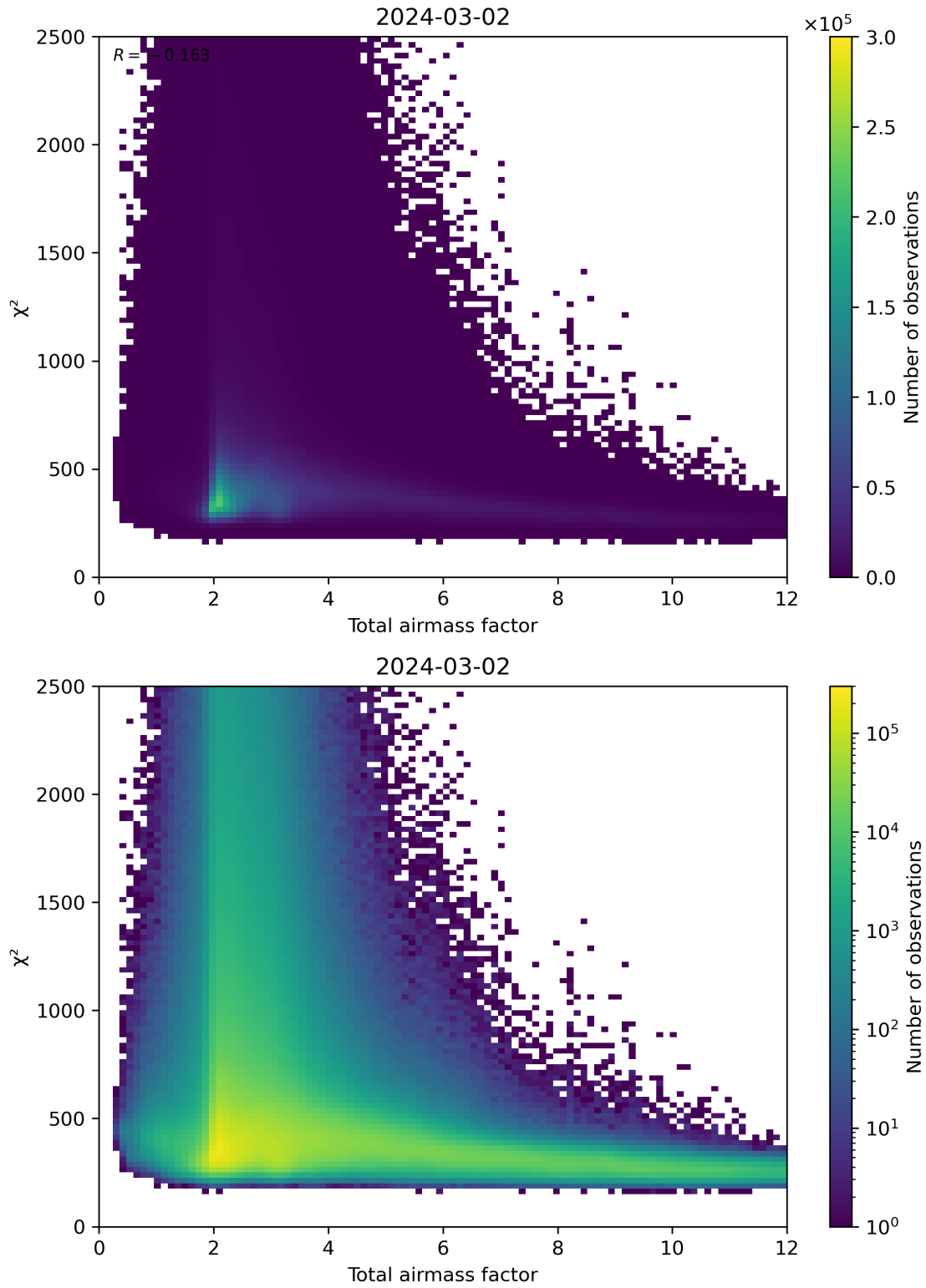
Figure 63: Scatter density plot of “Total airmass factor” against “ \chi^2 ” for 2024-03-01 to 2024-03-03.
