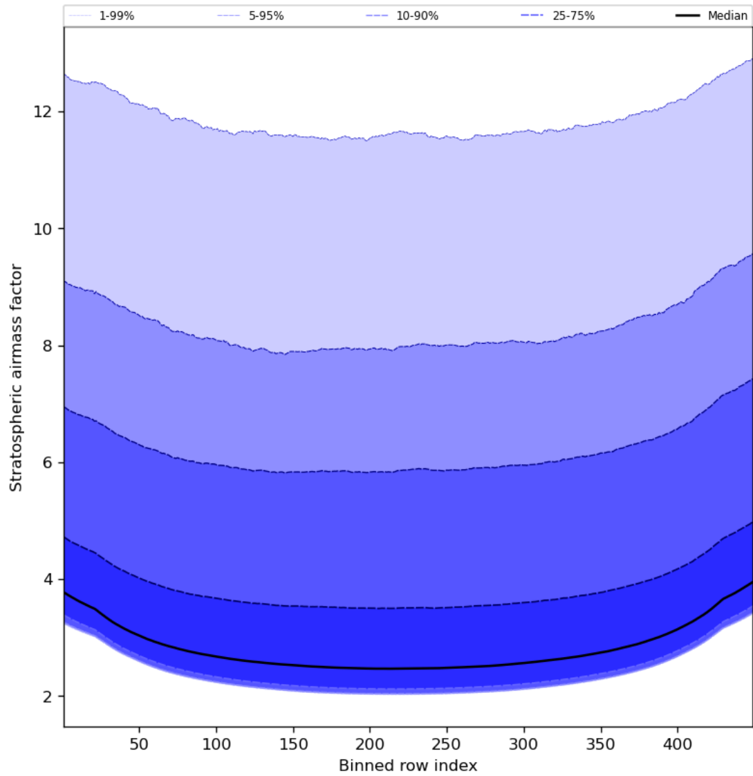
Figure 61: Along track statistics of “Stratospheric airmass factor” for 2024-03-01 to 2024-03-03
