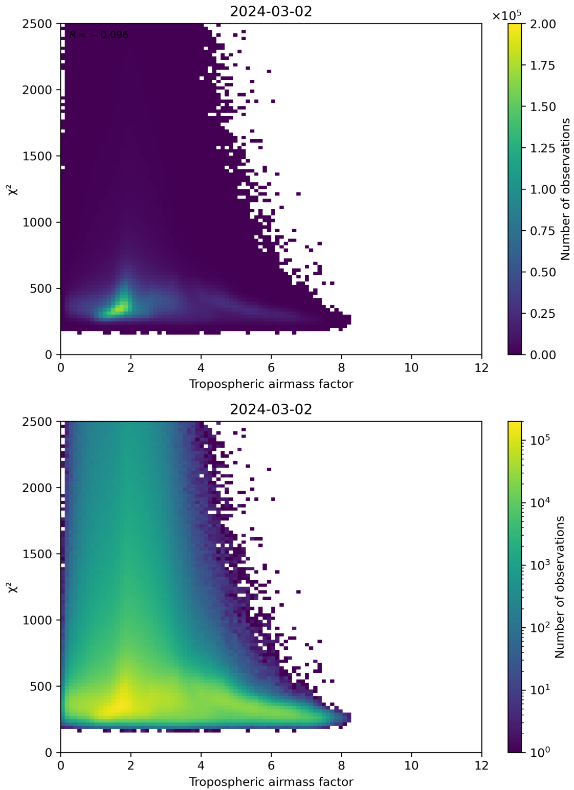
Figure 73: Scatter density plot of “Tropospheric airmass factor” against “ \chi^2 ” for 2024-03-01 to 2024-03-03.
