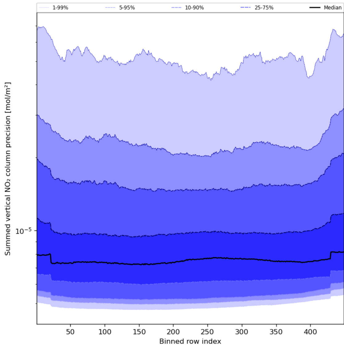
Figure 58: Along track statistics of “Summed vertical NO 2 column precision” for 2024-03-01 to 2024-03-03
