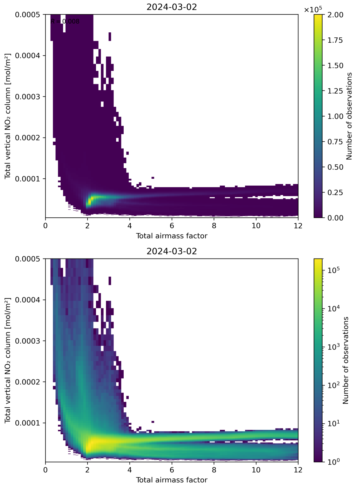
Figure 67: Scatter density plot of “Total airmass factor” against “Total vertical NO 2 column” for 2024-03-01 to 2024-03-03.
