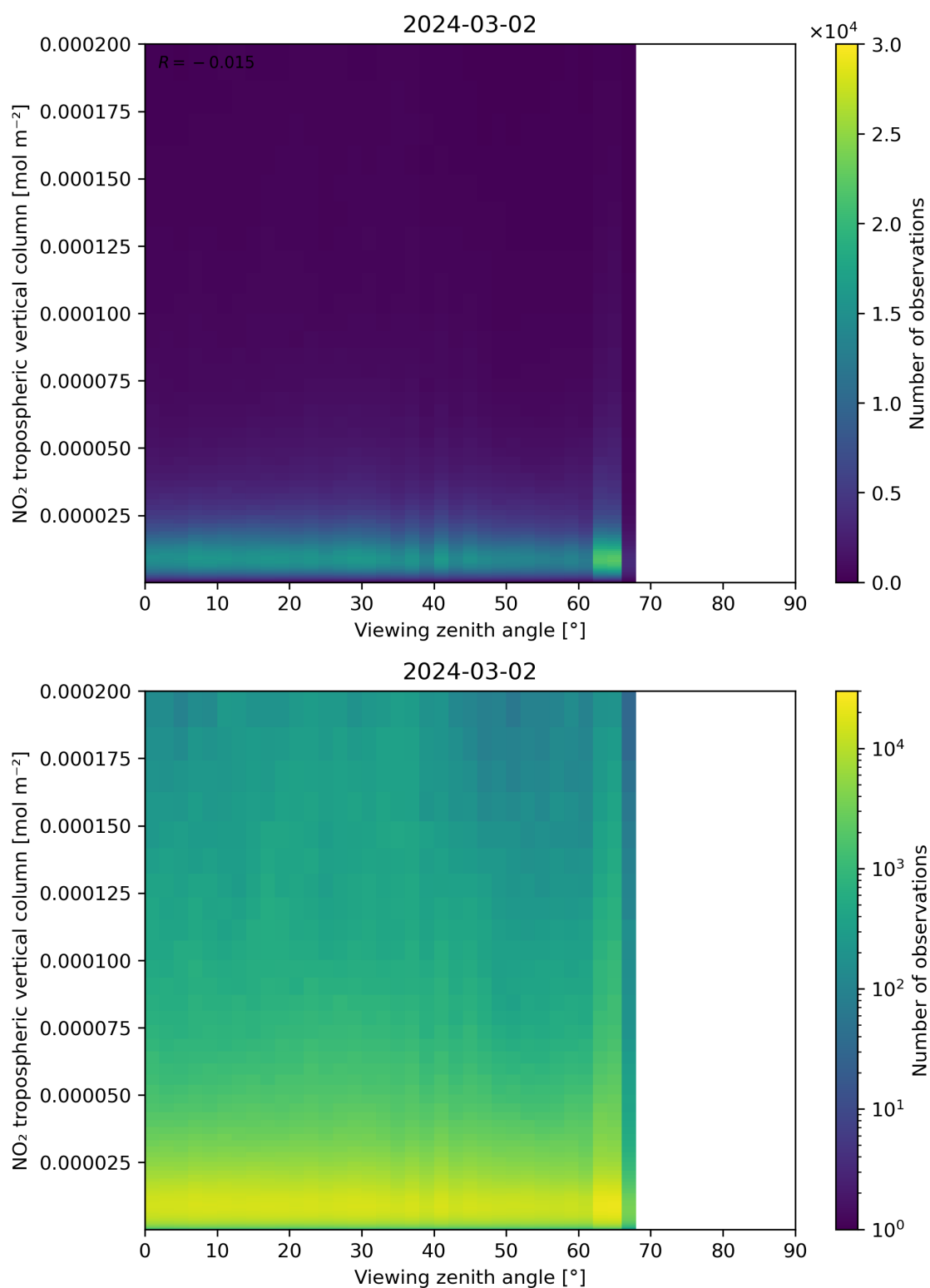
Figure 169: Scatter density plot of “Viewing zenith angle” against “NO 2 tropospheric vertical column” for 2024-03-01 to 2024-03-03.
