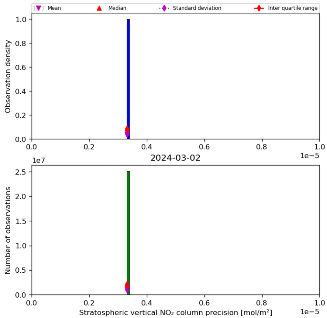
Figure 37: Histogram of “Stratospheric vertical NO 2 column precision” for 2024-03-01 to 2024-03-03
