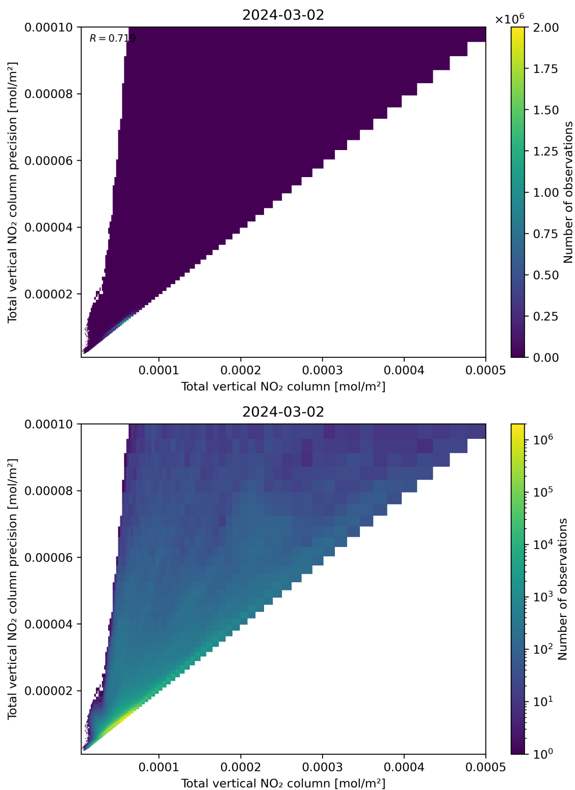
Figure 114: Scatter density plot of “Total vertical NO 2 column” against “Total vertical NO 2 column precision” for 2024-03-01 to 2024-03-03.
