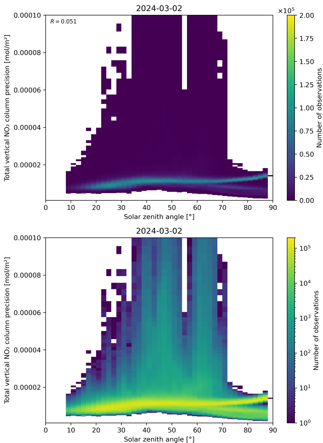
Figure 154: Scatter density plot of “Solar zenith angle” against “Total vertical NO 2 column precision” for 2024-03-01 to 2024-03-03.
