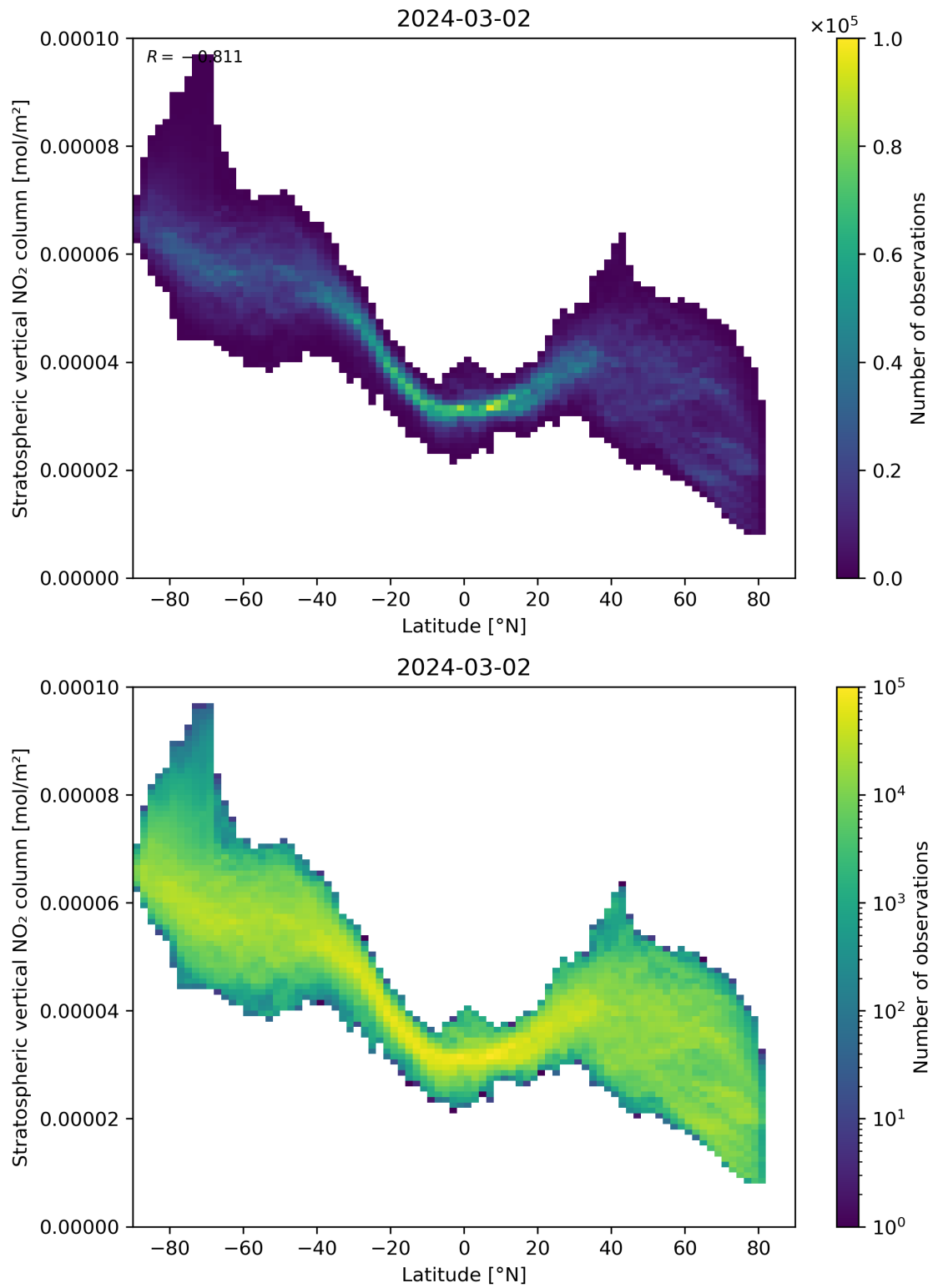
Figure 87: Scatter density plot of “Latitude” against “Stratospheric vertical NO 2 column” for 2024-03-01 to 2024-03-03.
