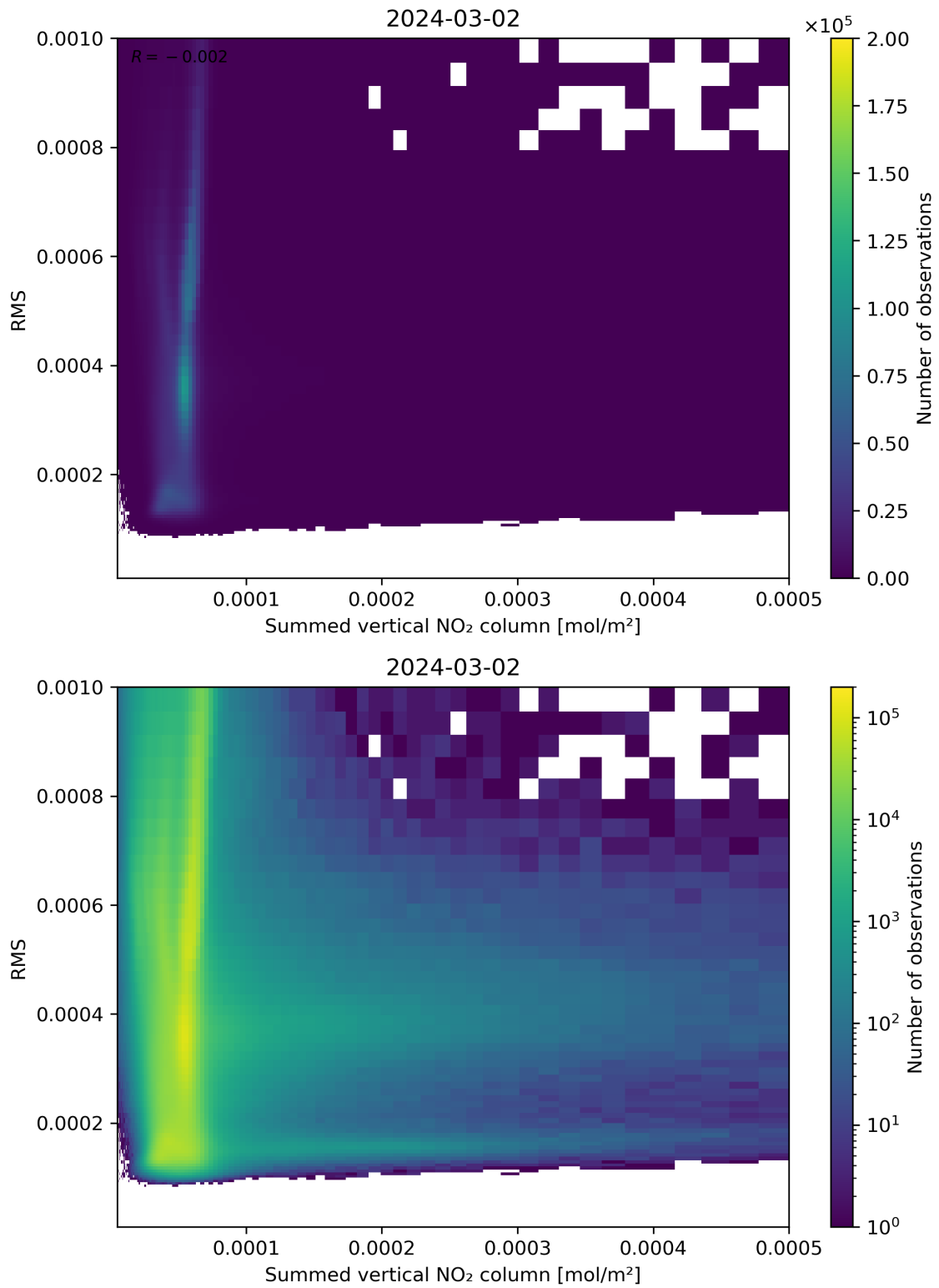
Figure 109: Scatter density plot of “Summed vertical NO 2 column” against “RMS” for 2024-03-01 to 2024-03-03.
