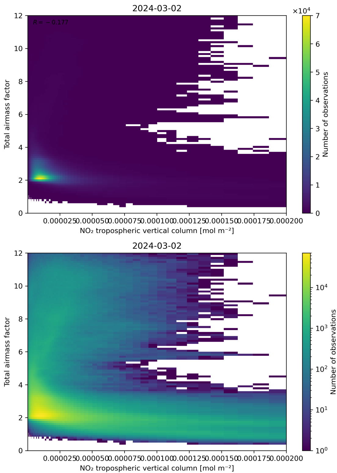
Figure 122: Scatter density plot of “NO 2 tropospheric vertical column” against “Total air mass factor” for 2024-03-01 to 2024-03-03.
