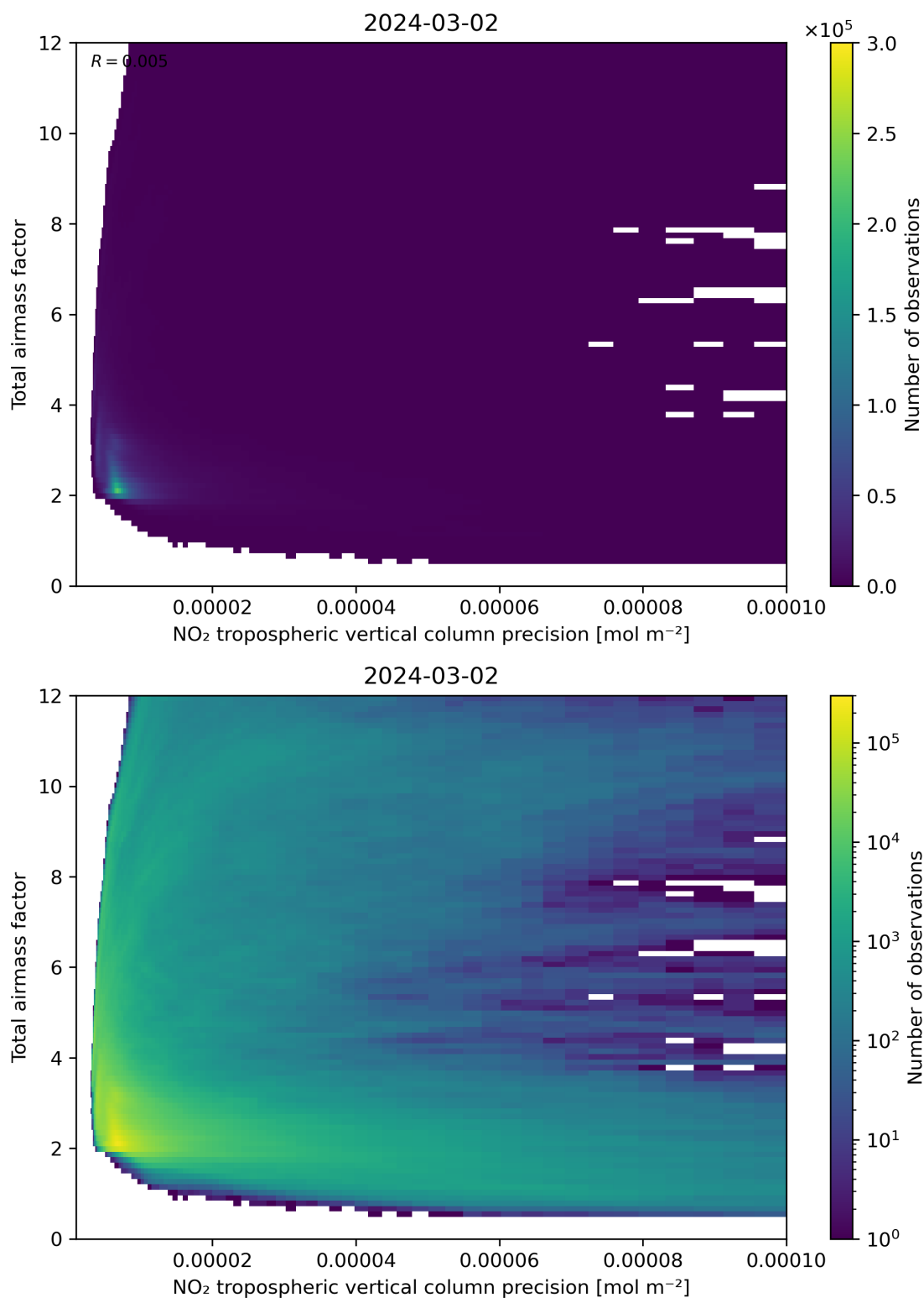
Figure 132: Scatter density plot of “NO 2 tropospheric vertical column precision” against “Total airmass factor” for 2024-03-01 to 2024-03-03.
