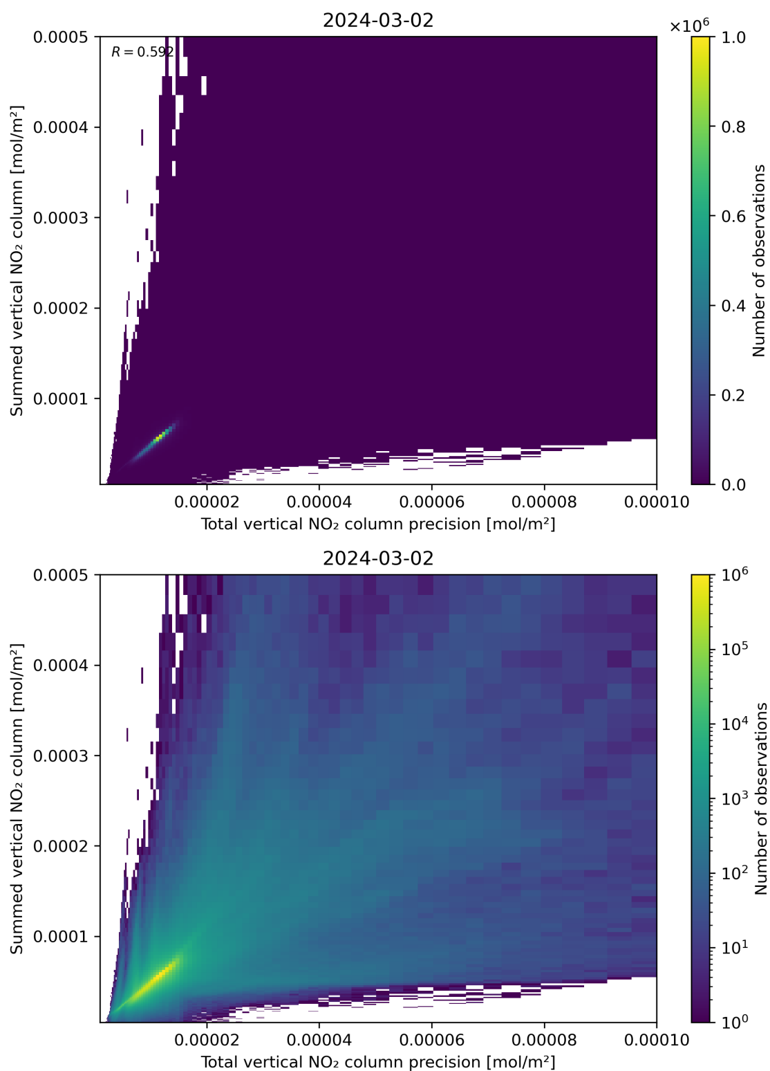
Figure 117: Scatter density plot of “Total vertical NO 2 column precision” against “Summed vertical NO 2 column” for 2024-03-01 to 2024-03-03.
