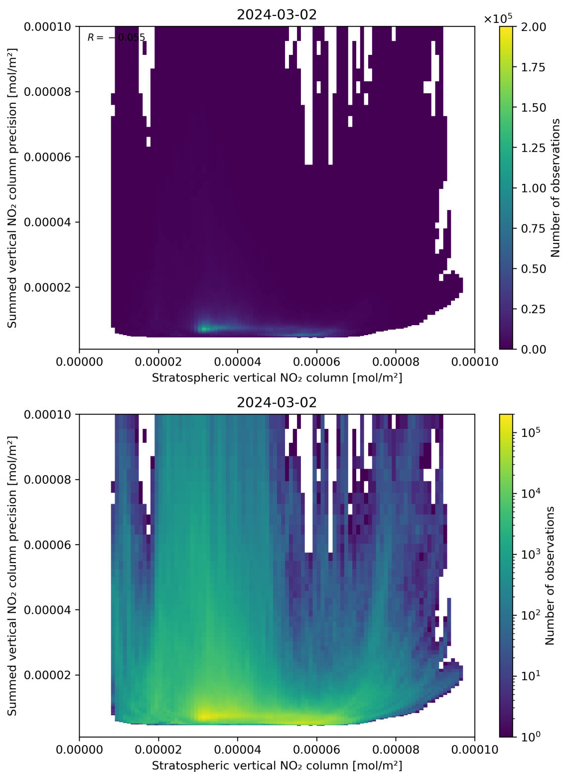
Figure 99: Scatter density plot of “Stratospheric vertical NO 2 column” against “Summed vertical NO 2 column precision” for 2024-03-01 to 2024-03-03.
