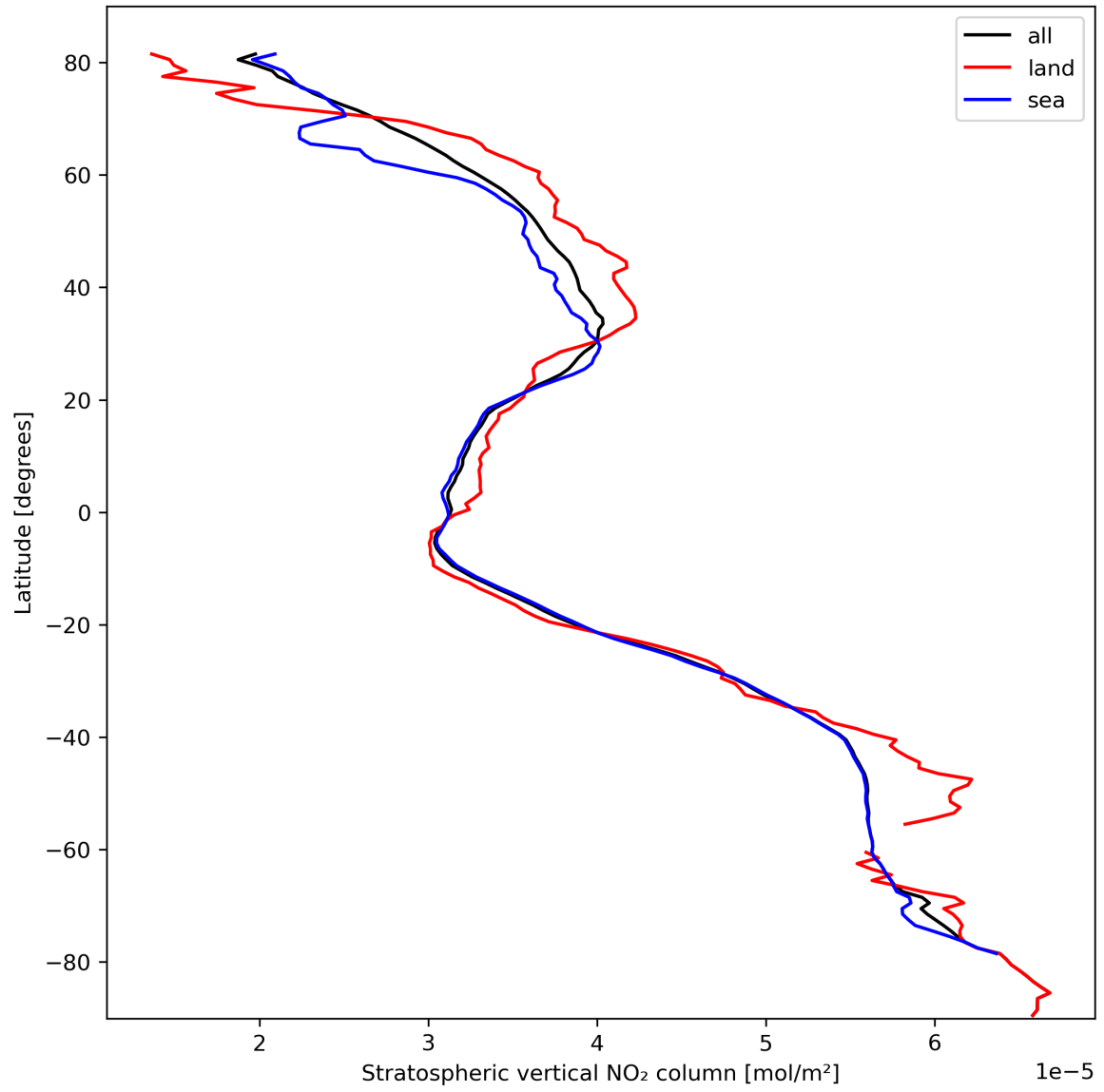
Figure 19: Zonal average of “Stratospheric vertical NO 2 column” for 2024-03-01 to 2024-03-03.
