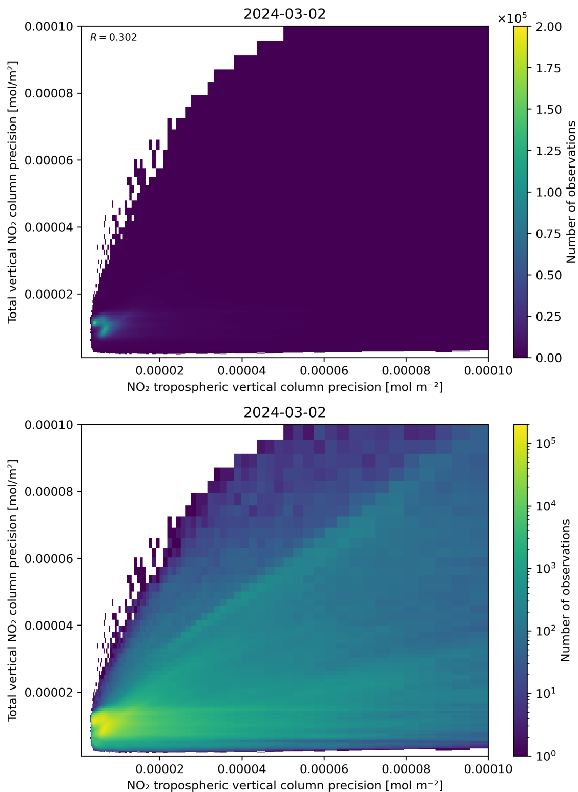
Figure 139: Scatter density plot of “NO 2 tropospheric vertical column precision” against “Total vertical NO 2 column precision” for 2024-03-01 to 2024-03-03.
