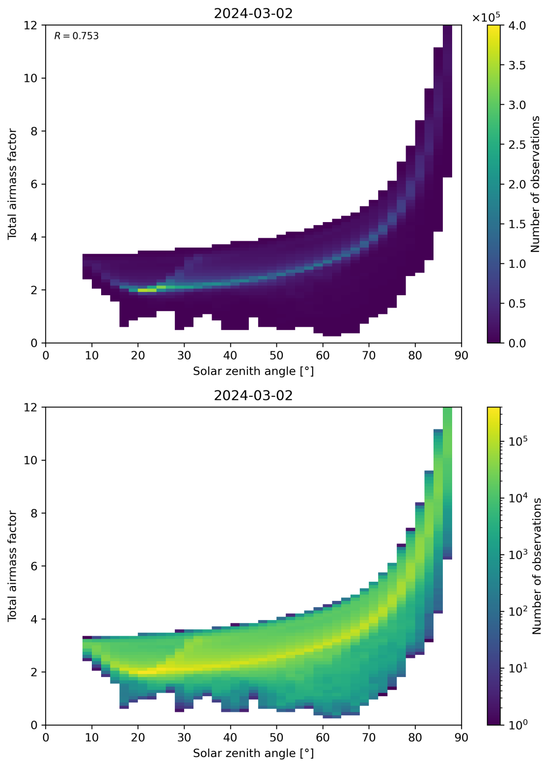
Figure 146: Scatter density plot of “Solar zenith angle” against “Total air mass factor” for 2024-03-01 to 2024-03-03.
