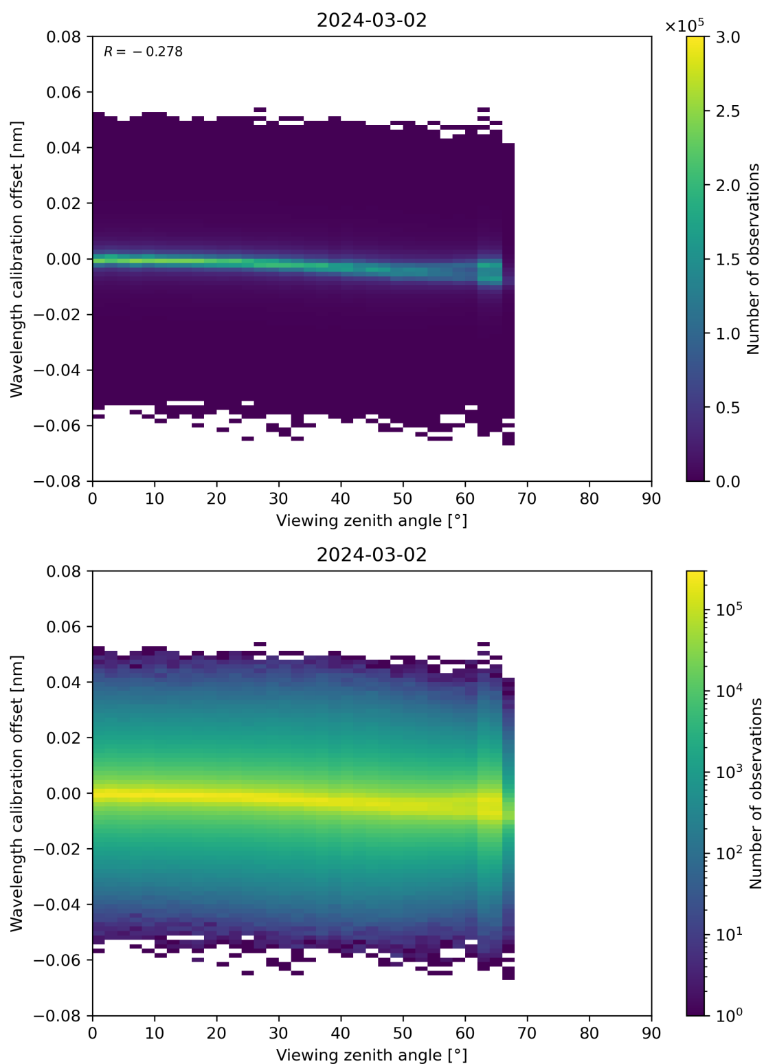
Figure 173: Scatter density plot of “Viewing zenith angle” against “Wavelength calibration offset” for 2024-03-01 to 2024-03-03.
