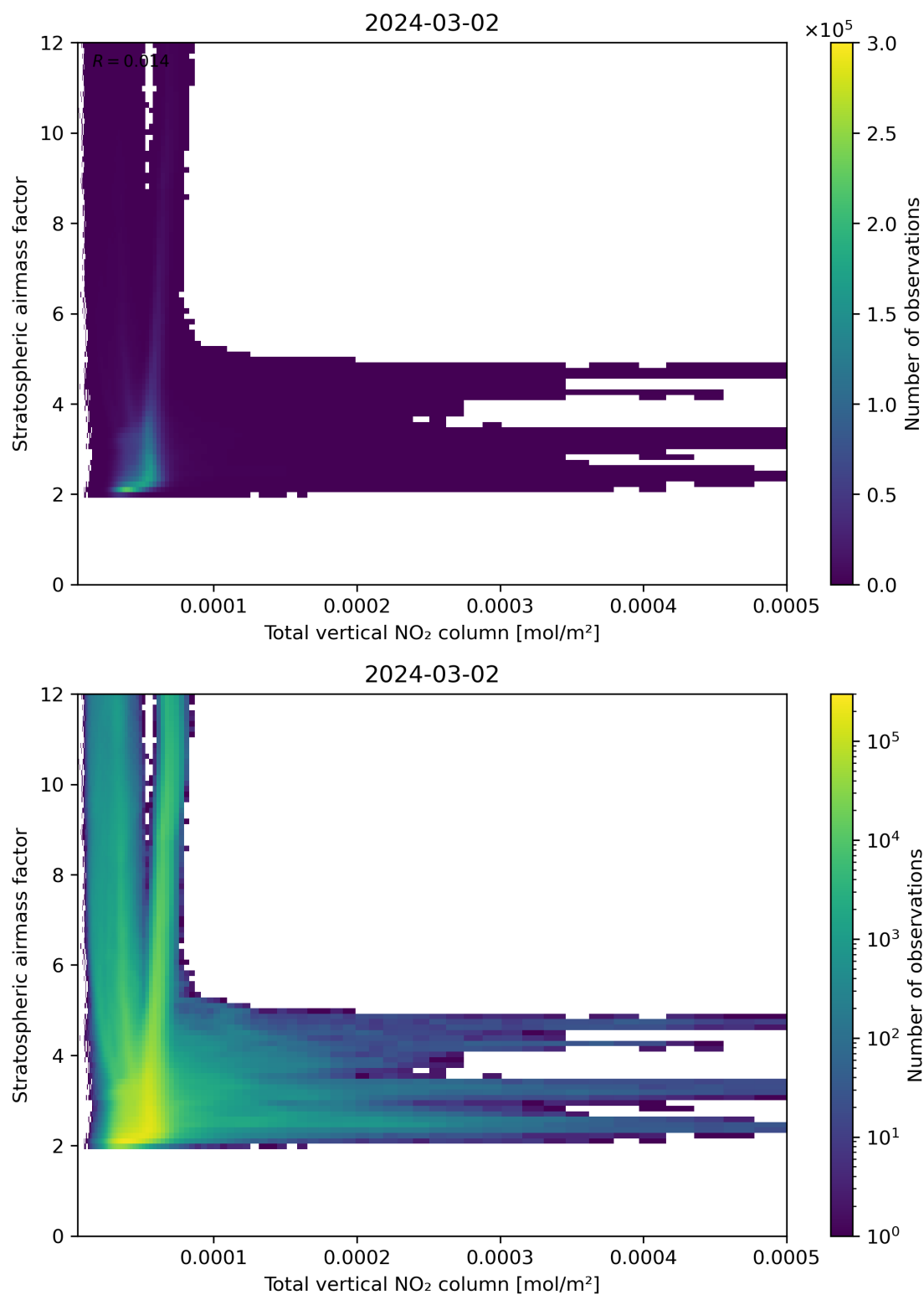
Figure 110: Scatter density plot of “Total vertical NO 2 column” against “Stratospheric airmass factor” for 2024-03-01 to 2024-03-03.
