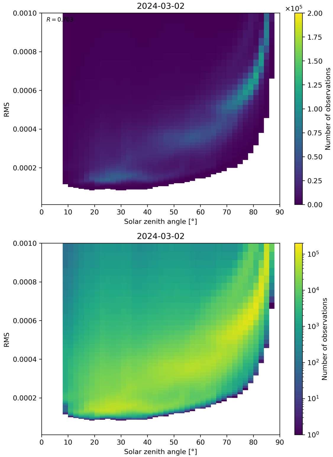
Figure 157: Scatter density plot of “Solar zenith angle” against “RMS” for 2024-03-01 to 2024-03-03.
