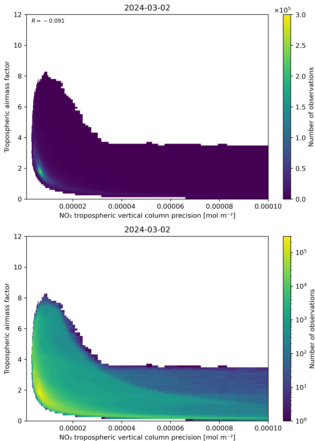
Figure 133: Scatter density plot of “NO 2 tropospheric vertical column precision” against “Tropospheric airmass factor” for 2024-03-01 to 2024-03-03.
