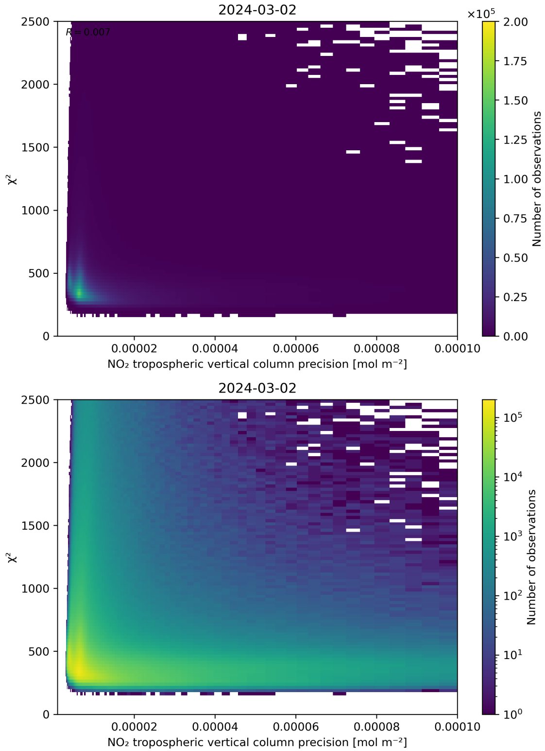
Figure 134: Scatter density plot of “NO 2 tropospheric vertical column precision” against “ \chi^2 ” for 2024-03-01 to 2024-03-03.
