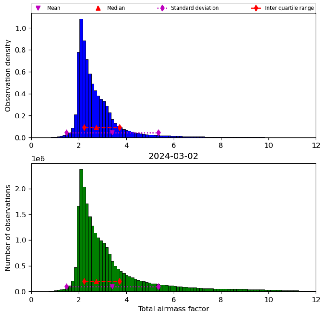
Figure 32: Histogram of “Total airmass factor” for 2024-03-01 to 2024-03-03
