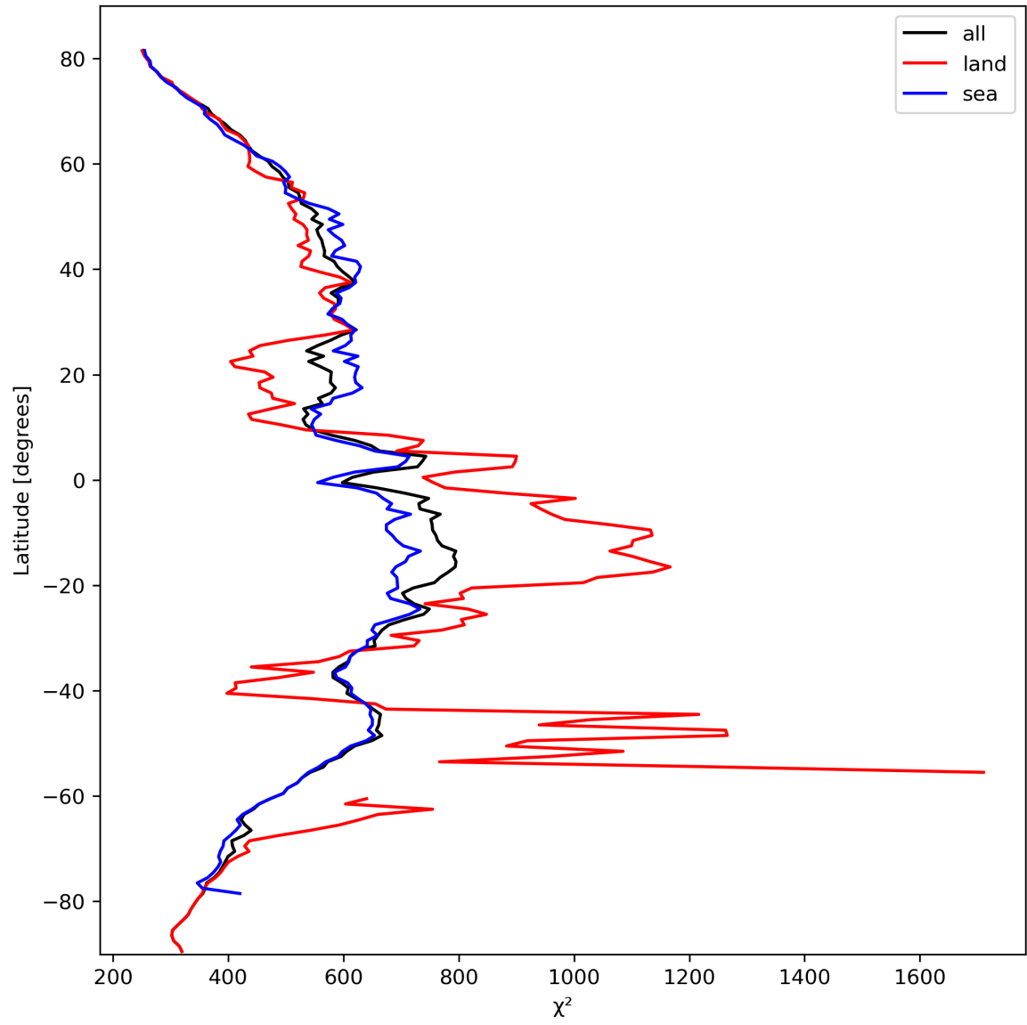
Figure 25: Zonal average of “ \chi^2 ” for 2024-03-01 to 2024-03-03.
