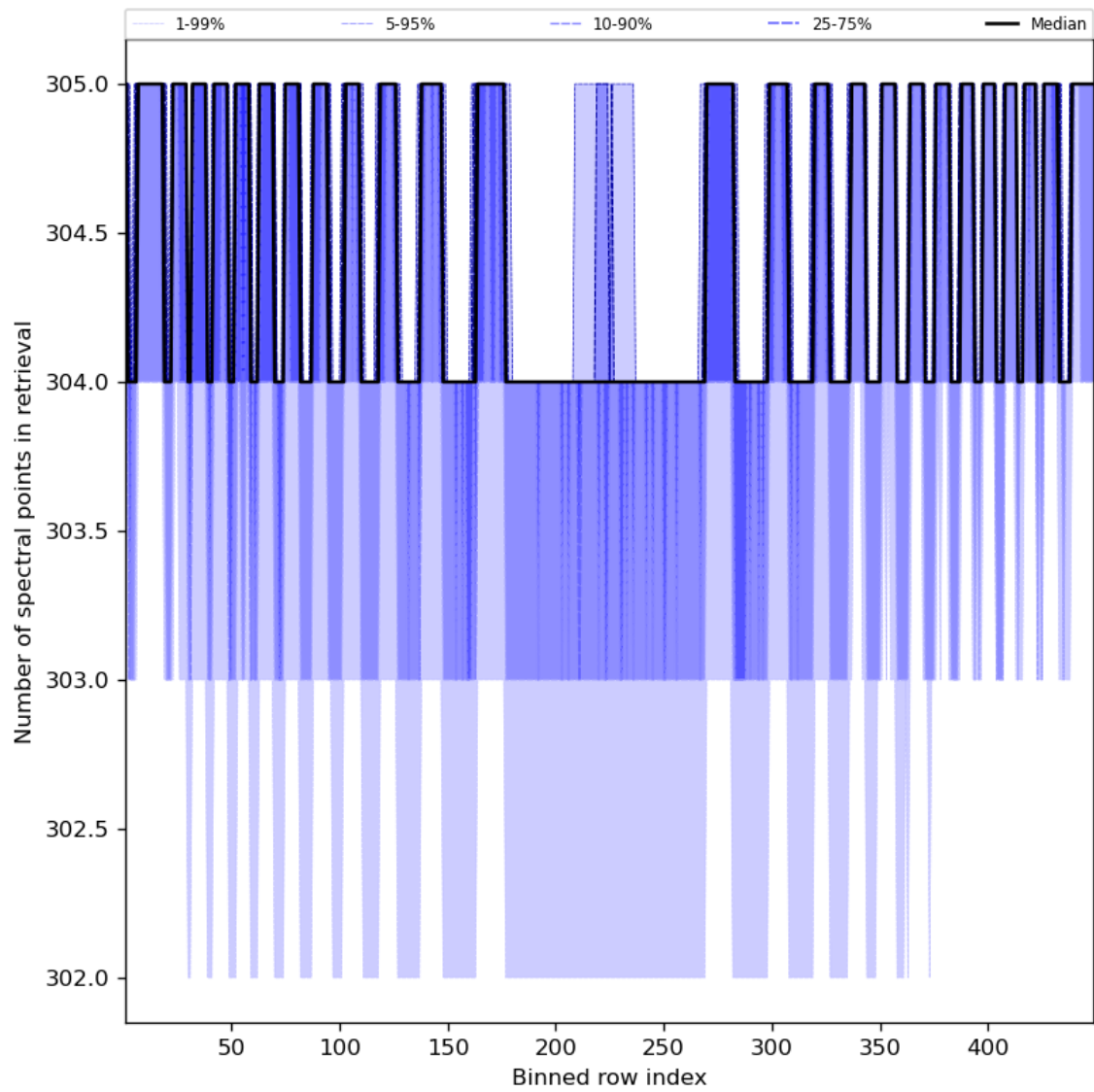
Figure 50: Along track statistics of “Number of spectral points in retrieval” for 2024-03-01 to 2024-03-03
