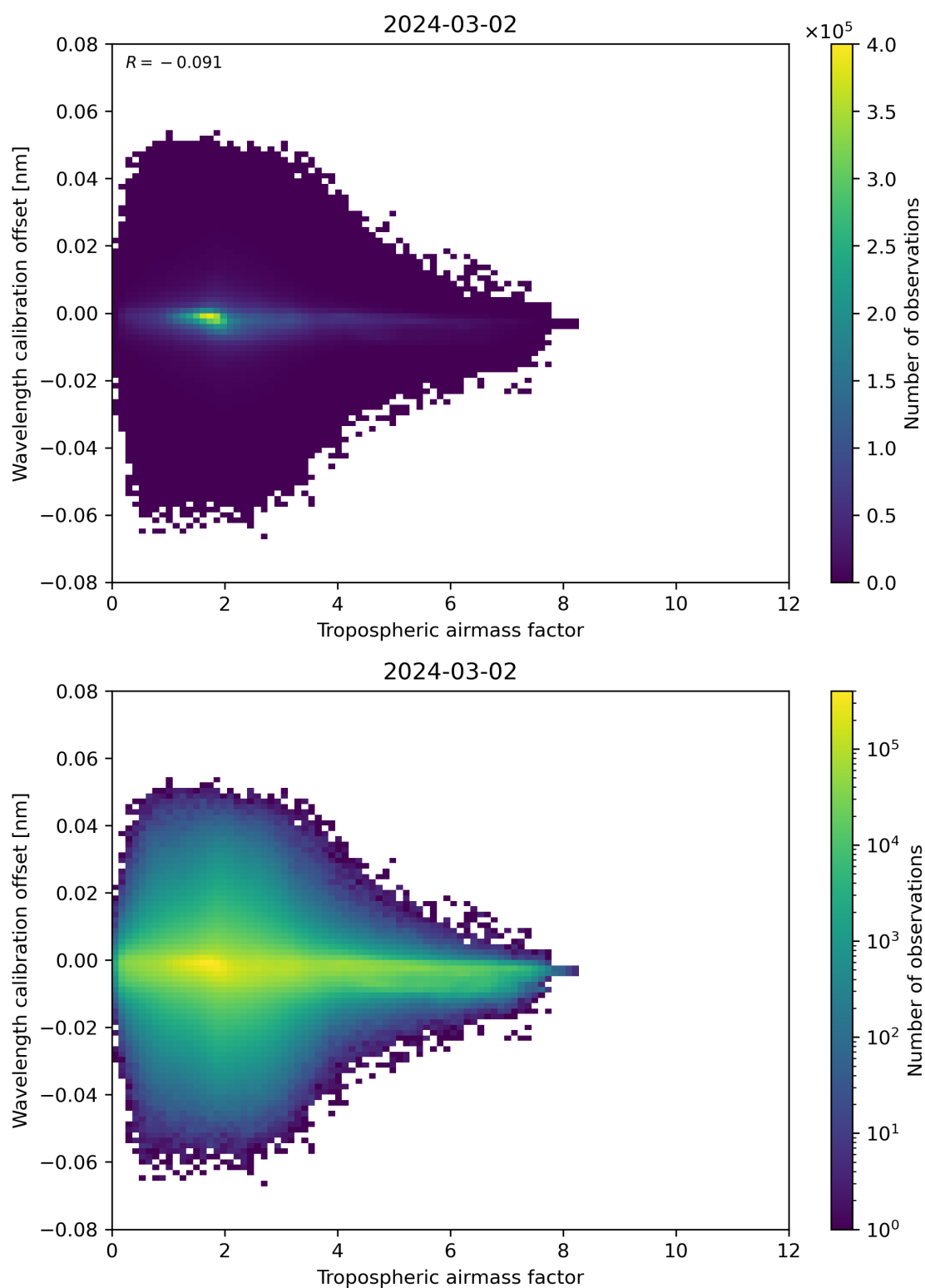
Figure 80: Scatter density plot of “Tropospheric airmass factor” against “Wavelength calibration offset” for 2024-03-01 to 2024-03-03.
