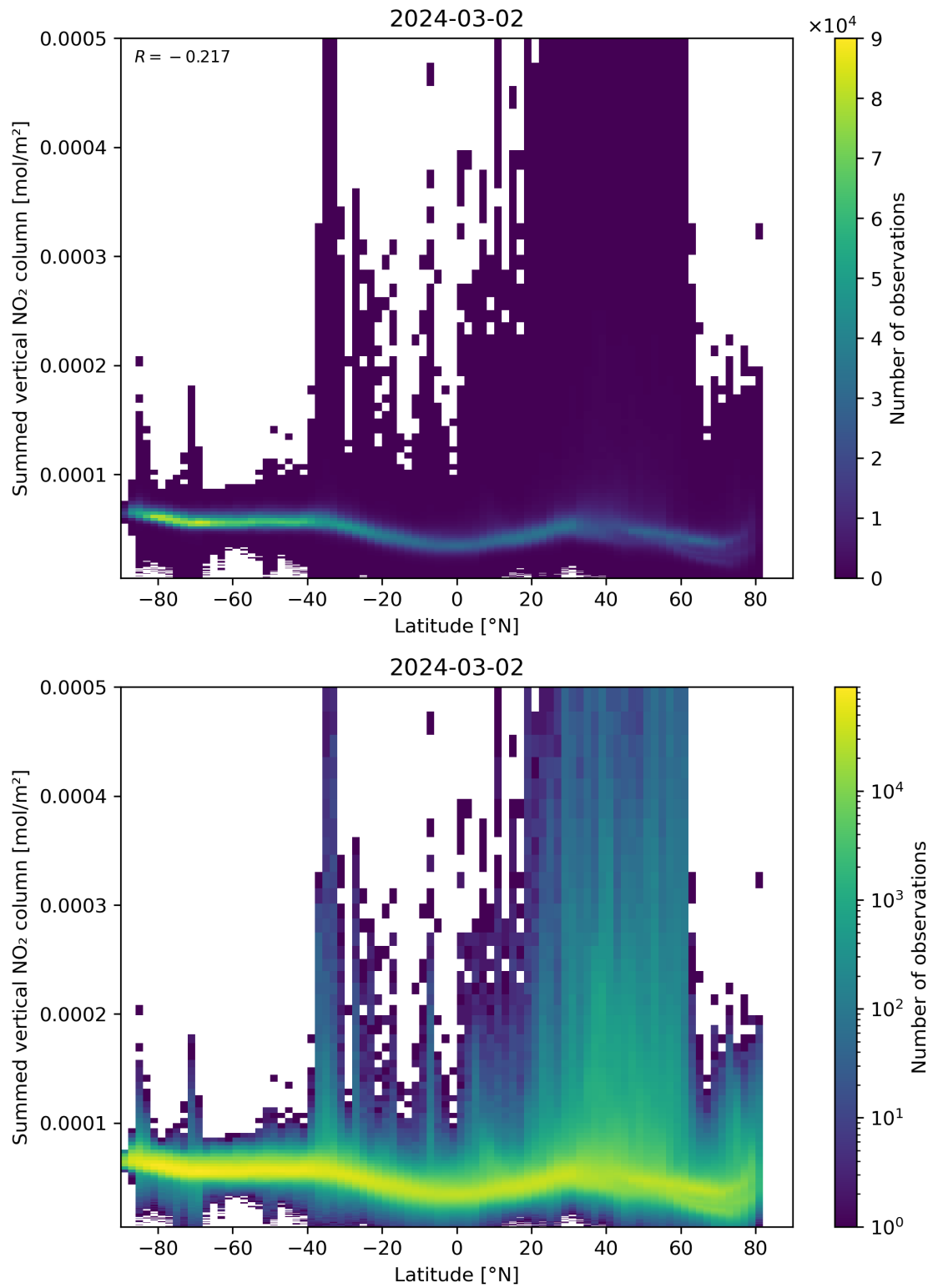
Figure 88: Scatter density plot of “Latitude” against “Summed vertical NO 2 column” for 2024-03-01 to 2024-03-03.
