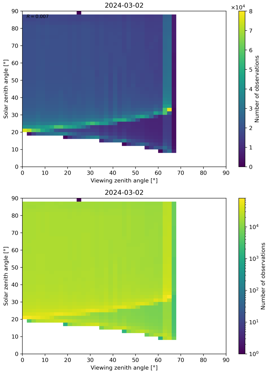
Figure 172: Scatter density plot of “Viewing zenith angle” against “Solar zenith angle” for 2024-03-01 to 2024-03-03.
