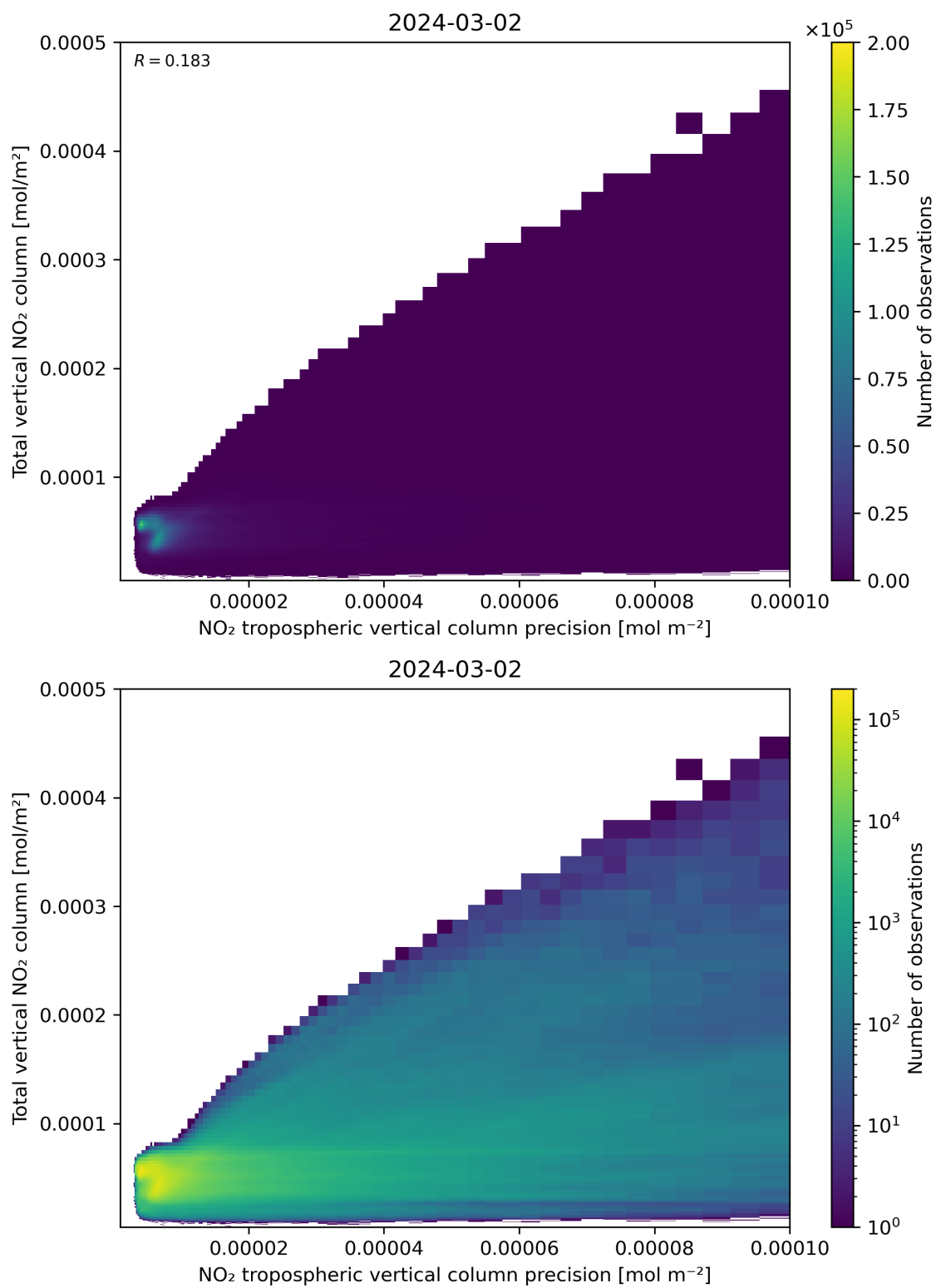
Figure 138: Scatter density plot of “NO 2 tropospheric vertical column precision” against “Total vertical NO 2 column” for 2024-03-01 to 2024-03-03.
