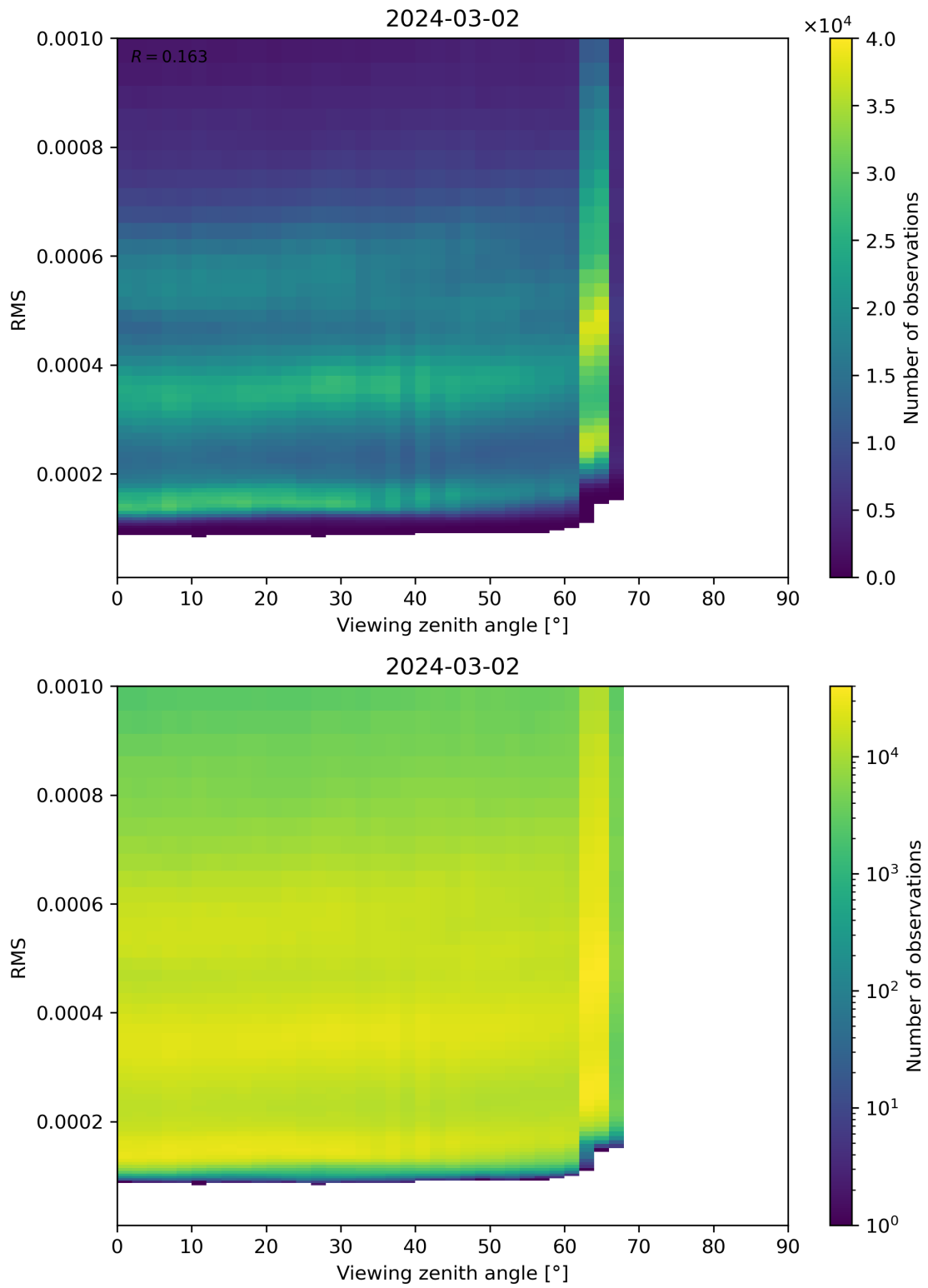
Figure 171: Scatter density plot of “Viewing zenith angle” against “RMS” for 2024-03-01 to 2024-03-03.
