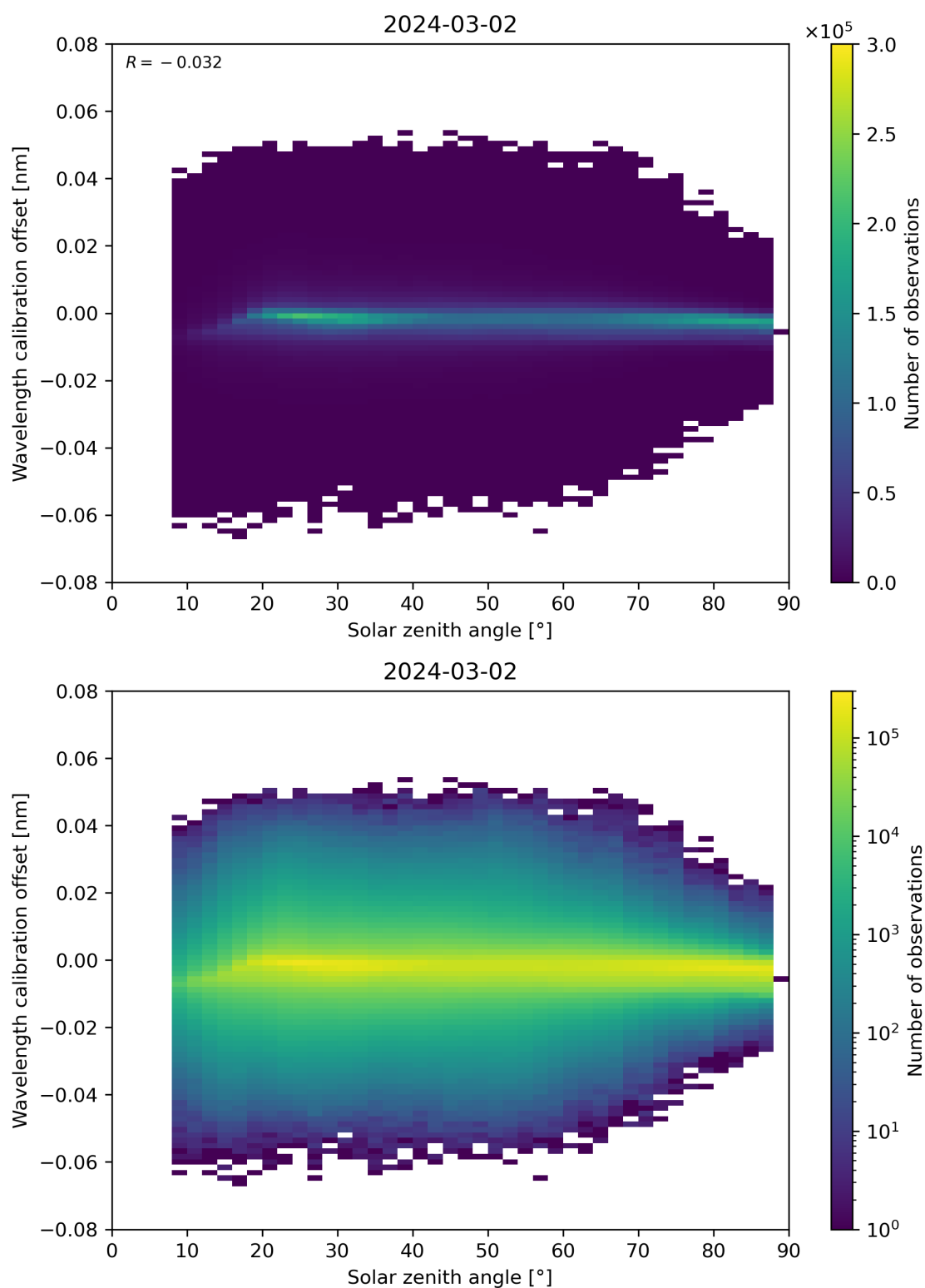
Figure 158: Scatter density plot of “Solar zenith angle” against “Wavelength calibration offset” for 2024-03-01 to 2024-03-03.
