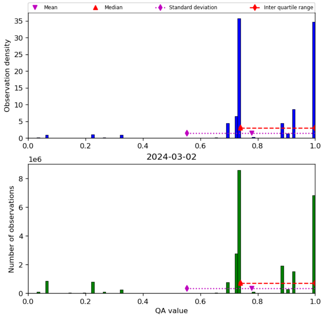
Figure 28: Histogram of “QA value” for 2024-03-01 to 2024-03-03
