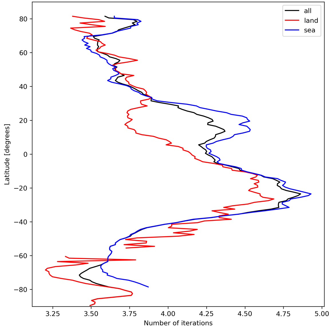
Figure 17: Zonal average of “Number of iterations” for 2024-03-01 to 2024-03-03.
