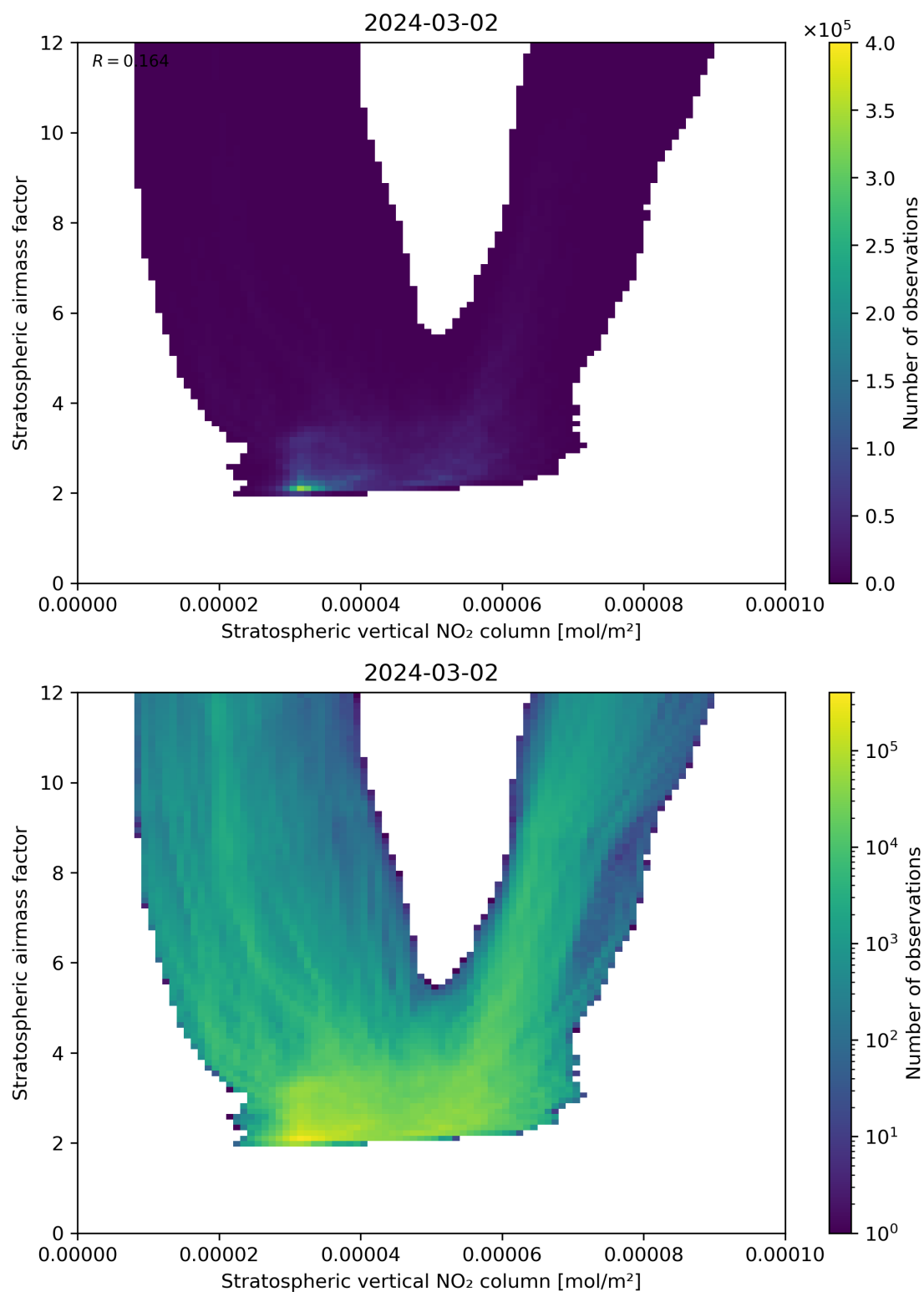
Figure 96: Scatter density plot of “Stratospheric vertical NO 2 column” against “Stratospheric airmass factor” for 2024-03-01 to 2024-03-03.
