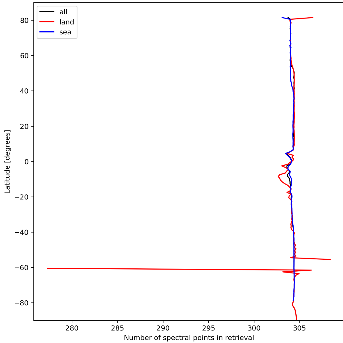
Figure 16: Zonal average of “Number of spectral points in retrieval” for 2024-03-01 to 2024-03-03.
