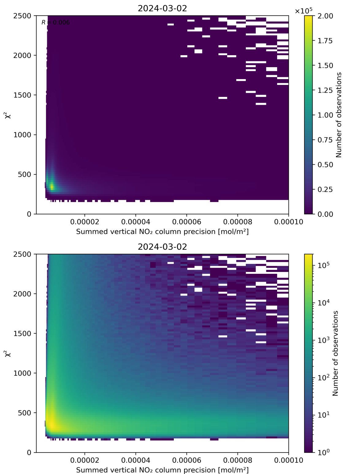
Figure 107: Scatter density plot of “Summed vertical NO 2 column precision” against “ \chi^2 ” for 2024-03-01 to 2024-03-03.
