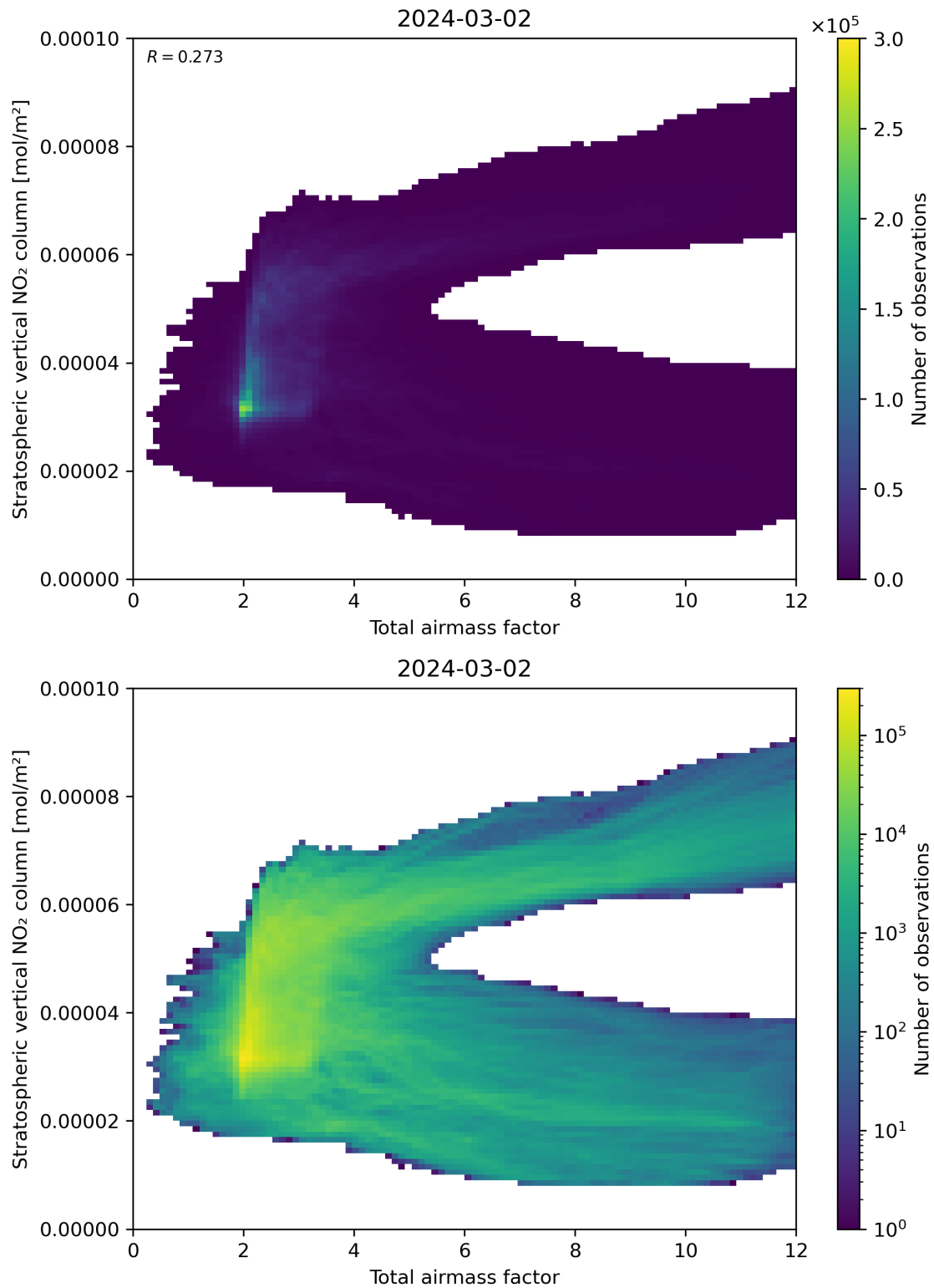
Figure 64: Scatter density plot of “Total airmass factor” against “Stratospheric vertical \text{NO}_2 column” for 2024-03-01 to 2024-03-03.
