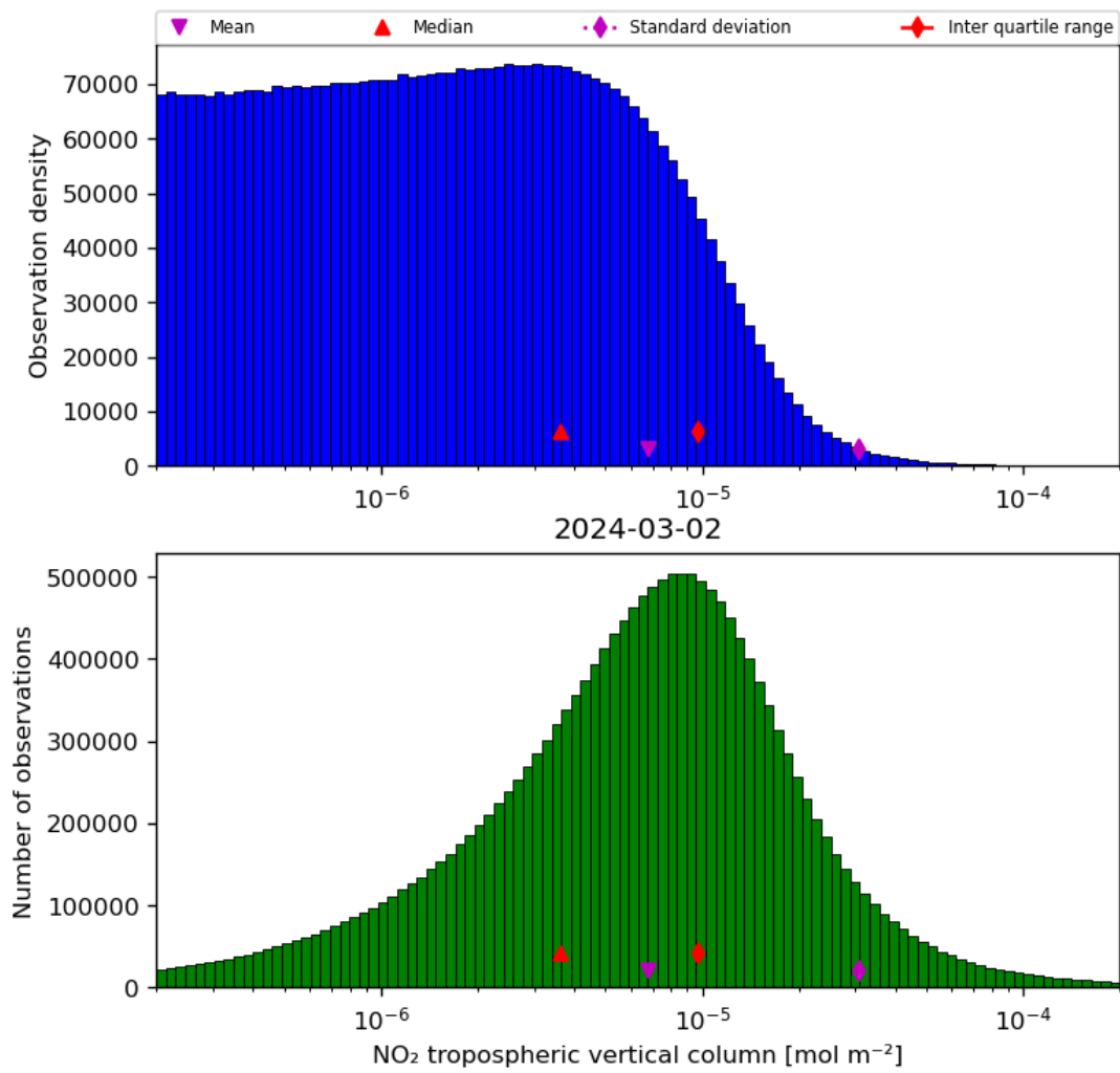
Figure 29: Histogram of “NO 2 tropospheric vertical column” for 2024-03-01 to 2024-03-03
