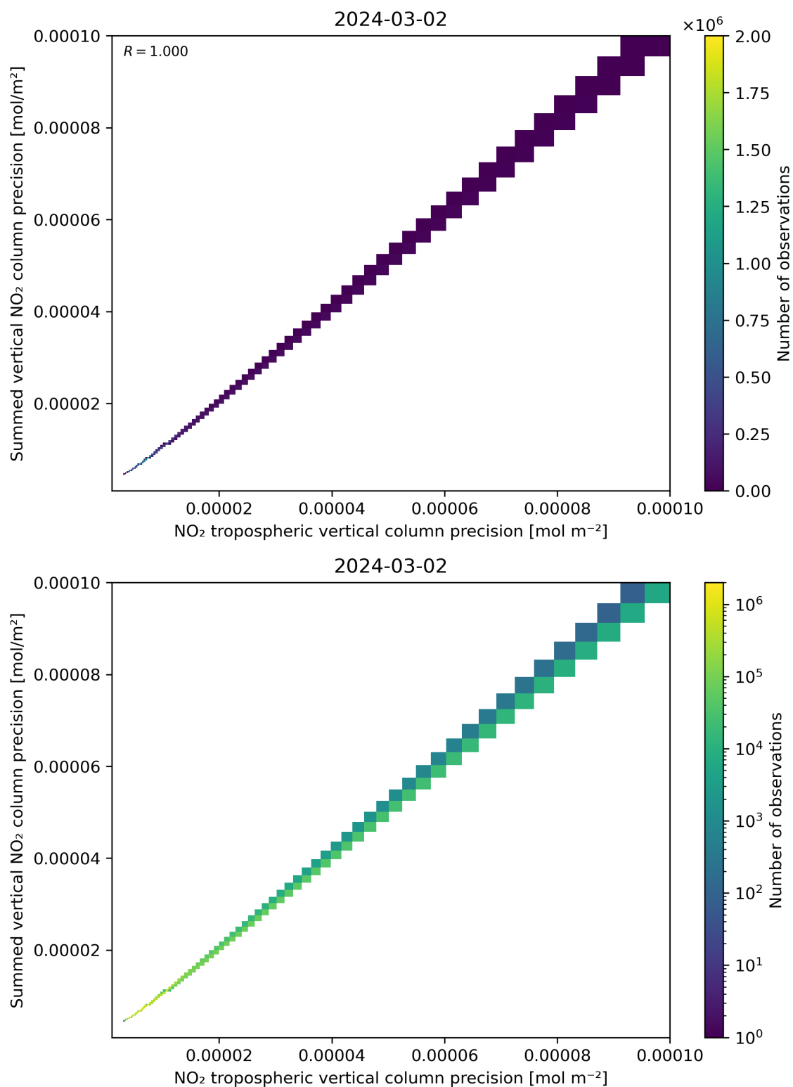
Figure 137: Scatter density plot of “NO 2 tropospheric vertical column precision” against “Summed vertical NO 2 column precision” for 2024-03-01 to 2024-03-03.
