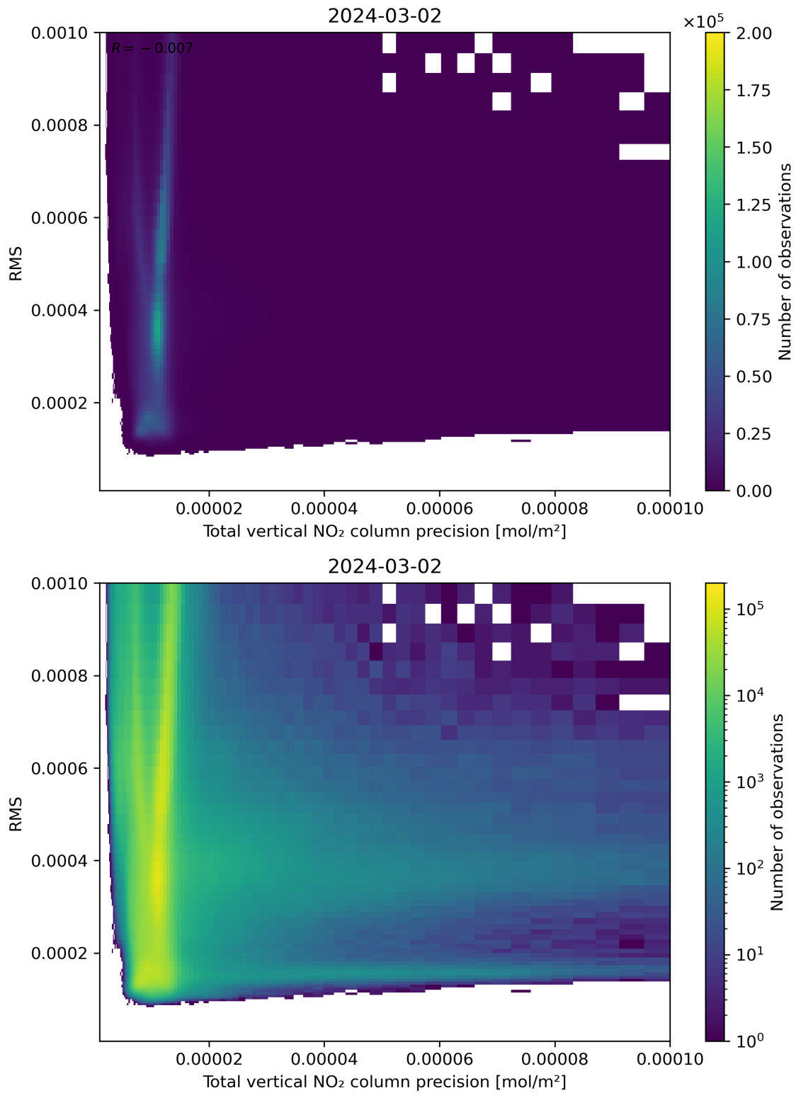
Figure 119: Scatter density plot of “Total vertical NO 2 column precision” against “RMS” for 2024-03-01 to 2024-03-03.
