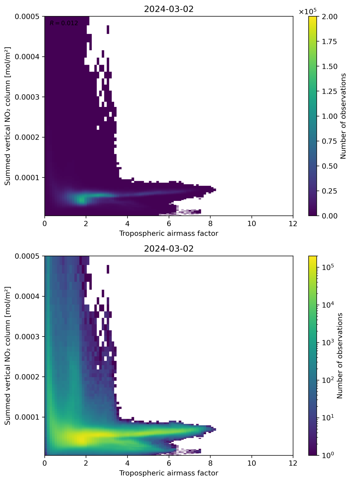
Figure 75: Scatter density plot of “Tropospheric air mass factor” against “Summed vertical NO 2 column” for 2024-03-01 to 2024-03-03.
