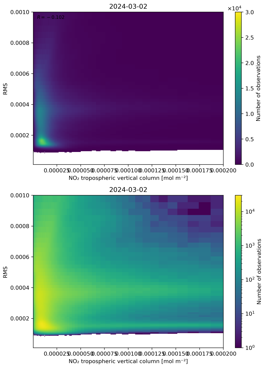
Figure 142: Scatter density plot of “NO 2 tropospheric vertical column” against “RMS” for 2024-03-01 to 2024-03-03.
