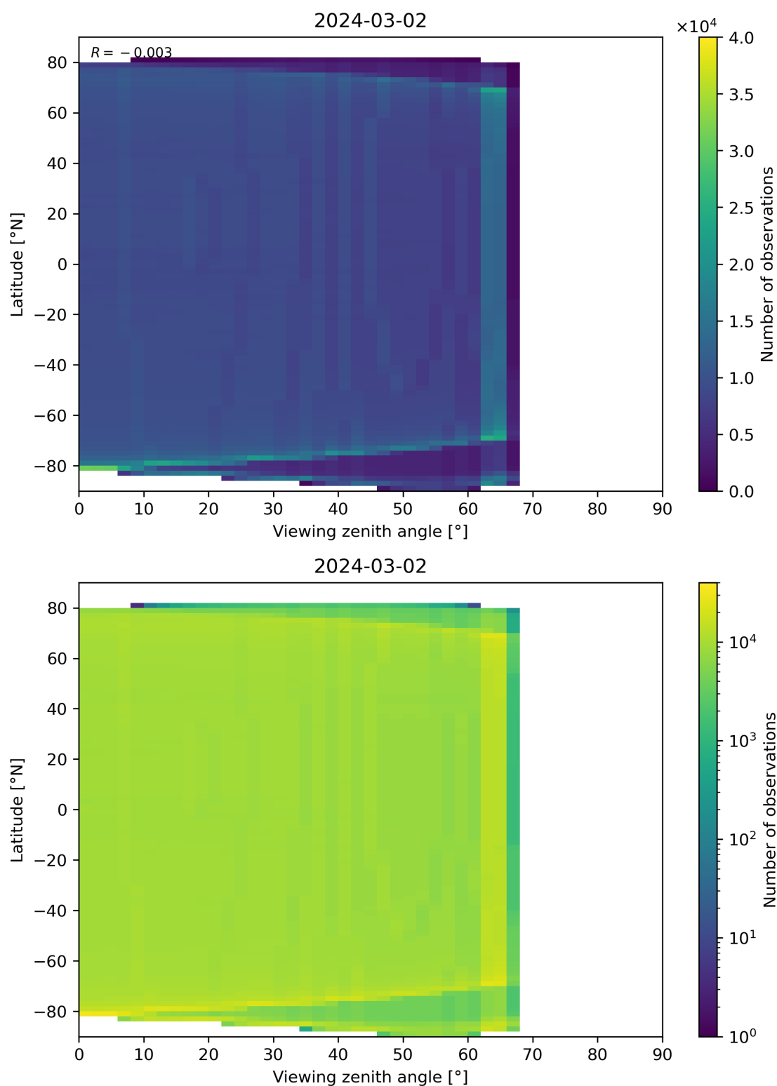
Figure 163: Scatter density plot of “Viewing zenith angle” against “Latitude” for 2024-03-01 to 2024-03-03.
