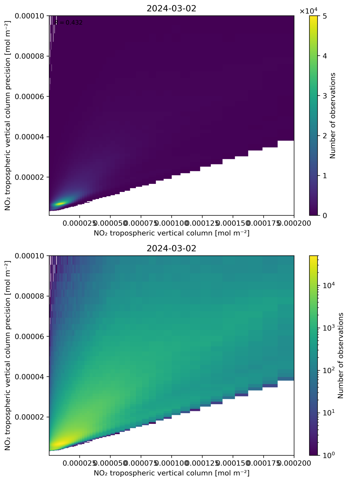
Figure 130: Scatter density plot of “NO 2 tropospheric vertical column” against “NO 2 tropospheric vertical column precision” for 2024-03-01 to 2024-03-03.
