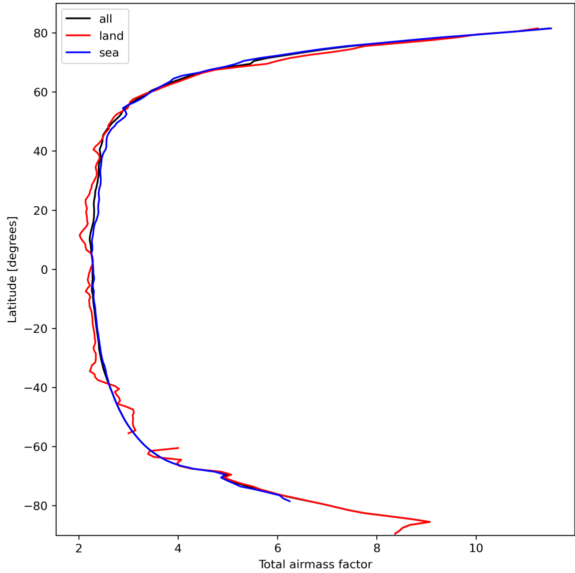
Figure 15: Zonal average of “Total airmass factor” for 2024-03-01 to 2024-03-03.
