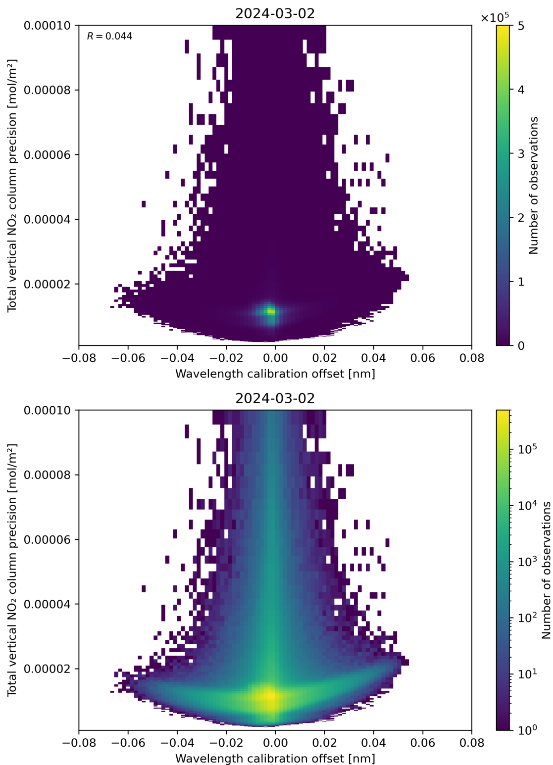
Figure 180: Scatter density plot of “Wavelength calibration offset” against “Total vertical NO 2 column precision” for 2024-03-01 to 2024-03-03.
