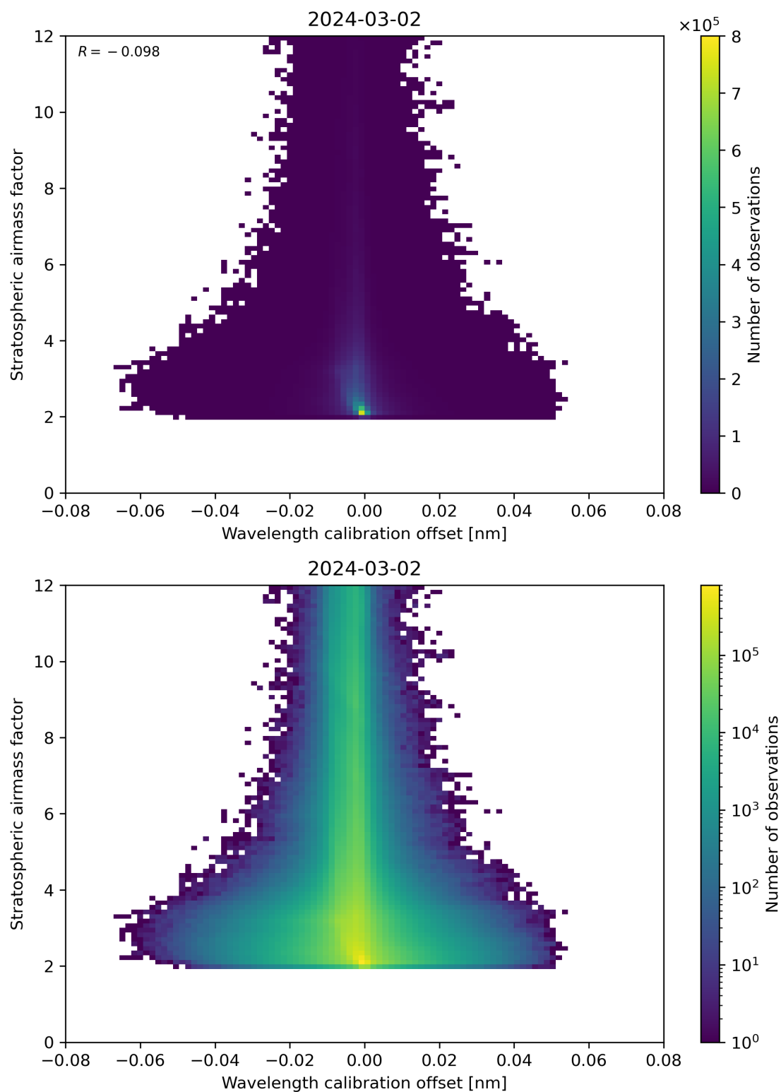
Figure 174: Scatter density plot of “Wavelength calibration offset” against “Stratospheric airmass factor” for 2024-03-01 to 2024-03-03.
