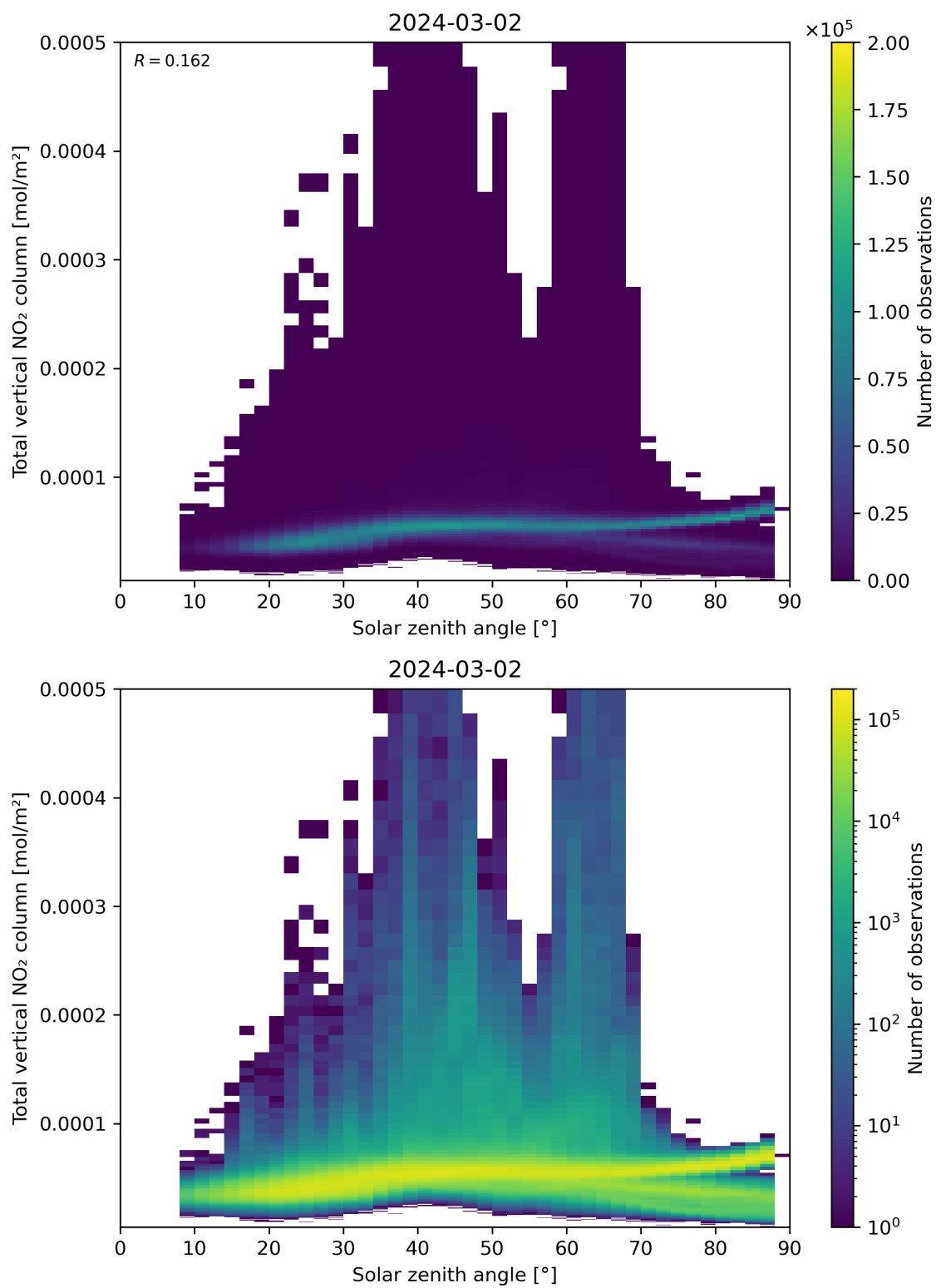
Figure 153: Scatter density plot of “Solar zenith angle” against “Total vertical NO 2 column” for 2024-03-01 to 2024-03-03.
