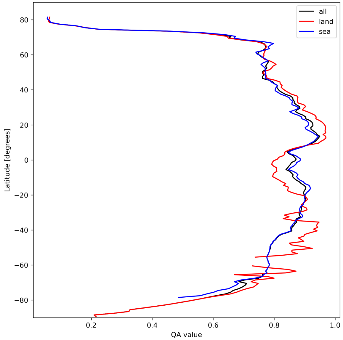
Figure 11: Zonal average of “QA value” for 2024-03-01 to 2024-03-03.
