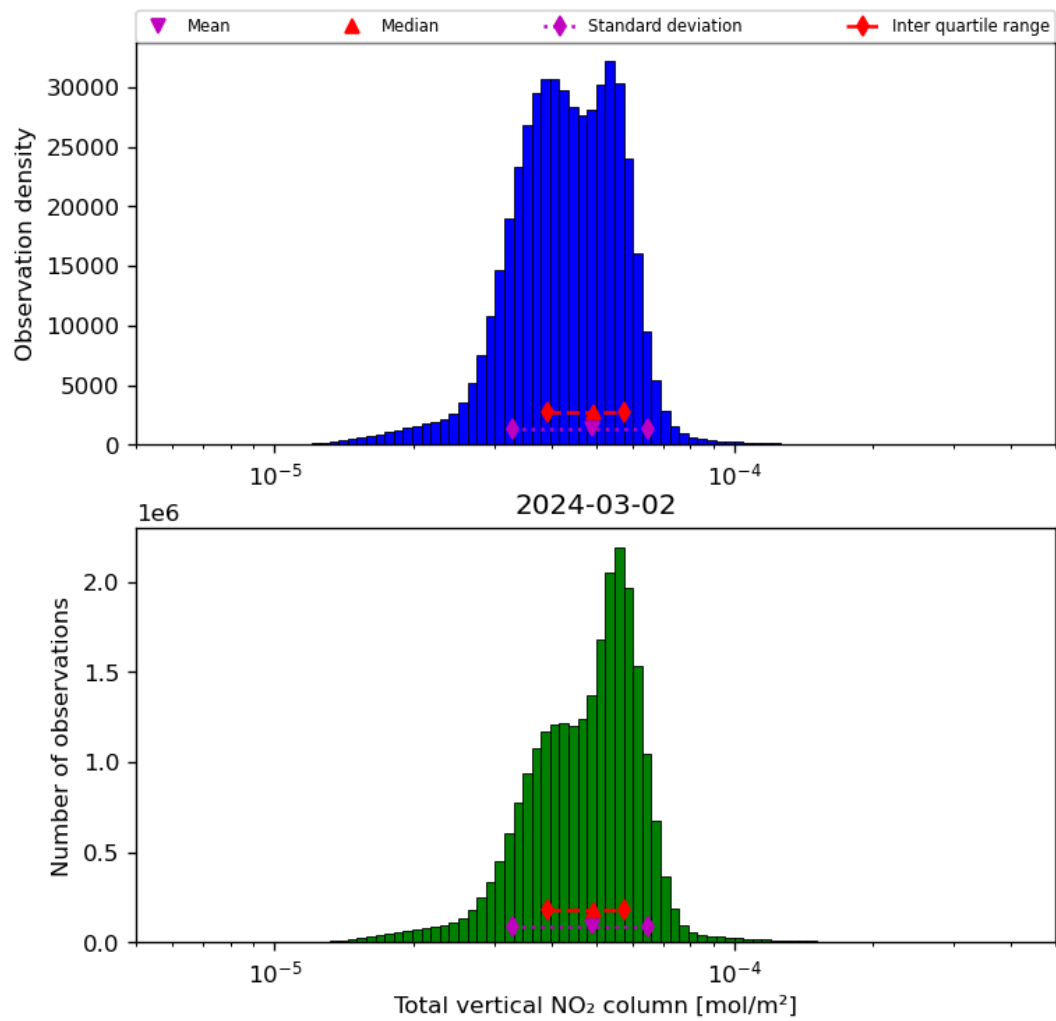
Figure 38: Histogram of “Total vertical NO 2 column” for 2024-03-01 to 2024-03-03
