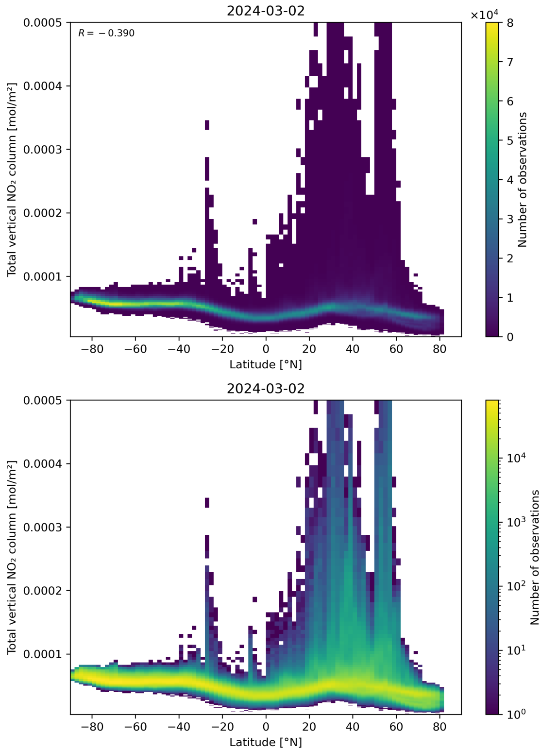
Figure 90: Scatter density plot of “Latitude” against “Total vertical NO 2 column” for 2024-03-01 to 2024-03-03.
