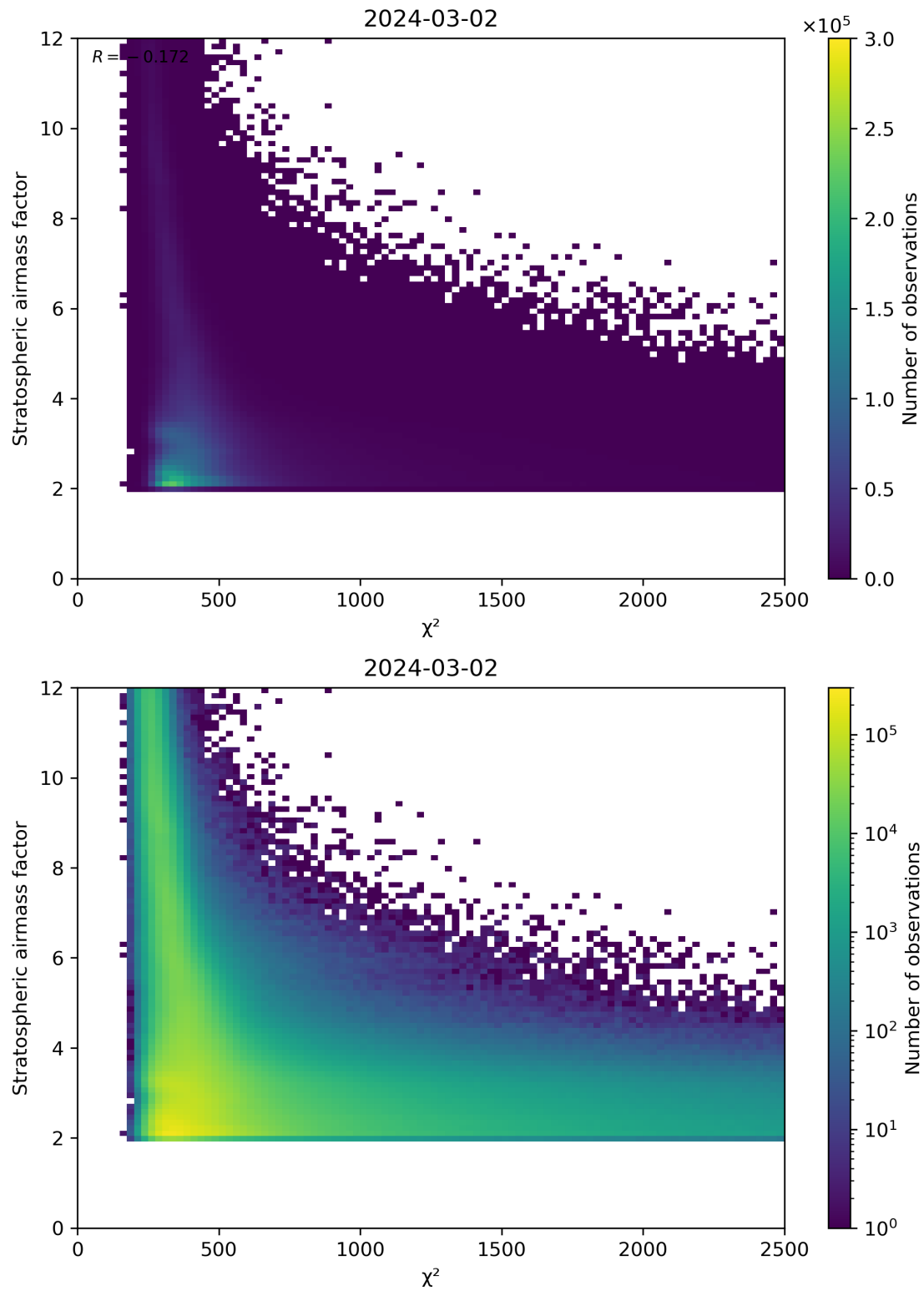
Figure 81: Scatter density plot of “ \chi^2 ” against “Stratospheric airmass factor” for 2024-03-01 to 2024-03-03.
