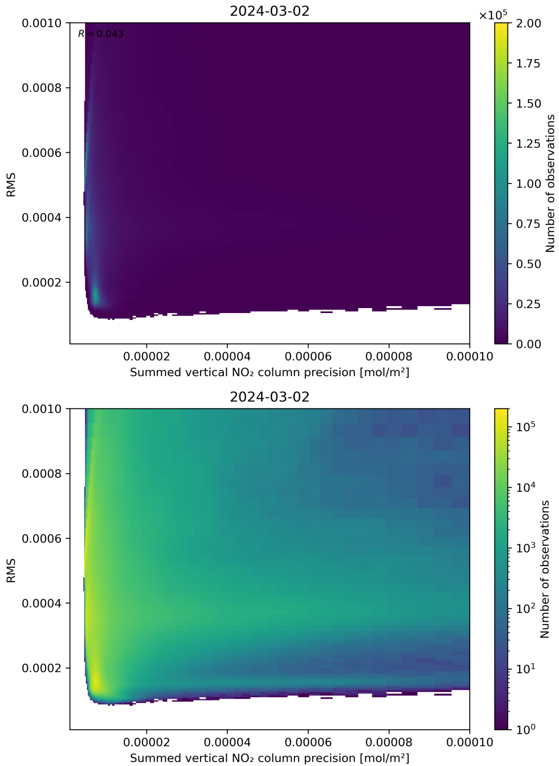
Figure 108: Scatter density plot of “Summed vertical NO 2 column precision” against “RMS” for 2024-03-01 to 2024-03-03.
