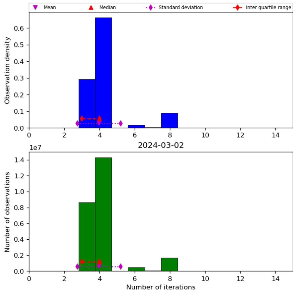
Figure 34: Histogram of “Number of iterations” for 2024-03-01 to 2024-03-03
