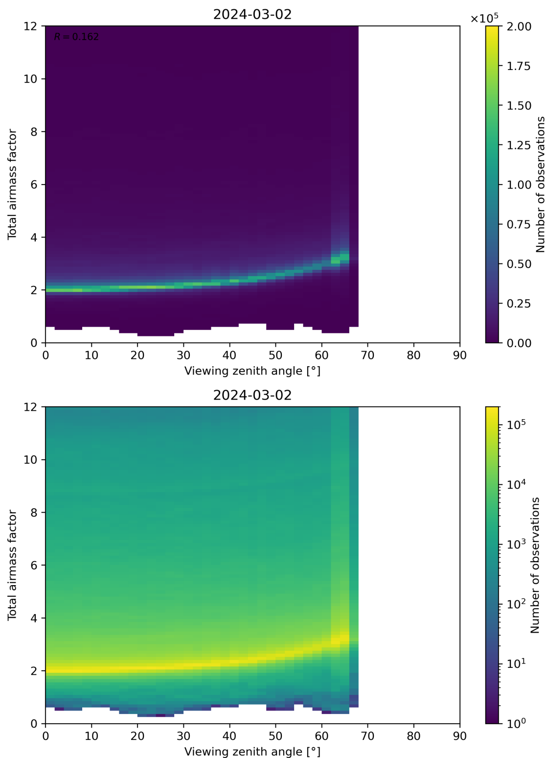
Figure 160: Scatter density plot of “Viewing zenith angle” against “Total airmass factor” for 2024-03-01 to 2024-03-03.
