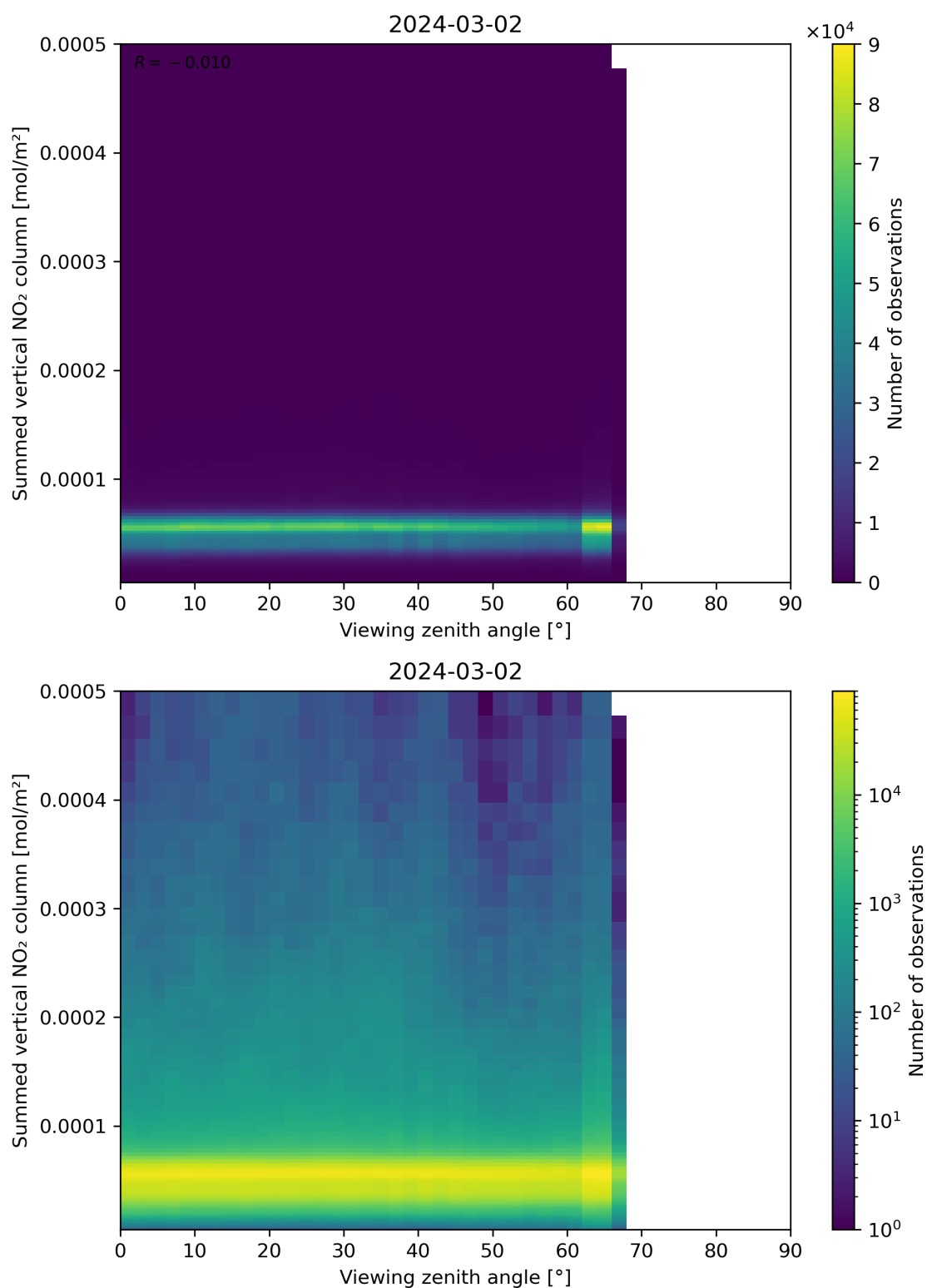
Figure 165: Scatter density plot of “Viewing zenith angle” against “Summed vertical NO 2 column” for 2024-03-01 to 2024-03-03.
