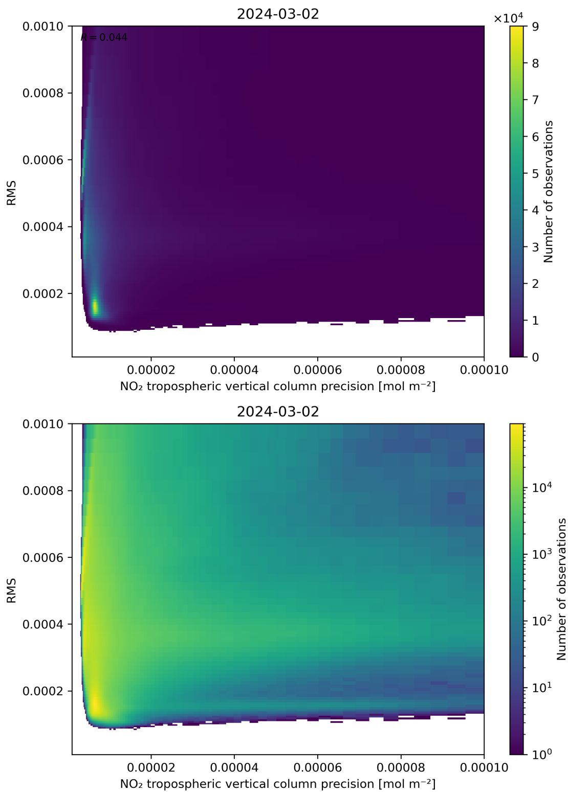
Figure 140: Scatter density plot of “NO 2 tropospheric vertical column precision” against “RMS” for 2024-03-01 to 2024-03-03.
