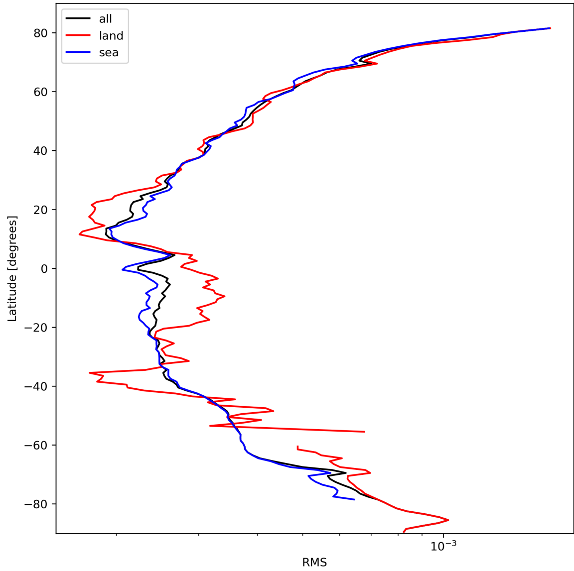
Figure 26: Zonal average of “RMS” for 2024-03-01 to 2024-03-03.
