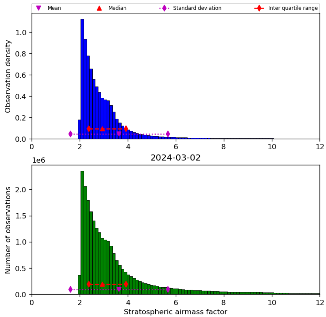
Figure 44: Histogram of “Stratospheric airmass factor” for 2024-03-01 to 2024-03-03
