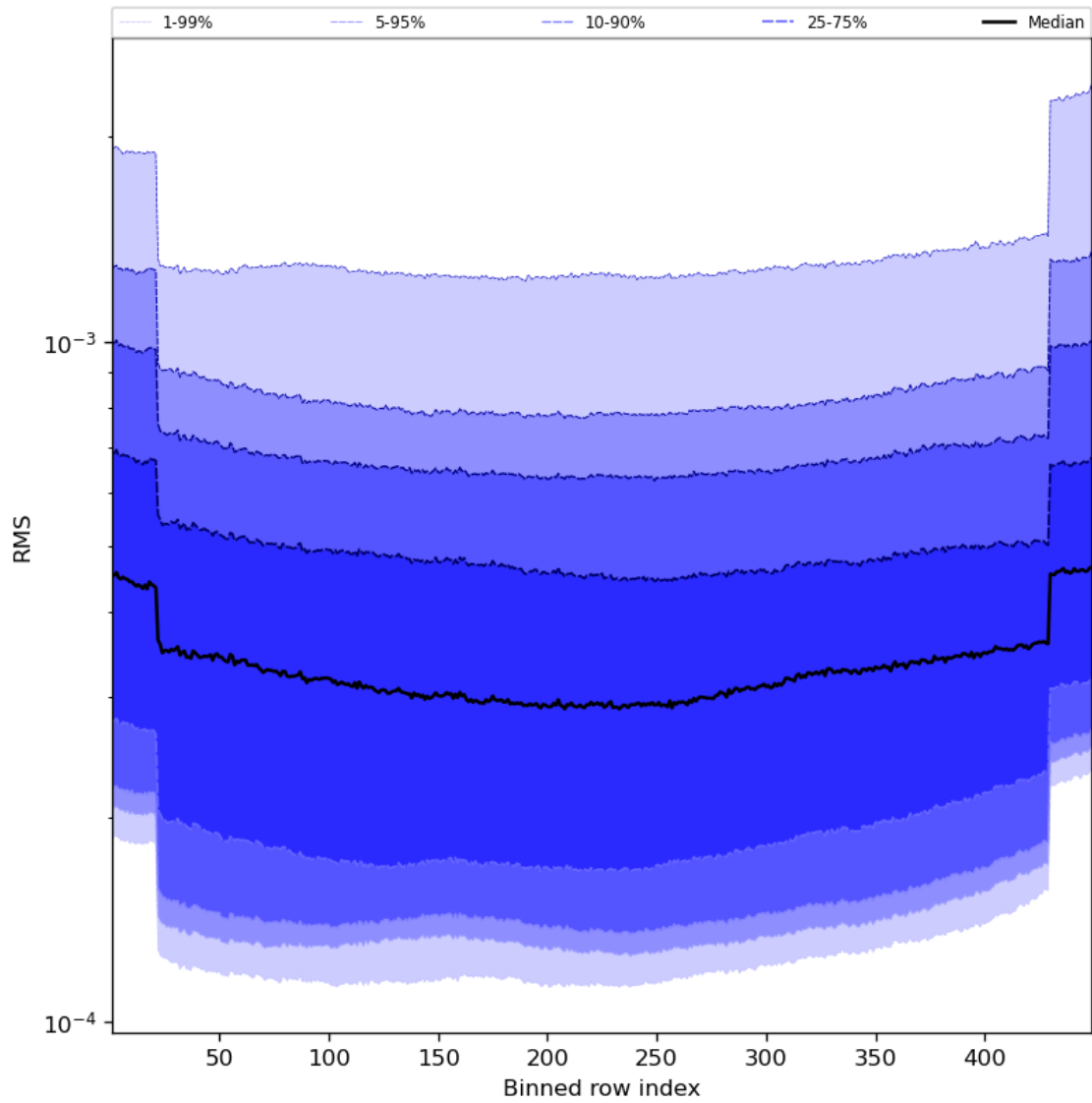
Figure 60: Along track statistics of “RMS” for 2024-03-01 to 2024-03-03
