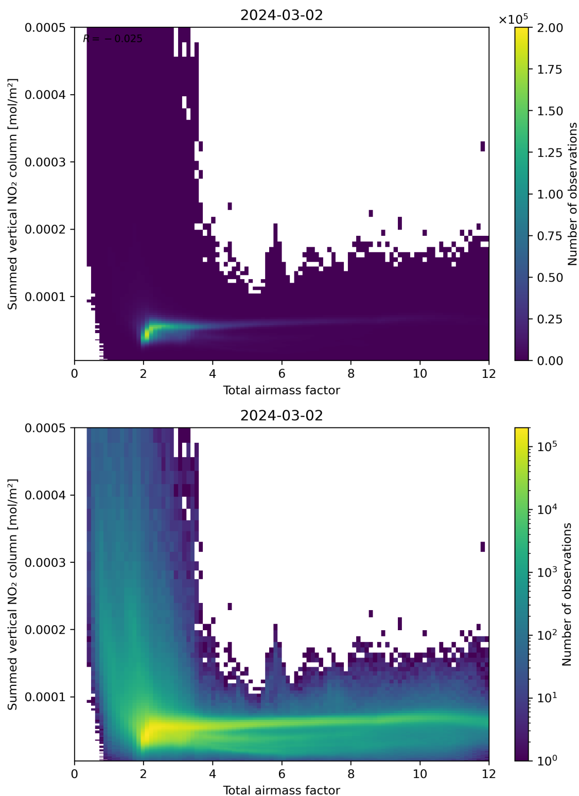
Figure 65: Scatter density plot of “Total airmass factor” against “Summed vertical NO 2 column” for 2024-03-01 to 2024-03-03.
