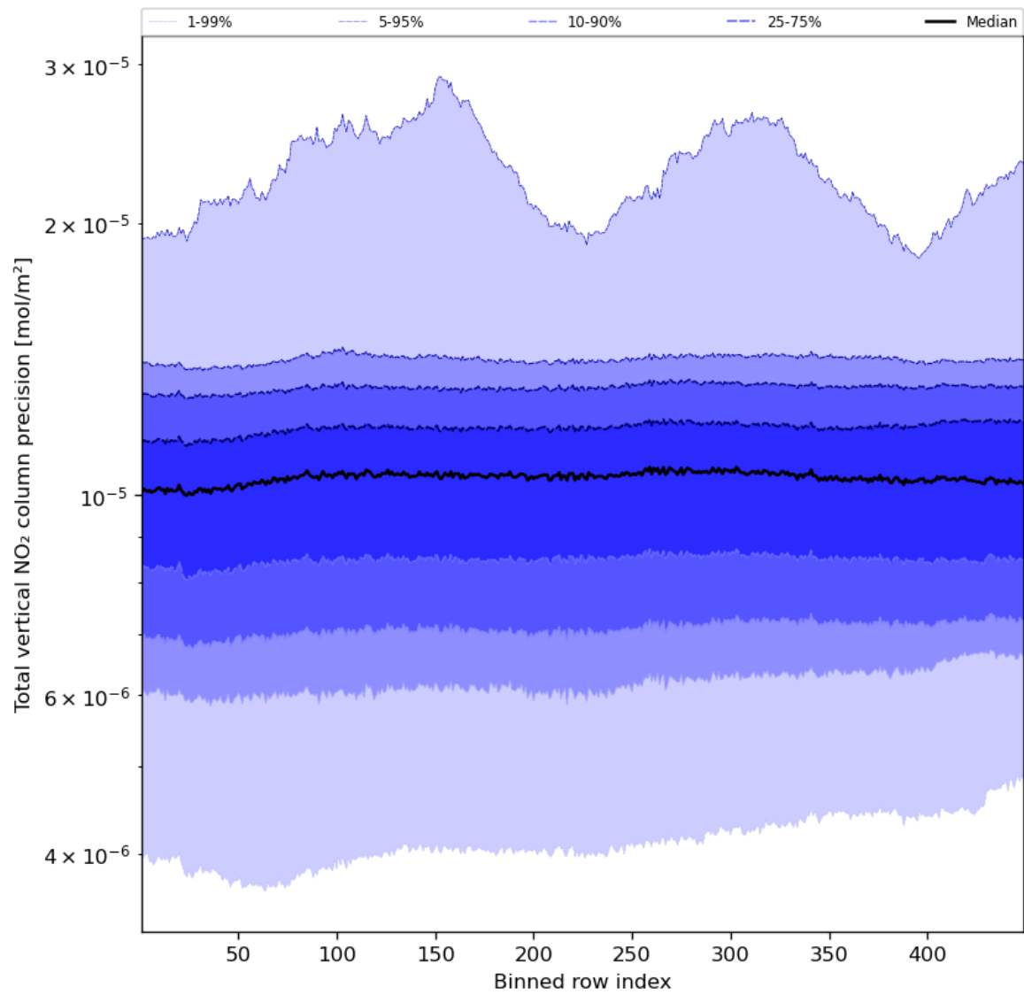
Figure 56: Along track statistics of “Total vertical NO 2 column precision” for 2024-03-01 to 2024-03-03
