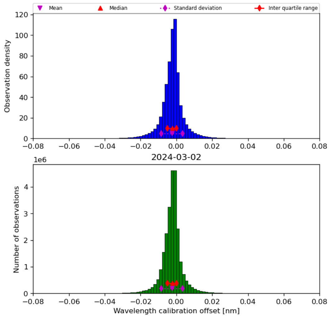
Figure 35: Histogram of “Wavelength calibration offset” for 2024-03-01 to 2024-03-03
