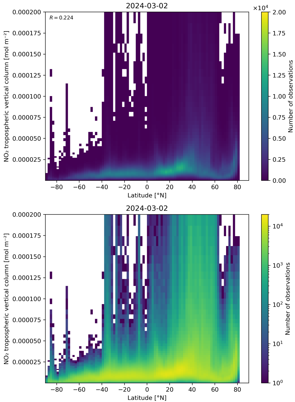
Figure 92: Scatter density plot of “Latitude” against “NO 2 tropospheric vertical column” for 2024-03-01 to 2024-03-03.
