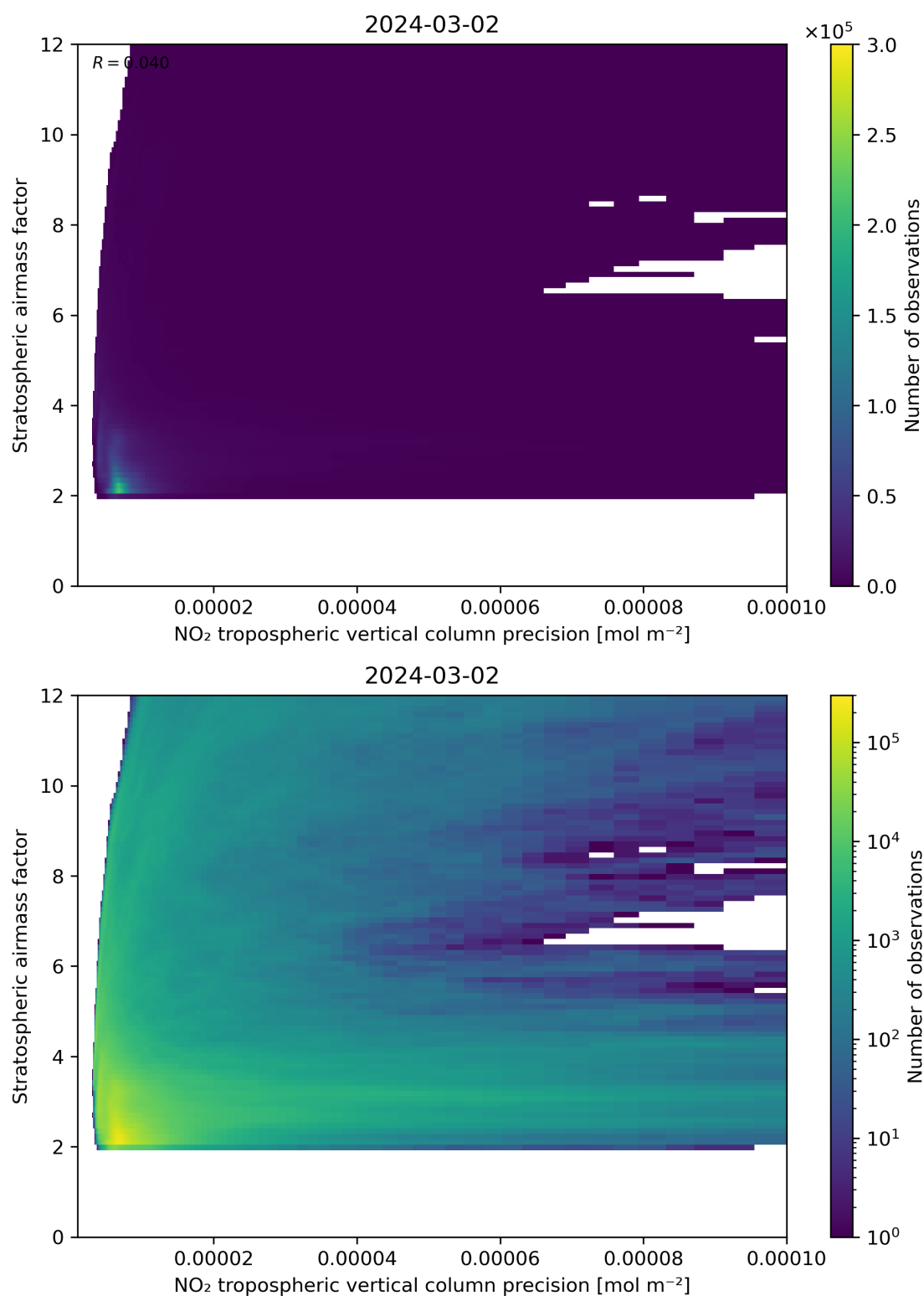
Figure 131: Scatter density plot of “NO 2 tropospheric vertical column precision” against “Stratospheric airmass factor” for 2024-03-01 to 2024-03-03.
