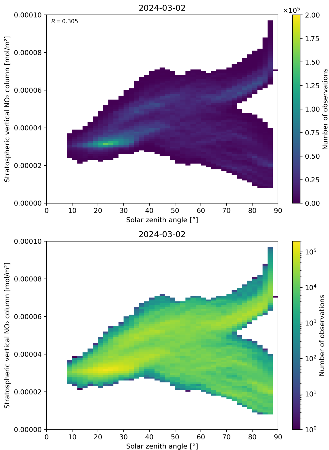
Figure 150: Scatter density plot of “Solar zenith angle” against “Stratospheric vertical NO 2 column” for 2024-03-01 to 2024-03-03.
