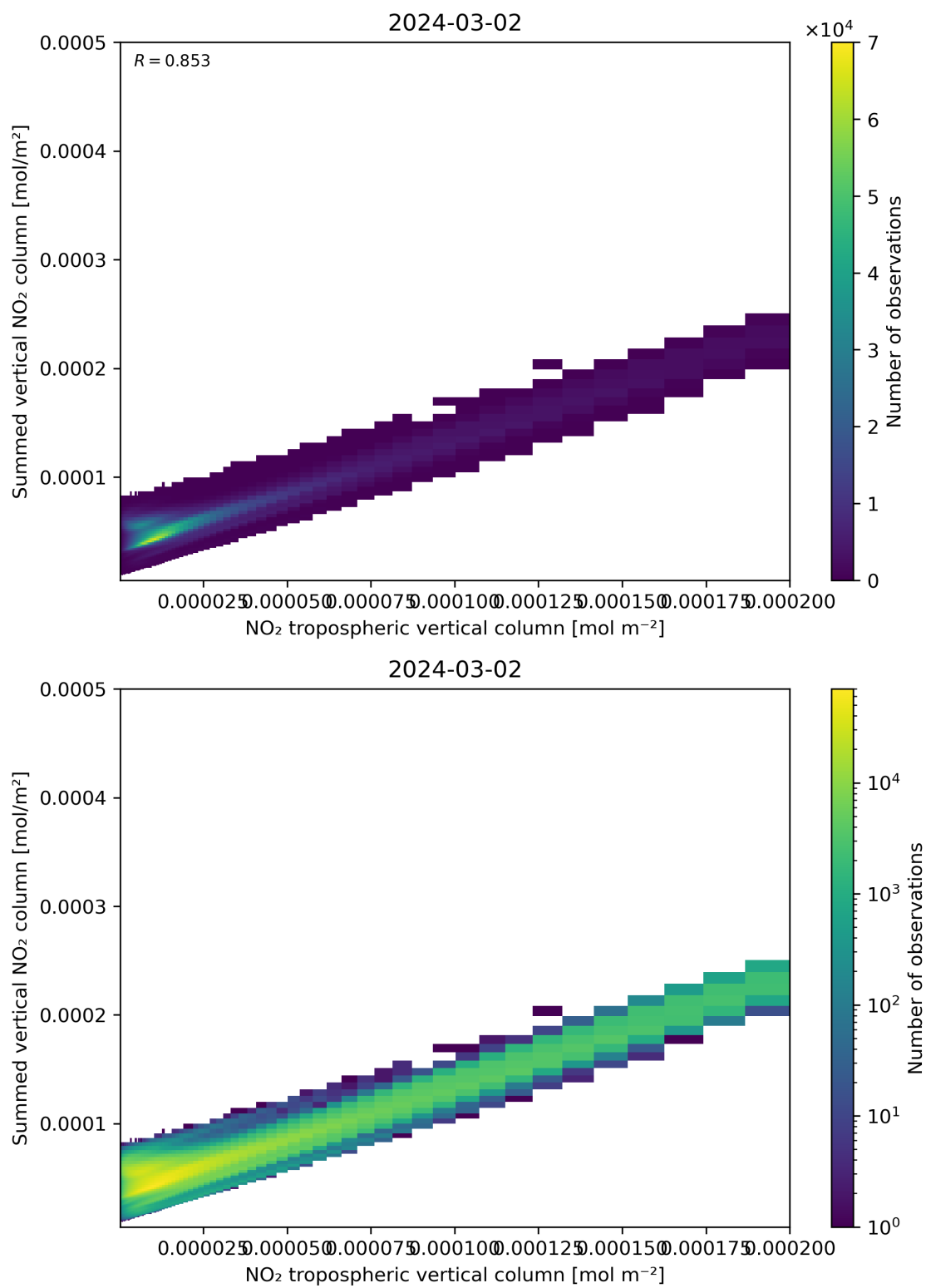
Figure 126: Scatter density plot of “NO 2 tropospheric vertical column” against “Summed vertical NO 2 column” for 2024-03-01 to 2024-03-03.
