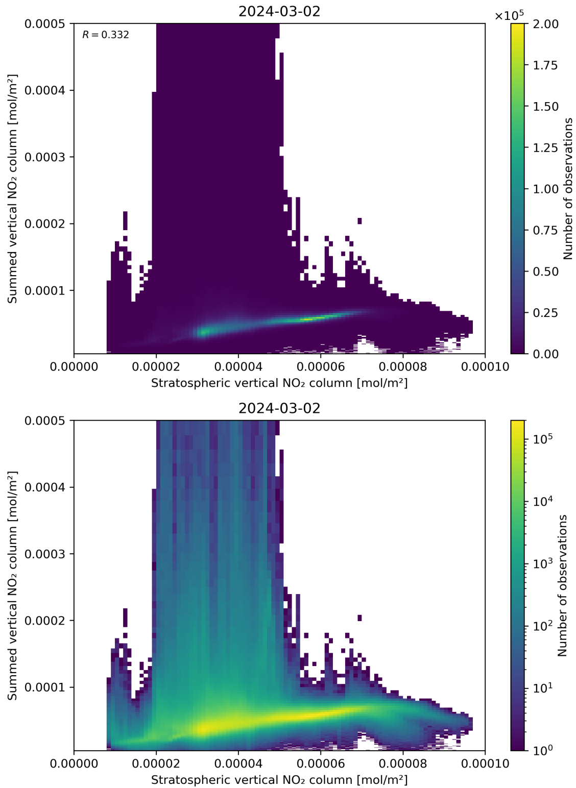
Figure 98: Scatter density plot of “Stratospheric vertical NO 2 column” against “Summed vertical NO 2 column” for 2024-03-01 to 2024-03-03.
