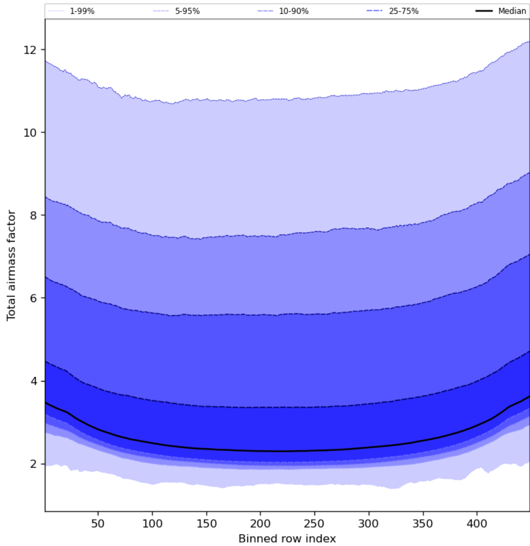
Figure 49: Along track statistics of “Total airmass factor” for 2024-03-01 to 2024-03-03
