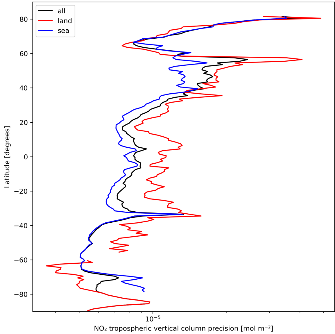
Figure 13: Zonal average of "NO 2 tropospheric vertical column precision" for 2024-03-01 to 2024-03-03.
