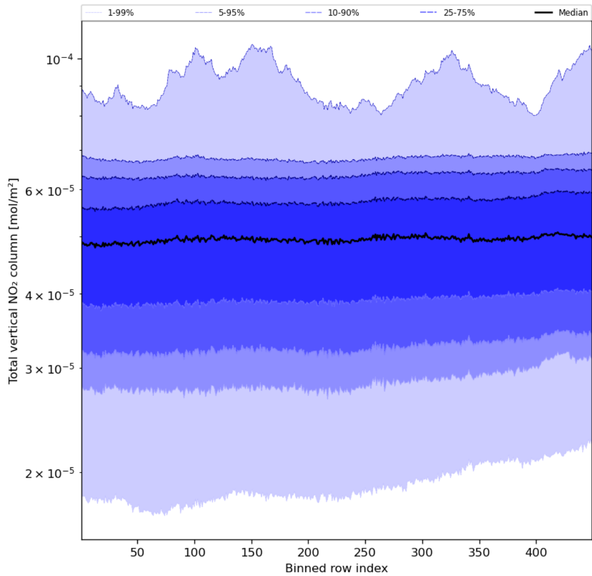
Figure 55: Along track statistics of “Total vertical NO 2 column” for 2024-03-01 to 2024-03-03
