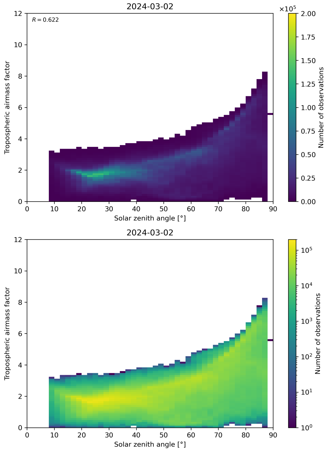
Figure 147: Scatter density plot of “Solar zenith angle” against “Tropospheric airmass factor” for 2024-03-01 to 2024-03-03.
