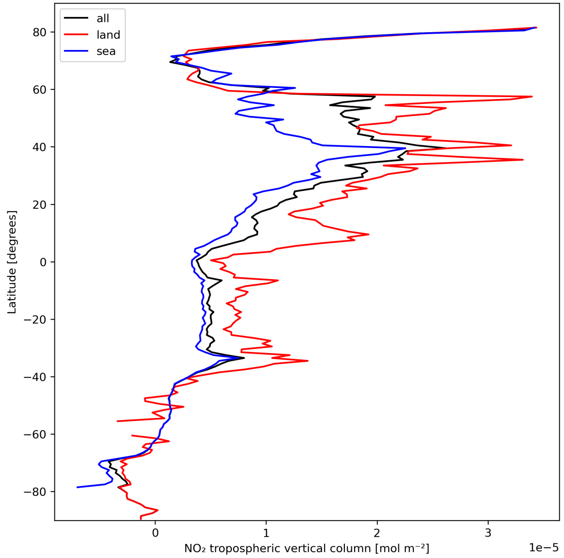
Figure 12: Zonal average of “NO 2 tropospheric vertical column” for 2024-03-01 to 2024-03-03.
