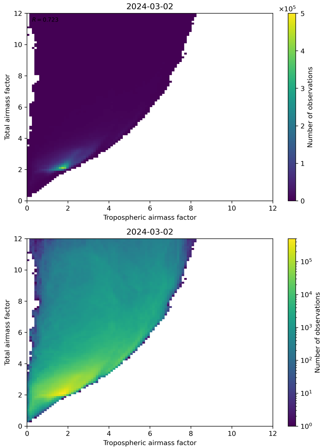
Figure 72: Scatter density plot of “Tropospheric airmass factor” against “Total airmass factor” for 2024-03-01 to 2024-03-03.
