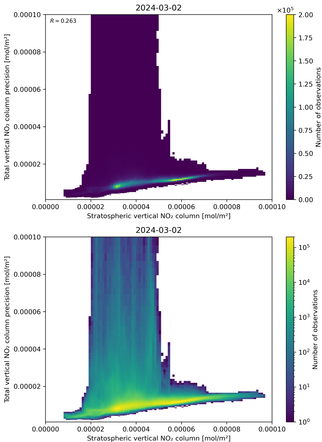
Figure 101: Scatter density plot of “Stratospheric vertical NO 2 column” against “Total vertical NO 2 column precision” for 2024-03-01 to 2024-03-03.
