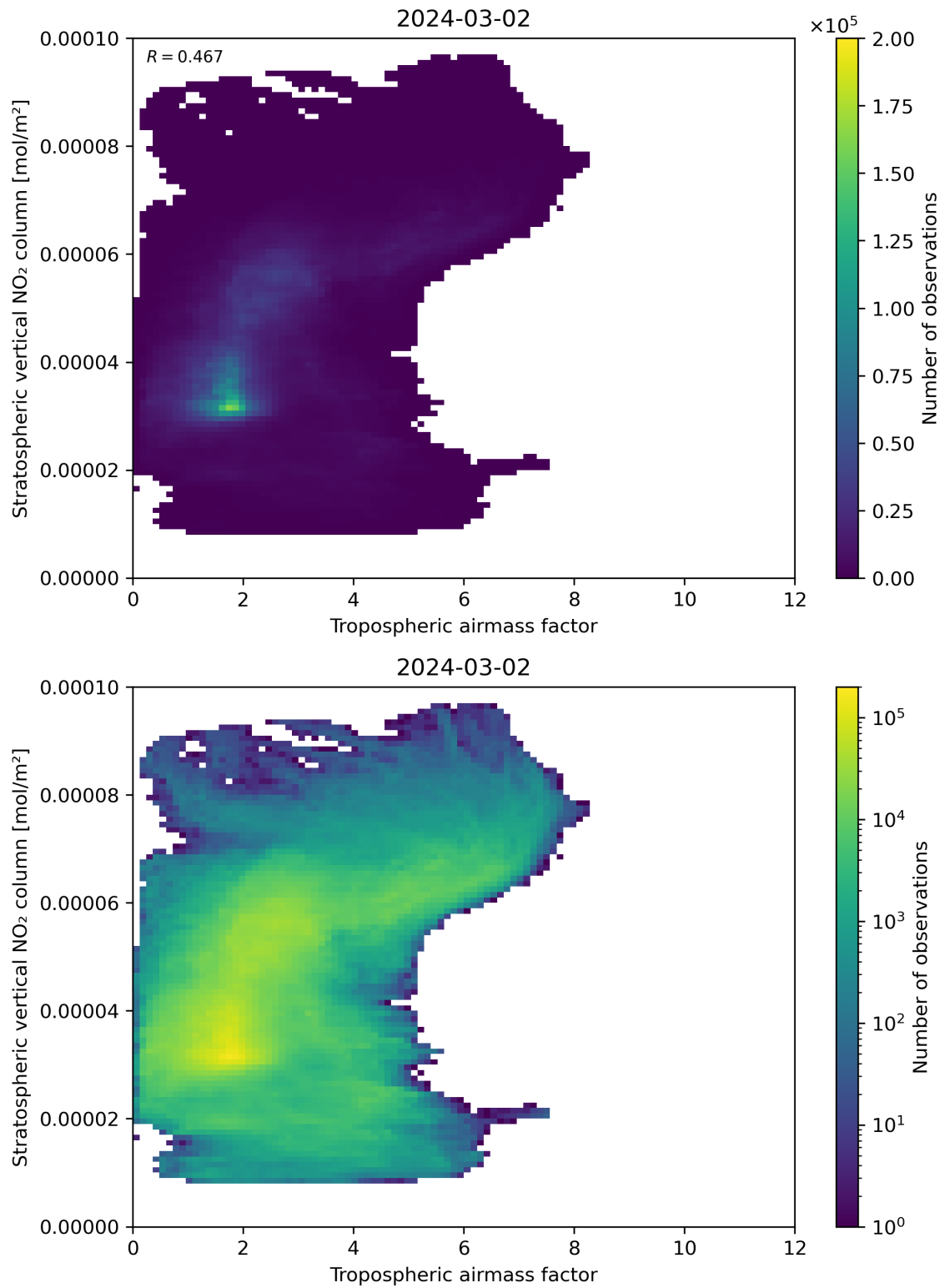
Figure 74: Scatter density plot of “Tropospheric air mass factor” against “Stratospheric vertical NO 2 column” for 2024-03-01 to 2024-03-03.
