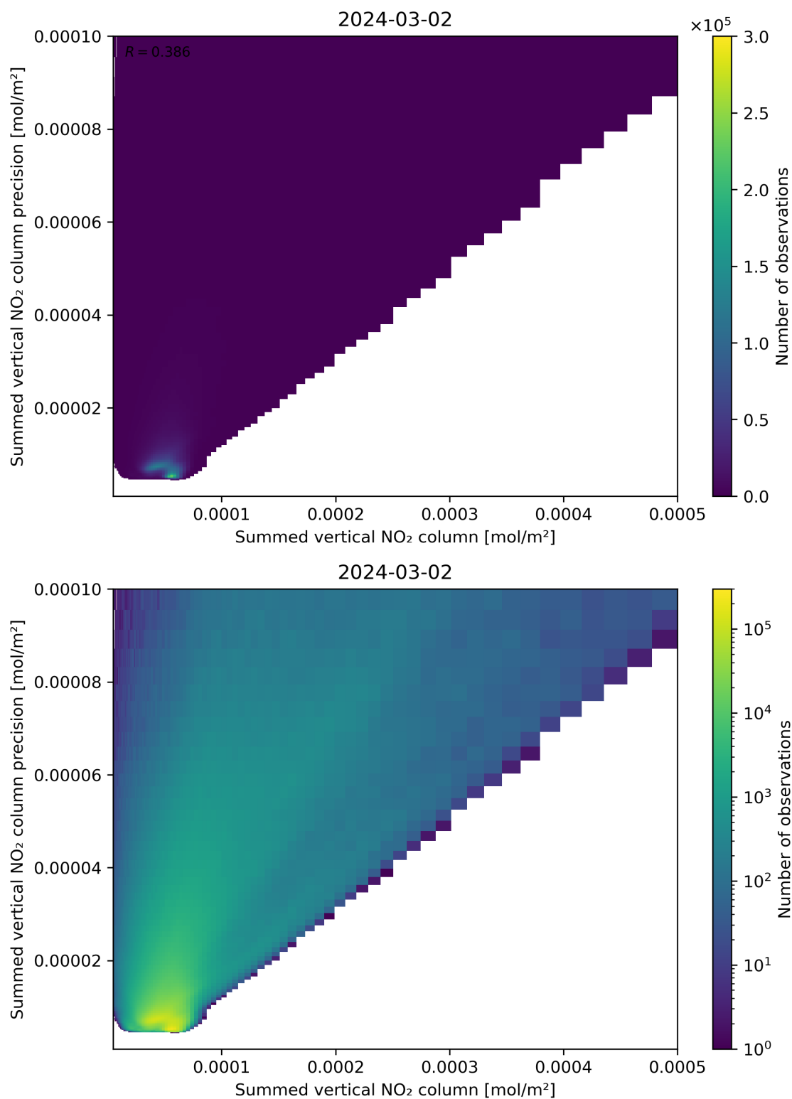
Figure 105: Scatter density plot of “Summed vertical NO 2 column” against “Summed vertical NO 2 column precision” for 2024-03-01 to 2024-03-03.
