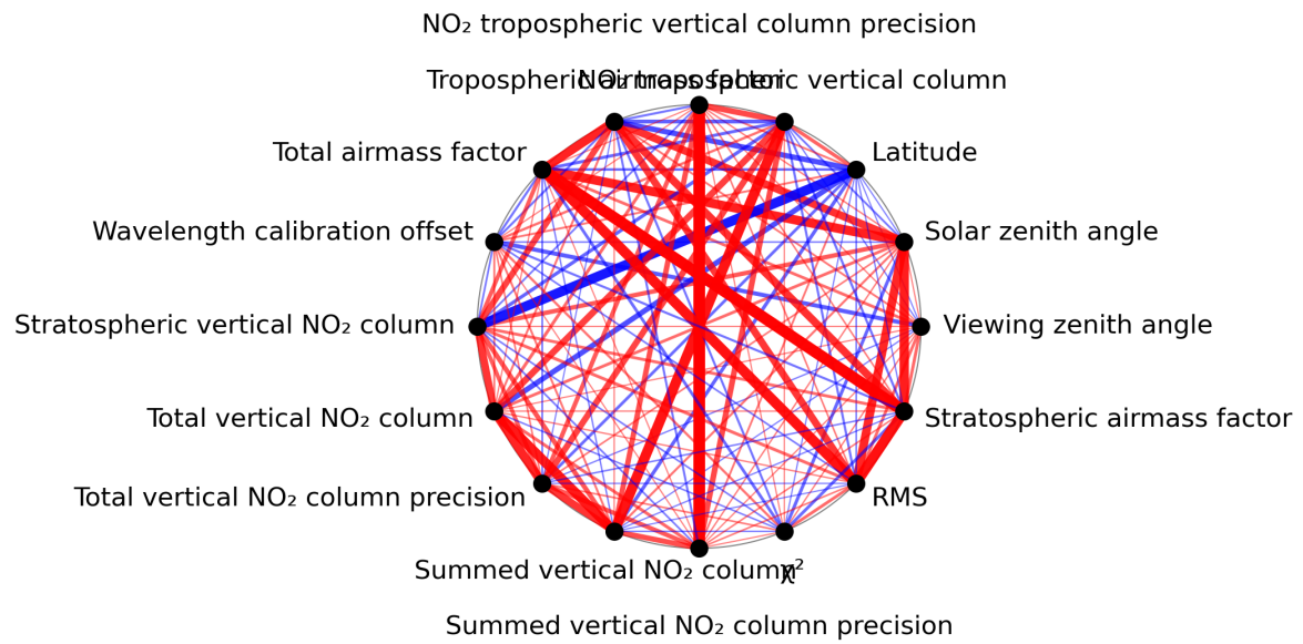
Figure 1: Map of correlation graph for 2024-03-01 to 2024-03-03.
