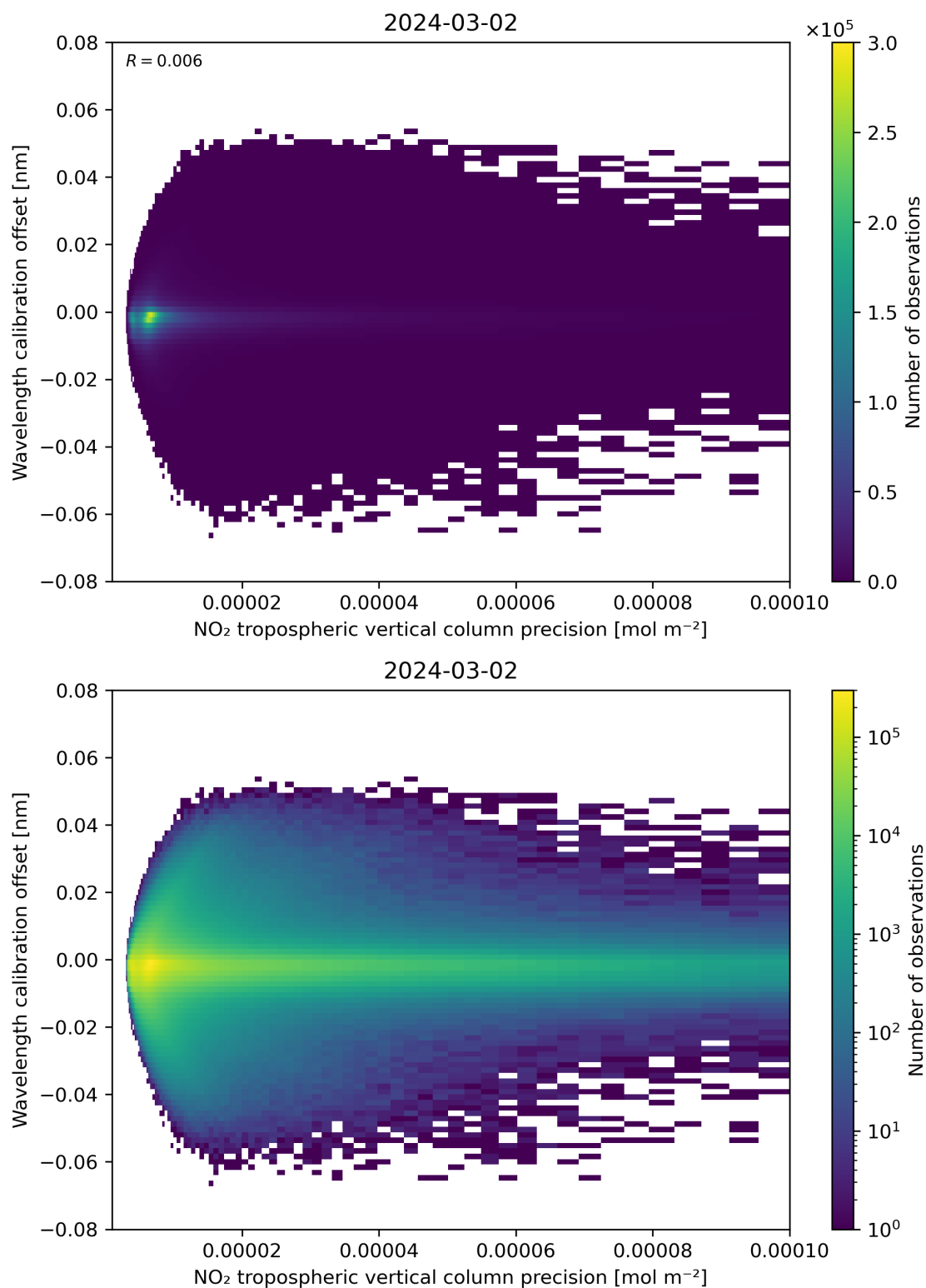
Figure 141: Scatter density plot of “NO 2 tropospheric vertical column precision” against “Wavelength calibration offset” for 2024-03-01 to 2024-03-03.
