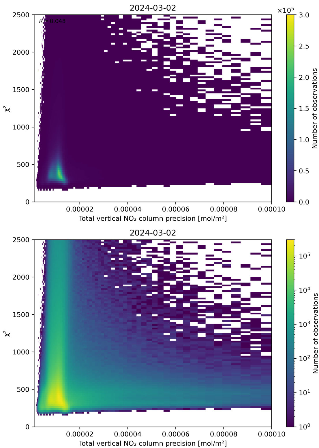
Figure 116: Scatter density plot of “Total vertical NO 2 column precision” against “ \chi^2 ” for 2024-03-01 to 2024-03-03.
