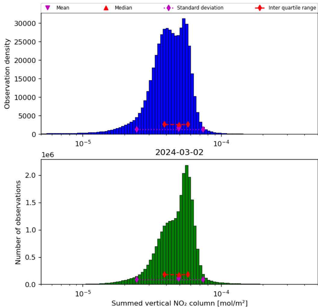
Figure 40: Histogram of “Summed vertical NO 2 column” for 2024-03-01 to 2024-03-03
