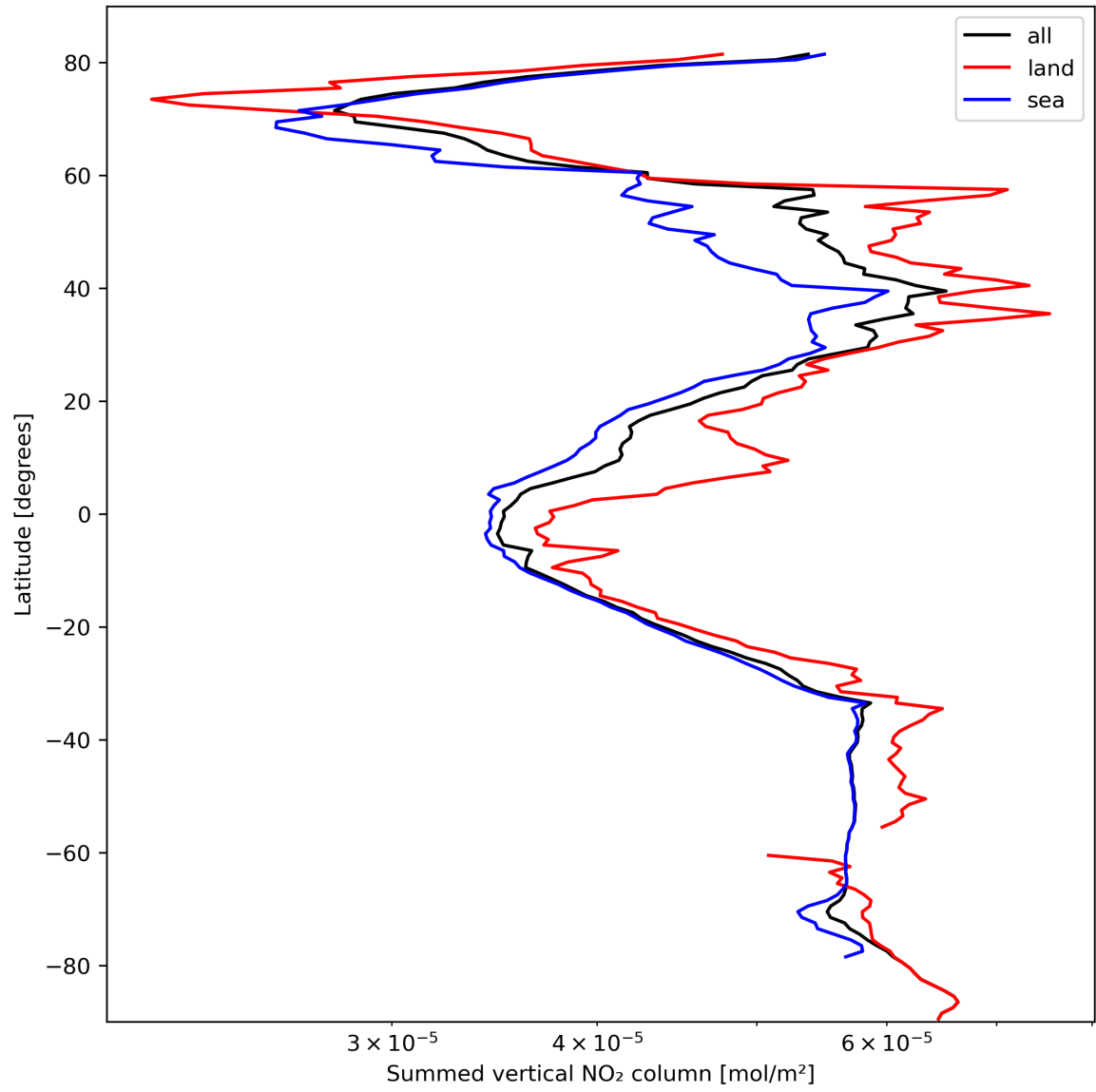
Figure 23: Zonal average of “Summed vertical NO 2 column” for 2024-03-01 to 2024-03-03.
