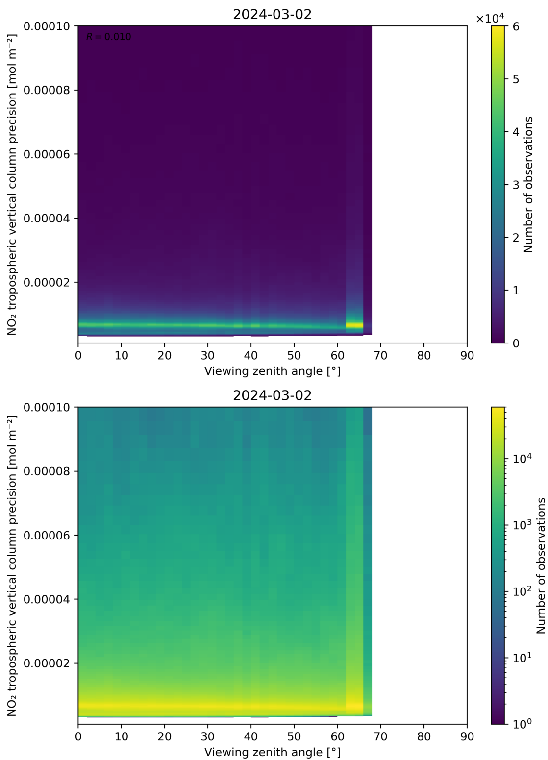
Figure 170: Scatter density plot of “Viewing zenith angle” against “NO 2 tropospheric vertical column precision” for 2024-03-01 to 2024-03-03.
