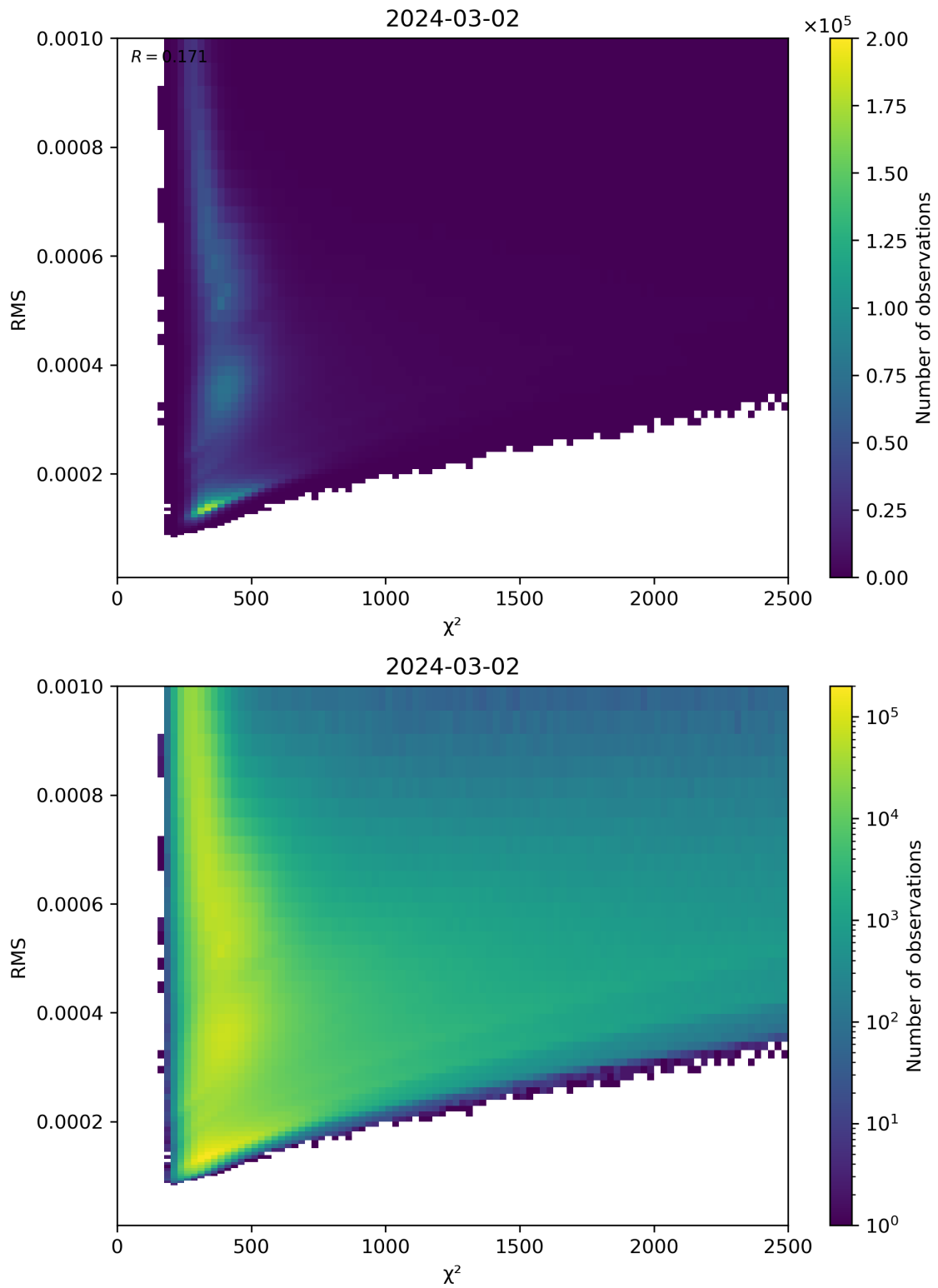
Figure 82: Scatter density plot of “ \chi^2 ” against “RMS” for 2024-03-01 to 2024-03-03.
