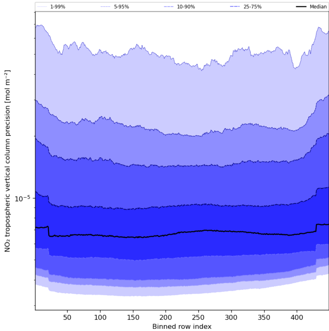
Figure 47: Along track statistics of “NO 2 tropospheric vertical column precision” for 2024-03-01 to 2024-03-03
