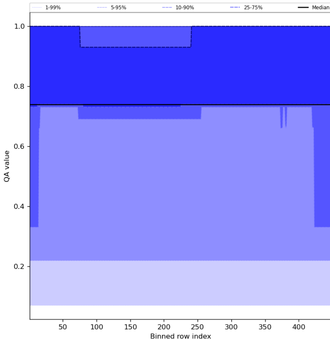
Figure 45: Along track statistics of “QA value” for 2024-03-01 to 2024-03-03
