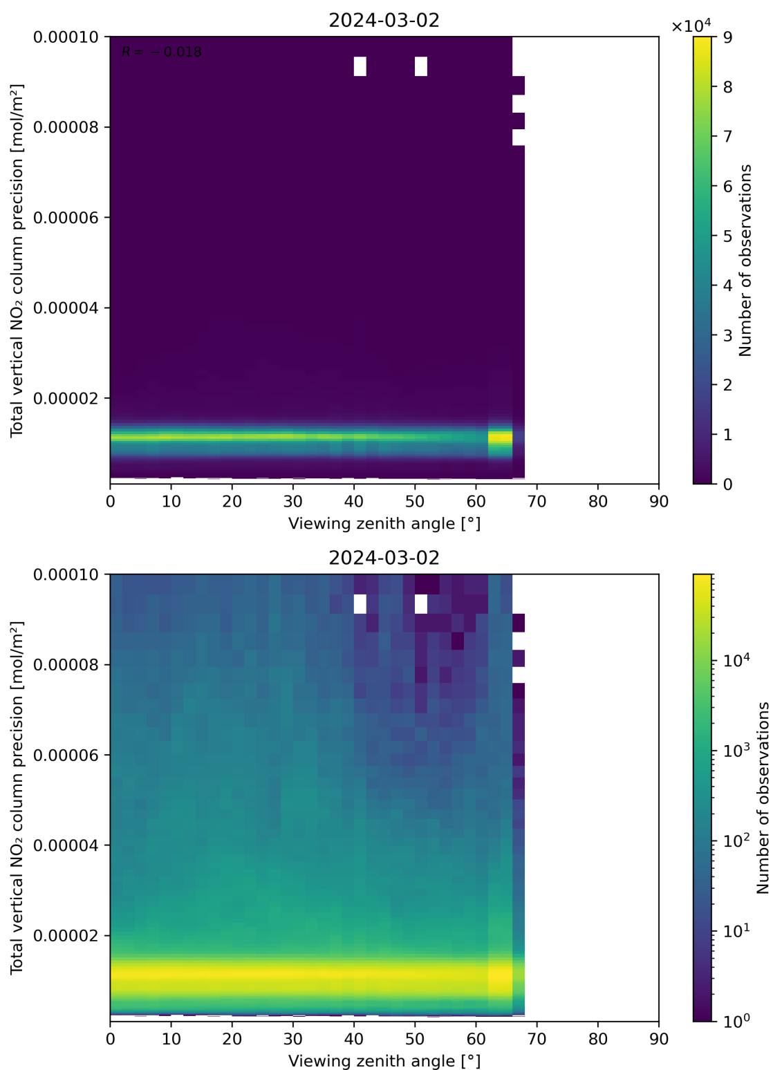
Figure 168: Scatter density plot of “Viewing zenith angle” against “Total vertical NO 2 column precision” for 2024-03-01 to 2024-03-03.
