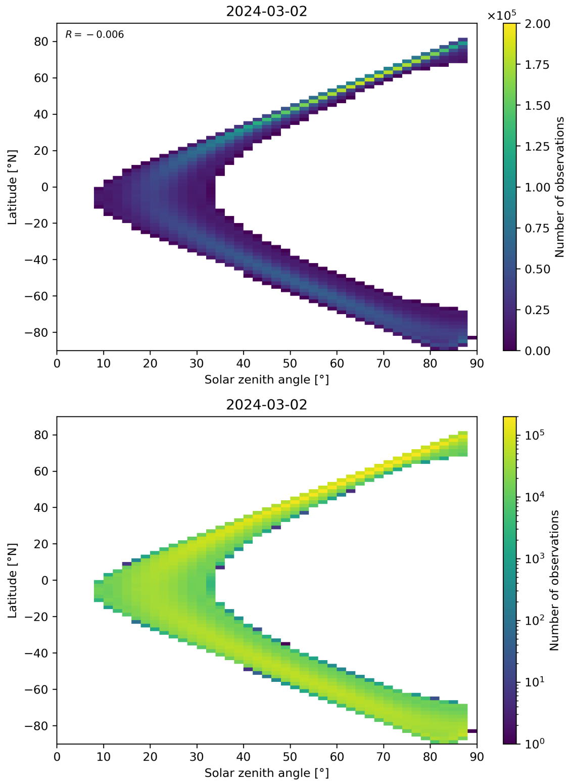
Figure 149: Scatter density plot of “Solar zenith angle” against “Latitude” for 2024-03-01 to 2024-03-03.
