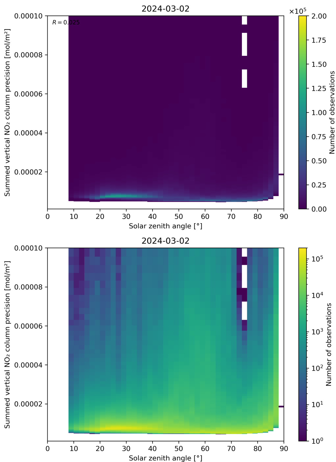
Figure 152: Scatter density plot of “Solar zenith angle” against “Summed vertical NO 2 column precision” for 2024-03-01 to 2024-03-03.
