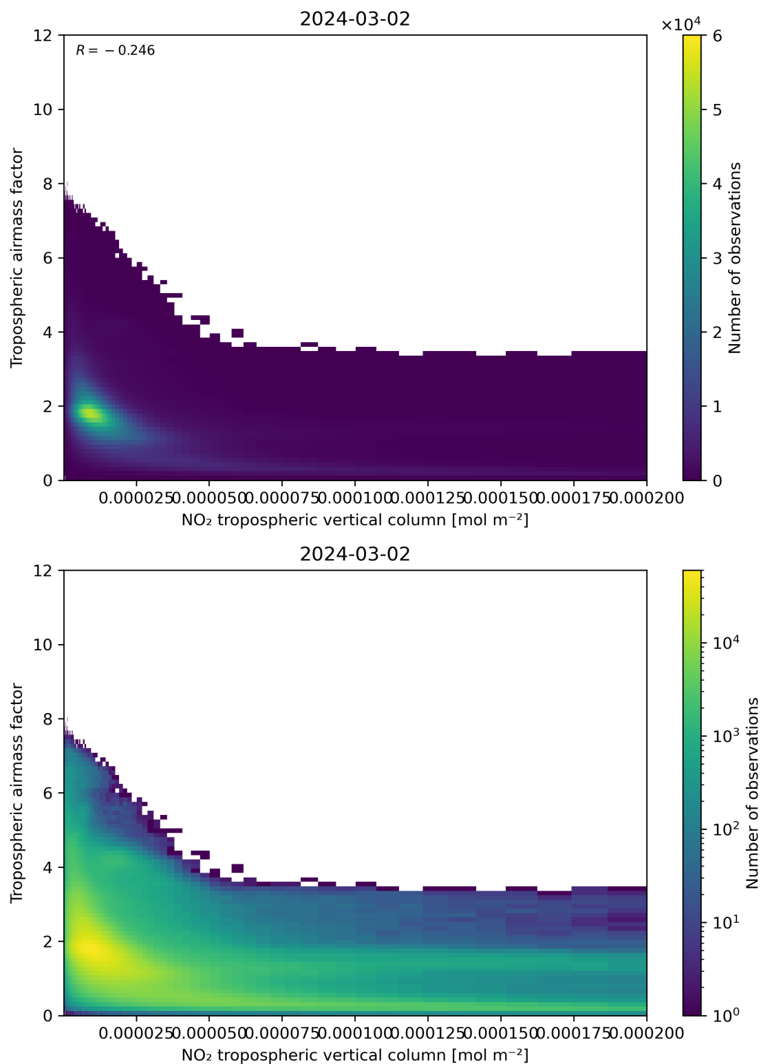
Figure 123: Scatter density plot of “NO 2 tropospheric vertical column” against “Tropospheric airmass factor” for 2024-03-01 to 2024-03-03.
