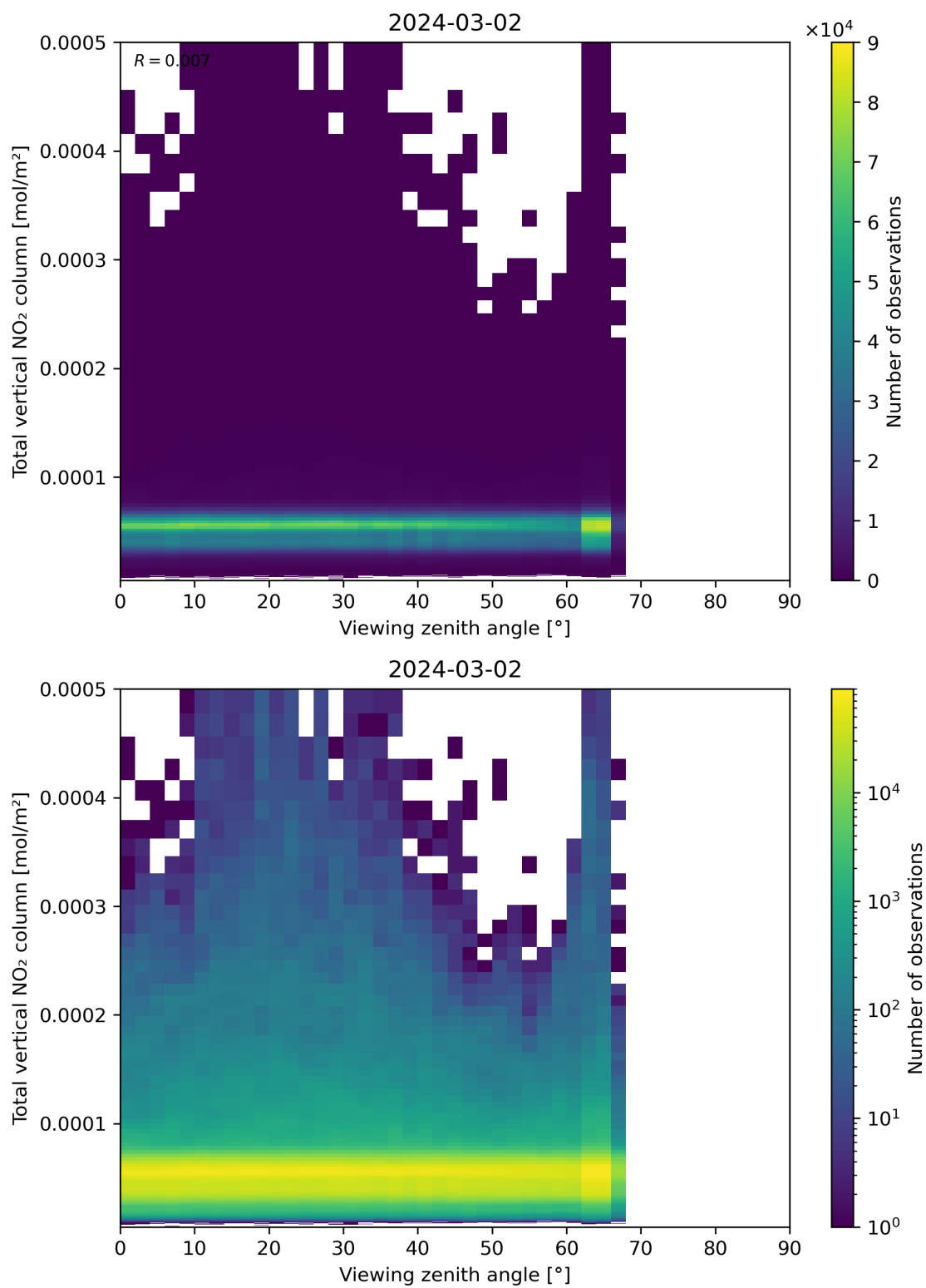
Figure 167: Scatter density plot of “Viewing zenith angle” against “Total vertical NO 2 column” for 2024-03-01 to 2024-03-03.
