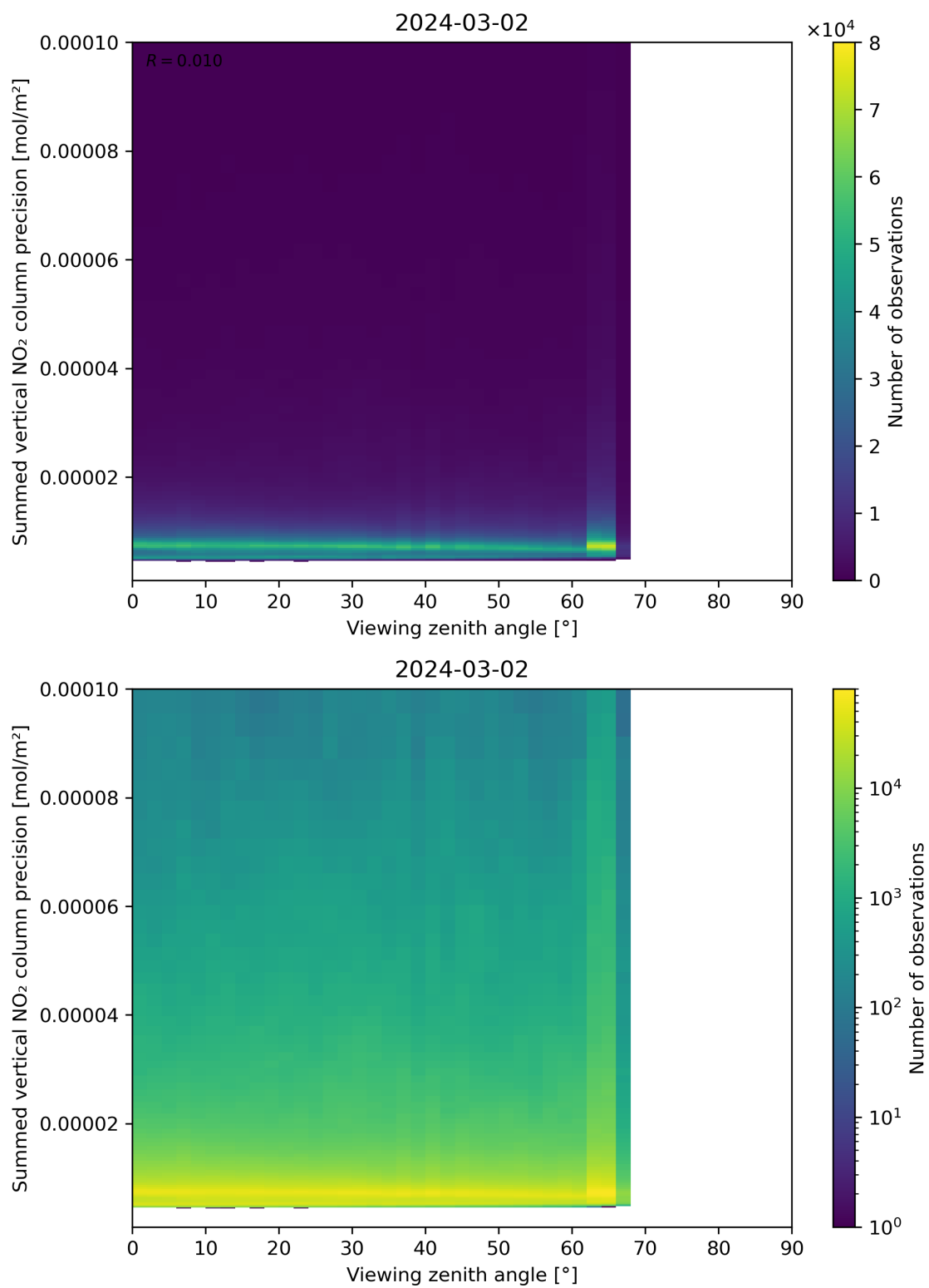
Figure 166: Scatter density plot of “Viewing zenith angle” against “Summed vertical NO 2 column precision” for 2024-03-01 to 2024-03-03.
