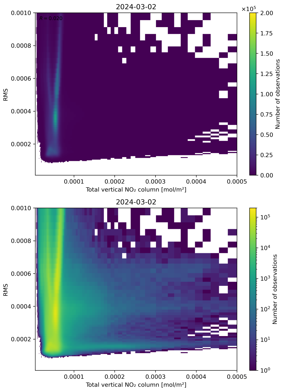
Figure 120: Scatter density plot of “Total vertical NO 2 column” against “RMS” for 2024-03-01 to 2024-03-03.
