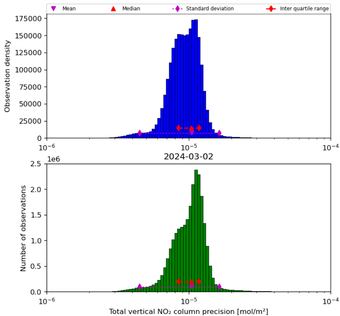
Figure 39: Histogram of “Total vertical NO 2 column precision” for 2024-03-01 to 2024-03-03
