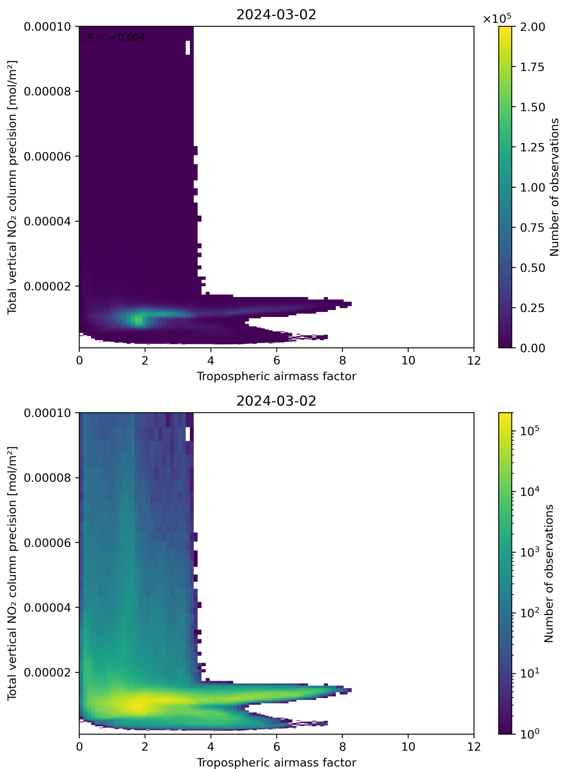
Figure 78: Scatter density plot of “Tropospheric air mass factor” against “Total vertical NO 2 column precision” for 2024-03-01 to 2024-03-03.
