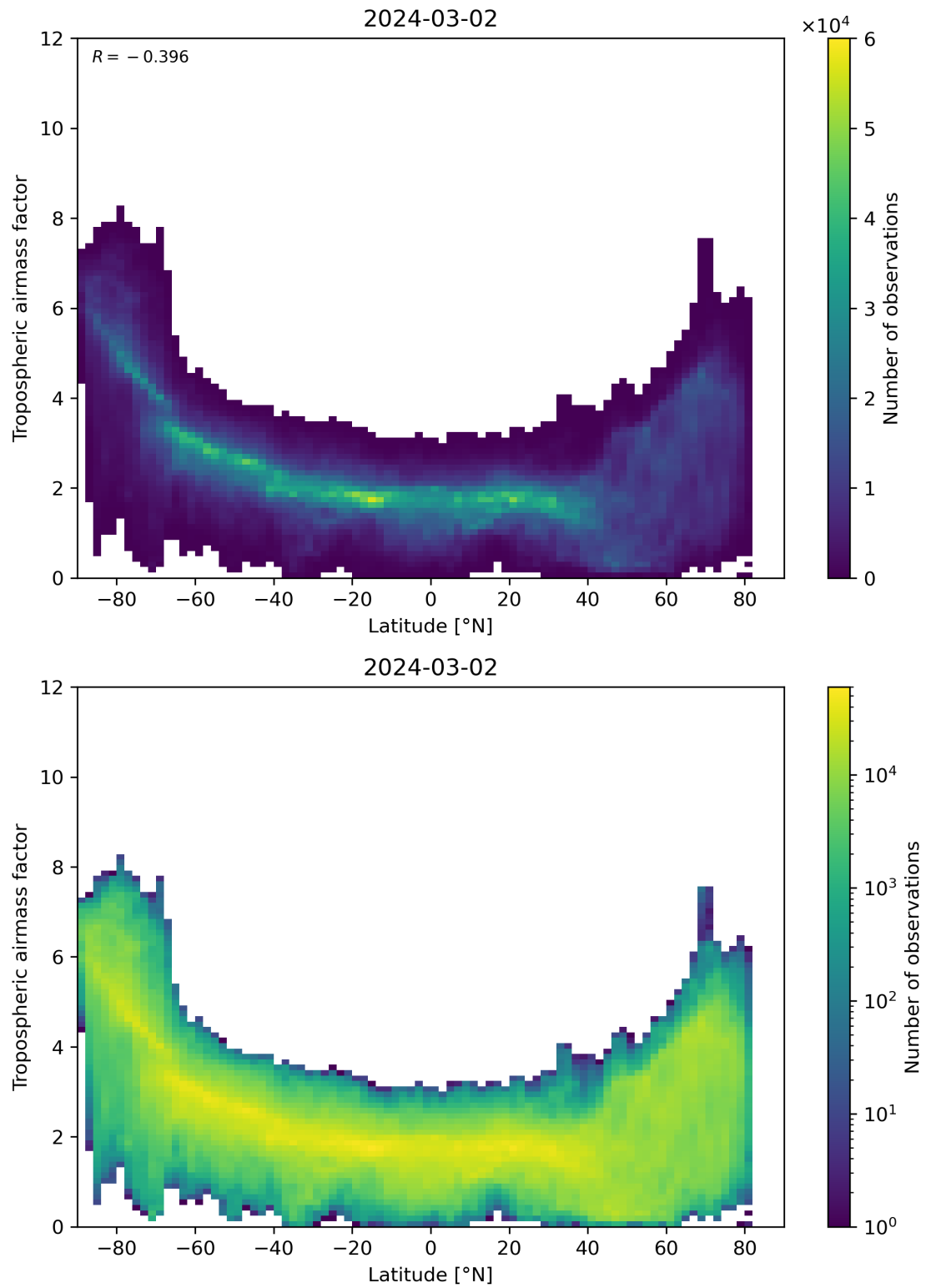
Figure 85: Scatter density plot of “Latitude” against “Tropospheric airmass factor” for 2024-03-01 to 2024-03-03.
