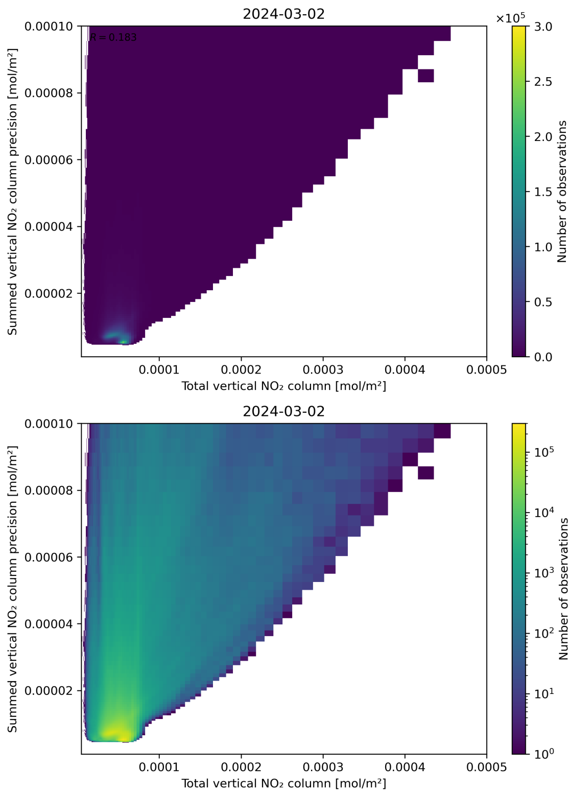
Figure 113: Scatter density plot of “Total vertical NO 2 column” against “Summed vertical NO 2 column precision” for 2024-03-01 to 2024-03-03.
