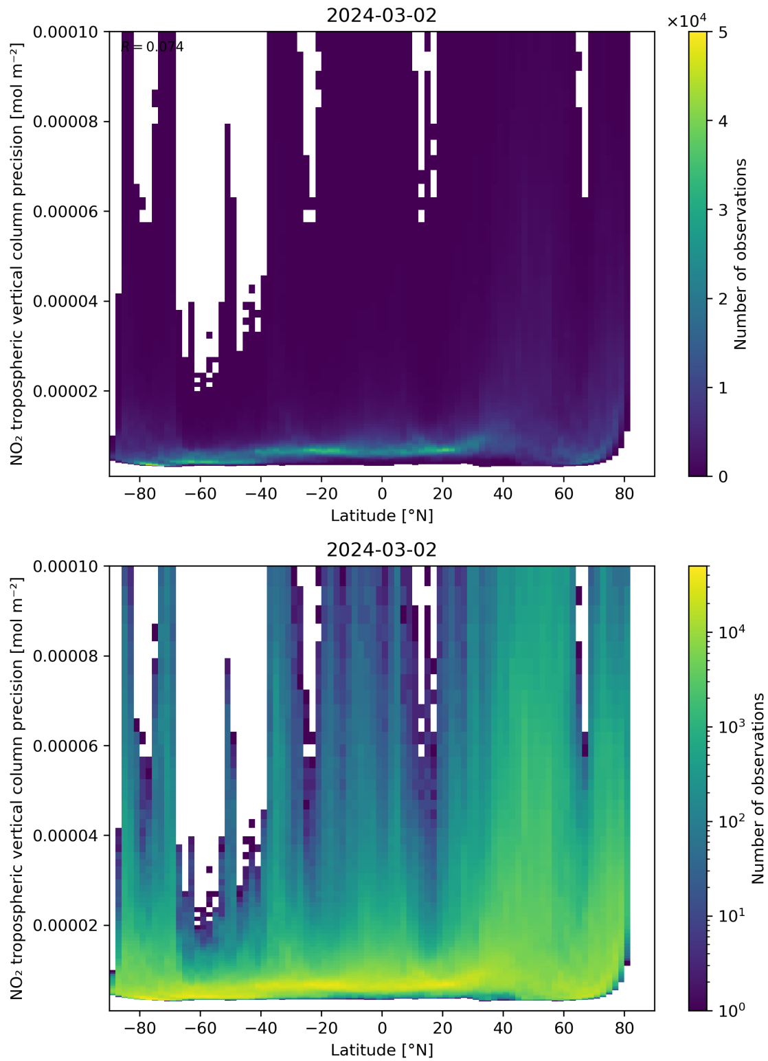
Figure 93: Scatter density plot of “Latitude” against “NO 2 tropospheric vertical column precision” for 2024-03-01 to 2024-03-03.
