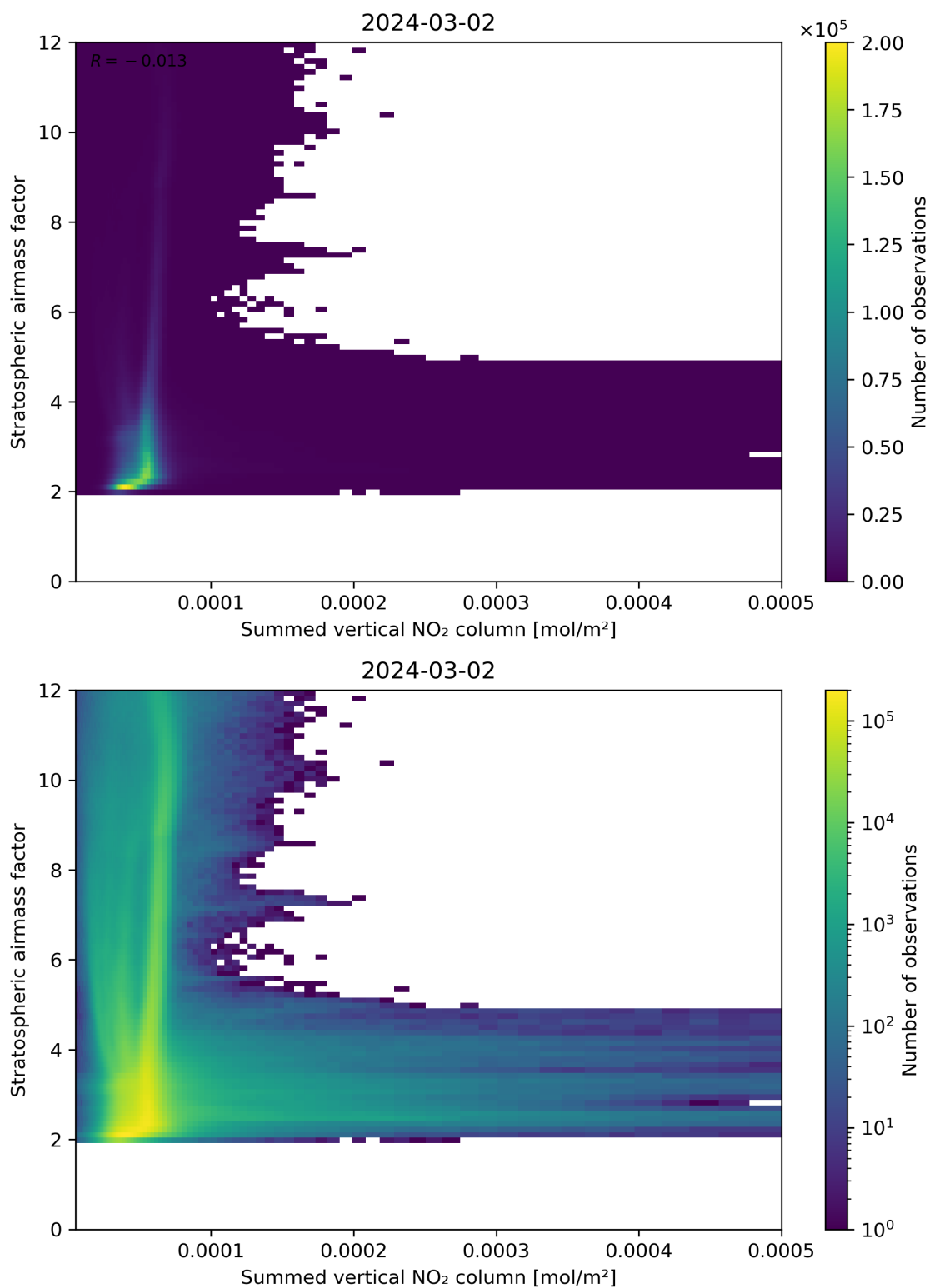
Figure 103: Scatter density plot of “Summed vertical NO 2 column” against “Stratospheric airmass factor” for 2024-03-01 to 2024-03-03.
