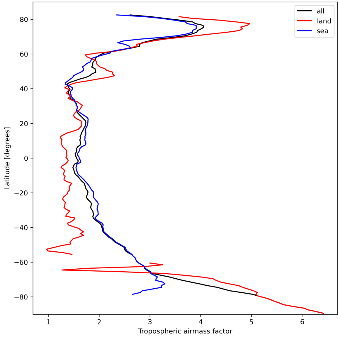
Figure 14: Zonal average of “Tropospheric airmass factor” for 2024-03-04 to 2024-03-05.
