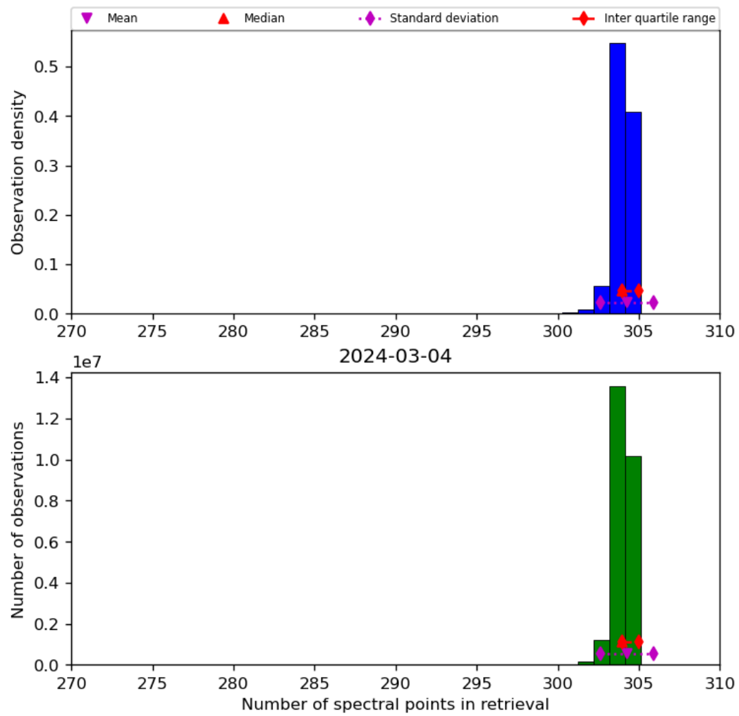
Figure 33: Histogram of “Number of spectral points in retrieval” for 2024-03-04 to 2024-03-05
