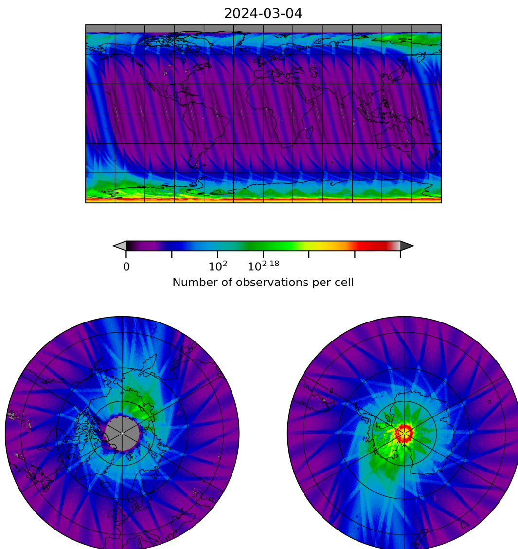
Figure 10: Map of the number of observations for 2024-03-04 to 2024-03-05
