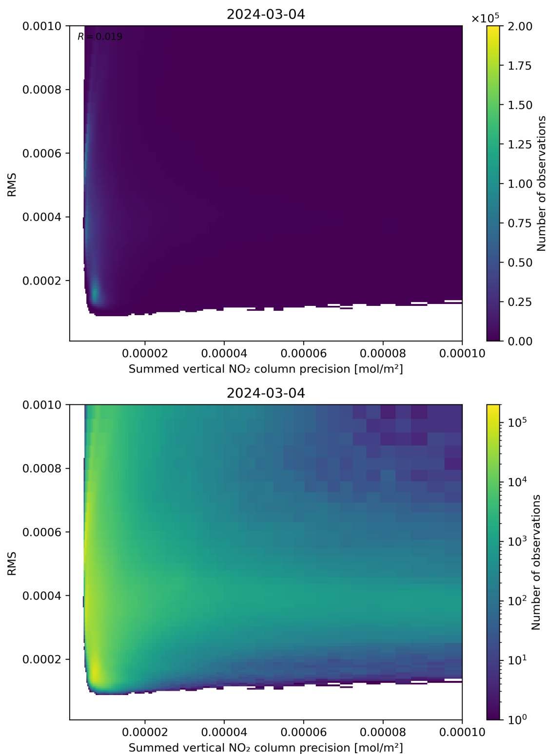
Figure 108: Scatter density plot of “Summed vertical NO 2 column precision” against “RMS” for 2024-03-04 to 2024-03-05.
