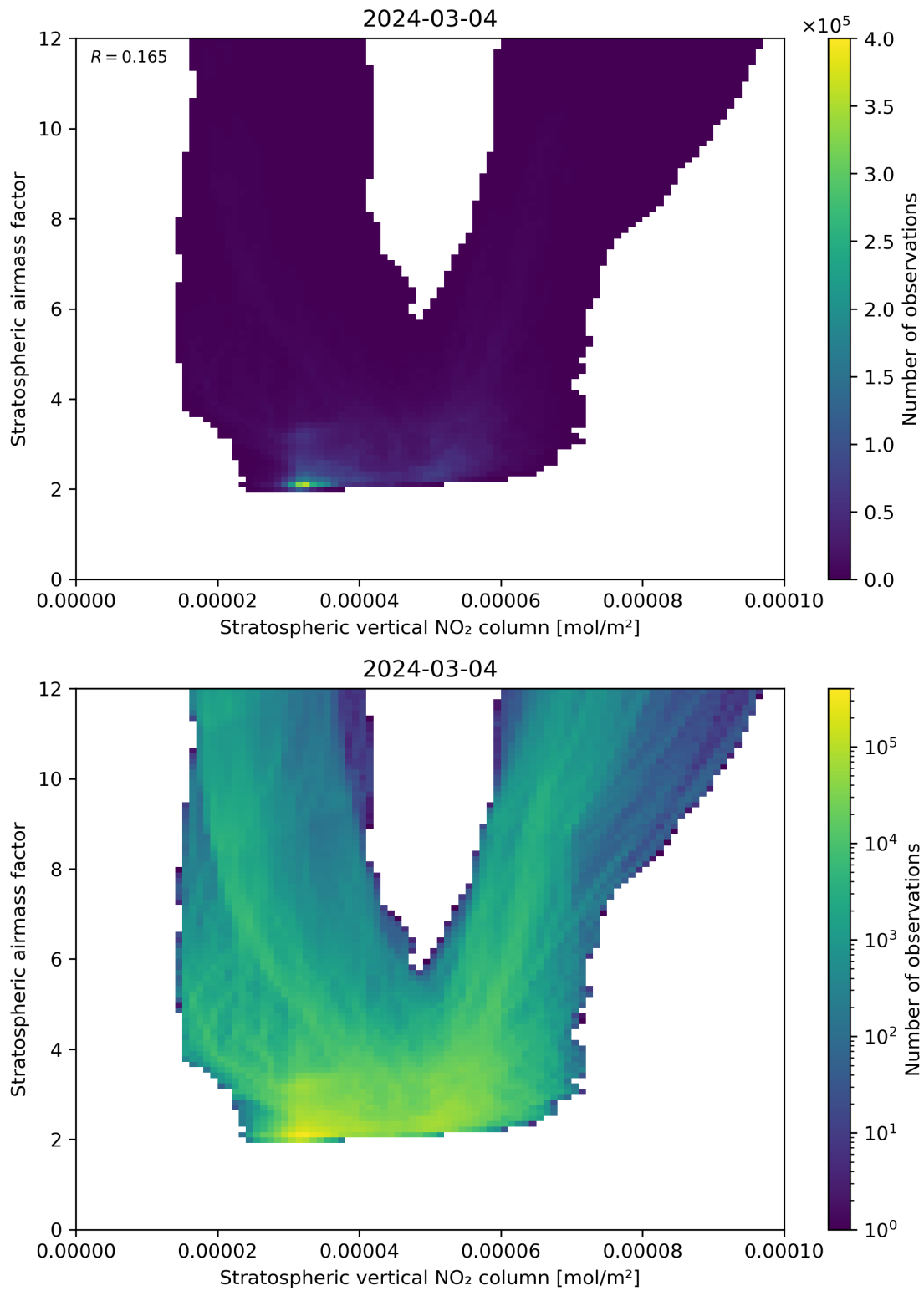
Figure 96: Scatter density plot of “Stratospheric vertical NO 2 column” against “Stratospheric airmass factor” for 2024-03-04 to 2024-03-05.
