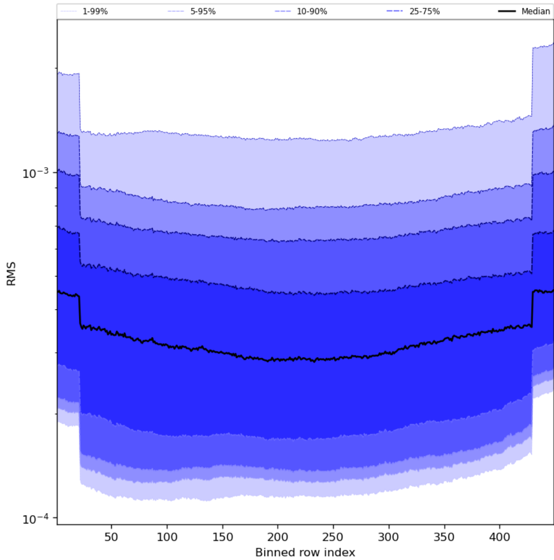
Figure 60: Along track statistics of “RMS” for 2024-03-04 to 2024-03-05
