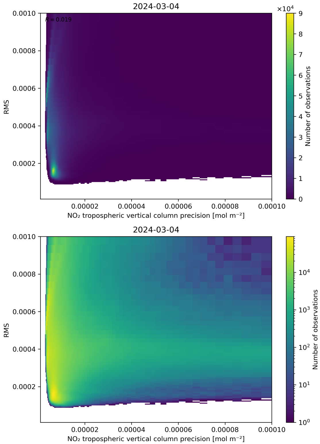
Figure 140: Scatter density plot of “NO 2 tropospheric vertical column precision” against “RMS” for 2024-03-04 to 2024-03-05.
