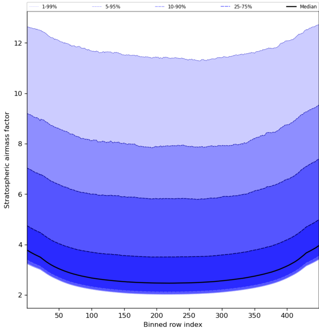
Figure 61: Along track statistics of “Stratospheric airmass factor” for 2024-03-04 to 2024-03-05
