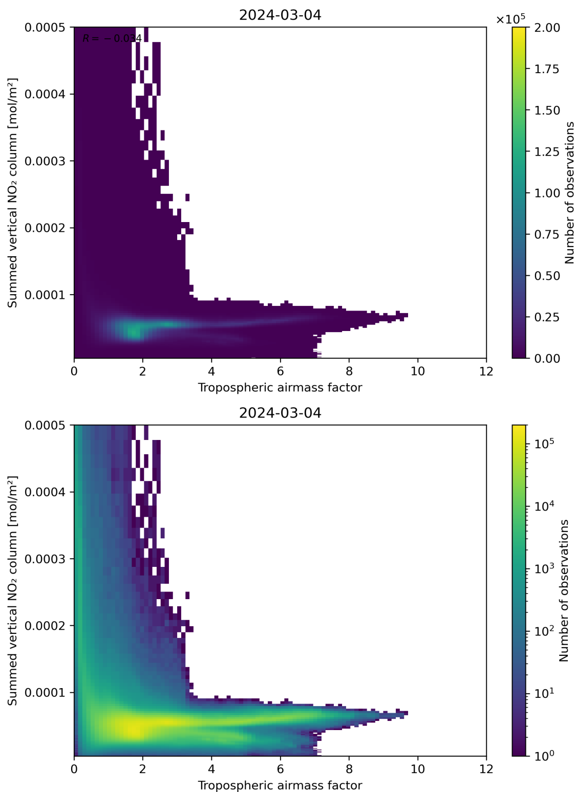
Figure 75: Scatter density plot of “Tropospheric air mass factor” against “Summed vertical NO 2 column” for 2024-03-04 to 2024-03-05.
