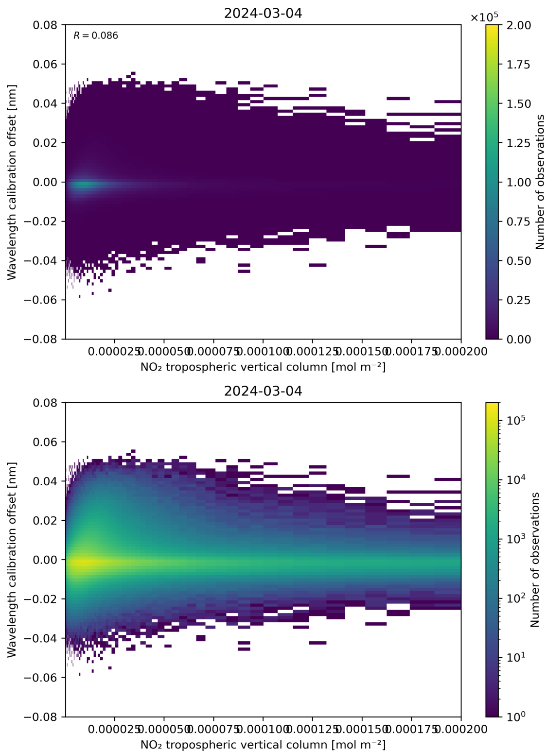
Figure 143: Scatter density plot of “NO 2 tropospheric vertical column” against “Wavelength calibration offset” for 2024-03-04 to 2024-03-05.
