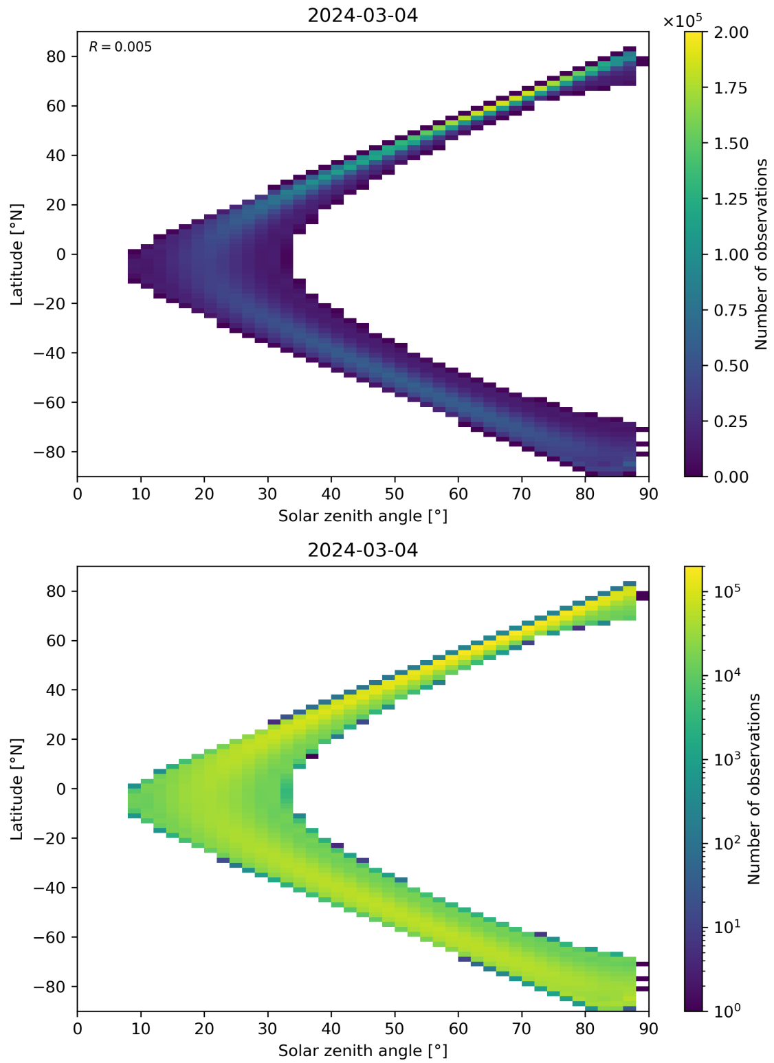
Figure 149: Scatter density plot of “Solar zenith angle” against “Latitude” for 2024-03-04 to 2024-03-05.
