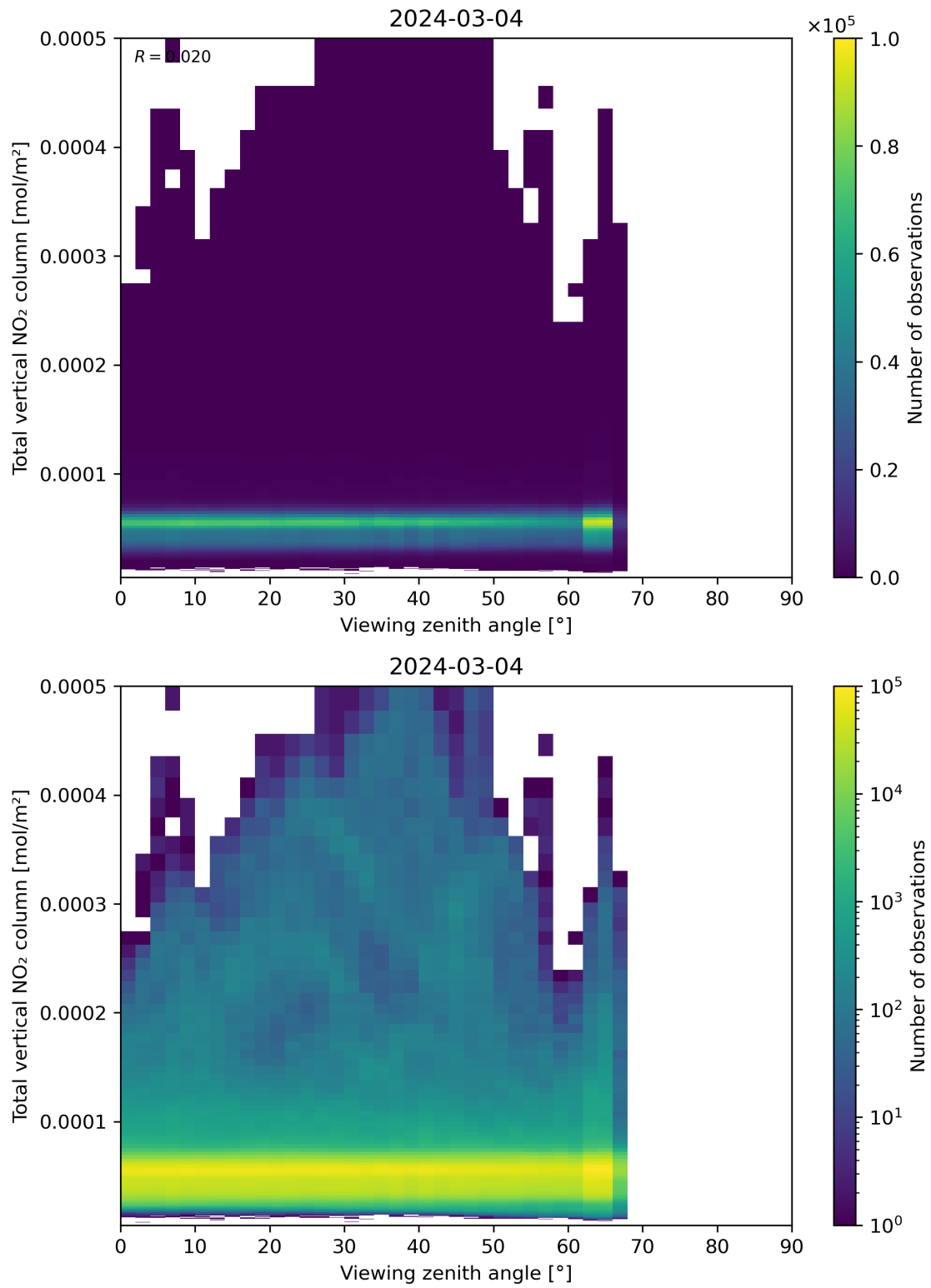
Figure 167: Scatter density plot of “Viewing zenith angle” against “Total vertical NO 2 column” for 2024-03-04 to 2024-03-05.
