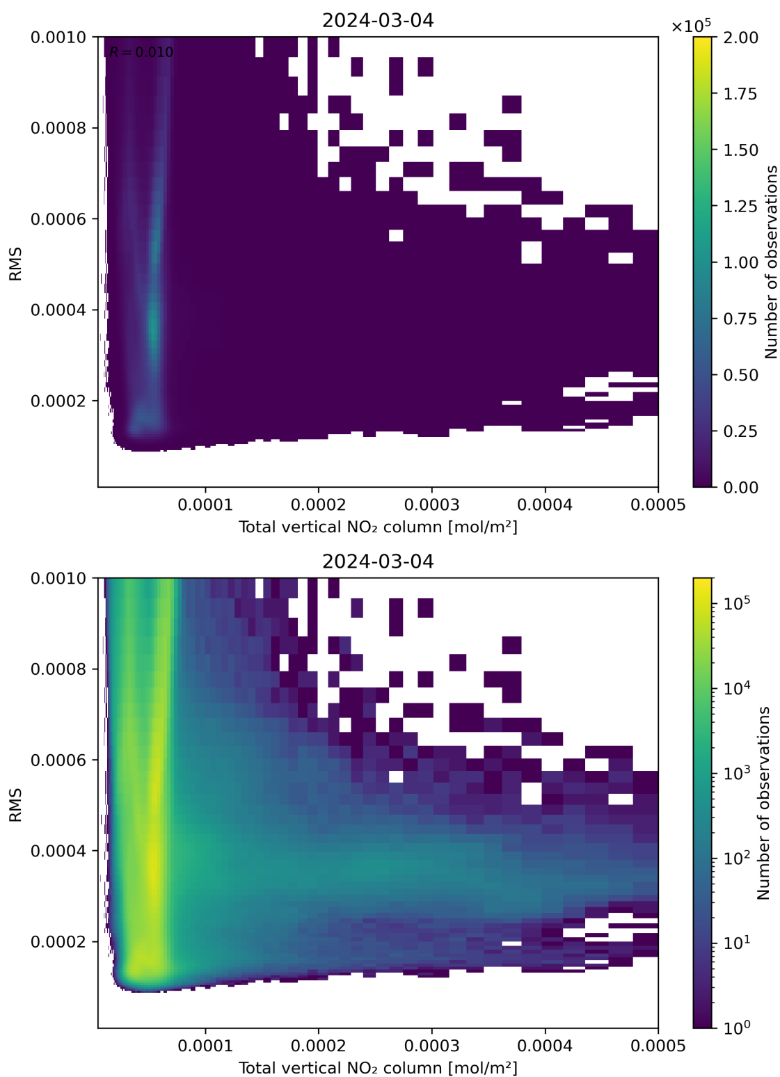
Figure 120: Scatter density plot of “Total vertical NO 2 column” against “RMS” for 2024-03-04 to 2024-03-05.
