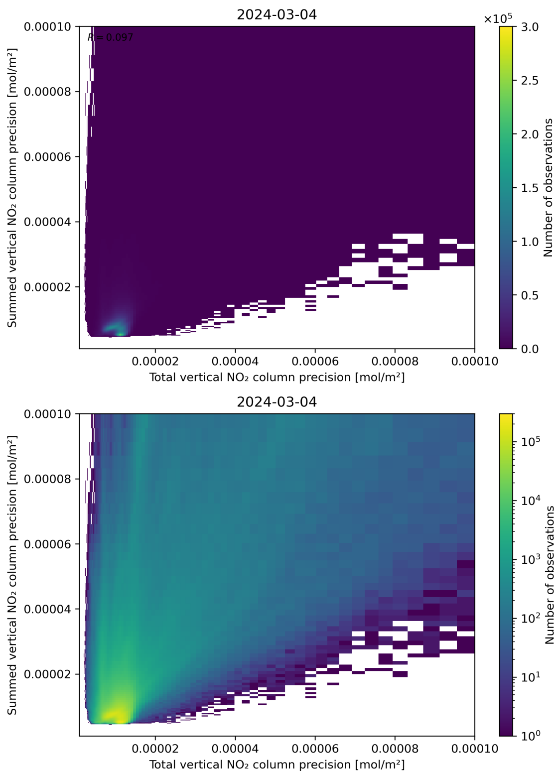
Figure 118: Scatter density plot of “Total vertical NO 2 column precision” against “Summed vertical NO 2 column precision” for 2024-03-04 to 2024-03-05.
