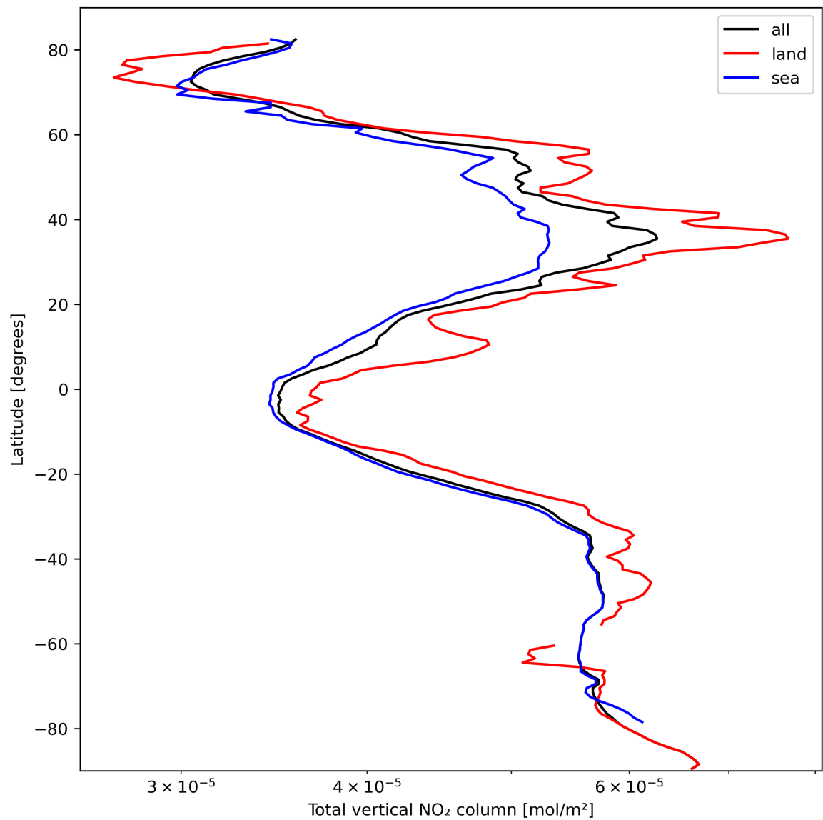
Figure 21: Zonal average of “Total vertical NO 2 column” for 2024-03-04 to 2024-03-05.
