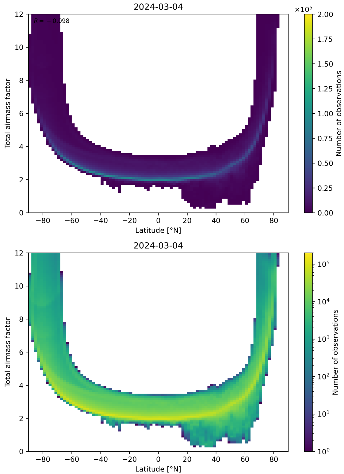
Figure 84: Scatter density plot of “Latitude” against “Total airmass factor” for 2024-03-04 to 2024-03-05.
