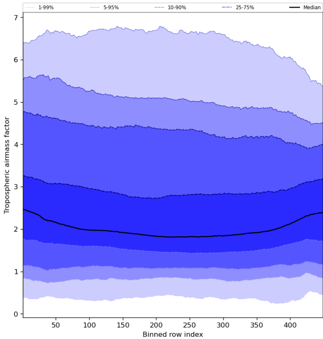
Figure 48: Along track statistics of “Tropospheric air mass factor” for 2024-03-04 to 2024-03-05
