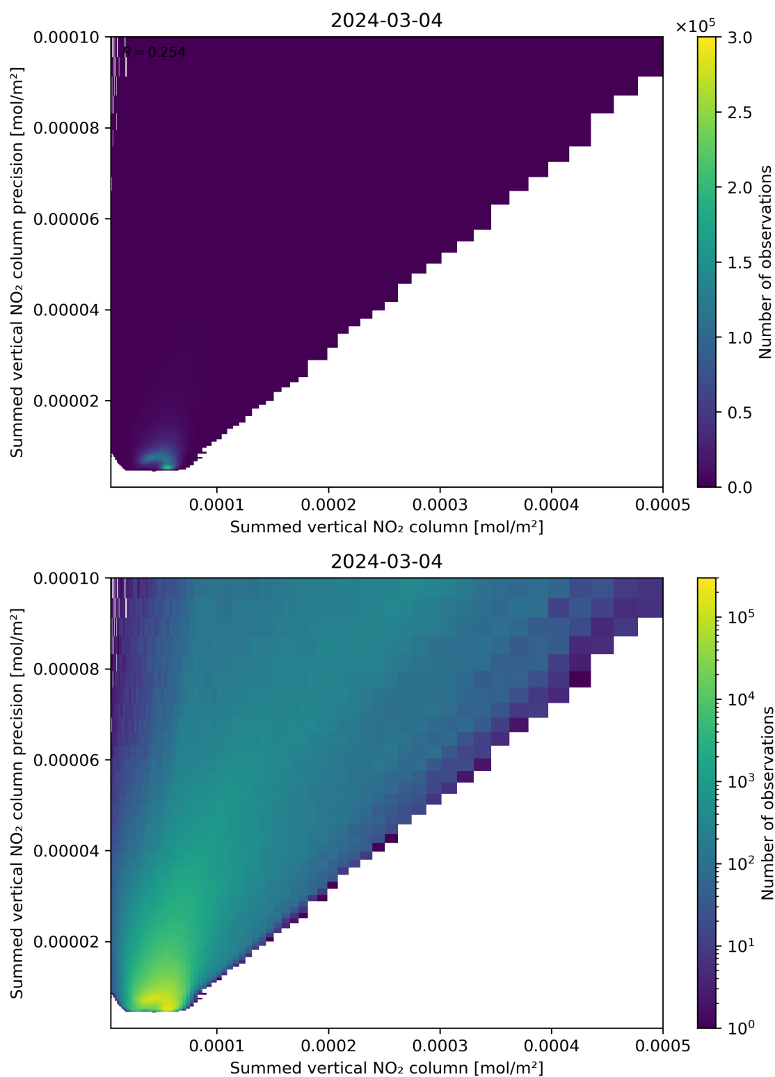
Figure 105: Scatter density plot of “Summed vertical NO 2 column” against “Summed vertical NO 2 column precision” for 2024-03-04 to 2024-03-05.
