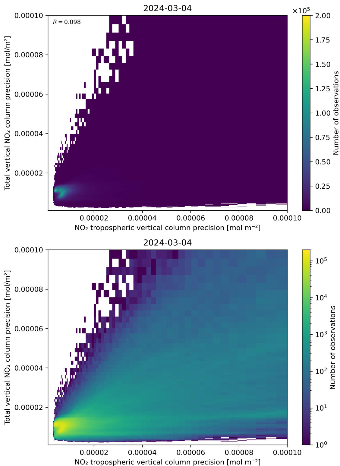
Figure 139: Scatter density plot of “NO 2 tropospheric vertical column precision” against “Total vertical NO 2 column precision” for 2024-03-04 to 2024-03-05.
