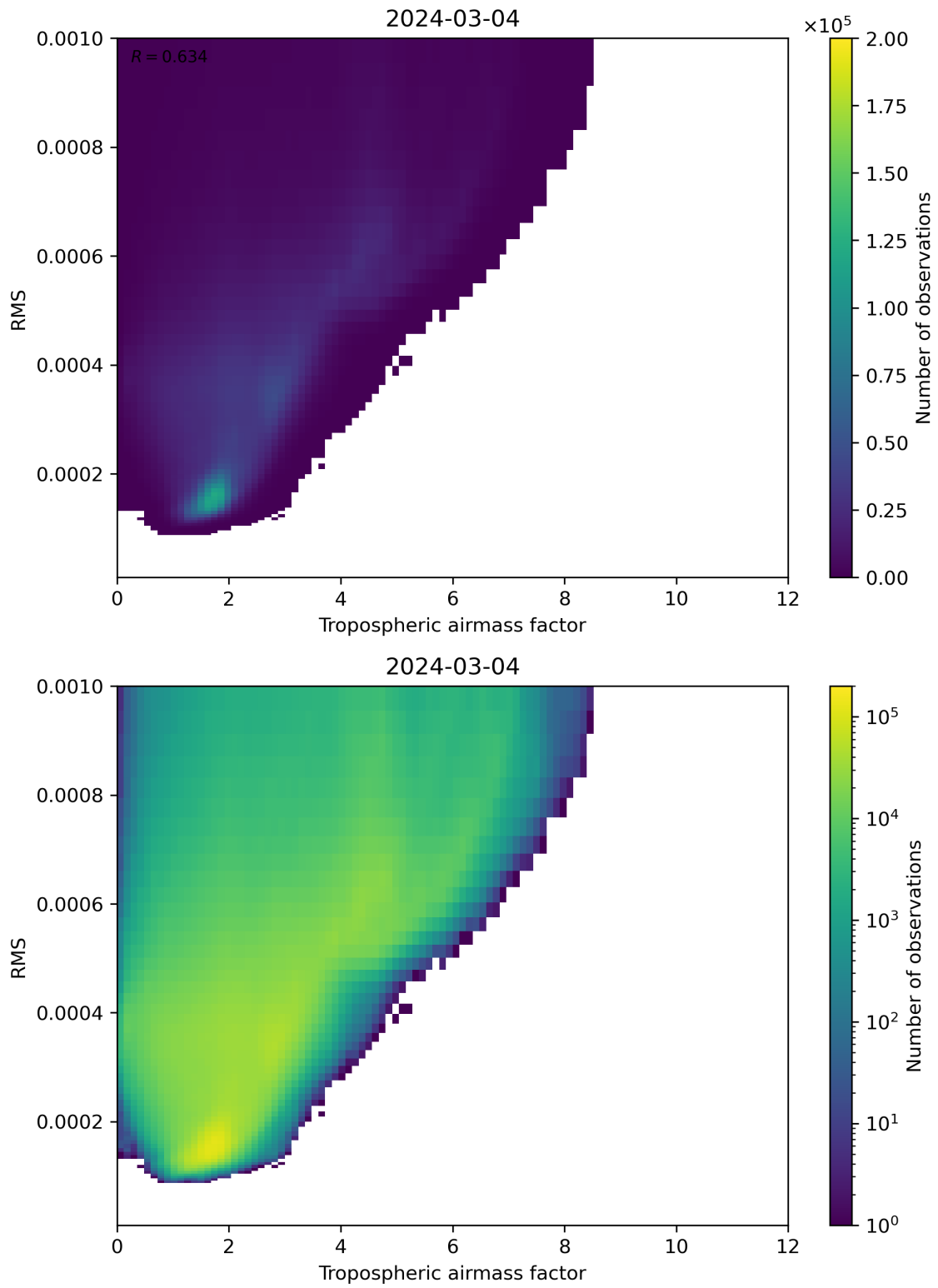
Figure 79: Scatter density plot of “Tropospheric airmass factor” against “RMS” for 2024-03-04 to 2024-03-05.
