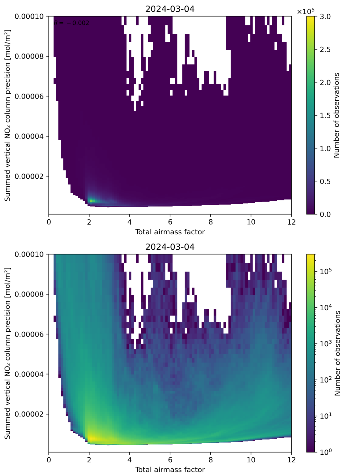
Figure 66: Scatter density plot of “Total airmass factor” against “Summed vertical NO 2 column precision” for 2024-03-04 to 2024-03-05.
