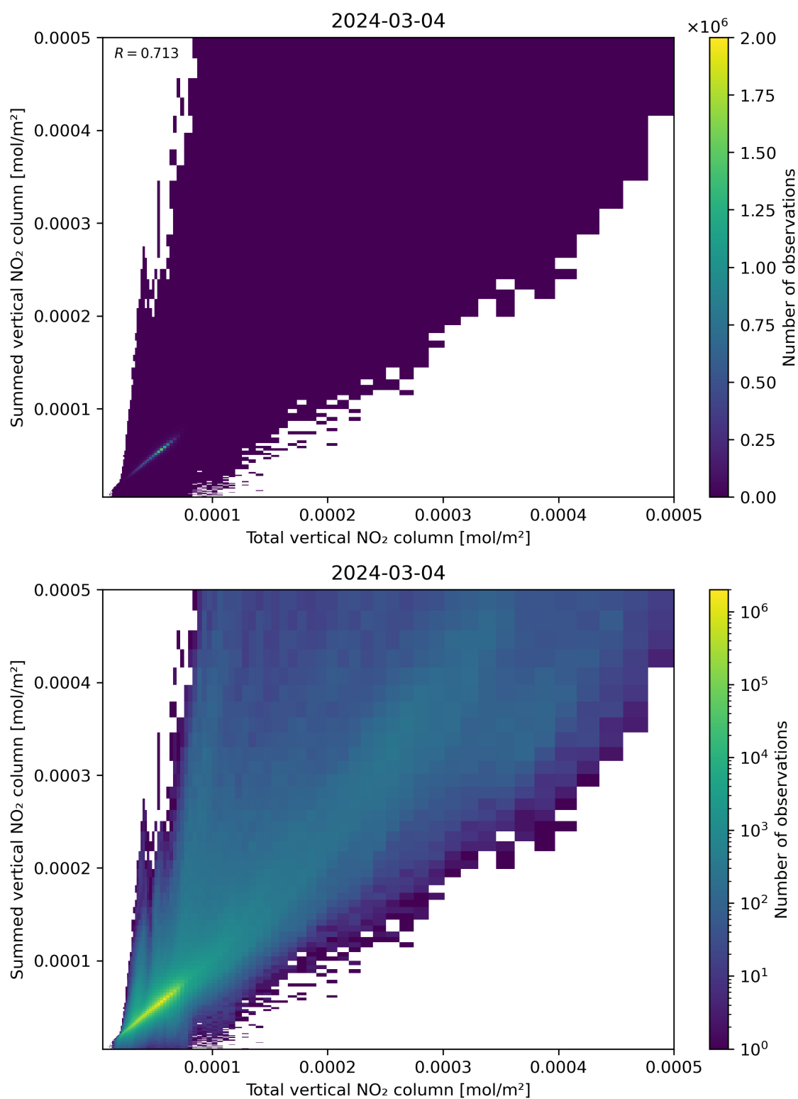
Figure 112: Scatter density plot of “Total vertical NO 2 column” against “Summed vertical NO 2 column” for 2024-03-04 to 2024-03-05.
