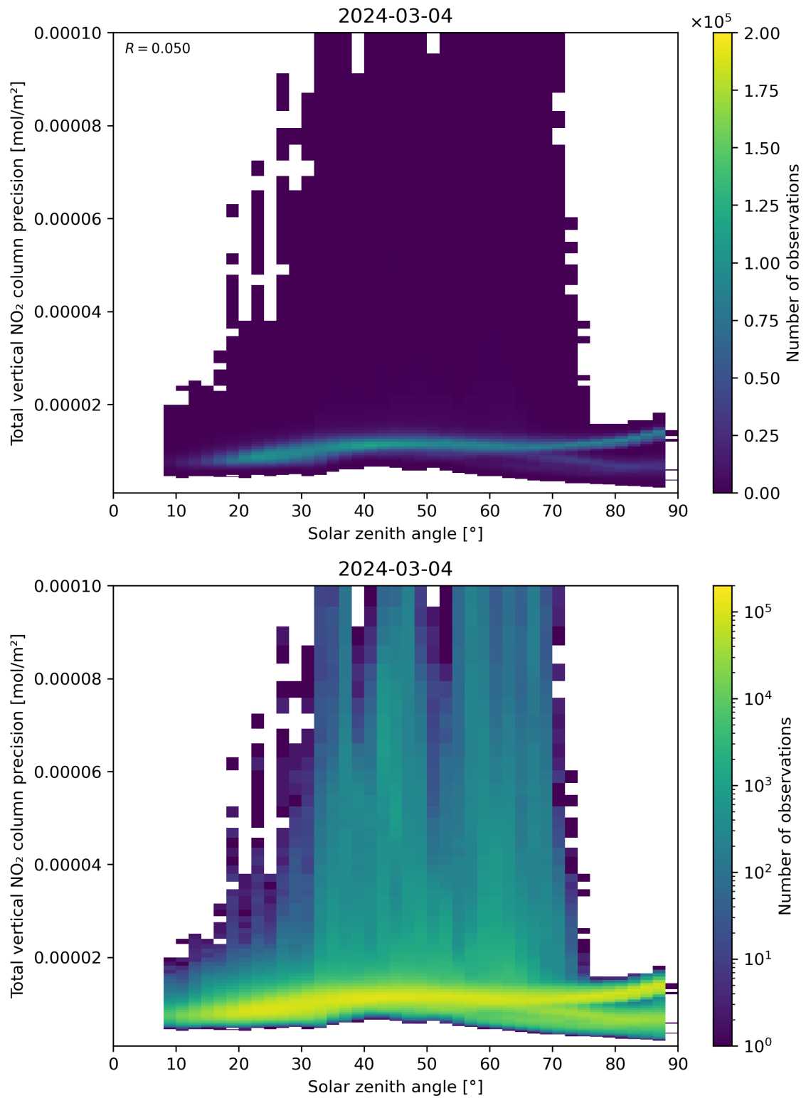
Figure 154: Scatter density plot of “Solar zenith angle” against “Total vertical NO 2 column precision” for 2024-03-04 to 2024-03-05.
