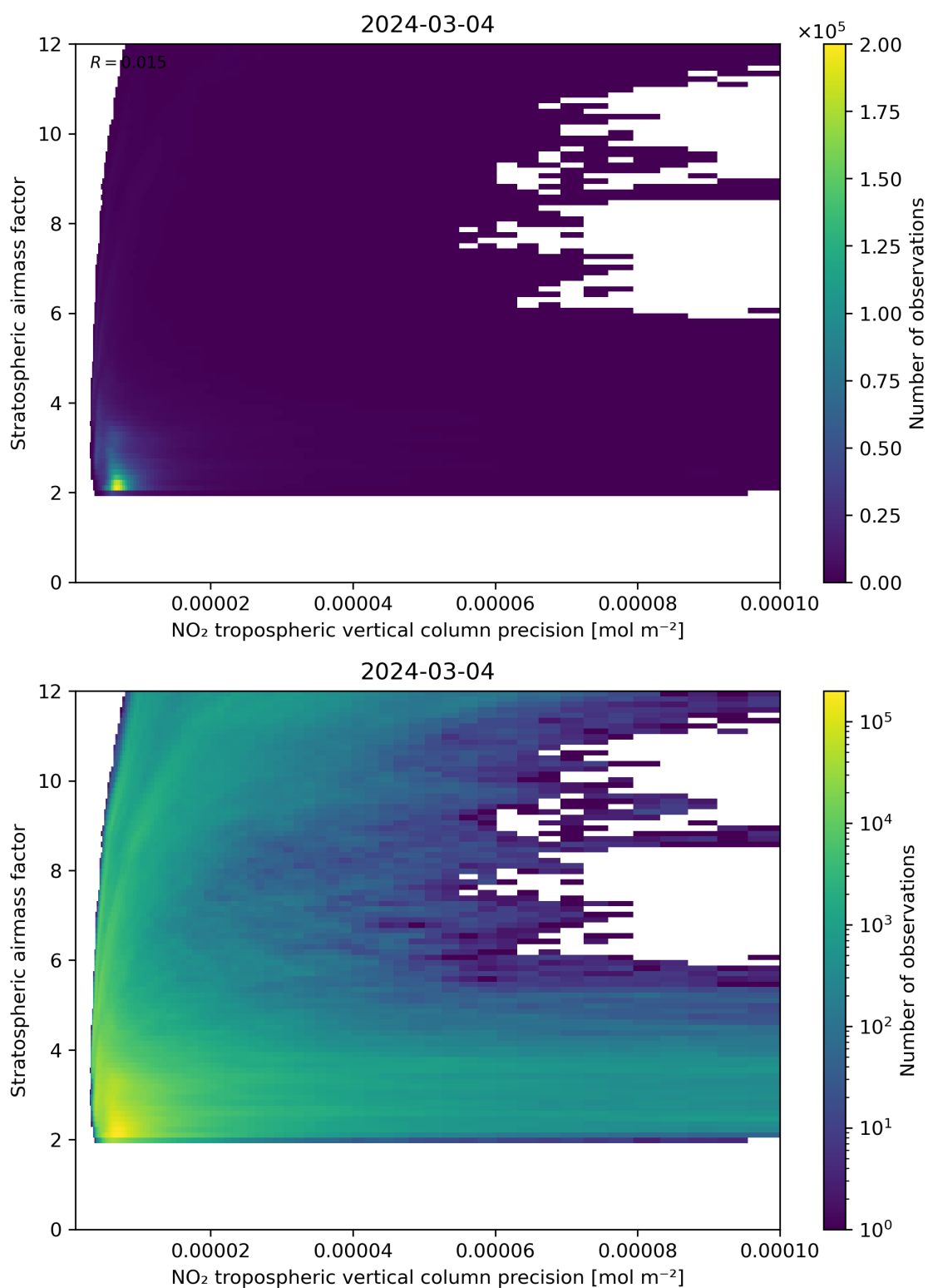
Figure 131: Scatter density plot of “NO 2 tropospheric vertical column precision” against “Stratospheric airmass factor” for 2024-03-04 to 2024-03-05.
