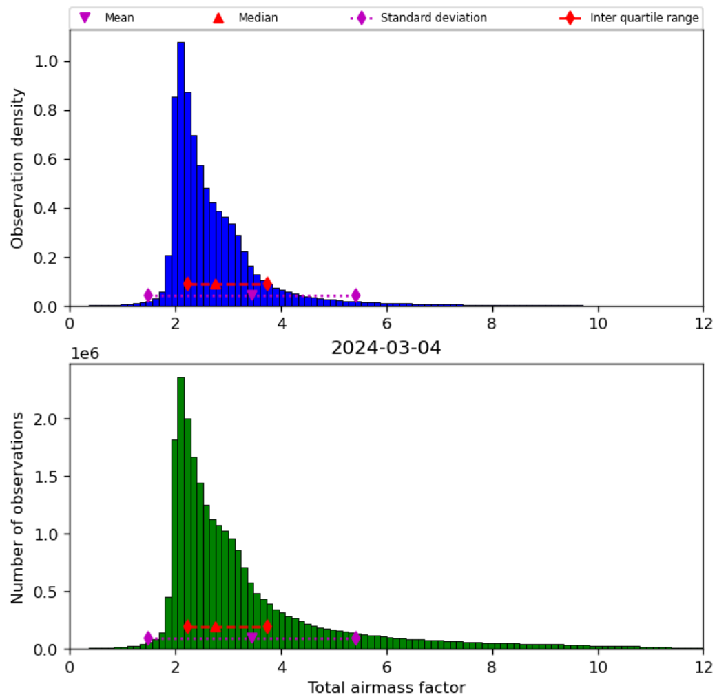
Figure 32: Histogram of “Total airmass factor” for 2024-03-04 to 2024-03-05
