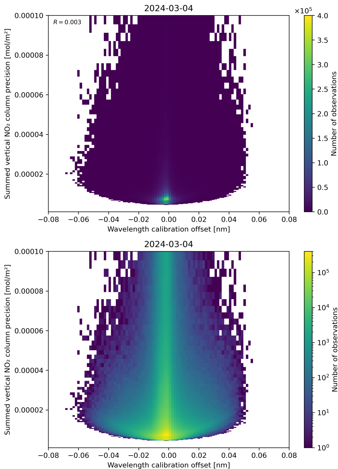
Figure 178: Scatter density plot of “Wavelength calibration offset” against “Summed vertical NO 2 column precision” for 2024-03-04 to 2024-03-05.
