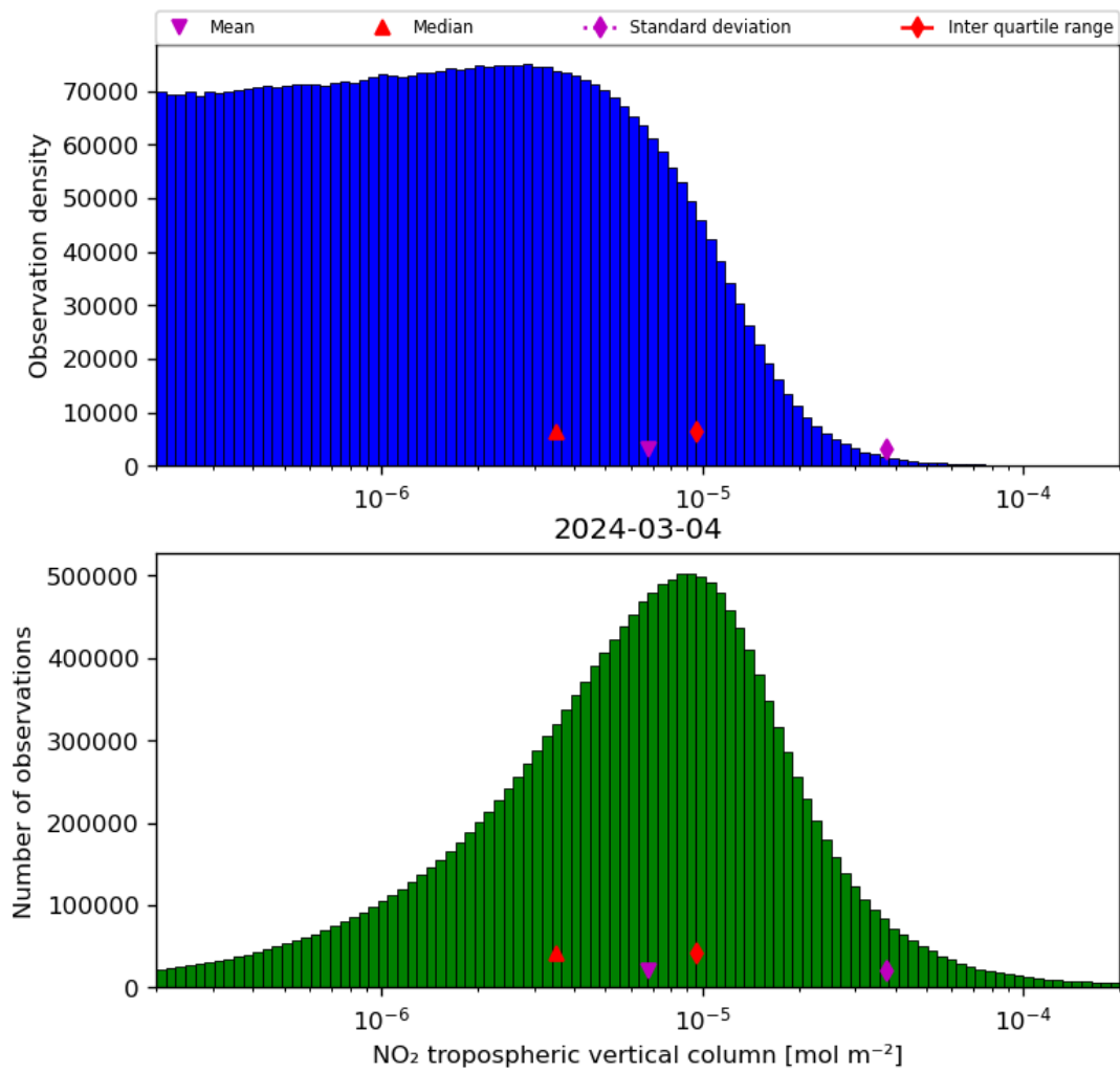
Figure 29: Histogram of “ \text{NO}_2 tropospheric vertical column” for 2024-03-04 to 2024-03-05
