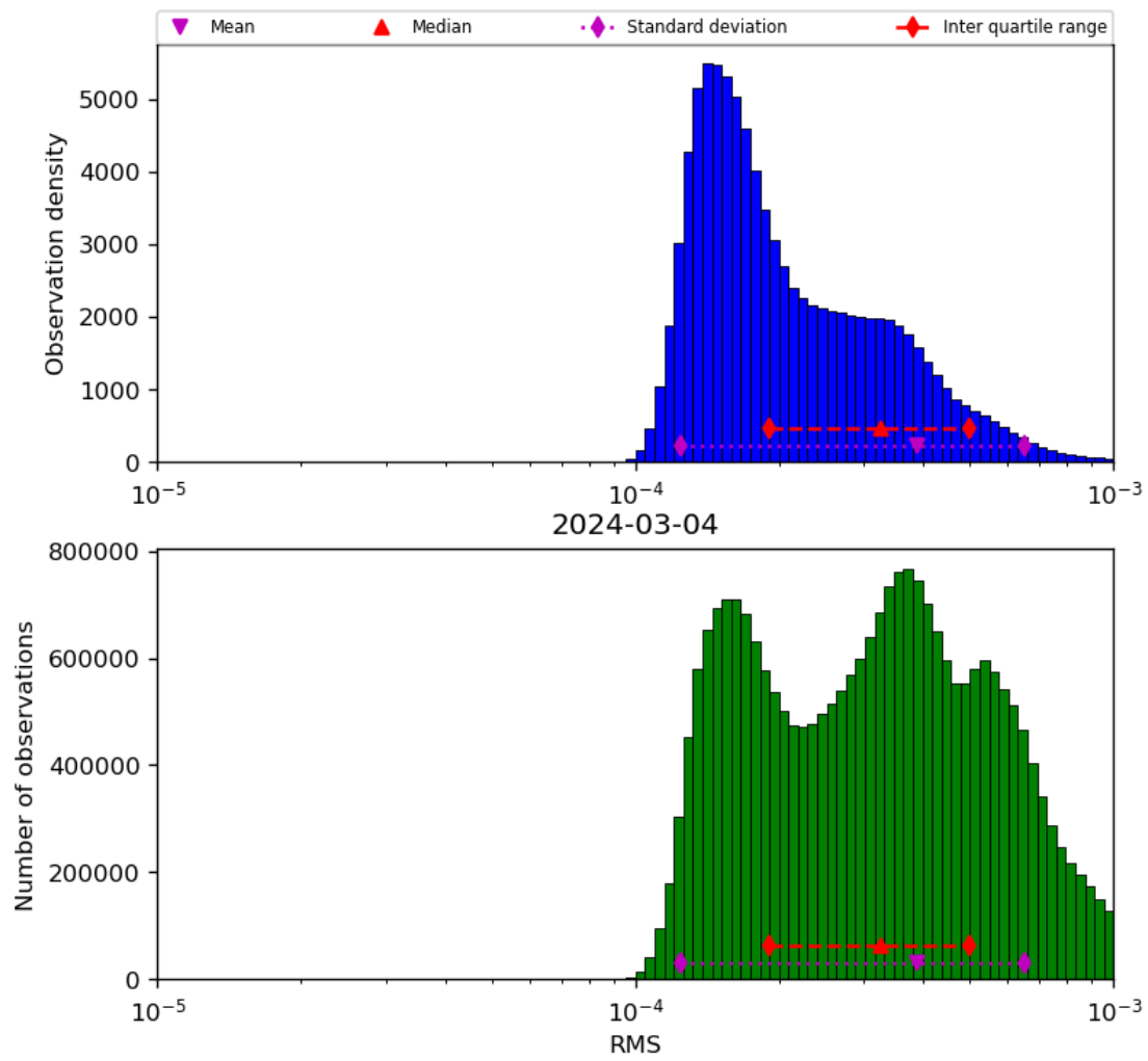
Figure 43: Histogram of “RMS” for 2024-03-04 to 2024-03-05
