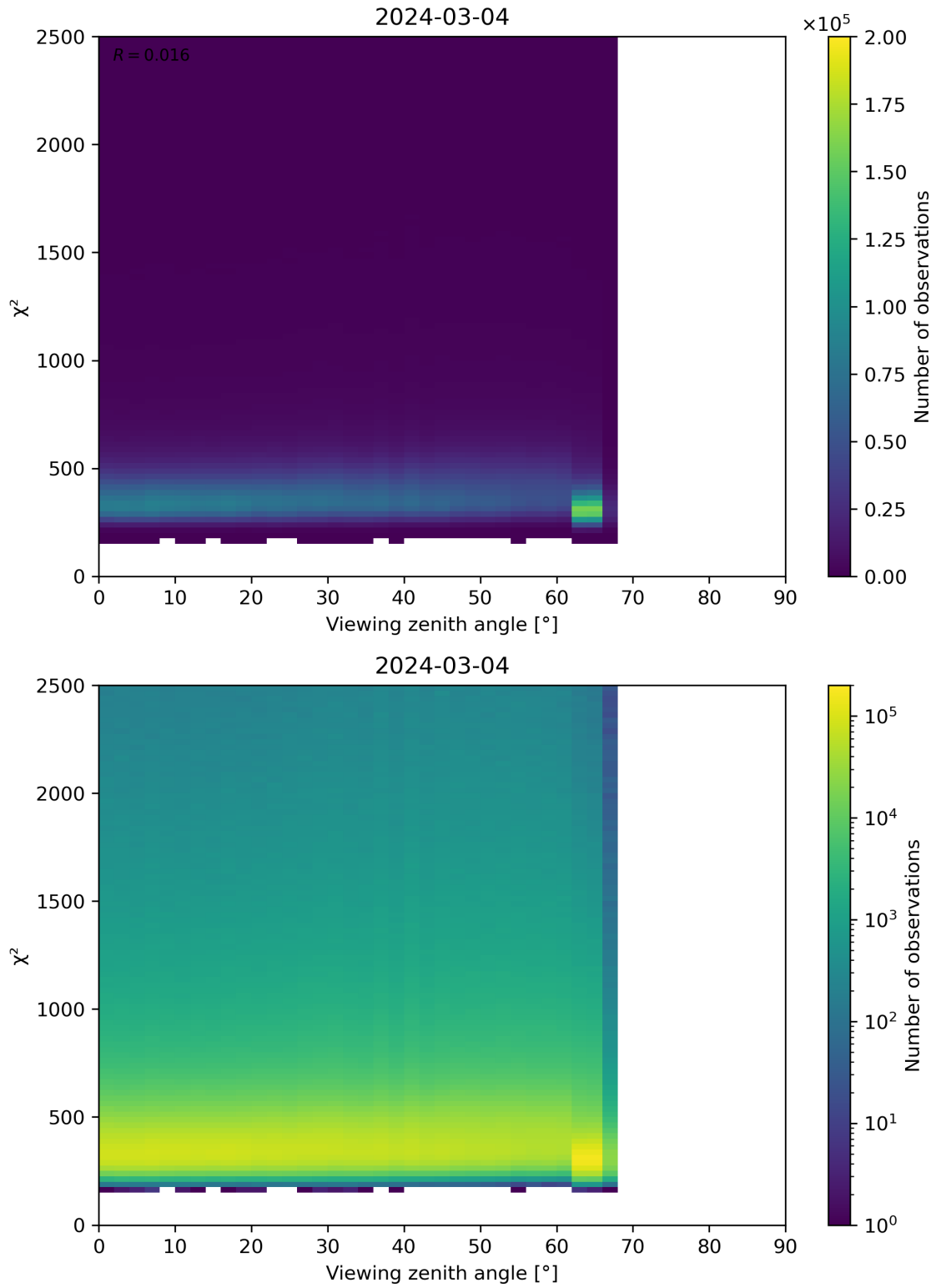
Figure 162: Scatter density plot of “Viewing zenith angle” against “ \chi^2 ” for 2024-03-04 to 2024-03-05.
