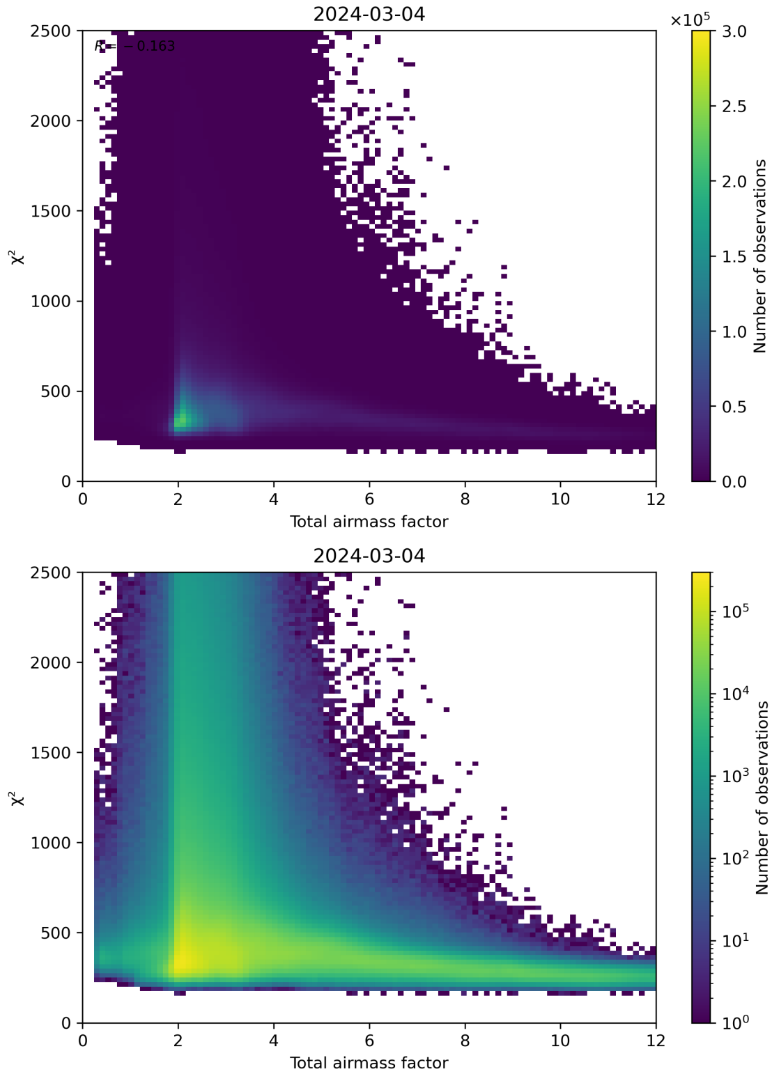
Figure 63: Scatter density plot of “Total airmass factor” against “ \chi^2 ” for 2024-03-04 to 2024-03-05.
