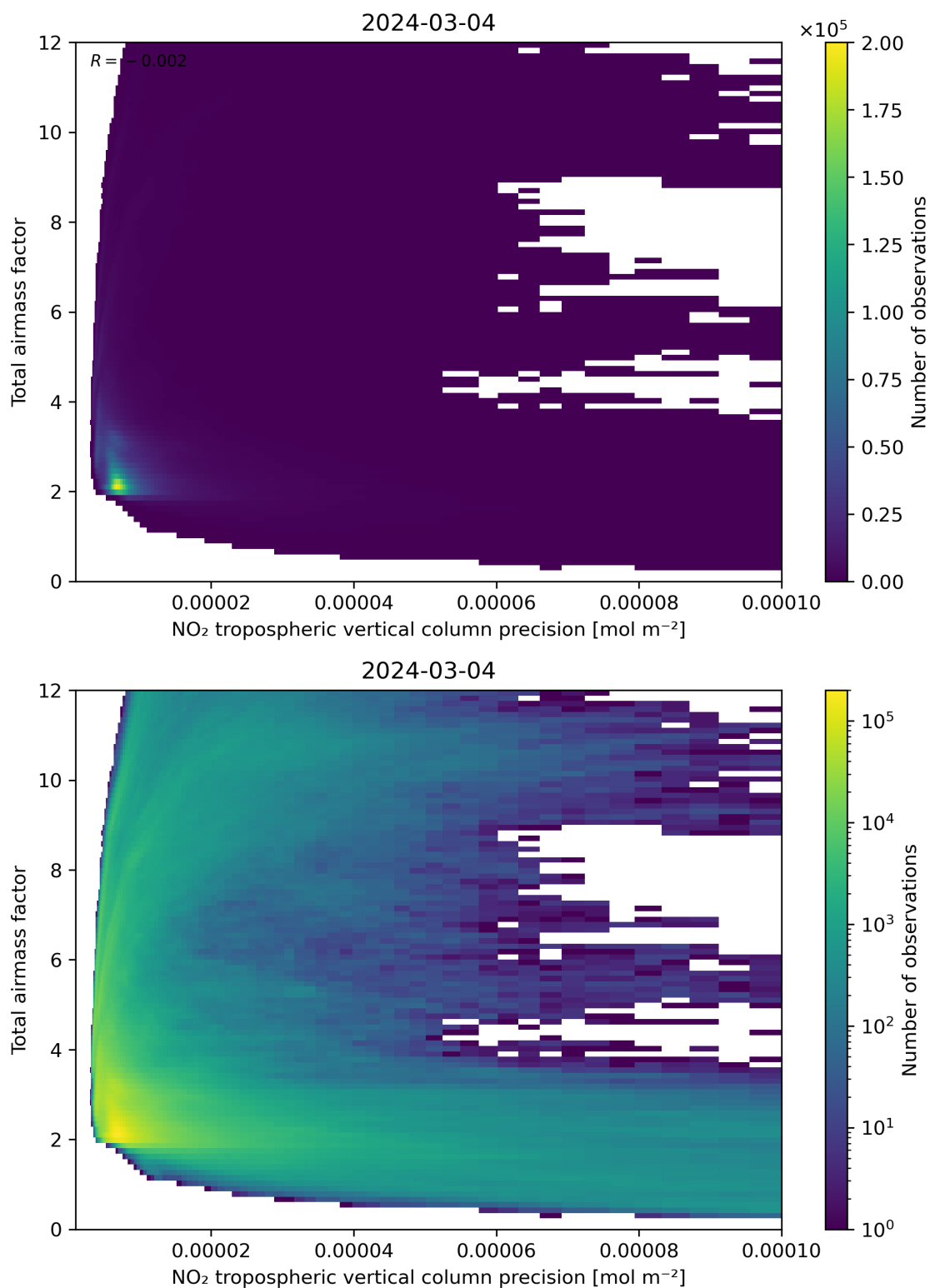
Figure 132: Scatter density plot of “NO 2 tropospheric vertical column precision” against “Total air mass factor” for 2024-03-04 to 2024-03-05.
