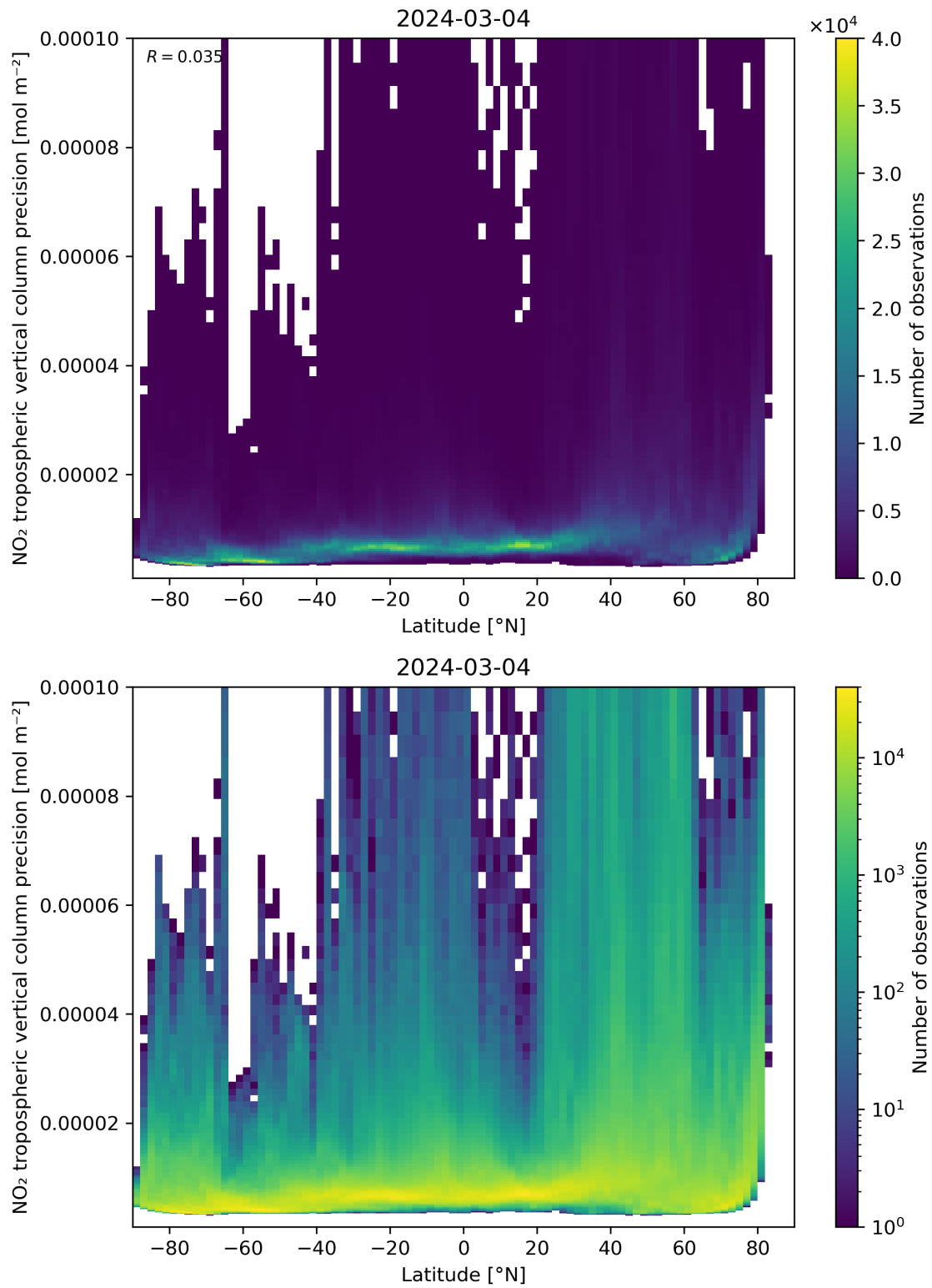
Figure 93: Scatter density plot of “Latitude” against “NO 2 tropospheric vertical column precision” for 2024-03-04 to 2024-03-05.
