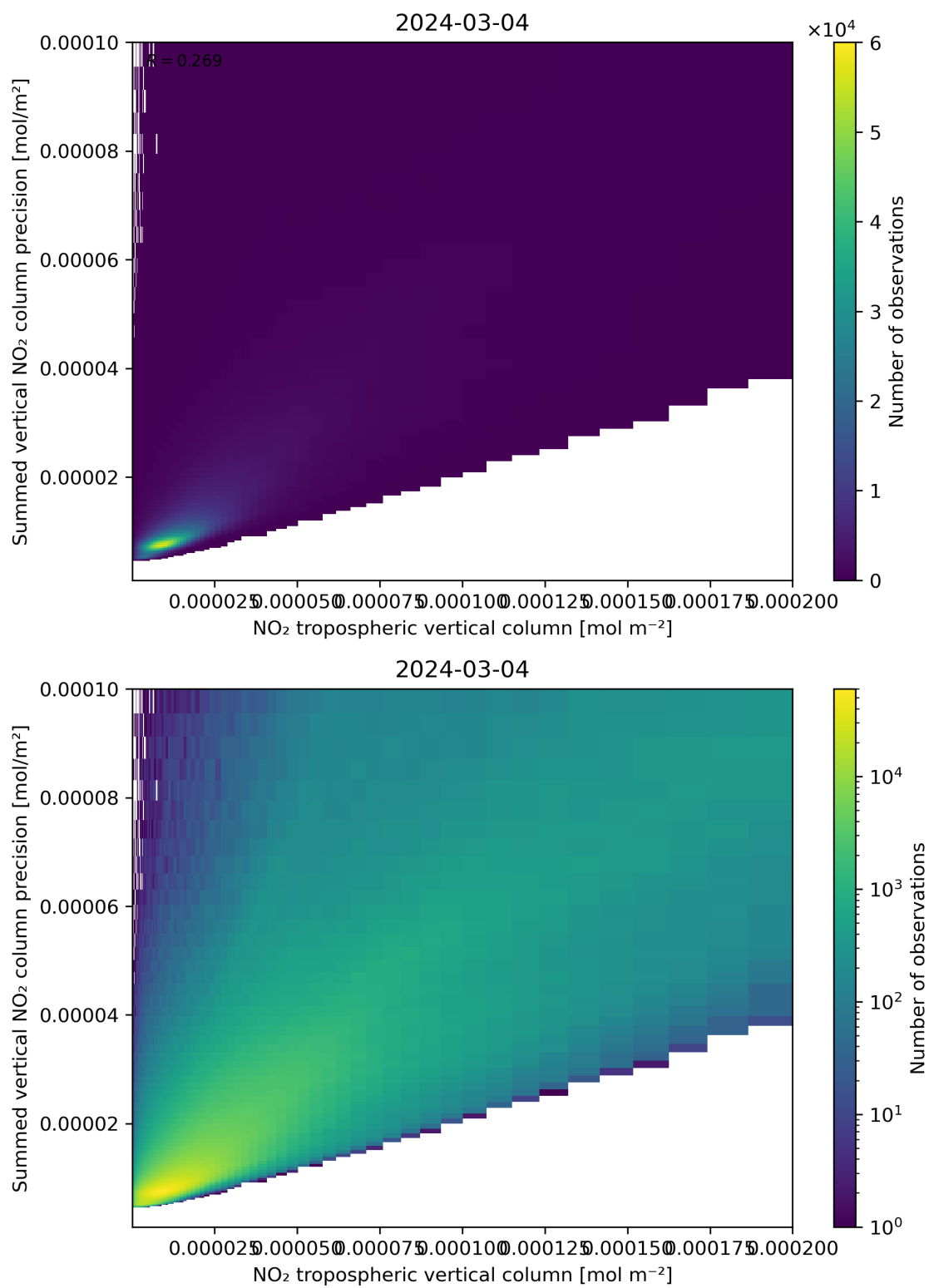
Figure 127: Scatter density plot of “NO 2 tropospheric vertical column” against “Summed vertical NO 2 column precision” for 2024-03-04 to 2024-03-05.
