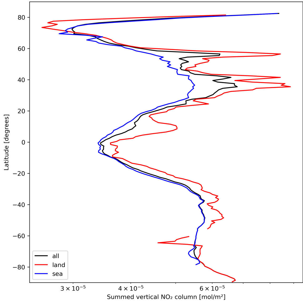
Figure 23: Zonal average of “Summed vertical NO 2 column” for 2024-03-04 to 2024-03-05.
