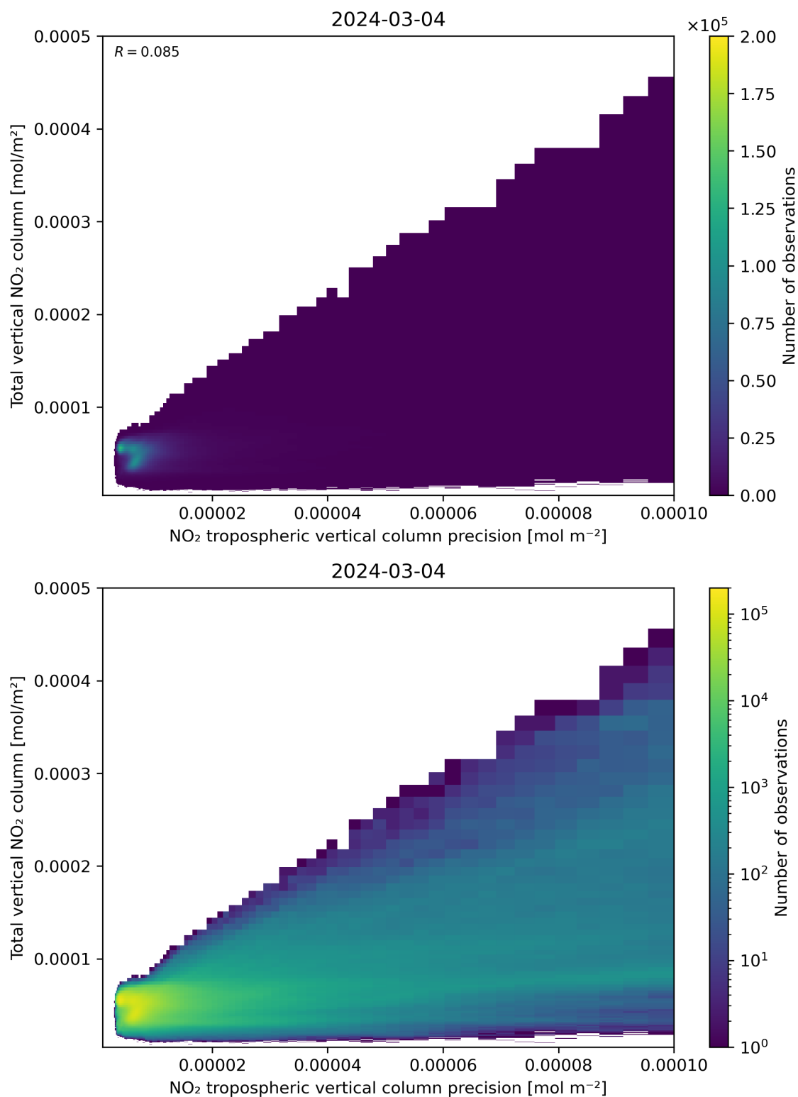
Figure 138: Scatter density plot of “NO 2 tropospheric vertical column precision” against “Total vertical NO 2 column” for 2024-03-04 to 2024-03-05.
