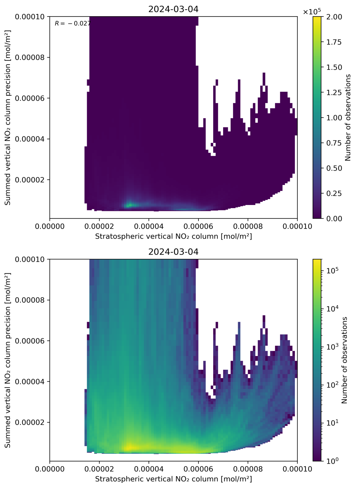
Figure 99: Scatter density plot of “Stratospheric vertical NO 2 column” against “Summed vertical NO 2 column precision” for 2024-03-04 to 2024-03-05.
