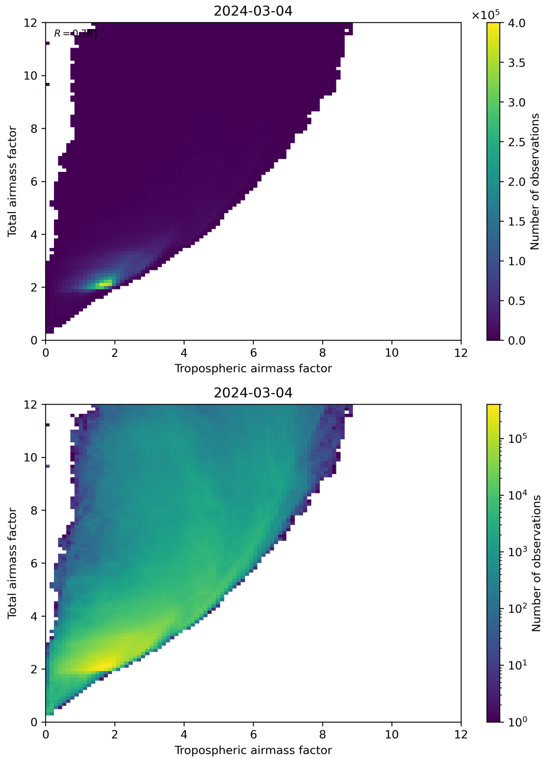
Figure 72: Scatter density plot of “Tropospheric airmass factor” against “Total airmass factor” for 2024-03-04 to 2024-03-05.
