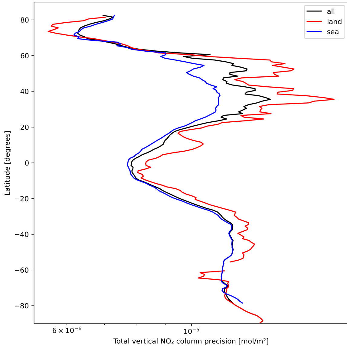
Figure 22: Zonal average of “Total vertical NO 2 column precision” for 2024-03-04 to 2024-03-05.
