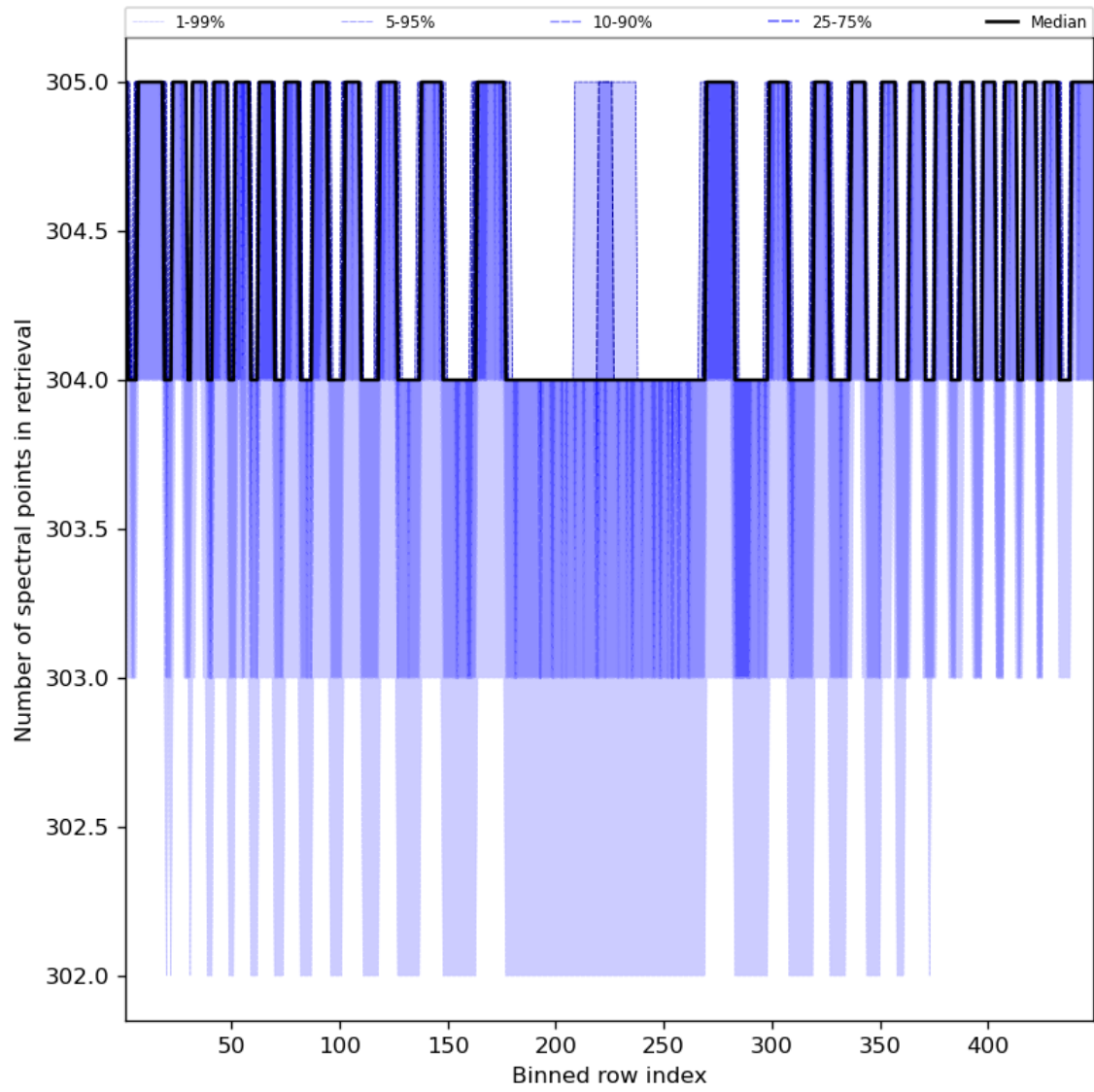
Figure 50: Along track statistics of “Number of spectral points in retrieval” for 2024-03-04 to 2024-03-05
