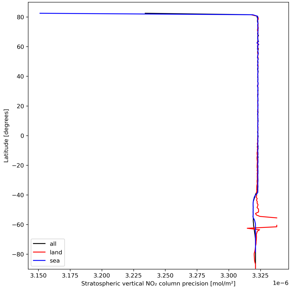
Figure 20: Zonal average of “Stratospheric vertical NO 2 column precision” for 2024-03-04 to 2024-03-05.
