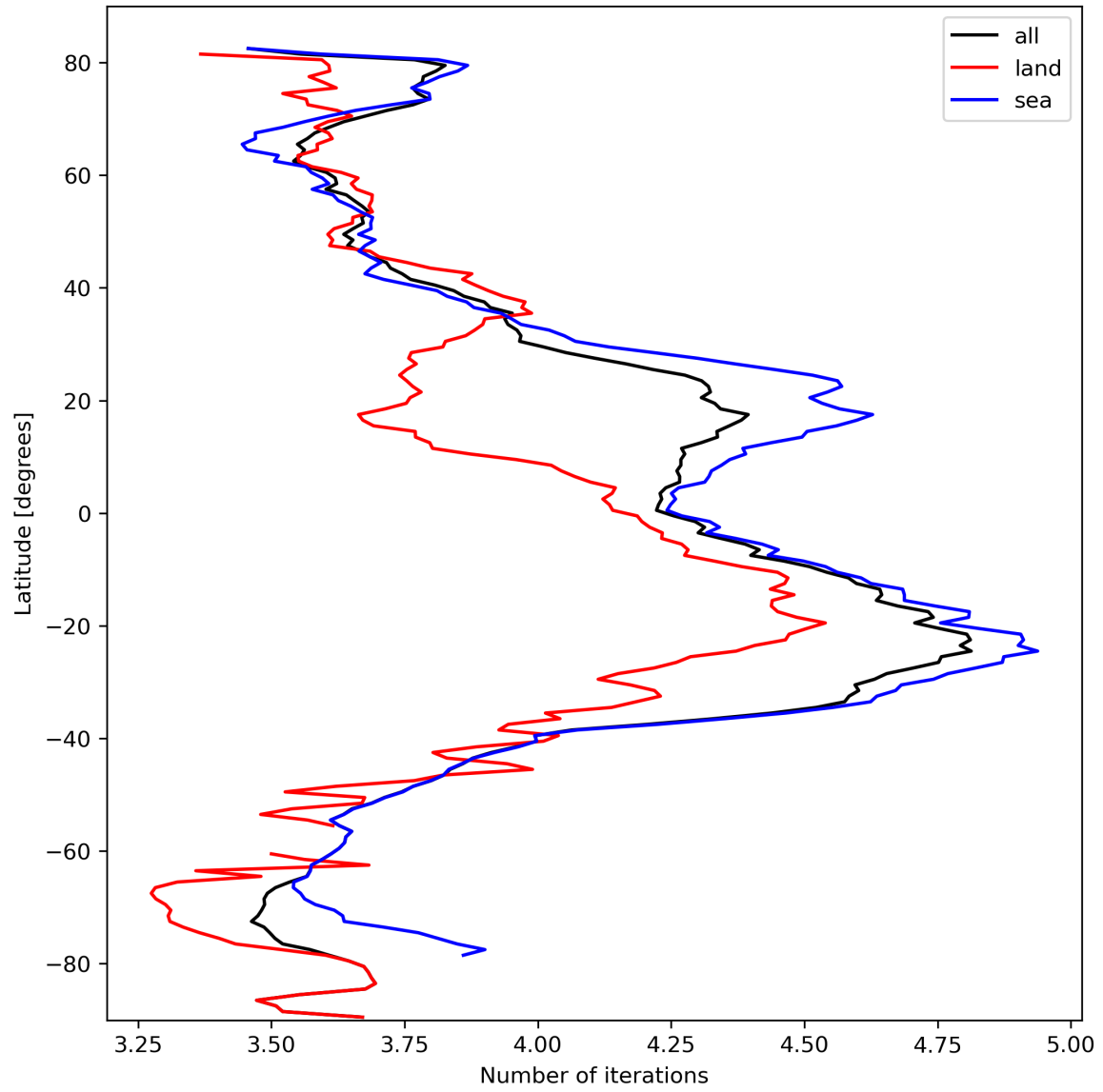
Figure 17: Zonal average of “Number of iterations” for 2024-03-04 to 2024-03-05.
