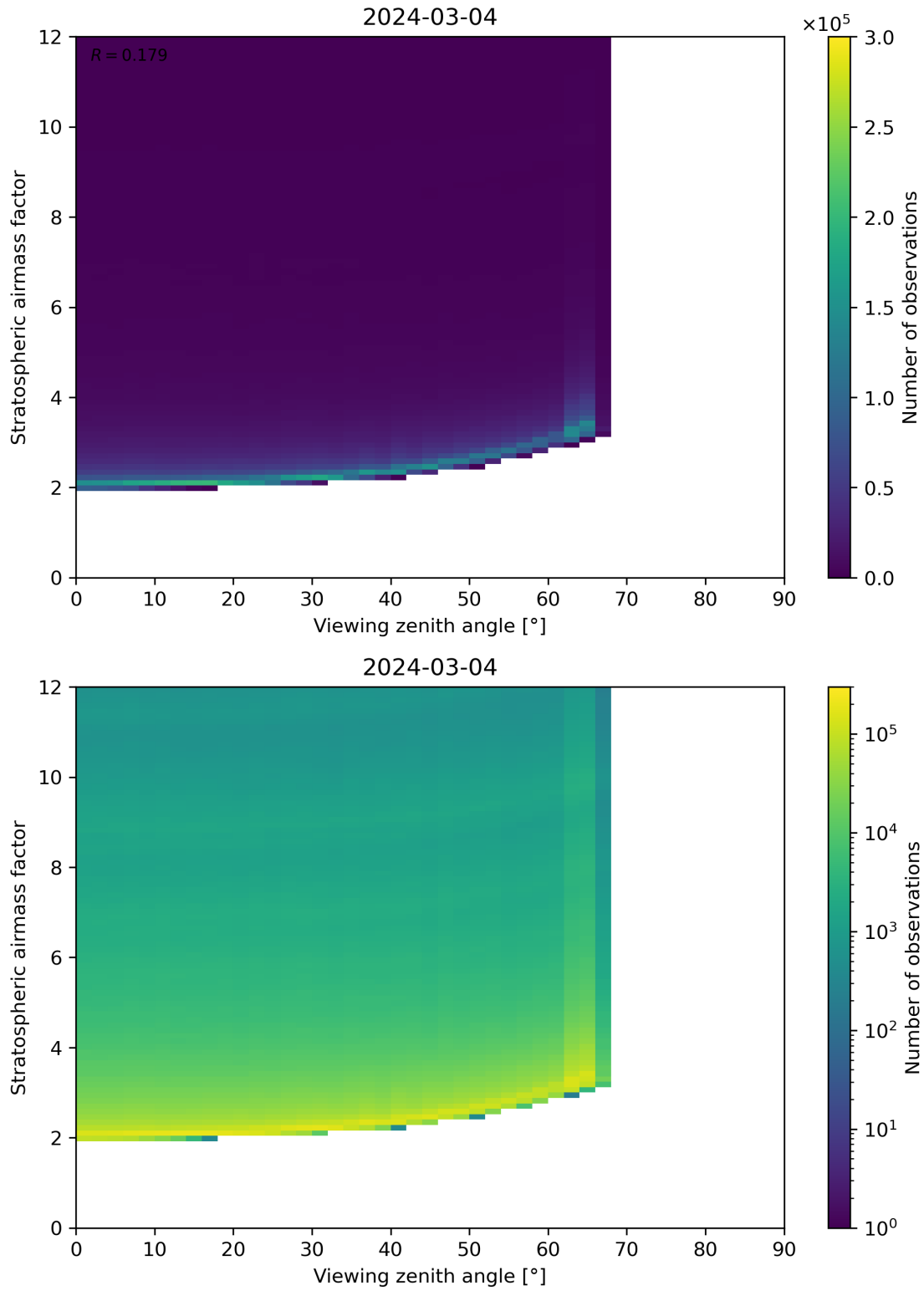
Figure 159: Scatter density plot of “Viewing zenith angle” against “Stratospheric airmass factor” for 2024-03-04 to 2024-03-05.
