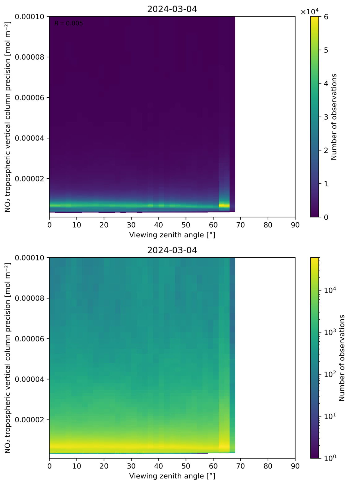
Figure 170: Scatter density plot of “Viewing zenith angle” against “NO 2 tropospheric vertical column precision” for 2024-03-04 to 2024-03-05.
