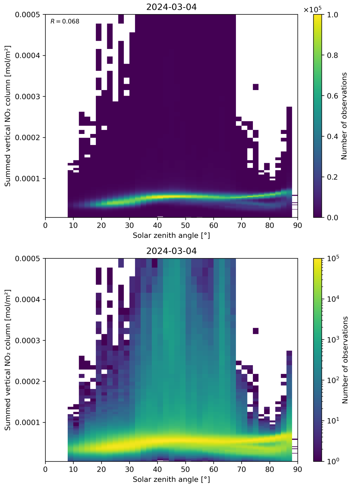
Figure 151: Scatter density plot of “Solar zenith angle” against “Summed vertical NO 2 column” for 2024-03-04 to 2024-03-05.
