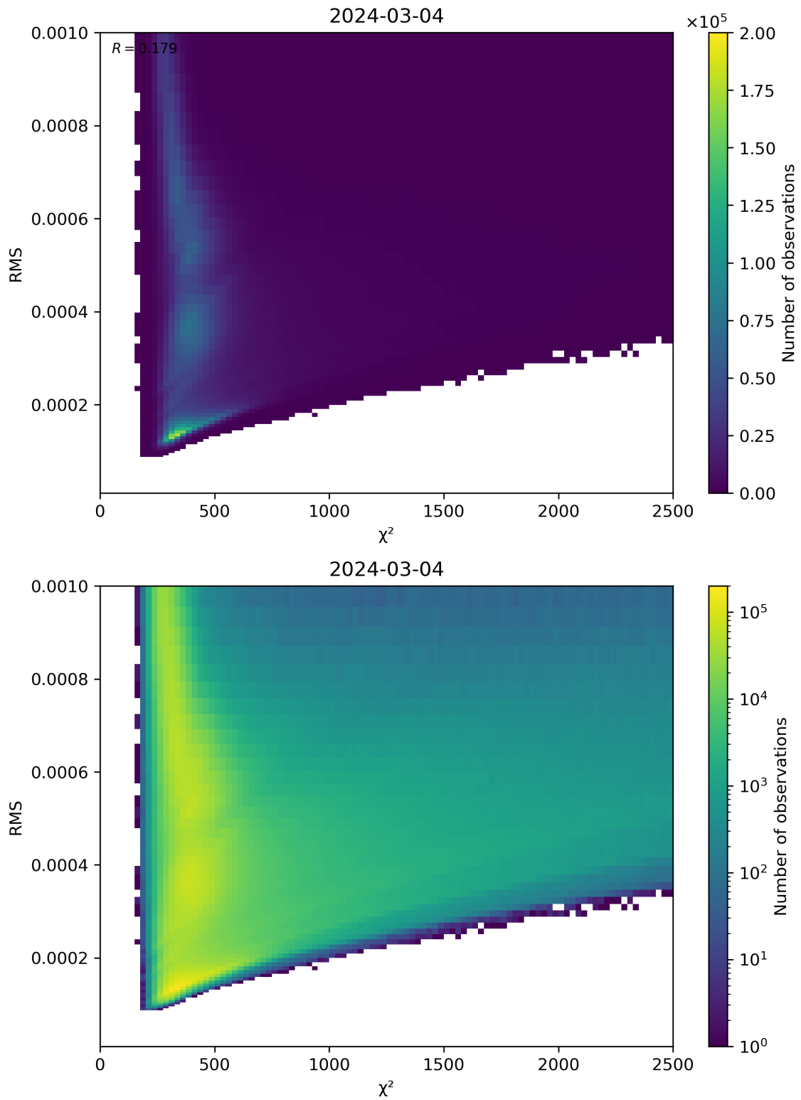
Figure 82: Scatter density plot of “ \chi^2 ” against “RMS” for 2024-03-04 to 2024-03-05.
