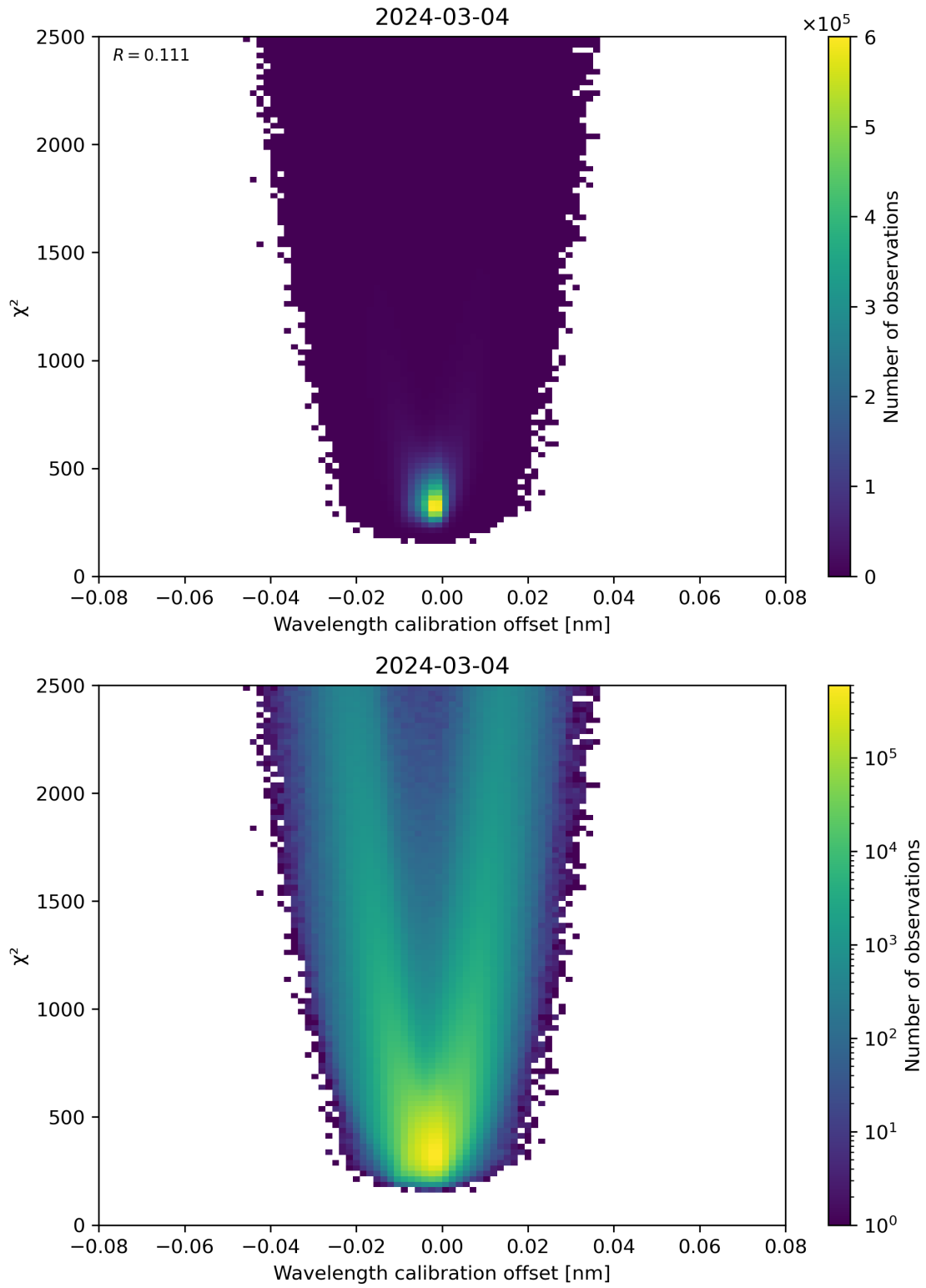
Figure 175: Scatter density plot of “Wavelength calibration offset” against “ \chi^2 ” for 2024-03-04 to 2024-03-05.
