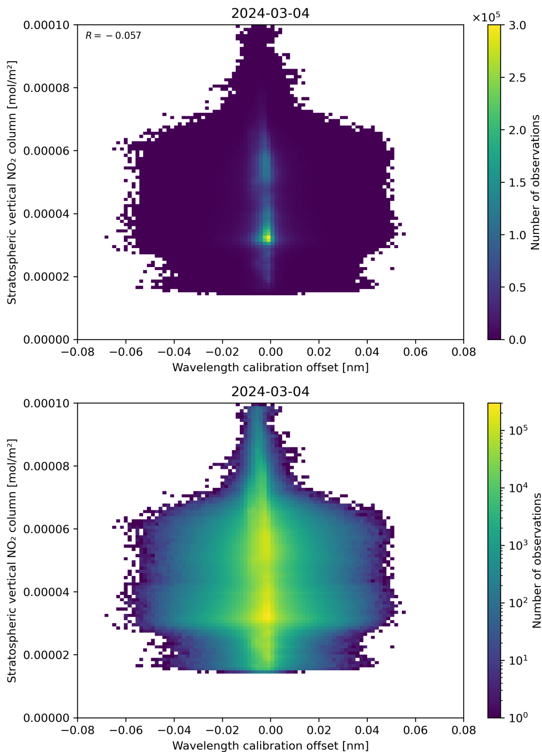
Figure 176: Scatter density plot of “Wavelength calibration offset” against “Stratospheric vertical NO 2 column” for 2024-03-04 to 2024-03-05.
