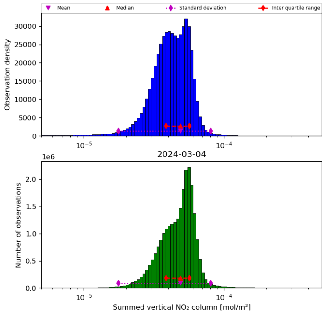
Figure 40: Histogram of “Summed vertical NO 2 column” for 2024-03-04 to 2024-03-05
