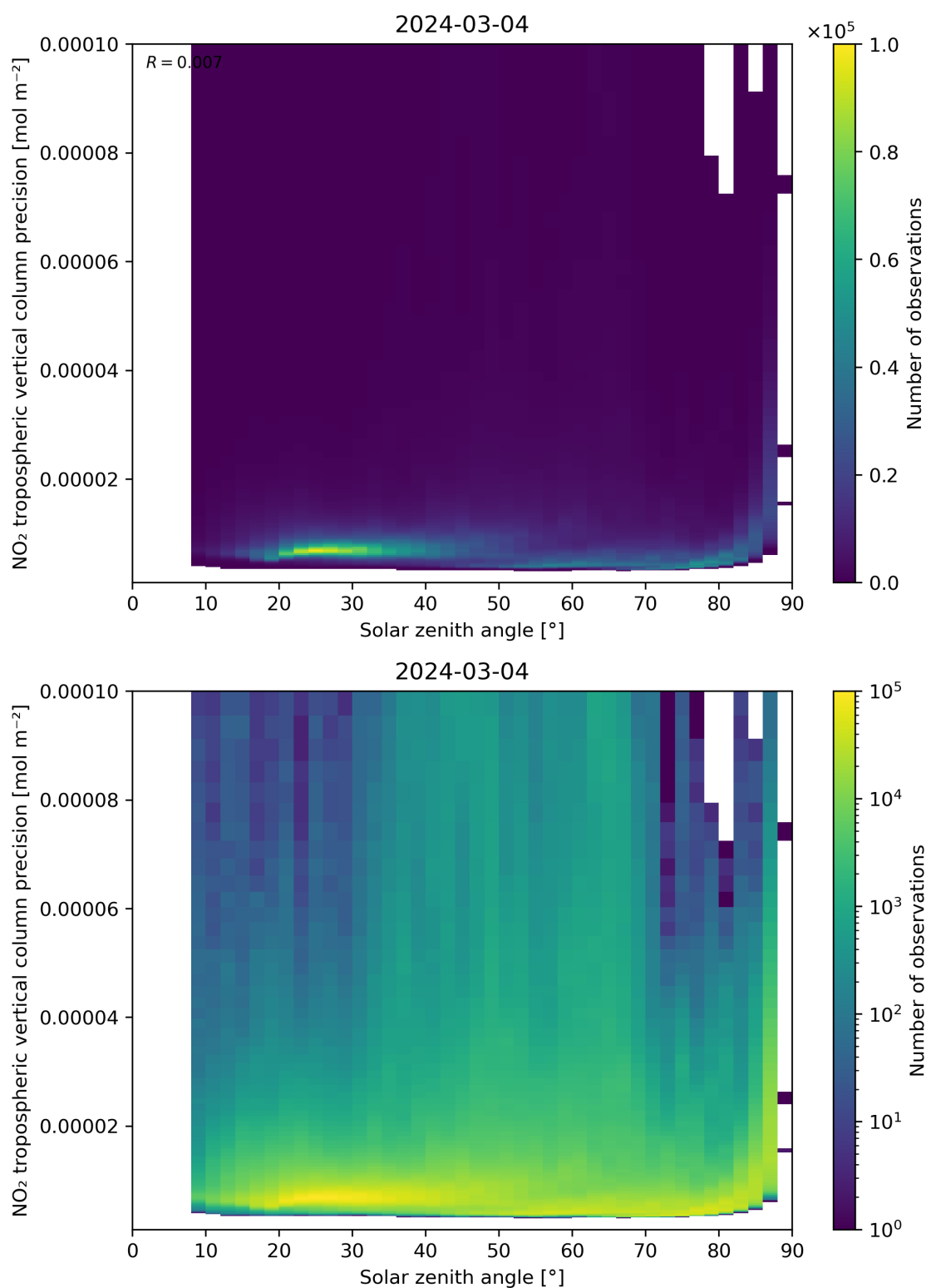
Figure 156: Scatter density plot of “Solar zenith angle” against “NO 2 tropospheric vertical column precision” for 2024-03-04 to 2024-03-05.
