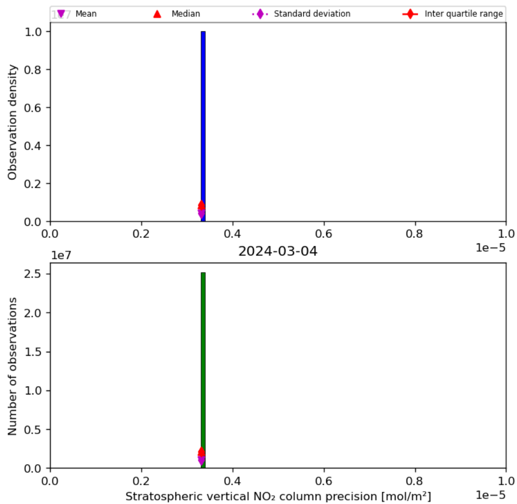
Figure 37: Histogram of “Stratospheric vertical NO 2 column precision” for 2024-03-04 to 2024-03-05
