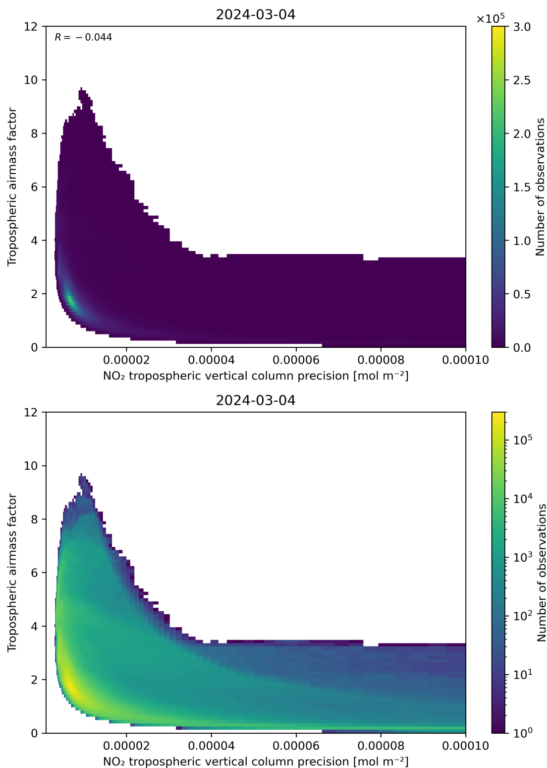
Figure 133: Scatter density plot of “NO 2 tropospheric vertical column precision” against “Tropospheric airmass factor” for 2024-03-04 to 2024-03-05.
