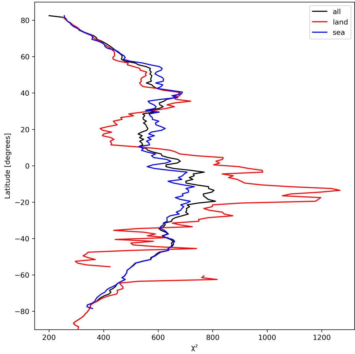
Figure 25: Zonal average of “ \chi^2 ” for 2024-03-04 to 2024-03-05.
