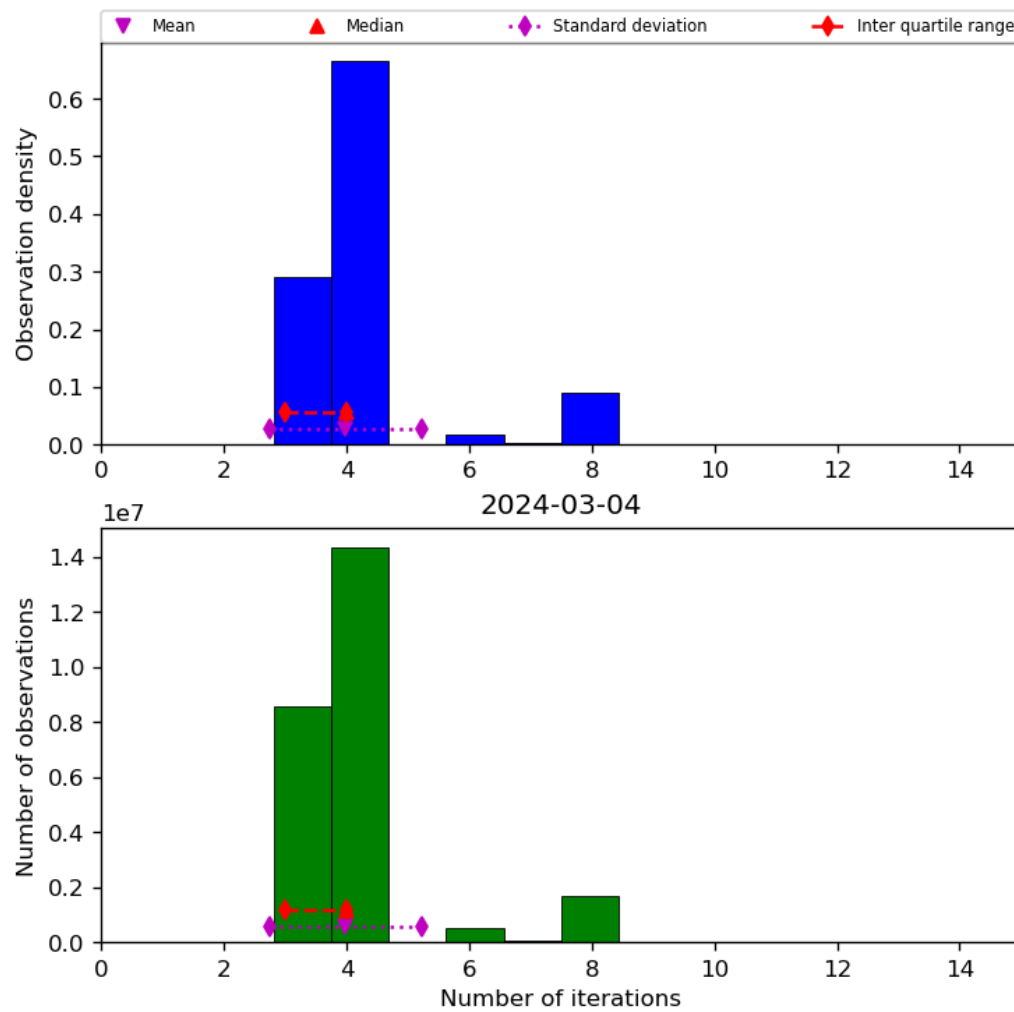
Figure 34: Histogram of “Number of iterations” for 2024-03-04 to 2024-03-05
