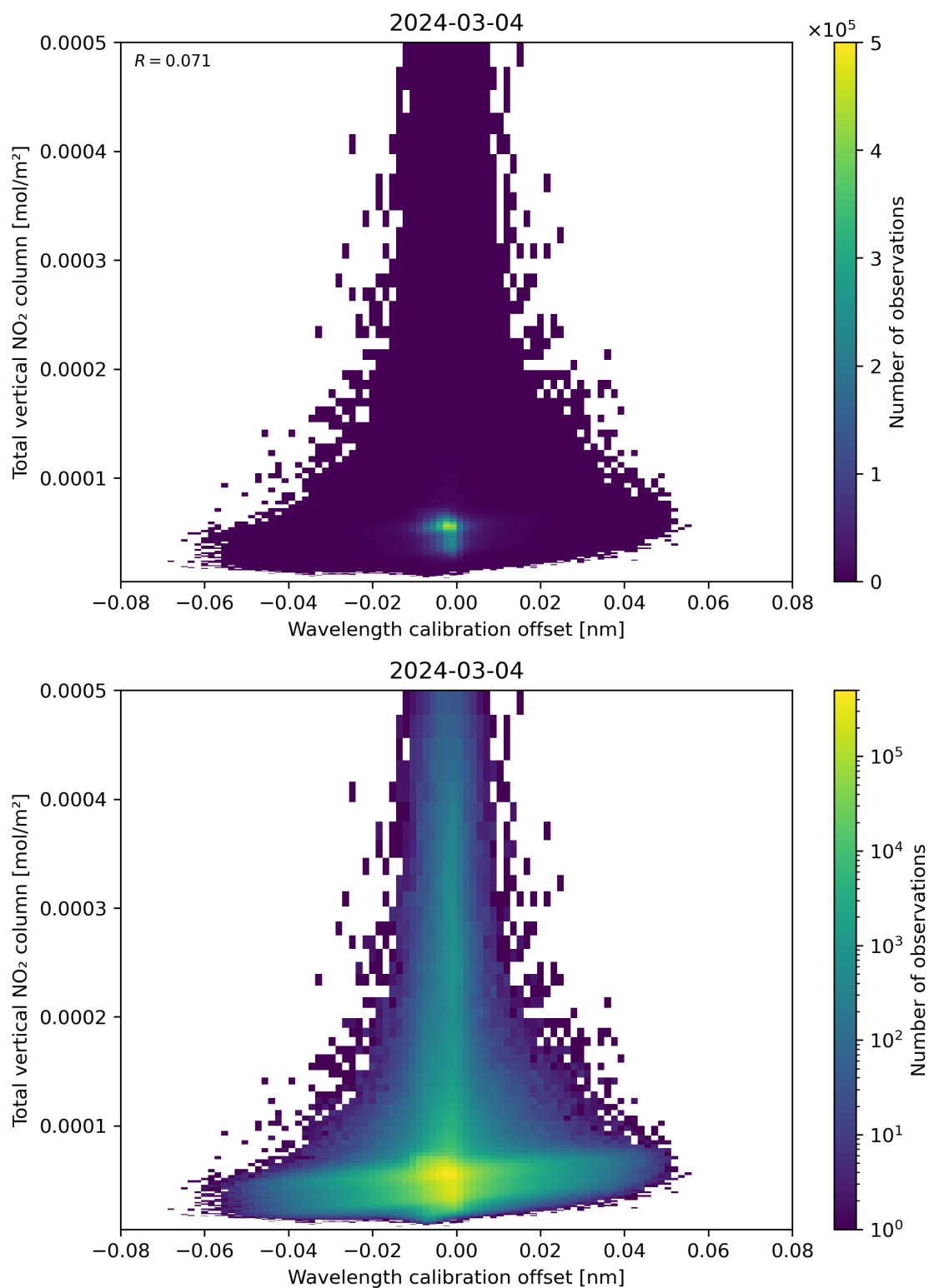
Figure 179: Scatter density plot of “Wavelength calibration offset” against “Total vertical NO 2 column” for 2024-03-04 to 2024-03-05.
