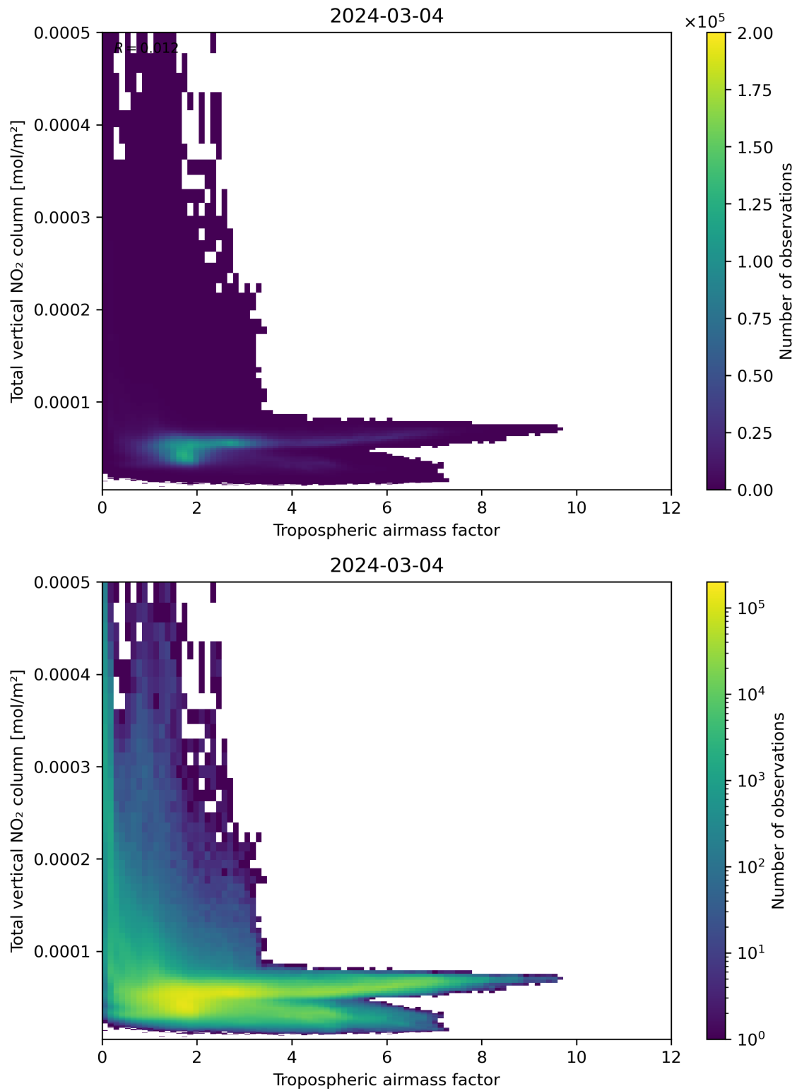
Figure 77: Scatter density plot of “Tropospheric airmass factor” against “Total vertical NO 2 column” for 2024-03-04 to 2024-03-05.
