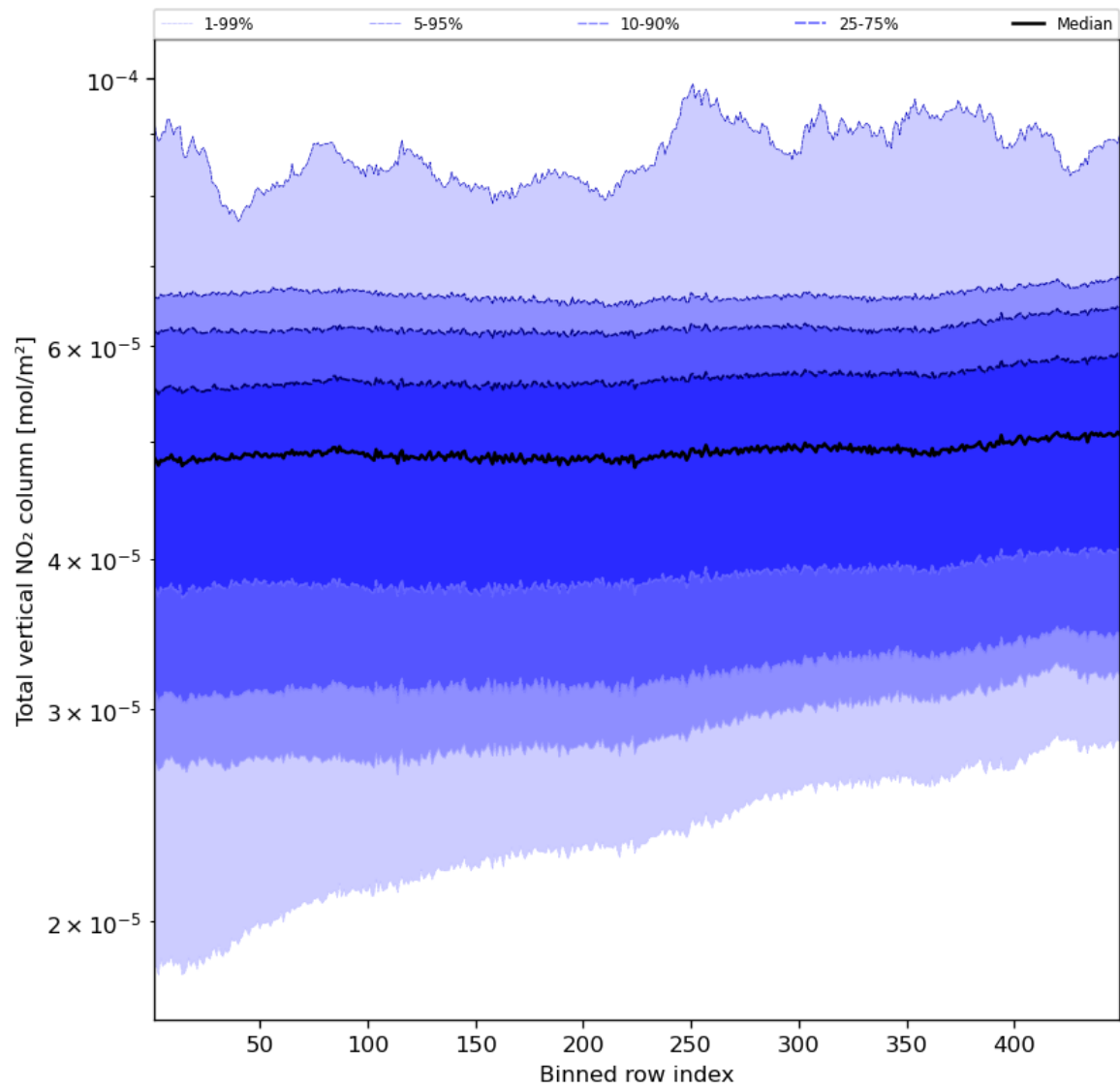
Figure 55: Along track statistics of “Total vertical NO 2 column” for 2024-03-04 to 2024-03-05
