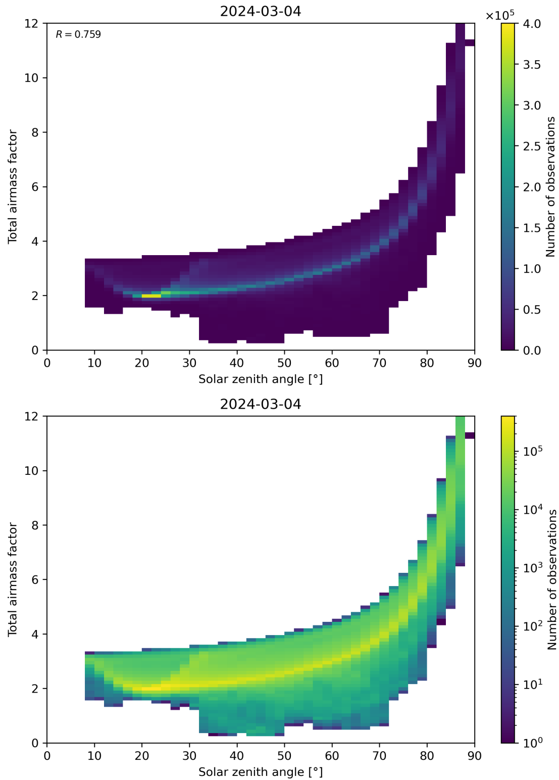
Figure 146: Scatter density plot of “Solar zenith angle” against “Total air mass factor” for 2024-03-04 to 2024-03-05.
