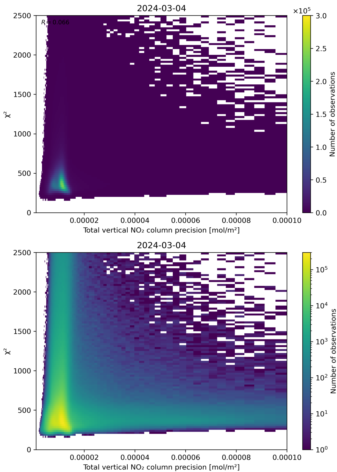
Figure 116: Scatter density plot of “Total vertical NO 2 column precision” against “ \chi^2 ” for 2024-03-04 to 2024-03-05.
