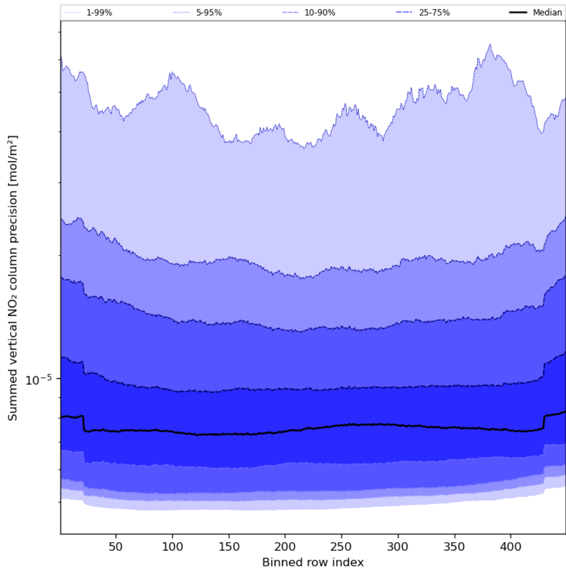
Figure 58: Along track statistics of “Summed vertical NO 2 column precision” for 2024-03-04 to 2024-03-05
