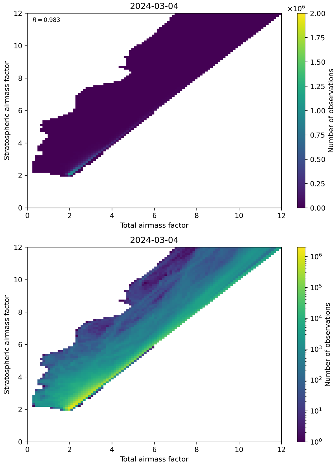
Figure 62: Scatter density plot of “Total airmass factor” against “Stratospheric airmass factor” for 2024-03-04 to 2024-03-05.
