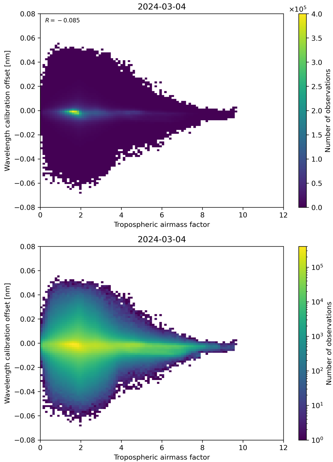
Figure 80: Scatter density plot of “Tropospheric airmass factor” against “Wavelength calibration offset” for 2024-03-04 to 2024-03-05.
