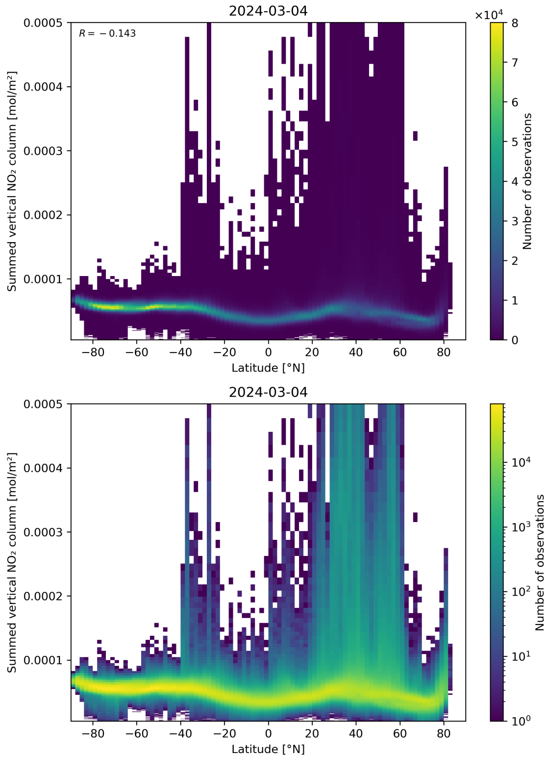
Figure 88: Scatter density plot of “Latitude” against “Summed vertical NO 2 column” for 2024-03-04 to 2024-03-05.
