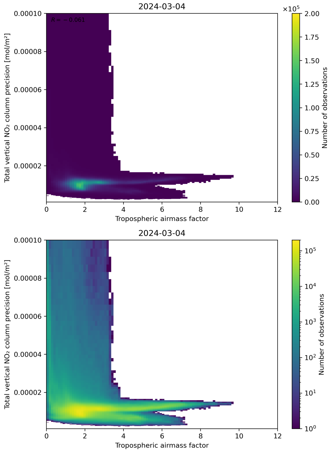
Figure 78: Scatter density plot of “Tropospheric air mass factor” against “Total vertical NO 2 column precision” for 2024-03-04 to 2024-03-05.
