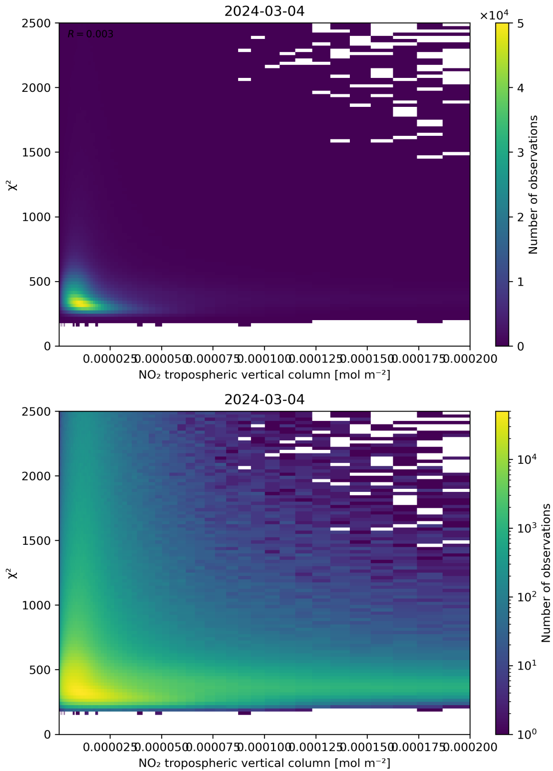
Figure 124: Scatter density plot of “NO 2 tropospheric vertical column” against “ \chi^2 ” for 2024-03-04 to 2024-03-05.
