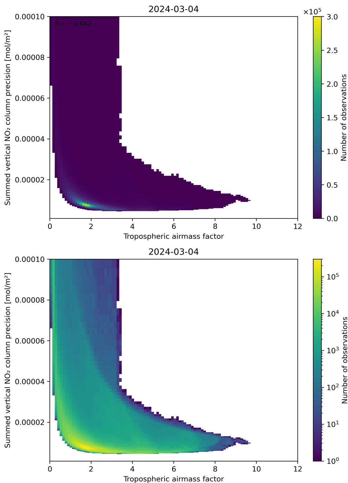
Figure 76: Scatter density plot of “Tropospheric air mass factor” against “Summed vertical NO 2 column precision” for 2024-03-04 to 2024-03-05.
