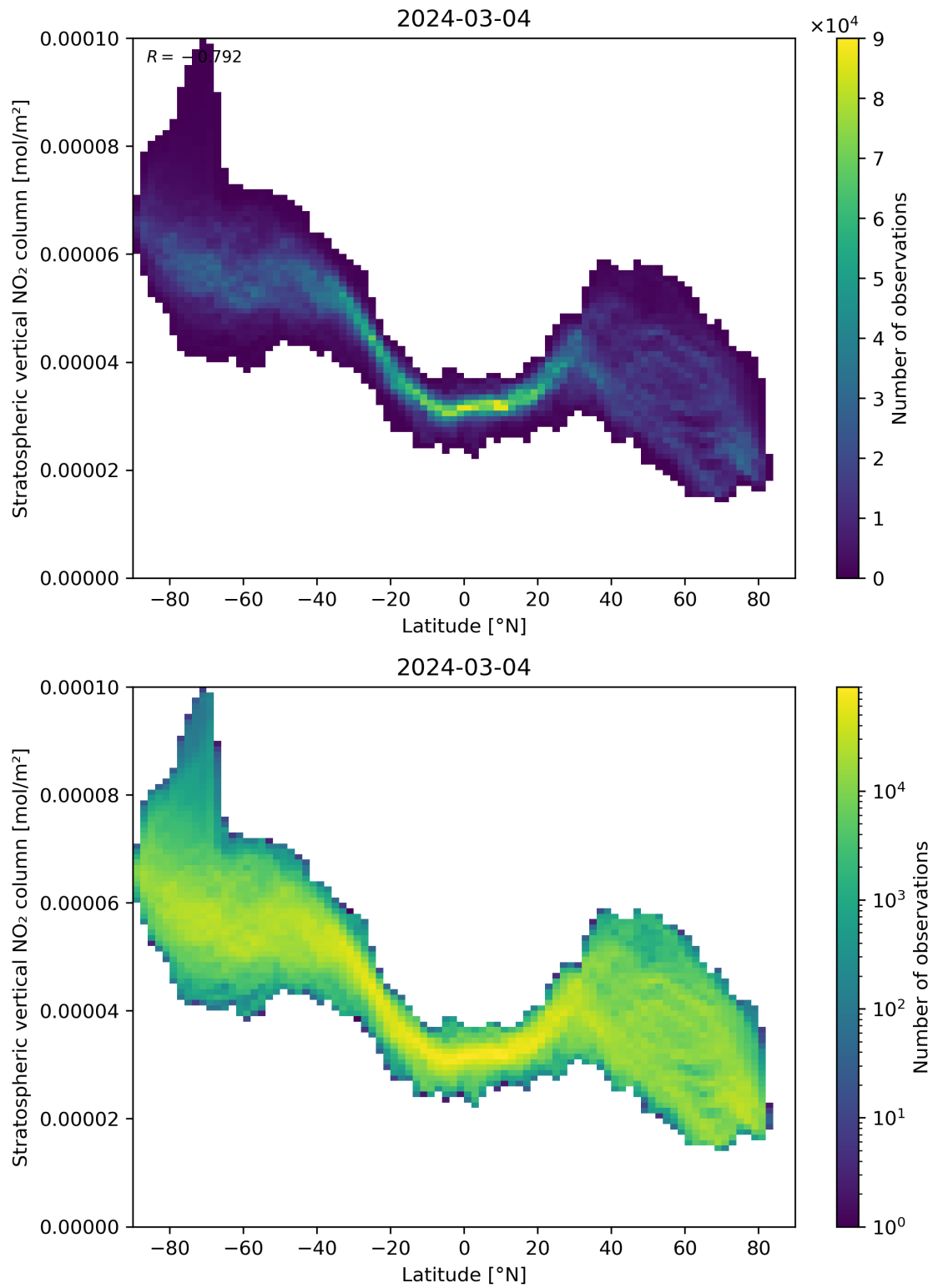
Figure 87: Scatter density plot of “Latitude” against “Stratospheric vertical NO 2 column” for 2024-03-04 to 2024-03-05.
