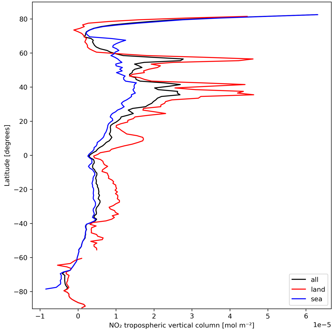
Figure 12: Zonal average of “NO 2 tropospheric vertical column” for 2024-03-04 to 2024-03-05.
