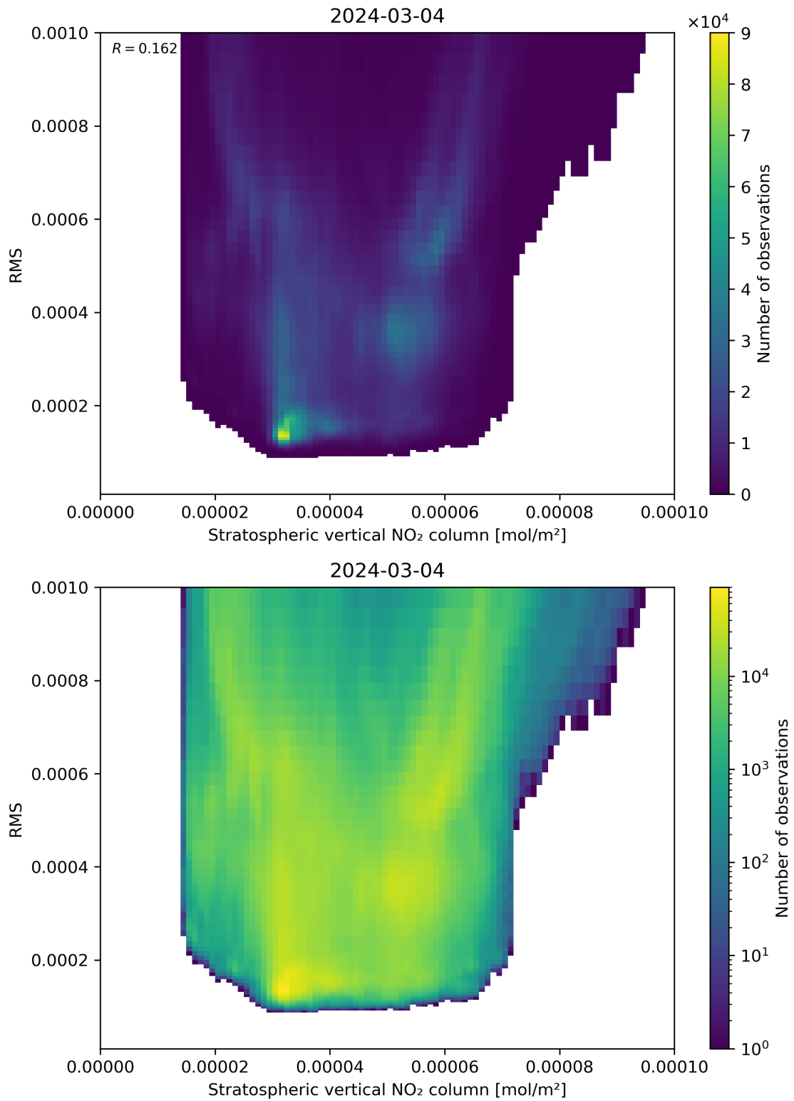
Figure 102: Scatter density plot of “Stratospheric vertical NO 2 column” against “RMS” for 2024-03-04 to 2024-03-05.
