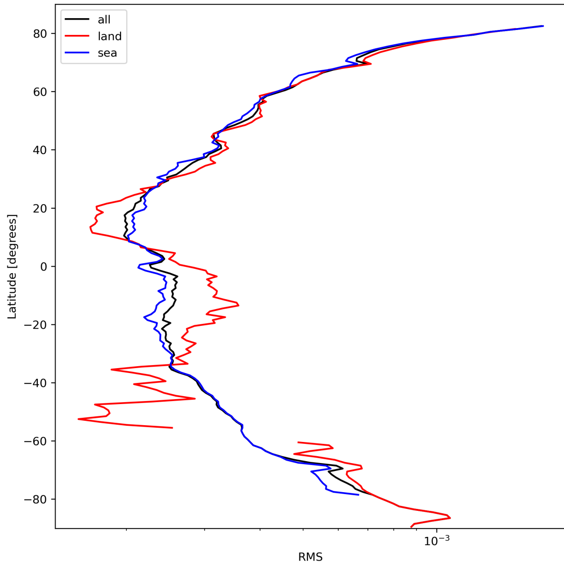
Figure 26: Zonal average of “RMS” for 2024-03-04 to 2024-03-05.
