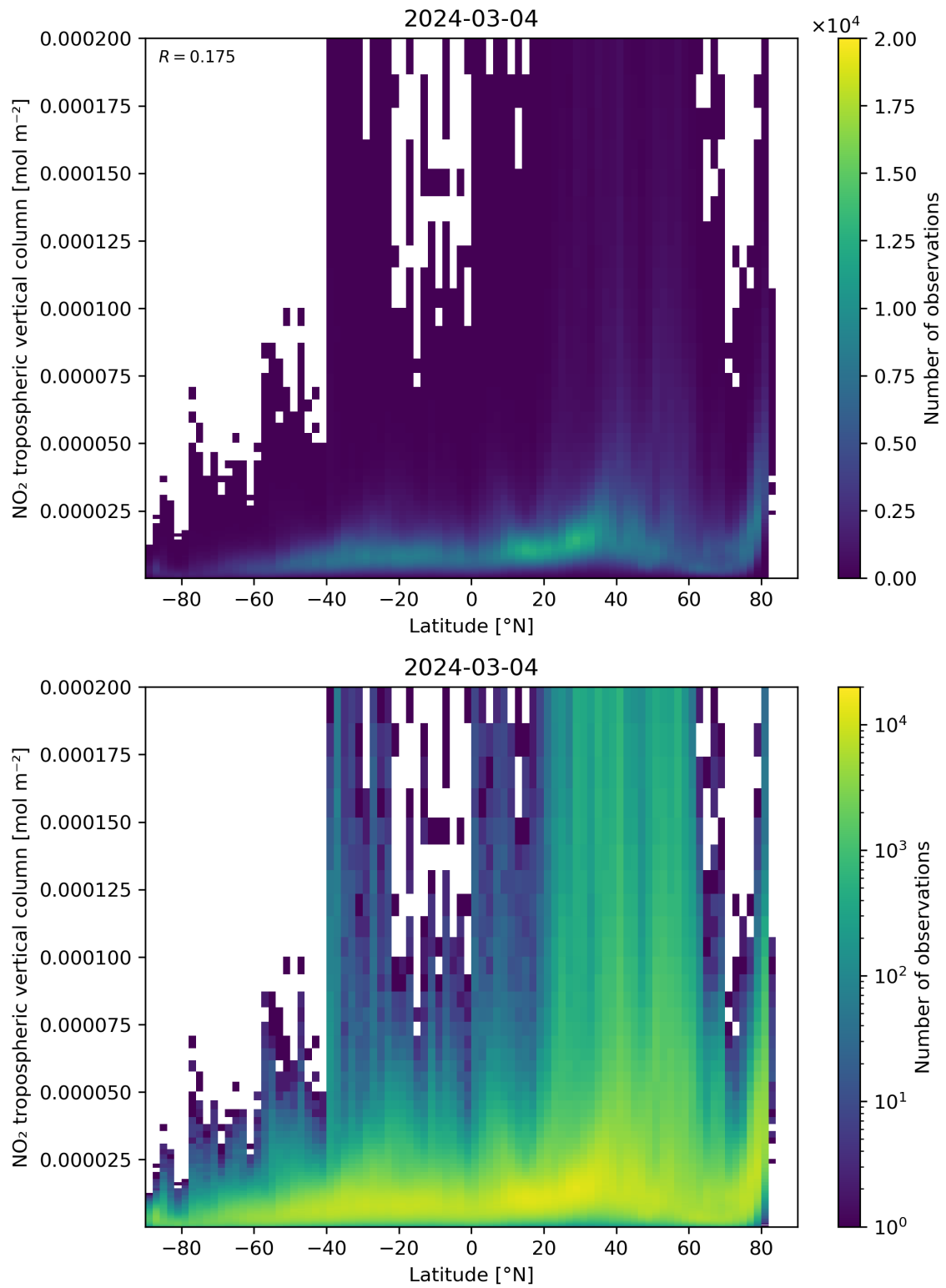
Figure 92: Scatter density plot of “Latitude” against “NO 2 tropospheric vertical column” for 2024-03-04 to 2024-03-05.
