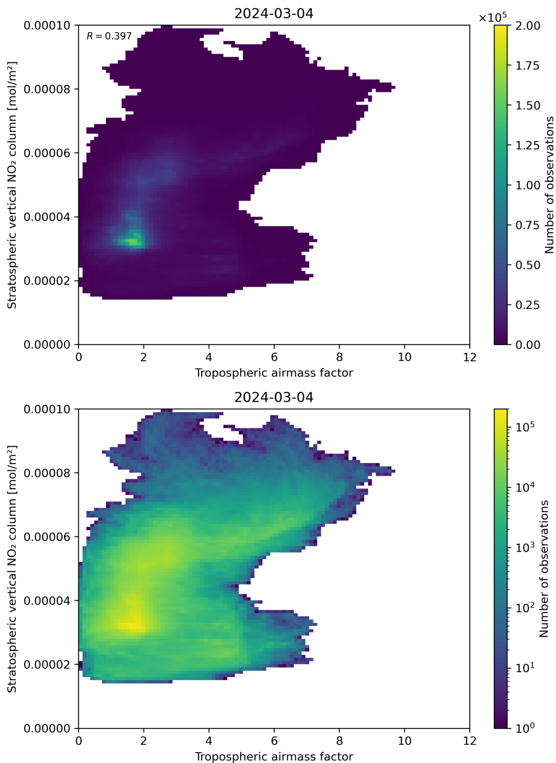
Figure 74: Scatter density plot of “Tropospheric air mass factor” against “Stratospheric vertical NO 2 column” for 2024-03-04 to 2024-03-05.
