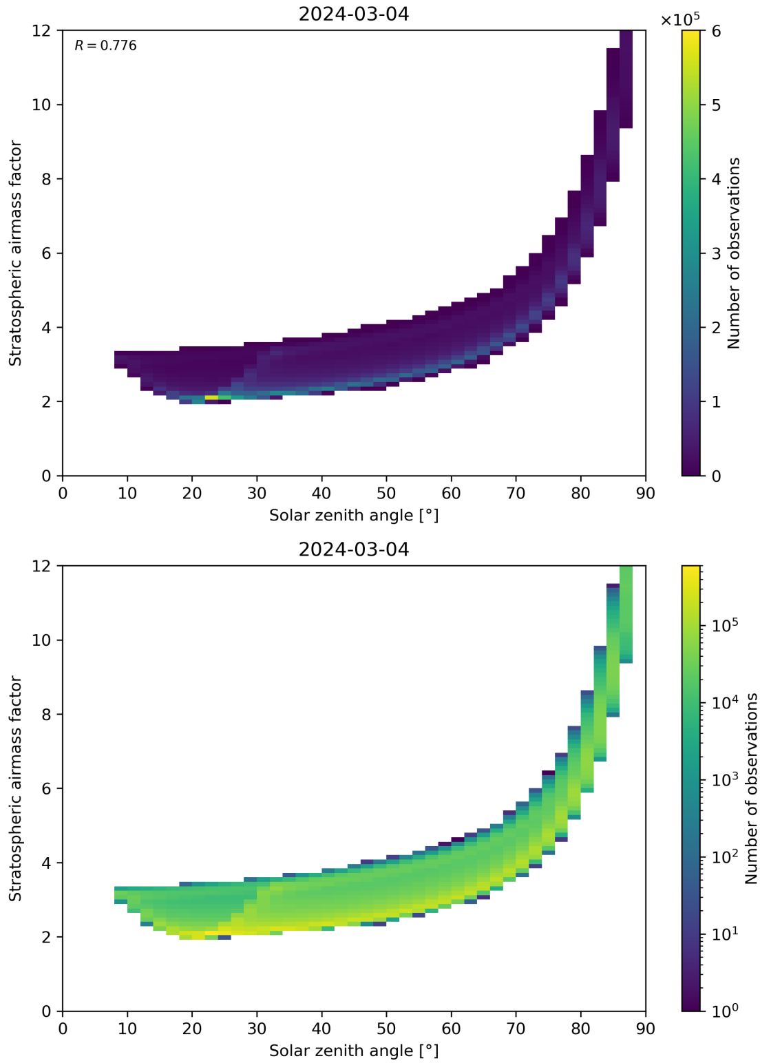
Figure 145: Scatter density plot of “Solar zenith angle” against “Stratospheric airmass factor” for 2024-03-04 to 2024-03-05.
