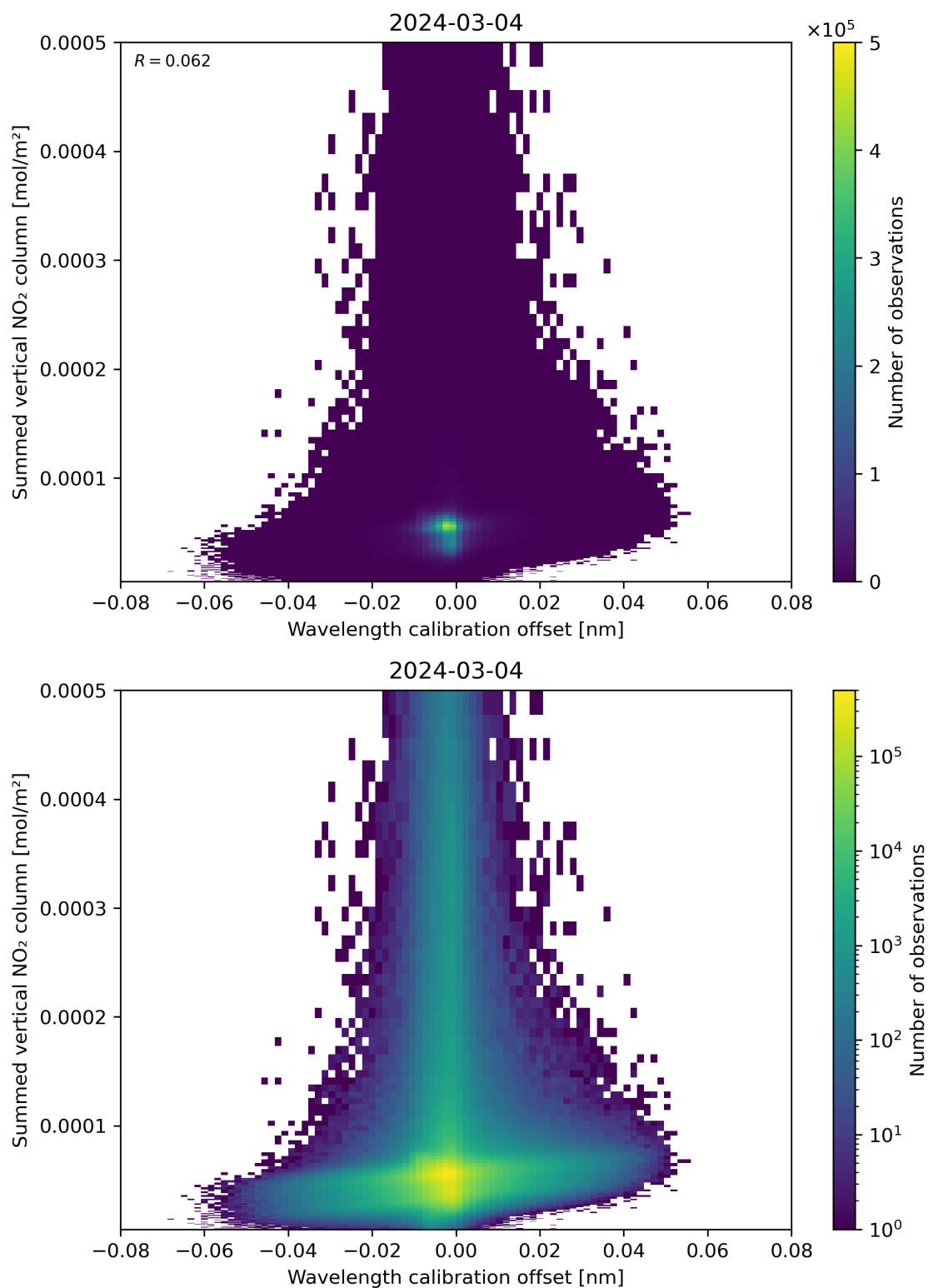
Figure 177: Scatter density plot of “Wavelength calibration offset” against “Summed vertical NO 2 column” for 2024-03-04 to 2024-03-05.
