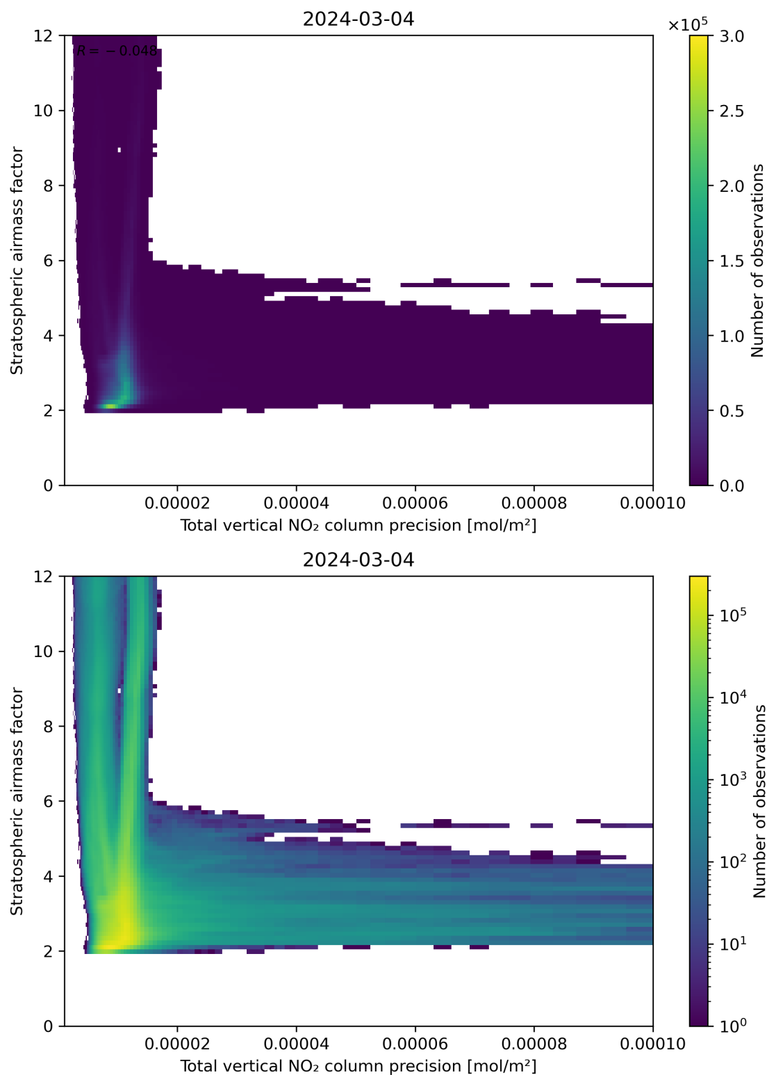
Figure 115: Scatter density plot of “Total vertical NO 2 column precision” against “Stratospheric air mass factor” for 2024-03-04 to 2024-03-05.
