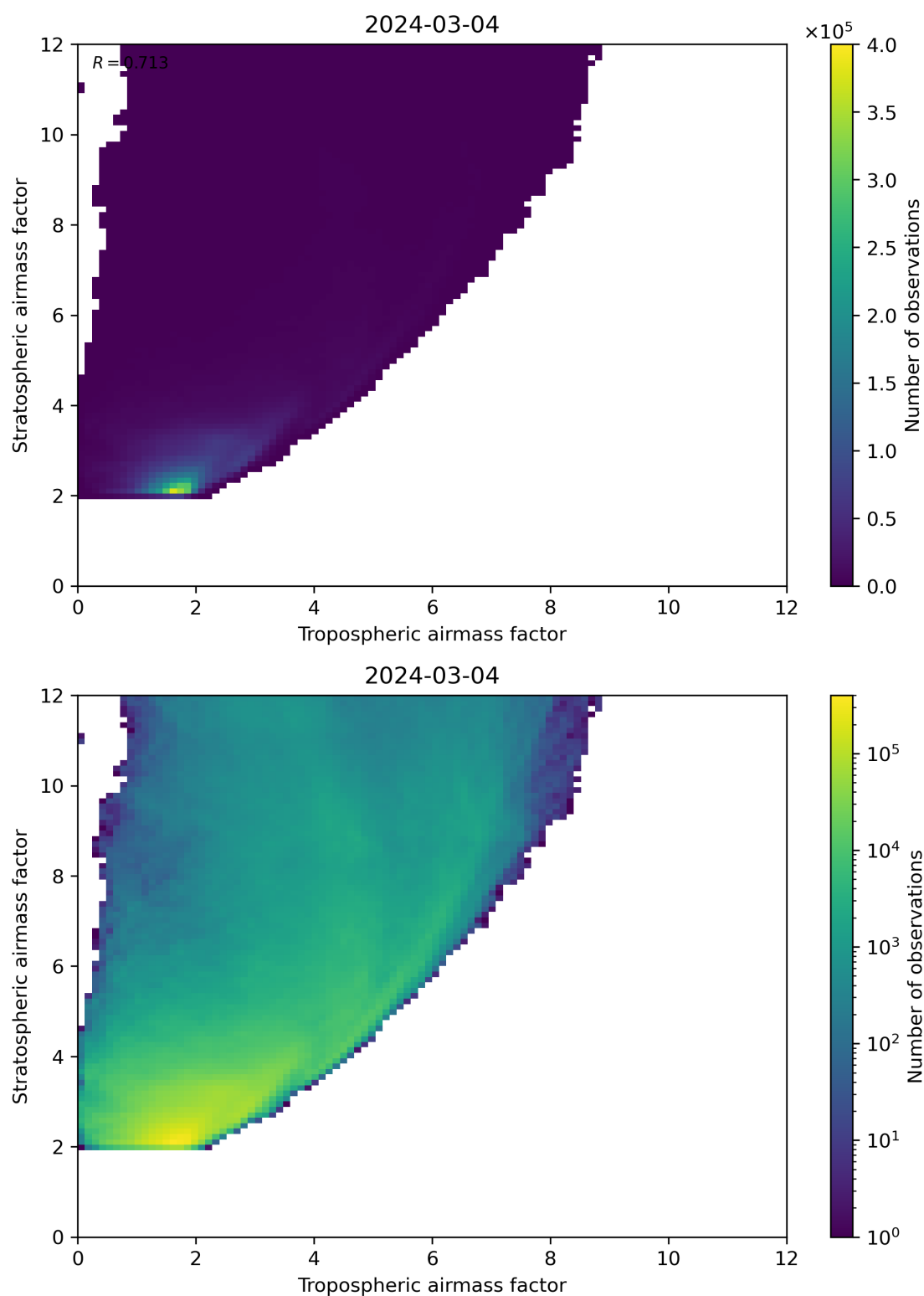
Figure 71: Scatter density plot of “Tropospheric airmass factor” against “Stratospheric airmass factor” for 2024-03-04 to 2024-03-05.
