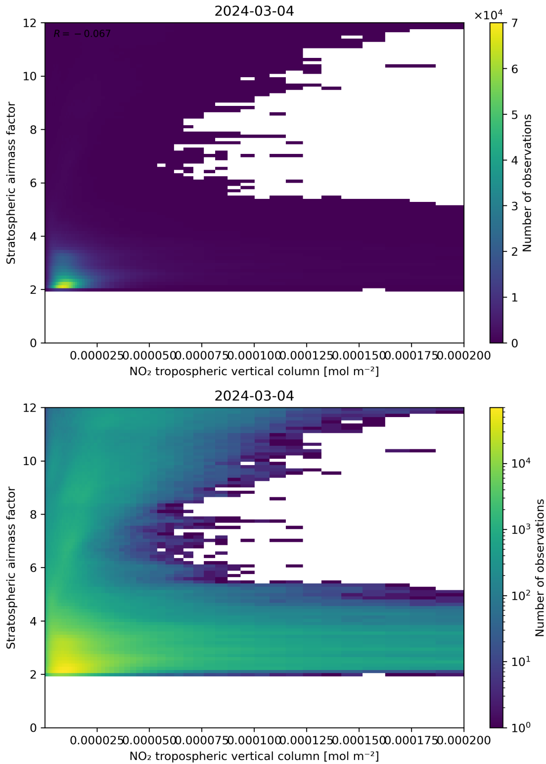
Figure 121: Scatter density plot of “NO 2 tropospheric vertical column” against “Stratospheric air mass factor” for 2024-03-04 to 2024-03-05.
