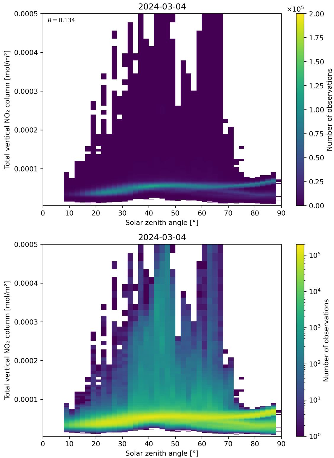
Figure 153: Scatter density plot of “Solar zenith angle” against “Total vertical NO 2 column” for 2024-03-04 to 2024-03-05.
