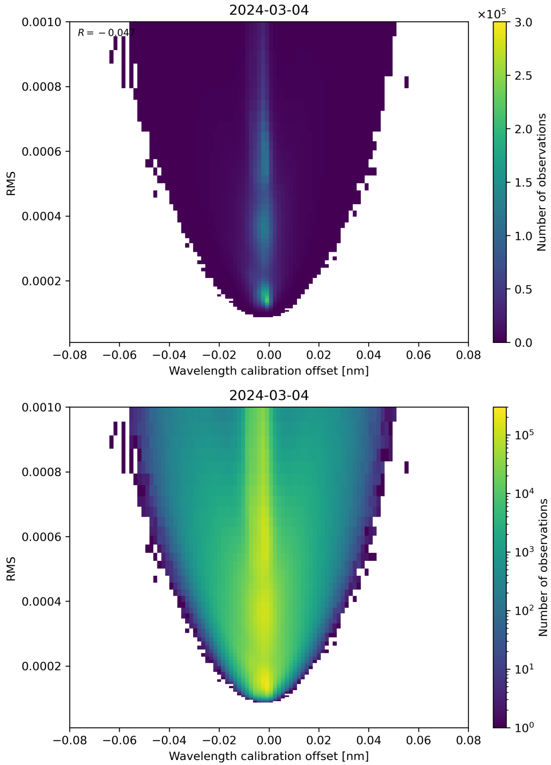
Figure 181: Scatter density plot of “Wavelength calibration offset” against “RMS” for 2024-03-04 to 2024-03-05.
