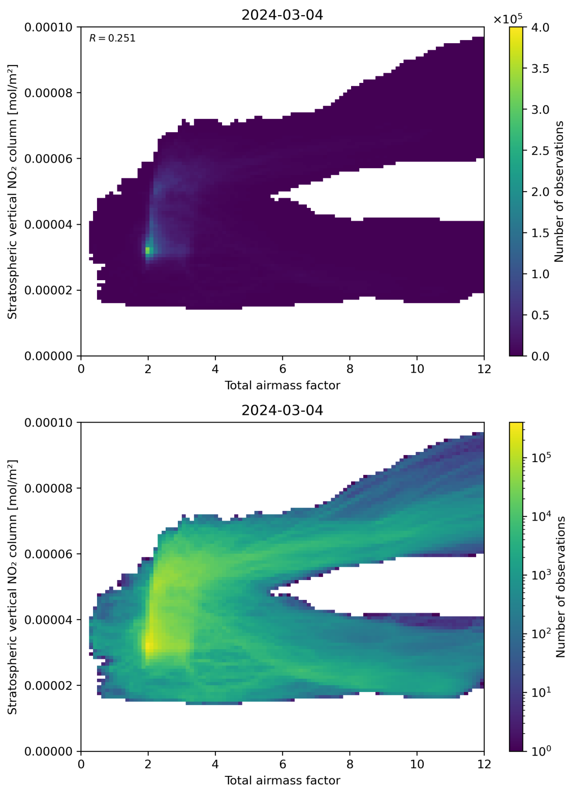
Figure 64: Scatter density plot of “Total airmass factor” against “Stratospheric vertical NO 2 column” for 2024-03-04 to 2024-03-05.
