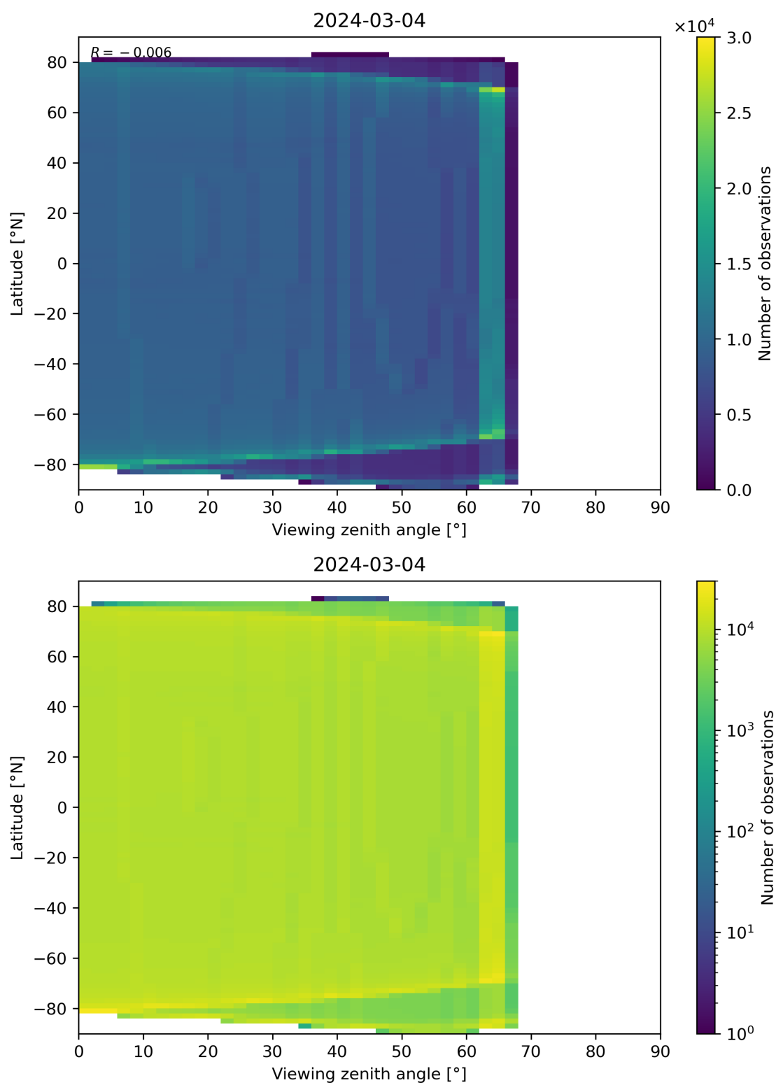
Figure 163: Scatter density plot of “Viewing zenith angle” against “Latitude” for 2024-03-04 to 2024-03-05.
