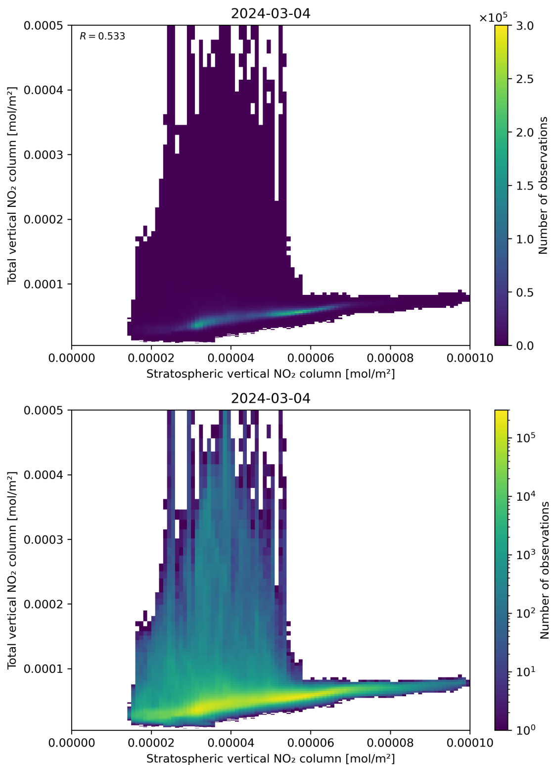
Figure 100: Scatter density plot of “Stratospheric vertical NO 2 column” against “Total vertical NO 2 column” for 2024-03-04 to 2024-03-05.
