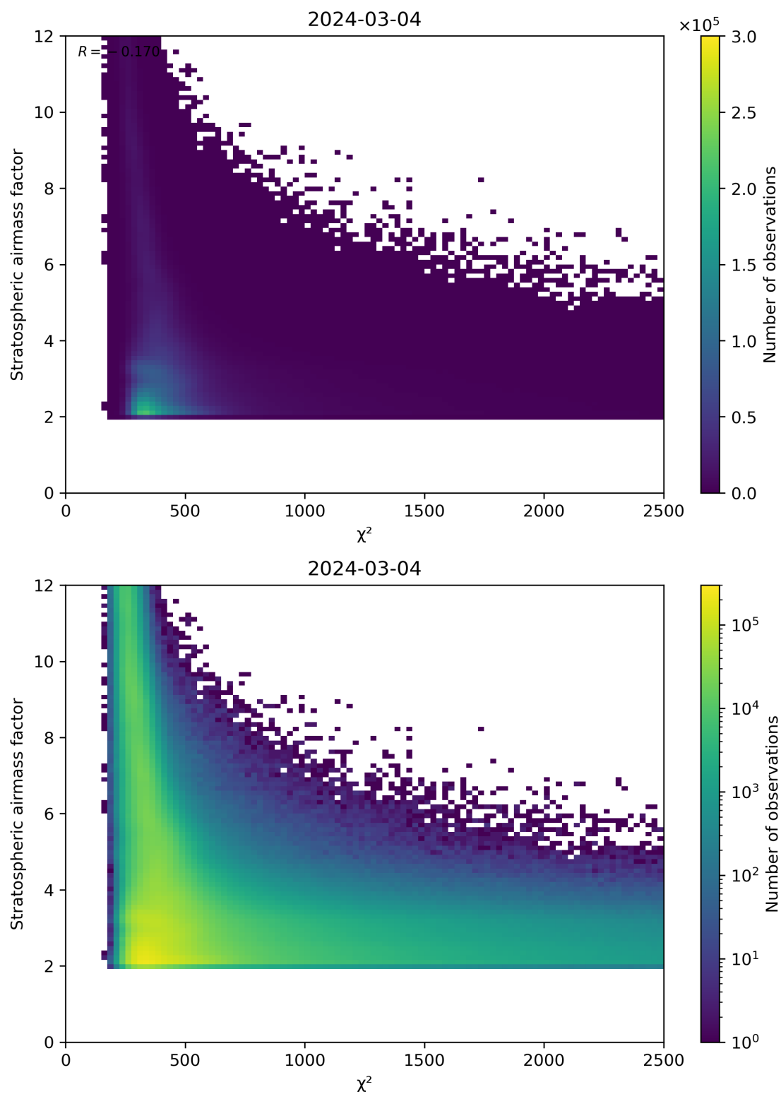
Figure 81: Scatter density plot of “ \chi^2 ” against “Stratospheric airmass factor” for 2024-03-04 to 2024-03-05.
