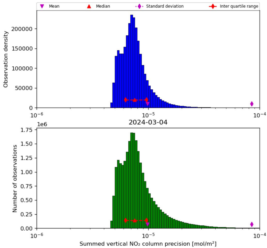
Figure 41: Histogram of “Summed vertical NO 2 column precision” for 2024-03-04 to 2024-03-05
