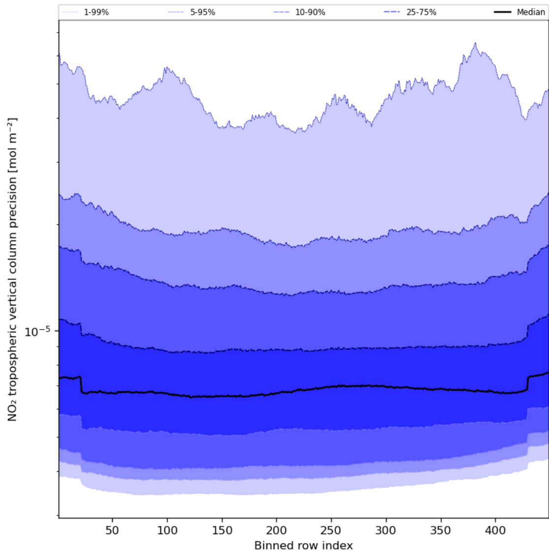
Figure 47: Along track statistics of “NO 2 tropospheric vertical column precision” for 2024-03-04 to 2024-03-05
