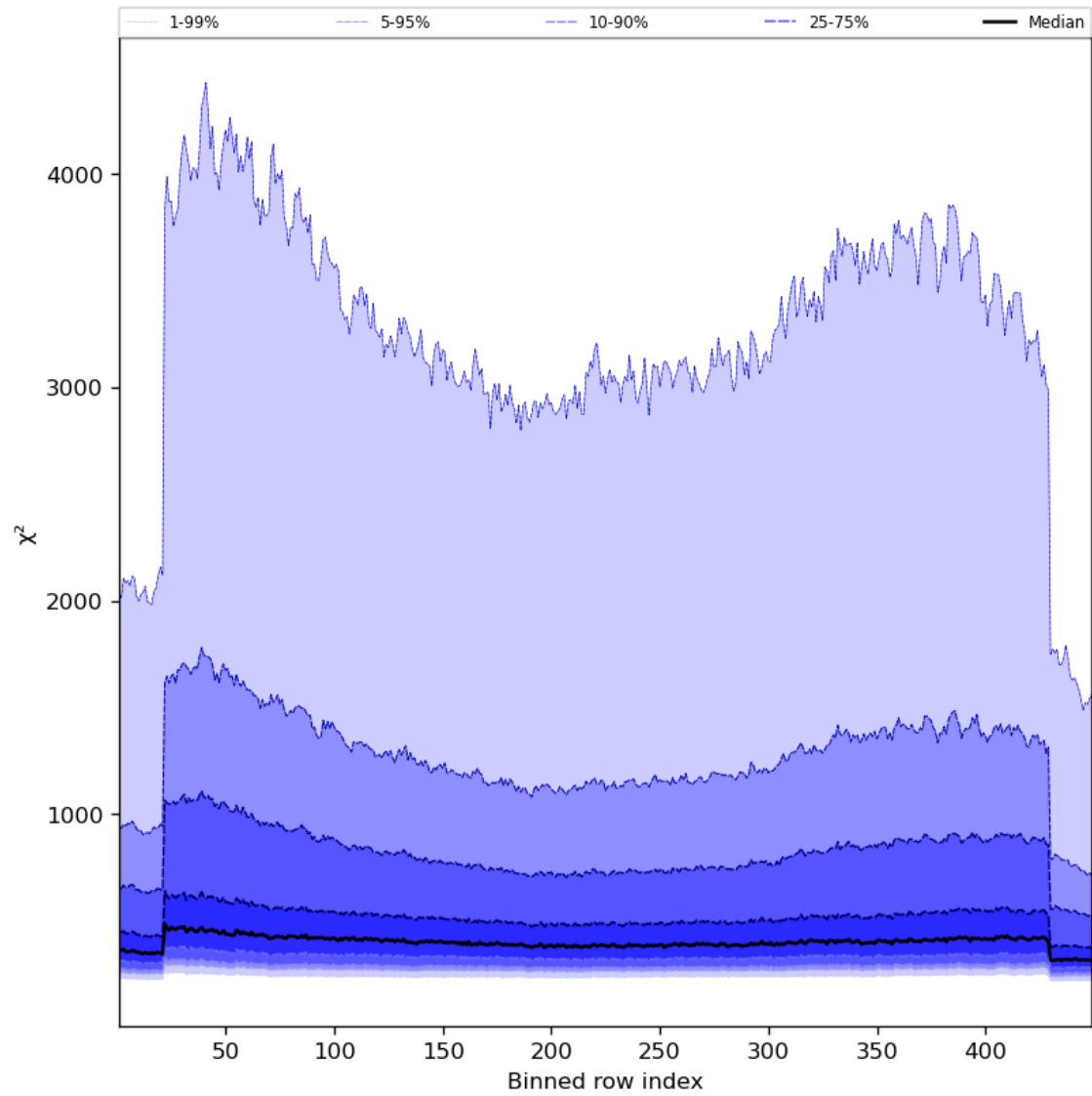
Figure 59: Along track statistics of “ \chi^2 ” for 2024-03-04 to 2024-03-05
