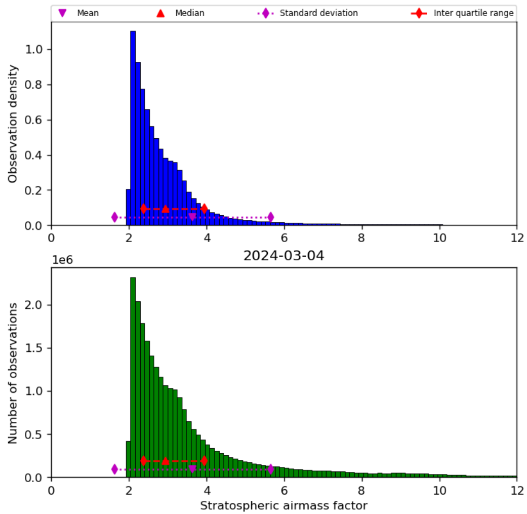
Figure 44: Histogram of “Stratospheric airmass factor” for 2024-03-04 to 2024-03-05
