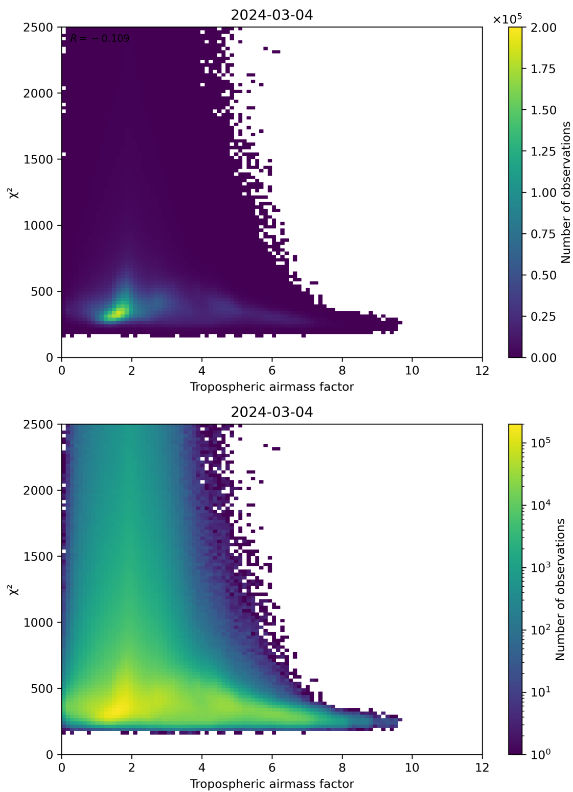
Figure 73: Scatter density plot of “Tropospheric airmass factor” against “ \chi^2 ” for 2024-03-04 to 2024-03-05.
