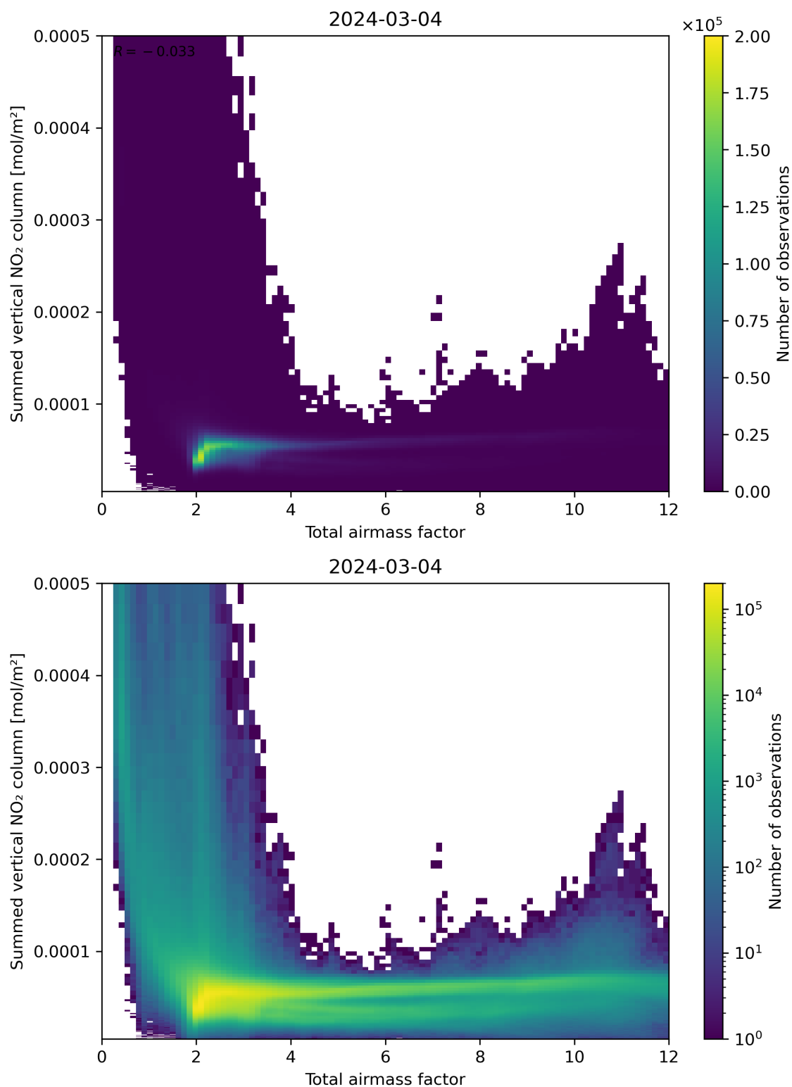
Figure 65: Scatter density plot of “Total airmass factor” against “Summed vertical NO 2 column” for 2024-03-04 to 2024-03-05.
