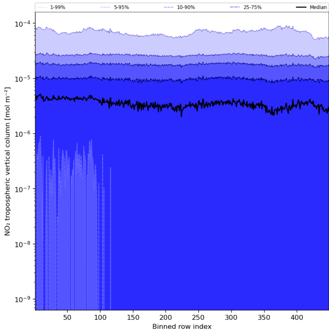
Figure 46: Along track statistics of “NO 2 tropospheric vertical column” for 2024-03-04 to 2024-03-05
