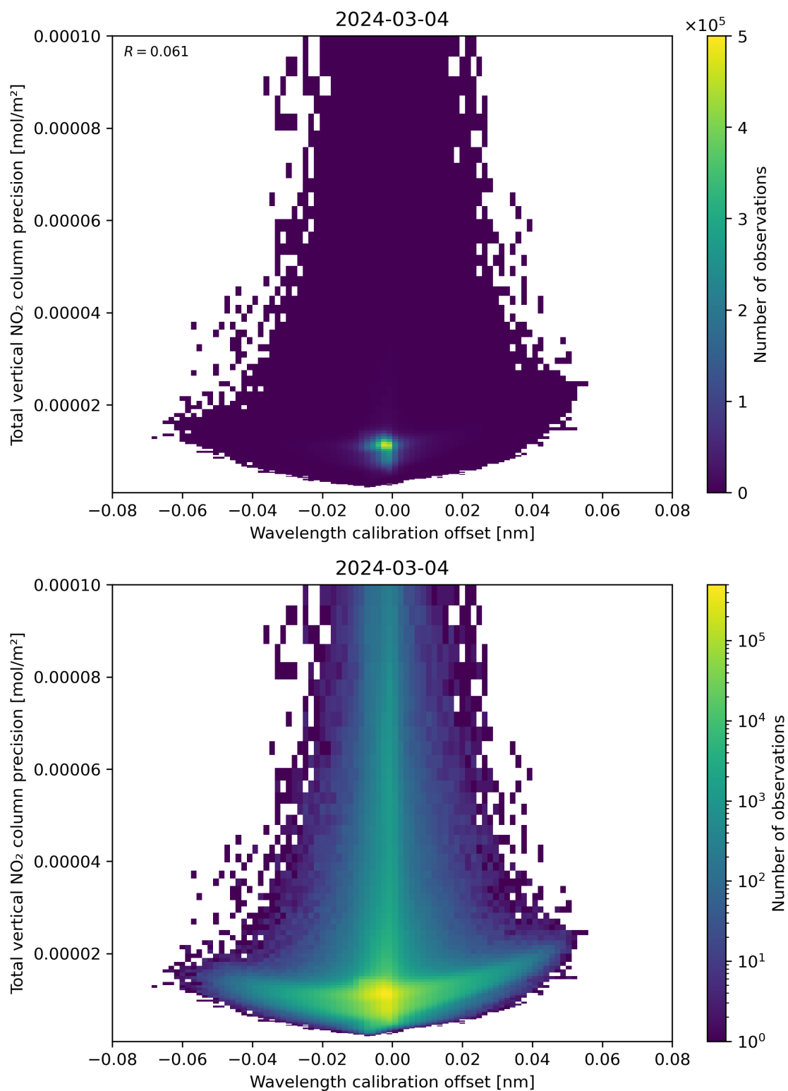
Figure 180: Scatter density plot of “Wavelength calibration offset” against “Total vertical NO 2 column precision” for 2024-03-04 to 2024-03-05.
