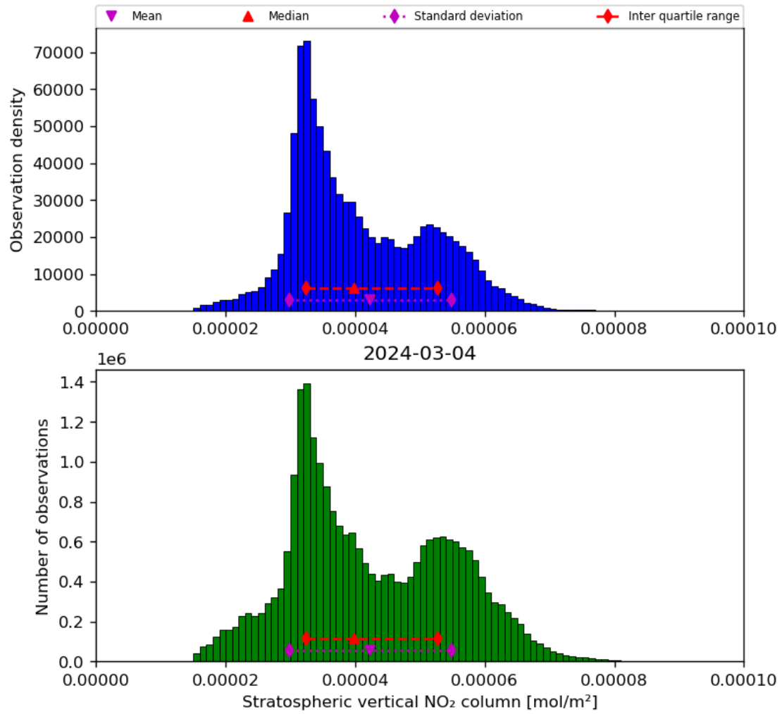
Figure 36: Histogram of “Stratospheric vertical NO 2 column” for 2024-03-04 to 2024-03-05
