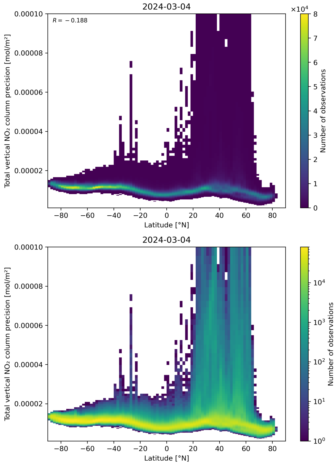
Figure 91: Scatter density plot of “Latitude” against “Total vertical NO 2 column precision” for 2024-03-04 to 2024-03-05.
