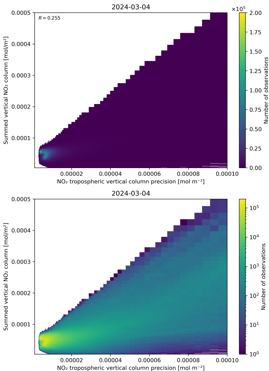
Figure 136: Scatter density plot of “NO 2 tropospheric vertical column precision” against “Summed vertical NO 2 column” for 2024-03-04 to 2024-03-05.
