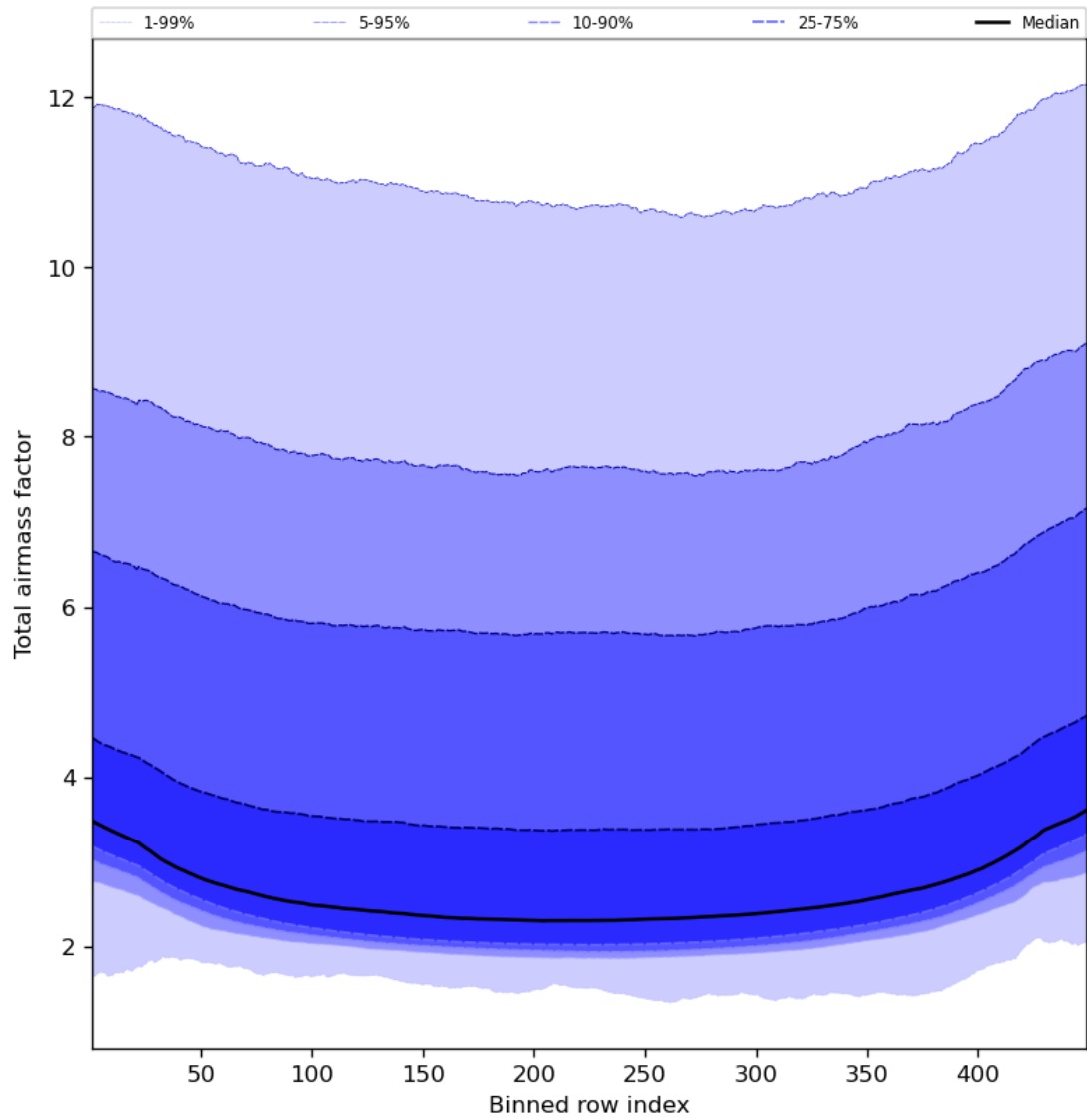
Figure 49: Along track statistics of “Total airmass factor” for 2024-03-04 to 2024-03-05
