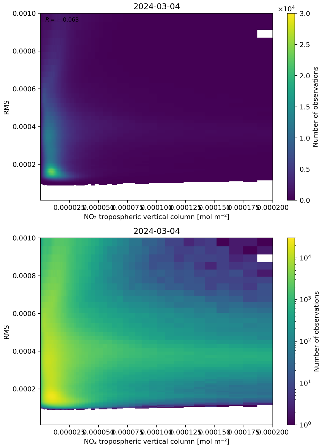
Figure 142: Scatter density plot of “NO 2 tropospheric vertical column” against “RMS” for 2024-03-04 to 2024-03-05.
