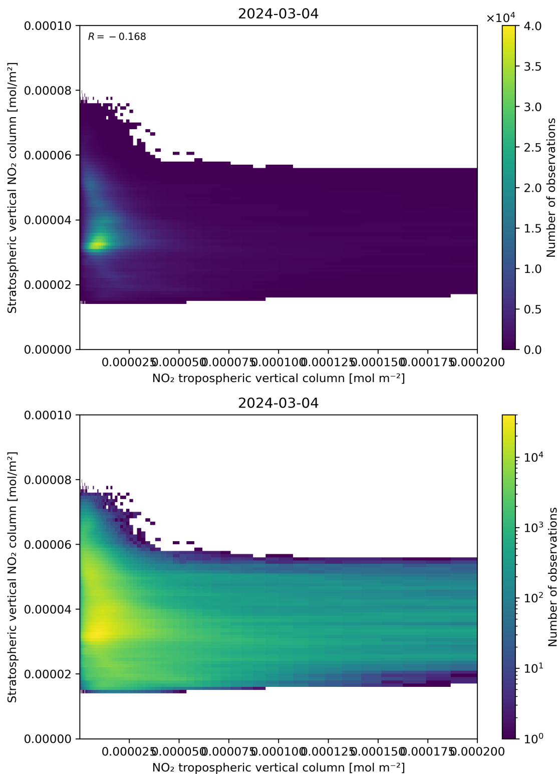
Figure 125: Scatter density plot of “NO 2 tropospheric vertical column” against “Stratospheric vertical NO 2 column” for 2024-03-04 to 2024-03-05.
