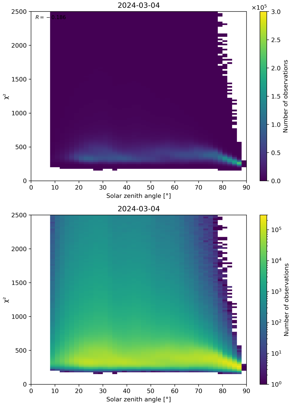
Figure 148: Scatter density plot of “Solar zenith angle” against “ \chi^2 ” for 2024-03-04 to 2024-03-05.
