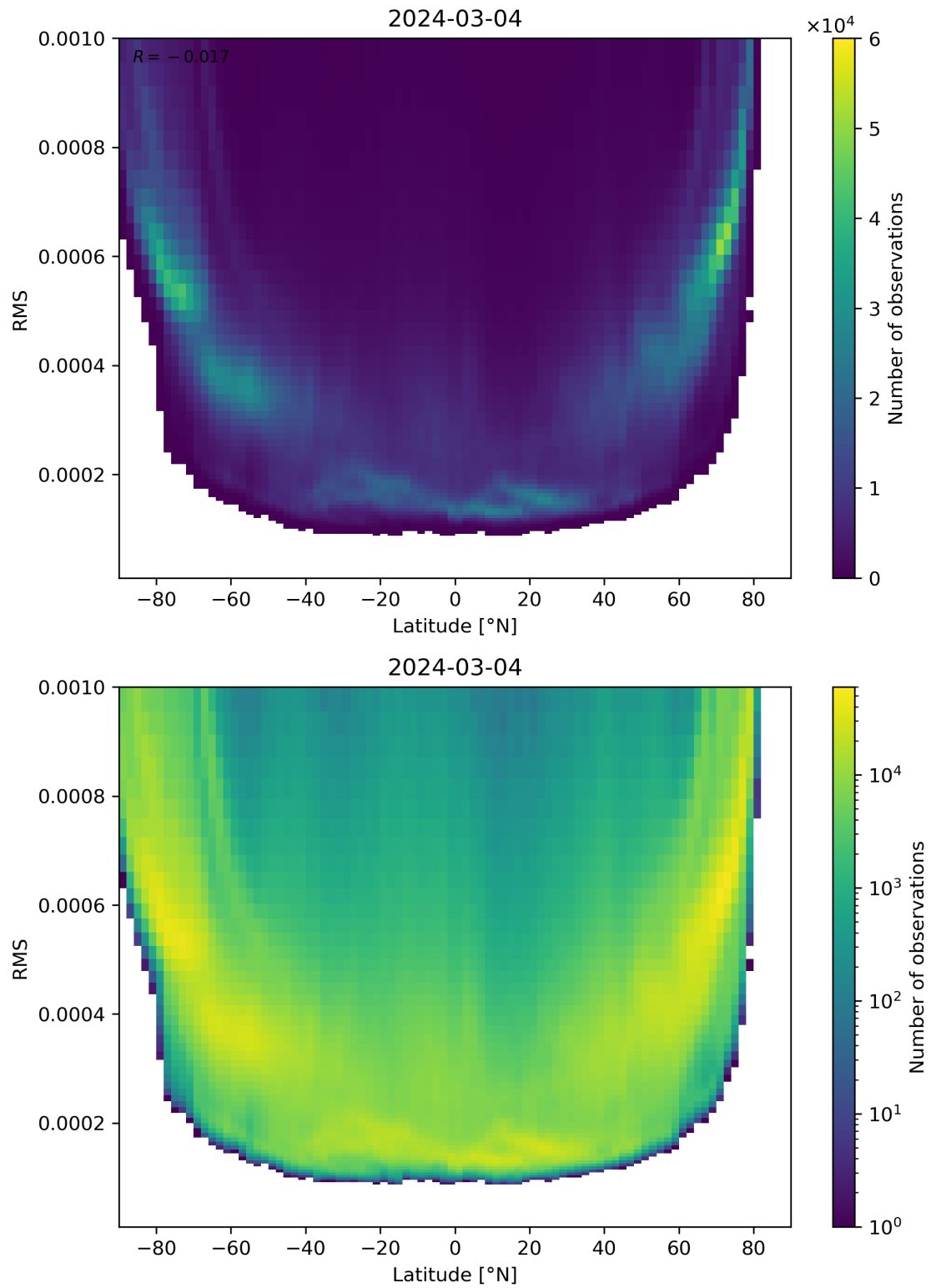
Figure 94: Scatter density plot of “Latitude” against “RMS” for 2024-03-04 to 2024-03-05.
