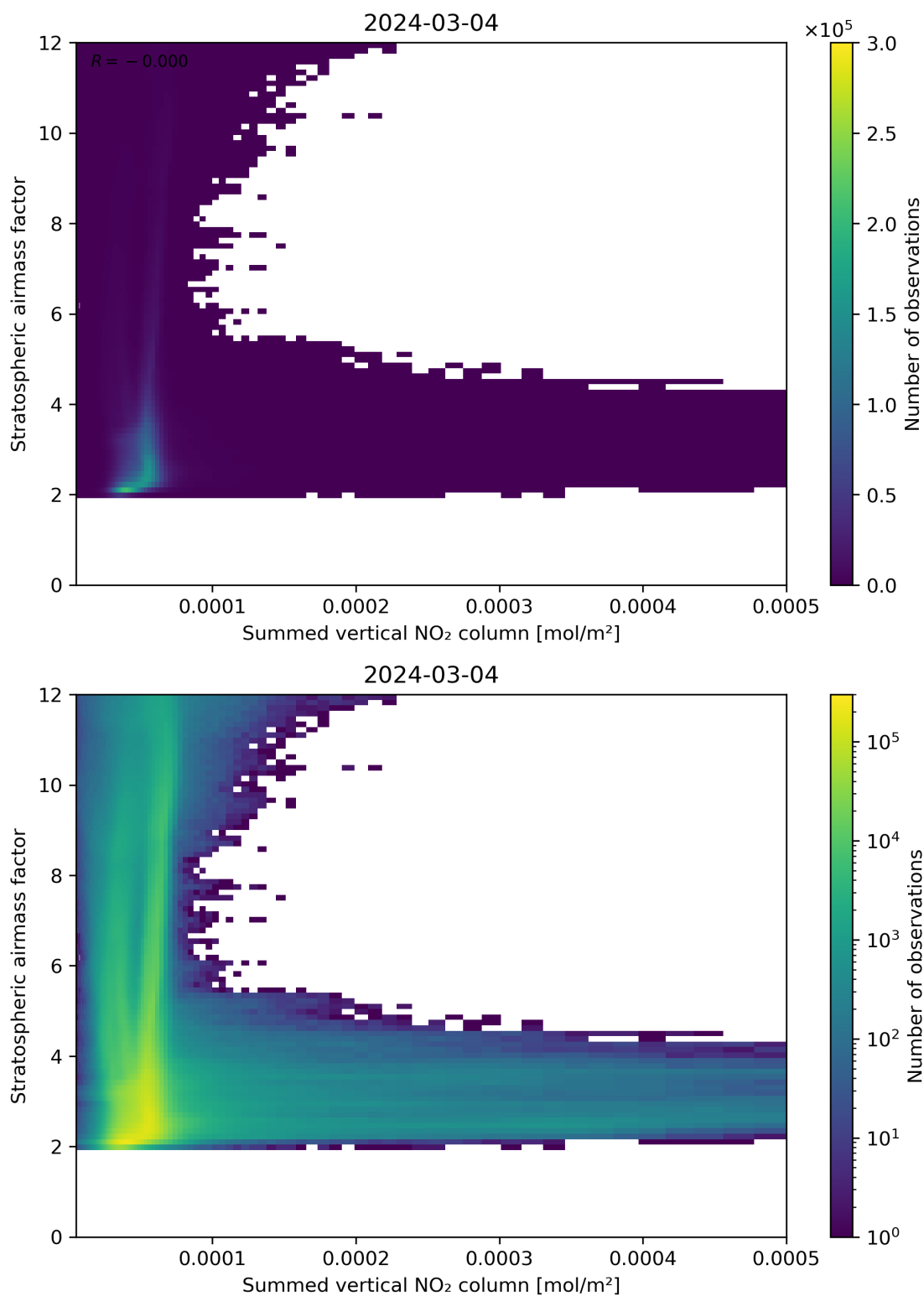
Figure 103: Scatter density plot of “Summed vertical NO 2 column” against “Stratospheric air mass factor” for 2024-03-04 to 2024-03-05.
