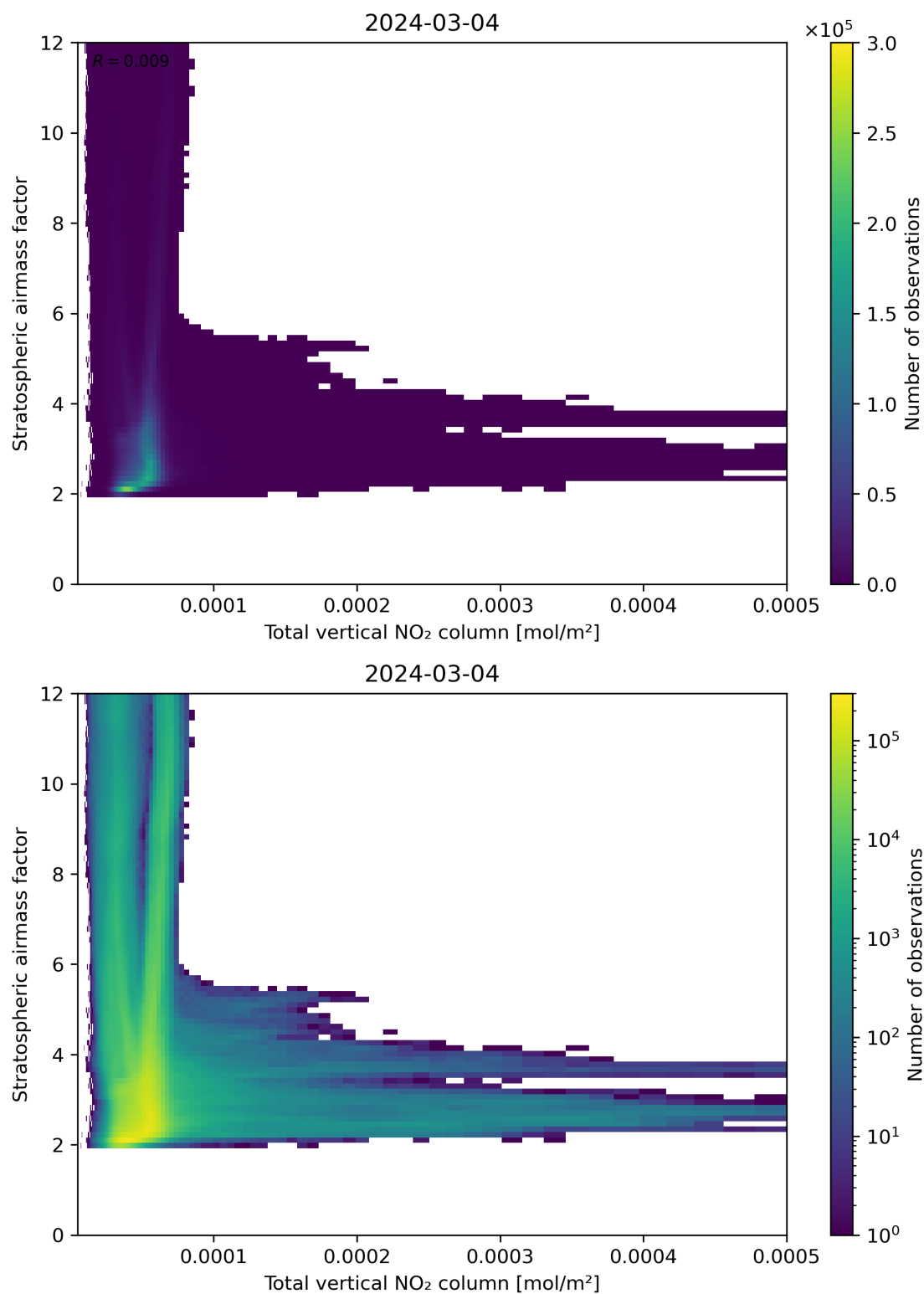
Figure 110: Scatter density plot of “Total vertical NO 2 column” against “Stratospheric air mass factor” for 2024-03-04 to 2024-03-05.
