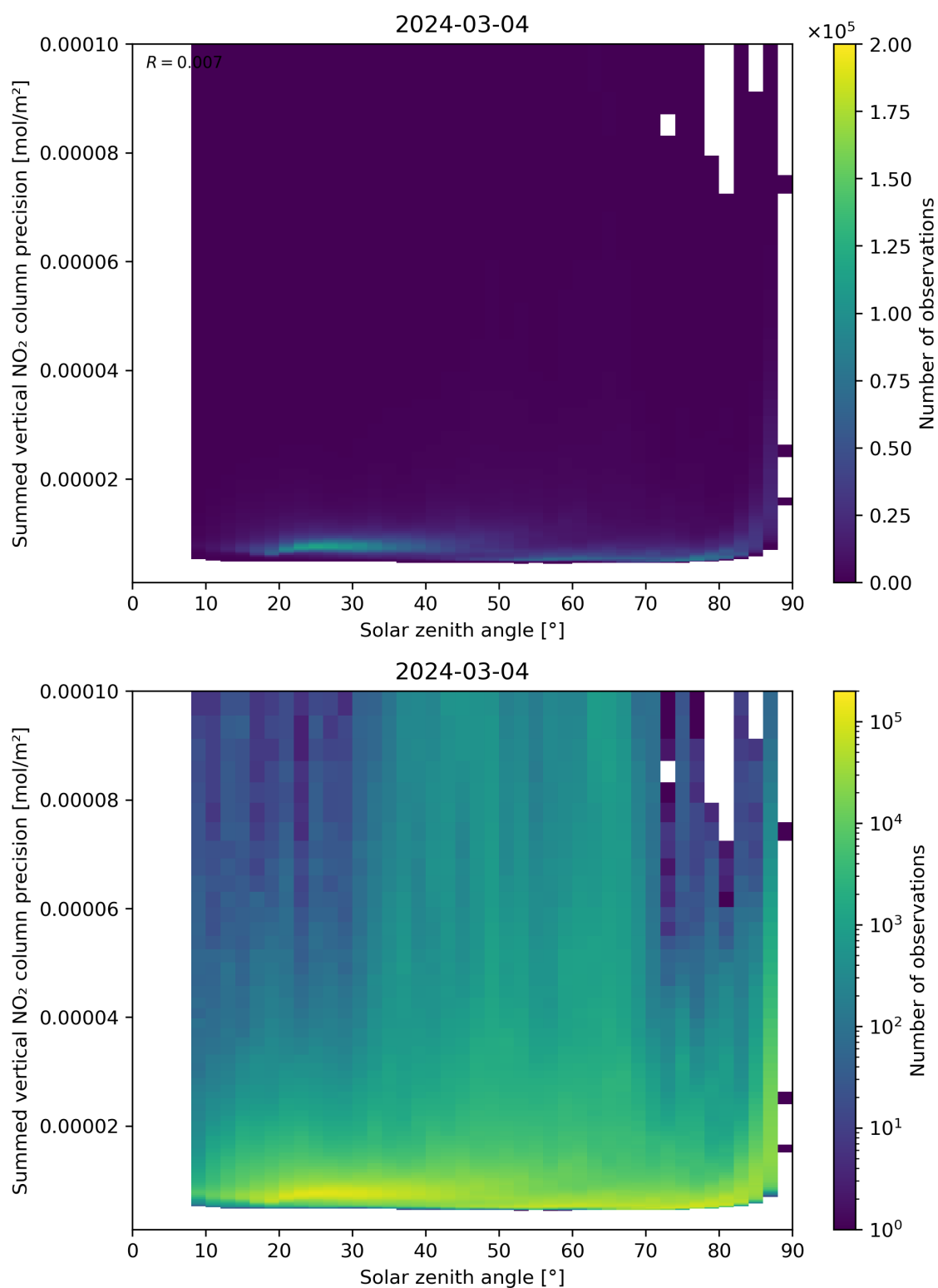
Figure 152: Scatter density plot of “Solar zenith angle” against “Summed vertical NO 2 column precision” for 2024-03-04 to 2024-03-05.
