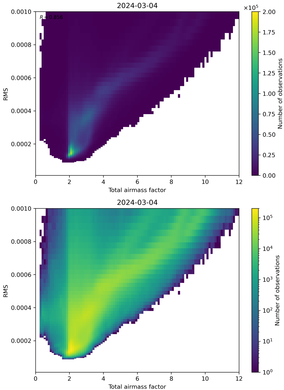
Figure 69: Scatter density plot of “Total airmass factor” against “RMS” for 2024-03-04 to 2024-03-05.
