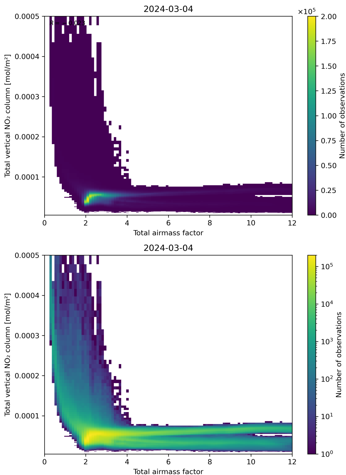
Figure 67: Scatter density plot of “Total airmass factor” against “Total vertical NO 2 column” for 2024-03-04 to 2024-03-05.
