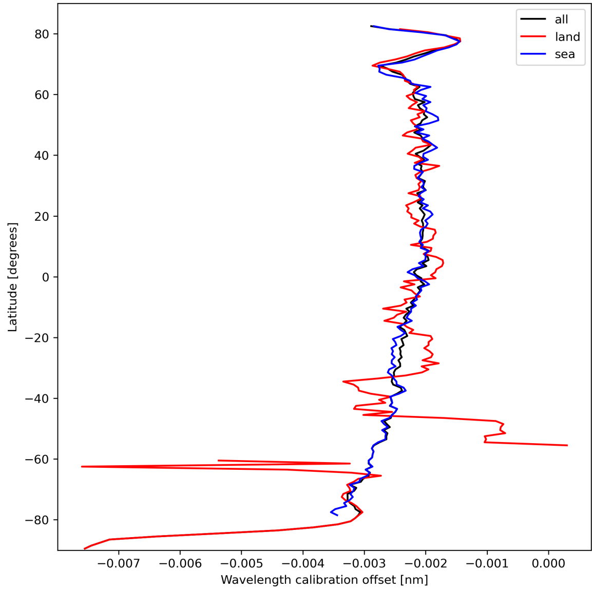
Figure 18: Zonal average of “Wavelength calibration offset” for 2024-03-04 to 2024-03-05.
