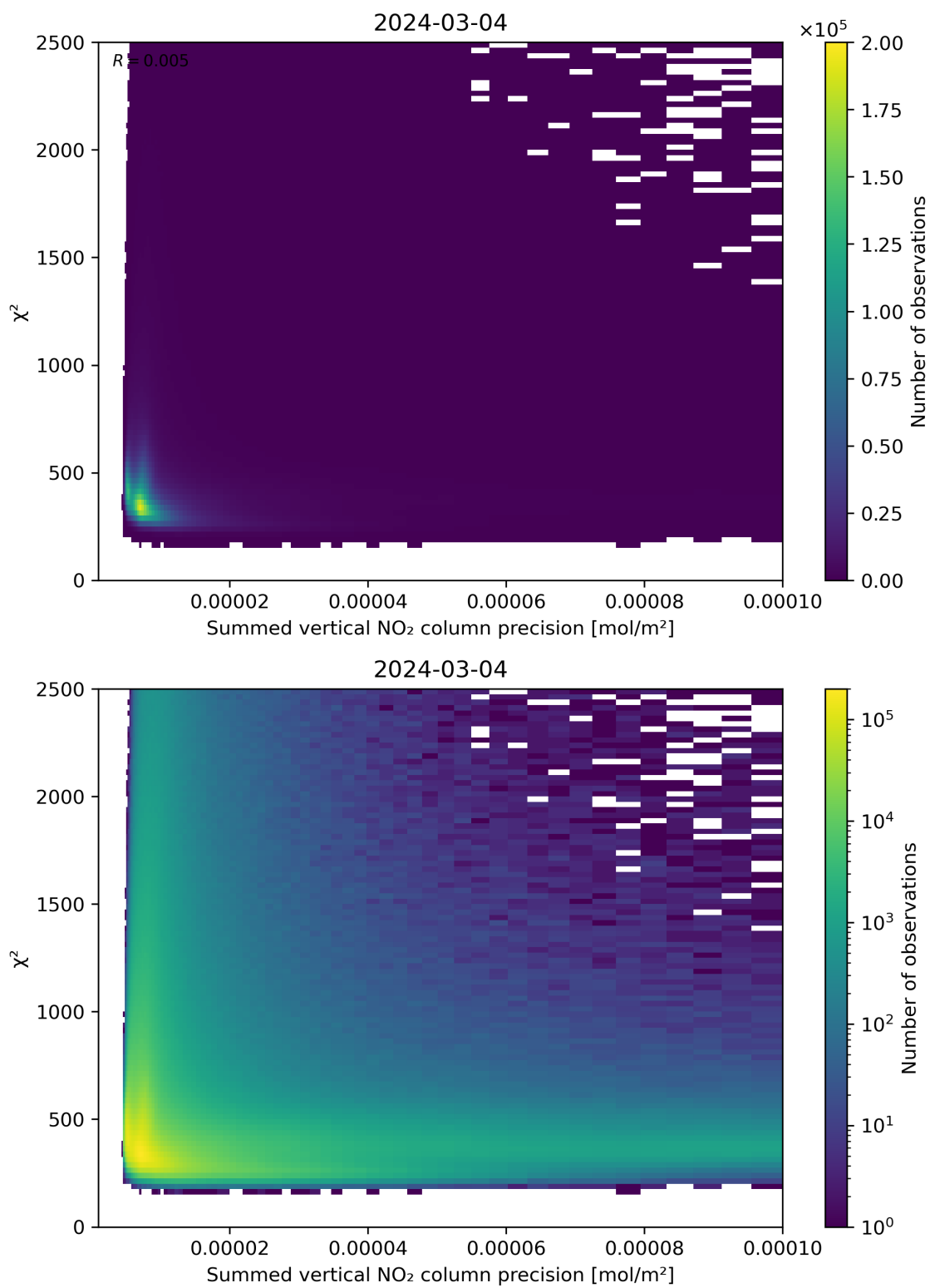
Figure 107: Scatter density plot of “Summed vertical NO 2 column precision” against “ \chi^2 ” for 2024-03-04 to 2024-03-05.
