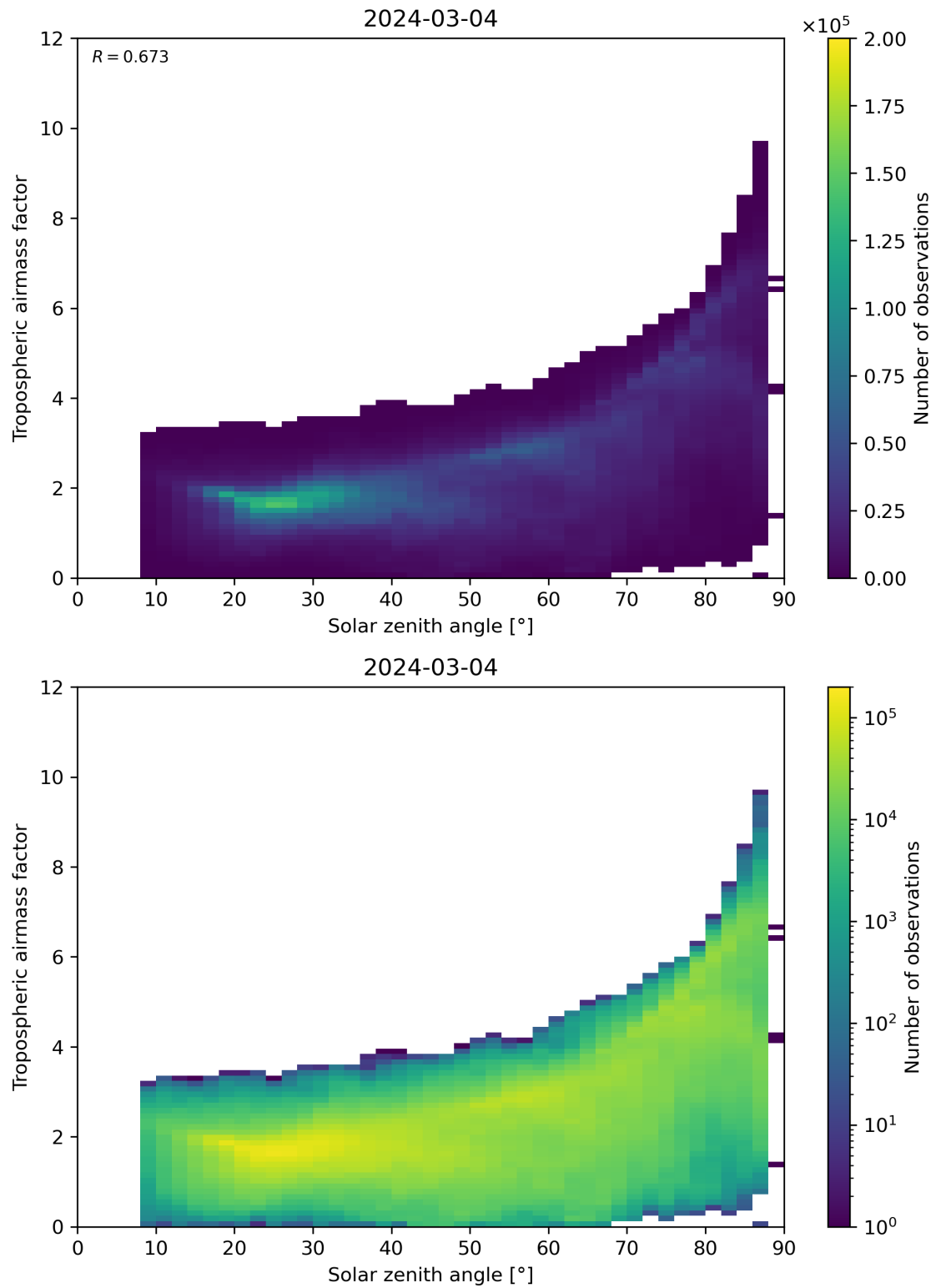
Figure 147: Scatter density plot of “Solar zenith angle” against “Tropospheric airmass factor” for 2024-03-04 to 2024-03-05.
