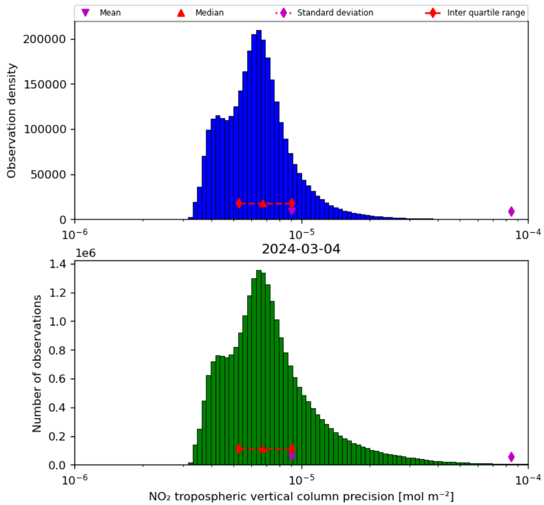
Figure 30: Histogram of “NO 2 tropospheric vertical column precision” for 2024-03-04 to 2024-03-05
