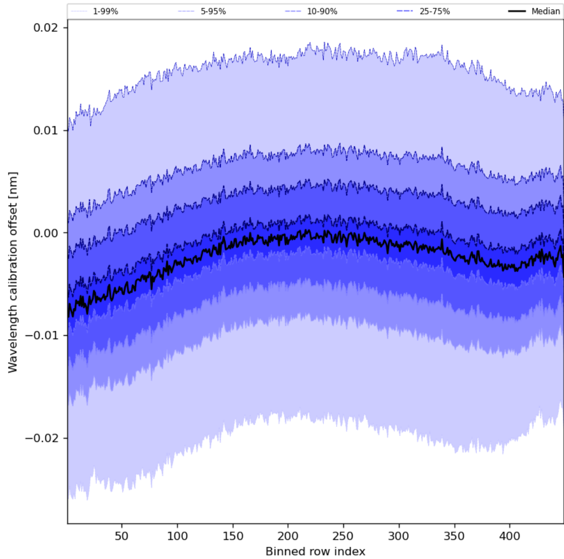
Figure 52: Along track statistics of “Wavelength calibration offset” for 2024-03-04 to 2024-03-05
