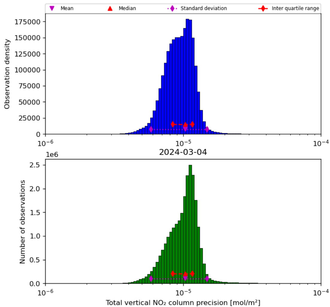
Figure 39: Histogram of “Total vertical NO 2 column precision” for 2024-03-04 to 2024-03-05
