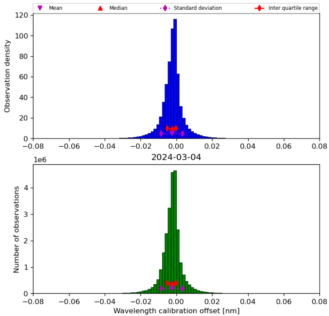
Figure 35: Histogram of “Wavelength calibration offset” for 2024-03-04 to 2024-03-05
