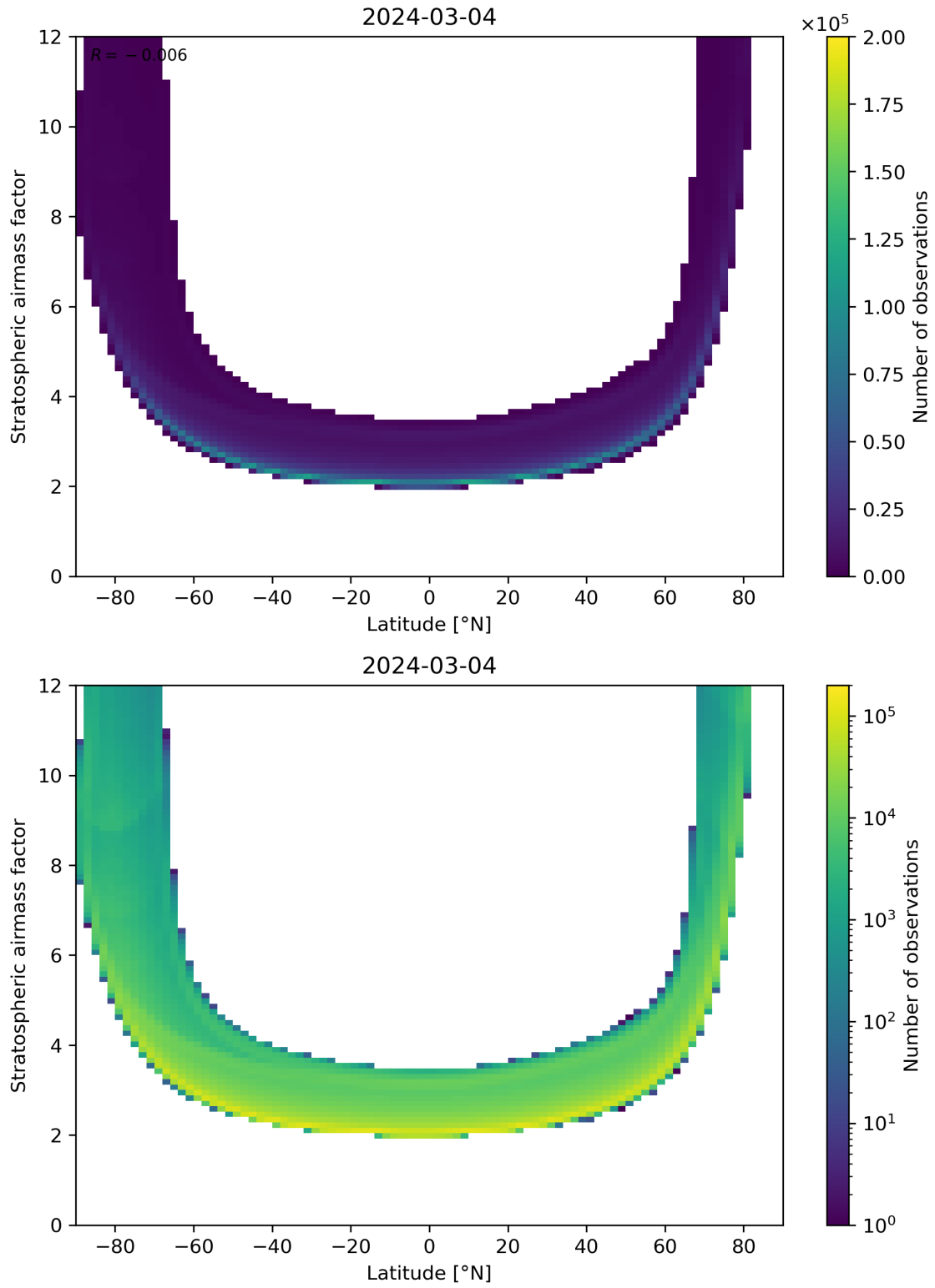
Figure 83: Scatter density plot of “Latitude” against “Stratospheric air mass factor” for 2024-03-04 to 2024-03-05.
