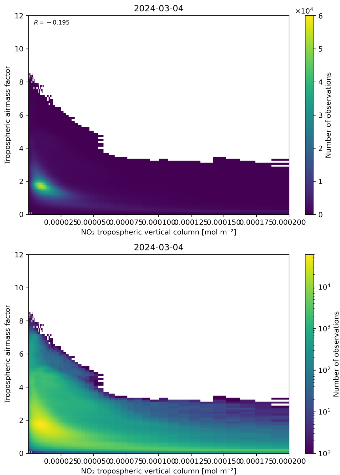
Figure 123: Scatter density plot of “NO 2 tropospheric vertical column” against “Tropospheric airmass factor” for 2024-03-04 to 2024-03-05.
