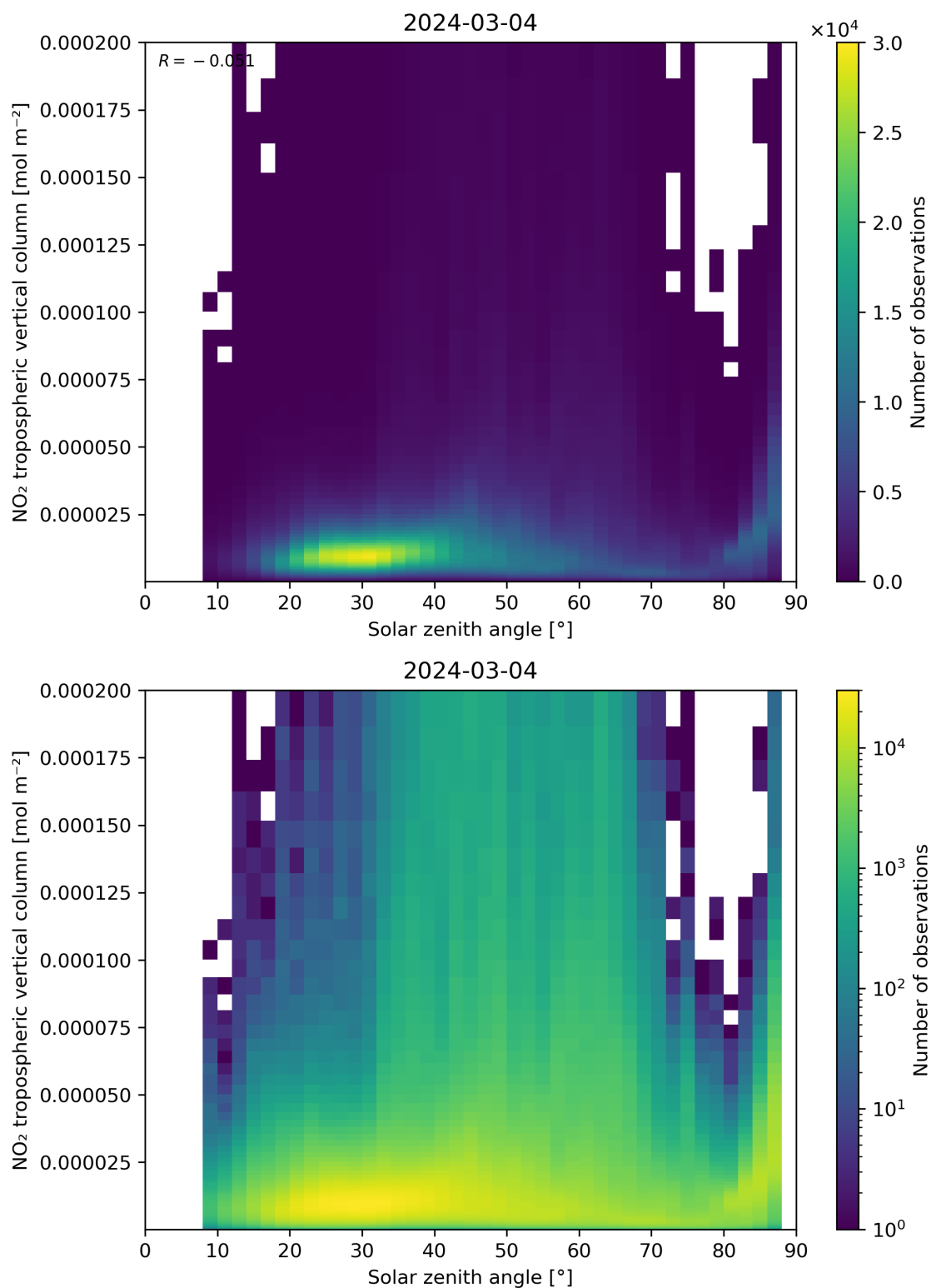
Figure 155: Scatter density plot of “Solar zenith angle” against “NO 2 tropospheric vertical column” for 2024-03-04 to 2024-03-05.
