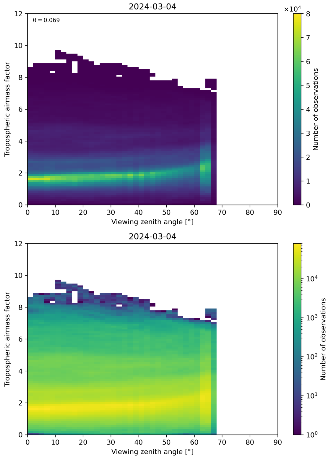
Figure 161: Scatter density plot of “Viewing zenith angle” against “Tropospheric airmass factor” for 2024-03-04 to 2024-03-05.
