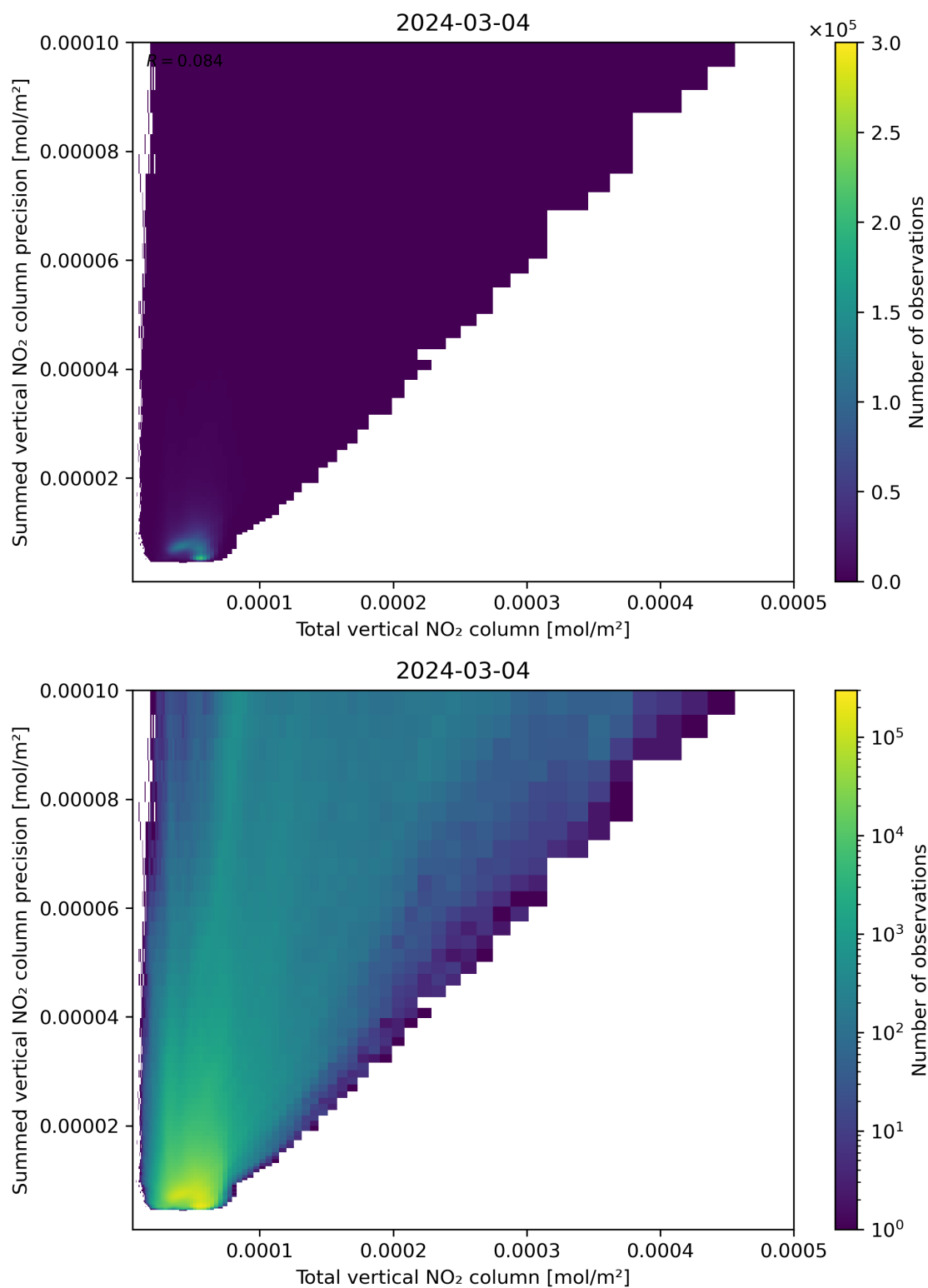
Figure 113: Scatter density plot of “Total vertical NO 2 column” against “Summed vertical NO 2 column precision” for 2024-03-04 to 2024-03-05.
