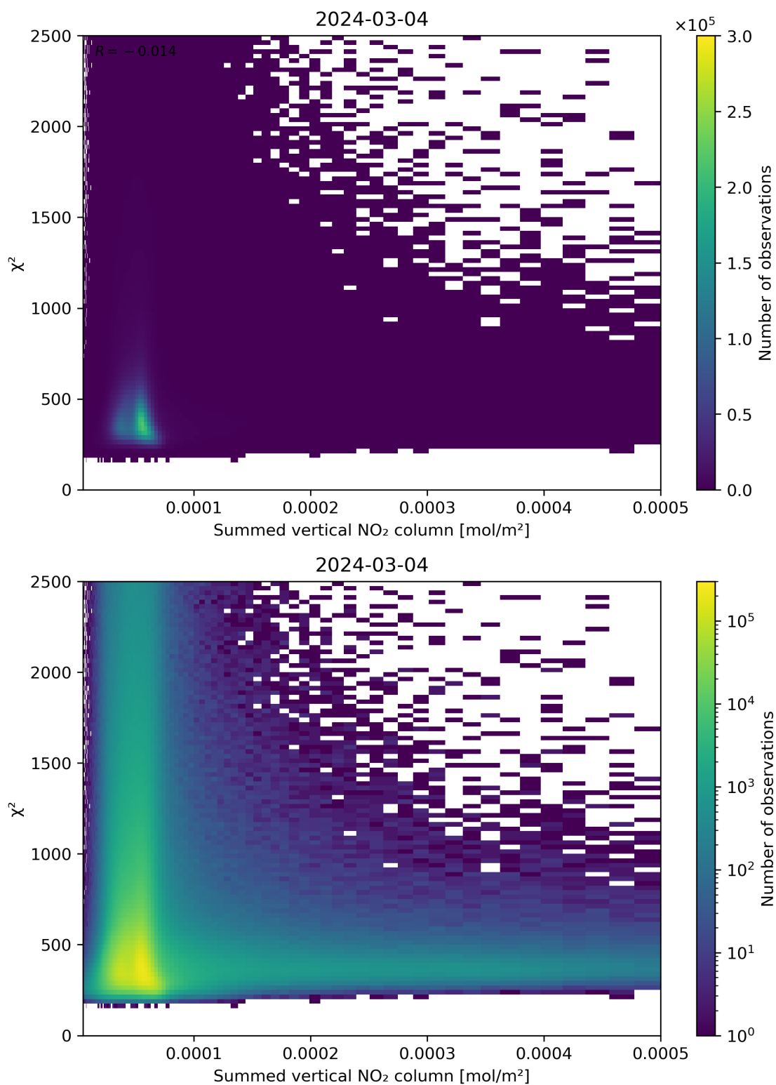
Figure 104: Scatter density plot of “Summed vertical NO 2 column” against “ \chi^2 ” for 2024-03-04 to 2024-03-05.
