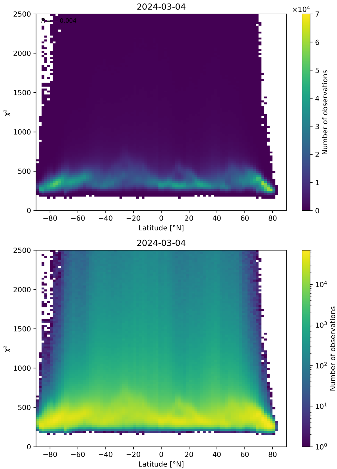
Figure 86: Scatter density plot of “Latitude” against “ \chi^2 ” for 2024-03-04 to 2024-03-05.
