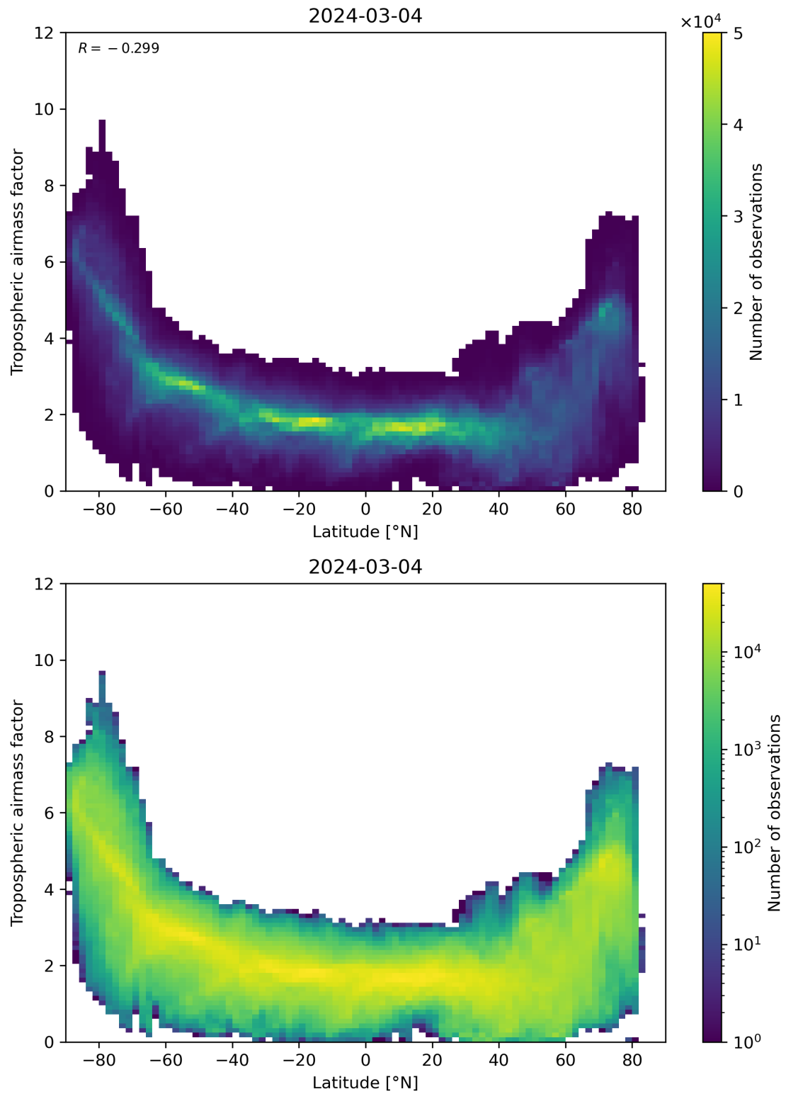
Figure 85: Scatter density plot of “Latitude” against “Tropospheric airmass factor” for 2024-03-04 to 2024-03-05.
