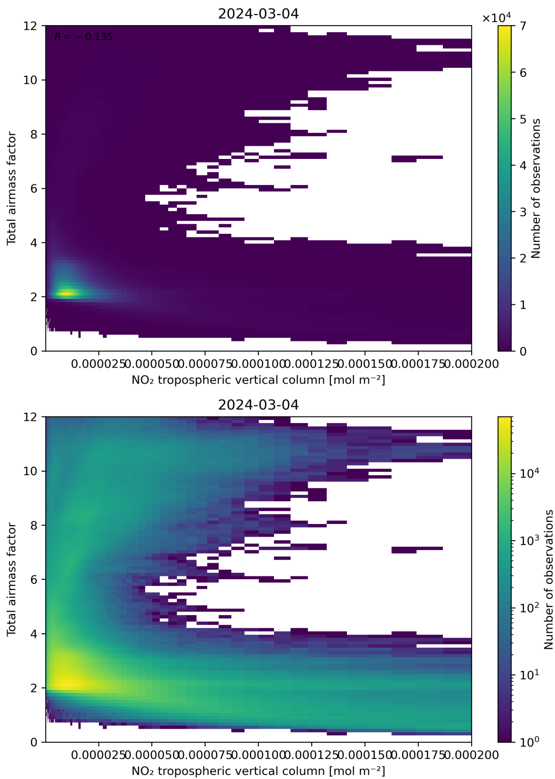
Figure 122: Scatter density plot of “NO 2 tropospheric vertical column” against “Total air mass factor” for 2024-03-04 to 2024-03-05.
