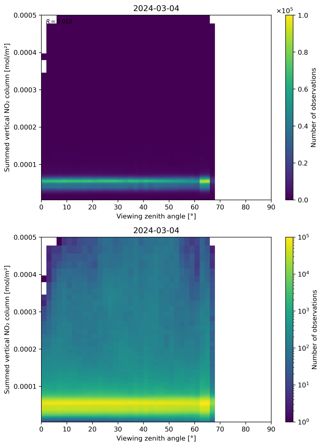
Figure 165: Scatter density plot of “Viewing zenith angle” against “Summed vertical NO 2 column” for 2024-03-04 to 2024-03-05.
