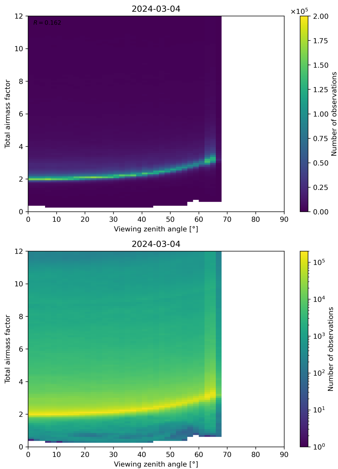
Figure 160: Scatter density plot of “Viewing zenith angle” against “Total airmass factor” for 2024-03-04 to 2024-03-05.
