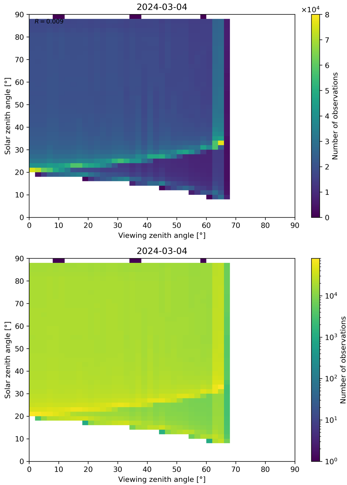
Figure 172: Scatter density plot of “Viewing zenith angle” against “Solar zenith angle” for 2024-03-04 to 2024-03-05.
