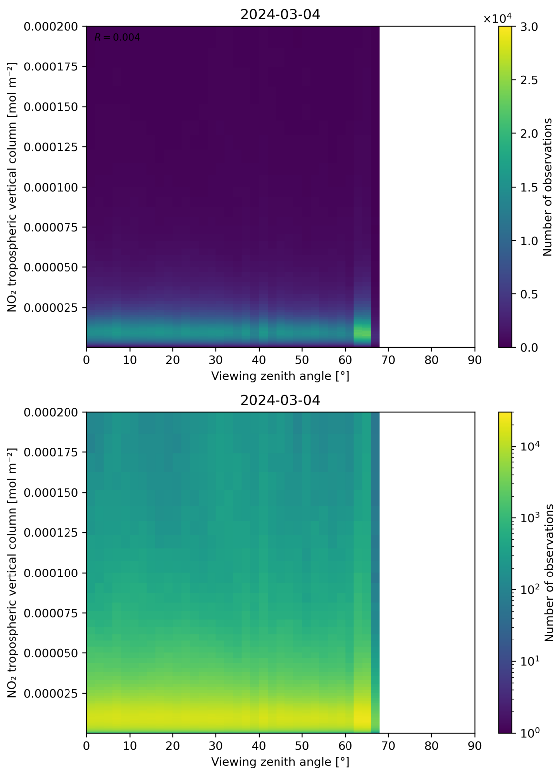
Figure 169: Scatter density plot of “Viewing zenith angle” against “NO 2 tropospheric vertical column” for 2024-03-04 to 2024-03-05.
