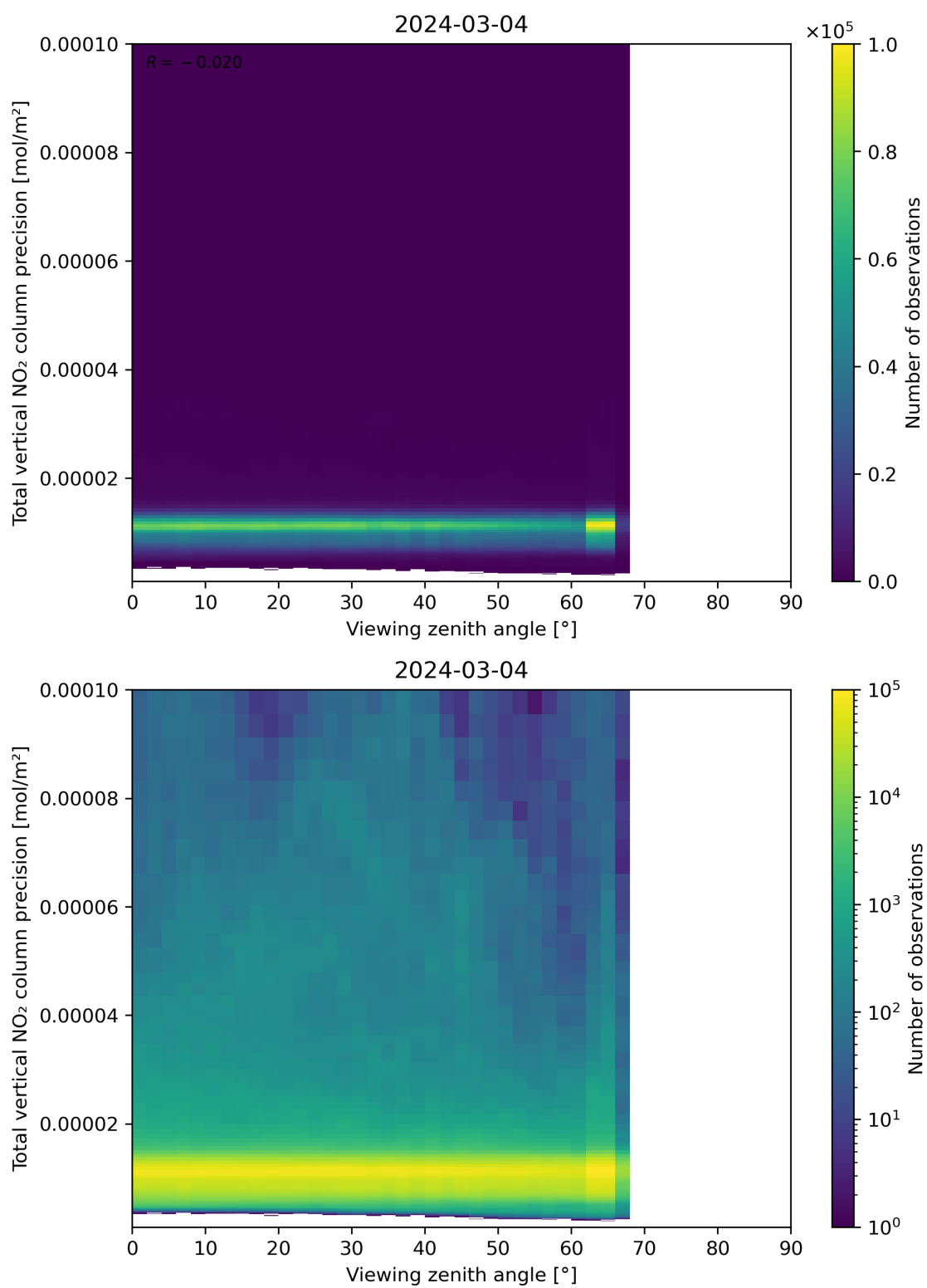
Figure 168: Scatter density plot of “Viewing zenith angle” against “Total vertical NO 2 column precision” for 2024-03-04 to 2024-03-05.
