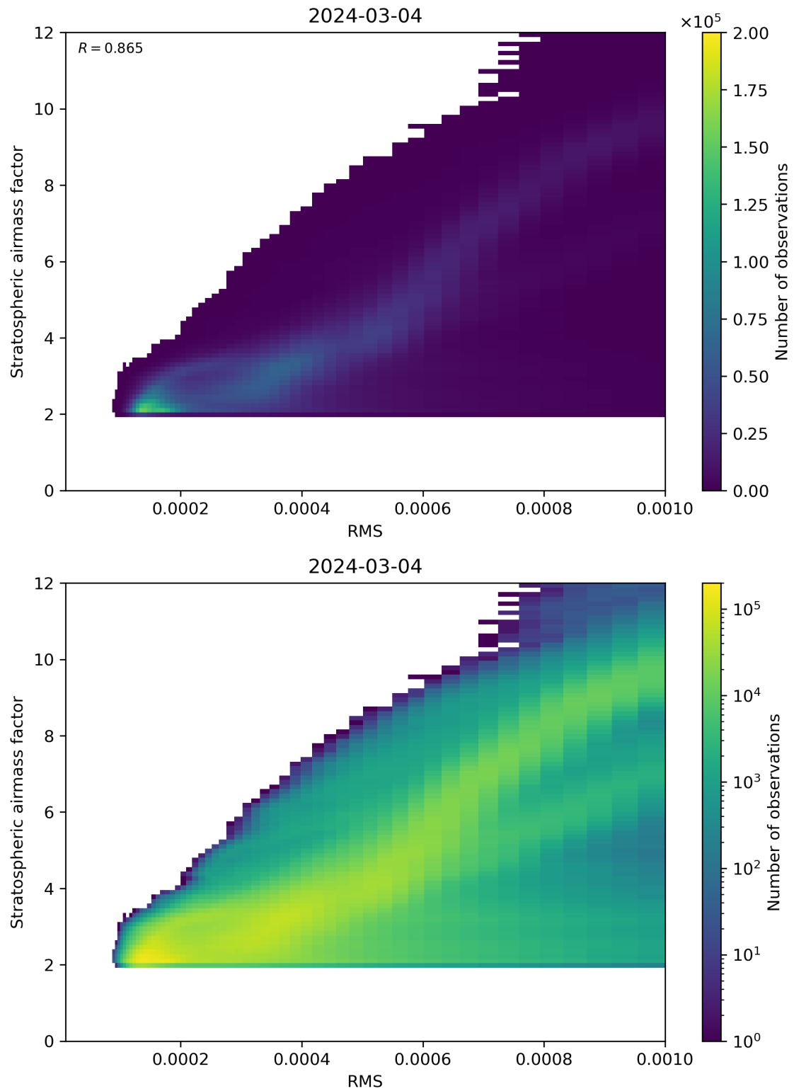
Figure 144: Scatter density plot of “RMS” against “Stratospheric airmass factor” for 2024-03-04 to 2024-03-05.
