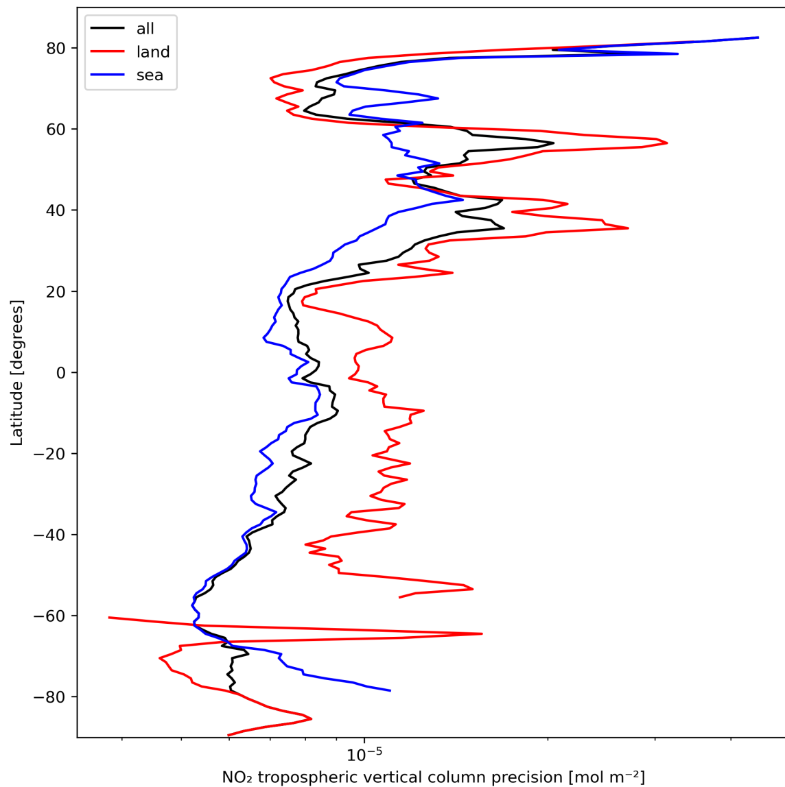
Figure 13: Zonal average of “NO 2 tropospheric vertical column precision” for 2024-03-04 to 2024-03-05.
