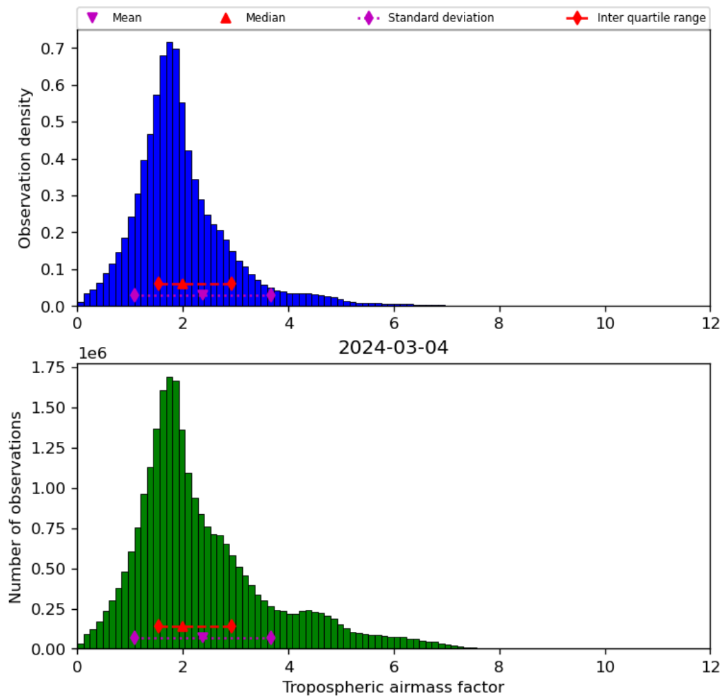
Figure 31: Histogram of “Tropospheric airmass factor” for 2024-03-04 to 2024-03-05
