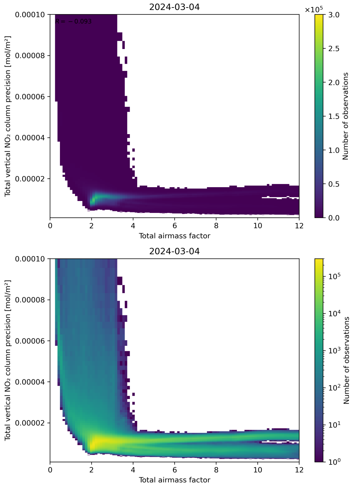
Figure 68: Scatter density plot of “Total airmass factor” against “Total vertical NO 2 column precision” for 2024-03-04 to 2024-03-05.
