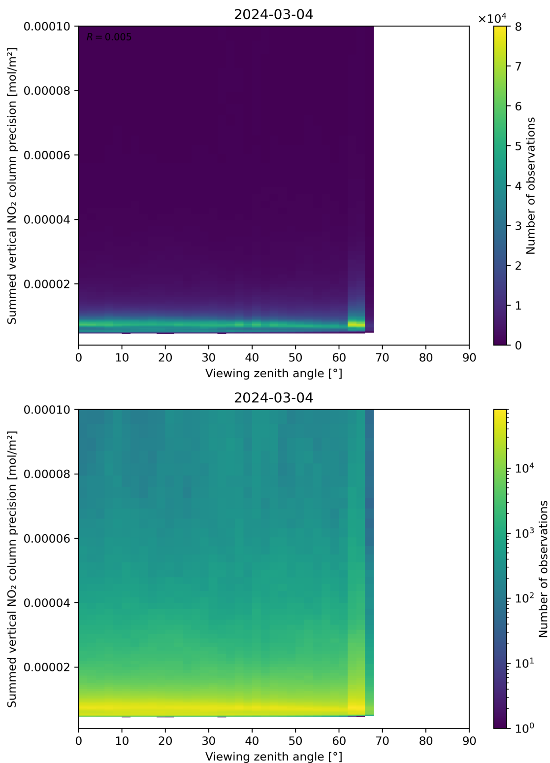
Figure 166: Scatter density plot of “Viewing zenith angle” against “Summed vertical NO 2 column precision” for 2024-03-04 to 2024-03-05.
