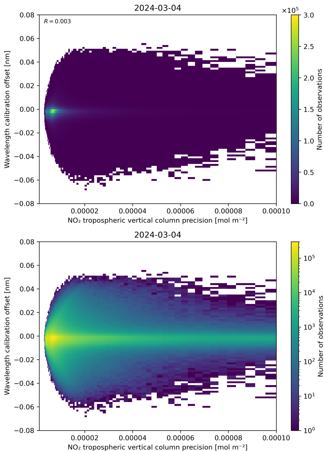
Figure 141: Scatter density plot of “NO 2 tropospheric vertical column precision” against “Wavelength calibration offset” for 2024-03-04 to 2024-03-05.
