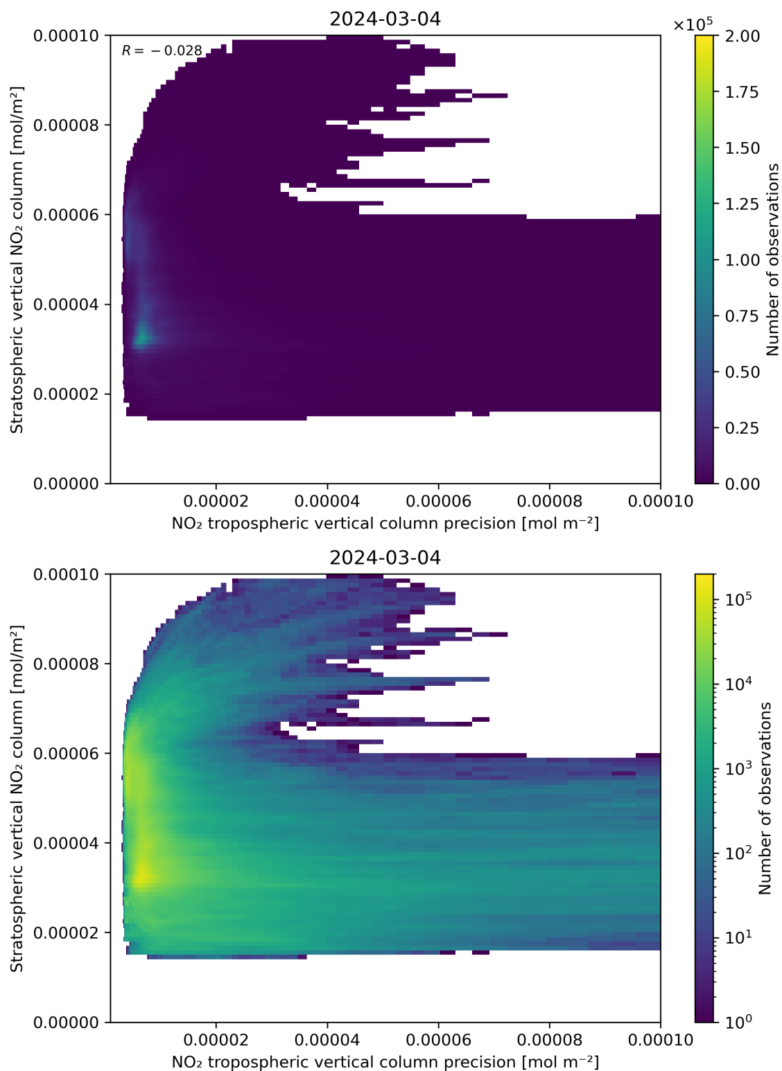
Figure 135: Scatter density plot of “NO 2 tropospheric vertical column precision” against “Stratospheric vertical NO 2 column” for 2024-03-04 to 2024-03-05.
