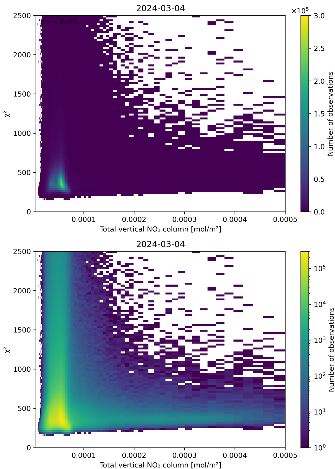
Figure 111: Scatter density plot of “Total vertical NO 2 column” against “ \chi^2 ” for 2024-03-04 to 2024-03-05.
