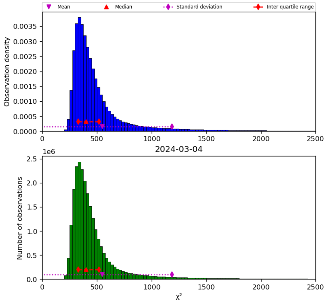
Figure 42: Histogram of “ \chi^2 ” for 2024-03-04 to 2024-03-05
