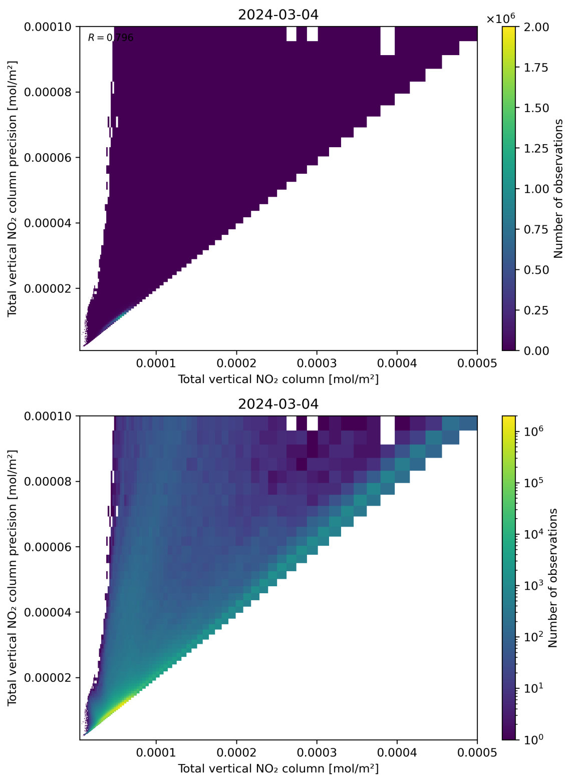
Figure 114: Scatter density plot of “Total vertical NO 2 column” against “Total vertical NO 2 column precision” for 2024-03-04 to 2024-03-05.
