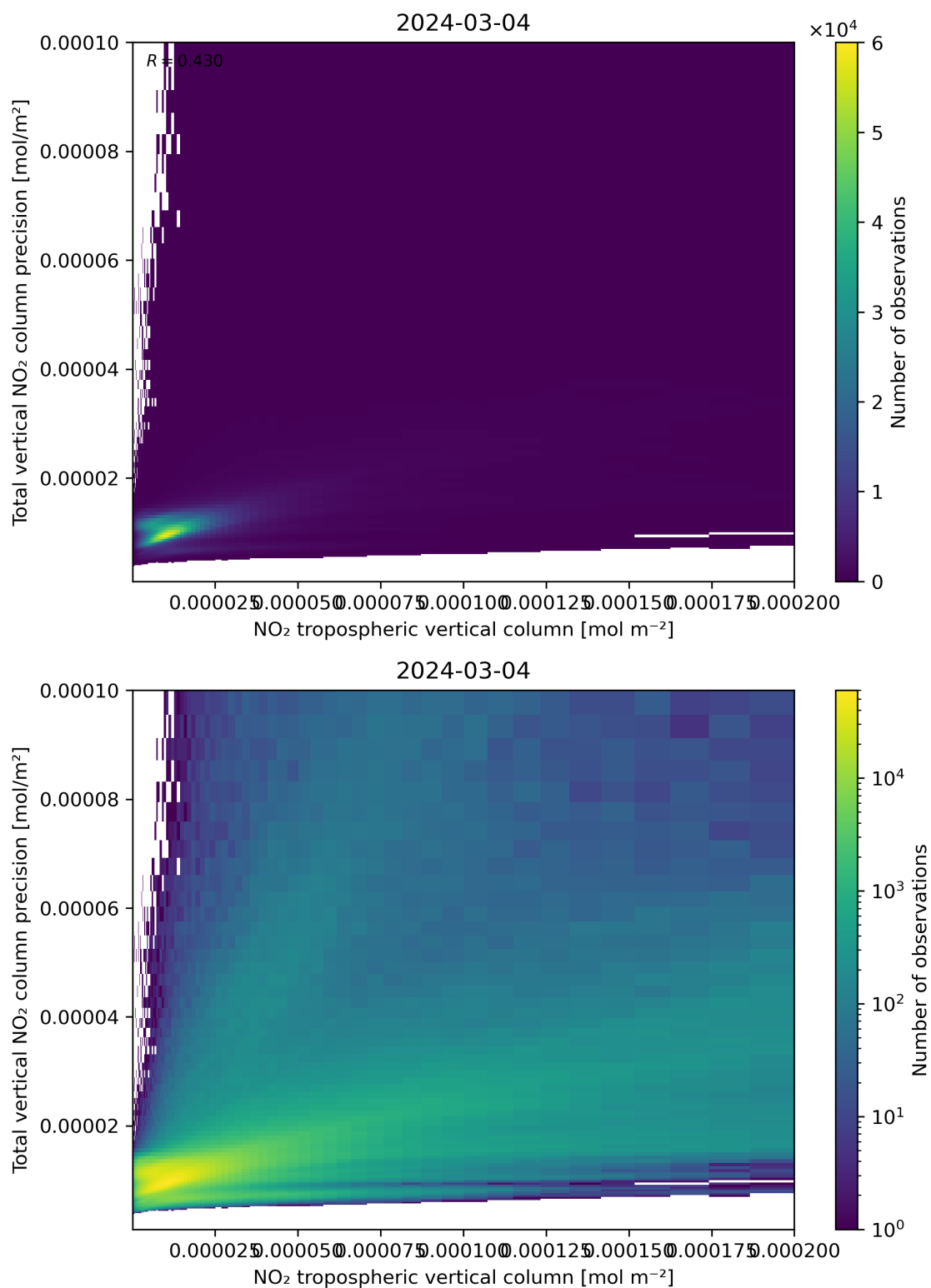
Figure 129: Scatter density plot of “NO 2 tropospheric vertical column” against “Total vertical NO 2 column precision” for 2024-03-04 to 2024-03-05.
