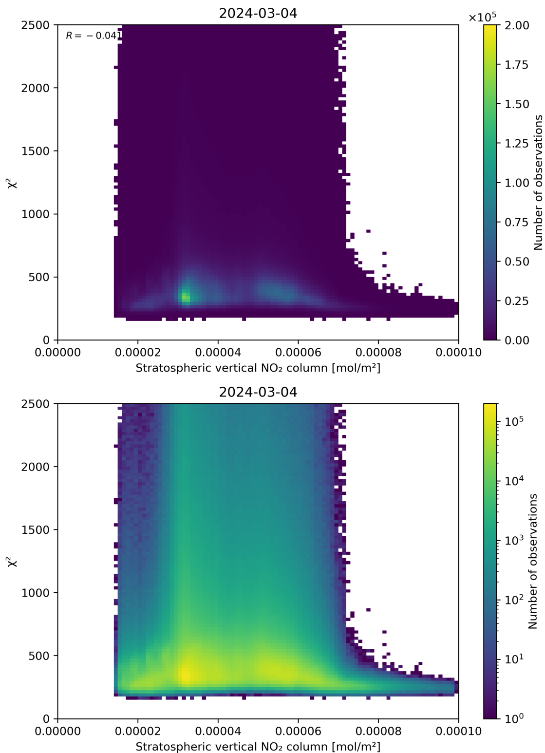
Figure 97: Scatter density plot of “Stratospheric vertical NO 2 column” against “ \chi^2 ” for 2024-03-04 to 2024-03-05.
