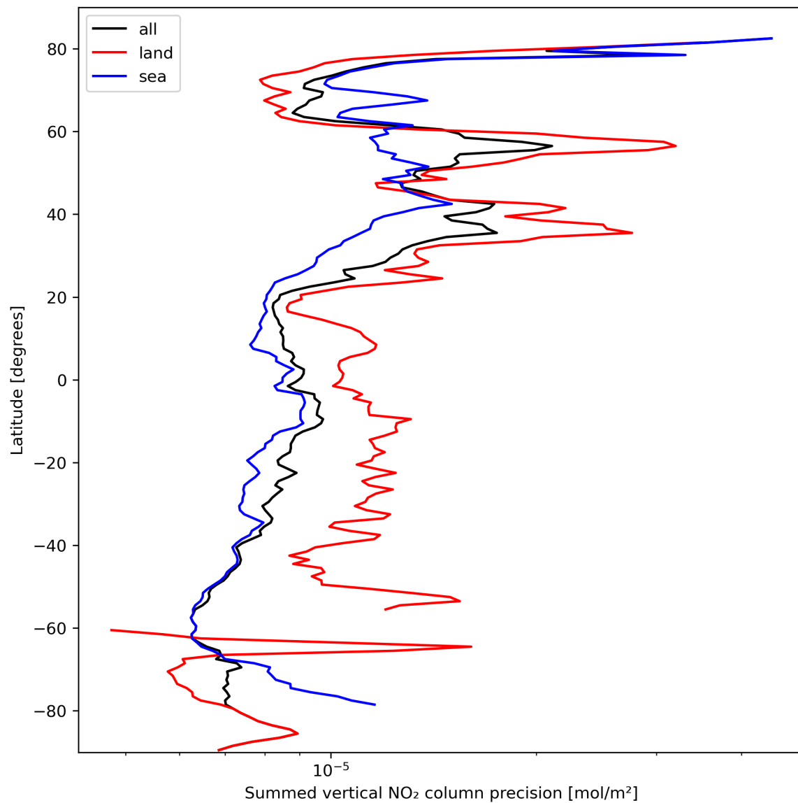
Figure 24: Zonal average of “Summed vertical NO 2 column precision” for 2024-03-04 to 2024-03-05.
