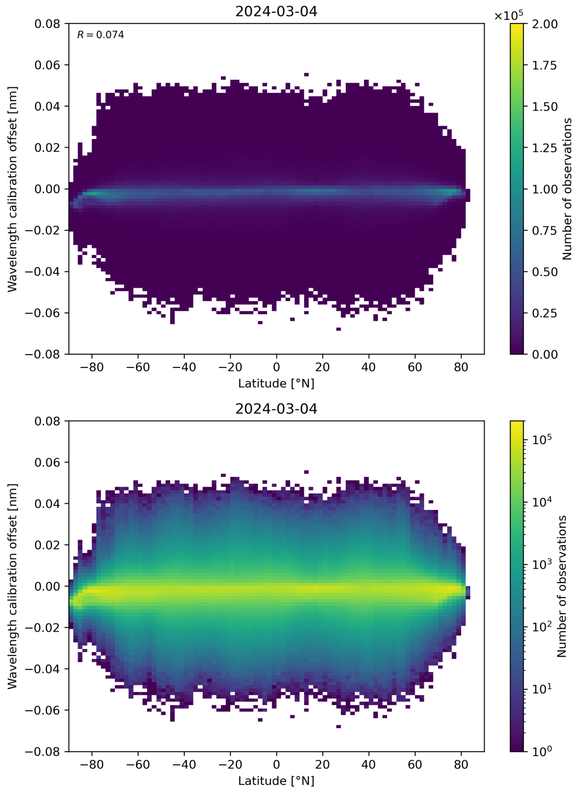
Figure 95: Scatter density plot of “Latitude” against “Wavelength calibration offset” for 2024-03-04 to 2024-03-05.
