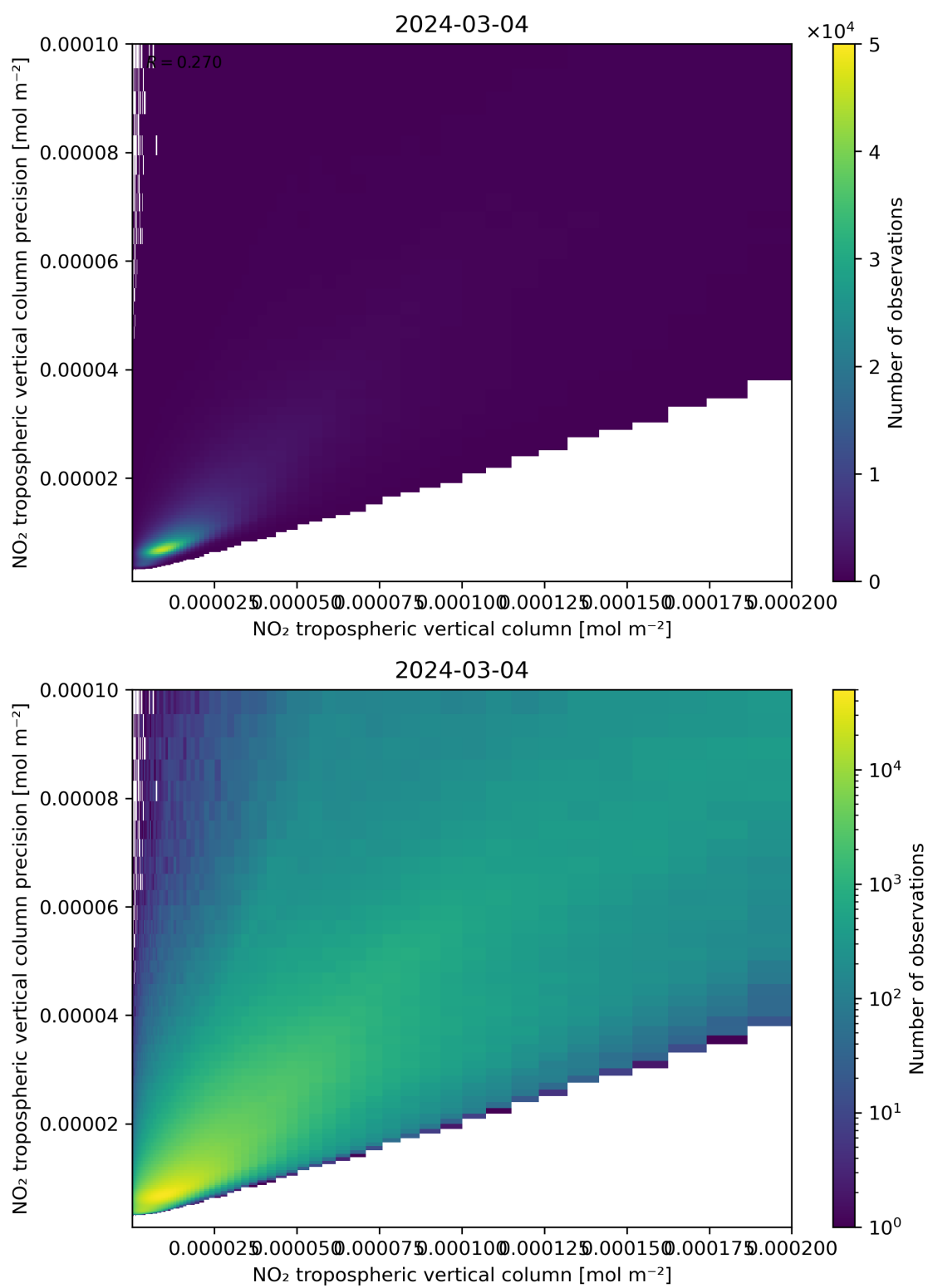
Figure 130: Scatter density plot of “NO 2 tropospheric vertical column” against “NO 2 tropospheric vertical column precision” for 2024-03-04 to 2024-03-05.
