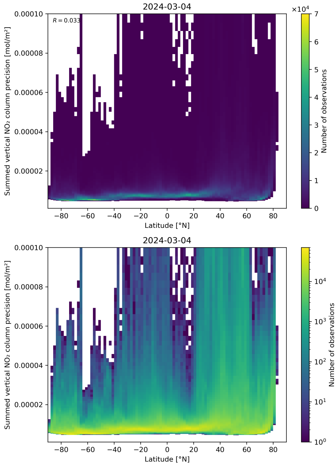
Figure 89: Scatter density plot of “Latitude” against “Summed vertical NO 2 column precision” for 2024-03-04 to 2024-03-05.
