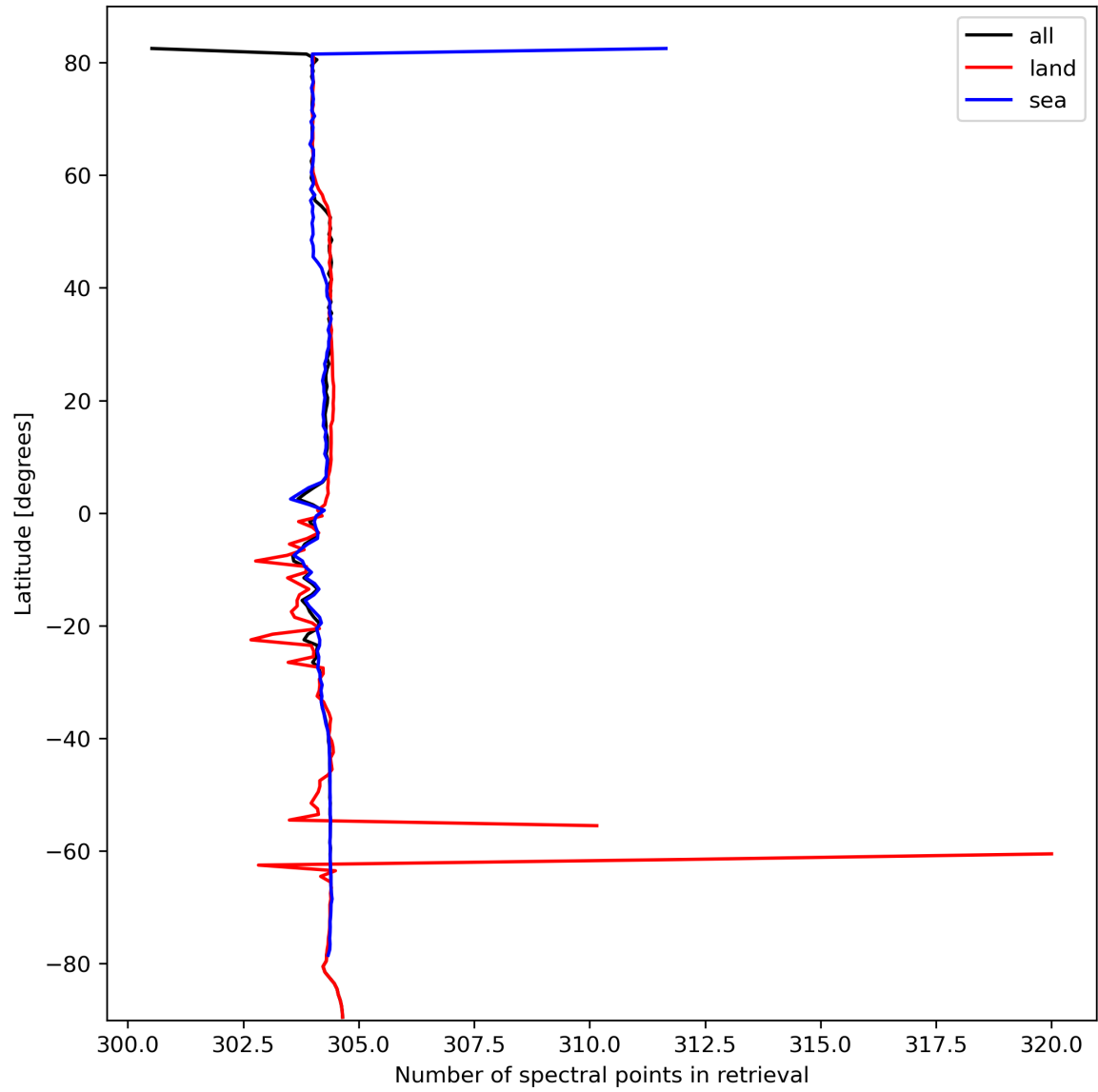
Figure 16: Zonal average of “Number of spectral points in retrieval” for 2024-03-04 to 2024-03-05.
