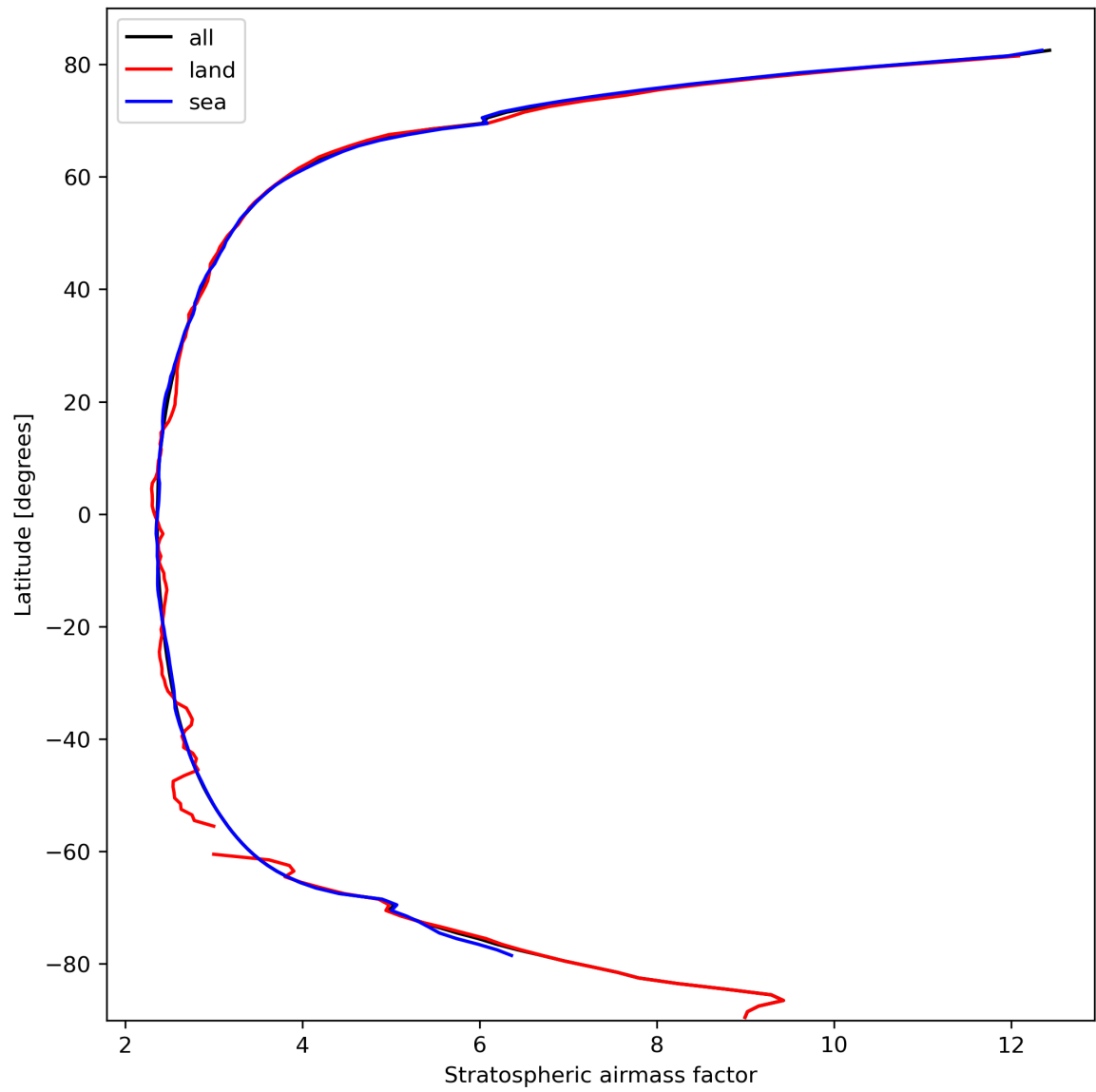
Figure 27: Zonal average of “Stratospheric air mass factor” for 2024-03-04 to 2024-03-05.
