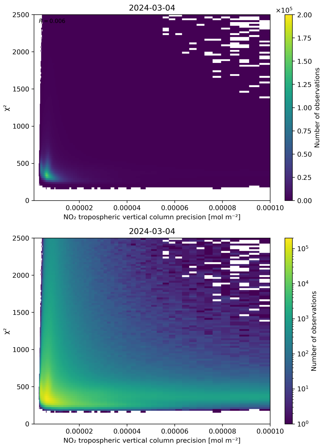
Figure 134: Scatter density plot of “NO 2 tropospheric vertical column precision” against “ \chi^2 ” for 2024-03-04 to 2024-03-05.
