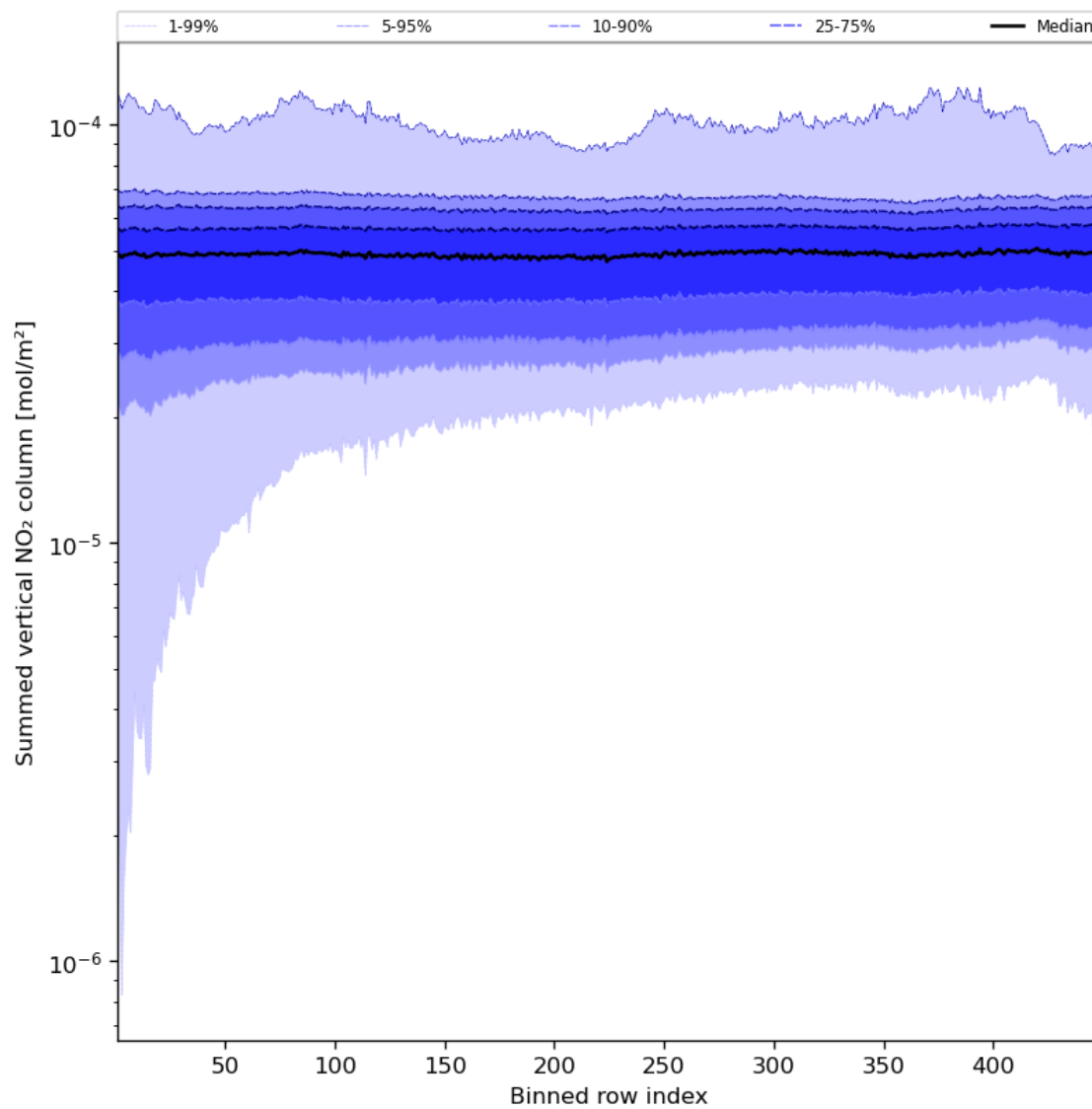
Figure 57: Along track statistics of “Summed vertical NO 2 column” for 2024-03-04 to 2024-03-05
