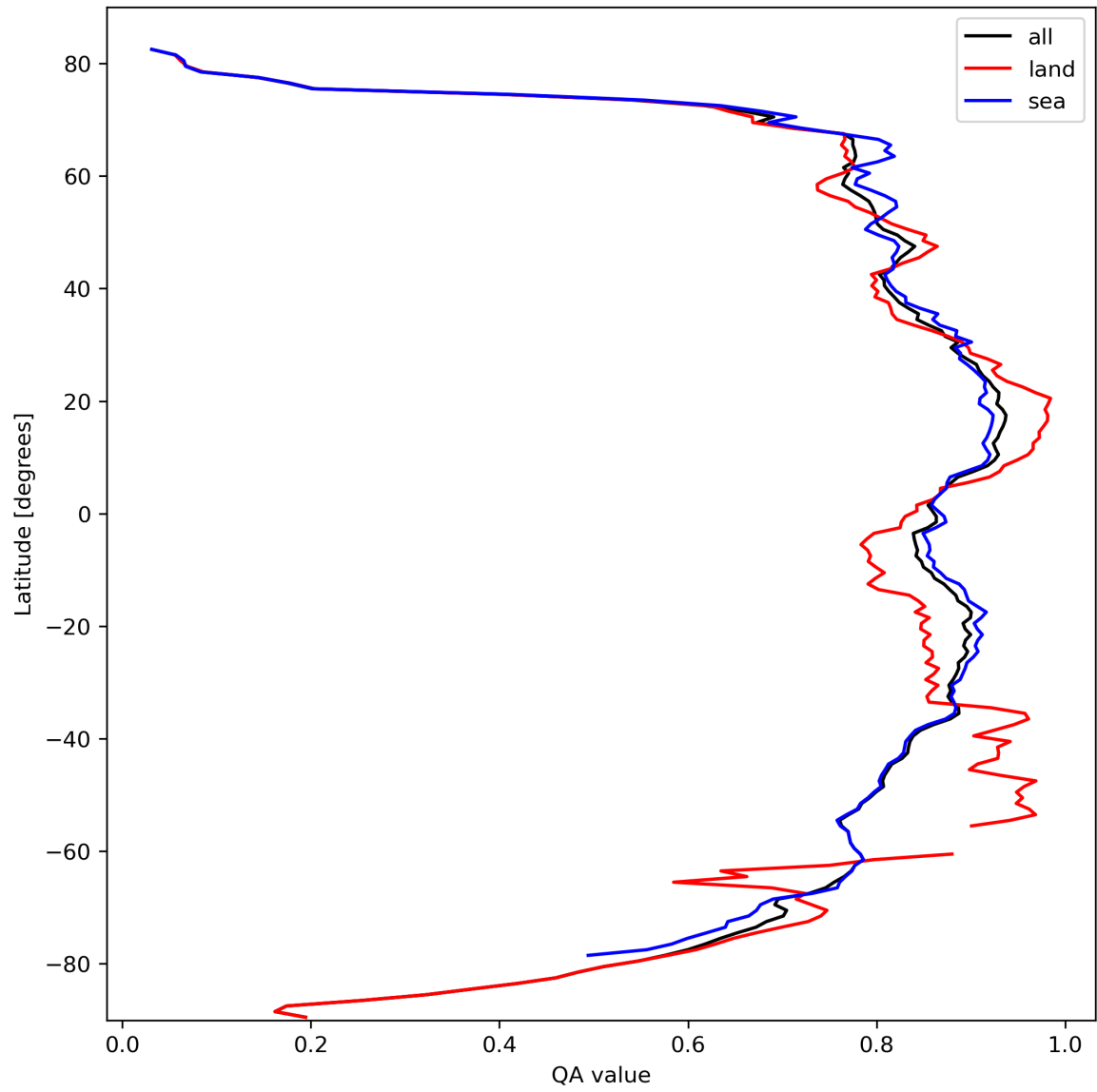
Figure 11: Zonal average of “QA value” for 2024-03-04 to 2024-03-05.
