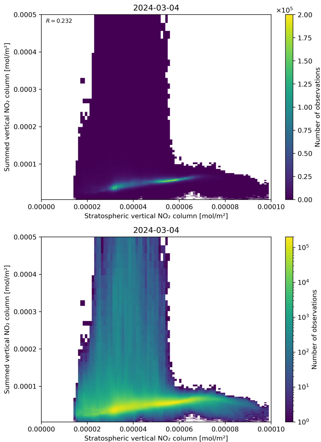
Figure 98: Scatter density plot of “Stratospheric vertical NO 2 column” against “Summed vertical NO 2 column” for 2024-03-04 to 2024-03-05.
