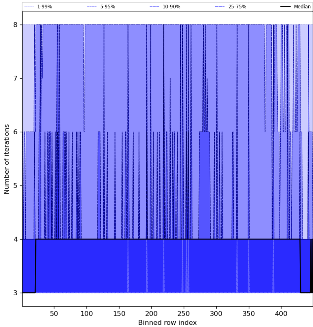
Figure 51: Along track statistics of “Number of iterations” for 2024-03-04 to 2024-03-05
