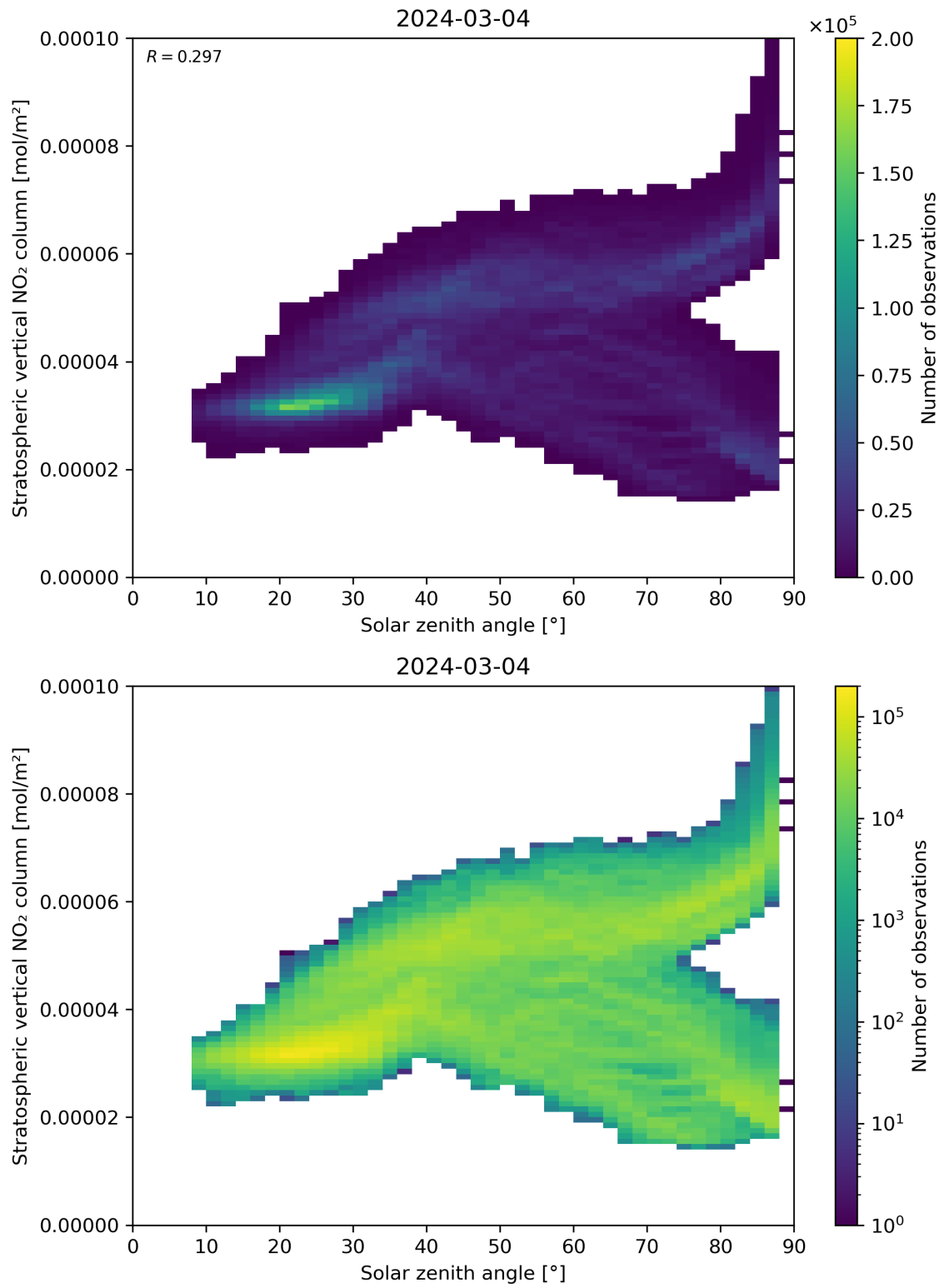
Figure 150: Scatter density plot of “Solar zenith angle” against “Stratospheric vertical NO 2 column” for 2024-03-04 to 2024-03-05.
