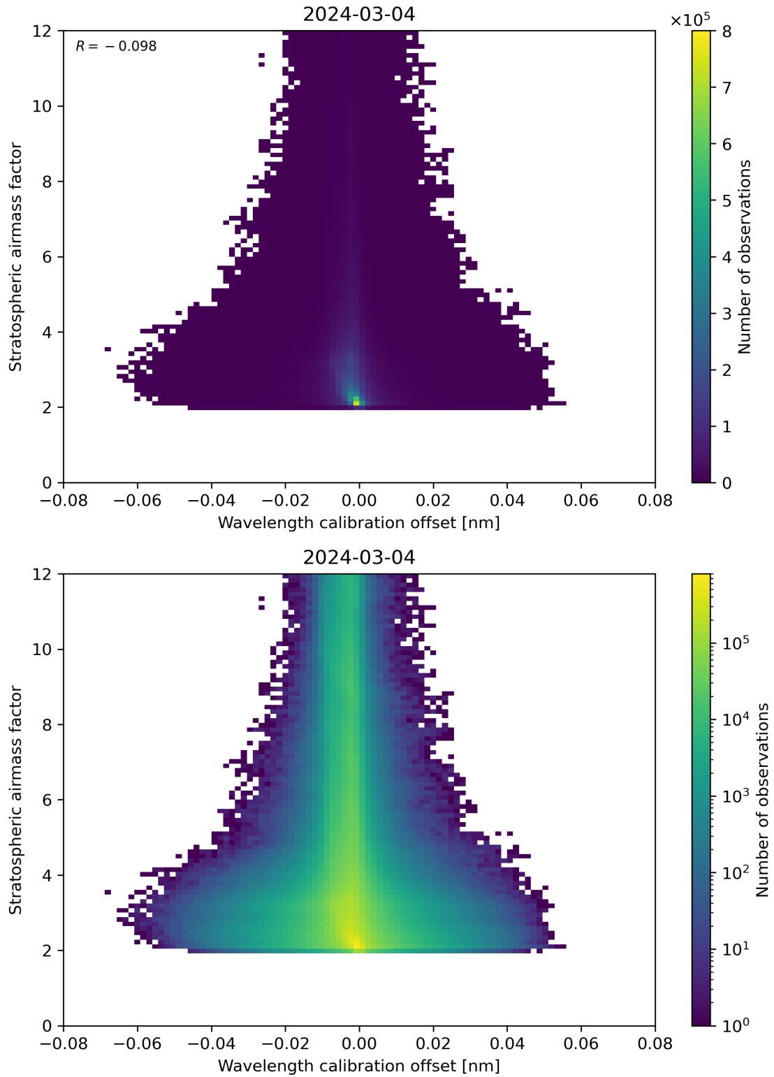
Figure 174: Scatter density plot of “Wavelength calibration offset” against “Stratospheric airmass factor” for 2024-03-04 to 2024-03-05.
