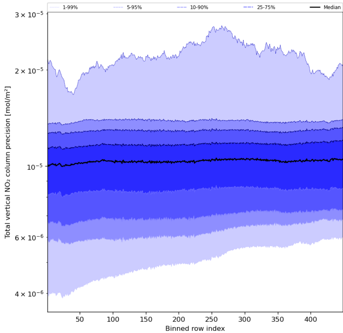
Figure 56: Along track statistics of “Total vertical NO 2 column precision” for 2024-03-04 to 2024-03-05
