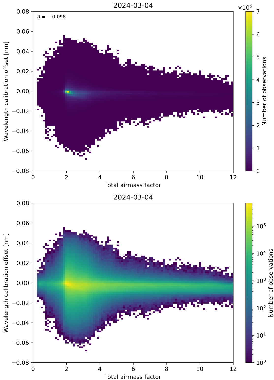
Figure 70: Scatter density plot of “Total airmass factor” against “Wavelength calibration offset” for 2024-03-04 to 2024-03-05.
