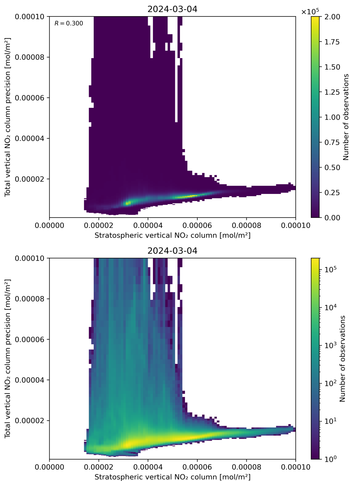
Figure 101: Scatter density plot of “Stratospheric vertical NO 2 column” against “Total vertical NO 2 column precision” for 2024-03-04 to 2024-03-05.
