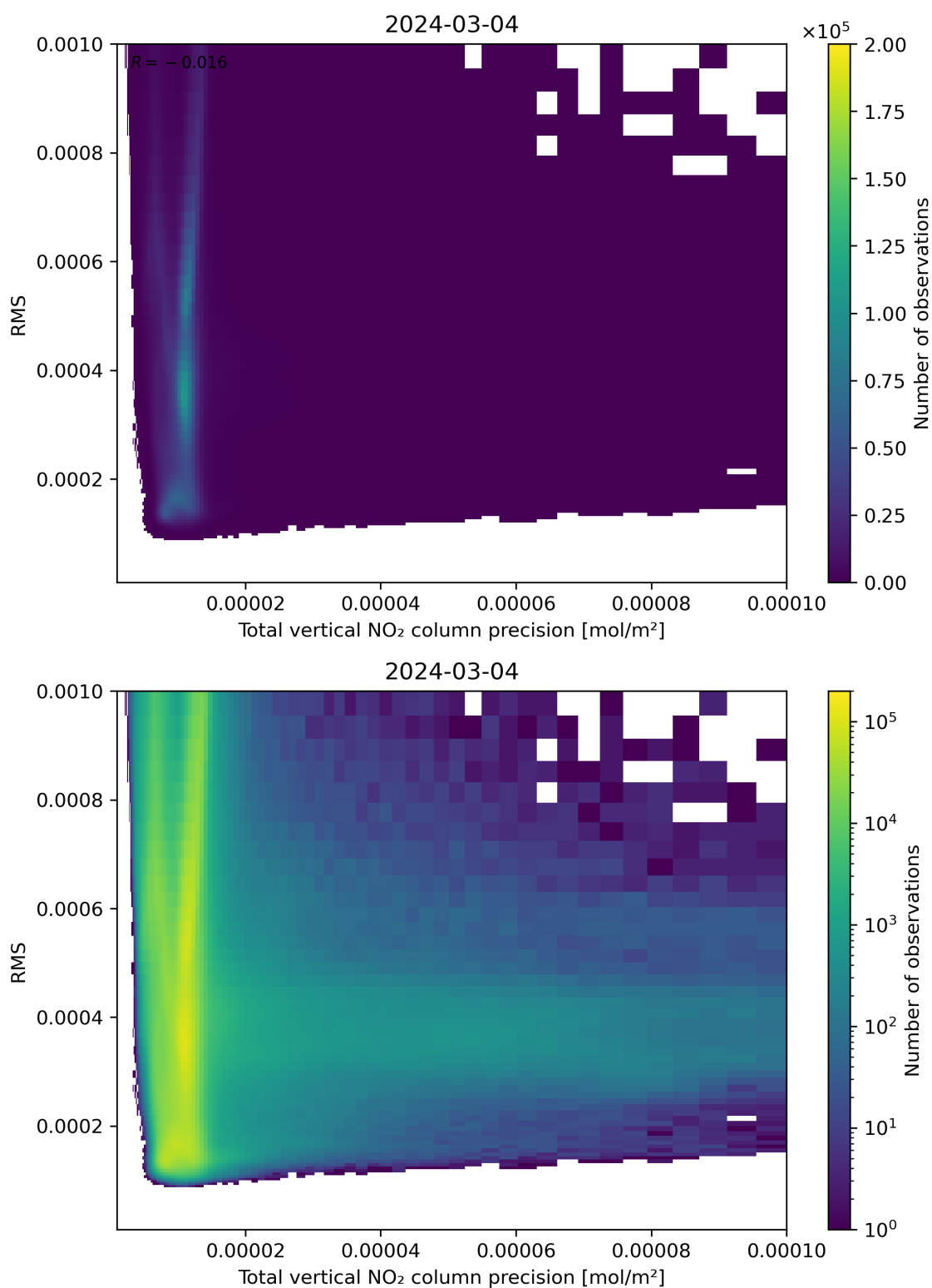
Figure 119: Scatter density plot of “Total vertical NO 2 column precision” against “RMS” for 2024-03-04 to 2024-03-05.
