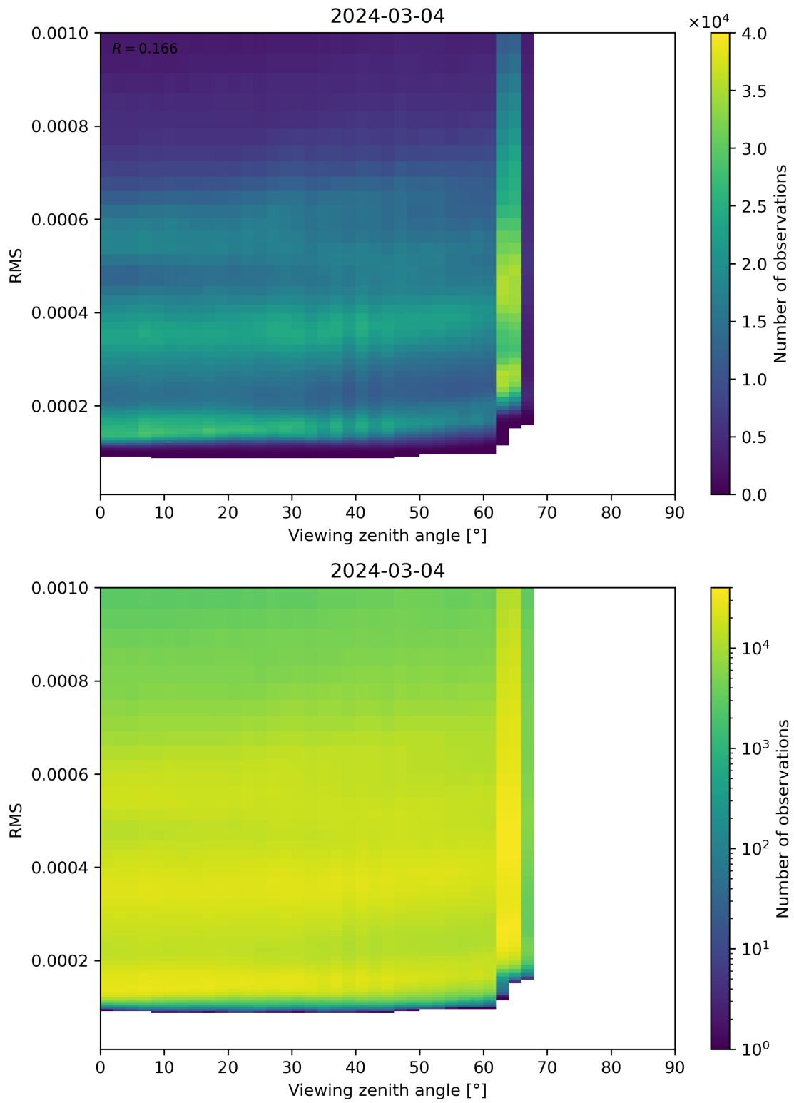
Figure 171: Scatter density plot of “Viewing zenith angle” against “RMS” for 2024-03-04 to 2024-03-05.
