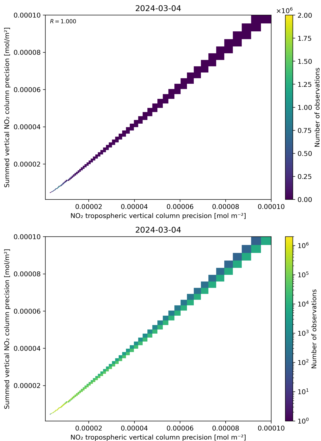
Figure 137: Scatter density plot of “NO 2 tropospheric vertical column precision” against “Summed vertical NO 2 column precision” for 2024-03-04 to 2024-03-05.
