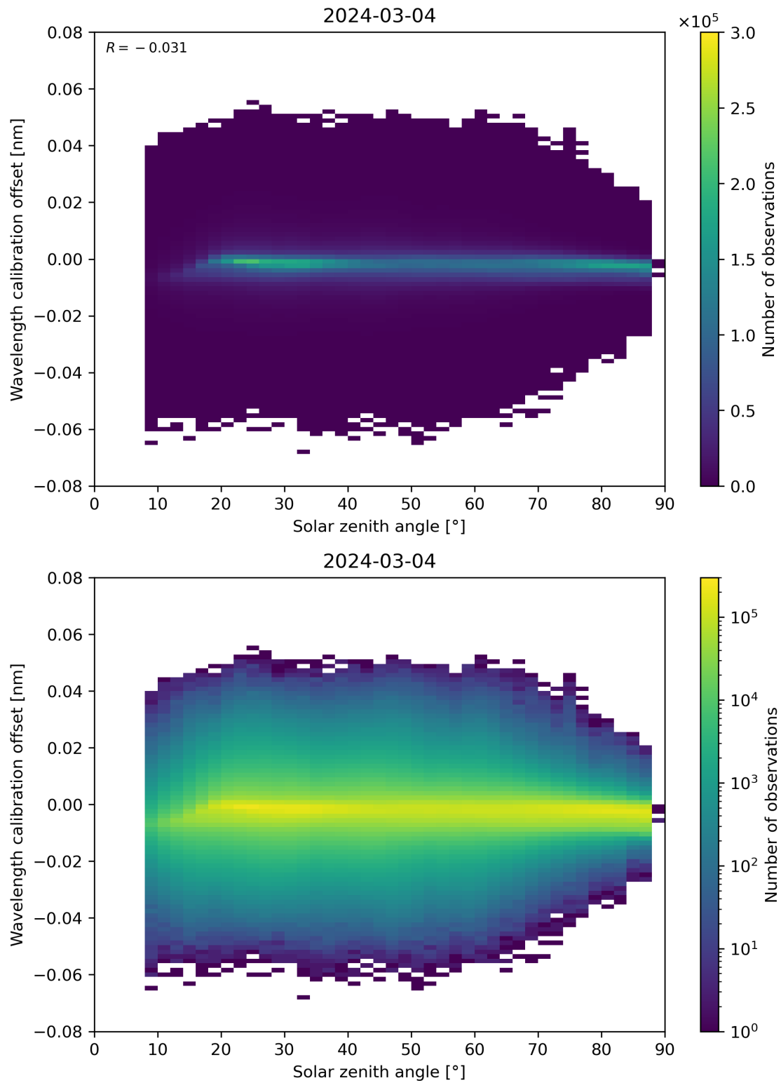
Figure 158: Scatter density plot of “Solar zenith angle” against “Wavelength calibration offset” for 2024-03-04 to 2024-03-05.
