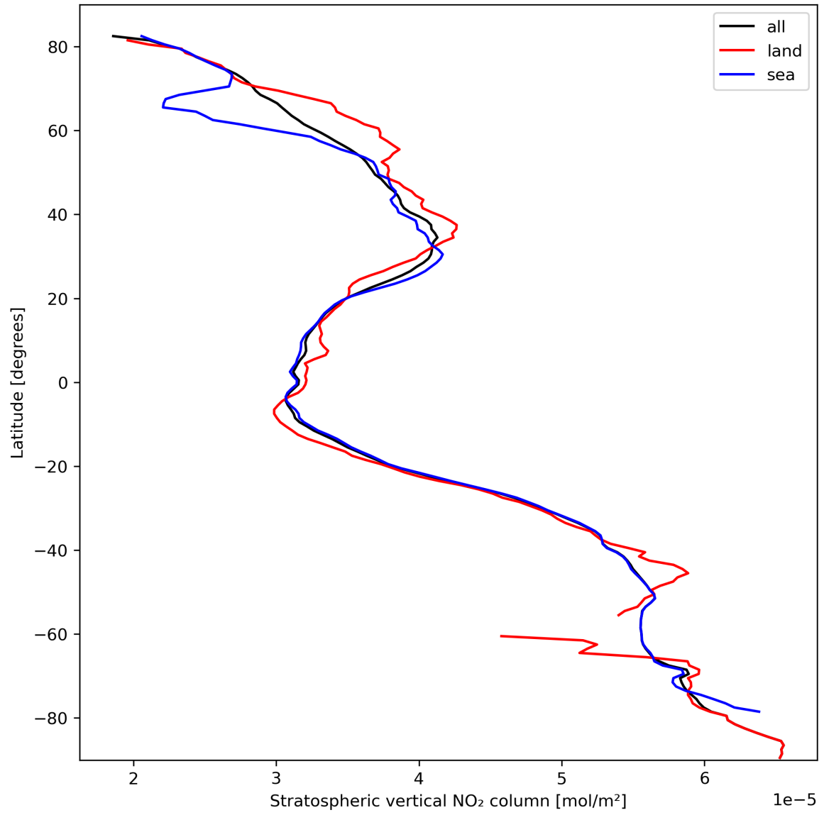
Figure 19: Zonal average of “Stratospheric vertical NO 2 column” for 2024-03-04 to 2024-03-05.
