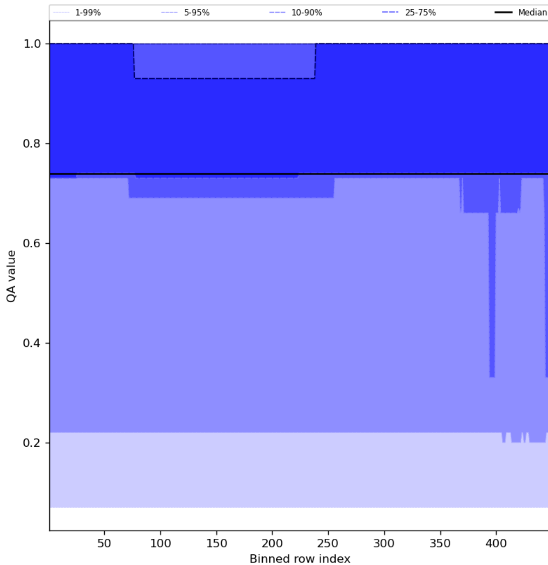
Figure 45: Along track statistics of “QA value” for 2024-03-04 to 2024-03-05
