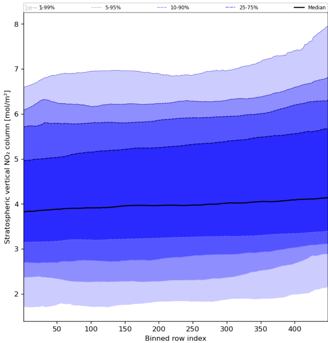
Figure 53: Along track statistics of “Stratospheric vertical NO 2 column” for 2024-03-04 to 2024-03-05
