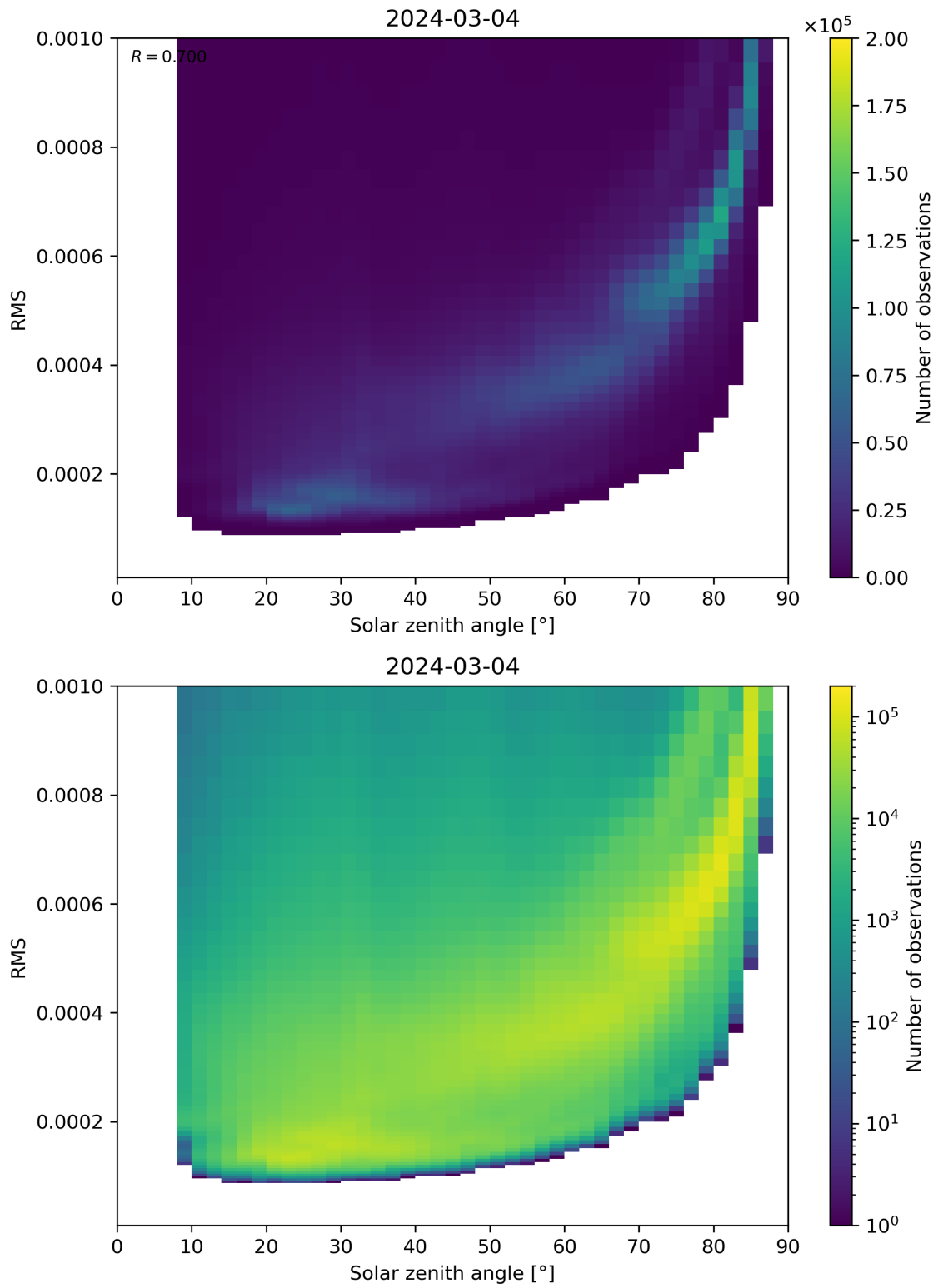
Figure 157: Scatter density plot of “Solar zenith angle” against “RMS” for 2024-03-04 to 2024-03-05.
