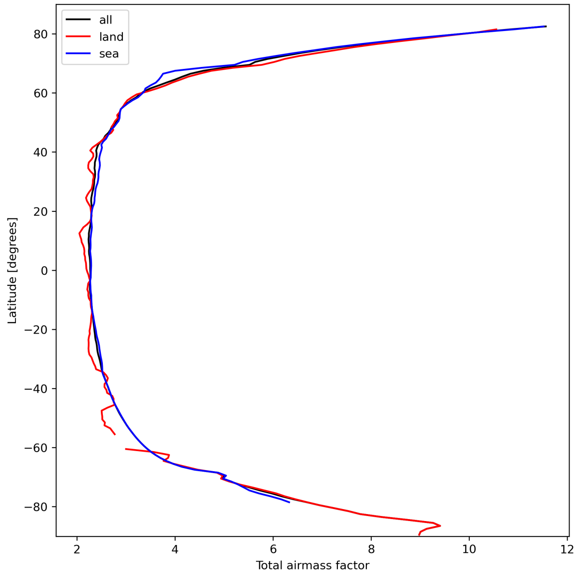
Figure 15: Zonal average of “Total airmass factor” for 2024-03-04 to 2024-03-05.
