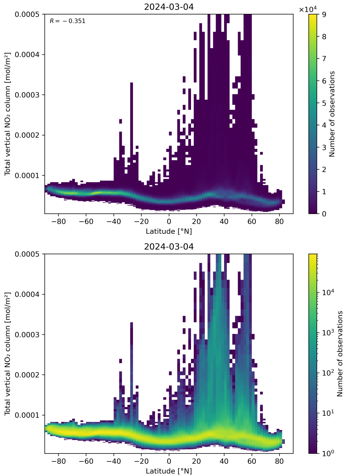
Figure 90: Scatter density plot of “Latitude” against “Total vertical NO 2 column” for 2024-03-04 to 2024-03-05.
