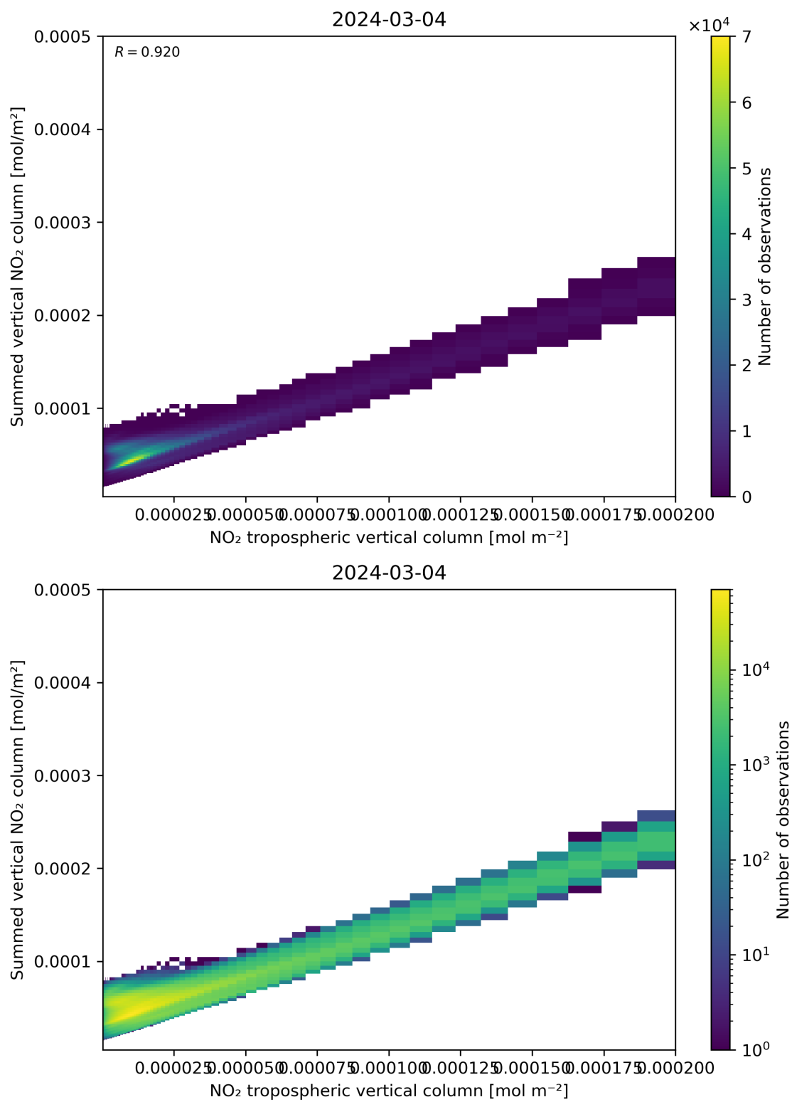
Figure 126: Scatter density plot of “NO 2 tropospheric vertical column” against “Summed vertical NO 2 column” for 2024-03-04 to 2024-03-05.
