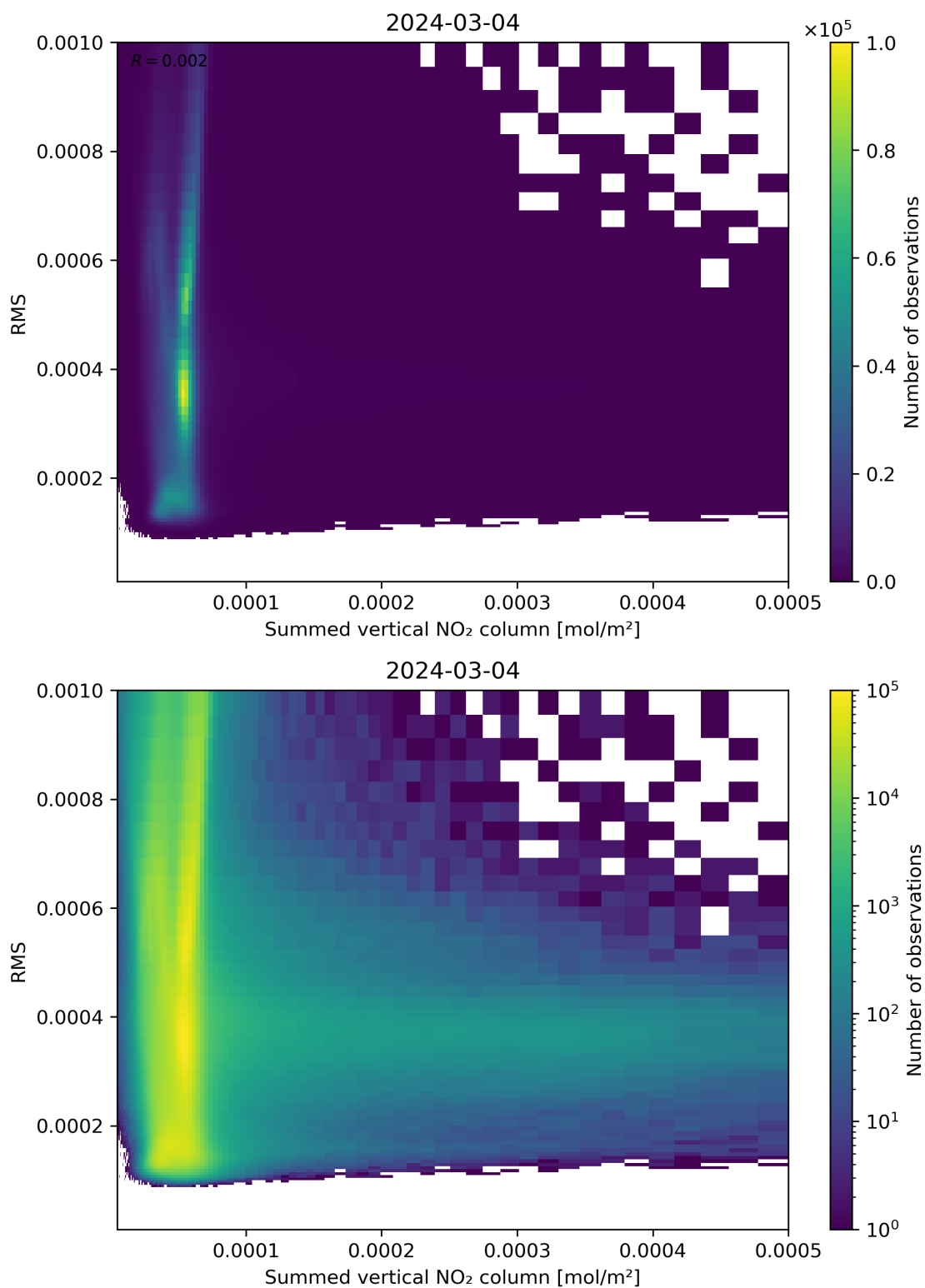
Figure 109: Scatter density plot of “Summed vertical NO 2 column” against “RMS” for 2024-03-04 to 2024-03-05.
