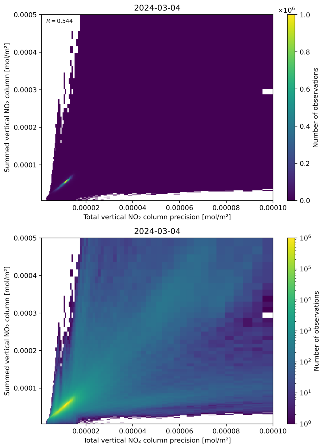
Figure 117: Scatter density plot of “Total vertical NO 2 column precision” against “Summed vertical NO 2 column” for 2024-03-04 to 2024-03-05.
