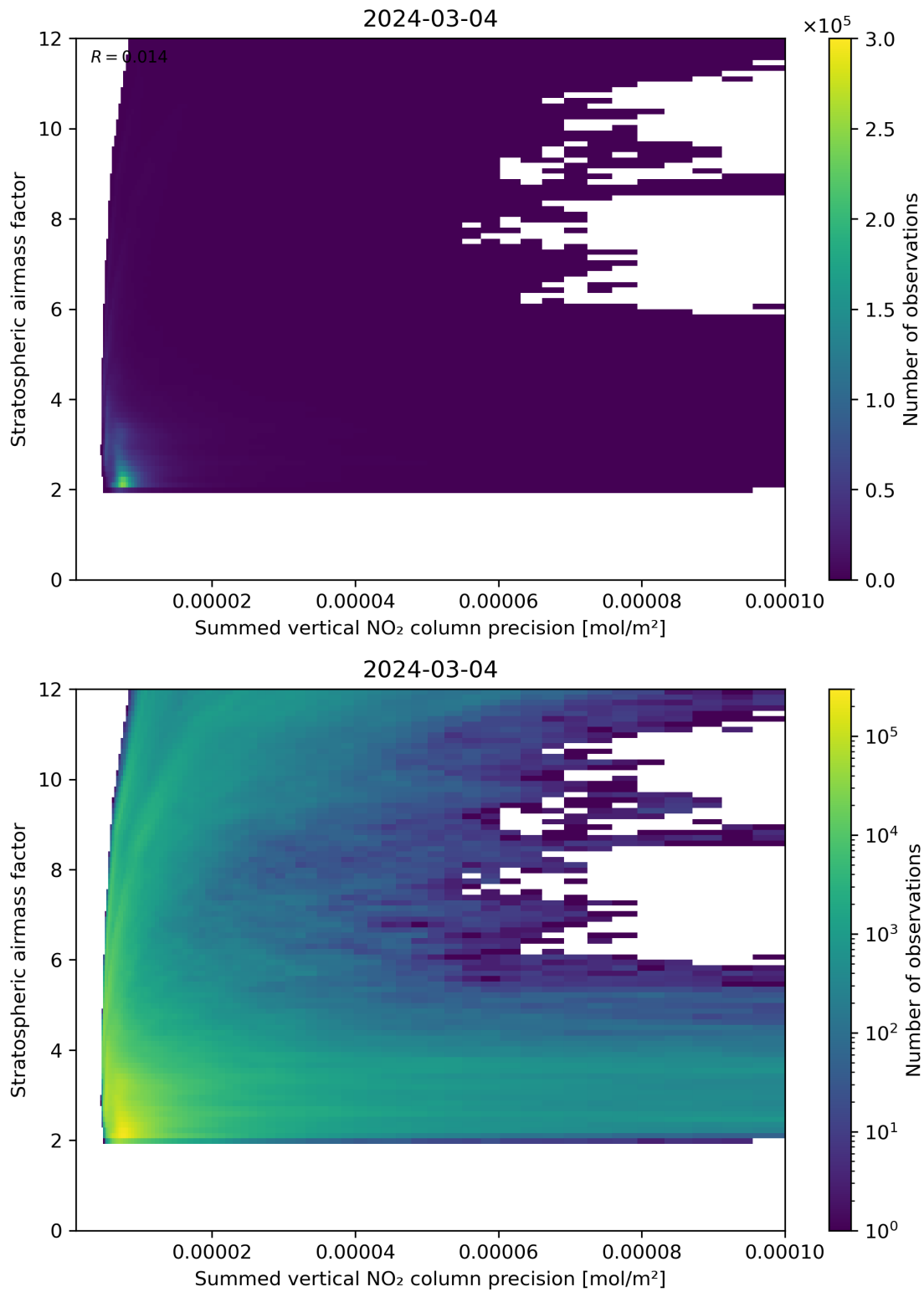
Figure 106: Scatter density plot of “Summed vertical NO 2 column precision” against “Stratospheric airmass factor” for 2024-03-04 to 2024-03-05.
