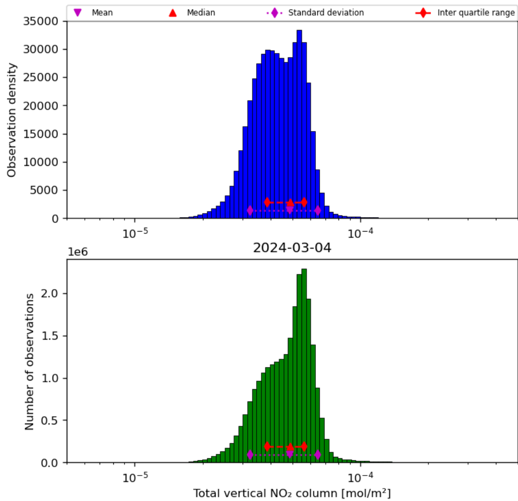
Figure 38: Histogram of “Total vertical NO 2 column” for 2024-03-04 to 2024-03-05
