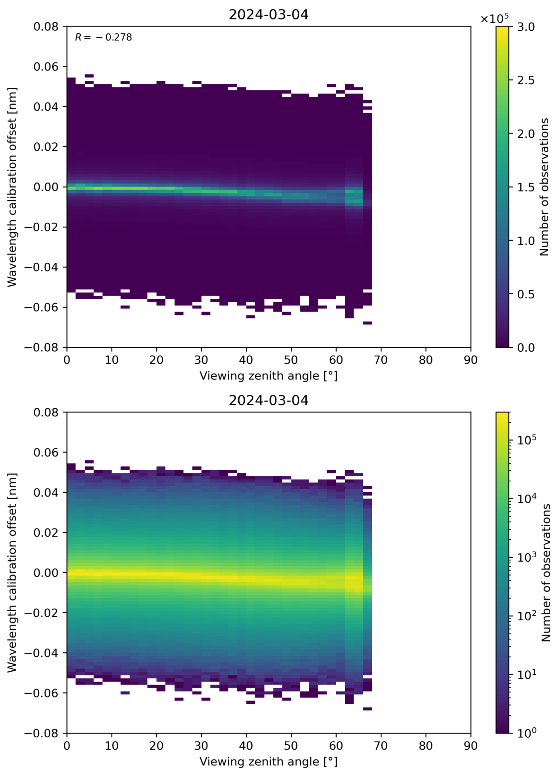
Figure 173: Scatter density plot of “Viewing zenith angle” against “Wavelength calibration offset” for 2024-03-04 to 2024-03-05.
