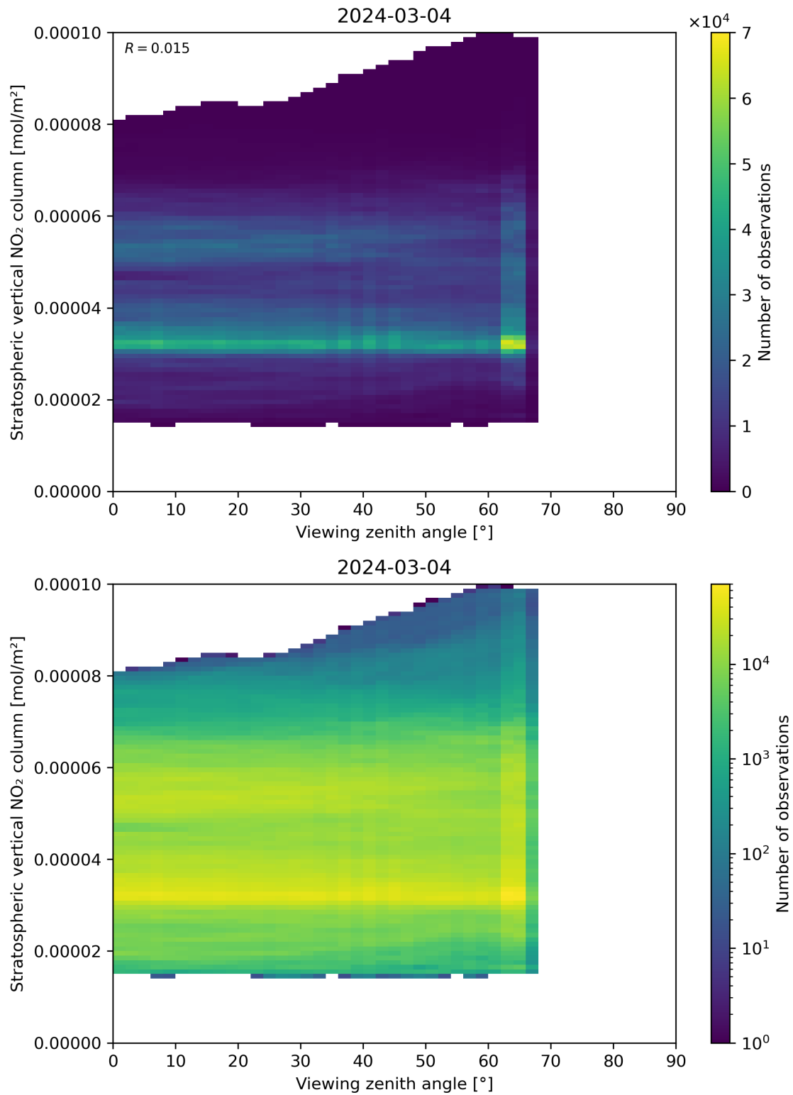
Figure 164: Scatter density plot of “Viewing zenith angle” against “Stratospheric vertical NO 2 column” for 2024-03-04 to 2024-03-05.
