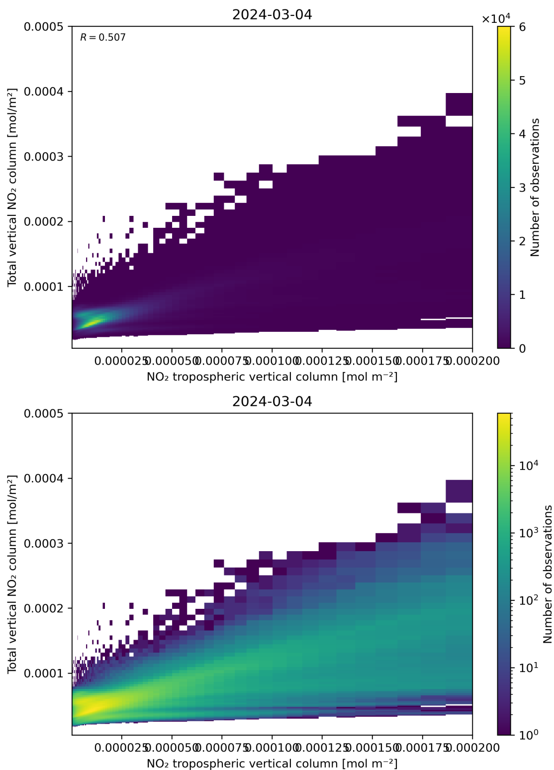
Figure 128: Scatter density plot of “NO 2 tropospheric vertical column” against “Total vertical NO 2 column” for 2024-03-04 to 2024-03-05.
