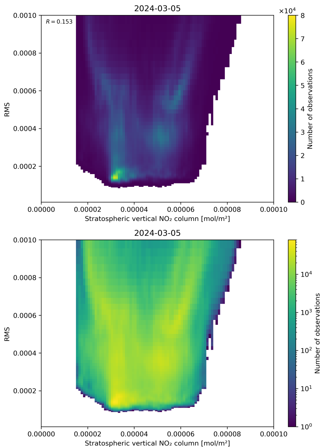
Figure 102: Scatter density plot of “Stratospheric vertical NO 2 column” against “RMS” for 2024-03-04 to 2024-03-06.
