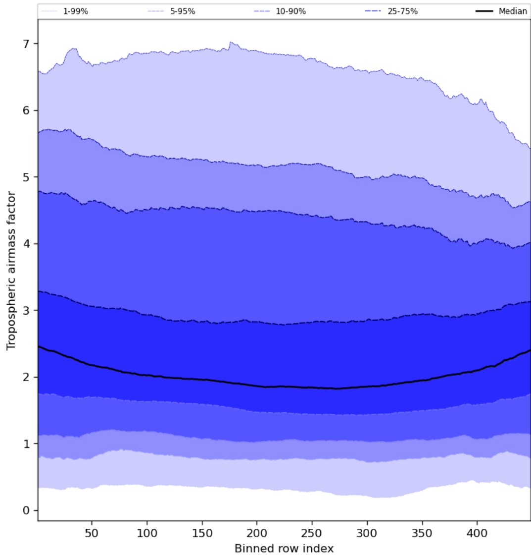
Figure 48: Along track statistics of “Tropospheric air mass factor” for 2024-03-04 to 2024-03-06
