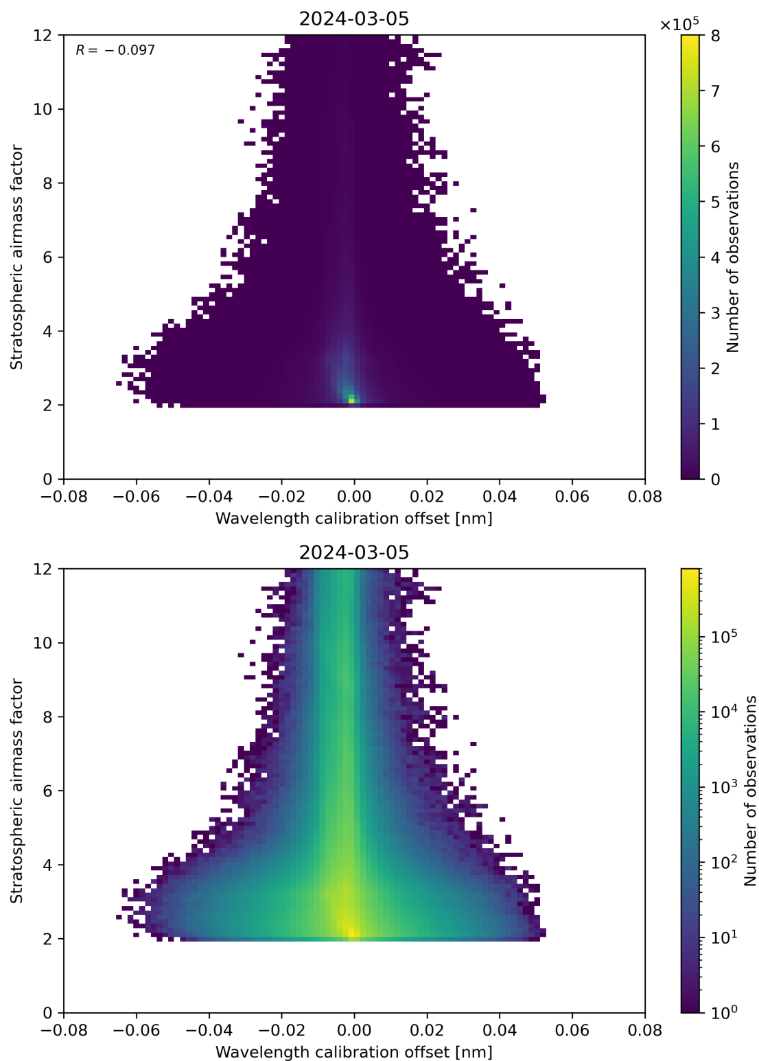
Figure 174: Scatter density plot of “Wavelength calibration offset” against “Stratospheric airmass factor” for 2024-03-04 to 2024-03-06.
