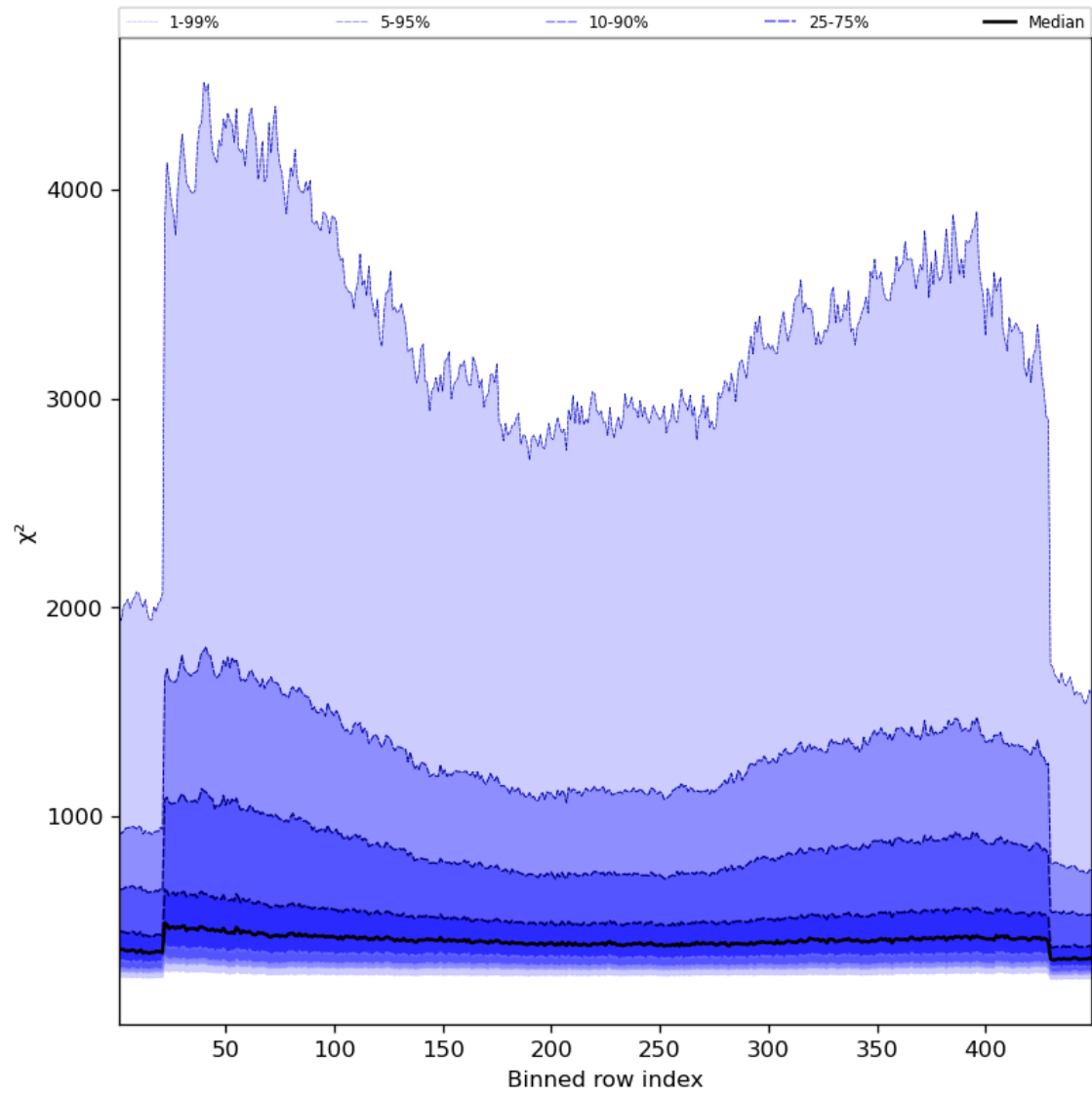
Figure 59: Along track statistics of “ \chi^2 ” for 2024-03-04 to 2024-03-06
