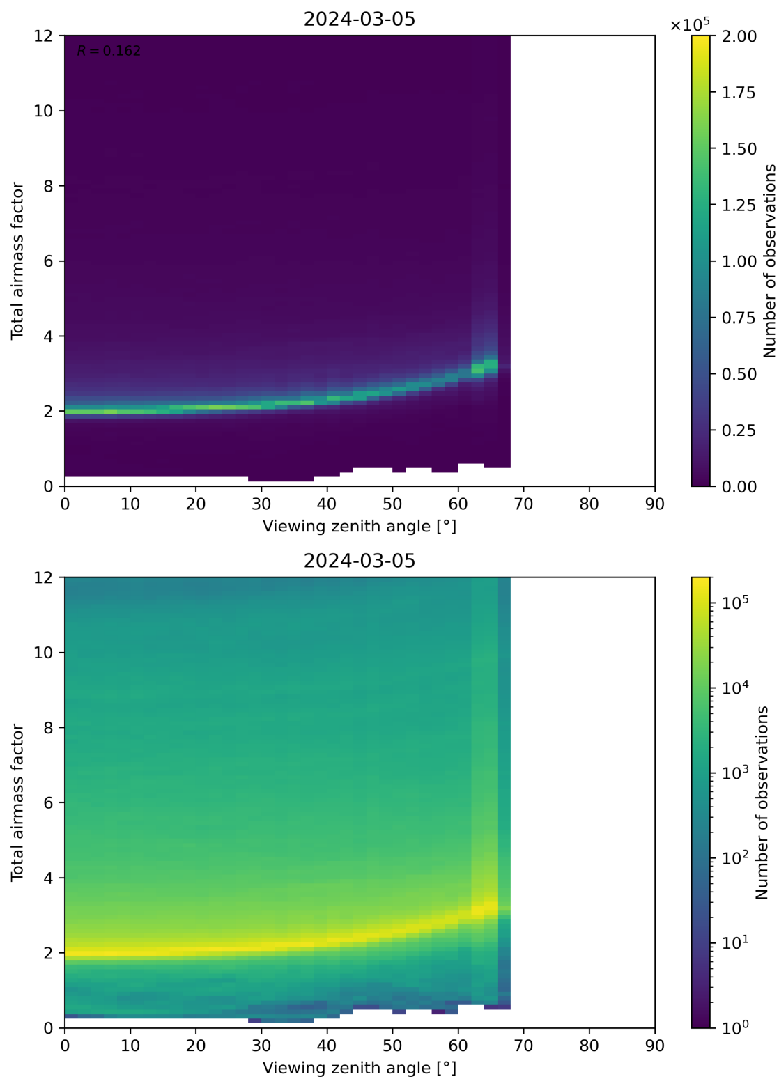
Figure 160: Scatter density plot of “Viewing zenith angle” against “Total airmass factor” for 2024-03-04 to 2024-03-06.
