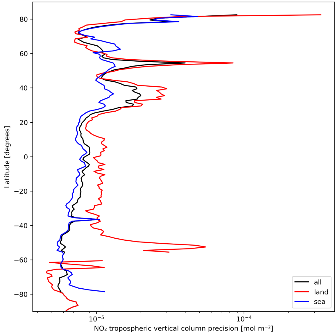
Figure 13: Zonal average of “NO 2 tropospheric vertical column precision” for 2024-03-04 to 2024-03-06.
