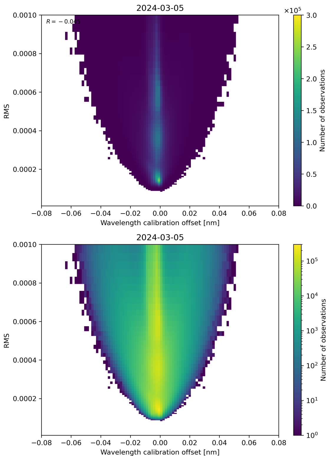
Figure 181: Scatter density plot of “Wavelength calibration offset” against “RMS” for 2024-03-04 to 2024-03-06.
