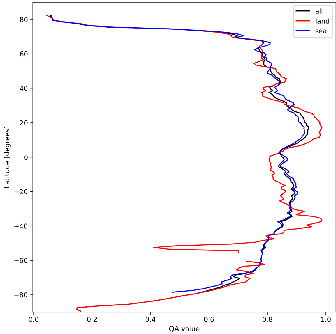
Figure 11: Zonal average of “QA value” for 2024-03-04 to 2024-03-06.
