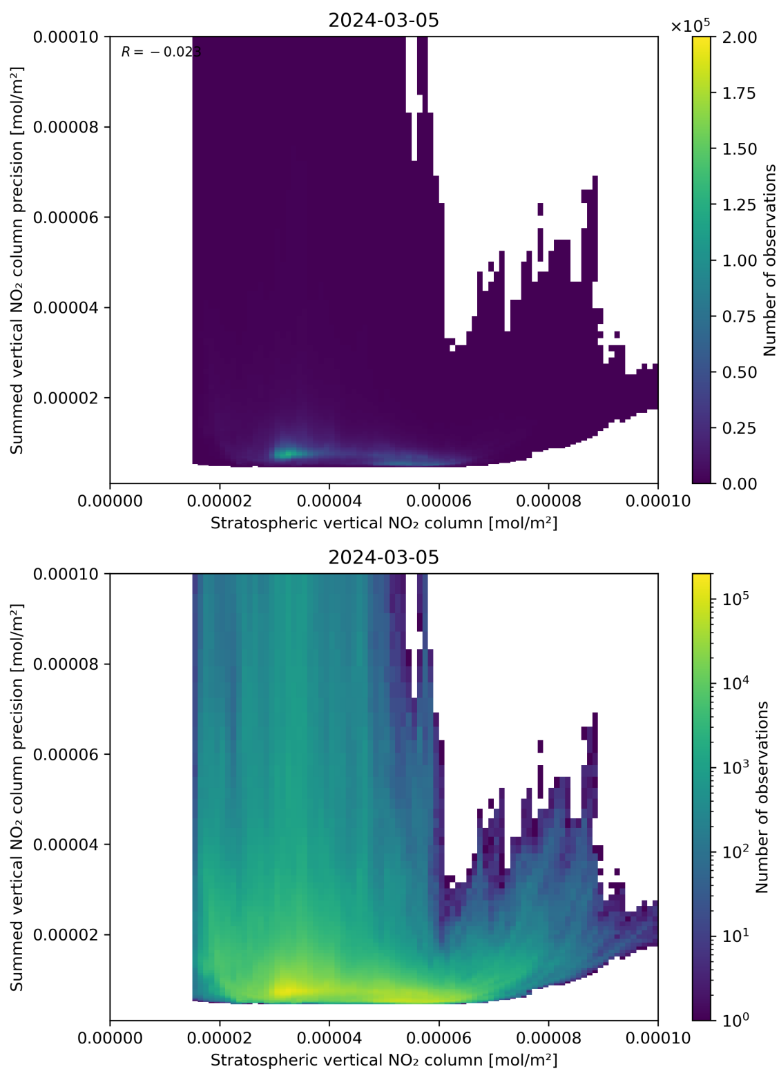
Figure 99: Scatter density plot of “Stratospheric vertical NO 2 column” against “Summed vertical NO 2 column precision” for 2024-03-04 to 2024-03-06.
