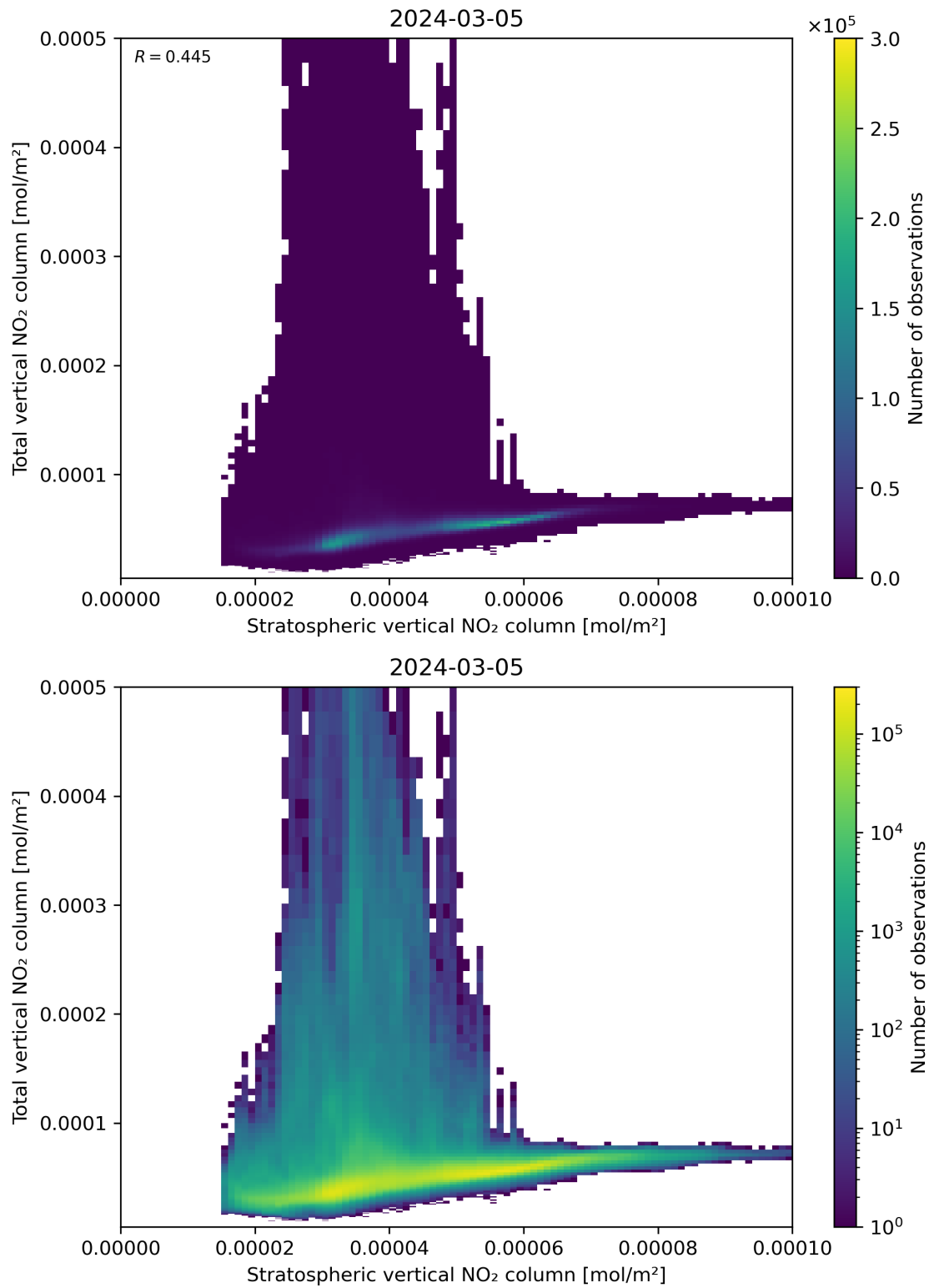
Figure 100: Scatter density plot of “Stratospheric vertical NO 2 column” against “Total vertical NO 2 column” for 2024-03-04 to 2024-03-06.
