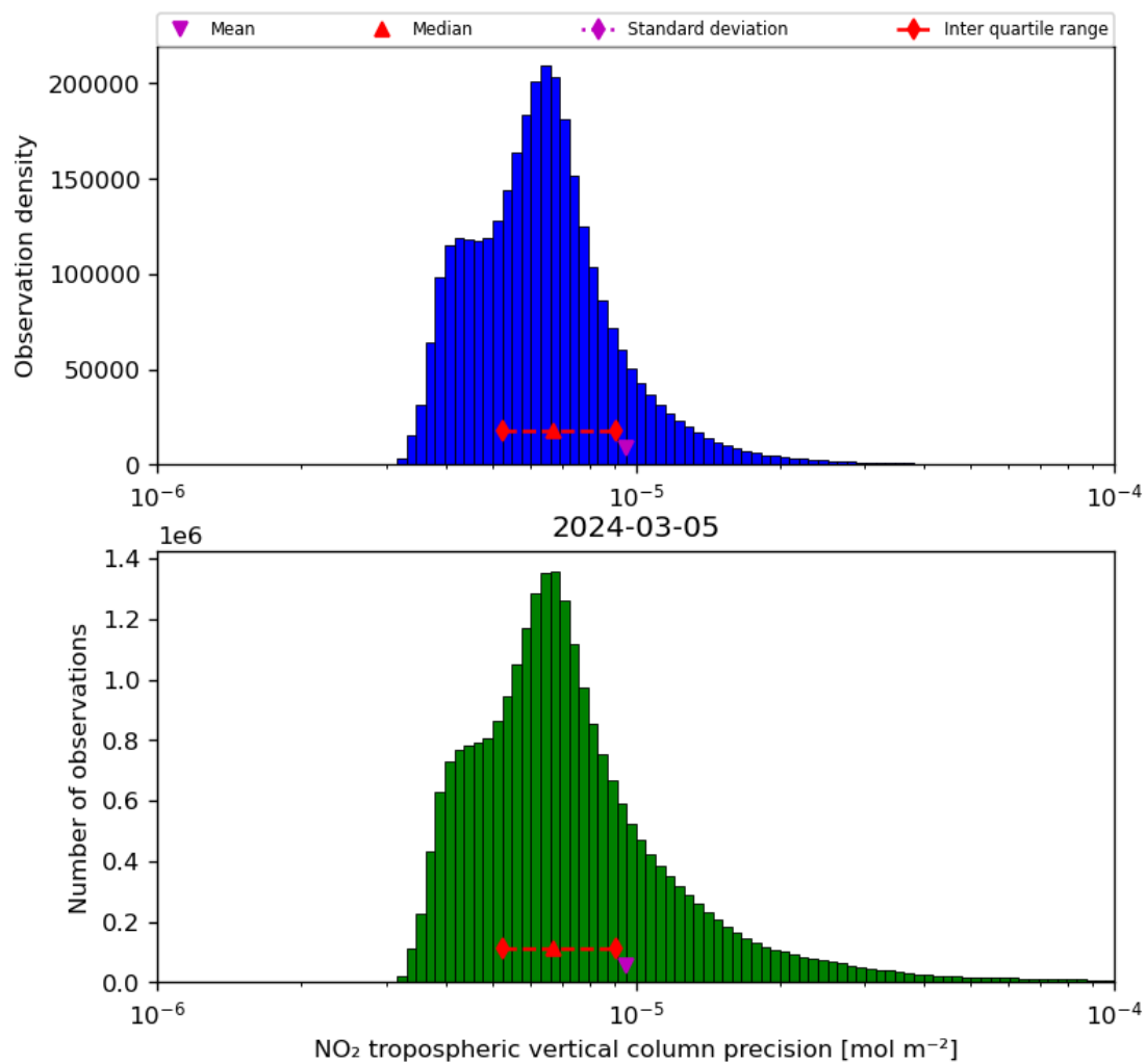
Figure 30: Histogram of “NO 2 tropospheric vertical column precision” for 2024-03-04 to 2024-03-06
