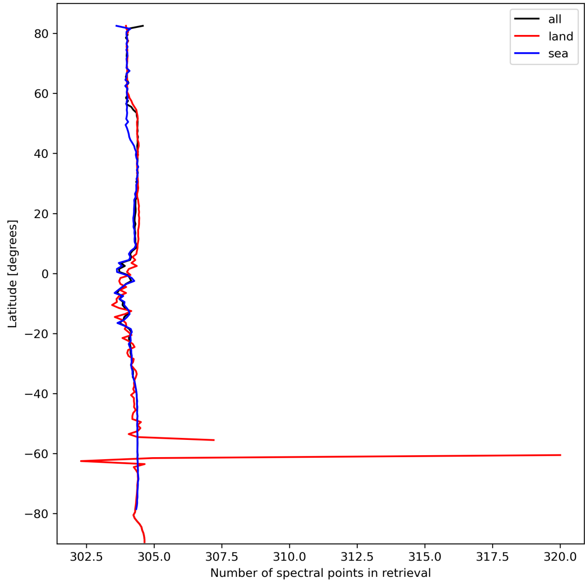
Figure 16: Zonal average of “Number of spectral points in retrieval” for 2024-03-04 to 2024-03-06.
