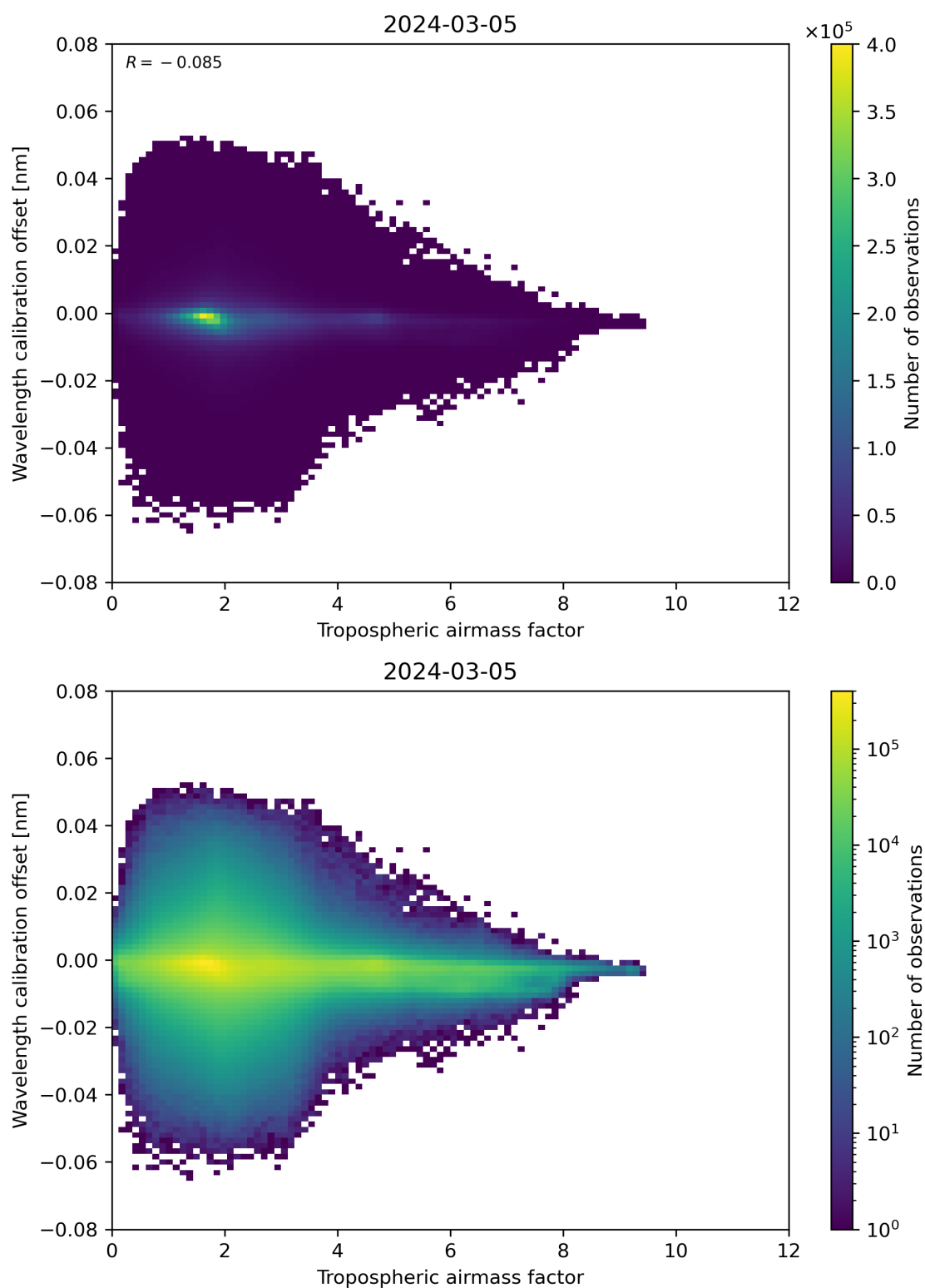
Figure 80: Scatter density plot of “Tropospheric airmass factor” against “Wavelength calibration offset” for 2024-03-04 to 2024-03-06.
