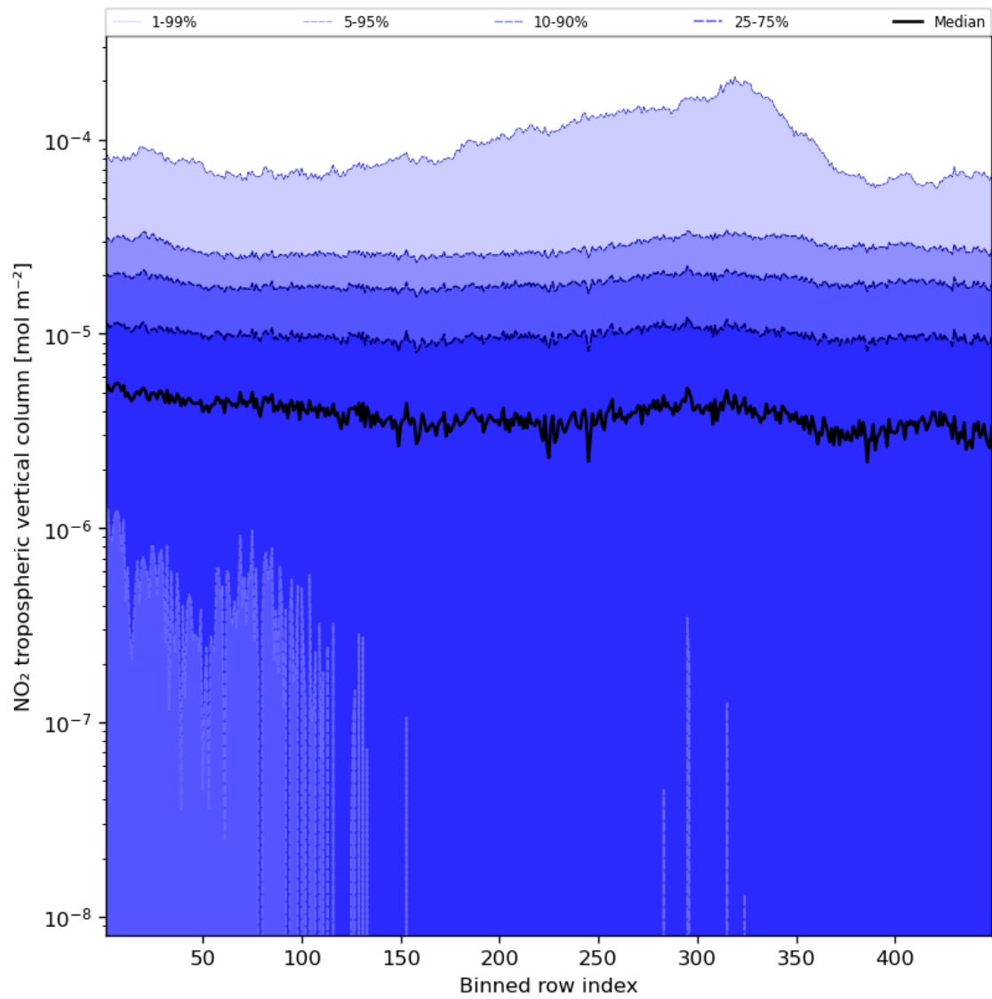
Figure 46: Along track statistics of “NO 2 tropospheric vertical column” for 2024-03-04 to 2024-03-06
