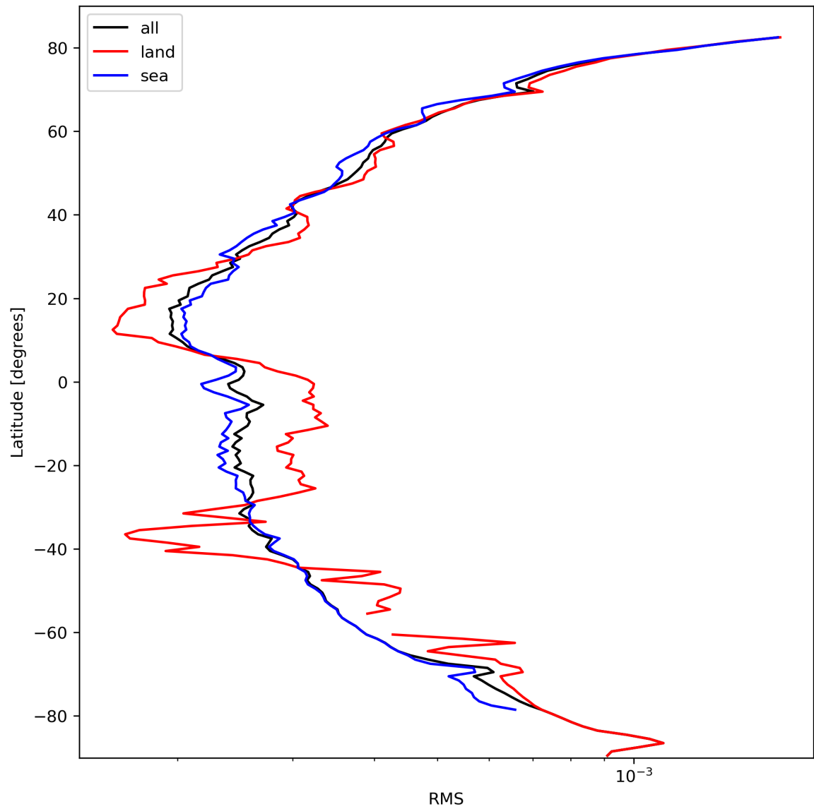
Figure 26: Zonal average of “RMS” for 2024-03-04 to 2024-03-06.
