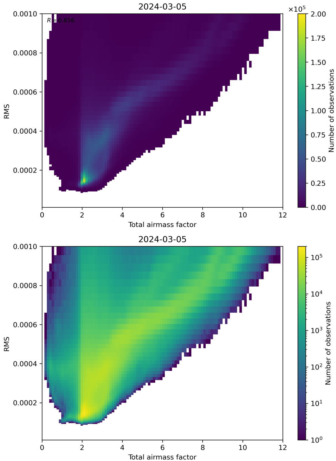
Figure 69: Scatter density plot of “Total airmass factor” against “RMS” for 2024-03-04 to 2024-03-06.
