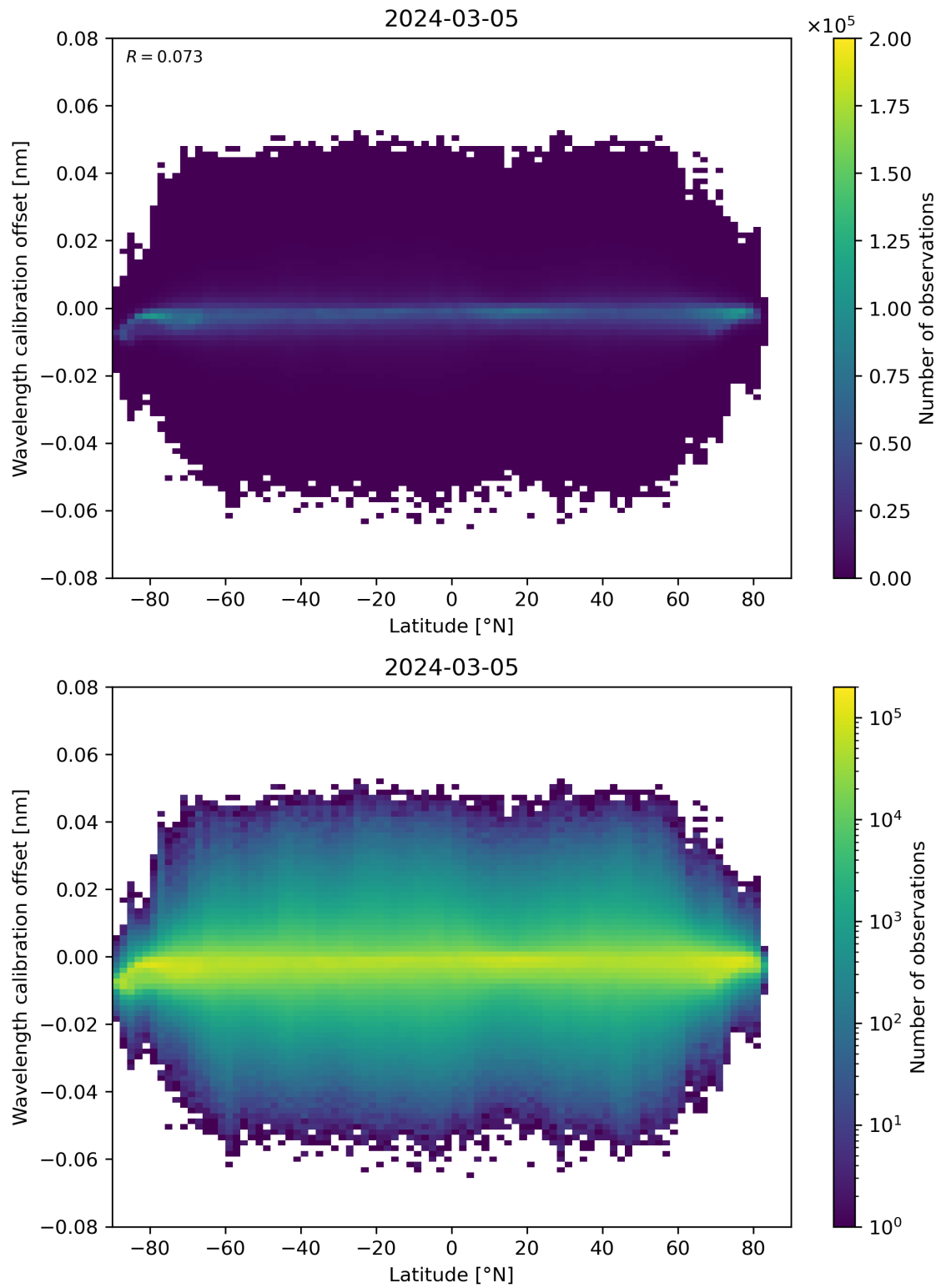
Figure 95: Scatter density plot of “Latitude” against “Wavelength calibration offset” for 2024-03-04 to 2024-03-06.
