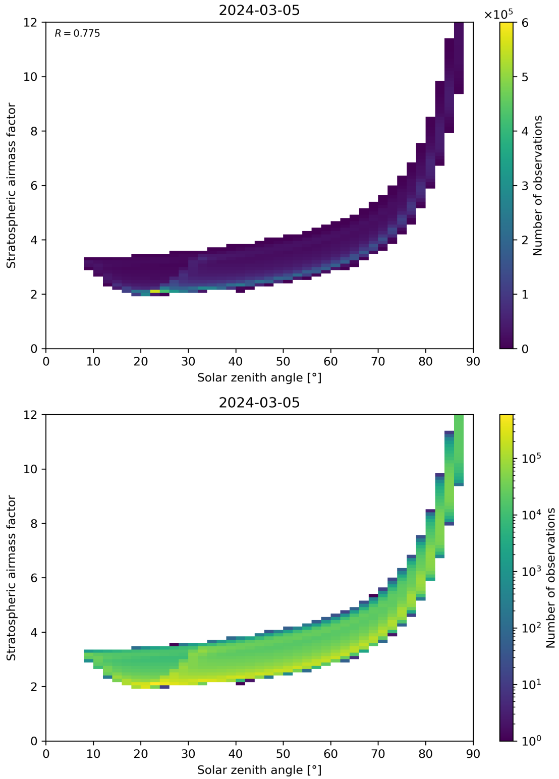
Figure 145: Scatter density plot of “Solar zenith angle” against “Stratospheric airmass factor” for 2024-03-04 to 2024-03-06.
