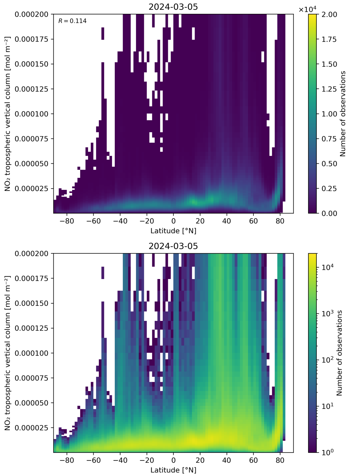
Figure 92: Scatter density plot of “Latitude” against “NO 2 tropospheric vertical column” for 2024-03-04 to 2024-03-06.
