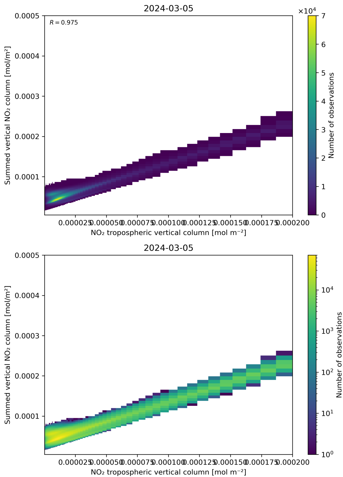
Figure 126: Scatter density plot of “NO 2 tropospheric vertical column” against “Summed vertical NO 2 column” for 2024-03-04 to 2024-03-06.
