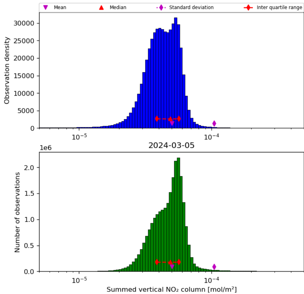
Figure 40: Histogram of “Summed vertical NO 2 column” for 2024-03-04 to 2024-03-06
