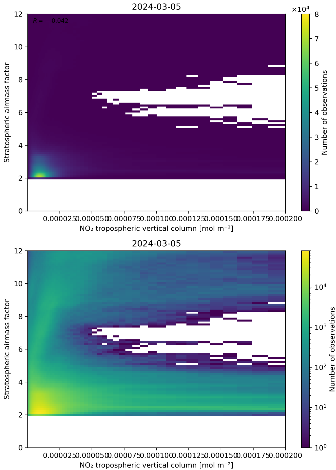
Figure 121: Scatter density plot of “NO 2 tropospheric vertical column” against “Stratospheric air mass factor” for 2024-03-04 to 2024-03-06.
