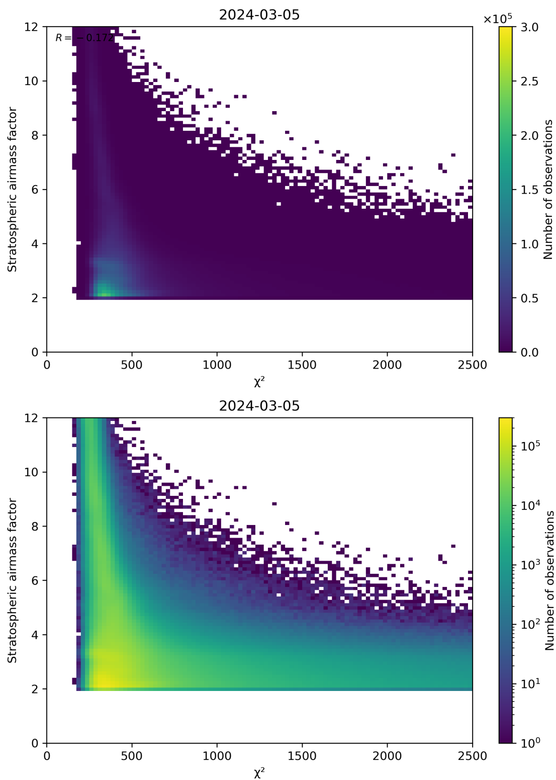
Figure 81: Scatter density plot of “ \chi^2 ” against “Stratospheric airmass factor” for 2024-03-04 to 2024-03-06.
