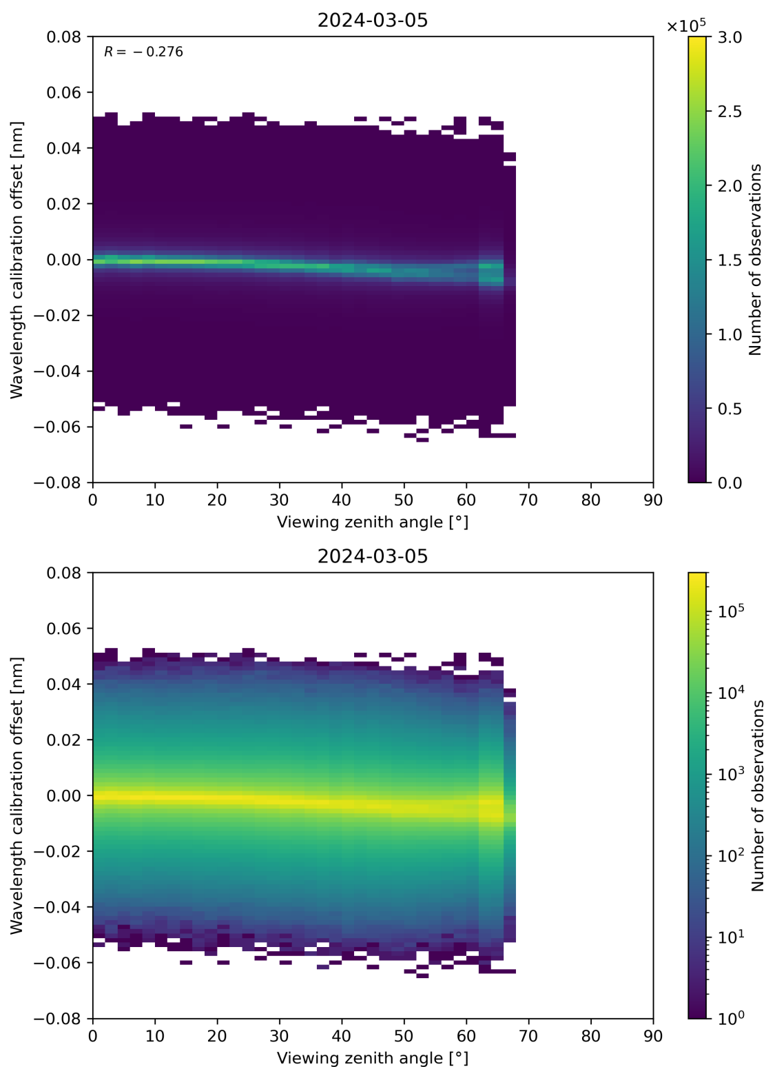
Figure 173: Scatter density plot of “Viewing zenith angle” against “Wavelength calibration offset” for 2024-03-04 to 2024-03-06.
