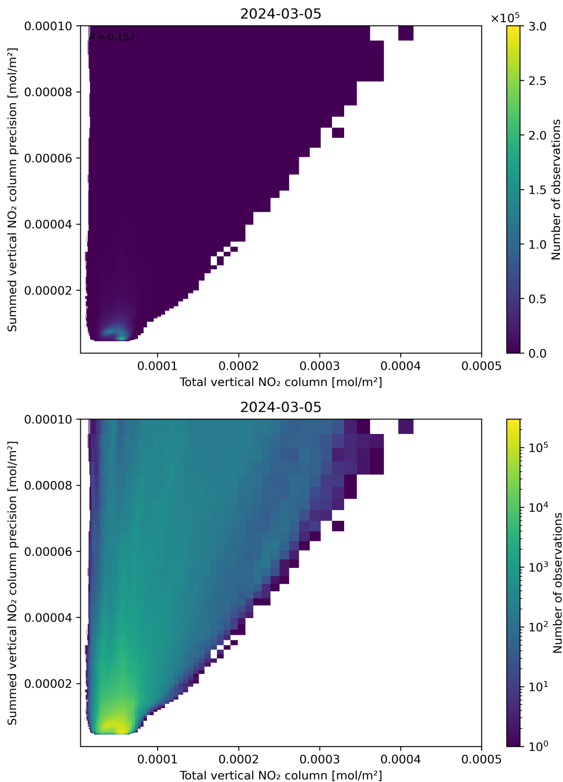
Figure 113: Scatter density plot of “Total vertical NO 2 column” against “Summed vertical NO 2 column precision” for 2024-03-04 to 2024-03-06.
