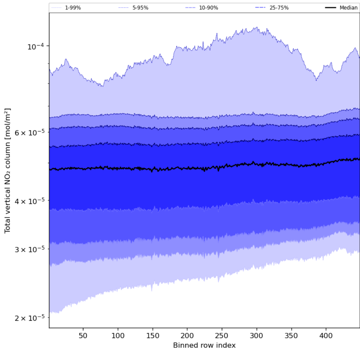
Figure 55: Along track statistics of “Total vertical NO 2 column” for 2024-03-04 to 2024-03-06
