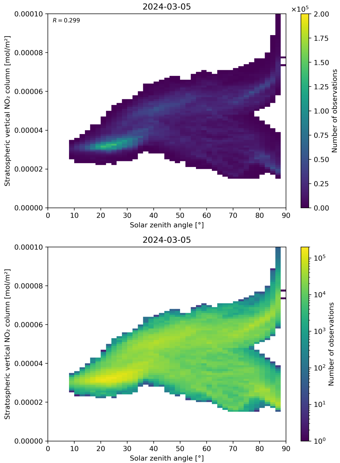
Figure 150: Scatter density plot of “Solar zenith angle” against “Stratospheric vertical NO 2 column” for 2024-03-04 to 2024-03-06.
