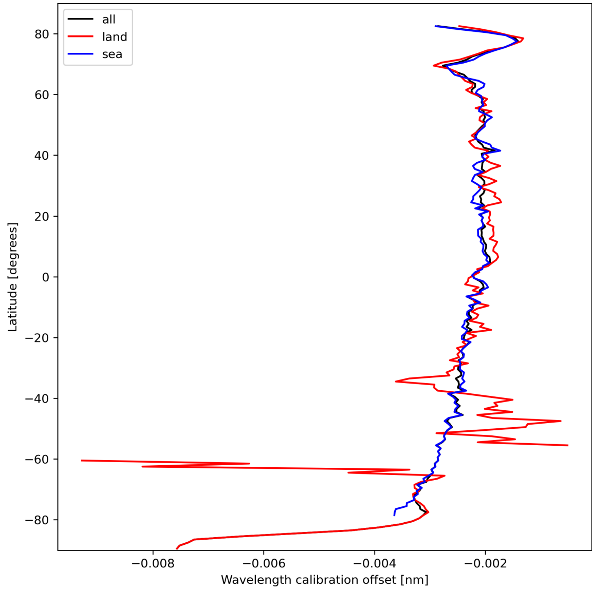
Figure 18: Zonal average of “Wavelength calibration offset” for 2024-03-04 to 2024-03-06.
