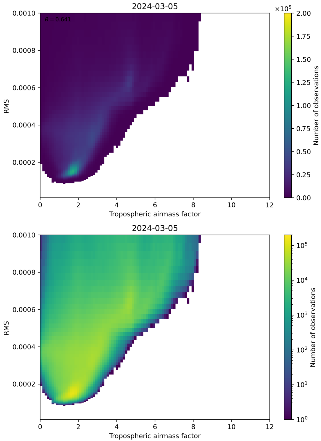
Figure 79: Scatter density plot of “Tropospheric airmass factor” against “RMS” for 2024-03-04 to 2024-03-06.
