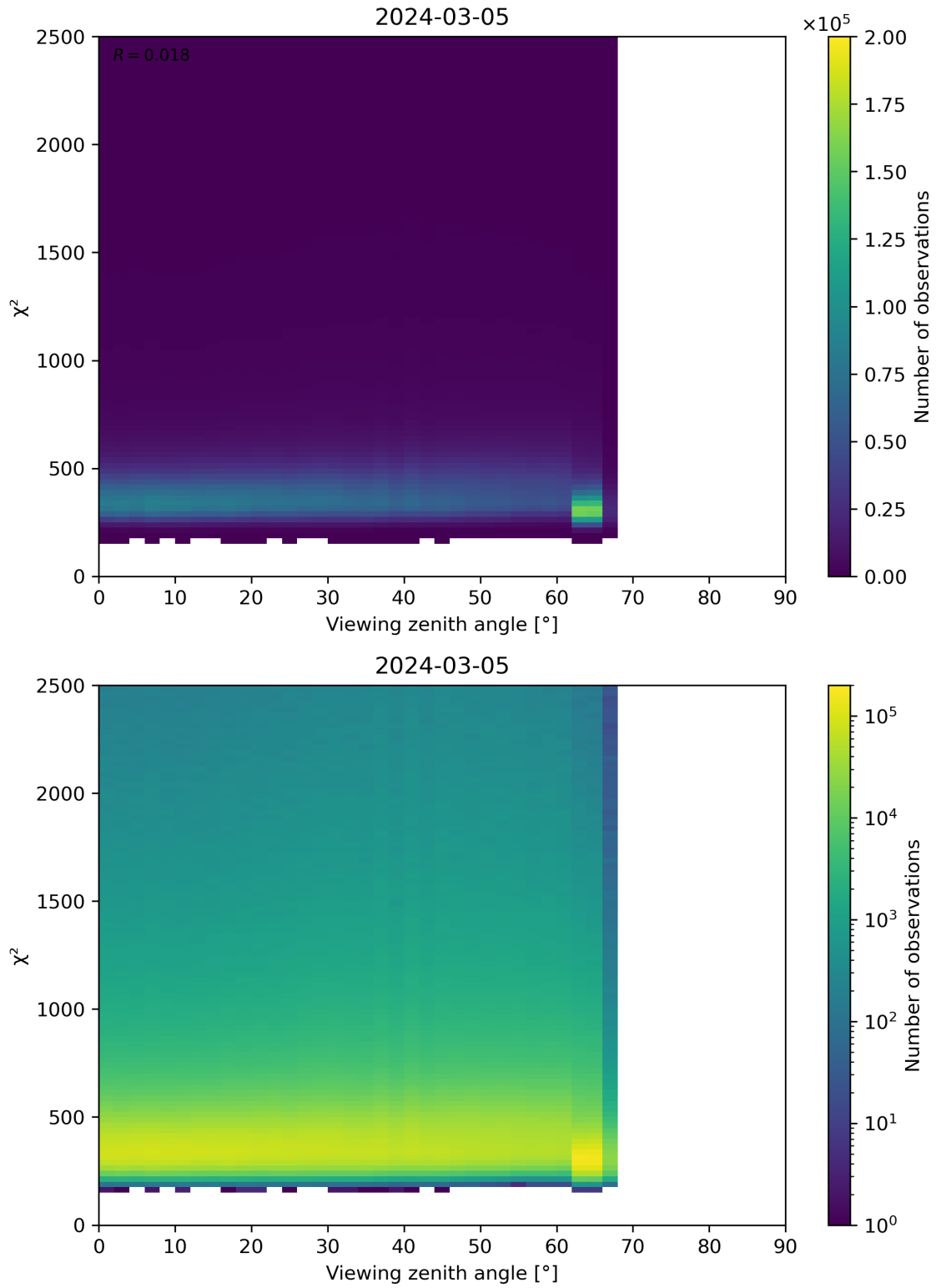
Figure 162: Scatter density plot of “Viewing zenith angle” against “ \chi^2 ” for 2024-03-04 to 2024-03-06.
