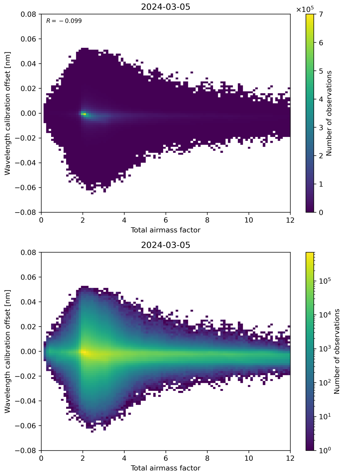
Figure 70: Scatter density plot of “Total airmass factor” against “Wavelength calibration offset” for 2024-03-04 to 2024-03-06.
