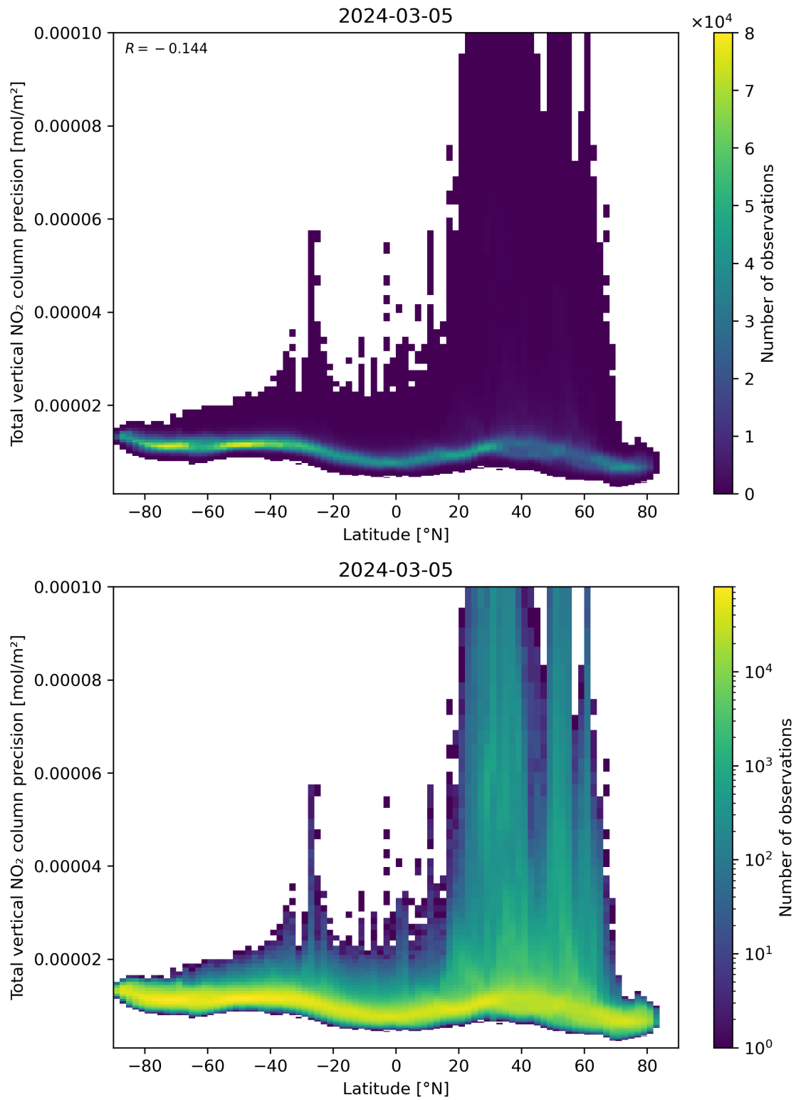
Figure 91: Scatter density plot of “Latitude” against “Total vertical NO 2 column precision” for 2024-03-04 to 2024-03-06.
