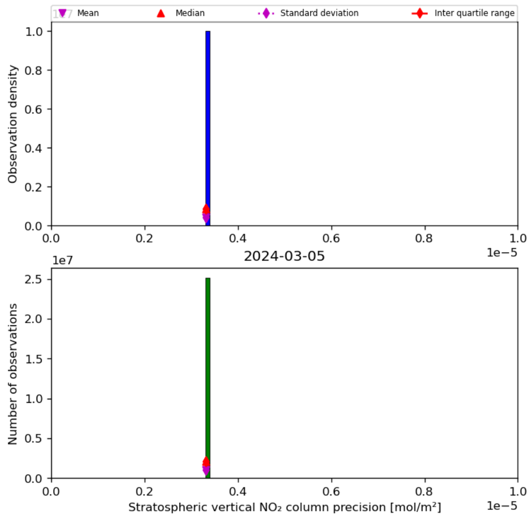
Figure 37: Histogram of “Stratospheric vertical NO 2 column precision” for 2024-03-04 to 2024-03-06
