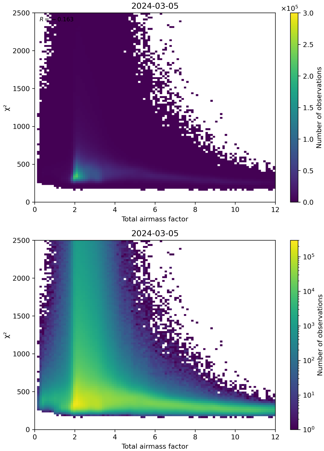
Figure 63: Scatter density plot of “Total airmass factor” against “ \chi^2 ” for 2024-03-04 to 2024-03-06.
