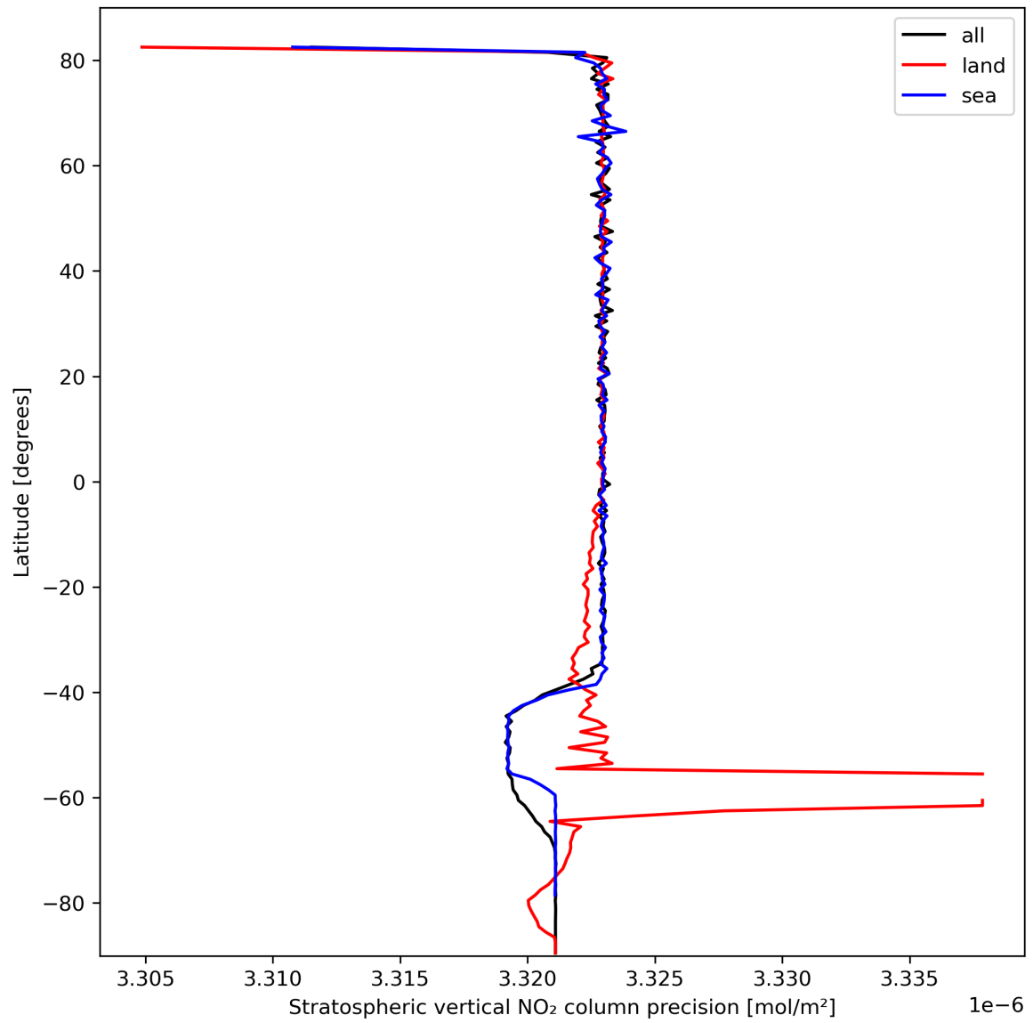
Figure 20: Zonal average of “Stratospheric vertical NO 2 column precision” for 2024-03-04 to 2024-03-06.
