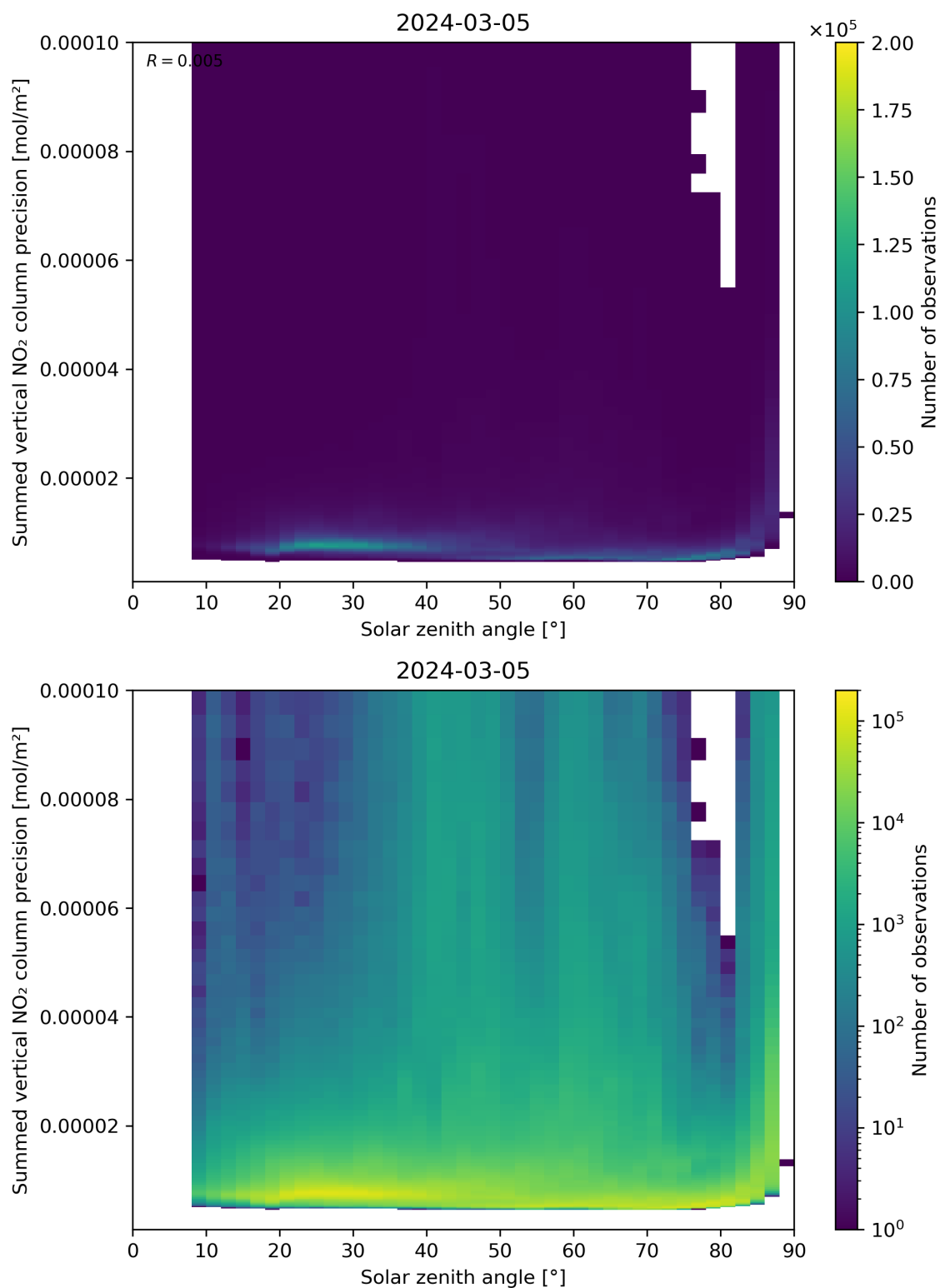
Figure 152: Scatter density plot of “Solar zenith angle” against “Summed vertical NO 2 column precision” for 2024-03-04 to 2024-03-06.
