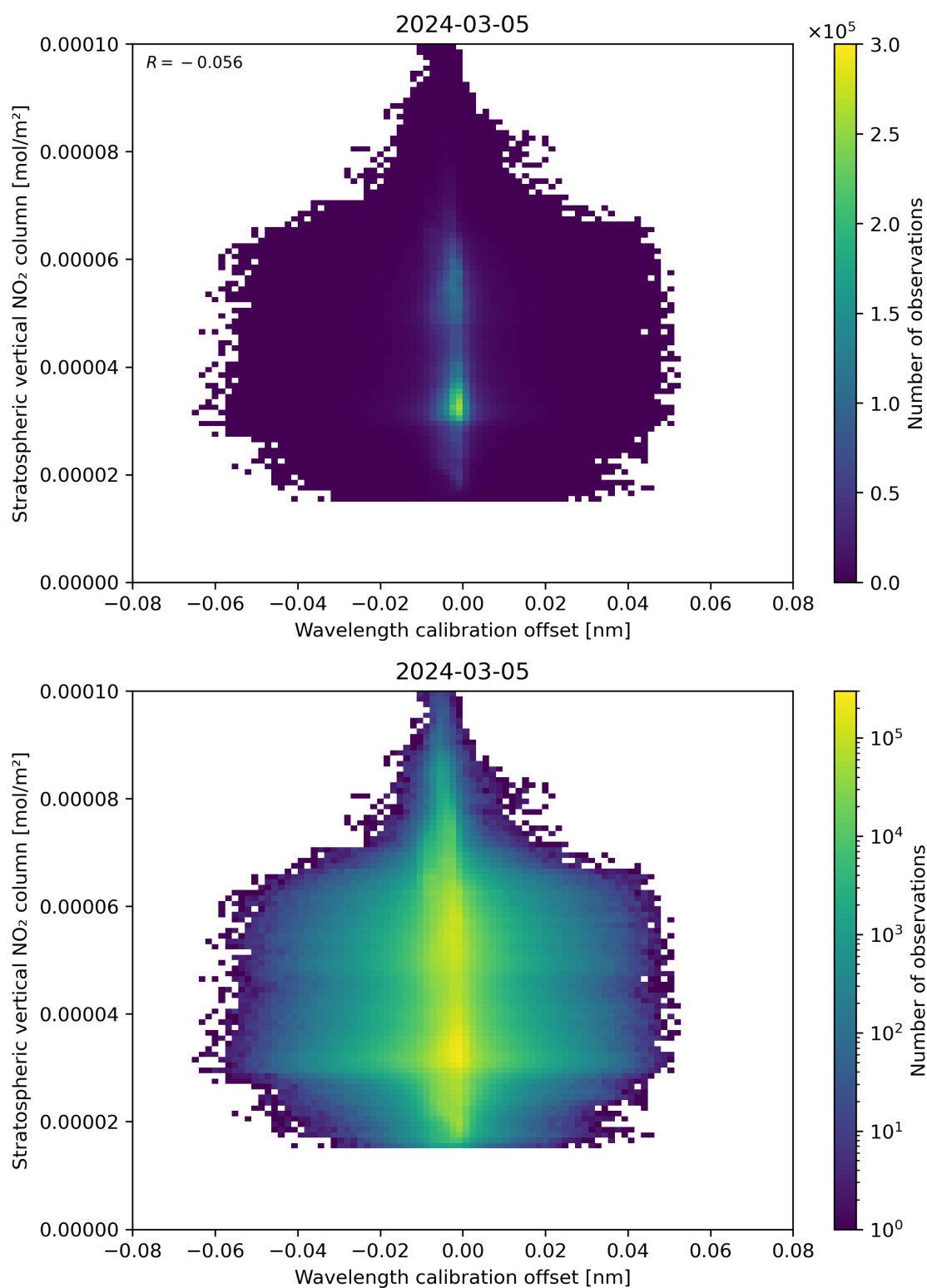
Figure 176: Scatter density plot of “Wavelength calibration offset” against “Stratospheric vertical NO 2 column” for 2024-03-04 to 2024-03-06.
