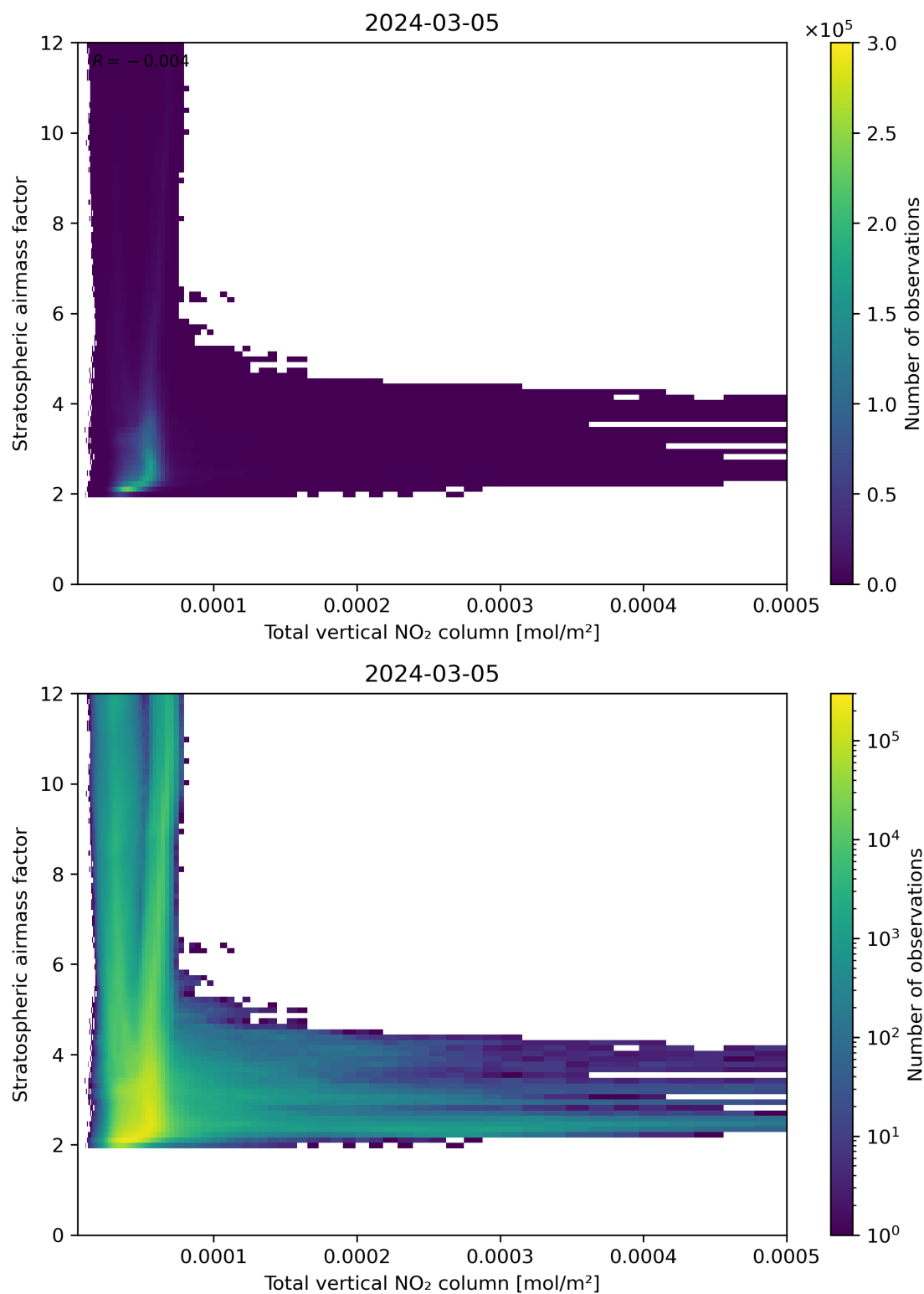
Figure 110: Scatter density plot of “Total vertical NO 2 column” against “Stratospheric airmass factor” for 2024-03-04 to 2024-03-06.
