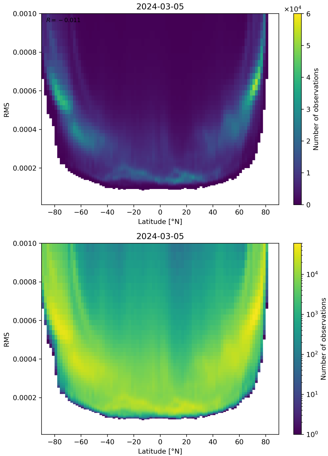
Figure 94: Scatter density plot of “Latitude” against “RMS” for 2024-03-04 to 2024-03-06.
