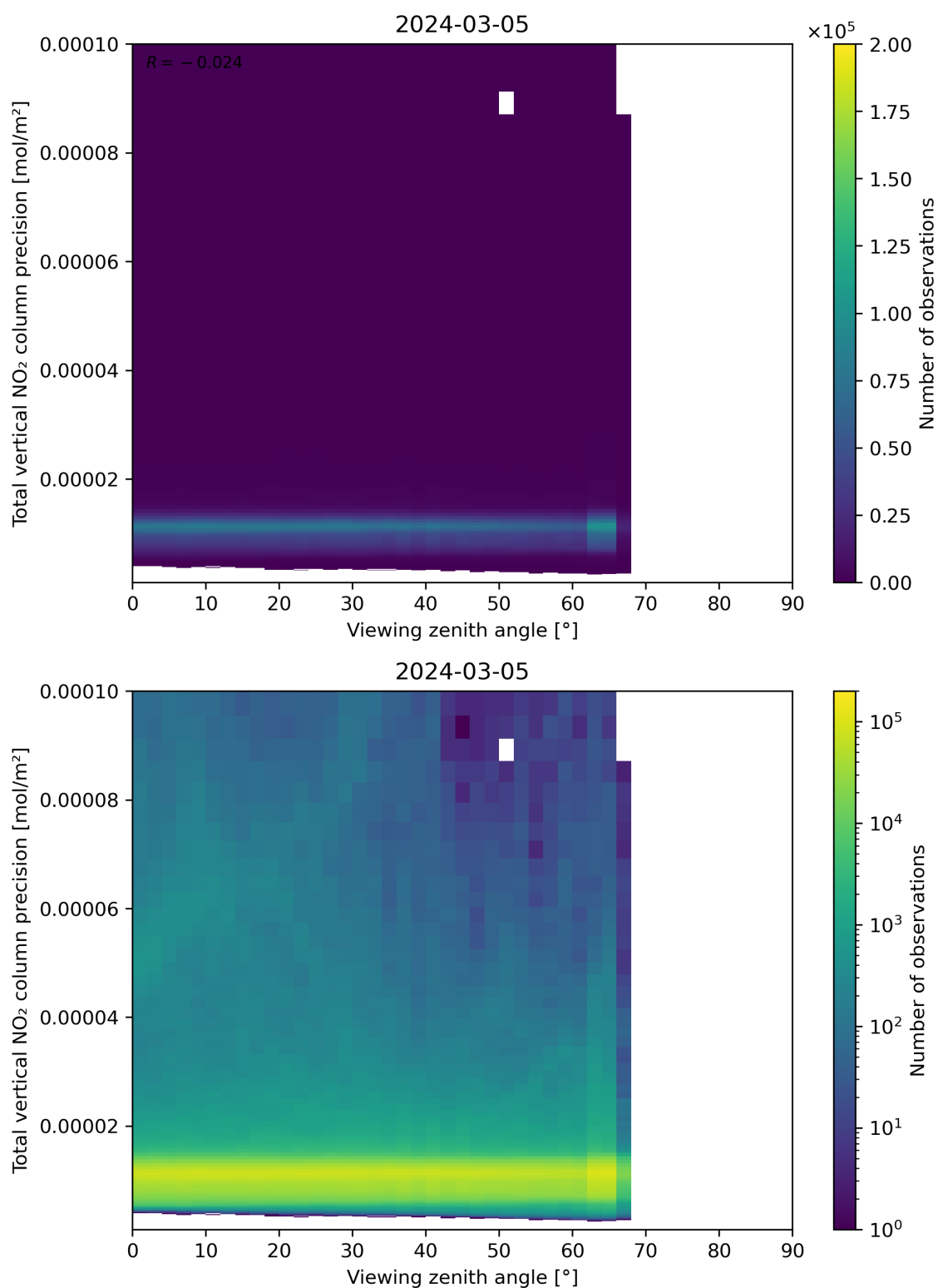
Figure 168: Scatter density plot of “Viewing zenith angle” against “Total vertical NO 2 column precision” for 2024-03-04 to 2024-03-06.
