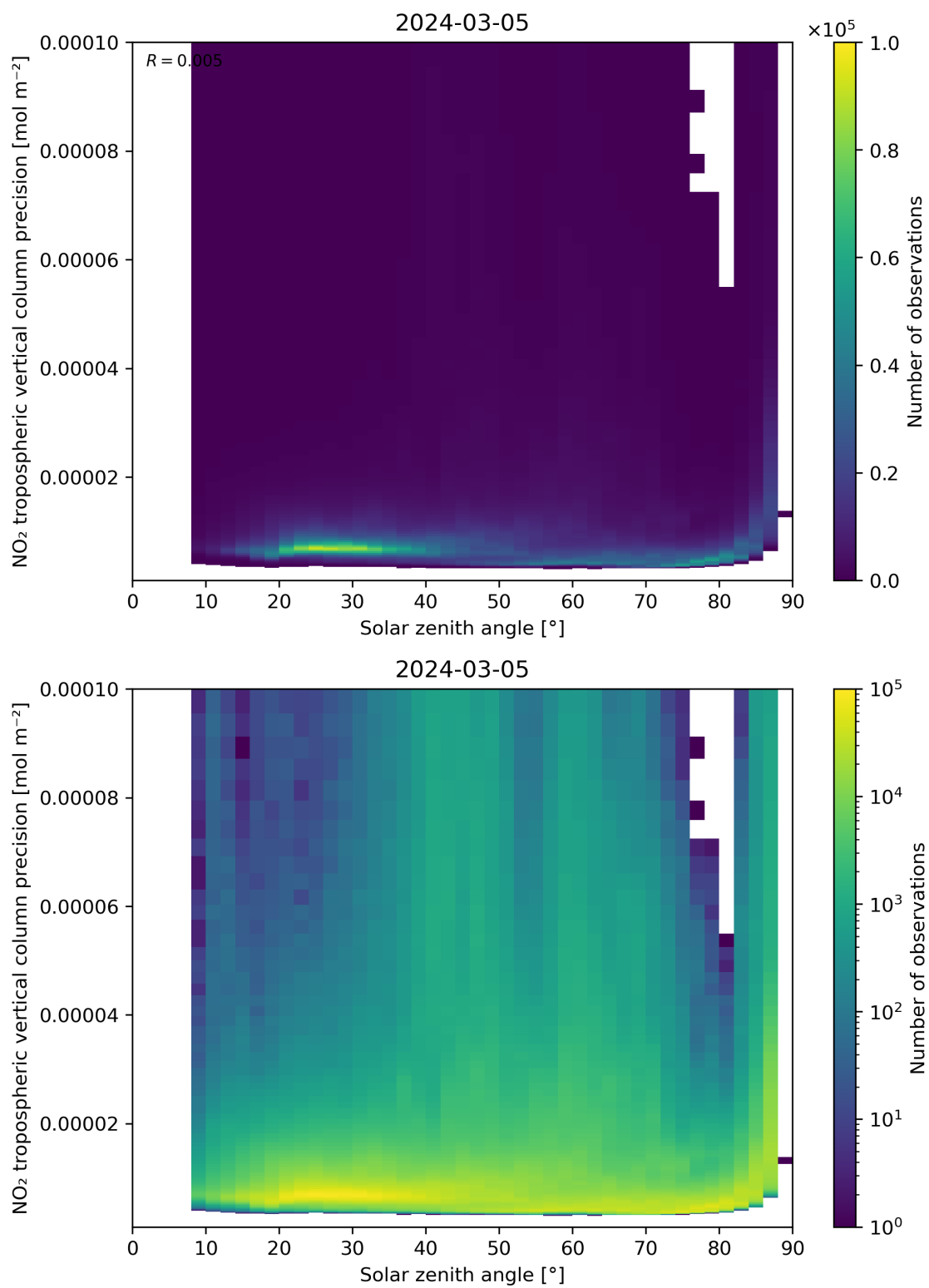
Figure 156: Scatter density plot of “Solar zenith angle” against “NO 2 tropospheric vertical column precision” for 2024-03-04 to 2024-03-06.
