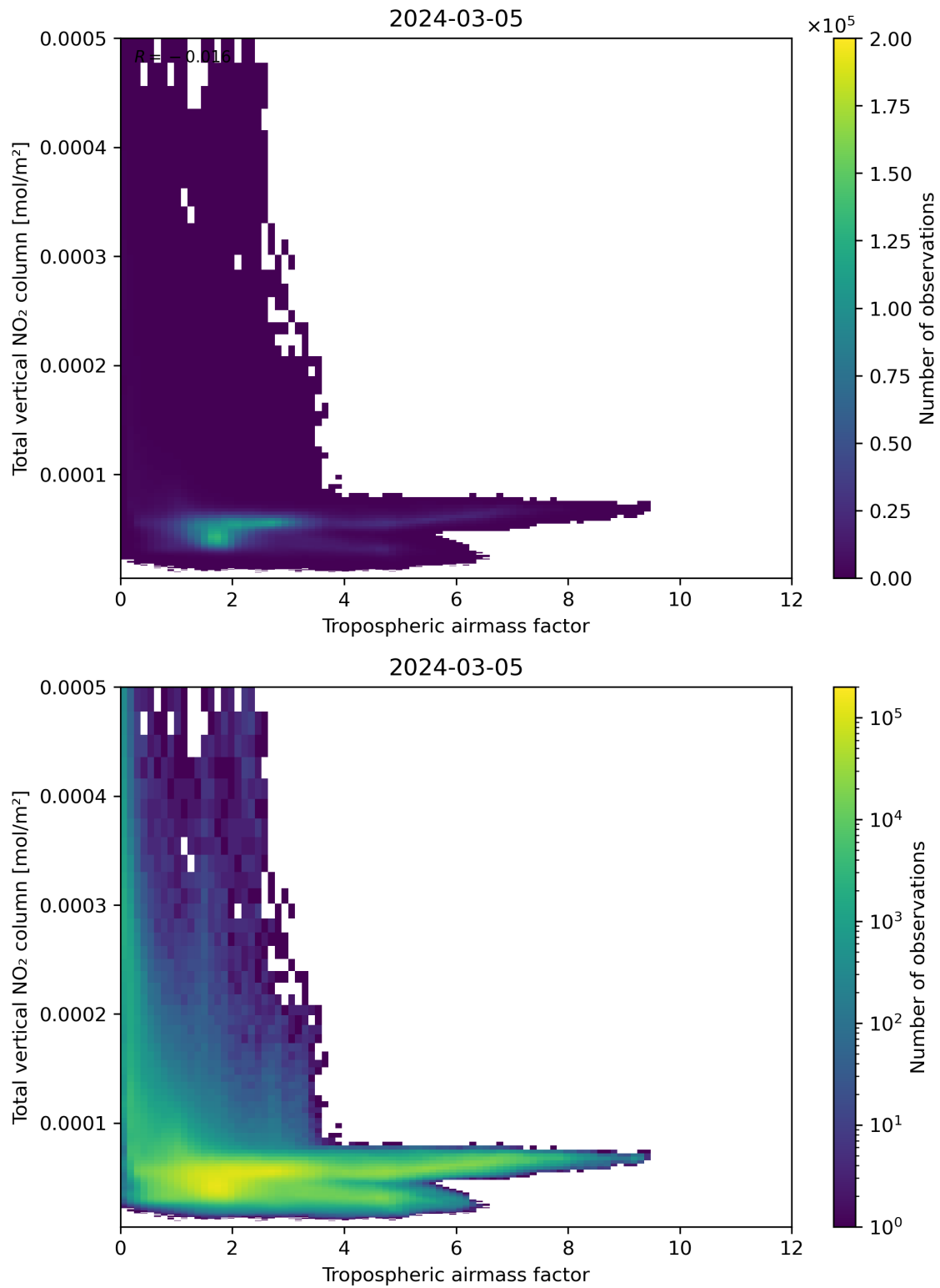
Figure 77: Scatter density plot of “Tropospheric airmass factor” against “Total vertical NO 2 column” for 2024-03-04 to 2024-03-06.
