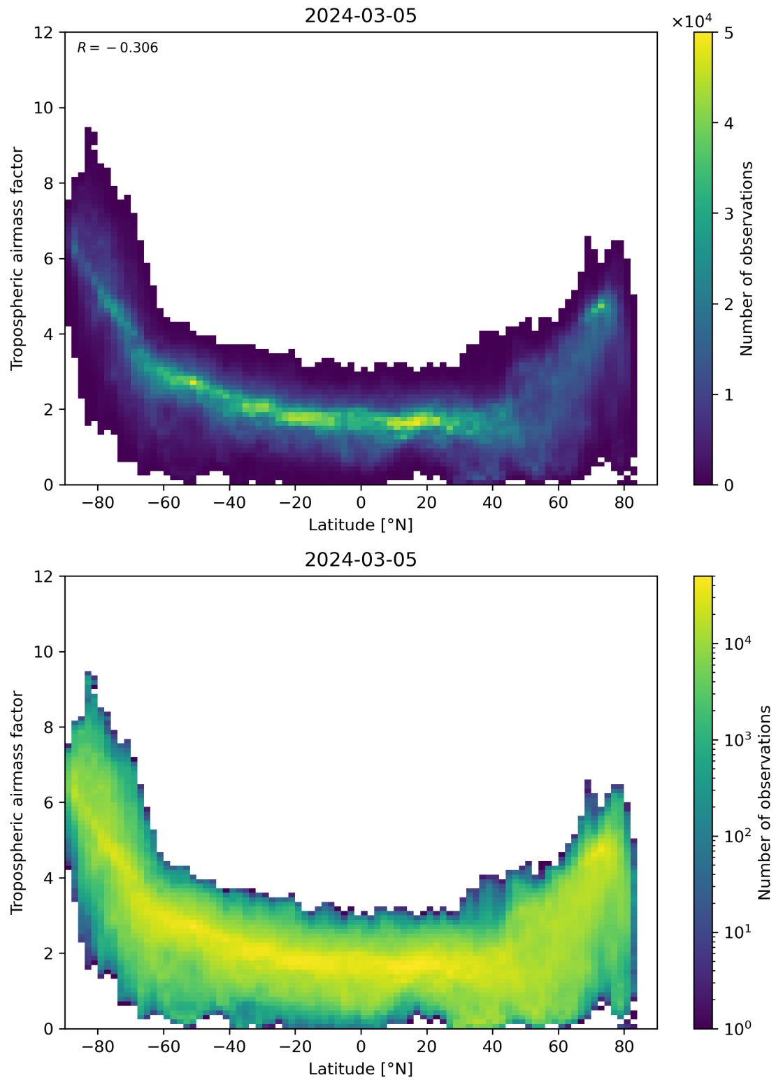
Figure 85: Scatter density plot of “Latitude” against “Tropospheric airmass factor” for 2024-03-04 to 2024-03-06.
