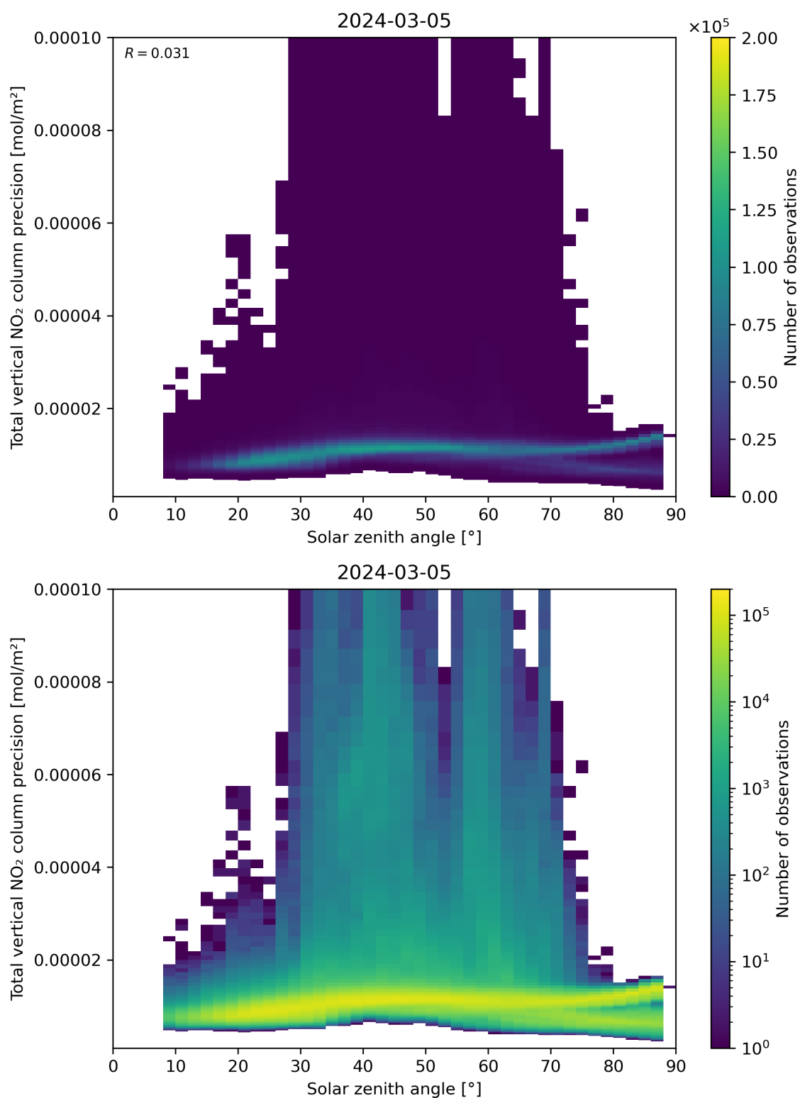
Figure 154: Scatter density plot of “Solar zenith angle” against “Total vertical NO 2 column precision” for 2024-03-04 to 2024-03-06.
