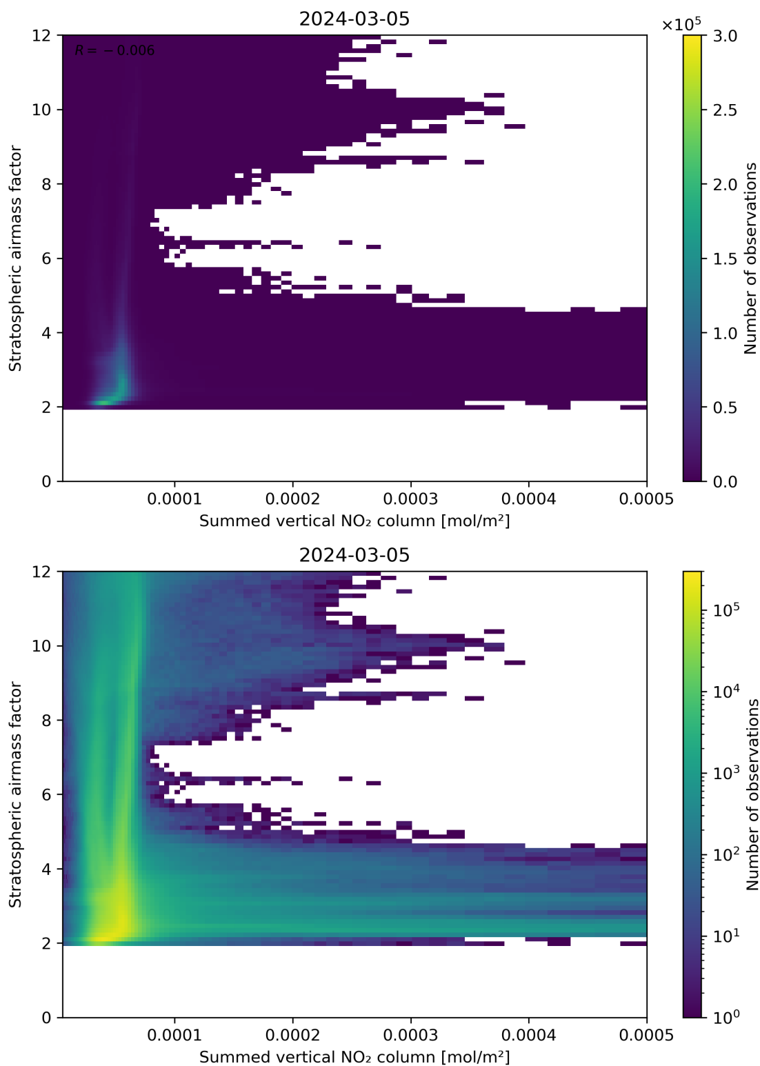
Figure 103: Scatter density plot of “Summed vertical NO 2 column” against “Stratospheric airmass factor” for 2024-03-04 to 2024-03-06.
