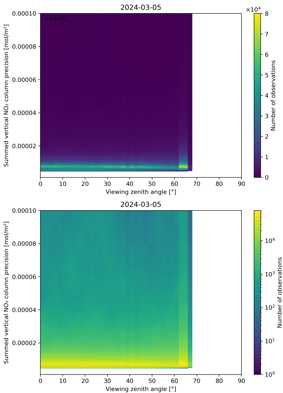
Figure 166: Scatter density plot of “Viewing zenith angle” against “Summed vertical NO 2 column precision” for 2024-03-04 to 2024-03-06.
