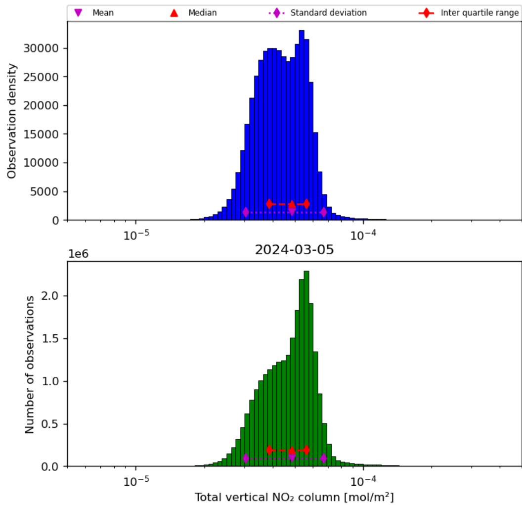
Figure 38: Histogram of “Total vertical NO 2 column” for 2024-03-04 to 2024-03-06
