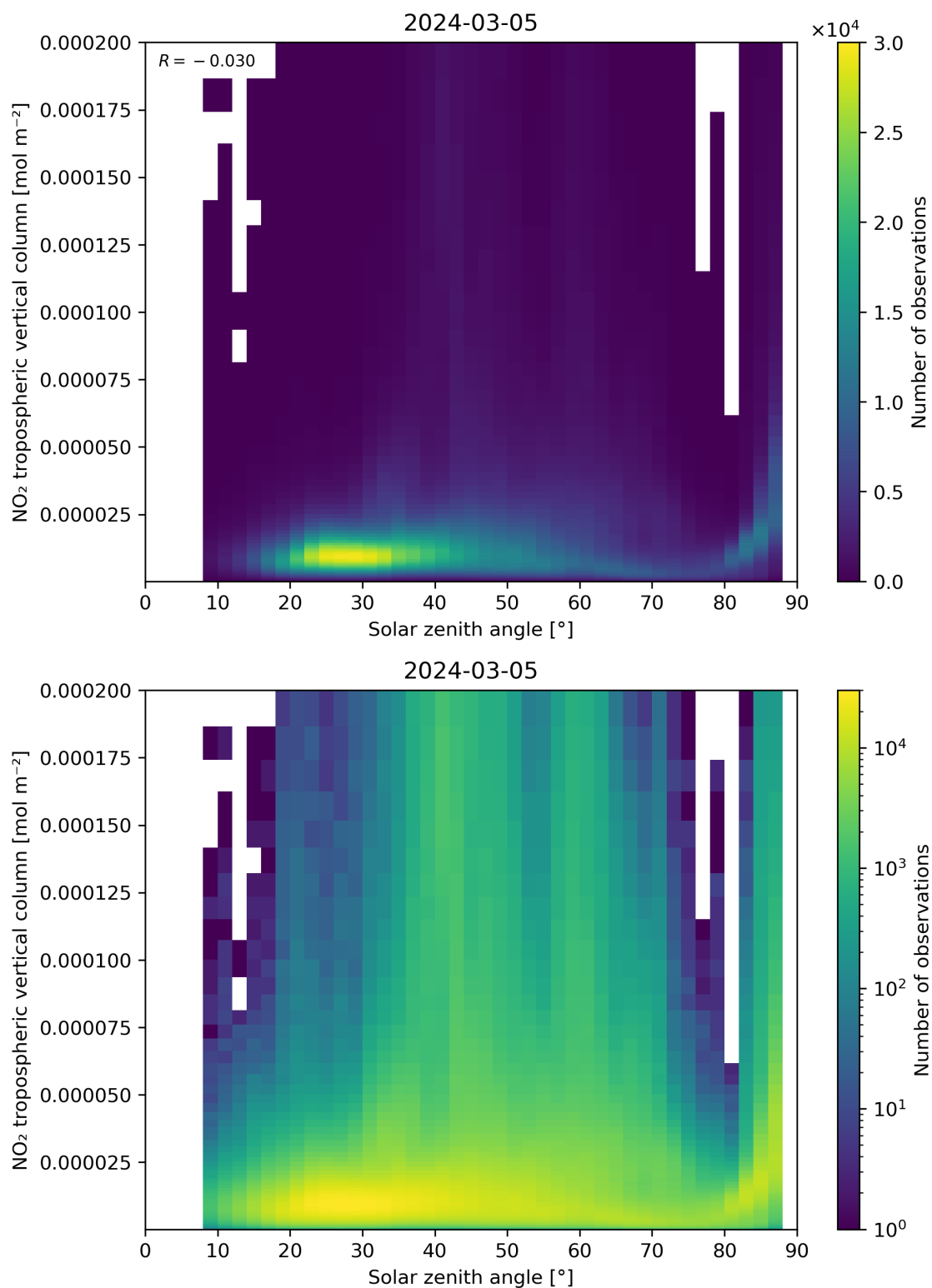
Figure 155: Scatter density plot of “Solar zenith angle” against “NO 2 tropospheric vertical column” for 2024-03-04 to 2024-03-06.
