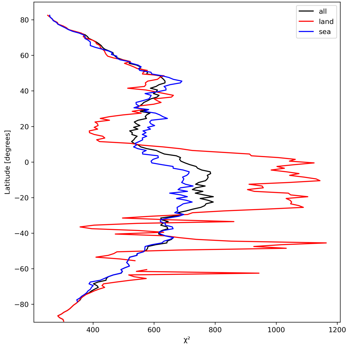
Figure 25: Zonal average of “ \chi^2 ” for 2024-03-04 to 2024-03-06.
