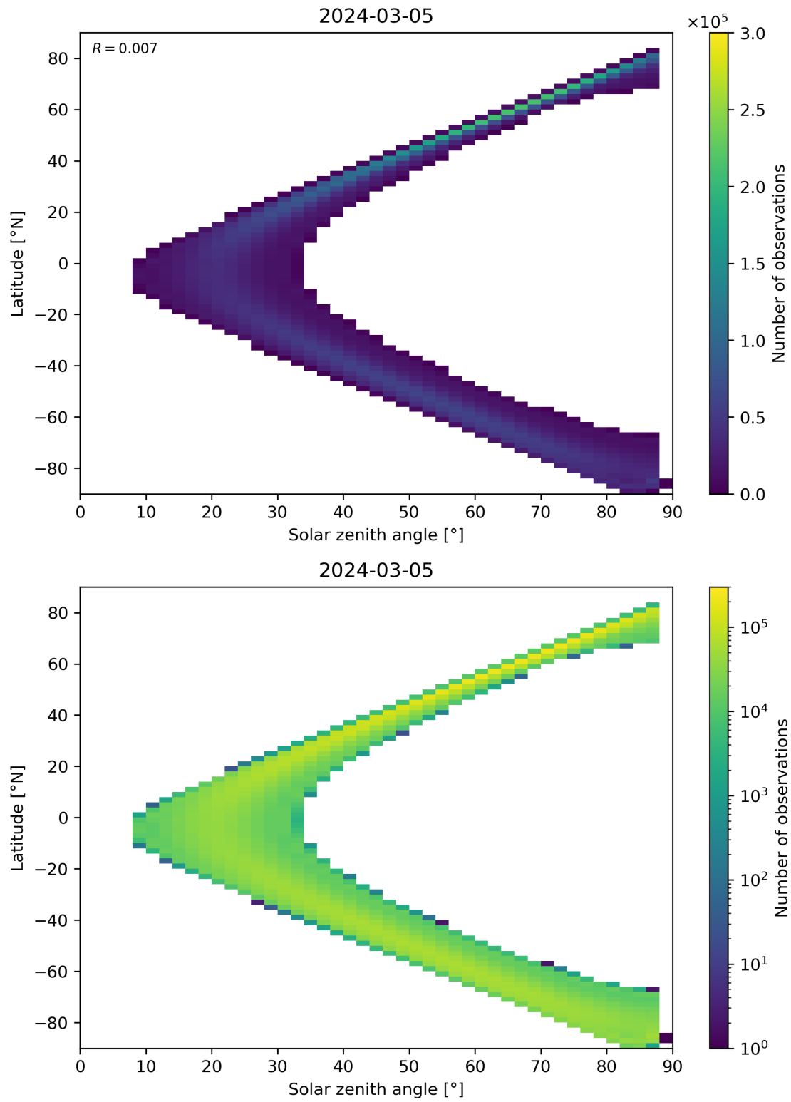
Figure 149: Scatter density plot of “Solar zenith angle” against “Latitude” for 2024-03-04 to 2024-03-06.
