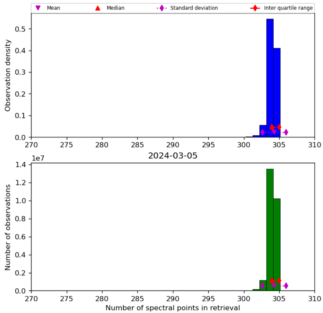
Figure 33: Histogram of “Number of spectral points in retrieval” for 2024-03-04 to 2024-03-06
