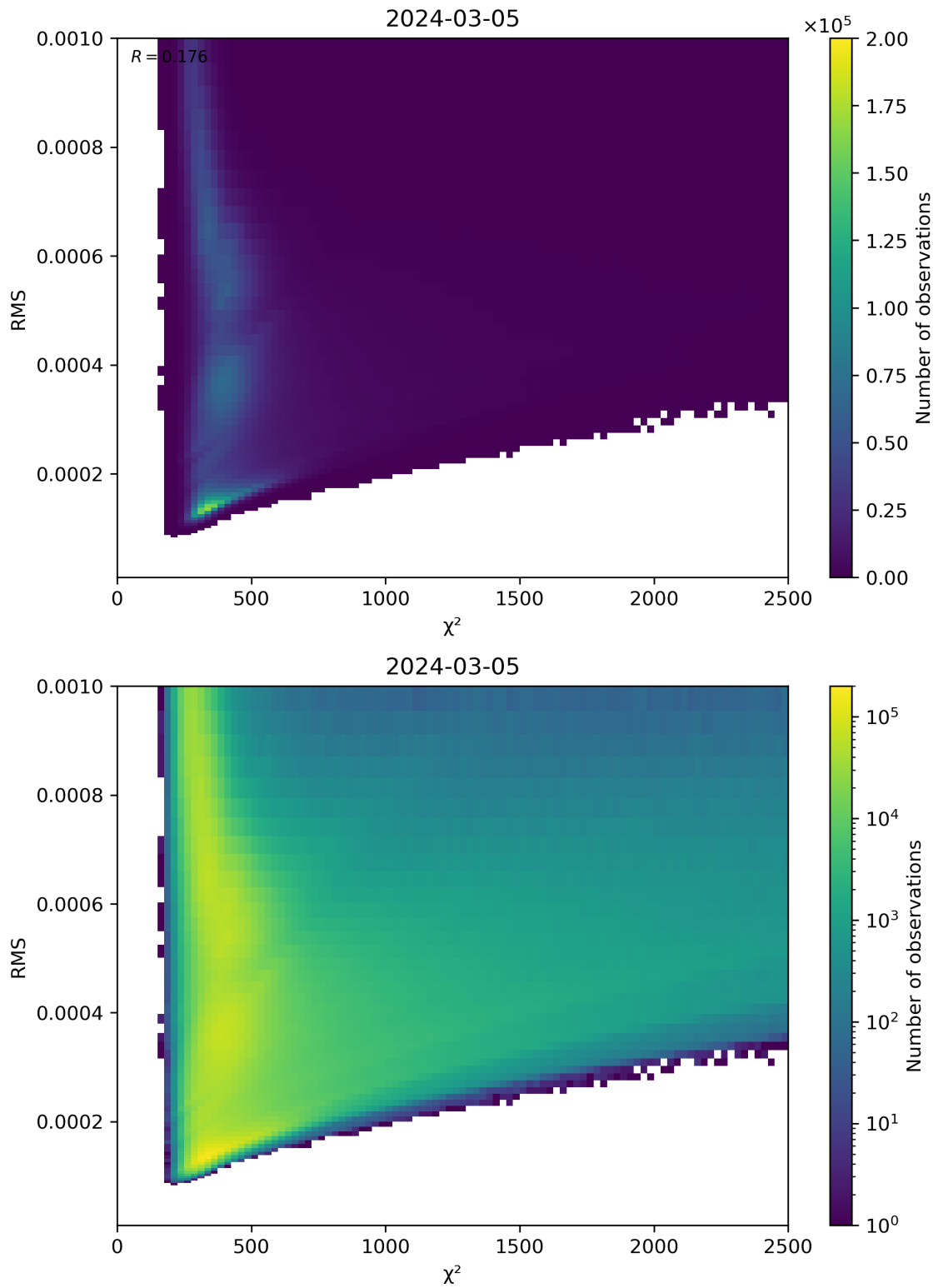
Figure 82: Scatter density plot of “ \chi^2 ” against “RMS” for 2024-03-04 to 2024-03-06.
