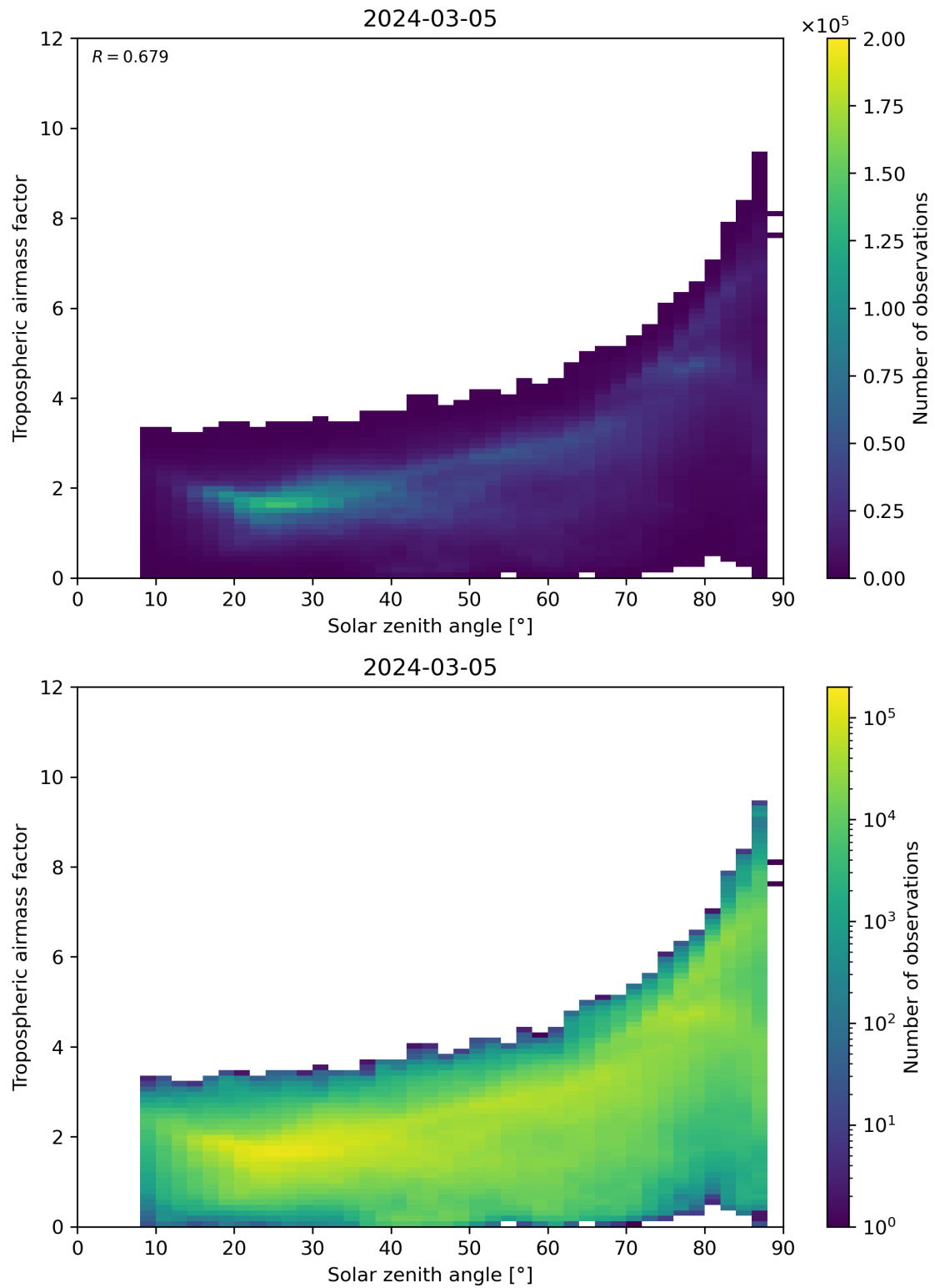
Figure 147: Scatter density plot of “Solar zenith angle” against “Tropospheric airmass factor” for 2024-03-04 to 2024-03-06.
