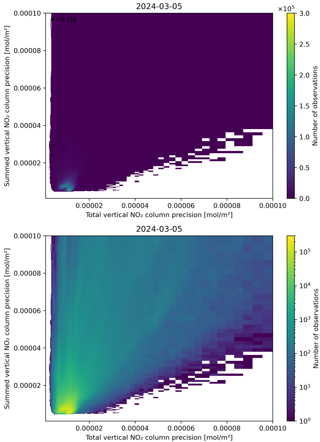
Figure 118: Scatter density plot of “Total vertical NO 2 column precision” against “Summed vertical NO 2 column precision” for 2024-03-04 to 2024-03-06.
