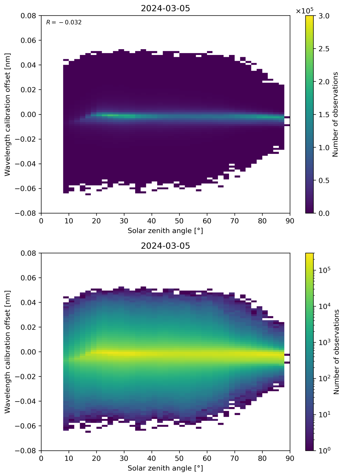
Figure 158: Scatter density plot of “Solar zenith angle” against “Wavelength calibration offset” for 2024-03-04 to 2024-03-06.
