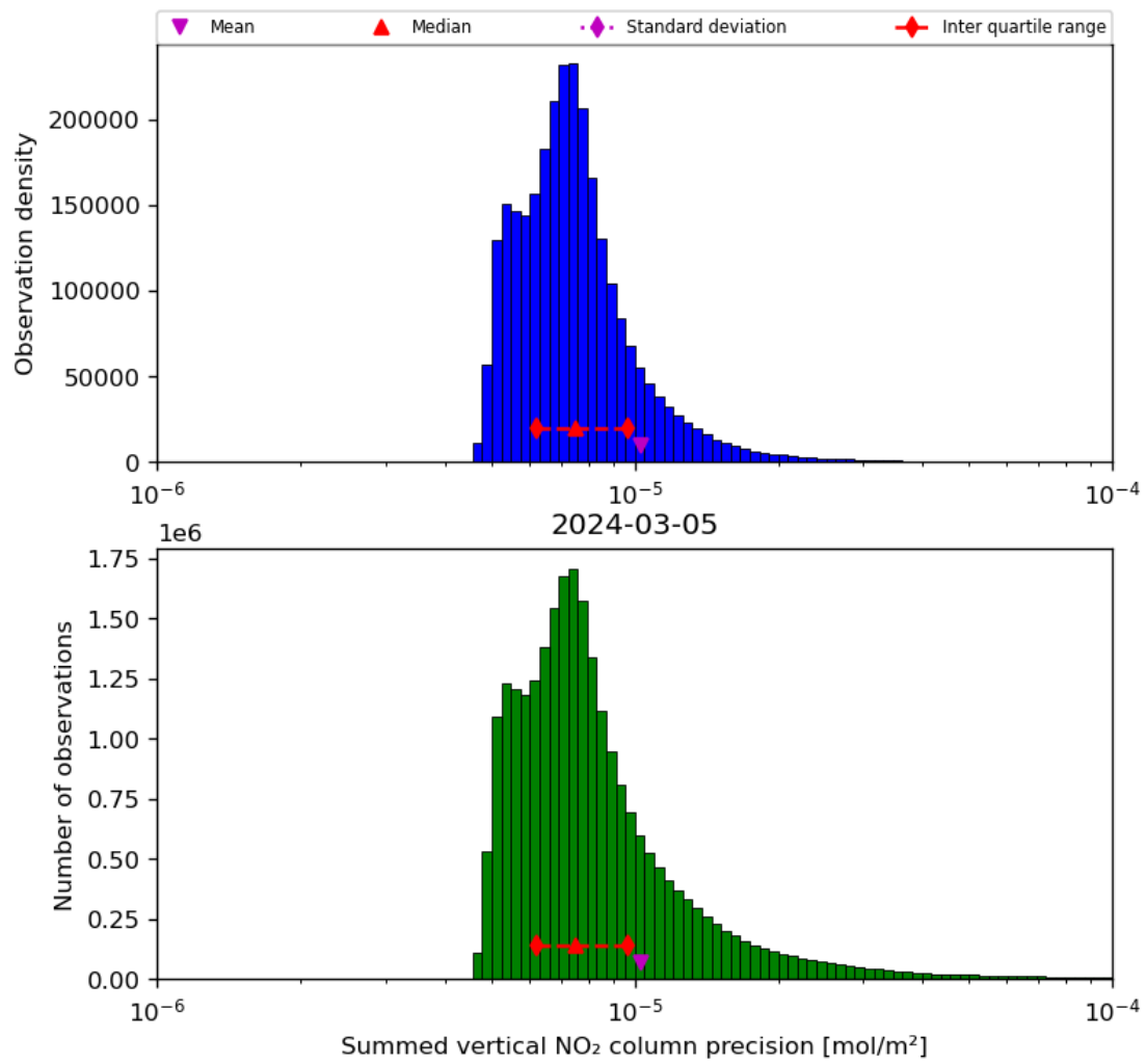
Figure 41: Histogram of "Summed vertical NO 2 column precision" for 2024-03-04 to 2024-03-06
