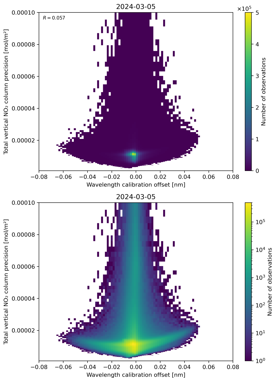
Figure 180: Scatter density plot of “Wavelength calibration offset” against “Total vertical NO 2 column precision” for 2024-03-04 to 2024-03-06.
