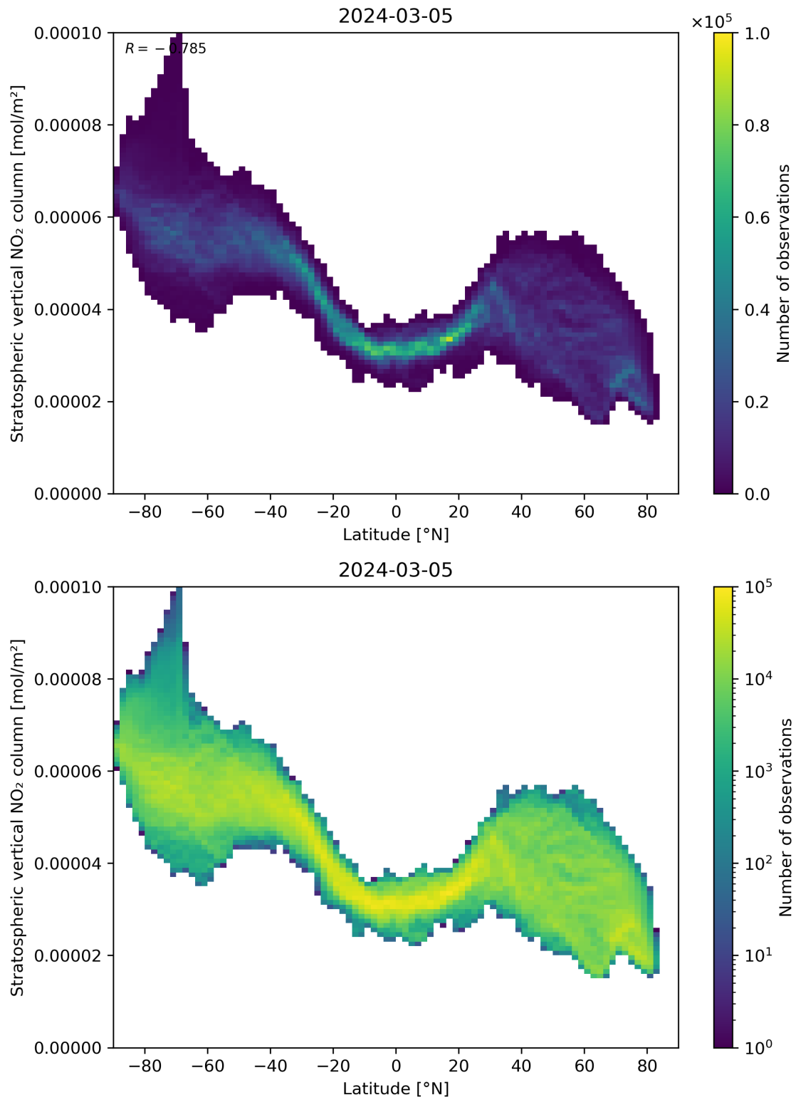
Figure 87: Scatter density plot of “Latitude” against “Stratospheric vertical NO 2 column” for 2024-03-04 to 2024-03-06.
