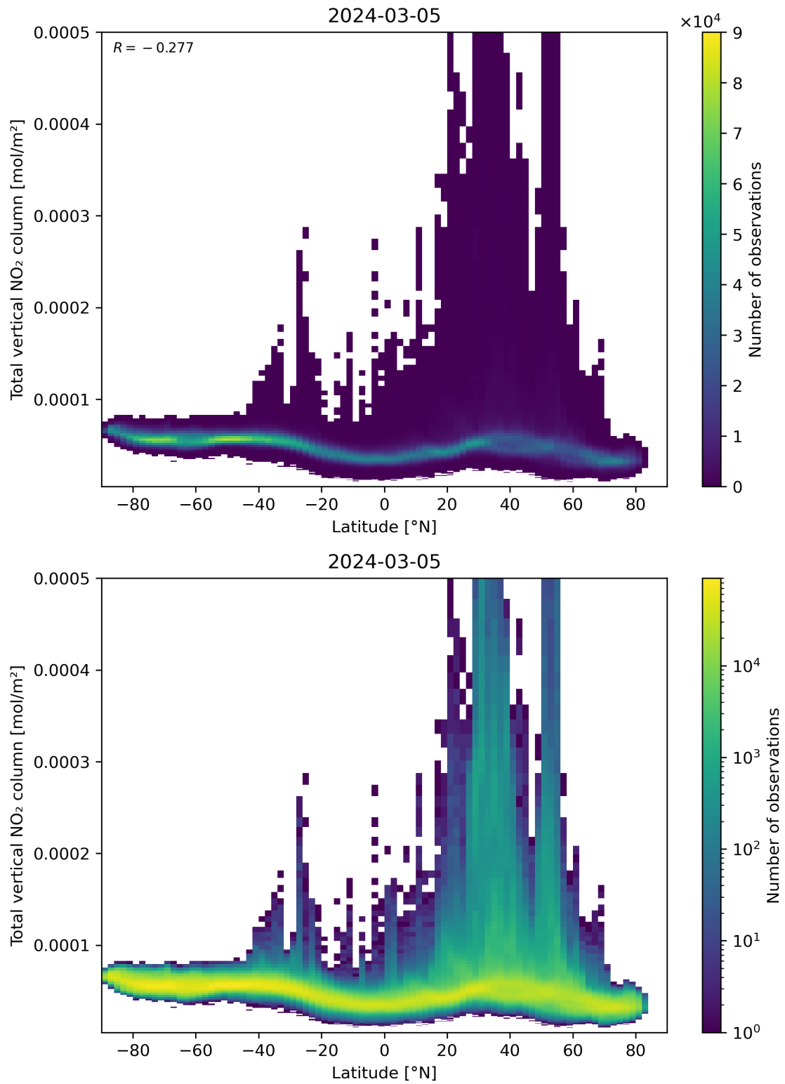
Figure 90: Scatter density plot of “Latitude” against “Total vertical NO 2 column” for 2024-03-04 to 2024-03-06.
