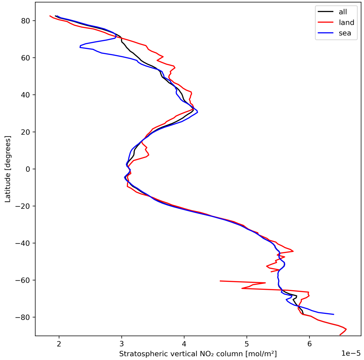
Figure 19: Zonal average of “Stratospheric vertical NO 2 column” for 2024-03-04 to 2024-03-06.
