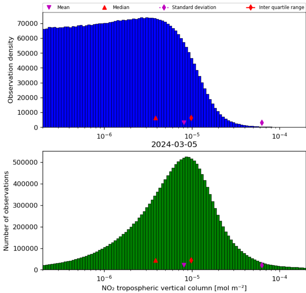
Figure 29: Histogram of “NO 2 tropospheric vertical column” for 2024-03-04 to 2024-03-06
