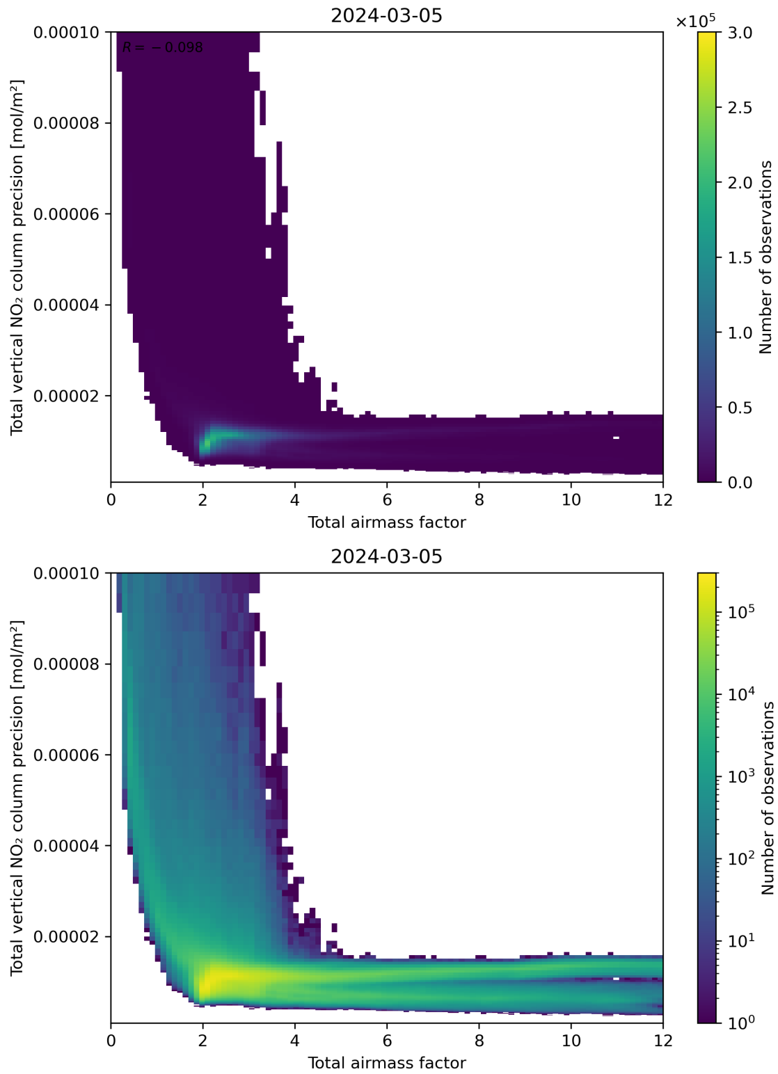
Figure 68: Scatter density plot of “Total airmass factor” against “Total vertical NO 2 column precision” for 2024-03-04 to 2024-03-06.
