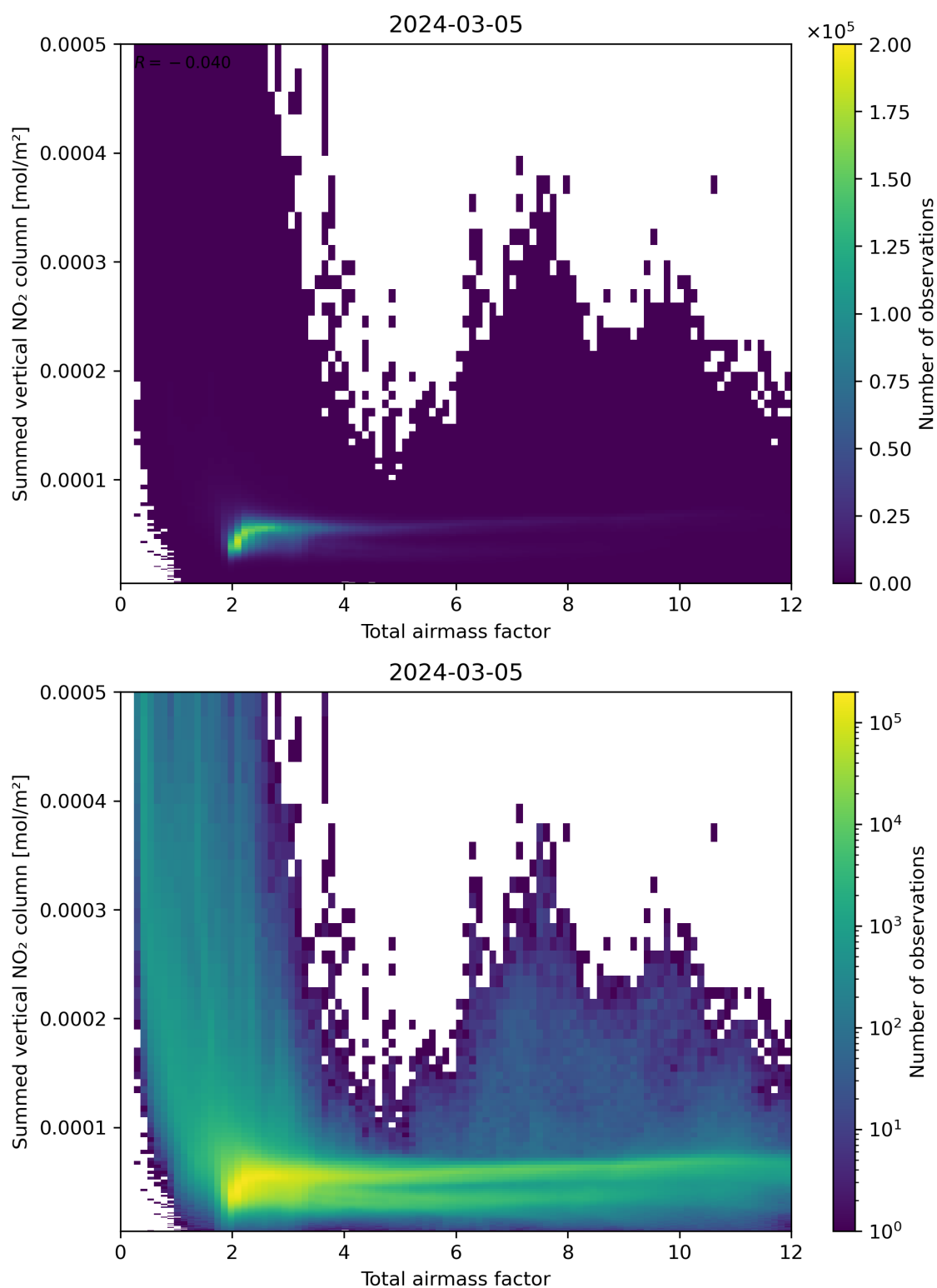
Figure 65: Scatter density plot of “Total airmass factor” against “Summed vertical NO 2 column” for 2024-03-04 to 2024-03-06.
