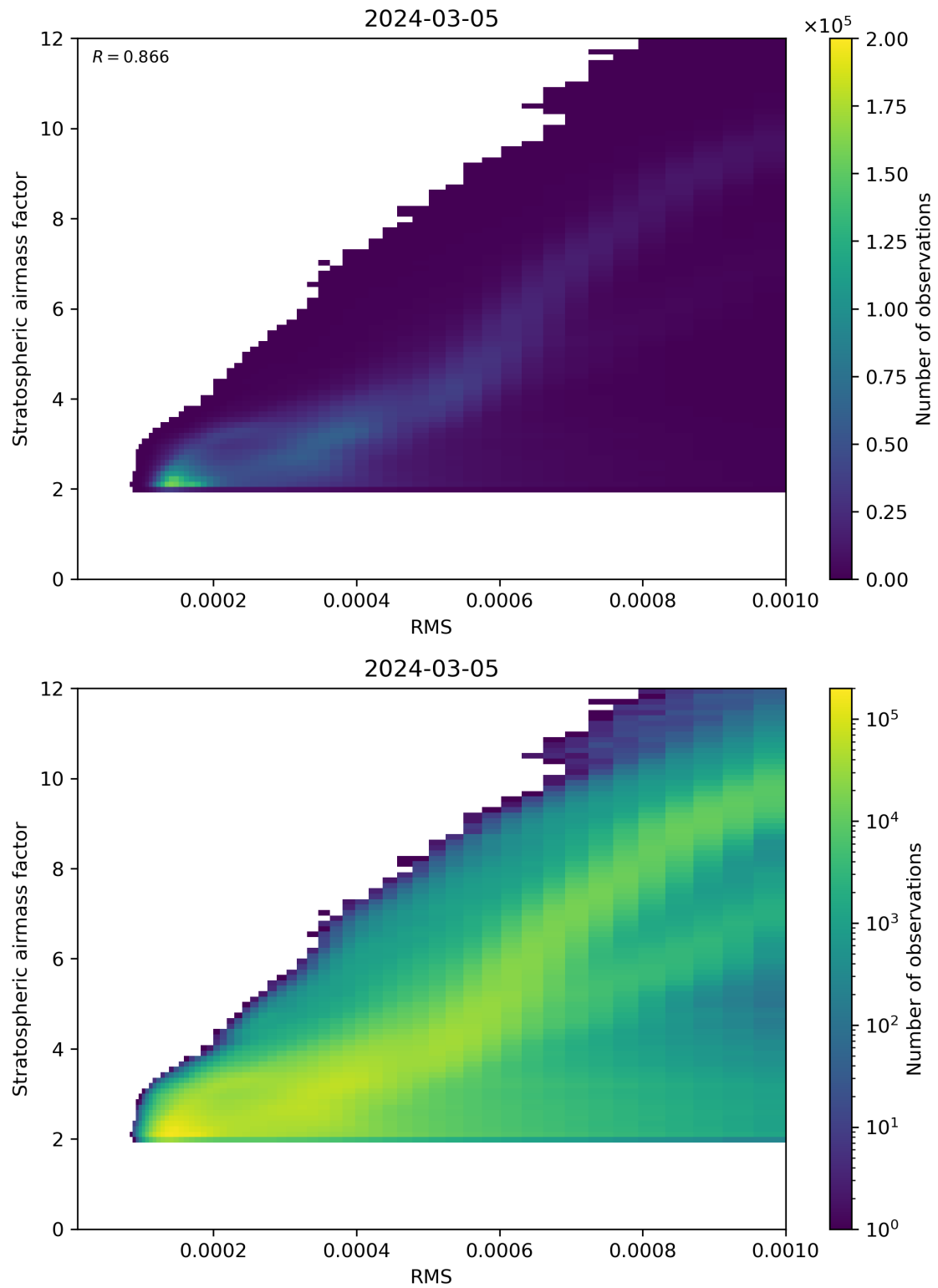
Figure 144: Scatter density plot of “RMS” against “Stratospheric airmass factor” for 2024-03-04 to 2024-03-06.
