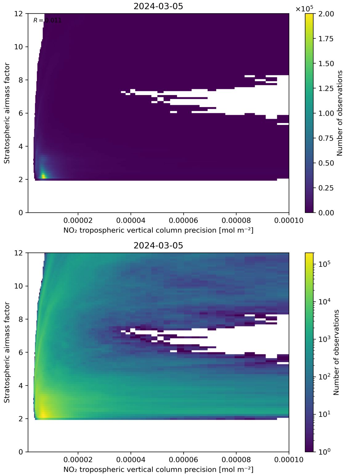
Figure 131: Scatter density plot of “NO 2 tropospheric vertical column precision” against “Stratospheric airmass factor” for 2024-03-04 to 2024-03-06.
