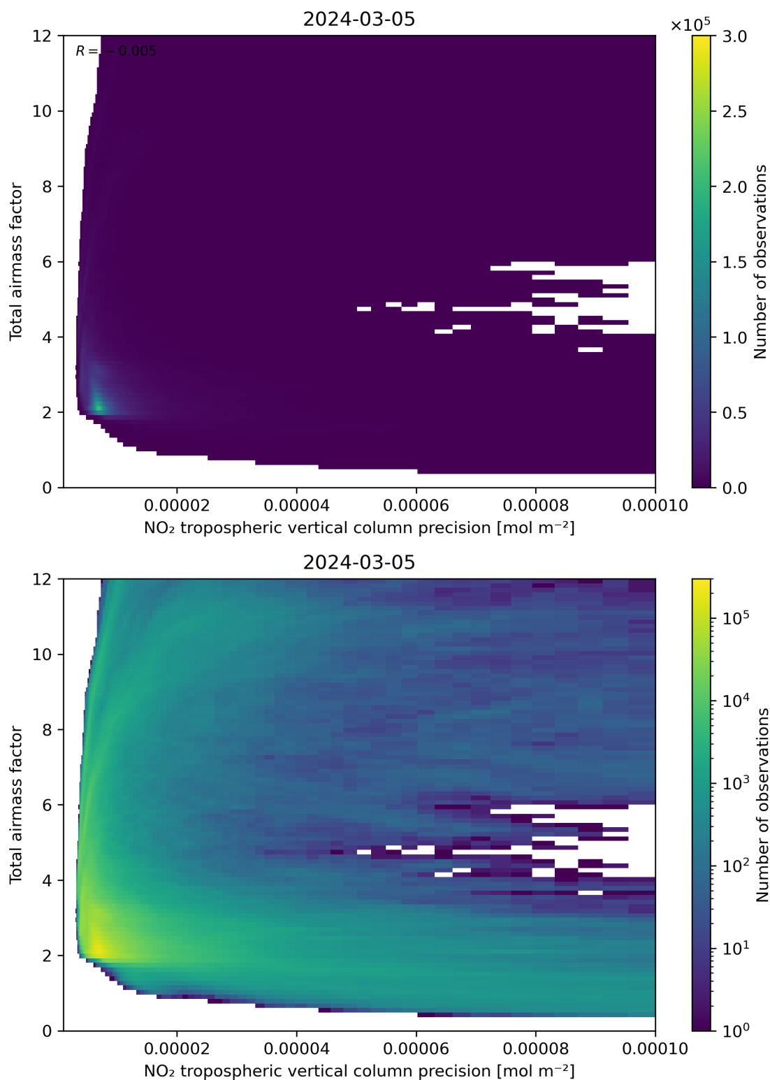
Figure 132: Scatter density plot of “NO 2 tropospheric vertical column precision” against “Total airmass factor” for 2024-03-04 to 2024-03-06.
