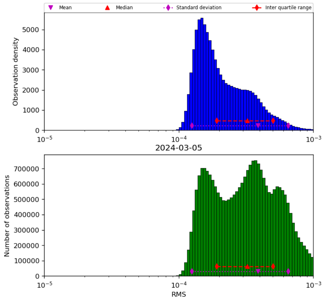
Figure 43: Histogram of “RMS” for 2024-03-04 to 2024-03-06
