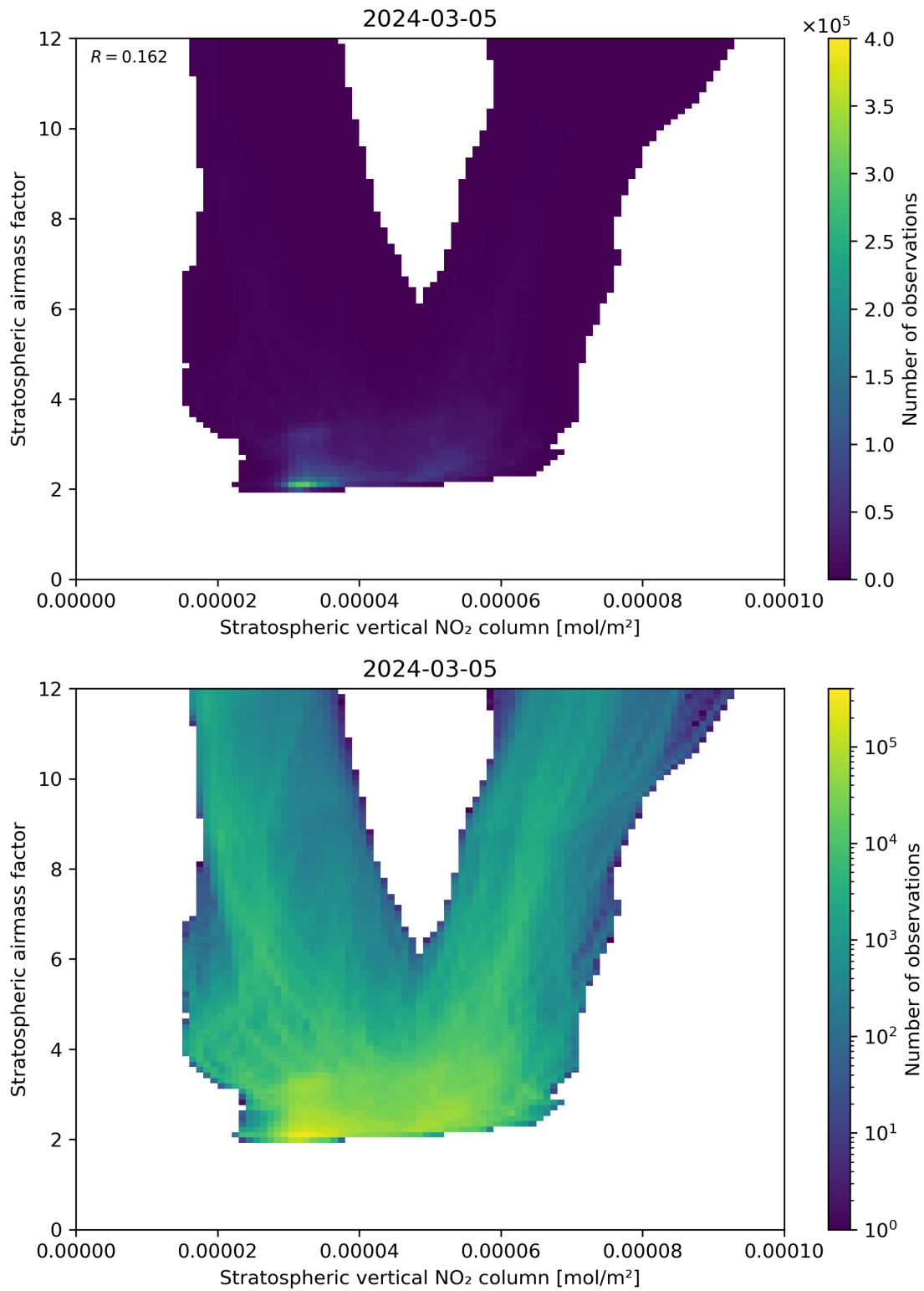
Figure 96: Scatter density plot of “Stratospheric vertical NO 2 column” against “Stratospheric airmass factor” for 2024-03-04 to 2024-03-06.
