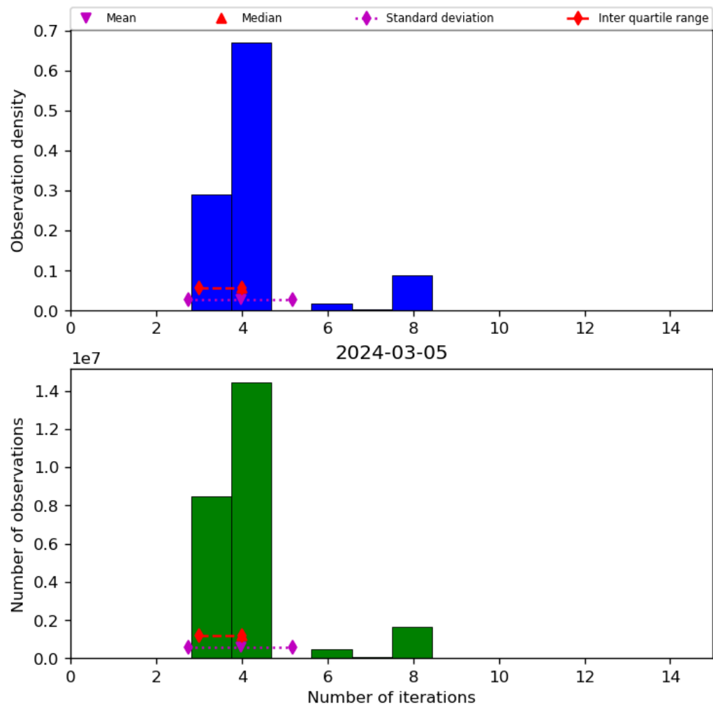
Figure 34: Histogram of “Number of iterations” for 2024-03-04 to 2024-03-06
