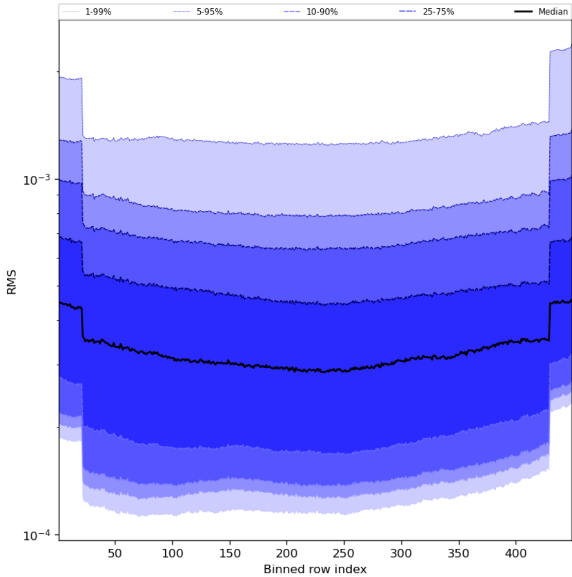
Figure 60: Along track statistics of “RMS” for 2024-03-04 to 2024-03-06
