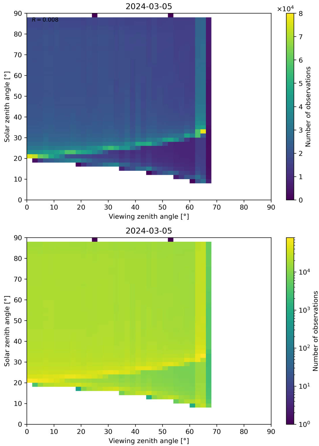
Figure 172: Scatter density plot of “Viewing zenith angle” against “Solar zenith angle” for 2024-03-04 to 2024-03-06.
