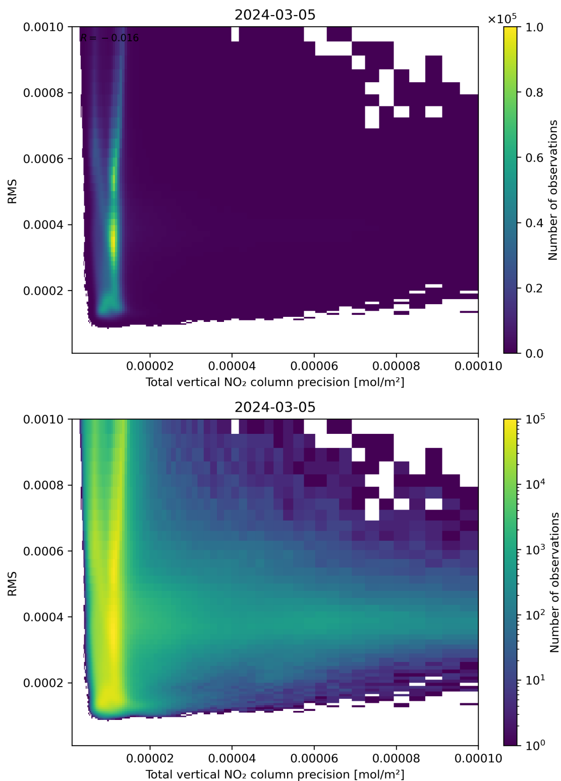
Figure 119: Scatter density plot of “Total vertical NO 2 column precision” against “RMS” for 2024-03-04 to 2024-03-06.
