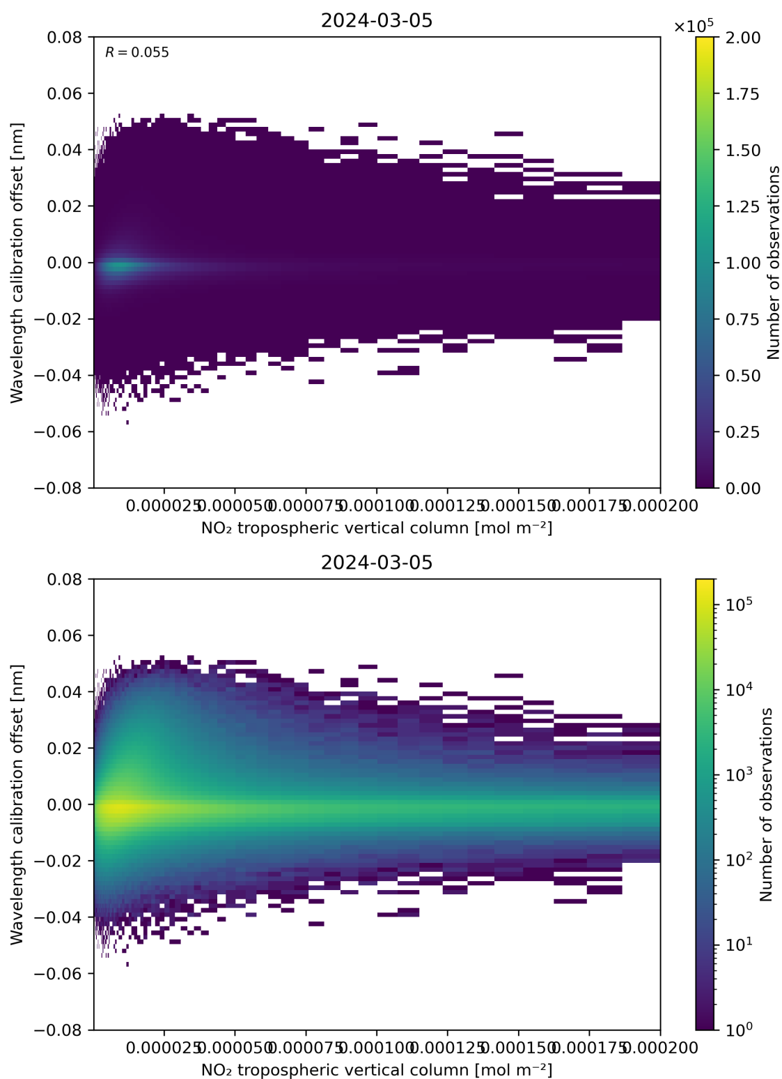
Figure 143: Scatter density plot of “NO 2 tropospheric vertical column” against “Wavelength calibration offset” for 2024-03-04 to 2024-03-06.
