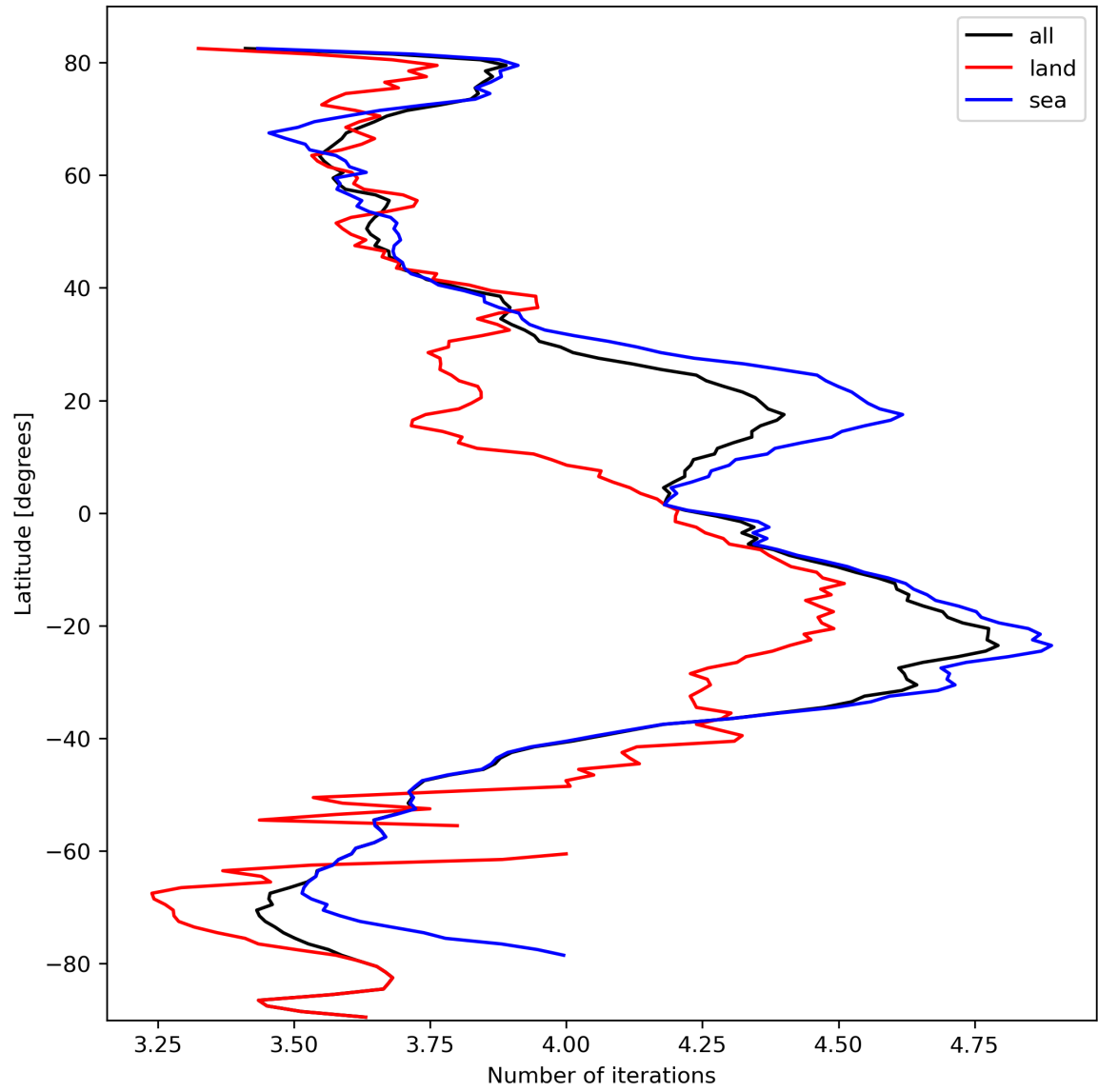
Figure 17: Zonal average of “Number of iterations” for 2024-03-04 to 2024-03-06.
