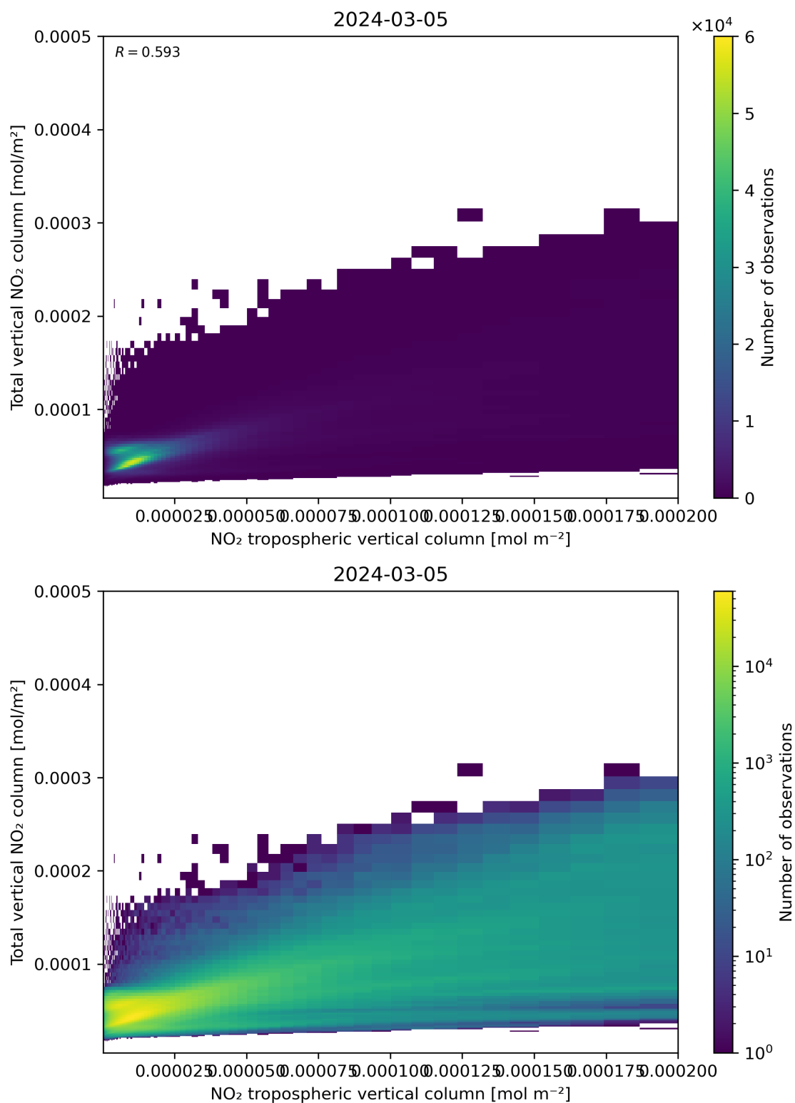
Figure 128: Scatter density plot of “NO 2 tropospheric vertical column” against “Total vertical NO 2 column” for 2024-03-04 to 2024-03-06.
