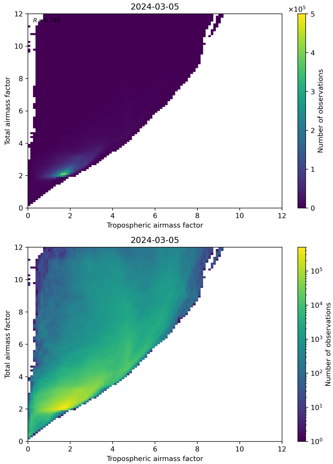
Figure 72: Scatter density plot of “Tropospheric airmass factor” against “Total airmass factor” for 2024-03-04 to 2024-03-06.
