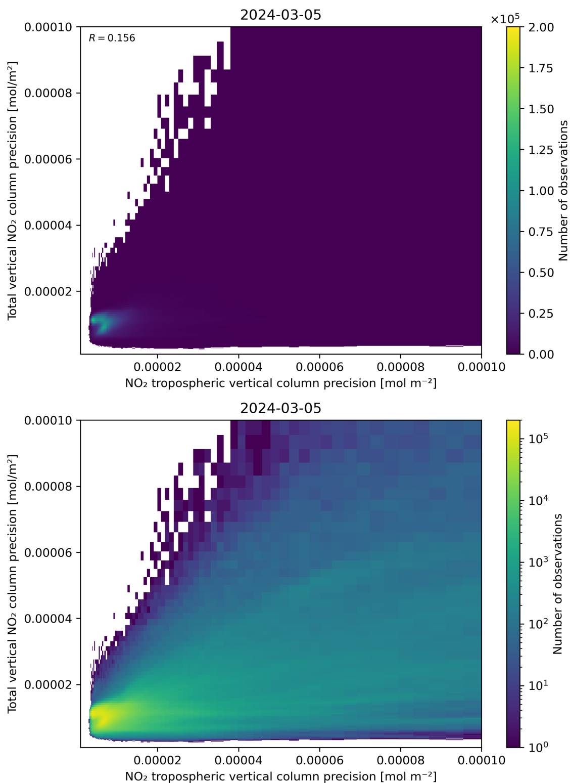
Figure 139: Scatter density plot of “NO 2 tropospheric vertical column precision” against “Total vertical NO 2 column precision” for 2024-03-04 to 2024-03-06.
