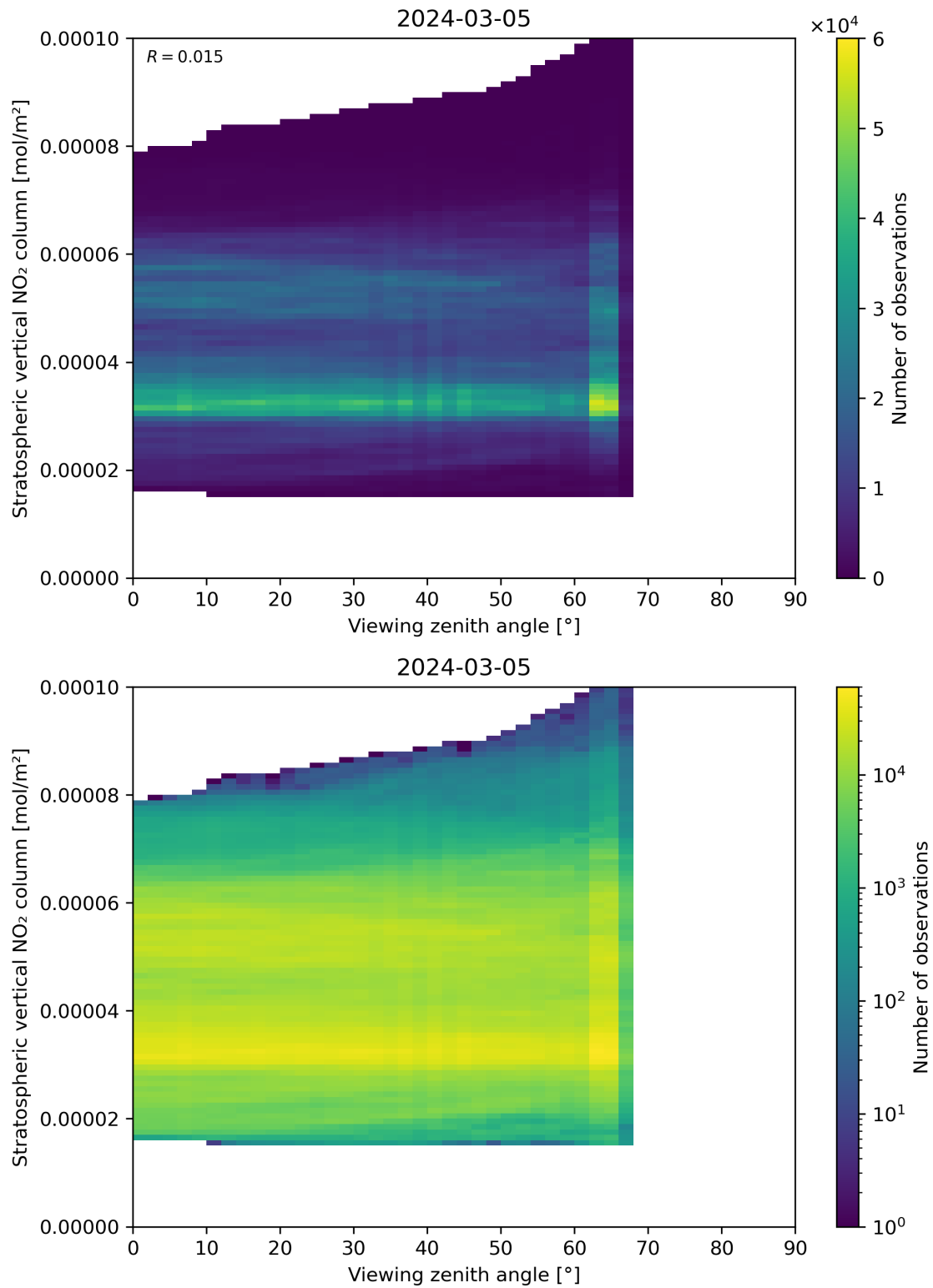
Figure 164: Scatter density plot of “Viewing zenith angle” against “Stratospheric vertical NO 2 column” for 2024-03-04 to 2024-03-06.
