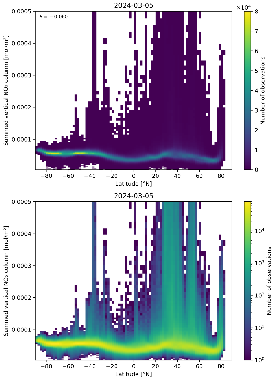
Figure 88: Scatter density plot of “Latitude” against “Summed vertical NO 2 column” for 2024-03-04 to 2024-03-06.
