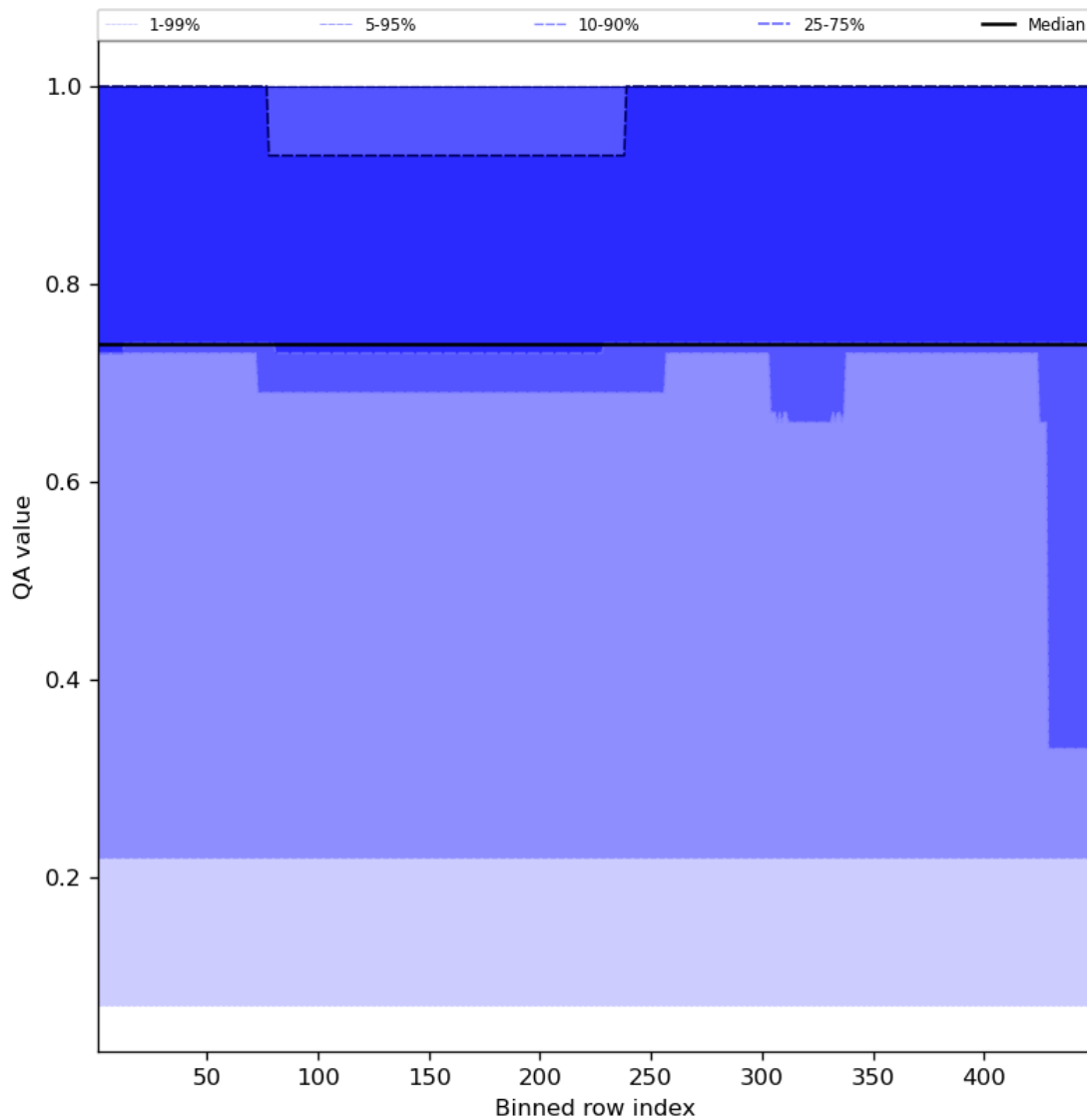
Figure 45: Along track statistics of “QA value” for 2024-03-04 to 2024-03-06
