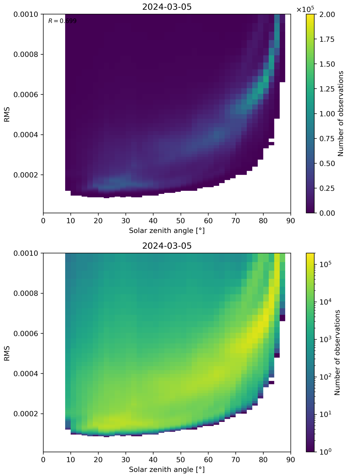
Figure 157: Scatter density plot of “Solar zenith angle” against “RMS” for 2024-03-04 to 2024-03-06.
