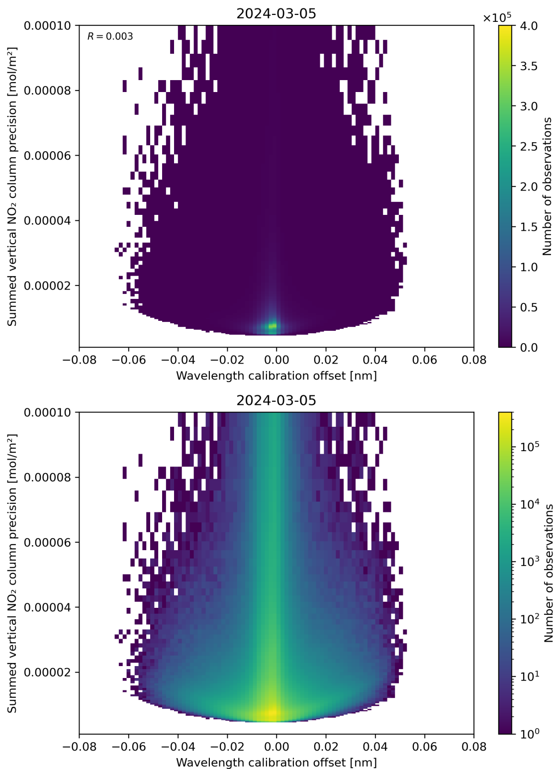
Figure 178: Scatter density plot of “Wavelength calibration offset” against “Summed vertical NO 2 column precision” for 2024-03-04 to 2024-03-06.
