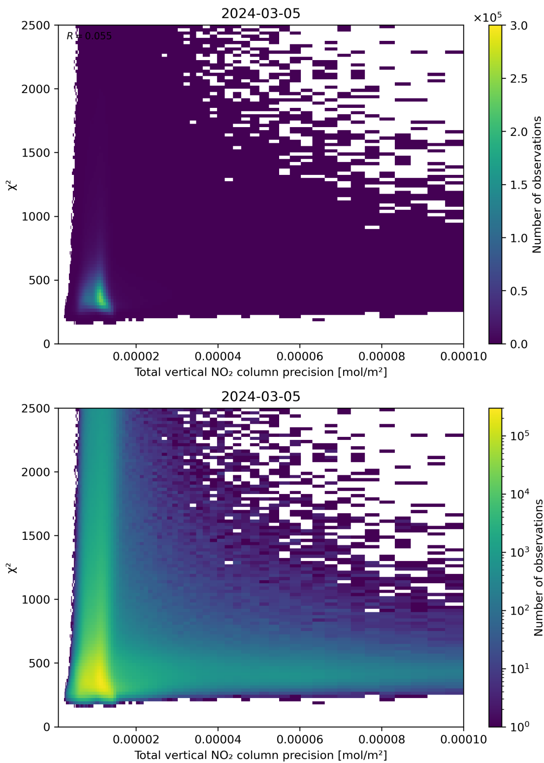
Figure 116: Scatter density plot of “Total vertical NO 2 column precision” against “ \chi^2 ” for 2024-03-04 to 2024-03-06.
