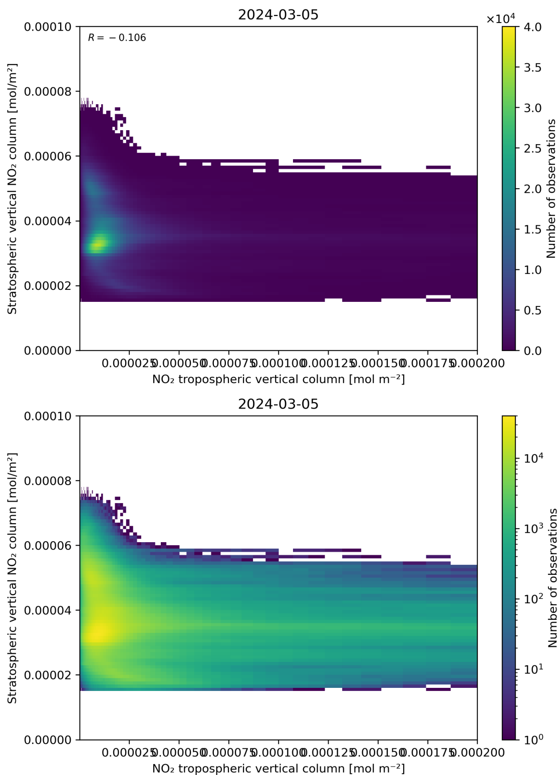
Figure 125: Scatter density plot of “NO 2 tropospheric vertical column” against “Stratospheric vertical NO 2 column” for 2024-03-04 to 2024-03-06.
