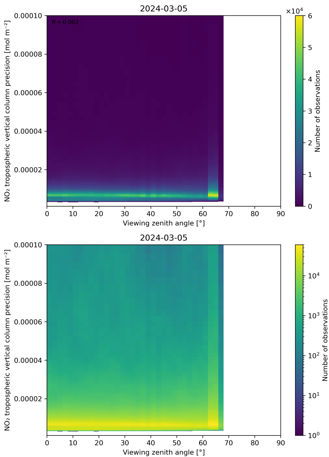
Figure 170: Scatter density plot of “Viewing zenith angle” against “NO 2 tropospheric vertical column precision” for 2024-03-04 to 2024-03-06.
