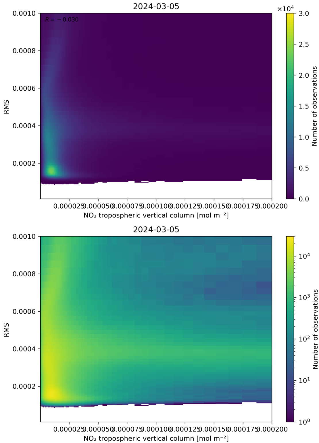
Figure 142: Scatter density plot of “NO 2 tropospheric vertical column” against “RMS” for 2024-03-04 to 2024-03-06.
