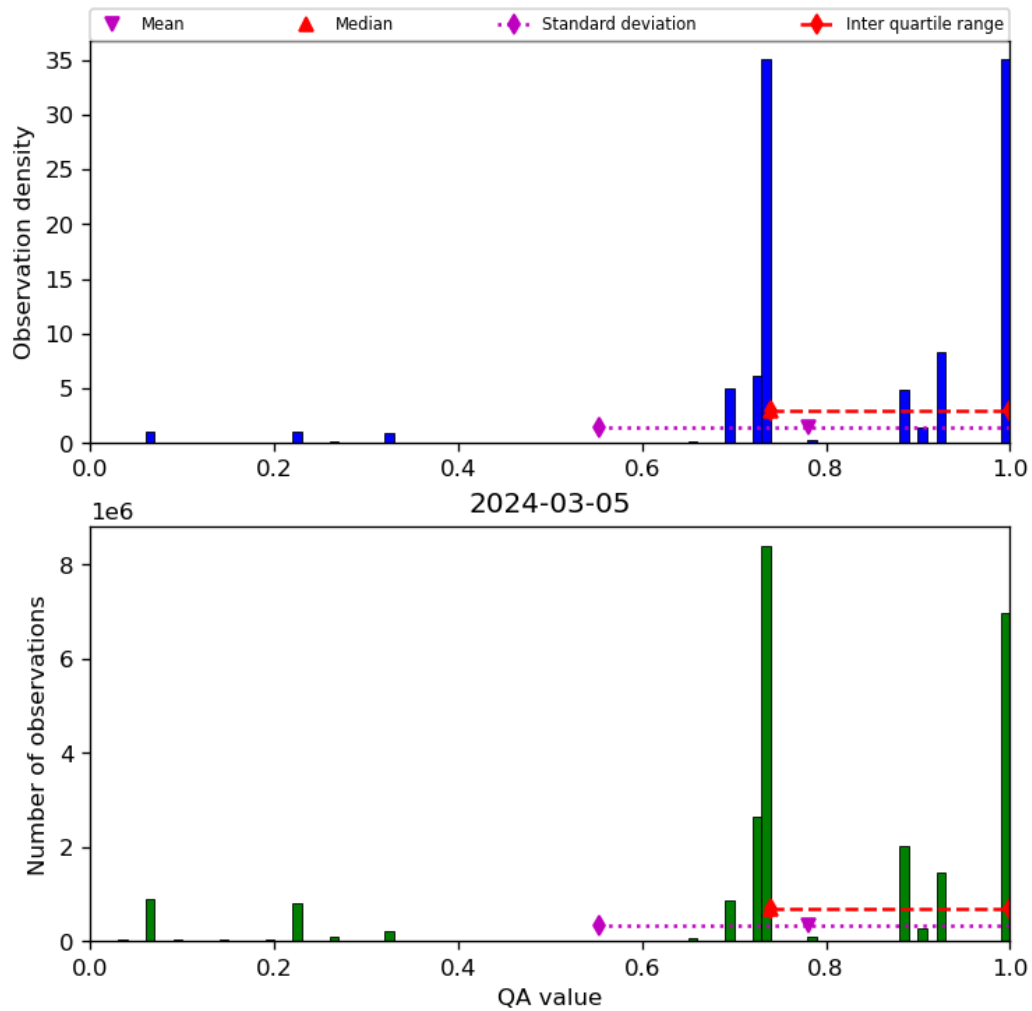
Figure 28: Histogram of “QA value” for 2024-03-04 to 2024-03-06
