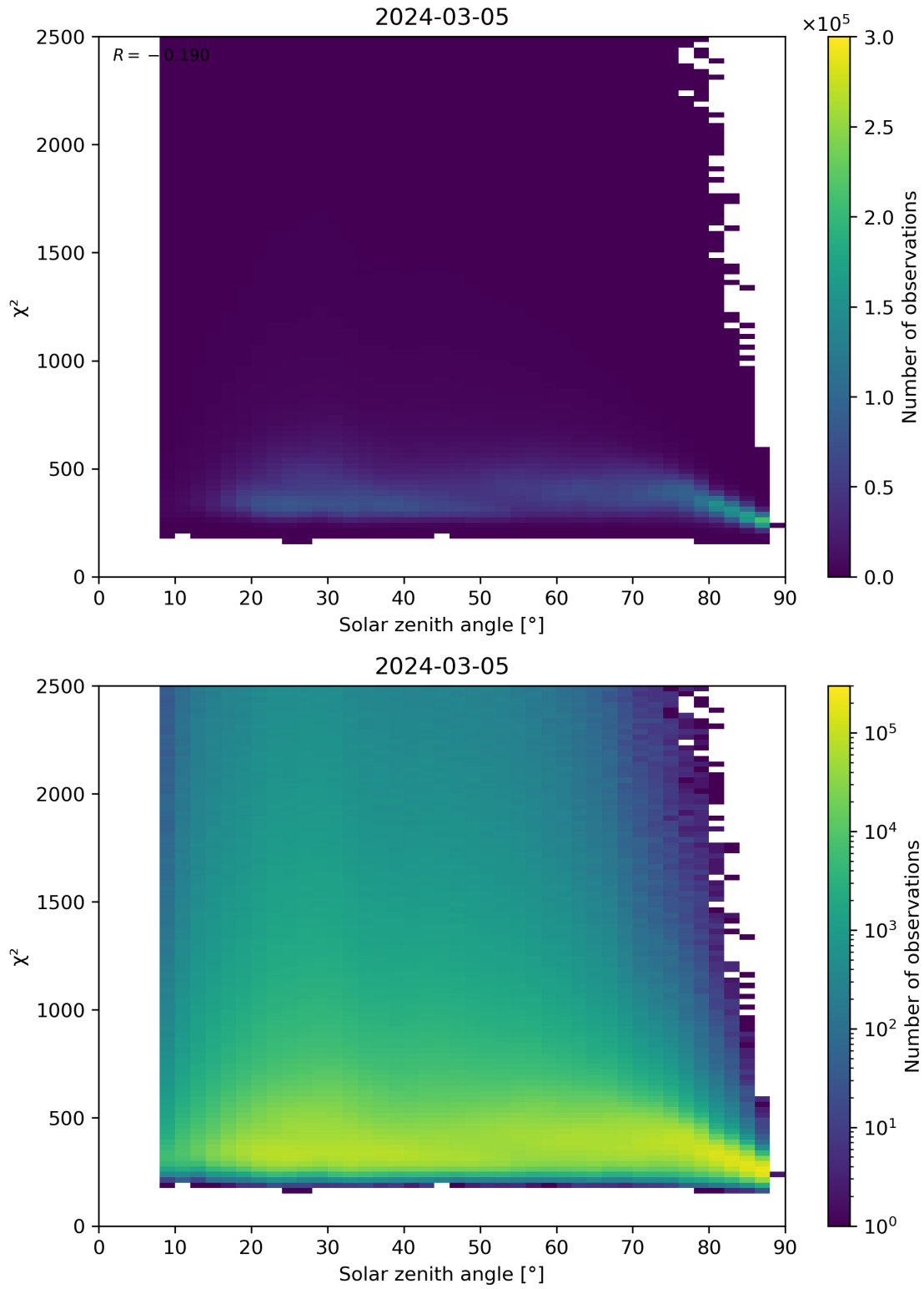
Figure 148: Scatter density plot of “Solar zenith angle” against “ \chi^2 ” for 2024-03-04 to 2024-03-06.
