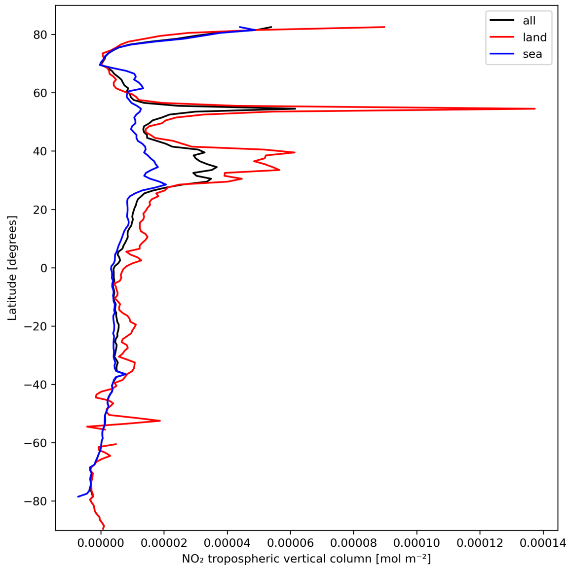
Figure 12: Zonal average of “NO 2 tropospheric vertical column” for 2024-03-04 to 2024-03-06.
