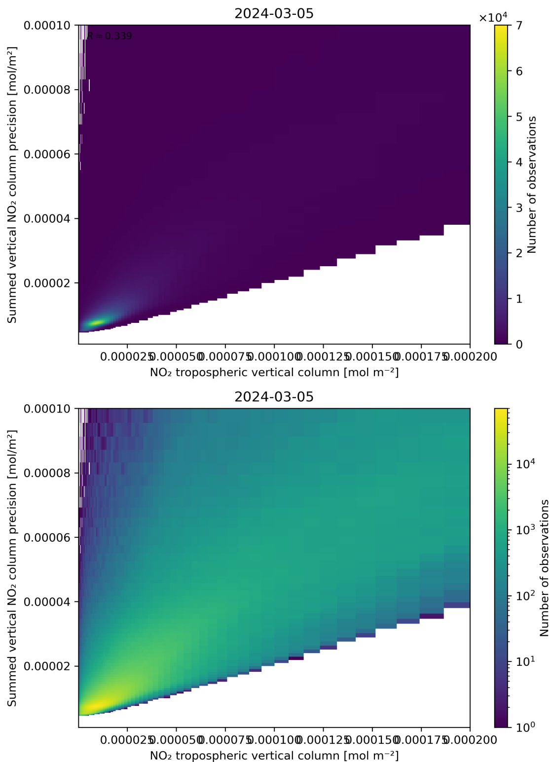
Figure 127: Scatter density plot of “NO 2 tropospheric vertical column” against “Summed vertical NO 2 column precision” for 2024-03-04 to 2024-03-06.
