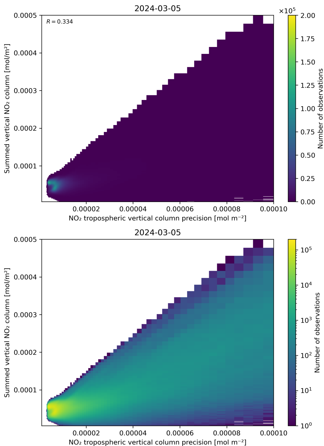
Figure 136: Scatter density plot of “NO 2 tropospheric vertical column precision” against “Summed vertical NO 2 column” for 2024-03-04 to 2024-03-06.
