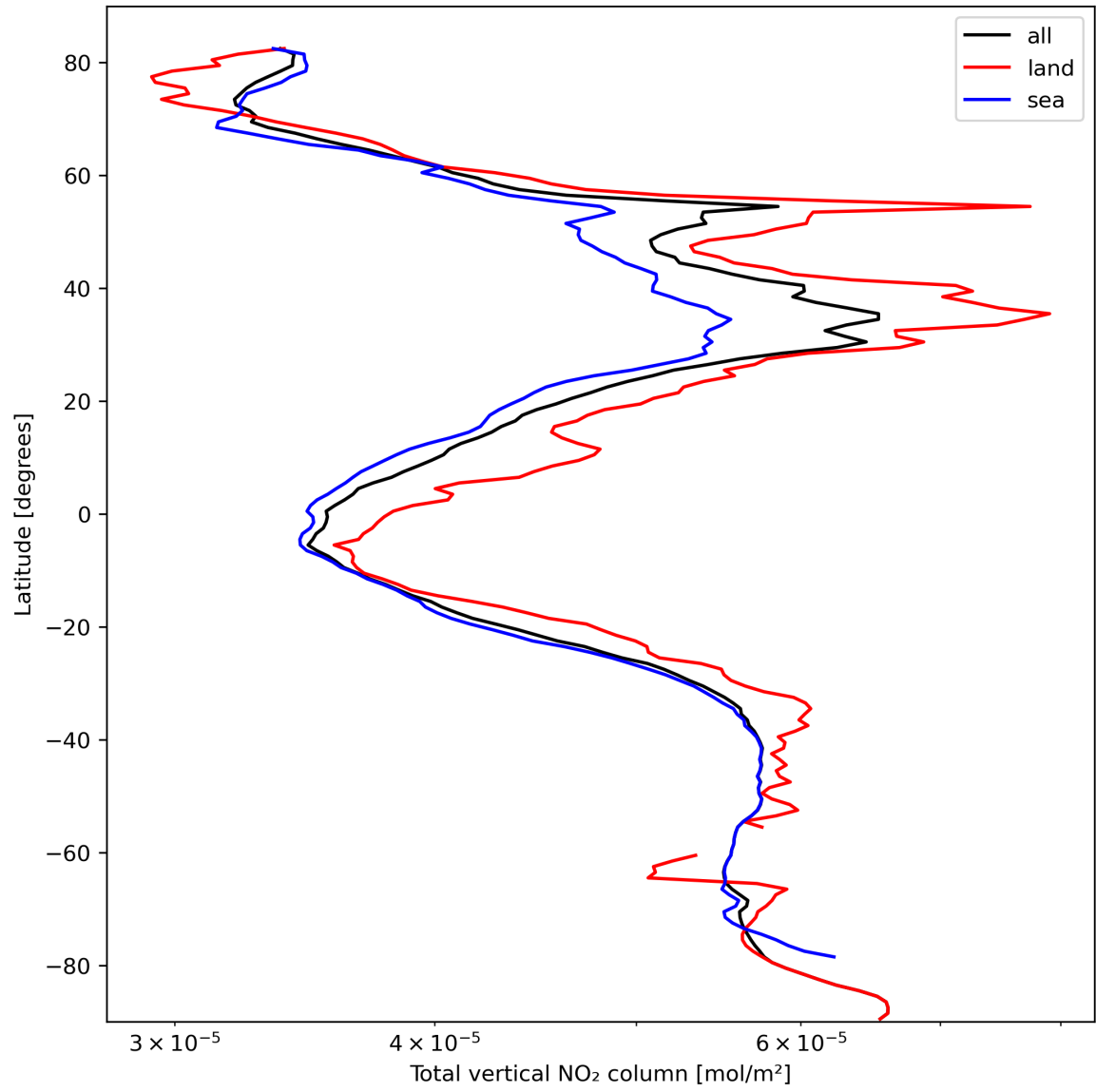
Figure 21: Zonal average of “Total vertical NO 2 column” for 2024-03-04 to 2024-03-06.
