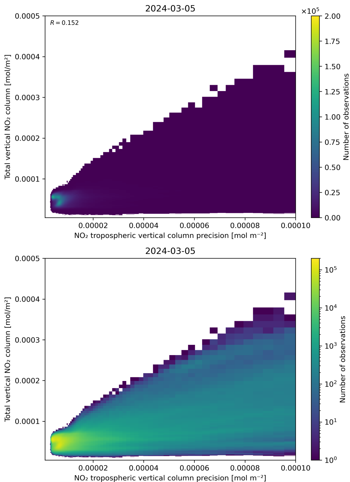
Figure 138: Scatter density plot of “NO 2 tropospheric vertical column precision” against “Total vertical NO 2 column” for 2024-03-04 to 2024-03-06.
