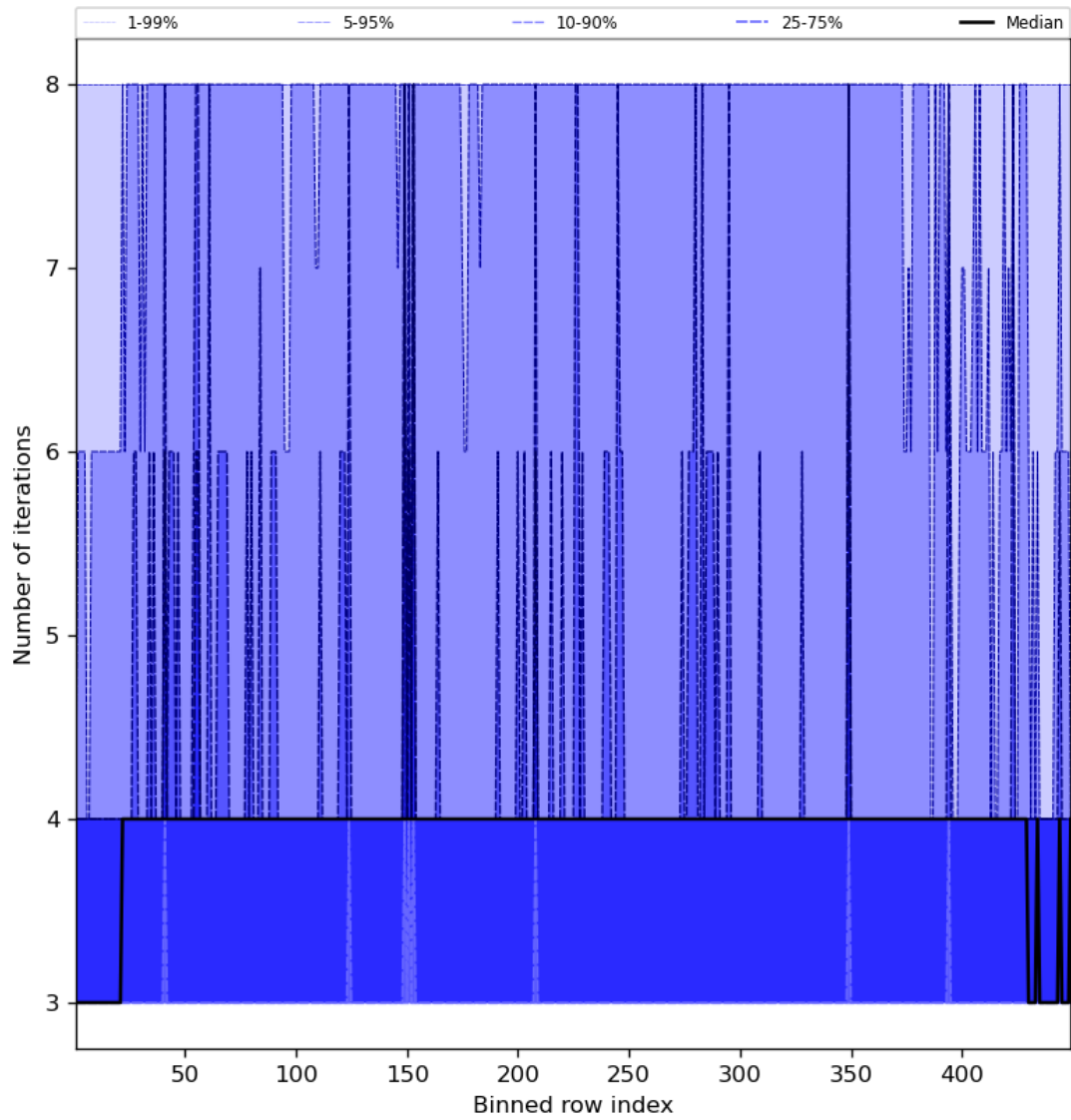
Figure 51: Along track statistics of “Number of iterations” for 2024-03-04 to 2024-03-06
