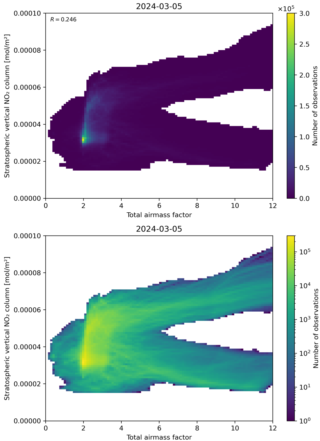
Figure 64: Scatter density plot of “Total airmass factor” against “Stratospheric vertical \text{NO}_2 column” for 2024-03-04 to 2024-03-06.
