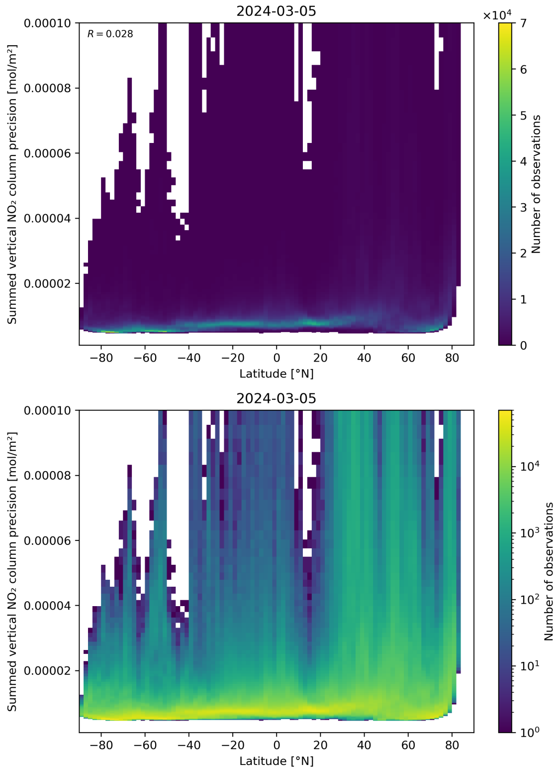
Figure 89: Scatter density plot of “Latitude” against “Summed vertical NO 2 column precision” for 2024-03-04 to 2024-03-06.
