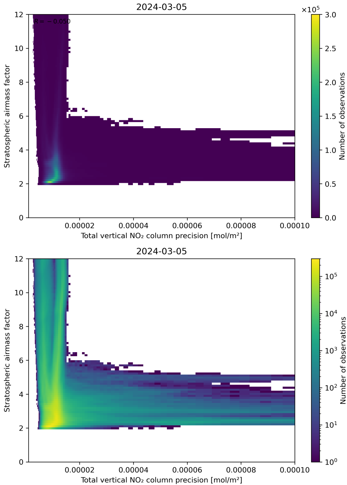
Figure 115: Scatter density plot of “Total vertical NO 2 column precision” against “Stratospheric air mass factor” for 2024-03-04 to 2024-03-06.
