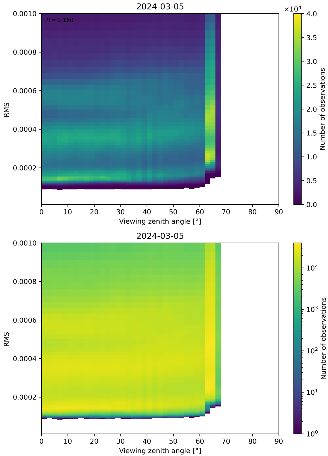
Figure 171: Scatter density plot of “Viewing zenith angle” against “RMS” for 2024-03-04 to 2024-03-06.
