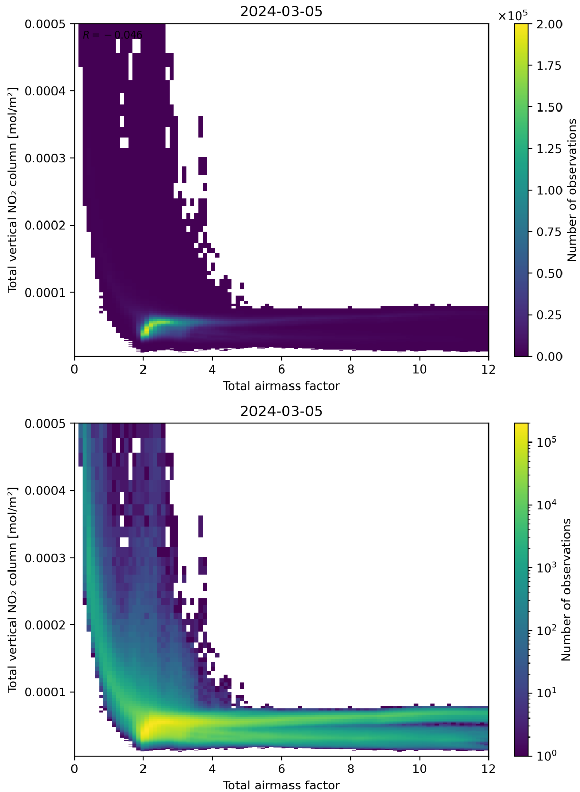
Figure 67: Scatter density plot of “Total airmass factor” against “Total vertical NO 2 column” for 2024-03-04 to 2024-03-06.
