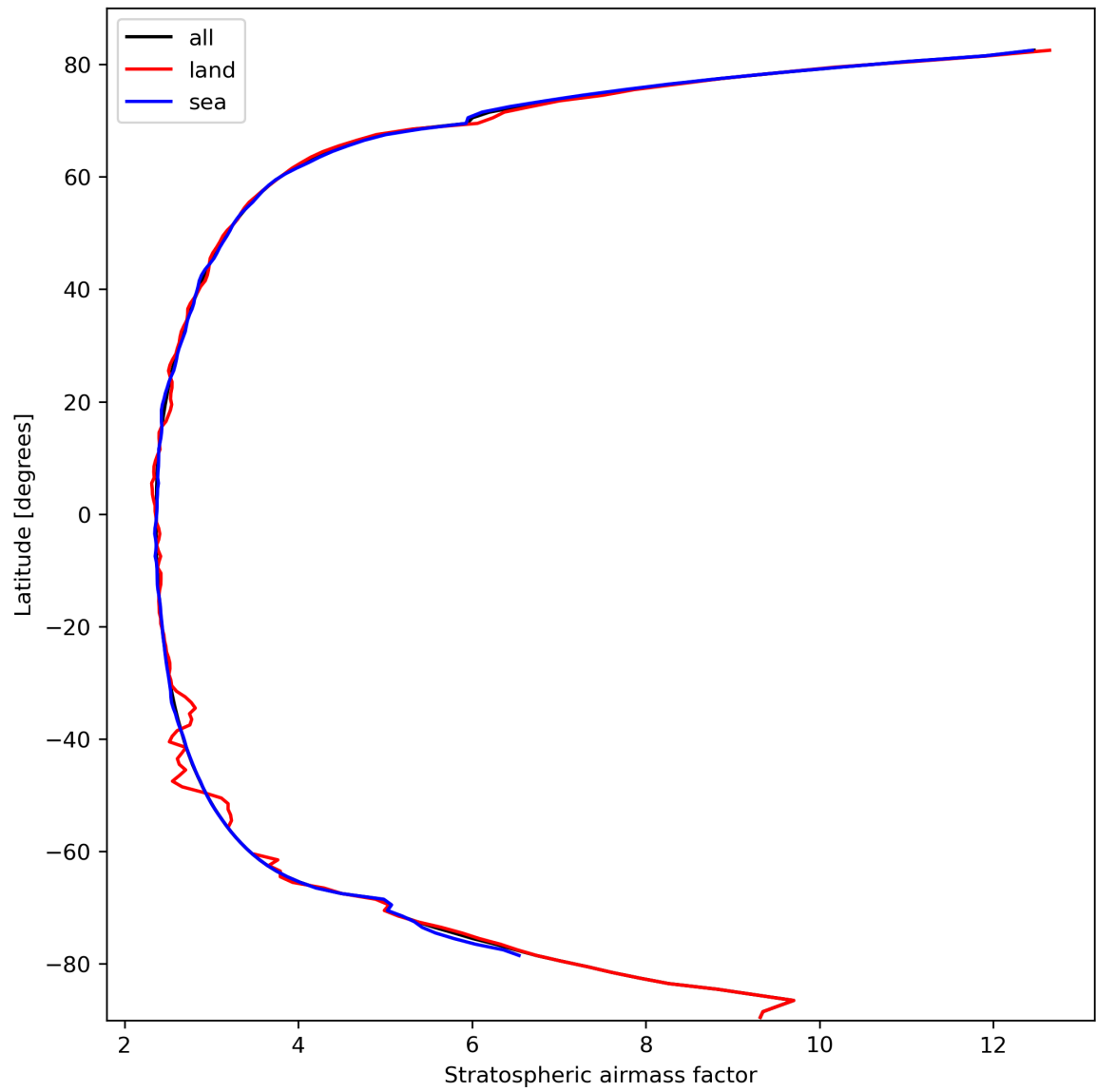
Figure 27: Zonal average of “Stratospheric air mass factor” for 2024-03-04 to 2024-03-06.
