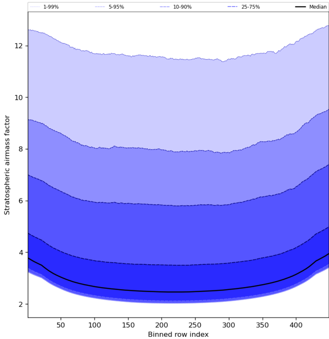
Figure 61: Along track statistics of “Stratospheric airmass factor” for 2024-03-04 to 2024-03-06
