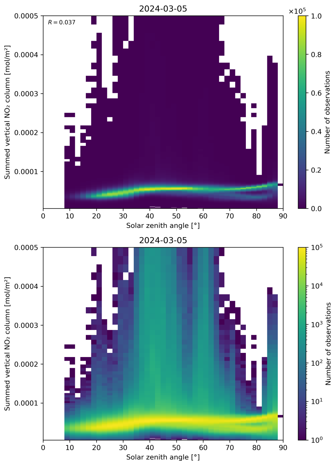
Figure 151: Scatter density plot of “Solar zenith angle” against “Summed vertical NO 2 column” for 2024-03-04 to 2024-03-06.
