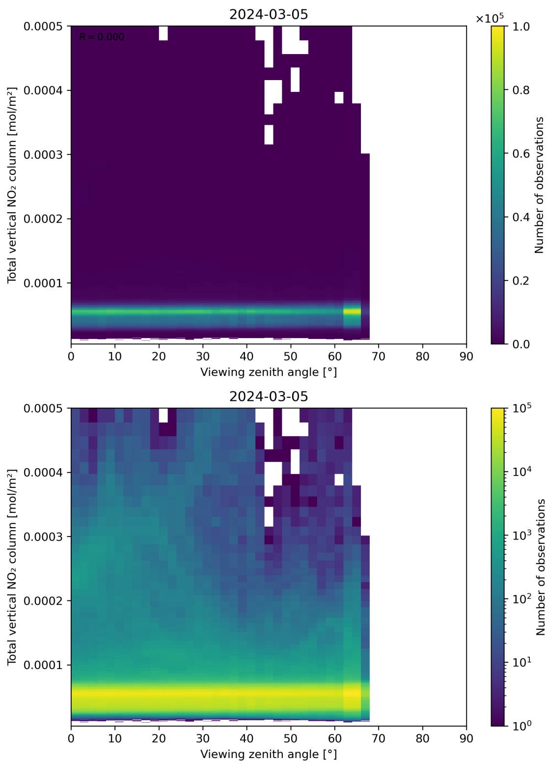
Figure 167: Scatter density plot of “Viewing zenith angle” against “Total vertical NO 2 column” for 2024-03-04 to 2024-03-06.
