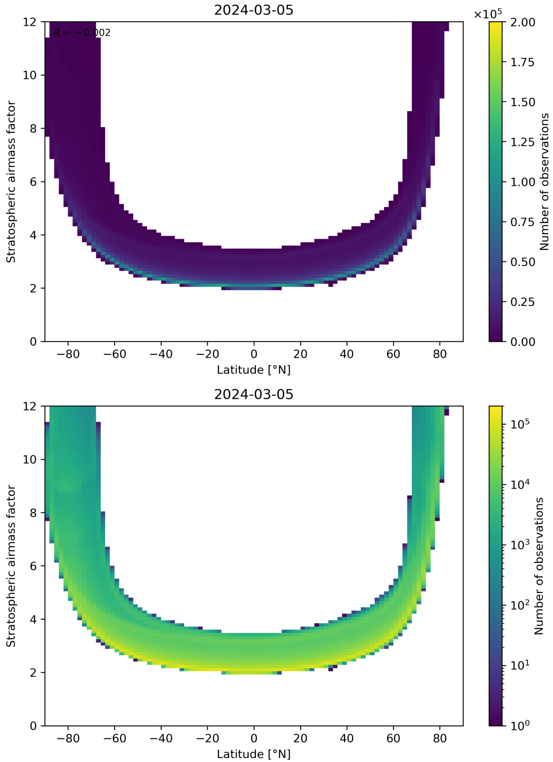
Figure 83: Scatter density plot of “Latitude” against “Stratospheric airmass factor” for 2024-03-04 to 2024-03-06.
