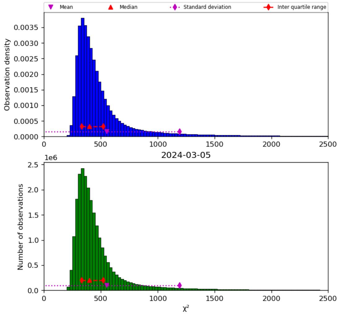
Figure 42: Histogram of “ \chi^2 ” for 2024-03-04 to 2024-03-06
