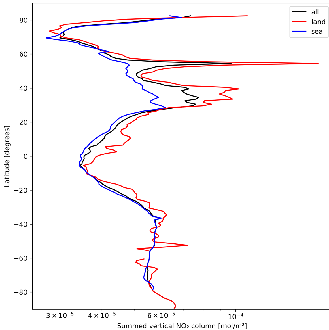
Figure 23: Zonal average of “Summed vertical NO 2 column” for 2024-03-04 to 2024-03-06.
