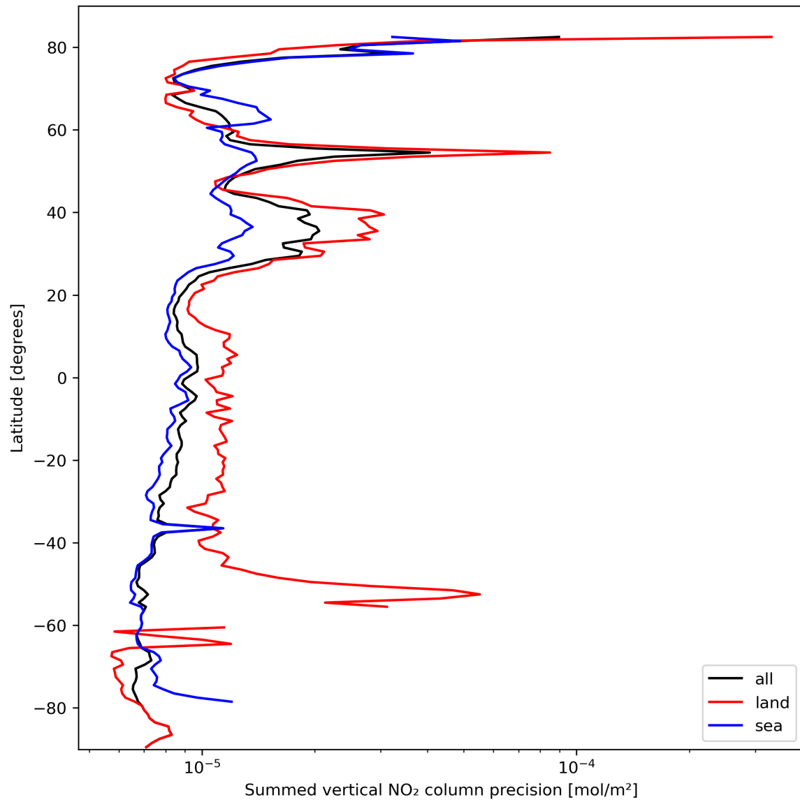
Figure 24: Zonal average of “Summed vertical NO 2 column precision” for 2024-03-04 to 2024-03-06.
