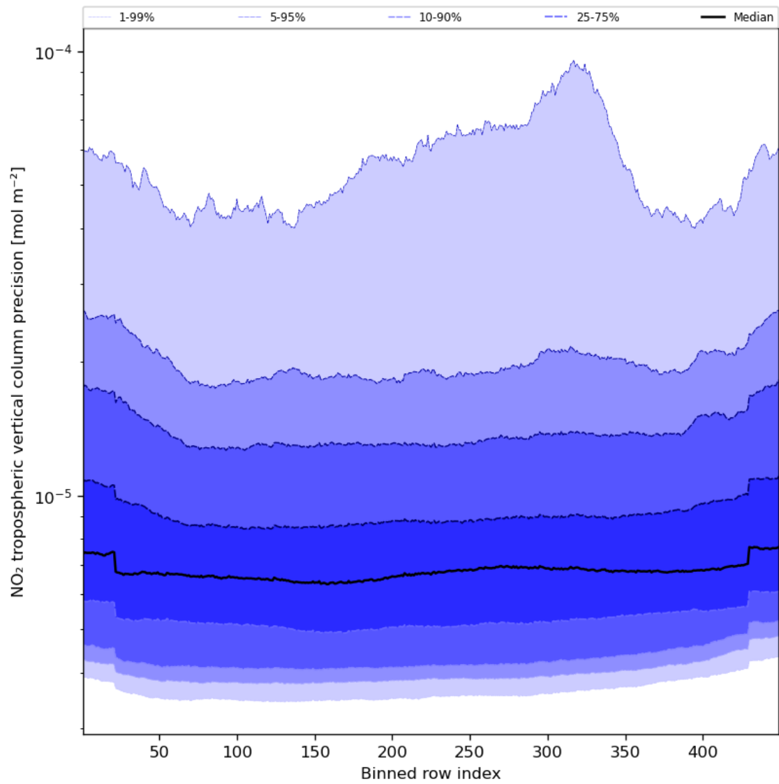
Figure 47: Along track statistics of “NO 2 tropospheric vertical column precision” for 2024-03-04 to 2024-03-06
