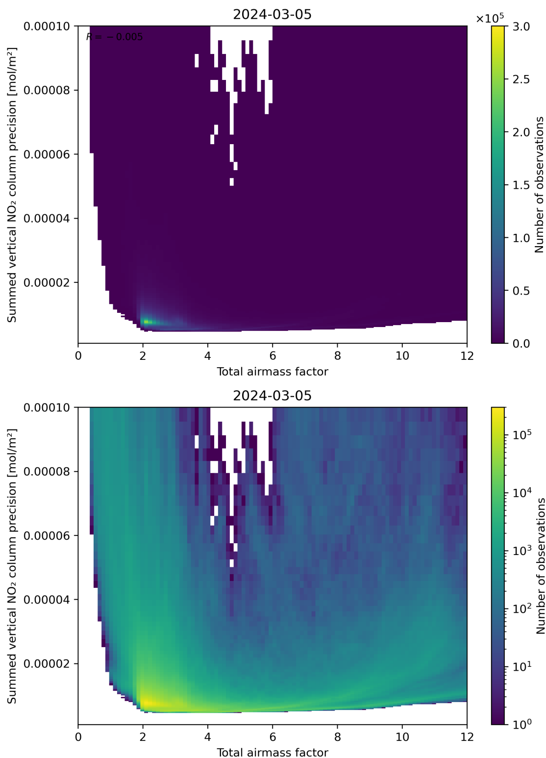
Figure 66: Scatter density plot of “Total airmass factor” against “Summed vertical NO 2 column precision” for 2024-03-04 to 2024-03-06.
