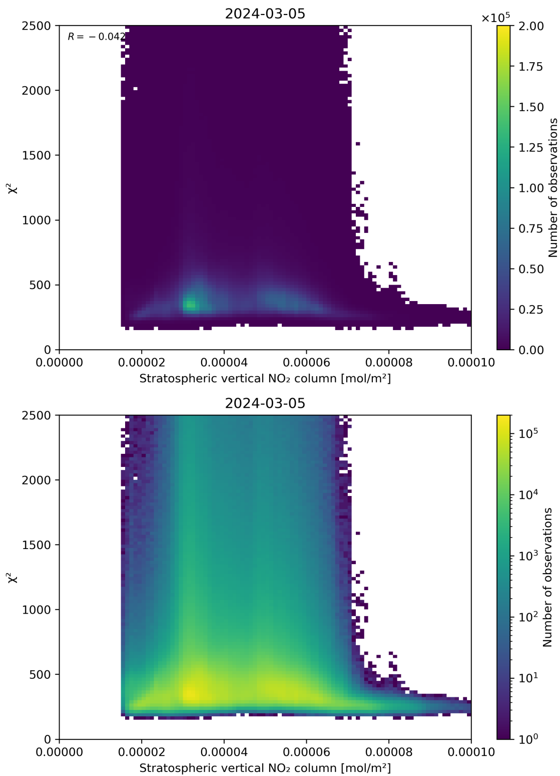
Figure 97: Scatter density plot of “Stratospheric vertical NO 2 column” against “ \chi^2 ” for 2024-03-04 to 2024-03-06.
