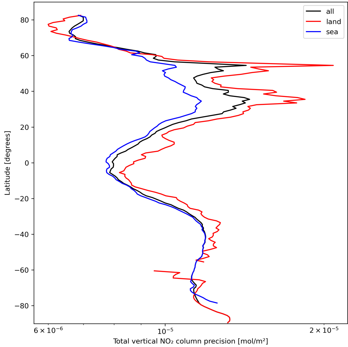
Figure 22: Zonal average of “Total vertical NO 2 column precision” for 2024-03-04 to 2024-03-06.
