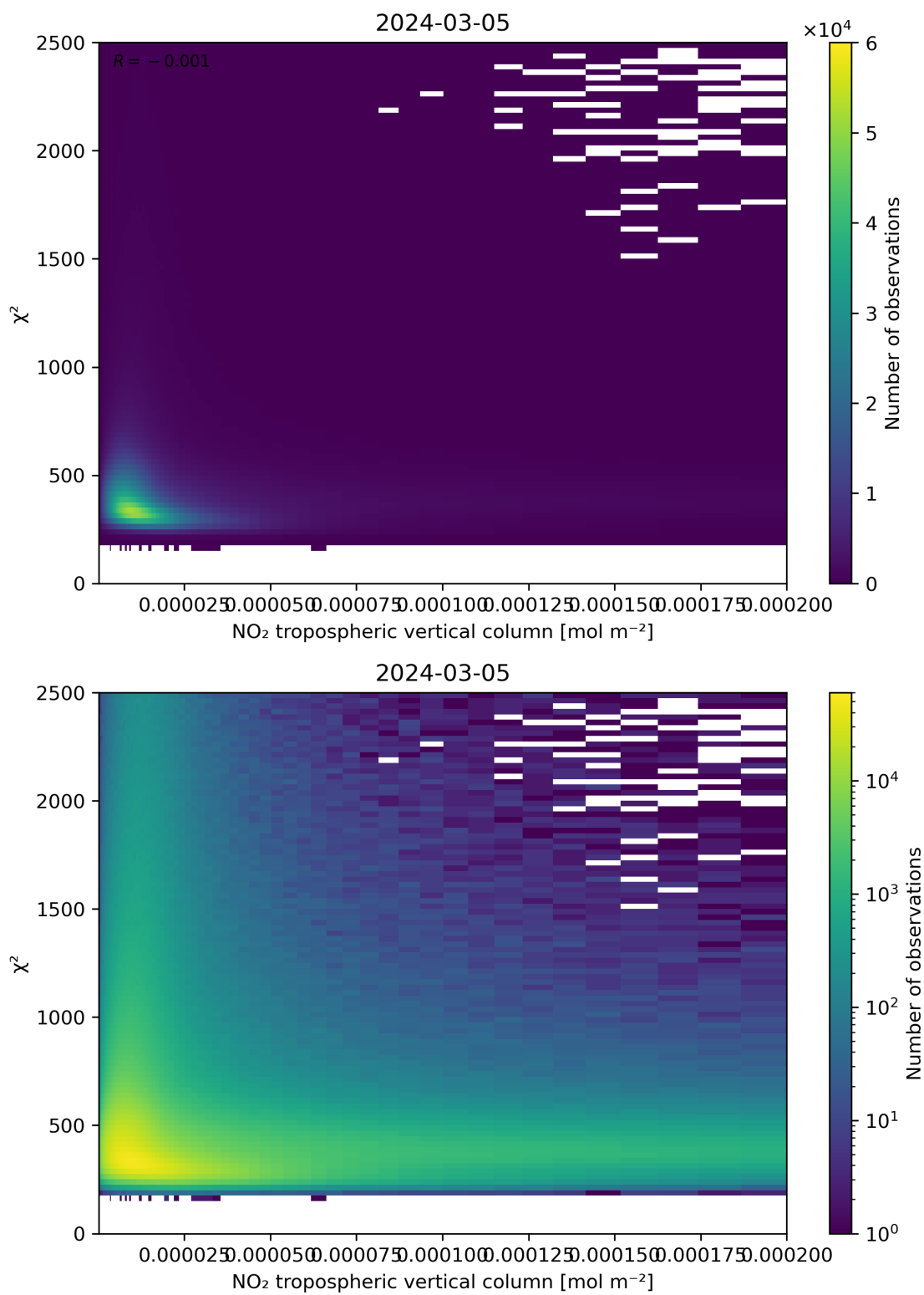
Figure 124: Scatter density plot of “NO 2 tropospheric vertical column” against “ \chi^2 ” for 2024-03-04 to 2024-03-06.
