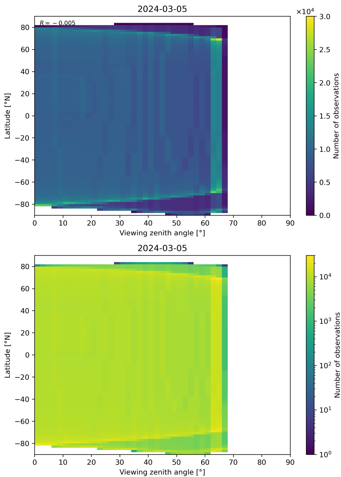
Figure 163: Scatter density plot of “Viewing zenith angle” against “Latitude” for 2024-03-04 to 2024-03-06.
