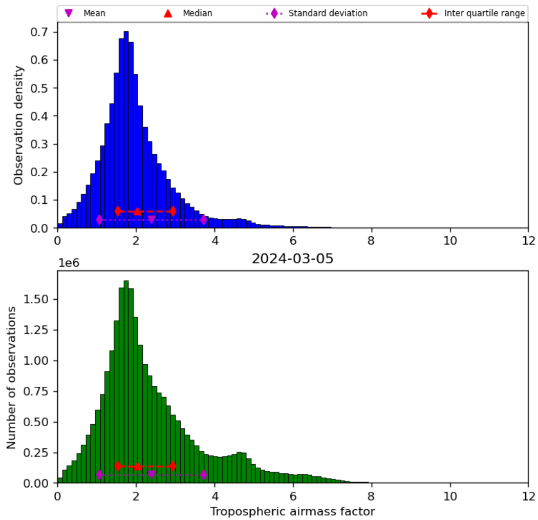
Figure 31: Histogram of “Tropospheric airmass factor” for 2024-03-04 to 2024-03-06
