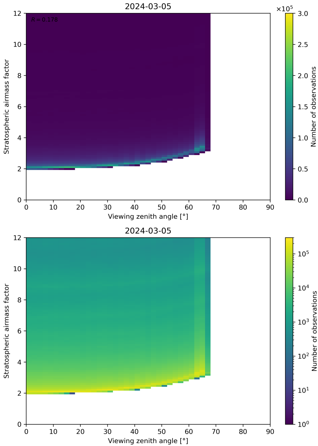
Figure 159: Scatter density plot of “Viewing zenith angle” against “Stratospheric airmass factor” for 2024-03-04 to 2024-03-06.
