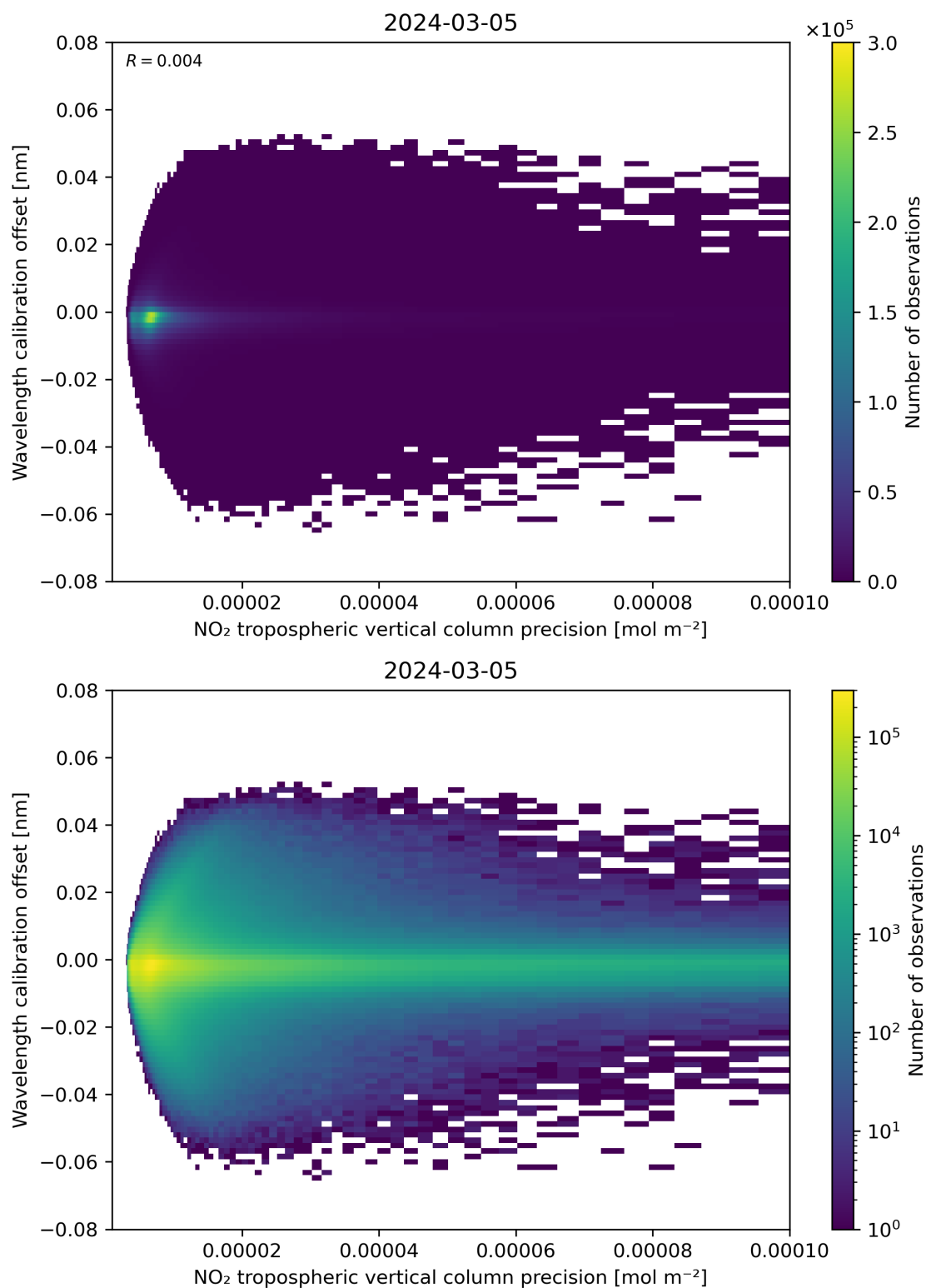
Figure 141: Scatter density plot of “NO 2 tropospheric vertical column precision” against “Wavelength calibration offset” for 2024-03-04 to 2024-03-06.
