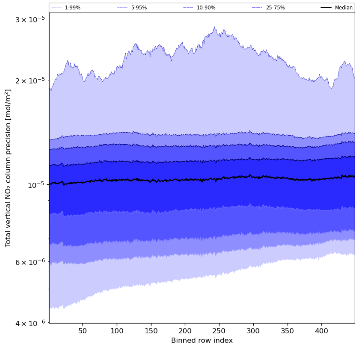
Figure 56: Along track statistics of “Total vertical NO 2 column precision” for 2024-03-04 to 2024-03-06
