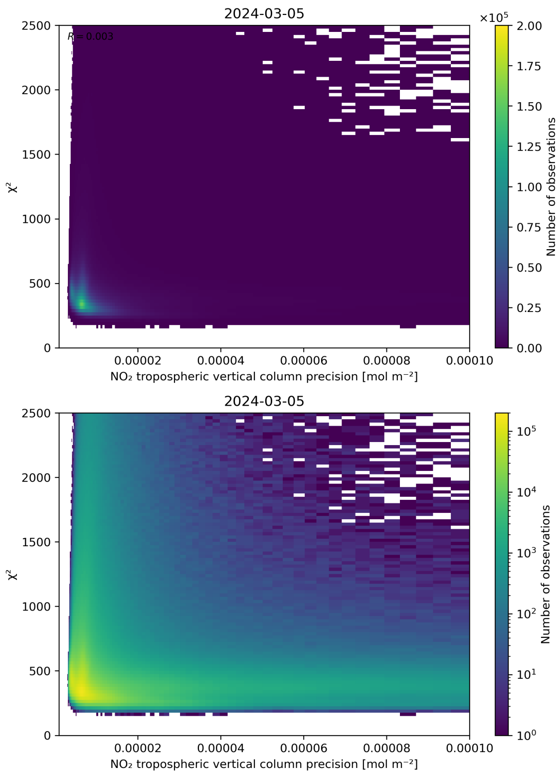
Figure 134: Scatter density plot of “NO 2 tropospheric vertical column precision” against “ \chi^2 ” for 2024-03-04 to 2024-03-06.
