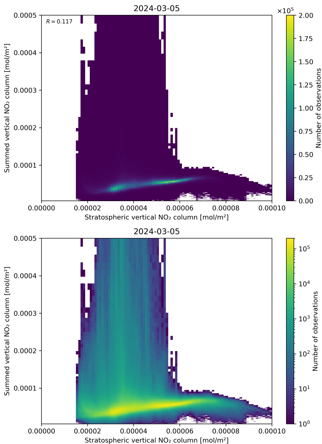
Figure 98: Scatter density plot of “Stratospheric vertical NO 2 column” against “Summed vertical NO 2 column” for 2024-03-04 to 2024-03-06.
