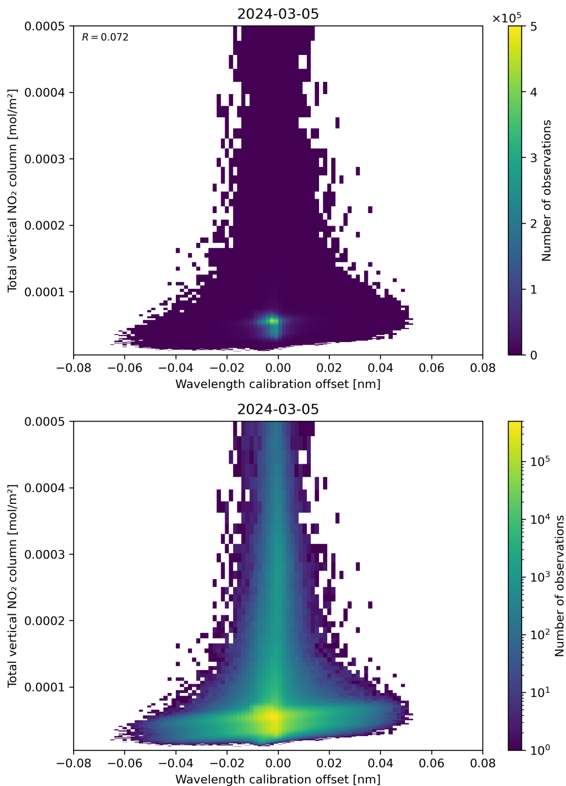
Figure 179: Scatter density plot of “Wavelength calibration offset” against “Total vertical NO 2 column” for 2024-03-04 to 2024-03-06.
