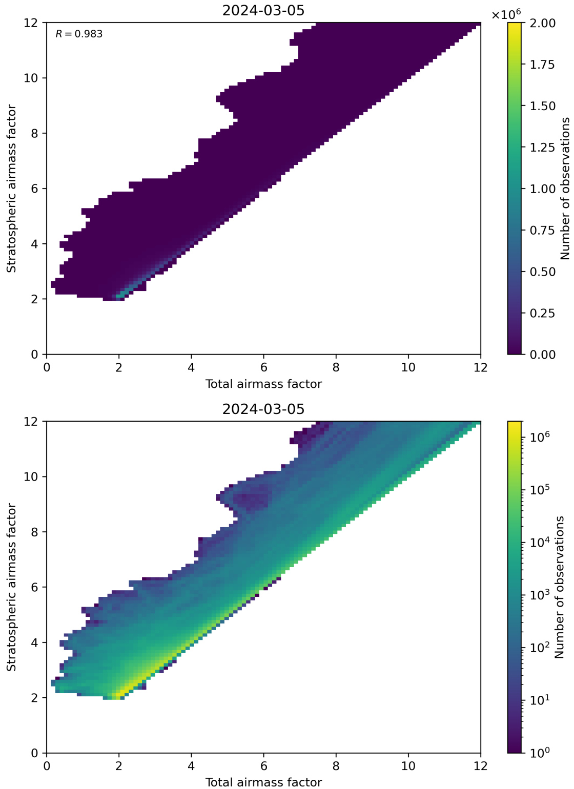
Figure 62: Scatter density plot of “Total airmass factor” against “Stratospheric airmass factor” for 2024-03-04 to 2024-03-06.
