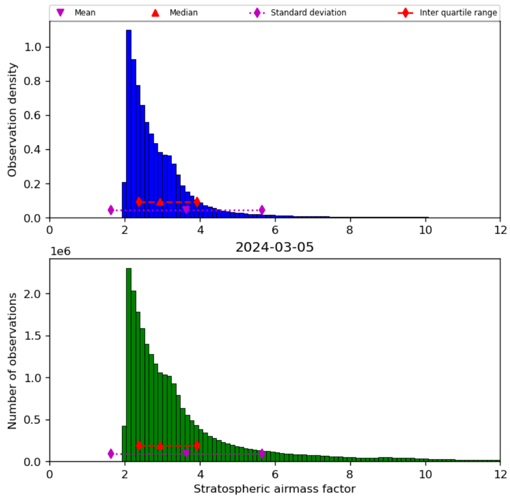
Figure 44: Histogram of “Stratospheric airmass factor” for 2024-03-04 to 2024-03-06
