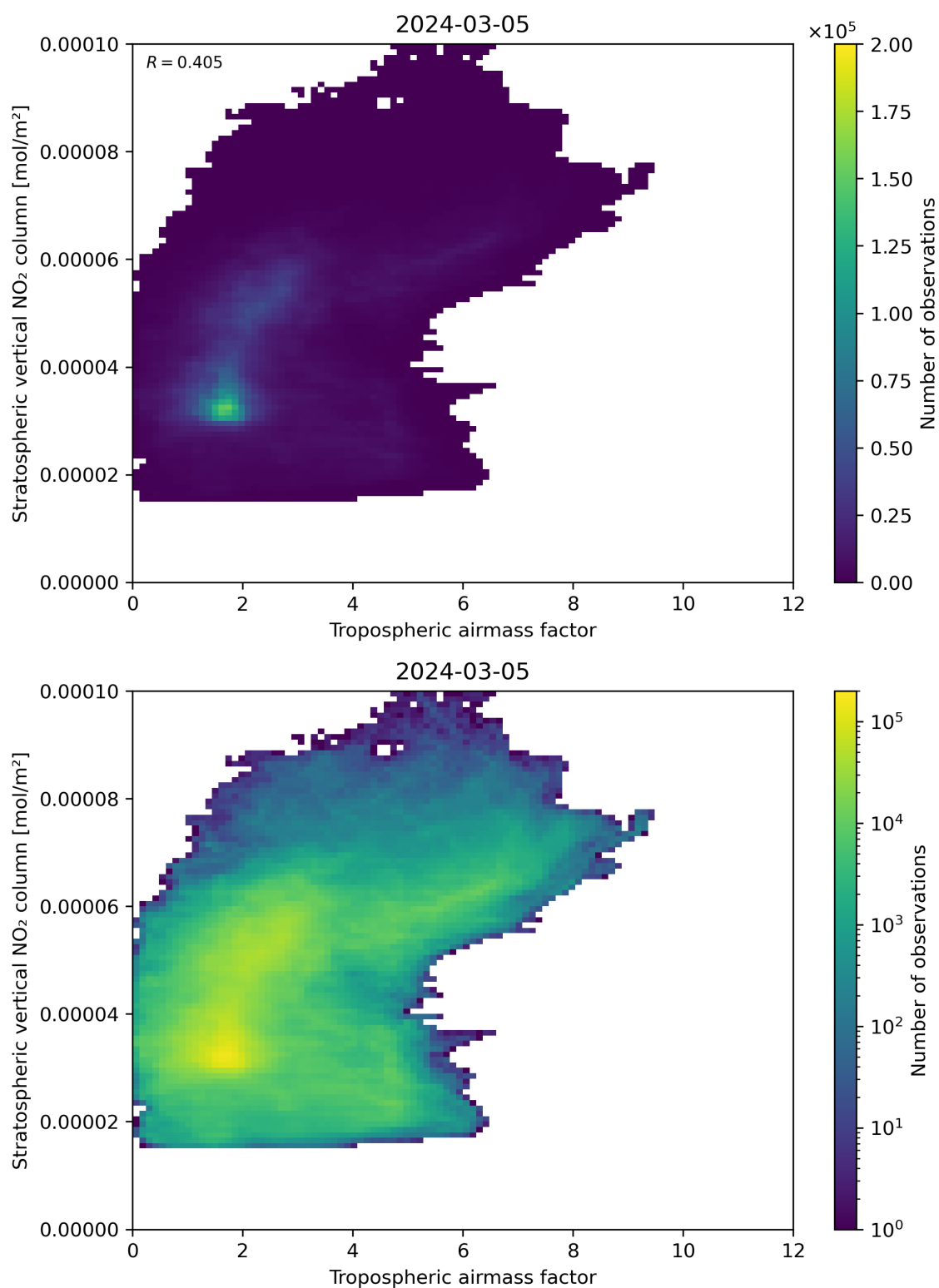
Figure 74: Scatter density plot of “Tropospheric air mass factor” against “Stratospheric vertical NO 2 column” for 2024-03-04 to 2024-03-06.
