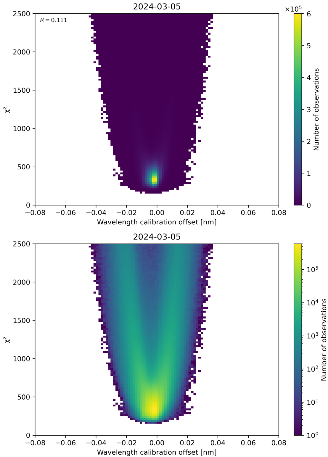
Figure 175: Scatter density plot of “Wavelength calibration offset” against “ \chi^2 ” for 2024-03-04 to 2024-03-06.
