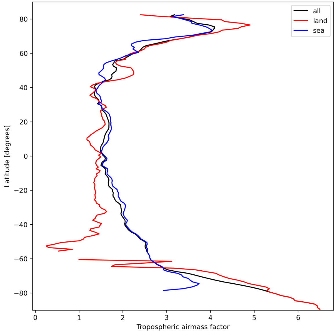
Figure 14: Zonal average of “Tropospheric airmass factor” for 2024-03-04 to 2024-03-06.
