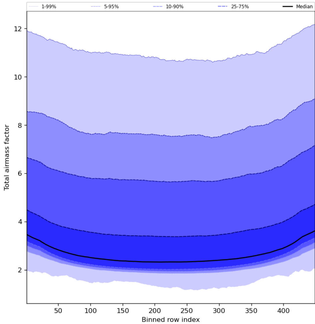
Figure 49: Along track statistics of “Total airmass factor” for 2024-03-04 to 2024-03-06
