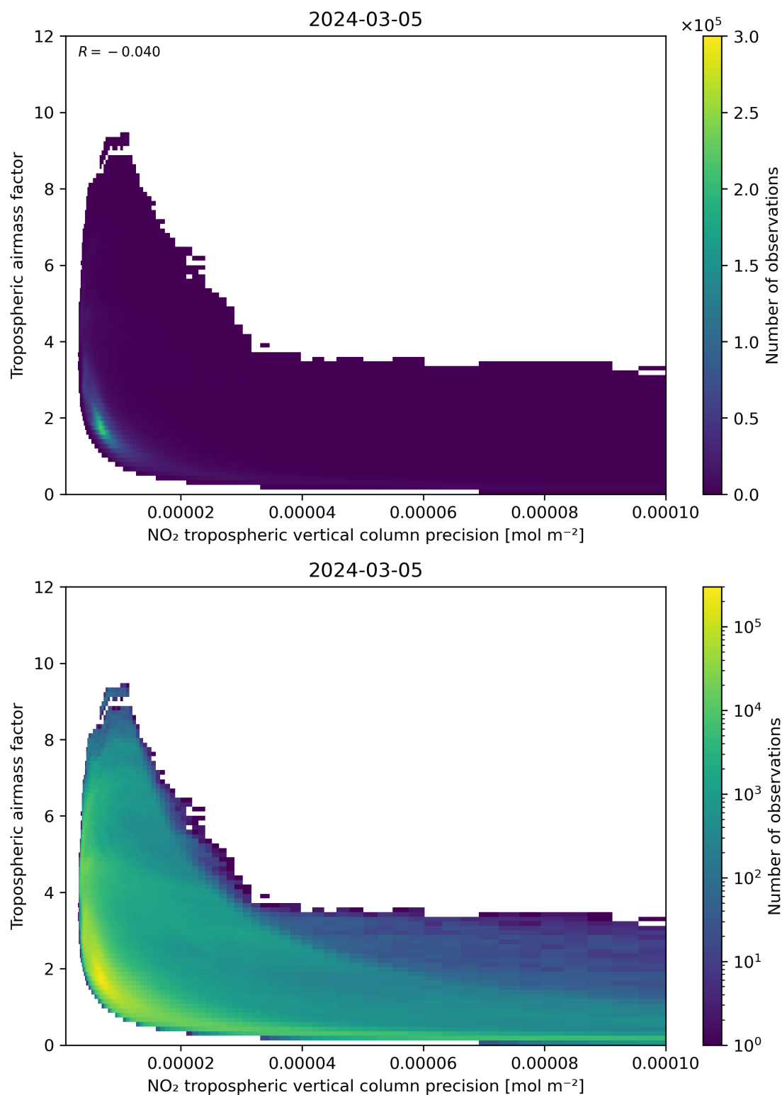
Figure 133: Scatter density plot of “NO 2 tropospheric vertical column precision” against “Tropospheric airmass factor” for 2024-03-04 to 2024-03-06.
