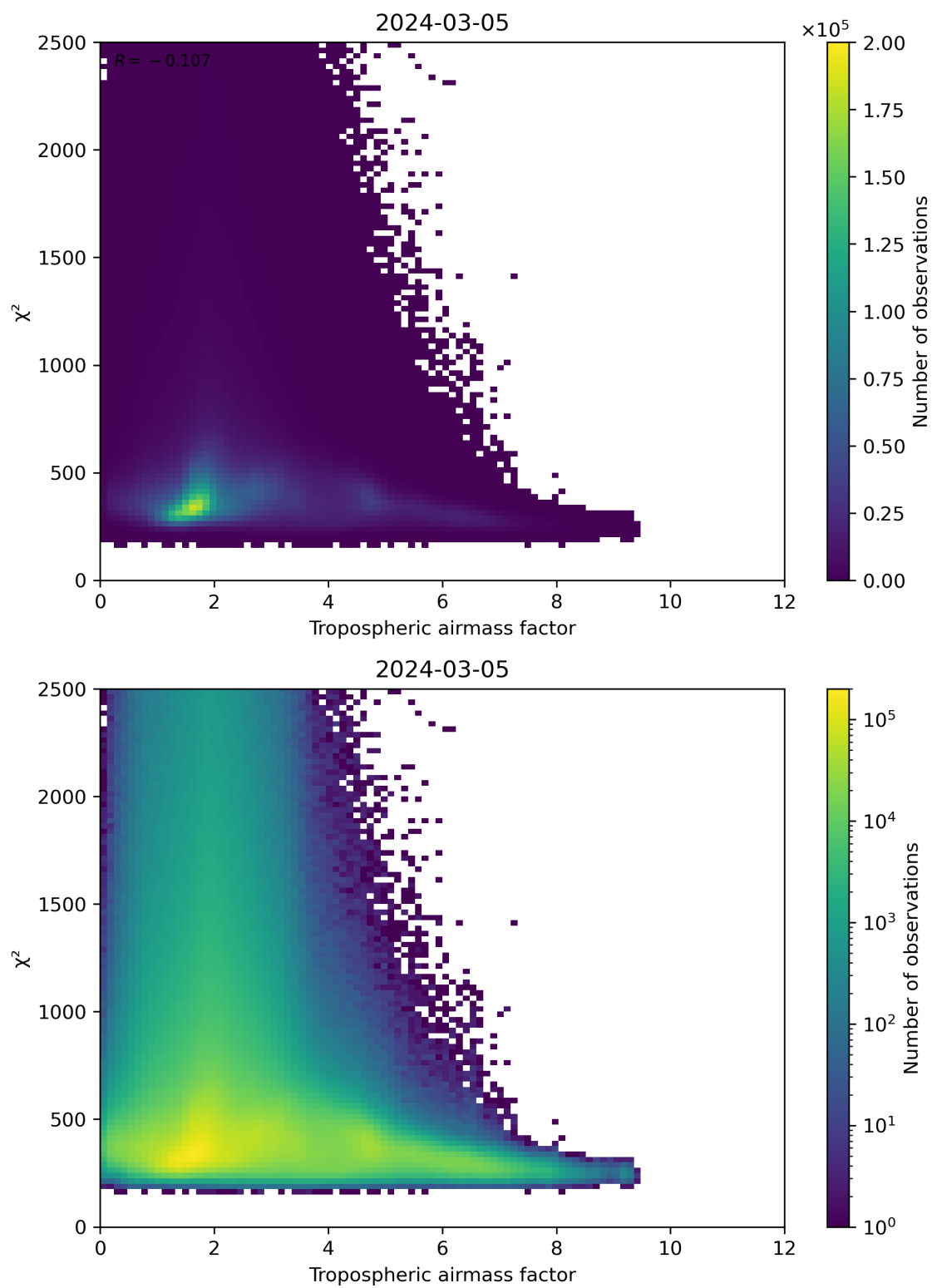
Figure 73: Scatter density plot of “Tropospheric airmass factor” against “ \chi^2 ” for 2024-03-04 to 2024-03-06.
