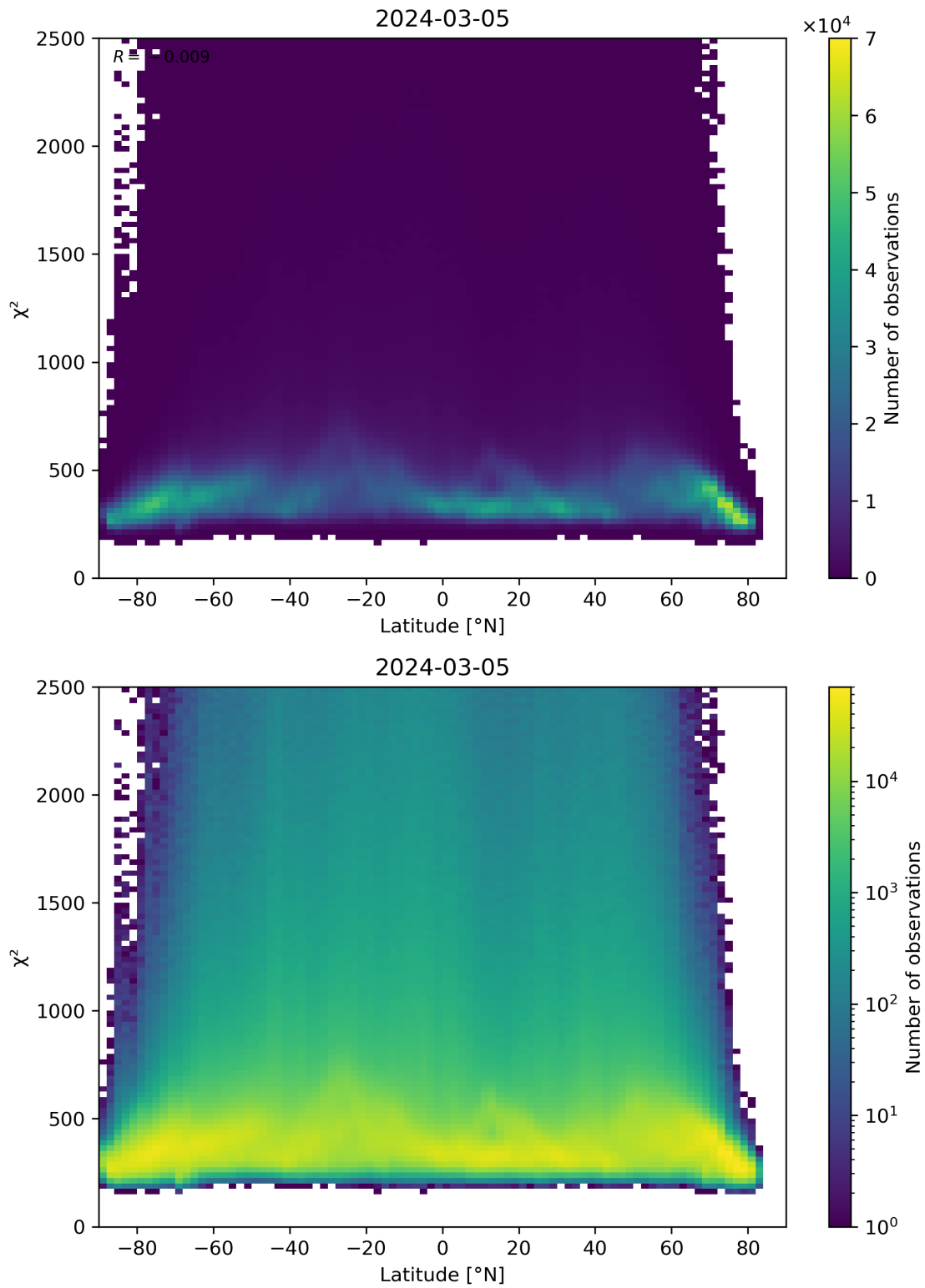
Figure 86: Scatter density plot of “Latitude” against “ \chi^2 ” for 2024-03-04 to 2024-03-06.
