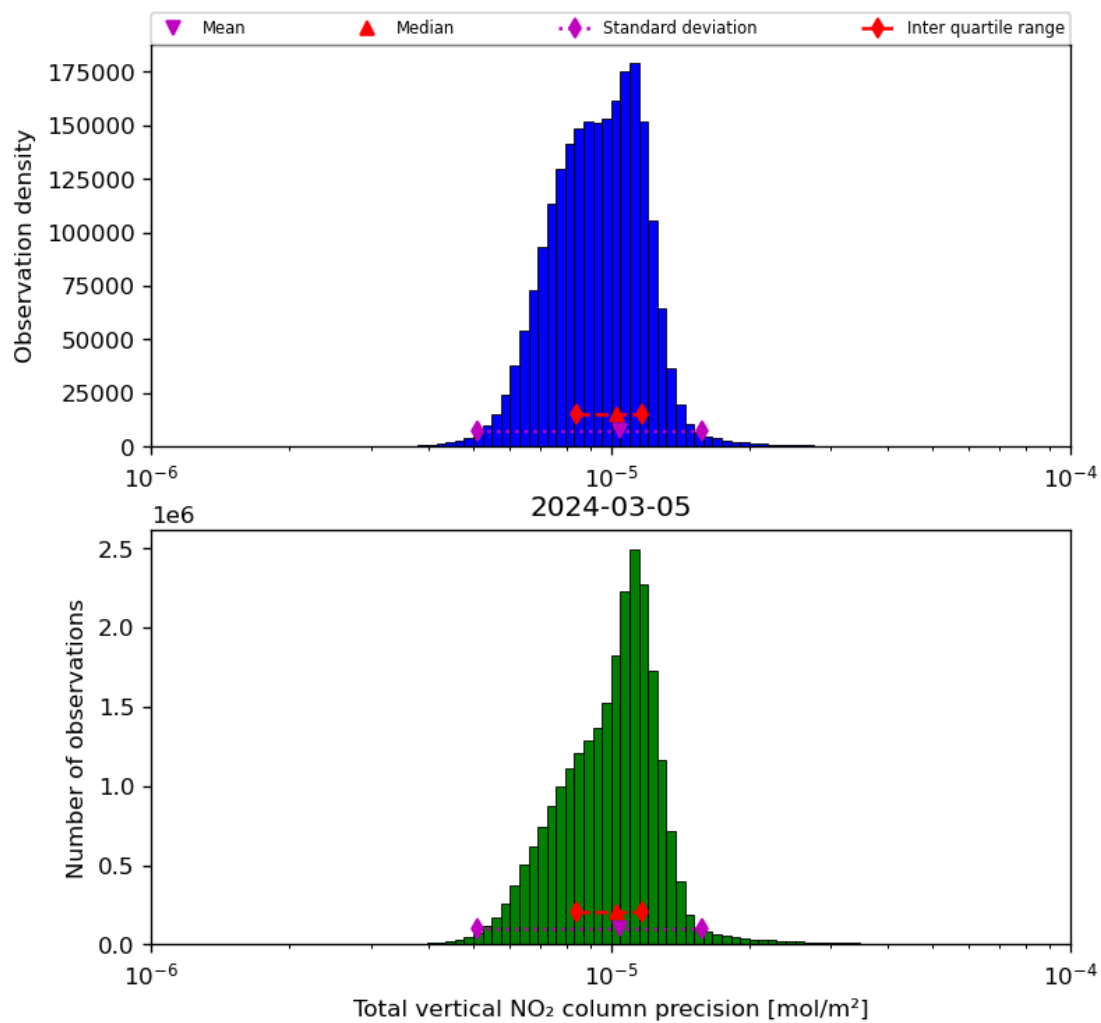
Figure 39: Histogram of “Total vertical NO 2 column precision” for 2024-03-04 to 2024-03-06
