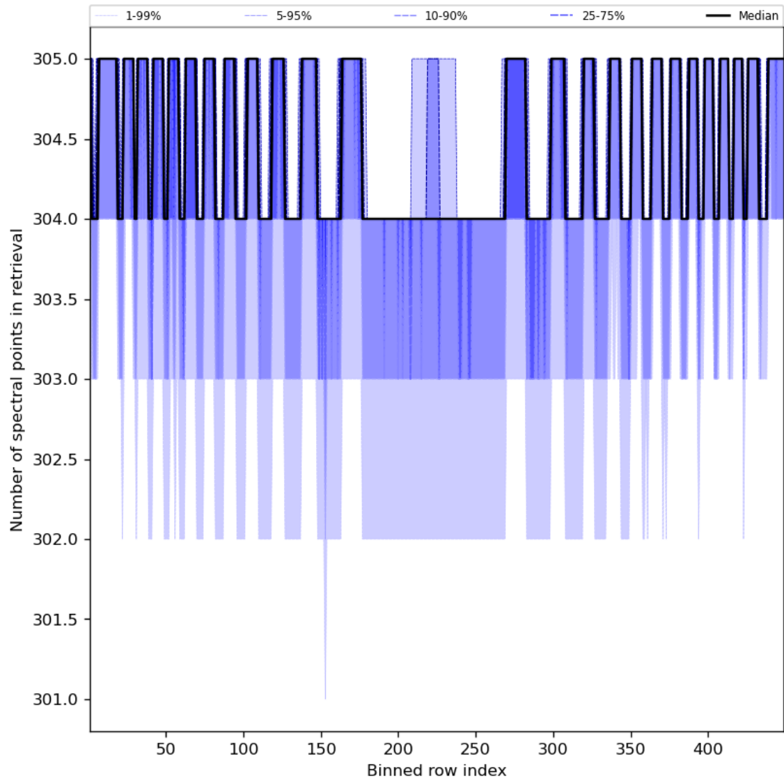
Figure 50: Along track statistics of “Number of spectral points in retrieval” for 2024-03-04 to 2024-03-06
