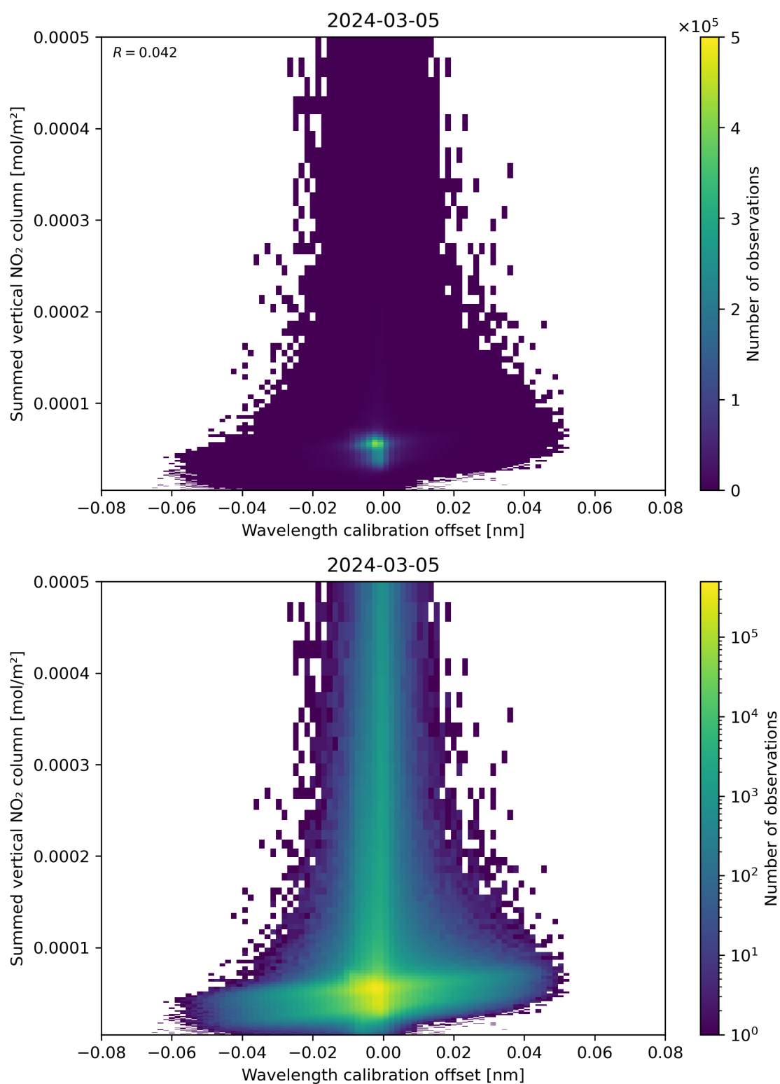
Figure 177: Scatter density plot of “Wavelength calibration offset” against “Summed vertical NO 2 column” for 2024-03-04 to 2024-03-06.
