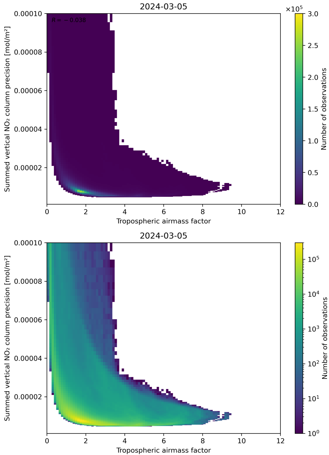
Figure 76: Scatter density plot of “Tropospheric air mass factor” against “Summed vertical NO 2 column precision” for 2024-03-04 to 2024-03-06.
