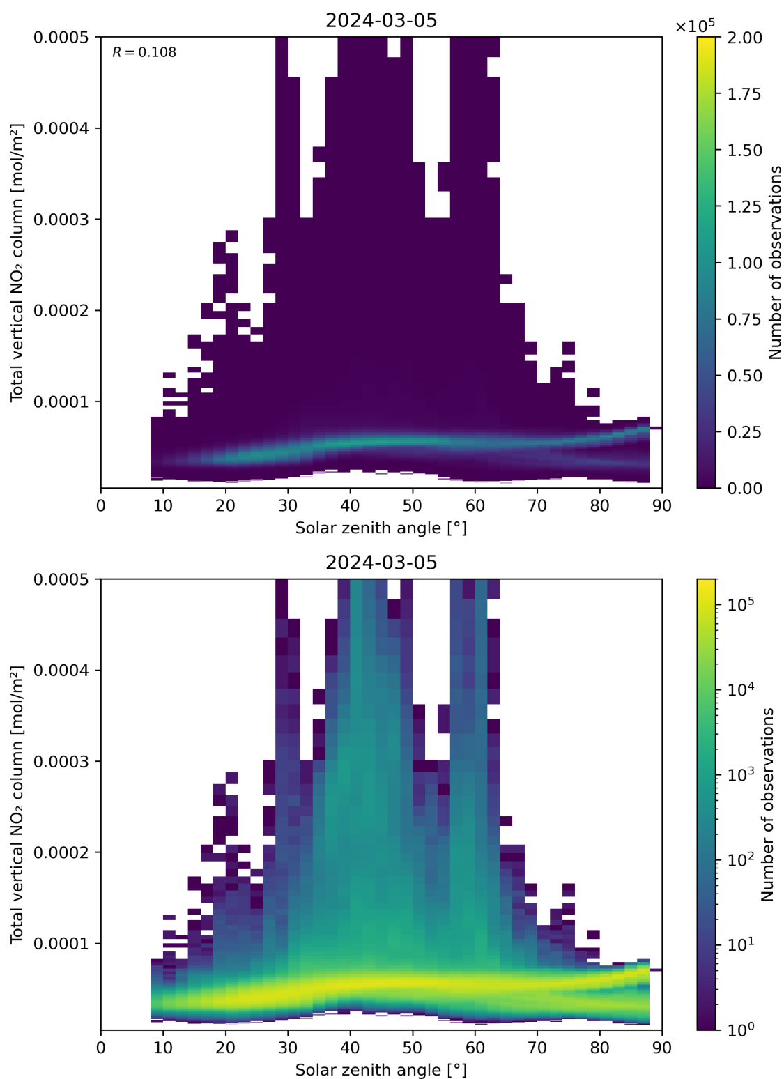
Figure 153: Scatter density plot of “Solar zenith angle” against “Total vertical NO 2 column” for 2024-03-04 to 2024-03-06.
