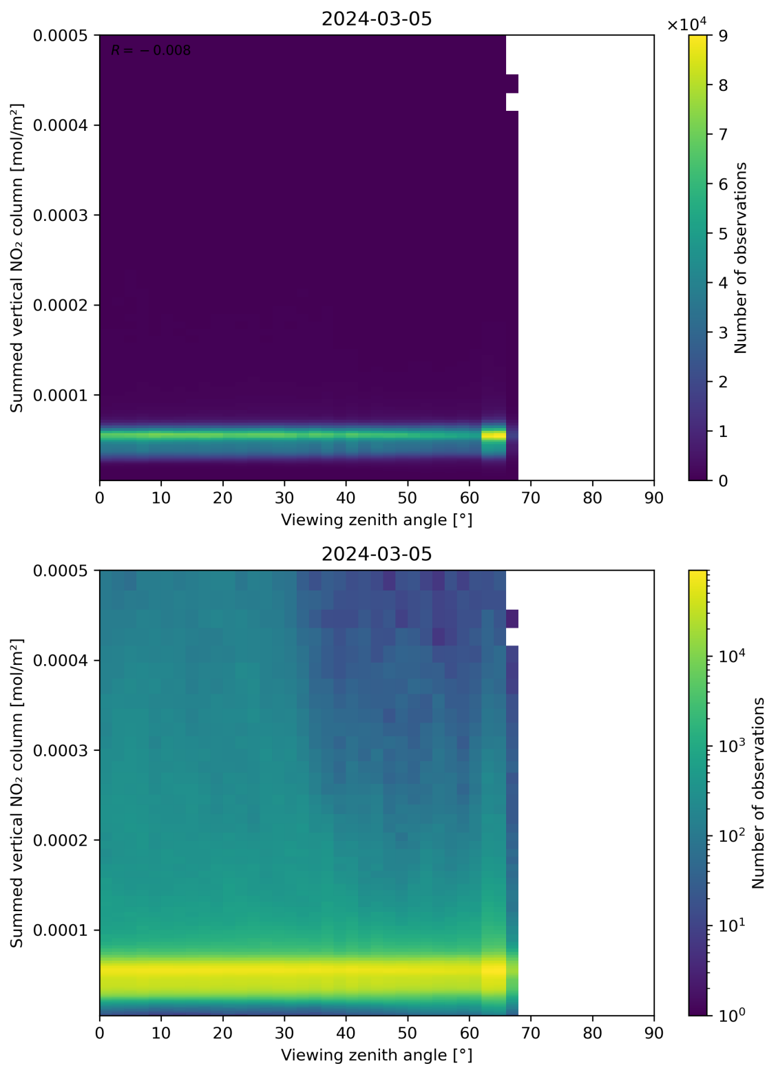
Figure 165: Scatter density plot of “Viewing zenith angle” against “Summed vertical NO 2 column” for 2024-03-04 to 2024-03-06.
