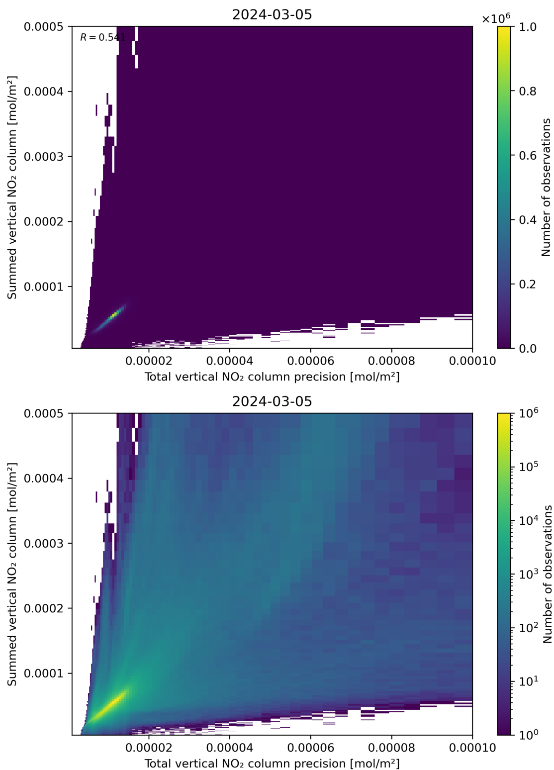
Figure 117: Scatter density plot of “Total vertical NO 2 column precision” against “Summed vertical NO 2 column” for 2024-03-04 to 2024-03-06.
