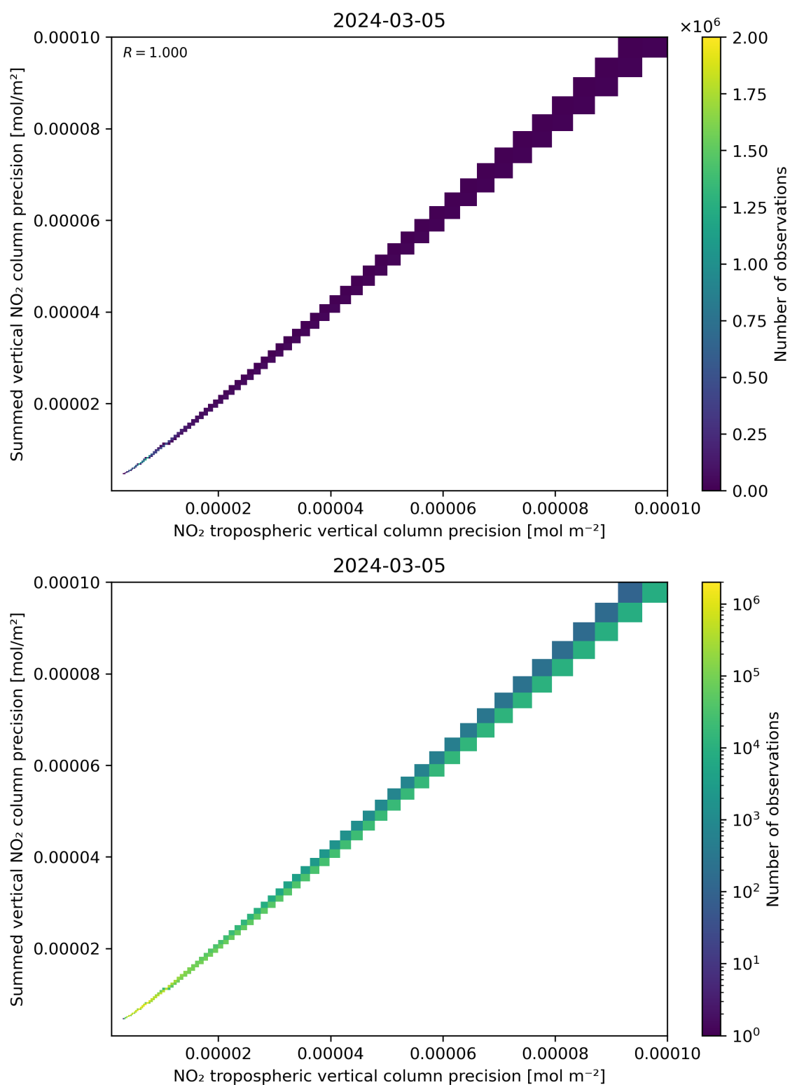
Figure 137: Scatter density plot of “NO 2 tropospheric vertical column precision” against “Summed vertical NO 2 column precision” for 2024-03-04 to 2024-03-06.
