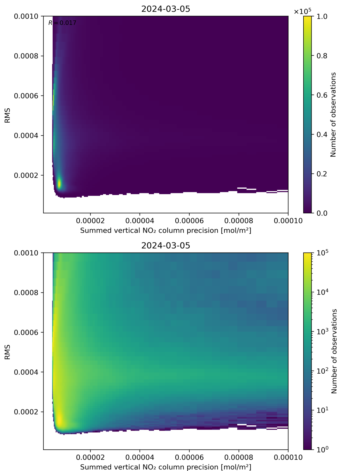
Figure 108: Scatter density plot of “Summed vertical NO 2 column precision” against “RMS” for 2024-03-04 to 2024-03-06.
