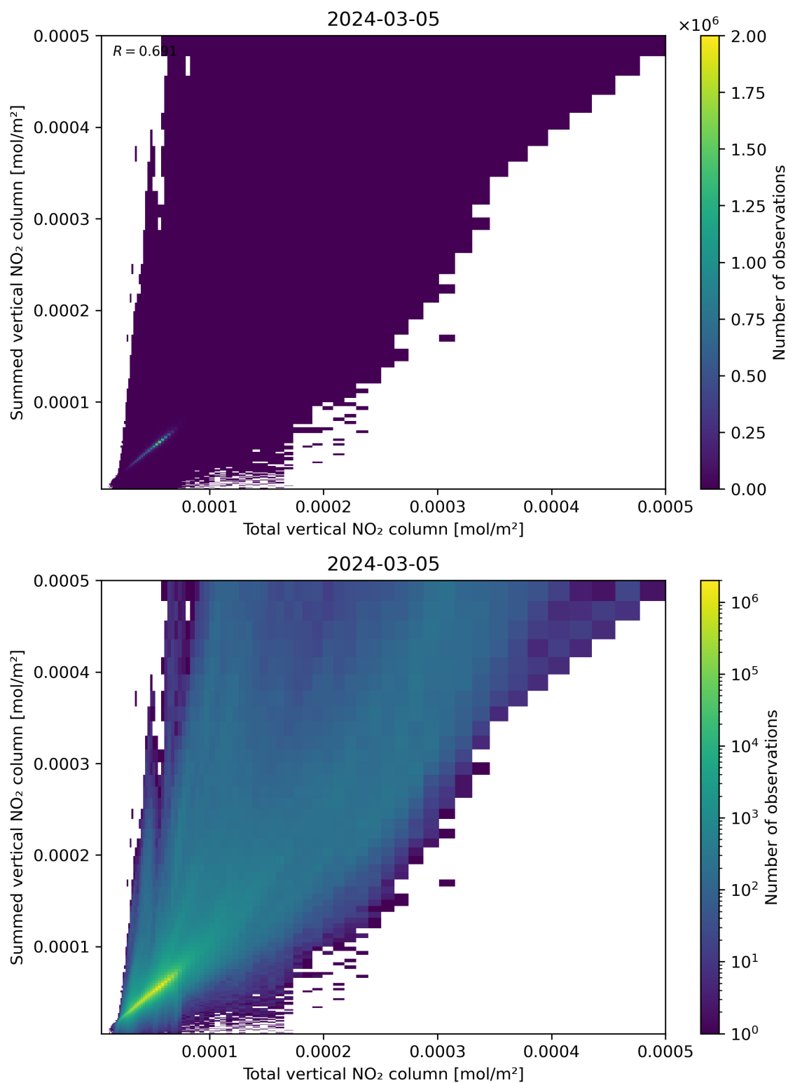
Figure 112: Scatter density plot of “Total vertical NO 2 column” against “Summed vertical NO 2 column” for 2024-03-04 to 2024-03-06.
