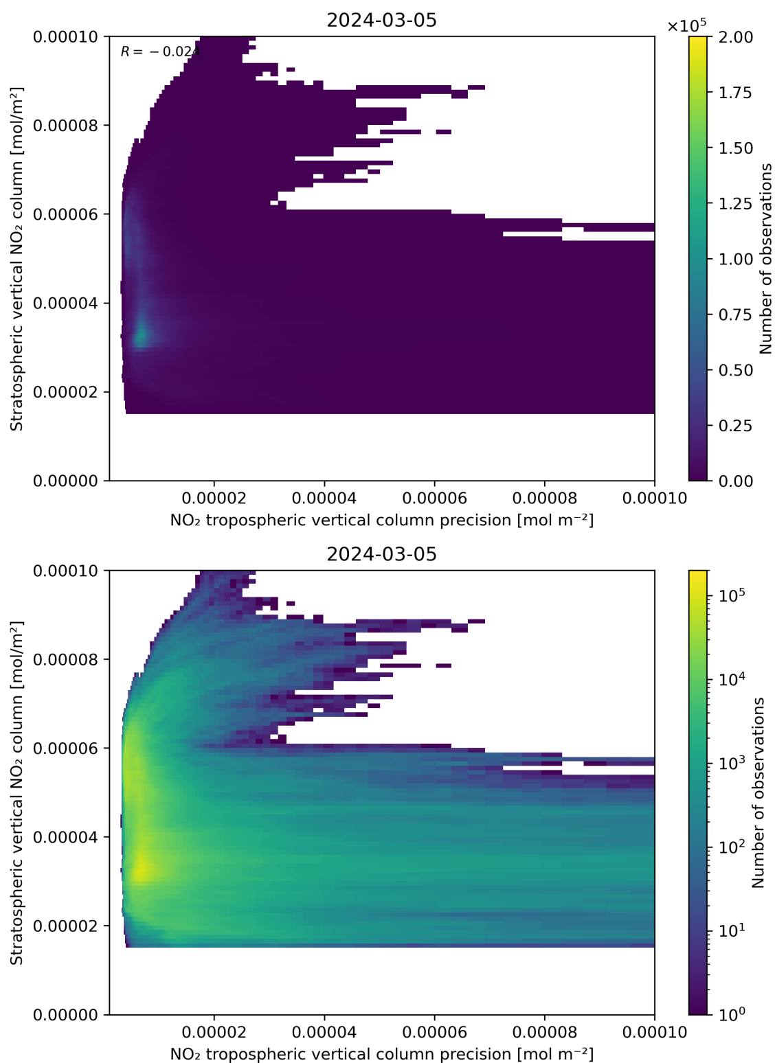
Figure 135: Scatter density plot of “NO 2 tropospheric vertical column precision” against “Stratospheric vertical NO 2 column” for 2024-03-04 to 2024-03-06.
