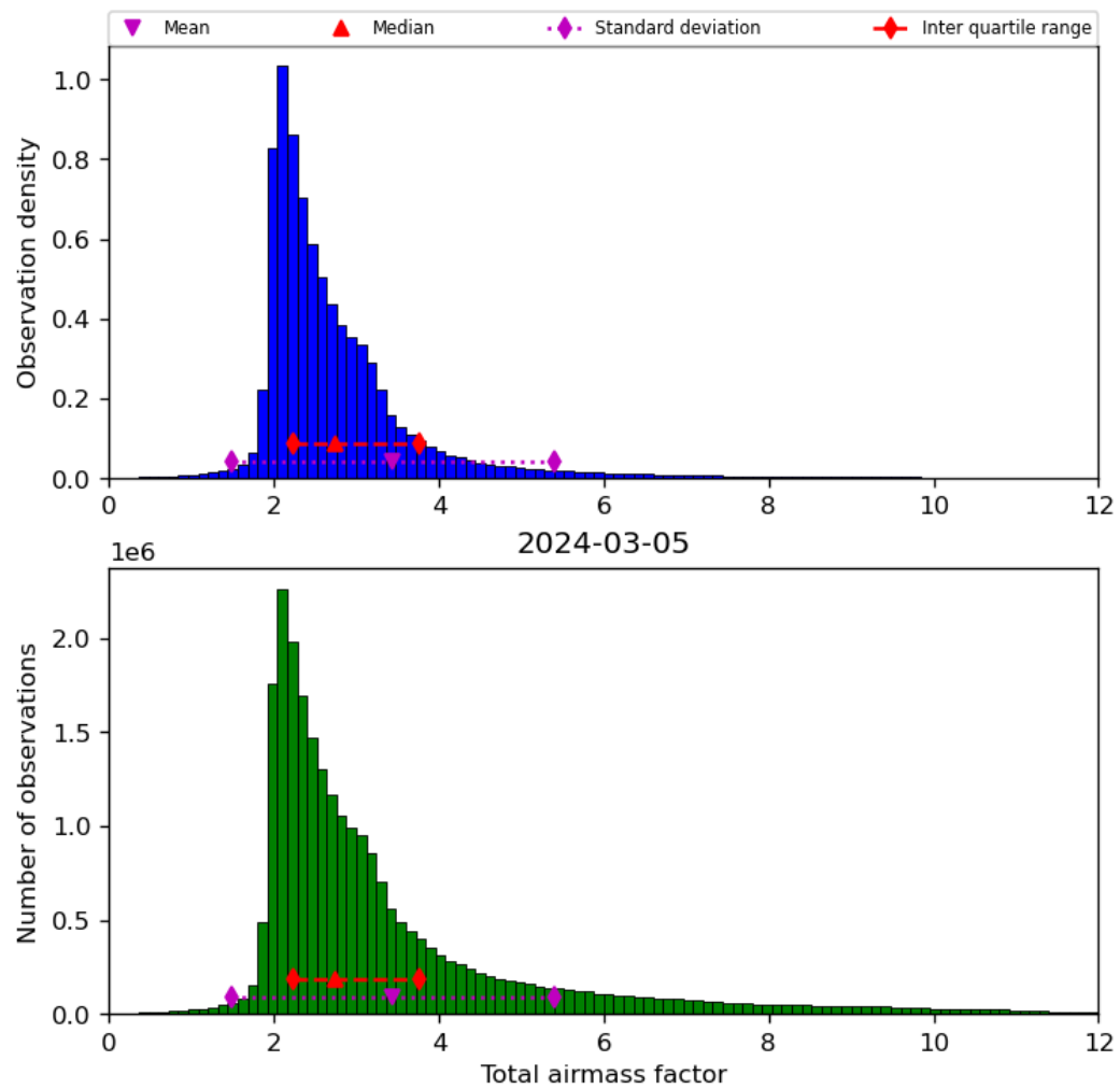
Figure 32: Histogram of “Total airmass factor” for 2024-03-04 to 2024-03-06
