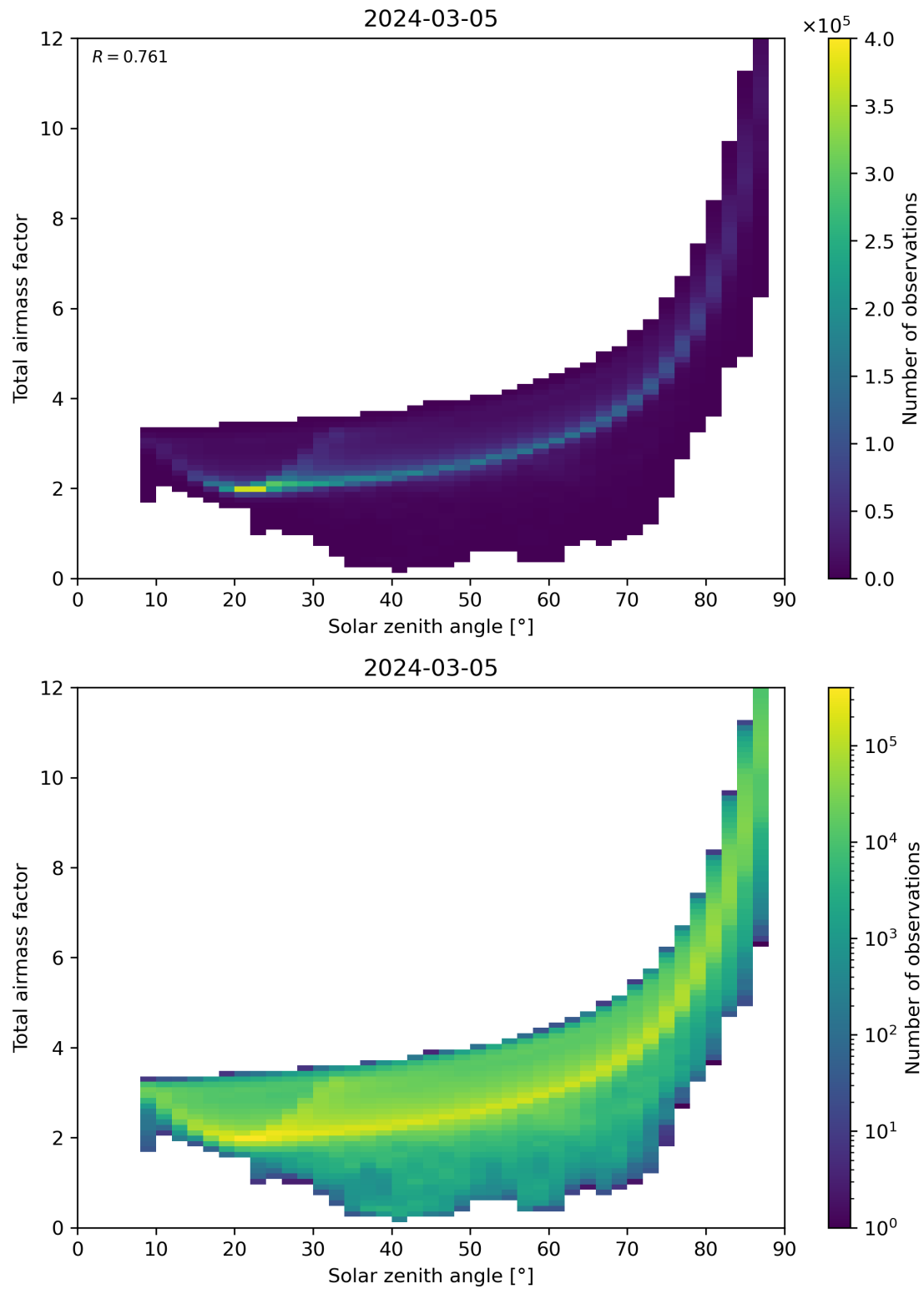
Figure 146: Scatter density plot of “Solar zenith angle” against “Total air mass factor” for 2024-03-04 to 2024-03-06.
