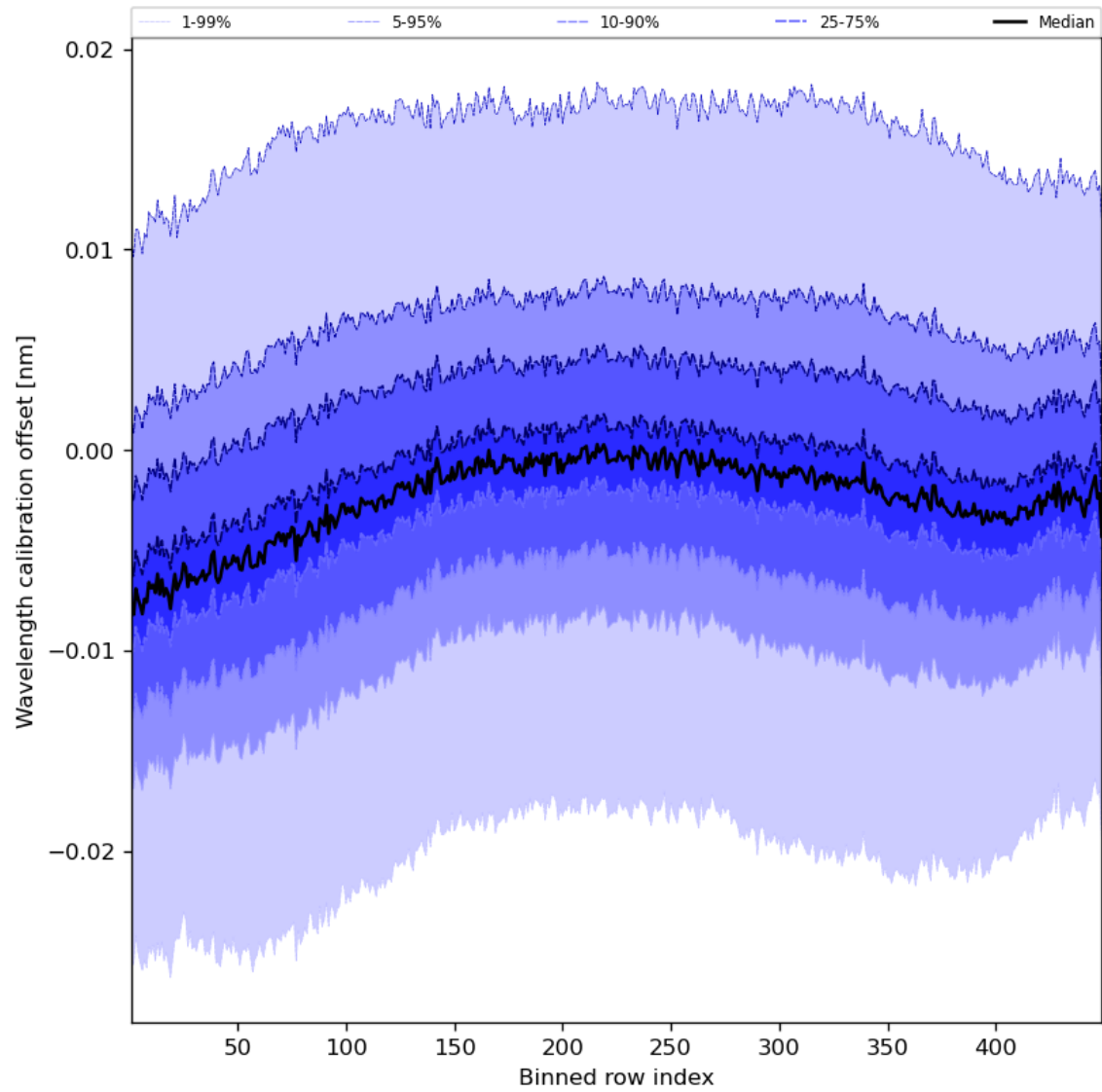
Figure 52: Along track statistics of “Wavelength calibration offset” for 2024-03-04 to 2024-03-06
