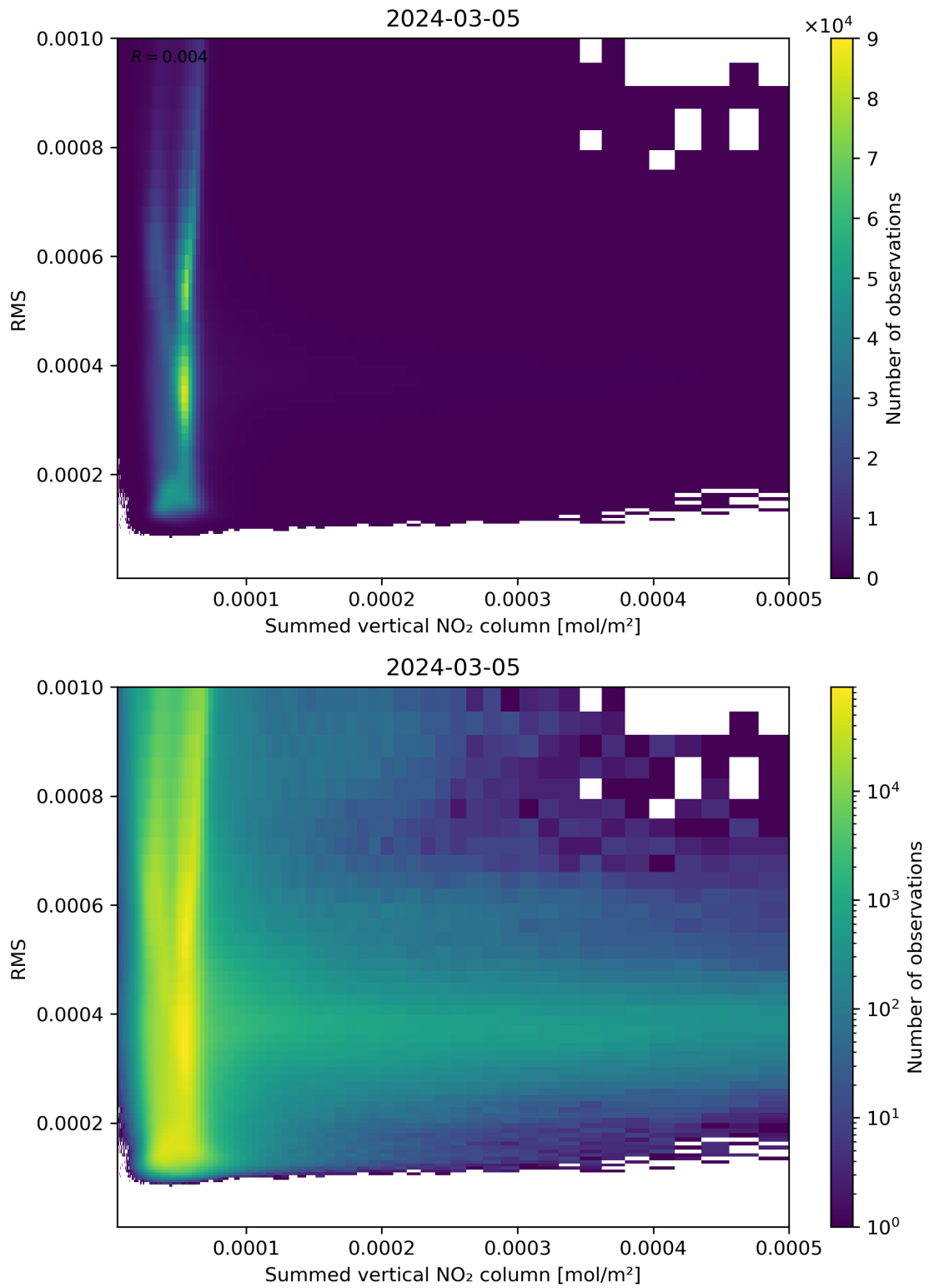
Figure 109: Scatter density plot of “Summed vertical NO 2 column” against “RMS” for 2024-03-04 to 2024-03-06.
