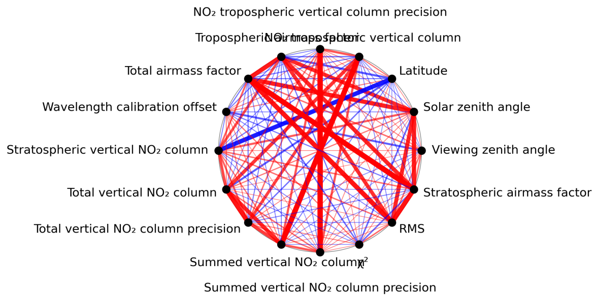
Figure 1: Map of correlation graph for 2024-03-04 to 2024-03-06.
