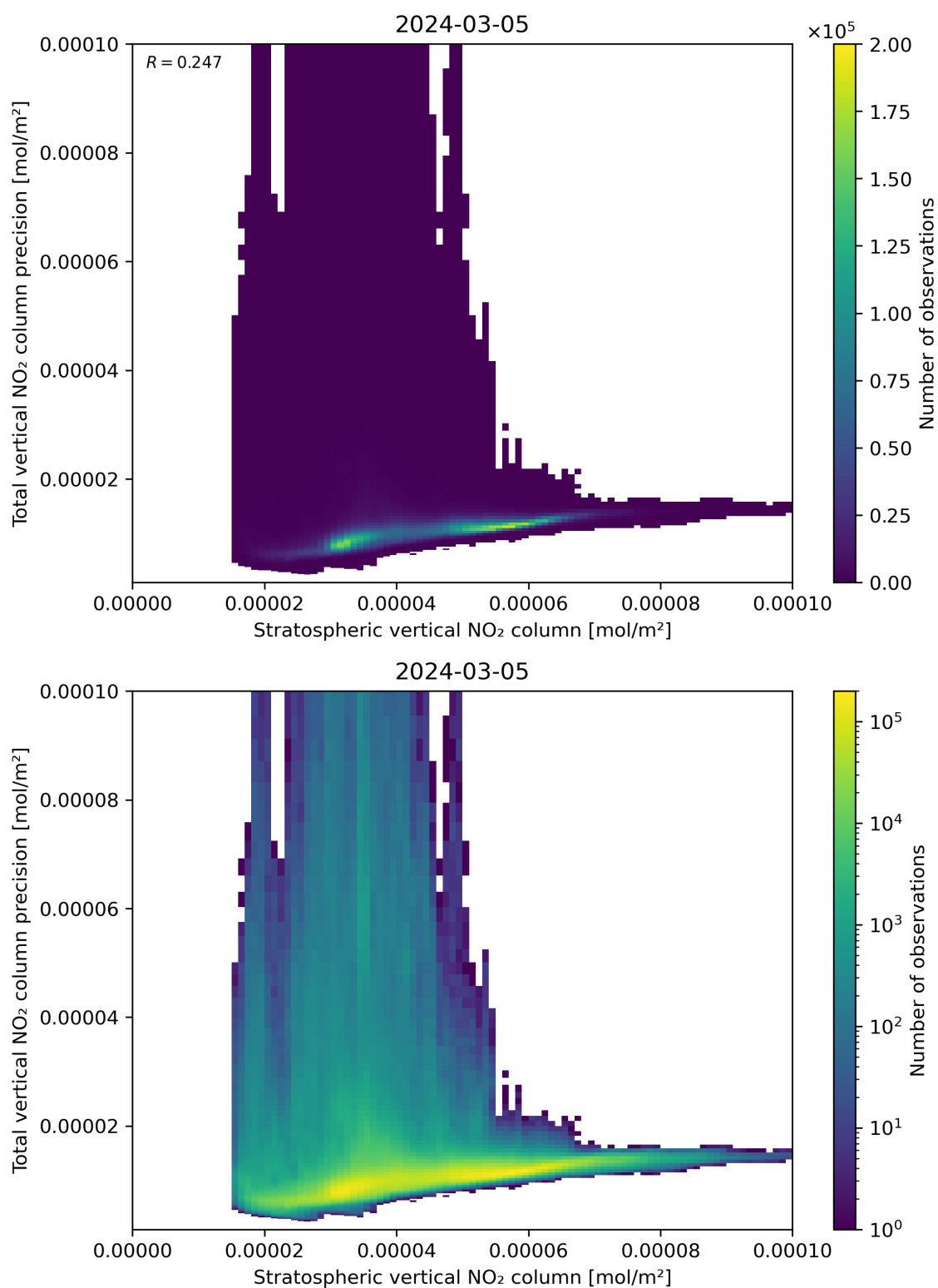
Figure 101: Scatter density plot of “Stratospheric vertical NO 2 column” against “Total vertical NO 2 column precision” for 2024-03-04 to 2024-03-06.
