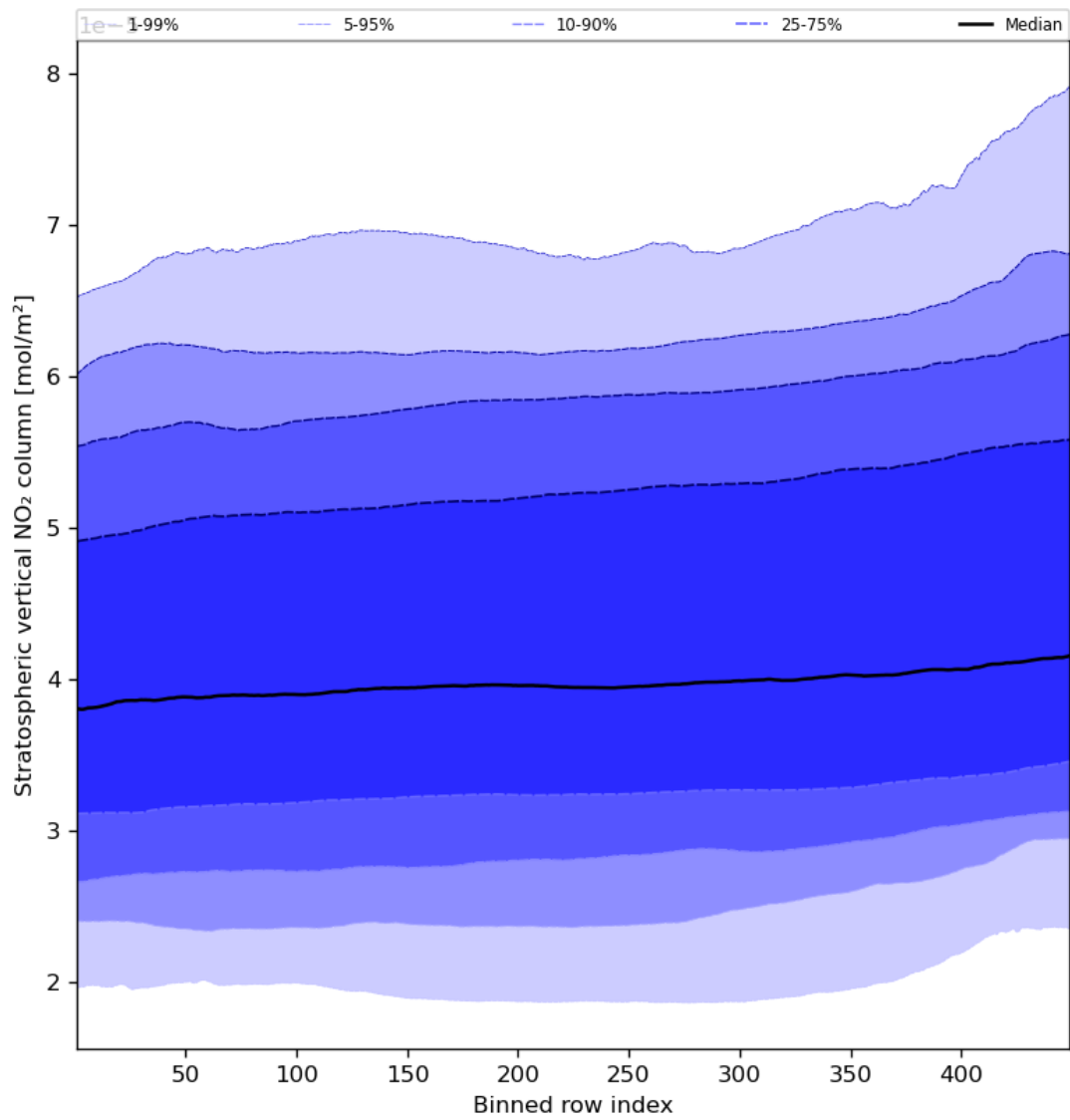
Figure 53: Along track statistics of “Stratospheric vertical NO 2 column” for 2024-03-04 to 2024-03-06
