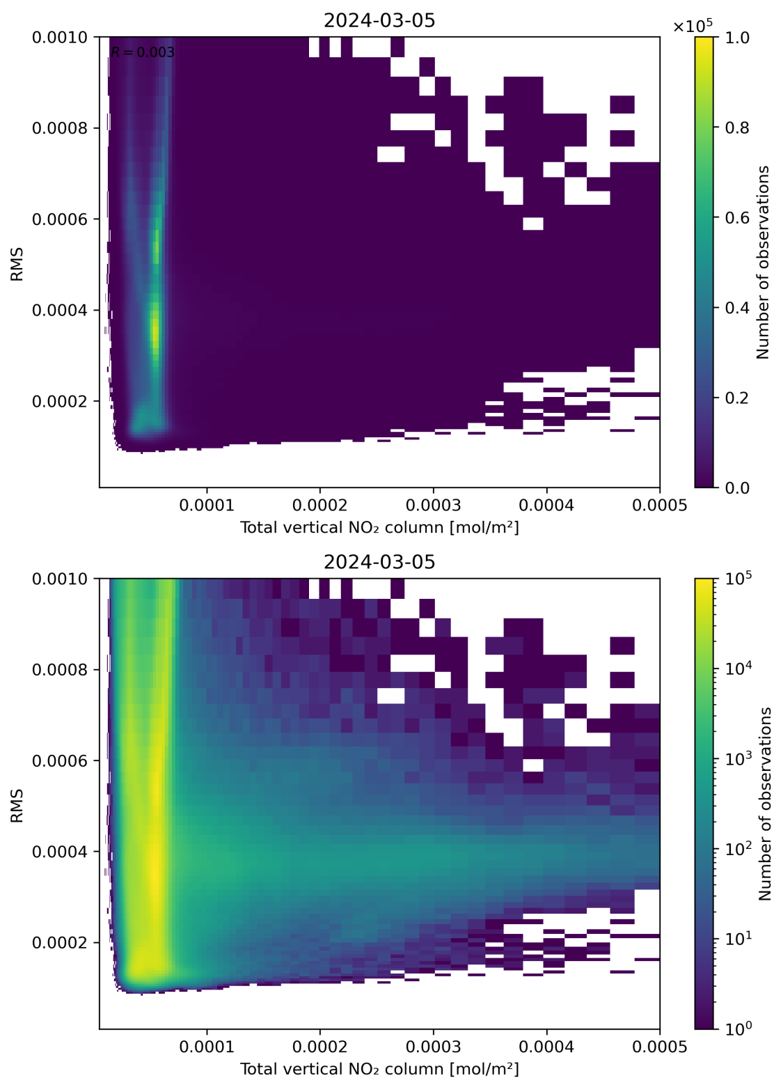
Figure 120: Scatter density plot of “Total vertical NO 2 column” against “RMS” for 2024-03-04 to 2024-03-06.
