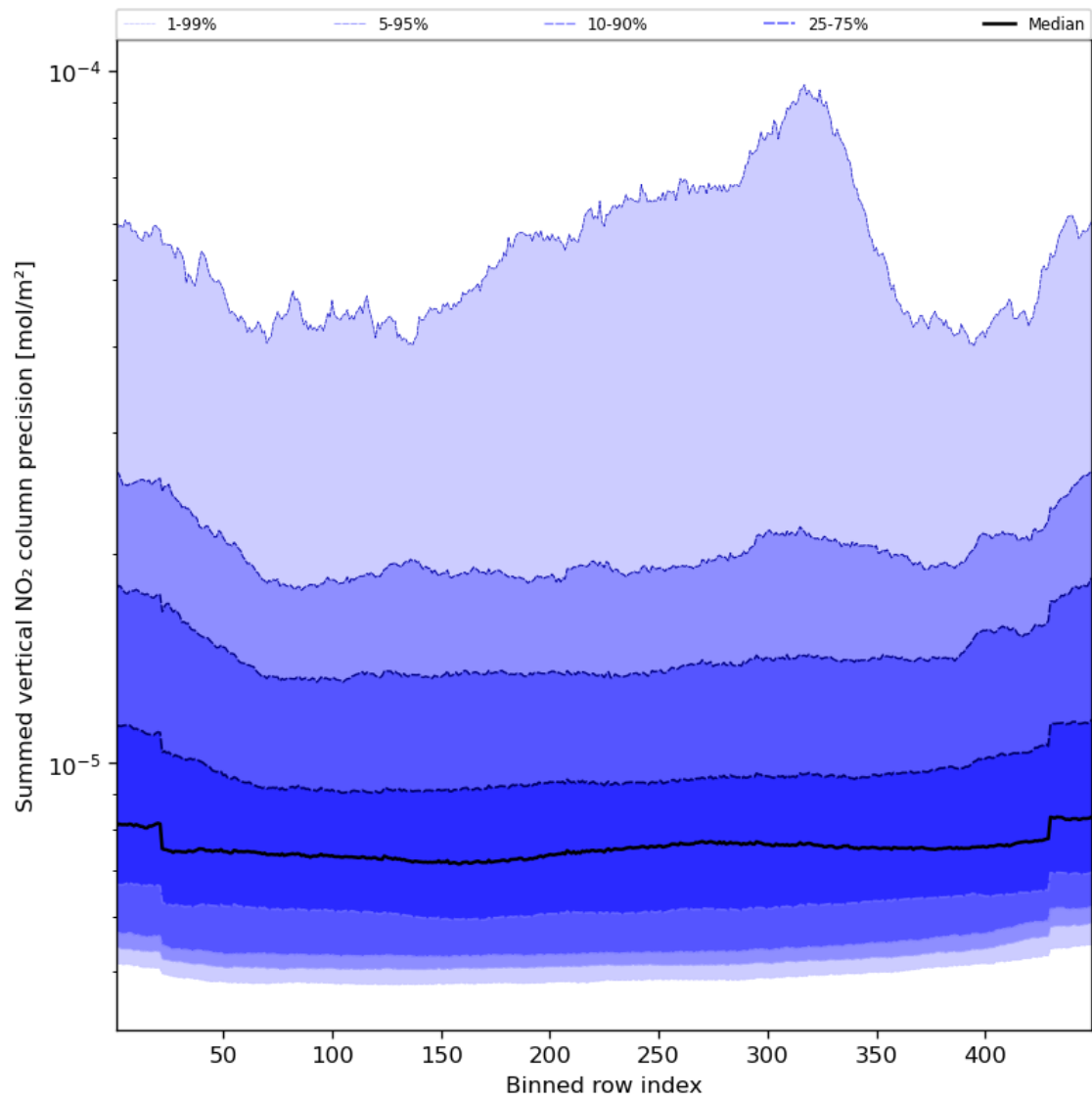
Figure 58: Along track statistics of “Summed vertical NO 2 column precision” for 2024-03-04 to 2024-03-06
