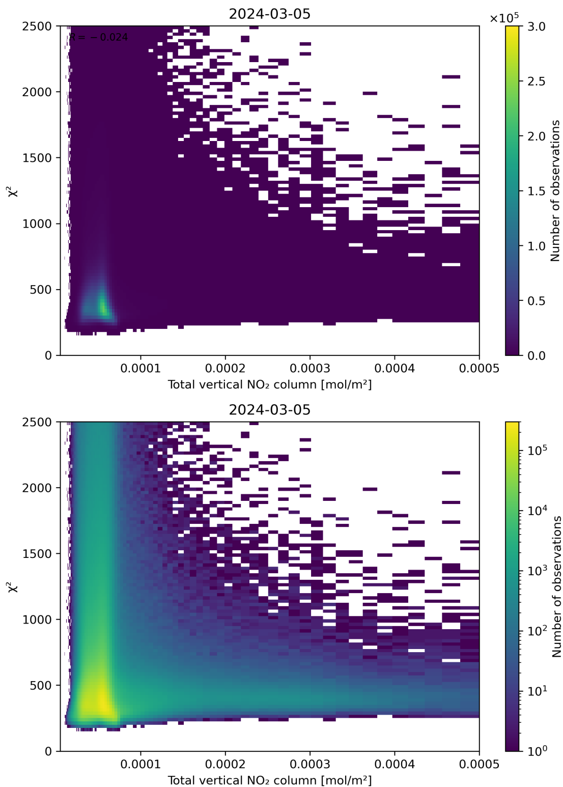
Figure 111: Scatter density plot of “Total vertical NO 2 column” against “ \chi^2 ” for 2024-03-04 to 2024-03-06.
