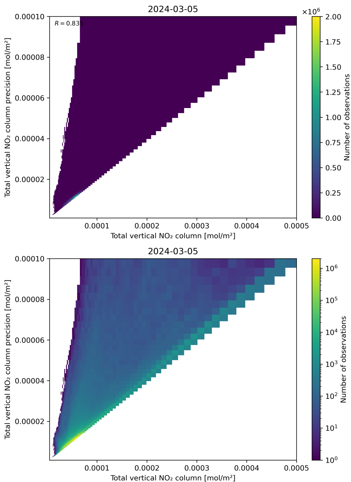
Figure 114: Scatter density plot of “Total vertical NO 2 column” against “Total vertical NO 2 column precision” for 2024-03-04 to 2024-03-06.
