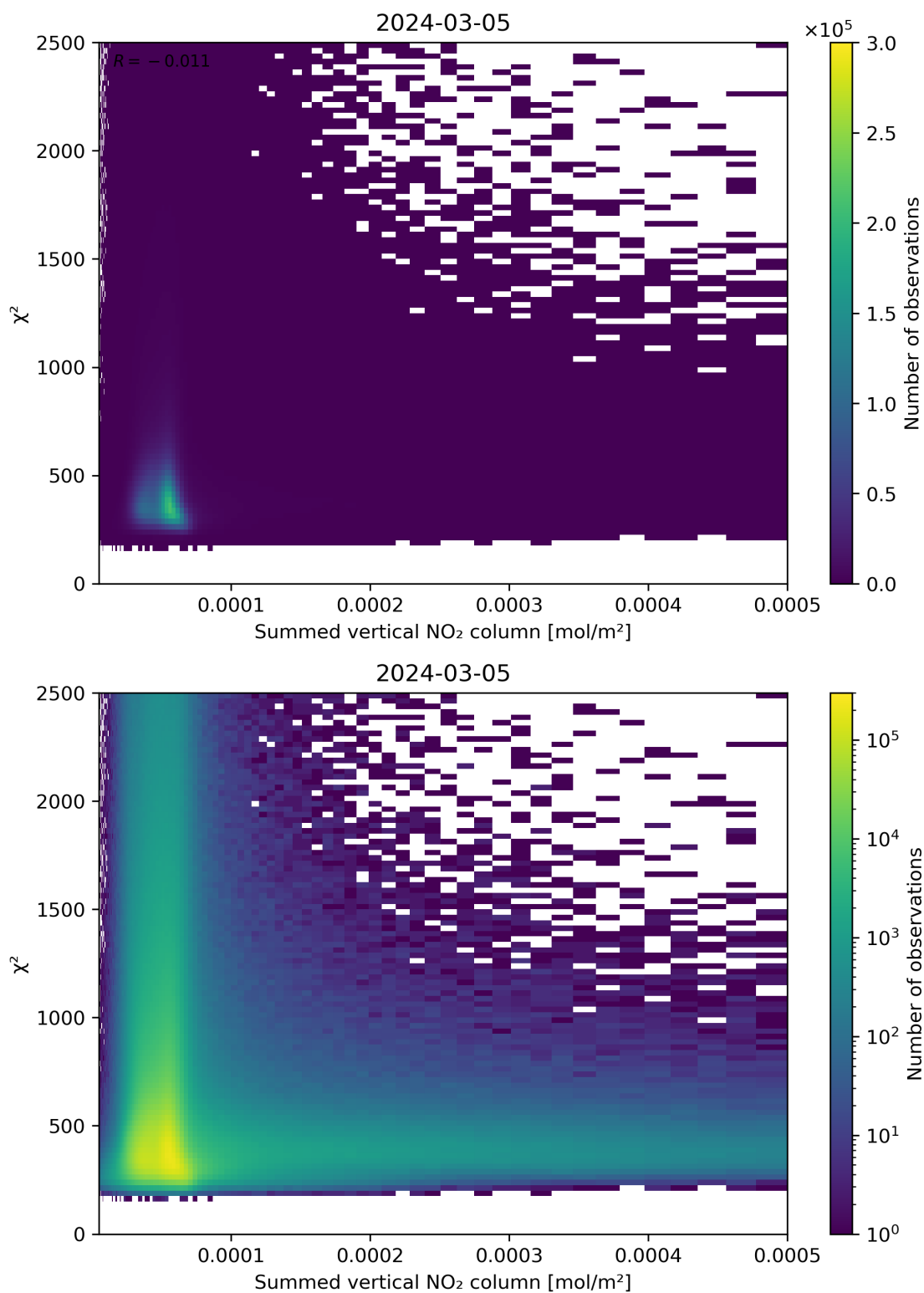
Figure 104: Scatter density plot of “Summed vertical NO 2 column” against “ \chi^2 ” for 2024-03-04 to 2024-03-06.
