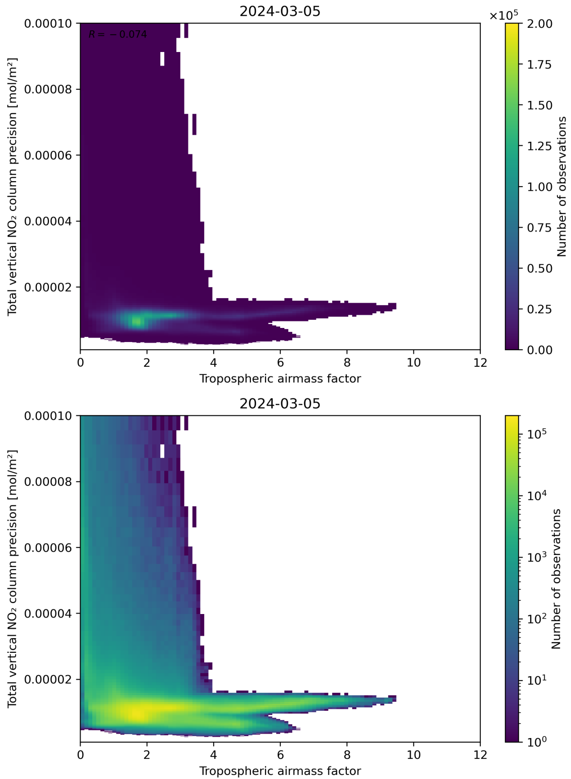
Figure 78: Scatter density plot of “Tropospheric air mass factor” against “Total vertical NO 2 column precision” for 2024-03-04 to 2024-03-06.
