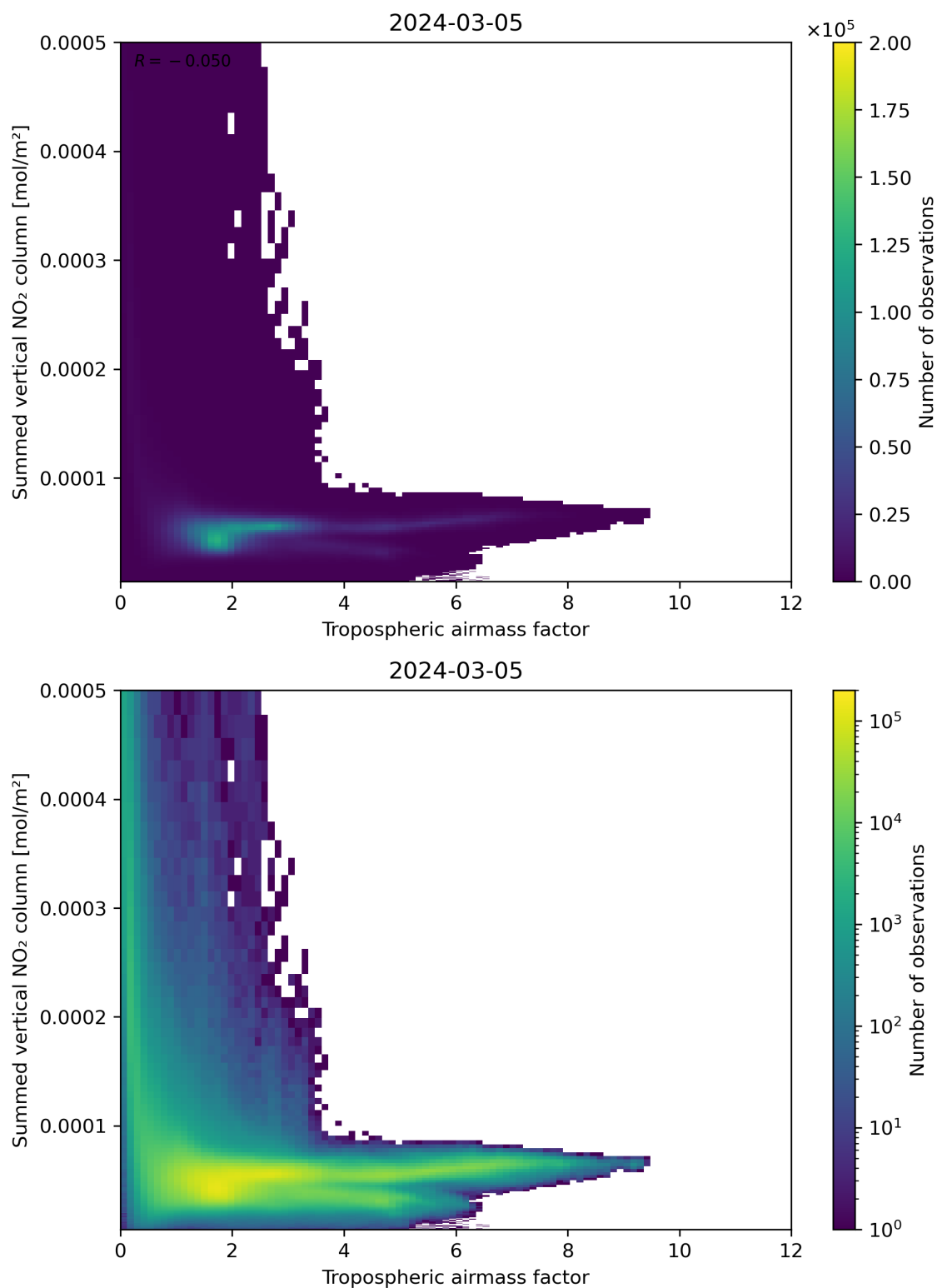
Figure 75: Scatter density plot of “Tropospheric airmass factor” against “Summed vertical NO 2 column” for 2024-03-04 to 2024-03-06.
