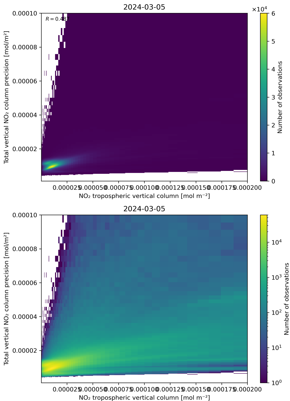
Figure 129: Scatter density plot of “NO 2 tropospheric vertical column” against “Total vertical NO 2 column precision” for 2024-03-04 to 2024-03-06.
