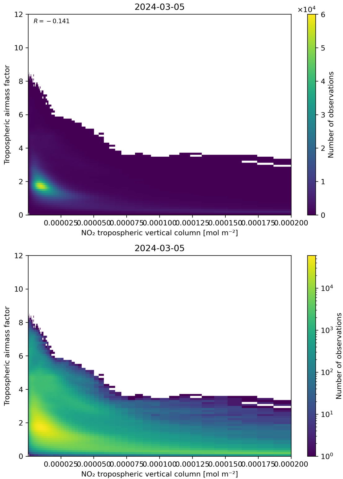
Figure 123: Scatter density plot of “NO 2 tropospheric vertical column” against “Tropospheric airmass factor” for 2024-03-04 to 2024-03-06.
