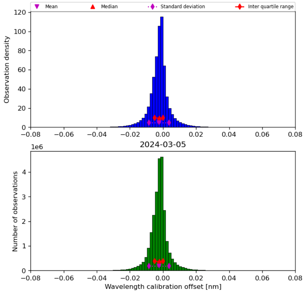
Figure 35: Histogram of “Wavelength calibration offset” for 2024-03-04 to 2024-03-06
