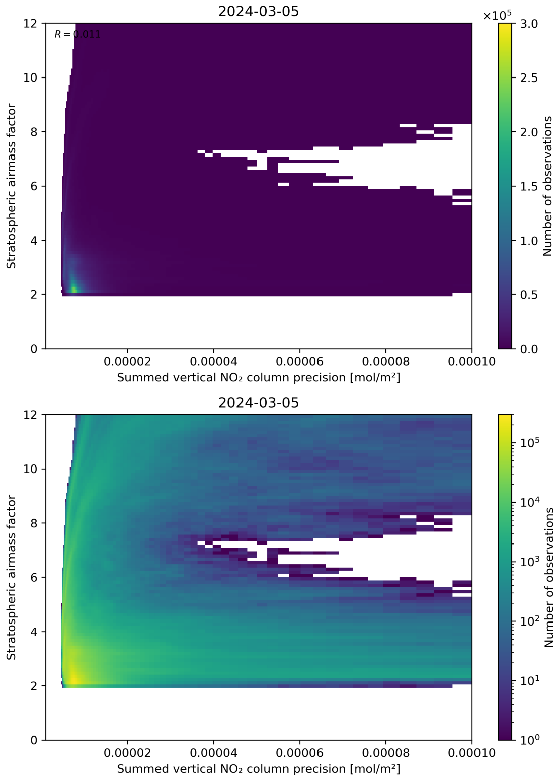
Figure 106: Scatter density plot of “Summed vertical NO 2 column precision” against “Stratospheric airmass factor” for 2024-03-04 to 2024-03-06.
