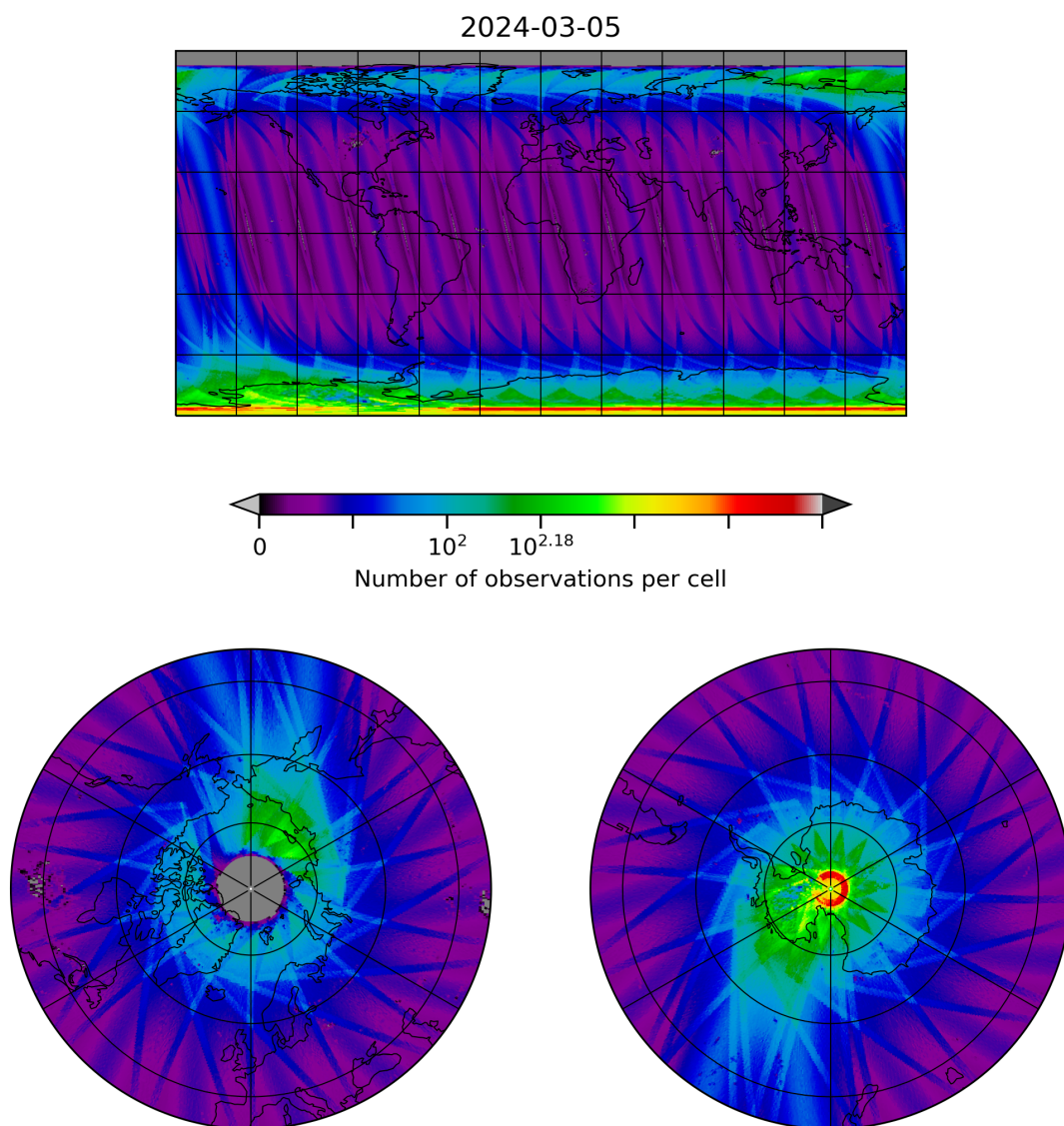
Figure 10: Map of the number of observations for 2024-03-04 to 2024-03-06
