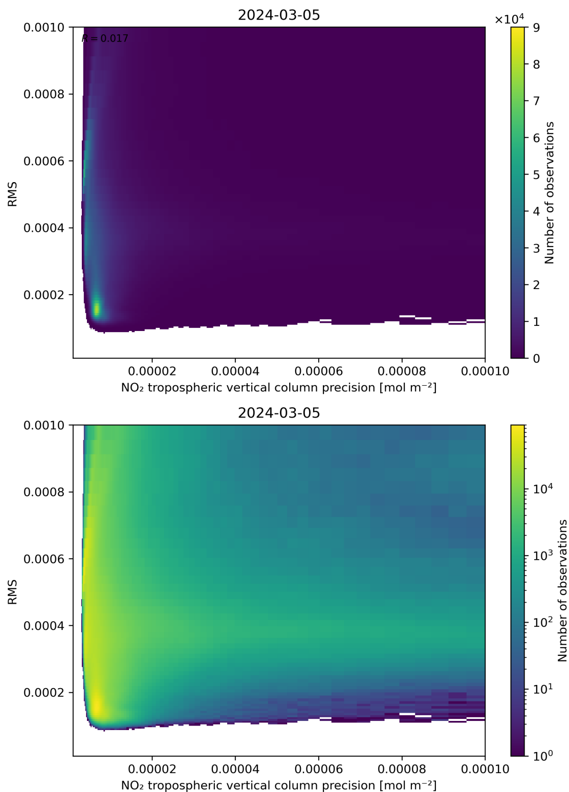
Figure 140: Scatter density plot of “NO 2 tropospheric vertical column precision” against “RMS” for 2024-03-04 to 2024-03-06.
