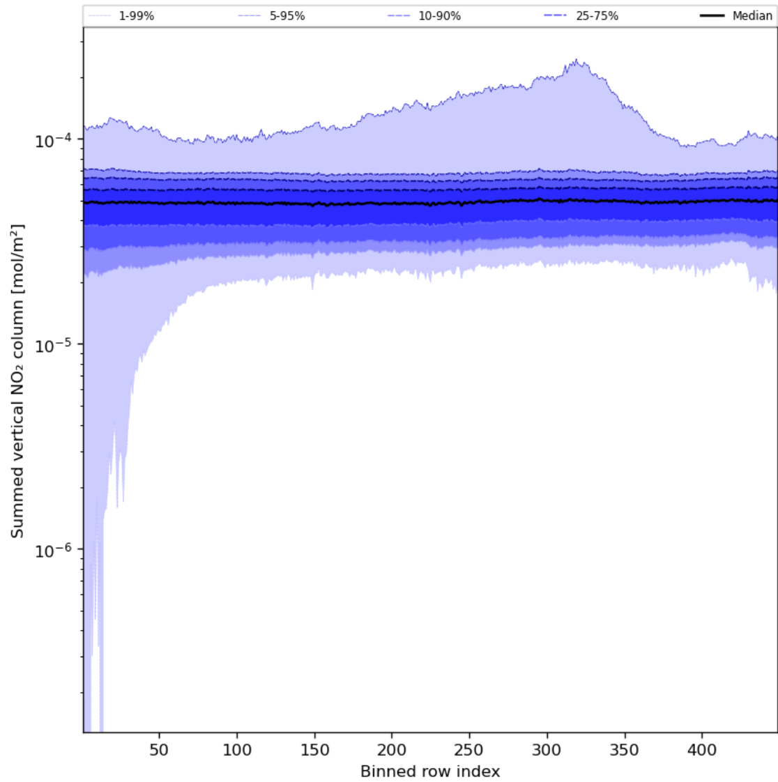
Figure 57: Along track statistics of “Summed vertical NO 2 column” for 2024-03-04 to 2024-03-06
