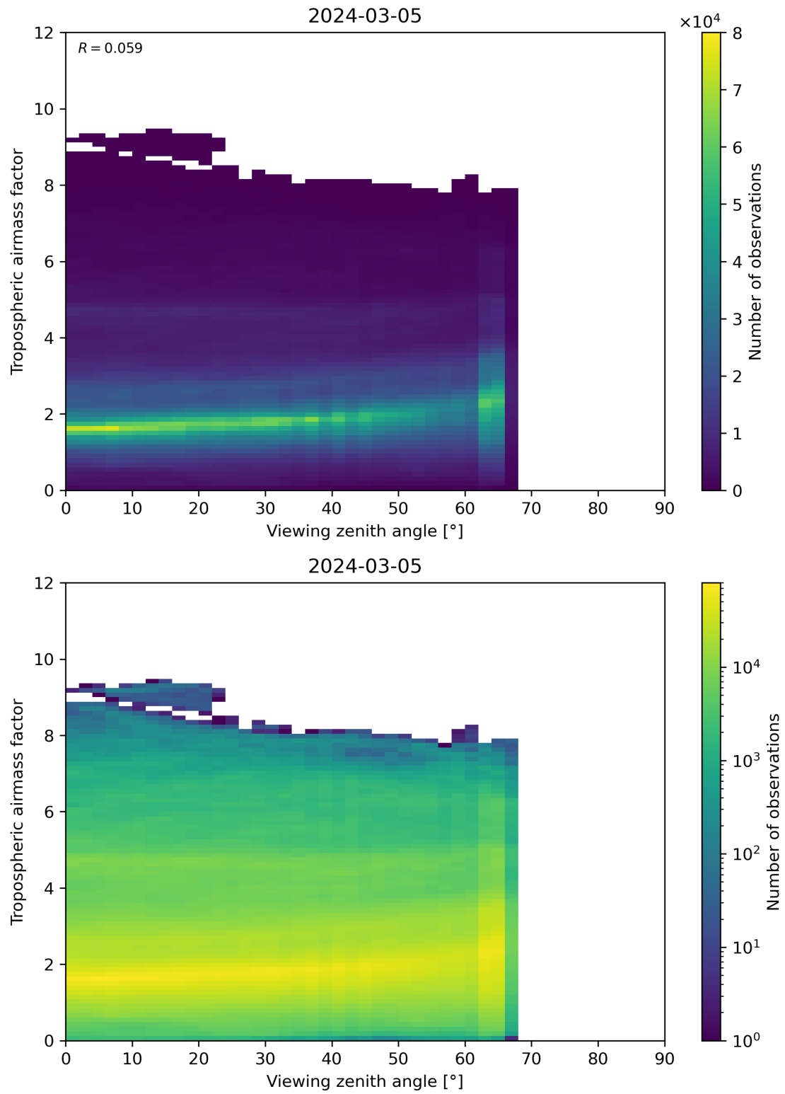
Figure 161: Scatter density plot of “Viewing zenith angle” against “Tropospheric airmass factor” for 2024-03-04 to 2024-03-06.
