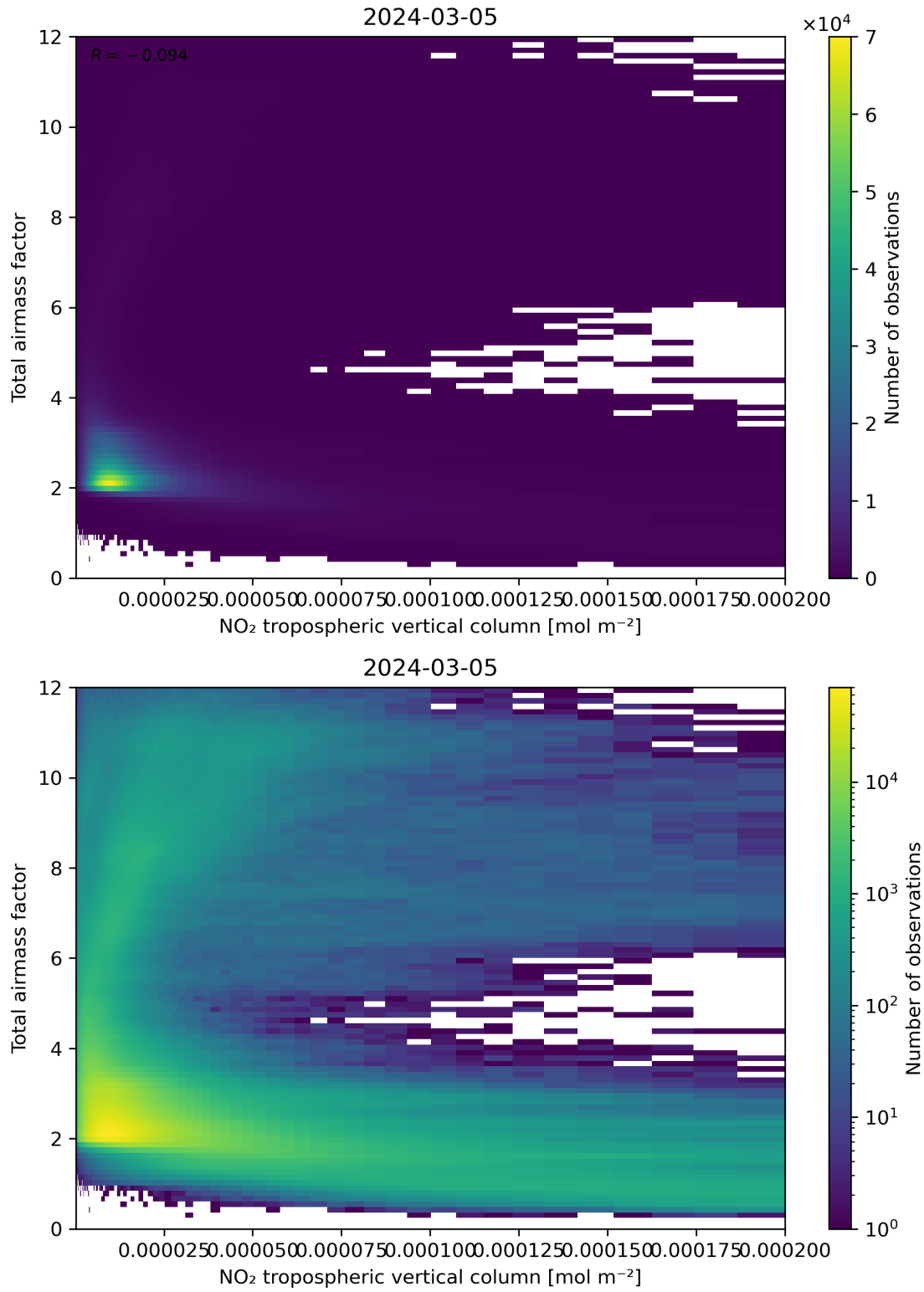
Figure 122: Scatter density plot of “NO 2 tropospheric vertical column” against “Total air mass factor” for 2024-03-04 to 2024-03-06.
