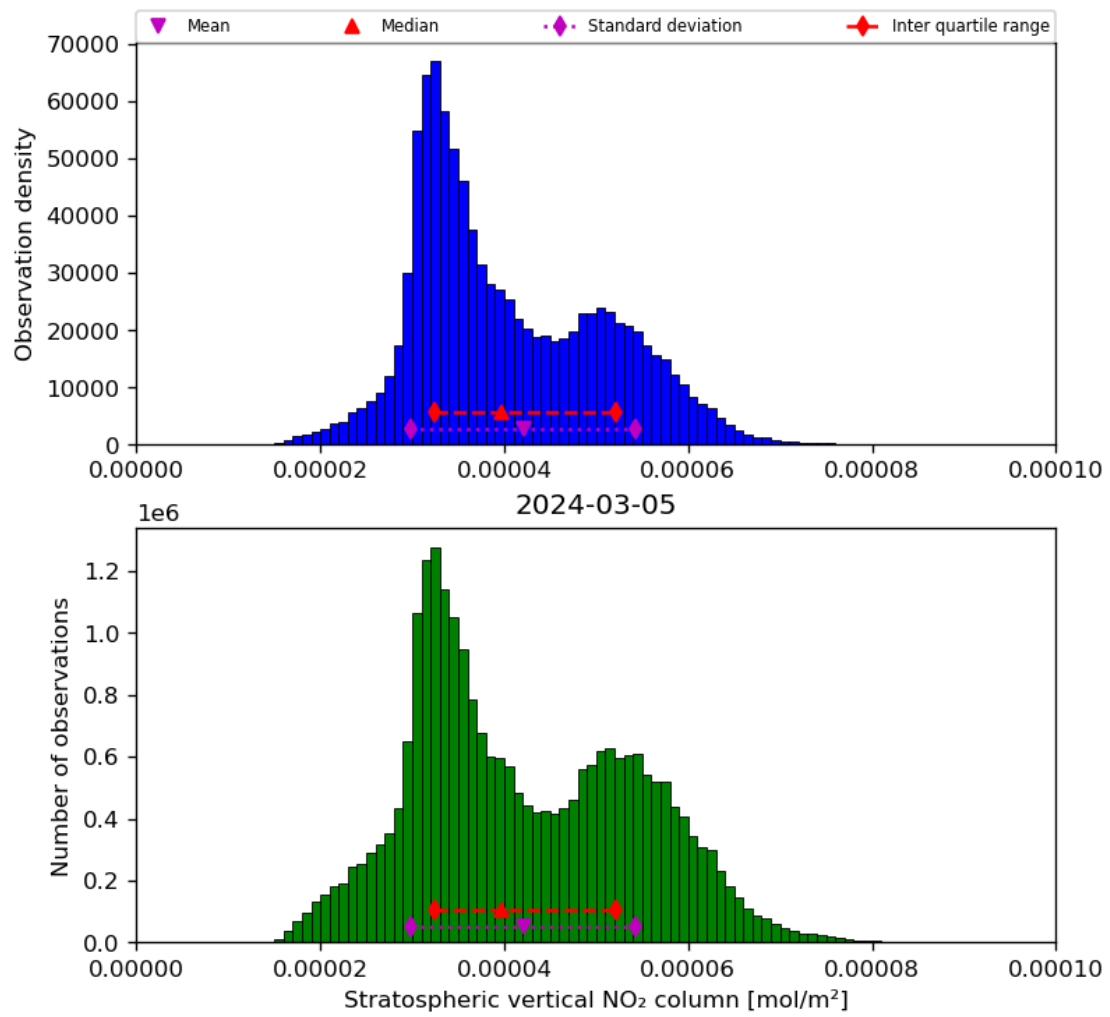
Figure 36: Histogram of “Stratospheric vertical NO 2 column” for 2024-03-04 to 2024-03-06
