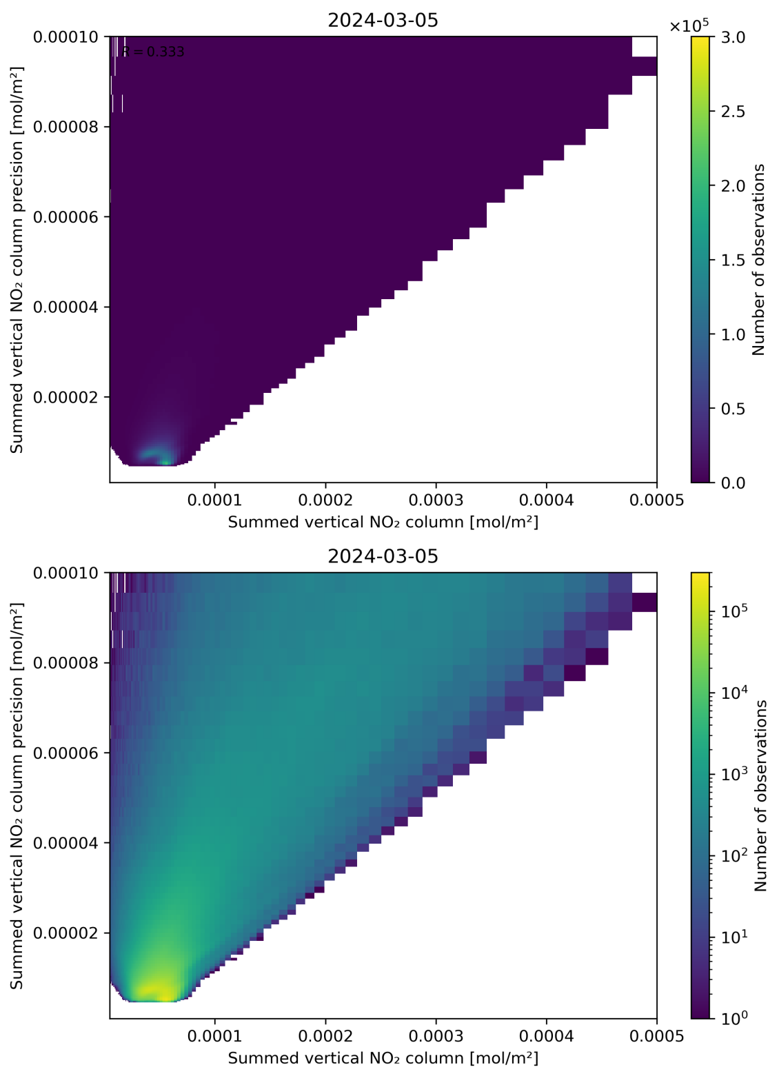
Figure 105: Scatter density plot of “Summed vertical NO 2 column” against “Summed vertical NO 2 column precision” for 2024-03-04 to 2024-03-06.
