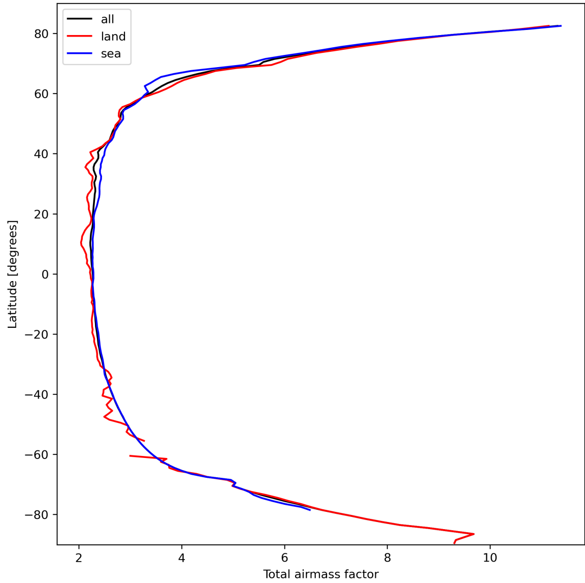
Figure 15: Zonal average of “Total airmass factor” for 2024-03-04 to 2024-03-06.
