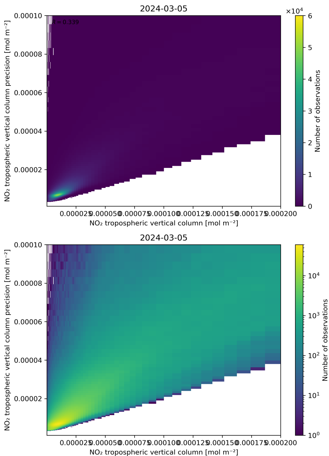
Figure 130: Scatter density plot of “NO 2 tropospheric vertical column” against “NO 2 tropospheric vertical column precision” for 2024-03-04 to 2024-03-06.
