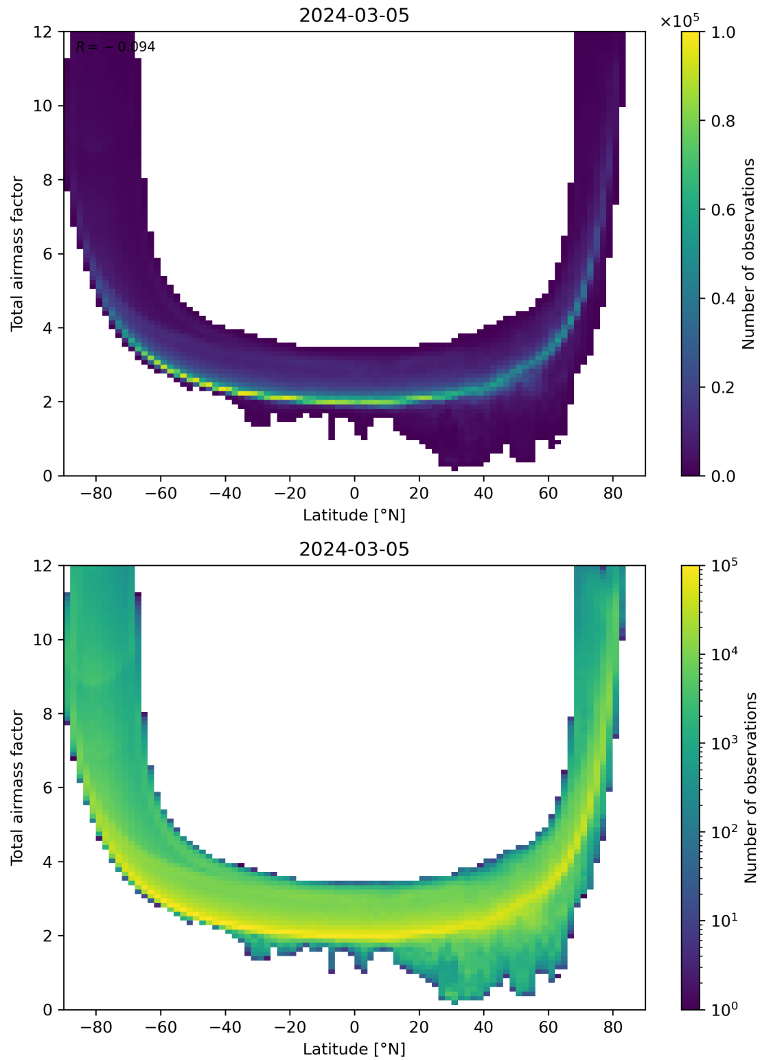
Figure 84: Scatter density plot of “Latitude” against “Total airmass factor” for 2024-03-04 to 2024-03-06.
