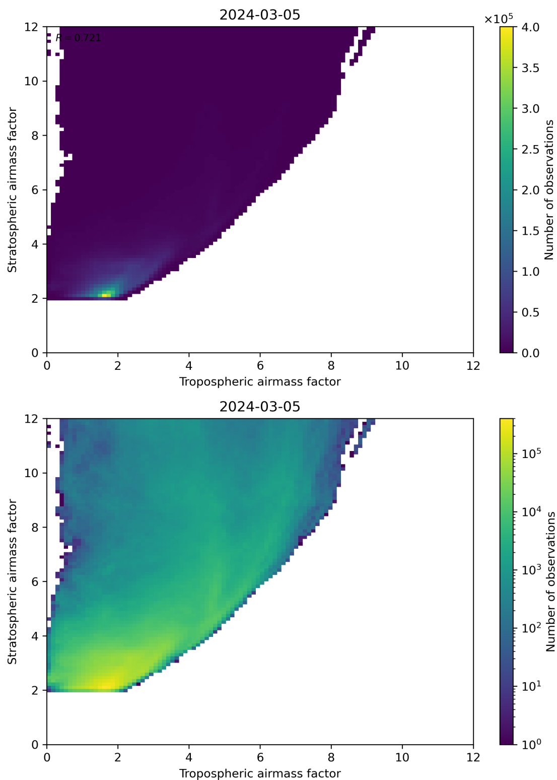
Figure 71: Scatter density plot of “Tropospheric airmass factor” against “Stratospheric airmass factor” for 2024-03-04 to 2024-03-06.
