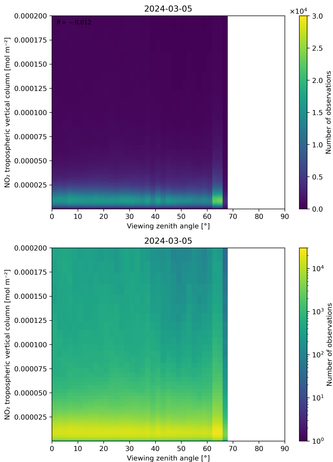
Figure 169: Scatter density plot of “Viewing zenith angle” against “NO 2 tropospheric vertical column” for 2024-03-04 to 2024-03-06.
