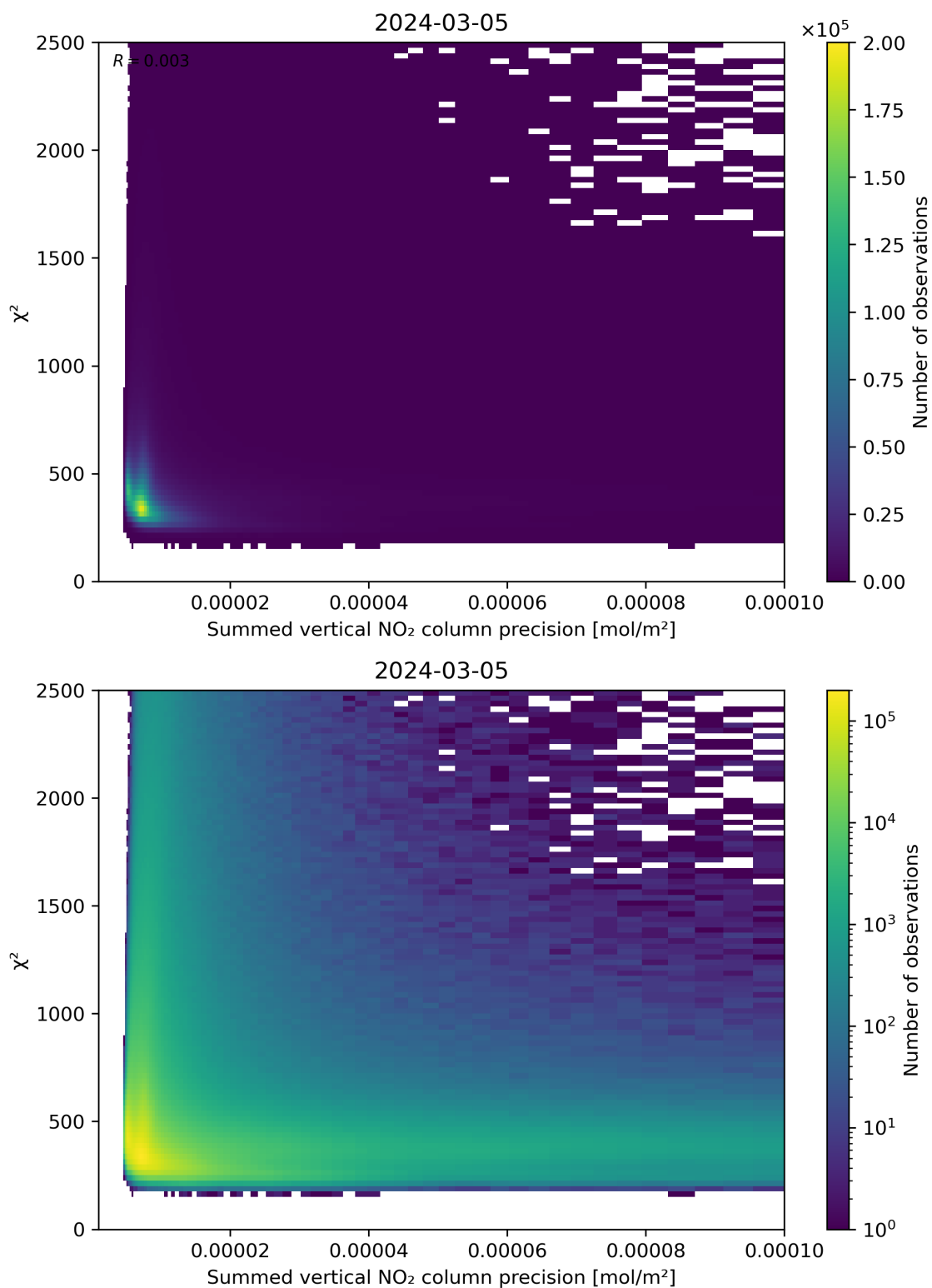
Figure 107: Scatter density plot of “Summed vertical NO 2 column precision” against “ \chi^2 ” for 2024-03-04 to 2024-03-06.
