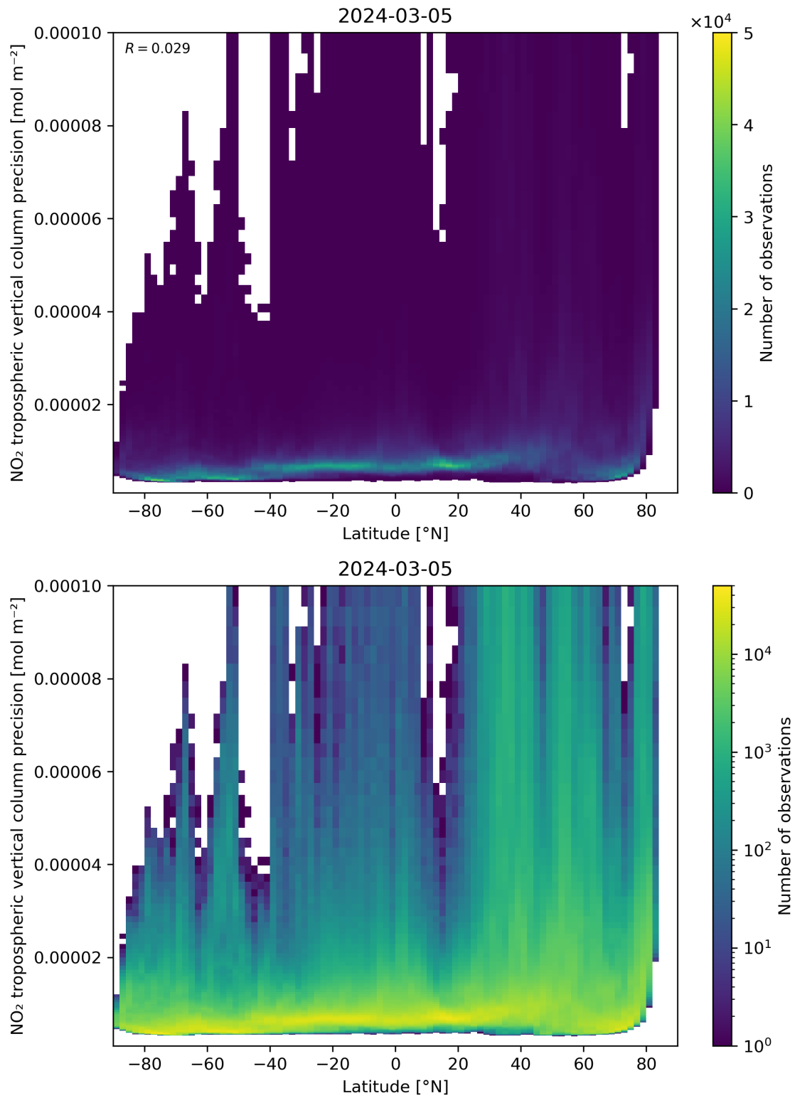
Figure 93: Scatter density plot of “Latitude” against “NO 2 tropospheric vertical column precision” for 2024-03-04 to 2024-03-06.
