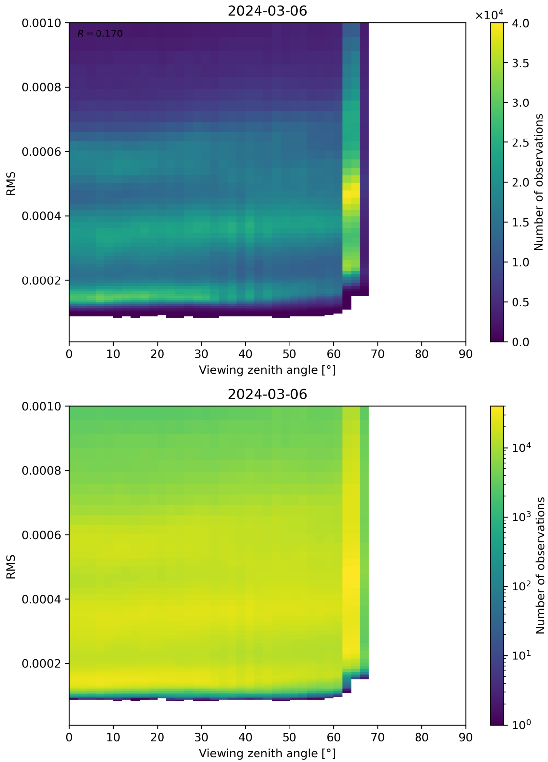
Figure 171: Scatter density plot of “Viewing zenith angle” against “RMS” for 2024-03-05 to 2024-03-07.
