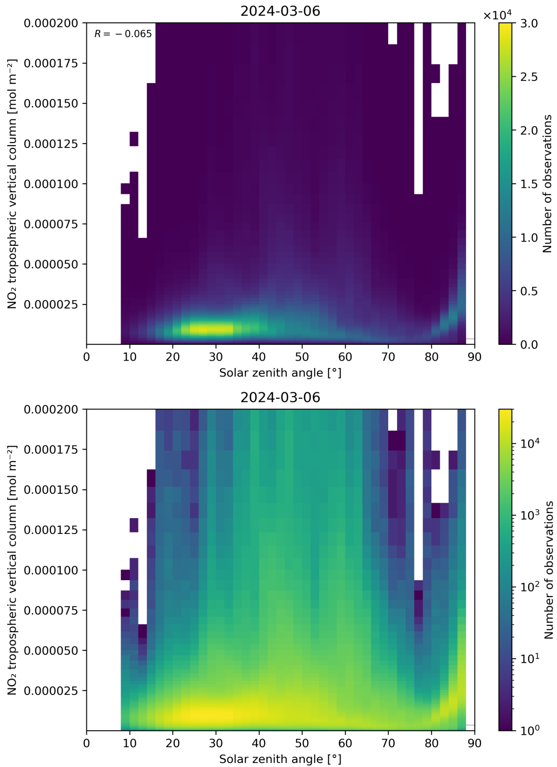
Figure 155: Scatter density plot of “Solar zenith angle” against “NO 2 tropospheric vertical column” for 2024-03-05 to 2024-03-07.
