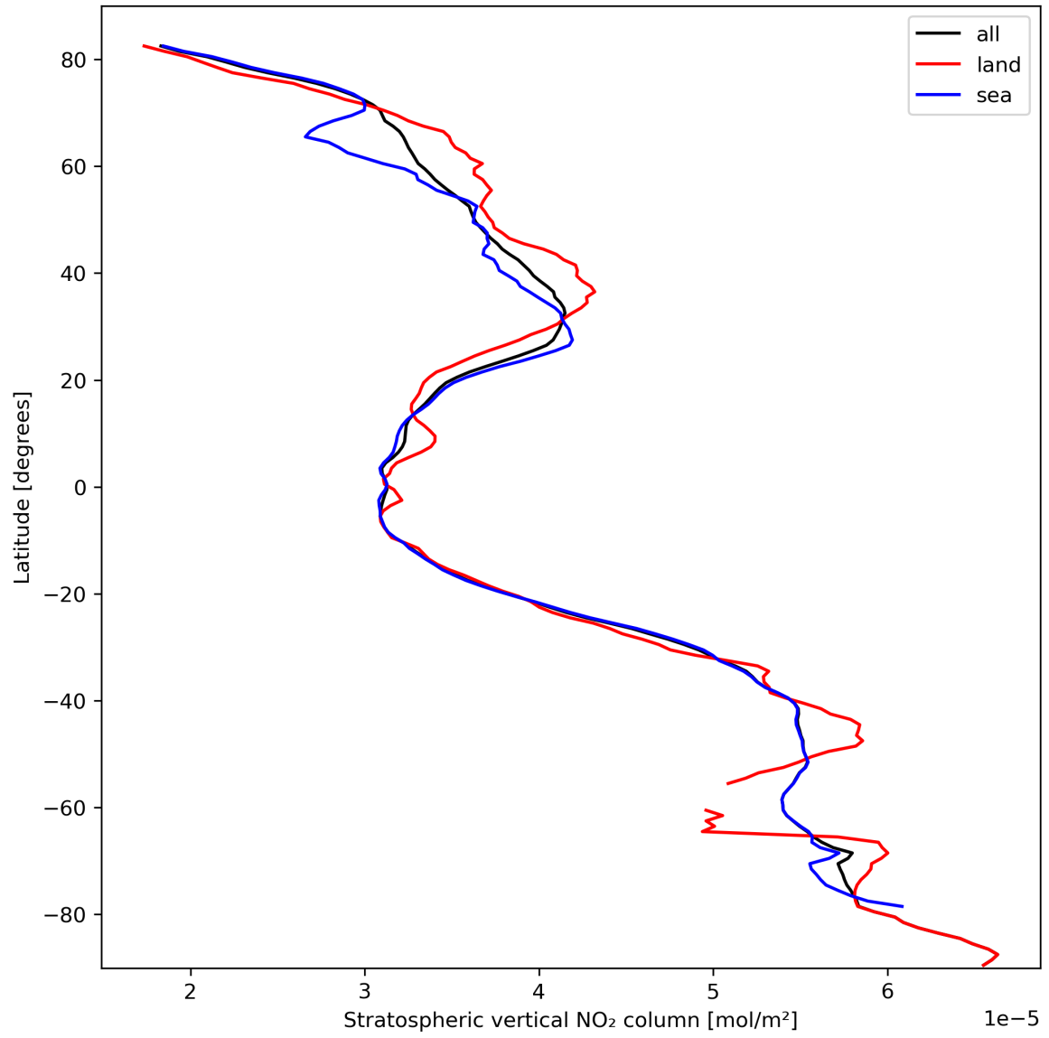
Figure 19: Zonal average of “Stratospheric vertical NO 2 column” for 2024-03-05 to 2024-03-07.
