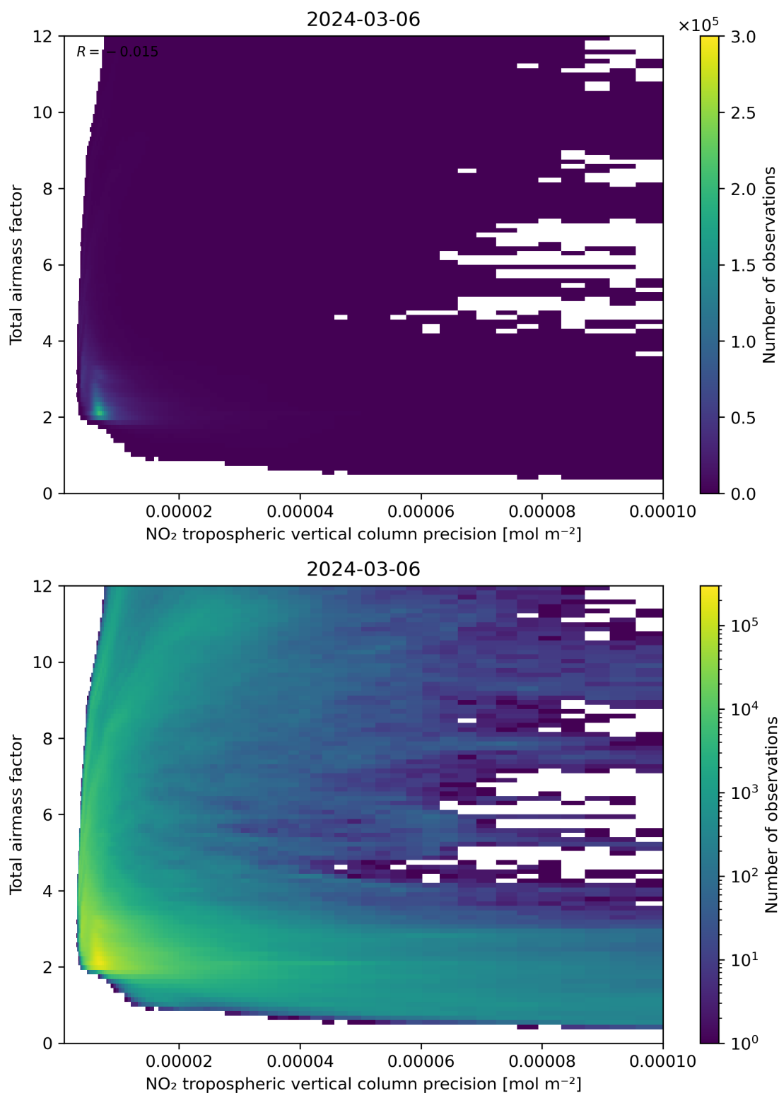
Figure 132: Scatter density plot of “NO 2 tropospheric vertical column precision” against “Total air mass factor” for 2024-03-05 to 2024-03-07.
