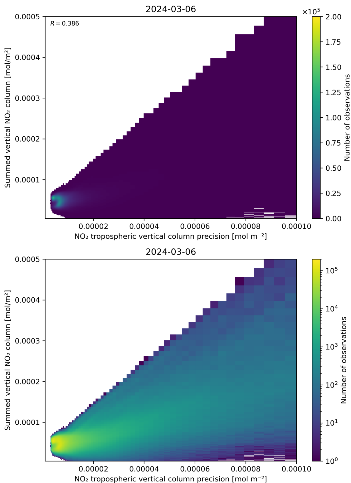
Figure 136: Scatter density plot of “NO 2 tropospheric vertical column precision” against “Summed vertical NO 2 column” for 2024-03-05 to 2024-03-07.
