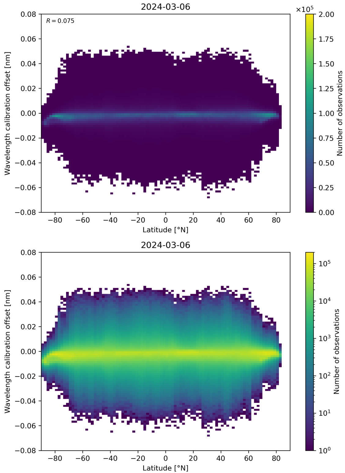
Figure 95: Scatter density plot of “Latitude” against “Wavelength calibration offset” for 2024-03-05 to 2024-03-07.
