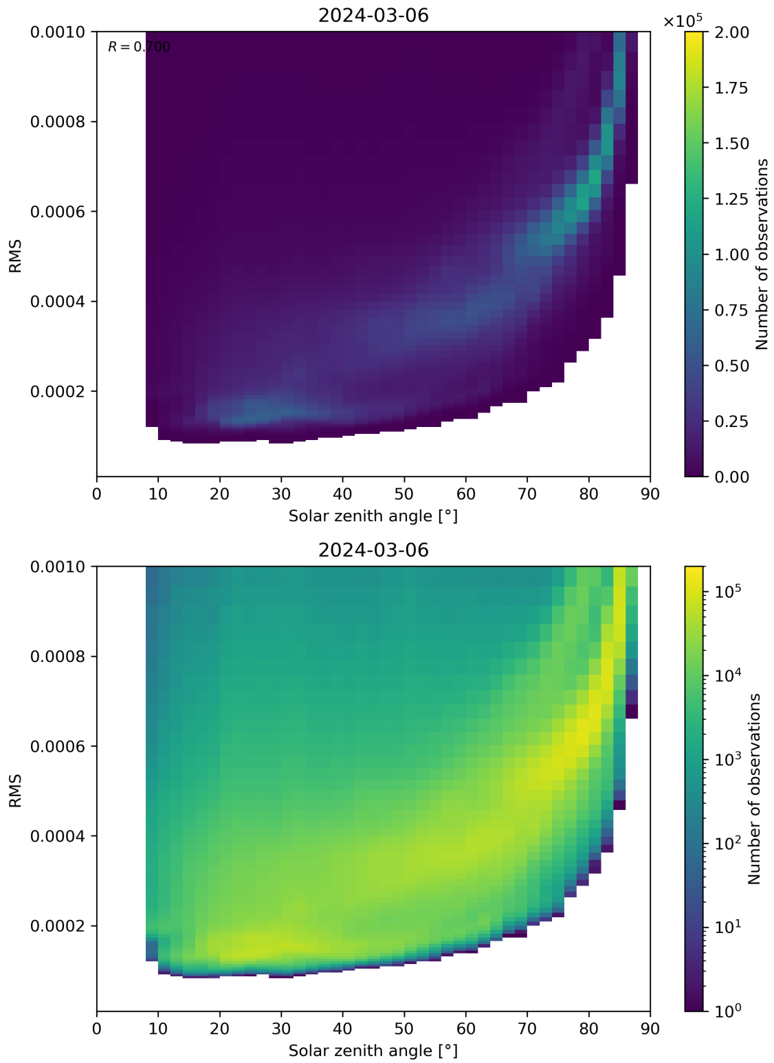
Figure 157: Scatter density plot of “Solar zenith angle” against “RMS” for 2024-03-05 to 2024-03-07.
