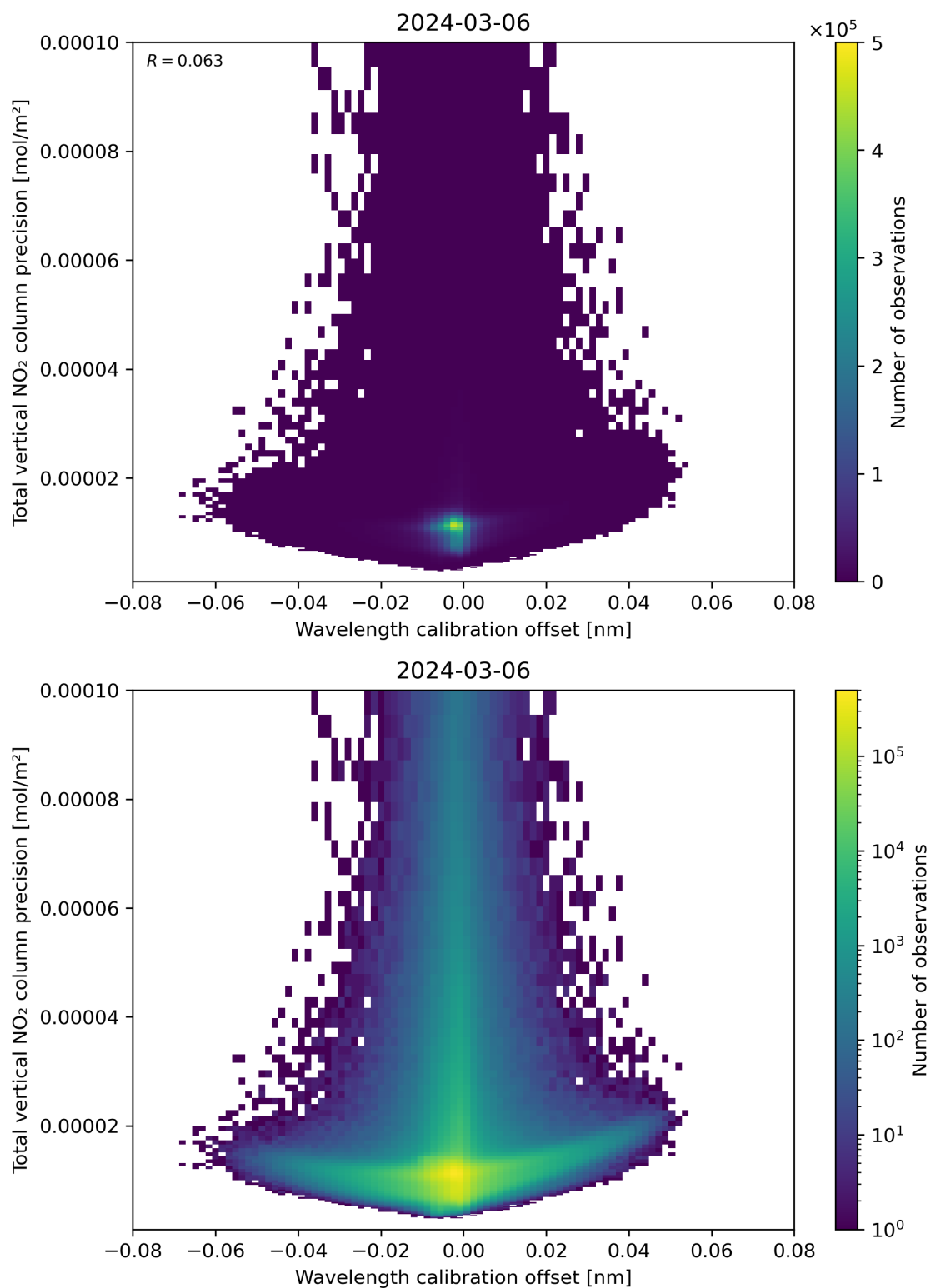
Figure 180: Scatter density plot of “Wavelength calibration offset” against “Total vertical NO 2 column precision” for 2024-03-05 to 2024-03-07.
