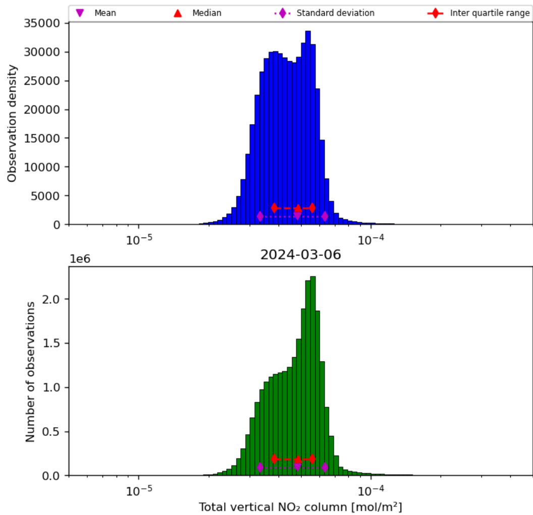
Figure 38: Histogram of “Total vertical NO 2 column” for 2024-03-05 to 2024-03-07
