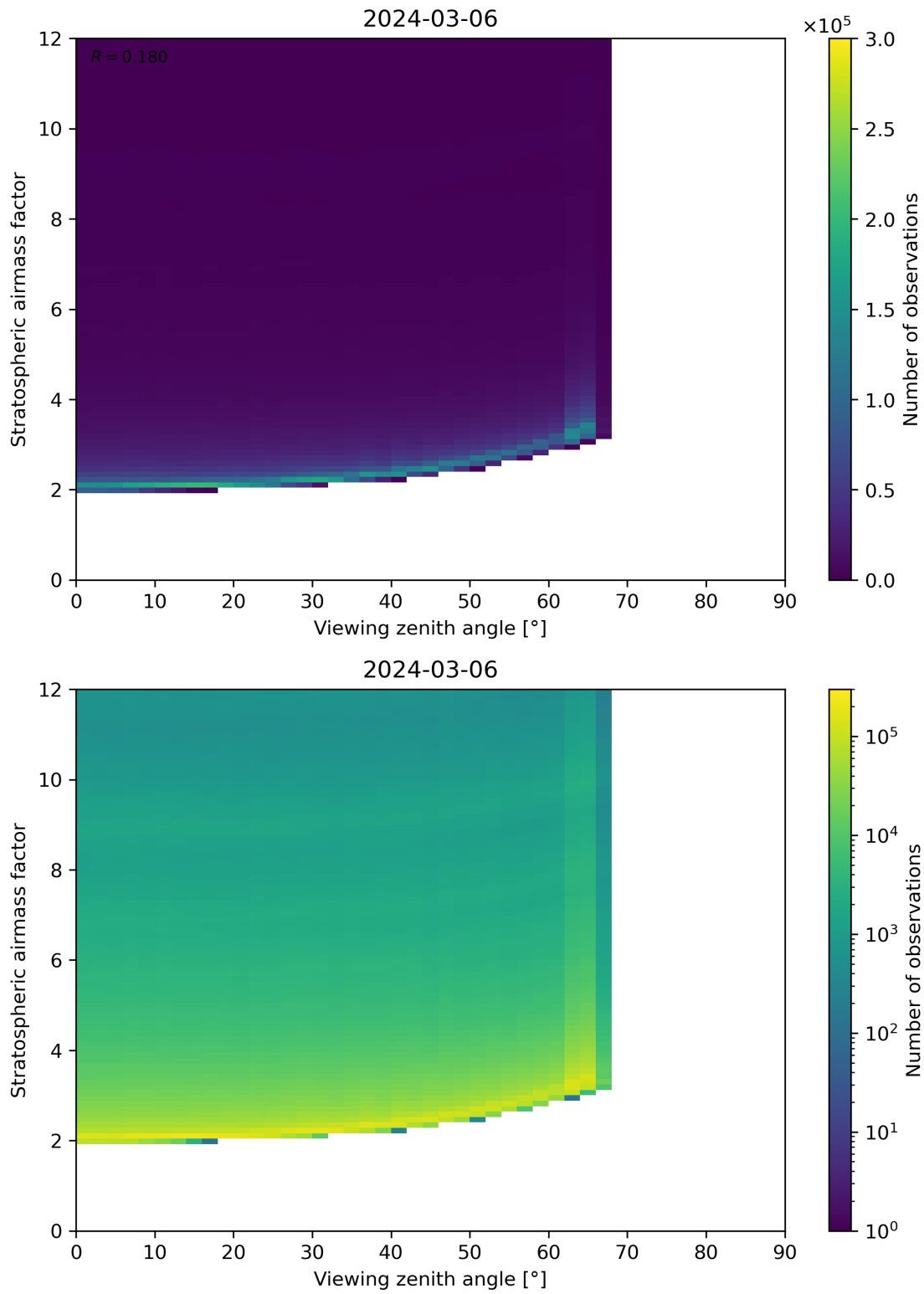
Figure 159: Scatter density plot of “Viewing zenith angle” against “Stratospheric airmass factor” for 2024-03-05 to 2024-03-07.
