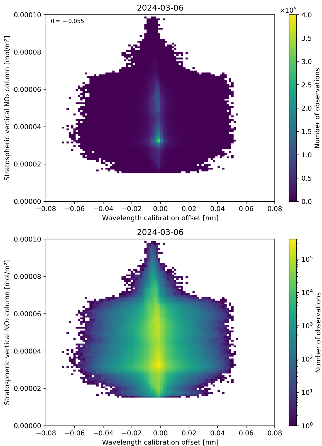
Figure 176: Scatter density plot of “Wavelength calibration offset” against “Stratospheric vertical NO 2 column” for 2024-03-05 to 2024-03-07.
