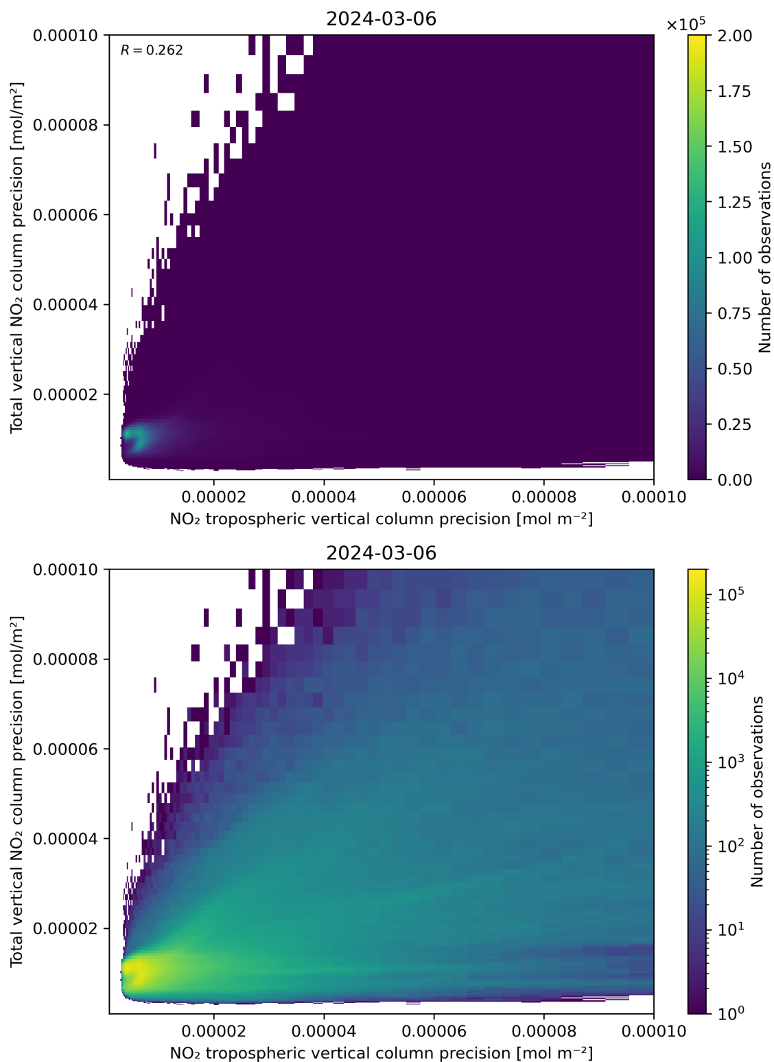
Figure 139: Scatter density plot of “NO 2 tropospheric vertical column precision” against “Total vertical NO 2 column precision” for 2024-03-05 to 2024-03-07.
