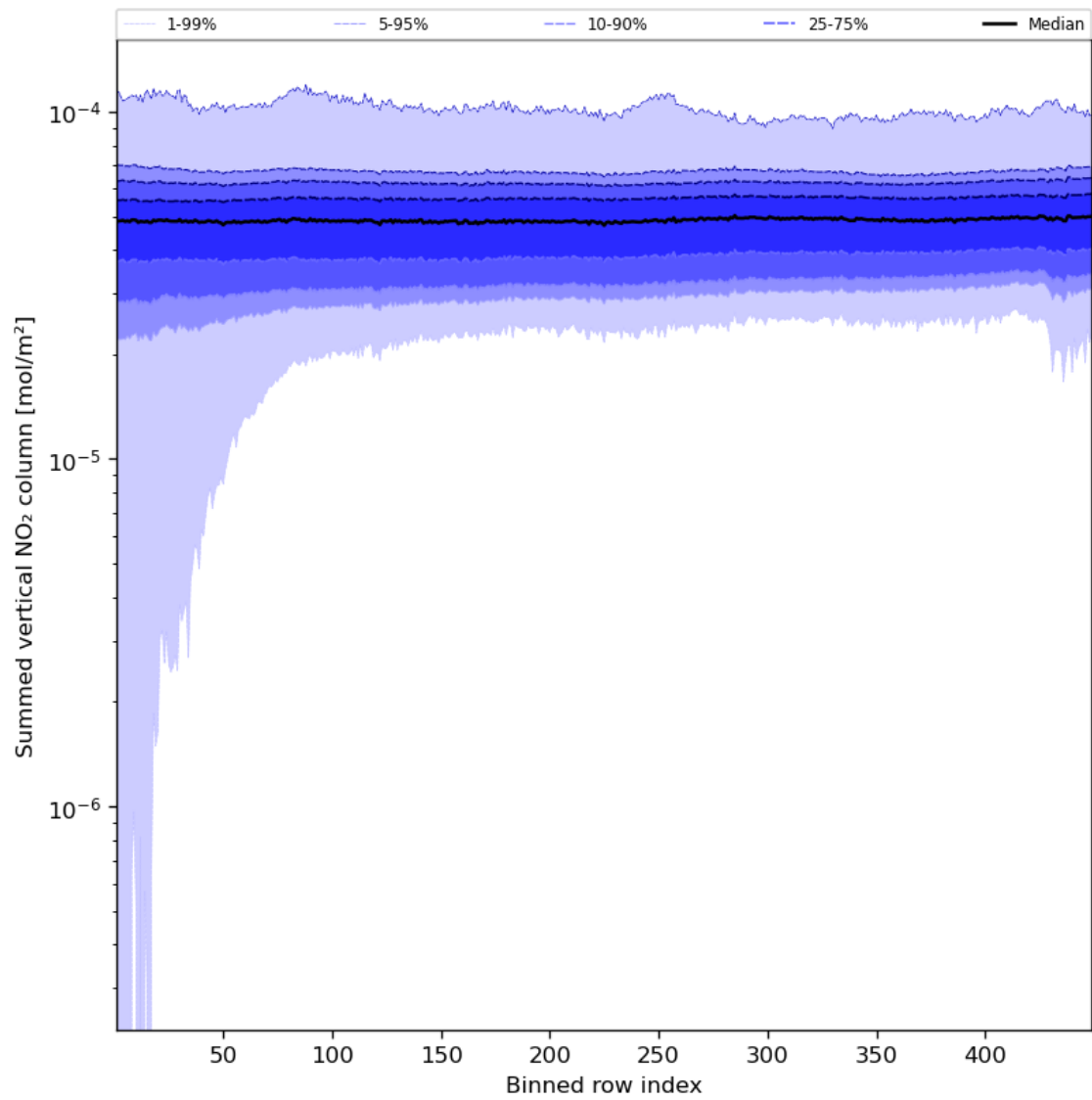
Figure 57: Along track statistics of “Summed vertical NO 2 column” for 2024-03-05 to 2024-03-07
