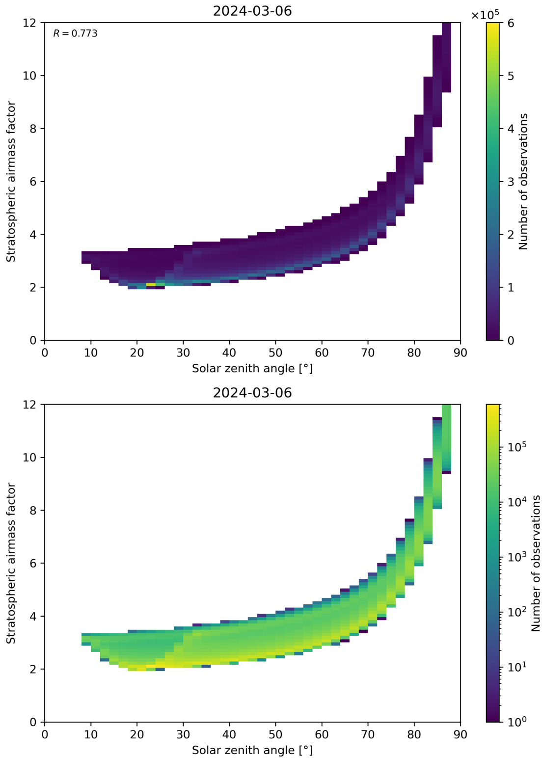
Figure 145: Scatter density plot of “Solar zenith angle” against “Stratospheric airmass factor” for 2024-03-05 to 2024-03-07.
