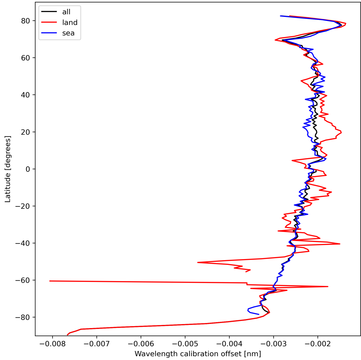
Figure 18: Zonal average of “Wavelength calibration offset” for 2024-03-05 to 2024-03-07.
