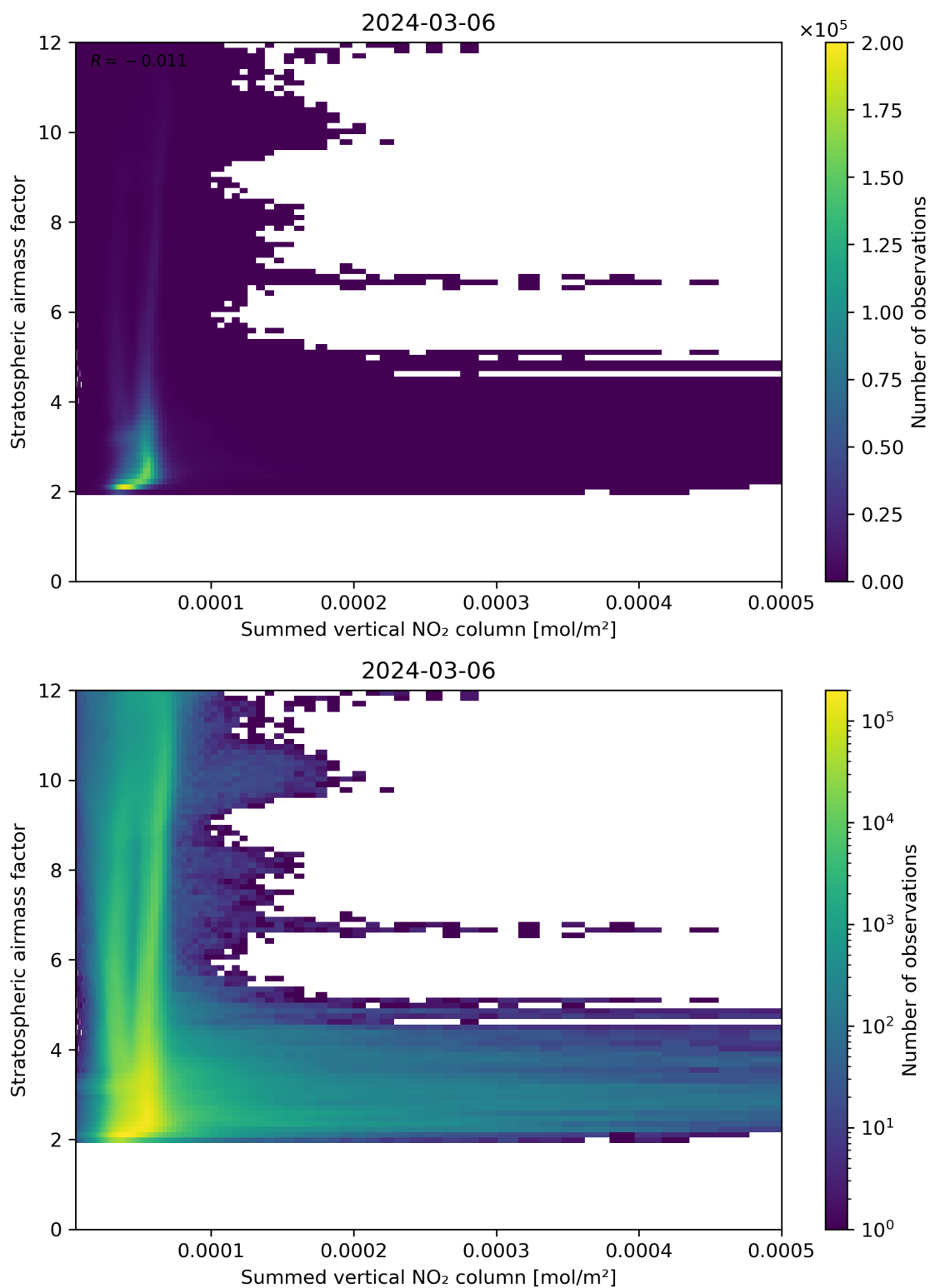
Figure 103: Scatter density plot of “Summed vertical NO 2 column” against “Stratospheric air mass factor” for 2024-03-05 to 2024-03-07.
