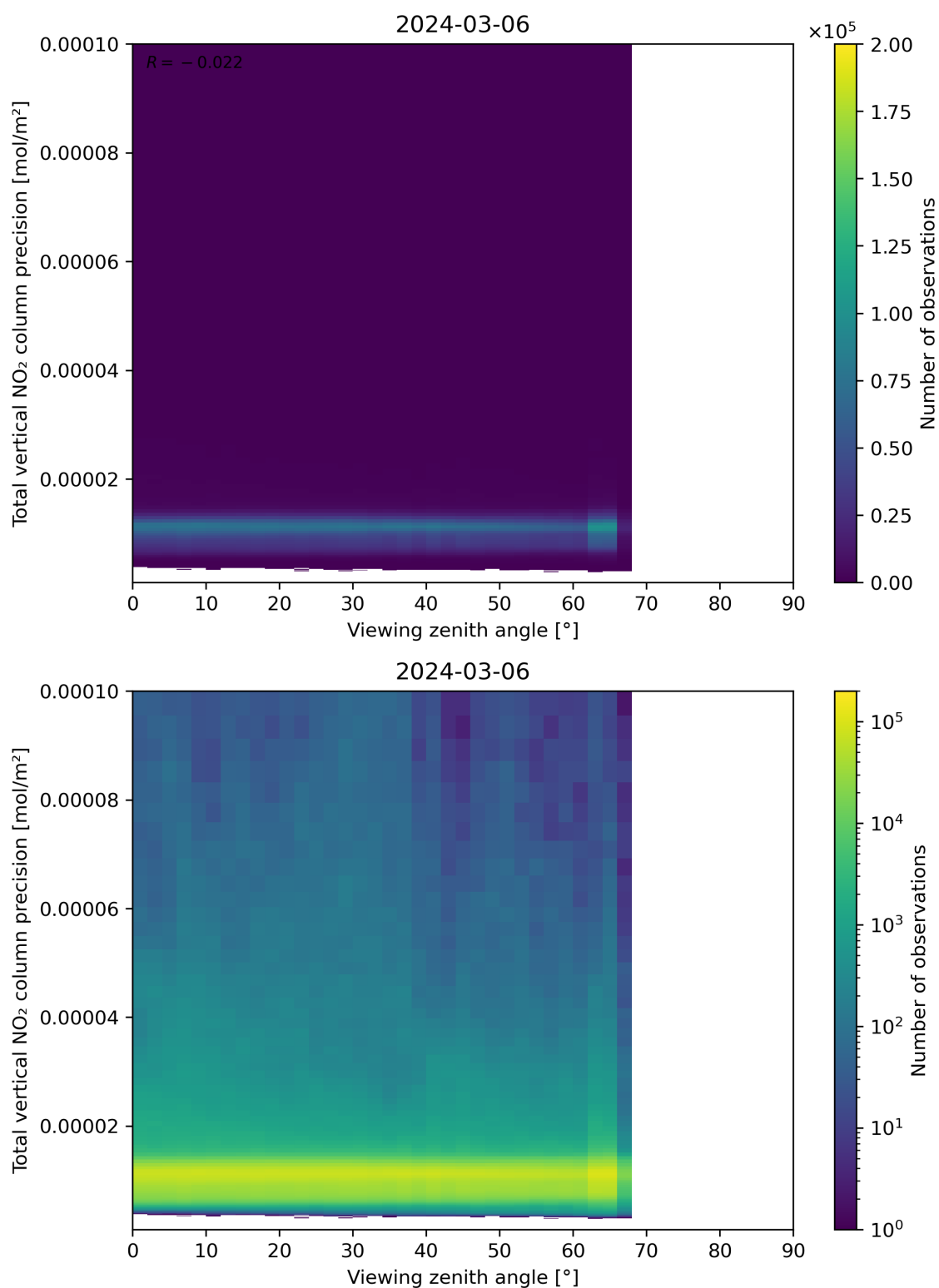
Figure 168: Scatter density plot of “Viewing zenith angle” against “Total vertical NO 2 column precision” for 2024-03-05 to 2024-03-07.
