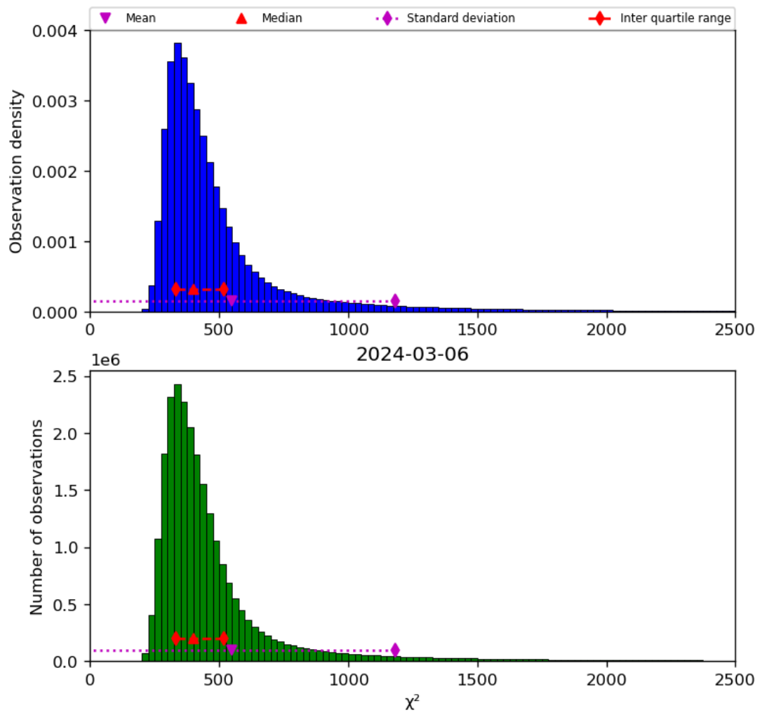
Figure 42: Histogram of “ \chi^2 ” for 2024-03-05 to 2024-03-07
