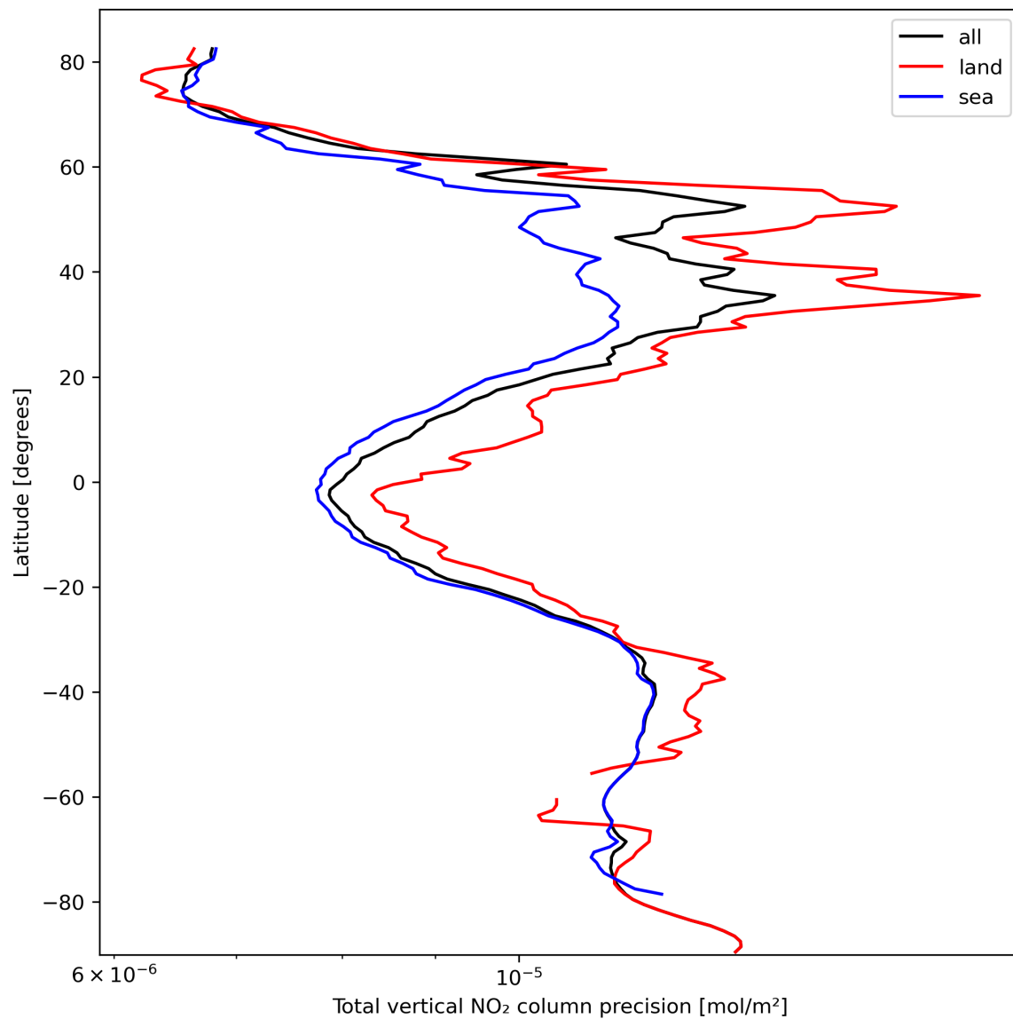
Figure 22: Zonal average of “Total vertical NO 2 column precision” for 2024-03-05 to 2024-03-07.
