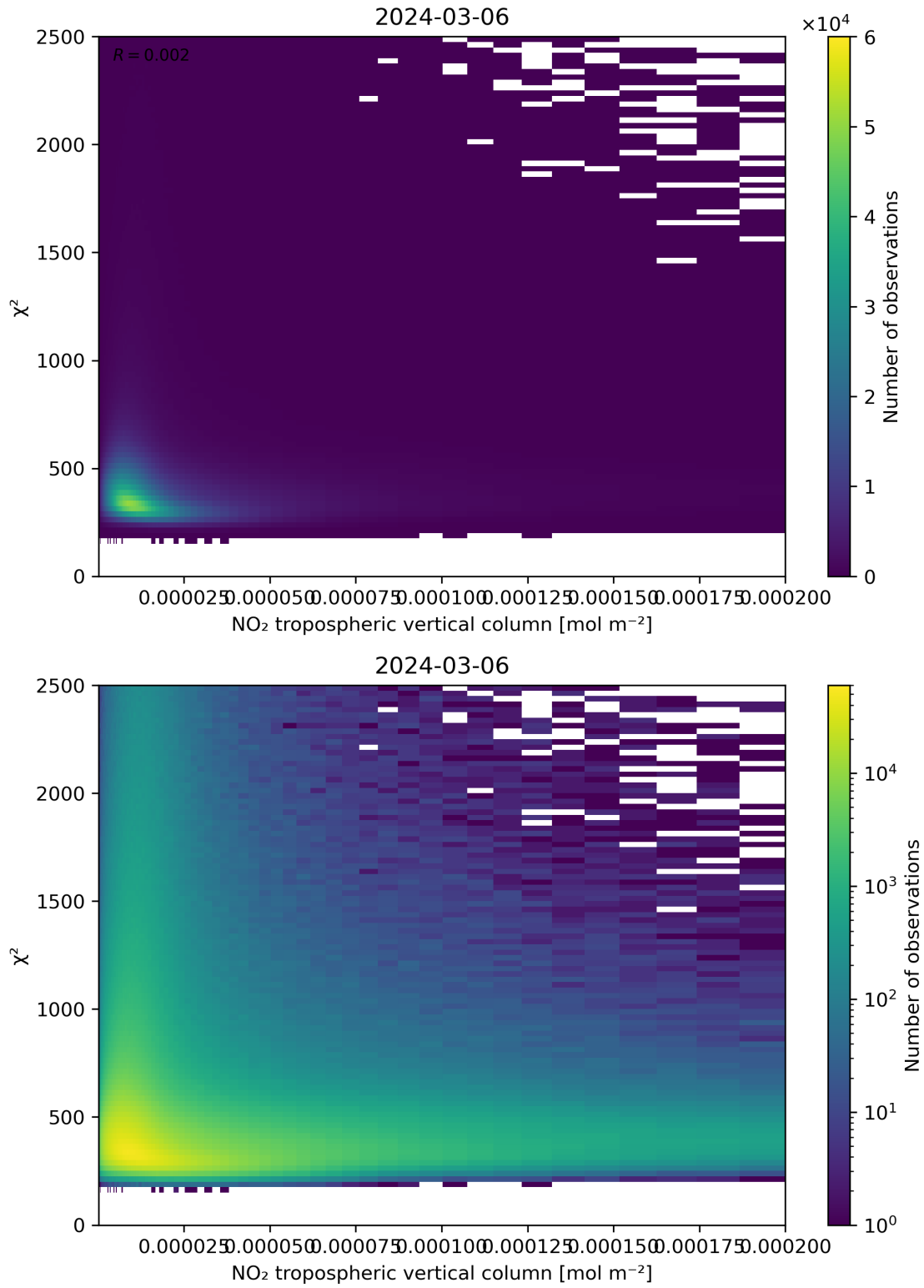
Figure 124: Scatter density plot of “NO 2 tropospheric vertical column” against “ \chi^2 ” for 2024-03-05 to 2024-03-07.
