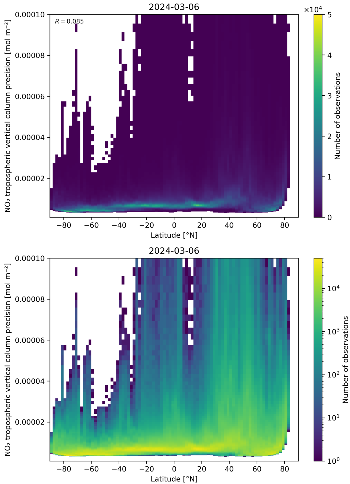
Figure 93: Scatter density plot of “Latitude” against “NO 2 tropospheric vertical column precision” for 2024-03-05 to 2024-03-07.
