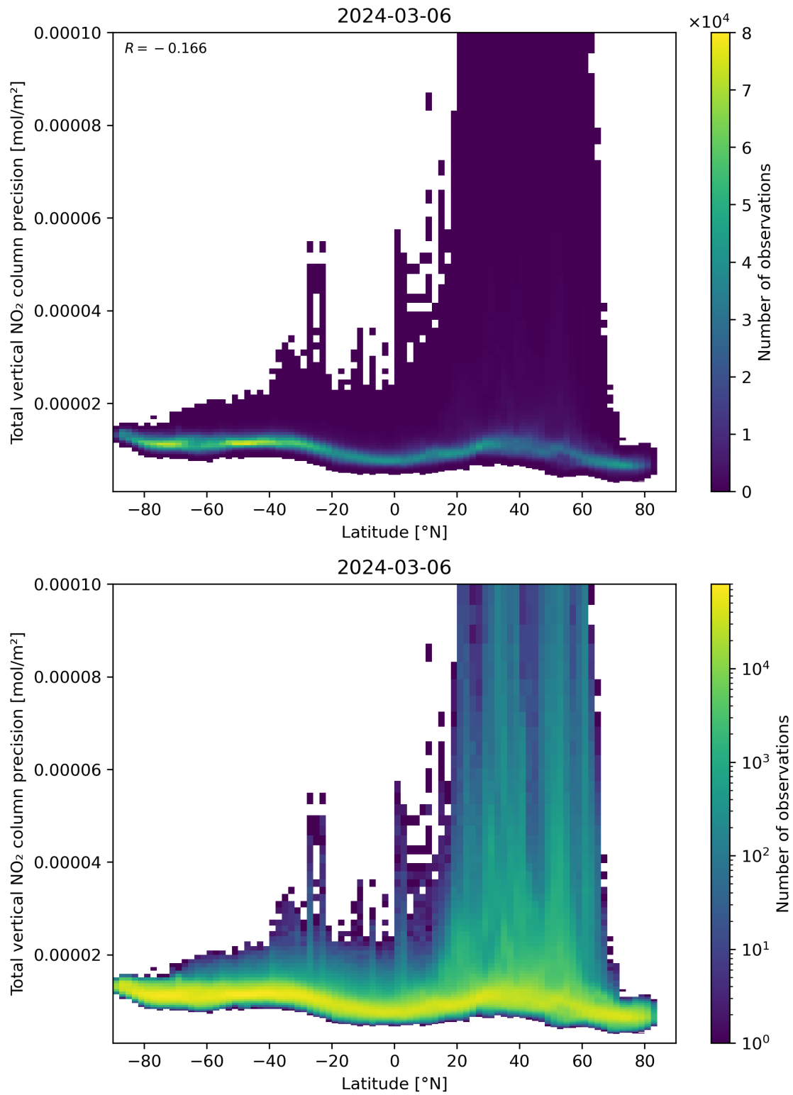
Figure 91: Scatter density plot of “Latitude” against “Total vertical NO 2 column precision” for 2024-03-05 to 2024-03-07.
