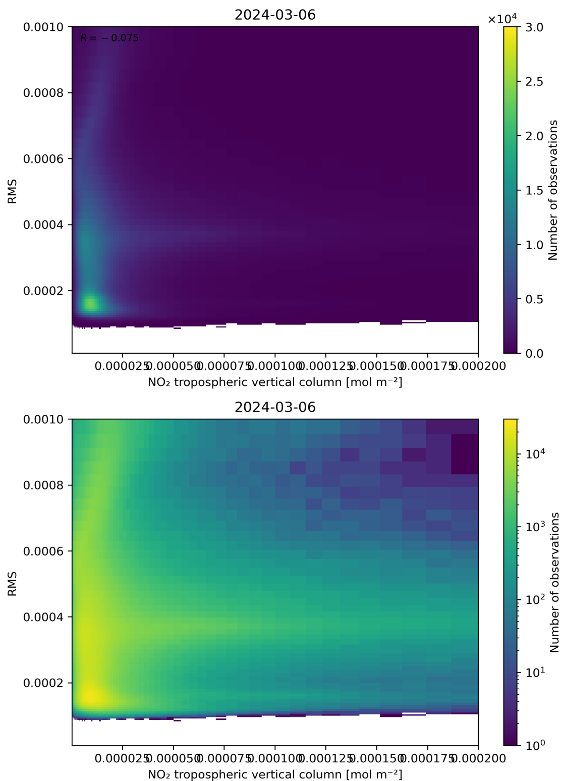
Figure 142: Scatter density plot of “NO 2 tropospheric vertical column” against “RMS” for 2024-03-05 to 2024-03-07.
