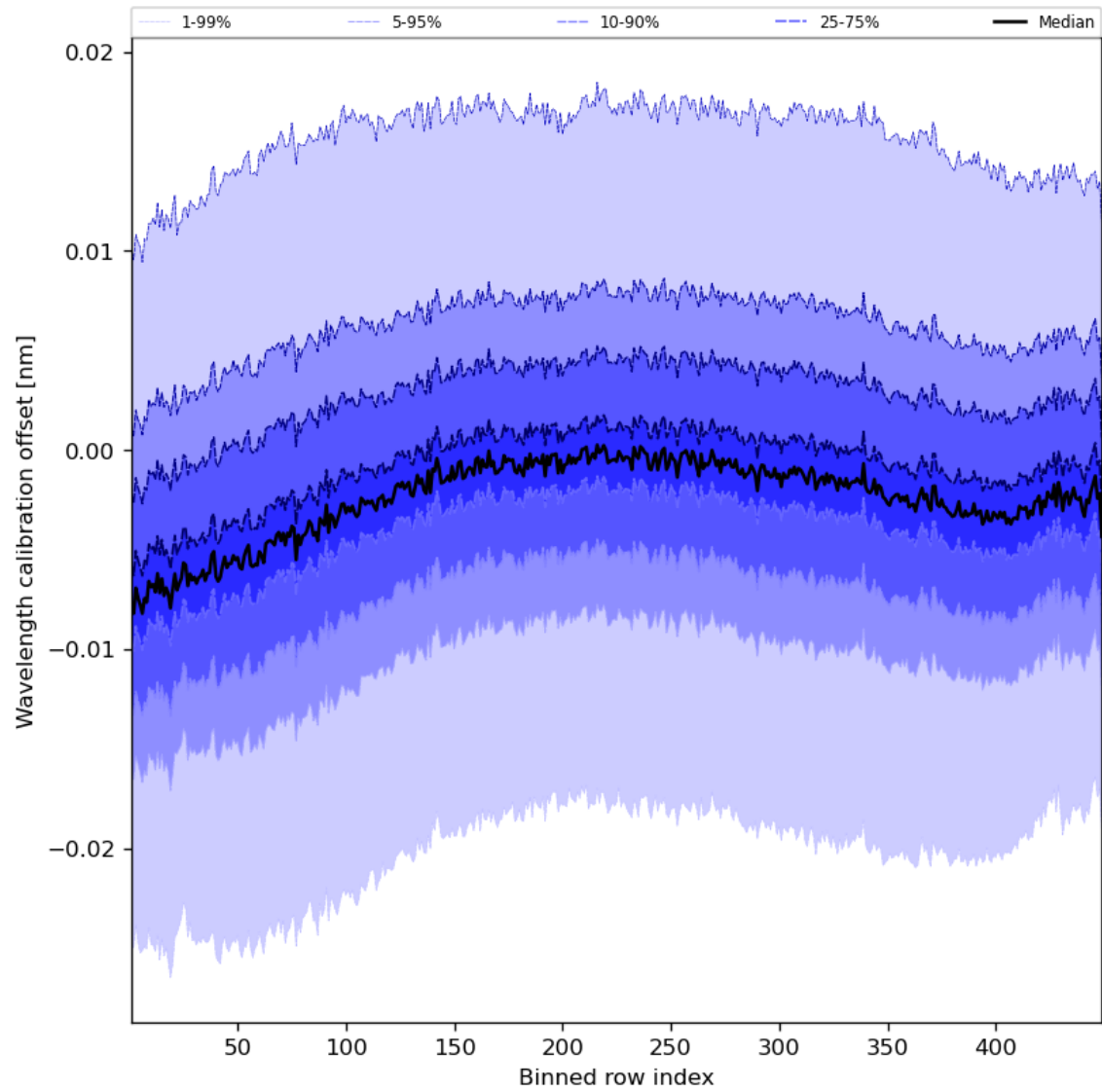
Figure 52: Along track statistics of “Wavelength calibration offset” for 2024-03-05 to 2024-03-07
