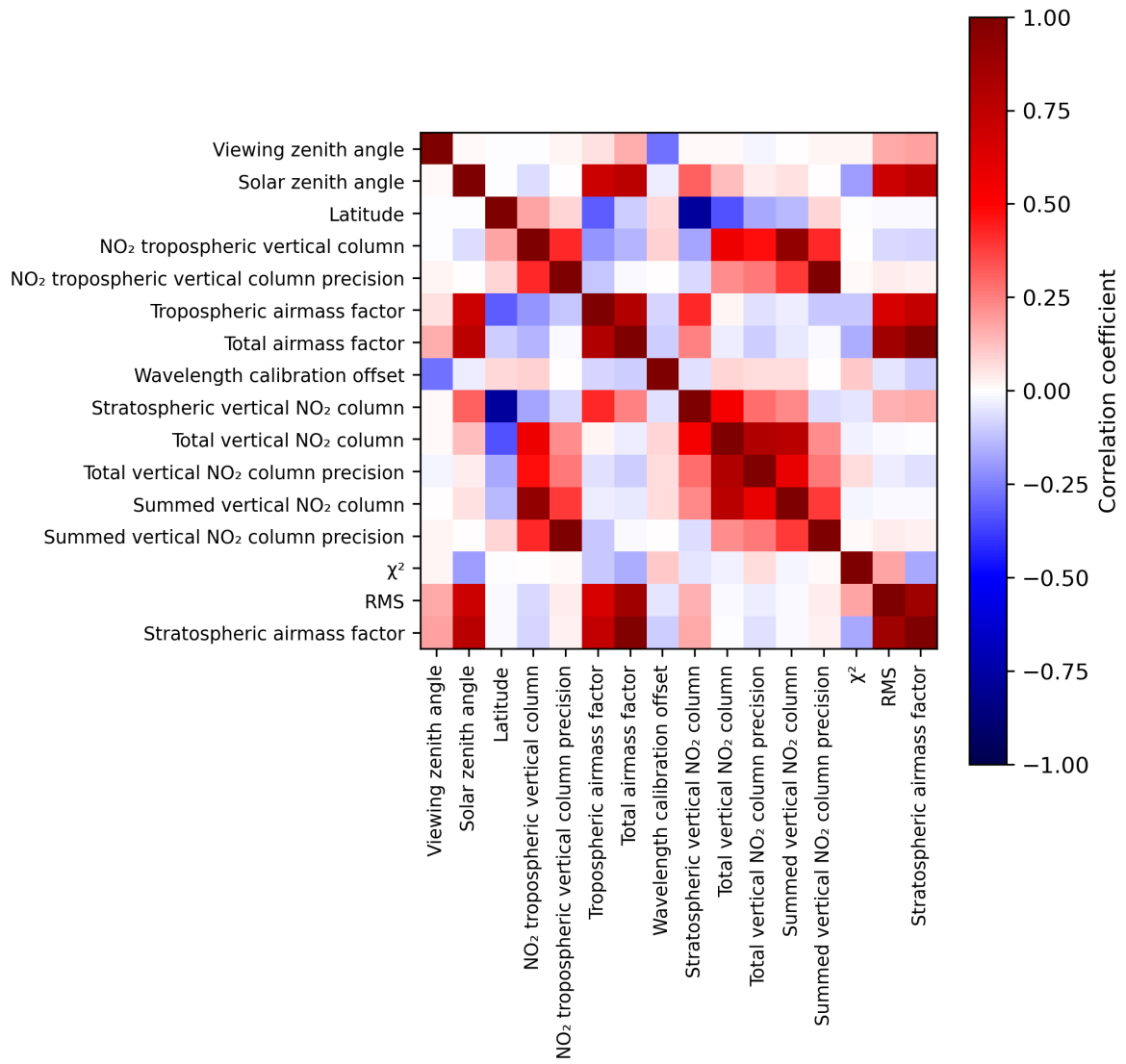
Figure 2: Map of correlation matrix for 2024-03-05 to 2024-03-07.
