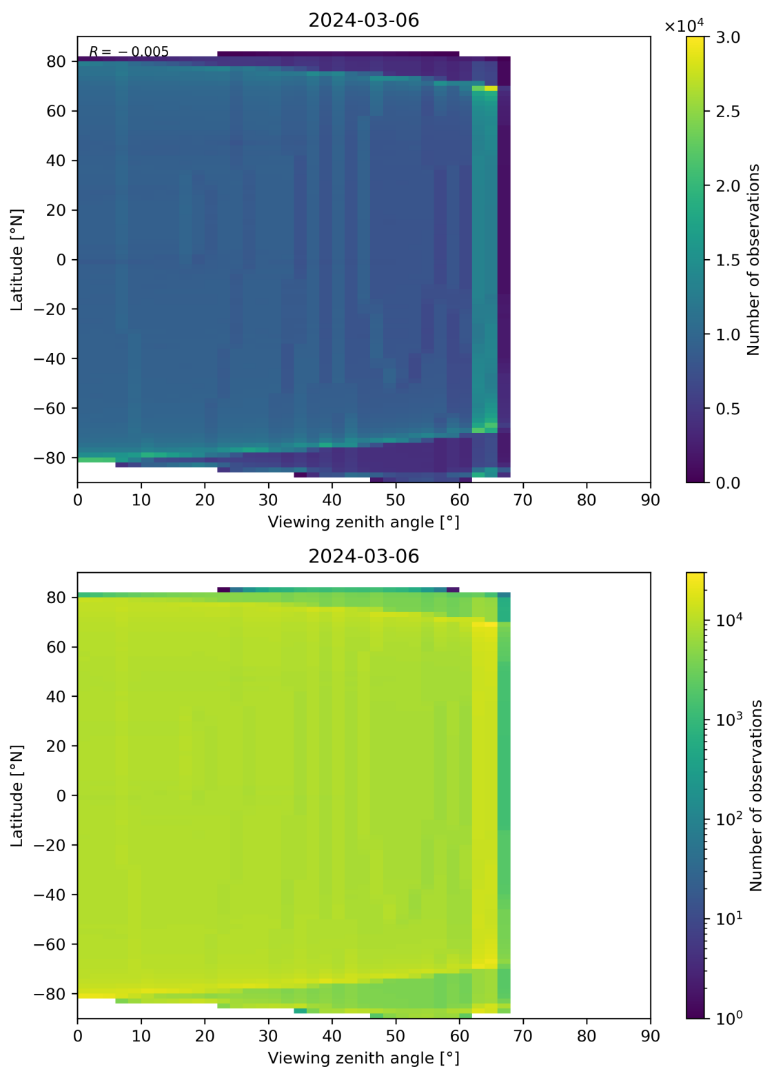
Figure 163: Scatter density plot of “Viewing zenith angle” against “Latitude” for 2024-03-05 to 2024-03-07.
