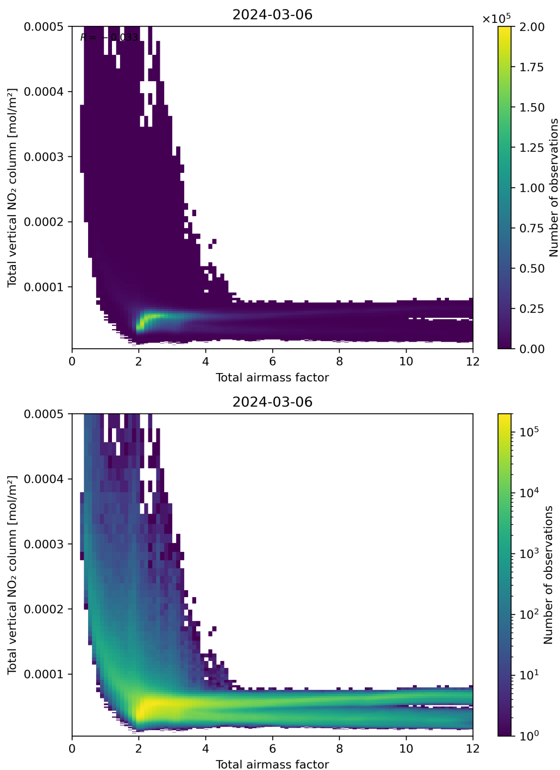
Figure 67: Scatter density plot of “Total airmass factor” against “Total vertical NO 2 column” for 2024-03-05 to 2024-03-07.
