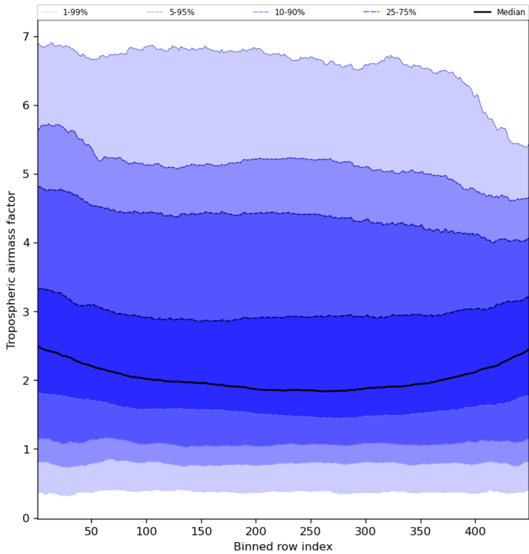
Figure 48: Along track statistics of “Tropospheric air mass factor” for 2024-03-05 to 2024-03-07
