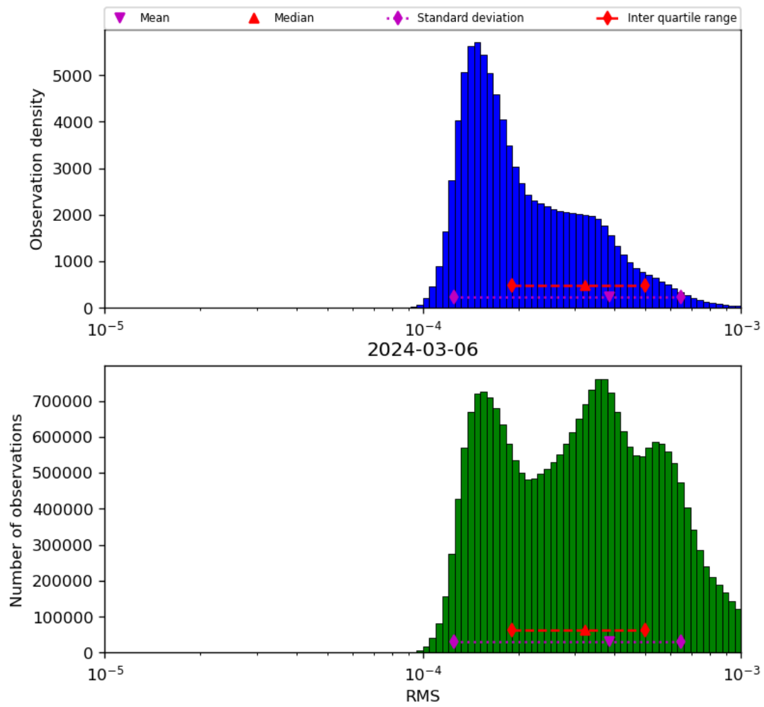
Figure 43: Histogram of “RMS” for 2024-03-05 to 2024-03-07
