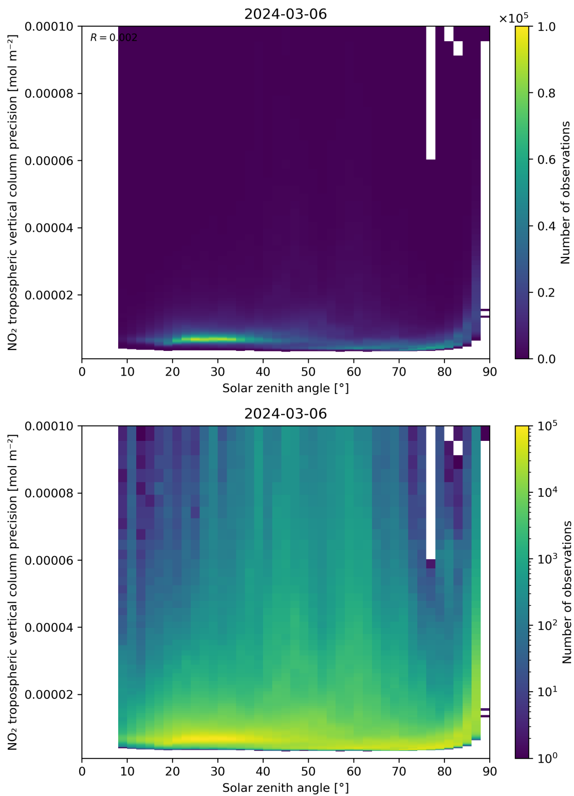
Figure 156: Scatter density plot of “Solar zenith angle” against “NO 2 tropospheric vertical column precision” for 2024-03-05 to 2024-03-07.
