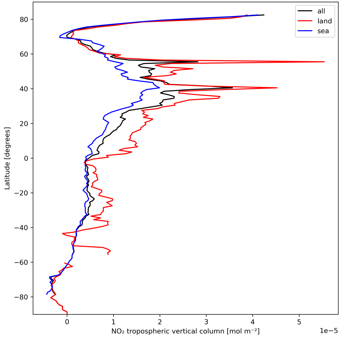
Figure 12: Zonal average of “NO 2 tropospheric vertical column” for 2024-03-05 to 2024-03-07.
