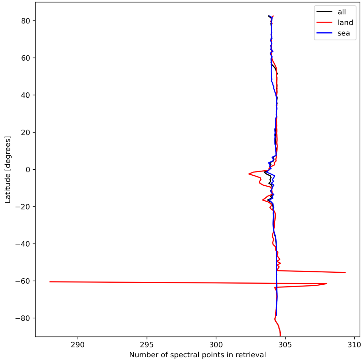
Figure 16: Zonal average of “Number of spectral points in retrieval” for 2024-03-05 to 2024-03-07.
