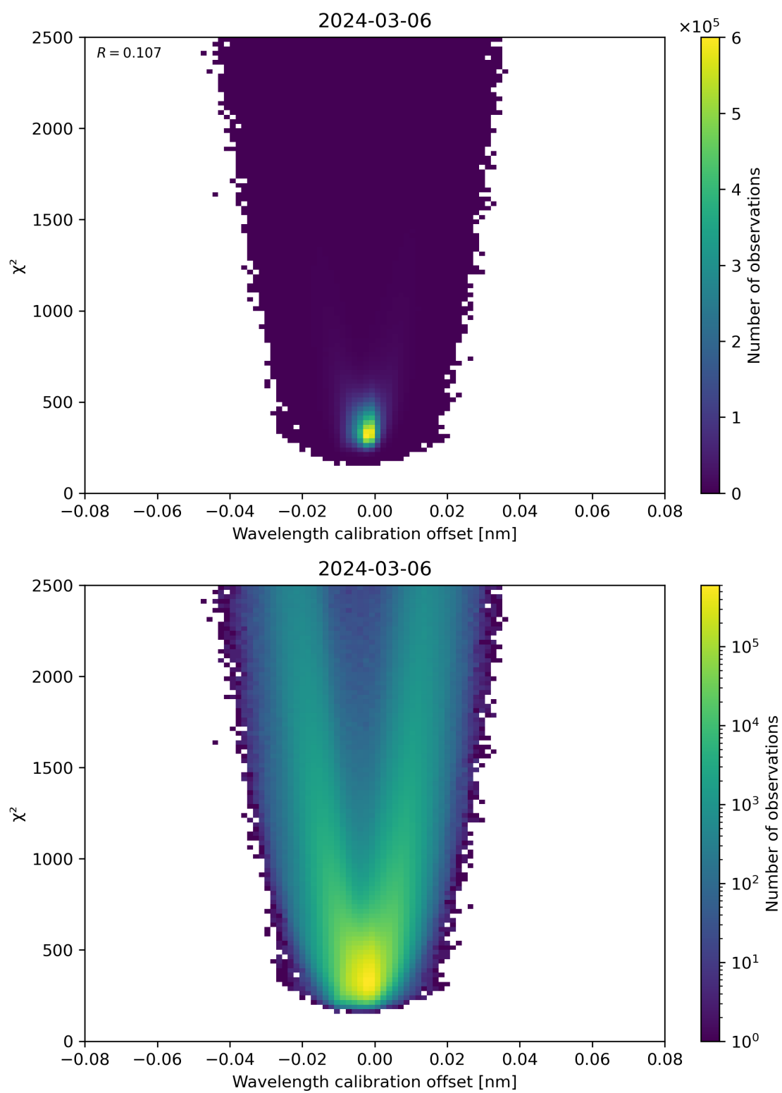
Figure 175: Scatter density plot of “Wavelength calibration offset” against “ \chi^2 ” for 2024-03-05 to 2024-03-07.
