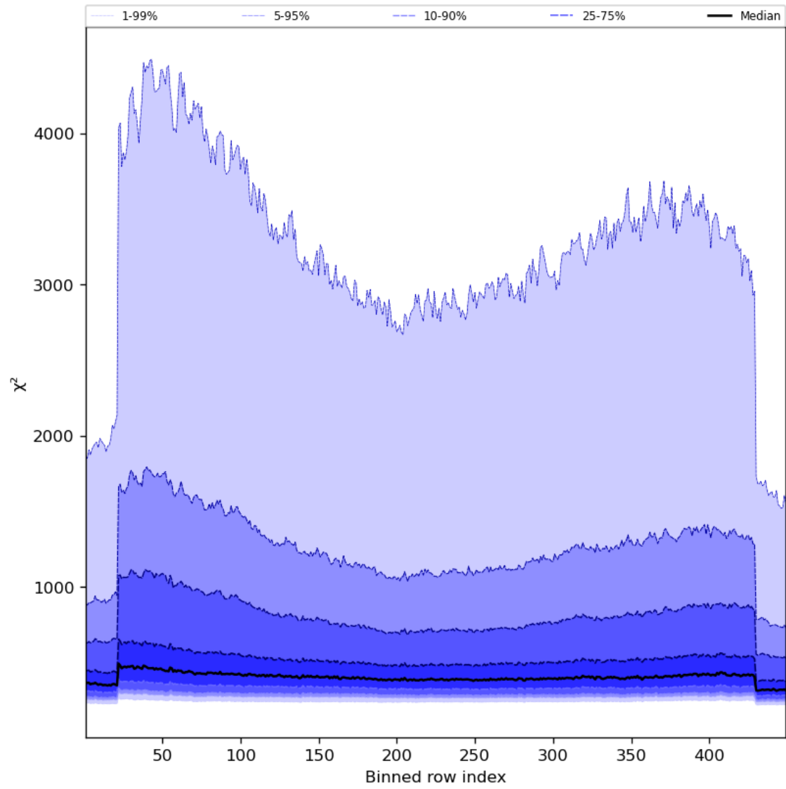
Figure 59: Along track statistics of “ \chi^2 ” for 2024-03-05 to 2024-03-07
