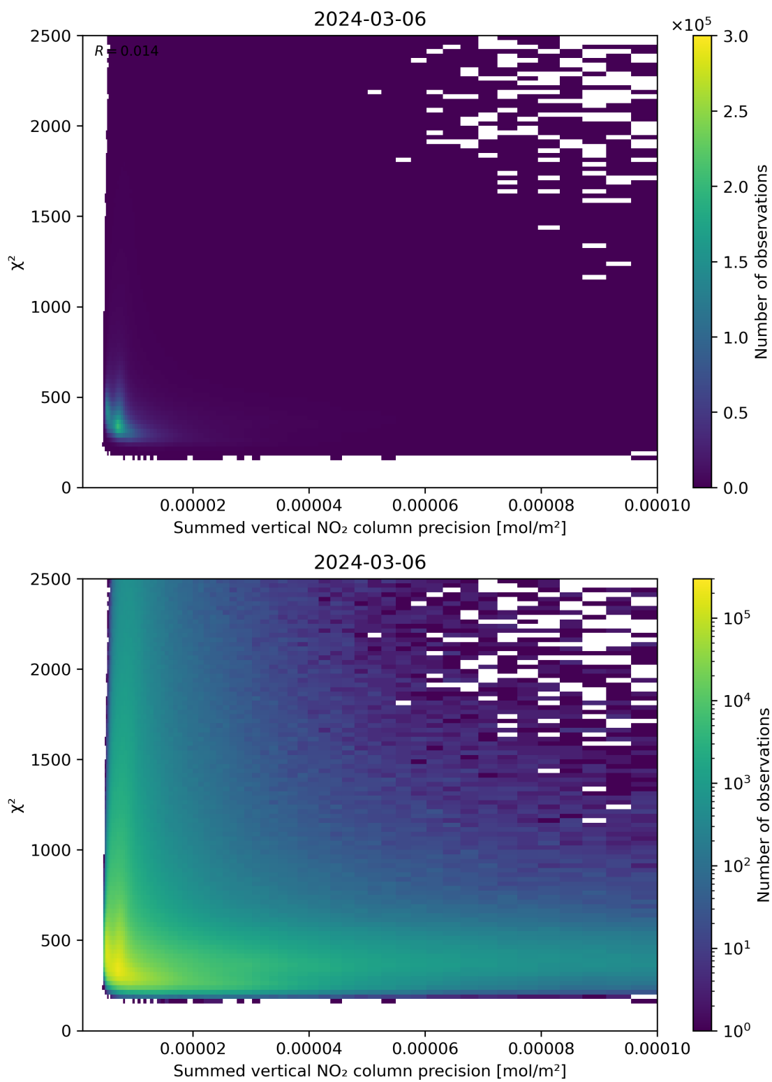
Figure 107: Scatter density plot of “Summed vertical NO 2 column precision” against “ \chi^2 ” for 2024-03-05 to 2024-03-07.
