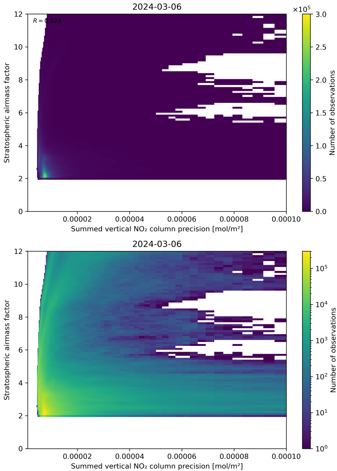
Figure 106: Scatter density plot of “Summed vertical NO 2 column precision” against “Stratospheric airmass factor” for 2024-03-05 to 2024-03-07.
