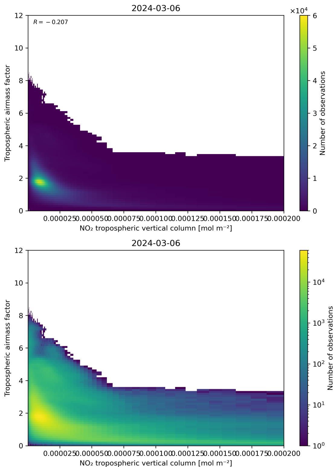
Figure 123: Scatter density plot of “NO 2 tropospheric vertical column” against “Tropospheric airmass factor” for 2024-03-05 to 2024-03-07.
