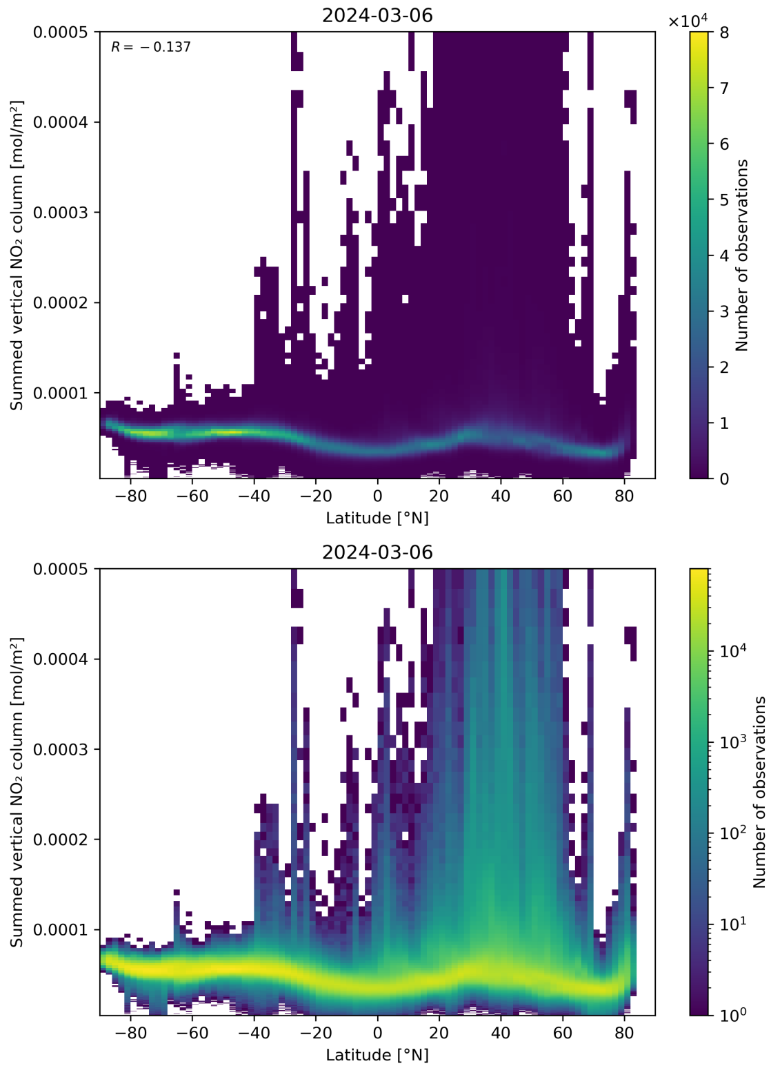
Figure 88: Scatter density plot of “Latitude” against “Summed vertical NO 2 column” for 2024-03-05 to 2024-03-07.
