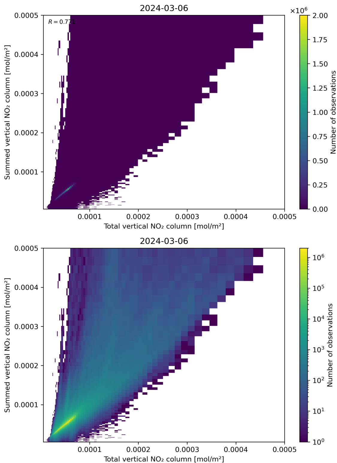
Figure 112: Scatter density plot of “Total vertical NO 2 column” against “Summed vertical NO 2 column” for 2024-03-05 to 2024-03-07.
