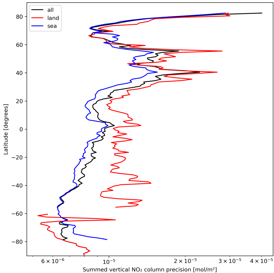
Figure 24: Zonal average of “Summed vertical NO 2 column precision” for 2024-03-05 to 2024-03-07.
