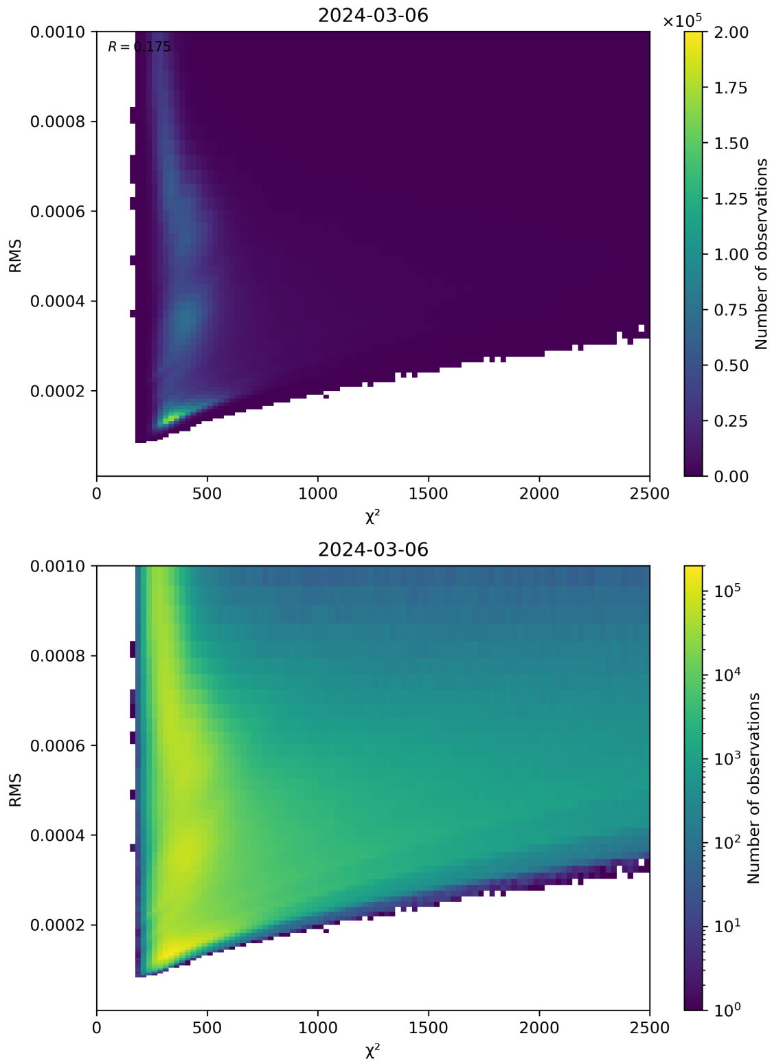
Figure 82: Scatter density plot of “ \chi^2 ” against “RMS” for 2024-03-05 to 2024-03-07.
