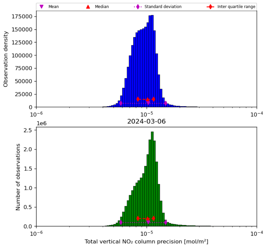
Figure 39: Histogram of “Total vertical NO 2 column precision” for 2024-03-05 to 2024-03-07
