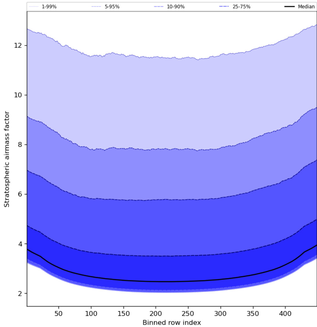
Figure 61: Along track statistics of “Stratospheric airmass factor” for 2024-03-05 to 2024-03-07
