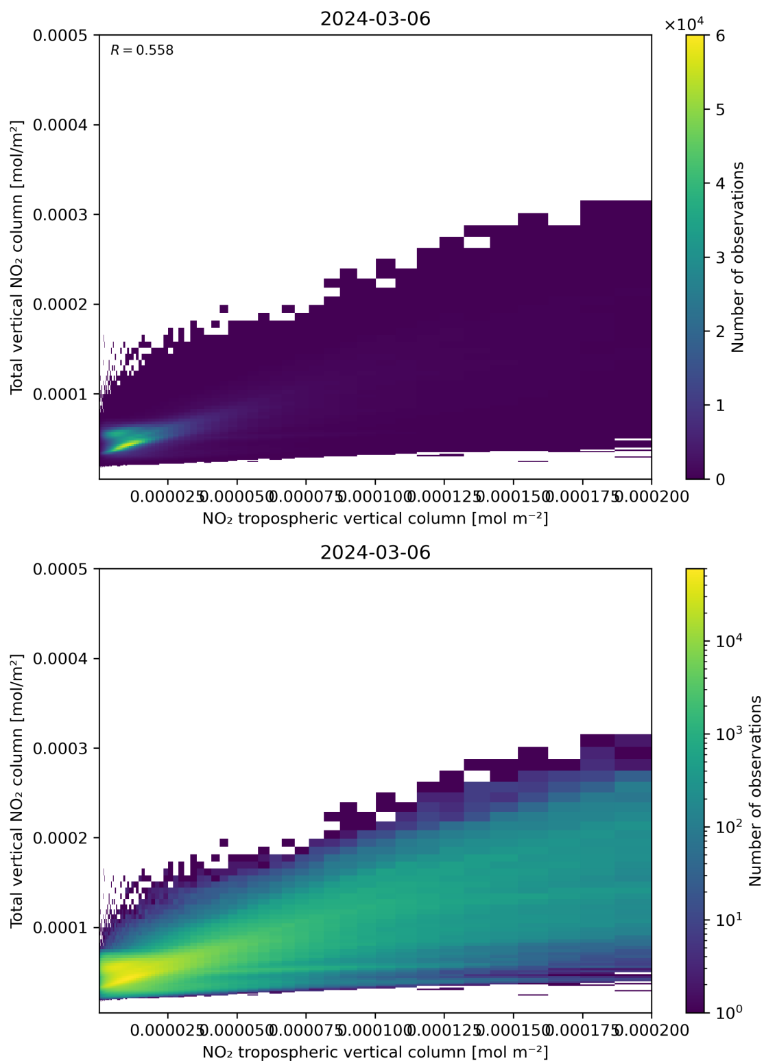
Figure 128: Scatter density plot of “NO 2 tropospheric vertical column” against “Total vertical NO 2 column” for 2024-03-05 to 2024-03-07.
