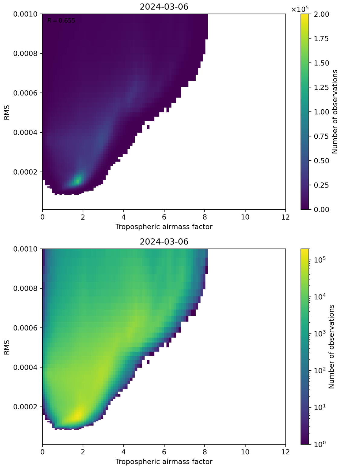
Figure 79: Scatter density plot of “Tropospheric airmass factor” against “RMS” for 2024-03-05 to 2024-03-07.
