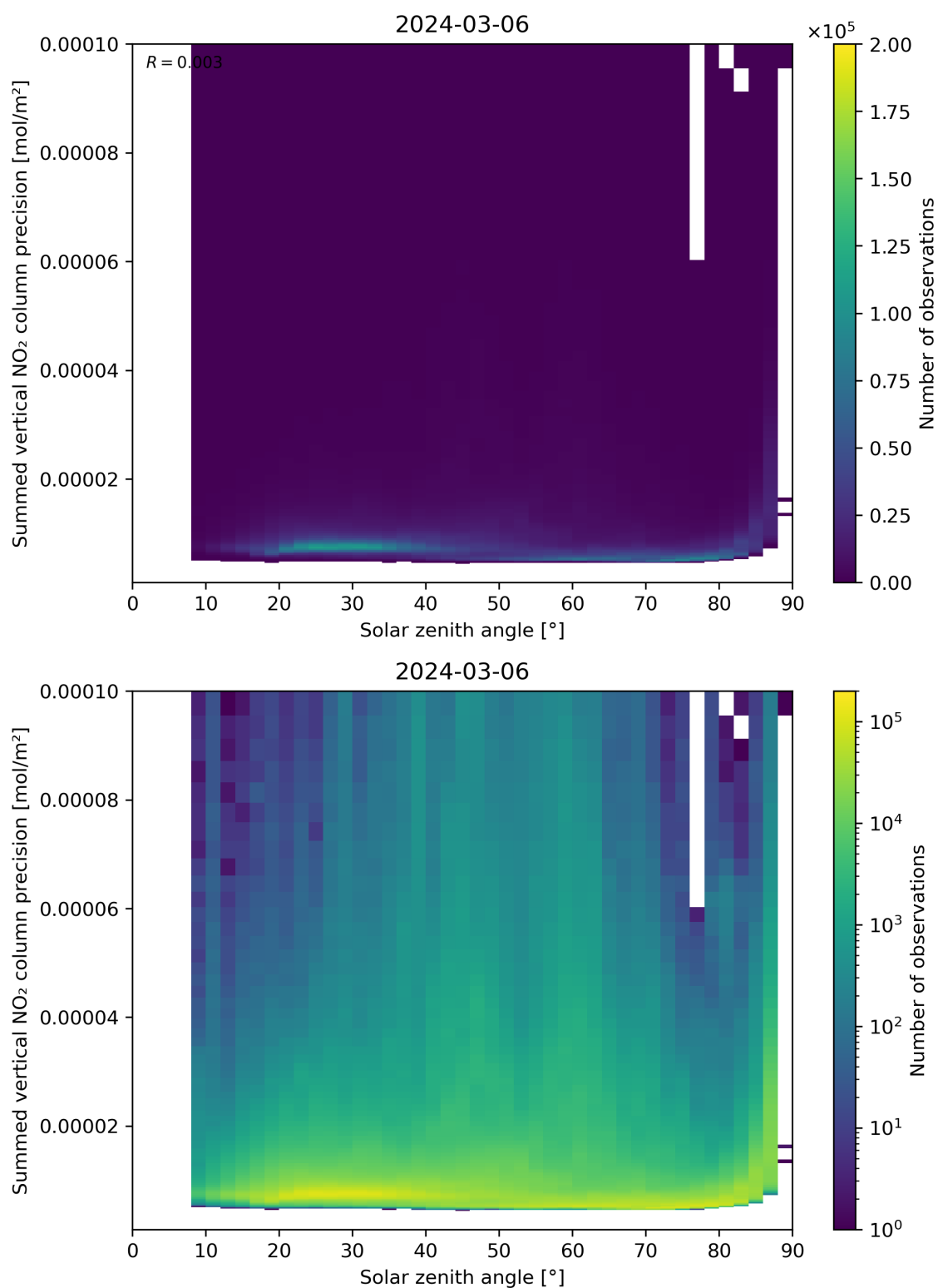
Figure 152: Scatter density plot of “Solar zenith angle” against “Summed vertical NO 2 column precision” for 2024-03-05 to 2024-03-07.
