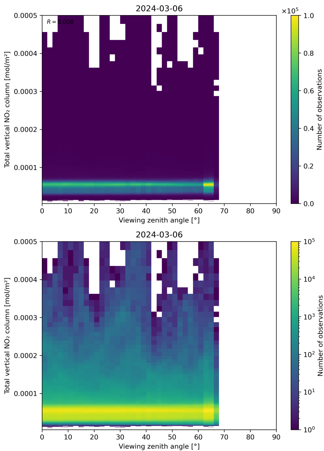
Figure 167: Scatter density plot of “Viewing zenith angle” against “Total vertical NO 2 column” for 2024-03-05 to 2024-03-07.
