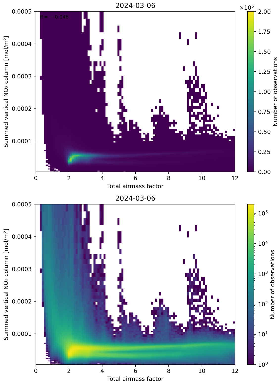
Figure 65: Scatter density plot of “Total airmass factor” against “Summed vertical NO 2 column” for 2024-03-05 to 2024-03-07.
