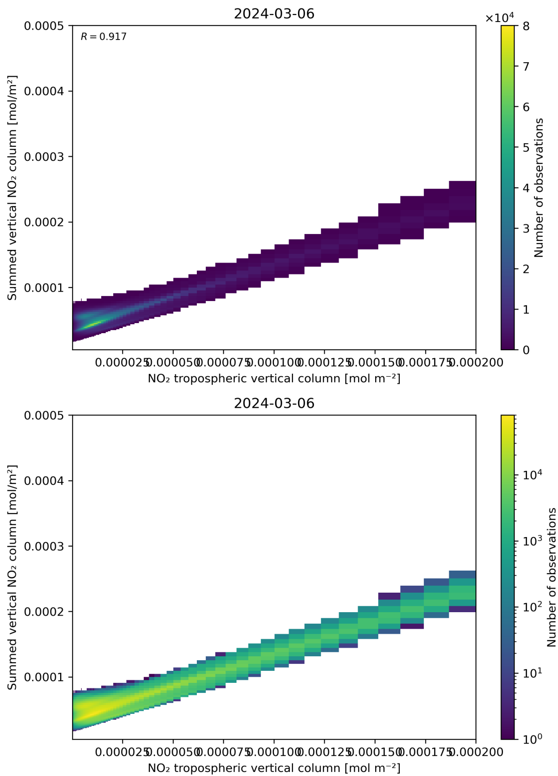
Figure 126: Scatter density plot of “NO 2 tropospheric vertical column” against “Summed vertical NO 2 column” for 2024-03-05 to 2024-03-07.
