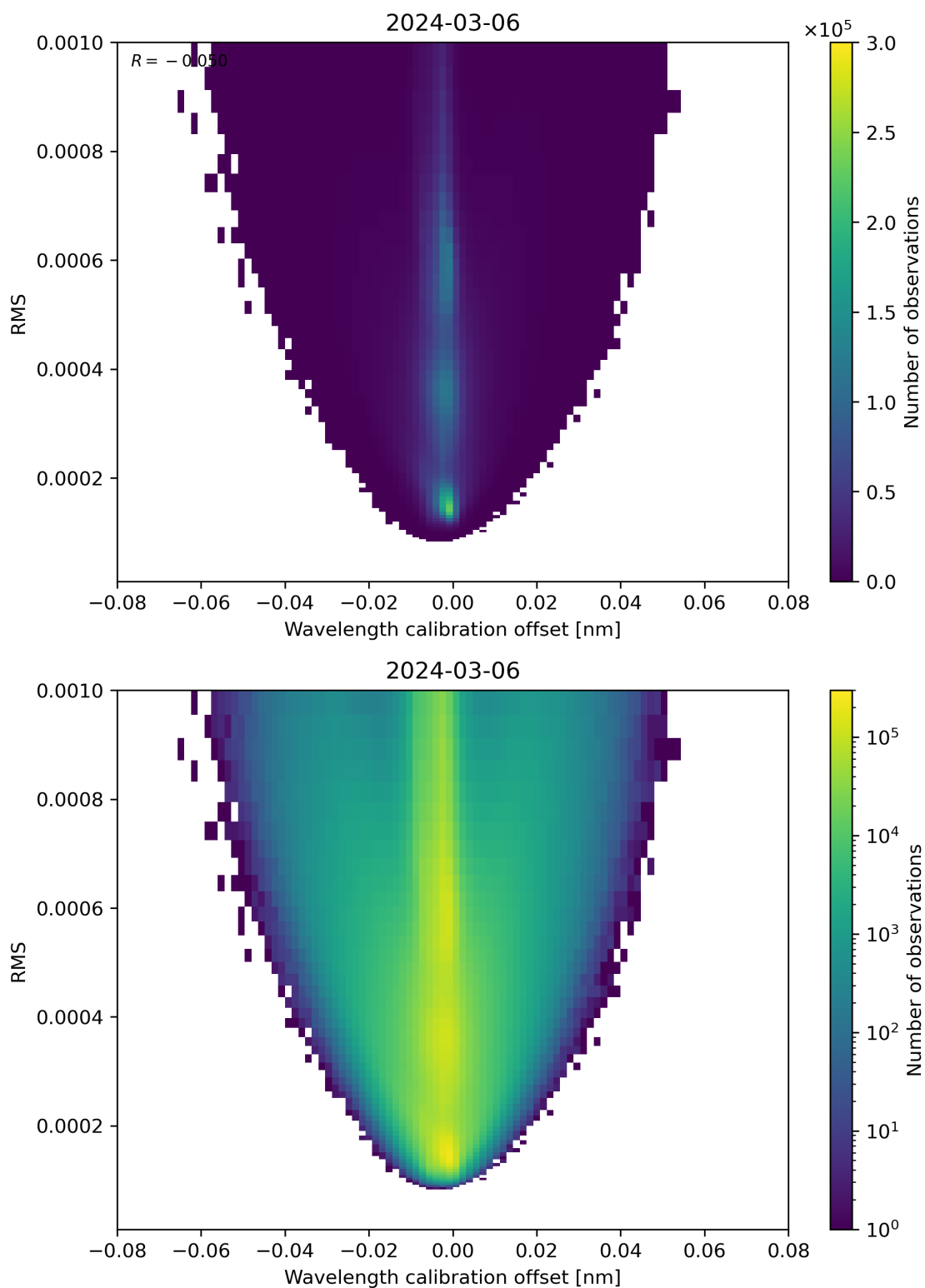
Figure 181: Scatter density plot of “Wavelength calibration offset” against “RMS” for 2024-03-05 to 2024-03-07.
