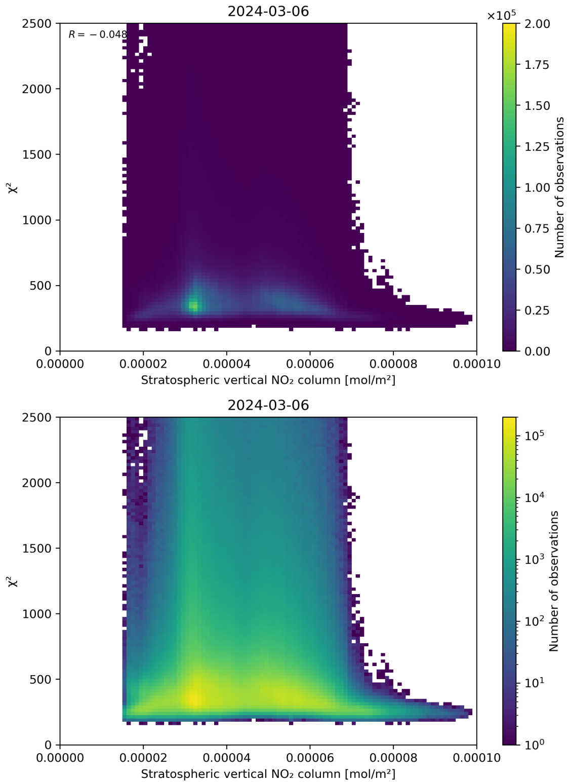
Figure 97: Scatter density plot of “Stratospheric vertical NO 2 column” against “ \chi^2 ” for 2024-03-05 to 2024-03-07.
