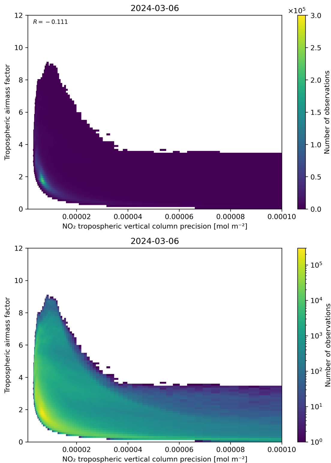
Figure 133: Scatter density plot of “NO 2 tropospheric vertical column precision” against “Tropospheric airmass factor” for 2024-03-05 to 2024-03-07.
