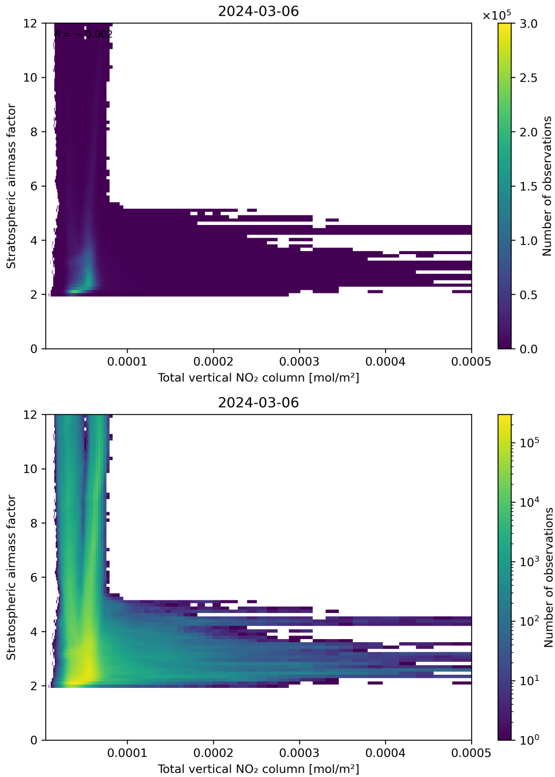
Figure 110: Scatter density plot of “Total vertical NO 2 column” against “Stratospheric air mass factor” for 2024-03-05 to 2024-03-07.
