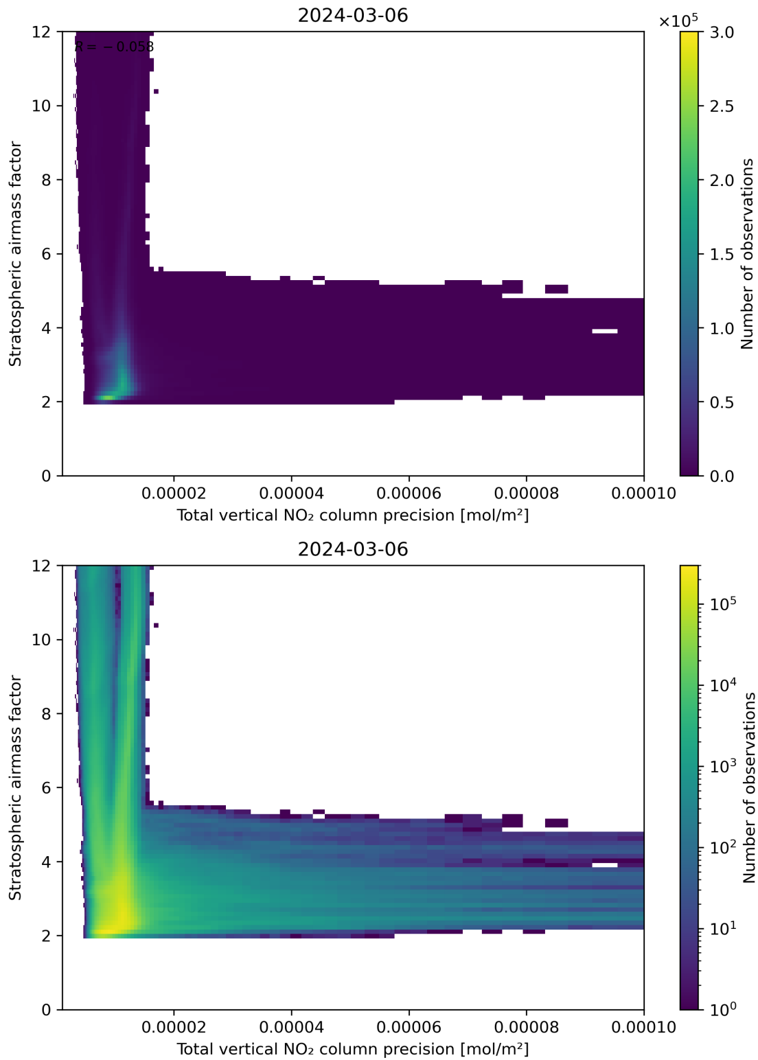
Figure 115: Scatter density plot of “Total vertical NO 2 column precision” against “Stratospheric air mass factor” for 2024-03-05 to 2024-03-07.
