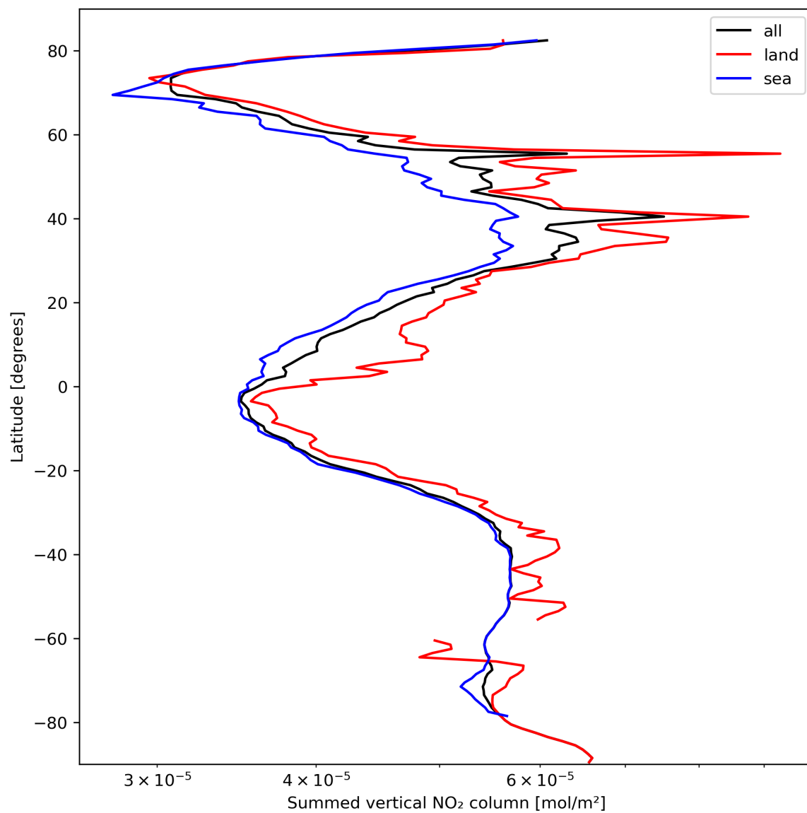
Figure 23: Zonal average of “Summed vertical NO 2 column” for 2024-03-05 to 2024-03-07.
