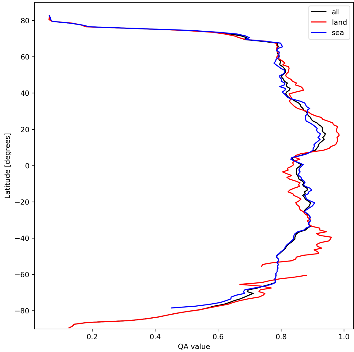
Figure 11: Zonal average of “QA value” for 2024-03-05 to 2024-03-07.
