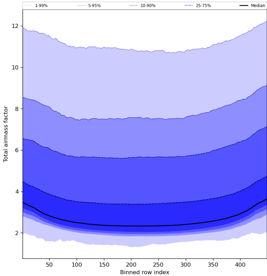
Figure 49: Along track statistics of “Total airmass factor” for 2024-03-05 to 2024-03-07
