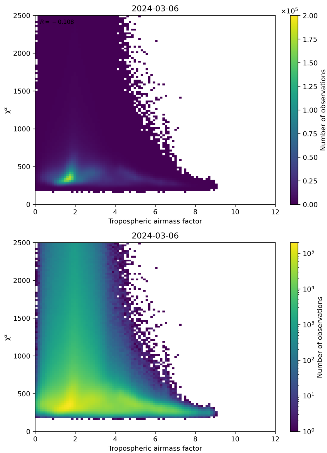
Figure 73: Scatter density plot of “Tropospheric airmass factor” against “ \chi^2 ” for 2024-03-05 to 2024-03-07.
