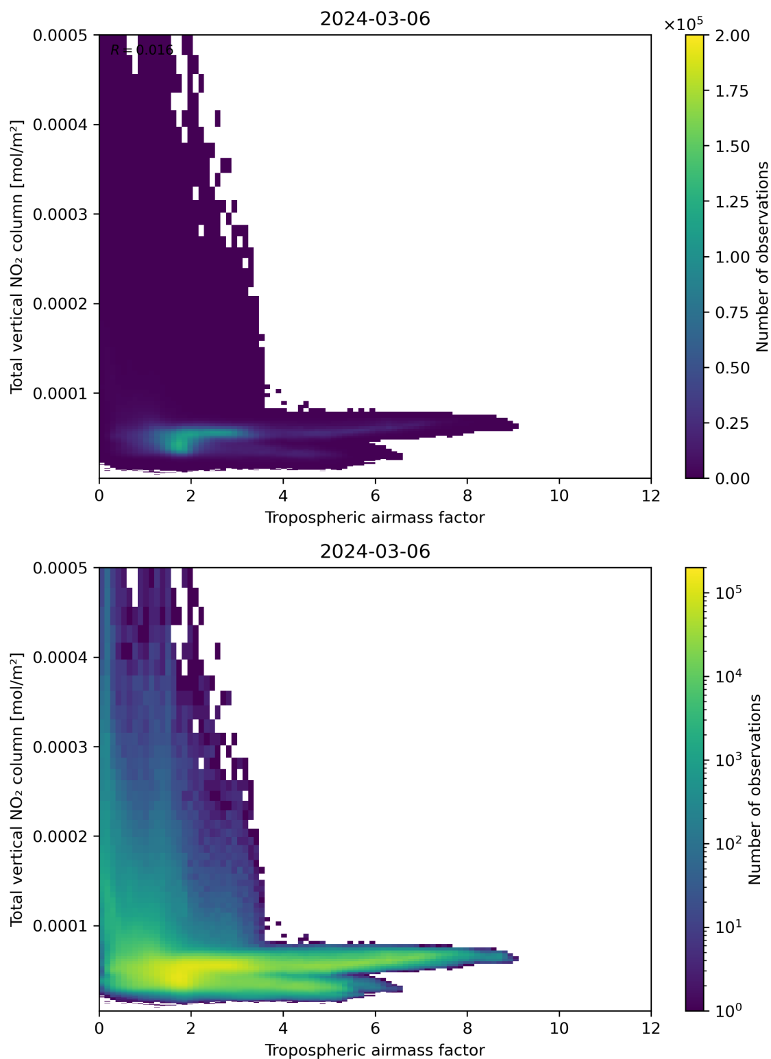
Figure 77: Scatter density plot of “Tropospheric airmass factor” against “Total vertical NO 2 column” for 2024-03-05 to 2024-03-07.
