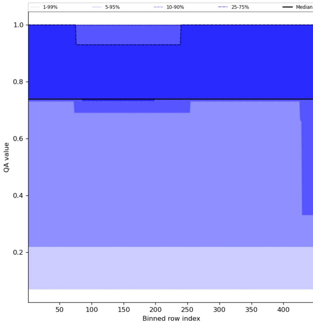
Figure 45: Along track statistics of “QA value” for 2024-03-05 to 2024-03-07
