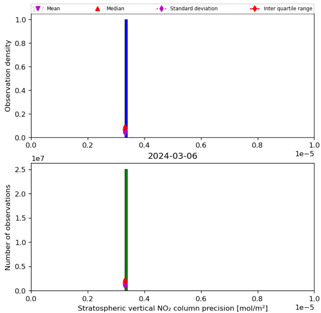
Figure 37: Histogram of “Stratospheric vertical NO 2 column precision” for 2024-03-05 to 2024-03-07
