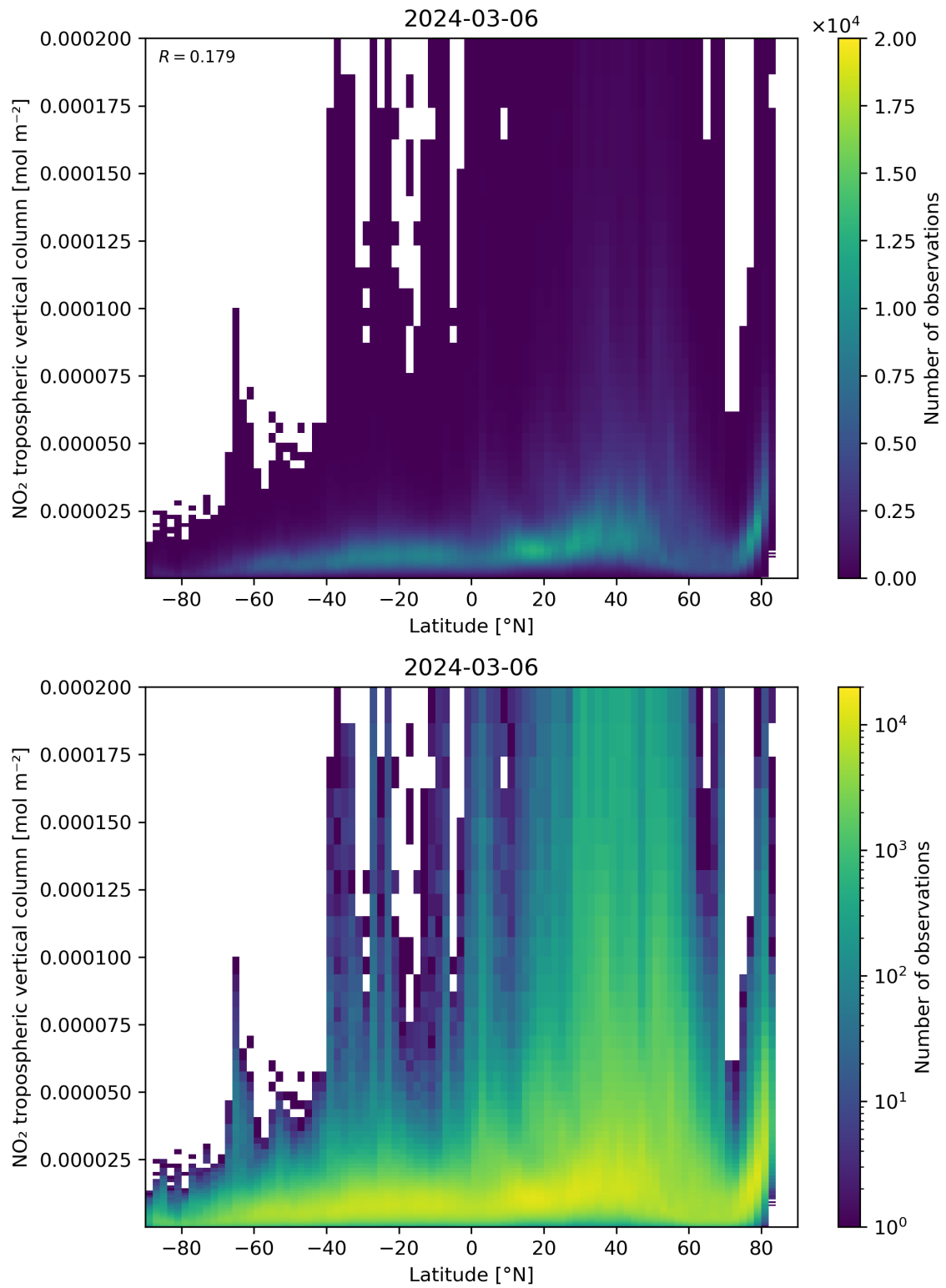
Figure 92: Scatter density plot of “Latitude” against “NO 2 tropospheric vertical column” for 2024-03-05 to 2024-03-07.
