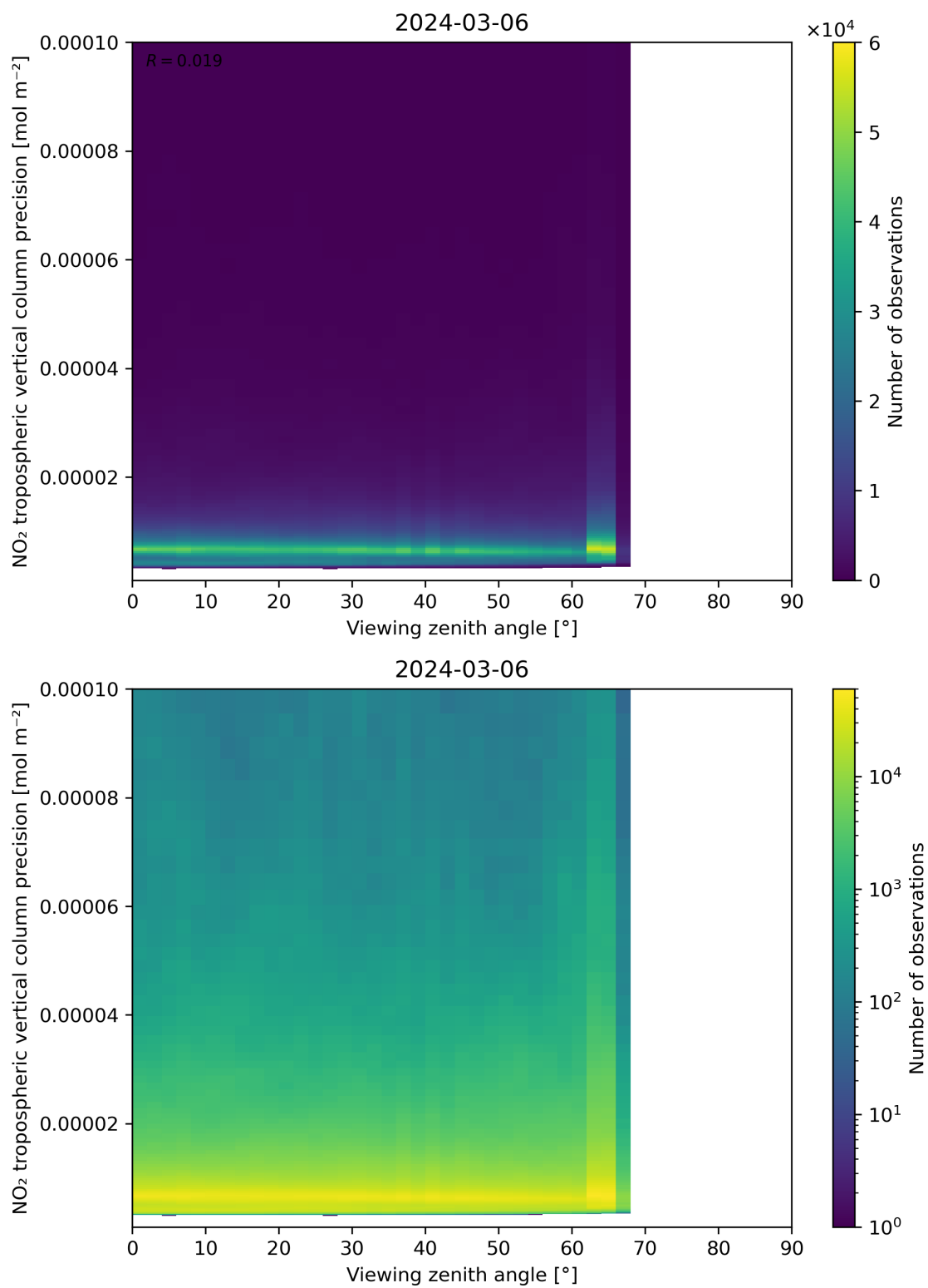
Figure 170: Scatter density plot of “Viewing zenith angle” against “NO 2 tropospheric vertical column precision” for 2024-03-05 to 2024-03-07.
