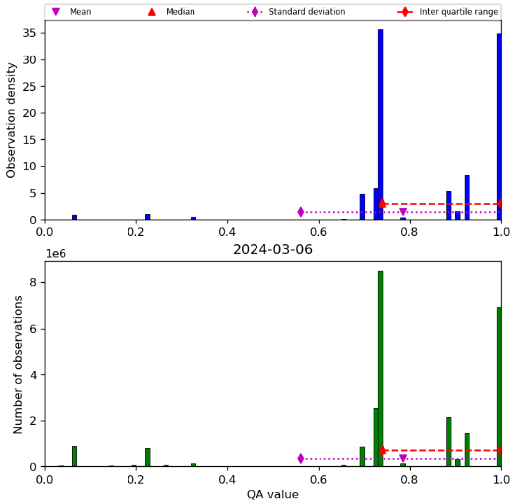
Figure 28: Histogram of “QA value” for 2024-03-05 to 2024-03-07
