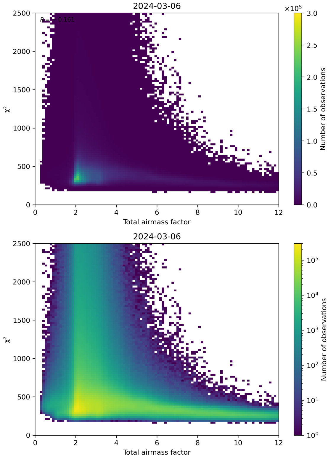
Figure 63: Scatter density plot of “Total airmass factor” against “ \chi^2 ” for 2024-03-05 to 2024-03-07.
