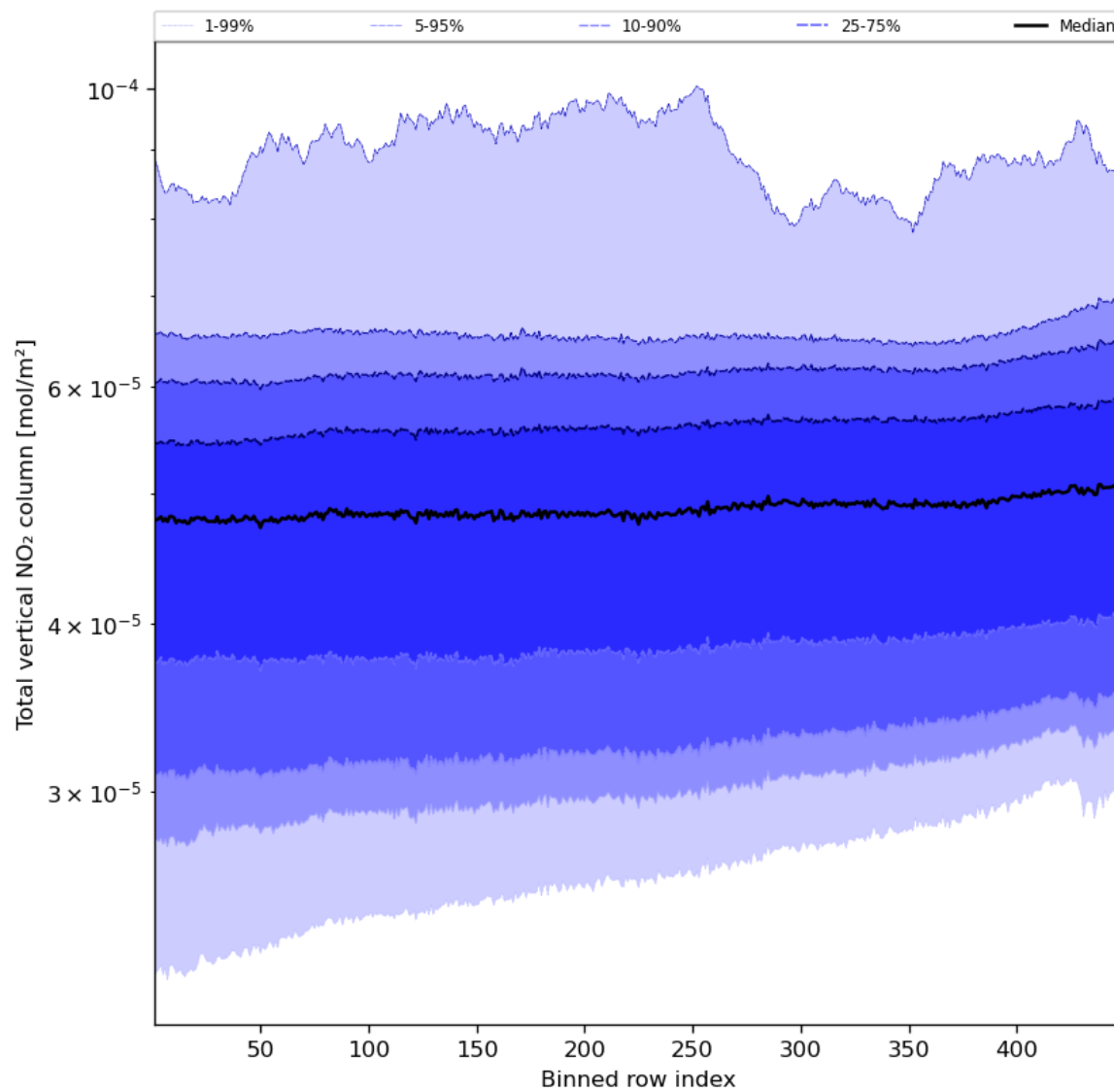
Figure 55: Along track statistics of “Total vertical NO 2 column” for 2024-03-05 to 2024-03-07
