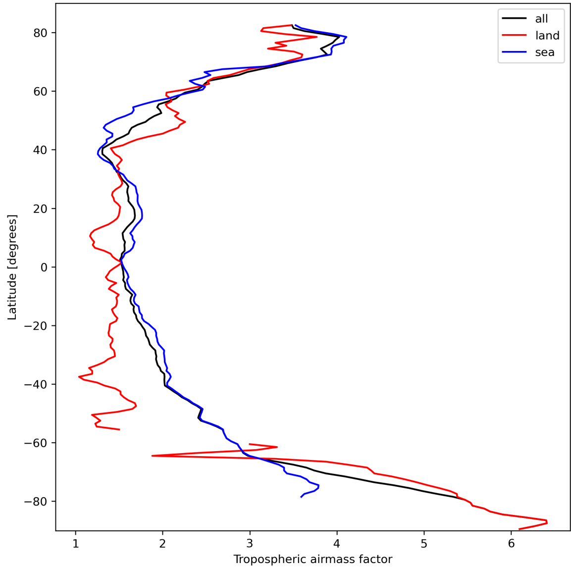
Figure 14: Zonal average of “Tropospheric airmass factor” for 2024-03-05 to 2024-03-07.
