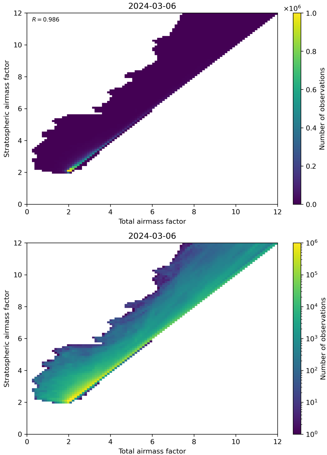
Figure 62: Scatter density plot of “Total airmass factor” against “Stratospheric airmass factor” for 2024-03-05 to 2024-03-07.
