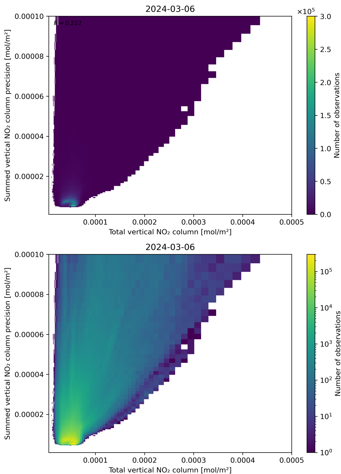
Figure 113: Scatter density plot of “Total vertical NO 2 column” against “Summed vertical NO 2 column precision” for 2024-03-05 to 2024-03-07.
