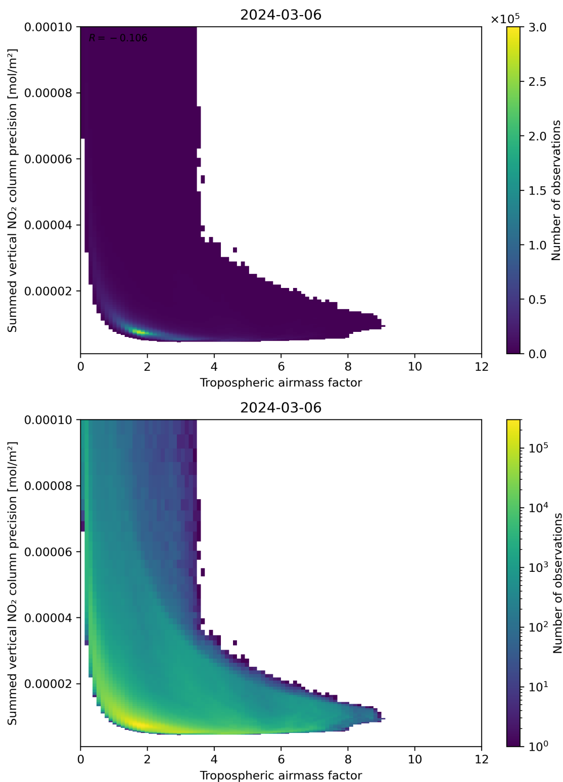
Figure 76: Scatter density plot of “Tropospheric air mass factor” against “Summed vertical NO 2 column precision” for 2024-03-05 to 2024-03-07.
