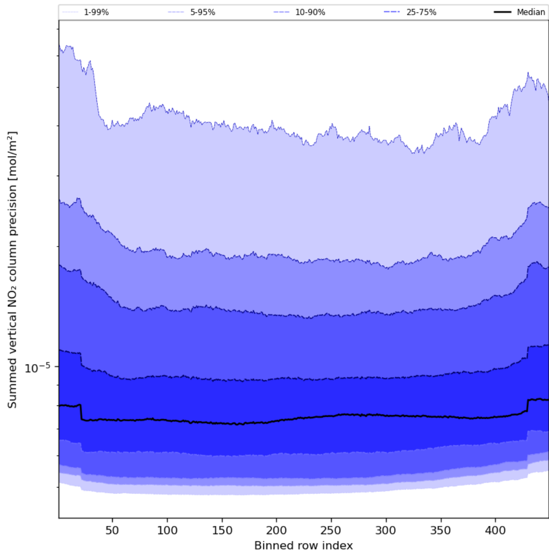
Figure 58: Along track statistics of “Summed vertical NO 2 column precision” for 2024-03-05 to 2024-03-07
