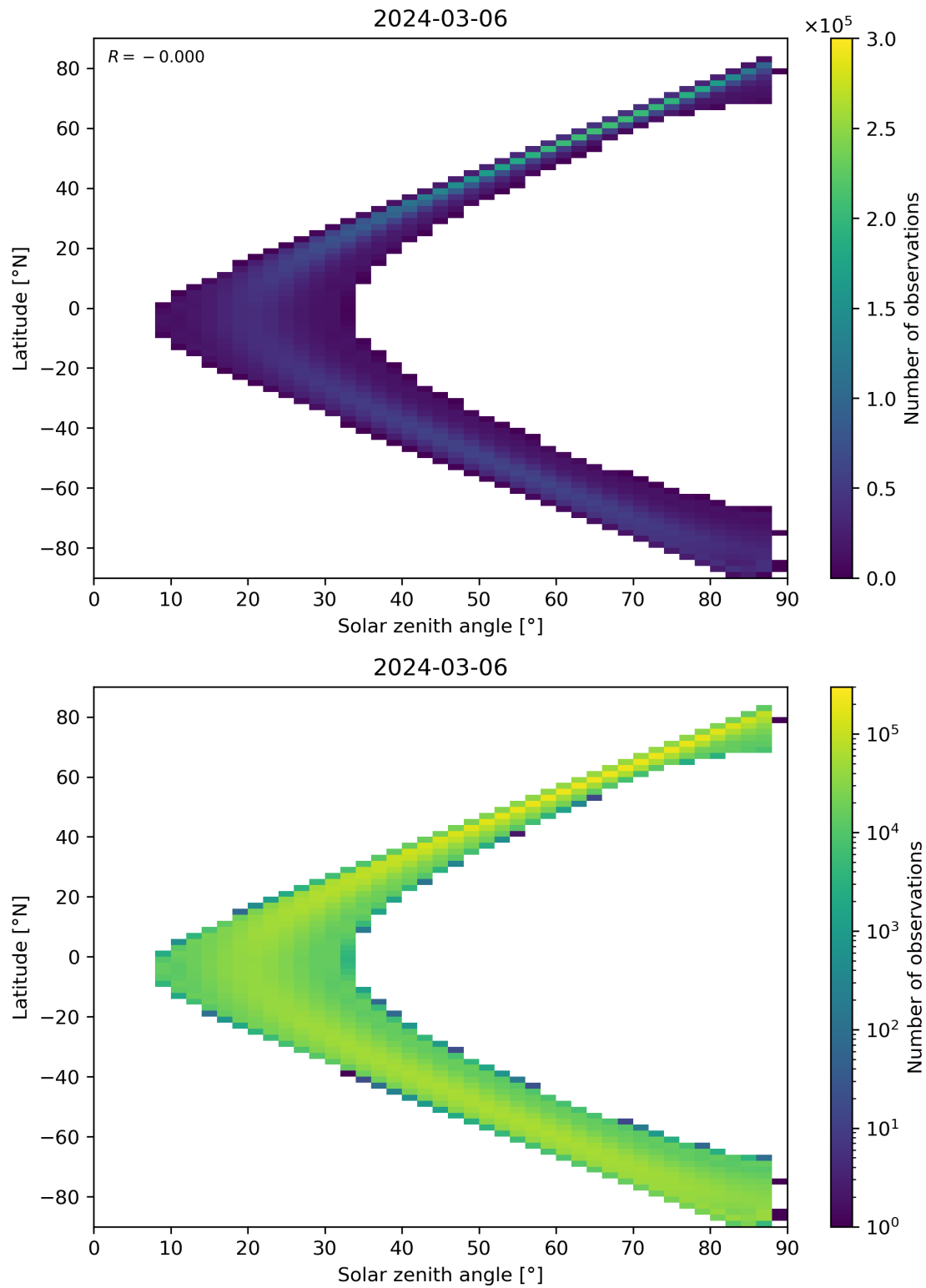
Figure 149: Scatter density plot of “Solar zenith angle” against “Latitude” for 2024-03-05 to 2024-03-07.
