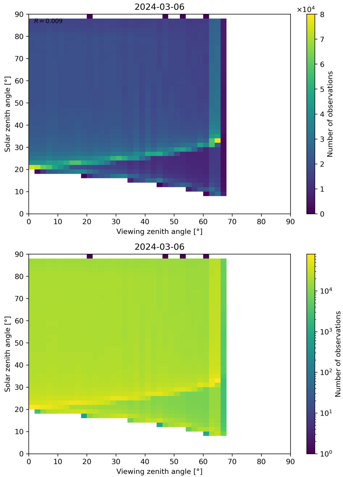
Figure 172: Scatter density plot of “Viewing zenith angle” against “Solar zenith angle” for 2024-03-05 to 2024-03-07.
