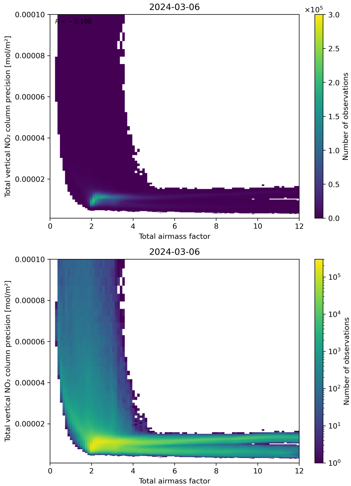
Figure 68: Scatter density plot of “Total airmass factor” against “Total vertical NO 2 column precision” for 2024-03-05 to 2024-03-07.
