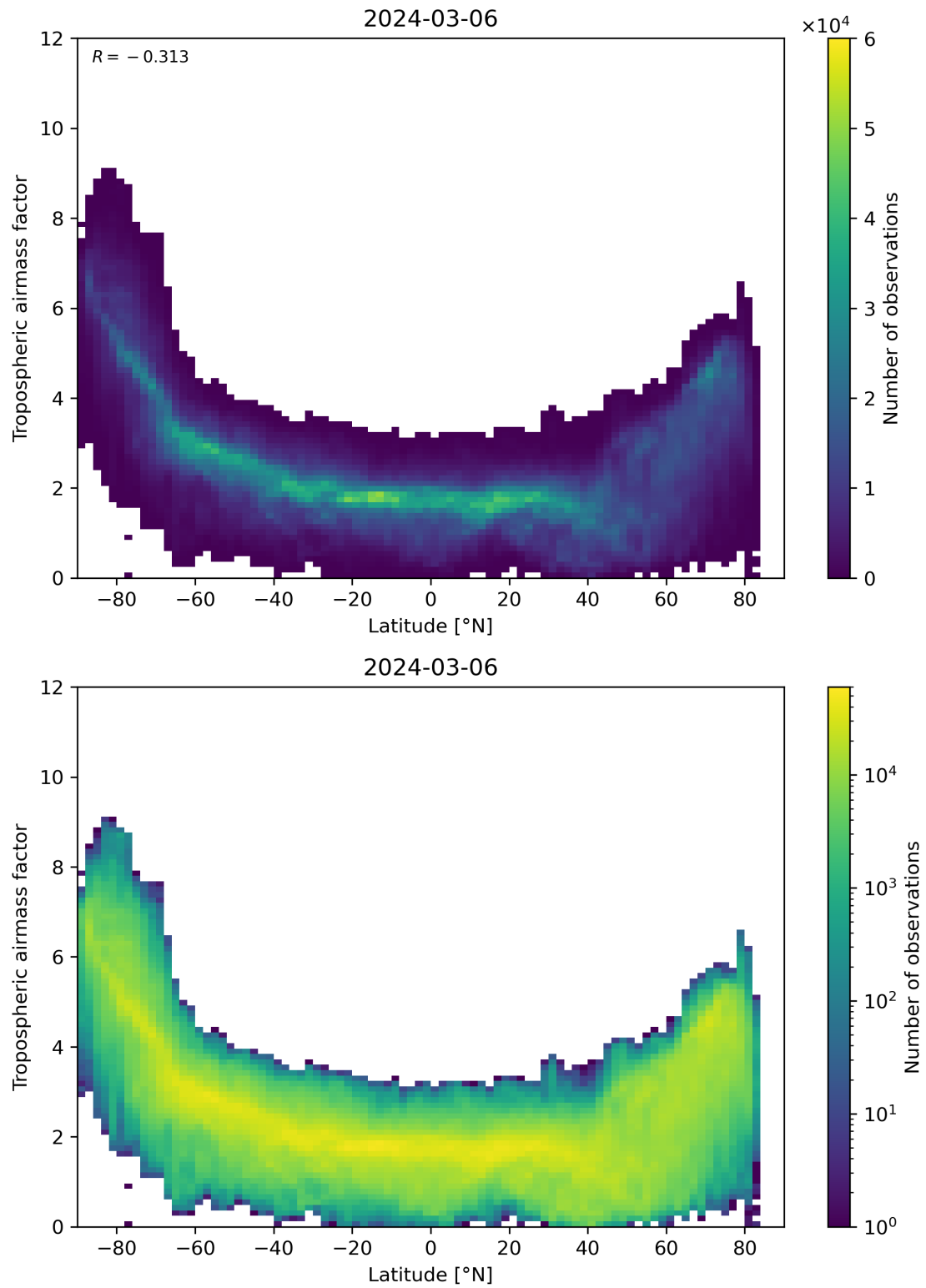
Figure 85: Scatter density plot of “Latitude” against “Tropospheric air mass factor” for 2024-03-05 to 2024-03-07.
