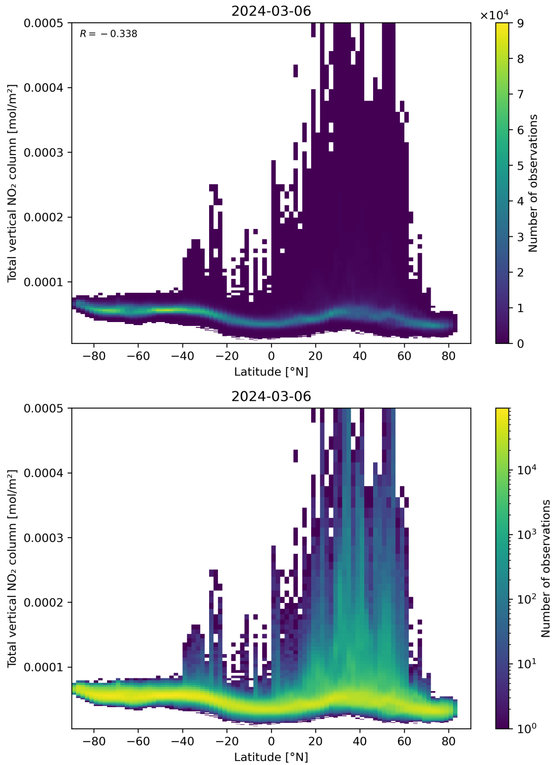
Figure 90: Scatter density plot of “Latitude” against “Total vertical NO 2 column” for 2024-03-05 to 2024-03-07.
