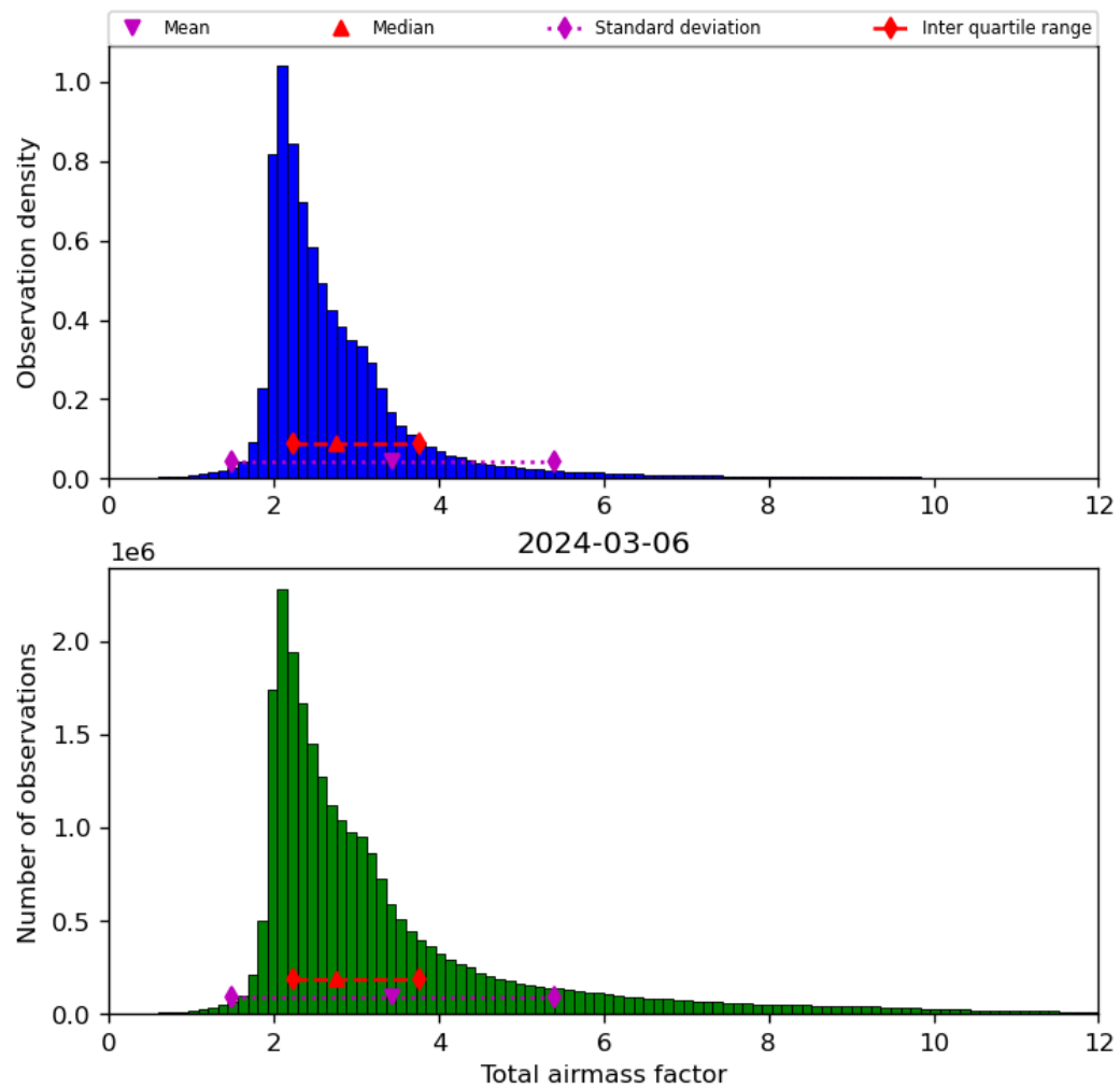
Figure 32: Histogram of “Total airmass factor” for 2024-03-05 to 2024-03-07
