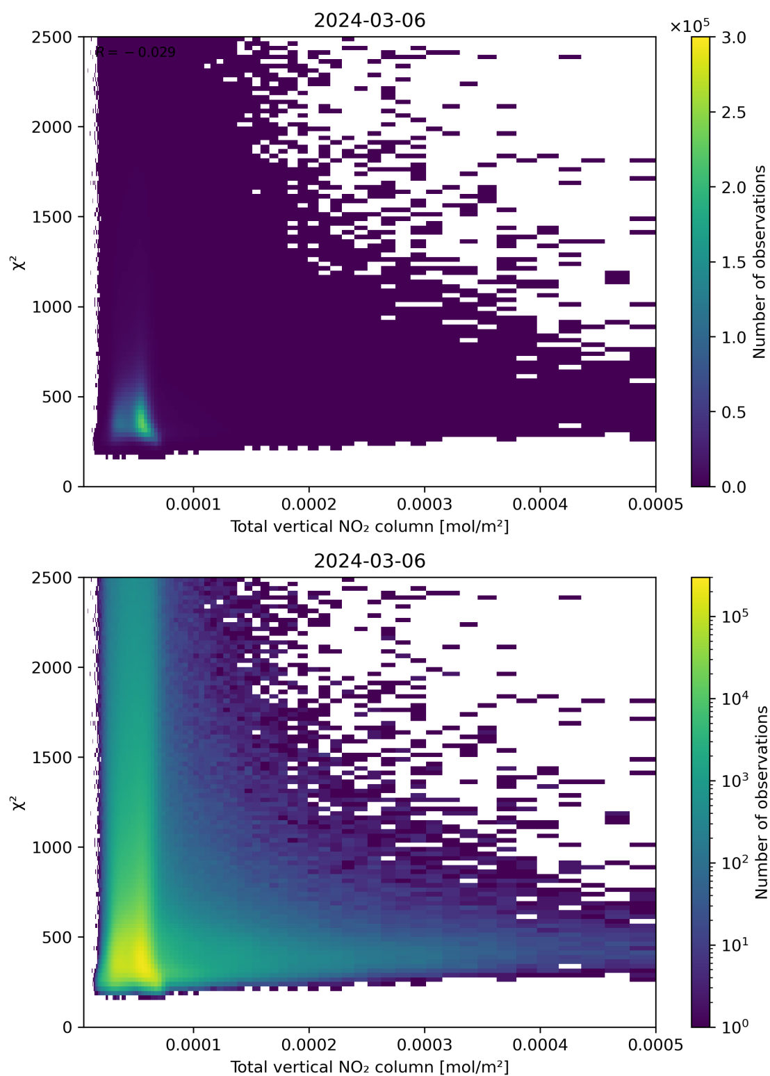
Figure 111: Scatter density plot of “Total vertical NO 2 column” against “ \chi^2 ” for 2024-03-05 to 2024-03-07.
