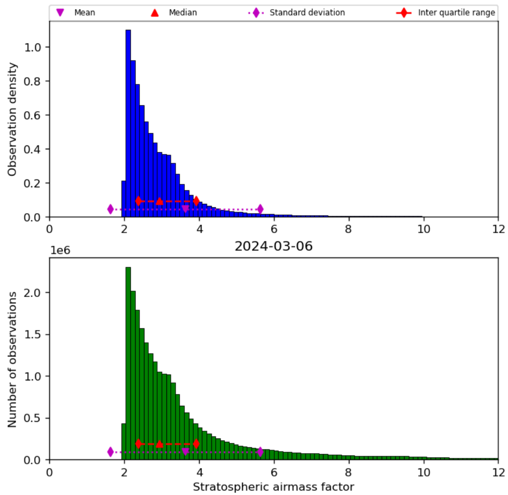
Figure 44: Histogram of “Stratospheric airmass factor” for 2024-03-05 to 2024-03-07
