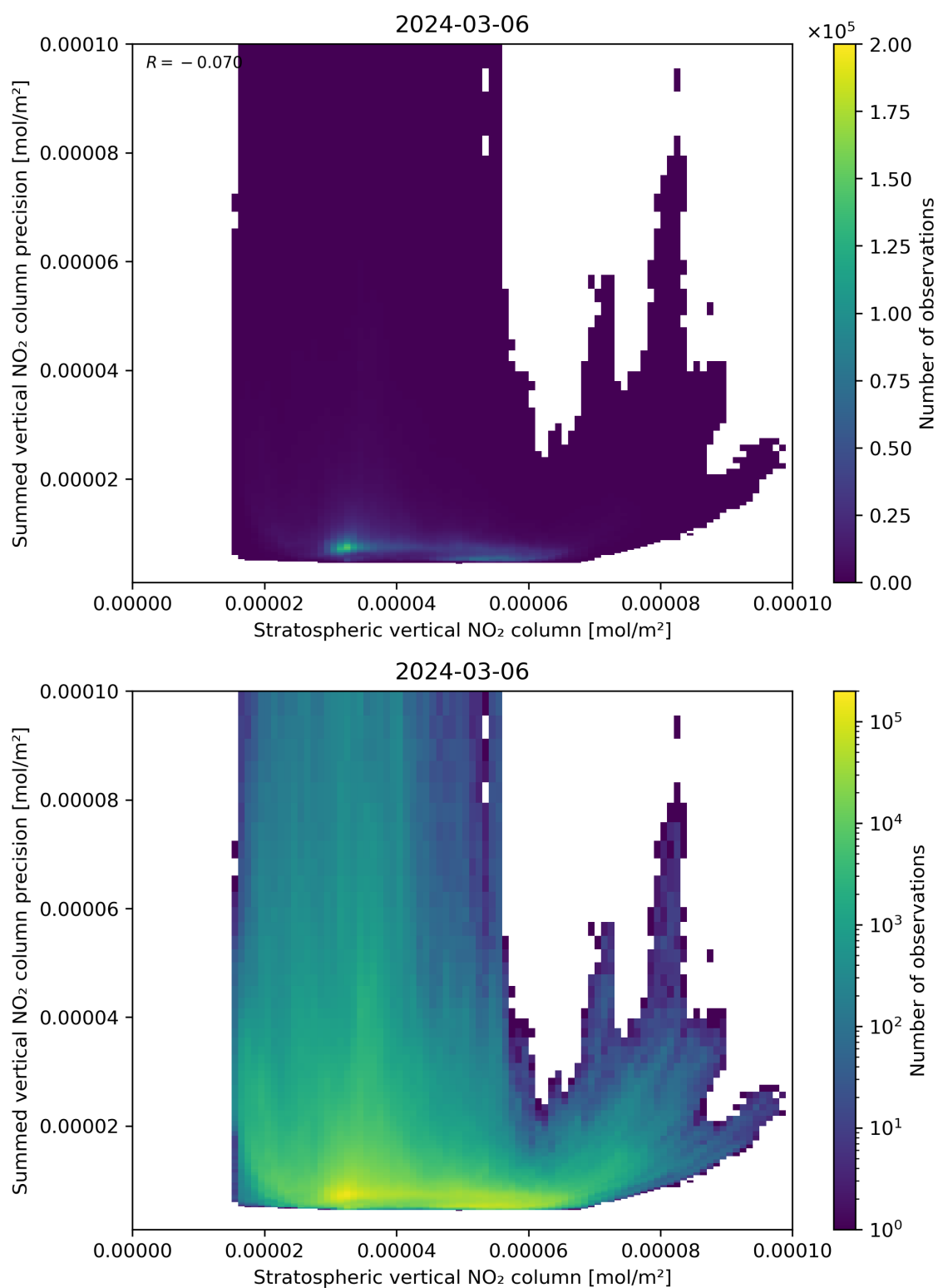
Figure 99: Scatter density plot of “Stratospheric vertical NO 2 column” against “Summed vertical NO 2 column precision” for 2024-03-05 to 2024-03-07.
