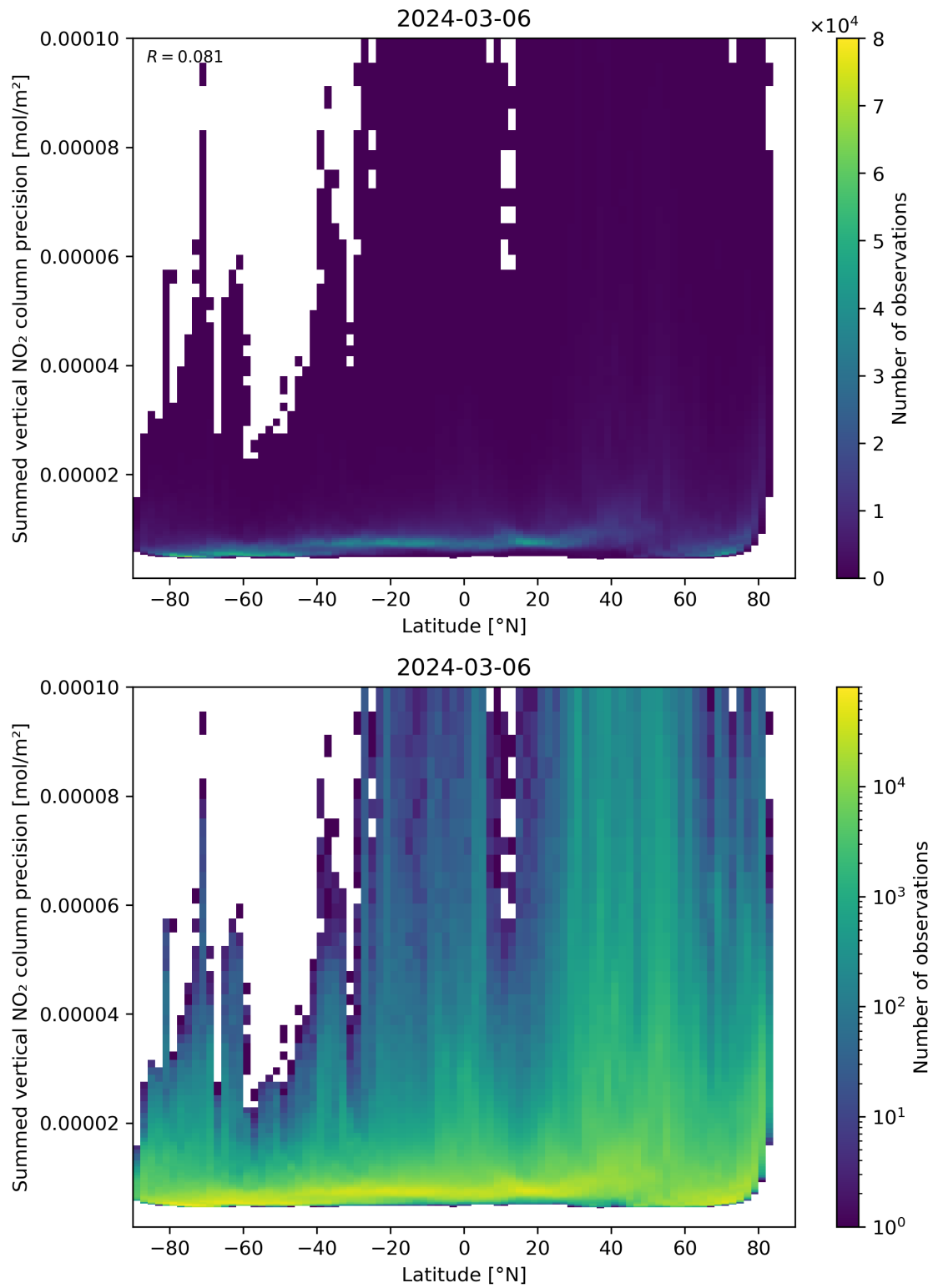
Figure 89: Scatter density plot of “Latitude” against “Summed vertical NO 2 column precision” for 2024-03-05 to 2024-03-07.
