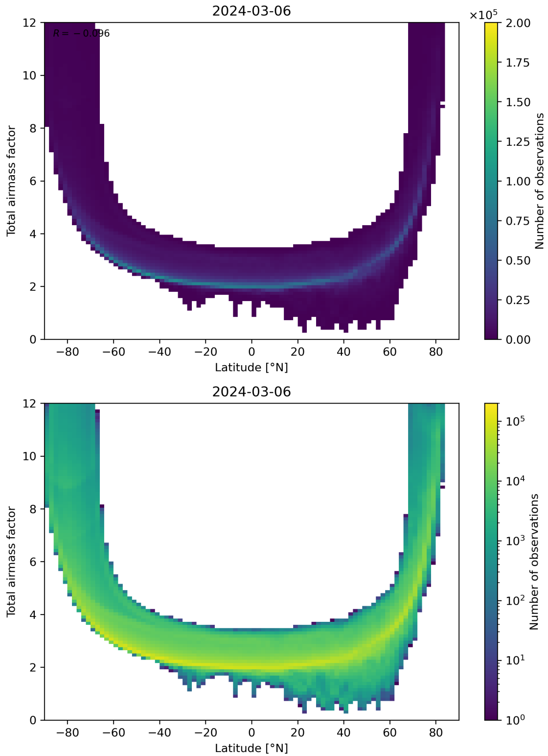
Figure 84: Scatter density plot of “Latitude” against “Total airmass factor” for 2024-03-05 to 2024-03-07.
