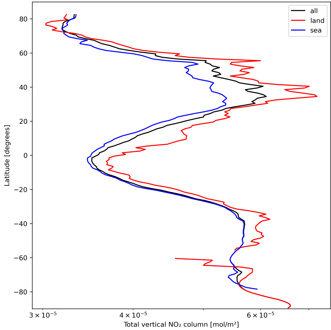
Figure 21: Zonal average of “Total vertical NO 2 column” for 2024-03-05 to 2024-03-07.
