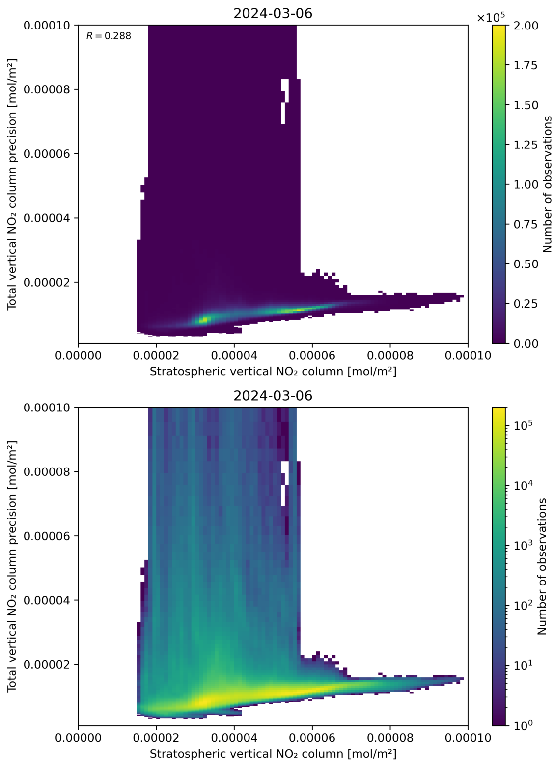
Figure 101: Scatter density plot of “Stratospheric vertical NO 2 column” against “Total vertical NO 2 column precision” for 2024-03-05 to 2024-03-07.
