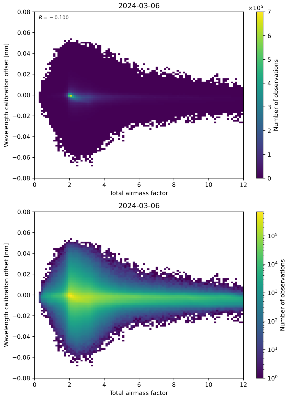
Figure 70: Scatter density plot of “Total airmass factor” against “Wavelength calibration offset” for 2024-03-05 to 2024-03-07.
