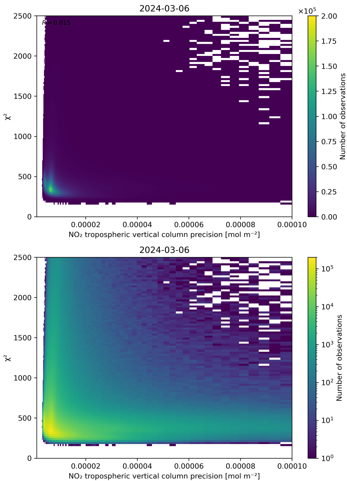
Figure 134: Scatter density plot of “NO 2 tropospheric vertical column precision” against “ \chi^2 ” for 2024-03-05 to 2024-03-07.
