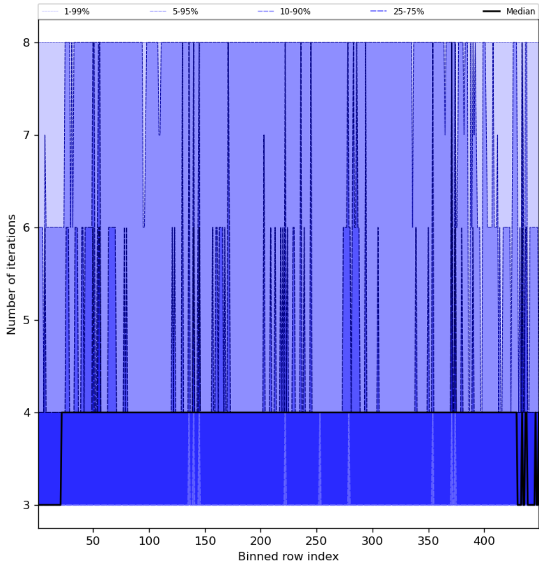
Figure 51: Along track statistics of “Number of iterations” for 2024-03-05 to 2024-03-07
