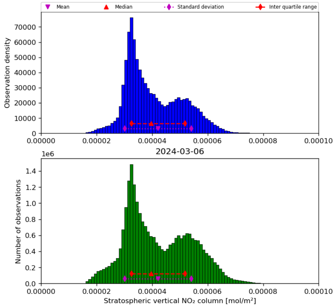
Figure 36: Histogram of “Stratospheric vertical NO 2 column” for 2024-03-05 to 2024-03-07
