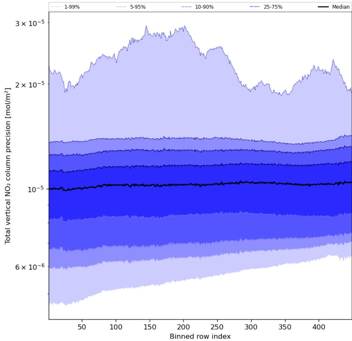
Figure 56: Along track statistics of “Total vertical NO 2 column precision” for 2024-03-05 to 2024-03-07
