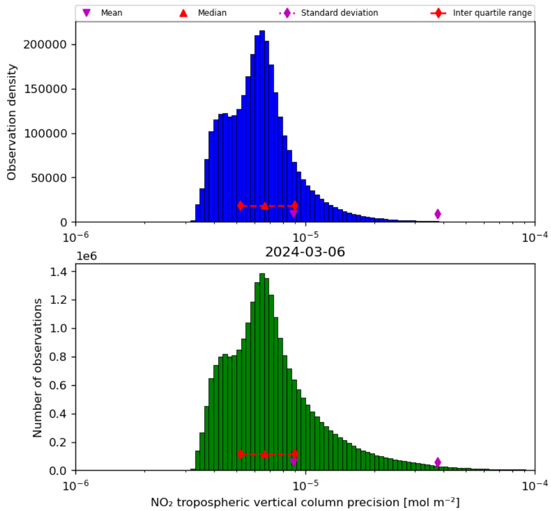
Figure 30: Histogram of “NO 2 tropospheric vertical column precision” for 2024-03-05 to 2024-03-07
