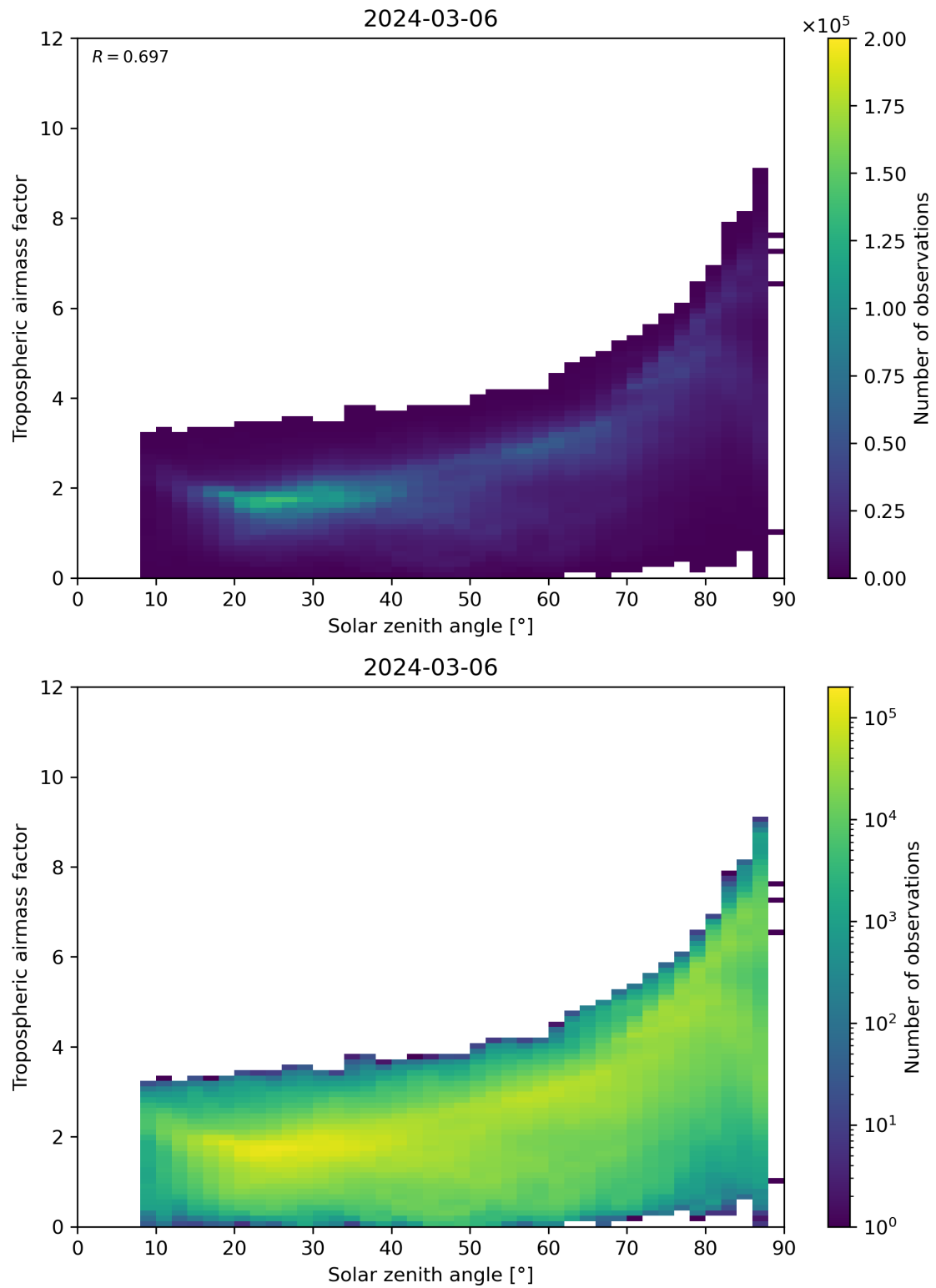
Figure 147: Scatter density plot of “Solar zenith angle” against “Tropospheric airmass factor” for 2024-03-05 to 2024-03-07.
