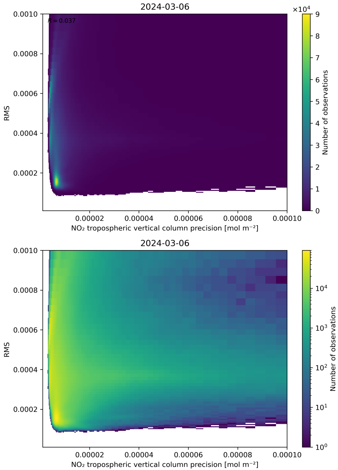
Figure 140: Scatter density plot of “NO 2 tropospheric vertical column precision” against “RMS” for 2024-03-05 to 2024-03-07.
