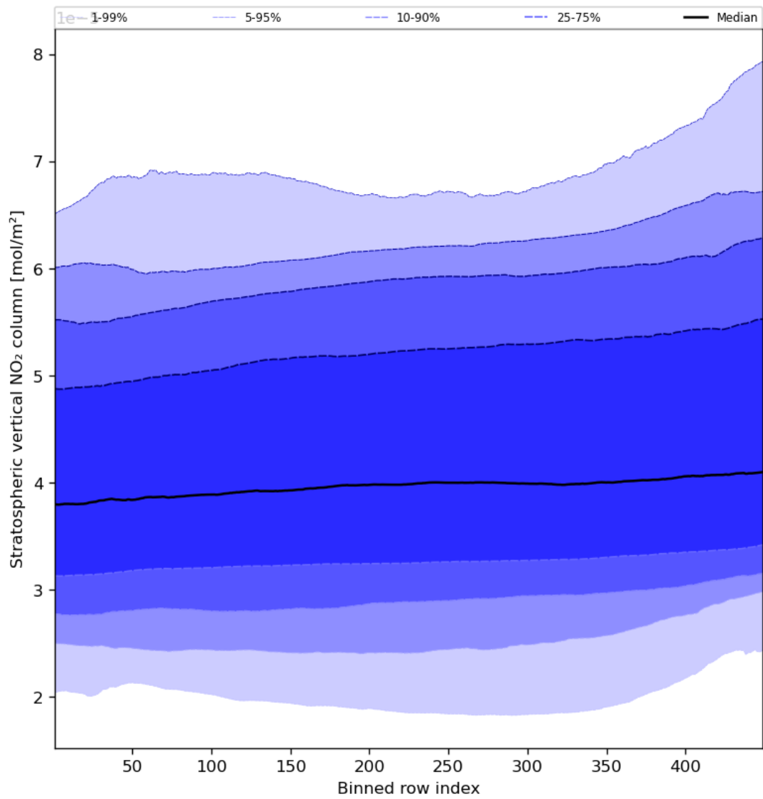
Figure 53: Along track statistics of “Stratospheric vertical NO 2 column” for 2024-03-05 to 2024-03-07
