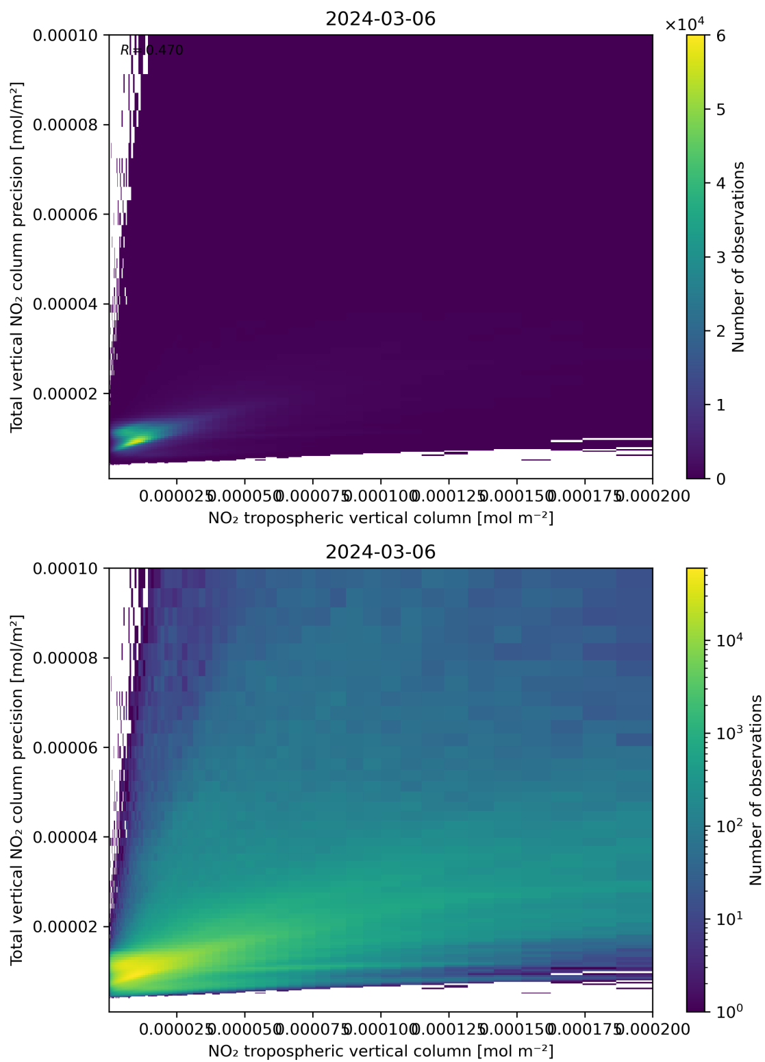
Figure 129: Scatter density plot of “NO 2 tropospheric vertical column” against “Total vertical NO 2 column precision” for 2024-03-05 to 2024-03-07.
