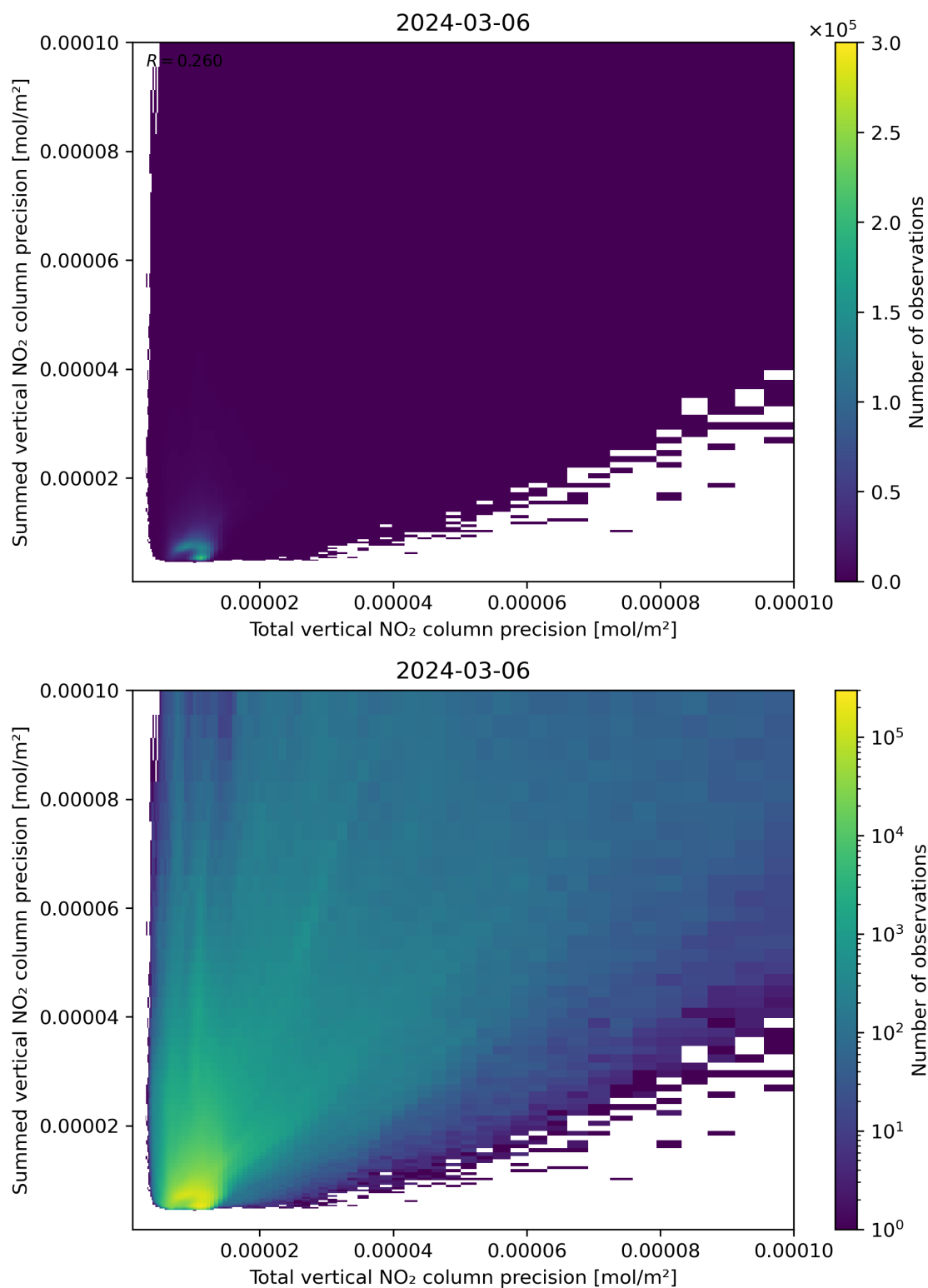
Figure 118: Scatter density plot of “Total vertical NO 2 column precision” against “Summed vertical NO 2 column precision” for 2024-03-05 to 2024-03-07.
