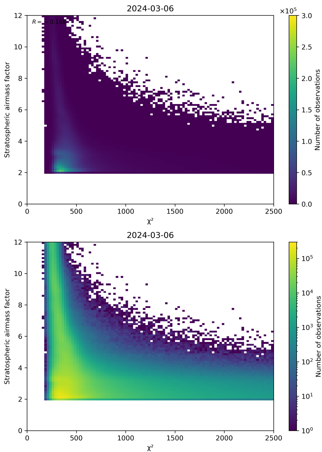
Figure 81: Scatter density plot of “ \chi^2 ” against “Stratospheric airmass factor” for 2024-03-05 to 2024-03-07.
