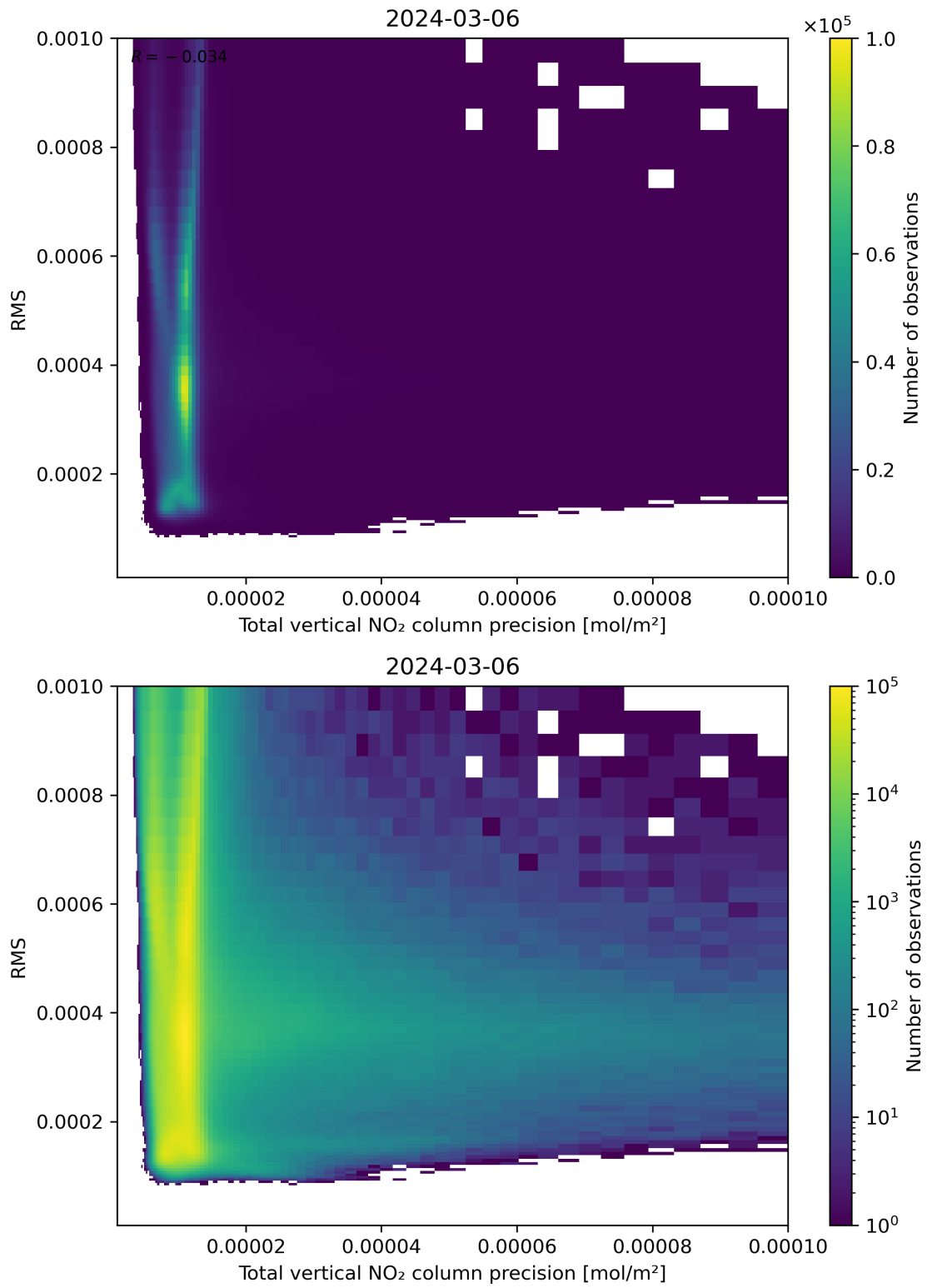
Figure 119: Scatter density plot of “Total vertical NO 2 column precision” against “RMS” for 2024-03-05 to 2024-03-07.
