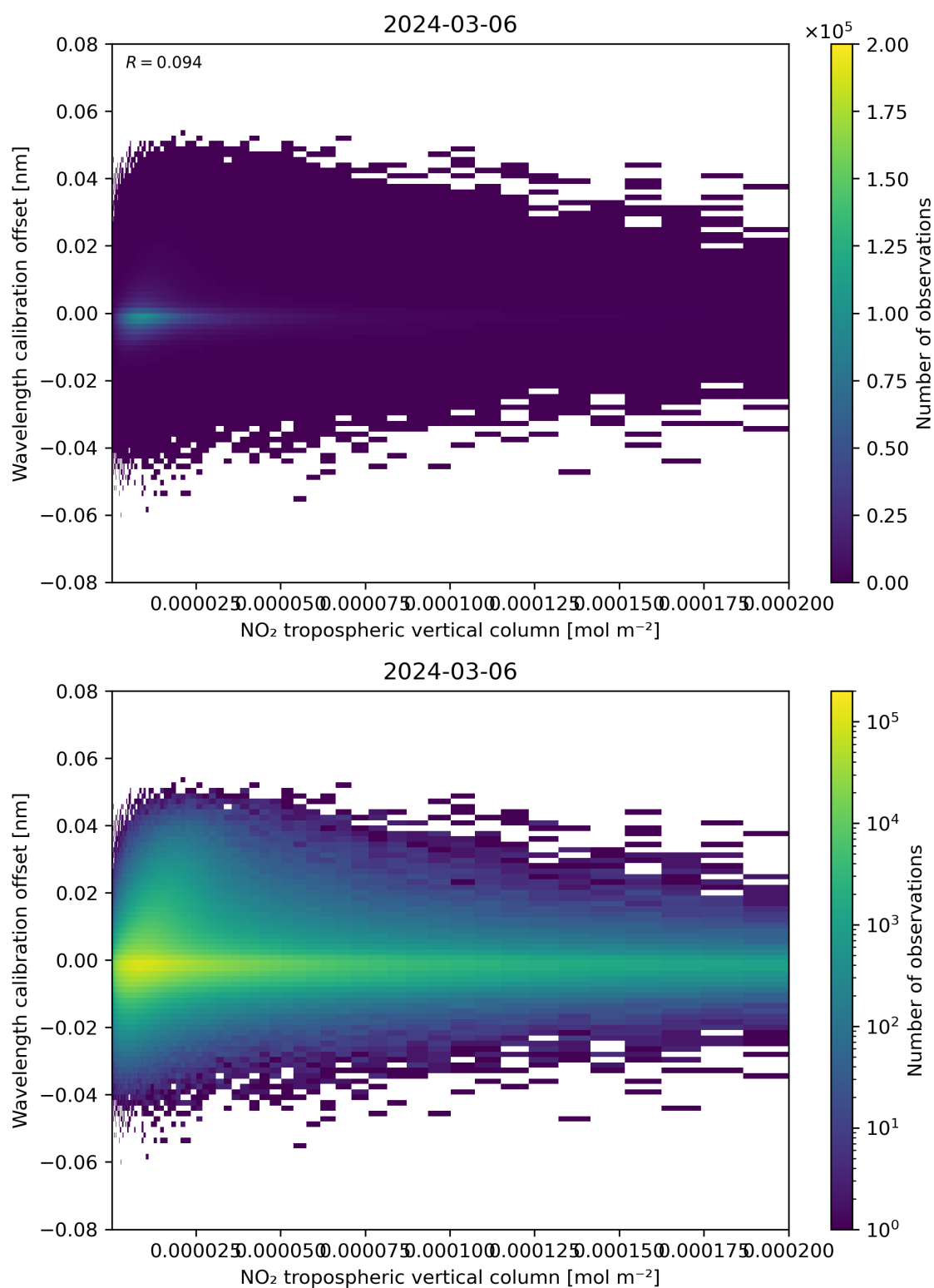
Figure 143: Scatter density plot of “NO 2 tropospheric vertical column” against “Wavelength calibration offset” for 2024-03-05 to 2024-03-07.
