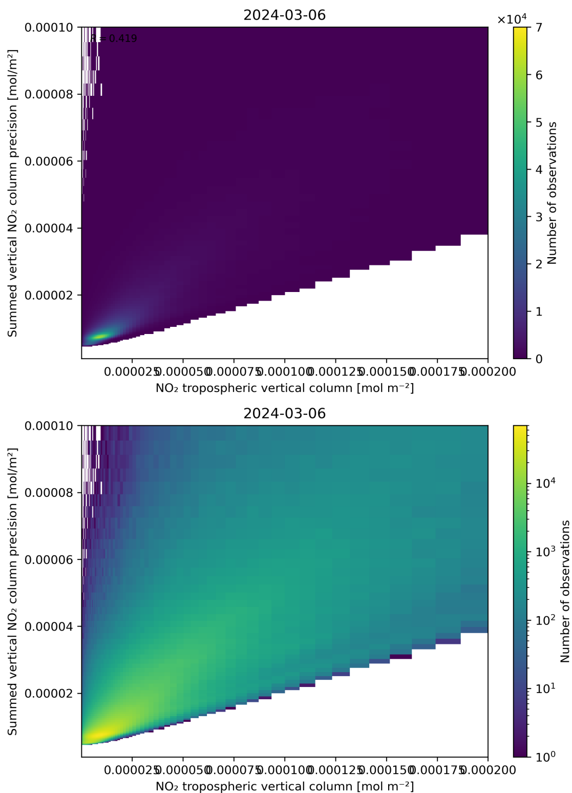
Figure 127: Scatter density plot of “NO 2 tropospheric vertical column” against “Summed vertical NO 2 column precision” for 2024-03-05 to 2024-03-07.
