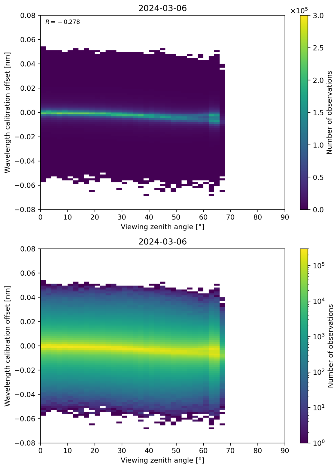
Figure 173: Scatter density plot of “Viewing zenith angle” against “Wavelength calibration offset” for 2024-03-05 to 2024-03-07.
