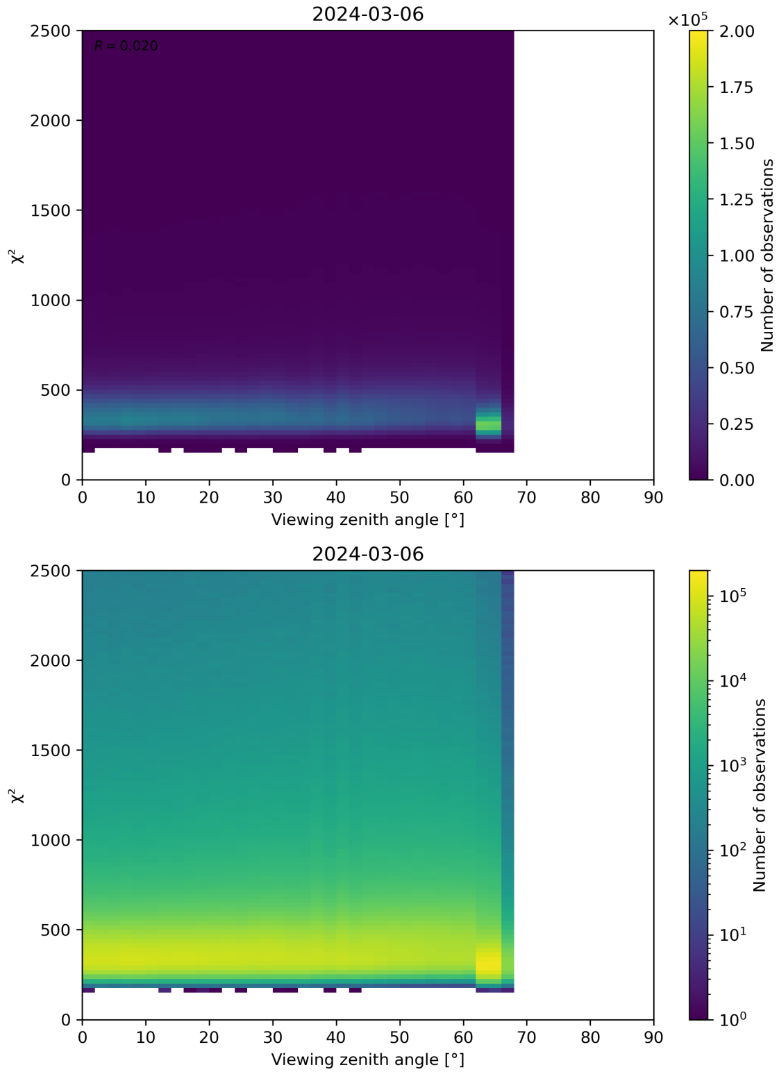
Figure 162: Scatter density plot of “Viewing zenith angle” against “ \chi^2 ” for 2024-03-05 to 2024-03-07.
