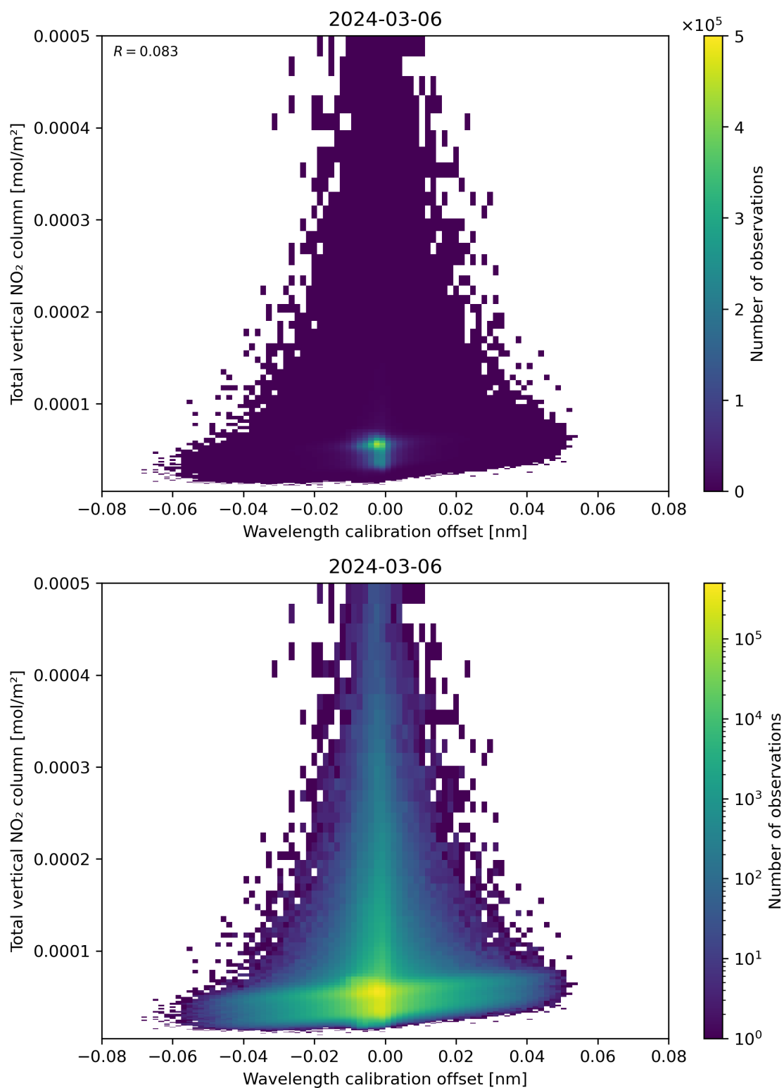
Figure 179: Scatter density plot of “Wavelength calibration offset” against “Total vertical NO 2 column” for 2024-03-05 to 2024-03-07.
