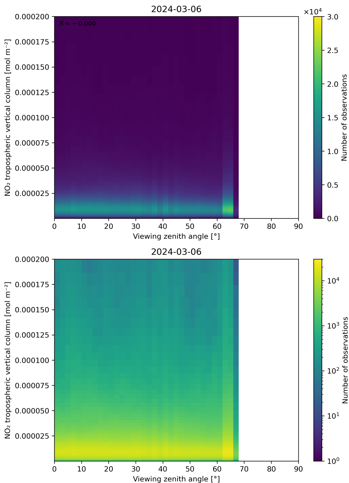
Figure 169: Scatter density plot of “Viewing zenith angle” against “NO 2 tropospheric vertical column” for 2024-03-05 to 2024-03-07.
