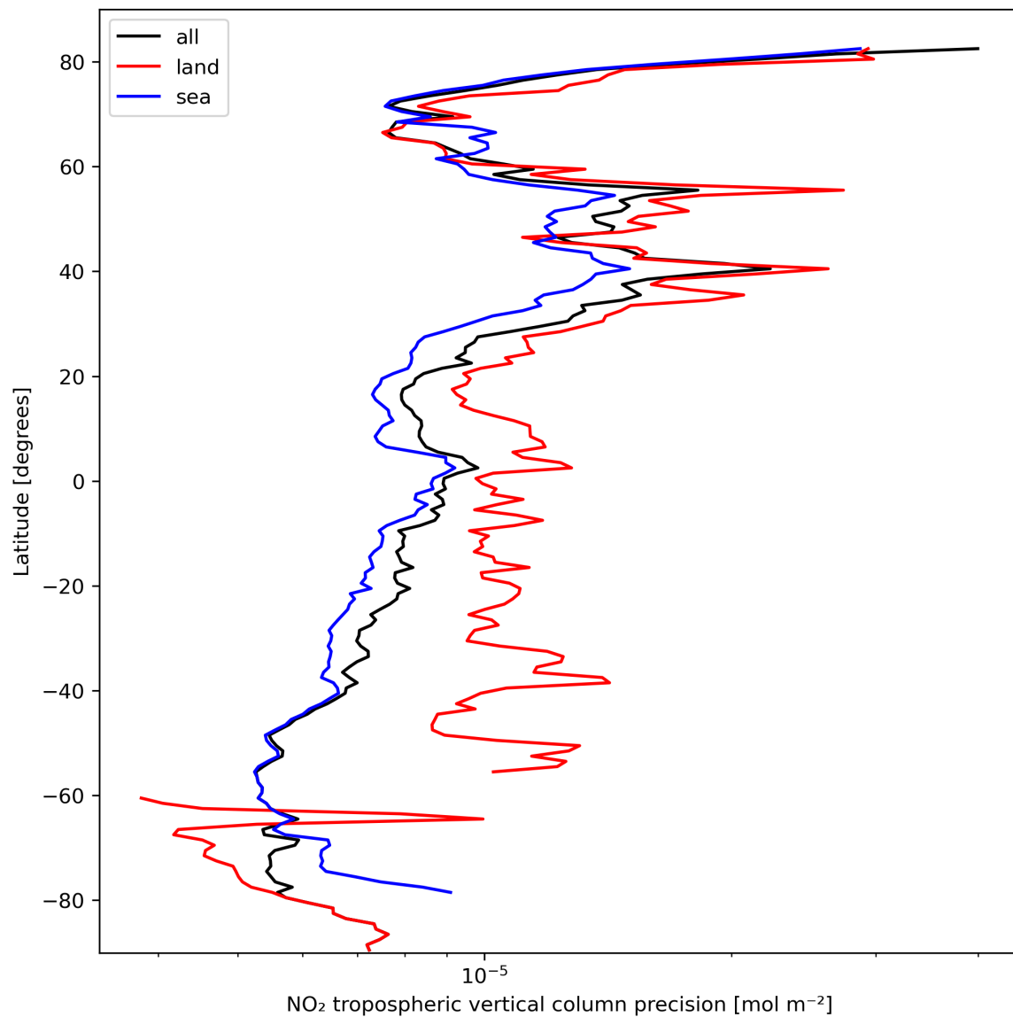
Figure 13: Zonal average of “NO 2 tropospheric vertical column precision” for 2024-03-05 to 2024-03-07.
