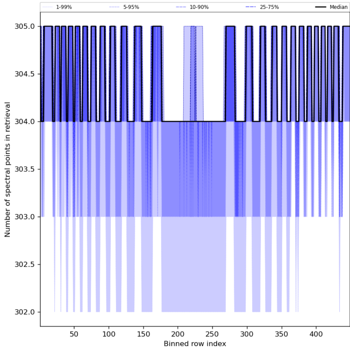
Figure 50: Along track statistics of “Number of spectral points in retrieval” for 2024-03-05 to 2024-03-07
