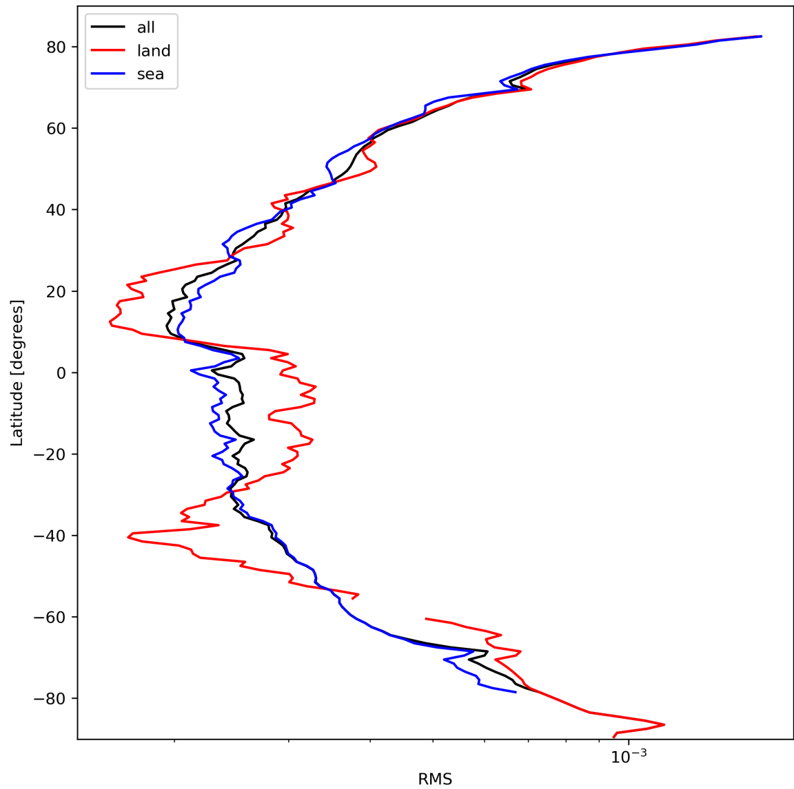
Figure 26: Zonal average of “RMS” for 2024-03-05 to 2024-03-07.
