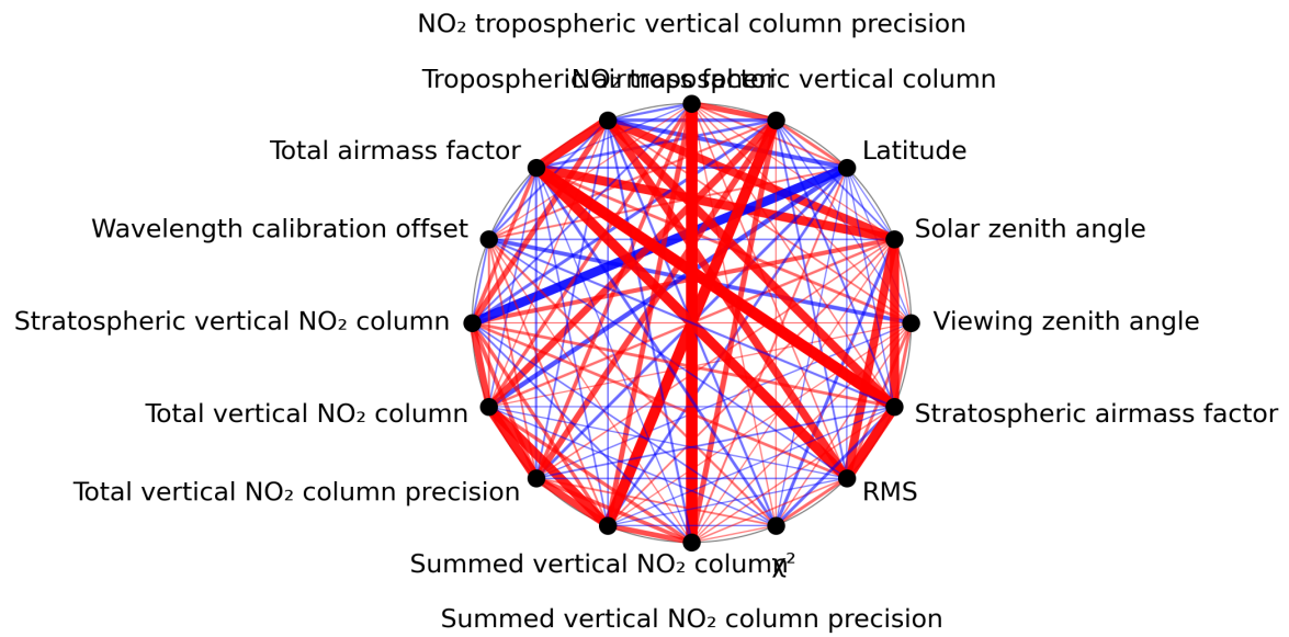
Figure 1: Map of correlation graph for 2024-03-05 to 2024-03-07.
