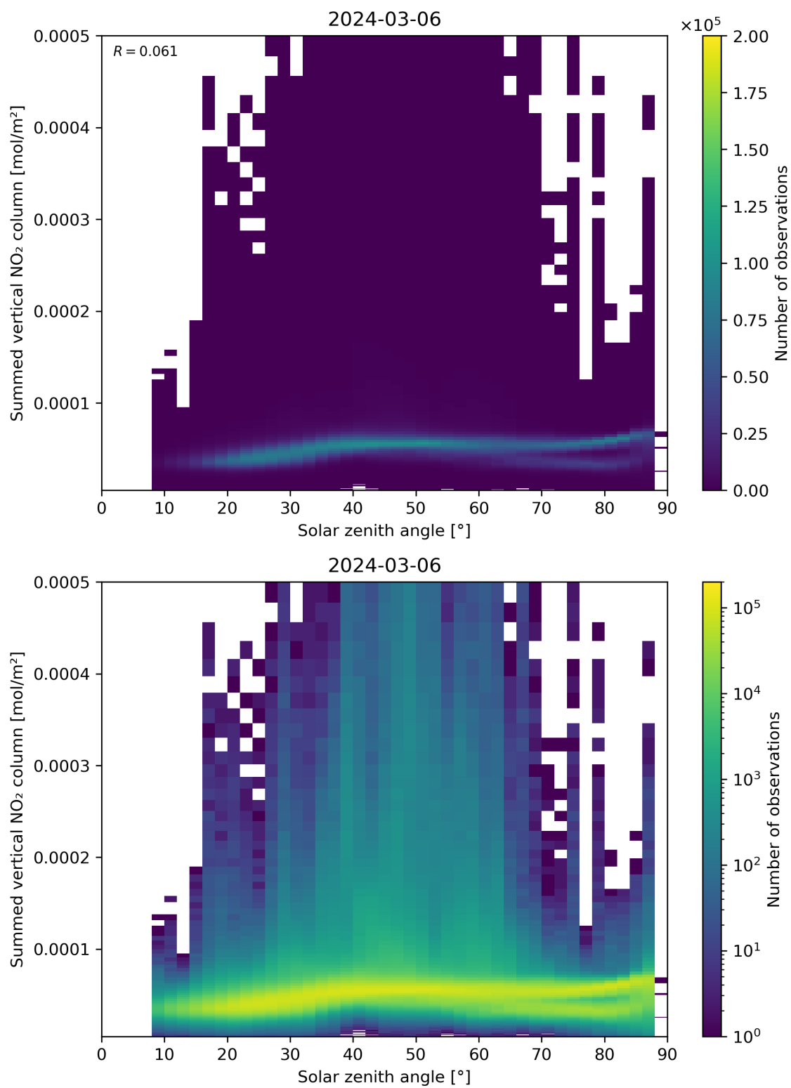
Figure 151: Scatter density plot of “Solar zenith angle” against “Summed vertical NO 2 column” for 2024-03-05 to 2024-03-07.
