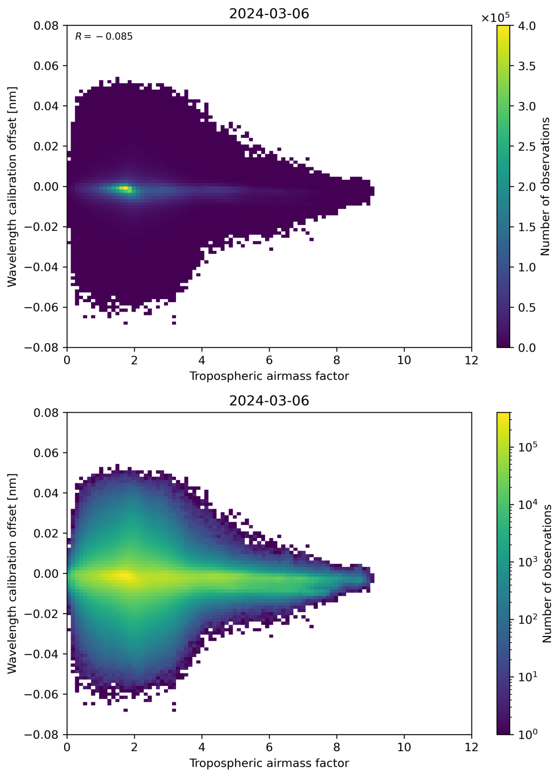
Figure 80: Scatter density plot of “Tropospheric airmass factor” against “Wavelength calibration offset” for 2024-03-05 to 2024-03-07.
