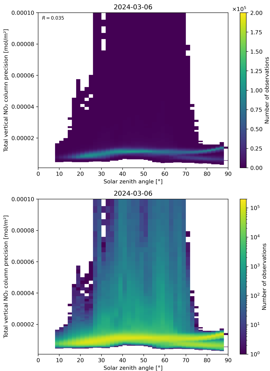
Figure 154: Scatter density plot of “Solar zenith angle” against “Total vertical NO 2 column precision” for 2024-03-05 to 2024-03-07.
