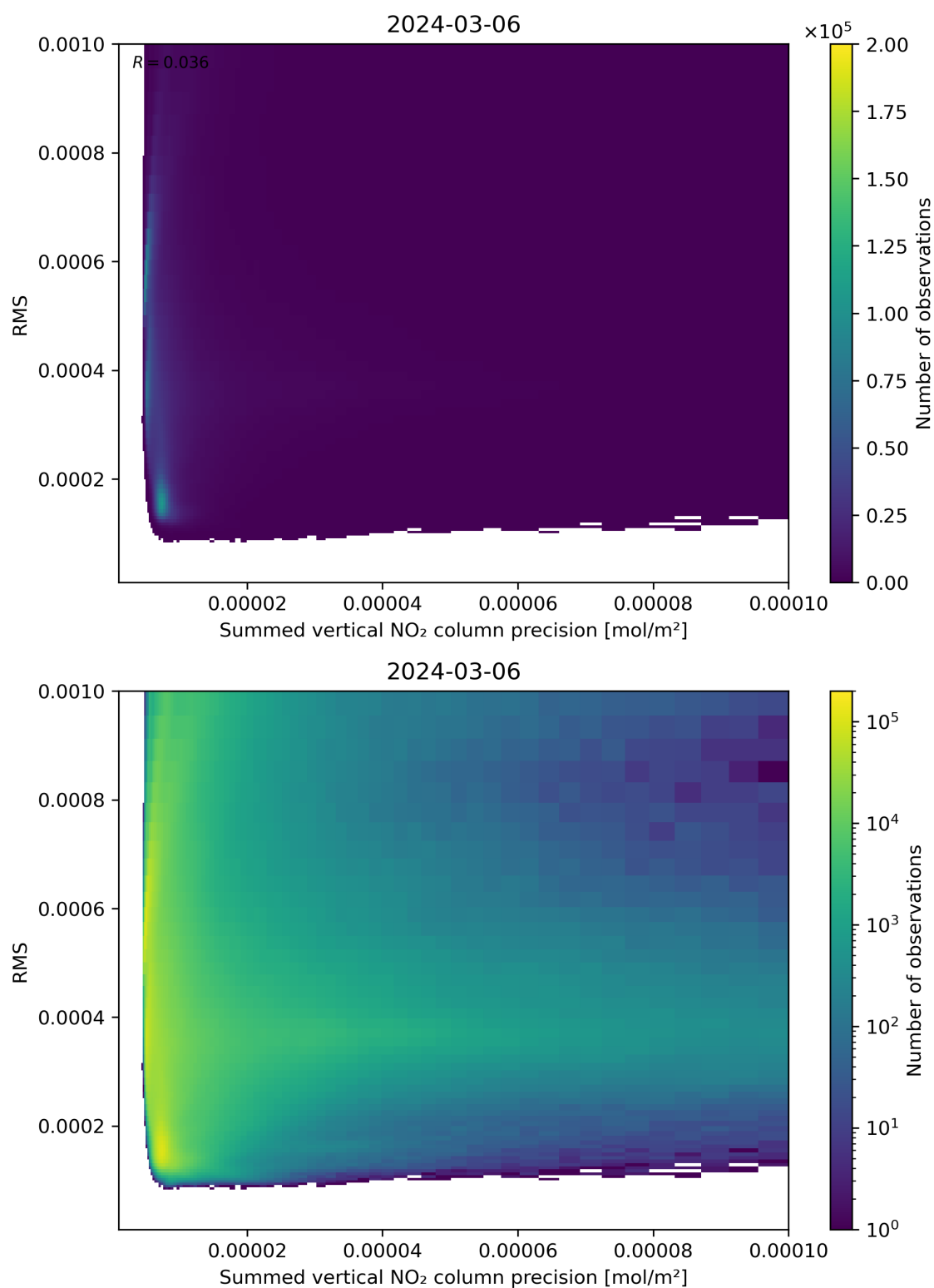
Figure 108: Scatter density plot of “Summed vertical NO 2 column precision” against “RMS” for 2024-03-05 to 2024-03-07.
