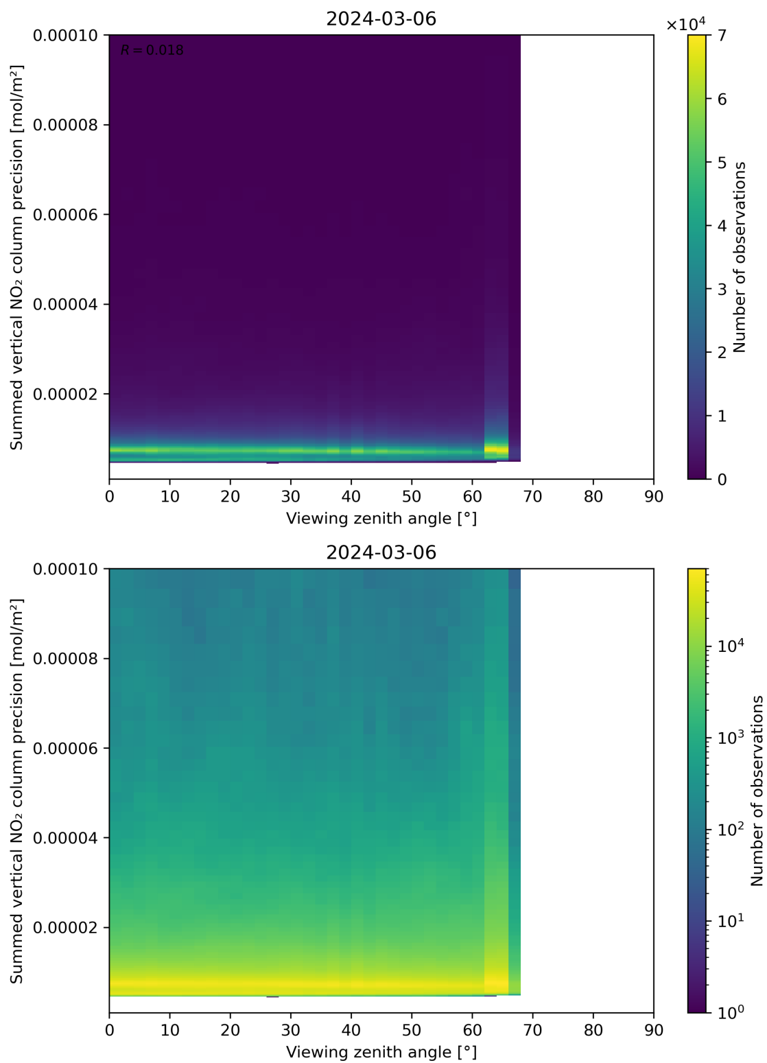
Figure 166: Scatter density plot of “Viewing zenith angle” against “Summed vertical NO 2 column precision” for 2024-03-05 to 2024-03-07.
