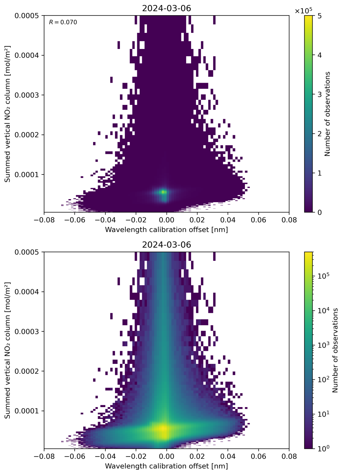
Figure 177: Scatter density plot of “Wavelength calibration offset” against “Summed vertical NO 2 column” for 2024-03-05 to 2024-03-07.
