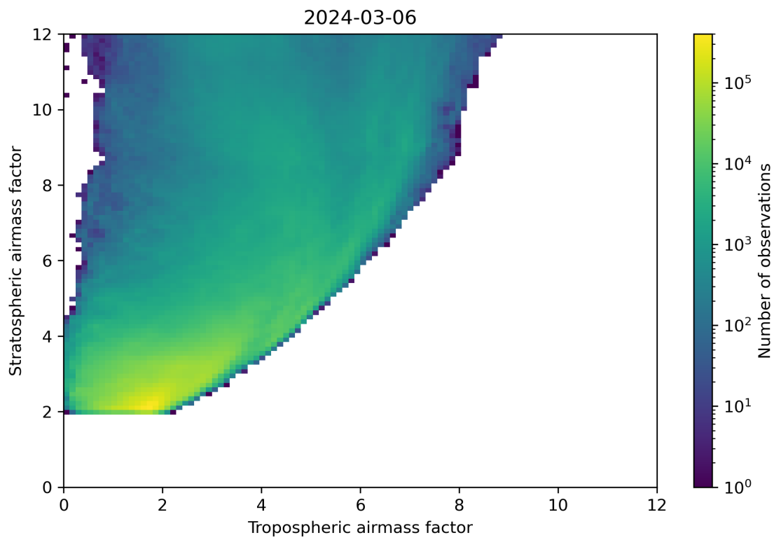
Figure 71: Scatter density plot of “Tropospheric airmass factor” against “Stratospheric airmass factor” for 2024-03-05 to 2024-03-07.
