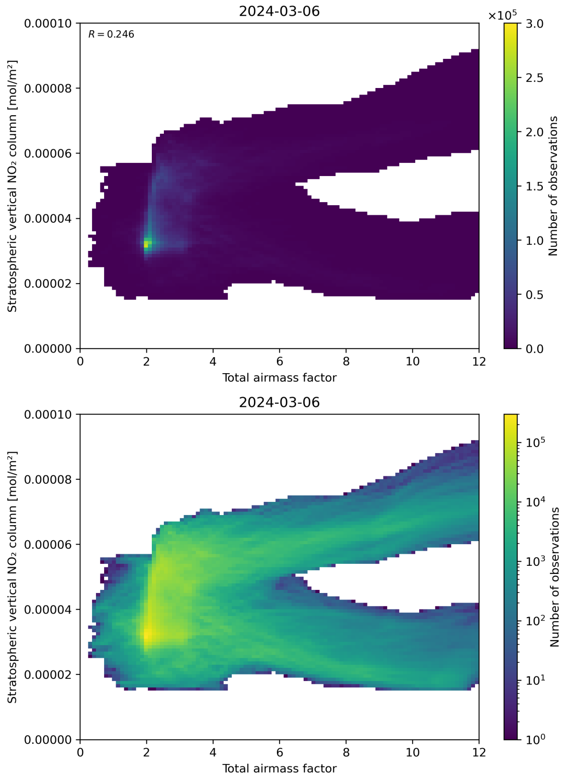
Figure 64: Scatter density plot of “Total airmass factor” against “Stratospheric vertical \text{NO}_2 column” for 2024-03-05 to 2024-03-07.
