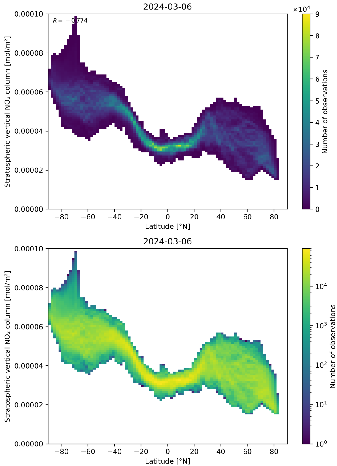
Figure 87: Scatter density plot of “Latitude” against “Stratospheric vertical NO 2 column” for 2024-03-05 to 2024-03-07.
