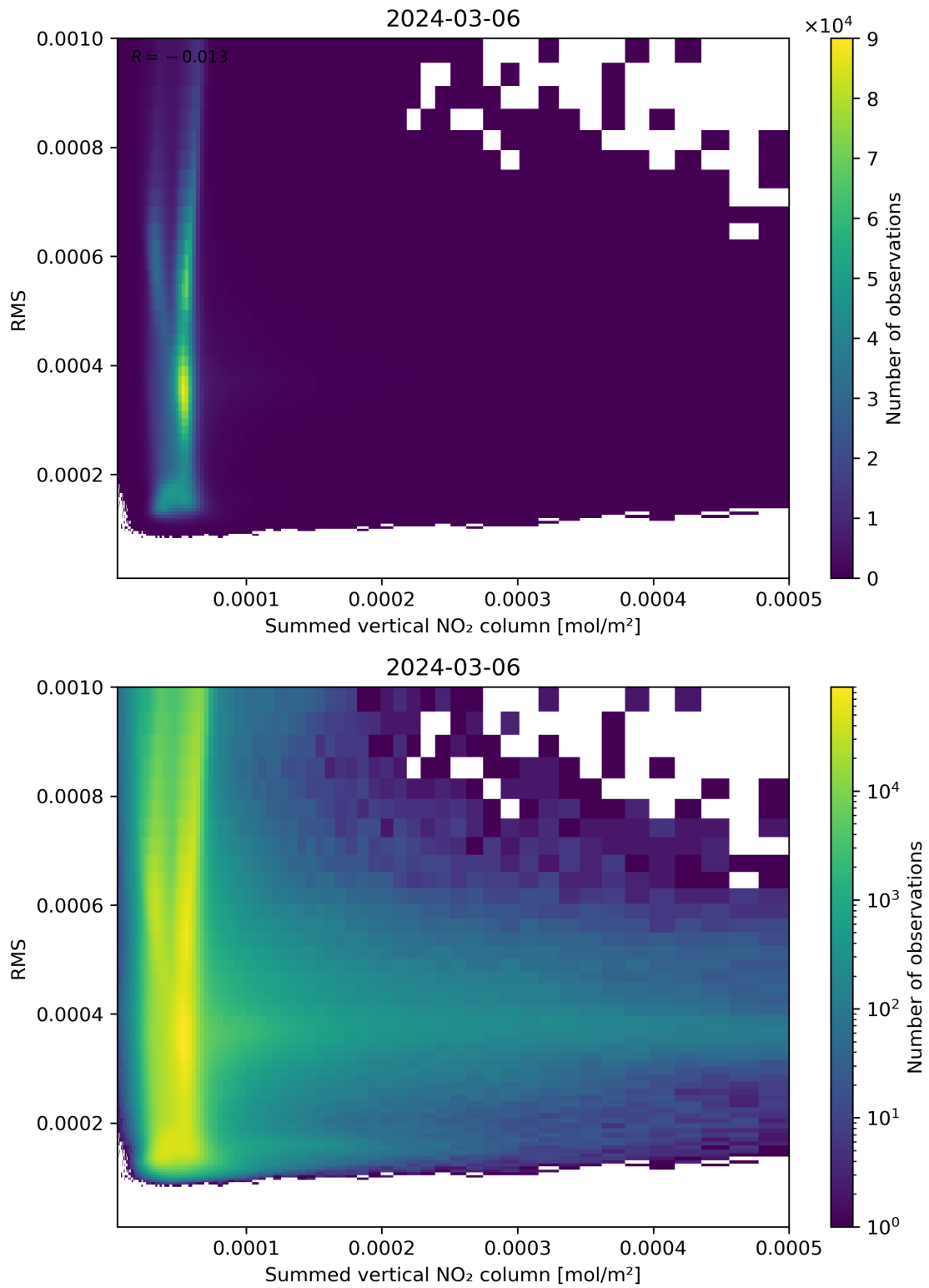
Figure 109: Scatter density plot of “Summed vertical NO 2 column” against “RMS” for 2024-03-05 to 2024-03-07.
