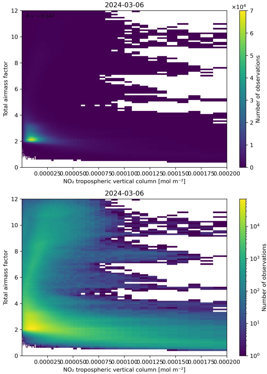
Figure 122: Scatter density plot of “NO 2 tropospheric vertical column” against “Total air mass factor” for 2024-03-05 to 2024-03-07.
