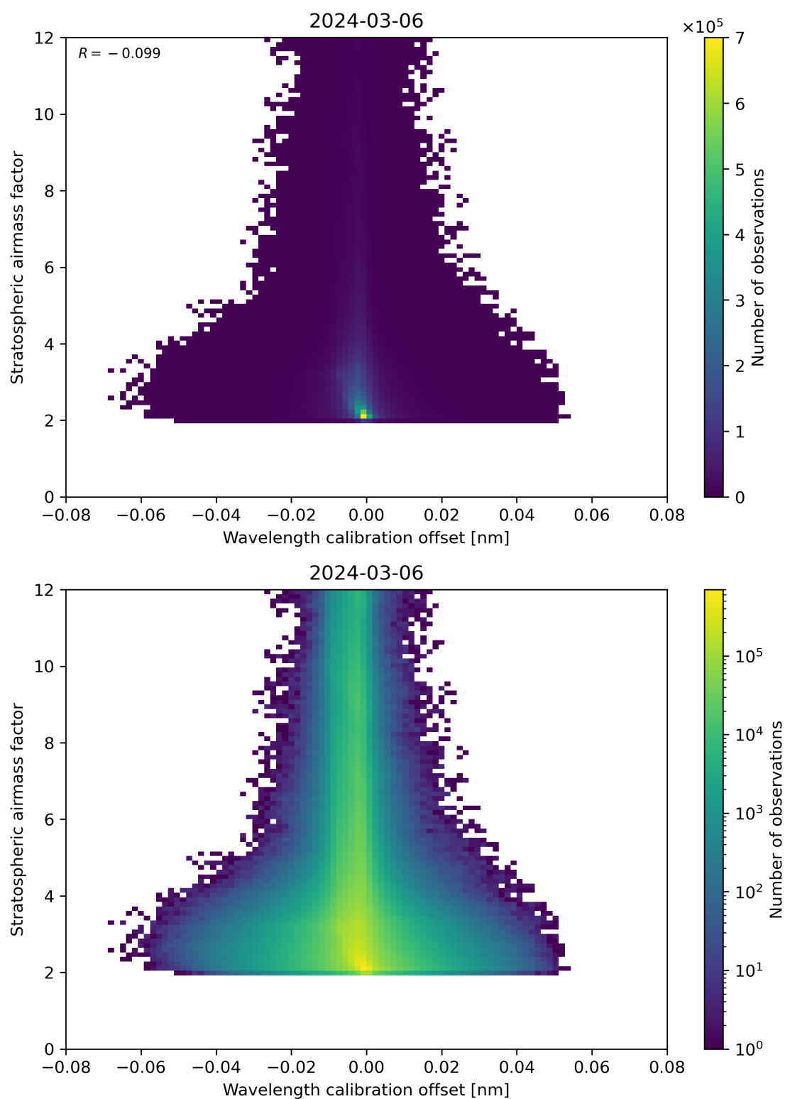
Figure 174: Scatter density plot of “Wavelength calibration offset” against “Stratospheric air mass factor” for 2024-03-05 to 2024-03-07.
