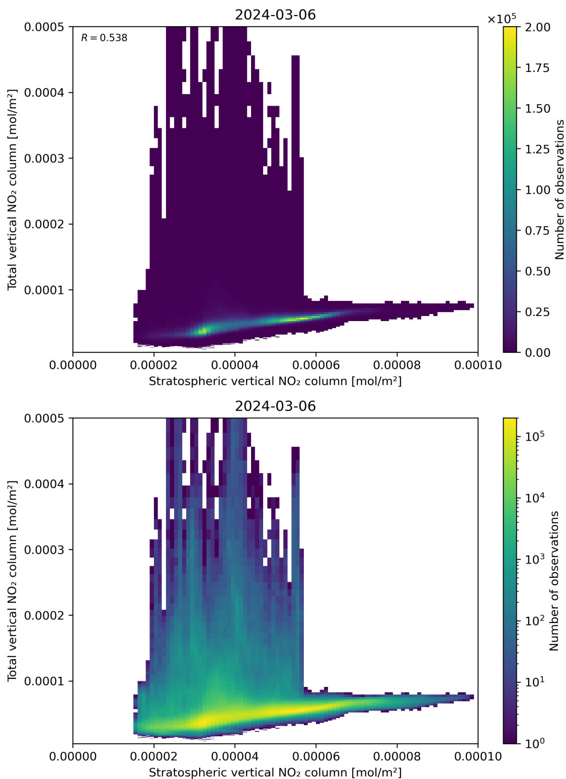
Figure 100: Scatter density plot of “Stratospheric vertical NO 2 column” against “Total vertical NO 2 column” for 2024-03-05 to 2024-03-07.
