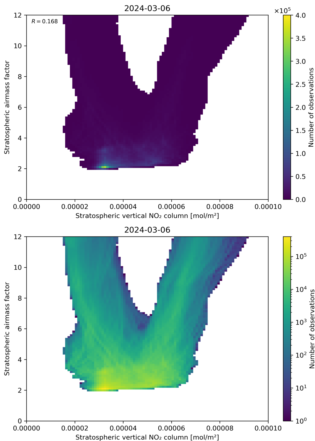
Figure 96: Scatter density plot of “Stratospheric vertical NO 2 column” against “Stratospheric airmass factor” for 2024-03-05 to 2024-03-07.
