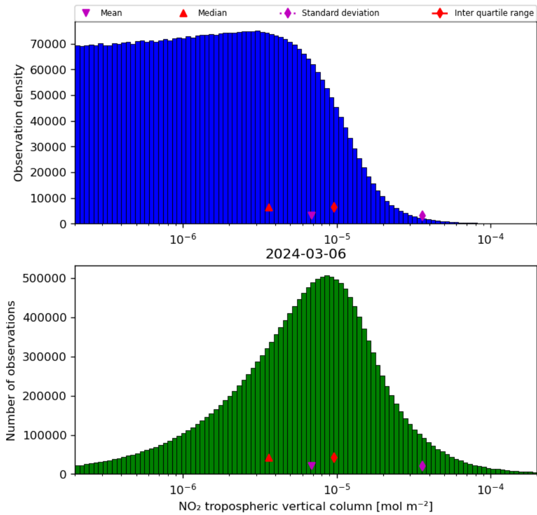
Figure 29: Histogram of “NO 2 tropospheric vertical column” for 2024-03-05 to 2024-03-07
