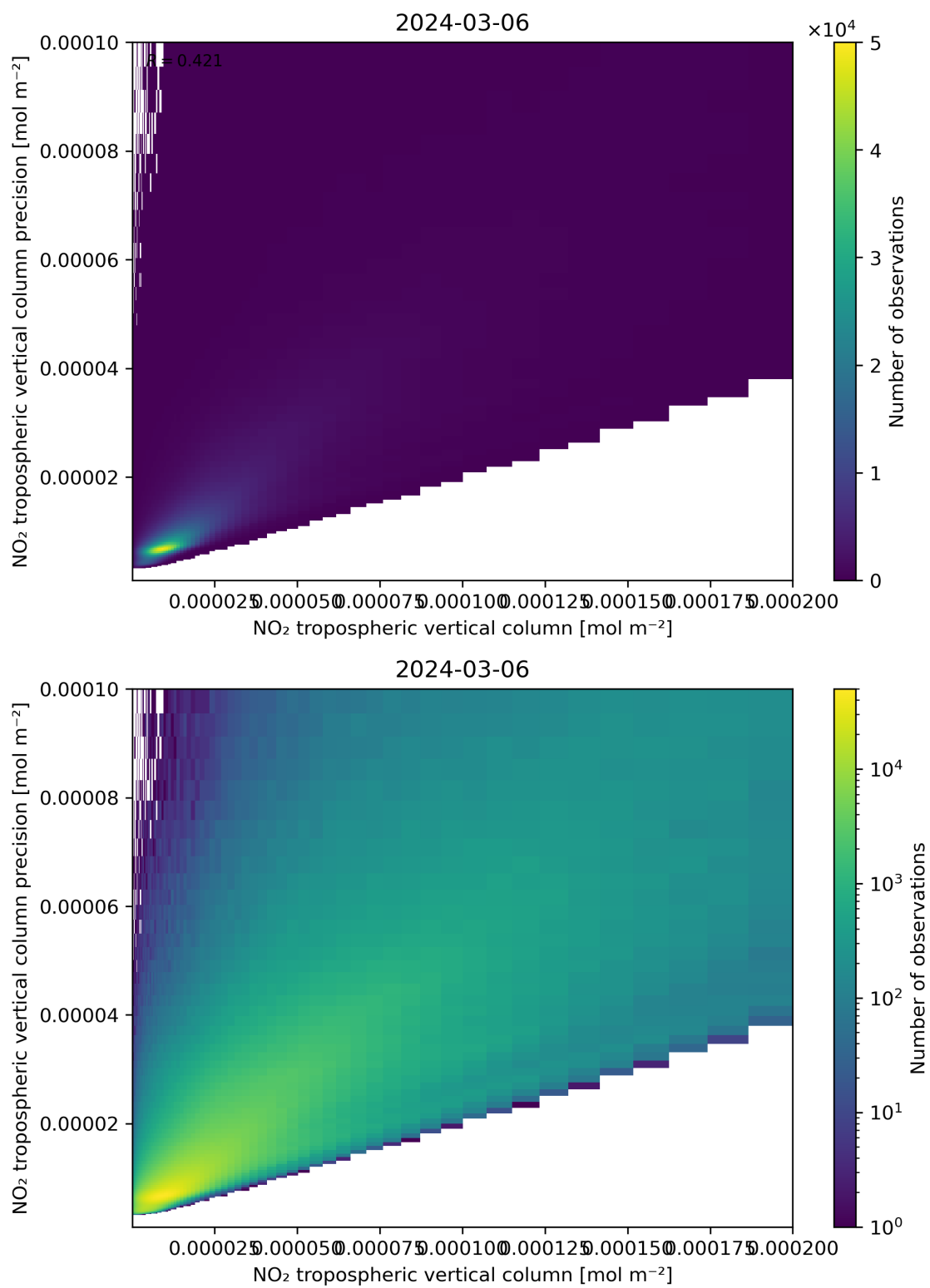
Figure 130: Scatter density plot of “NO 2 tropospheric vertical column” against “NO 2 tropospheric vertical column precision” for 2024-03-05 to 2024-03-07.
