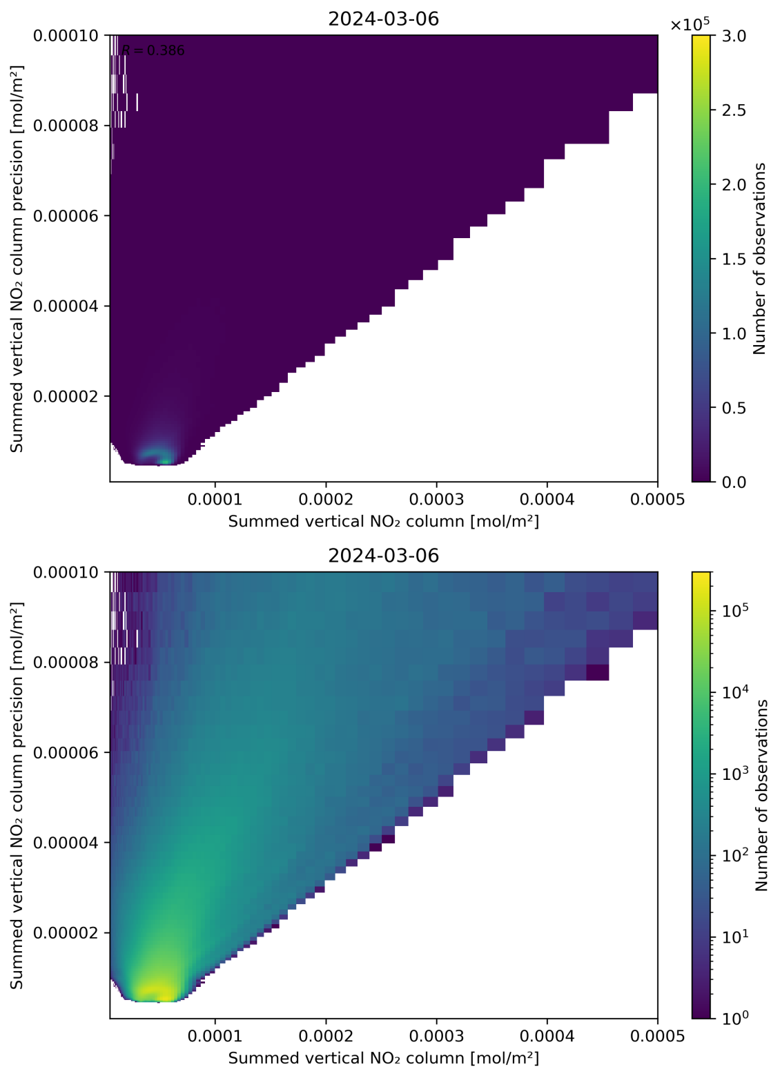
Figure 105: Scatter density plot of “Summed vertical NO 2 column” against “Summed vertical NO 2 column precision” for 2024-03-05 to 2024-03-07.
