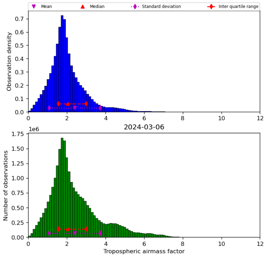
Figure 31: Histogram of “Tropospheric airmass factor” for 2024-03-05 to 2024-03-07
