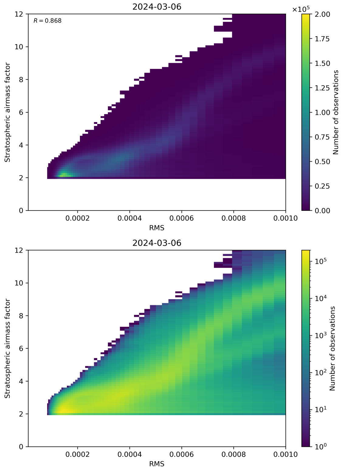
Figure 144: Scatter density plot of “RMS” against “Stratospheric airmass factor” for 2024-03-05 to 2024-03-07.
