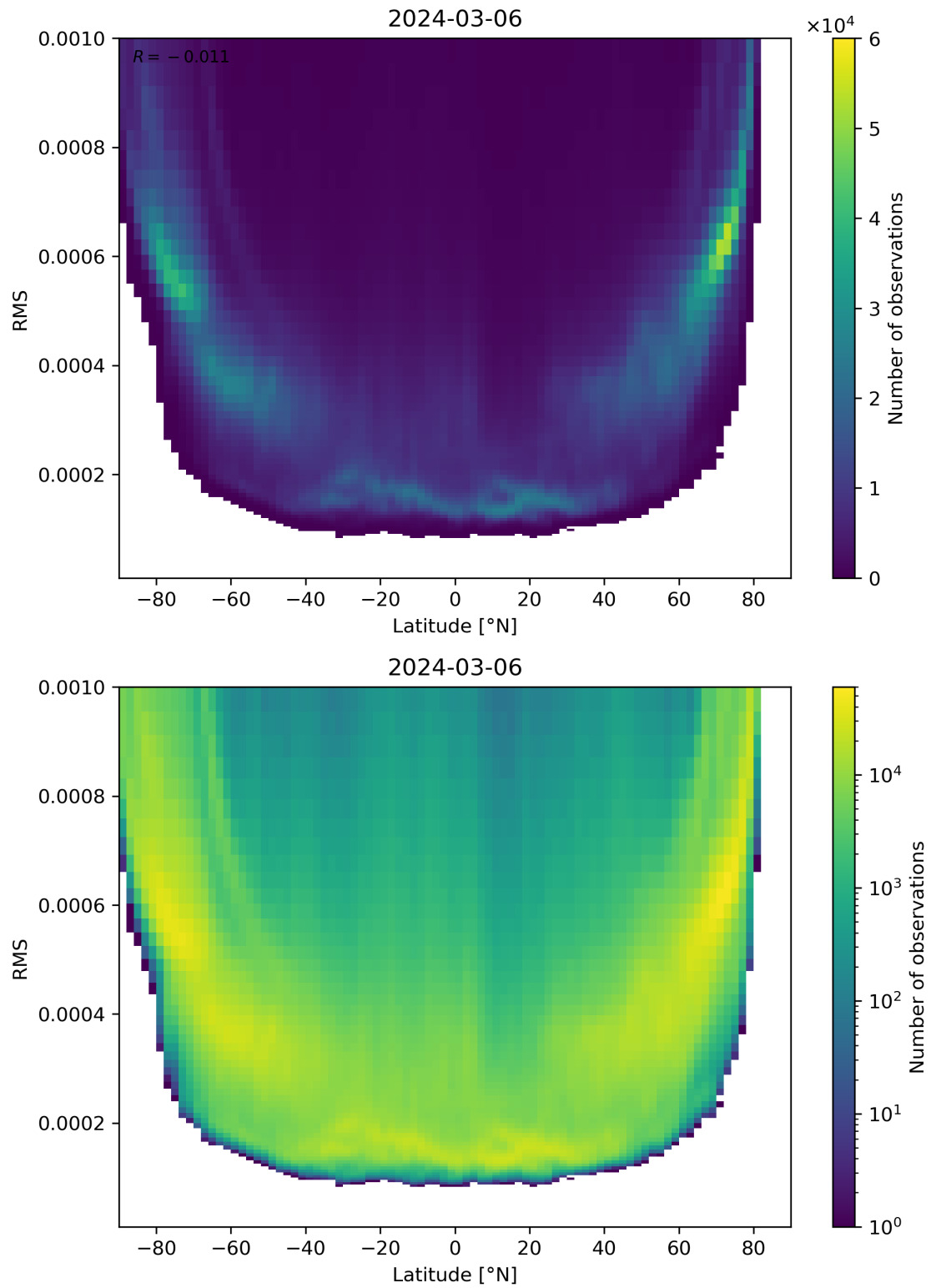
Figure 94: Scatter density plot of “Latitude” against “RMS” for 2024-03-05 to 2024-03-07.
