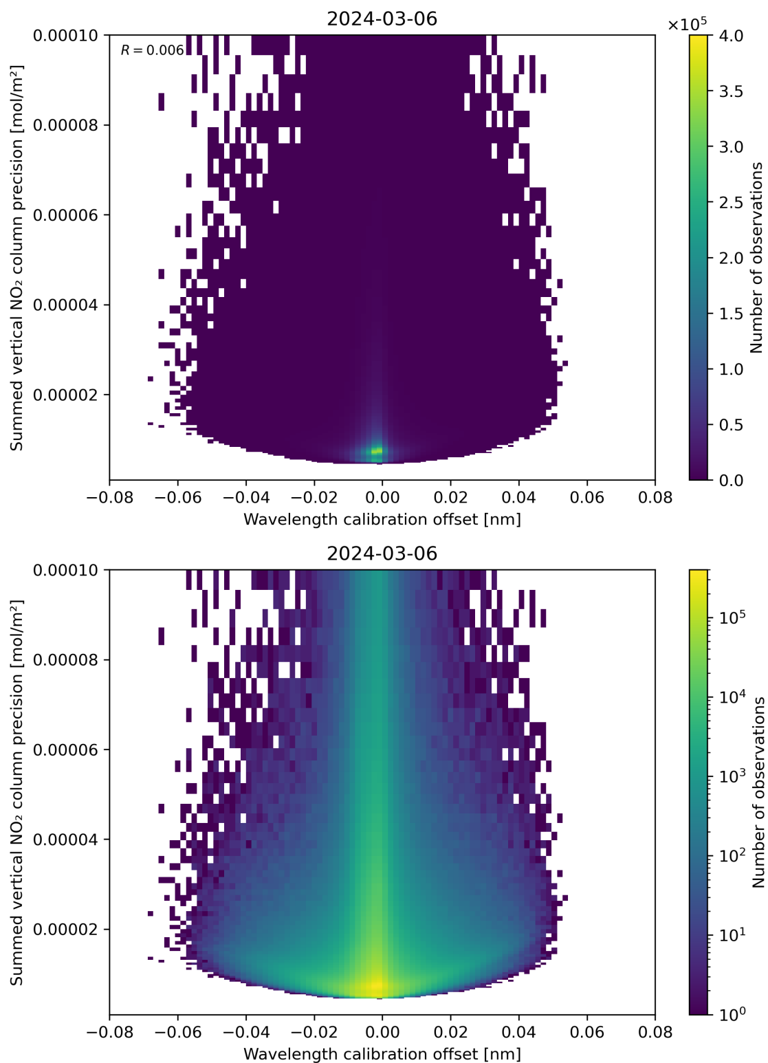
Figure 178: Scatter density plot of “Wavelength calibration offset” against “Summed vertical NO 2 column precision” for 2024-03-05 to 2024-03-07.
