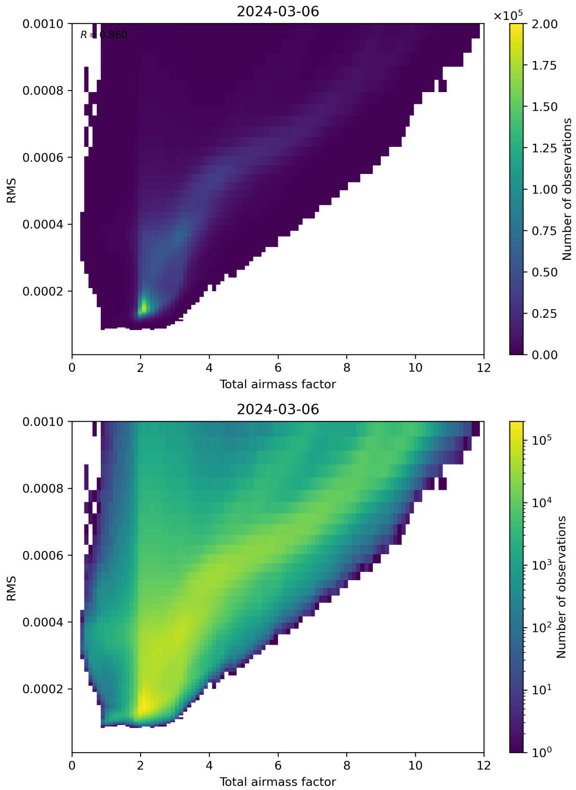
Figure 69: Scatter density plot of “Total airmass factor” against “RMS” for 2024-03-05 to 2024-03-07.
