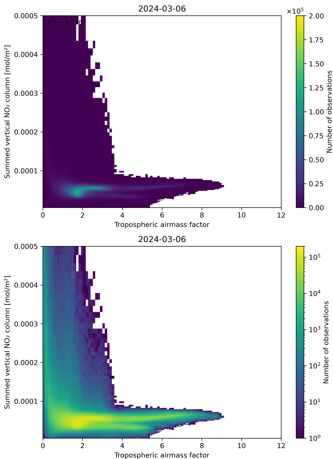
Figure 75: Scatter density plot of “Tropospheric air mass factor” against “Summed vertical NO 2 column” for 2024-03-05 to 2024-03-07.
