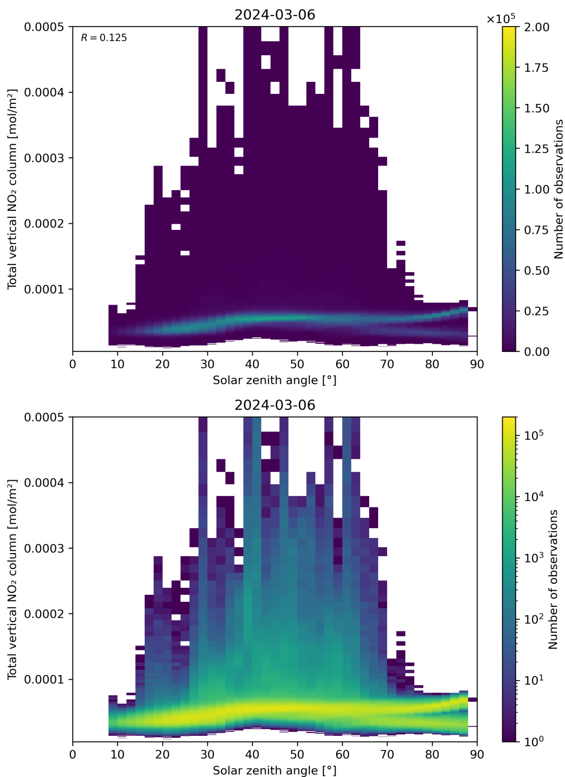
Figure 153: Scatter density plot of “Solar zenith angle” against “Total vertical NO 2 column” for 2024-03-05 to 2024-03-07.
