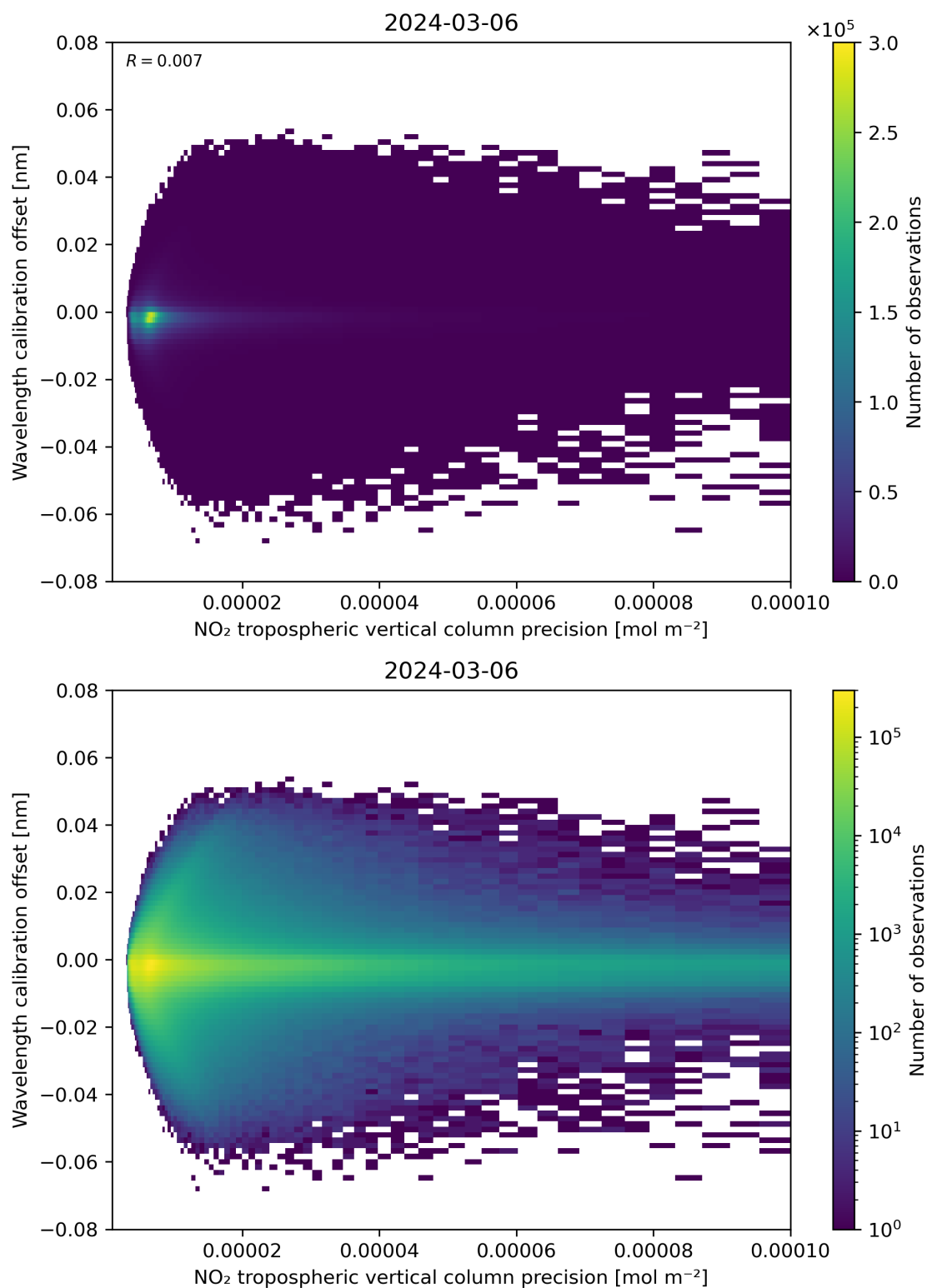
Figure 141: Scatter density plot of “NO 2 tropospheric vertical column precision” against “Wavelength calibration offset” for 2024-03-05 to 2024-03-07.
