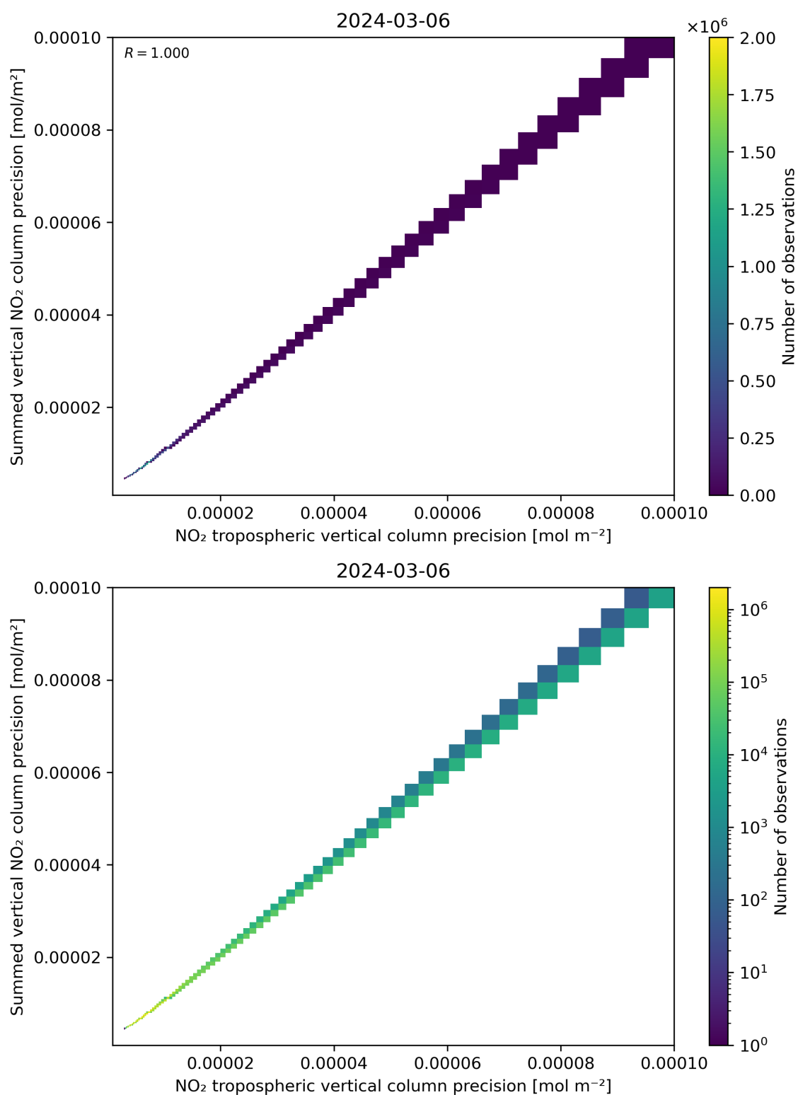
Figure 137: Scatter density plot of “NO 2 tropospheric vertical column precision” against “Summed vertical NO 2 column precision” for 2024-03-05 to 2024-03-07.
