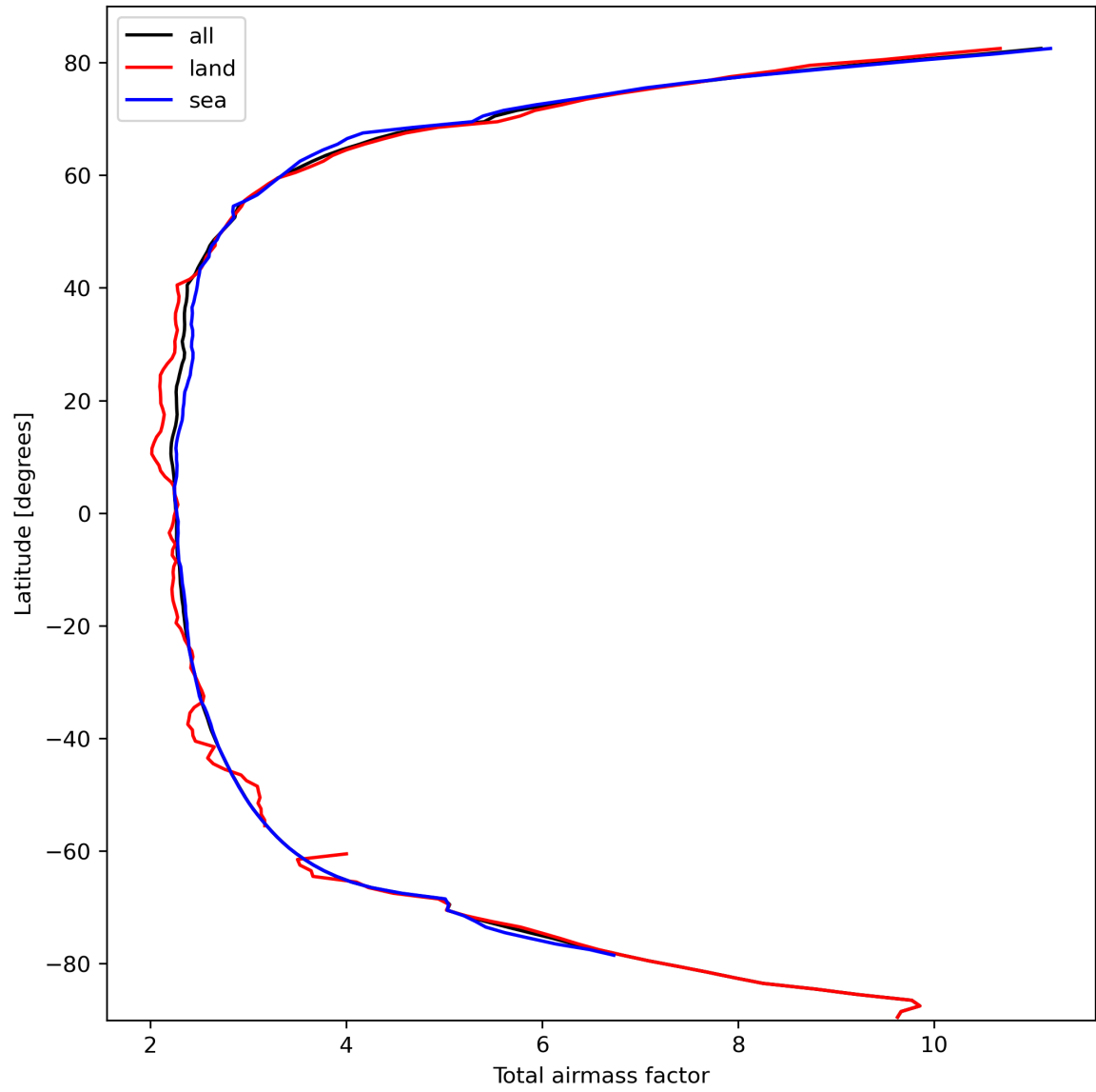
Figure 15: Zonal average of “Total airmass factor” for 2024-03-05 to 2024-03-07.
