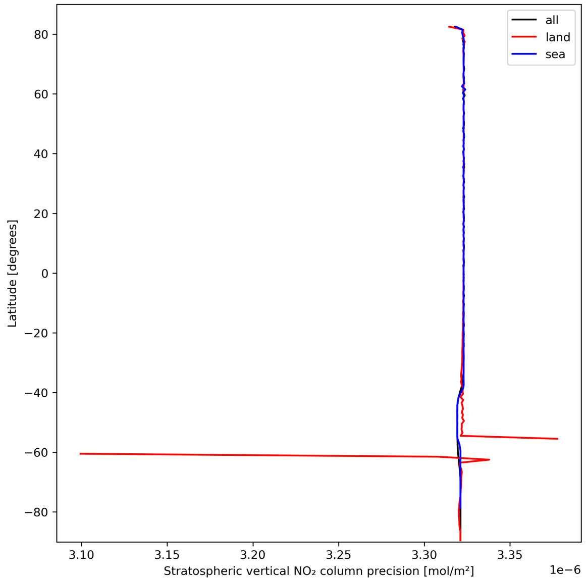
Figure 20: Zonal average of “Stratospheric vertical NO 2 column precision” for 2024-03-05 to 2024-03-07.
