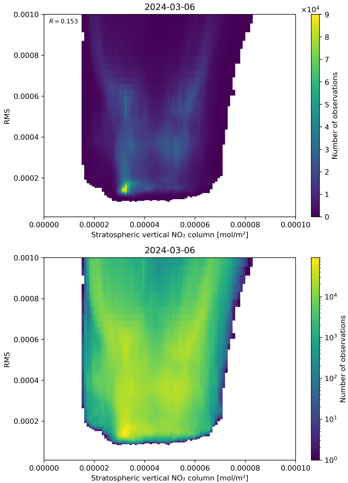
Figure 102: Scatter density plot of “Stratospheric vertical NO 2 column” against “RMS” for 2024-03-05 to 2024-03-07.
