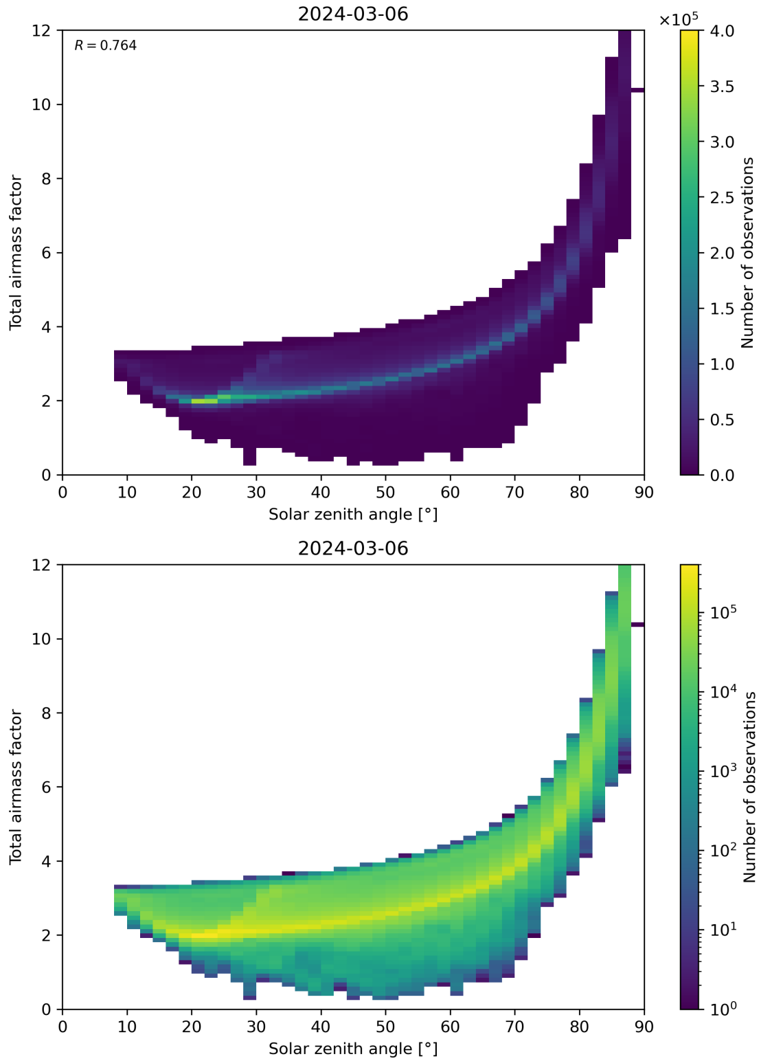
Figure 146: Scatter density plot of “Solar zenith angle” against “Total air mass factor” for 2024-03-05 to 2024-03-07.
