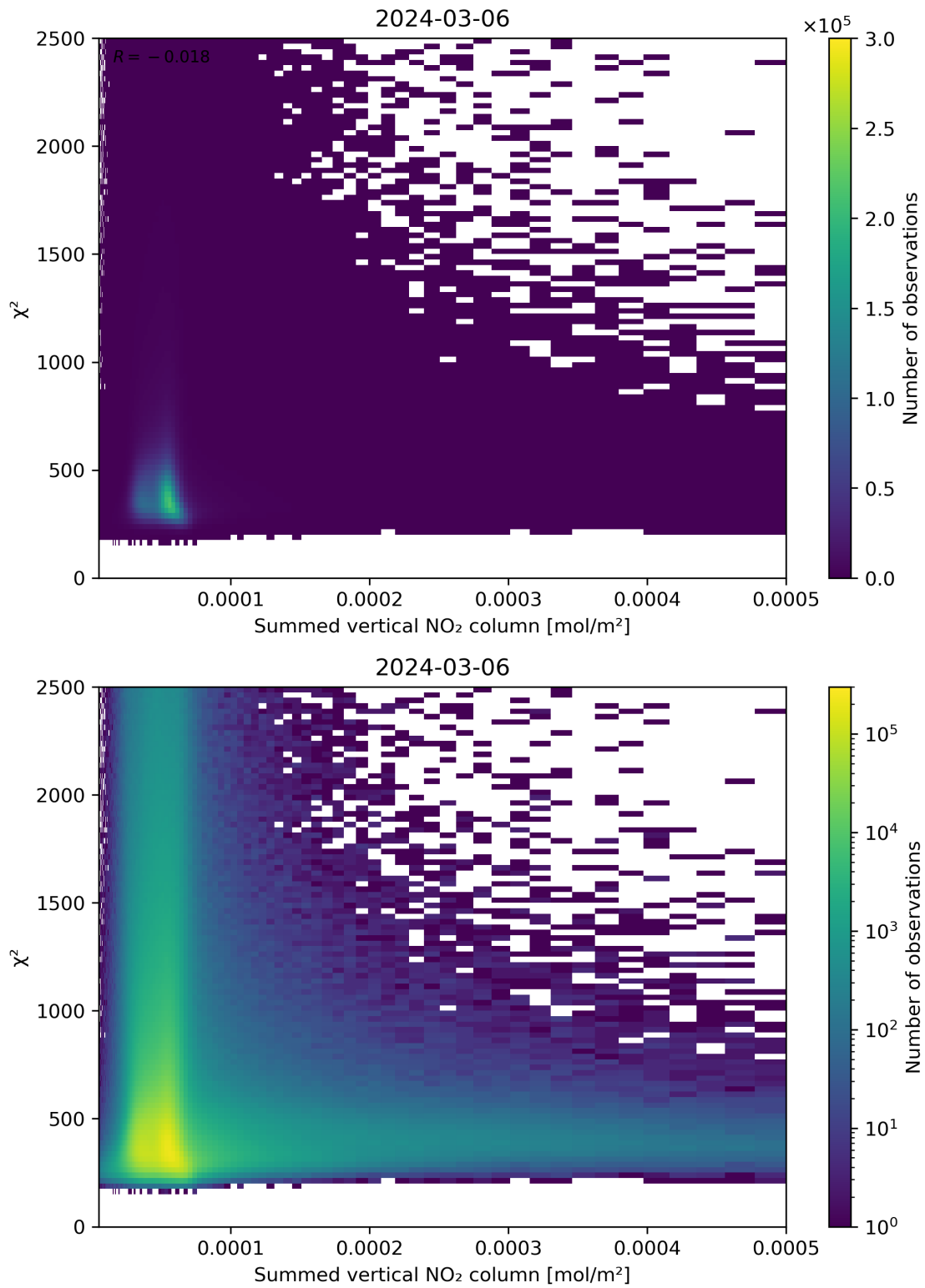
Figure 104: Scatter density plot of “Summed vertical NO 2 column” against “ \chi^2 ” for 2024-03-05 to 2024-03-07.
