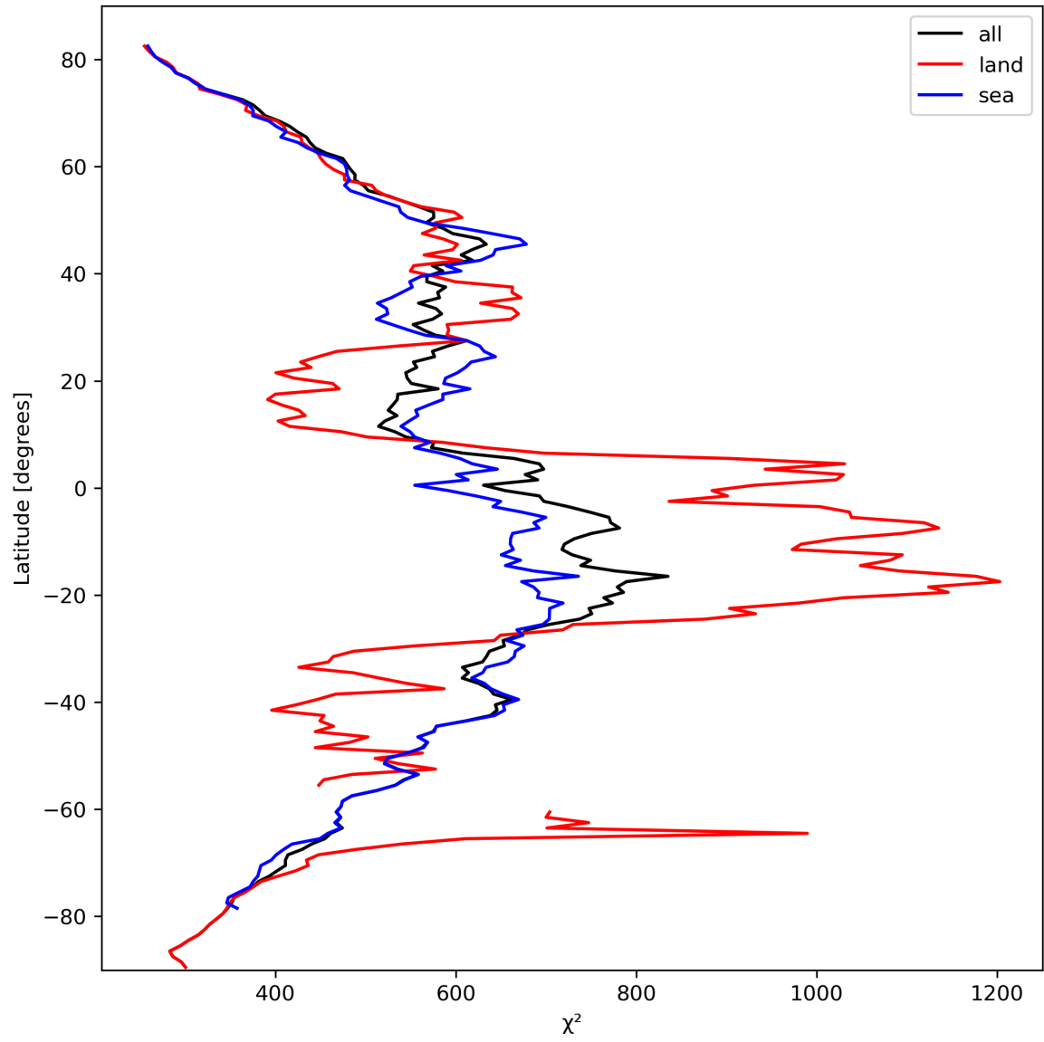
Figure 25: Zonal average of “ \chi^2 ” for 2024-03-05 to 2024-03-07.
