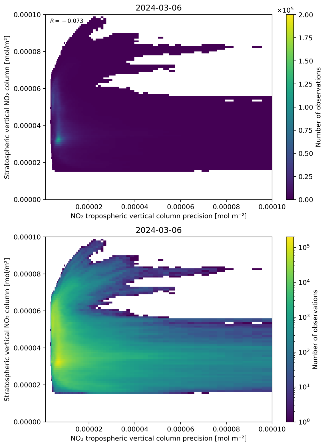
Figure 135: Scatter density plot of “NO 2 tropospheric vertical column precision” against “Stratospheric vertical NO 2 column” for 2024-03-05 to 2024-03-07.
