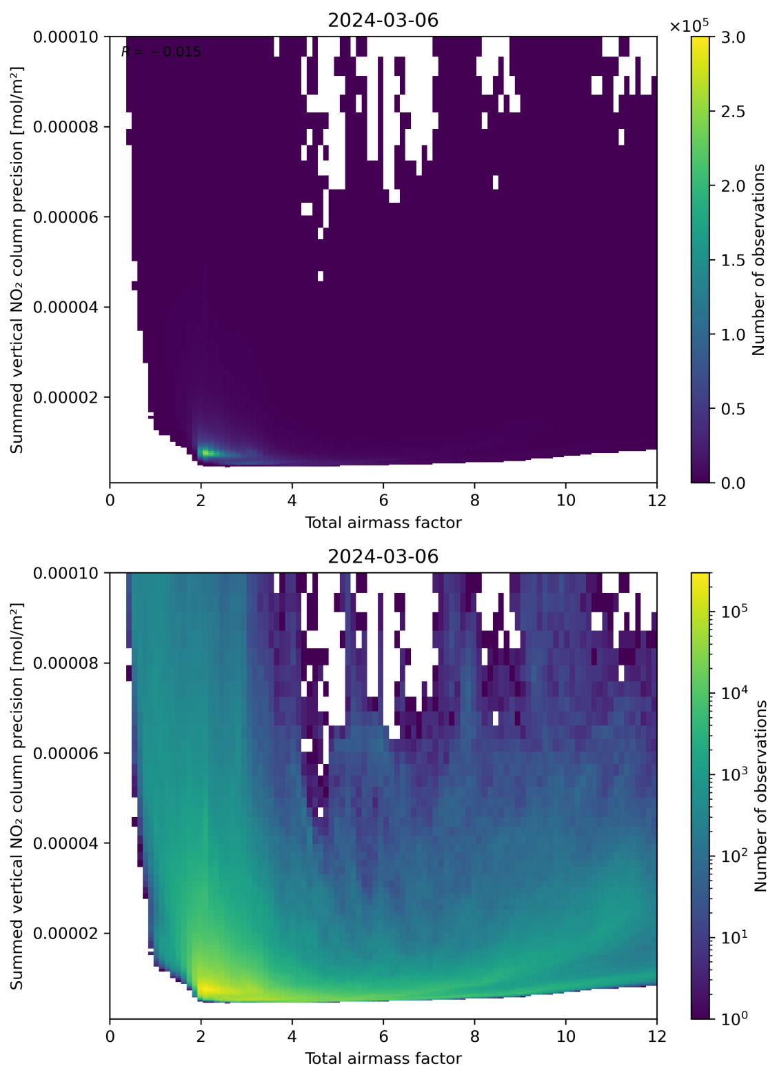
Figure 66: Scatter density plot of “Total airmass factor” against “Summed vertical NO 2 column precision” for 2024-03-05 to 2024-03-07.
