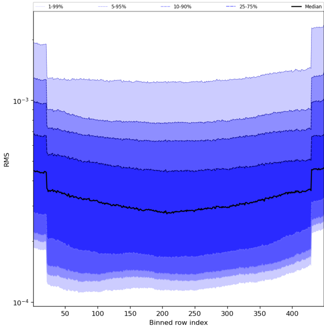
Figure 60: Along track statistics of “RMS” for 2024-03-05 to 2024-03-07
