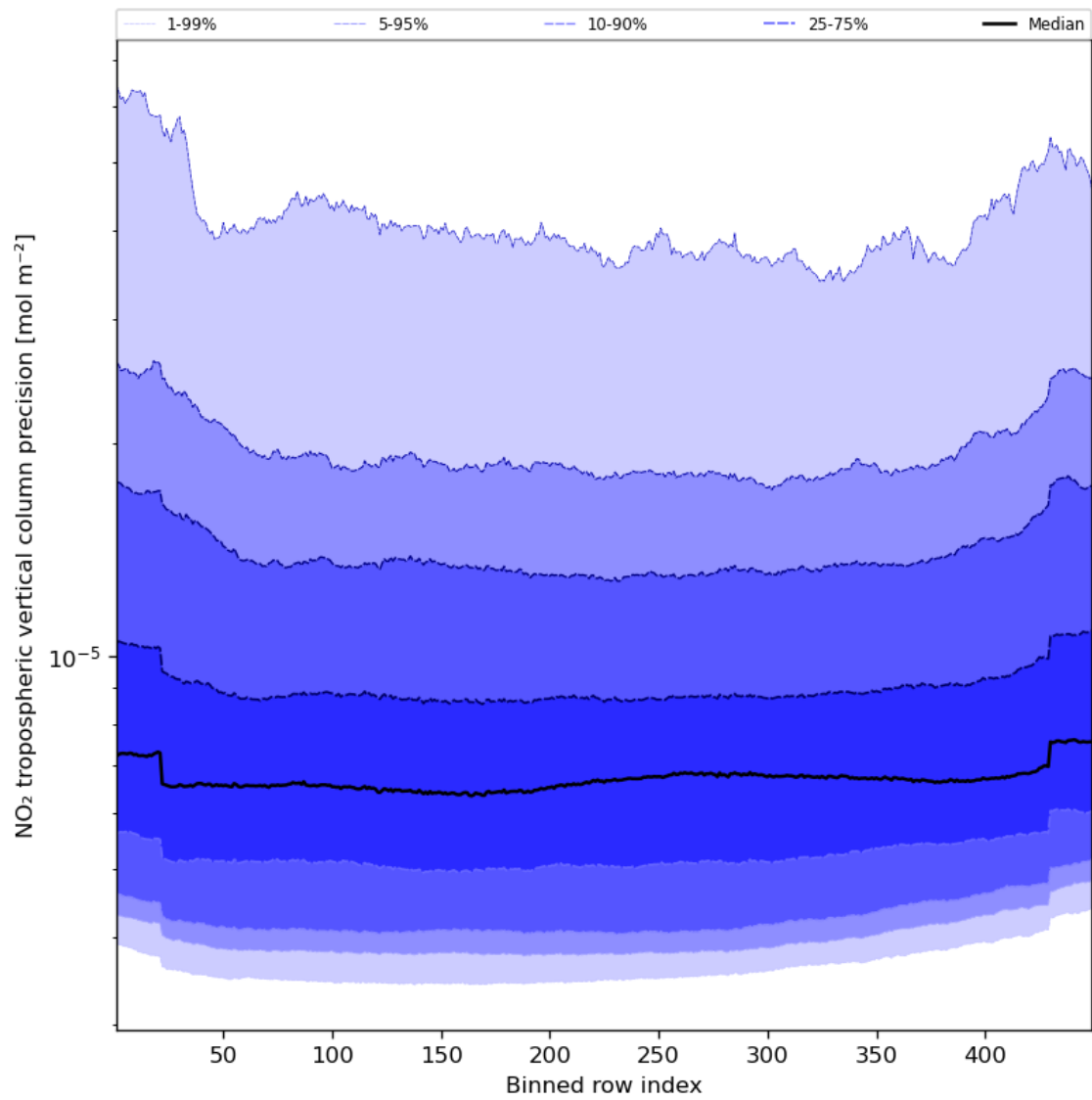
Figure 47: Along track statistics of “NO 2 tropospheric vertical column precision” for 2024-03-05 to 2024-03-07
