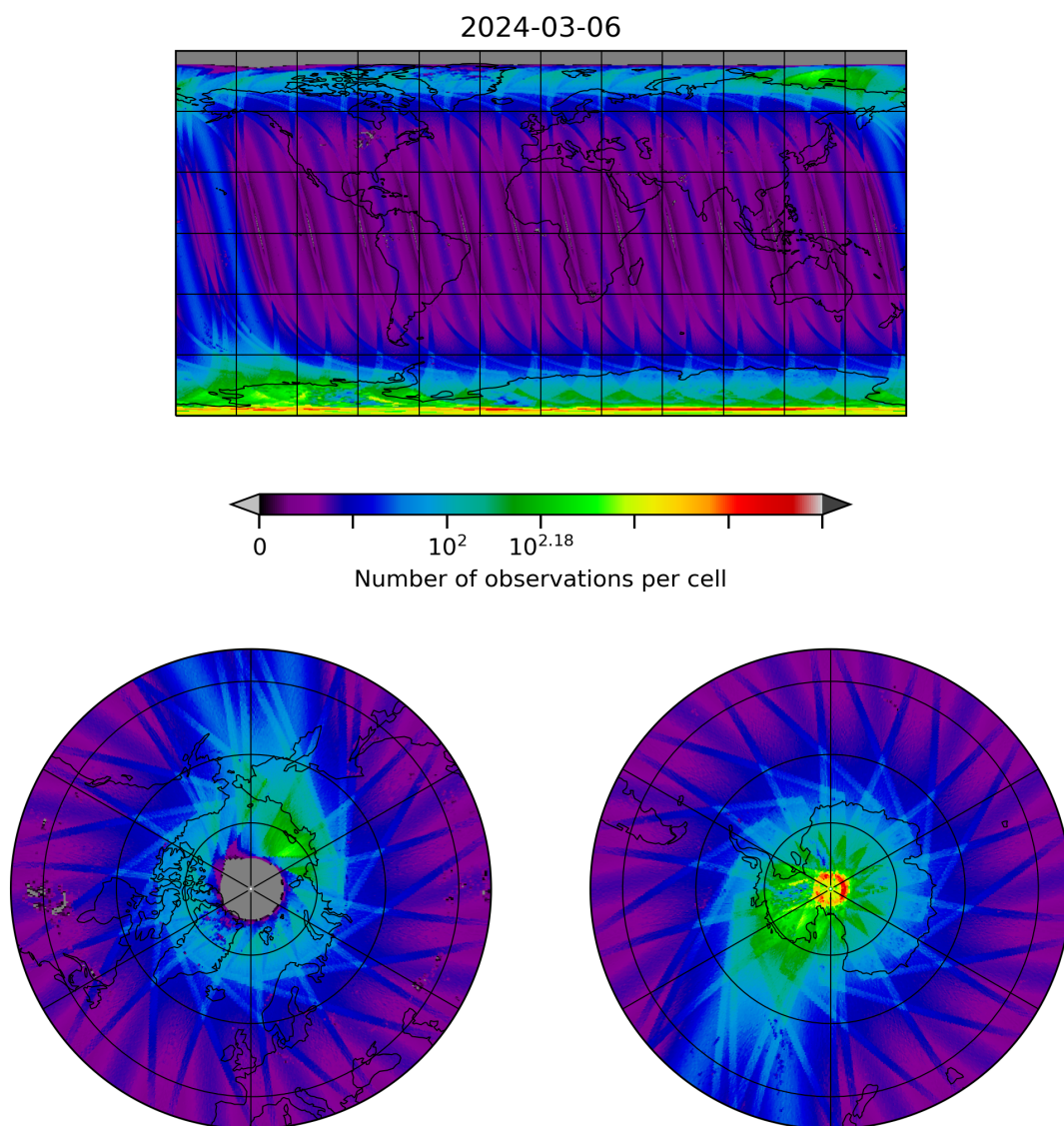
Figure 10: Map of the number of observations for 2024-03-05 to 2024-03-07
