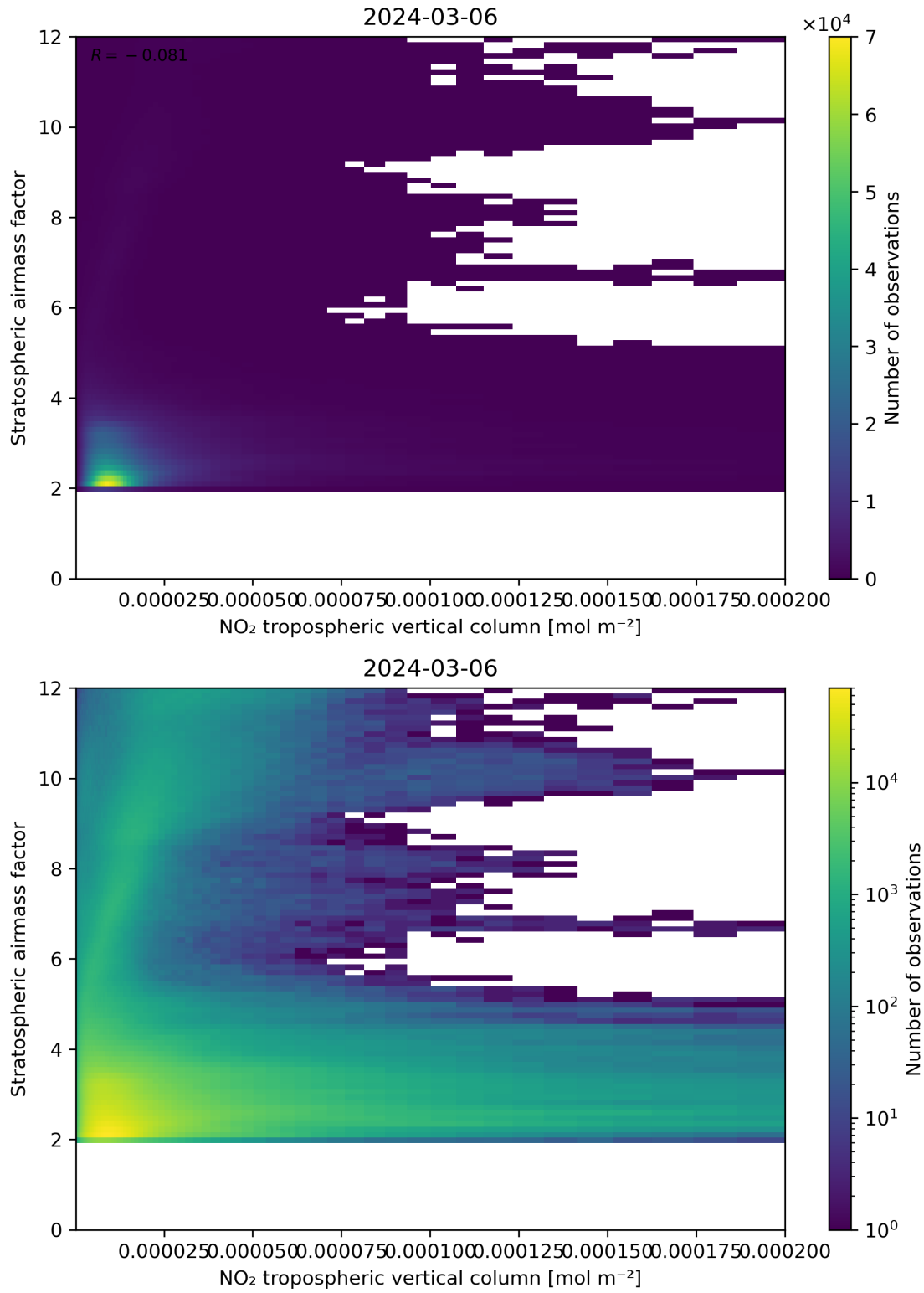
Figure 121: Scatter density plot of “NO 2 tropospheric vertical column” against “Stratospheric air mass factor” for 2024-03-05 to 2024-03-07.
