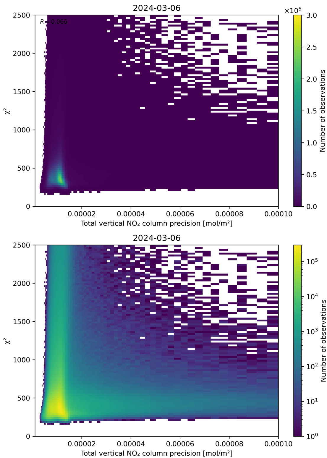
Figure 116: Scatter density plot of “Total vertical NO 2 column precision” against “ \chi^2 ” for 2024-03-05 to 2024-03-07.
