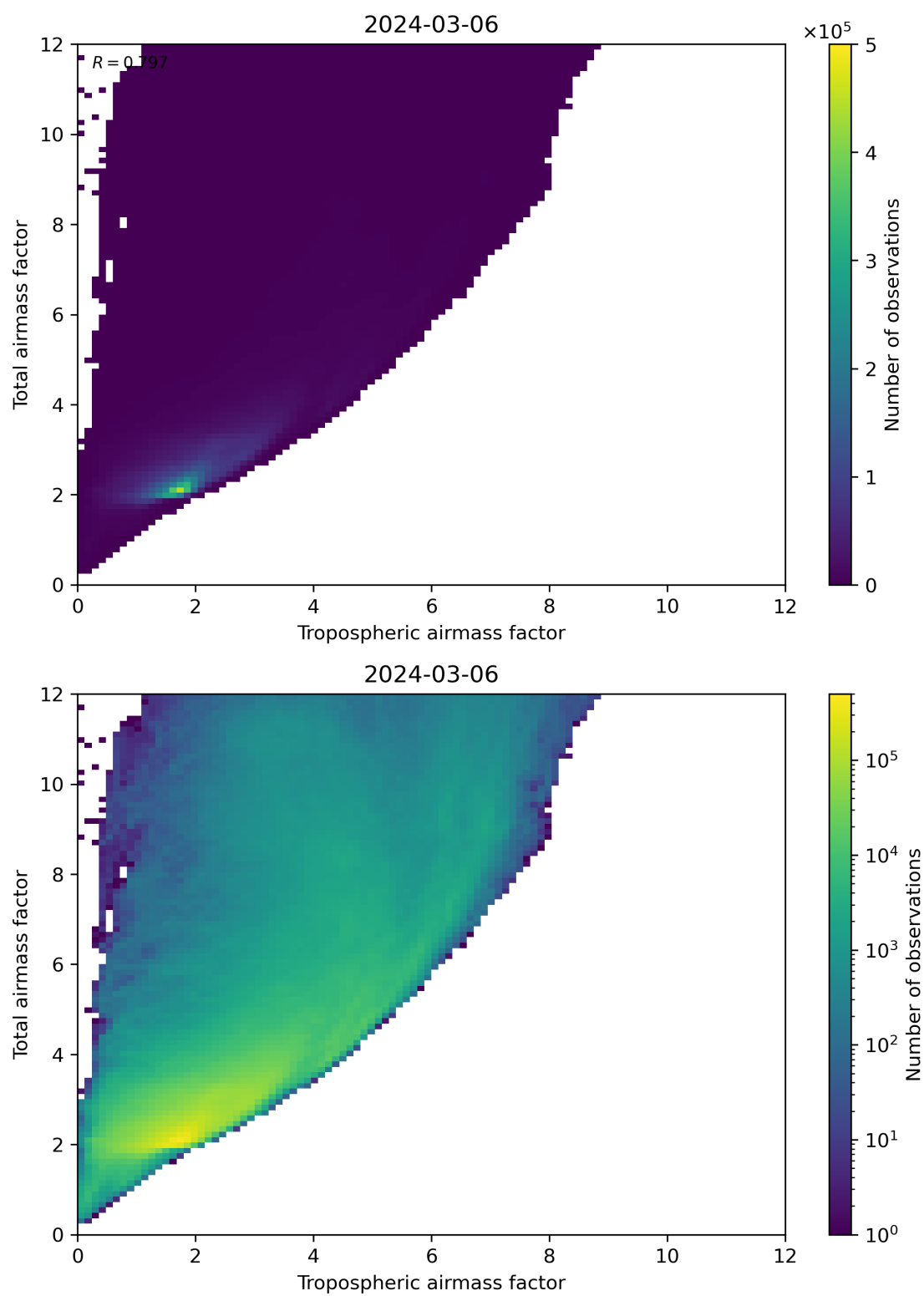
Figure 72: Scatter density plot of “Tropospheric airmass factor” against “Total airmass factor” for 2024-03-05 to 2024-03-07.
