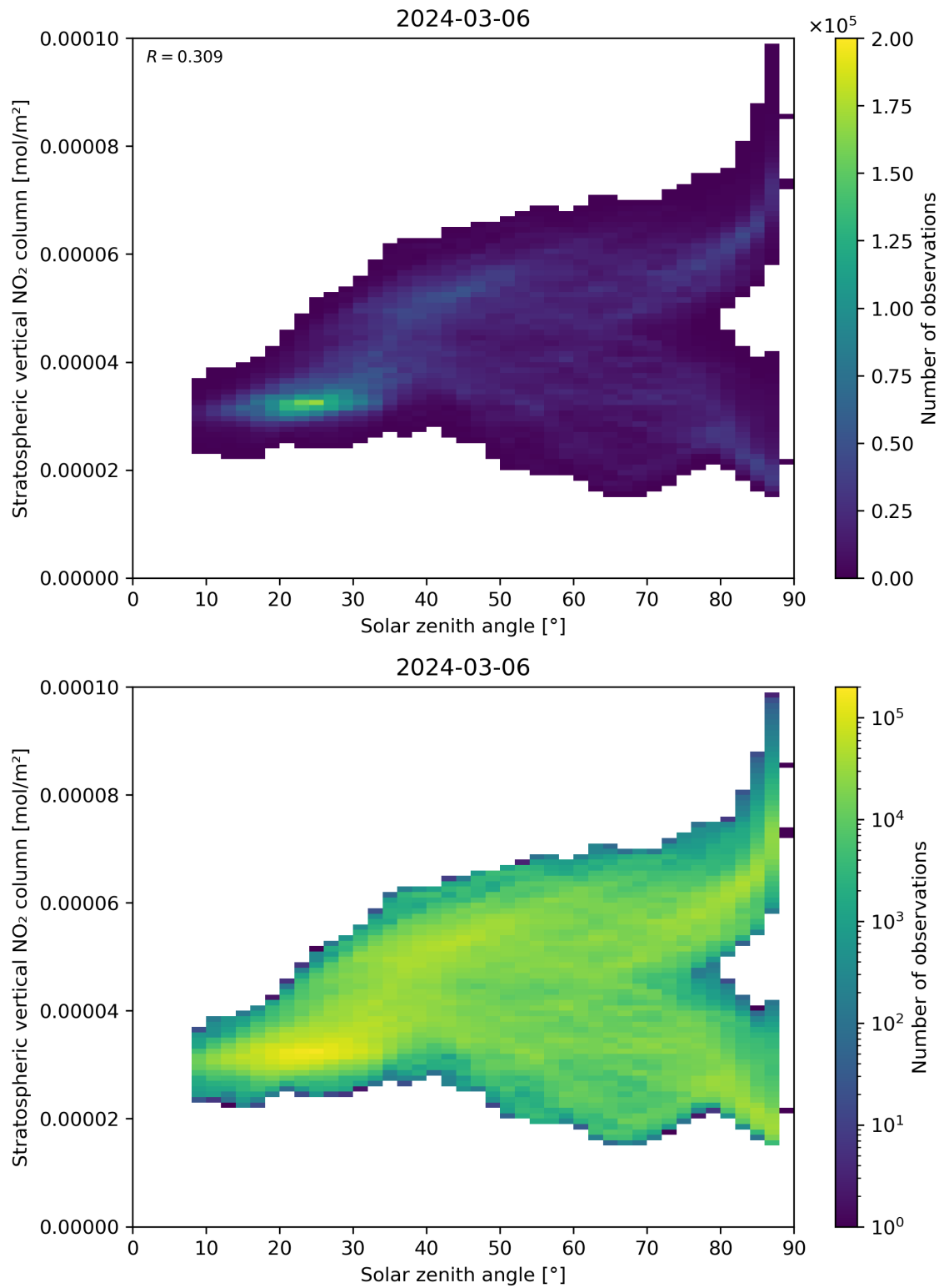
Figure 150: Scatter density plot of “Solar zenith angle” against “Stratospheric vertical NO 2 column” for 2024-03-05 to 2024-03-07.
