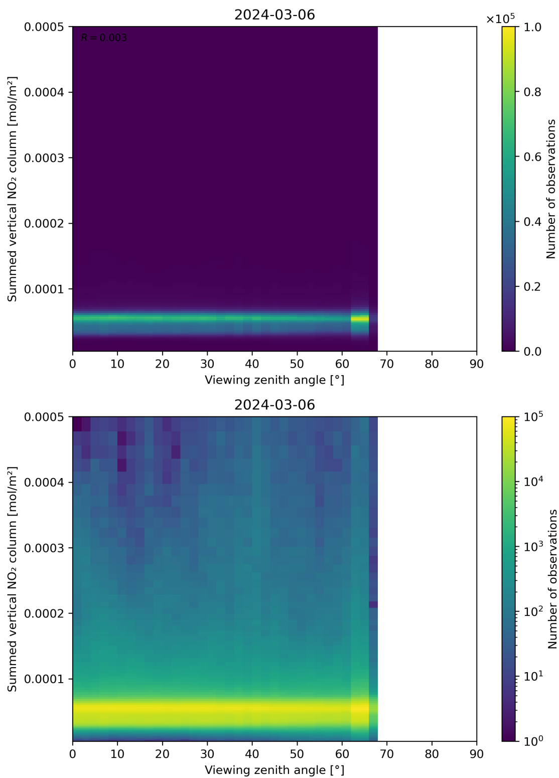
Figure 165: Scatter density plot of “Viewing zenith angle” against “Summed vertical NO 2 column” for 2024-03-05 to 2024-03-07.
