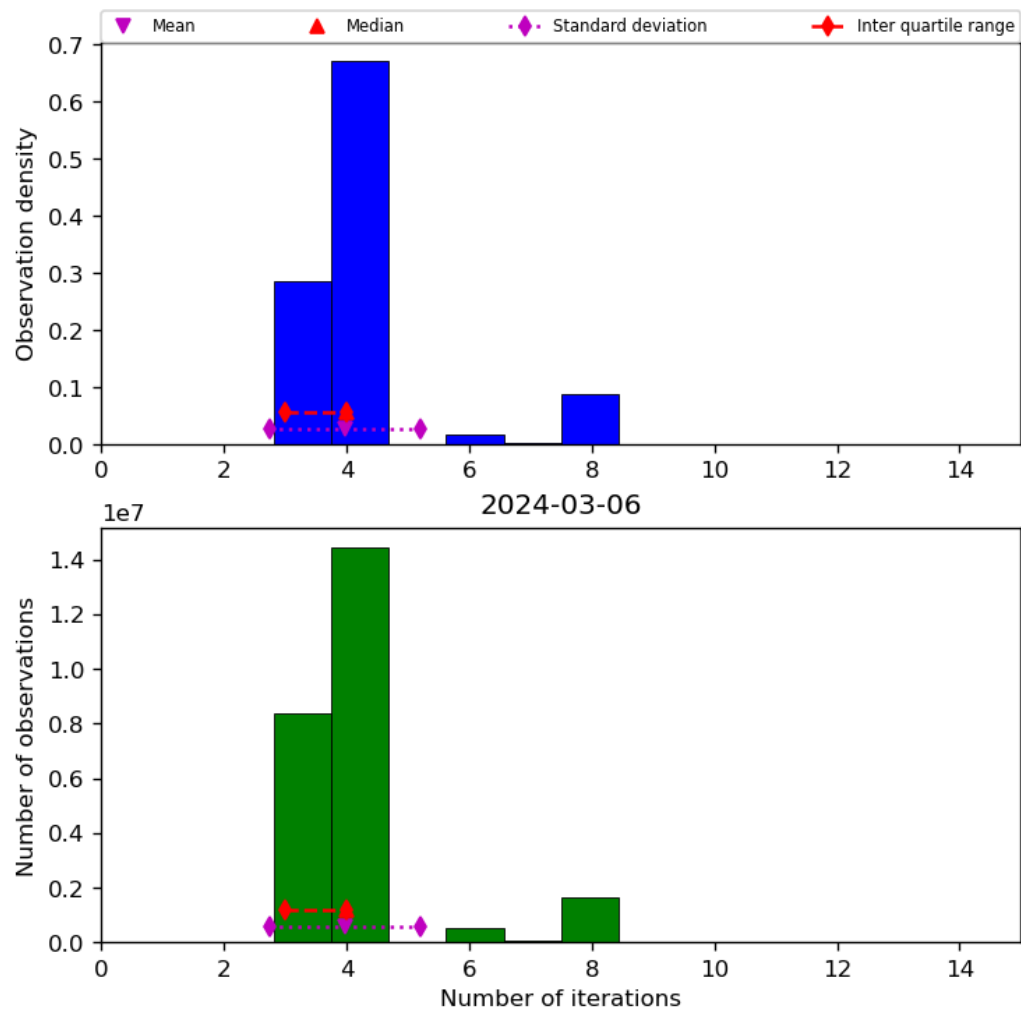
Figure 34: Histogram of “Number of iterations” for 2024-03-05 to 2024-03-07
