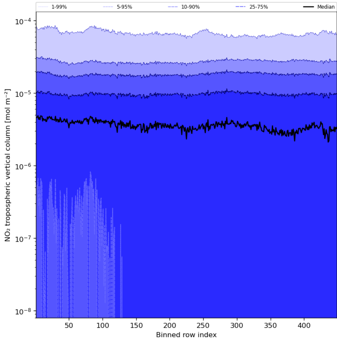
Figure 46: Along track statistics of “NO 2 tropospheric vertical column” for 2024-03-05 to 2024-03-07
