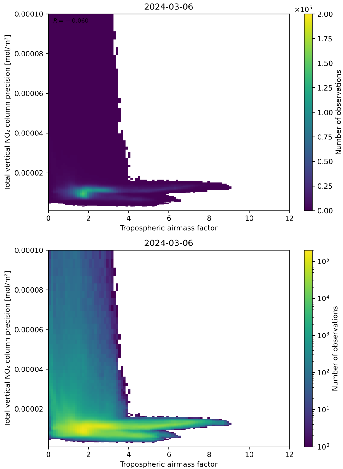
Figure 78: Scatter density plot of “Tropospheric air mass factor” against “Total vertical NO 2 column precision” for 2024-03-05 to 2024-03-07.
