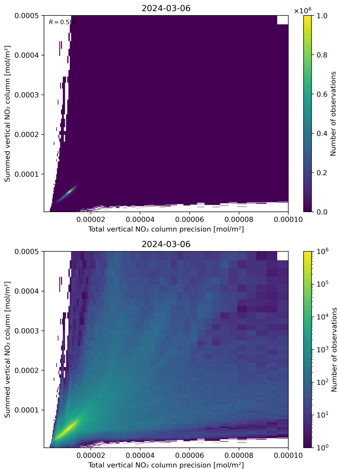
Figure 117: Scatter density plot of “Total vertical NO 2 column precision” against “Summed vertical NO 2 column” for 2024-03-05 to 2024-03-07.
