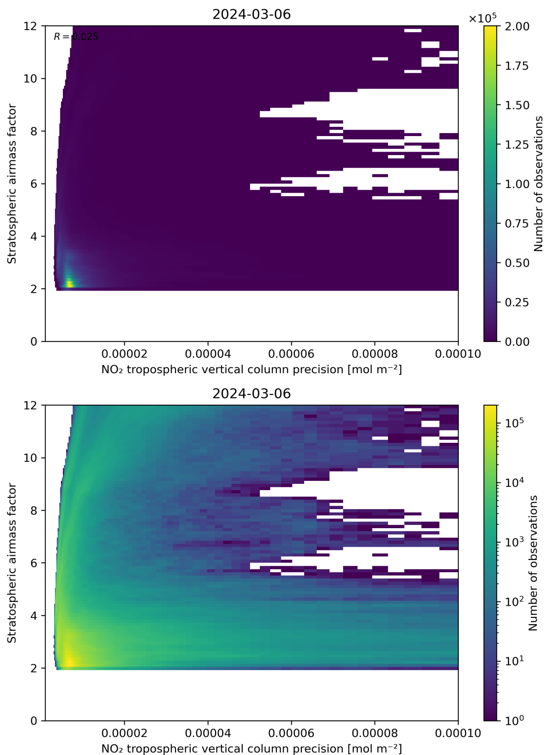
Figure 131: Scatter density plot of “NO 2 tropospheric vertical column precision” against “Stratospheric airmass factor” for 2024-03-05 to 2024-03-07.
