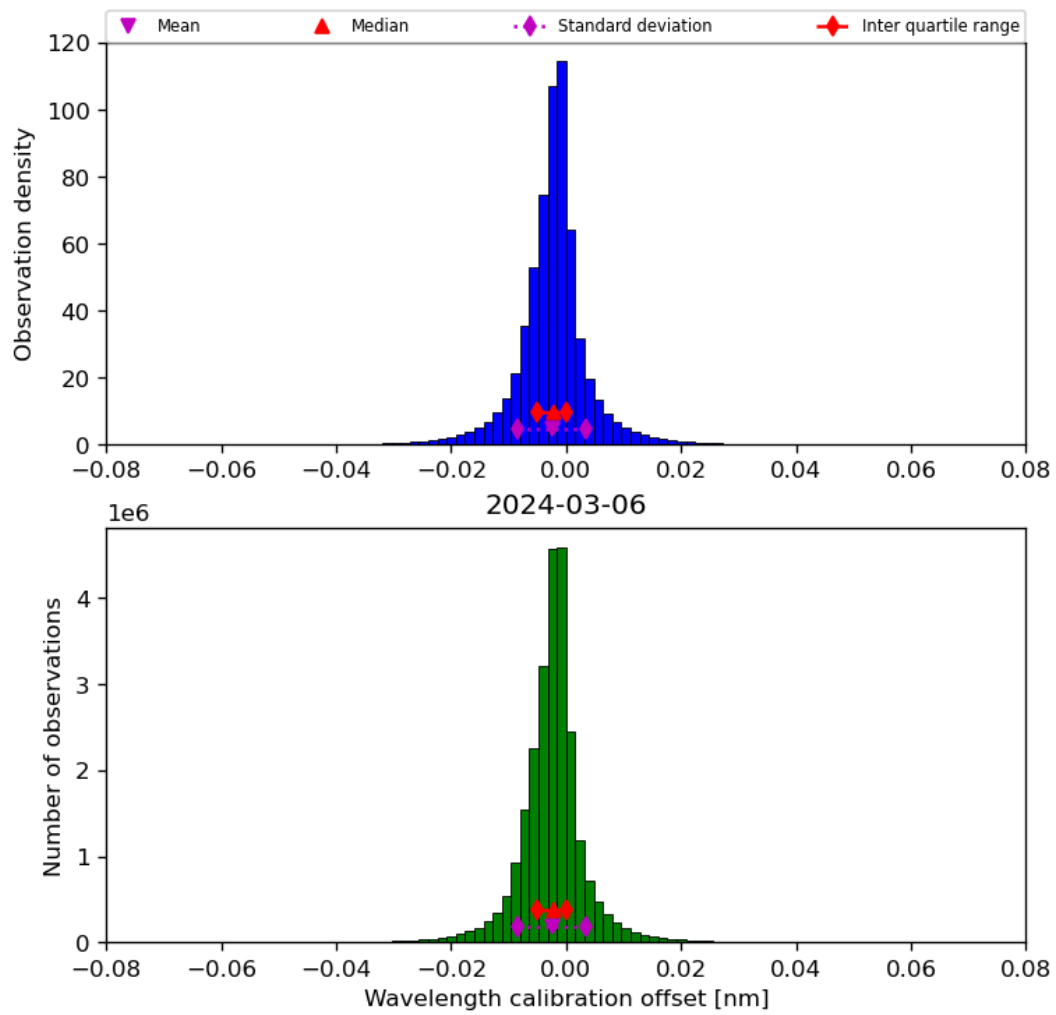
Figure 35: Histogram of “Wavelength calibration offset” for 2024-03-05 to 2024-03-07
