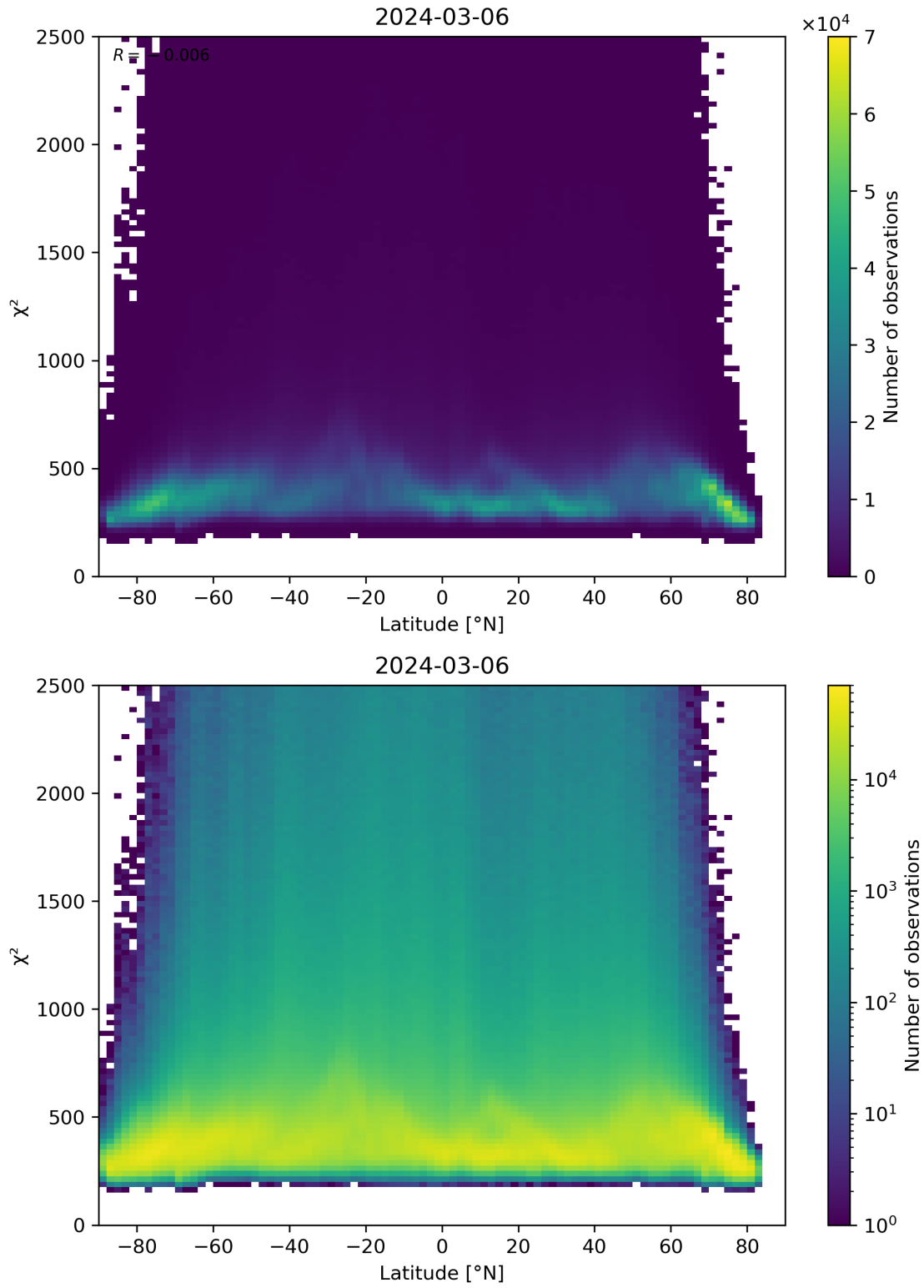
Figure 86: Scatter density plot of “Latitude” against “ \chi^2 ” for 2024-03-05 to 2024-03-07.
