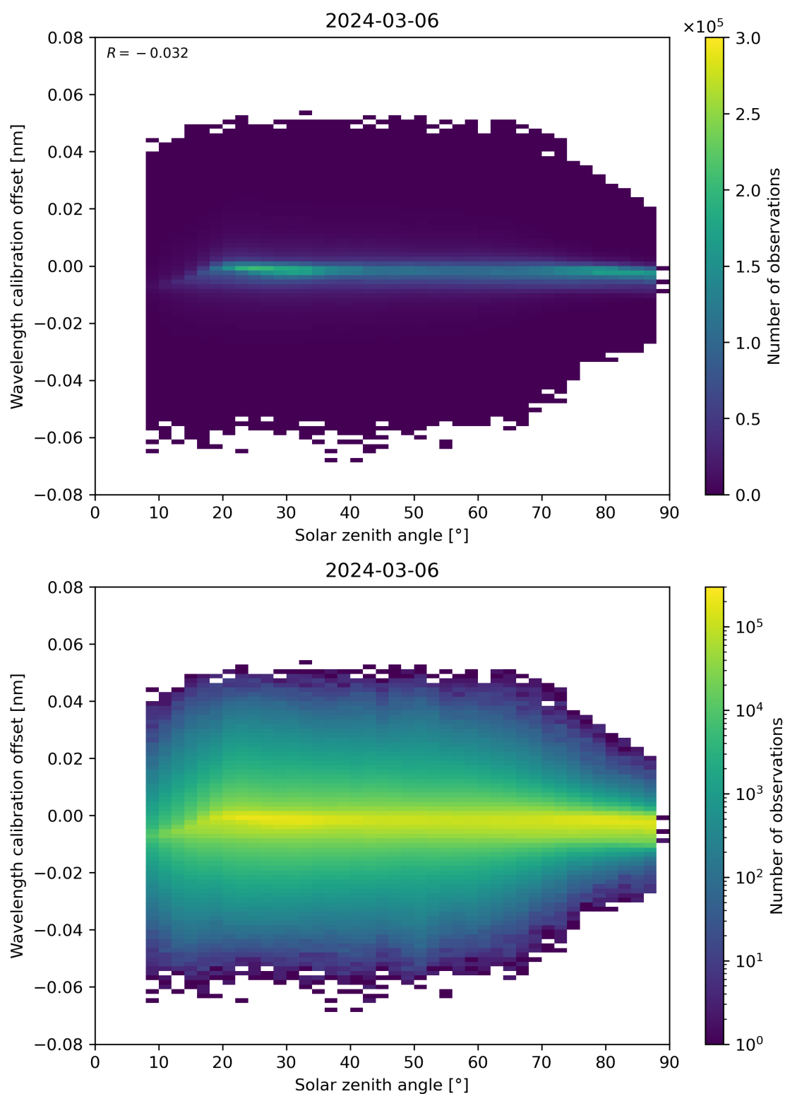
Figure 158: Scatter density plot of “Solar zenith angle” against “Wavelength calibration offset” for 2024-03-05 to 2024-03-07.
