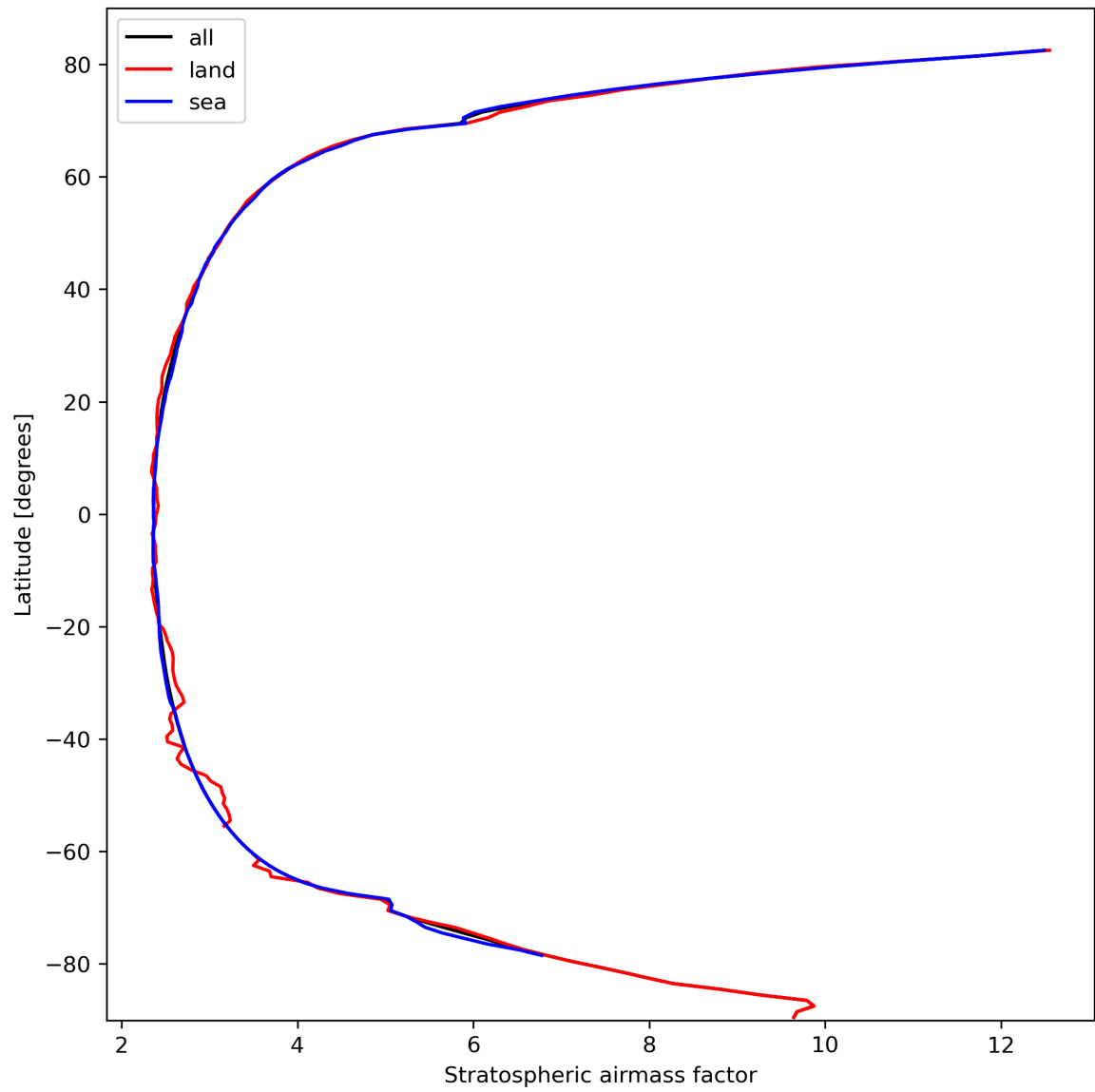
Figure 27: Zonal average of “Stratospheric air mass factor” for 2024-03-05 to 2024-03-07.
