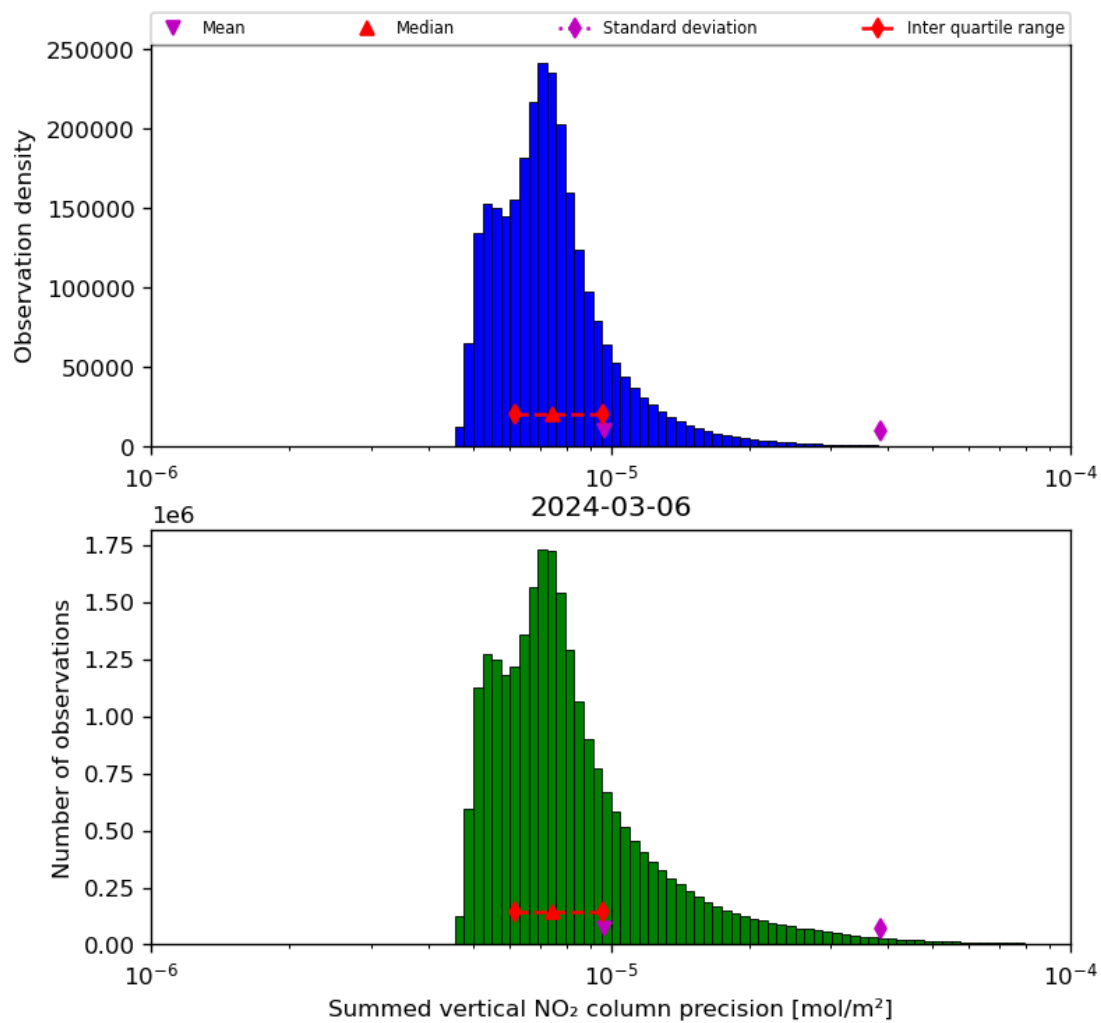
Figure 41: Histogram of "Summed vertical NO 2 column precision" for 2024-03-05 to 2024-03-07
