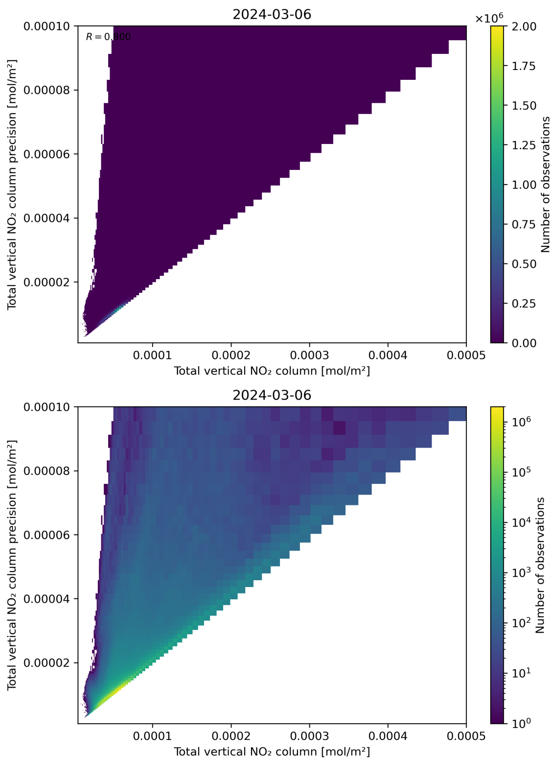
Figure 114: Scatter density plot of “Total vertical NO 2 column” against “Total vertical NO 2 column precision” for 2024-03-05 to 2024-03-07.
