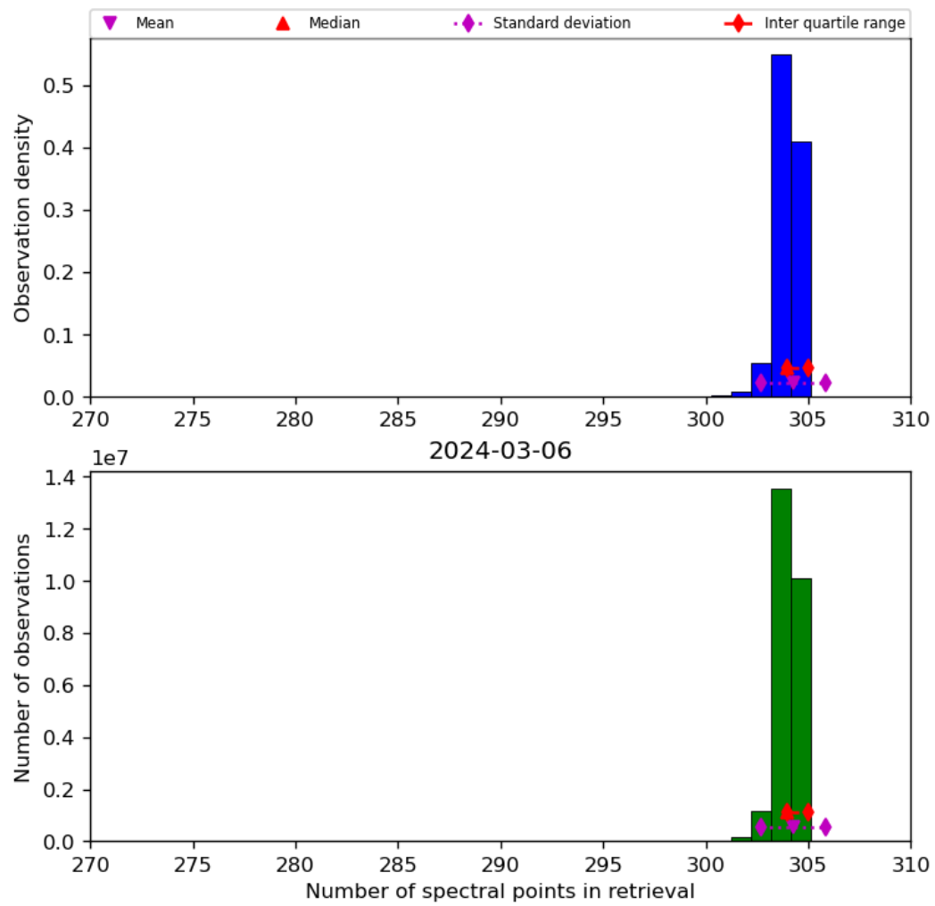
Figure 33: Histogram of “Number of spectral points in retrieval” for 2024-03-05 to 2024-03-07
