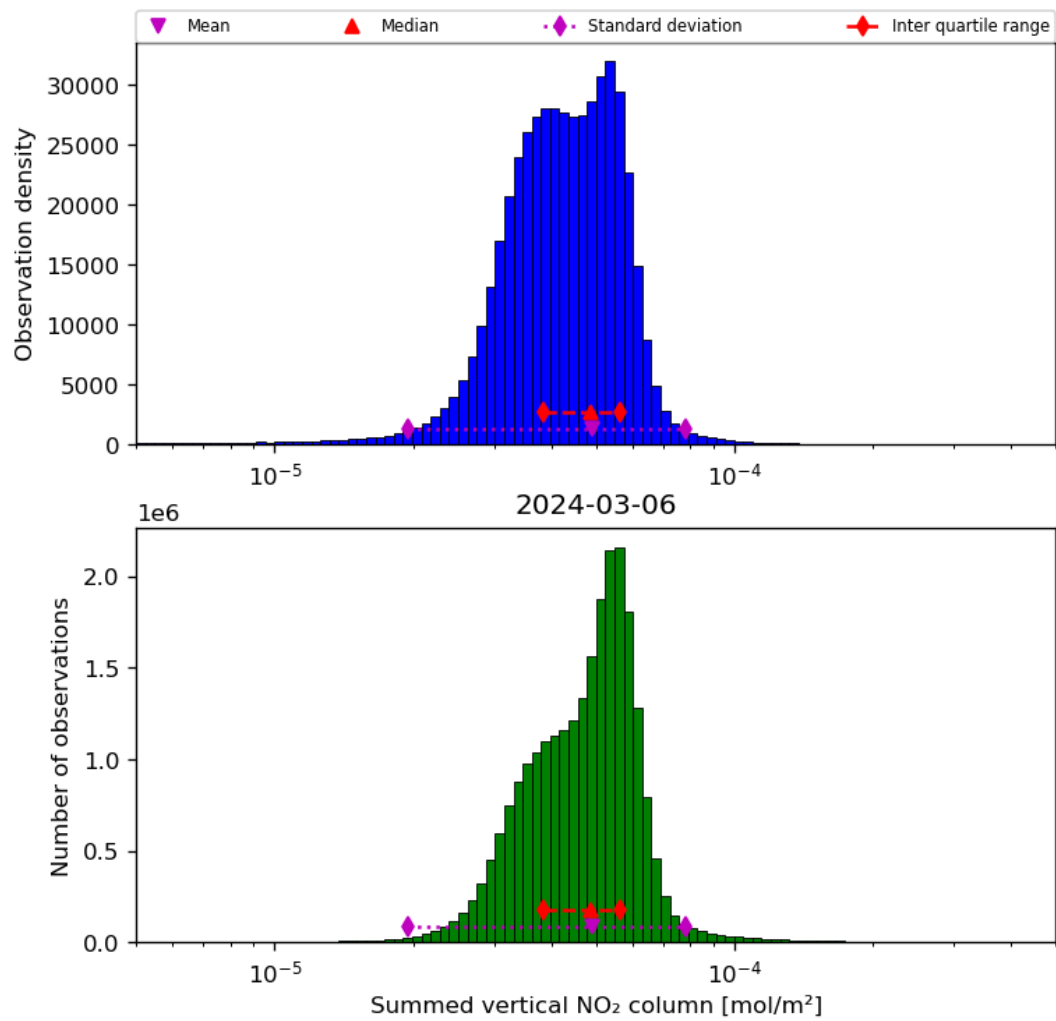
Figure 40: Histogram of “Summed vertical NO 2 column” for 2024-03-05 to 2024-03-07
