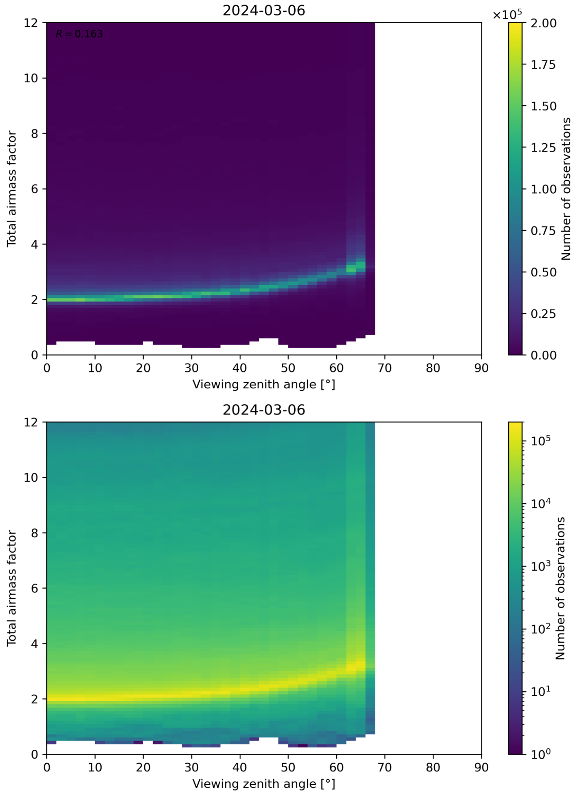
Figure 160: Scatter density plot of “Viewing zenith angle” against “Total airmass factor” for 2024-03-05 to 2024-03-07.
