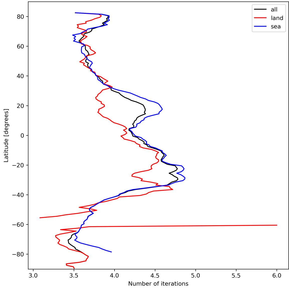
Figure 17: Zonal average of “Number of iterations” for 2024-03-05 to 2024-03-07.
