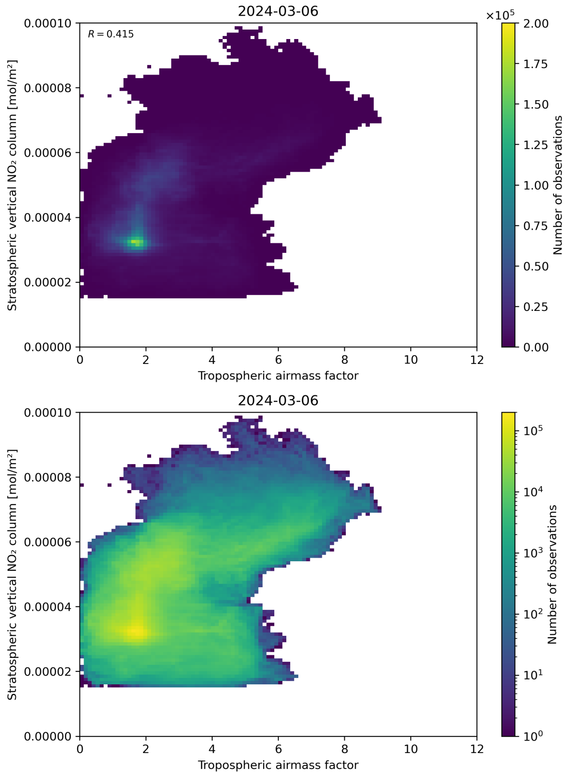
Figure 74: Scatter density plot of “Tropospheric air mass factor” against “Stratospheric vertical NO 2 column” for 2024-03-05 to 2024-03-07.
