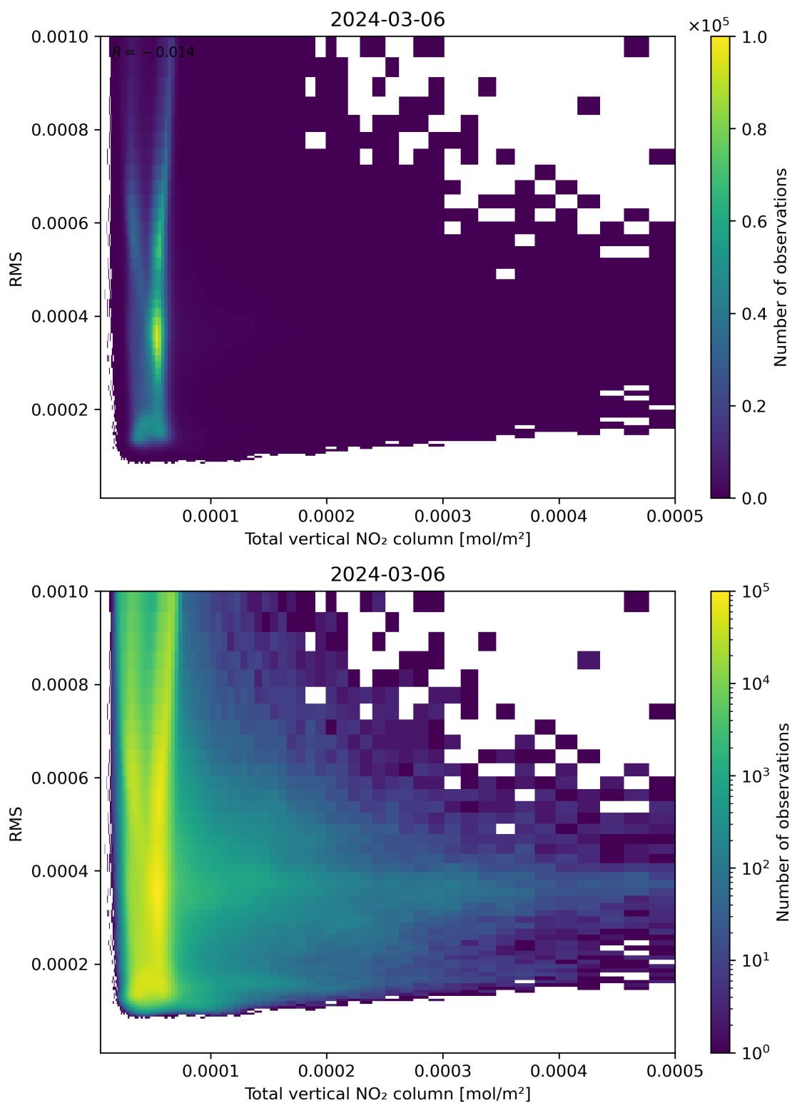
Figure 120: Scatter density plot of “Total vertical NO 2 column” against “RMS” for 2024-03-05 to 2024-03-07.
