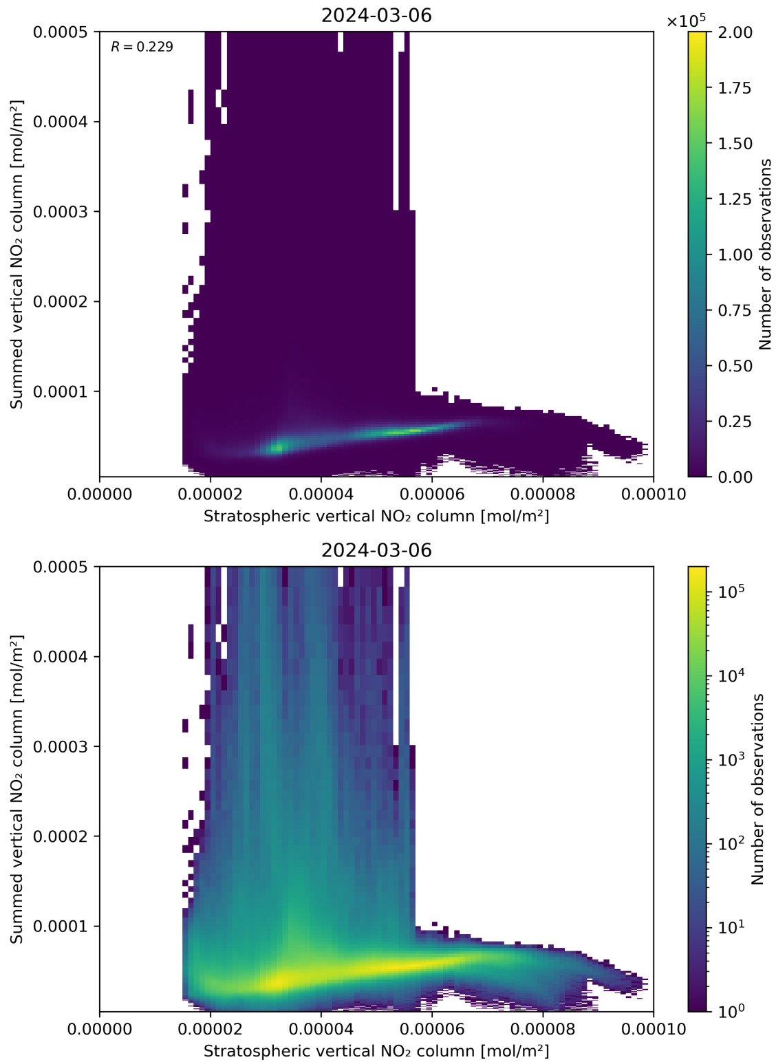
Figure 98: Scatter density plot of “Stratospheric vertical NO 2 column” against “Summed vertical NO 2 column” for 2024-03-05 to 2024-03-07.
