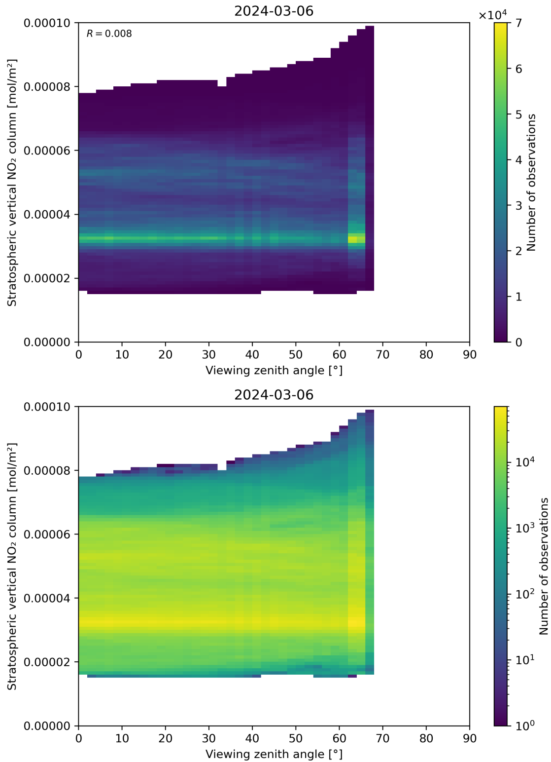
Figure 164: Scatter density plot of “Viewing zenith angle” against “Stratospheric vertical NO 2 column” for 2024-03-05 to 2024-03-07.
