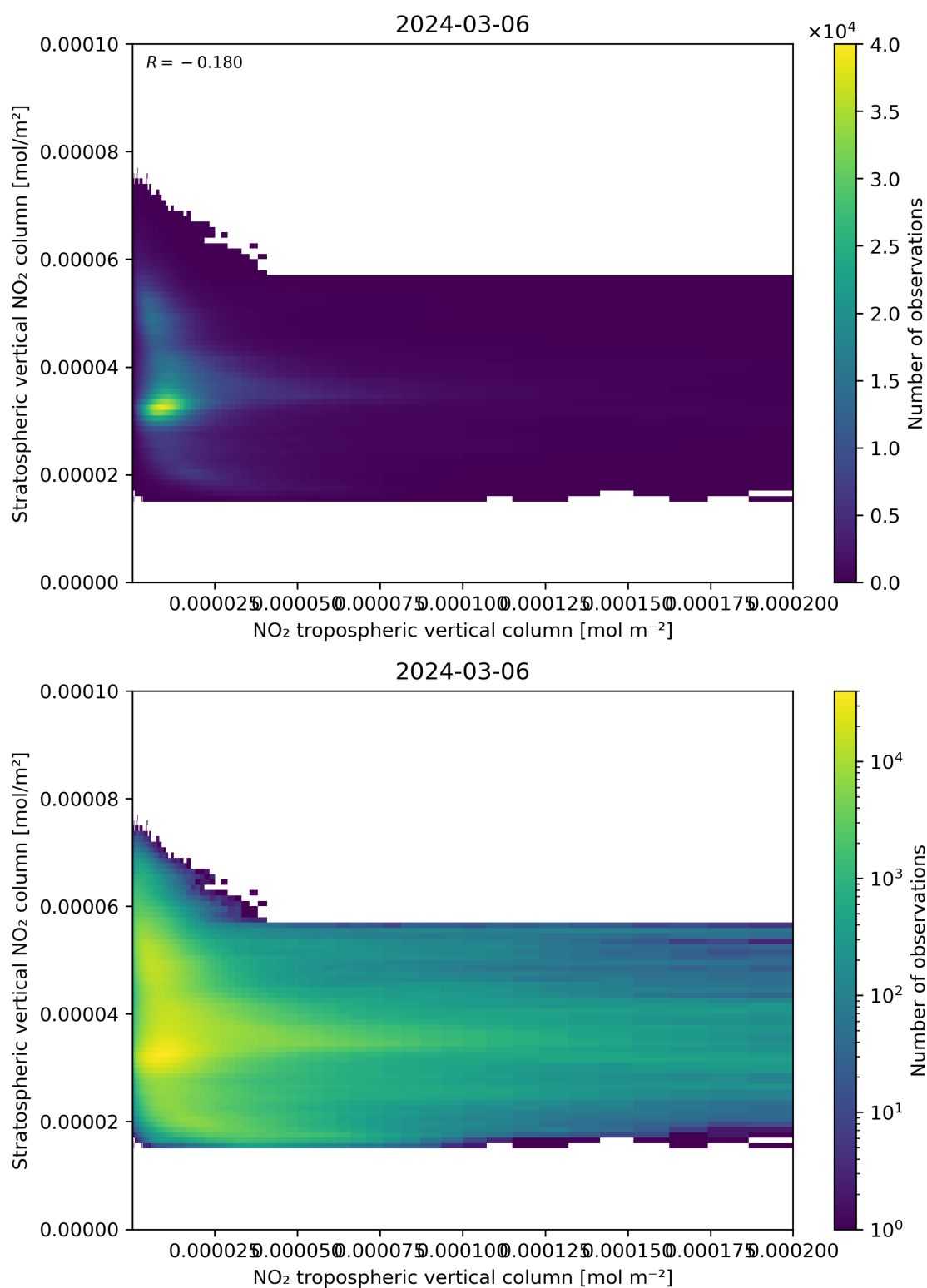
Figure 125: Scatter density plot of “NO 2 tropospheric vertical column” against “Stratospheric vertical NO 2 column” for 2024-03-05 to 2024-03-07.
