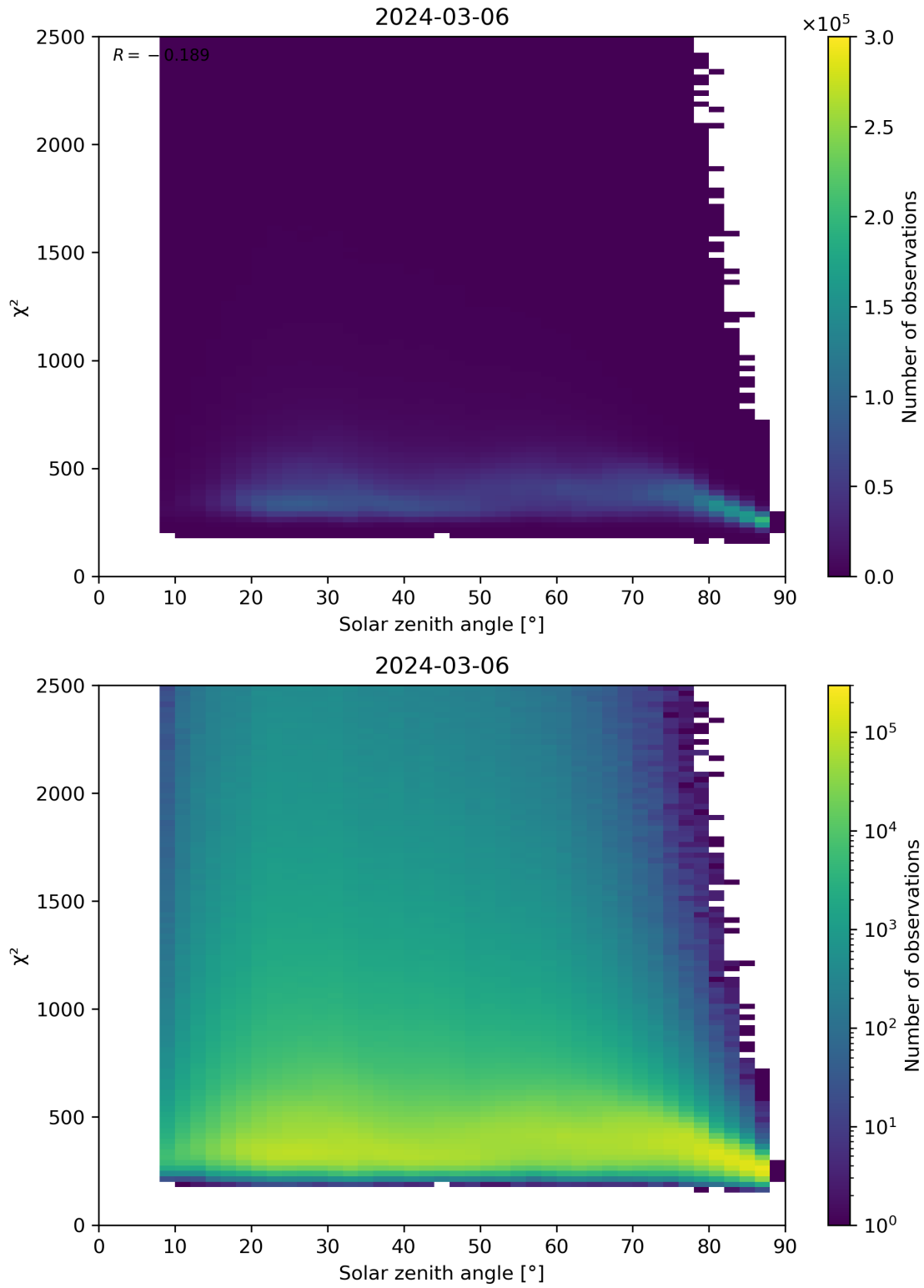
Figure 148: Scatter density plot of “Solar zenith angle” against “ \chi^2 ” for 2024-03-05 to 2024-03-07.
