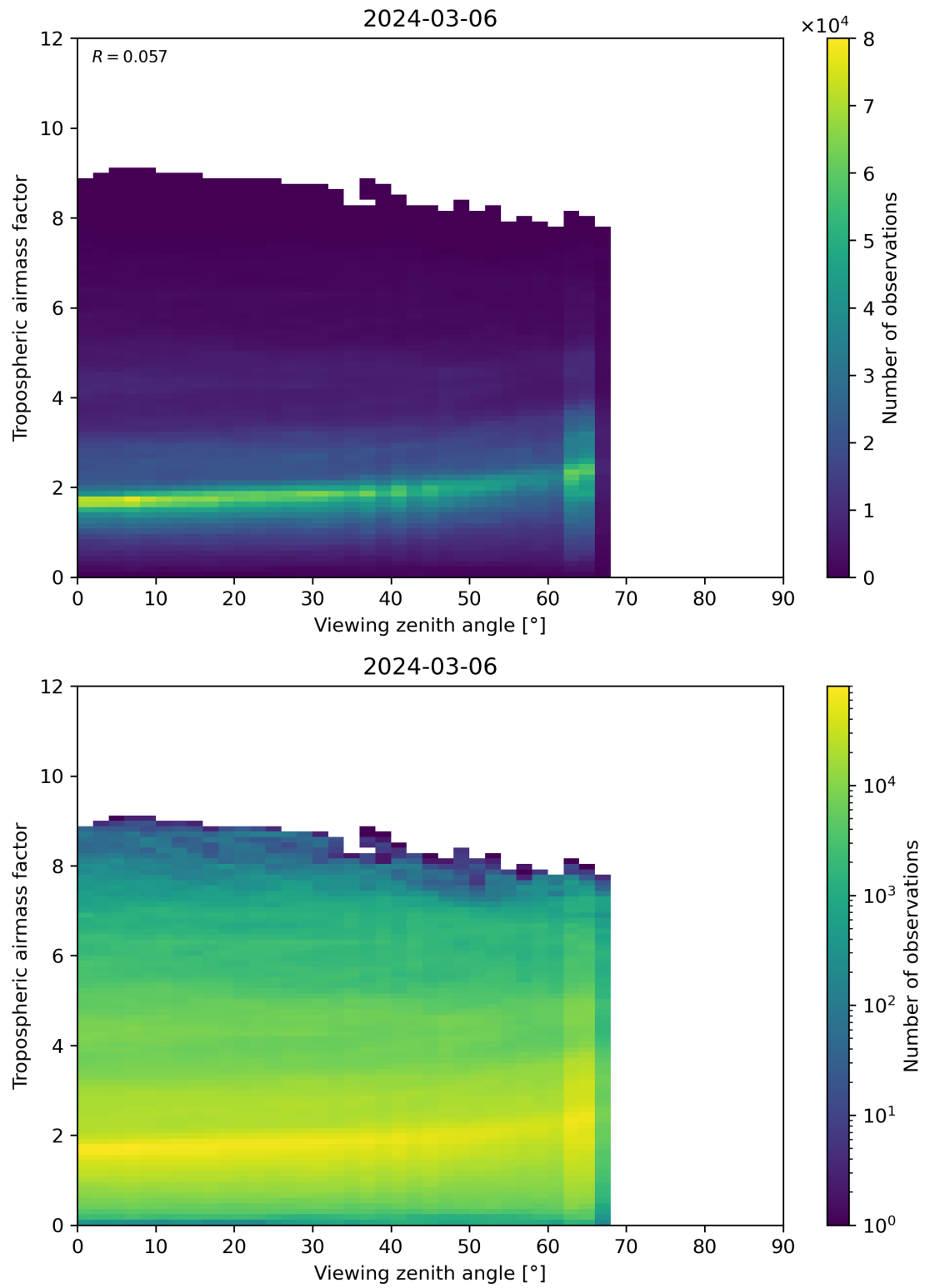
Figure 161: Scatter density plot of “Viewing zenith angle” against “Tropospheric airmass factor” for 2024-03-05 to 2024-03-07.
