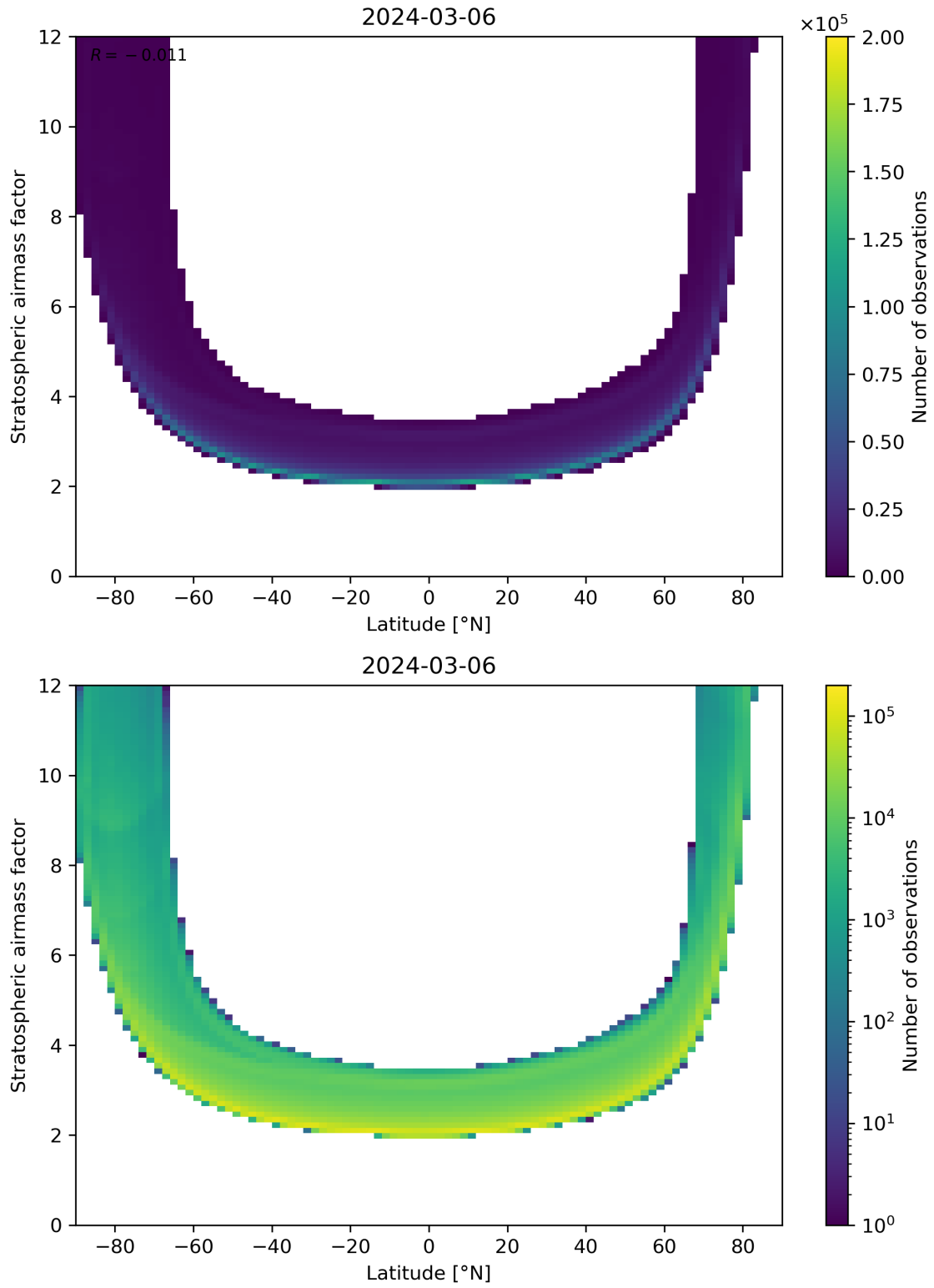
Figure 83: Scatter density plot of “Latitude” against “Stratospheric airmass factor” for 2024-03-05 to 2024-03-07.
