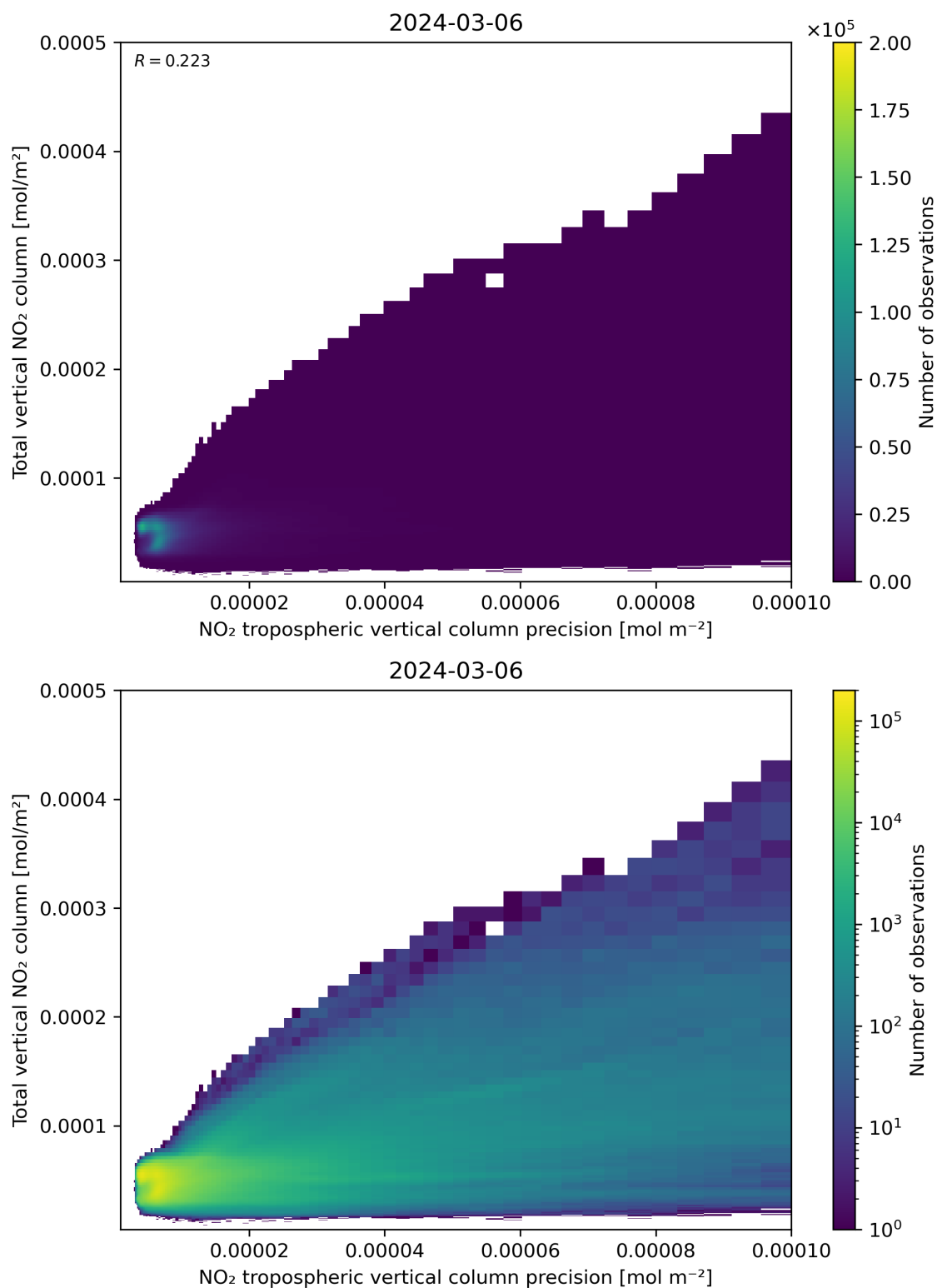
Figure 138: Scatter density plot of “NO 2 tropospheric vertical column precision” against “Total vertical NO 2 column” for 2024-03-05 to 2024-03-07.
