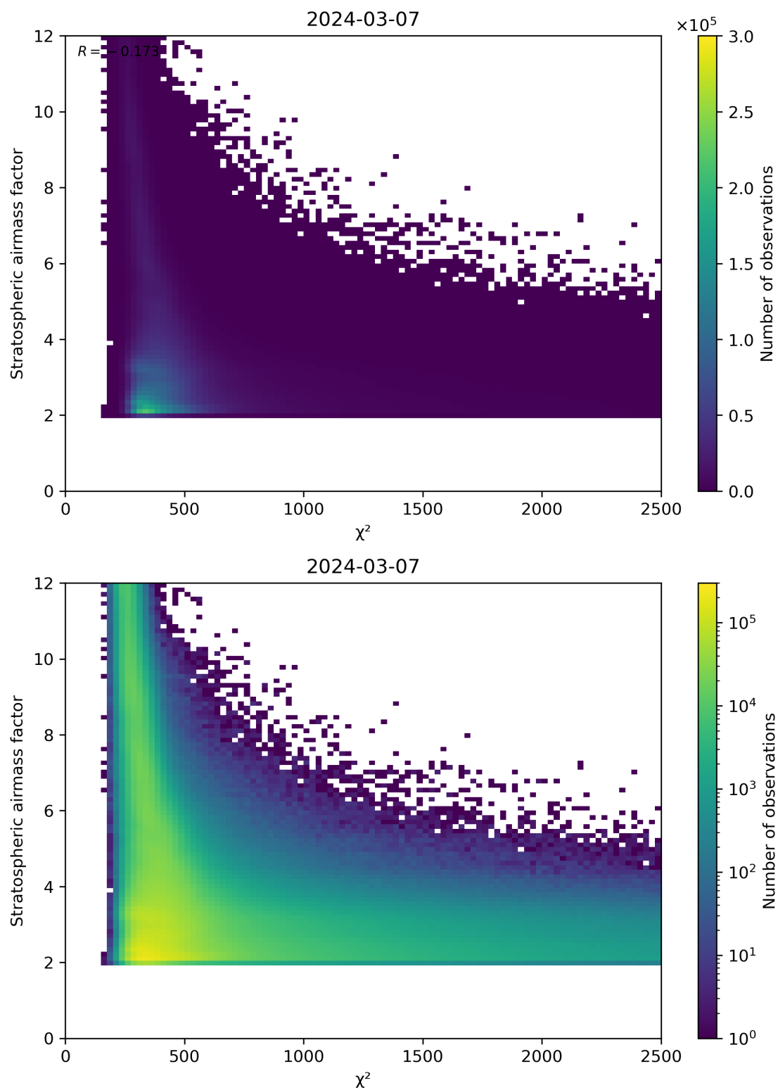
Figure 81: Scatter density plot of “ \chi^2 ” against “Stratospheric airmass factor” for 2024-03-06 to 2024-03-08.
