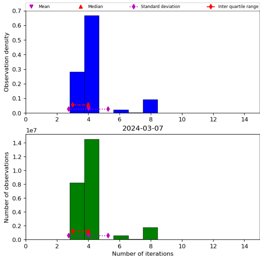
Figure 34: Histogram of “Number of iterations” for 2024-03-06 to 2024-03-08
