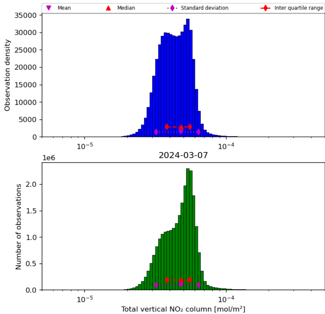
Figure 38: Histogram of “Total vertical NO 2 column” for 2024-03-06 to 2024-03-08
