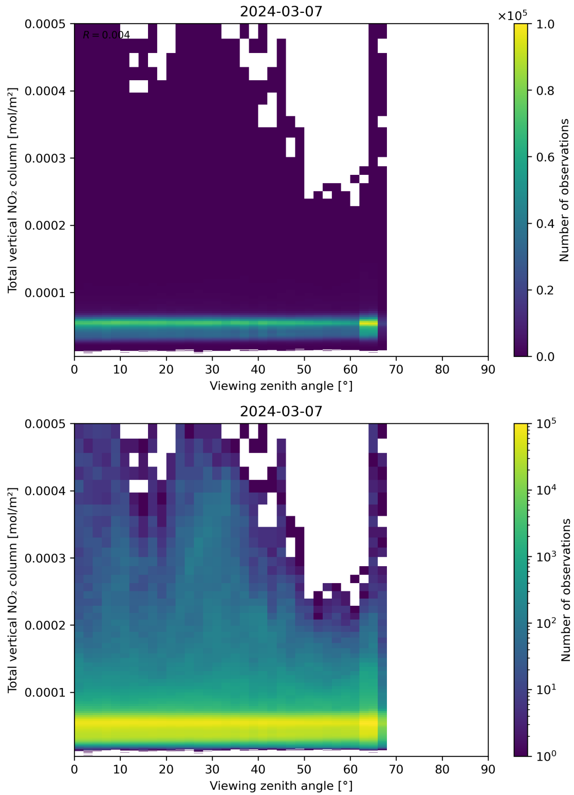
Figure 167: Scatter density plot of “Viewing zenith angle” against “Total vertical NO 2 column” for 2024-03-06 to 2024-03-08.
