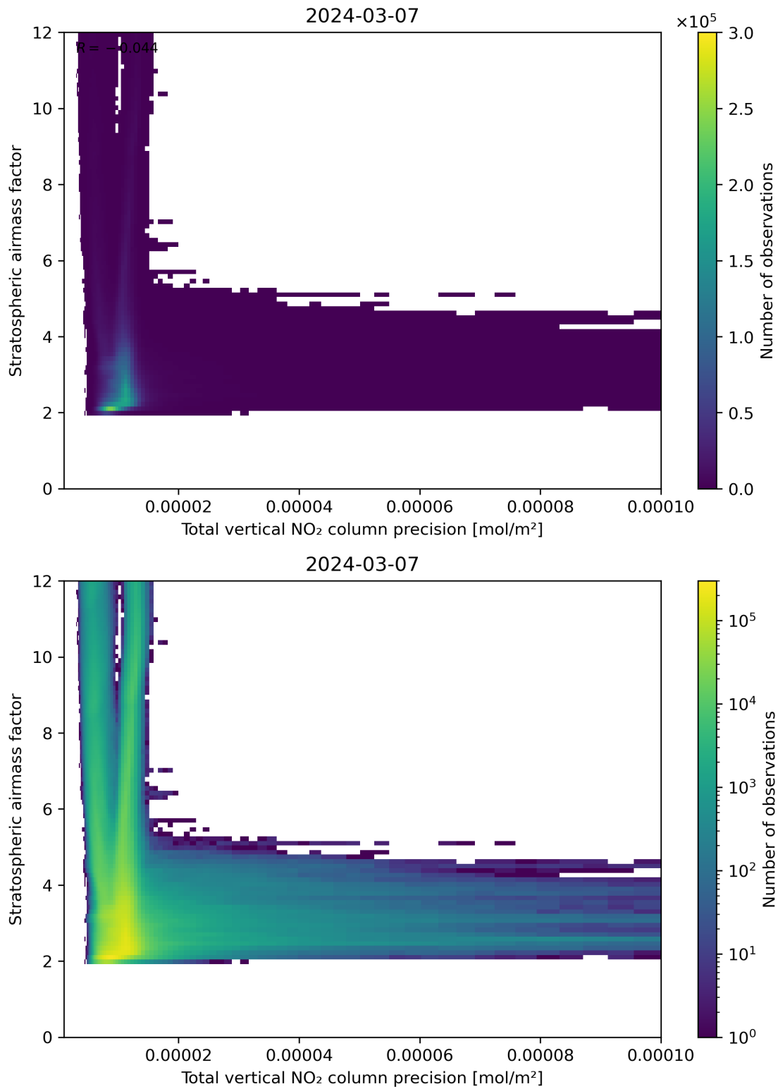
Figure 115: Scatter density plot of “Total vertical NO 2 column precision” against “Stratospheric airmass factor” for 2024-03-06 to 2024-03-08.
