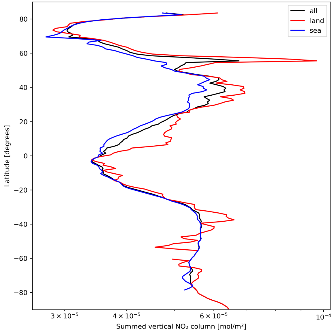
Figure 23: Zonal average of “Summed vertical NO 2 column” for 2024-03-06 to 2024-03-08.
