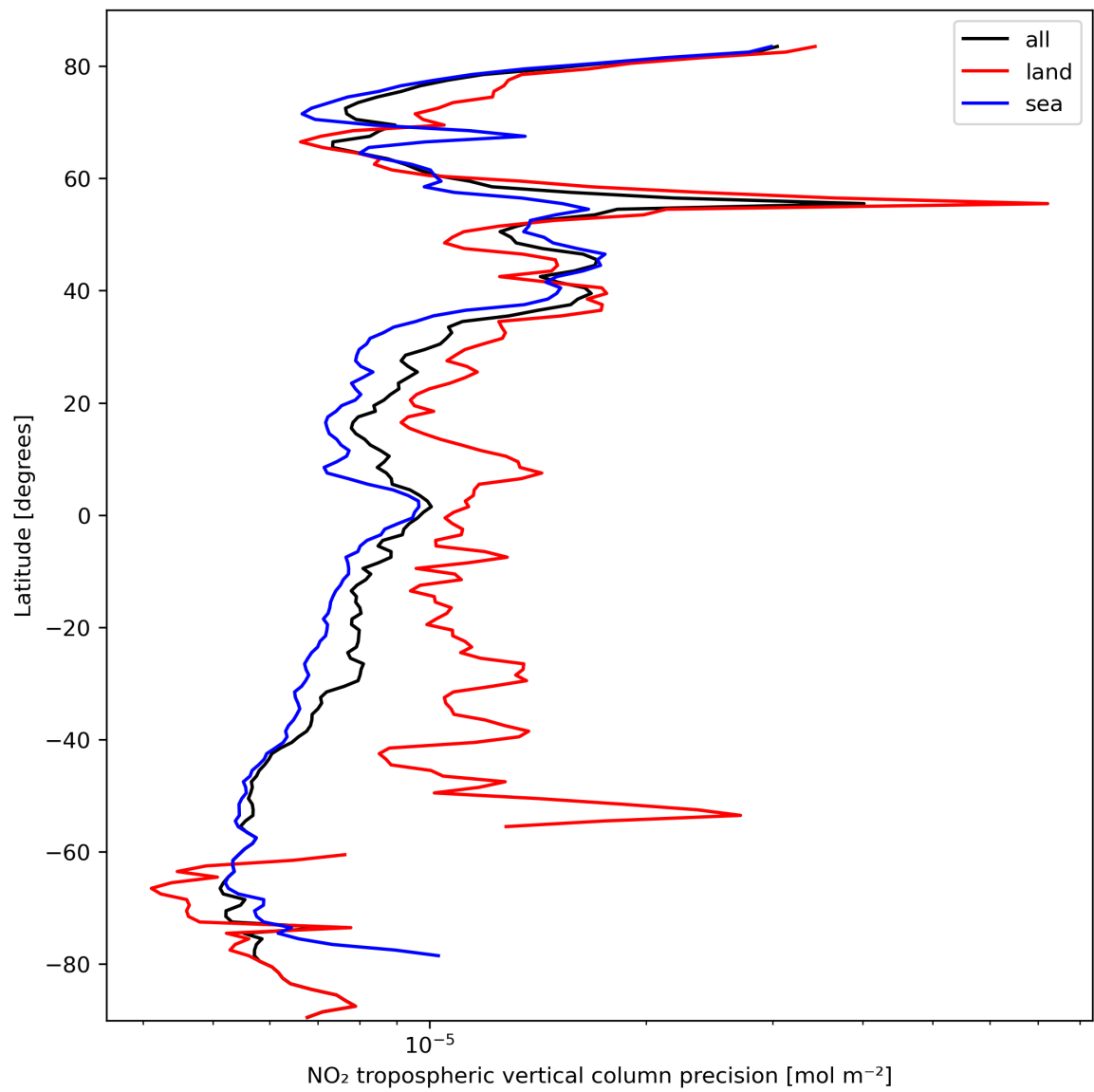
Figure 13: Zonal average of “NO 2 tropospheric vertical column precision” for 2024-03-06 to 2024-03-08.
