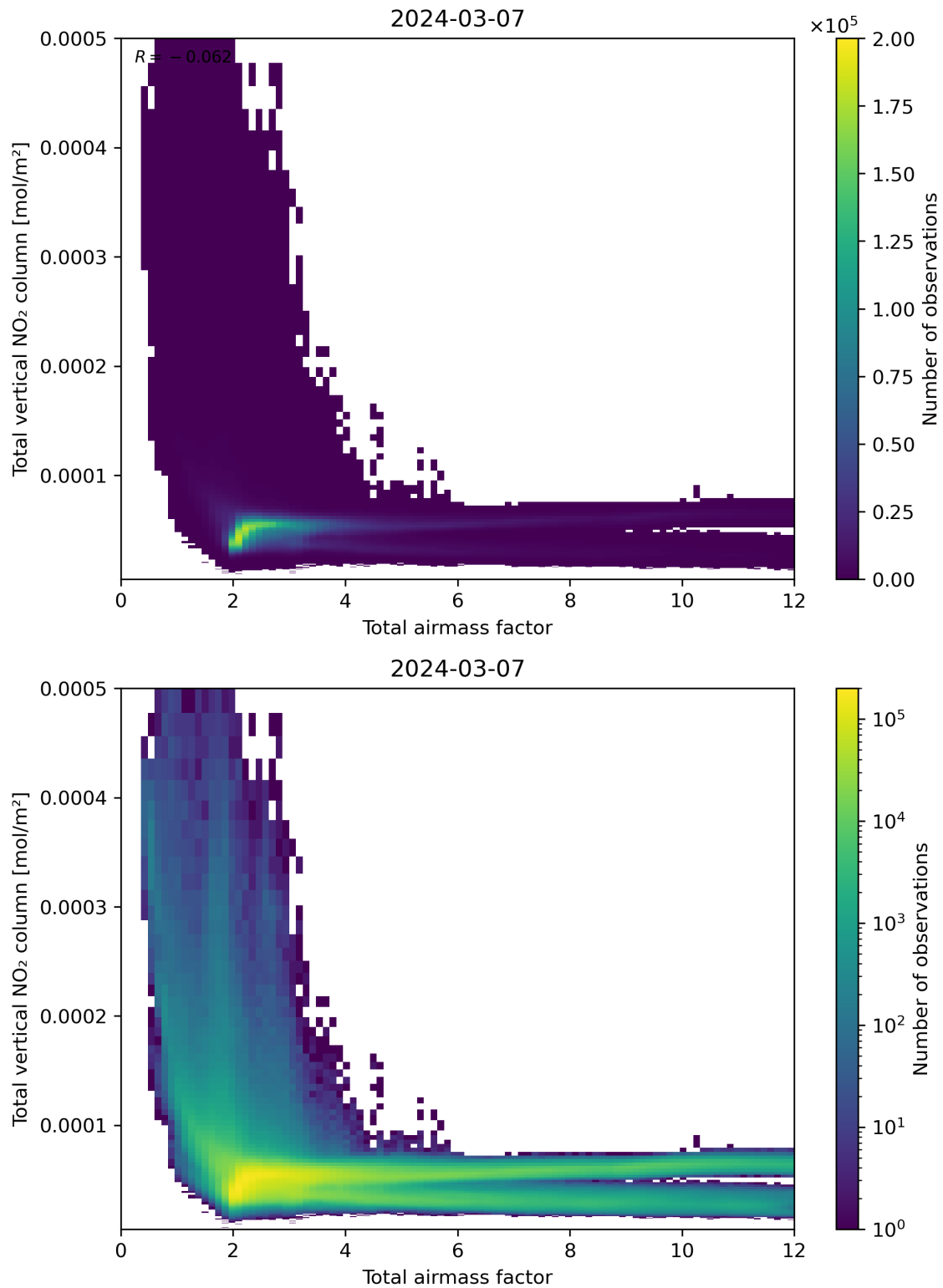
Figure 67: Scatter density plot of “Total airmass factor” against “Total vertical NO 2 column” for 2024-03-06 to 2024-03-08.
