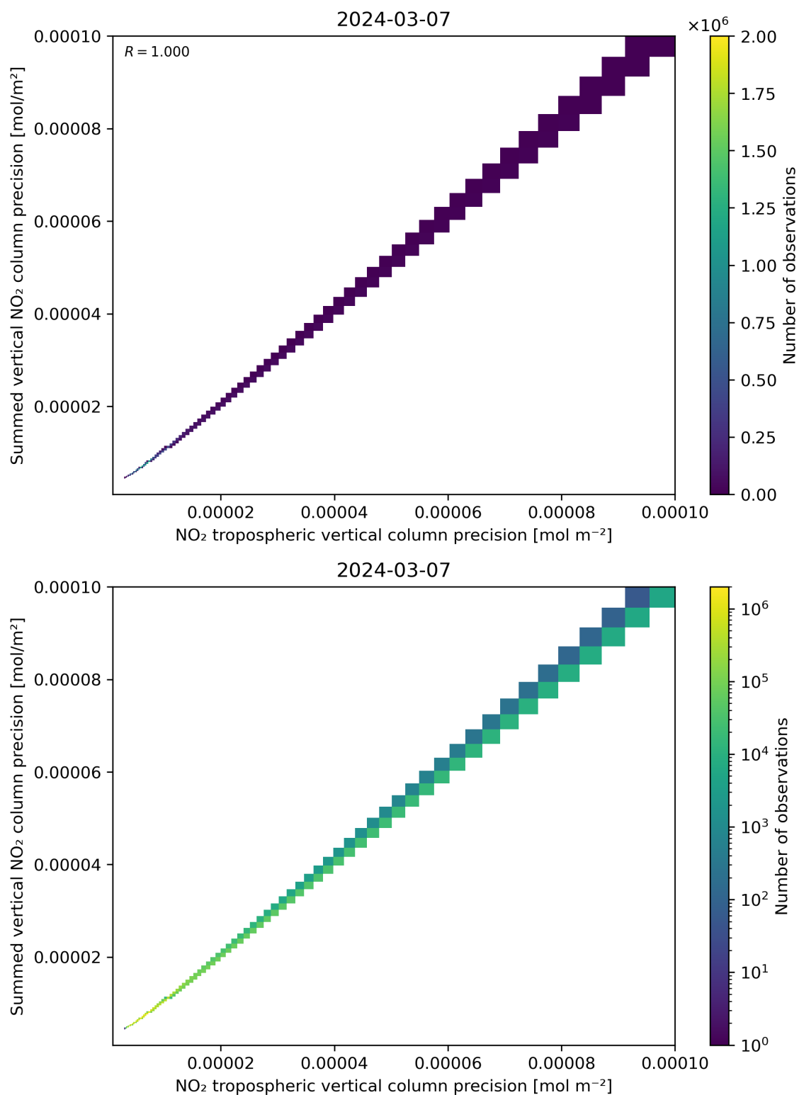
Figure 137: Scatter density plot of “NO 2 tropospheric vertical column precision” against “Summed vertical NO 2 column precision” for 2024-03-06 to 2024-03-08.
