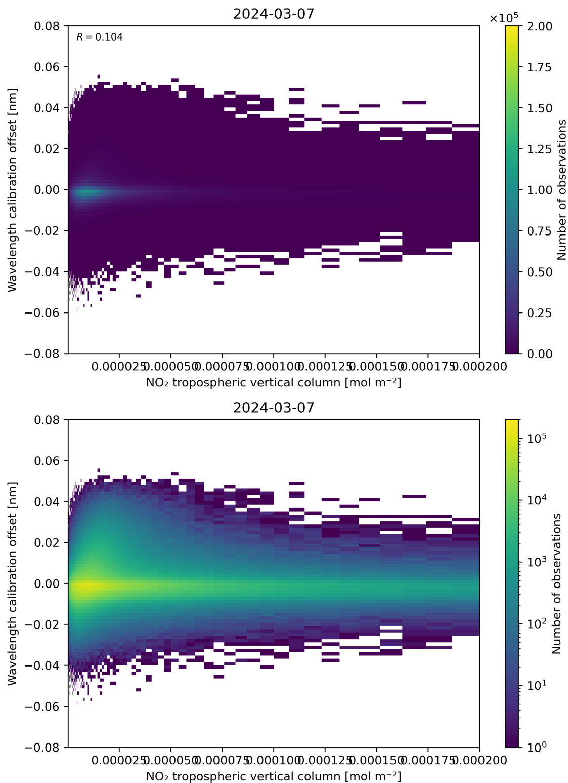
Figure 143: Scatter density plot of “NO 2 tropospheric vertical column” against “Wavelength calibration offset” for 2024-03-06 to 2024-03-08.
