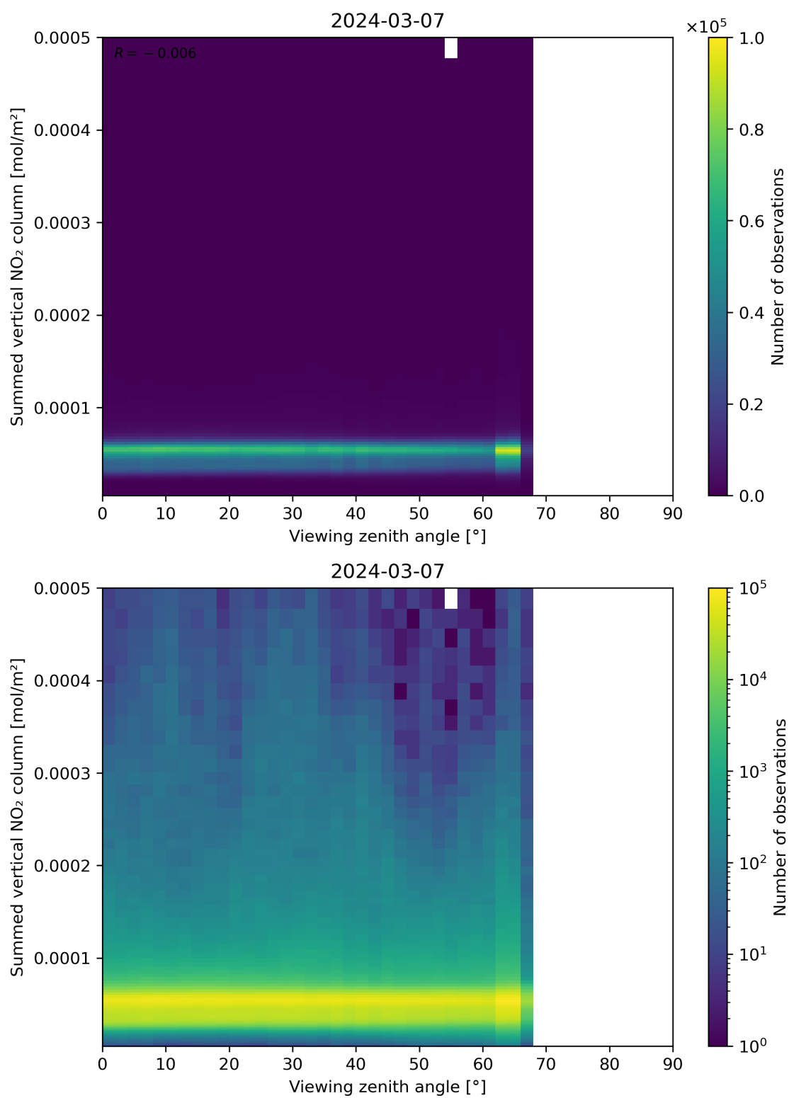
Figure 165: Scatter density plot of “Viewing zenith angle” against “Summed vertical NO 2 column” for 2024-03-06 to 2024-03-08.
