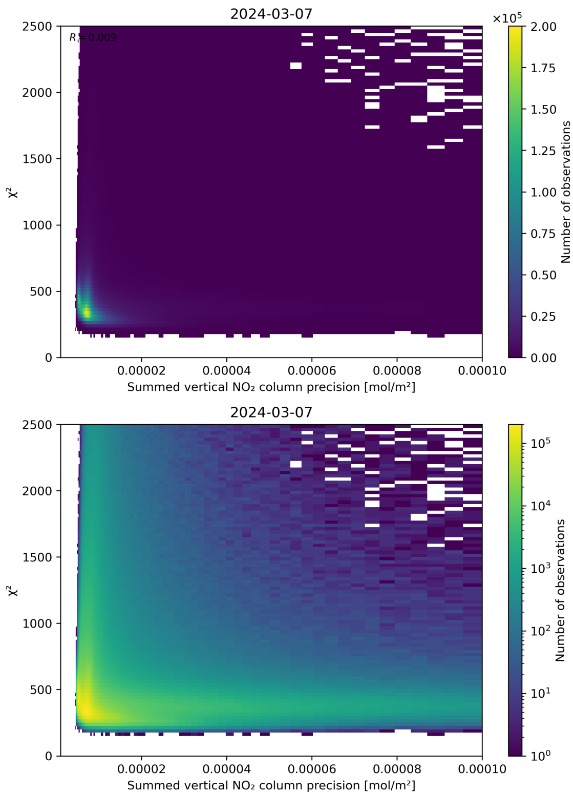
Figure 107: Scatter density plot of “Summed vertical NO 2 column precision” against “ \chi^2 ” for 2024-03-06 to 2024-03-08.
