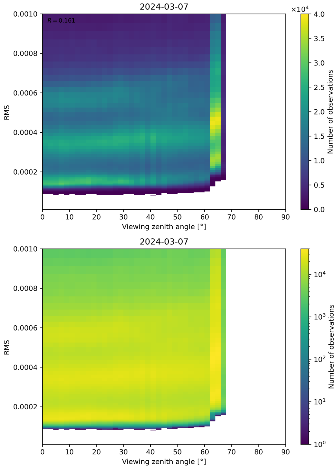
Figure 171: Scatter density plot of “Viewing zenith angle” against “RMS” for 2024-03-06 to 2024-03-08.
