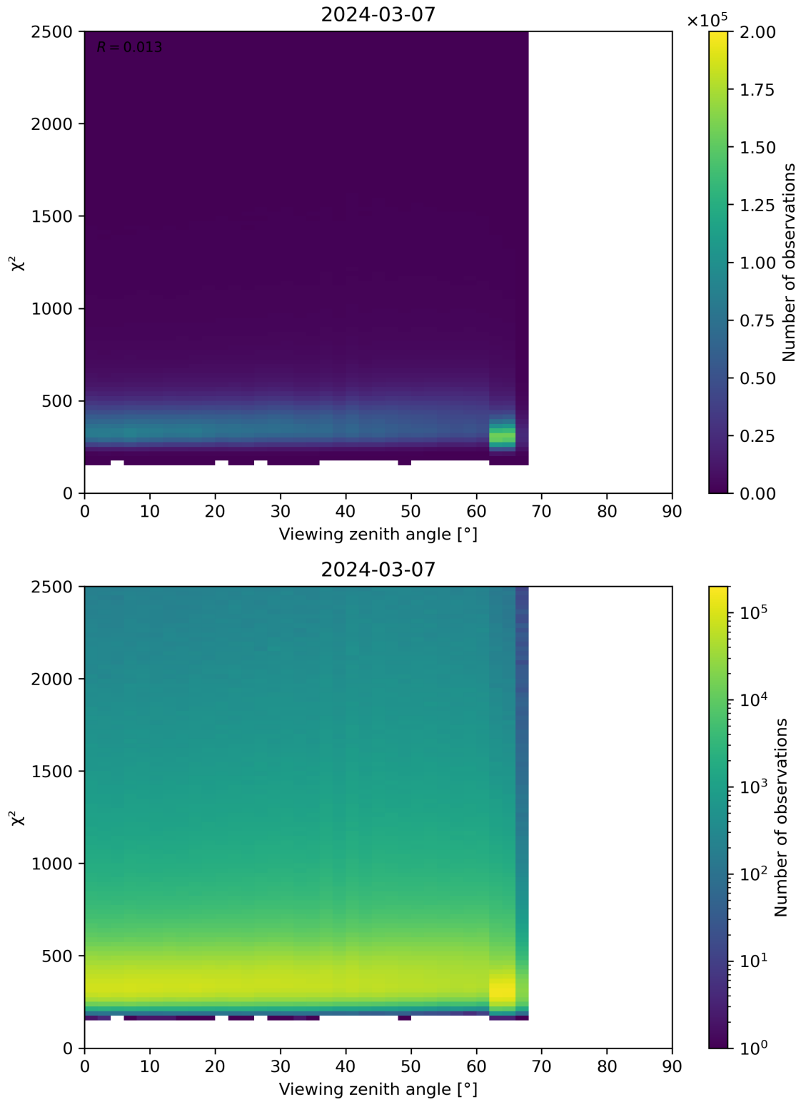
Figure 162: Scatter density plot of “Viewing zenith angle” against “ \chi^2 ” for 2024-03-06 to 2024-03-08.
