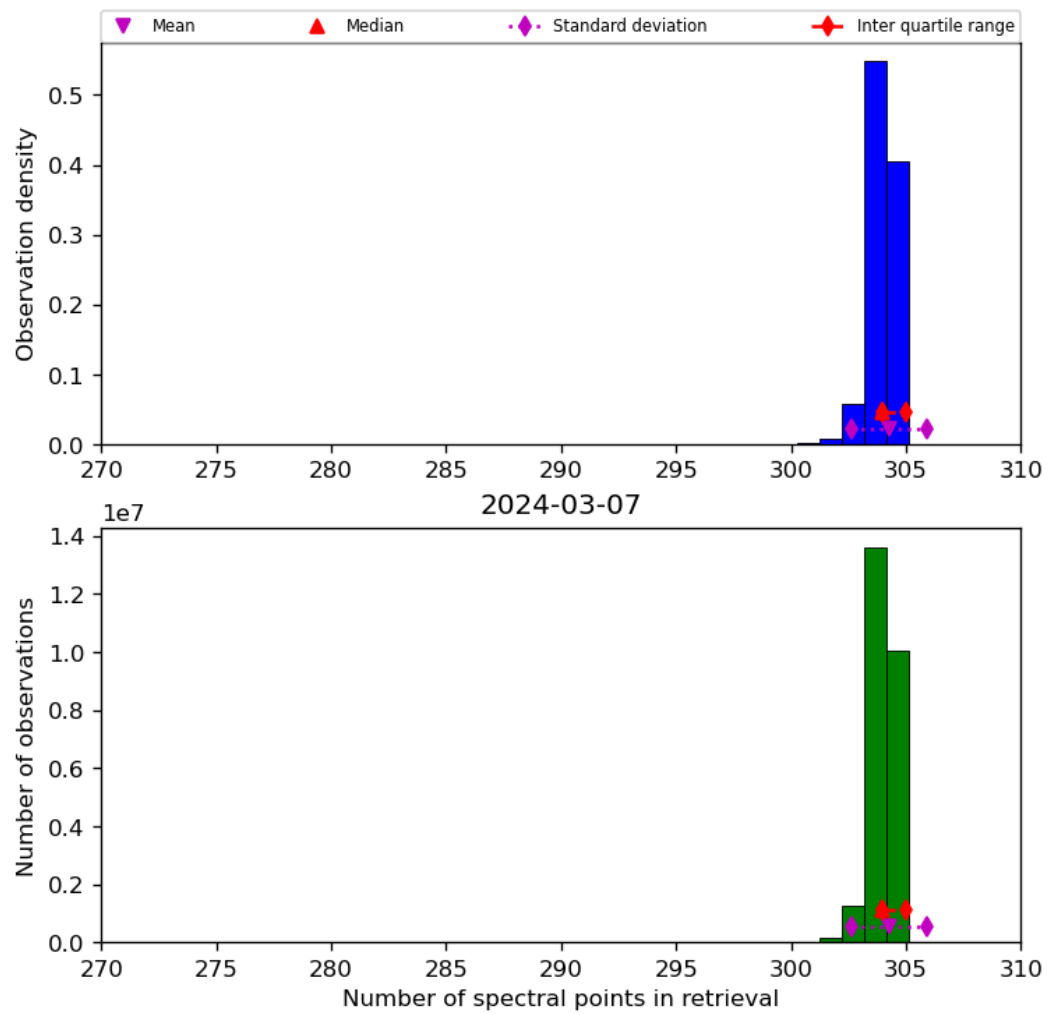
Figure 33: Histogram of “Number of spectral points in retrieval” for 2024-03-06 to 2024-03-08
