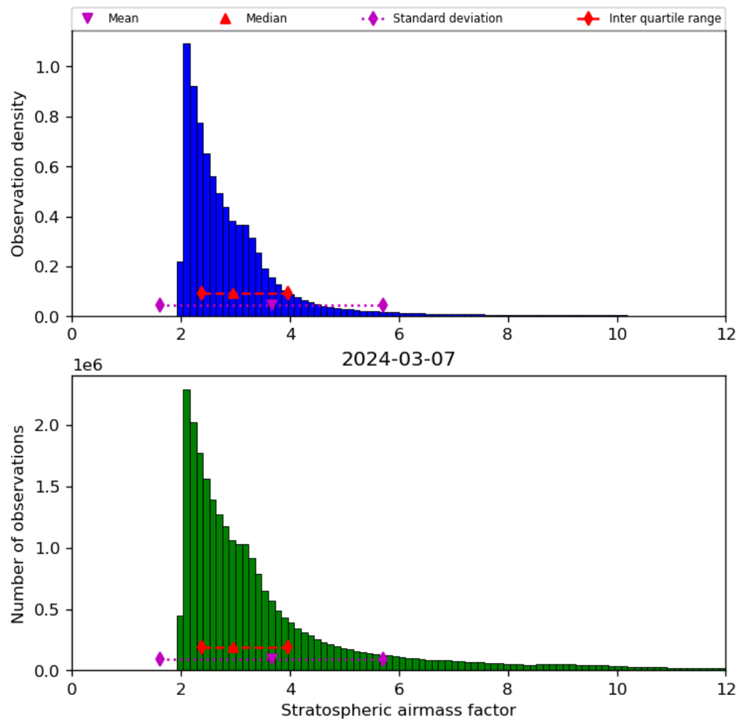
Figure 44: Histogram of “Stratospheric airmass factor” for 2024-03-06 to 2024-03-08
