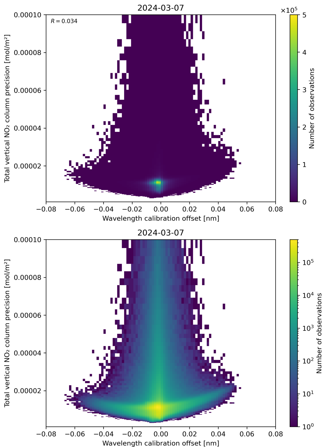
Figure 180: Scatter density plot of “Wavelength calibration offset” against “Total vertical NO 2 column precision” for 2024-03-06 to 2024-03-08.
