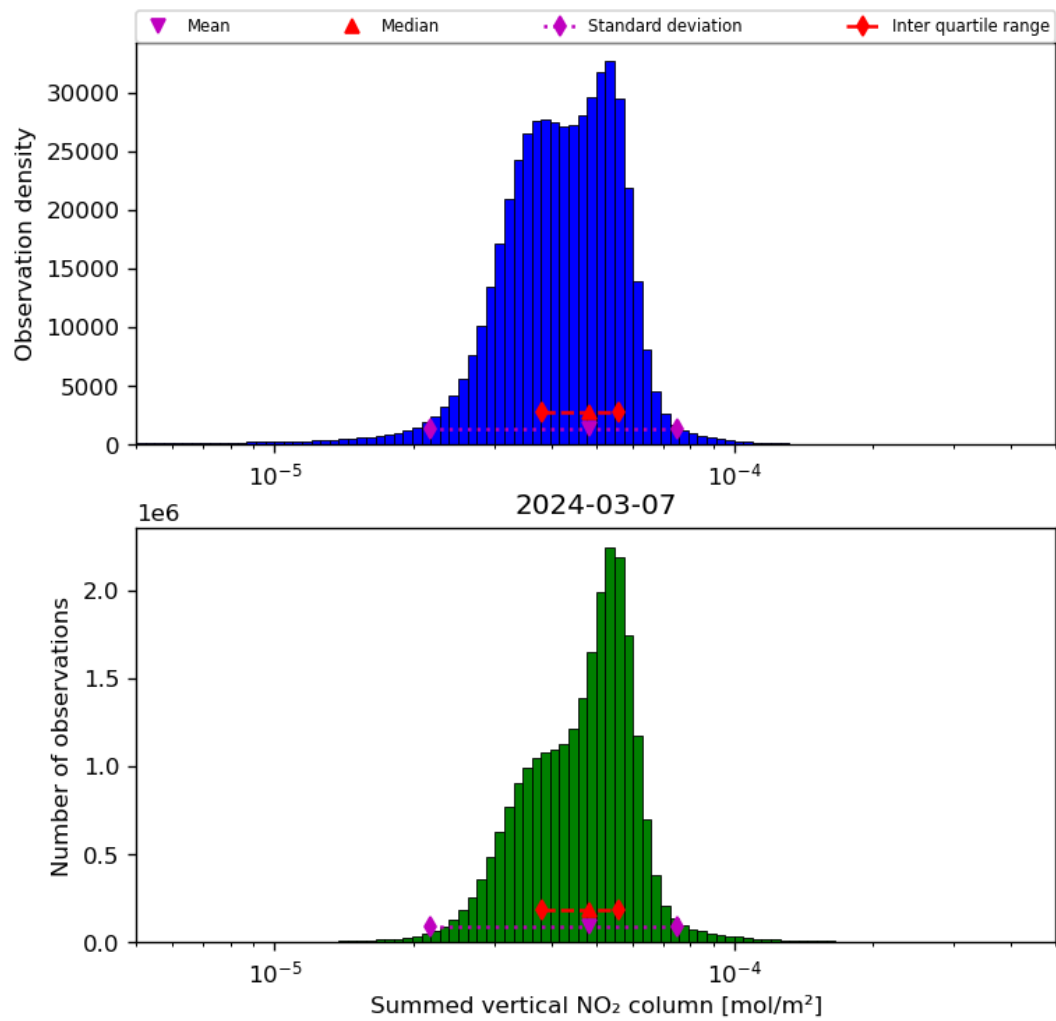
Figure 40: Histogram of “Summed vertical NO 2 column” for 2024-03-06 to 2024-03-08
