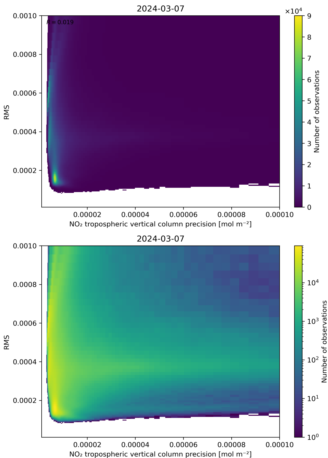
Figure 140: Scatter density plot of “NO 2 tropospheric vertical column precision” against “RMS” for 2024-03-06 to 2024-03-08.
