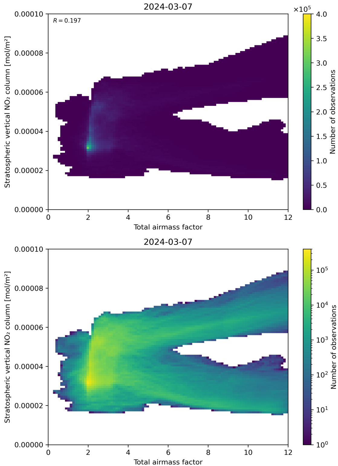
Figure 64: Scatter density plot of “Total airmass factor” against “Stratospheric vertical NO 2 column” for 2024-03-06 to 2024-03-08.
