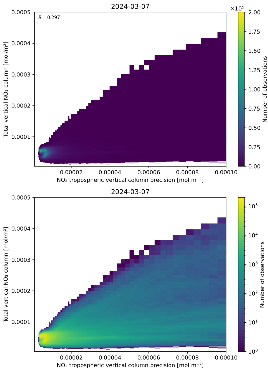
Figure 138: Scatter density plot of “NO 2 tropospheric vertical column precision” against “Total vertical NO 2 column” for 2024-03-06 to 2024-03-08.
