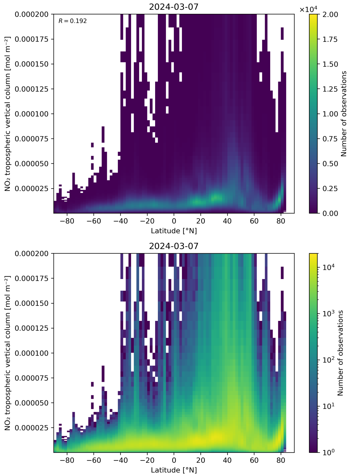
Figure 92: Scatter density plot of “Latitude” against “NO 2 tropospheric vertical column” for 2024-03-06 to 2024-03-08.
