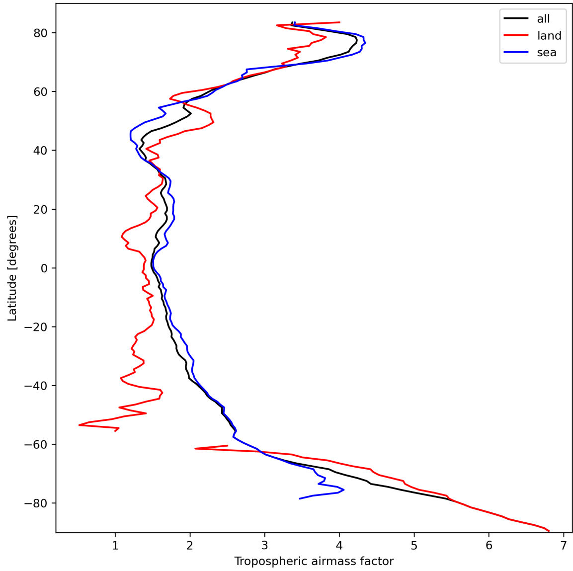
Figure 14: Zonal average of “Tropospheric airmass factor” for 2024-03-06 to 2024-03-08.
