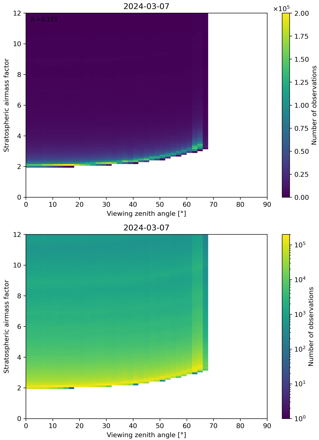
Figure 159: Scatter density plot of “Viewing zenith angle” against “Stratospheric airmass factor” for 2024-03-06 to 2024-03-08.
