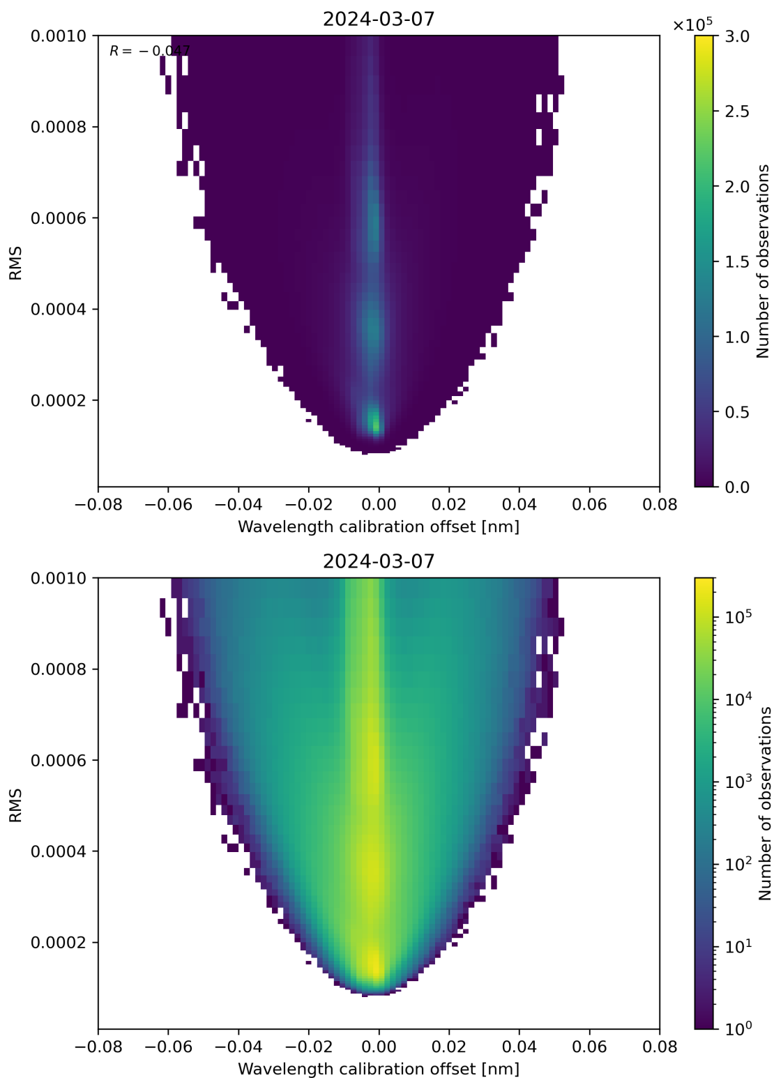
Figure 181: Scatter density plot of “Wavelength calibration offset” against “RMS” for 2024-03-06 to 2024-03-08.
