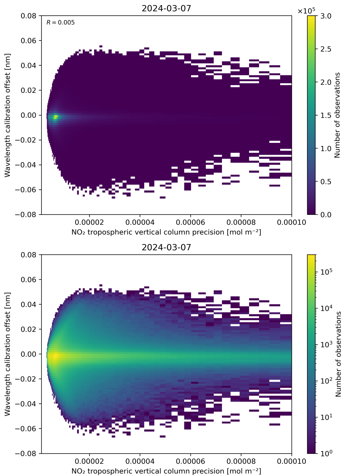
Figure 141: Scatter density plot of “NO 2 tropospheric vertical column precision” against “Wavelength calibration offset” for 2024-03-06 to 2024-03-08.
