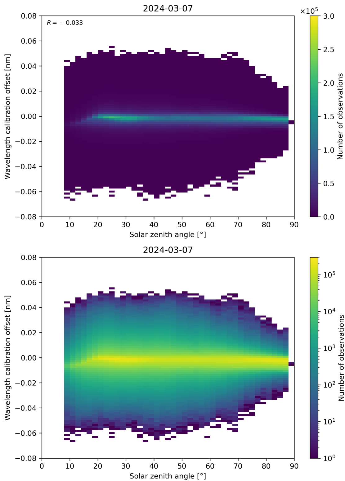
Figure 158: Scatter density plot of “Solar zenith angle” against “Wavelength calibration offset” for 2024-03-06 to 2024-03-08.
