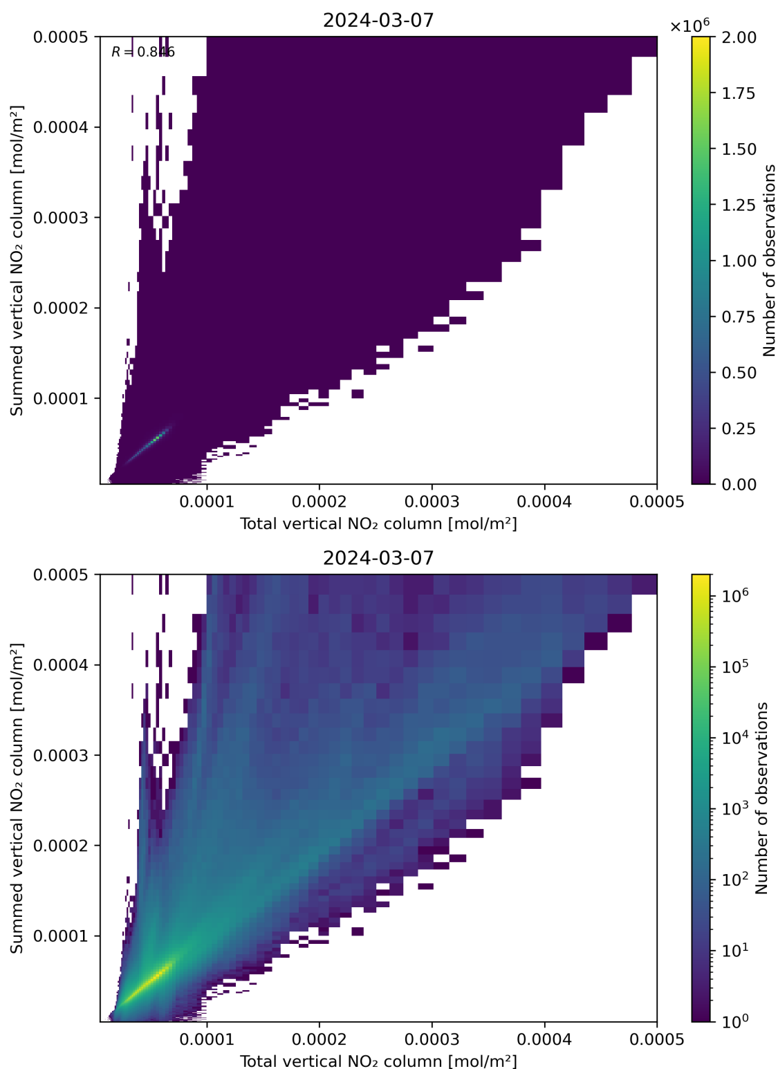
Figure 112: Scatter density plot of “Total vertical NO 2 column” against “Summed vertical NO 2 column” for 2024-03-06 to 2024-03-08.
