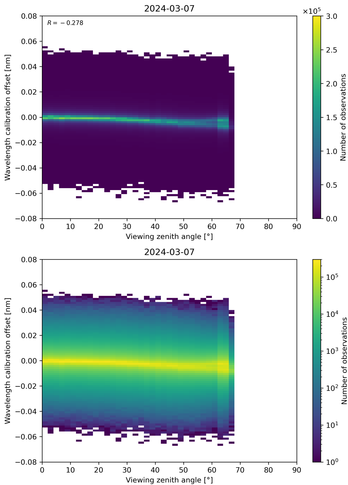
Figure 173: Scatter density plot of “Viewing zenith angle” against “Wavelength calibration offset” for 2024-03-06 to 2024-03-08.
