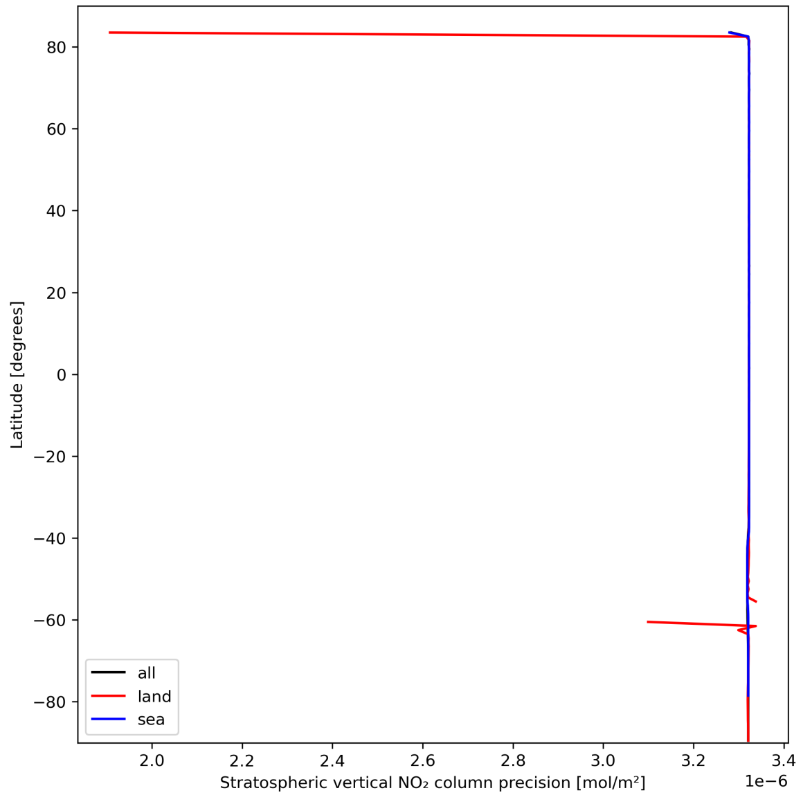
Figure 20: Zonal average of “Stratospheric vertical NO 2 column precision” for 2024-03-06 to 2024-03-08.
