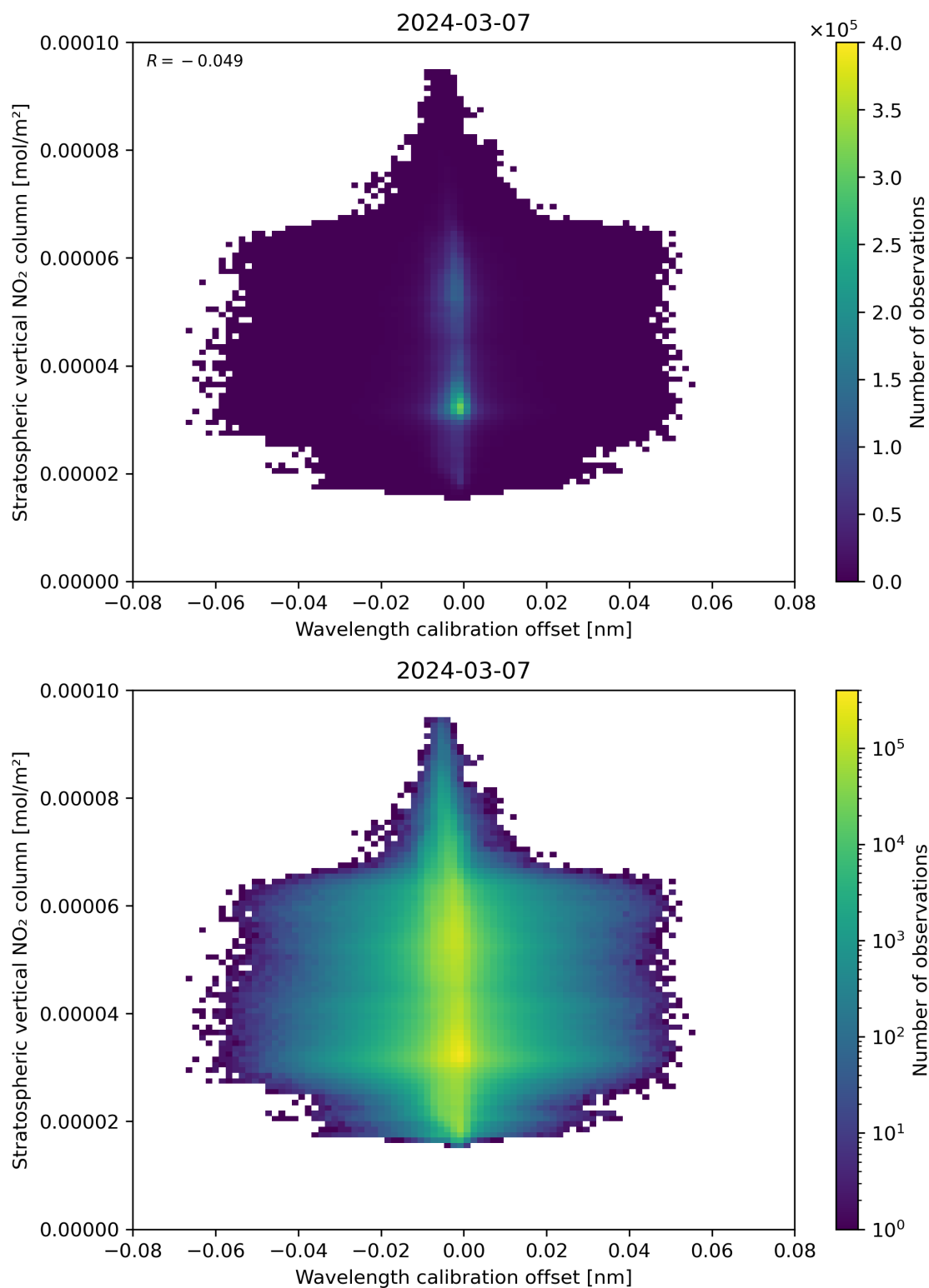
Figure 176: Scatter density plot of “Wavelength calibration offset” against “Stratospheric vertical NO 2 column” for 2024-03-06 to 2024-03-08.
