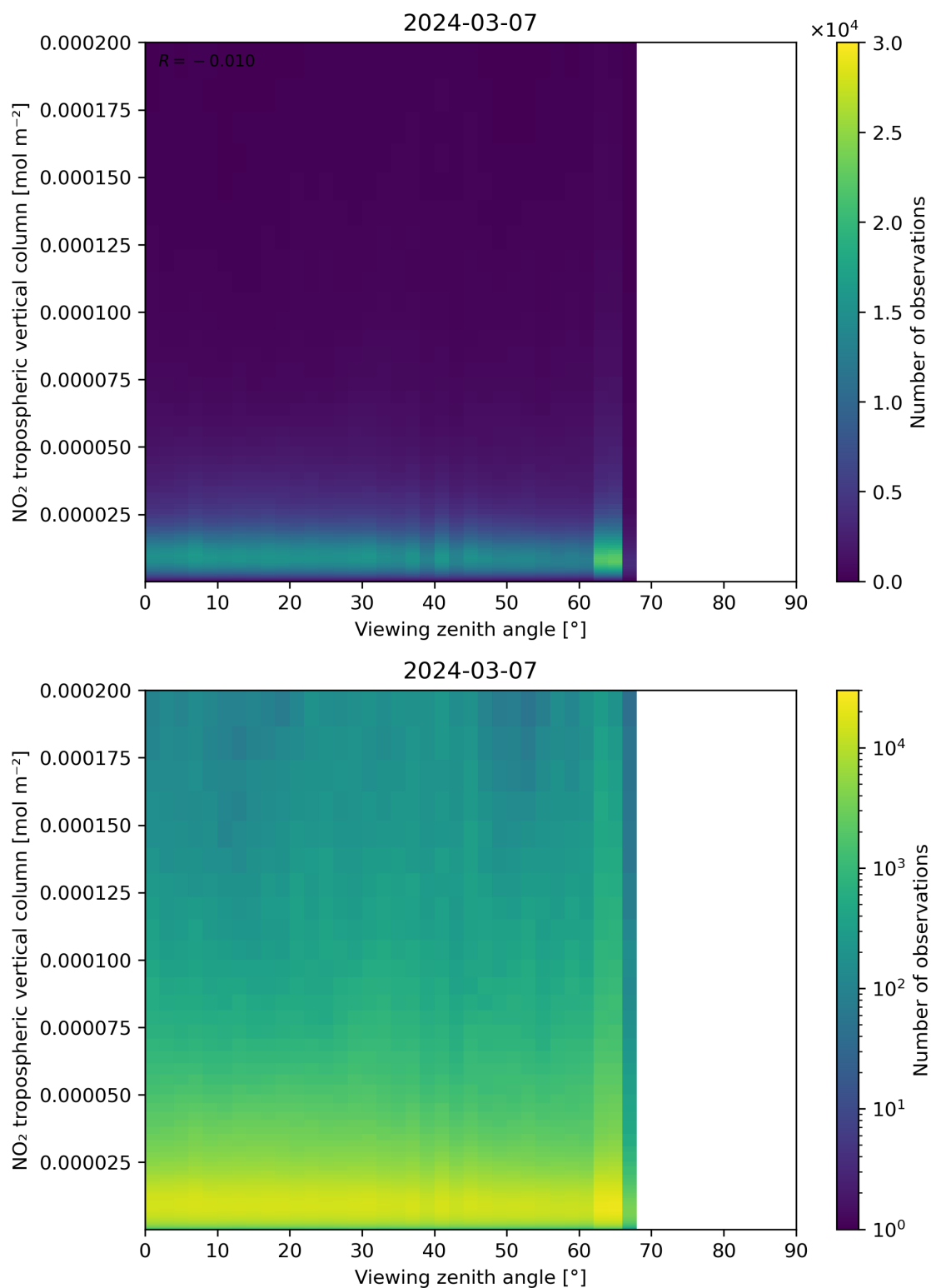
Figure 169: Scatter density plot of “Viewing zenith angle” against “NO 2 tropospheric vertical column” for 2024-03-06 to 2024-03-08.
