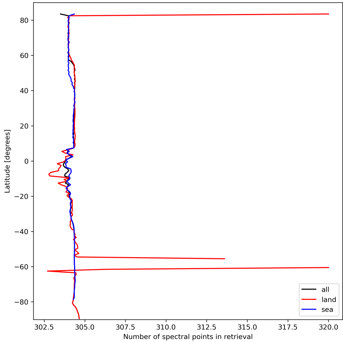
Figure 16: Zonal average of “Number of spectral points in retrieval” for 2024-03-06 to 2024-03-08.
