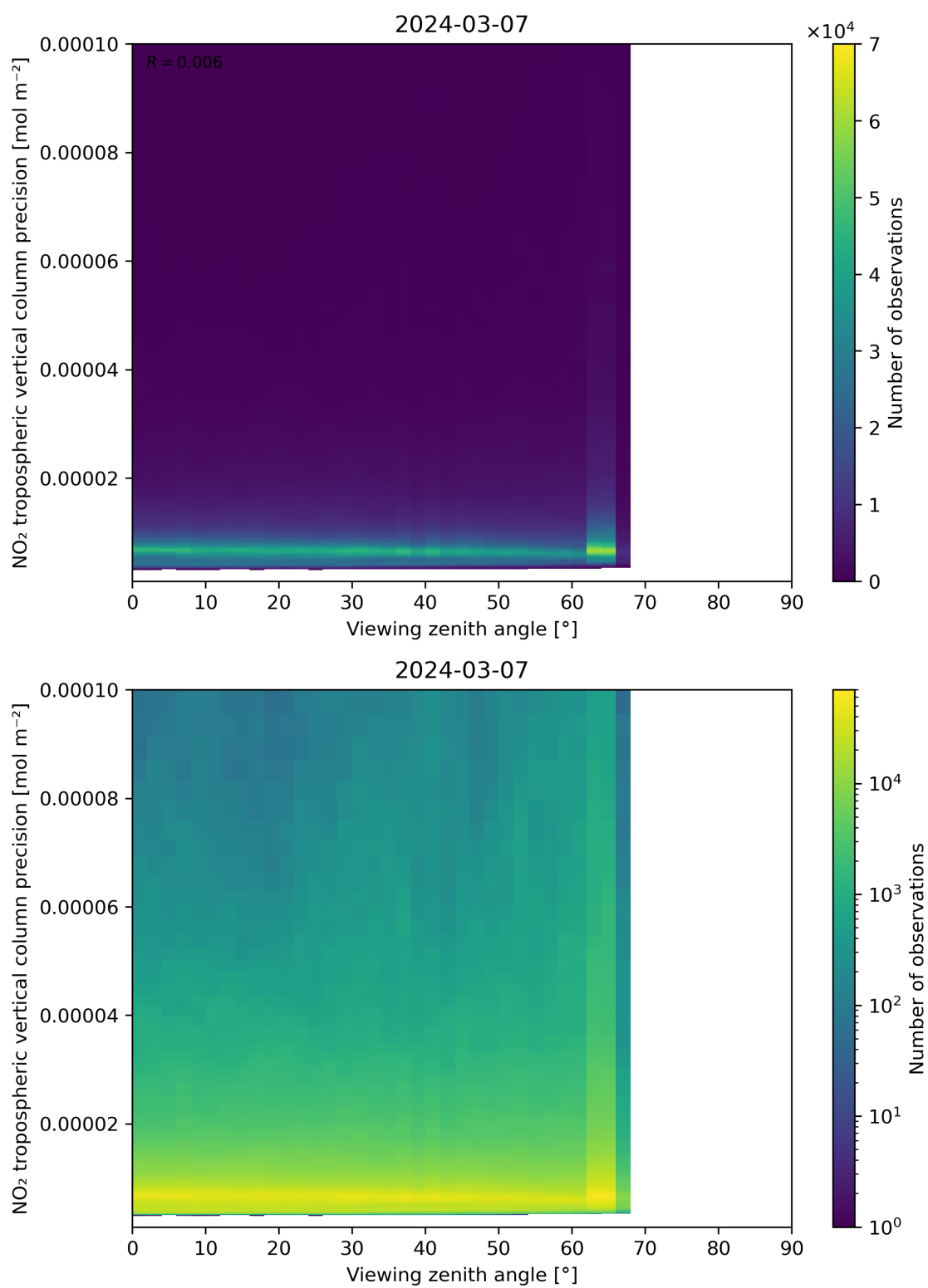
Figure 170: Scatter density plot of “Viewing zenith angle” against “NO 2 tropospheric vertical column precision” for 2024-03-06 to 2024-03-08.
