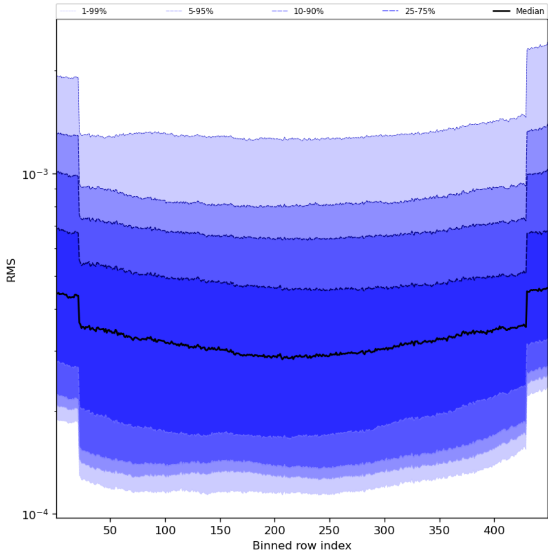
Figure 60: Along track statistics of “RMS” for 2024-03-06 to 2024-03-08
