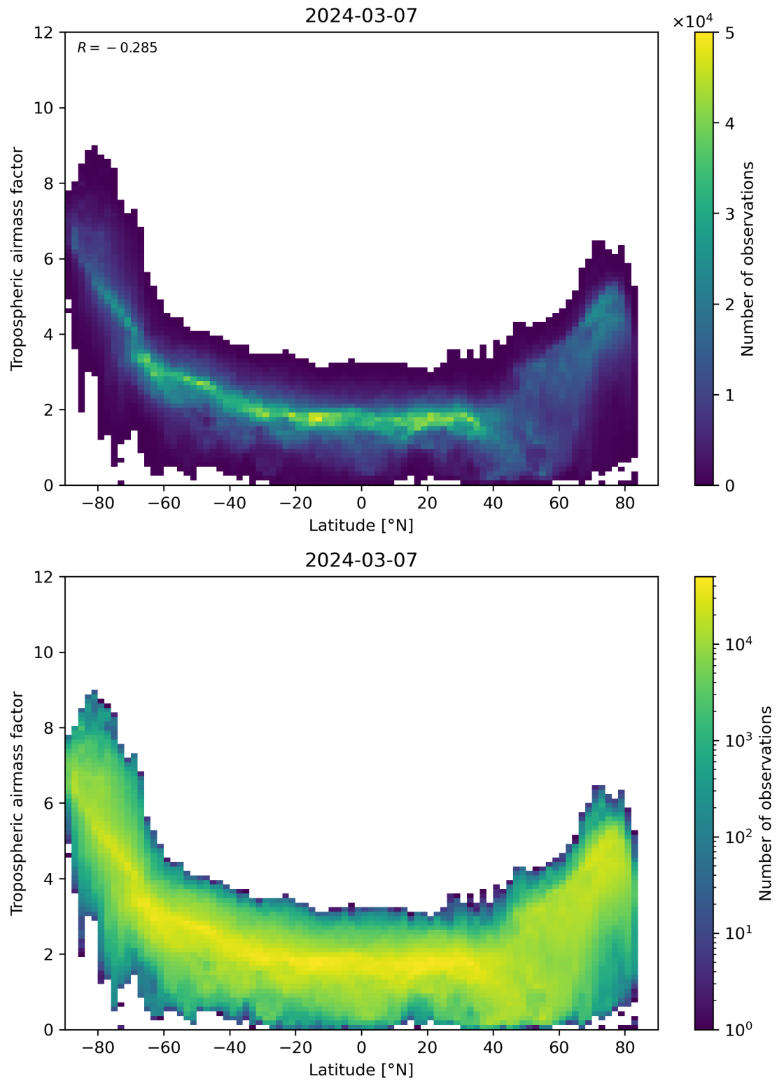
Figure 85: Scatter density plot of “Latitude” against “Tropospheric airmass factor” for 2024-03-06 to 2024-03-08.
