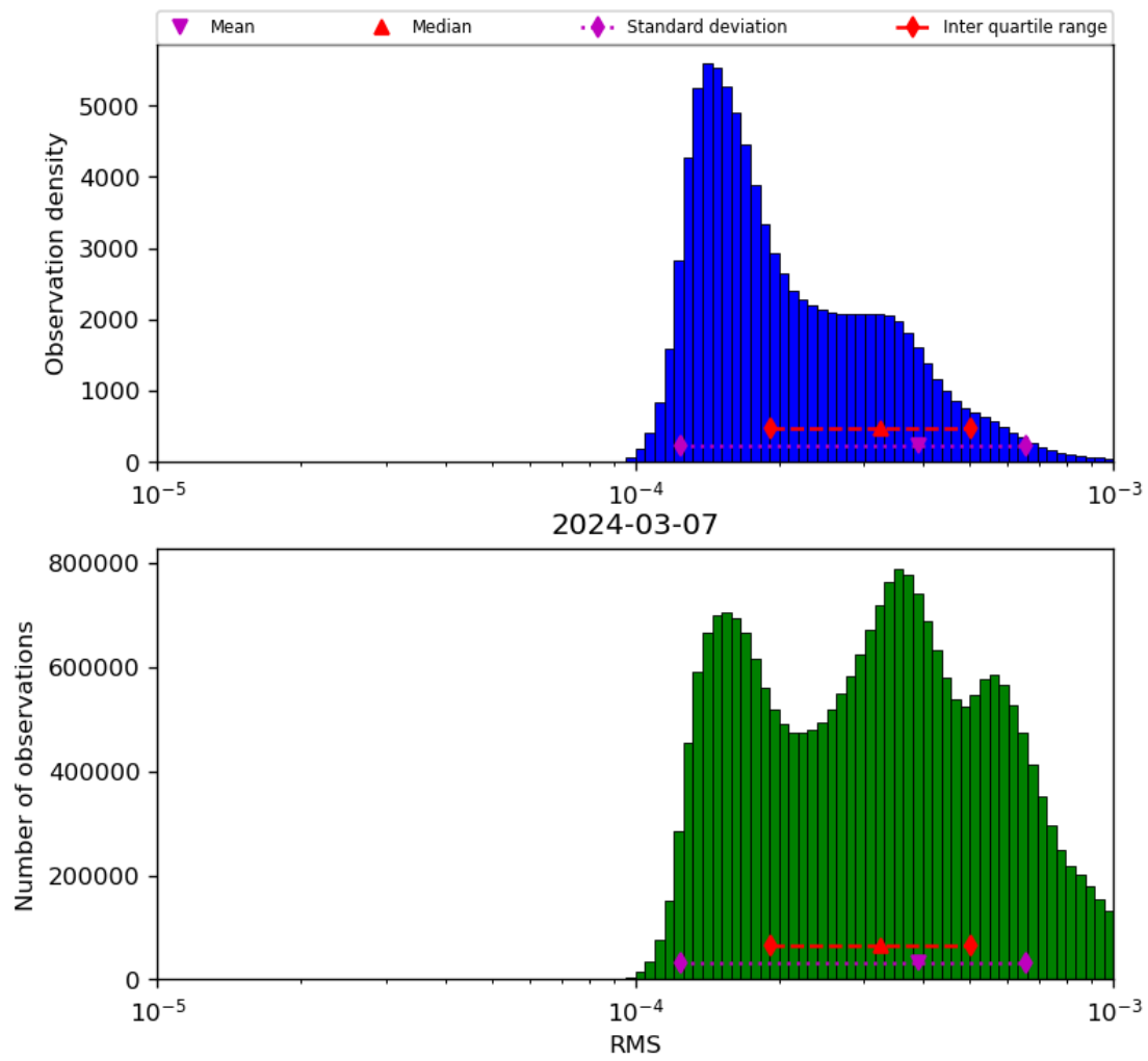
Figure 43: Histogram of “RMS” for 2024-03-06 to 2024-03-08
