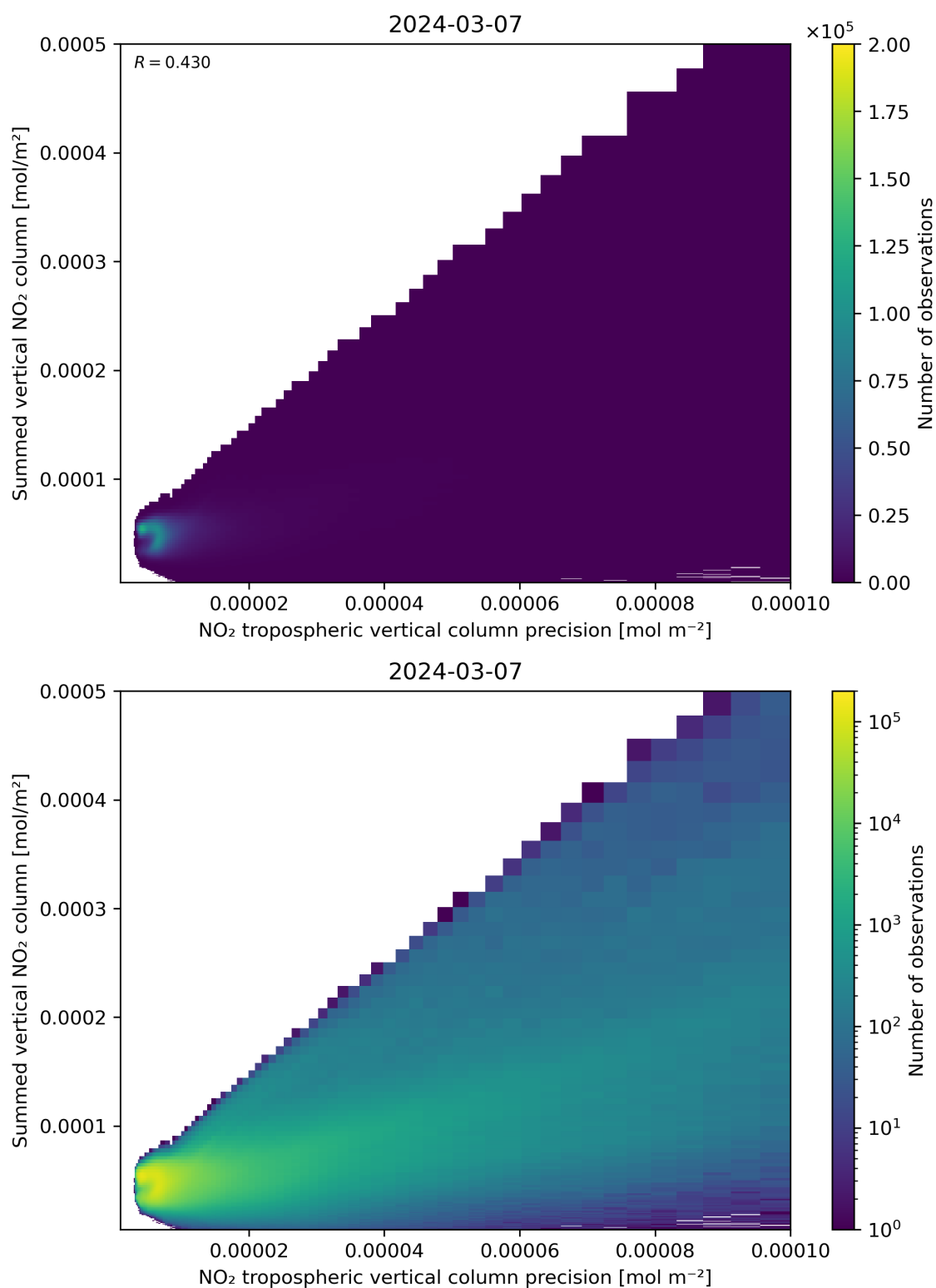
Figure 136: Scatter density plot of “NO 2 tropospheric vertical column precision” against “Summed vertical NO 2 column” for 2024-03-06 to 2024-03-08.
