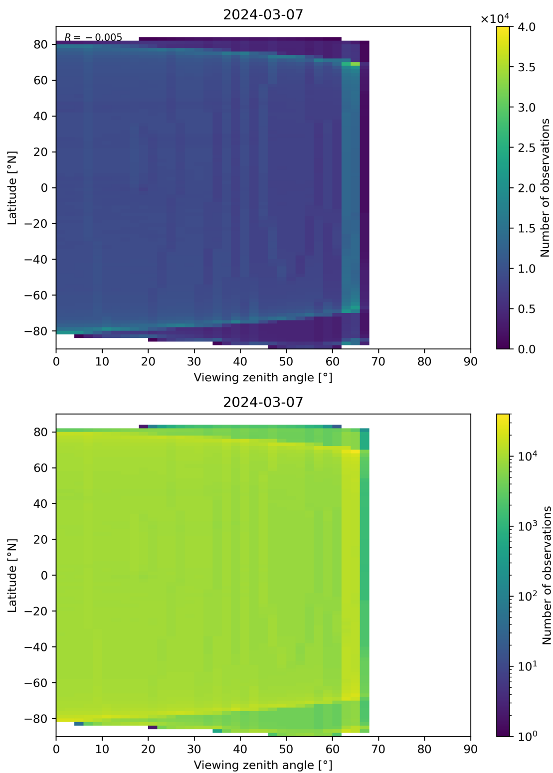
Figure 163: Scatter density plot of “Viewing zenith angle” against “Latitude” for 2024-03-06 to 2024-03-08.
