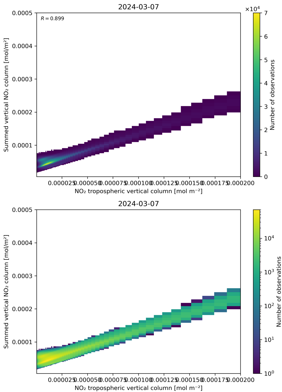
Figure 126: Scatter density plot of “NO 2 tropospheric vertical column” against “Summed vertical NO 2 column” for 2024-03-06 to 2024-03-08.
