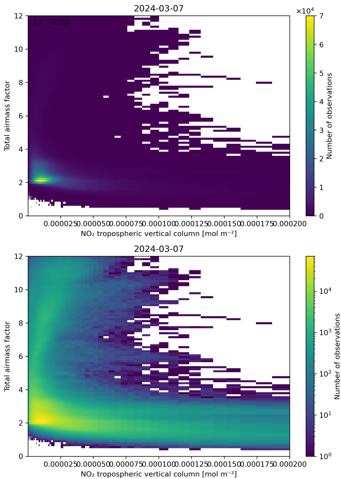
Figure 122: Scatter density plot of “NO 2 tropospheric vertical column” against “Total air mass factor” for 2024-03-06 to 2024-03-08.
