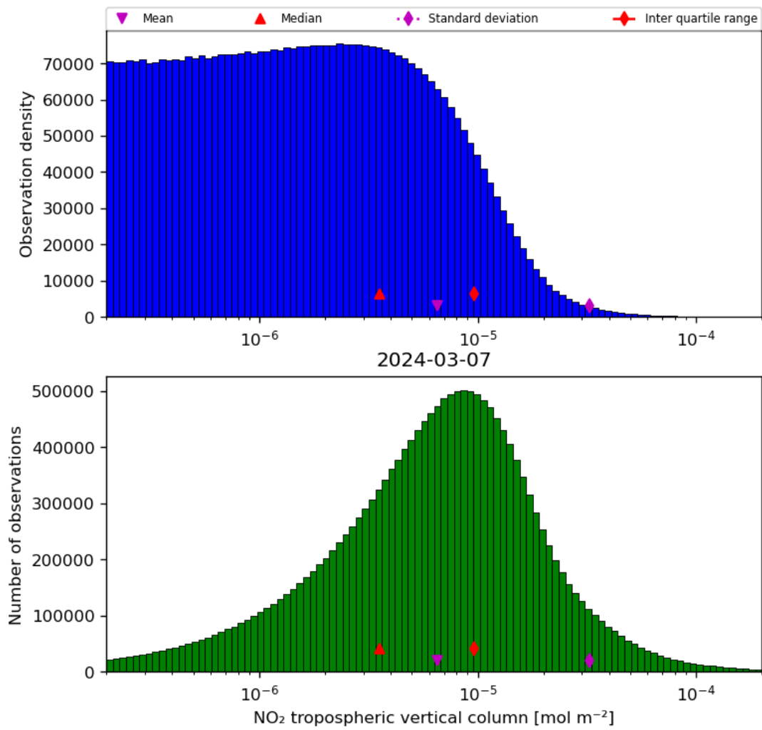
Figure 29: Histogram of “NO 2 tropospheric vertical column” for 2024-03-06 to 2024-03-08
