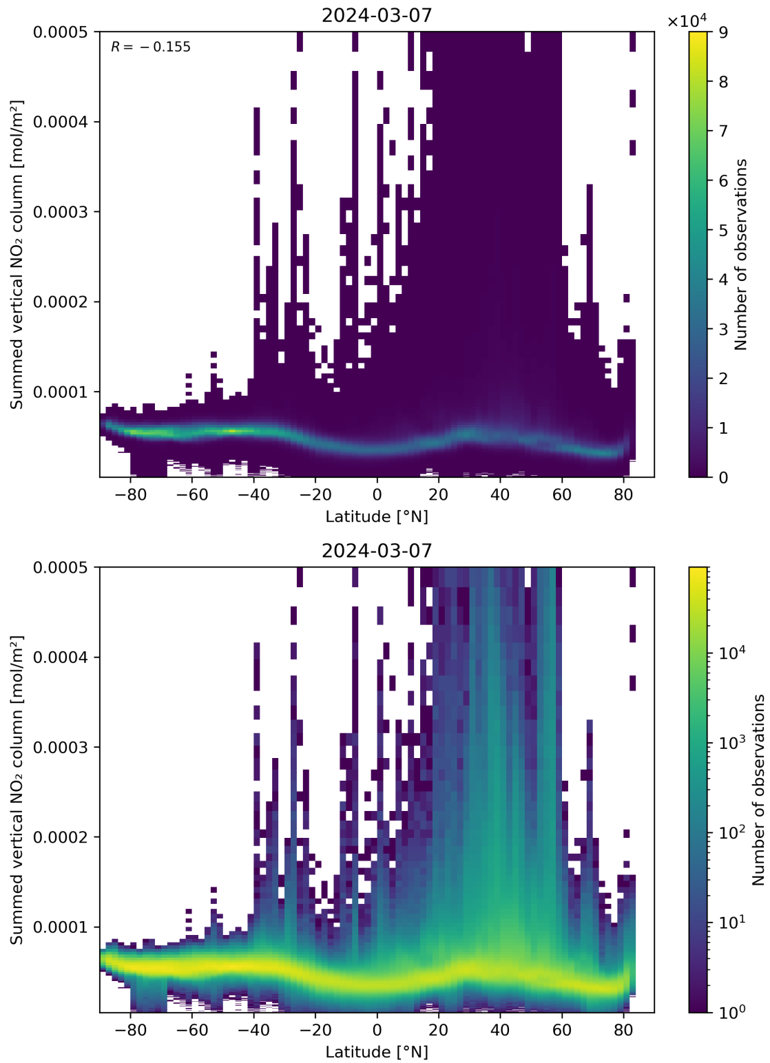
Figure 88: Scatter density plot of “Latitude” against “Summed vertical NO 2 column” for 2024-03-06 to 2024-03-08.
