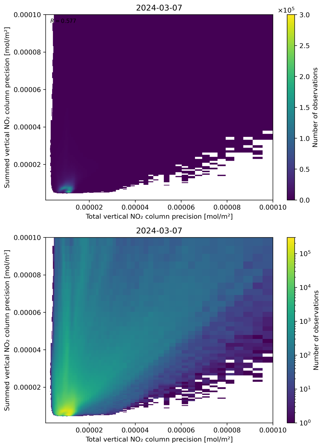
Figure 118: Scatter density plot of “Total vertical NO 2 column precision” against “Summed vertical NO 2 column precision” for 2024-03-06 to 2024-03-08.
