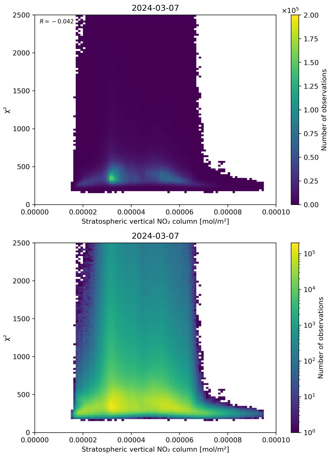
Figure 97: Scatter density plot of “Stratospheric vertical NO 2 column” against “ \chi^2 ” for 2024-03-06 to 2024-03-08.
