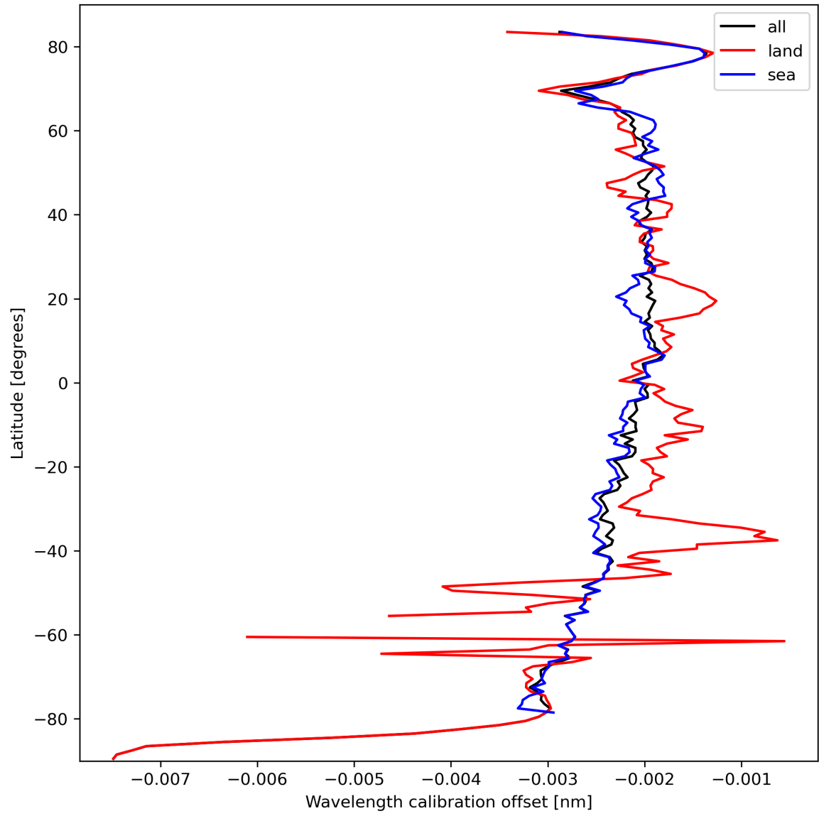
Figure 18: Zonal average of “Wavelength calibration offset” for 2024-03-06 to 2024-03-08.
