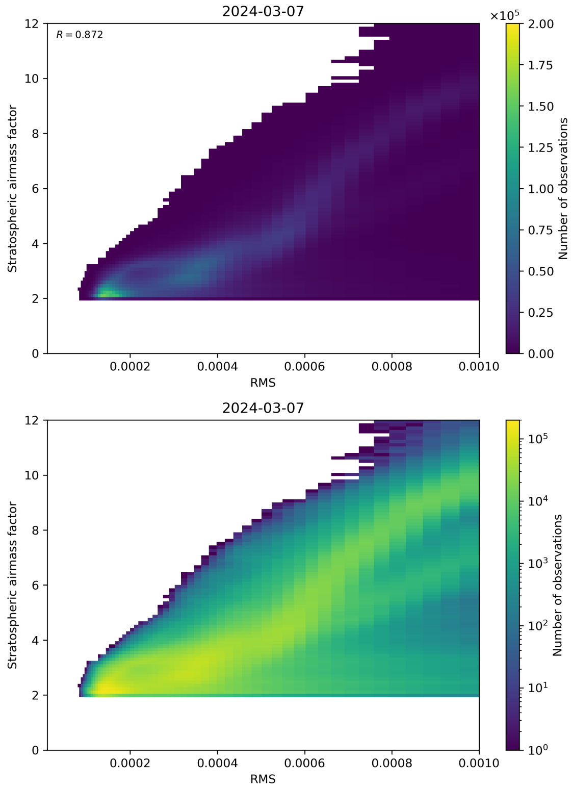
Figure 144: Scatter density plot of “RMS” against “Stratospheric airmass factor” for 2024-03-06 to 2024-03-08.
