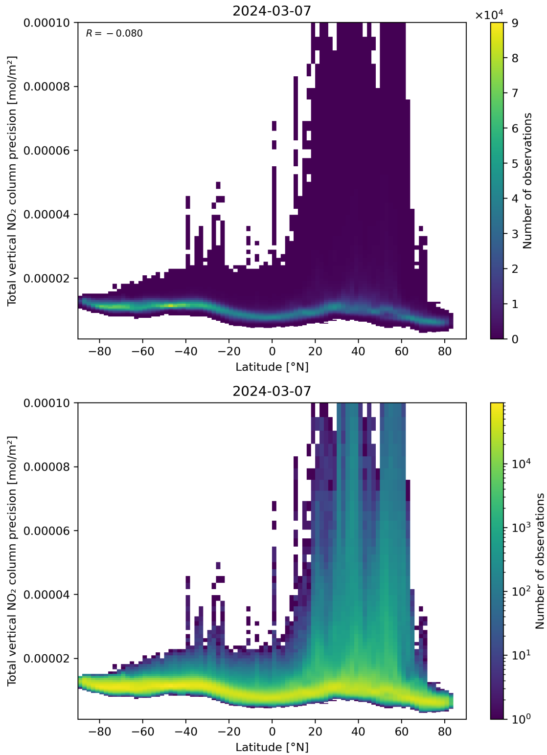
Figure 91: Scatter density plot of “Latitude” against “Total vertical NO 2 column precision” for 2024-03-06 to 2024-03-08.
