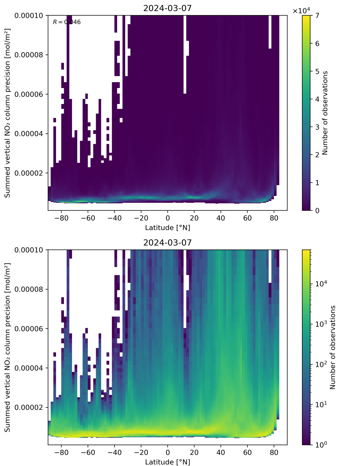
Figure 89: Scatter density plot of “Latitude” against “Summed vertical NO 2 column precision” for 2024-03-06 to 2024-03-08.
