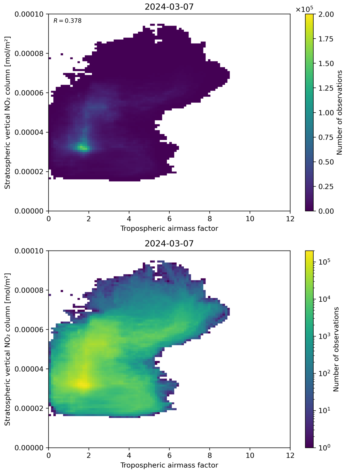
Figure 74: Scatter density plot of “Tropospheric airmass factor” against “Stratospheric vertical NO 2 column” for 2024-03-06 to 2024-03-08.
