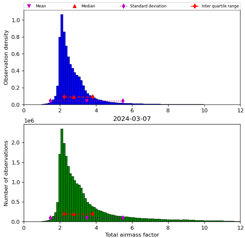
Figure 32: Histogram of “Total airmass factor” for 2024-03-06 to 2024-03-08
