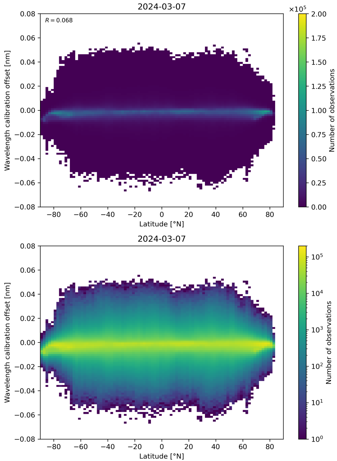
Figure 95: Scatter density plot of “Latitude” against “Wavelength calibration offset” for 2024-03-06 to 2024-03-08.
