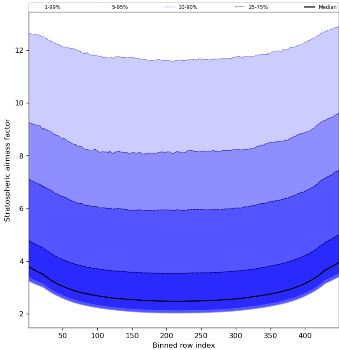
Figure 61: Along track statistics of “Stratospheric airmass factor” for 2024-03-06 to 2024-03-08
