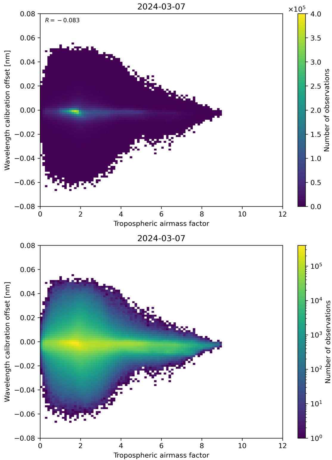
Figure 80: Scatter density plot of “Tropospheric airmass factor” against “Wavelength calibration offset” for 2024-03-06 to 2024-03-08.
