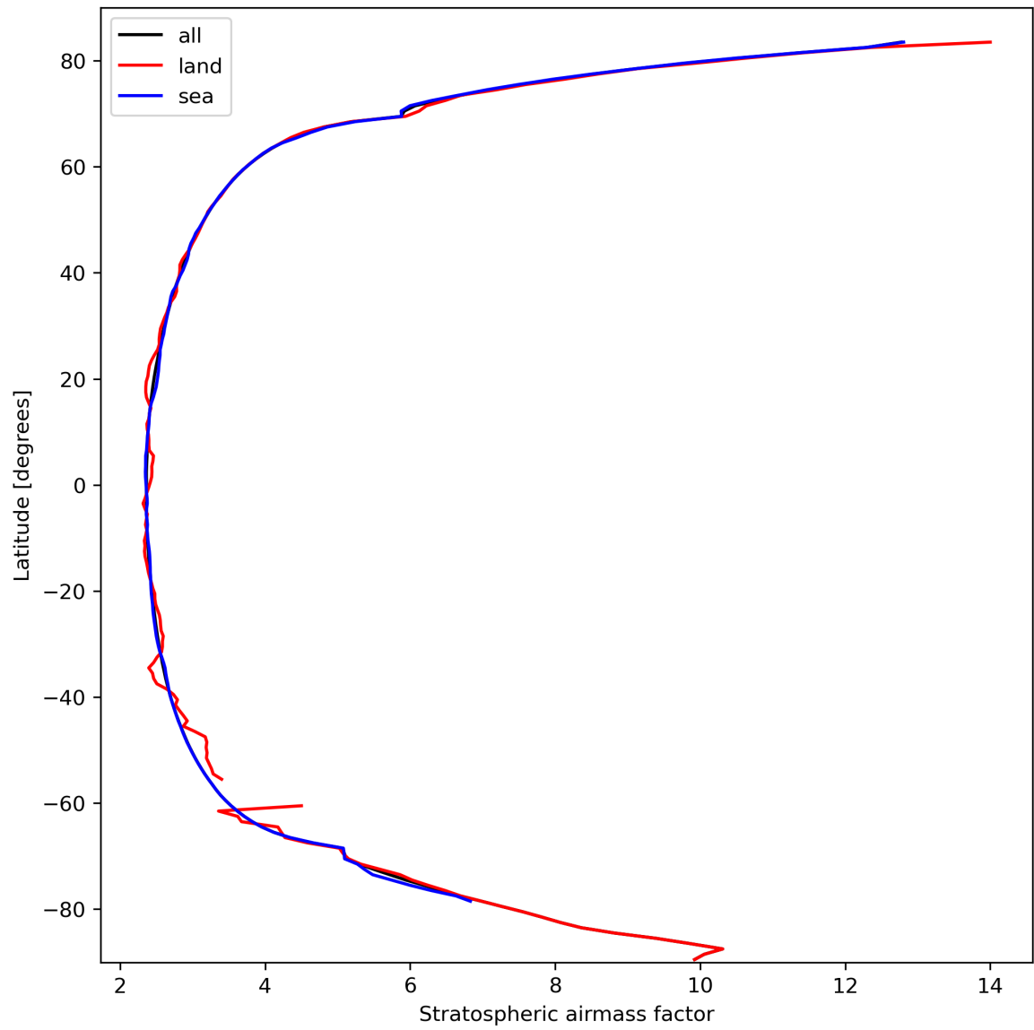
Figure 27: Zonal average of “Stratospheric air mass factor” for 2024-03-06 to 2024-03-08.
