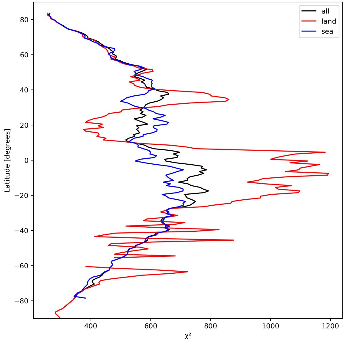
Figure 25: Zonal average of “ \chi^2 ” for 2024-03-06 to 2024-03-08.
