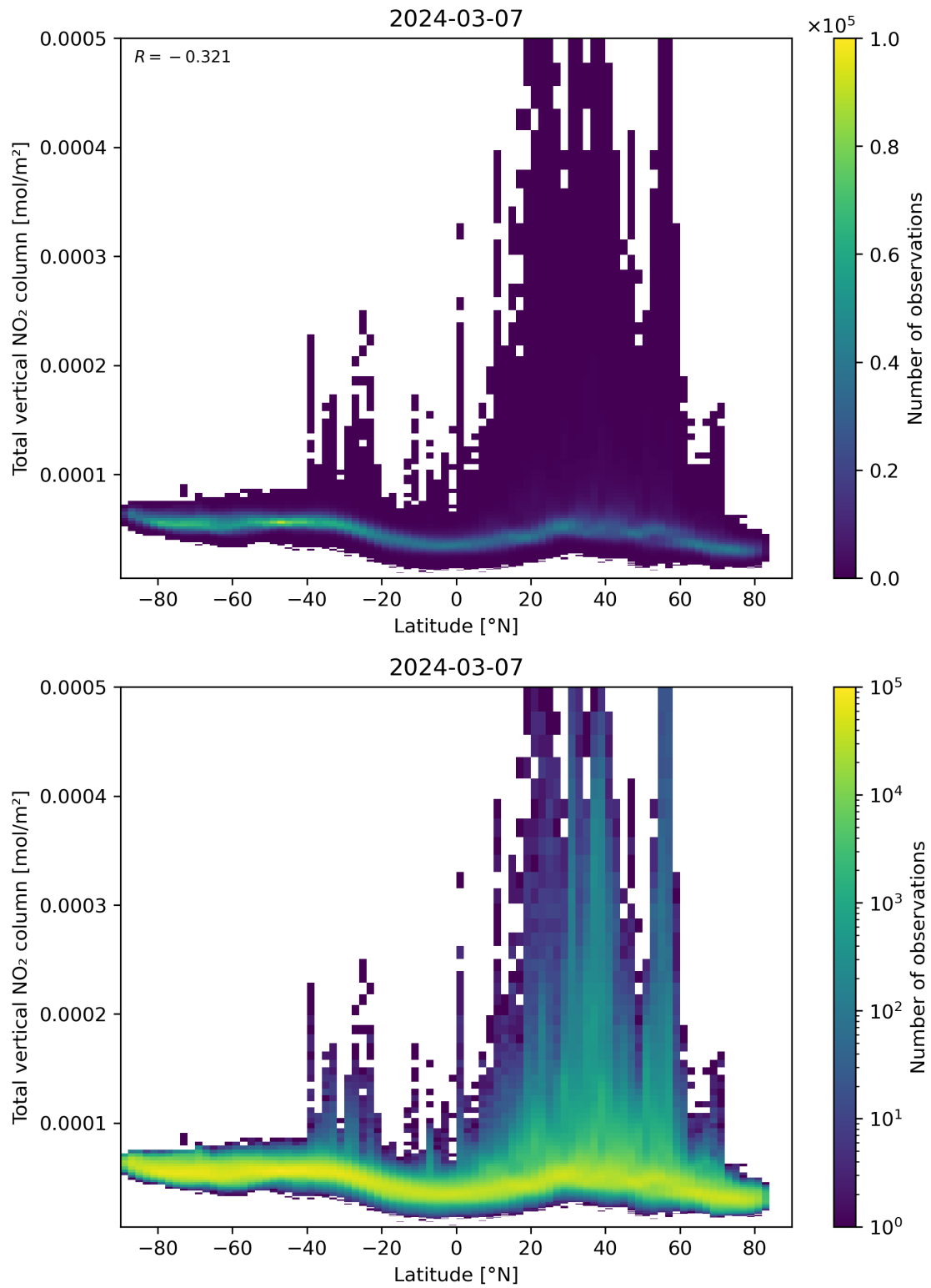
Figure 90: Scatter density plot of “Latitude” against “Total vertical NO 2 column” for 2024-03-06 to 2024-03-08.
