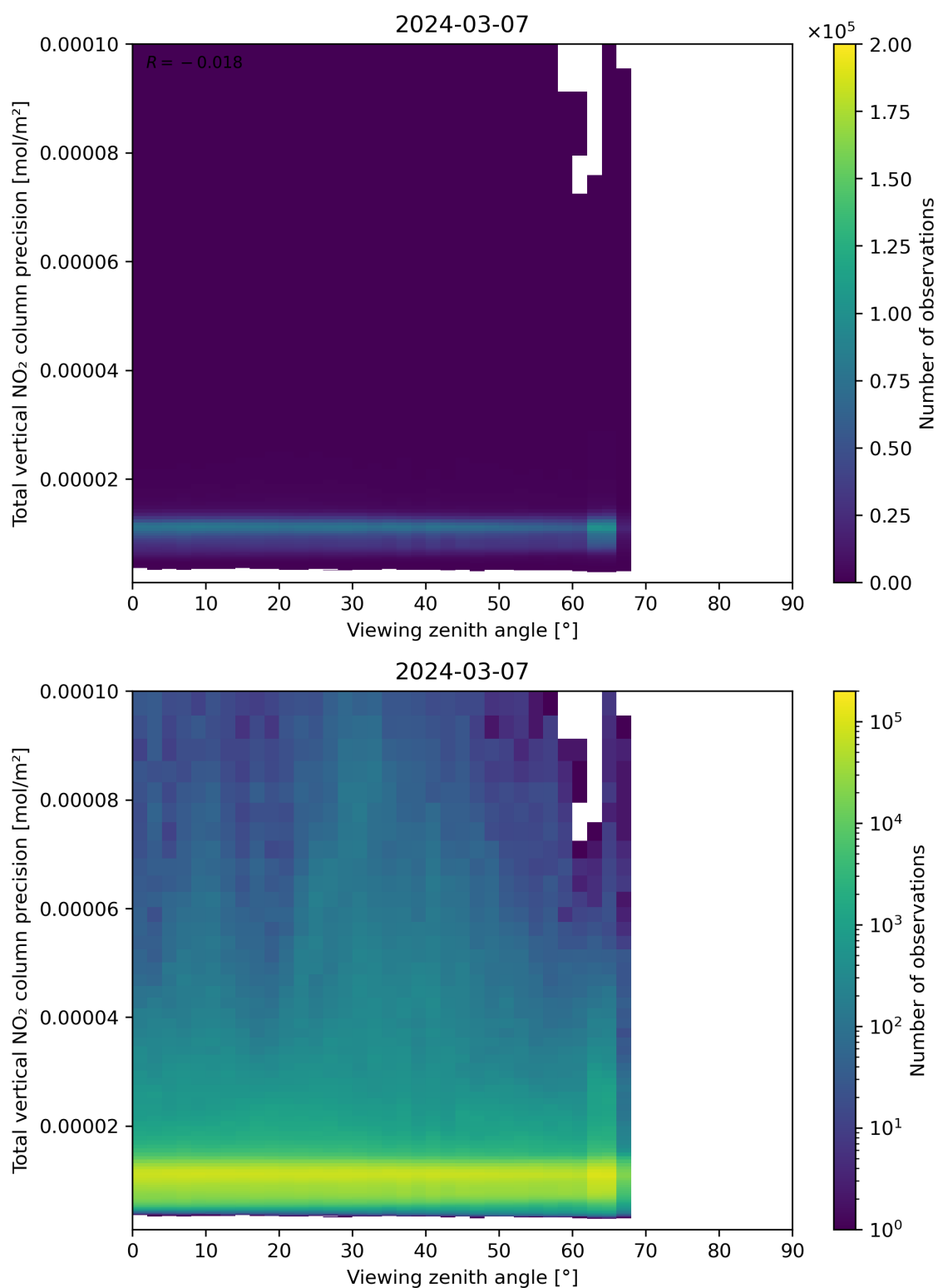
Figure 168: Scatter density plot of “Viewing zenith angle” against “Total vertical NO 2 column precision” for 2024-03-06 to 2024-03-08.
