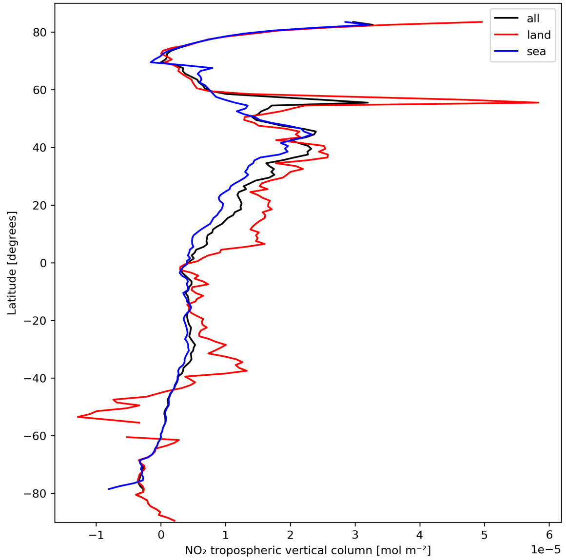
Figure 12: Zonal average of “NO 2 tropospheric vertical column” for 2024-03-06 to 2024-03-08.
