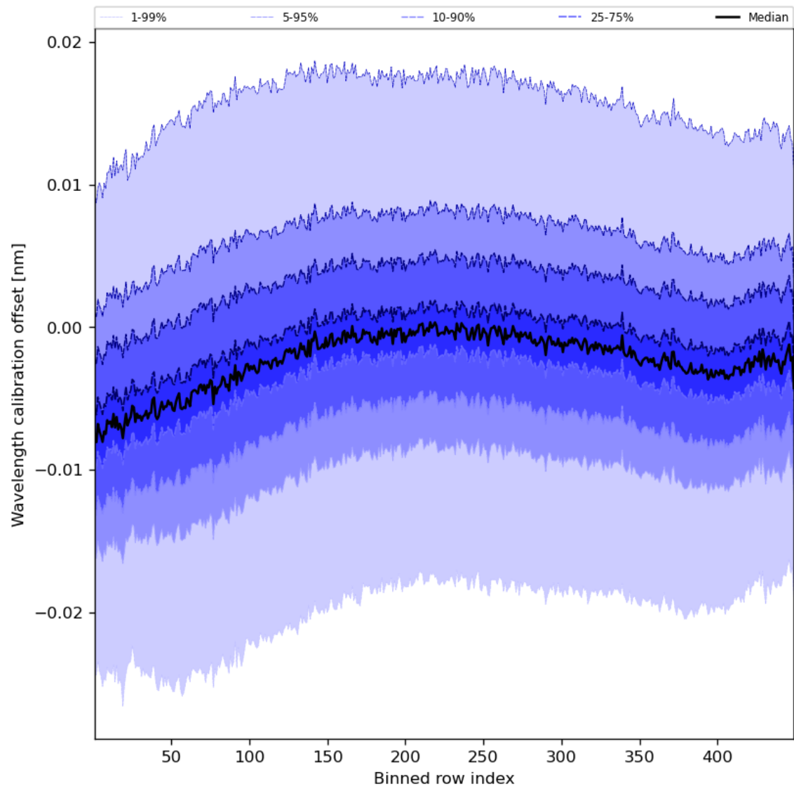
Figure 52: Along track statistics of “Wavelength calibration offset” for 2024-03-06 to 2024-03-08
