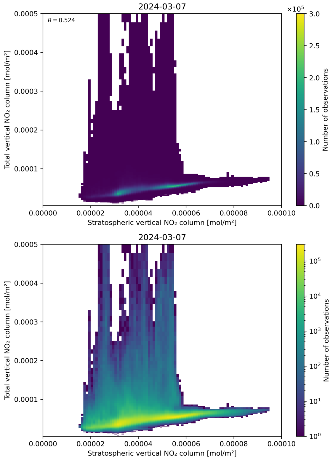
Figure 100: Scatter density plot of “Stratospheric vertical NO 2 column” against “Total vertical NO 2 column” for 2024-03-06 to 2024-03-08.
