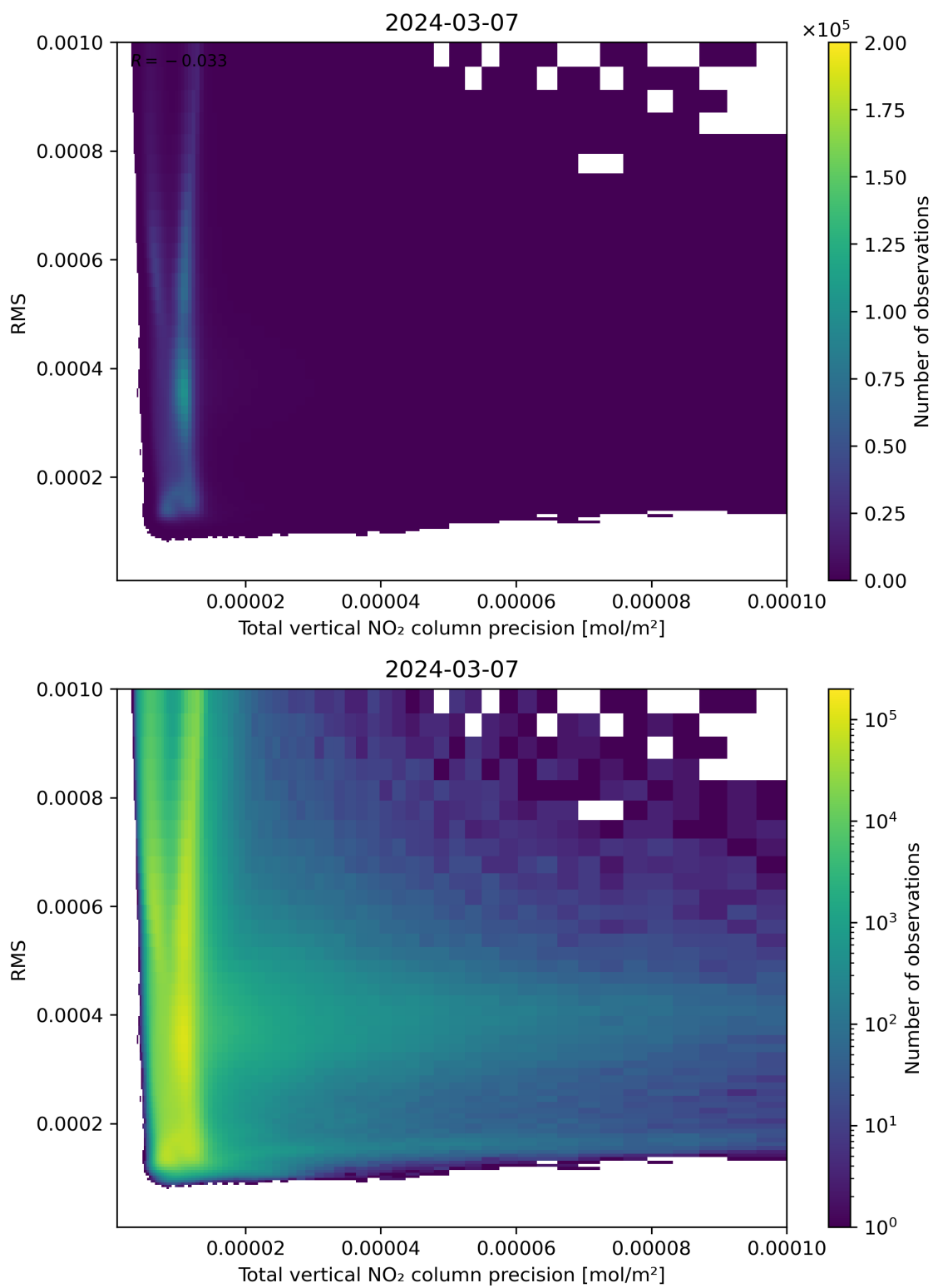
Figure 119: Scatter density plot of “Total vertical NO 2 column precision” against “RMS” for 2024-03-06 to 2024-03-08.
