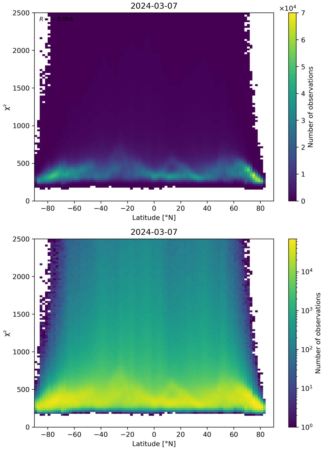
Figure 86: Scatter density plot of “Latitude” against “ \chi^2 ” for 2024-03-06 to 2024-03-08.
