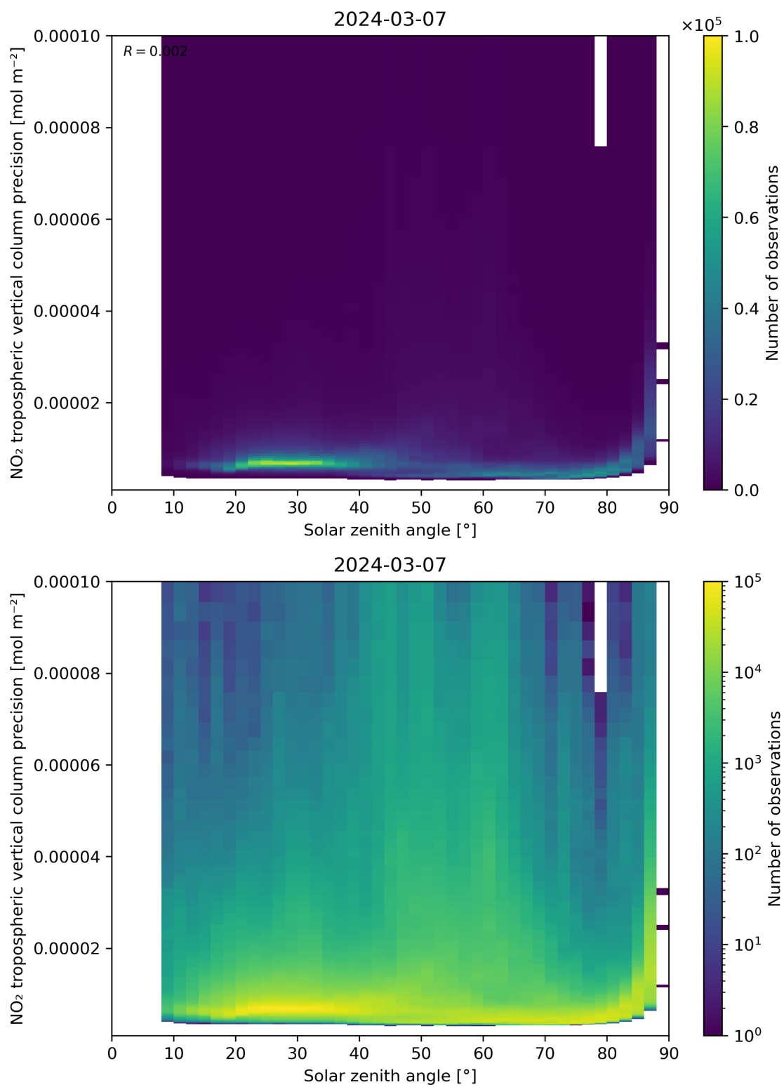
Figure 156: Scatter density plot of “Solar zenith angle” against “NO 2 tropospheric vertical column precision” for 2024-03-06 to 2024-03-08.
