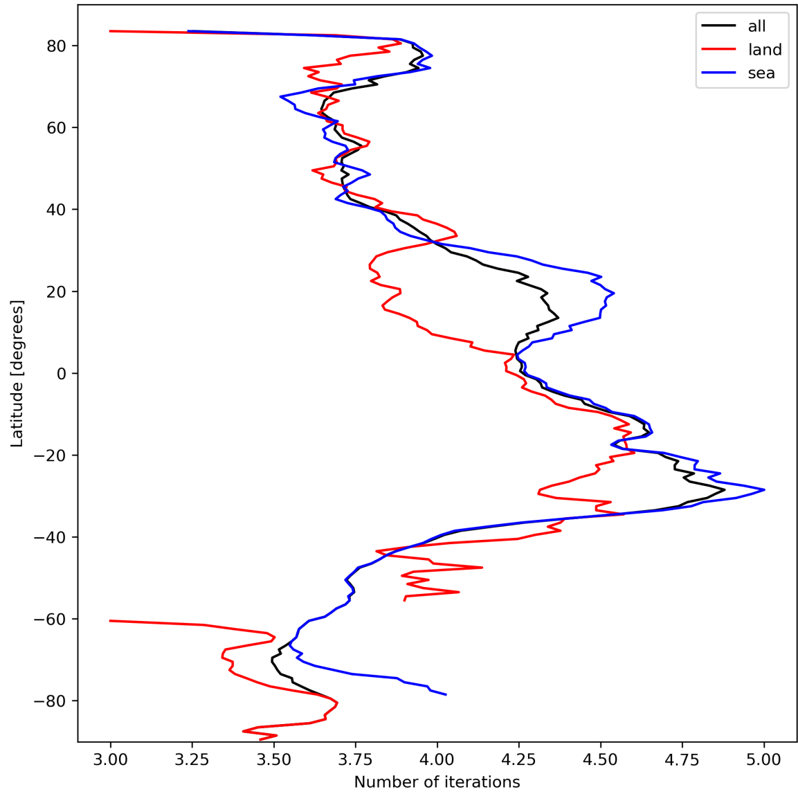
Figure 17: Zonal average of “Number of iterations” for 2024-03-06 to 2024-03-08.
