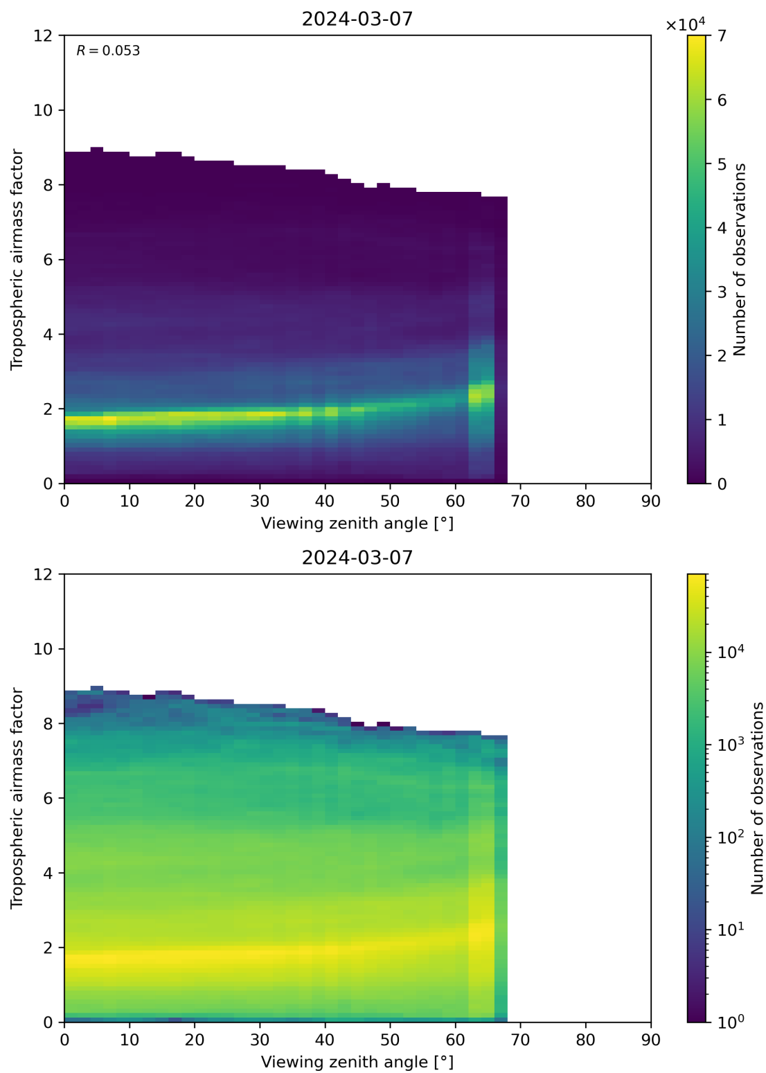
Figure 161: Scatter density plot of “Viewing zenith angle” against “Tropospheric airmass factor” for 2024-03-06 to 2024-03-08.
