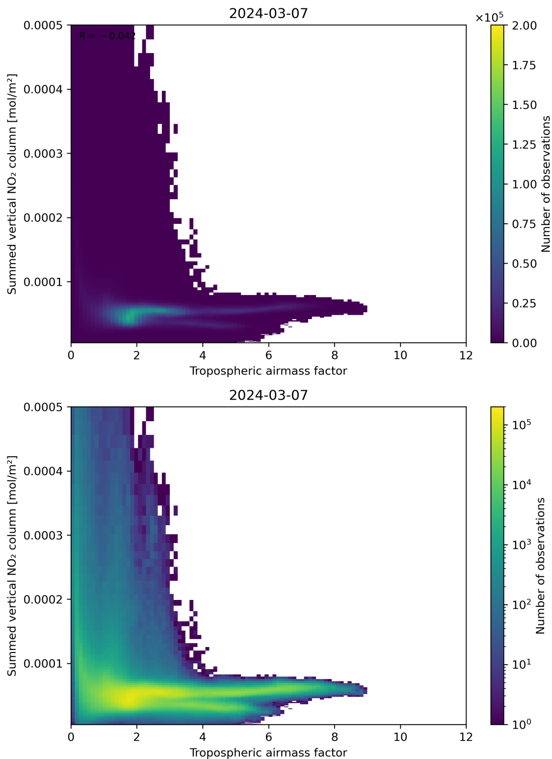
Figure 75: Scatter density plot of “Tropospheric airmass factor” against “Summed vertical NO 2 column” for 2024-03-06 to 2024-03-08.
