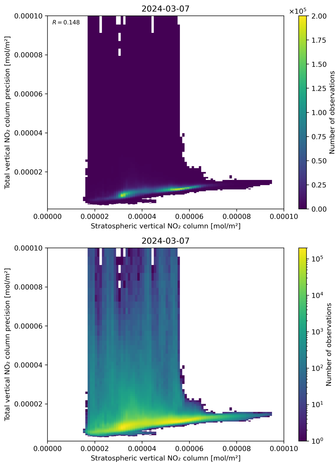
Figure 101: Scatter density plot of “Stratospheric vertical NO 2 column” against “Total vertical NO 2 column precision” for 2024-03-06 to 2024-03-08.
