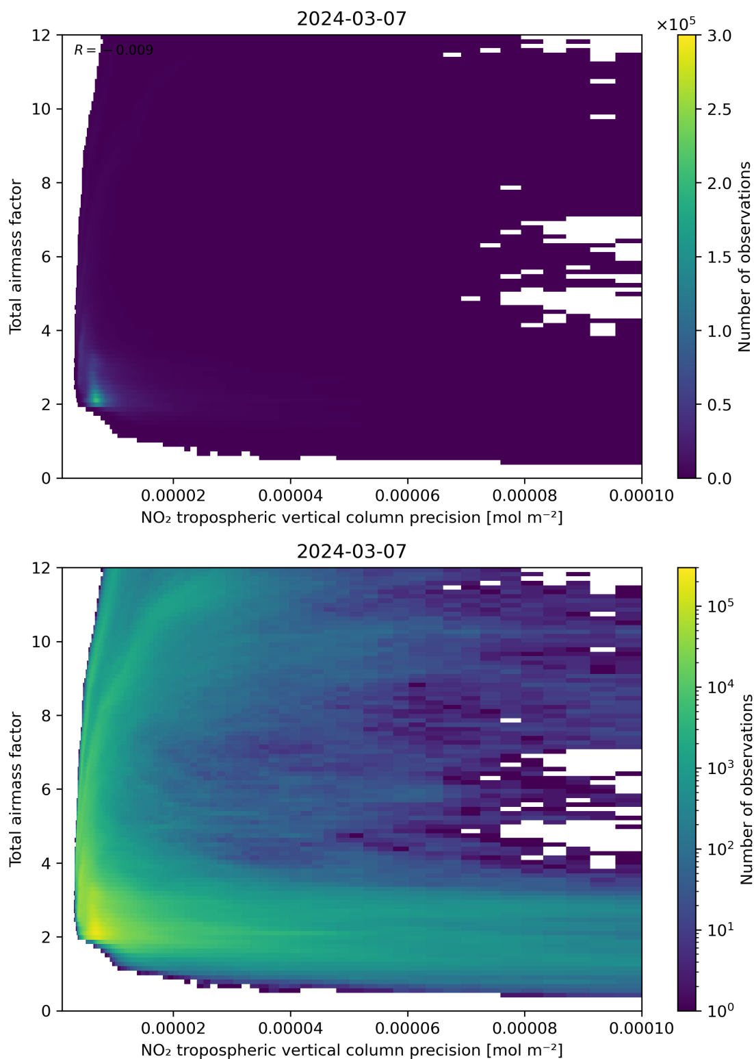
Figure 132: Scatter density plot of “NO 2 tropospheric vertical column precision” against “Total air mass factor” for 2024-03-06 to 2024-03-08.
