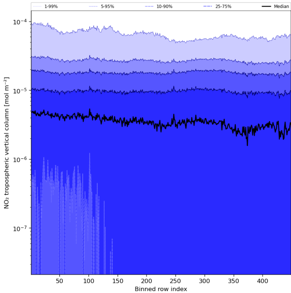
Figure 46: Along track statistics of “NO 2 tropospheric vertical column” for 2024-03-06 to 2024-03-08
