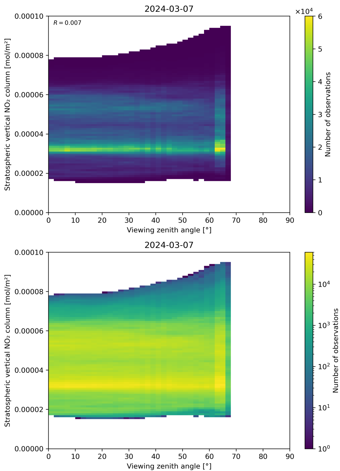
Figure 164: Scatter density plot of “Viewing zenith angle” against “Stratospheric vertical NO 2 column” for 2024-03-06 to 2024-03-08.
