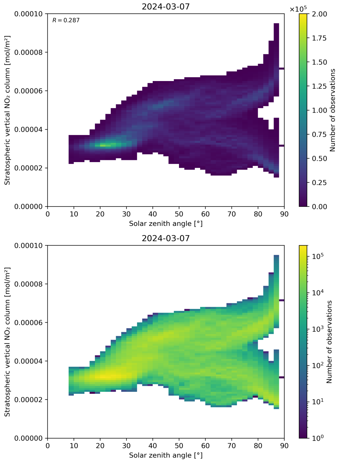
Figure 150: Scatter density plot of “Solar zenith angle” against “Stratospheric vertical \text{NO}_2 column” for 2024-03-06 to 2024-03-08.
