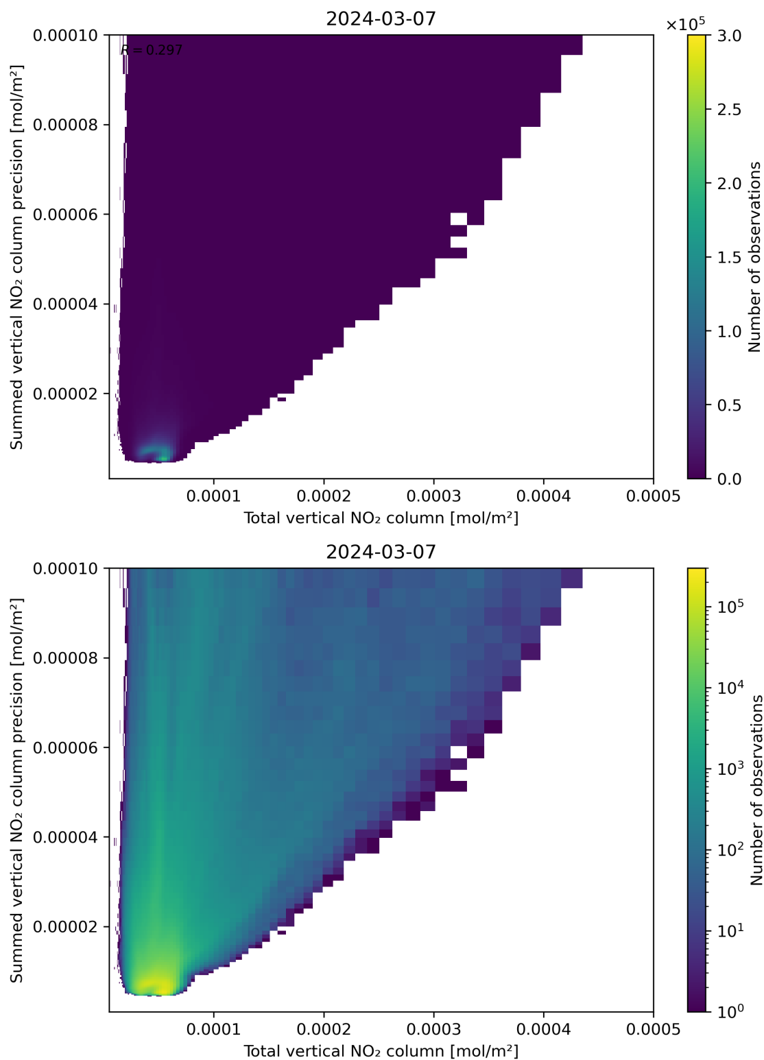
Figure 113: Scatter density plot of “Total vertical NO 2 column” against “Summed vertical NO 2 column precision” for 2024-03-06 to 2024-03-08.
