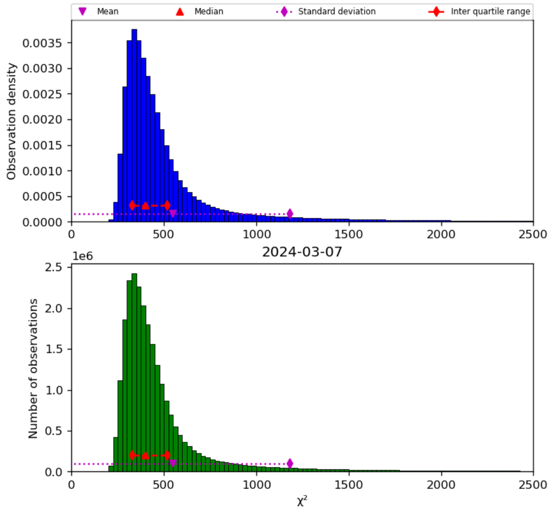
Figure 42: Histogram of “ \chi^2 ” for 2024-03-06 to 2024-03-08
