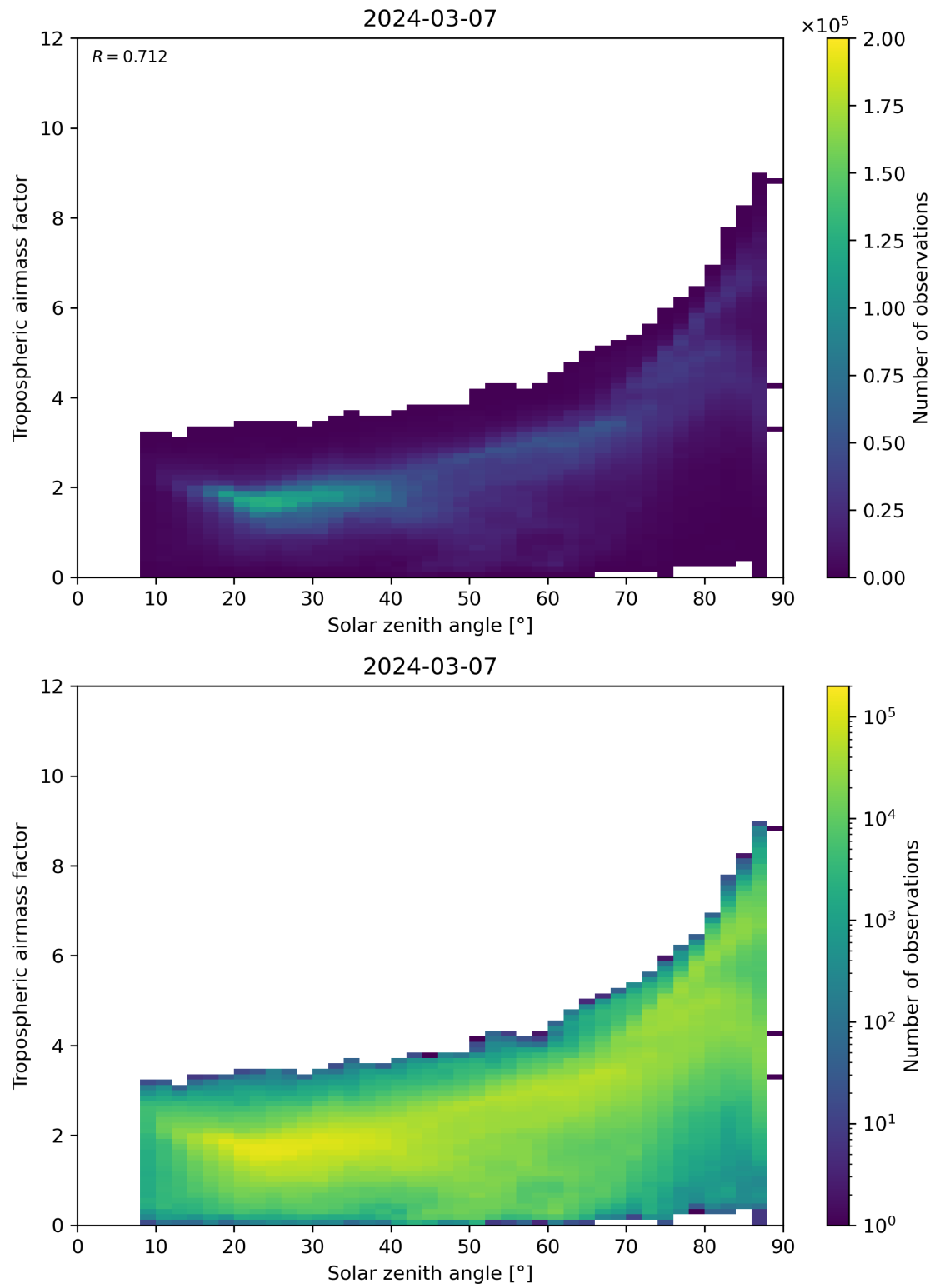
Figure 147: Scatter density plot of “Solar zenith angle” against “Tropospheric airmass factor” for 2024-03-06 to 2024-03-08.
