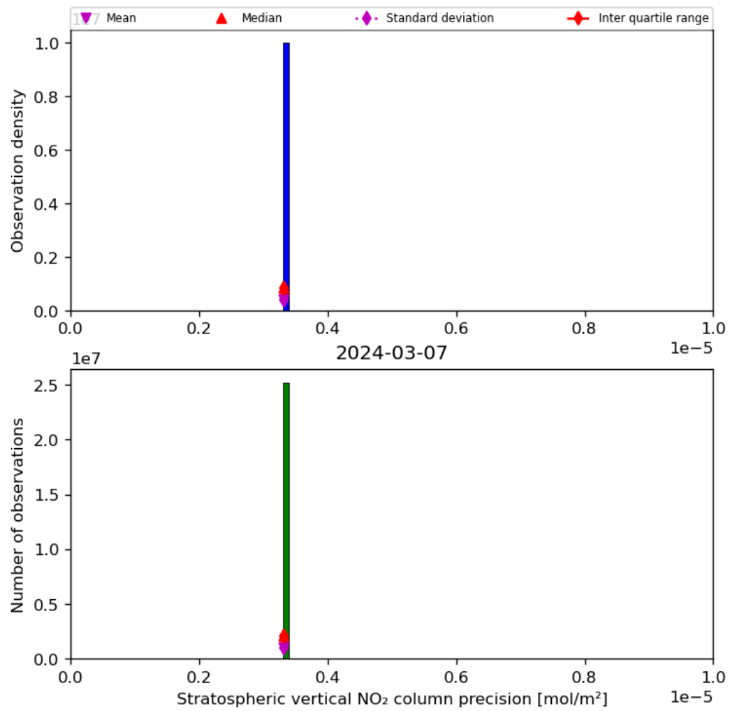
Figure 37: Histogram of “Stratospheric vertical NO 2 column precision” for 2024-03-06 to 2024-03-08
