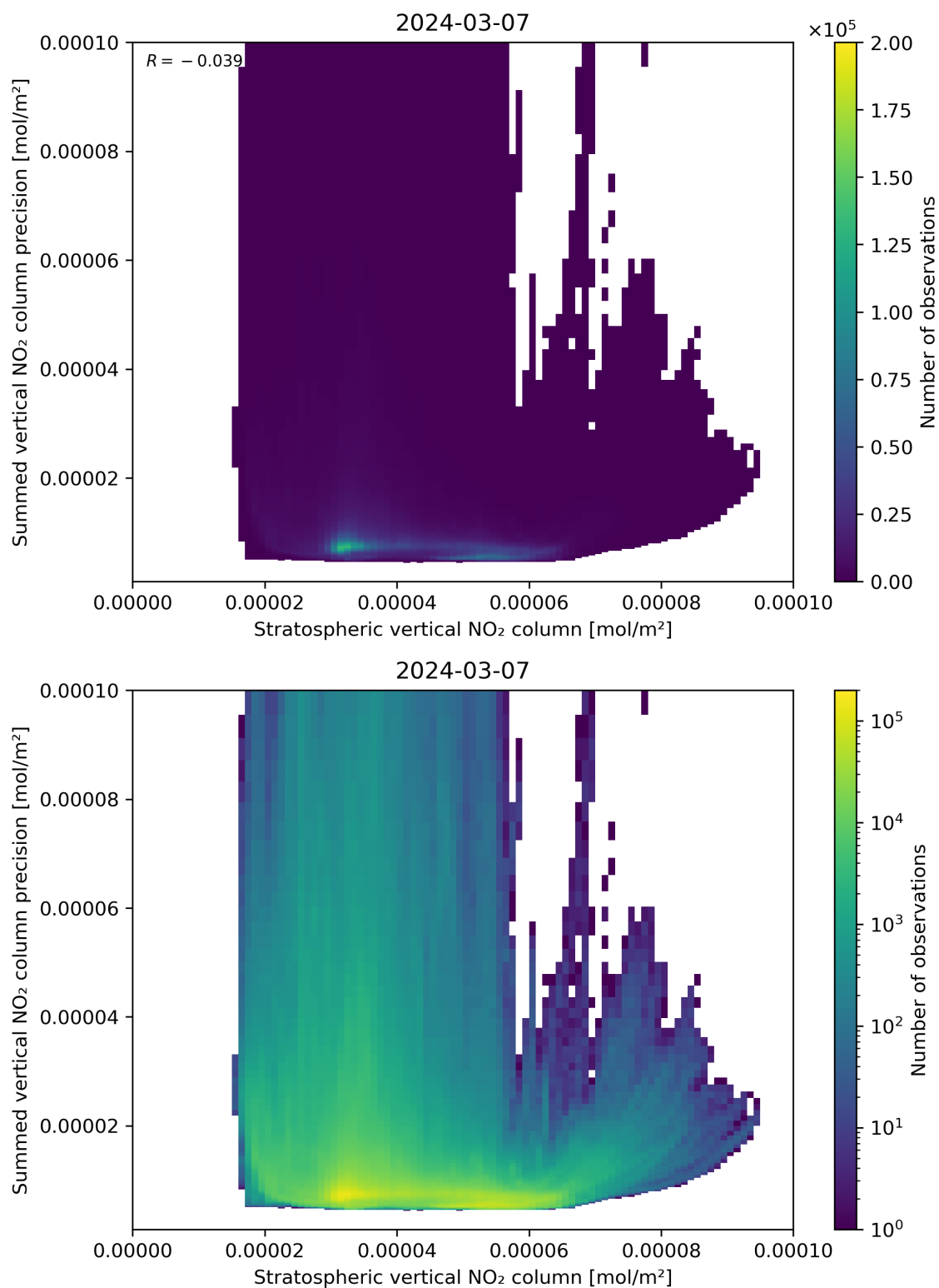
Figure 99: Scatter density plot of “Stratospheric vertical NO 2 column” against “Summed vertical NO 2 column precision” for 2024-03-06 to 2024-03-08.
