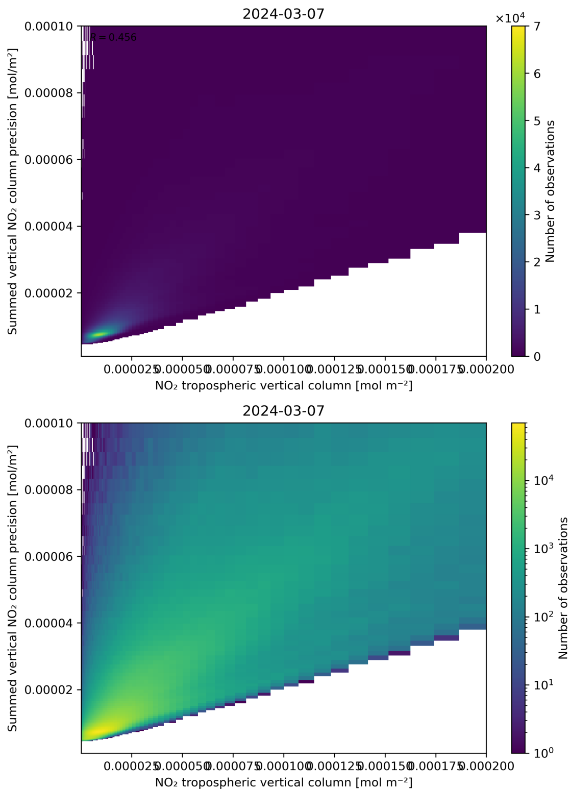
Figure 127: Scatter density plot of “NO 2 tropospheric vertical column” against “Summed vertical NO 2 column precision” for 2024-03-06 to 2024-03-08.
