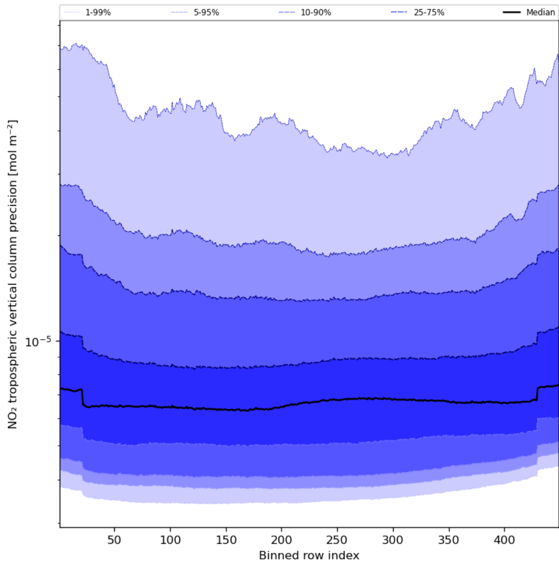
Figure 47: Along track statistics of “NO 2 tropospheric vertical column precision” for 2024-03-06 to 2024-03-08
