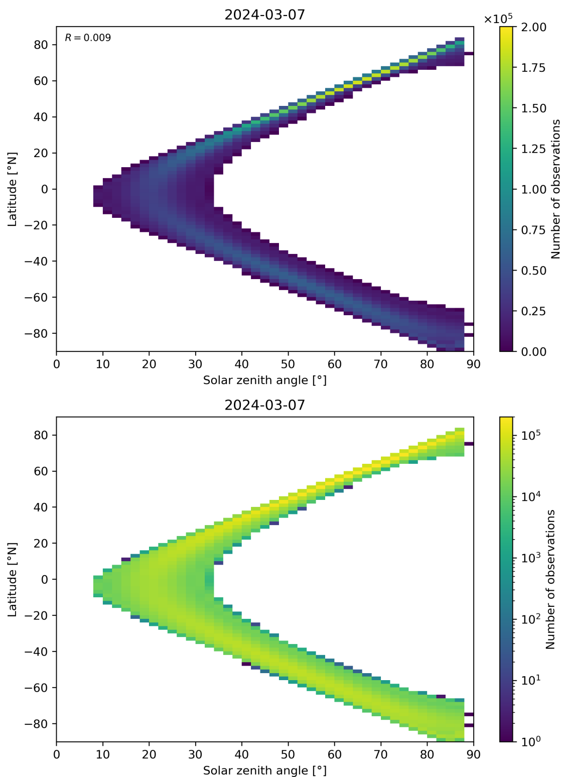
Figure 149: Scatter density plot of “Solar zenith angle” against “Latitude” for 2024-03-06 to 2024-03-08.
