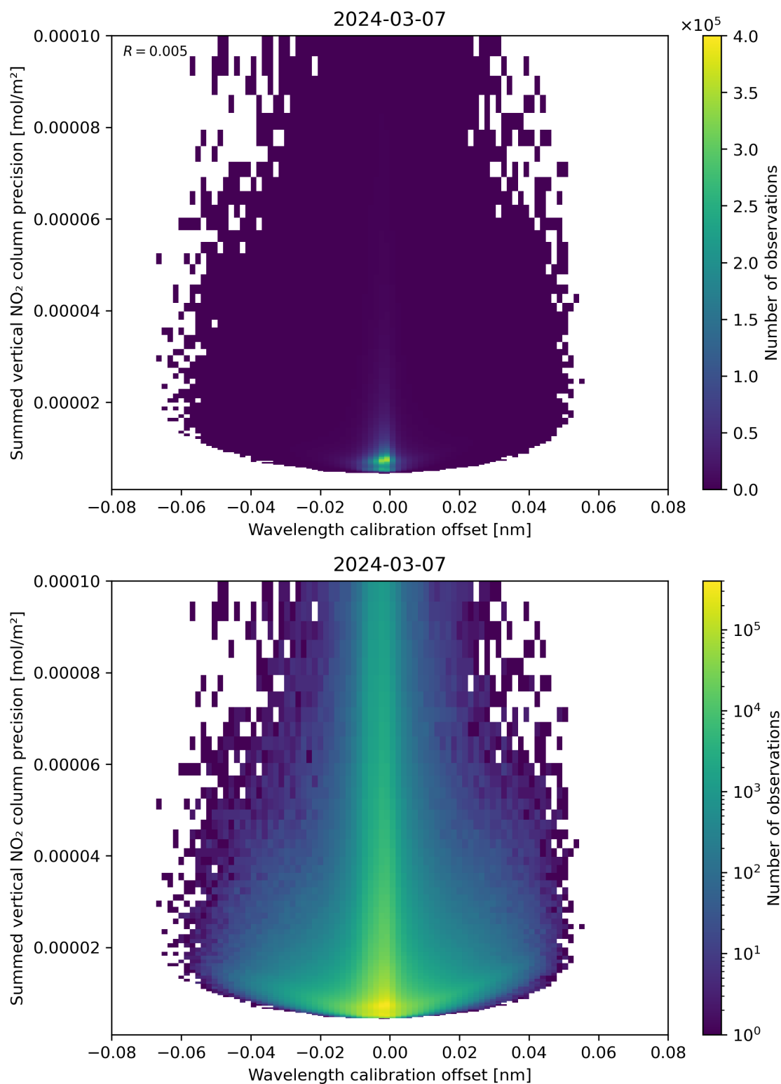
Figure 178: Scatter density plot of “Wavelength calibration offset” against “Summed vertical NO 2 column precision” for 2024-03-06 to 2024-03-08.
