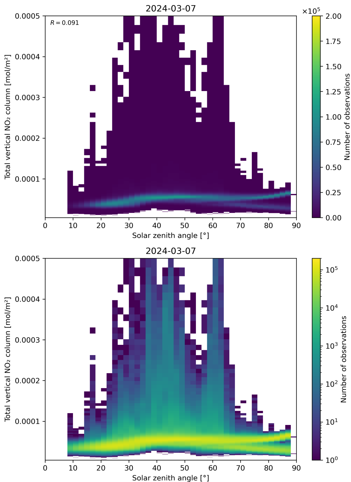
Figure 153: Scatter density plot of “Solar zenith angle” against “Total vertical NO 2 column” for 2024-03-06 to 2024-03-08.
