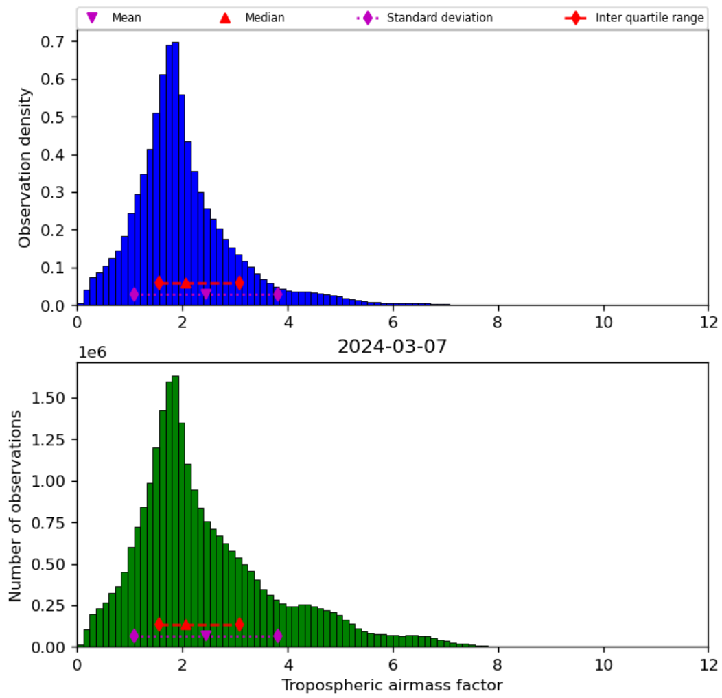
Figure 31: Histogram of “Tropospheric airmass factor” for 2024-03-06 to 2024-03-08
