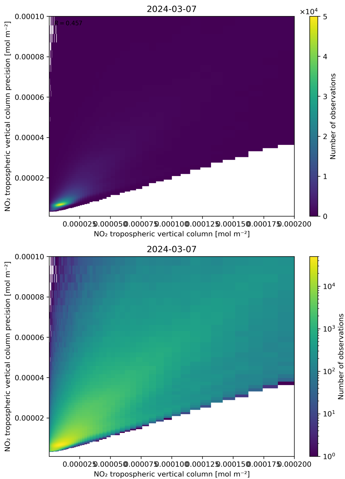
Figure 130: Scatter density plot of “NO 2 tropospheric vertical column” against “NO 2 tropospheric vertical column precision” for 2024-03-06 to 2024-03-08.
