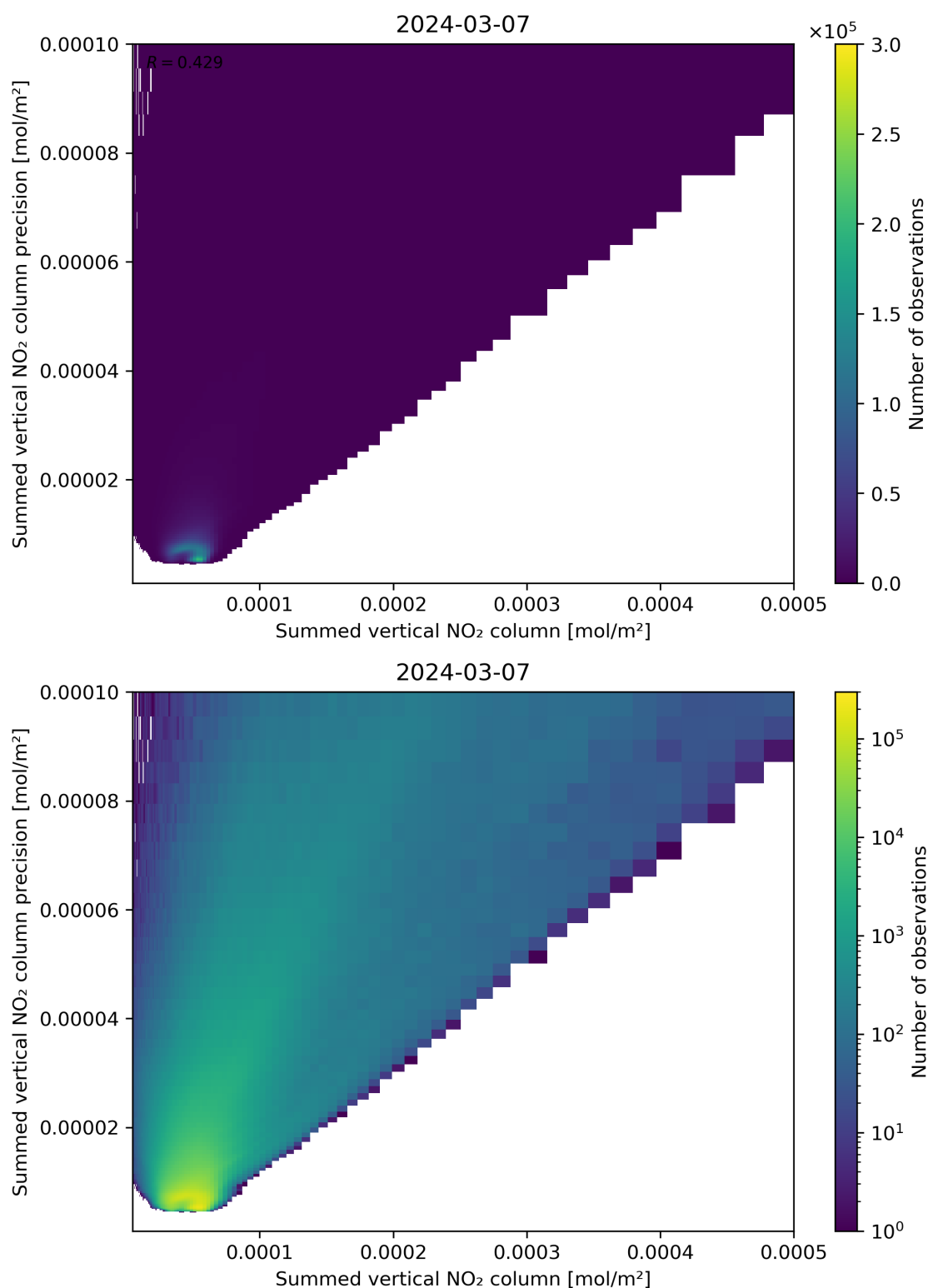
Figure 105: Scatter density plot of “Summed vertical NO 2 column” against “Summed vertical NO 2 column precision” for 2024-03-06 to 2024-03-08.
