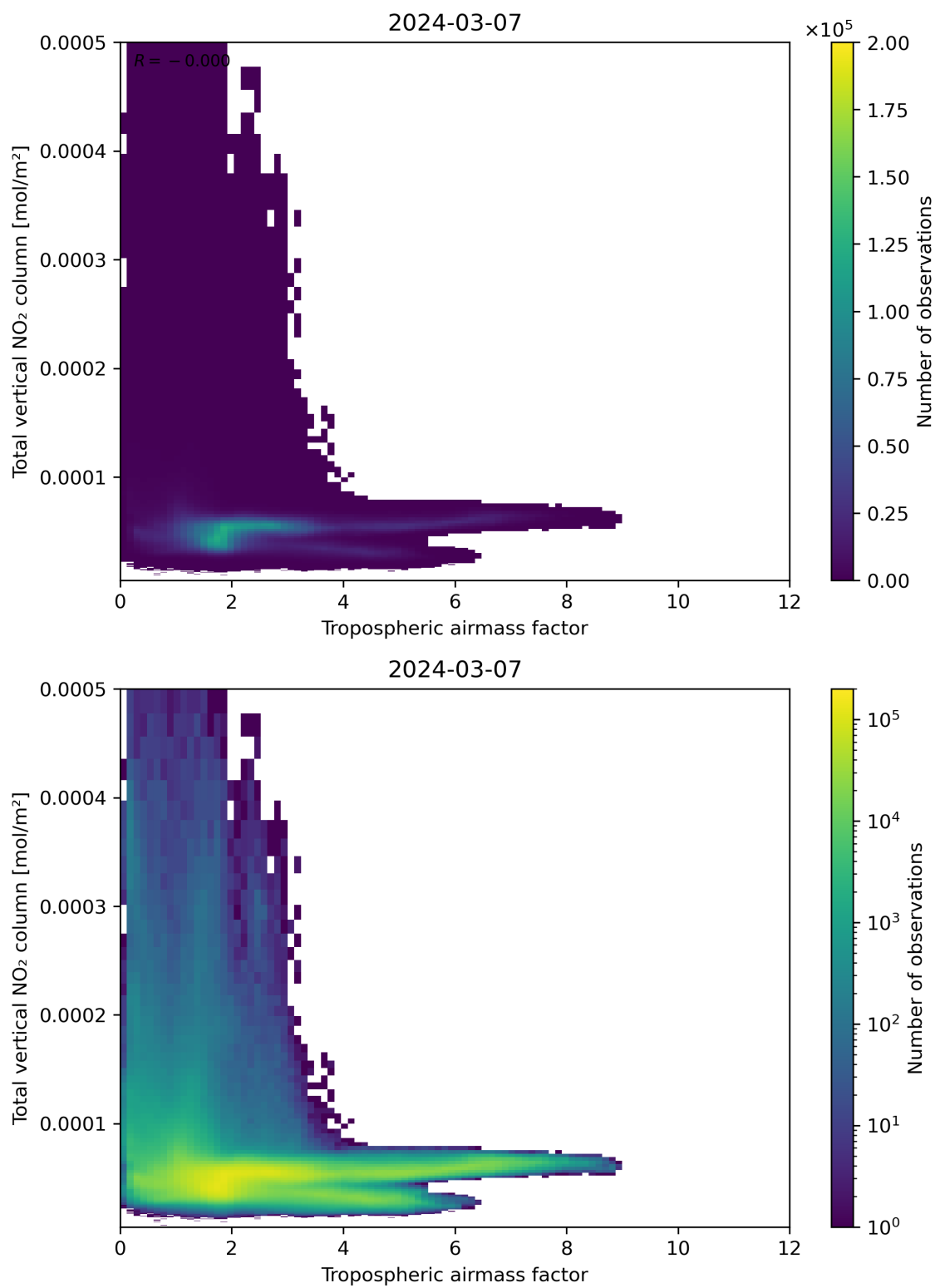
Figure 77: Scatter density plot of “Tropospheric airmass factor” against “Total vertical NO 2 column” for 2024-03-06 to 2024-03-08.
