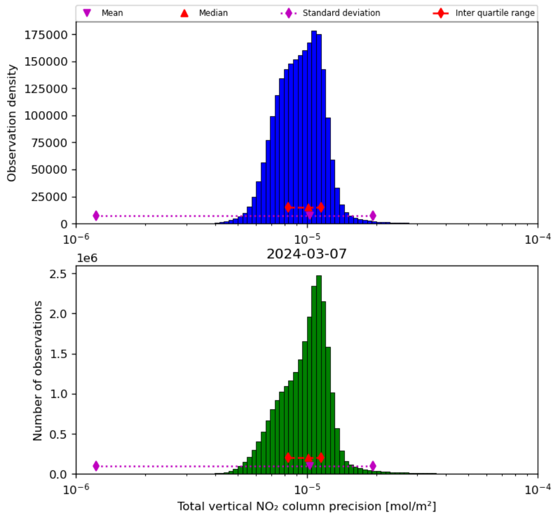
Figure 39: Histogram of “Total vertical NO 2 column precision” for 2024-03-06 to 2024-03-08
