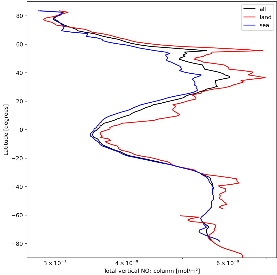
Figure 21: Zonal average of “Total vertical NO 2 column” for 2024-03-06 to 2024-03-08.
