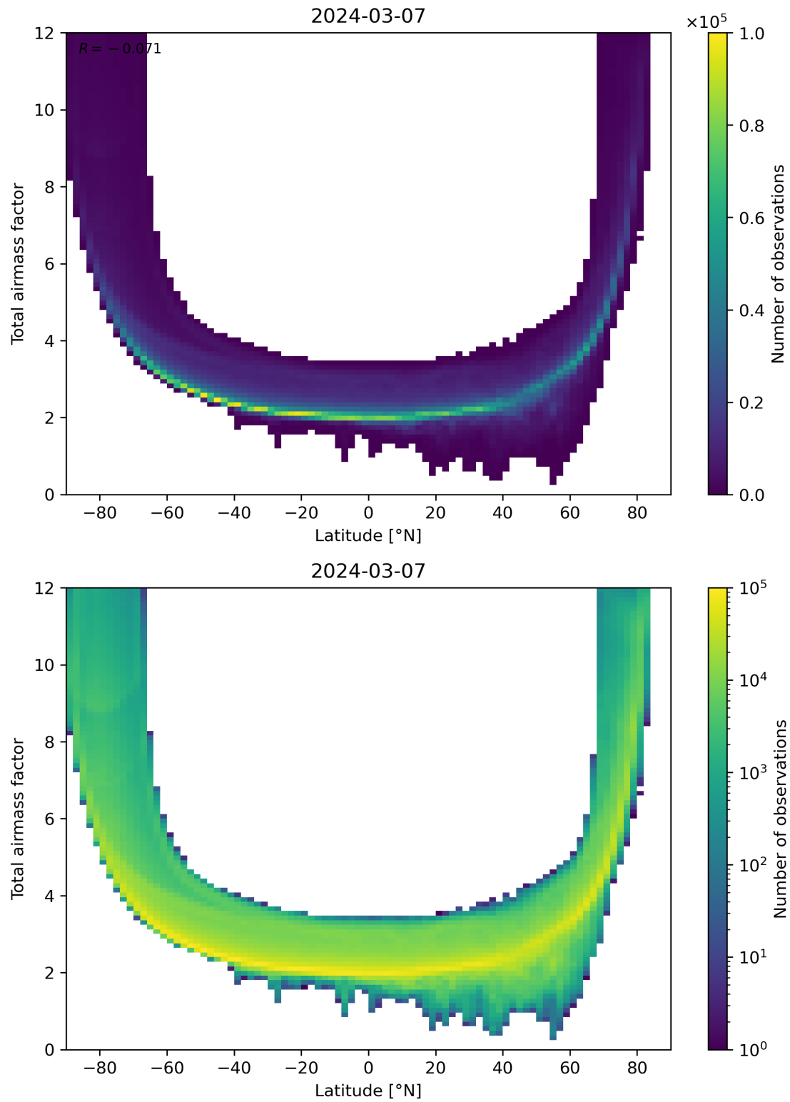
Figure 84: Scatter density plot of “Latitude” against “Total airmass factor” for 2024-03-06 to 2024-03-08.
