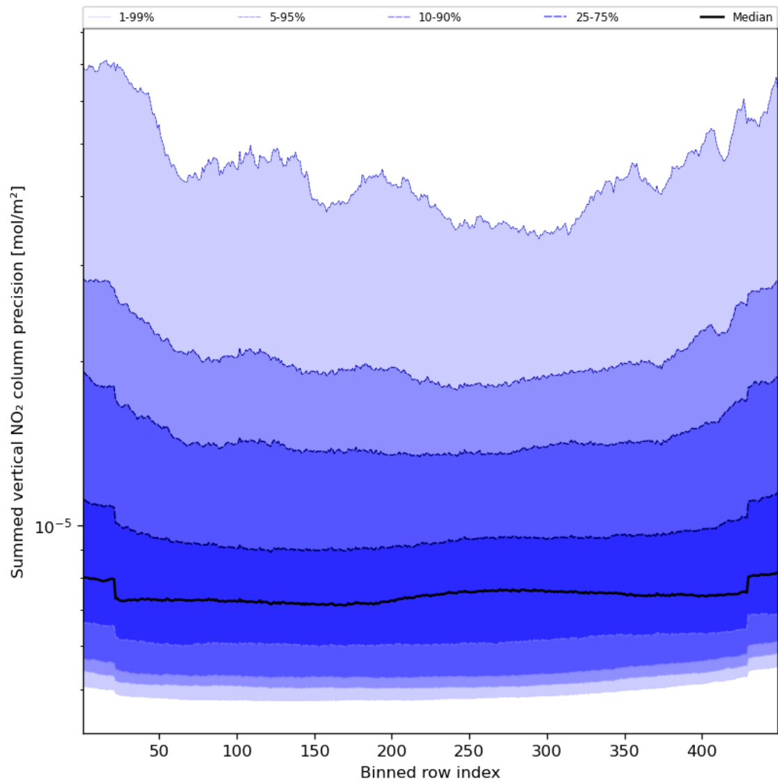
Figure 58: Along track statistics of “Summed vertical NO 2 column precision” for 2024-03-06 to 2024-03-08
