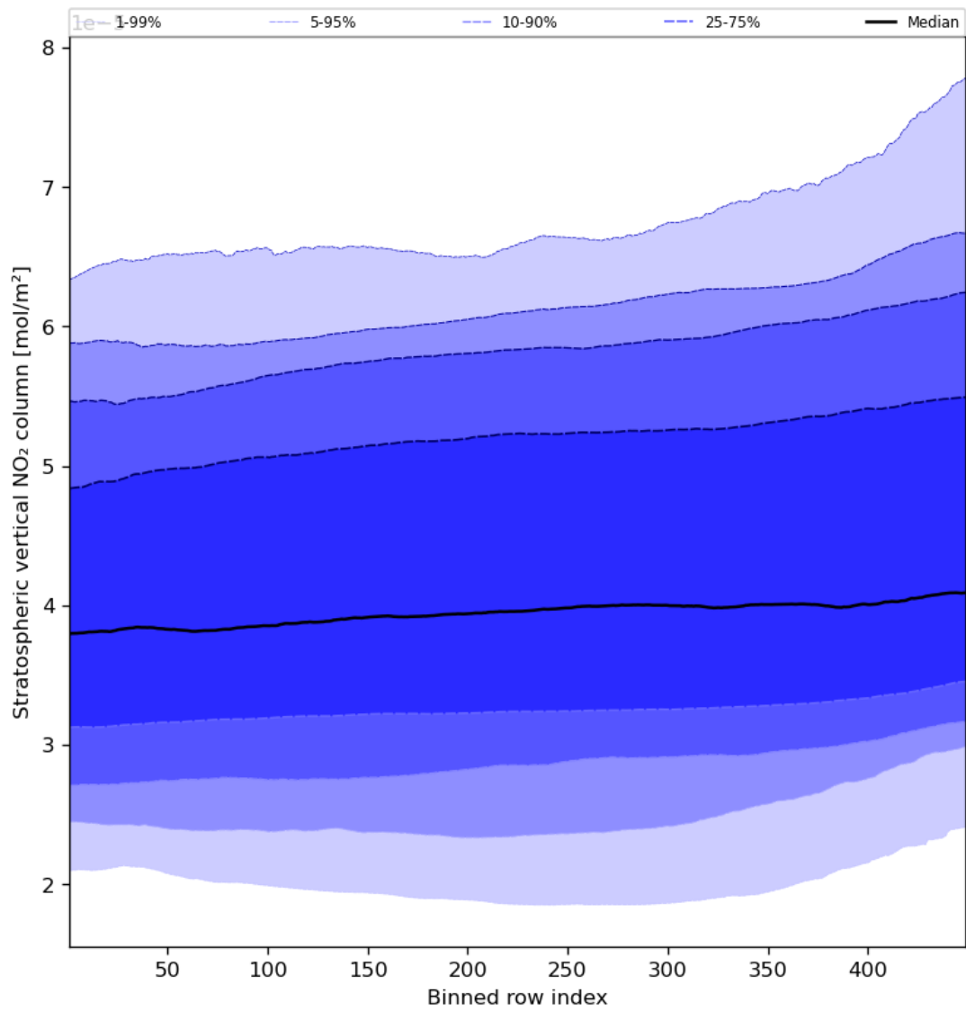
Figure 53: Along track statistics of “Stratospheric vertical NO 2 column” for 2024-03-06 to 2024-03-08
