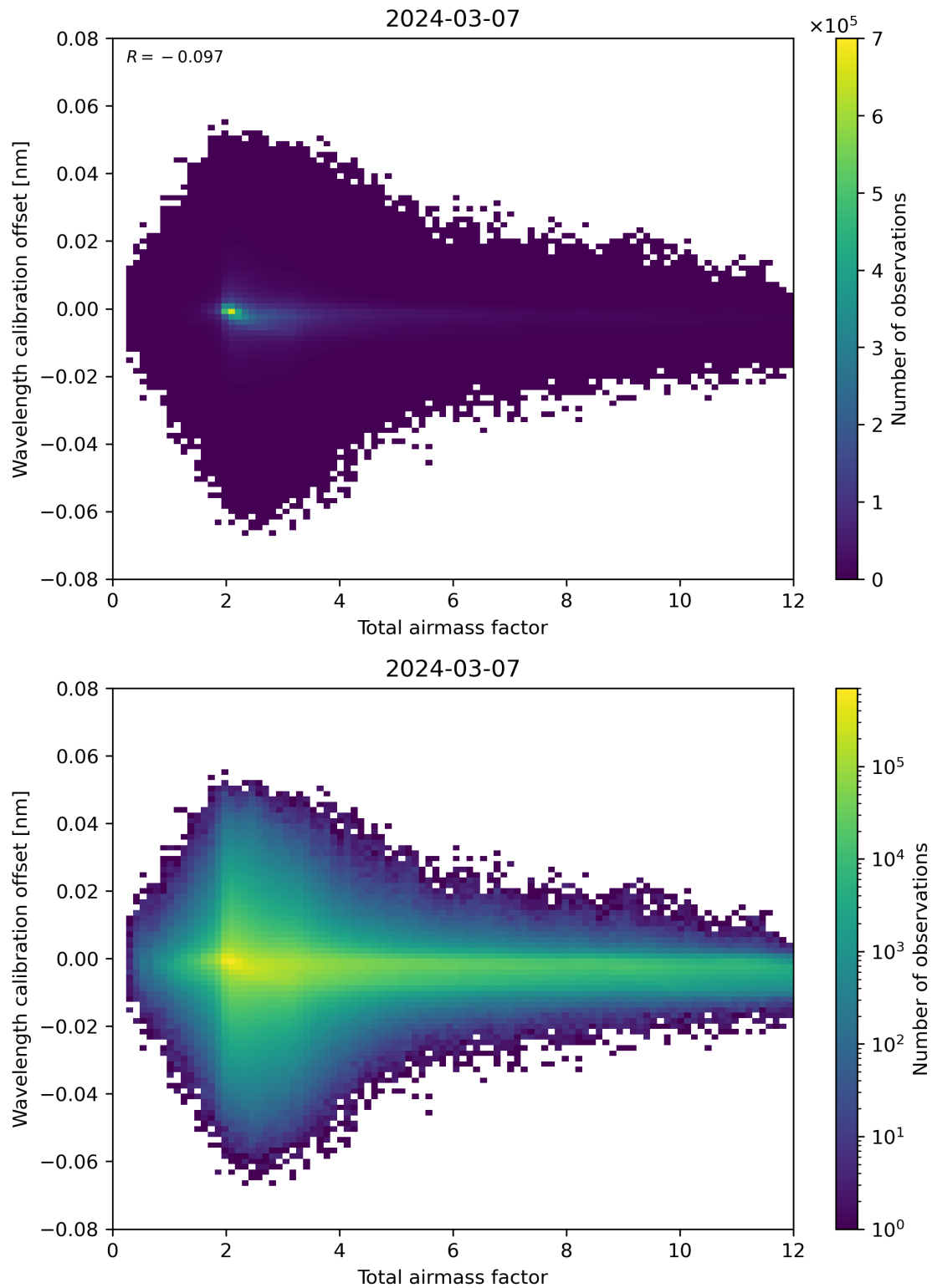
Figure 70: Scatter density plot of “Total airmass factor” against “Wavelength calibration offset” for 2024-03-06 to 2024-03-08.
