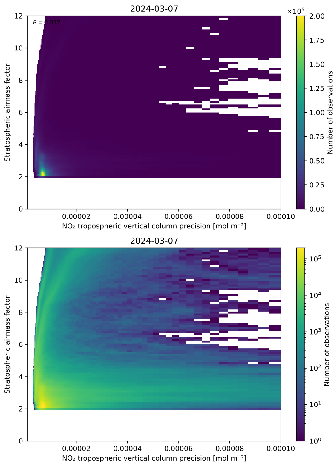
Figure 131: Scatter density plot of “NO 2 tropospheric vertical column precision” against “Stratospheric airmass factor” for 2024-03-06 to 2024-03-08.
