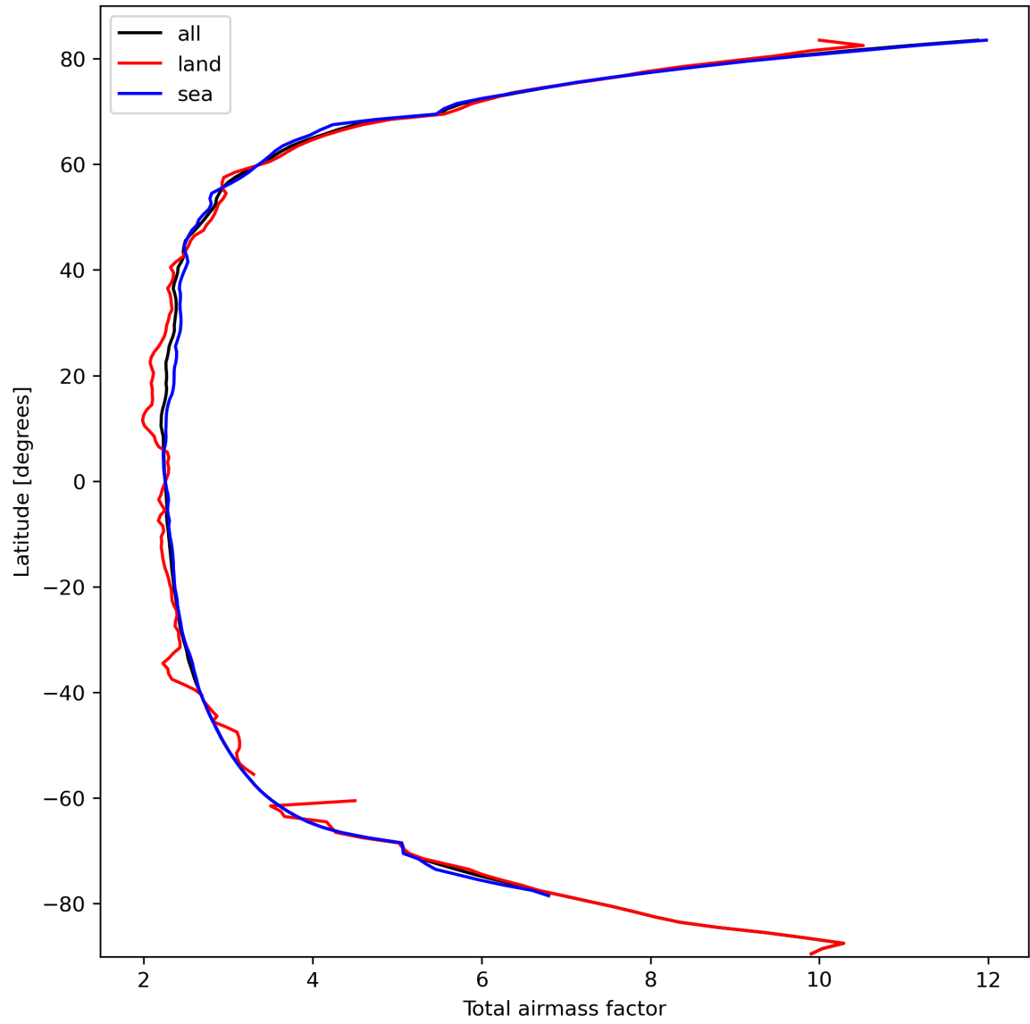
Figure 15: Zonal average of “Total airmass factor” for 2024-03-06 to 2024-03-08.
