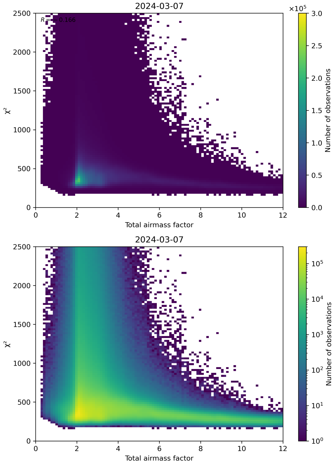
Figure 63: Scatter density plot of “Total airmass factor” against “ \chi^2 ” for 2024-03-06 to 2024-03-08.
