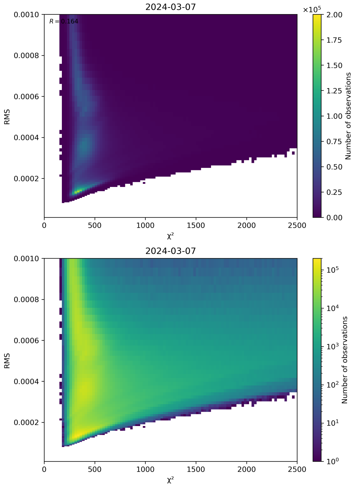
Figure 82: Scatter density plot of “ \chi^2 ” against “RMS” for 2024-03-06 to 2024-03-08.
