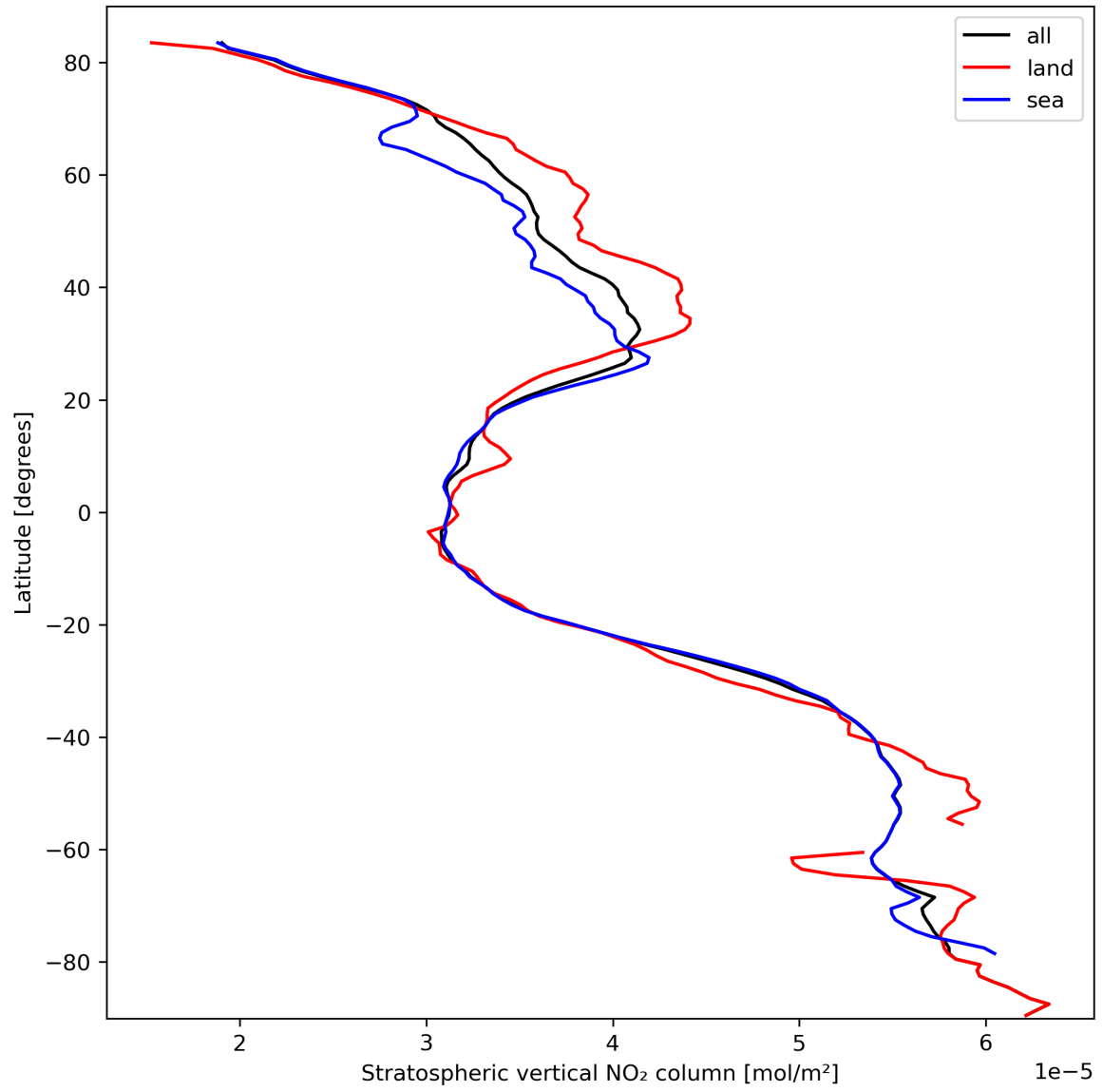
Figure 19: Zonal average of “Stratospheric vertical NO 2 column” for 2024-03-06 to 2024-03-08.
