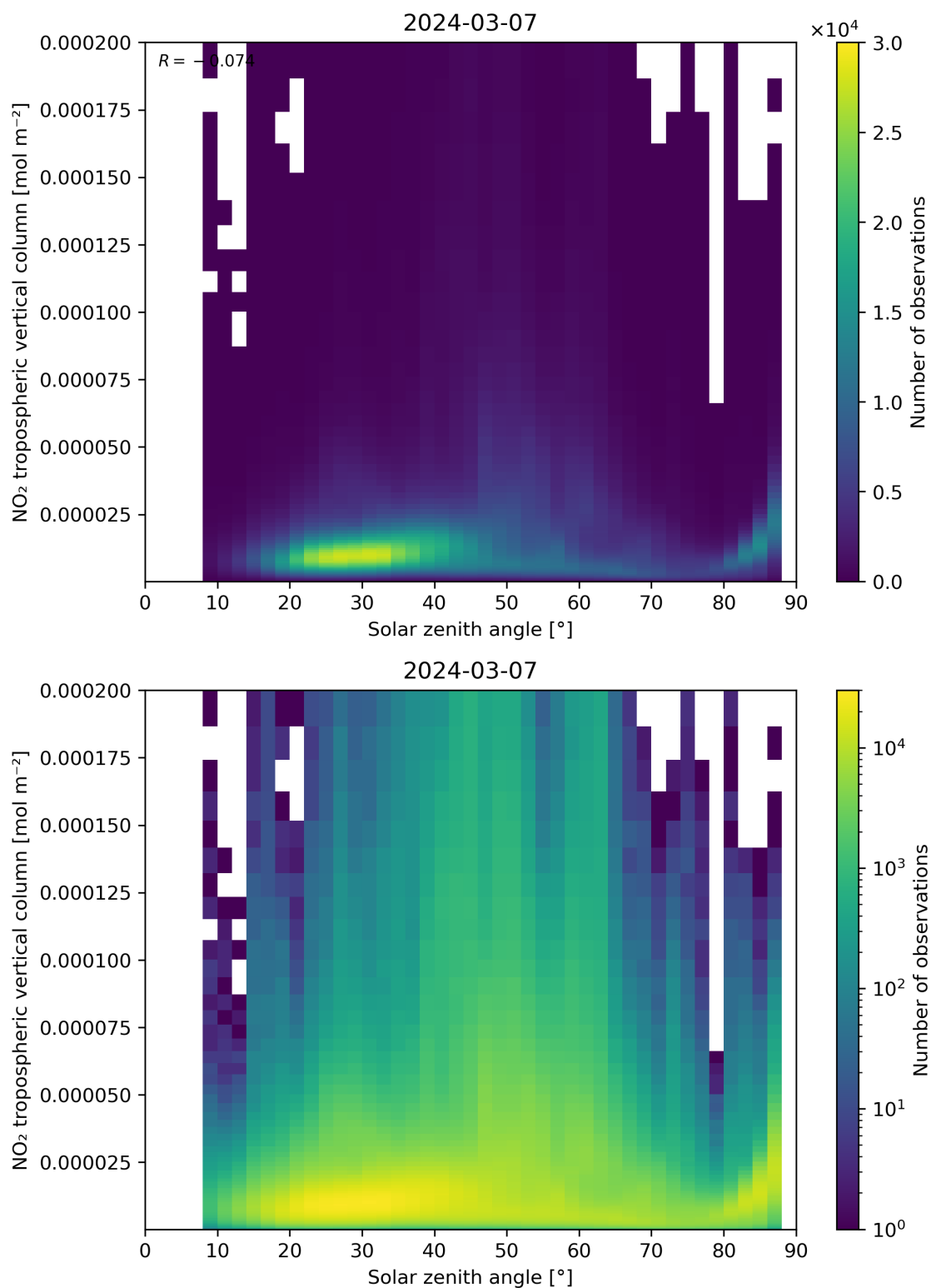
Figure 155: Scatter density plot of “Solar zenith angle” against “NO 2 tropospheric vertical column” for 2024-03-06 to 2024-03-08.
