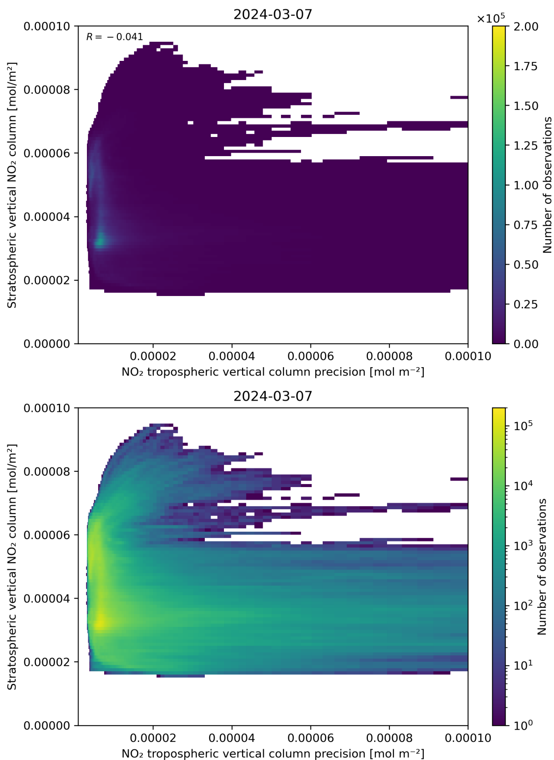
Figure 135: Scatter density plot of “NO 2 tropospheric vertical column precision” against “Stratospheric vertical NO 2 column” for 2024-03-06 to 2024-03-08.
