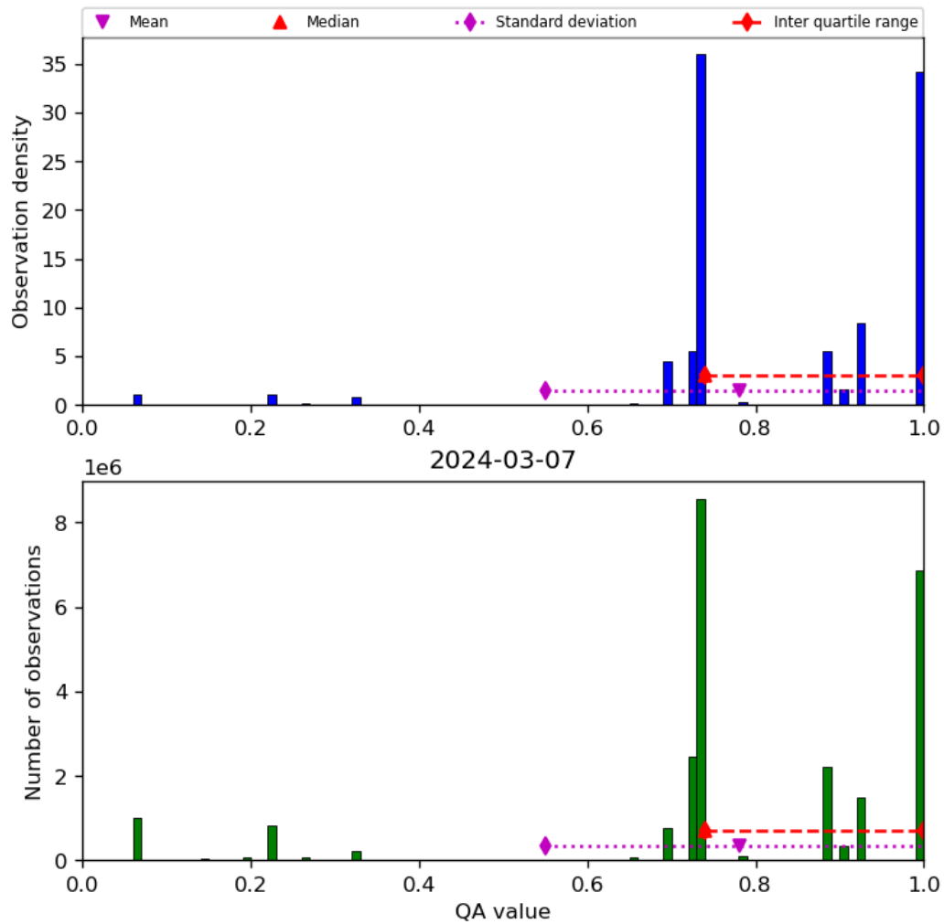
Figure 28: Histogram of “QA value” for 2024-03-06 to 2024-03-08
