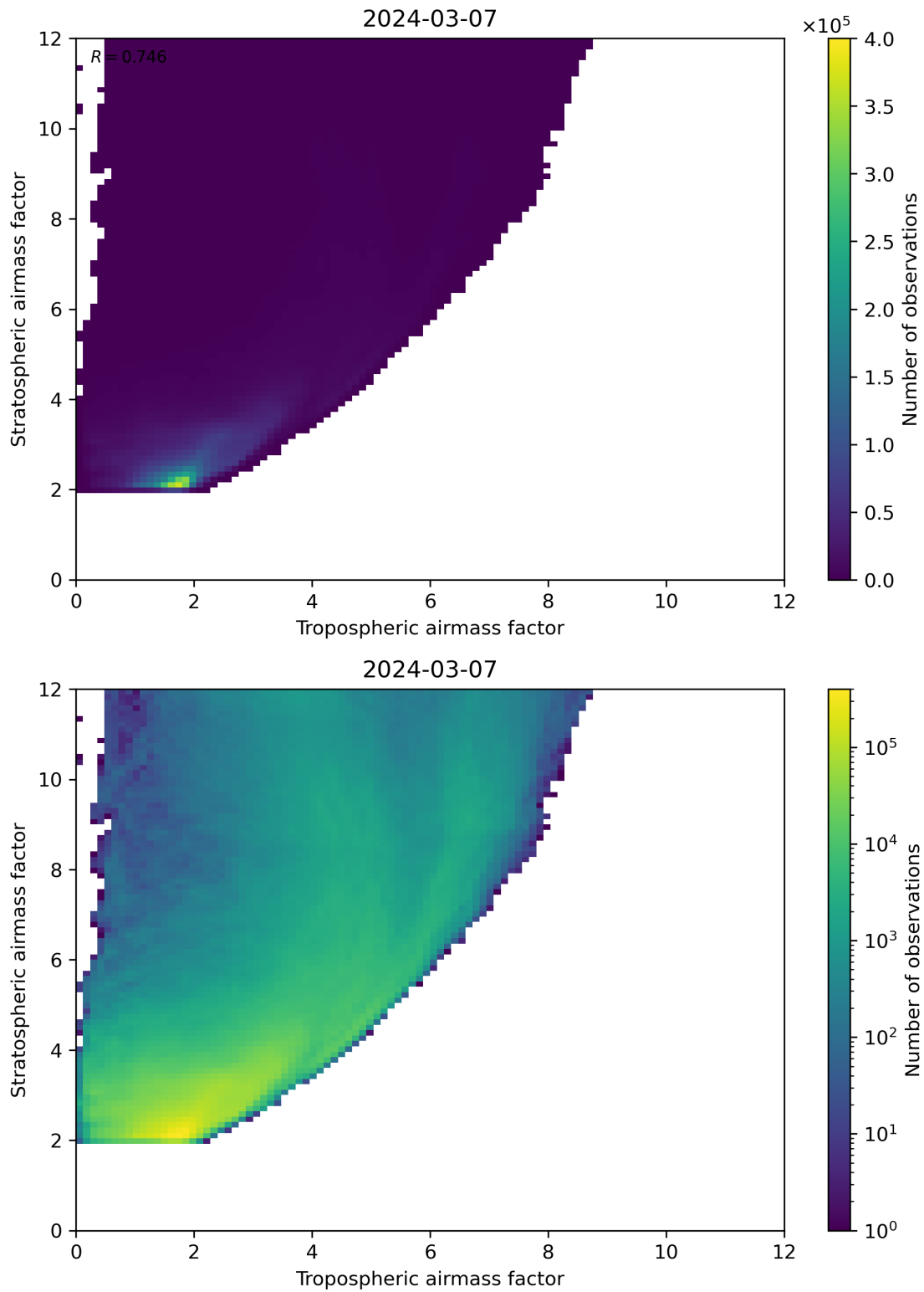
Figure 71: Scatter density plot of “Tropospheric airmass factor” against “Stratospheric airmass factor” for 2024-03-06 to 2024-03-08.
