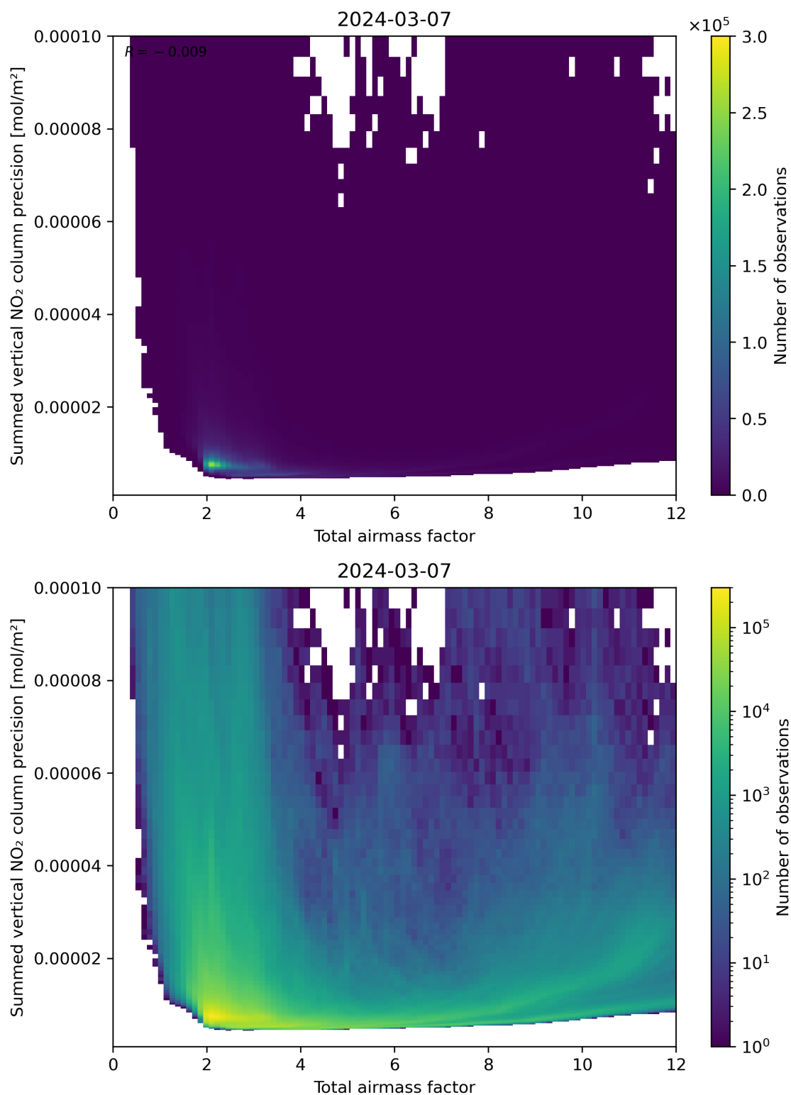
Figure 66: Scatter density plot of “Total airmass factor” against “Summed vertical NO 2 column precision” for 2024-03-06 to 2024-03-08.
