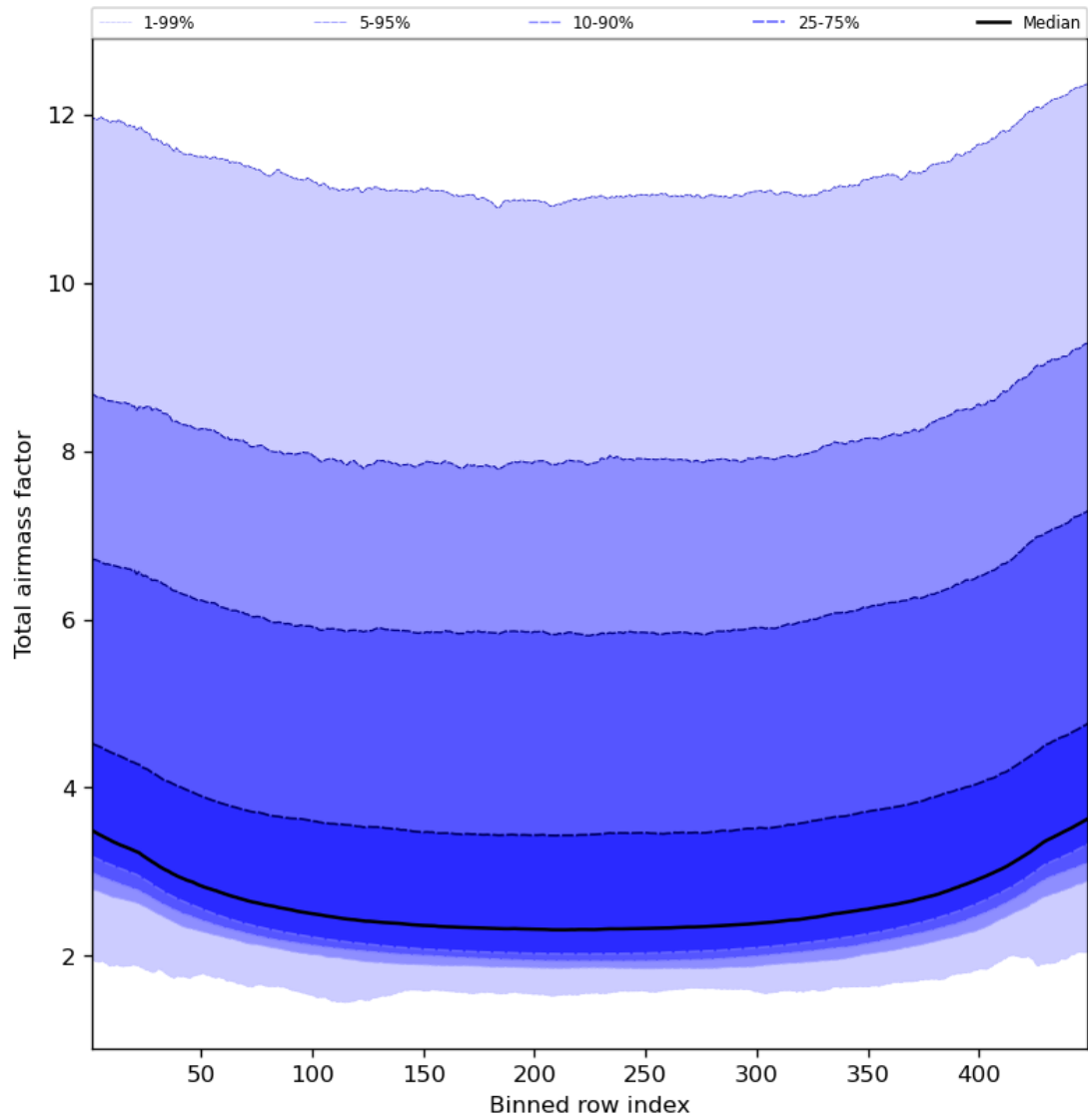
Figure 49: Along track statistics of “Total airmass factor” for 2024-03-06 to 2024-03-08
