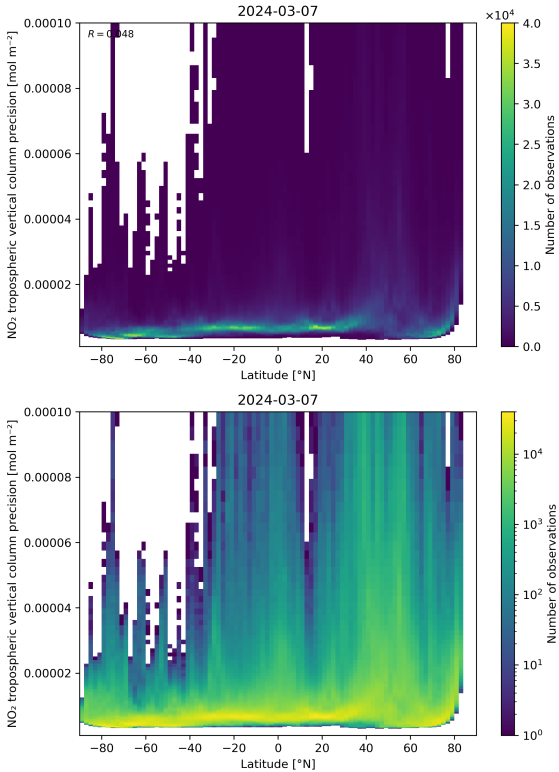
Figure 93: Scatter density plot of “Latitude” against “NO 2 tropospheric vertical column precision” for 2024-03-06 to 2024-03-08.
