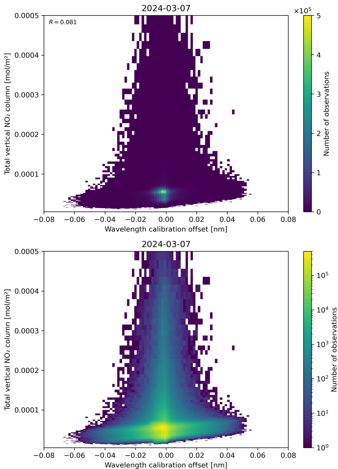
Figure 179: Scatter density plot of “Wavelength calibration offset” against “Total vertical NO 2 column” for 2024-03-06 to 2024-03-08.
