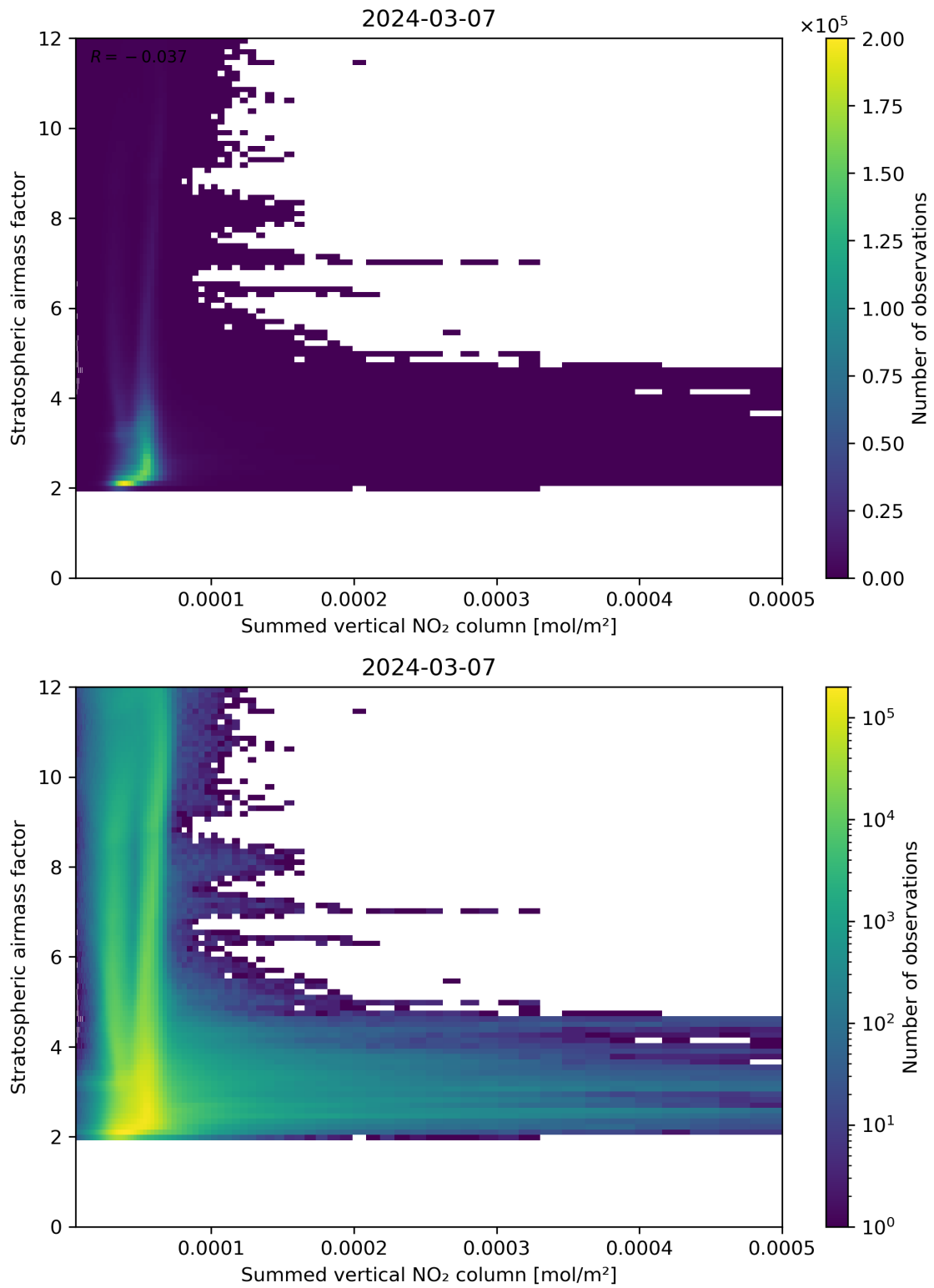
Figure 103: Scatter density plot of “Summed vertical NO 2 column” against “Stratospheric air mass factor” for 2024-03-06 to 2024-03-08.
