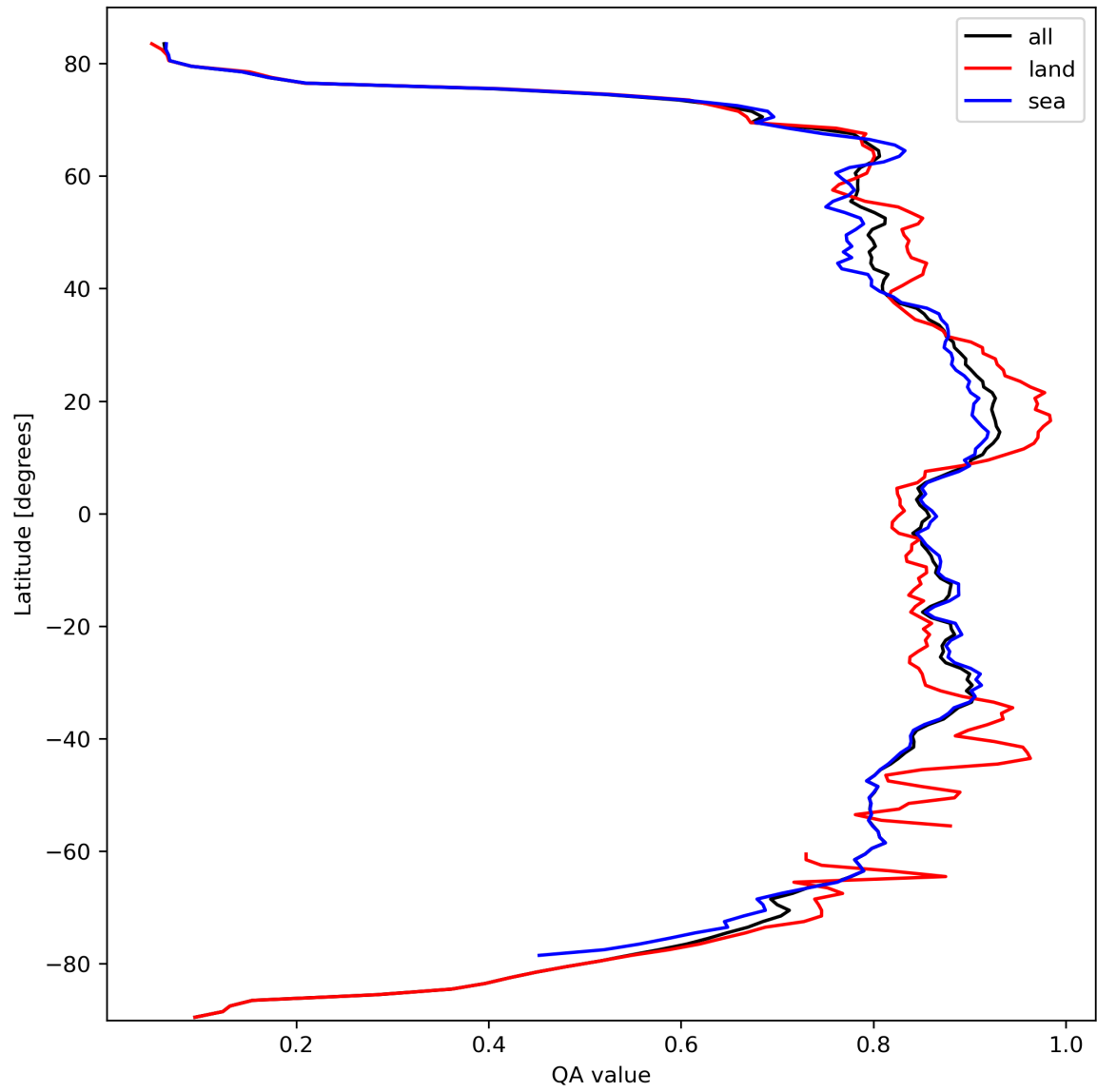
Figure 11: Zonal average of “QA value” for 2024-03-06 to 2024-03-08.
