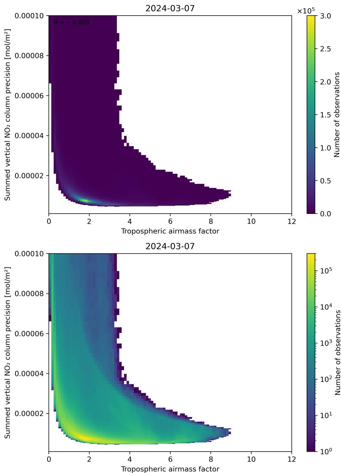
Figure 76: Scatter density plot of “Tropospheric air mass factor” against “Summed vertical NO 2 column precision” for 2024-03-06 to 2024-03-08.
