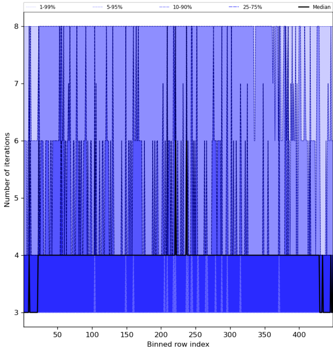
Figure 51: Along track statistics of “Number of iterations” for 2024-03-06 to 2024-03-08
