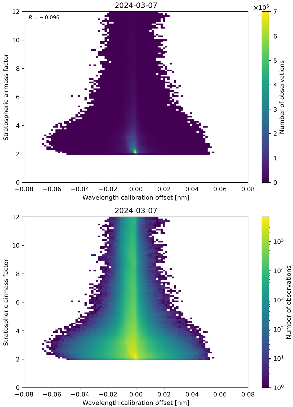
Figure 174: Scatter density plot of “Wavelength calibration offset” against “Stratospheric air mass factor” for 2024-03-06 to 2024-03-08.
