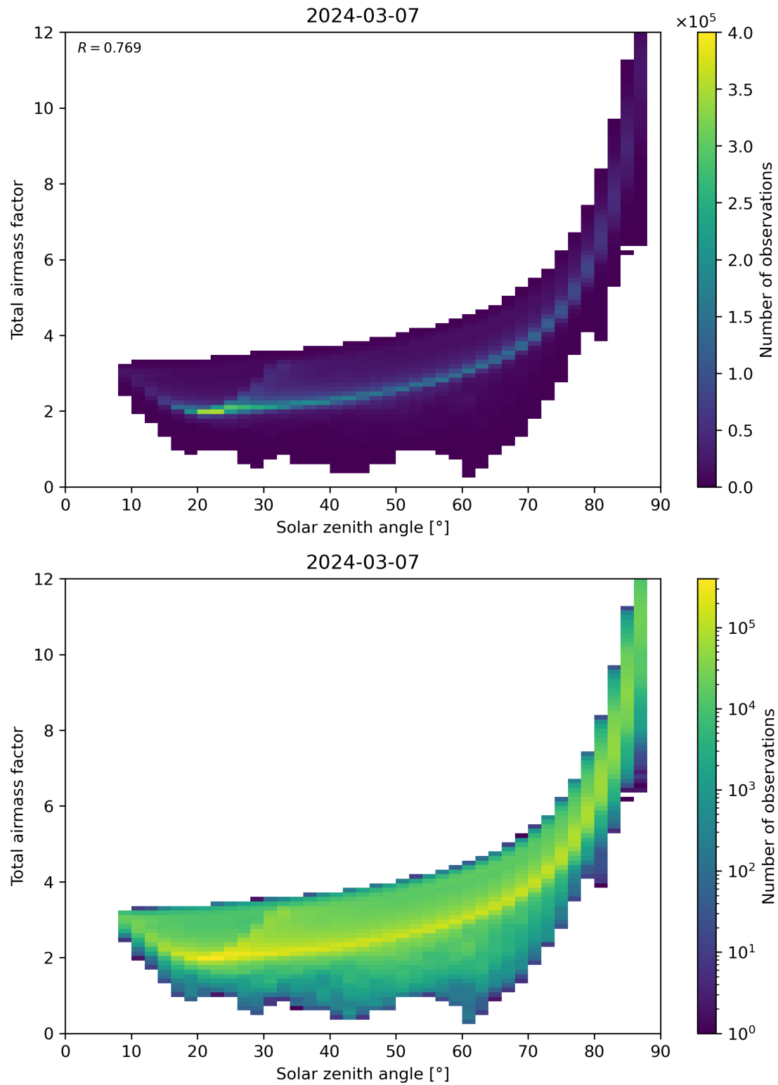
Figure 146: Scatter density plot of “Solar zenith angle” against “Total air mass factor” for 2024-03-06 to 2024-03-08.
