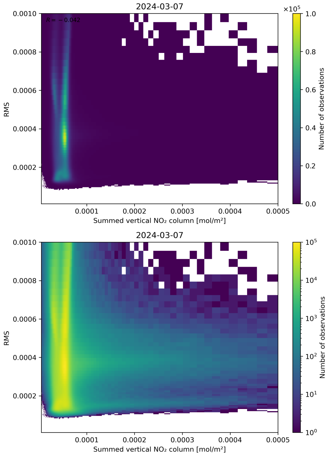
Figure 109: Scatter density plot of “Summed vertical NO 2 column” against “RMS” for 2024-03-06 to 2024-03-08.
