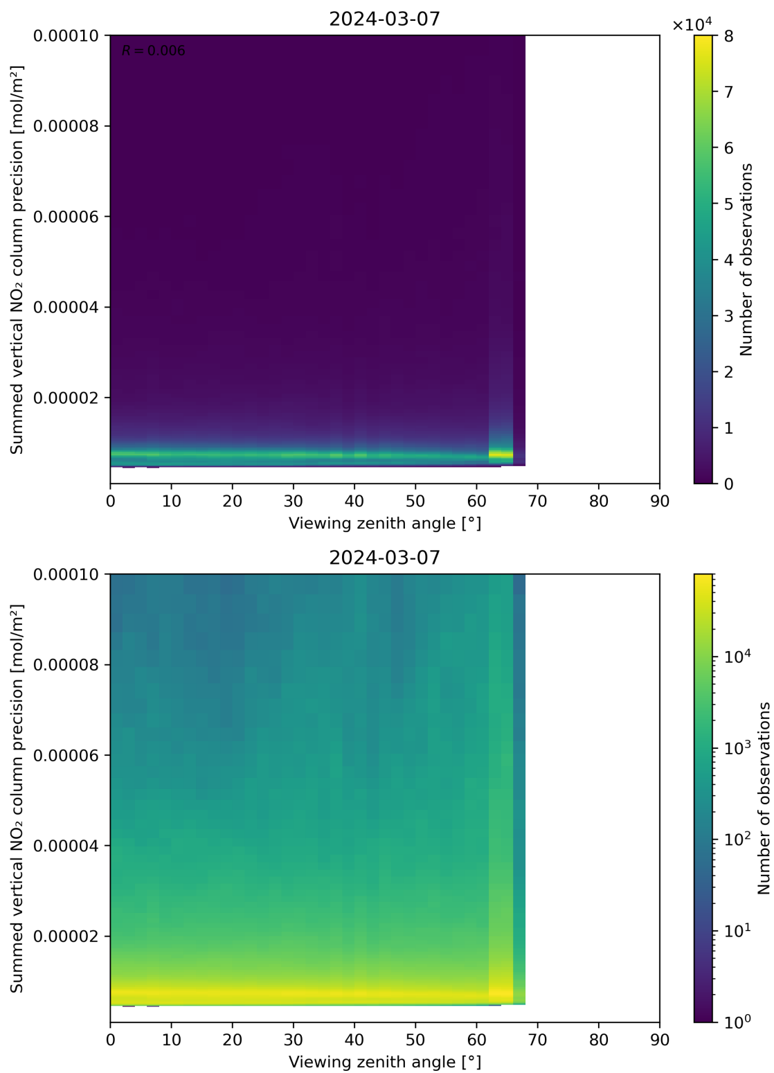
Figure 166: Scatter density plot of “Viewing zenith angle” against “Summed vertical NO 2 column precision” for 2024-03-06 to 2024-03-08.
