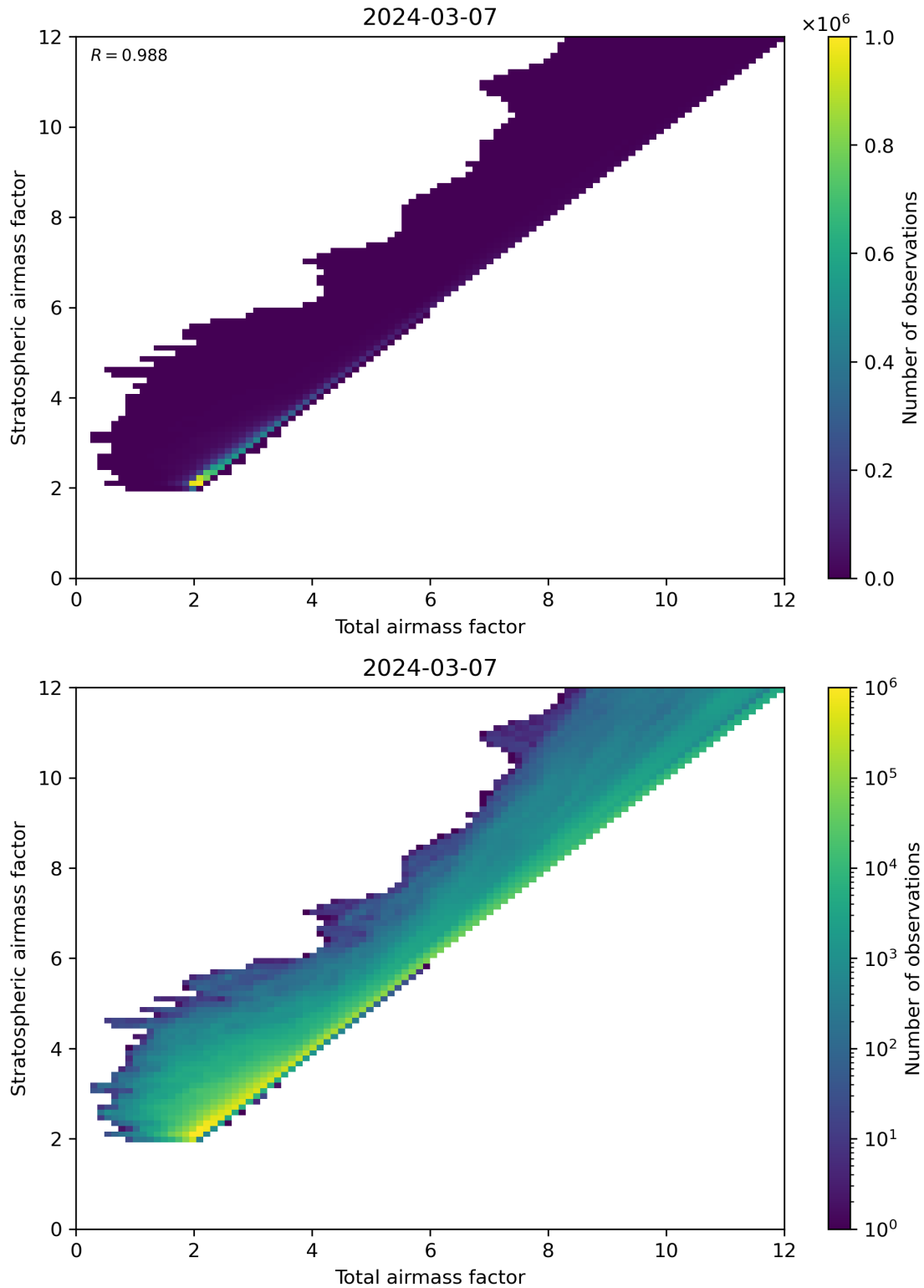
Figure 62: Scatter density plot of “Total airmass factor” against “Stratospheric airmass factor” for 2024-03-06 to 2024-03-08.
