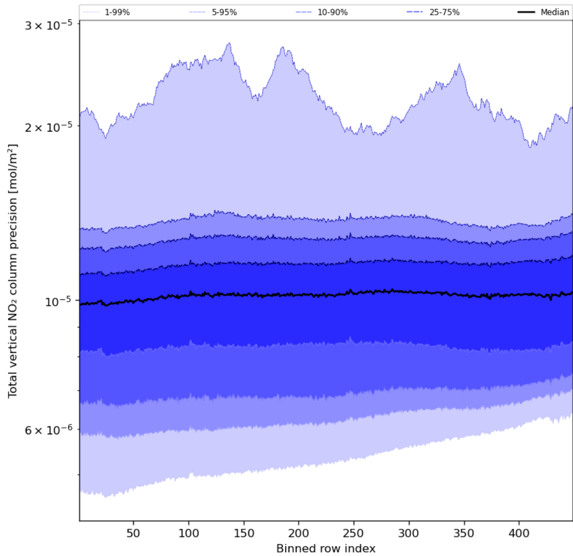
Figure 56: Along track statistics of “Total vertical NO 2 column precision” for 2024-03-06 to 2024-03-08
