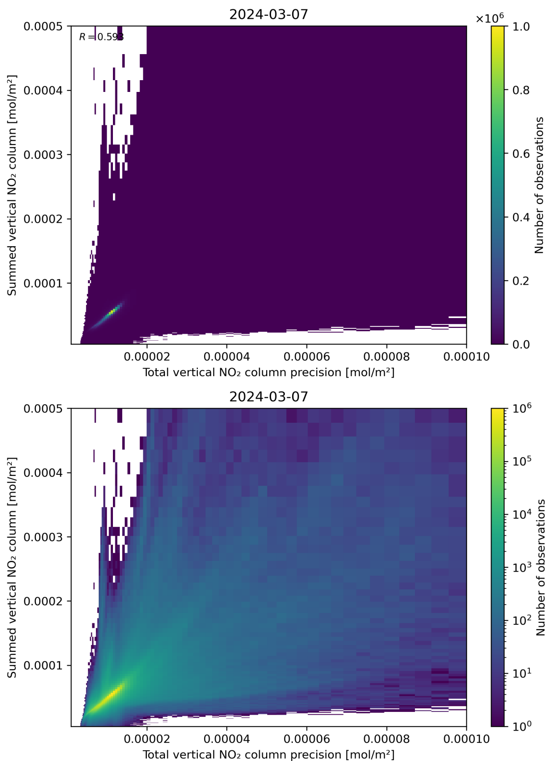
Figure 117: Scatter density plot of “Total vertical NO 2 column precision” against “Summed vertical NO 2 column” for 2024-03-06 to 2024-03-08.
