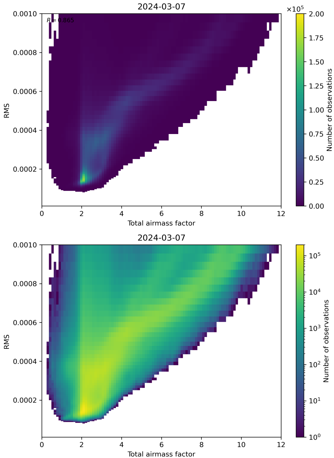
Figure 69: Scatter density plot of “Total airmass factor” against “RMS” for 2024-03-06 to 2024-03-08.
