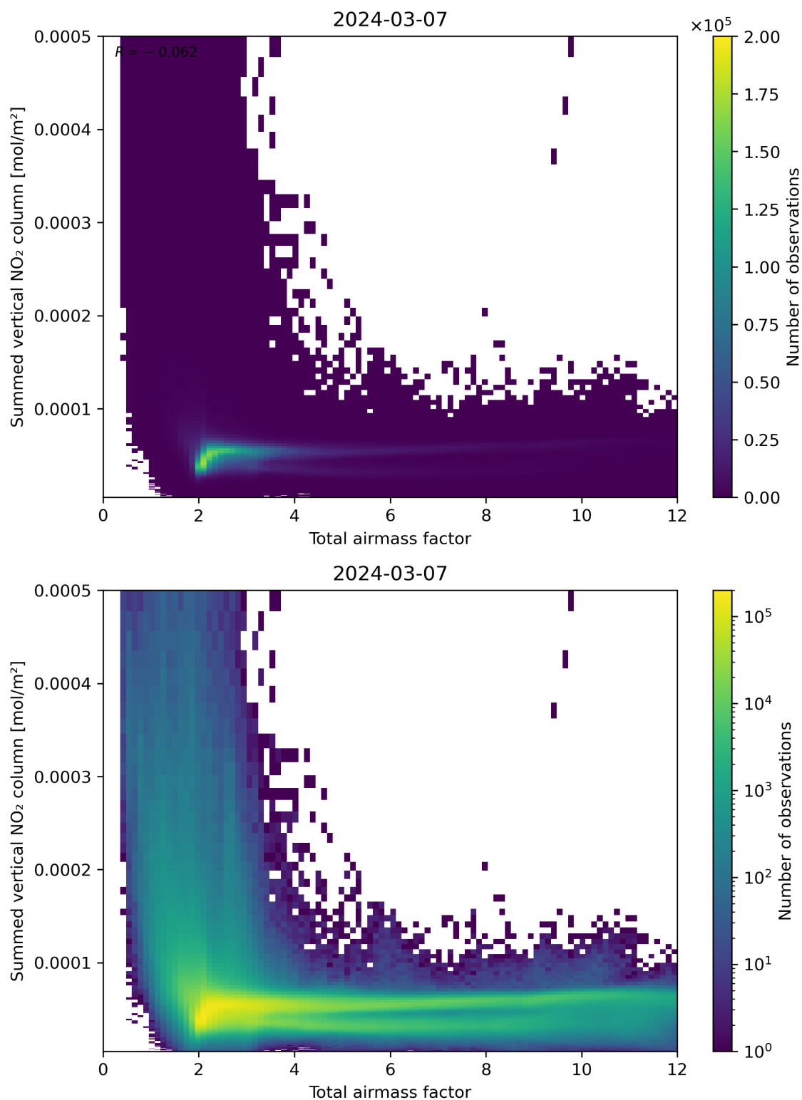
Figure 65: Scatter density plot of “Total airmass factor” against “Summed vertical NO 2 column” for 2024-03-06 to 2024-03-08.
