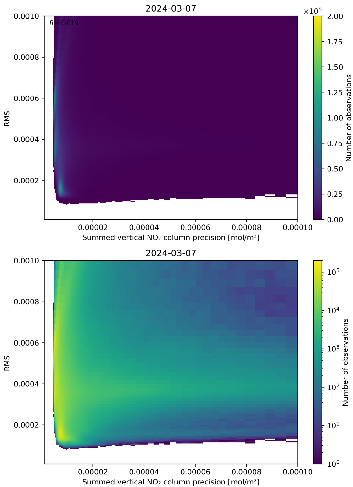
Figure 108: Scatter density plot of “Summed vertical NO 2 column precision” against “RMS” for 2024-03-06 to 2024-03-08.
