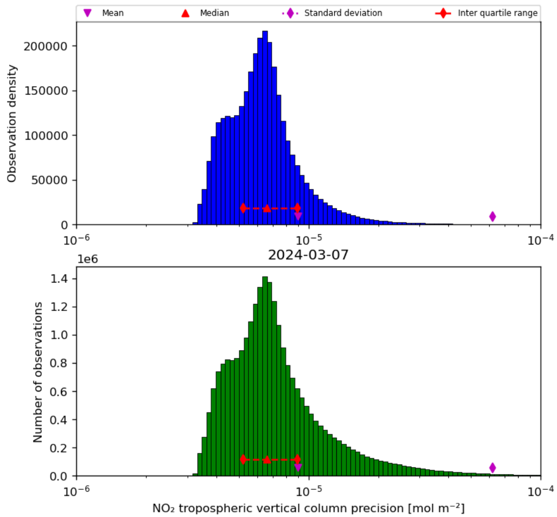
Figure 30: Histogram of “NO 2 tropospheric vertical column precision” for 2024-03-06 to 2024-03-08
