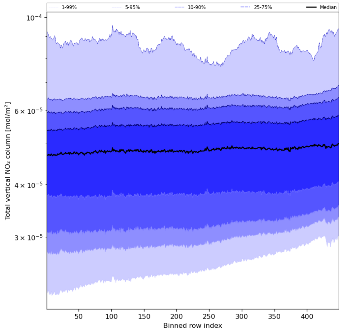
Figure 55: Along track statistics of “Total vertical NO 2 column” for 2024-03-06 to 2024-03-08
