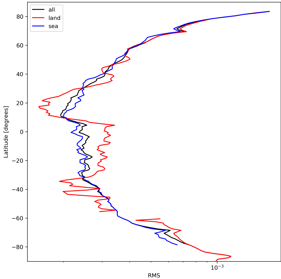
Figure 26: Zonal average of “RMS” for 2024-03-06 to 2024-03-08.
