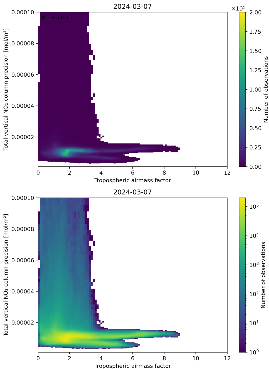
Figure 78: Scatter density plot of “Tropospheric air mass factor” against “Total vertical NO 2 column precision” for 2024-03-06 to 2024-03-08.
