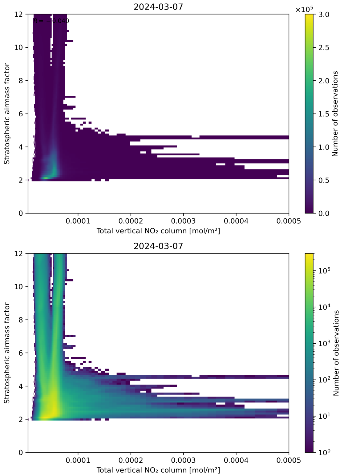
Figure 110: Scatter density plot of “Total vertical NO 2 column” against “Stratospheric air mass factor” for 2024-03-06 to 2024-03-08.
