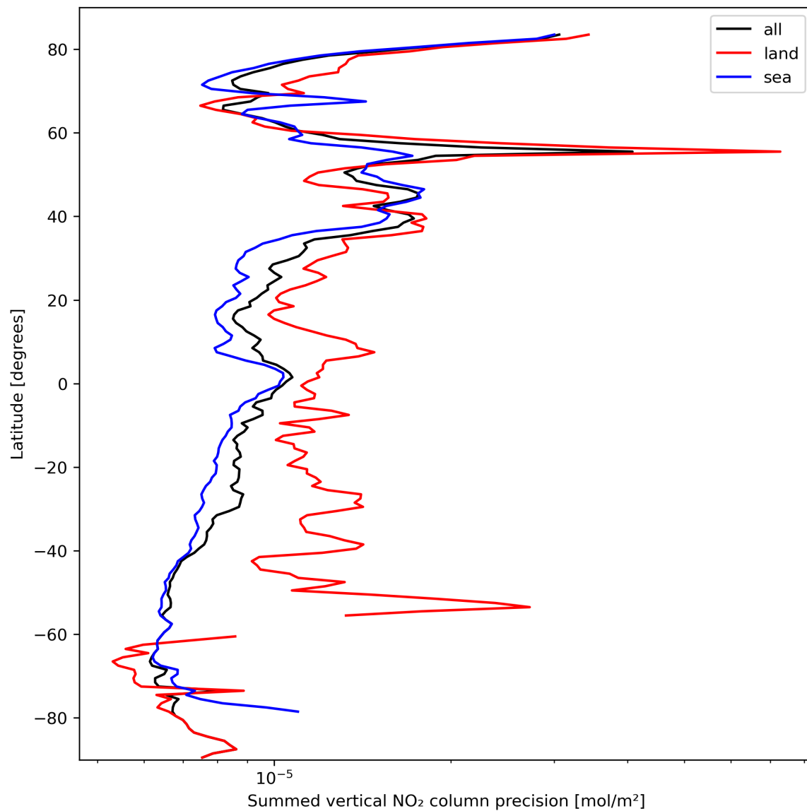
Figure 24: Zonal average of “Summed vertical NO 2 column precision” for 2024-03-06 to 2024-03-08.
