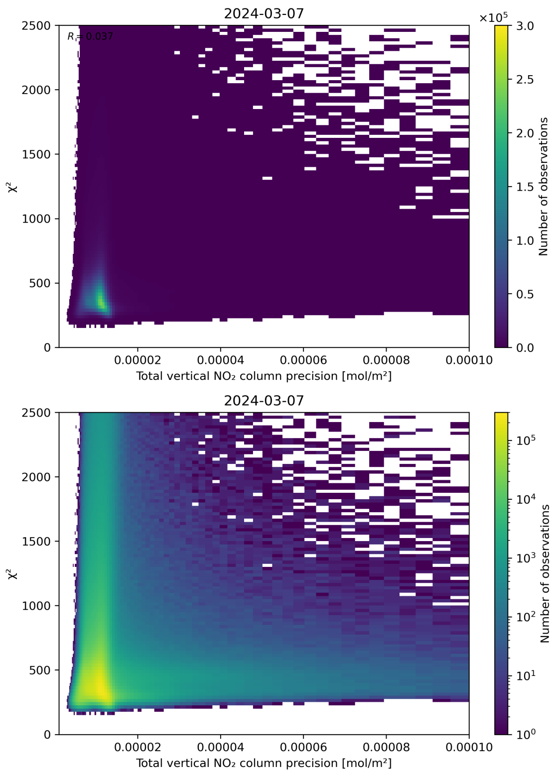
Figure 116: Scatter density plot of “Total vertical NO 2 column precision” against “ \chi^2 ” for 2024-03-06 to 2024-03-08.
