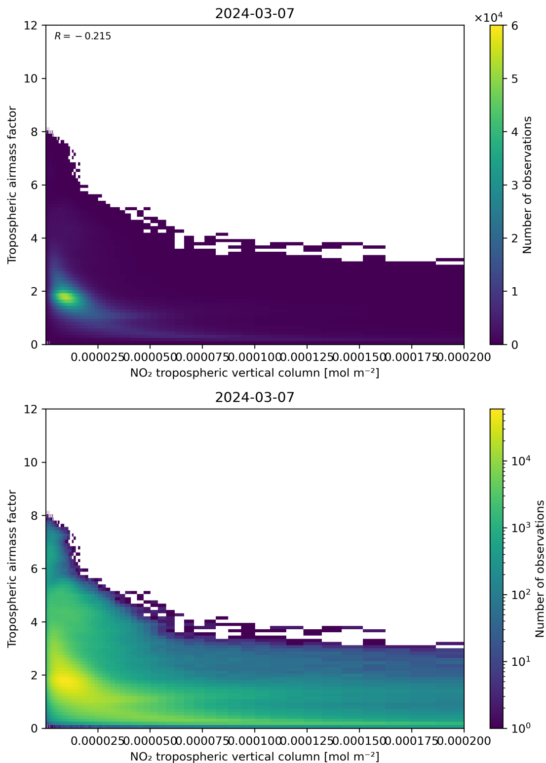
Figure 123: Scatter density plot of “NO 2 tropospheric vertical column” against “Tropospheric airmass factor” for 2024-03-06 to 2024-03-08.
