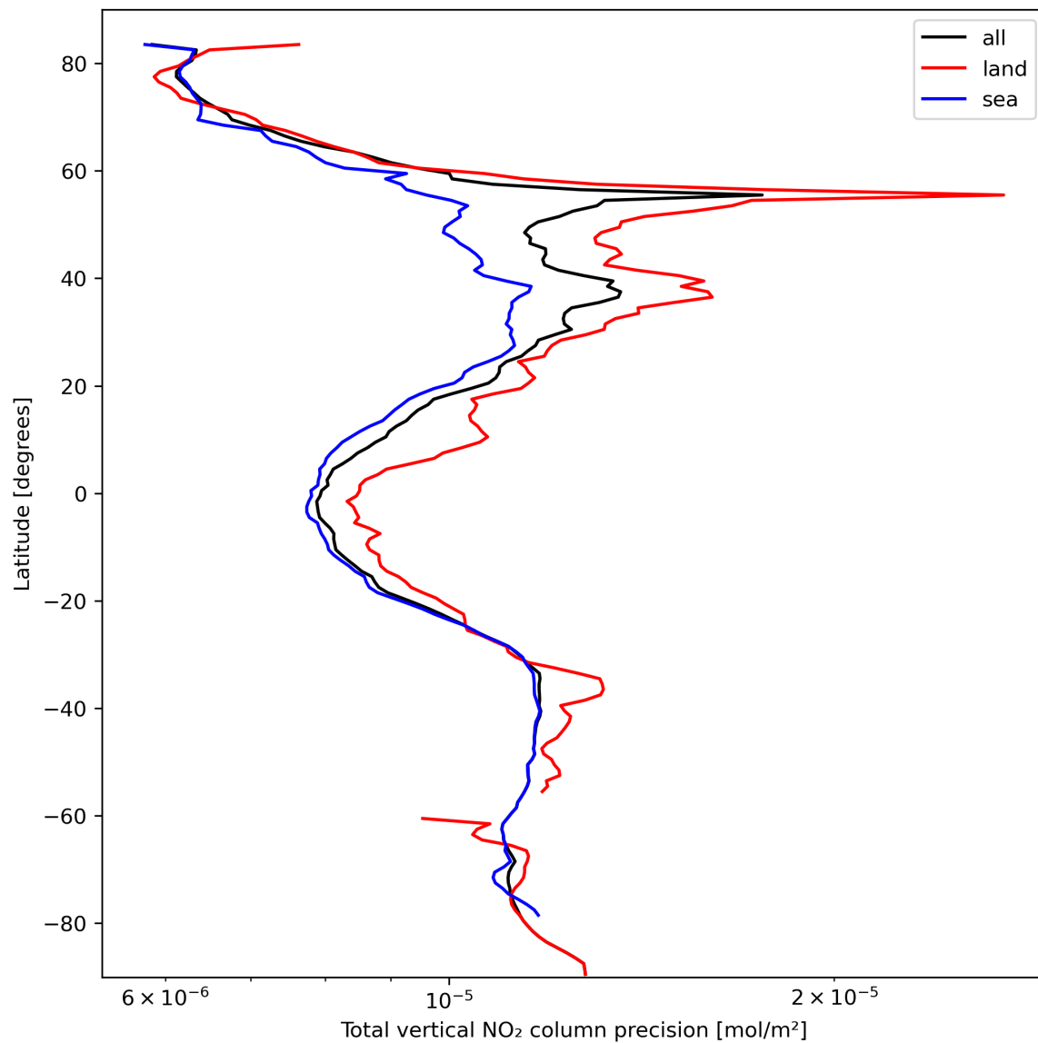
Figure 22: Zonal average of "Total vertical NO 2 column precision" for 2024-03-06 to 2024-03-08.
