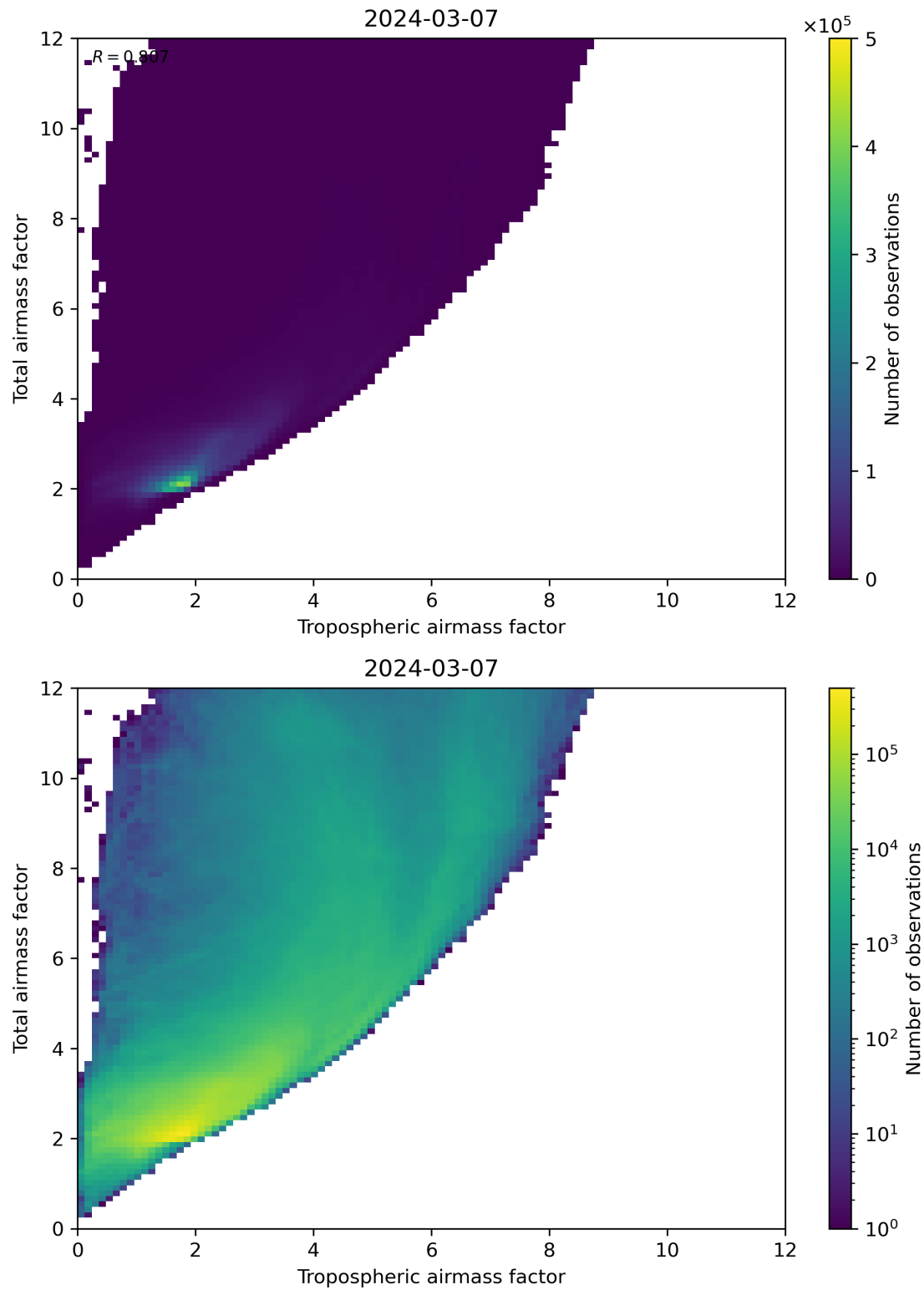
Figure 72: Scatter density plot of “Tropospheric airmass factor” against “Total airmass factor” for 2024-03-06 to 2024-03-08.
