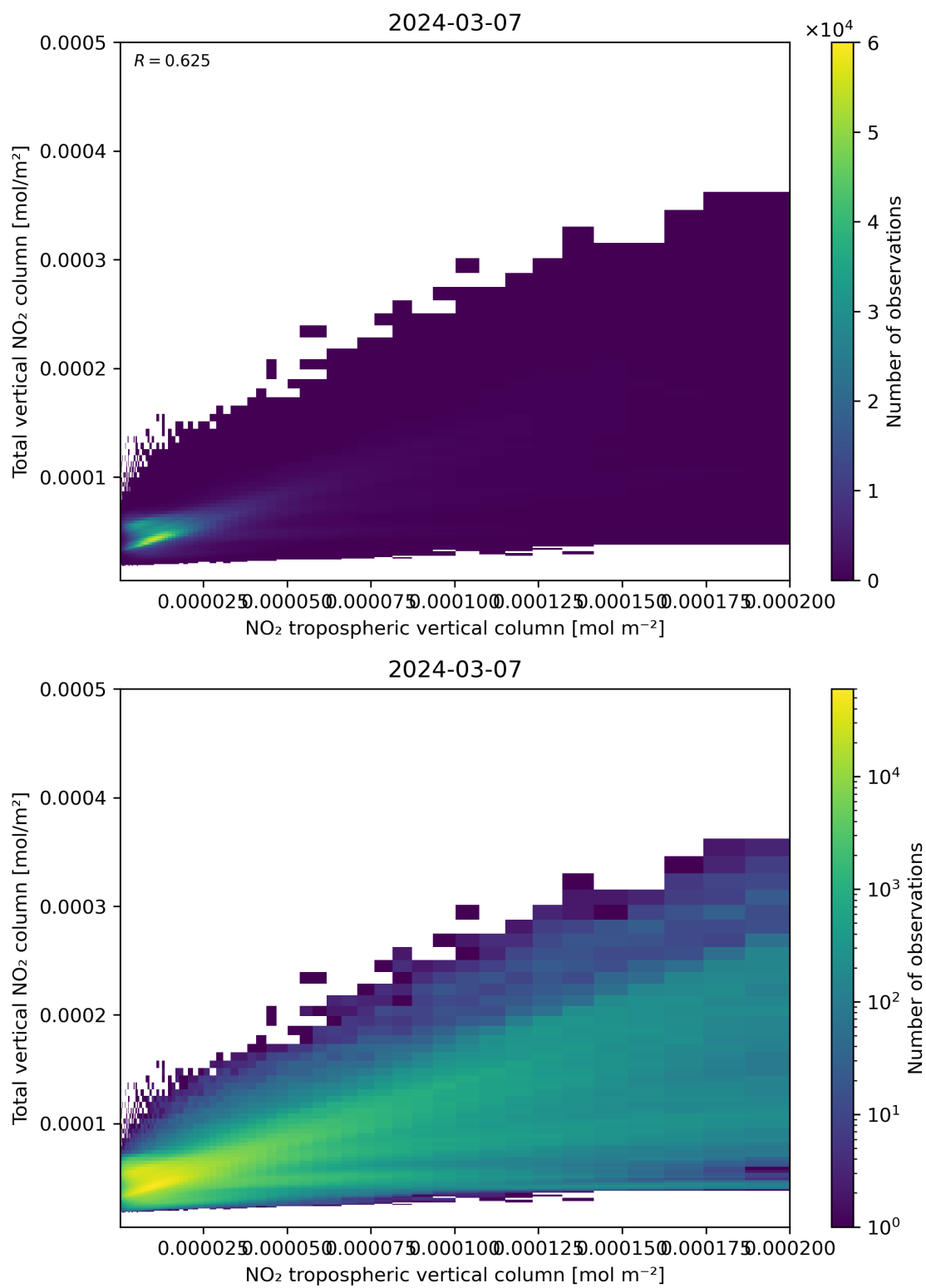
Figure 128: Scatter density plot of “NO 2 tropospheric vertical column” against “Total vertical NO 2 column” for 2024-03-06 to 2024-03-08.
