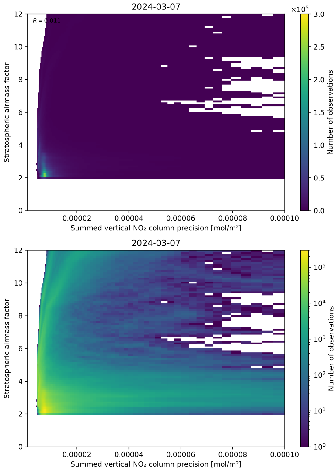
Figure 106: Scatter density plot of “Summed vertical NO 2 column precision” against “Stratospheric airmass factor” for 2024-03-06 to 2024-03-08.
