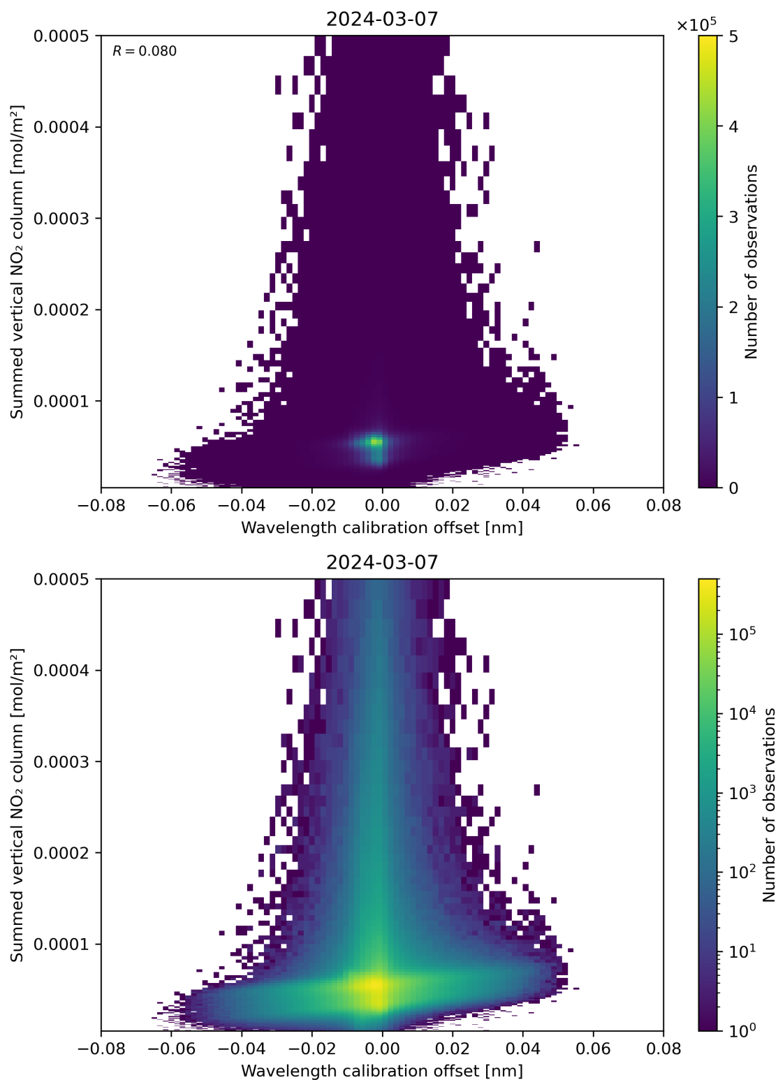
Figure 177: Scatter density plot of “Wavelength calibration offset” against “Summed vertical NO 2 column” for 2024-03-06 to 2024-03-08.
