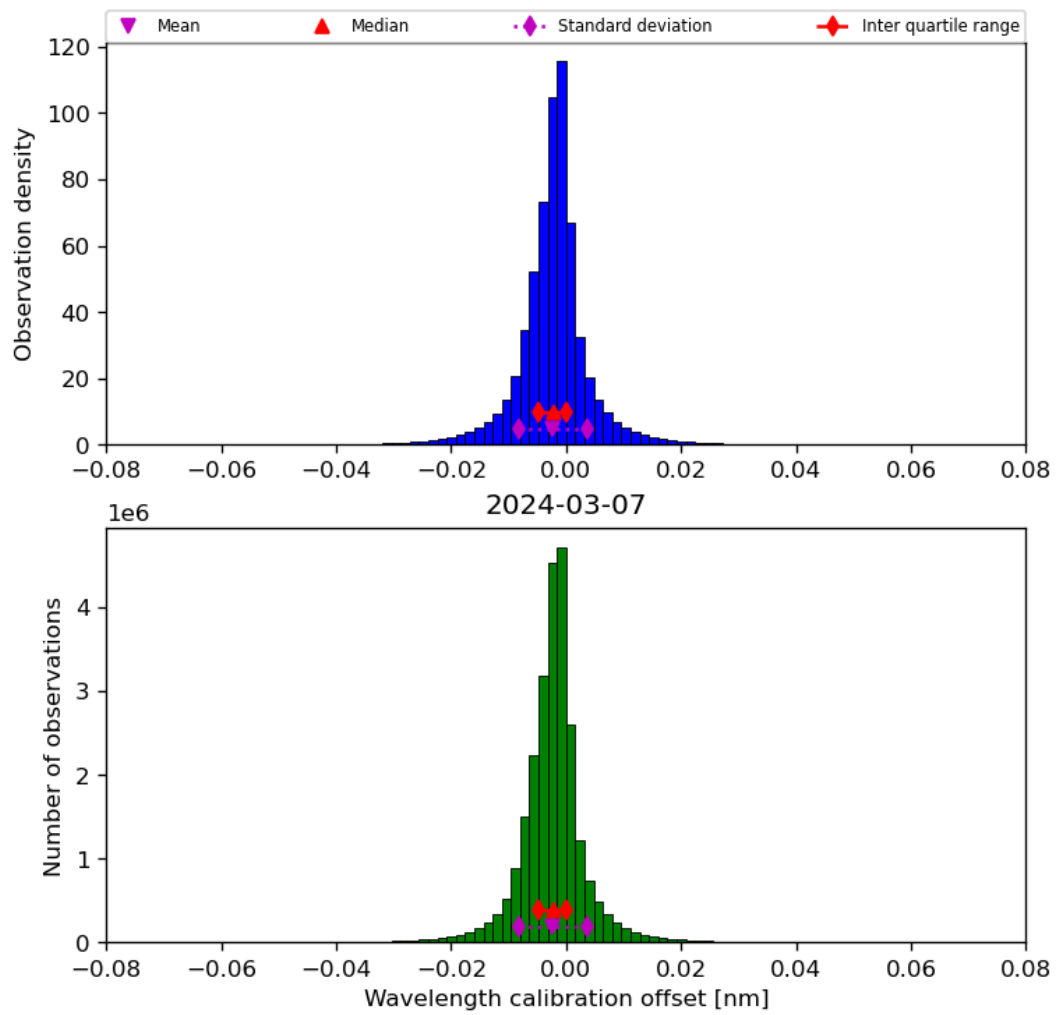
Figure 35: Histogram of “Wavelength calibration offset” for 2024-03-06 to 2024-03-08
