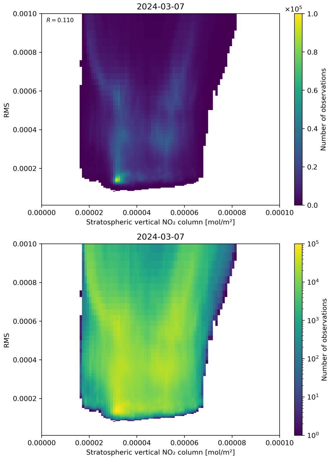
Figure 102: Scatter density plot of “Stratospheric vertical NO 2 column” against “RMS” for 2024-03-06 to 2024-03-08.
