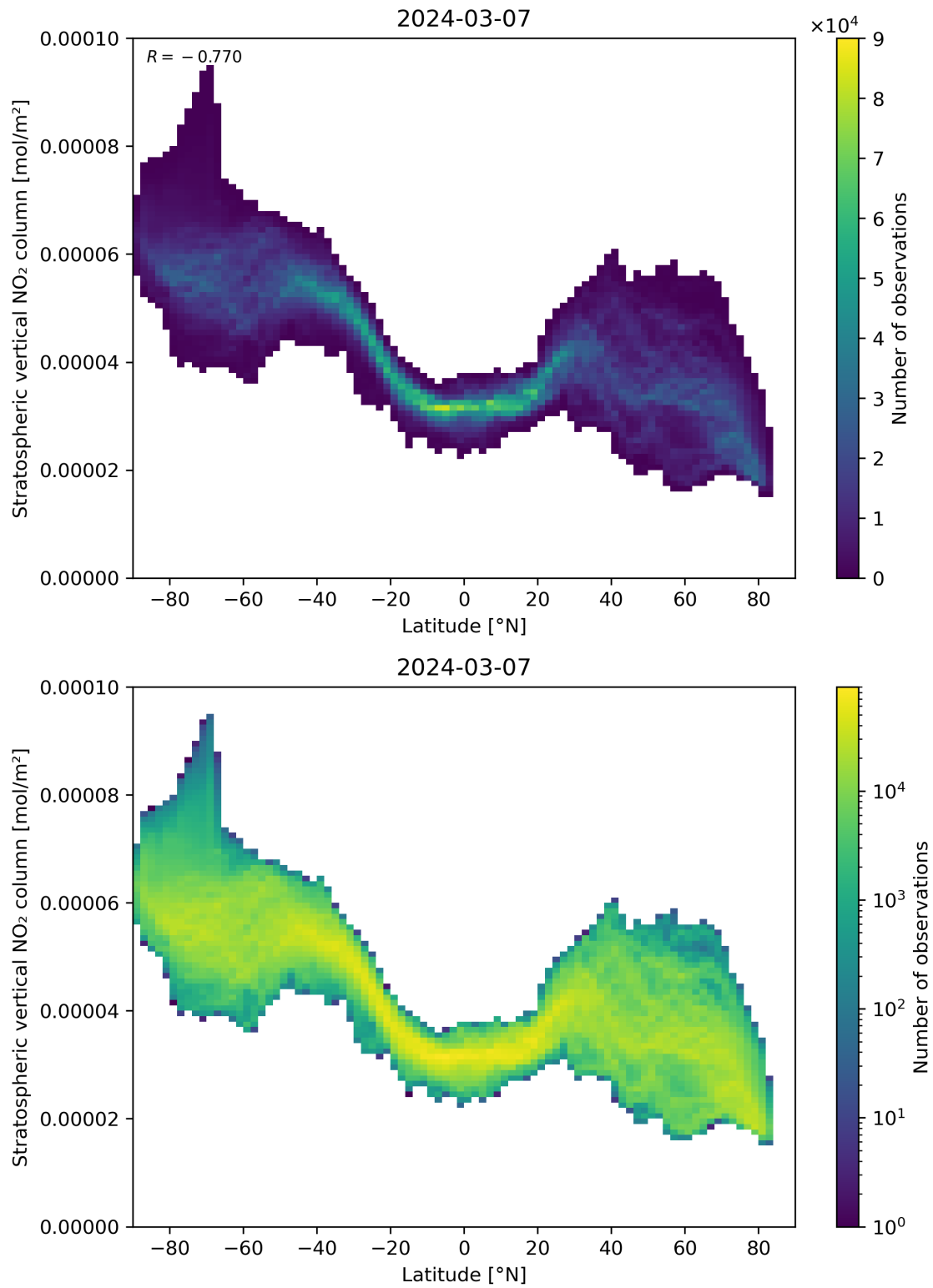
Figure 87: Scatter density plot of “Latitude” against “Stratospheric vertical NO 2 column” for 2024-03-06 to 2024-03-08.
