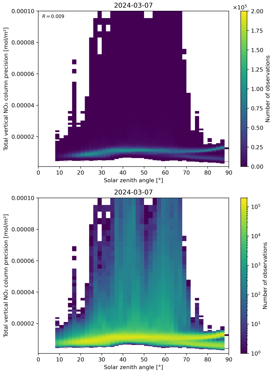
Figure 154: Scatter density plot of “Solar zenith angle” against “Total vertical NO 2 column precision” for 2024-03-06 to 2024-03-08.
