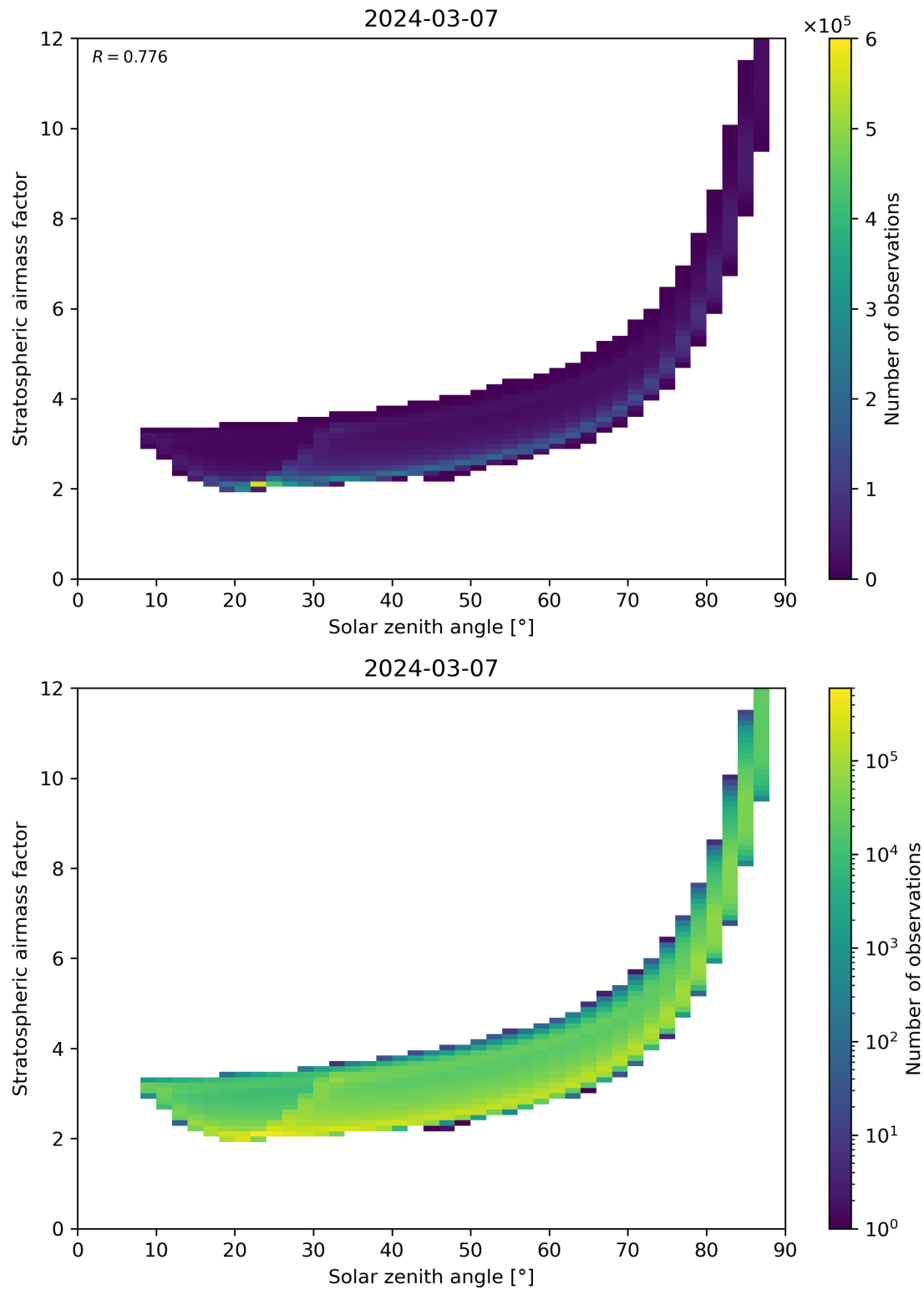
Figure 145: Scatter density plot of “Solar zenith angle” against “Stratospheric airmass factor” for 2024-03-06 to 2024-03-08.
