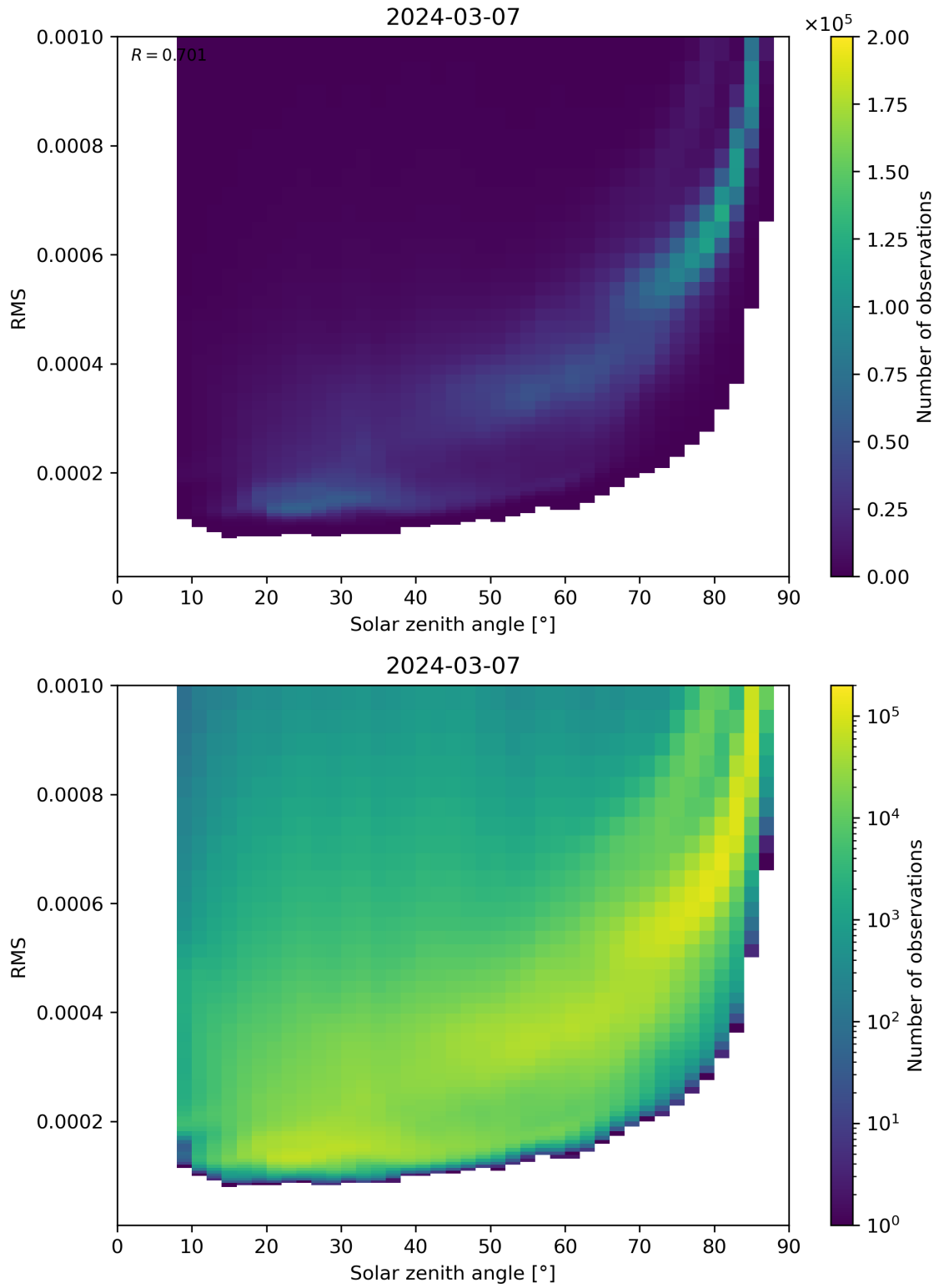
Figure 157: Scatter density plot of “Solar zenith angle” against “RMS” for 2024-03-06 to 2024-03-08.
