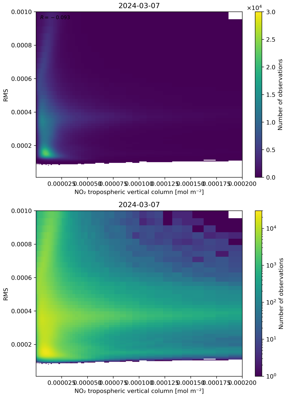
Figure 142: Scatter density plot of “NO 2 tropospheric vertical column” against “RMS” for 2024-03-06 to 2024-03-08.
