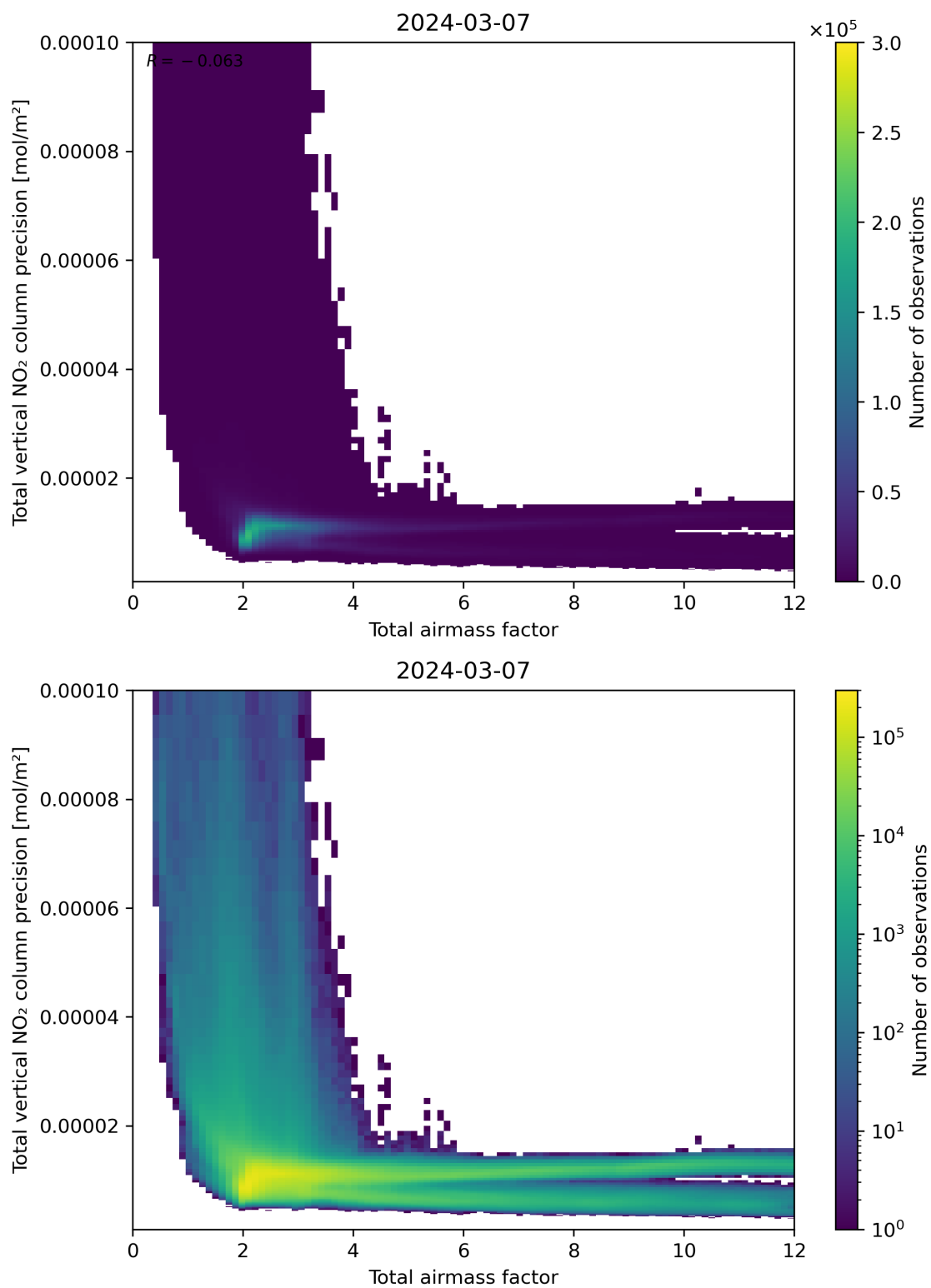
Figure 68: Scatter density plot of “Total airmass factor” against “Total vertical NO 2 column precision” for 2024-03-06 to 2024-03-08.
