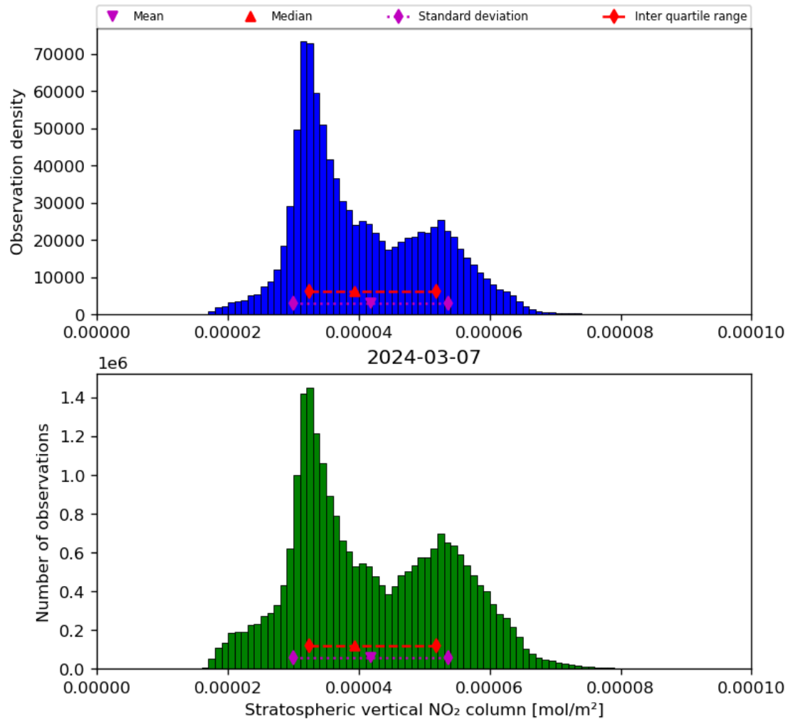
Figure 36: Histogram of “Stratospheric vertical NO 2 column” for 2024-03-06 to 2024-03-08
