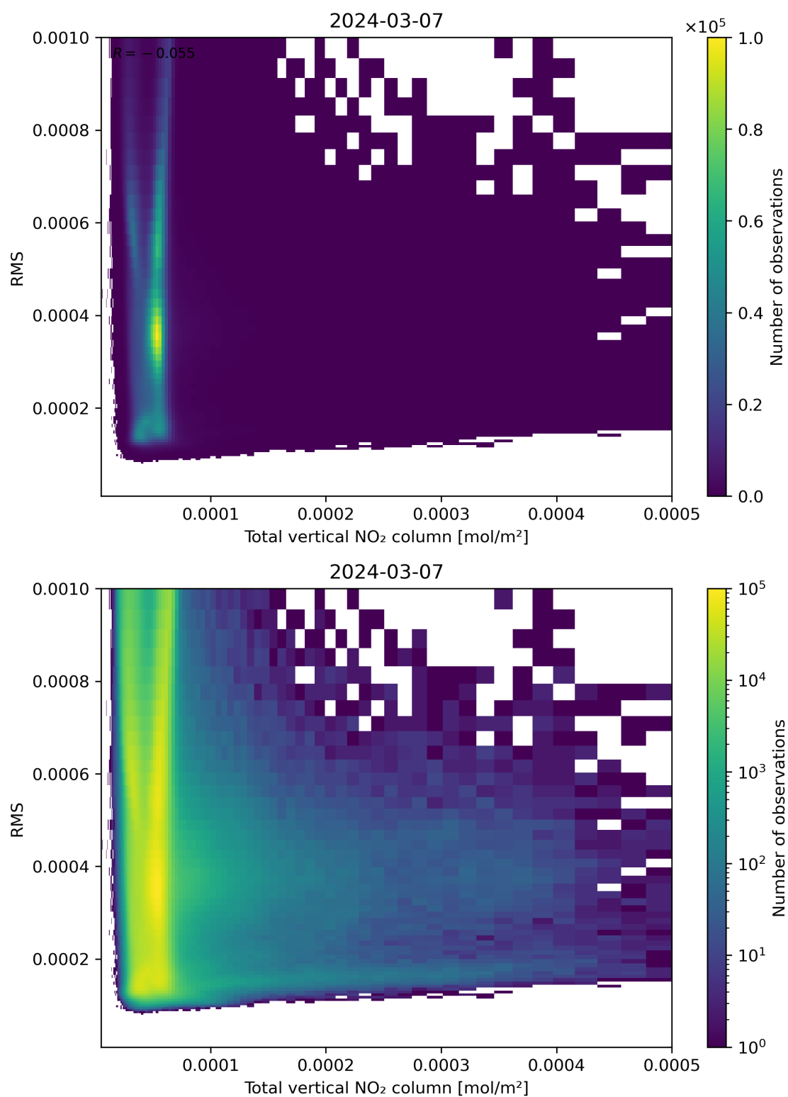
Figure 120: Scatter density plot of “Total vertical NO 2 column” against “RMS” for 2024-03-06 to 2024-03-08.
