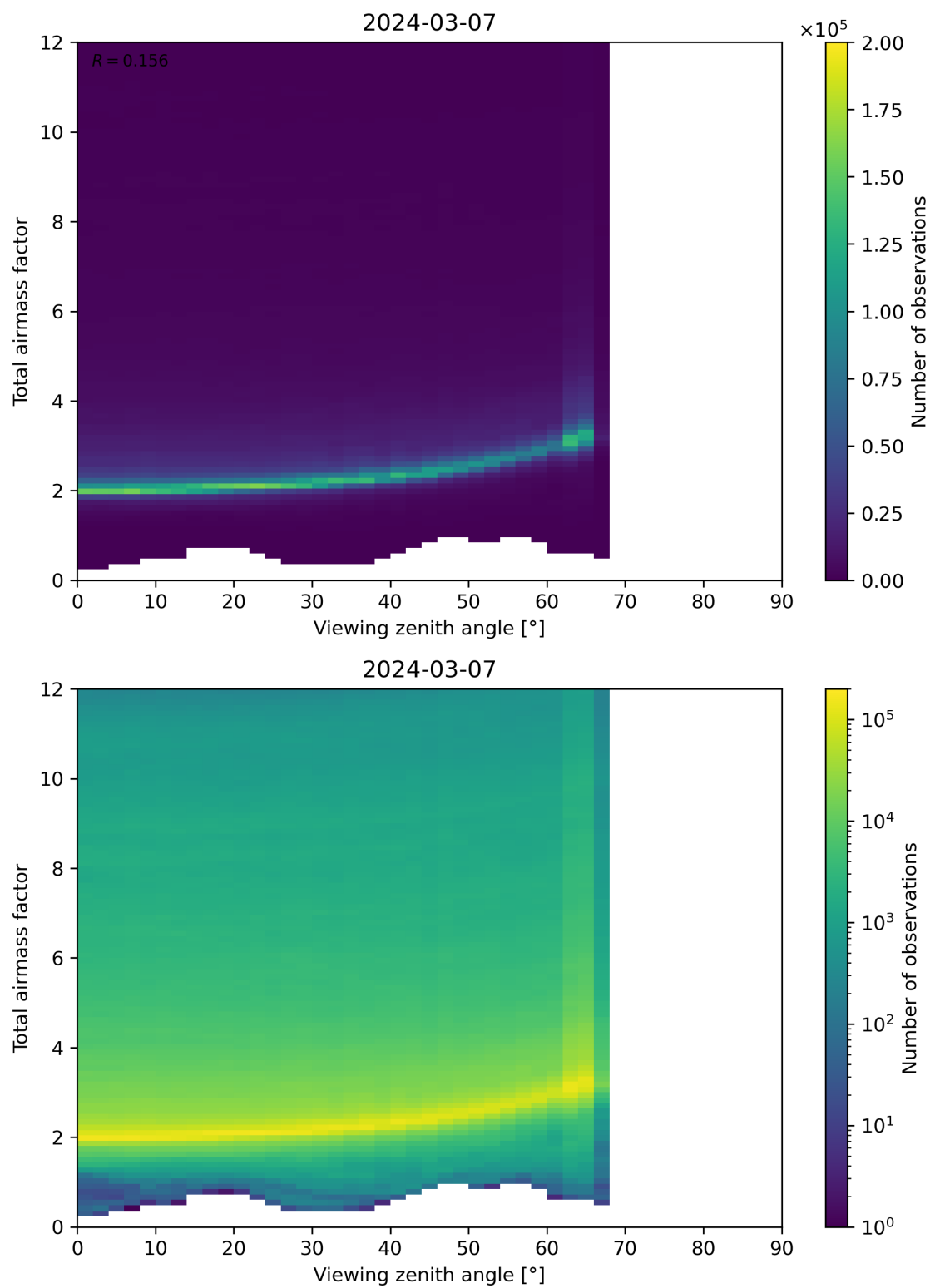
Figure 160: Scatter density plot of “Viewing zenith angle” against “Total airmass factor” for 2024-03-06 to 2024-03-08.
