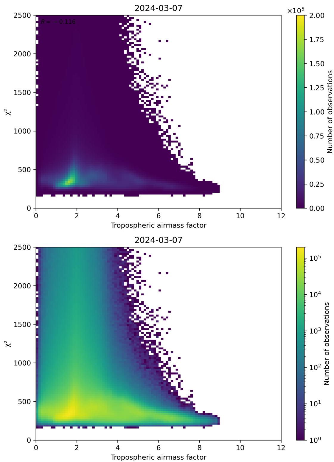
Figure 73: Scatter density plot of “Tropospheric airmass factor” against “ \chi^2 ” for 2024-03-06 to 2024-03-08.
