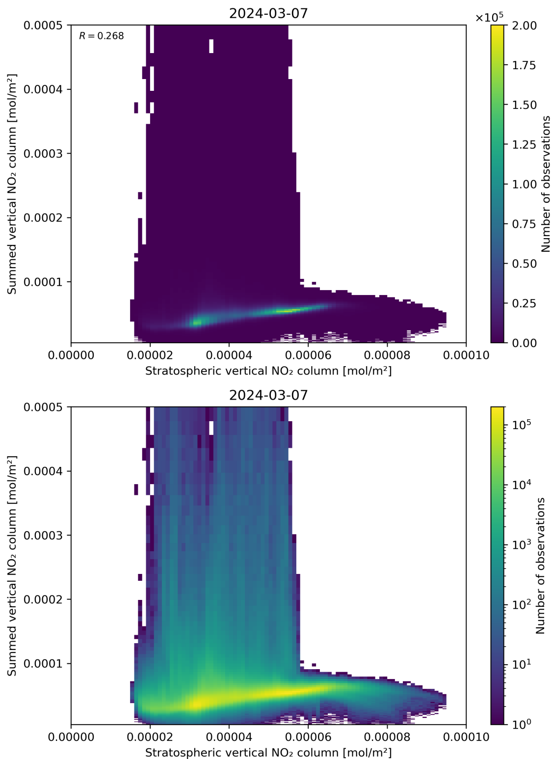
Figure 98: Scatter density plot of “Stratospheric vertical NO 2 column” against “Summed vertical NO 2 column” for 2024-03-06 to 2024-03-08.
