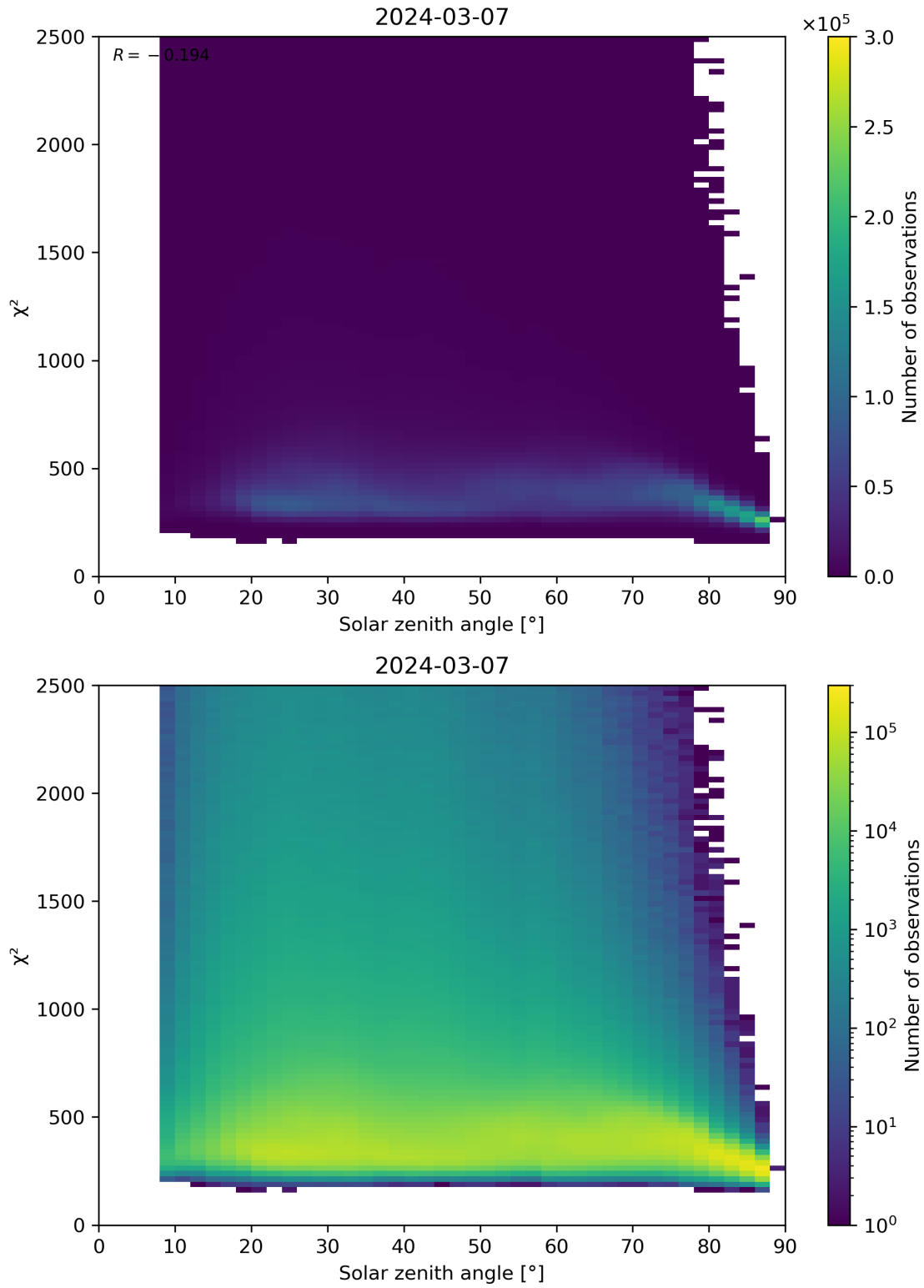
Figure 148: Scatter density plot of “Solar zenith angle” against “ \chi^2 ” for 2024-03-06 to 2024-03-08.
