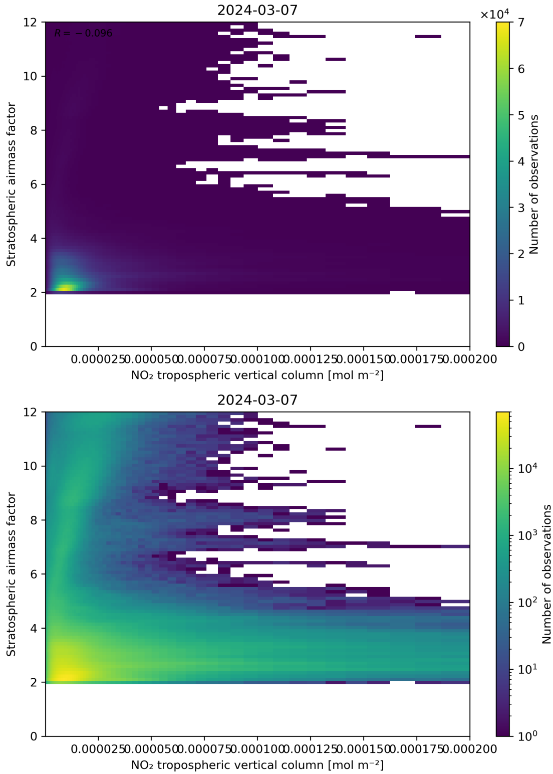
Figure 121: Scatter density plot of “NO 2 tropospheric vertical column” against “Stratospheric air mass factor” for 2024-03-06 to 2024-03-08.
