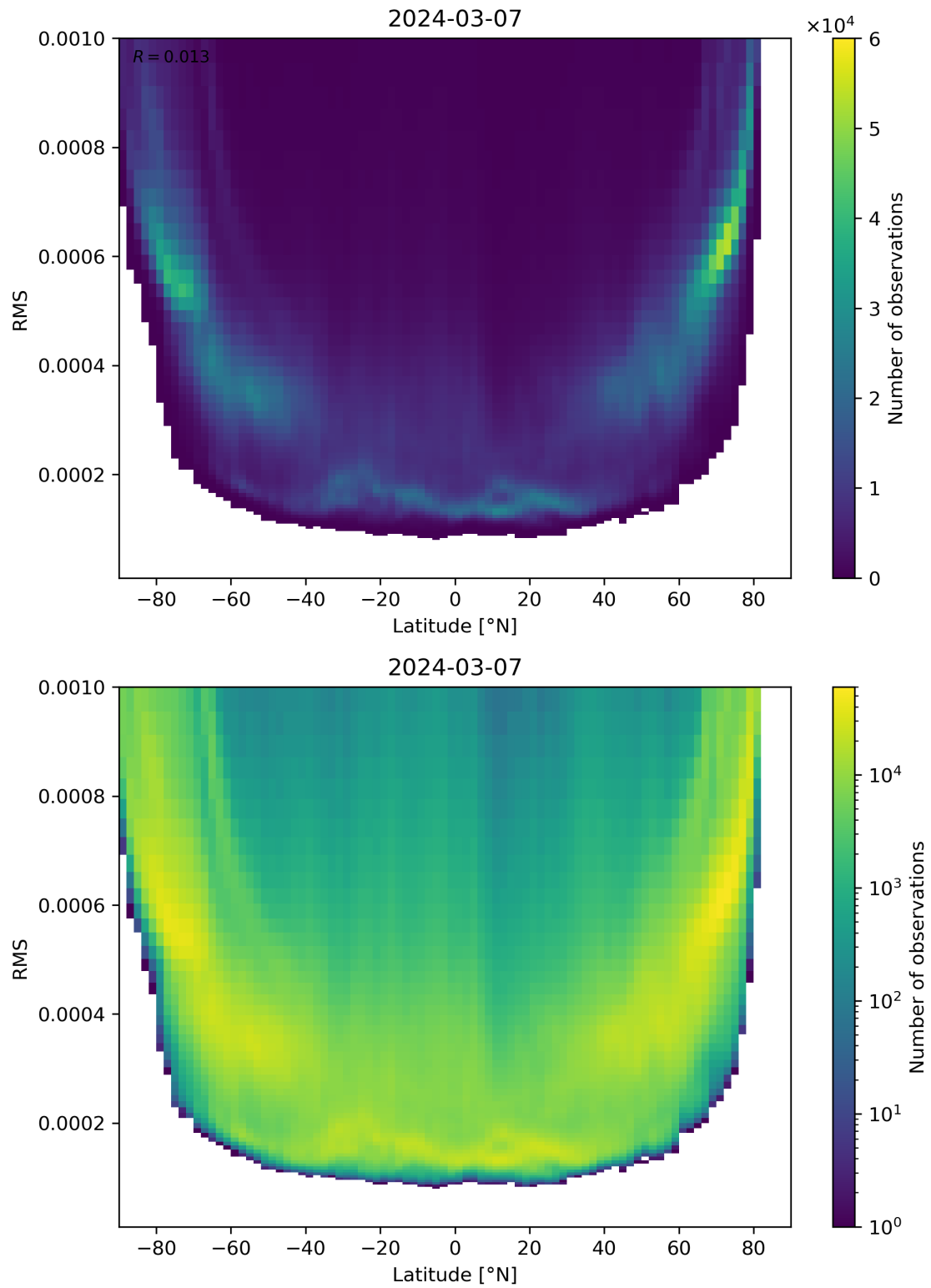
Figure 94: Scatter density plot of “Latitude” against “RMS” for 2024-03-06 to 2024-03-08.
