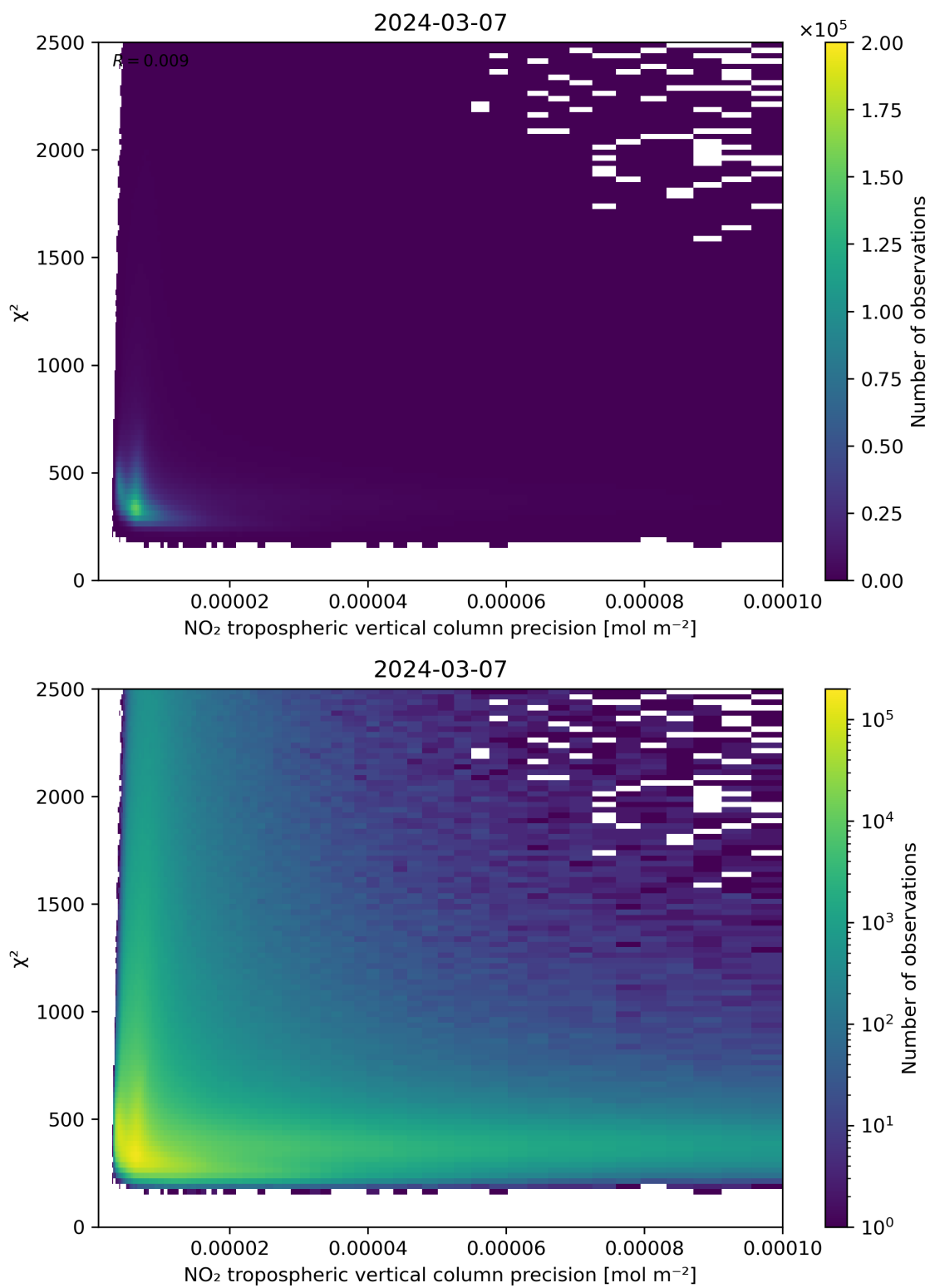
Figure 134: Scatter density plot of “NO 2 tropospheric vertical column precision” against “ \chi^2 ” for 2024-03-06 to 2024-03-08.
