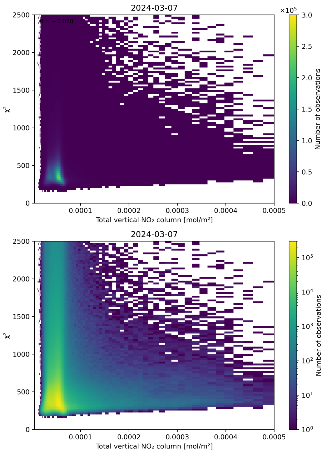
Figure 111: Scatter density plot of “Total vertical NO 2 column” against “ \chi^2 ” for 2024-03-06 to 2024-03-08.
