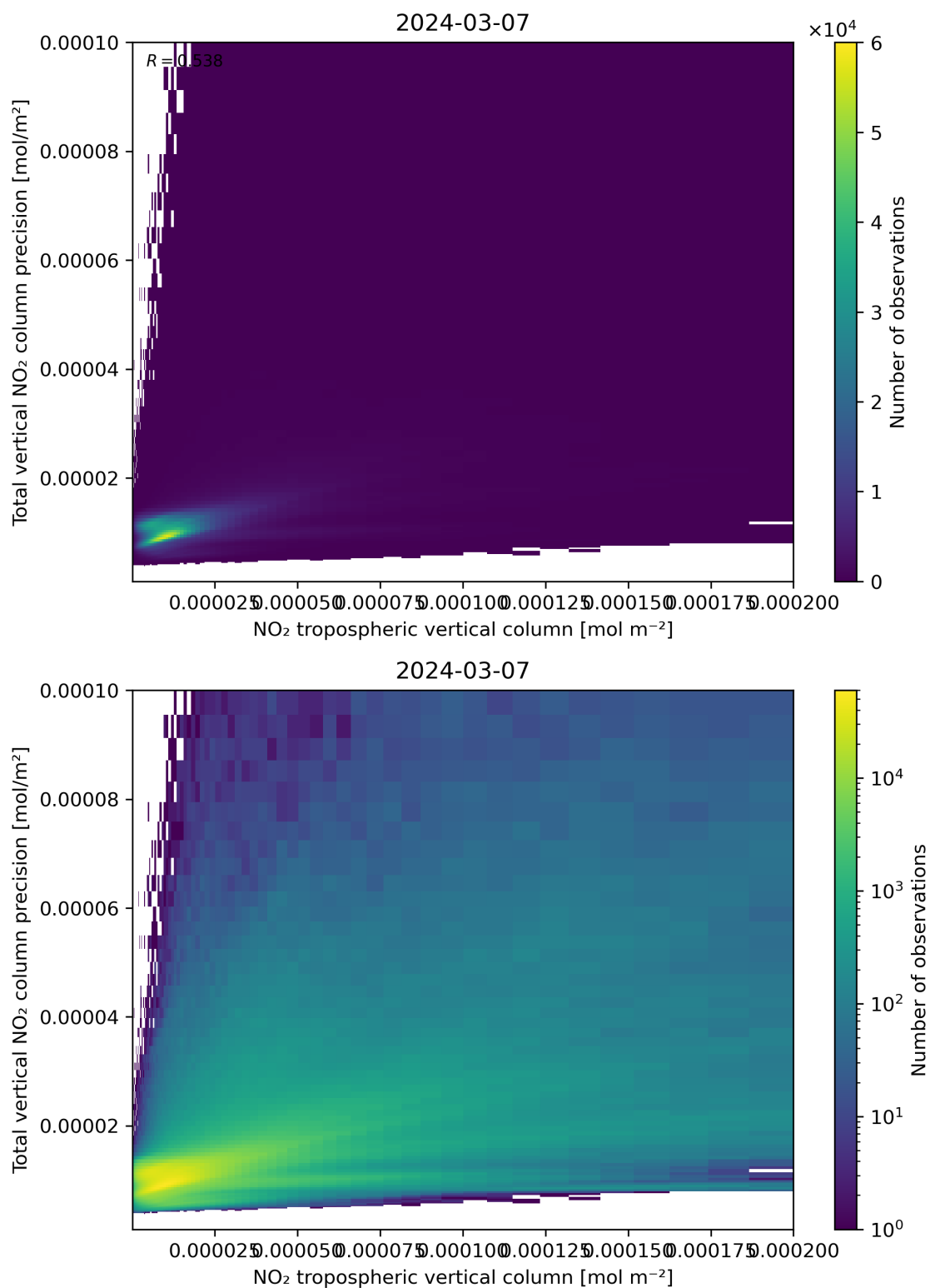
Figure 129: Scatter density plot of “NO 2 tropospheric vertical column” against “Total vertical NO 2 column precision” for 2024-03-06 to 2024-03-08.
