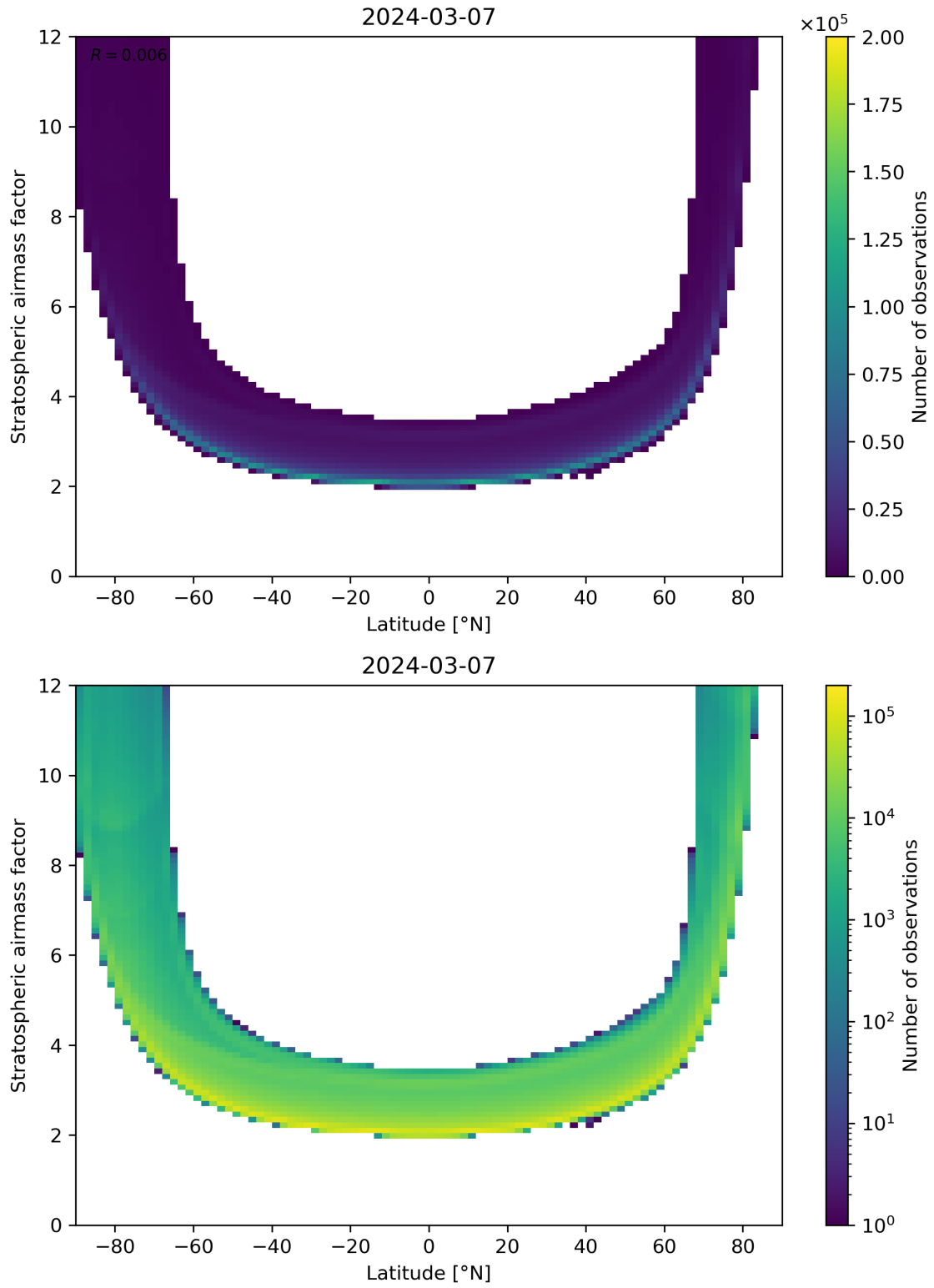
Figure 83: Scatter density plot of “Latitude” against “Stratospheric airmass factor” for 2024-03-06 to 2024-03-08.
