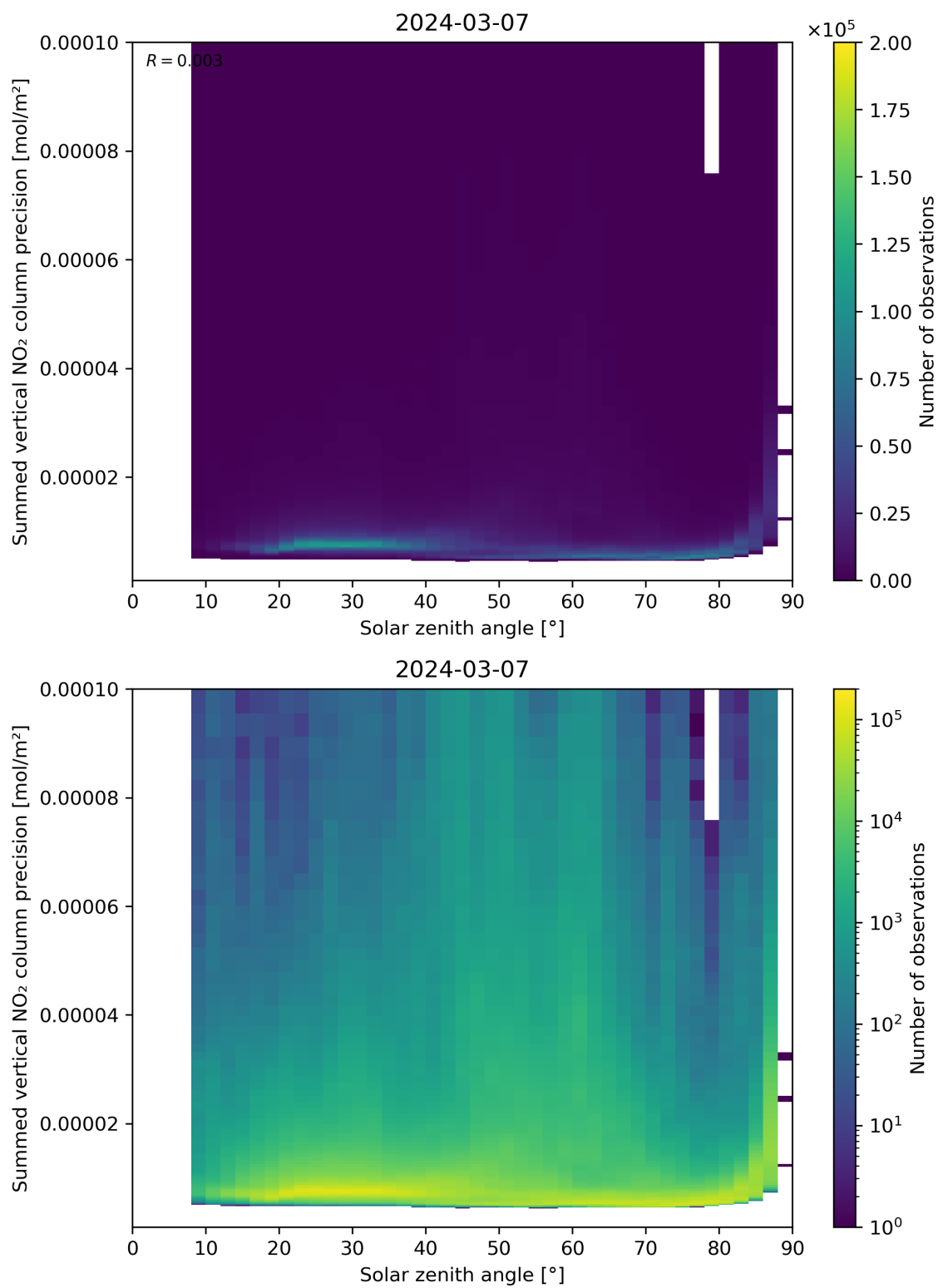
Figure 152: Scatter density plot of “Solar zenith angle” against “Summed vertical NO 2 column precision” for 2024-03-06 to 2024-03-08.
