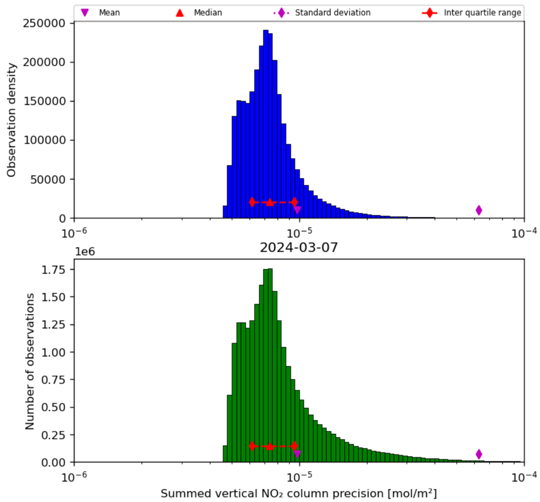
Figure 41: Histogram of "Summed vertical NO 2 column precision" for 2024-03-06 to 2024-03-08
