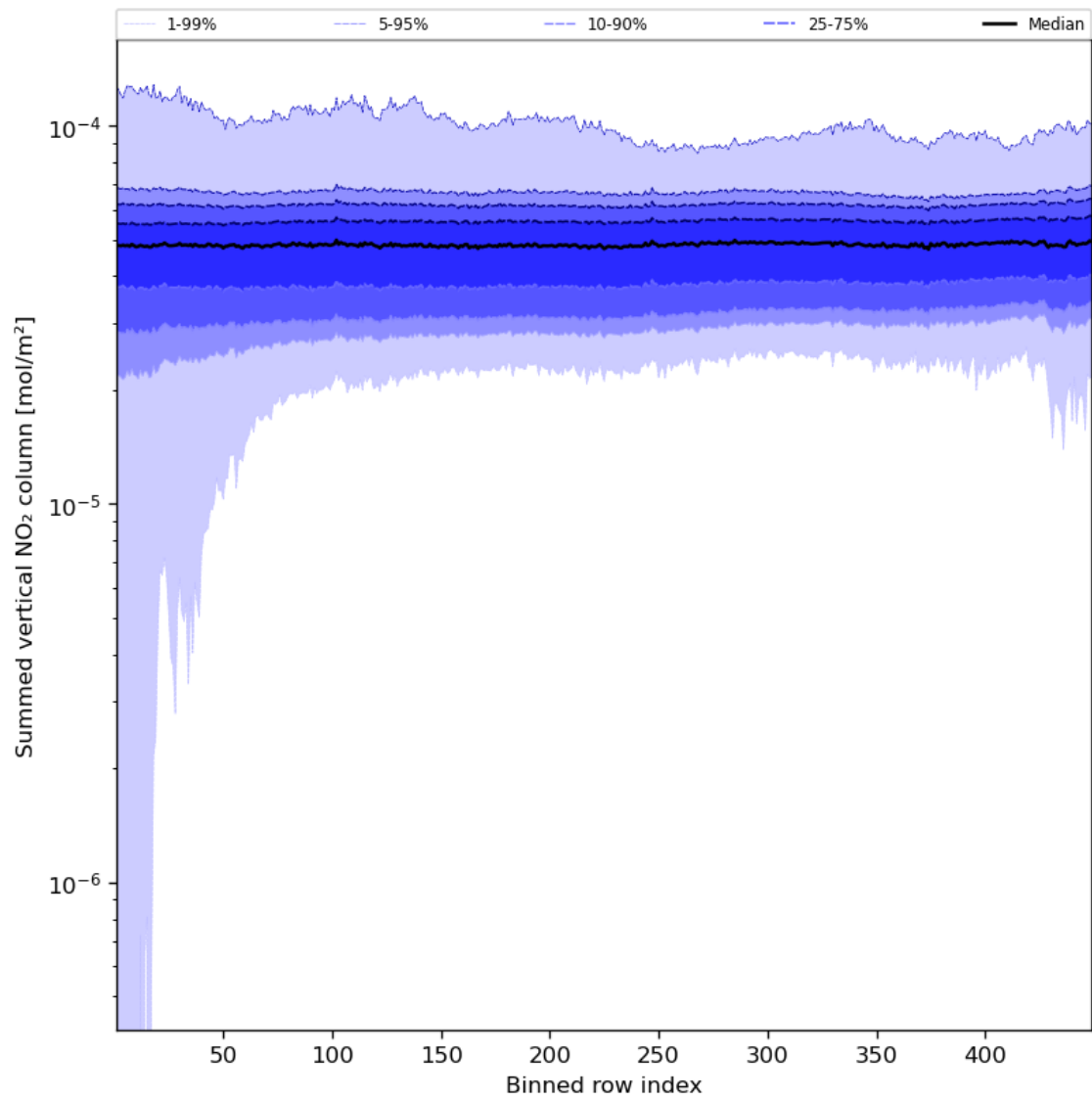
Figure 57: Along track statistics of “Summed vertical NO 2 column” for 2024-03-06 to 2024-03-08
