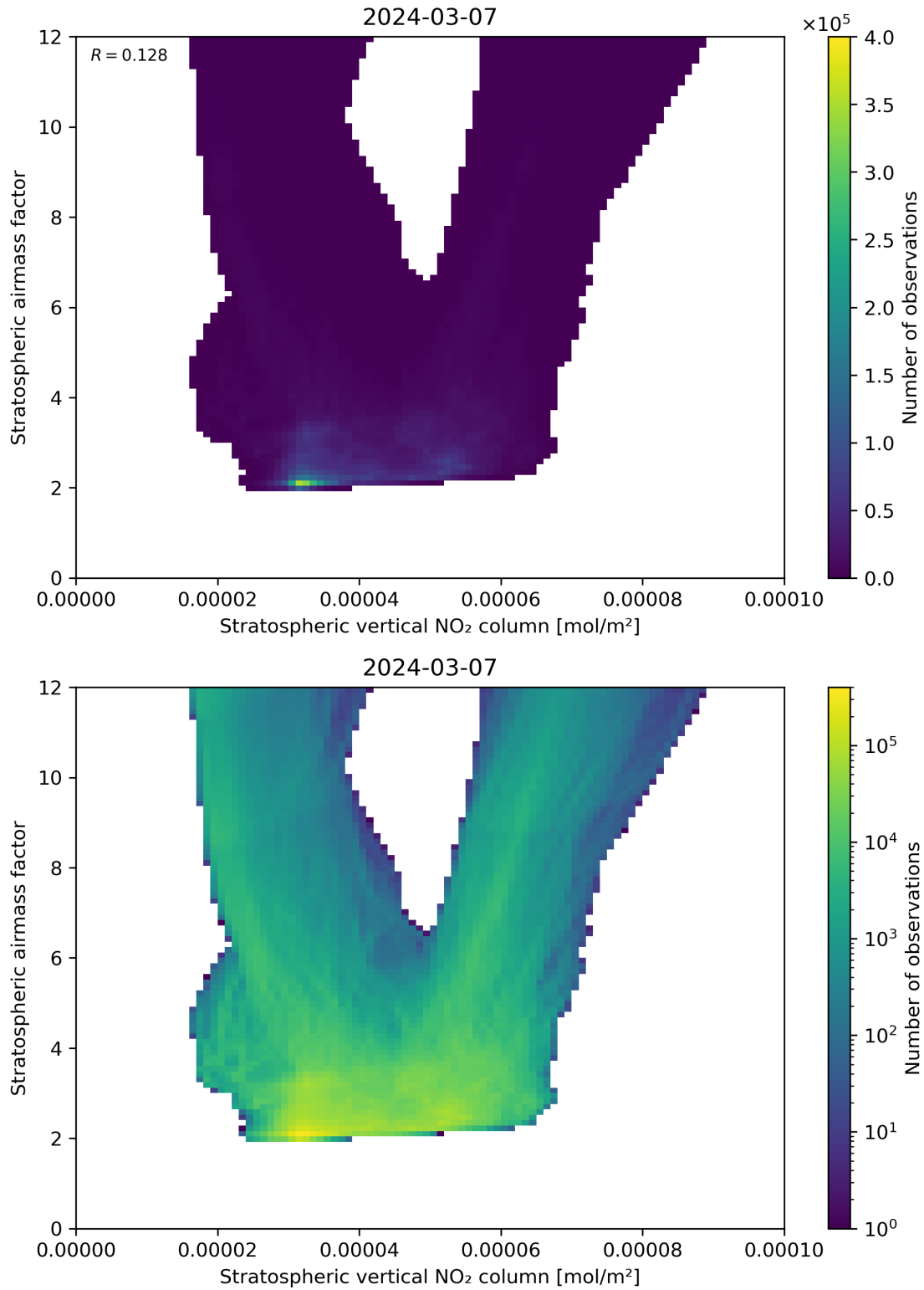
Figure 96: Scatter density plot of “Stratospheric vertical NO 2 column” against “Stratospheric airmass factor” for 2024-03-06 to 2024-03-08.
