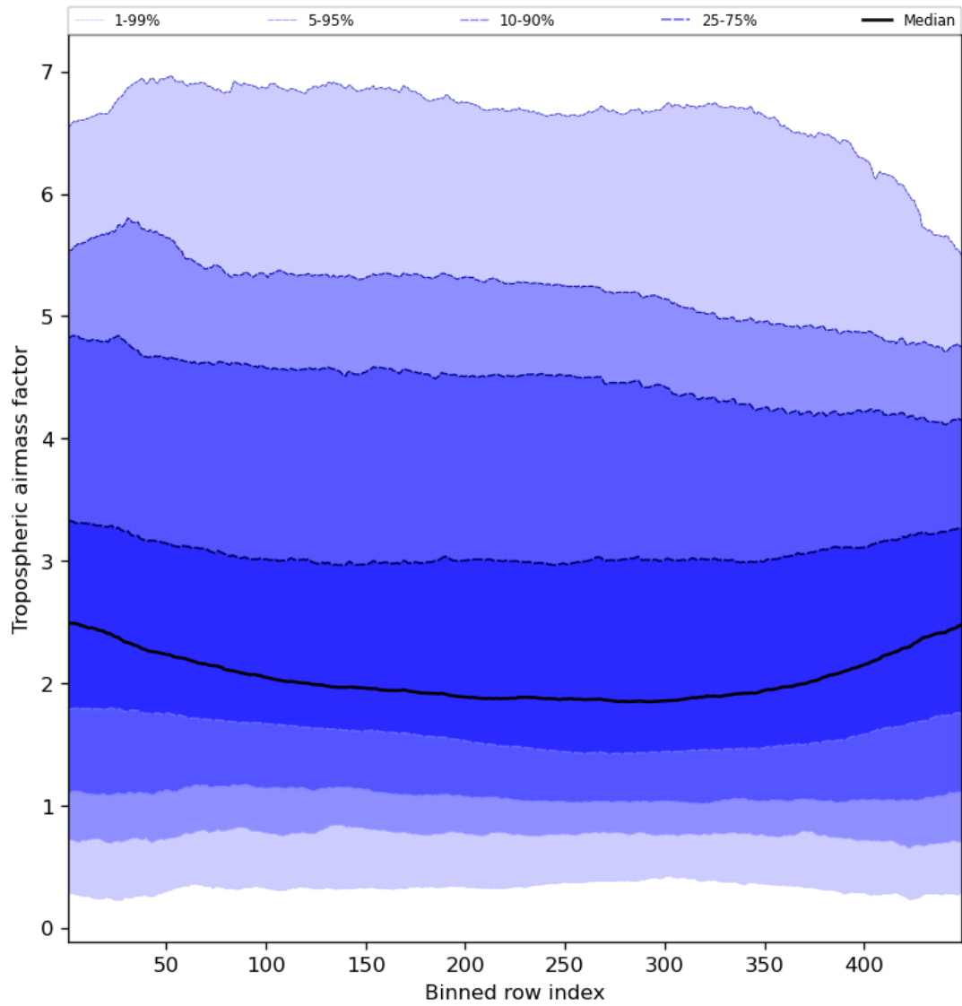
Figure 48: Along track statistics of “Tropospheric air mass factor” for 2024-03-06 to 2024-03-08
