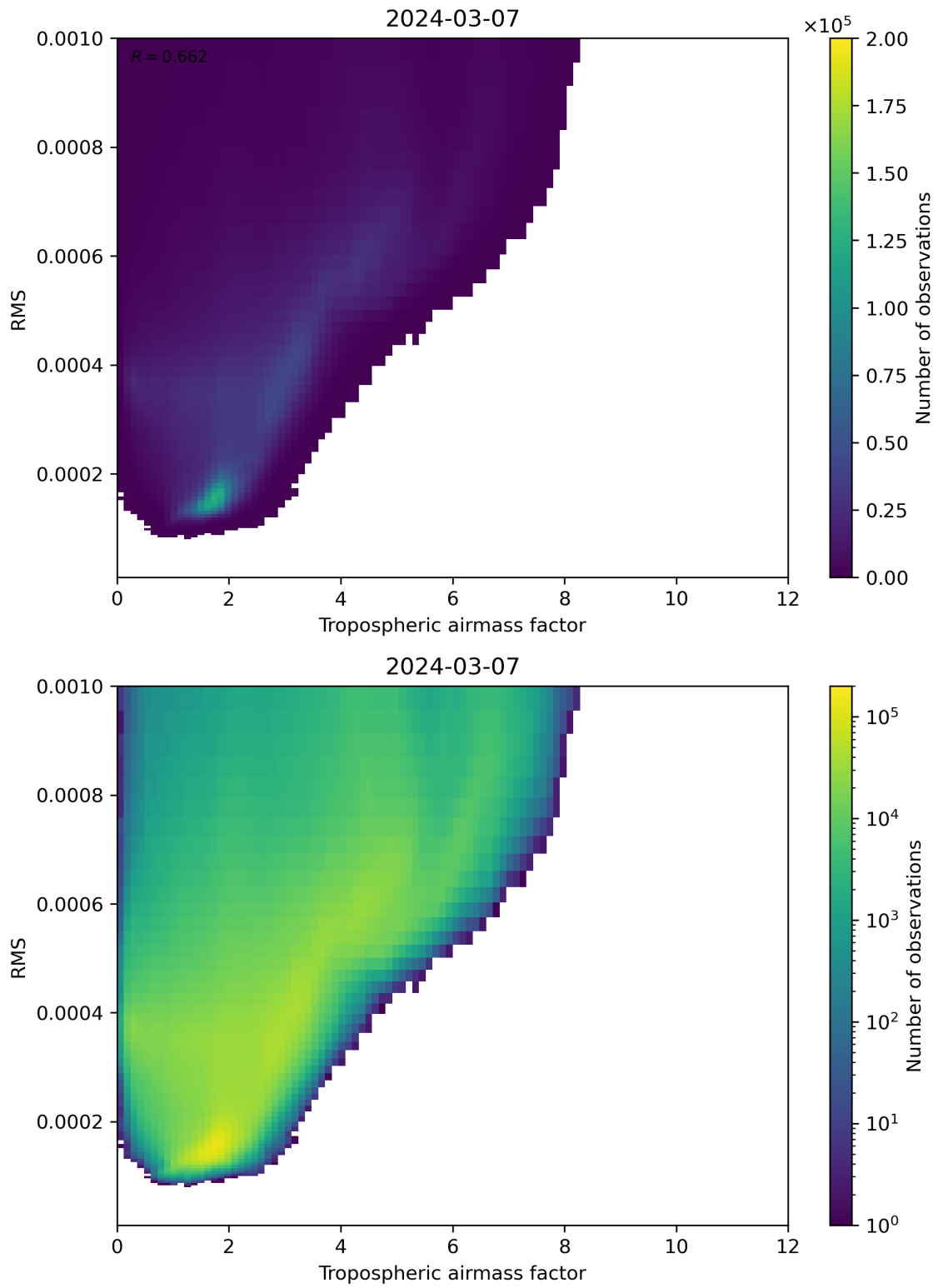
Figure 79: Scatter density plot of “Tropospheric airmass factor” against “RMS” for 2024-03-06 to 2024-03-08.
