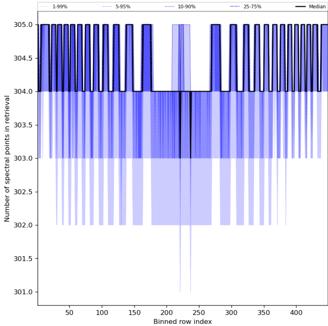
Figure 50: Along track statistics of “Number of spectral points in retrieval” for 2024-03-06 to 2024-03-08
