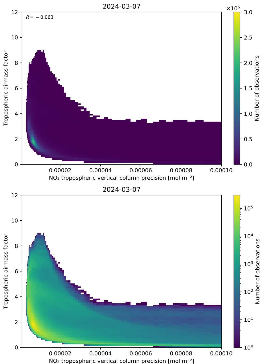
Figure 133: Scatter density plot of “NO 2 tropospheric vertical column precision” against “Tropospheric airmass factor” for 2024-03-06 to 2024-03-08.
