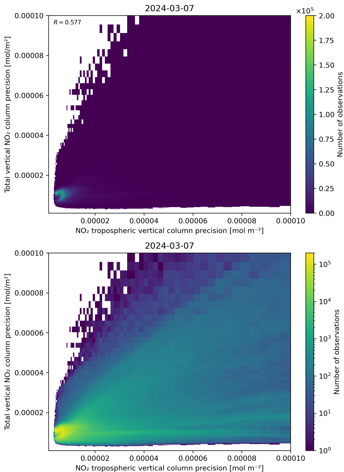
Figure 139: Scatter density plot of “NO 2 tropospheric vertical column precision” against “Total vertical NO 2 column precision” for 2024-03-06 to 2024-03-08.
