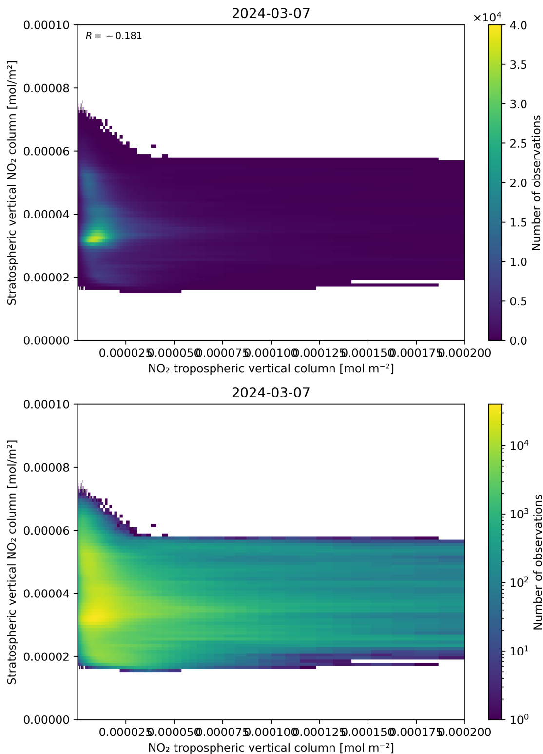
Figure 125: Scatter density plot of “NO 2 tropospheric vertical column” against “Stratospheric vertical NO 2 column” for 2024-03-06 to 2024-03-08.
