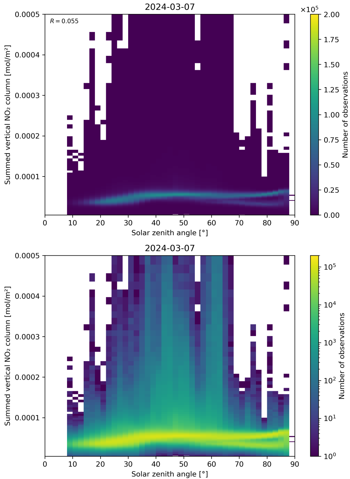
Figure 151: Scatter density plot of “Solar zenith angle” against “Summed vertical NO 2 column” for 2024-03-06 to 2024-03-08.
