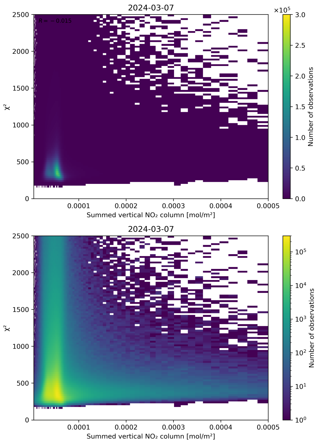
Figure 104: Scatter density plot of “Summed vertical NO 2 column” against “ \chi^2 ” for 2024-03-06 to 2024-03-08.
