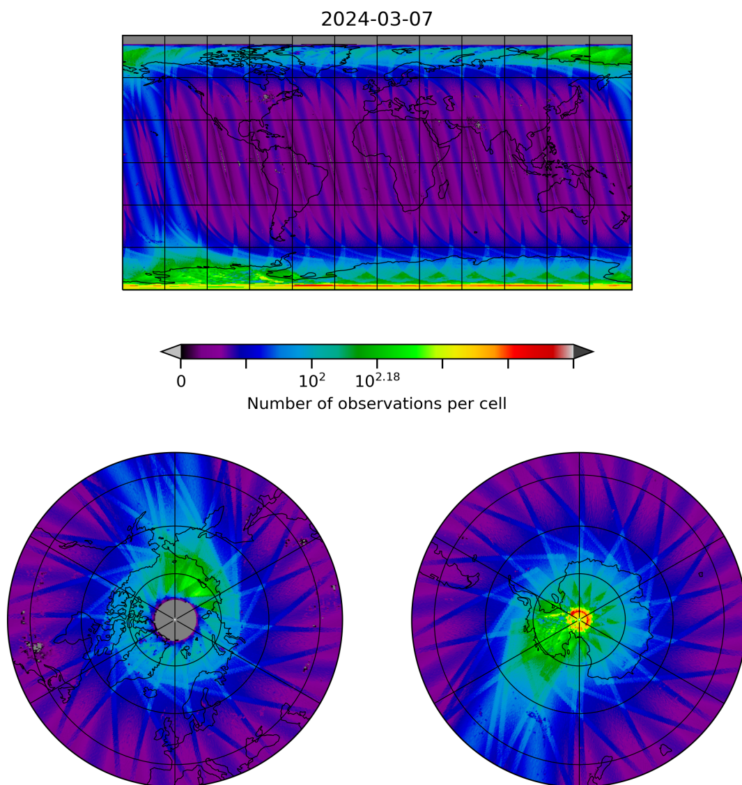
Figure 10: Map of the number of observations for 2024-03-06 to 2024-03-08
