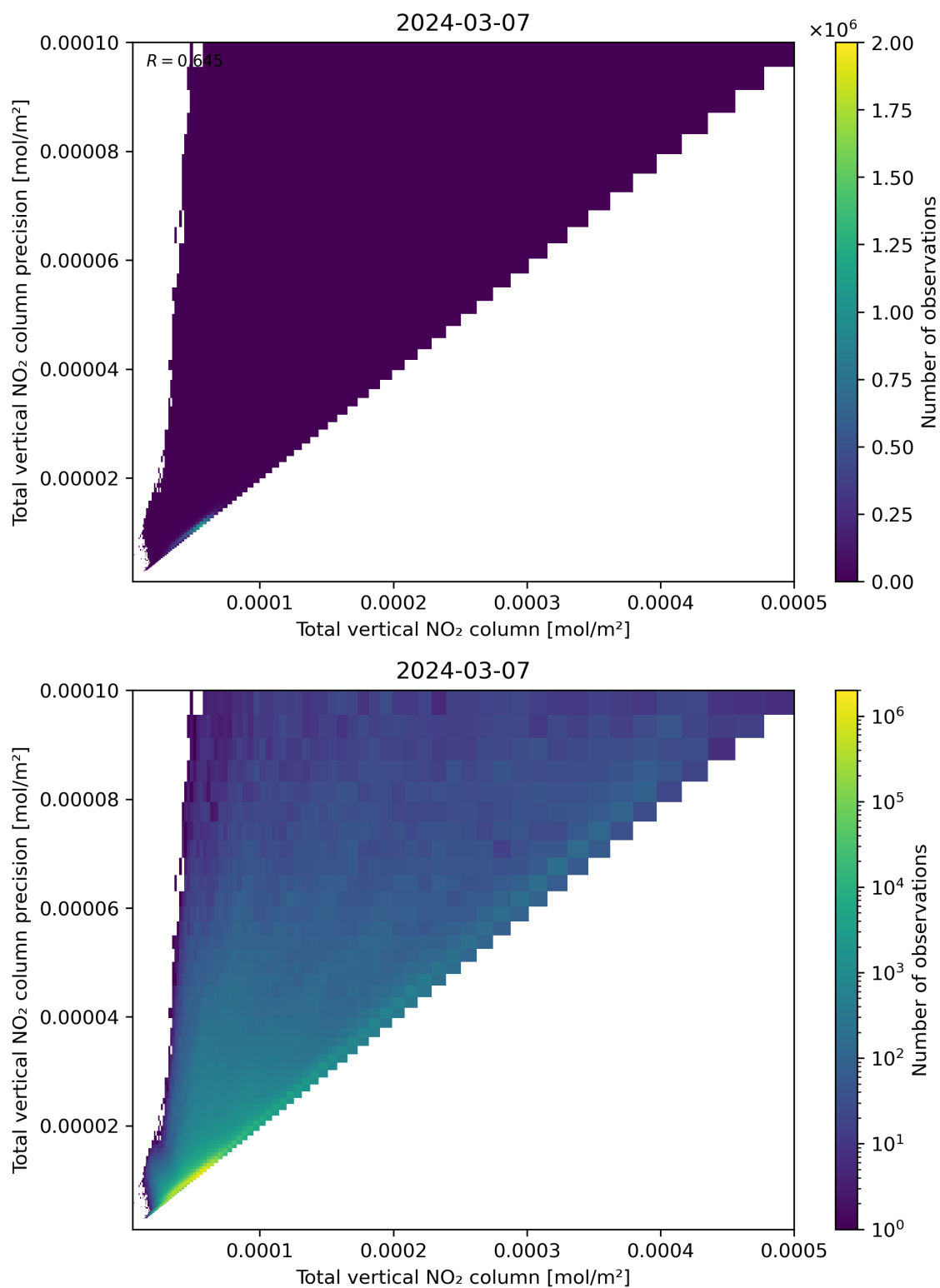
Figure 114: Scatter density plot of “Total vertical NO 2 column” against “Total vertical NO 2 column precision” for 2024-03-06 to 2024-03-08.
