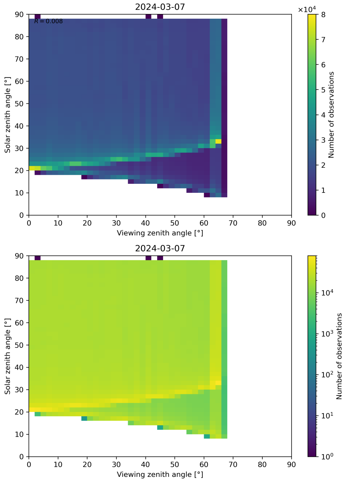
Figure 172: Scatter density plot of “Viewing zenith angle” against “Solar zenith angle” for 2024-03-06 to 2024-03-08.
