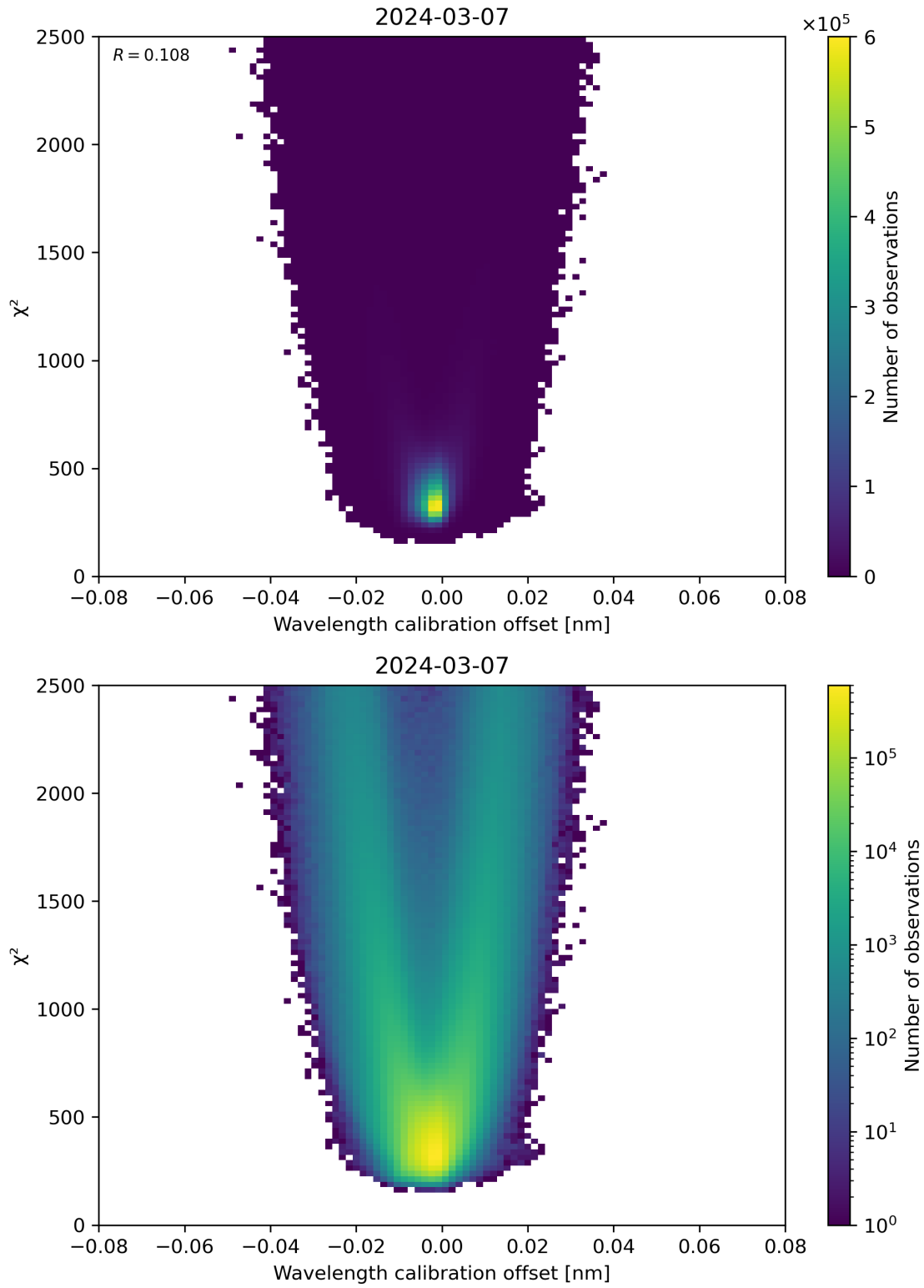
Figure 175: Scatter density plot of “Wavelength calibration offset” against “ \chi^2 ” for 2024-03-06 to 2024-03-08.
