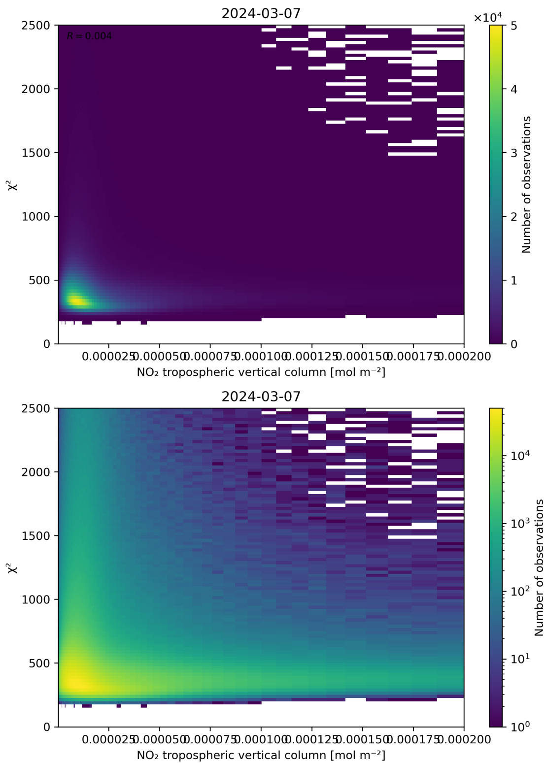
Figure 124: Scatter density plot of “NO 2 tropospheric vertical column” against “ \chi^2 ” for 2024-03-06 to 2024-03-08.
