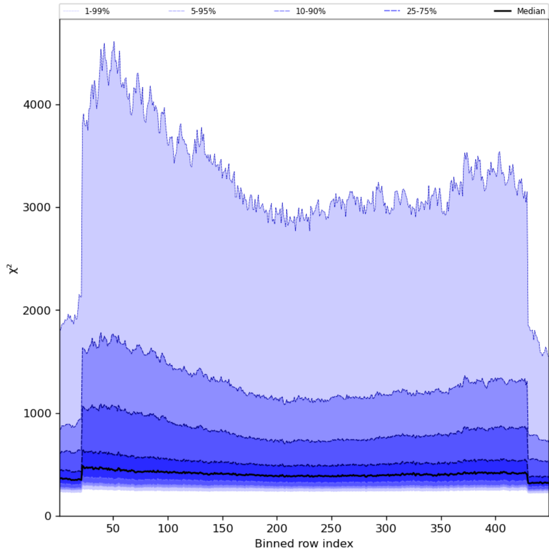
Figure 59: Along track statistics of “ \chi^2 ” for 2024-03-06 to 2024-03-08
