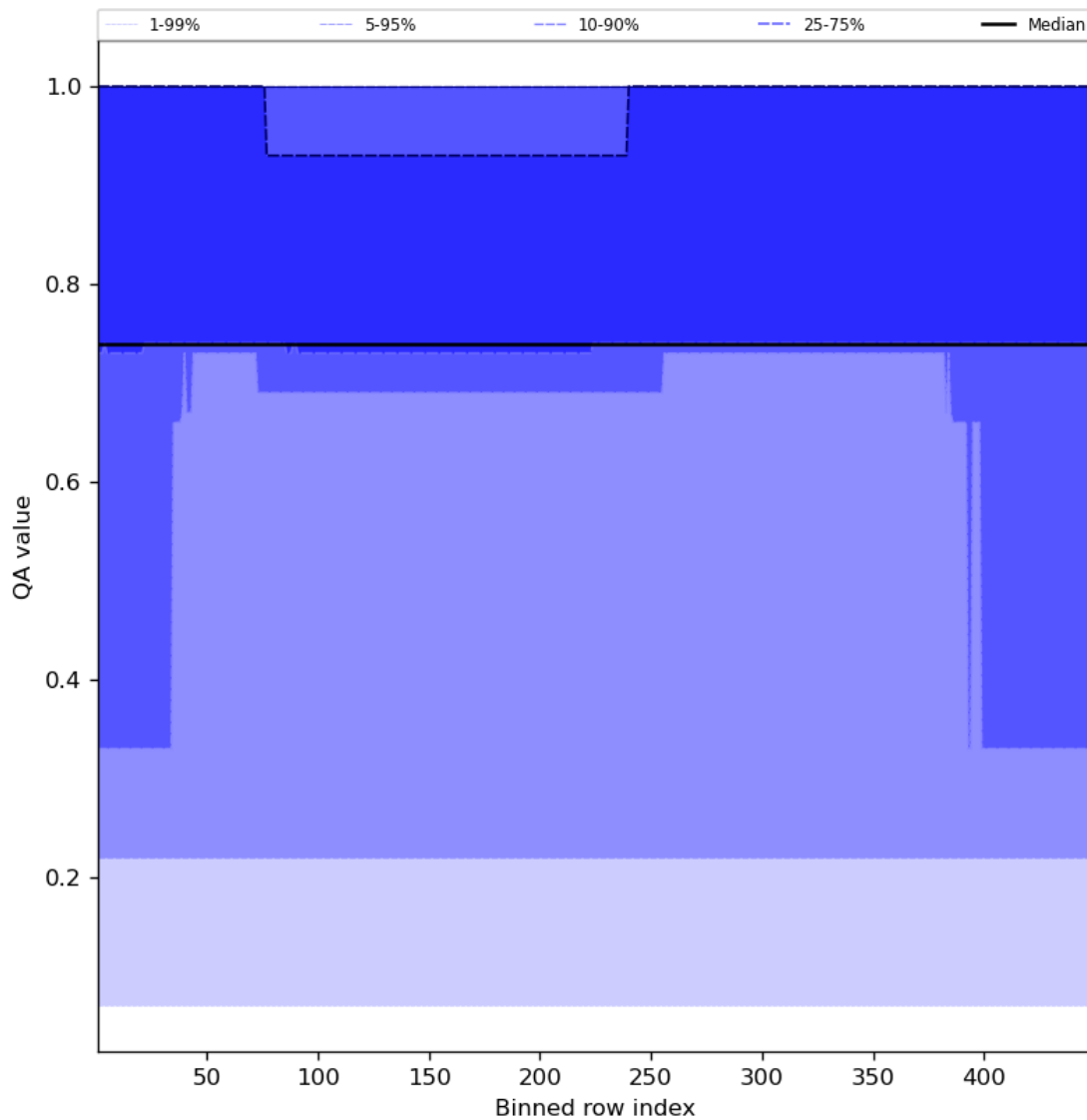
Figure 45: Along track statistics of “QA value” for 2024-03-06 to 2024-03-08
