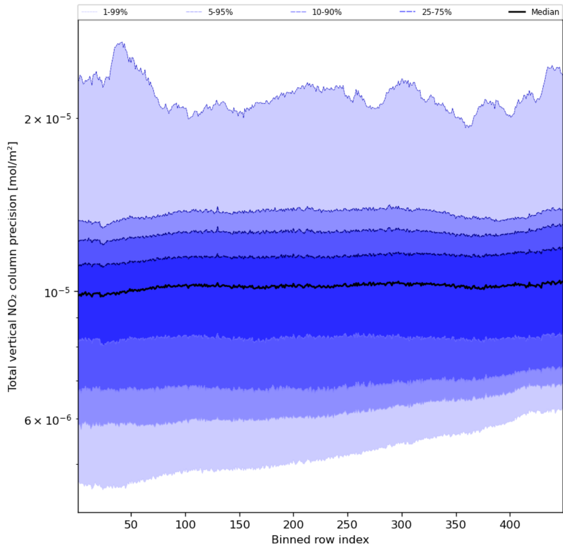
Figure 56: Along track statistics of “Total vertical NO 2 column precision” for 2024-03-07 to 2024-03-09
