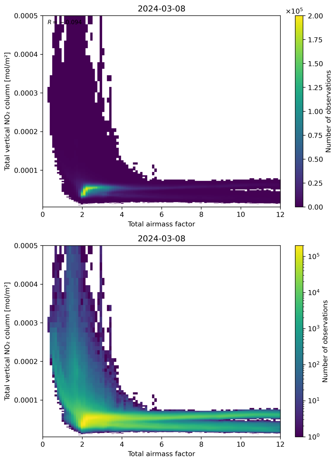
Figure 67: Scatter density plot of “Total airmass factor” against “Total vertical NO 2 column” for 2024-03-07 to 2024-03-09.
