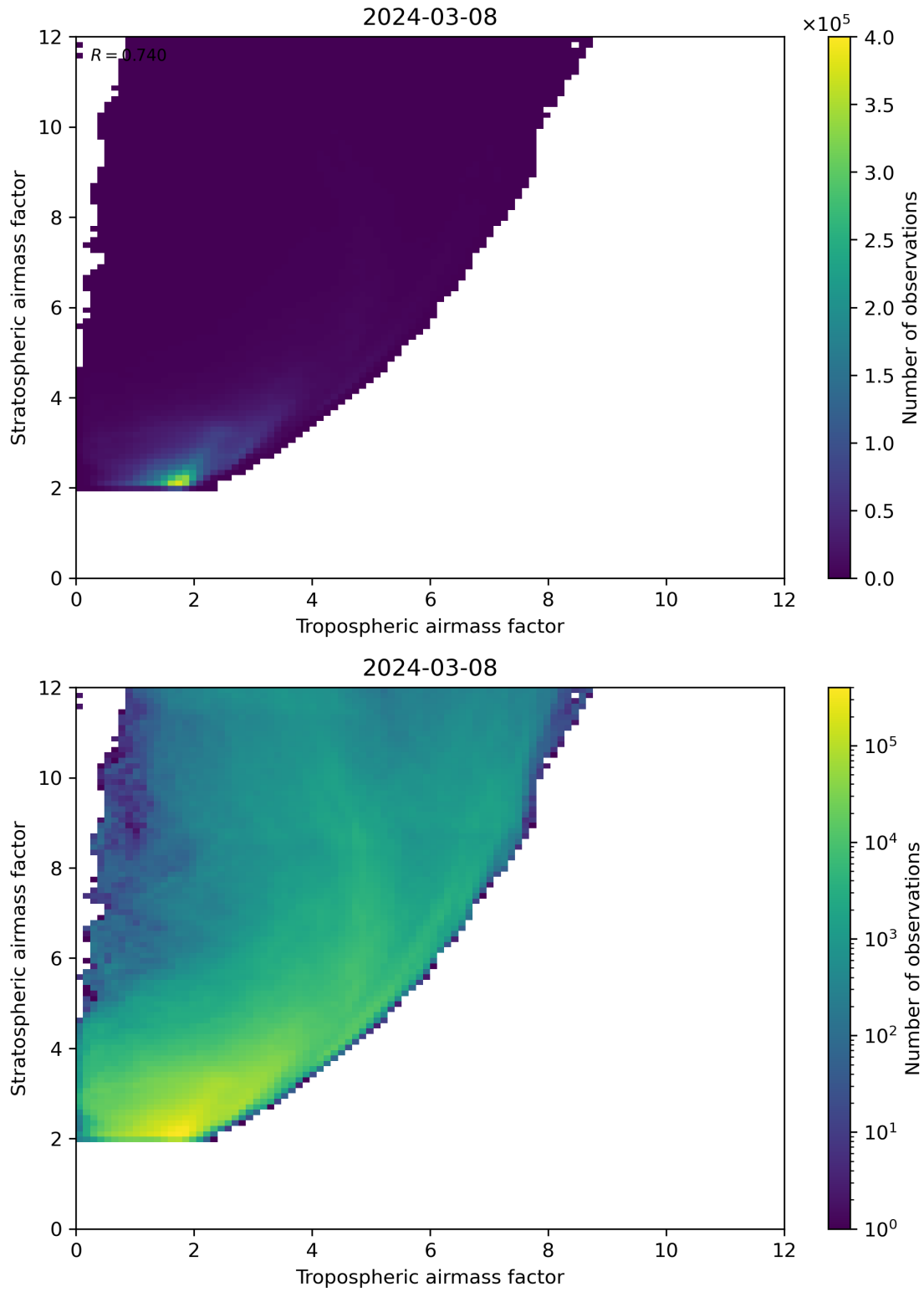
Figure 71: Scatter density plot of “Tropospheric airmass factor” against “Stratospheric airmass factor” for 2024-03-07 to 2024-03-09.
