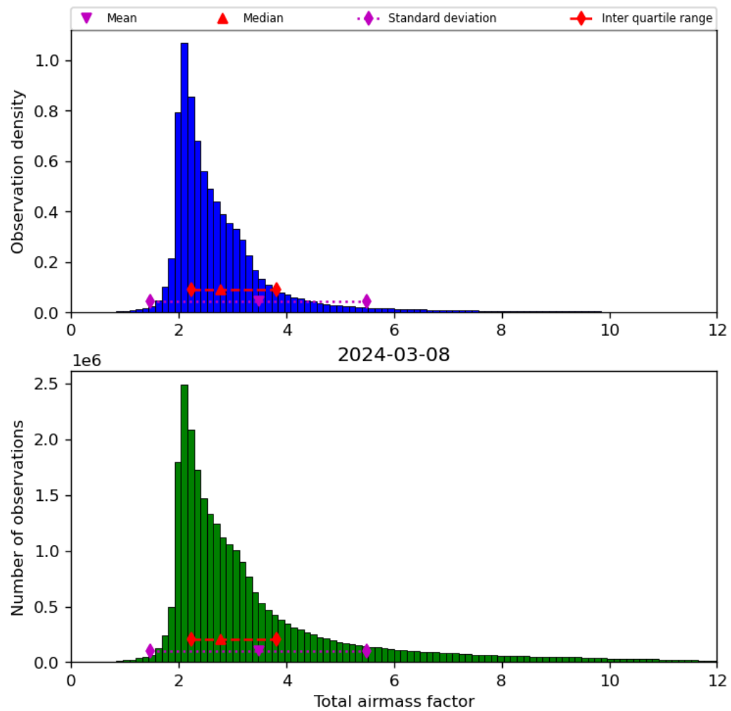
Figure 32: Histogram of “Total airmass factor” for 2024-03-07 to 2024-03-09
