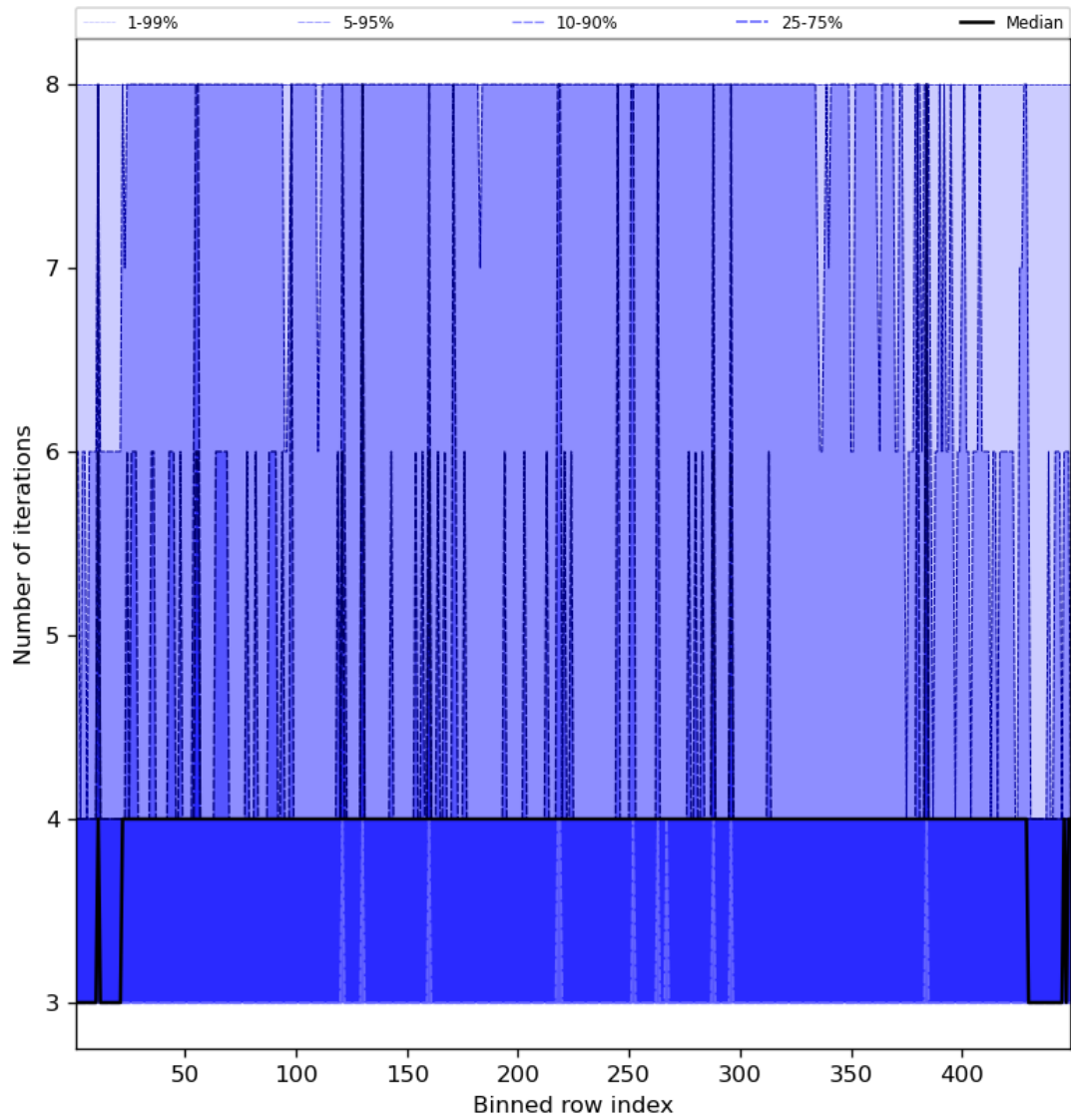
Figure 51: Along track statistics of “Number of iterations” for 2024-03-07 to 2024-03-09
