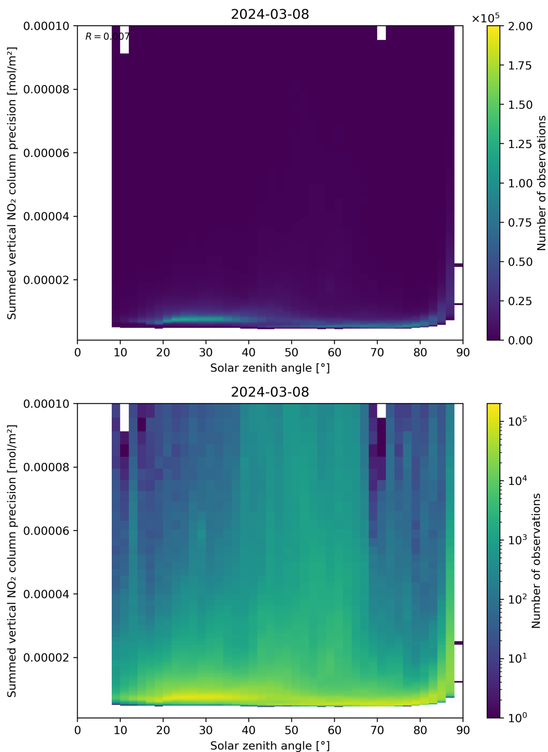
Figure 152: Scatter density plot of “Solar zenith angle” against “Summed vertical NO 2 column precision” for 2024-03-07 to 2024-03-09.
