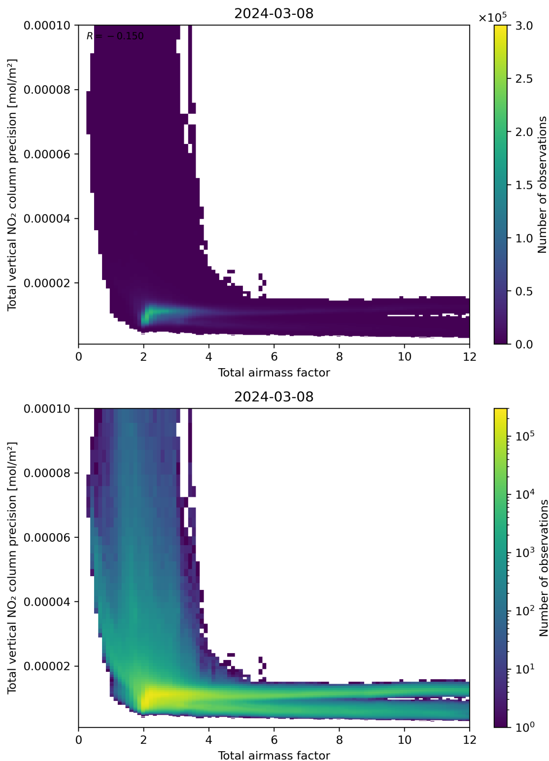
Figure 68: Scatter density plot of “Total airmass factor” against “Total vertical NO 2 column precision” for 2024-03-07 to 2024-03-09.
