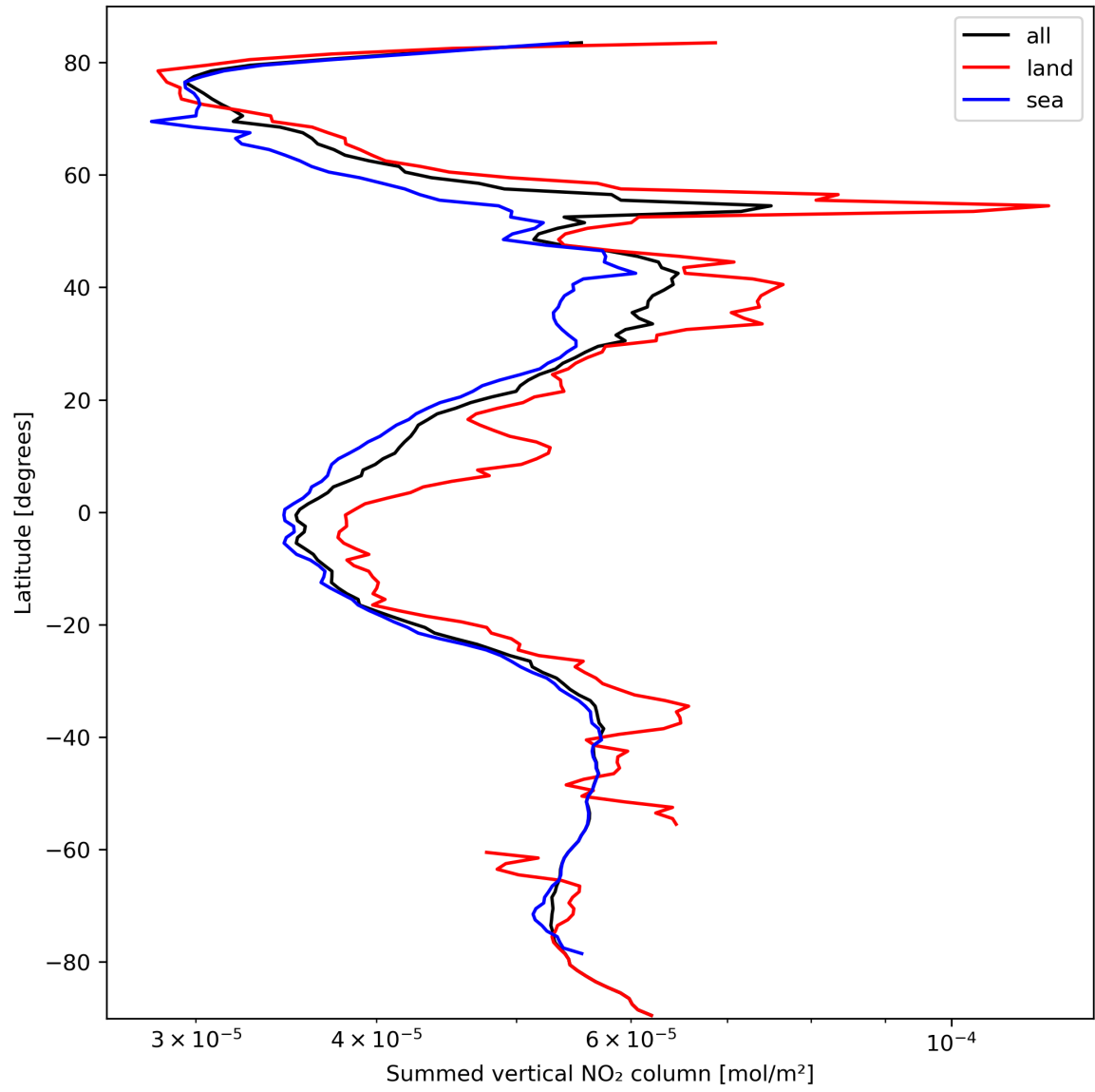
Figure 23: Zonal average of “Summed vertical NO 2 column” for 2024-03-07 to 2024-03-09.
