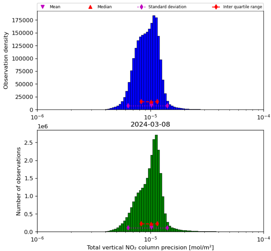
Figure 39: Histogram of “Total vertical NO 2 column precision” for 2024-03-07 to 2024-03-09
