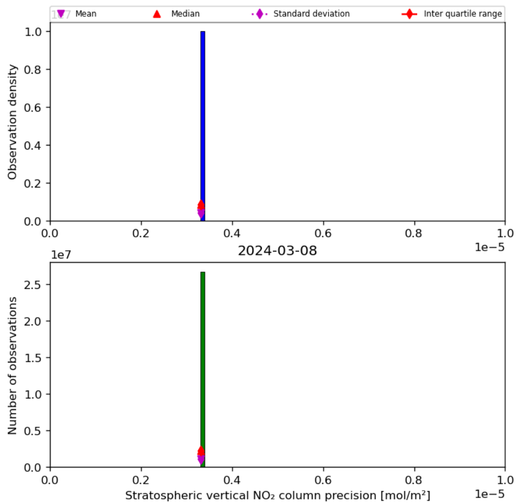
Figure 37: Histogram of “Stratospheric vertical NO 2 column precision” for 2024-03-07 to 2024-03-09
