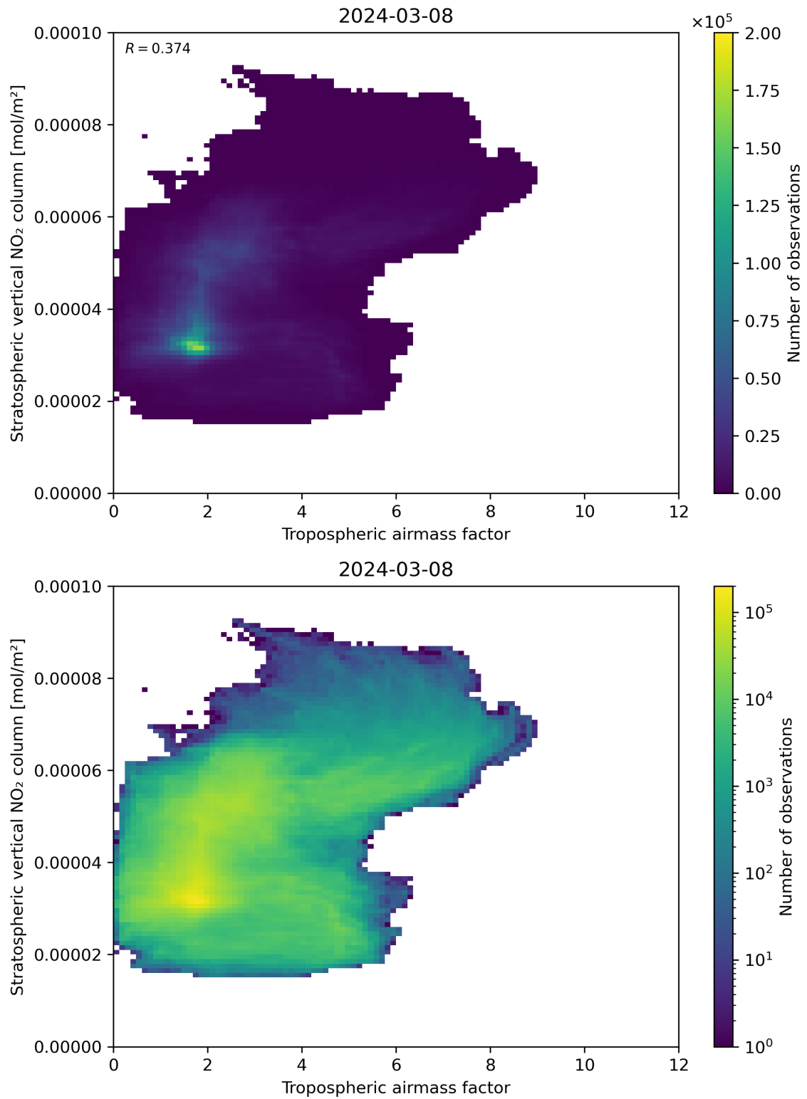
Figure 74: Scatter density plot of “Tropospheric air mass factor” against “Stratospheric vertical NO 2 column” for 2024-03-07 to 2024-03-09.
