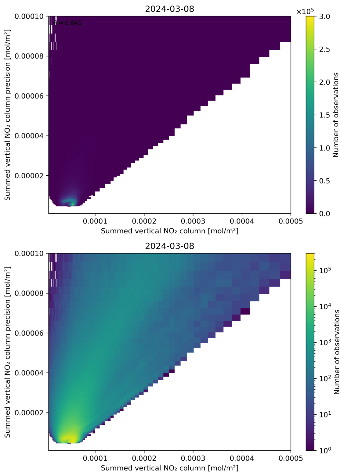
Figure 105: Scatter density plot of “Summed vertical NO 2 column” against “Summed vertical NO 2 column precision” for 2024-03-07 to 2024-03-09.
