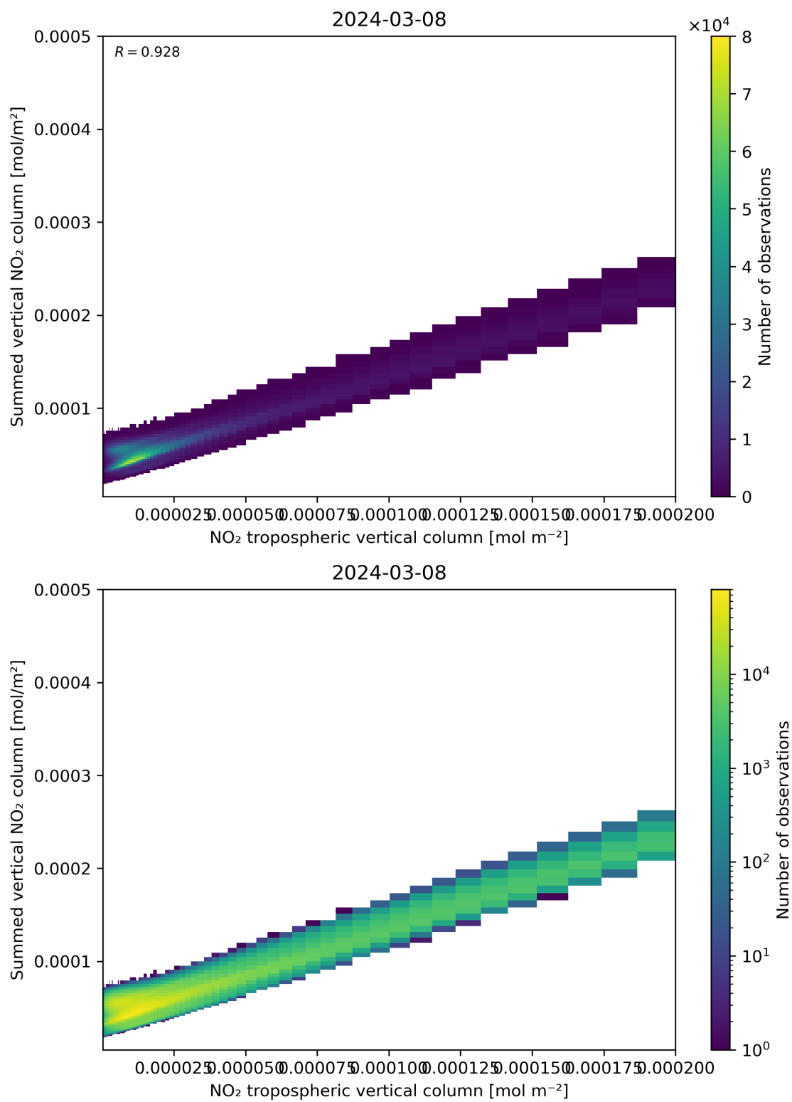
Figure 126: Scatter density plot of “NO 2 tropospheric vertical column” against “Summed vertical NO 2 column” for 2024-03-07 to 2024-03-09.
