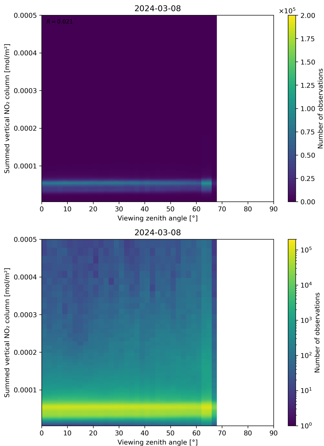
Figure 165: Scatter density plot of “Viewing zenith angle” against “Summed vertical NO 2 column” for 2024-03-07 to 2024-03-09.
