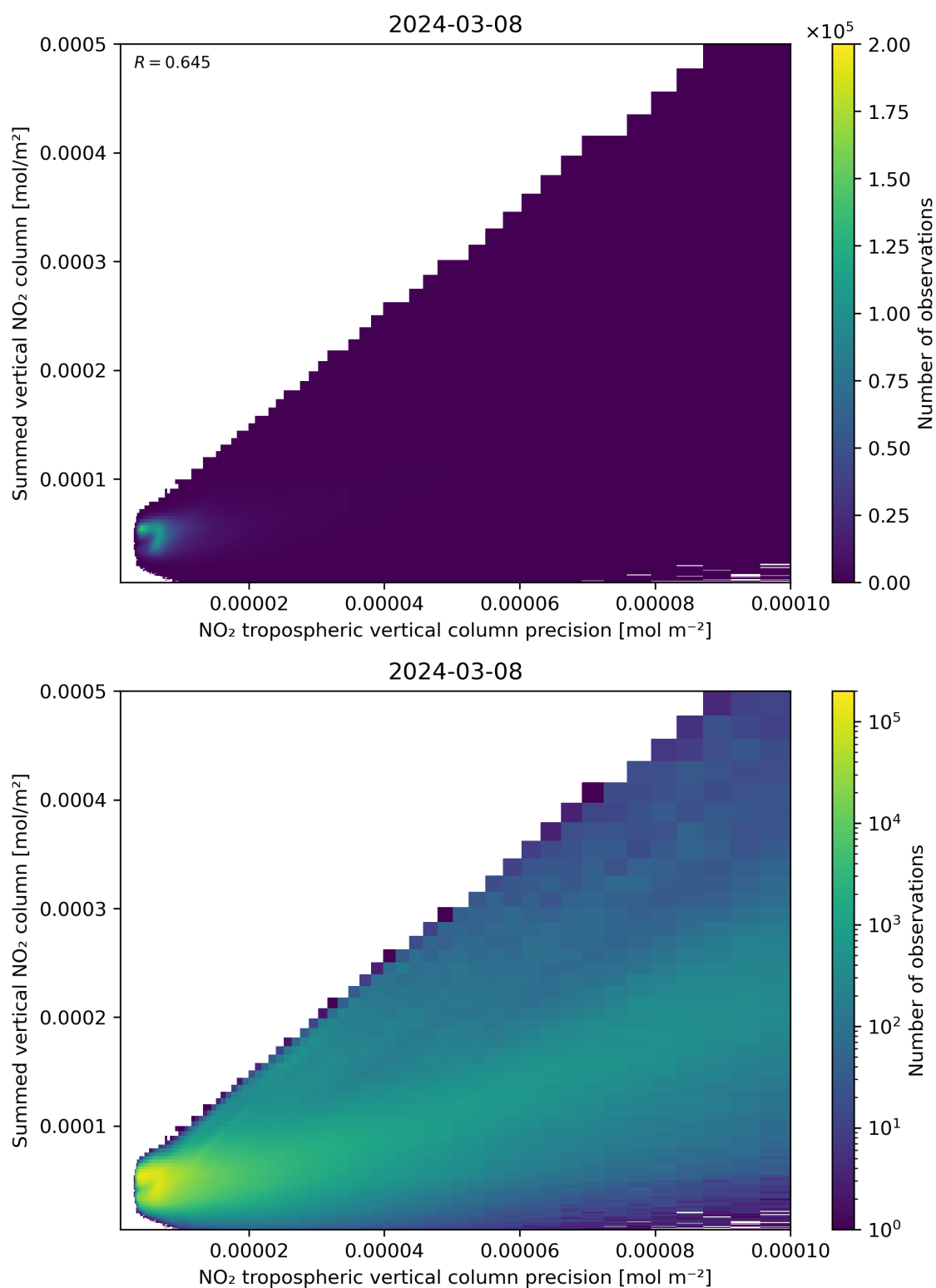
Figure 136: Scatter density plot of “NO 2 tropospheric vertical column precision” against “Summed vertical NO 2 column” for 2024-03-07 to 2024-03-09.
