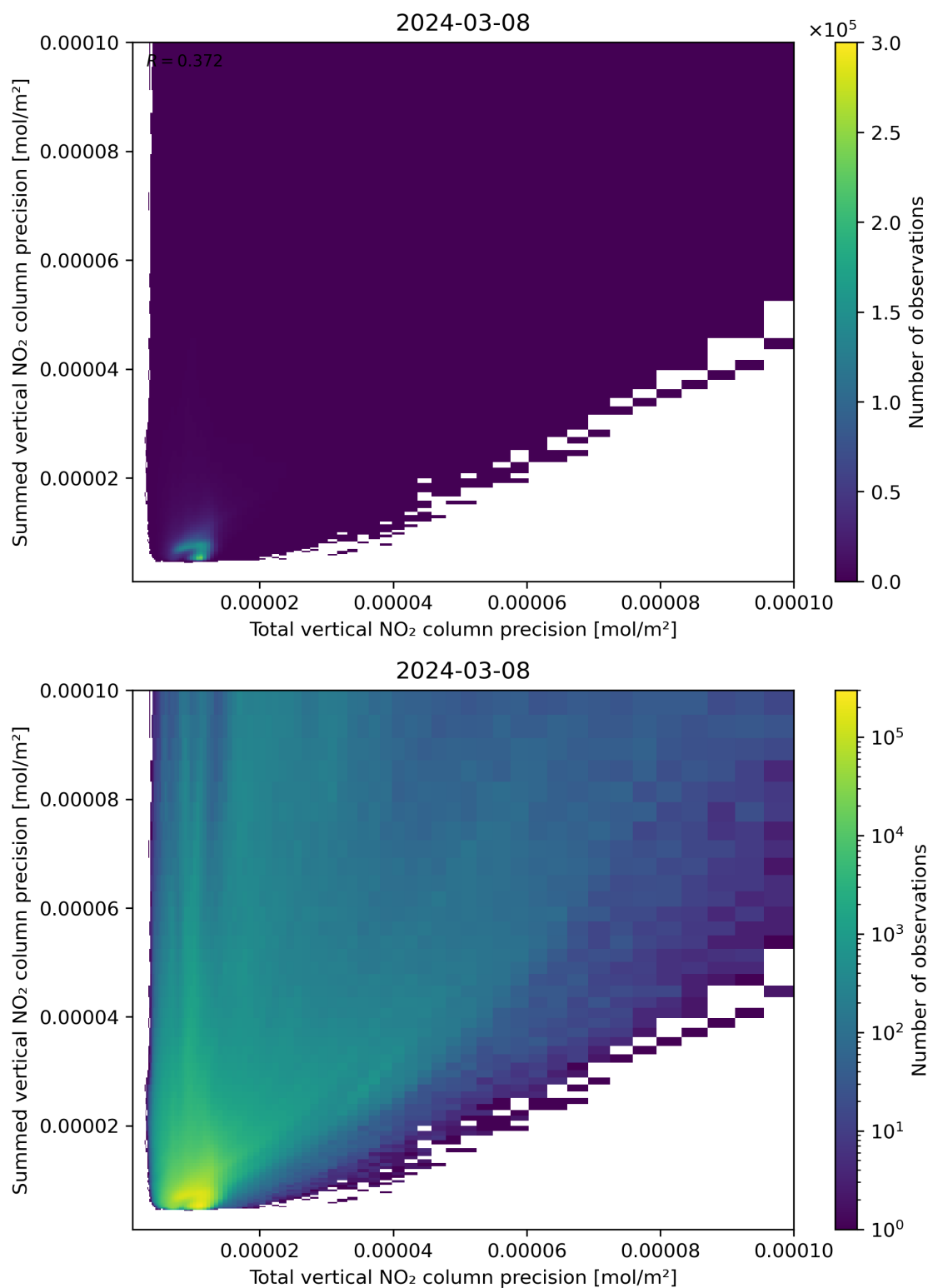
Figure 118: Scatter density plot of “Total vertical NO 2 column precision” against “Summed vertical NO 2 column precision” for 2024-03-07 to 2024-03-09.
