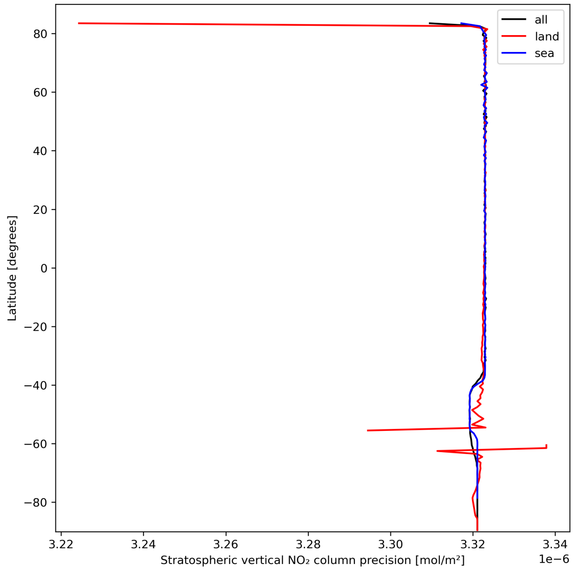
Figure 20: Zonal average of “Stratospheric vertical NO 2 column precision” for 2024-03-07 to 2024-03-09.
