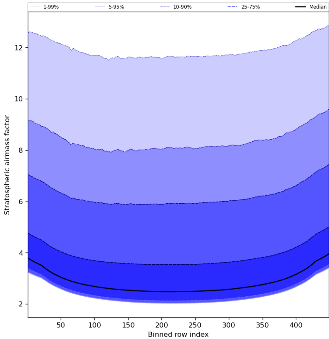
Figure 61: Along track statistics of “Stratospheric airmass factor” for 2024-03-07 to 2024-03-09
