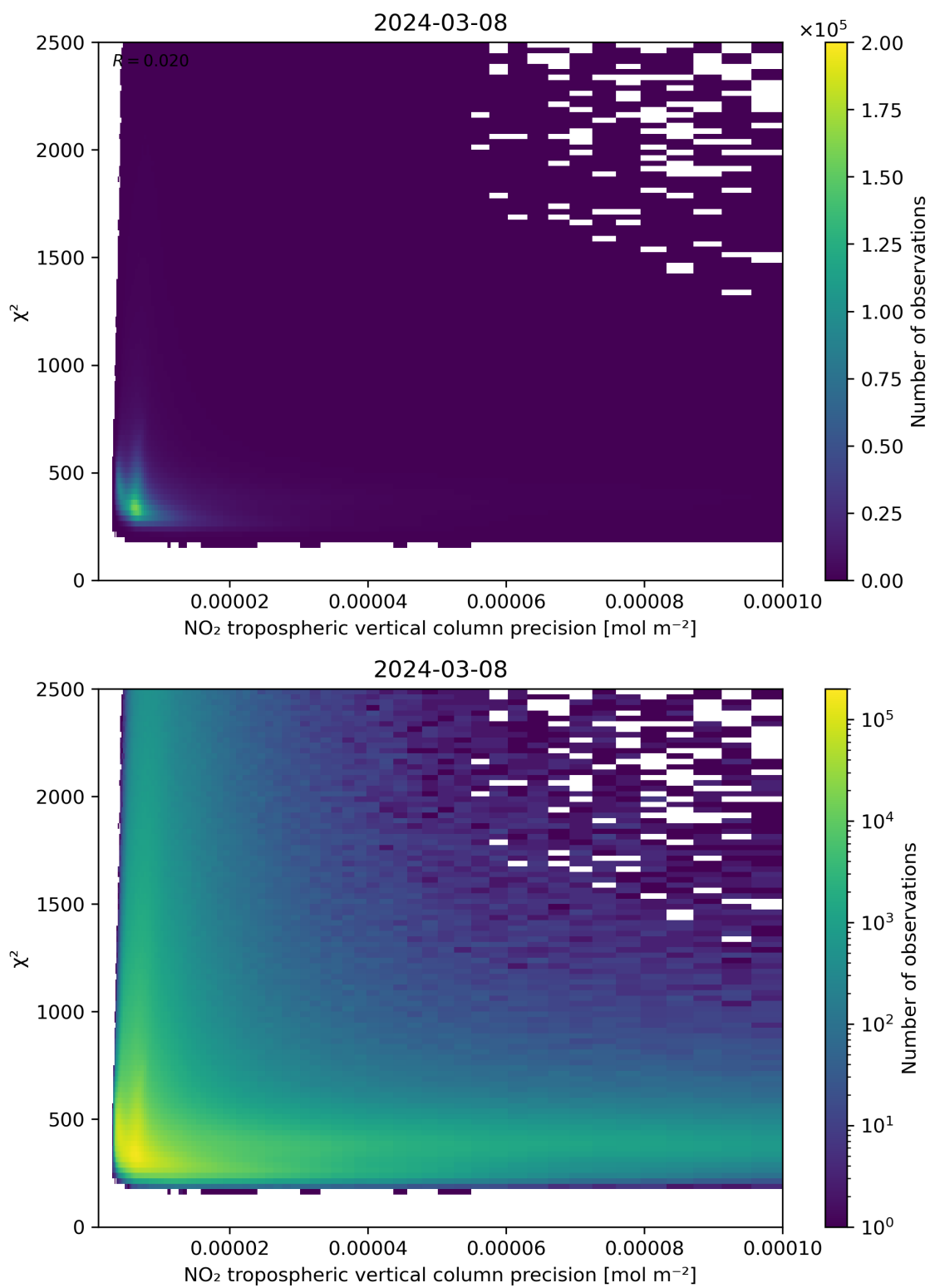
Figure 134: Scatter density plot of “NO 2 tropospheric vertical column precision” against “ \chi^2 ” for 2024-03-07 to 2024-03-09.
