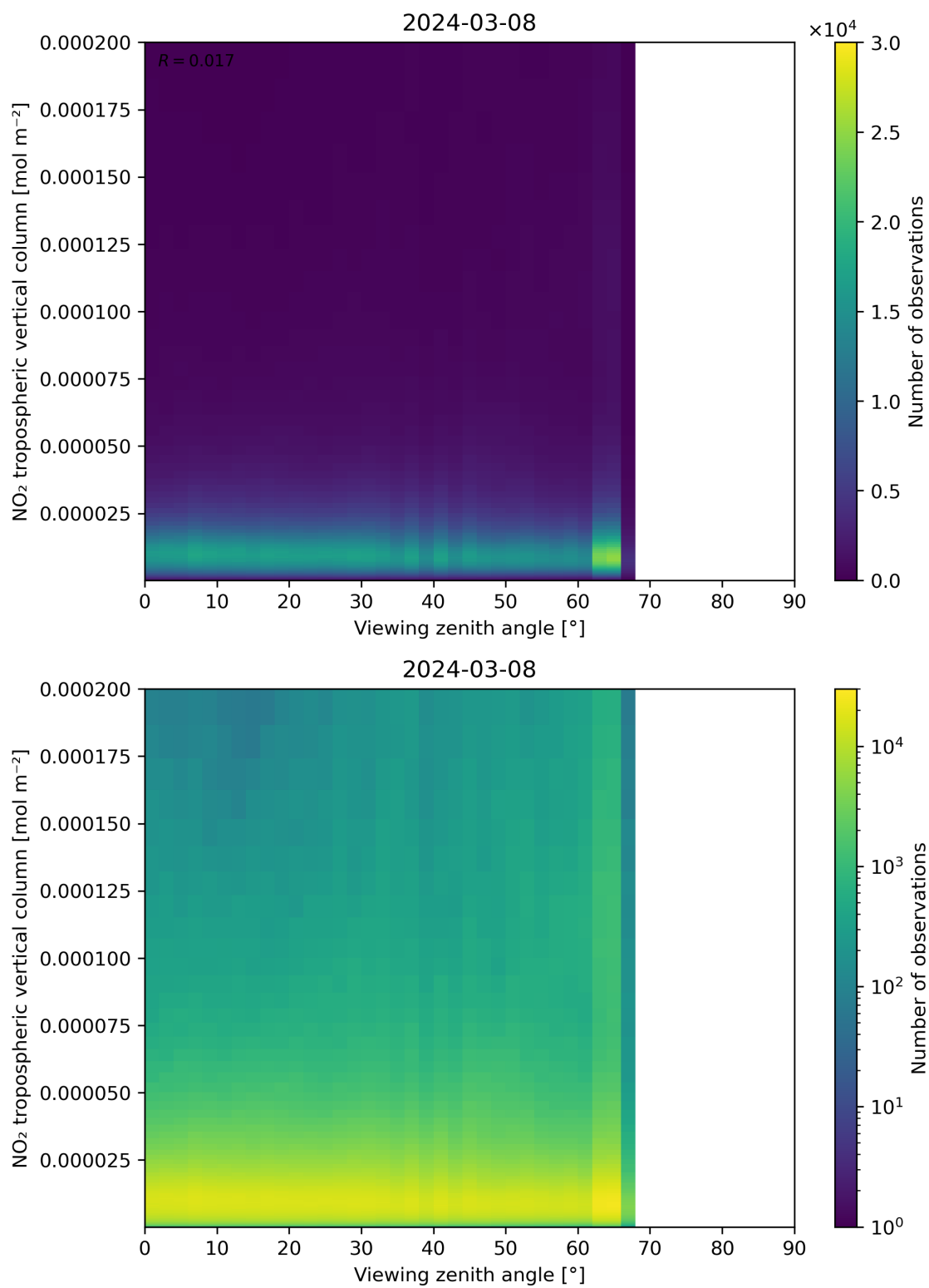
Figure 169: Scatter density plot of “Viewing zenith angle” against “NO 2 tropospheric vertical column” for 2024-03-07 to 2024-03-09.
