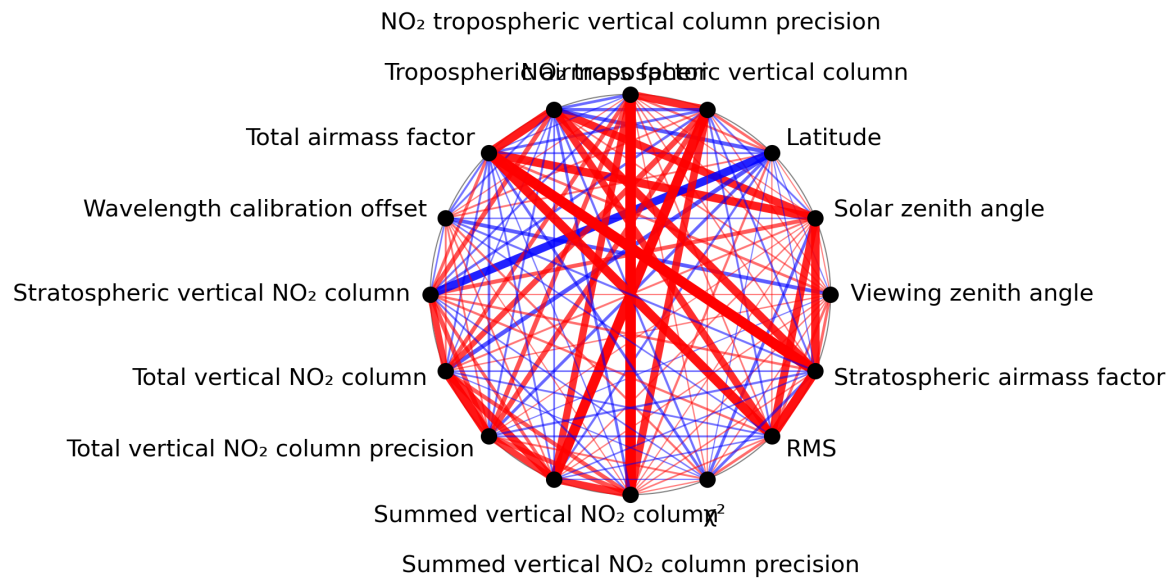
Figure 1: Map of correlation graph for 2024-03-07 to 2024-03-09.
