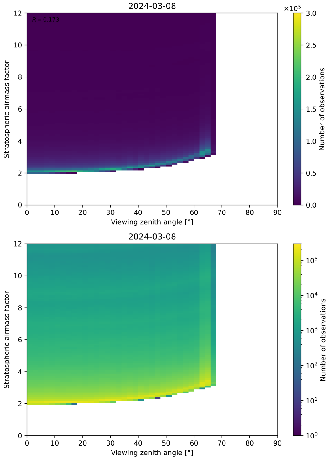
Figure 159: Scatter density plot of “Viewing zenith angle” against “Stratospheric airmass factor” for 2024-03-07 to 2024-03-09.
