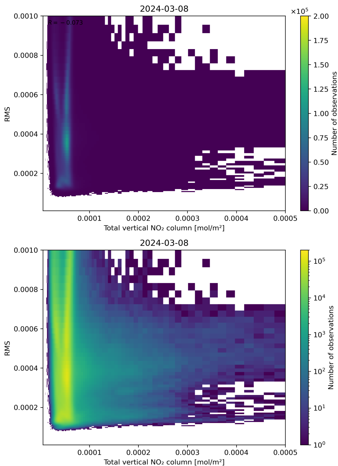
Figure 120: Scatter density plot of “Total vertical NO 2 column” against “RMS” for 2024-03-07 to 2024-03-09.
