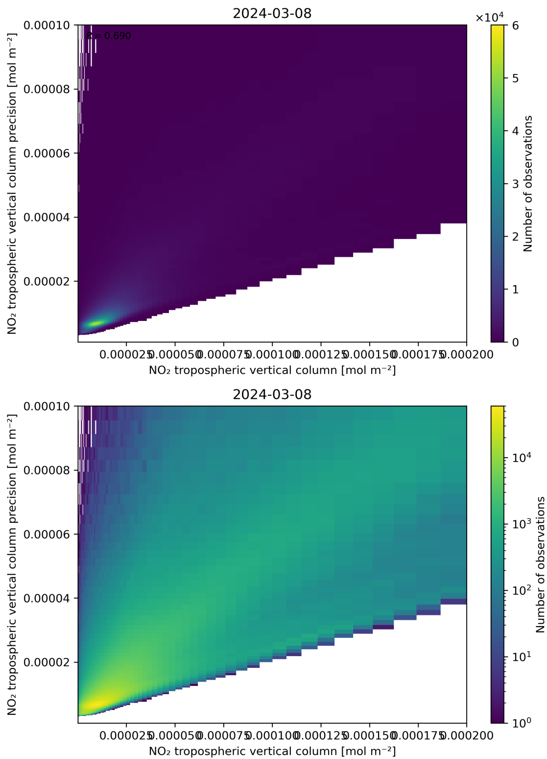
Figure 130: Scatter density plot of “NO 2 tropospheric vertical column” against “NO 2 tropospheric vertical column precision” for 2024-03-07 to 2024-03-09.
