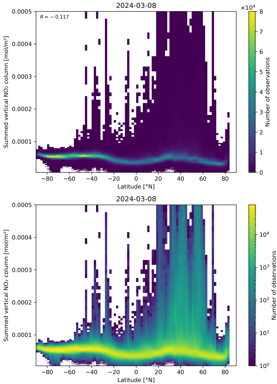
Figure 88: Scatter density plot of “Latitude” against “Summed vertical NO 2 column” for 2024-03-07 to 2024-03-09.
