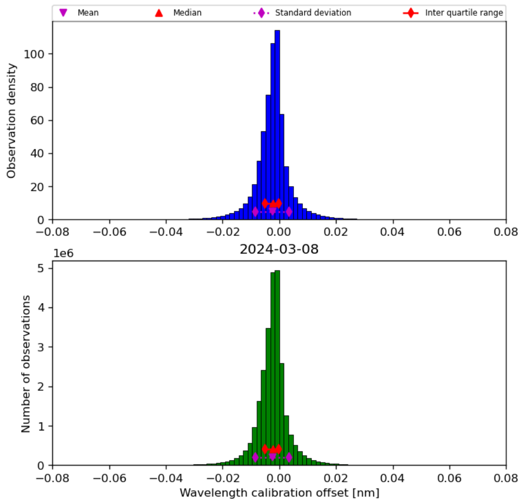
Figure 35: Histogram of “Wavelength calibration offset” for 2024-03-07 to 2024-03-09
