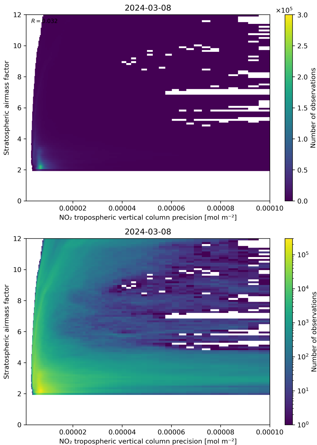
Figure 131: Scatter density plot of “NO 2 tropospheric vertical column precision” against “Stratospheric airmass factor” for 2024-03-07 to 2024-03-09.
