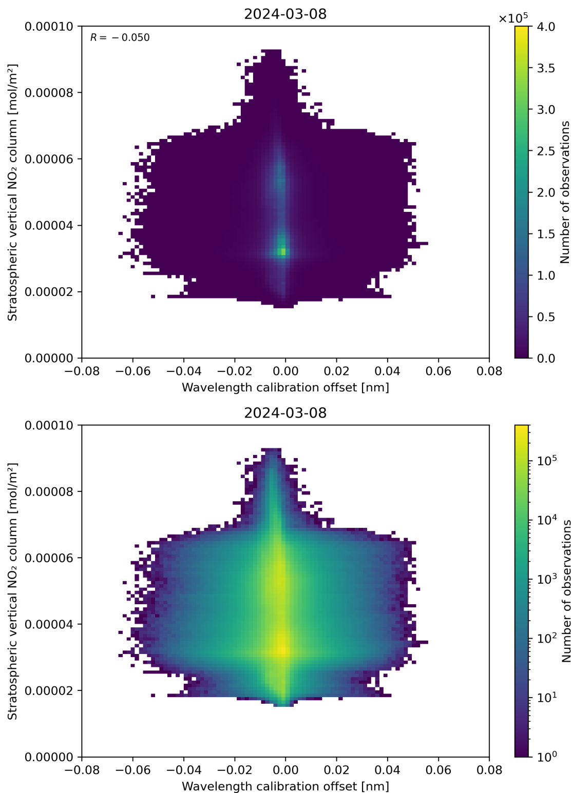
Figure 176: Scatter density plot of “Wavelength calibration offset” against “Stratospheric vertical NO 2 column” for 2024-03-07 to 2024-03-09.
