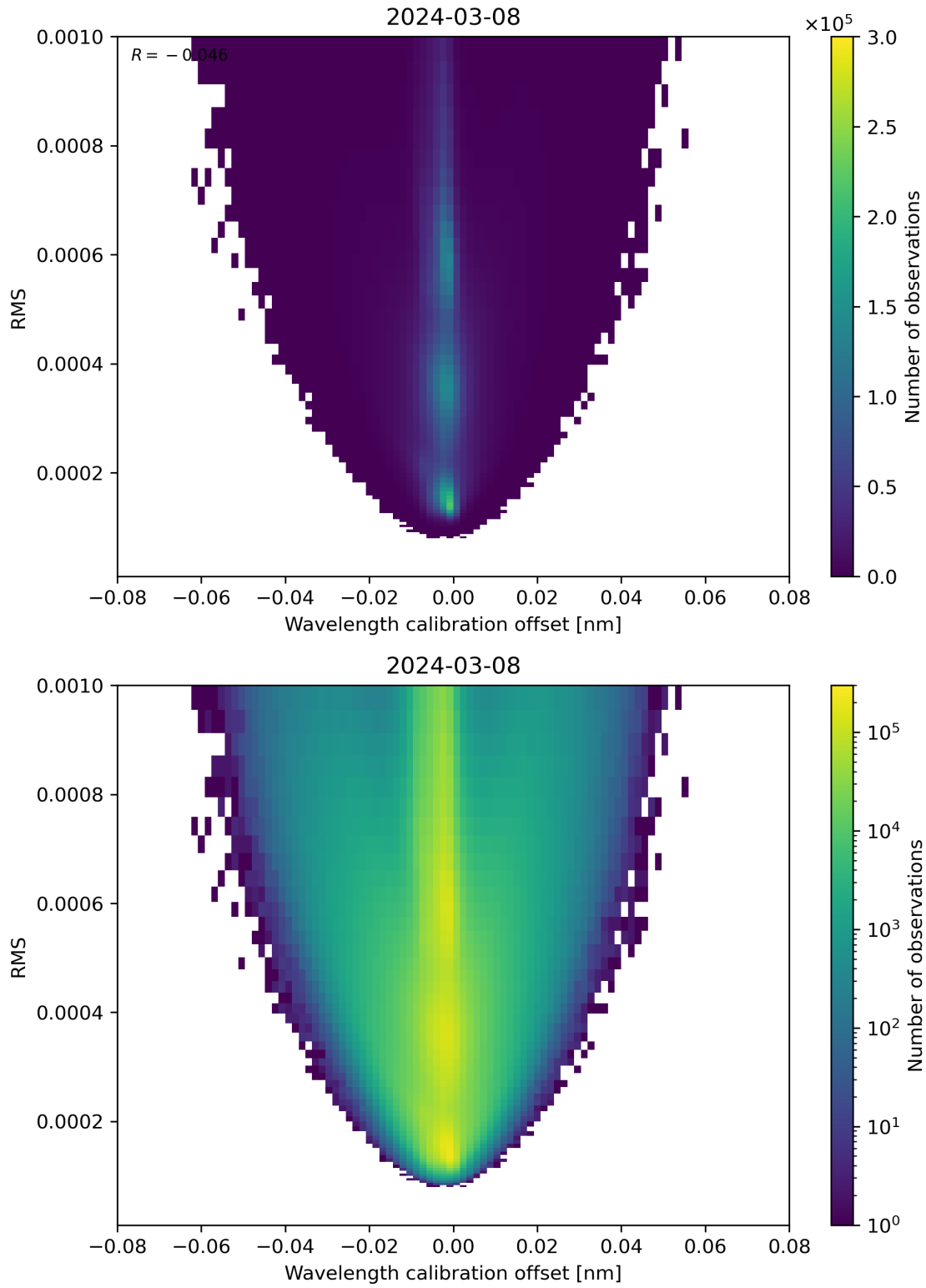
Figure 181: Scatter density plot of “Wavelength calibration offset” against “RMS” for 2024-03-07 to 2024-03-09.
