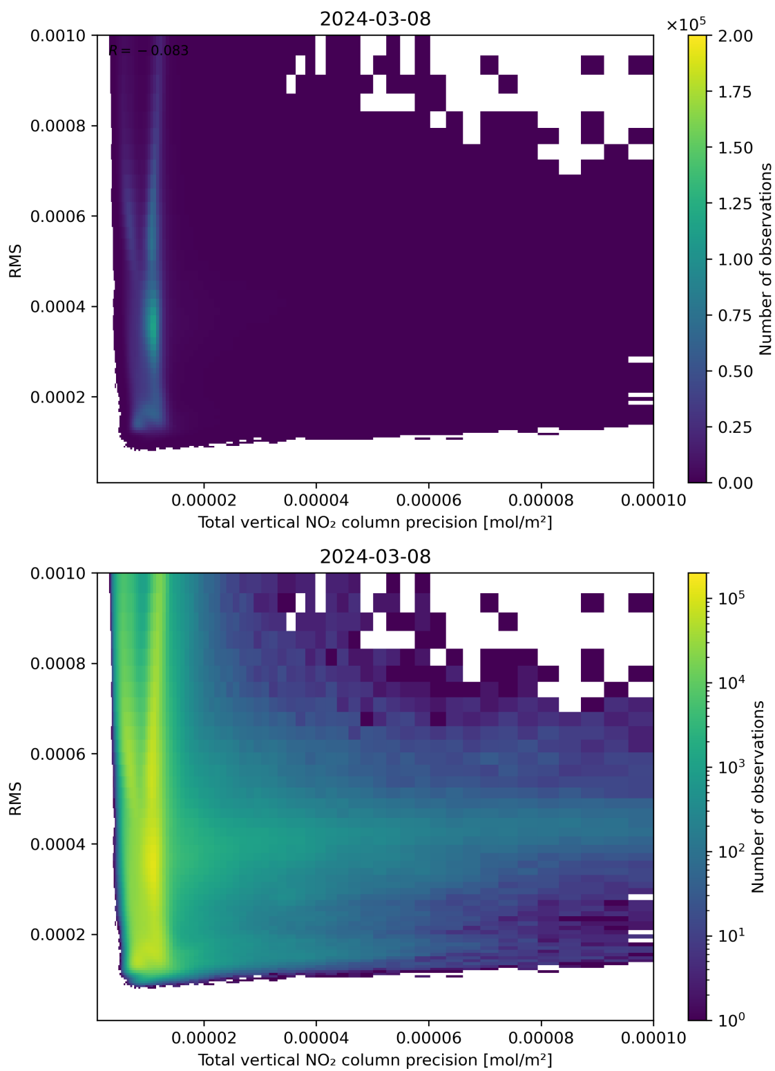
Figure 119: Scatter density plot of “Total vertical NO 2 column precision” against “RMS” for 2024-03-07 to 2024-03-09.
