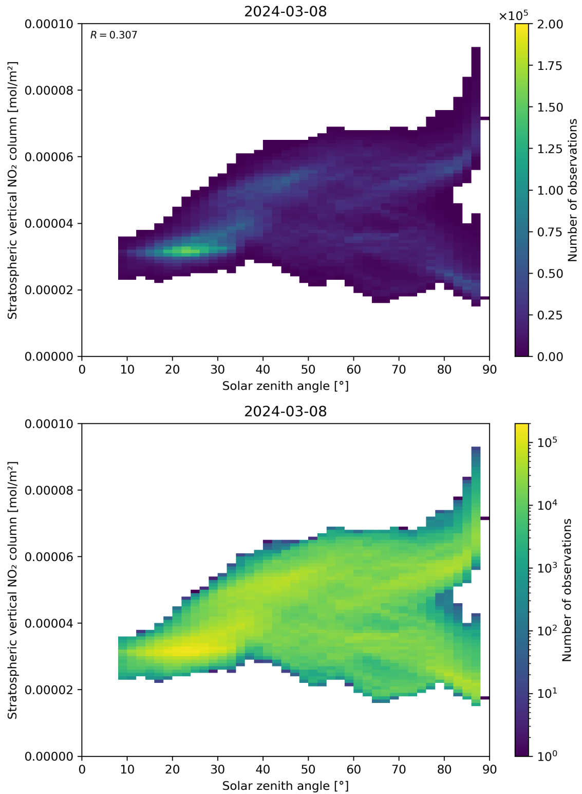
Figure 150: Scatter density plot of “Solar zenith angle” against “Stratospheric vertical \text{NO}_2 column” for 2024-03-07 to 2024-03-09.
