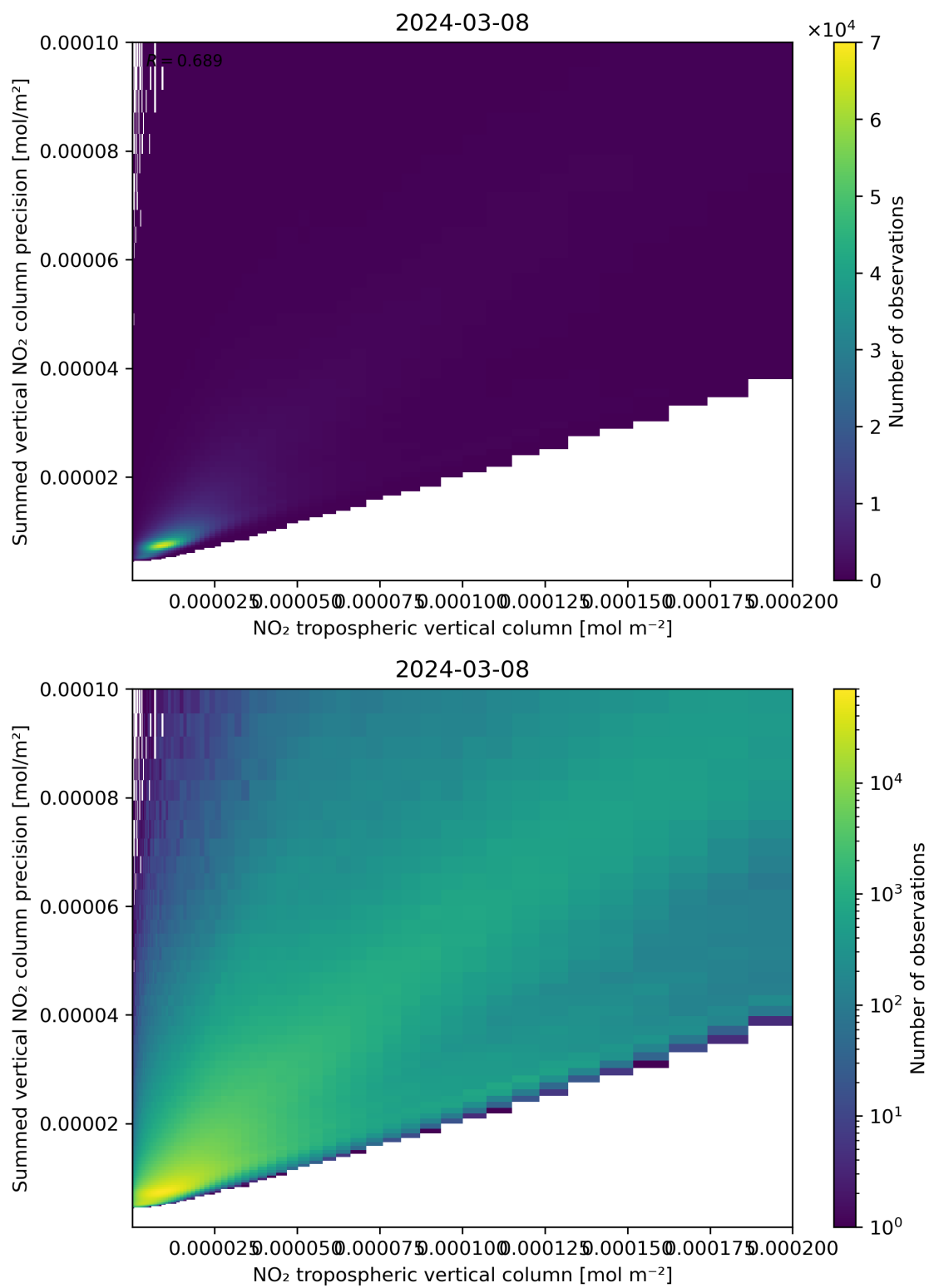
Figure 127: Scatter density plot of “NO 2 tropospheric vertical column” against “Summed vertical NO 2 column precision” for 2024-03-07 to 2024-03-09.
