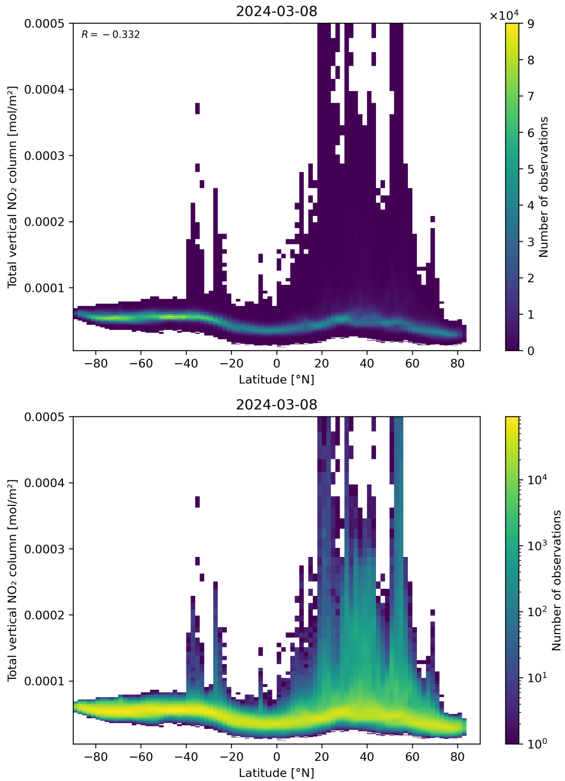
Figure 90: Scatter density plot of “Latitude” against “Total vertical NO 2 column” for 2024-03-07 to 2024-03-09.
