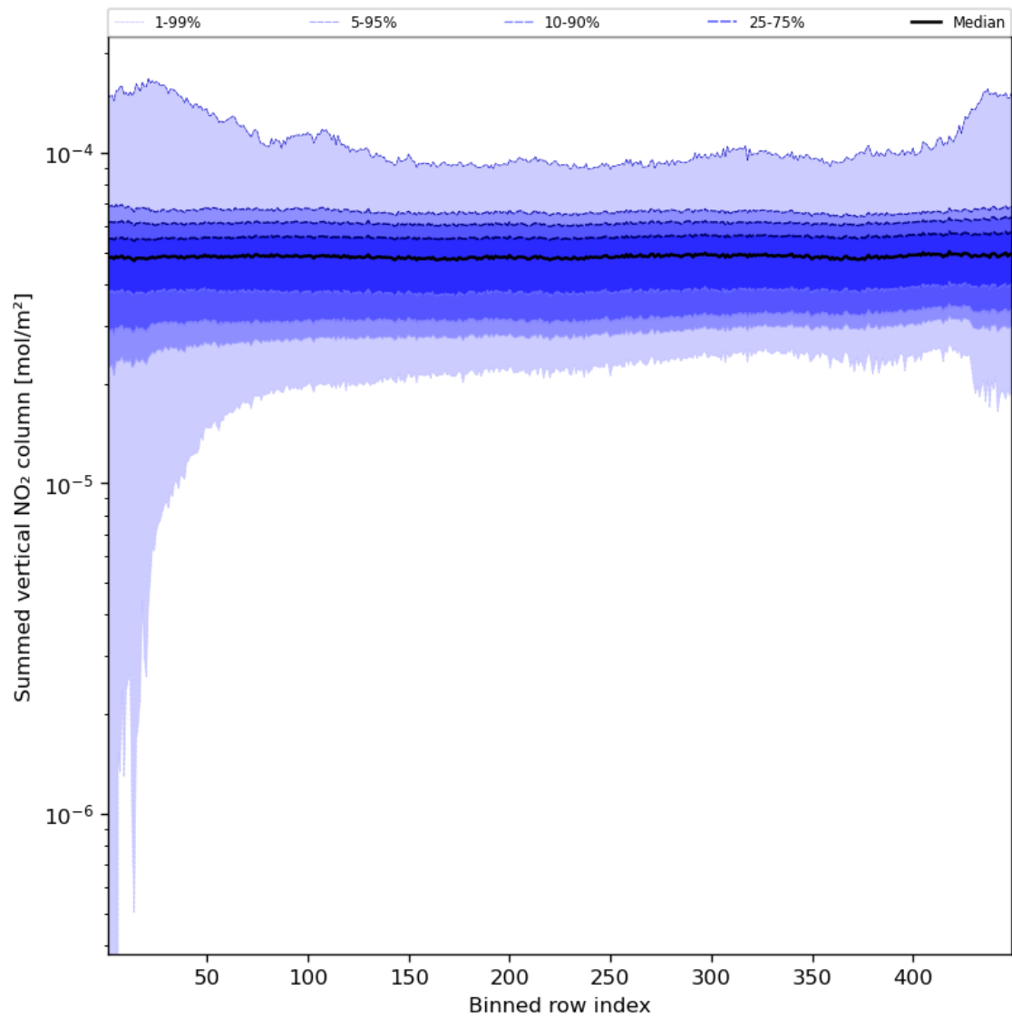
Figure 57: Along track statistics of “Summed vertical NO 2 column” for 2024-03-07 to 2024-03-09
