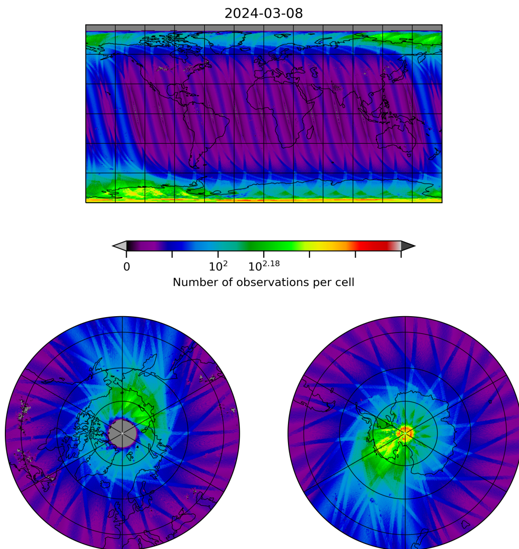
Figure 10: Map of the number of observations for 2024-03-07 to 2024-03-09
