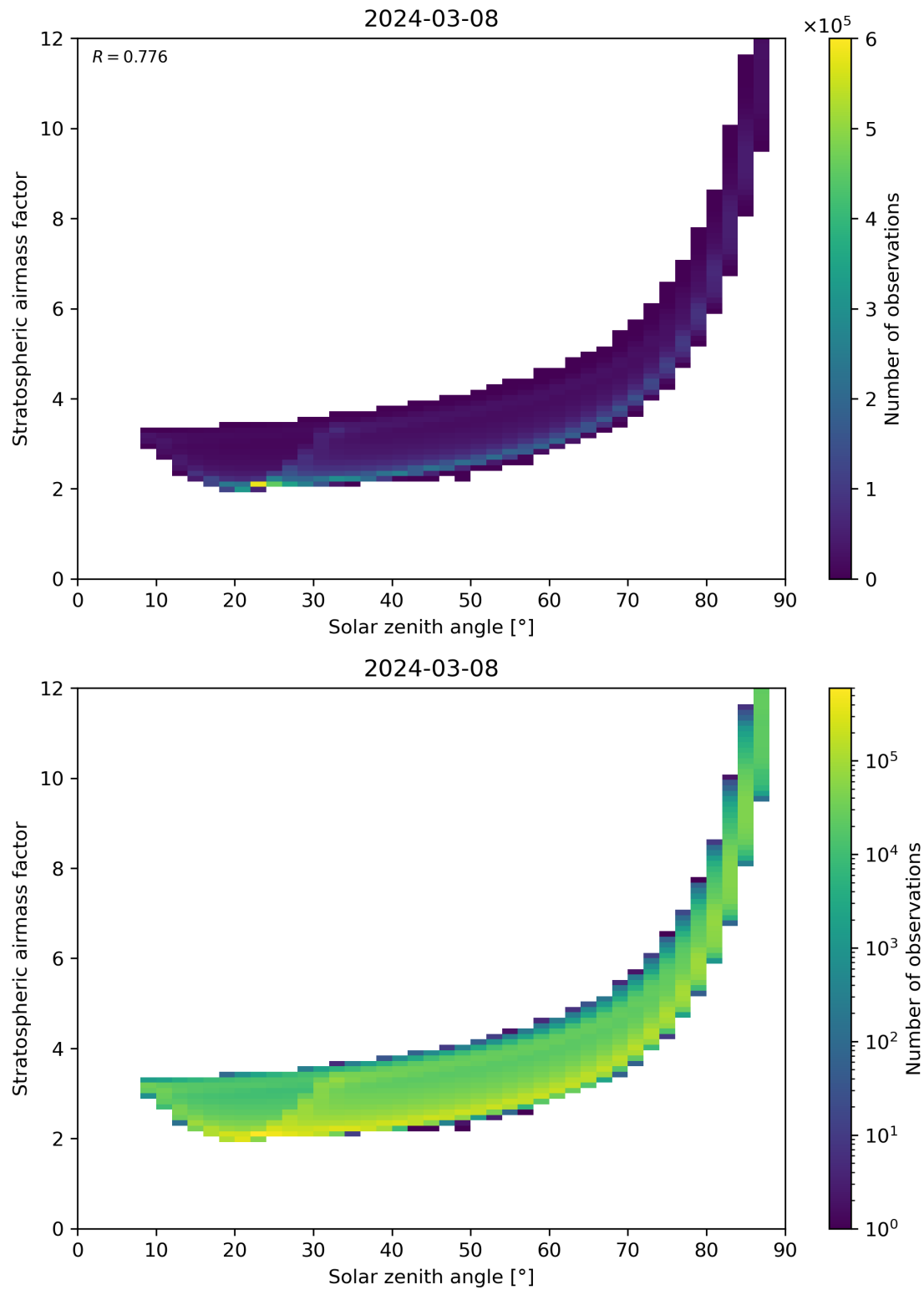
Figure 145: Scatter density plot of “Solar zenith angle” against “Stratospheric airmass factor” for 2024-03-07 to 2024-03-09.
