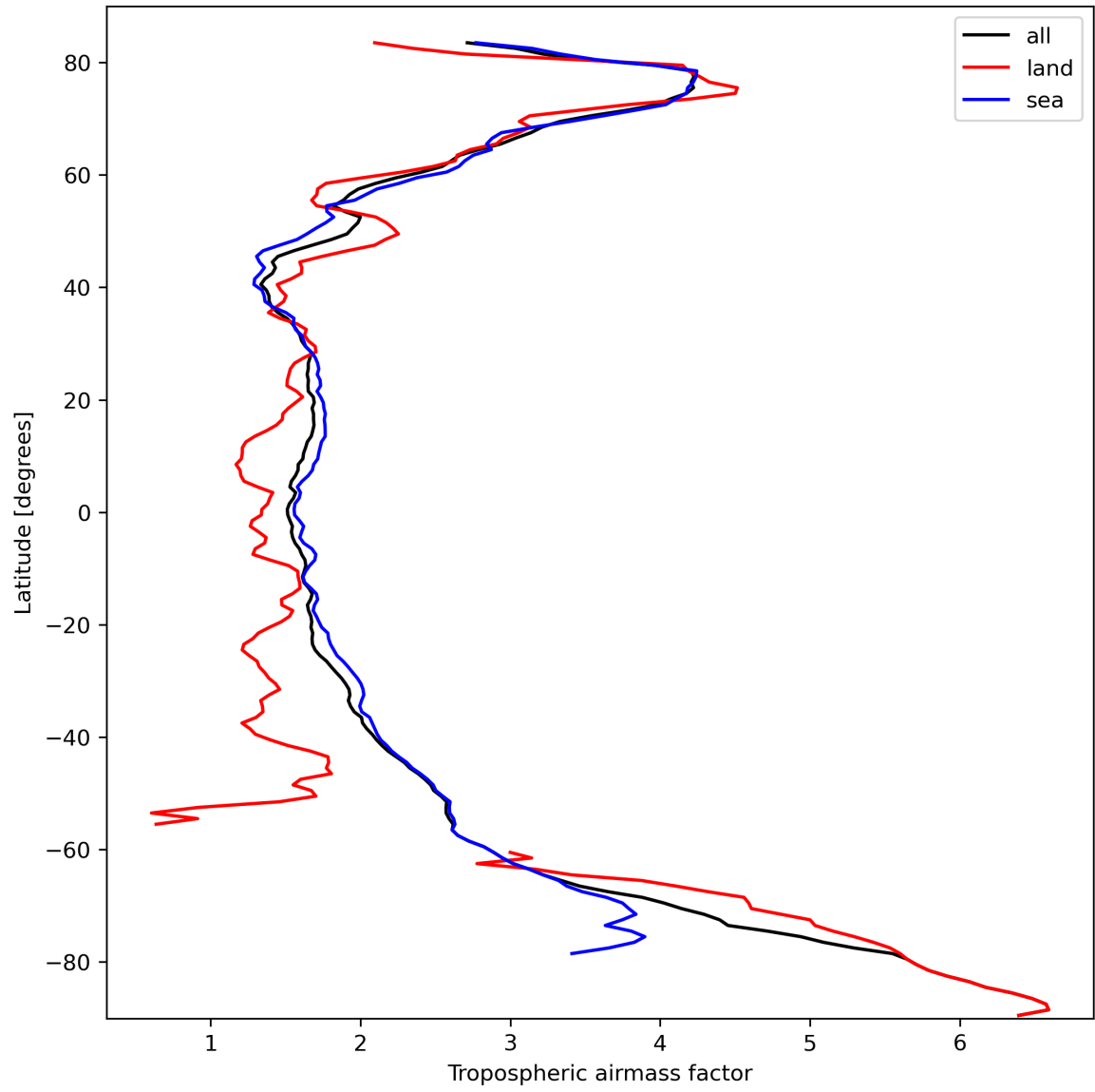
Figure 14: Zonal average of “Tropospheric airmass factor” for 2024-03-07 to 2024-03-09.
