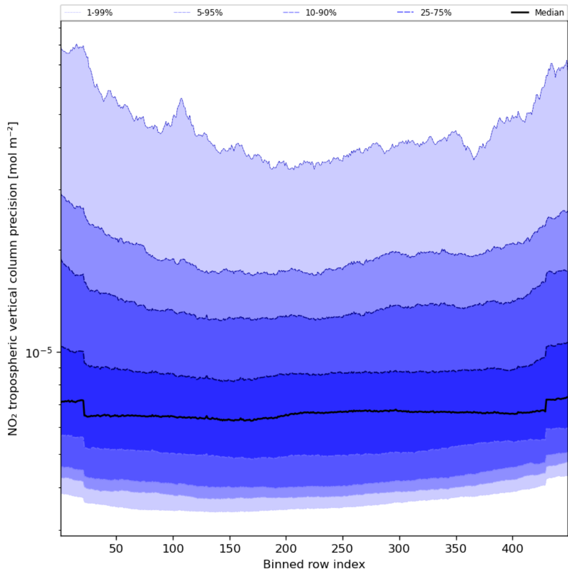
Figure 47: Along track statistics of “NO 2 tropospheric vertical column precision” for 2024-03-07 to 2024-03-09
