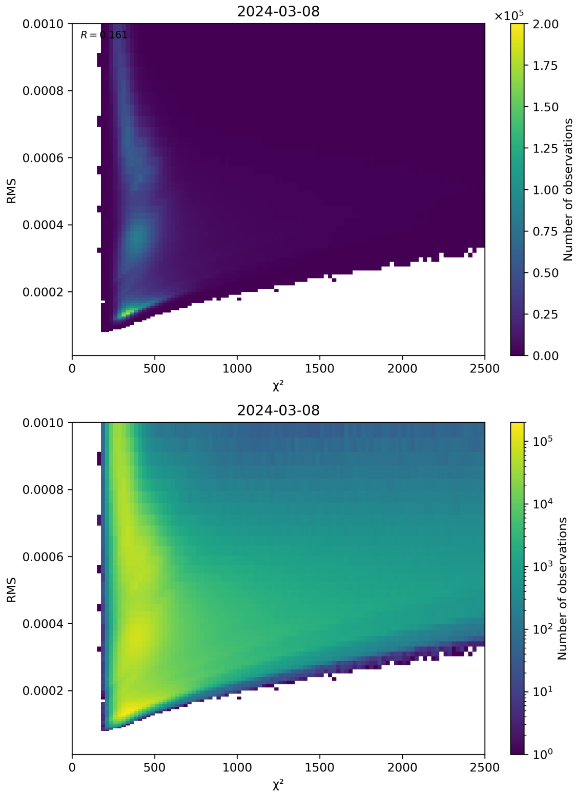
Figure 82: Scatter density plot of “ \chi^2 ” against “RMS” for 2024-03-07 to 2024-03-09.
