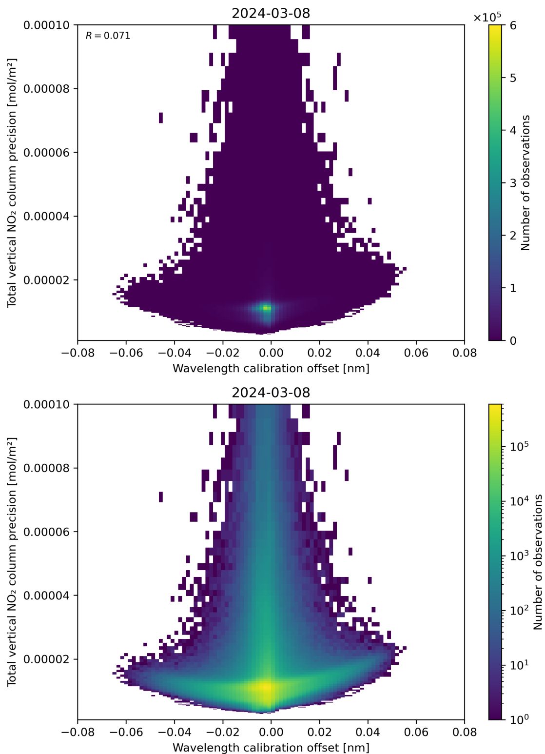
Figure 180: Scatter density plot of “Wavelength calibration offset” against “Total vertical NO 2 column precision” for 2024-03-07 to 2024-03-09.
