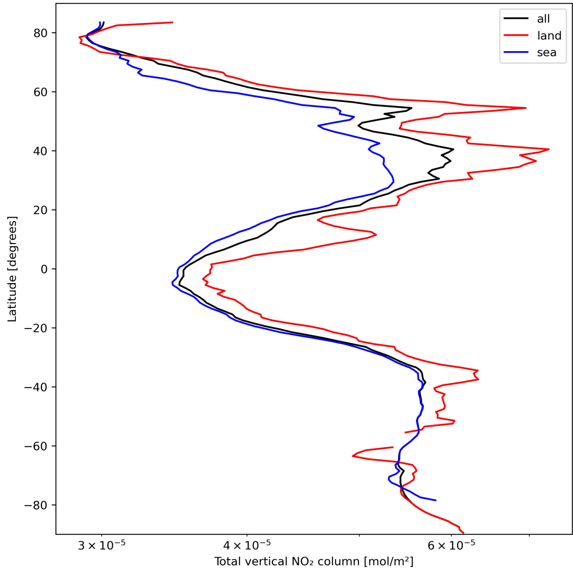
Figure 21: Zonal average of “Total vertical NO 2 column” for 2024-03-07 to 2024-03-09.
