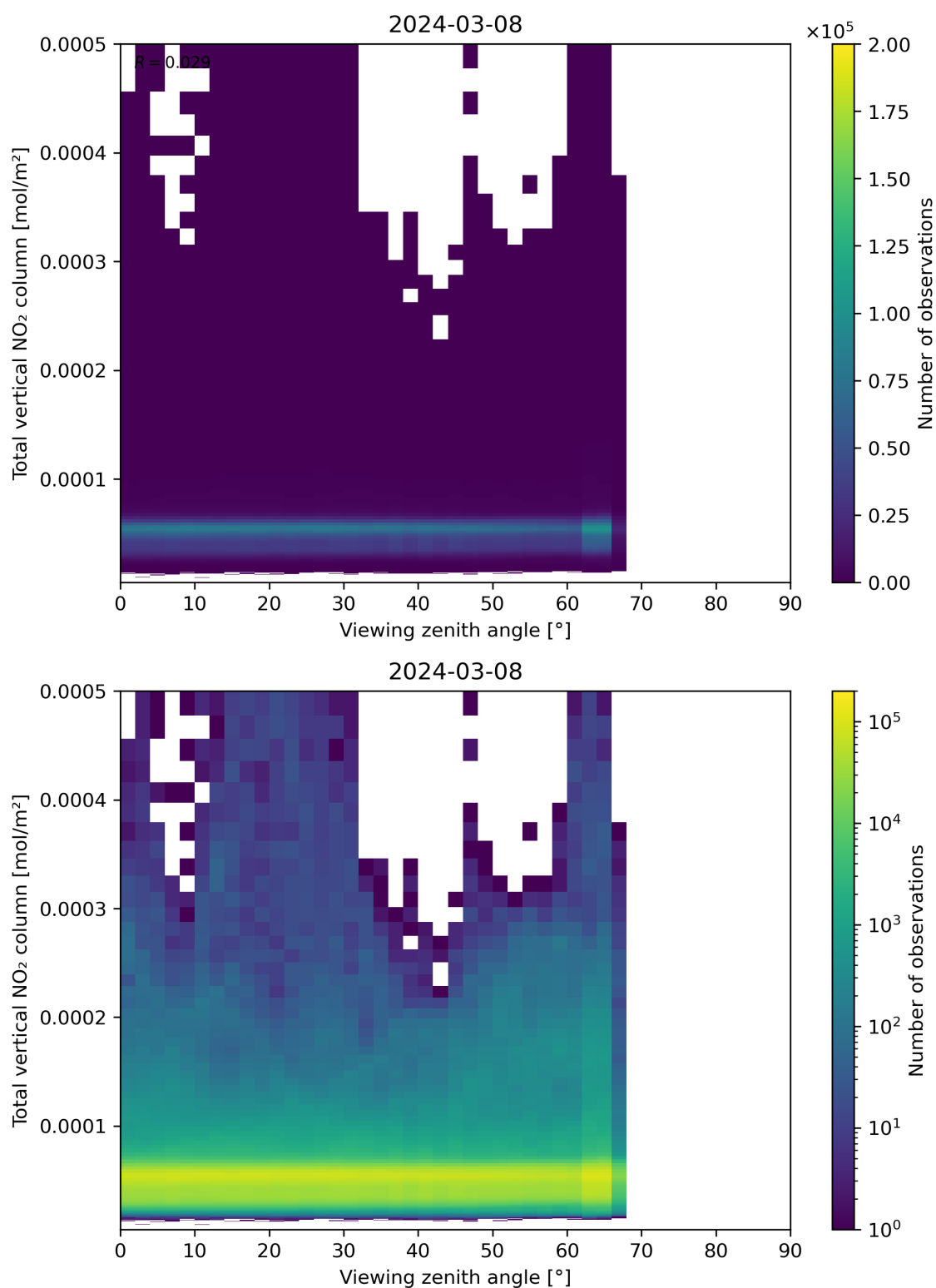
Figure 167: Scatter density plot of “Viewing zenith angle” against “Total vertical NO 2 column” for 2024-03-07 to 2024-03-09.
