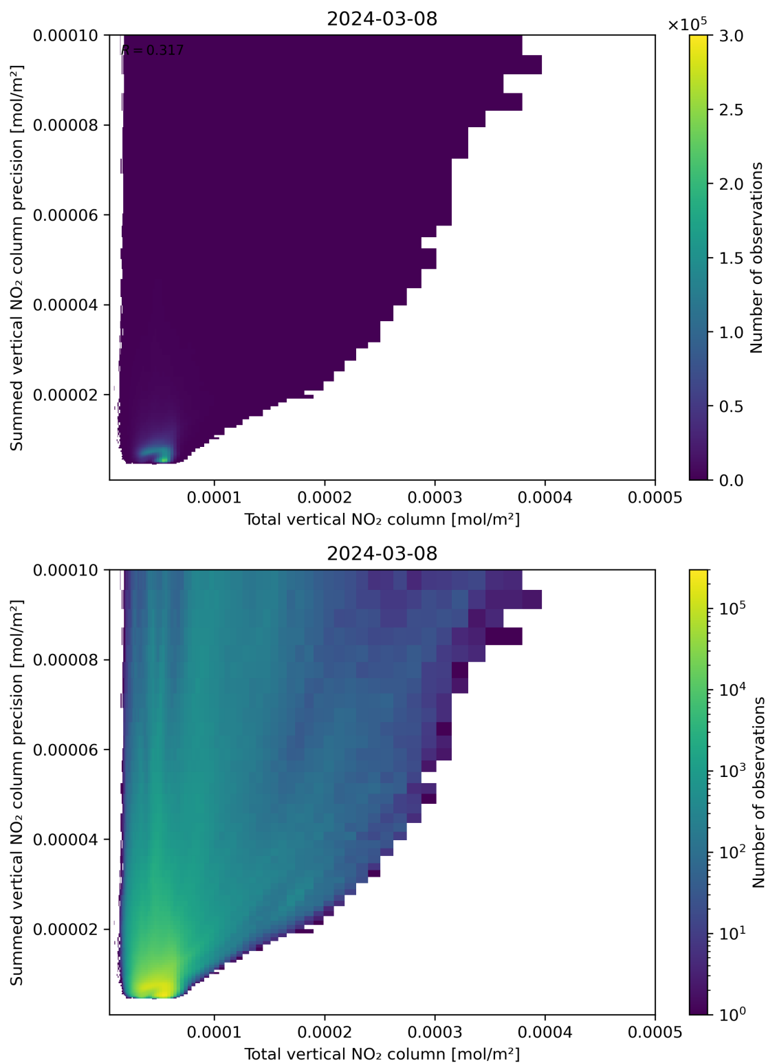
Figure 113: Scatter density plot of “Total vertical NO 2 column” against “Summed vertical NO 2 column precision” for 2024-03-07 to 2024-03-09.
