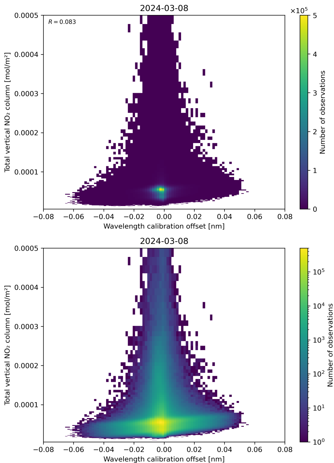
Figure 179: Scatter density plot of “Wavelength calibration offset” against “Total vertical NO 2 column” for 2024-03-07 to 2024-03-09.
