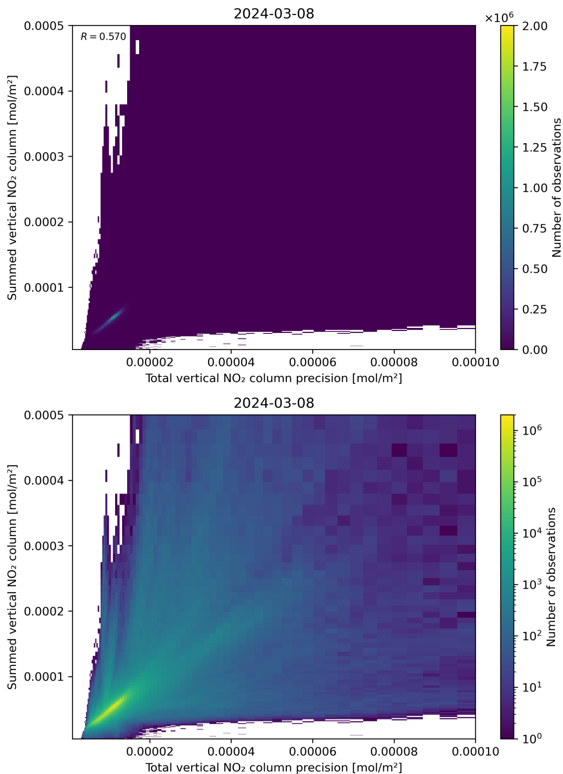
Figure 117: Scatter density plot of “Total vertical NO 2 column precision” against “Summed vertical NO 2 column” for 2024-03-07 to 2024-03-09.
