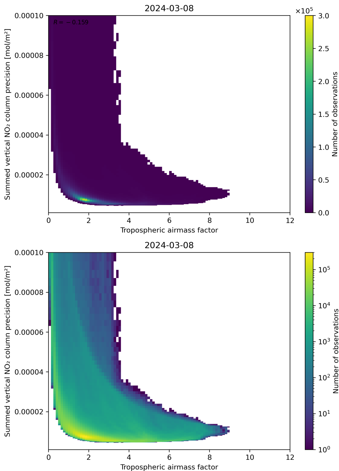
Figure 76: Scatter density plot of “Tropospheric air mass factor” against “Summed vertical NO 2 column precision” for 2024-03-07 to 2024-03-09.
