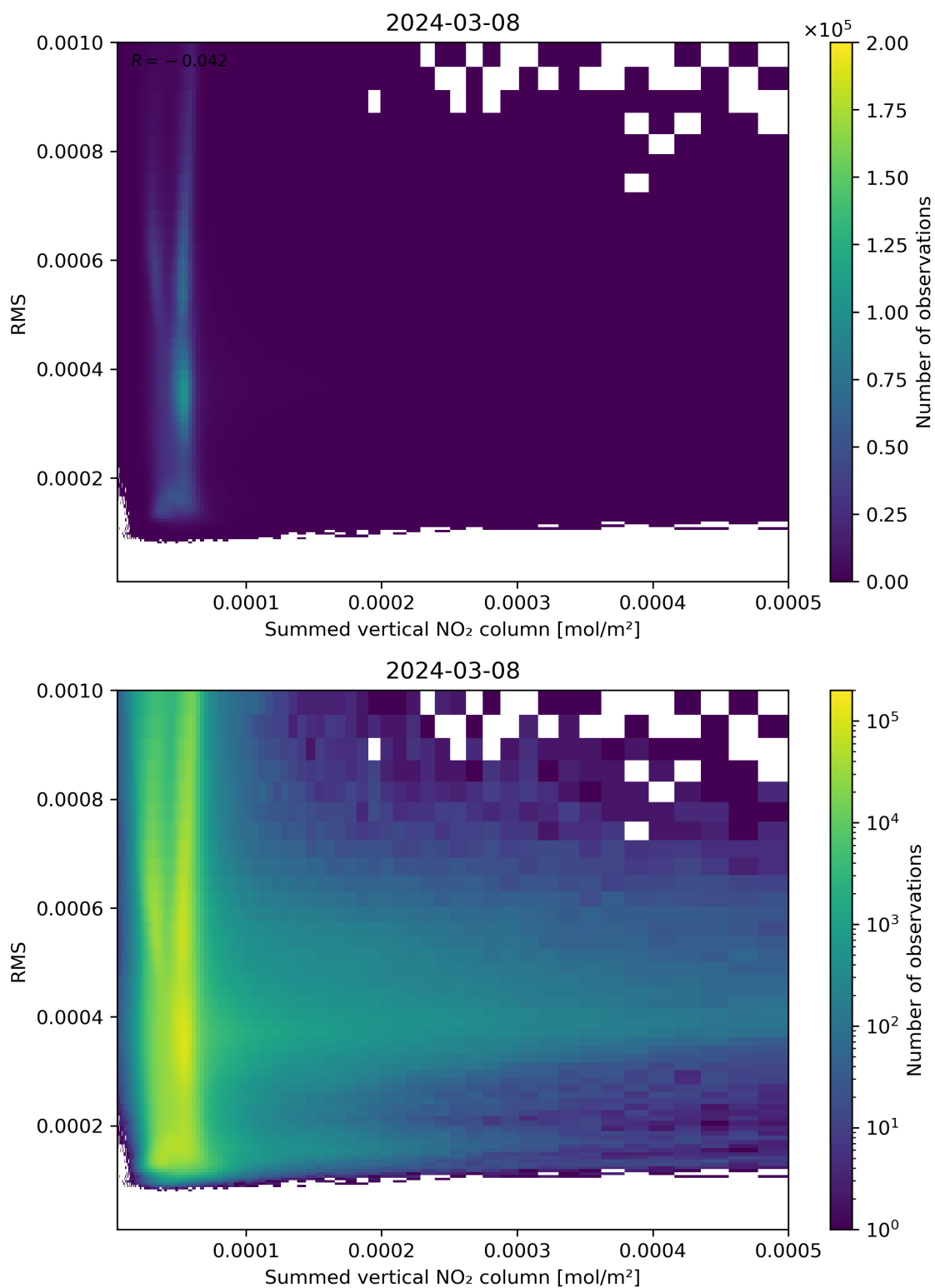
Figure 109: Scatter density plot of “Summed vertical NO 2 column” against “RMS” for 2024-03-07 to 2024-03-09.
