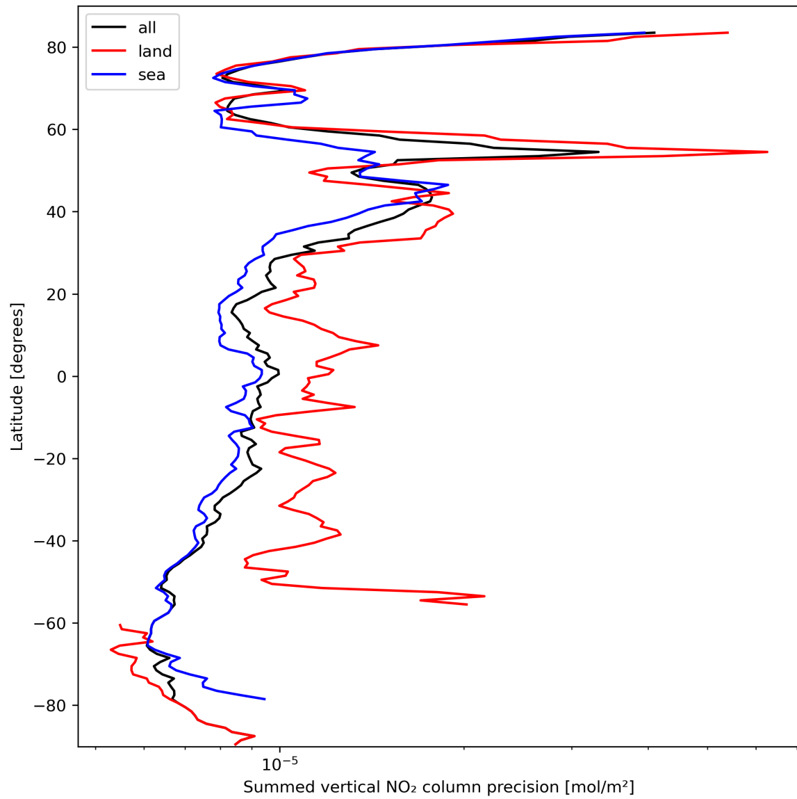
Figure 24: Zonal average of “Summed vertical NO 2 column precision” for 2024-03-07 to 2024-03-09.
