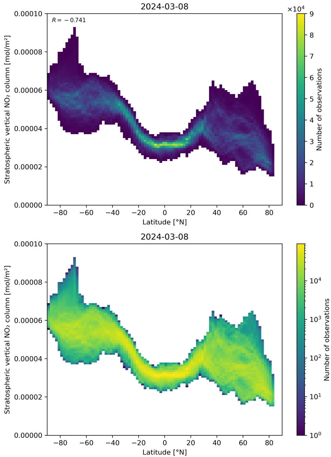
Figure 87: Scatter density plot of “Latitude” against “Stratospheric vertical NO 2 column” for 2024-03-07 to 2024-03-09.
