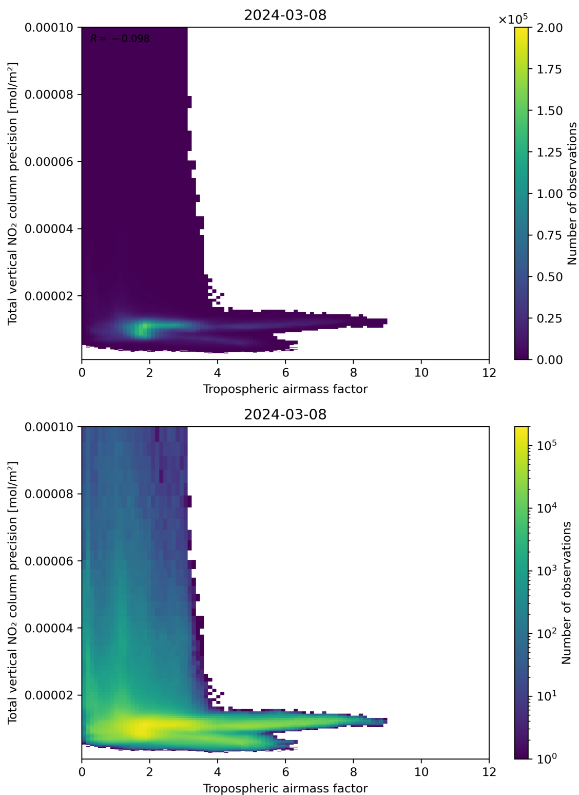
Figure 78: Scatter density plot of “Tropospheric air mass factor” against “Total vertical NO 2 column precision” for 2024-03-07 to 2024-03-09.
