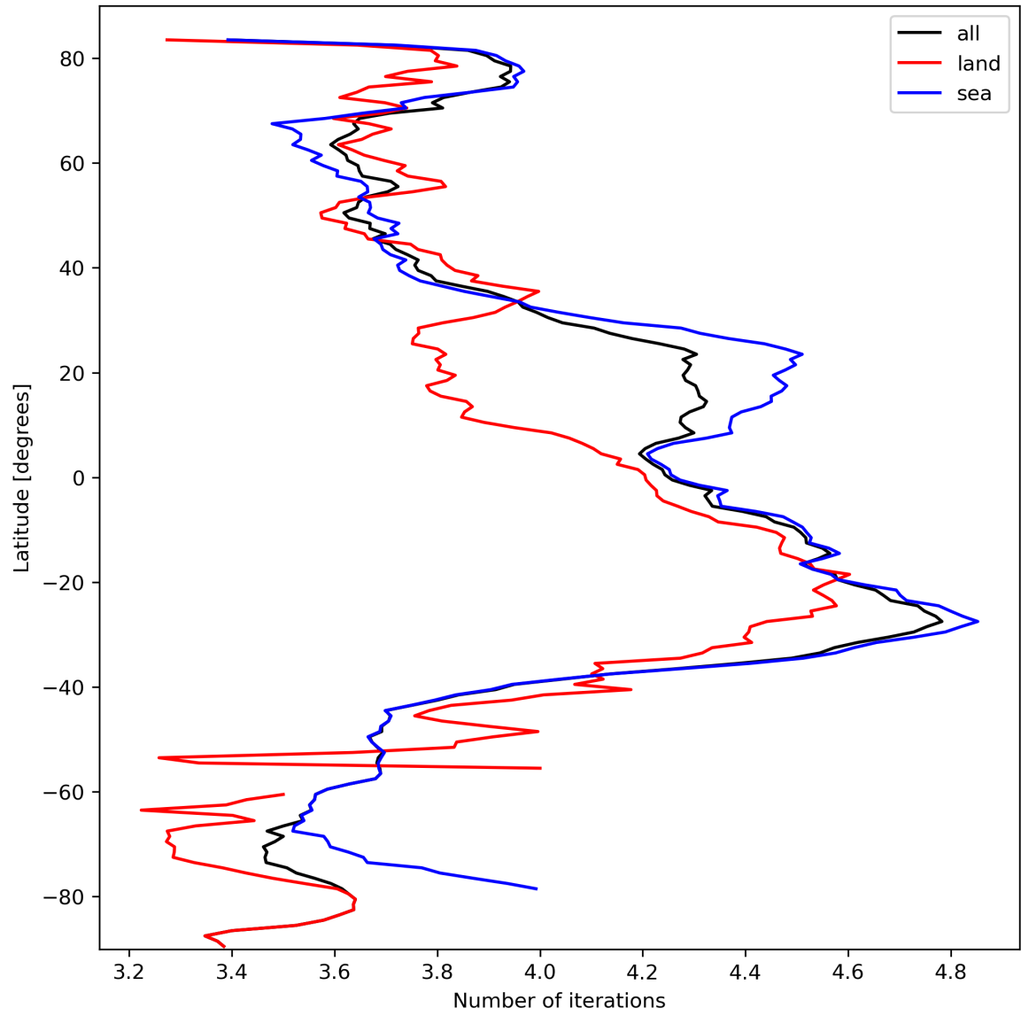
Figure 17: Zonal average of “Number of iterations” for 2024-03-07 to 2024-03-09.
