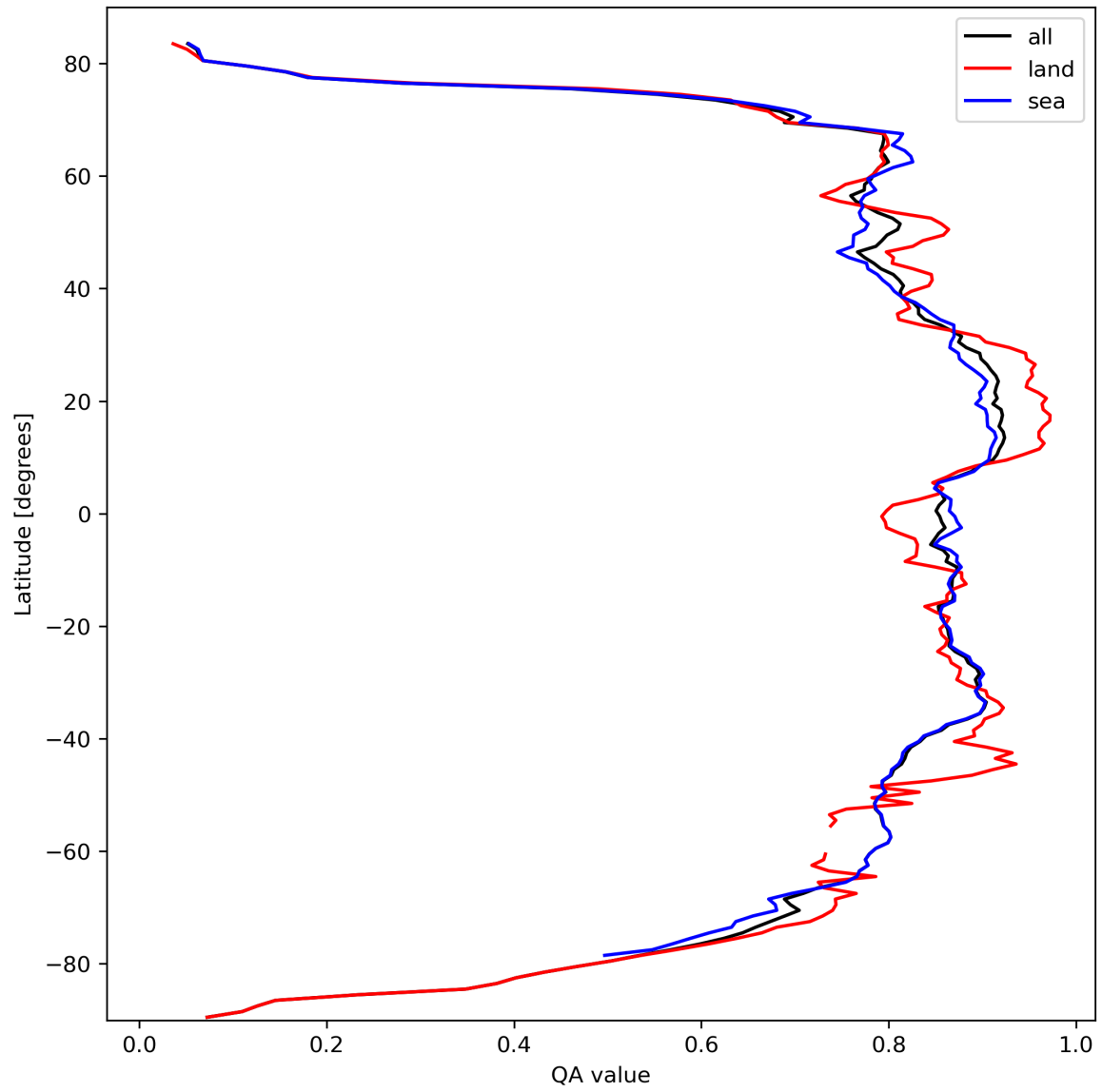
Figure 11: Zonal average of “QA value” for 2024-03-07 to 2024-03-09.
