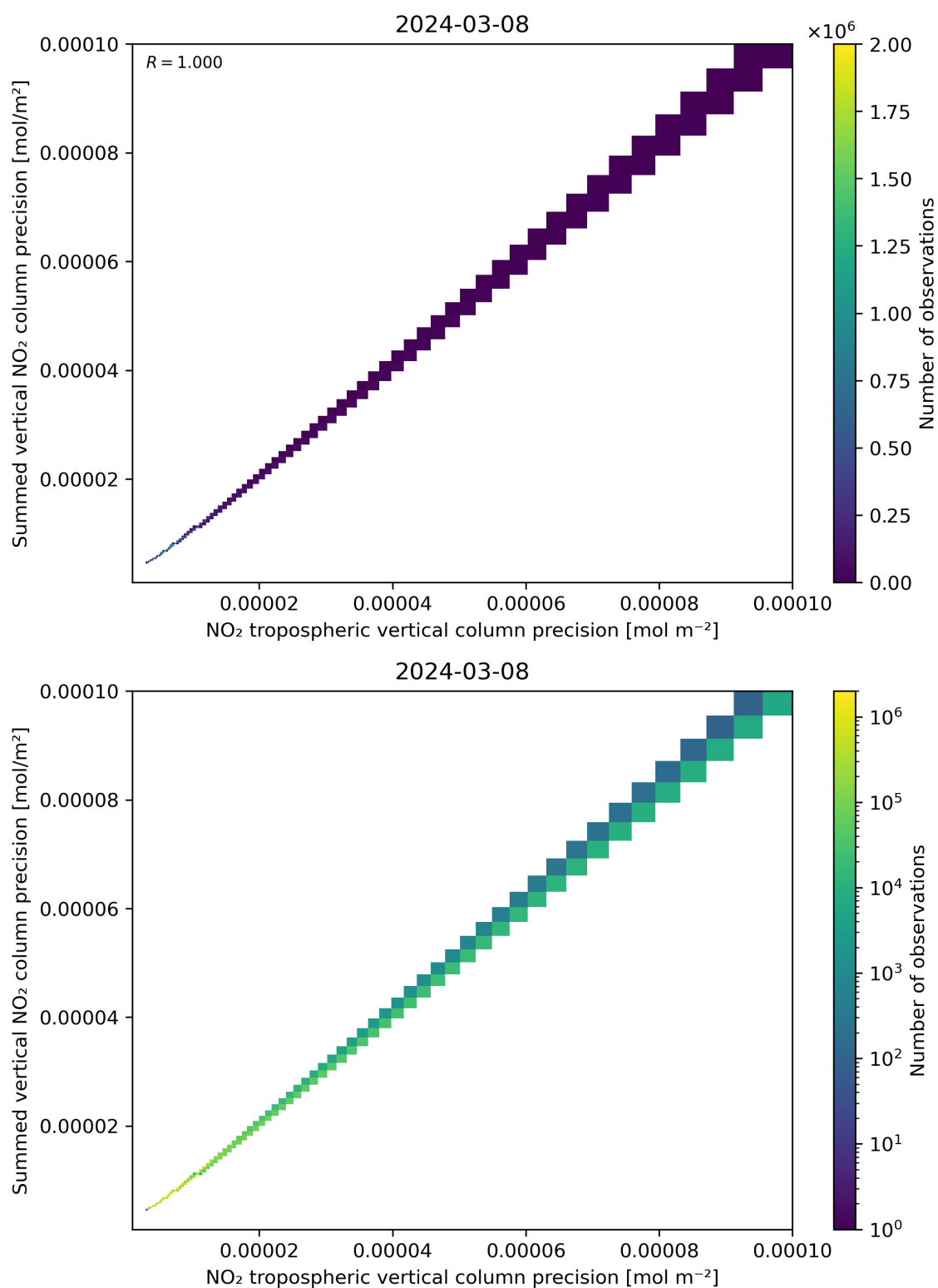
Figure 137: Scatter density plot of “NO 2 tropospheric vertical column precision” against “Summed vertical NO 2 column precision” for 2024-03-07 to 2024-03-09.
