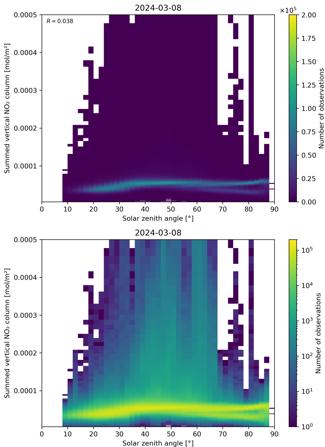
Figure 151: Scatter density plot of “Solar zenith angle” against “Summed vertical NO 2 column” for 2024-03-07 to 2024-03-09.
