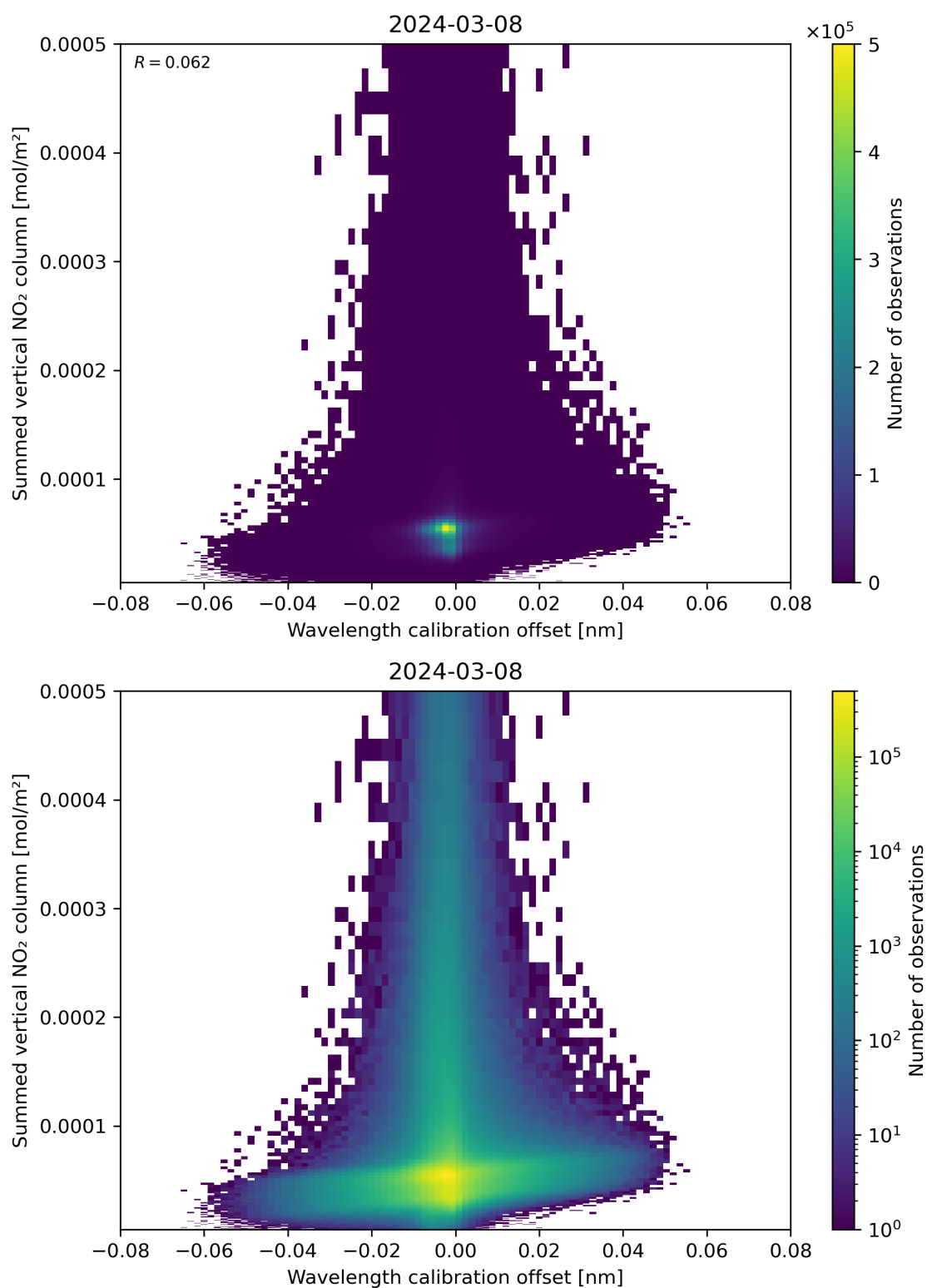
Figure 177: Scatter density plot of “Wavelength calibration offset” against “Summed vertical NO 2 column” for 2024-03-07 to 2024-03-09.
