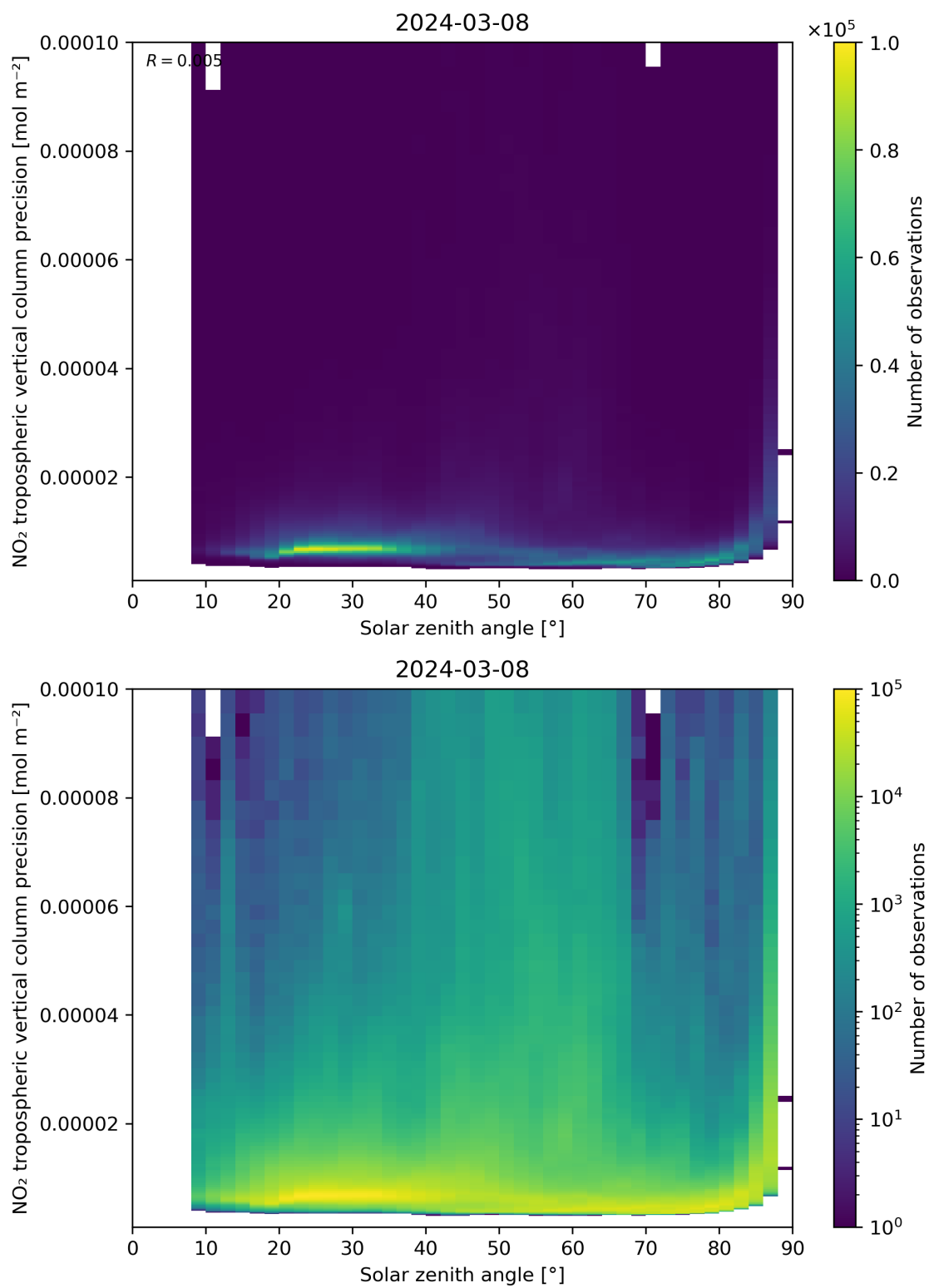
Figure 156: Scatter density plot of “Solar zenith angle” against “NO 2 tropospheric vertical column precision” for 2024-03-07 to 2024-03-09.
