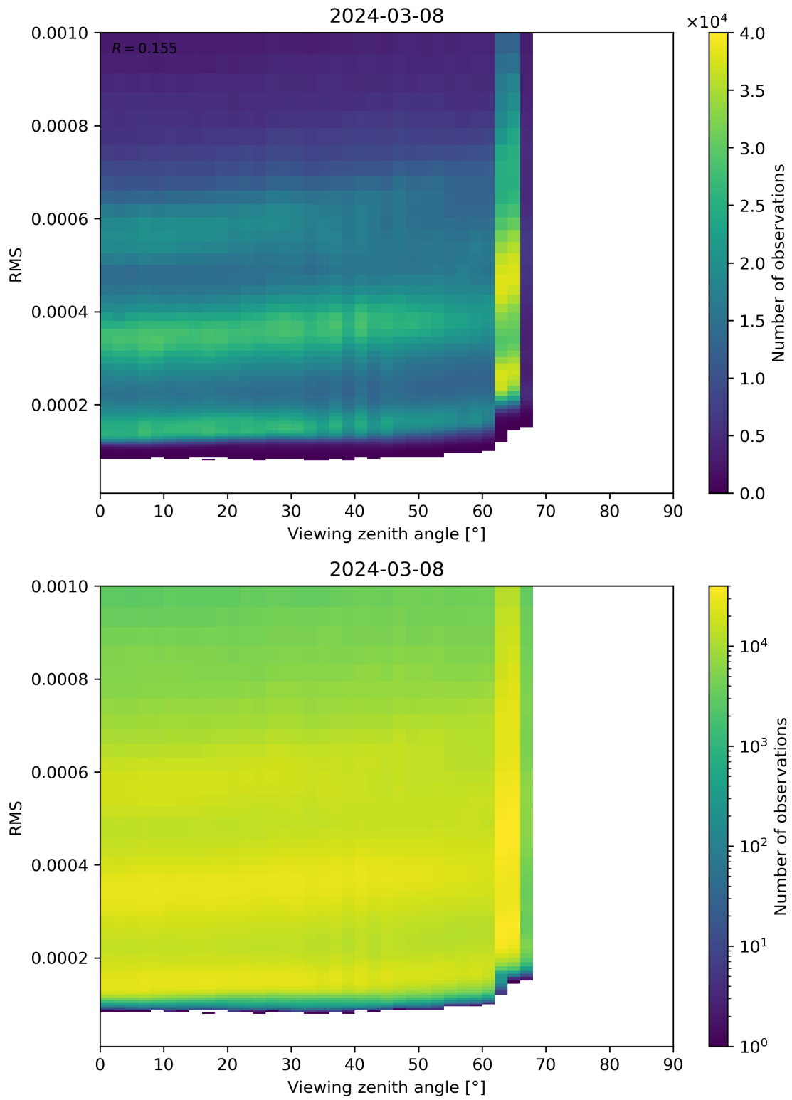
Figure 171: Scatter density plot of “Viewing zenith angle” against “RMS” for 2024-03-07 to 2024-03-09.
