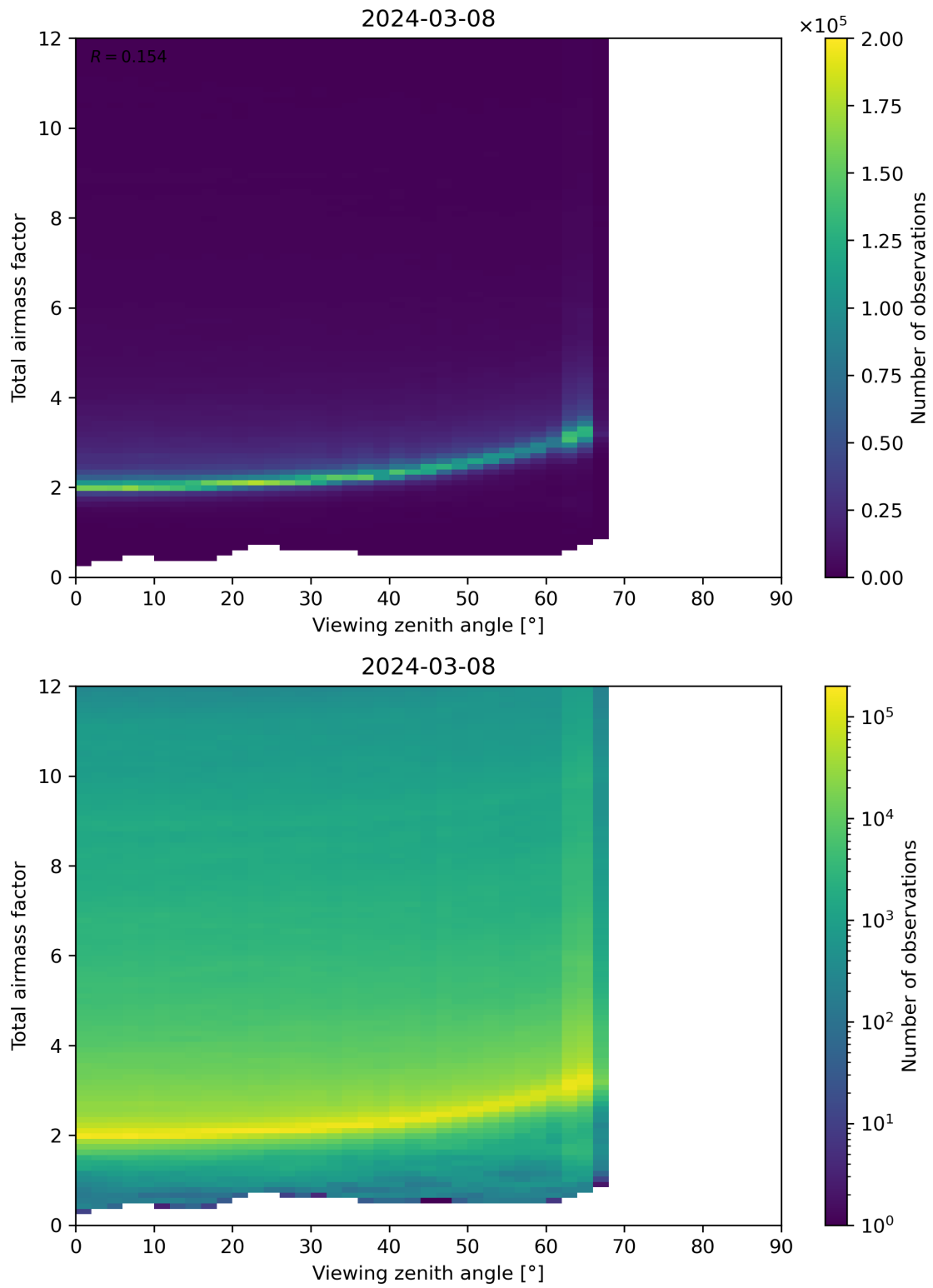
Figure 160: Scatter density plot of “Viewing zenith angle” against “Total airmass factor” for 2024-03-07 to 2024-03-09.
