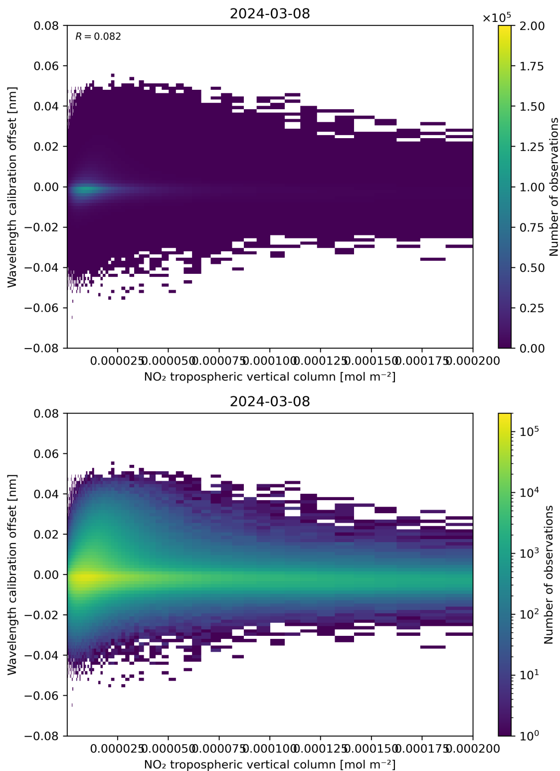
Figure 143: Scatter density plot of “NO 2 tropospheric vertical column” against “Wavelength calibration offset” for 2024-03-07 to 2024-03-09.
