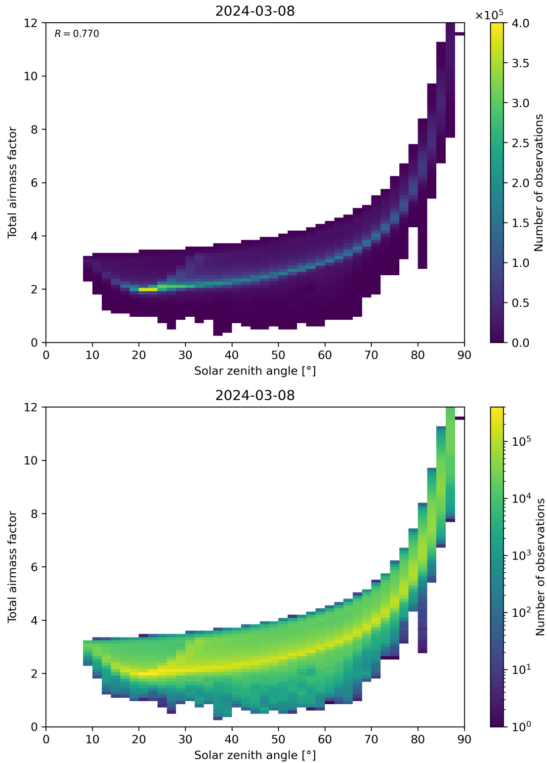
Figure 146: Scatter density plot of “Solar zenith angle” against “Total air mass factor” for 2024-03-07 to 2024-03-09.
