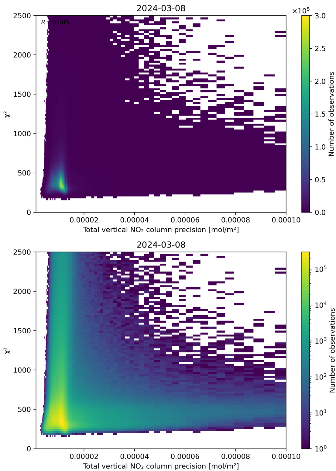
Figure 116: Scatter density plot of “Total vertical NO 2 column precision” against “ \chi^2 ” for 2024-03-07 to 2024-03-09.
