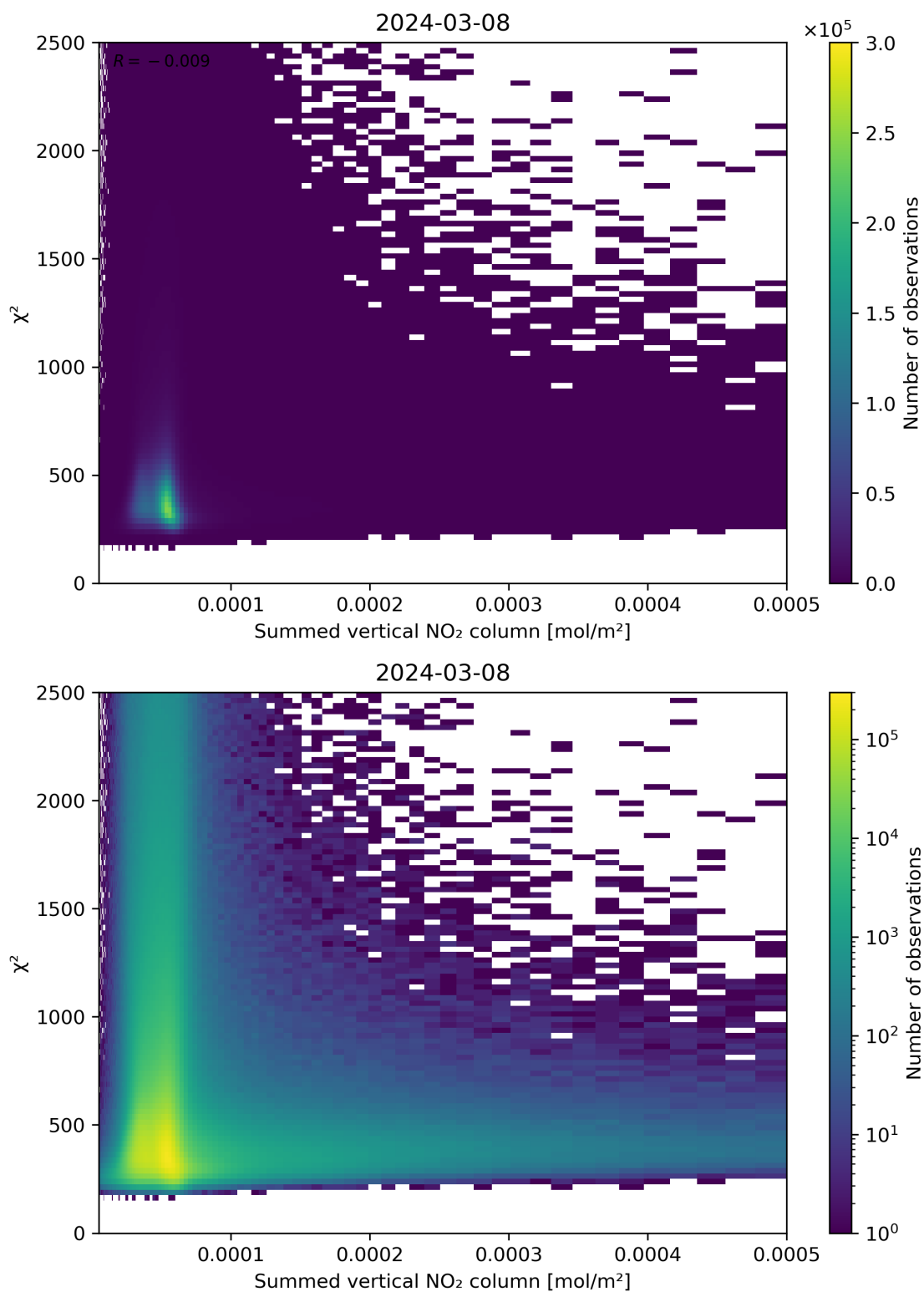
Figure 104: Scatter density plot of “Summed vertical NO 2 column” against “ \chi^2 ” for 2024-03-07 to 2024-03-09.
