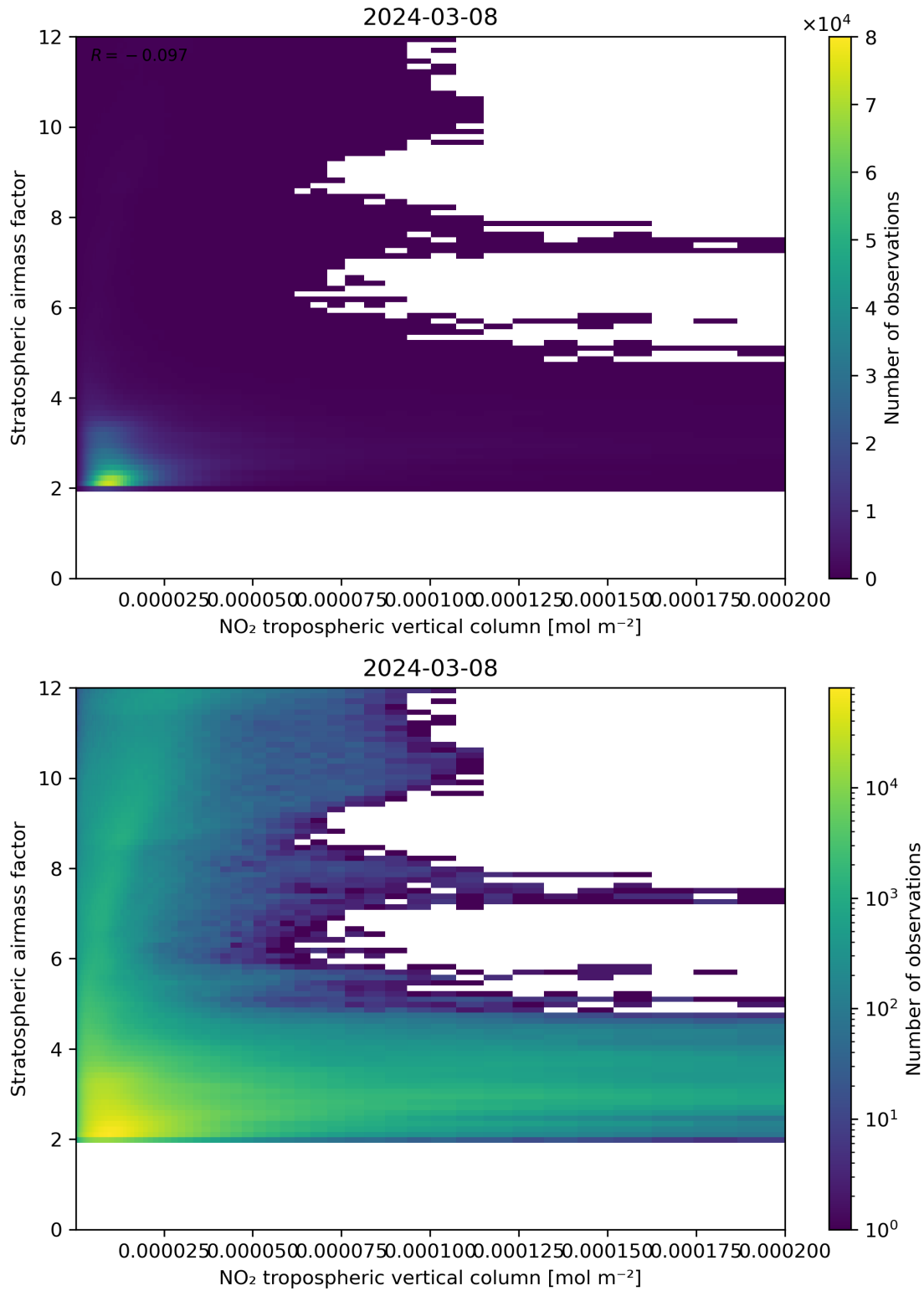
Figure 121: Scatter density plot of “NO 2 tropospheric vertical column” against “Stratospheric air mass factor” for 2024-03-07 to 2024-03-09.
