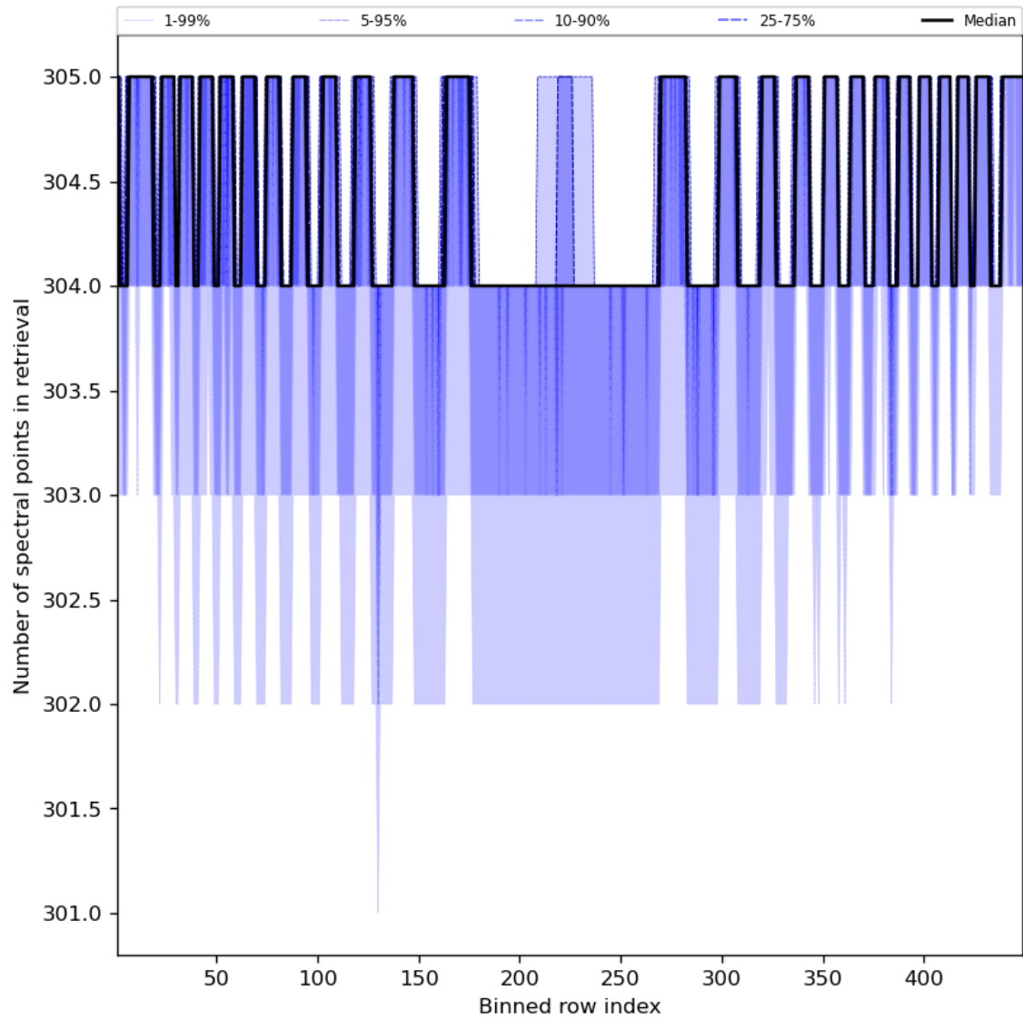
Figure 50: Along track statistics of “Number of spectral points in retrieval” for 2024-03-07 to 2024-03-09
