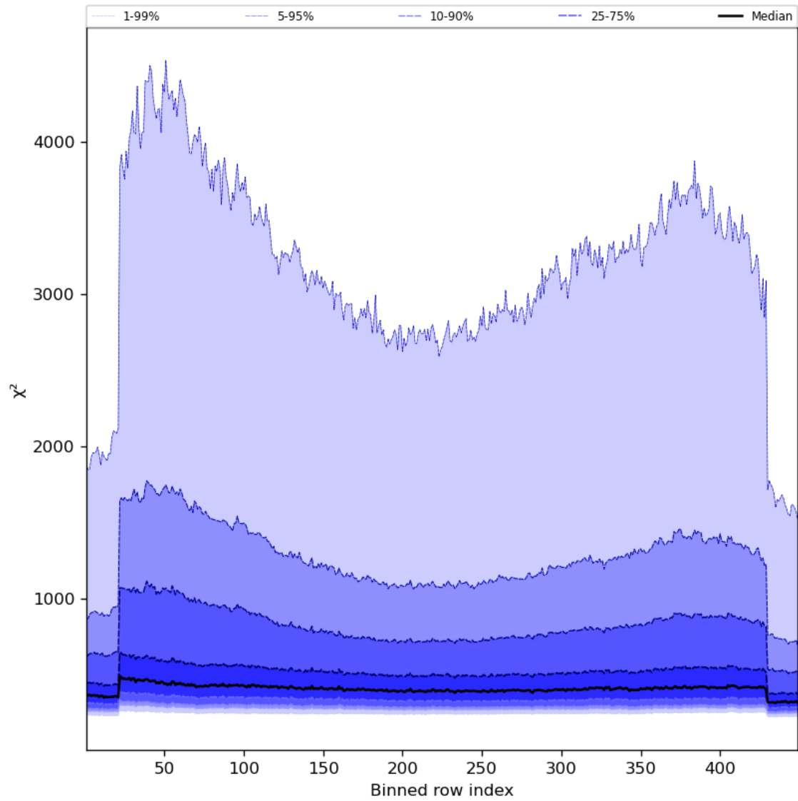
Figure 59: Along track statistics of “ \chi^2 ” for 2024-03-07 to 2024-03-09
