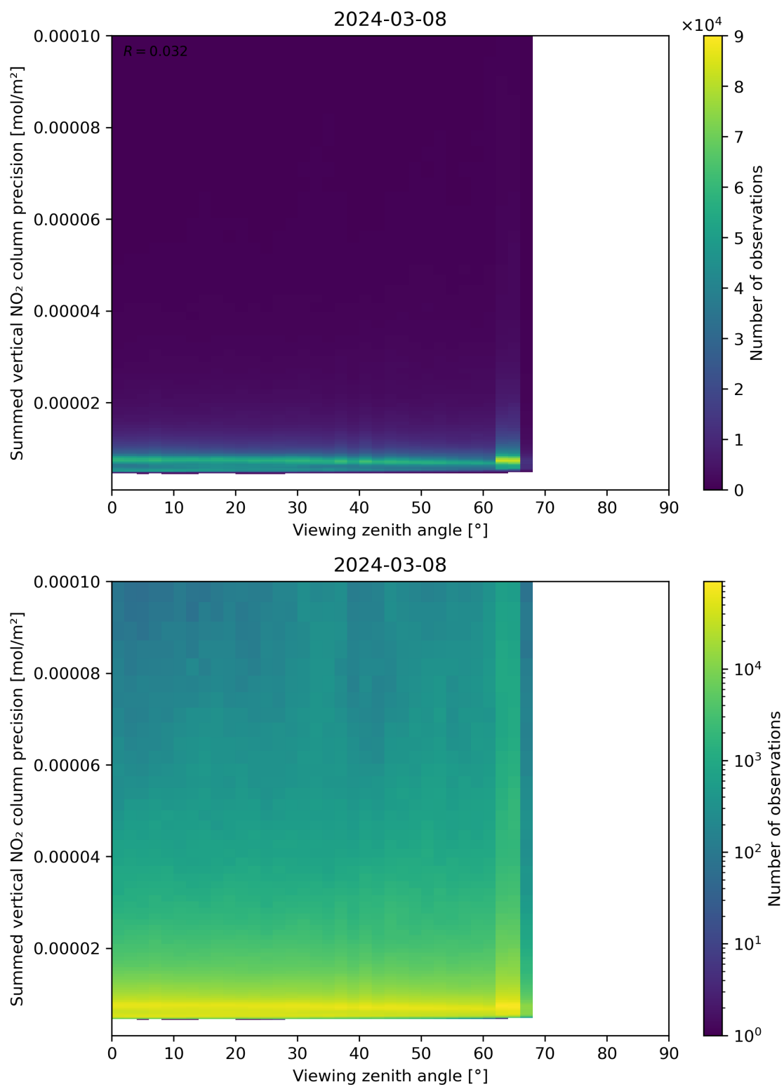
Figure 166: Scatter density plot of “Viewing zenith angle” against “Summed vertical NO 2 column precision” for 2024-03-07 to 2024-03-09.
