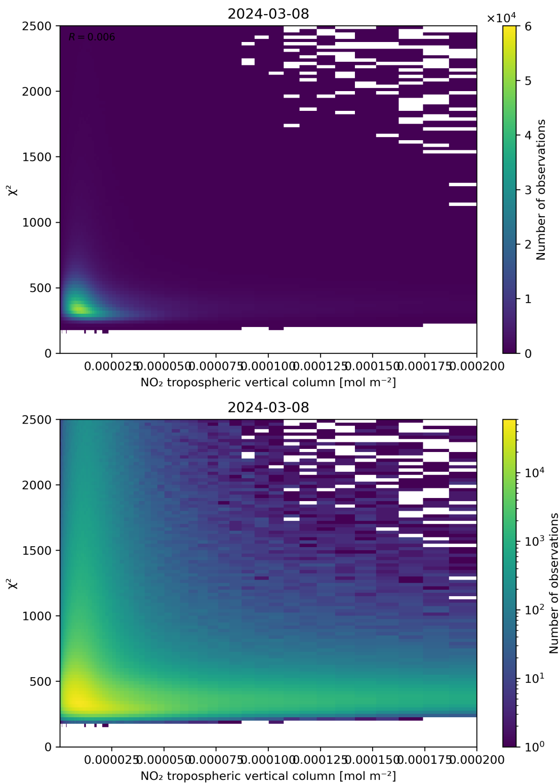
Figure 124: Scatter density plot of “NO 2 tropospheric vertical column” against “ \chi^2 ” for 2024-03-07 to 2024-03-09.
