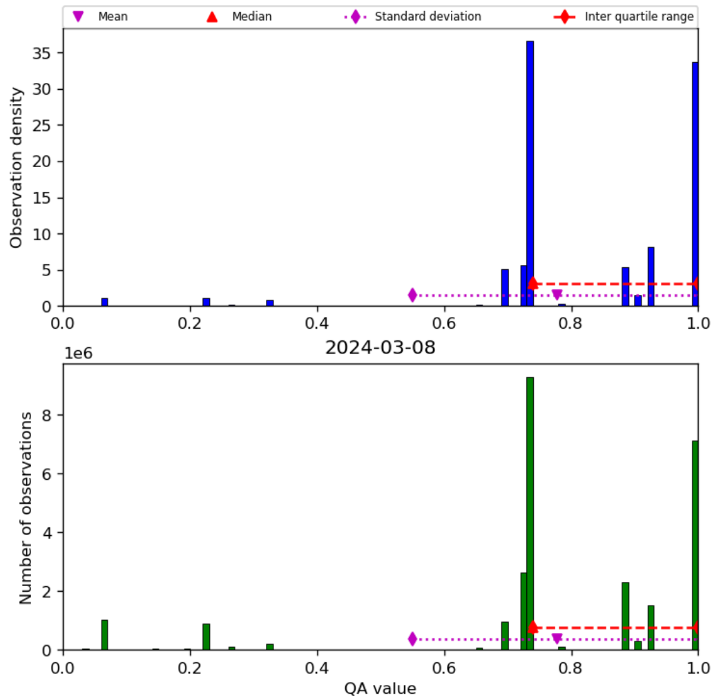
Figure 28: Histogram of “QA value” for 2024-03-07 to 2024-03-09
