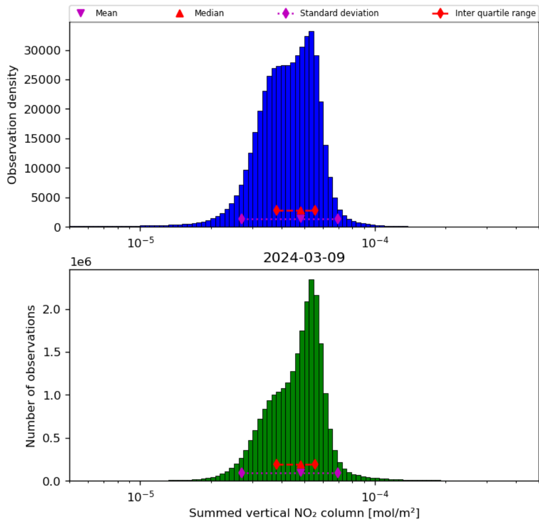
Figure 40: Histogram of “Summed vertical NO 2 column” for 2024-03-09 to 2024-03-10
