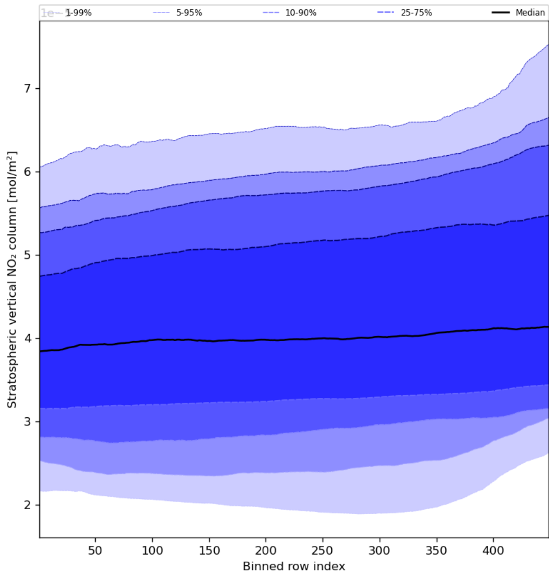
Figure 53: Along track statistics of “Stratospheric vertical NO 2 column” for 2024-03-09 to 2024-03-10
