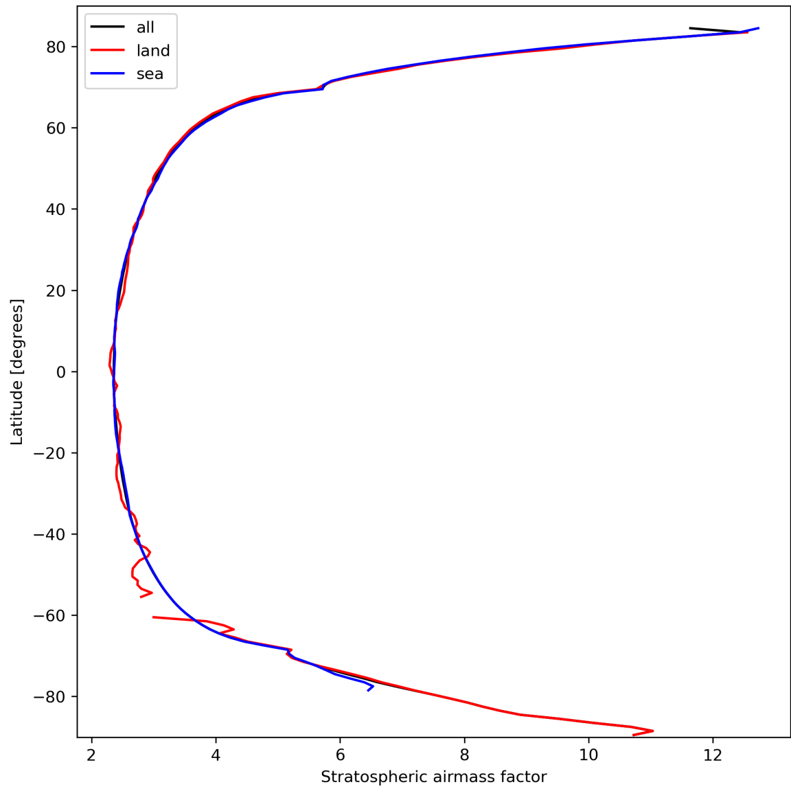
Figure 27: Zonal average of “Stratospheric airmass factor” for 2024-03-09 to 2024-03-10.
