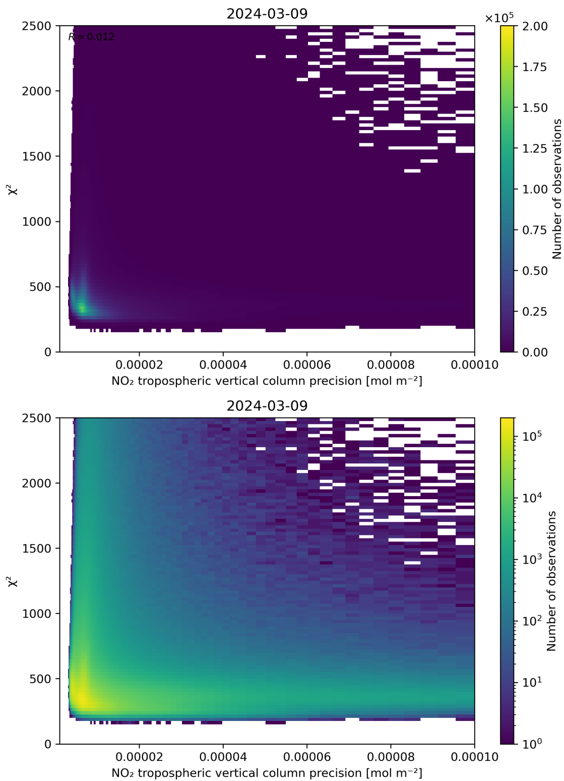
Figure 134: Scatter density plot of “NO 2 tropospheric vertical column precision” against “ \chi^2 ” for 2024-03-09 to 2024-03-10.
