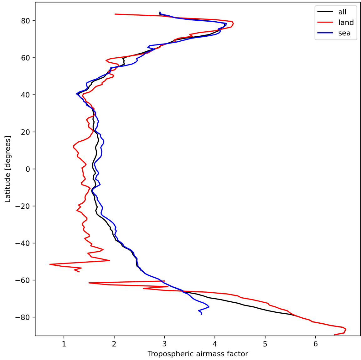
Figure 14: Zonal average of “Tropospheric airmass factor” for 2024-03-09 to 2024-03-10.
