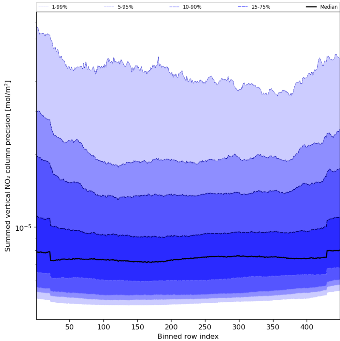
Figure 58: Along track statistics of “Summed vertical NO 2 column precision” for 2024-03-09 to 2024-03-10
