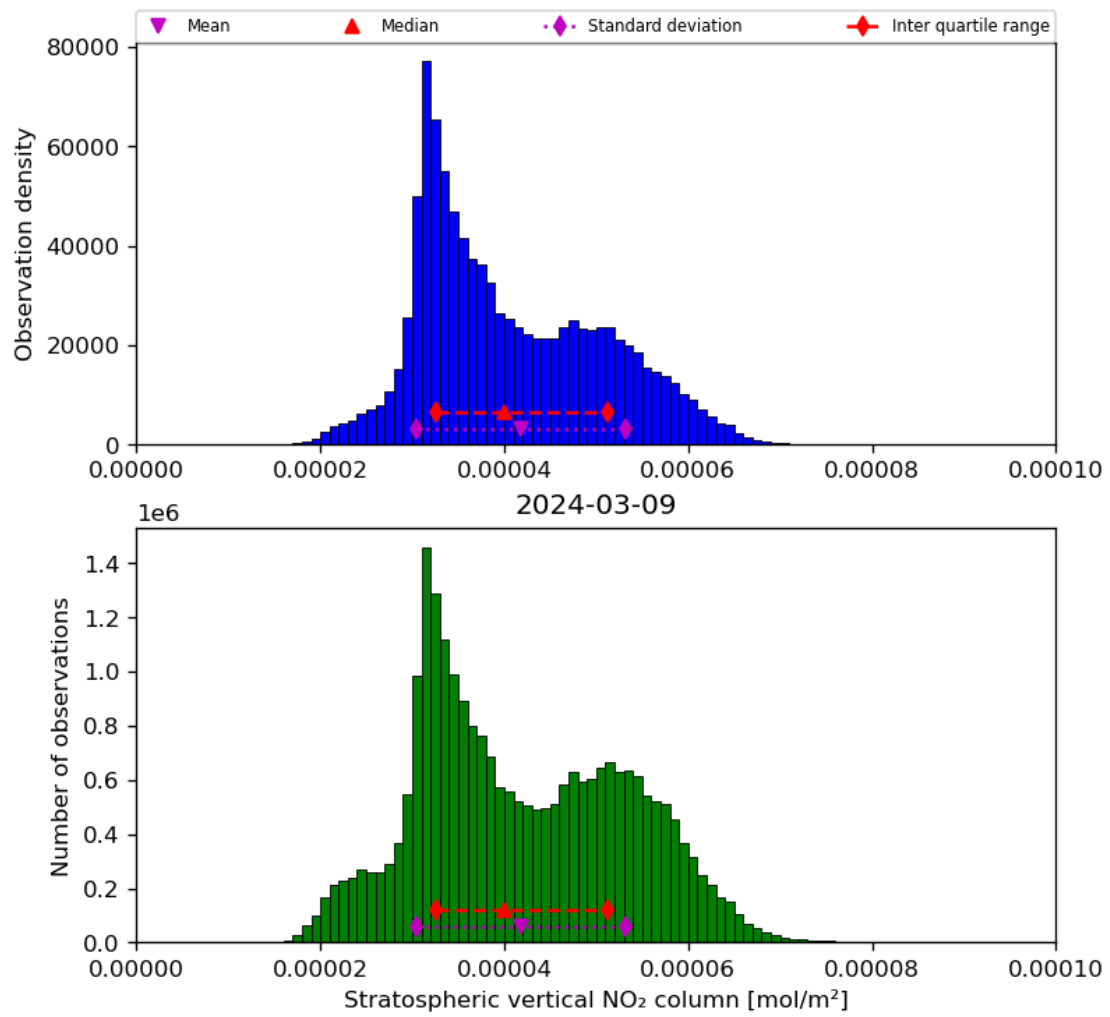
Figure 36: Histogram of “Stratospheric vertical NO 2 column” for 2024-03-09 to 2024-03-10
