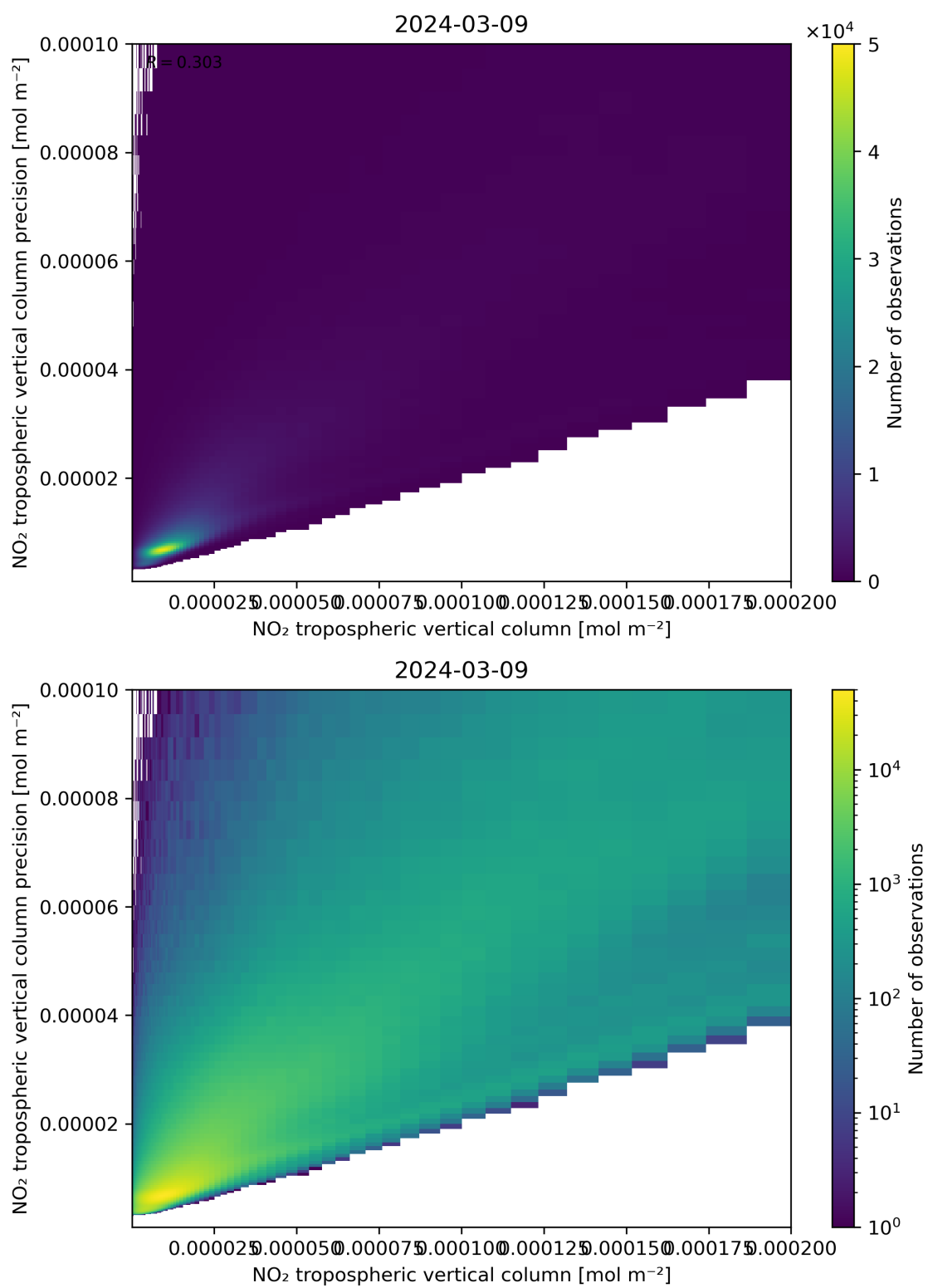
Figure 130: Scatter density plot of “NO 2 tropospheric vertical column” against “NO 2 tropospheric vertical column precision” for 2024-03-09 to 2024-03-10.
