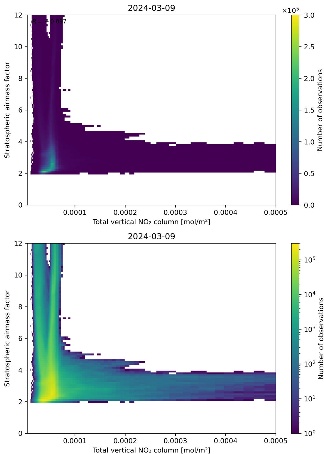
Figure 110: Scatter density plot of “Total vertical NO 2 column” against “Stratospheric airmass factor” for 2024-03-09 to 2024-03-10.
