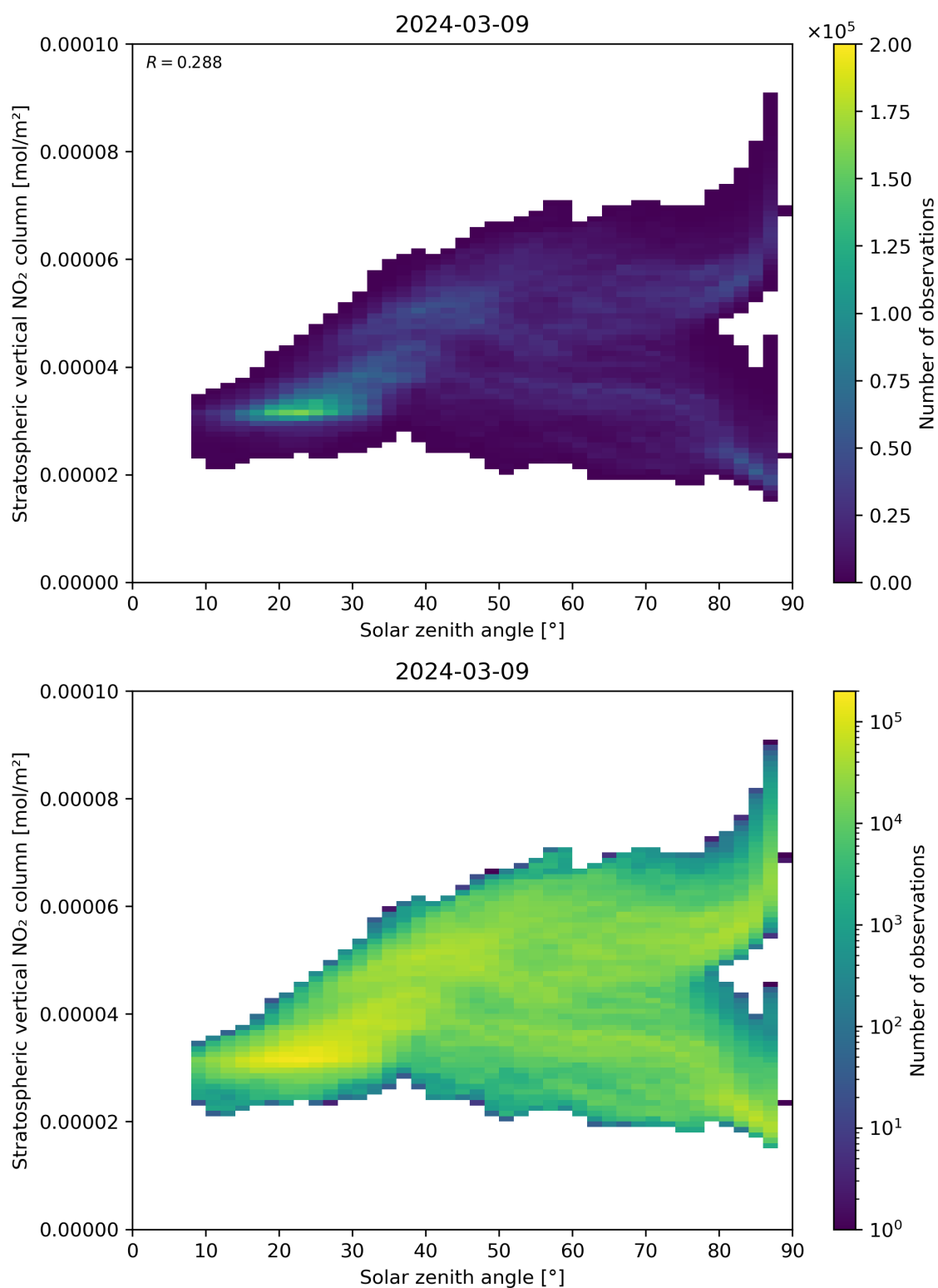
Figure 150: Scatter density plot of “Solar zenith angle” against “Stratospheric vertical NO 2 column” for 2024-03-09 to 2024-03-10.
