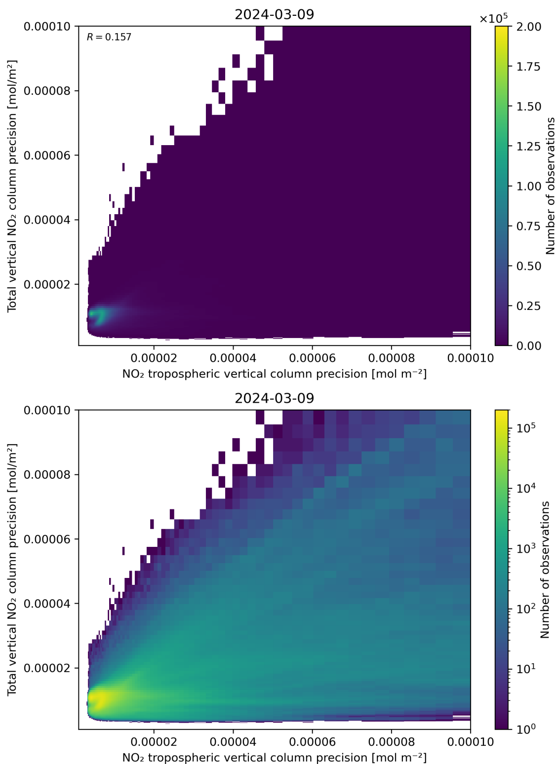
Figure 139: Scatter density plot of “NO 2 tropospheric vertical column precision” against “Total vertical NO 2 column precision” for 2024-03-09 to 2024-03-10.
