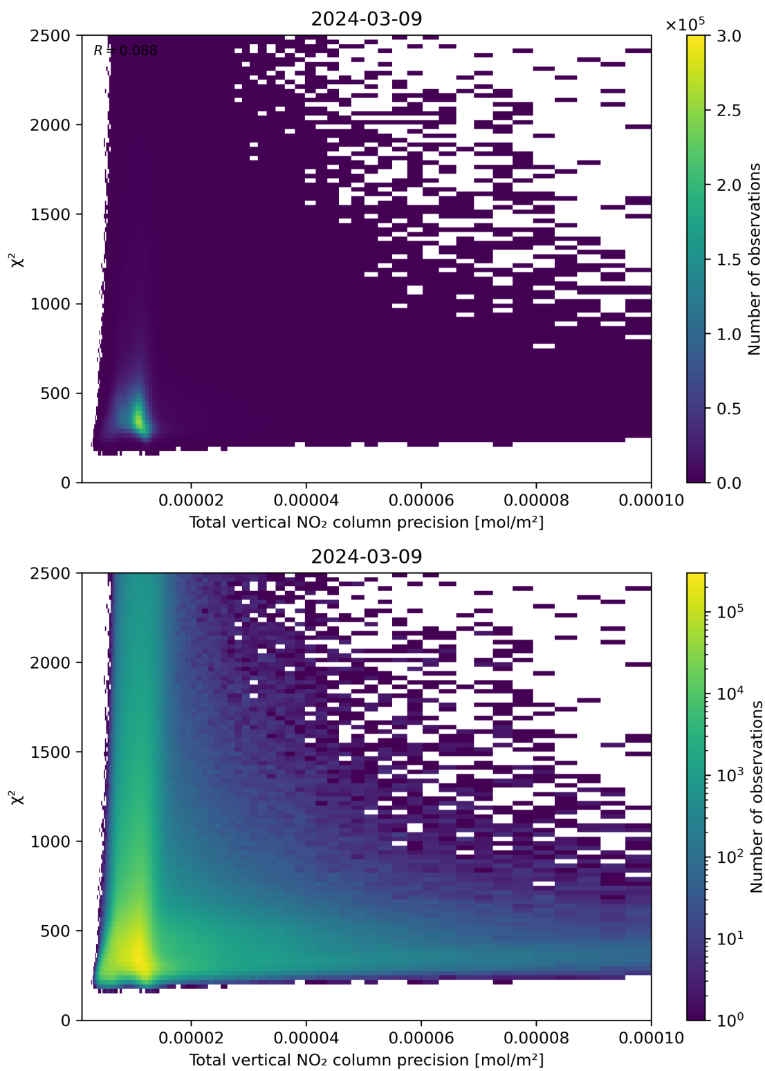
Figure 116: Scatter density plot of “Total vertical NO 2 column precision” against “ \chi^2 ” for 2024-03-09 to 2024-03-10.
