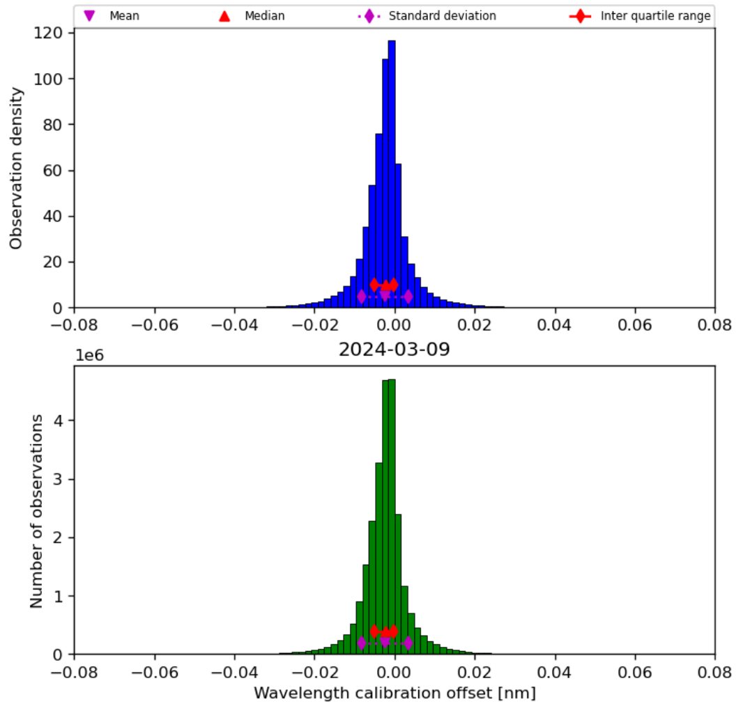
Figure 35: Histogram of “Wavelength calibration offset” for 2024-03-09 to 2024-03-10
