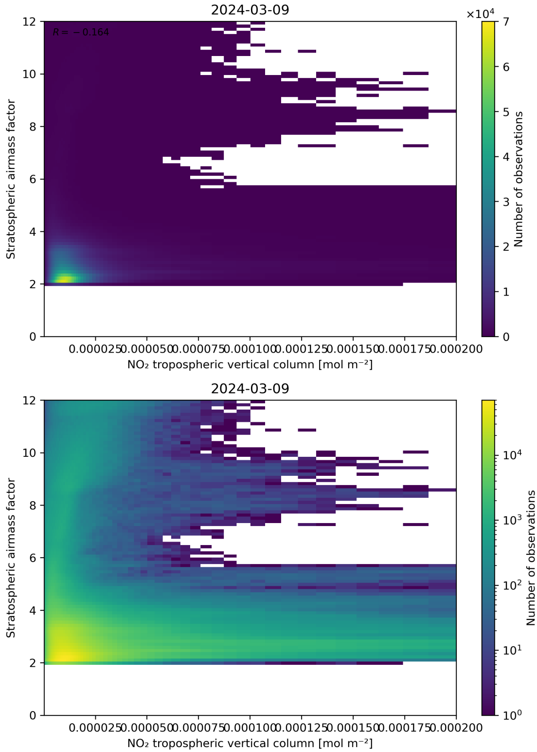
Figure 121: Scatter density plot of “NO 2 tropospheric vertical column” against “Stratospheric air mass factor” for 2024-03-09 to 2024-03-10.
