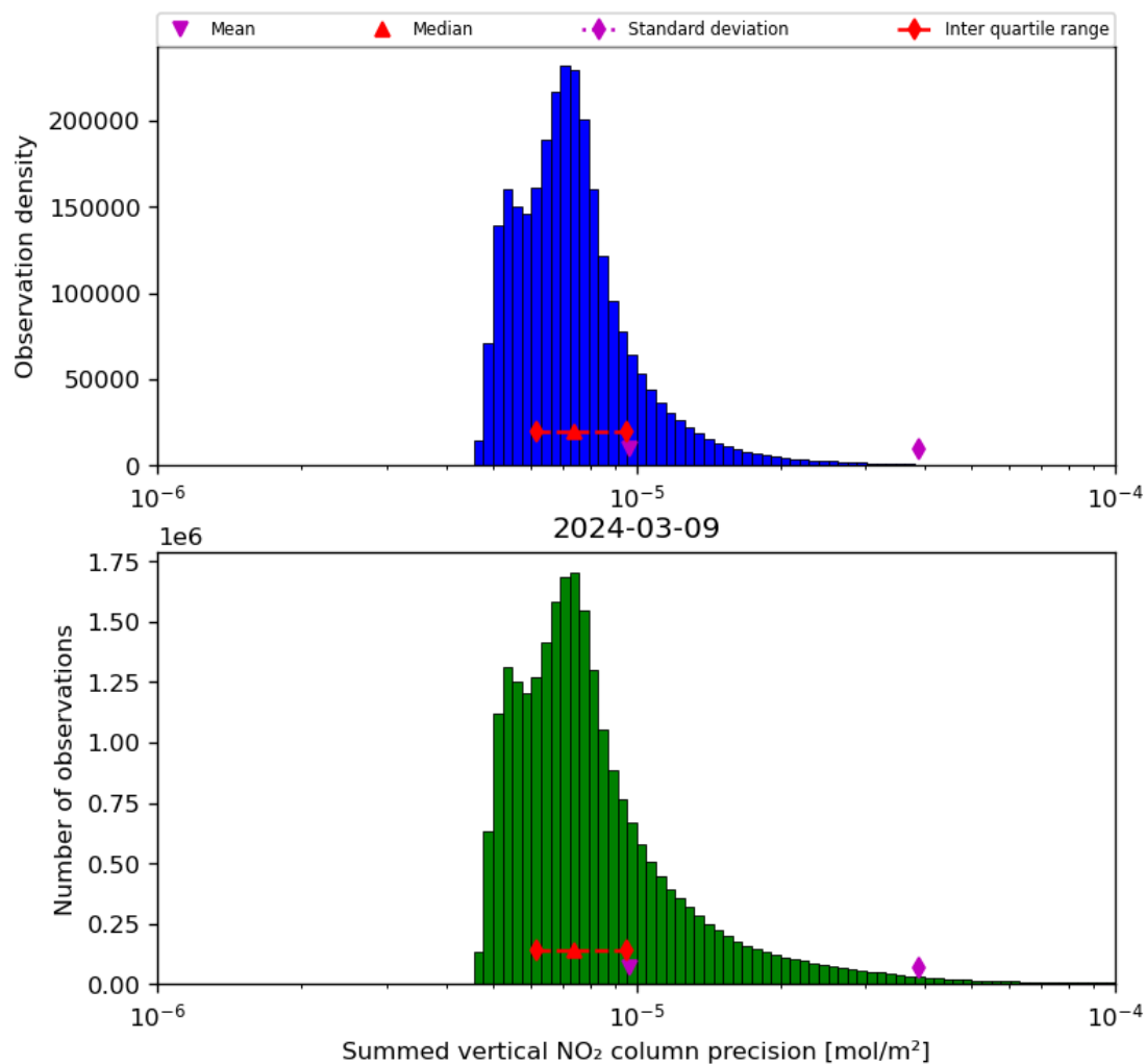
Figure 41: Histogram of “Summed vertical NO 2 column precision” for 2024-03-09 to 2024-03-10
