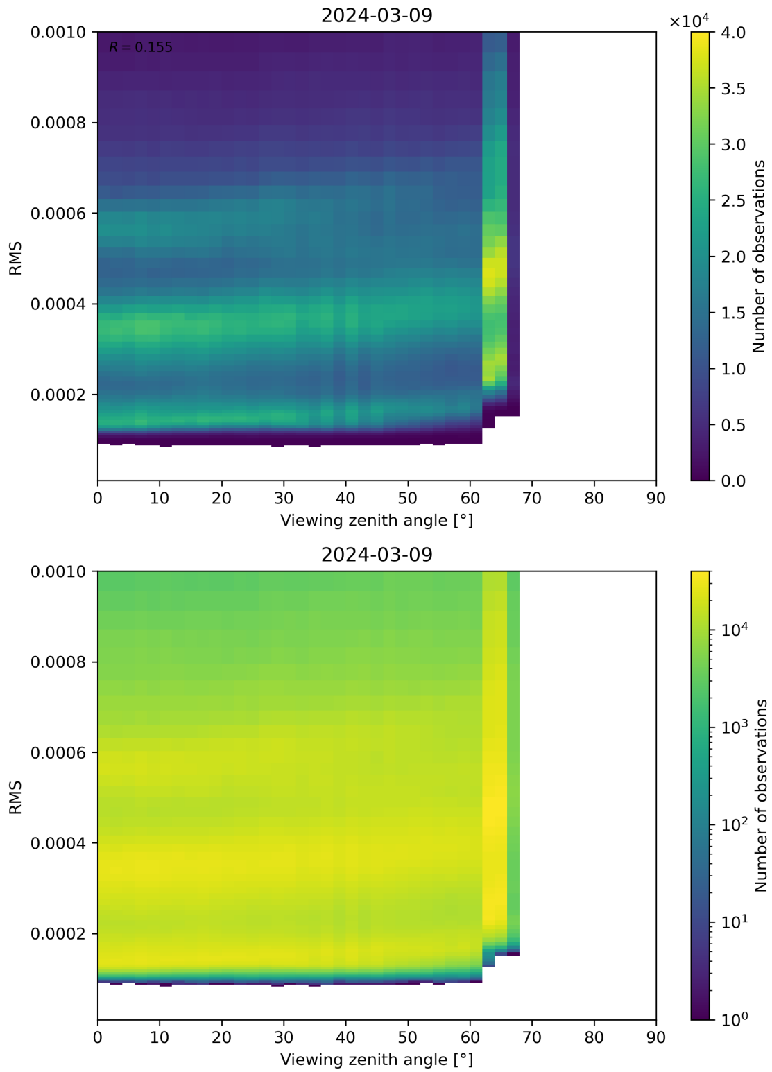
Figure 171: Scatter density plot of “Viewing zenith angle” against “RMS” for 2024-03-09 to 2024-03-10.
