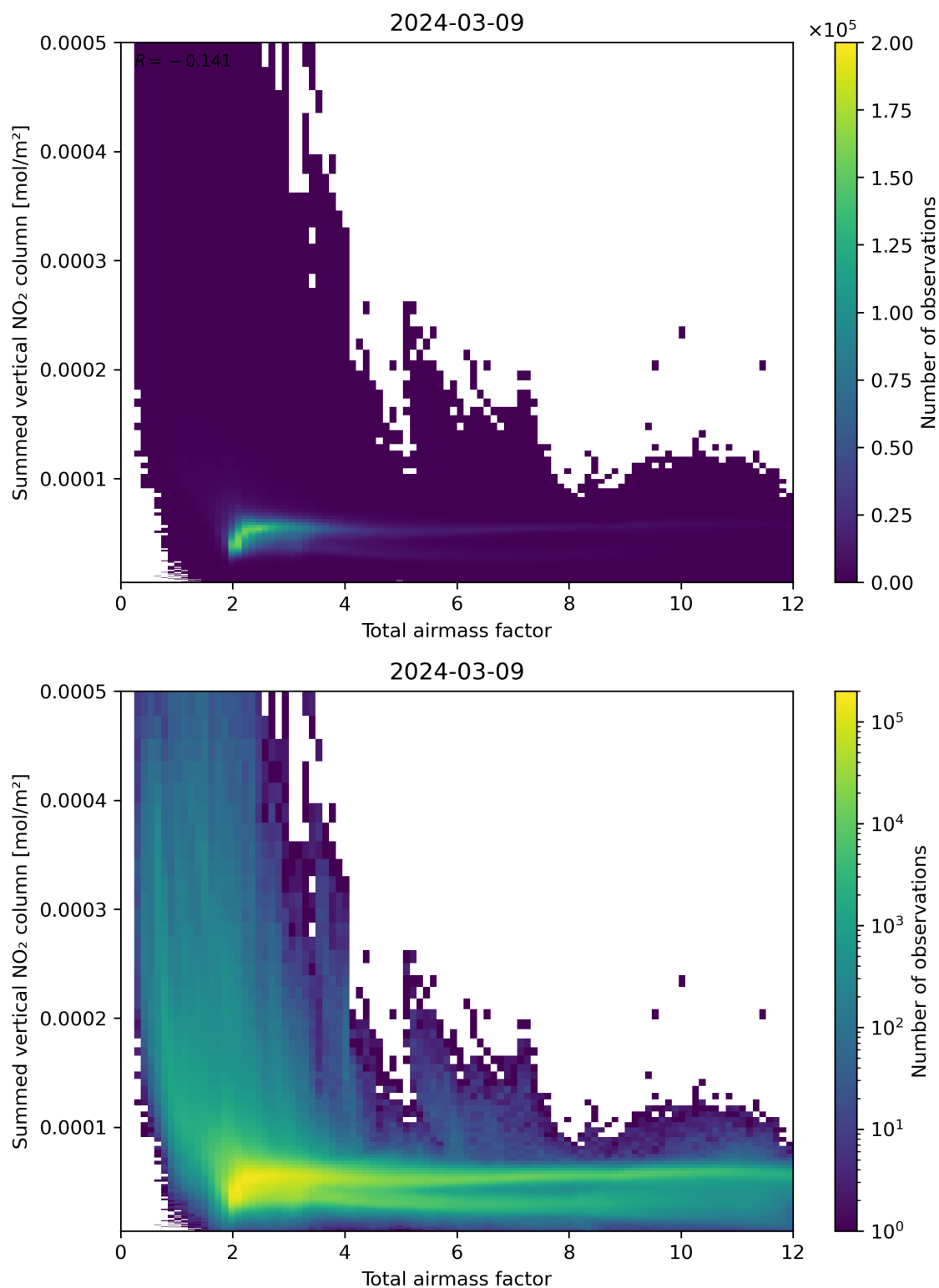
Figure 65: Scatter density plot of “Total airmass factor” against “Summed vertical NO 2 column” for 2024-03-09 to 2024-03-10.
