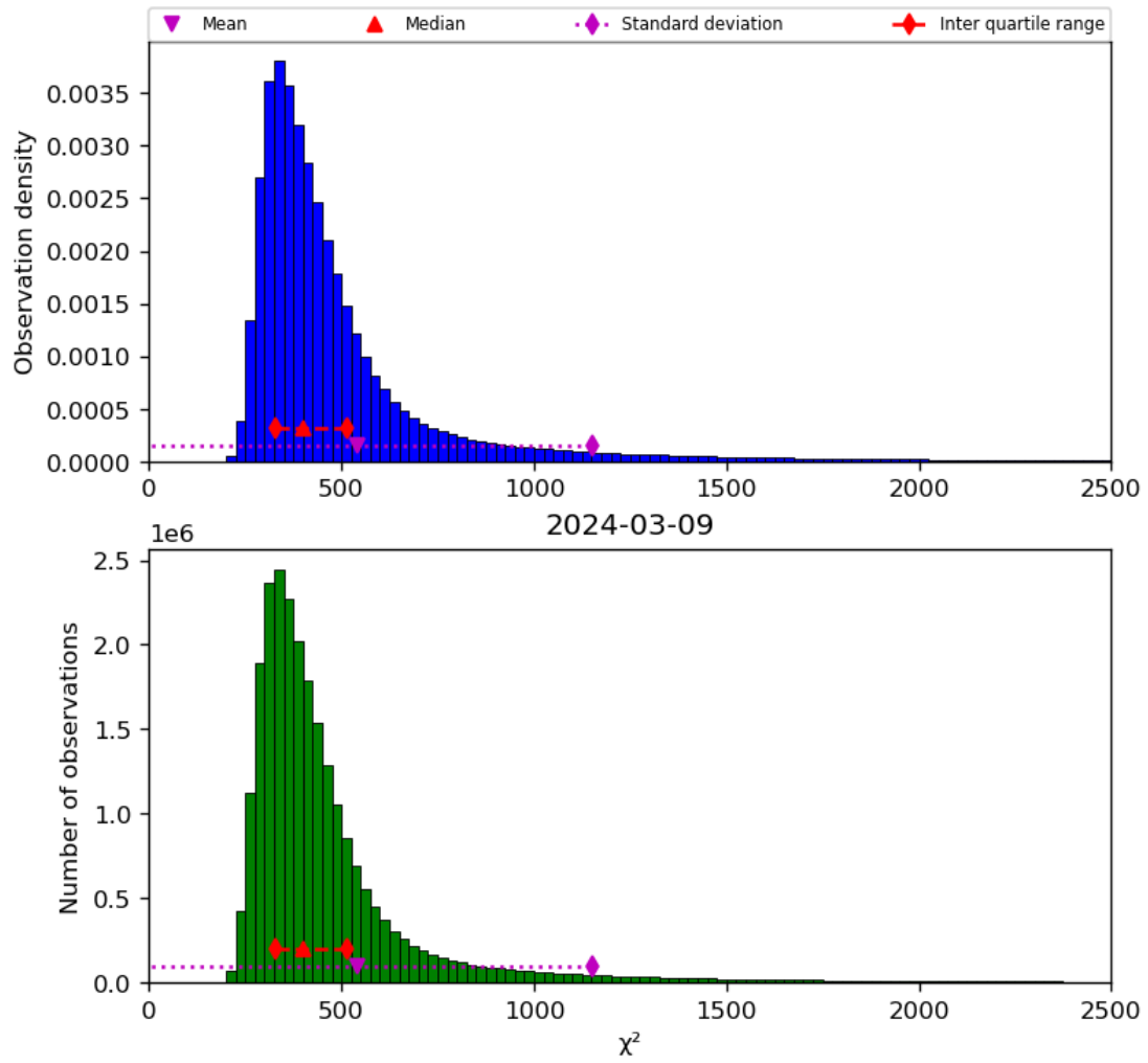
Figure 42: Histogram of “ \chi^2 ” for 2024-03-09 to 2024-03-10
