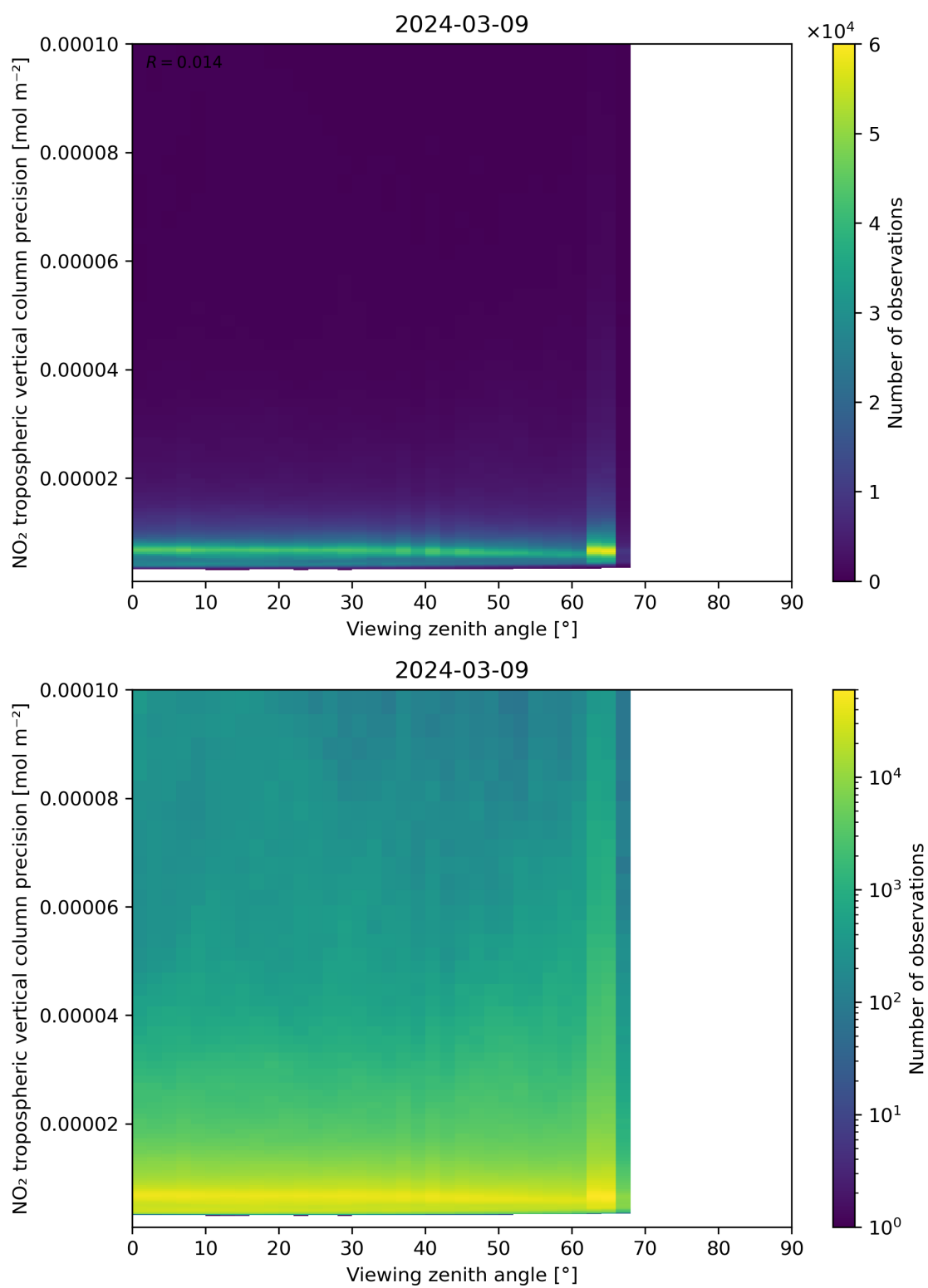
Figure 170: Scatter density plot of “Viewing zenith angle” against “NO 2 tropospheric vertical column precision” for 2024-03-09 to 2024-03-10.
