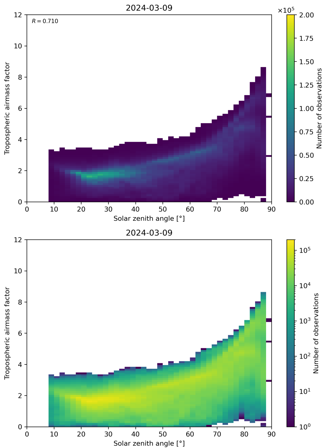
Figure 147: Scatter density plot of “Solar zenith angle” against “Tropospheric airmass factor” for 2024-03-09 to 2024-03-10.
