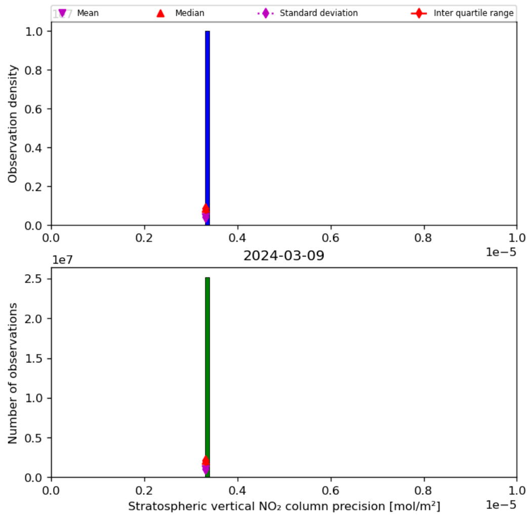
Figure 37: Histogram of “Stratospheric vertical NO 2 column precision” for 2024-03-09 to 2024-03-10
