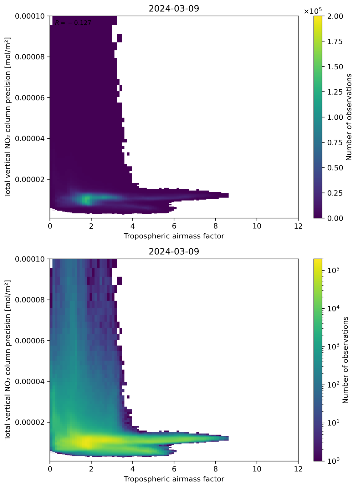
Figure 78: Scatter density plot of “Tropospheric air mass factor” against “Total vertical NO 2 column precision” for 2024-03-09 to 2024-03-10.
