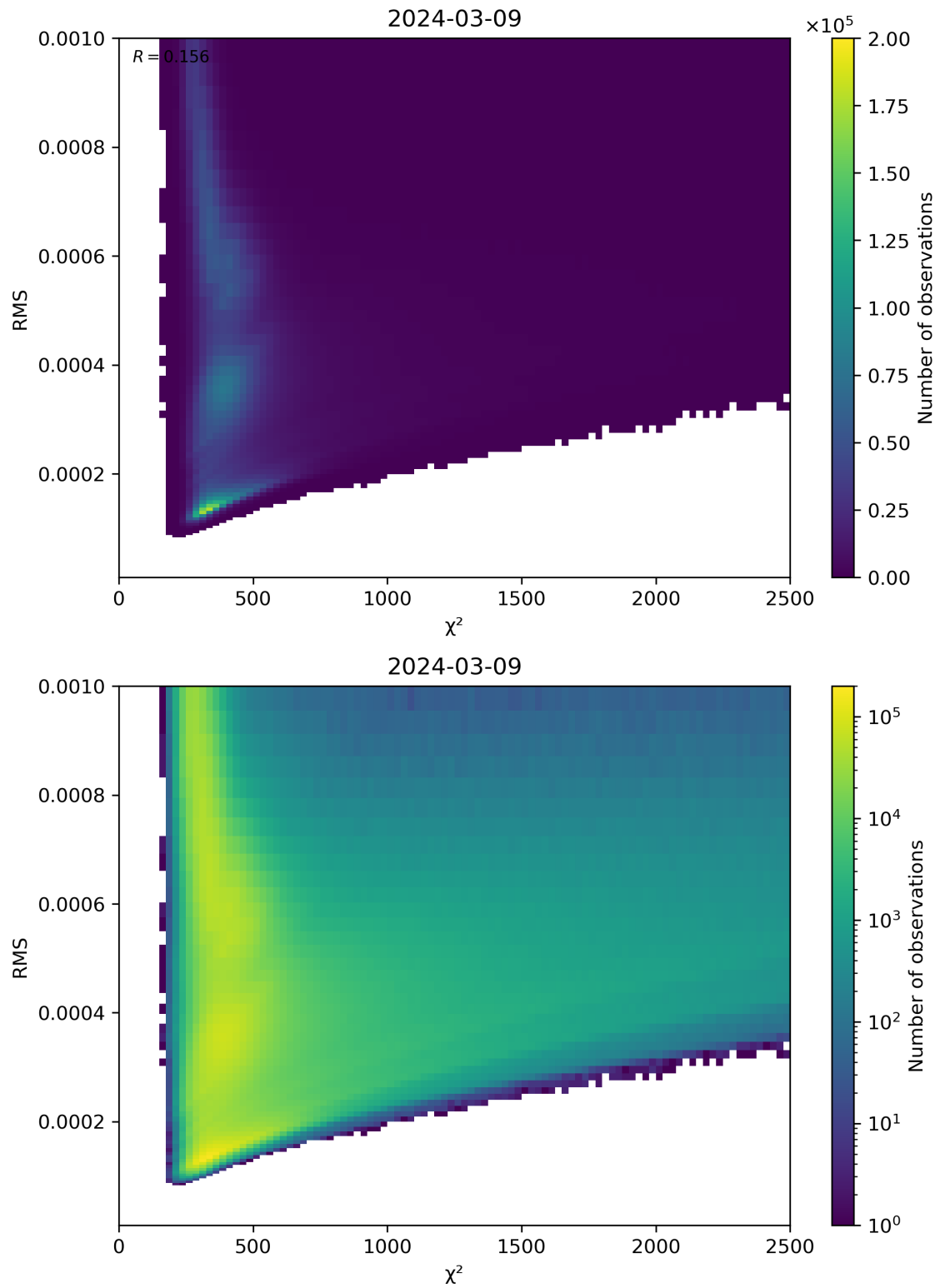
Figure 82: Scatter density plot of “ \chi^2 ” against “RMS” for 2024-03-09 to 2024-03-10.
