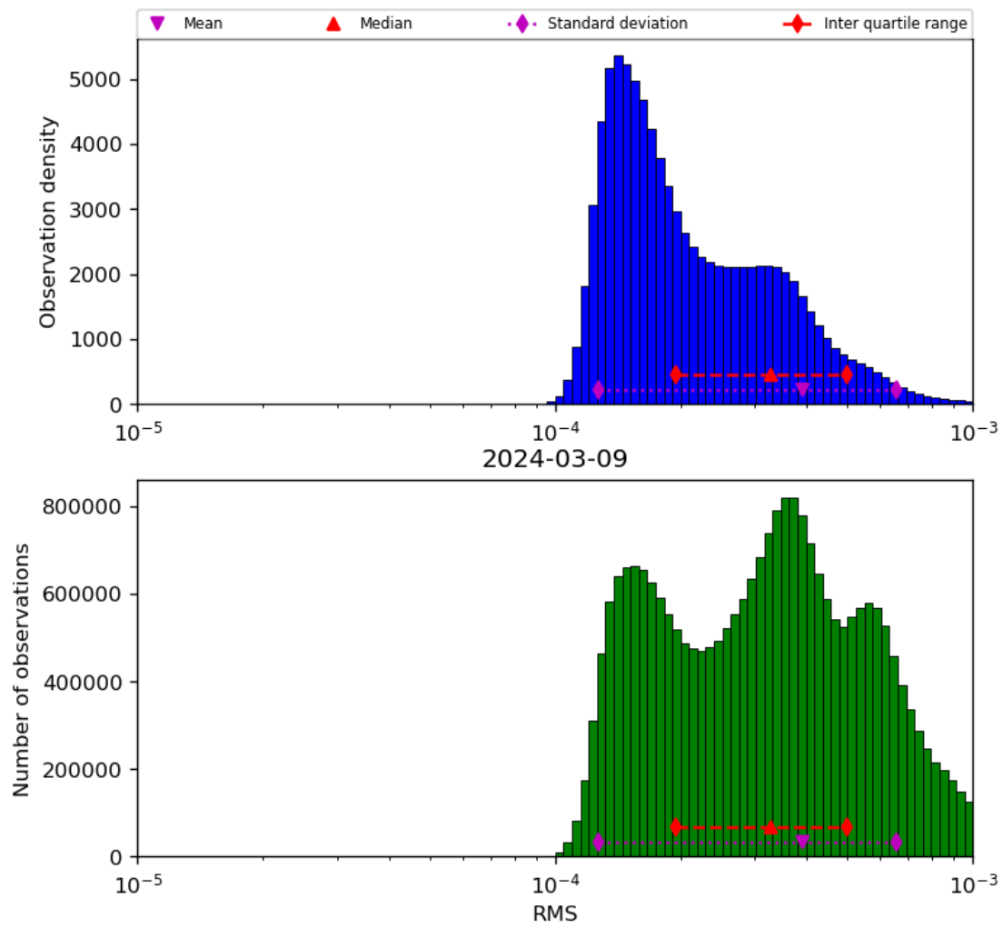
Figure 43: Histogram of “RMS” for 2024-03-09 to 2024-03-10
