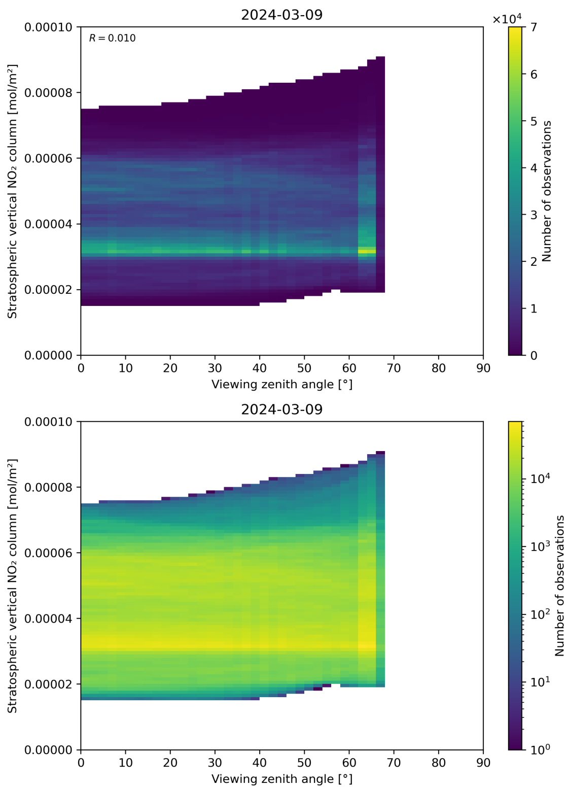
Figure 164: Scatter density plot of “Viewing zenith angle” against “Stratospheric vertical NO 2 column” for 2024-03-09 to 2024-03-10.
