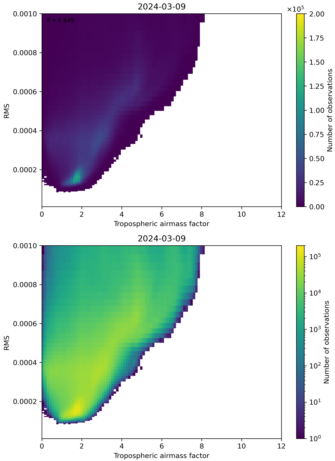
Figure 79: Scatter density plot of “Tropospheric airmass factor” against “RMS” for 2024-03-09 to 2024-03-10.
