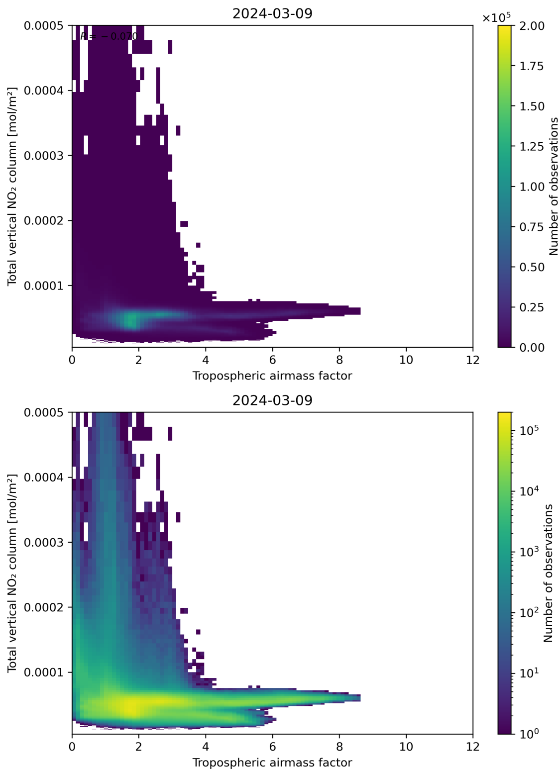
Figure 77: Scatter density plot of “Tropospheric airmass factor” against “Total vertical NO 2 column” for 2024-03-09 to 2024-03-10.
