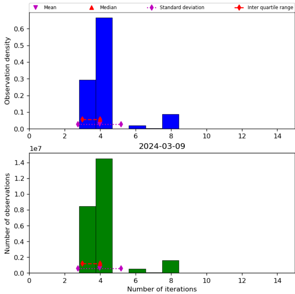
Figure 34: Histogram of “Number of iterations” for 2024-03-09 to 2024-03-10
