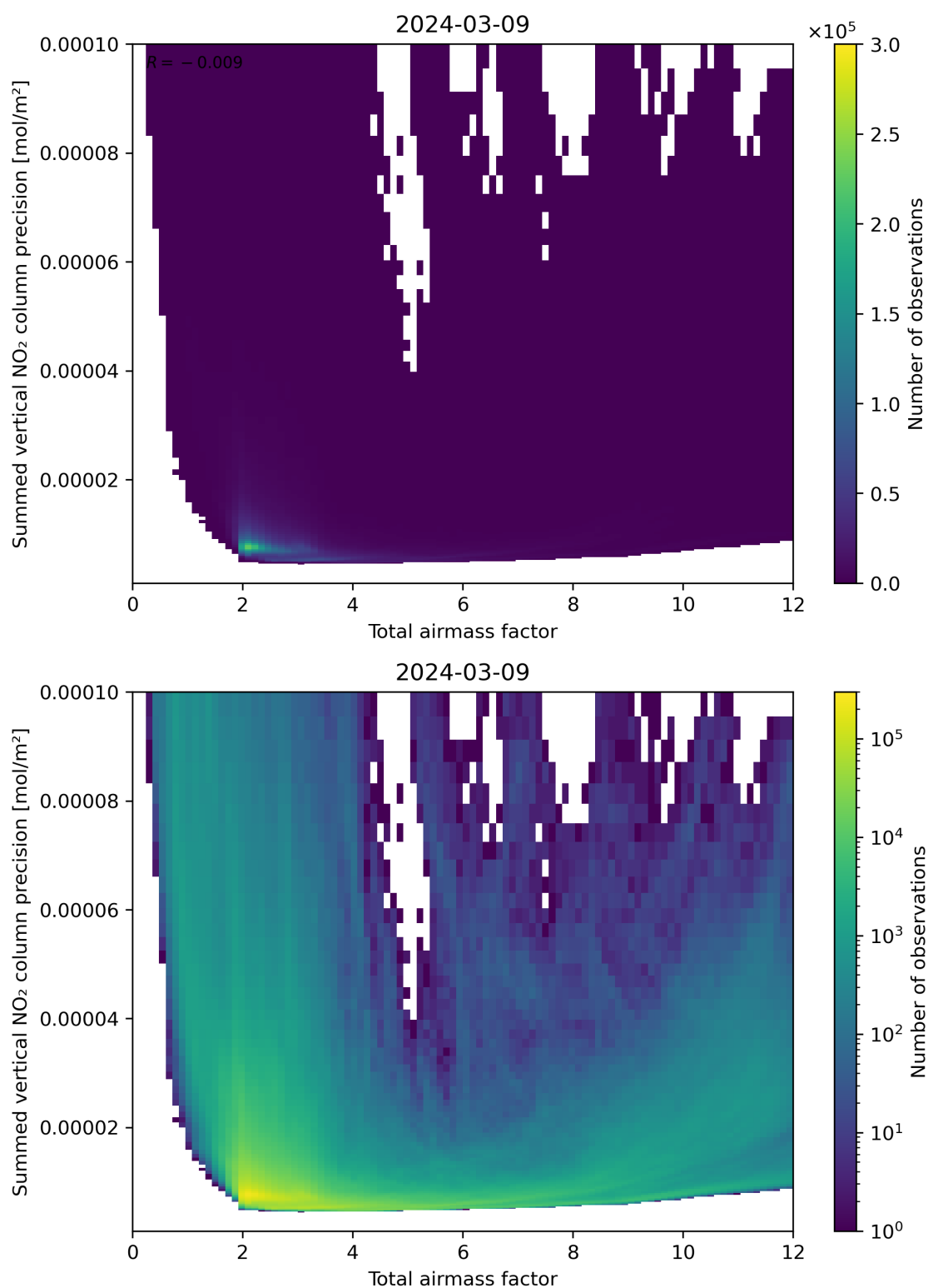
Figure 66: Scatter density plot of “Total airmass factor” against “Summed vertical NO 2 column precision” for 2024-03-09 to 2024-03-10.
