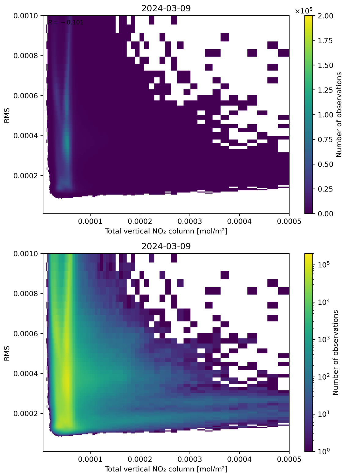
Figure 120: Scatter density plot of “Total vertical NO 2 column” against “RMS” for 2024-03-09 to 2024-03-10.
