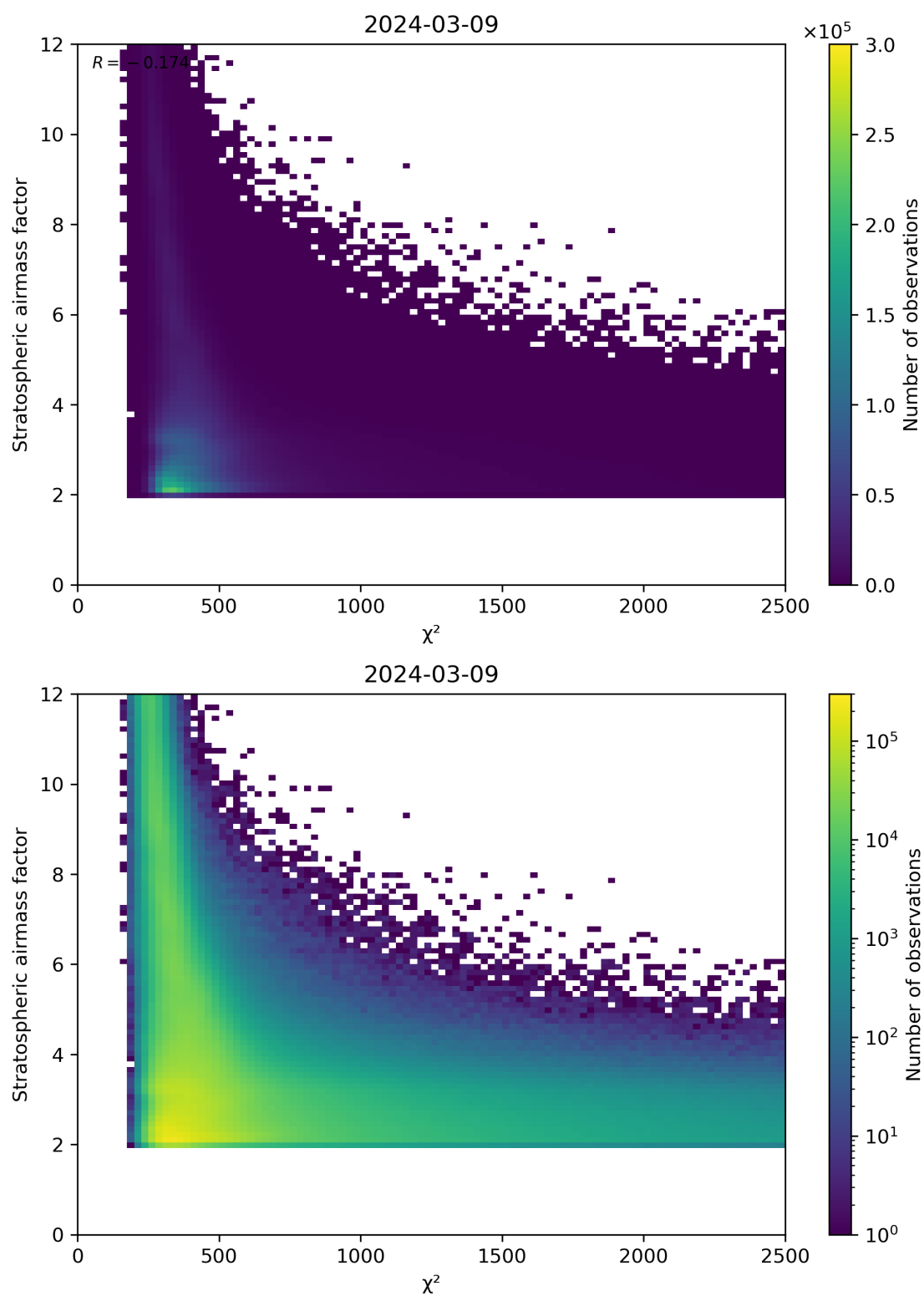
Figure 81: Scatter density plot of “ \chi^2 ” against “Stratospheric airmass factor” for 2024-03-09 to 2024-03-10.
