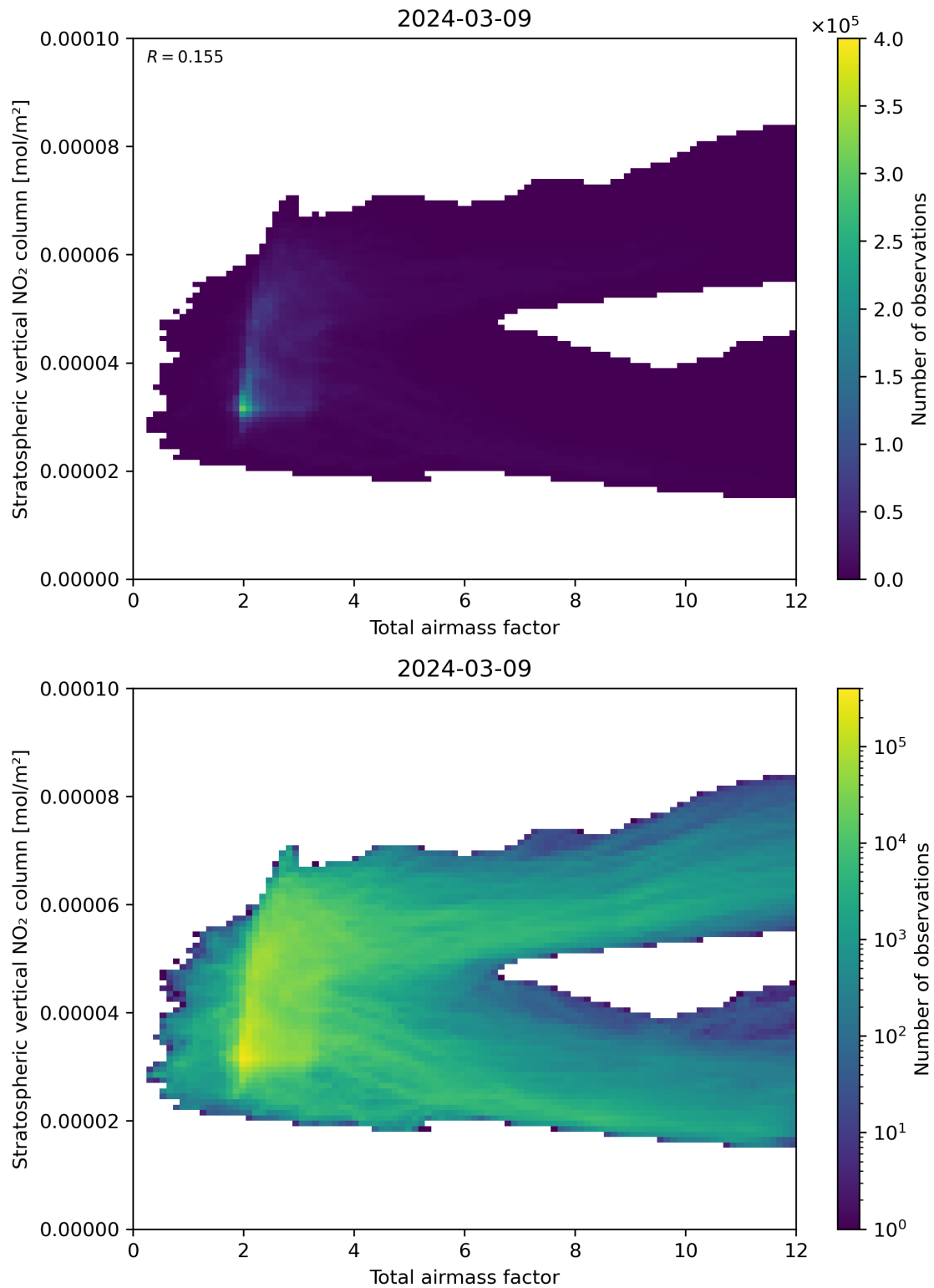
Figure 64: Scatter density plot of “Total airmass factor” against “Stratospheric vertical NO 2 column” for 2024-03-09 to 2024-03-10.
