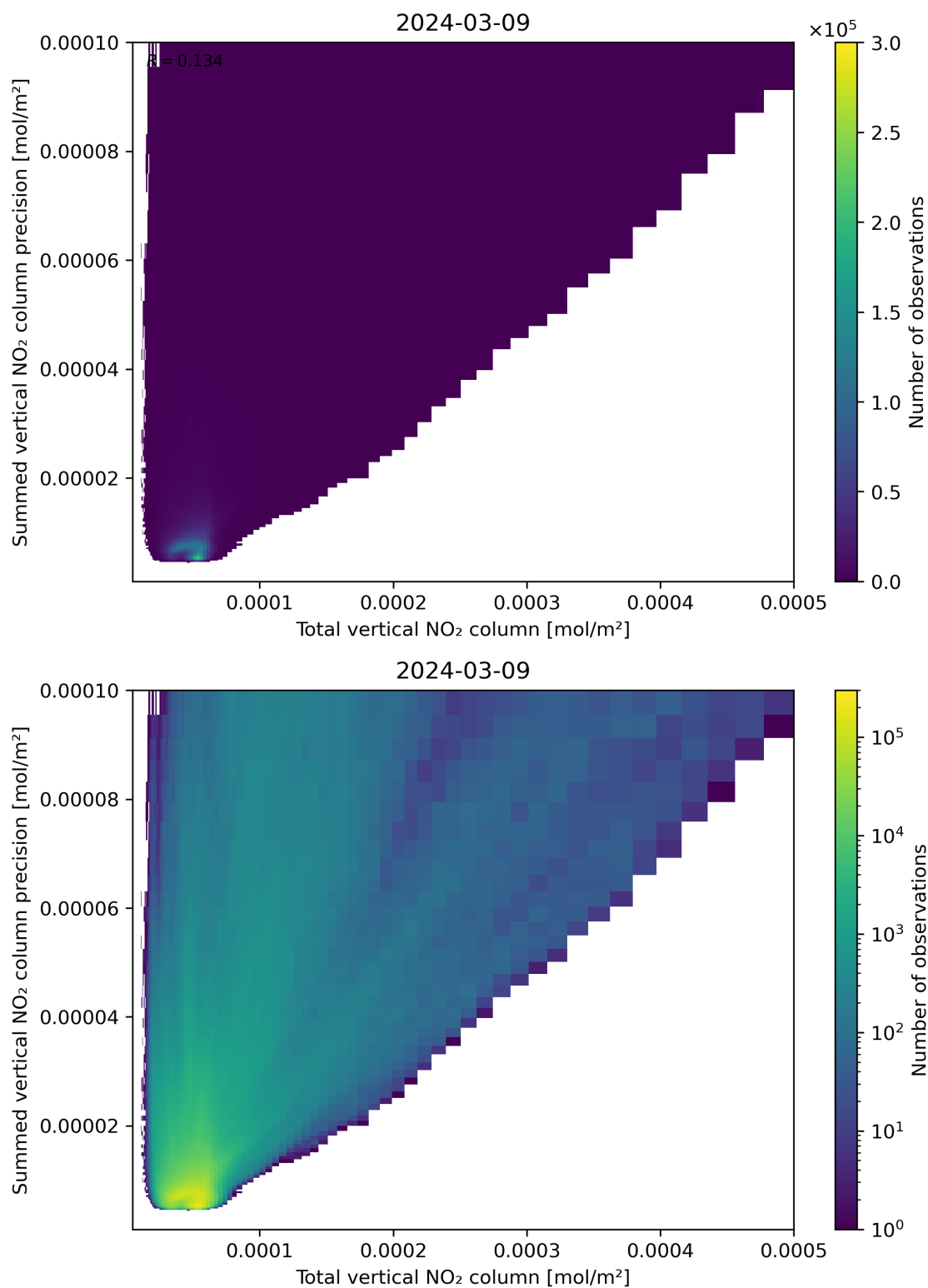
Figure 113: Scatter density plot of “Total vertical NO 2 column” against “Summed vertical NO 2 column precision” for 2024-03-09 to 2024-03-10.
