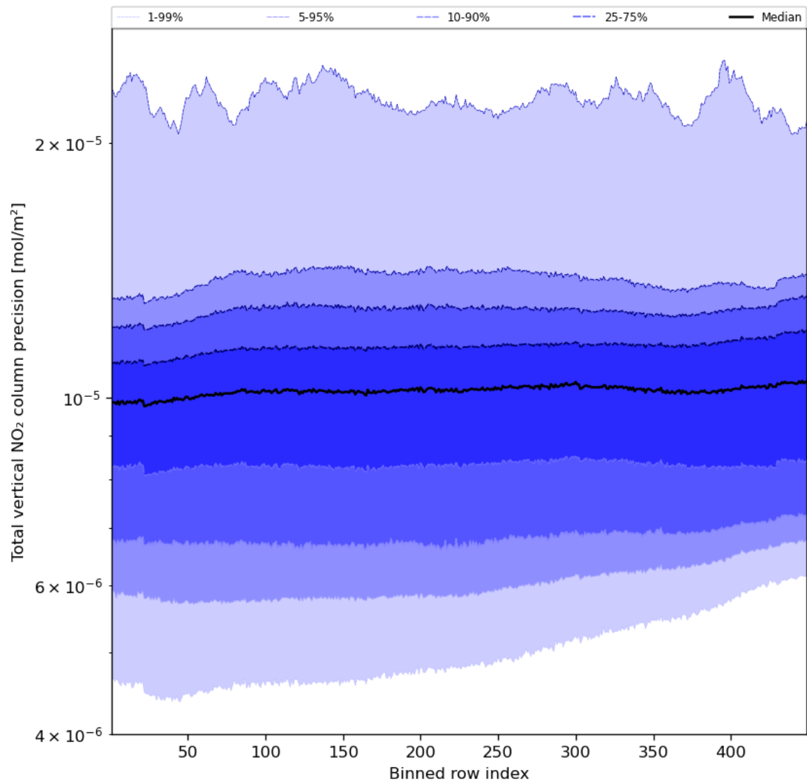
Figure 56: Along track statistics of “Total vertical NO 2 column precision” for 2024-03-09 to 2024-03-10
