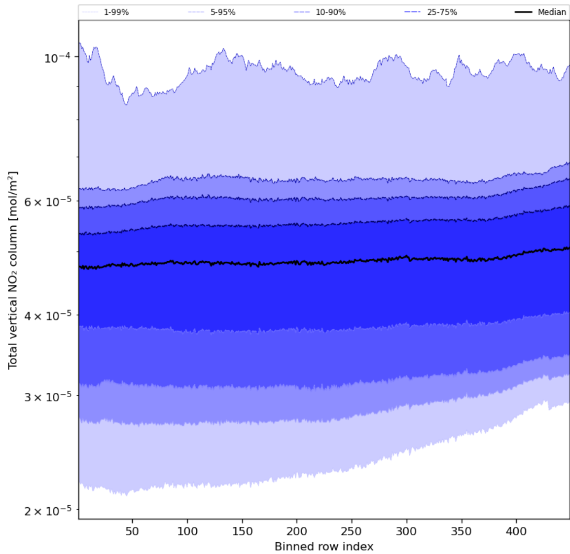
Figure 55: Along track statistics of “Total vertical NO 2 column” for 2024-03-09 to 2024-03-10
