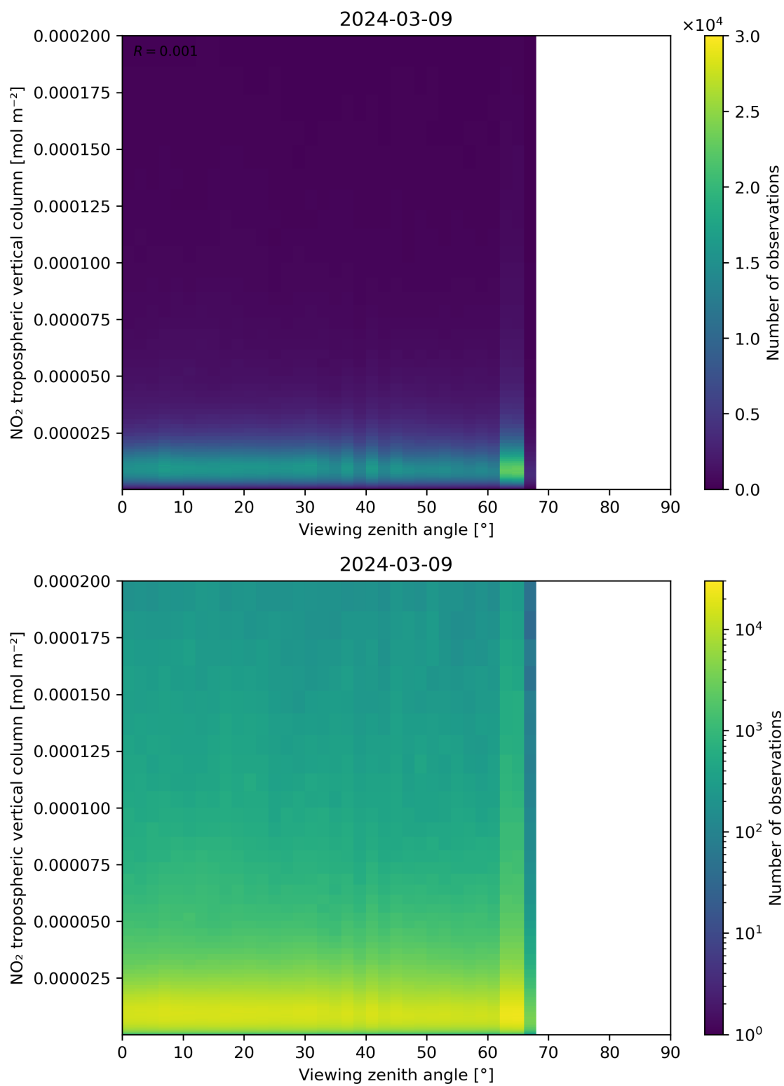
Figure 169: Scatter density plot of “Viewing zenith angle” against “NO 2 tropospheric vertical column” for 2024-03-09 to 2024-03-10.
