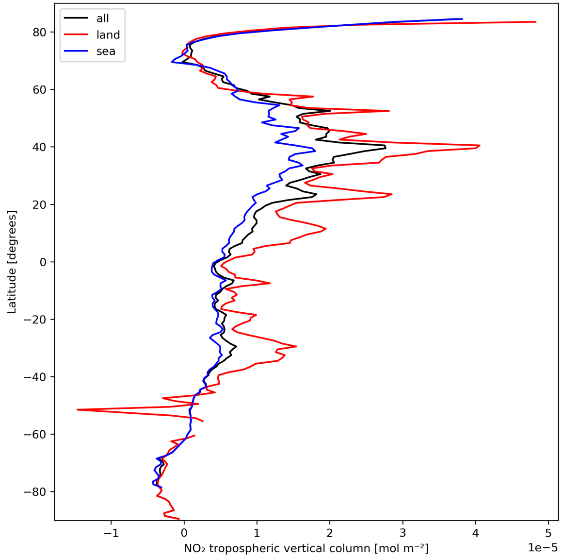
Figure 12: Zonal average of “NO 2 tropospheric vertical column” for 2024-03-09 to 2024-03-10.
