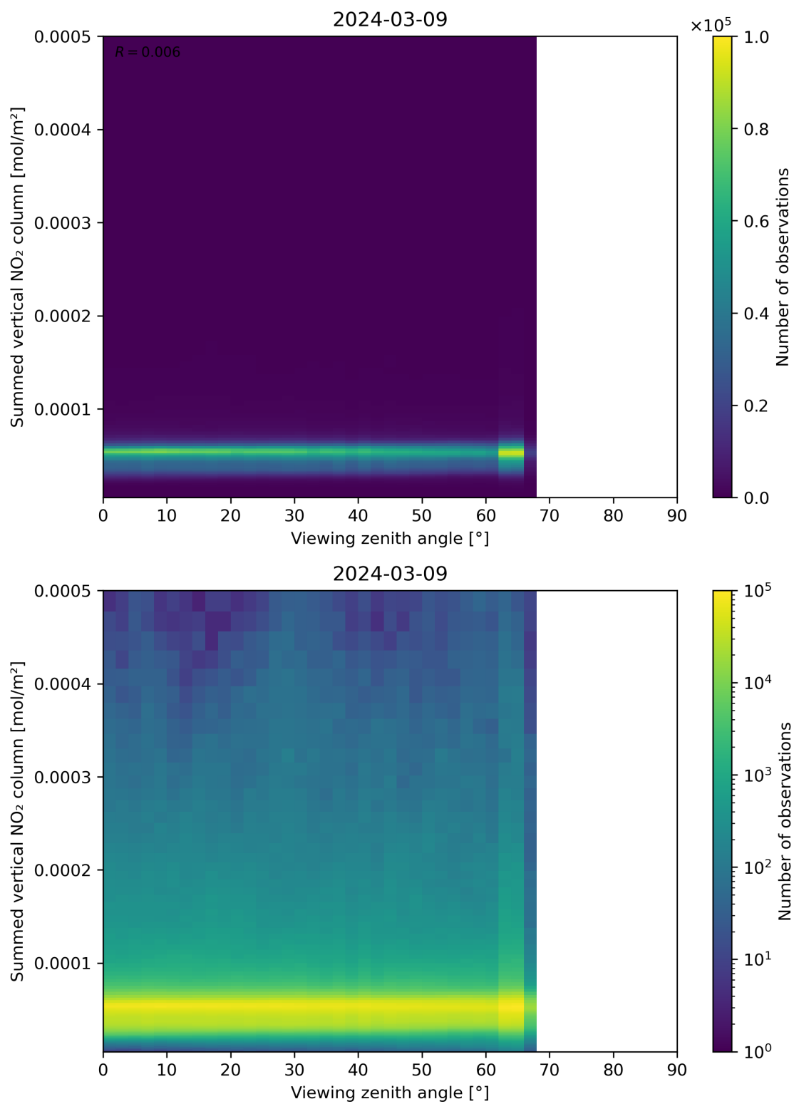
Figure 165: Scatter density plot of “Viewing zenith angle” against “Summed vertical NO 2 column” for 2024-03-09 to 2024-03-10.
