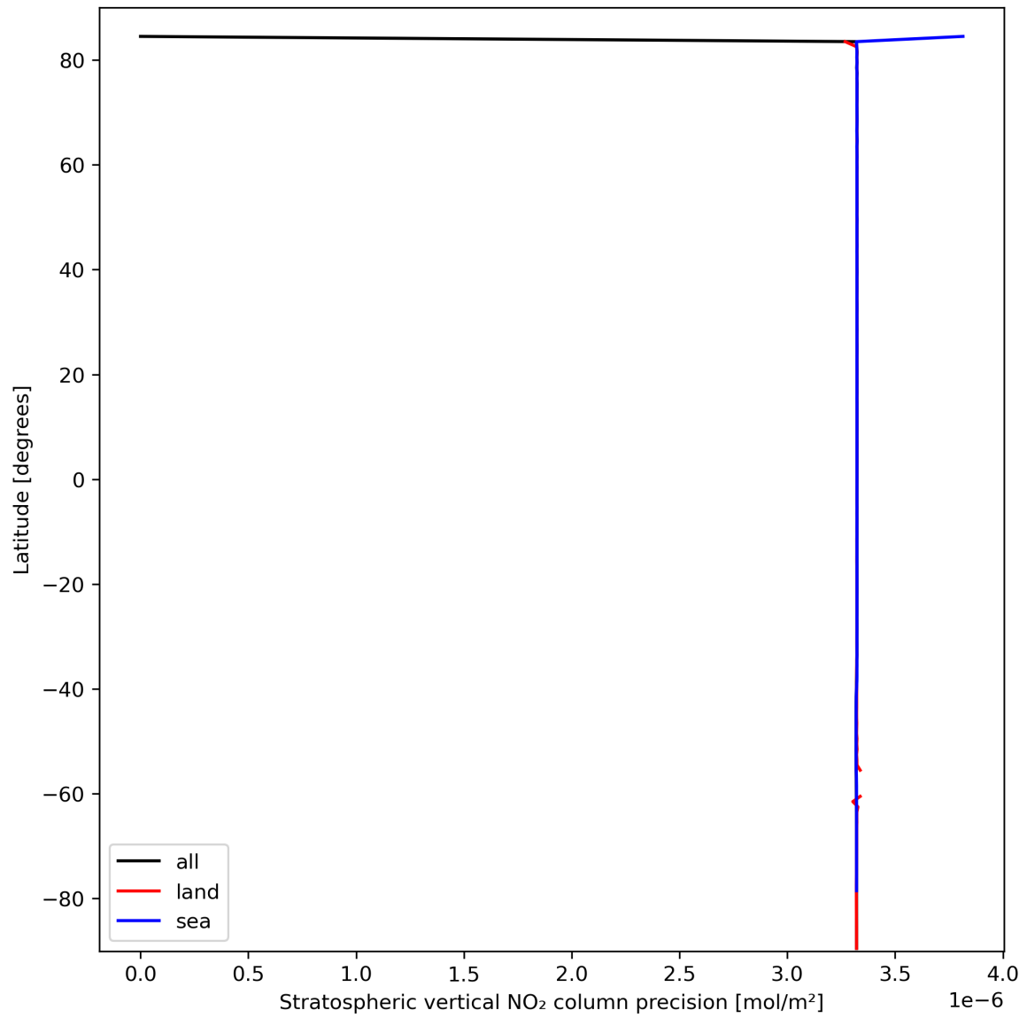
Figure 20: Zonal average of “Stratospheric vertical NO 2 column precision” for 2024-03-09 to 2024-03-10.
