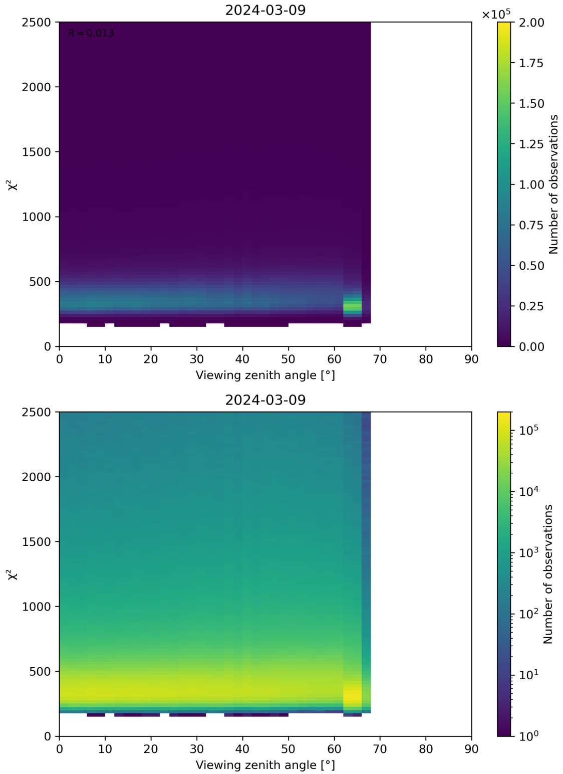
Figure 162: Scatter density plot of “Viewing zenith angle” against “ \chi^2 ” for 2024-03-09 to 2024-03-10.
