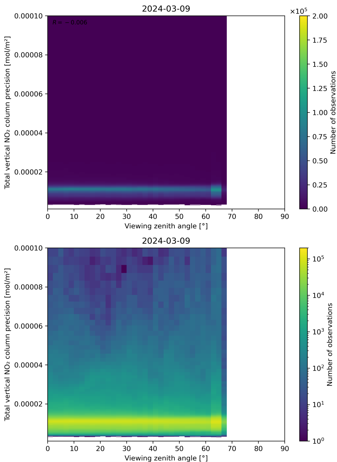
Figure 168: Scatter density plot of “Viewing zenith angle” against “Total vertical NO 2 column precision” for 2024-03-09 to 2024-03-10.
