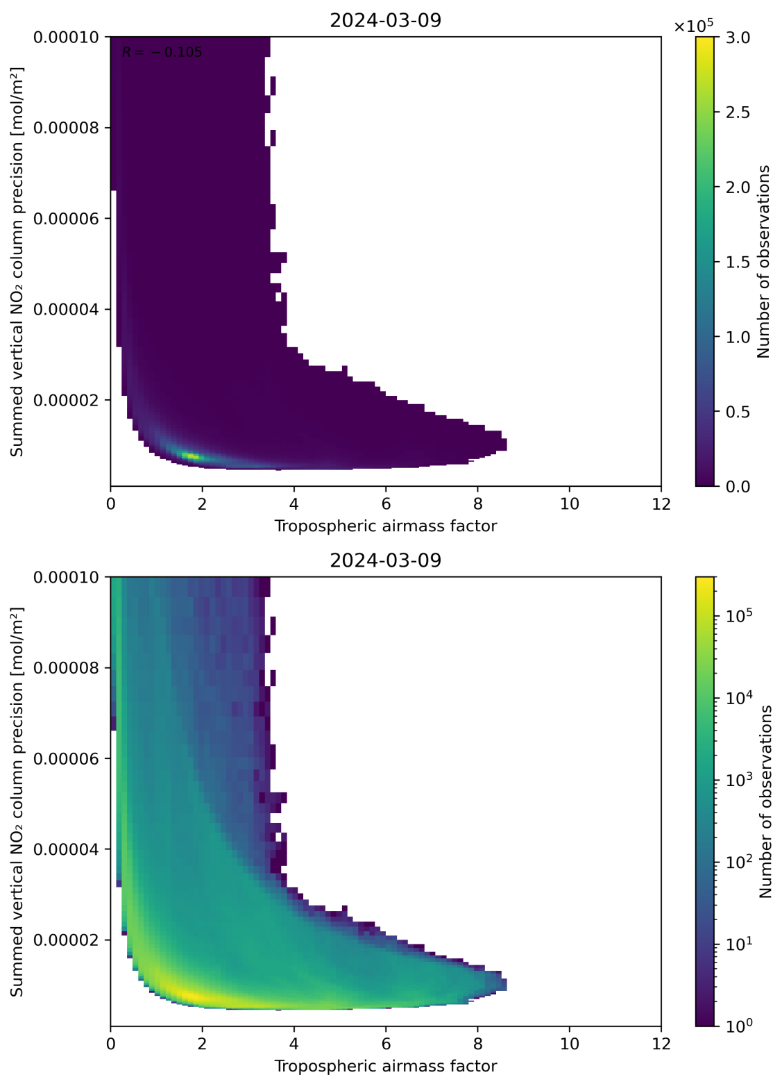
Figure 76: Scatter density plot of “Tropospheric air mass factor” against “Summed vertical NO 2 column precision” for 2024-03-09 to 2024-03-10.
