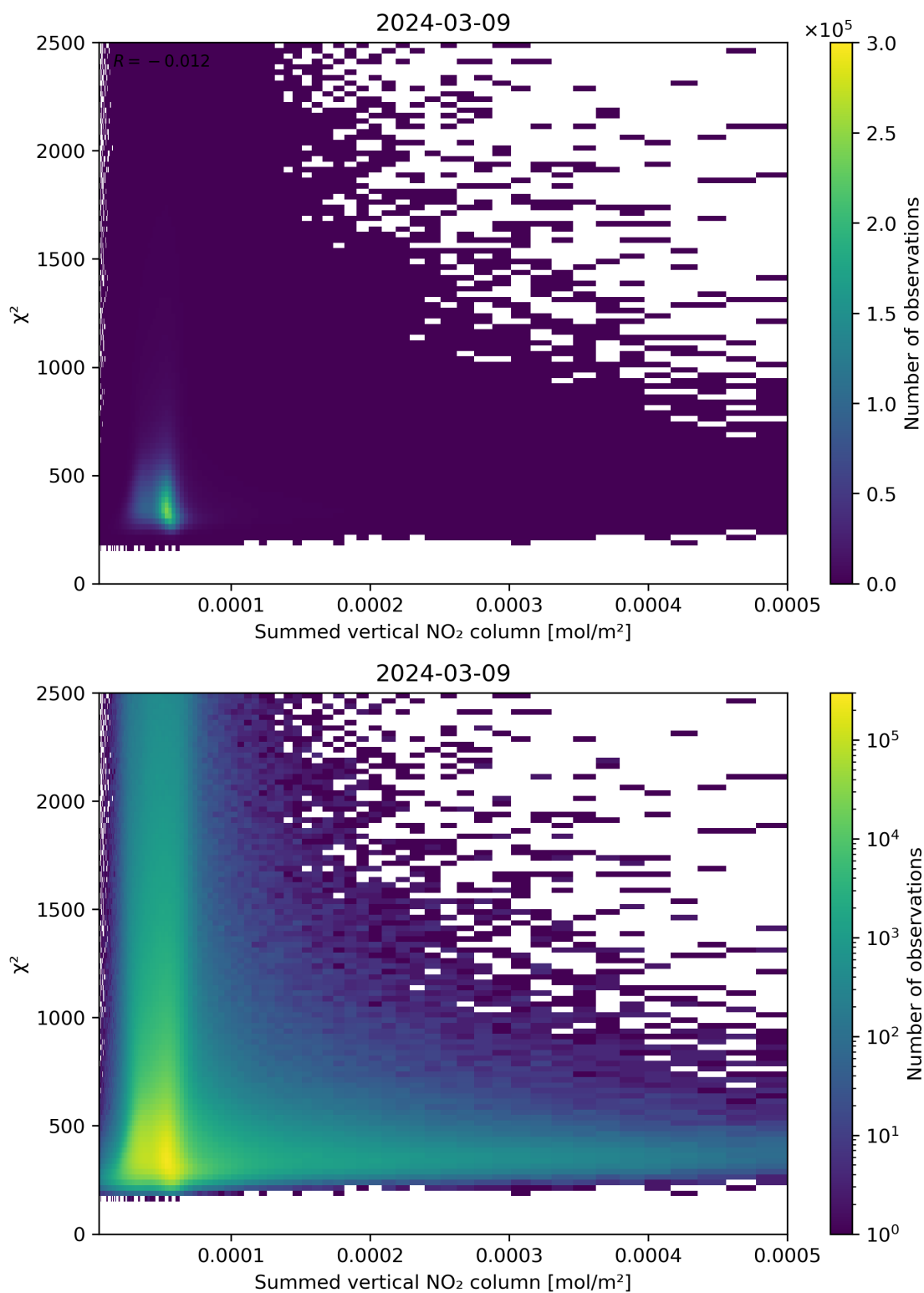
Figure 104: Scatter density plot of “Summed vertical NO 2 column” against “ \chi^2 ” for 2024-03-09 to 2024-03-10.
