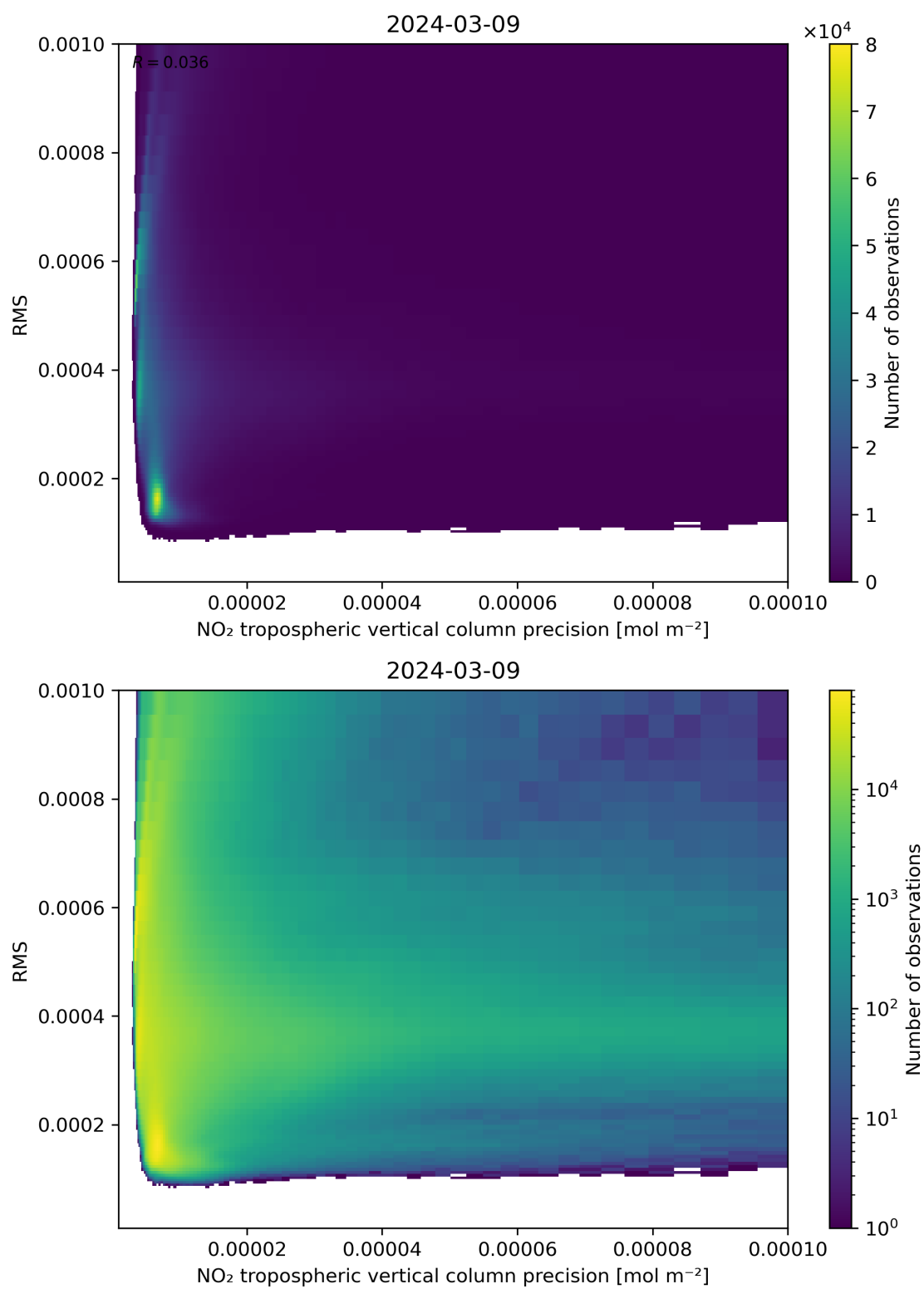
Figure 140: Scatter density plot of “NO 2 tropospheric vertical column precision” against “RMS” for 2024-03-09 to 2024-03-10.
