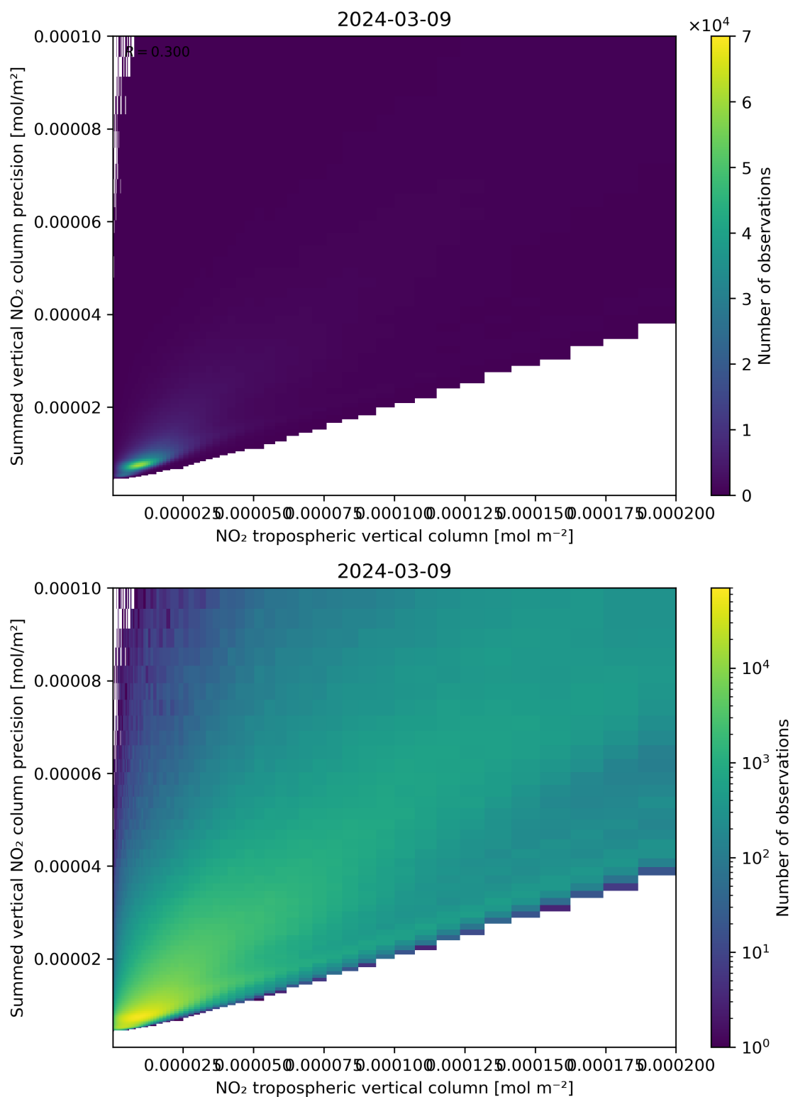
Figure 127: Scatter density plot of “NO 2 tropospheric vertical column” against “Summed vertical NO 2 column precision” for 2024-03-09 to 2024-03-10.
