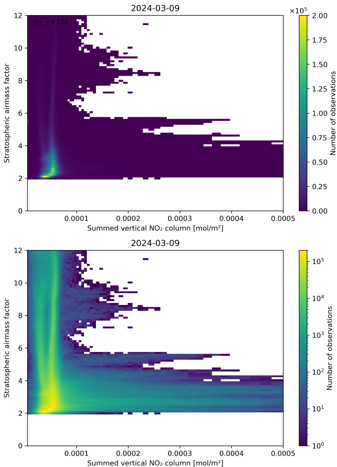
Figure 103: Scatter density plot of “Summed vertical NO 2 column” against “Stratospheric air mass factor” for 2024-03-09 to 2024-03-10.
