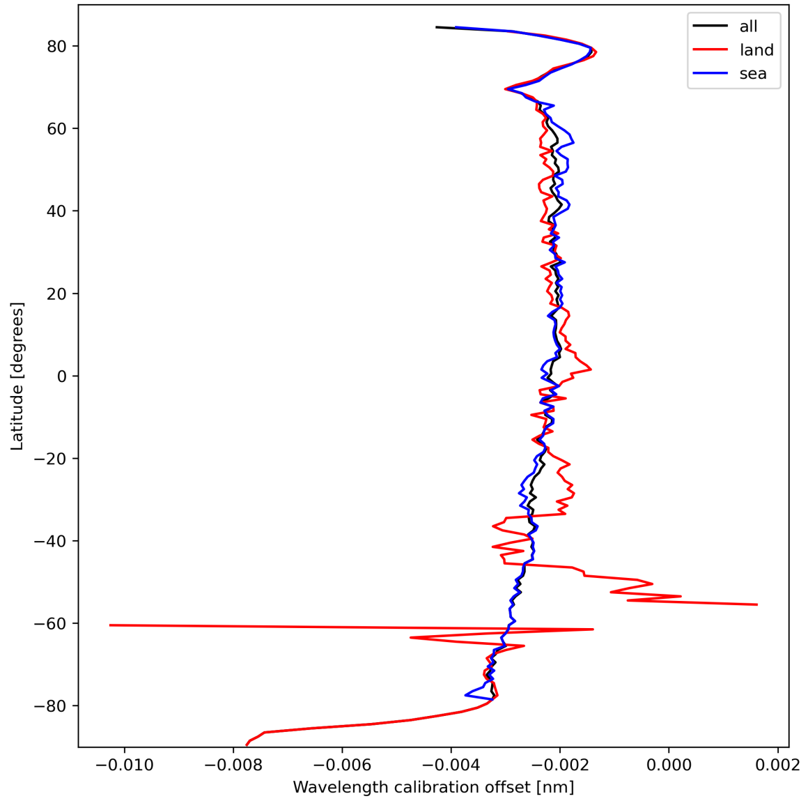
Figure 18: Zonal average of “Wavelength calibration offset” for 2024-03-09 to 2024-03-10.
