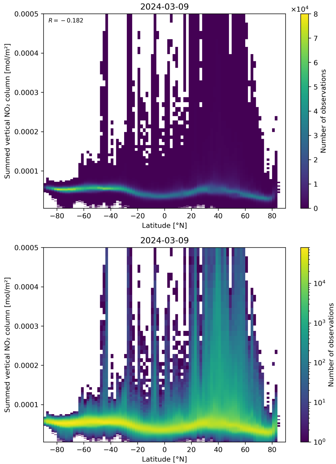
Figure 88: Scatter density plot of “Latitude” against “Summed vertical NO 2 column” for 2024-03-09 to 2024-03-10.
