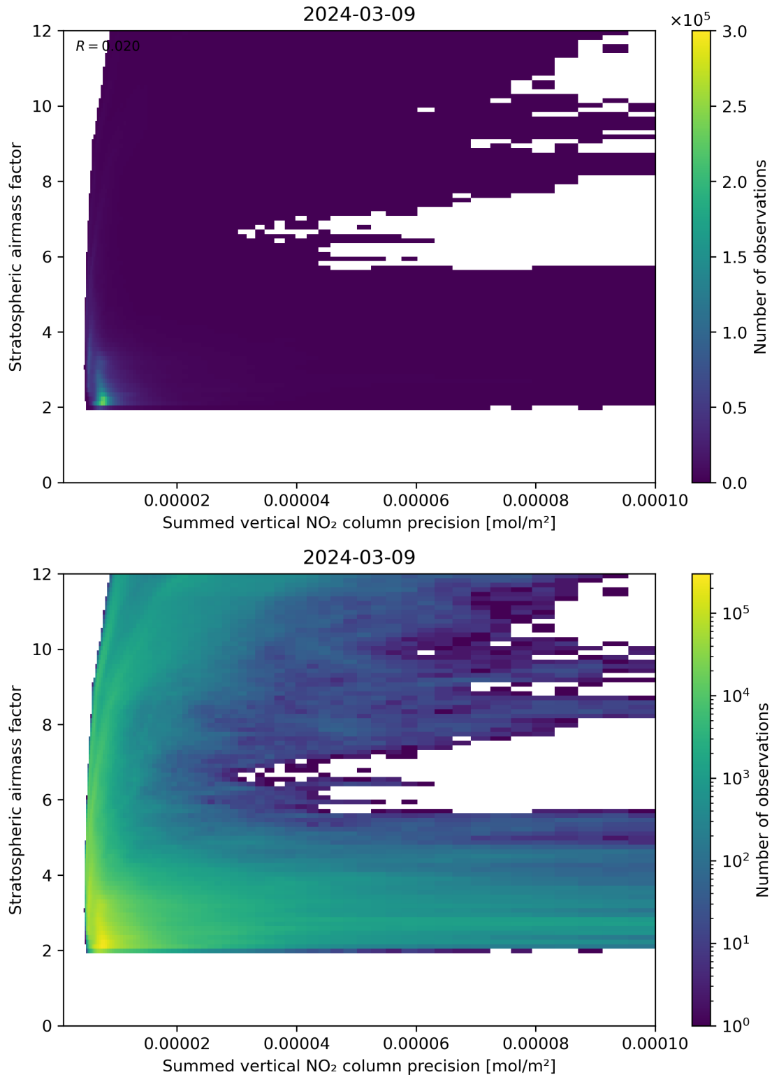
Figure 106: Scatter density plot of “Summed vertical NO 2 column precision” against “Stratospheric airmass factor” for 2024-03-09 to 2024-03-10.
