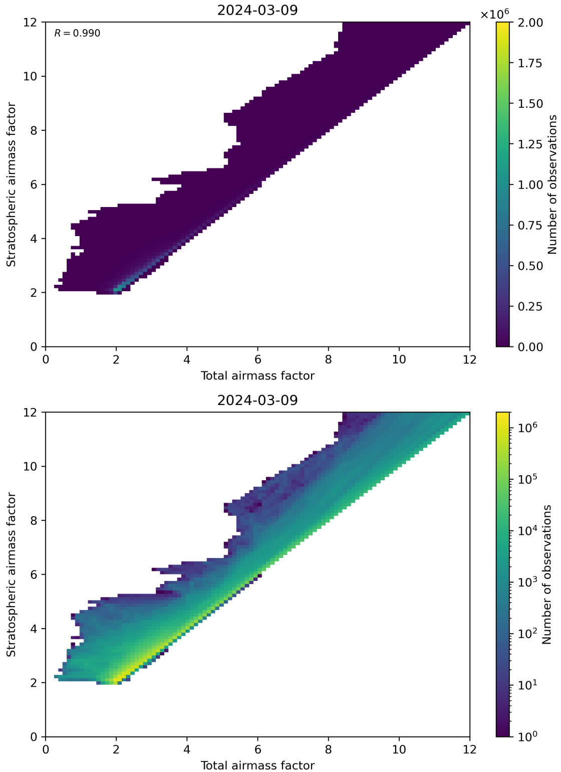
Figure 62: Scatter density plot of “Total airmass factor” against “Stratospheric airmass factor” for 2024-03-09 to 2024-03-10.
