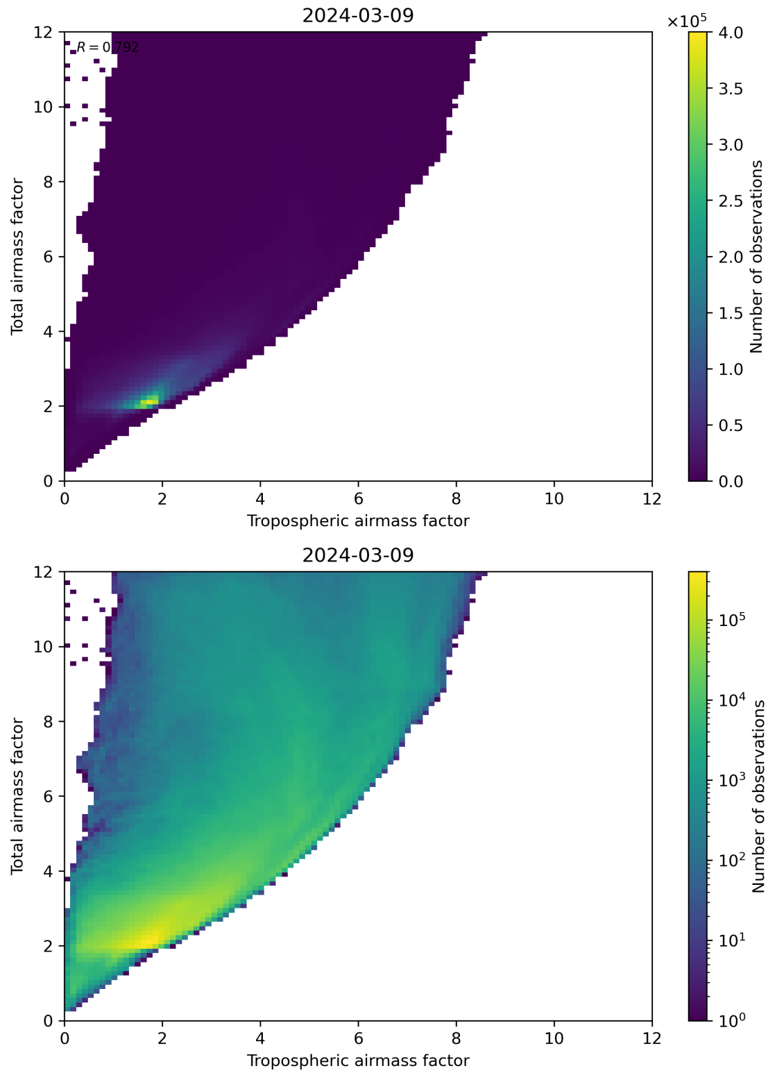
Figure 72: Scatter density plot of “Tropospheric airmass factor” against “Total airmass factor” for 2024-03-09 to 2024-03-10.
