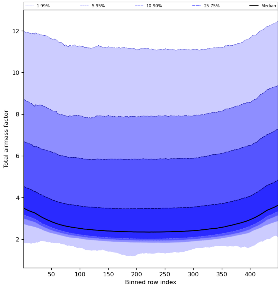
Figure 49: Along track statistics of “Total airmass factor” for 2024-03-09 to 2024-03-10
