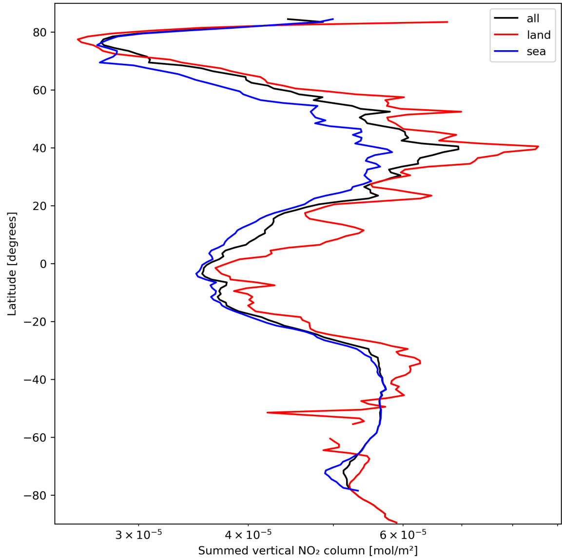
Figure 23: Zonal average of “Summed vertical NO 2 column” for 2024-03-09 to 2024-03-10.
