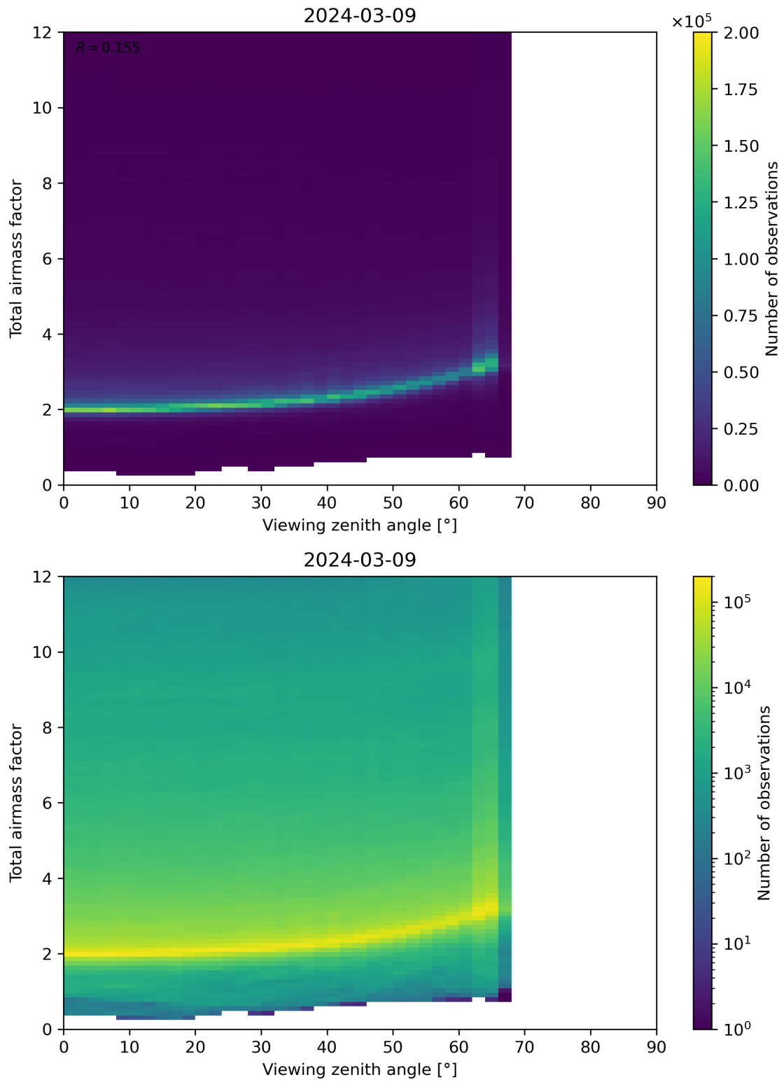
Figure 160: Scatter density plot of “Viewing zenith angle” against “Total airmass factor” for 2024-03-09 to 2024-03-10.
