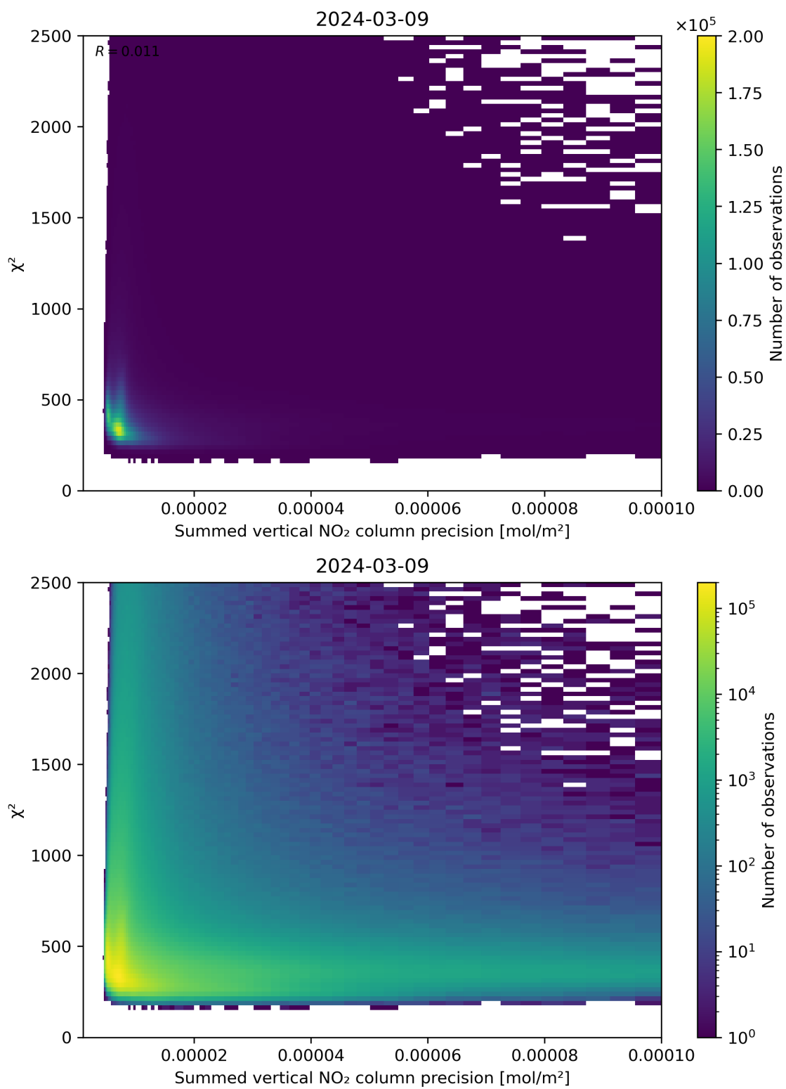
Figure 107: Scatter density plot of “Summed vertical NO 2 column precision” against “ \chi^2 ” for 2024-03-09 to 2024-03-10.
