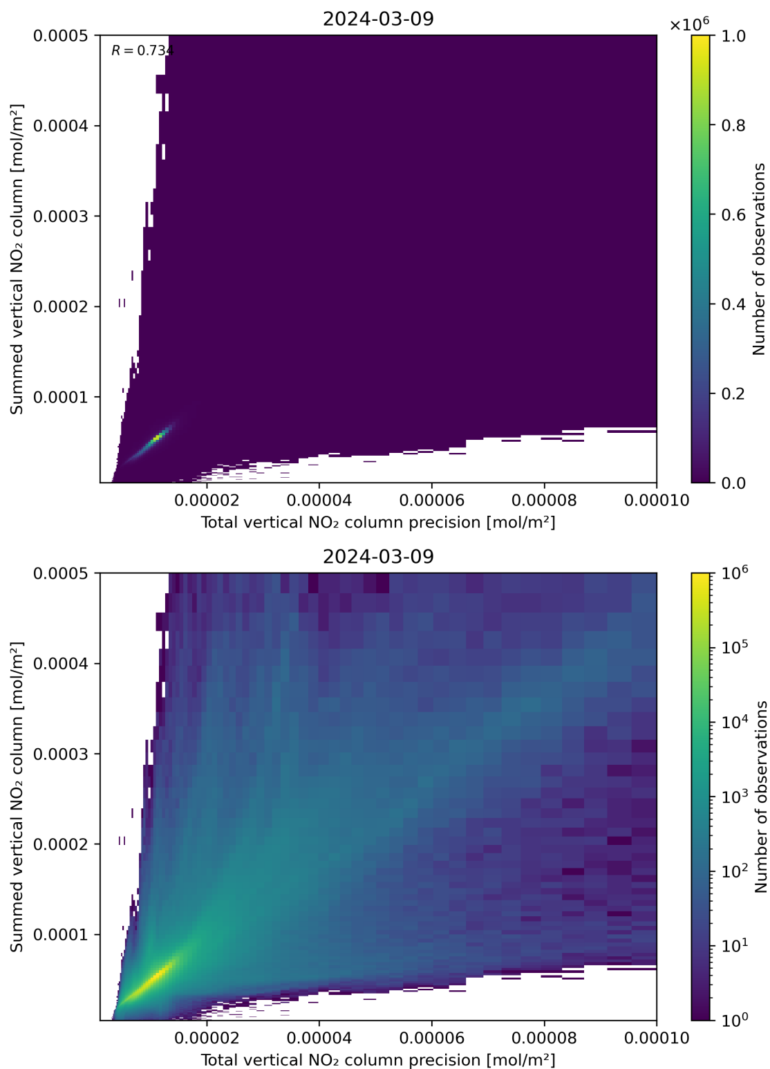
Figure 117: Scatter density plot of “Total vertical NO 2 column precision” against “Summed vertical NO 2 column” for 2024-03-09 to 2024-03-10.
