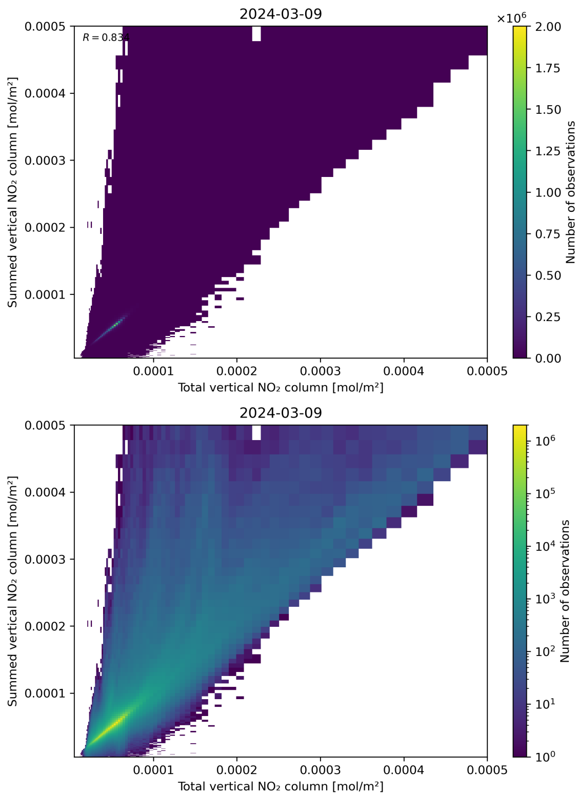
Figure 112: Scatter density plot of “Total vertical NO 2 column” against “Summed vertical NO 2 column” for 2024-03-09 to 2024-03-10.
