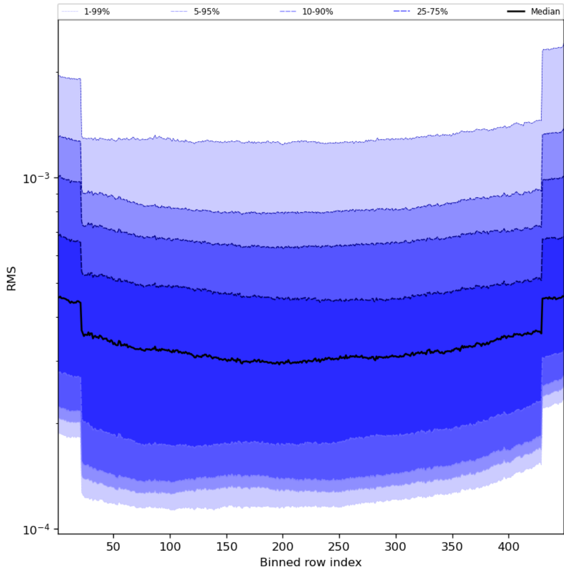
Figure 60: Along track statistics of “RMS” for 2024-03-09 to 2024-03-10
