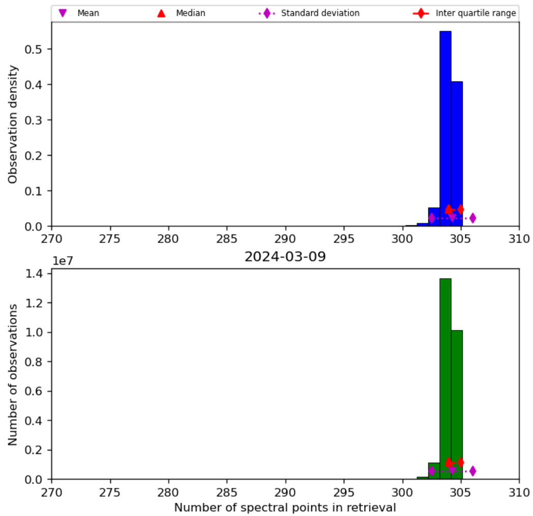
Figure 33: Histogram of “Number of spectral points in retrieval” for 2024-03-09 to 2024-03-10
