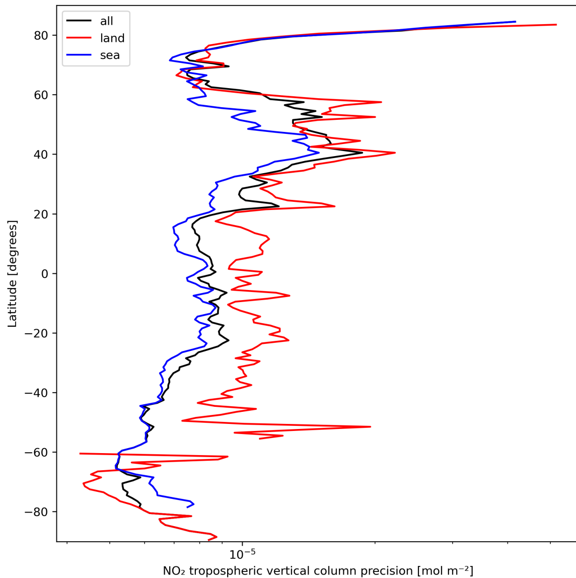
Figure 13: Zonal average of “NO 2 tropospheric vertical column precision” for 2024-03-09 to 2024-03-10.
