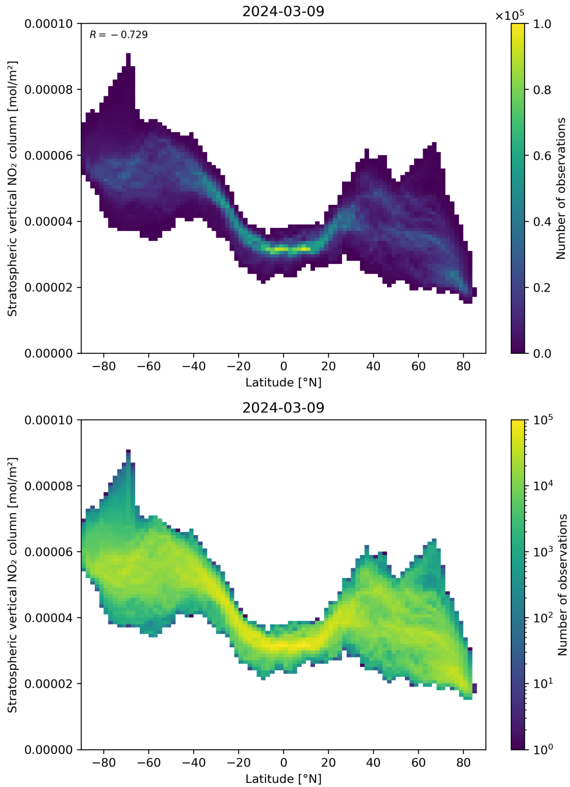
Figure 87: Scatter density plot of “Latitude” against “Stratospheric vertical NO 2 column” for 2024-03-09 to 2024-03-10.
