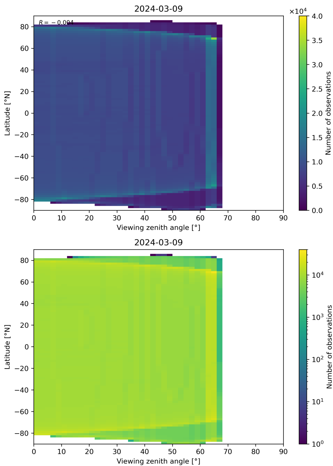
Figure 163: Scatter density plot of “Viewing zenith angle” against “Latitude” for 2024-03-09 to 2024-03-10.
