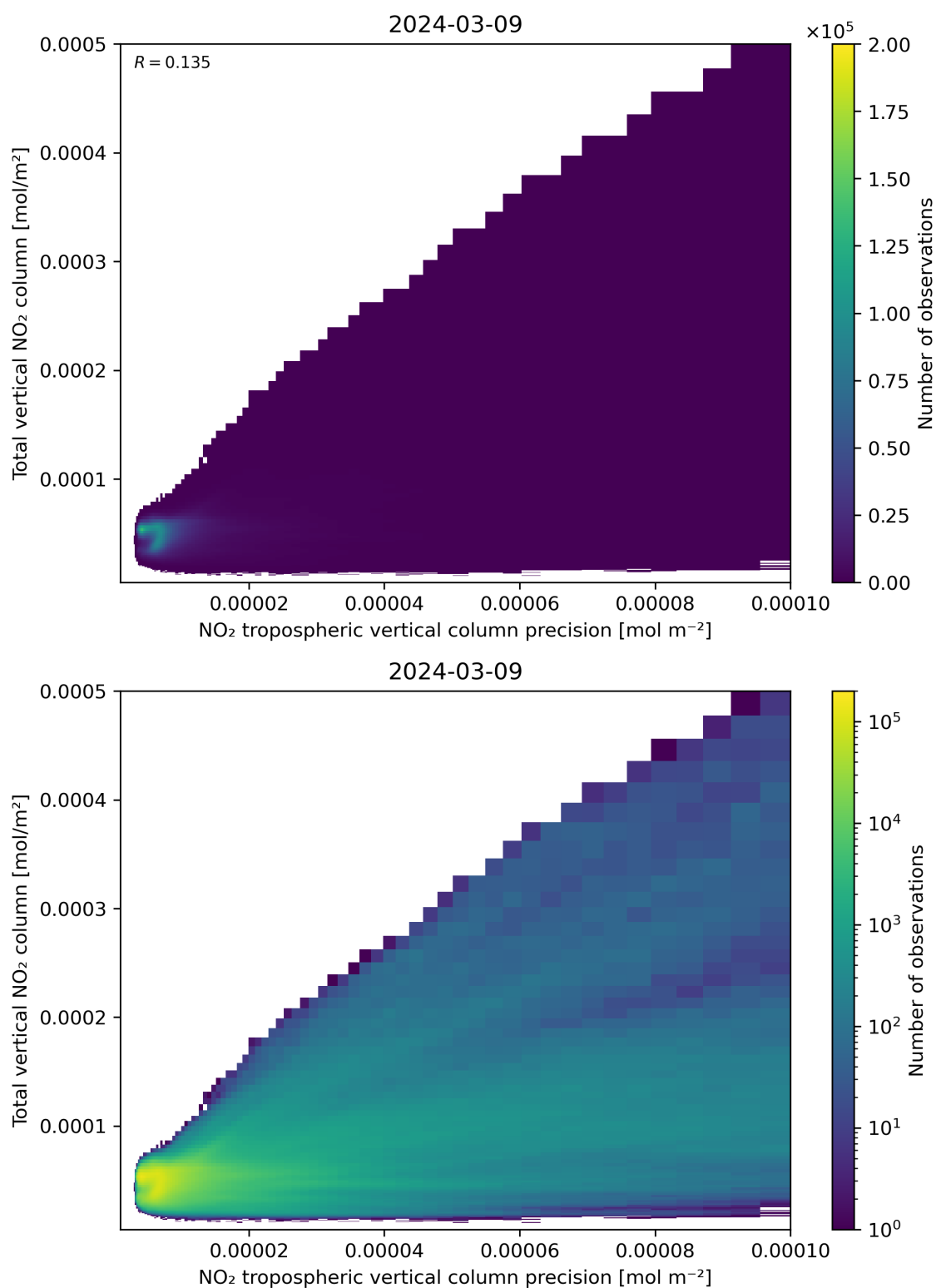
Figure 138: Scatter density plot of “NO 2 tropospheric vertical column precision” against “Total vertical NO 2 column” for 2024-03-09 to 2024-03-10.
