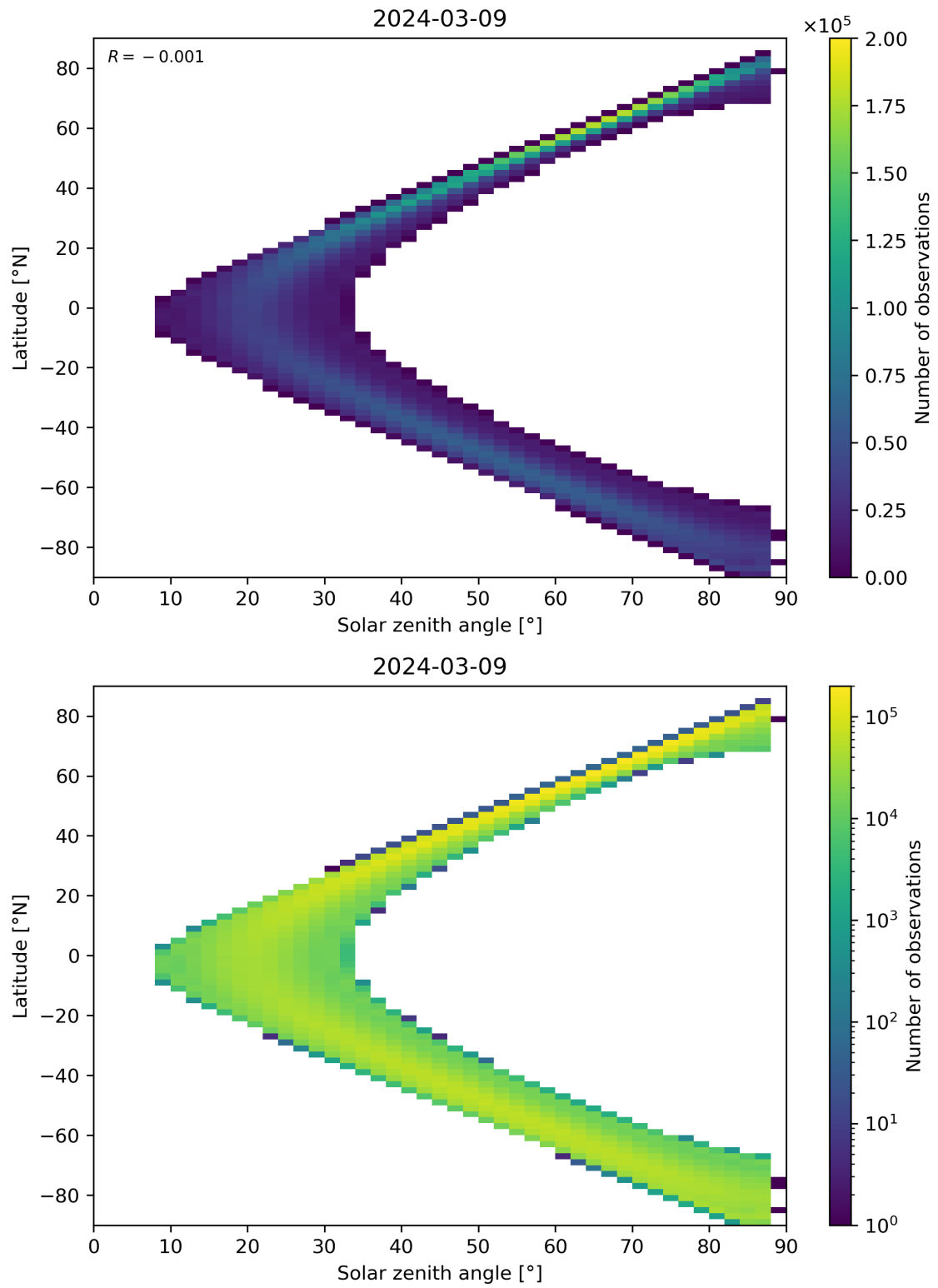
Figure 149: Scatter density plot of “Solar zenith angle” against “Latitude” for 2024-03-09 to 2024-03-10.
