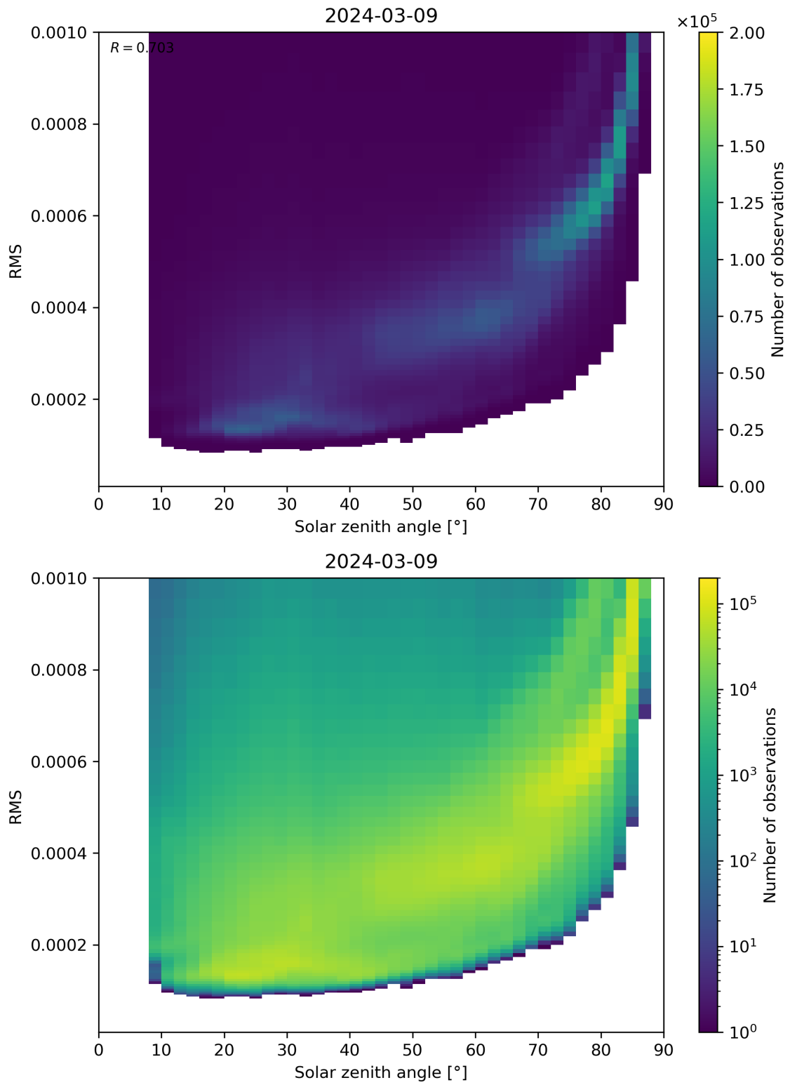
Figure 157: Scatter density plot of “Solar zenith angle” against “RMS” for 2024-03-09 to 2024-03-10.
