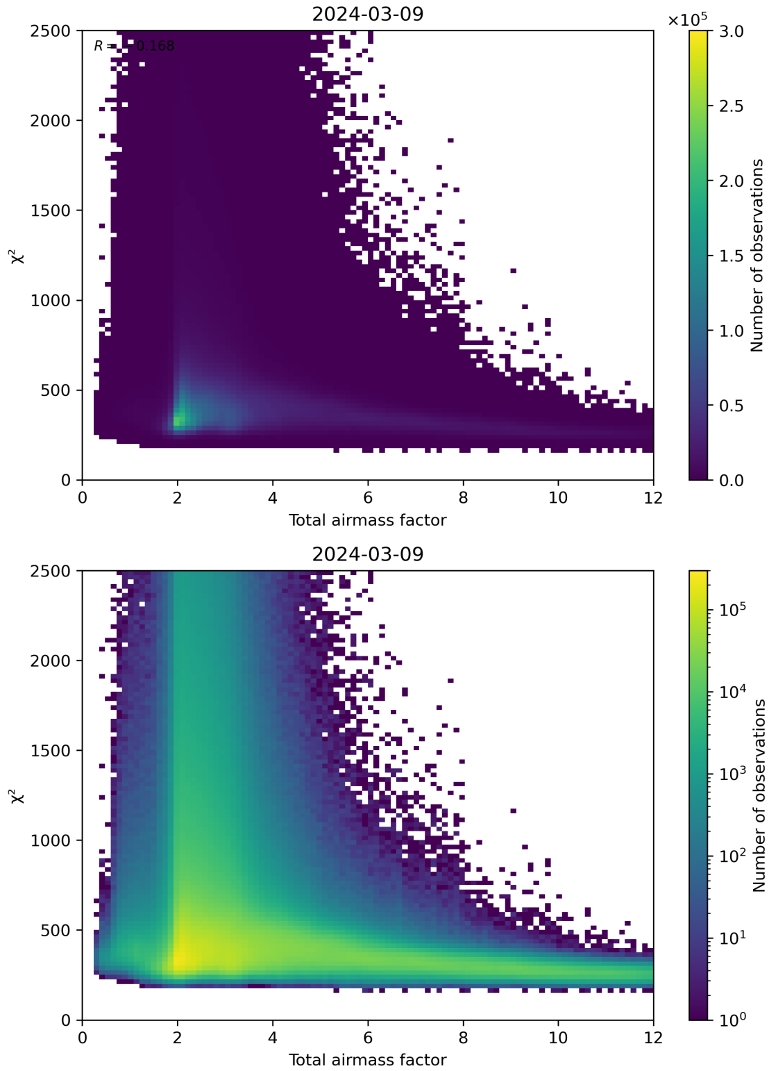
Figure 63: Scatter density plot of “Total airmass factor” against “ \chi^2 ” for 2024-03-09 to 2024-03-10.
