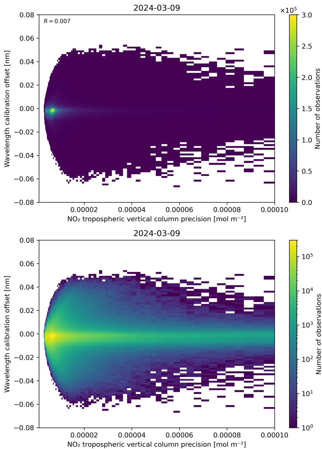
Figure 141: Scatter density plot of “NO 2 tropospheric vertical column precision” against “Wavelength calibration offset” for 2024-03-09 to 2024-03-10.
