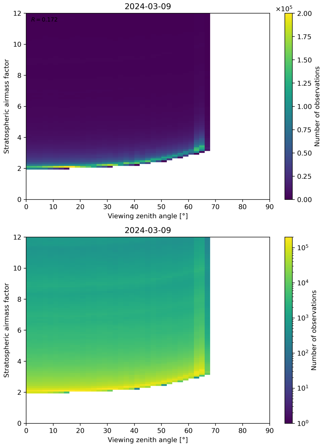
Figure 159: Scatter density plot of “Viewing zenith angle” against “Stratospheric airmass factor” for 2024-03-09 to 2024-03-10.
