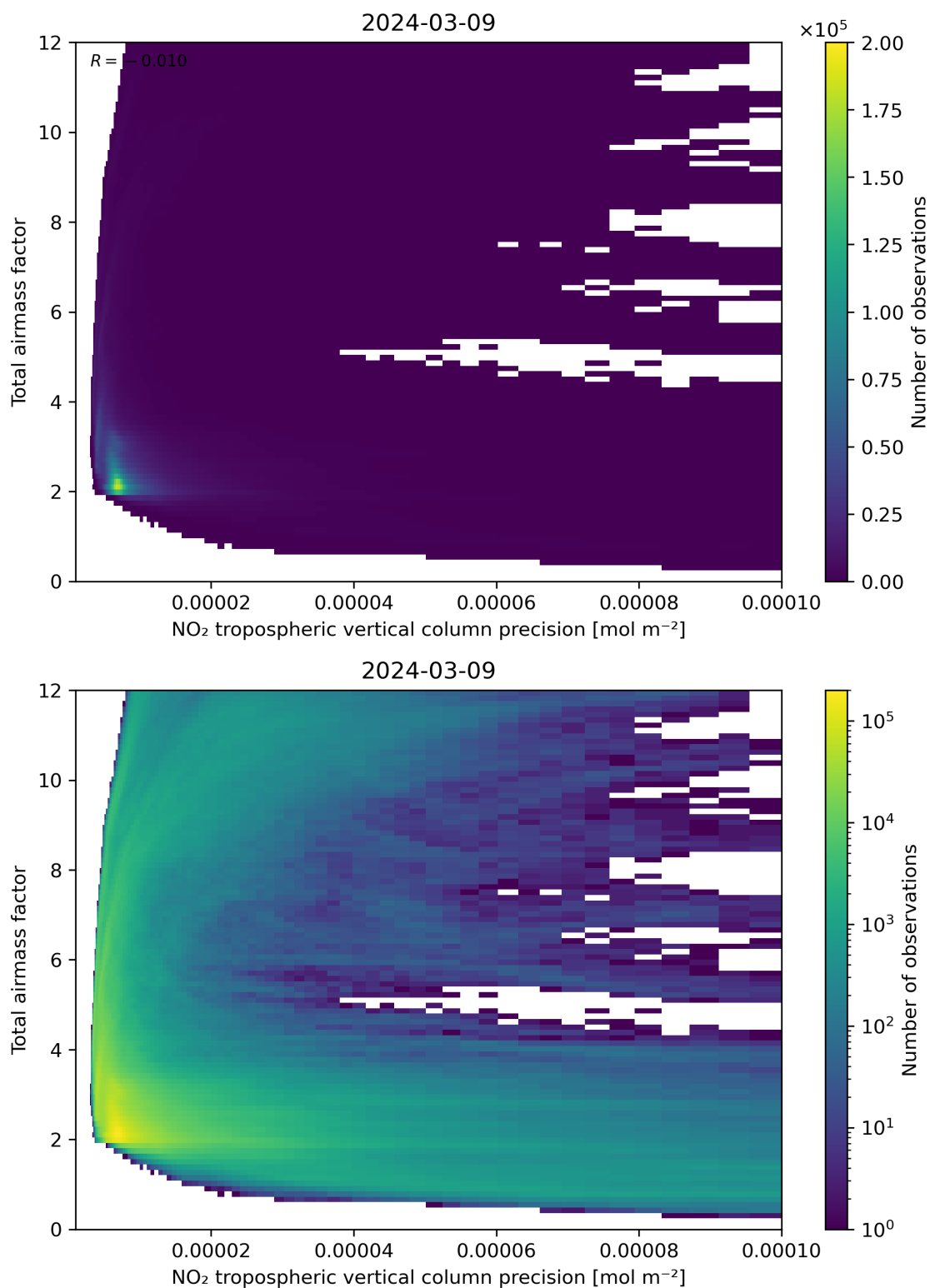
Figure 132: Scatter density plot of “NO 2 tropospheric vertical column precision” against “Total air mass factor” for 2024-03-09 to 2024-03-10.
