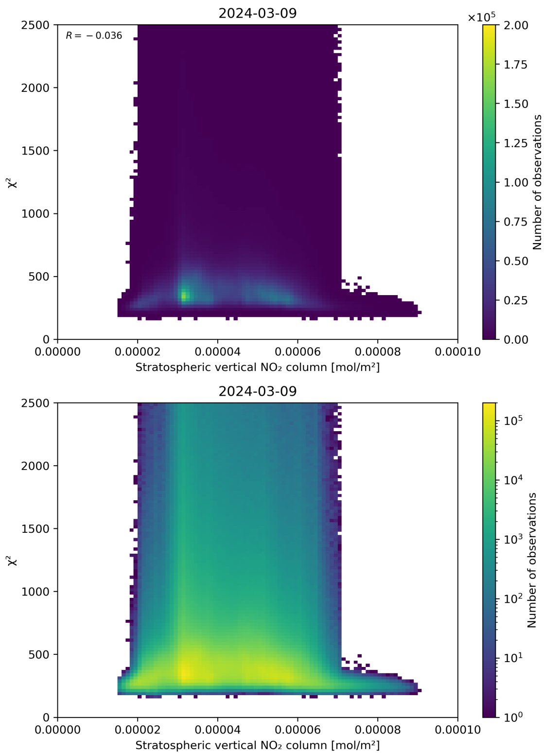
Figure 97: Scatter density plot of “Stratospheric vertical NO 2 column” against “ \chi^2 ” for 2024-03-09 to 2024-03-10.
