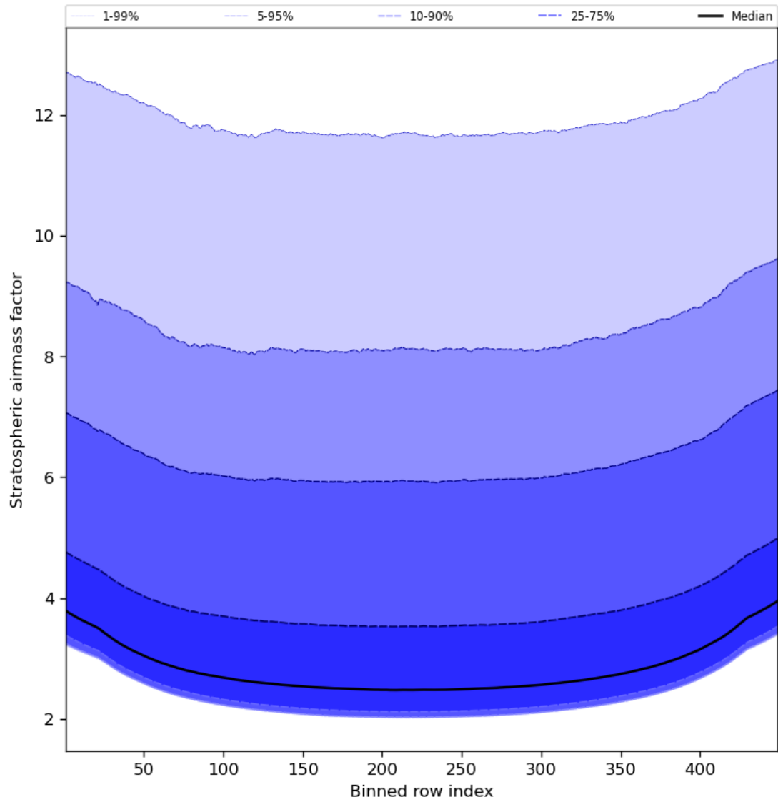
Figure 61: Along track statistics of “Stratospheric airmass factor” for 2024-03-09 to 2024-03-10
