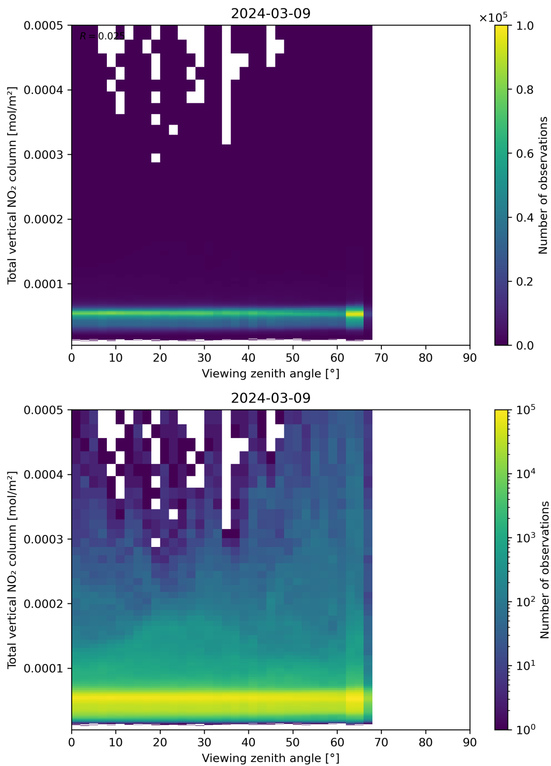
Figure 167: Scatter density plot of “Viewing zenith angle” against “Total vertical NO 2 column” for 2024-03-09 to 2024-03-10.
