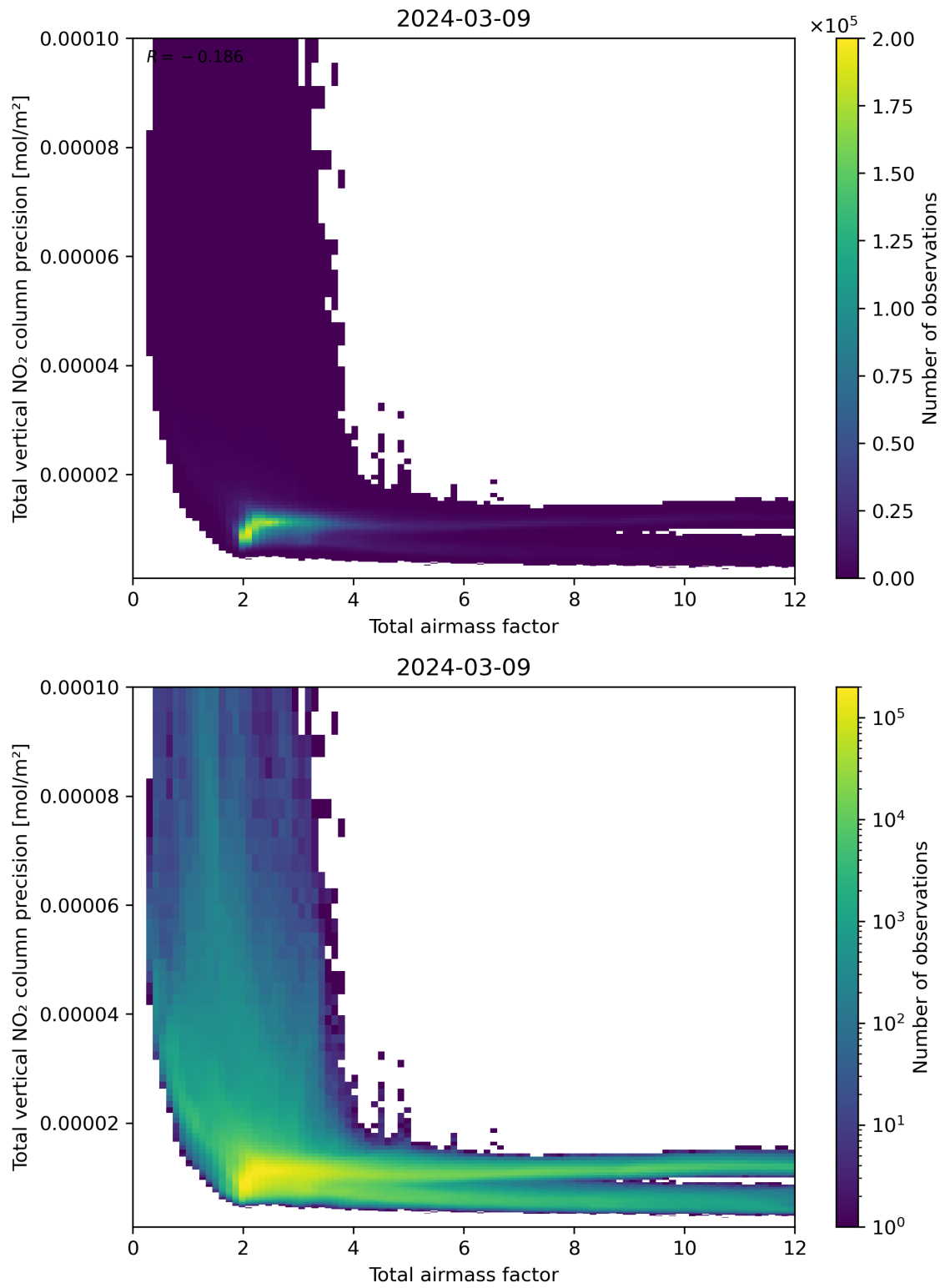
Figure 68: Scatter density plot of “Total airmass factor” against “Total vertical NO 2 column precision” for 2024-03-09 to 2024-03-10.
