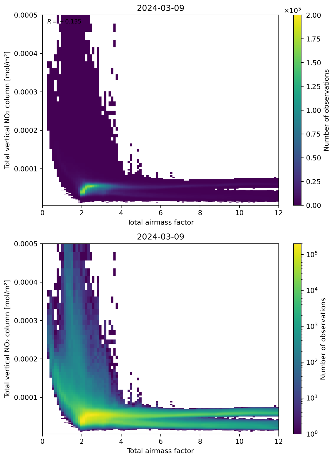
Figure 67: Scatter density plot of “Total airmass factor” against “Total vertical NO 2 column” for 2024-03-09 to 2024-03-10.
