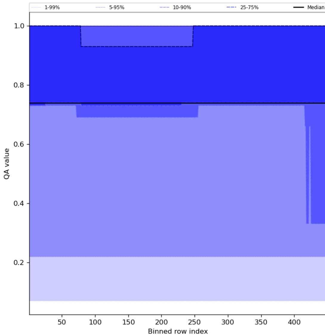
Figure 45: Along track statistics of “QA value” for 2024-03-09 to 2024-03-10
