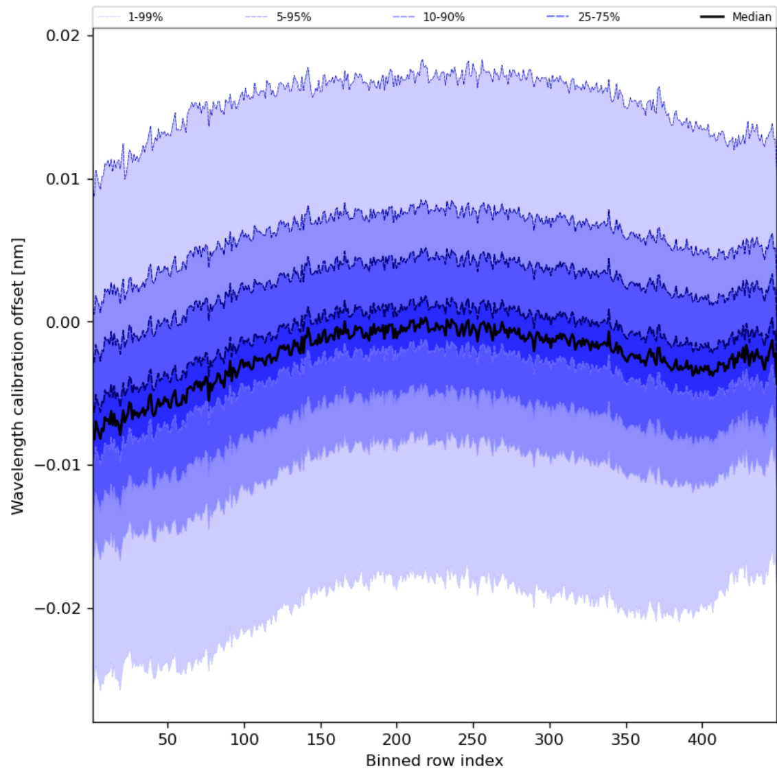
Figure 52: Along track statistics of “Wavelength calibration offset” for 2024-03-09 to 2024-03-10
