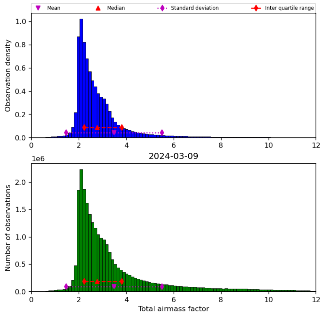
Figure 32: Histogram of “Total airmass factor” for 2024-03-09 to 2024-03-10
