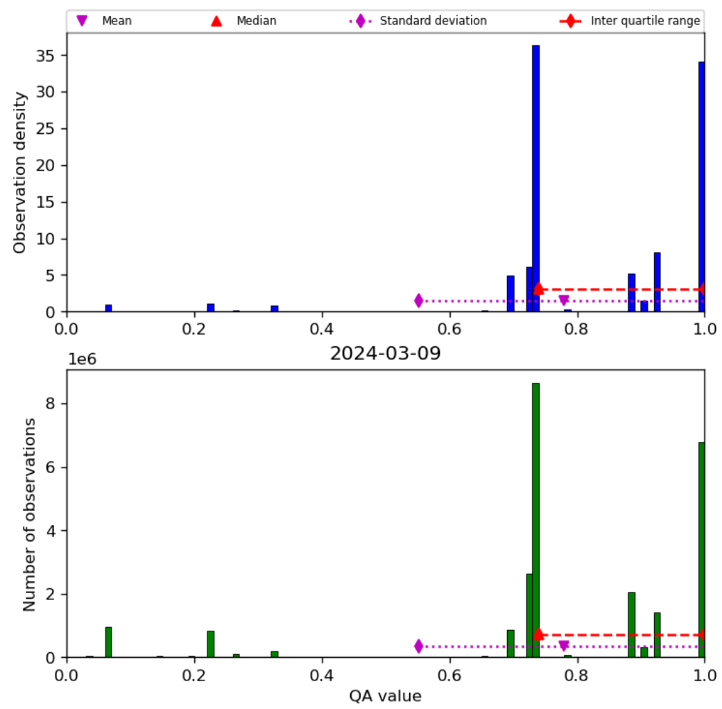
Figure 28: Histogram of “QA value” for 2024-03-09 to 2024-03-10
