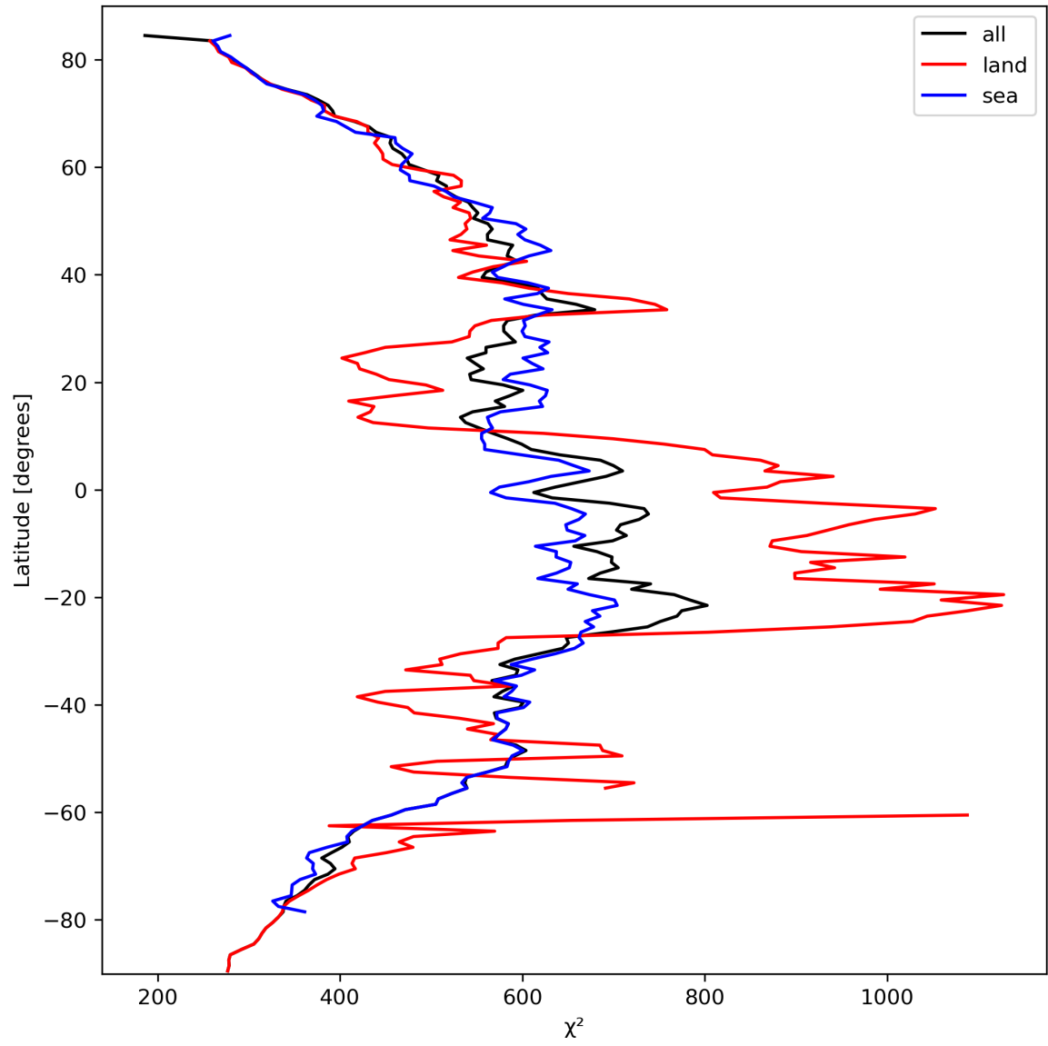
Figure 25: Zonal average of “ \chi^2 ” for 2024-03-09 to 2024-03-10.
