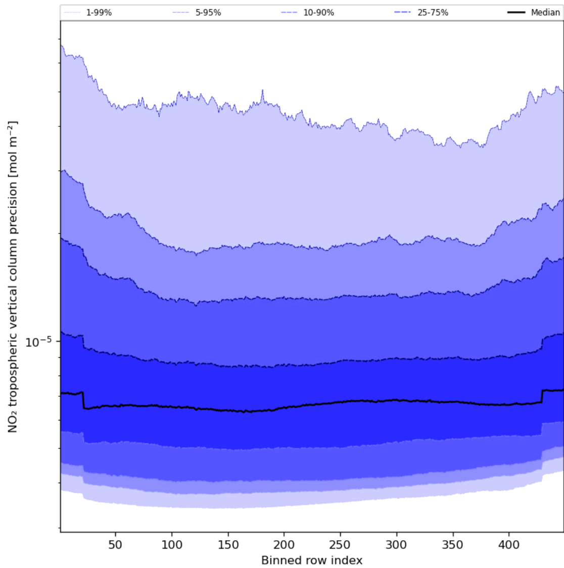
Figure 47: Along track statistics of “NO 2 tropospheric vertical column precision” for 2024-03-09 to 2024-03-10
