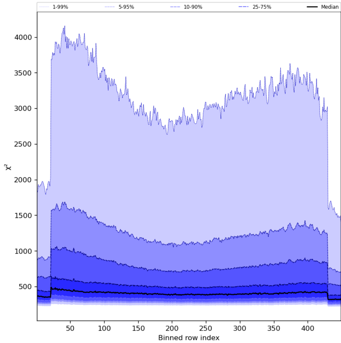
Figure 59: Along track statistics of “ \chi^2 ” for 2024-03-09 to 2024-03-10
