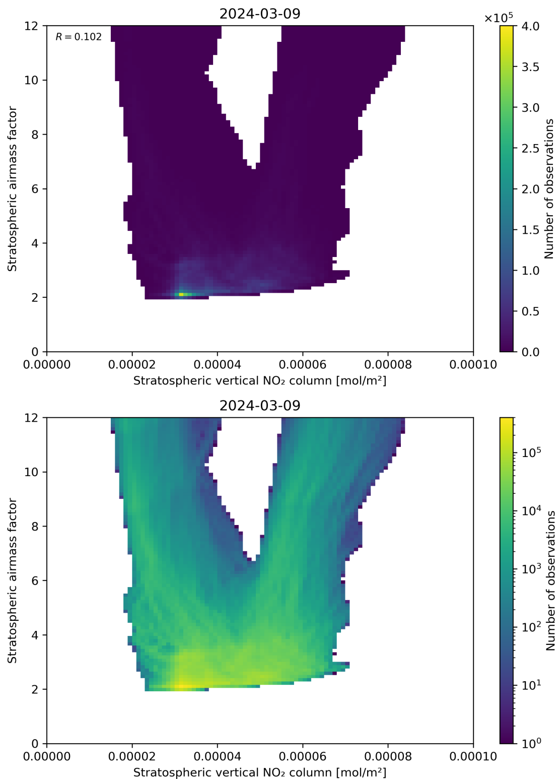
Figure 96: Scatter density plot of “Stratospheric vertical NO 2 column” against “Stratospheric airmass factor” for 2024-03-09 to 2024-03-10.
