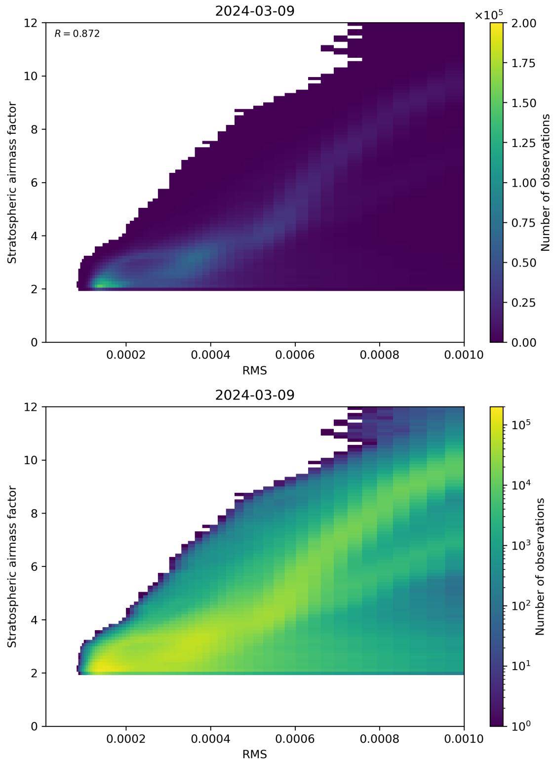
Figure 144: Scatter density plot of “RMS” against “Stratospheric airmass factor” for 2024-03-09 to 2024-03-10.
