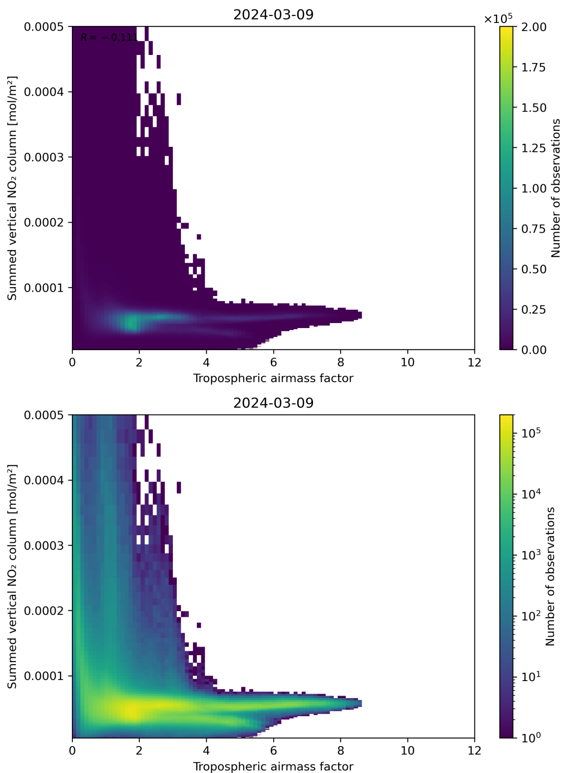
Figure 75: Scatter density plot of “Tropospheric airmass factor” against “Summed vertical NO 2 column” for 2024-03-09 to 2024-03-10.
