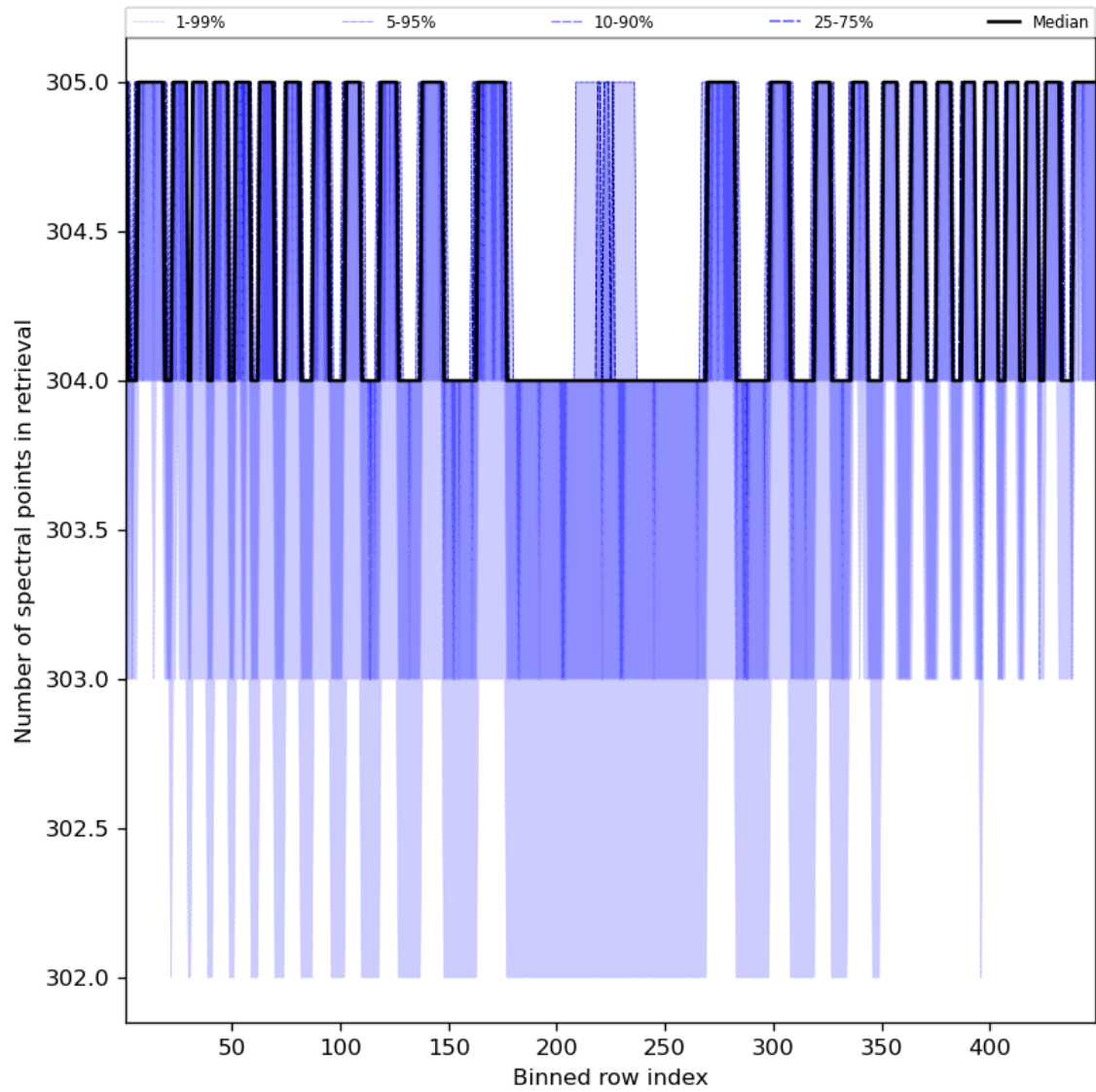
Figure 50: Along track statistics of “Number of spectral points in retrieval” for 2024-03-09 to 2024-03-10
