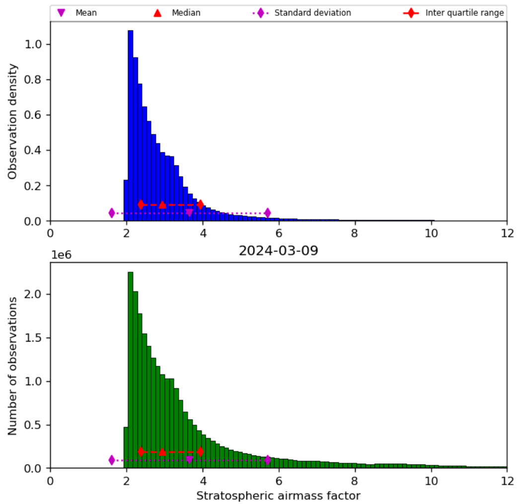
Figure 44: Histogram of “Stratospheric airmass factor” for 2024-03-09 to 2024-03-10
