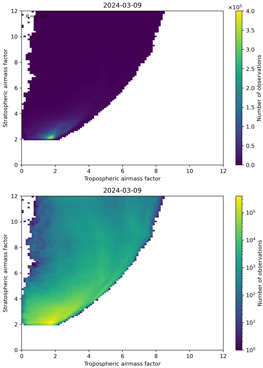
Figure 71: Scatter density plot of “Tropospheric airmass factor” against “Stratospheric airmass factor” for 2024-03-09 to 2024-03-10.
