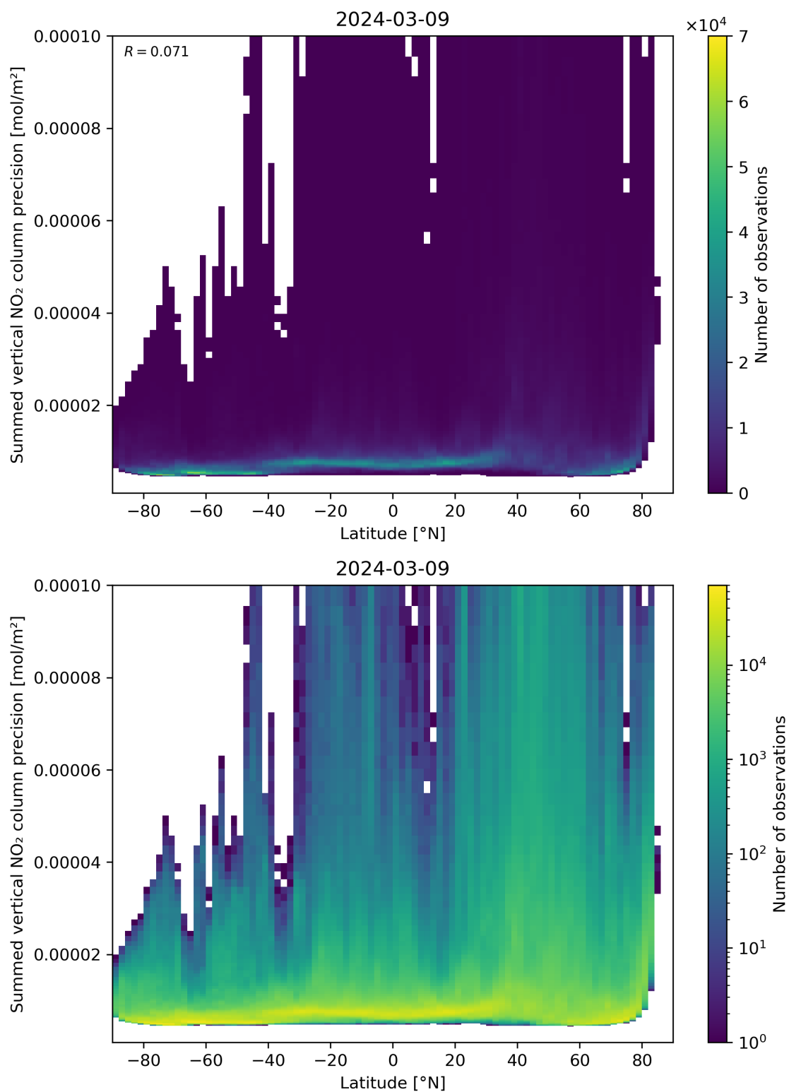
Figure 89: Scatter density plot of “Latitude” against “Summed vertical NO 2 column precision” for 2024-03-09 to 2024-03-10.
