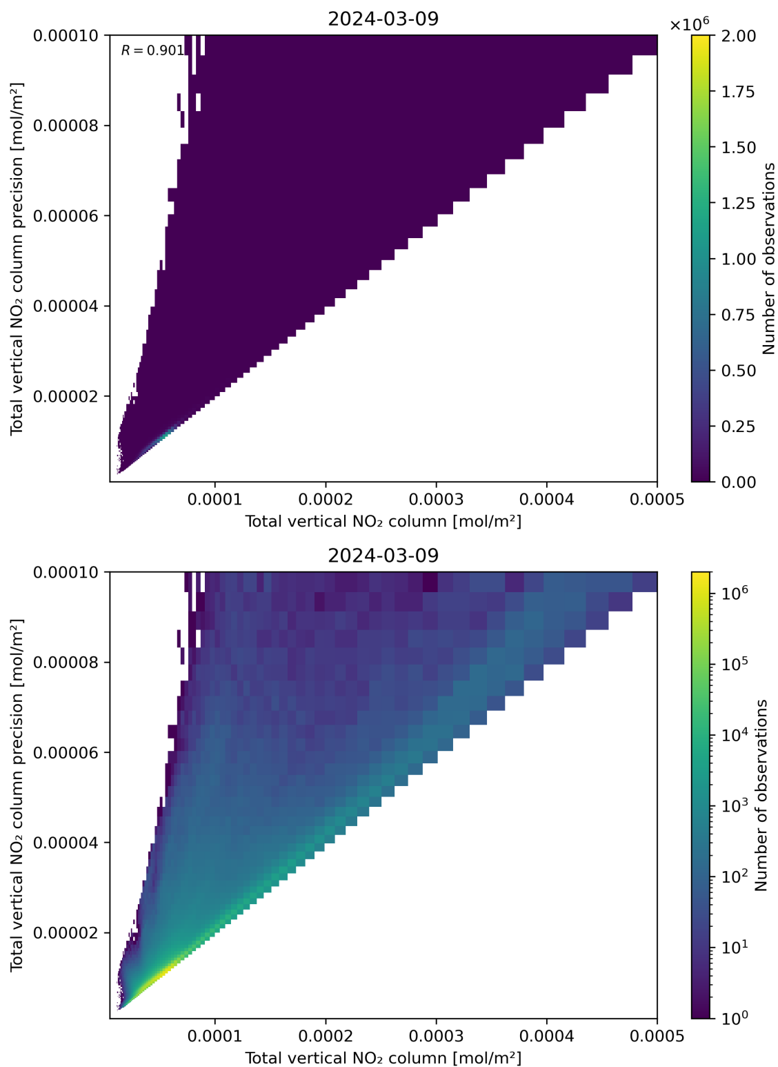
Figure 114: Scatter density plot of “Total vertical NO 2 column” against “Total vertical NO 2 column precision” for 2024-03-09 to 2024-03-10.
