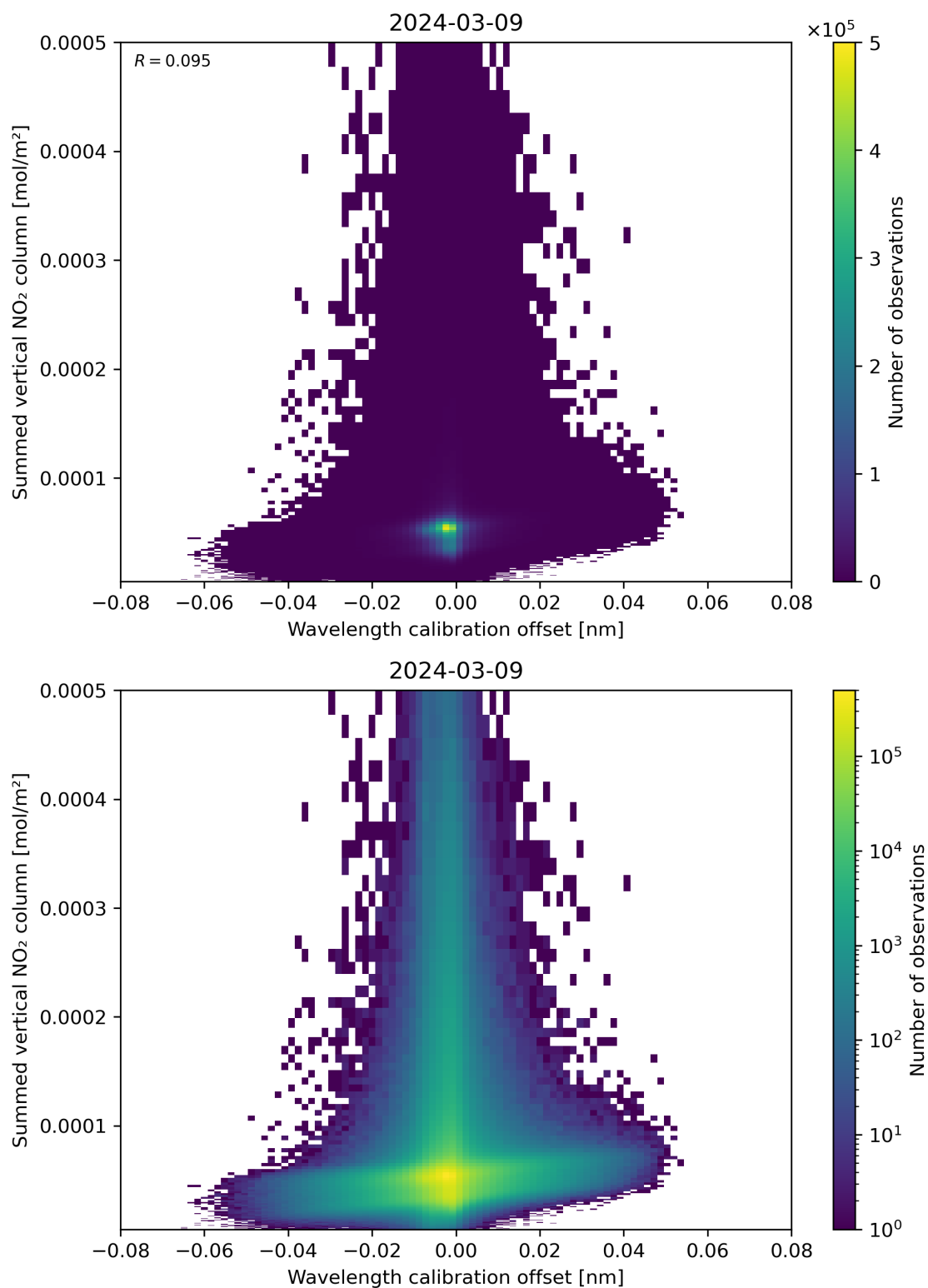
Figure 177: Scatter density plot of “Wavelength calibration offset” against “Summed vertical NO 2 column” for 2024-03-09 to 2024-03-10.
