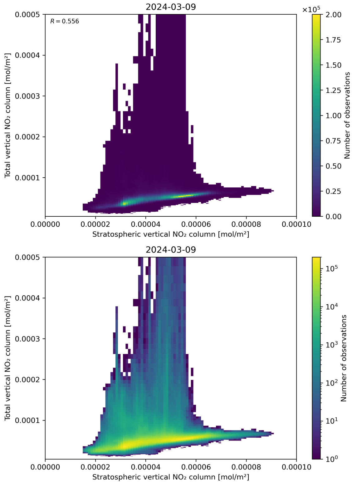
Figure 100: Scatter density plot of “Stratospheric vertical NO 2 column” against “Total vertical NO 2 column” for 2024-03-09 to 2024-03-10.
