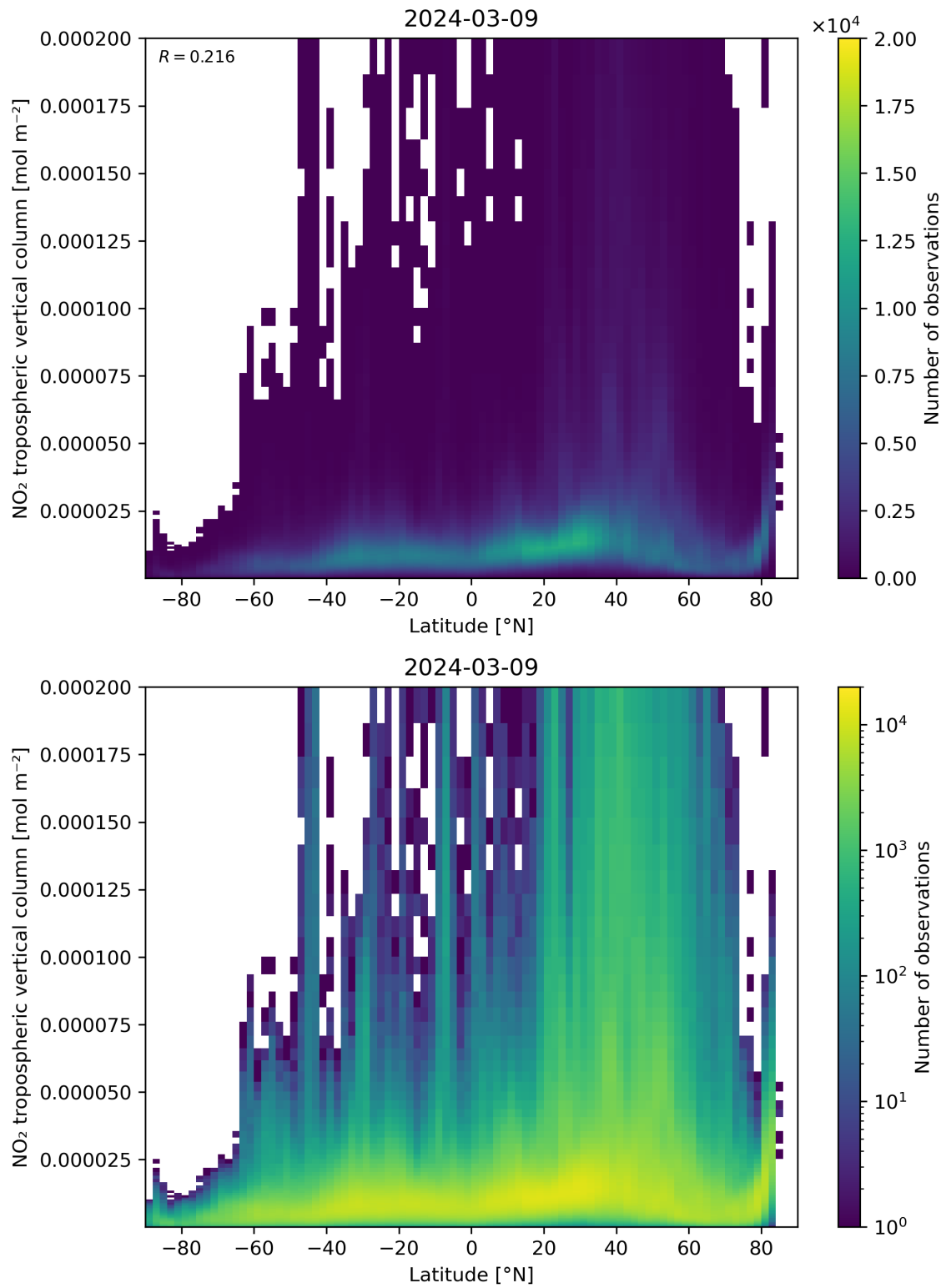
Figure 92: Scatter density plot of “Latitude” against “NO 2 tropospheric vertical column” for 2024-03-09 to 2024-03-10.
