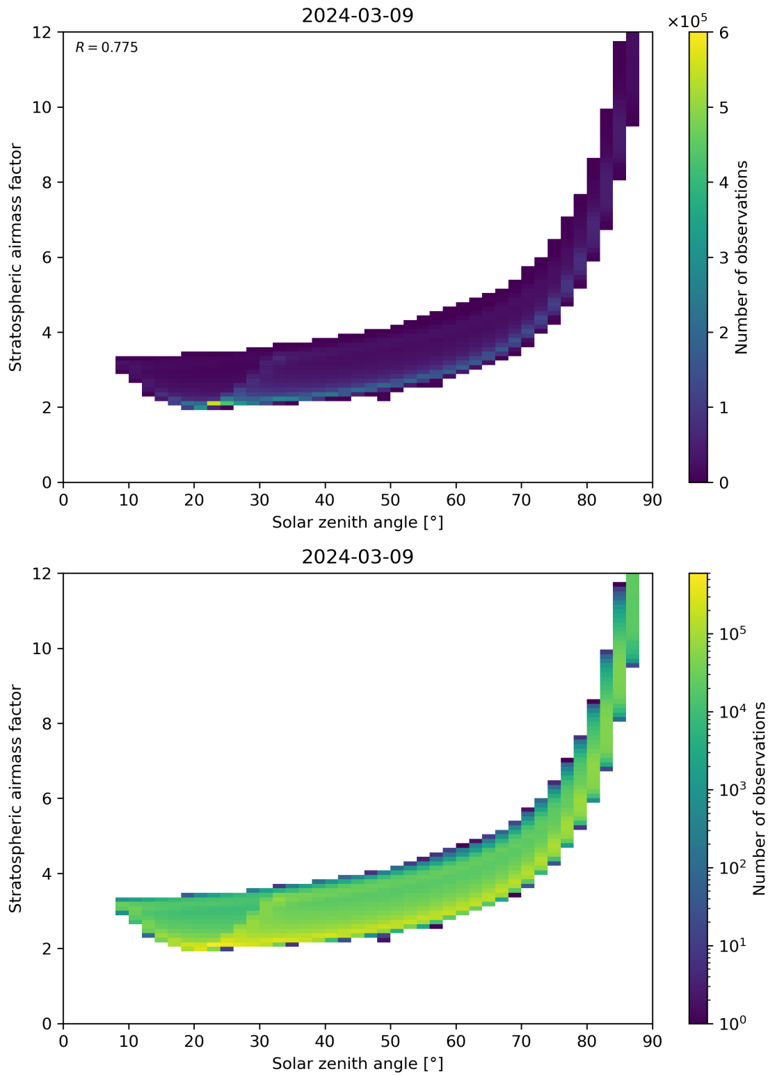
Figure 145: Scatter density plot of “Solar zenith angle” against “Stratospheric airmass factor” for 2024-03-09 to 2024-03-10.
