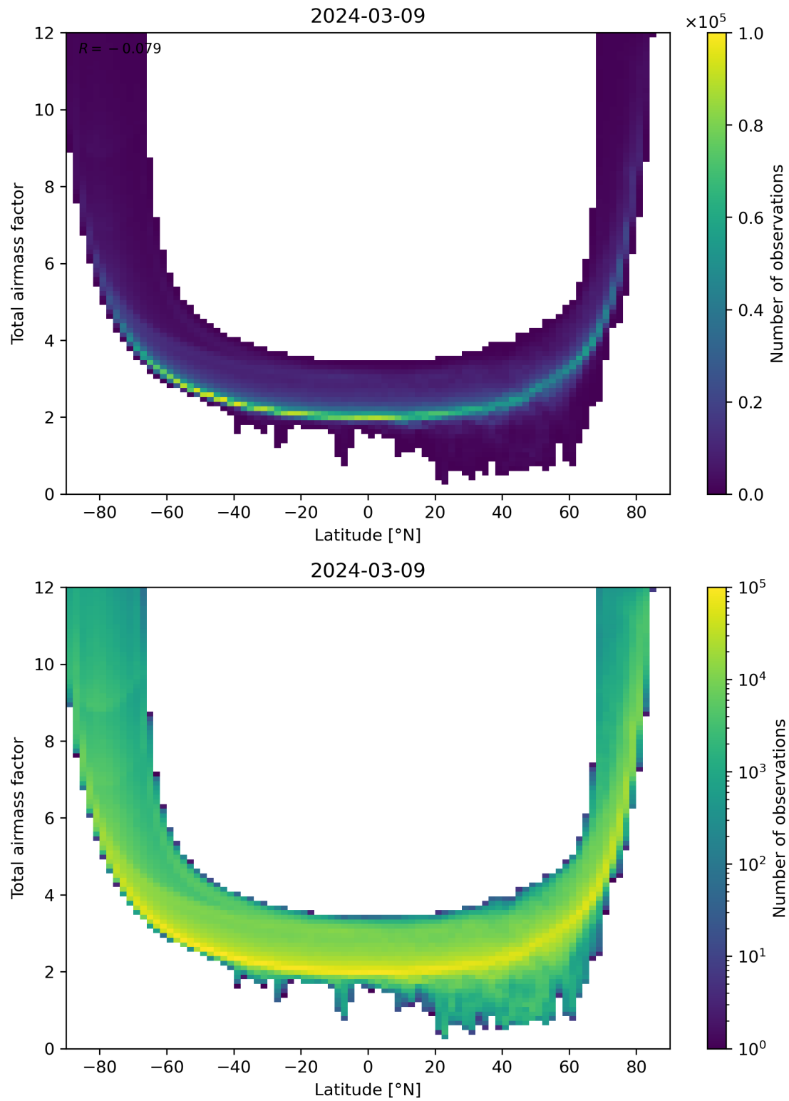
Figure 84: Scatter density plot of “Latitude” against “Total airmass factor” for 2024-03-09 to 2024-03-10.
