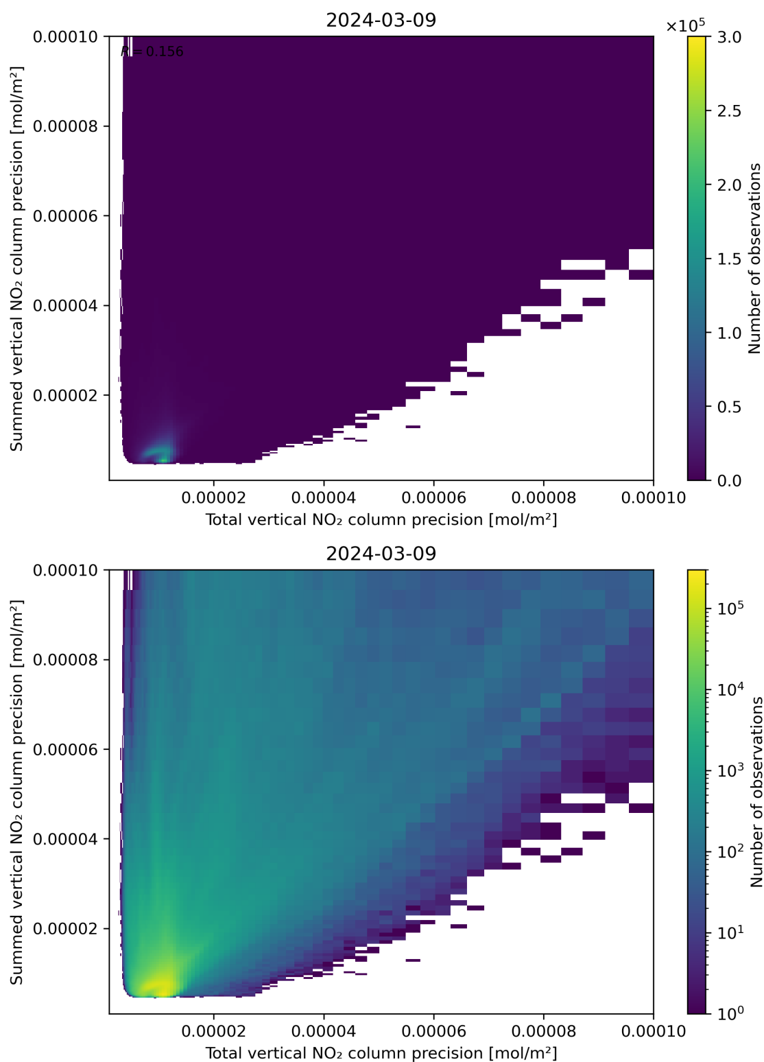
Figure 118: Scatter density plot of “Total vertical NO 2 column precision” against “Summed vertical NO 2 column precision” for 2024-03-09 to 2024-03-10.
