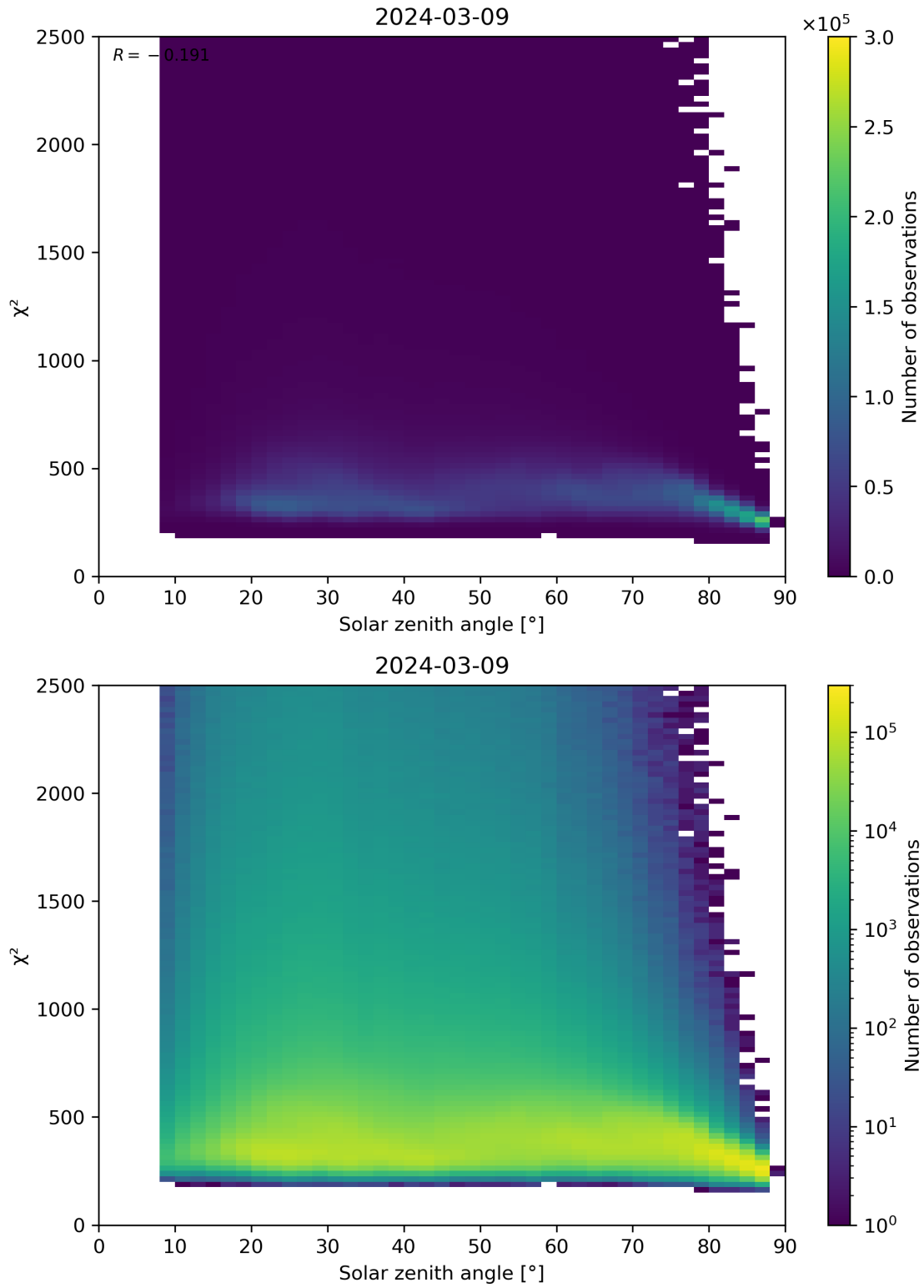
Figure 148: Scatter density plot of “Solar zenith angle” against “ \chi^2 ” for 2024-03-09 to 2024-03-10.
