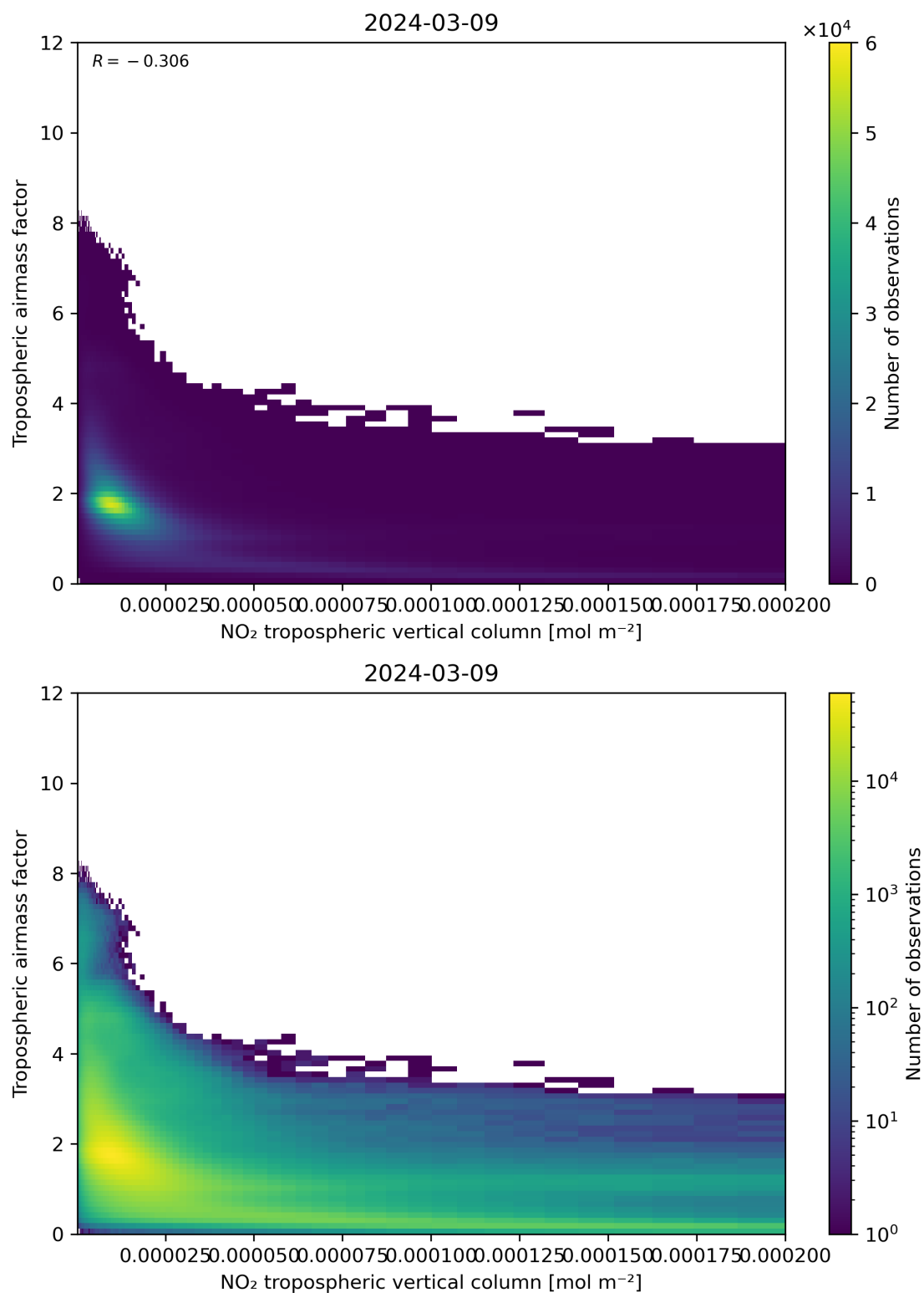
Figure 123: Scatter density plot of “NO 2 tropospheric vertical column” against “Tropospheric air mass factor” for 2024-03-09 to 2024-03-10.
