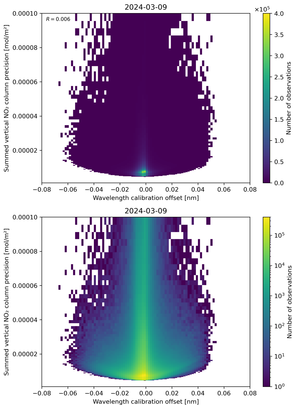
Figure 178: Scatter density plot of “Wavelength calibration offset” against “Summed vertical NO 2 column precision” for 2024-03-09 to 2024-03-10.
