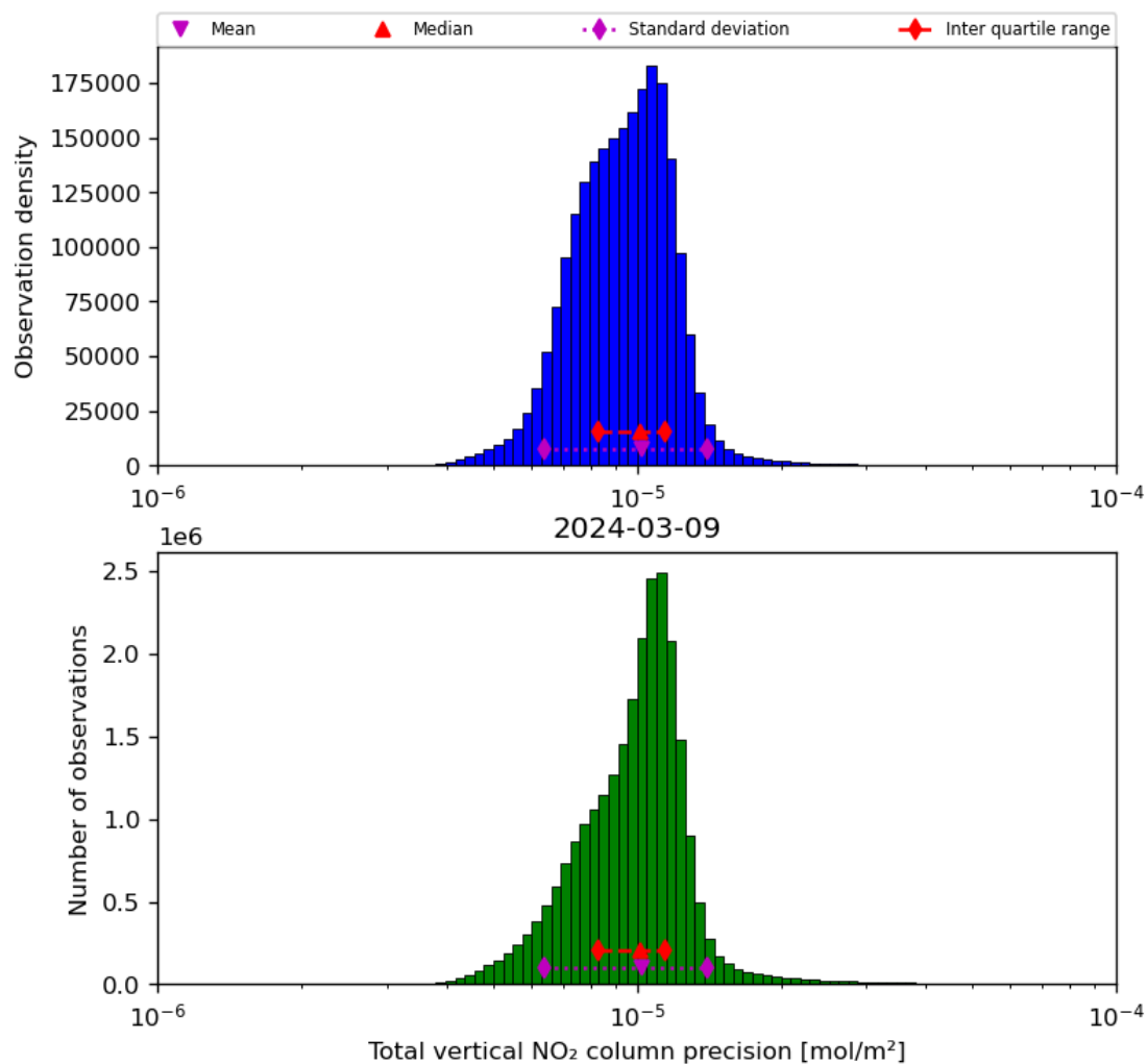
Figure 39: Histogram of “Total vertical NO 2 column precision” for 2024-03-09 to 2024-03-10
