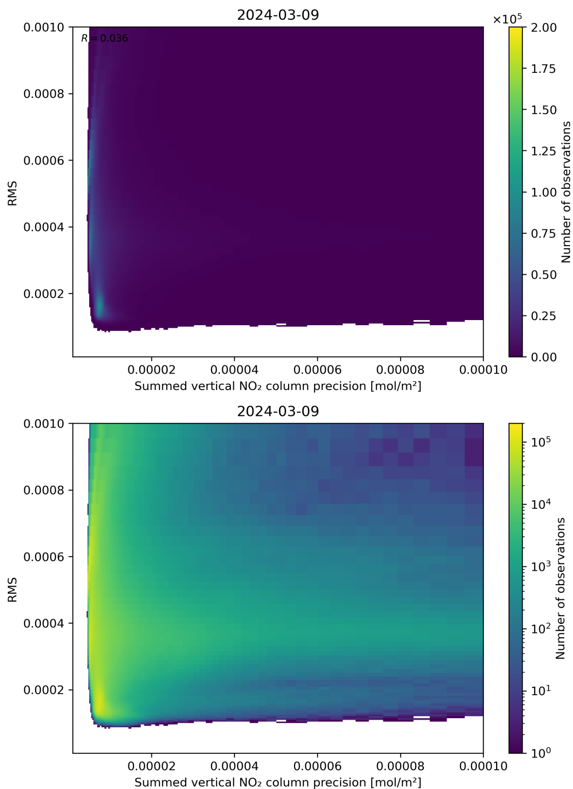
Figure 108: Scatter density plot of “Summed vertical NO 2 column precision” against “RMS” for 2024-03-09 to 2024-03-10.
