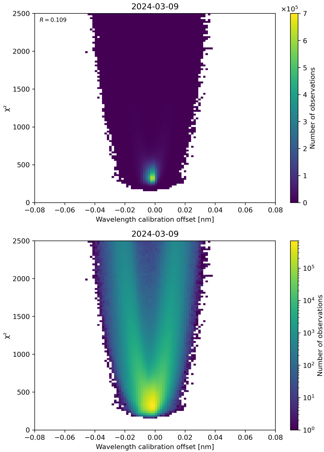
Figure 175: Scatter density plot of “Wavelength calibration offset” against “ \chi^2 ” for 2024-03-09 to 2024-03-10.
