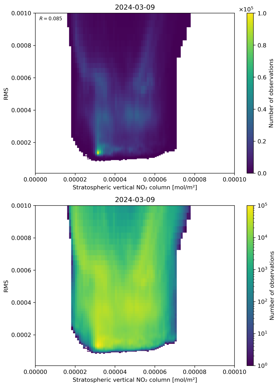
Figure 102: Scatter density plot of “Stratospheric vertical NO 2 column” against “RMS” for 2024-03-09 to 2024-03-10.
