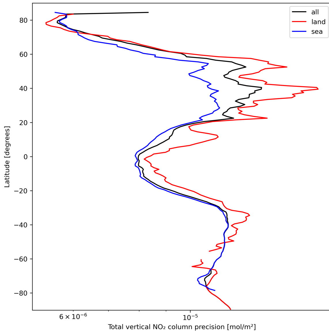
Figure 22: Zonal average of “Total vertical NO 2 column precision” for 2024-03-09 to 2024-03-10.
