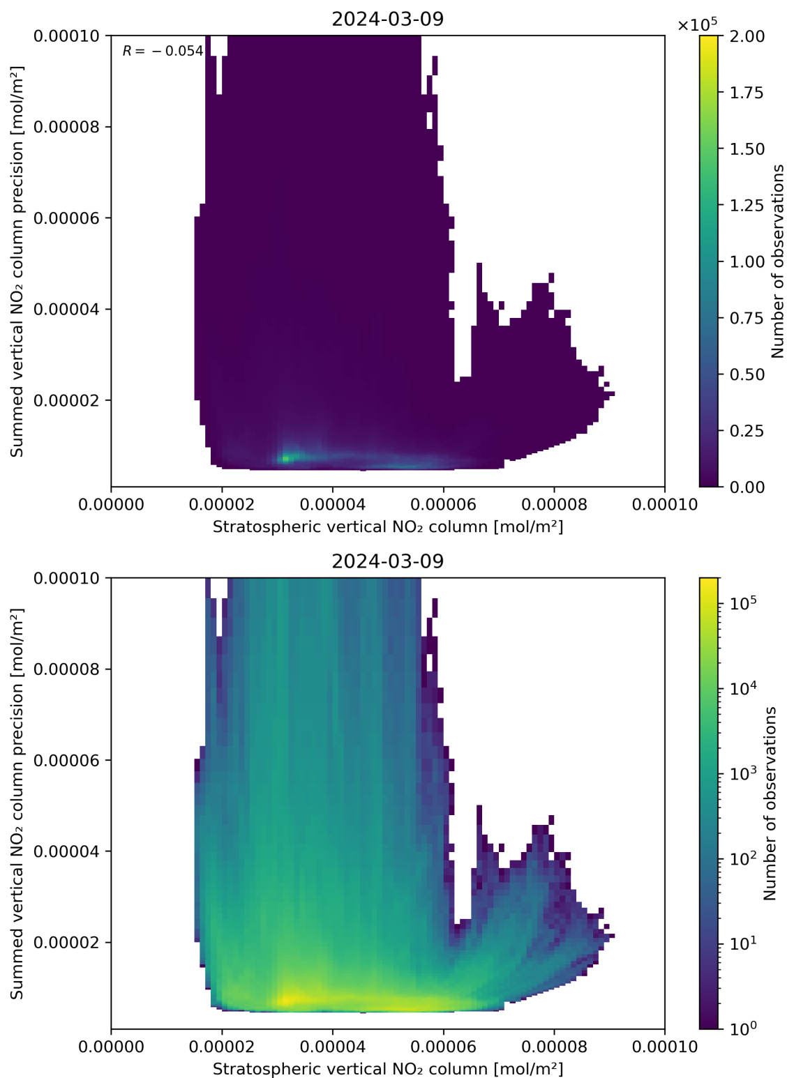
Figure 99: Scatter density plot of “Stratospheric vertical NO 2 column” against “Summed vertical NO 2 column precision” for 2024-03-09 to 2024-03-10.
