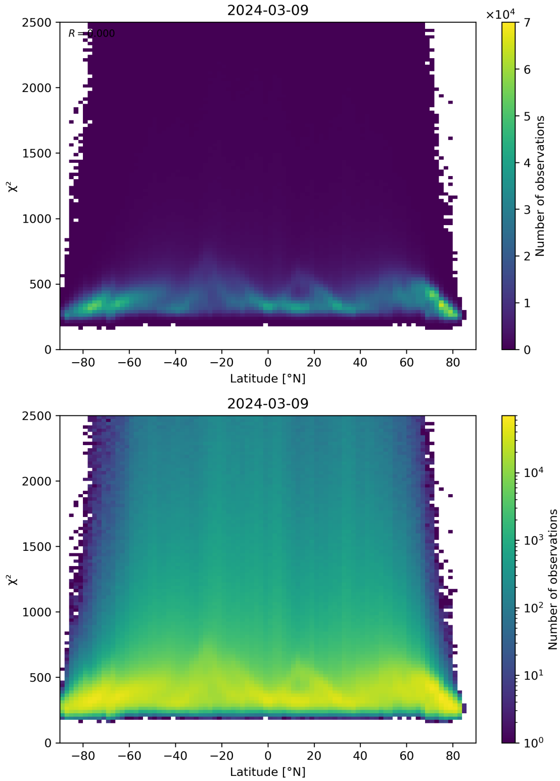
Figure 86: Scatter density plot of “Latitude” against “ \chi^2 ” for 2024-03-09 to 2024-03-10.
