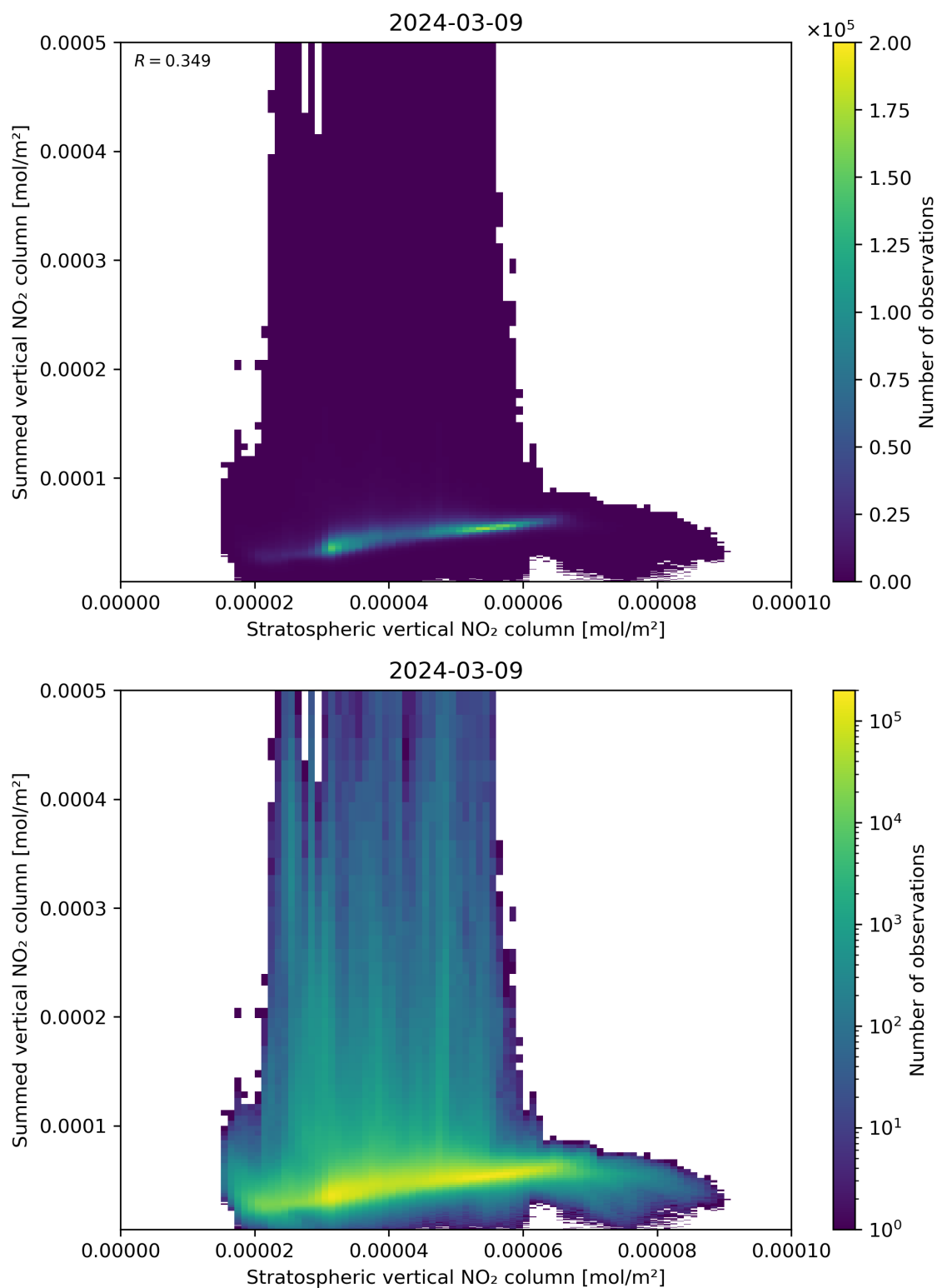
Figure 98: Scatter density plot of “Stratospheric vertical NO 2 column” against “Summed vertical NO 2 column” for 2024-03-09 to 2024-03-10.
