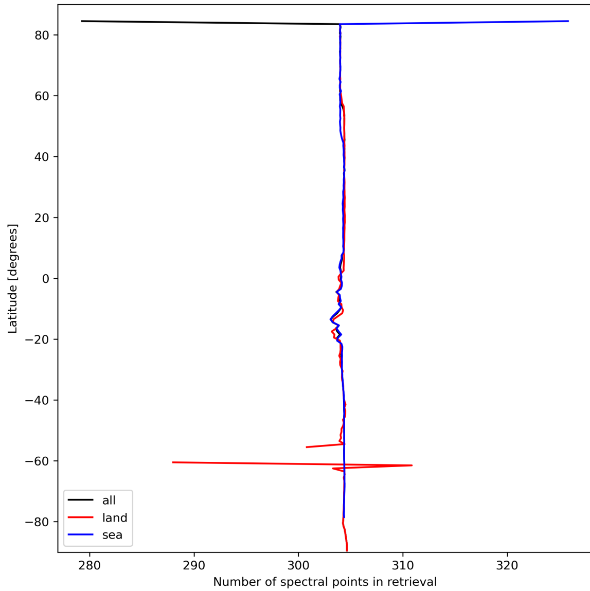
Figure 16: Zonal average of “Number of spectral points in retrieval” for 2024-03-09 to 2024-03-10.
