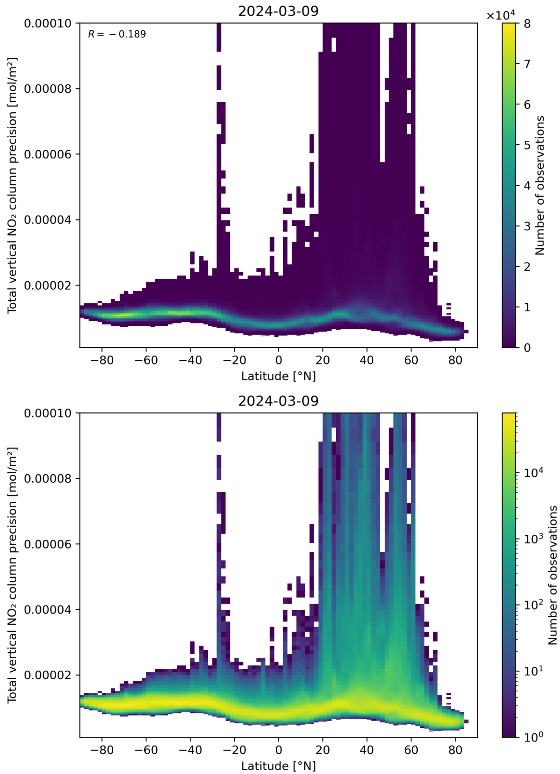
Figure 91: Scatter density plot of “Latitude” against “Total vertical NO 2 column precision” for 2024-03-09 to 2024-03-10.
