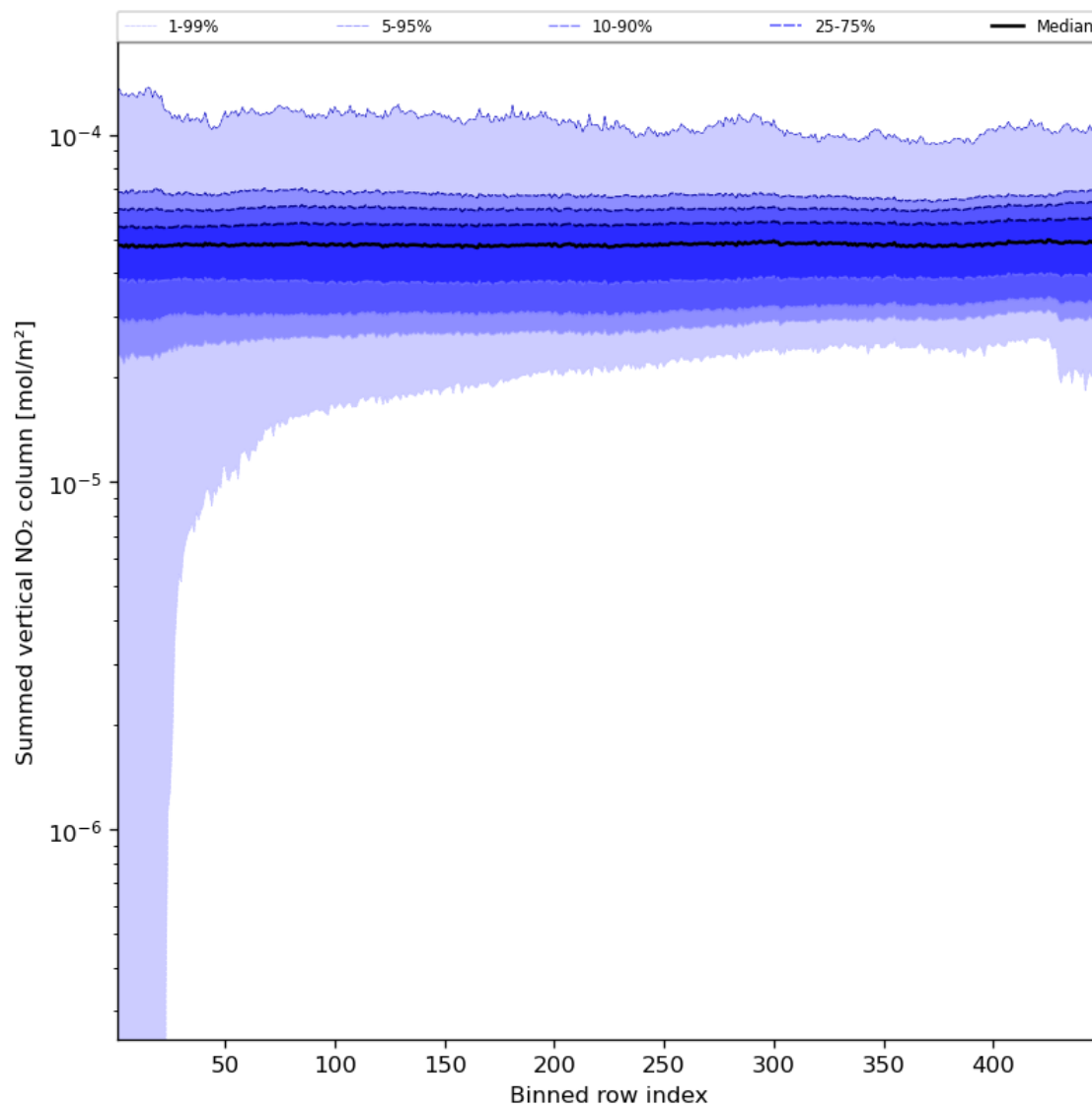
Figure 57: Along track statistics of “Summed vertical NO 2 column” for 2024-03-09 to 2024-03-10
