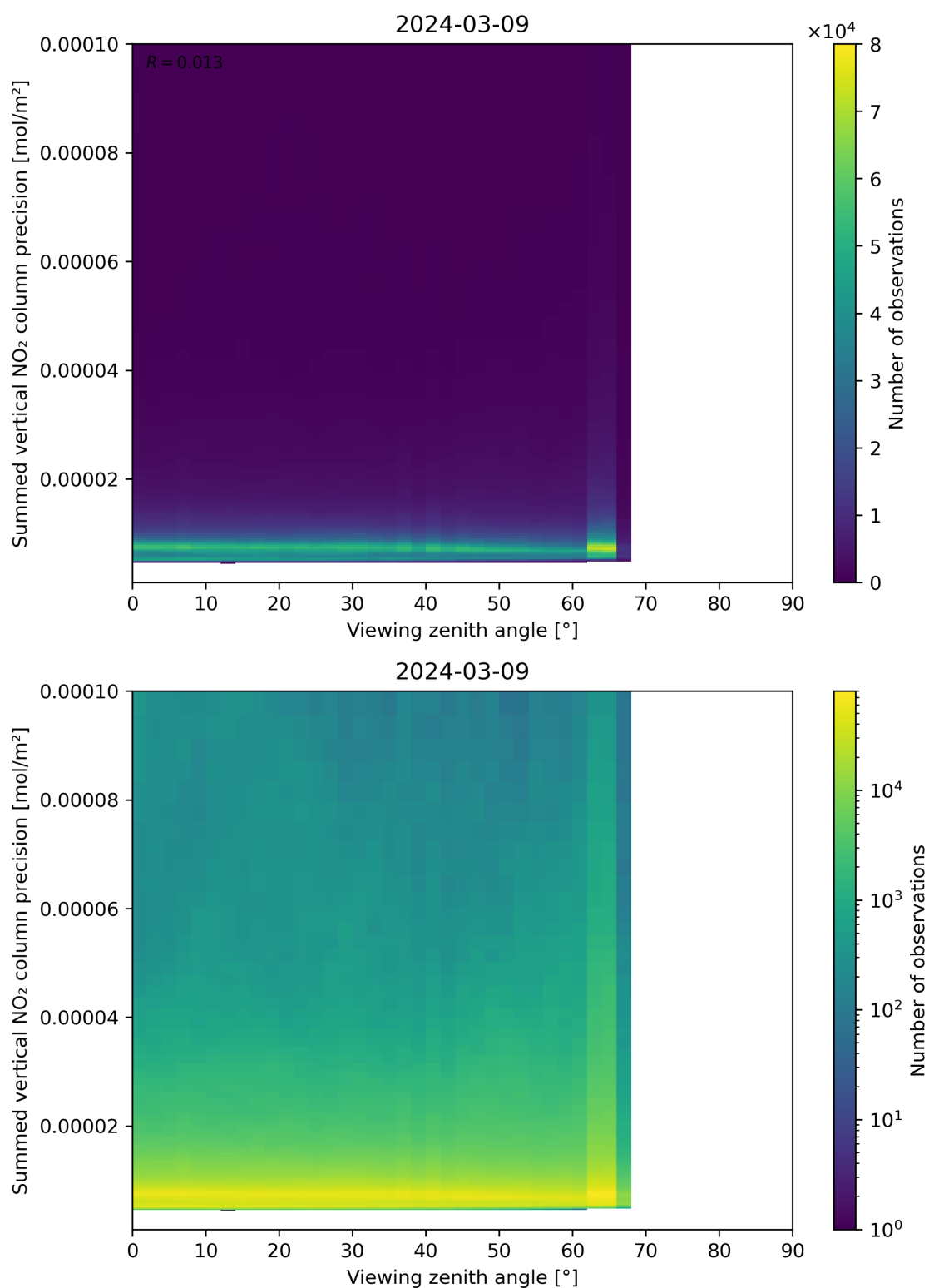
Figure 166: Scatter density plot of “Viewing zenith angle” against “Summed vertical NO 2 column precision” for 2024-03-09 to 2024-03-10.
