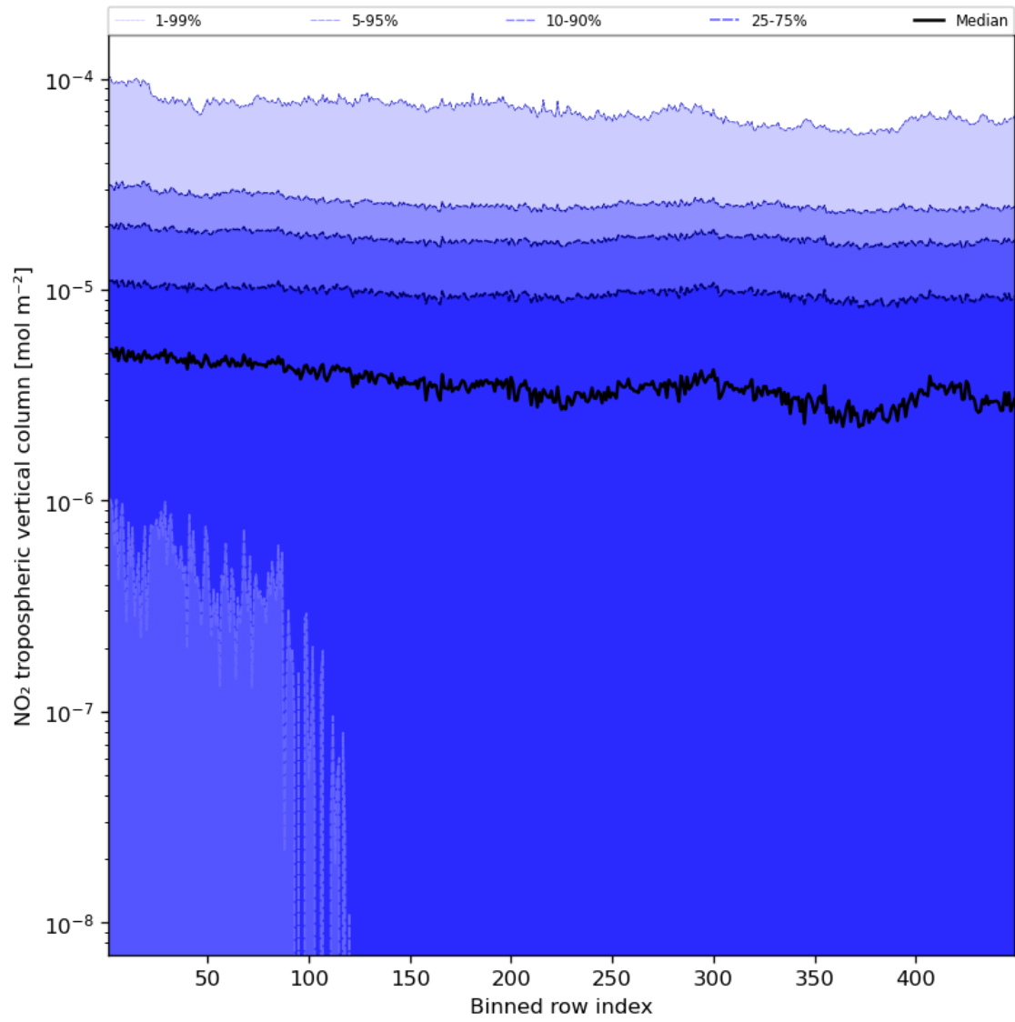
Figure 46: Along track statistics of “NO 2 tropospheric vertical column” for 2024-03-09 to 2024-03-10
