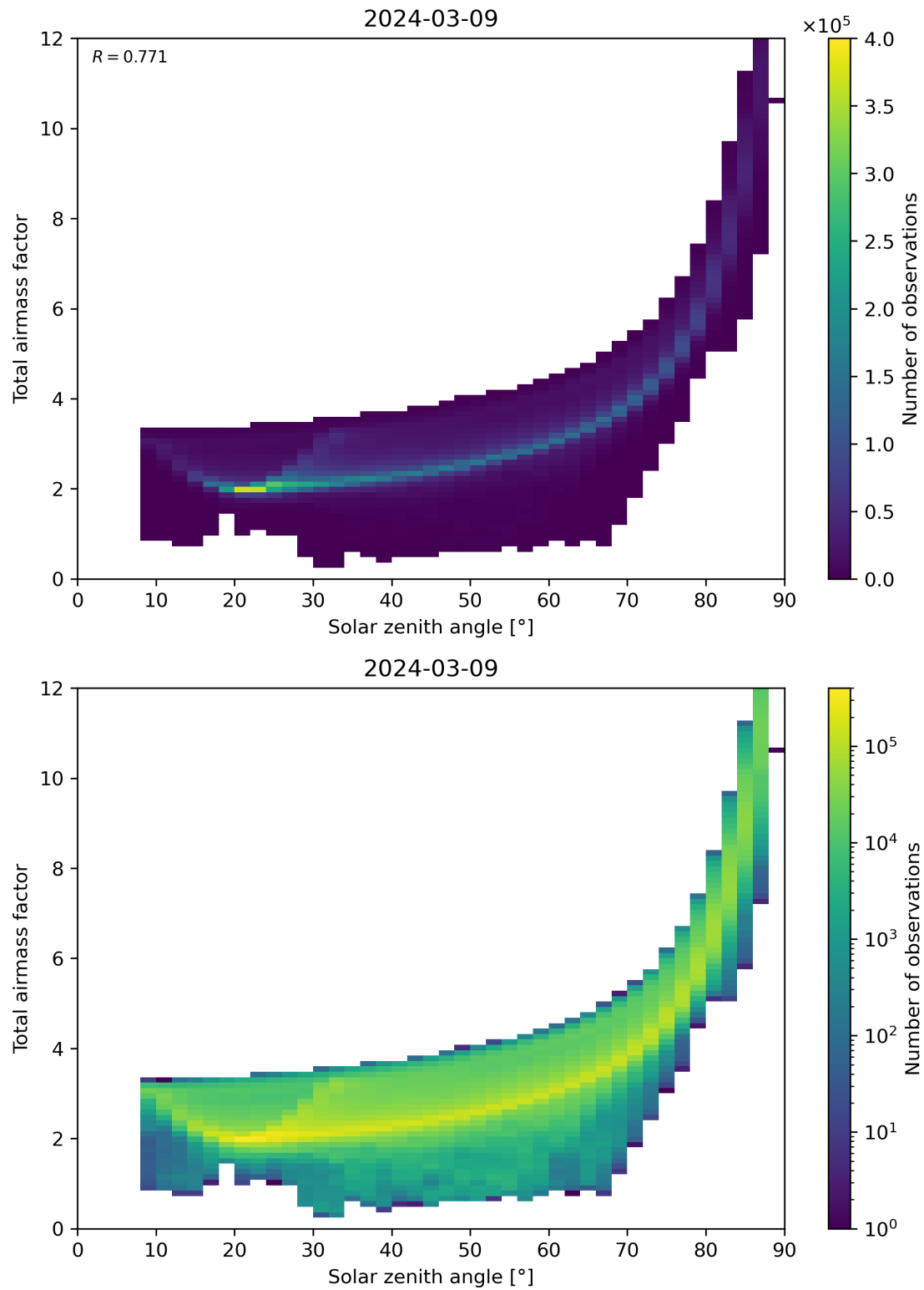
Figure 146: Scatter density plot of “Solar zenith angle” against “Total air mass factor” for 2024-03-09 to 2024-03-10.
