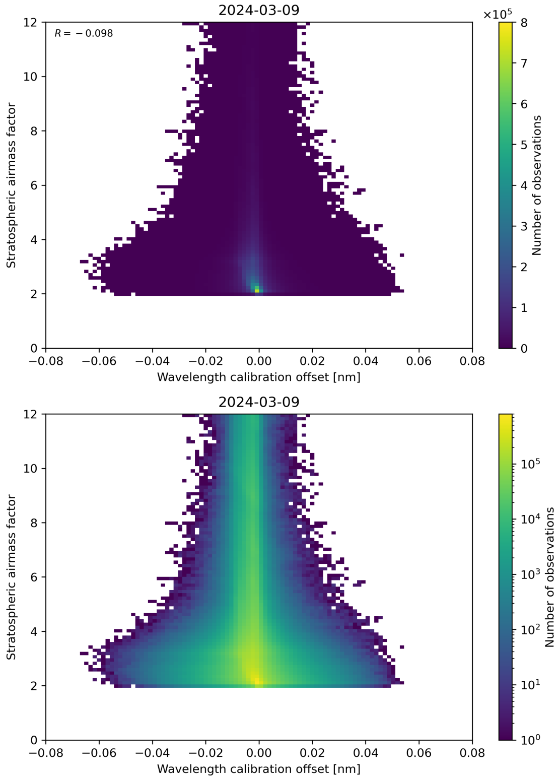
Figure 174: Scatter density plot of “Wavelength calibration offset” against “Stratospheric air mass factor” for 2024-03-09 to 2024-03-10.
