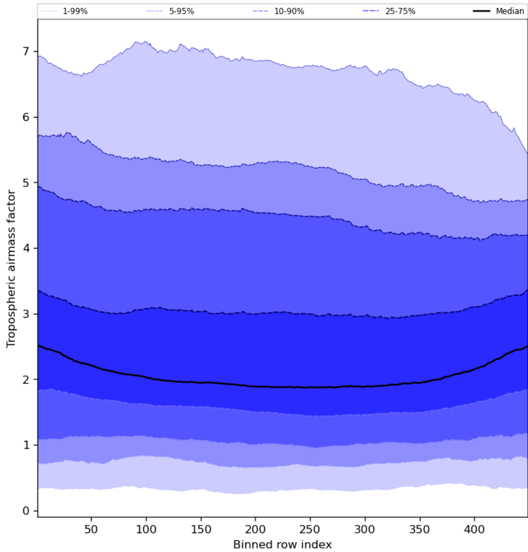
Figure 48: Along track statistics of “Tropospheric air mass factor” for 2024-03-09 to 2024-03-10
