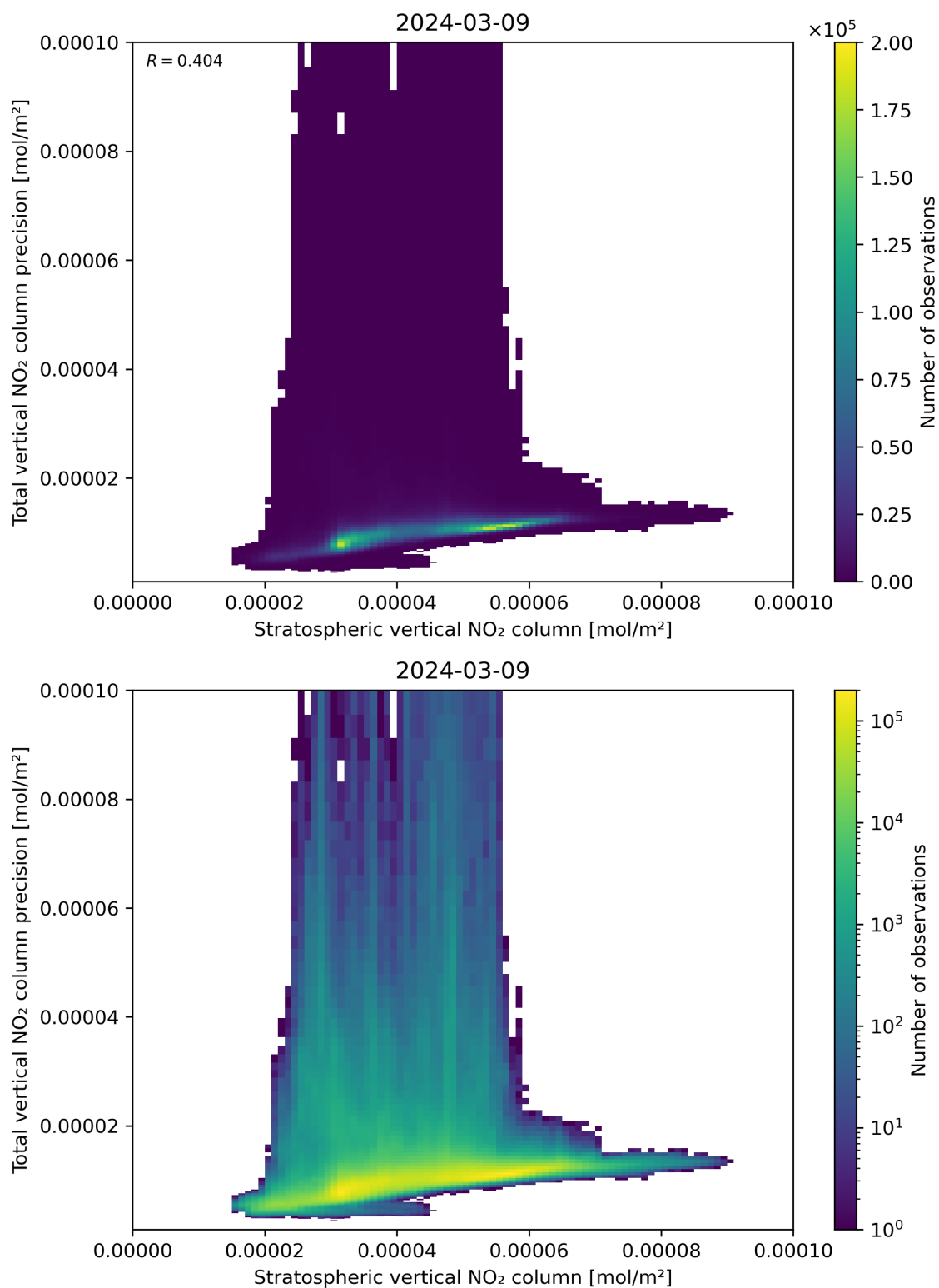
Figure 101: Scatter density plot of “Stratospheric vertical NO 2 column” against “Total vertical NO 2 column precision” for 2024-03-09 to 2024-03-10.
