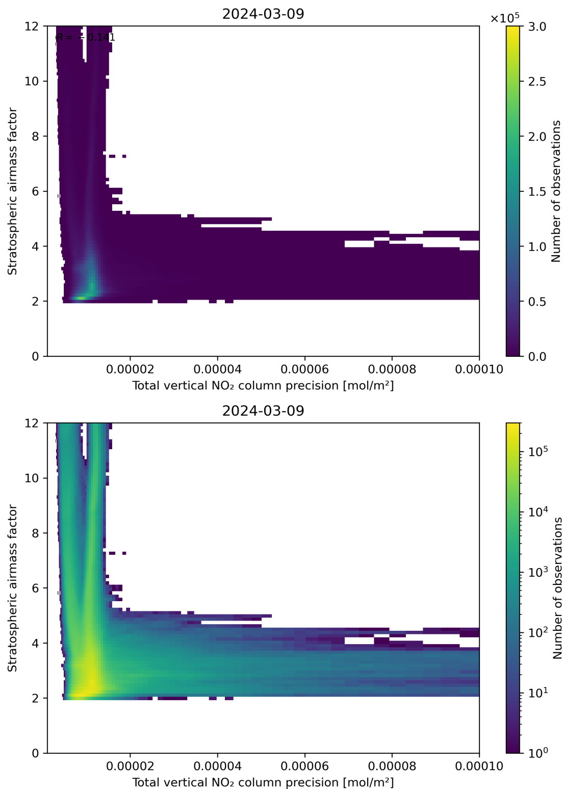
Figure 115: Scatter density plot of “Total vertical NO 2 column precision” against “Stratospheric air mass factor” for 2024-03-09 to 2024-03-10.
