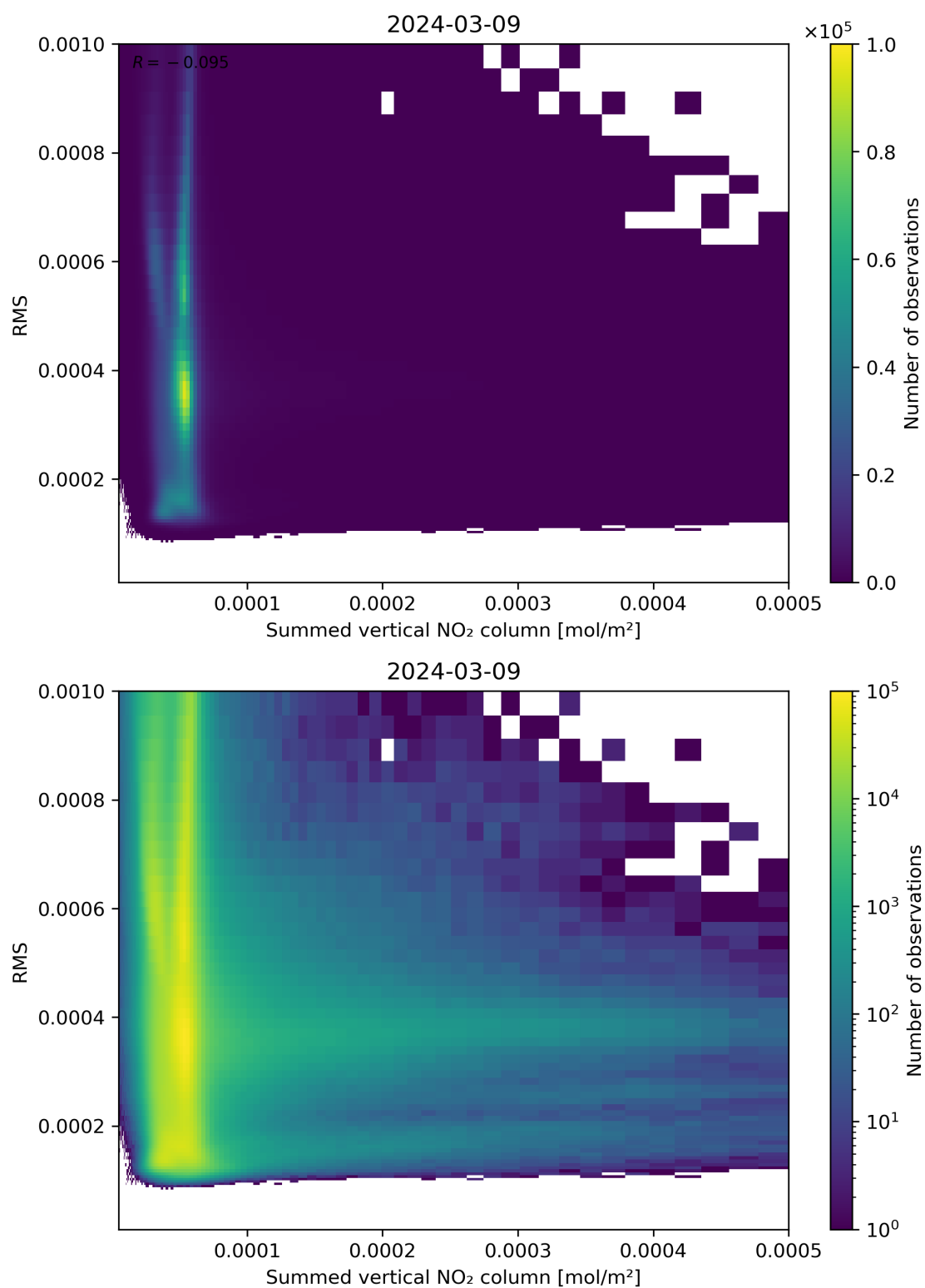
Figure 109: Scatter density plot of “Summed vertical NO 2 column” against “RMS” for 2024-03-09 to 2024-03-10.
