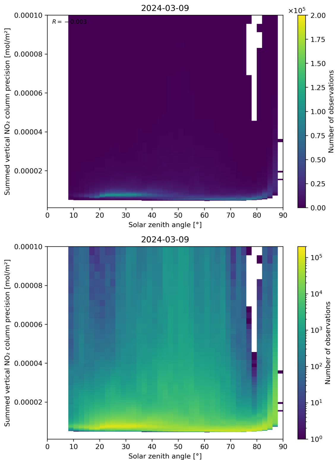
Figure 152: Scatter density plot of “Solar zenith angle” against “Summed vertical NO 2 column precision” for 2024-03-09 to 2024-03-10.
