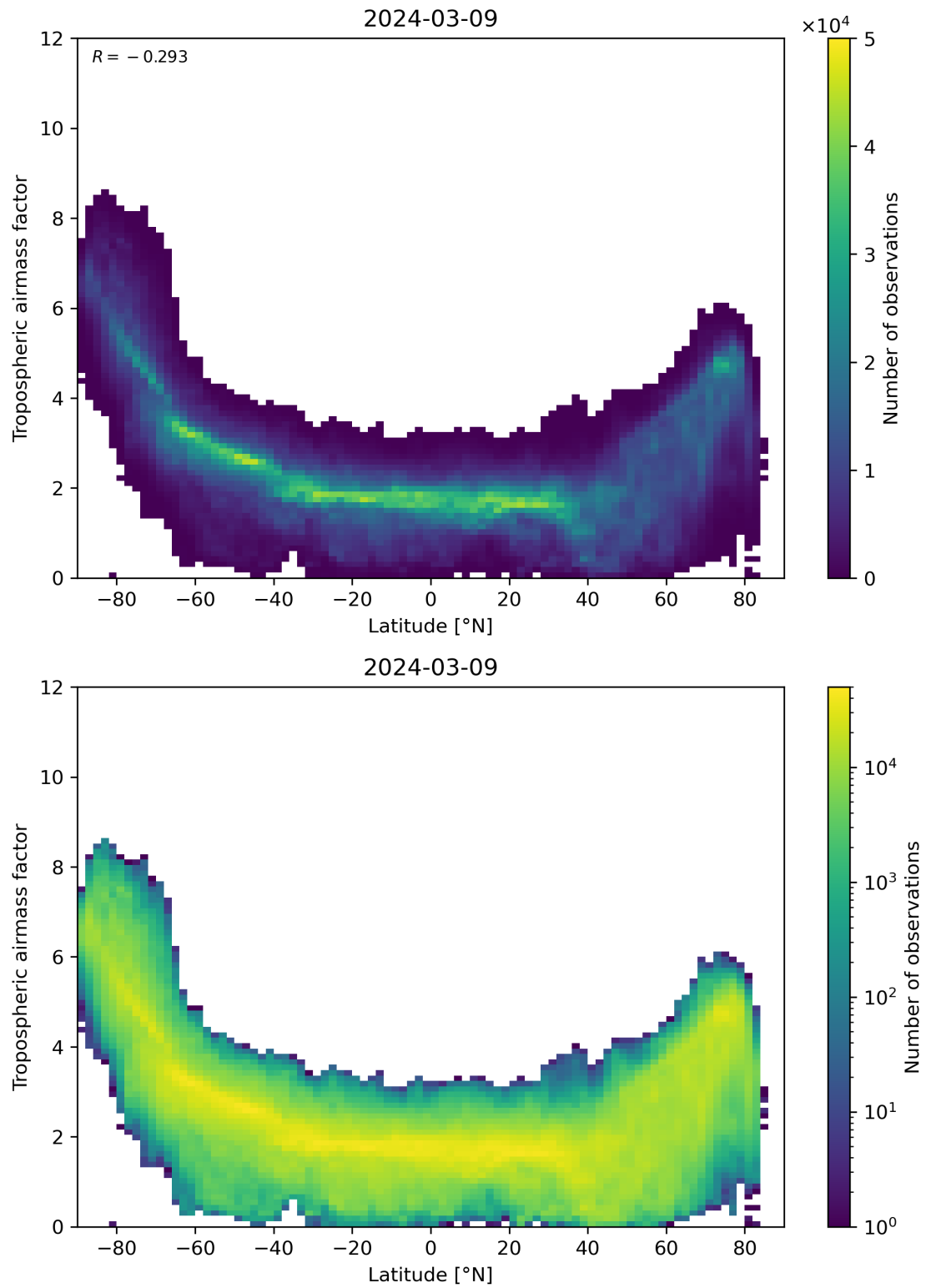
Figure 85: Scatter density plot of “Latitude” against “Tropospheric airmass factor” for 2024-03-09 to 2024-03-10.
