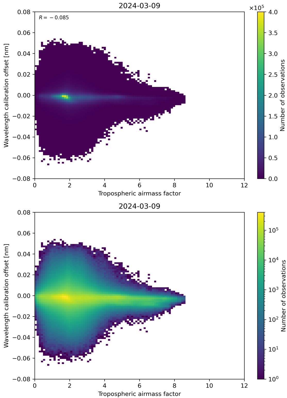
Figure 80: Scatter density plot of “Tropospheric airmass factor” against “Wavelength calibration offset” for 2024-03-09 to 2024-03-10.
