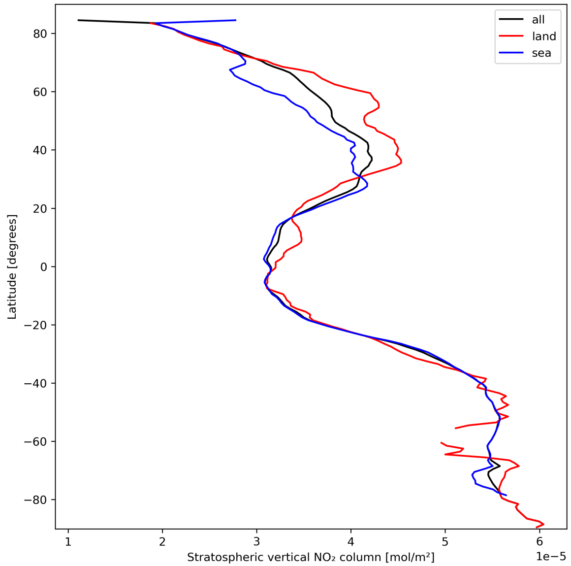
Figure 19: Zonal average of “Stratospheric vertical NO 2 column” for 2024-03-09 to 2024-03-10.
