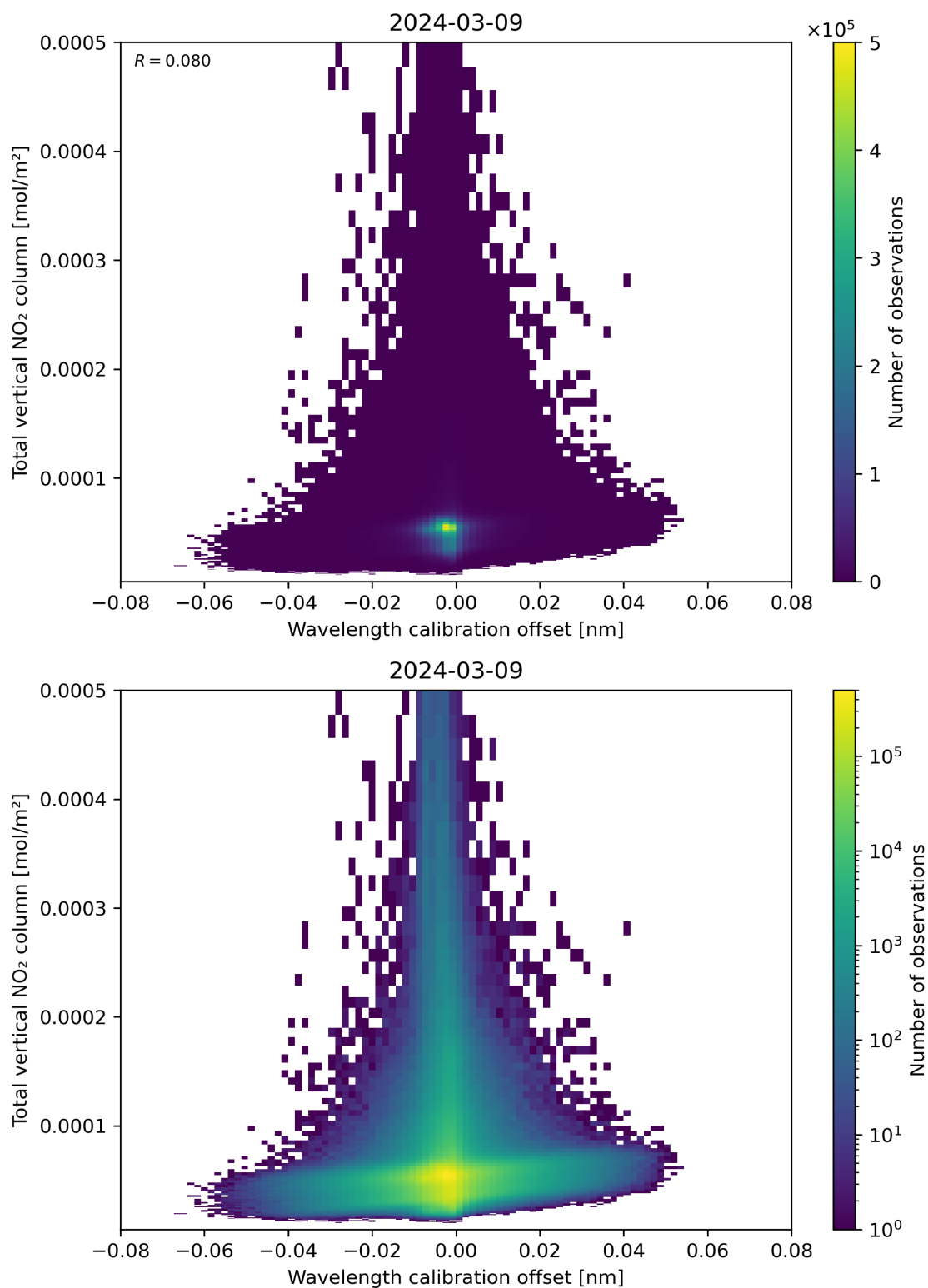
Figure 179: Scatter density plot of “Wavelength calibration offset” against “Total vertical NO 2 column” for 2024-03-09 to 2024-03-10.
