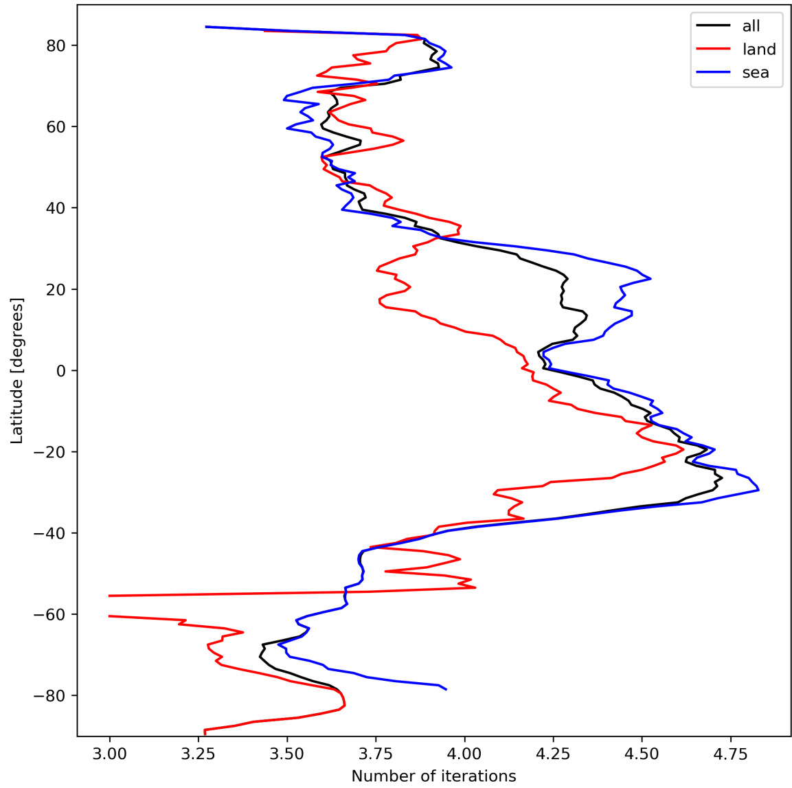
Figure 17: Zonal average of “Number of iterations” for 2024-03-09 to 2024-03-10.
