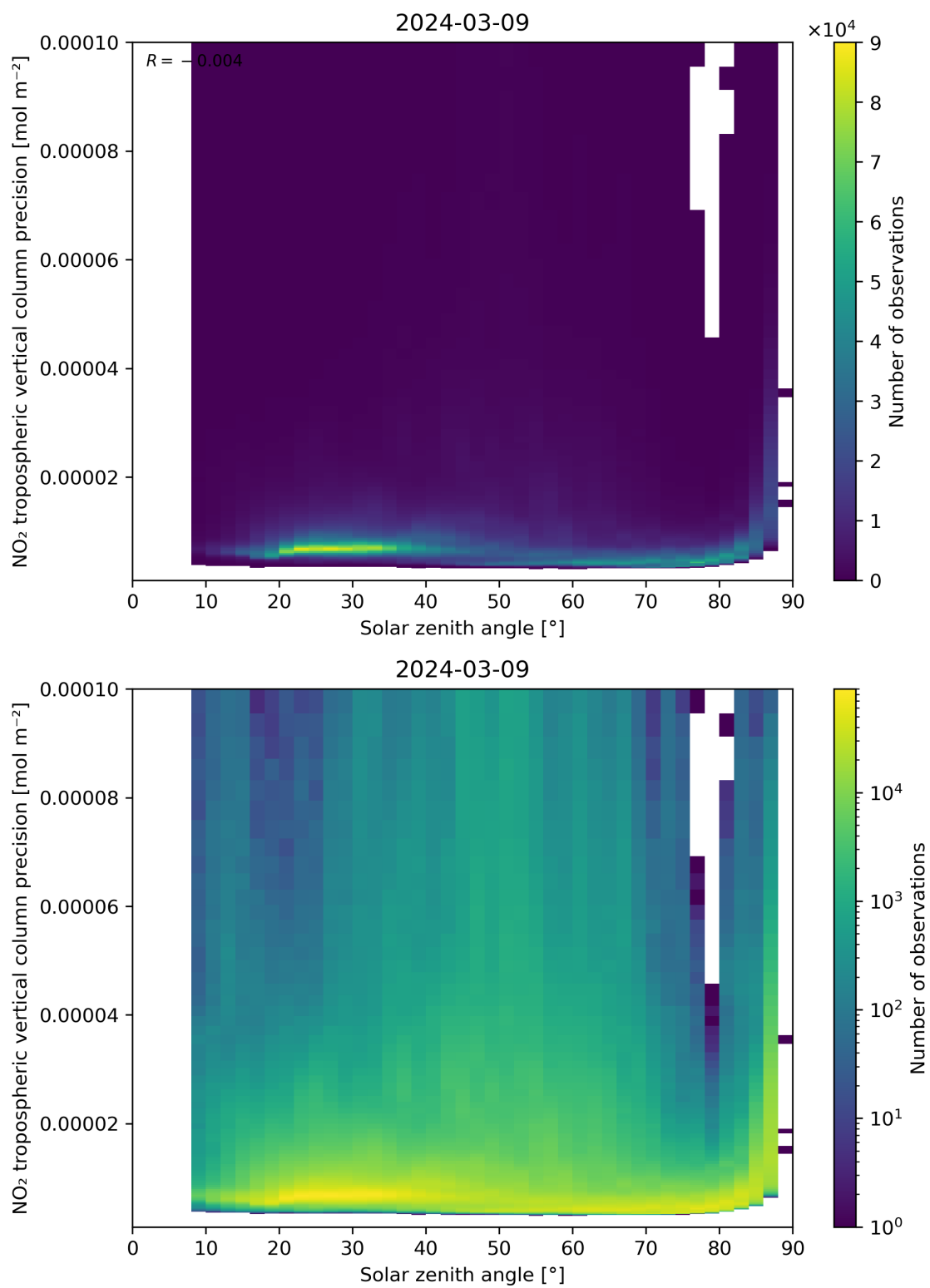
Figure 156: Scatter density plot of “Solar zenith angle” against “NO 2 tropospheric vertical column precision” for 2024-03-09 to 2024-03-10.
