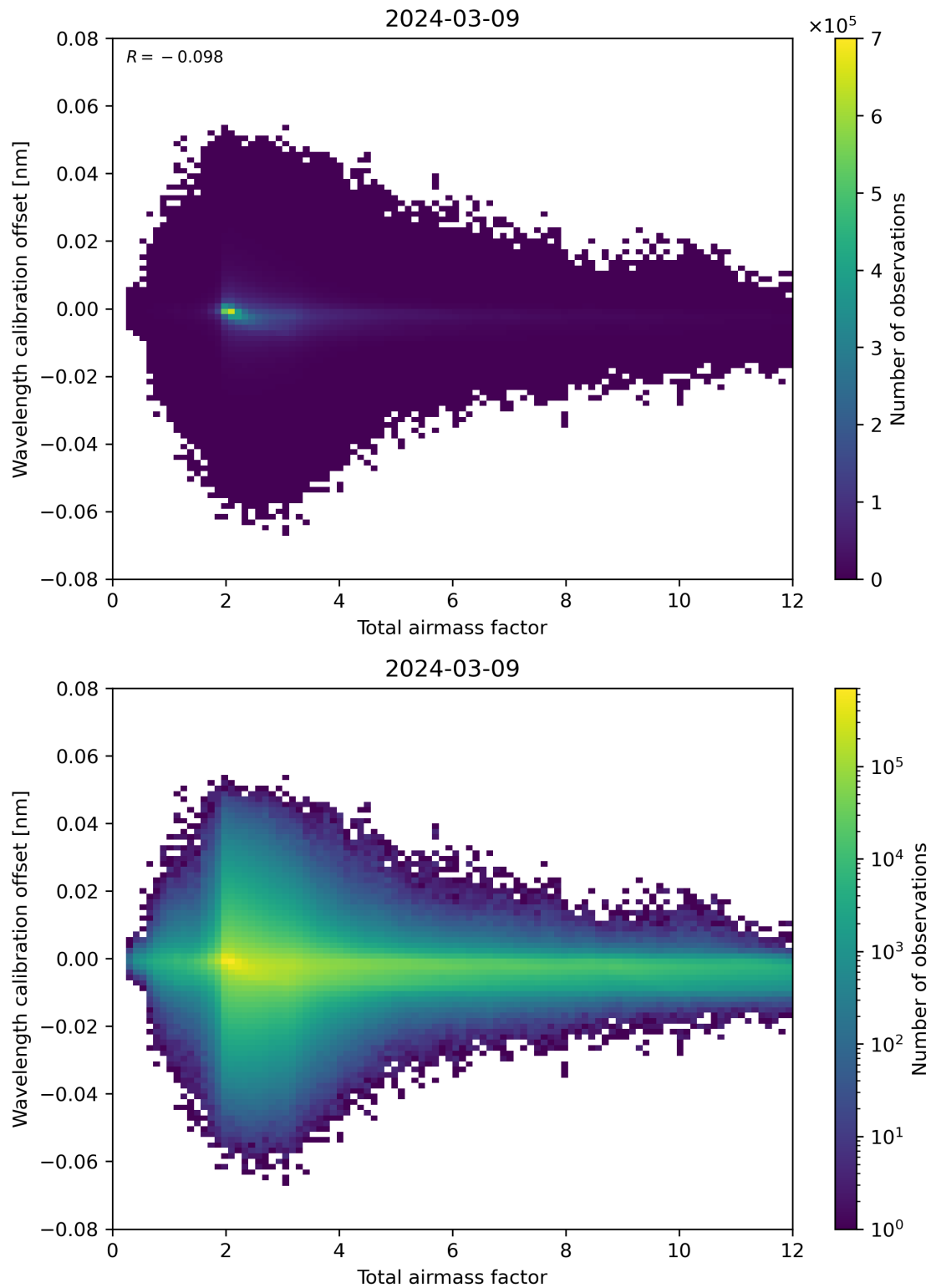
Figure 70: Scatter density plot of “Total airmass factor” against “Wavelength calibration offset” for 2024-03-09 to 2024-03-10.
