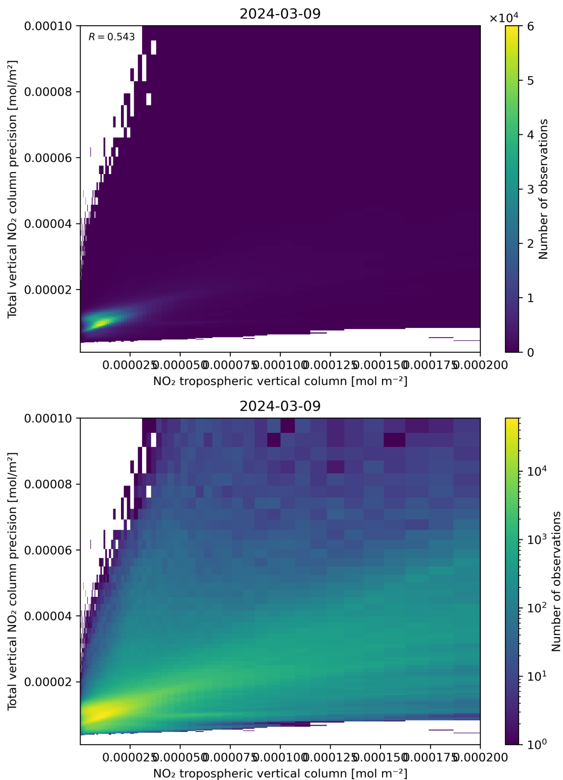
Figure 129: Scatter density plot of “NO 2 tropospheric vertical column” against “Total vertical NO 2 column precision” for 2024-03-09 to 2024-03-10.
