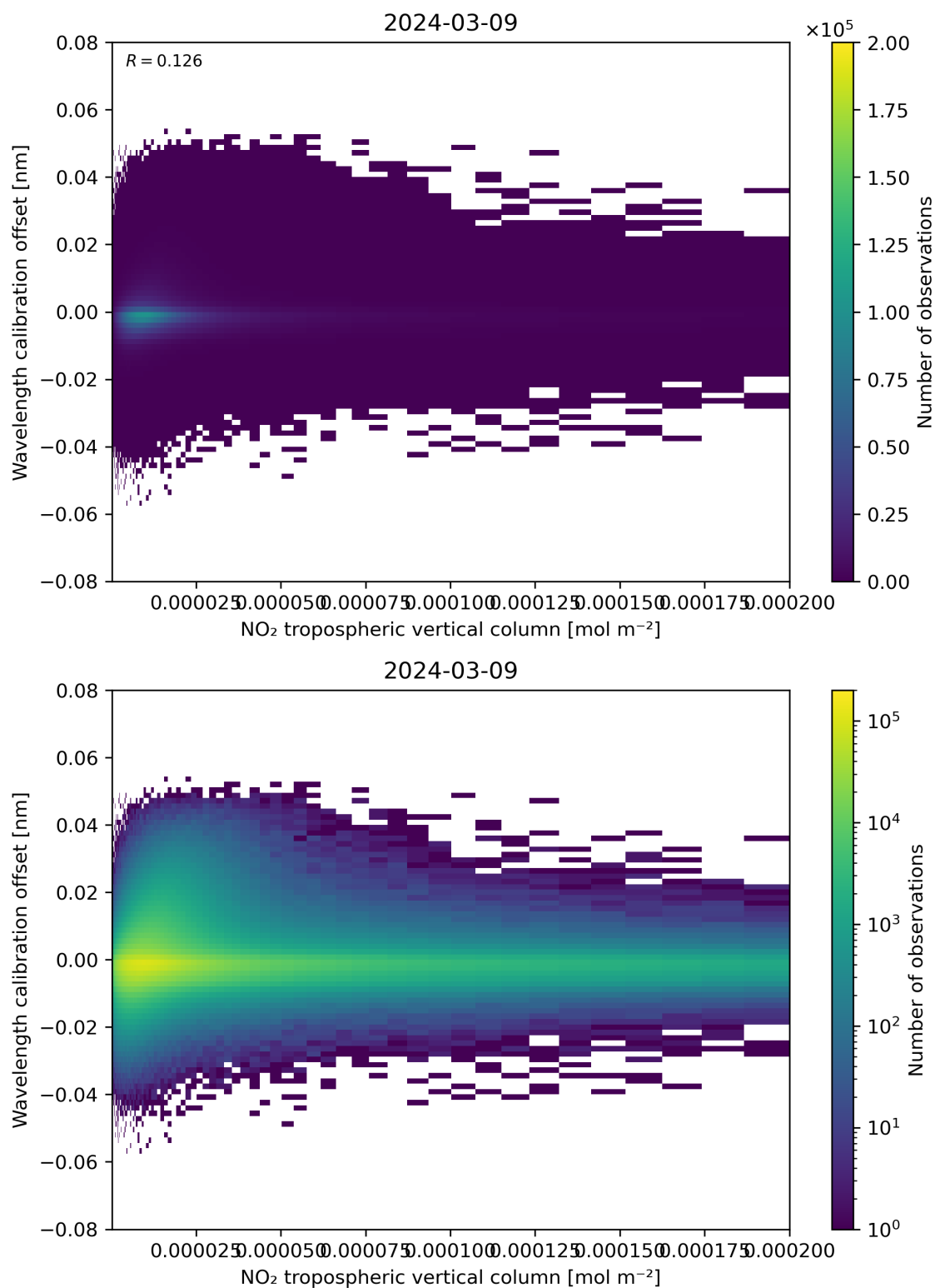
Figure 143: Scatter density plot of “NO 2 tropospheric vertical column” against “Wavelength calibration offset” for 2024-03-09 to 2024-03-10.
