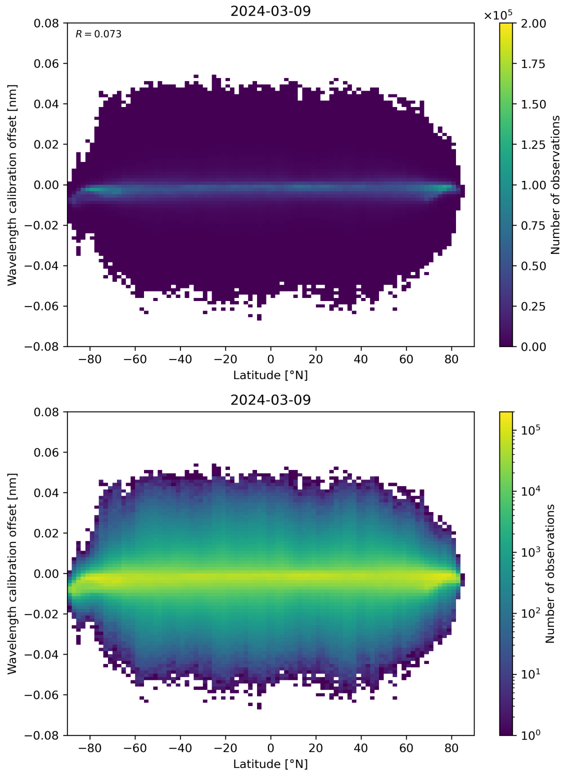
Figure 95: Scatter density plot of “Latitude” against “Wavelength calibration offset” for 2024-03-09 to 2024-03-10.
