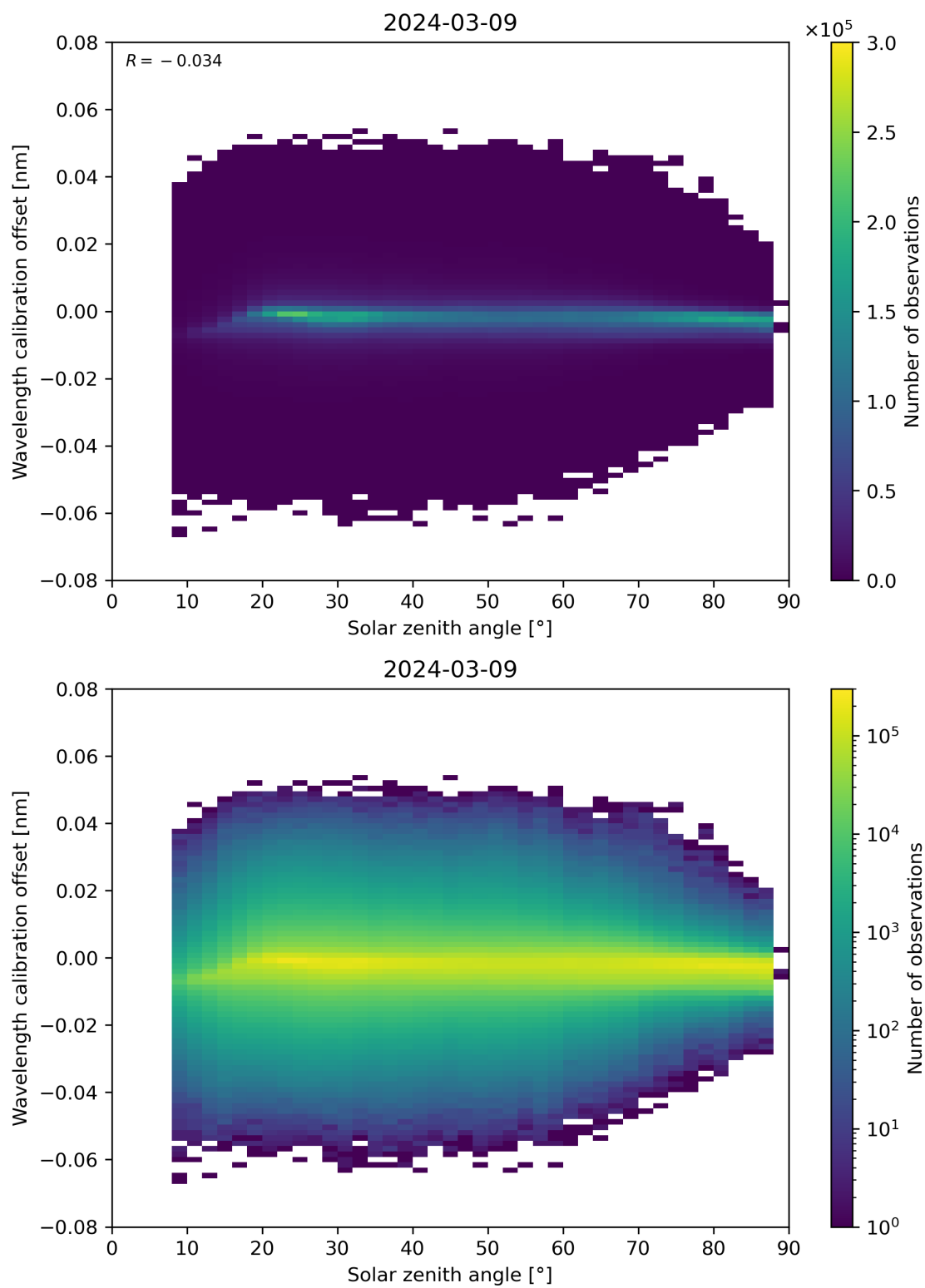
Figure 158: Scatter density plot of “Solar zenith angle” against “Wavelength calibration offset” for 2024-03-09 to 2024-03-10.
