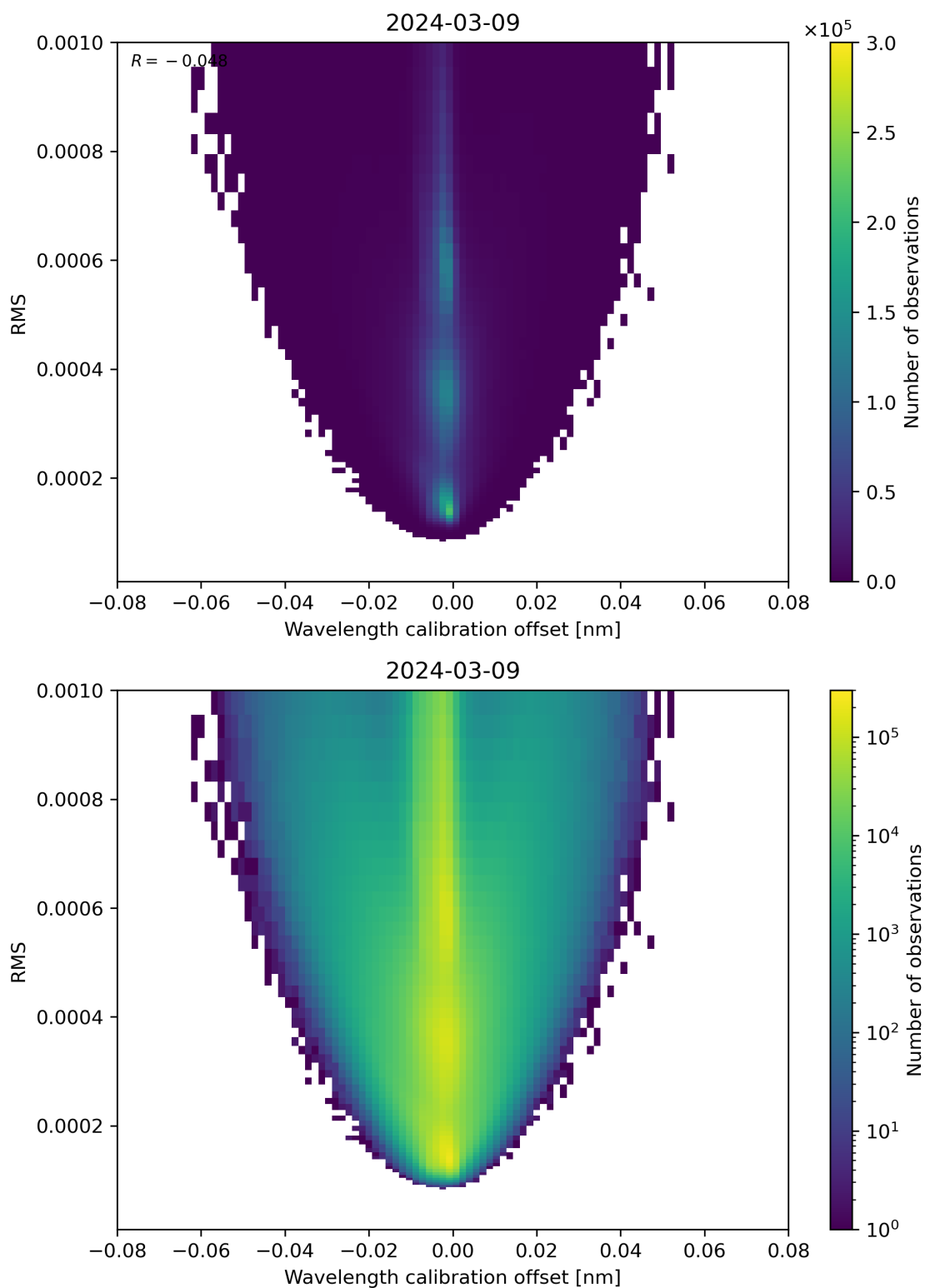
Figure 181: Scatter density plot of “Wavelength calibration offset” against “RMS” for 2024-03-09 to 2024-03-10.
