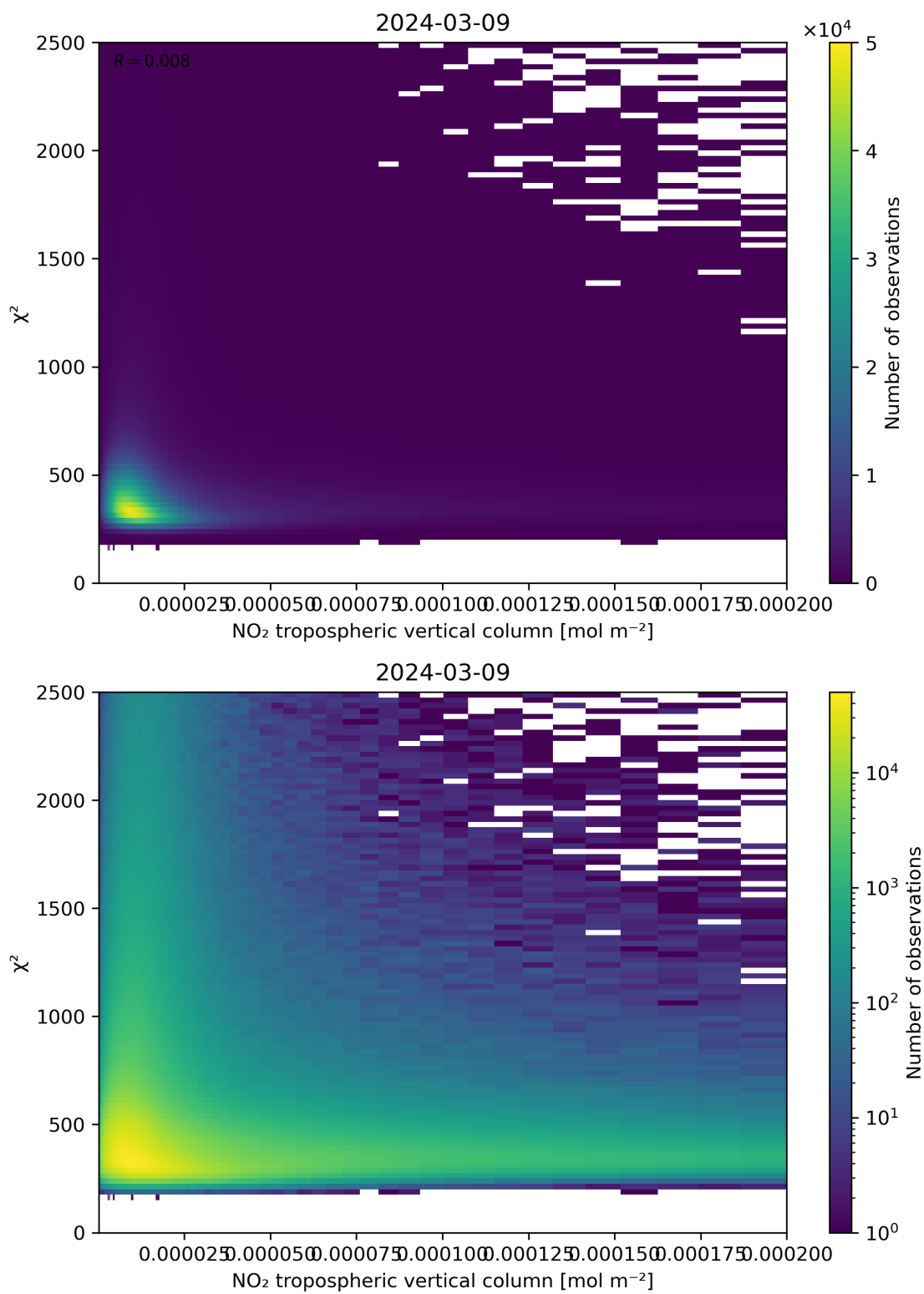
Figure 124: Scatter density plot of “NO 2 tropospheric vertical column” against “ \chi^2 ” for 2024-03-09 to 2024-03-10.
