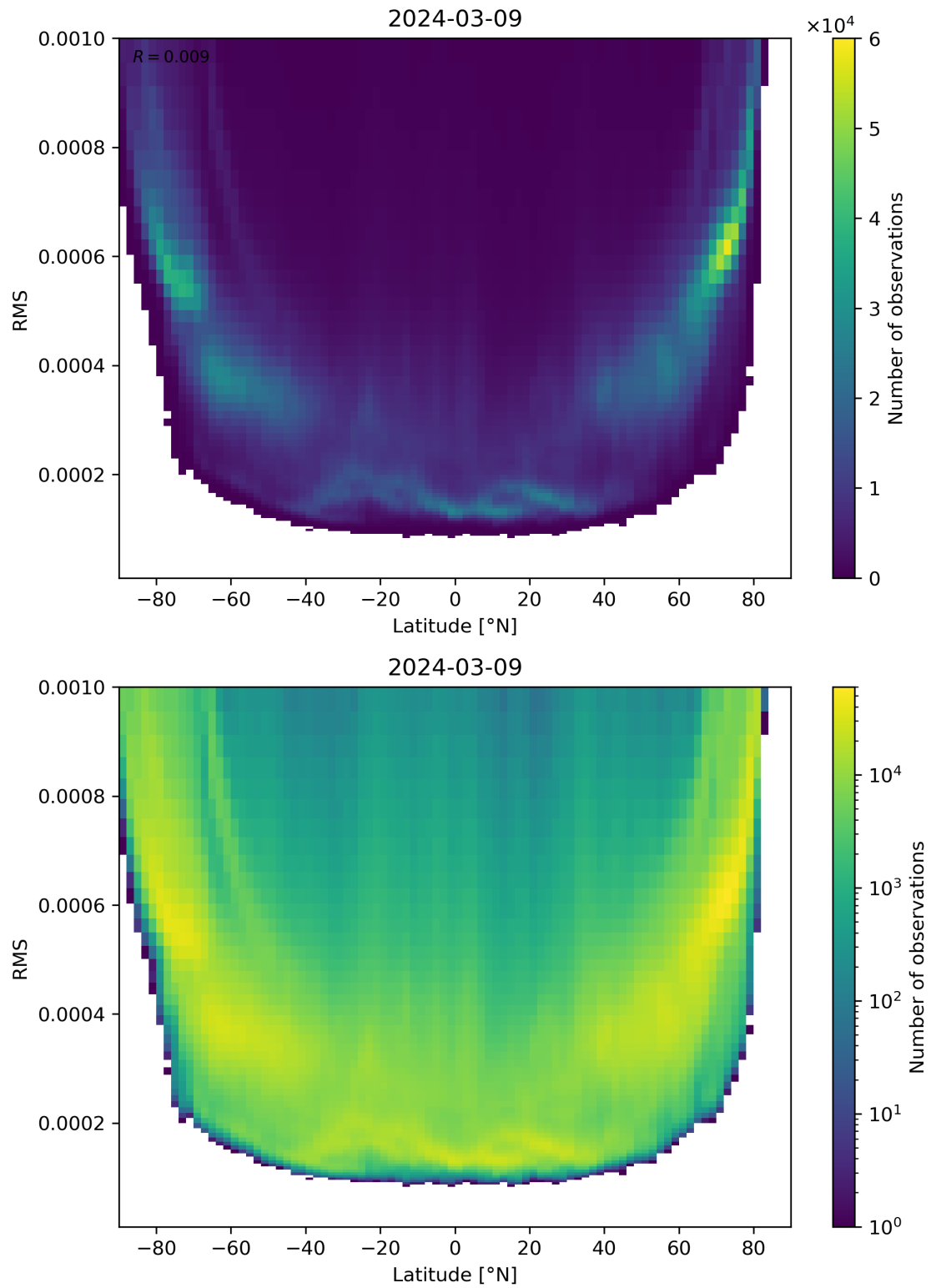
Figure 94: Scatter density plot of “Latitude” against “RMS” for 2024-03-09 to 2024-03-10.
