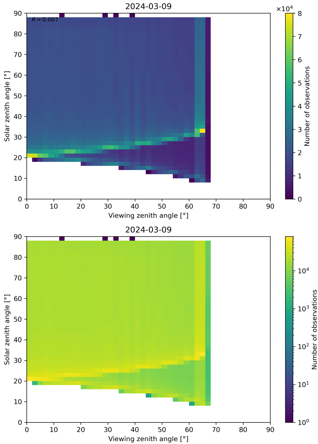
Figure 172: Scatter density plot of “Viewing zenith angle” against “Solar zenith angle” for 2024-03-09 to 2024-03-10.
