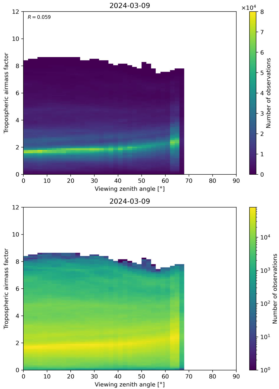
Figure 161: Scatter density plot of “Viewing zenith angle” against “Tropospheric airmass factor” for 2024-03-09 to 2024-03-10.
