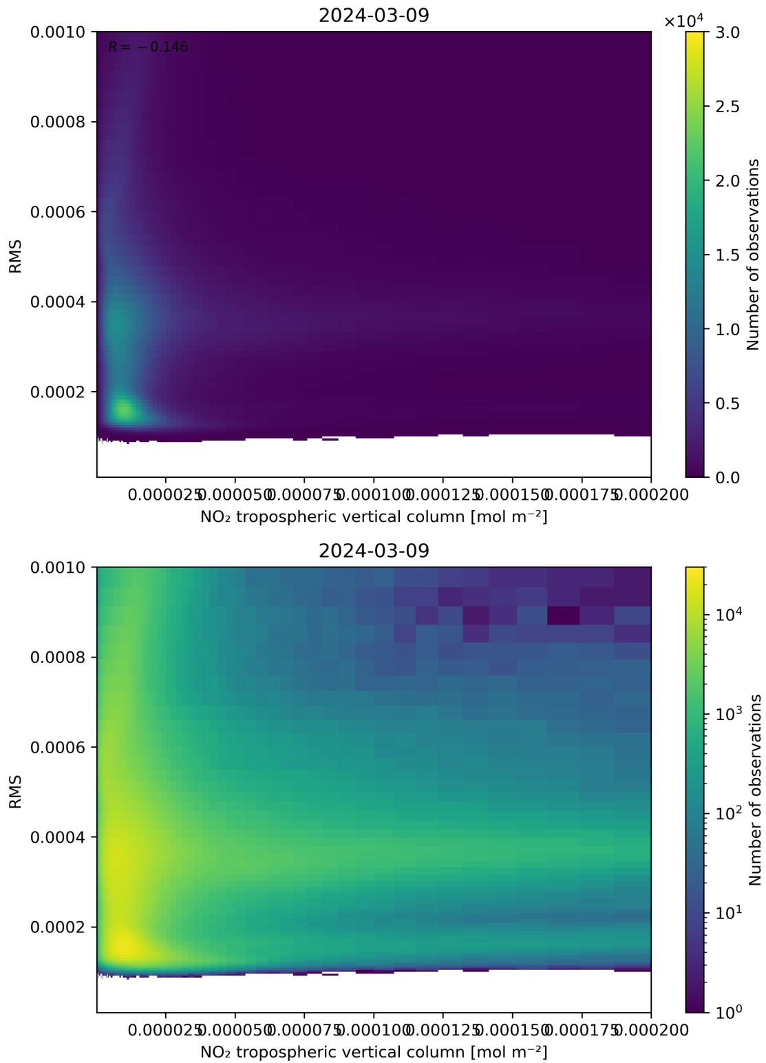
Figure 142: Scatter density plot of “NO 2 tropospheric vertical column” against “RMS” for 2024-03-09 to 2024-03-10.
