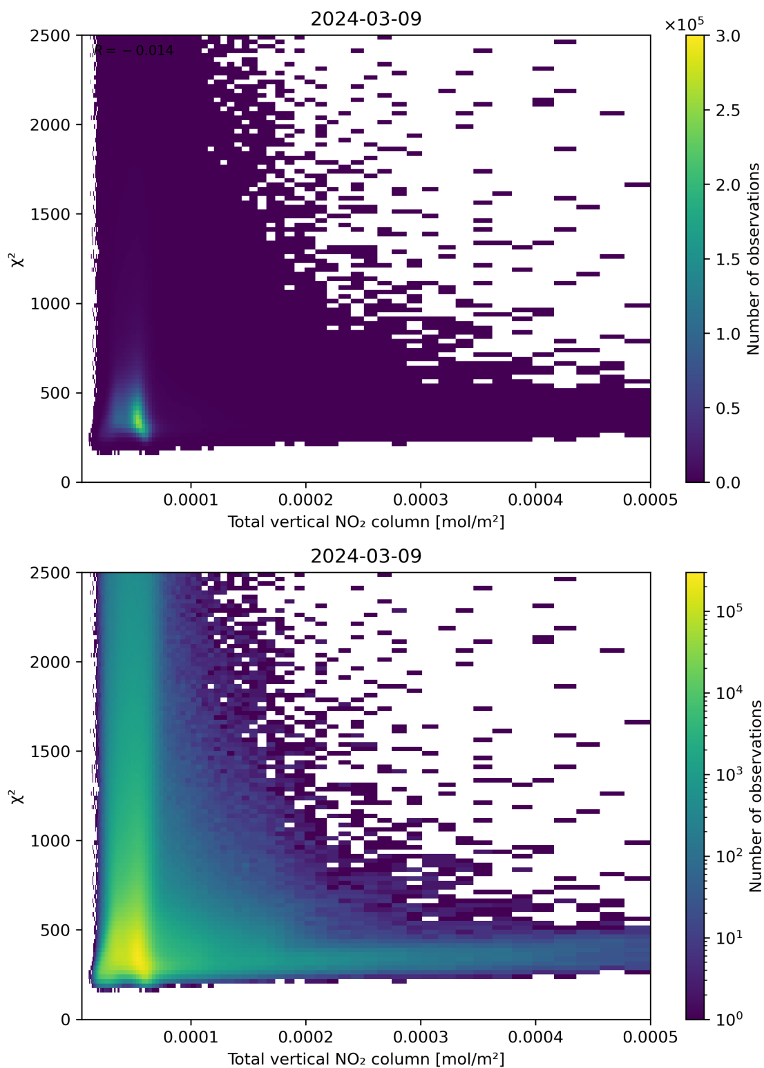
Figure 111: Scatter density plot of “Total vertical NO 2 column” against “ \chi^2 ” for 2024-03-09 to 2024-03-10.
