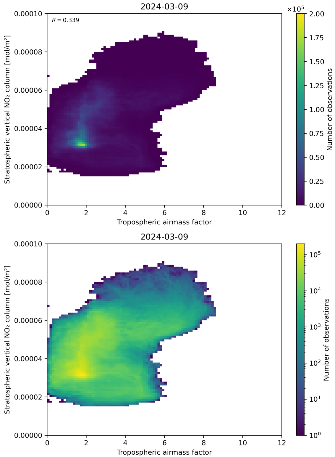
Figure 74: Scatter density plot of “Tropospheric airmass factor” against “Stratospheric vertical NO 2 column” for 2024-03-09 to 2024-03-10.
