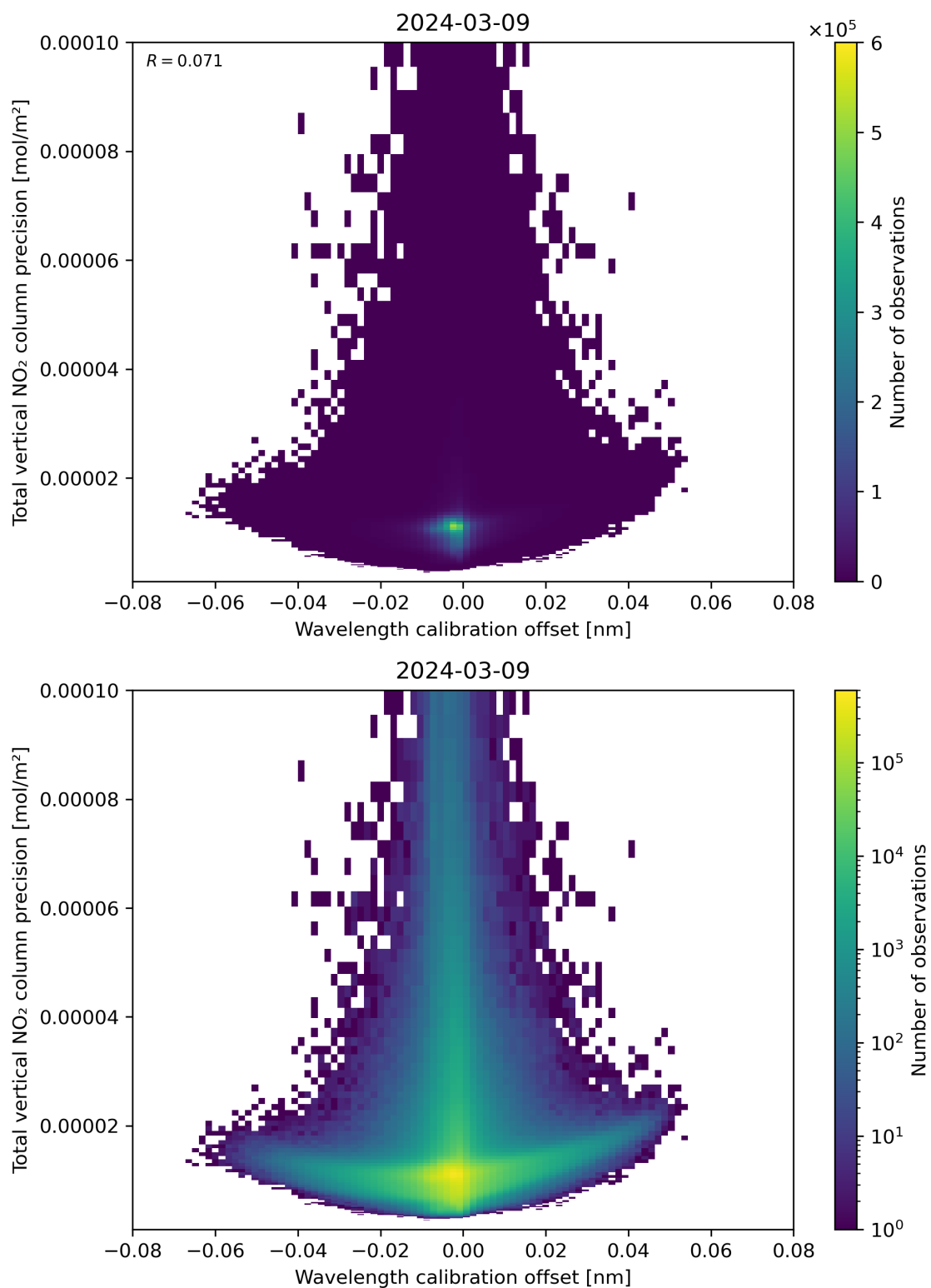
Figure 180: Scatter density plot of “Wavelength calibration offset” against “Total vertical NO 2 column precision” for 2024-03-09 to 2024-03-10.
