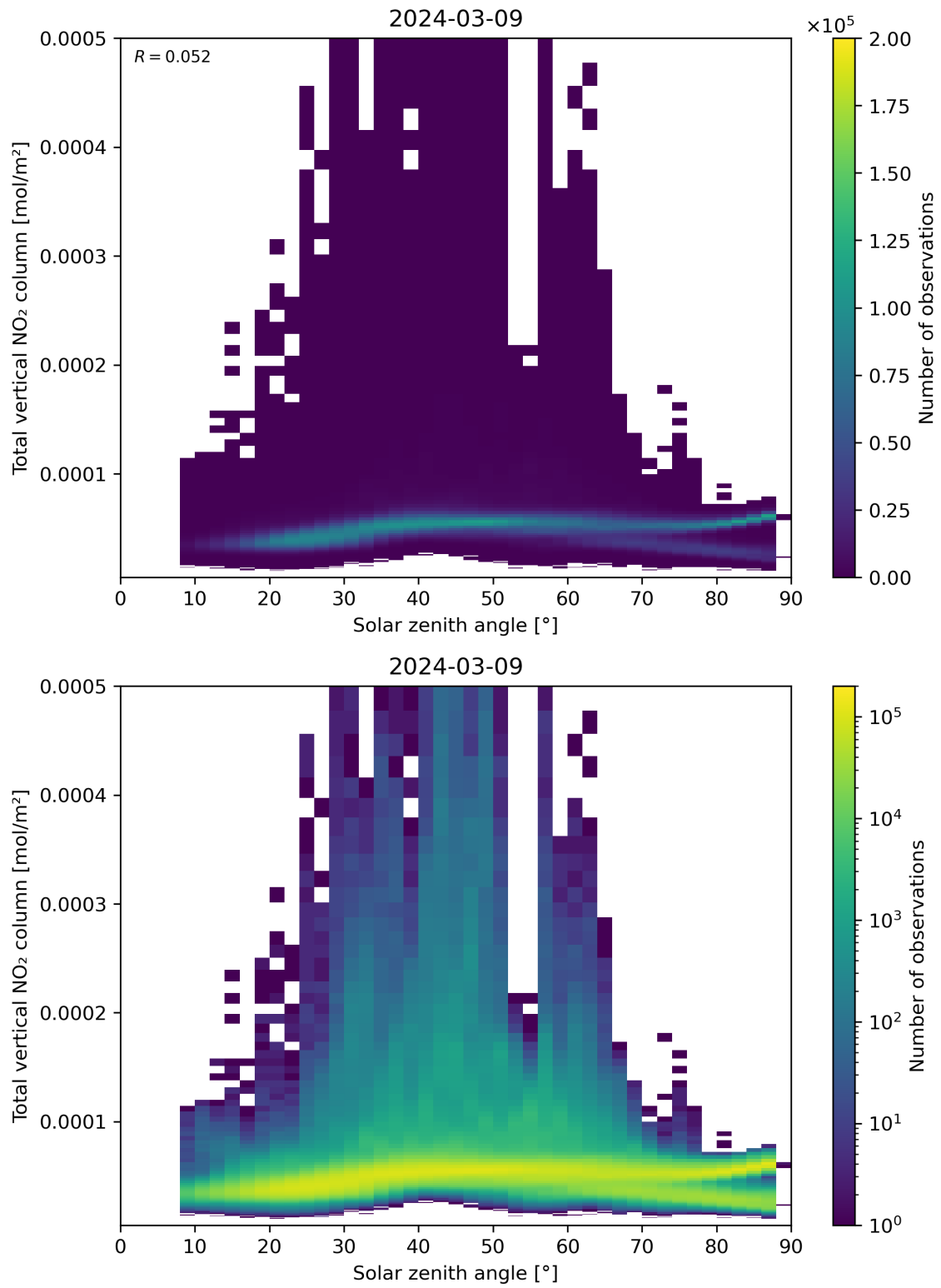
Figure 153: Scatter density plot of “Solar zenith angle” against “Total vertical NO 2 column” for 2024-03-09 to 2024-03-10.
