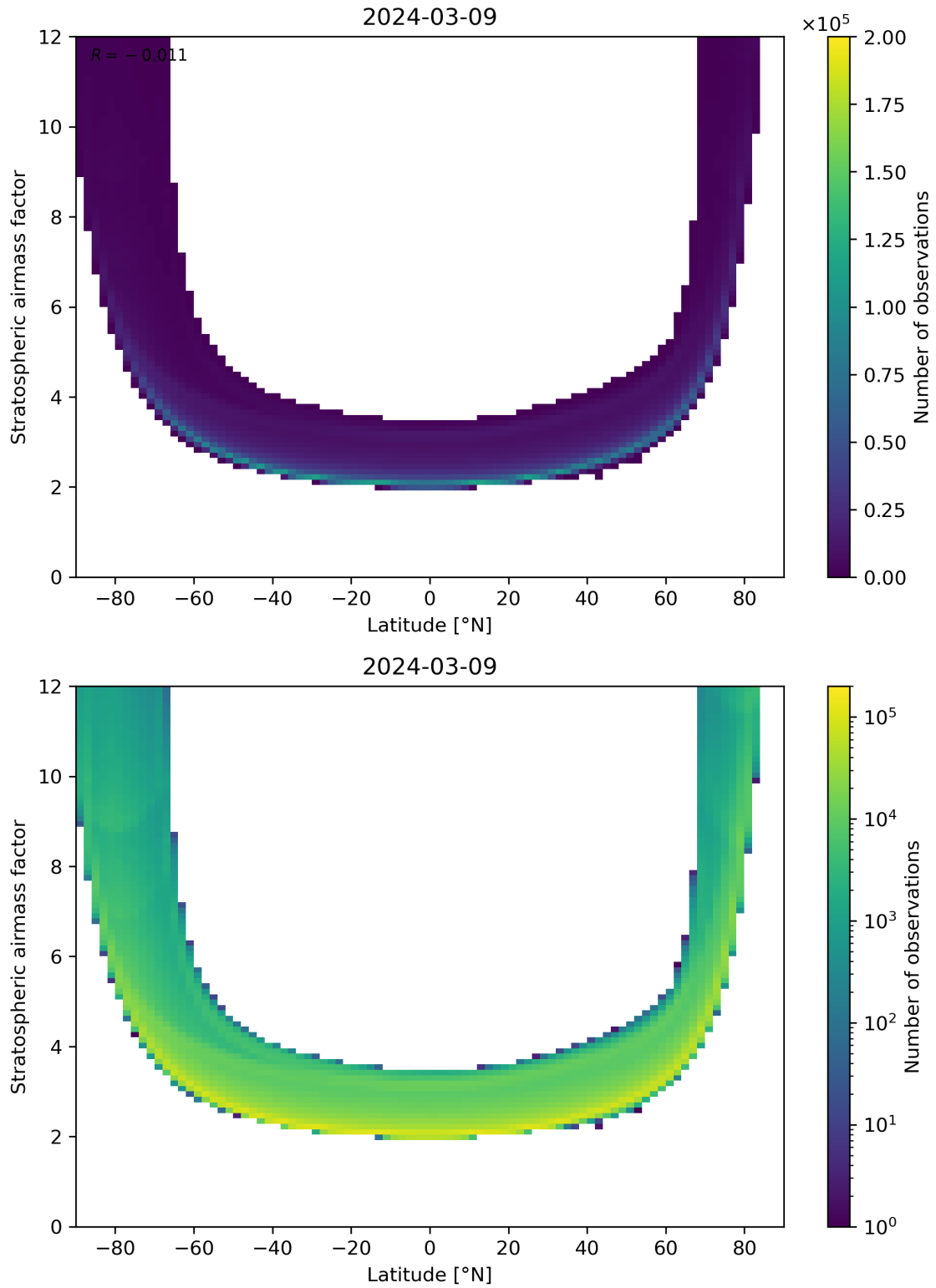
Figure 83: Scatter density plot of “Latitude” against “Stratospheric air mass factor” for 2024-03-09 to 2024-03-10.
