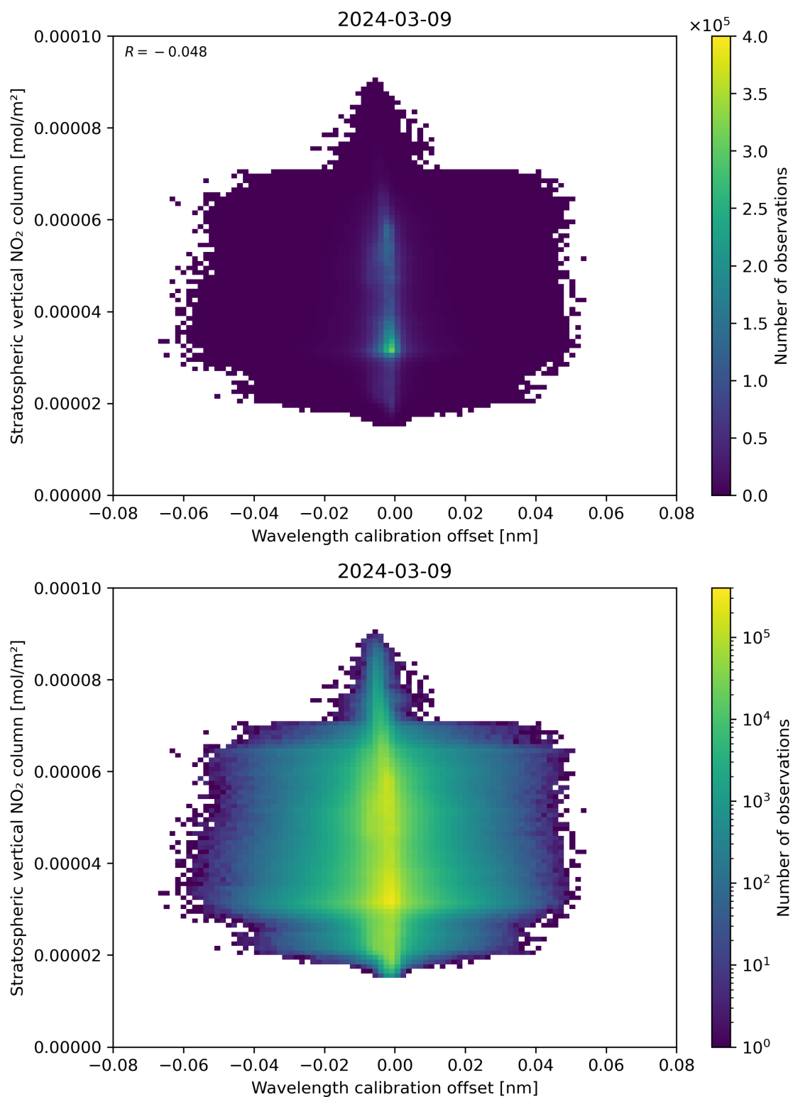
Figure 176: Scatter density plot of “Wavelength calibration offset” against “Stratospheric vertical NO 2 column” for 2024-03-09 to 2024-03-10.
