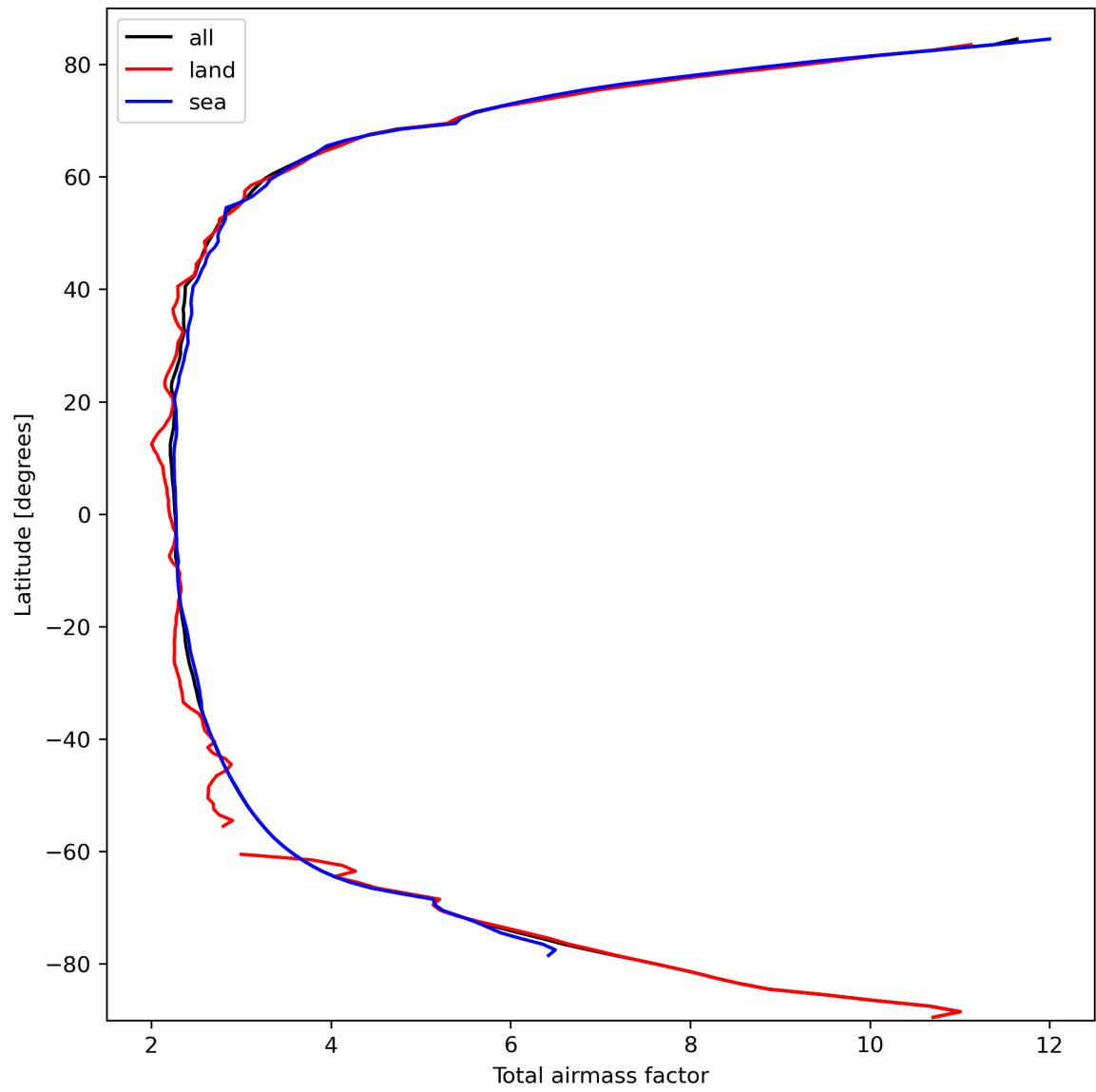
Figure 15: Zonal average of “Total airmass factor” for 2024-03-09 to 2024-03-10.
