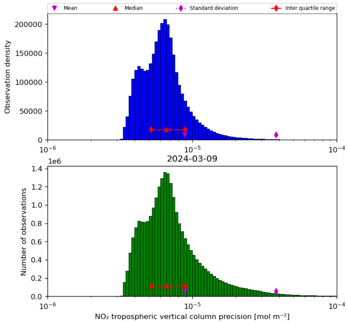
Figure 30: Histogram of “NO 2 tropospheric vertical column precision” for 2024-03-09 to 2024-03-10
