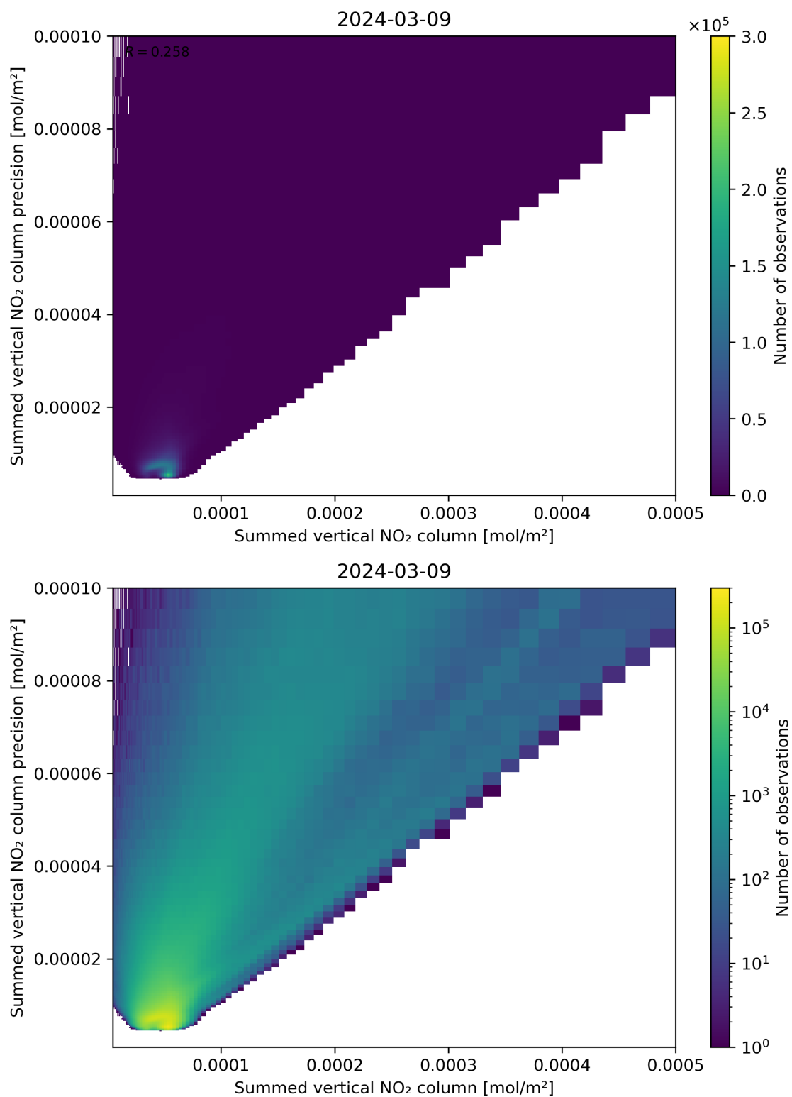
Figure 105: Scatter density plot of “Summed vertical NO 2 column” against “Summed vertical NO 2 column precision” for 2024-03-09 to 2024-03-10.
