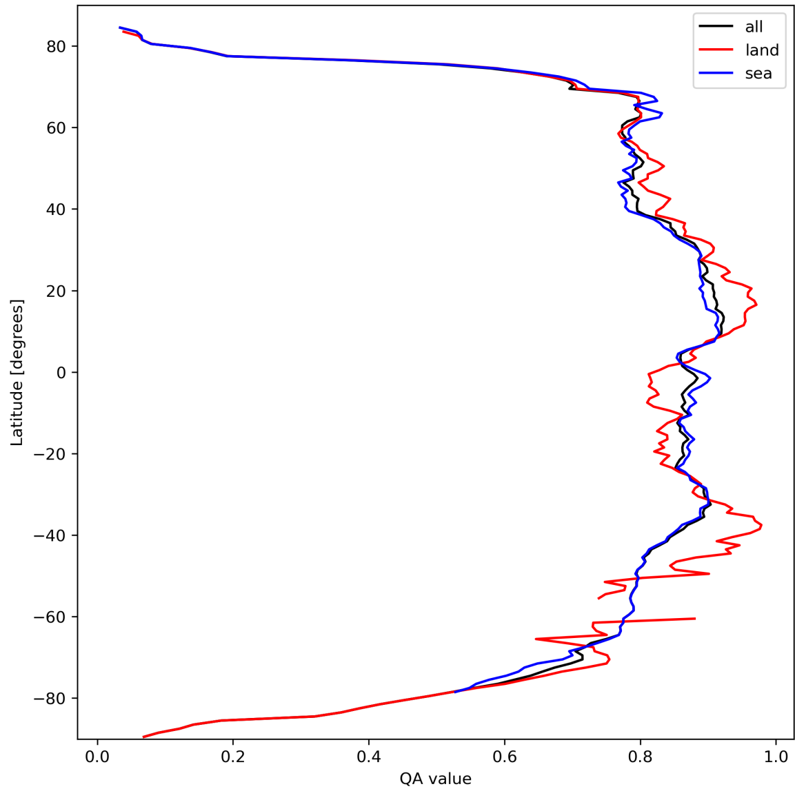
Figure 11: Zonal average of “QA value” for 2024-03-09 to 2024-03-10.
