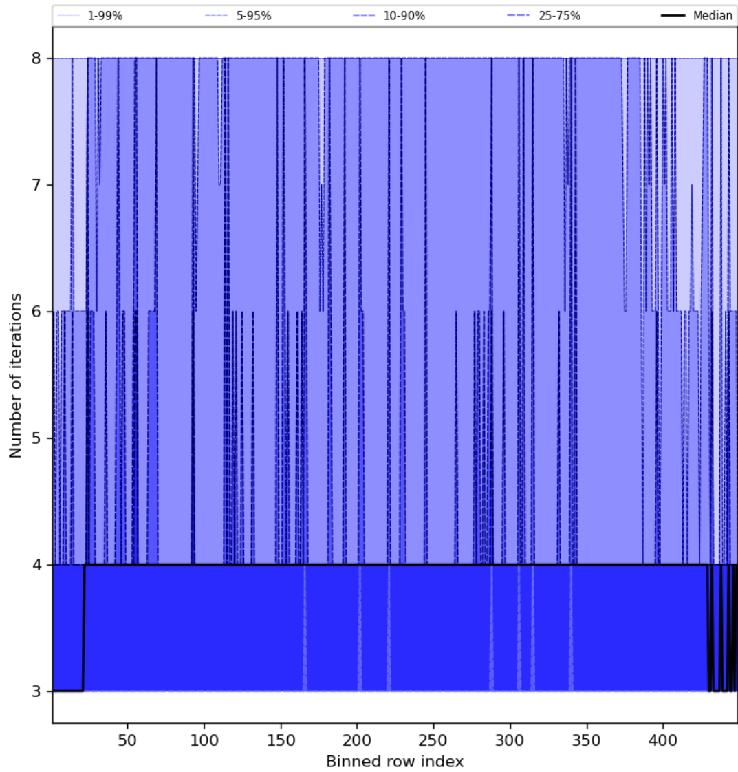
Figure 51: Along track statistics of “Number of iterations” for 2024-03-09 to 2024-03-10
