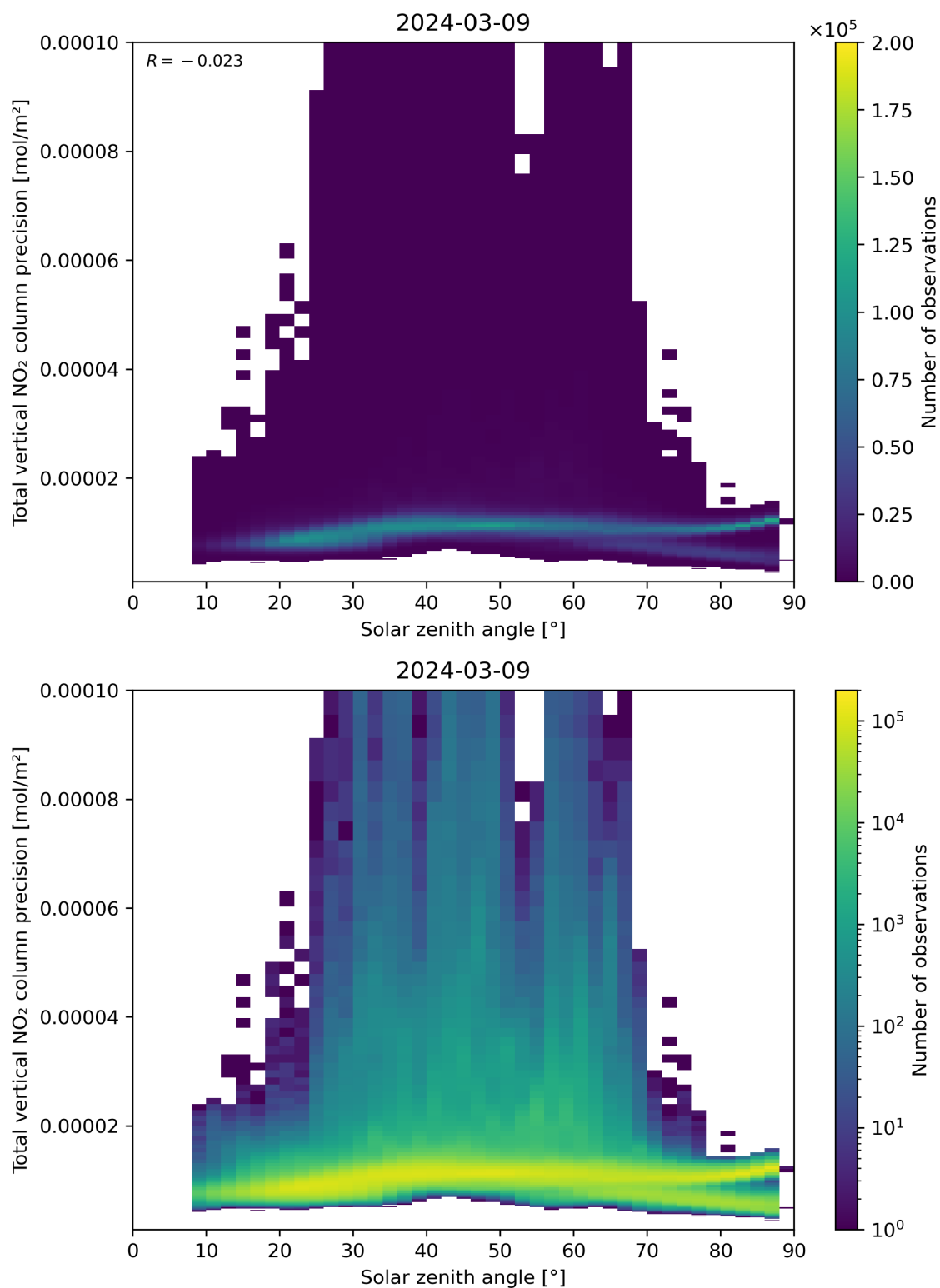
Figure 154: Scatter density plot of “Solar zenith angle” against “Total vertical NO 2 column precision” for 2024-03-09 to 2024-03-10.
