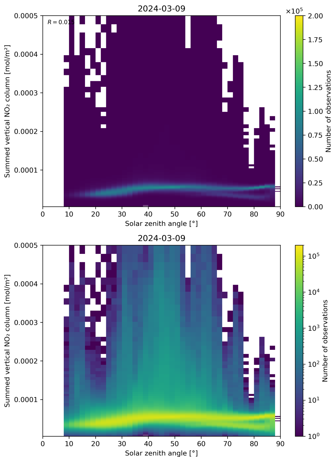
Figure 151: Scatter density plot of “Solar zenith angle” against “Summed vertical NO 2 column” for 2024-03-09 to 2024-03-10.
