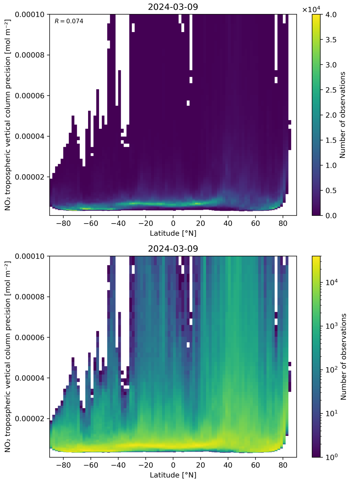
Figure 93: Scatter density plot of “Latitude” against “NO 2 tropospheric vertical column precision” for 2024-03-09 to 2024-03-10.
