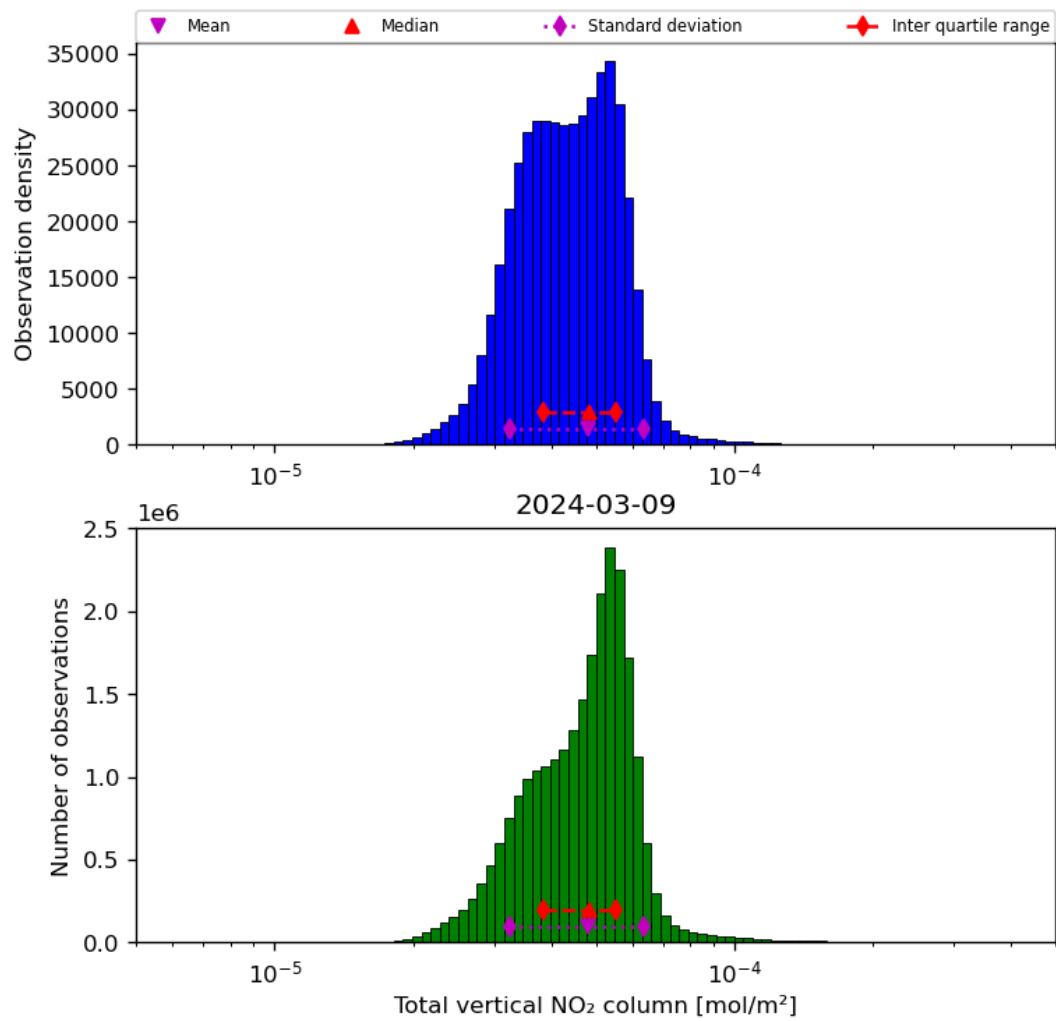
Figure 38: Histogram of “Total vertical NO 2 column” for 2024-03-09 to 2024-03-10
