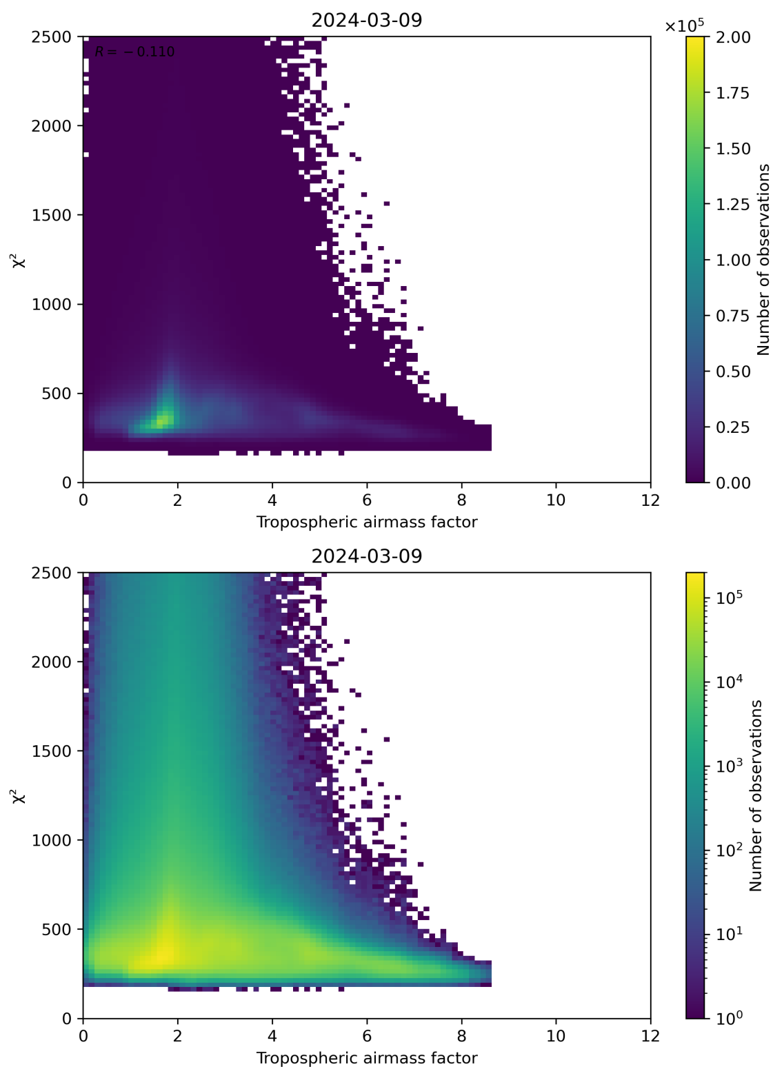
Figure 73: Scatter density plot of “Tropospheric airmass factor” against “ \chi^2 ” for 2024-03-09 to 2024-03-10.
