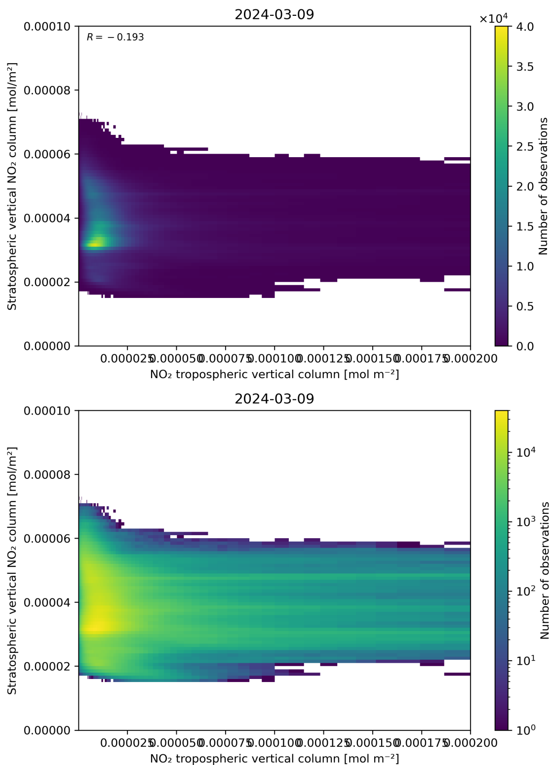
Figure 125: Scatter density plot of “NO 2 tropospheric vertical column” against “Stratospheric vertical NO 2 column” for 2024-03-09 to 2024-03-10.
