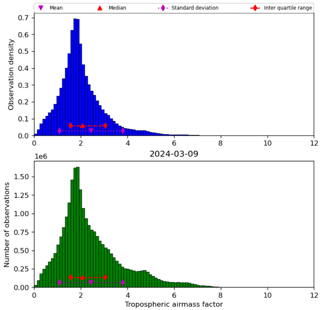
Figure 31: Histogram of “Tropospheric airmass factor” for 2024-03-09 to 2024-03-10
