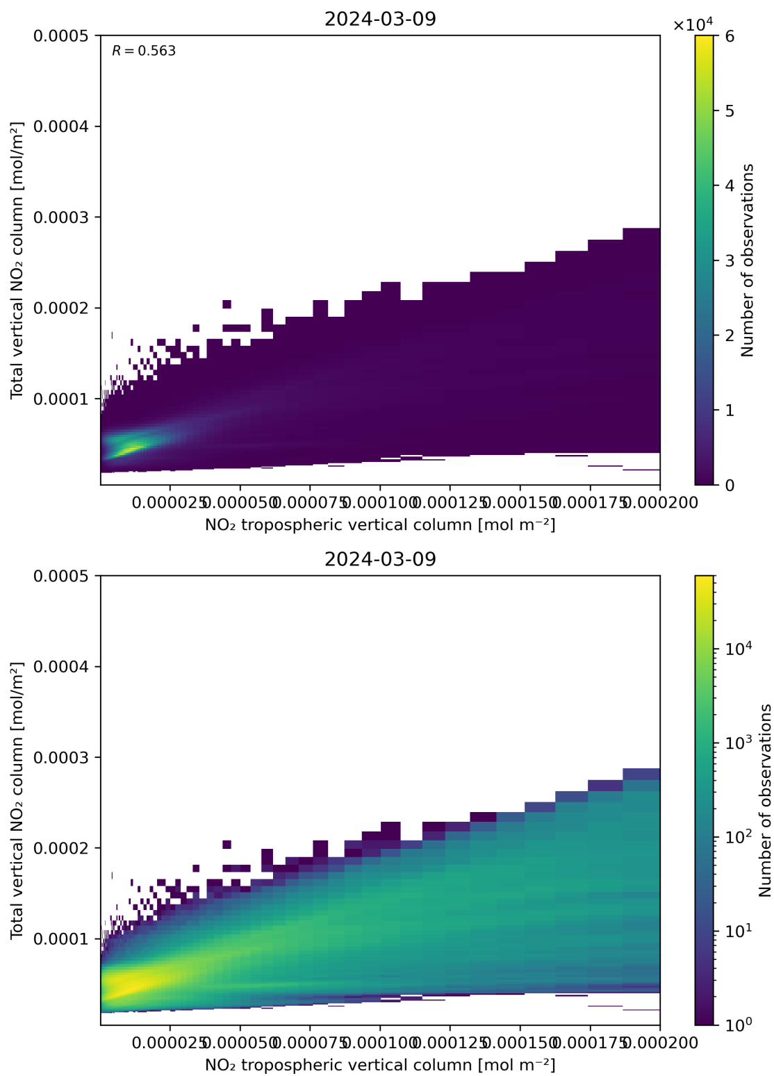
Figure 128: Scatter density plot of “NO 2 tropospheric vertical column” against “Total vertical NO 2 column” for 2024-03-09 to 2024-03-10.
