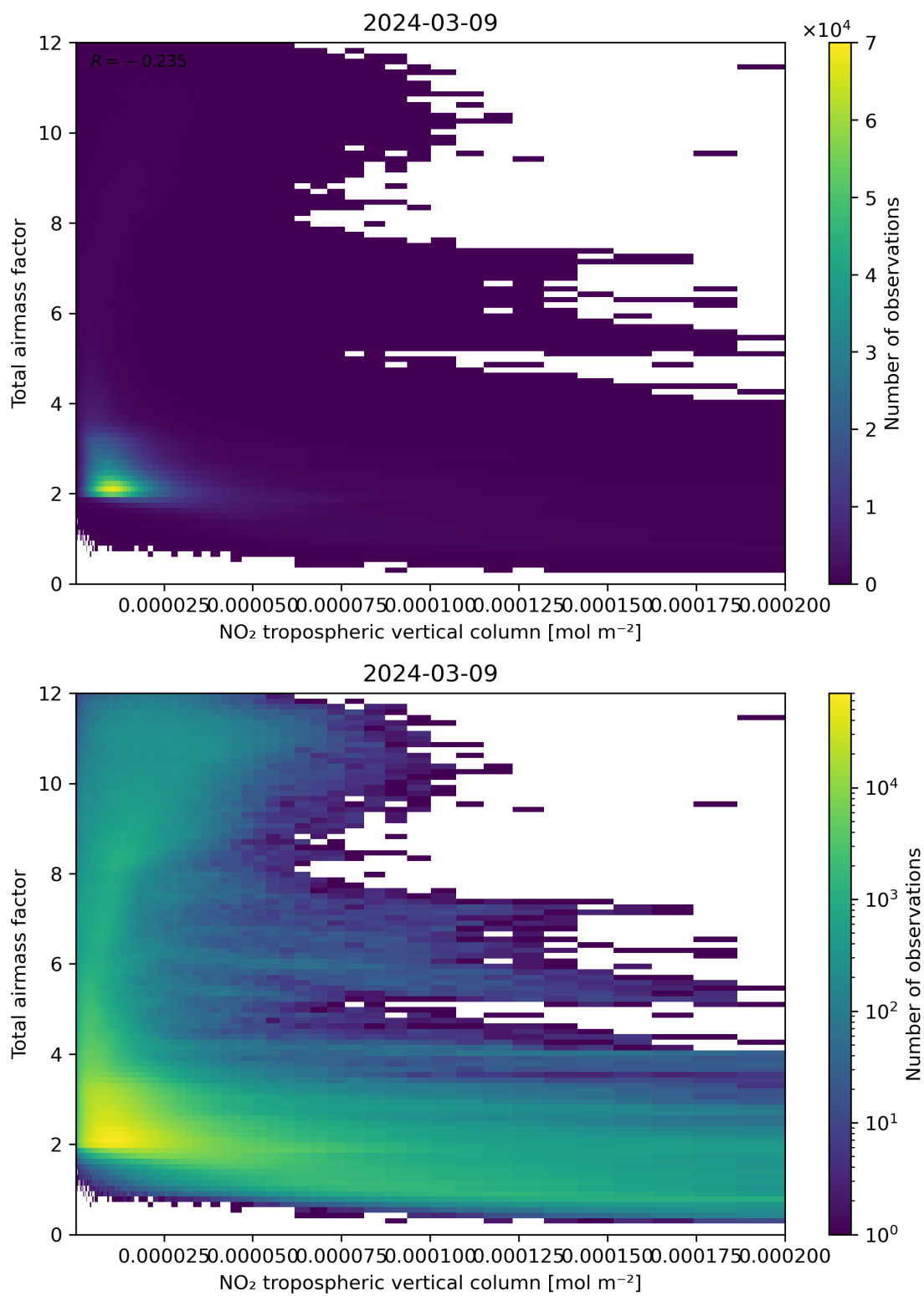
Figure 122: Scatter density plot of “NO 2 tropospheric vertical column” against “Total air mass factor” for 2024-03-09 to 2024-03-10.
