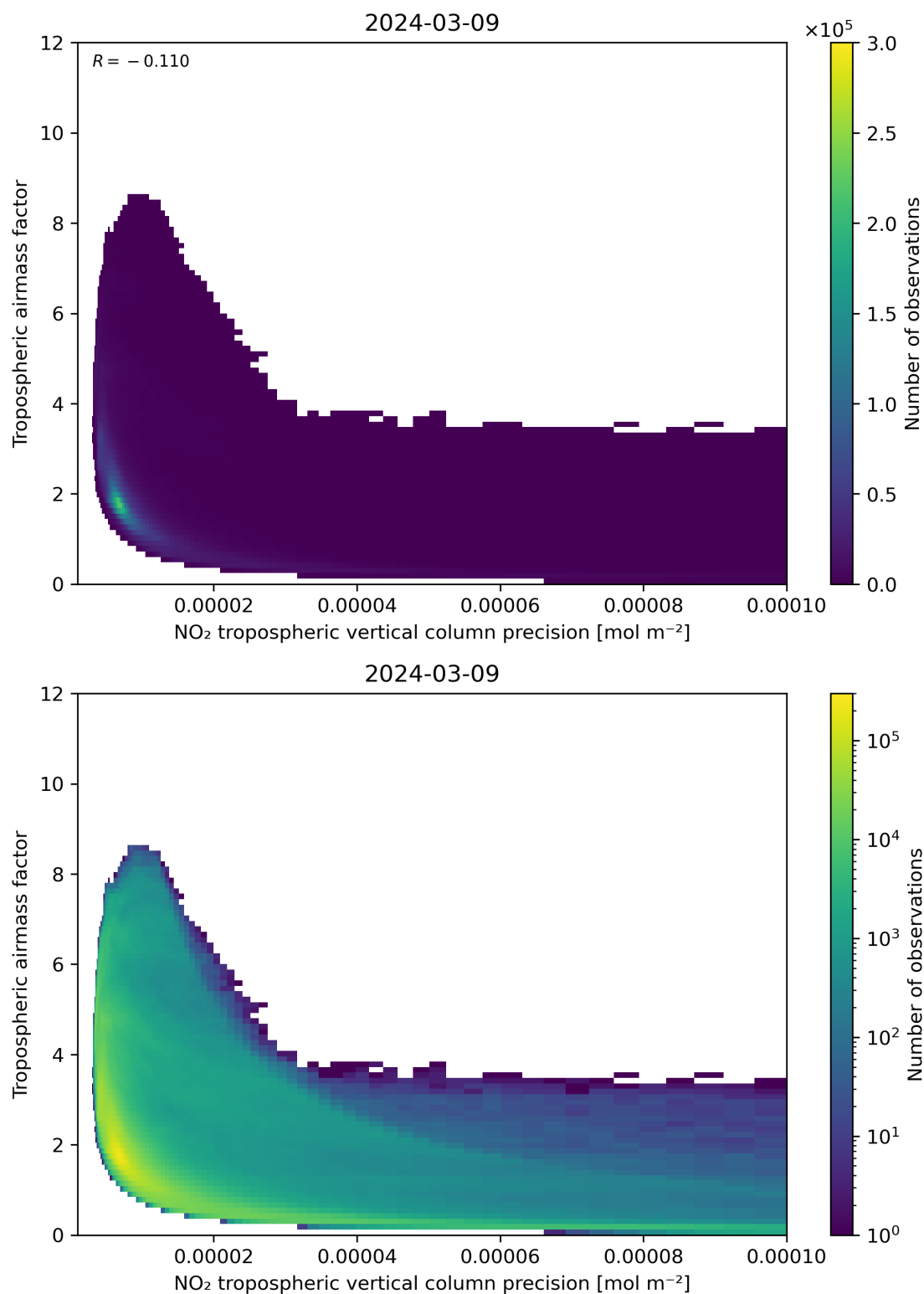
Figure 133: Scatter density plot of “NO 2 tropospheric vertical column precision” against “Tropospheric airmass factor” for 2024-03-09 to 2024-03-10.
