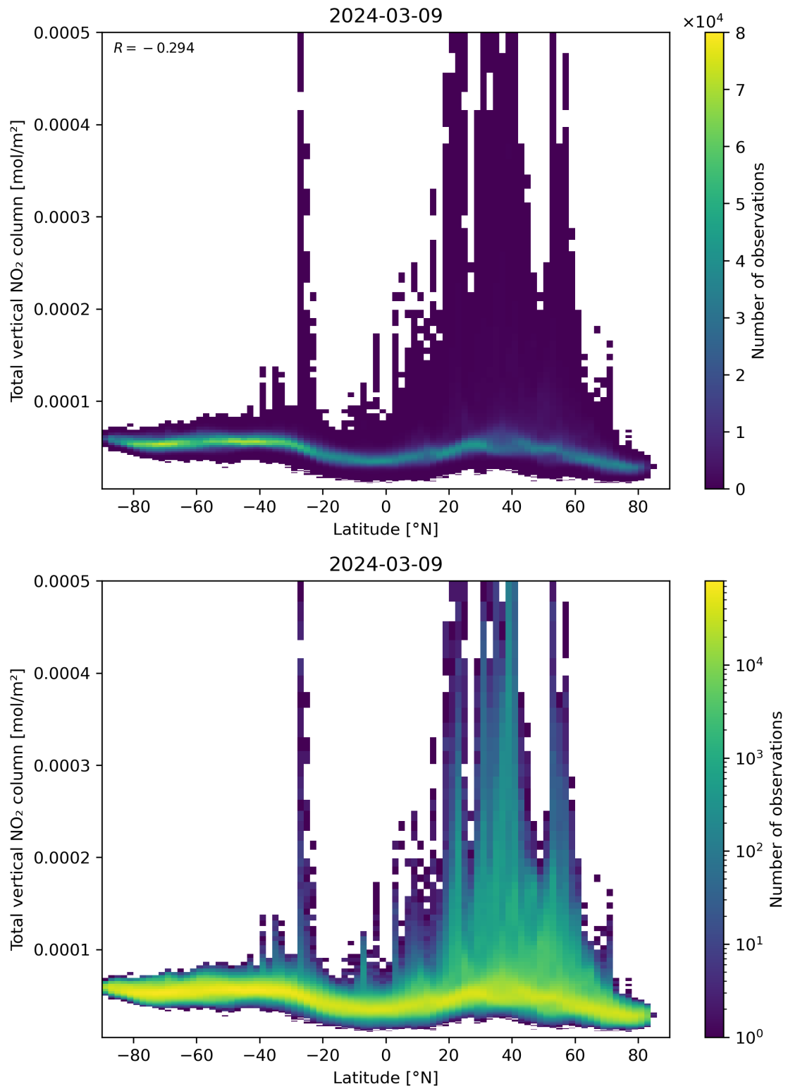
Figure 90: Scatter density plot of “Latitude” against “Total vertical NO 2 column” for 2024-03-09 to 2024-03-10.
