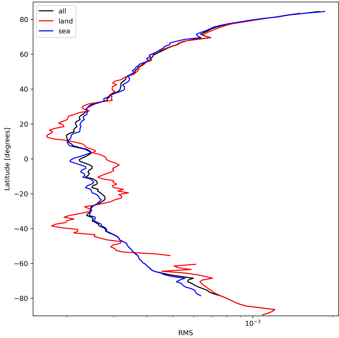
Figure 26: Zonal average of “RMS” for 2024-03-09 to 2024-03-10.
