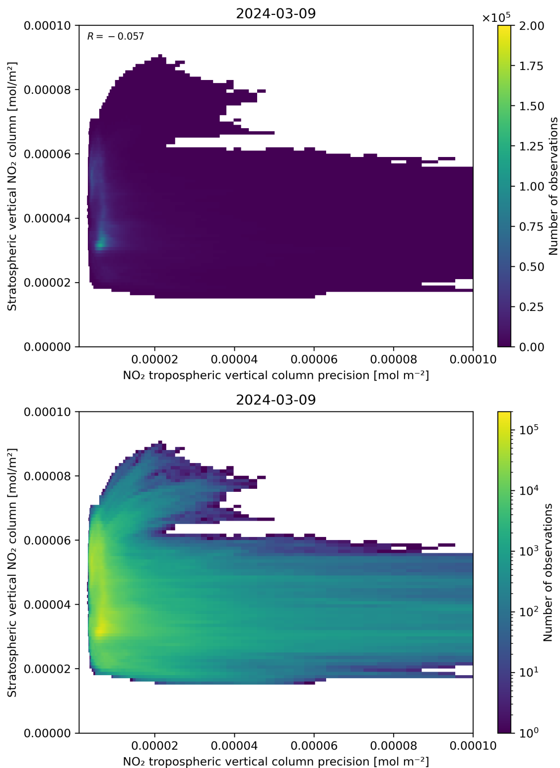
Figure 135: Scatter density plot of “NO 2 tropospheric vertical column precision” against “Stratospheric vertical NO 2 column” for 2024-03-09 to 2024-03-10.
