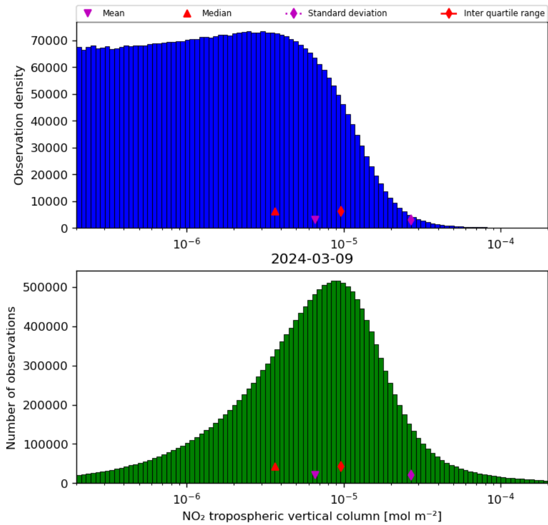
Figure 29: Histogram of “NO 2 tropospheric vertical column” for 2024-03-09 to 2024-03-10
