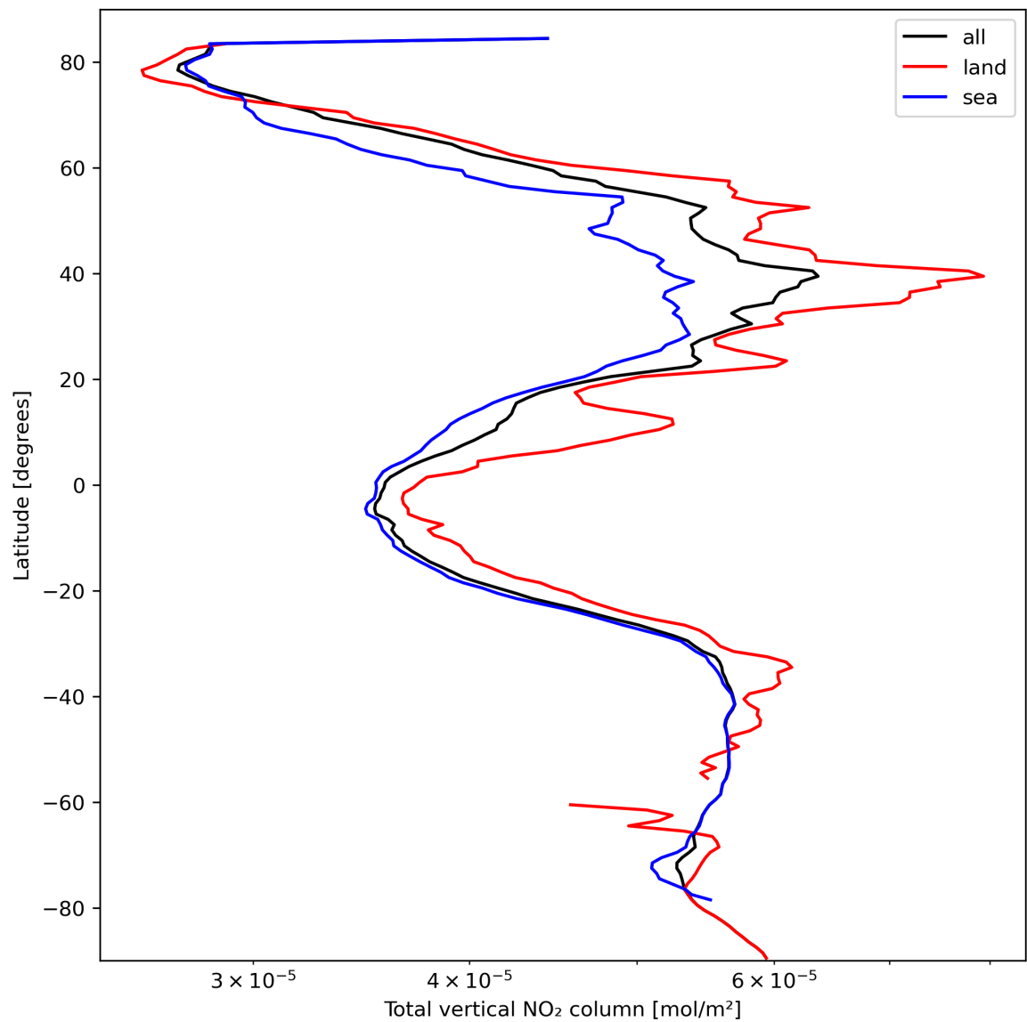
Figure 21: Zonal average of “Total vertical NO 2 column” for 2024-03-09 to 2024-03-10.
