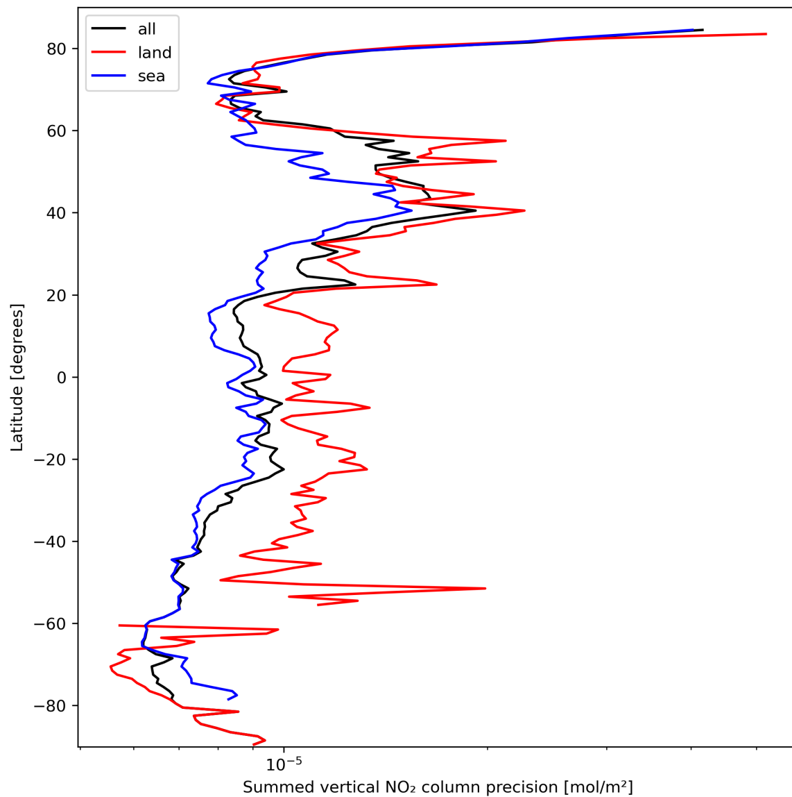
Figure 24: Zonal average of “Summed vertical NO 2 column precision” for 2024-03-09 to 2024-03-10.
