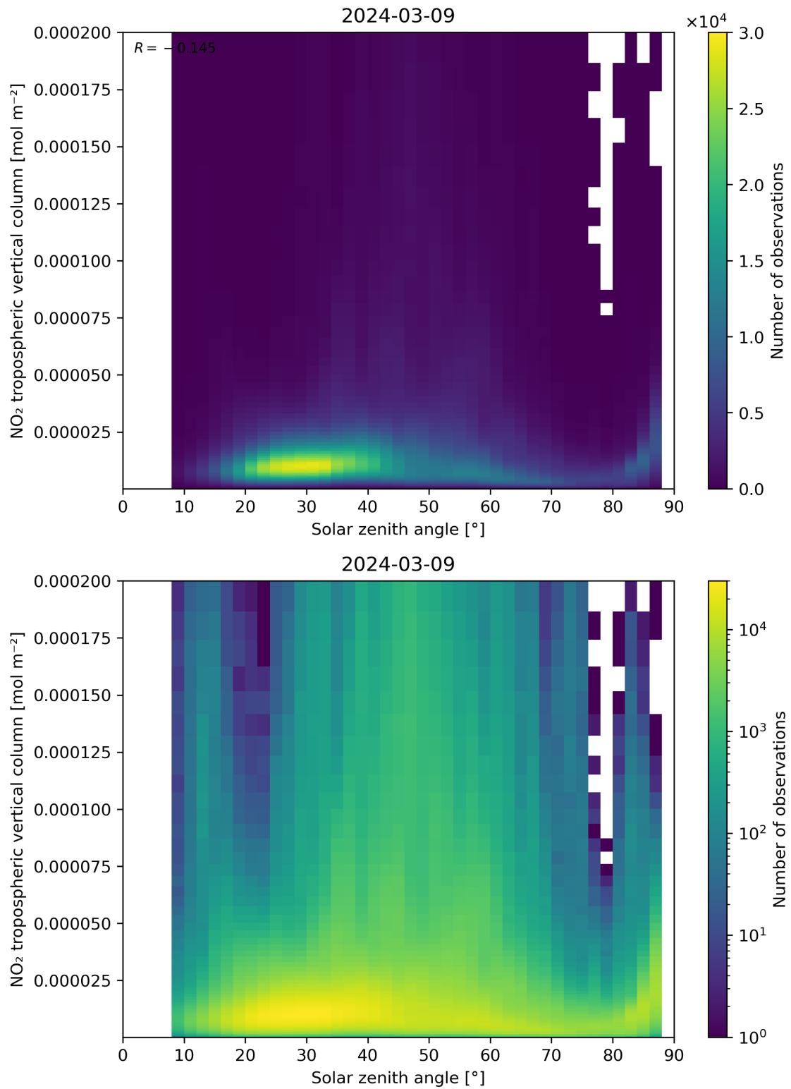
Figure 155: Scatter density plot of “Solar zenith angle” against “NO 2 tropospheric vertical column” for 2024-03-09 to 2024-03-10.
