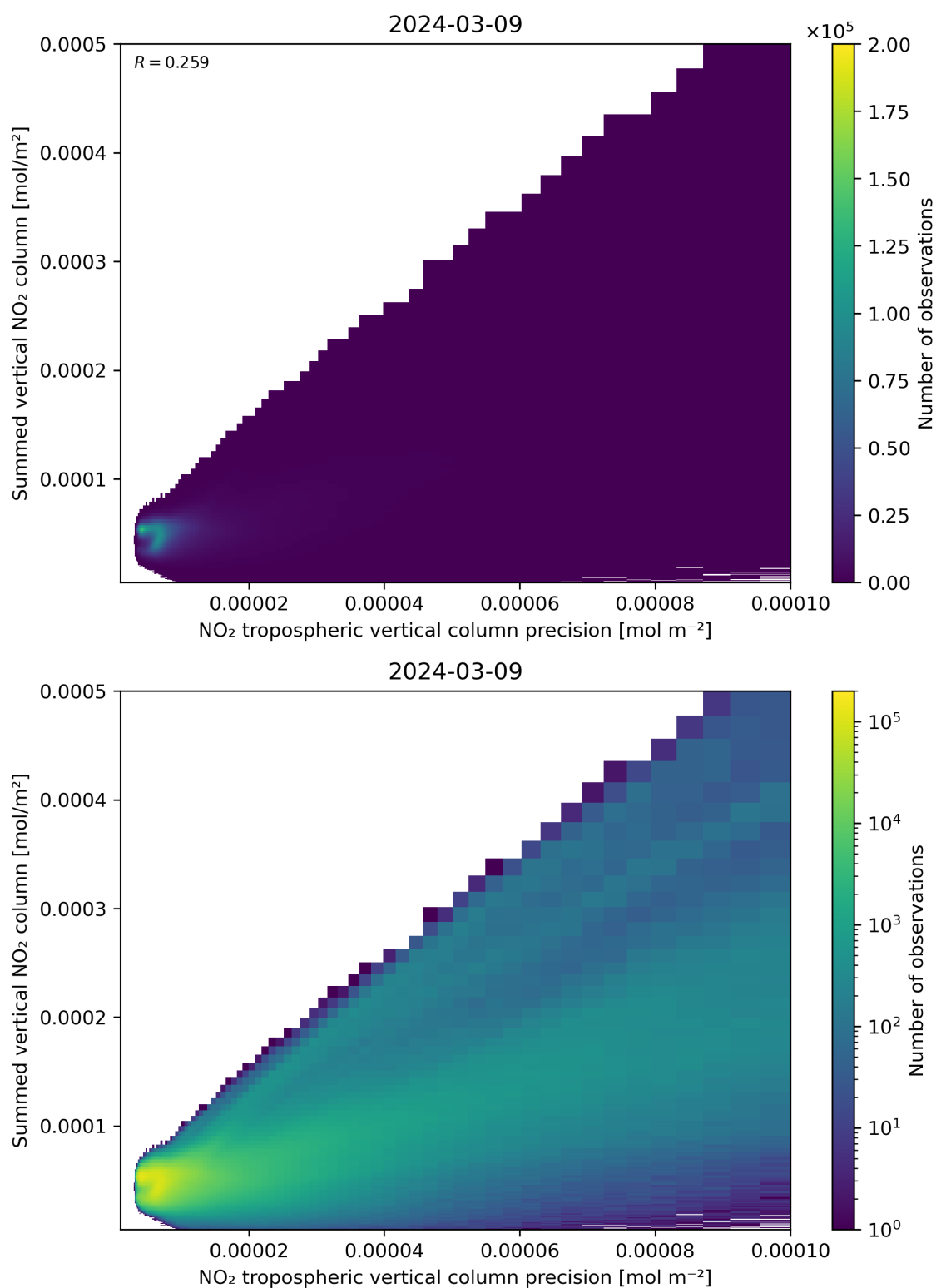
Figure 136: Scatter density plot of “NO 2 tropospheric vertical column precision” against “Summed vertical NO 2 column” for 2024-03-09 to 2024-03-10.
