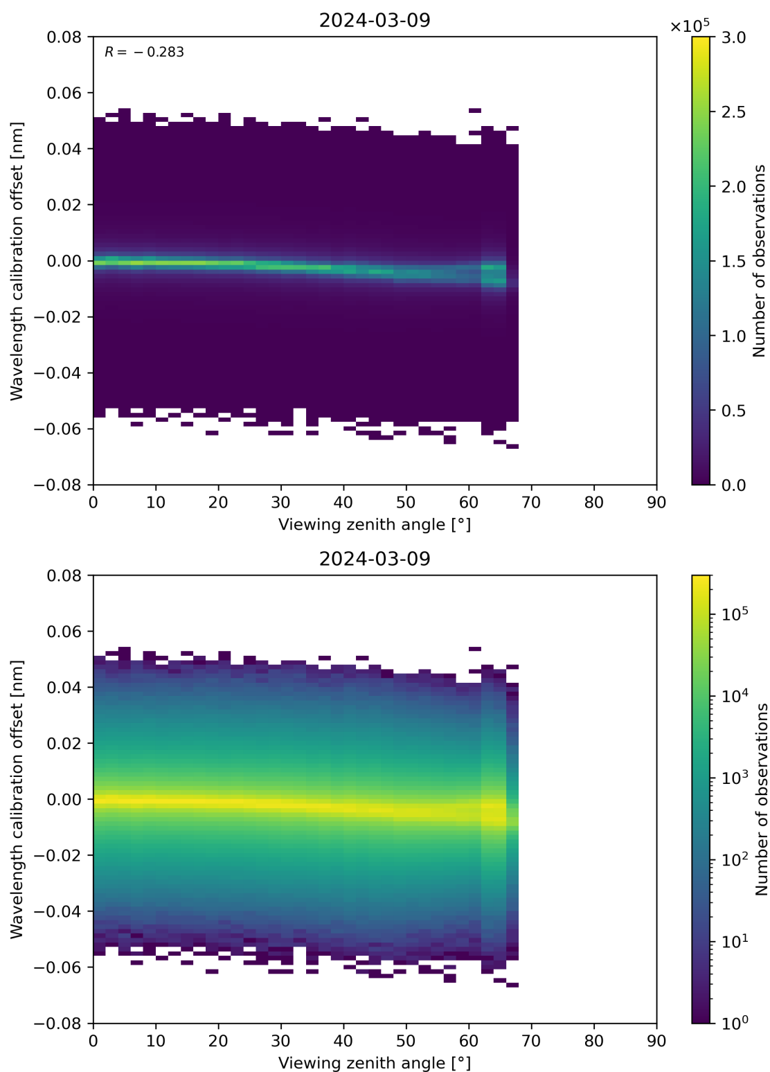
Figure 173: Scatter density plot of “Viewing zenith angle” against “Wavelength calibration offset” for 2024-03-09 to 2024-03-10.
