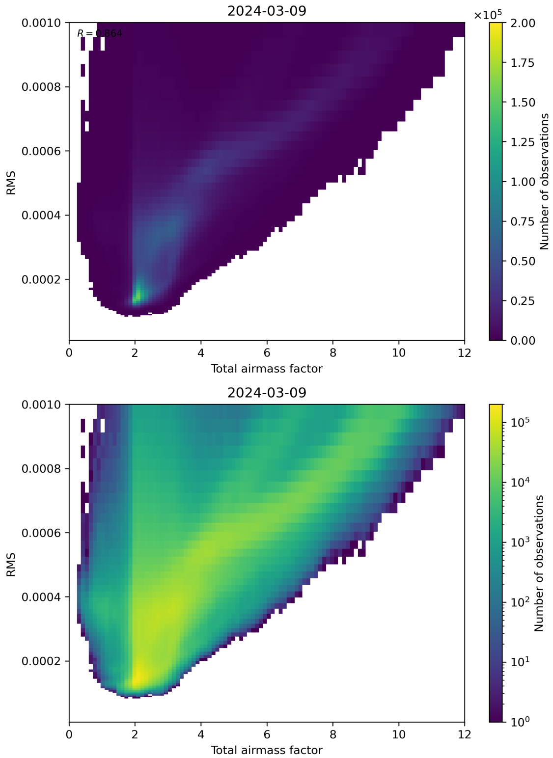
Figure 69: Scatter density plot of “Total airmass factor” against “RMS” for 2024-03-09 to 2024-03-10.
