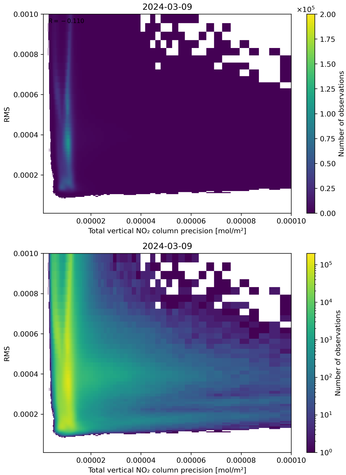
Figure 119: Scatter density plot of “Total vertical NO 2 column precision” against “RMS” for 2024-03-09 to 2024-03-10.
