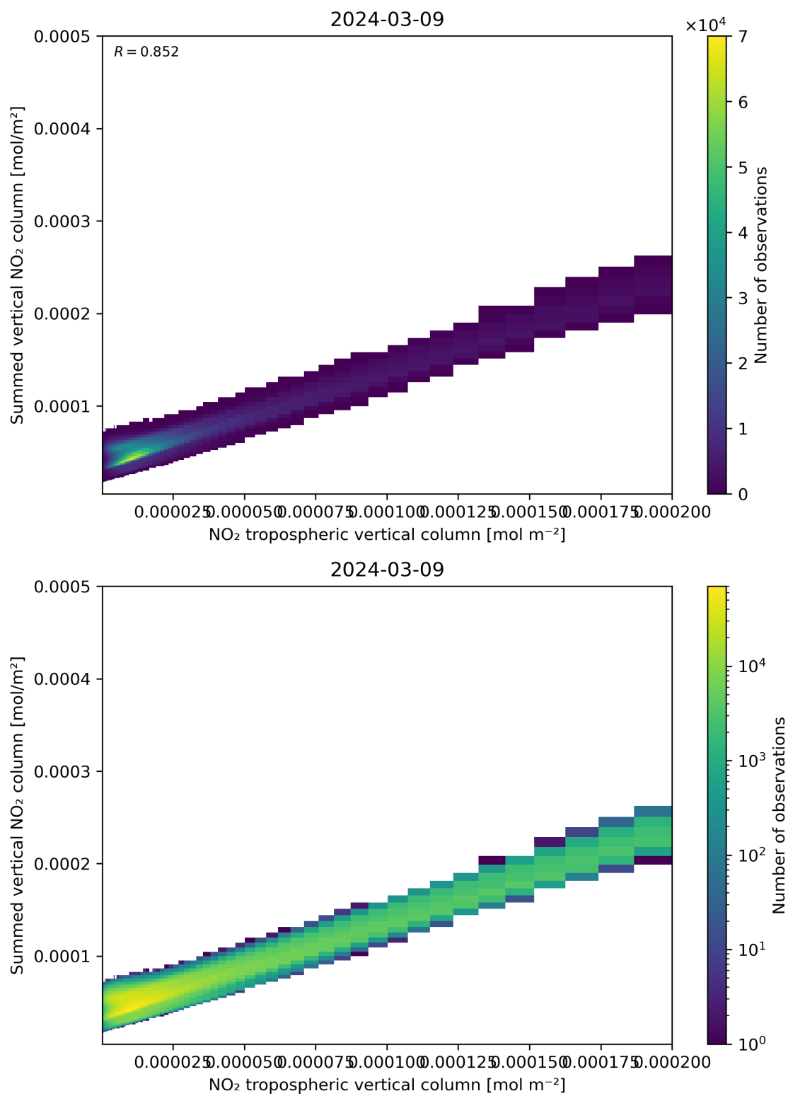
Figure 126: Scatter density plot of “NO 2 tropospheric vertical column” against “Summed vertical NO 2 column” for 2024-03-09 to 2024-03-10.
