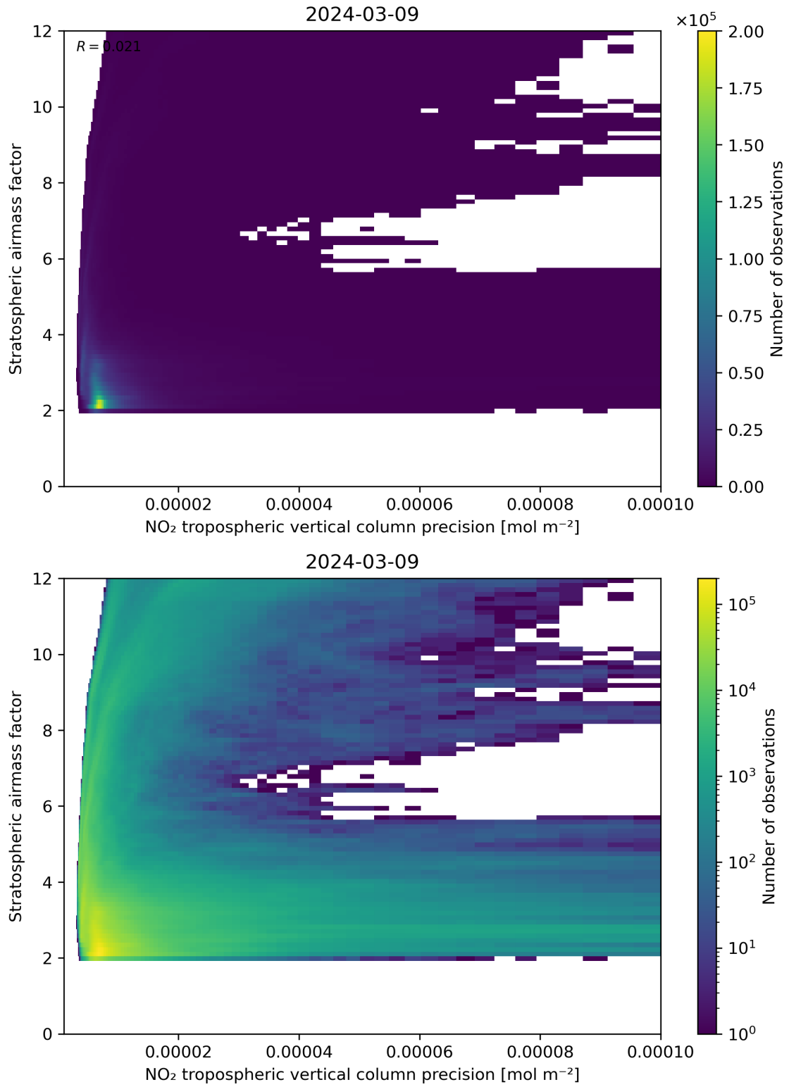
Figure 131: Scatter density plot of “NO 2 tropospheric vertical column precision” against “Stratospheric airmass factor” for 2024-03-09 to 2024-03-10.
