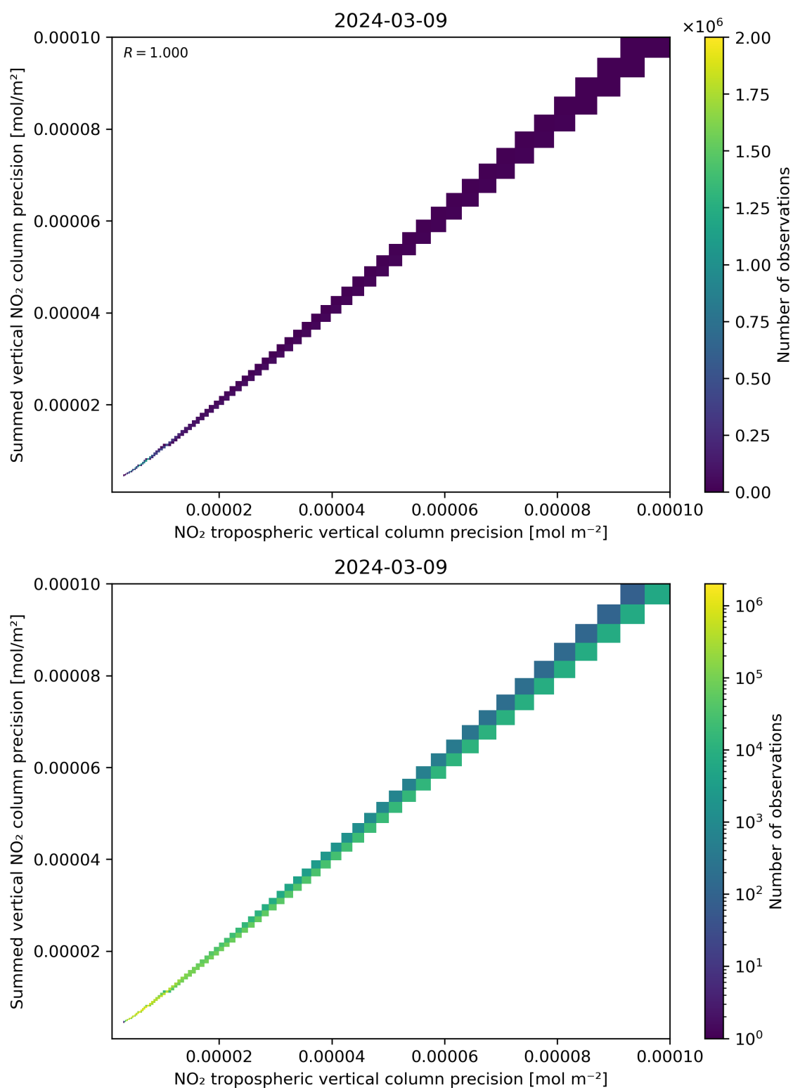
Figure 137: Scatter density plot of “NO 2 tropospheric vertical column precision” against “Summed vertical NO 2 column precision” for 2024-03-09 to 2024-03-10.
