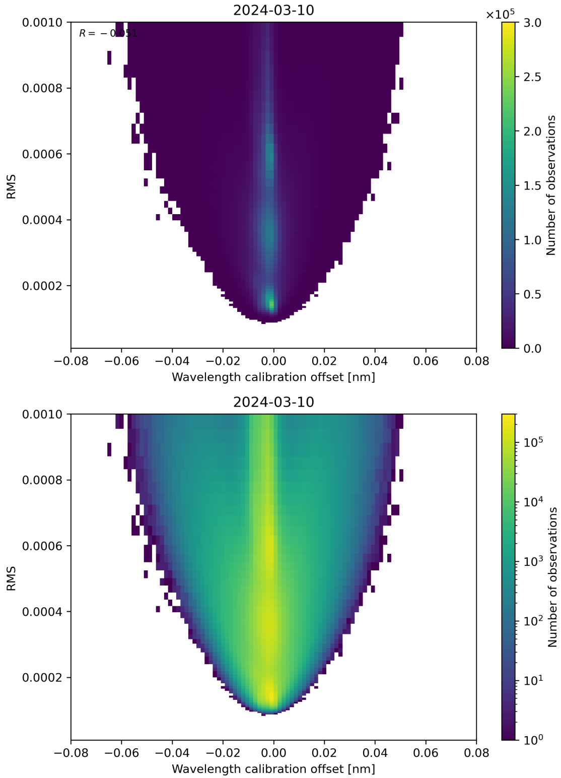
Figure 181: Scatter density plot of “Wavelength calibration offset” against “RMS” for 2024-03-09 to 2024-03-11.
