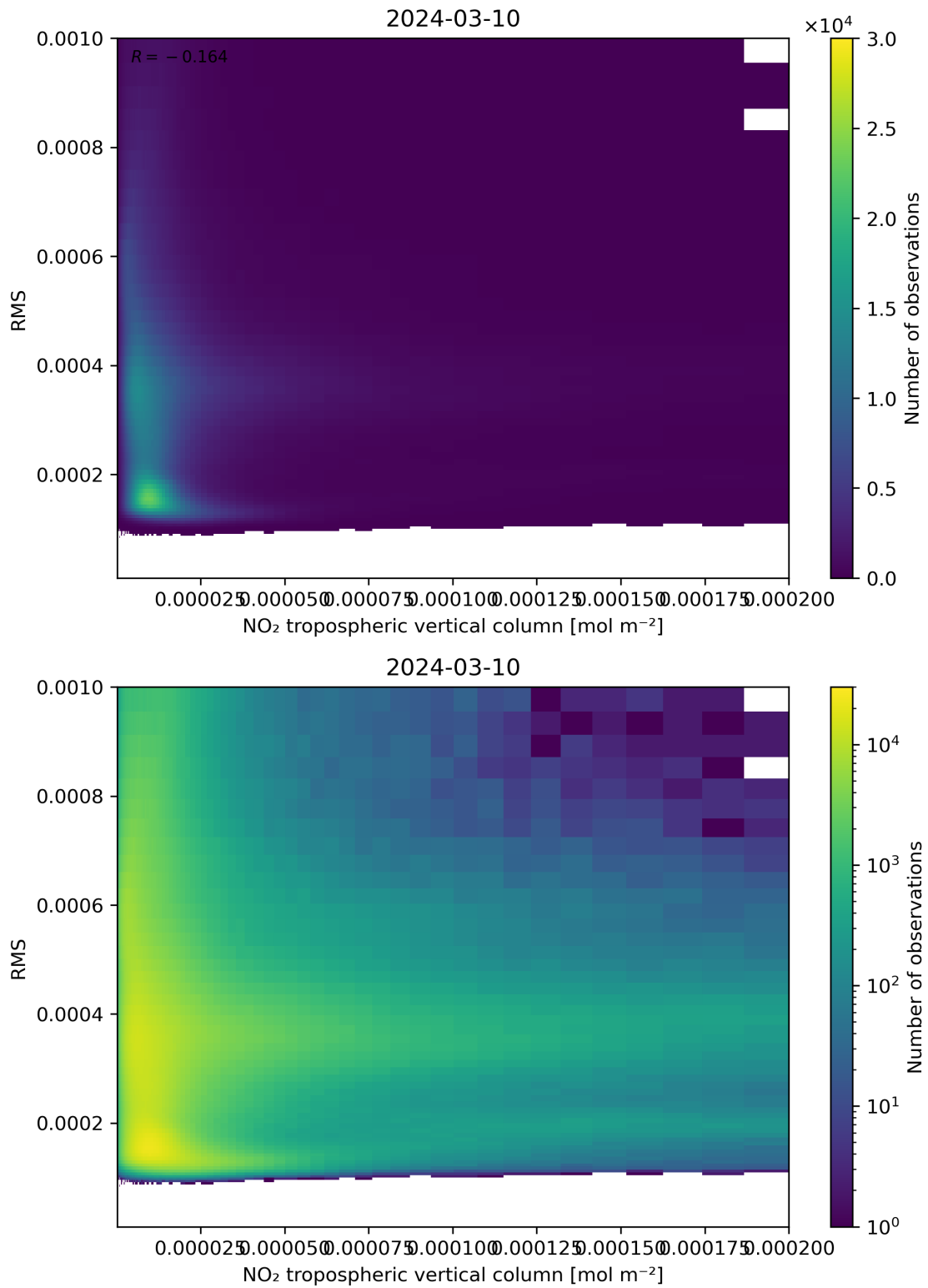
Figure 142: Scatter density plot of “NO 2 tropospheric vertical column” against “RMS” for 2024-03-09 to 2024-03-11.
