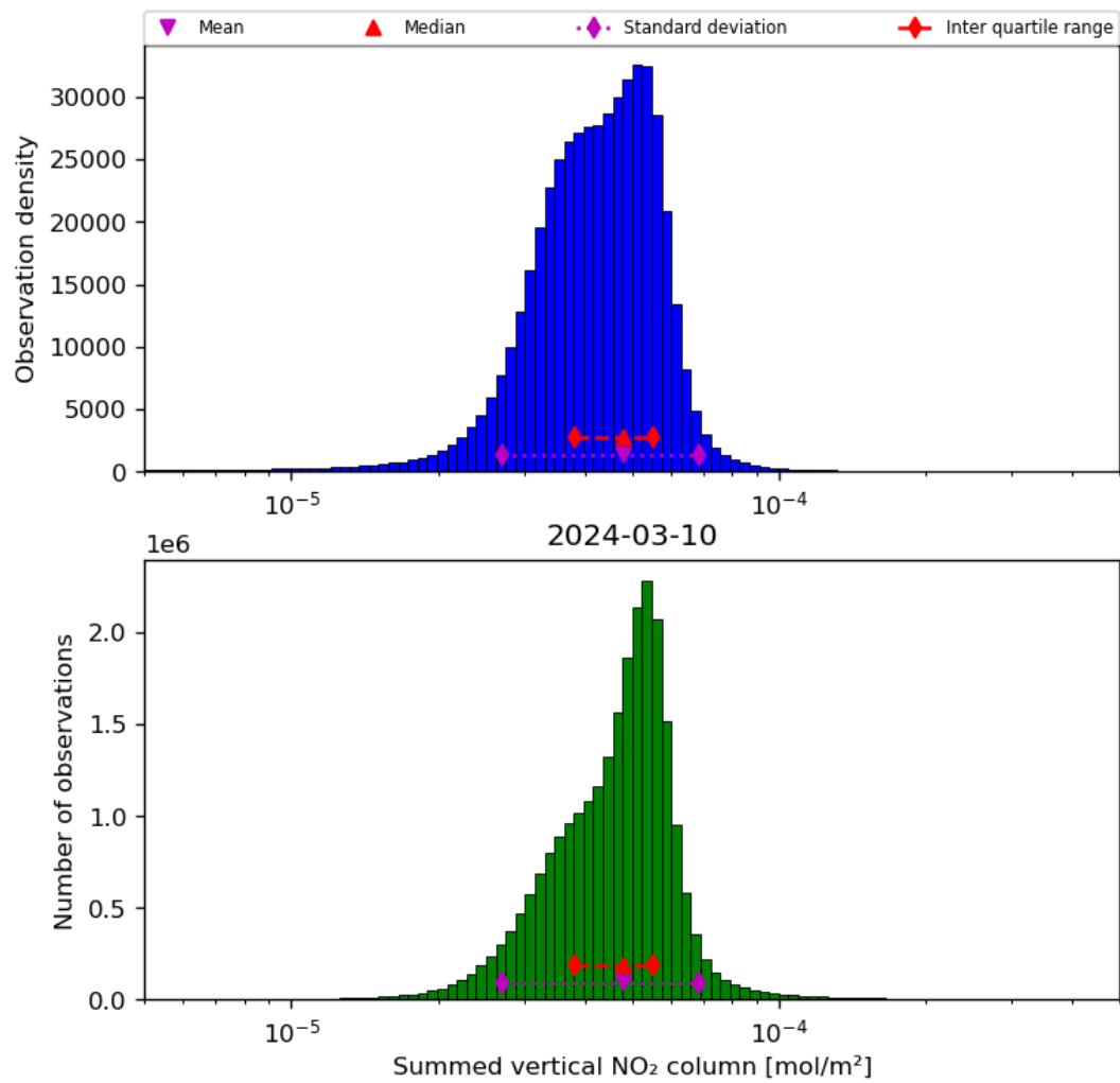
Figure 40: Histogram of “Summed vertical NO 2 column” for 2024-03-09 to 2024-03-11
