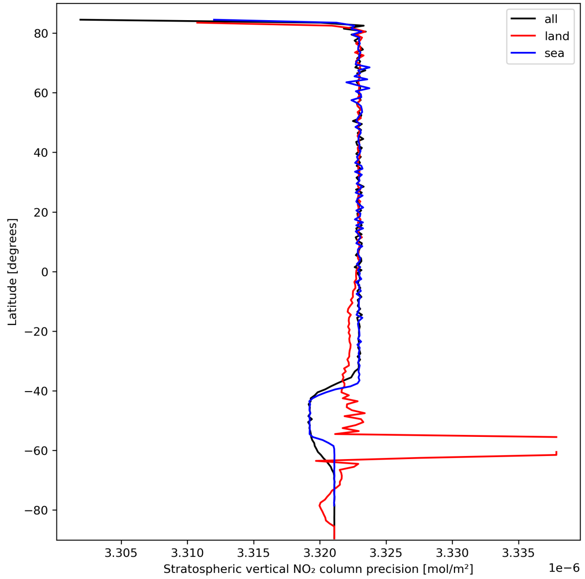
Figure 20: Zonal average of “Stratospheric vertical NO 2 column precision” for 2024-03-09 to 2024-03-11.
