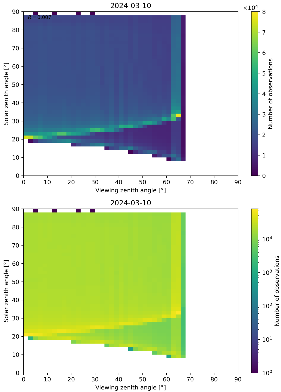
Figure 172: Scatter density plot of “Viewing zenith angle” against “Solar zenith angle” for 2024-03-09 to 2024-03-11.
