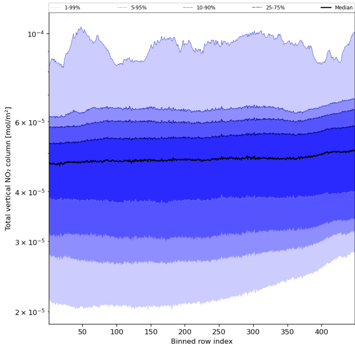
Figure 55: Along track statistics of “Total vertical NO 2 column” for 2024-03-09 to 2024-03-11
