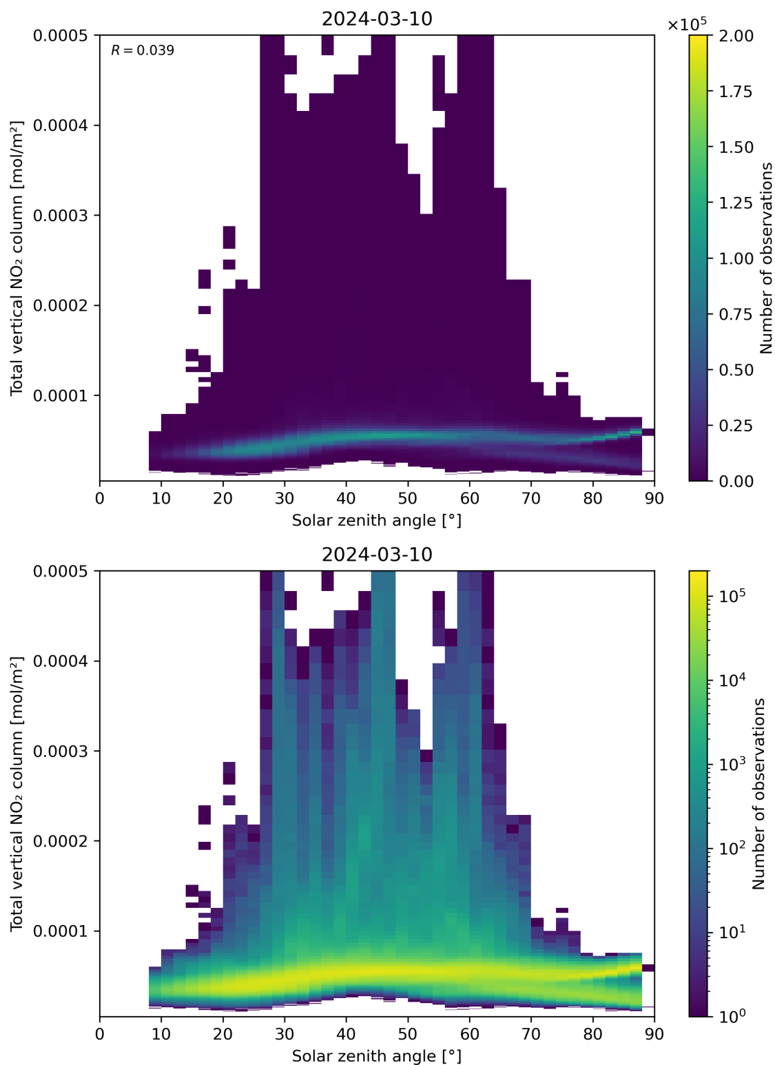
Figure 153: Scatter density plot of “Solar zenith angle” against “Total vertical NO 2 column” for 2024-03-09 to 2024-03-11.
