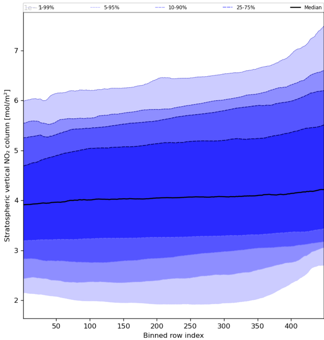
Figure 53: Along track statistics of “Stratospheric vertical NO 2 column” for 2024-03-09 to 2024-03-11
