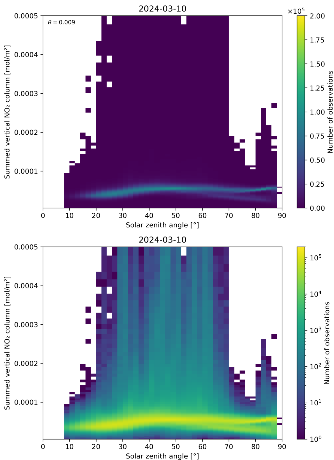
Figure 151: Scatter density plot of “Solar zenith angle” against “Summed vertical NO 2 column” for 2024-03-09 to 2024-03-11.
