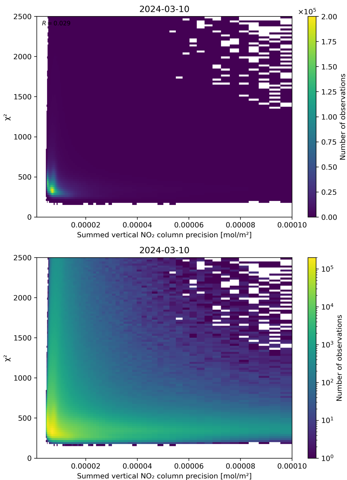
Figure 107: Scatter density plot of “Summed vertical NO 2 column precision” against “ \chi^2 ” for 2024-03-09 to 2024-03-11.
