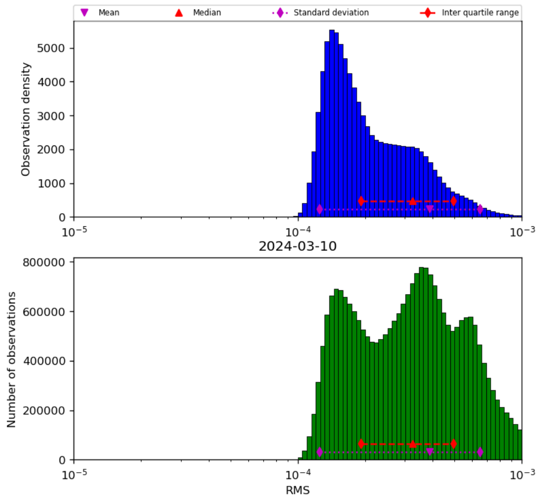
Figure 43: Histogram of “RMS” for 2024-03-09 to 2024-03-11
