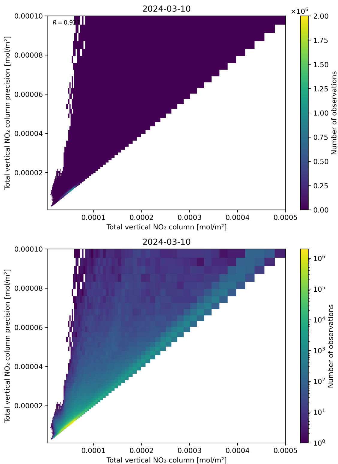
Figure 114: Scatter density plot of “Total vertical NO 2 column” against “Total vertical NO 2 column precision” for 2024-03-09 to 2024-03-11.
