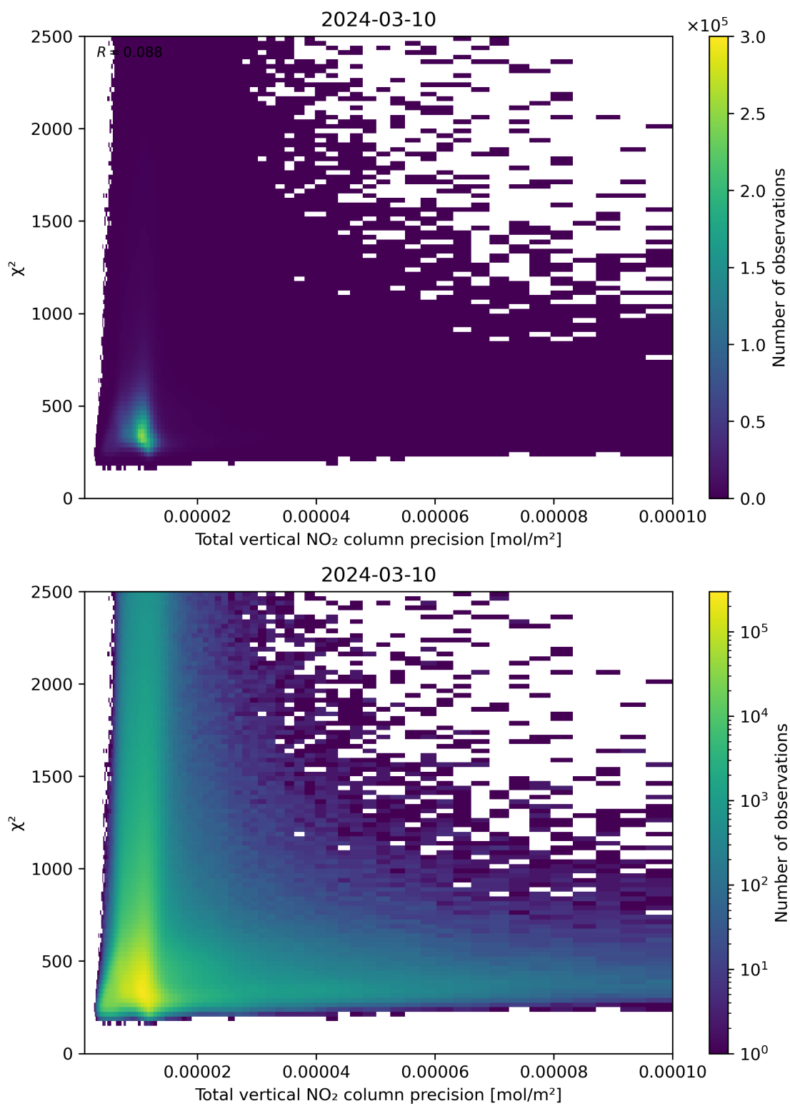
Figure 116: Scatter density plot of “Total vertical NO 2 column precision” against “ \chi^2 ” for 2024-03-09 to 2024-03-11.
