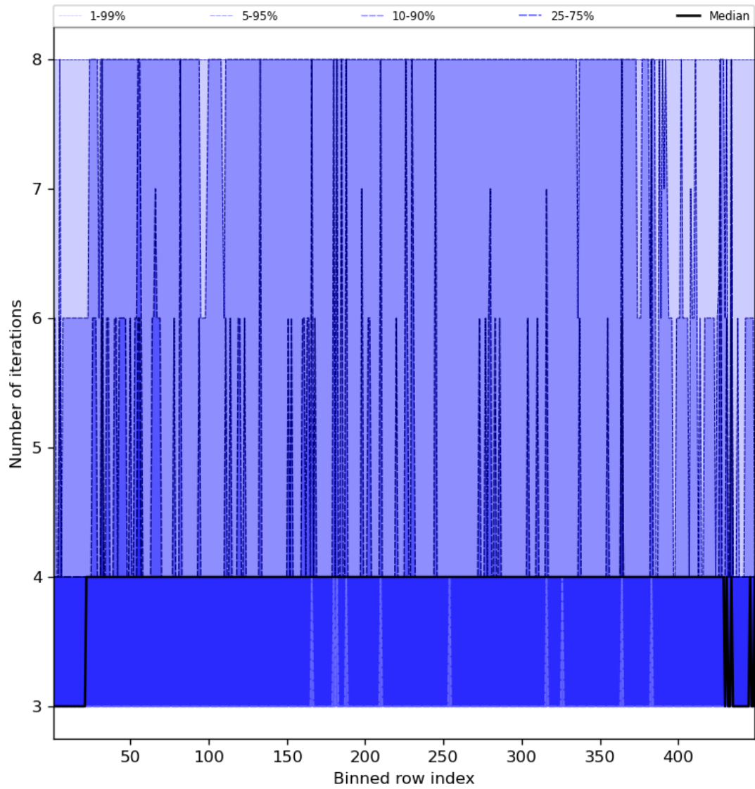
Figure 51: Along track statistics of “Number of iterations” for 2024-03-09 to 2024-03-11
