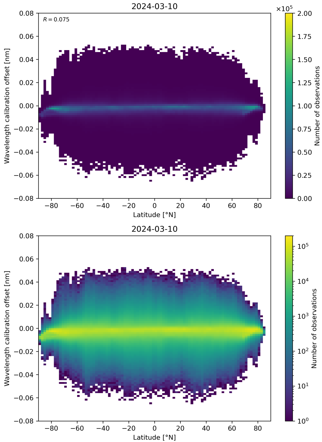
Figure 95: Scatter density plot of “Latitude” against “Wavelength calibration offset” for 2024-03-09 to 2024-03-11.
