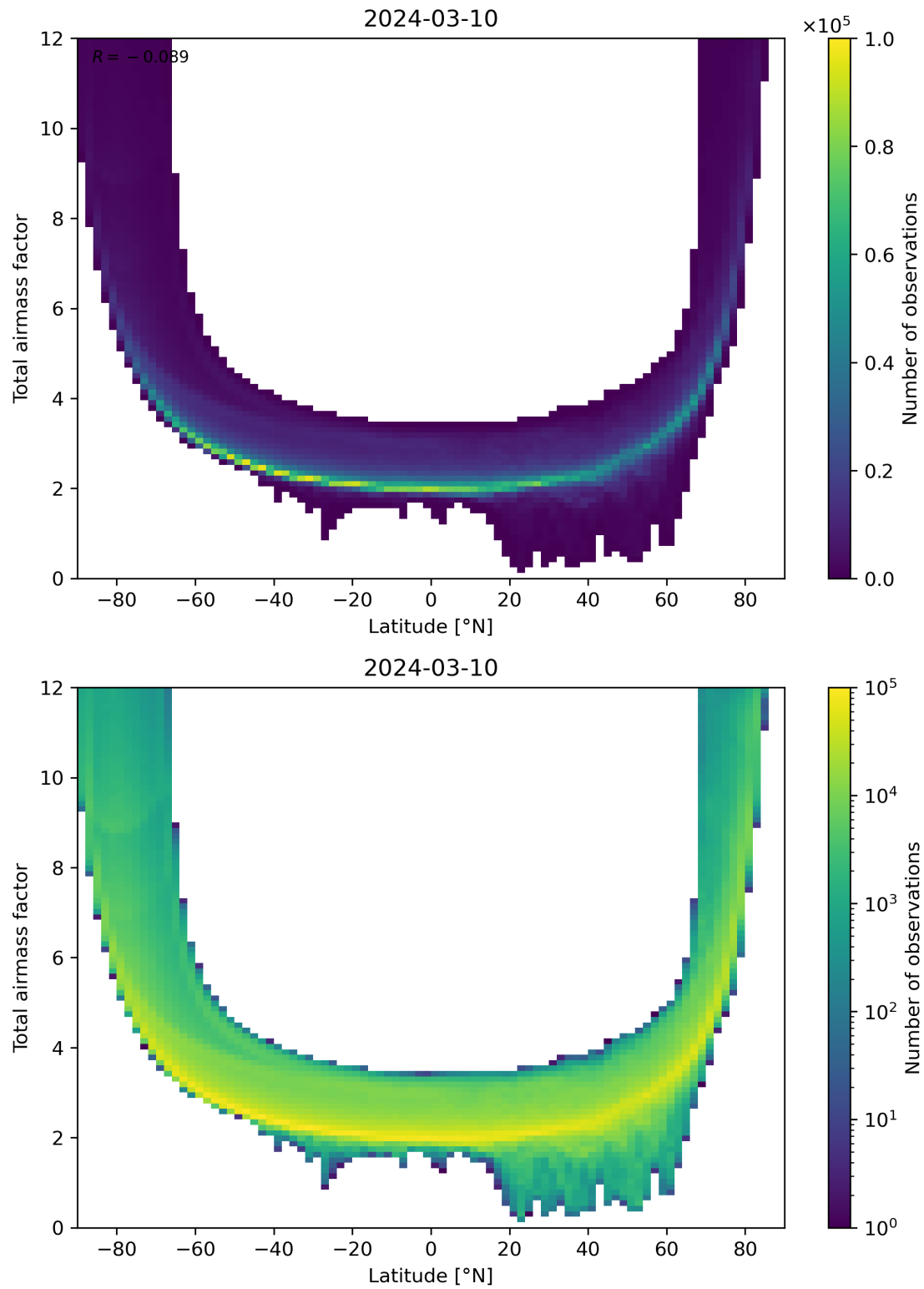
Figure 84: Scatter density plot of “Latitude” against “Total air mass factor” for 2024-03-09 to 2024-03-11.
