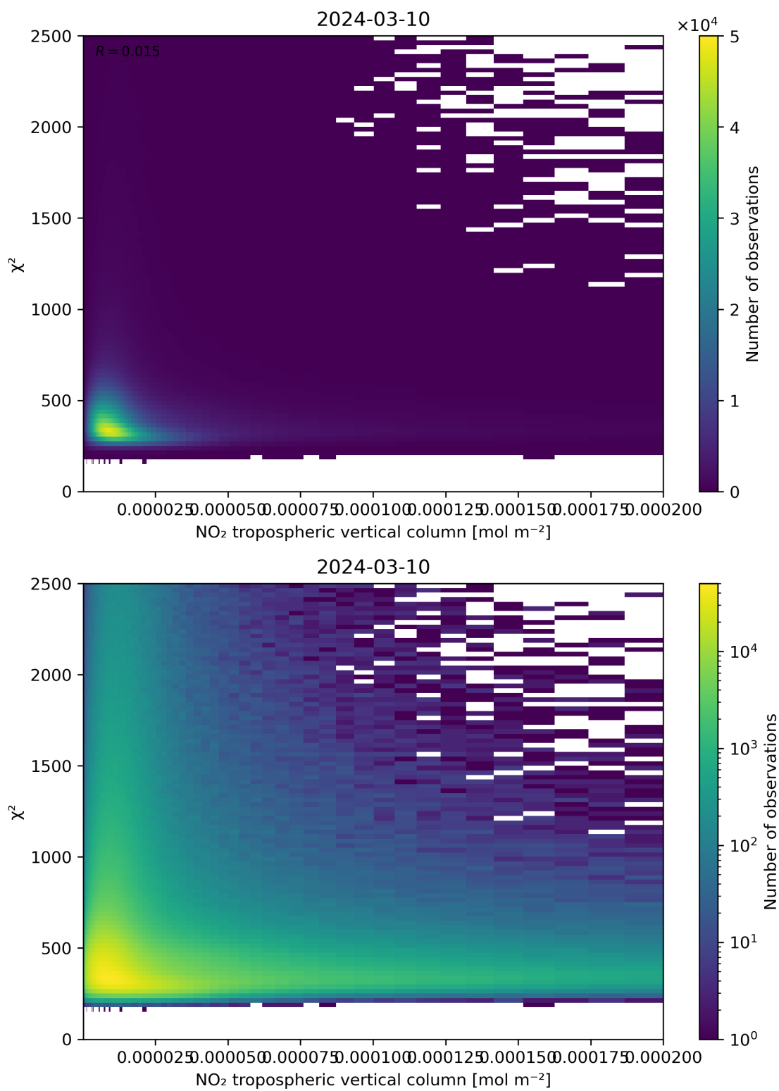
Figure 124: Scatter density plot of “NO 2 tropospheric vertical column” against “ \chi^2 ” for 2024-03-09 to 2024-03-11.
