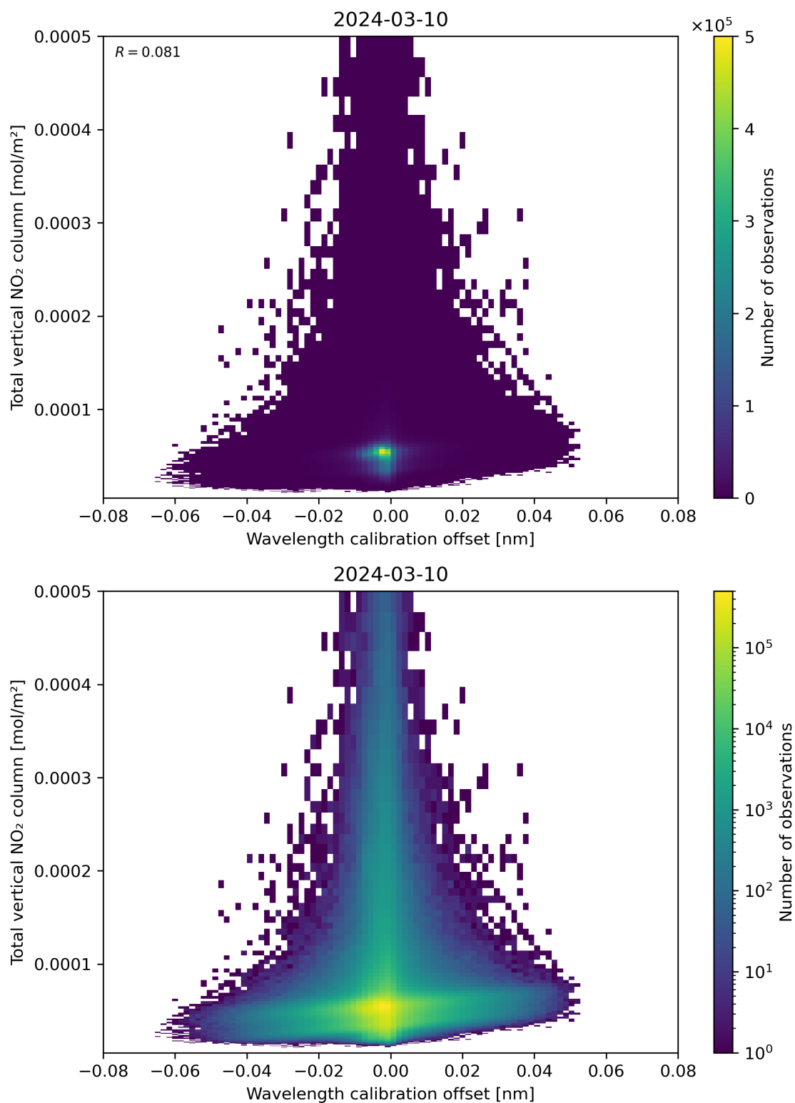
Figure 179: Scatter density plot of “Wavelength calibration offset” against “Total vertical NO 2 column” for 2024-03-09 to 2024-03-11.
