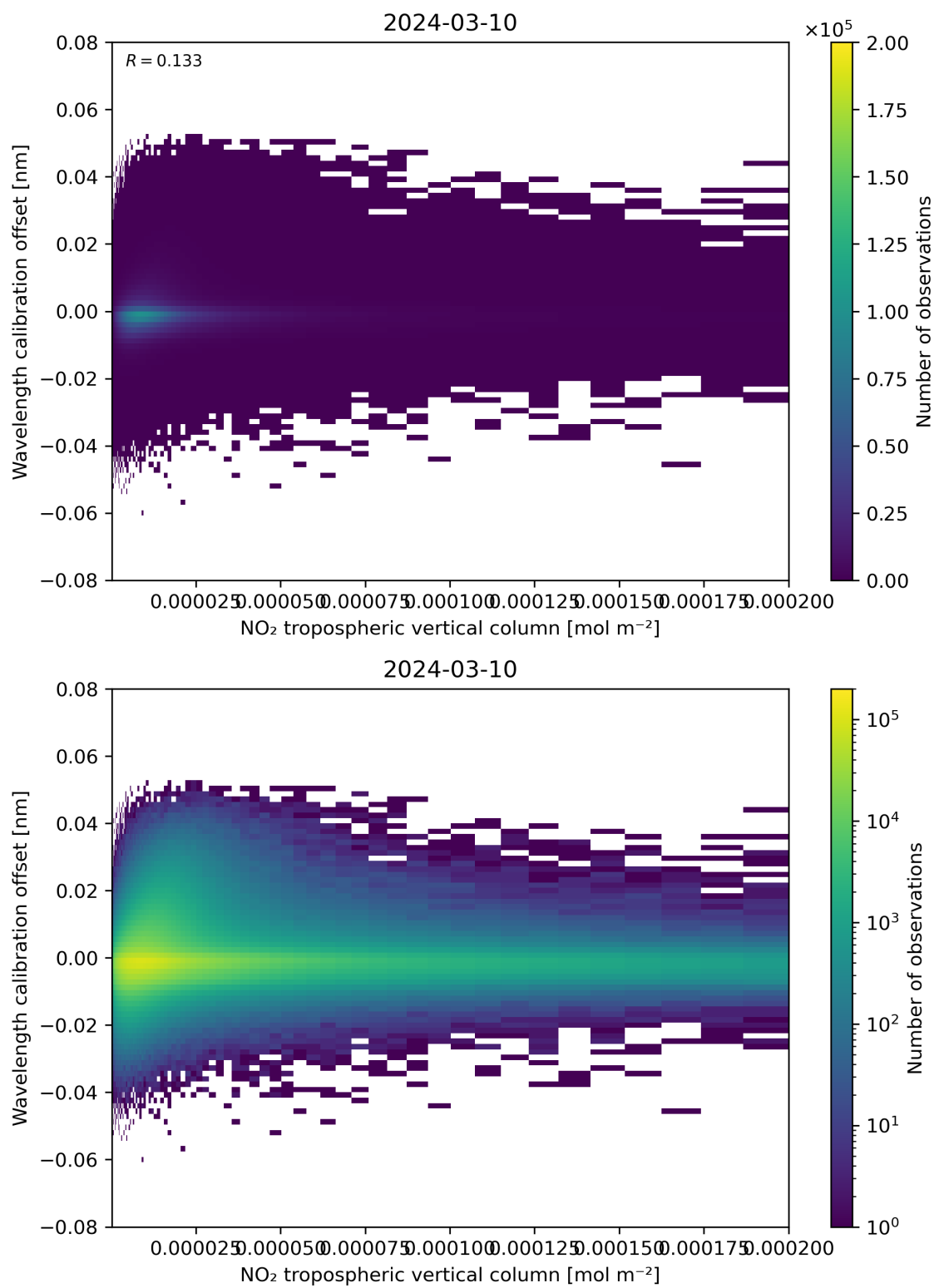
Figure 143: Scatter density plot of “NO 2 tropospheric vertical column” against “Wavelength calibration offset” for 2024-03-09 to 2024-03-11.
