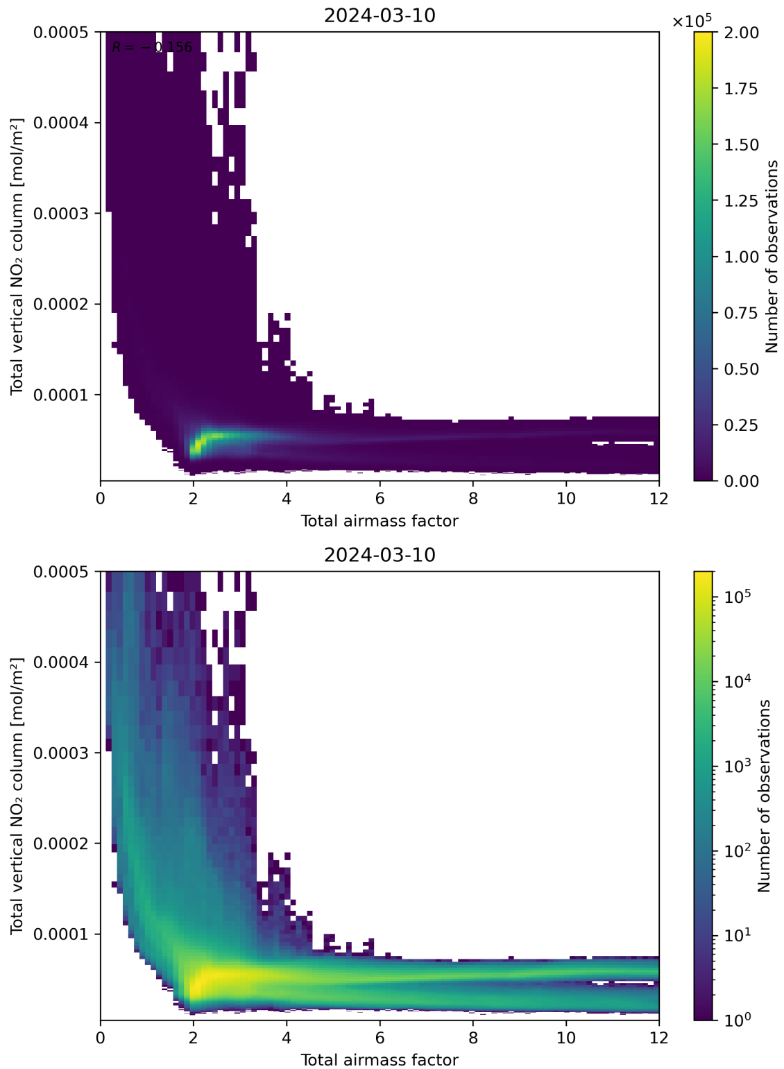
Figure 67: Scatter density plot of “Total airmass factor” against “Total vertical NO 2 column” for 2024-03-09 to 2024-03-11.
