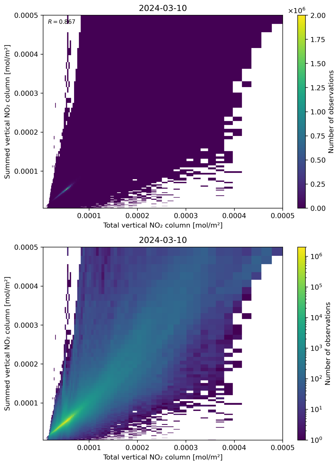
Figure 112: Scatter density plot of “Total vertical NO 2 column” against “Summed vertical NO 2 column” for 2024-03-09 to 2024-03-11.
