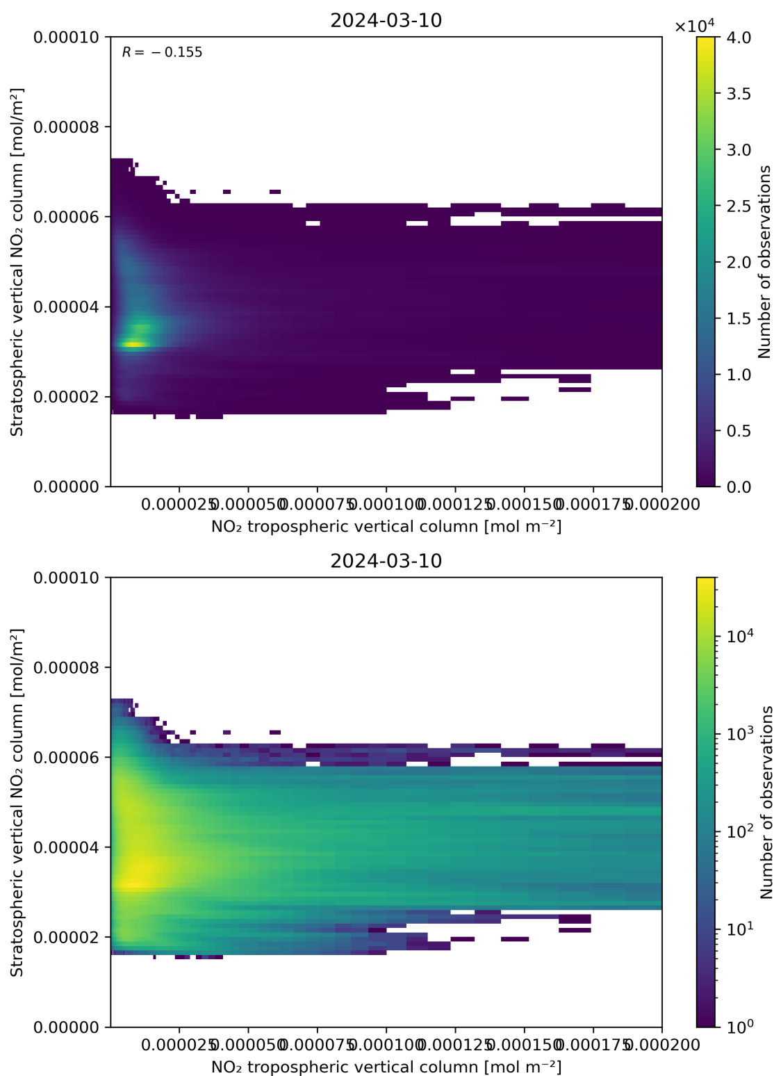
Figure 125: Scatter density plot of “NO 2 tropospheric vertical column” against “Stratospheric vertical NO 2 column” for 2024-03-09 to 2024-03-11.
