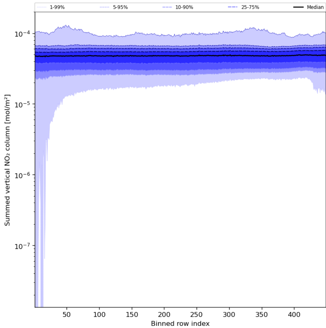
Figure 57: Along track statistics of “Summed vertical NO 2 column” for 2024-03-09 to 2024-03-11
