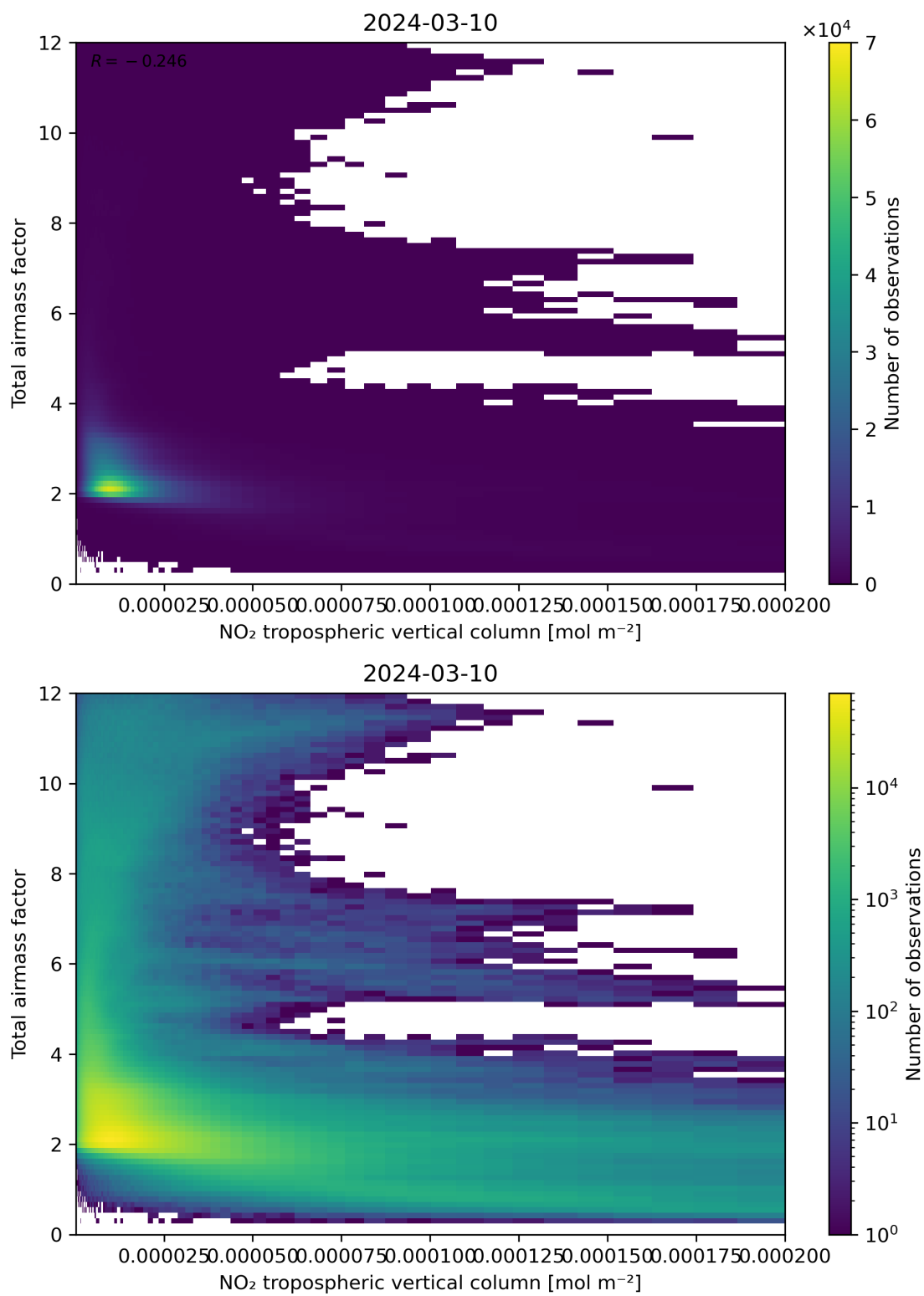
Figure 122: Scatter density plot of “NO 2 tropospheric vertical column” against “Total air mass factor” for 2024-03-09 to 2024-03-11.
