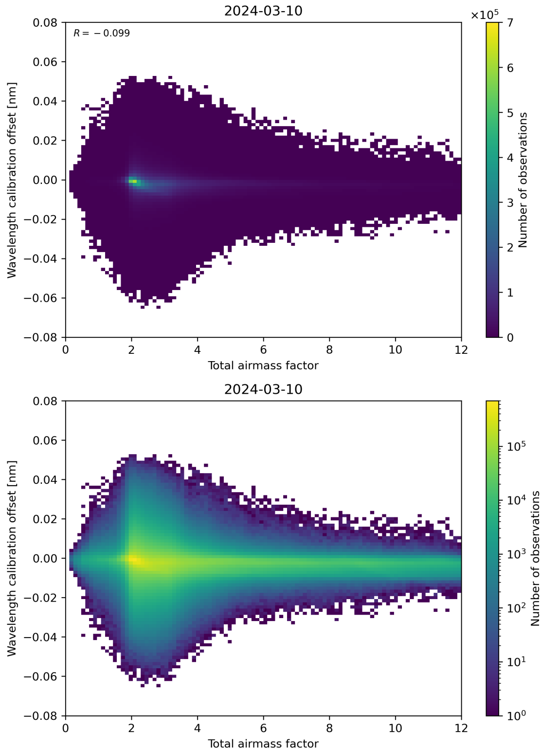
Figure 70: Scatter density plot of “Total airmass factor” against “Wavelength calibration offset” for 2024-03-09 to 2024-03-11.
