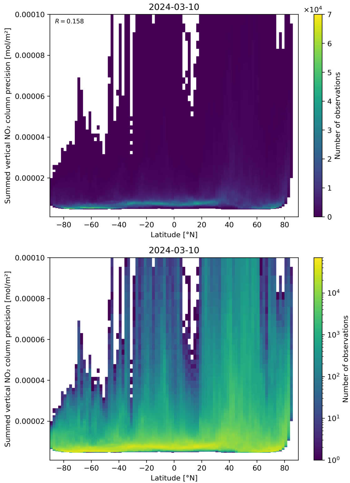
Figure 89: Scatter density plot of “Latitude” against “Summed vertical NO 2 column precision” for 2024-03-09 to 2024-03-11.
