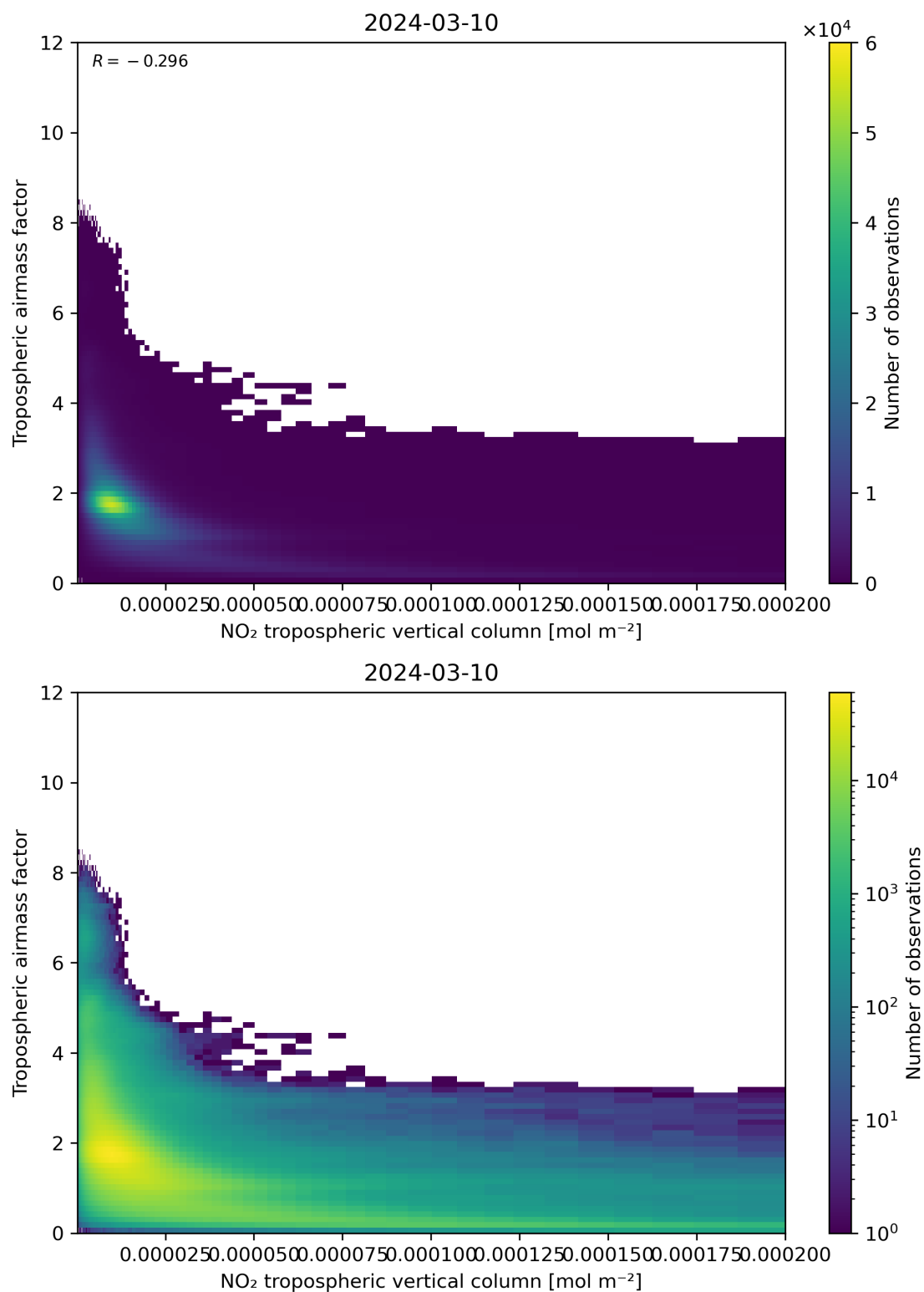
Figure 123: Scatter density plot of “NO 2 tropospheric vertical column” against “Tropospheric air mass factor” for 2024-03-09 to 2024-03-11.
