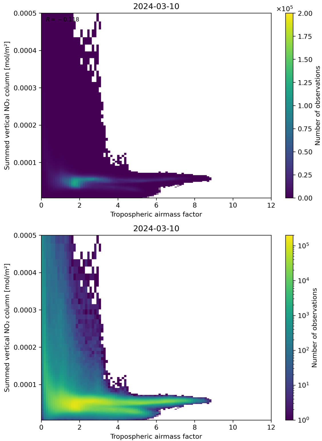
Figure 75: Scatter density plot of “Tropospheric air mass factor” against “Summed vertical NO 2 column” for 2024-03-09 to 2024-03-11.
