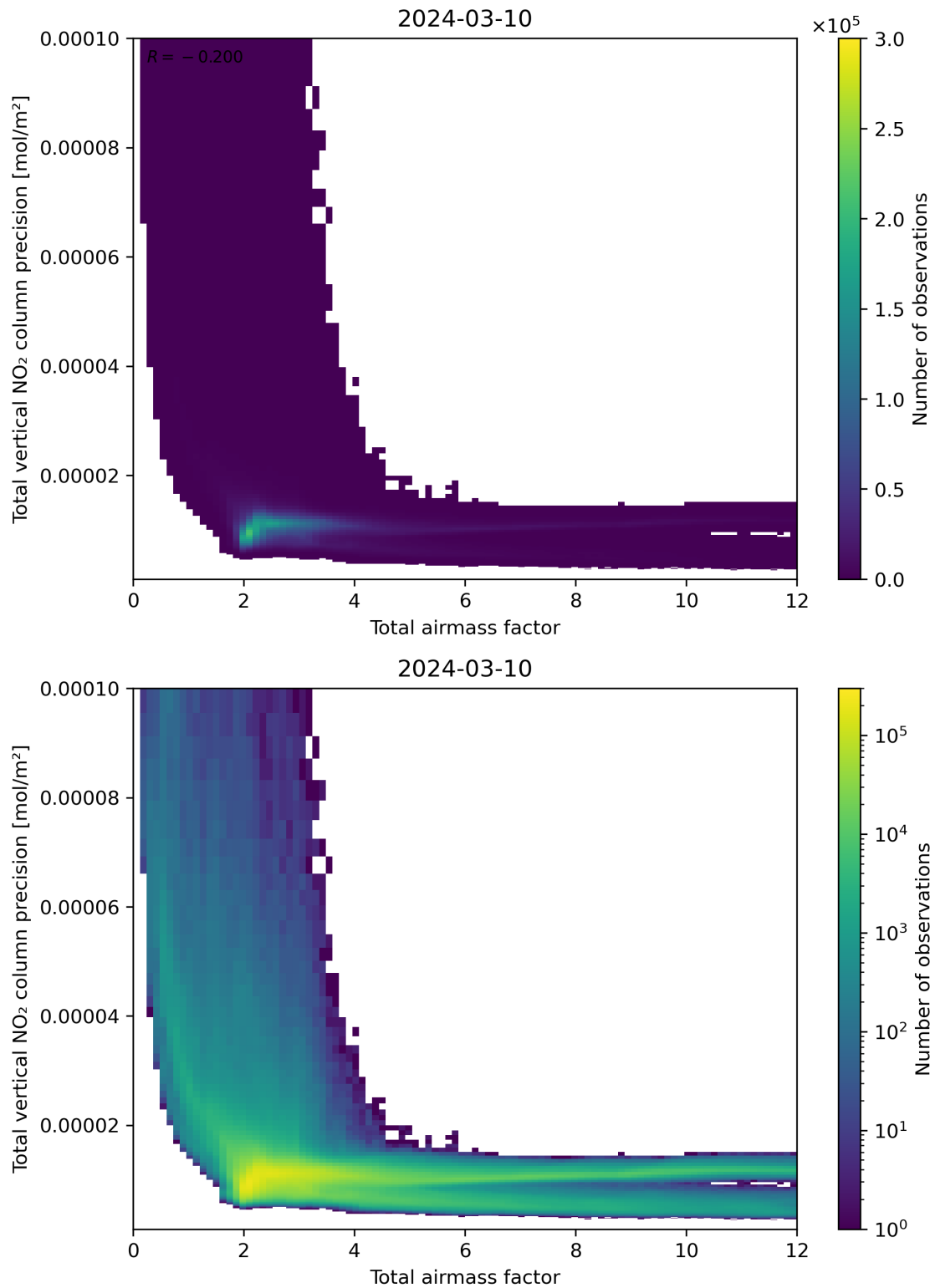
Figure 68: Scatter density plot of “Total airmass factor” against “Total vertical NO 2 column precision” for 2024-03-09 to 2024-03-11.
