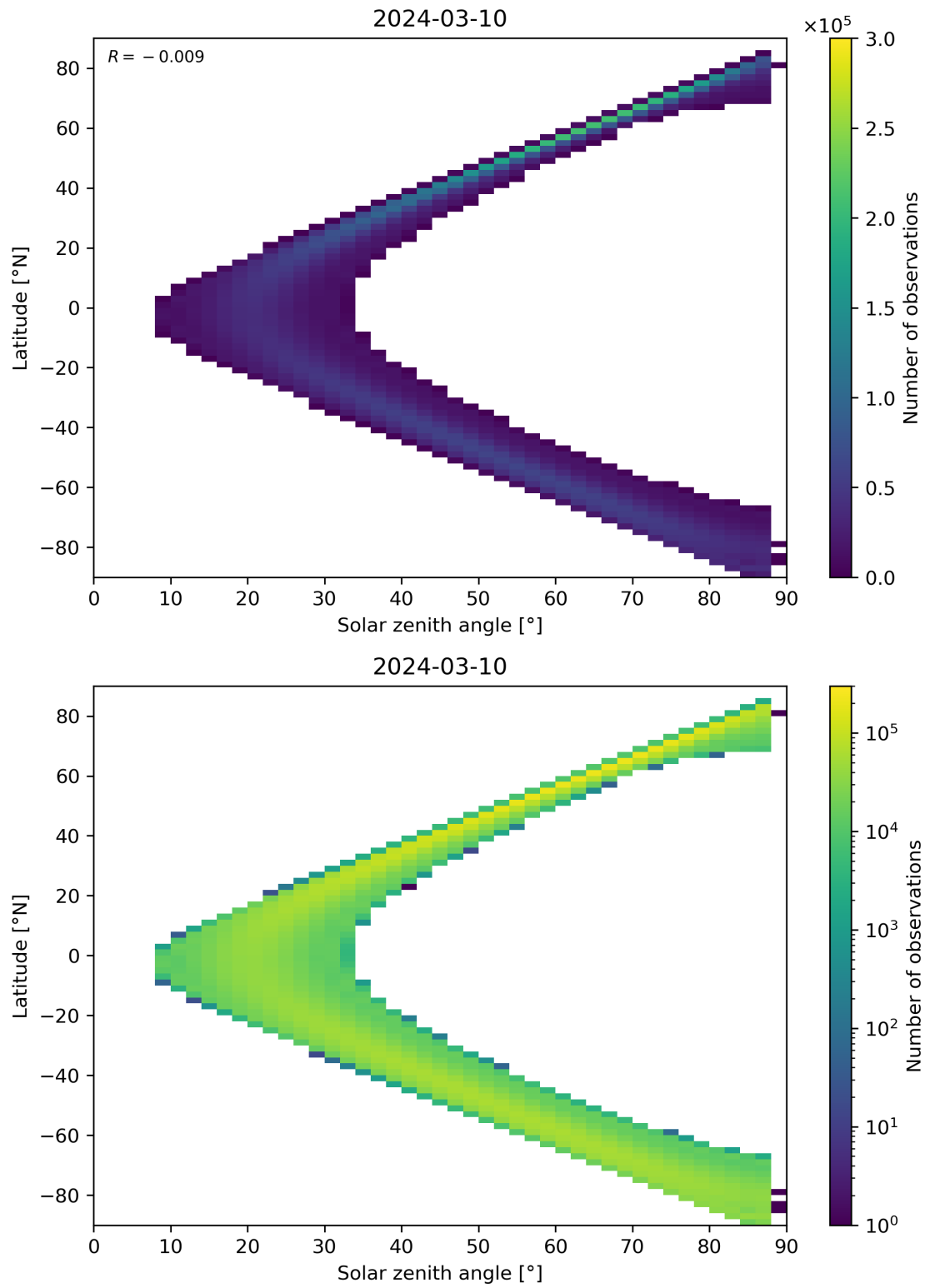
Figure 149: Scatter density plot of “Solar zenith angle” against “Latitude” for 2024-03-09 to 2024-03-11.
