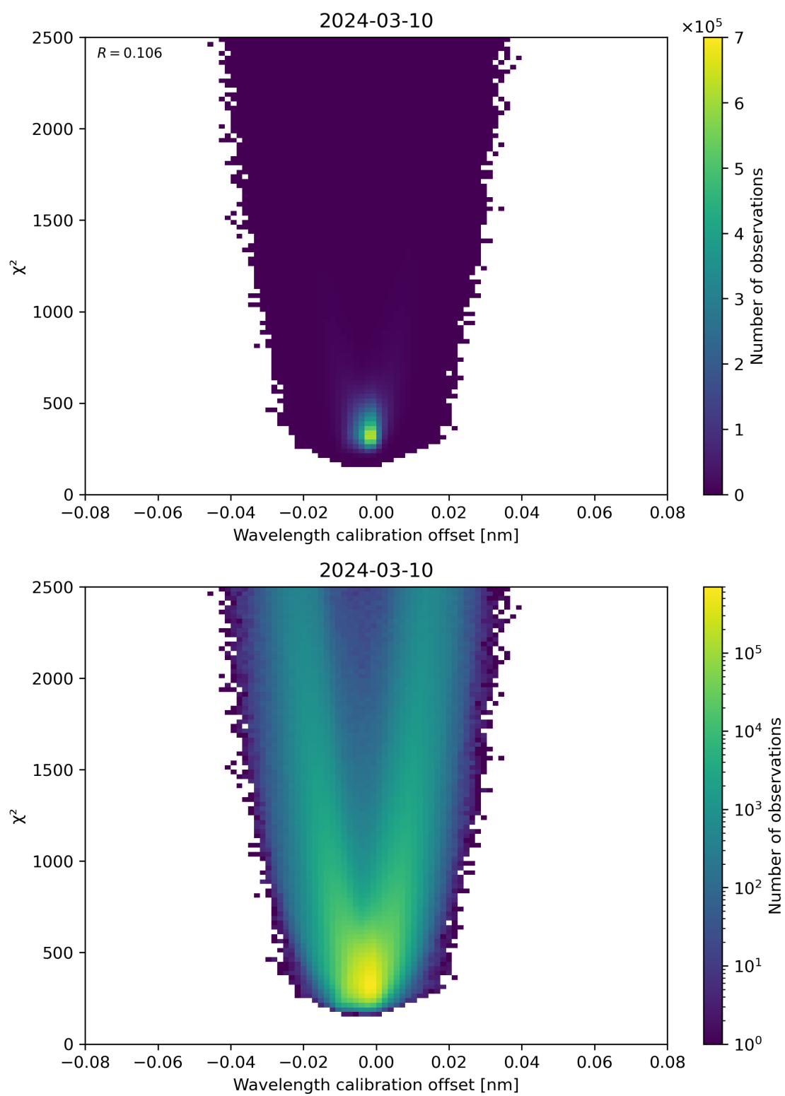
Figure 175: Scatter density plot of “Wavelength calibration offset” against “ \chi^2 ” for 2024-03-09 to 2024-03-11.
