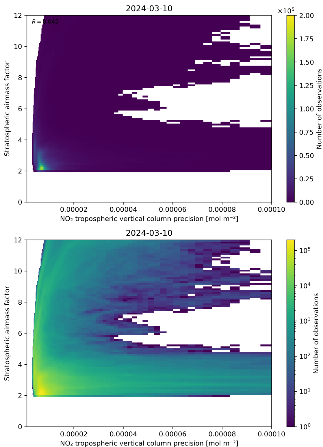
Figure 131: Scatter density plot of “NO 2 tropospheric vertical column precision” against “Stratospheric airmass factor” for 2024-03-09 to 2024-03-11.
