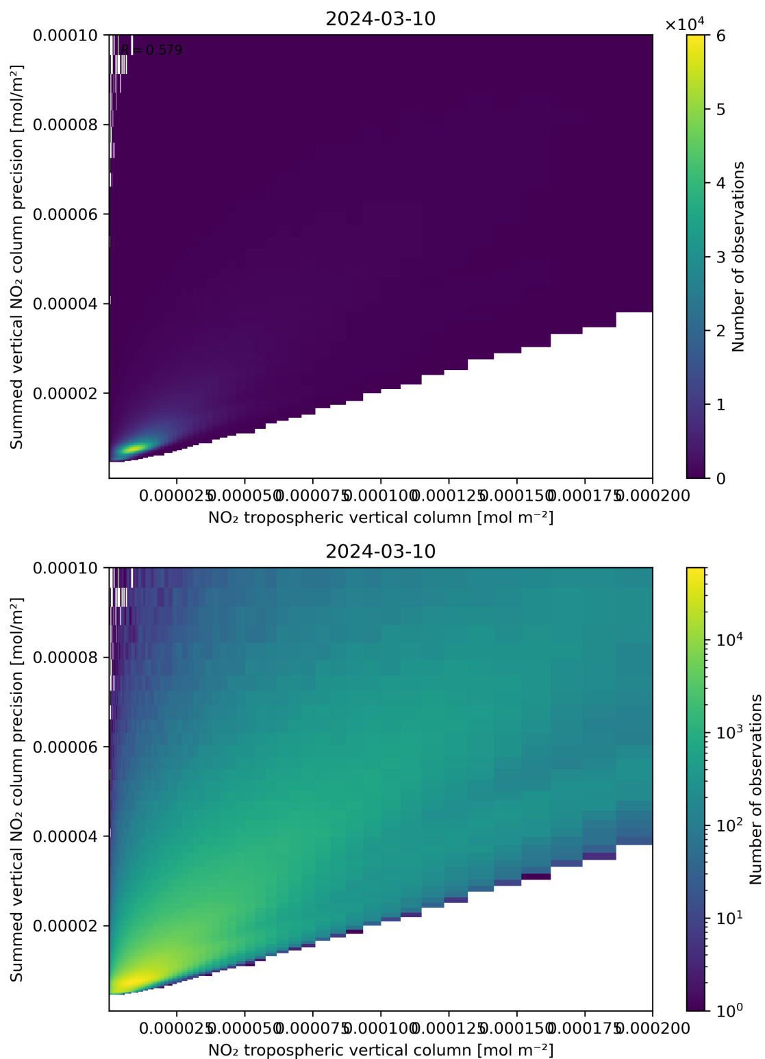
Figure 127: Scatter density plot of “NO 2 tropospheric vertical column” against “Summed vertical NO 2 column precision” for 2024-03-09 to 2024-03-11.
