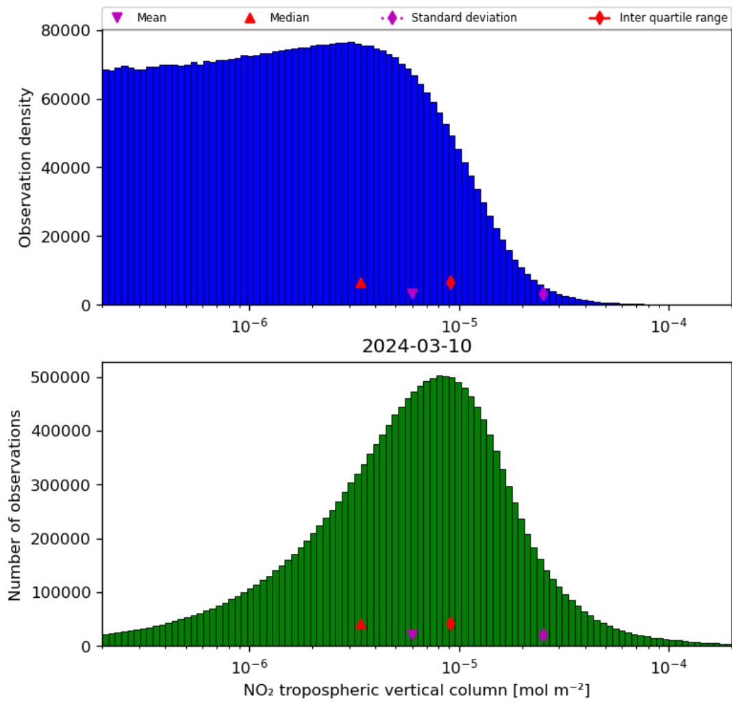
Figure 29: Histogram of “NO 2 tropospheric vertical column” for 2024-03-09 to 2024-03-11
