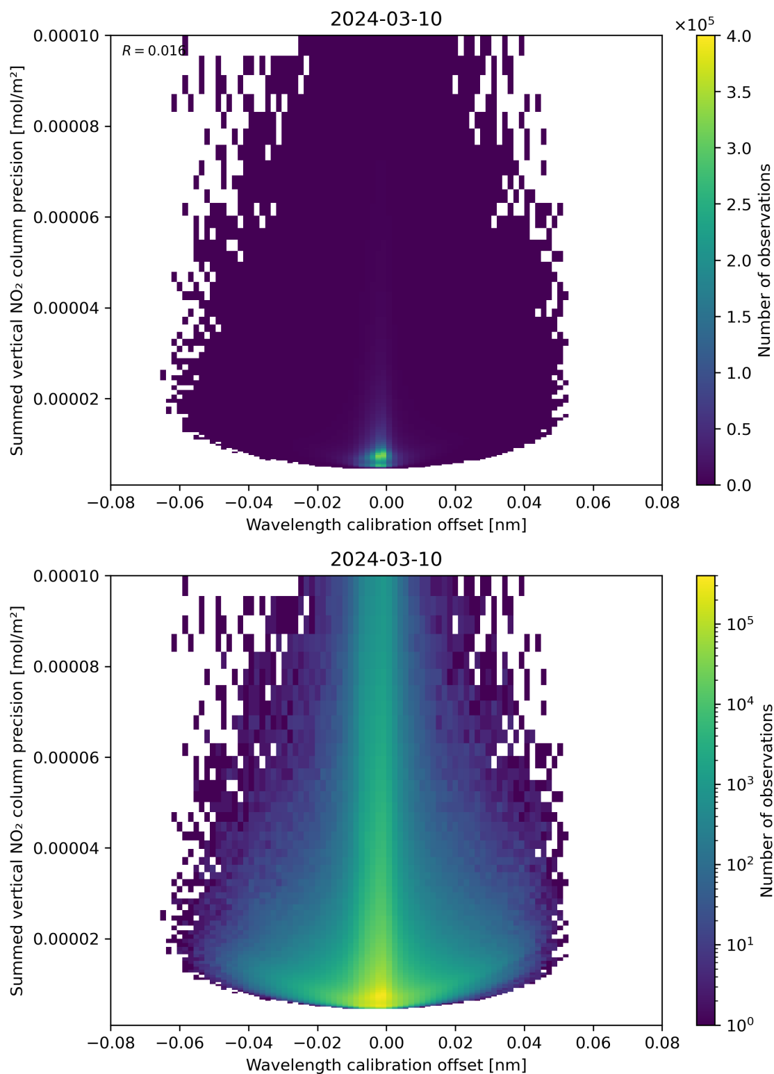
Figure 178: Scatter density plot of “Wavelength calibration offset” against “Summed vertical NO 2 column precision” for 2024-03-09 to 2024-03-11.
