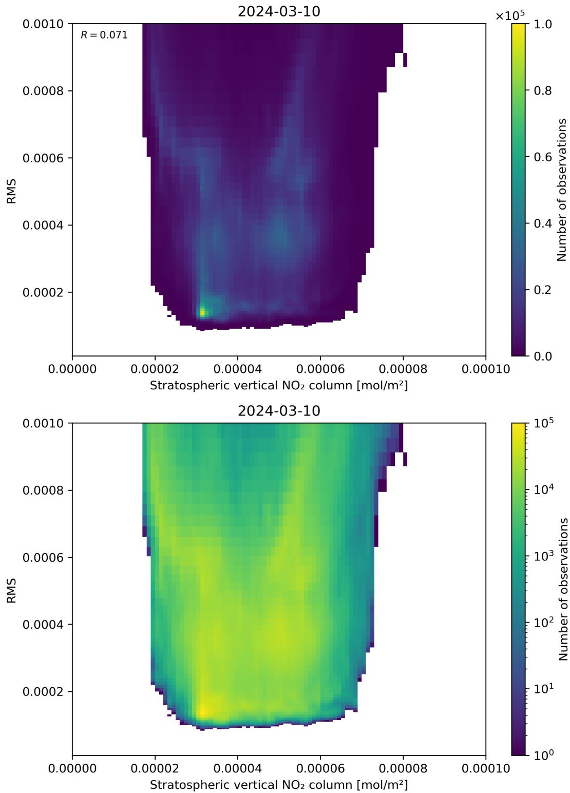
Figure 102: Scatter density plot of “Stratospheric vertical NO 2 column” against “RMS” for 2024-03-09 to 2024-03-11.
