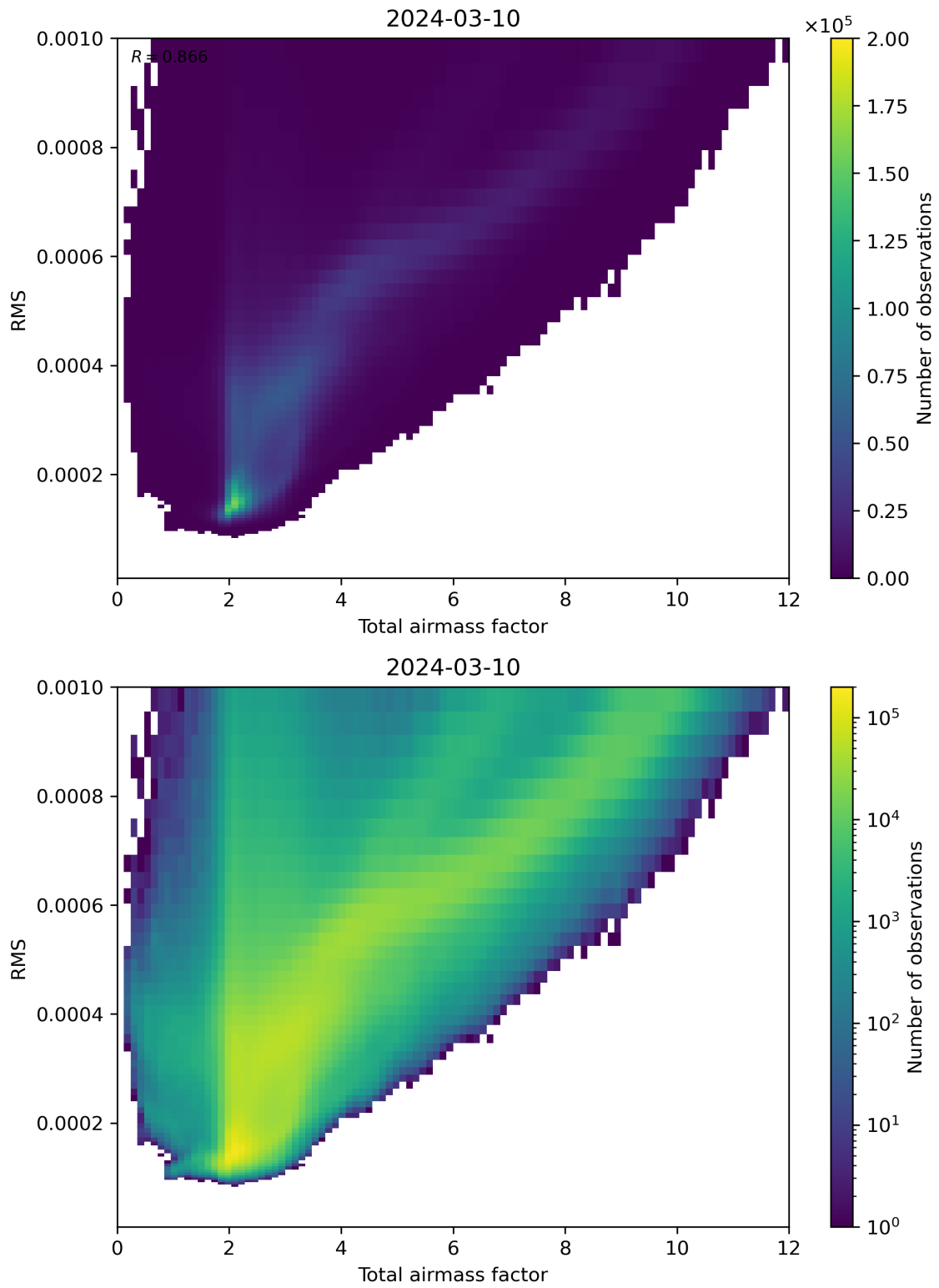
Figure 69: Scatter density plot of “Total airmass factor” against “RMS” for 2024-03-09 to 2024-03-11.
