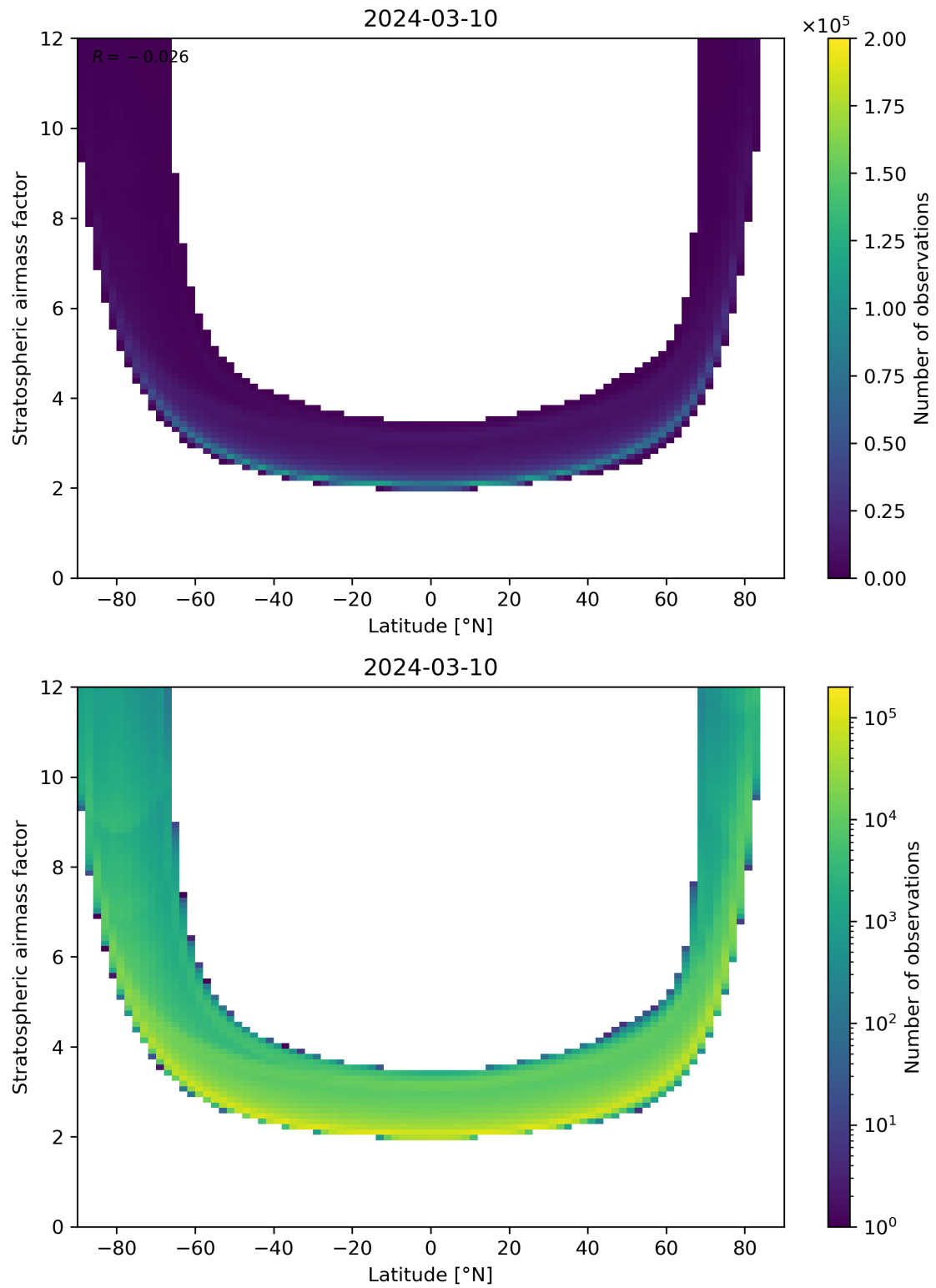
Figure 83: Scatter density plot of “Latitude” against “Stratospheric air mass factor” for 2024-03-09 to 2024-03-11.
