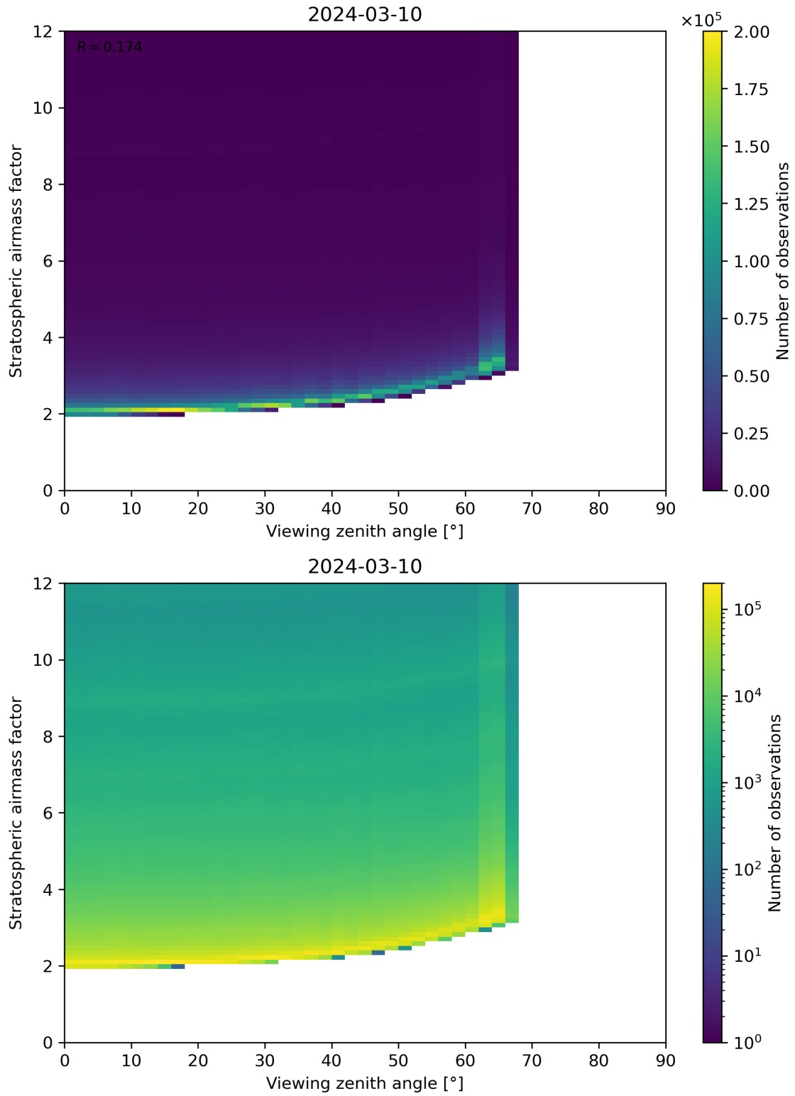
Figure 159: Scatter density plot of “Viewing zenith angle” against “Stratospheric airmass factor” for 2024-03-09 to 2024-03-11.
