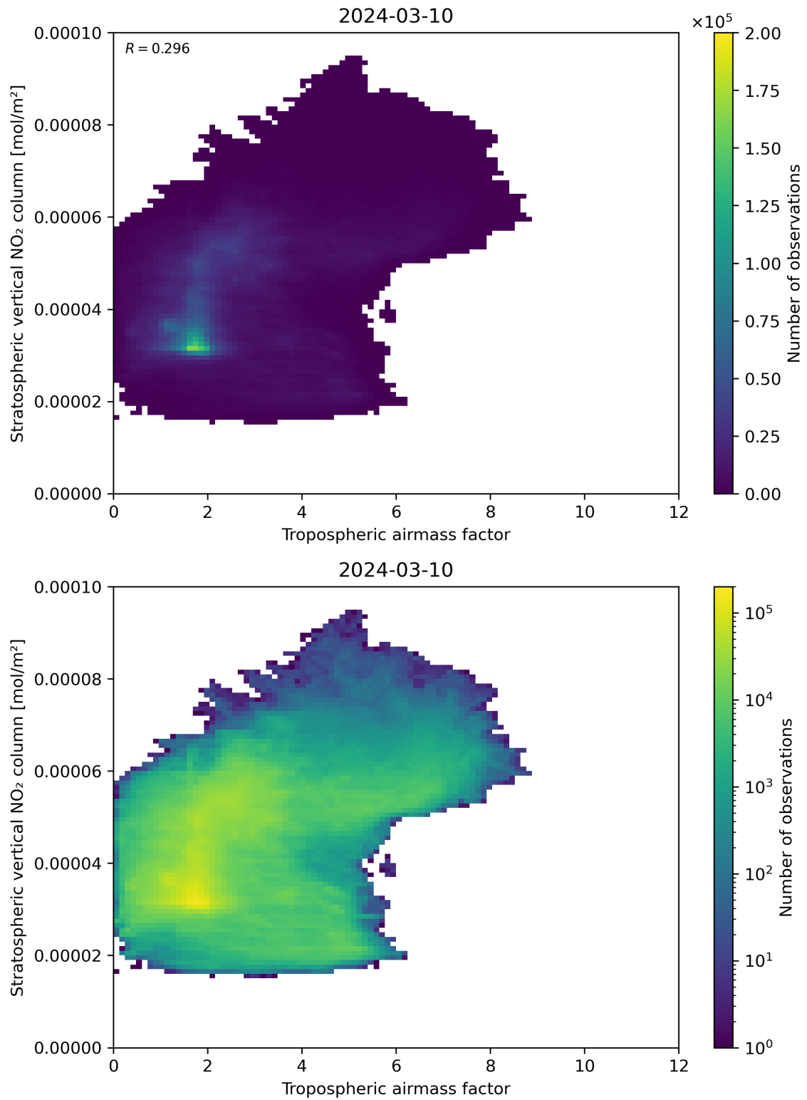
Figure 74: Scatter density plot of “Tropospheric air mass factor” against “Stratospheric vertical NO 2 column” for 2024-03-09 to 2024-03-11.
