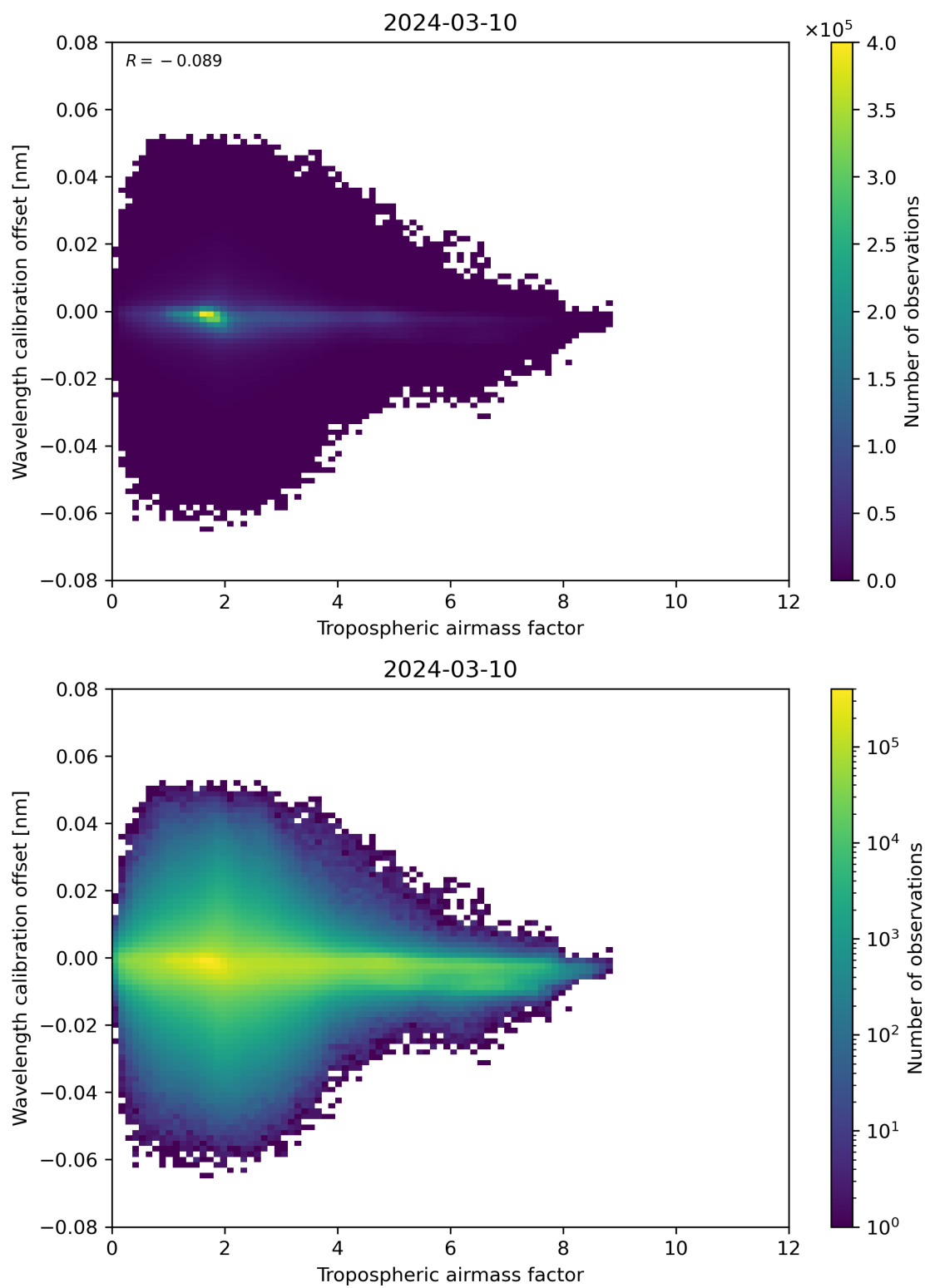
Figure 80: Scatter density plot of “Tropospheric airmass factor” against “Wavelength calibration offset” for 2024-03-09 to 2024-03-11.
