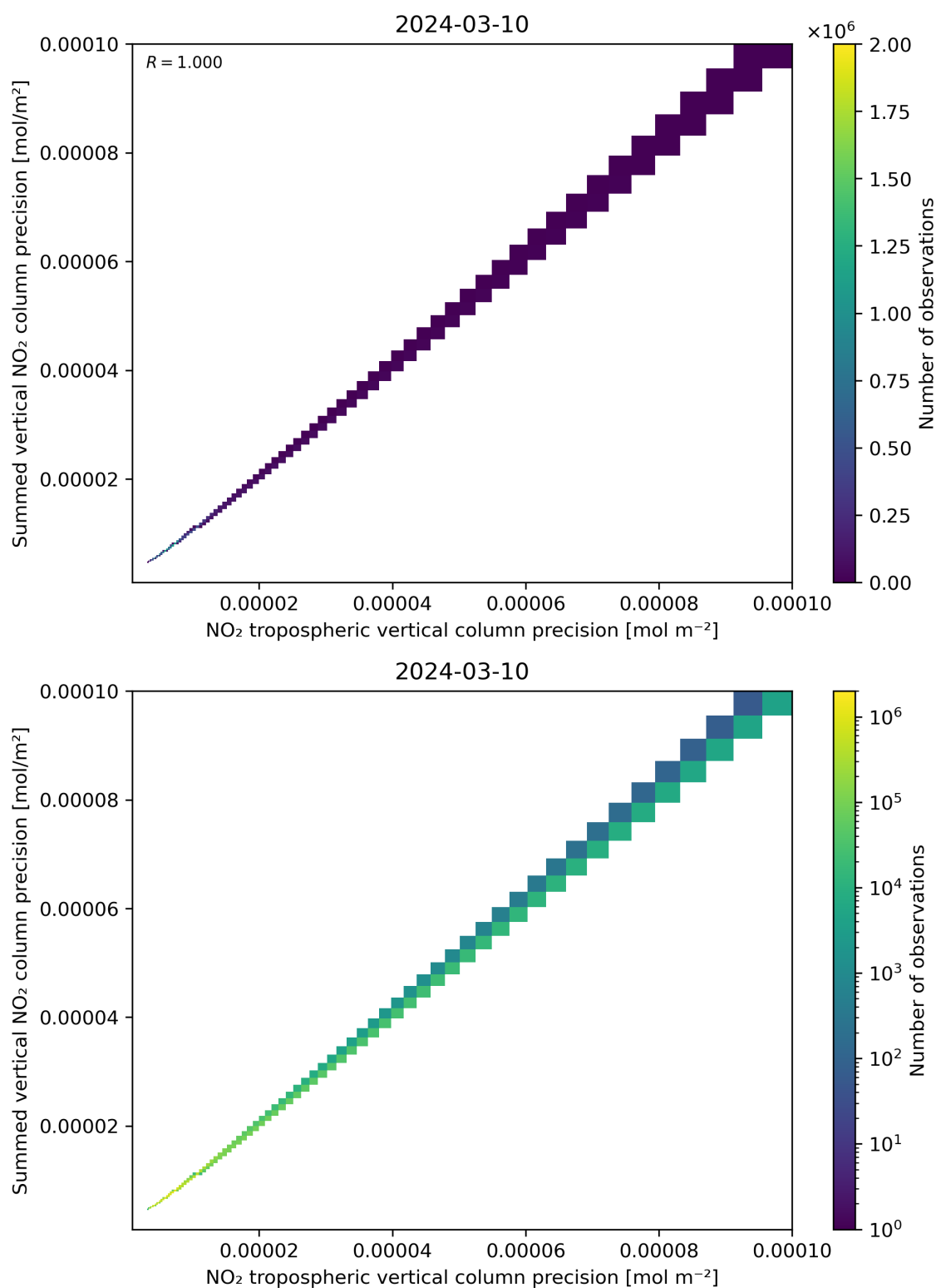
Figure 137: Scatter density plot of “NO 2 tropospheric vertical column precision” against “Summed vertical NO 2 column precision” for 2024-03-09 to 2024-03-11.
