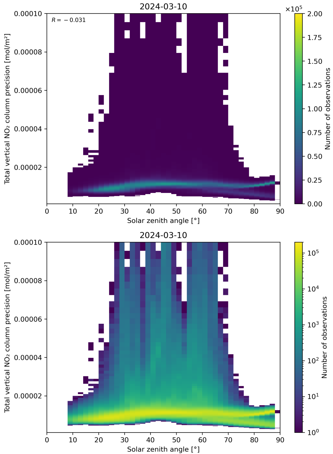
Figure 154: Scatter density plot of “Solar zenith angle” against “Total vertical NO 2 column precision” for 2024-03-09 to 2024-03-11.
