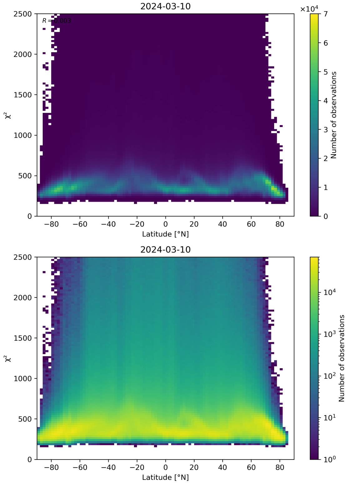
Figure 86: Scatter density plot of “Latitude” against “ \chi^2 ” for 2024-03-09 to 2024-03-11.
