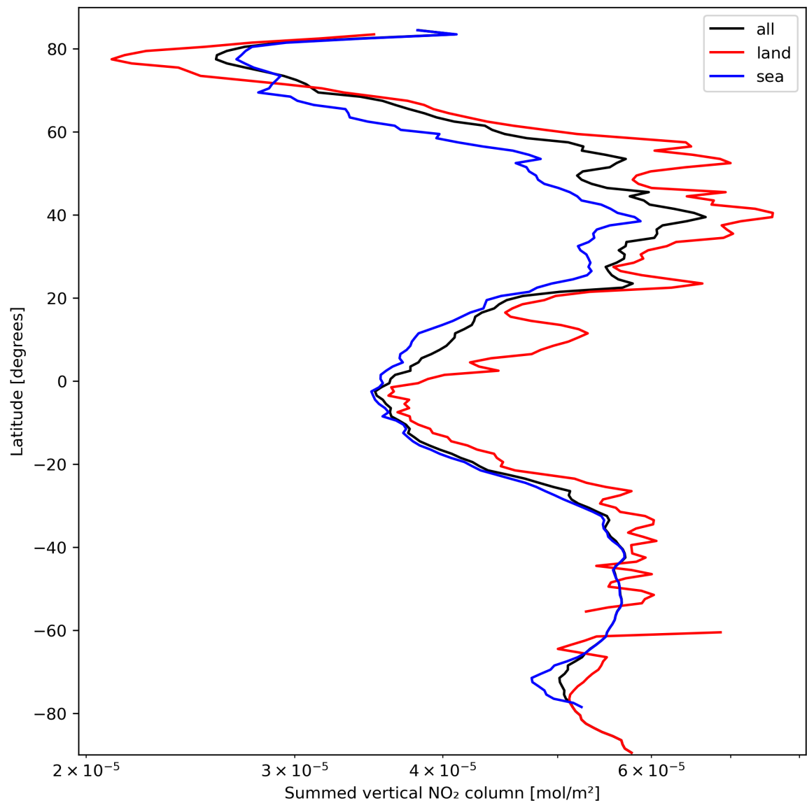
Figure 23: Zonal average of “Summed vertical NO 2 column” for 2024-03-09 to 2024-03-11.
