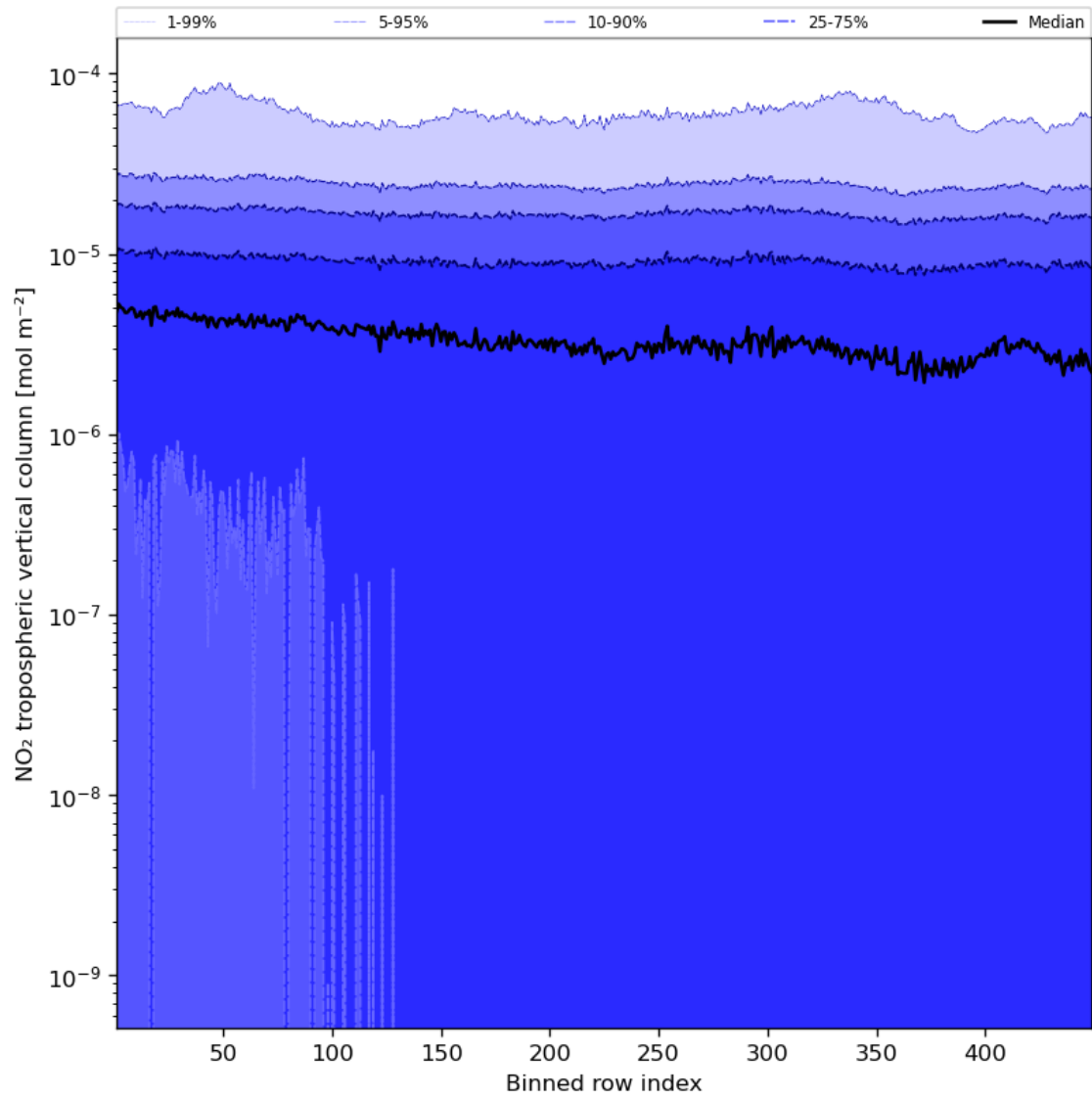
Figure 46: Along track statistics of “NO 2 tropospheric vertical column” for 2024-03-09 to 2024-03-11
