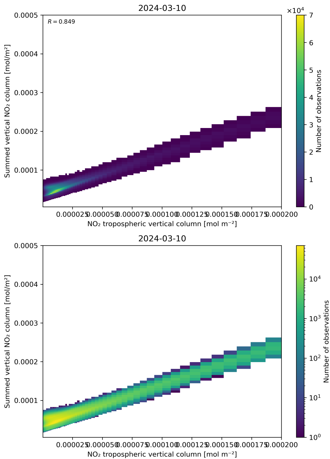
Figure 126: Scatter density plot of “NO 2 tropospheric vertical column” against “Summed vertical NO 2 column” for 2024-03-09 to 2024-03-11.
