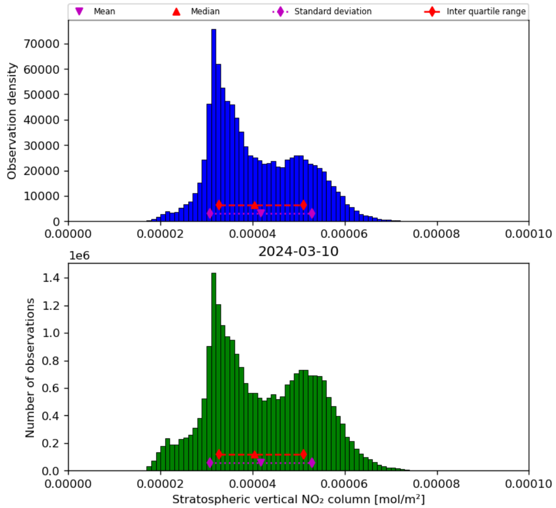
Figure 36: Histogram of “Stratospheric vertical NO 2 column” for 2024-03-09 to 2024-03-11
