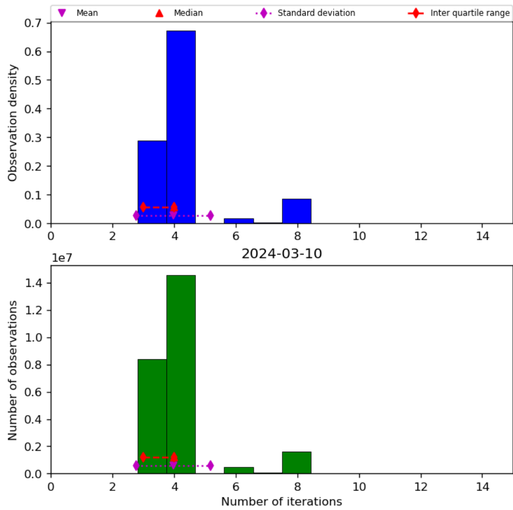
Figure 34: Histogram of “Number of iterations” for 2024-03-09 to 2024-03-11
