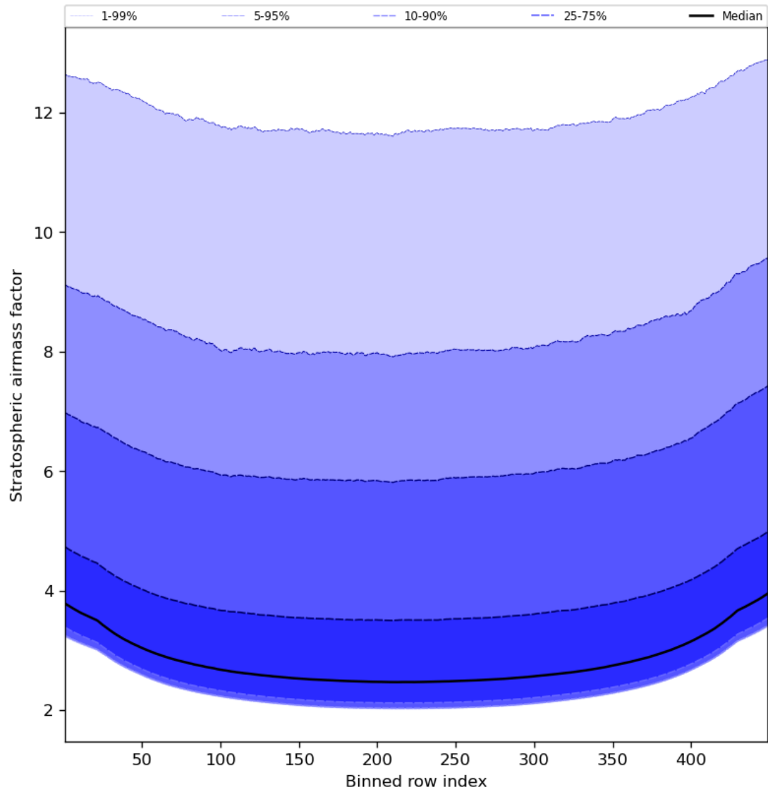
Figure 61: Along track statistics of “Stratospheric airmass factor” for 2024-03-09 to 2024-03-11
