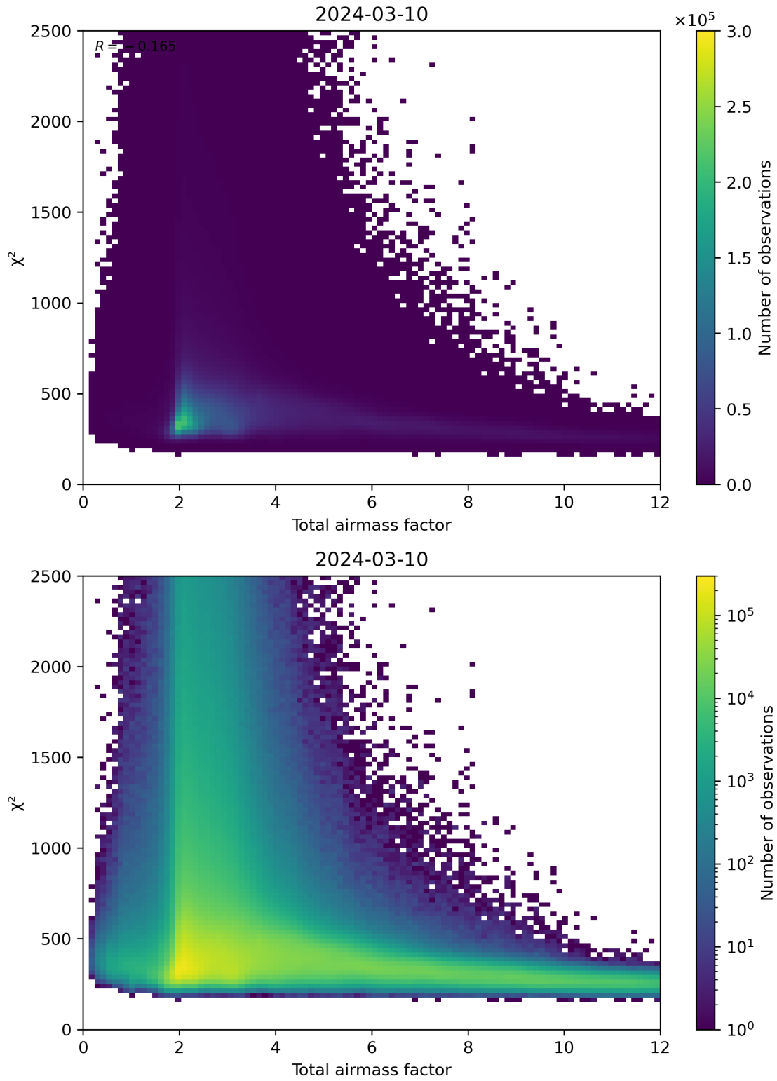
Figure 63: Scatter density plot of “Total airmass factor” against “ \chi^2 ” for 2024-03-09 to 2024-03-11.
