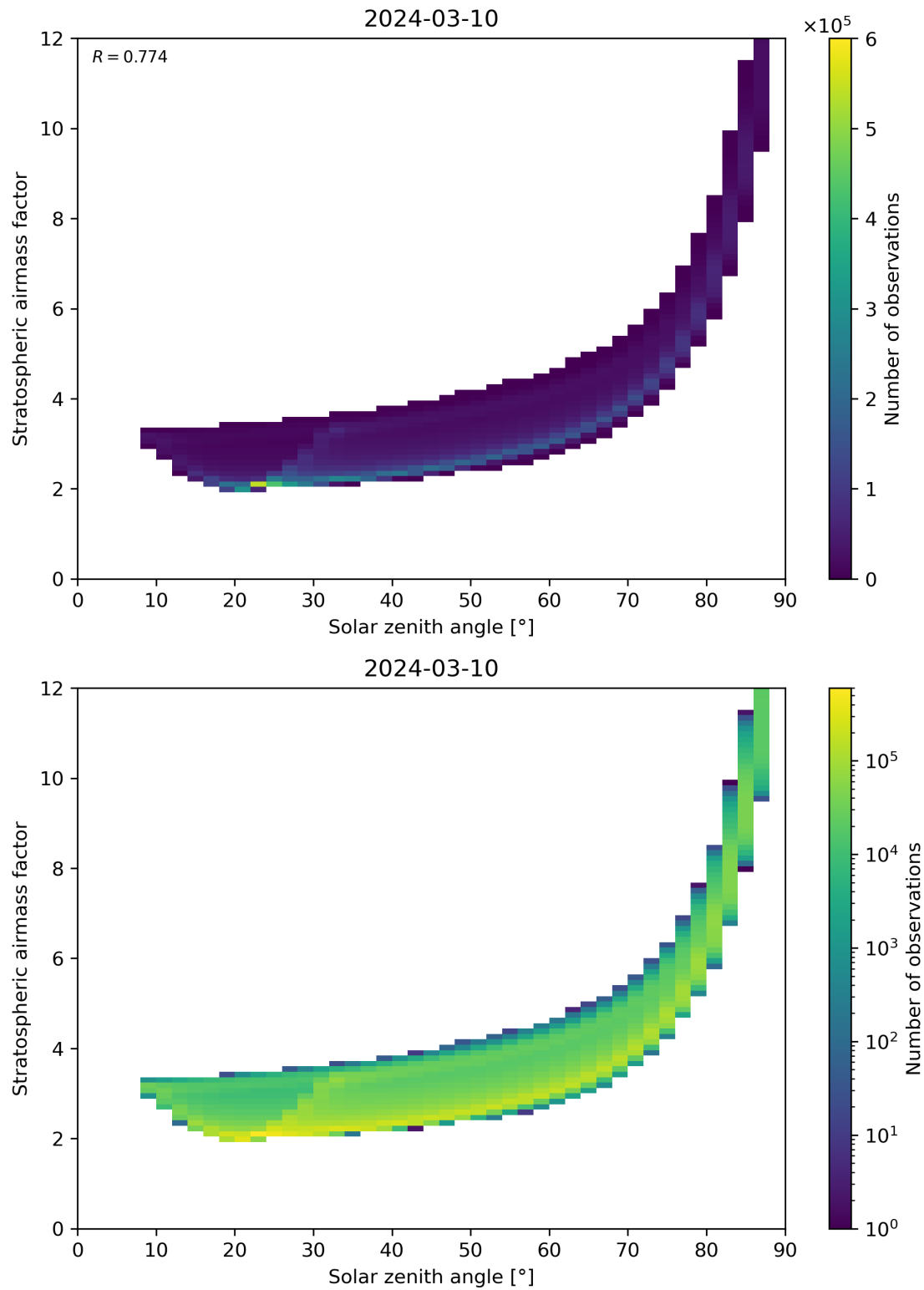
Figure 145: Scatter density plot of “Solar zenith angle” against “Stratospheric airmass factor” for 2024-03-09 to 2024-03-11.
