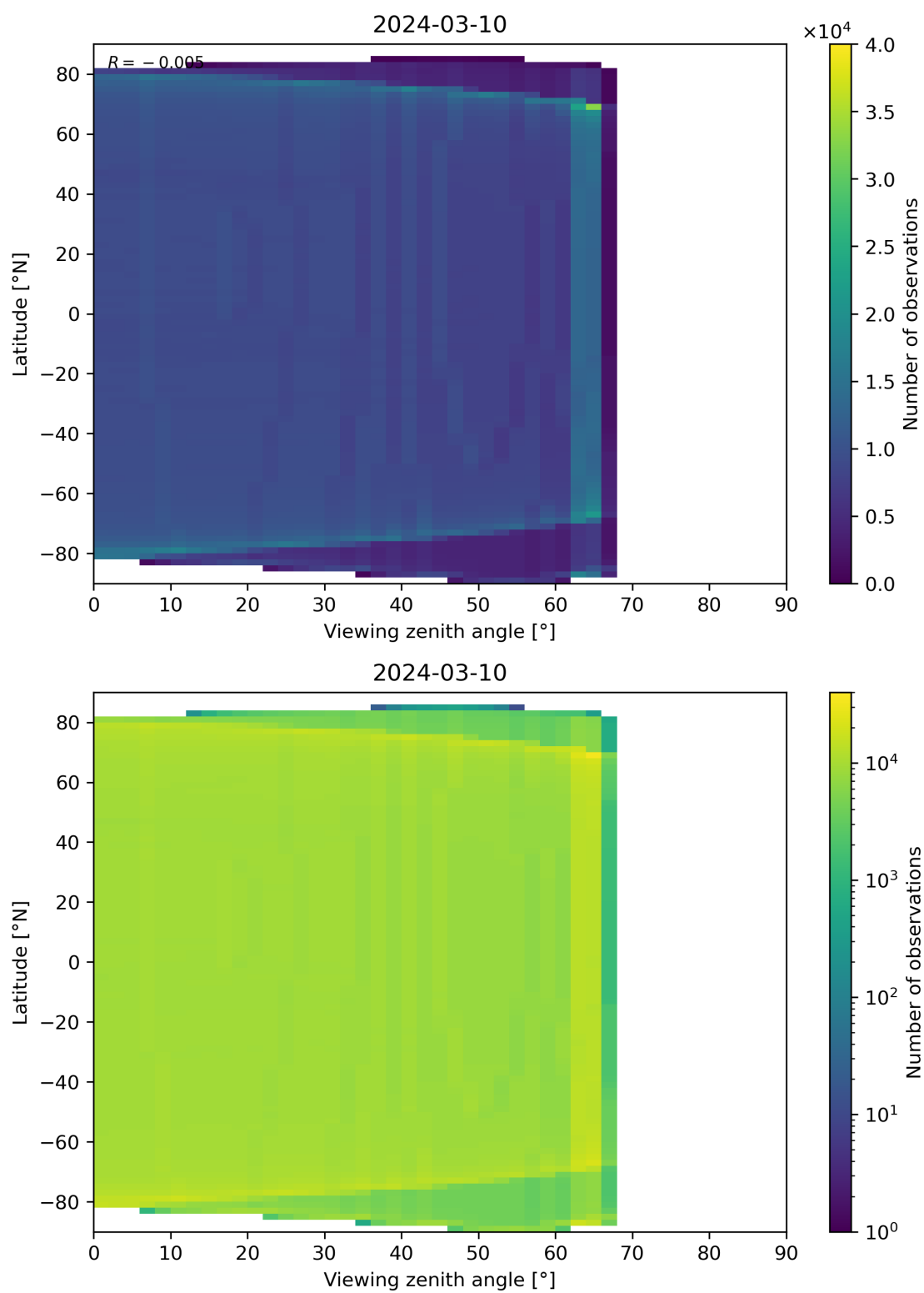
Figure 163: Scatter density plot of “Viewing zenith angle” against “Latitude” for 2024-03-09 to 2024-03-11.
