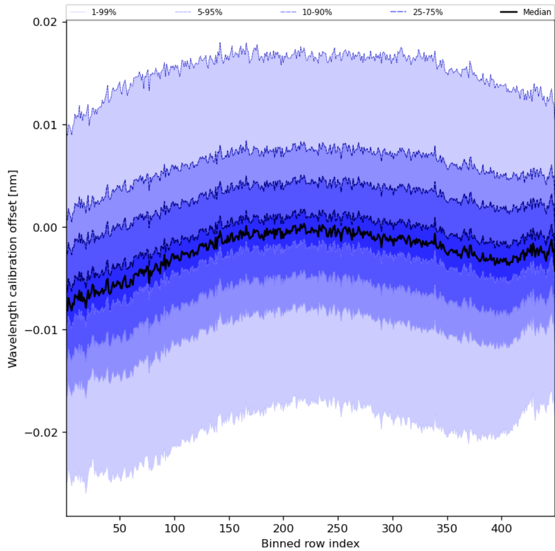
Figure 52: Along track statistics of “Wavelength calibration offset” for 2024-03-09 to 2024-03-11
