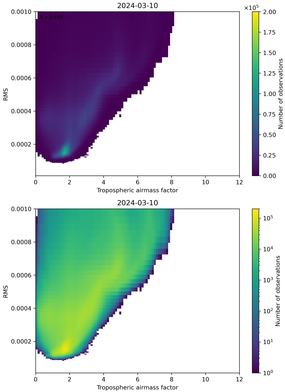
Figure 79: Scatter density plot of “Tropospheric airmass factor” against “RMS” for 2024-03-09 to 2024-03-11.
