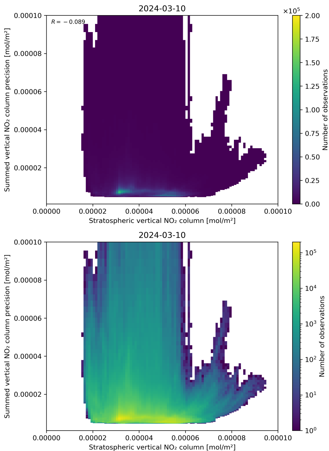
Figure 99: Scatter density plot of “Stratospheric vertical NO 2 column” against “Summed vertical NO 2 column precision” for 2024-03-09 to 2024-03-11.
