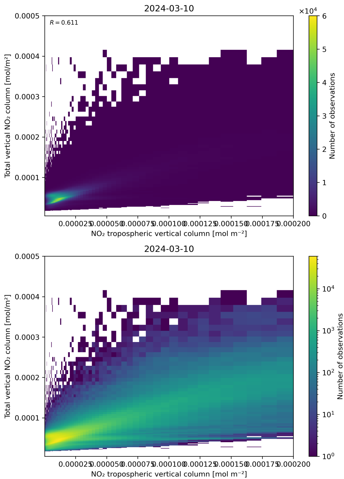
Figure 128: Scatter density plot of “NO 2 tropospheric vertical column” against “Total vertical NO 2 column” for 2024-03-09 to 2024-03-11.
