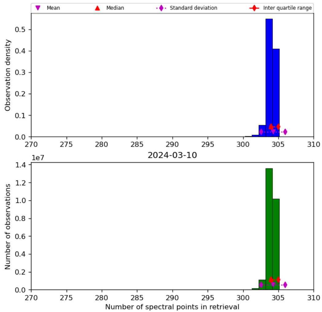
Figure 33: Histogram of “Number of spectral points in retrieval” for 2024-03-09 to 2024-03-11
