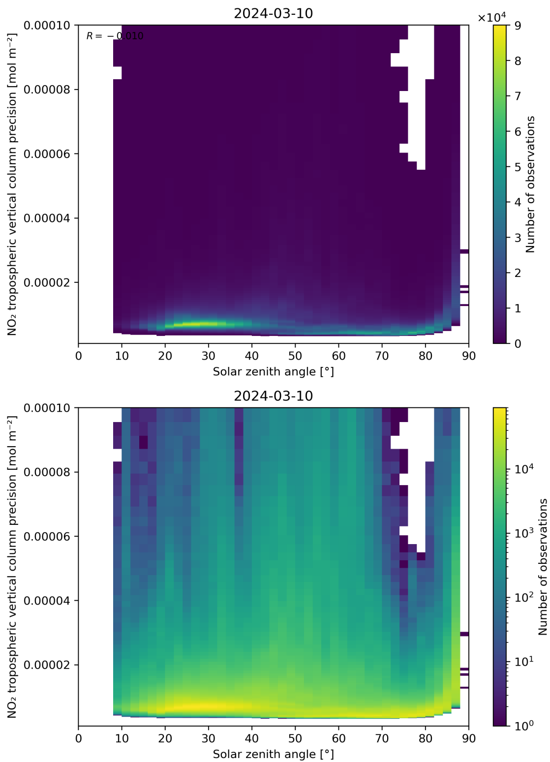
Figure 156: Scatter density plot of “Solar zenith angle” against “NO 2 tropospheric vertical column precision” for 2024-03-09 to 2024-03-11.
