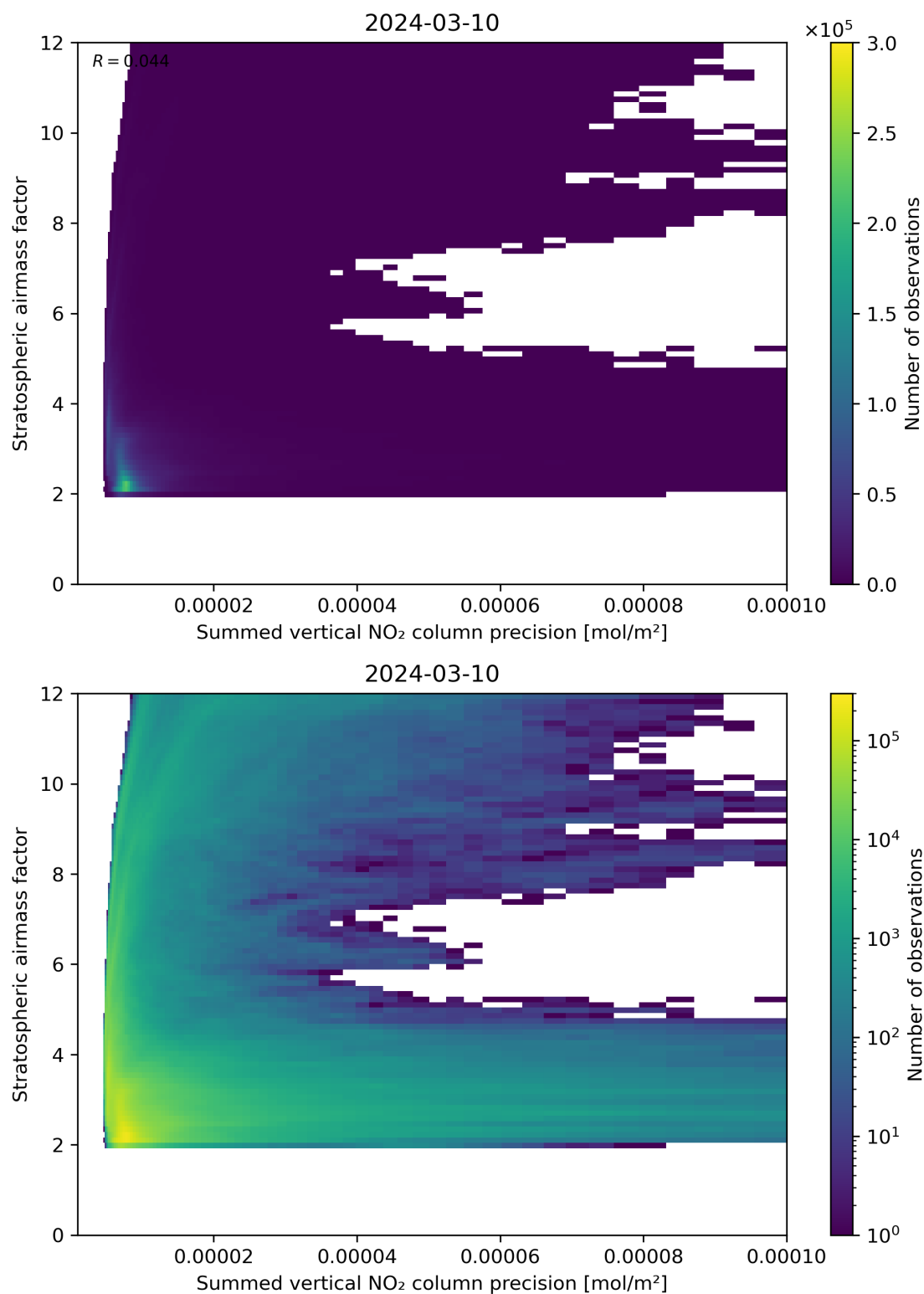
Figure 106: Scatter density plot of “Summed vertical NO 2 column precision” against “Stratospheric airmass factor” for 2024-03-09 to 2024-03-11.
