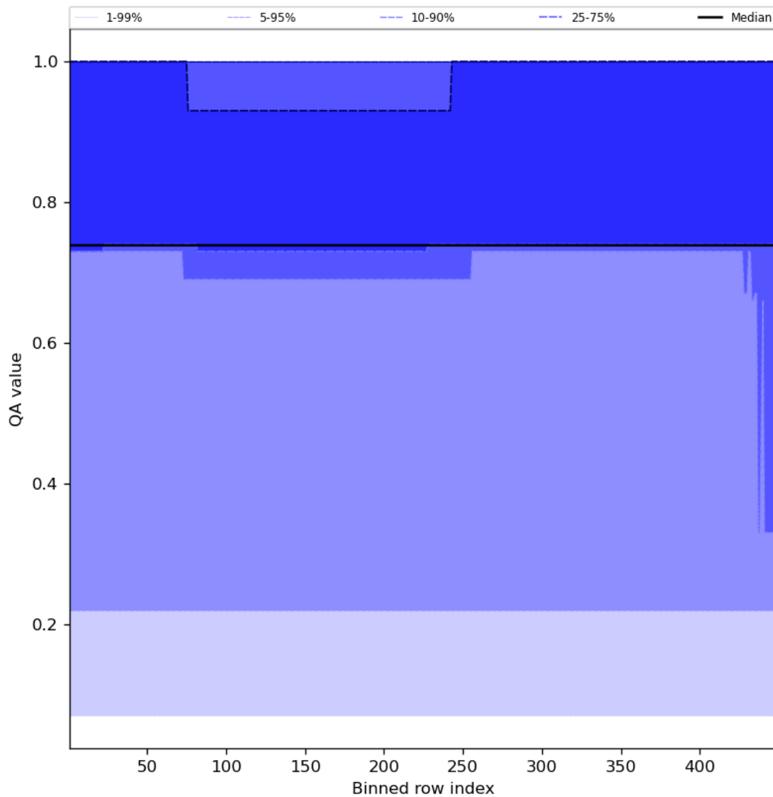
Figure 45: Along track statistics of “QA value” for 2024-03-09 to 2024-03-11
