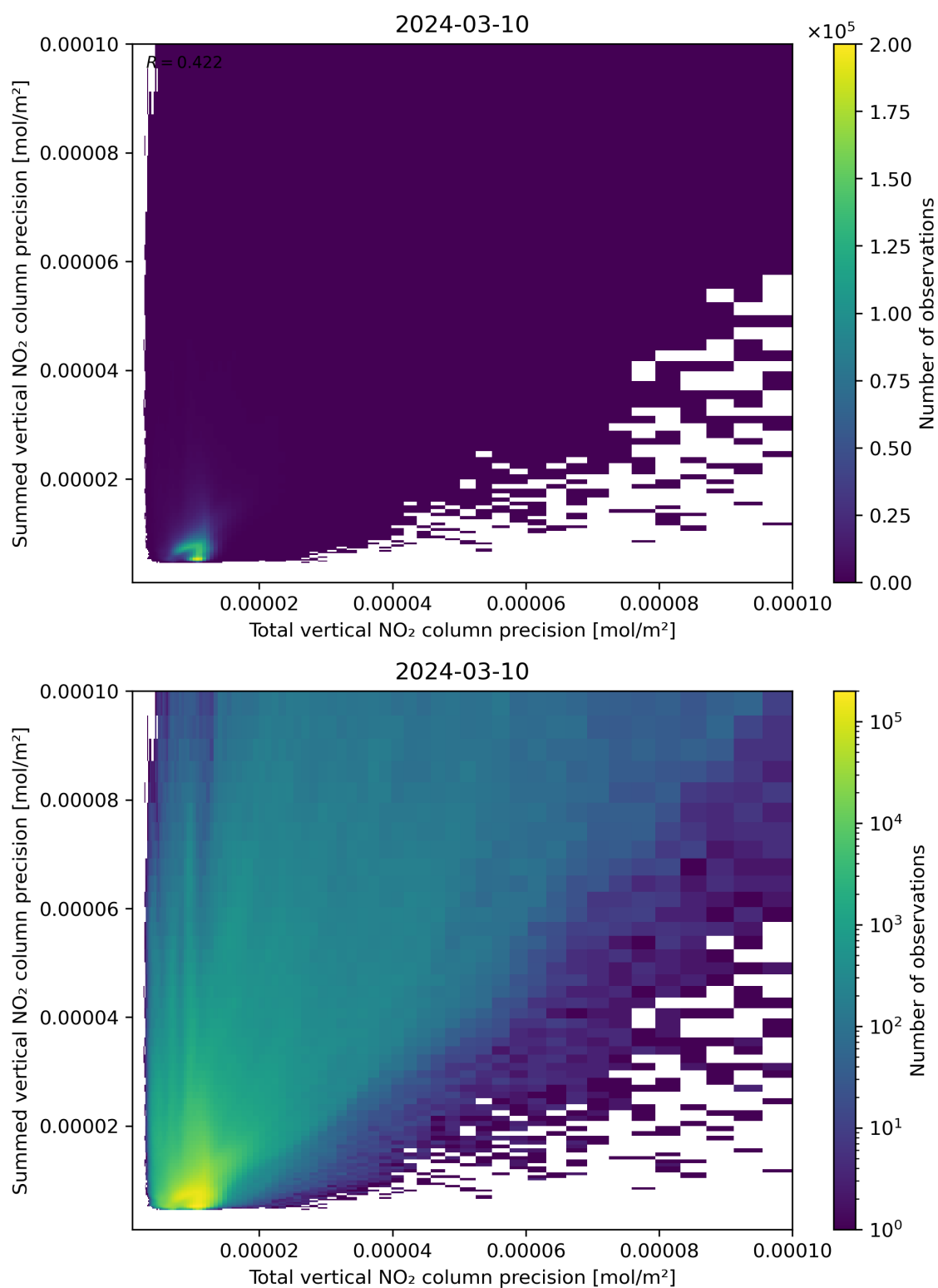
Figure 118: Scatter density plot of “Total vertical NO 2 column precision” against “Summed vertical NO 2 column precision” for 2024-03-09 to 2024-03-11.
