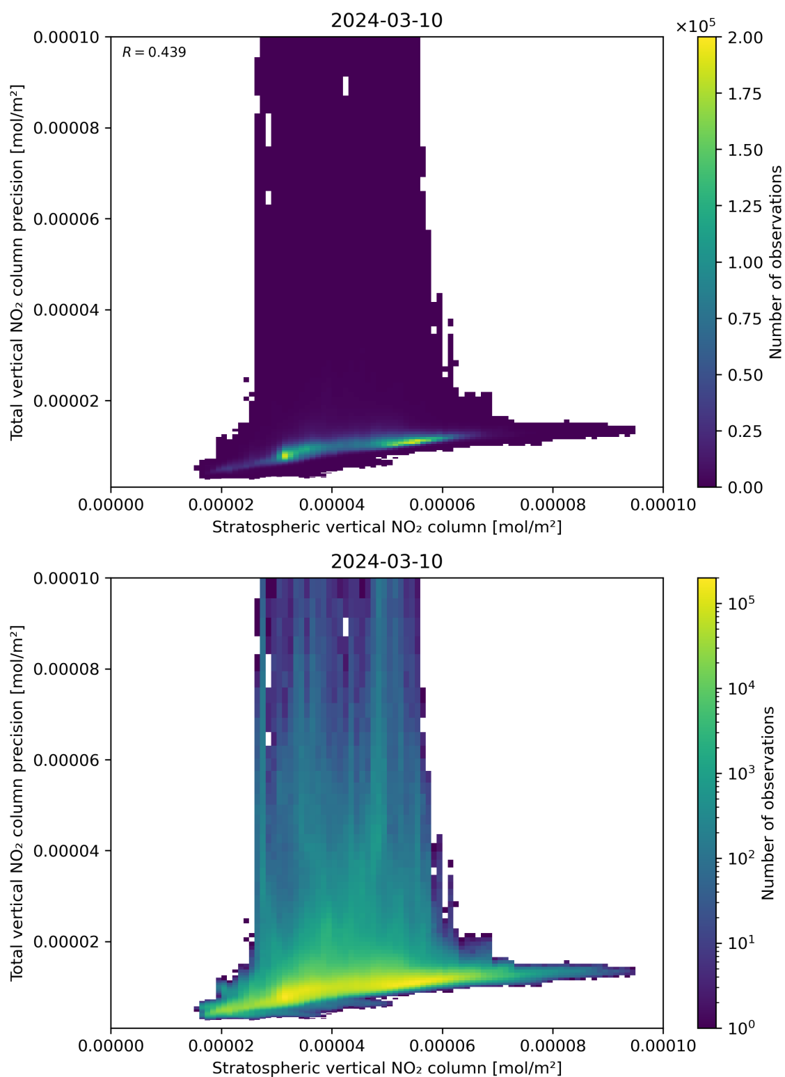
Figure 101: Scatter density plot of “Stratospheric vertical NO 2 column” against “Total vertical NO 2 column precision” for 2024-03-09 to 2024-03-11.
