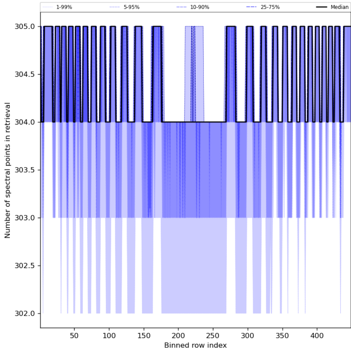
Figure 50: Along track statistics of “Number of spectral points in retrieval” for 2024-03-09 to 2024-03-11
