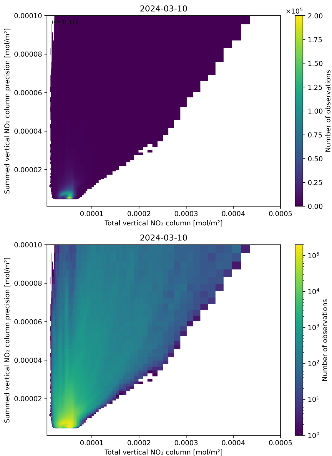
Figure 113: Scatter density plot of “Total vertical NO 2 column” against “Summed vertical NO 2 column precision” for 2024-03-09 to 2024-03-11.
