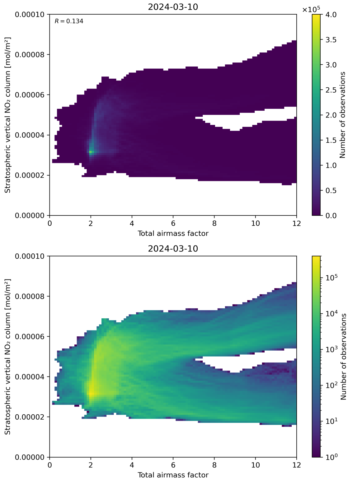
Figure 64: Scatter density plot of “Total airmass factor” against “Stratospheric vertical NO 2 column” for 2024-03-09 to 2024-03-11.
