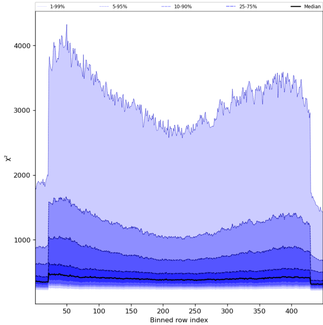
Figure 59: Along track statistics of “ \chi^2 ” for 2024-03-09 to 2024-03-11
