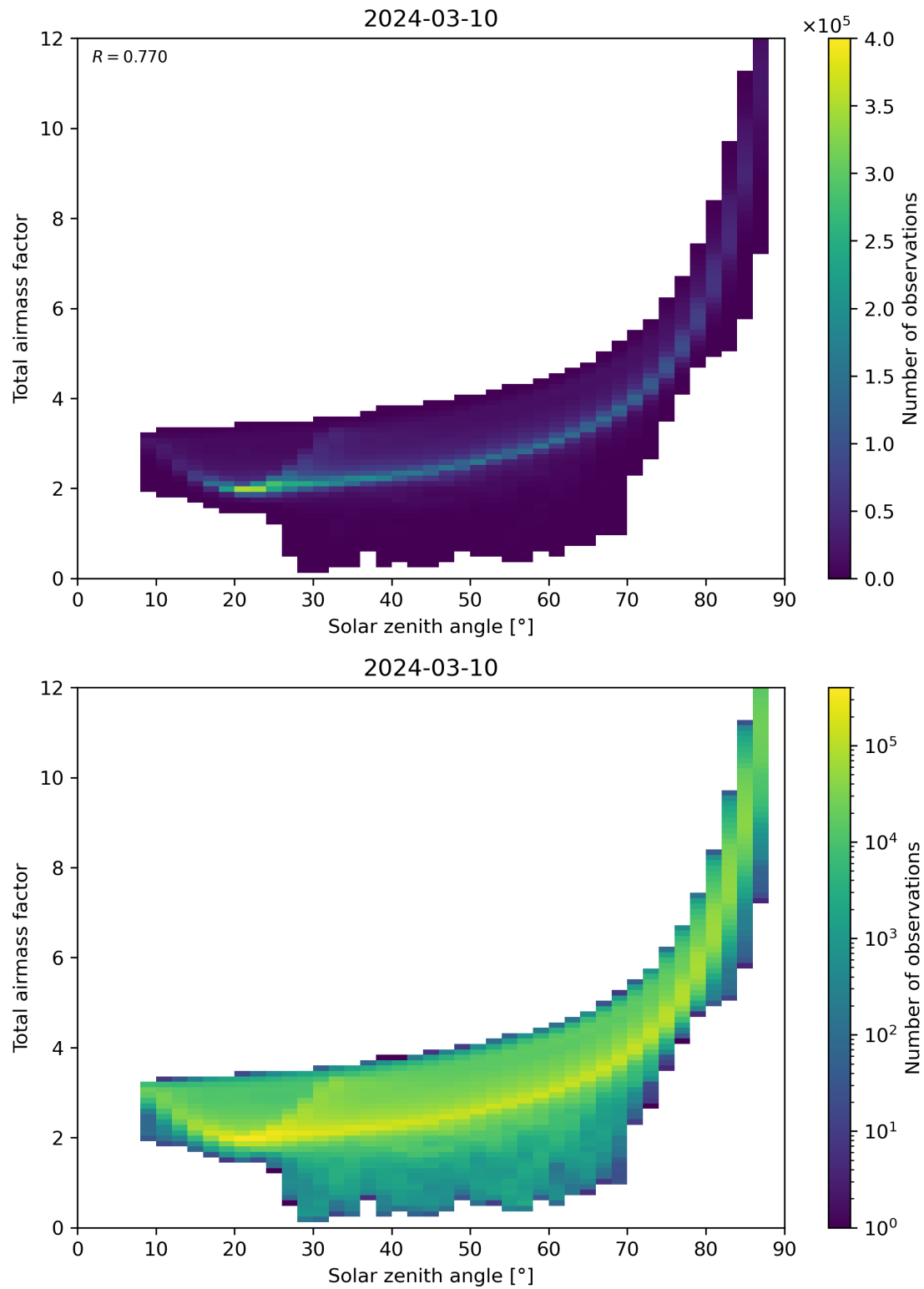
Figure 146: Scatter density plot of “Solar zenith angle” against “Total air mass factor” for 2024-03-09 to 2024-03-11.
