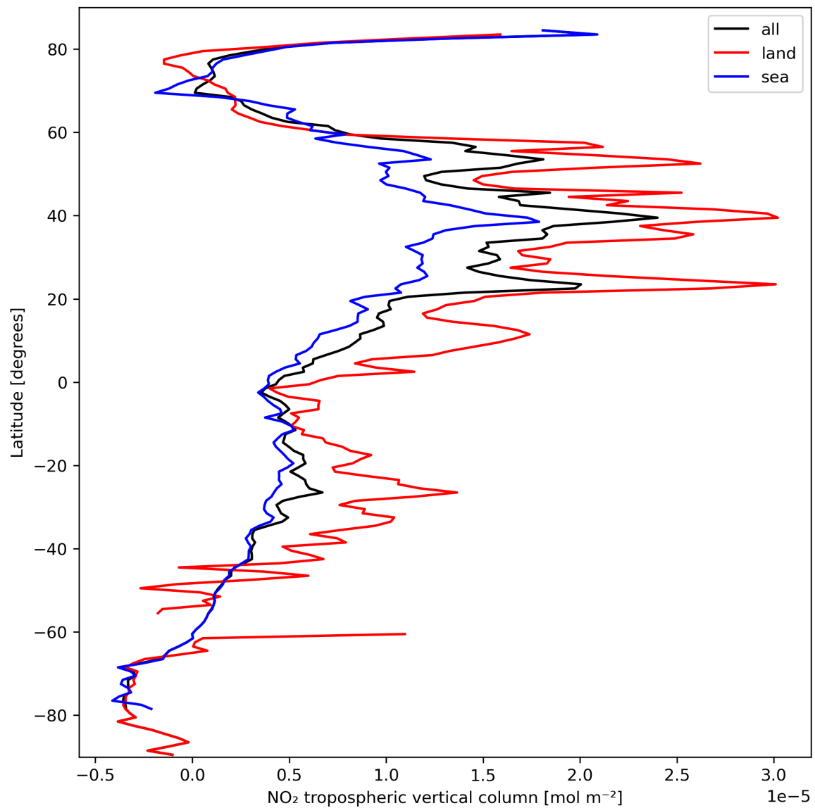
Figure 12: Zonal average of “NO 2 tropospheric vertical column” for 2024-03-09 to 2024-03-11.
