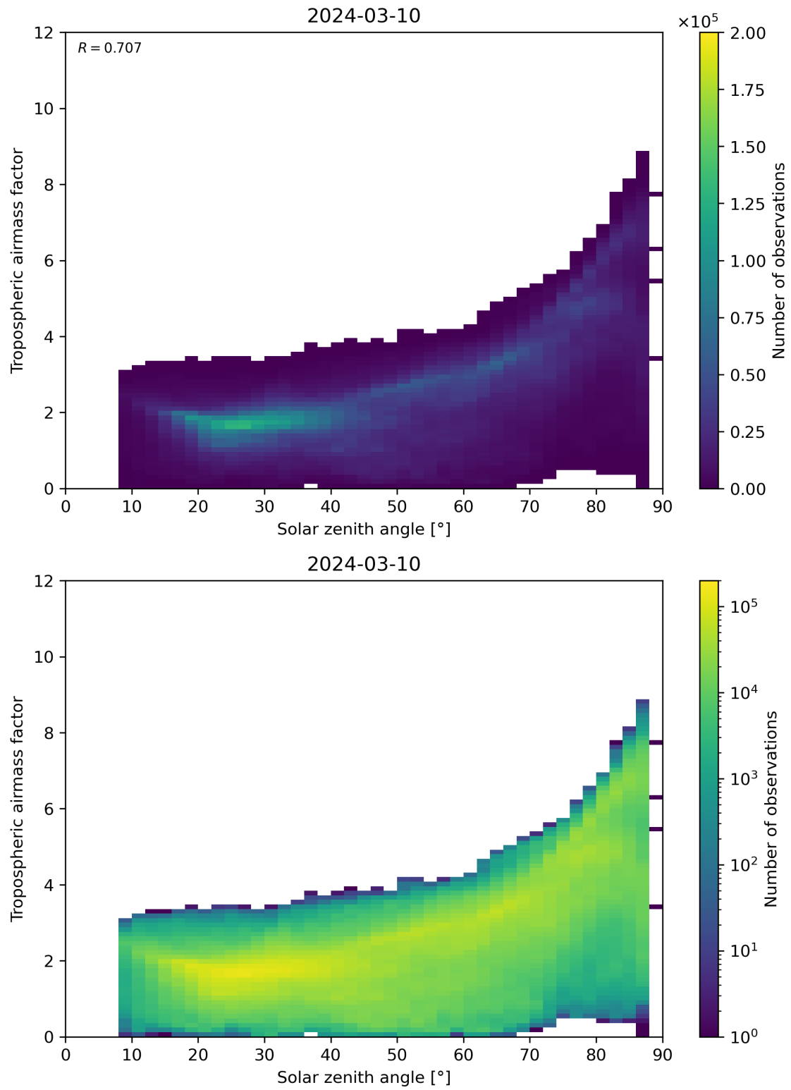
Figure 147: Scatter density plot of “Solar zenith angle” against “Tropospheric airmass factor” for 2024-03-09 to 2024-03-11.
