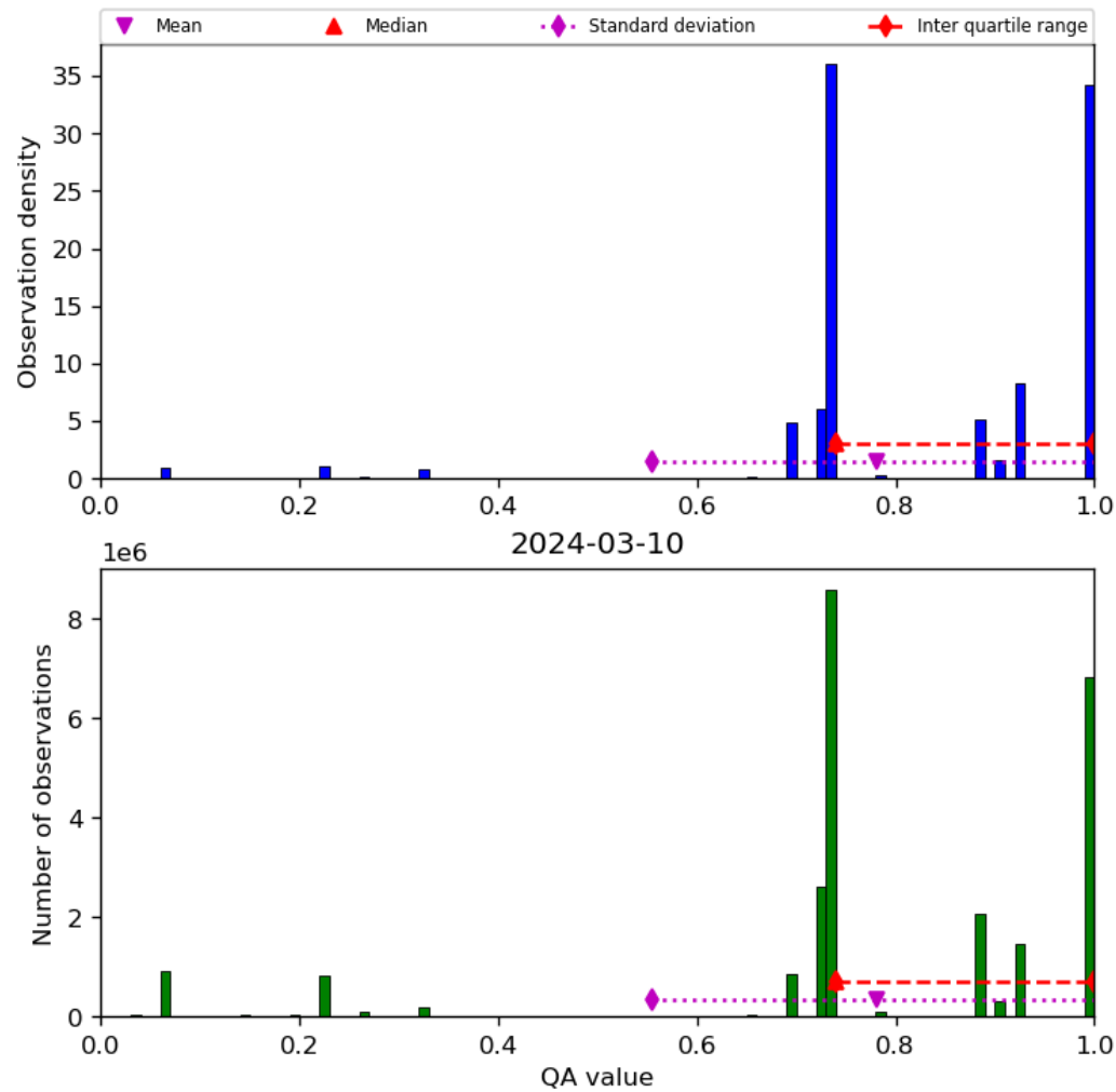
Figure 28: Histogram of “QA value” for 2024-03-09 to 2024-03-11
