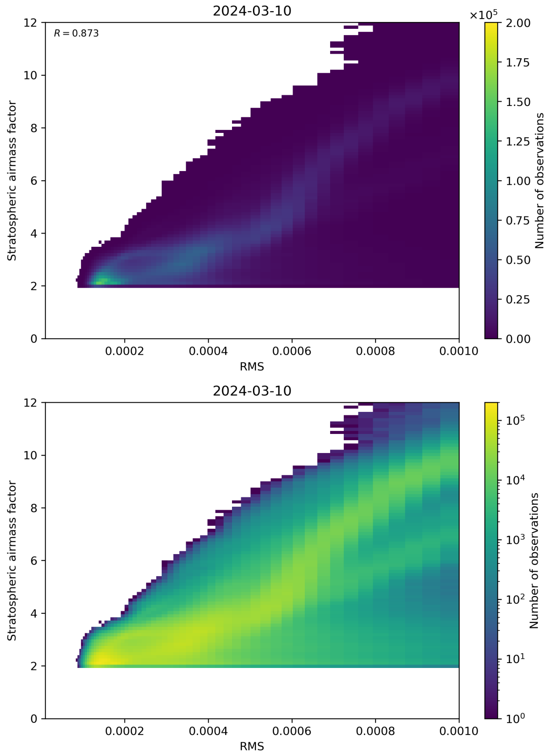
Figure 144: Scatter density plot of “RMS” against “Stratospheric airmass factor” for 2024-03-09 to 2024-03-11.
