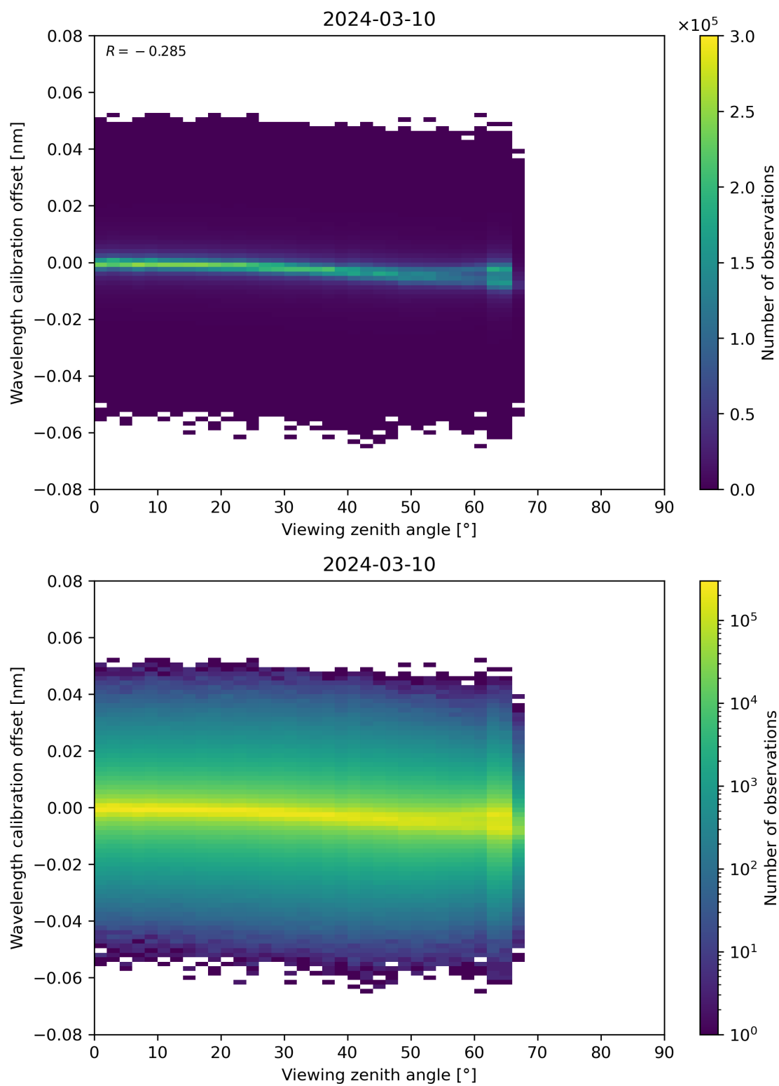
Figure 173: Scatter density plot of “Viewing zenith angle” against “Wavelength calibration offset” for 2024-03-09 to 2024-03-11.
