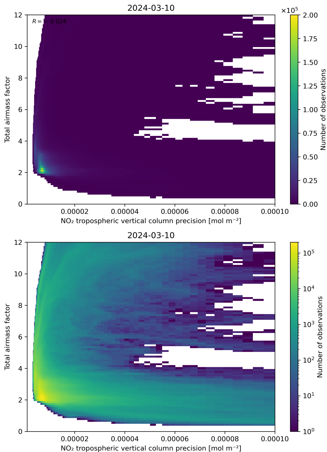
Figure 132: Scatter density plot of “NO 2 tropospheric vertical column precision” against “Total airmass factor” for 2024-03-09 to 2024-03-11.
