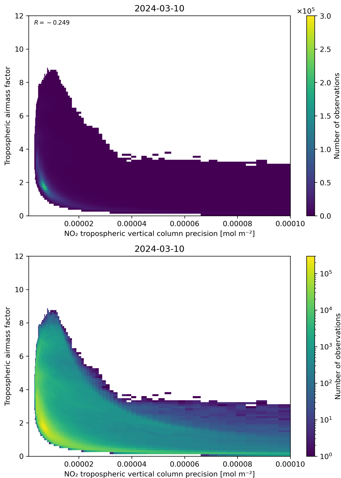
Figure 133: Scatter density plot of “NO 2 tropospheric vertical column precision” against “Tropospheric airmass factor” for 2024-03-09 to 2024-03-11.
