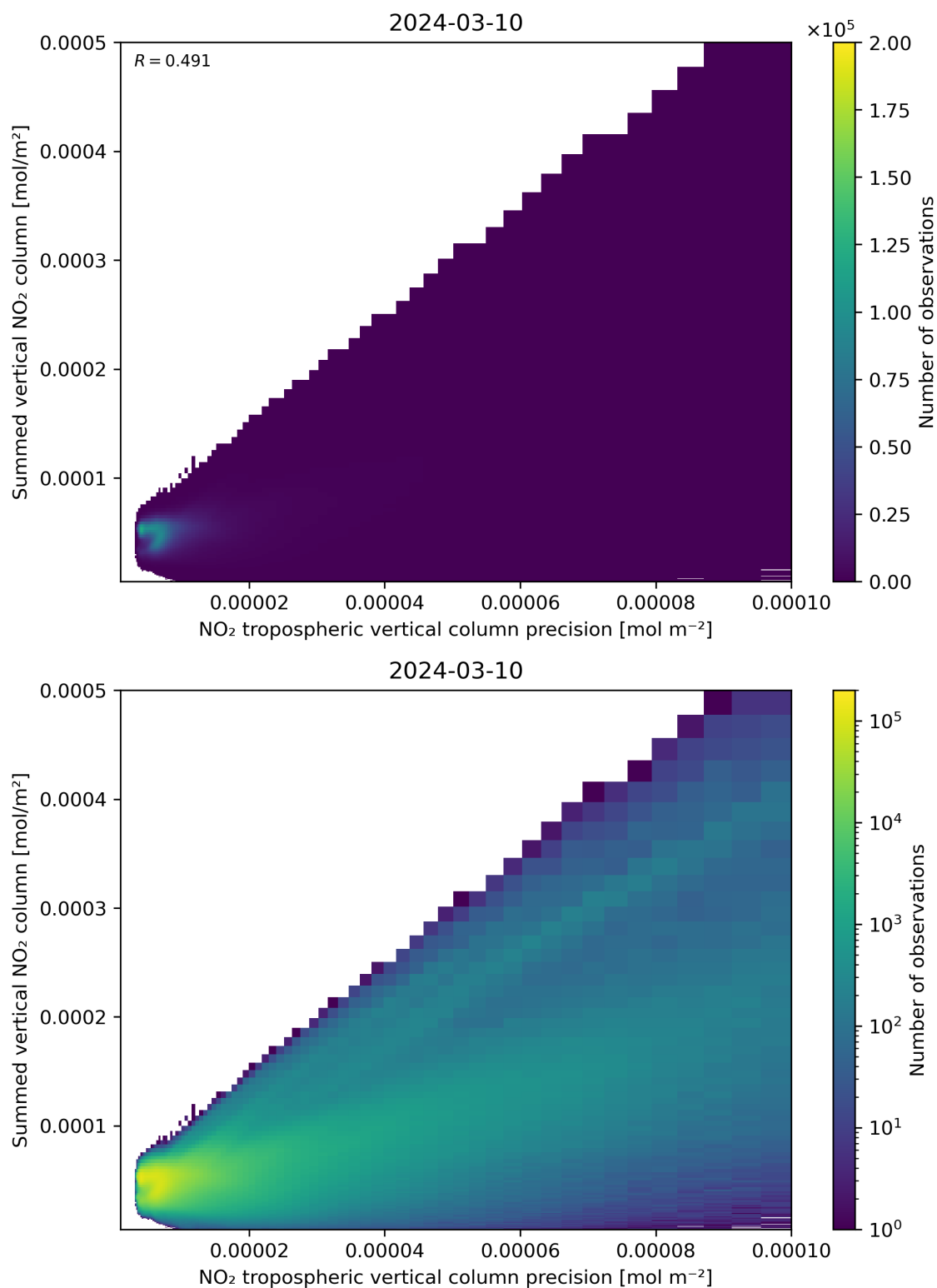
Figure 136: Scatter density plot of “NO 2 tropospheric vertical column precision” against “Summed vertical NO 2 column” for 2024-03-09 to 2024-03-11.
