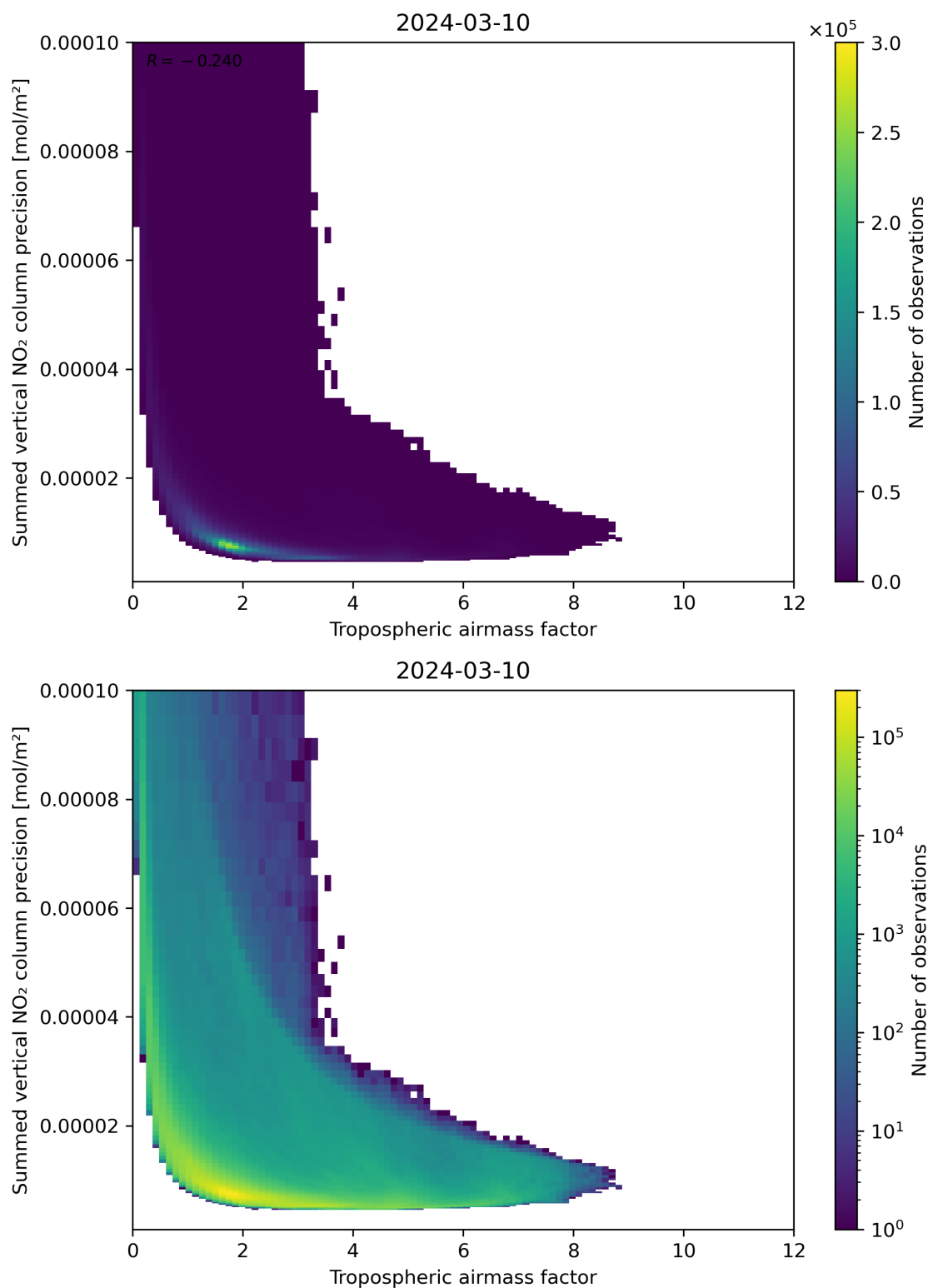
Figure 76: Scatter density plot of “Tropospheric air mass factor” against “Summed vertical NO 2 column precision” for 2024-03-09 to 2024-03-11.
