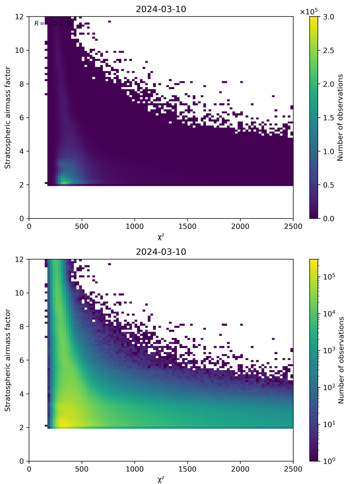
Figure 81: Scatter density plot of “ \chi^2 ” against “Stratospheric airmass factor” for 2024-03-09 to 2024-03-11.
