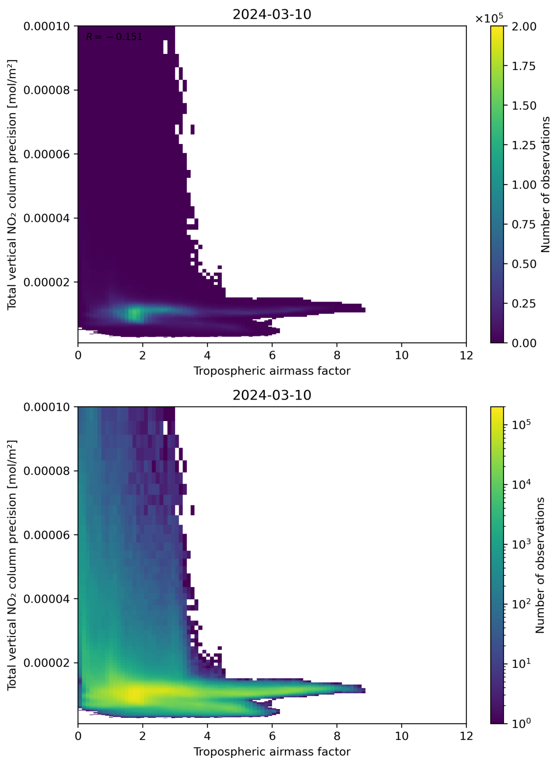
Figure 78: Scatter density plot of “Tropospheric air mass factor” against “Total vertical NO 2 column precision” for 2024-03-09 to 2024-03-11.
