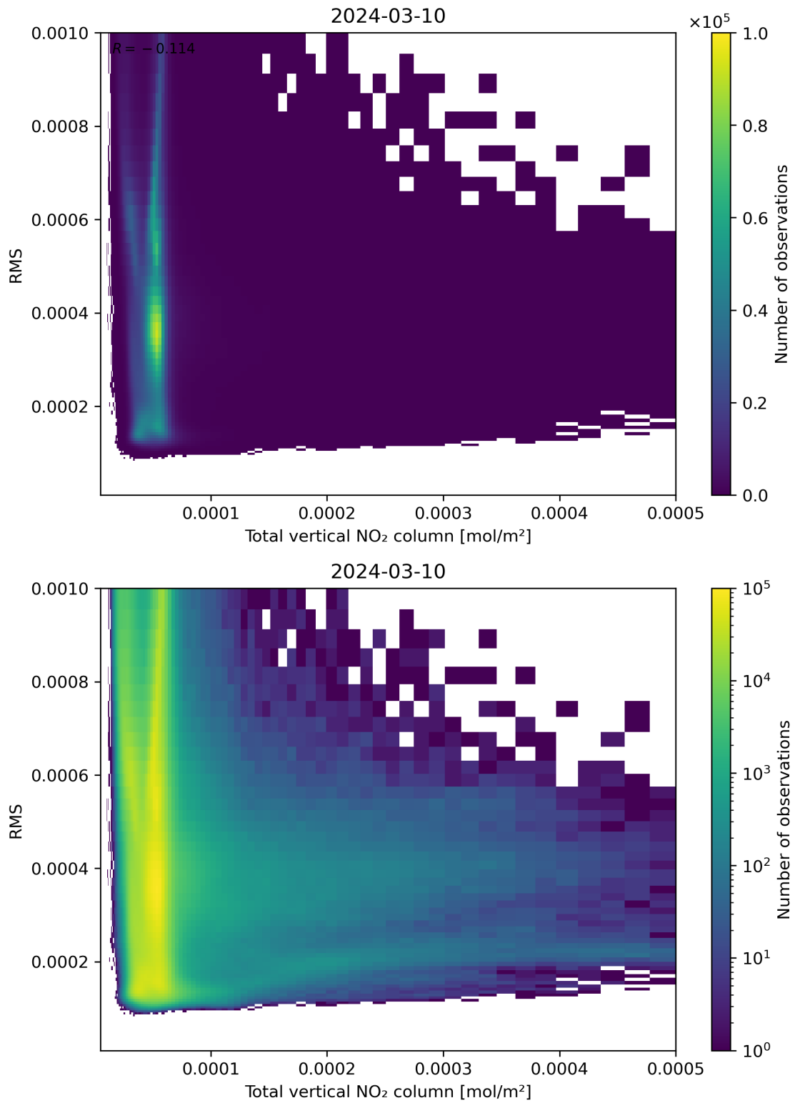
Figure 120: Scatter density plot of “Total vertical NO 2 column” against “RMS” for 2024-03-09 to 2024-03-11.
