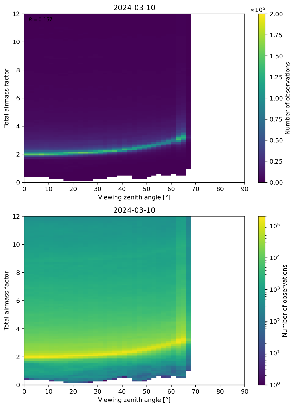
Figure 160: Scatter density plot of “Viewing zenith angle” against “Total airmass factor” for 2024-03-09 to 2024-03-11.
