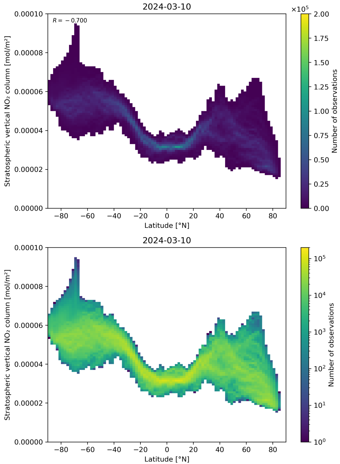
Figure 87: Scatter density plot of “Latitude” against “Stratospheric vertical NO 2 column” for 2024-03-09 to 2024-03-11.
