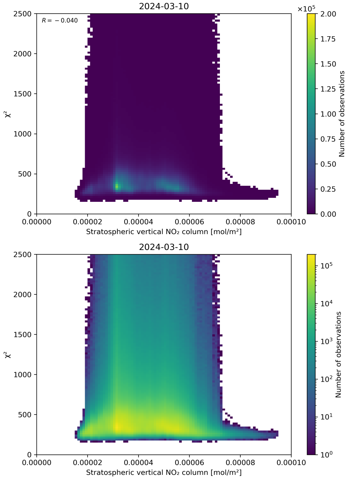
Figure 97: Scatter density plot of “Stratospheric vertical NO 2 column” against “ \chi^2 ” for 2024-03-09 to 2024-03-11.
