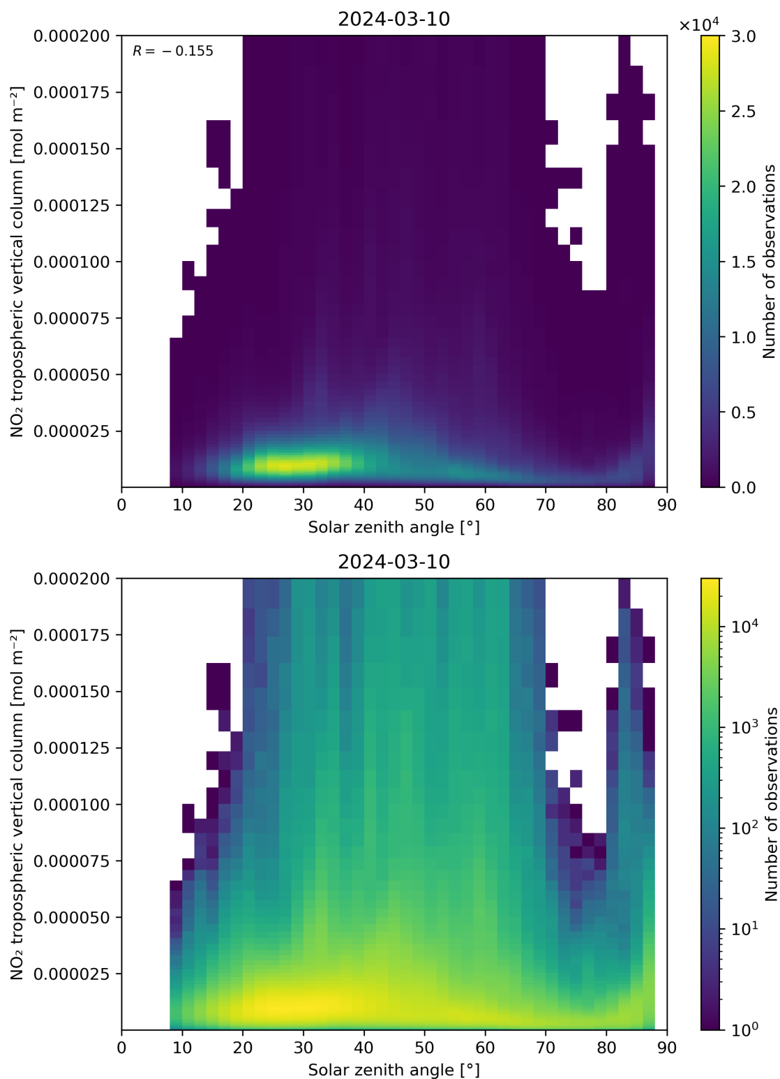
Figure 155: Scatter density plot of “Solar zenith angle” against “NO 2 tropospheric vertical column” for 2024-03-09 to 2024-03-11.
