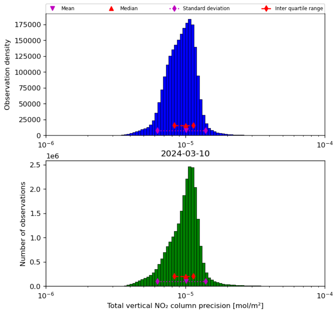
Figure 39: Histogram of "Total vertical NO 2 column precision" for 2024-03-09 to 2024-03-11
