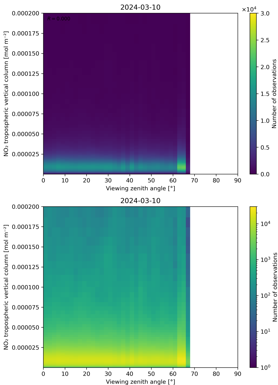
Figure 169: Scatter density plot of “Viewing zenith angle” against “NO 2 tropospheric vertical column” for 2024-03-09 to 2024-03-11.
