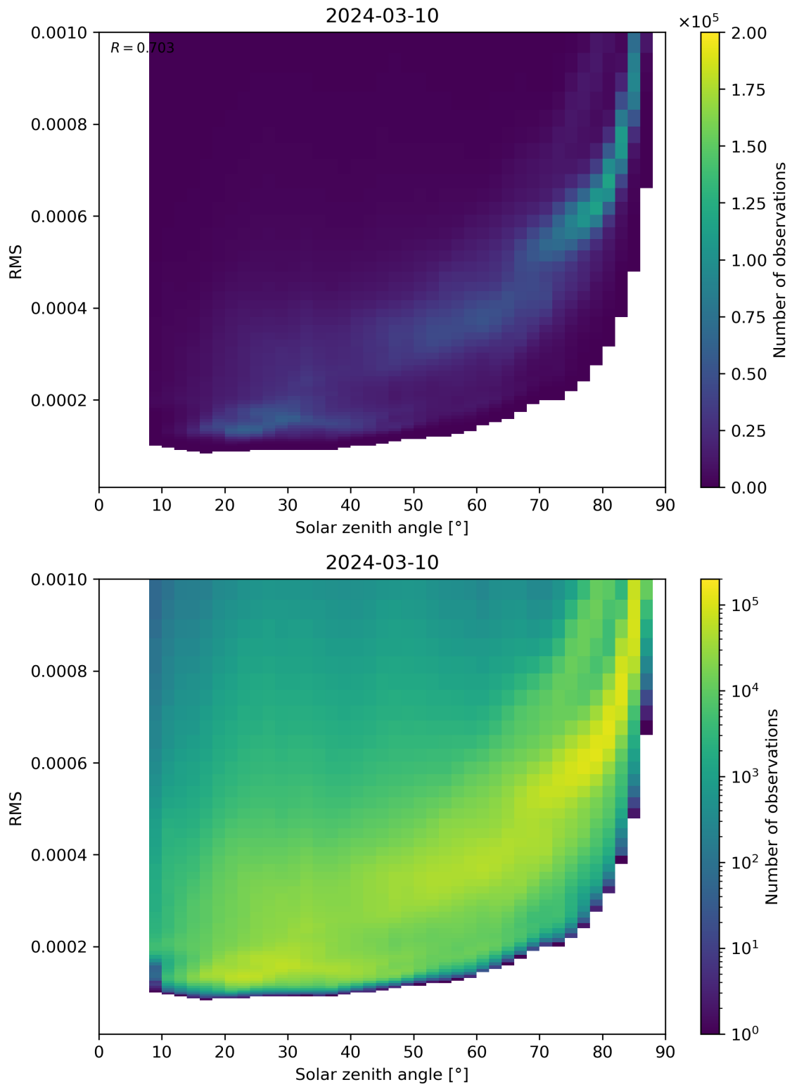
Figure 157: Scatter density plot of “Solar zenith angle” against “RMS” for 2024-03-09 to 2024-03-11.
