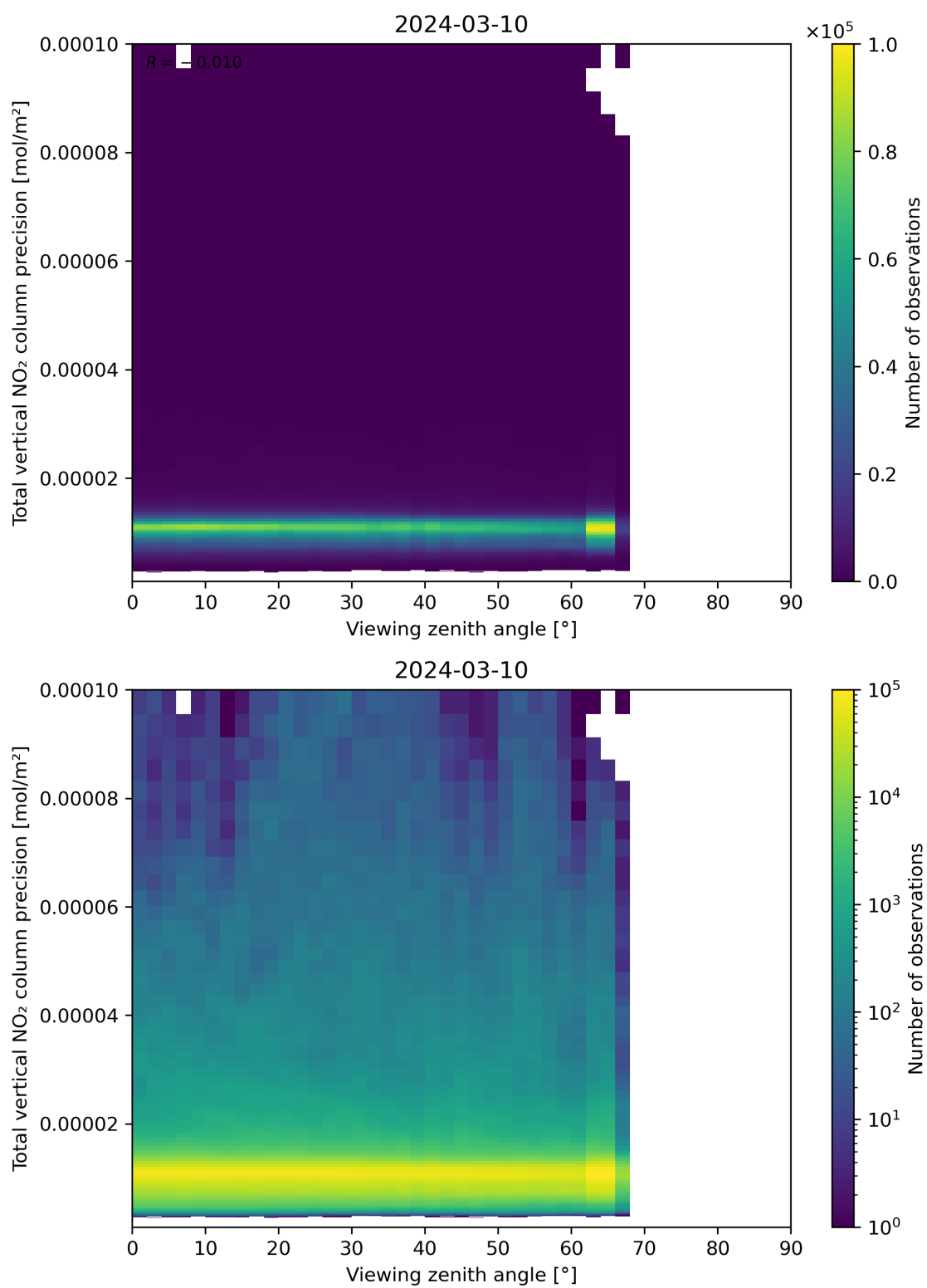
Figure 168: Scatter density plot of “Viewing zenith angle” against “Total vertical NO 2 column precision” for 2024-03-09 to 2024-03-11.
