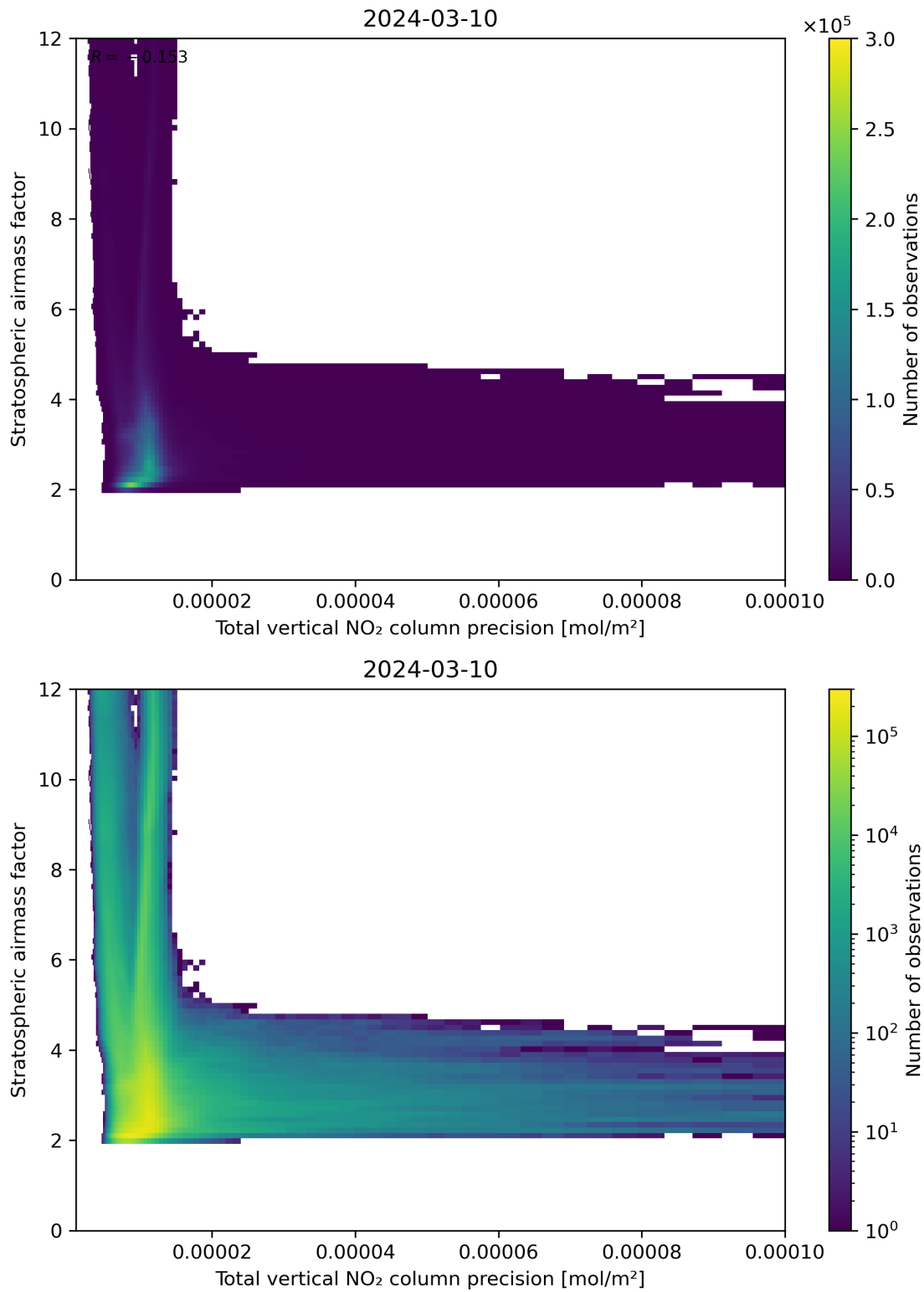
Figure 115: Scatter density plot of “Total vertical NO 2 column precision” against “Stratospheric airmass factor” for 2024-03-09 to 2024-03-11.
