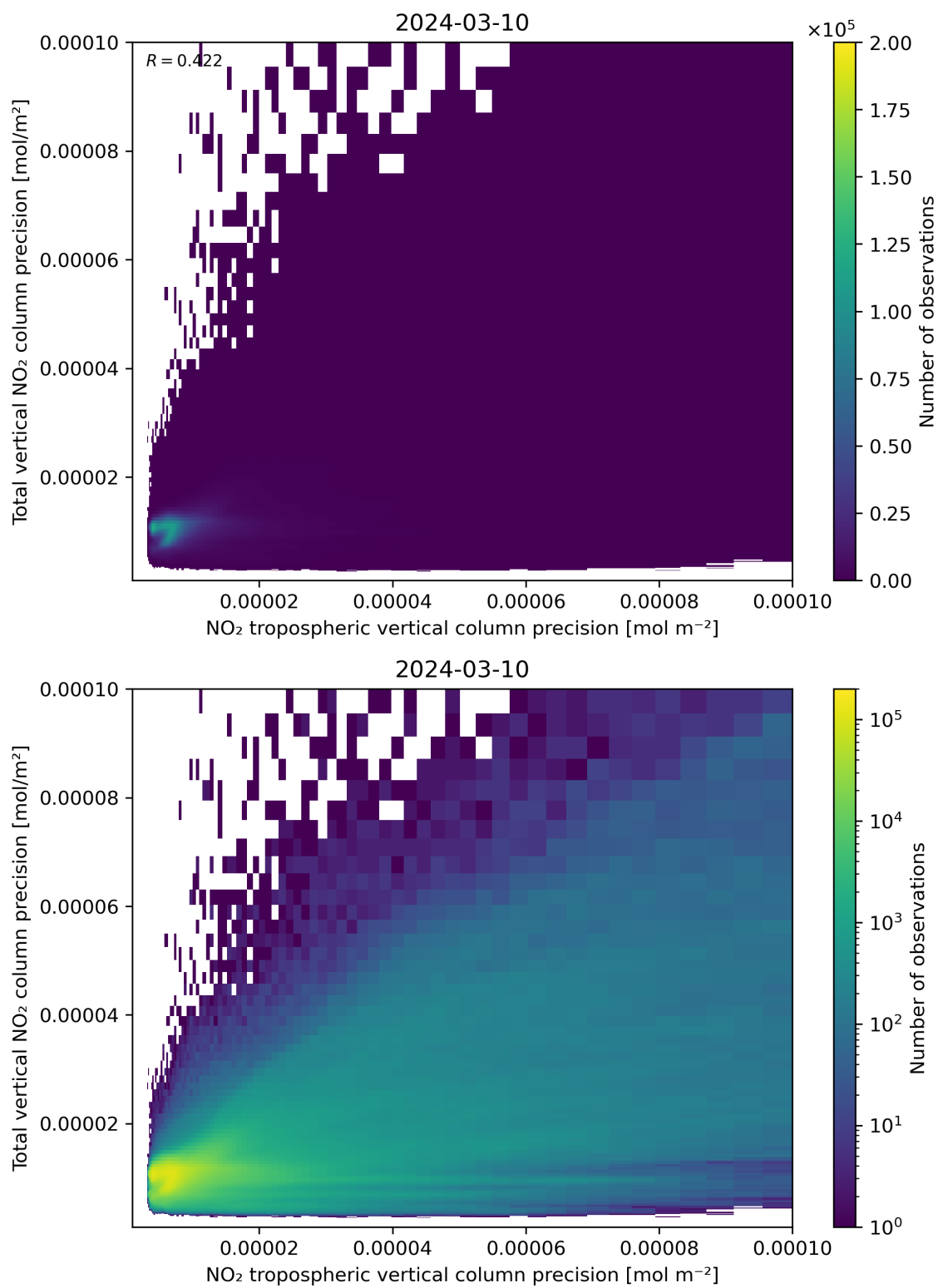
Figure 139: Scatter density plot of “NO 2 tropospheric vertical column precision” against “Total vertical NO 2 column precision” for 2024-03-09 to 2024-03-11.
