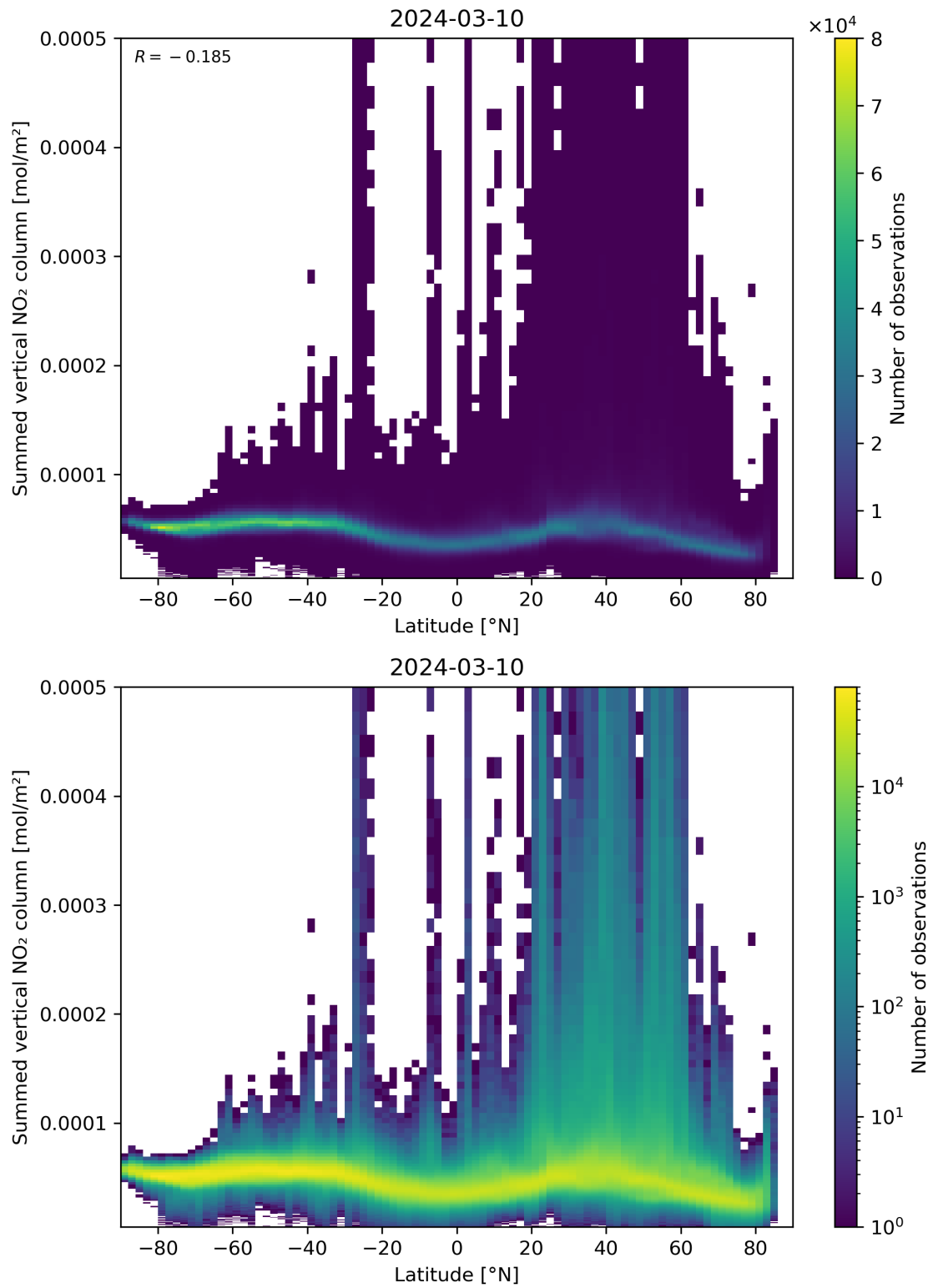
Figure 88: Scatter density plot of “Latitude” against “Summed vertical NO 2 column” for 2024-03-09 to 2024-03-11.
