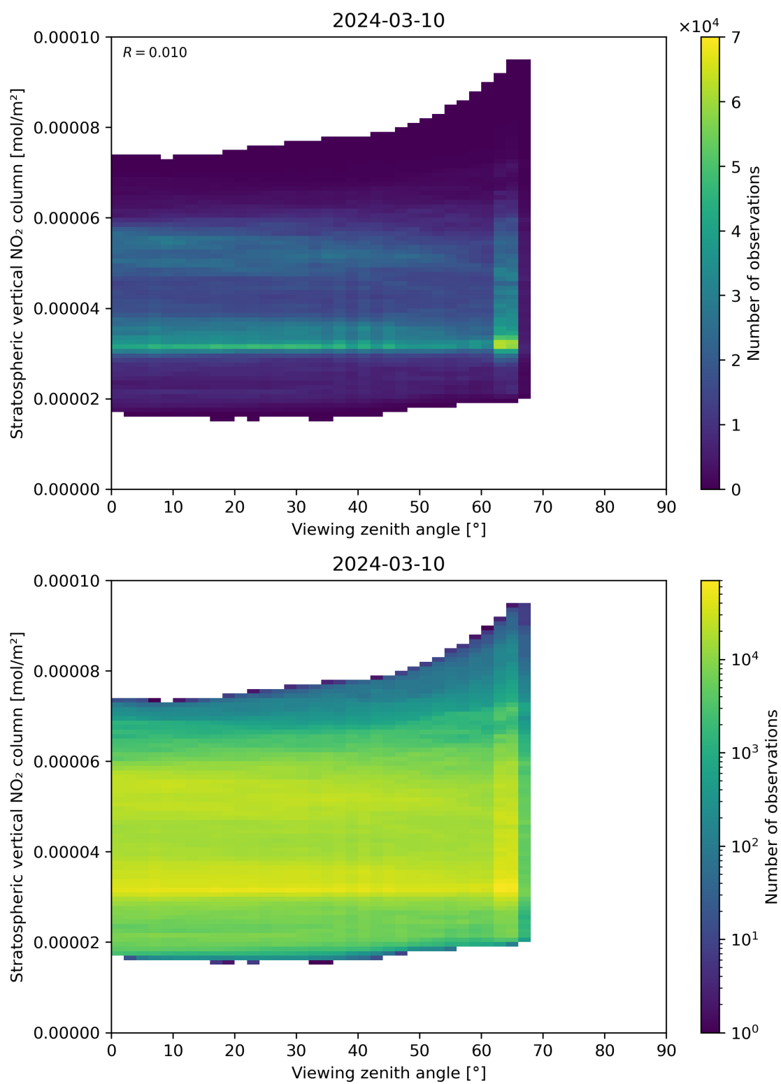
Figure 164: Scatter density plot of “Viewing zenith angle” against “Stratospheric vertical NO 2 column” for 2024-03-09 to 2024-03-11.
