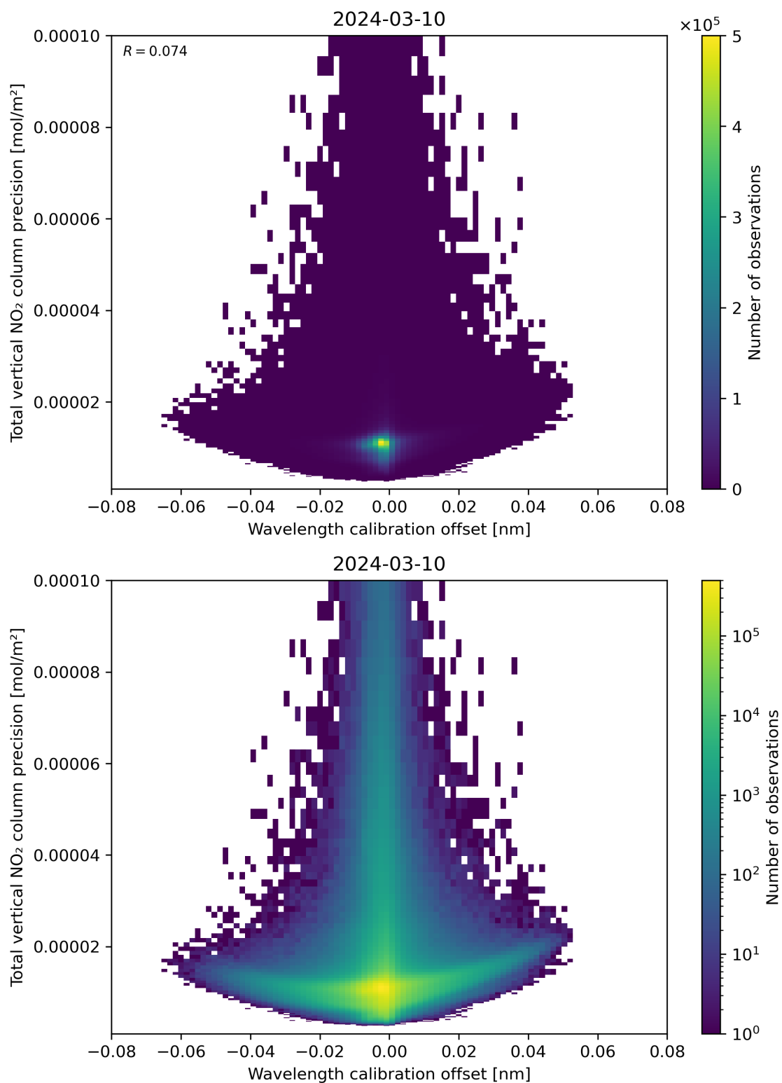
Figure 180: Scatter density plot of “Wavelength calibration offset” against “Total vertical NO 2 column precision” for 2024-03-09 to 2024-03-11.
