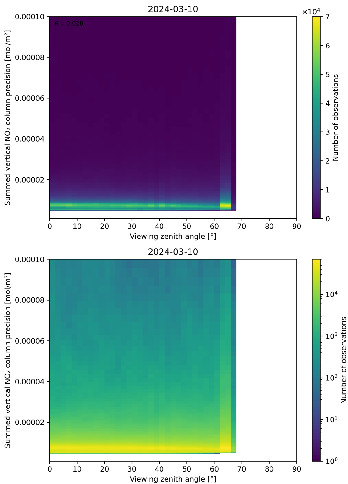
Figure 166: Scatter density plot of “Viewing zenith angle” against “Summed vertical NO 2 column precision” for 2024-03-09 to 2024-03-11.
