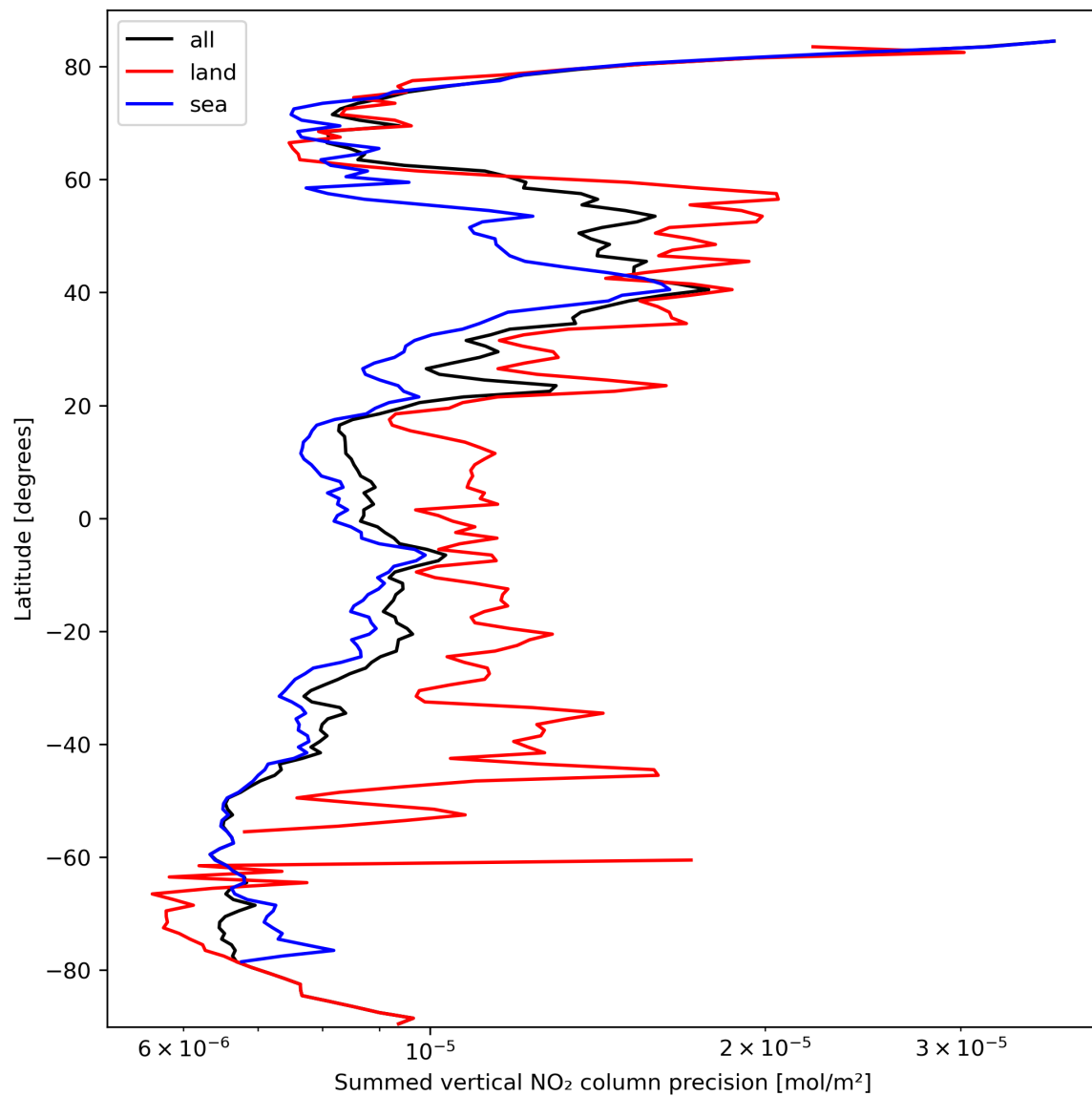
Figure 24: Zonal average of “Summed vertical NO 2 column precision” for 2024-03-09 to 2024-03-11.
