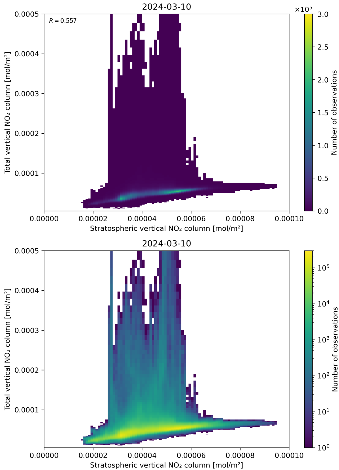
Figure 100: Scatter density plot of “Stratospheric vertical NO 2 column” against “Total vertical NO 2 column” for 2024-03-09 to 2024-03-11.
