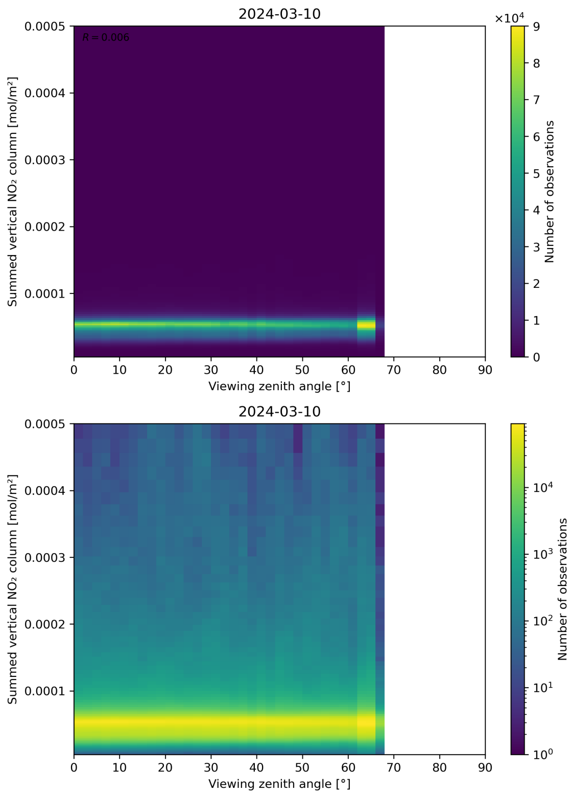
Figure 165: Scatter density plot of “Viewing zenith angle” against “Summed vertical NO 2 column” for 2024-03-09 to 2024-03-11.
