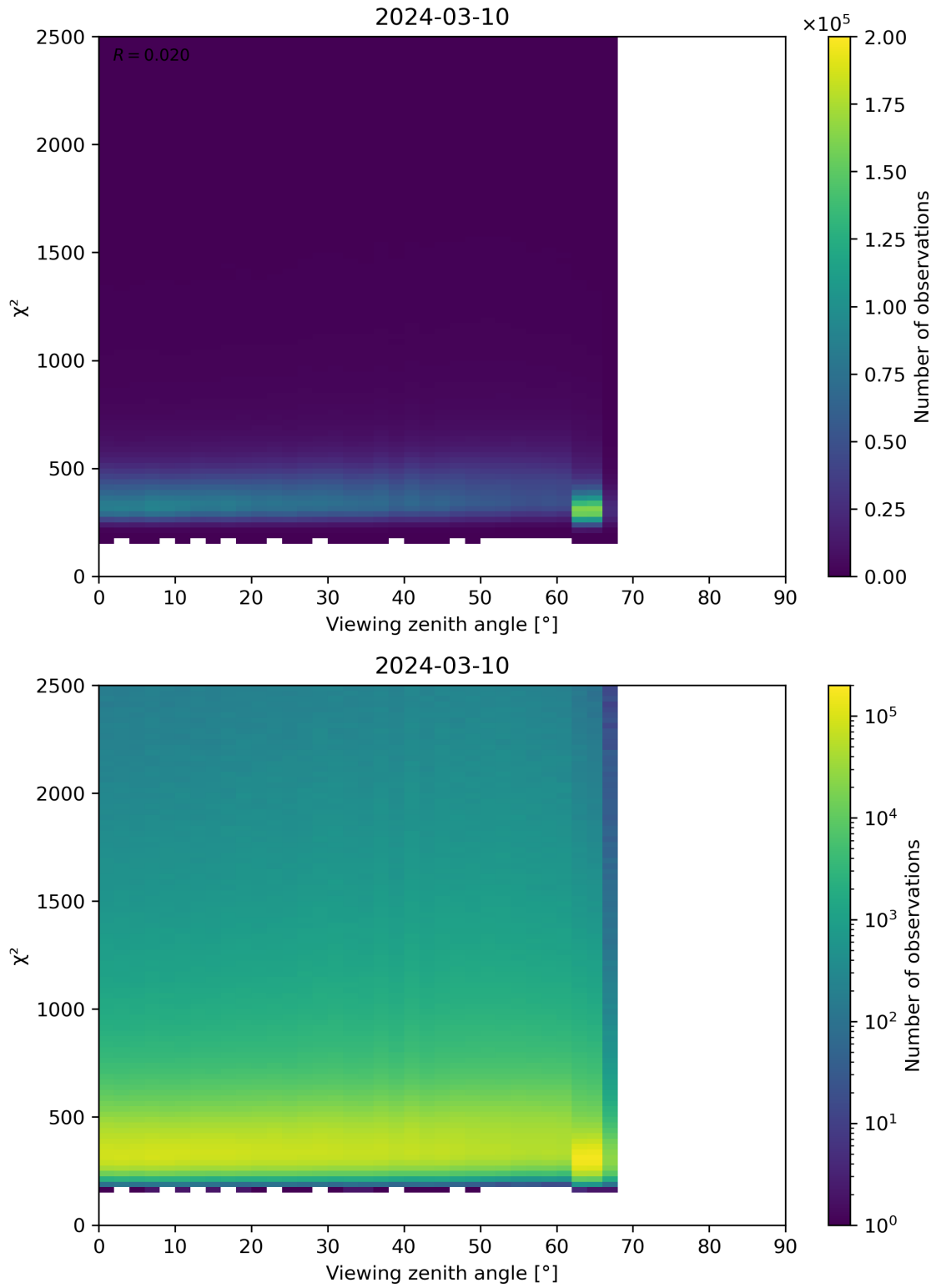
Figure 162: Scatter density plot of “Viewing zenith angle” against “ \chi^2 ” for 2024-03-09 to 2024-03-11.
