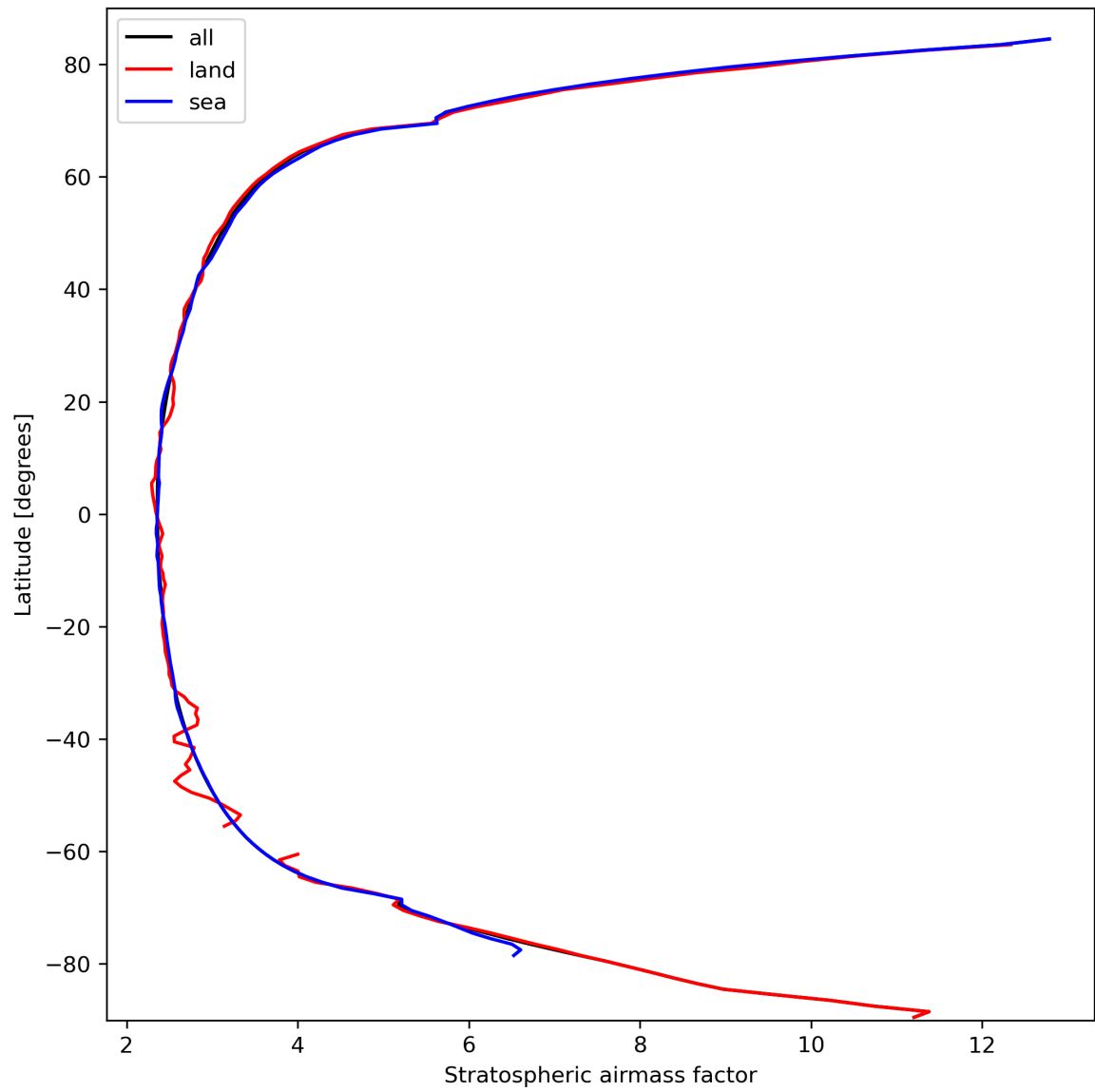
Figure 27: Zonal average of “Stratospheric air mass factor” for 2024-03-09 to 2024-03-11.
