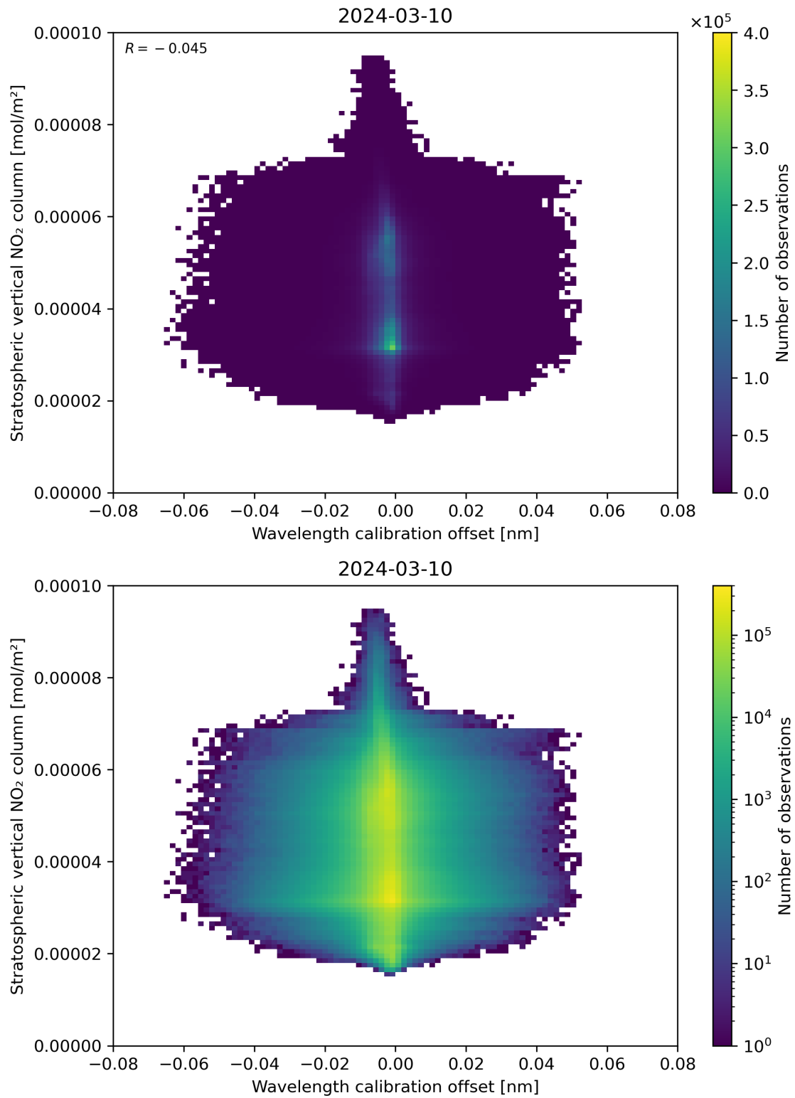
Figure 176: Scatter density plot of “Wavelength calibration offset” against “Stratospheric vertical NO 2 column” for 2024-03-09 to 2024-03-11.
