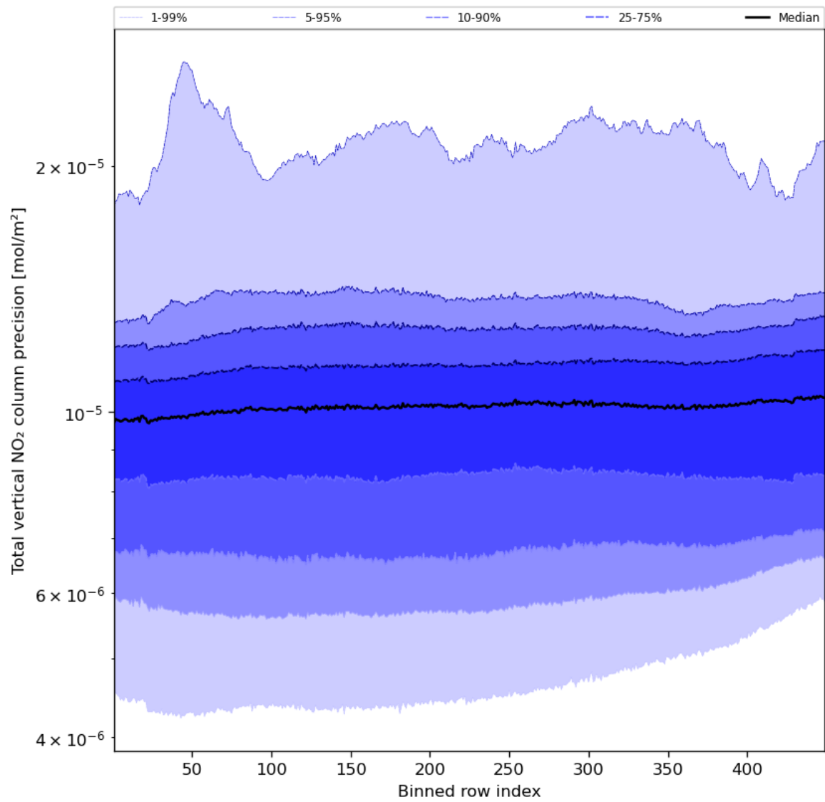
Figure 56: Along track statistics of “Total vertical NO 2 column precision” for 2024-03-09 to 2024-03-11
