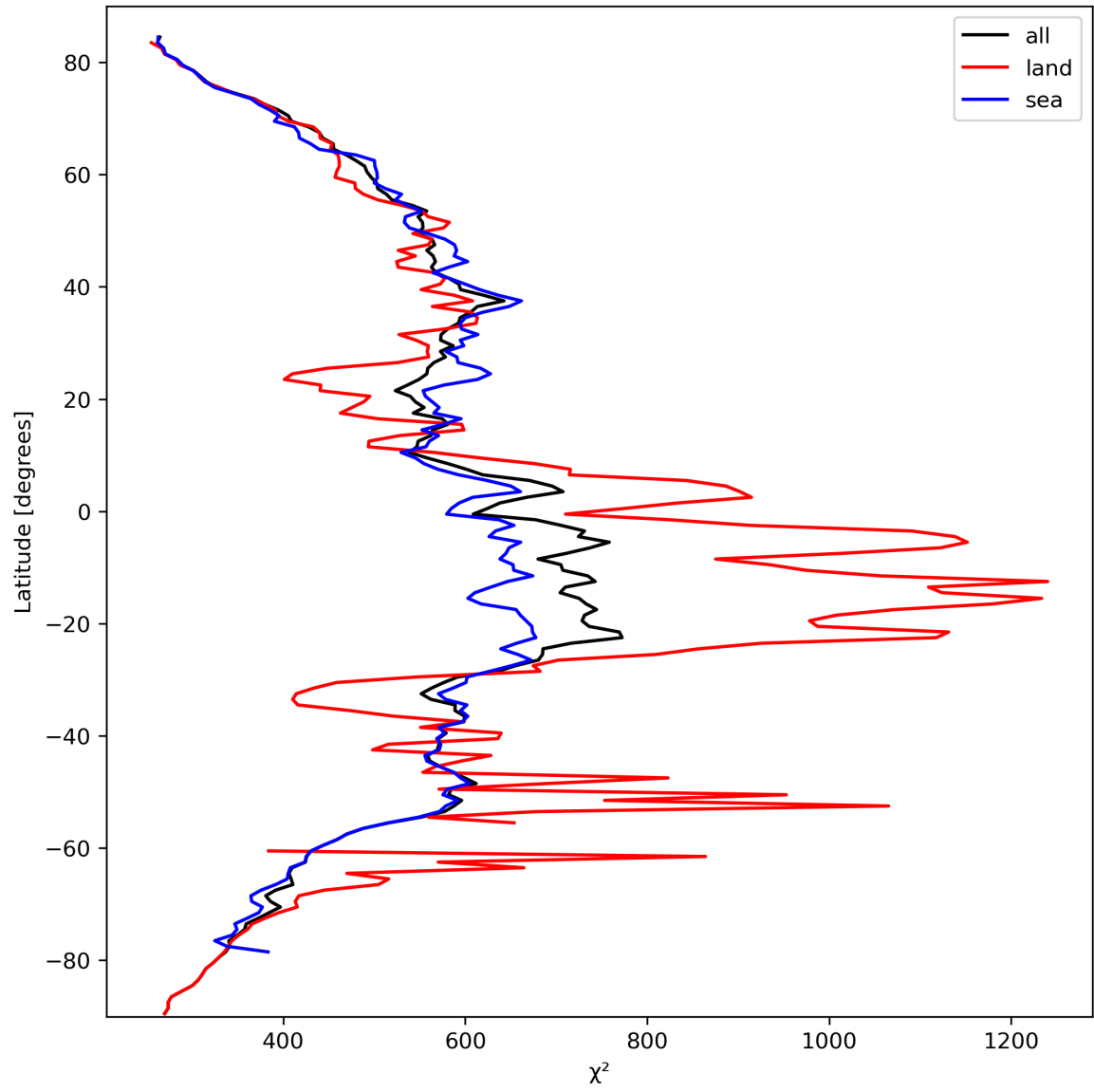
Figure 25: Zonal average of “ \chi^2 ” for 2024-03-09 to 2024-03-11.
