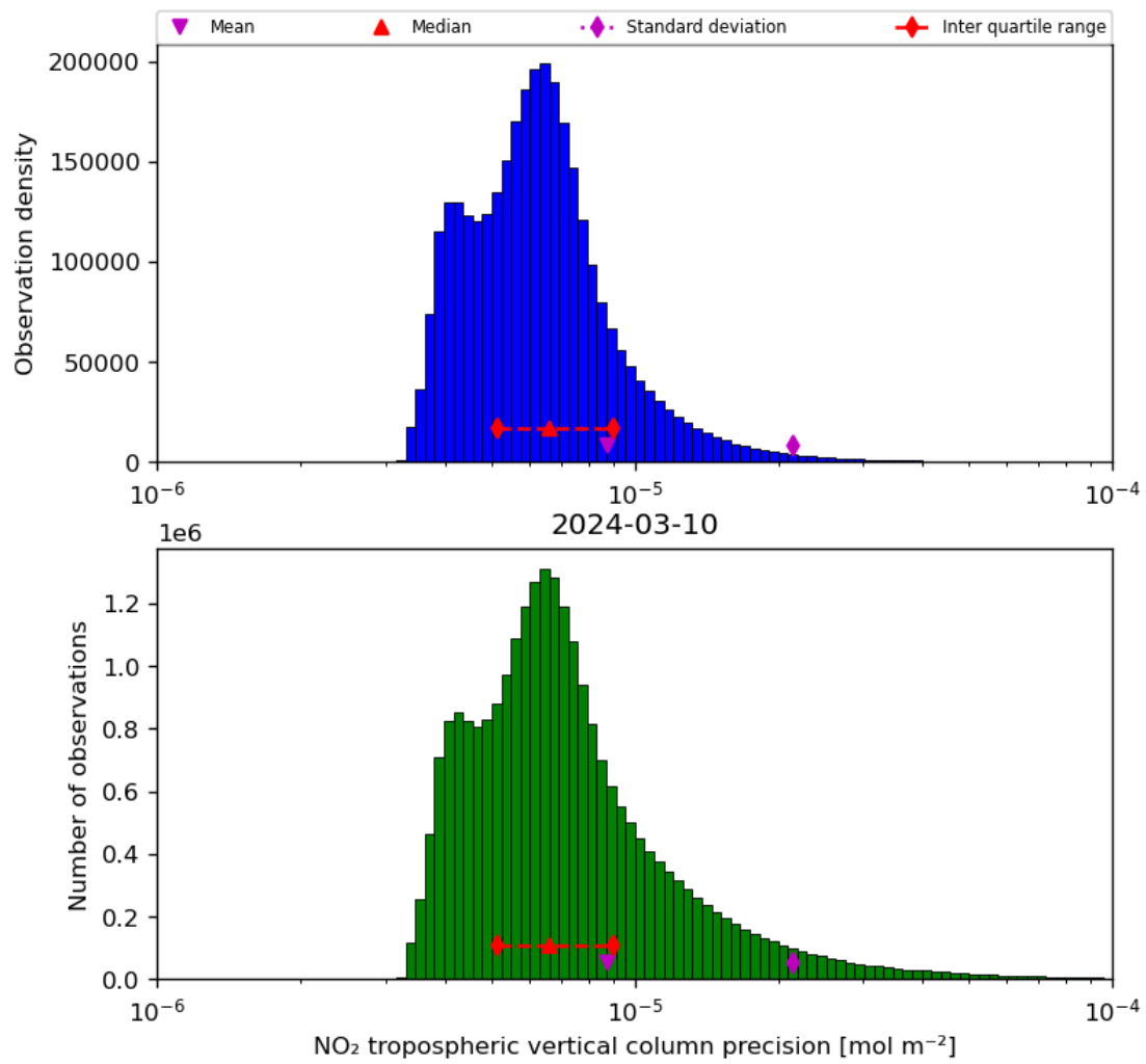
Figure 30: Histogram of “NO 2 tropospheric vertical column precision” for 2024-03-09 to 2024-03-11
