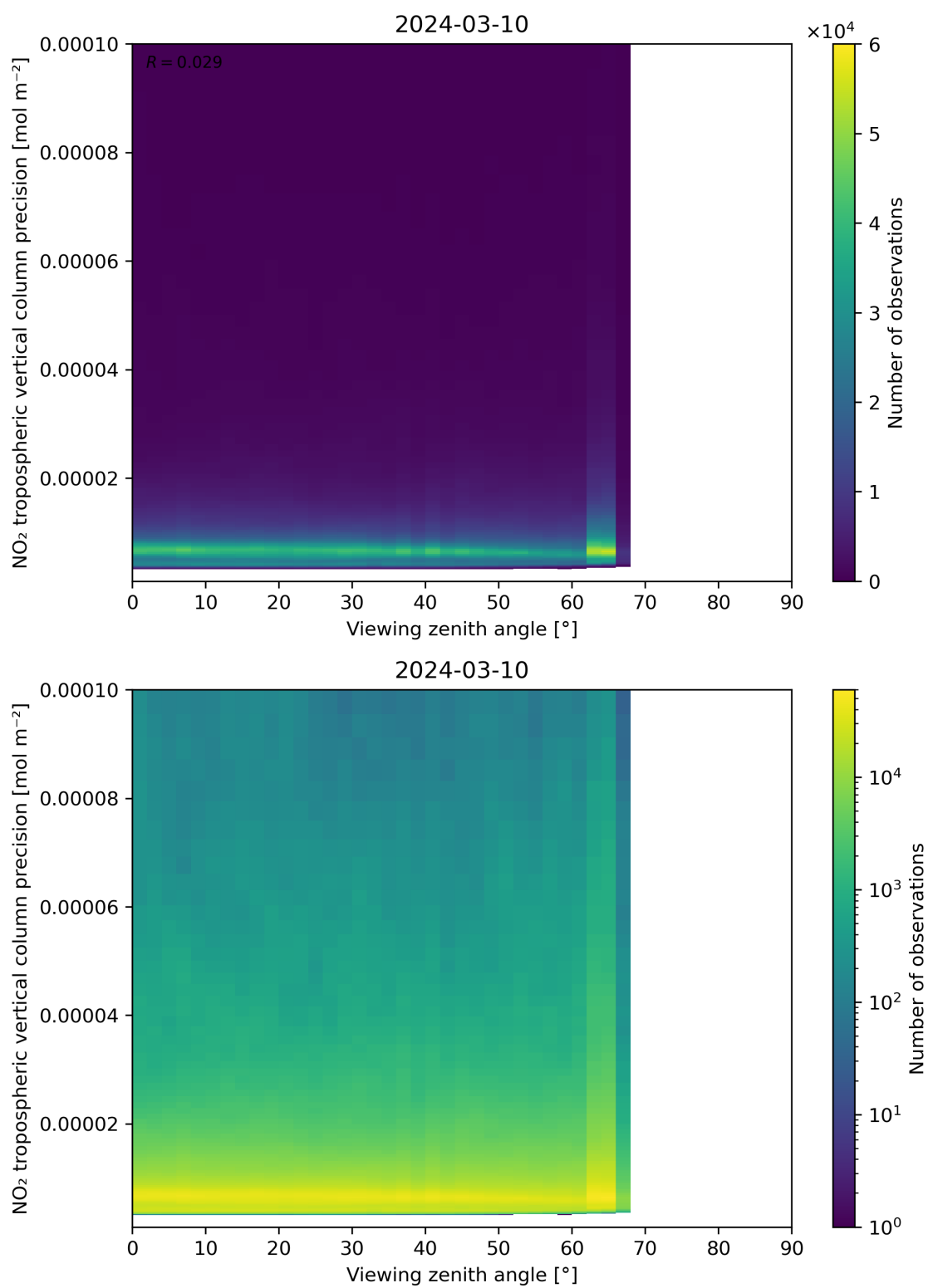
Figure 170: Scatter density plot of “Viewing zenith angle” against “NO 2 tropospheric vertical column precision” for 2024-03-09 to 2024-03-11.
