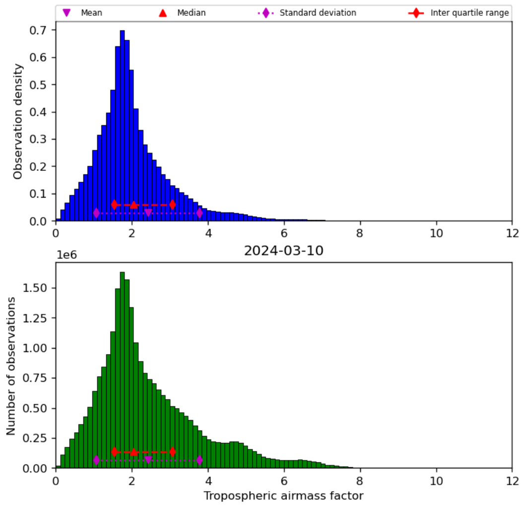
Figure 31: Histogram of “Tropospheric airmass factor” for 2024-03-09 to 2024-03-11
