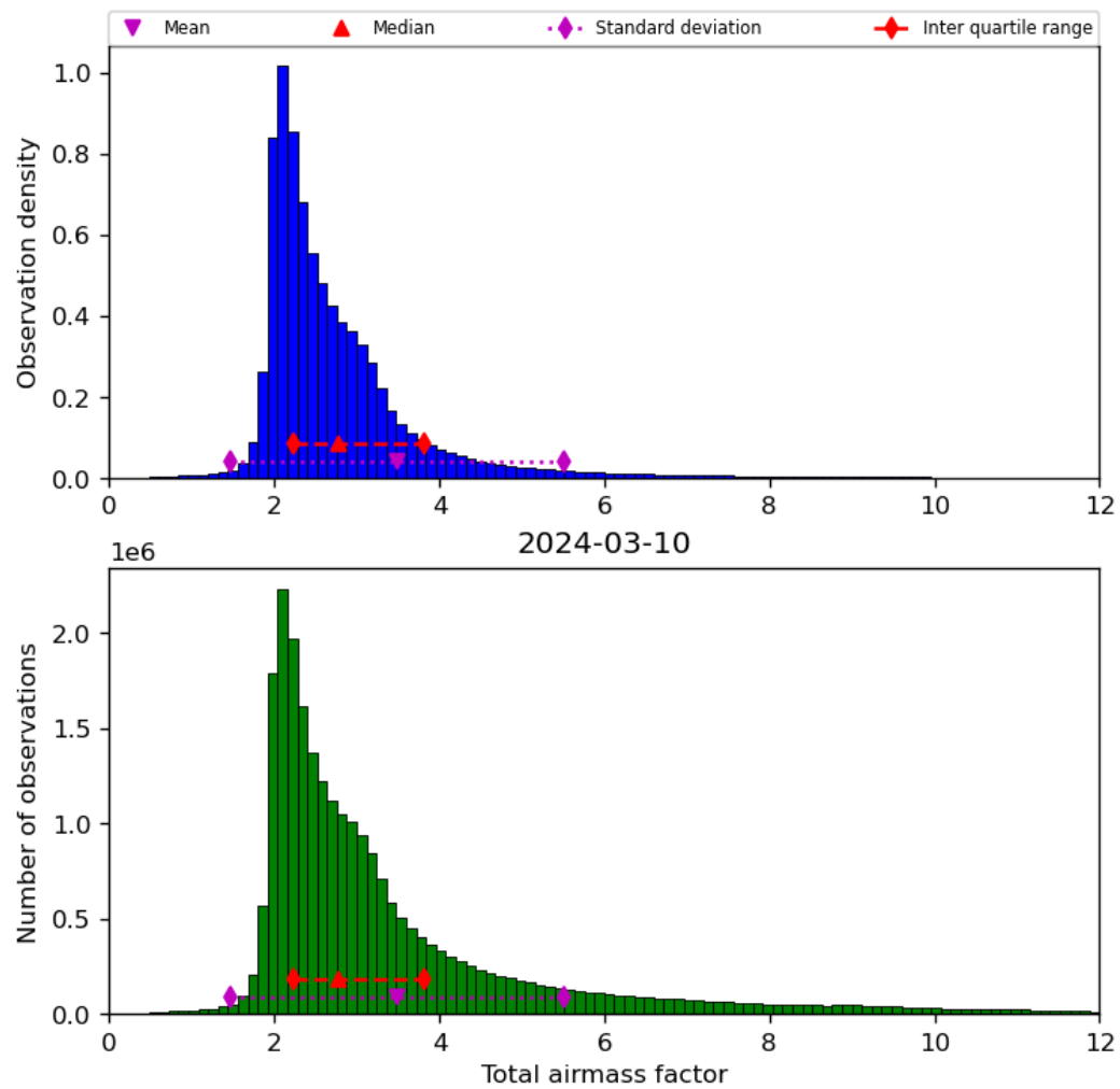
Figure 32: Histogram of “Total airmass factor” for 2024-03-09 to 2024-03-11
