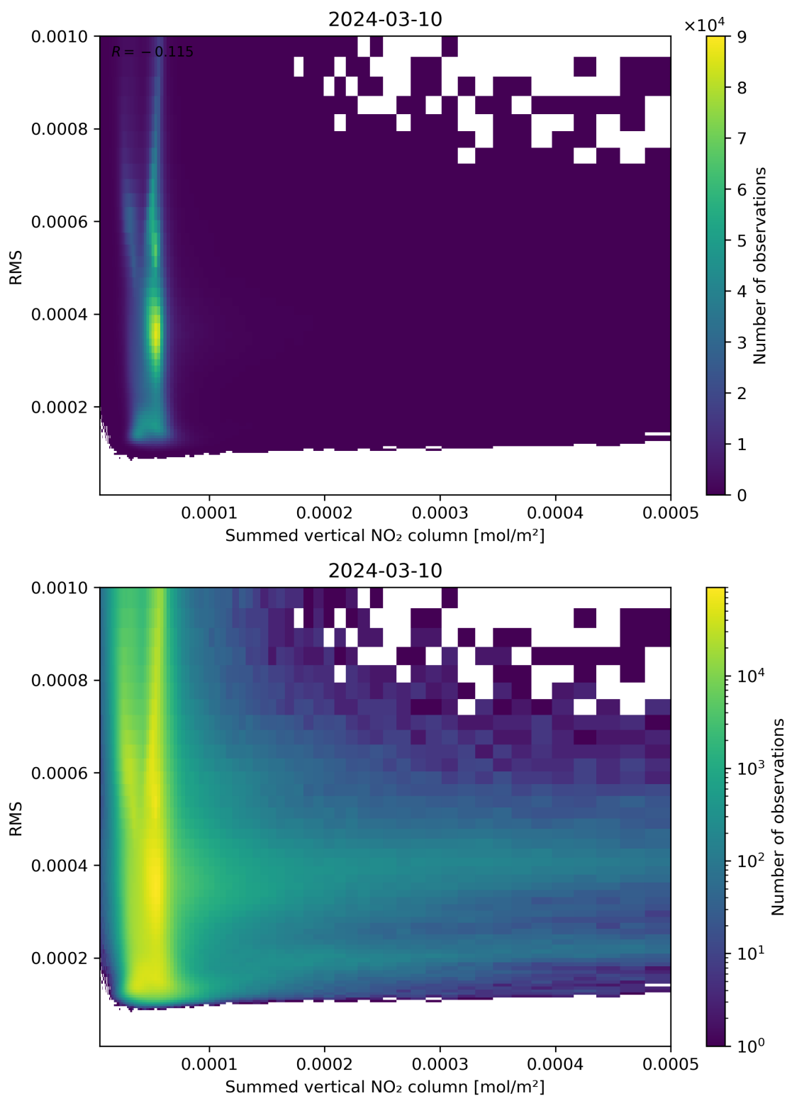
Figure 109: Scatter density plot of “Summed vertical NO 2 column” against “RMS” for 2024-03-09 to 2024-03-11.
