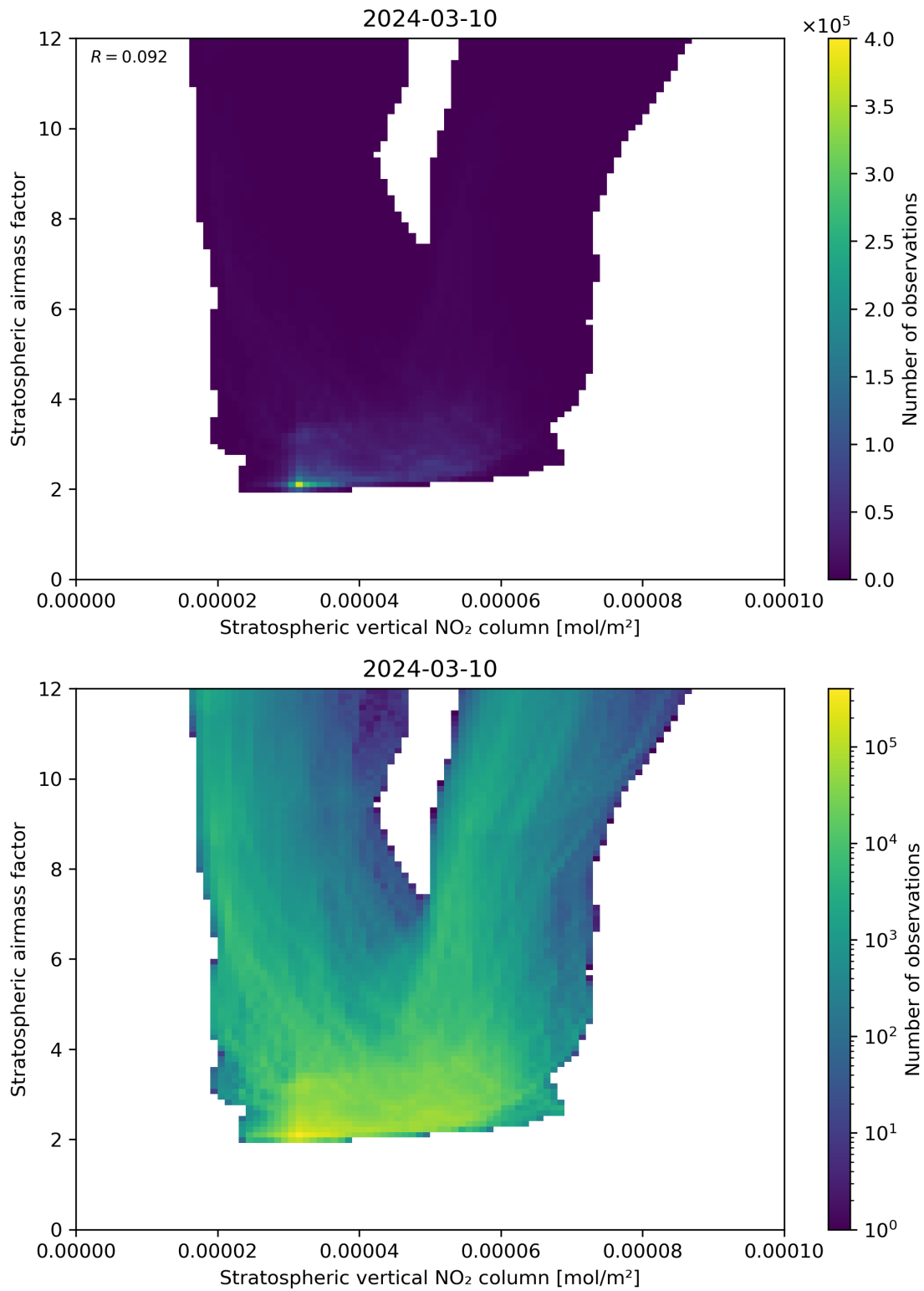
Figure 96: Scatter density plot of “Stratospheric vertical NO 2 column” against “Stratospheric airmass factor” for 2024-03-09 to 2024-03-11.
