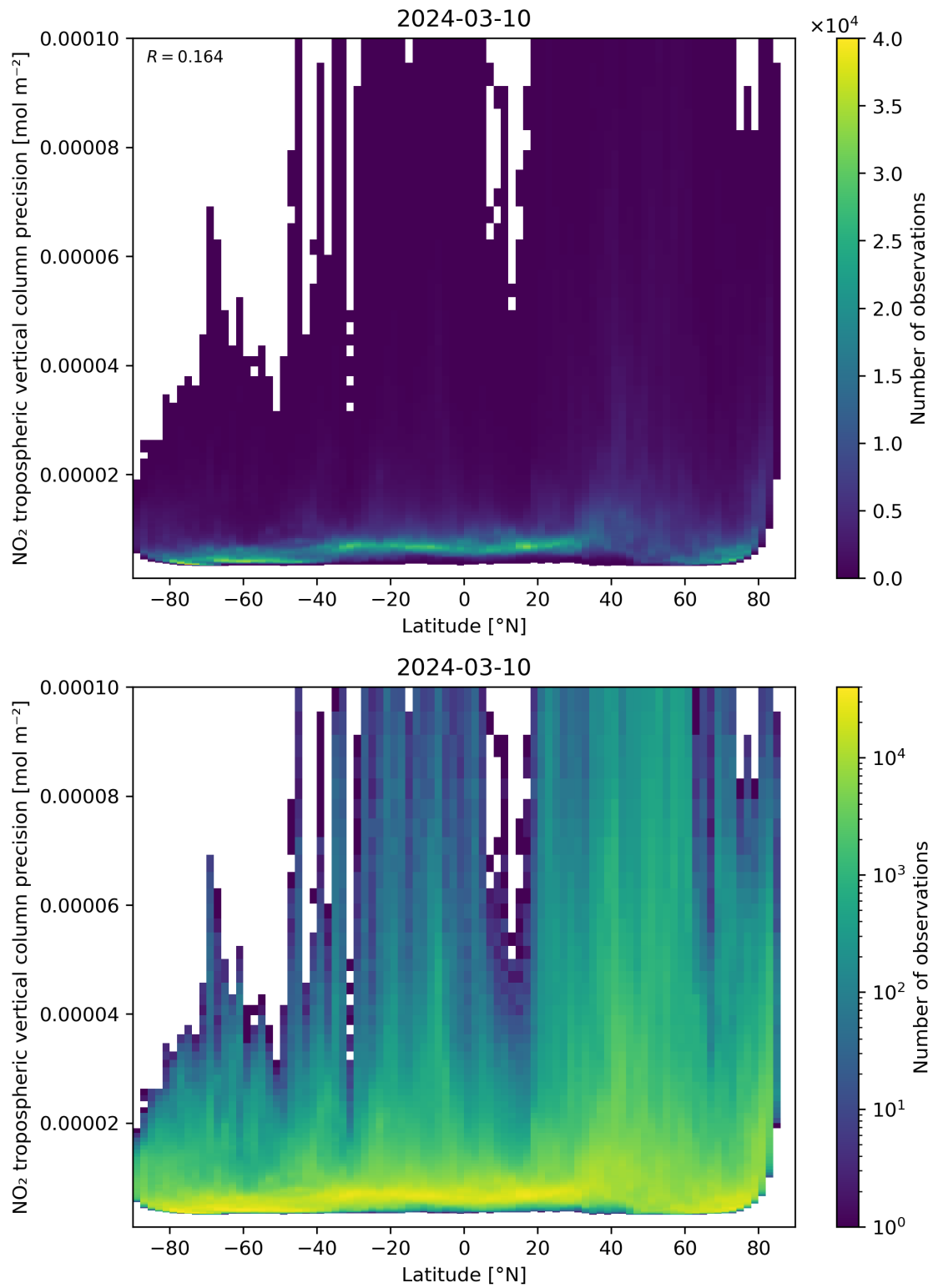
Figure 93: Scatter density plot of “Latitude” against “NO 2 tropospheric vertical column precision” for 2024-03-09 to 2024-03-11.
