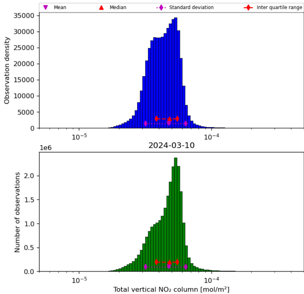
Figure 38: Histogram of “Total vertical NO 2 column” for 2024-03-09 to 2024-03-11
