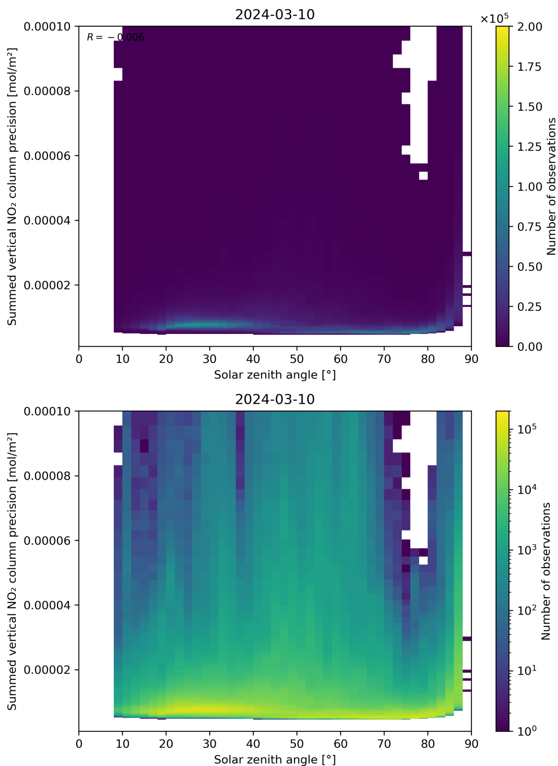
Figure 152: Scatter density plot of “Solar zenith angle” against “Summed vertical NO 2 column precision” for 2024-03-09 to 2024-03-11.
