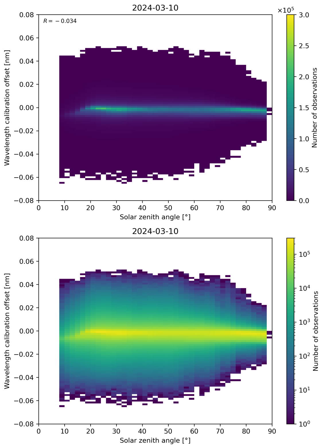
Figure 158: Scatter density plot of “Solar zenith angle” against “Wavelength calibration offset” for 2024-03-09 to 2024-03-11.
