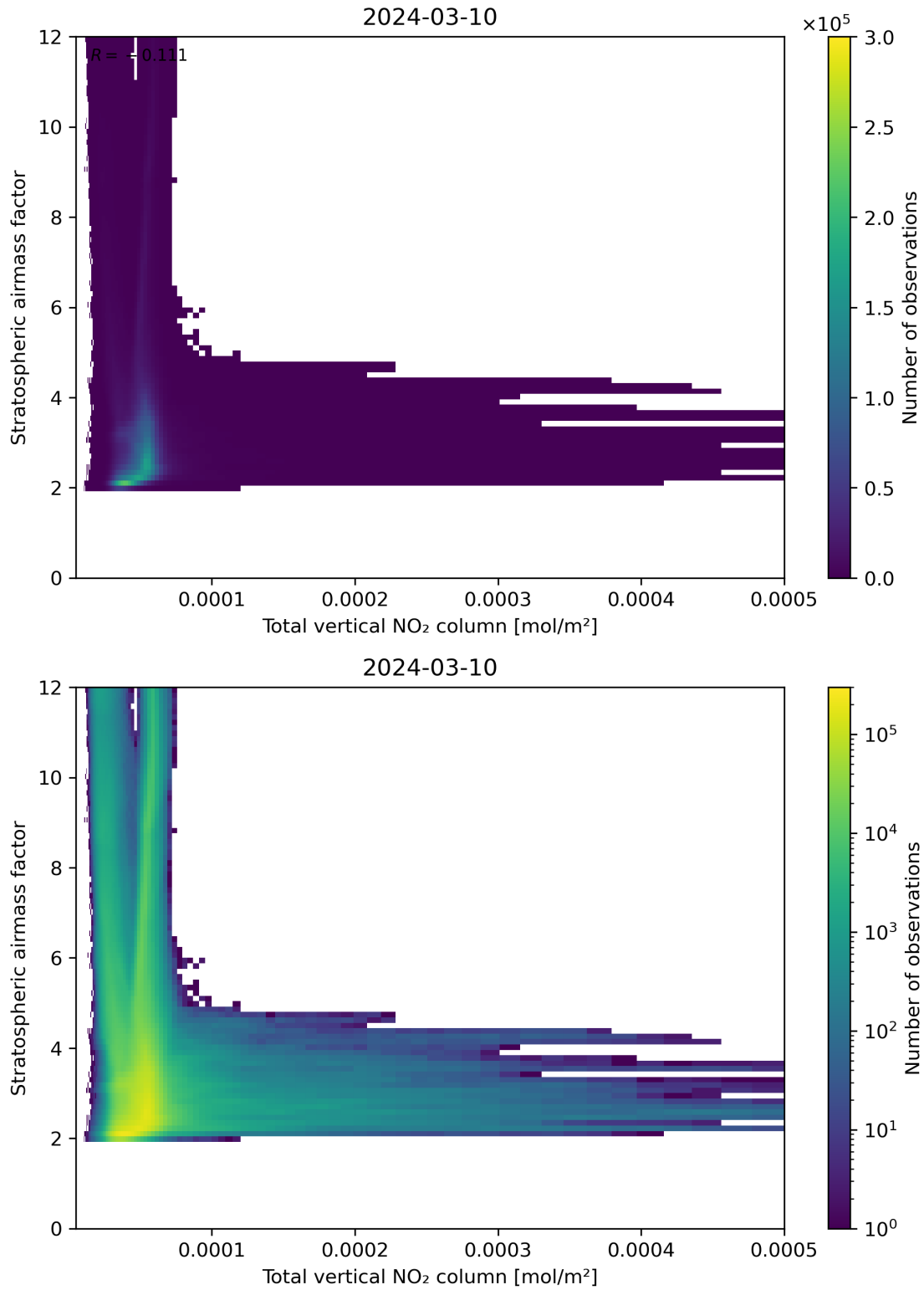
Figure 110: Scatter density plot of “Total vertical NO 2 column” against “Stratospheric airmass factor” for 2024-03-09 to 2024-03-11.
