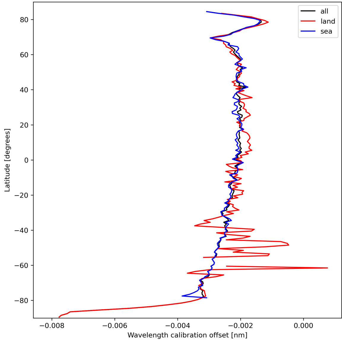
Figure 18: Zonal average of “Wavelength calibration offset” for 2024-03-09 to 2024-03-11.
