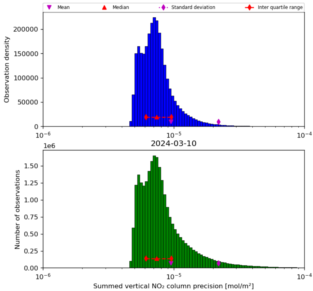
Figure 41: Histogram of “Summed vertical NO 2 column precision” for 2024-03-09 to 2024-03-11
