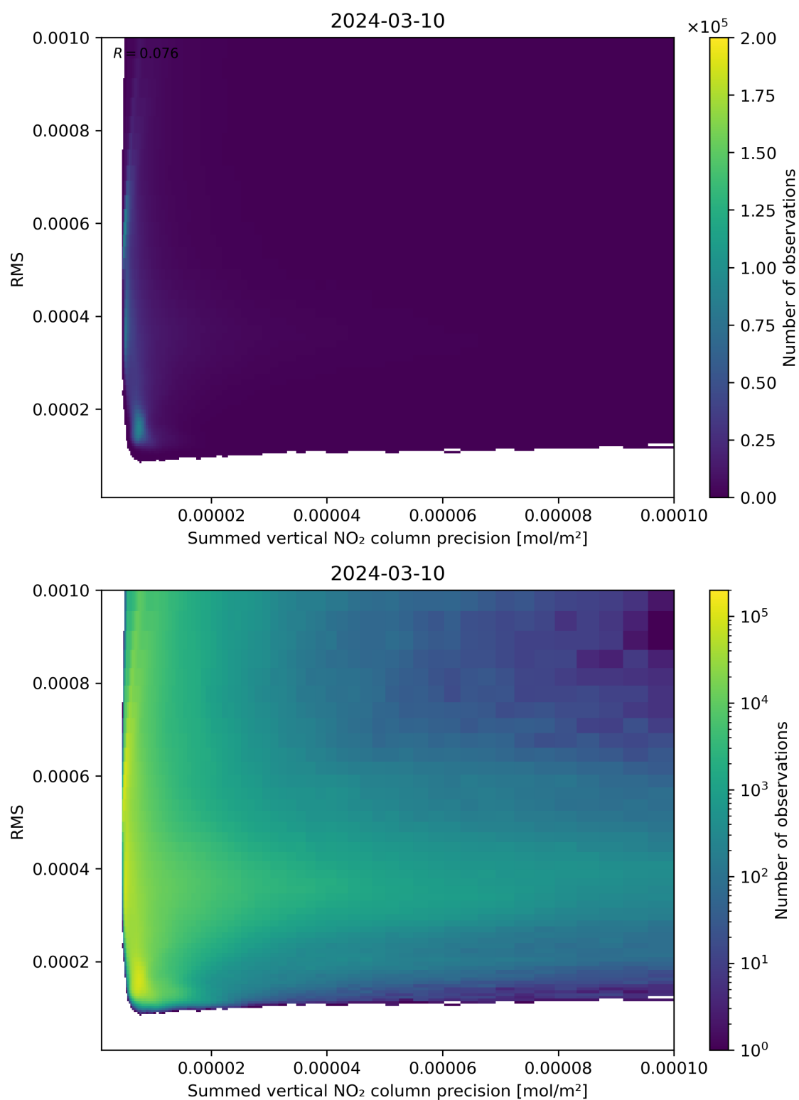
Figure 108: Scatter density plot of “Summed vertical NO 2 column precision” against “RMS” for 2024-03-09 to 2024-03-11.
