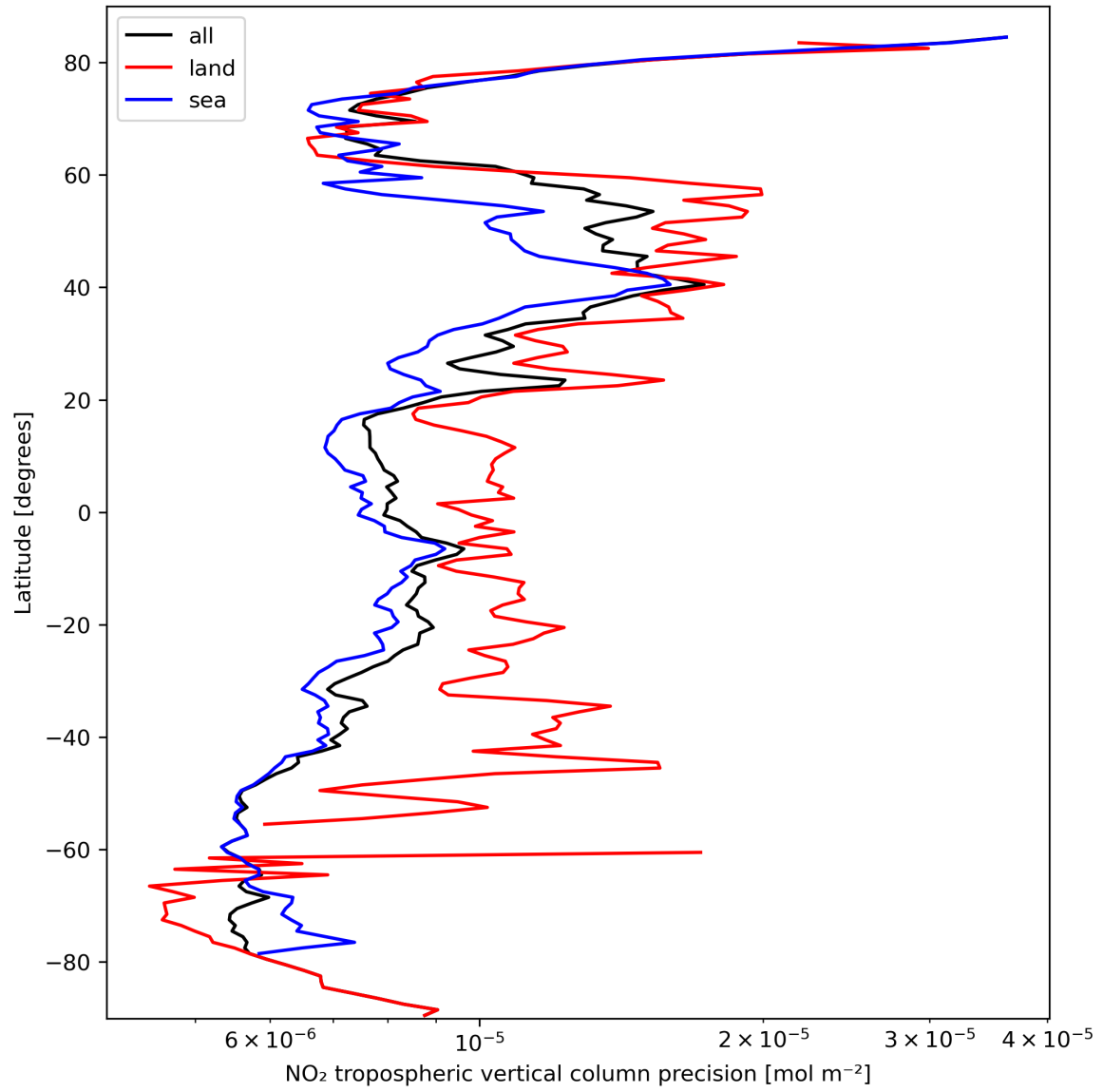
Figure 13: Zonal average of “NO 2 tropospheric vertical column precision” for 2024-03-09 to 2024-03-11.
