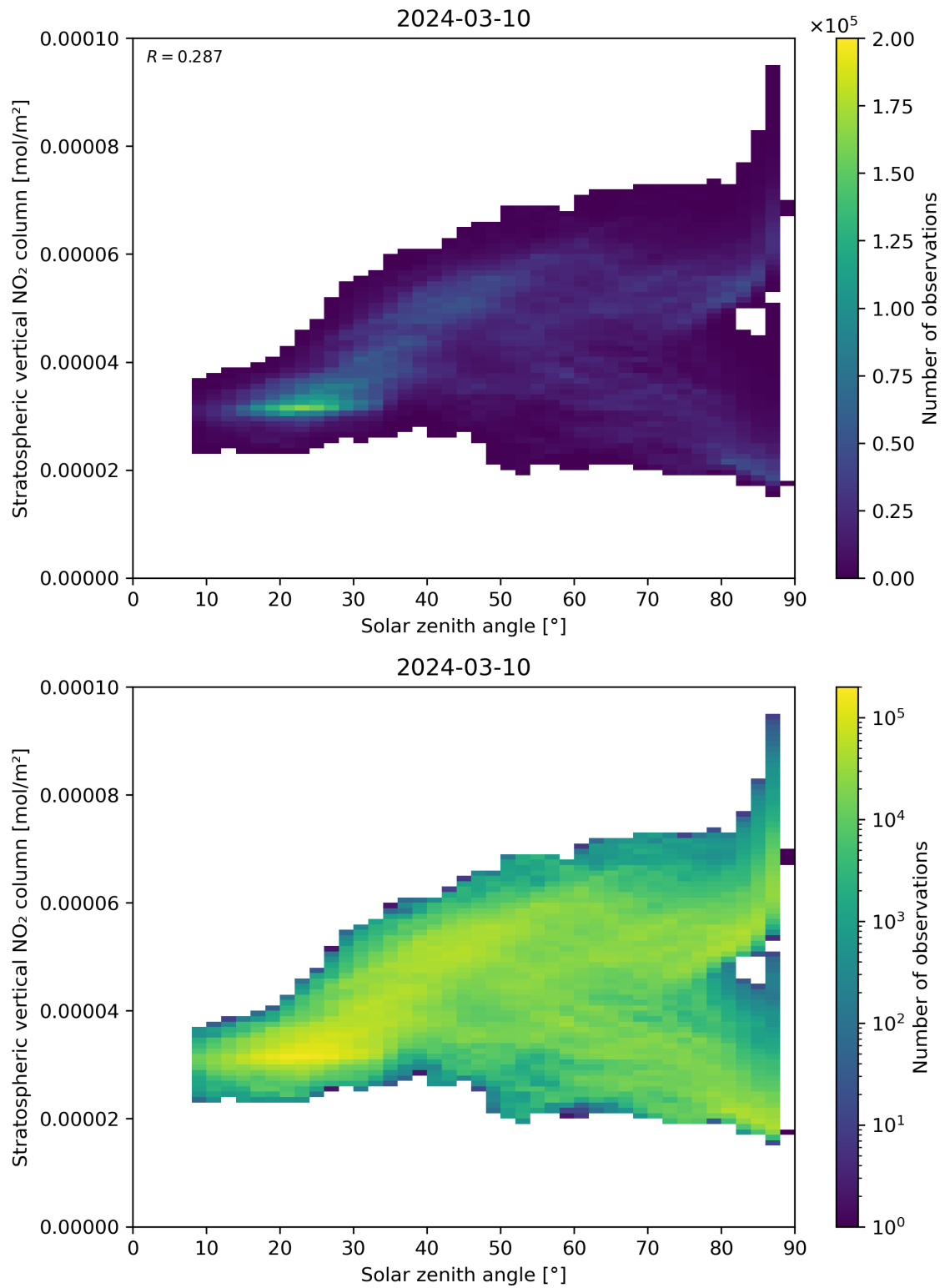
Figure 150: Scatter density plot of “Solar zenith angle” against “Stratospheric vertical NO 2 column” for 2024-03-09 to 2024-03-11.
