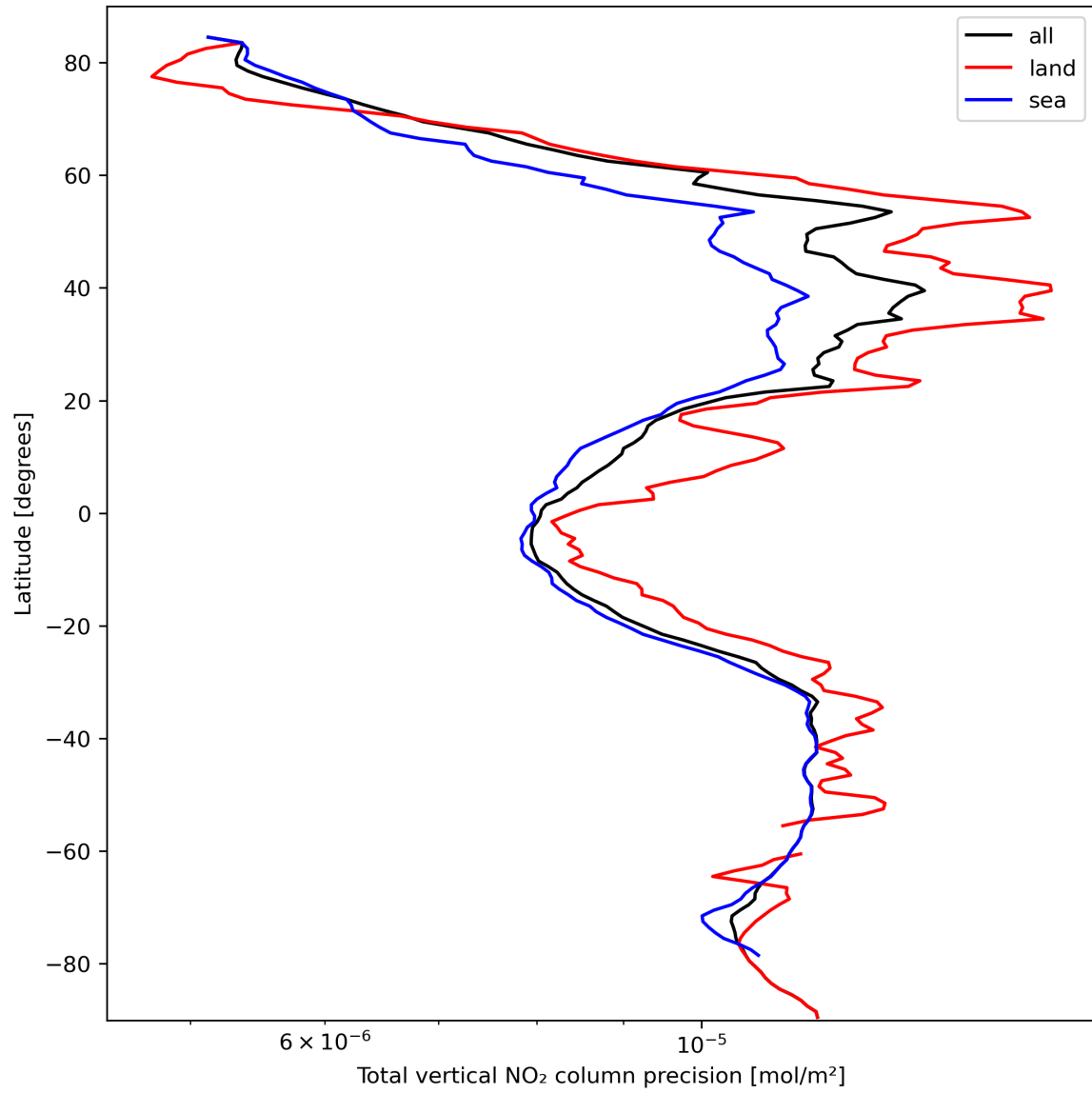
Figure 22: Zonal average of “Total vertical NO 2 column precision” for 2024-03-09 to 2024-03-11.
