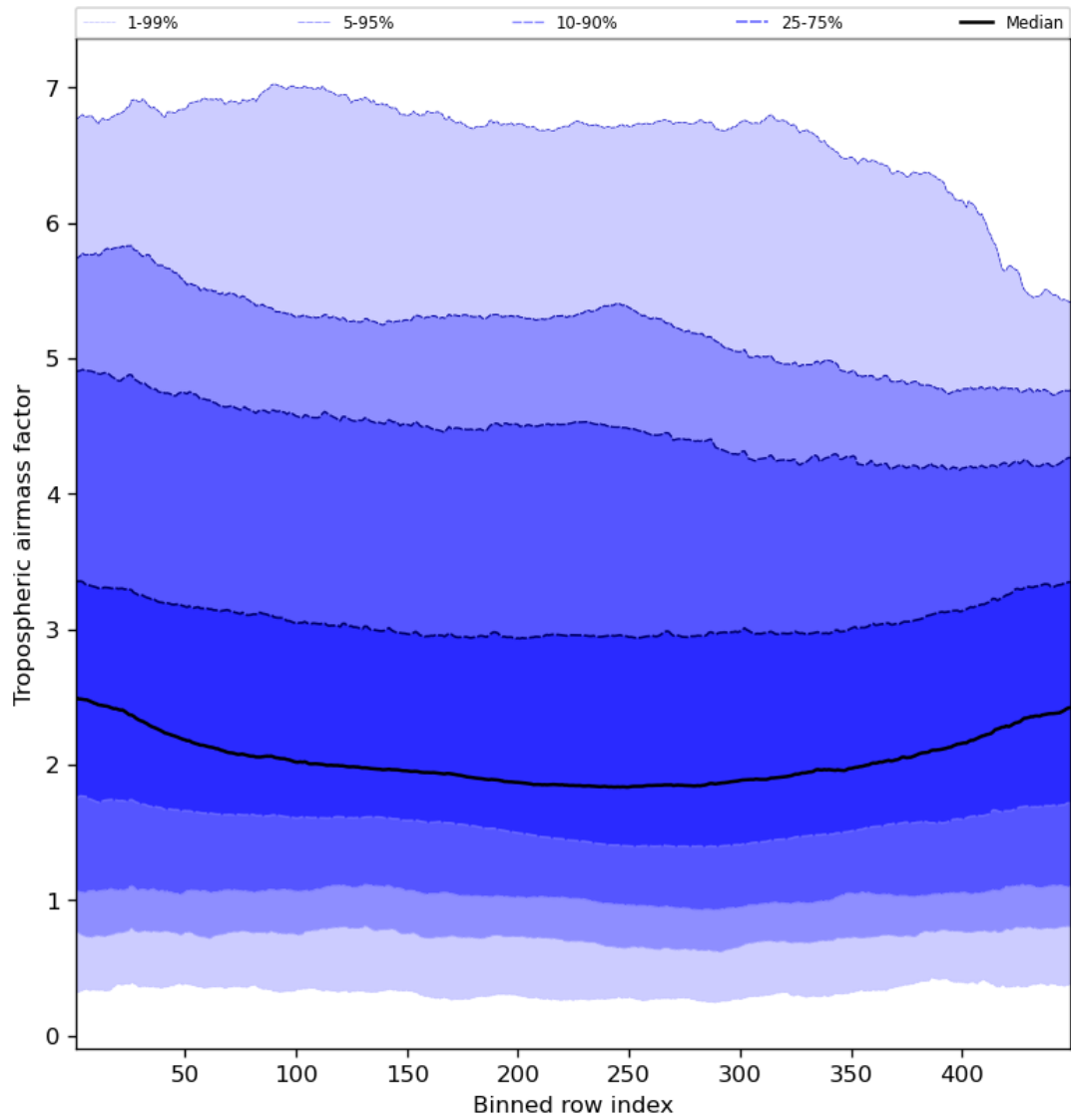
Figure 48: Along track statistics of “Tropospheric air mass factor” for 2024-03-09 to 2024-03-11
