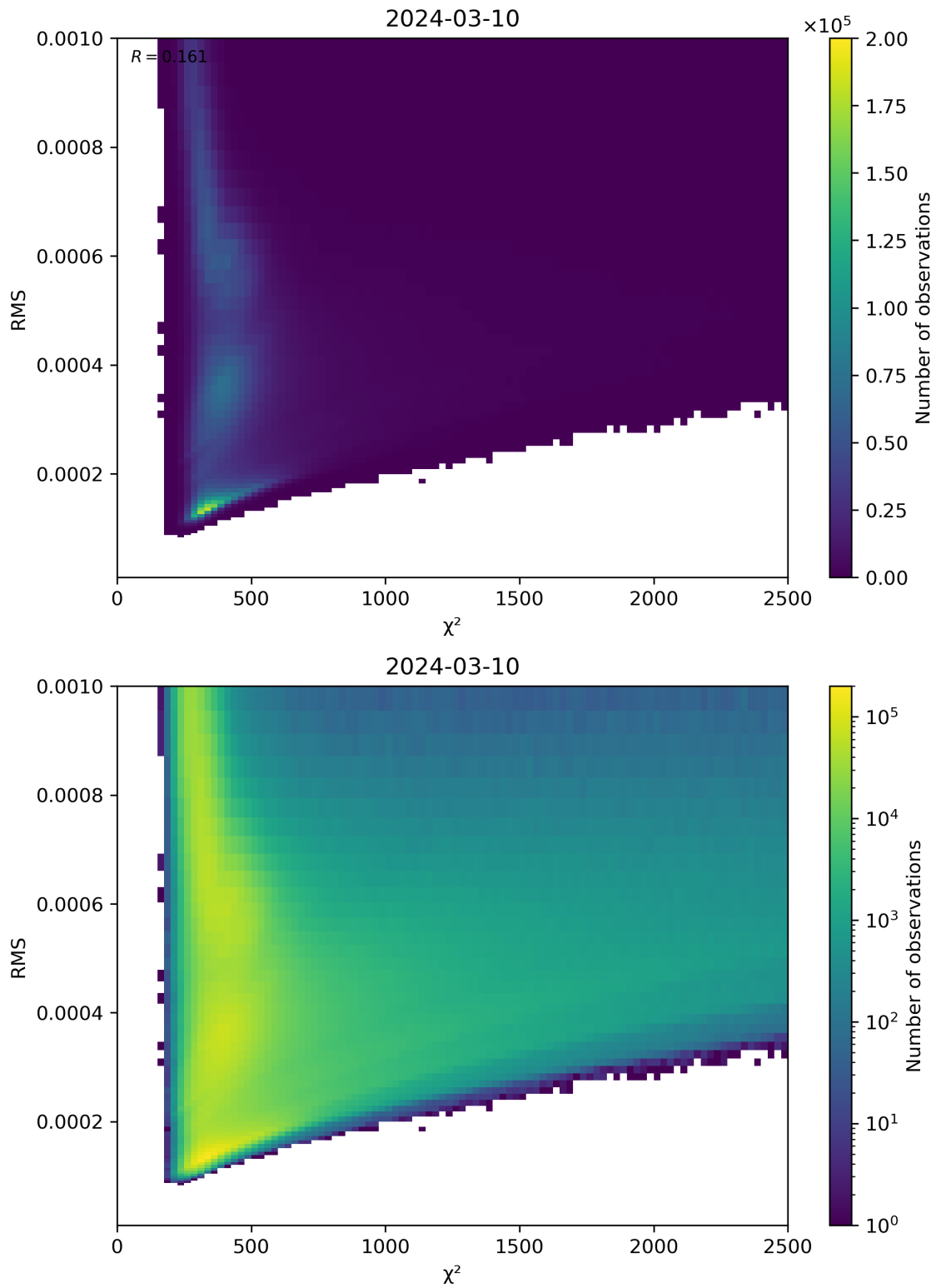
Figure 82: Scatter density plot of “ \chi^2 ” against “RMS” for 2024-03-09 to 2024-03-11.
