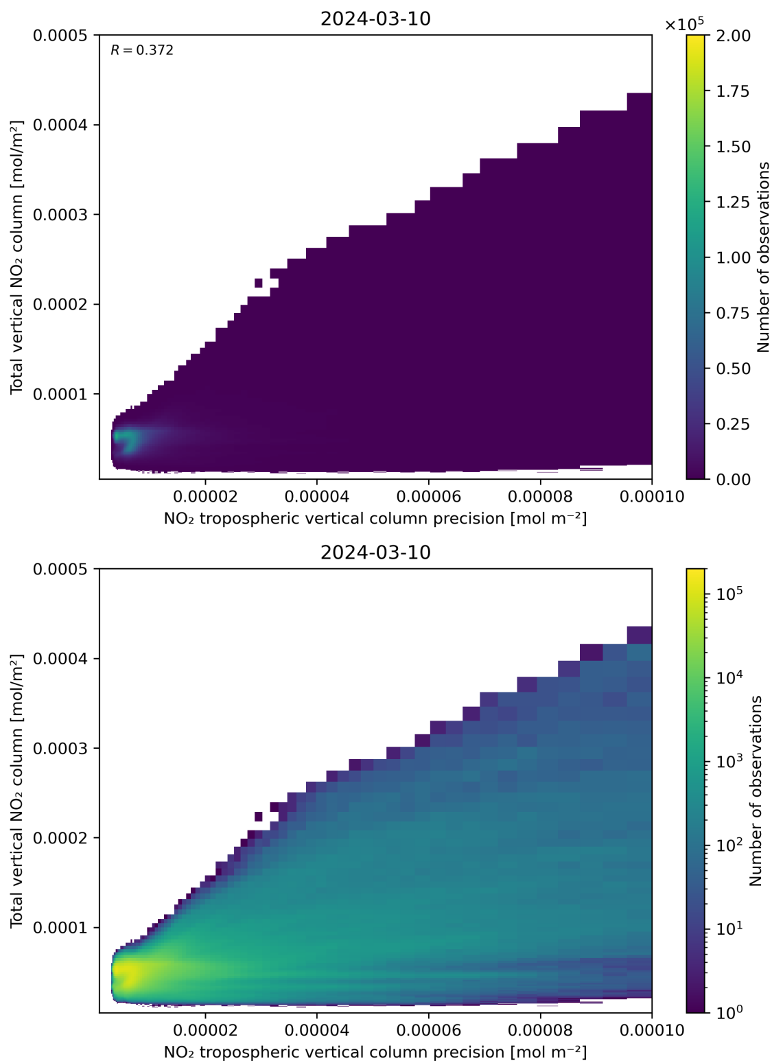
Figure 138: Scatter density plot of “NO 2 tropospheric vertical column precision” against “Total vertical NO 2 column” for 2024-03-09 to 2024-03-11.
