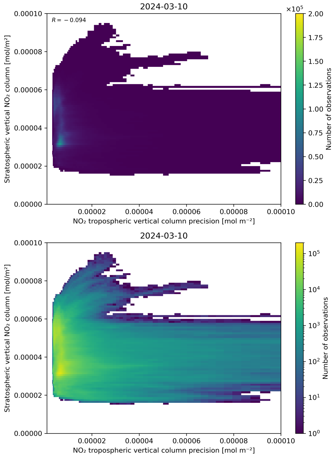
Figure 135: Scatter density plot of “NO 2 tropospheric vertical column precision” against “Stratospheric vertical NO 2 column” for 2024-03-09 to 2024-03-11.
