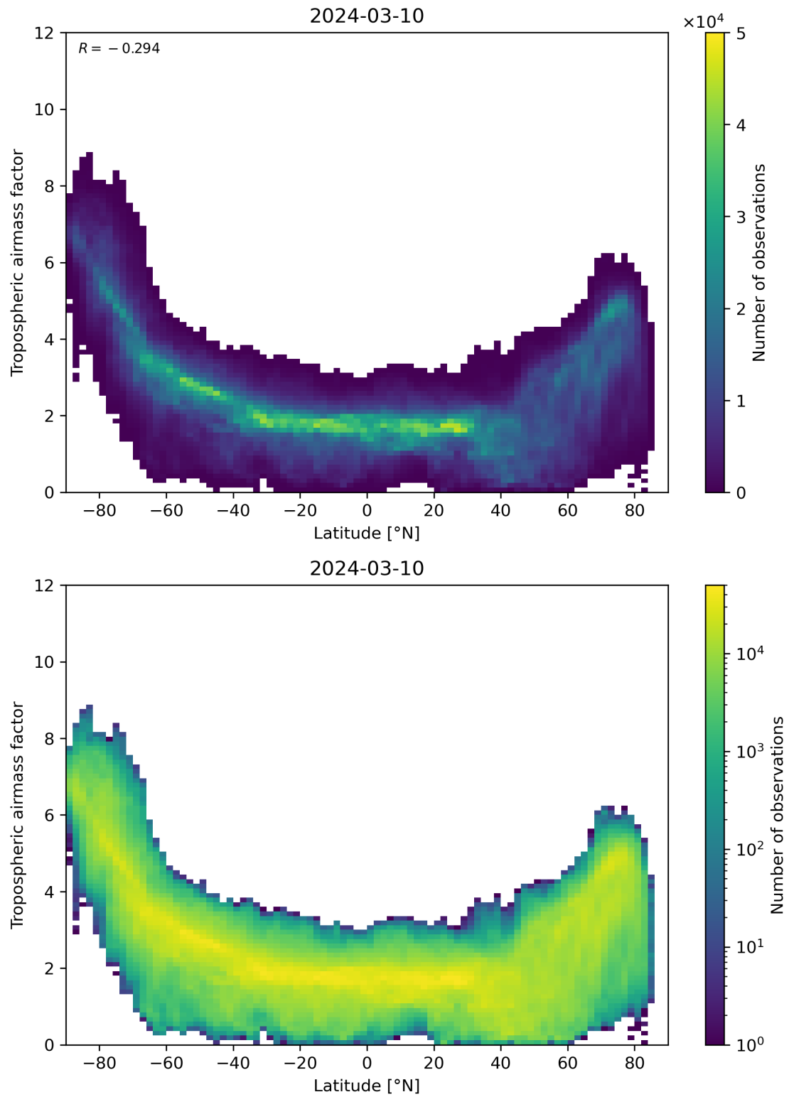
Figure 85: Scatter density plot of “Latitude” against “Tropospheric airmass factor” for 2024-03-09 to 2024-03-11.
