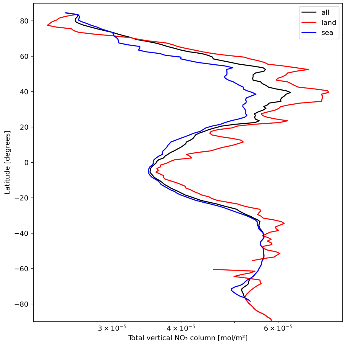
Figure 21: Zonal average of “Total vertical NO 2 column” for 2024-03-09 to 2024-03-11.
