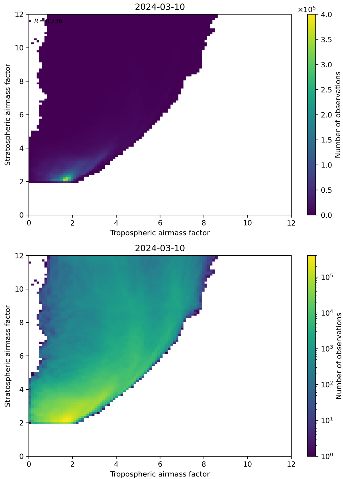
Figure 71: Scatter density plot of “Tropospheric airmass factor” against “Stratospheric airmass factor” for 2024-03-09 to 2024-03-11.
