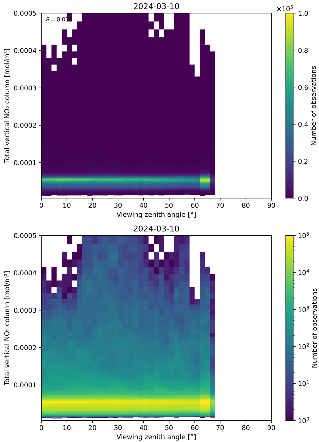
Figure 167: Scatter density plot of “Viewing zenith angle” against “Total vertical NO 2 column” for 2024-03-09 to 2024-03-11.
