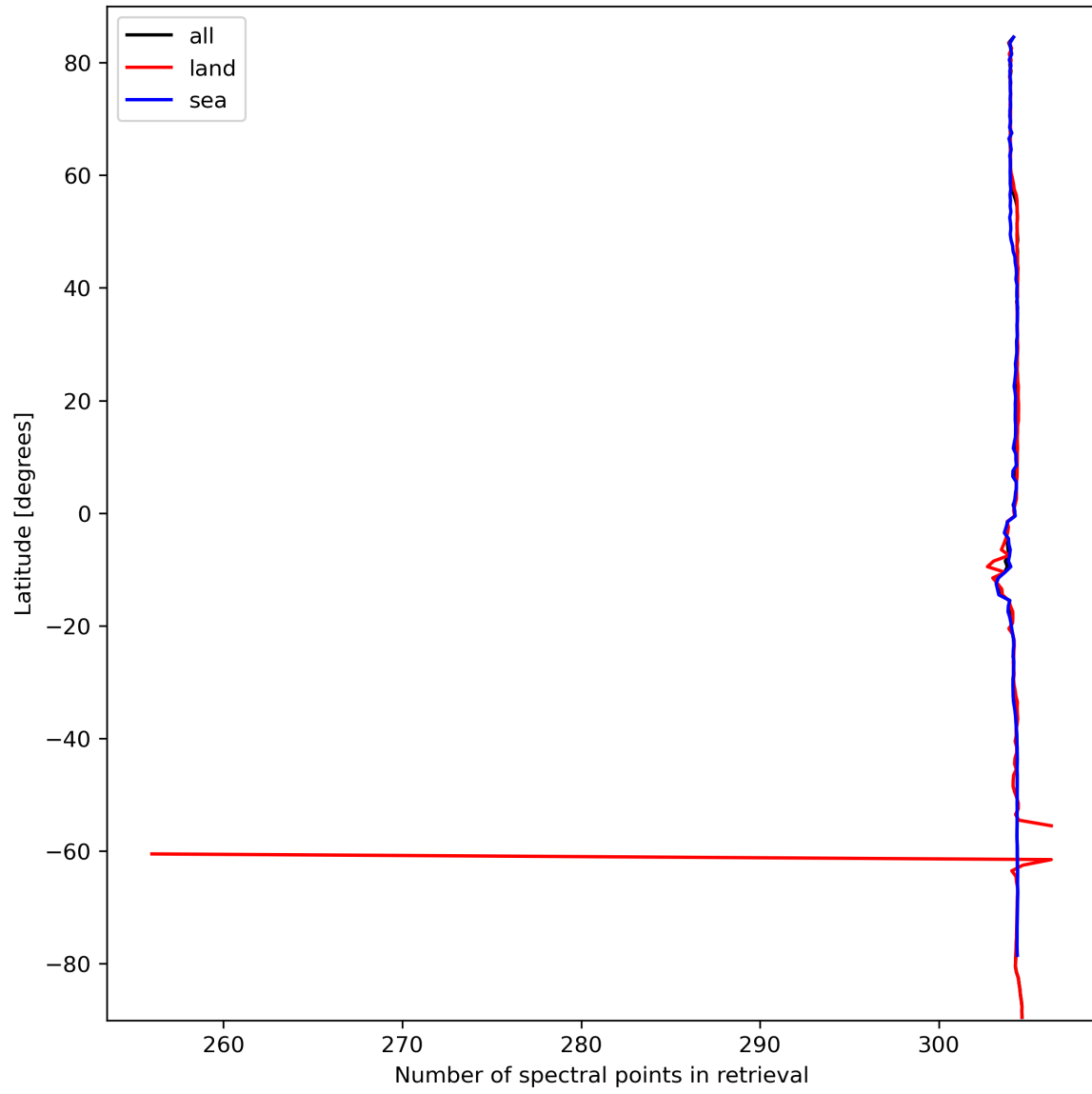
Figure 16: Zonal average of “Number of spectral points in retrieval” for 2024-03-09 to 2024-03-11.
