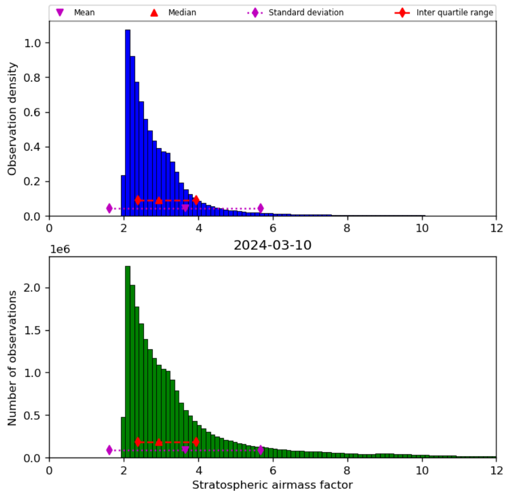
Figure 44: Histogram of “Stratospheric airmass factor” for 2024-03-09 to 2024-03-11
