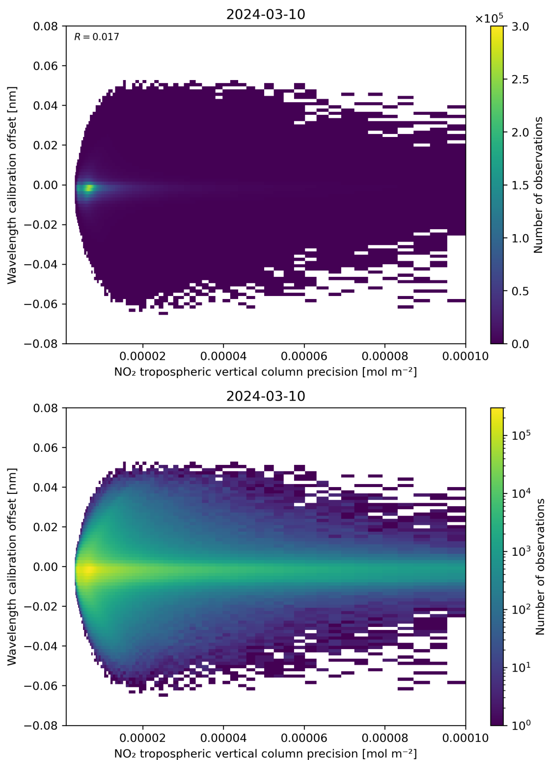
Figure 141: Scatter density plot of “NO 2 tropospheric vertical column precision” against “Wavelength calibration offset” for 2024-03-09 to 2024-03-11.
