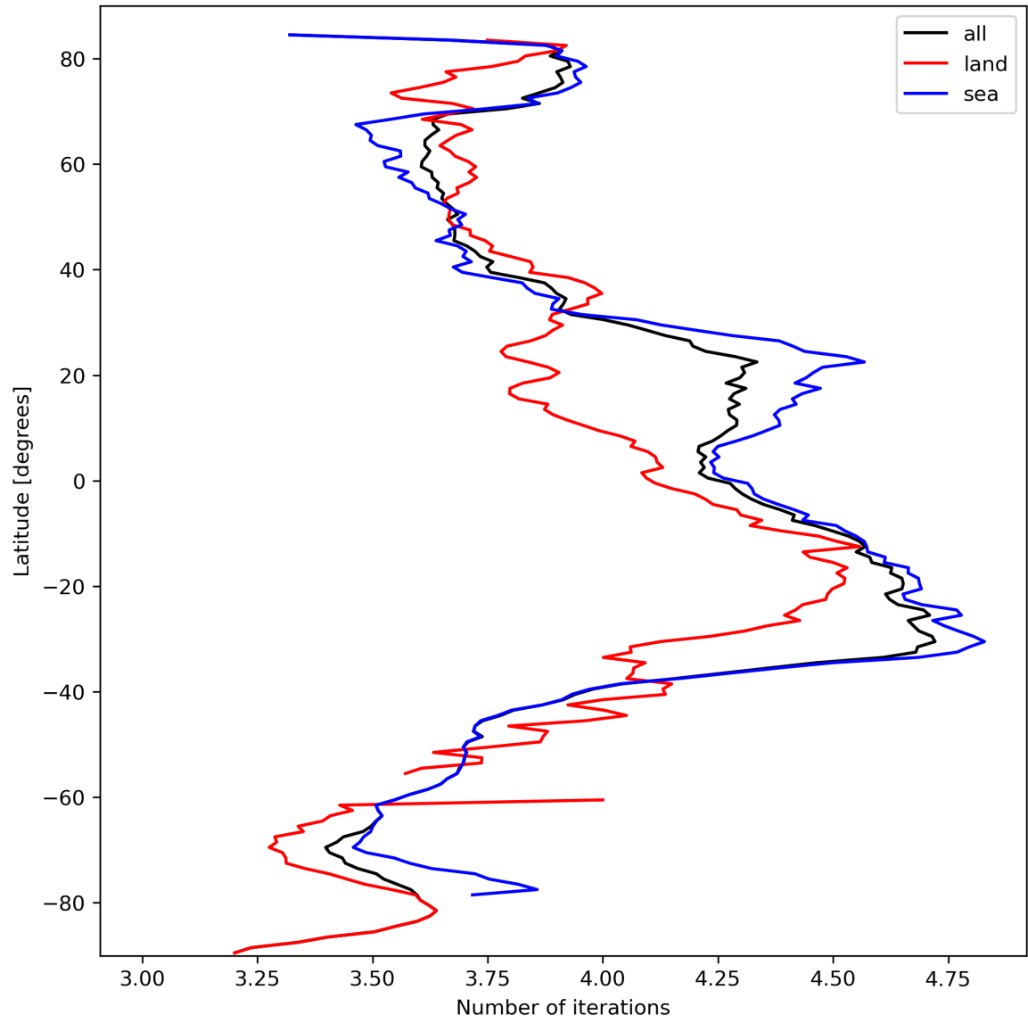
Figure 17: Zonal average of “Number of iterations” for 2024-03-09 to 2024-03-11.
