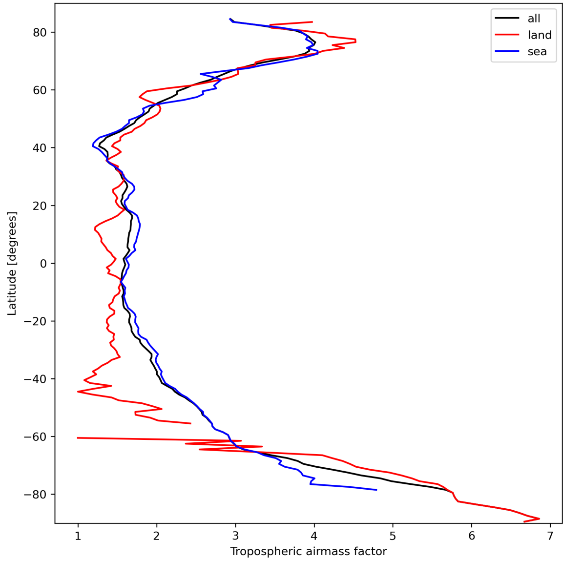
Figure 14: Zonal average of “Tropospheric air mass factor” for 2024-03-09 to 2024-03-11.
