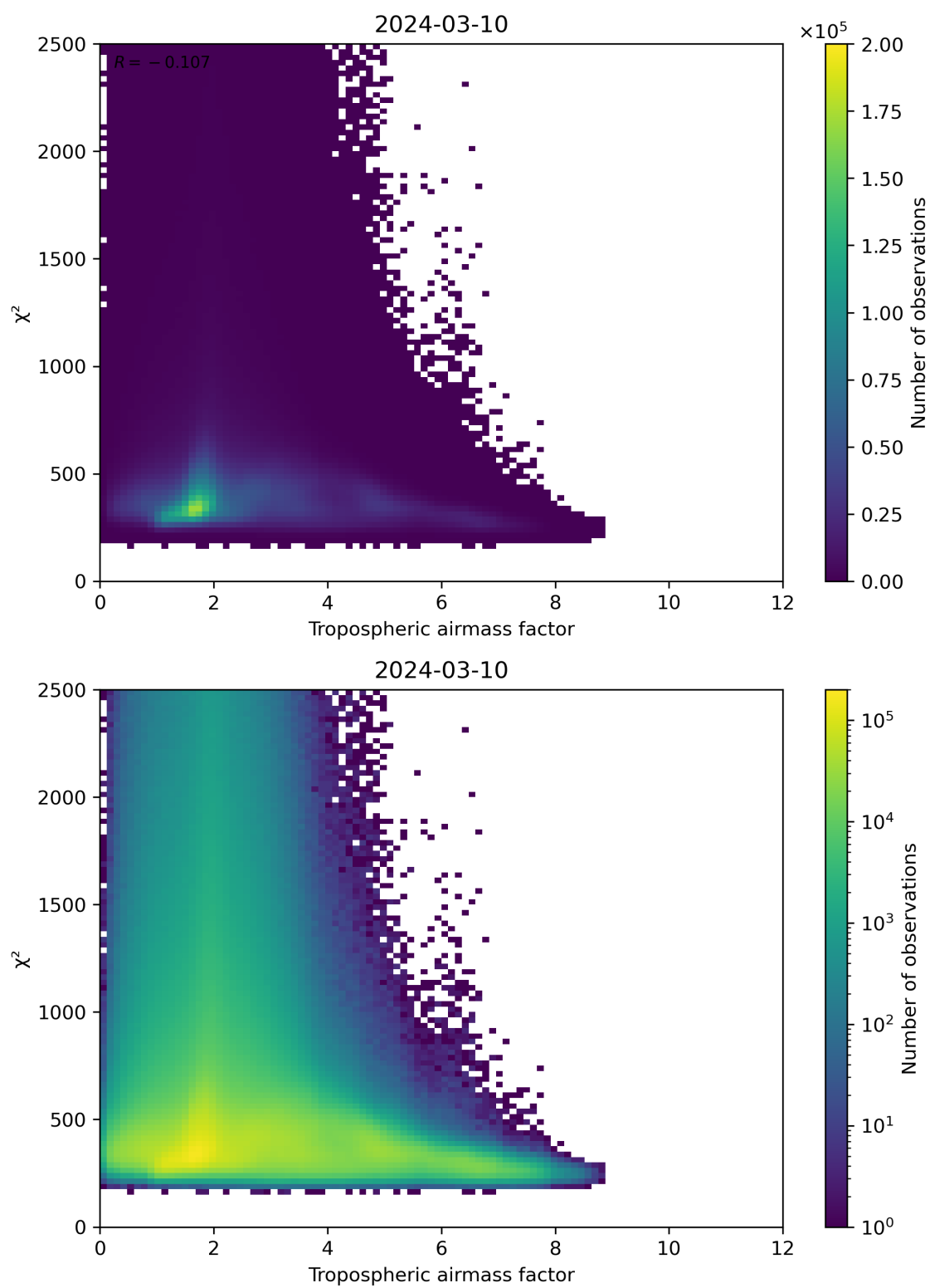
Figure 73: Scatter density plot of “Tropospheric airmass factor” against “ \chi^2 ” for 2024-03-09 to 2024-03-11.
