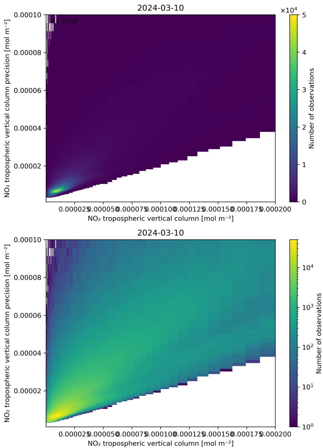
Figure 130: Scatter density plot of “NO 2 tropospheric vertical column” against “NO 2 tropospheric vertical column precision” for 2024-03-09 to 2024-03-11.
