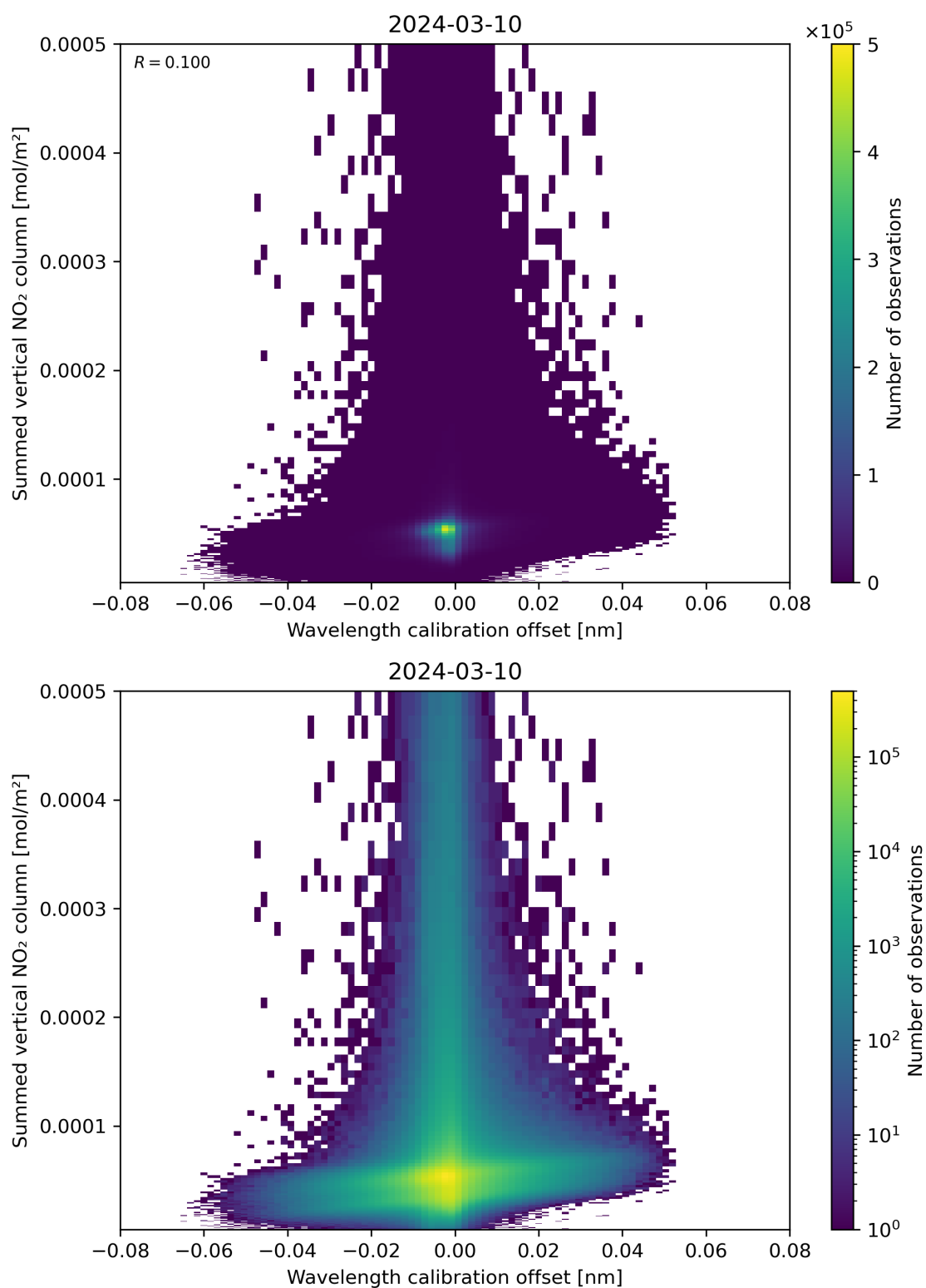
Figure 177: Scatter density plot of “Wavelength calibration offset” against “Summed vertical NO 2 column” for 2024-03-09 to 2024-03-11.
