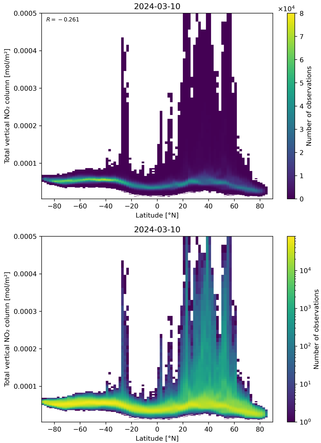
Figure 90: Scatter density plot of “Latitude” against “Total vertical NO 2 column” for 2024-03-09 to 2024-03-11.
