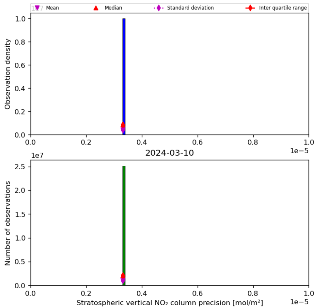
Figure 37: Histogram of “Stratospheric vertical NO 2 column precision” for 2024-03-09 to 2024-03-11
