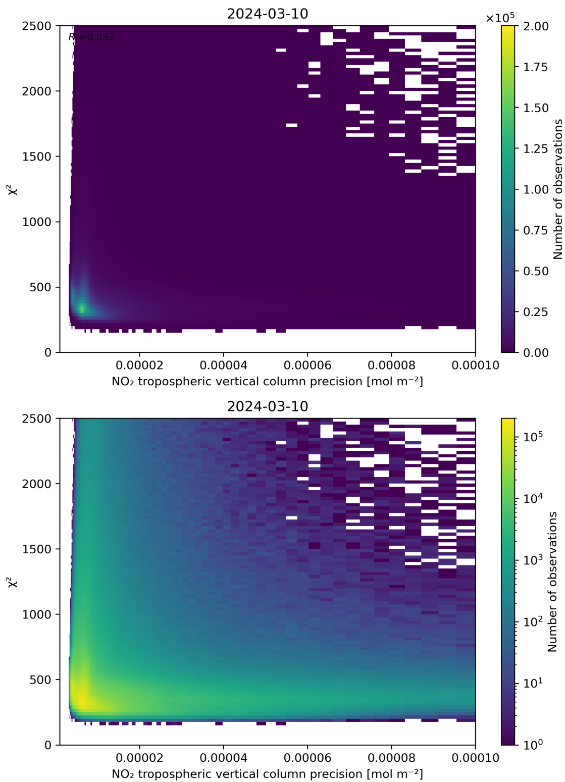
Figure 134: Scatter density plot of “NO 2 tropospheric vertical column precision” against “ \chi^2 ” for 2024-03-09 to 2024-03-11.
