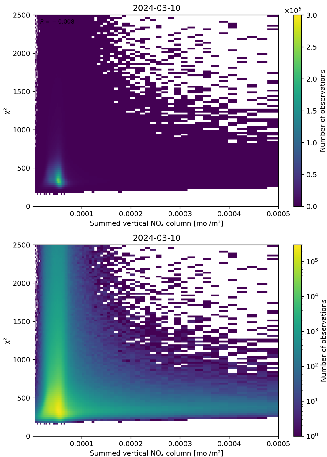
Figure 104: Scatter density plot of “Summed vertical NO 2 column” against “ \chi^2 ” for 2024-03-09 to 2024-03-11.
