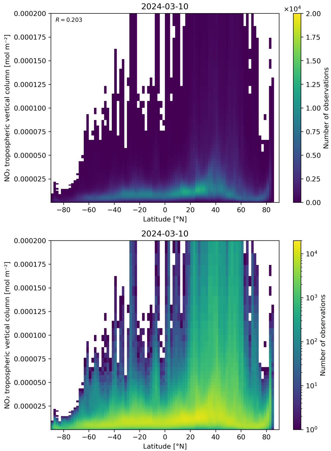
Figure 92: Scatter density plot of “Latitude” against “NO 2 tropospheric vertical column” for 2024-03-09 to 2024-03-11.
