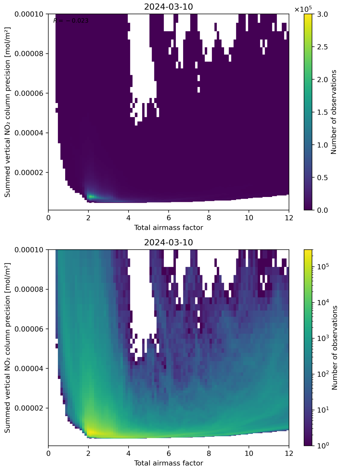
Figure 66: Scatter density plot of “Total airmass factor” against “Summed vertical NO 2 column precision” for 2024-03-09 to 2024-03-11.
