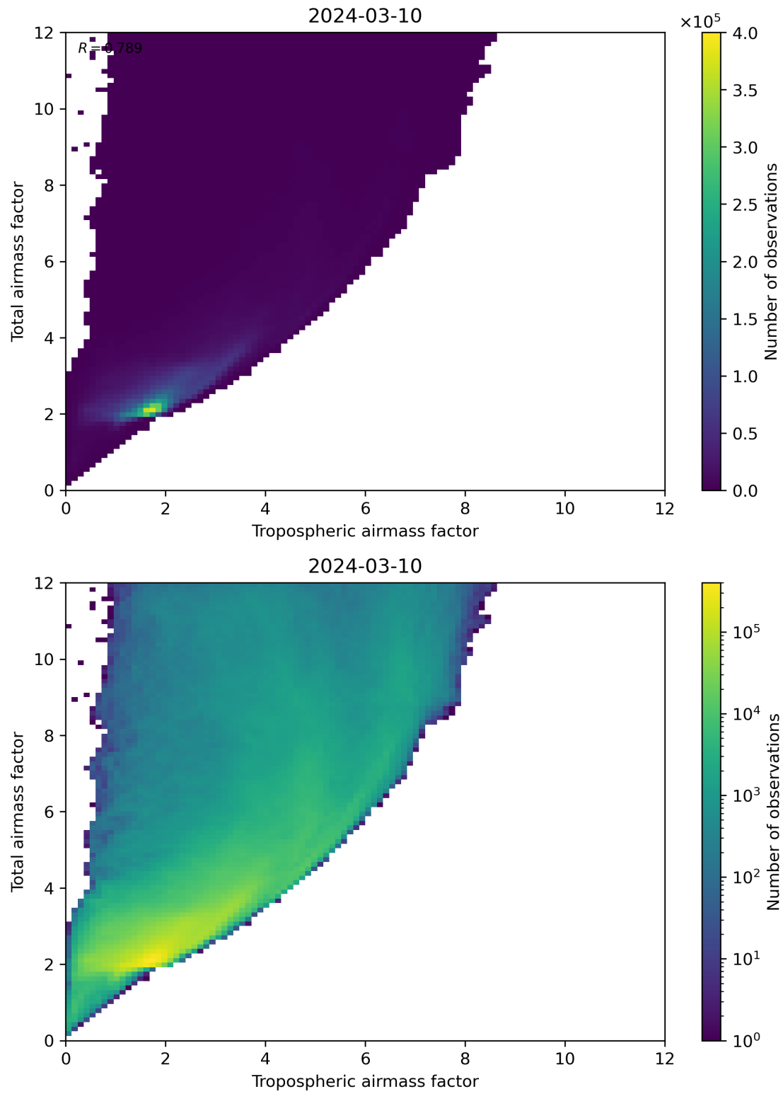
Figure 72: Scatter density plot of “Tropospheric airmass factor” against “Total airmass factor” for 2024-03-09 to 2024-03-11.
