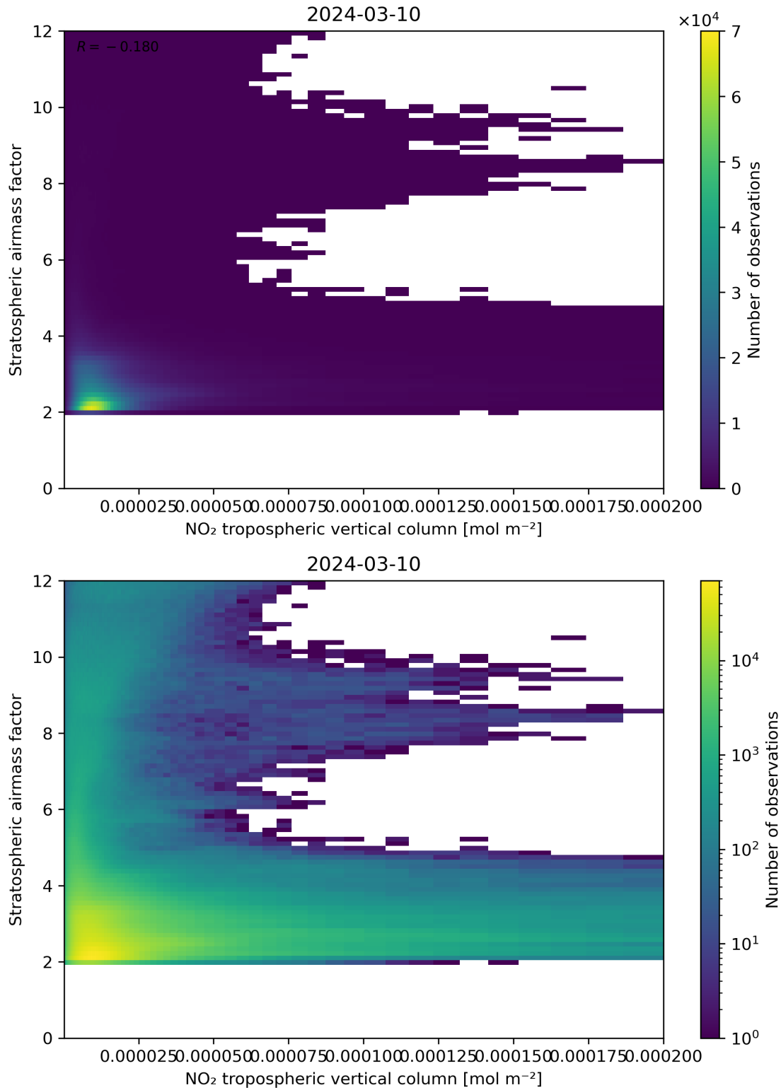
Figure 121: Scatter density plot of “NO 2 tropospheric vertical column” against “Stratospheric air mass factor” for 2024-03-09 to 2024-03-11.
