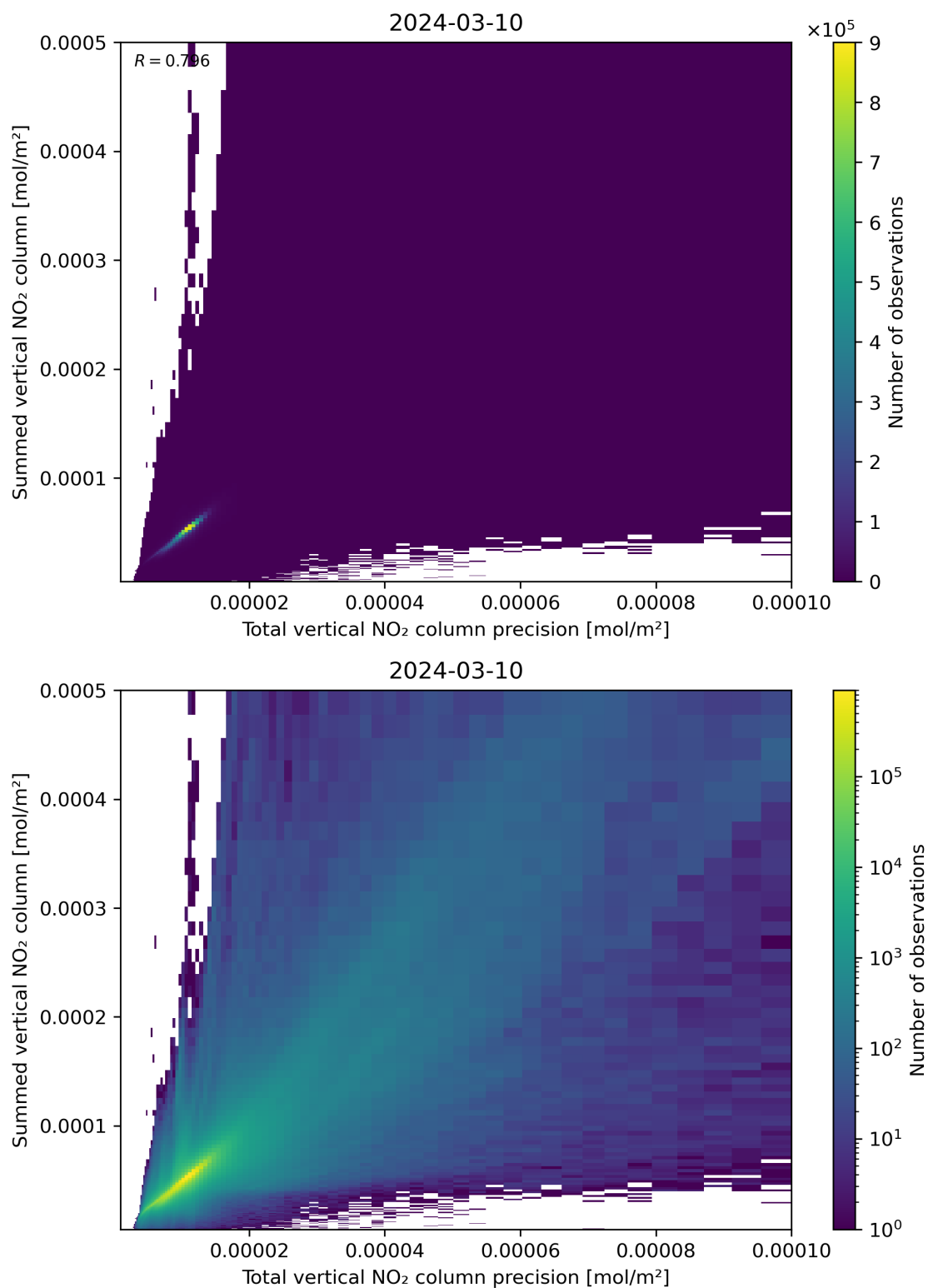
Figure 117: Scatter density plot of “Total vertical NO 2 column precision” against “Summed vertical NO 2 column” for 2024-03-09 to 2024-03-11.
