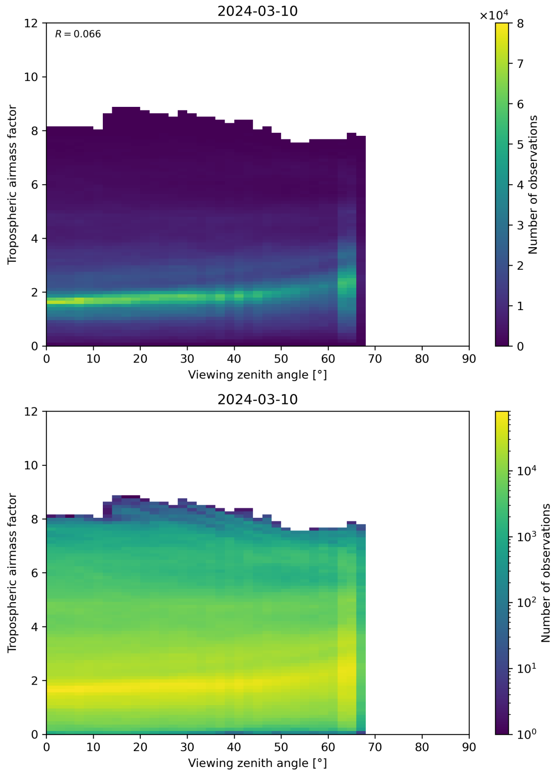
Figure 161: Scatter density plot of “Viewing zenith angle” against “Tropospheric airmass factor” for 2024-03-09 to 2024-03-11.
