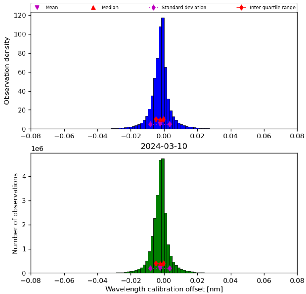
Figure 35: Histogram of “Wavelength calibration offset” for 2024-03-09 to 2024-03-11
