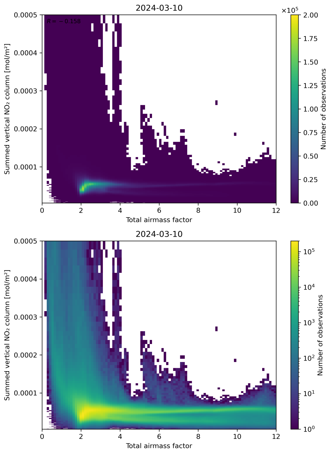
Figure 65: Scatter density plot of “Total airmass factor” against “Summed vertical NO 2 column” for 2024-03-09 to 2024-03-11.
