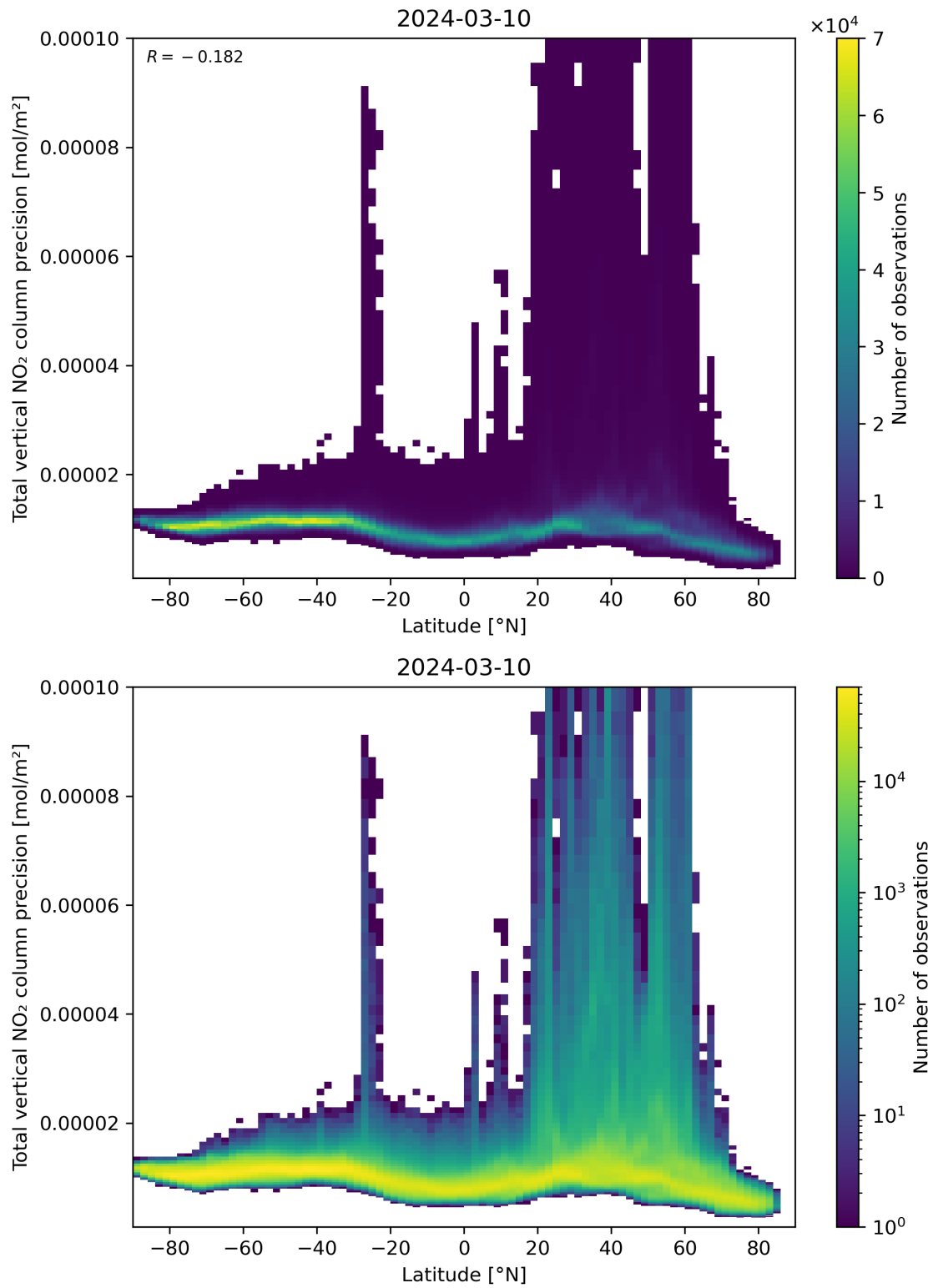
Figure 91: Scatter density plot of “Latitude” against “Total vertical NO 2 column precision” for 2024-03-09 to 2024-03-11.
