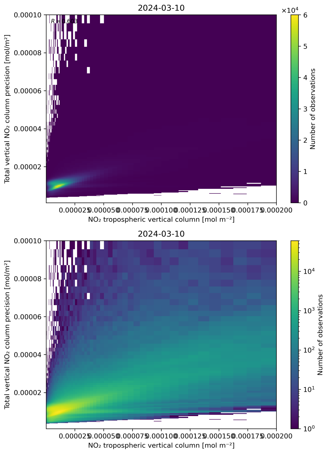
Figure 129: Scatter density plot of “NO 2 tropospheric vertical column” against “Total vertical NO 2 column precision” for 2024-03-09 to 2024-03-11.
