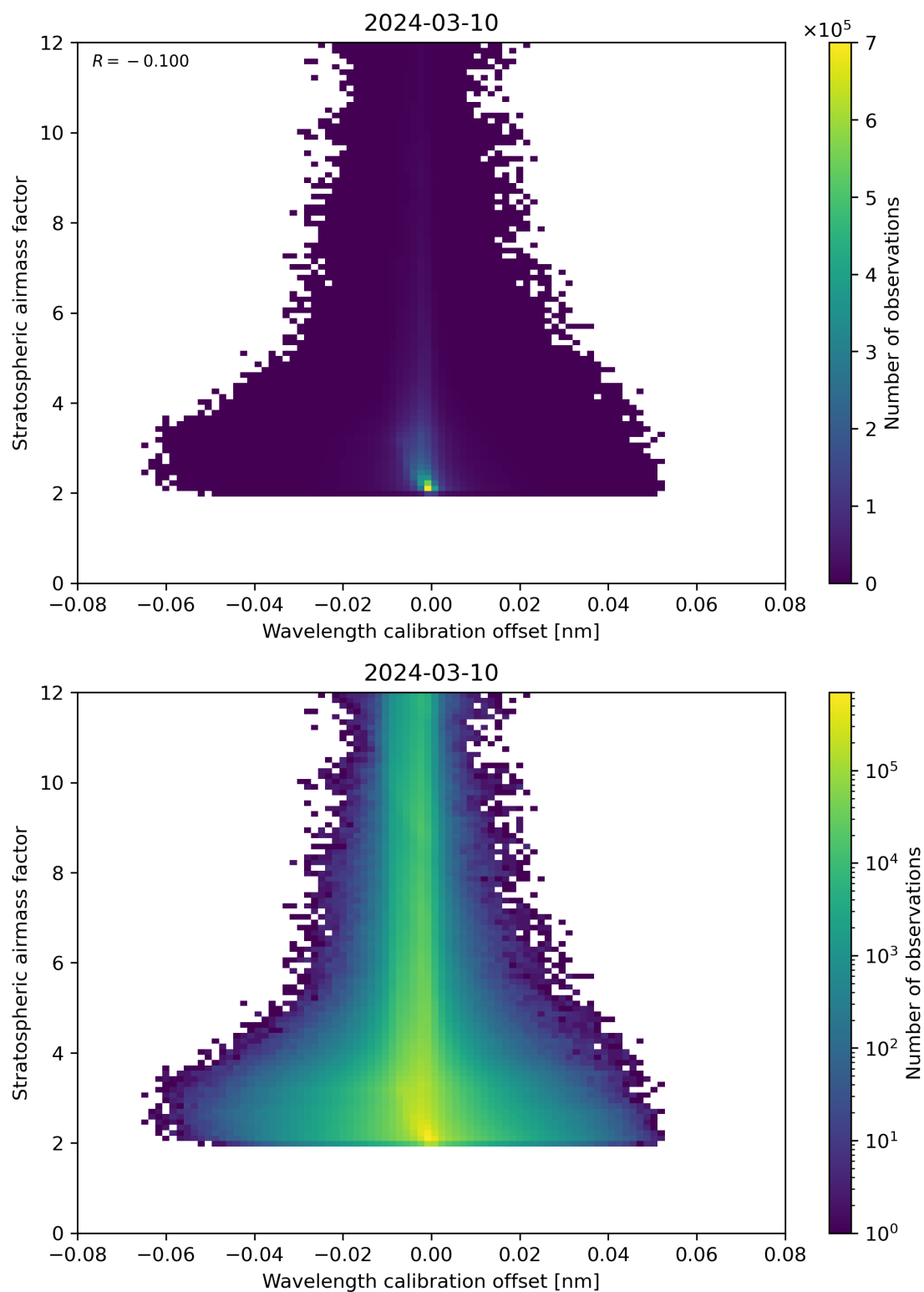
Figure 174: Scatter density plot of “Wavelength calibration offset” against “Stratospheric airmass factor” for 2024-03-09 to 2024-03-11.
