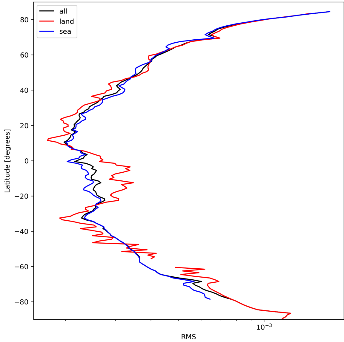
Figure 26: Zonal average of “RMS” for 2024-03-09 to 2024-03-11.
