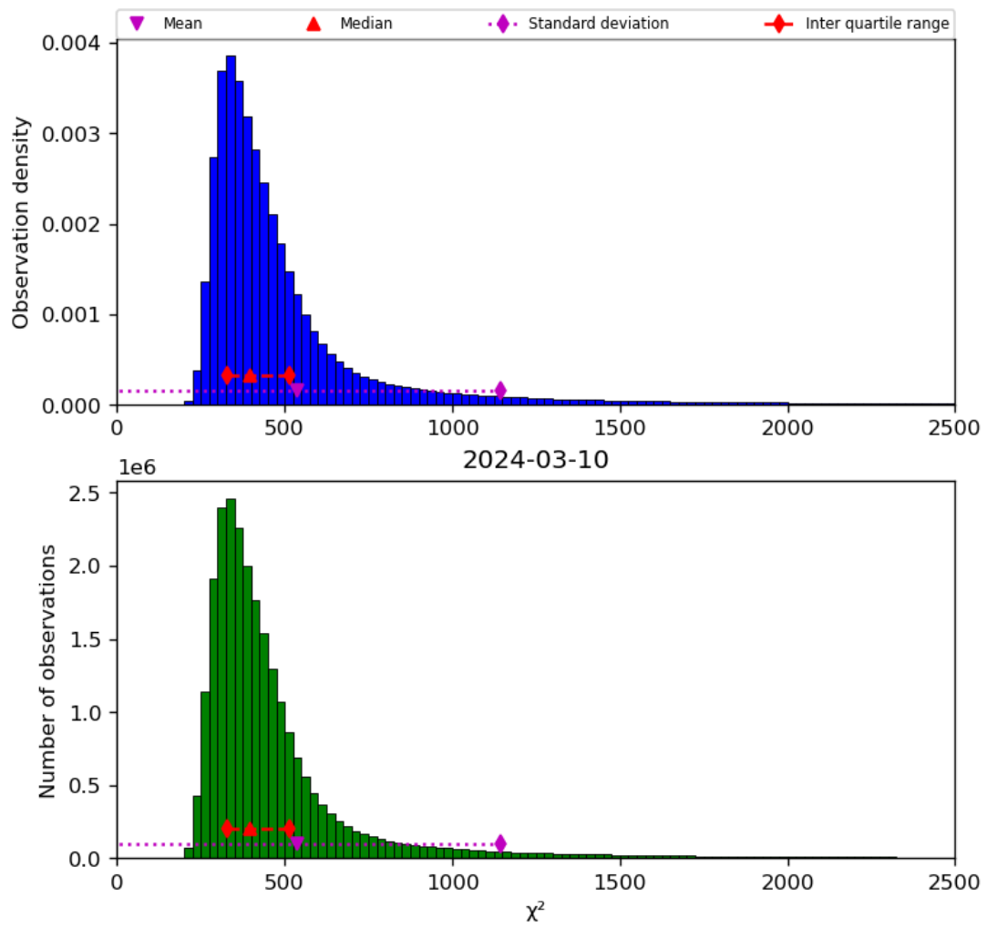
Figure 42: Histogram of “ \chi^2 ” for 2024-03-09 to 2024-03-11
