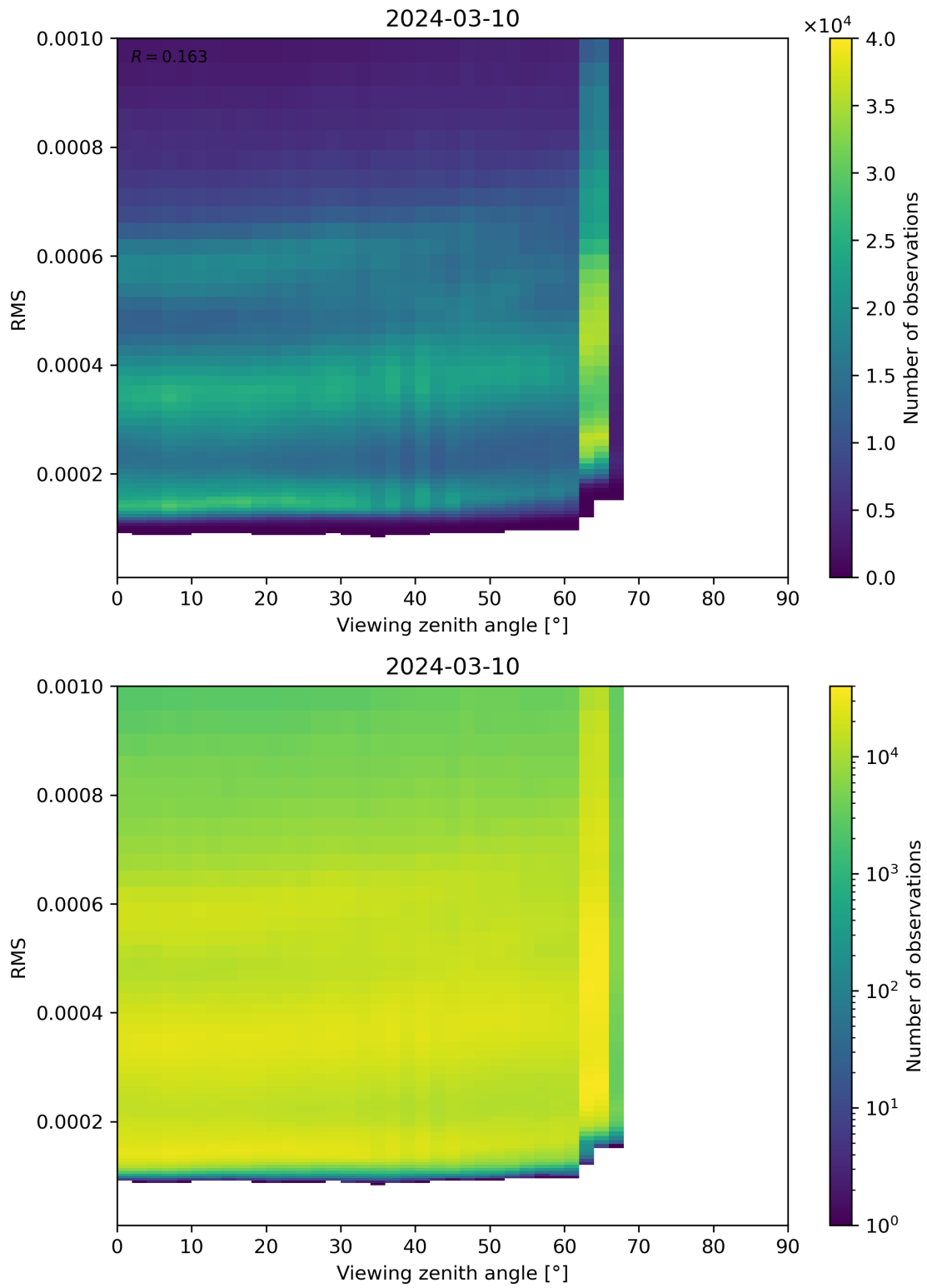
Figure 171: Scatter density plot of “Viewing zenith angle” against “RMS” for 2024-03-09 to 2024-03-11.
