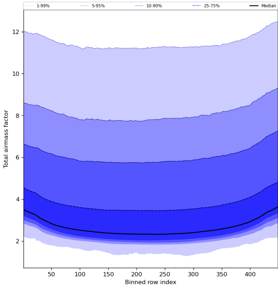
Figure 49: Along track statistics of “Total airmass factor” for 2024-03-09 to 2024-03-11
