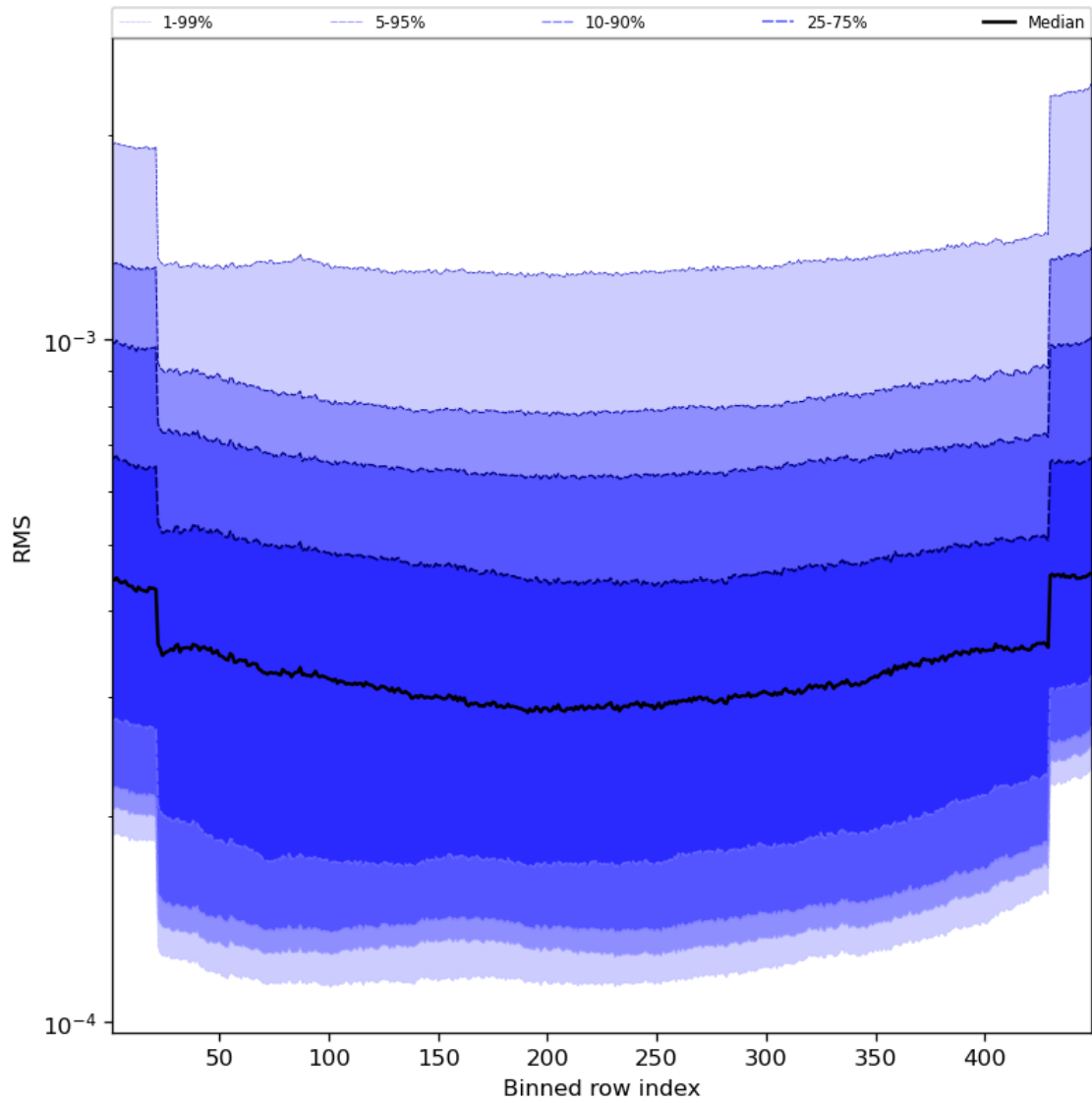
Figure 60: Along track statistics of “RMS” for 2024-03-09 to 2024-03-11
